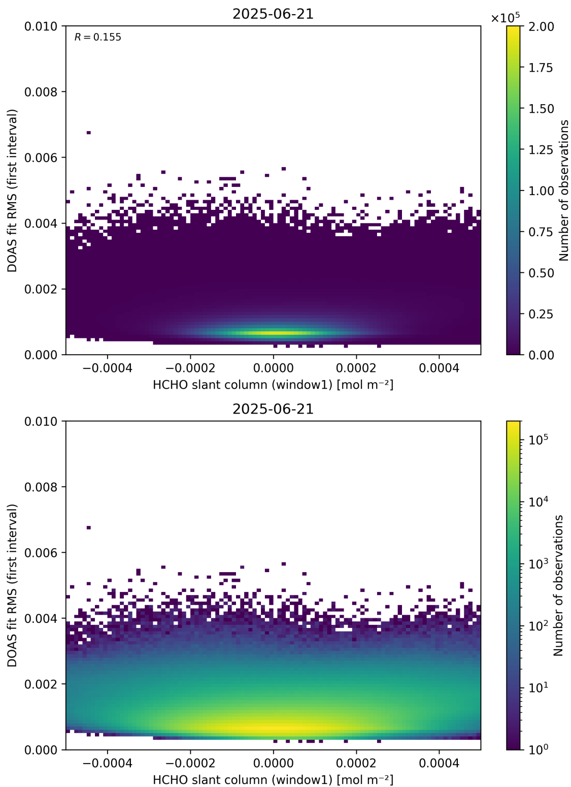
Figure 78: Scatter density plot of “HCHO slant column (window1)” against “DOAS fit RMS (first interval)” for 2025-06-20 to 2025-06-22.
