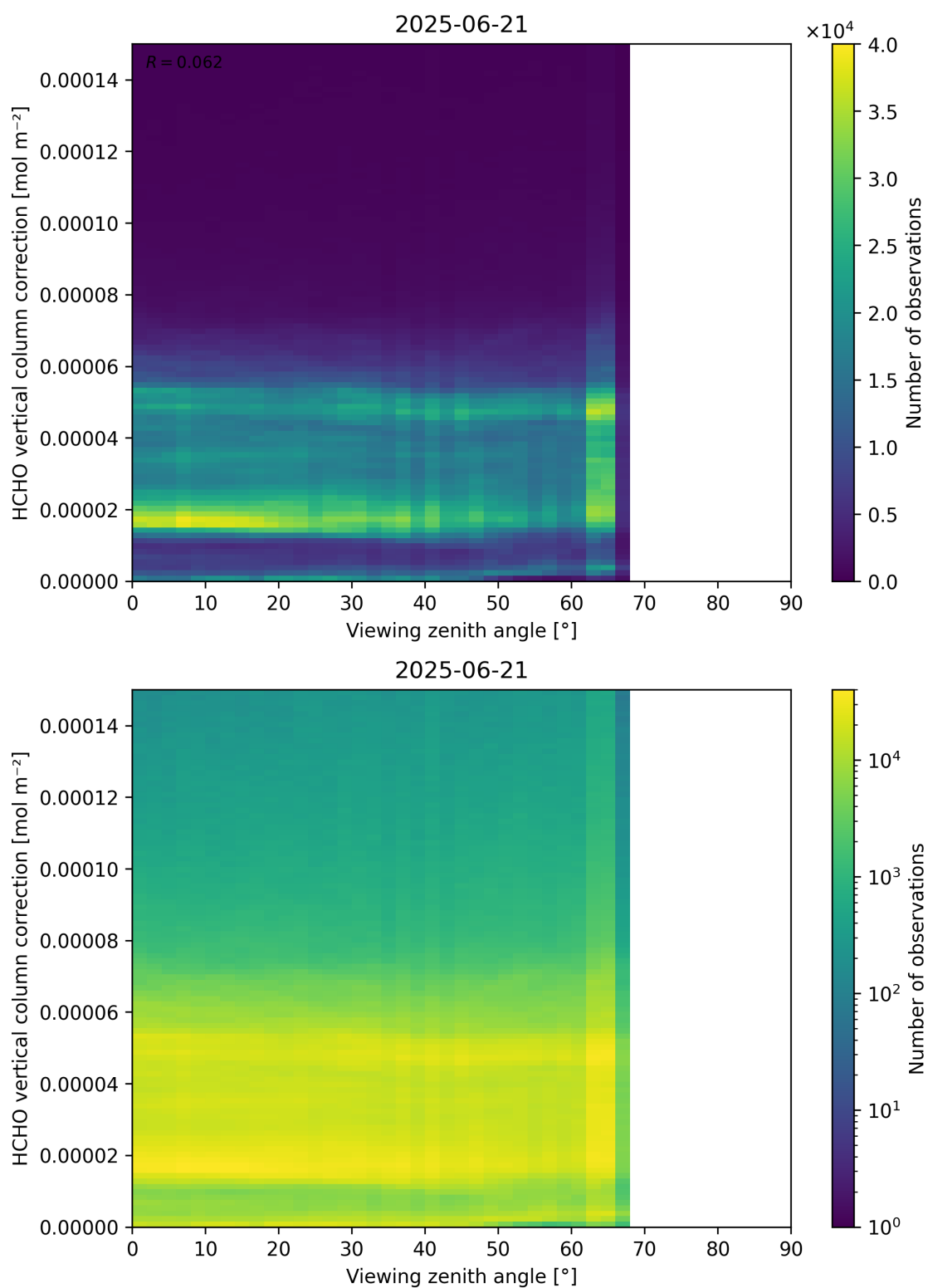
Figure 193: Scatter density plot of “Viewing zenith angle” against “HCHO vertical column correction” for 2025-06-20 to 2025-06-22.
