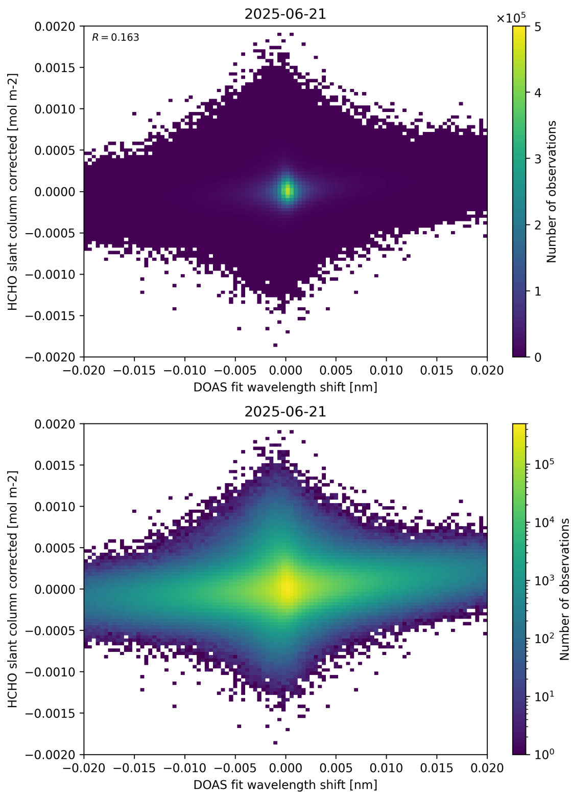
Figure 66: Scatter density plot of “DOAS fit wavelength shift” against “HCHO slant column corrected” for 2025-06-20 to 2025-06-22.
