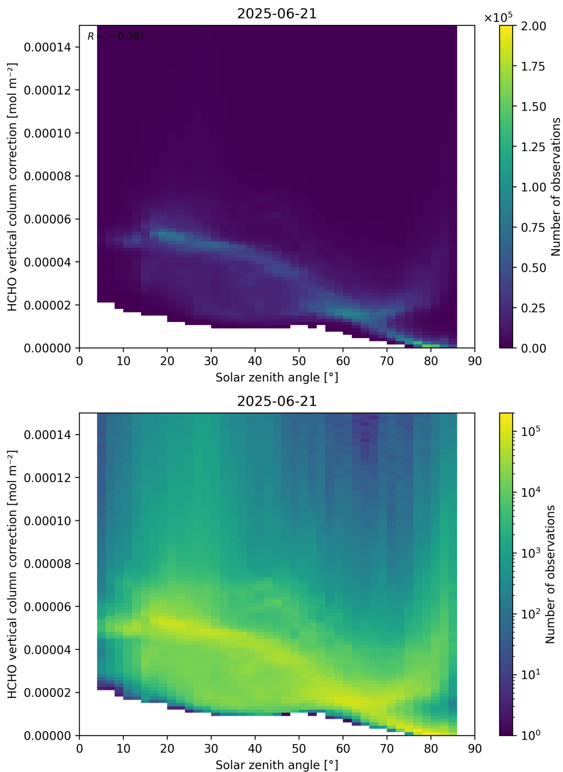
Figure 178: Scatter density plot of “Solar zenith angle” against “HCHO vertical column correction” for 2025-06-20 to 2025-06-22.
