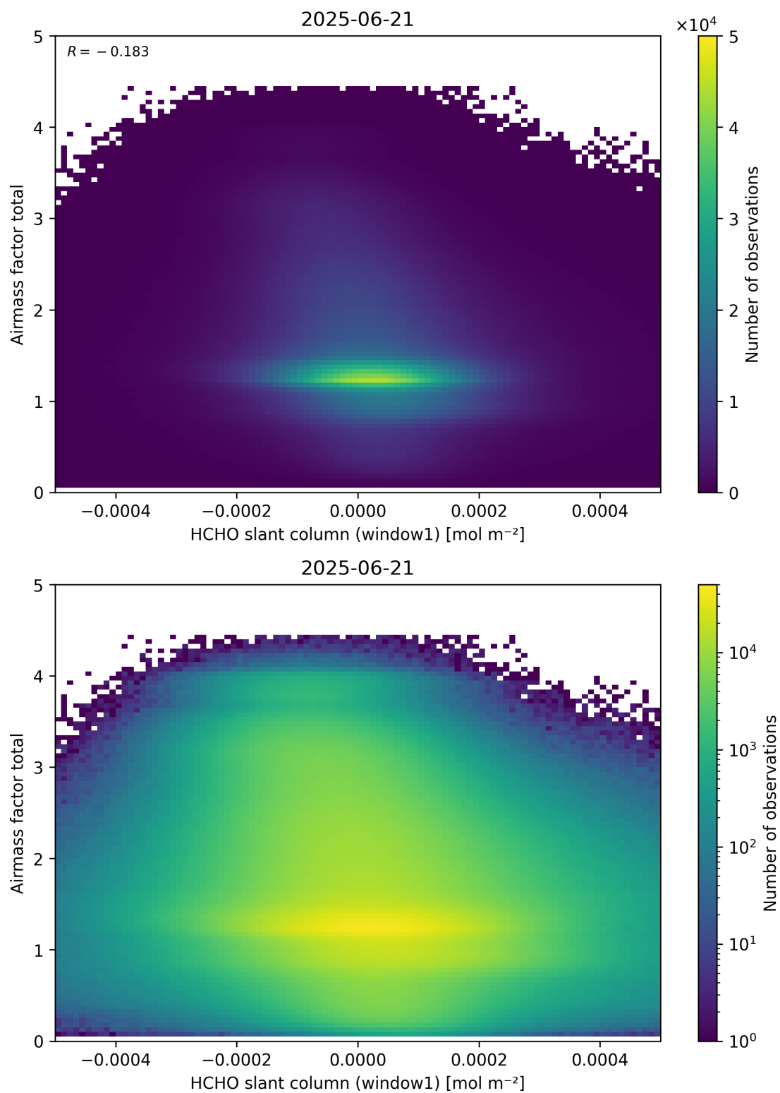
Figure 85: Scatter density plot of “HCHO slant column (window1)” against “Airmass factor total” for 2025-06-20 to 2025-06-22.
