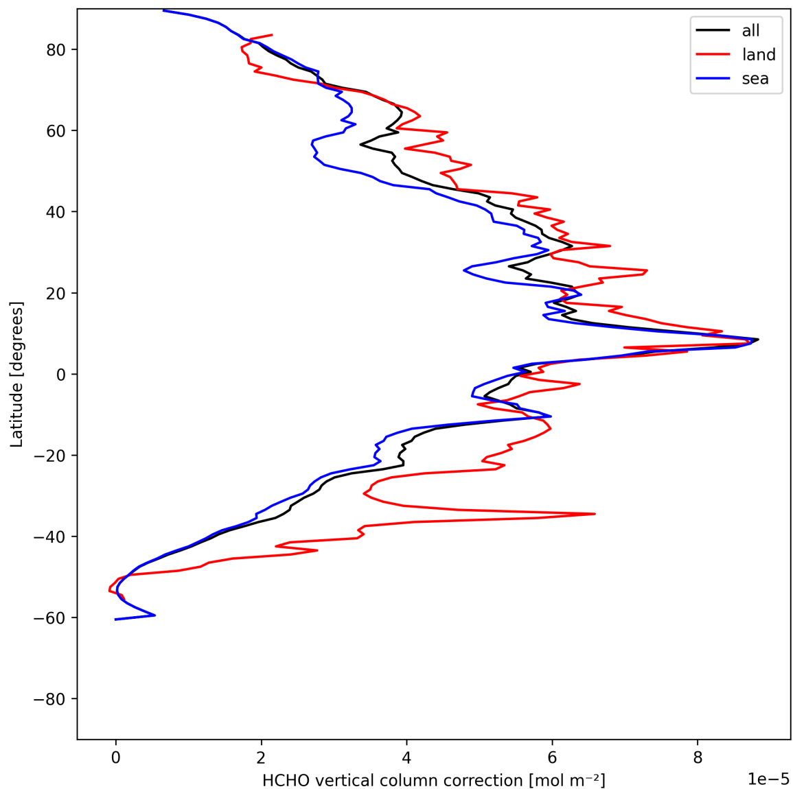
Figure 23: Zonal average of “HCHO vertical column correction” for 2025-06-20 to 2025-06-22.
