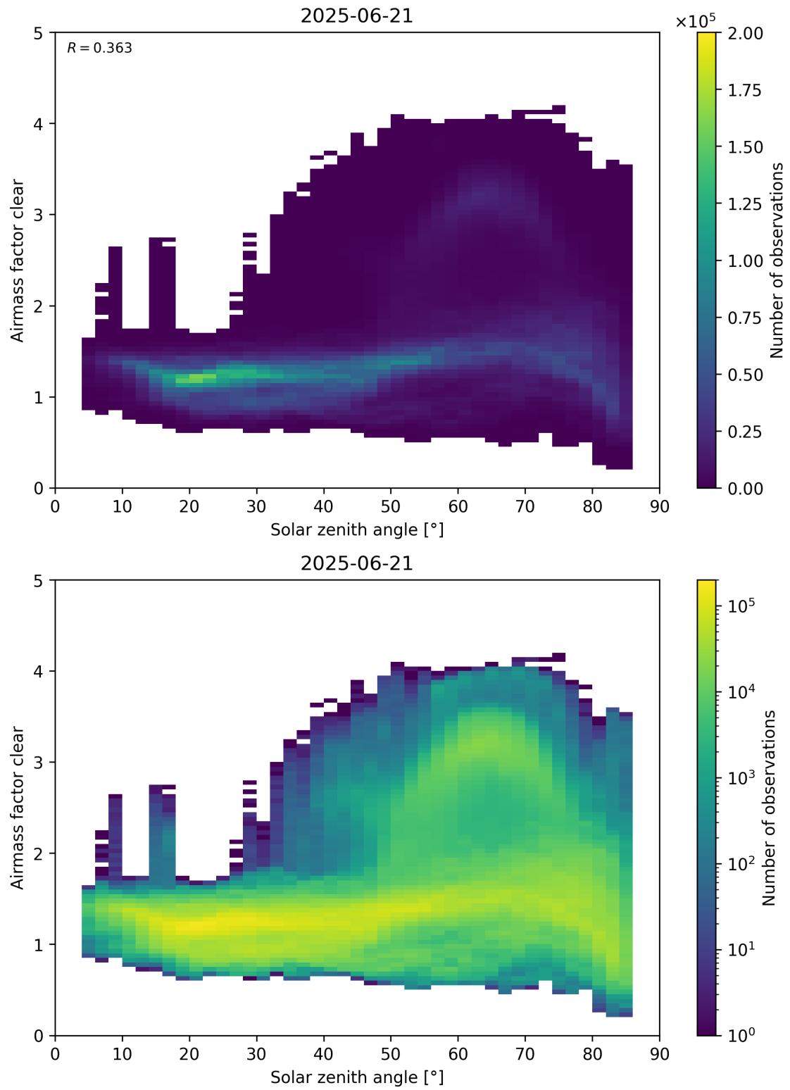
Figure 170: Scatter density plot of “Solar zenith angle” against “Airmass factor clear” for 2025-06-20 to 2025-06-22.
