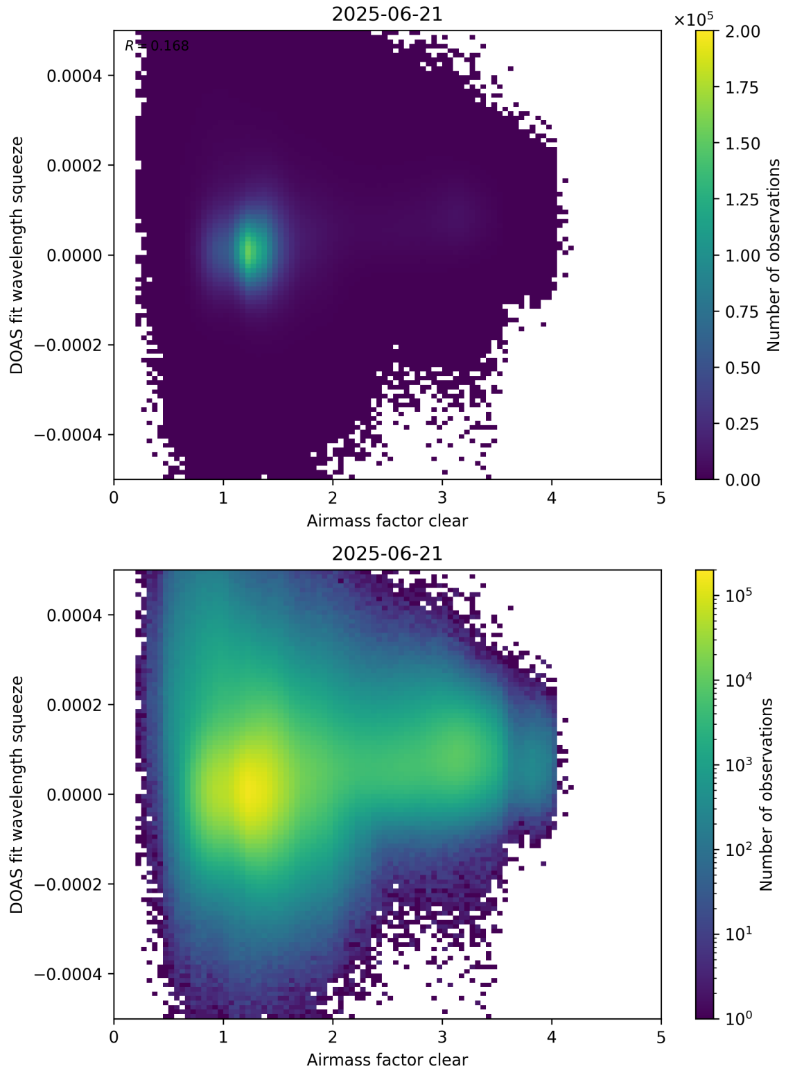
Figure 73: Scatter density plot of “Airmass factor clear” against “DOAS fit wavelength squeeze” for 2025-06-20 to 2025-06-22.
