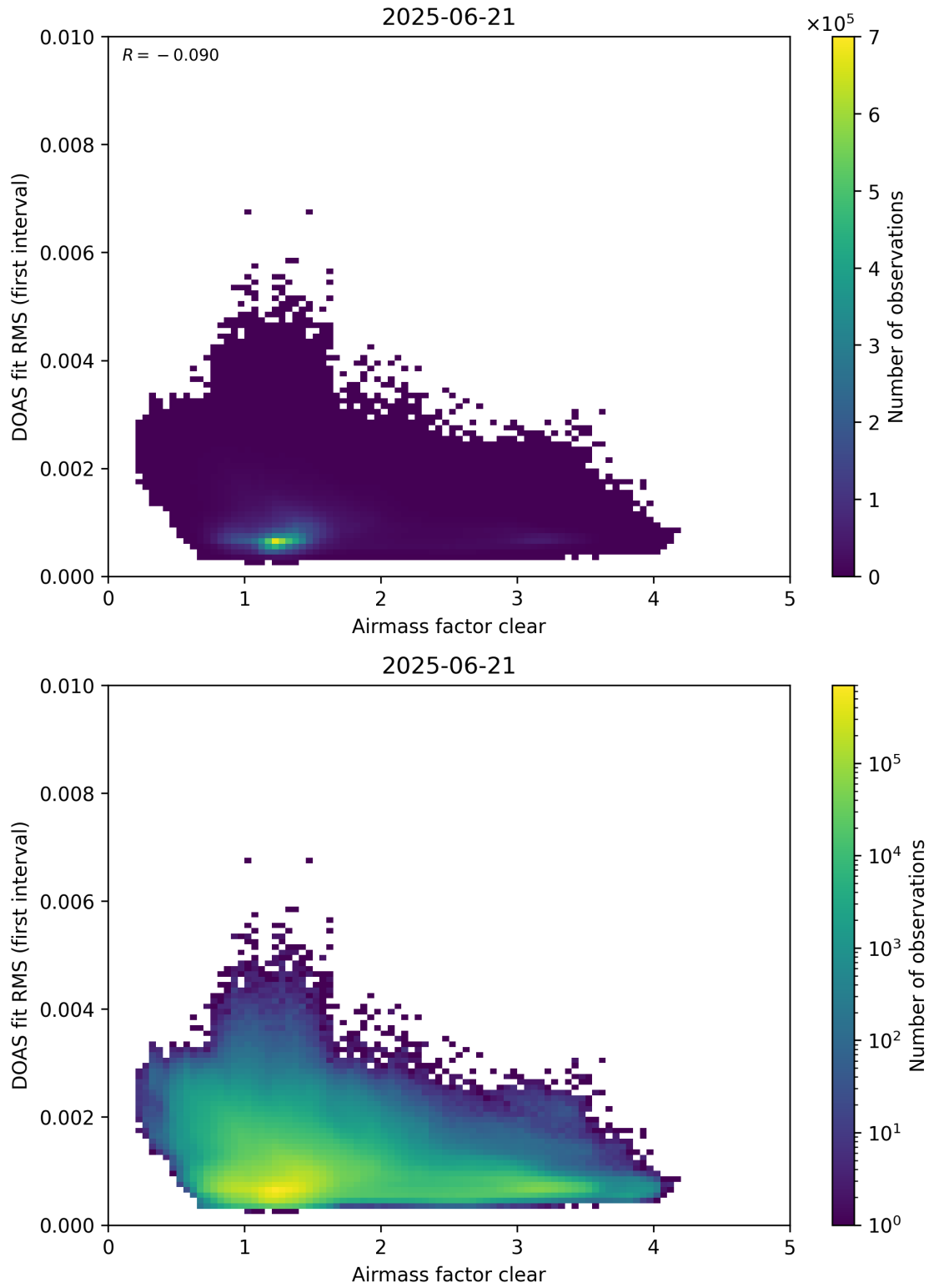
Figure 71: Scatter density plot of “Airmass factor clear” against “DOAS fit RMS (first interval)” for 2025-06-20 to 2025-06-22.
