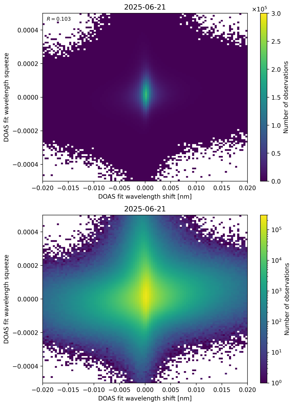
Figure 65: Scatter density plot of “DOAS fit wavelength shift” against “DOAS fit wavelength squeeze” for 2025-06-20 to 2025-06-22.
