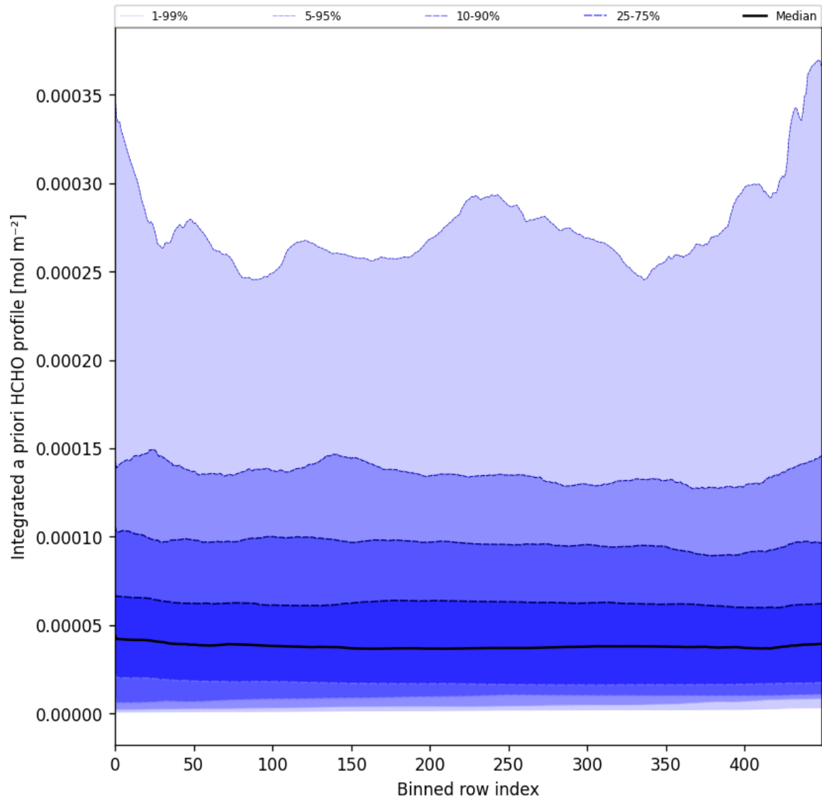
Figure 57: Along track statistics of “Integrated a priori HCHO profile” for 2025-06-20 to 2025-06-22
