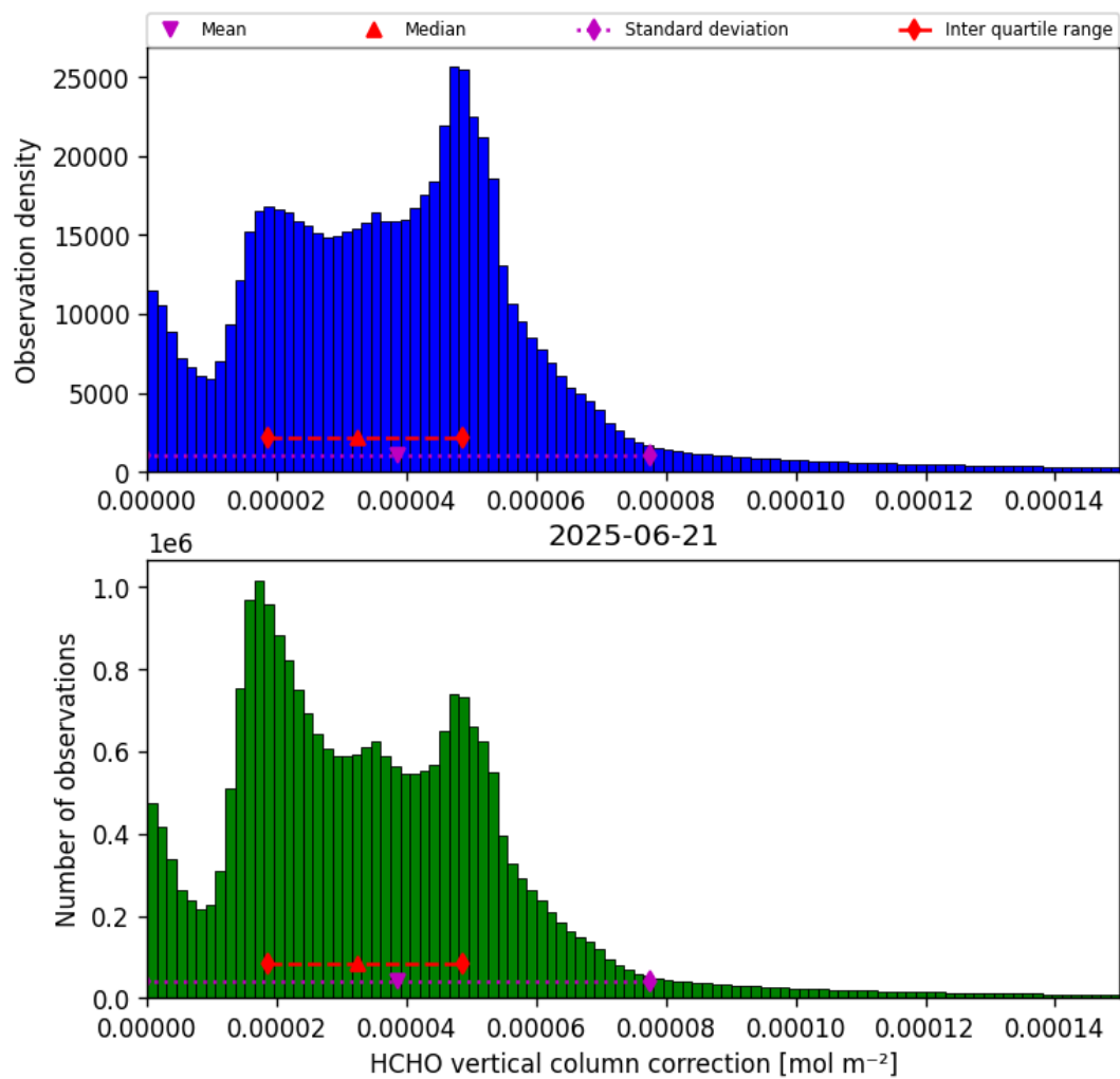
Figure 37: Histogram of “HCHO vertical column correction” for 2025-06-20 to 2025-06-22
