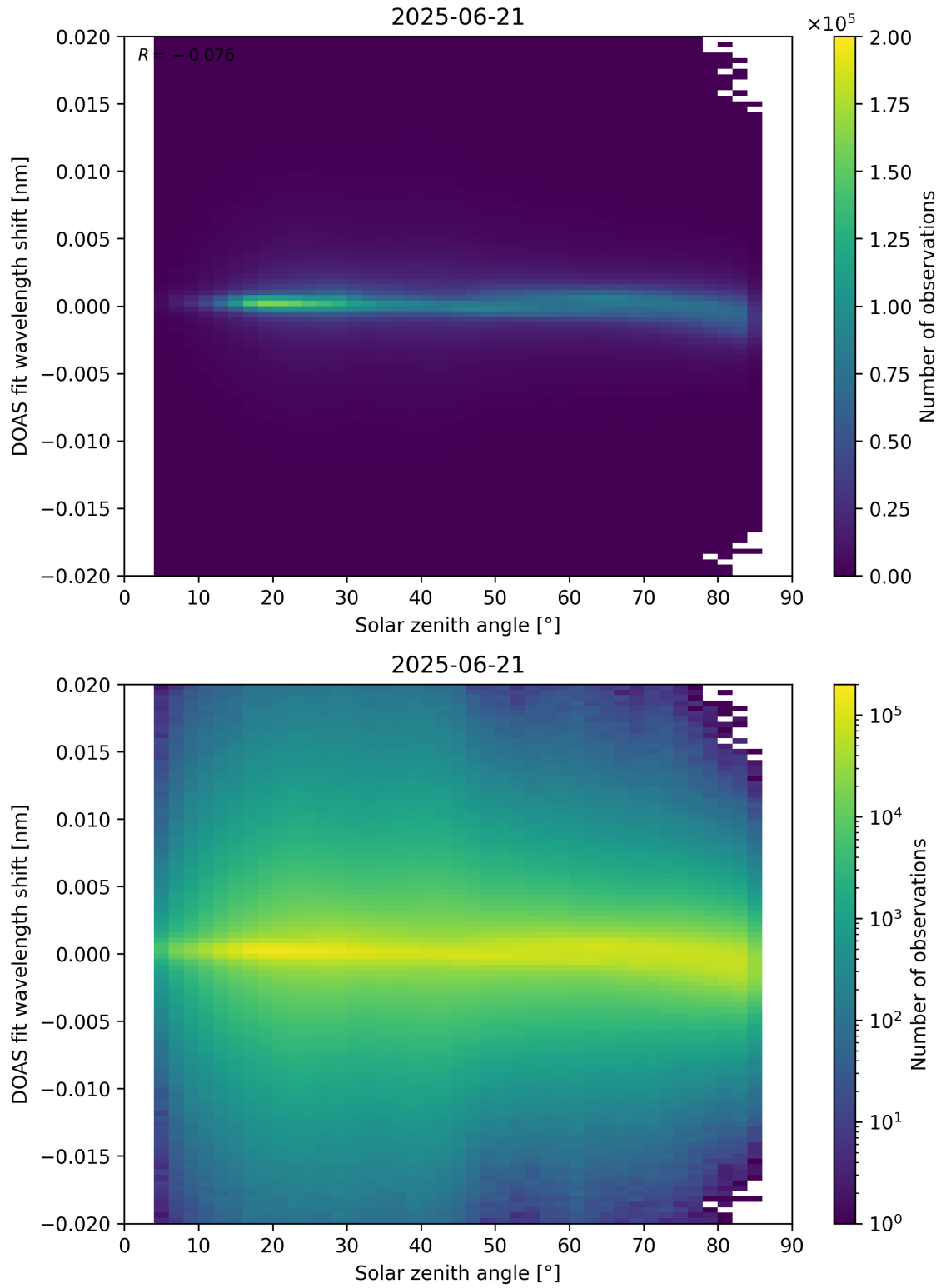
Figure 168: Scatter density plot of “Solar zenith angle” against “DOAS fit wavelength shift” for 2025-06-20 to 2025-06-22.
