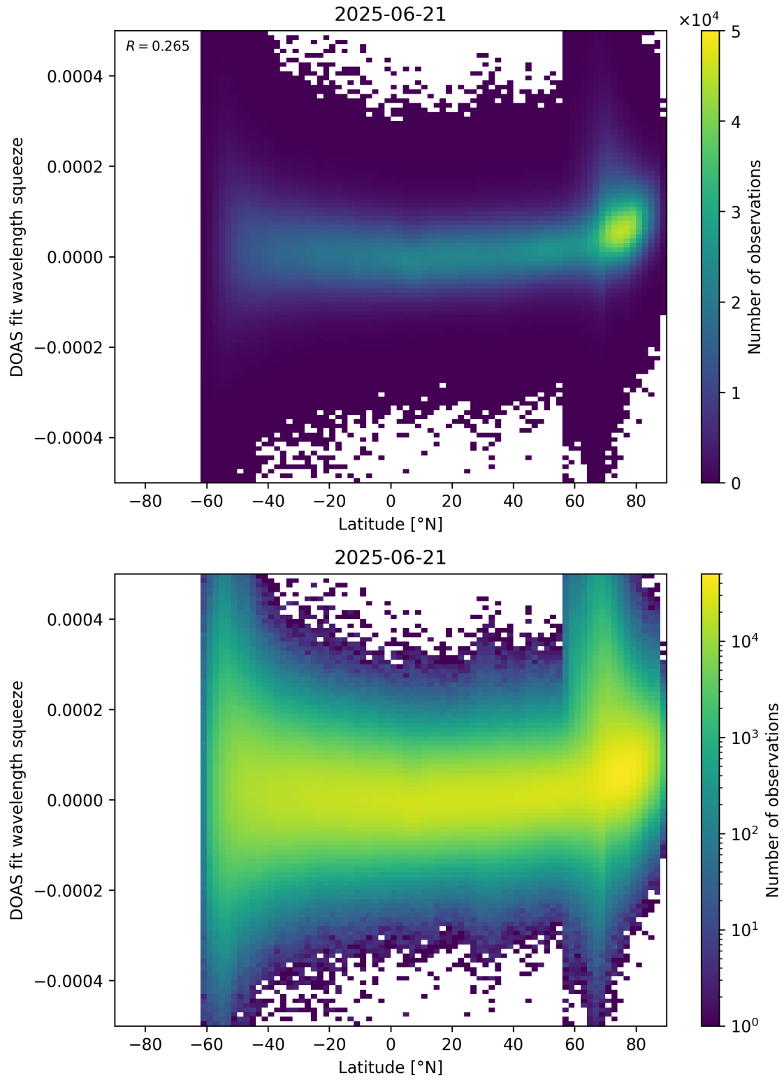
Figure 155: Scatter density plot of “Latitude” against “DOAS fit wavelength squeeze” for 2025-06-20 to 2025-06-22.
