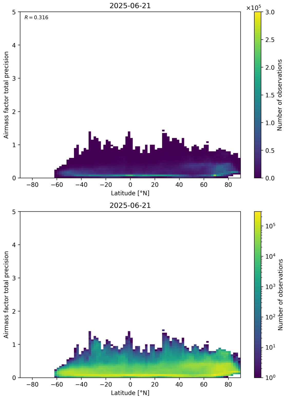
Figure 162: Scatter density plot of “Latitude” against “Airmass factor total precision” for 2025-06-20 to 2025-06-22.
