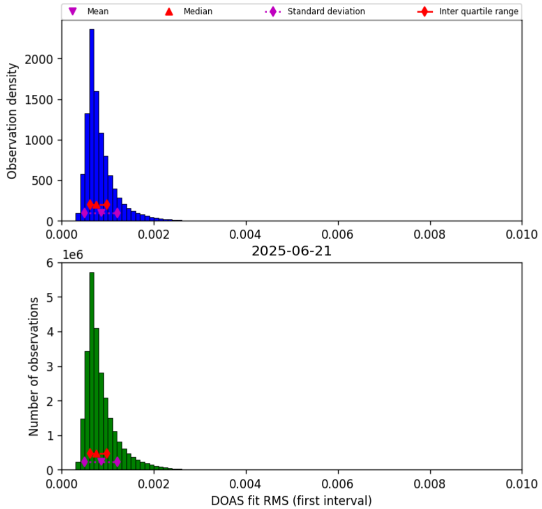
Figure 46: Histogram of “DOAS fit RMS (first interval)” for 2025-06-20 to 2025-06-22
