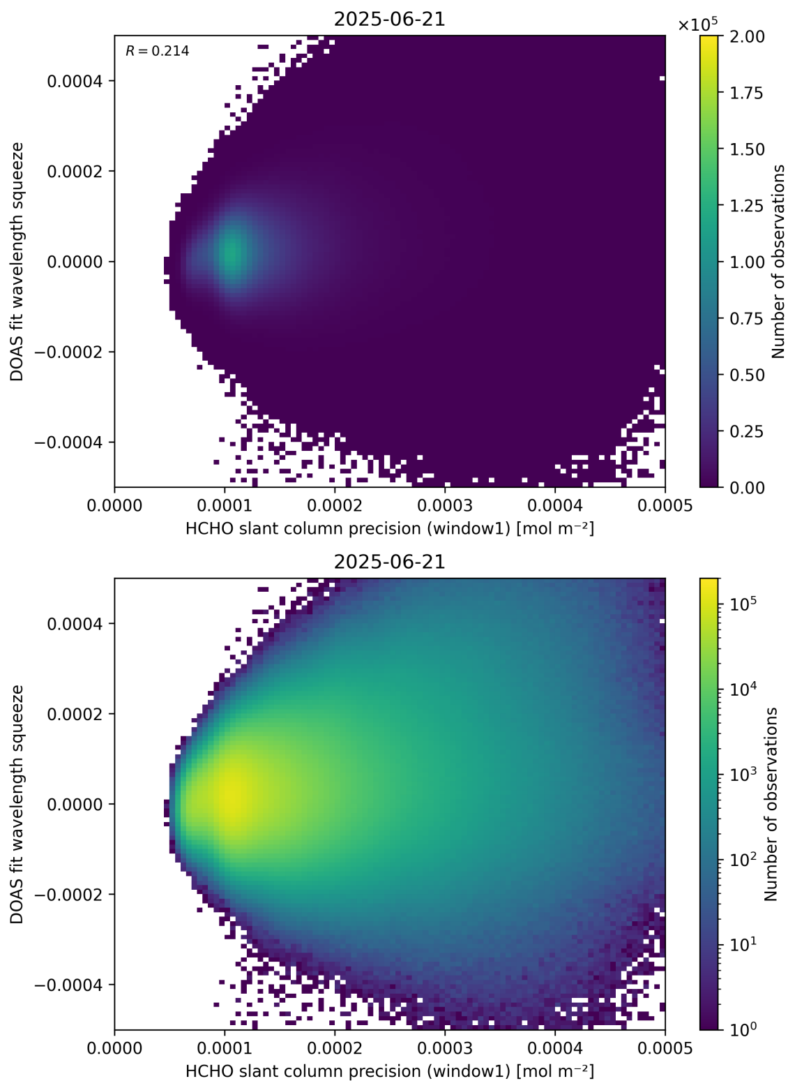
Figure 90: Scatter density plot of “HCHO slant column precision (window1)” against “DOAS fit wavelength squeeze” for 2025-06-20 to 2025-06-22.
