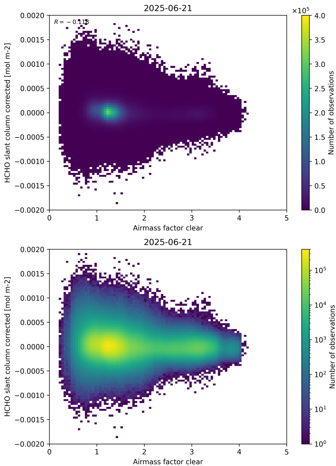
Figure 74: Scatter density plot of “Airmass factor clear” against “HCHO slant column corrected” for 2025-06-20 to 2025-06-22.
