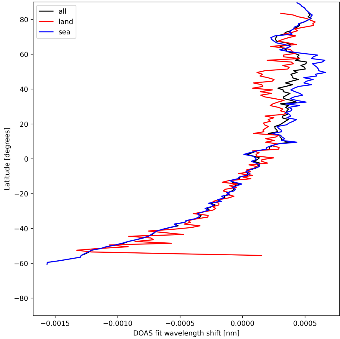
Figure 30: Zonal average of “DOAS fit wavelength shift” for 2025-06-20 to 2025-06-22.
