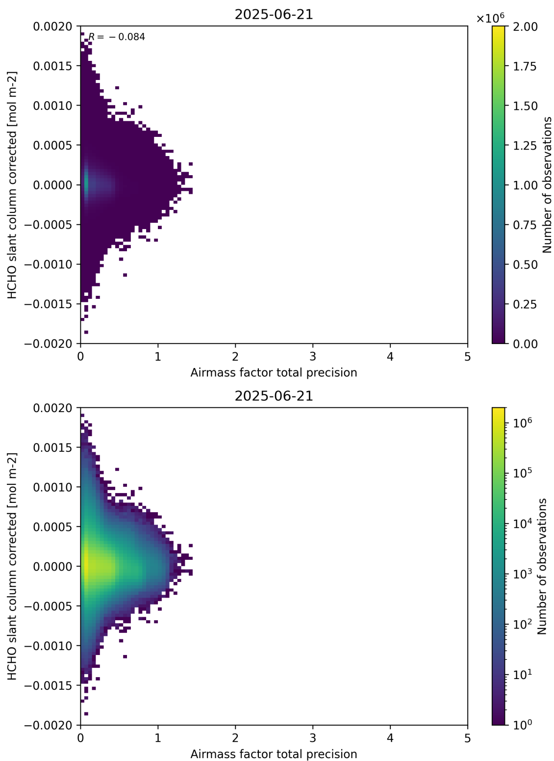
Figure 109: Scatter density plot of “Airmass factor total precision” against “HCHO slant column corrected” for 2025-06-20 to 2025-06-22.
