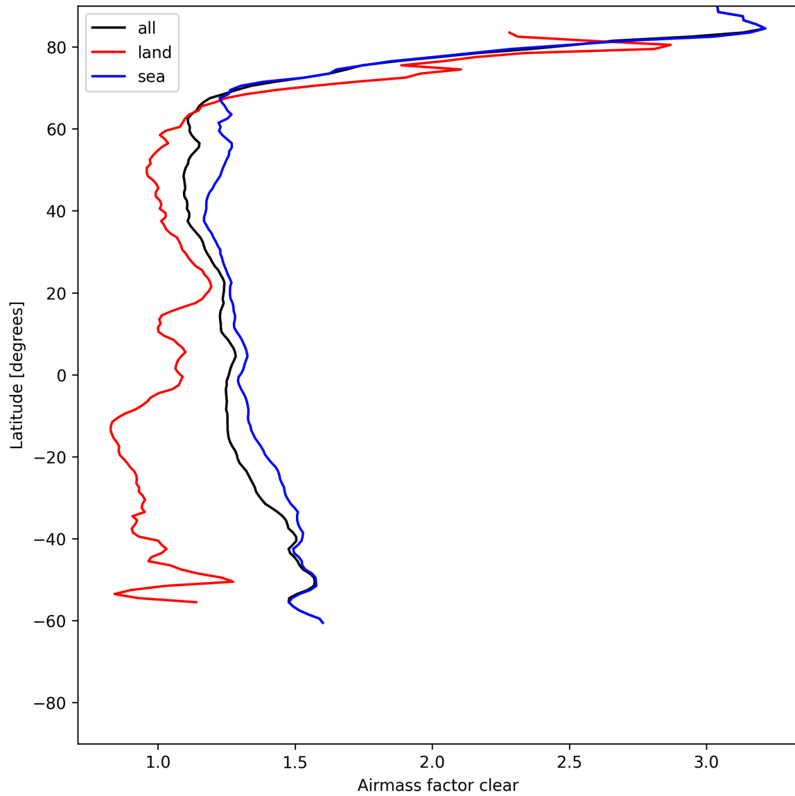
Figure 28: Zonal average of “Airmass factor clear” for 2025-06-20 to 2025-06-22.
