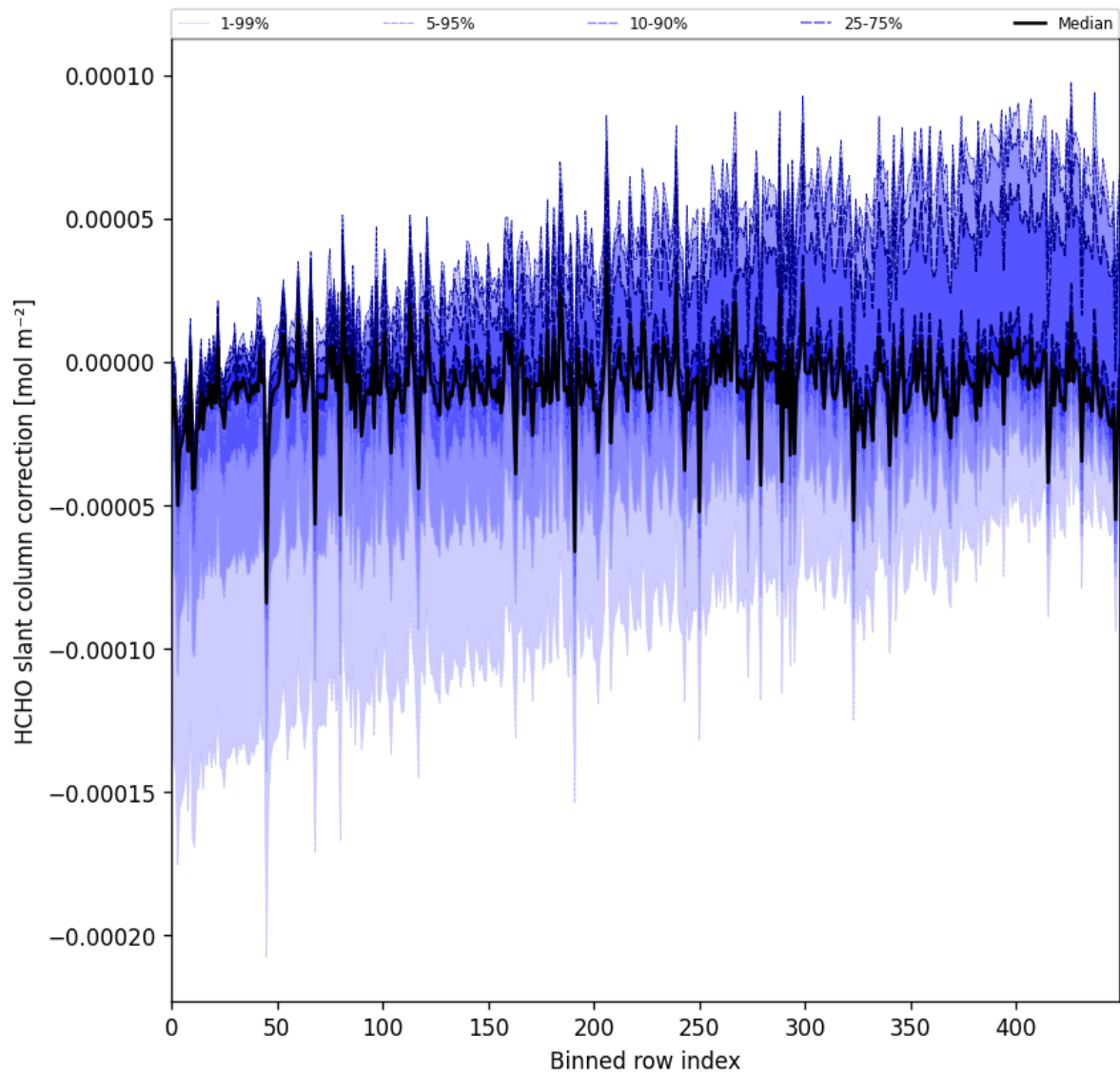
Figure 61: Along track statistics of “HCHO slant column correction” for 2025-06-20 to 2025-06-22
