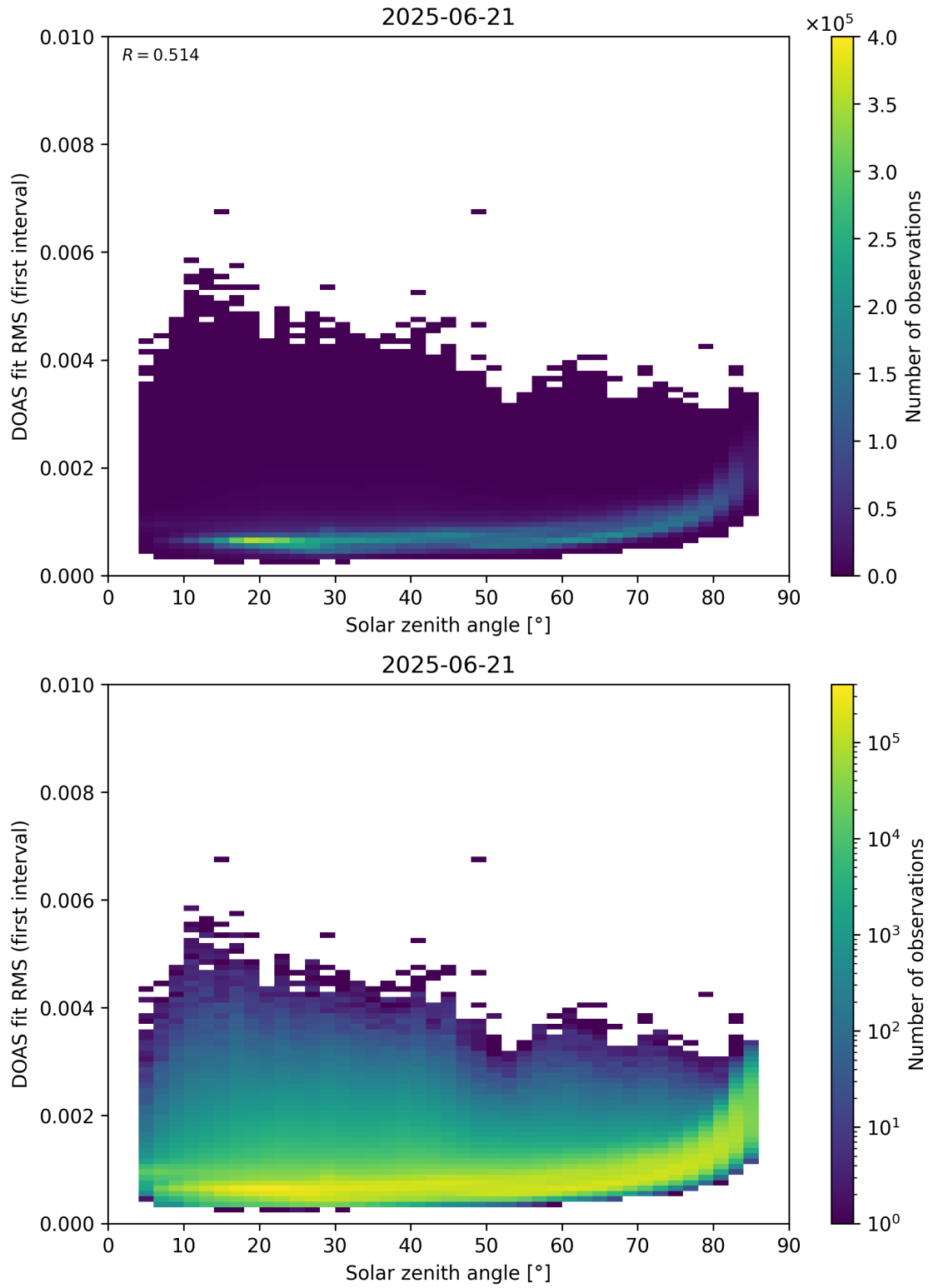
Figure 167: Scatter density plot of “Solar zenith angle” against “DOAS fit RMS (first interval)” for 2025-06-20 to 2025-06-22.
