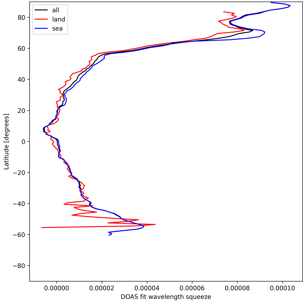
Figure 31: Zonal average of “DOAS fit wavelength squeeze” for 2025-06-20 to 2025-06-22.
