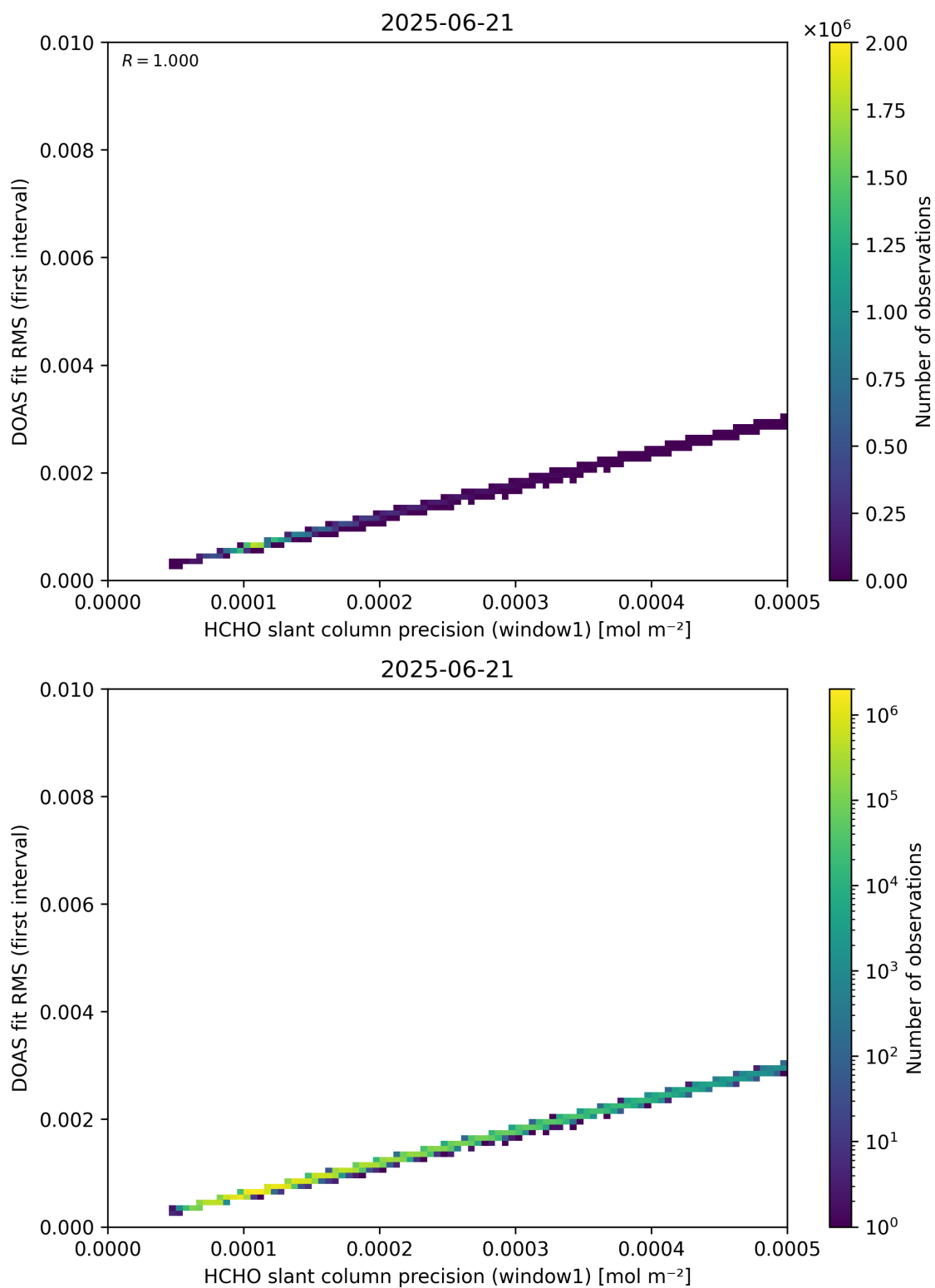
Figure 88: Scatter density plot of “HCHO slant column precision (window1)” against “DOAS fit RMS (first interval)” for 2025-06-20 to 2025-06-22.
