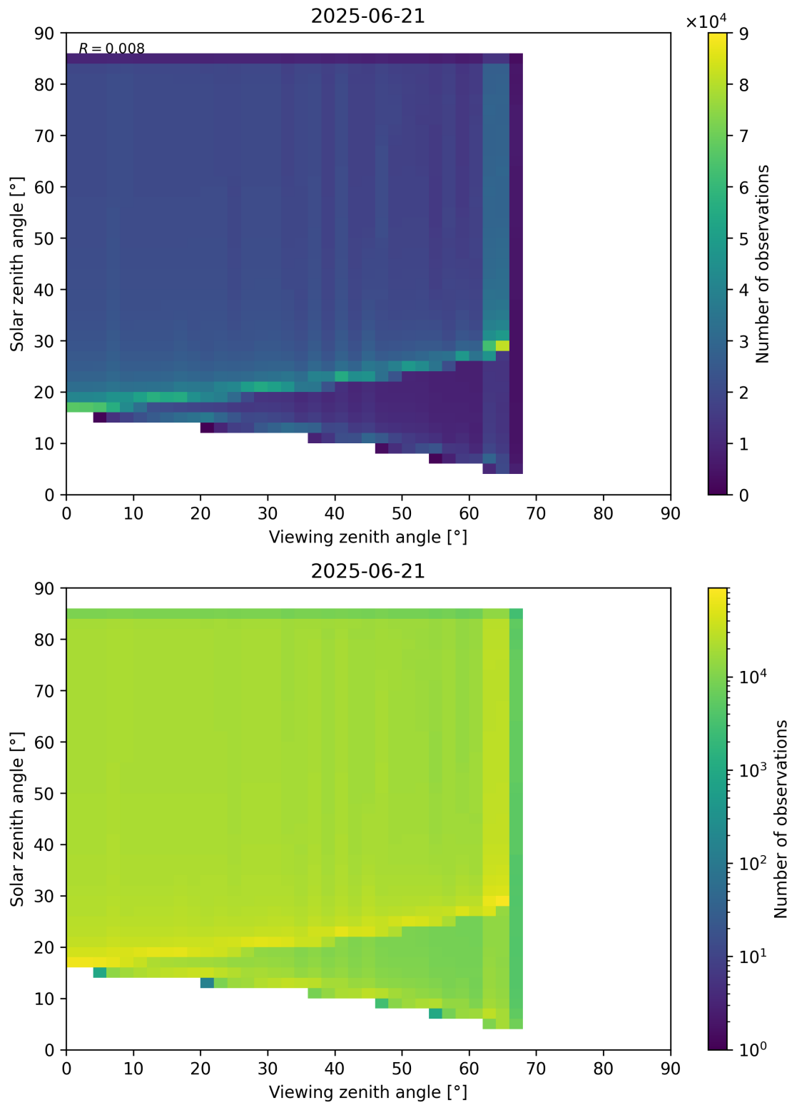
Figure 197: Scatter density plot of “Viewing zenith angle” against “Solar zenith angle” for 2025-06-20 to 2025-06-22.
