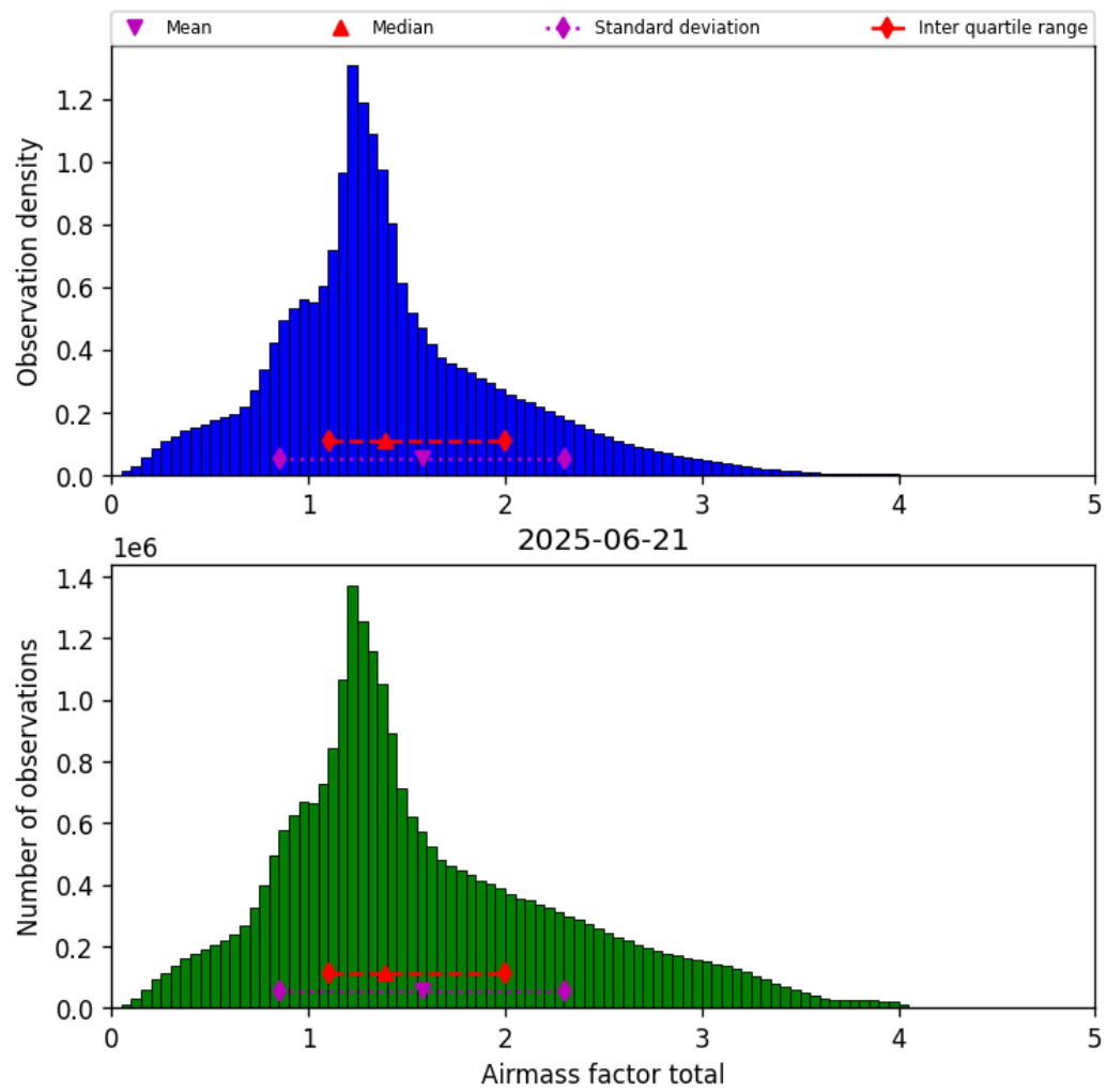
Figure 40: Histogram of “Airmass factor total” for 2025-06-20 to 2025-06-22
