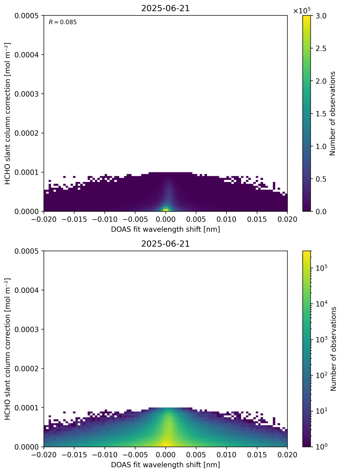
Figure 67: Scatter density plot of “DOAS fit wavelength shift” against “HCHO slant column correction” for 2025-06-20 to 2025-06-22.
