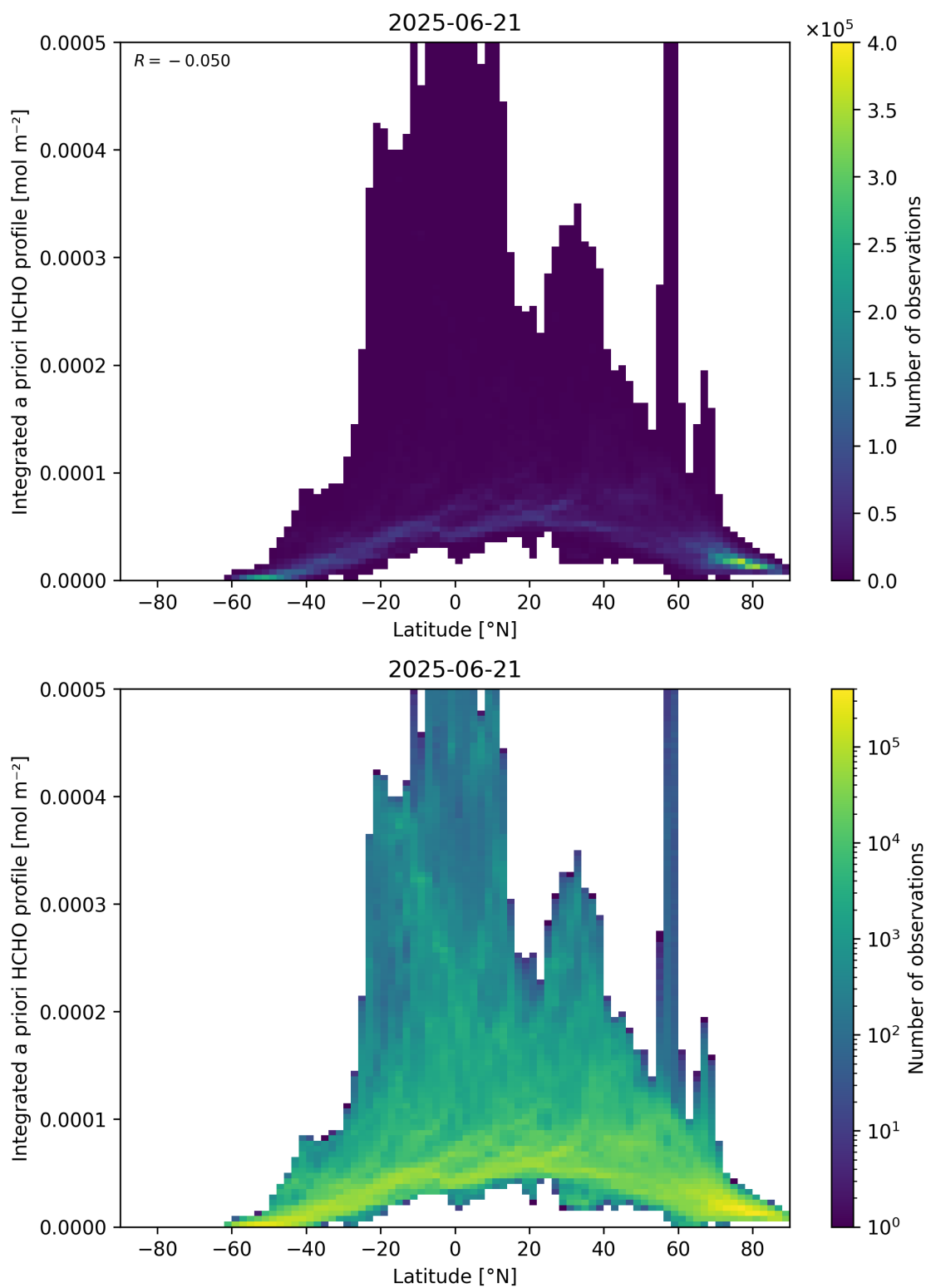
Figure 166: Scatter density plot of “Latitude” against “Integrated a priori HCHO profile” for 2025-06-20 to 2025-06-22.
