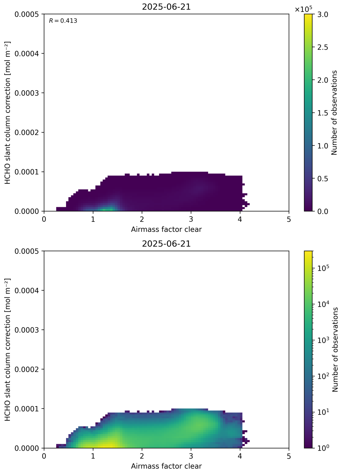
Figure 75: Scatter density plot of “Airmass factor clear” against “HCHO slant column correction” for 2025-06-20 to 2025-06-22.
