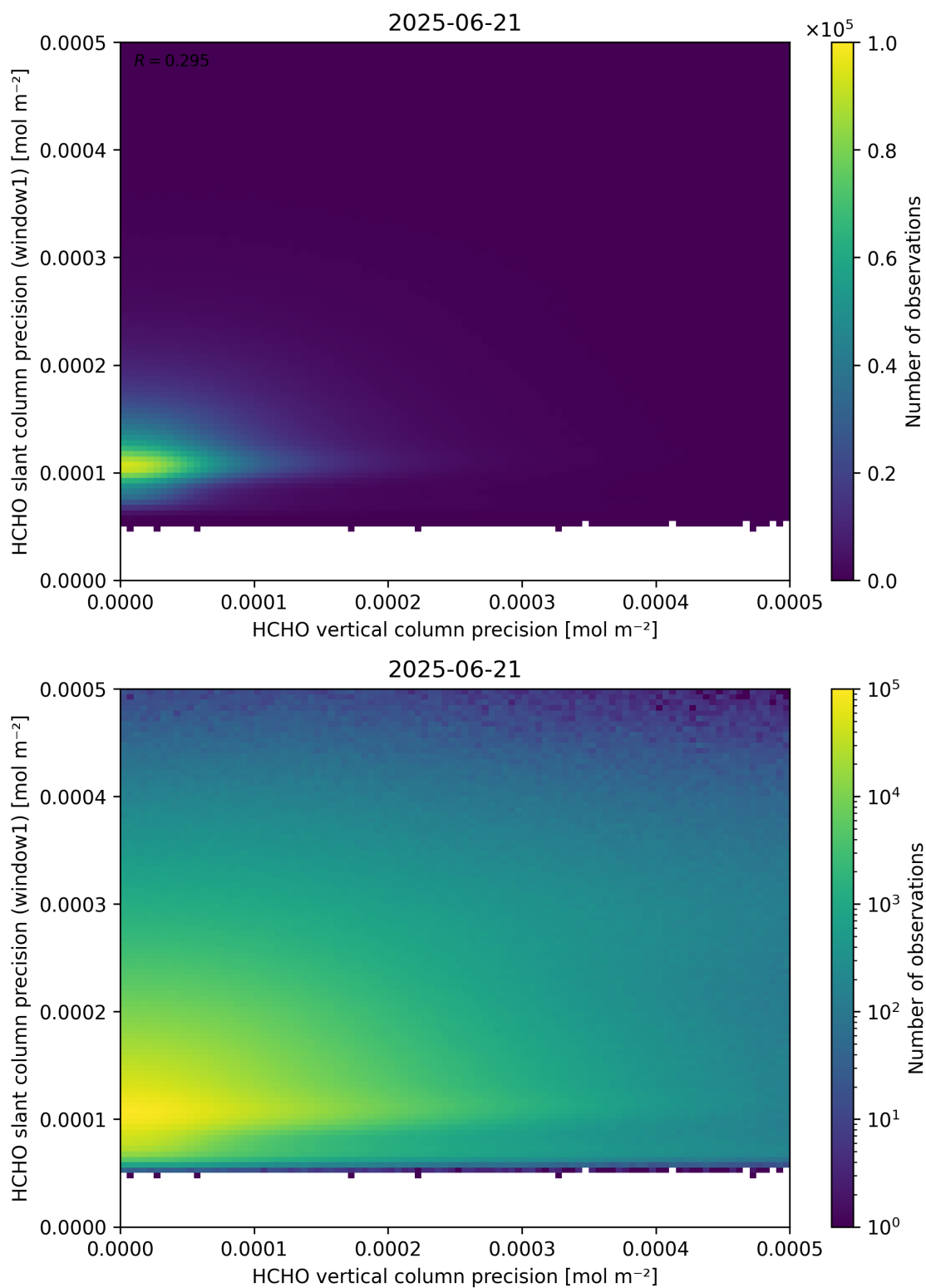
Figure 143: Scatter density plot of “HCHO vertical column precision” against “HCHO slant column precision (window1)” for 2025-06-20 to 2025-06-22.
