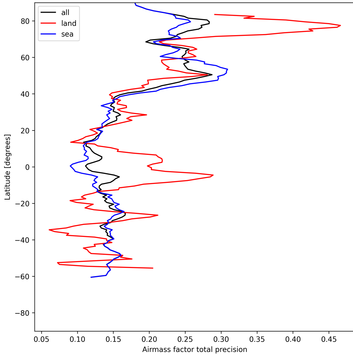
Figure 27: Zonal average of “Airmass factor total precision” for 2025-06-20 to 2025-06-22.
