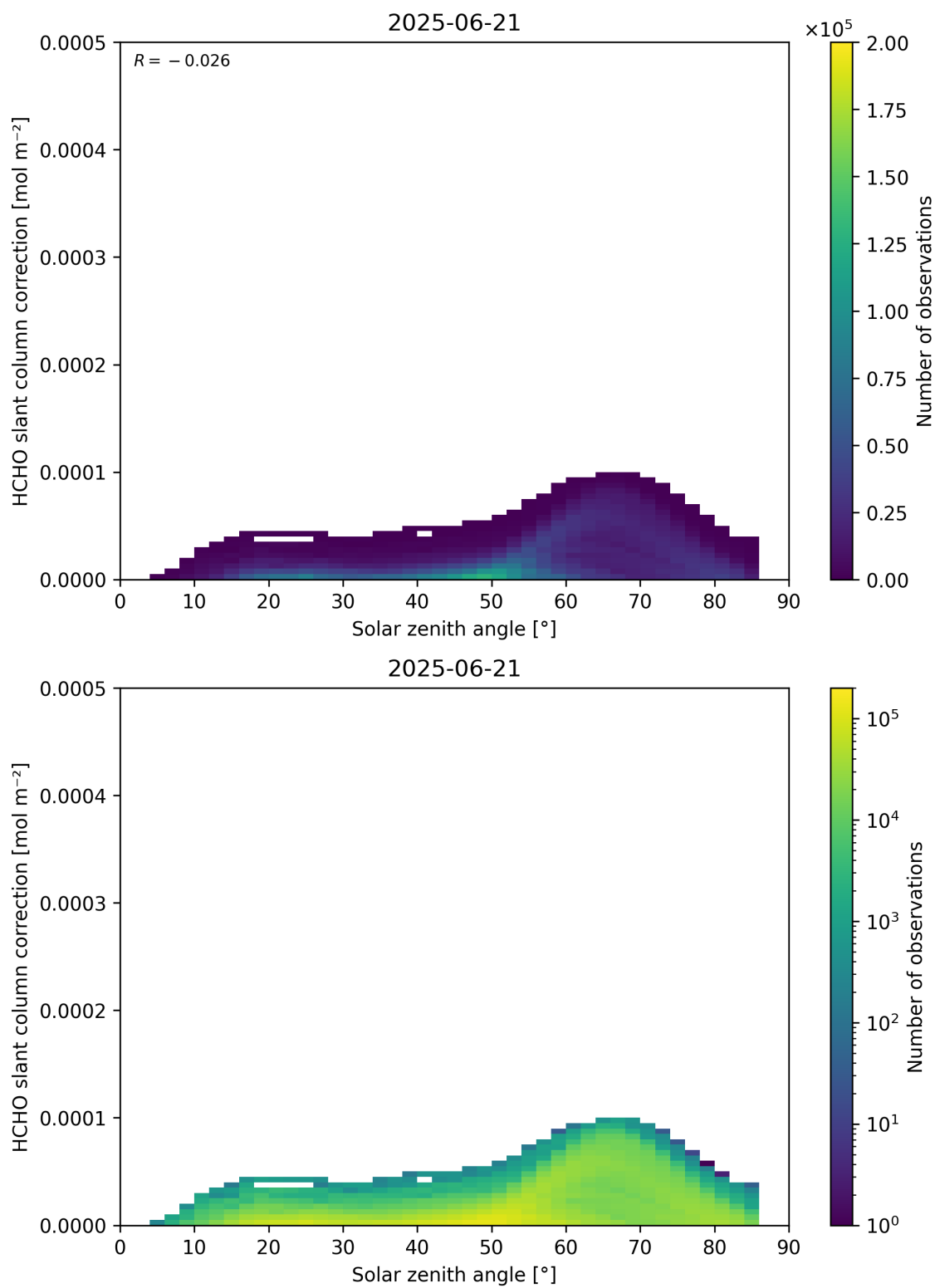
Figure 172: Scatter density plot of “Solar zenith angle” against “HCHO slant column correction” for 2025-06-20 to 2025-06-22.
