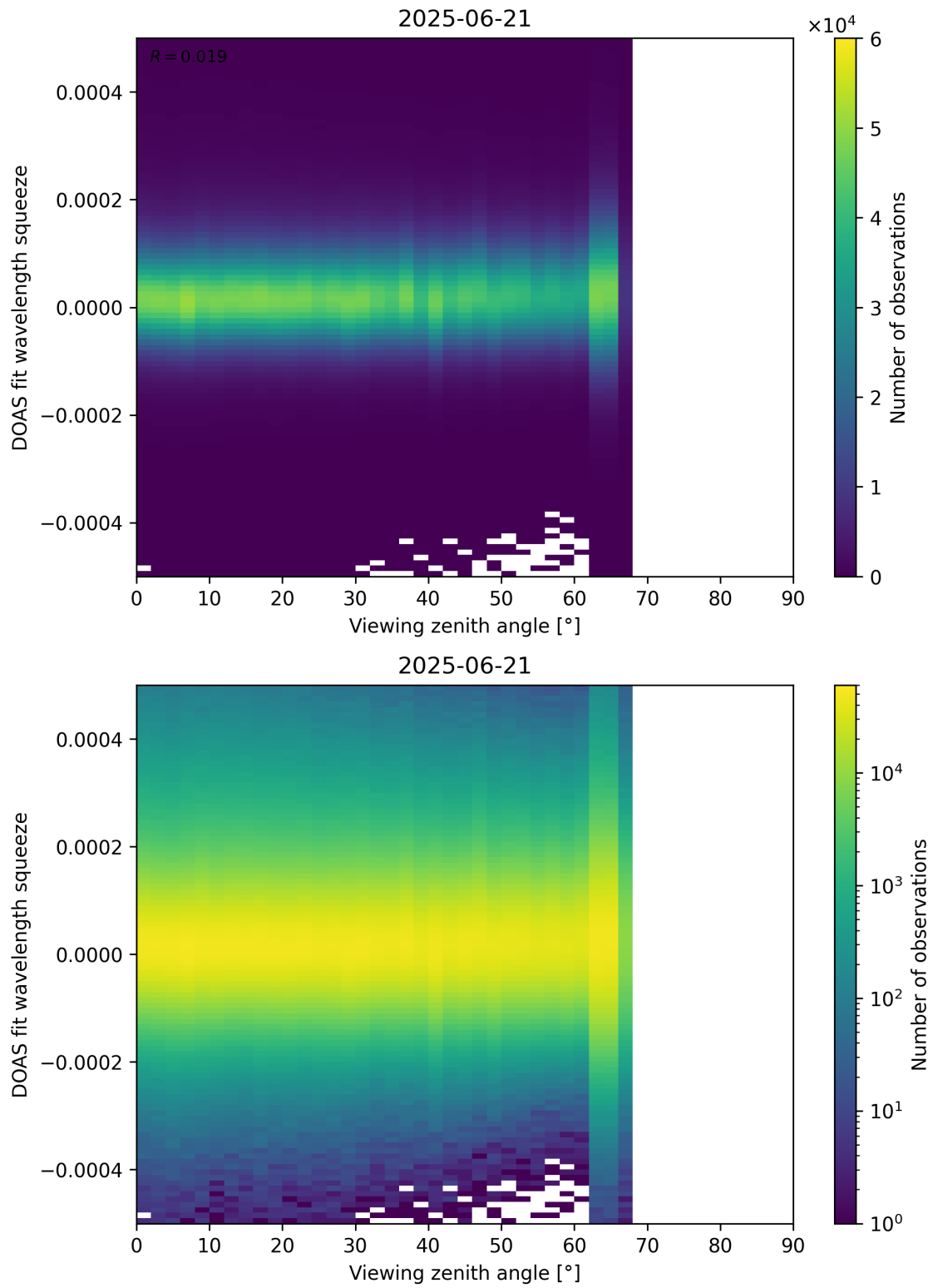
Figure 184: Scatter density plot of “Viewing zenith angle” against “DOAS fit wavelength squeeze” for 2025-06-20 to 2025-06-22.
