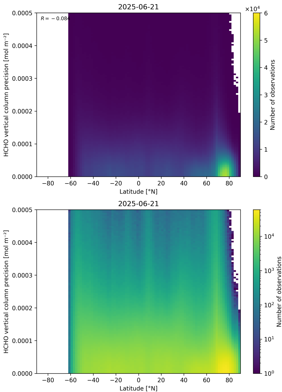
Figure 165: Scatter density plot of “Latitude” against “HCHO vertical column precision” for 2025-06-20 to 2025-06-22.
