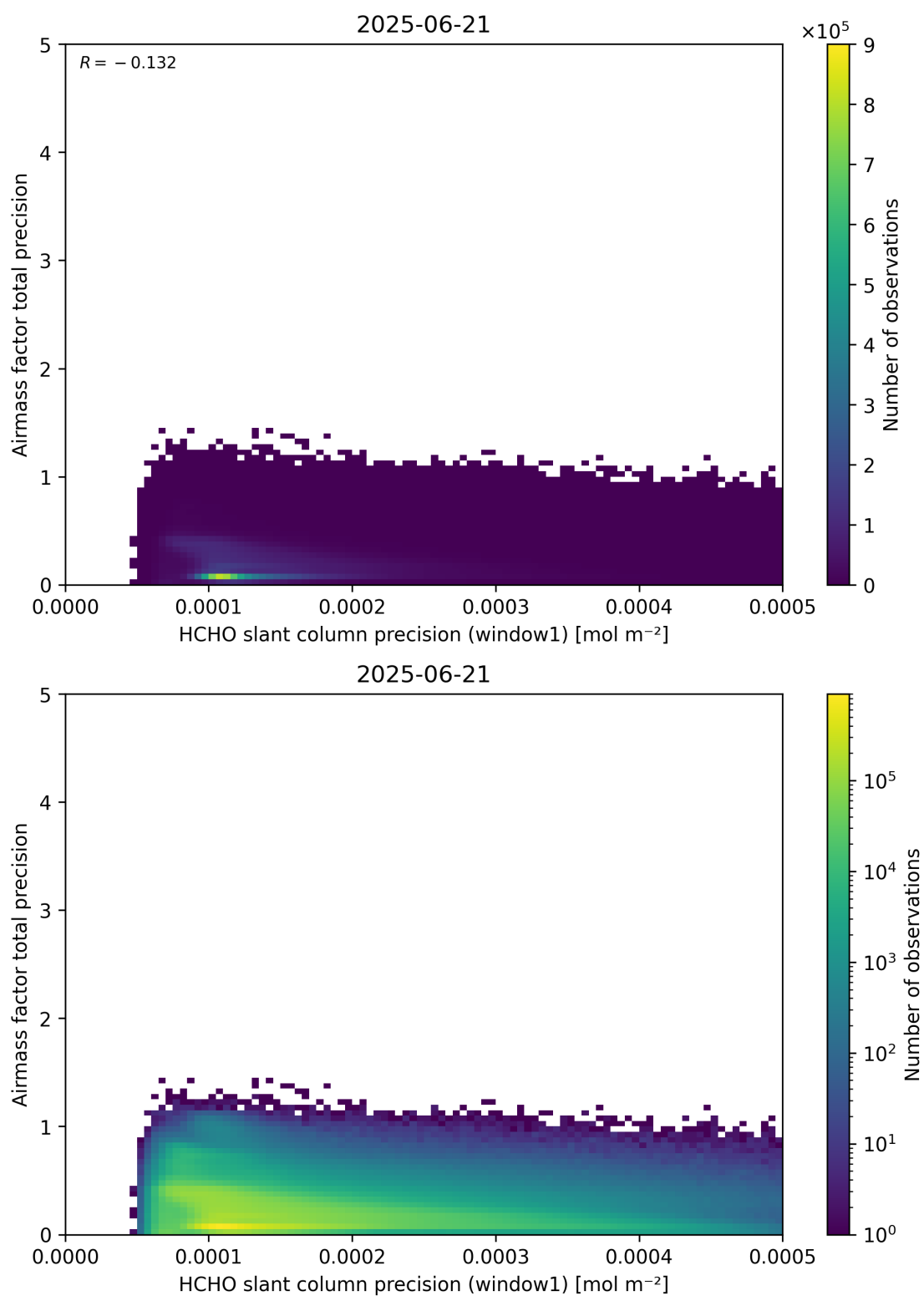
Figure 95: Scatter density plot of “HCHO slant column precision (window1)” against “Airmass factor total precision” for 2025-06-20 to 2025-06-22.
