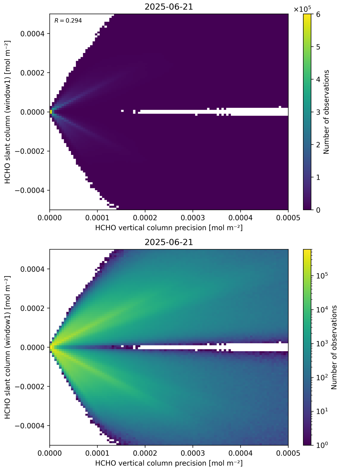
Figure 142: Scatter density plot of “HCHO vertical column precision” against “HCHO slant column (window1)” for 2025-06-20 to 2025-06-22.
