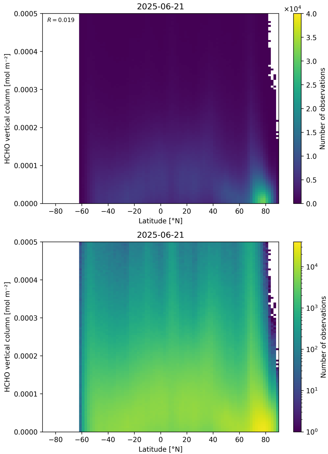
Figure 163: Scatter density plot of “Latitude” against “HCHO vertical column” for 2025-06-20 to 2025-06-22.
