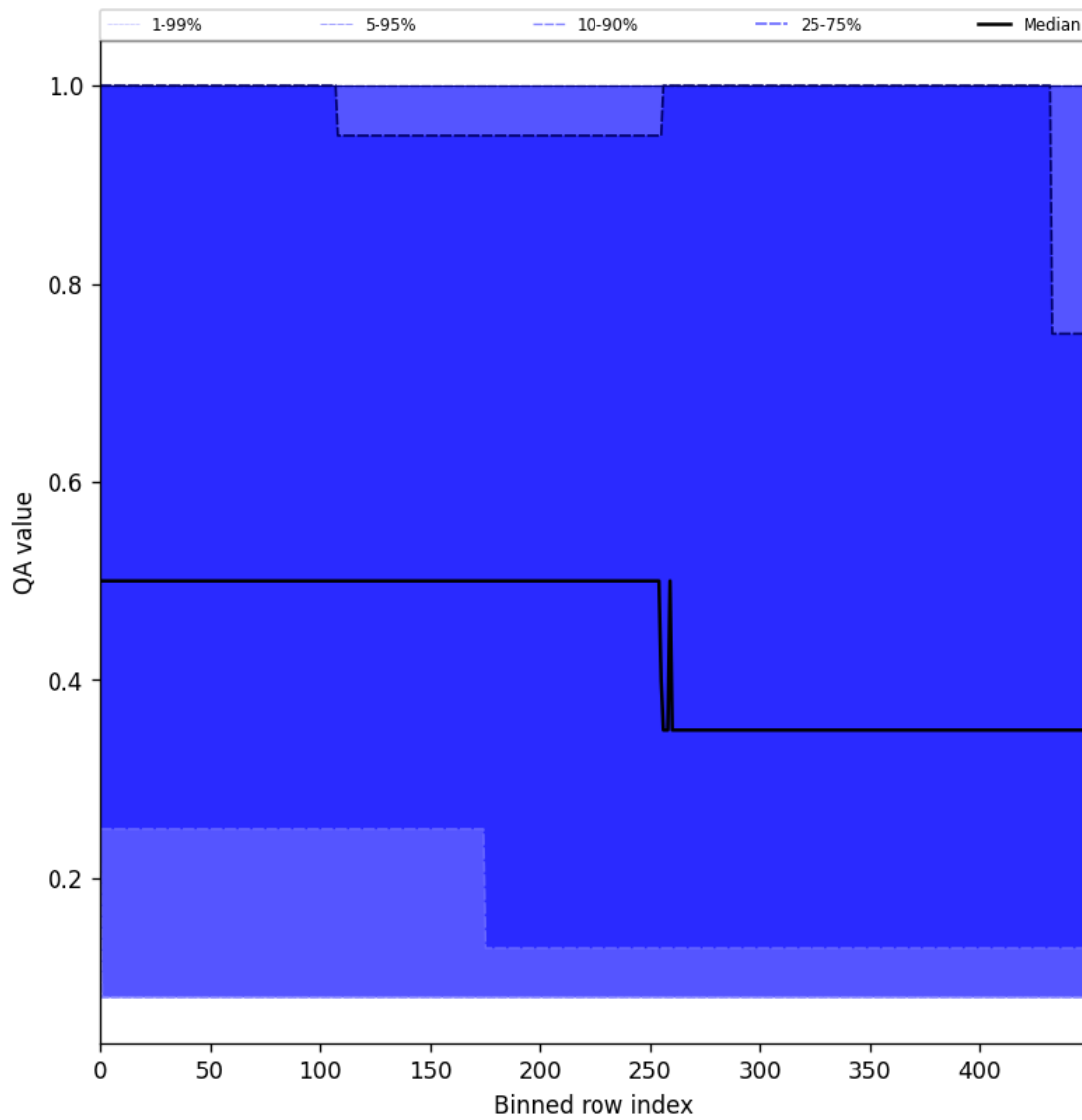
Figure 48: Along track statistics of “QA value” for 2025-06-20 to 2025-06-22
