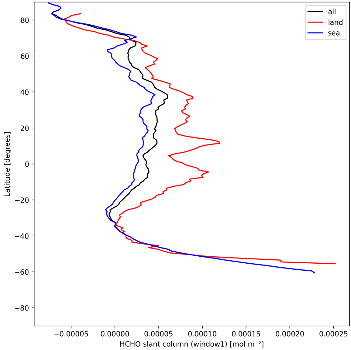
Figure 24: Zonal average of “HCHO slant column (window1)” for 2025-06-20 to 2025-06-22.
