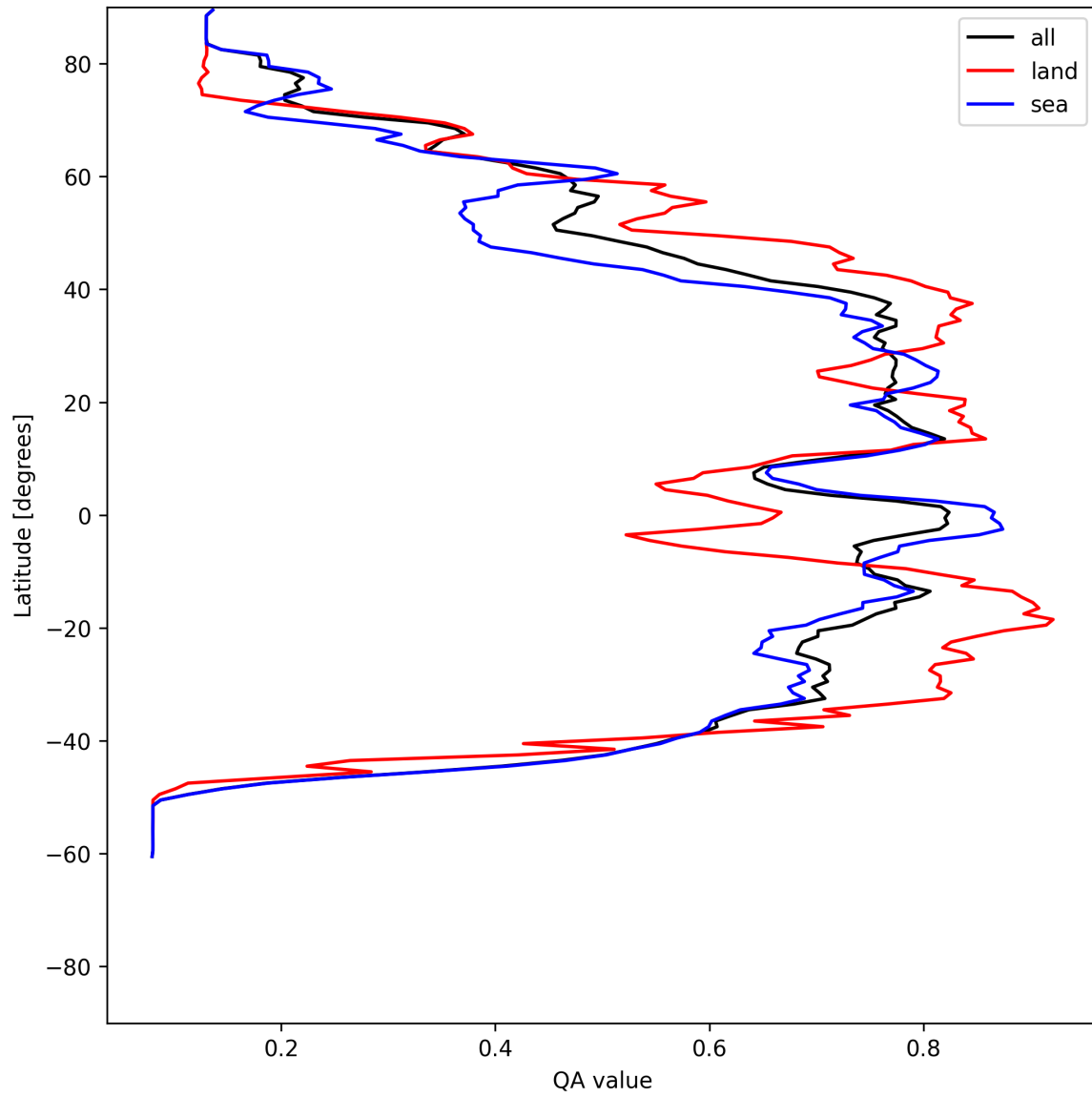
Figure 20: Zonal average of “QA value” for 2025-06-20 to 2025-06-22.
