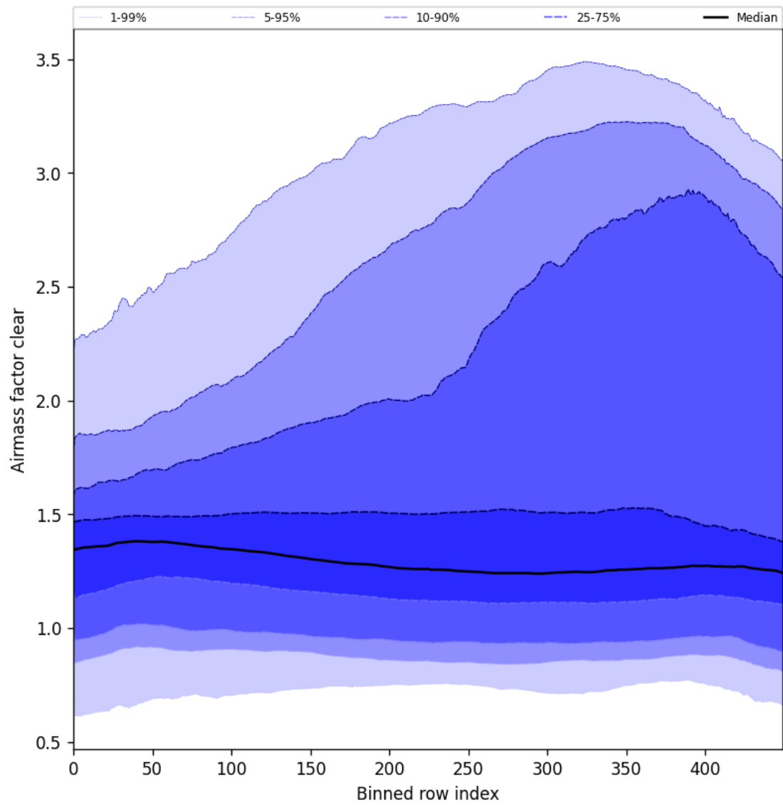
Figure 56: Along track statistics of “Air mass factor clear” for 2025-06-20 to 2025-06-22
