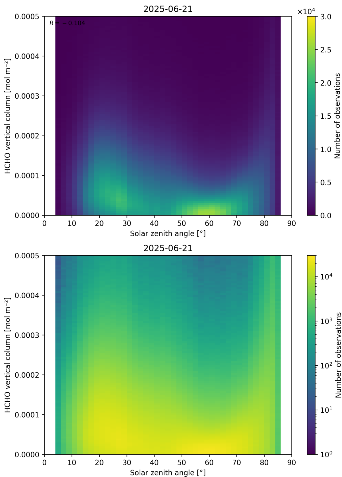
Figure 177: Scatter density plot of “Solar zenith angle” against “HCHO vertical column” for 2025-06-20 to 2025-06-22.
