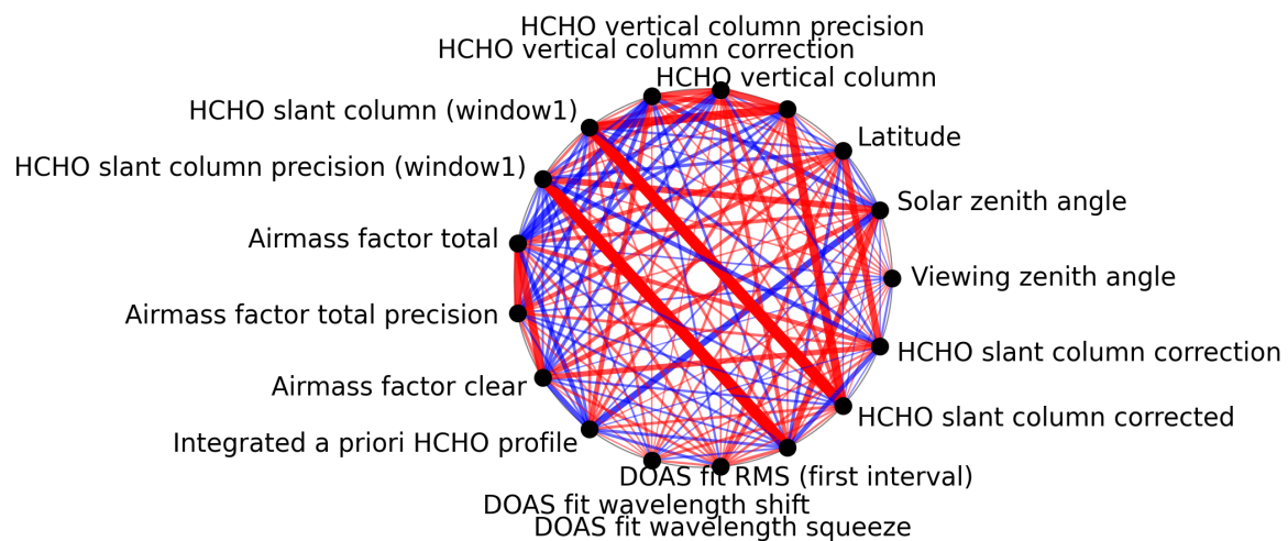
Figure 1: Map of correlation graph for 2025-06-20 to 2025-06-22.
