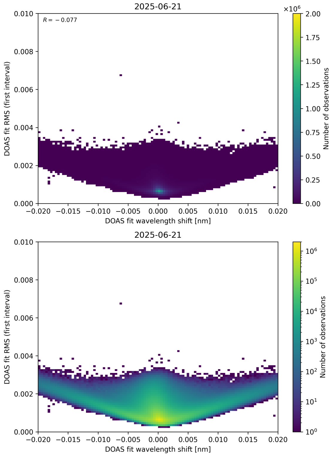
Figure 64: Scatter density plot of “DOAS fit wavelength shift” against “DOAS fit RMS (first interval)” for 2025-06-20 to 2025-06-22.
