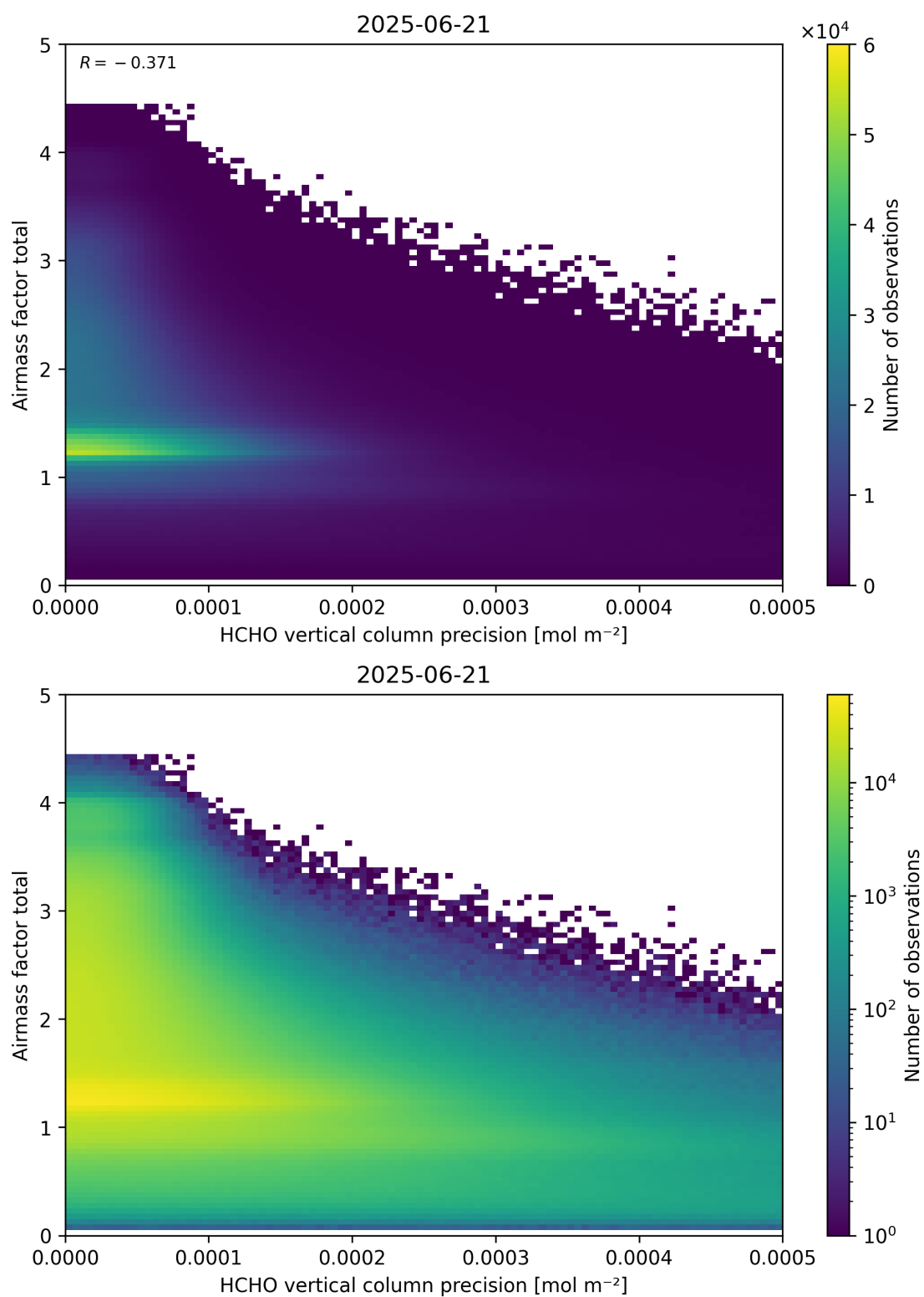
Figure 144: Scatter density plot of “HCHO vertical column precision” against “Airmass factor total” for 2025-06-20 to 2025-06-22.
