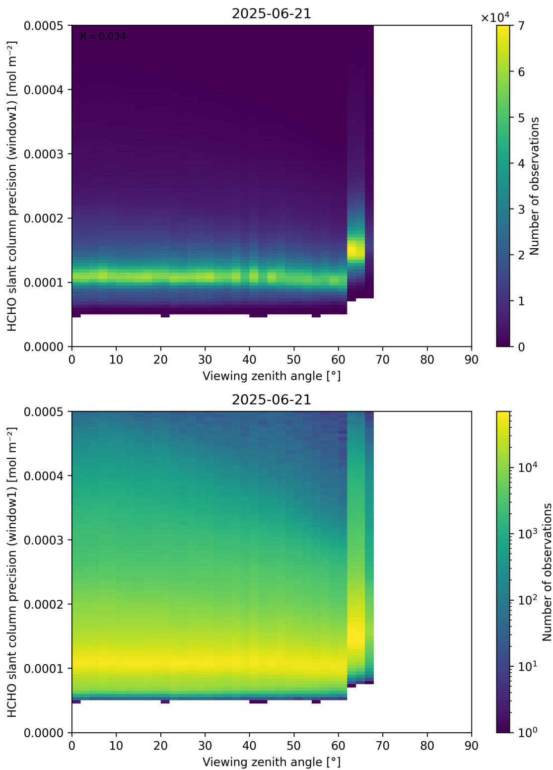
Figure 189: Scatter density plot of “Viewing zenith angle” against “HCHO slant column precision (window1)” for 2025-06-20 to 2025-06-22.
