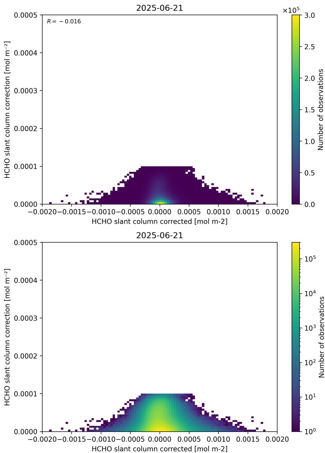
Figure 77: Scatter density plot of “HCHO slant column corrected” against “HCHO slant column correction” for 2025-06-20 to 2025-06-22.
