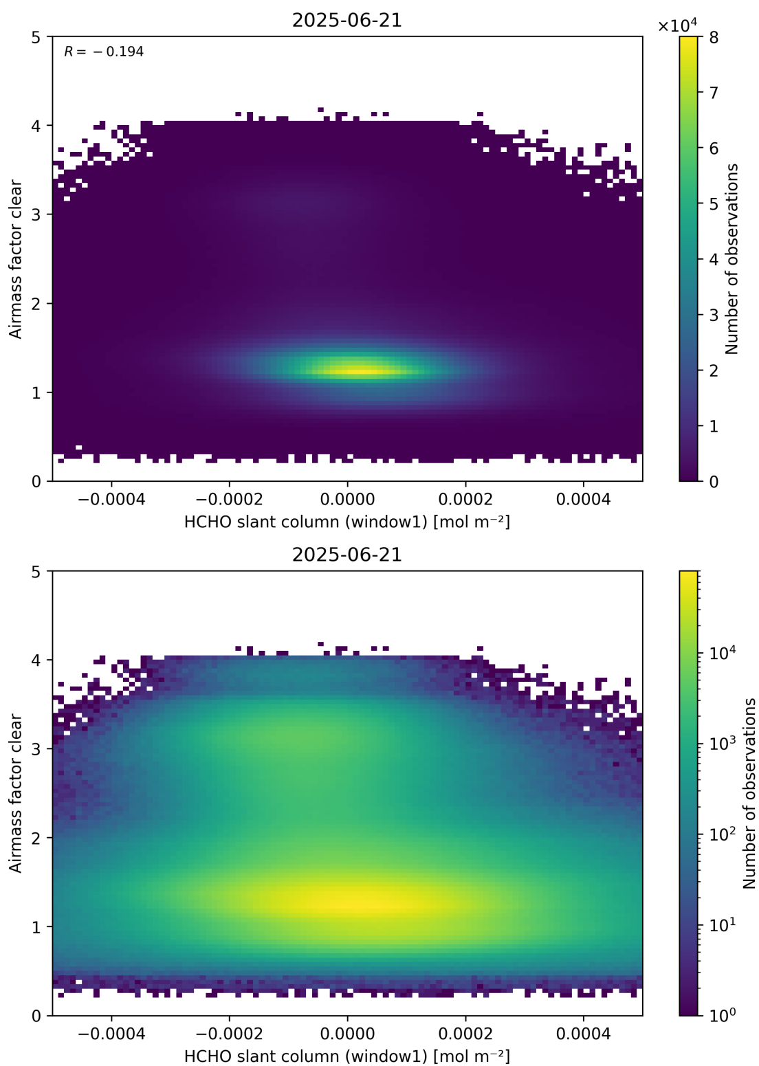
Figure 81: Scatter density plot of “HCHO slant column (window1)” against “Airmass factor clear” for 2025-06-20 to 2025-06-22.
