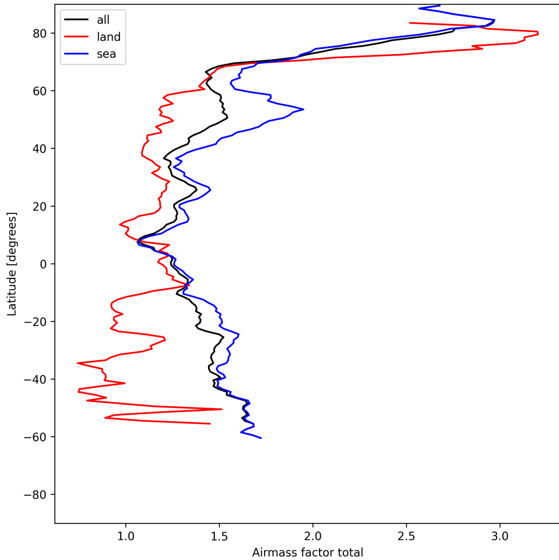
Figure 26: Zonal average of “Airmass factor total” for 2025-06-20 to 2025-06-22.
