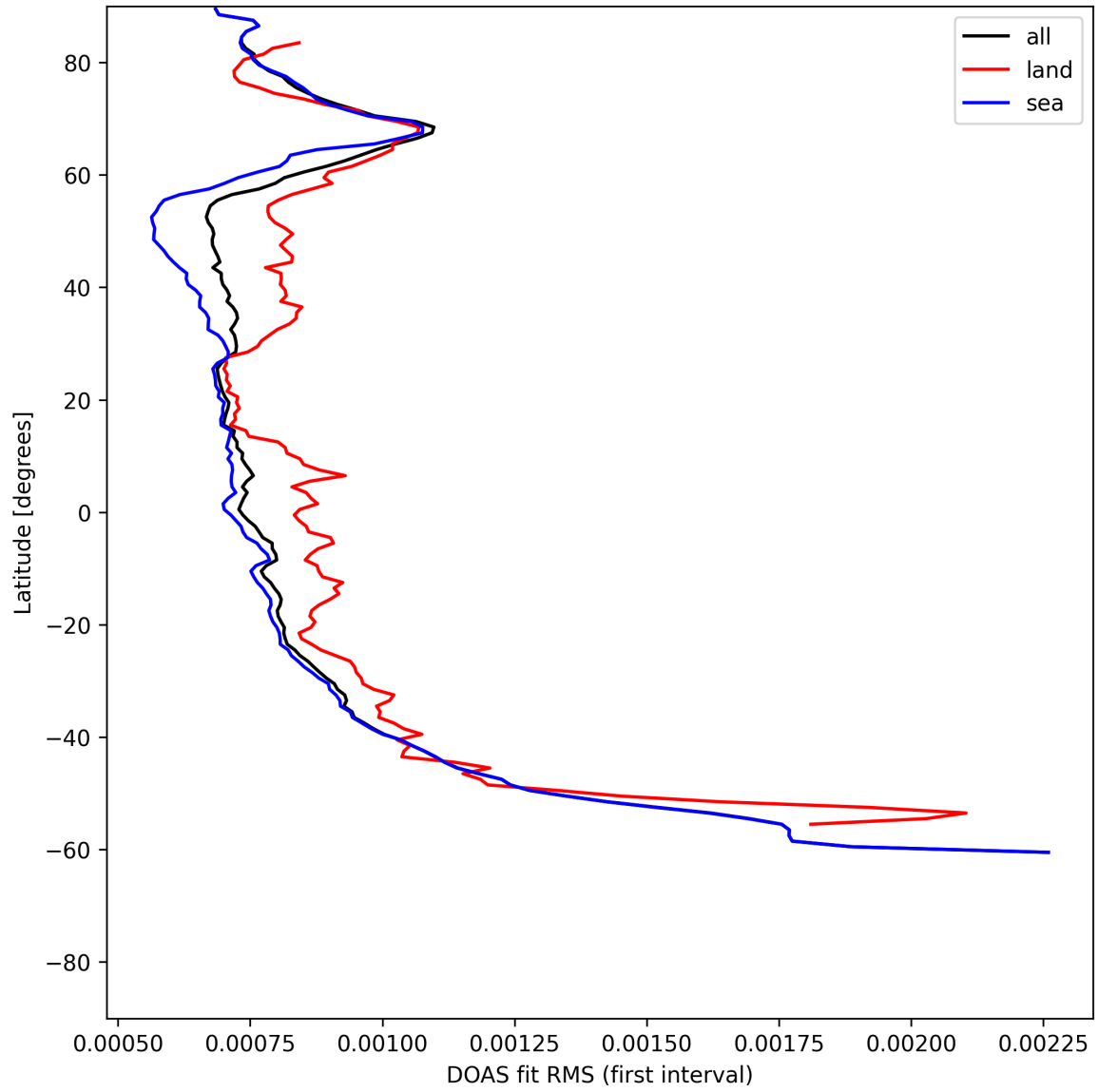
Figure 32: Zonal average of "DOAS fit RMS (first interval)" for 2025-06-20 to 2025-06-22.
