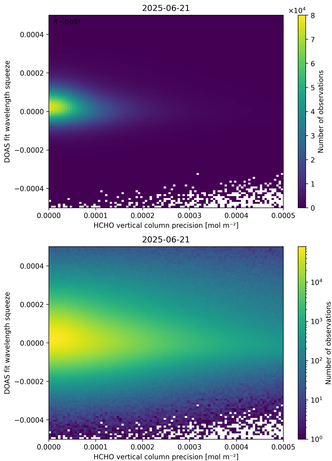
Figure 138: Scatter density plot of “HCHO vertical column precision” against “DOAS fit wavelength squeeze” for 2025-06-20 to 2025-06-22.
