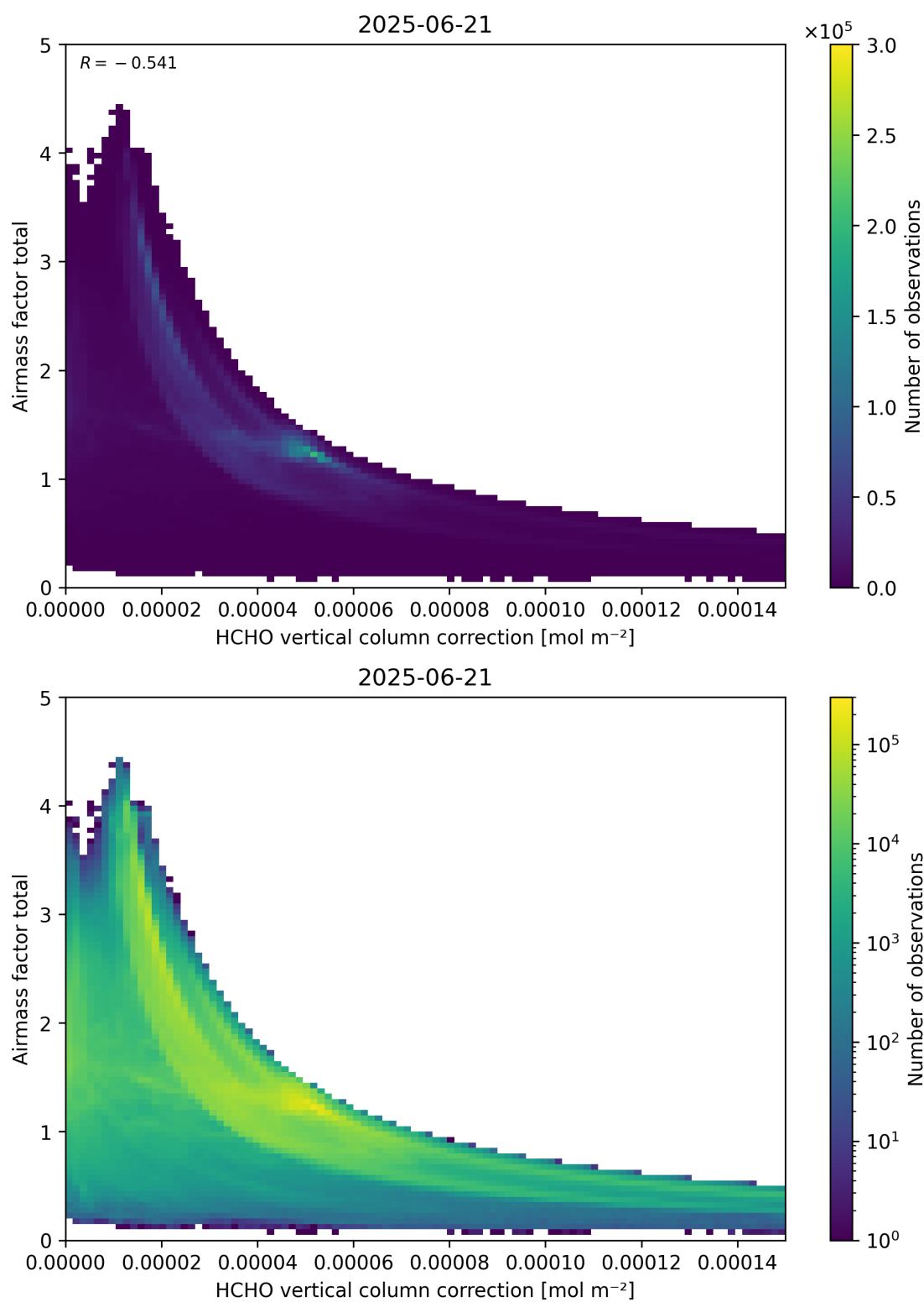
Figure 120: Scatter density plot of “HCHO vertical column correction” against “Airmass factor total” for 2025-06-20 to 2025-06-22.
