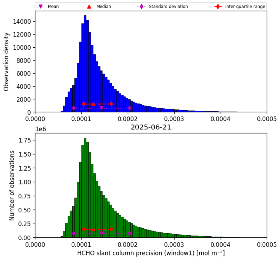
Figure 39: Histogram of “HCHO slant column precision (window1)” for 2025-06-20 to 2025-06-22
