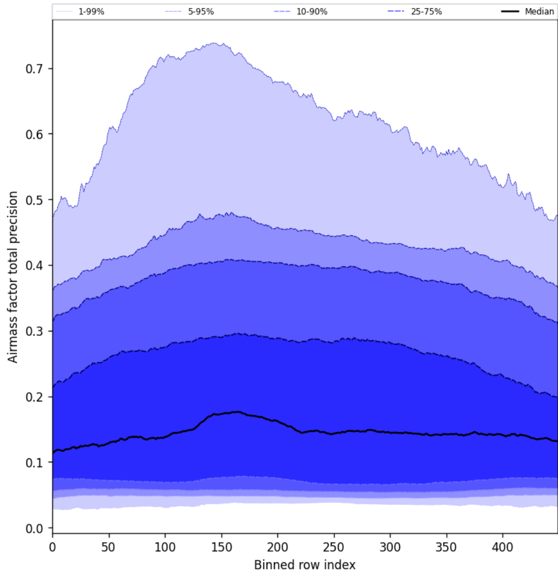
Figure 55: Along track statistics of “Airmass factor total precision” for 2025-06-20 to 2025-06-22
