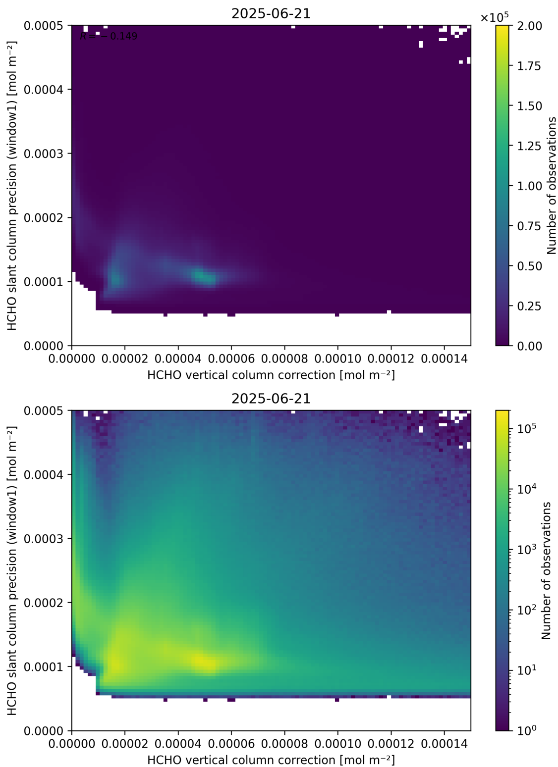
Figure 119: Scatter density plot of “HCHO vertical column correction” against “HCHO slant column precision (window1)” for 2025-06-20 to 2025-06-22.
