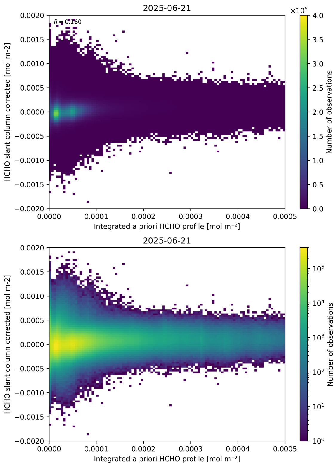
Figure 151: Scatter density plot of “Integrated a priori HCHO profile” against “HCHO slant column corrected” for 2025-06-20 to 2025-06-22.
