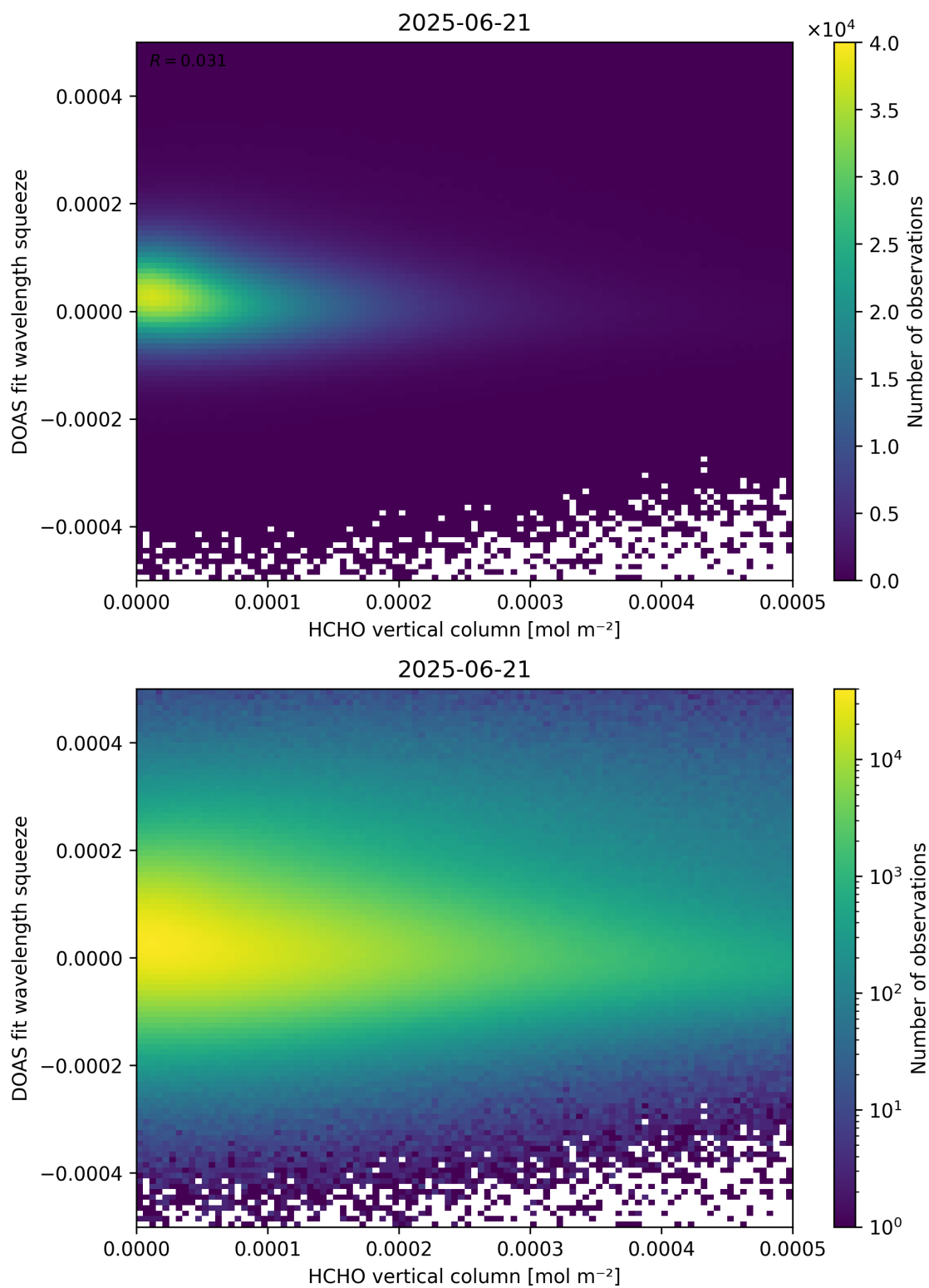
Figure 125: Scatter density plot of “HCHO vertical column” against “DOAS fit wavelength squeeze” for 2025-06-20 to 2025-06-22.
