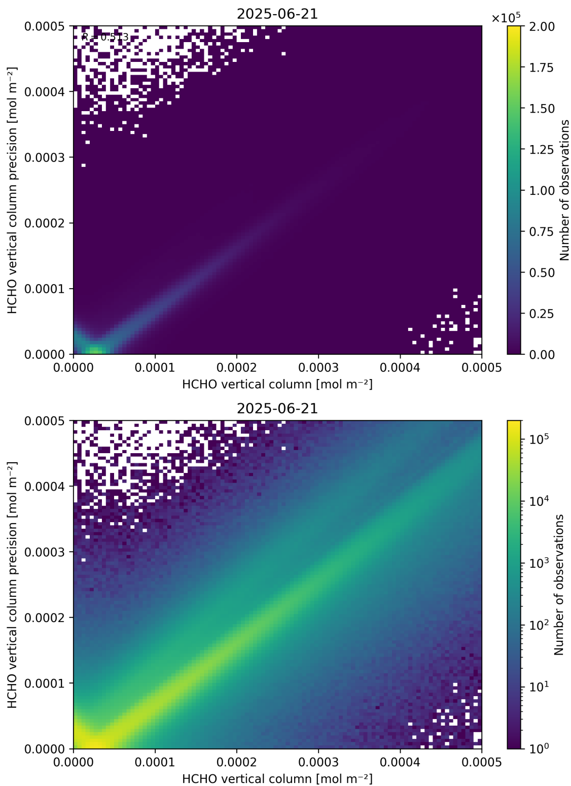
Figure 134: Scatter density plot of “HCHO vertical column” against “HCHO vertical column precision” for 2025-06-20 to 2025-06-22.
