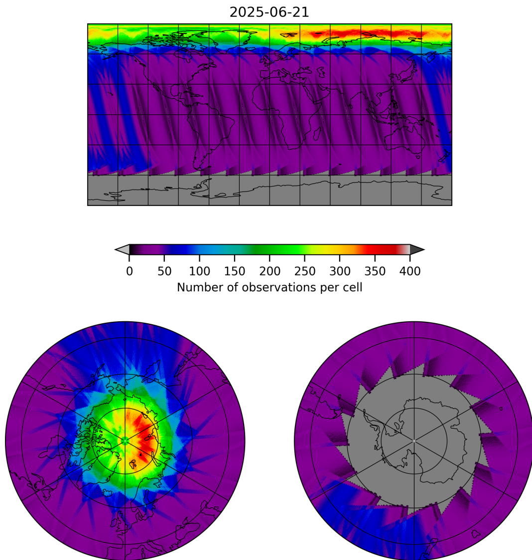
Figure 19: Map of the number of observations for 2025-06-20 to 2025-06-22
