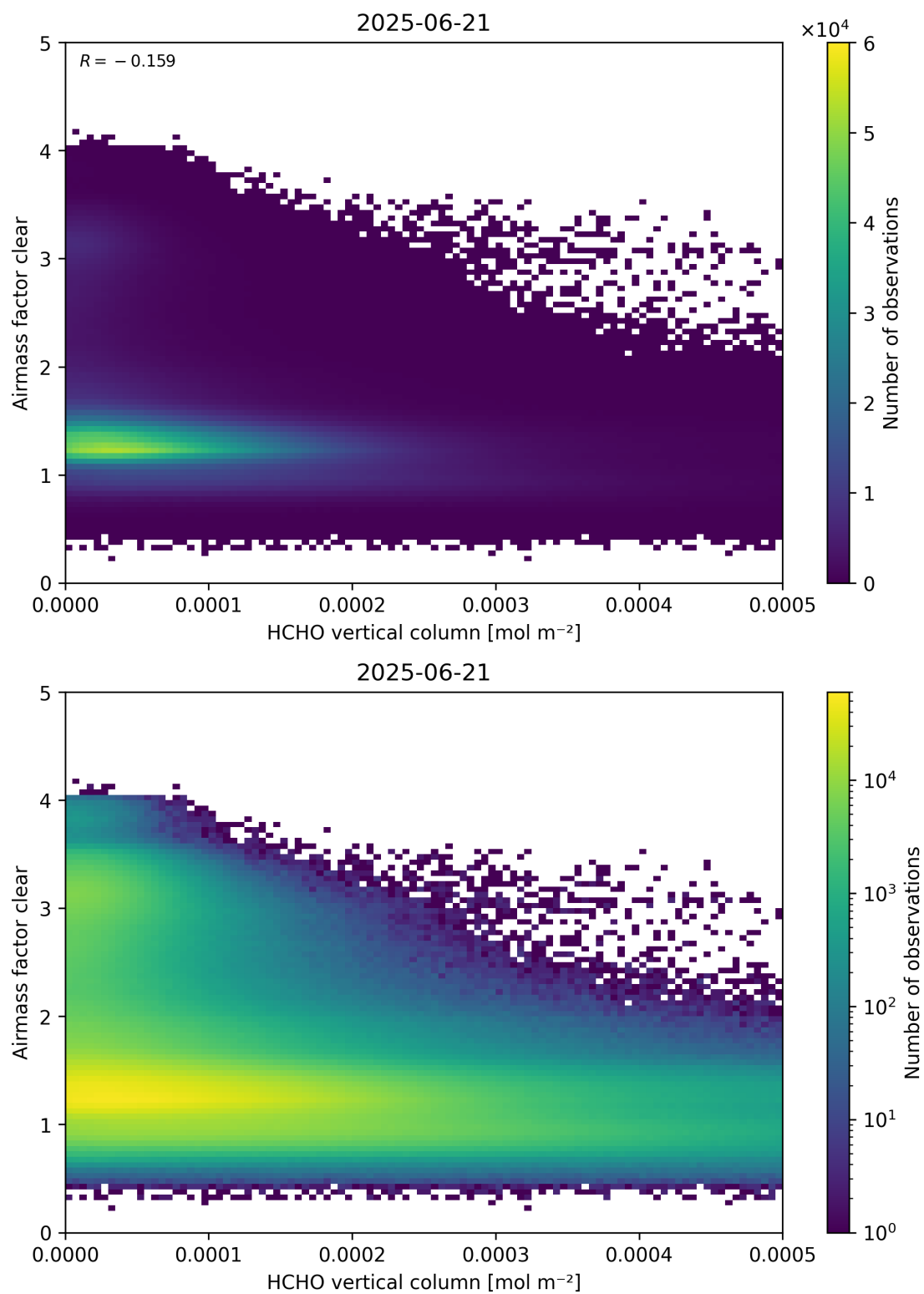
Figure 126: Scatter density plot of “HCHO vertical column” against “Airmass factor clear” for 2025-06-20 to 2025-06-22.
