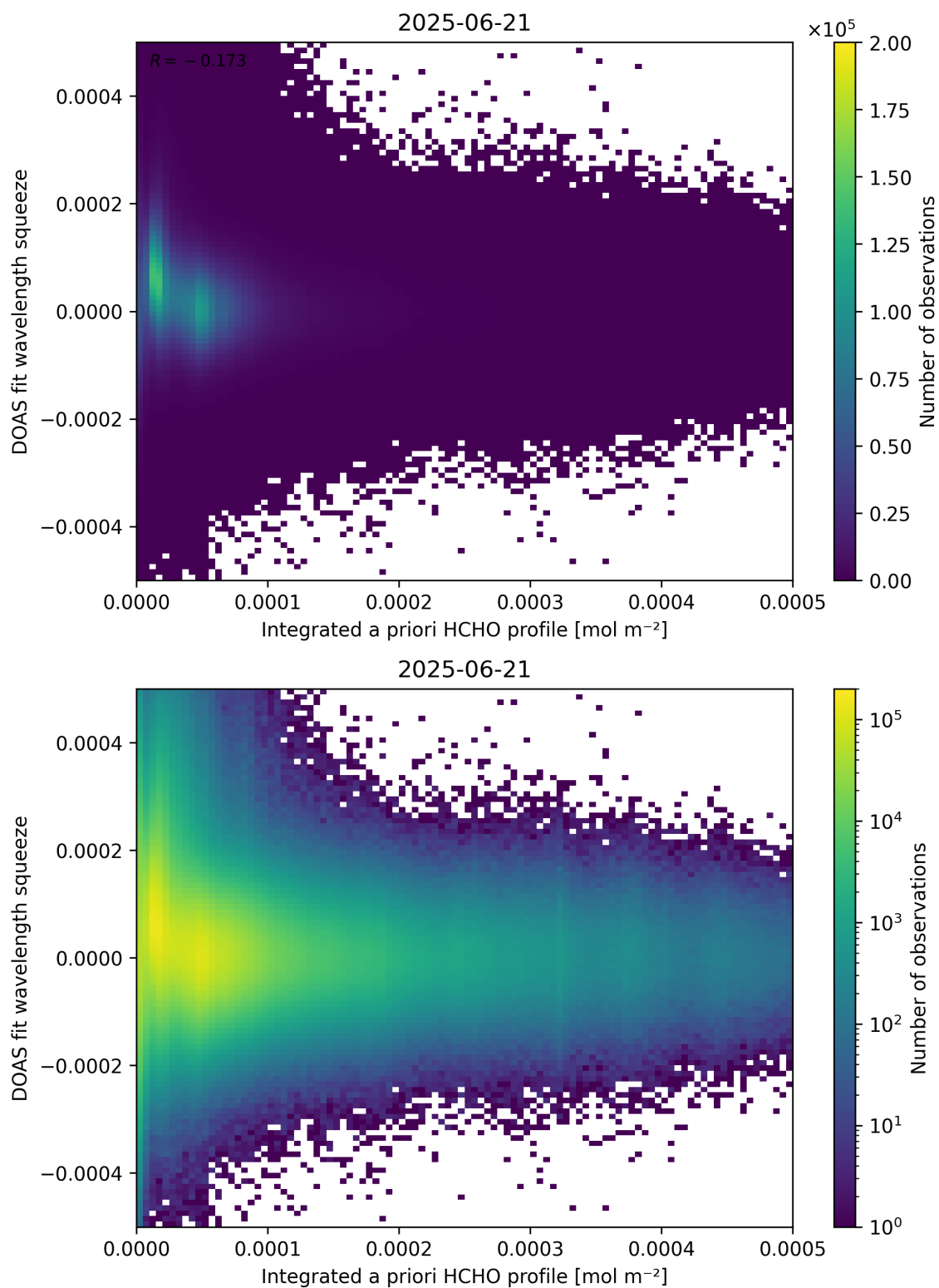
Figure 150: Scatter density plot of “Integrated a priori HCHO profile” against “DOAS fit wavelength squeeze” for 2025-06-20 to 2025-06-22.
