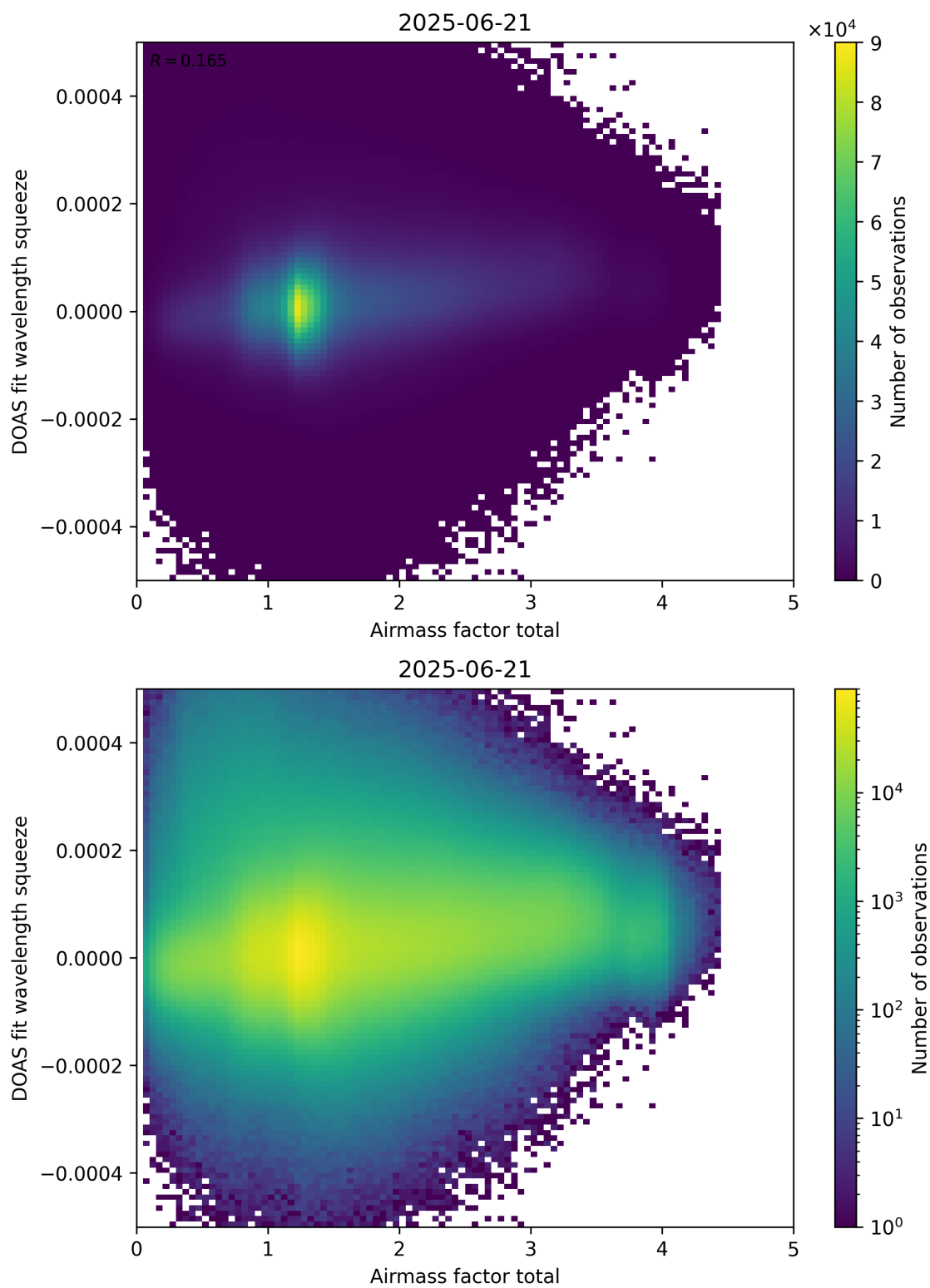
Figure 99: Scatter density plot of “Airmass factor total” against “DOAS fit wavelength squeeze” for 2025-06-20 to 2025-06-22.
