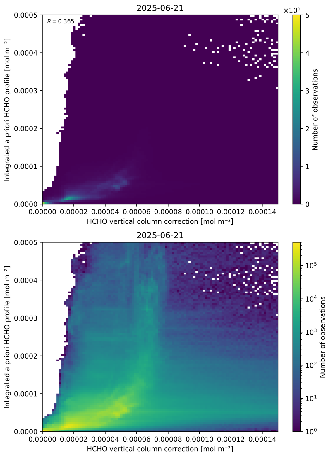
Figure 122: Scatter density plot of “HCHO vertical column correction” against “Integrated a priori HCHO profile” for 2025-06-20 to 2025-06-22.
