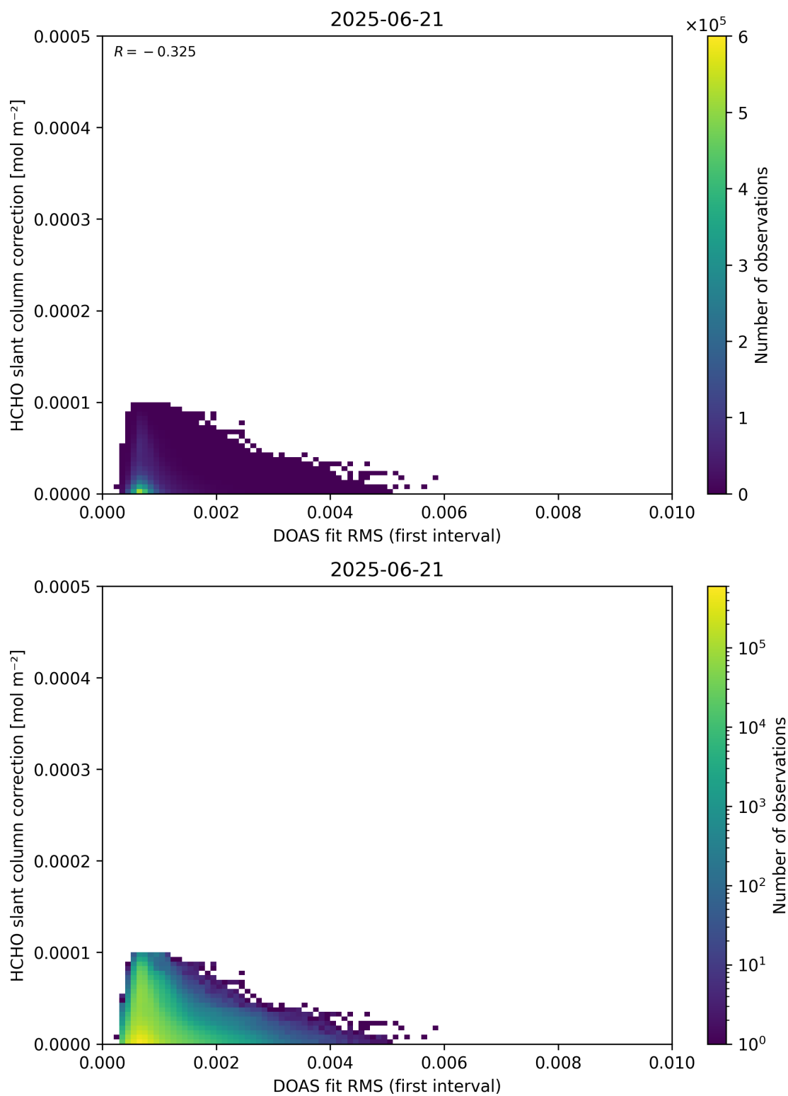
Figure 63: Scatter density plot of “DOAS fit RMS (first interval)” against “HCHO slant column correction” for 2025-06-20 to 2025-06-22.
