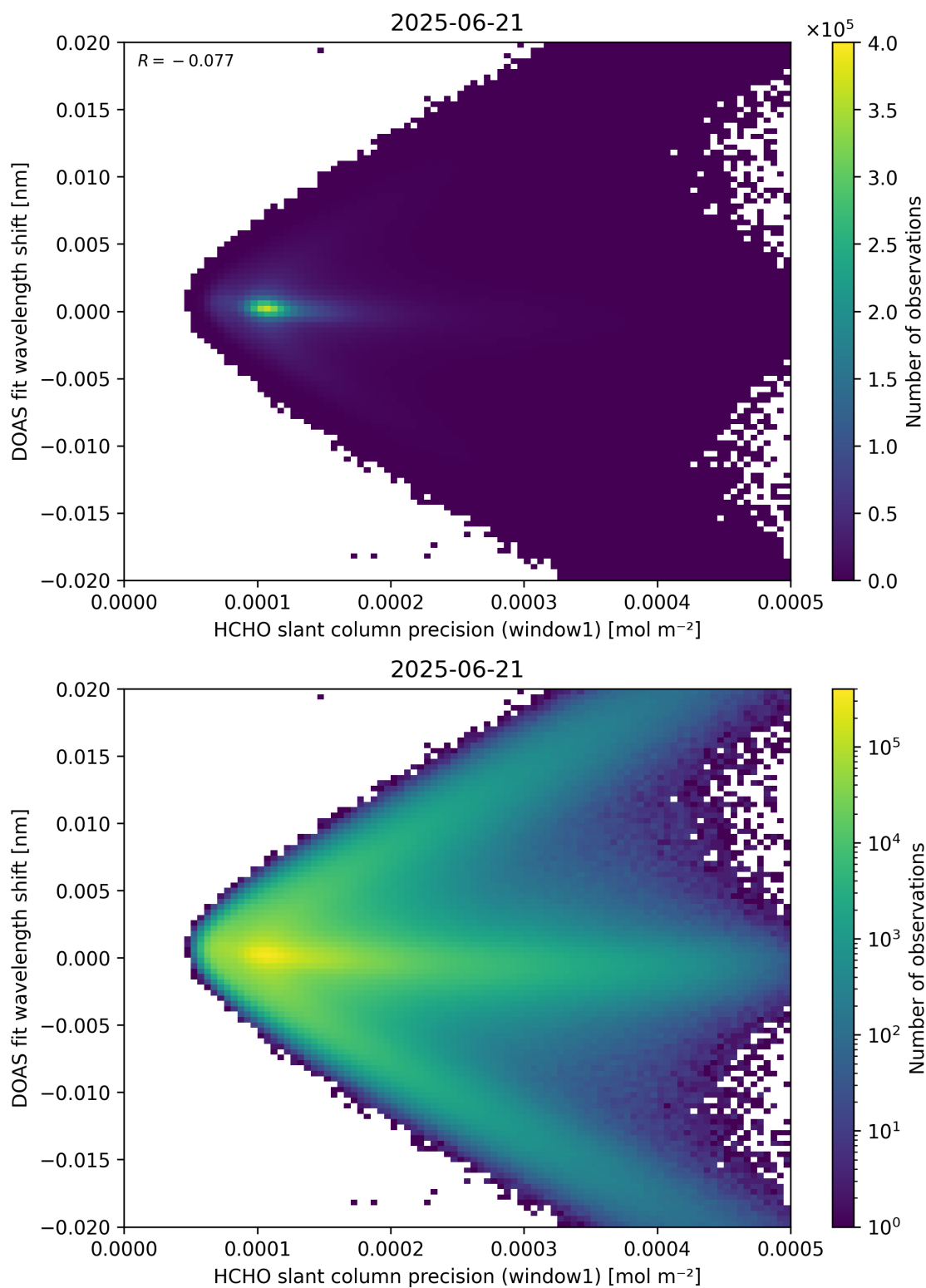
Figure 89: Scatter density plot of “HCHO slant column precision (window1)” against “DOAS fit wavelength shift” for 2025-06-20 to 2025-06-22.
