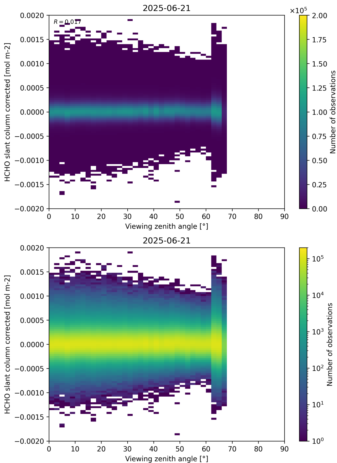
Figure 186: Scatter density plot of “Viewing zenith angle” against “HCHO slant column corrected” for 2025-06-20 to 2025-06-22.
