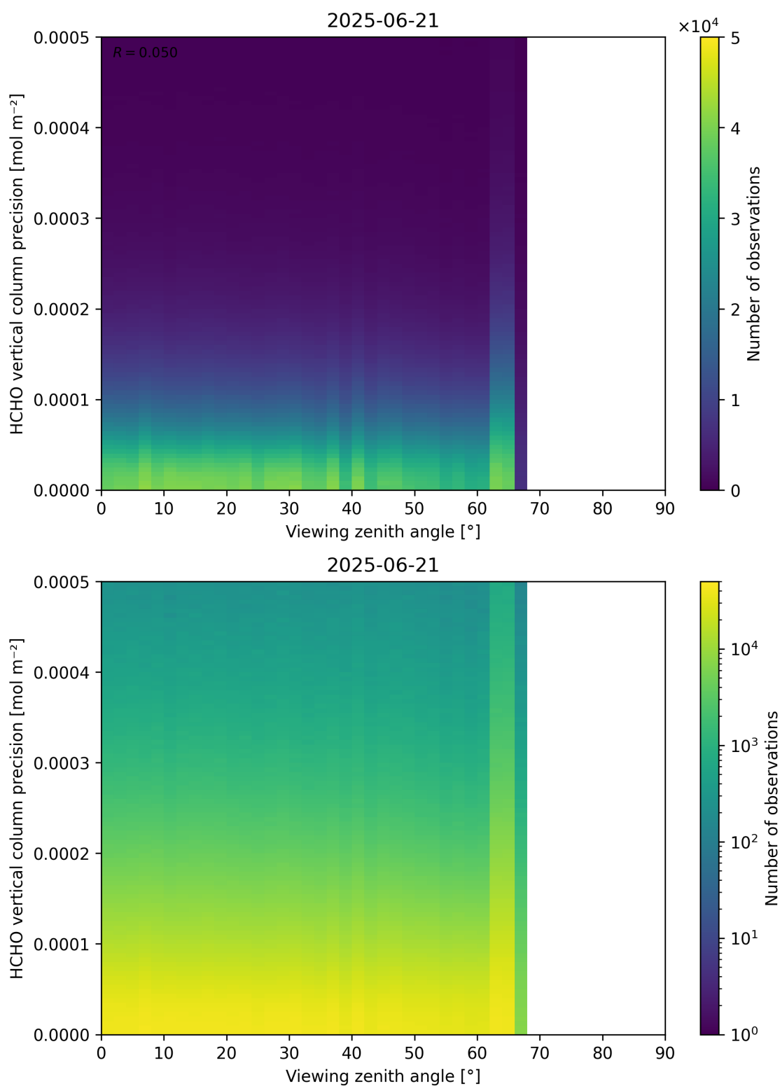
Figure 194: Scatter density plot of “Viewing zenith angle” against “HCHO vertical column precision” for 2025-06-20 to 2025-06-22.
