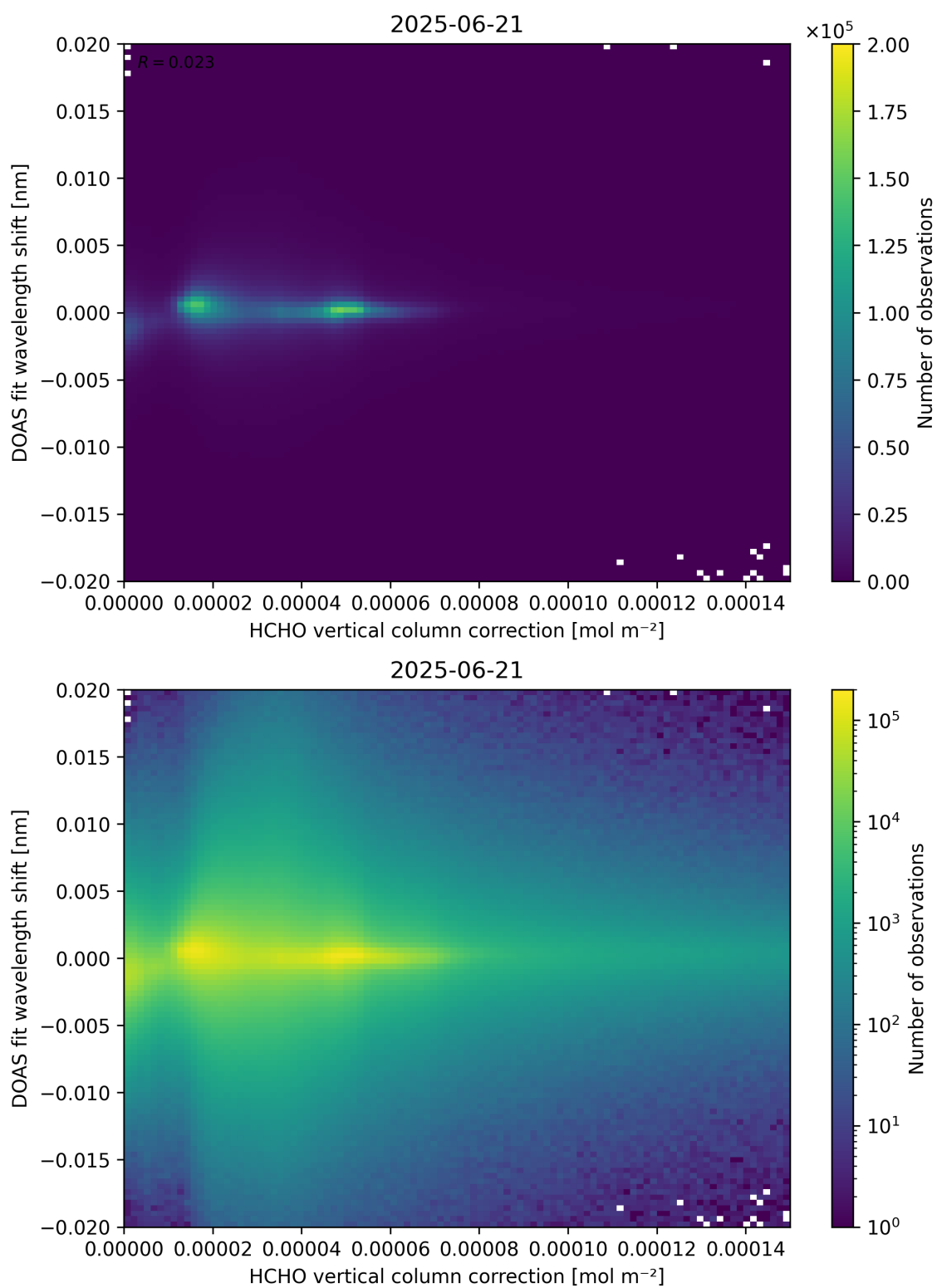
Figure 113: Scatter density plot of “HCHO vertical column correction” against “DOAS fit wavelength shift” for 2025-06-20 to 2025-06-22.
