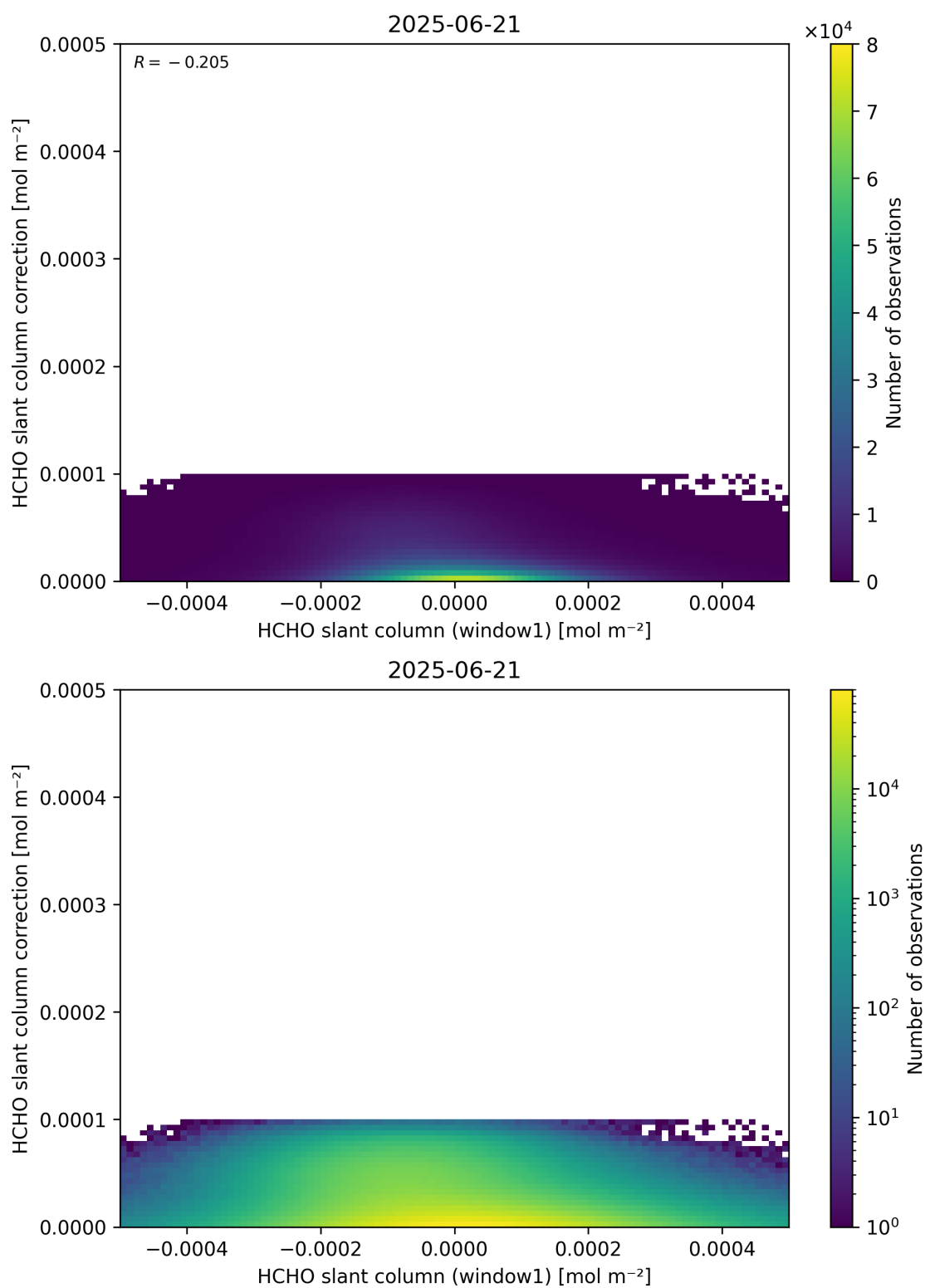
Figure 83: Scatter density plot of “HCHO slant column (window1)” against “HCHO slant column correction” for 2025-06-20 to 2025-06-22.
