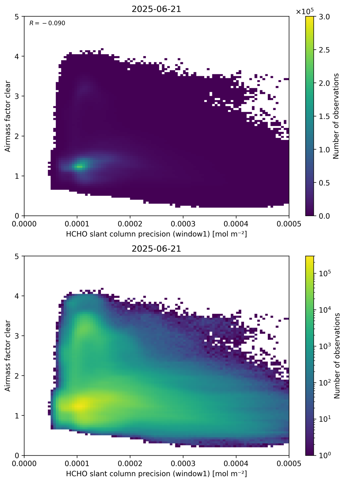
Figure 91: Scatter density plot of “HCHO slant column precision (window1)” against “Airmass factor clear” for 2025-06-20 to 2025-06-22.
