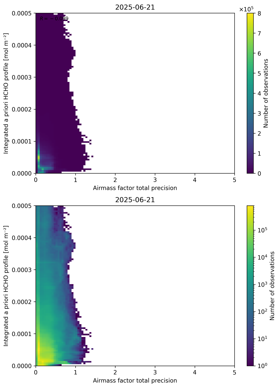
Figure 111: Scatter density plot of “Airmass factor total precision” against “Integrated a priori HCHO profile” for 2025-06-20 to 2025-06-22.
