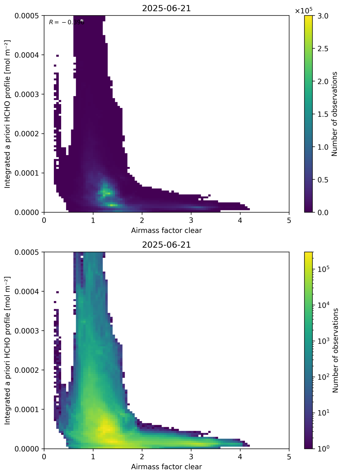
Figure 76: Scatter density plot of “Airmass factor clear” against “Integrated a priori HCHO profile” for 2025-06-20 to 2025-06-22.
