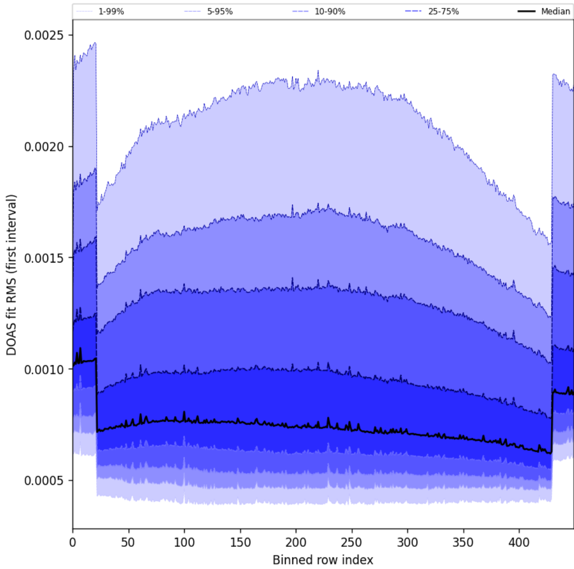
Figure 60: Along track statistics of “DOAS fit RMS (first interval)” for 2025-06-20 to 2025-06-22
