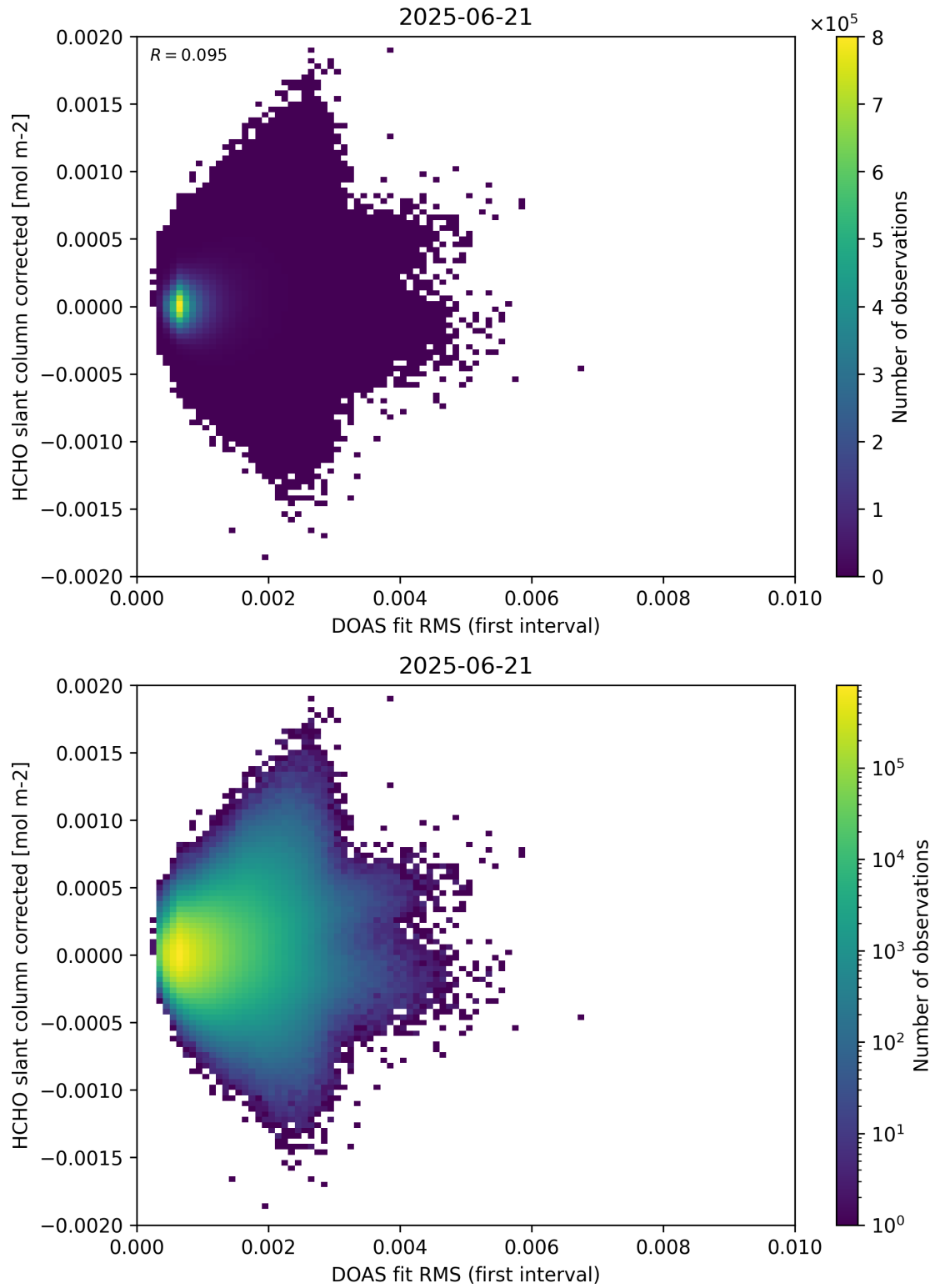
Figure 62: Scatter density plot of “DOAS fit RMS (first interval)” against “HCHO slant column corrected” for 2025-06-20 to 2025-06-22.
