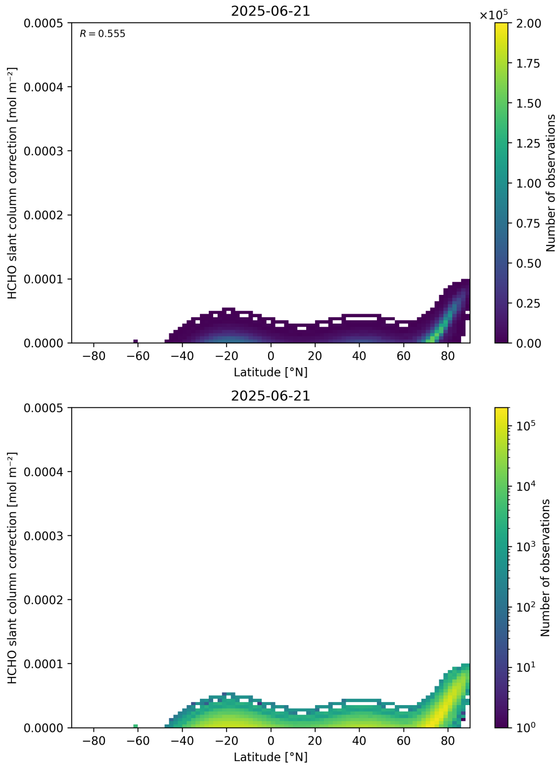
Figure 158: Scatter density plot of “Latitude” against “HCHO slant column correction” for 2025-06-20 to 2025-06-22.
