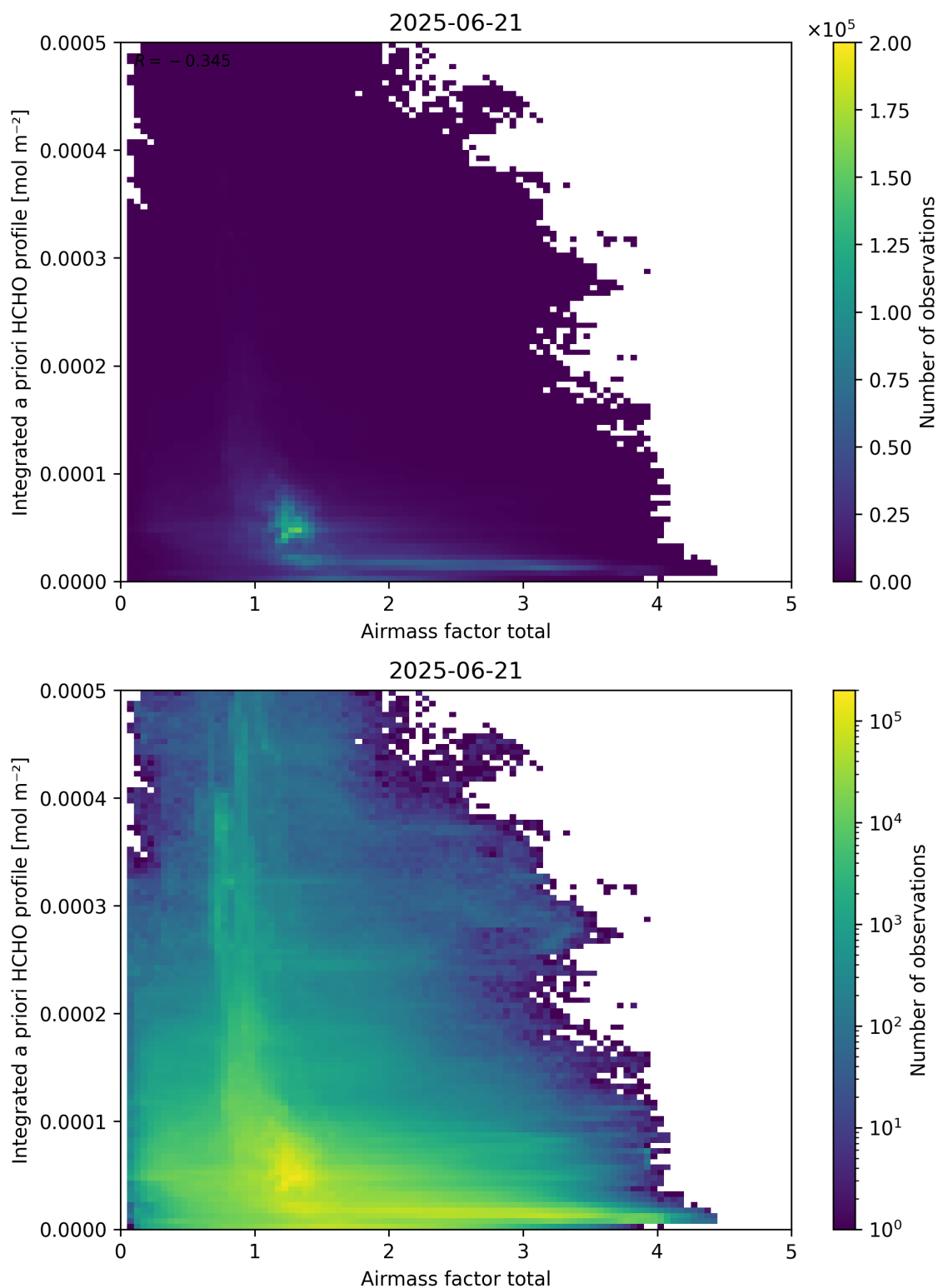
Figure 104: Scatter density plot of “Airmass factor total” against “Integrated a priori HCHO profile” for 2025-06-20 to 2025-06-22.
