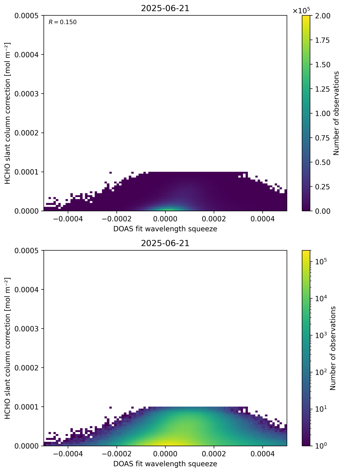
Figure 70: Scatter density plot of “DOAS fit wavelength squeeze” against “HCHO slant column correction” for 2025-06-20 to 2025-06-22.
