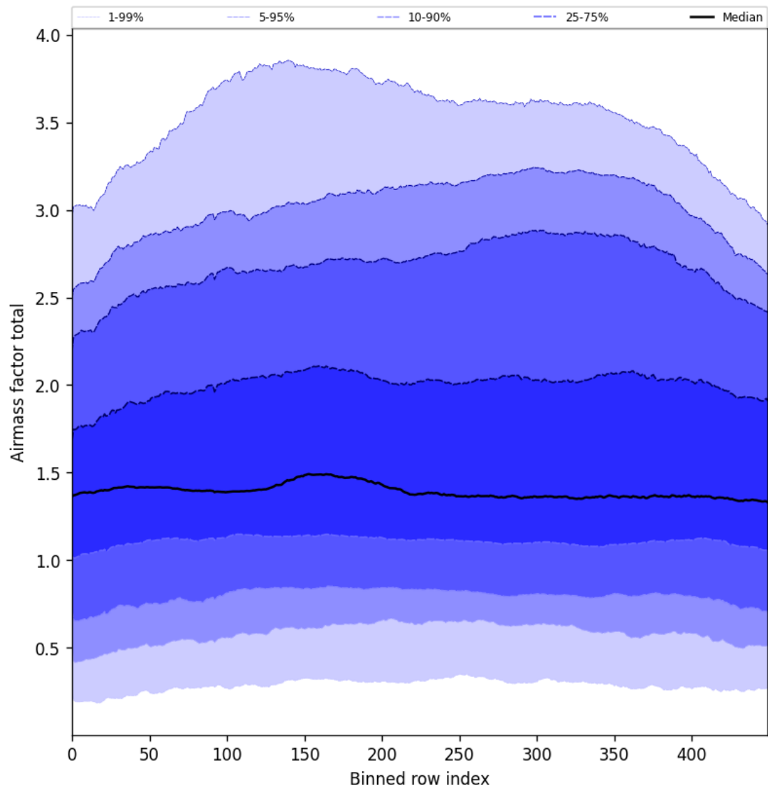
Figure 54: Along track statistics of “Airmass factor total” for 2025-06-20 to 2025-06-22
