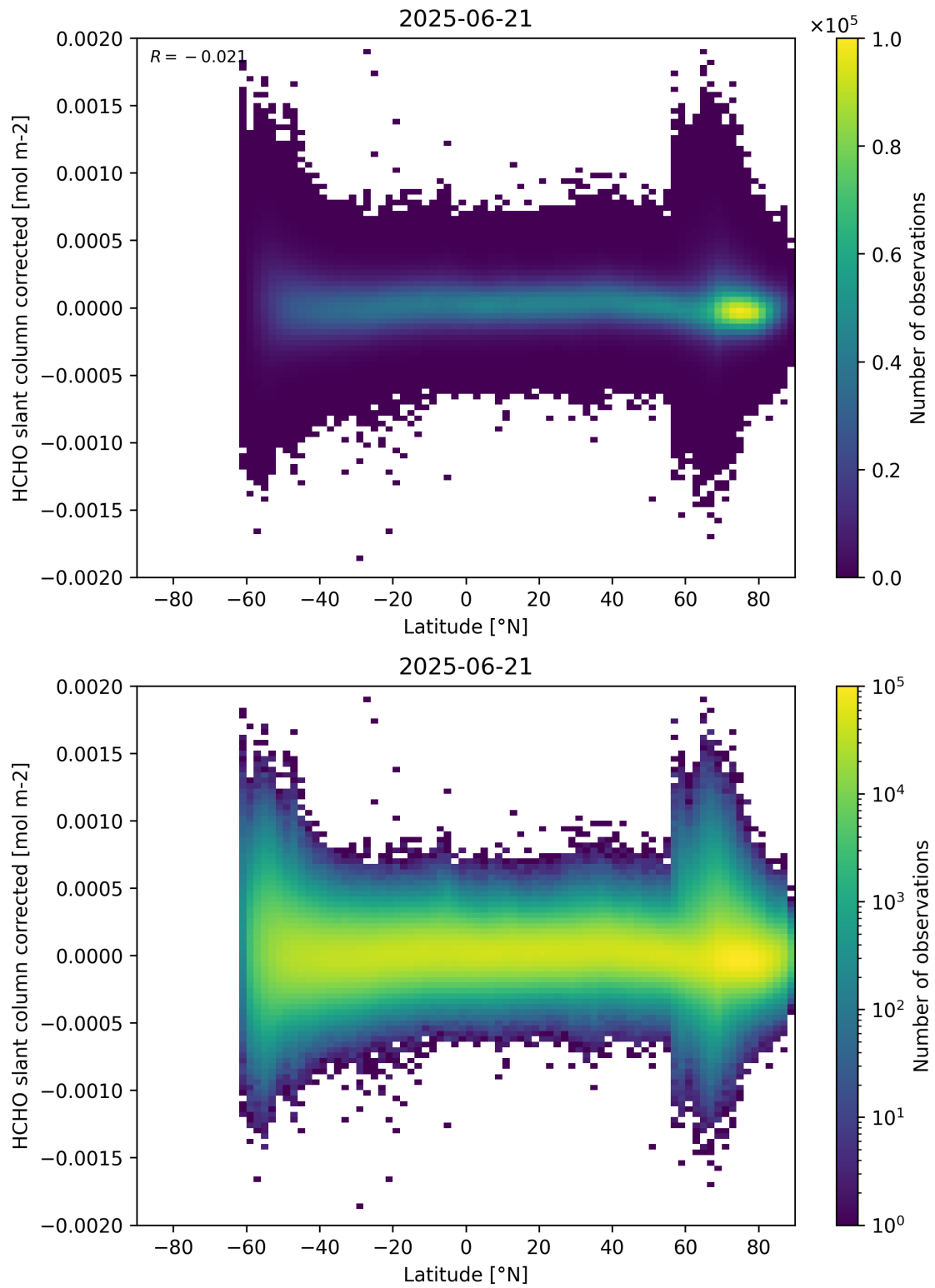
Figure 157: Scatter density plot of “Latitude” against “HCHO slant column corrected” for 2025-06-20 to 2025-06-22.
