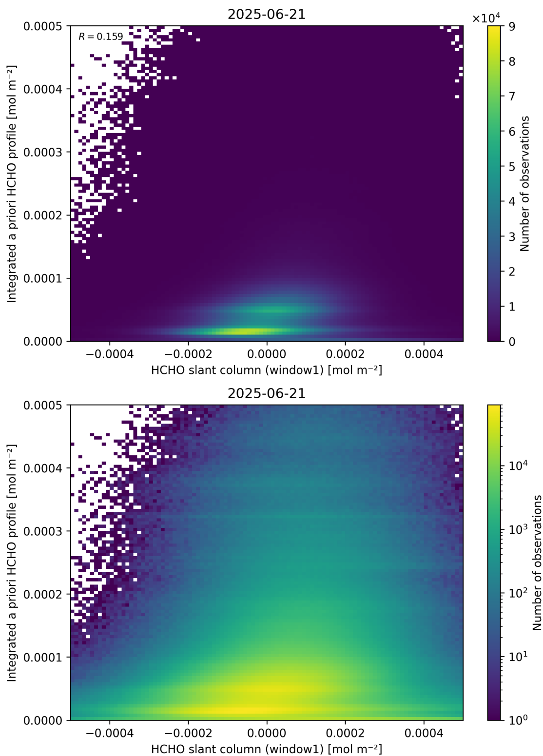
Figure 87: Scatter density plot of “HCHO slant column (window1)” against “Integrated a priori HCHO profile” for 2025-06-20 to 2025-06-22.
