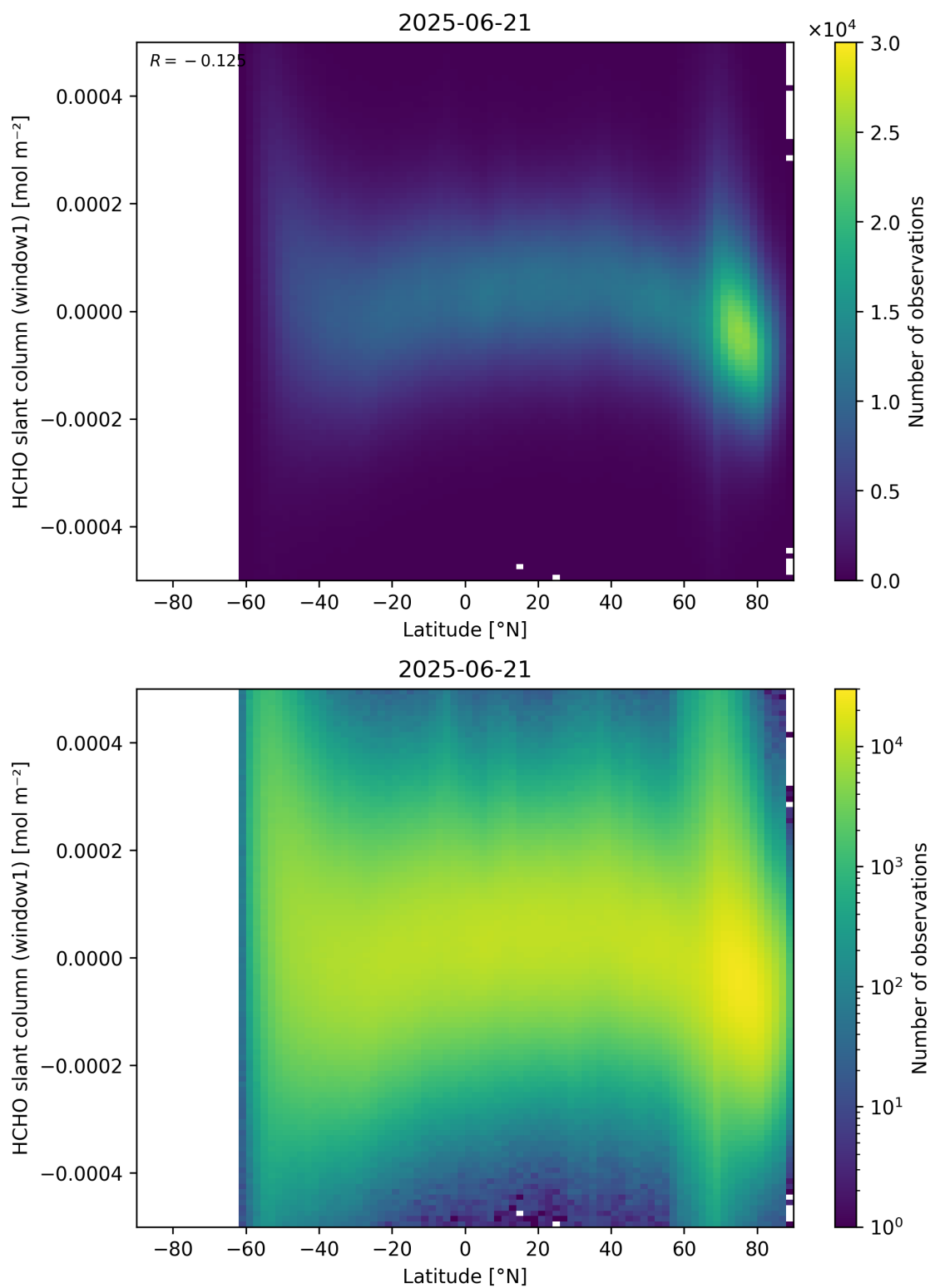
Figure 159: Scatter density plot of “Latitude” against “HCHO slant column (window1)” for 2025-06-20 to 2025-06-22.
