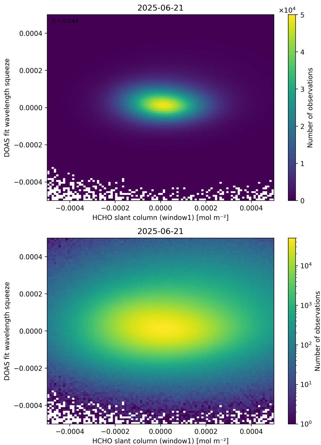
Figure 80: Scatter density plot of “HCHO slant column (window1)” against “DOAS fit wavelength squeeze” for 2025-06-20 to 2025-06-22.
