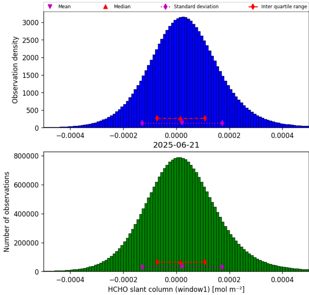
Figure 38: Histogram of “HCHO slant column (window1)” for 2025-06-20 to 2025-06-22
