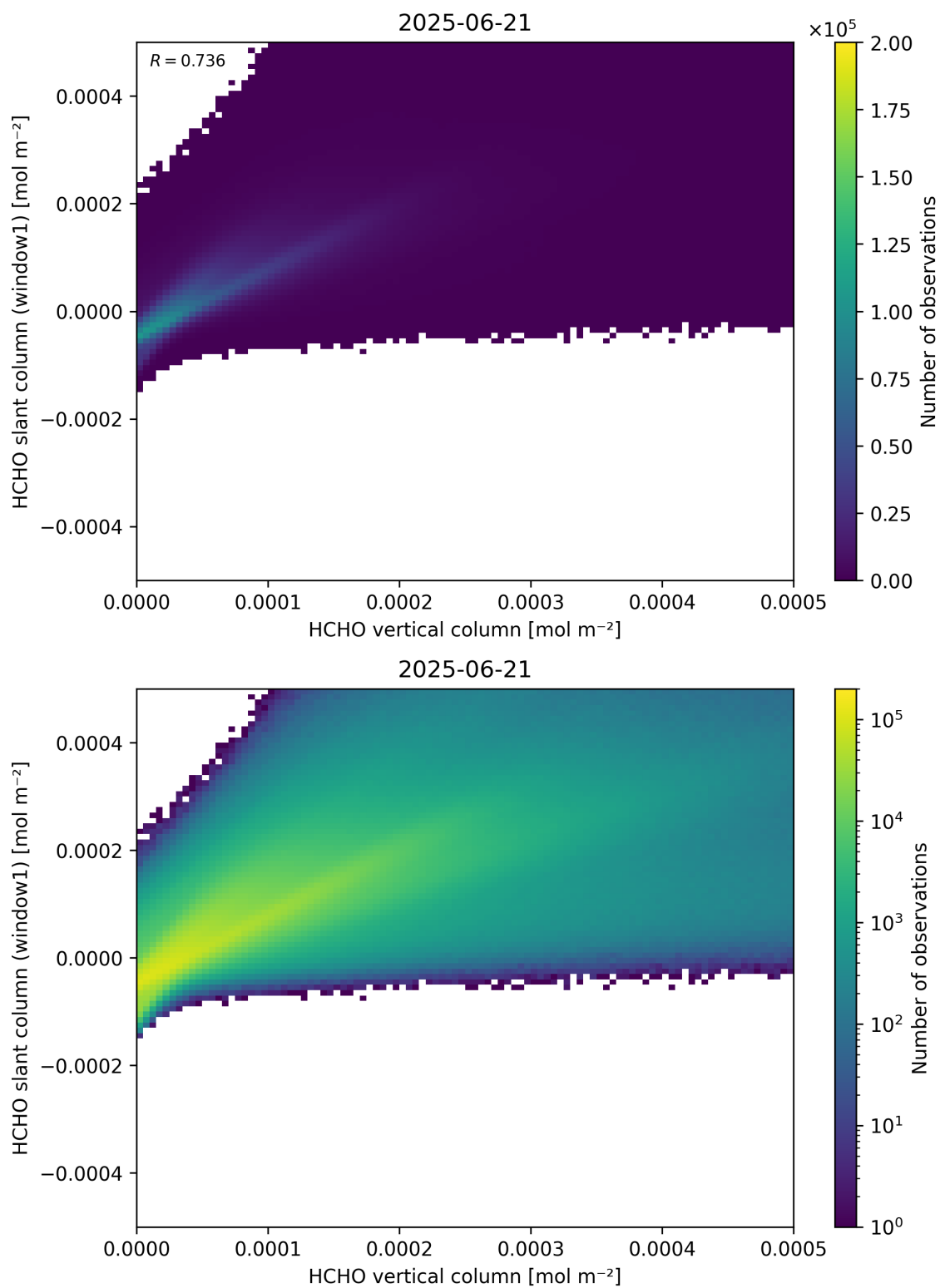
Figure 129: Scatter density plot of “HCHO vertical column” against “HCHO slant column (window1)” for 2025-06-20 to 2025-06-22.
