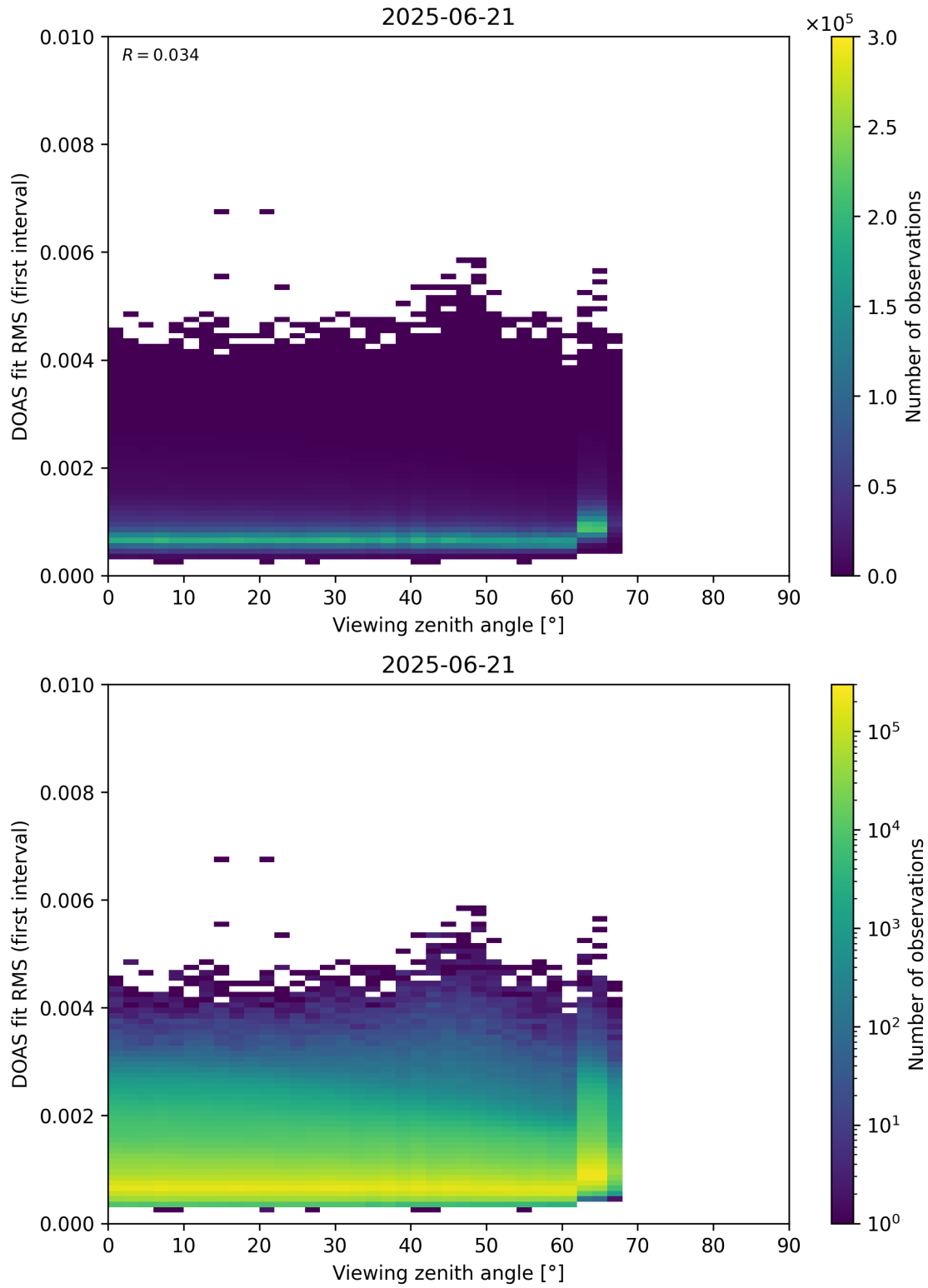
Figure 182: Scatter density plot of “Viewing zenith angle” against “DOAS fit RMS (first interval)” for 2025-06-20 to 2025-06-22.
