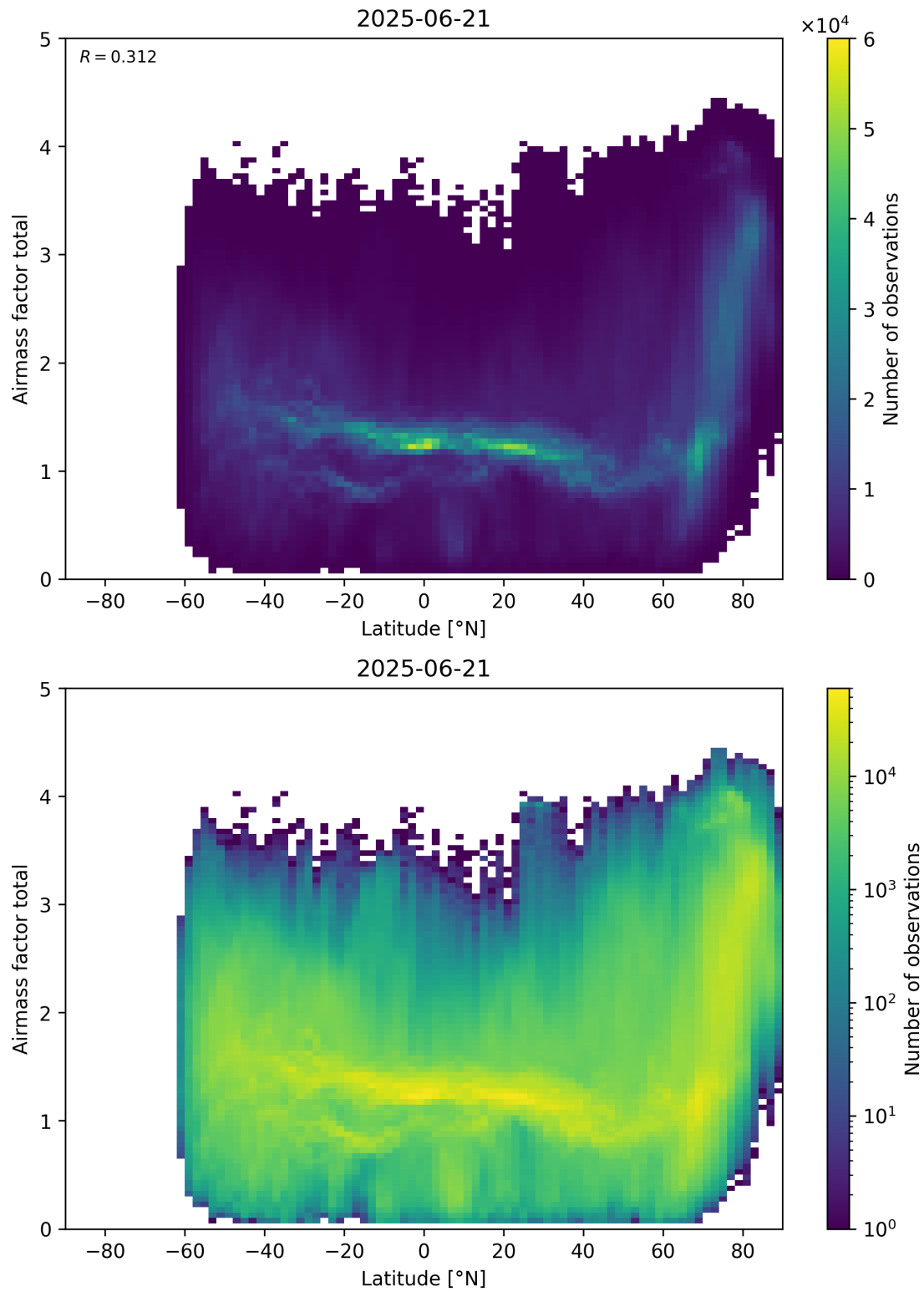
Figure 161: Scatter density plot of “Latitude” against “Airmass factor total” for 2025-06-20 to 2025-06-22.
