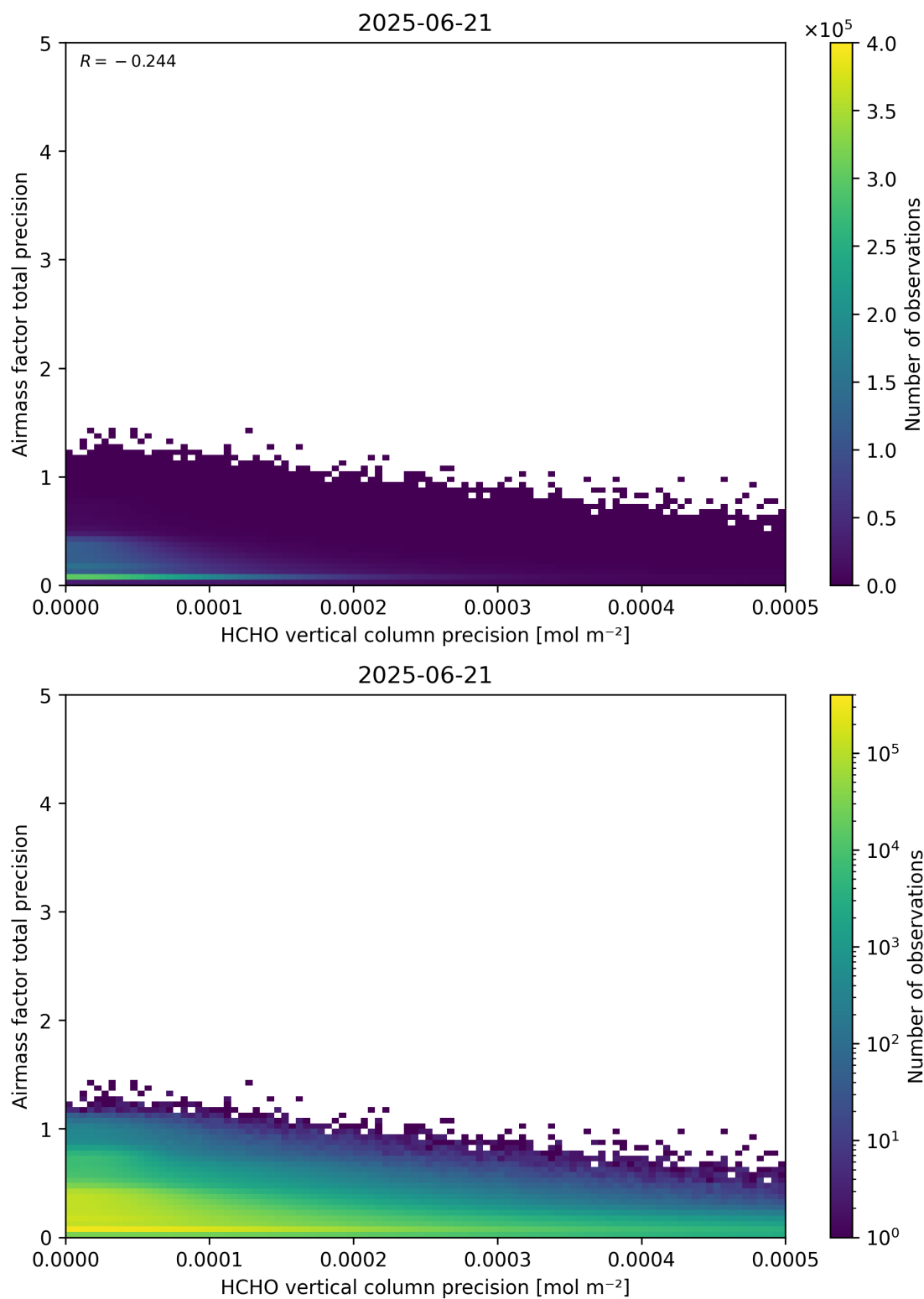
Figure 145: Scatter density plot of “HCHO vertical column precision” against “Airmass factor total precision” for 2025-06-20 to 2025-06-22.
