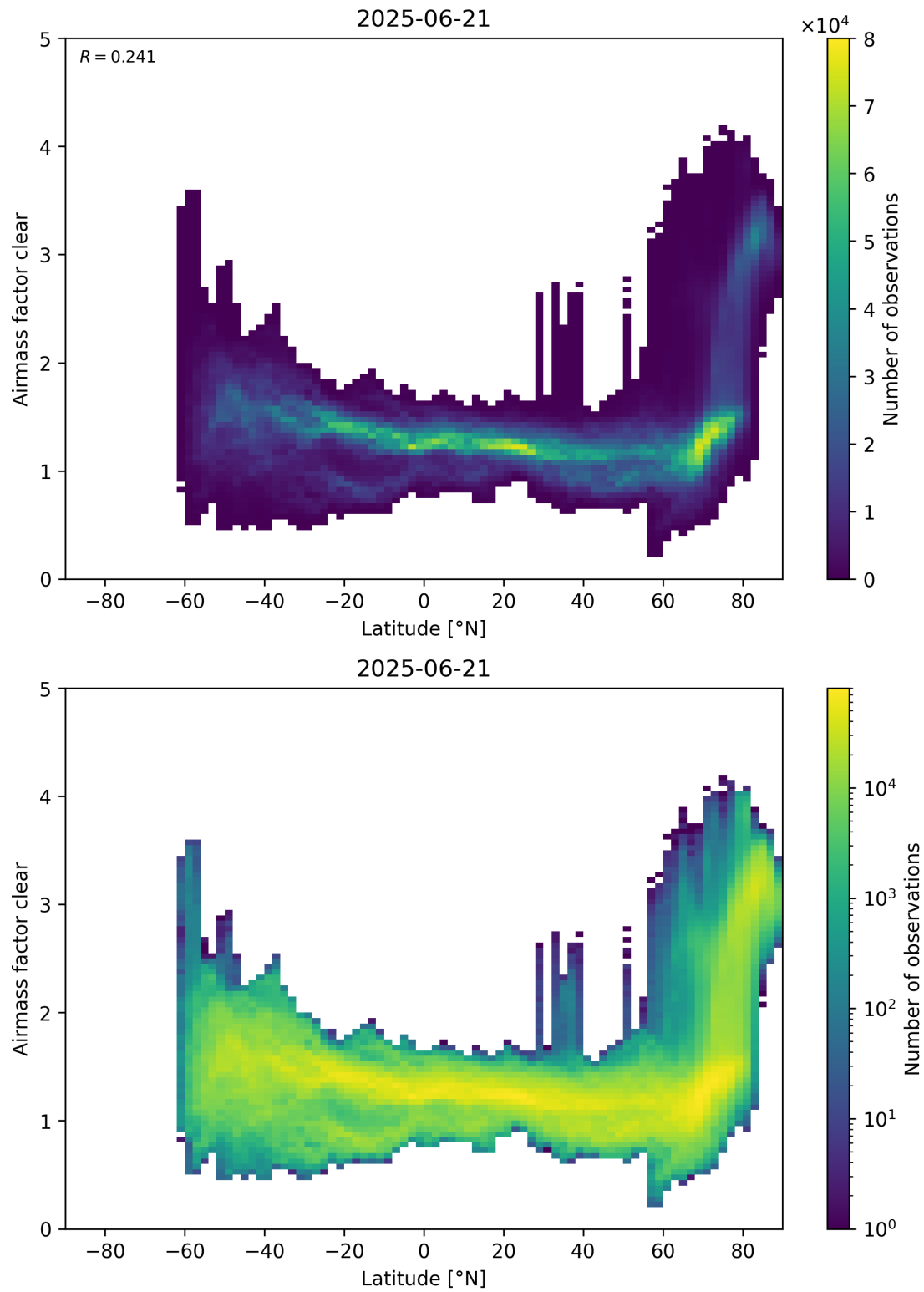
Figure 156: Scatter density plot of “Latitude” against “Airmass factor clear” for 2025-06-20 to 2025-06-22.
