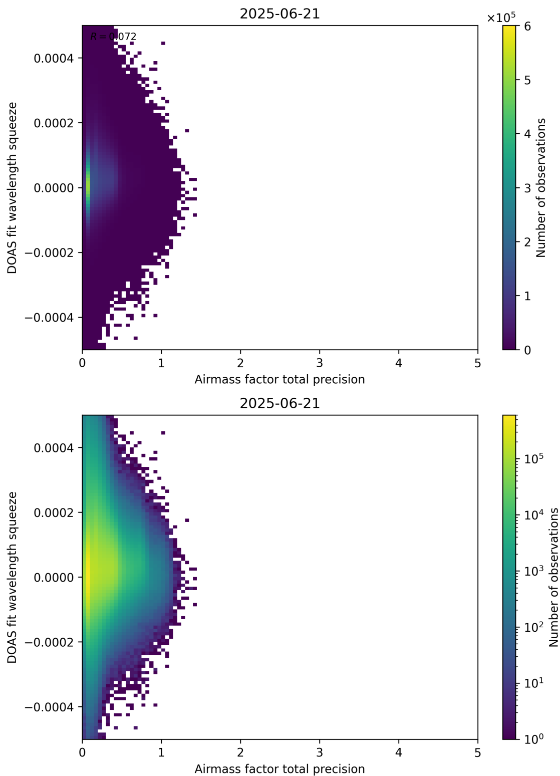
Figure 107: Scatter density plot of “Airmass factor total precision” against “DOAS fit wavelength squeeze” for 2025-06-20 to 2025-06-22.
