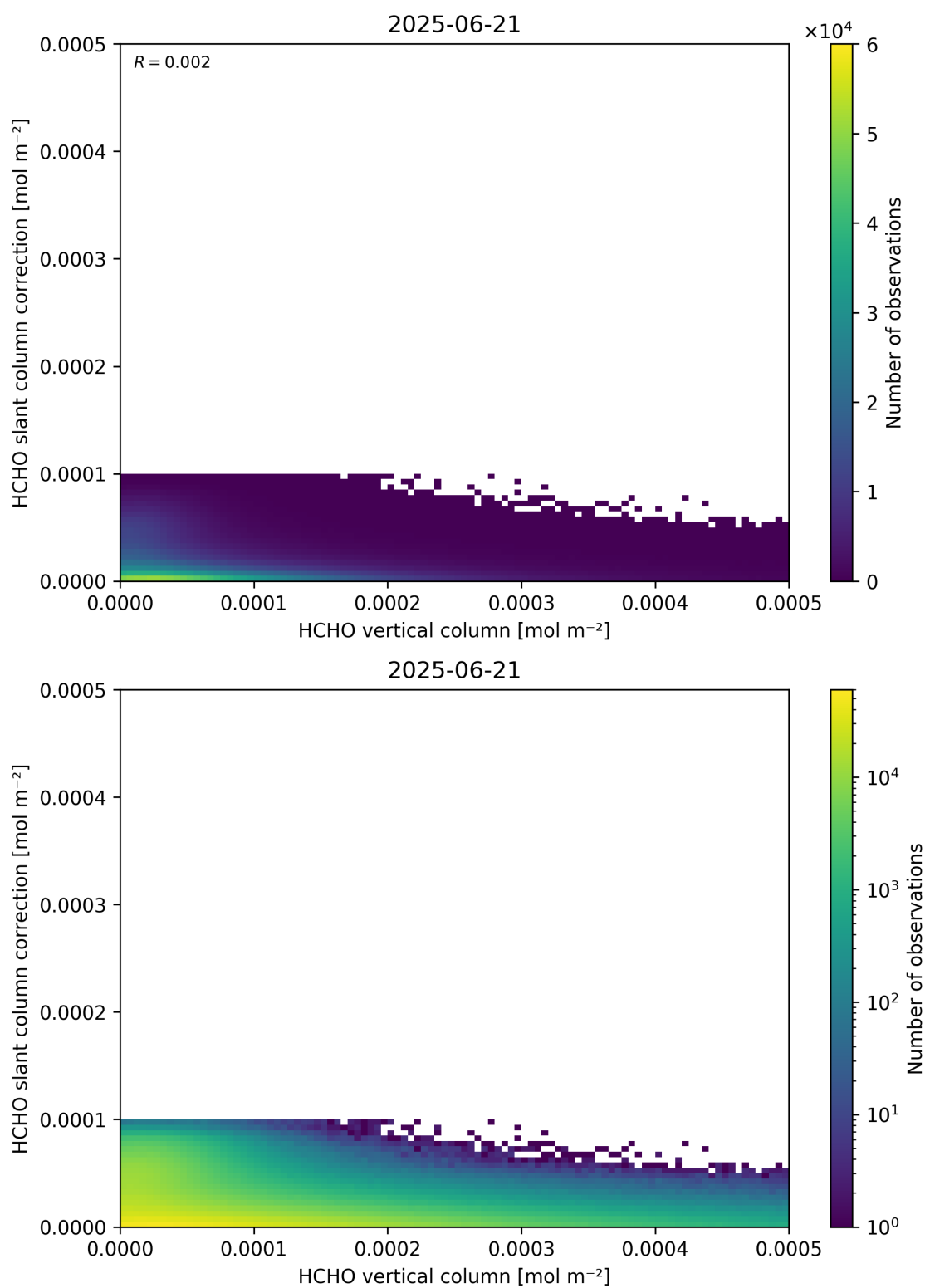
Figure 128: Scatter density plot of “HCHO vertical column” against “HCHO slant column correction” for 2025-06-20 to 2025-06-22.
