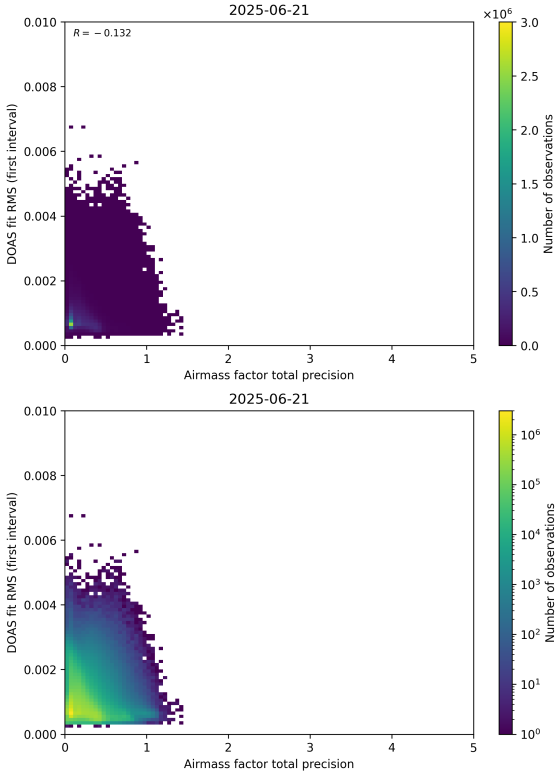
Figure 105: Scatter density plot of “Airmass factor total precision” against “DOAS fit RMS (first interval)” for 2025-06-20 to 2025-06-22.
