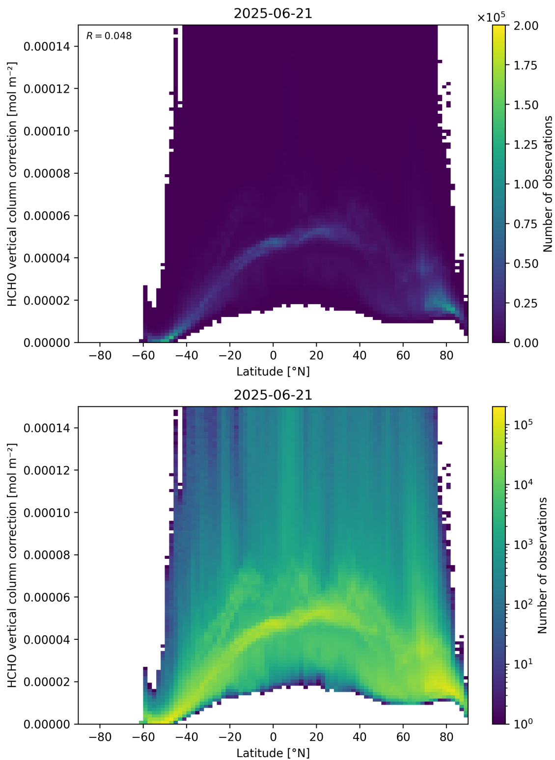
Figure 164: Scatter density plot of “Latitude” against “HCHO vertical column correction” for 2025-06-20 to 2025-06-22.
