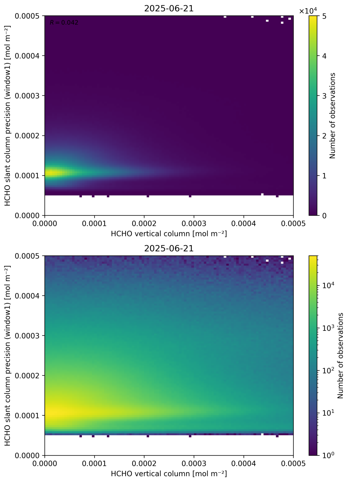
Figure 130: Scatter density plot of “HCHO vertical column” against “HCHO slant column precision (window1)” for 2025-06-20 to 2025-06-22.
