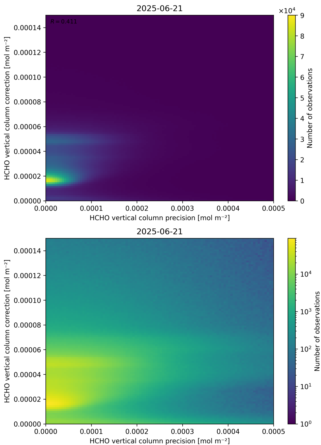
Figure 146: Scatter density plot of “HCHO vertical column precision” against “HCHO vertical column correction” for 2025-06-20 to 2025-06-22.
