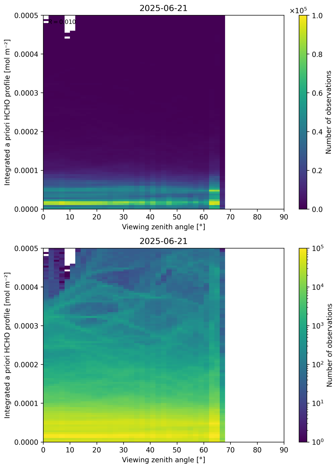
Figure 195: Scatter density plot of “Viewing zenith angle” against “Integrated a priori HCHO profile” for 2025-06-20 to 2025-06-22.
