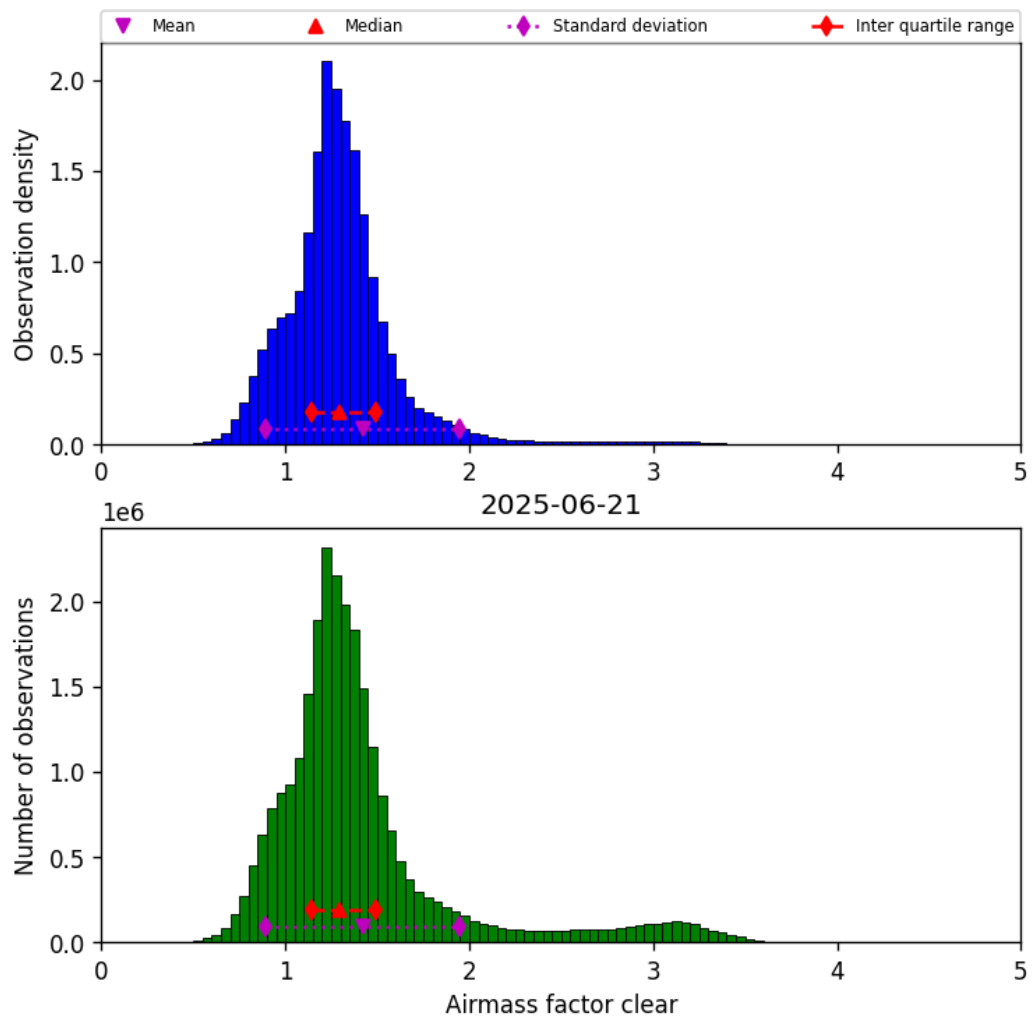
Figure 42: Histogram of “Airmass factor clear” for 2025-06-20 to 2025-06-22
