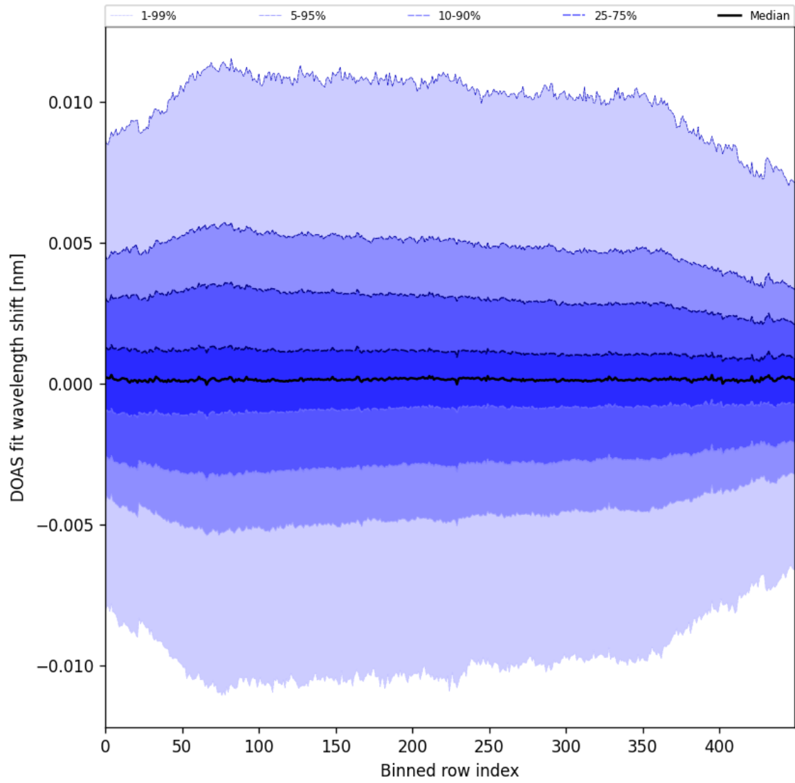
Figure 58: Along track statistics of “DOAS fit wavelength shift” for 2025-06-20 to 2025-06-22
