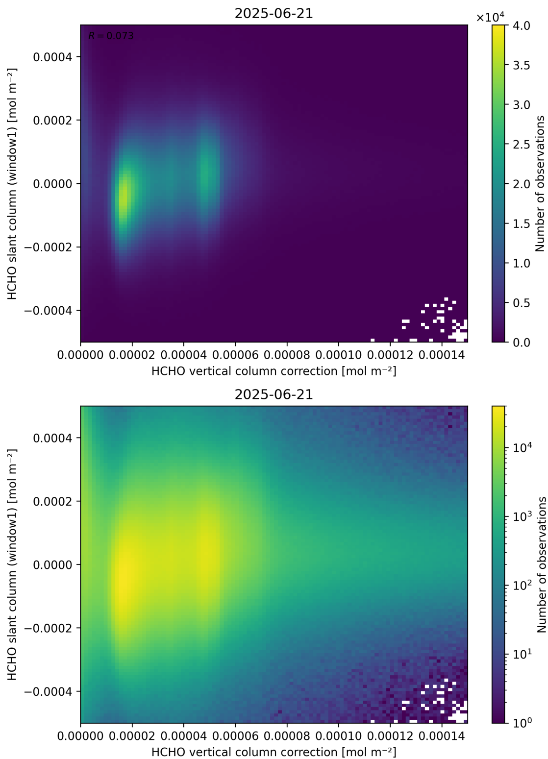
Figure 118: Scatter density plot of “HCHO vertical column correction” against “HCHO slant column (window1)” for 2025-06-20 to 2025-06-22.
