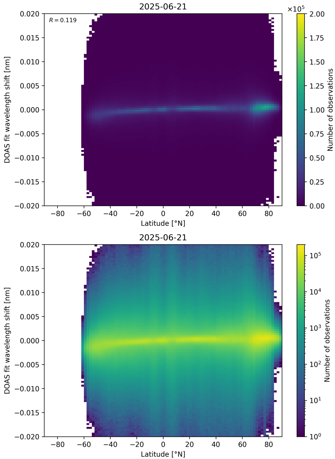
Figure 154: Scatter density plot of “Latitude” against “DOAS fit wavelength shift” for 2025-06-20 to 2025-06-22.
