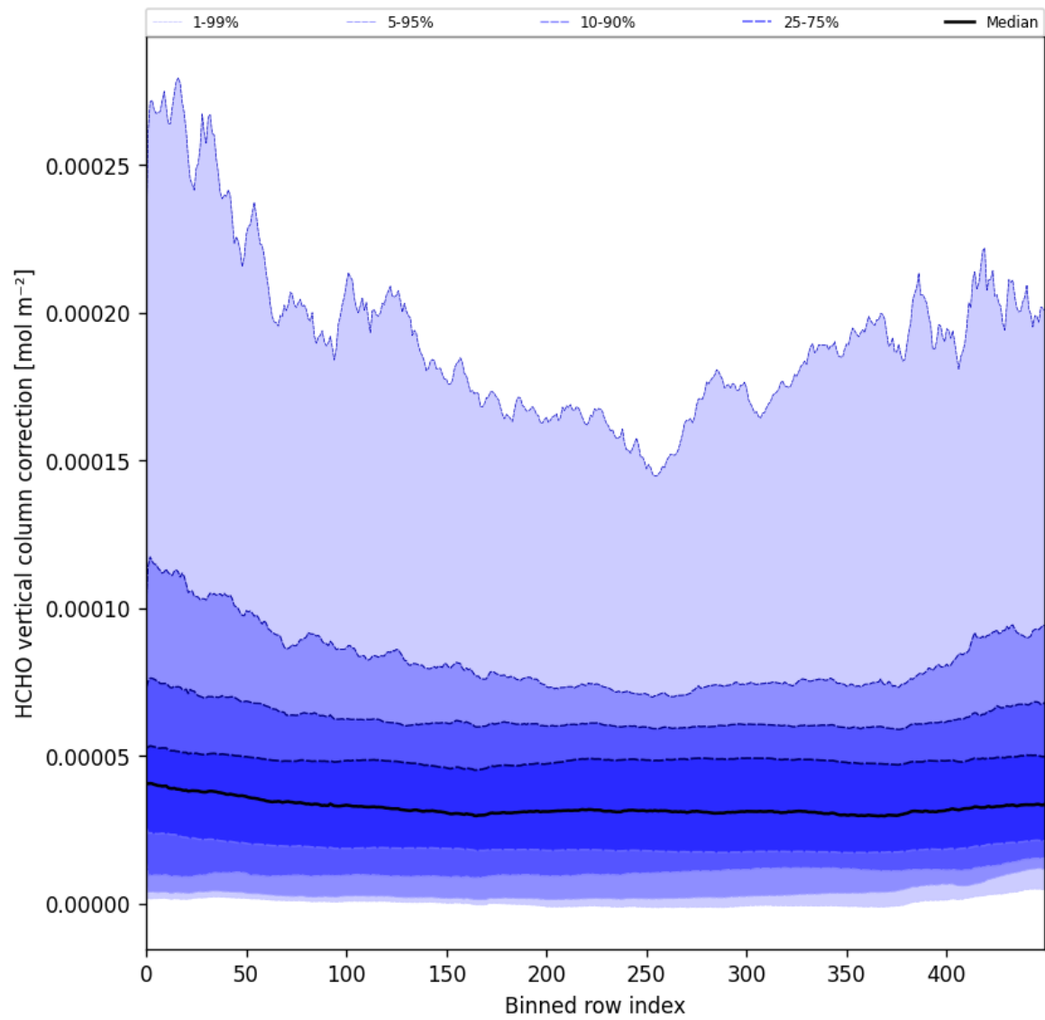
Figure 51: Along track statistics of “HCHO vertical column correction” for 2025-06-20 to 2025-06-22
