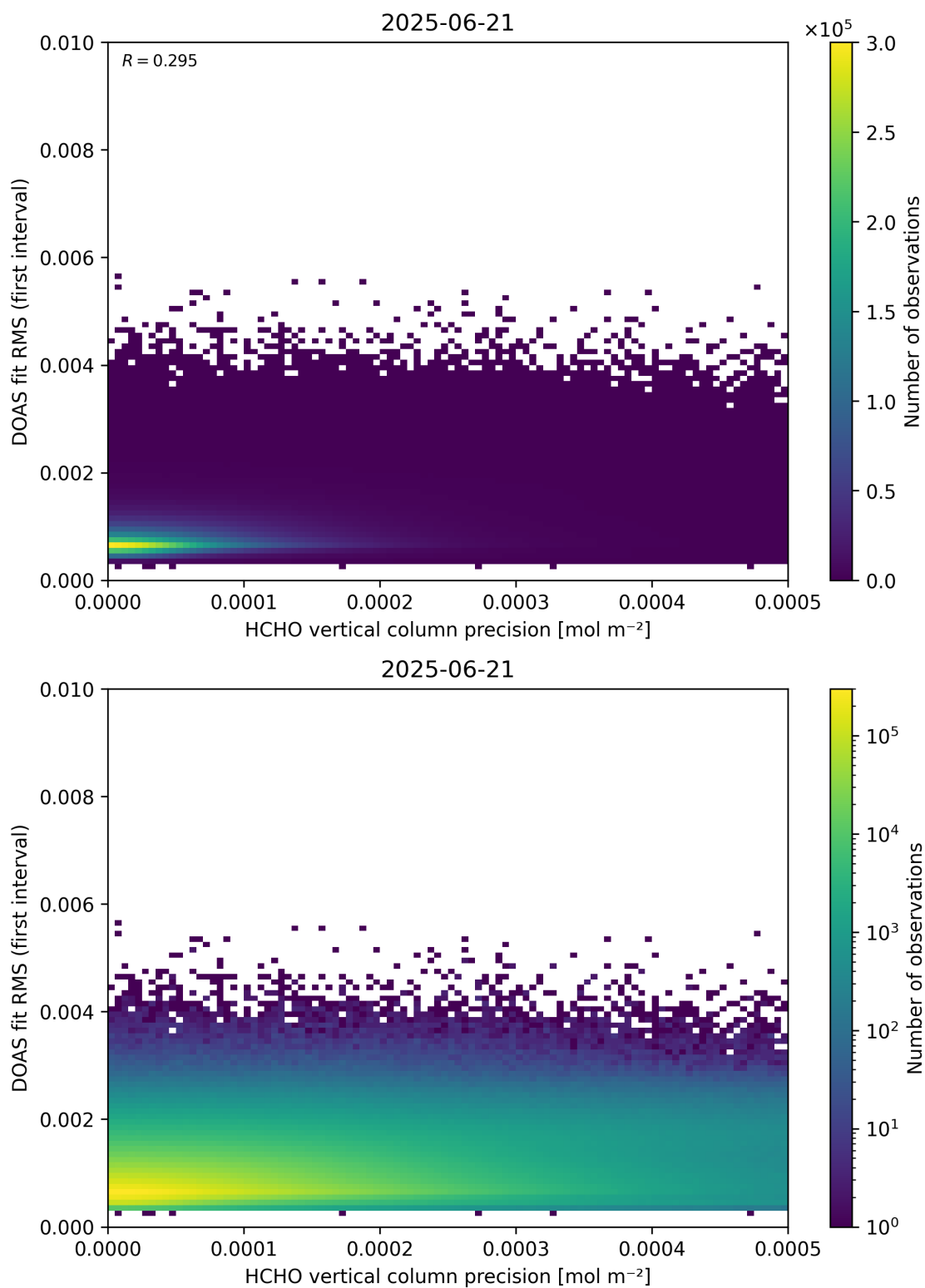
Figure 136: Scatter density plot of “HCHO vertical column precision” against “DOAS fit RMS (first interval)” for 2025-06-20 to 2025-06-22.
