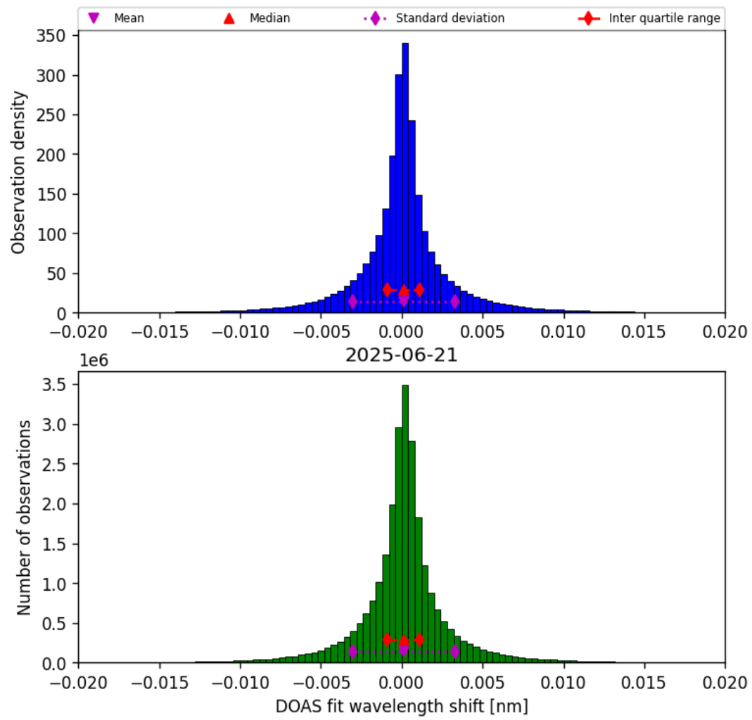
Figure 44: Histogram of “DOAS fit wavelength shift” for 2025-06-20 to 2025-06-22
