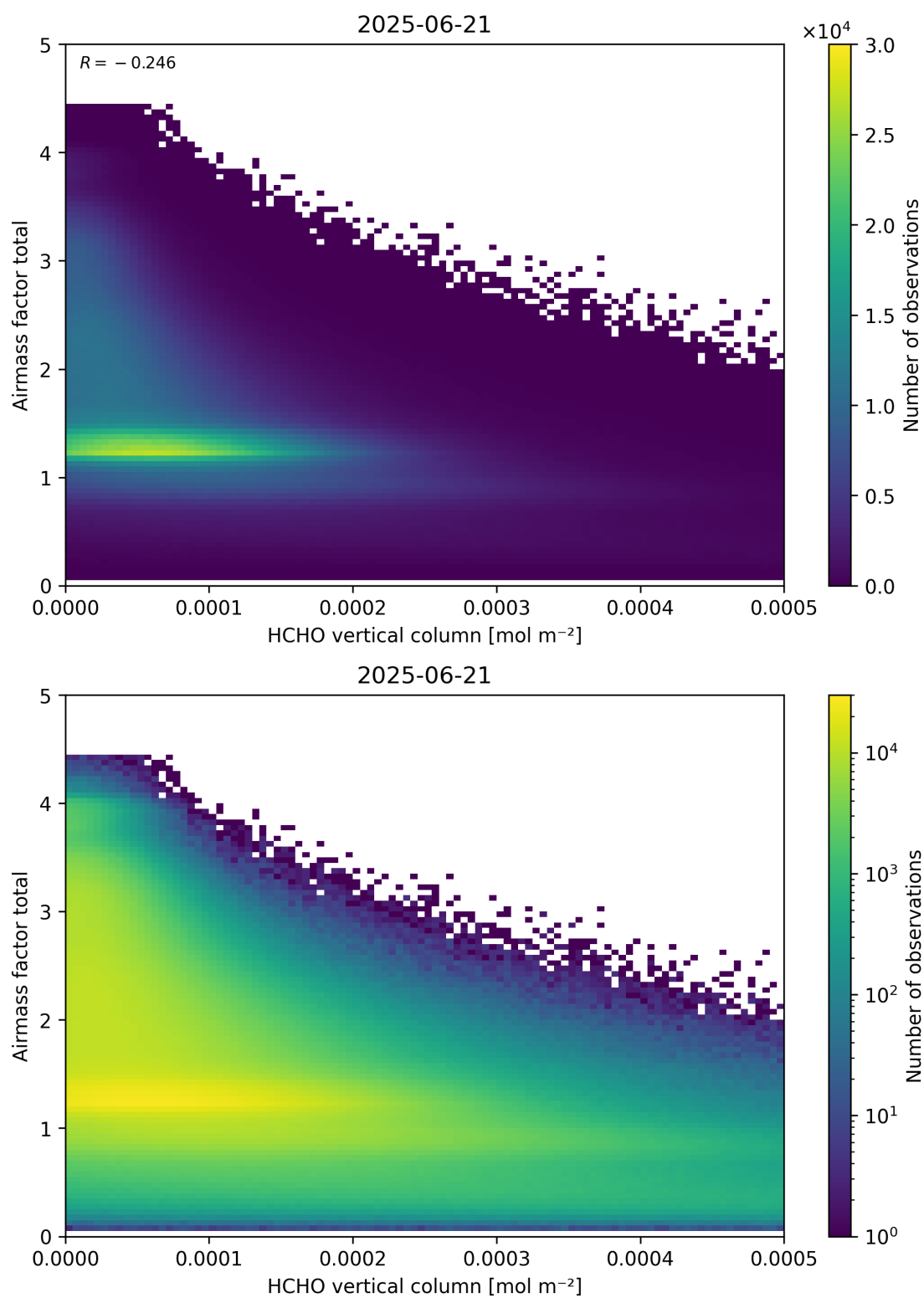
Figure 131: Scatter density plot of “HCHO vertical column” against “Airmass factor total” for 2025-06-20 to 2025-06-22.
