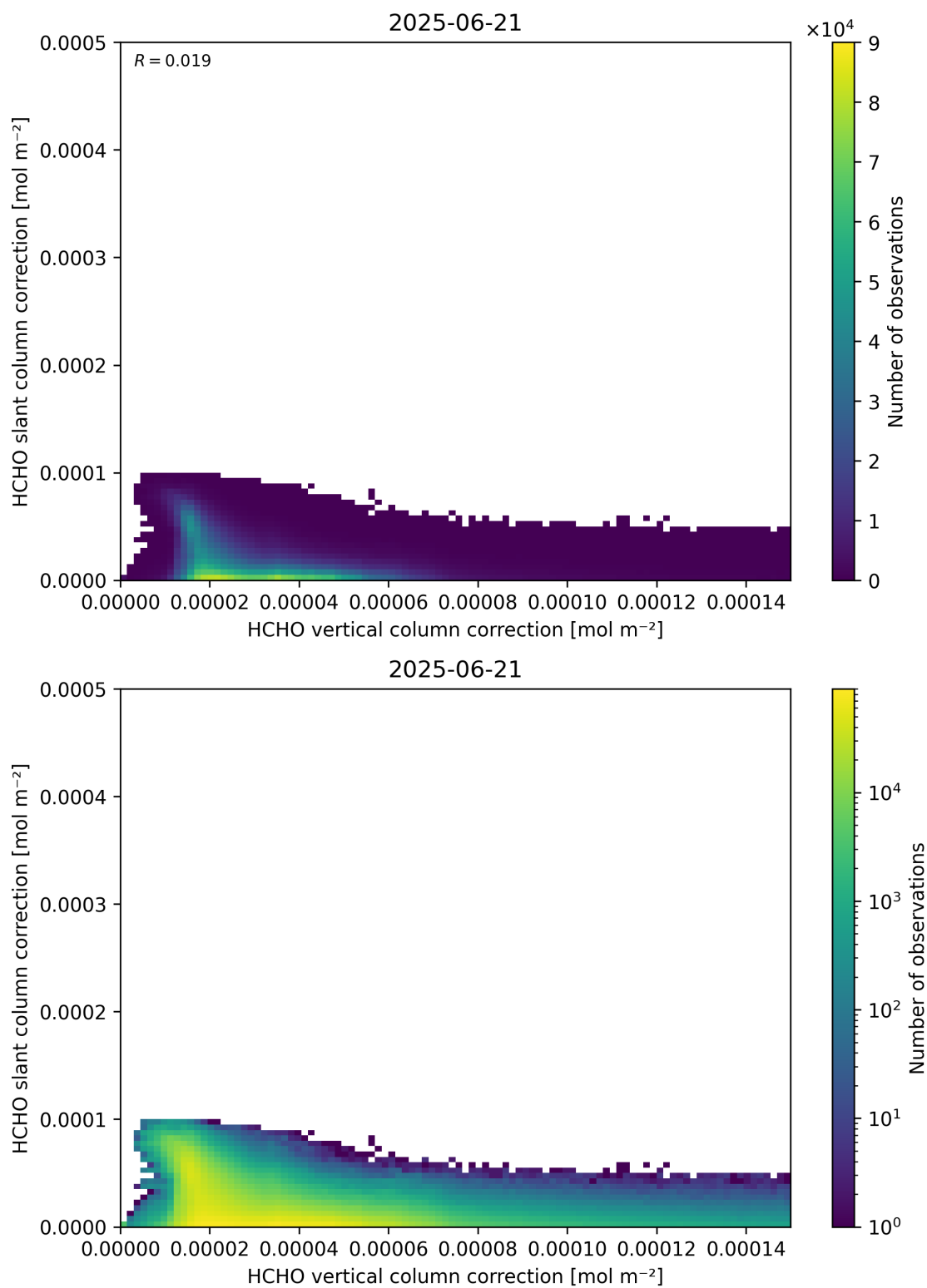
Figure 117: Scatter density plot of “HCHO vertical column correction” against “HCHO slant column correction” for 2025-06-20 to 2025-06-22.
