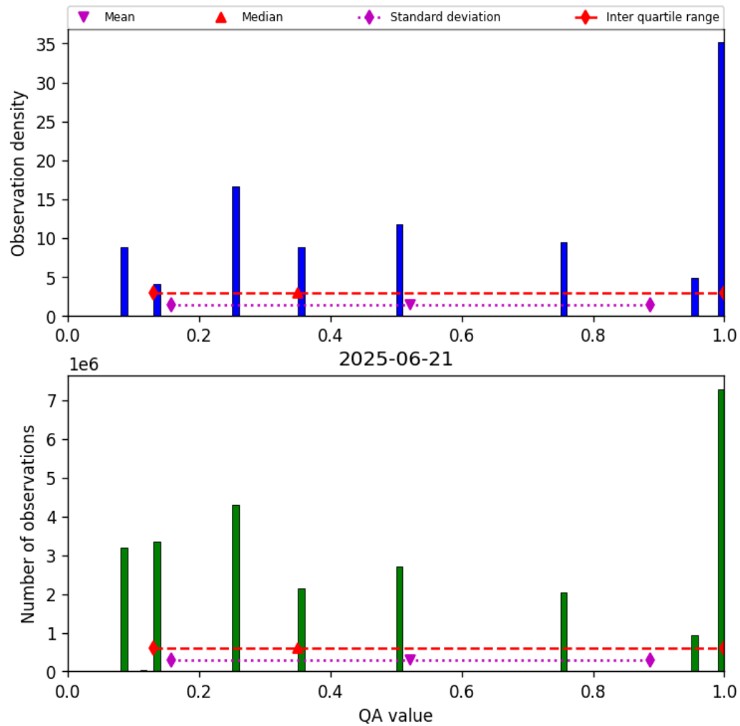
Figure 34: Histogram of “QA value” for 2025-06-20 to 2025-06-22
