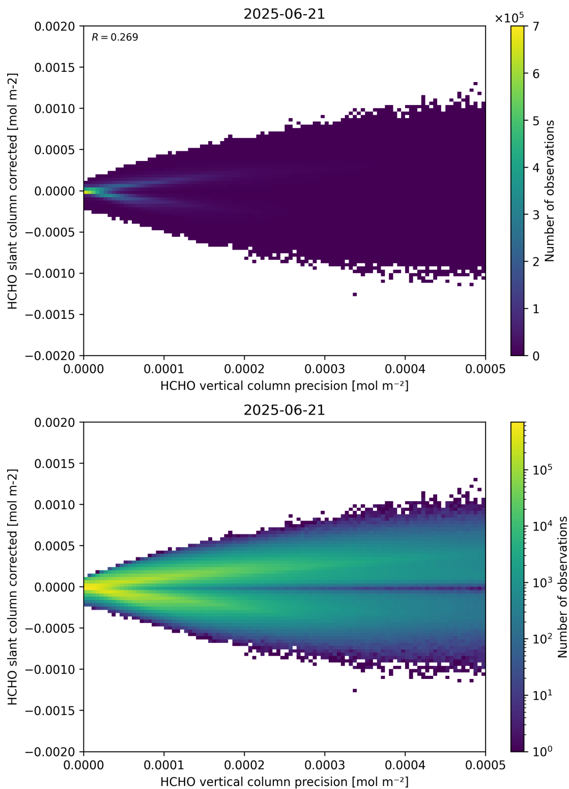
Figure 140: Scatter density plot of “HCHO vertical column precision” against “HCHO slant column corrected” for 2025-06-20 to 2025-06-22.
