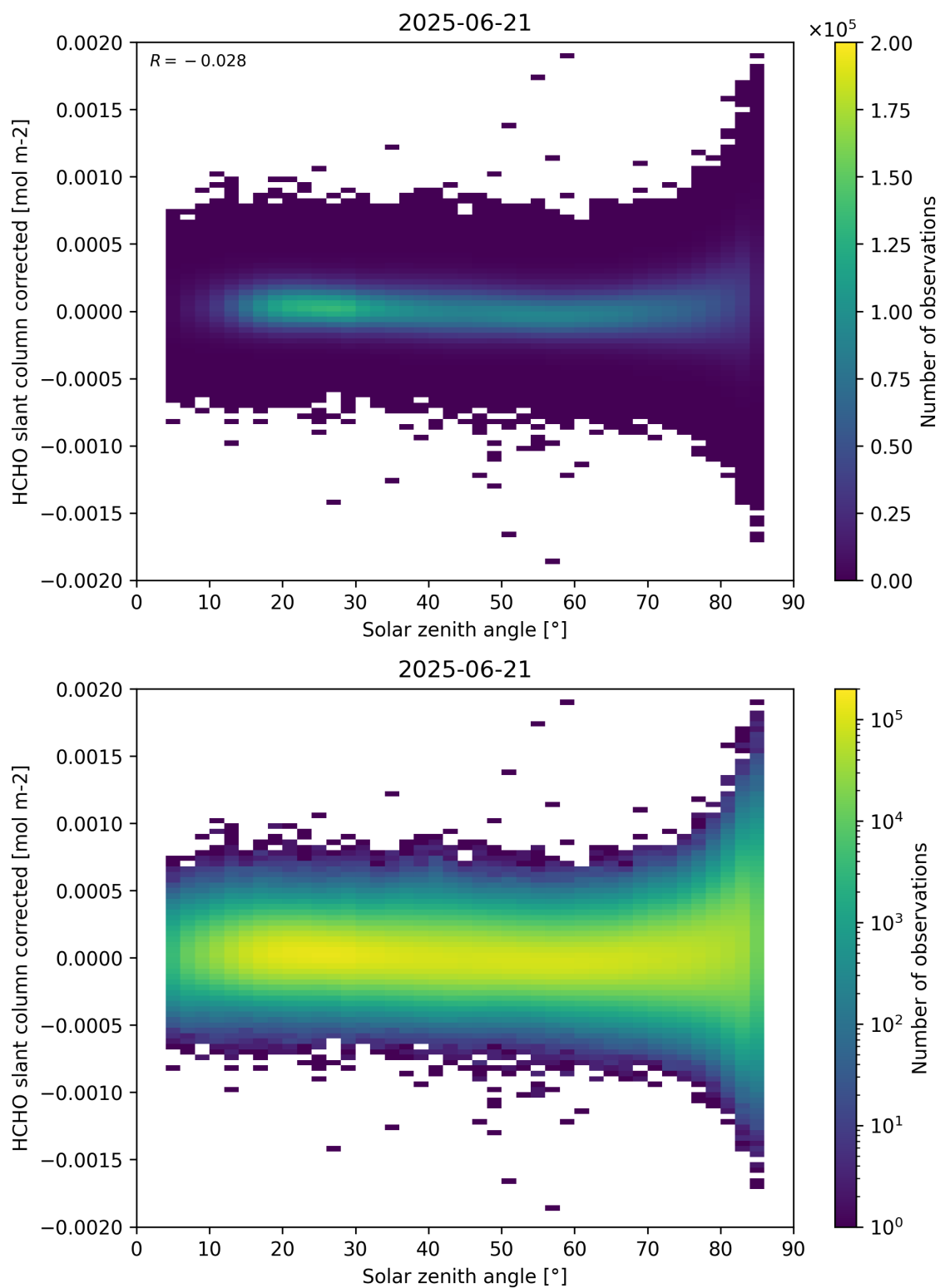
Figure 171: Scatter density plot of “Solar zenith angle” against “HCHO slant column corrected” for 2025-06-20 to 2025-06-22.
