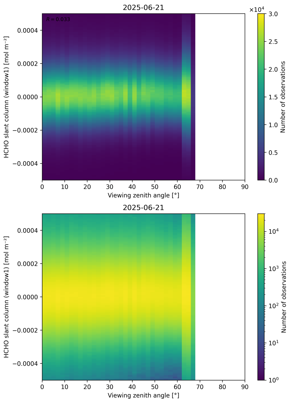
Figure 188: Scatter density plot of “Viewing zenith angle” against “HCHO slant column (window1)” for 2025-06-20 to 2025-06-22.
