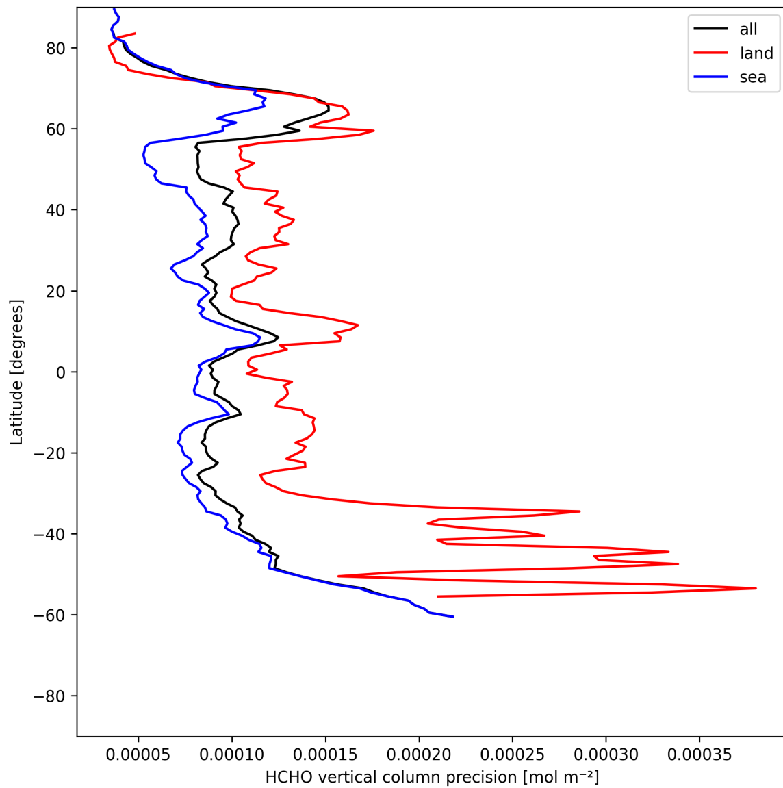
Figure 22: Zonal average of “HCHO vertical column precision” for 2025-06-20 to 2025-06-22.
