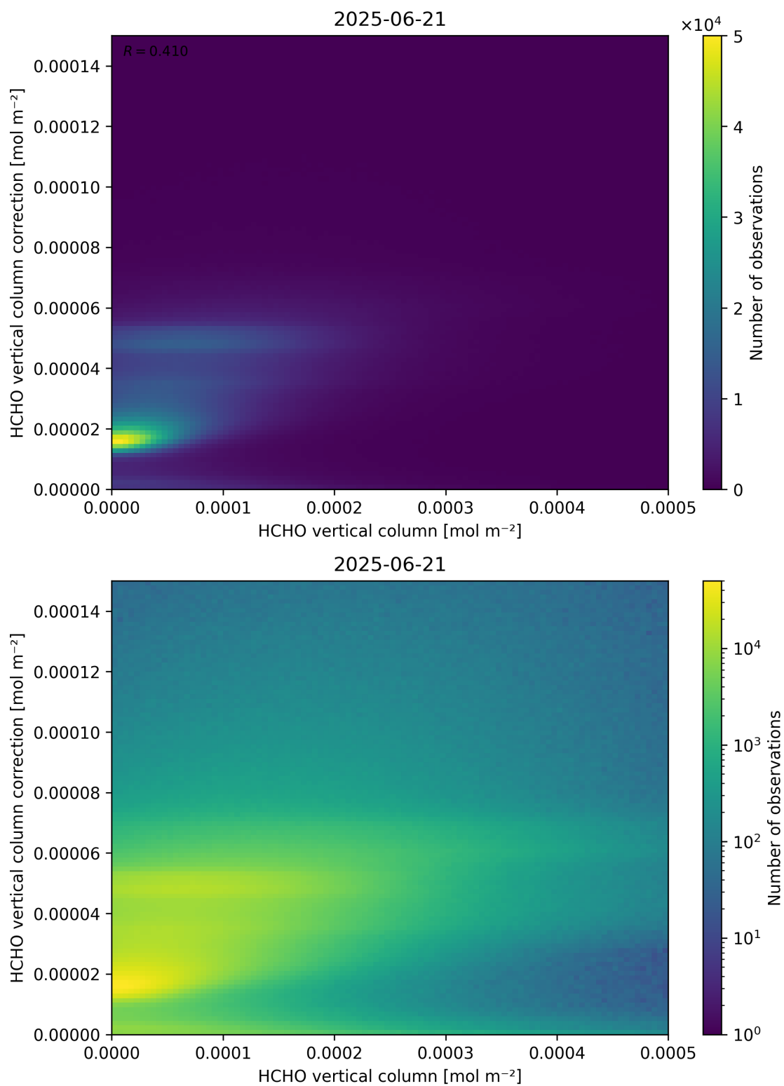
Figure 133: Scatter density plot of “HCHO vertical column” against “HCHO vertical column correction” for 2025-06-20 to 2025-06-22.
