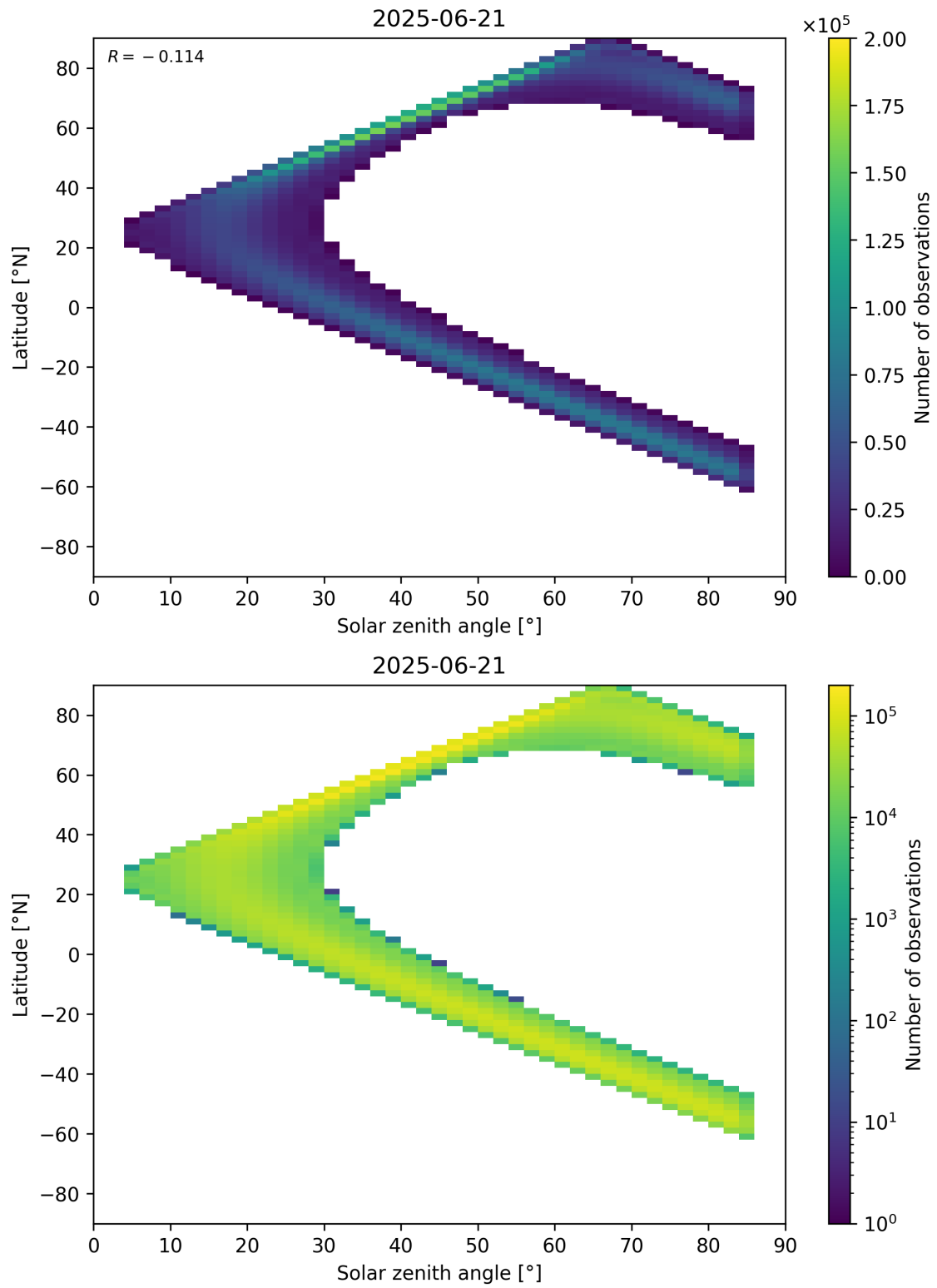
Figure 181: Scatter density plot of “Solar zenith angle” against “Latitude” for 2025-06-20 to 2025-06-22.
