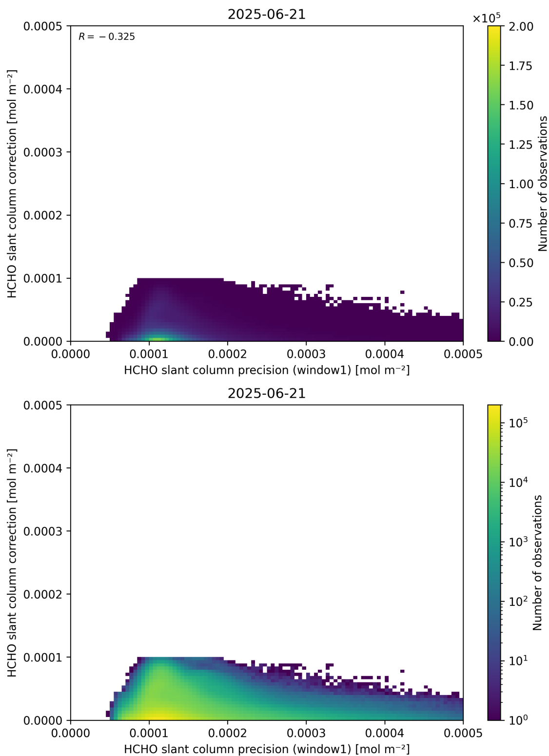
Figure 93: Scatter density plot of “HCHO slant column precision (window1)” against “HCHO slant column correction” for 2025-06-20 to 2025-06-22.
