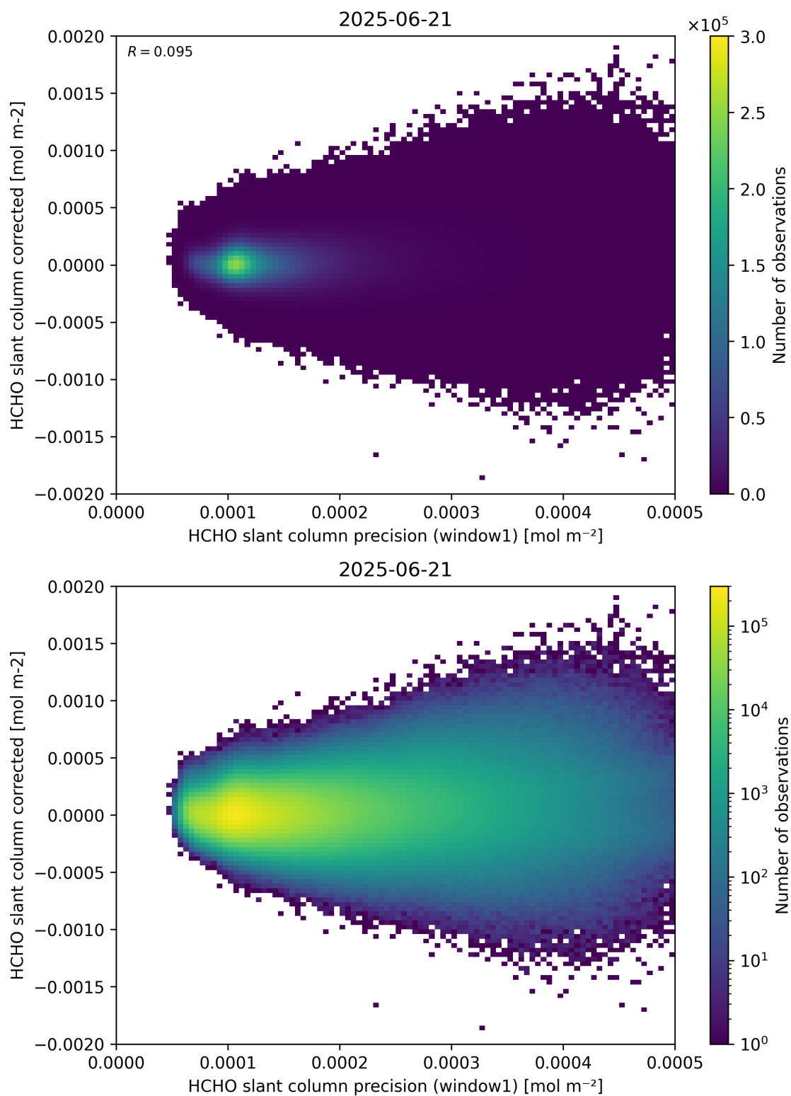
Figure 92: Scatter density plot of “HCHO slant column precision (window1)” against “HCHO slant column corrected” for 2025-06-20 to 2025-06-22.
