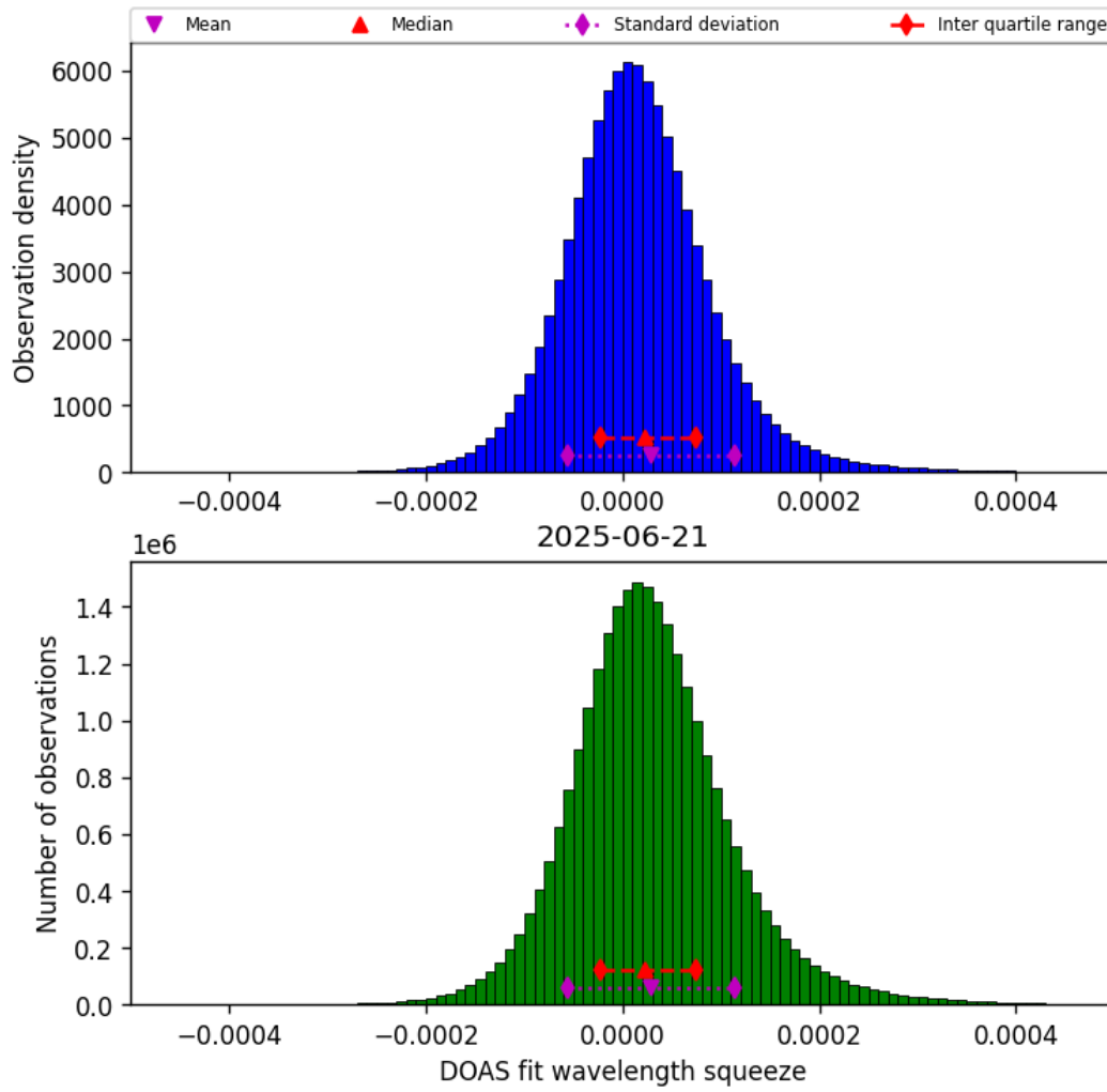
Figure 45: Histogram of “DOAS fit wavelength squeeze” for 2025-06-20 to 2025-06-22
