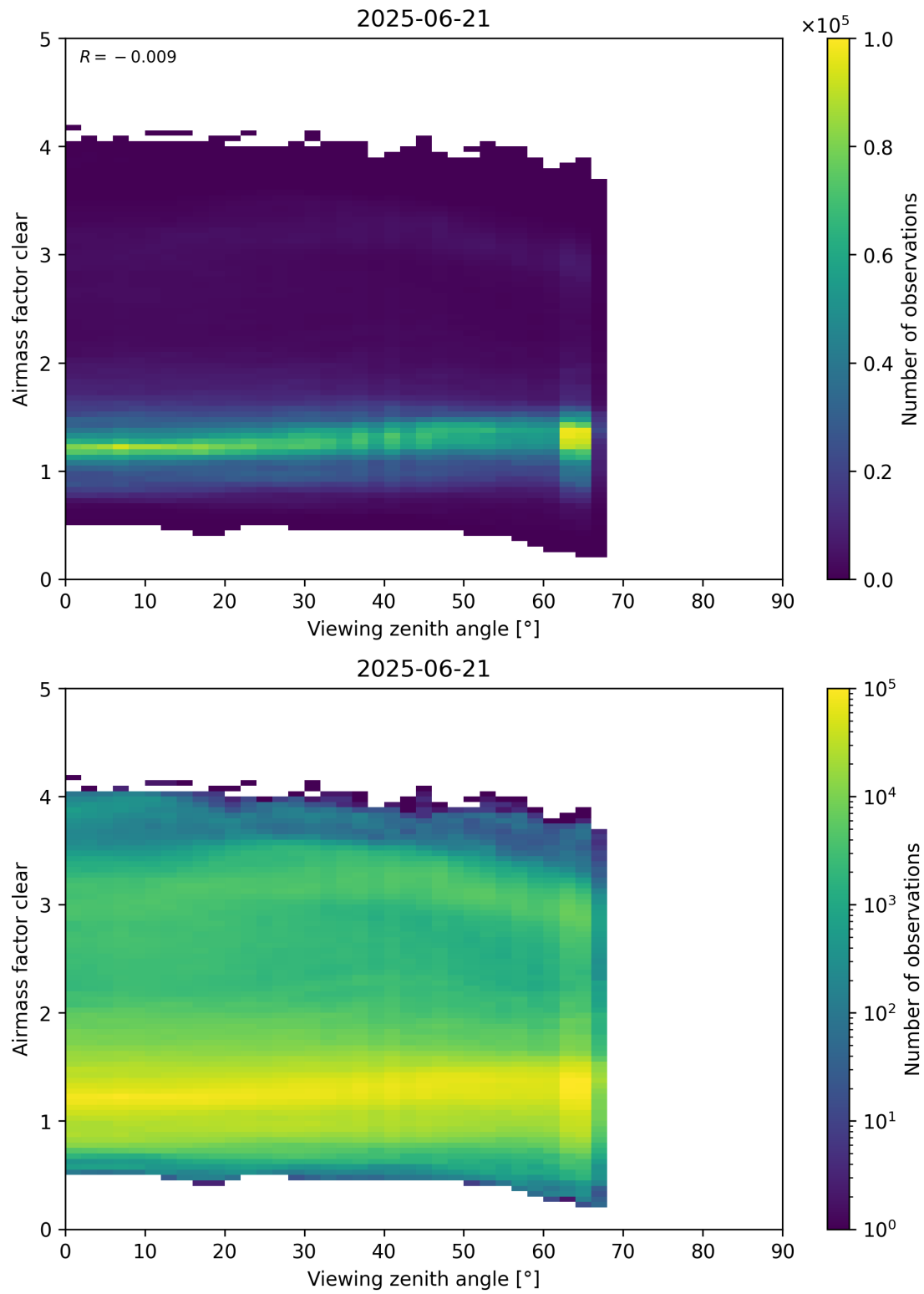
Figure 185: Scatter density plot of “Viewing zenith angle” against “Airmass factor clear” for 2025-06-20 to 2025-06-22.
