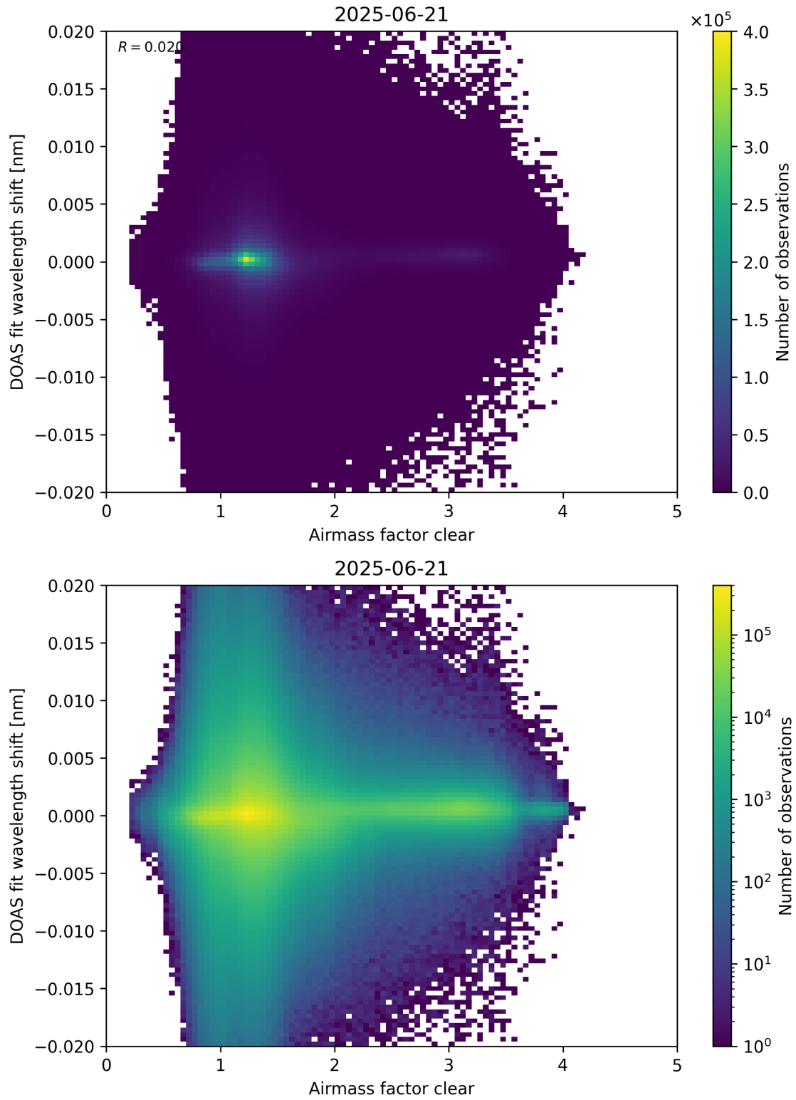
Figure 72: Scatter density plot of “Airmass factor clear” against “DOAS fit wavelength shift” for 2025-06-20 to 2025-06-22.
