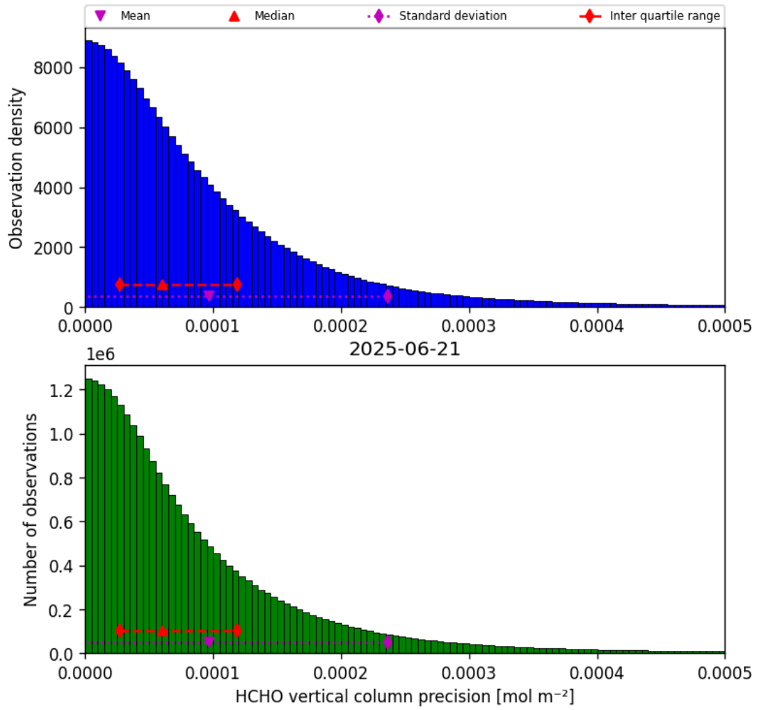
Figure 36: Histogram of “HCHO vertical column precision” for 2025-06-20 to 2025-06-22
