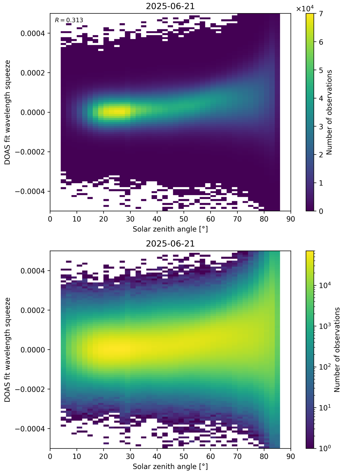
Figure 169: Scatter density plot of “Solar zenith angle” against “DOAS fit wavelength squeeze” for 2025-06-20 to 2025-06-22.
