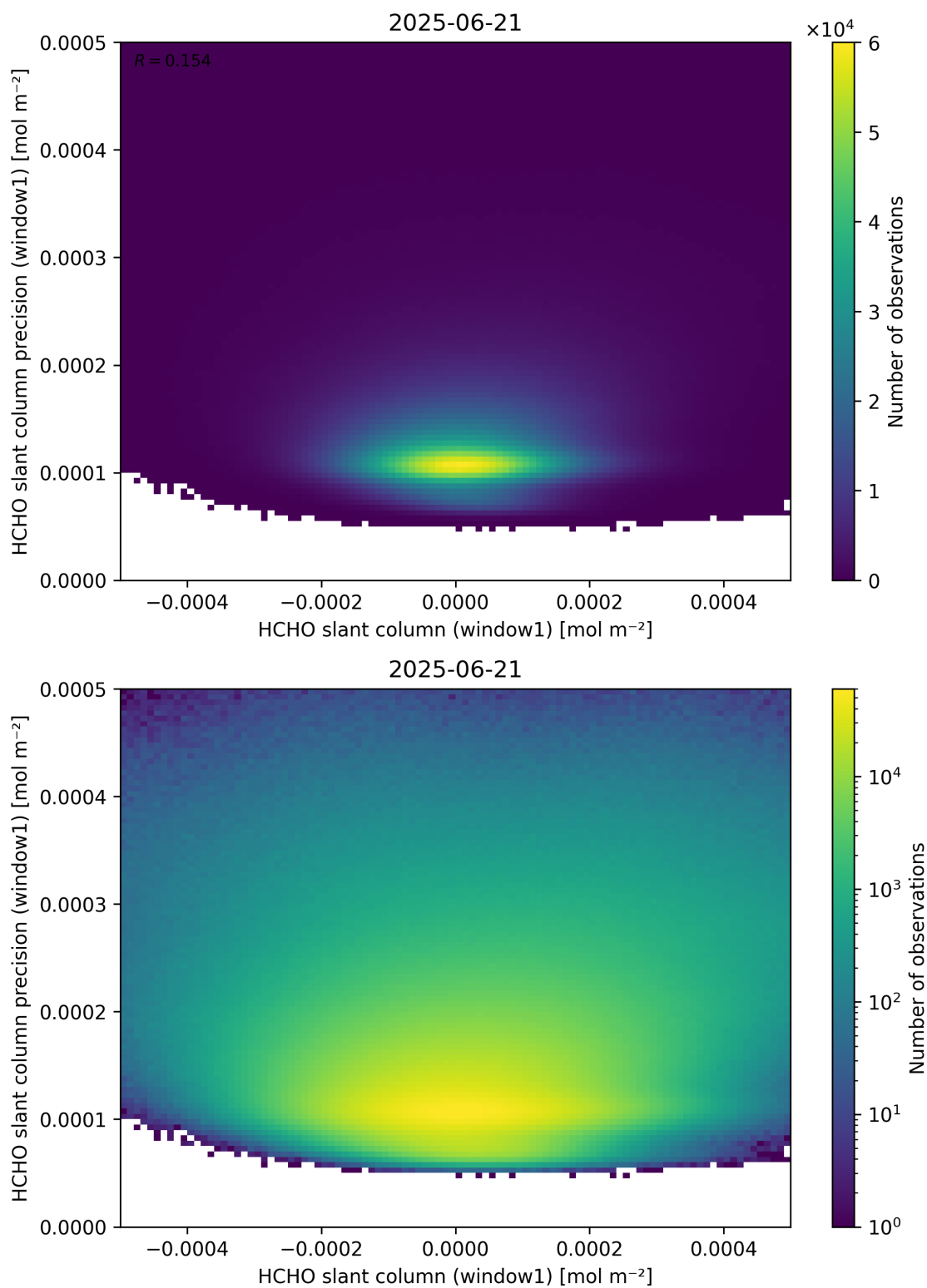
Figure 84: Scatter density plot of “HCHO slant column (window1)” against “HCHO slant column precision (window1)” for 2025-06-20 to 2025-06-22.
