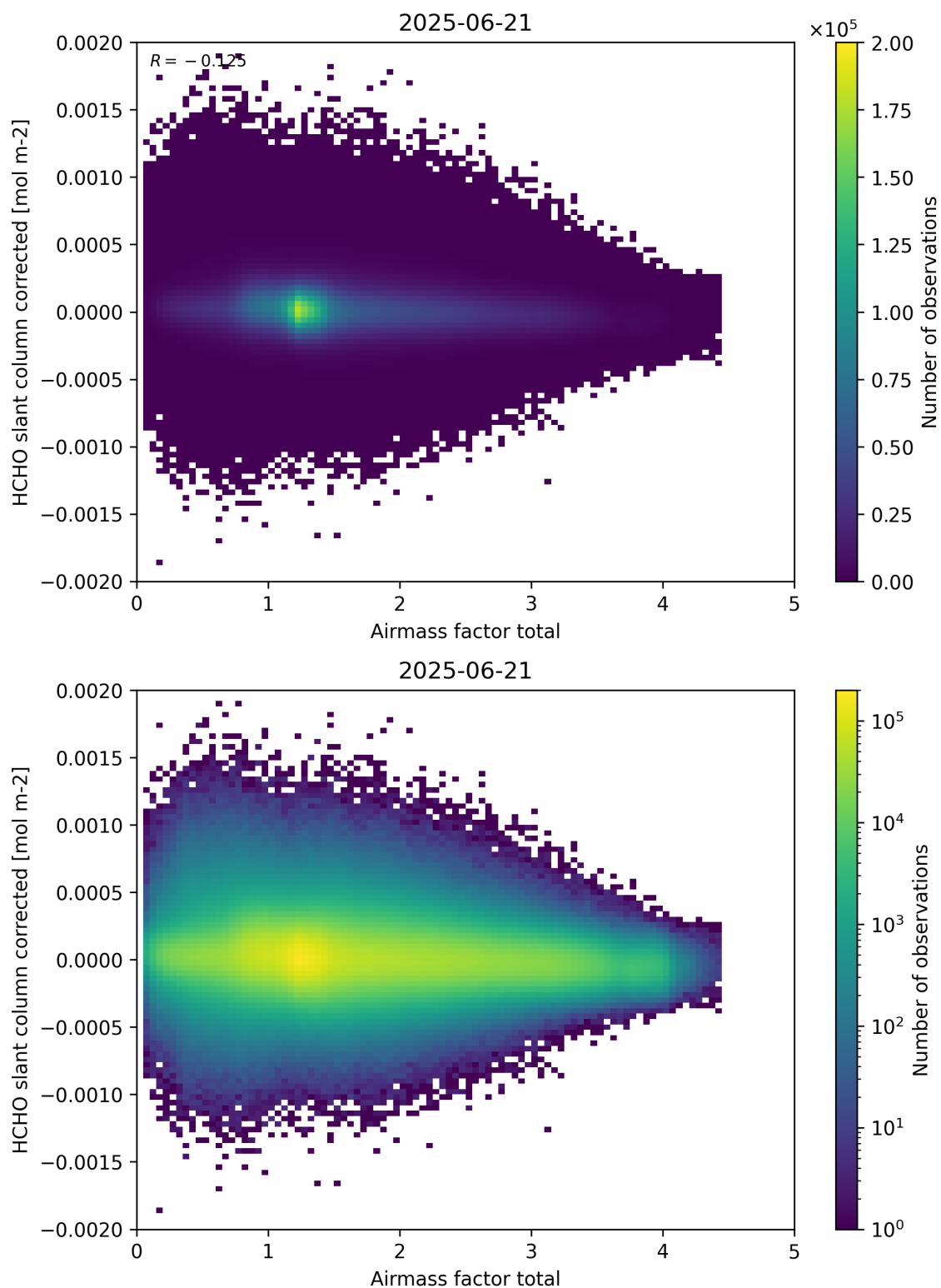
Figure 101: Scatter density plot of “Airmass factor total” against “HCHO slant column corrected” for 2025-06-20 to 2025-06-22.
