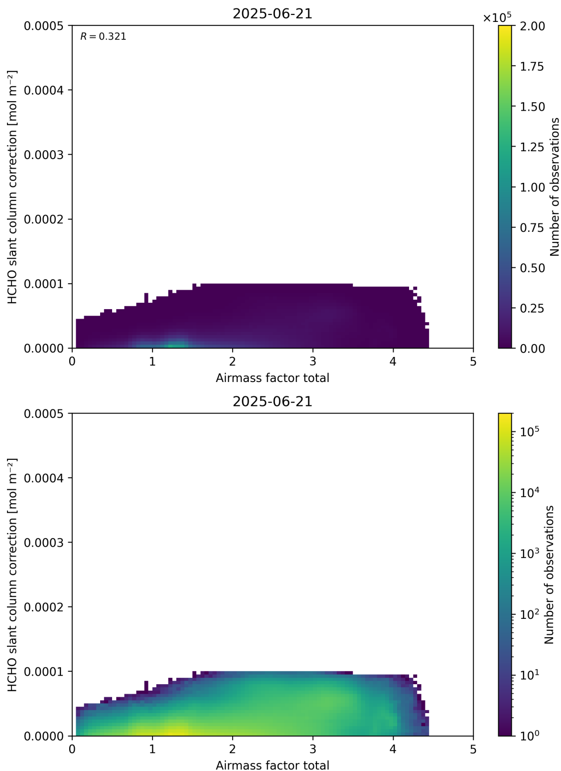
Figure 102: Scatter density plot of “Airmass factor total” against “HCHO slant column correction” for 2025-06-20 to 2025-06-22.
