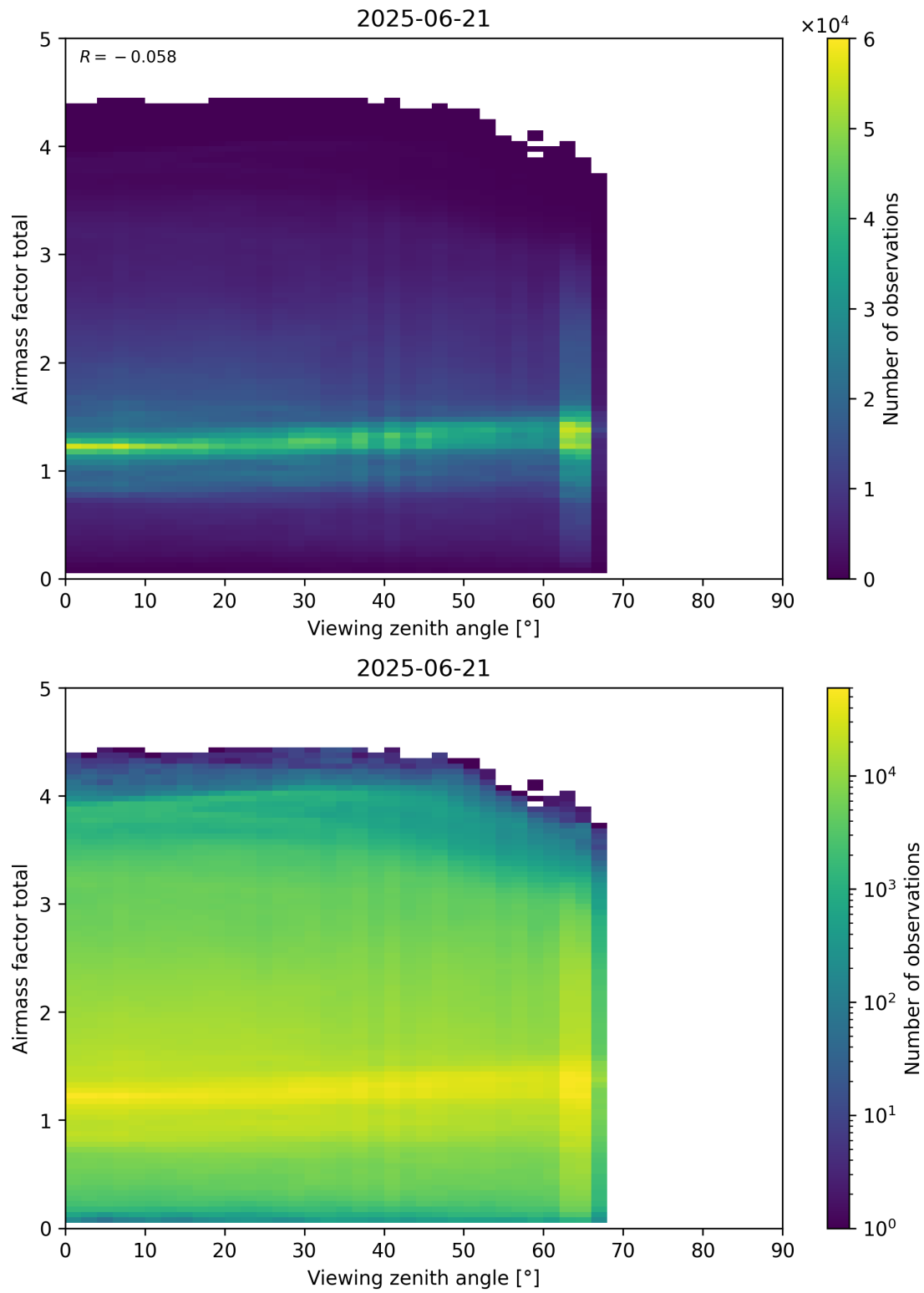
Figure 190: Scatter density plot of “Viewing zenith angle” against “Airmass factor total” for 2025-06-20 to 2025-06-22.
