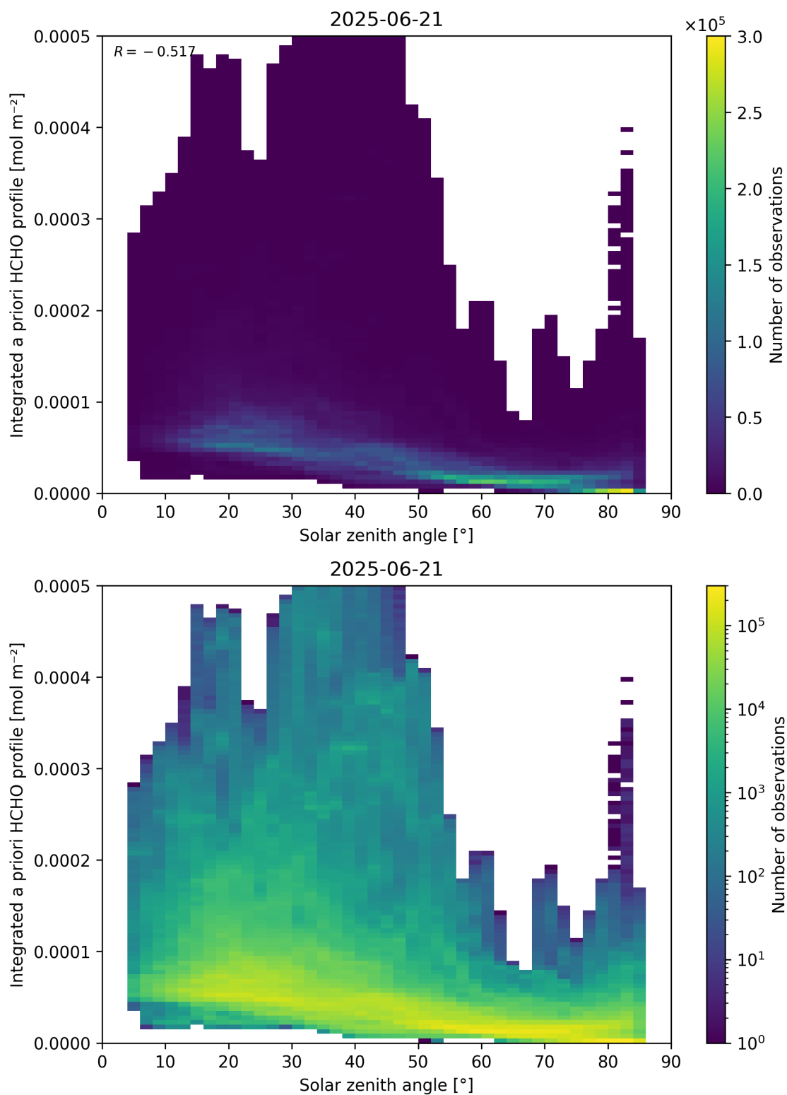
Figure 180: Scatter density plot of “Solar zenith angle” against “Integrated a priori HCHO profile” for 2025-06-20 to 2025-06-22.
