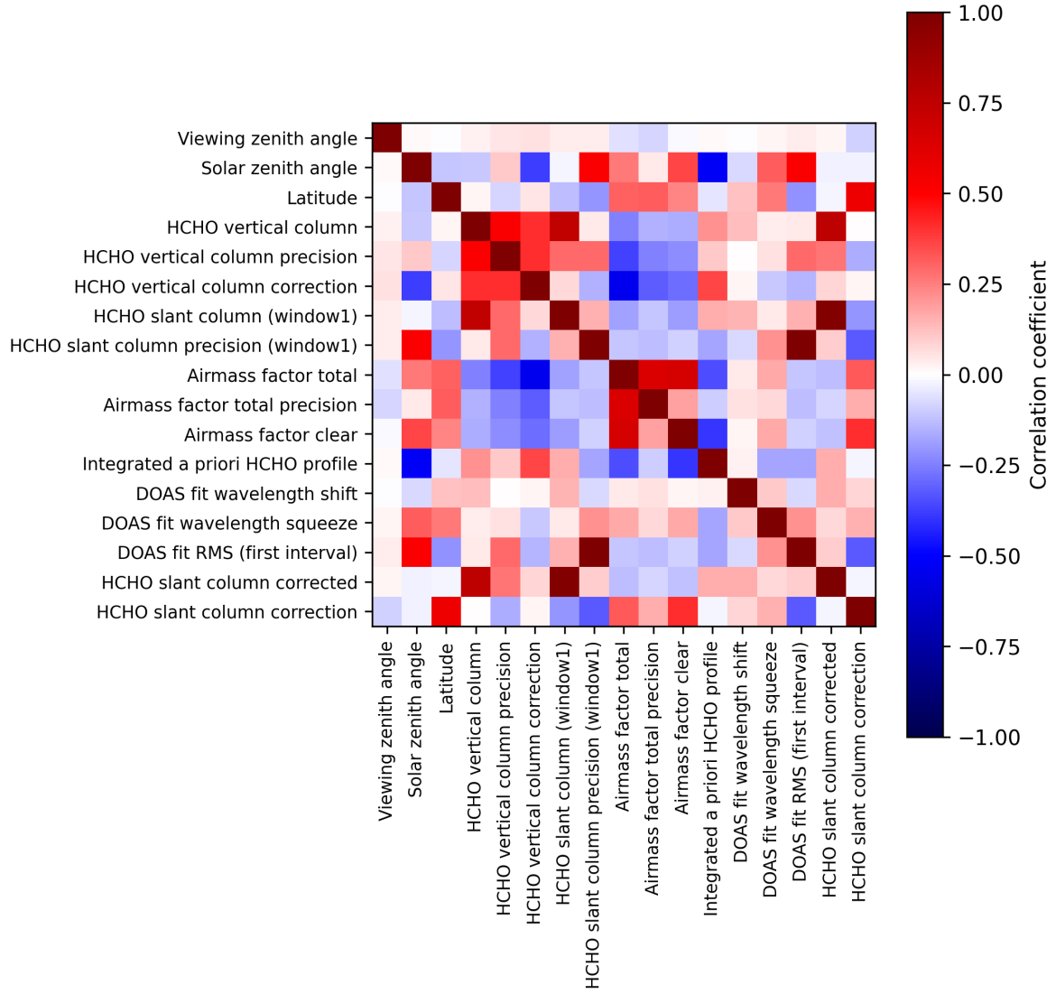
Figure 2: Map of correlation matrix for 2025-06-20 to 2025-06-22.
