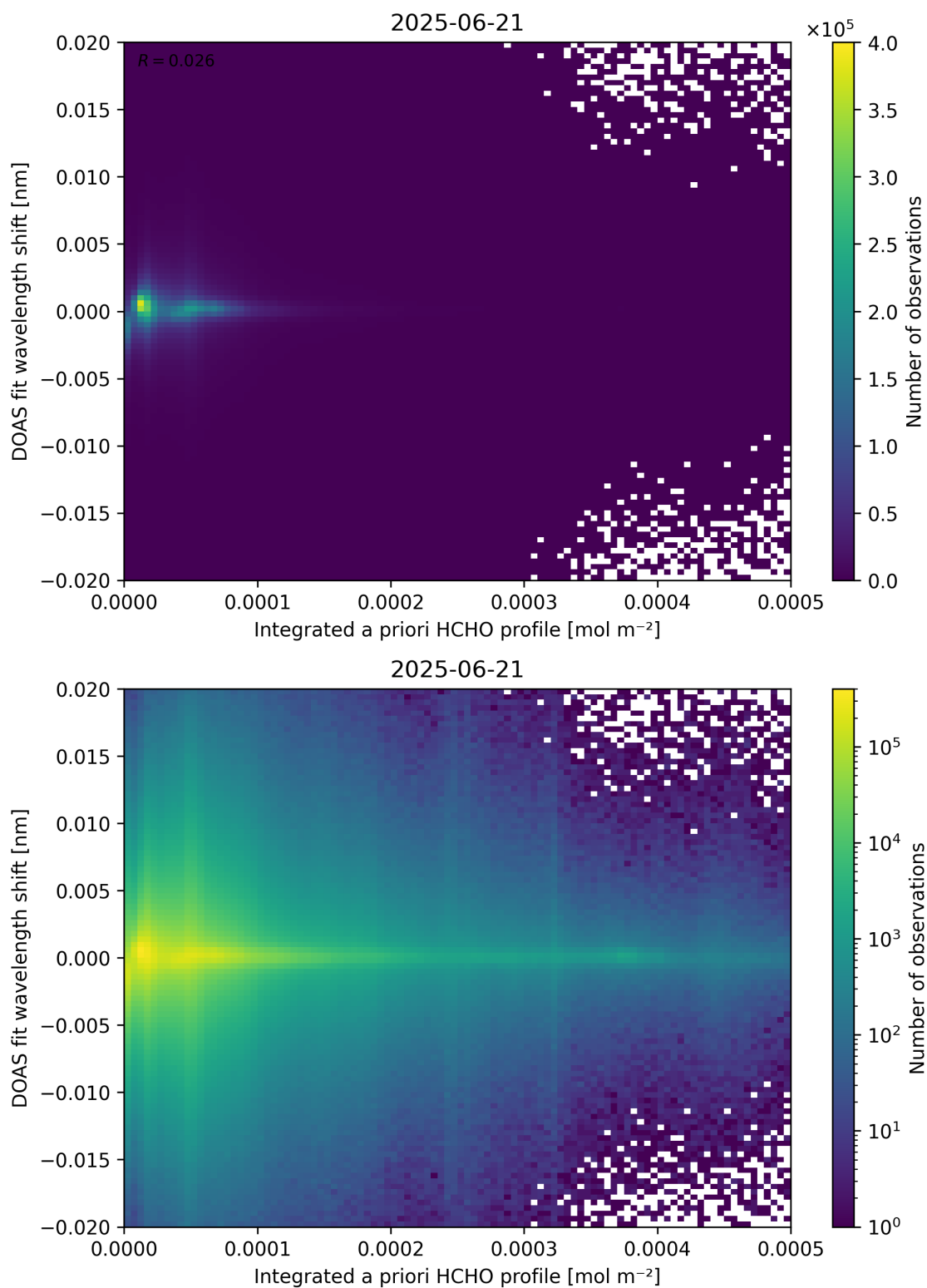
Figure 149: Scatter density plot of “Integrated a priori HCHO profile” against “DOAS fit wavelength shift” for 2025-06-20 to 2025-06-22.
