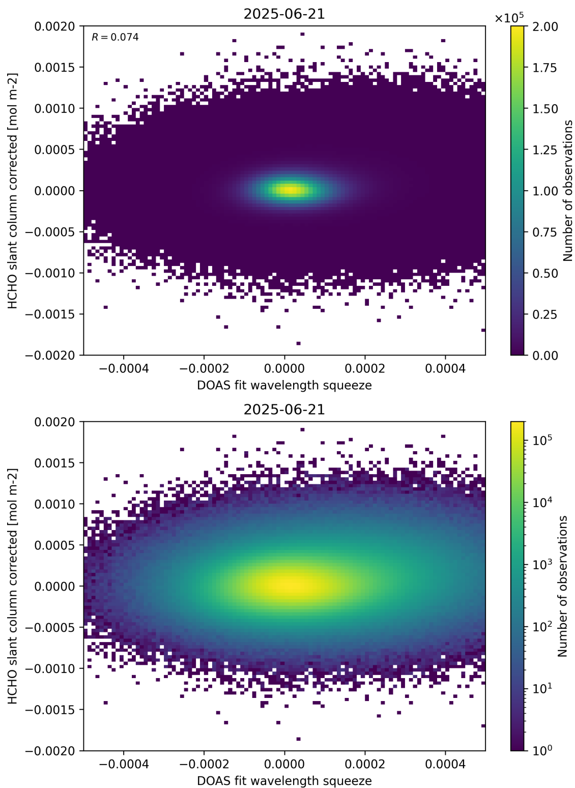
Figure 69: Scatter density plot of “DOAS fit wavelength squeeze” against “HCHO slant column corrected” for 2025-06-20 to 2025-06-22.
