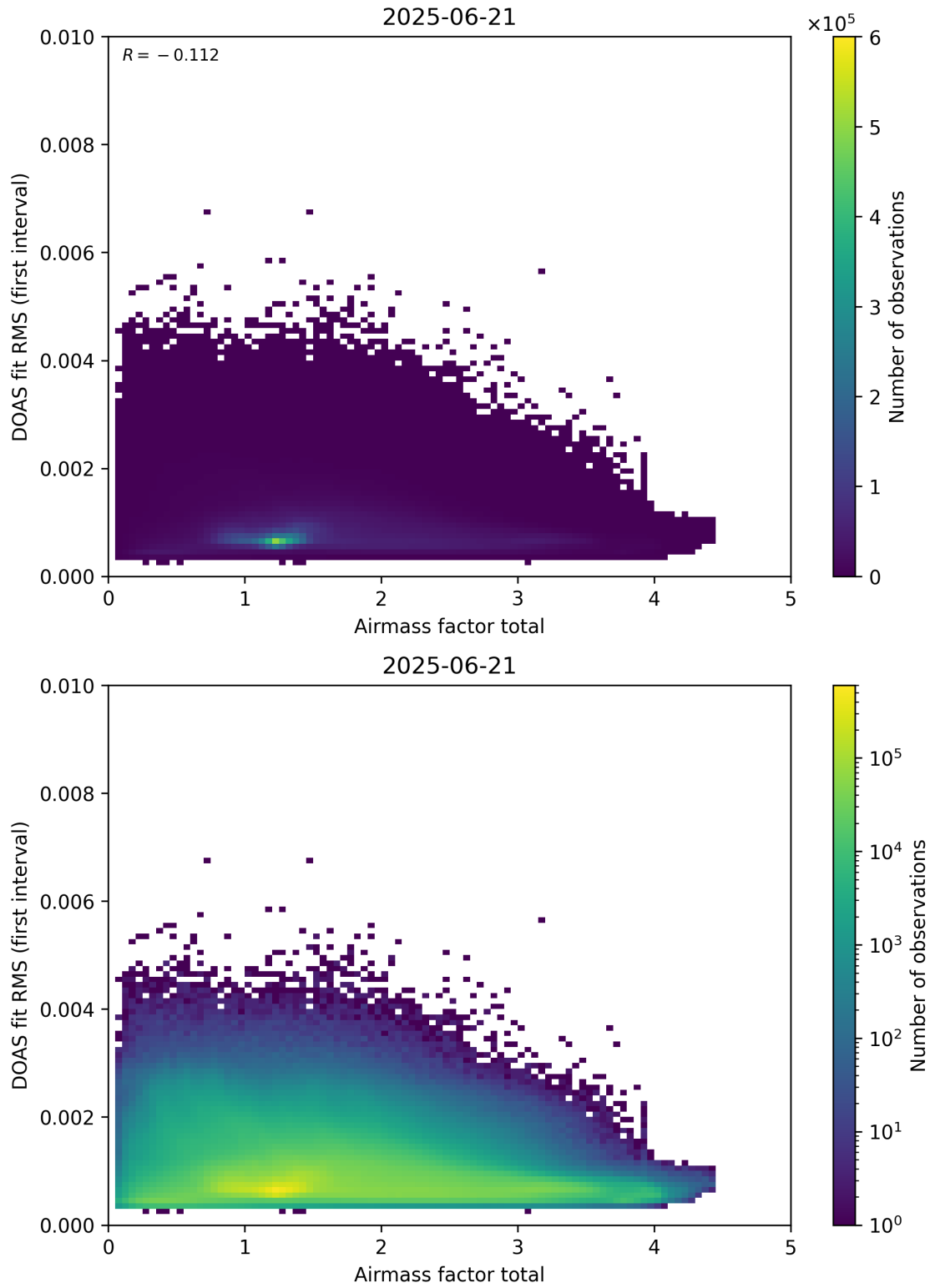
Figure 97: Scatter density plot of “Airmass factor total” against “DOAS fit RMS (first interval)” for 2025-06-20 to 2025-06-22.
