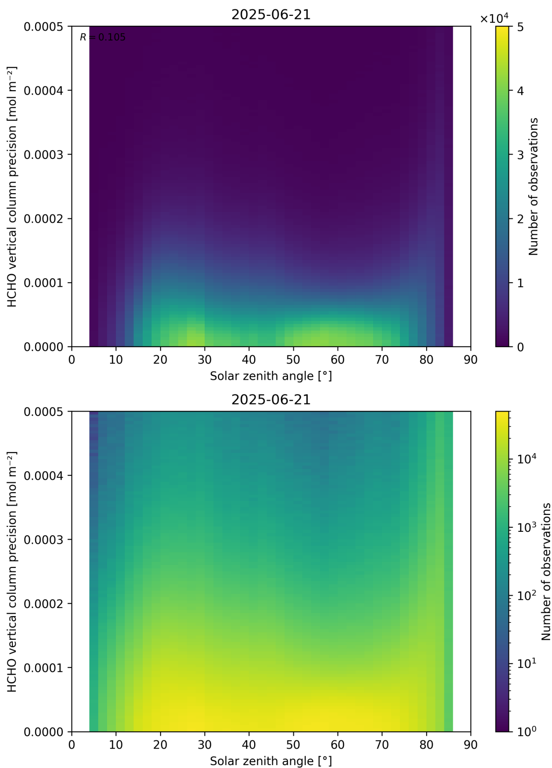
Figure 179: Scatter density plot of “Solar zenith angle” against “HCHO vertical column precision” for 2025-06-20 to 2025-06-22.
