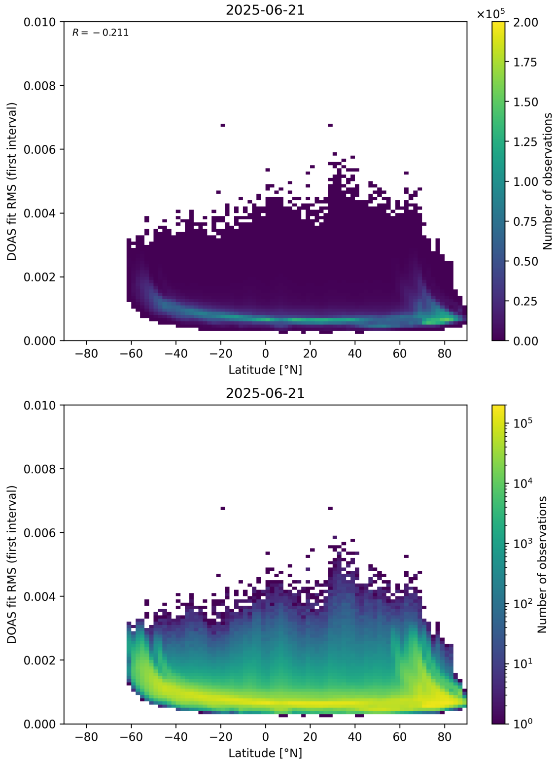
Figure 153: Scatter density plot of “Latitude” against “DOAS fit RMS (first interval)” for 2025-06-20 to 2025-06-22.
