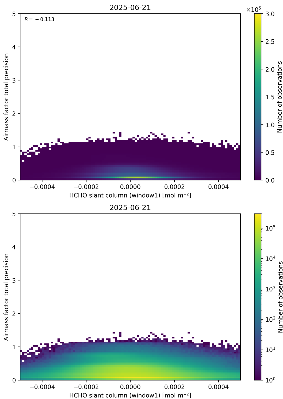
Figure 86: Scatter density plot of “HCHO slant column (window1)” against “Airmass factor total precision” for 2025-06-20 to 2025-06-22.
