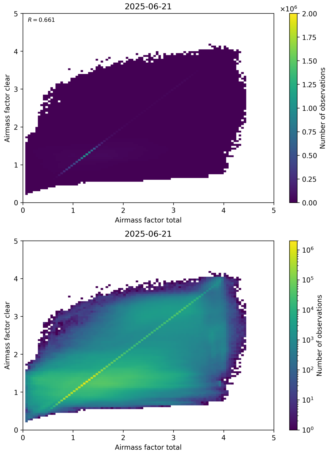
Figure 100: Scatter density plot of “Airmass factor total” against “Airmass factor clear” for 2025-06-20 to 2025-06-22.
