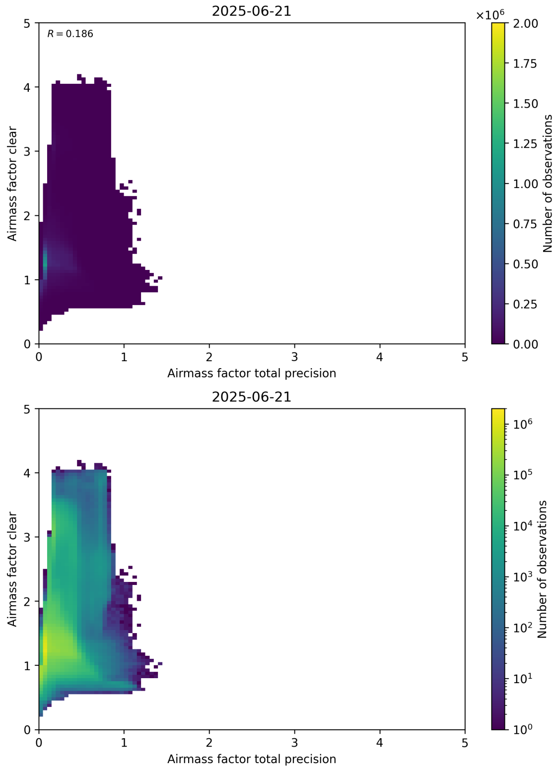
Figure 108: Scatter density plot of “Airmass factor total precision” against “Airmass factor clear” for 2025-06-20 to 2025-06-22.
