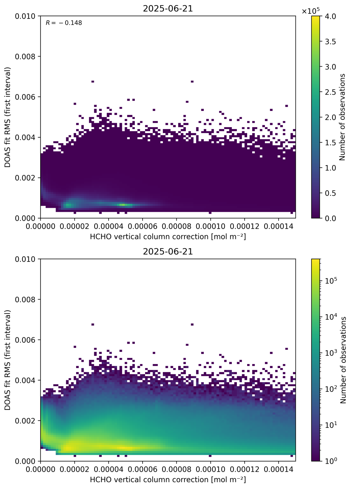
Figure 112: Scatter density plot of “HCHO vertical column correction” against “DOAS fit RMS (first interval)” for 2025-06-20 to 2025-06-22.
