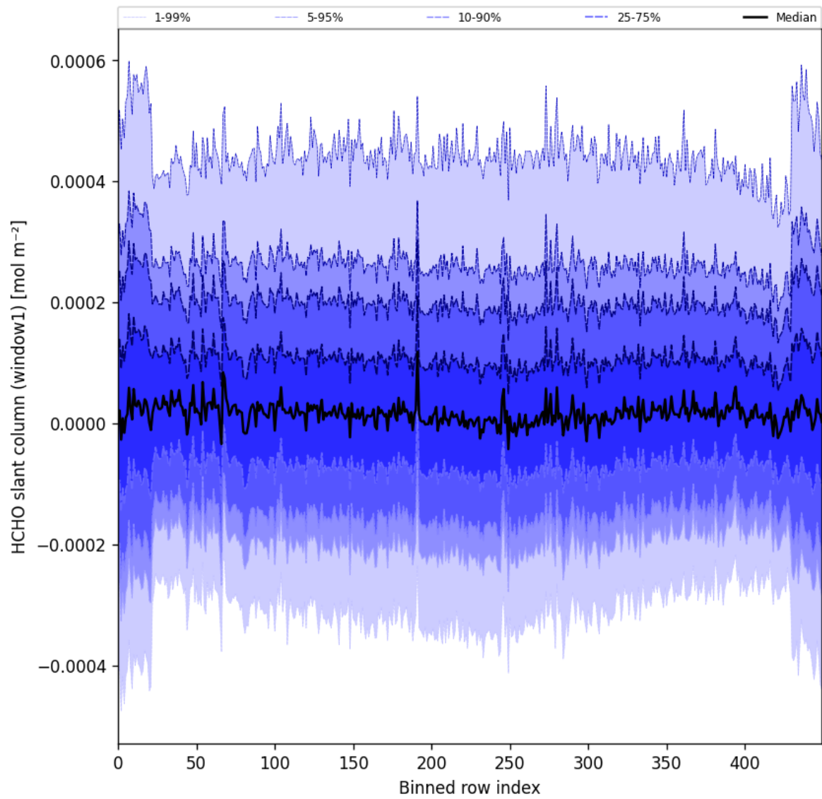
Figure 52: Along track statistics of "HCHO slant column (window1)" for 2025-06-20 to 2025-06-22
