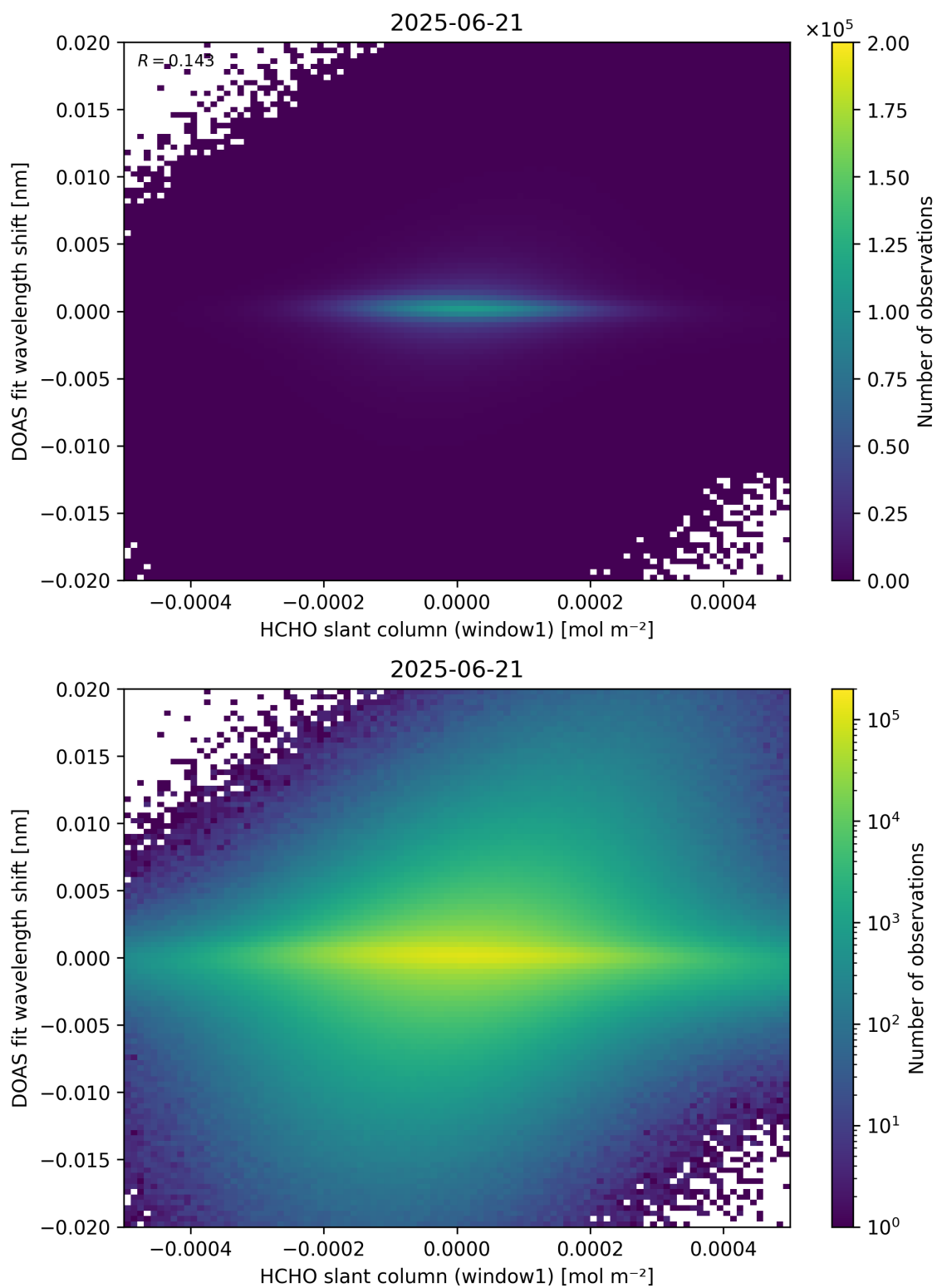
Figure 79: Scatter density plot of “HCHO slant column (window1)” against “DOAS fit wavelength shift” for 2025-06-20 to 2025-06-22.
