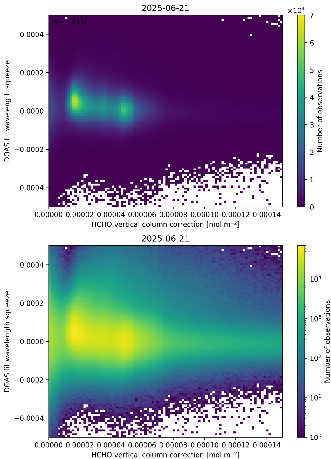
Figure 114: Scatter density plot of “HCHO vertical column correction” against “DOAS fit wavelength squeeze” for 2025-06-20 to 2025-06-22.
