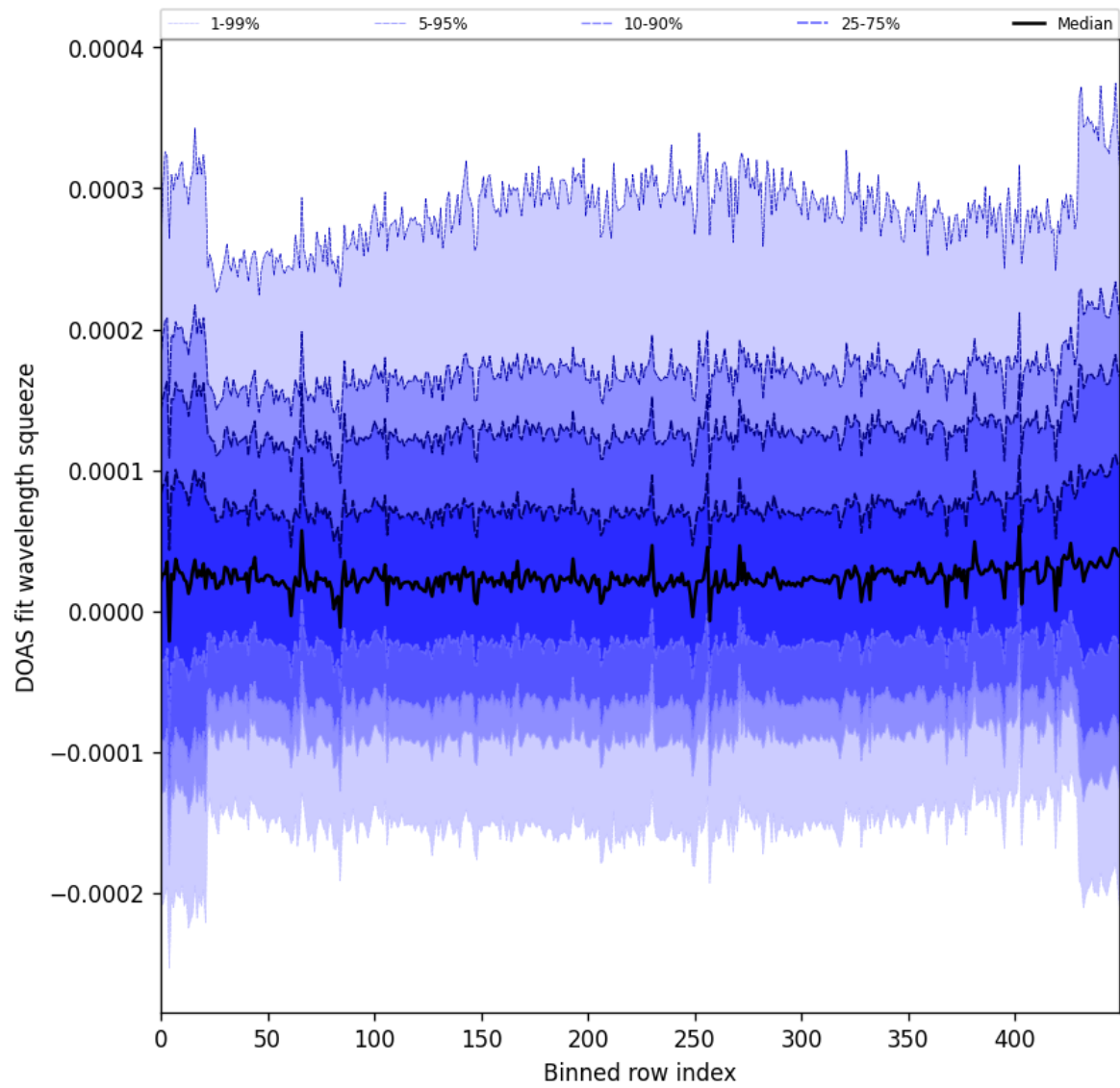
Figure 59: Along track statistics of “DOAS fit wavelength squeeze” for 2025-06-20 to 2025-06-22
