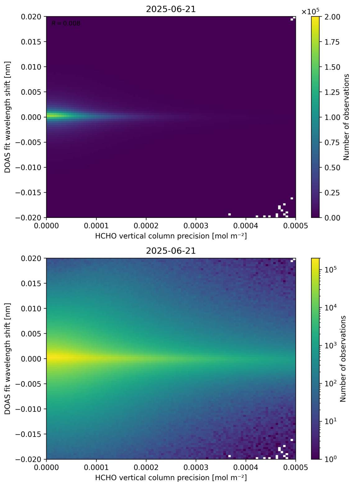
Figure 137: Scatter density plot of “HCHO vertical column precision” against “DOAS fit wavelength shift” for 2025-06-20 to 2025-06-22.
