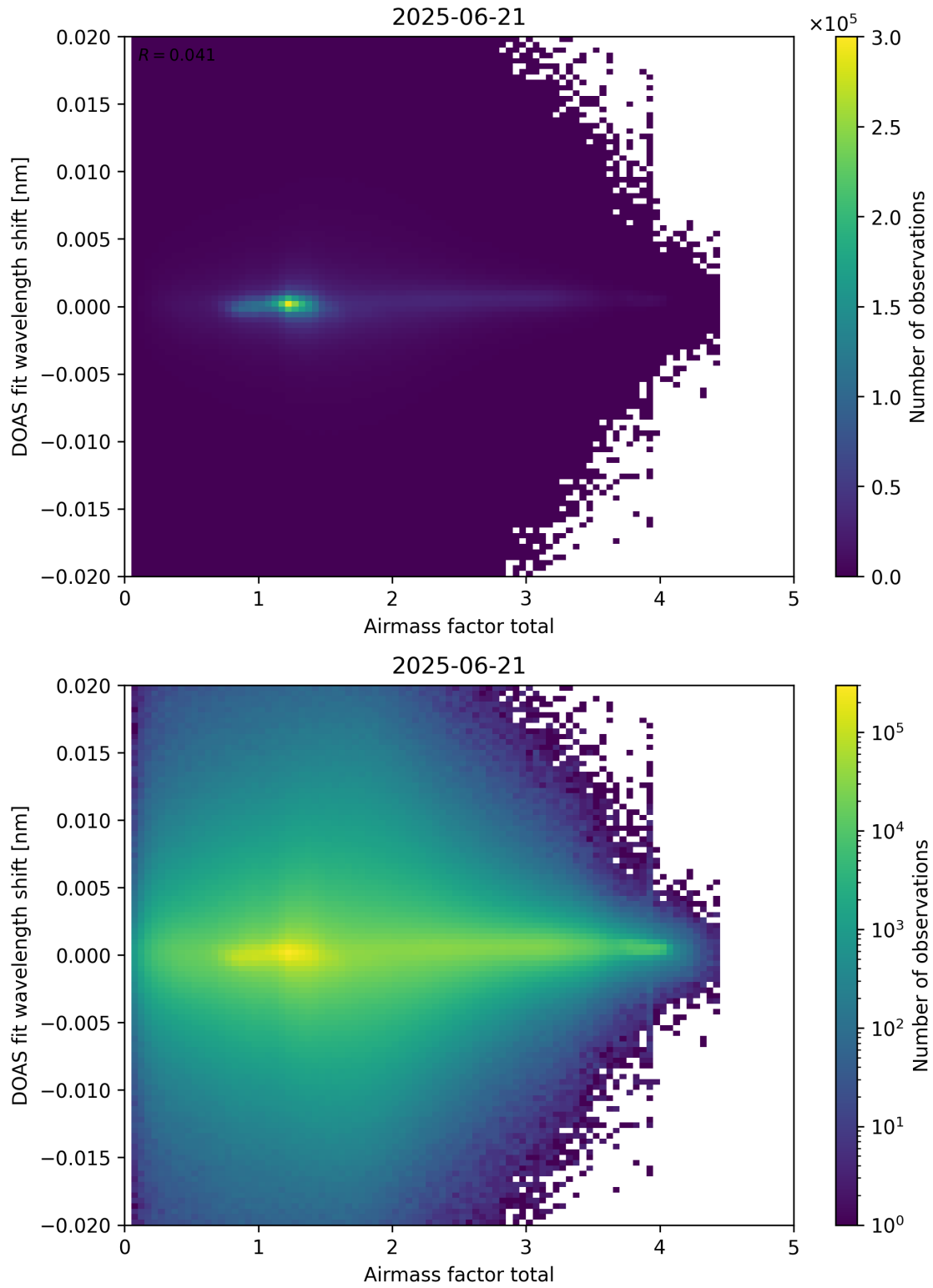
Figure 98: Scatter density plot of “Airmass factor total” against “DOAS fit wavelength shift” for 2025-06-20 to 2025-06-22.
