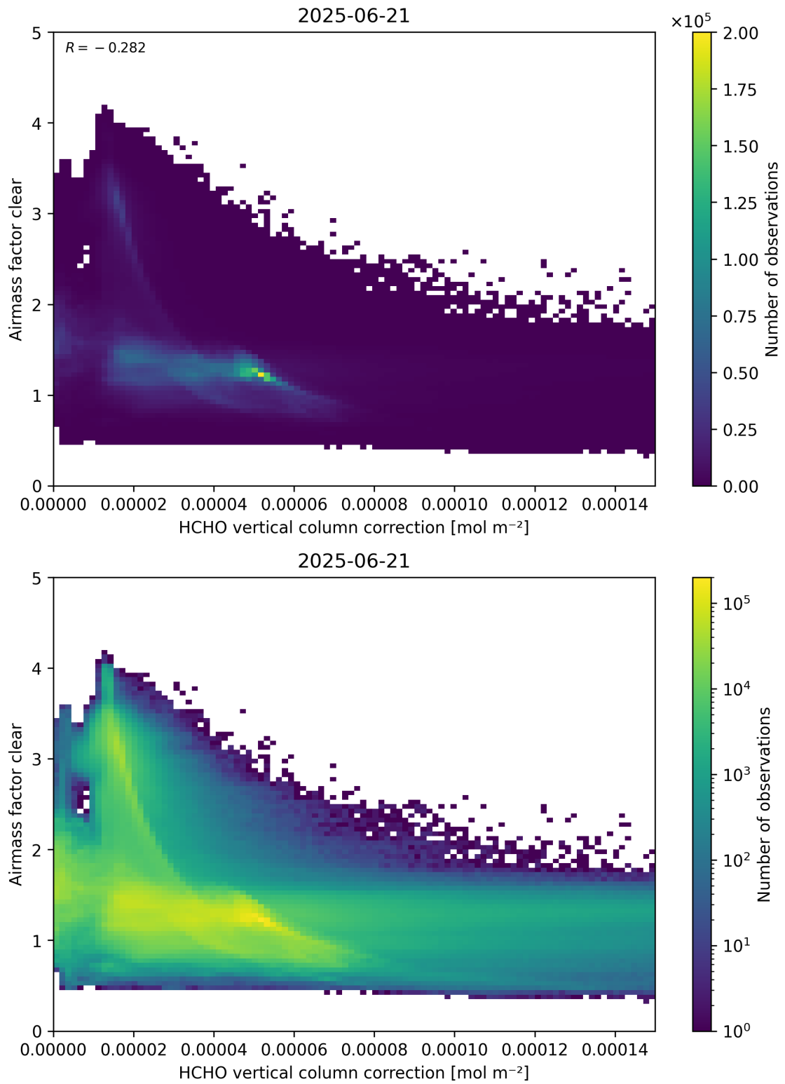
Figure 115: Scatter density plot of “HCHO vertical column correction” against “Airmass factor clear” for 2025-06-20 to 2025-06-22.
