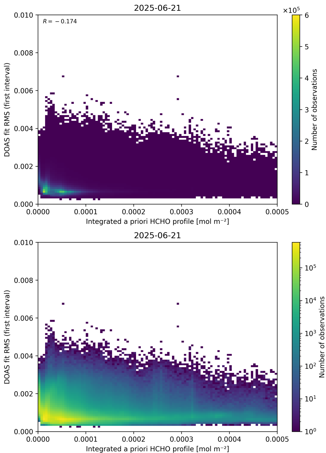
Figure 148: Scatter density plot of “Integrated a priori HCHO profile” against “DOAS fit RMS (first interval)” for 2025-06-20 to 2025-06-22.
