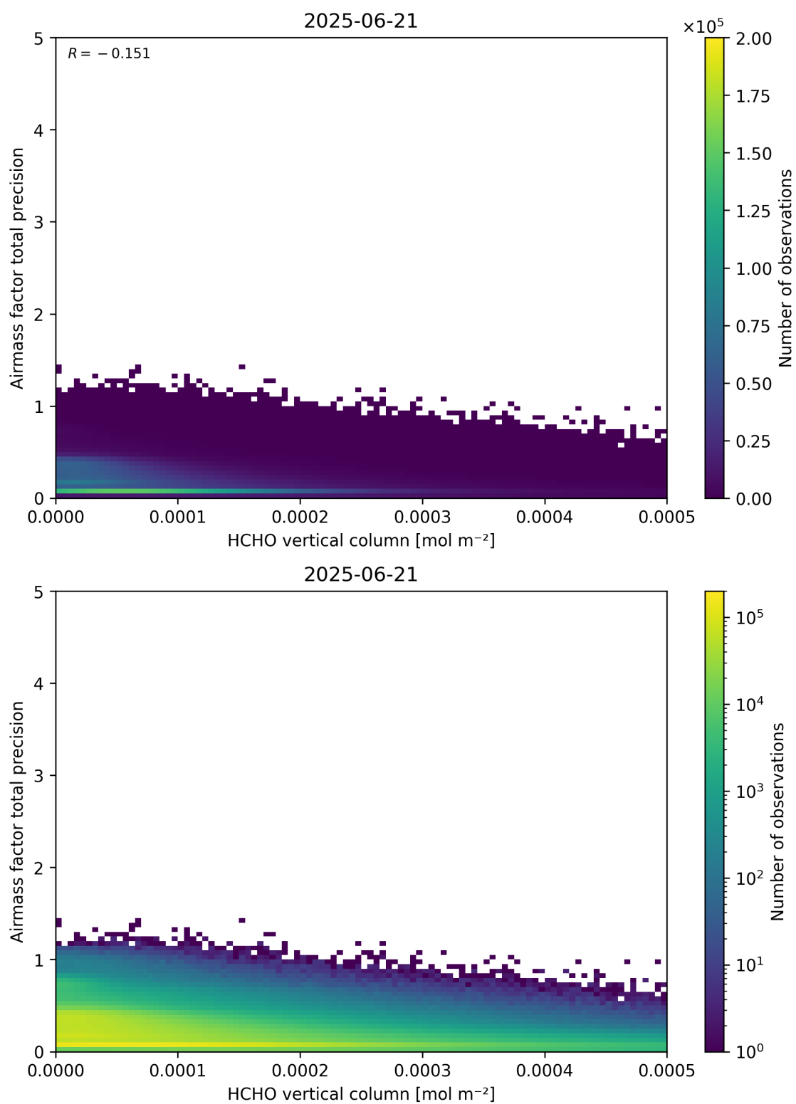
Figure 132: Scatter density plot of “HCHO vertical column” against “Airmass factor total precision” for 2025-06-20 to 2025-06-22.
