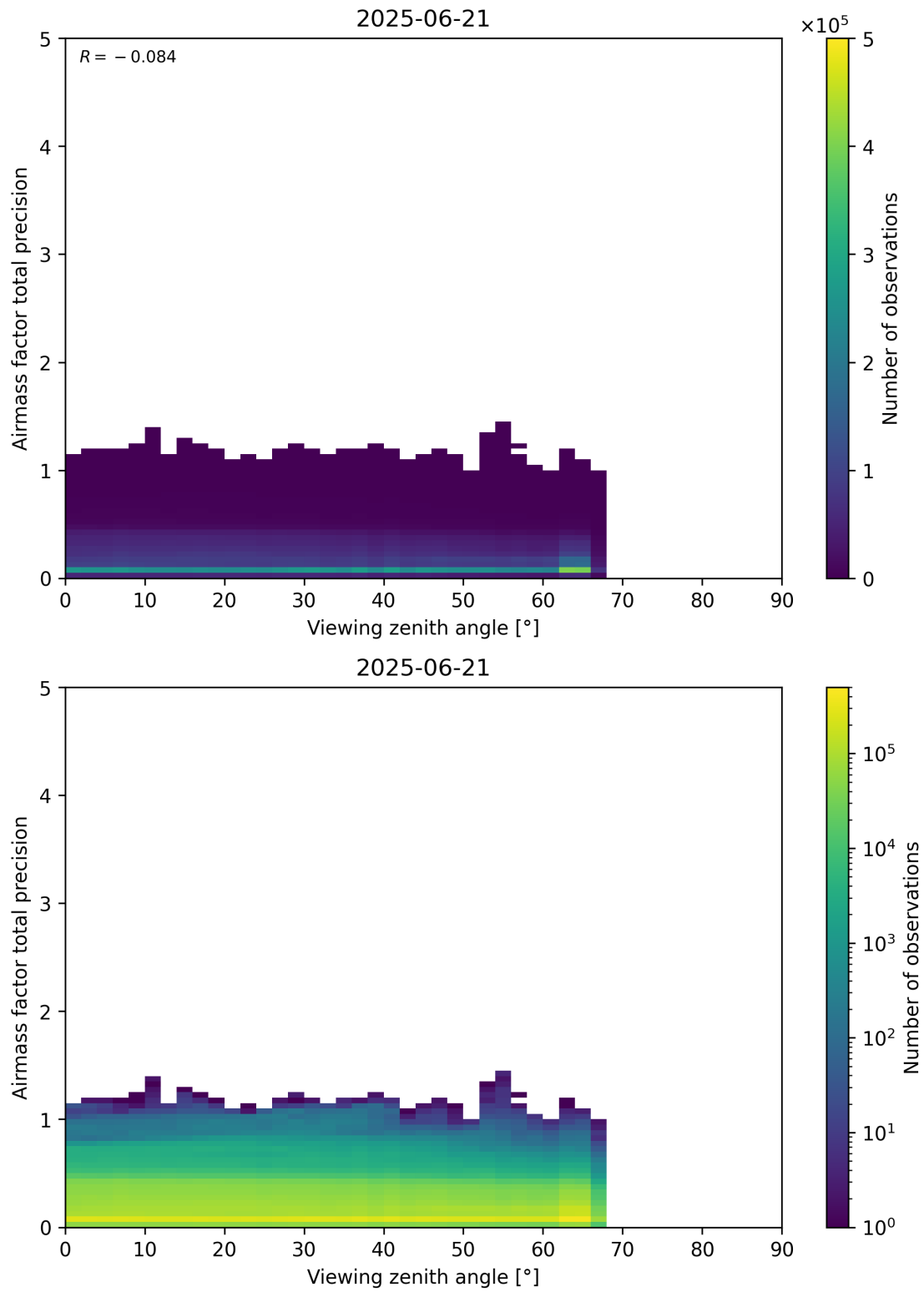
Figure 191: Scatter density plot of “Viewing zenith angle” against “Airmass factor total precision” for 2025-06-20 to 2025-06-22.
