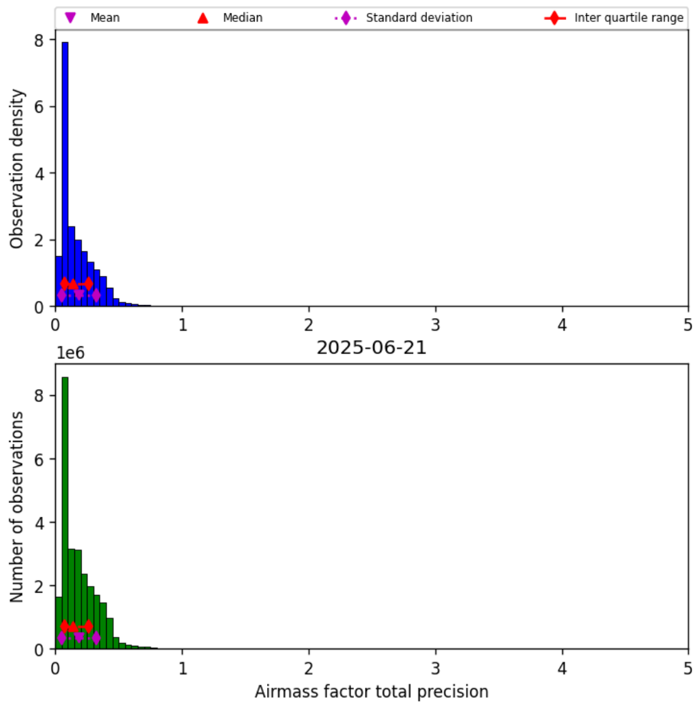
Figure 41: Histogram of “Airmass factor total precision” for 2025-06-20 to 2025-06-22
