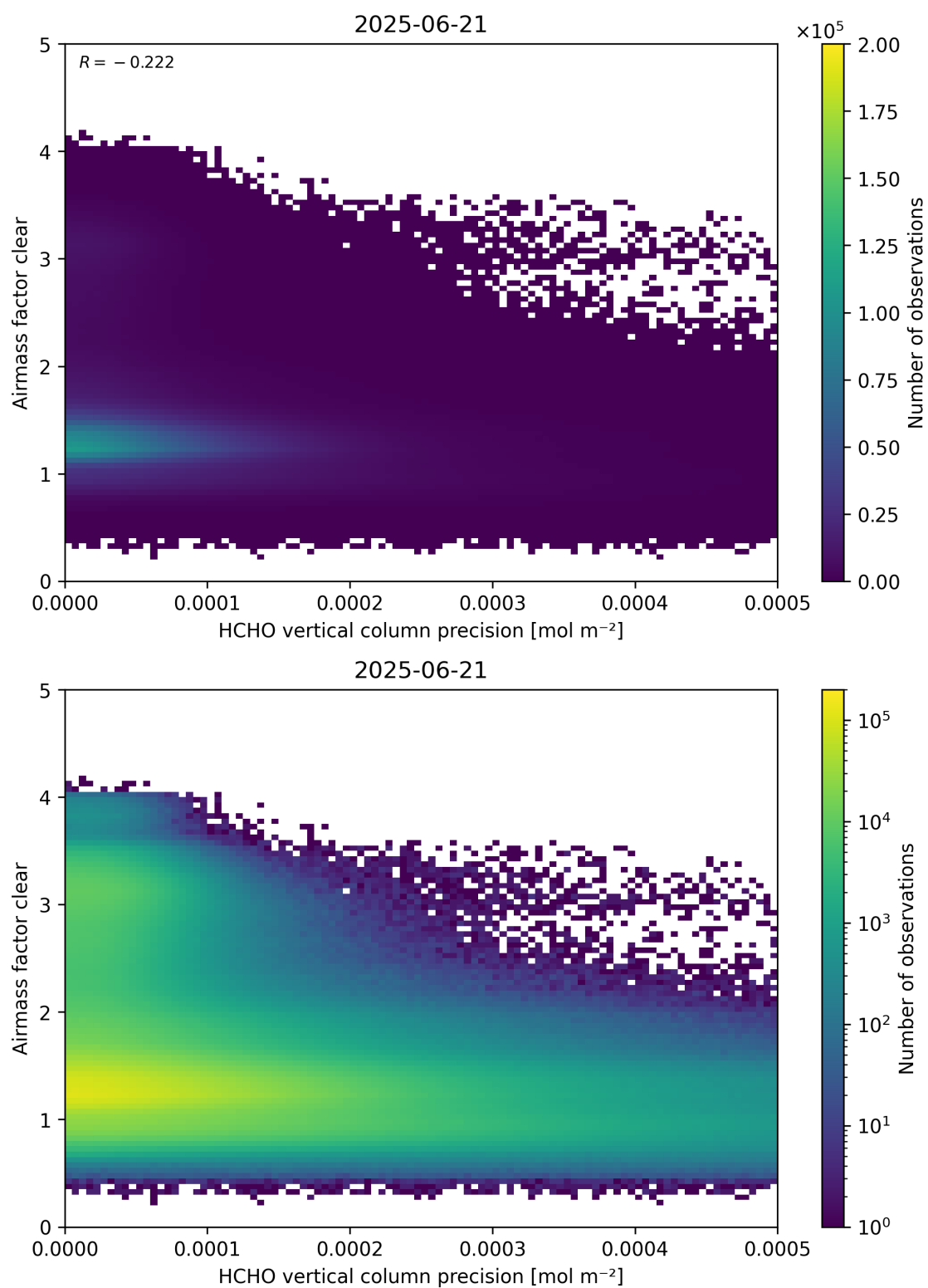
Figure 139: Scatter density plot of “HCHO vertical column precision” against “Airmass factor clear” for 2025-06-20 to 2025-06-22.
