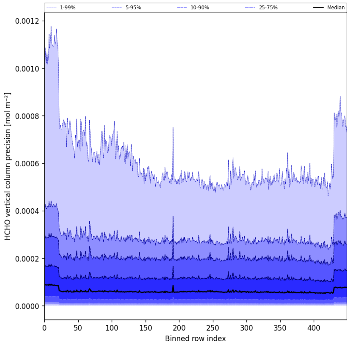
Figure 50: Along track statistics of “HCHO vertical column precision” for 2025-06-20 to 2025-06-22
