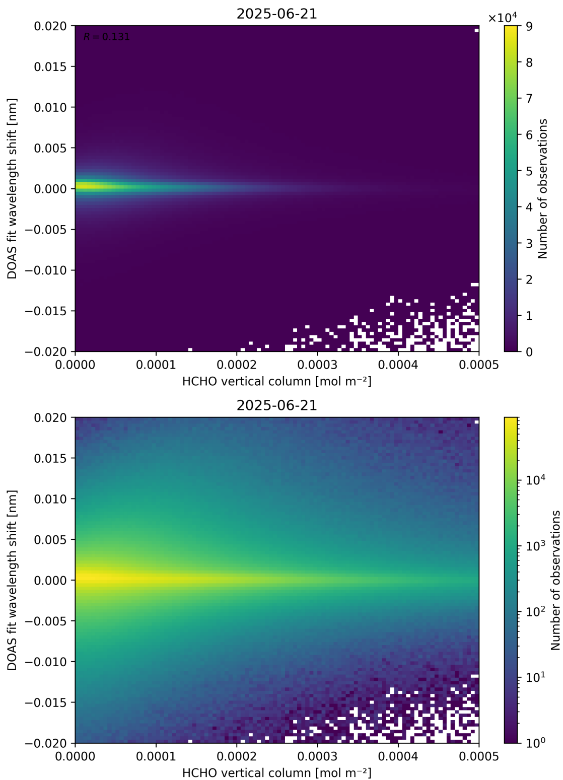
Figure 124: Scatter density plot of “HCHO vertical column” against “DOAS fit wavelength shift” for 2025-06-20 to 2025-06-22.
