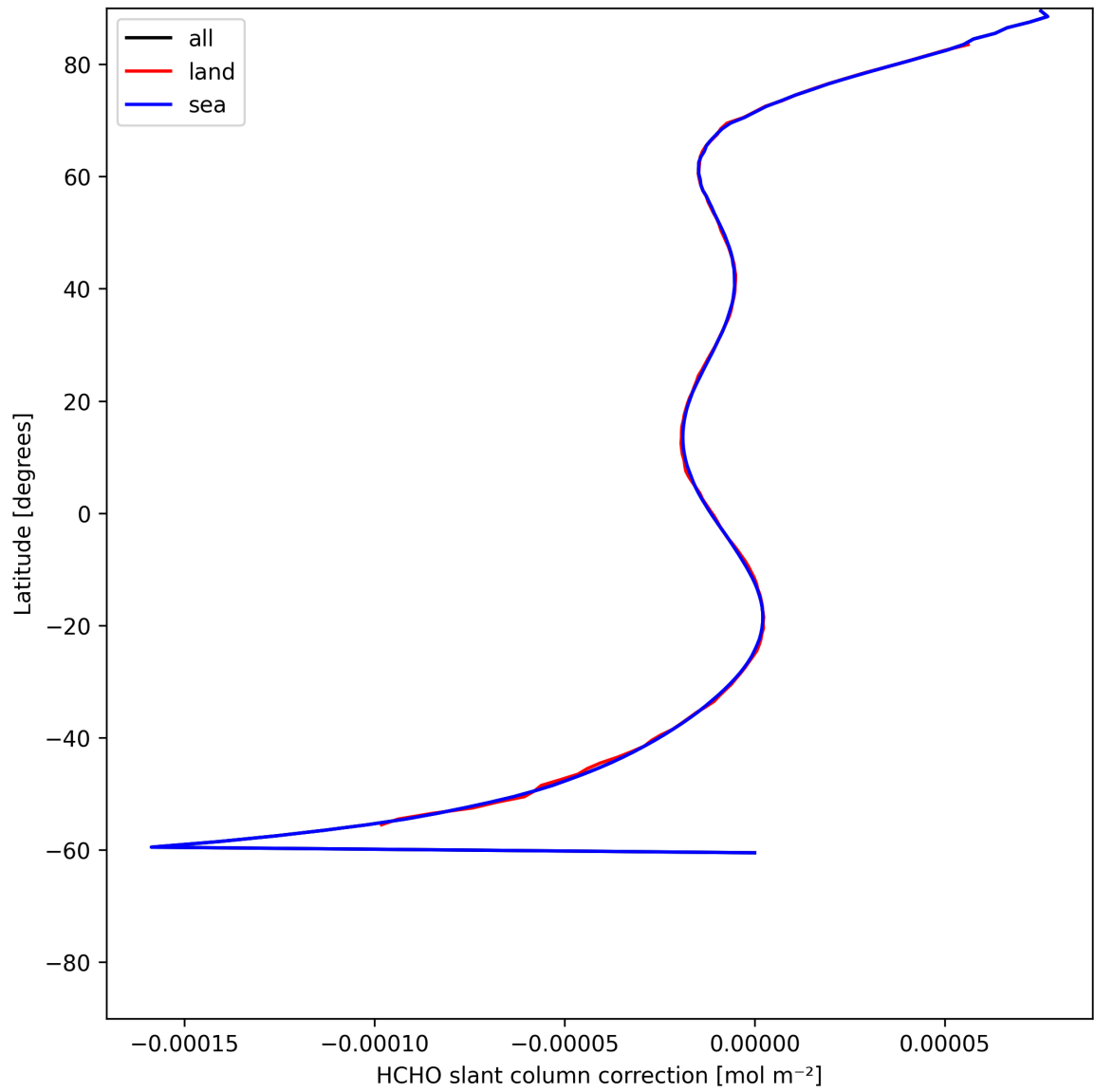
Figure 33: Zonal average of “HCHO slant column correction” for 2025-06-20 to 2025-06-22.
