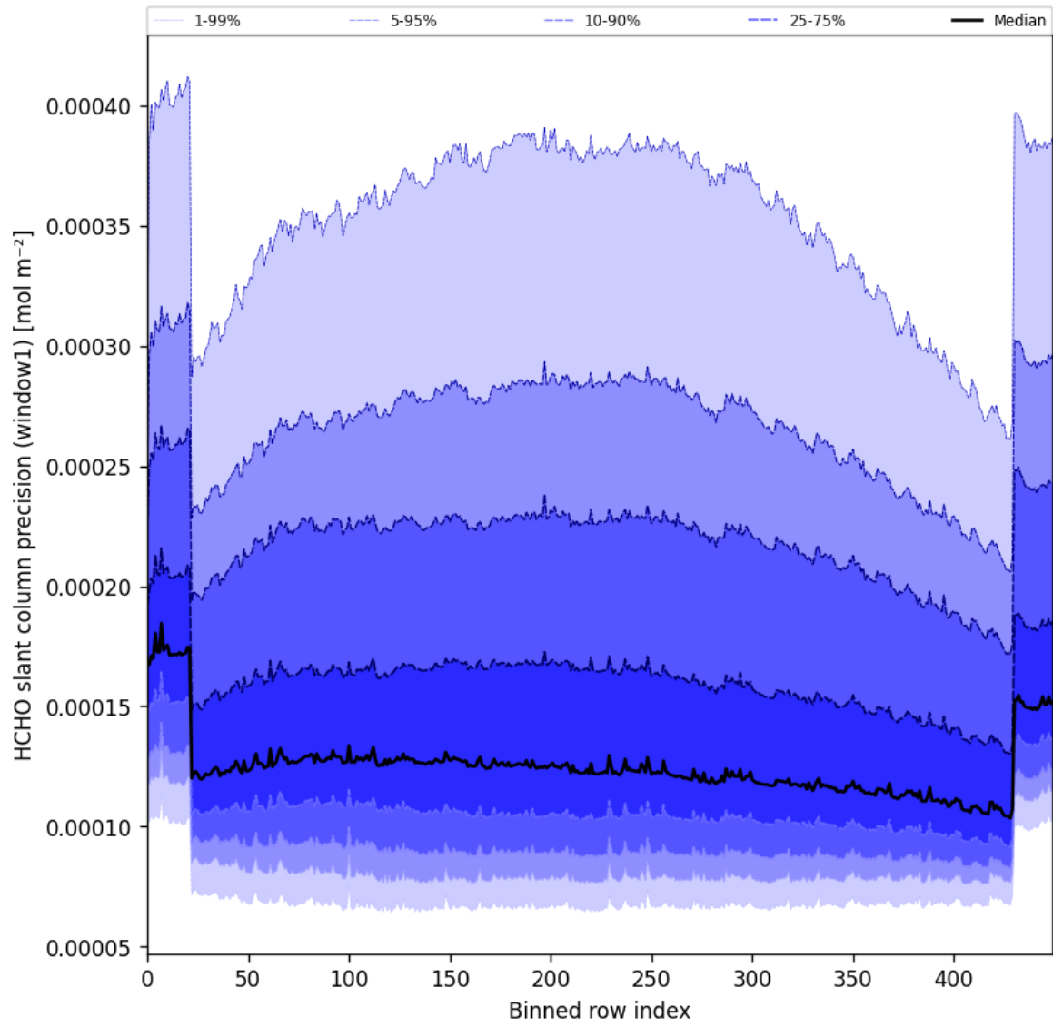
Figure 53: Along track statistics of “HCHO slant column precision (window1)” for 2025-06-20 to 2025-06-22
