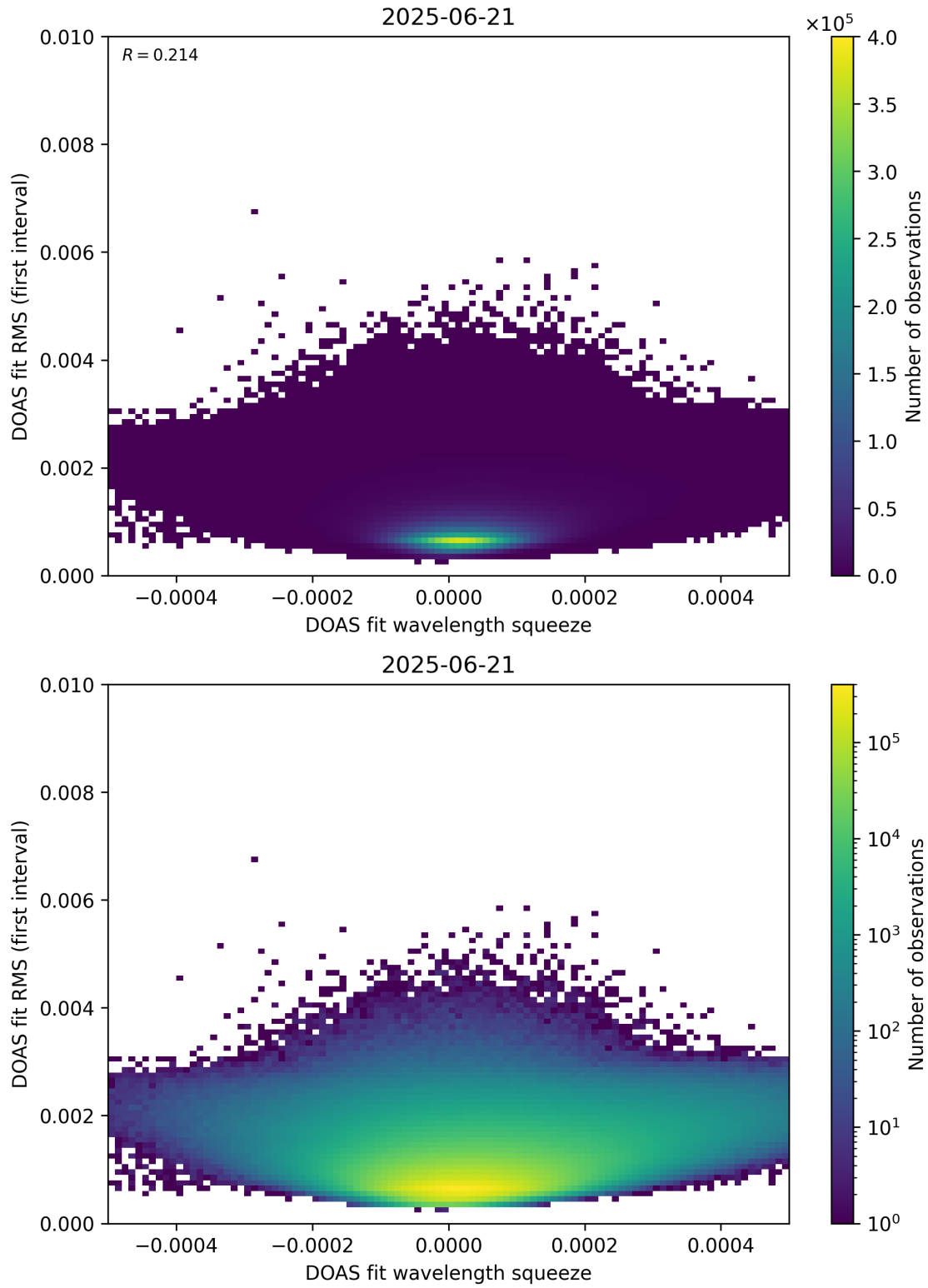
Figure 68: Scatter density plot of “DOAS fit wavelength squeeze” against “DOAS fit RMS (first interval)” for 2025-06-20 to 2025-06-22.
