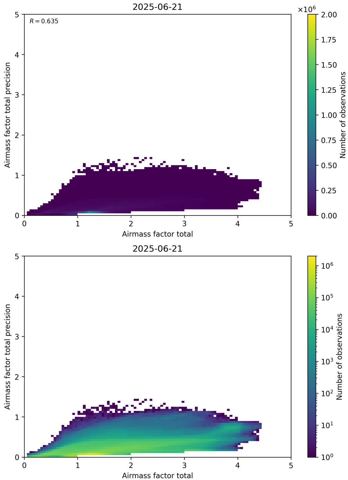
Figure 103: Scatter density plot of “Airmass factor total” against “Airmass factor total precision” for 2025-06-20 to 2025-06-22.
