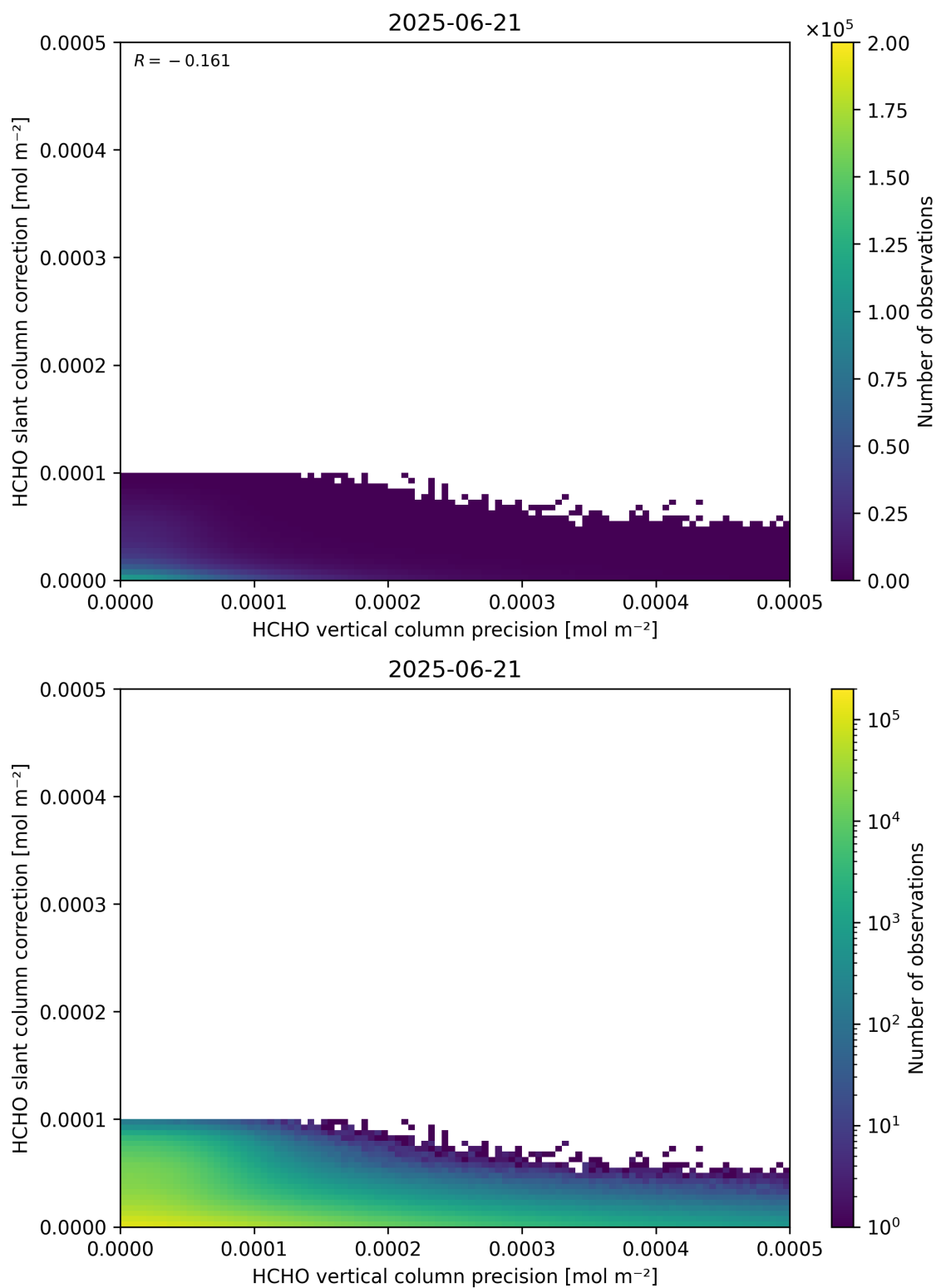
Figure 141: Scatter density plot of “HCHO vertical column precision” against “HCHO slant column correction” for 2025-06-20 to 2025-06-22.
