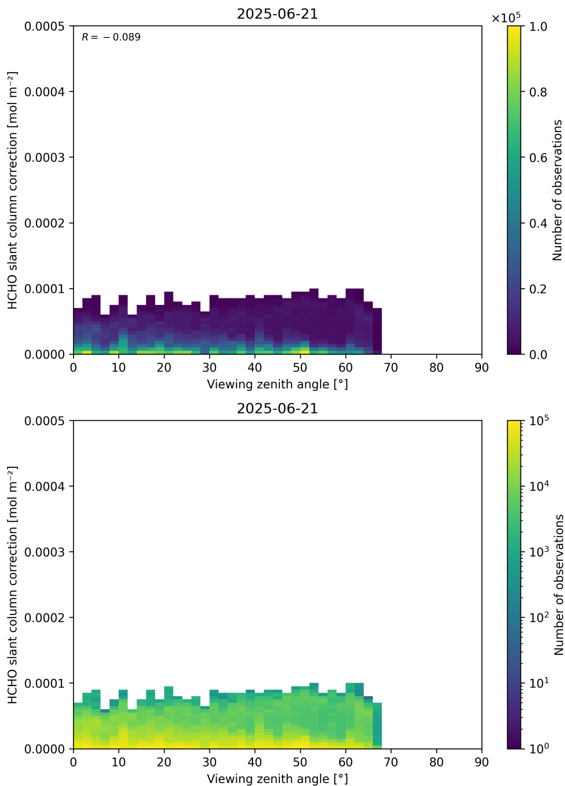
Figure 187: Scatter density plot of “Viewing zenith angle” against “HCHO slant column correction” for 2025-06-20 to 2025-06-22.
