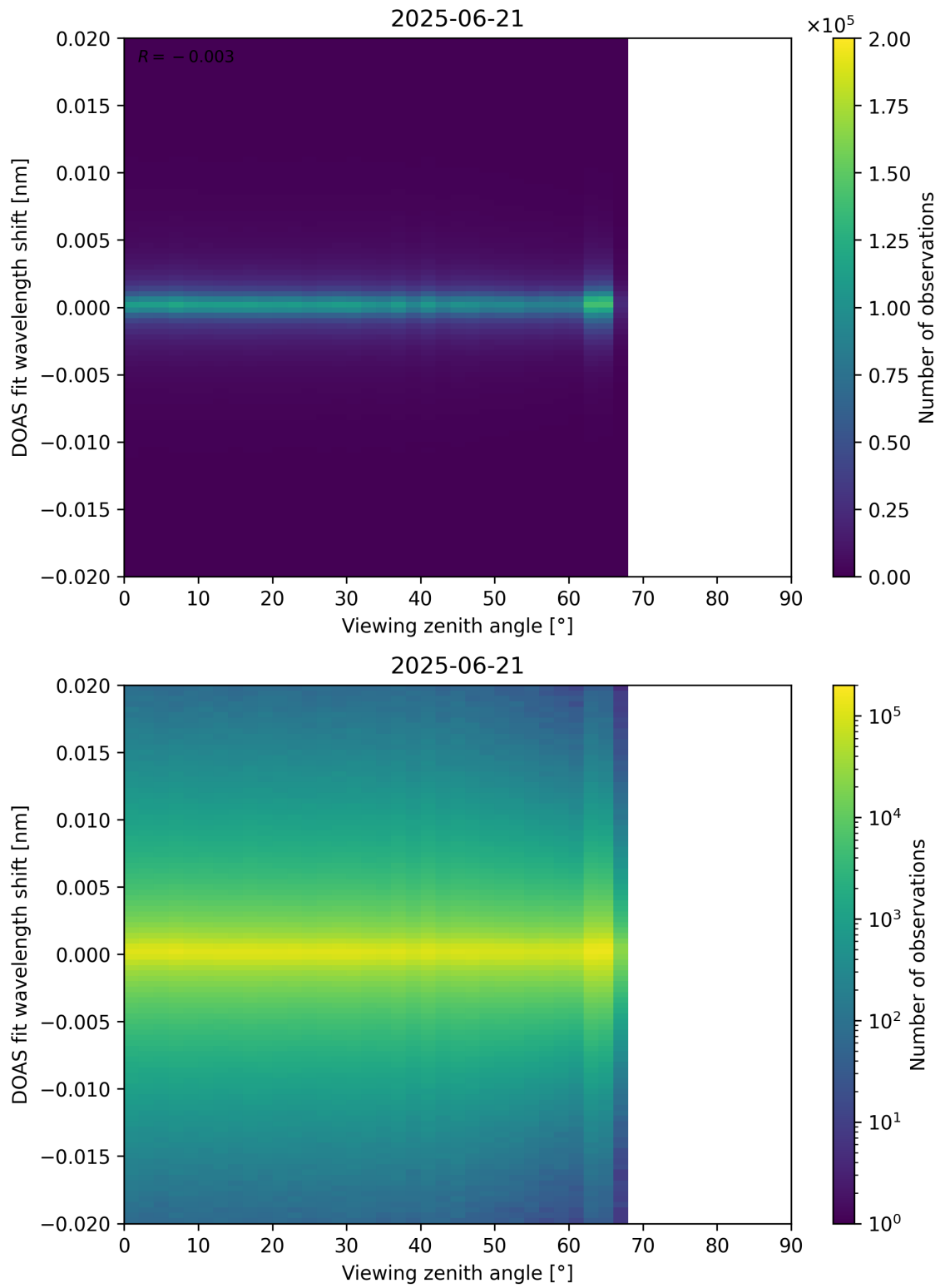
Figure 183: Scatter density plot of “Viewing zenith angle” against “DOAS fit wavelength shift” for 2025-06-20 to 2025-06-22.
