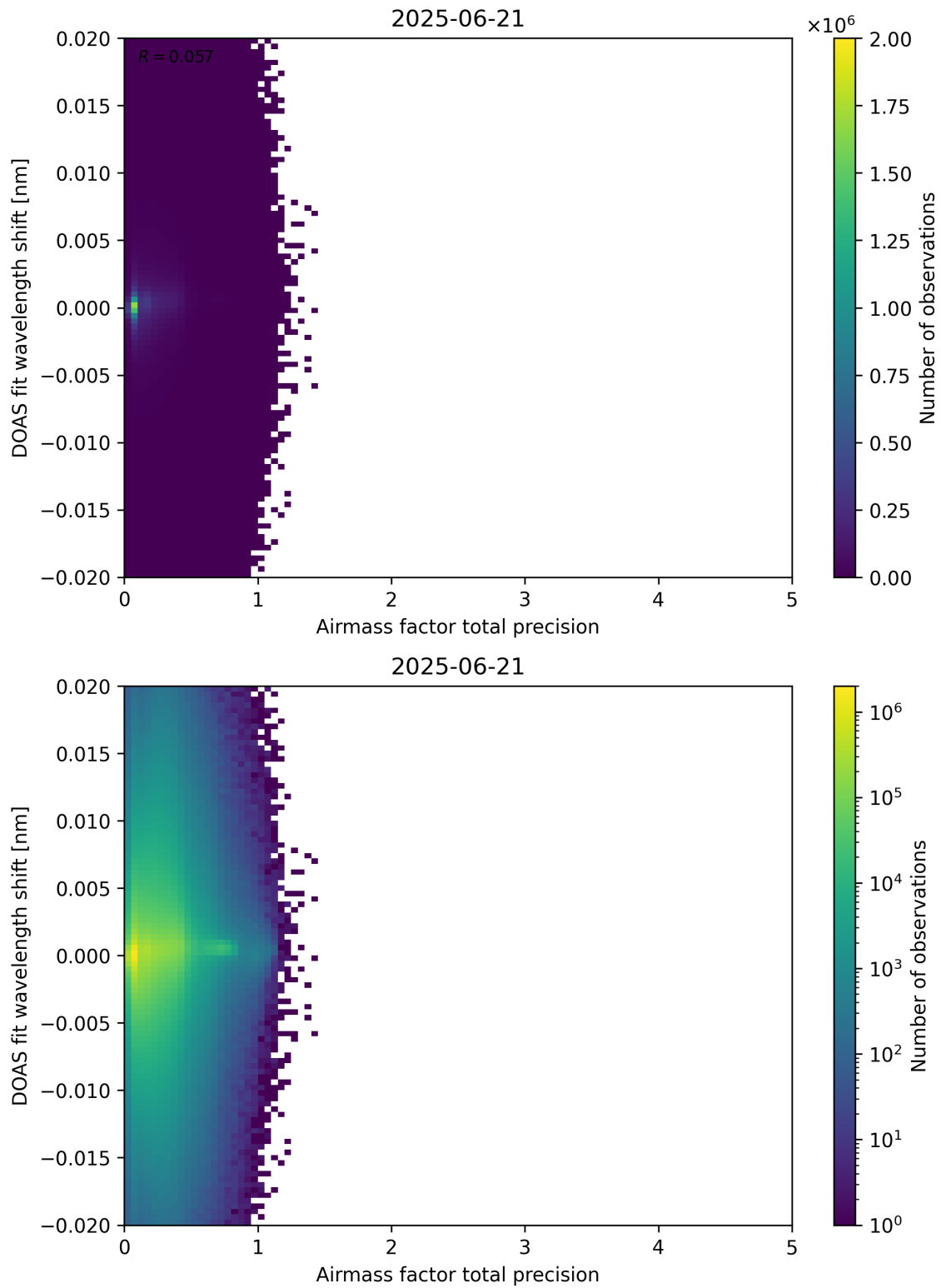
Figure 106: Scatter density plot of “Airmass factor total precision” against “DOAS fit wavelength shift” for 2025-06-20 to 2025-06-22.
