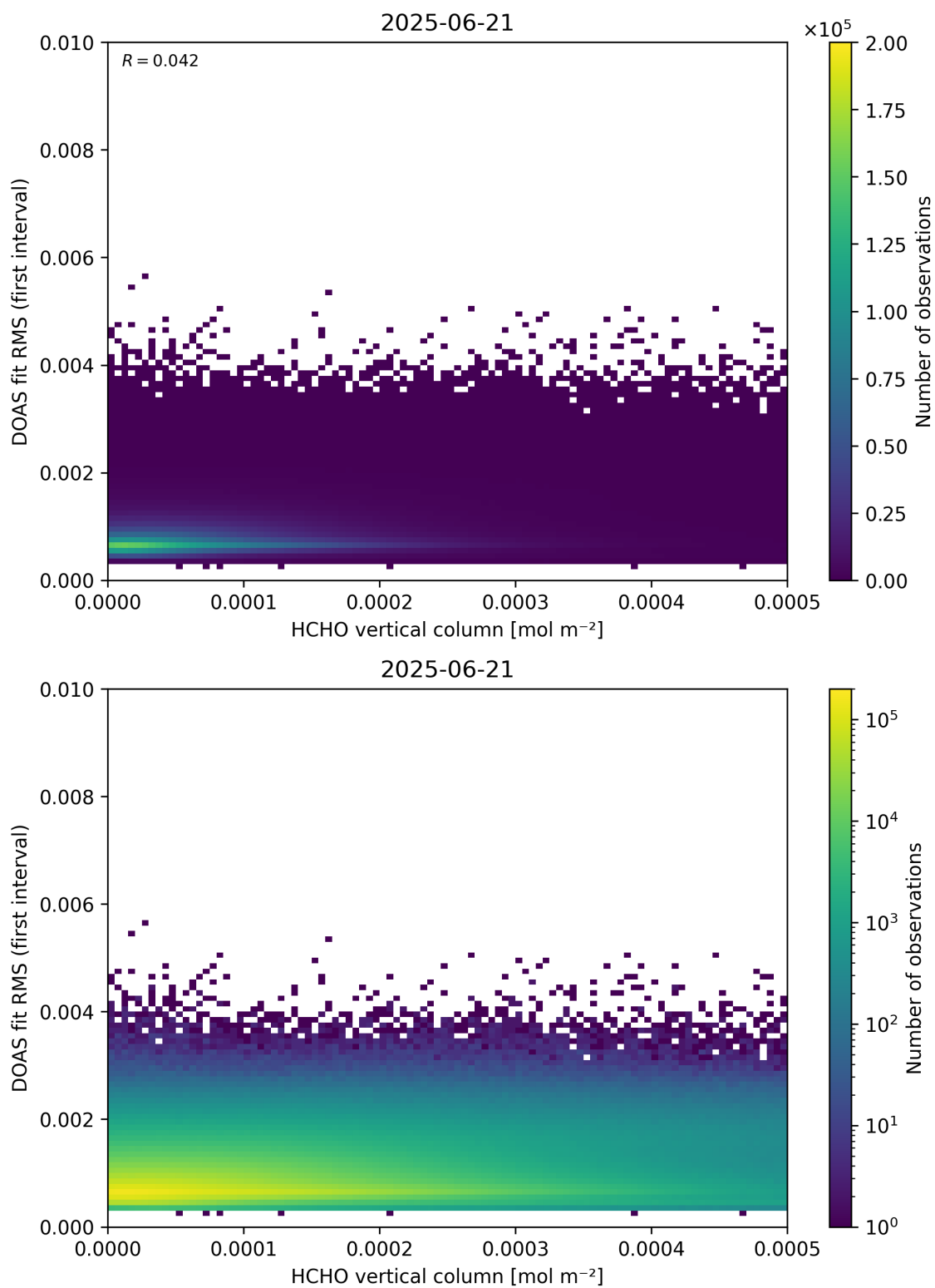
Figure 123: Scatter density plot of “HCHO vertical column” against “DOAS fit RMS (first interval)” for 2025-06-20 to 2025-06-22.
