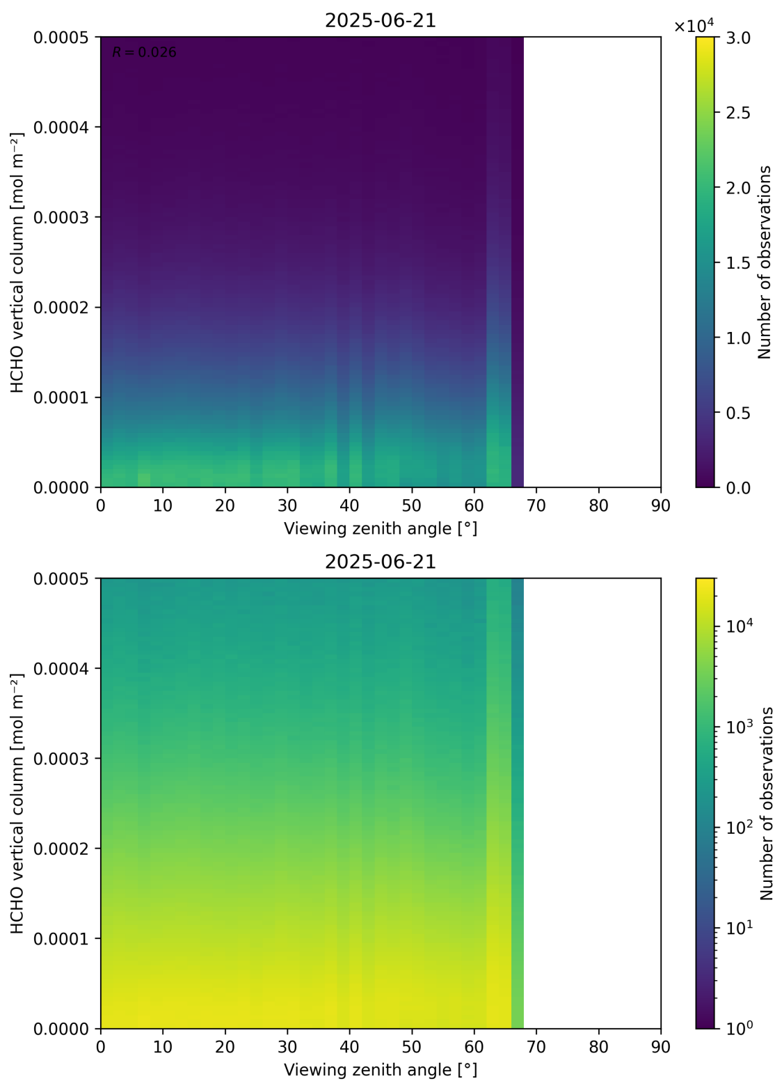
Figure 192: Scatter density plot of “Viewing zenith angle” against “HCHO vertical column” for 2025-06-20 to 2025-06-22.
