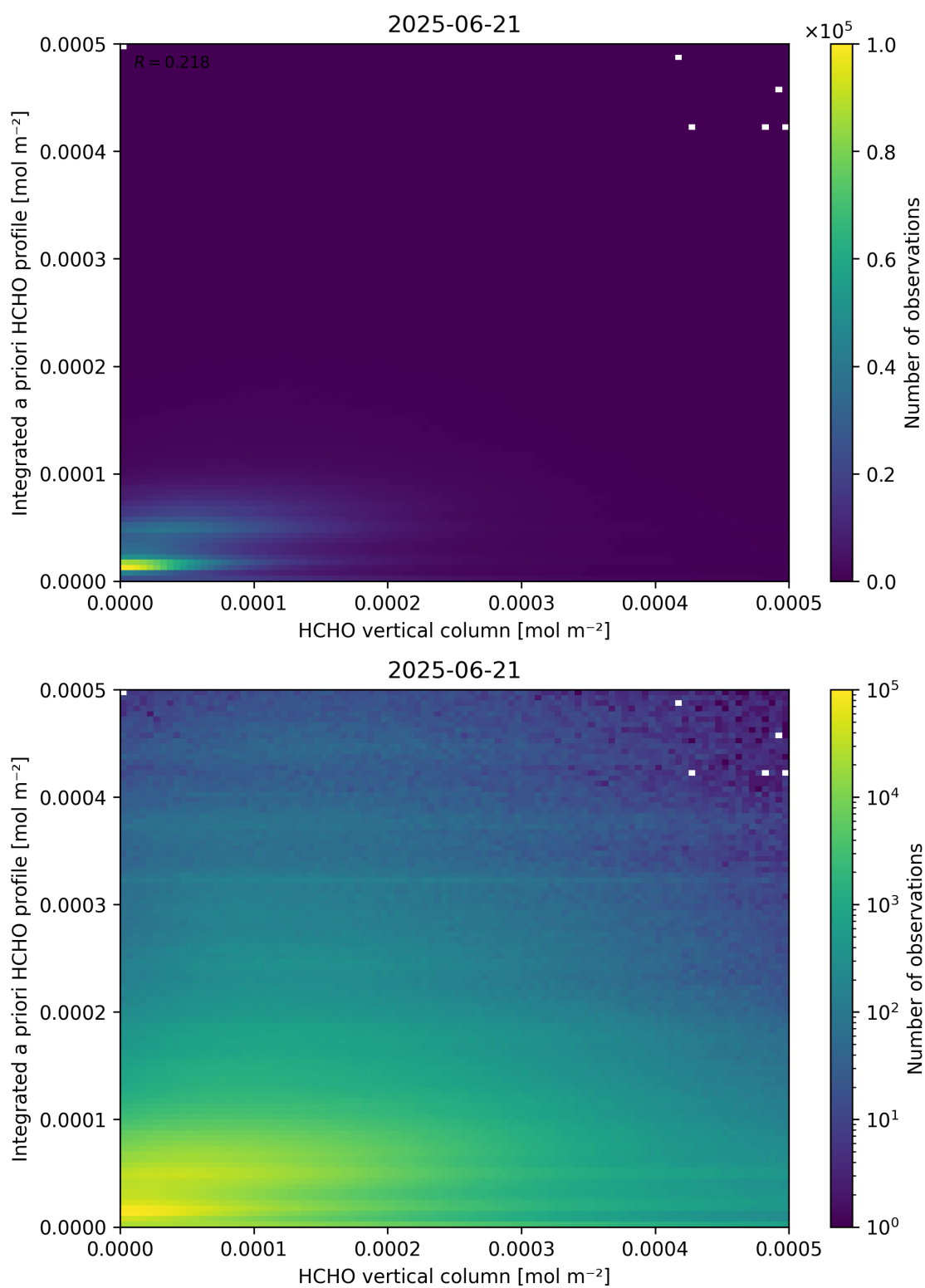
Figure 135: Scatter density plot of “HCHO vertical column” against “Integrated a priori HCHO profile” for 2025-06-20 to 2025-06-22.
