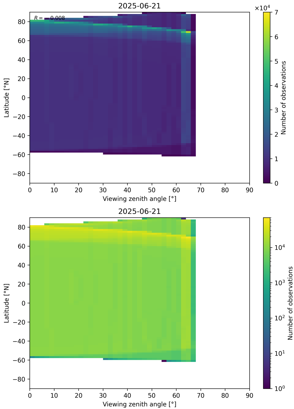
Figure 196: Scatter density plot of “Viewing zenith angle” against “Latitude” for 2025-06-20 to 2025-06-22.
