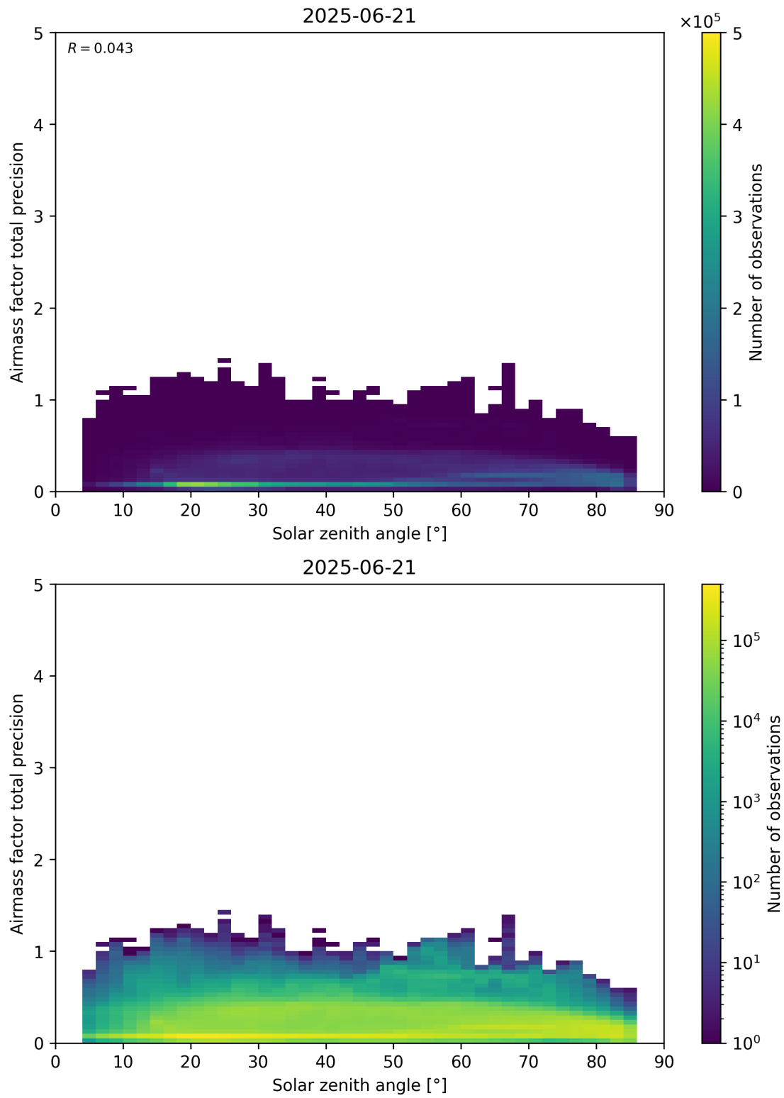
Figure 176: Scatter density plot of “Solar zenith angle” against “Airmass factor total precision” for 2025-06-20 to 2025-06-22.
