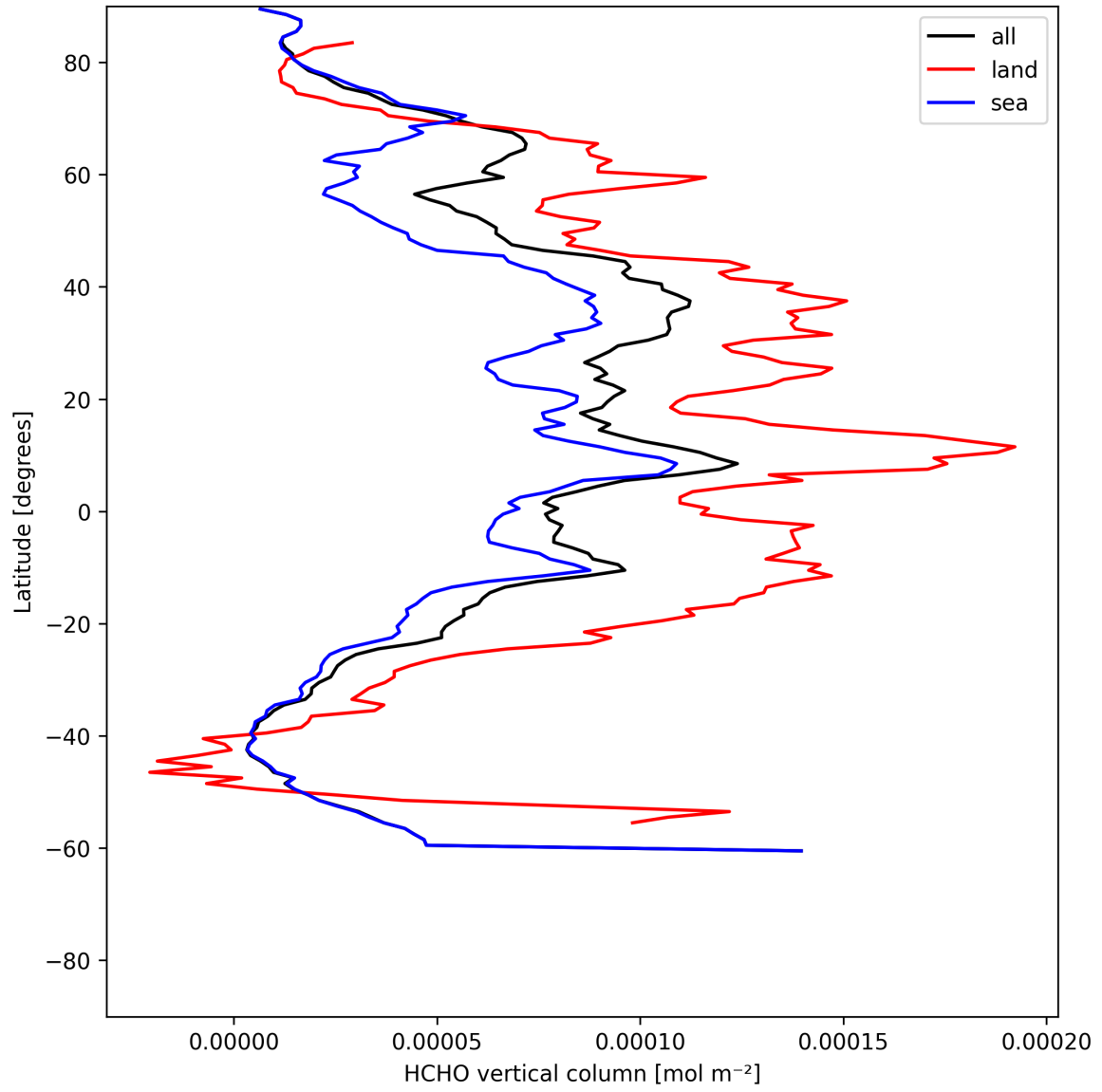
Figure 21: Zonal average of “HCHO vertical column” for 2025-06-20 to 2025-06-22.
