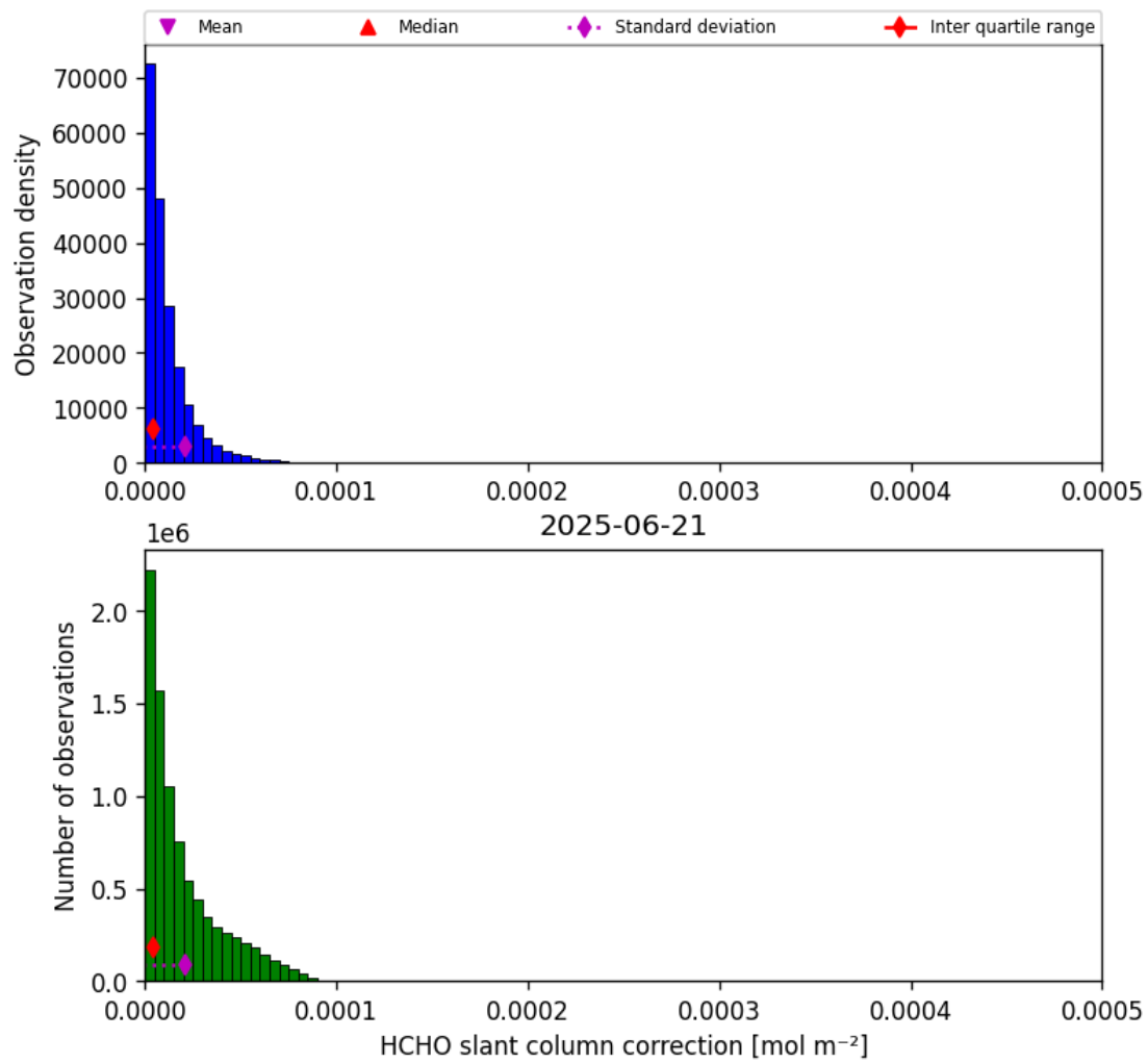
Figure 47: Histogram of "HCHO slant column correction" for 2025-06-20 to 2025-06-22
