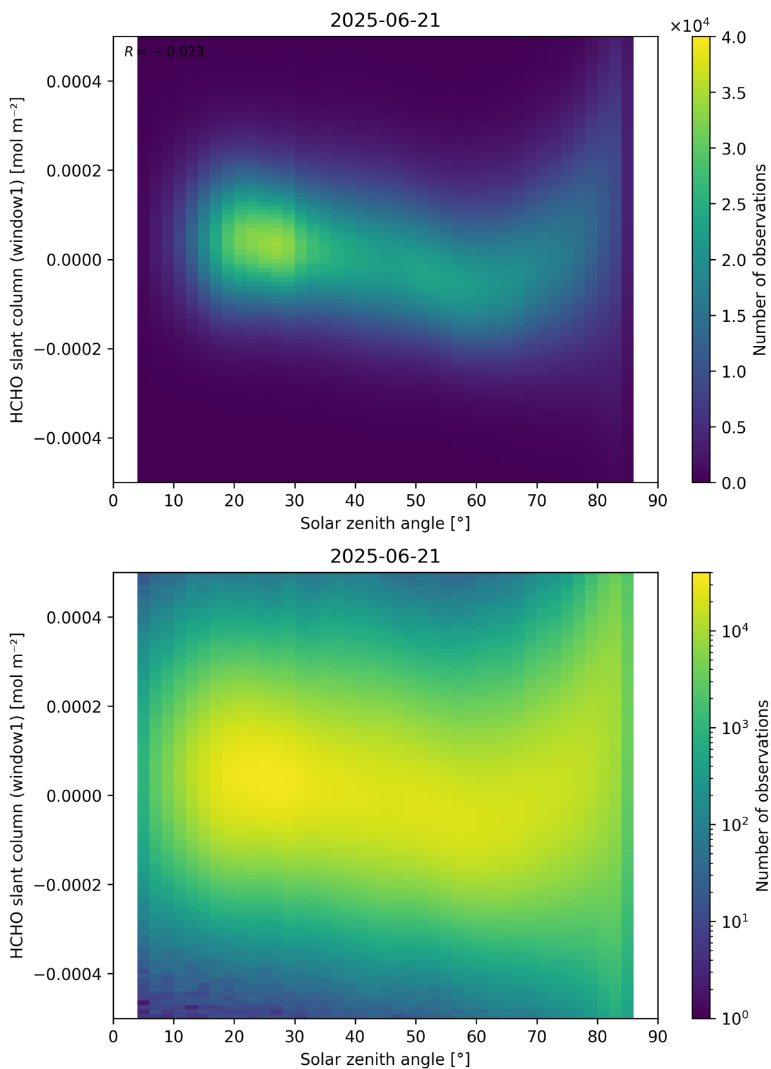
Figure 173: Scatter density plot of “Solar zenith angle” against “HCHO slant column (window1)” for 2025-06-20 to 2025-06-22.
