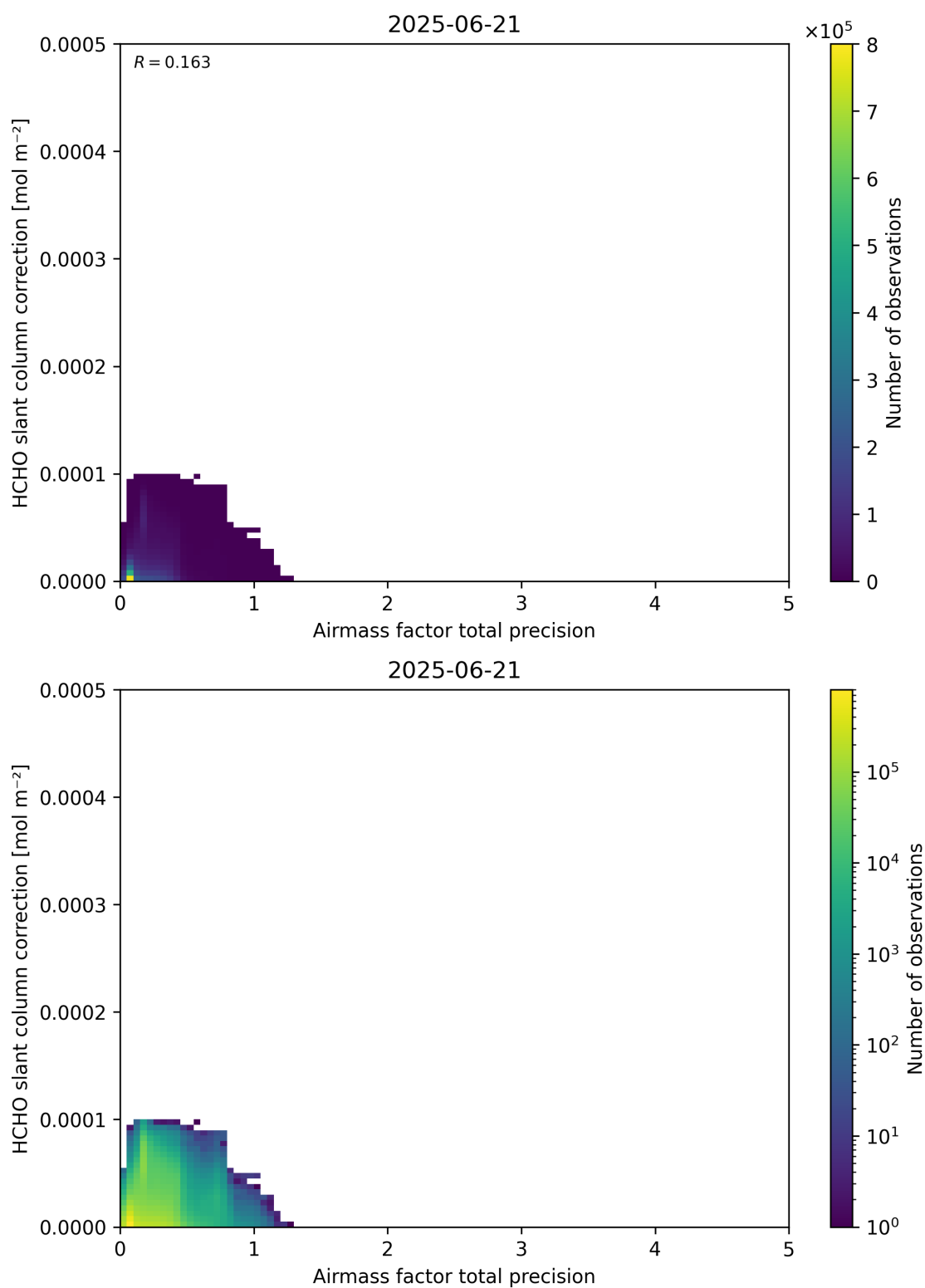
Figure 110: Scatter density plot of “Airmass factor total precision” against “HCHO slant column correction” for 2025-06-20 to 2025-06-22.
