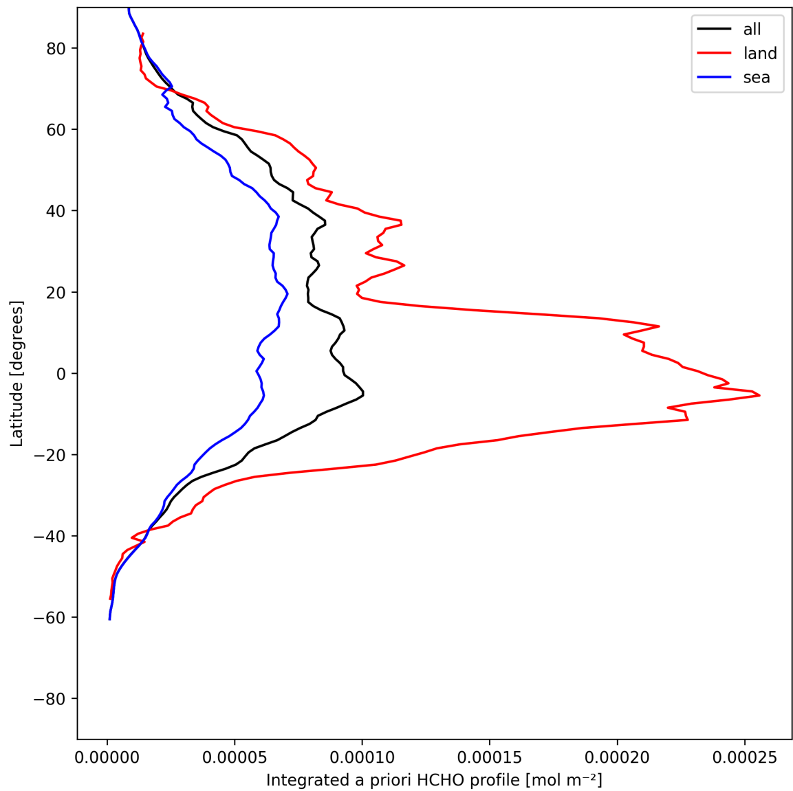
Figure 29: Zonal average of “Integrated a priori HCHO profile” for 2025-06-20 to 2025-06-22.
