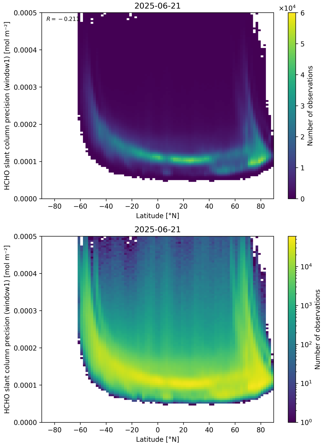
Figure 160: Scatter density plot of “Latitude” against “HCHO slant column precision (window1)” for 2025-06-20 to 2025-06-22.
