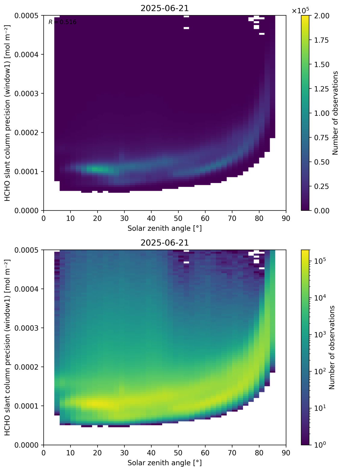
Figure 174: Scatter density plot of “Solar zenith angle” against “HCHO slant column precision (window1)” for 2025-06-20 to 2025-06-22.
