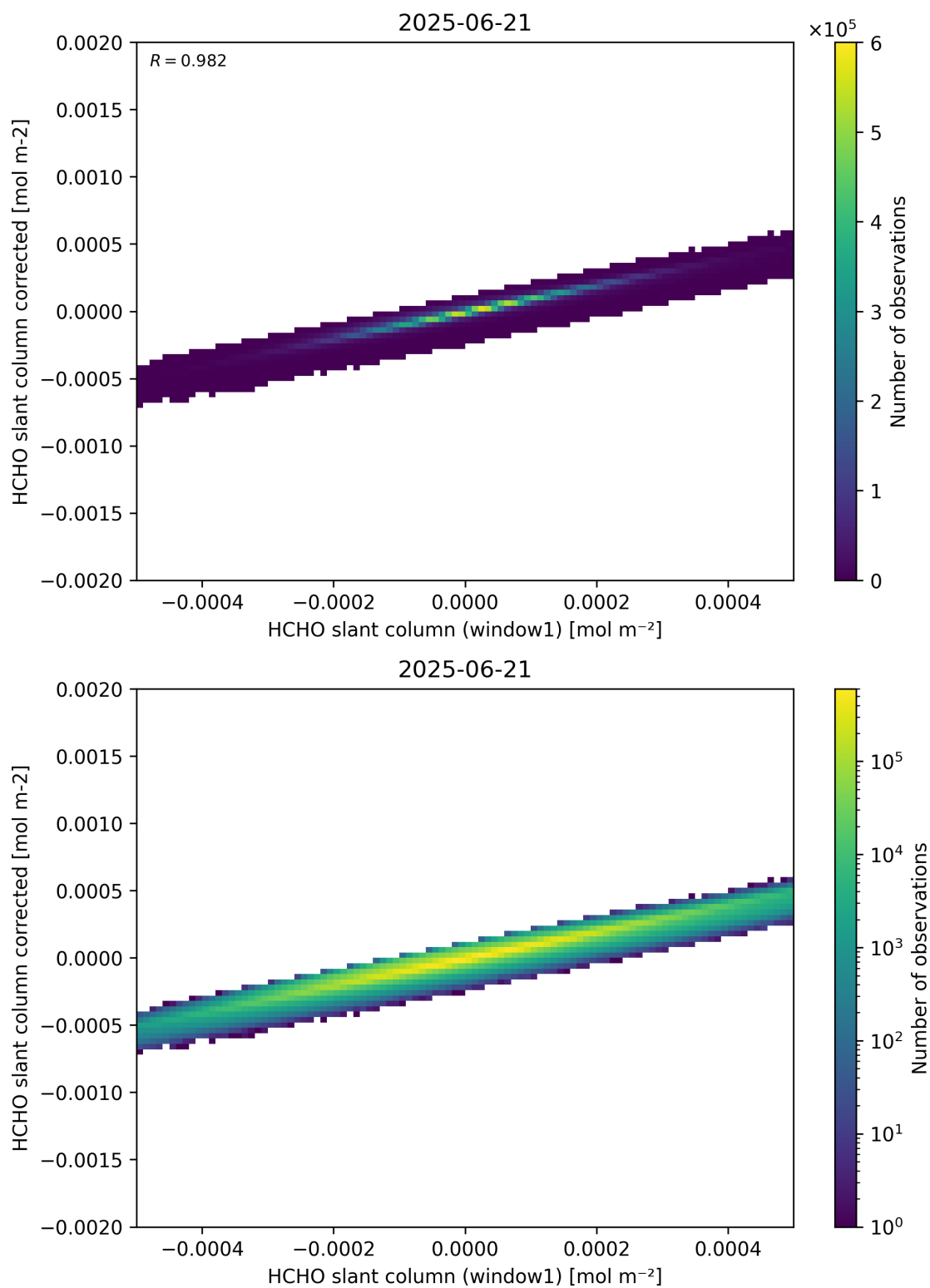
Figure 82: Scatter density plot of “HCHO slant column (window1)” against “HCHO slant column corrected” for 2025-06-20 to 2025-06-22.
