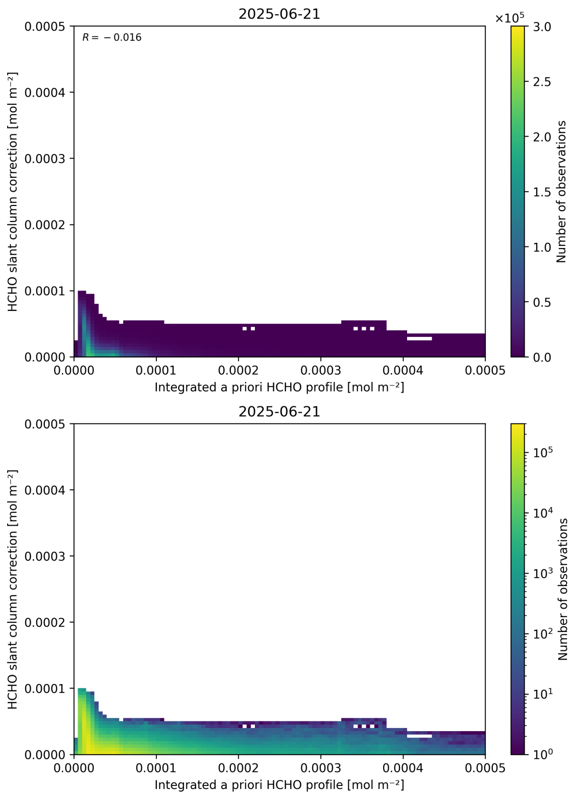
Figure 152: Scatter density plot of “Integrated a priori HCHO profile” against “HCHO slant column correction” for 2025-06-20 to 2025-06-22.
