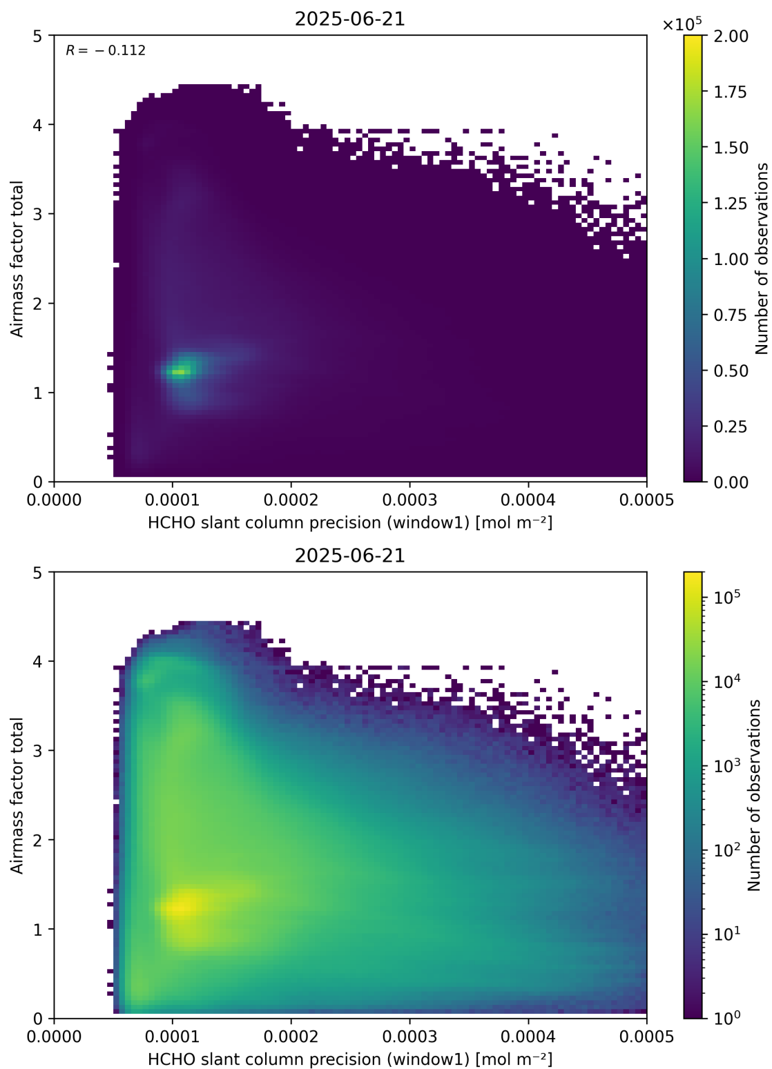
Figure 94: Scatter density plot of “HCHO slant column precision (window1)” against “Airmass factor total” for 2025-06-20 to 2025-06-22.
