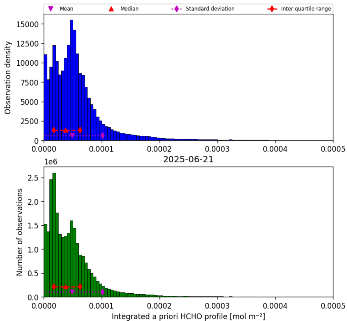
Figure 43: Histogram of “Integrated a priori HCHO profile” for 2025-06-20 to 2025-06-22
