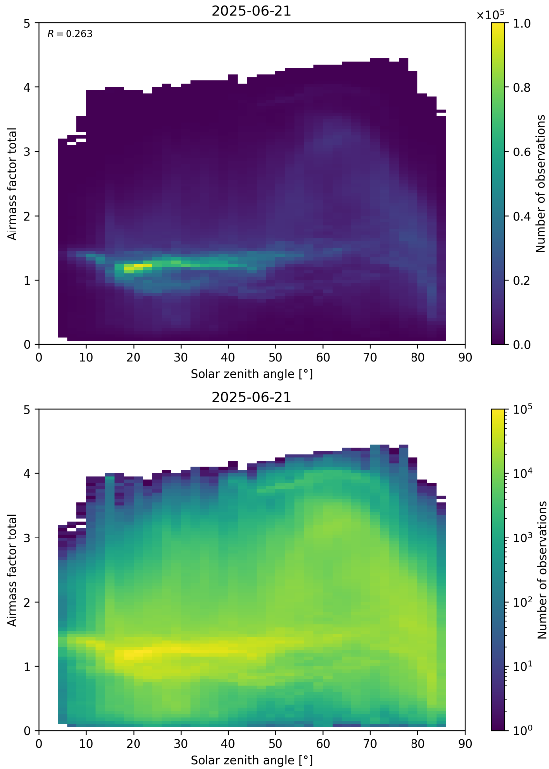
Figure 175: Scatter density plot of “Solar zenith angle” against “Airmass factor total” for 2025-06-20 to 2025-06-22.
