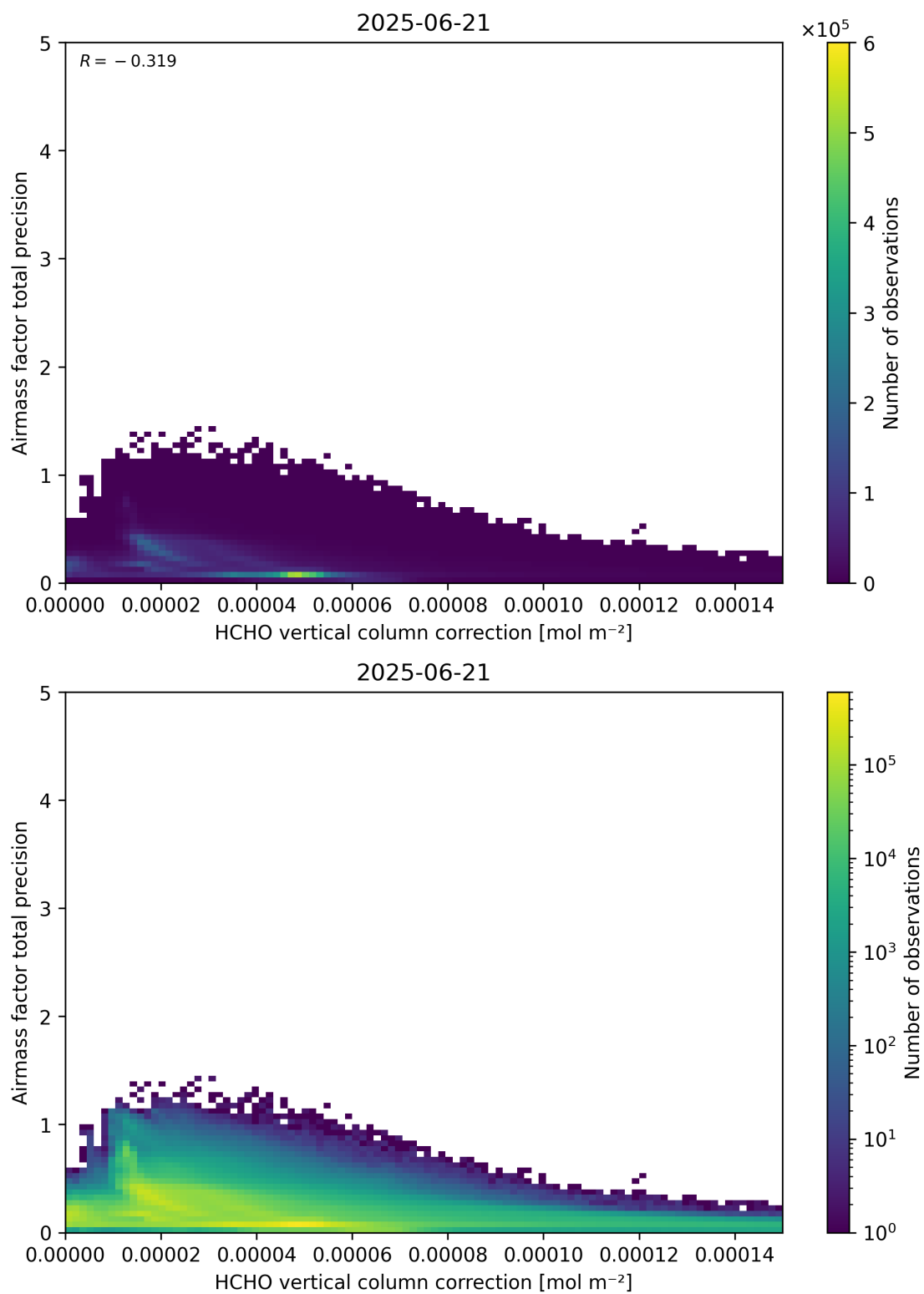
Figure 121: Scatter density plot of “HCHO vertical column correction” against “Airmass factor total precision” for 2025-06-20 to 2025-06-22.
