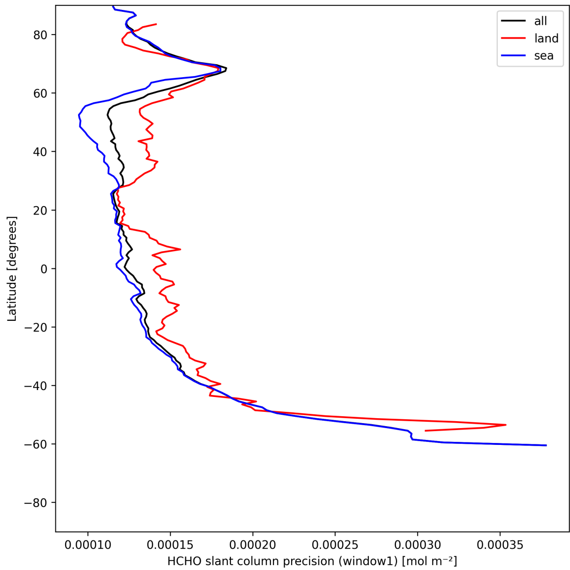
Figure 25: Zonal average of “HCHO slant column precision (window1)” for 2025-06-20 to 2025-06-22.
