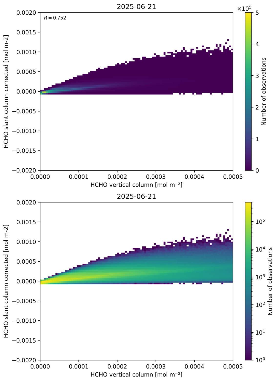
Figure 127: Scatter density plot of “HCHO vertical column” against “HCHO slant column corrected” for 2025-06-20 to 2025-06-22.
