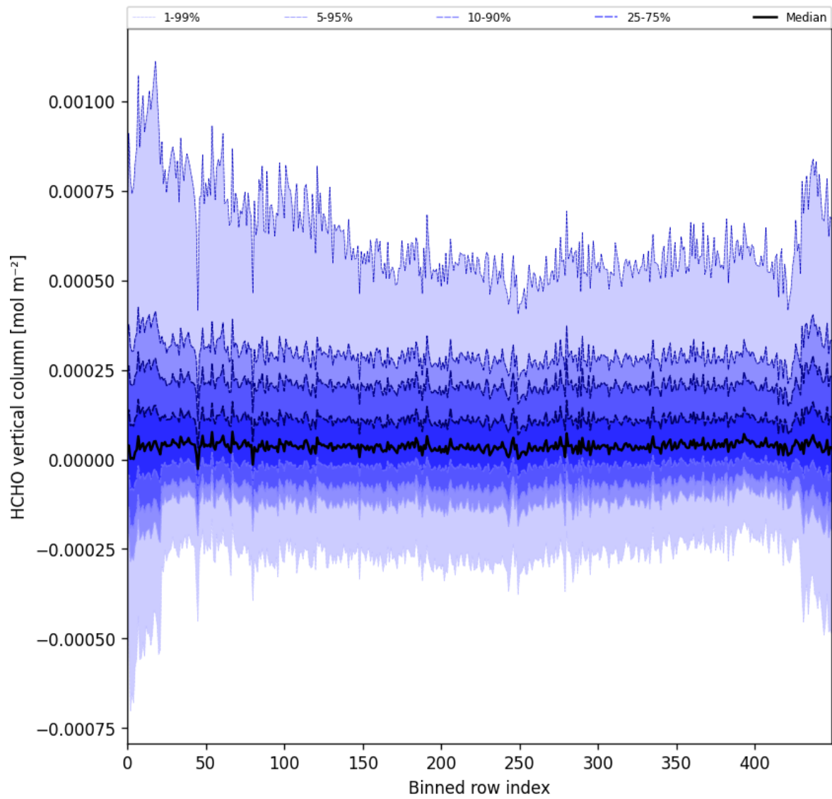
Figure 49: Along track statistics of “HCHO vertical column” for 2025-06-20 to 2025-06-22
