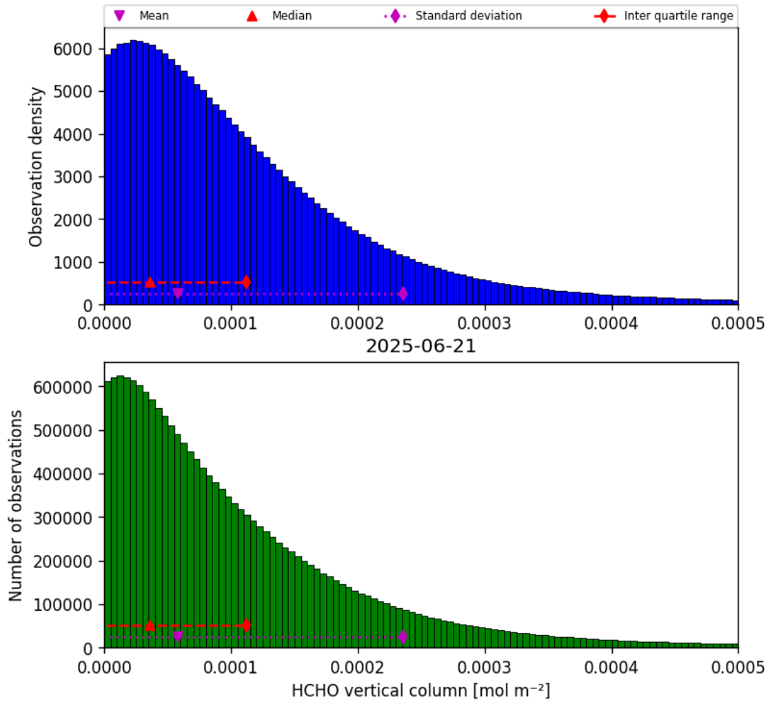
Figure 35: Histogram of “HCHO vertical column” for 2025-06-20 to 2025-06-22
