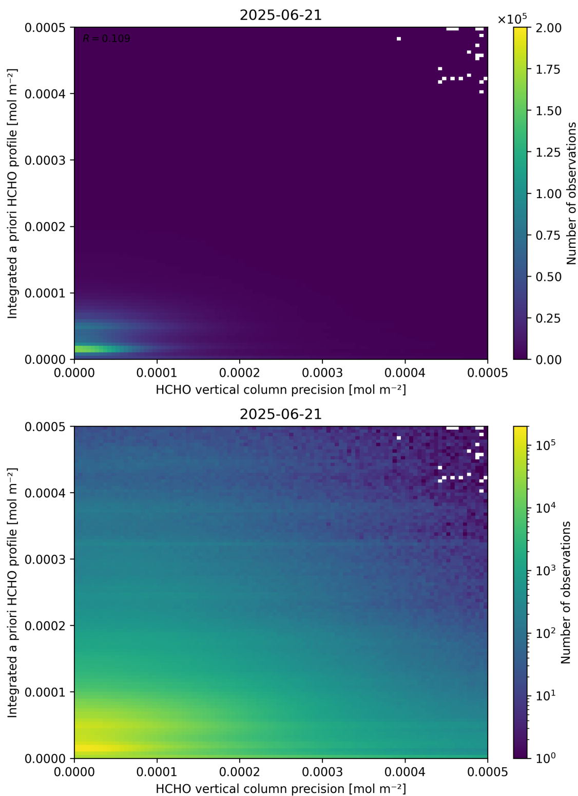
Figure 147: Scatter density plot of “HCHO vertical column precision” against “Integrated a priori HCHO profile” for 2025-06-20 to 2025-06-22.
