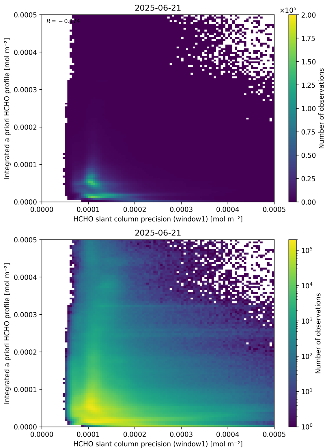
Figure 96: Scatter density plot of “HCHO slant column precision (window1)” against “Integrated a priori HCHO profile” for 2025-06-20 to 2025-06-22.
