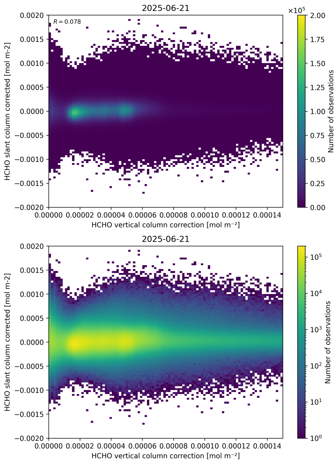
Figure 116: Scatter density plot of “HCHO vertical column correction” against “HCHO slant column corrected” for 2025-06-20 to 2025-06-22.
