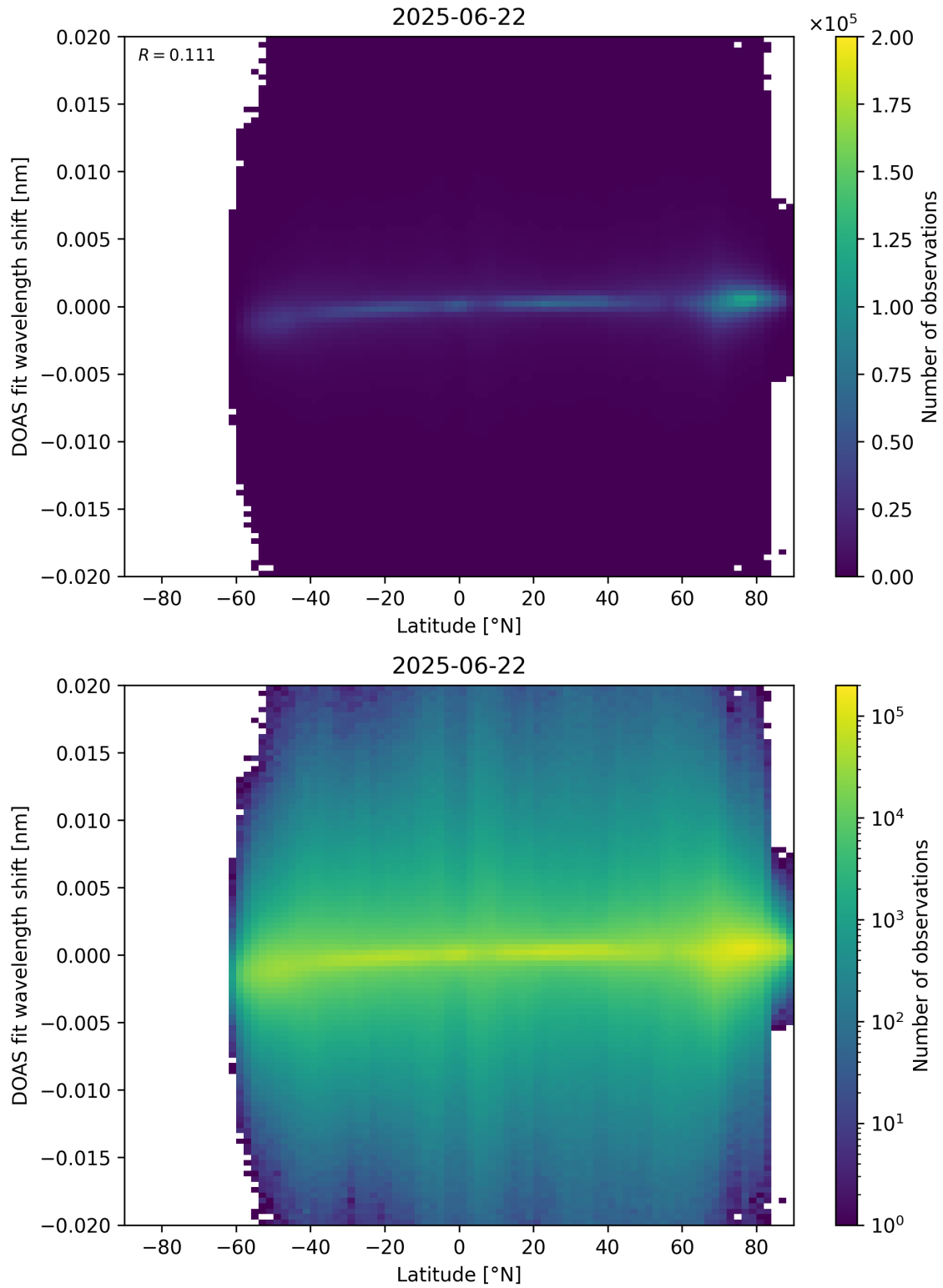
Figure 154: Scatter density plot of “Latitude” against “DOAS fit wavelength shift” for 2025-06-22 to 2025-06-23.
