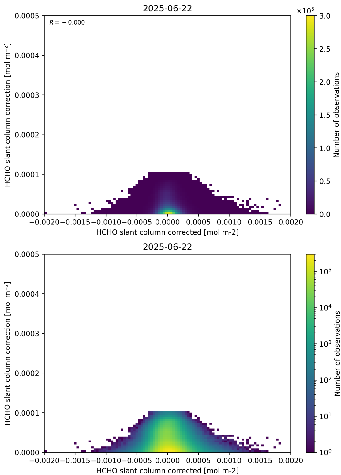
Figure 77: Scatter density plot of “HCHO slant column corrected” against “HCHO slant column correction” for 2025-06-22 to 2025-06-23.
