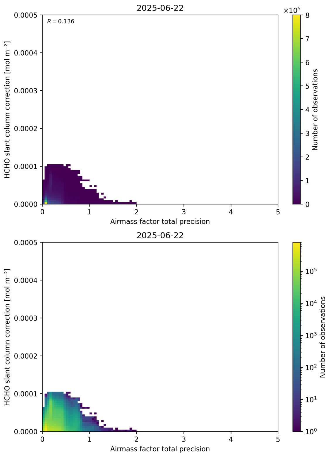
Figure 110: Scatter density plot of “Airmass factor total precision” against “HCHO slant column correction” for 2025-06-22 to 2025-06-23.
