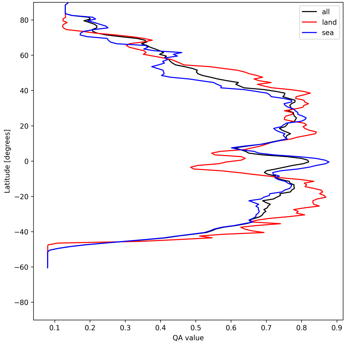
Figure 20: Zonal average of “QA value” for 2025-06-22 to 2025-06-23.
