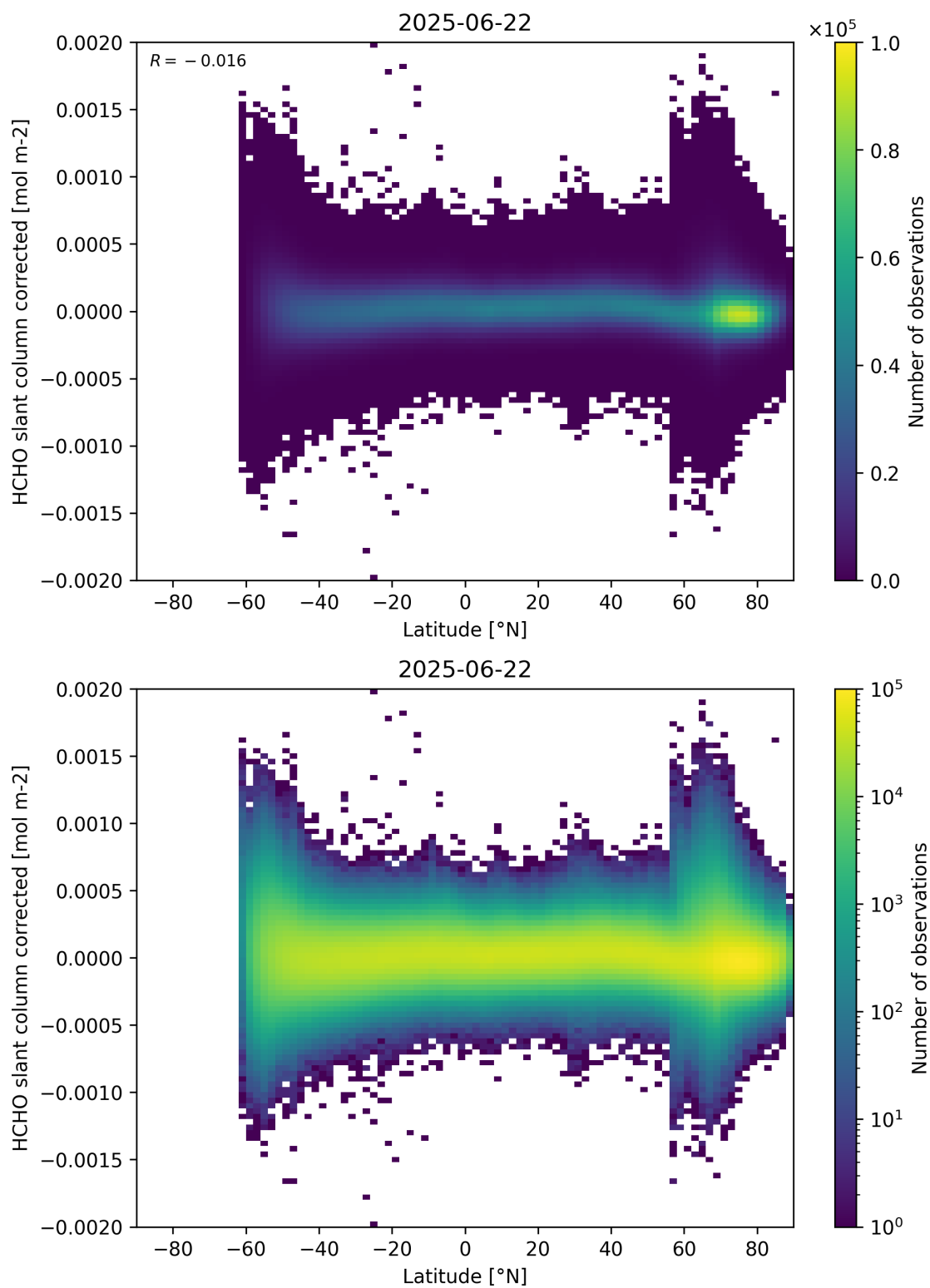
Figure 157: Scatter density plot of “Latitude” against “HCHO slant column corrected” for 2025-06-22 to 2025-06-23.
