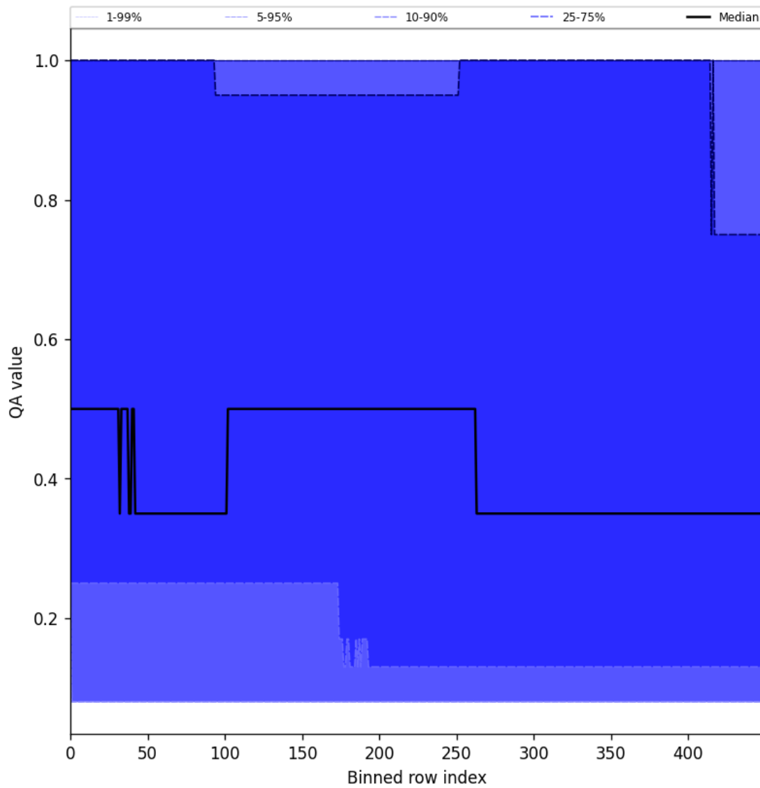
Figure 48: Along track statistics of “QA value” for 2025-06-22 to 2025-06-23
