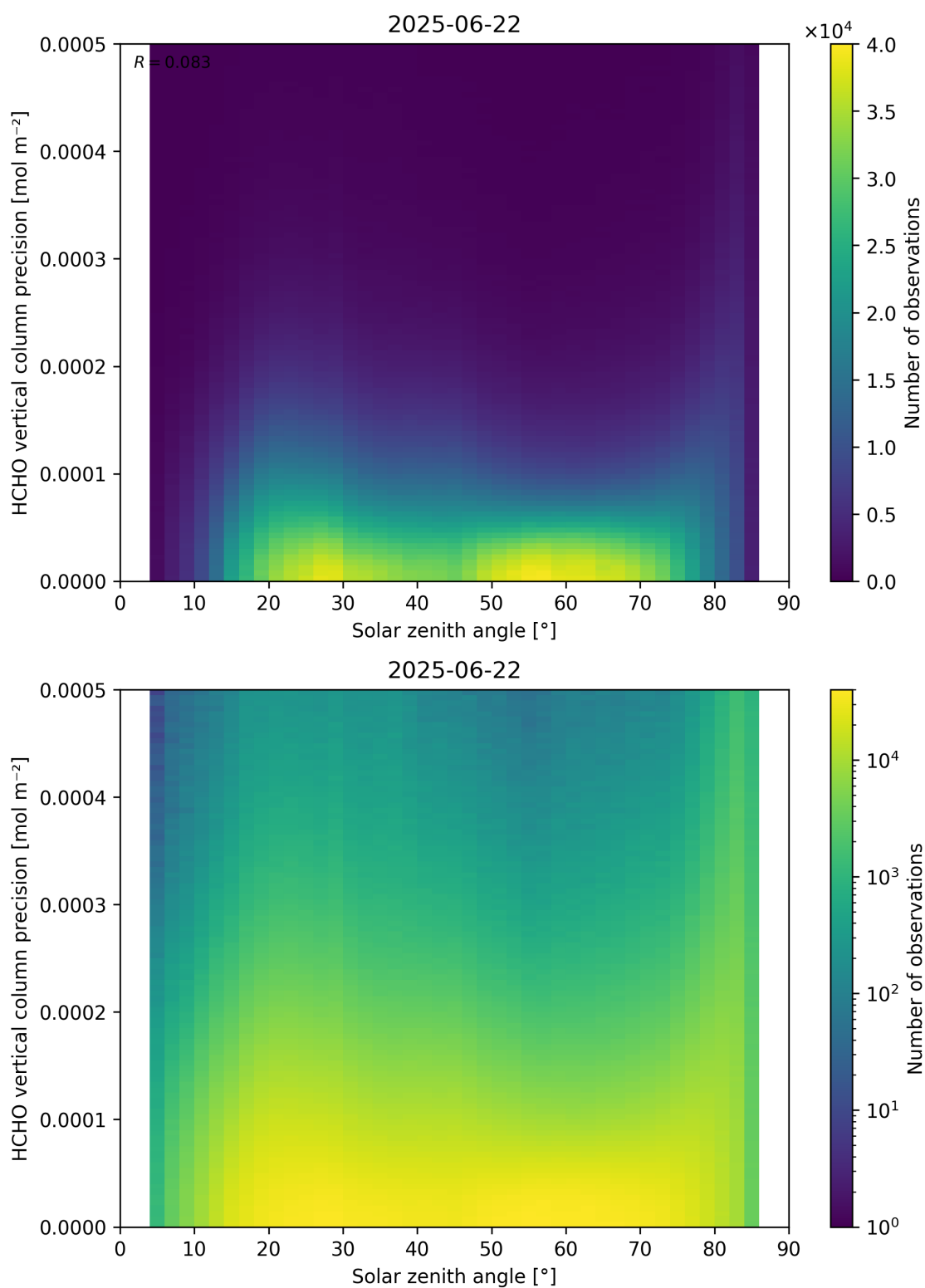
Figure 179: Scatter density plot of “Solar zenith angle” against “HCHO vertical column precision” for 2025-06-22 to 2025-06-23.
