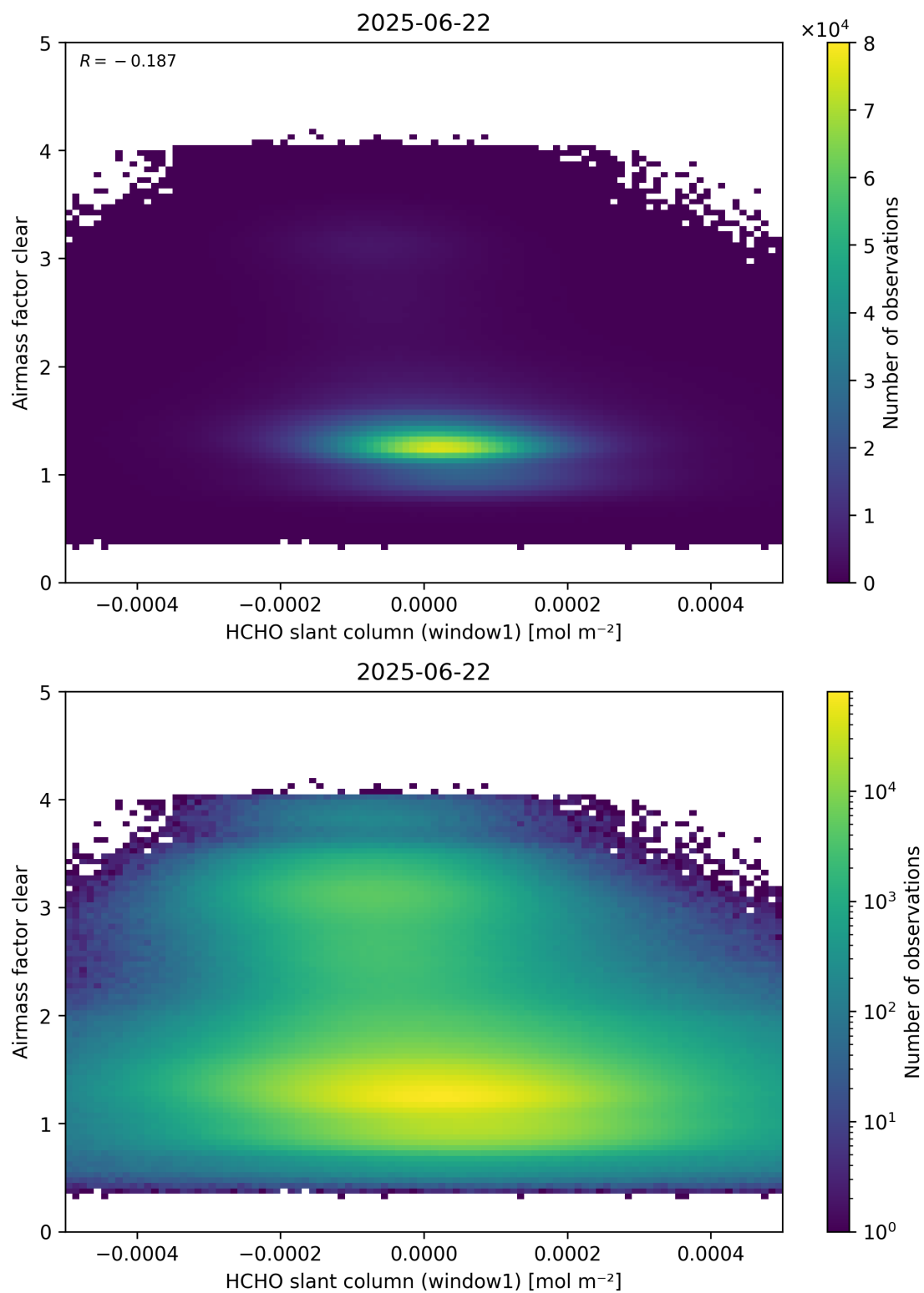
Figure 81: Scatter density plot of “HCHO slant column (window1)” against “Airmass factor clear” for 2025-06-22 to 2025-06-23.
