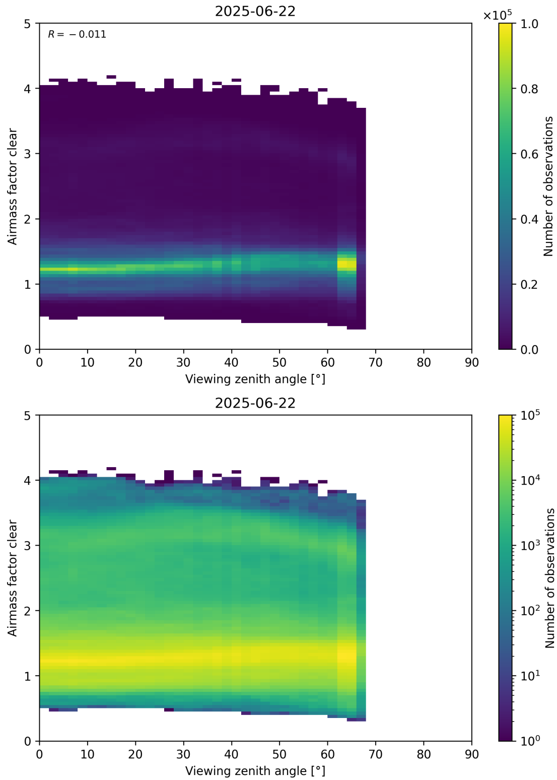
Figure 185: Scatter density plot of “Viewing zenith angle” against “Airmass factor clear” for 2025-06-22 to 2025-06-23.
