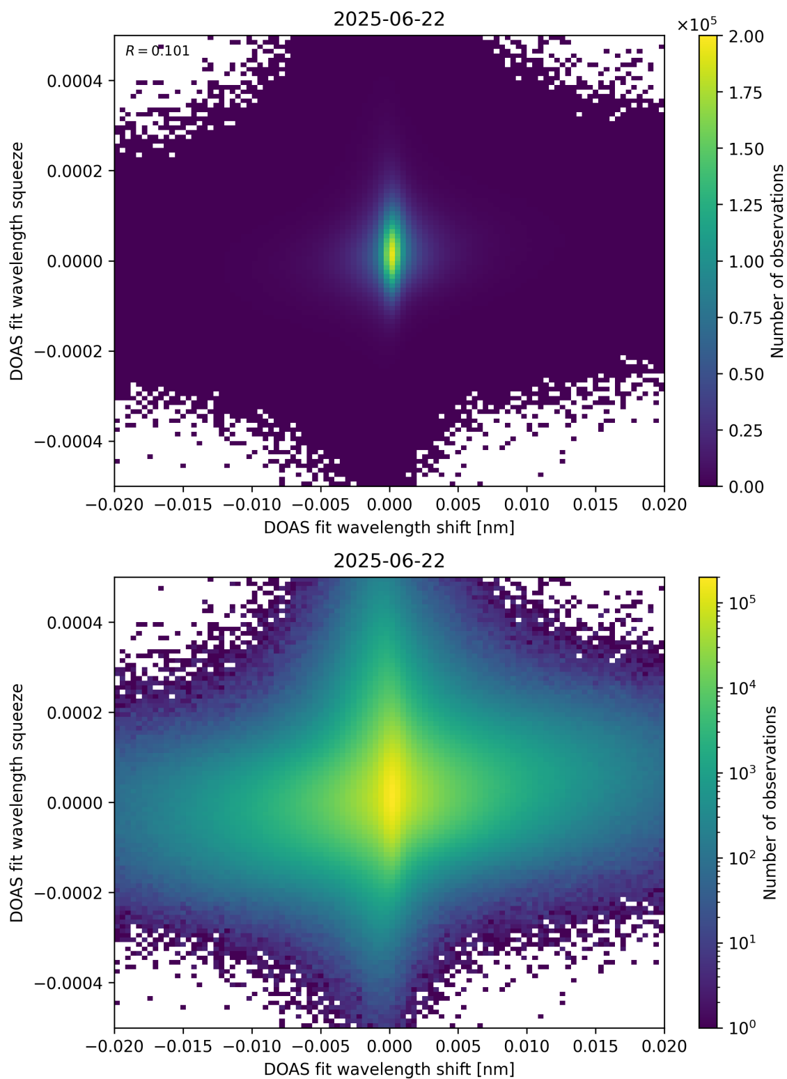
Figure 65: Scatter density plot of “DOAS fit wavelength shift” against “DOAS fit wavelength squeeze” for 2025-06-22 to 2025-06-23.
