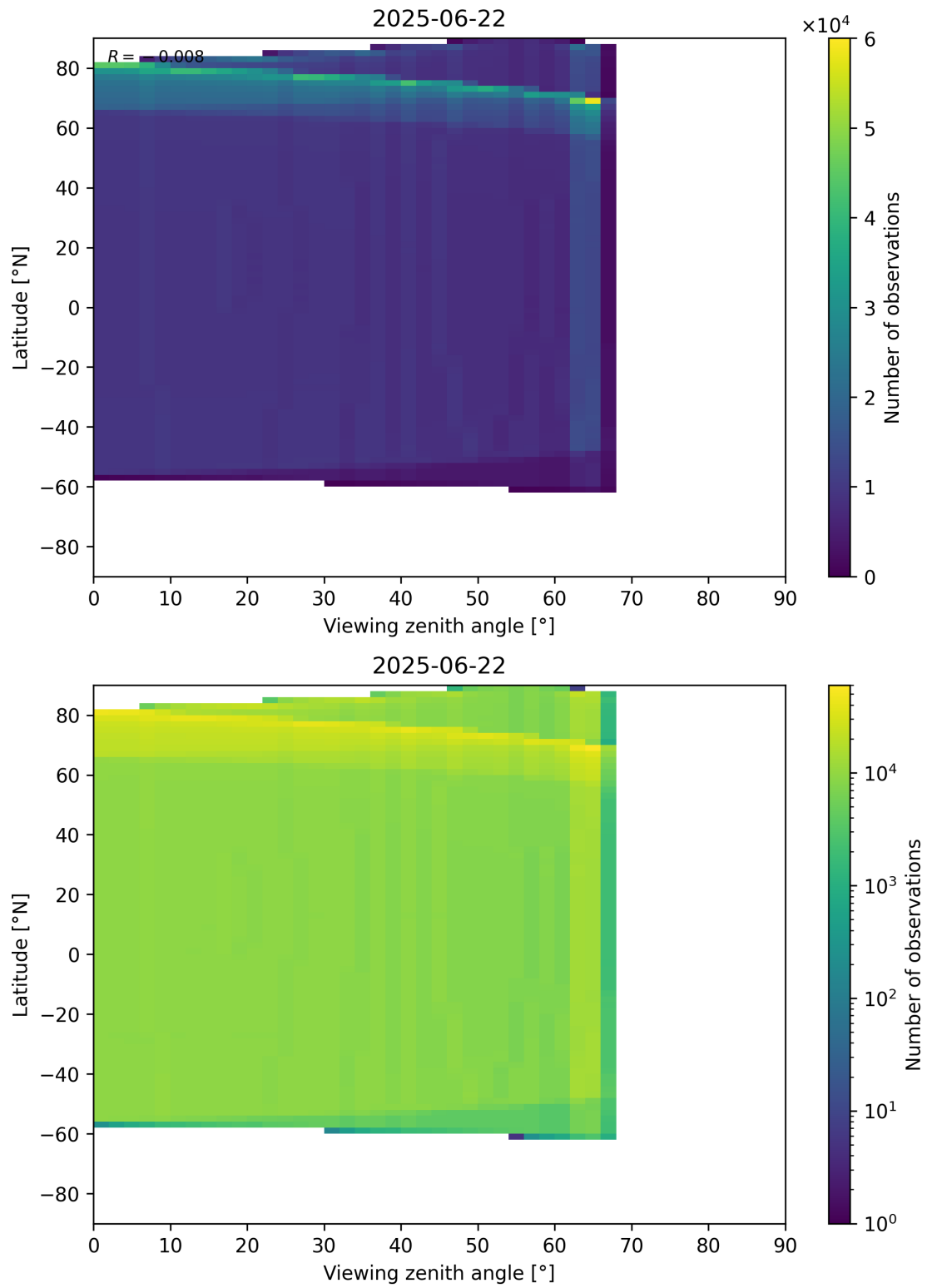
Figure 196: Scatter density plot of “Viewing zenith angle” against “Latitude” for 2025-06-22 to 2025-06-23.
