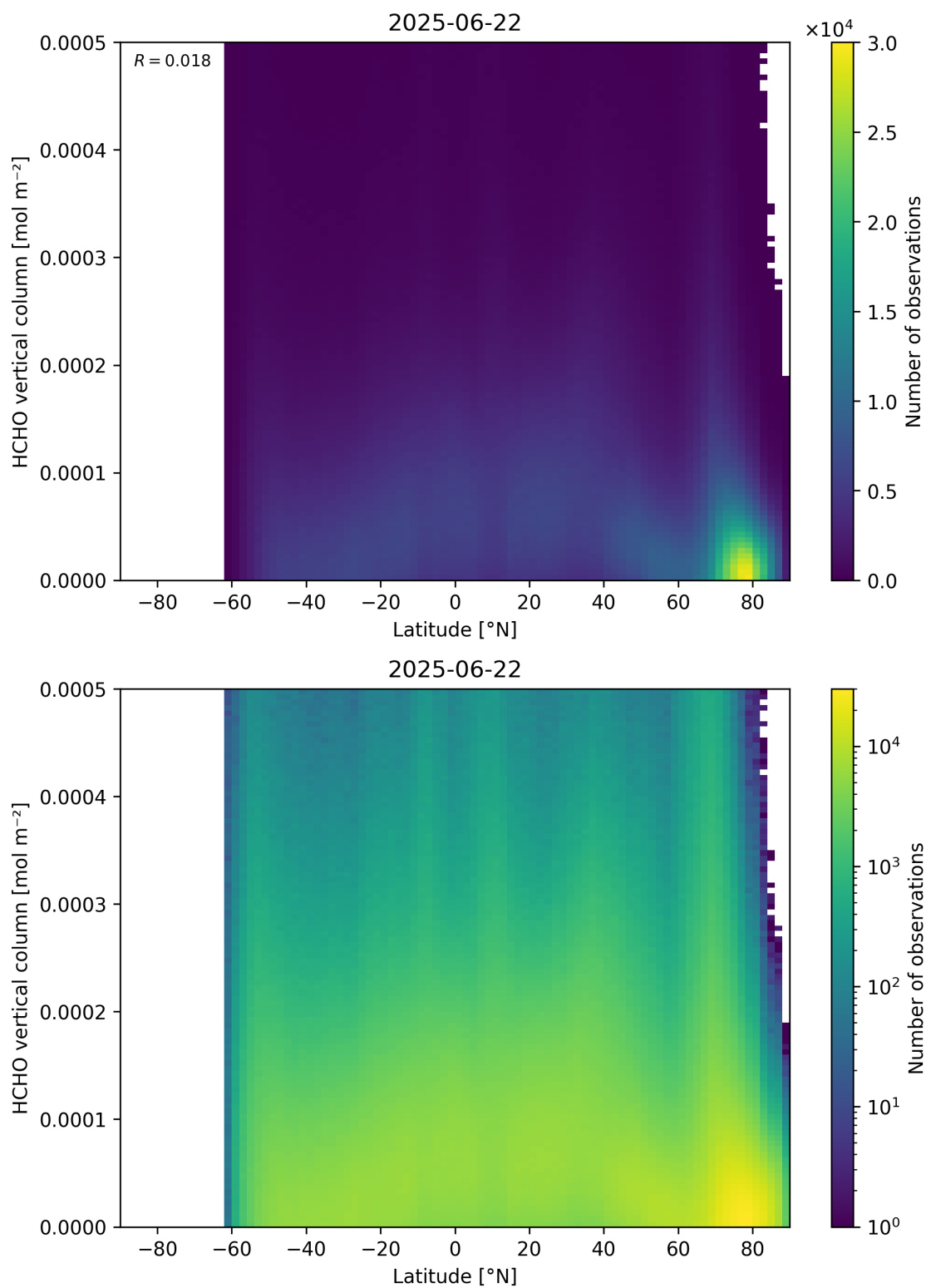
Figure 163: Scatter density plot of “Latitude” against “HCHO vertical column” for 2025-06-22 to 2025-06-23.
