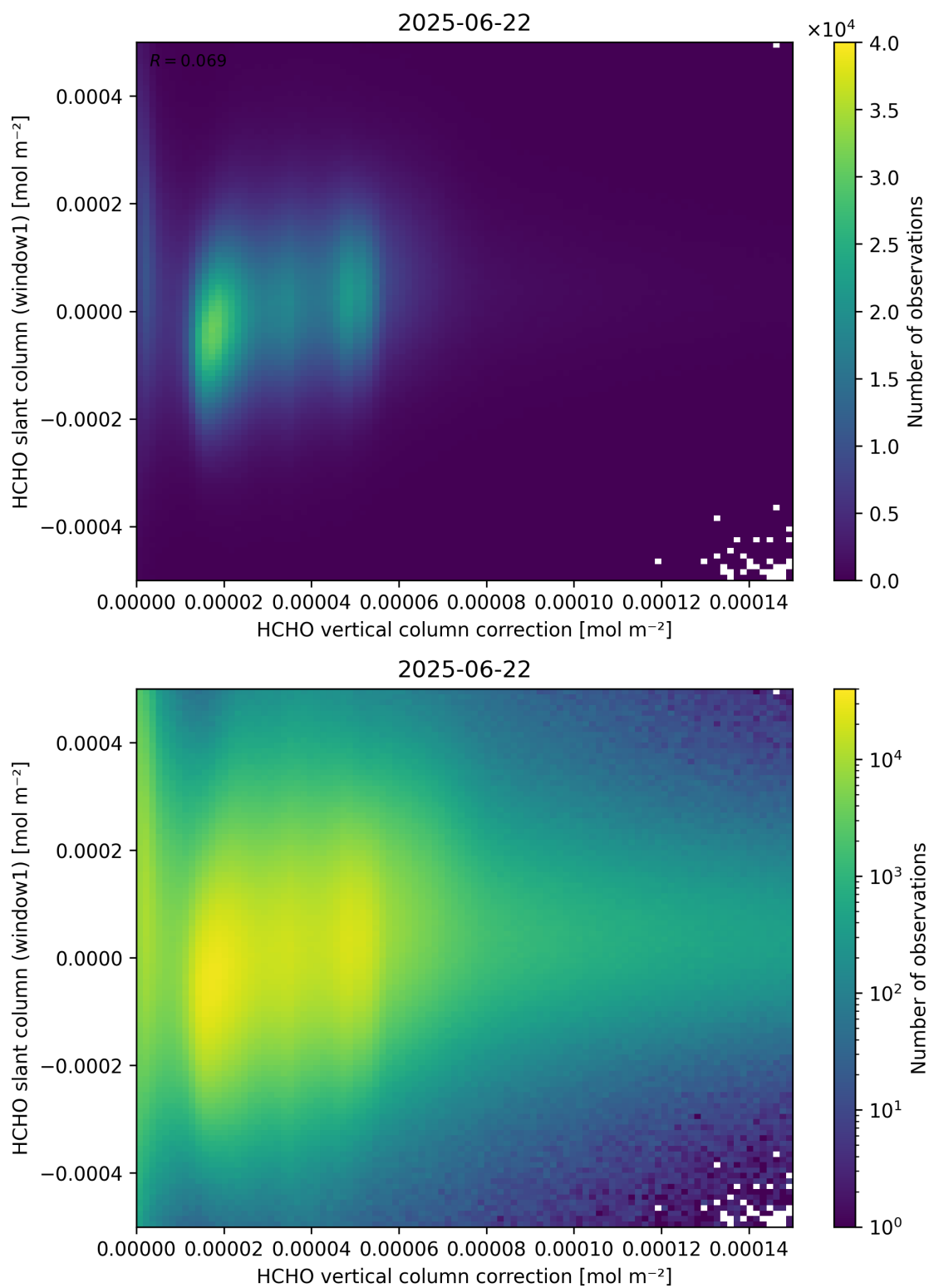
Figure 118: Scatter density plot of “HCHO vertical column correction” against “HCHO slant column (window1)” for 2025-06-22 to 2025-06-23.
