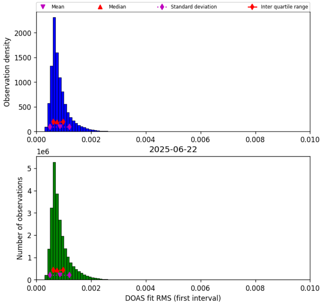
Figure 46: Histogram of “DOAS fit RMS (first interval)” for 2025-06-22 to 2025-06-23
