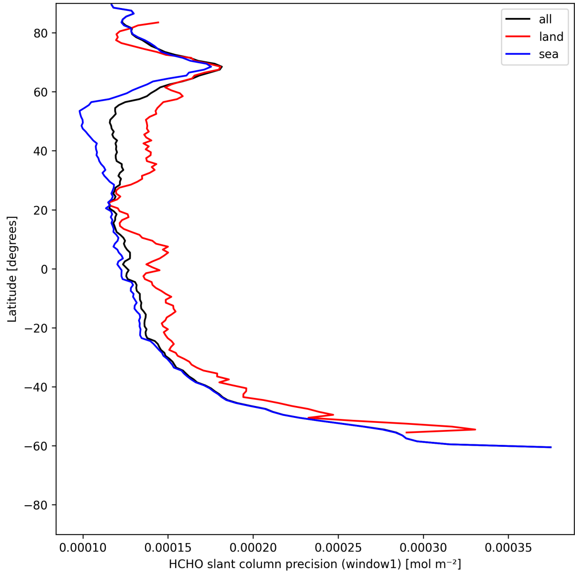
Figure 25: Zonal average of “HCHO slant column precision (window1)” for 2025-06-22 to 2025-06-23.
