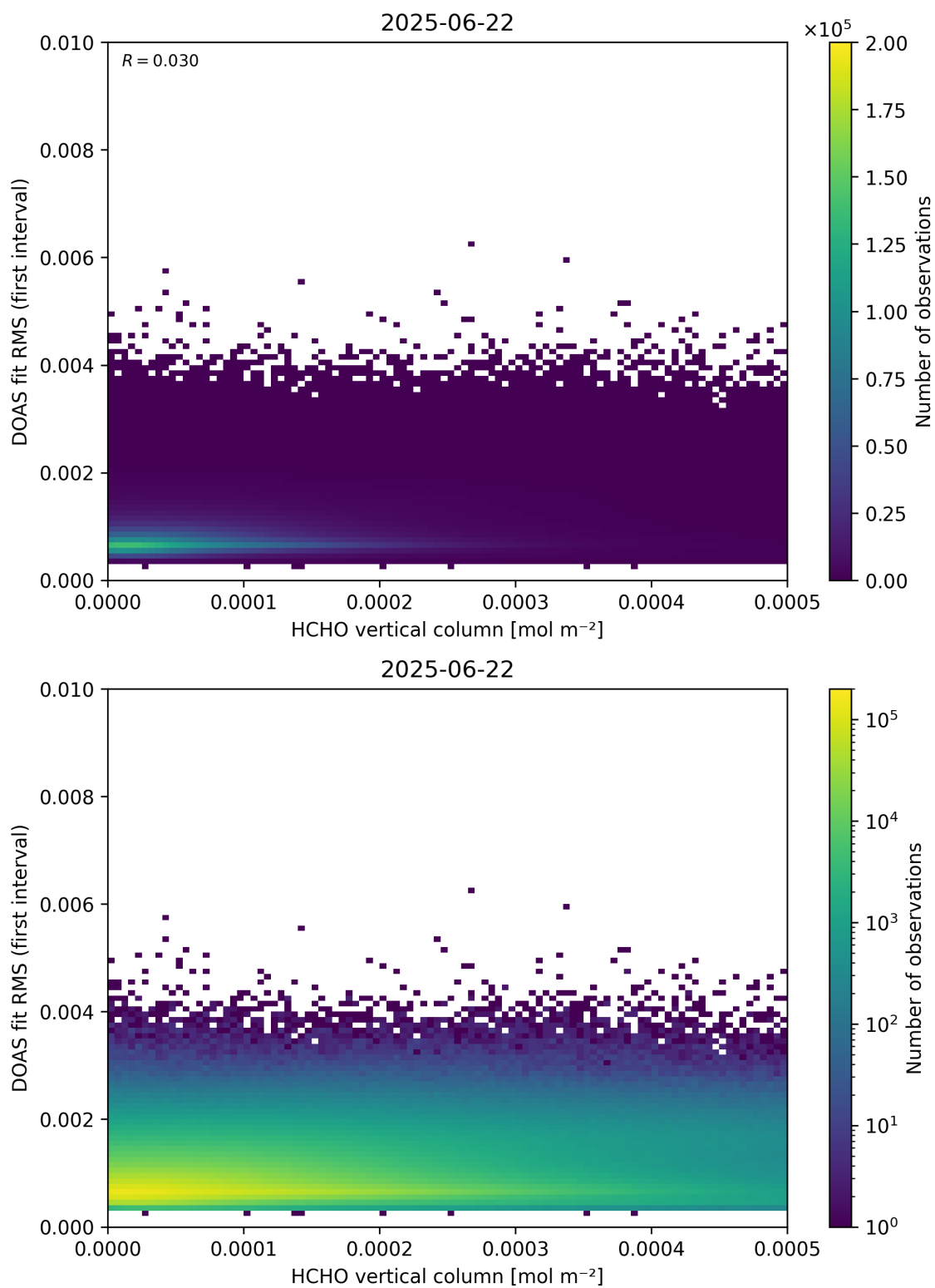
Figure 123: Scatter density plot of “HCHO vertical column” against “DOAS fit RMS (first interval)” for 2025-06-22 to 2025-06-23.
