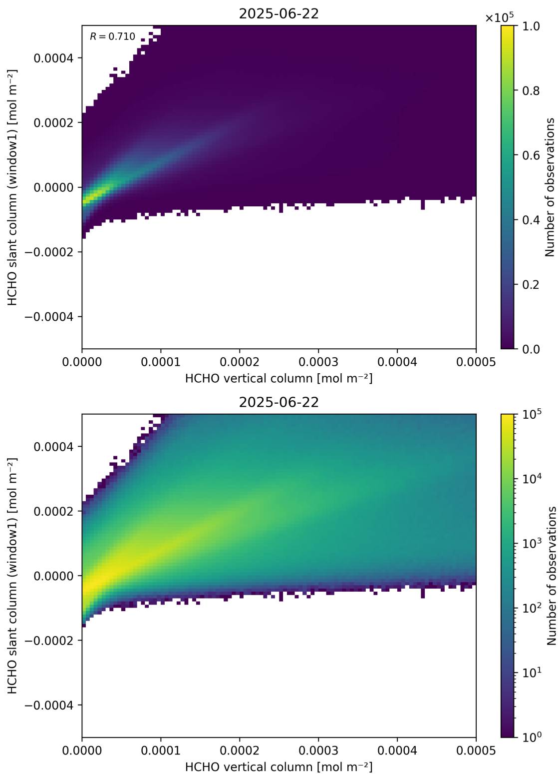
Figure 129: Scatter density plot of “HCHO vertical column” against “HCHO slant column (window1)” for 2025-06-22 to 2025-06-23.
