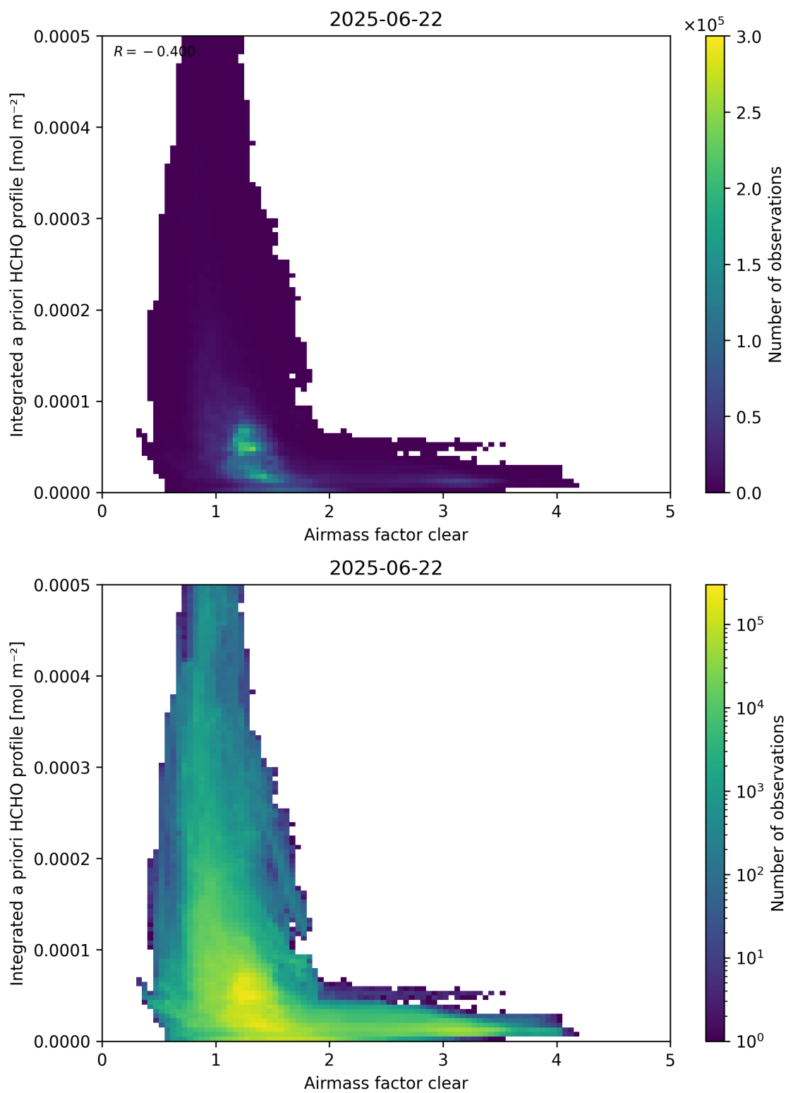
Figure 76: Scatter density plot of “Airmass factor clear” against “Integrated a priori HCHO profile” for 2025-06-22 to 2025-06-23.
