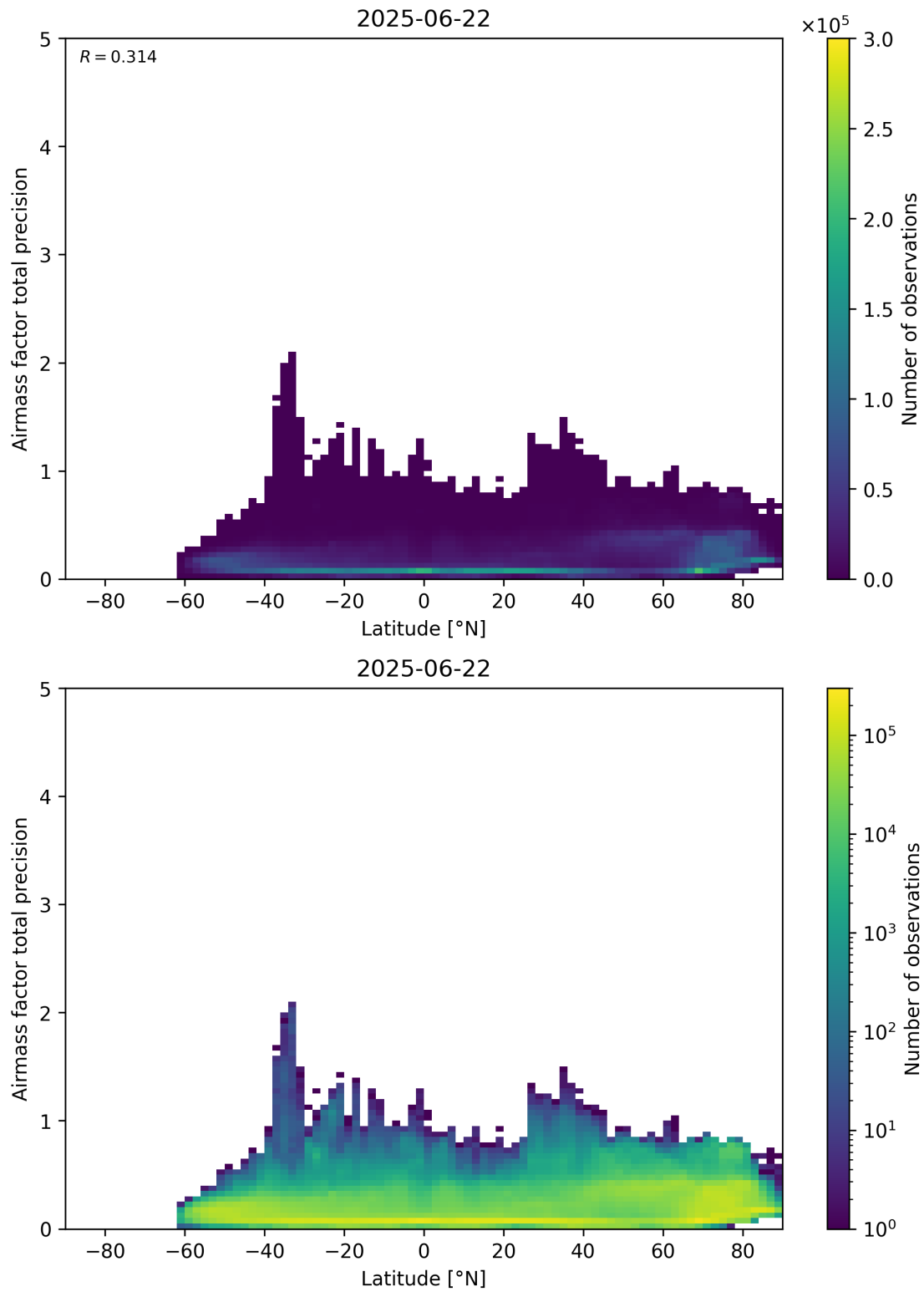
Figure 162: Scatter density plot of “Latitude” against “Airmass factor total precision” for 2025-06-22 to 2025-06-23.
