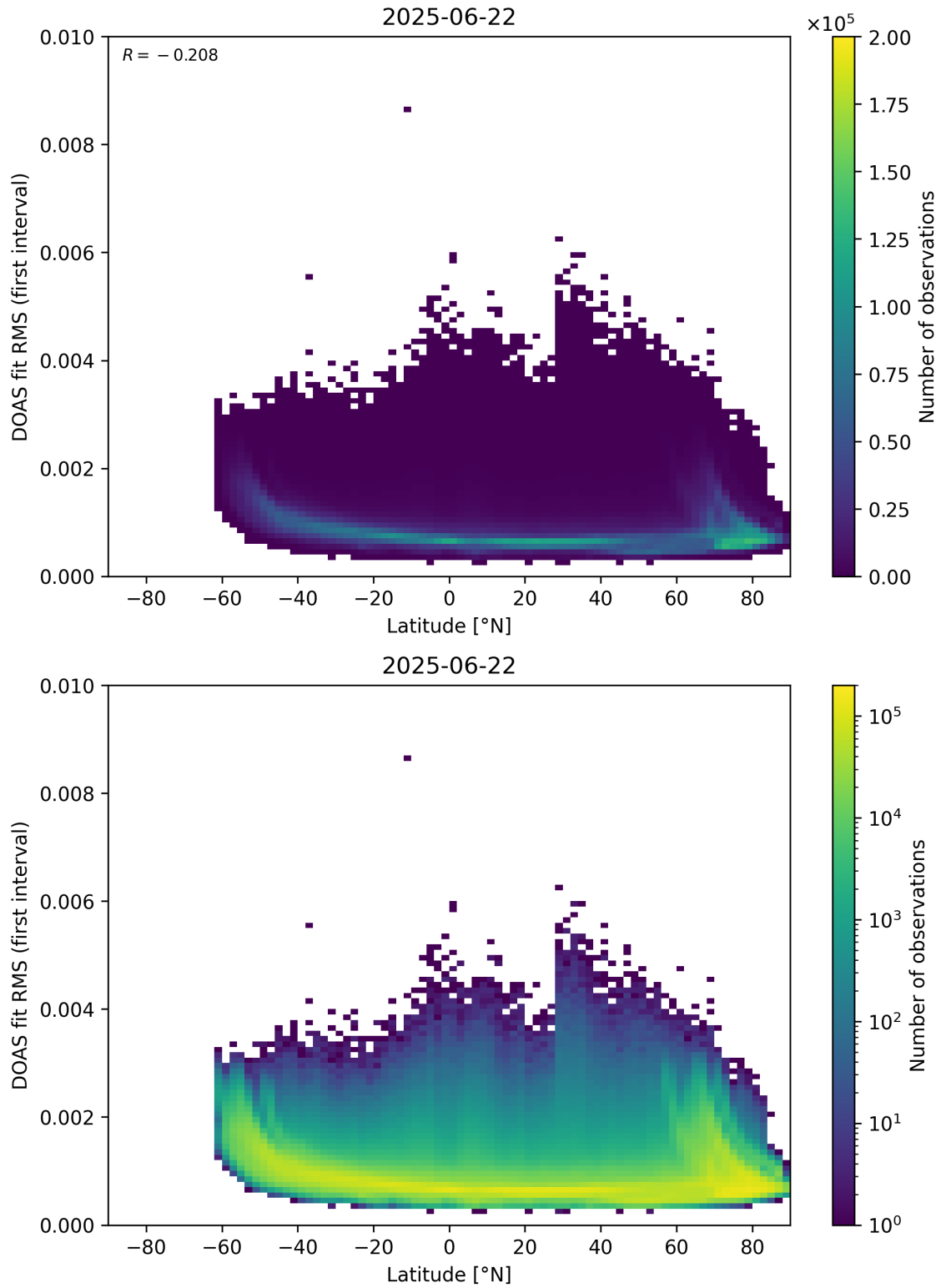
Figure 153: Scatter density plot of “Latitude” against “DOAS fit RMS (first interval)” for 2025-06-22 to 2025-06-23.
