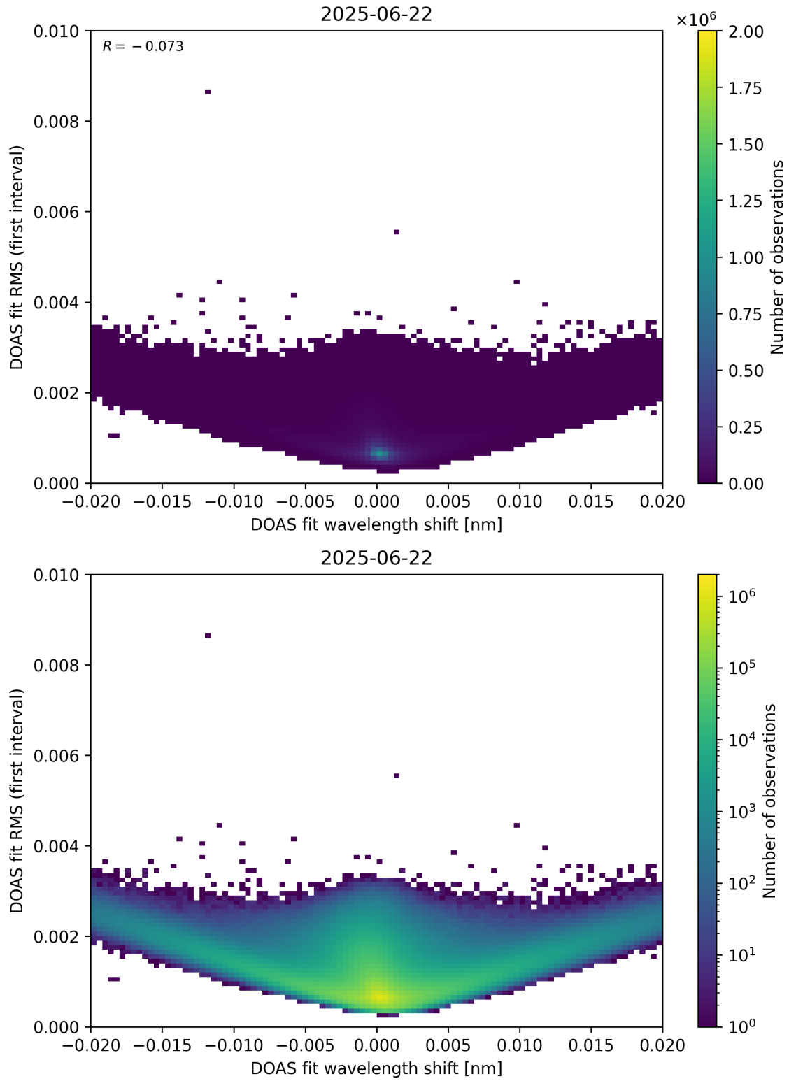
Figure 64: Scatter density plot of “DOAS fit wavelength shift” against “DOAS fit RMS (first interval)” for 2025-06-22 to 2025-06-23.
