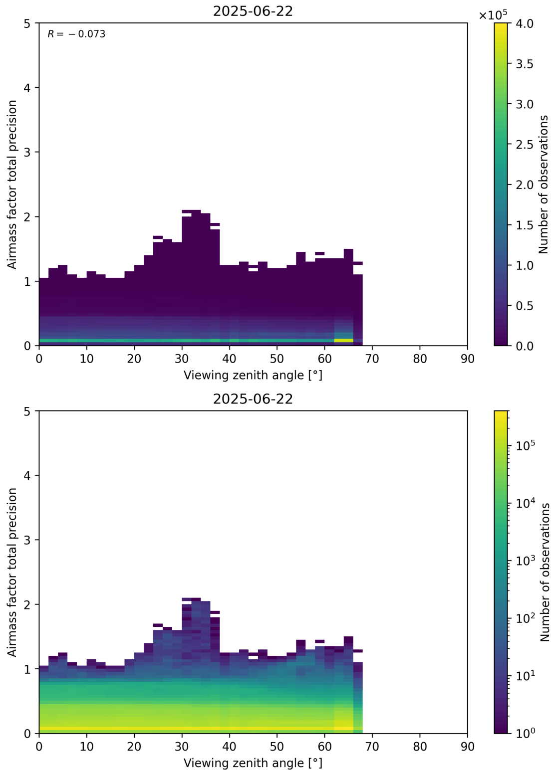
Figure 191: Scatter density plot of “Viewing zenith angle” against “Airmass factor total precision” for 2025-06-22 to 2025-06-23.
