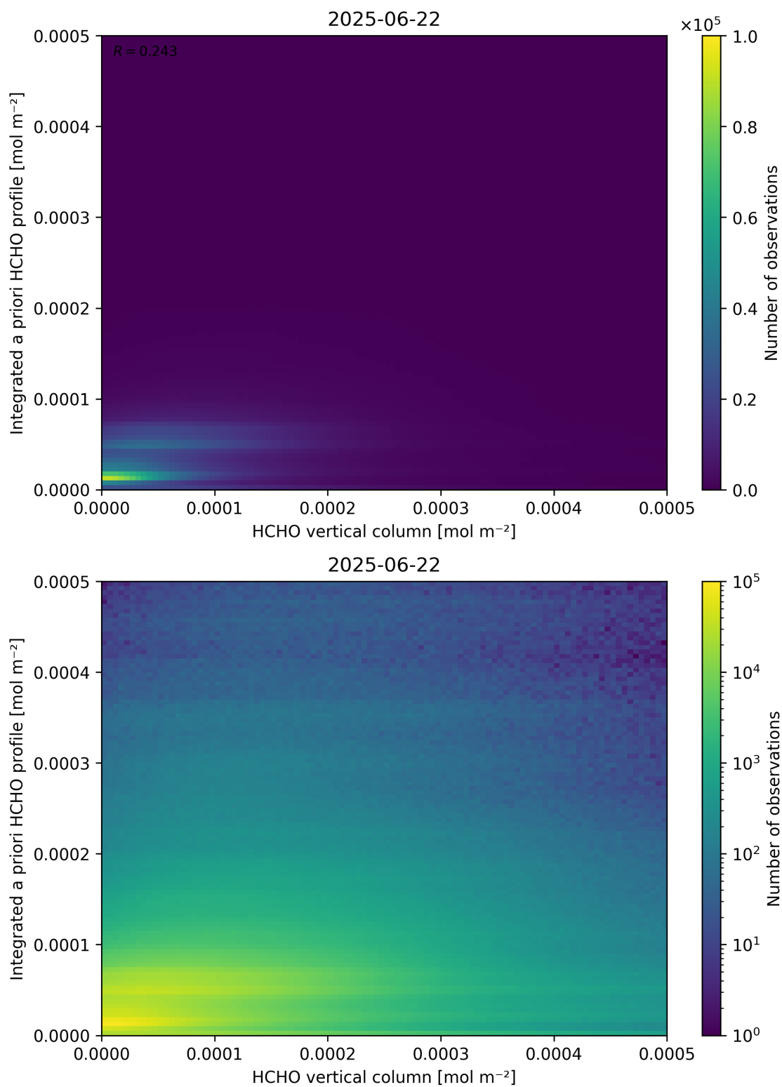
Figure 135: Scatter density plot of “HCHO vertical column” against “Integrated a priori HCHO profile” for 2025-06-22 to 2025-06-23.
