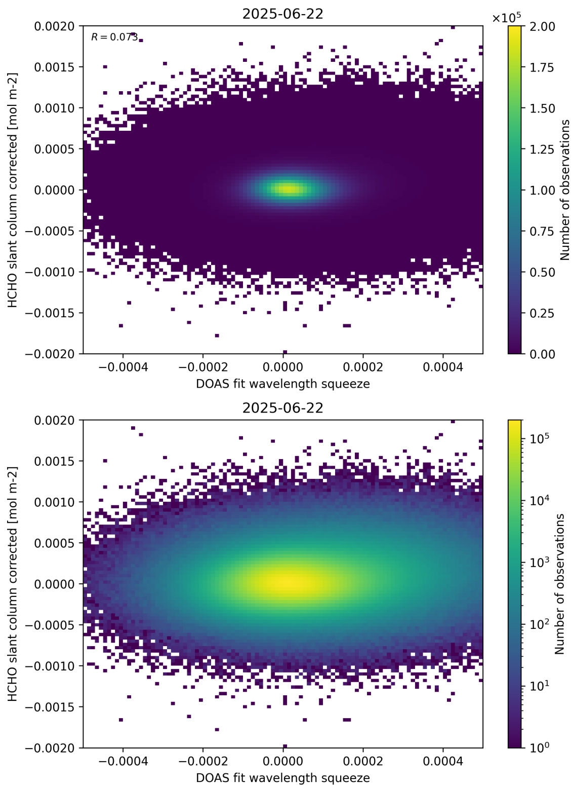
Figure 69: Scatter density plot of “DOAS fit wavelength squeeze” against “HCHO slant column corrected” for 2025-06-22 to 2025-06-23.
