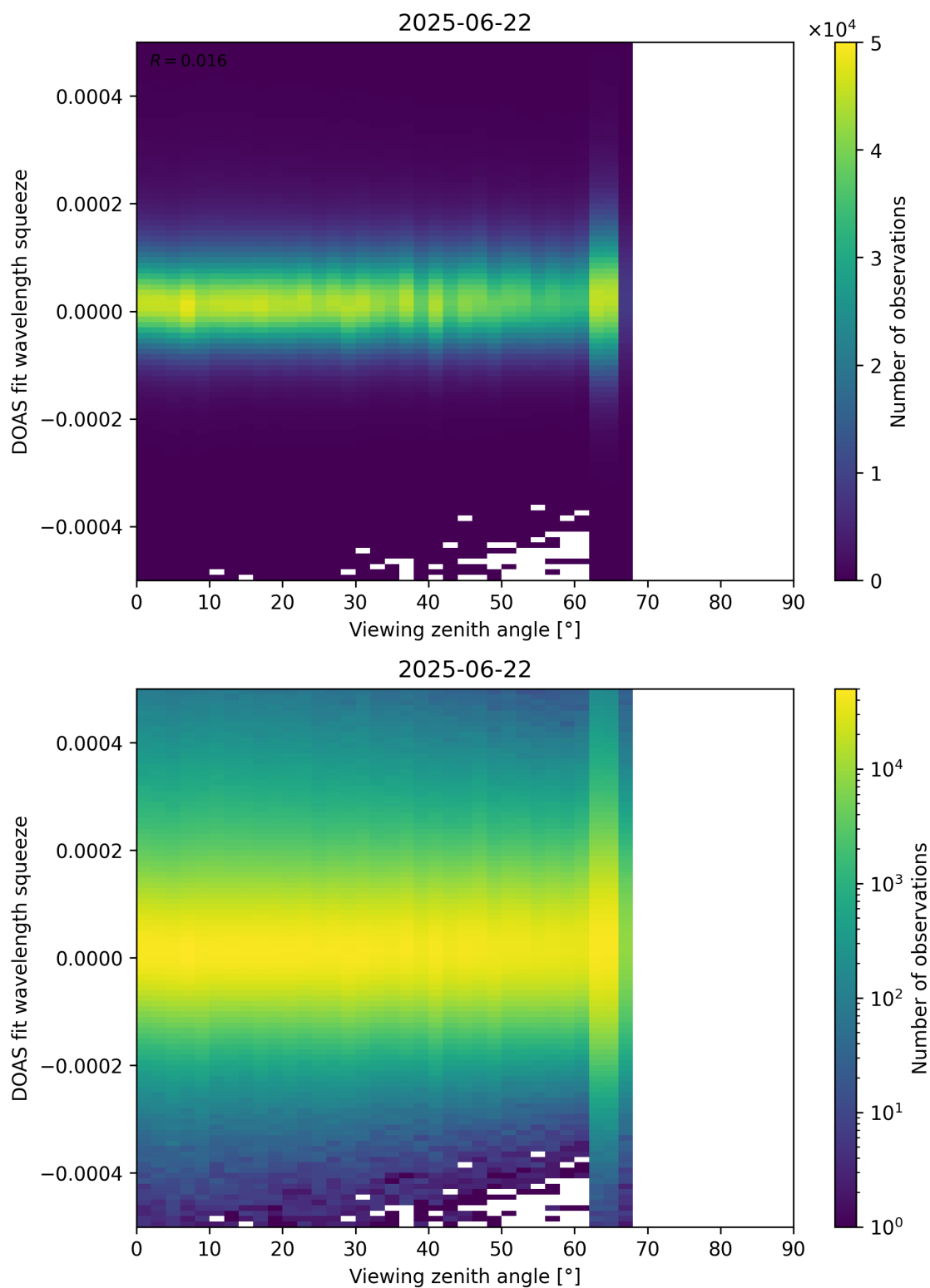
Figure 184: Scatter density plot of “Viewing zenith angle” against “DOAS fit wavelength squeeze” for 2025-06-22 to 2025-06-23.
