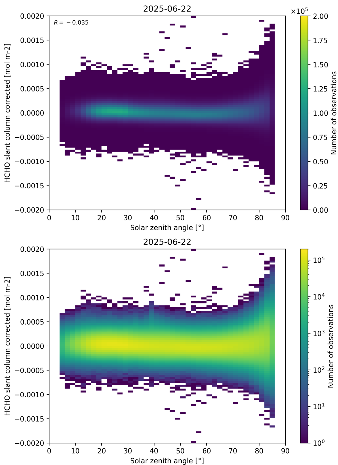
Figure 171: Scatter density plot of “Solar zenith angle” against “HCHO slant column corrected” for 2025-06-22 to 2025-06-23.
