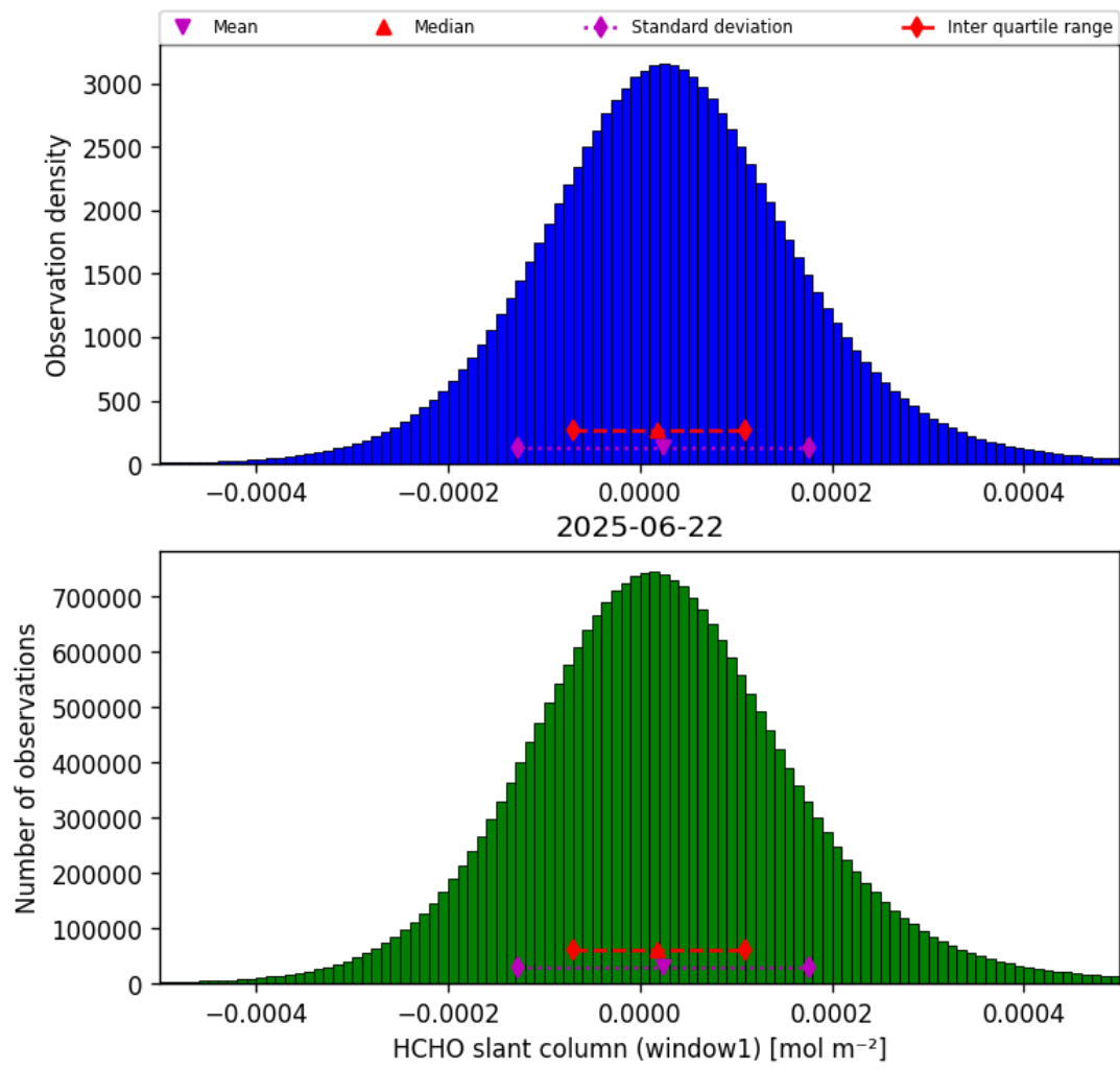
Figure 38: Histogram of “HCHO slant column (window1)” for 2025-06-22 to 2025-06-23
