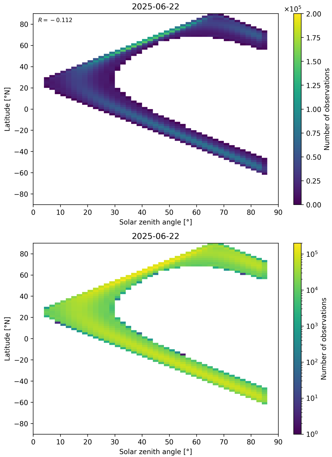
Figure 181: Scatter density plot of “Solar zenith angle” against “Latitude” for 2025-06-22 to 2025-06-23.
