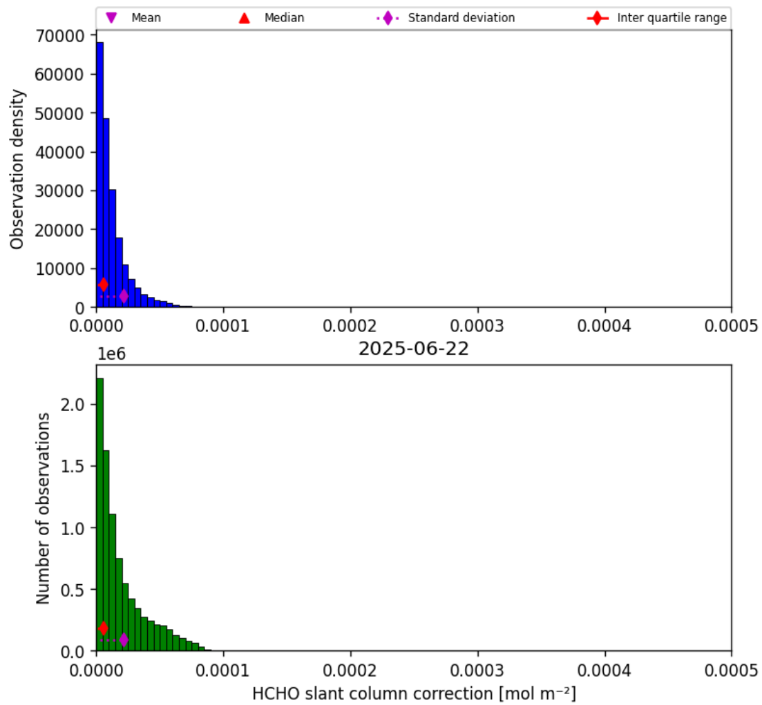
Figure 47: Histogram of “HCHO slant column correction” for 2025-06-22 to 2025-06-23
