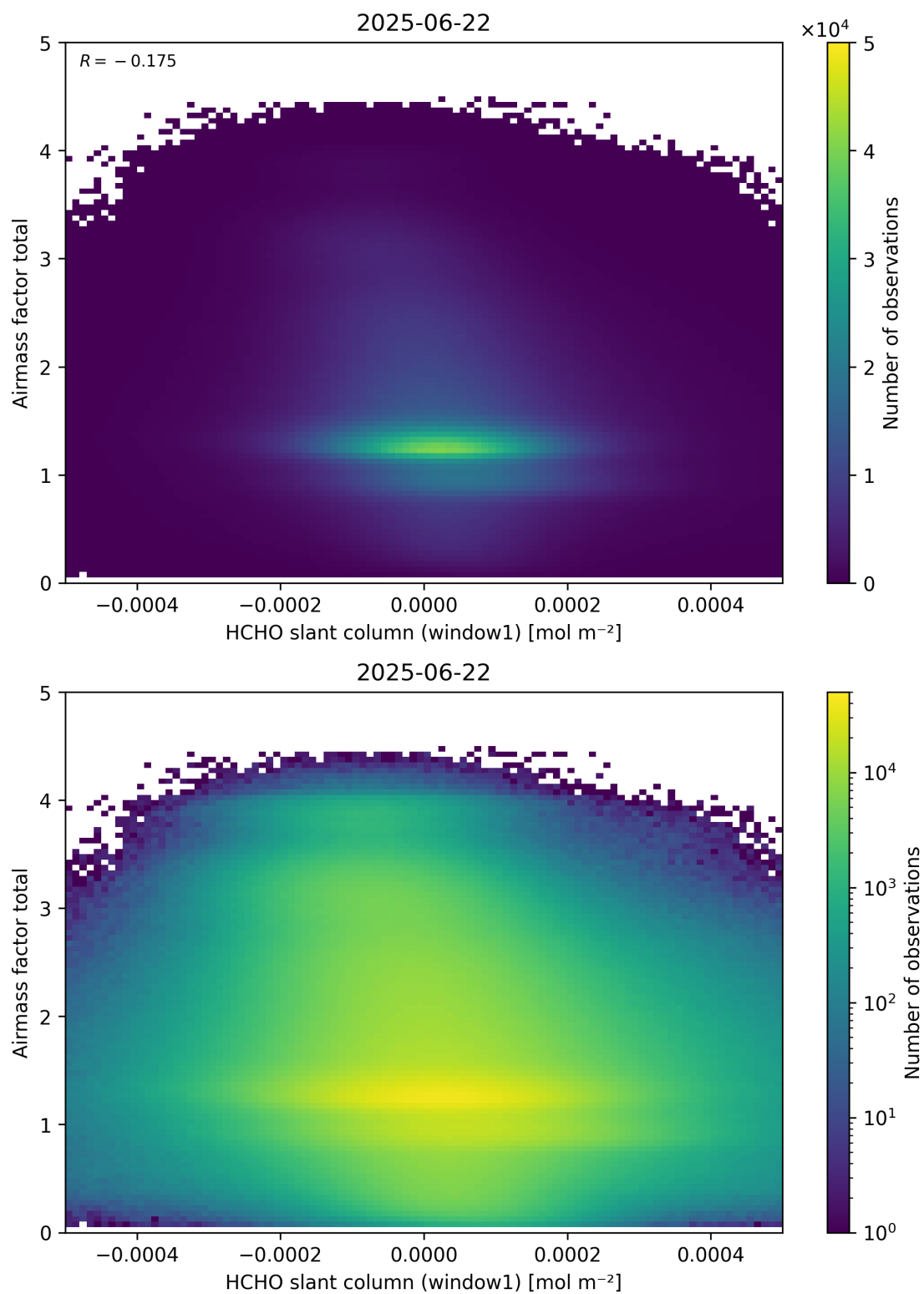
Figure 85: Scatter density plot of “HCHO slant column (window1)” against “Airmass factor total” for 2025-06-22 to 2025-06-23.
