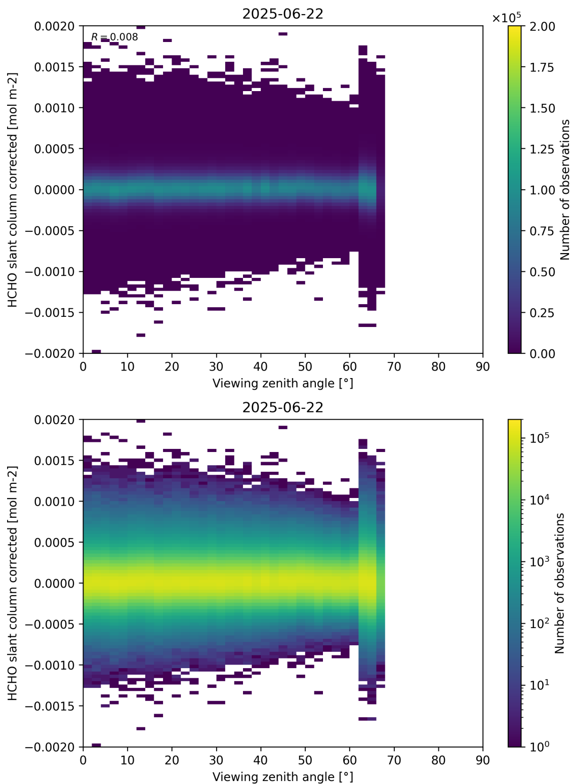
Figure 186: Scatter density plot of “Viewing zenith angle” against “HCHO slant column corrected” for 2025-06-22 to 2025-06-23.
