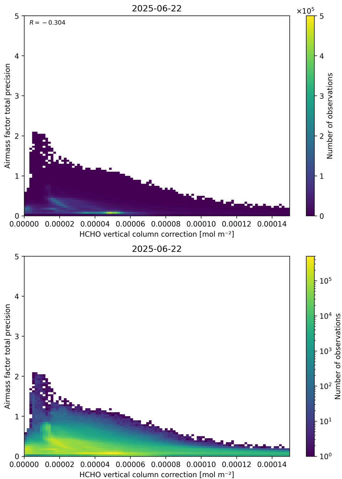
Figure 121: Scatter density plot of “HCHO vertical column correction” against “Airmass factor total precision” for 2025-06-22 to 2025-06-23.
