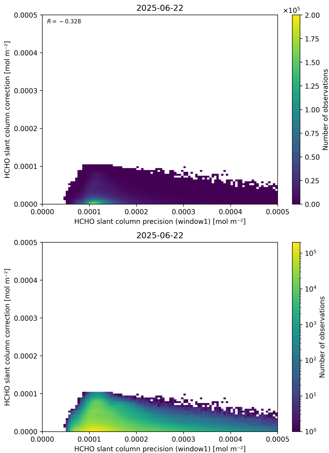
Figure 93: Scatter density plot of “HCHO slant column precision (window1)” against “HCHO slant column correction” for 2025-06-22 to 2025-06-23.
