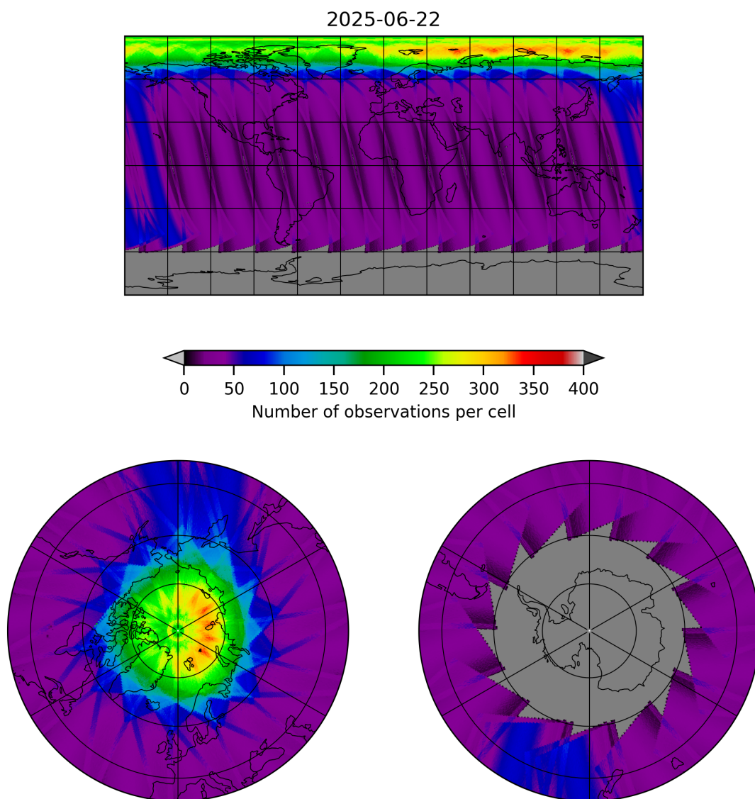
Figure 19: Map of the number of observations for 2025-06-22 to 2025-06-23
