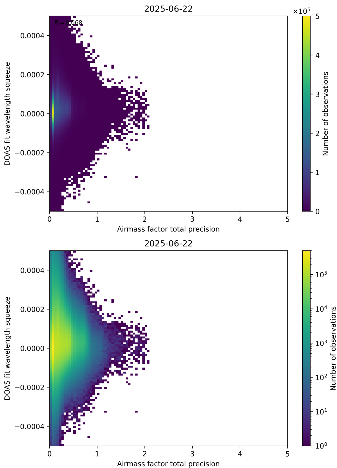
Figure 107: Scatter density plot of “Airmass factor total precision” against “DOAS fit wavelength squeeze” for 2025-06-22 to 2025-06-23.
