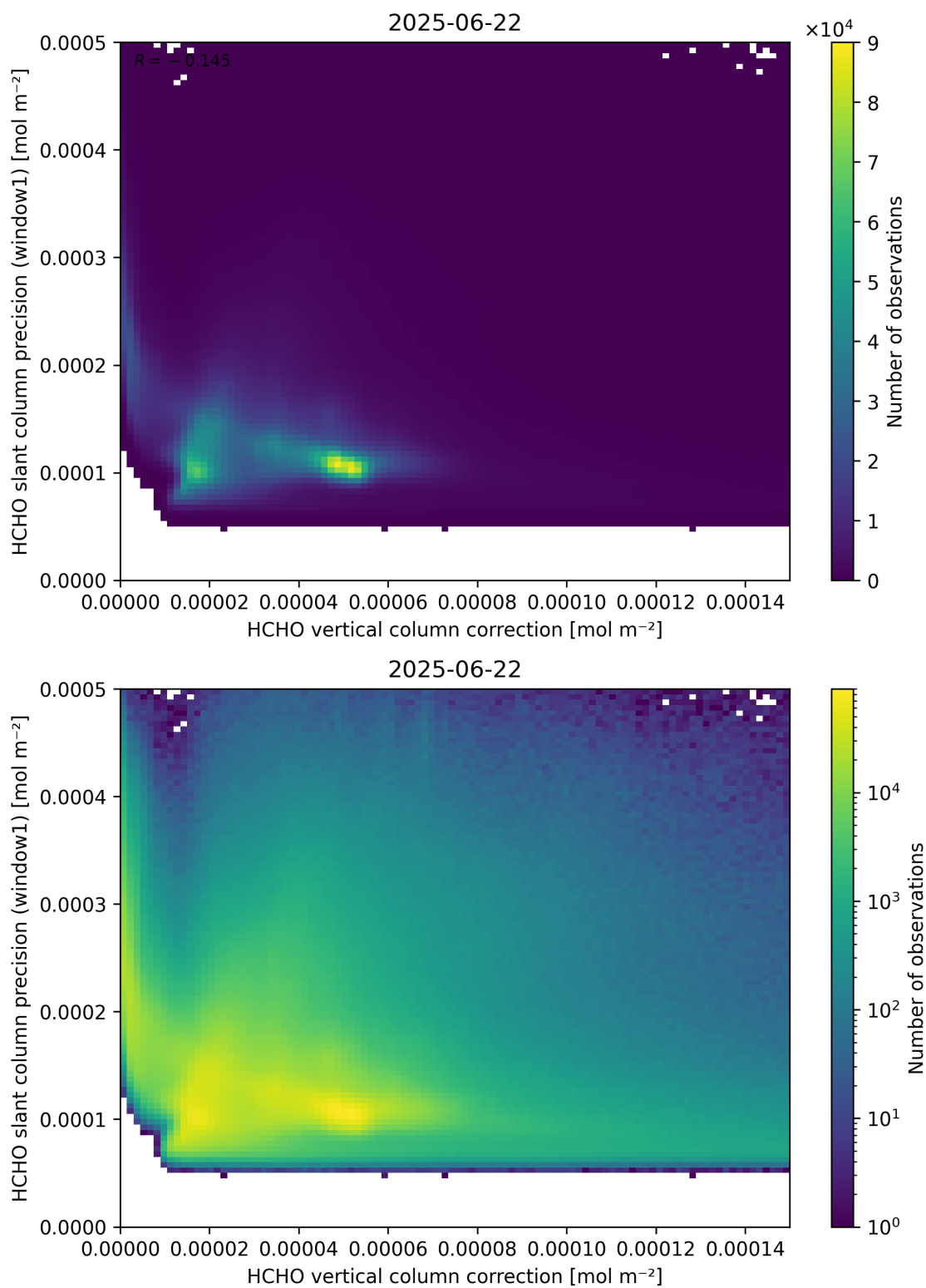
Figure 119: Scatter density plot of “HCHO vertical column correction” against “HCHO slant column precision (window1)” for 2025-06-22 to 2025-06-23.
