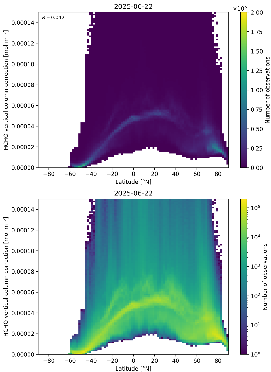
Figure 164: Scatter density plot of “Latitude” against “HCHO vertical column correction” for 2025-06-22 to 2025-06-23.
