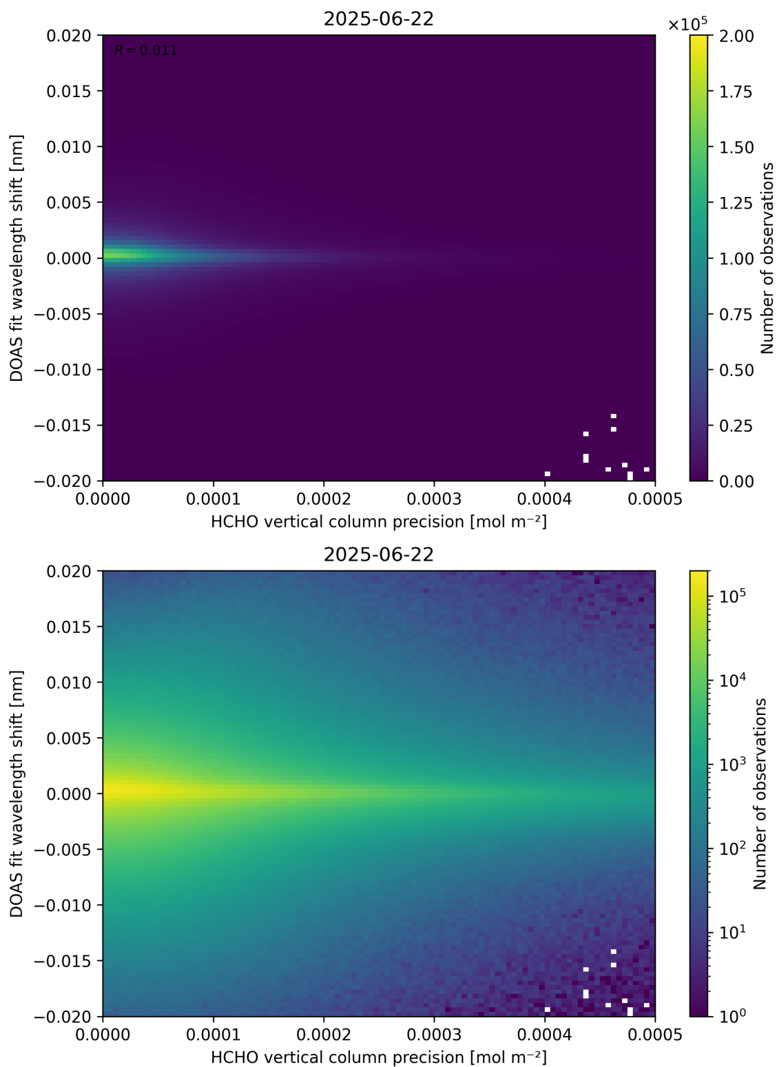
Figure 137: Scatter density plot of “HCHO vertical column precision” against “DOAS fit wavelength shift” for 2025-06-22 to 2025-06-23.
