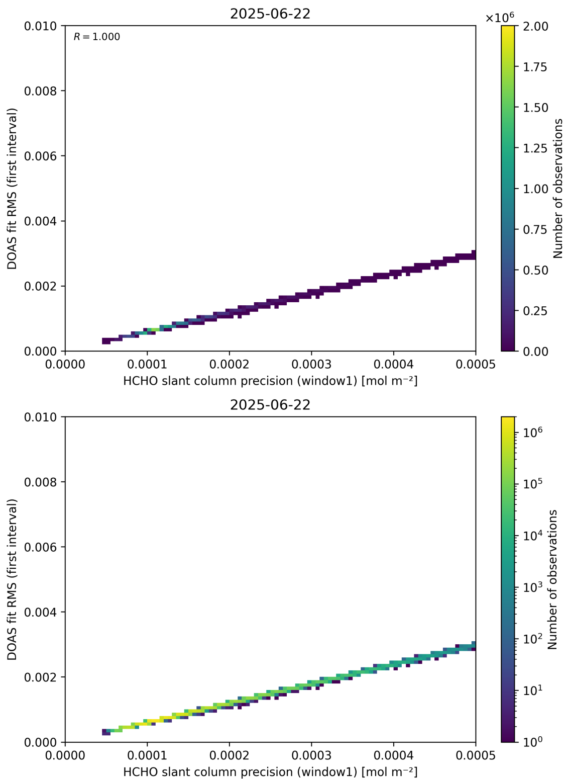
Figure 88: Scatter density plot of “HCHO slant column precision (window1)” against “DOAS fit RMS (first interval)” for 2025-06-22 to 2025-06-23.
