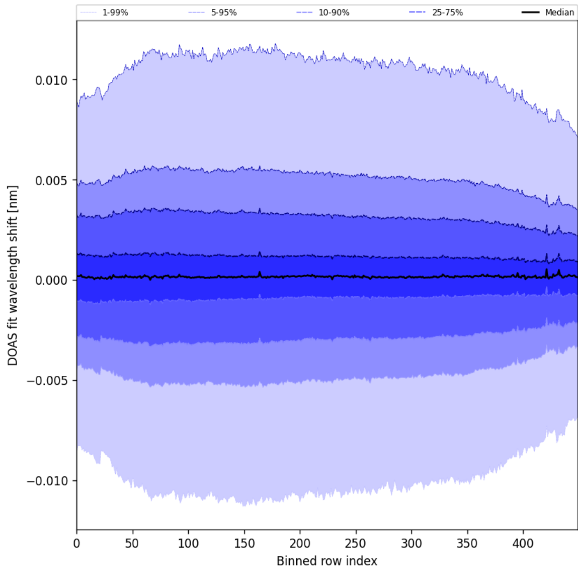
Figure 58: Along track statistics of “DOAS fit wavelength shift” for 2025-06-22 to 2025-06-23
