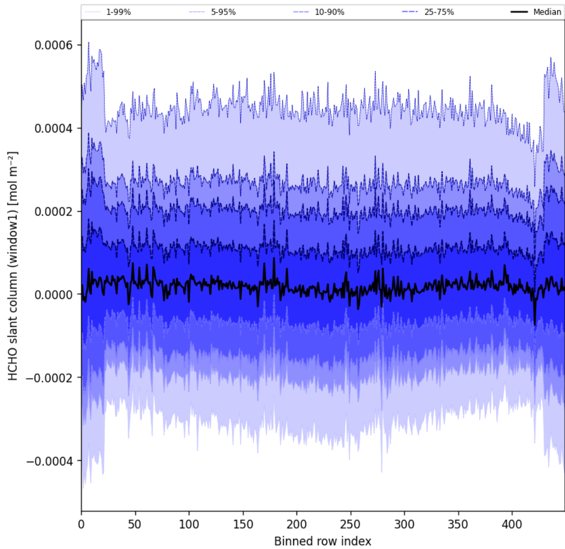
Figure 52: Along track statistics of “HCHO slant column (window1)” for 2025-06-22 to 2025-06-23
