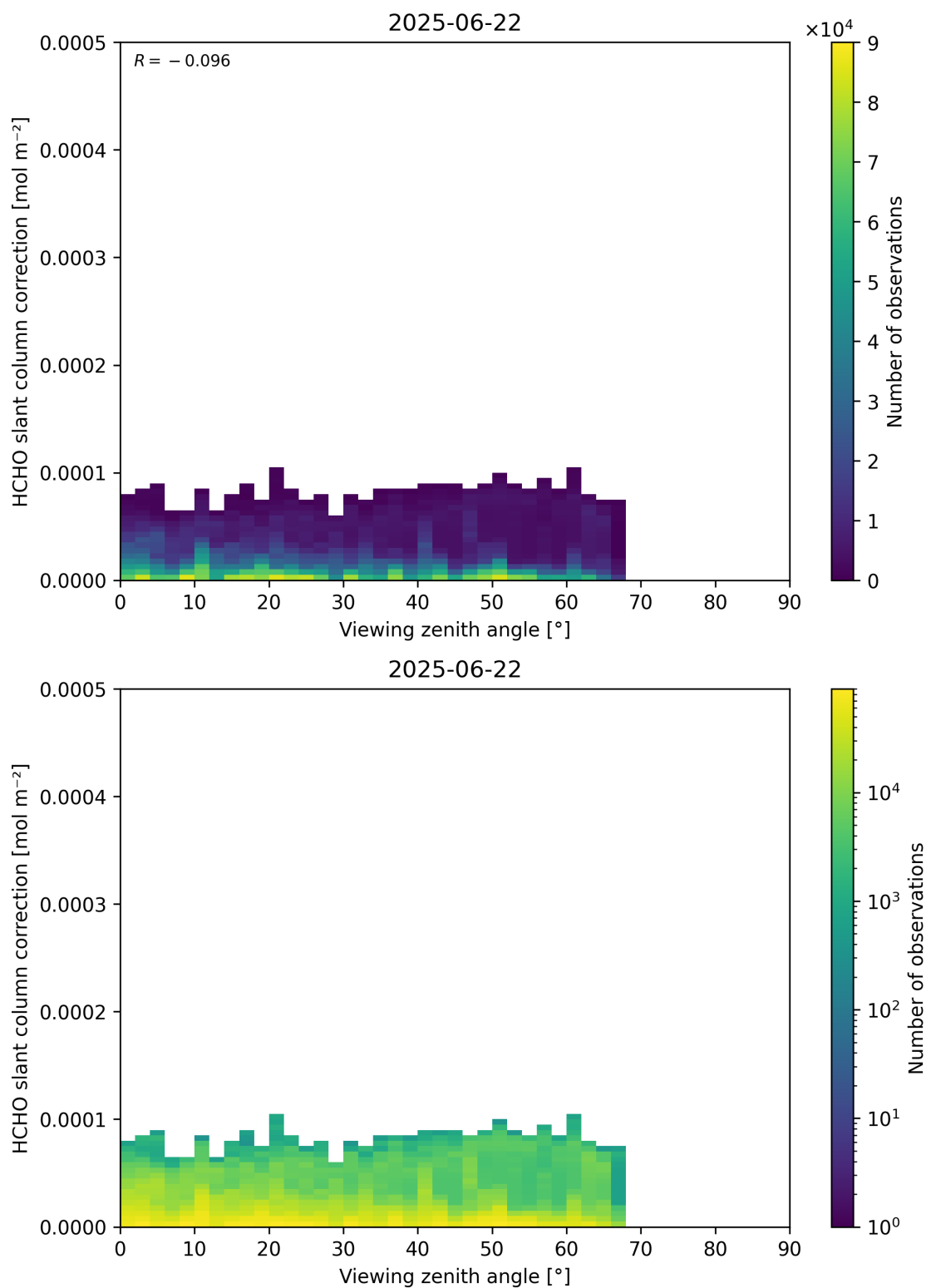
Figure 187: Scatter density plot of “Viewing zenith angle” against “HCHO slant column correction” for 2025-06-22 to 2025-06-23.
