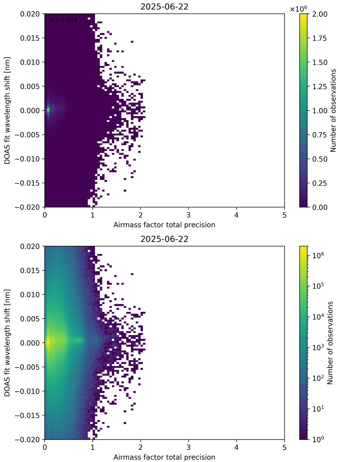
Figure 106: Scatter density plot of “Airmass factor total precision” against “DOAS fit wavelength shift” for 2025-06-22 to 2025-06-23.
