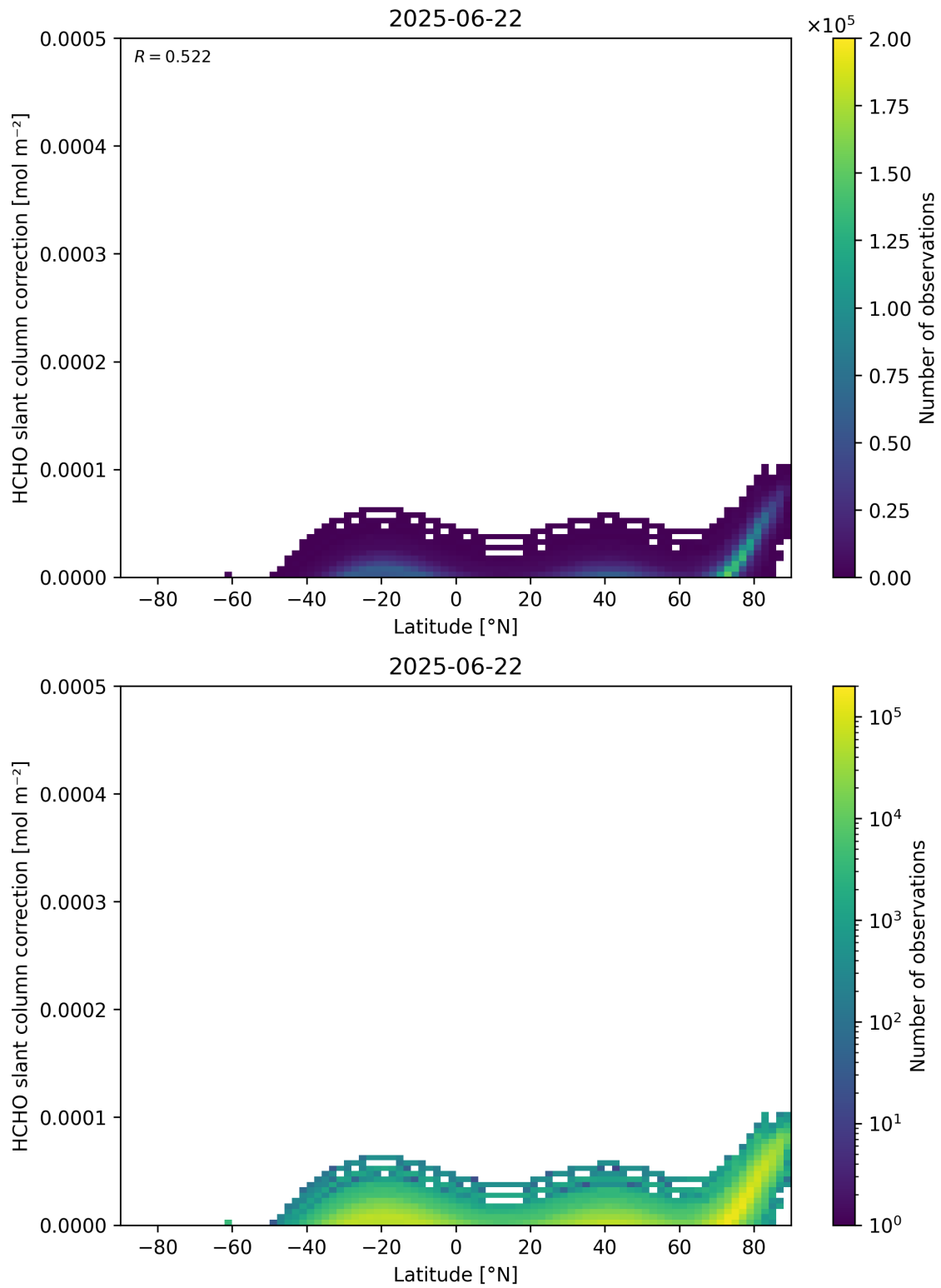
Figure 158: Scatter density plot of “Latitude” against “HCHO slant column correction” for 2025-06-22 to 2025-06-23.
