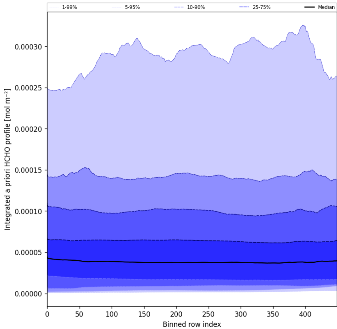
Figure 57: Along track statistics of “Integrated a priori HCHO profile” for 2025-06-22 to 2025-06-23
