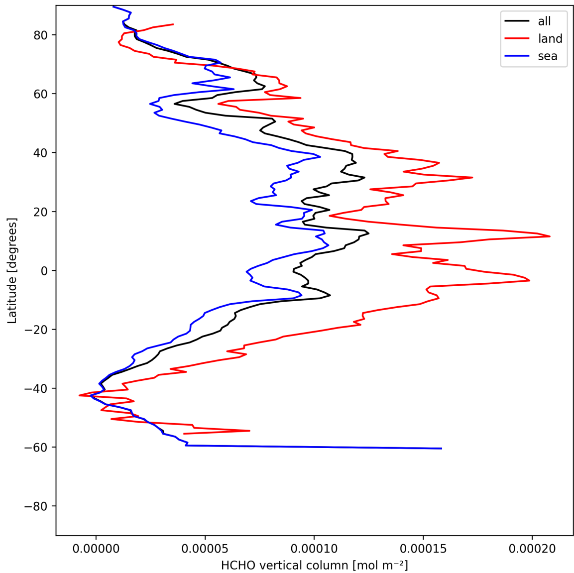
Figure 21: Zonal average of “HCHO vertical column” for 2025-06-22 to 2025-06-23.
