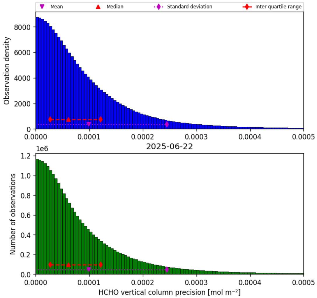
Figure 36: Histogram of “HCHO vertical column precision” for 2025-06-22 to 2025-06-23
