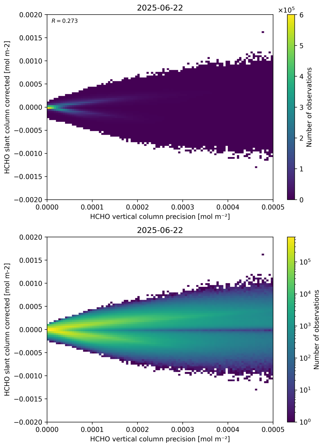
Figure 140: Scatter density plot of “HCHO vertical column precision” against “HCHO slant column corrected” for 2025-06-22 to 2025-06-23.
