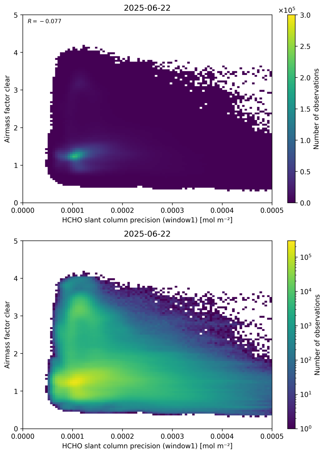
Figure 91: Scatter density plot of “HCHO slant column precision (window1)” against “Airmass factor clear” for 2025-06-22 to 2025-06-23.
