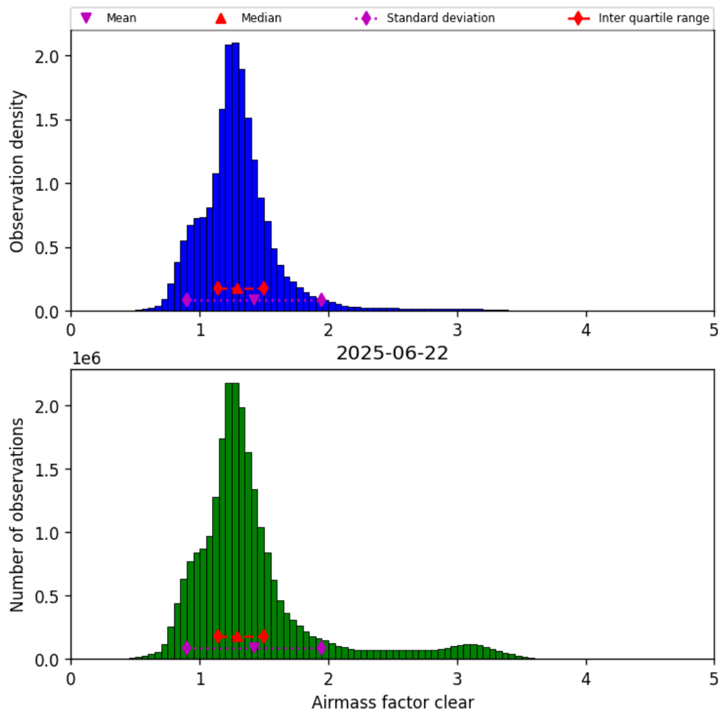
Figure 42: Histogram of “Airmass factor clear” for 2025-06-22 to 2025-06-23
