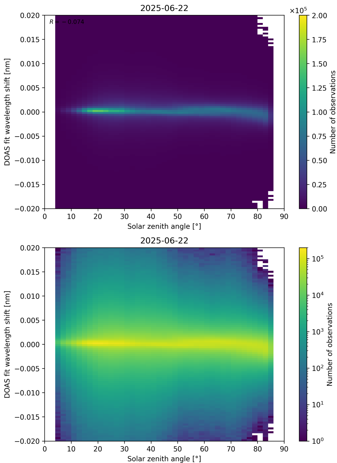
Figure 168: Scatter density plot of “Solar zenith angle” against “DOAS fit wavelength shift” for 2025-06-22 to 2025-06-23.
