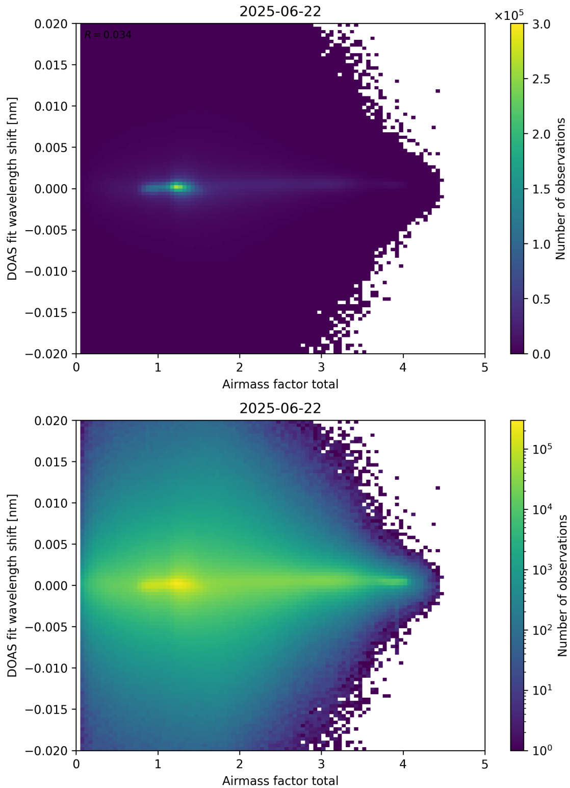
Figure 98: Scatter density plot of “Airmass factor total” against “DOAS fit wavelength shift” for 2025-06-22 to 2025-06-23.
