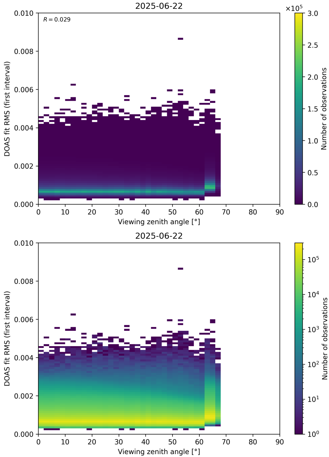
Figure 182: Scatter density plot of “Viewing zenith angle” against “DOAS fit RMS (first interval)” for 2025-06-22 to 2025-06-23.
