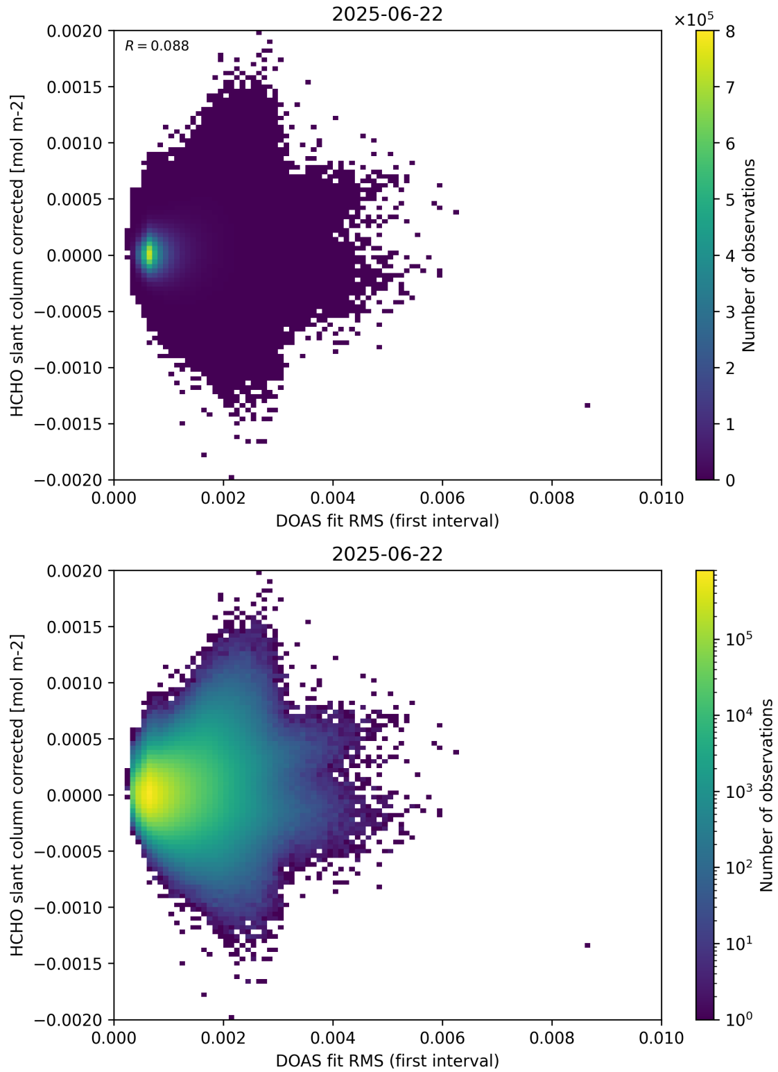
Figure 62: Scatter density plot of “DOAS fit RMS (first interval)” against “HCHO slant column corrected” for 2025-06-22 to 2025-06-23.
