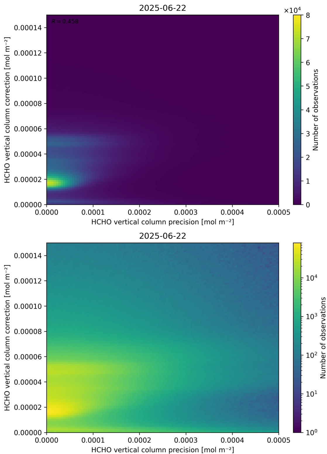
Figure 146: Scatter density plot of “HCHO vertical column precision” against “HCHO vertical column correction” for 2025-06-22 to 2025-06-23.
