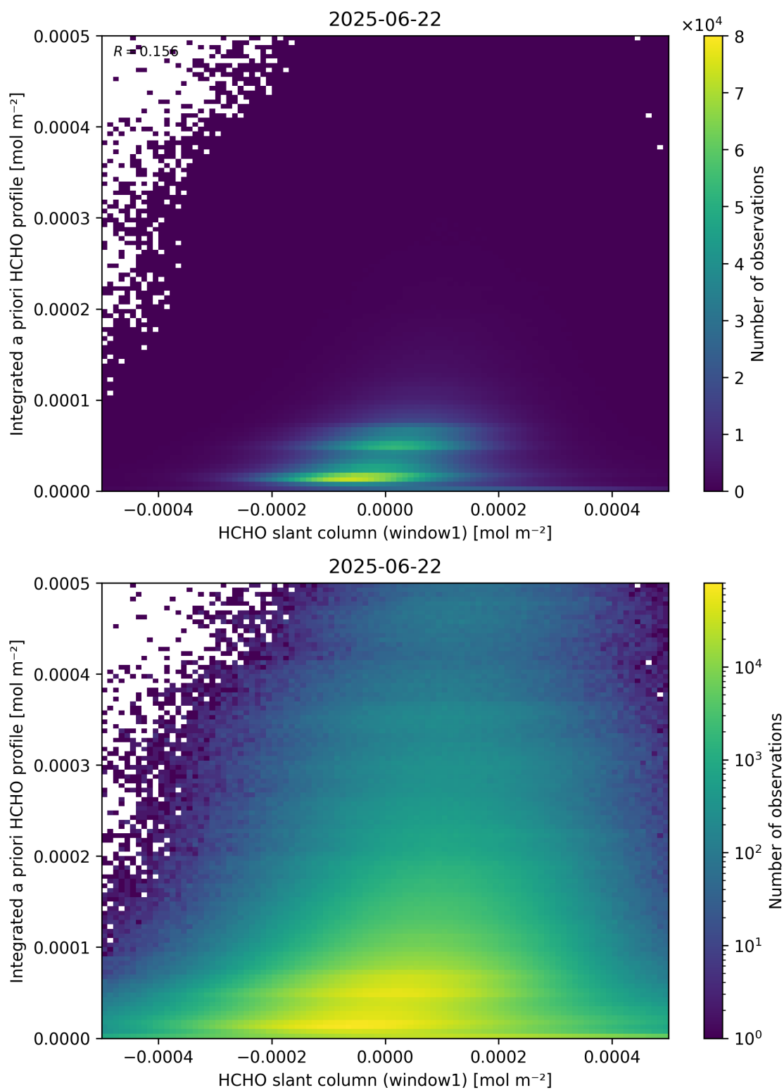
Figure 87: Scatter density plot of “HCHO slant column (window1)” against “Integrated a priori HCHO profile” for 2025-06-22 to 2025-06-23.
