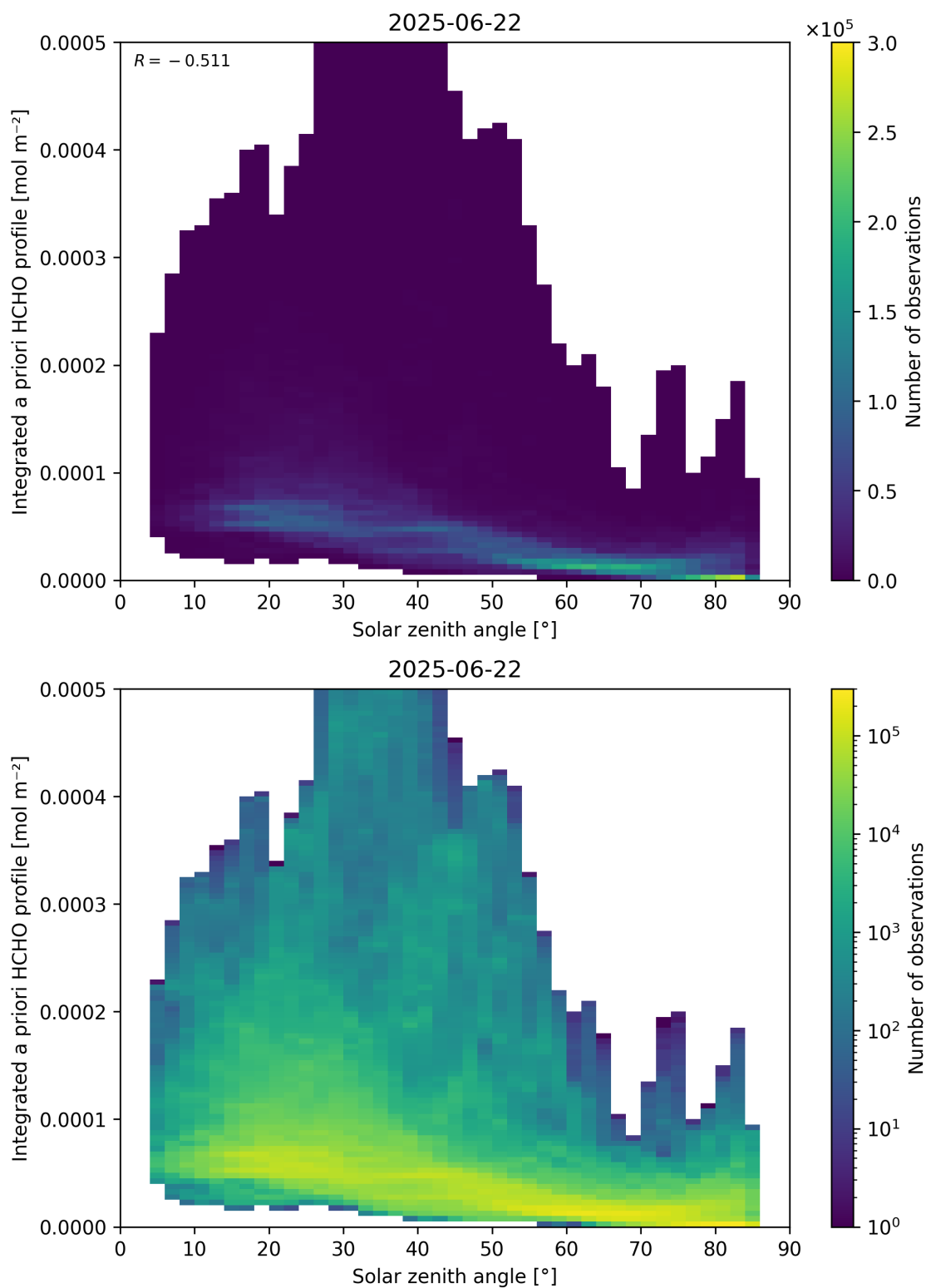
Figure 180: Scatter density plot of “Solar zenith angle” against “Integrated a priori HCHO profile” for 2025-06-22 to 2025-06-23.
