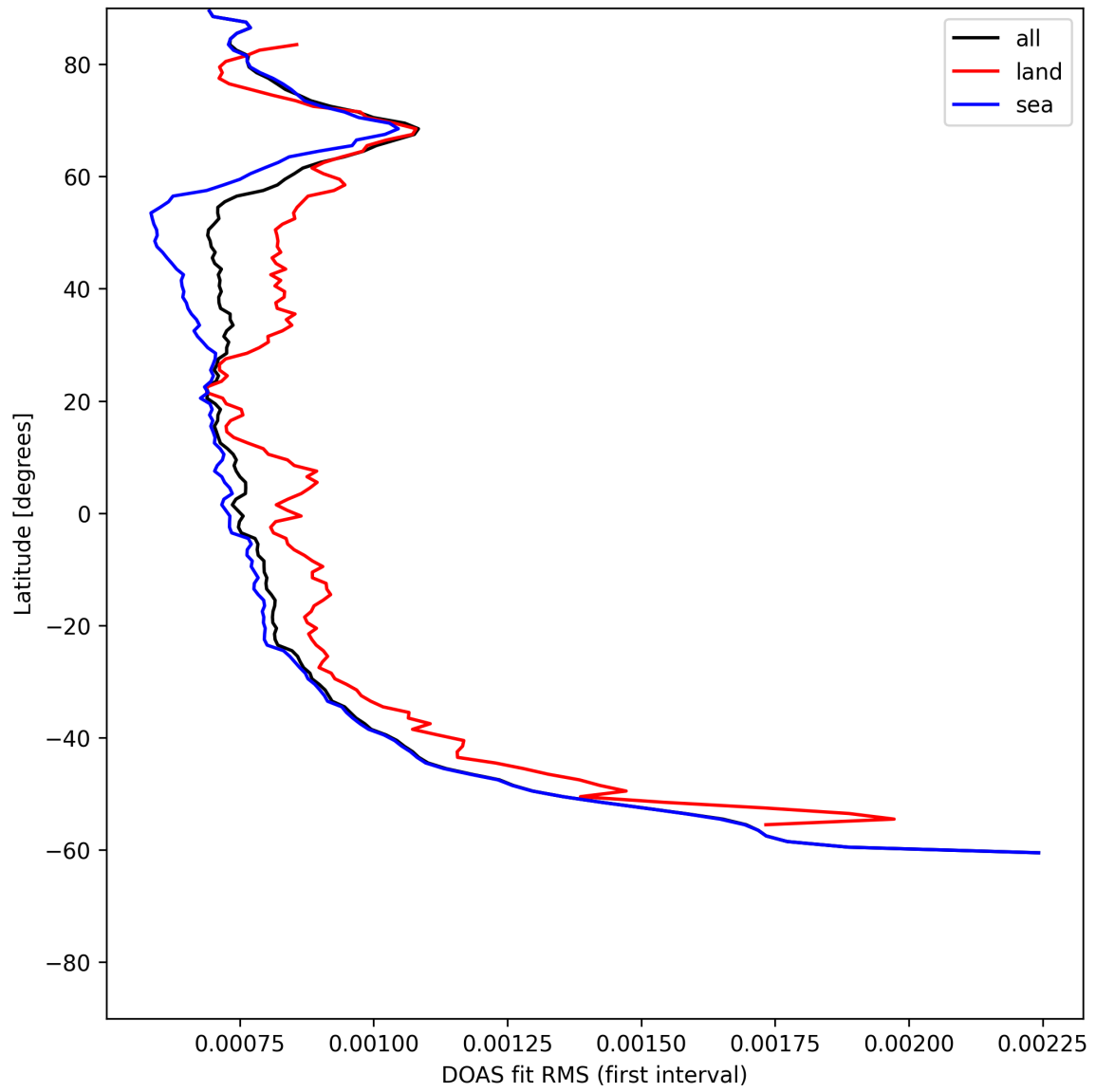
Figure 32: Zonal average of “DOAS fit RMS (first interval)” for 2025-06-22 to 2025-06-23.
