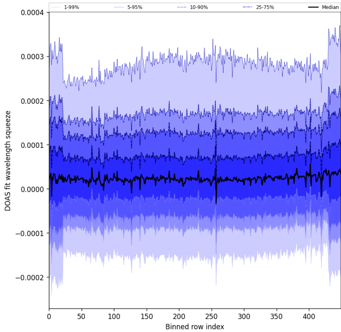
Figure 59: Along track statistics of “DOAS fit wavelength squeeze” for 2025-06-22 to 2025-06-23
