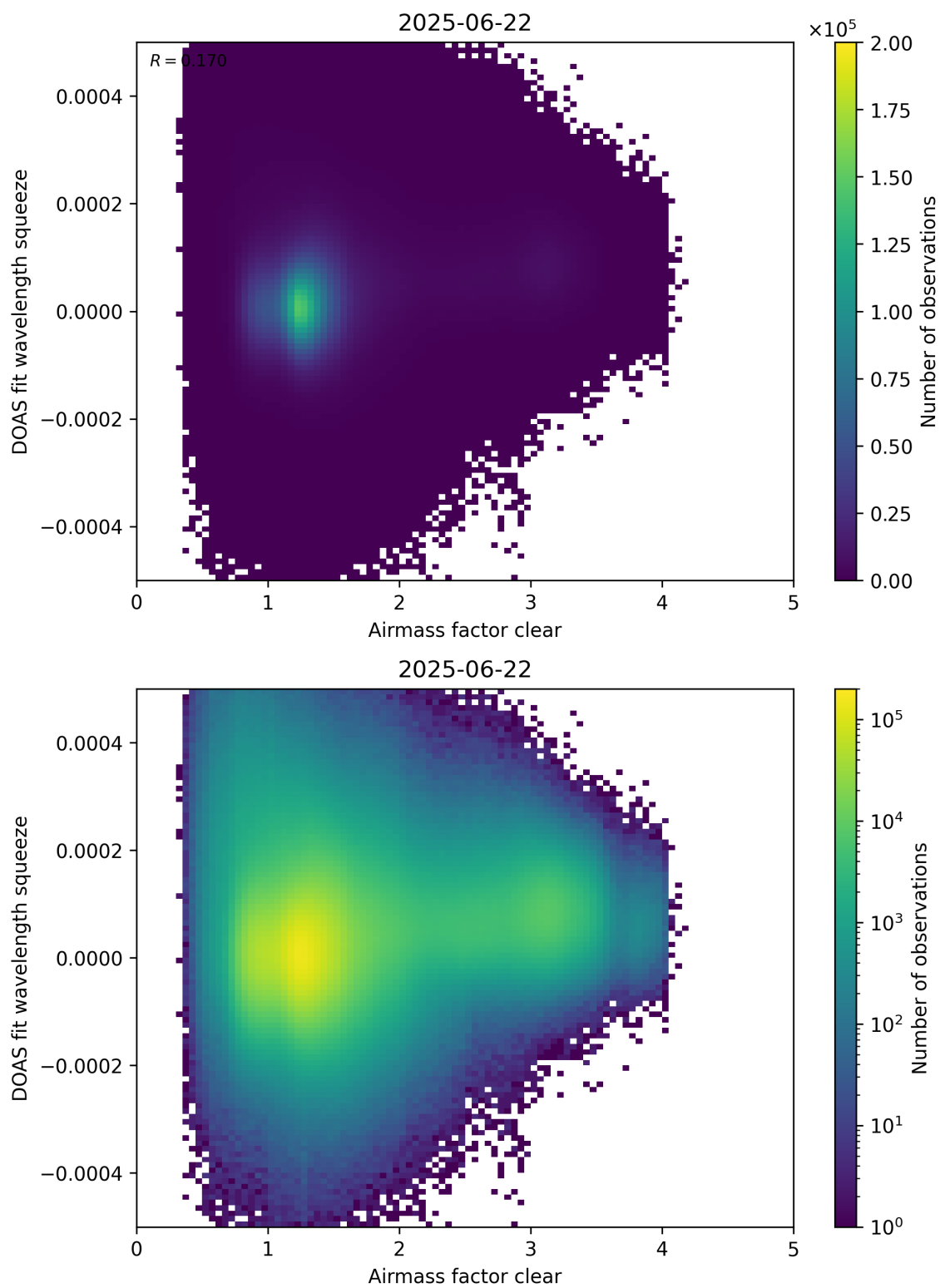
Figure 73: Scatter density plot of “Airmass factor clear” against “DOAS fit wavelength squeeze” for 2025-06-22 to 2025-06-23.
