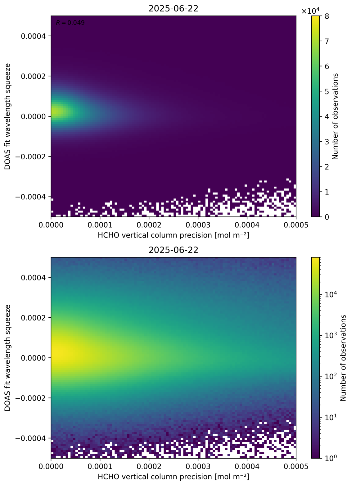
Figure 138: Scatter density plot of “HCHO vertical column precision” against “DOAS fit wavelength squeeze” for 2025-06-22 to 2025-06-23.
