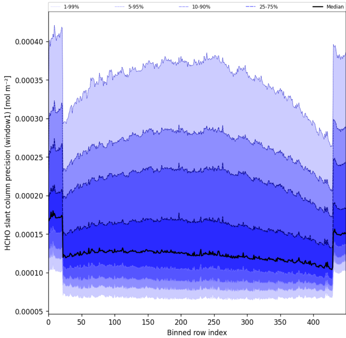
Figure 53: Along track statistics of “HCHO slant column precision (window1)” for 2025-06-22 to 2025-06-23
