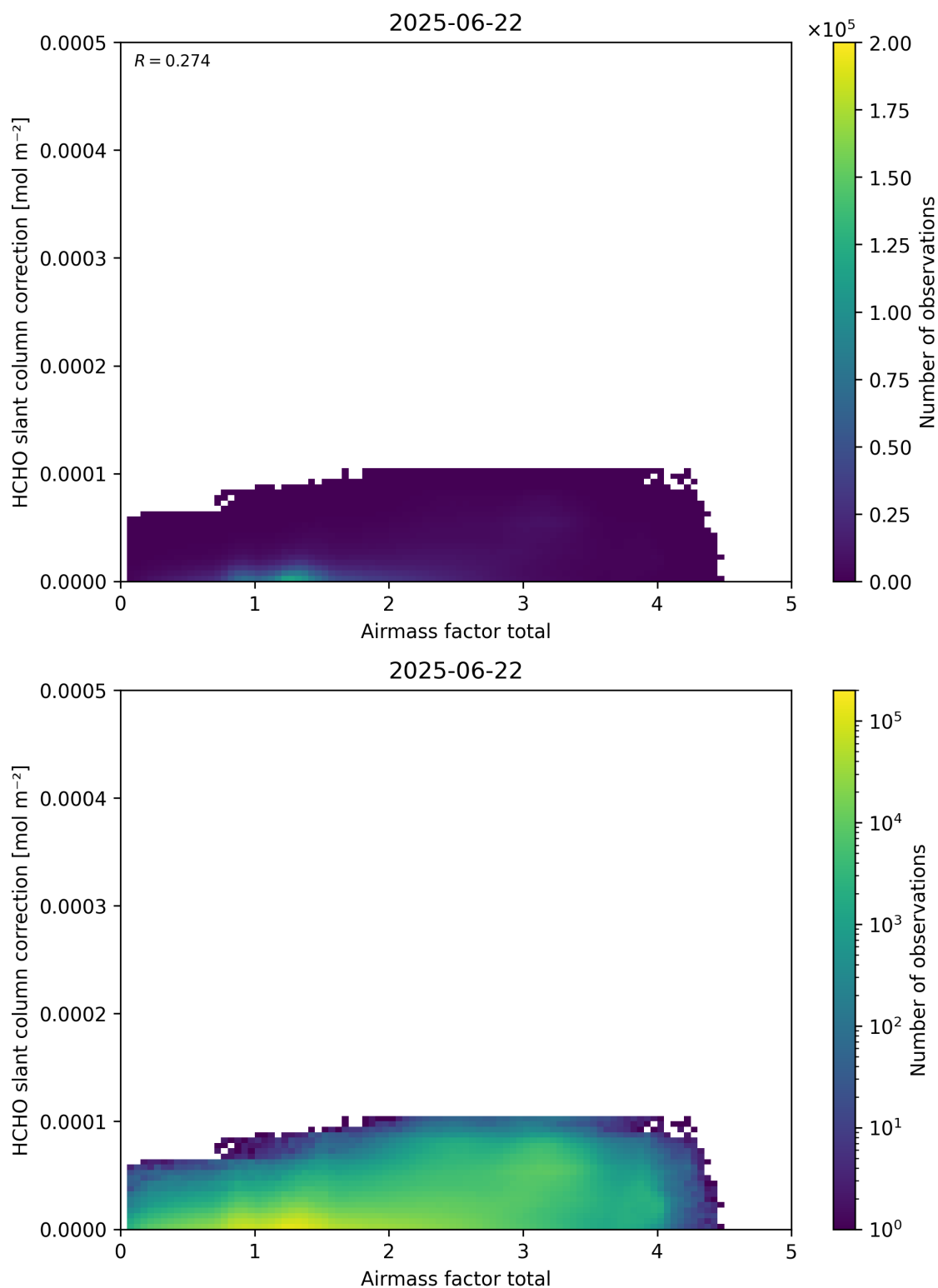
Figure 102: Scatter density plot of “Airmass factor total” against “HCHO slant column correction” for 2025-06-22 to 2025-06-23.
