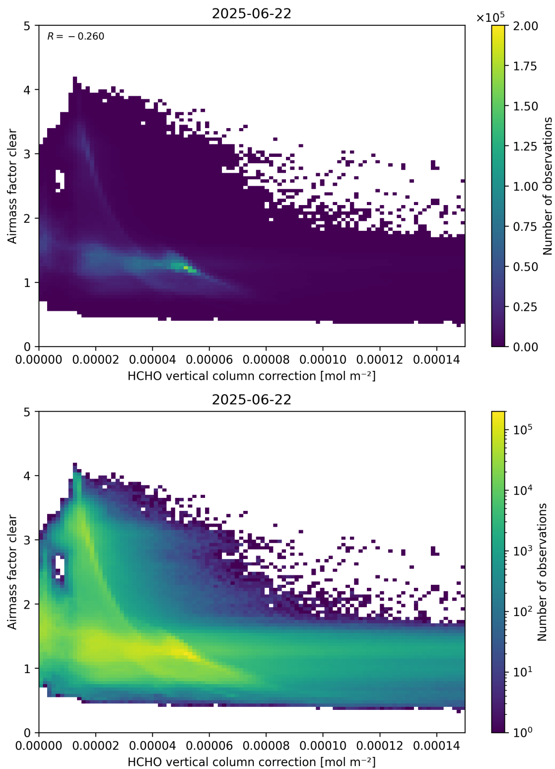
Figure 115: Scatter density plot of “HCHO vertical column correction” against “Airmass factor clear” for 2025-06-22 to 2025-06-23.
