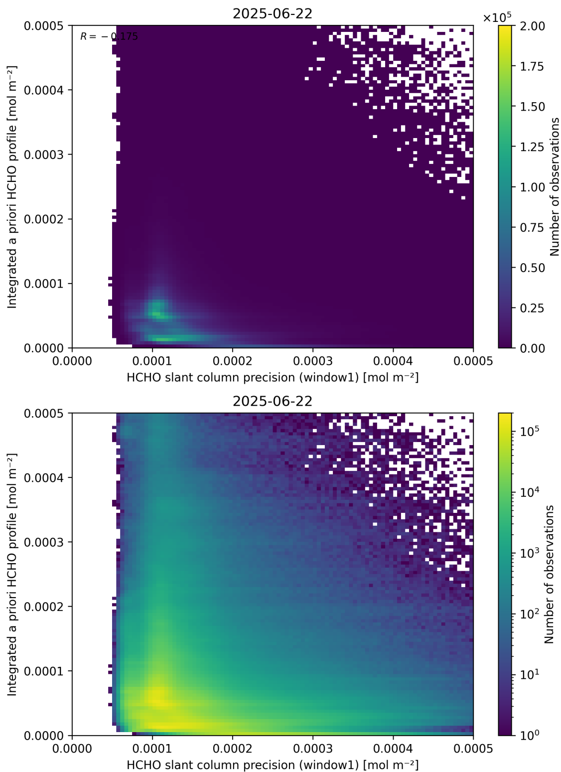
Figure 96: Scatter density plot of “HCHO slant column precision (window1)” against “Integrated a priori HCHO profile” for 2025-06-22 to 2025-06-23.
