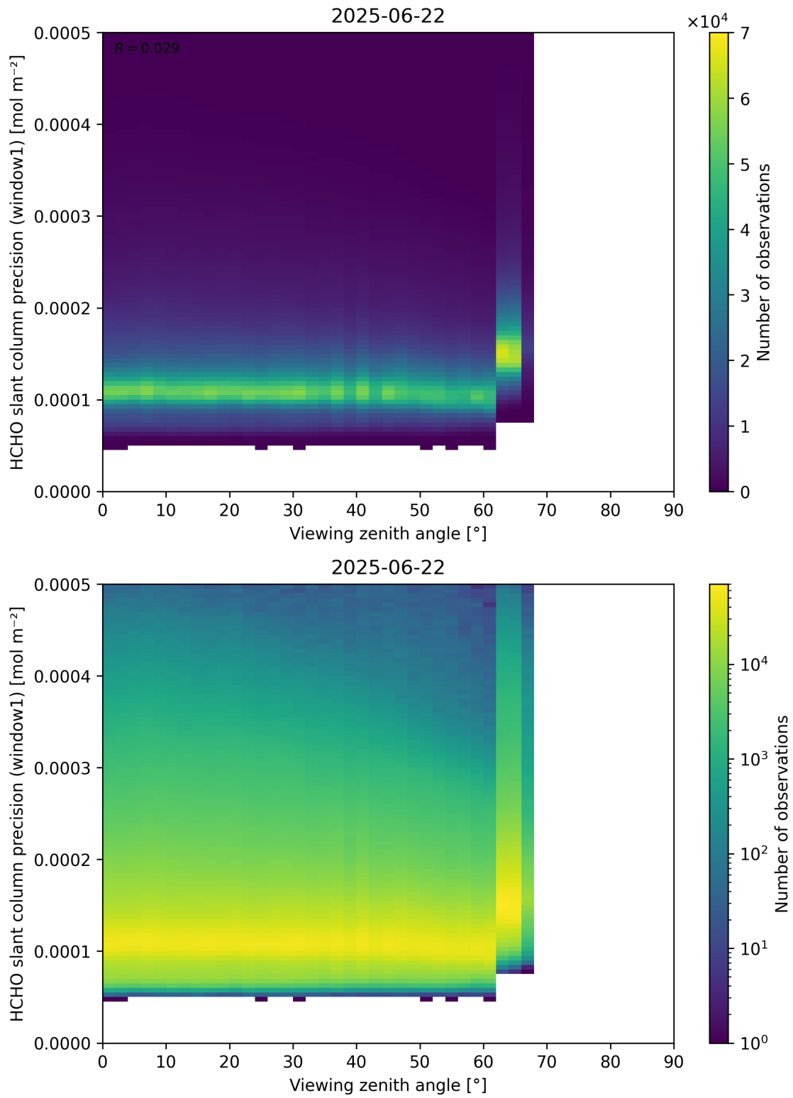
Figure 189: Scatter density plot of “Viewing zenith angle” against “HCHO slant column precision (window1)” for 2025-06-22 to 2025-06-23.
