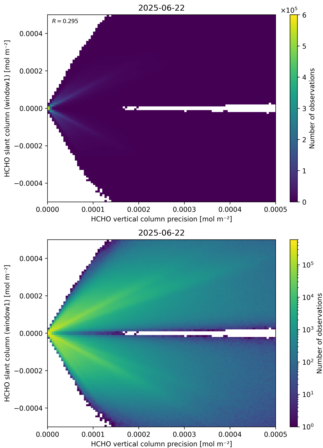
Figure 142: Scatter density plot of “HCHO vertical column precision” against “HCHO slant column (window1)” for 2025-06-22 to 2025-06-23.
