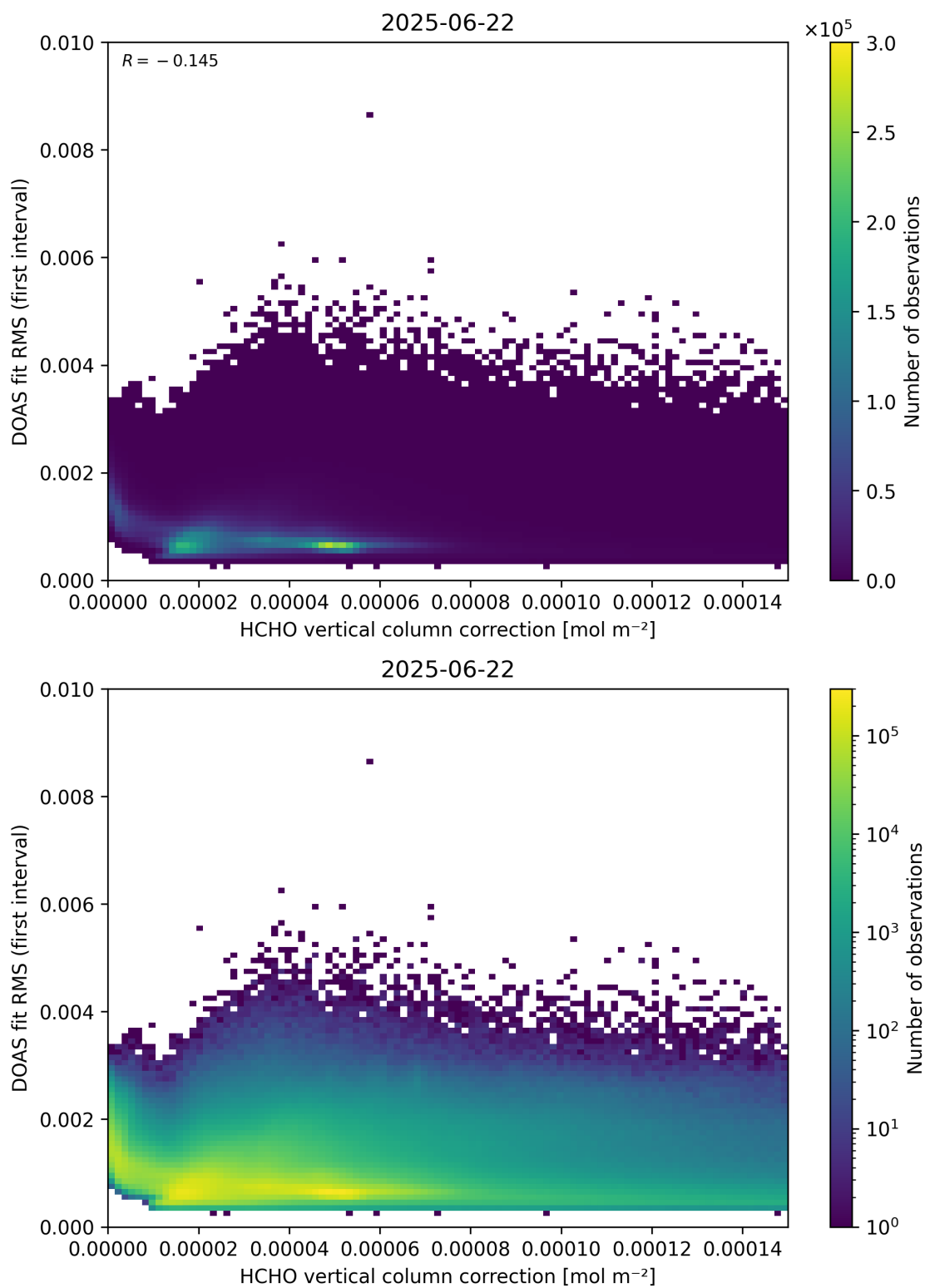
Figure 112: Scatter density plot of “HCHO vertical column correction” against “DOAS fit RMS (first interval)” for 2025-06-22 to 2025-06-23.
