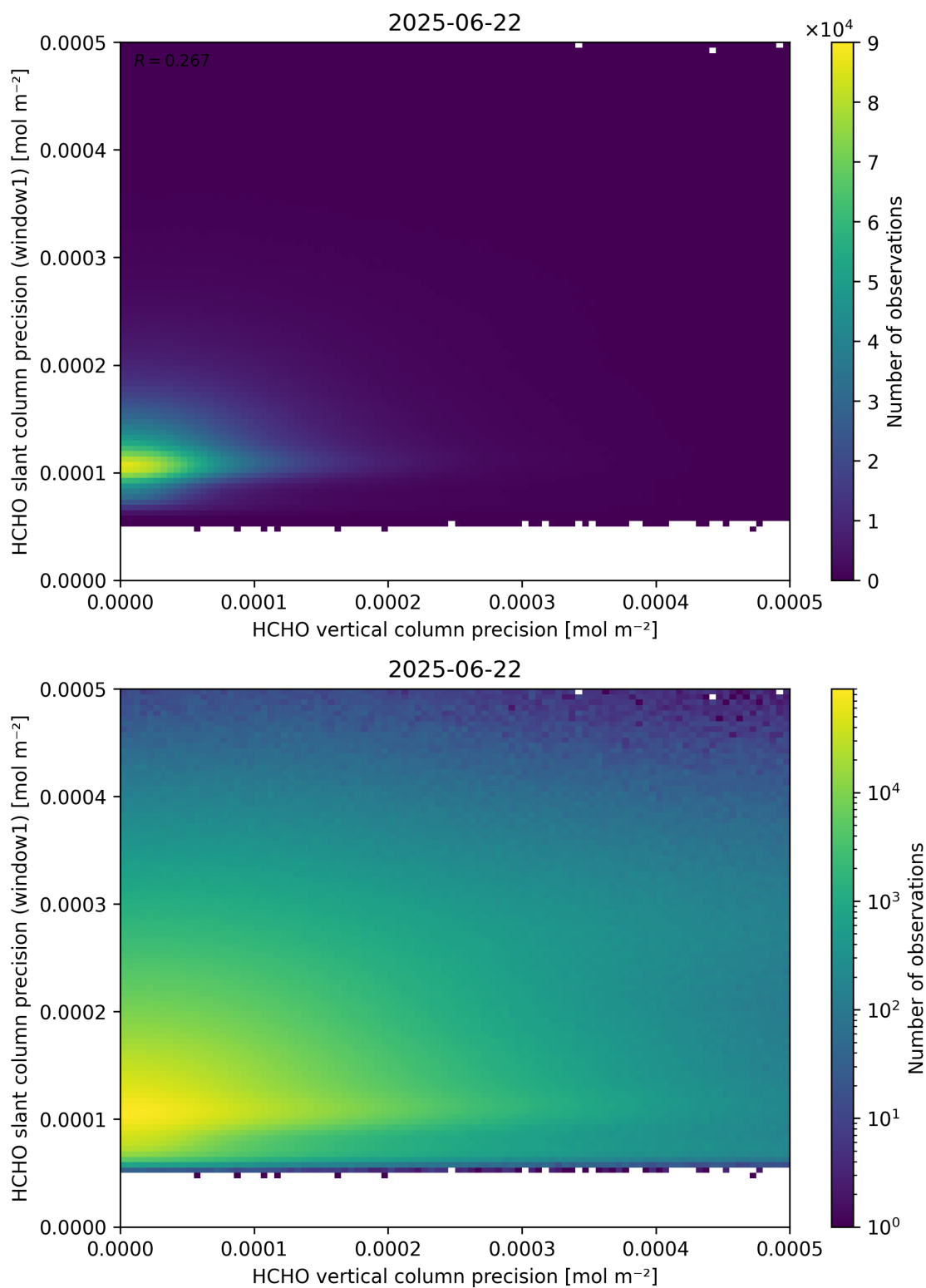
Figure 143: Scatter density plot of “HCHO vertical column precision” against “HCHO slant column precision (window1)” for 2025-06-22 to 2025-06-23.
