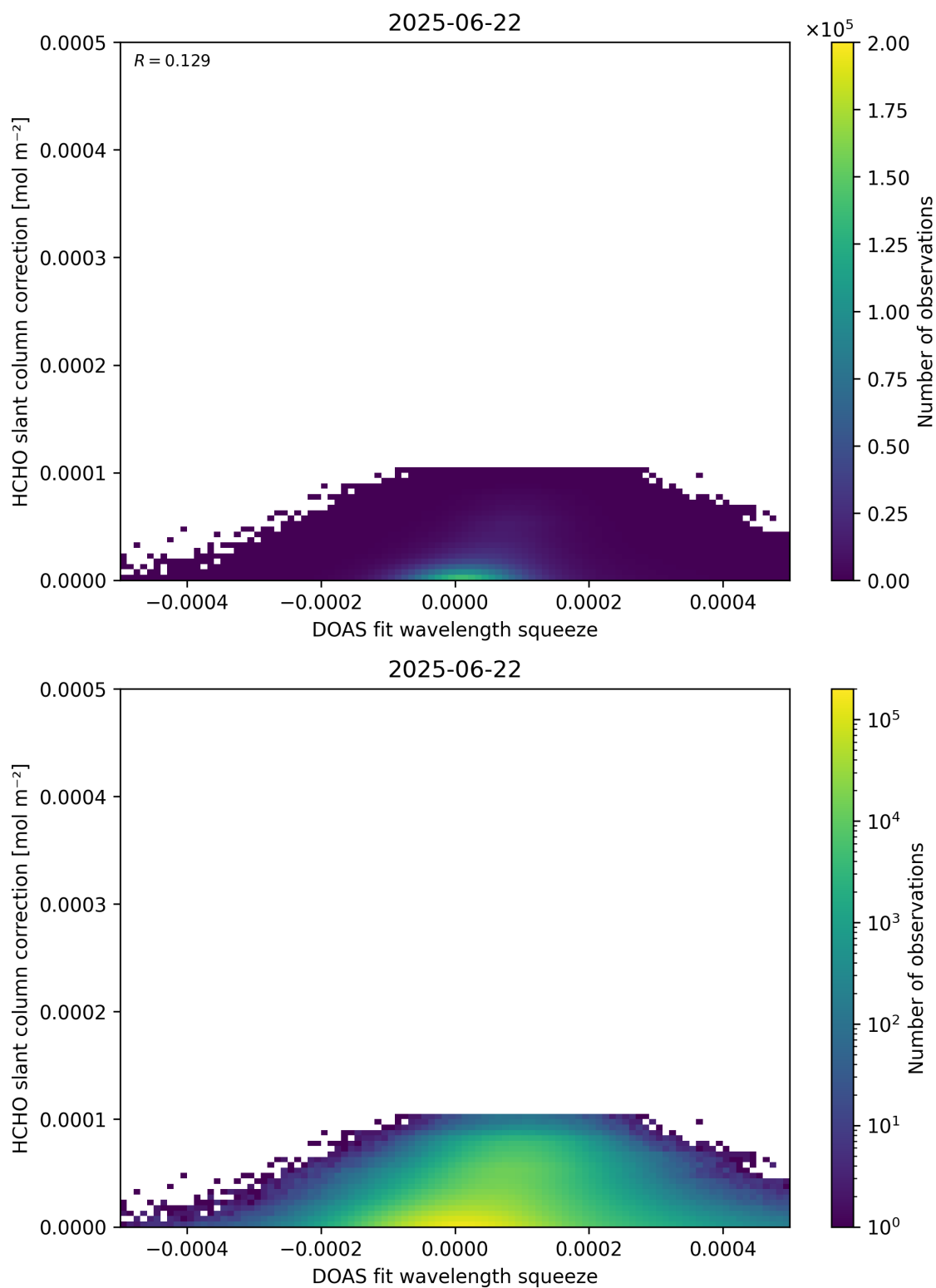
Figure 70: Scatter density plot of “DOAS fit wavelength squeeze” against “HCHO slant column correction” for 2025-06-22 to 2025-06-23.
