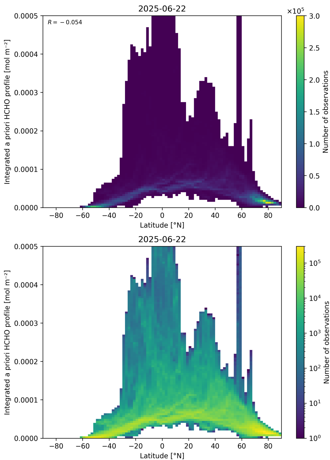
Figure 166: Scatter density plot of “Latitude” against “Integrated a priori HCHO profile” for 2025-06-22 to 2025-06-23.
