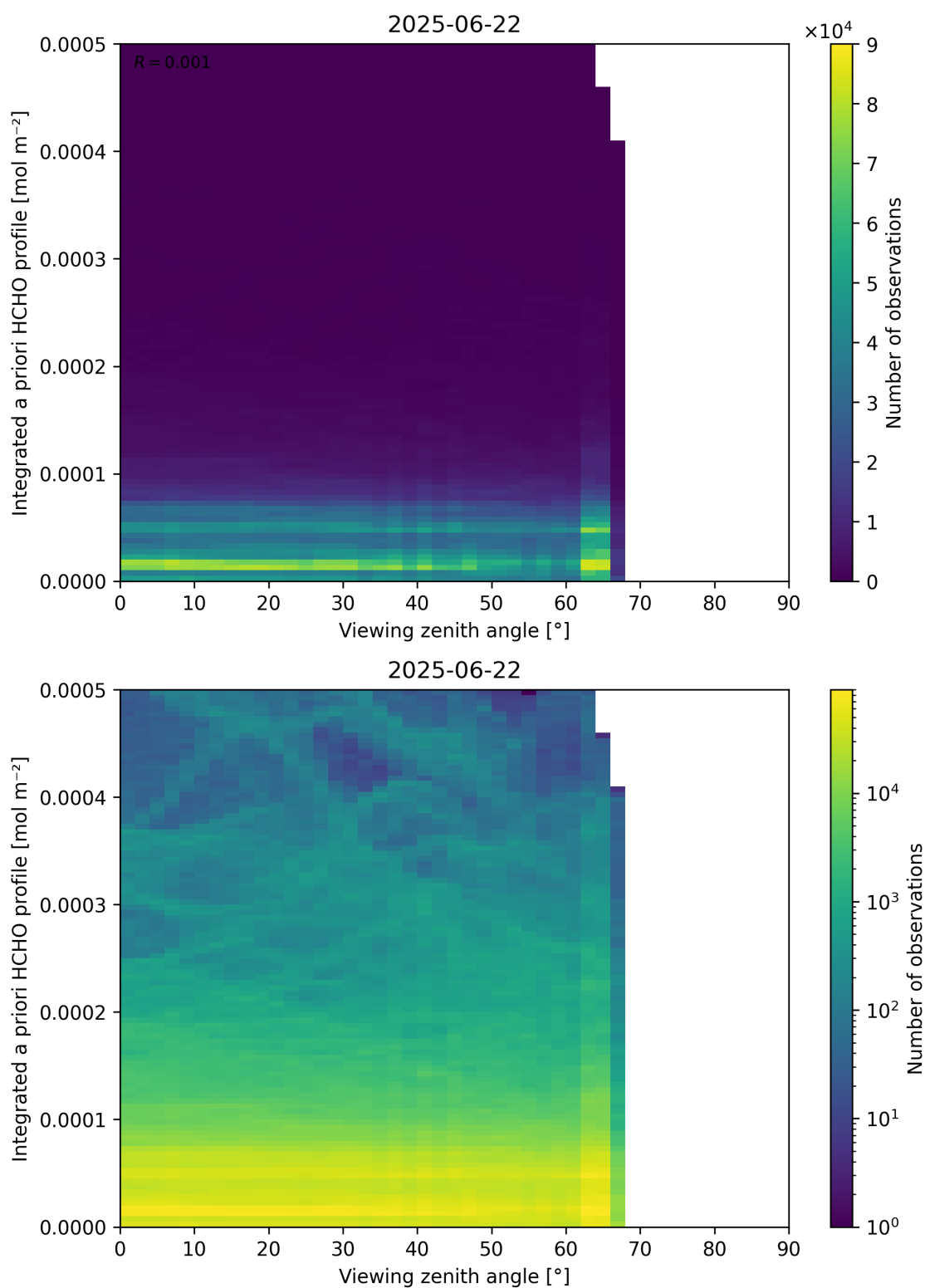
Figure 195: Scatter density plot of “Viewing zenith angle” against “Integrated a priori HCHO profile” for 2025-06-22 to 2025-06-23.
