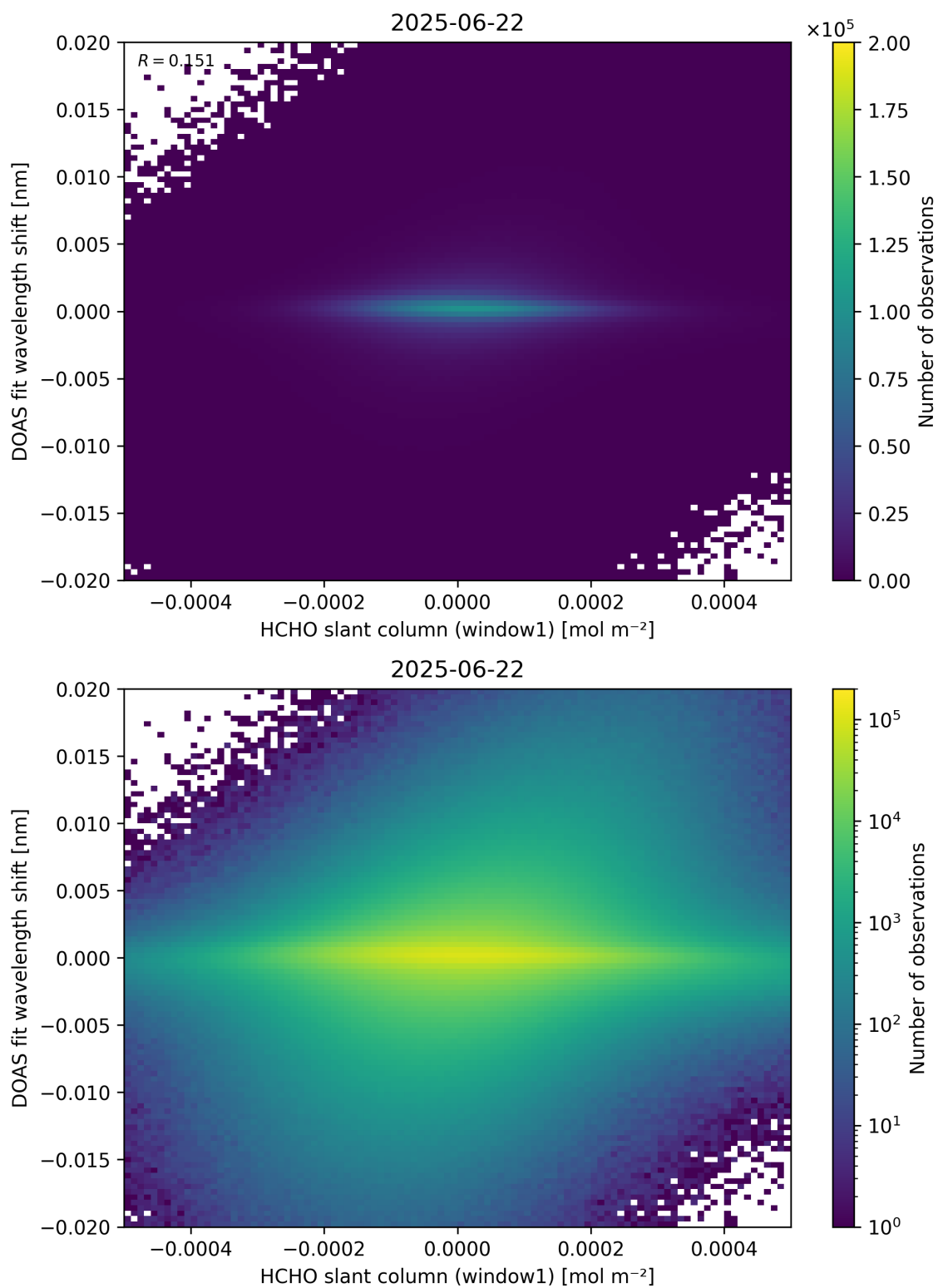
Figure 79: Scatter density plot of “HCHO slant column (window1)” against “DOAS fit wavelength shift” for 2025-06-22 to 2025-06-23.
