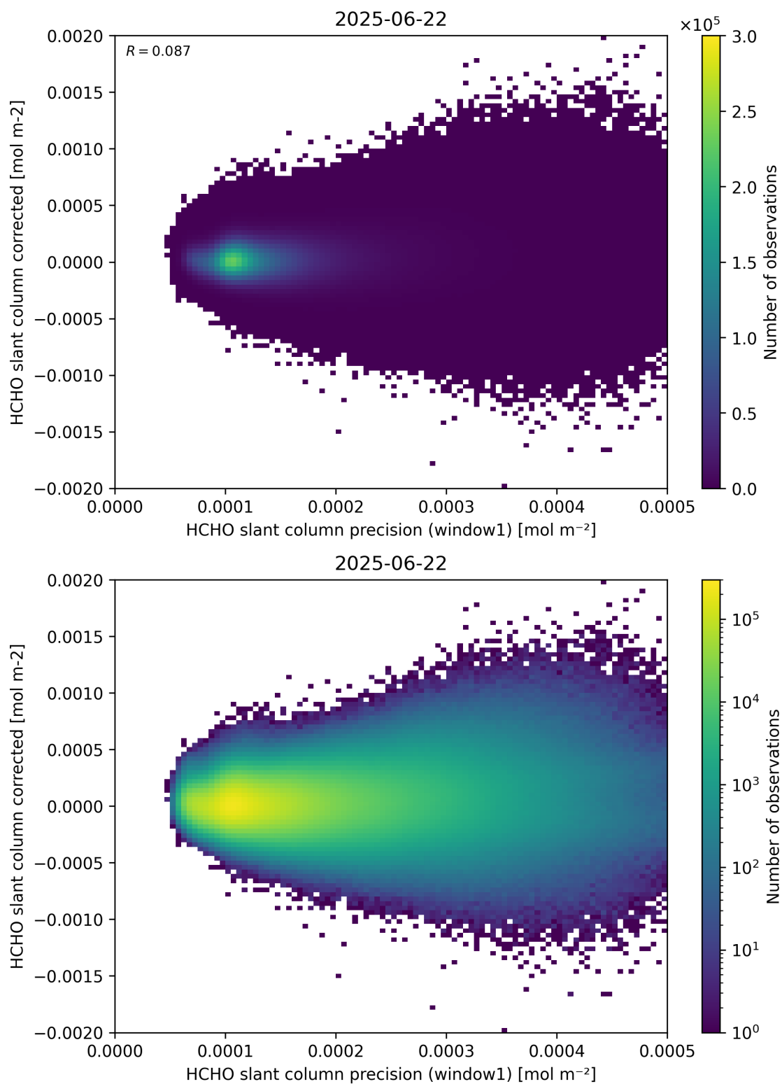
Figure 92: Scatter density plot of “HCHO slant column precision (window1)” against “HCHO slant column corrected” for 2025-06-22 to 2025-06-23.
