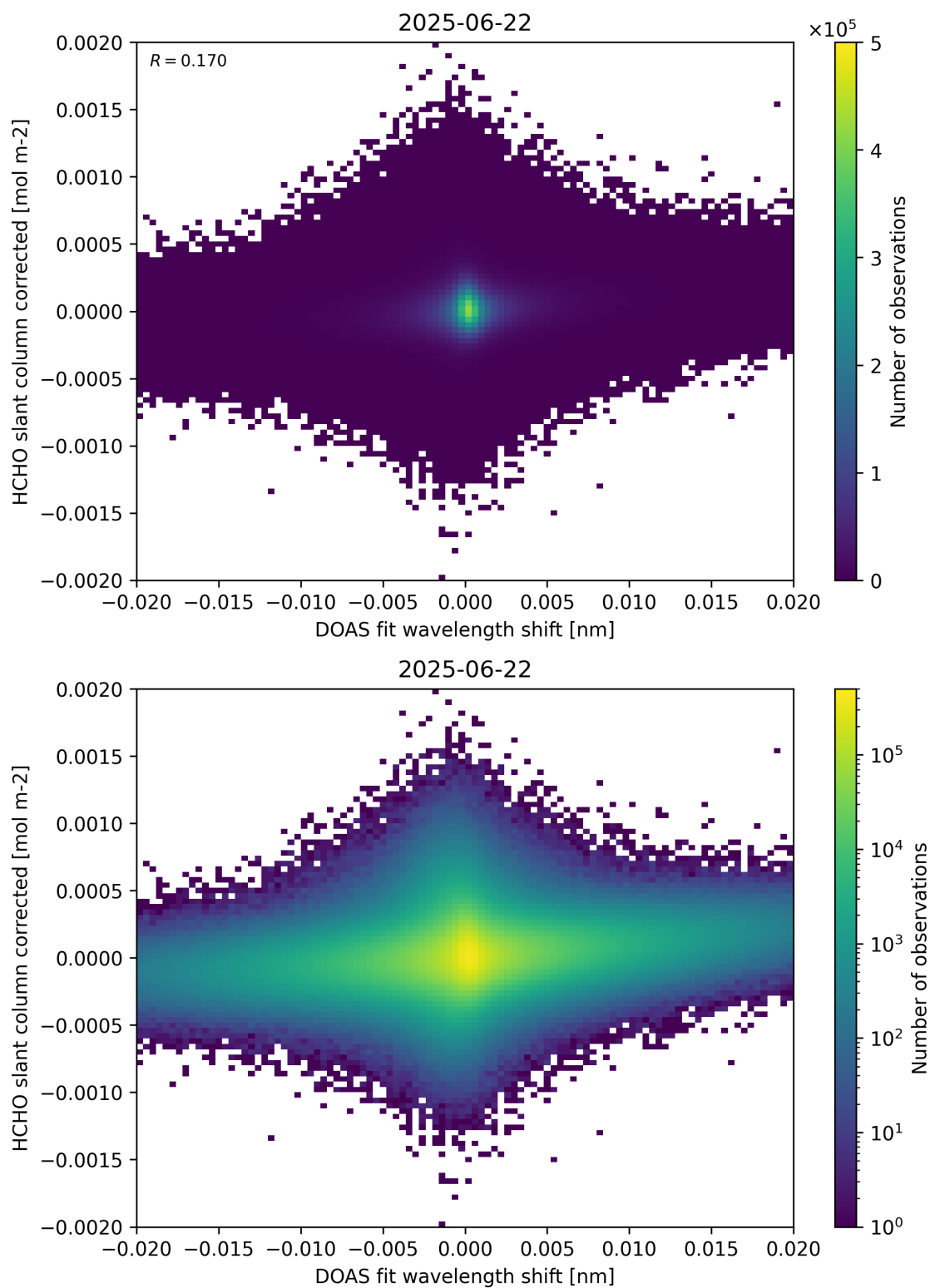
Figure 66: Scatter density plot of “DOAS fit wavelength shift” against “HCHO slant column corrected” for 2025-06-22 to 2025-06-23.
