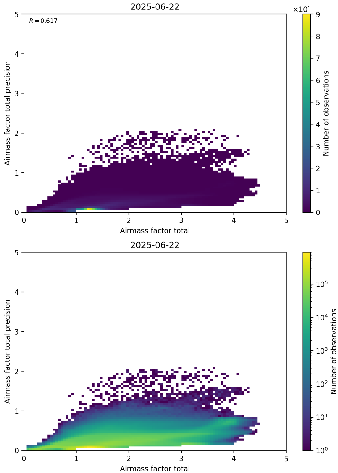
Figure 103: Scatter density plot of “Airmass factor total” against “Airmass factor total precision” for 2025-06-22 to 2025-06-23.
