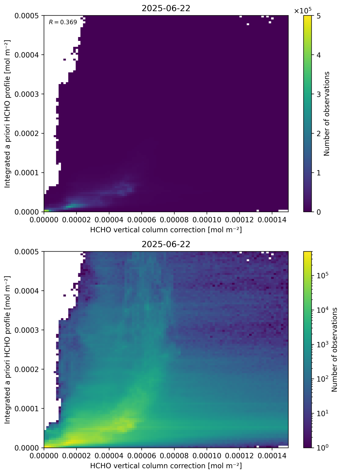
Figure 122: Scatter density plot of “HCHO vertical column correction” against “Integrated a priori HCHO profile” for 2025-06-22 to 2025-06-23.
