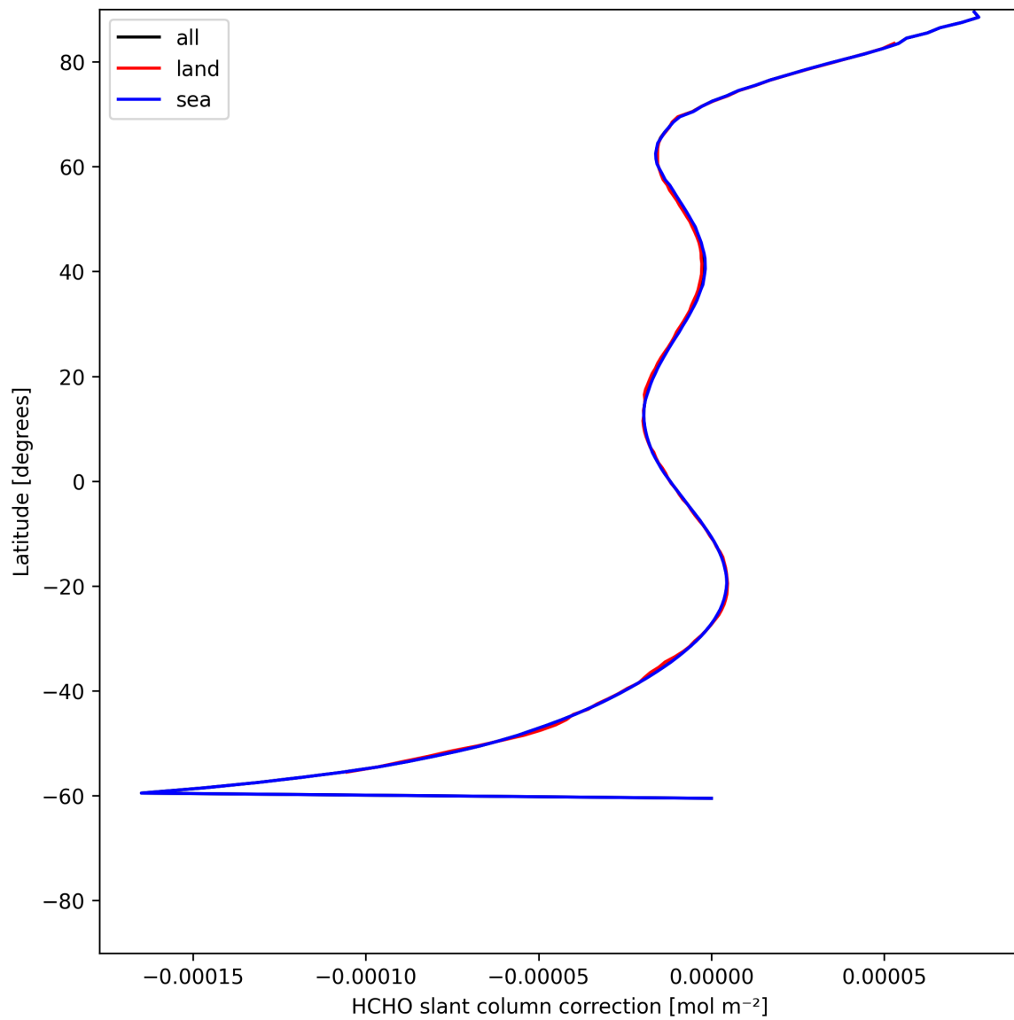
Figure 33: Zonal average of “HCHO slant column correction” for 2025-06-22 to 2025-06-23.
