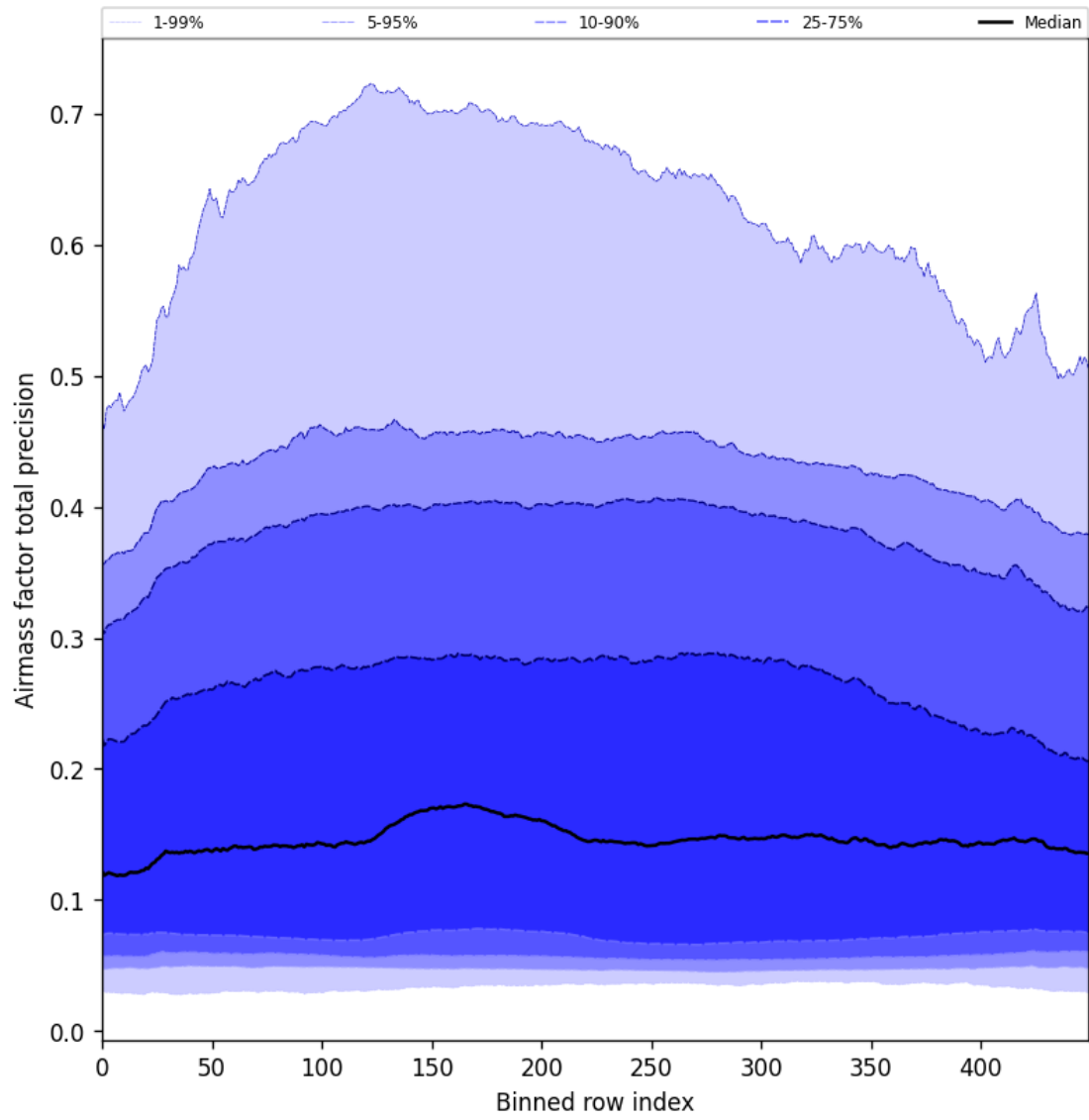
Figure 55: Along track statistics of “Airmass factor total precision” for 2025-06-22 to 2025-06-23
