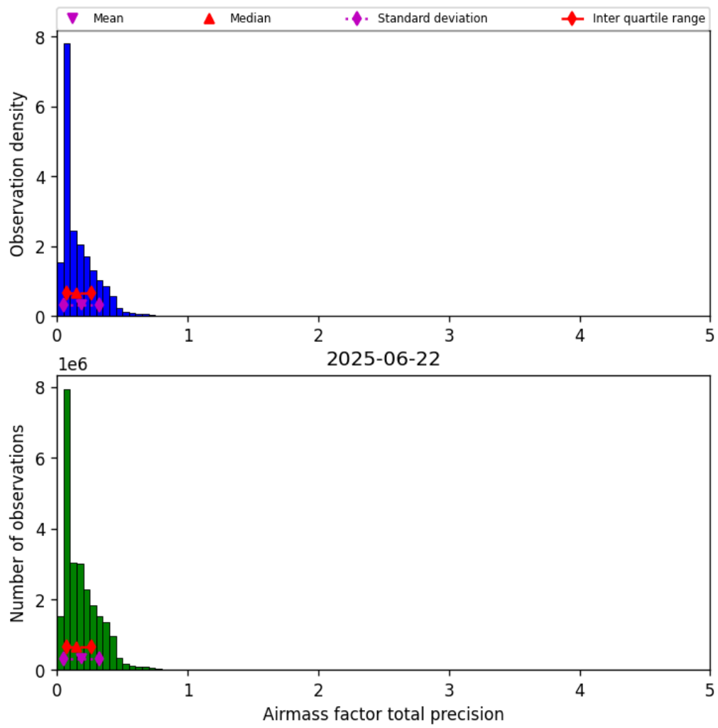
Figure 41: Histogram of “Airmass factor total precision” for 2025-06-22 to 2025-06-23
