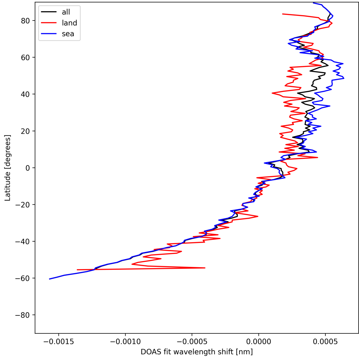
Figure 30: Zonal average of “DOAS fit wavelength shift” for 2025-06-22 to 2025-06-23.
