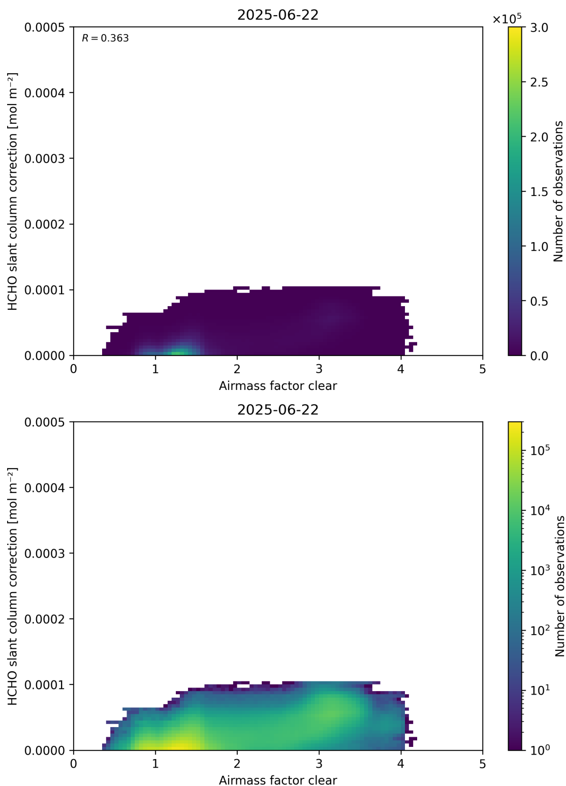
Figure 75: Scatter density plot of “Airmass factor clear” against “HCHO slant column correction” for 2025-06-22 to 2025-06-23.
