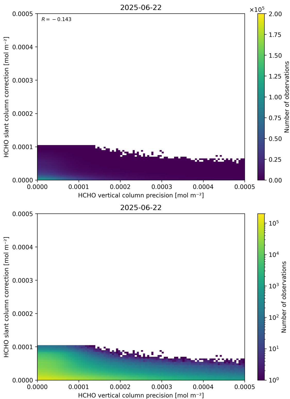
Figure 141: Scatter density plot of “HCHO vertical column precision” against “HCHO slant column correction” for 2025-06-22 to 2025-06-23.
