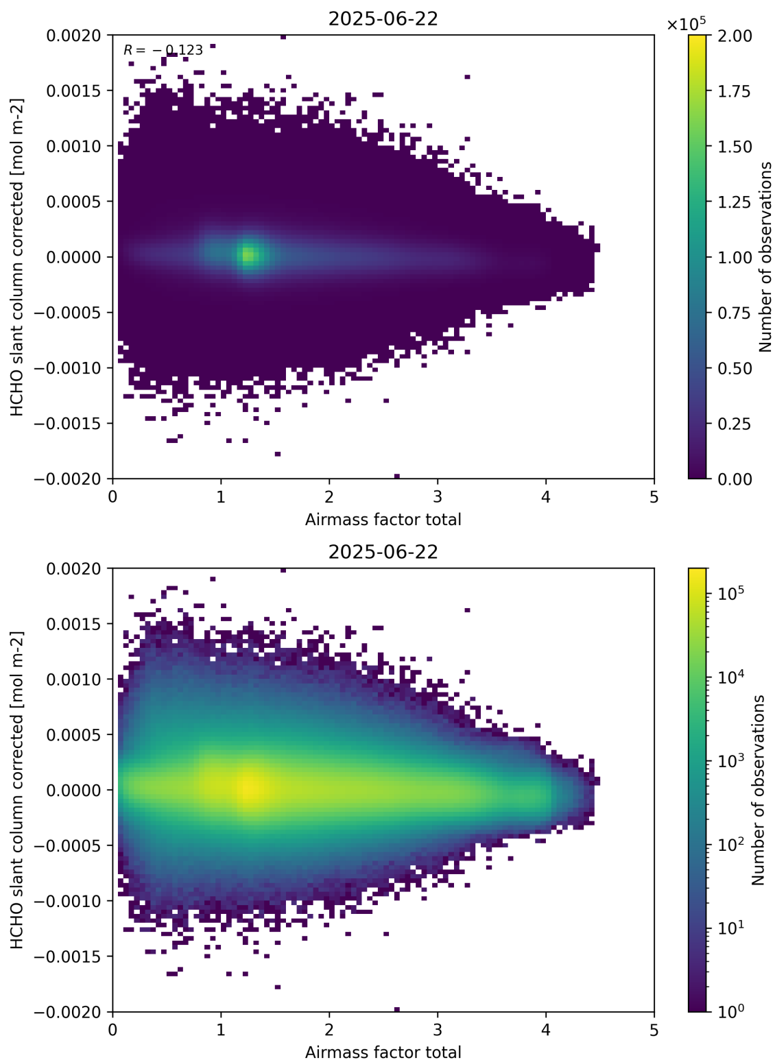
Figure 101: Scatter density plot of “Airmass factor total” against “HCHO slant column corrected” for 2025-06-22 to 2025-06-23.
