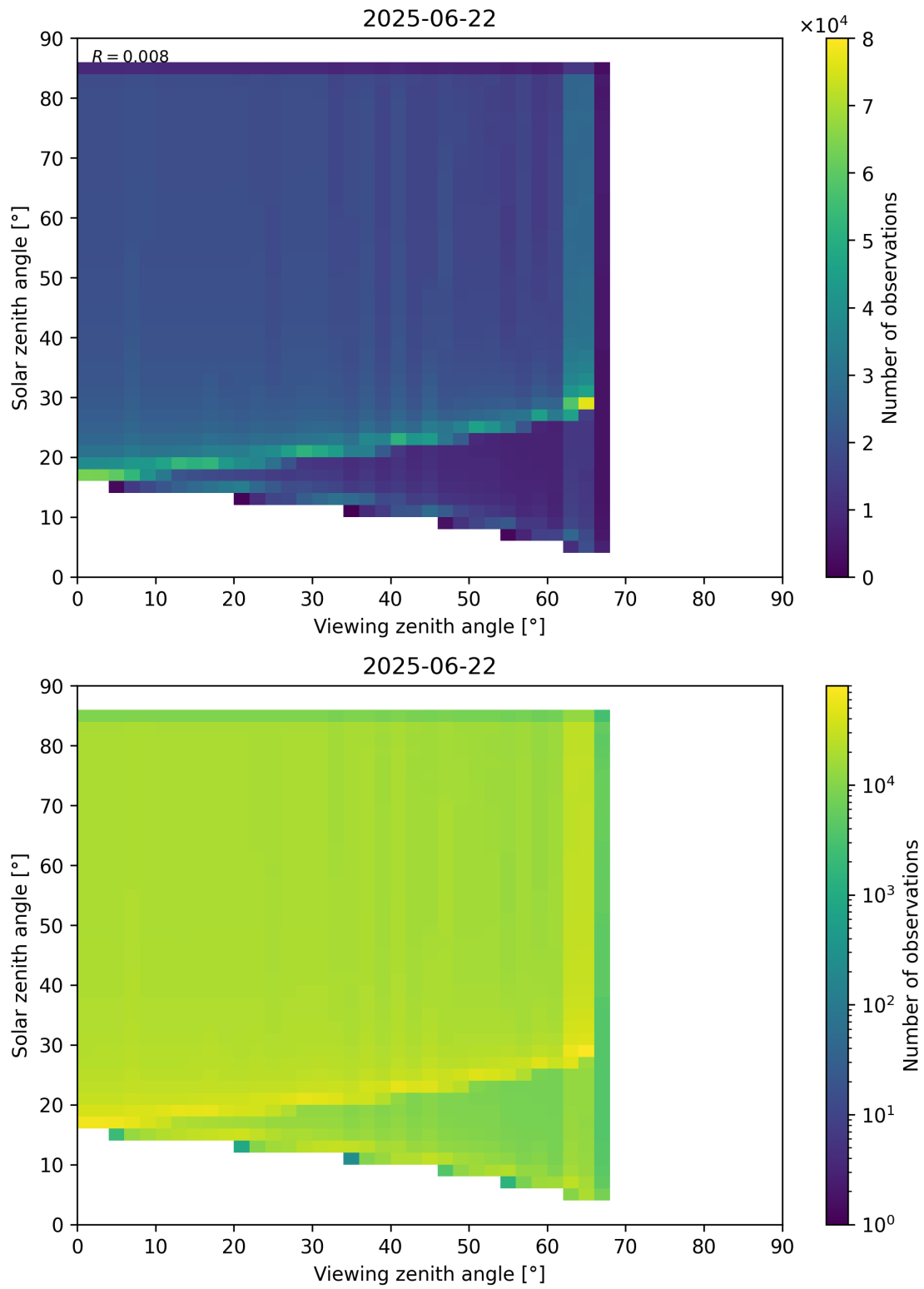
Figure 197: Scatter density plot of “Viewing zenith angle” against “Solar zenith angle” for 2025-06-22 to 2025-06-23.
