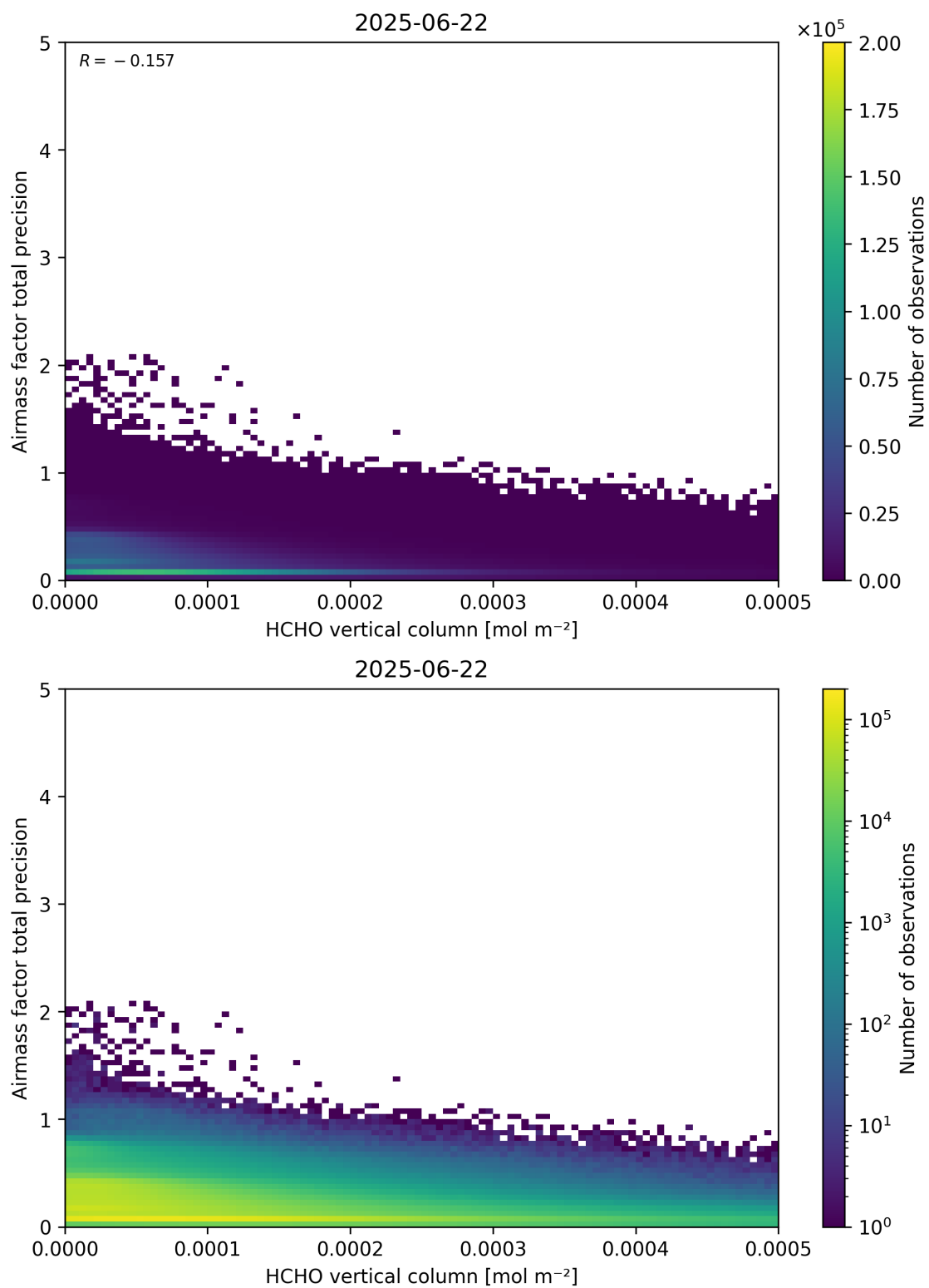
Figure 132: Scatter density plot of “HCHO vertical column” against “Airmass factor total precision” for 2025-06-22 to 2025-06-23.
