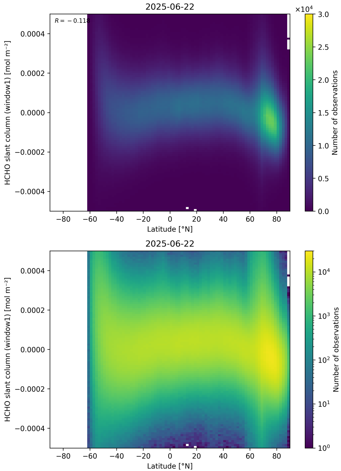
Figure 159: Scatter density plot of “Latitude” against “HCHO slant column (window1)” for 2025-06-22 to 2025-06-23.
