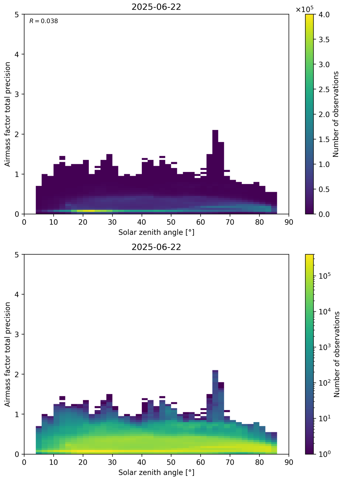
Figure 176: Scatter density plot of “Solar zenith angle” against “Airmass factor total precision” for 2025-06-22 to 2025-06-23.
