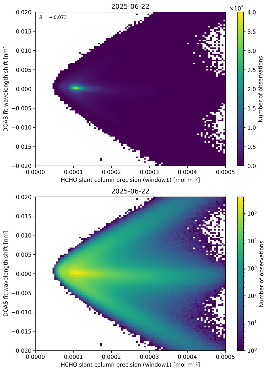
Figure 89: Scatter density plot of “HCHO slant column precision (window1)” against “DOAS fit wavelength shift” for 2025-06-22 to 2025-06-23.
