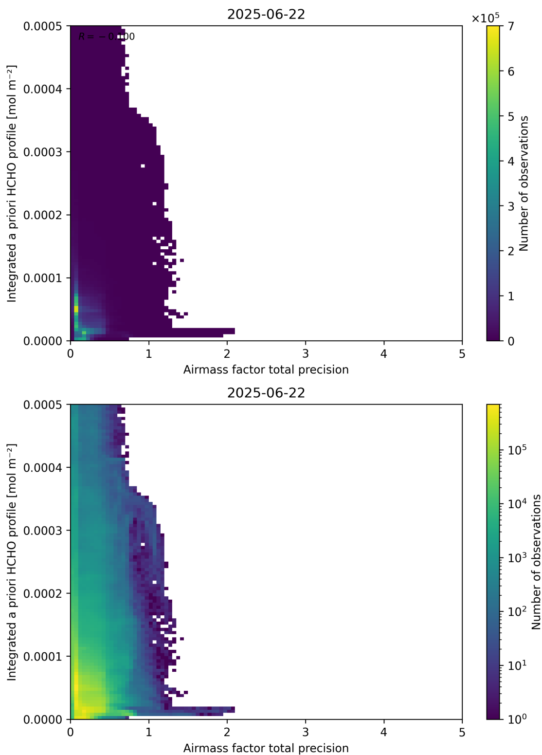
Figure 111: Scatter density plot of “Airmass factor total precision” against “Integrated a priori HCHO profile” for 2025-06-22 to 2025-06-23.
