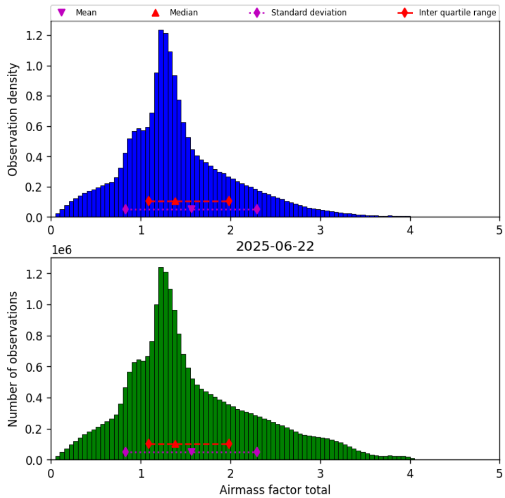
Figure 40: Histogram of “Airmass factor total” for 2025-06-22 to 2025-06-23
