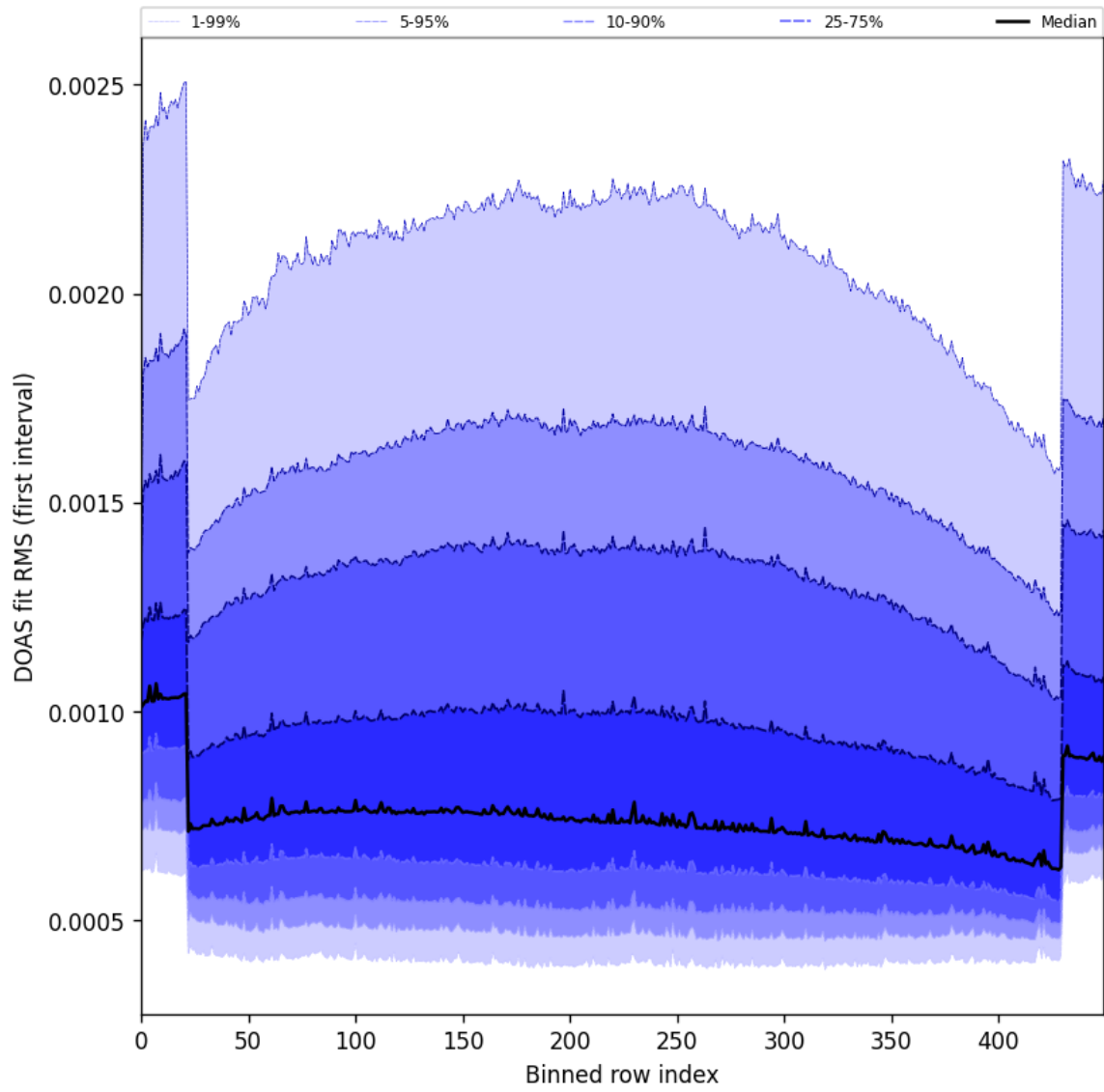
Figure 60: Along track statistics of “DOAS fit RMS (first interval)” for 2025-06-22 to 2025-06-23
