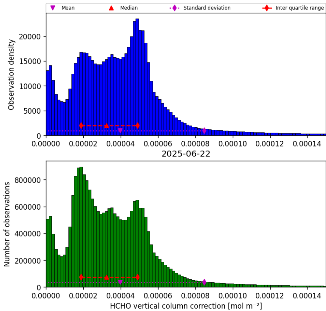
Figure 37: Histogram of “HCHO vertical column correction” for 2025-06-22 to 2025-06-23
