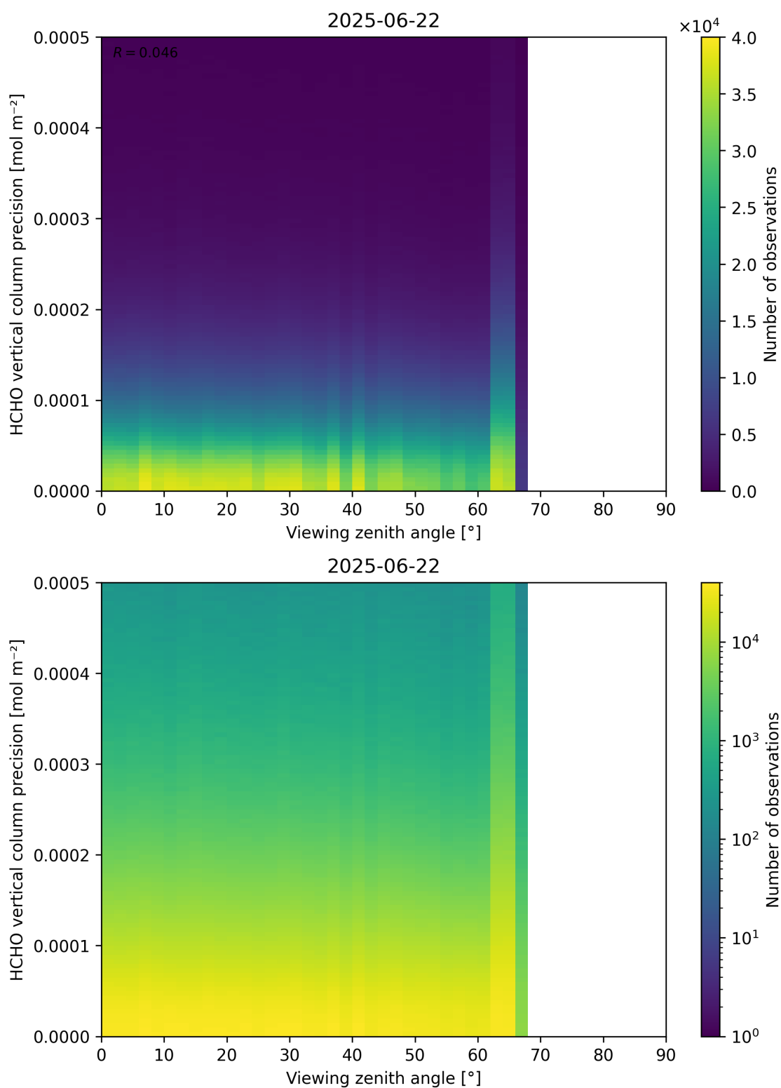
Figure 194: Scatter density plot of “Viewing zenith angle” against “HCHO vertical column precision” for 2025-06-22 to 2025-06-23.
