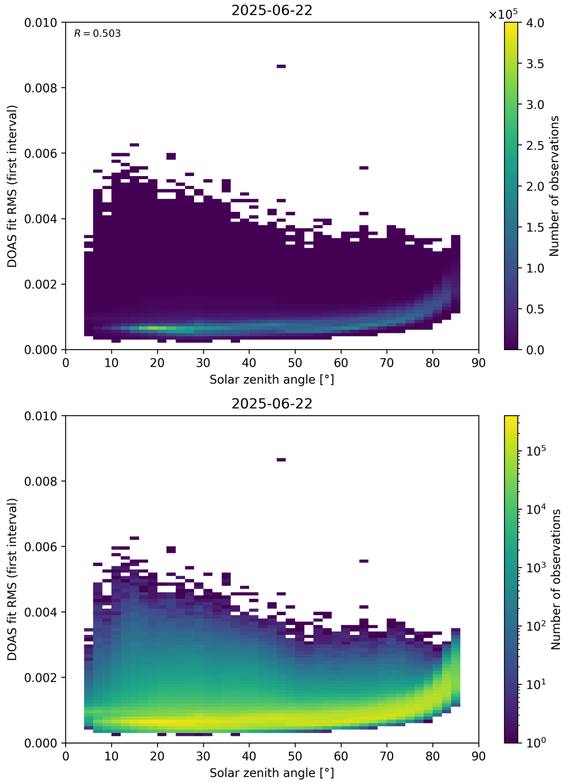
Figure 167: Scatter density plot of “Solar zenith angle” against “DOAS fit RMS (first interval)” for 2025-06-22 to 2025-06-23.
