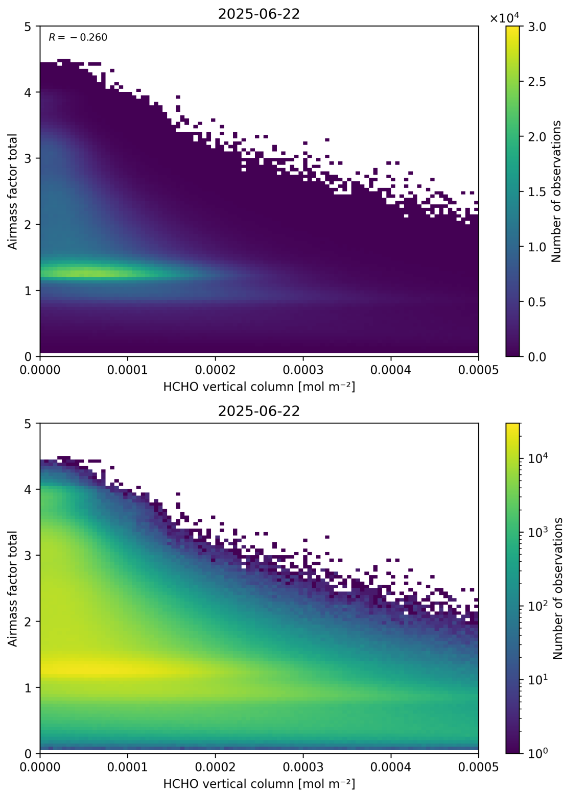
Figure 131: Scatter density plot of “HCHO vertical column” against “Airmass factor total” for 2025-06-22 to 2025-06-23.
