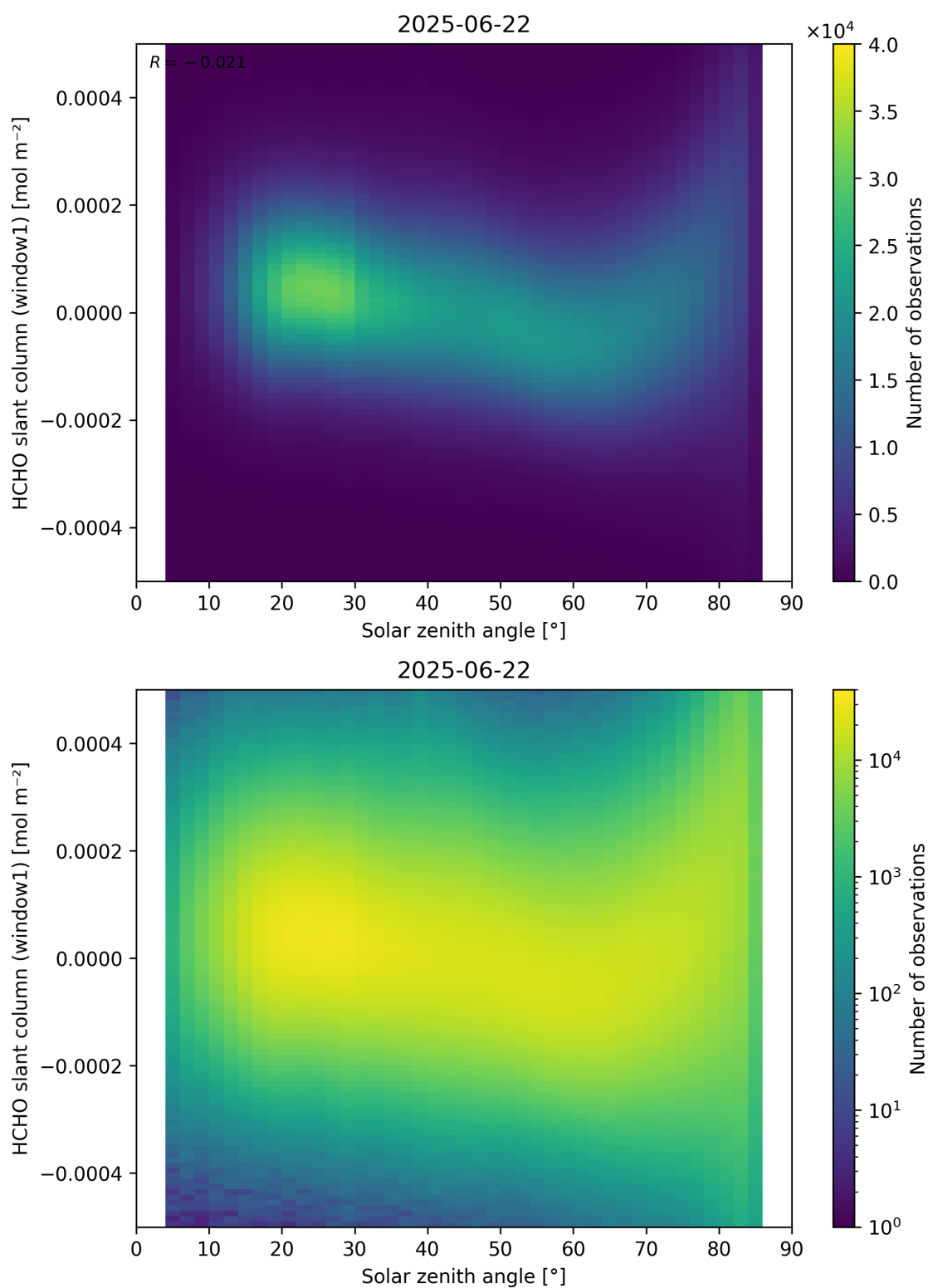
Figure 173: Scatter density plot of “Solar zenith angle” against “HCHO slant column (window1)” for 2025-06-22 to 2025-06-23.
