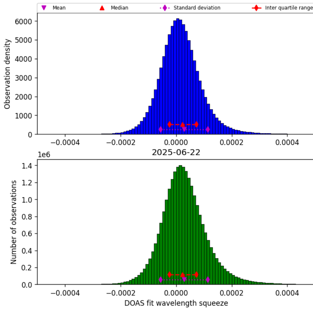
Figure 45: Histogram of “DOAS fit wavelength squeeze” for 2025-06-22 to 2025-06-23
