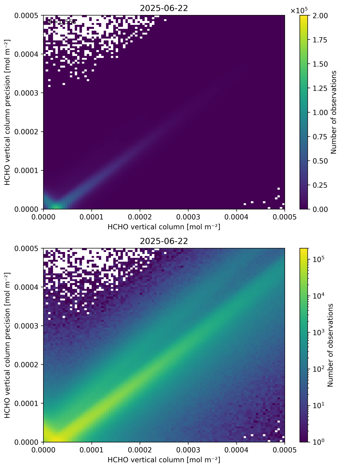
Figure 134: Scatter density plot of “HCHO vertical column” against “HCHO vertical column precision” for 2025-06-22 to 2025-06-23.
