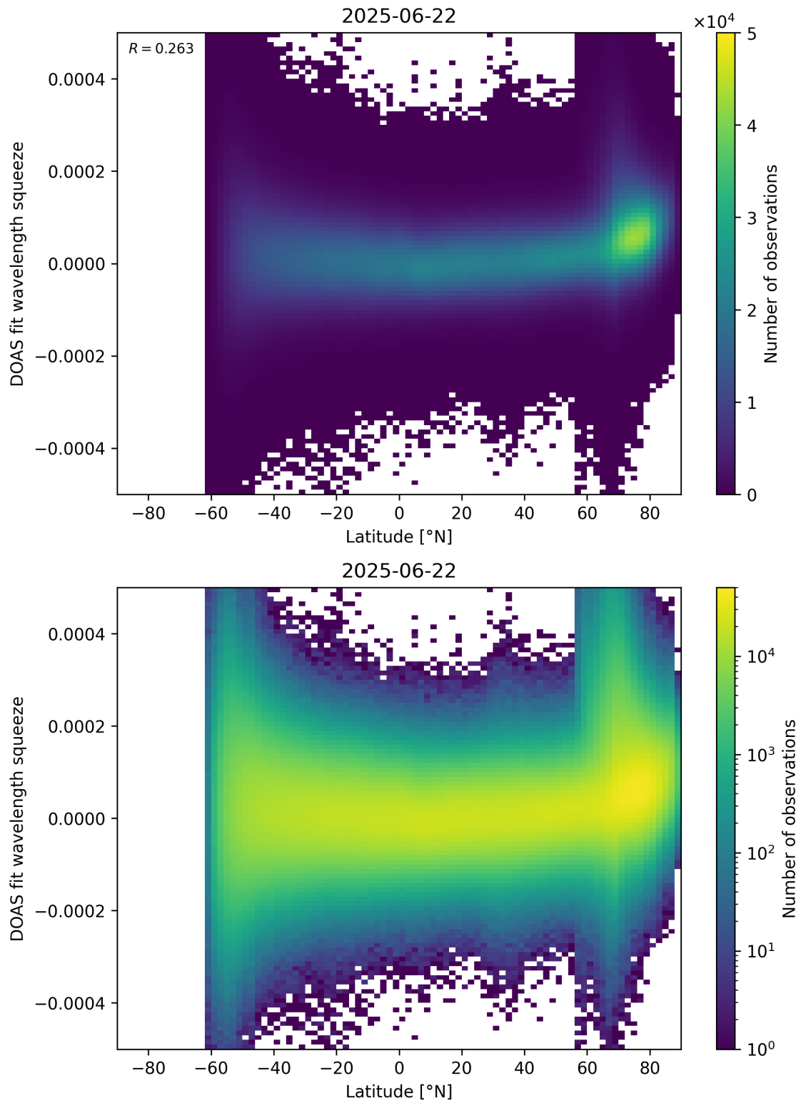
Figure 155: Scatter density plot of “Latitude” against “DOAS fit wavelength squeeze” for 2025-06-22 to 2025-06-23.
