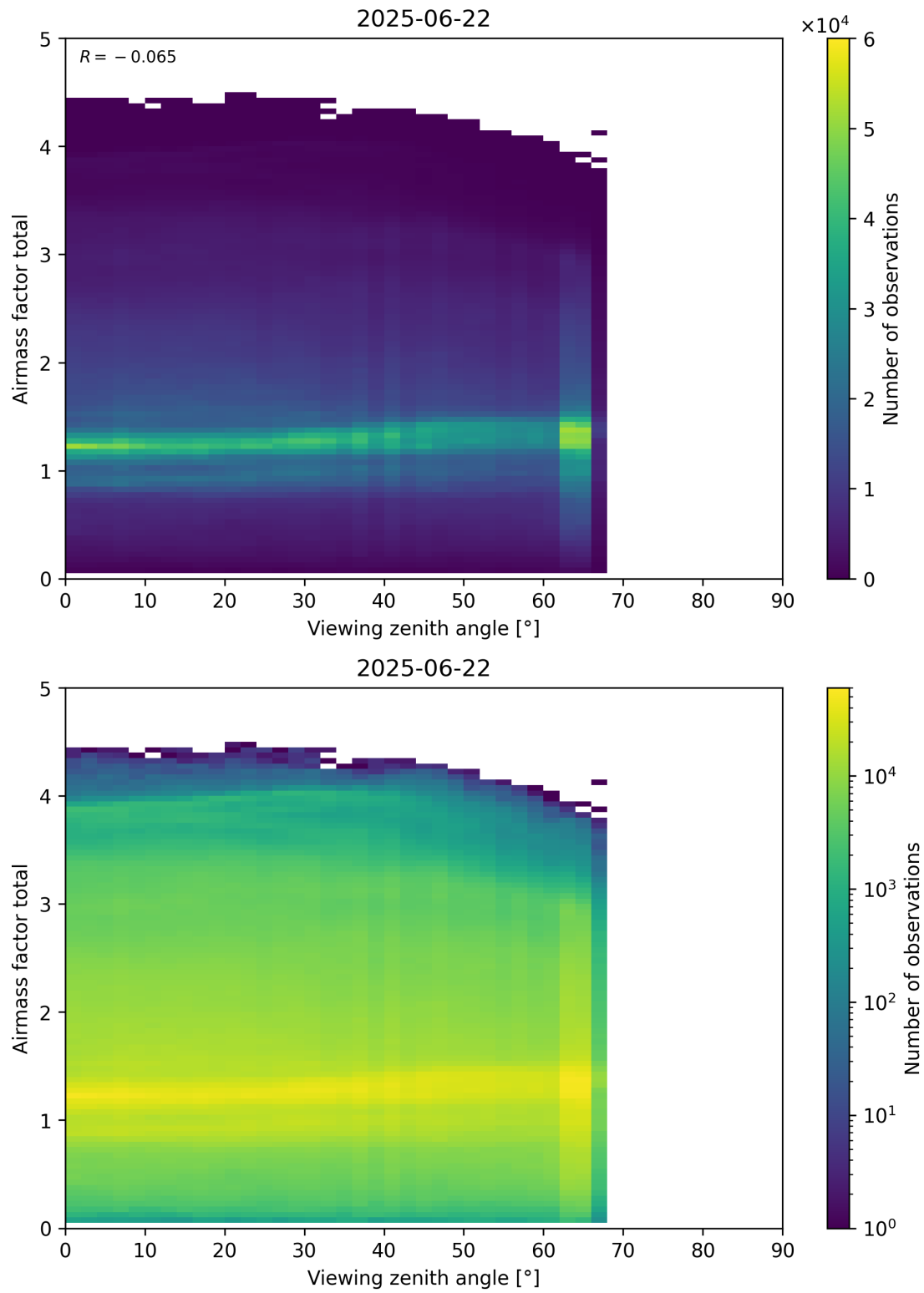
Figure 190: Scatter density plot of “Viewing zenith angle” against “Airmass factor total” for 2025-06-22 to 2025-06-23.
