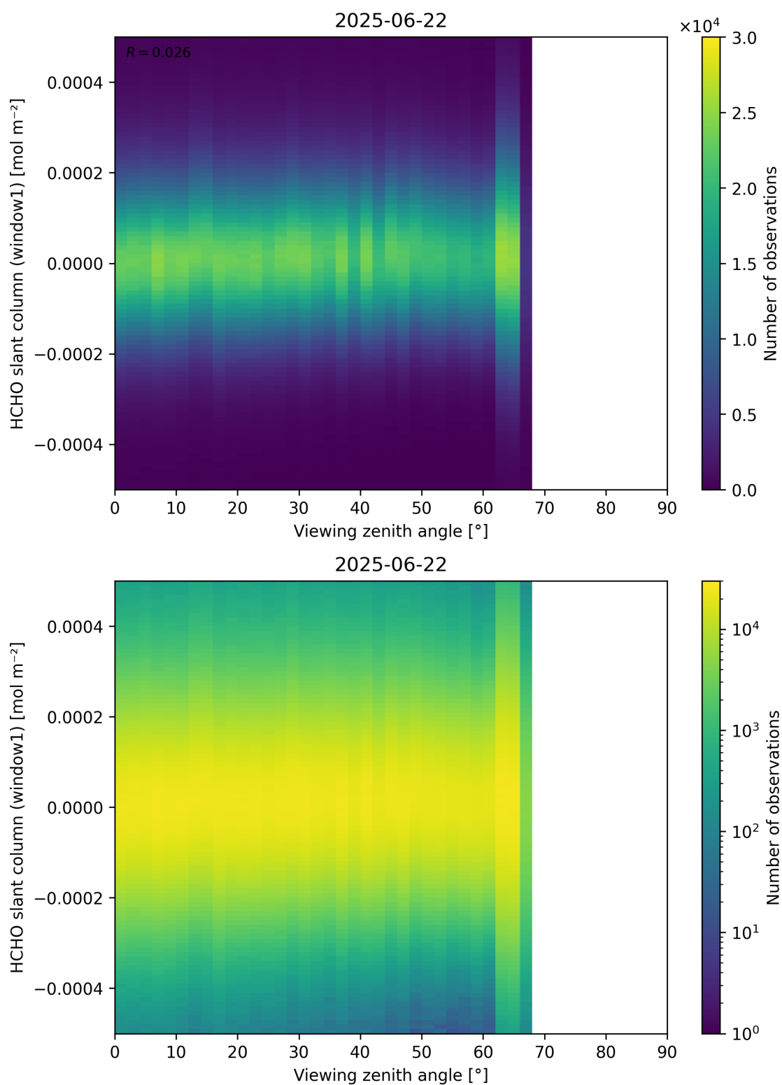
Figure 188: Scatter density plot of “Viewing zenith angle” against “HCHO slant column (window1)” for 2025-06-22 to 2025-06-23.
