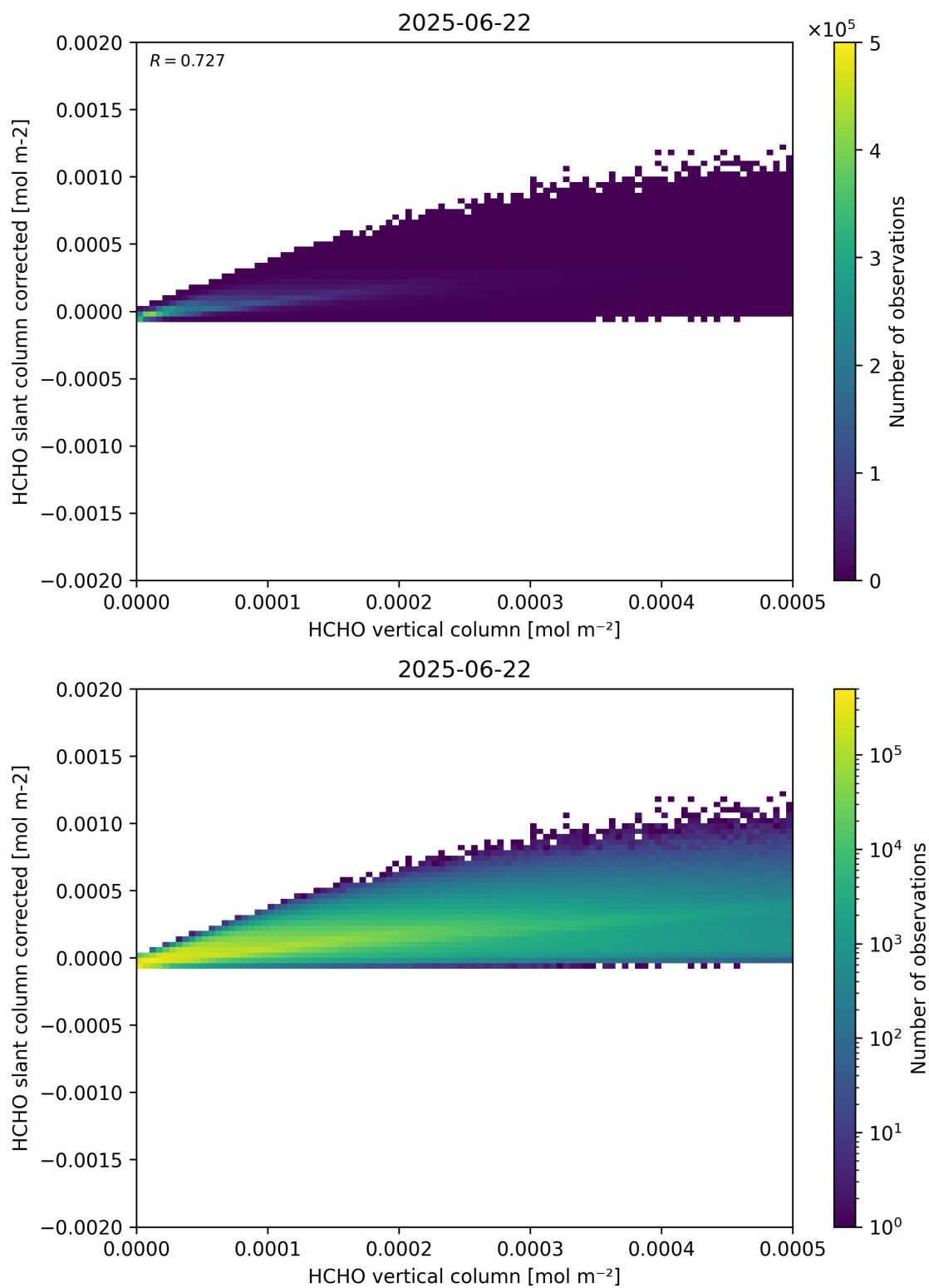
Figure 127: Scatter density plot of “HCHO vertical column” against “HCHO slant column corrected” for 2025-06-22 to 2025-06-23.
