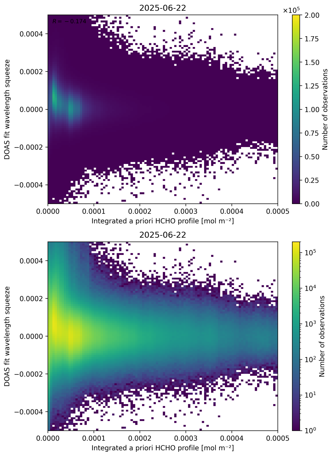
Figure 150: Scatter density plot of “Integrated a priori HCHO profile” against “DOAS fit wavelength squeeze” for 2025-06-22 to 2025-06-23.
