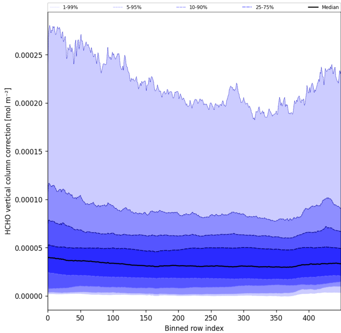
Figure 51: Along track statistics of “HCHO vertical column correction” for 2025-06-22 to 2025-06-23
