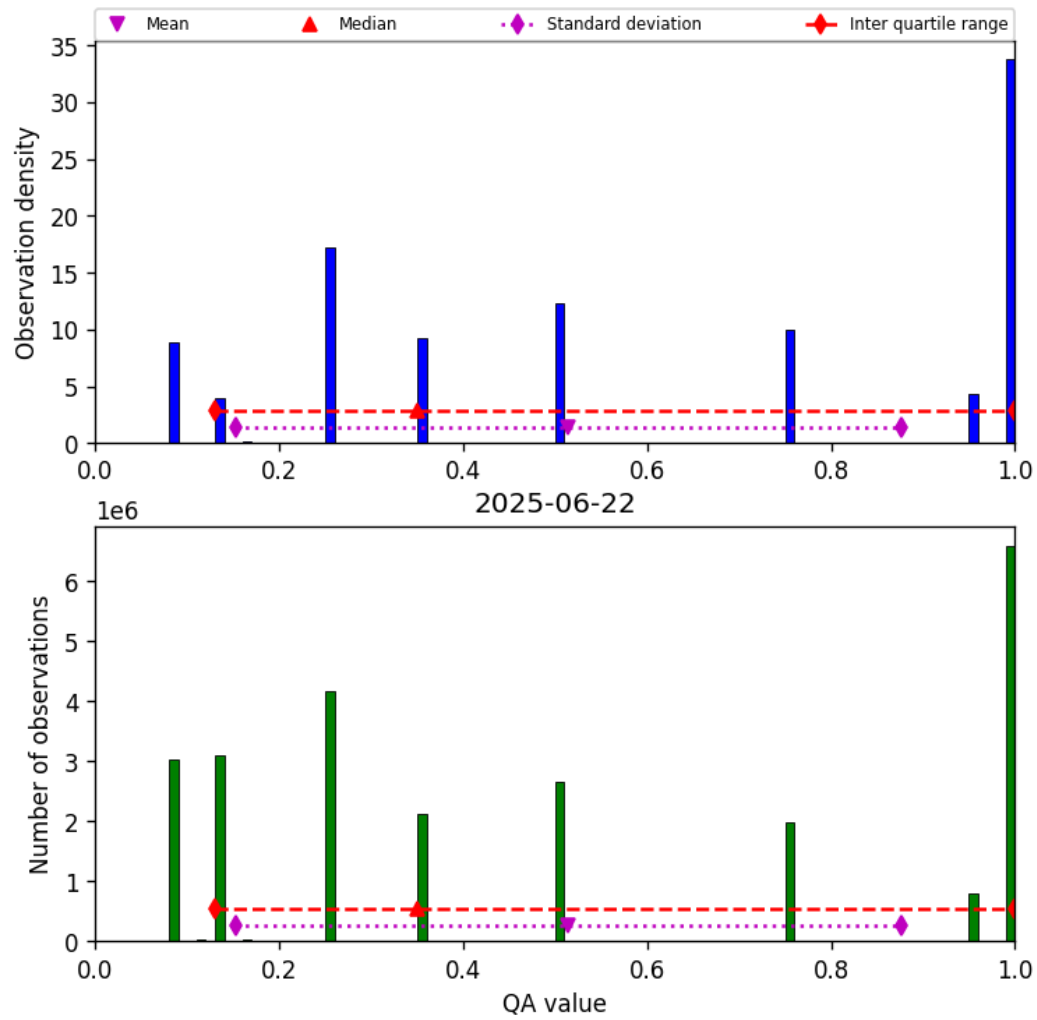
Figure 34: Histogram of “QA value” for 2025-06-22 to 2025-06-23
