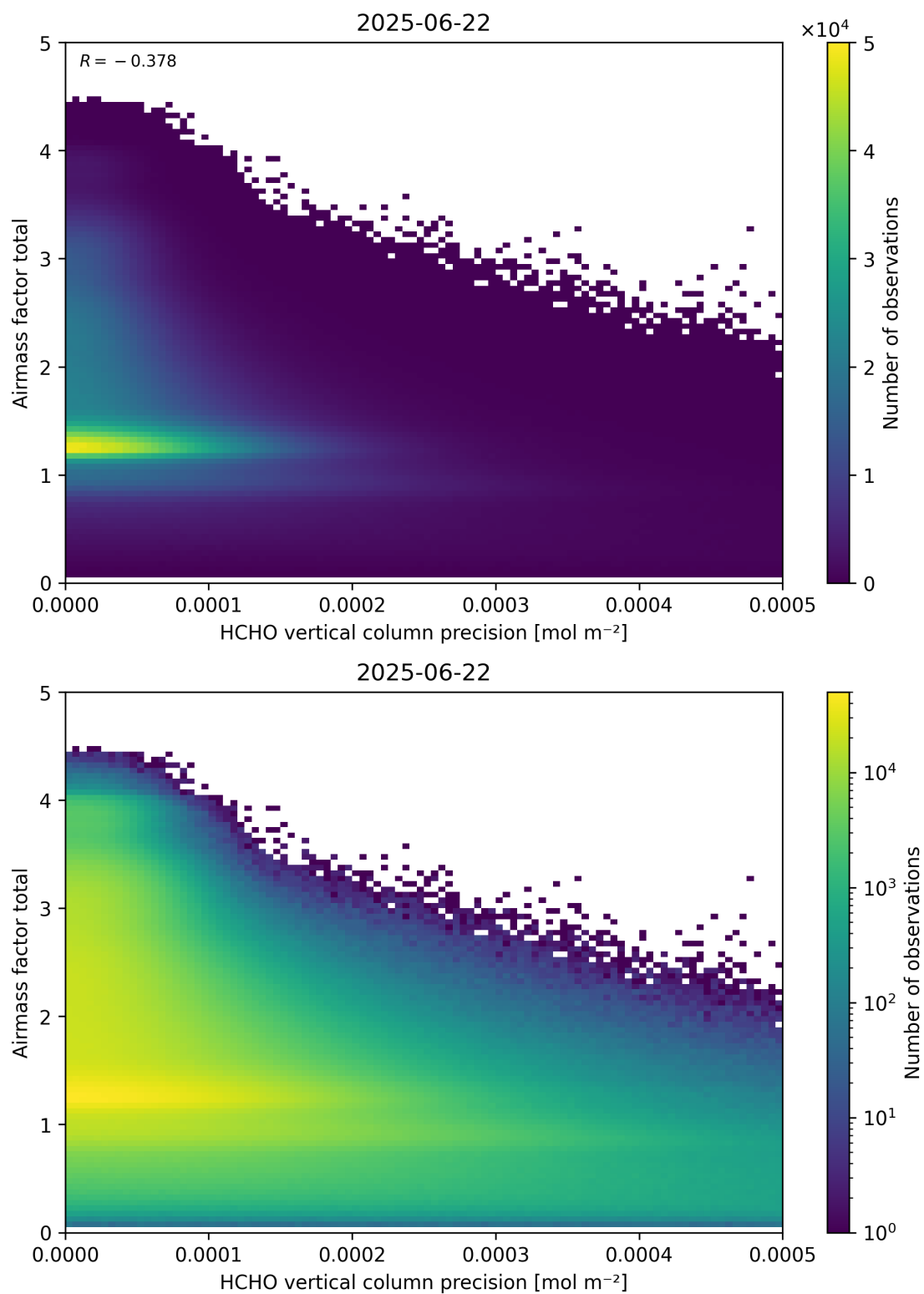
Figure 144: Scatter density plot of “HCHO vertical column precision” against “Airmass factor total” for 2025-06-22 to 2025-06-23.
