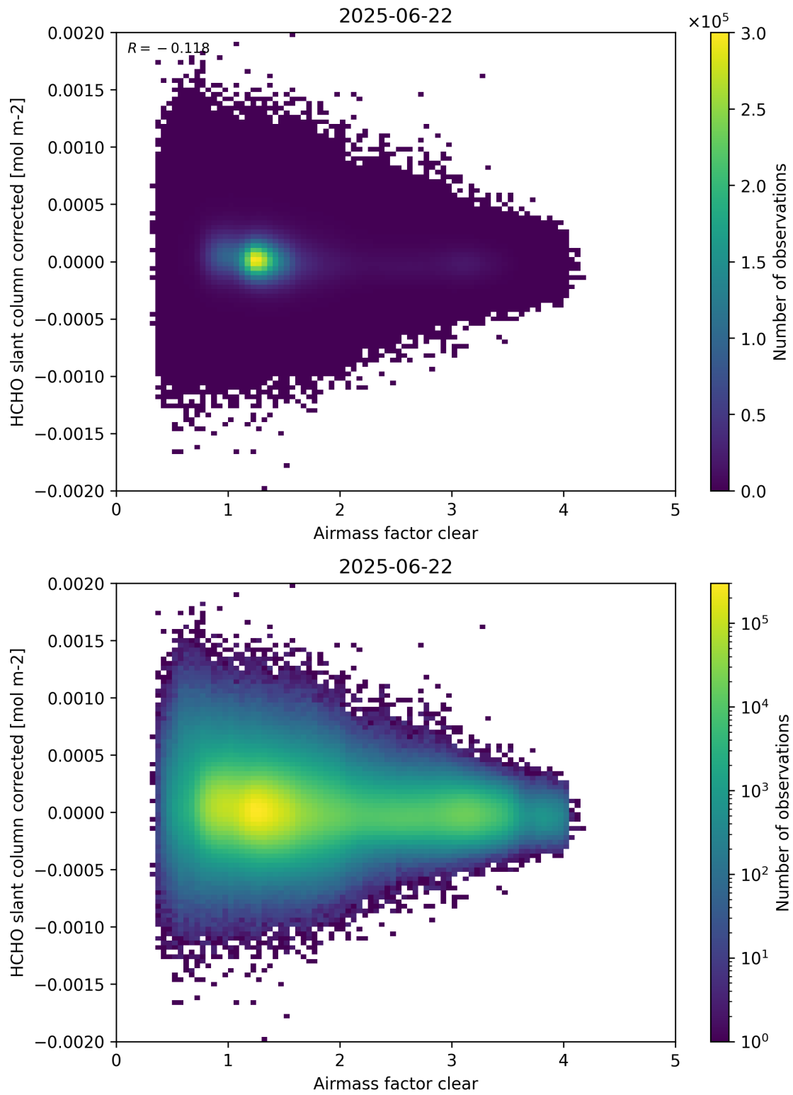
Figure 74: Scatter density plot of “Airmass factor clear” against “HCHO slant column corrected” for 2025-06-22 to 2025-06-23.
