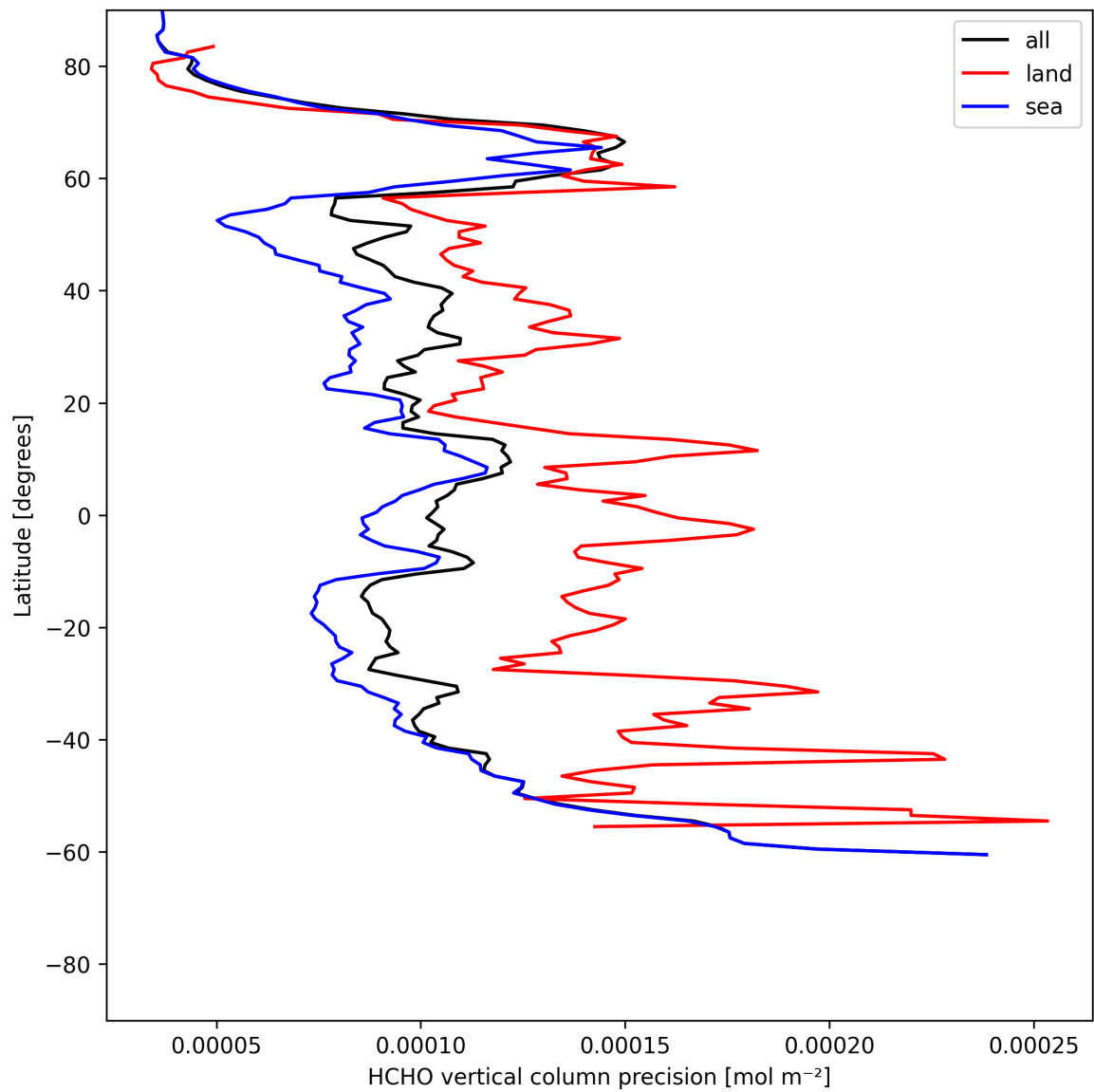
Figure 22: Zonal average of “HCHO vertical column precision” for 2025-06-22 to 2025-06-23.
