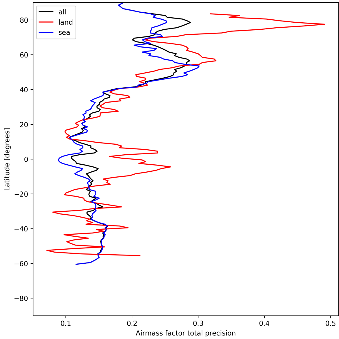
Figure 27: Zonal average of “Airmass factor total precision” for 2025-06-22 to 2025-06-23.
