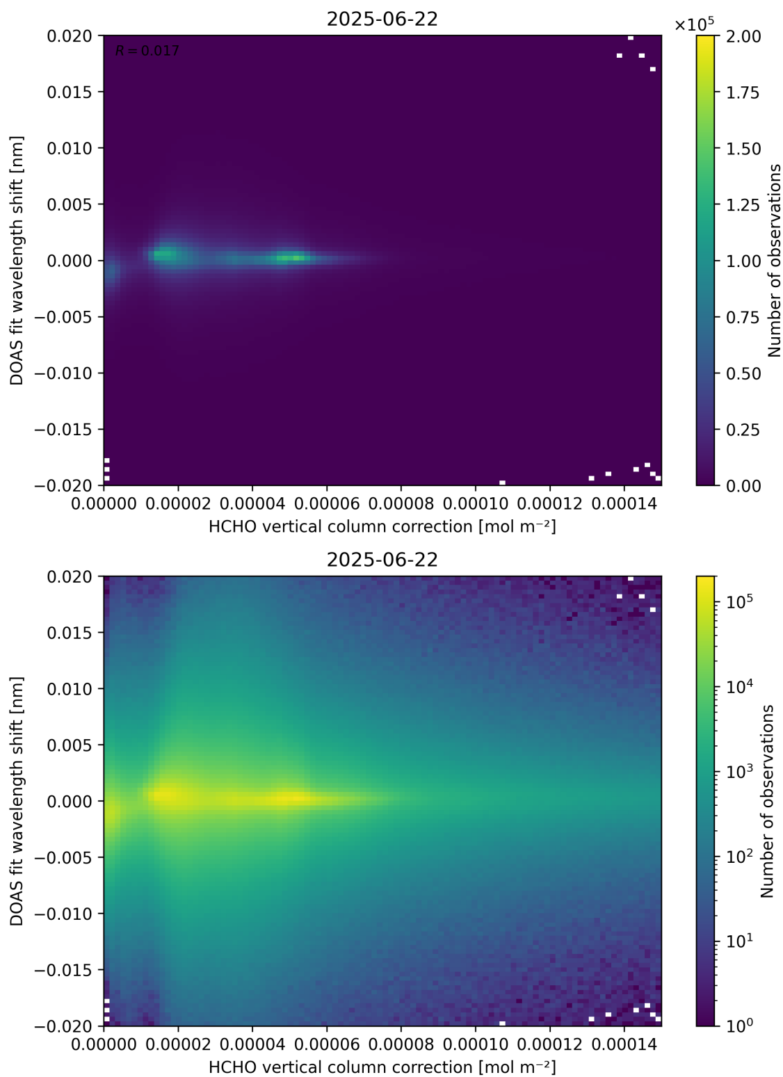
Figure 113: Scatter density plot of “HCHO vertical column correction” against “DOAS fit wavelength shift” for 2025-06-22 to 2025-06-23.
