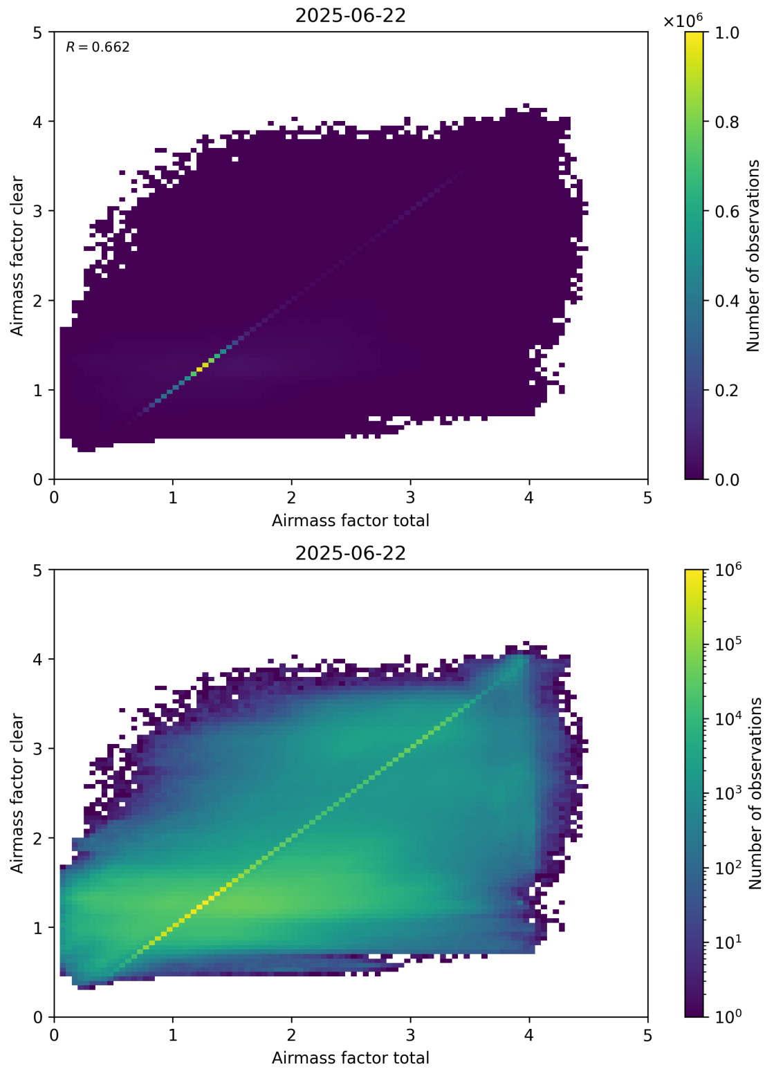
Figure 100: Scatter density plot of “Airmass factor total” against “Airmass factor clear” for 2025-06-22 to 2025-06-23.
