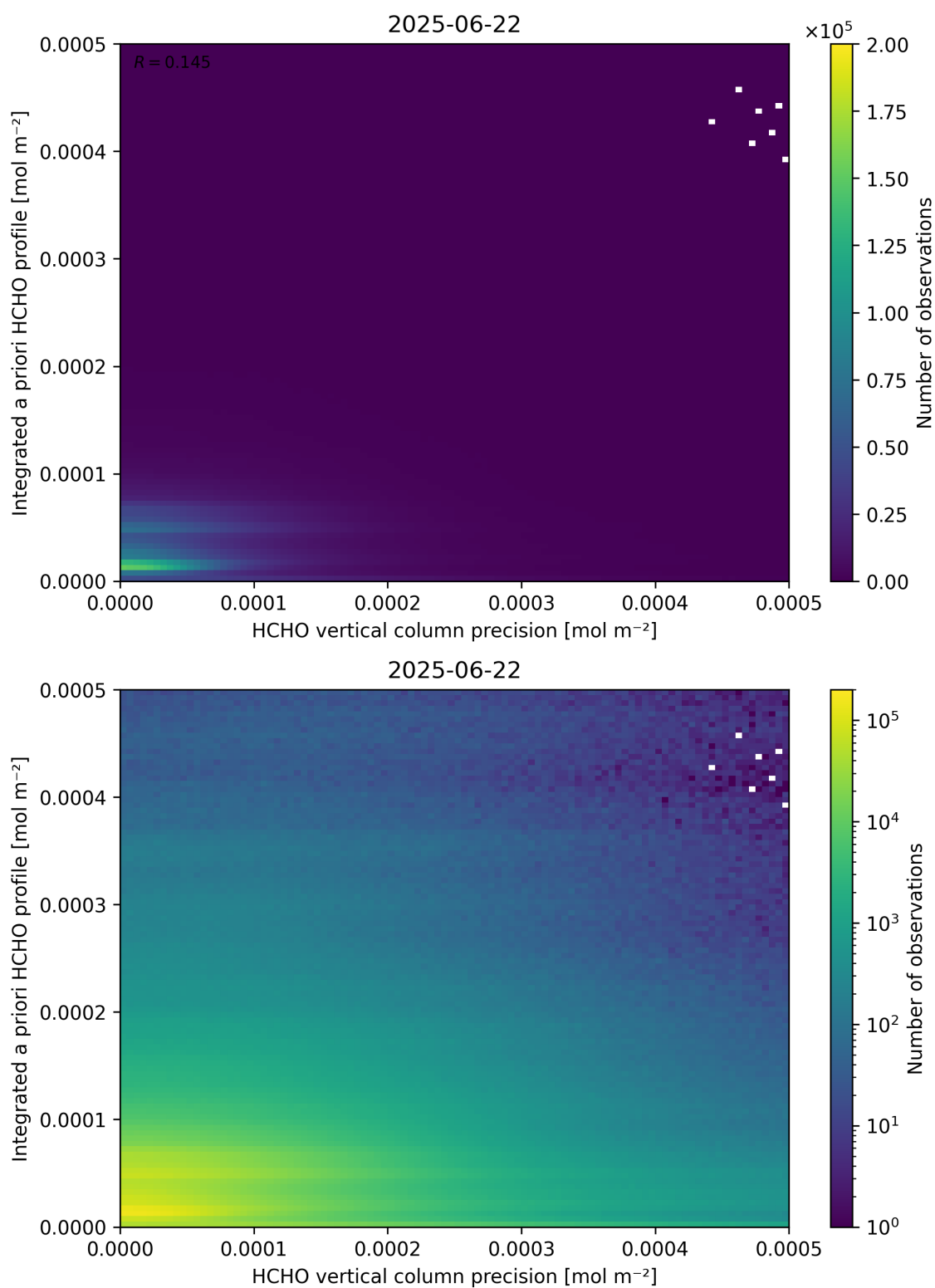
Figure 147: Scatter density plot of “HCHO vertical column precision” against “Integrated a priori HCHO profile” for 2025-06-22 to 2025-06-23.
