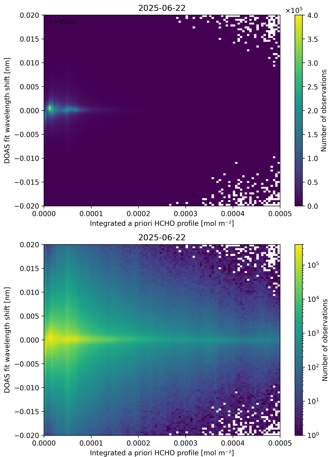
Figure 149: Scatter density plot of “Integrated a priori HCHO profile” against “DOAS fit wavelength shift” for 2025-06-22 to 2025-06-23.
