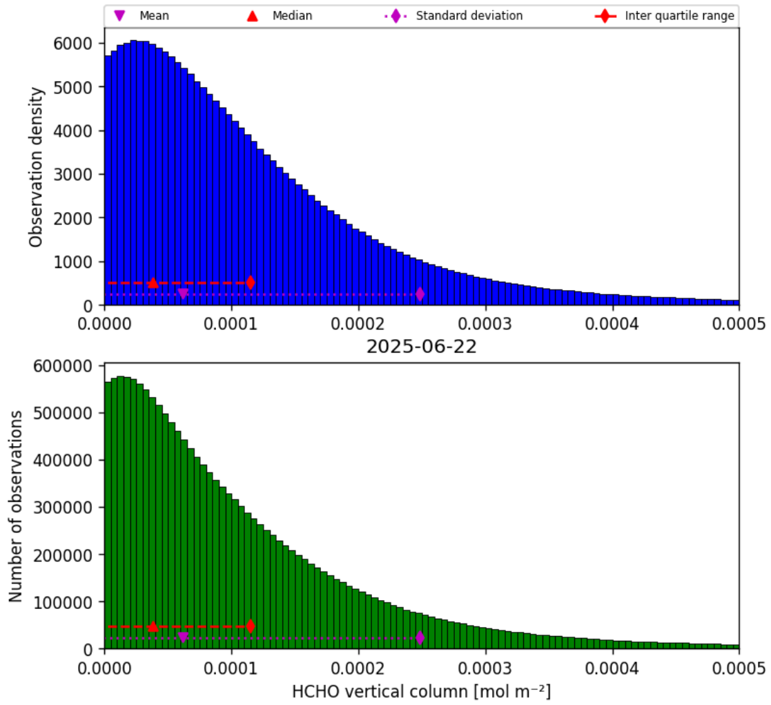
Figure 35: Histogram of “HCHO vertical column” for 2025-06-22 to 2025-06-23
