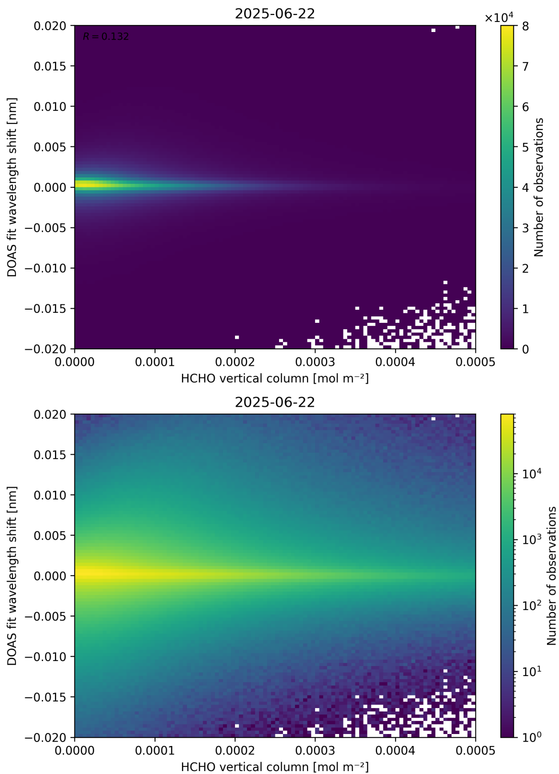
Figure 124: Scatter density plot of “HCHO vertical column” against “DOAS fit wavelength shift” for 2025-06-22 to 2025-06-23.
