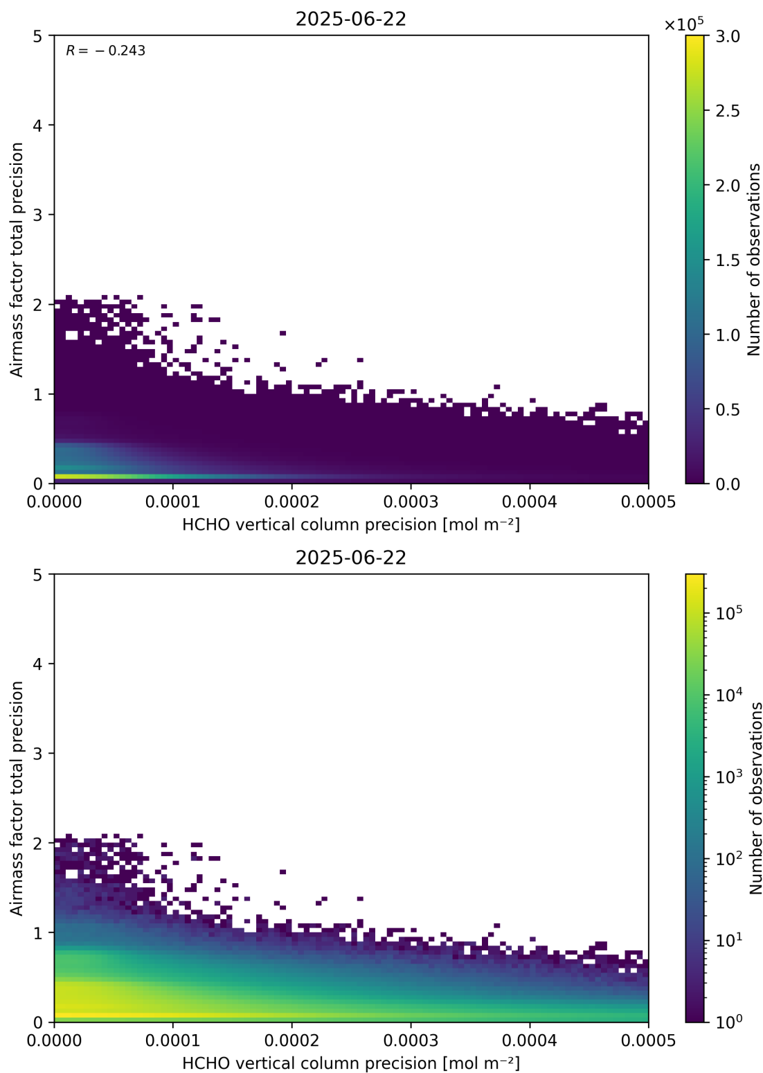
Figure 145: Scatter density plot of “HCHO vertical column precision” against “Airmass factor total precision” for 2025-06-22 to 2025-06-23.
