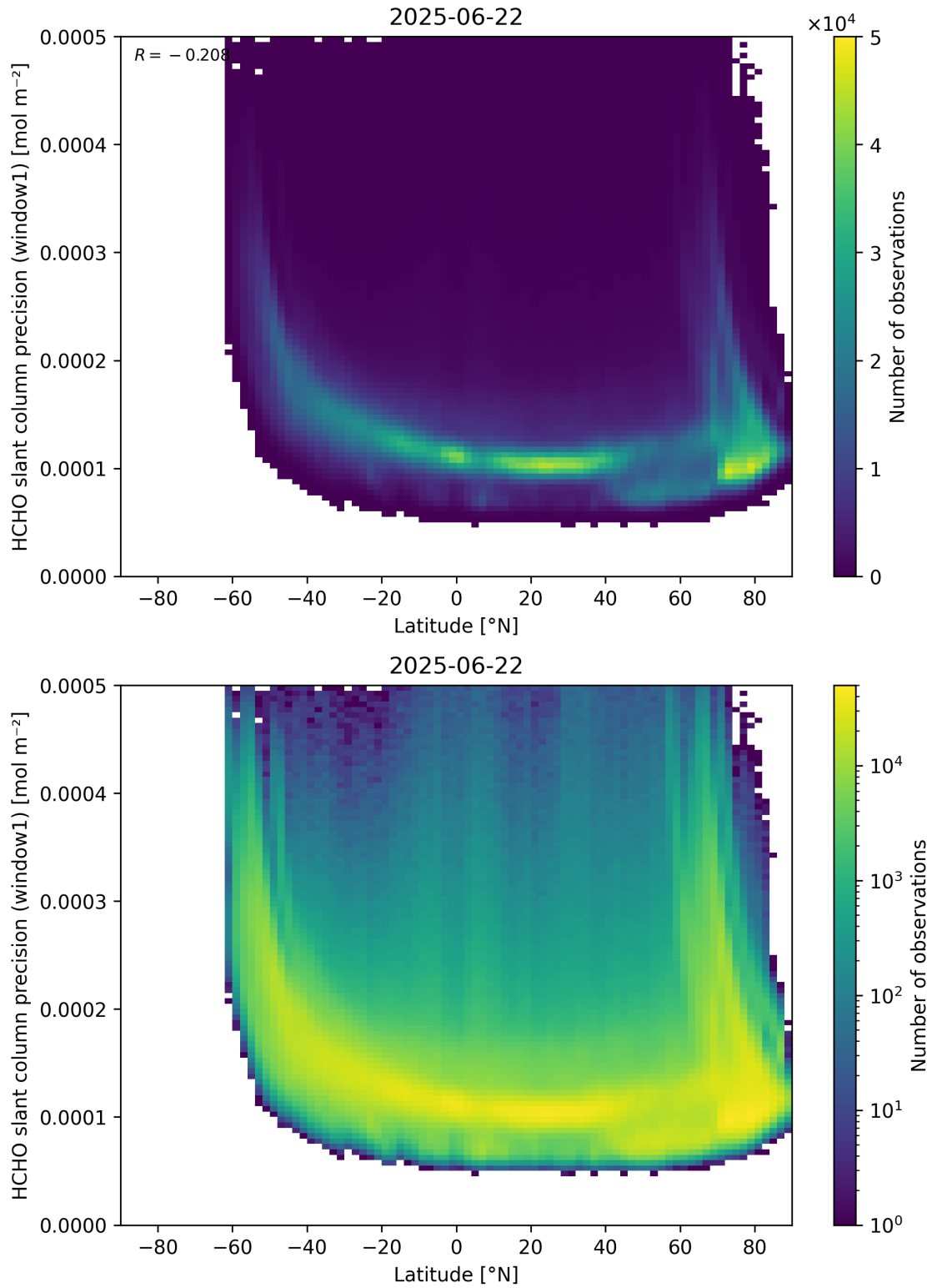
Figure 160: Scatter density plot of “Latitude” against “HCHO slant column precision (window1)” for 2025-06-22 to 2025-06-23.
