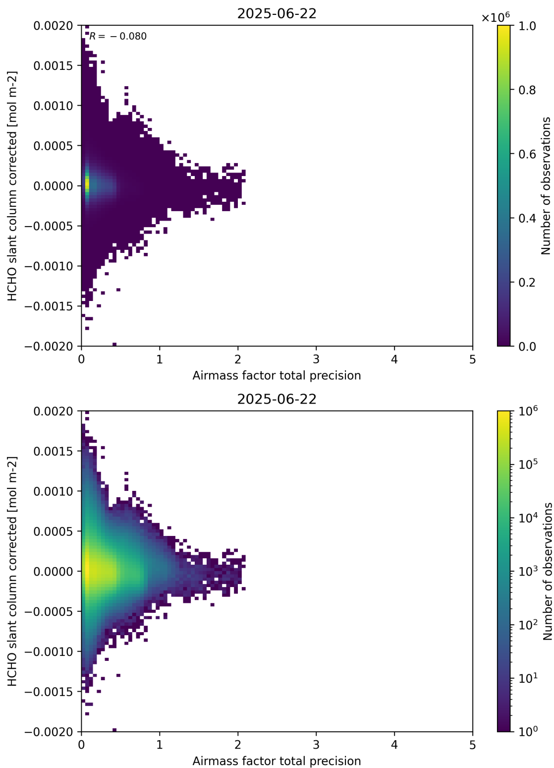
Figure 109: Scatter density plot of “Airmass factor total precision” against “HCHO slant column corrected” for 2025-06-22 to 2025-06-23.
