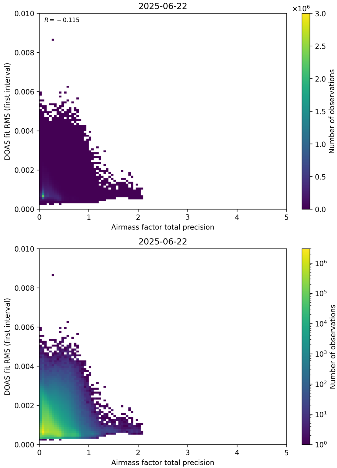
Figure 105: Scatter density plot of “Airmass factor total precision” against “DOAS fit RMS (first interval)” for 2025-06-22 to 2025-06-23.
