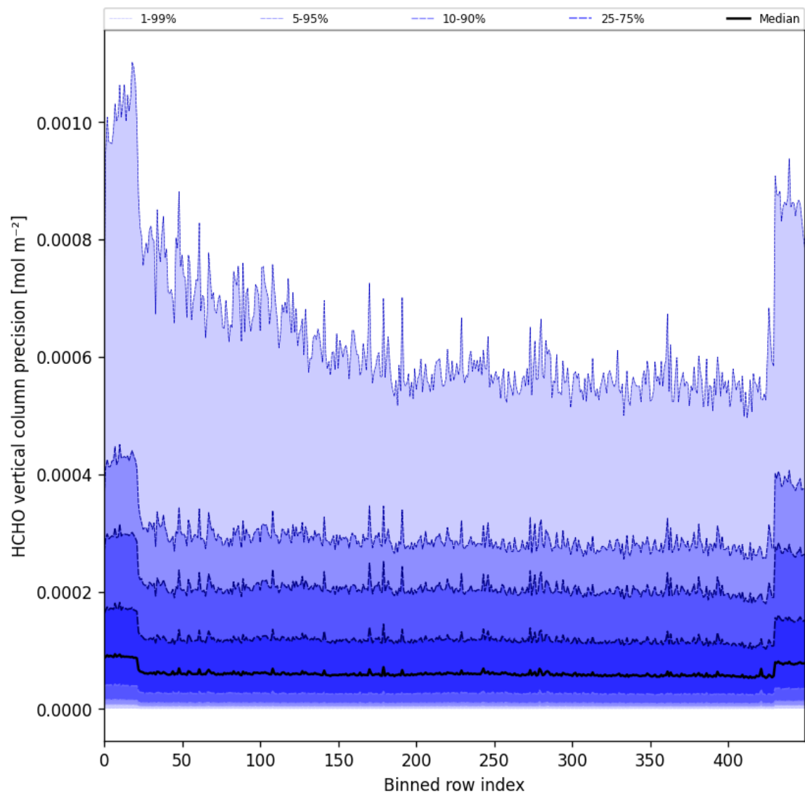
Figure 50: Along track statistics of “HCHO vertical column precision” for 2025-06-22 to 2025-06-23
