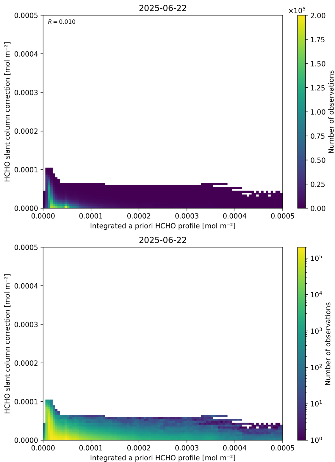
Figure 152: Scatter density plot of “Integrated a priori HCHO profile” against “HCHO slant column correction” for 2025-06-22 to 2025-06-23.
