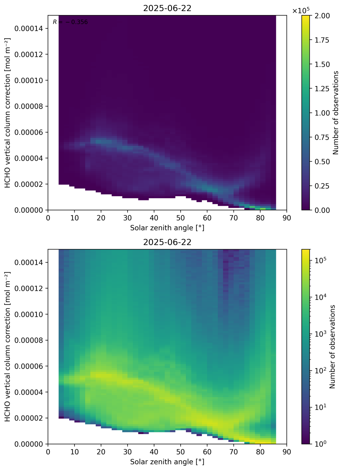
Figure 178: Scatter density plot of “Solar zenith angle” against “HCHO vertical column correction” for 2025-06-22 to 2025-06-23.
