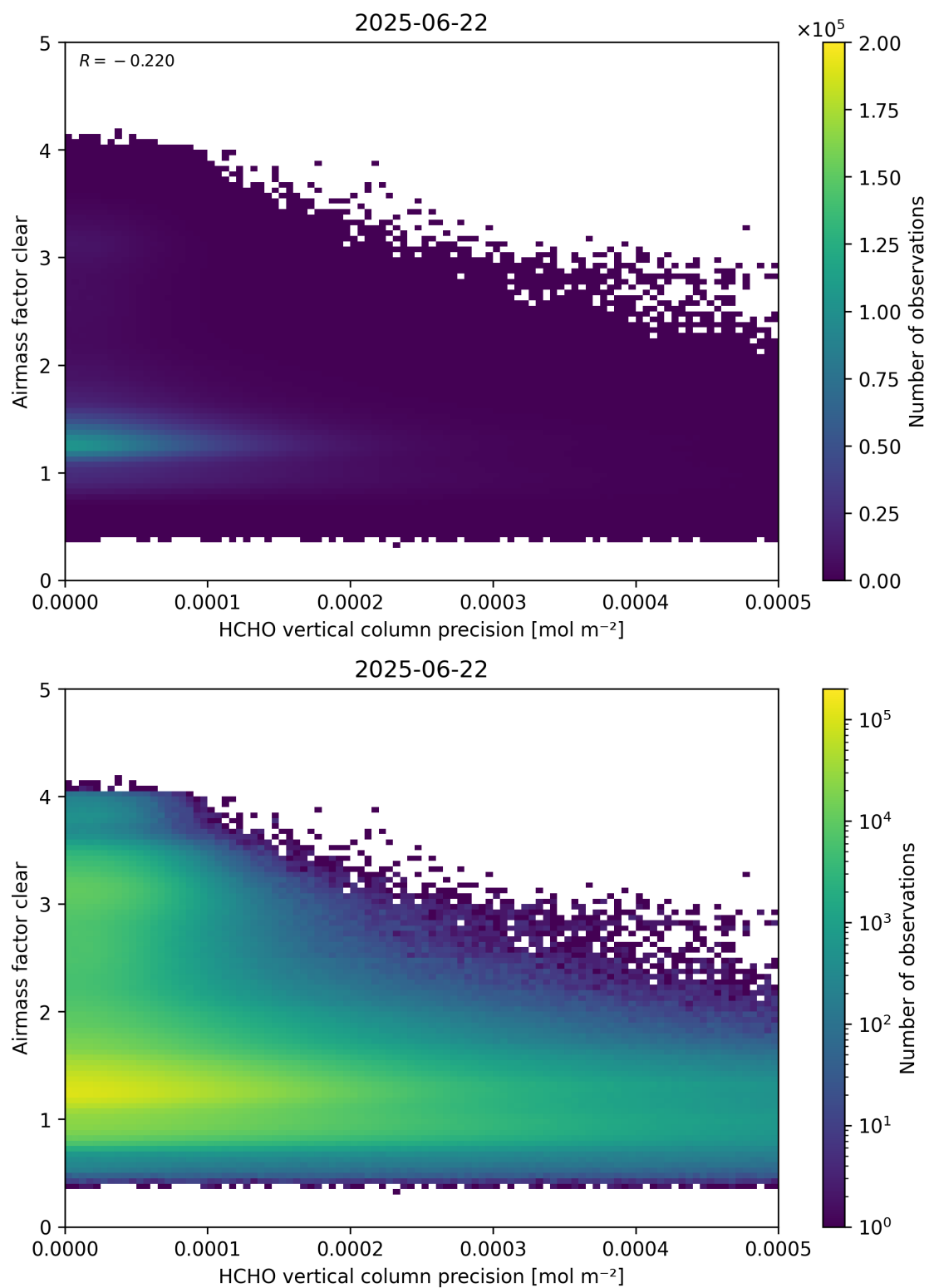
Figure 139: Scatter density plot of “HCHO vertical column precision” against “Airmass factor clear” for 2025-06-22 to 2025-06-23.
