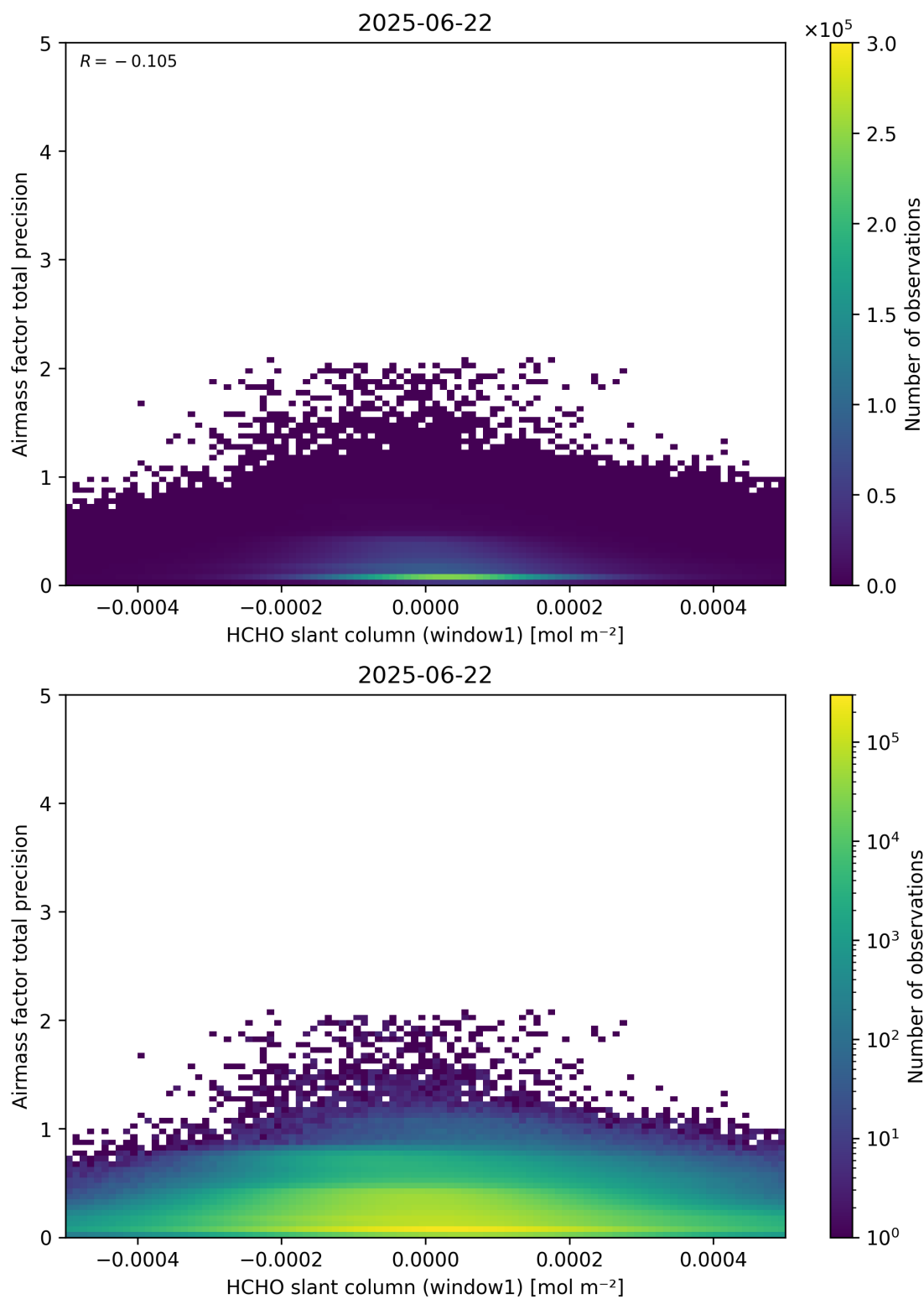
Figure 86: Scatter density plot of “HCHO slant column (window1)” against “Airmass factor total precision” for 2025-06-22 to 2025-06-23.
