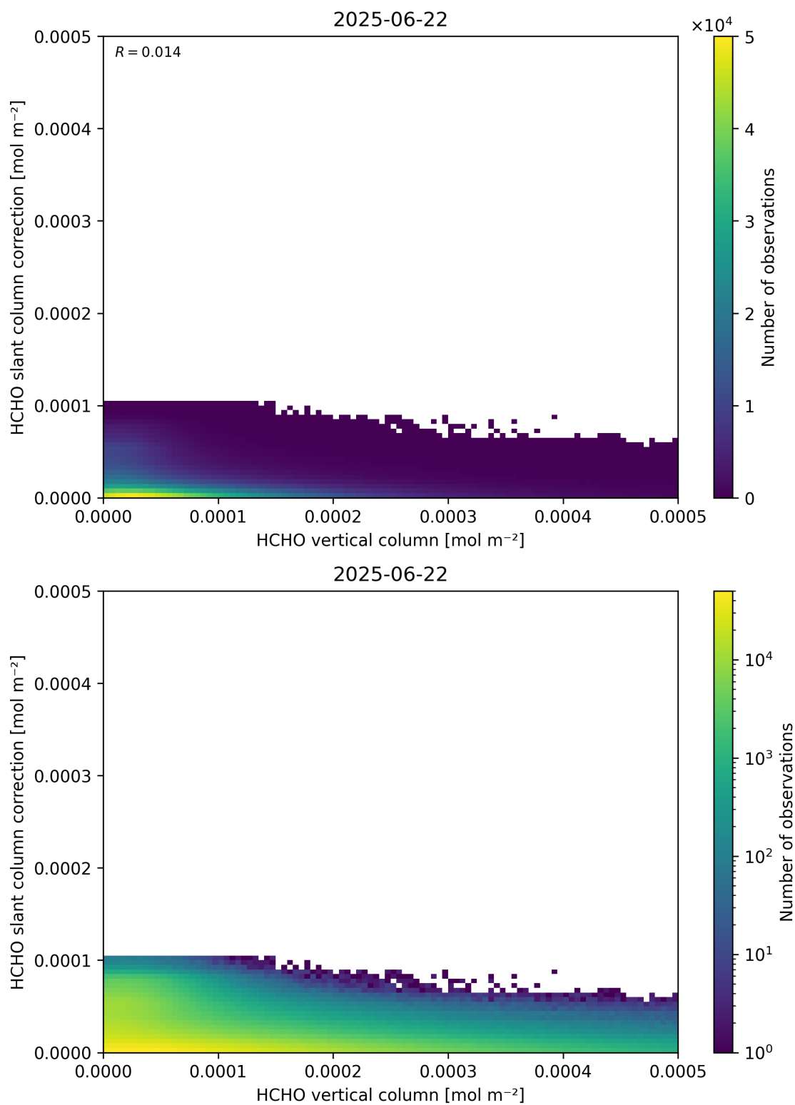
Figure 128: Scatter density plot of “HCHO vertical column” against “HCHO slant column correction” for 2025-06-22 to 2025-06-23.
