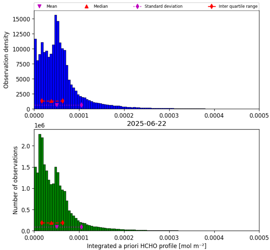
Figure 43: Histogram of “Integrated a priori HCHO profile” for 2025-06-22 to 2025-06-23
