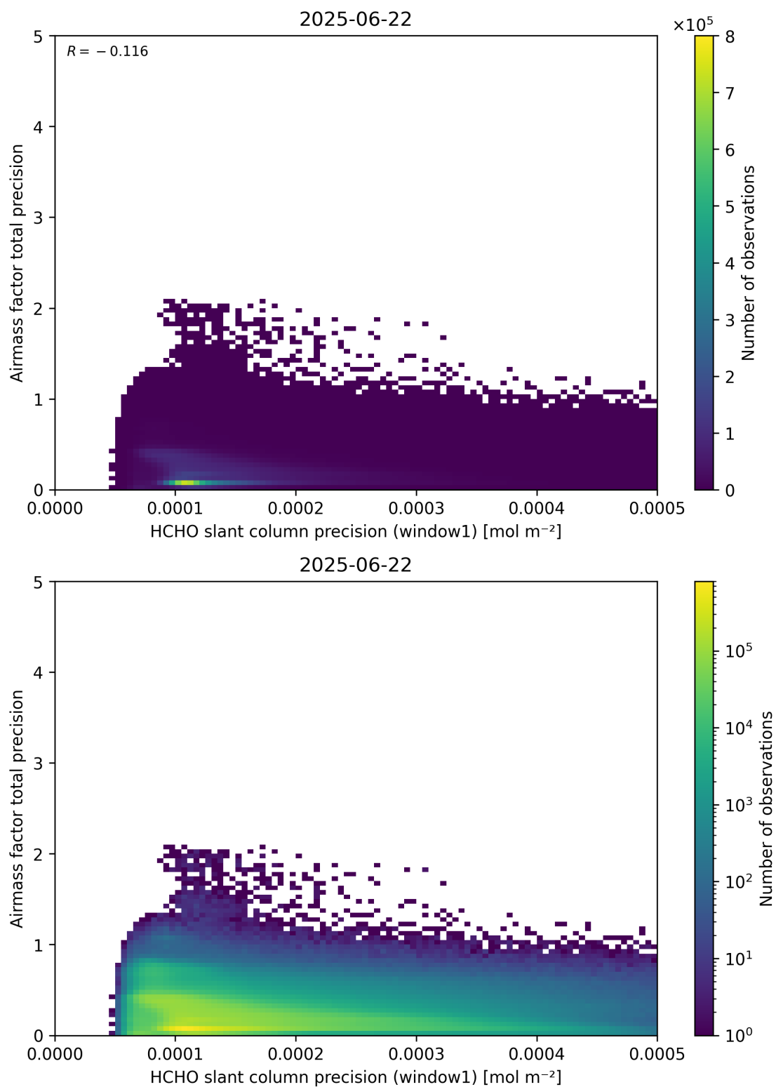
Figure 95: Scatter density plot of “HCHO slant column precision (window1)” against “Airmass factor total precision” for 2025-06-22 to 2025-06-23.
