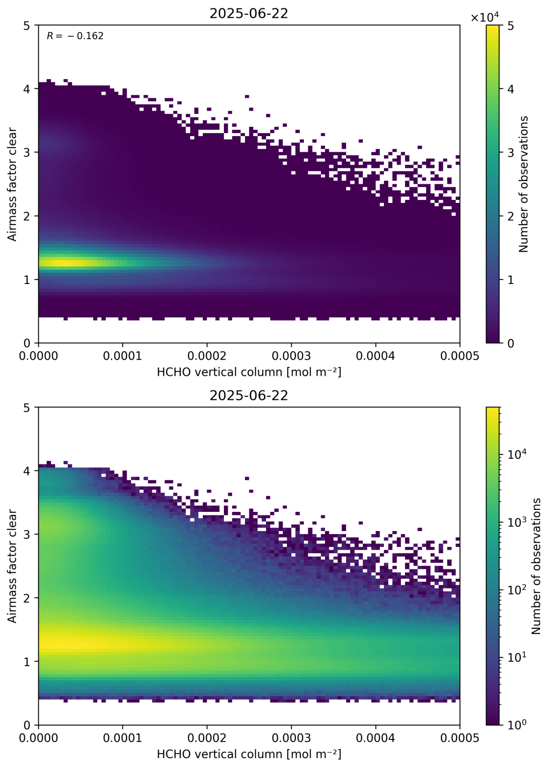
Figure 126: Scatter density plot of “HCHO vertical column” against “Airmass factor clear” for 2025-06-22 to 2025-06-23.
