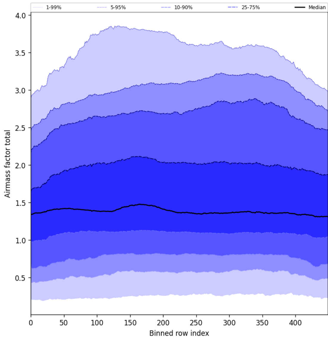
Figure 54: Along track statistics of “Airmass factor total” for 2025-06-22 to 2025-06-23
