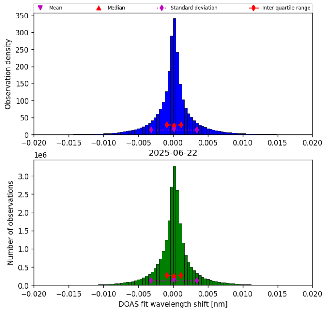
Figure 44: Histogram of “DOAS fit wavelength shift” for 2025-06-22 to 2025-06-23
