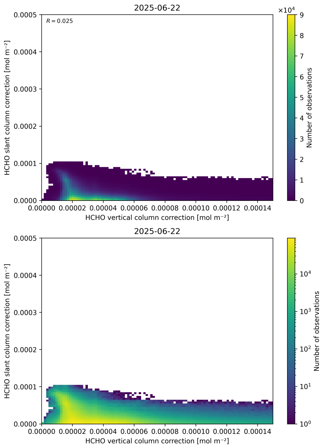
Figure 117: Scatter density plot of “HCHO vertical column correction” against “HCHO slant column correction” for 2025-06-22 to 2025-06-23.
