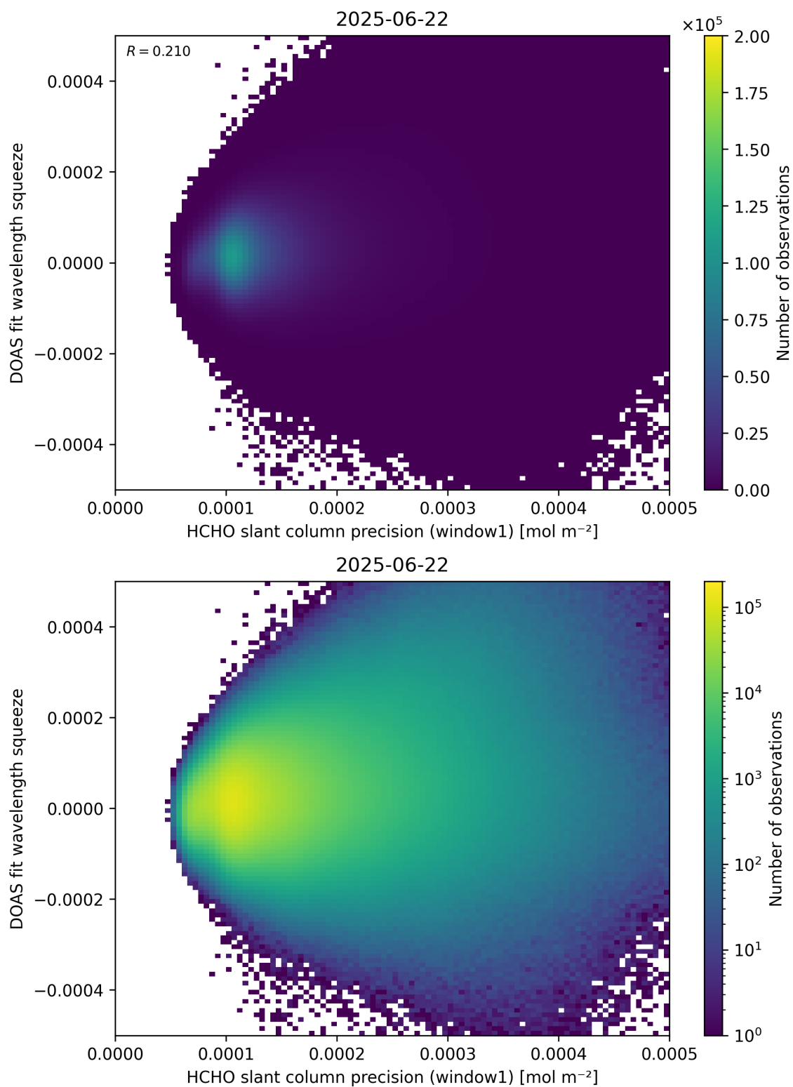
Figure 90: Scatter density plot of “HCHO slant column precision (window1)” against “DOAS fit wavelength squeeze” for 2025-06-22 to 2025-06-23.
