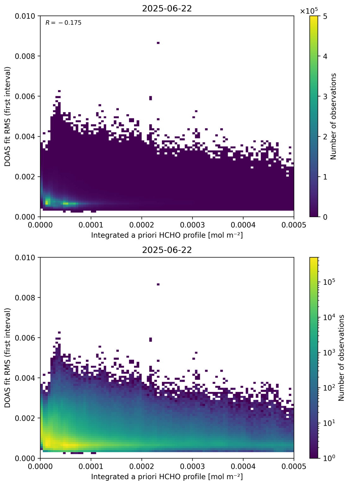
Figure 148: Scatter density plot of “Integrated a priori HCHO profile” against “DOAS fit RMS (first interval)” for 2025-06-22 to 2025-06-23.
