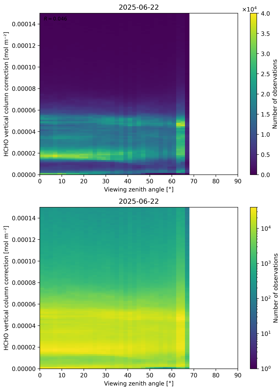
Figure 193: Scatter density plot of “Viewing zenith angle” against “HCHO vertical column correction” for 2025-06-22 to 2025-06-23.
