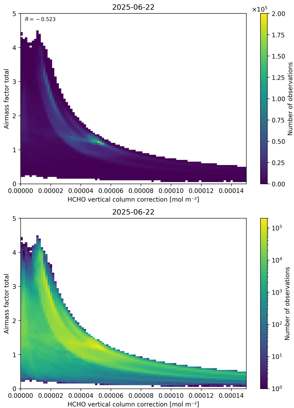
Figure 120: Scatter density plot of “HCHO vertical column correction” against “Airmass factor total” for 2025-06-22 to 2025-06-23.
