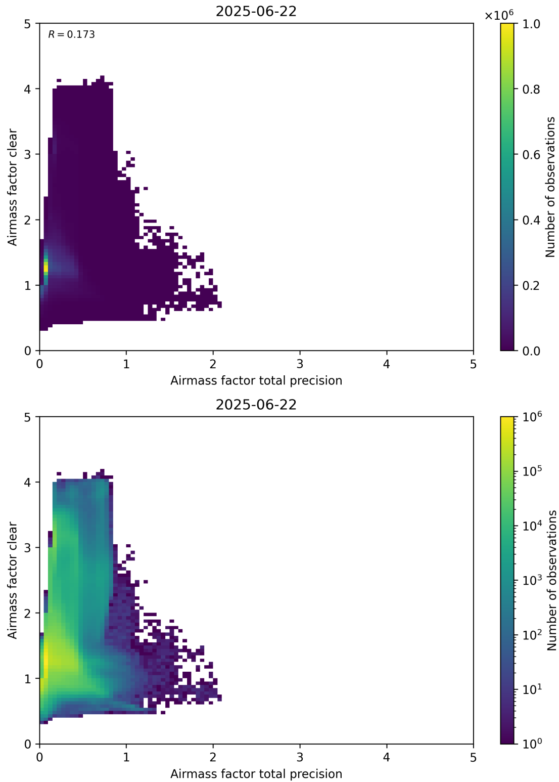
Figure 108: Scatter density plot of “Airmass factor total precision” against “Airmass factor clear” for 2025-06-22 to 2025-06-23.
