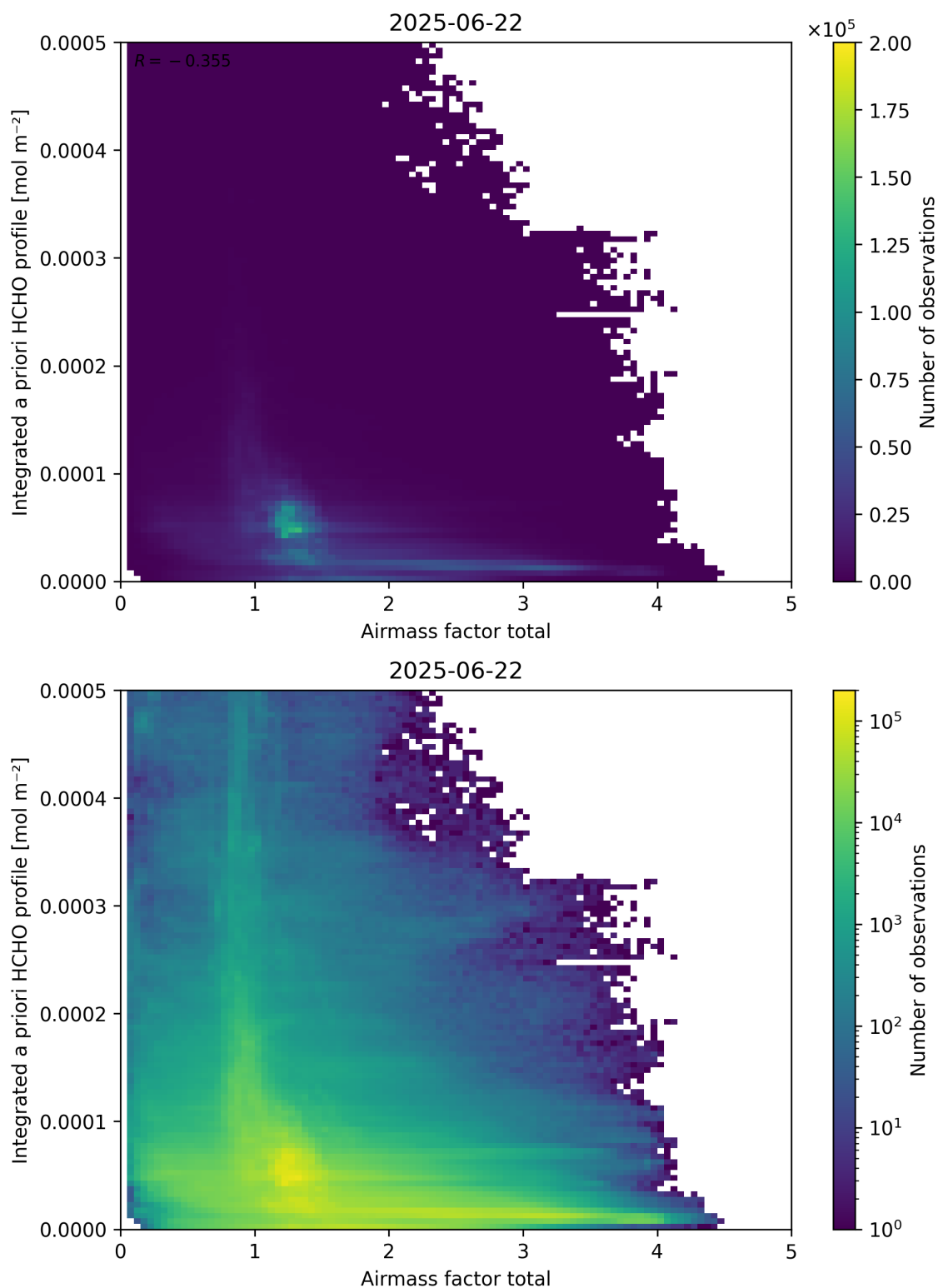
Figure 104: Scatter density plot of “Airmass factor total” against “Integrated a priori HCHO profile” for 2025-06-22 to 2025-06-23.
