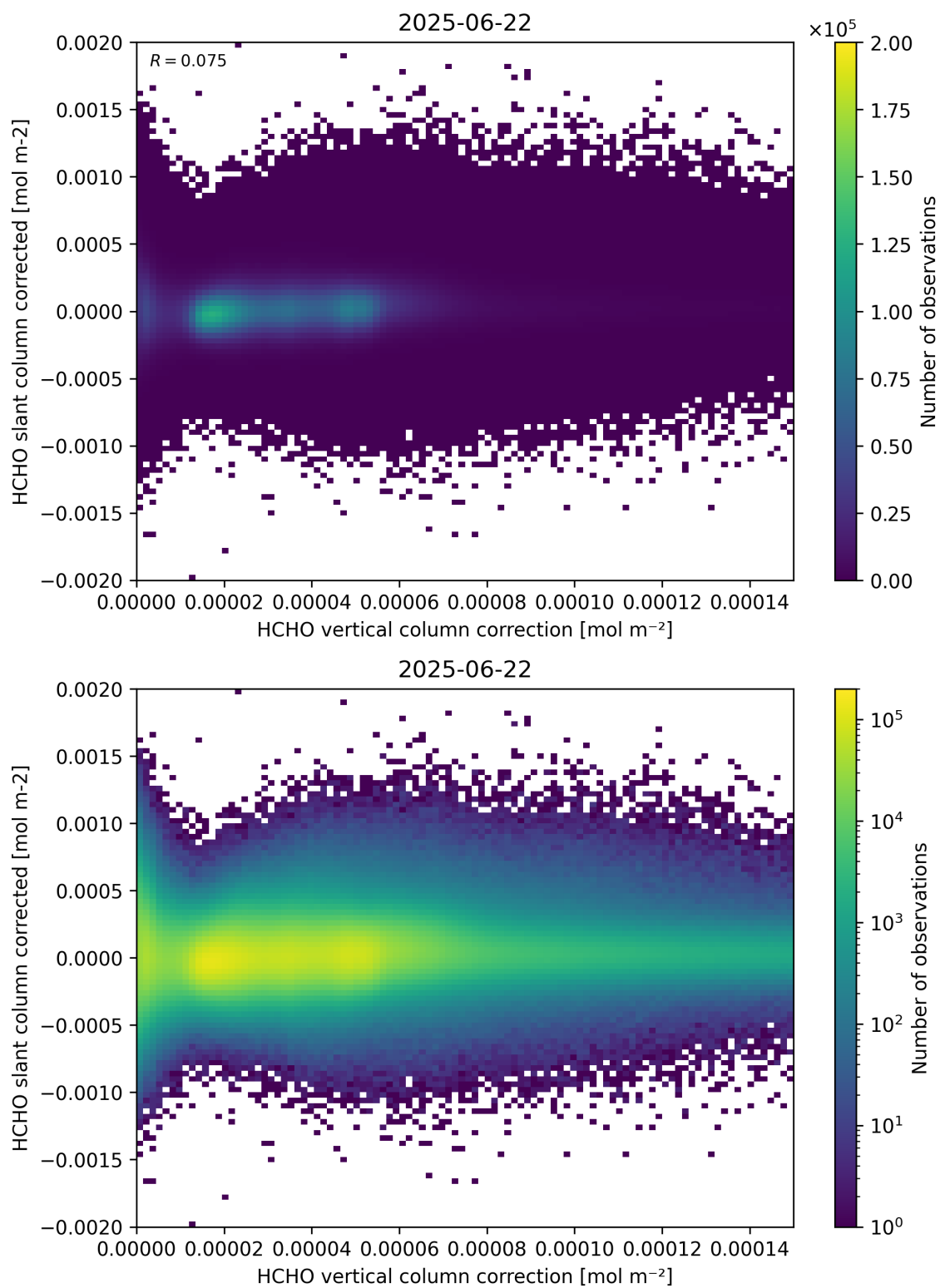
Figure 116: Scatter density plot of “HCHO vertical column correction” against “HCHO slant column corrected” for 2025-06-22 to 2025-06-23.
