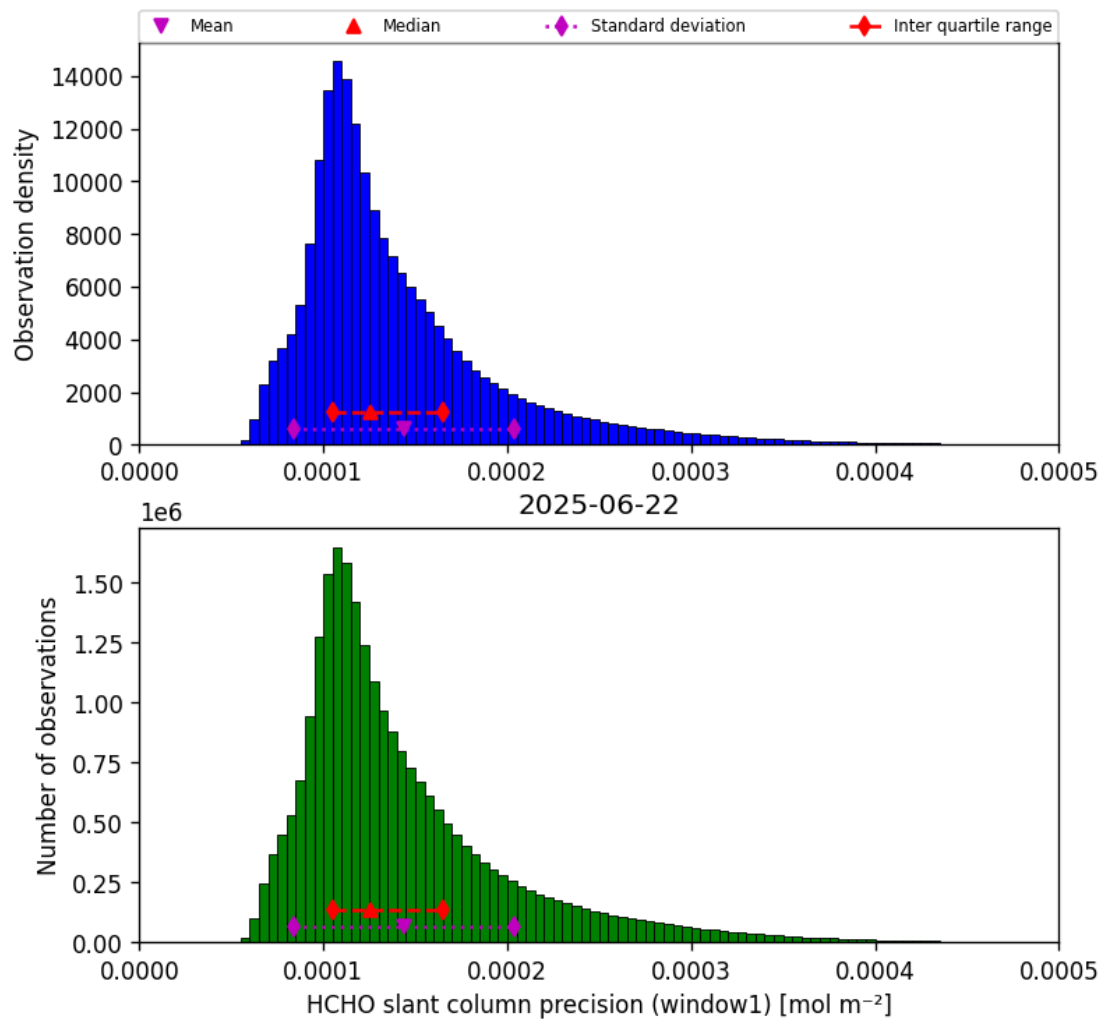
Figure 39: Histogram of “HCHO slant column precision (window1)” for 2025-06-22 to 2025-06-23
