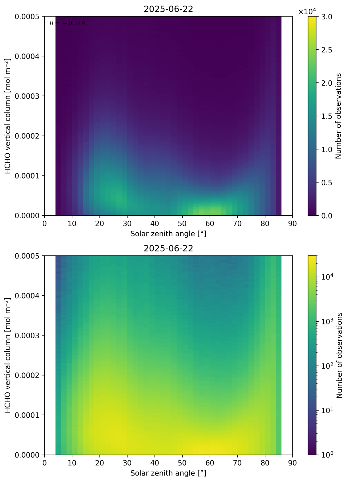
Figure 177: Scatter density plot of “Solar zenith angle” against “HCHO vertical column” for 2025-06-22 to 2025-06-23.
