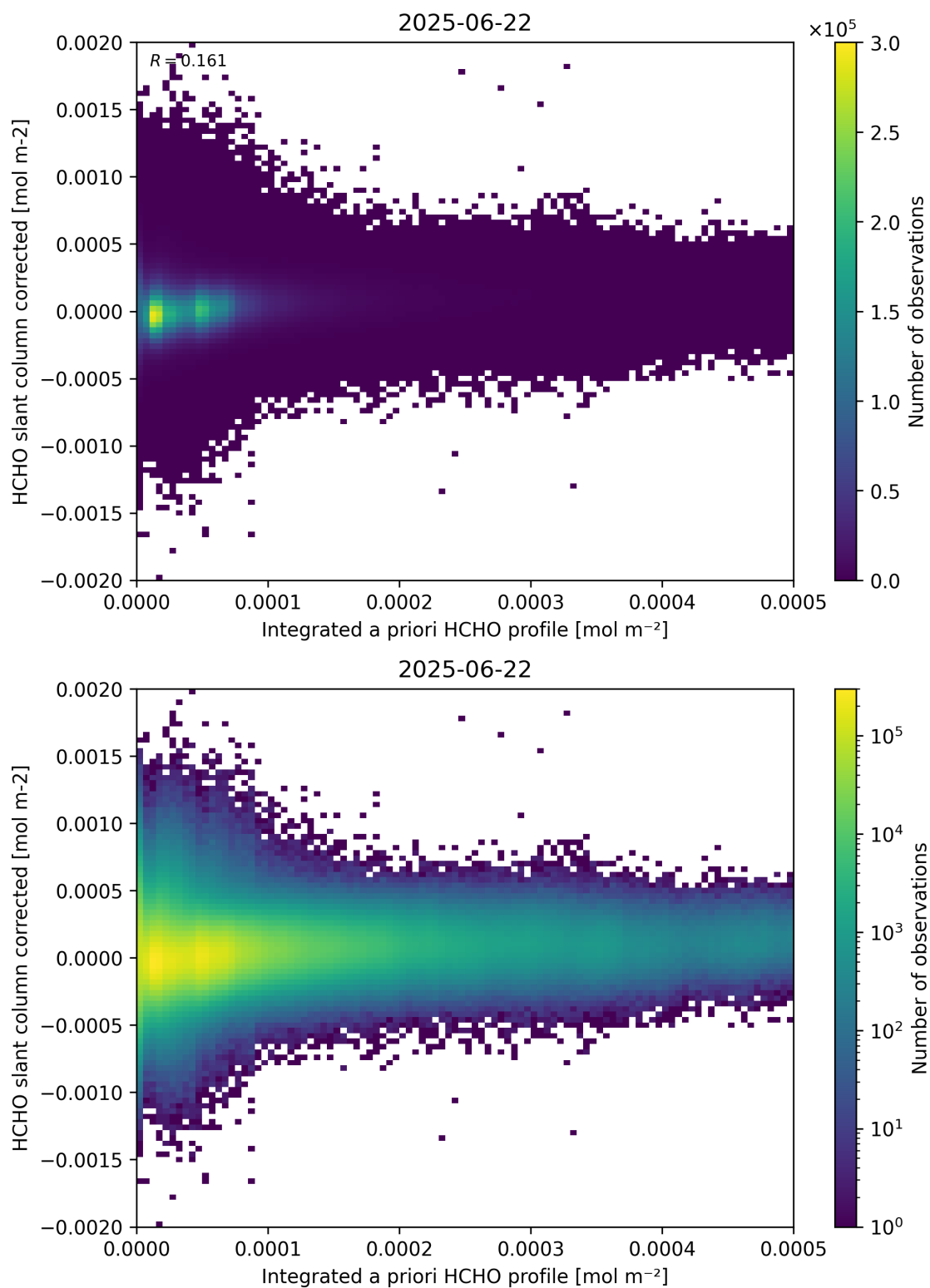
Figure 151: Scatter density plot of “Integrated a priori HCHO profile” against “HCHO slant column corrected” for 2025-06-22 to 2025-06-23.
