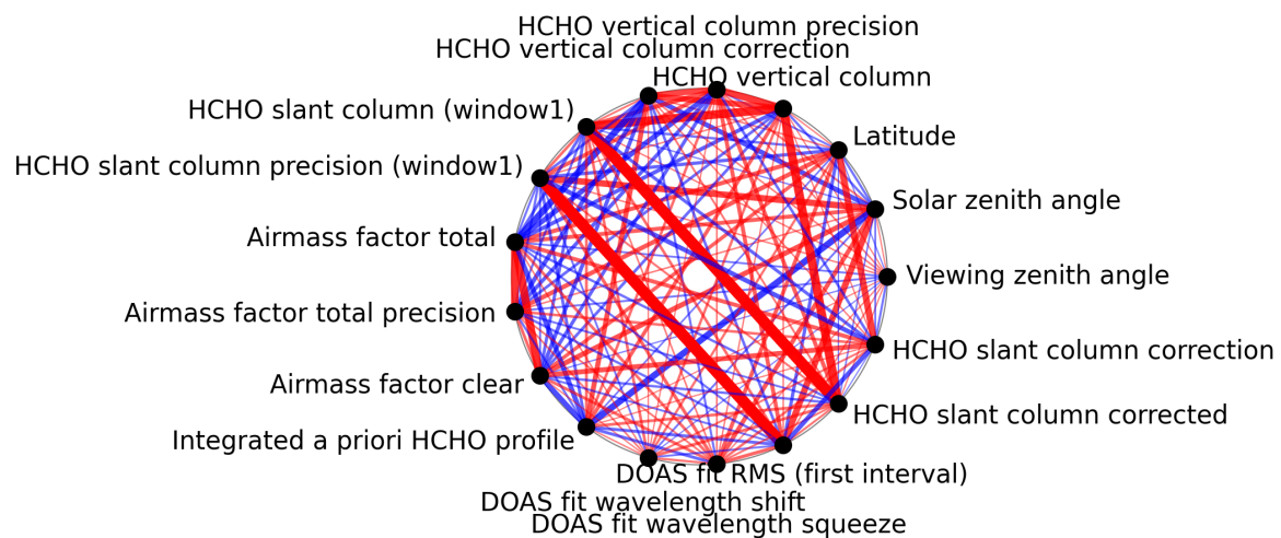
Figure 1: Map of correlation graph for 2025-06-22 to 2025-06-23.
