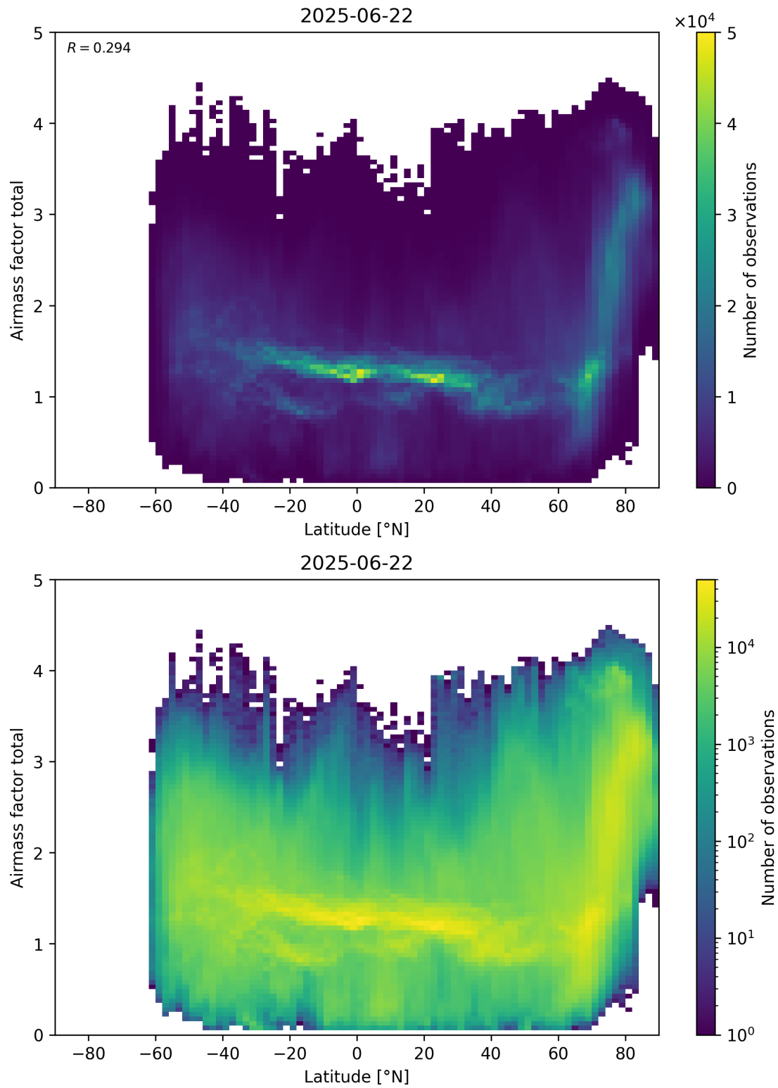
Figure 161: Scatter density plot of “Latitude” against “Airmass factor total” for 2025-06-22 to 2025-06-23.
