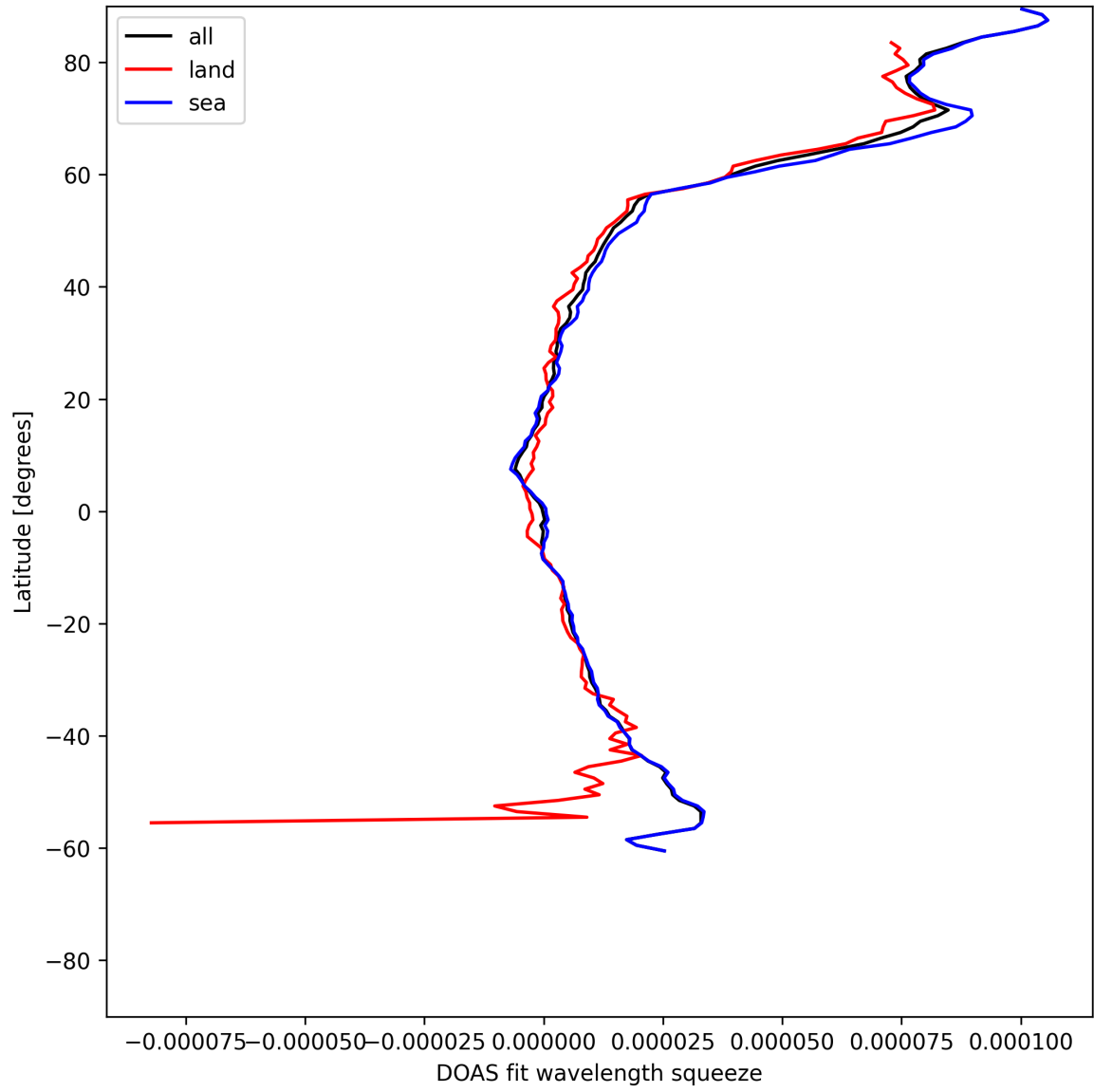
Figure 31: Zonal average of “DOAS fit wavelength squeeze” for 2025-06-22 to 2025-06-23.
