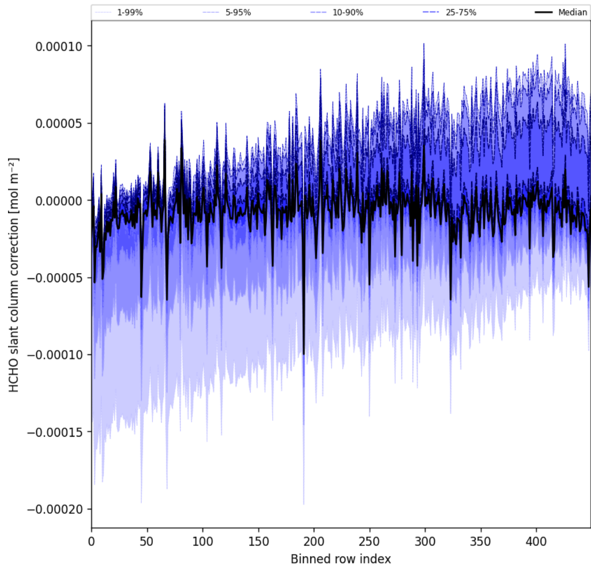
Figure 61: Along track statistics of “HCHO slant column correction” for 2025-06-22 to 2025-06-23
