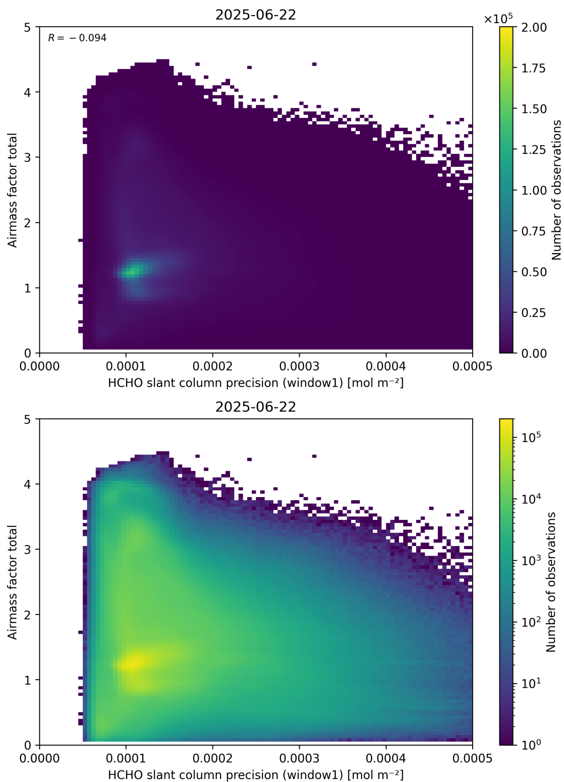
Figure 94: Scatter density plot of “HCHO slant column precision (window1)” against “Airmass factor total” for 2025-06-22 to 2025-06-23.
