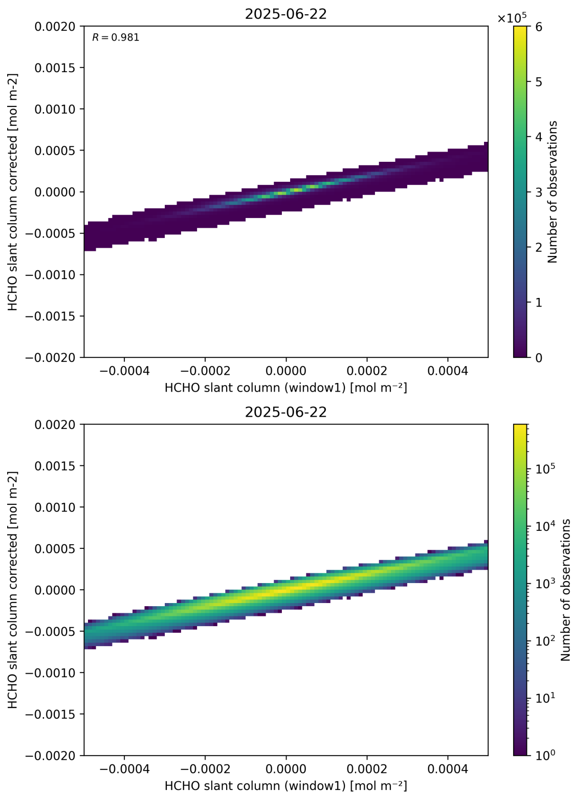
Figure 82: Scatter density plot of “HCHO slant column (window1)” against “HCHO slant column corrected” for 2025-06-22 to 2025-06-23.
