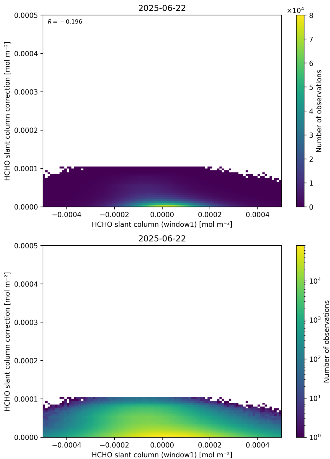
Figure 83: Scatter density plot of “HCHO slant column (window1)” against “HCHO slant column correction” for 2025-06-22 to 2025-06-23.
