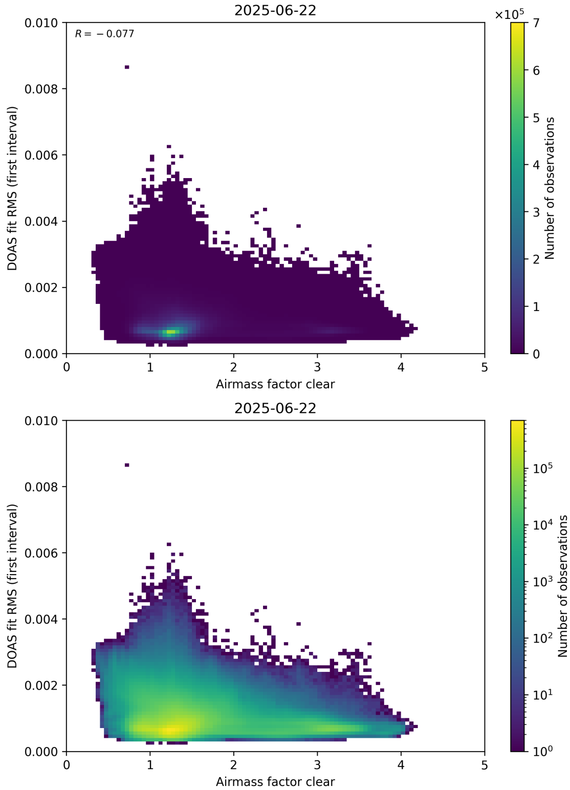
Figure 71: Scatter density plot of “Airmass factor clear” against “DOAS fit RMS (first interval)” for 2025-06-22 to 2025-06-23.
