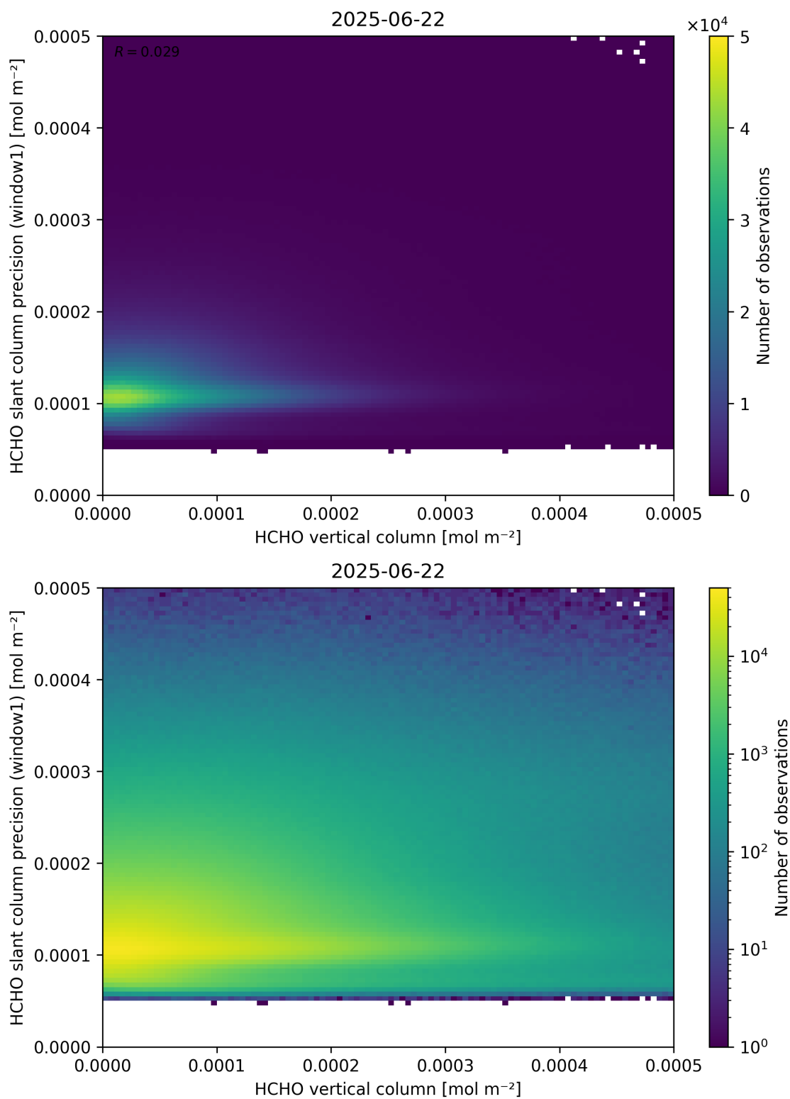
Figure 130: Scatter density plot of “HCHO vertical column” against “HCHO slant column precision (window1)” for 2025-06-22 to 2025-06-23.
