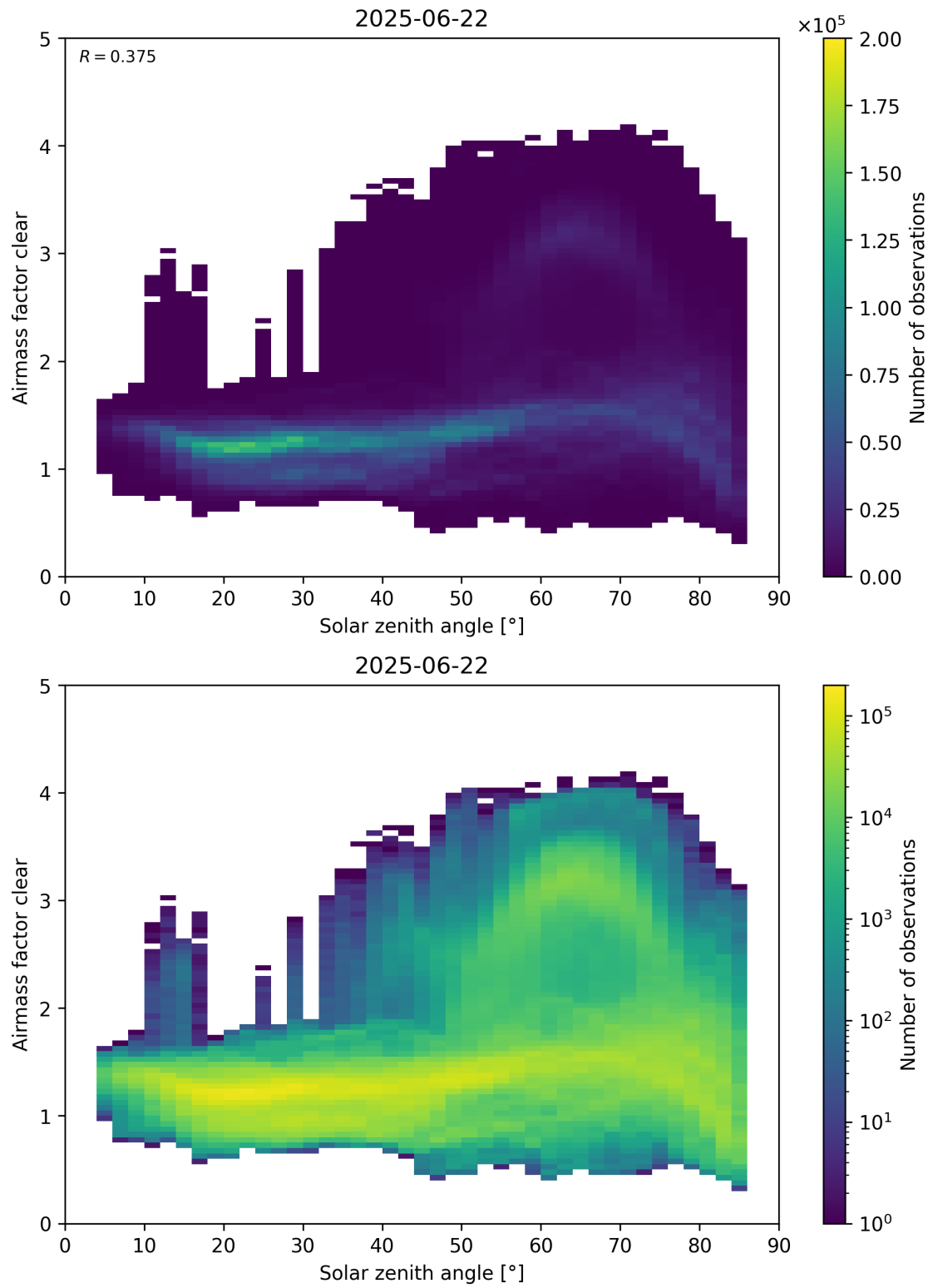
Figure 170: Scatter density plot of “Solar zenith angle” against “Airmass factor clear” for 2025-06-22 to 2025-06-23.
