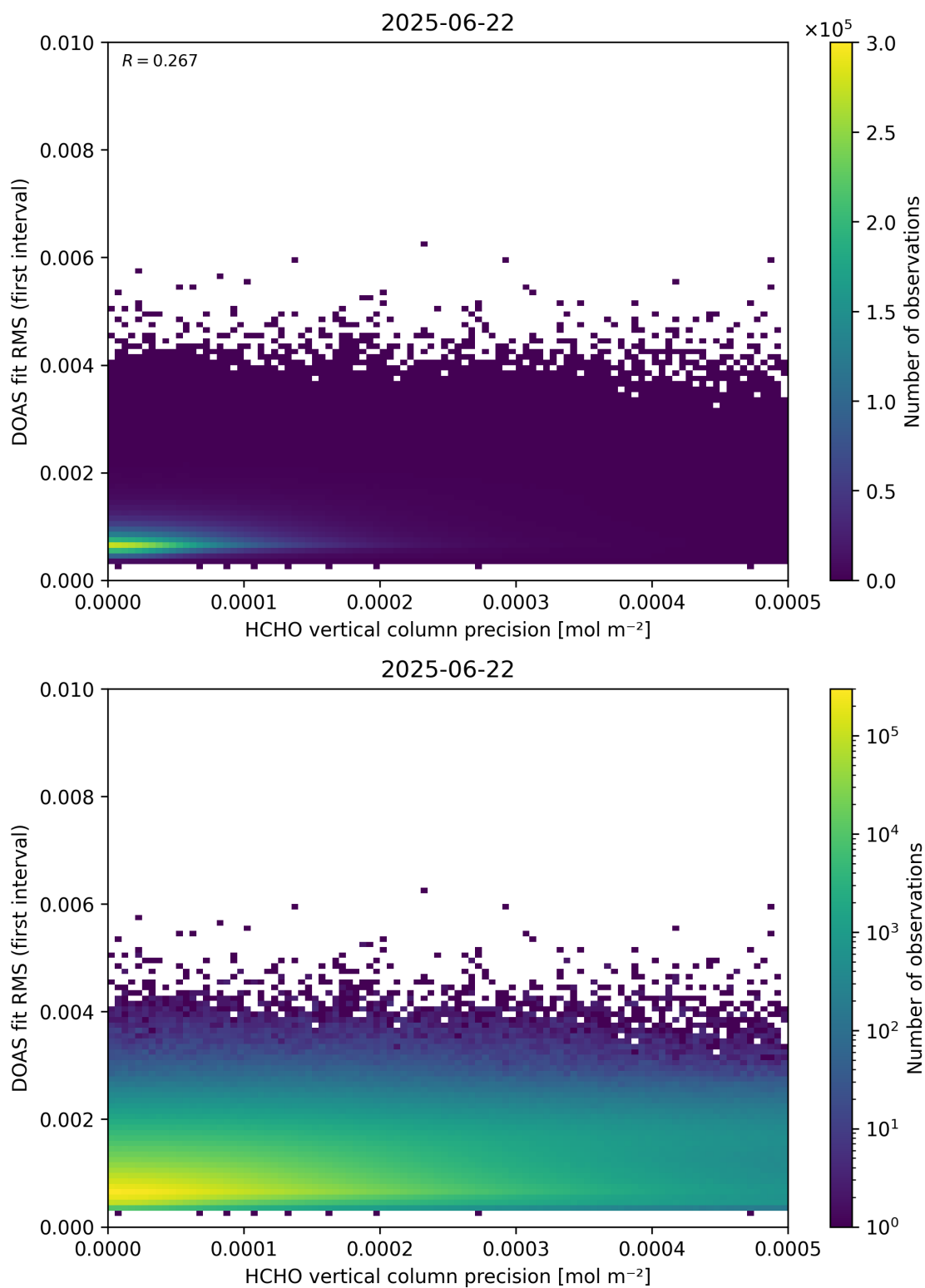
Figure 136: Scatter density plot of “HCHO vertical column precision” against “DOAS fit RMS (first interval)” for 2025-06-22 to 2025-06-23.
