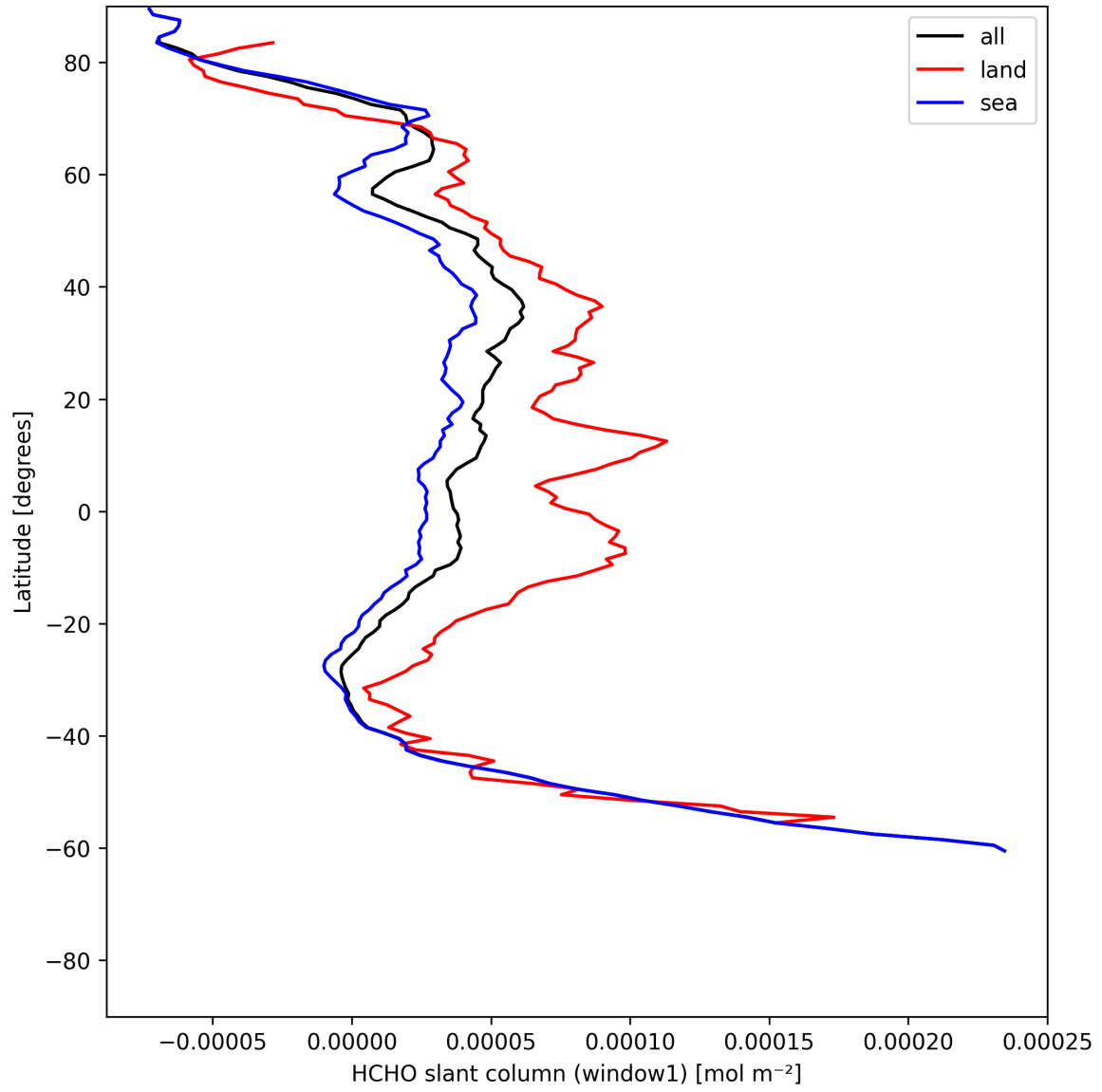
Figure 24: Zonal average of “HCHO slant column (window1)” for 2025-06-22 to 2025-06-23.
