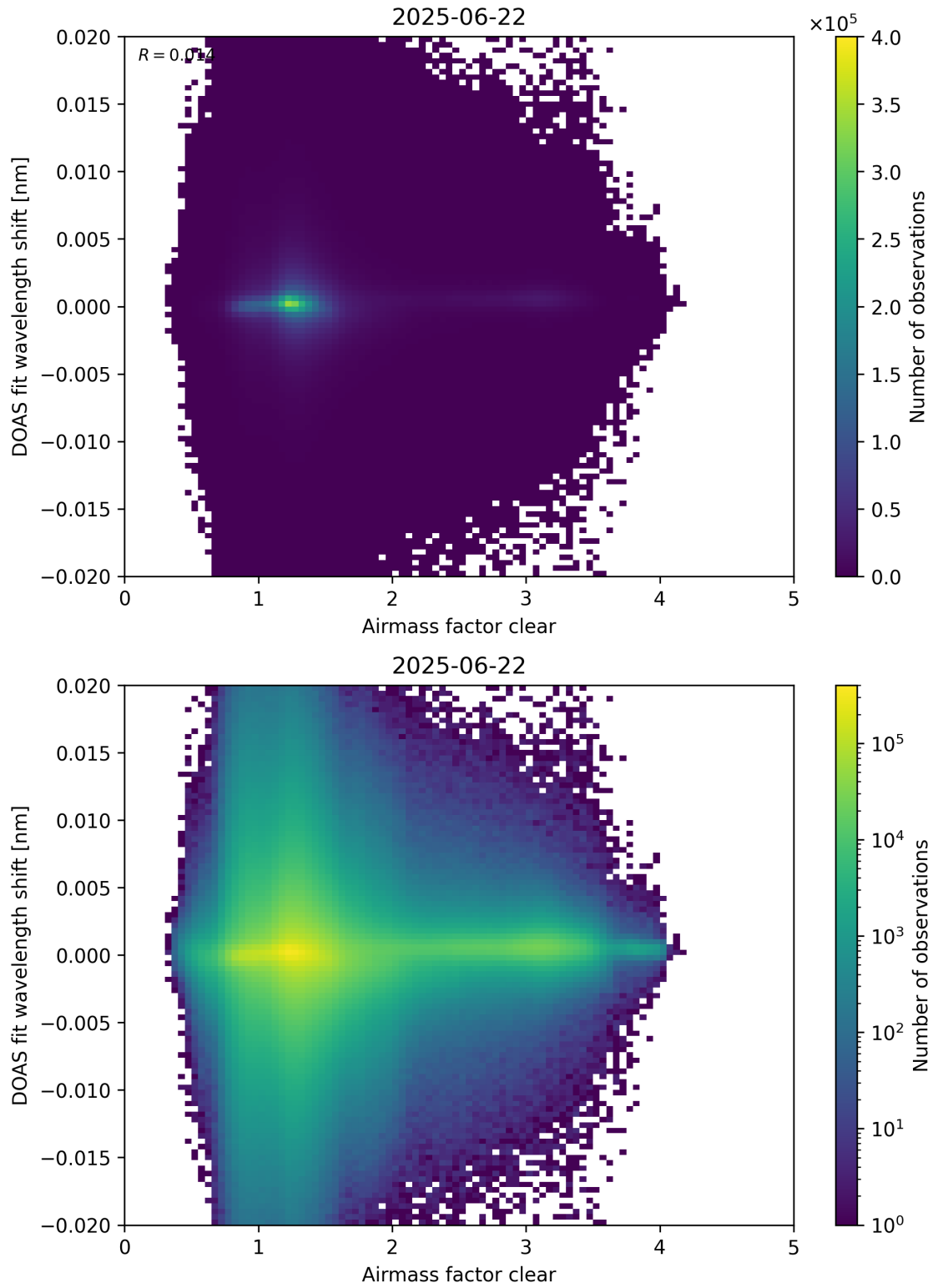
Figure 72: Scatter density plot of “Airmass factor clear” against “DOAS fit wavelength shift” for 2025-06-22 to 2025-06-23.
