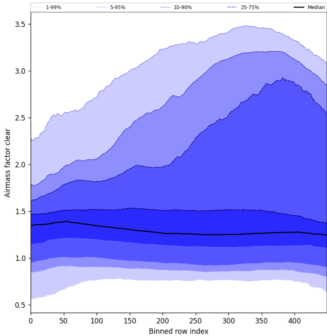
Figure 56: Along track statistics of “Air mass factor clear” for 2025-06-22 to 2025-06-23
