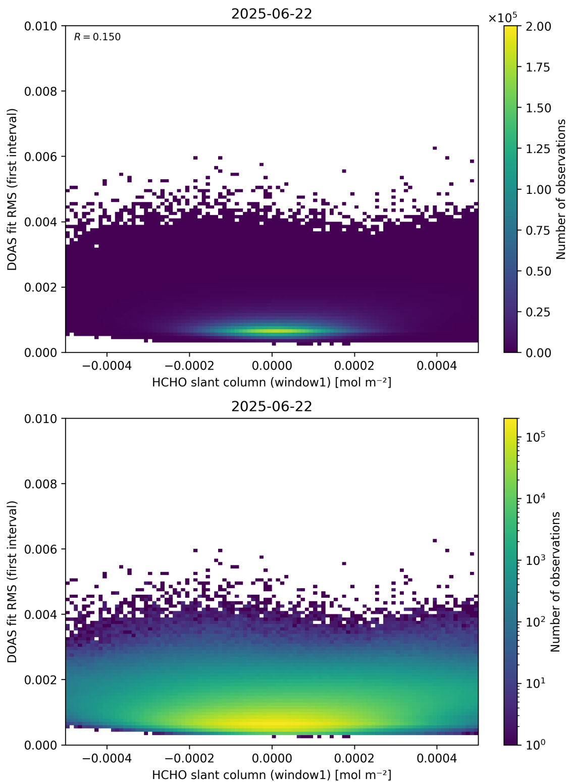
Figure 78: Scatter density plot of “HCHO slant column (window1)” against “DOAS fit RMS (first interval)” for 2025-06-22 to 2025-06-23.
