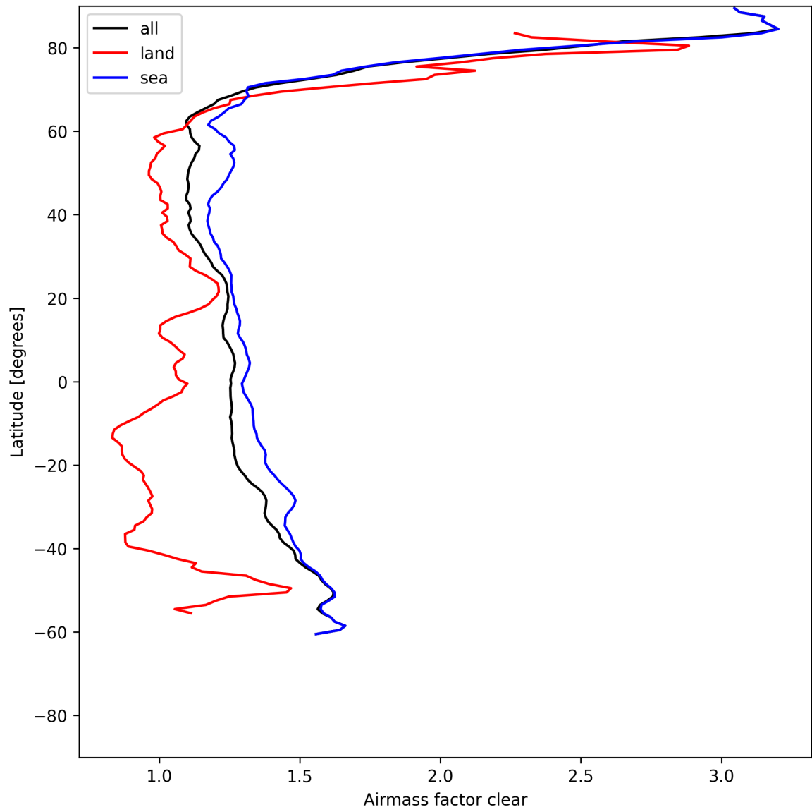
Figure 28: Zonal average of “Airmass factor clear” for 2025-06-22 to 2025-06-23.
