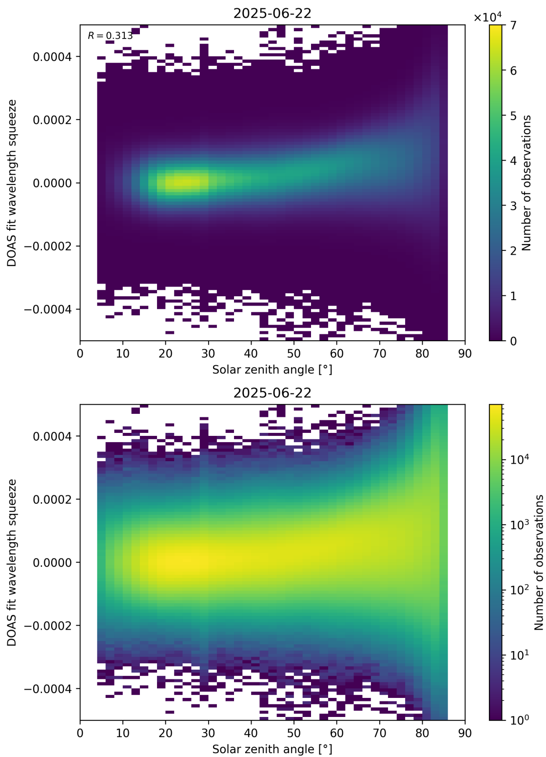
Figure 169: Scatter density plot of “Solar zenith angle” against “DOAS fit wavelength squeeze” for 2025-06-22 to 2025-06-23.
