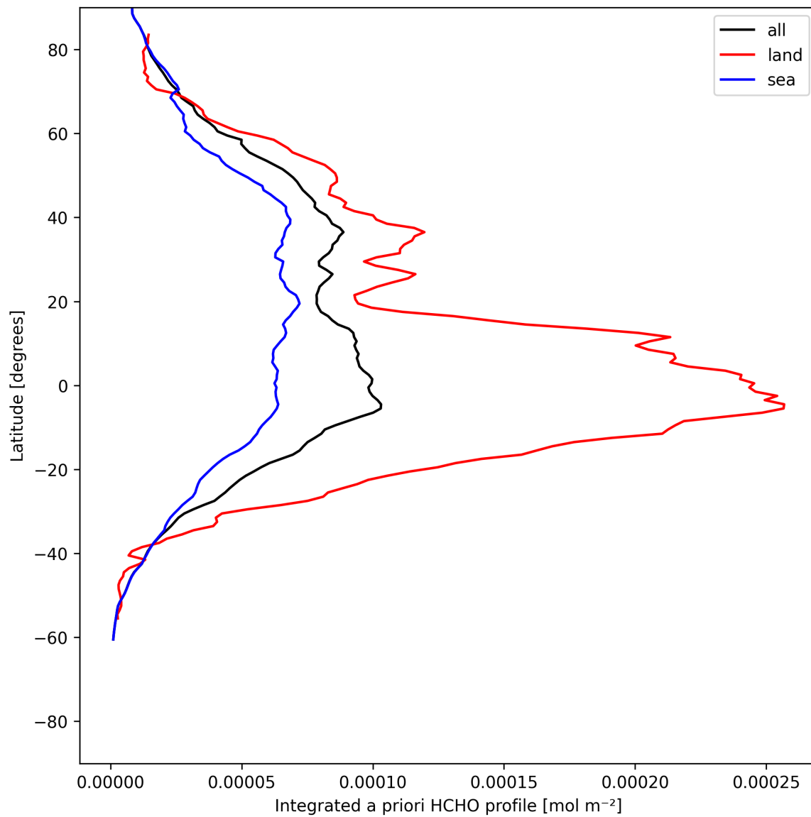
Figure 29: Zonal average of “Integrated a priori HCHO profile” for 2025-06-22 to 2025-06-23.
