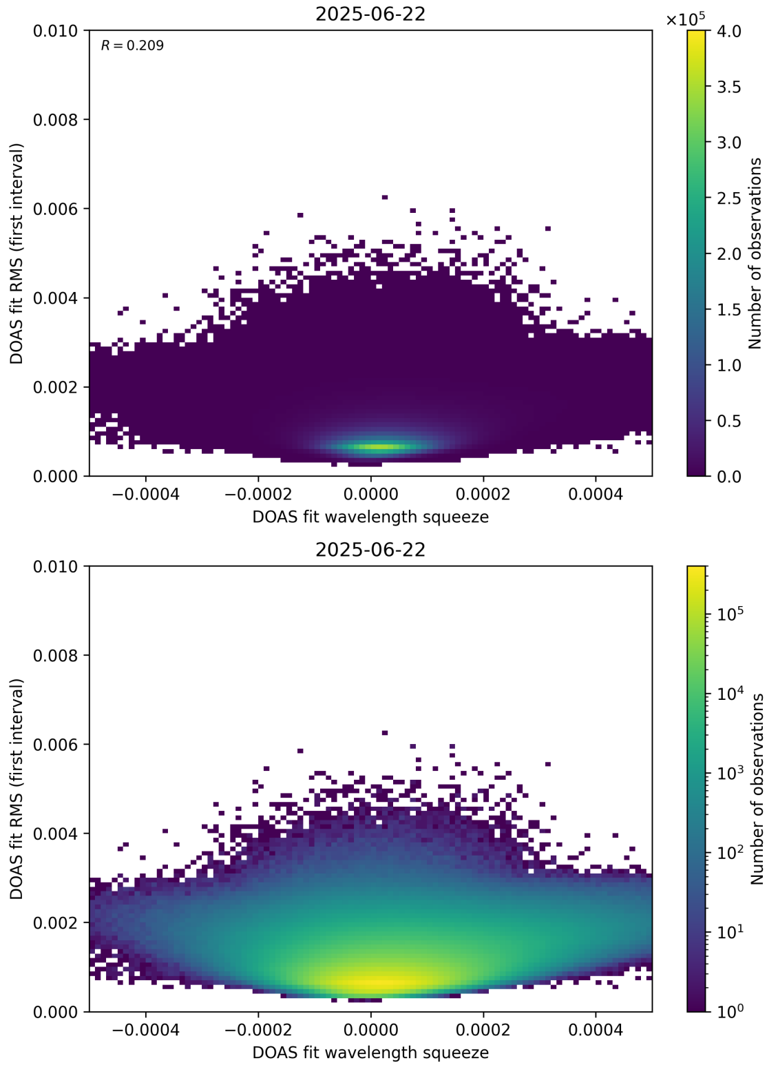
Figure 68: Scatter density plot of “DOAS fit wavelength squeeze” against “DOAS fit RMS (first interval)” for 2025-06-22 to 2025-06-23.
