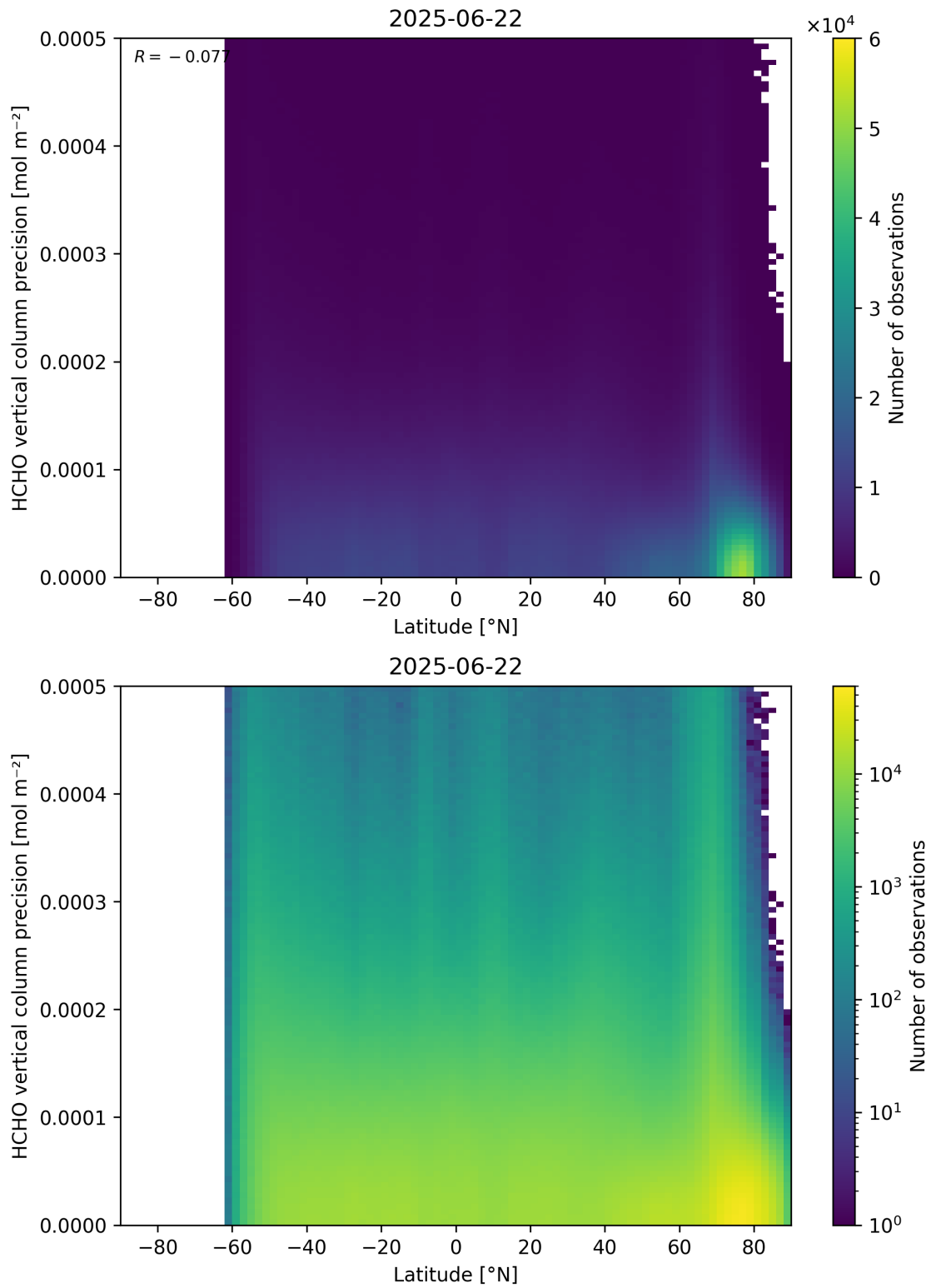
Figure 165: Scatter density plot of “Latitude” against “HCHO vertical column precision” for 2025-06-22 to 2025-06-23.
