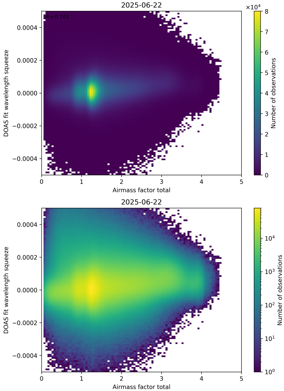
Figure 99: Scatter density plot of “Airmass factor total” against “DOAS fit wavelength squeeze” for 2025-06-22 to 2025-06-23.
