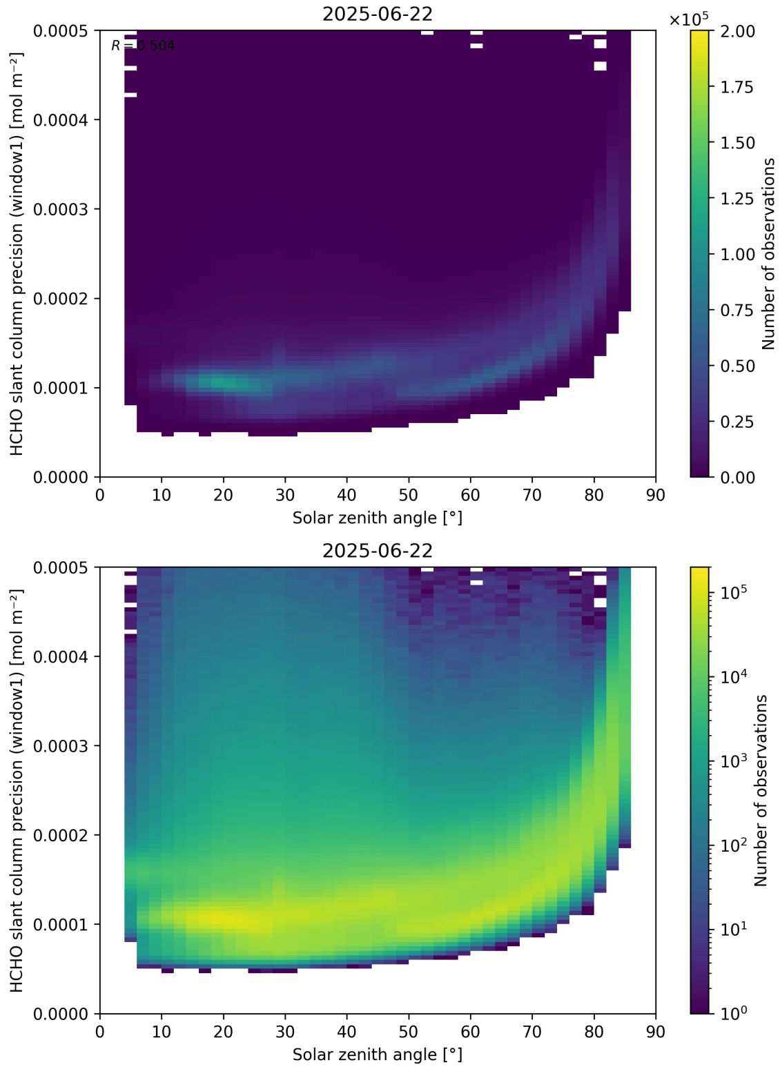
Figure 174: Scatter density plot of “Solar zenith angle” against “HCHO slant column precision (window1)” for 2025-06-22 to 2025-06-23.
