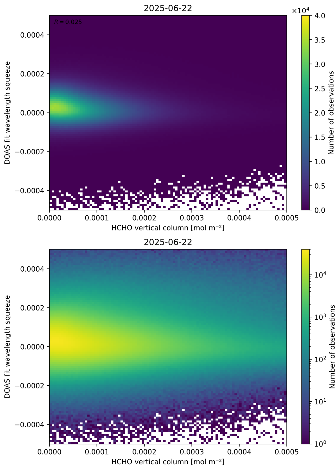
Figure 125: Scatter density plot of “HCHO vertical column” against “DOAS fit wavelength squeeze” for 2025-06-22 to 2025-06-23.
