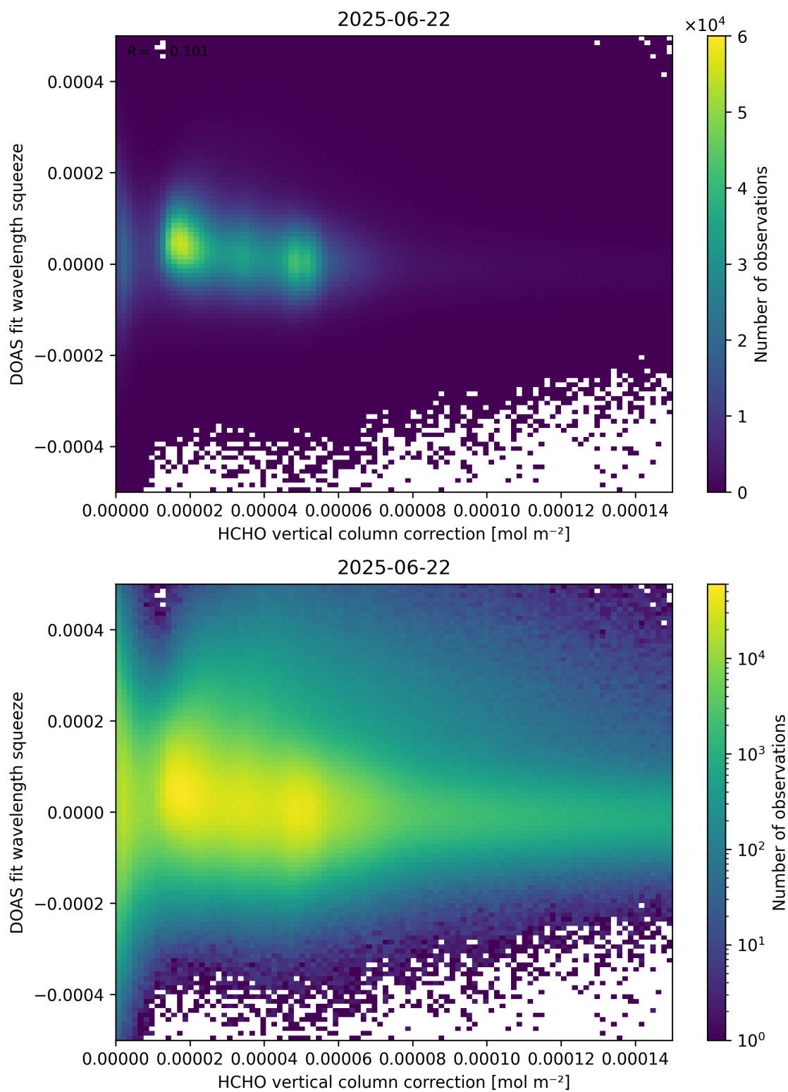
Figure 114: Scatter density plot of “HCHO vertical column correction” against “DOAS fit wavelength squeeze” for 2025-06-22 to 2025-06-23.
