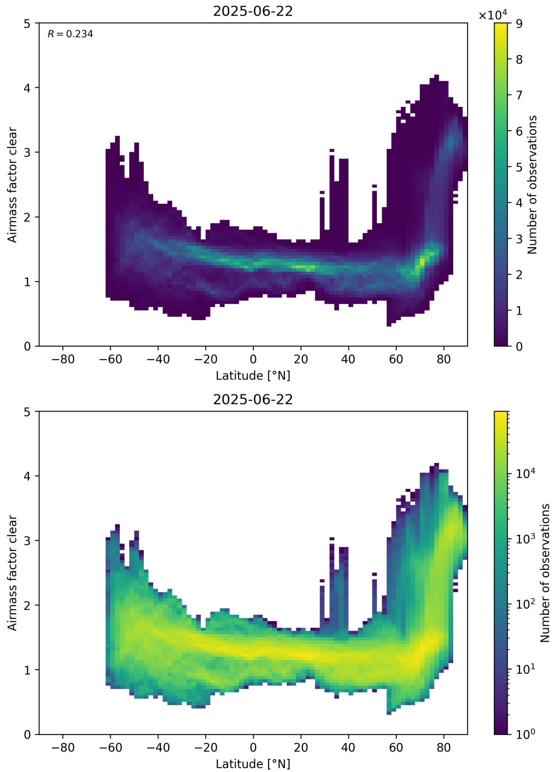
Figure 156: Scatter density plot of “Latitude” against “Airmass factor clear” for 2025-06-22 to 2025-06-23.
