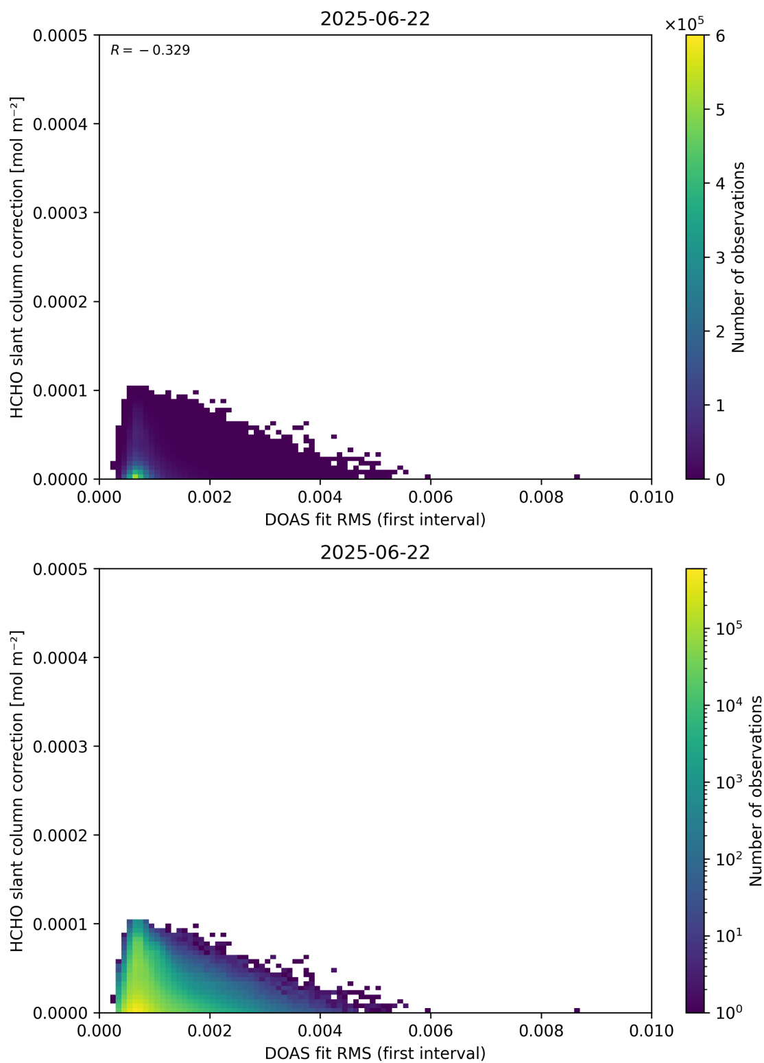
Figure 63: Scatter density plot of “DOAS fit RMS (first interval)” against “HCHO slant column correction” for 2025-06-22 to 2025-06-23.
