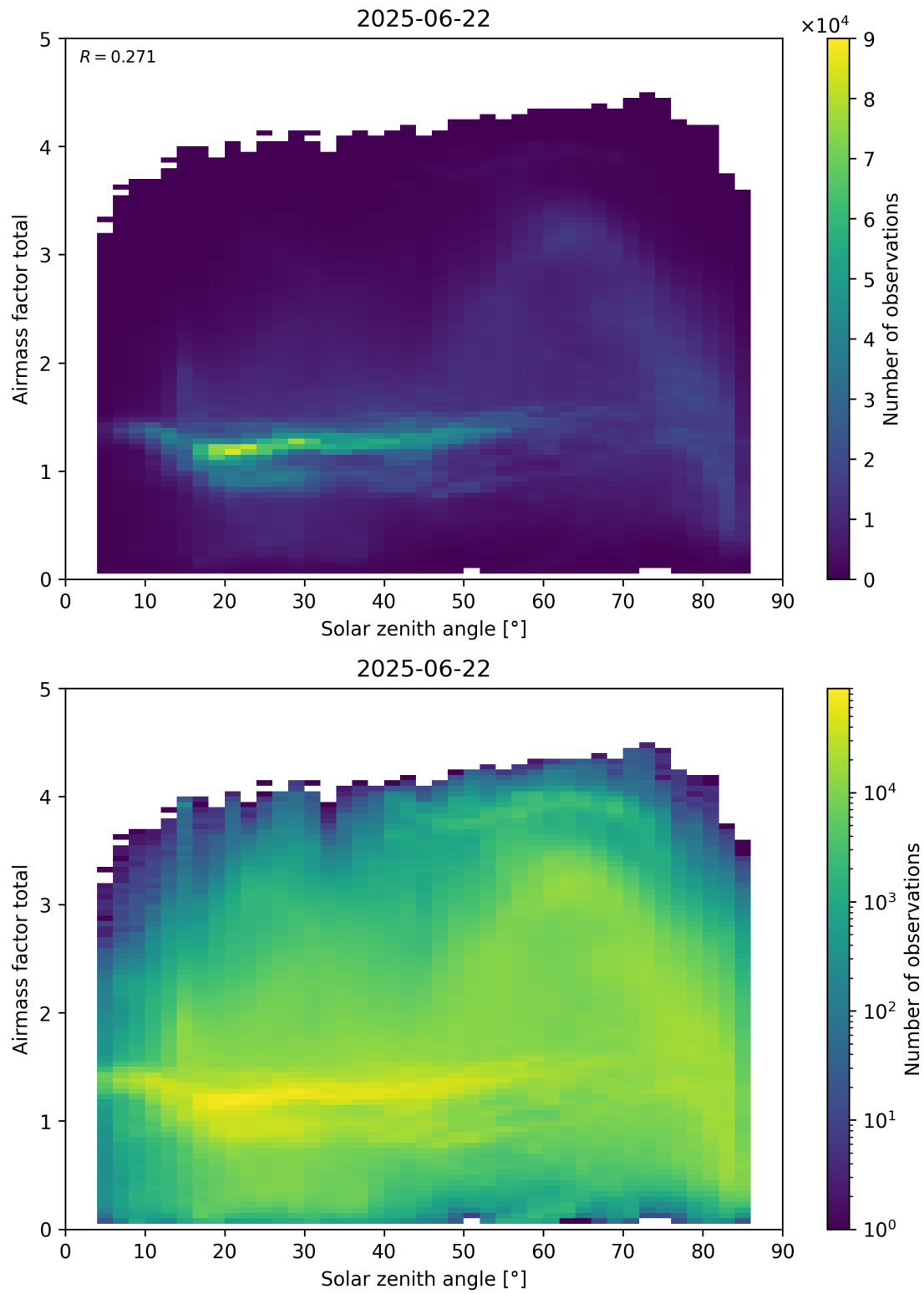
Figure 175: Scatter density plot of “Solar zenith angle” against “Airmass factor total” for 2025-06-22 to 2025-06-23.
