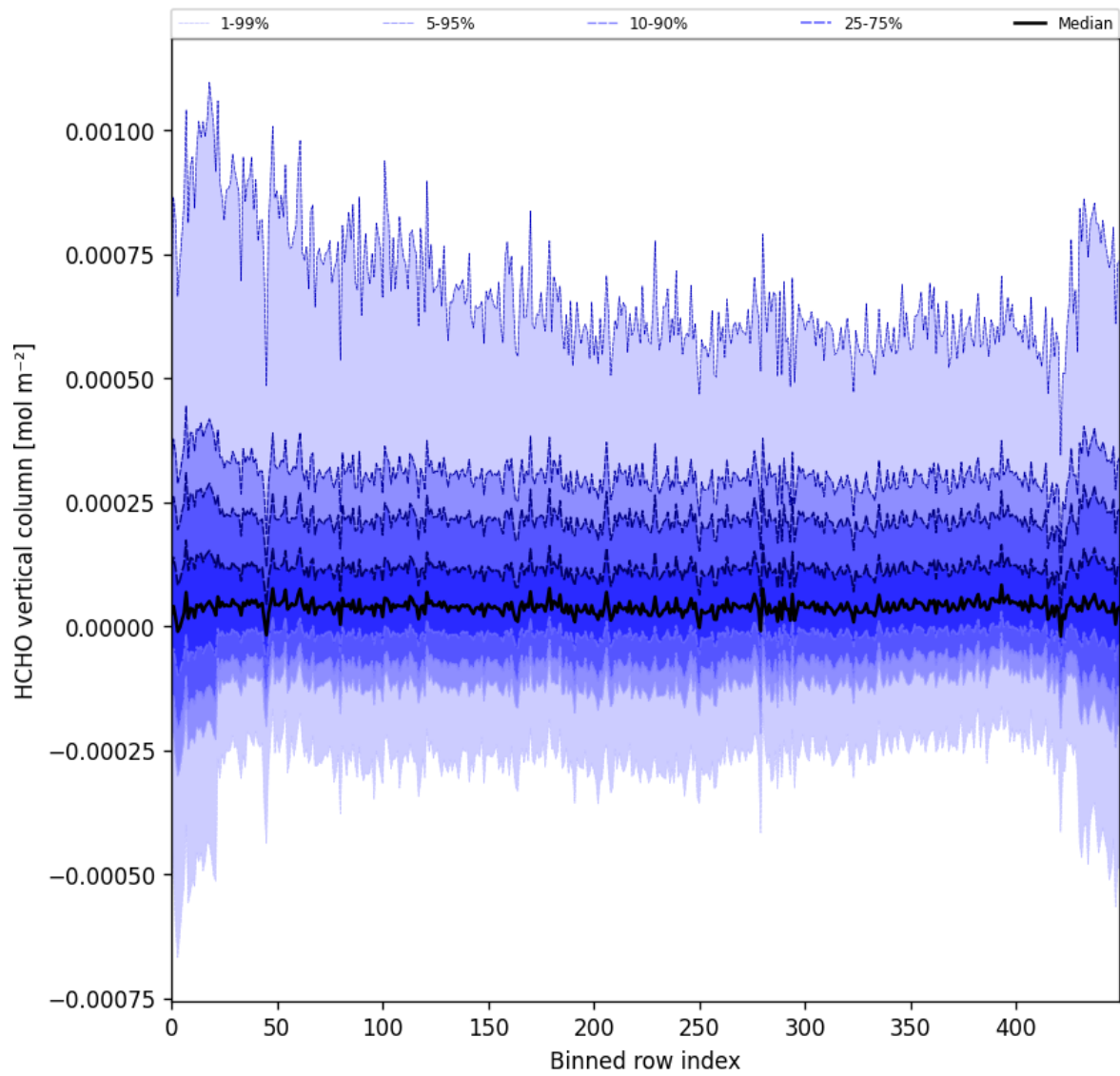
Figure 49: Along track statistics of “HCHO vertical column” for 2025-06-22 to 2025-06-23
