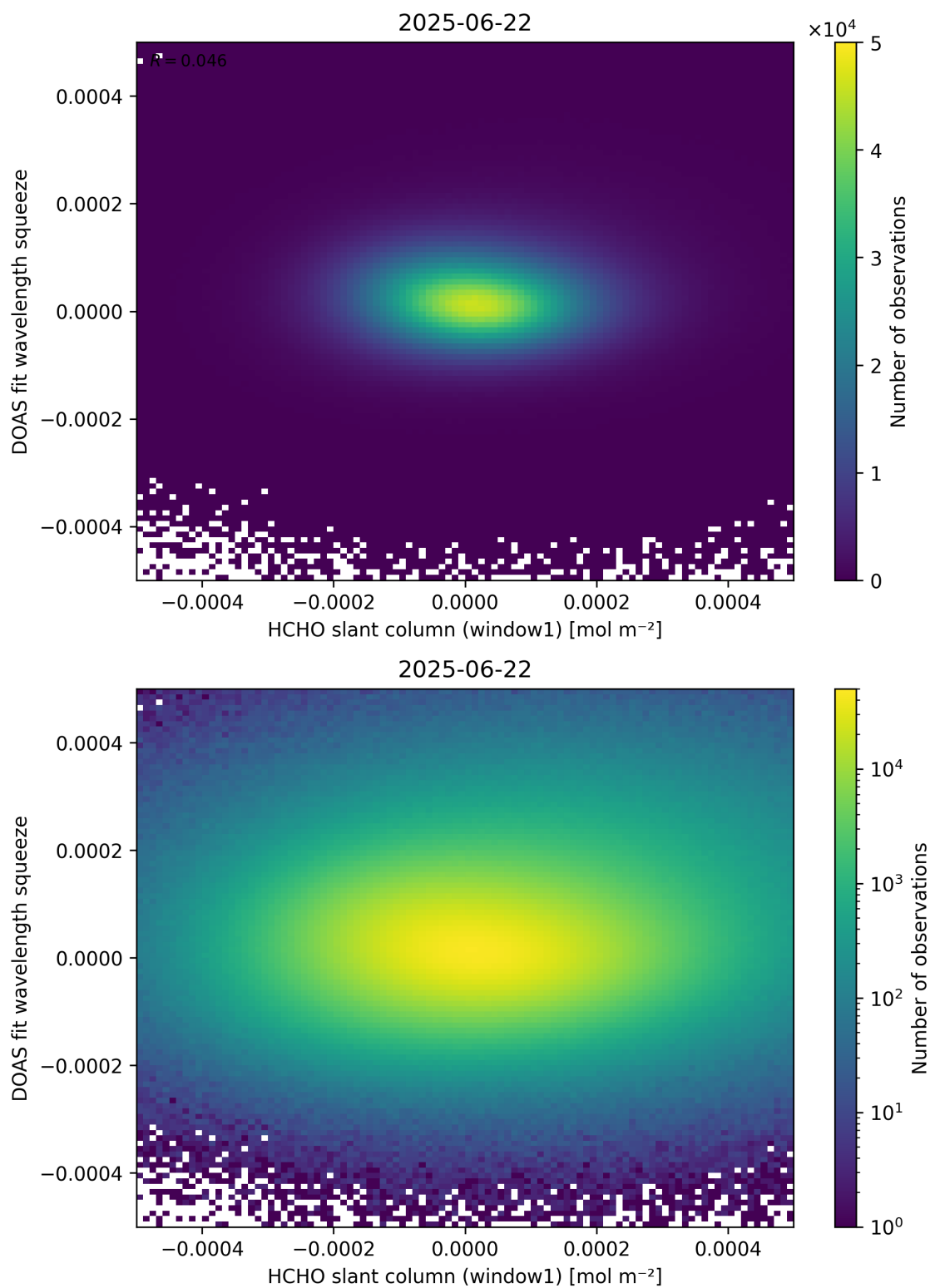
Figure 80: Scatter density plot of “HCHO slant column (window1)” against “DOAS fit wavelength squeeze” for 2025-06-22 to 2025-06-23.
