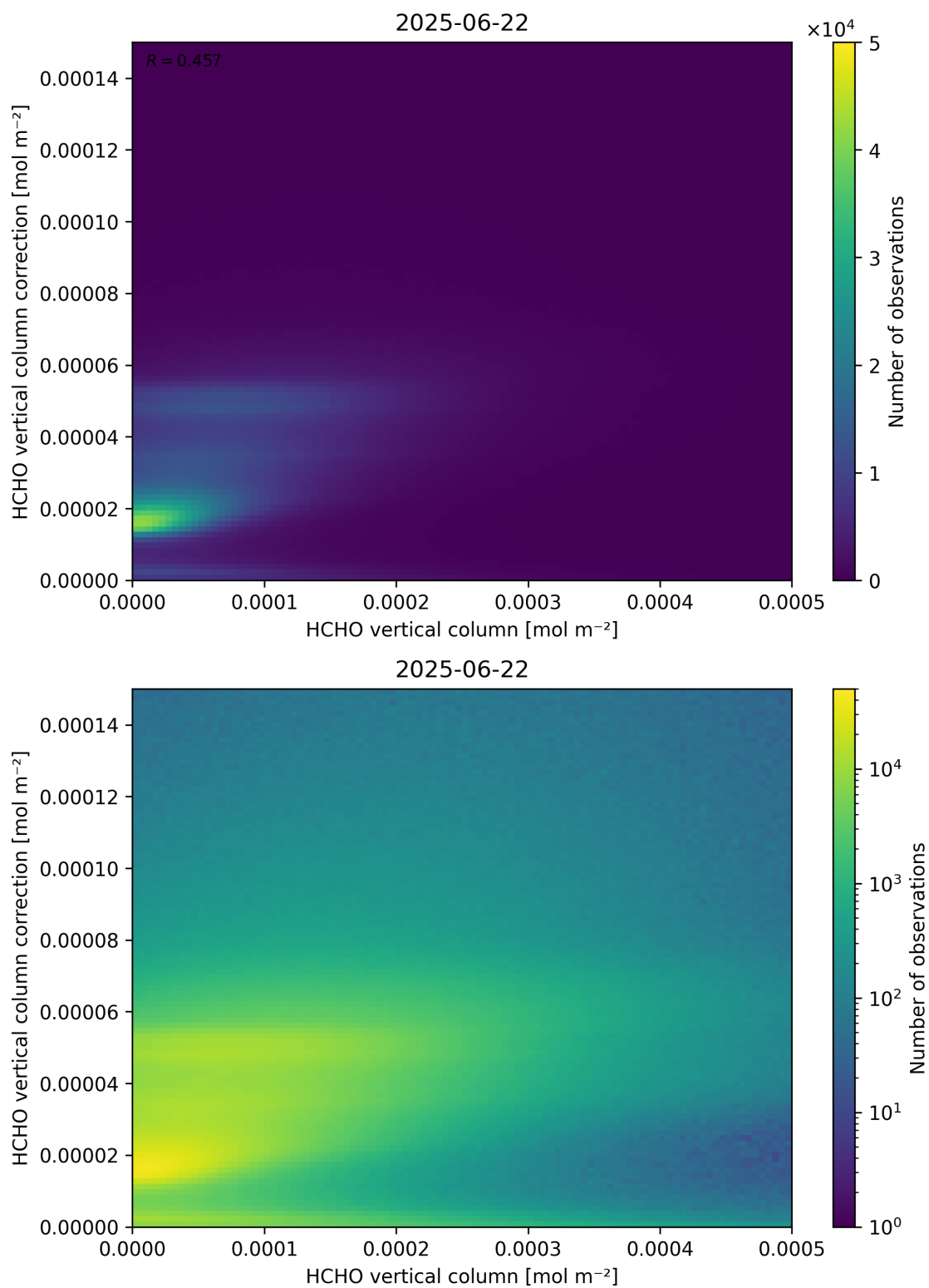
Figure 133: Scatter density plot of “HCHO vertical column” against “HCHO vertical column correction” for 2025-06-22 to 2025-06-23.
