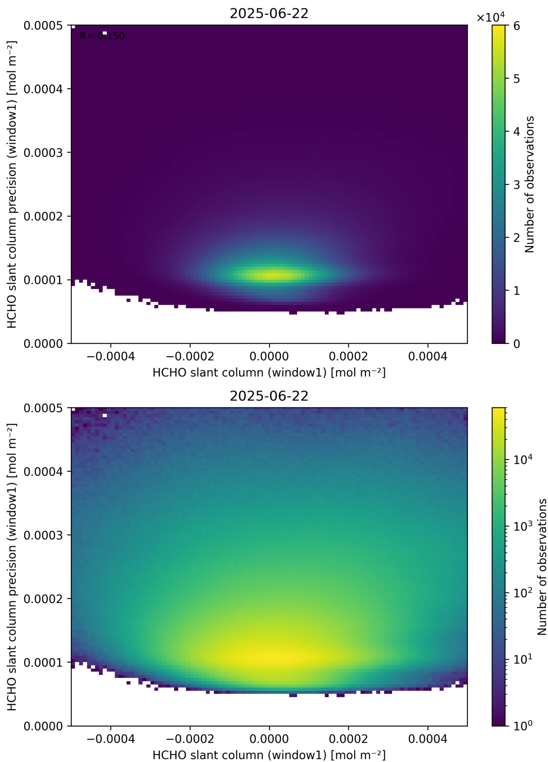
Figure 84: Scatter density plot of “HCHO slant column (window1)” against “HCHO slant column precision (window1)” for 2025-06-22 to 2025-06-23.
