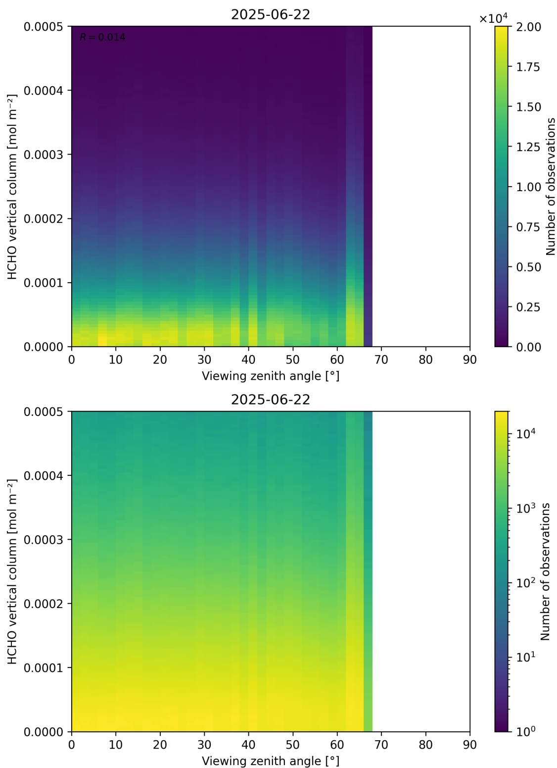
Figure 192: Scatter density plot of “Viewing zenith angle” against “HCHO vertical column” for 2025-06-22 to 2025-06-23.
