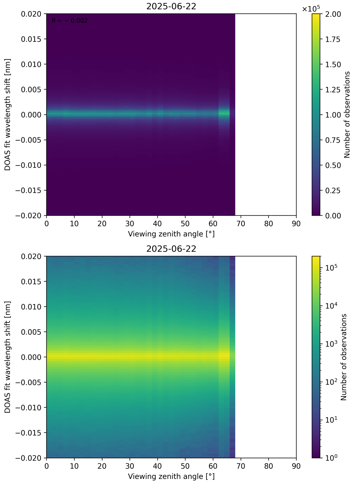
Figure 183: Scatter density plot of “Viewing zenith angle” against “DOAS fit wavelength shift” for 2025-06-22 to 2025-06-23.
