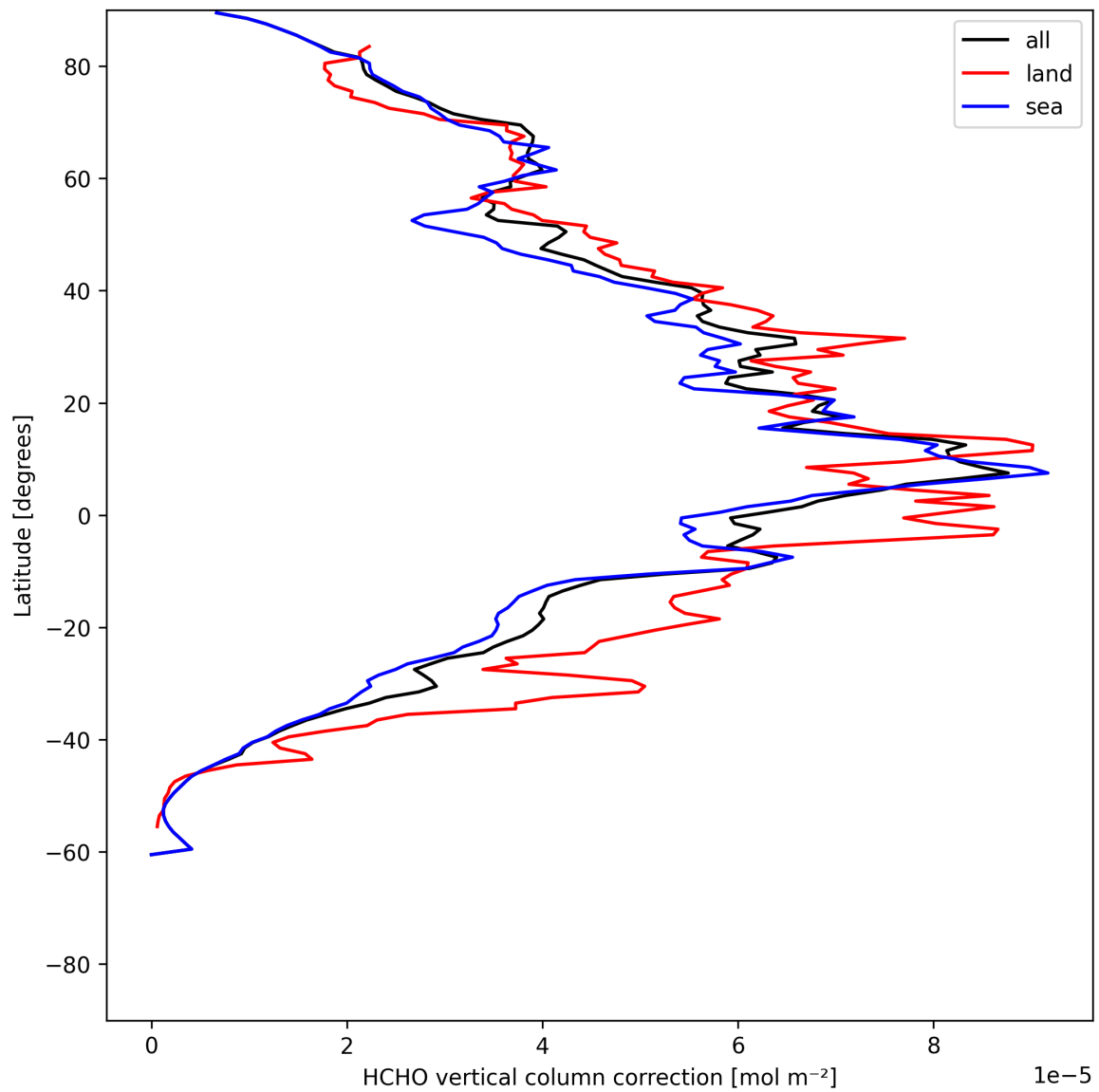
Figure 23: Zonal average of “HCHO vertical column correction” for 2025-06-22 to 2025-06-23.
