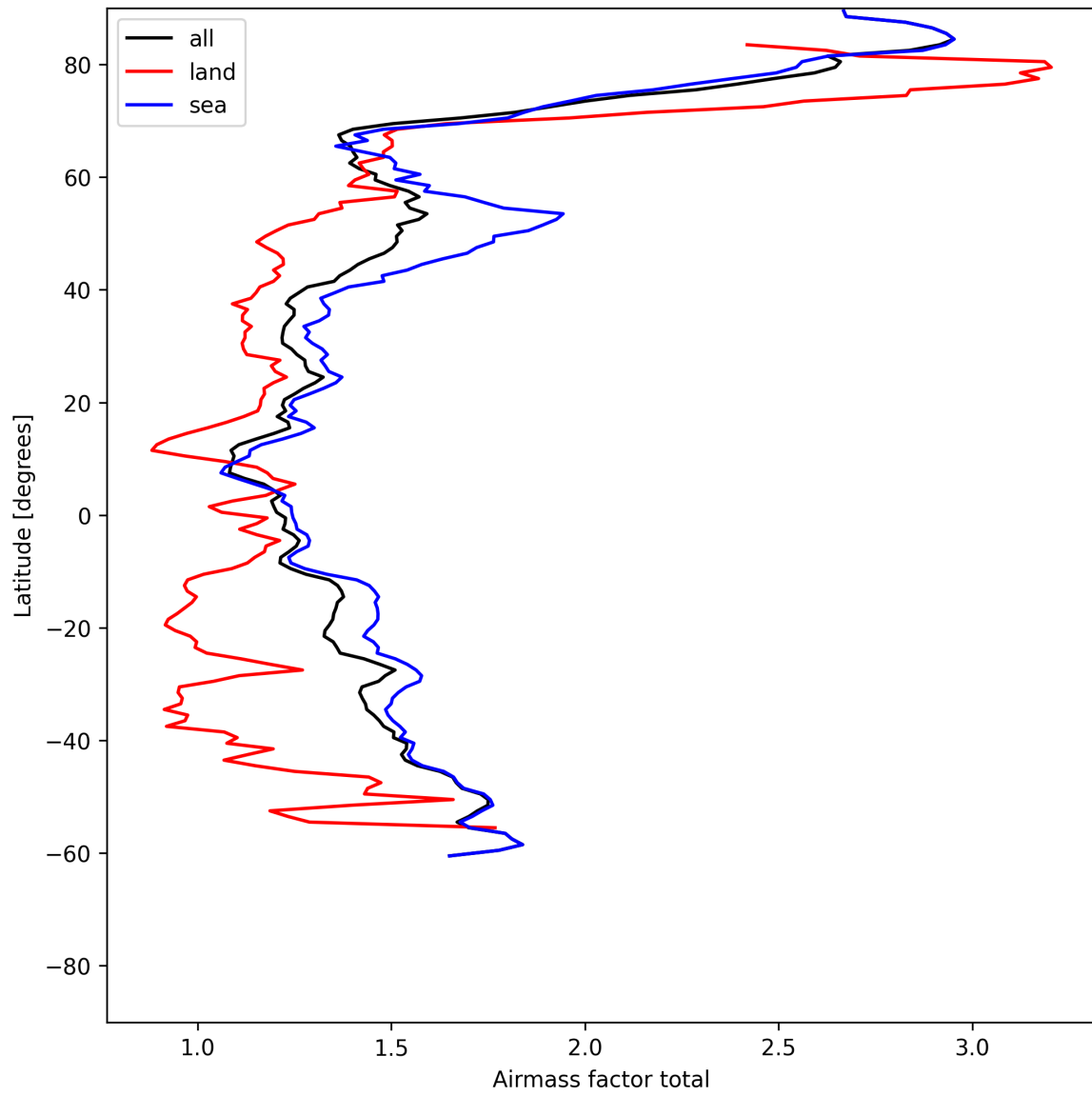
Figure 26: Zonal average of “Airmass factor total” for 2025-06-22 to 2025-06-23.
