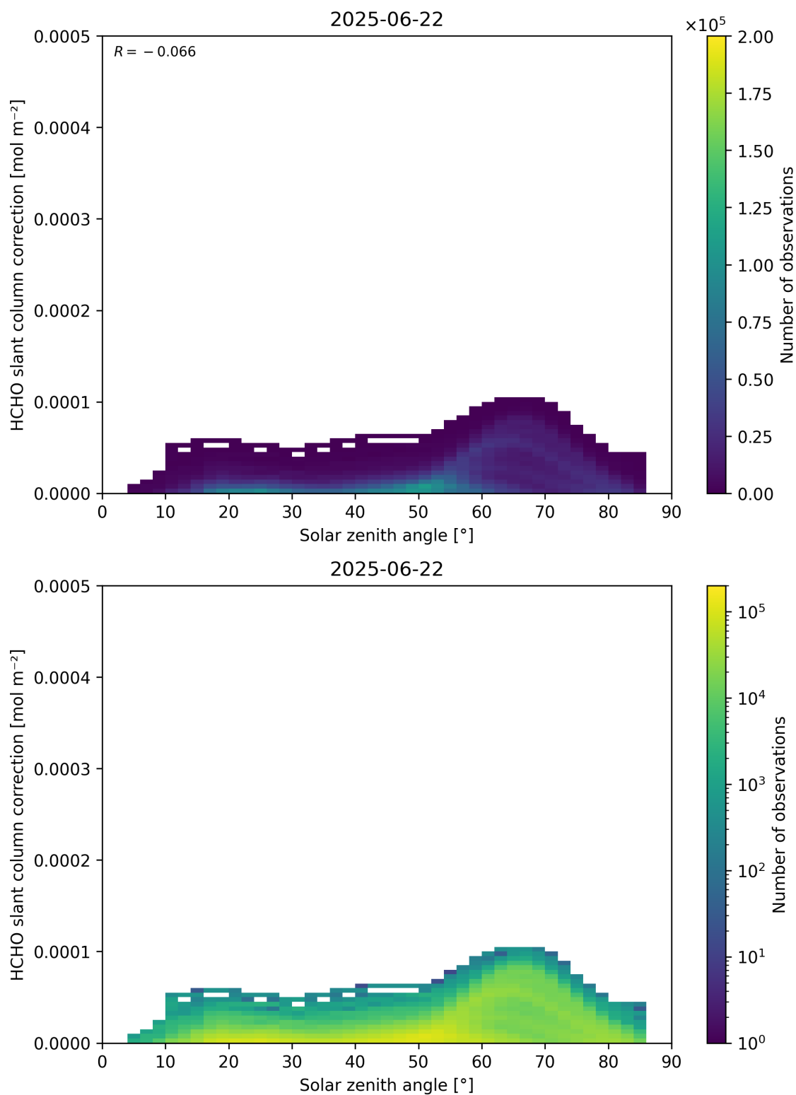
Figure 172: Scatter density plot of “Solar zenith angle” against “HCHO slant column correction” for 2025-06-22 to 2025-06-23.
