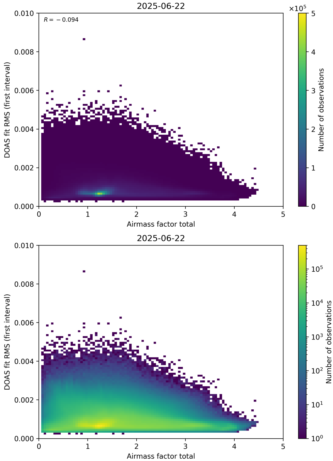
Figure 97: Scatter density plot of “Airmass factor total” against “DOAS fit RMS (first interval)” for 2025-06-22 to 2025-06-23.
