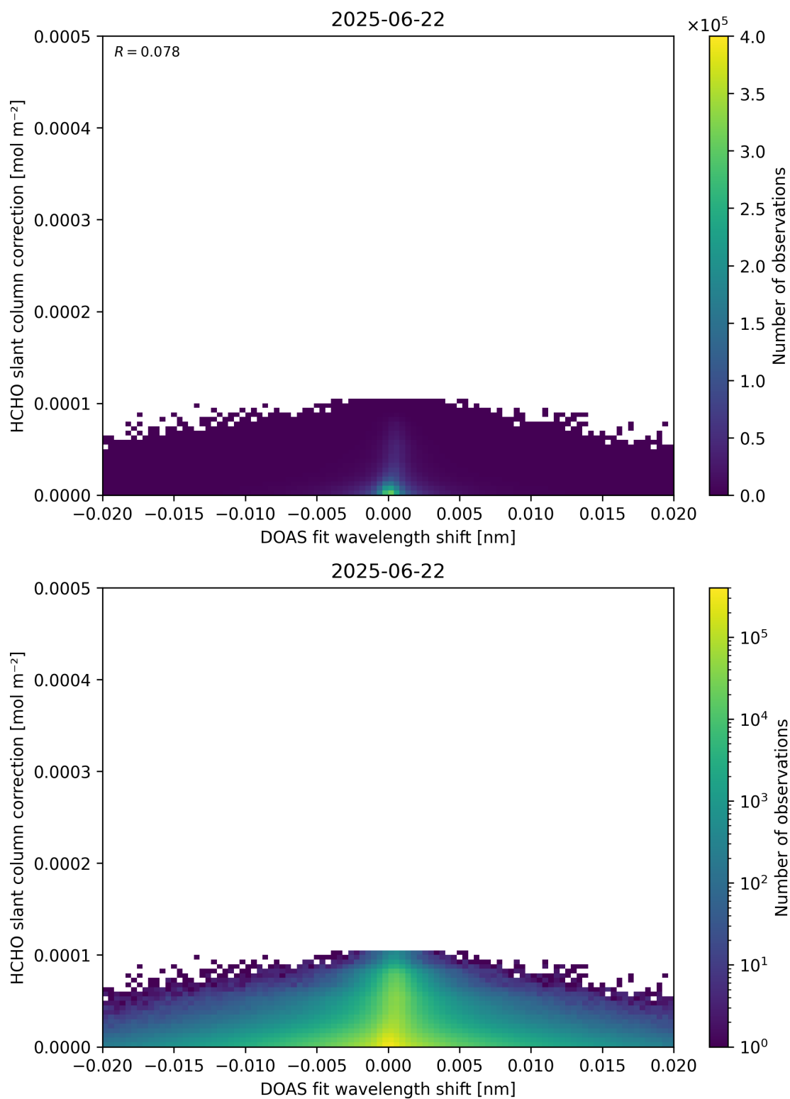
Figure 67: Scatter density plot of “DOAS fit wavelength shift” against “HCHO slant column correction” for 2025-06-22 to 2025-06-23.
