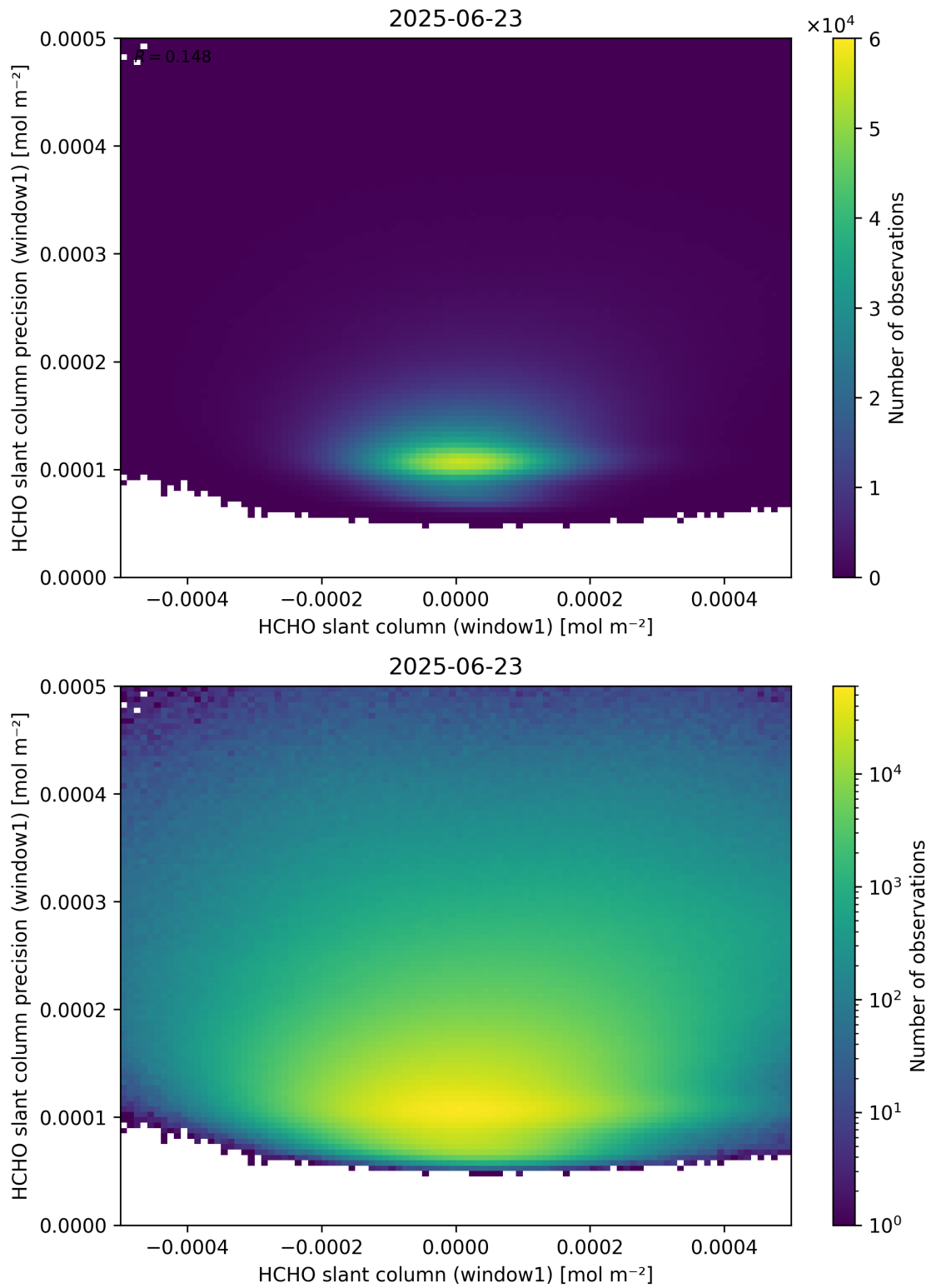
Figure 84: Scatter density plot of “HCHO slant column (window1)” against “HCHO slant column precision (window1)” for 2025-06-22 to 2025-06-24.
