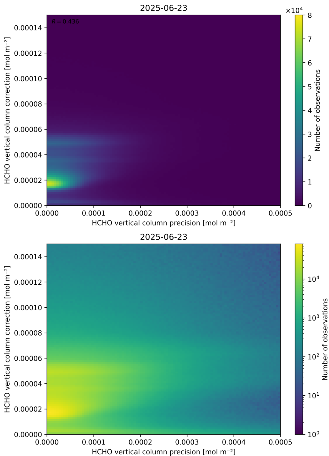
Figure 146: Scatter density plot of “HCHO vertical column precision” against “HCHO vertical column correction” for 2025-06-22 to 2025-06-24.
