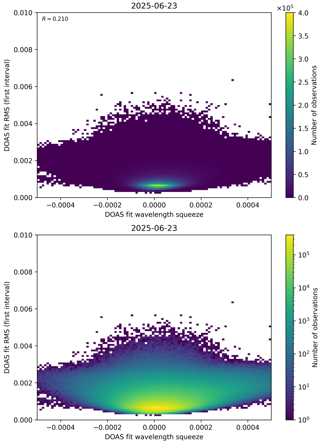
Figure 68: Scatter density plot of “DOAS fit wavelength squeeze” against “DOAS fit RMS (first interval)” for 2025-06-22 to 2025-06-24.
