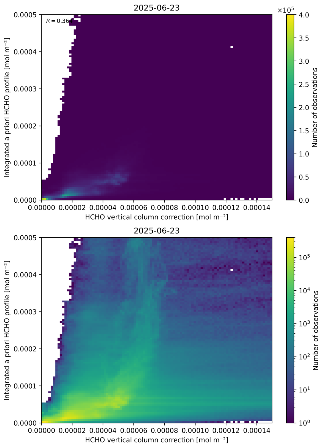
Figure 122: Scatter density plot of “HCHO vertical column correction” against “Integrated a priori HCHO profile” for 2025-06-22 to 2025-06-24.
