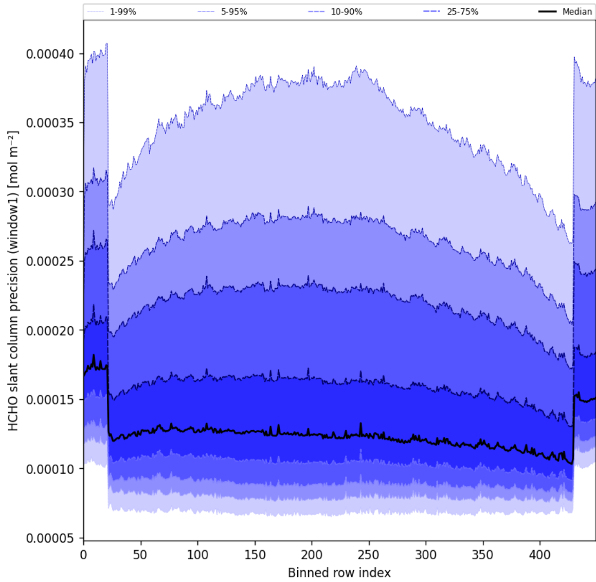
Figure 53: Along track statistics of “HCHO slant column precision (window1)” for 2025-06-22 to 2025-06-24
