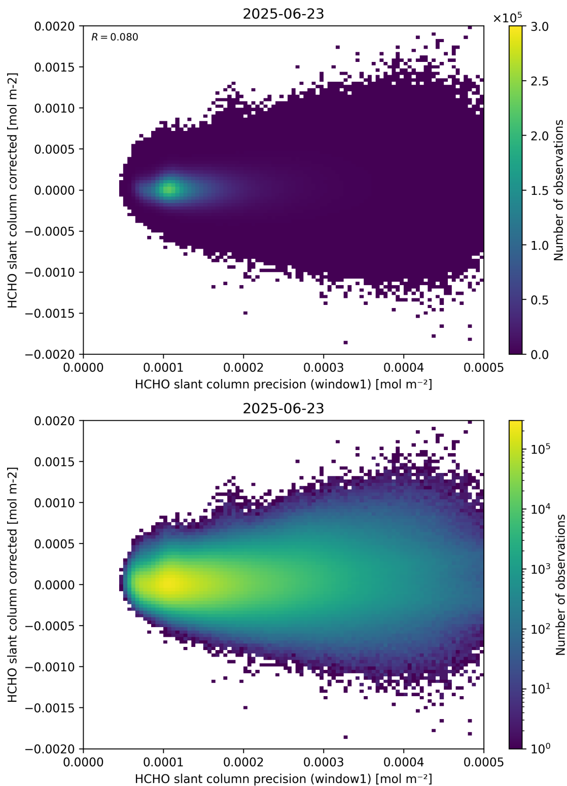
Figure 92: Scatter density plot of “HCHO slant column precision (window1)” against “HCHO slant column corrected” for 2025-06-22 to 2025-06-24.
