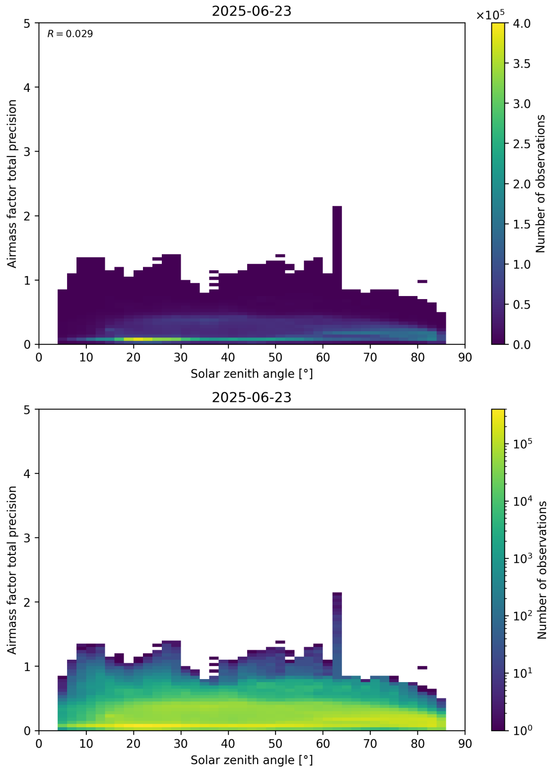
Figure 176: Scatter density plot of “Solar zenith angle” against “Airmass factor total precision” for 2025-06-22 to 2025-06-24.
