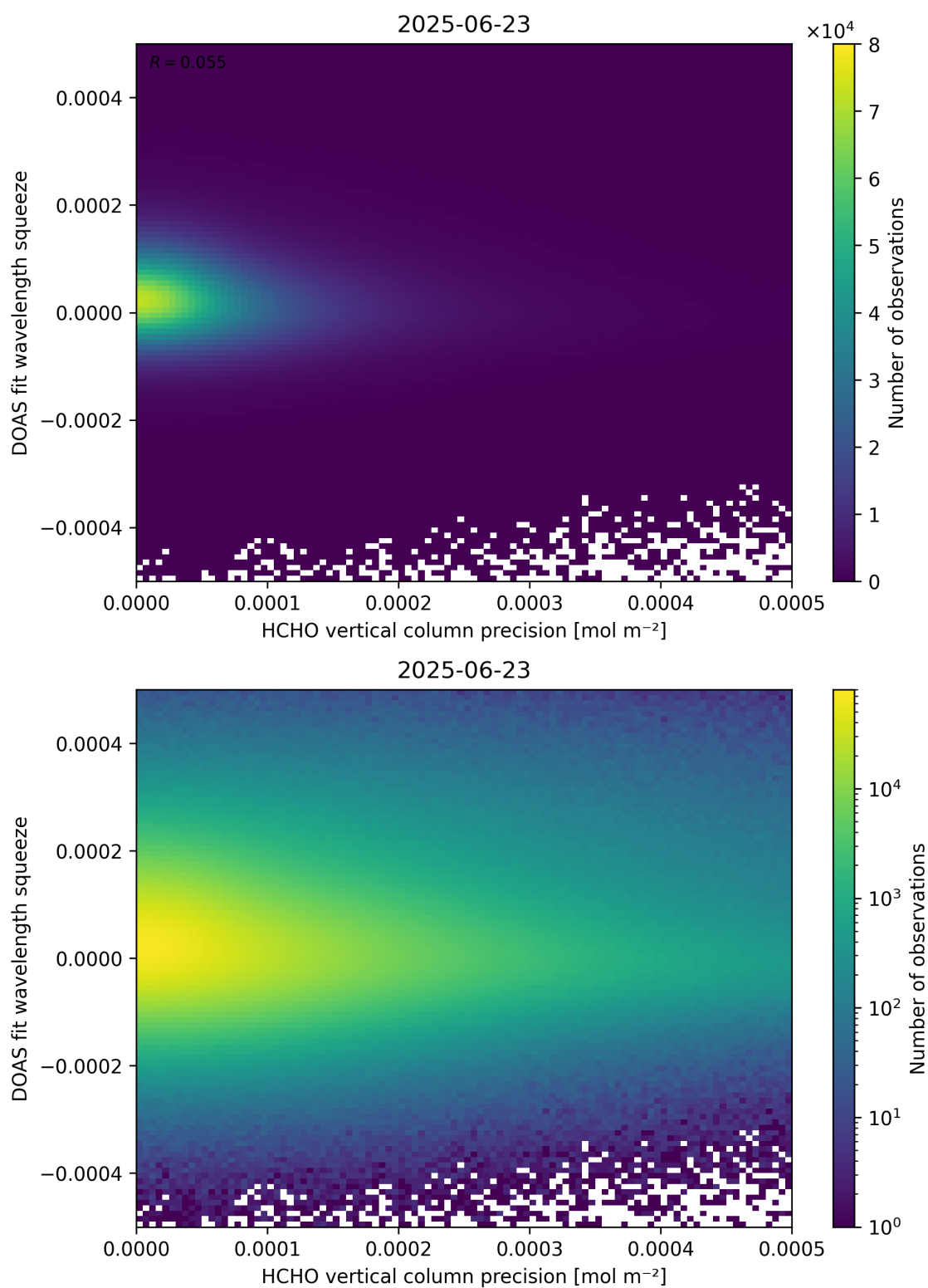
Figure 138: Scatter density plot of “HCHO vertical column precision” against “DOAS fit wavelength squeeze” for 2025-06-22 to 2025-06-24.
