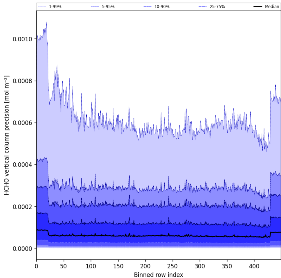
Figure 50: Along track statistics of “HCHO vertical column precision” for 2025-06-22 to 2025-06-24
