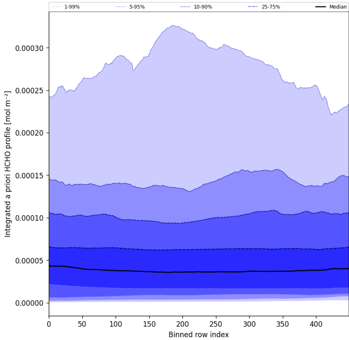
Figure 57: Along track statistics of "Integrated a priori HCHO profile" for 2025-06-22 to 2025-06-24
