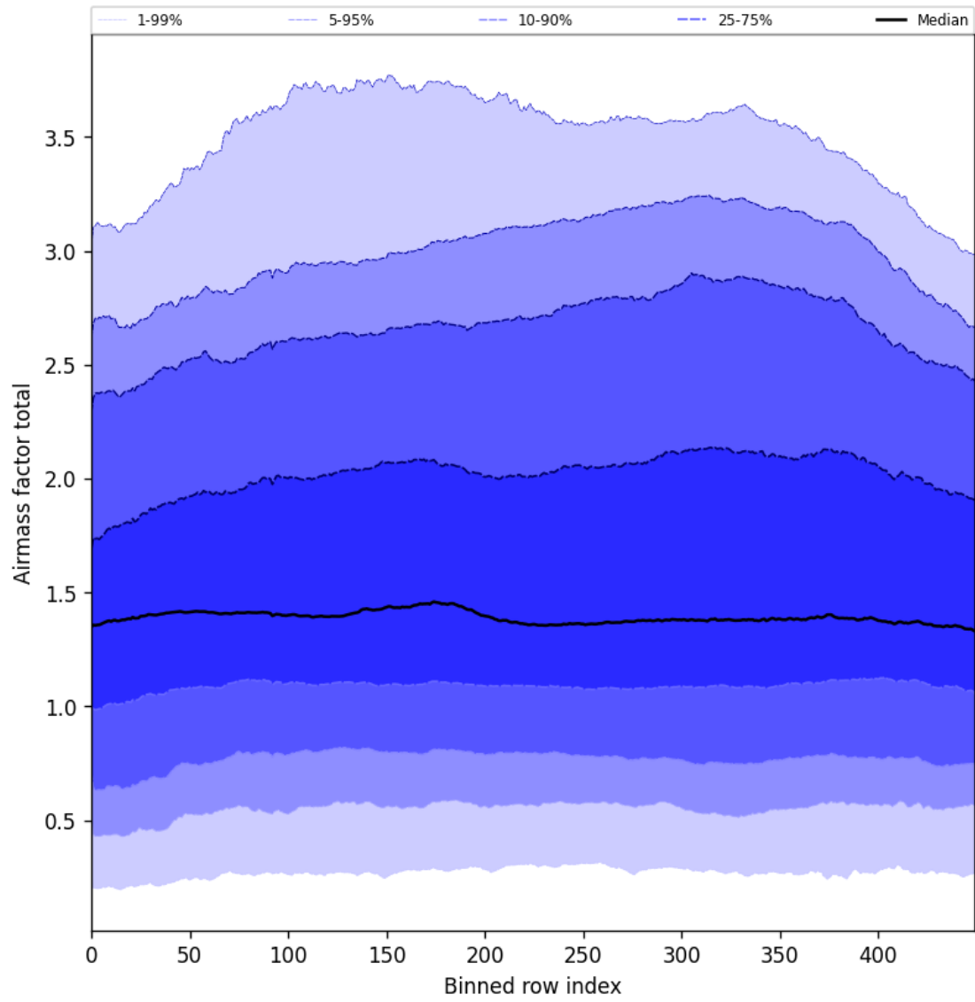
Figure 54: Along track statistics of “Airmass factor total” for 2025-06-22 to 2025-06-24
