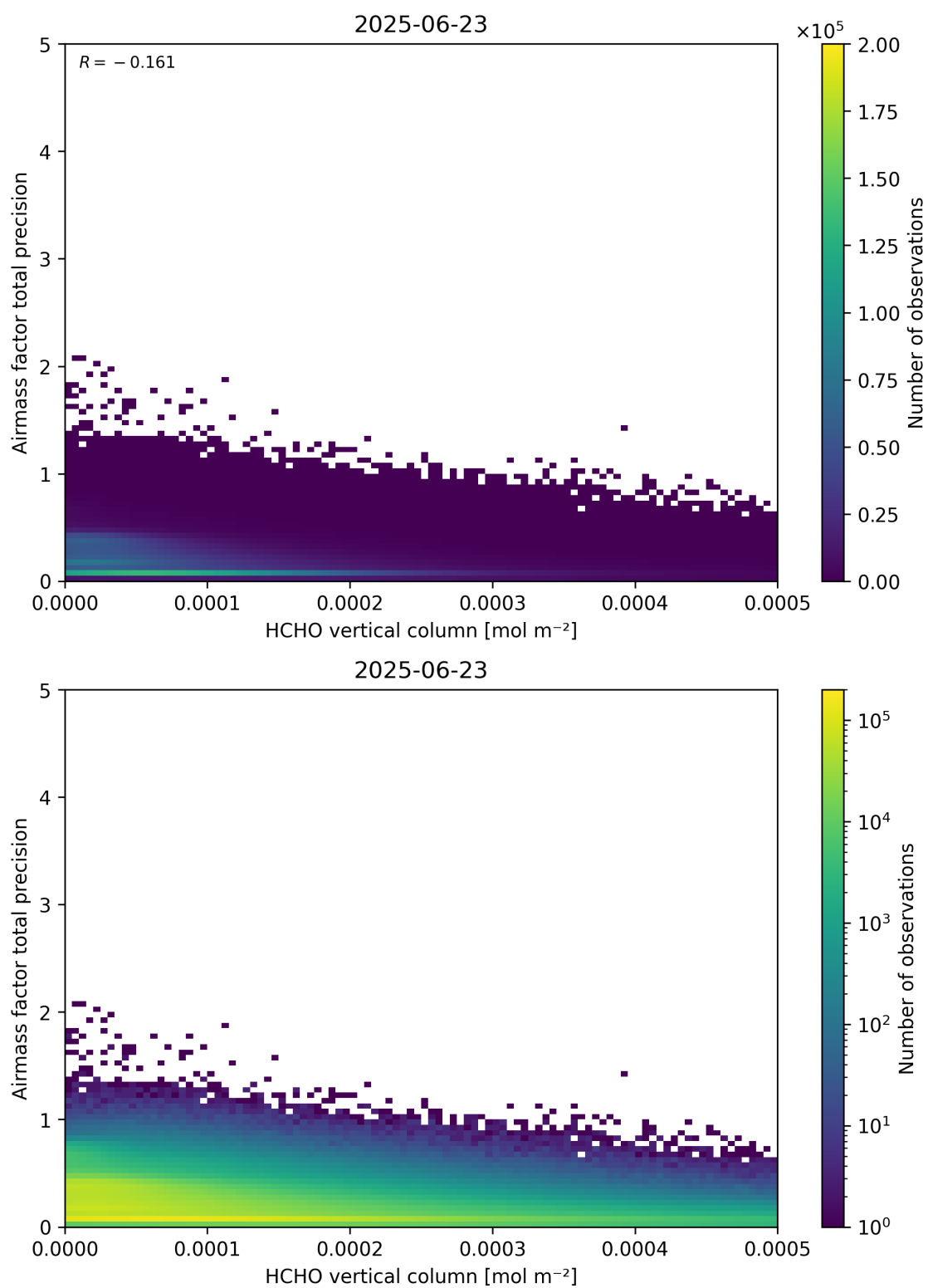
Figure 132: Scatter density plot of “HCHO vertical column” against “Airmass factor total precision” for 2025-06-22 to 2025-06-24.
