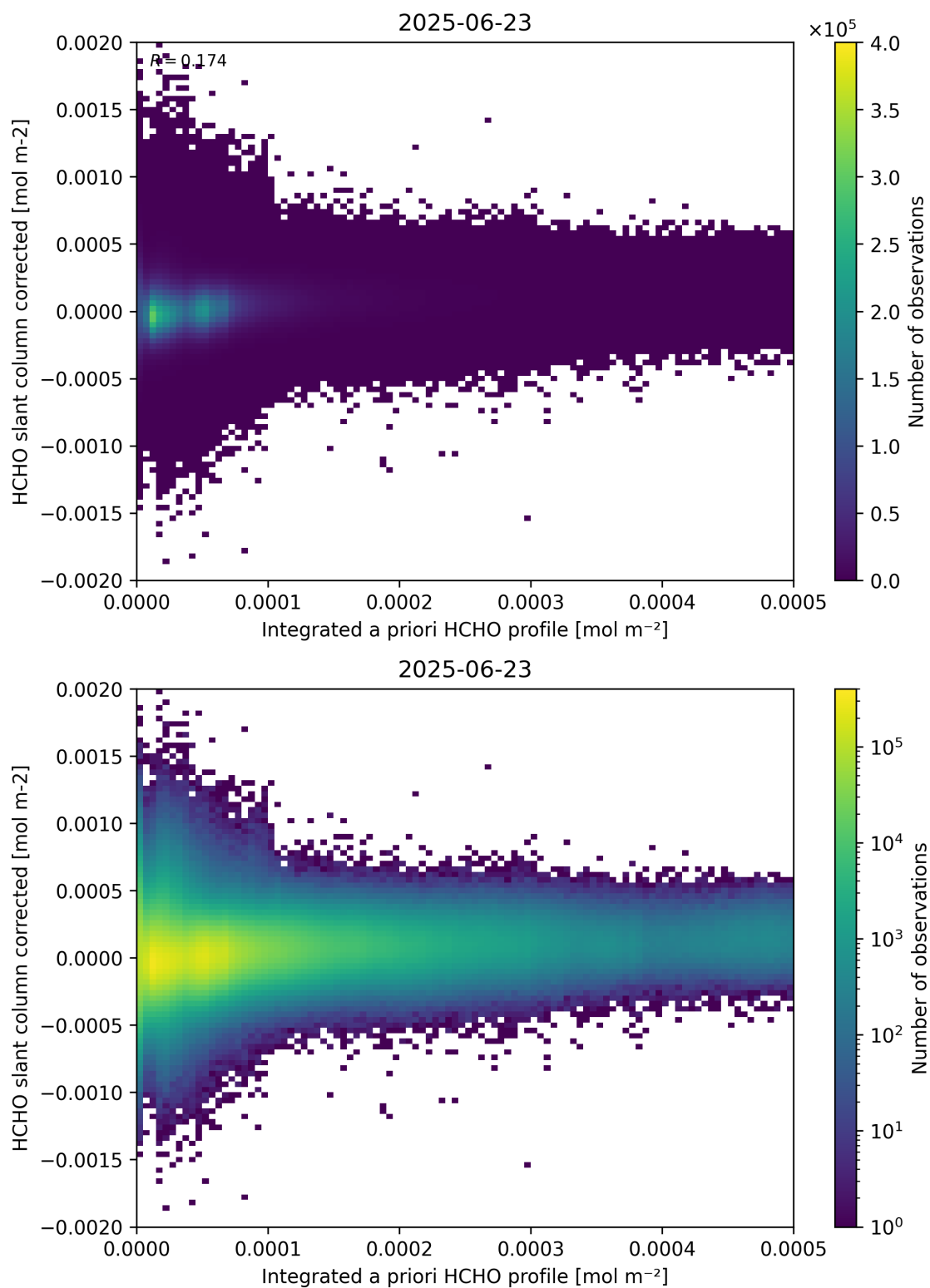
Figure 151: Scatter density plot of “Integrated a priori HCHO profile” against “HCHO slant column corrected” for 2025-06-22 to 2025-06-24.
