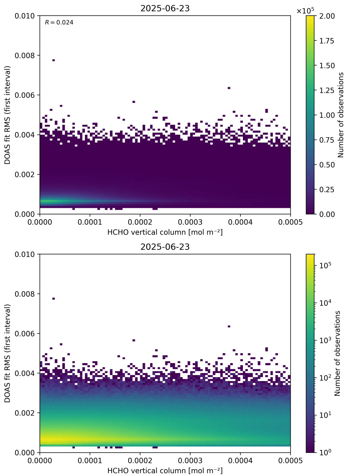
Figure 123: Scatter density plot of “HCHO vertical column” against “DOAS fit RMS (first interval)” for 2025-06-22 to 2025-06-24.
