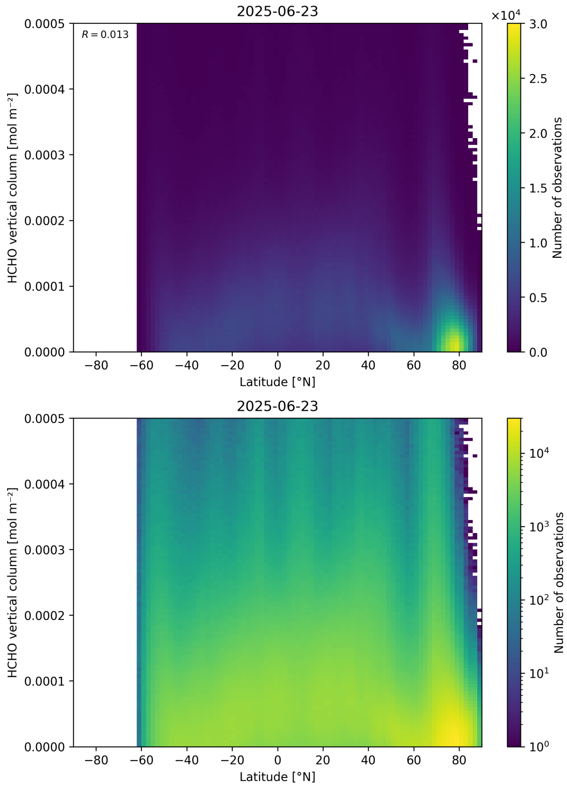
Figure 163: Scatter density plot of “Latitude” against “HCHO vertical column” for 2025-06-22 to 2025-06-24.
