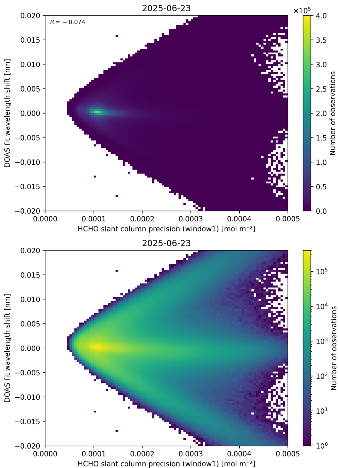
Figure 89: Scatter density plot of “HCHO slant column precision (window1)” against “DOAS fit wavelength shift” for 2025-06-22 to 2025-06-24.
