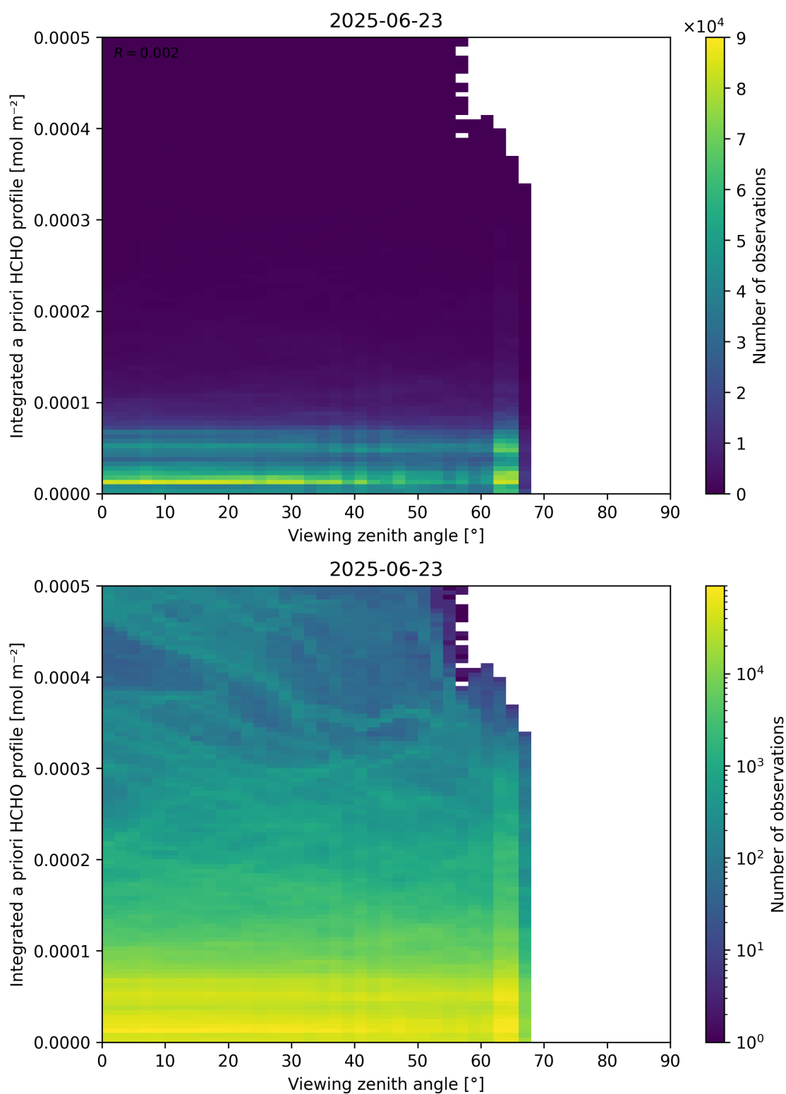
Figure 195: Scatter density plot of “Viewing zenith angle” against “Integrated a priori HCHO profile” for 2025-06-22 to 2025-06-24.
