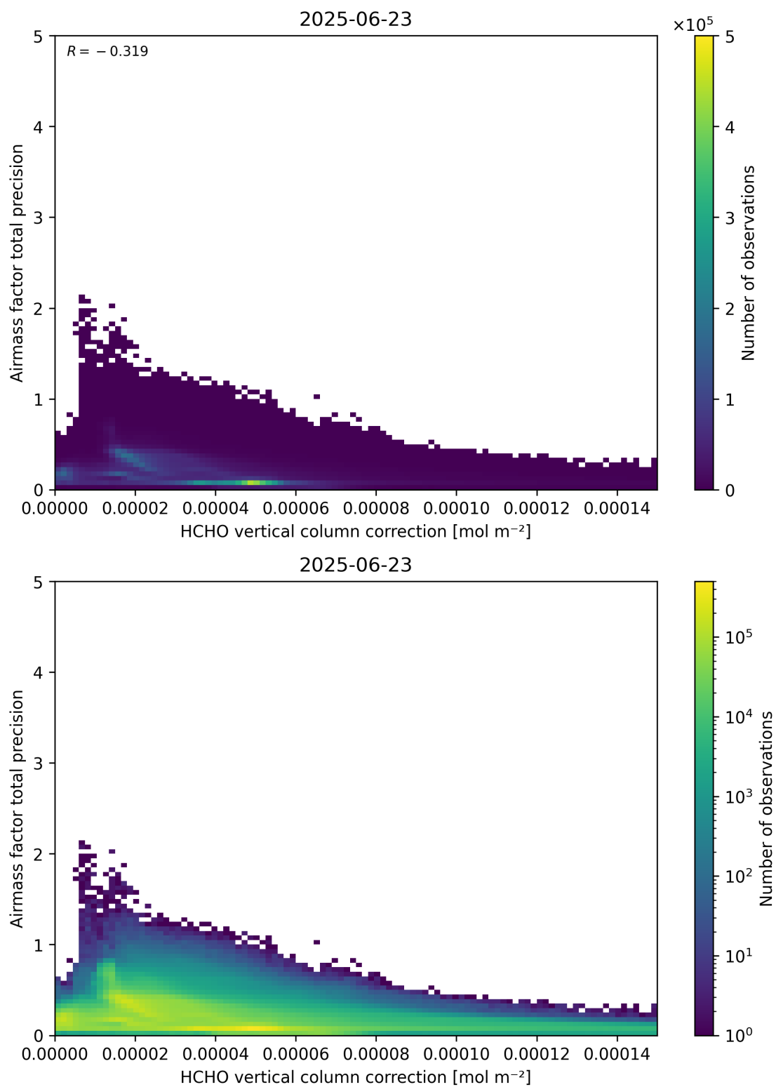
Figure 121: Scatter density plot of “HCHO vertical column correction” against “Airmass factor total precision” for 2025-06-22 to 2025-06-24.
