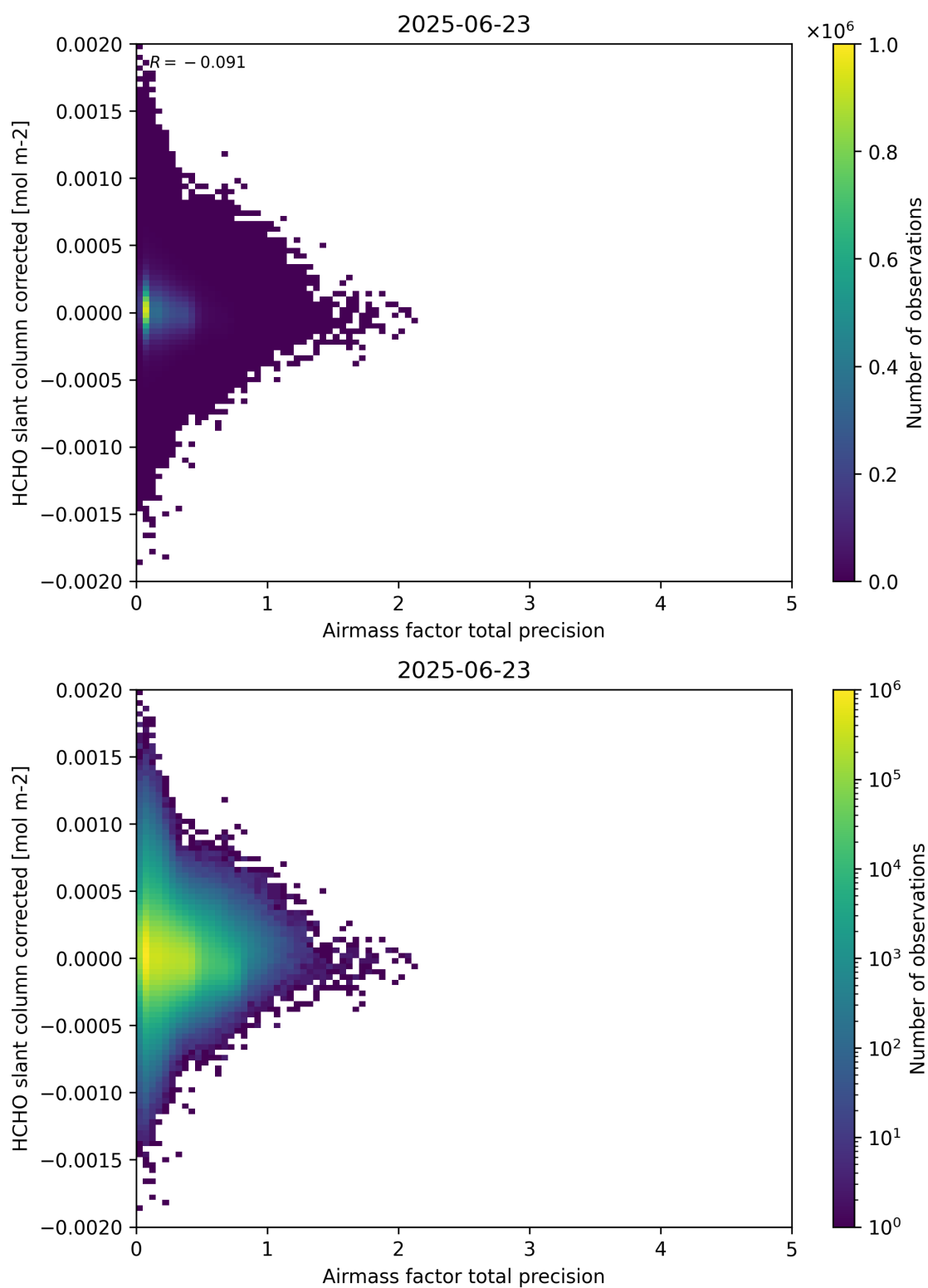
Figure 109: Scatter density plot of “Airmass factor total precision” against “HCHO slant column corrected” for 2025-06-22 to 2025-06-24.
