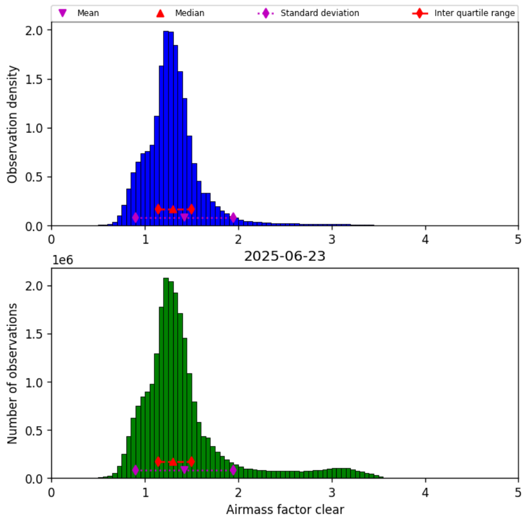
Figure 42: Histogram of “Airmass factor clear” for 2025-06-22 to 2025-06-24
