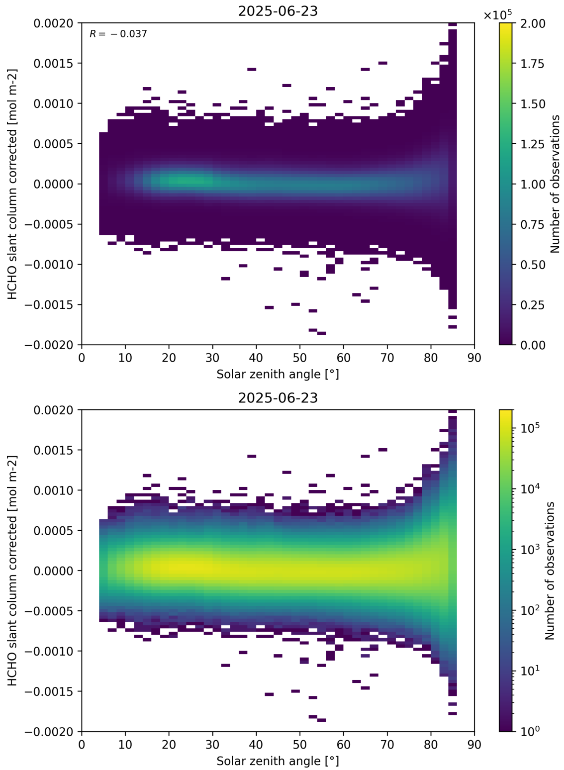
Figure 171: Scatter density plot of “Solar zenith angle” against “HCHO slant column corrected” for 2025-06-22 to 2025-06-24.
