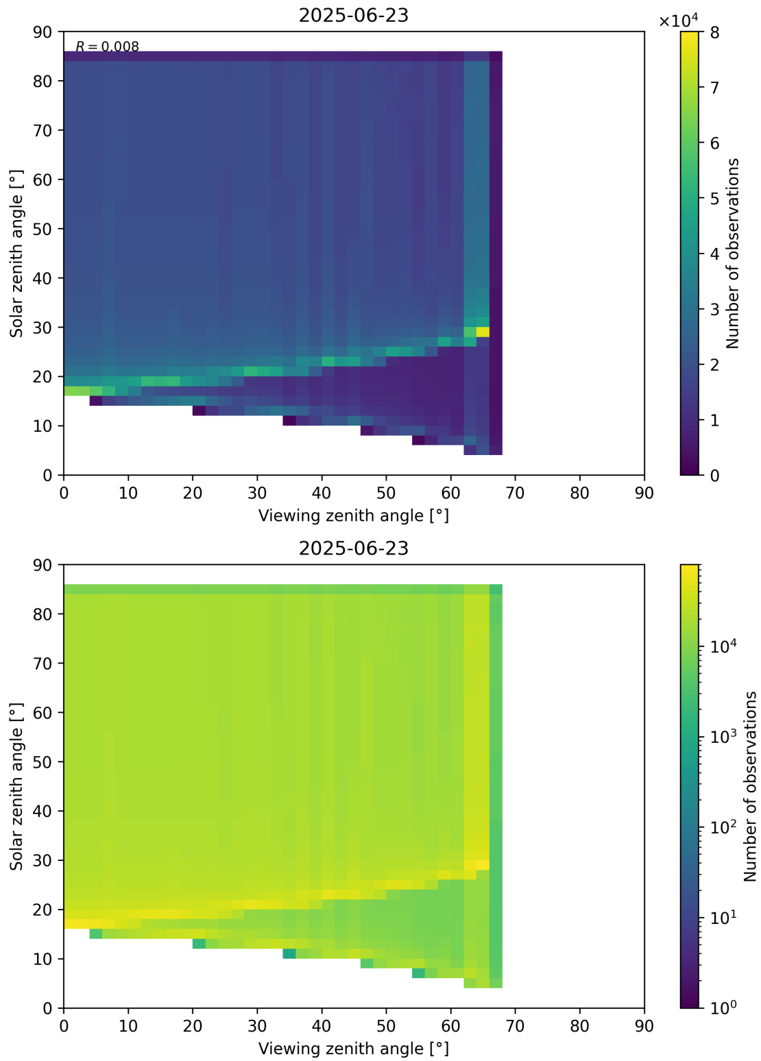
Figure 197: Scatter density plot of “Viewing zenith angle” against “Solar zenith angle” for 2025-06-22 to 2025-06-24.
