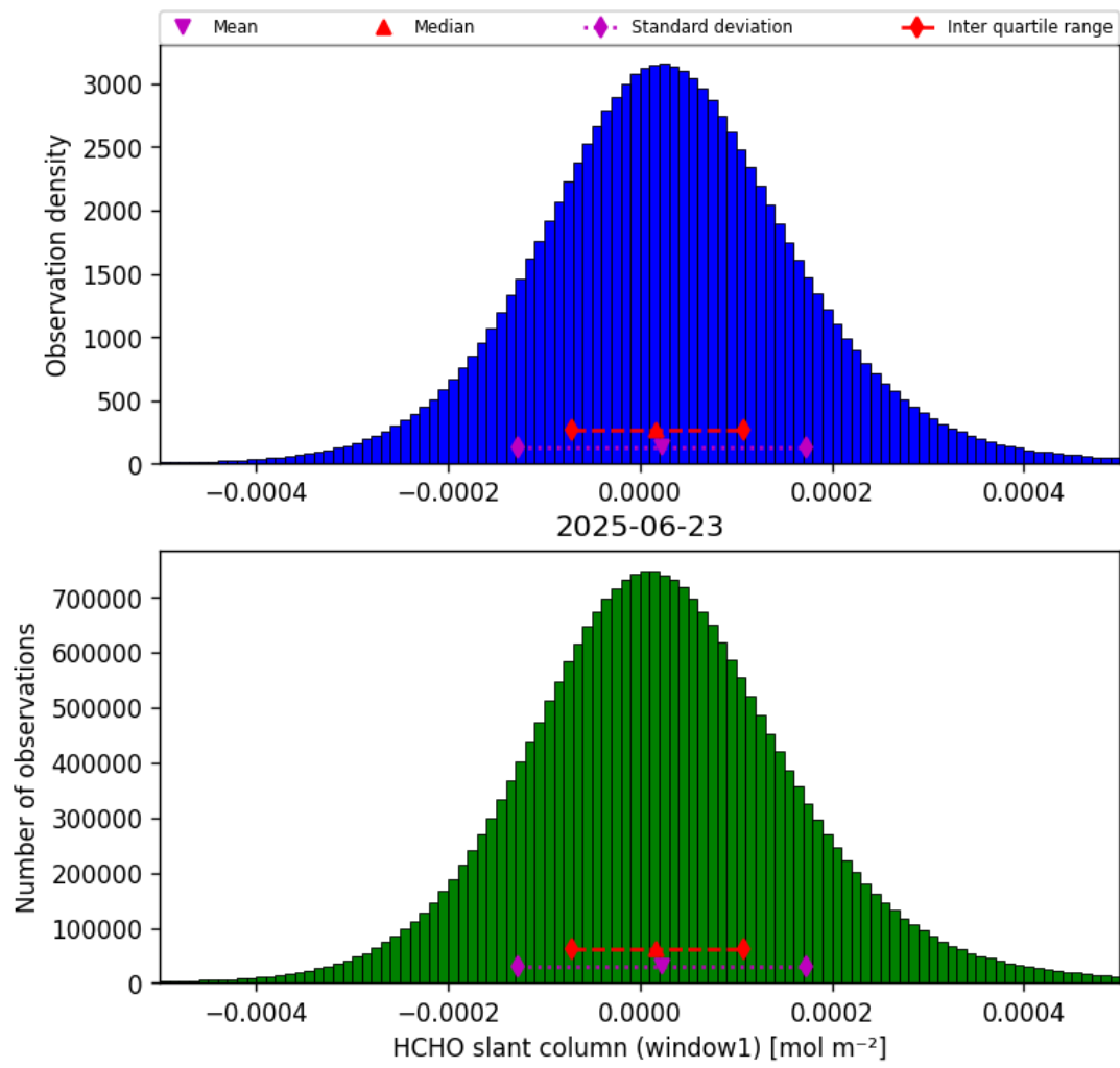
Figure 38: Histogram of “HCHO slant column (window1)” for 2025-06-22 to 2025-06-24
