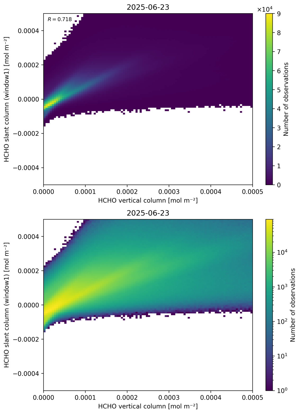
Figure 129: Scatter density plot of “HCHO vertical column” against “HCHO slant column (window1)” for 2025-06-22 to 2025-06-24.
