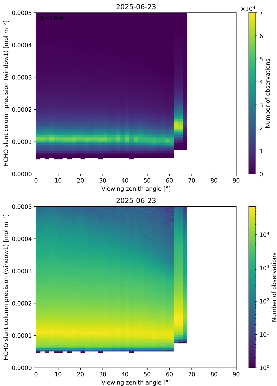
Figure 189: Scatter density plot of “Viewing zenith angle” against “HCHO slant column precision (window1)” for 2025-06-22 to 2025-06-24.
