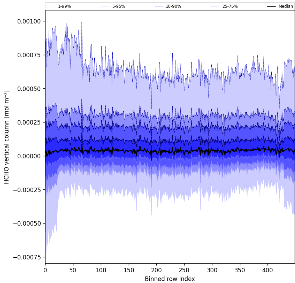
Figure 49: Along track statistics of “HCHO vertical column” for 2025-06-22 to 2025-06-24
