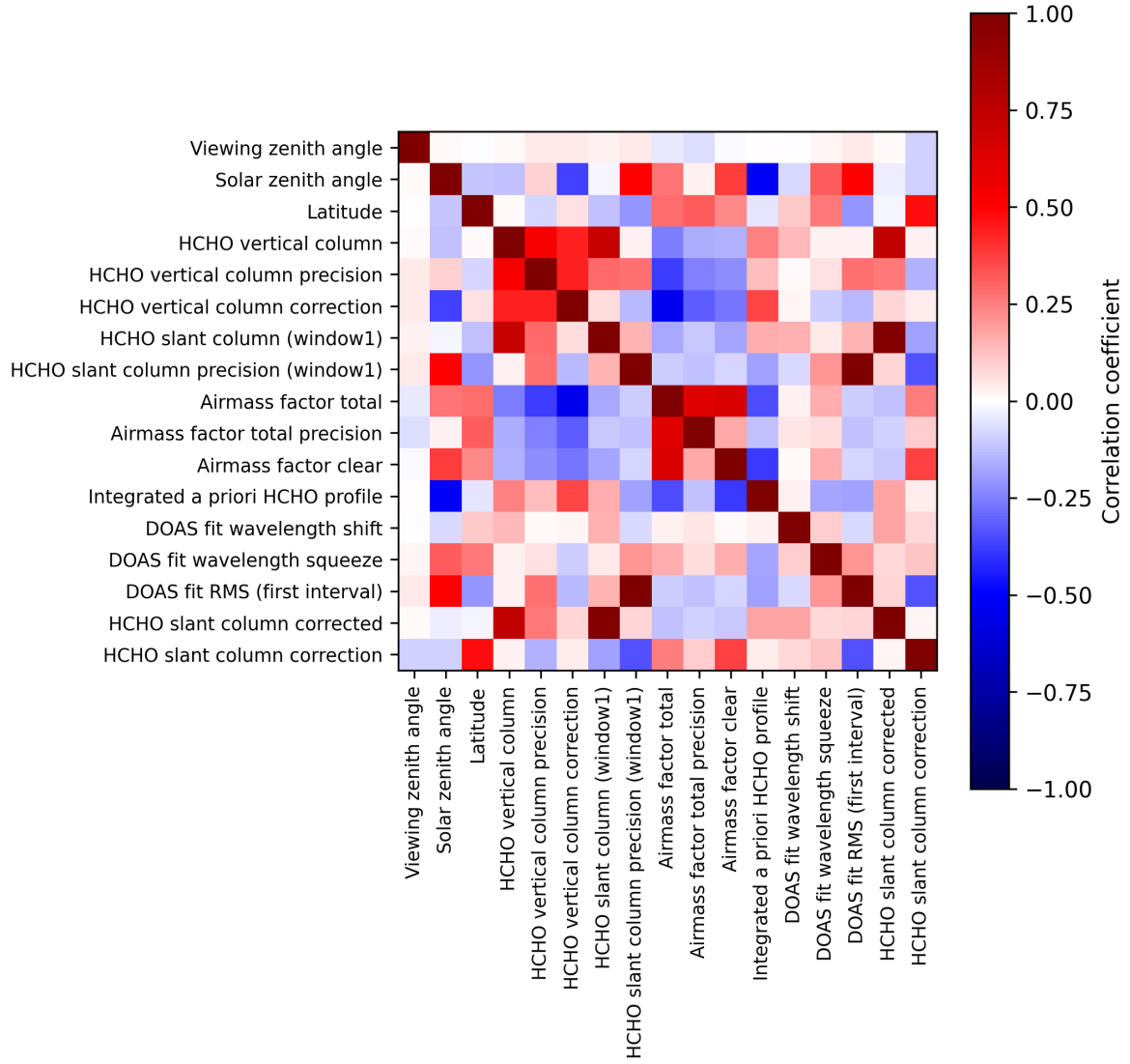
Figure 2: Map of correlation matrix for 2025-06-22 to 2025-06-24.
