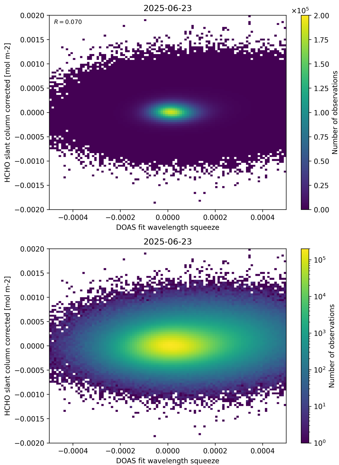
Figure 69: Scatter density plot of “DOAS fit wavelength squeeze” against “HCHO slant column corrected” for 2025-06-22 to 2025-06-24.
