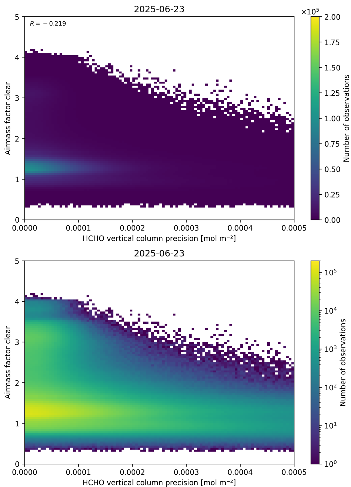
Figure 139: Scatter density plot of “HCHO vertical column precision” against “Airmass factor clear” for 2025-06-22 to 2025-06-24.
