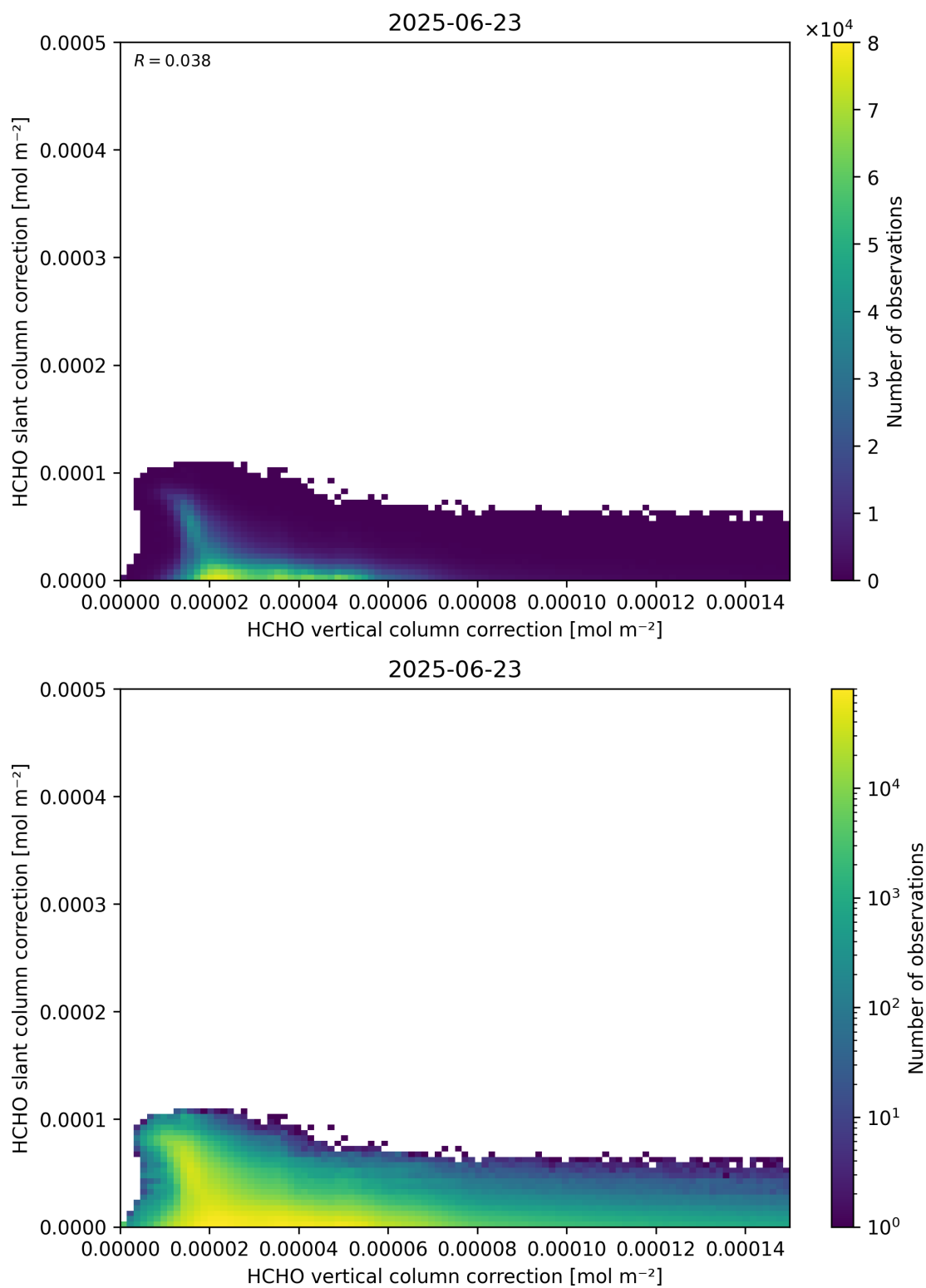
Figure 117: Scatter density plot of “HCHO vertical column correction” against “HCHO slant column correction” for 2025-06-22 to 2025-06-24.
