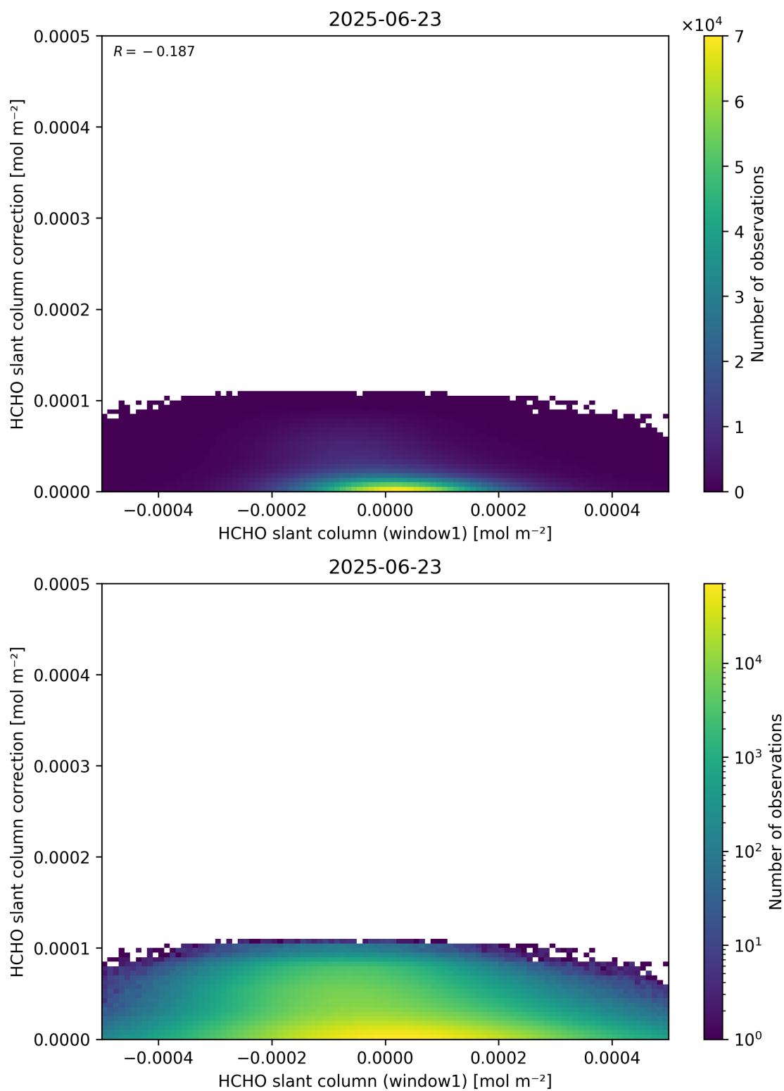
Figure 83: Scatter density plot of “HCHO slant column (window1)” against “HCHO slant column correction” for 2025-06-22 to 2025-06-24.
