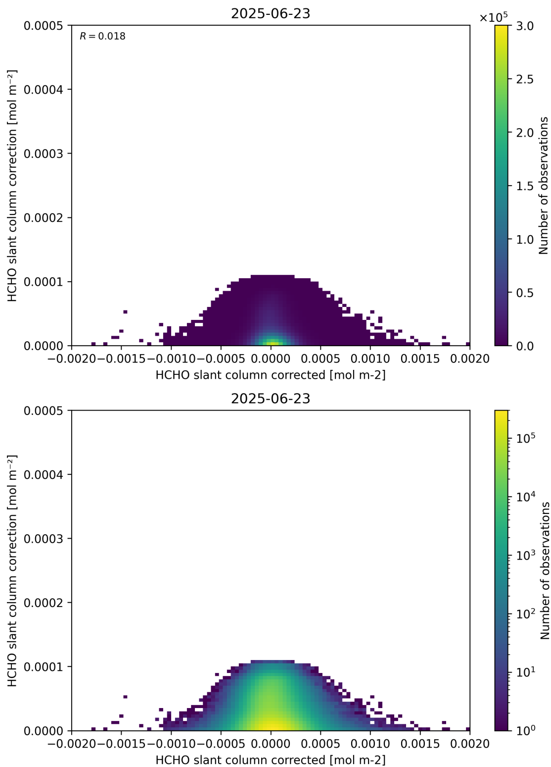
Figure 77: Scatter density plot of “HCHO slant column corrected” against “HCHO slant column correction” for 2025-06-22 to 2025-06-24.
