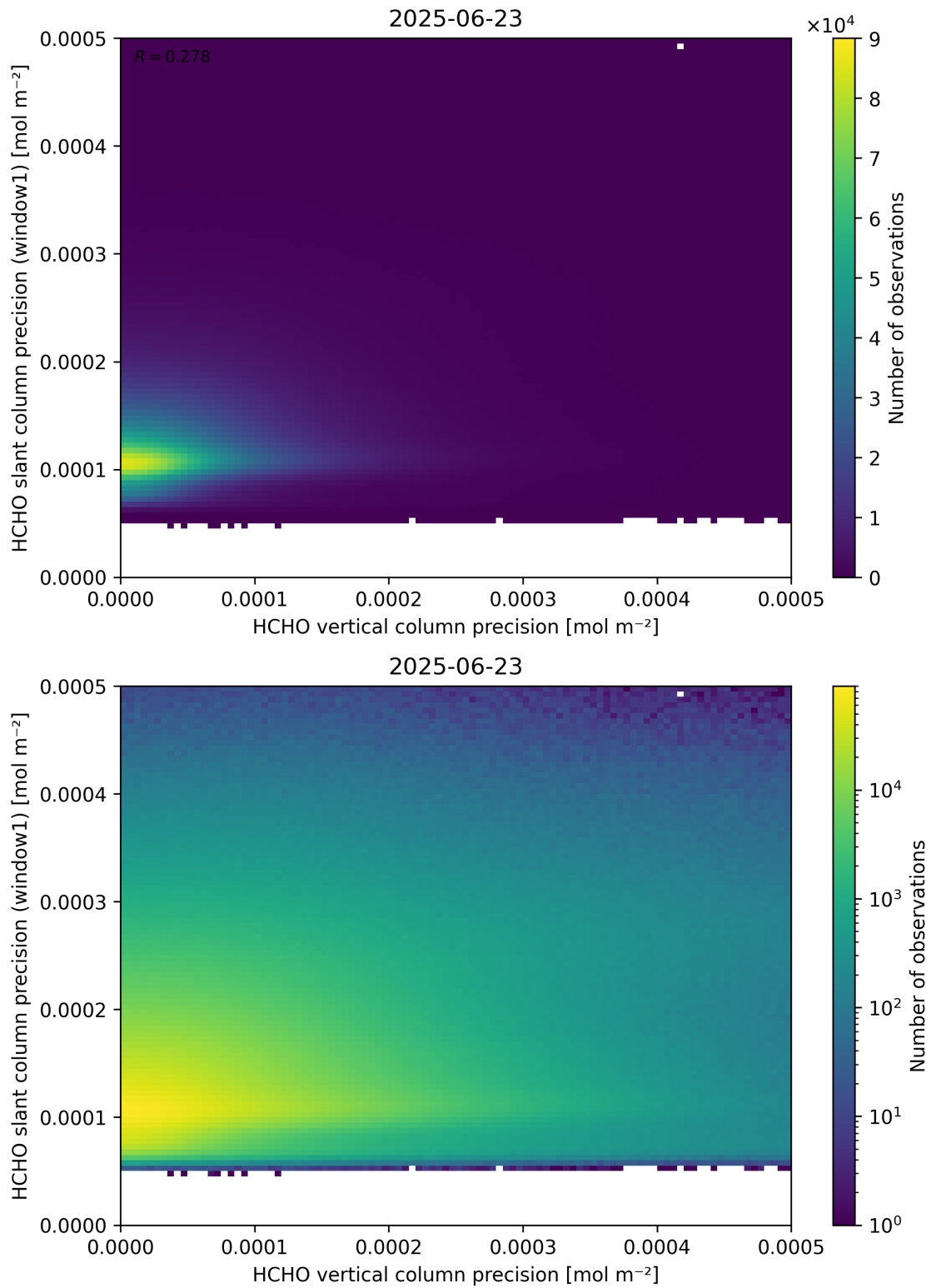
Figure 143: Scatter density plot of “HCHO vertical column precision” against “HCHO slant column precision (window1)” for 2025-06-22 to 2025-06-24.
