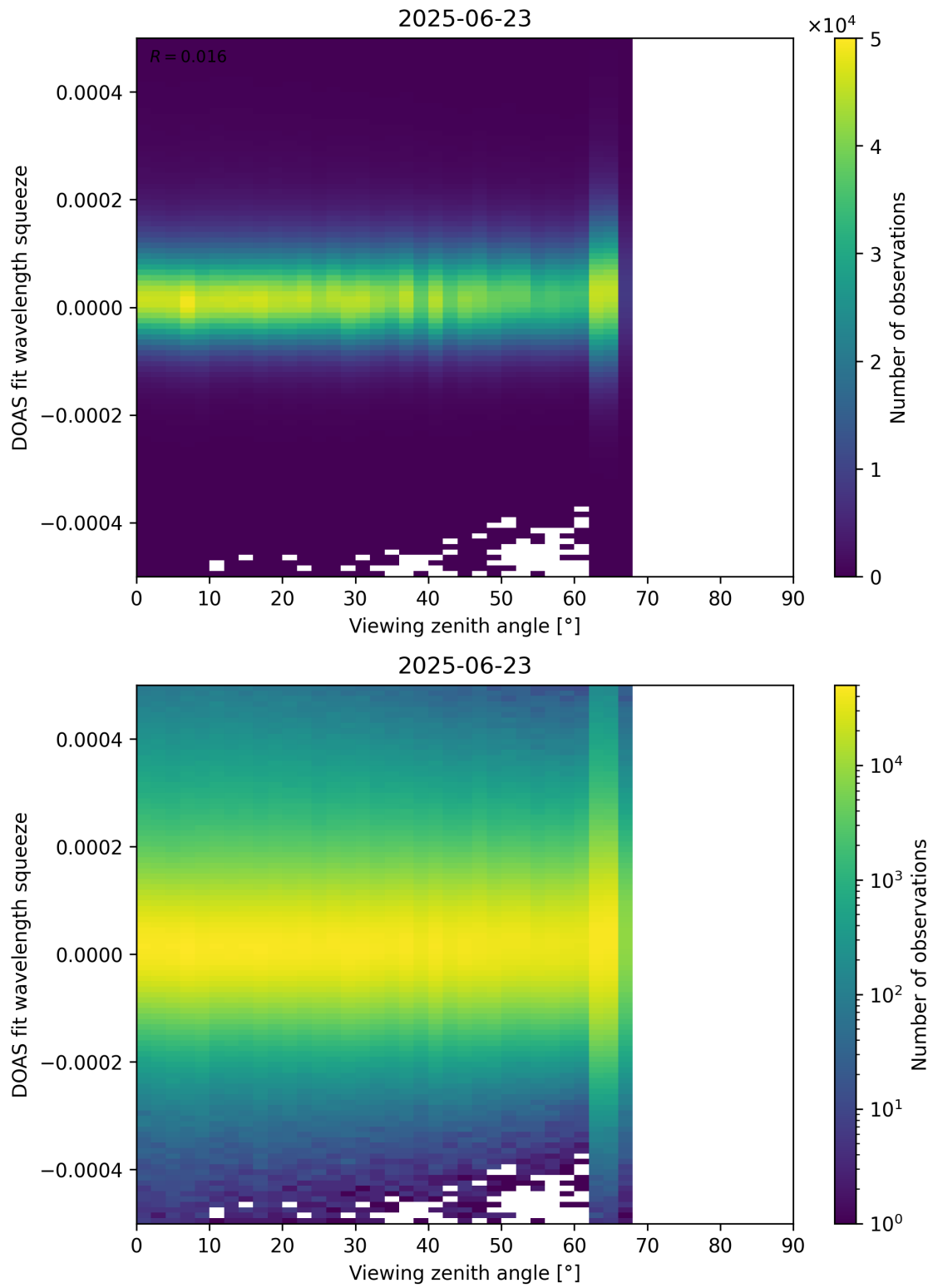
Figure 184: Scatter density plot of “Viewing zenith angle” against “DOAS fit wavelength squeeze” for 2025-06-22 to 2025-06-24.
