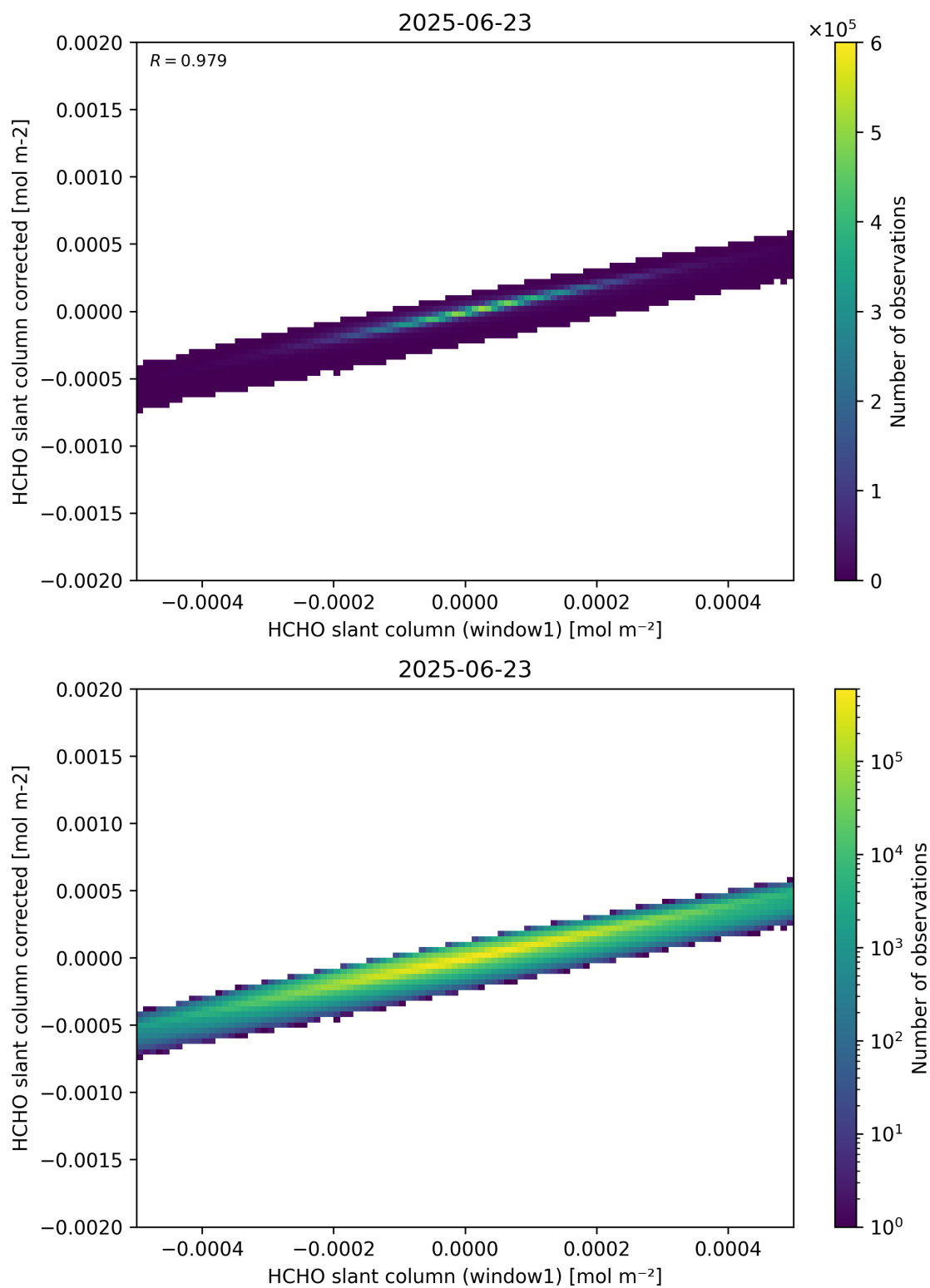
Figure 82: Scatter density plot of “HCHO slant column (window1)” against “HCHO slant column corrected” for 2025-06-22 to 2025-06-24.
