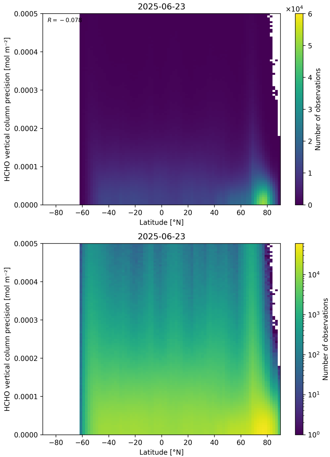
Figure 165: Scatter density plot of “Latitude” against “HCHO vertical column precision” for 2025-06-22 to 2025-06-24.
