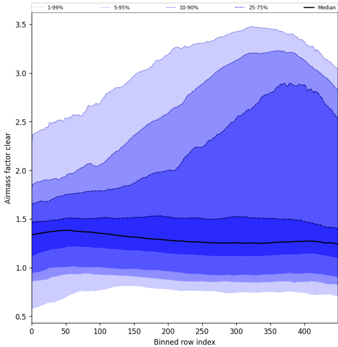
Figure 56: Along track statistics of “Air mass factor clear” for 2025-06-22 to 2025-06-24
