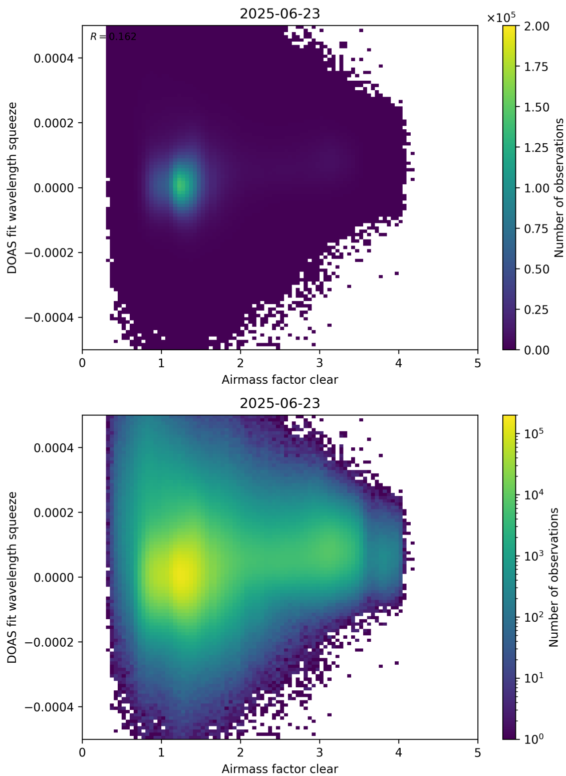
Figure 73: Scatter density plot of “Airmass factor clear” against “DOAS fit wavelength squeeze” for 2025-06-22 to 2025-06-24.
