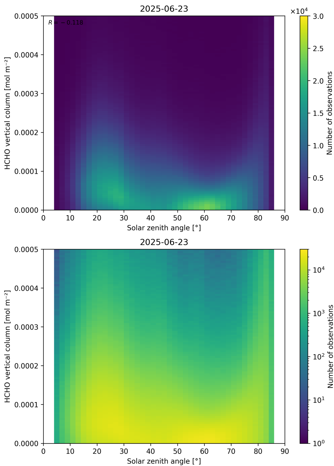
Figure 177: Scatter density plot of “Solar zenith angle” against “HCHO vertical column” for 2025-06-22 to 2025-06-24.
