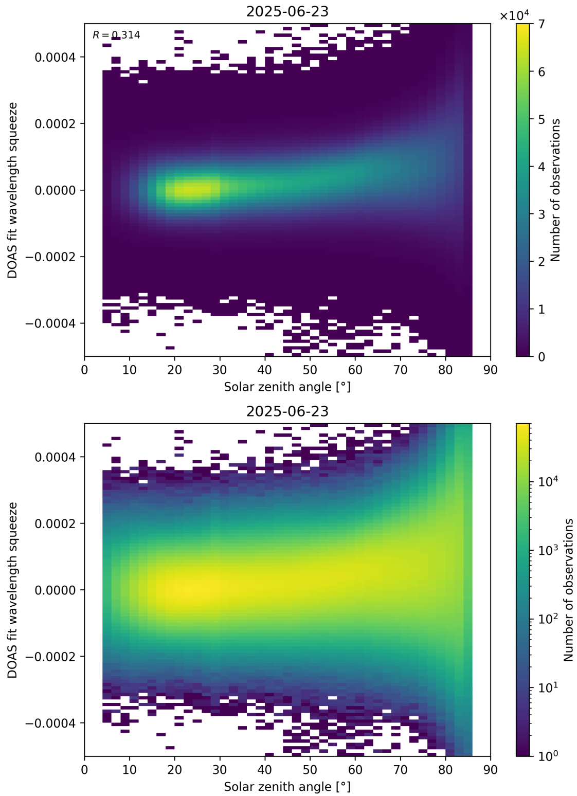
Figure 169: Scatter density plot of “Solar zenith angle” against “DOAS fit wavelength squeeze” for 2025-06-22 to 2025-06-24.
