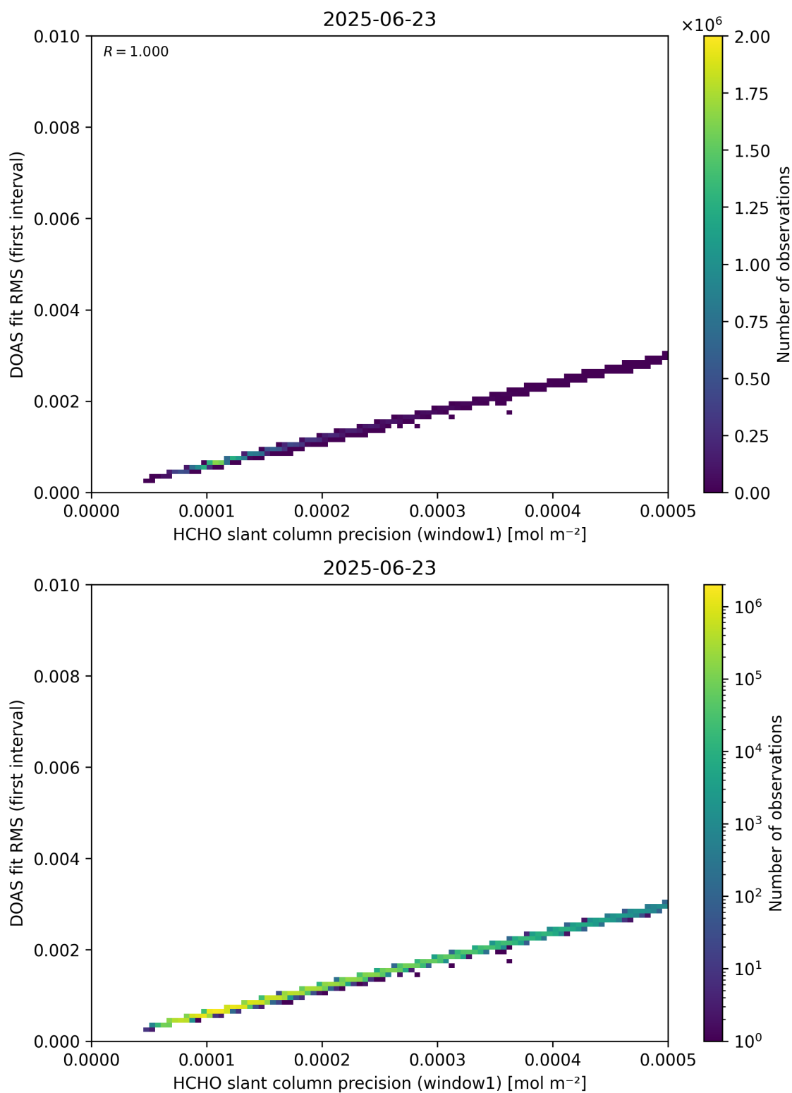
Figure 88: Scatter density plot of “HCHO slant column precision (window1)” against “DOAS fit RMS (first interval)” for 2025-06-22 to 2025-06-24.
