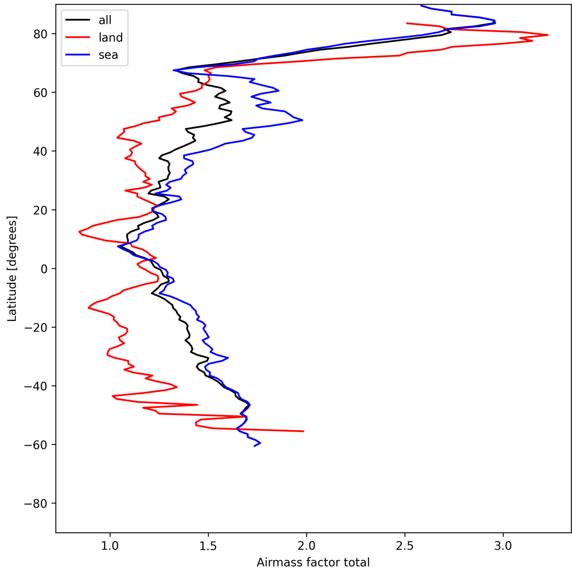
Figure 26: Zonal average of “Airmass factor total” for 2025-06-22 to 2025-06-24.
