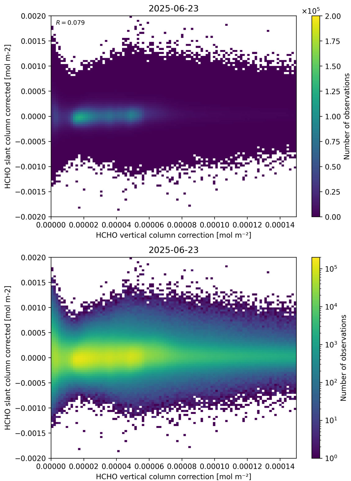
Figure 116: Scatter density plot of “HCHO vertical column correction” against “HCHO slant column corrected” for 2025-06-22 to 2025-06-24.
