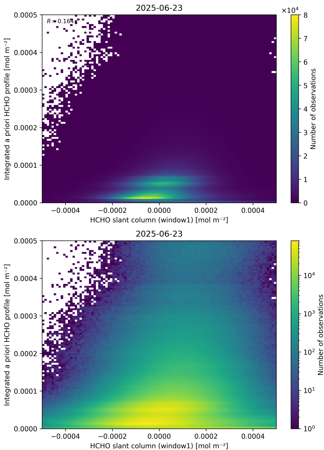
Figure 87: Scatter density plot of “HCHO slant column (window1)” against “Integrated a priori HCHO profile” for 2025-06-22 to 2025-06-24.
