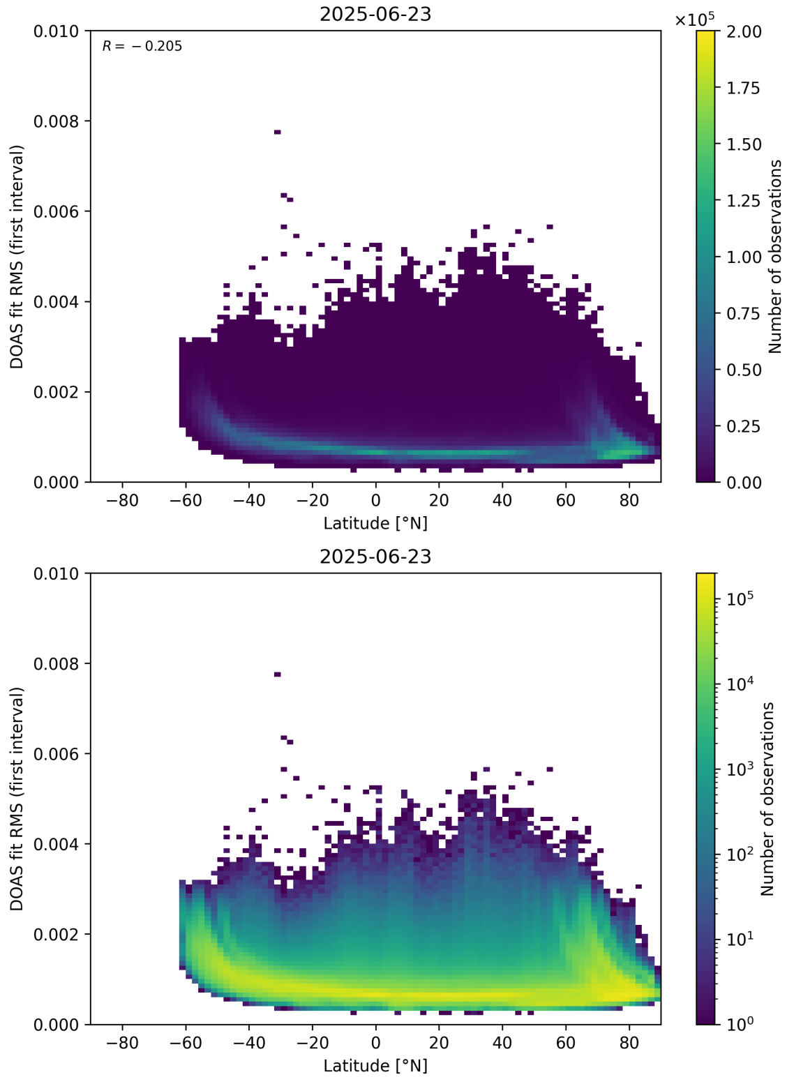
Figure 153: Scatter density plot of “Latitude” against “DOAS fit RMS (first interval)” for 2025-06-22 to 2025-06-24.
