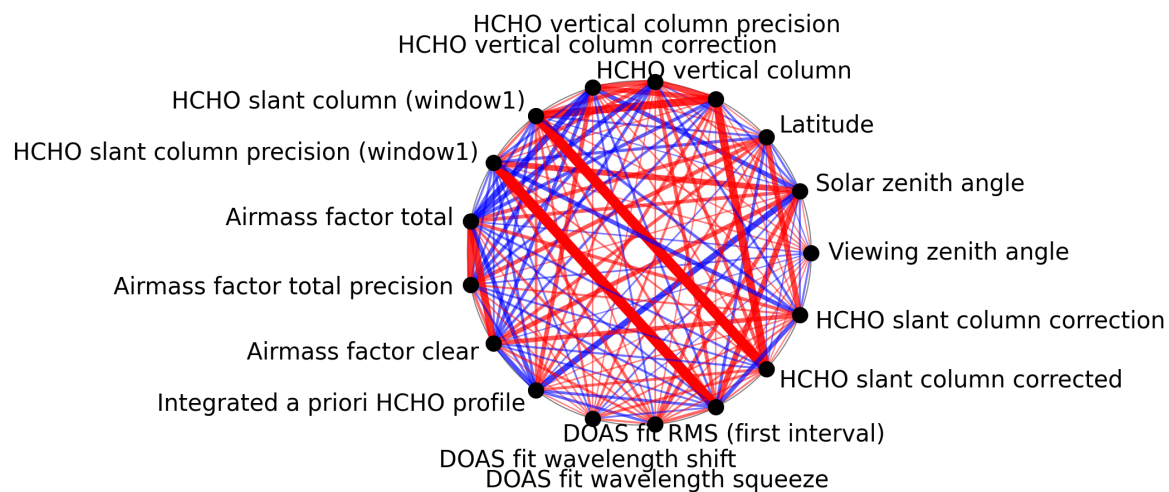
Figure 1: Map of correlation graph for 2025-06-22 to 2025-06-24.
