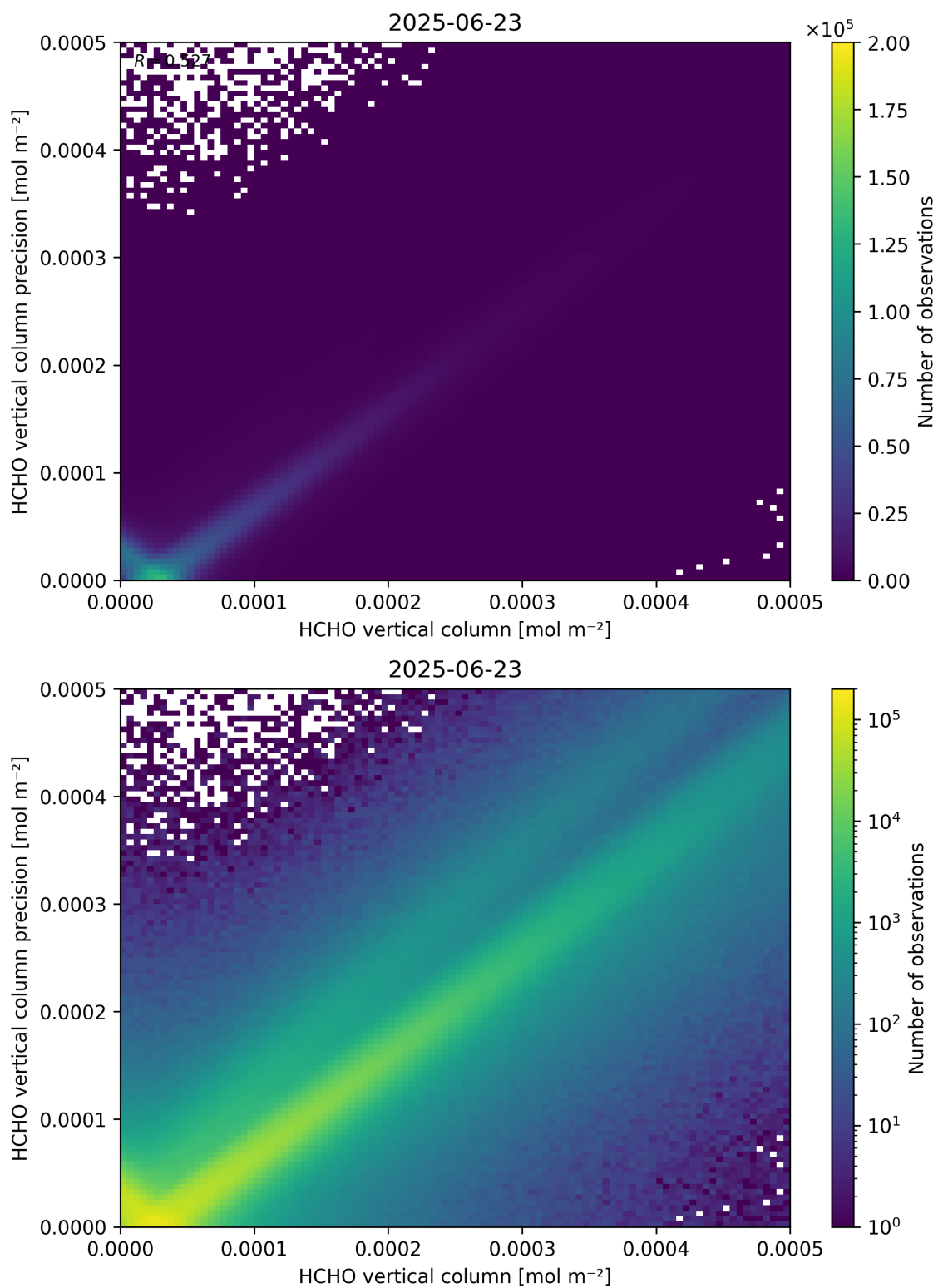
Figure 134: Scatter density plot of “HCHO vertical column” against “HCHO vertical column precision” for 2025-06-22 to 2025-06-24.
