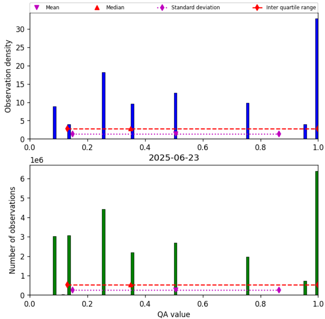
Figure 34: Histogram of “QA value” for 2025-06-22 to 2025-06-24
