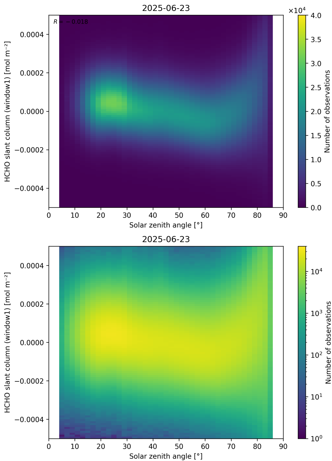
Figure 173: Scatter density plot of “Solar zenith angle” against “HCHO slant column (window1)” for 2025-06-22 to 2025-06-24.
