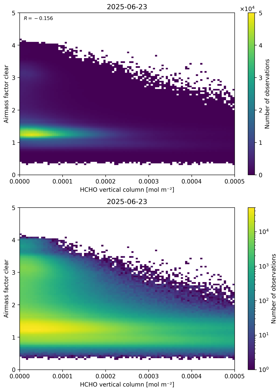
Figure 126: Scatter density plot of “HCHO vertical column” against “Airmass factor clear” for 2025-06-22 to 2025-06-24.
