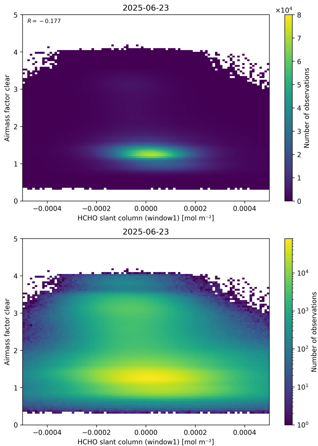
Figure 81: Scatter density plot of “HCHO slant column (window1)” against “Airmass factor clear” for 2025-06-22 to 2025-06-24.
