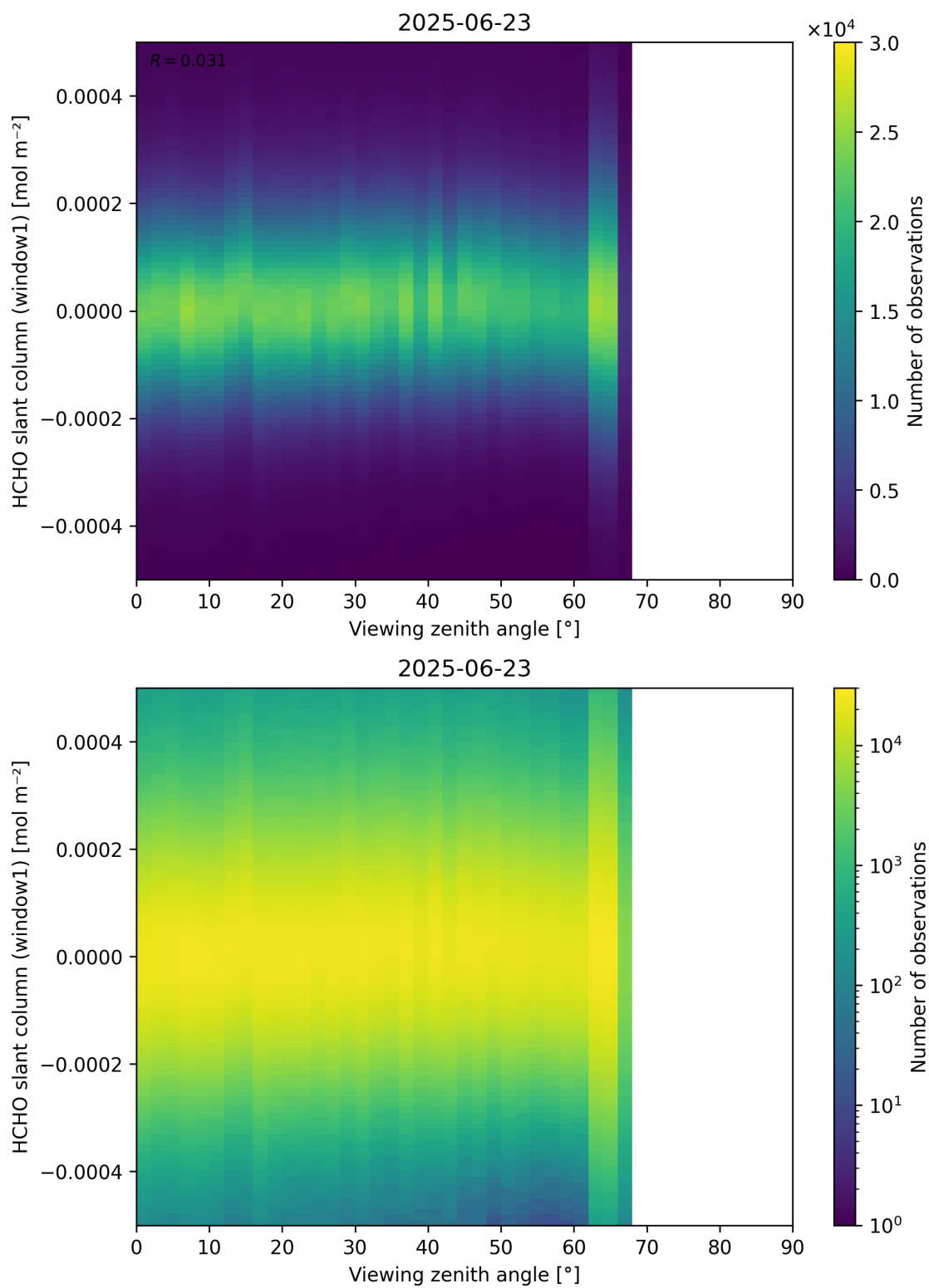
Figure 188: Scatter density plot of “Viewing zenith angle” against “HCHO slant column (window1)” for 2025-06-22 to 2025-06-24.
