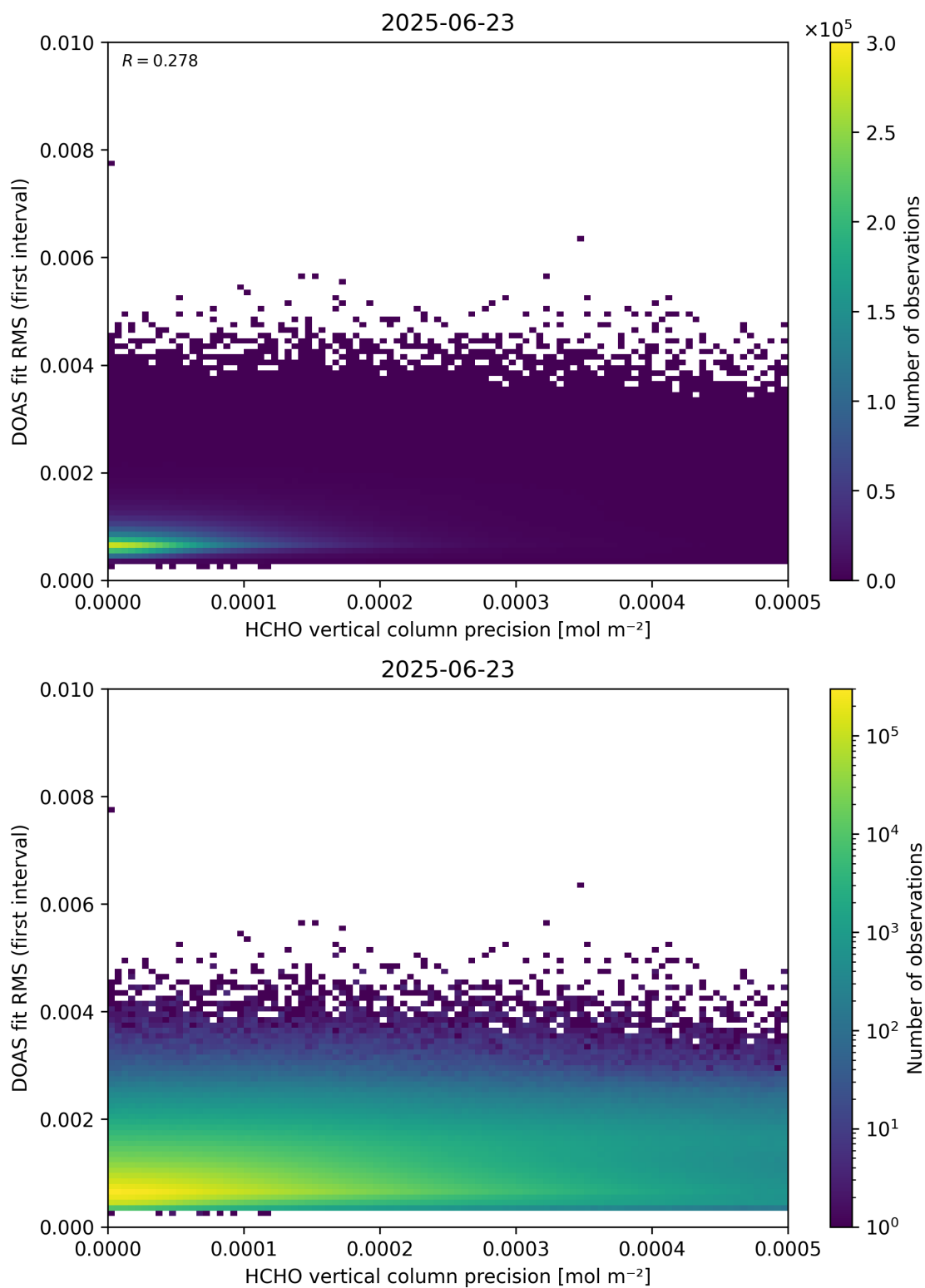
Figure 136: Scatter density plot of “HCHO vertical column precision” against “DOAS fit RMS (first interval)” for 2025-06-22 to 2025-06-24.
