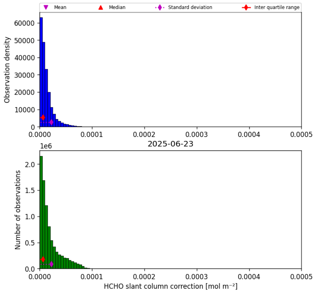
Figure 47: Histogram of “HCHO slant column correction” for 2025-06-22 to 2025-06-24
