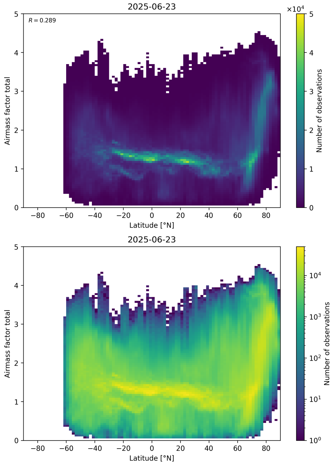
Figure 161: Scatter density plot of “Latitude” against “Airmass factor total” for 2025-06-22 to 2025-06-24.
