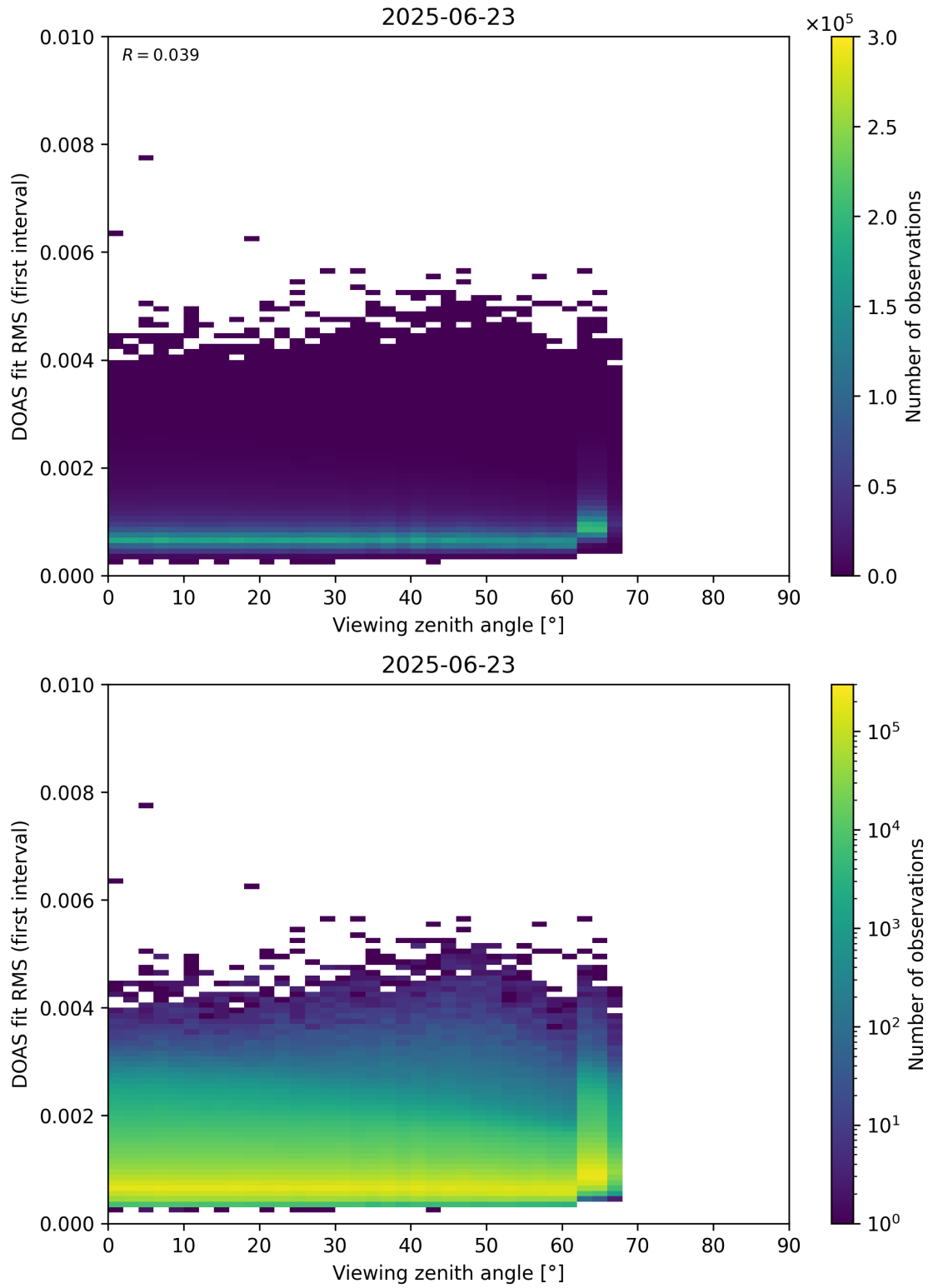
Figure 182: Scatter density plot of “Viewing zenith angle” against “DOAS fit RMS (first interval)” for 2025-06-22 to 2025-06-24.
