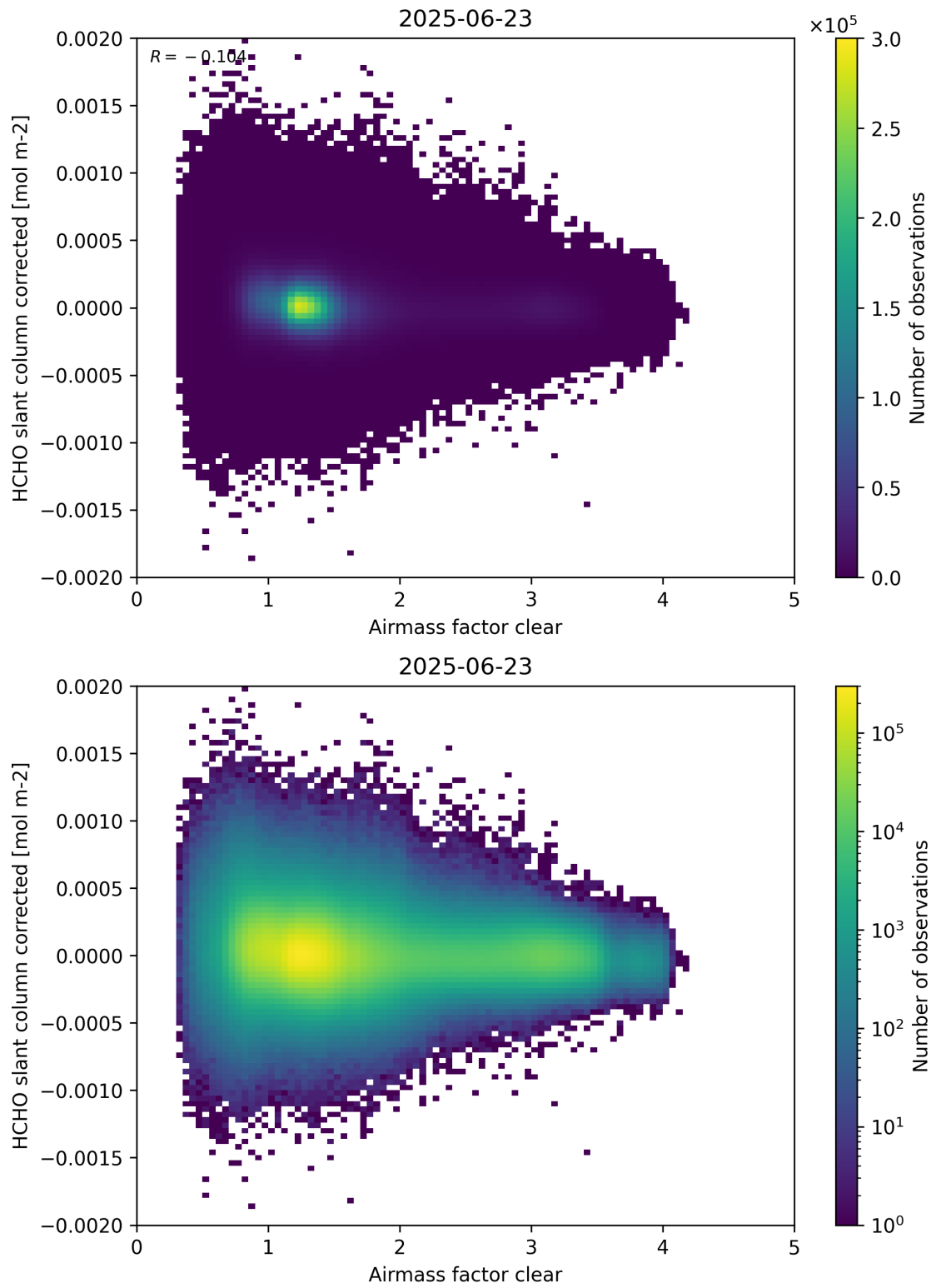
Figure 74: Scatter density plot of “Airmass factor clear” against “HCHO slant column corrected” for 2025-06-22 to 2025-06-24.
