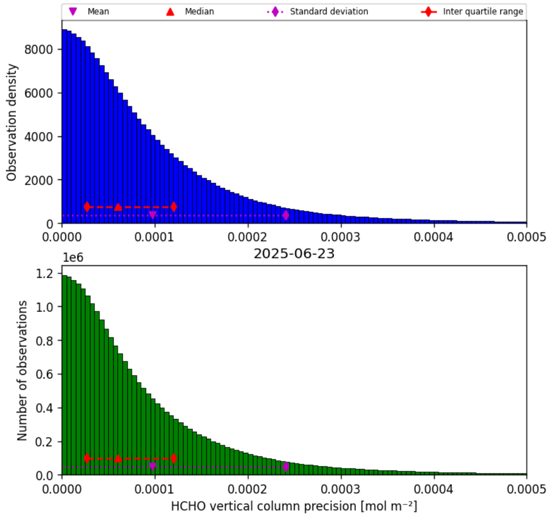
Figure 36: Histogram of “HCHO vertical column precision” for 2025-06-22 to 2025-06-24
