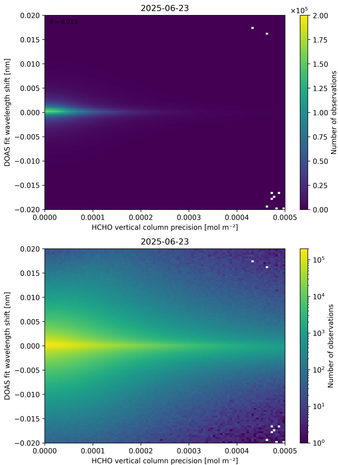
Figure 137: Scatter density plot of “HCHO vertical column precision” against “DOAS fit wavelength shift” for 2025-06-22 to 2025-06-24.
