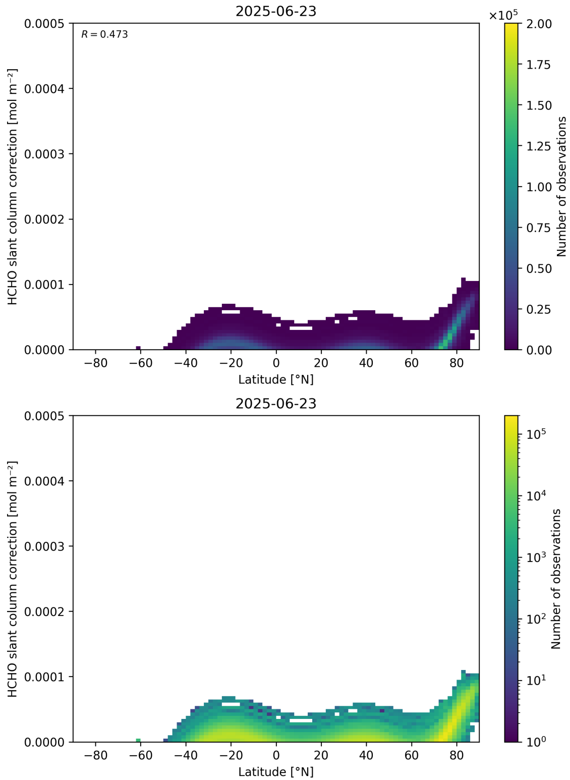
Figure 158: Scatter density plot of “Latitude” against “HCHO slant column correction” for 2025-06-22 to 2025-06-24.
