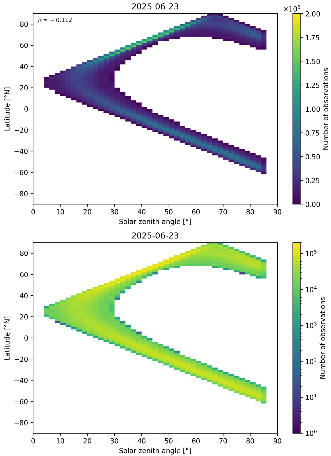
Figure 181: Scatter density plot of “Solar zenith angle” against “Latitude” for 2025-06-22 to 2025-06-24.
