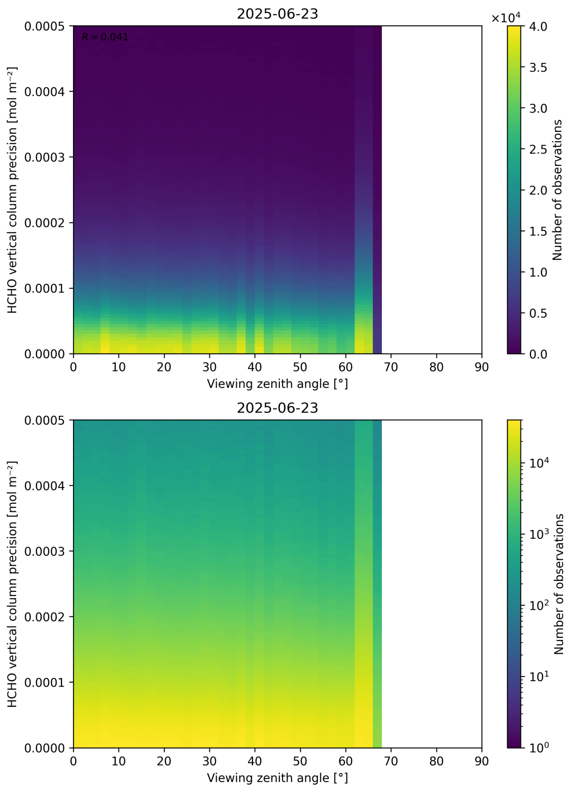
Figure 194: Scatter density plot of “Viewing zenith angle” against “HCHO vertical column precision” for 2025-06-22 to 2025-06-24.
