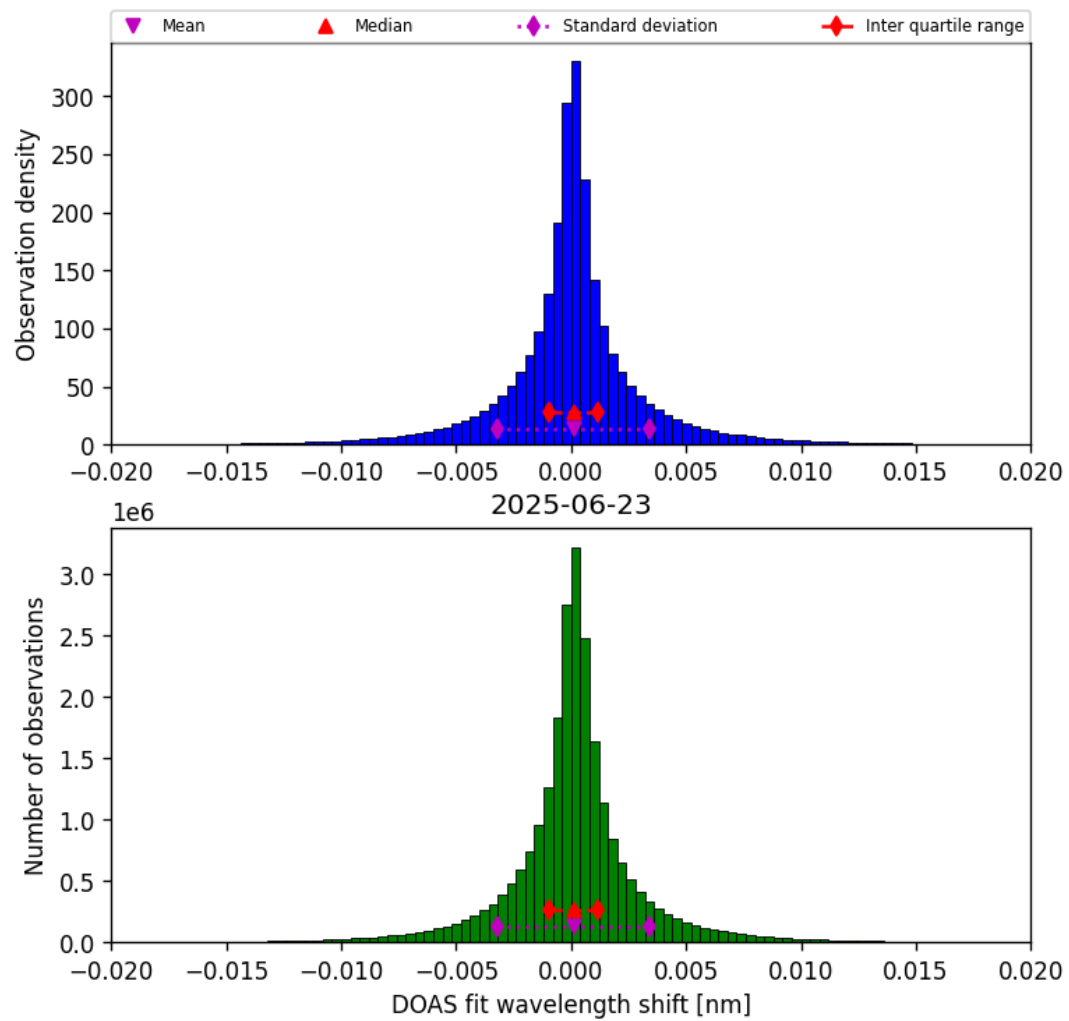
Figure 44: Histogram of “DOAS fit wavelength shift” for 2025-06-22 to 2025-06-24
