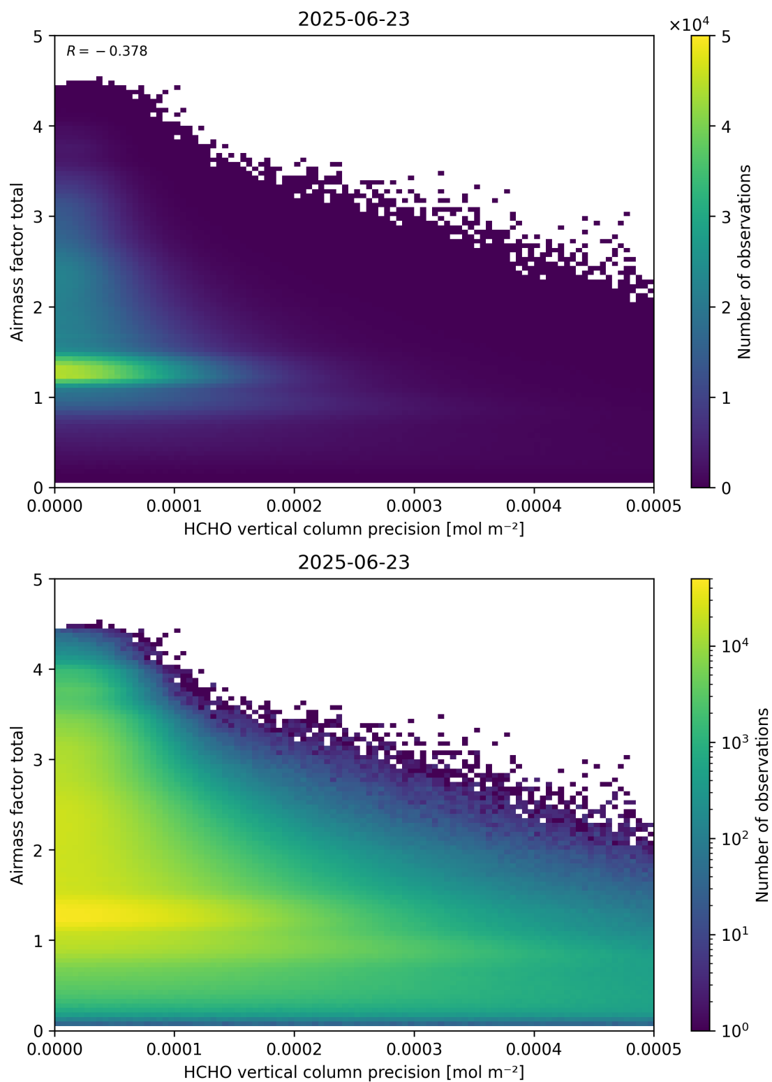
Figure 144: Scatter density plot of “HCHO vertical column precision” against “Airmass factor total” for 2025-06-22 to 2025-06-24.
