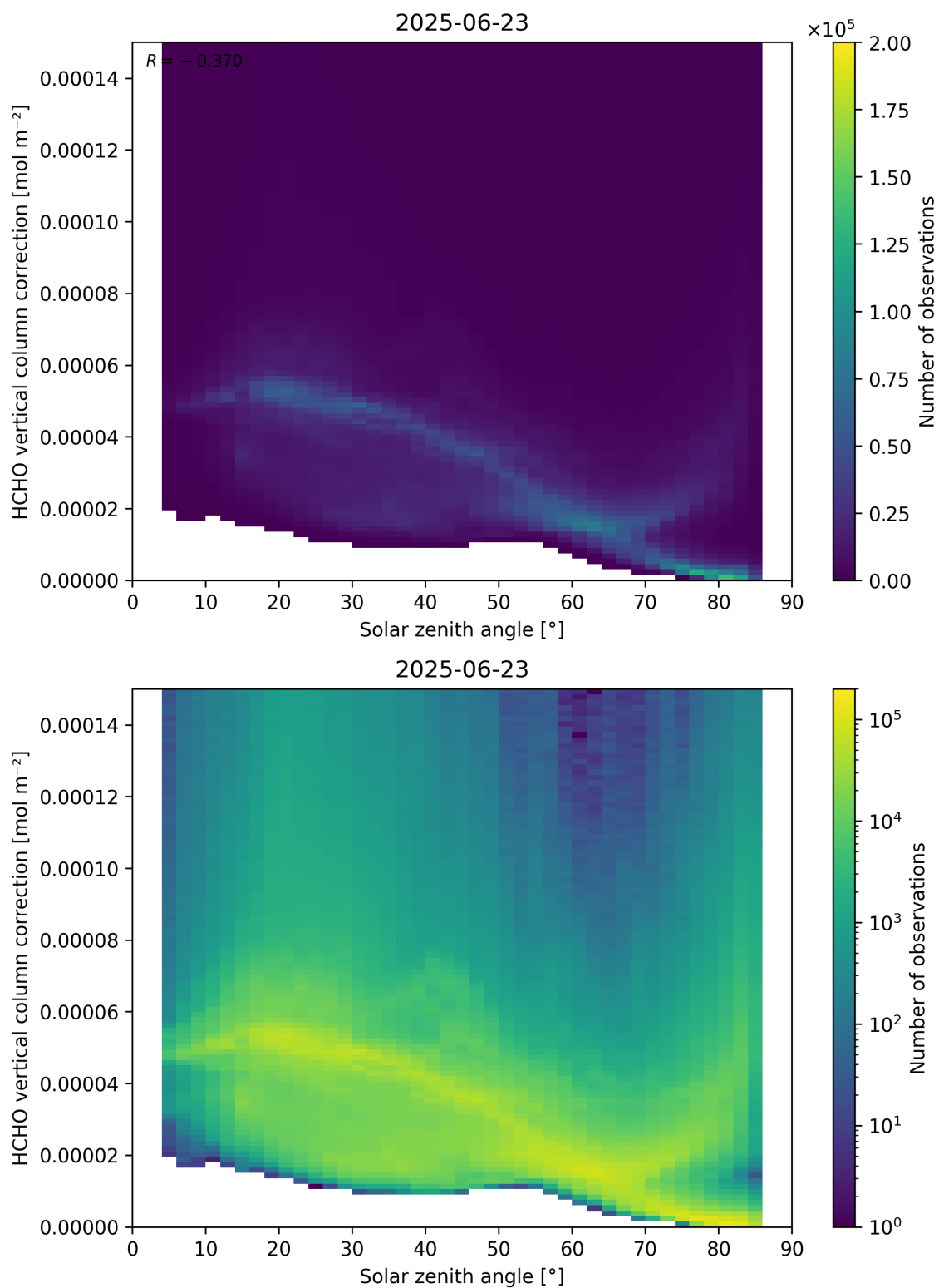
Figure 178: Scatter density plot of “Solar zenith angle” against “HCHO vertical column correction” for 2025-06-22 to 2025-06-24.
