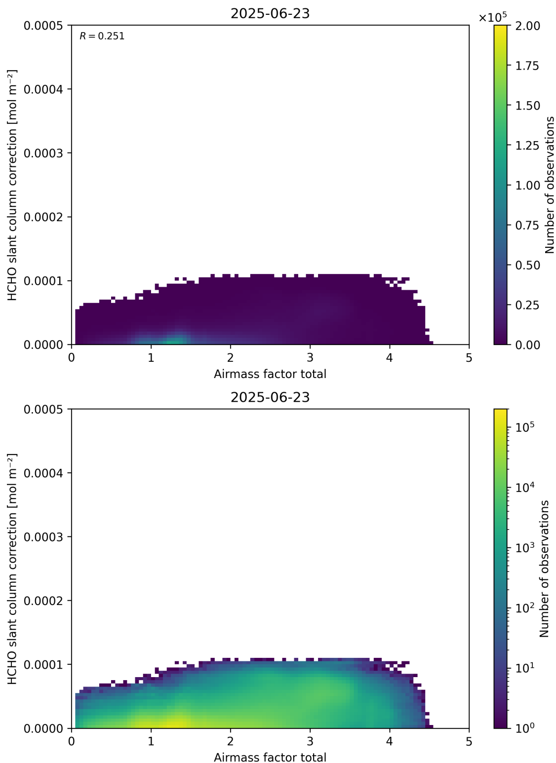
Figure 102: Scatter density plot of “Airmass factor total” against “HCHO slant column correction” for 2025-06-22 to 2025-06-24.
