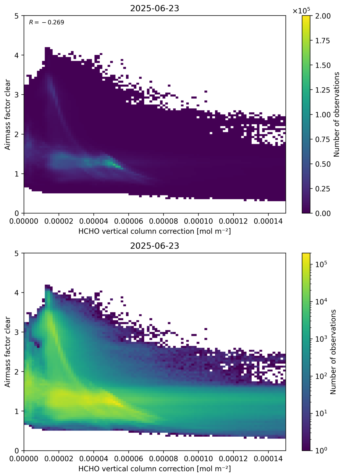
Figure 115: Scatter density plot of “HCHO vertical column correction” against “Airmass factor clear” for 2025-06-22 to 2025-06-24.
