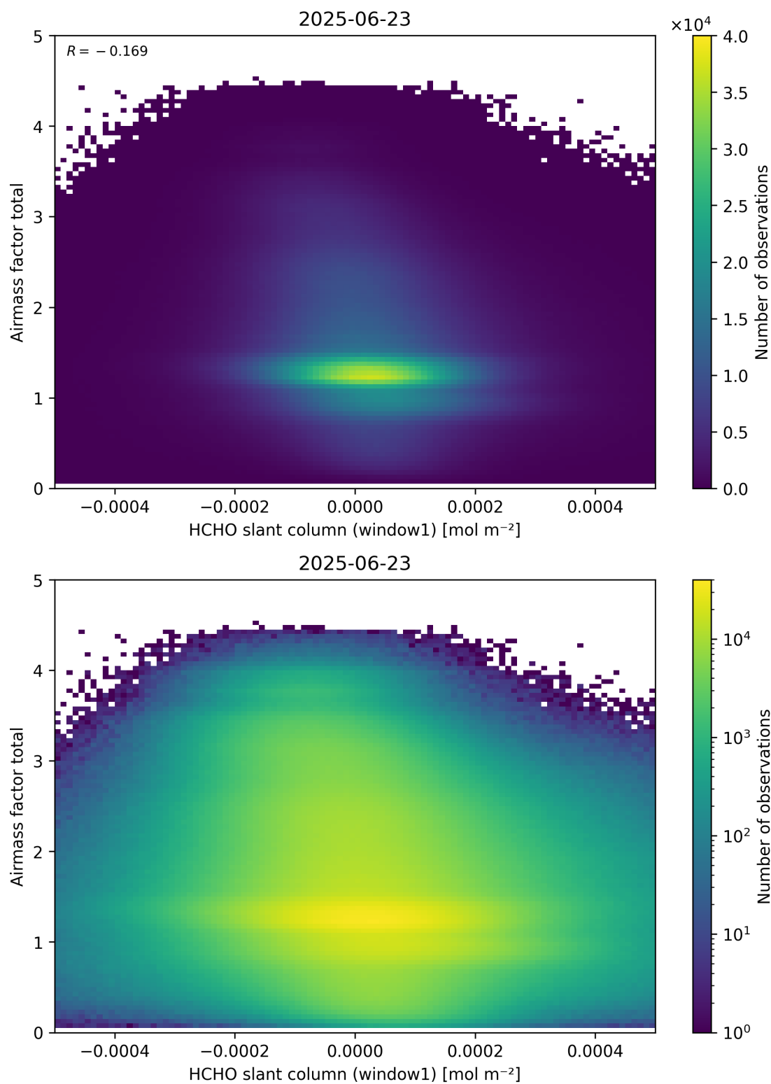
Figure 85: Scatter density plot of “HCHO slant column (window1)” against “Airmass factor total” for 2025-06-22 to 2025-06-24.
