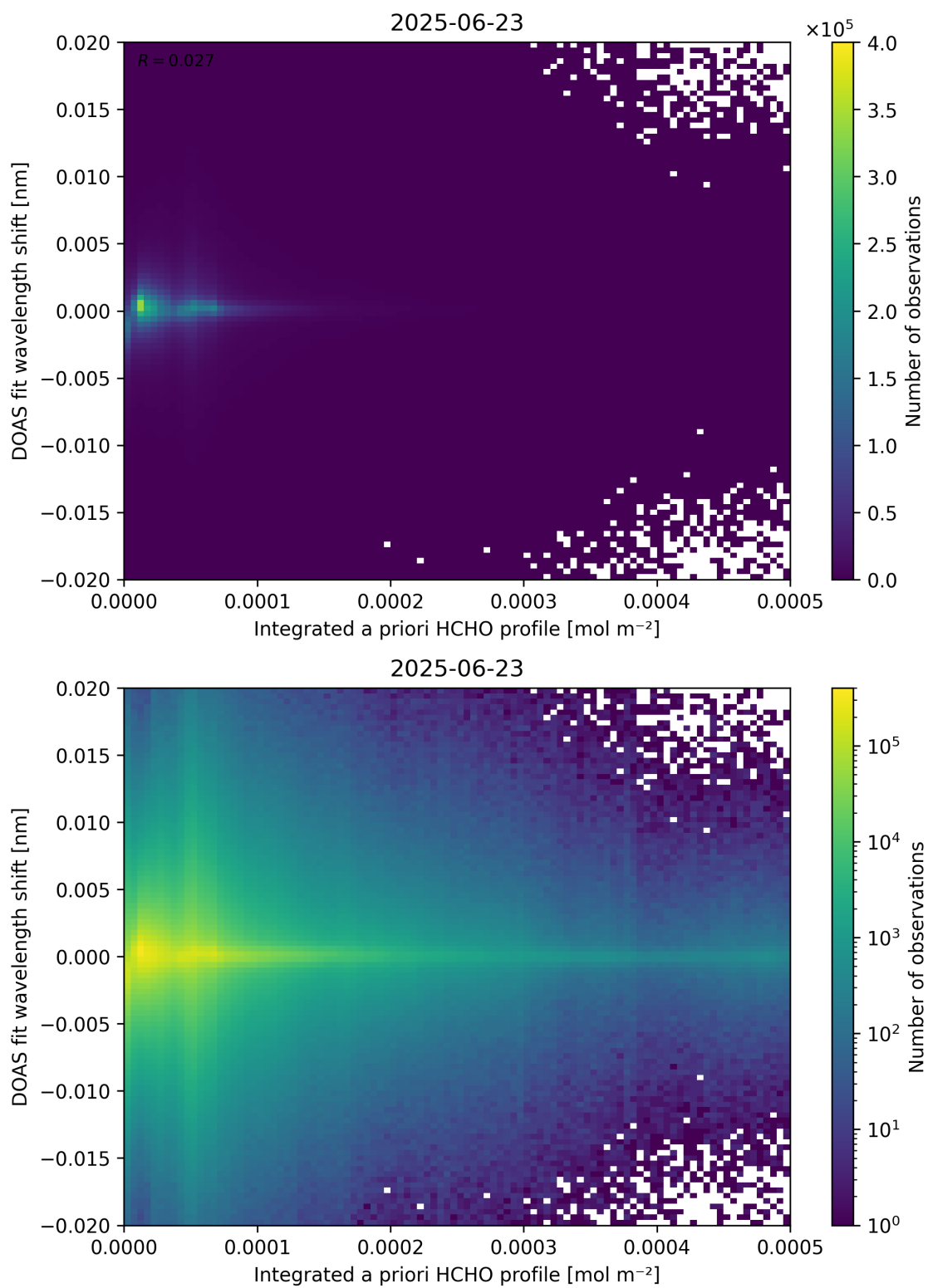
Figure 149: Scatter density plot of “Integrated a priori HCHO profile” against “DOAS fit wavelength shift” for 2025-06-22 to 2025-06-24.
