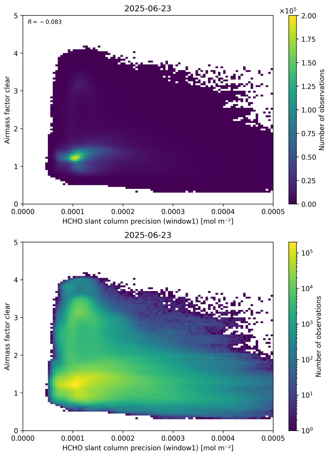
Figure 91: Scatter density plot of “HCHO slant column precision (window1)” against “Airmass factor clear” for 2025-06-22 to 2025-06-24.
