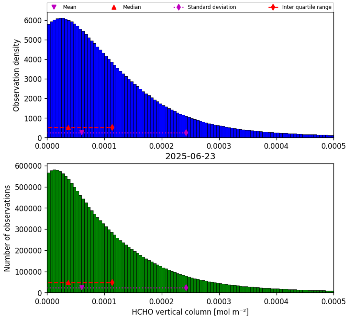
Figure 35: Histogram of “HCHO vertical column” for 2025-06-22 to 2025-06-24
