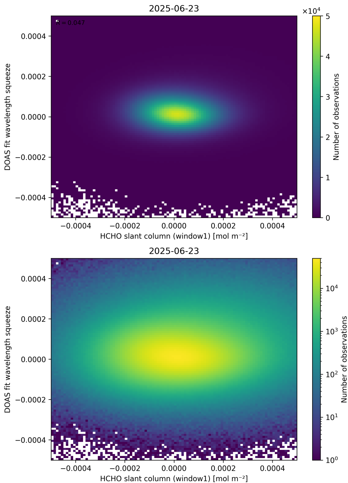
Figure 80: Scatter density plot of “HCHO slant column (window1)” against “DOAS fit wavelength squeeze” for 2025-06-22 to 2025-06-24.
