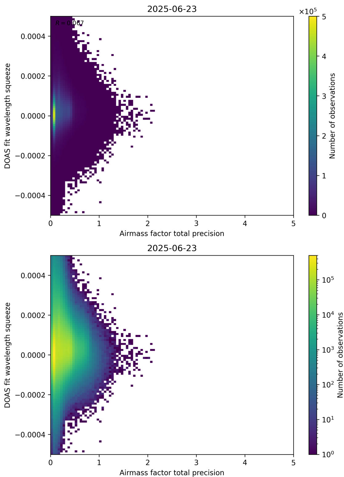
Figure 107: Scatter density plot of “Airmass factor total precision” against “DOAS fit wavelength squeeze” for 2025-06-22 to 2025-06-24.
