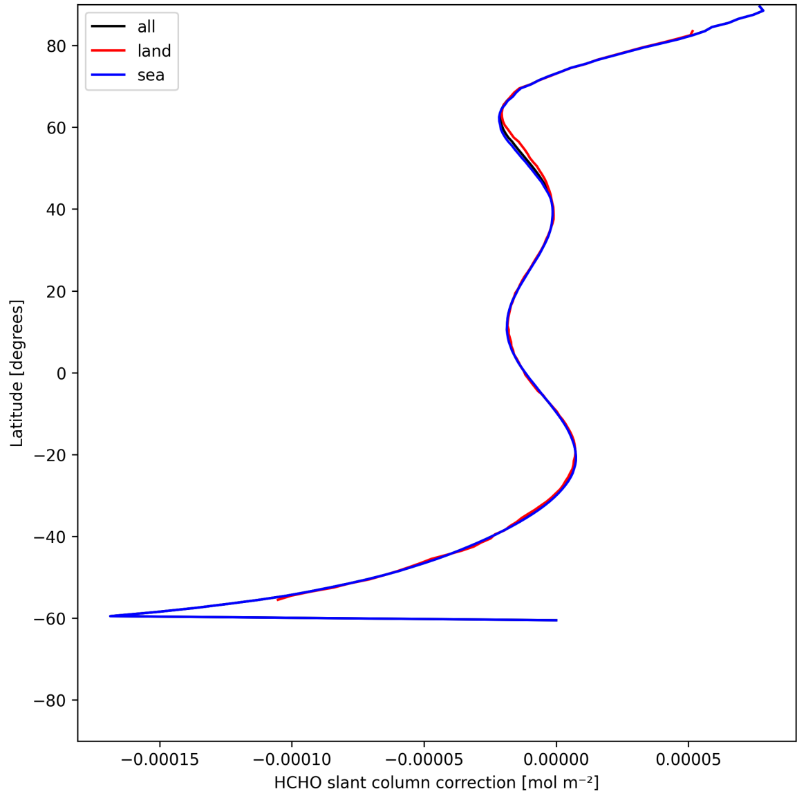
Figure 33: Zonal average of “HCHO slant column correction” for 2025-06-22 to 2025-06-24.
