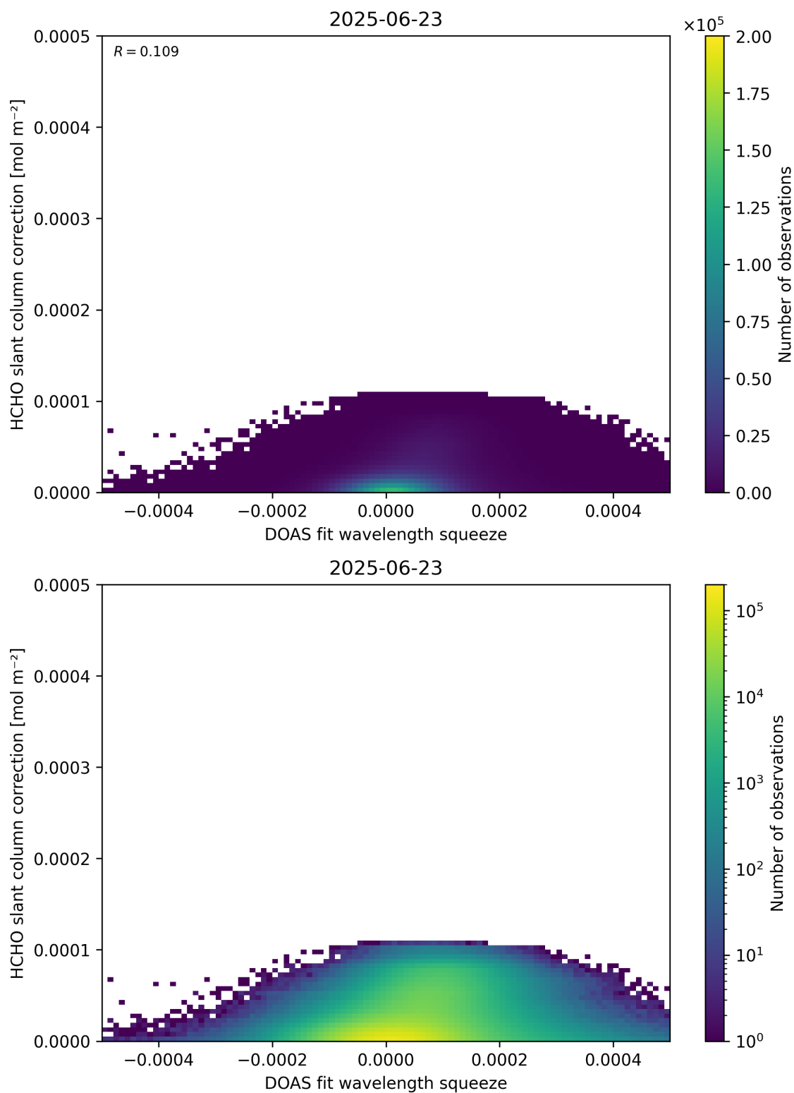
Figure 70: Scatter density plot of “DOAS fit wavelength squeeze” against “HCHO slant column correction” for 2025-06-22 to 2025-06-24.
