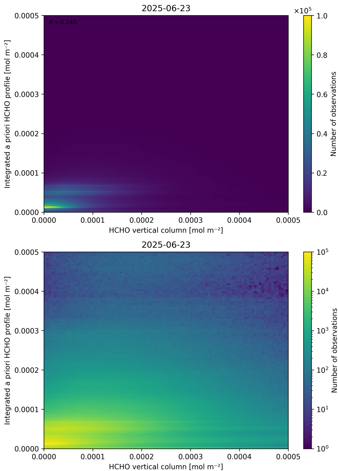
Figure 135: Scatter density plot of “HCHO vertical column” against “Integrated a priori HCHO profile” for 2025-06-22 to 2025-06-24.
