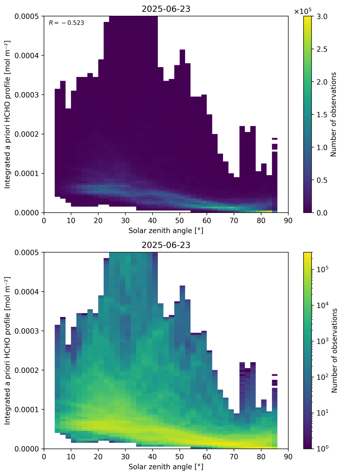
Figure 180: Scatter density plot of “Solar zenith angle” against “Integrated a priori HCHO profile” for 2025-06-22 to 2025-06-24.
