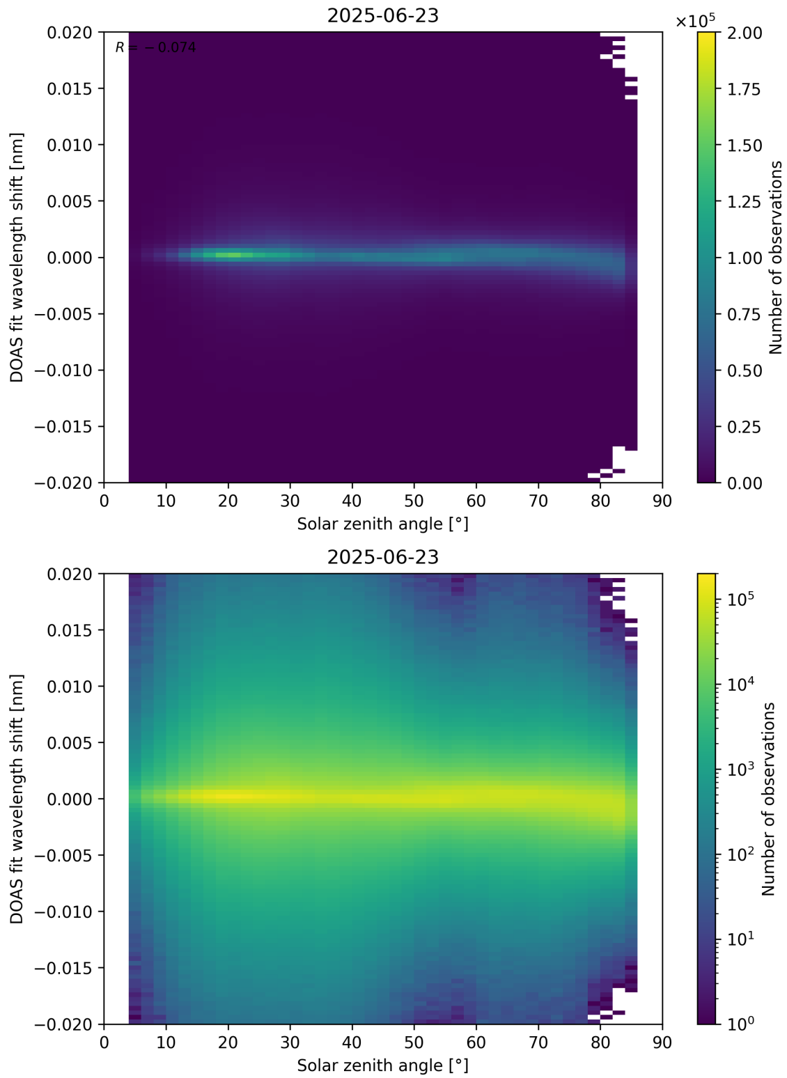
Figure 168: Scatter density plot of “Solar zenith angle” against “DOAS fit wavelength shift” for 2025-06-22 to 2025-06-24.
