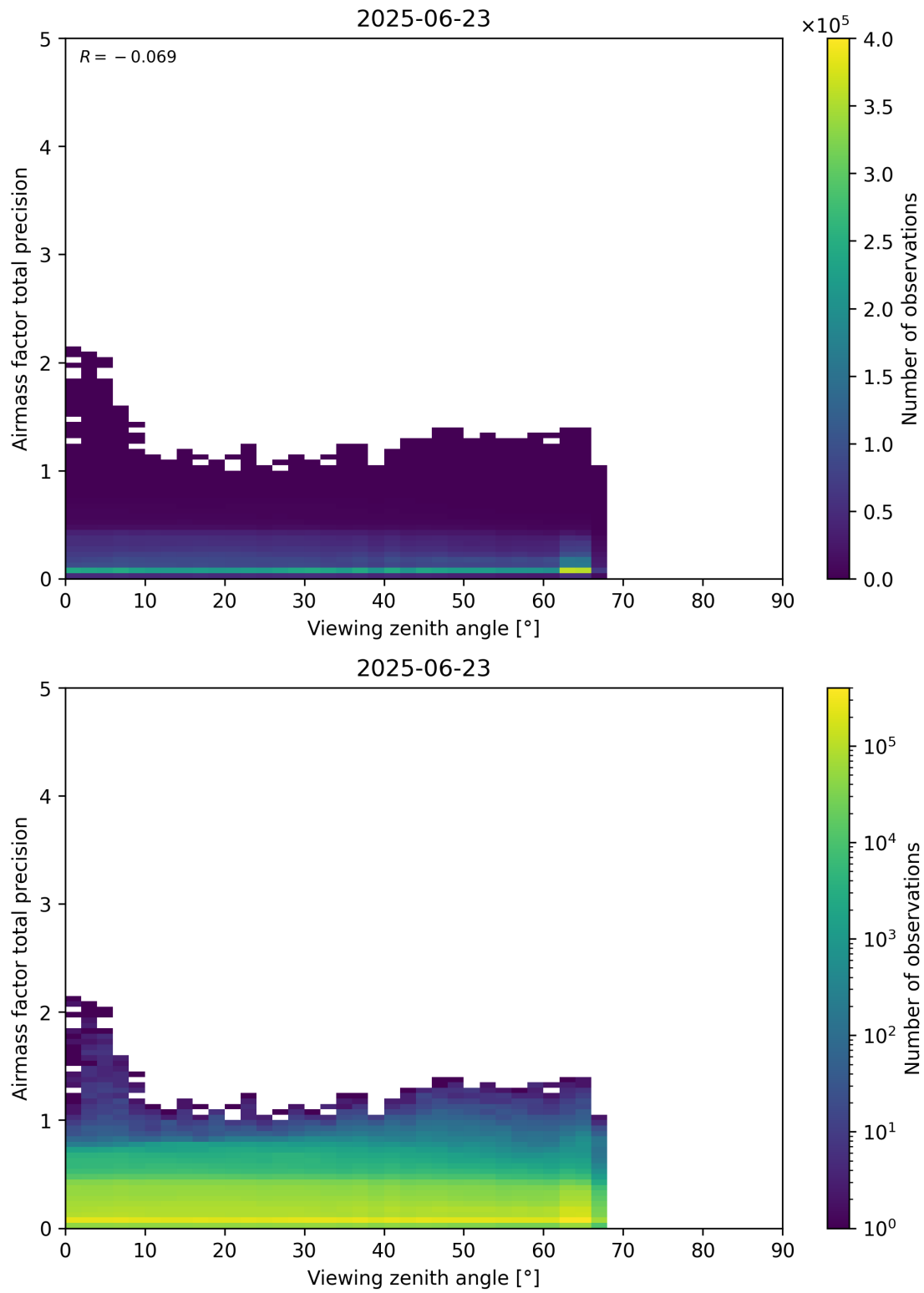
Figure 191: Scatter density plot of “Viewing zenith angle” against “Airmass factor total precision” for 2025-06-22 to 2025-06-24.
