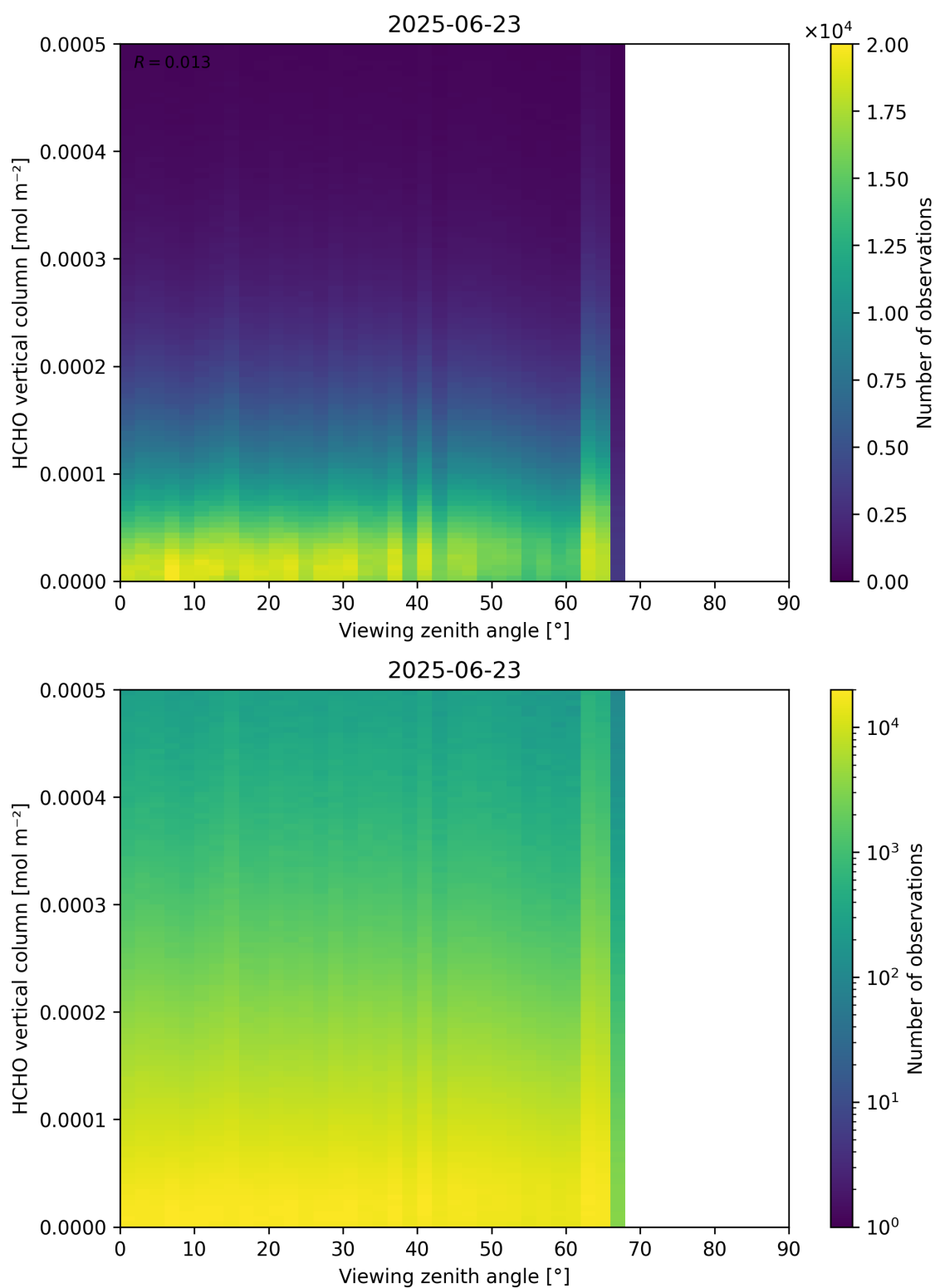
Figure 192: Scatter density plot of “Viewing zenith angle” against “HCHO vertical column” for 2025-06-22 to 2025-06-24.
