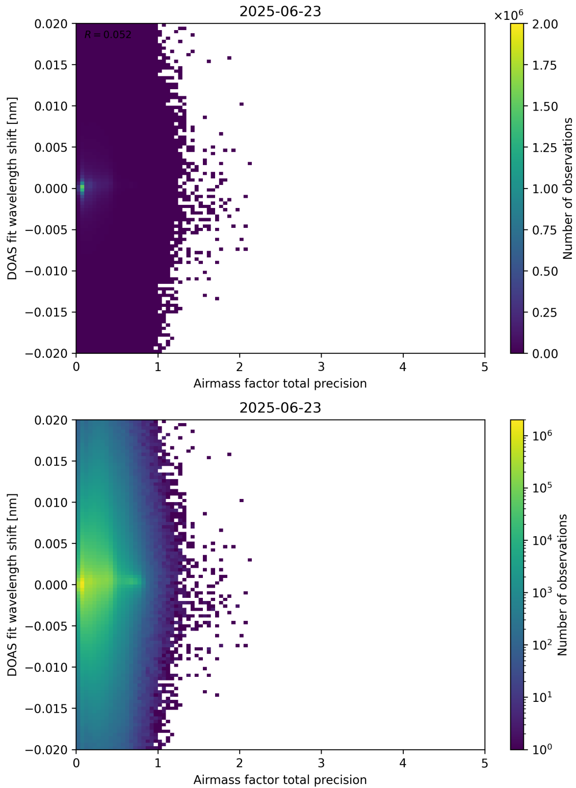
Figure 106: Scatter density plot of “Airmass factor total precision” against “DOAS fit wavelength shift” for 2025-06-22 to 2025-06-24.
