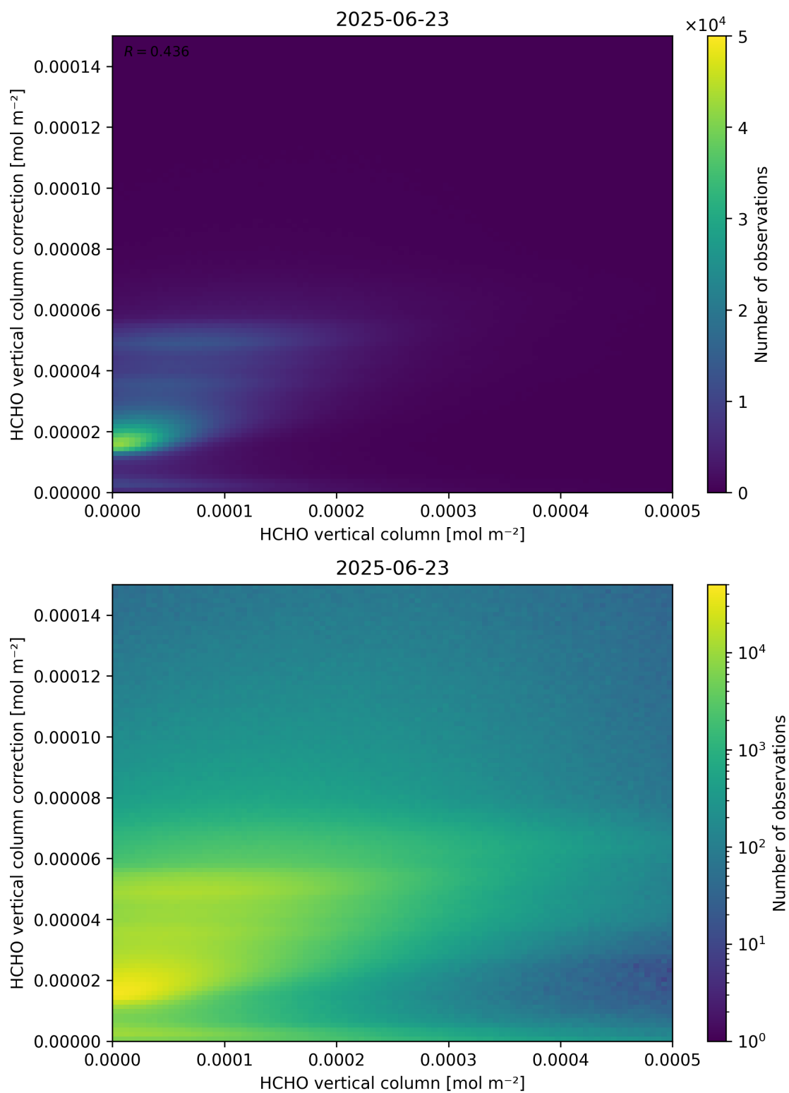
Figure 133: Scatter density plot of “HCHO vertical column” against “HCHO vertical column correction” for 2025-06-22 to 2025-06-24.
