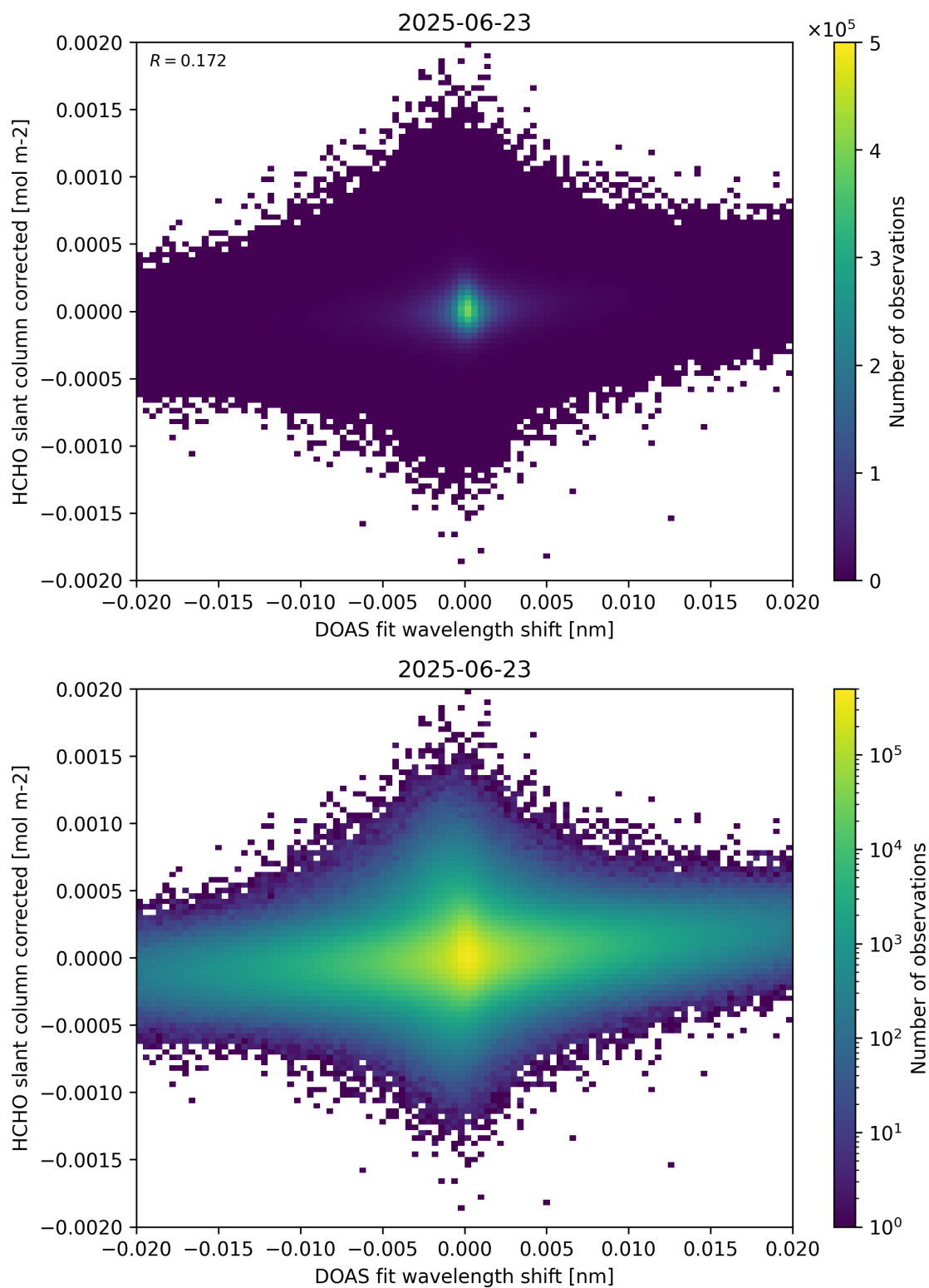
Figure 66: Scatter density plot of “DOAS fit wavelength shift” against “HCHO slant column corrected” for 2025-06-22 to 2025-06-24.
