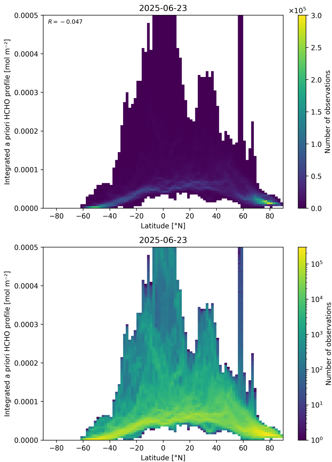
Figure 166: Scatter density plot of “Latitude” against “Integrated a priori HCHO profile” for 2025-06-22 to 2025-06-24.
