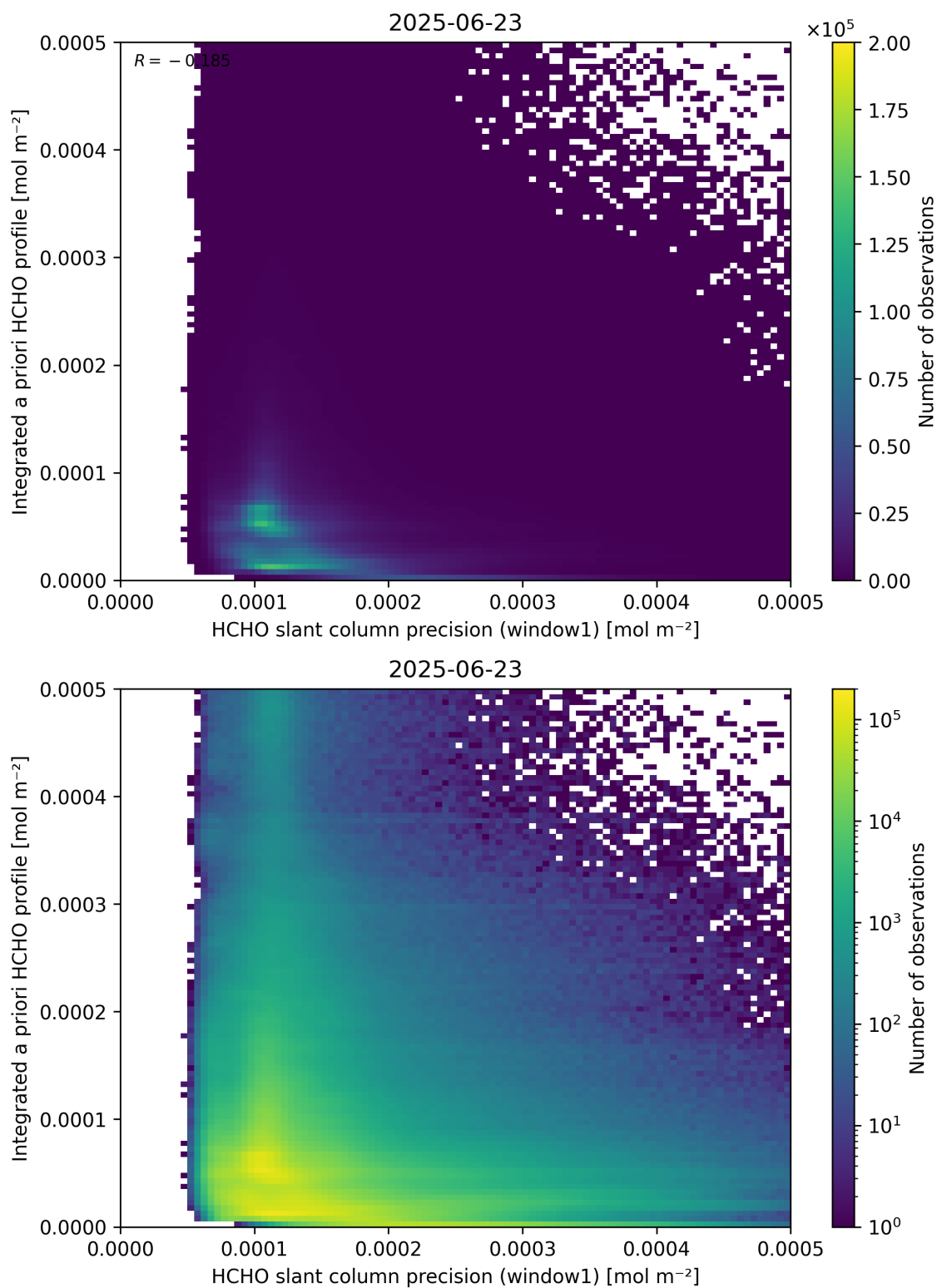
Figure 96: Scatter density plot of “HCHO slant column precision (window1)” against “Integrated a priori HCHO profile” for 2025-06-22 to 2025-06-24.
