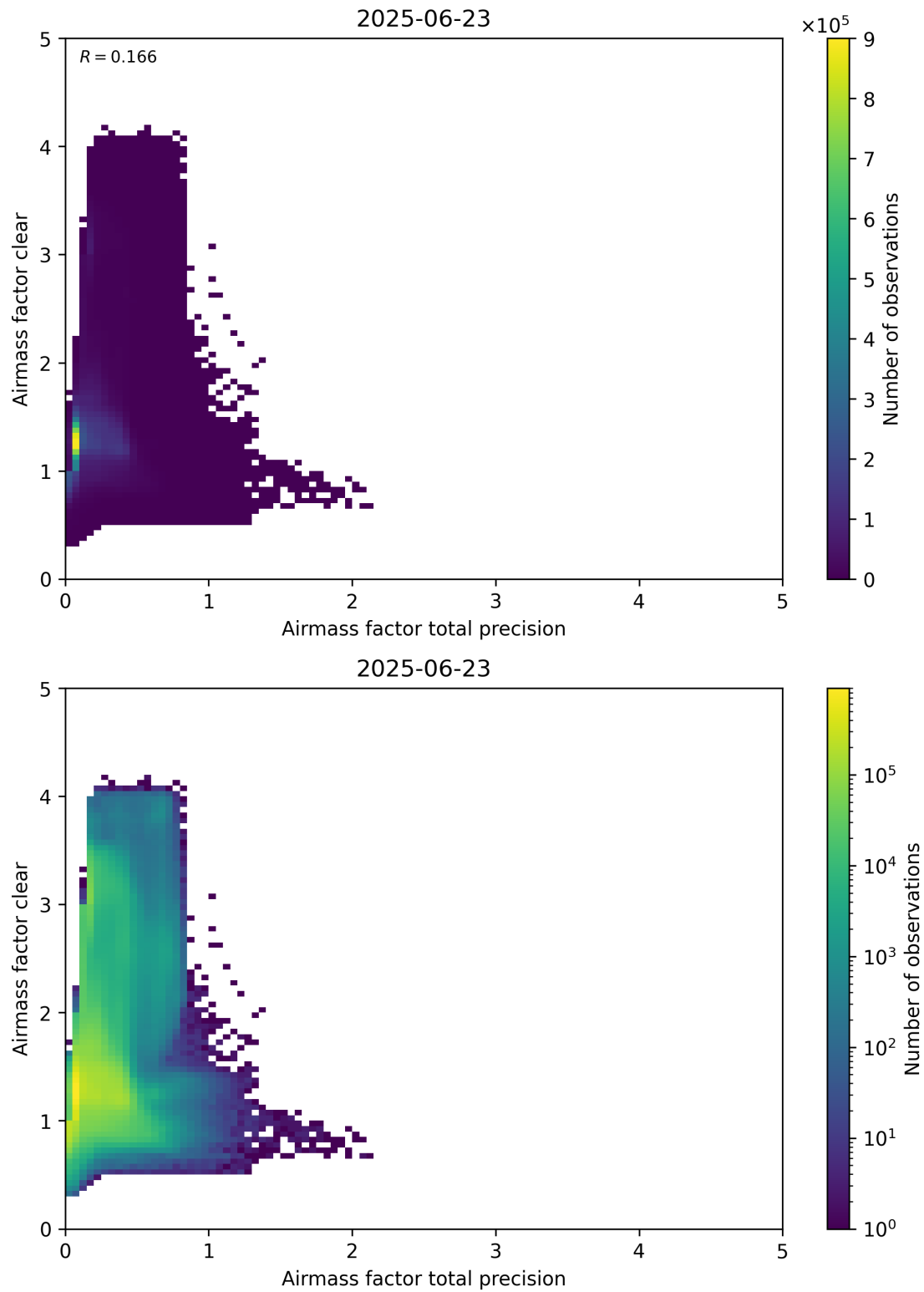
Figure 108: Scatter density plot of “Airmass factor total precision” against “Airmass factor clear” for 2025-06-22 to 2025-06-24.
