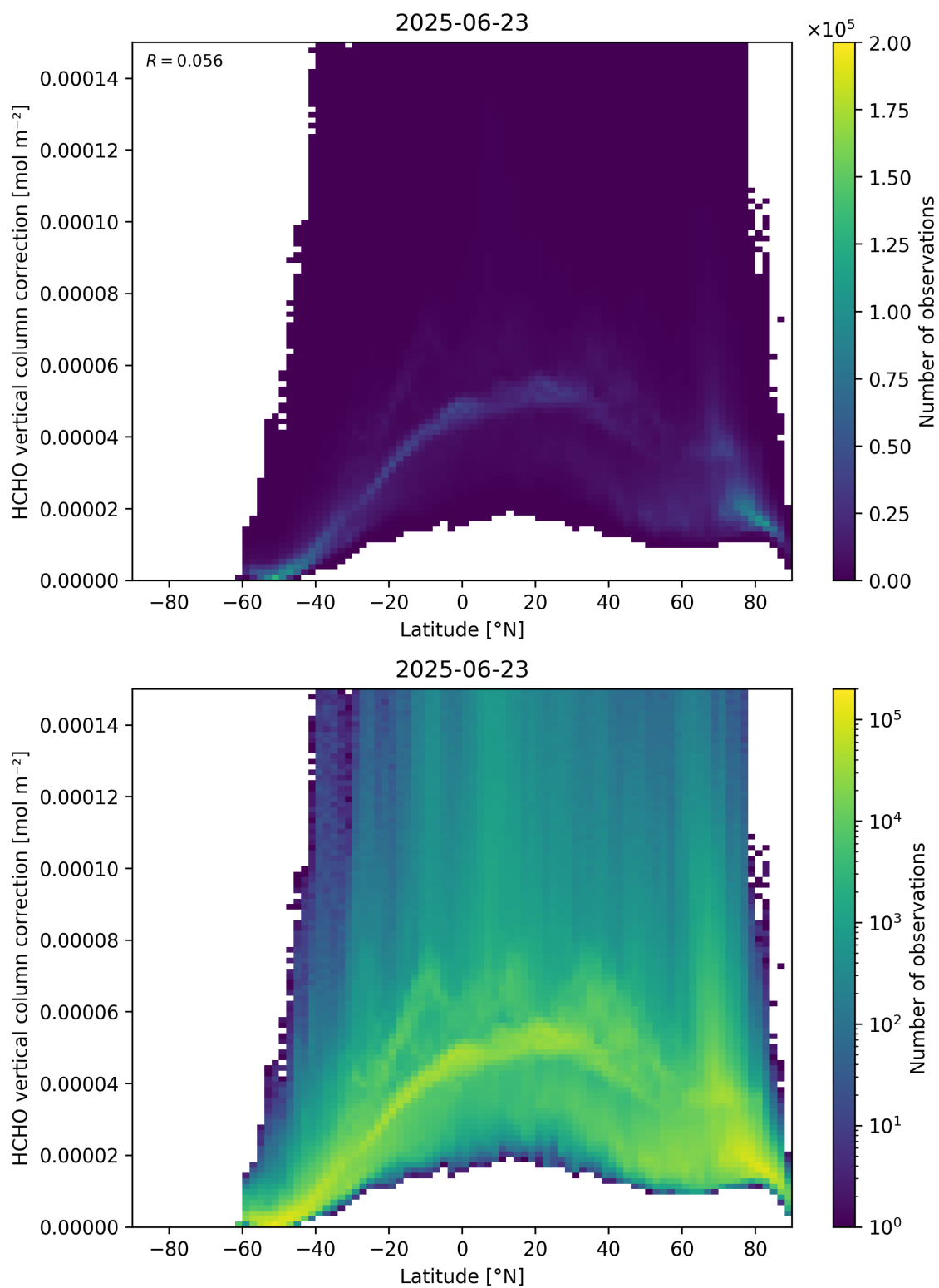
Figure 164: Scatter density plot of “Latitude” against “HCHO vertical column correction” for 2025-06-22 to 2025-06-24.
