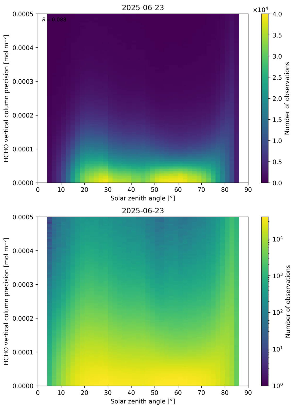
Figure 179: Scatter density plot of “Solar zenith angle” against “HCHO vertical column precision” for 2025-06-22 to 2025-06-24.
