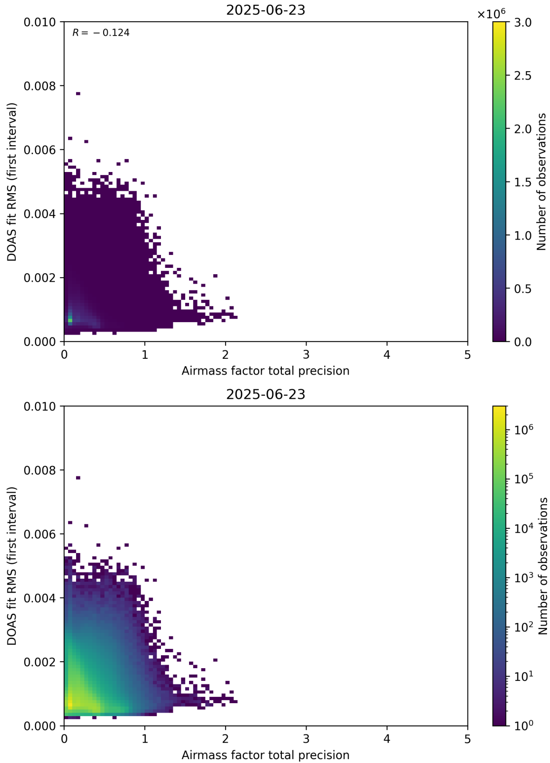
Figure 105: Scatter density plot of “Airmass factor total precision” against “DOAS fit RMS (first interval)” for 2025-06-22 to 2025-06-24.
