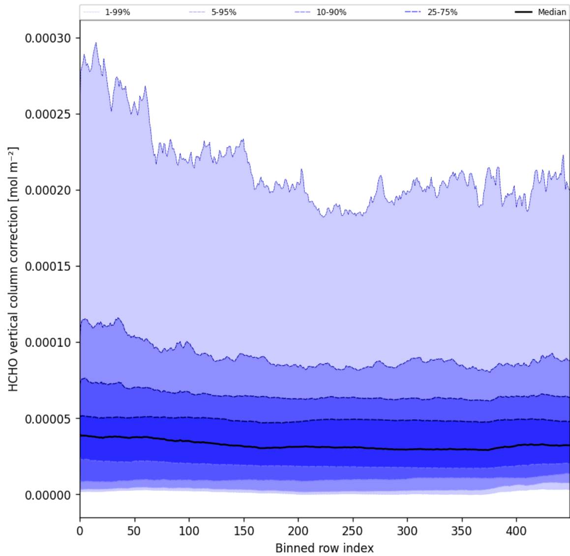
Figure 51: Along track statistics of “HCHO vertical column correction” for 2025-06-22 to 2025-06-24
