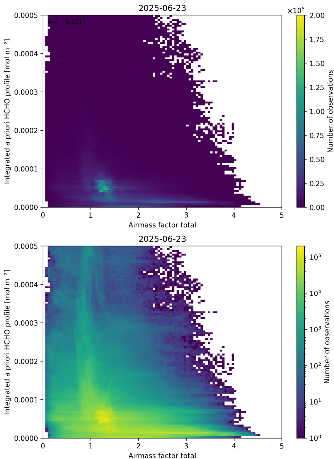
Figure 104: Scatter density plot of “Airmass factor total” against “Integrated a priori HCHO profile” for 2025-06-22 to 2025-06-24.
