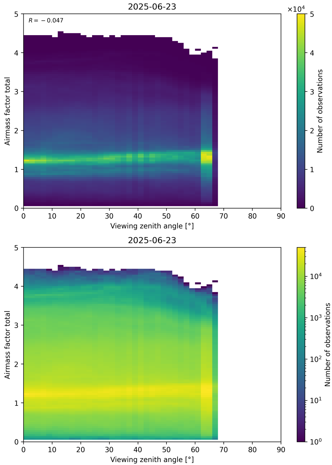
Figure 190: Scatter density plot of “Viewing zenith angle” against “Airmass factor total” for 2025-06-22 to 2025-06-24.
