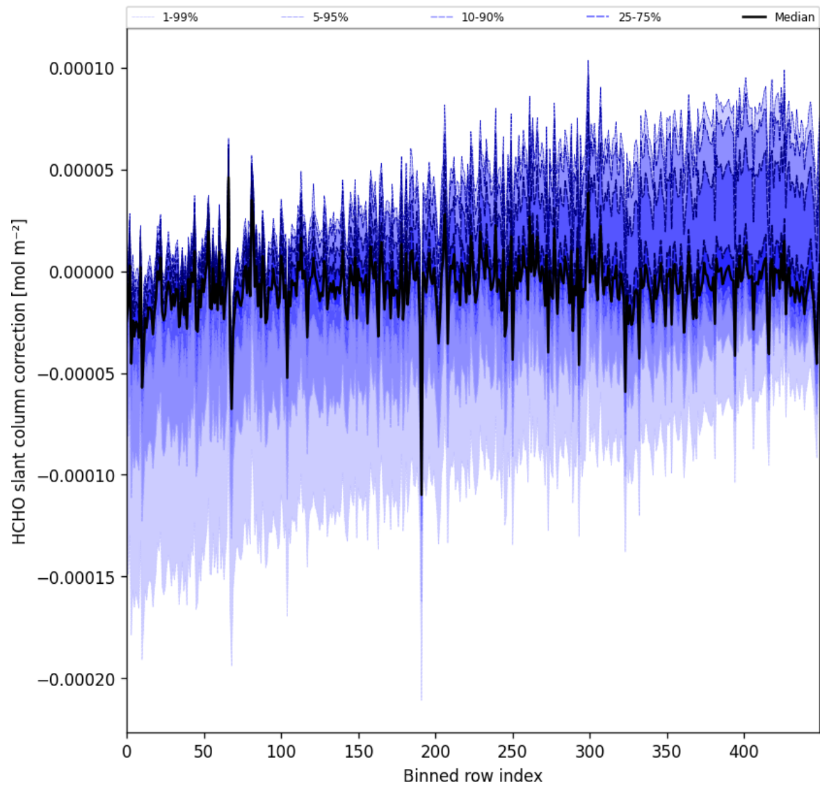
Figure 61: Along track statistics of “HCHO slant column correction” for 2025-06-22 to 2025-06-24
