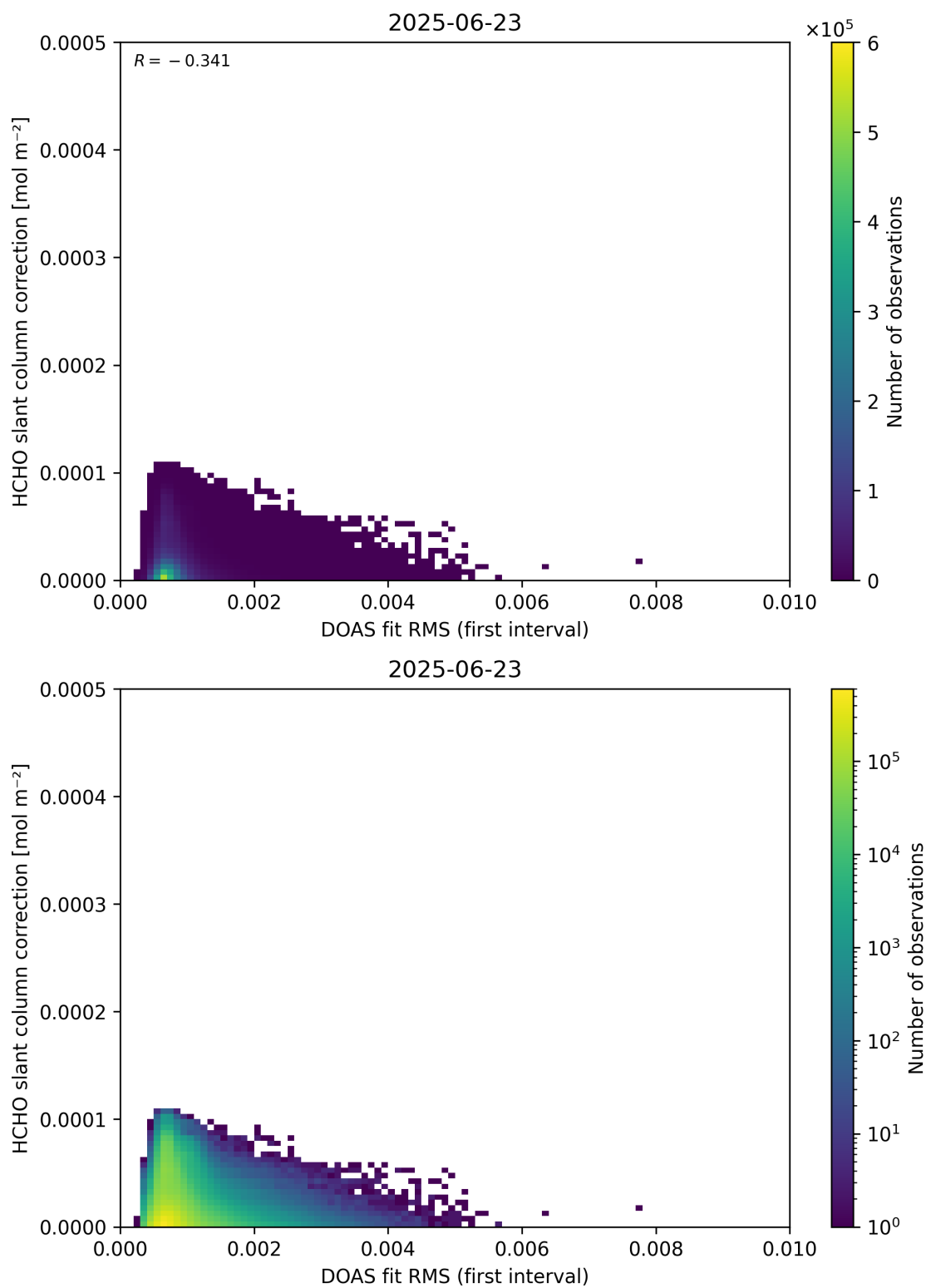
Figure 63: Scatter density plot of “DOAS fit RMS (first interval)” against “HCHO slant column correction” for 2025-06-22 to 2025-06-24.
