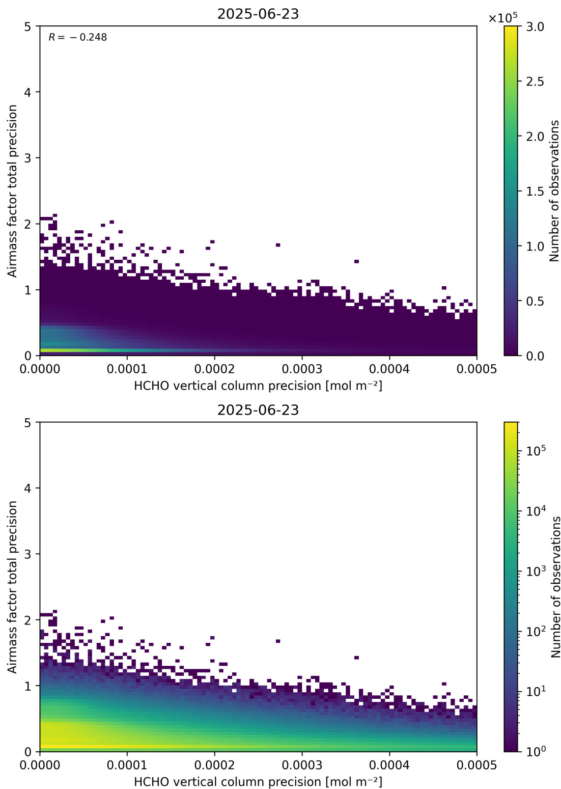
Figure 145: Scatter density plot of “HCHO vertical column precision” against “Airmass factor total precision” for 2025-06-22 to 2025-06-24.
