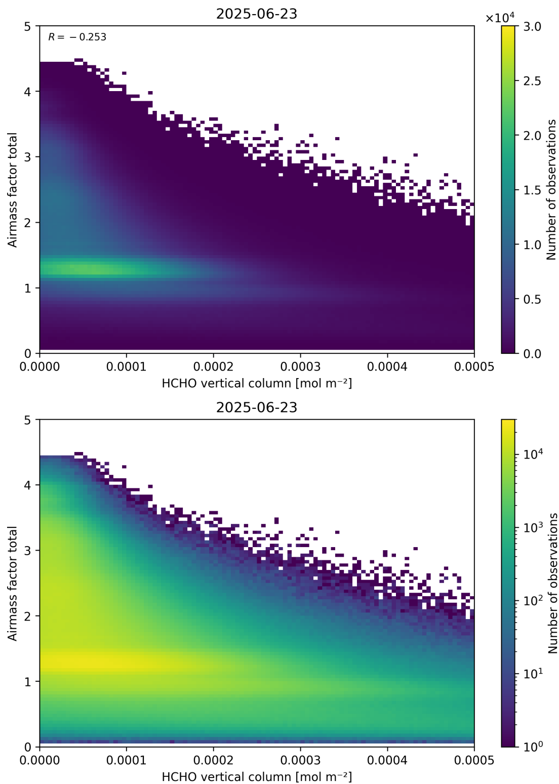
Figure 131: Scatter density plot of “HCHO vertical column” against “Airmass factor total” for 2025-06-22 to 2025-06-24.
