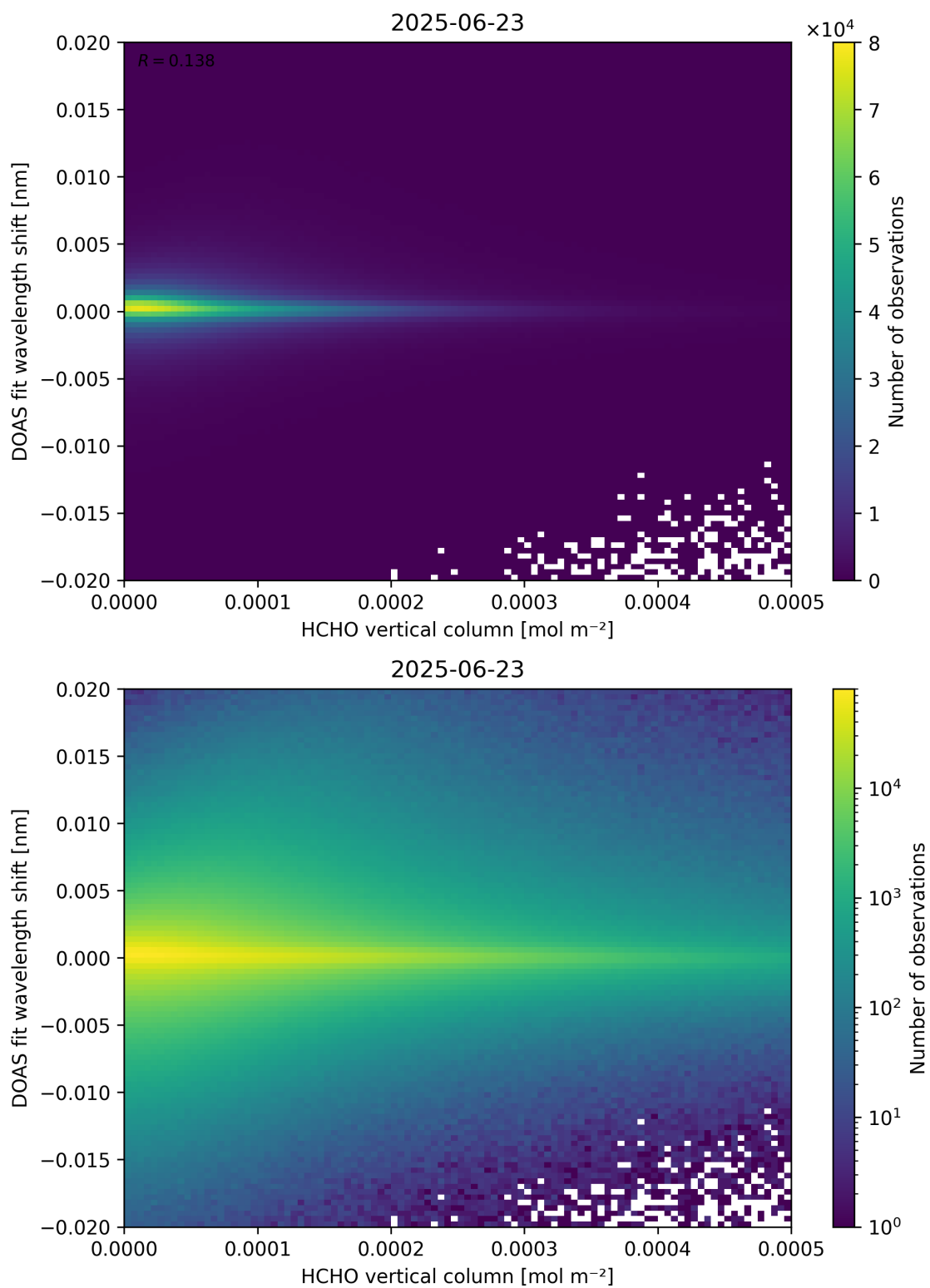
Figure 124: Scatter density plot of “HCHO vertical column” against “DOAS fit wavelength shift” for 2025-06-22 to 2025-06-24.
