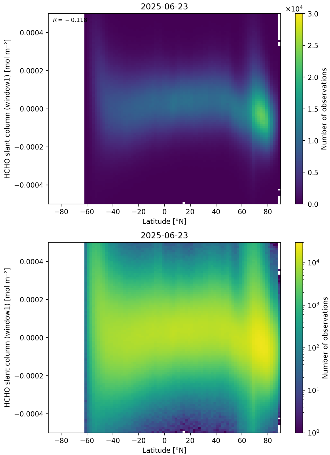
Figure 159: Scatter density plot of “Latitude” against “HCHO slant column (window1)” for 2025-06-22 to 2025-06-24.
