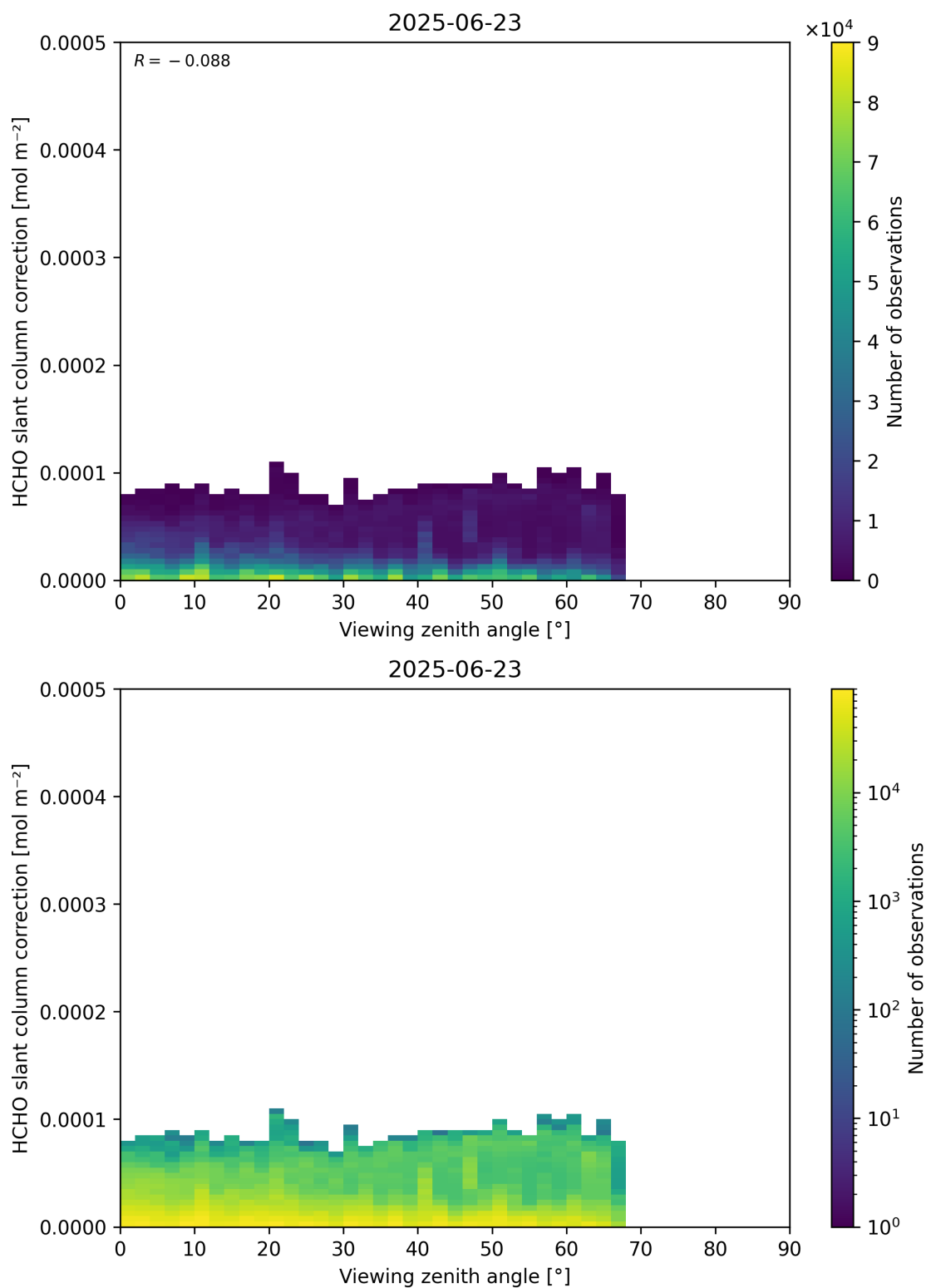
Figure 187: Scatter density plot of “Viewing zenith angle” against “HCHO slant column correction” for 2025-06-22 to 2025-06-24.
