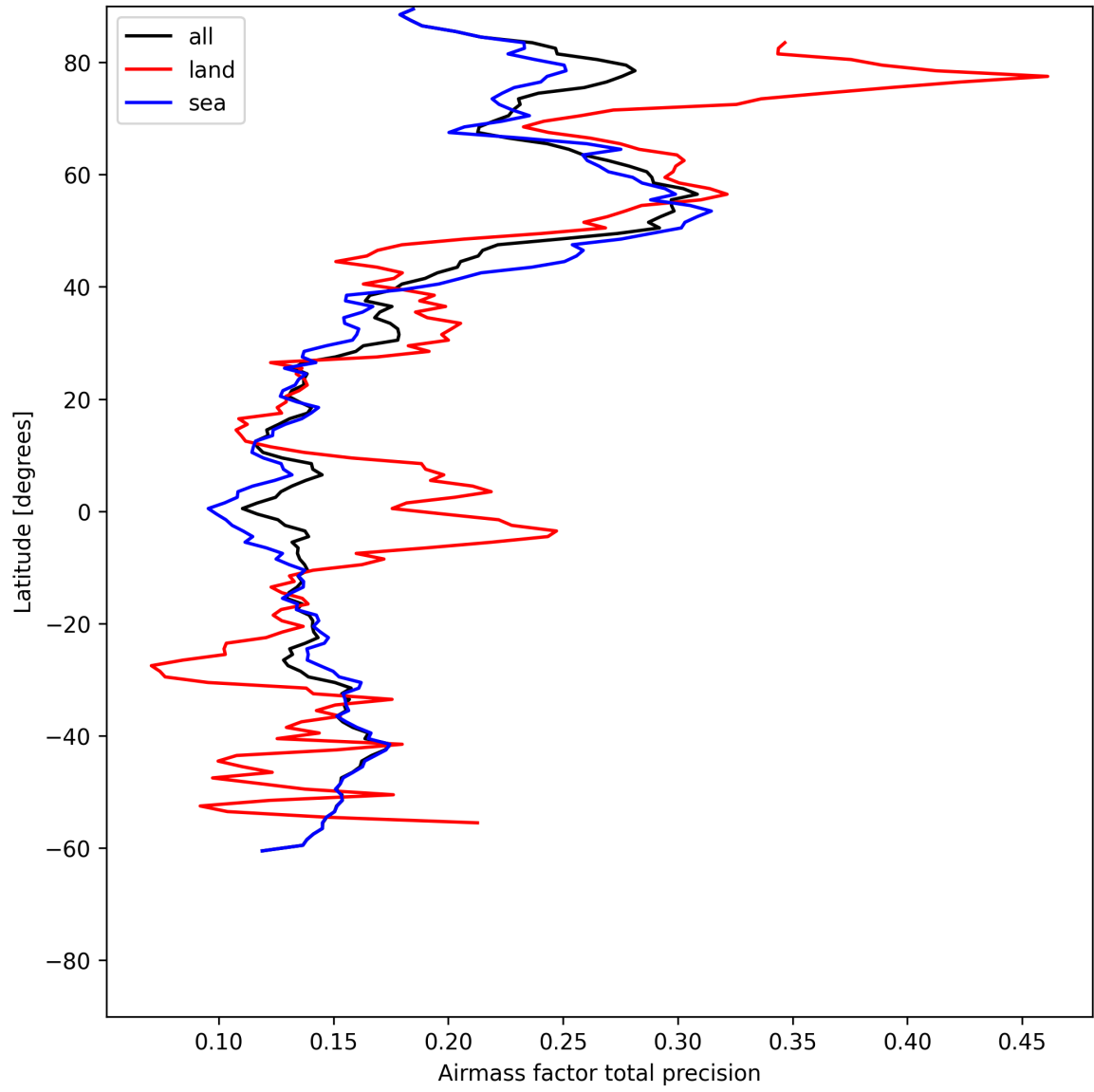
Figure 27: Zonal average of “Airmass factor total precision” for 2025-06-22 to 2025-06-24.
