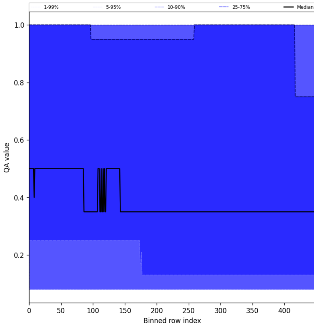
Figure 48: Along track statistics of “QA value” for 2025-06-22 to 2025-06-24
