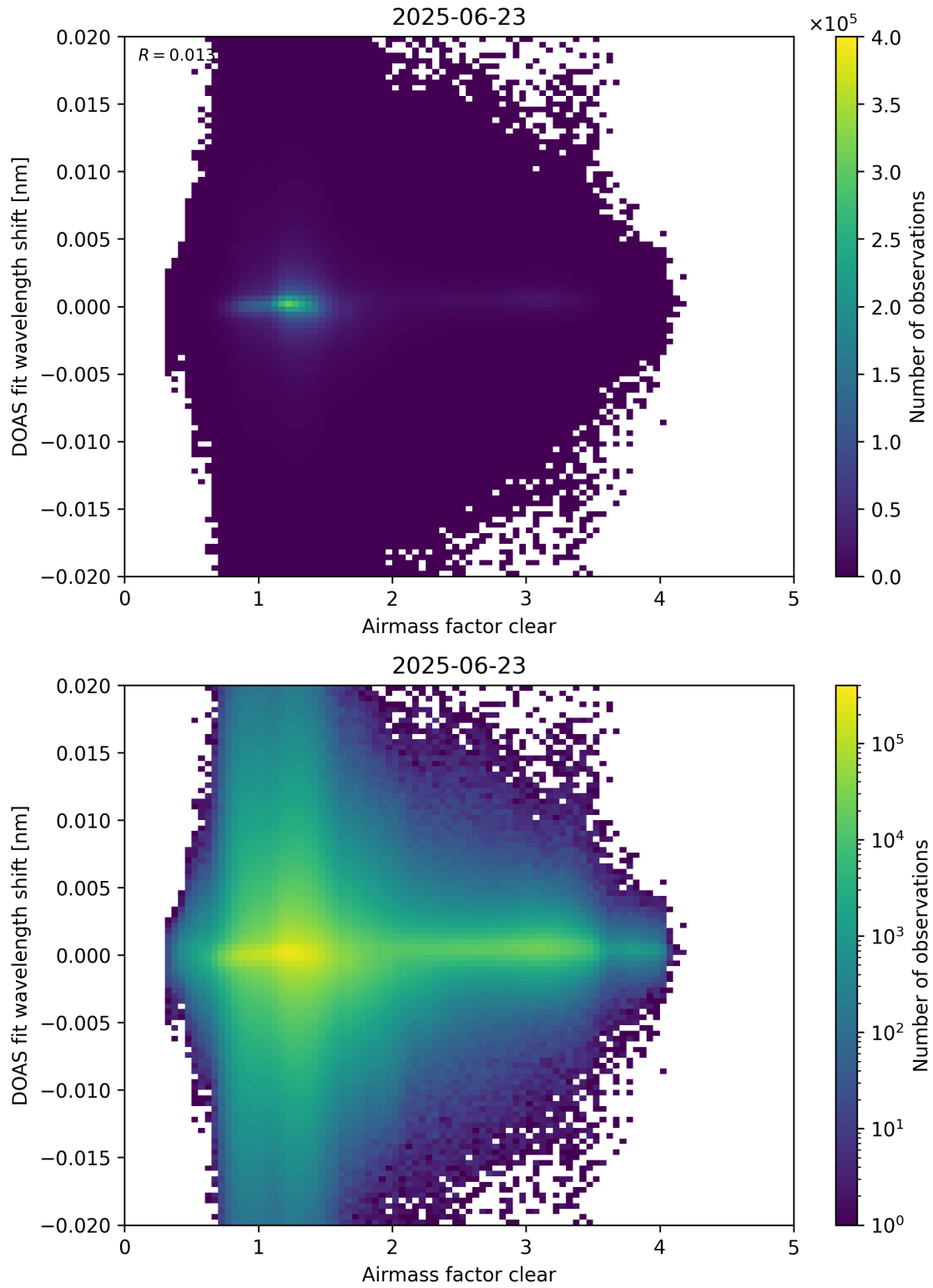
Figure 72: Scatter density plot of “Airmass factor clear” against “DOAS fit wavelength shift” for 2025-06-22 to 2025-06-24.
