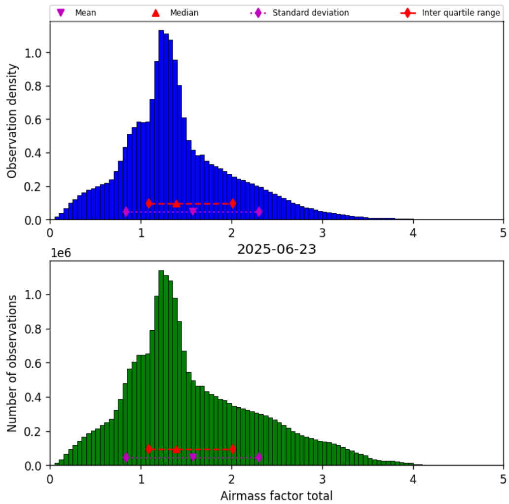
Figure 40: Histogram of “Airmass factor total” for 2025-06-22 to 2025-06-24
