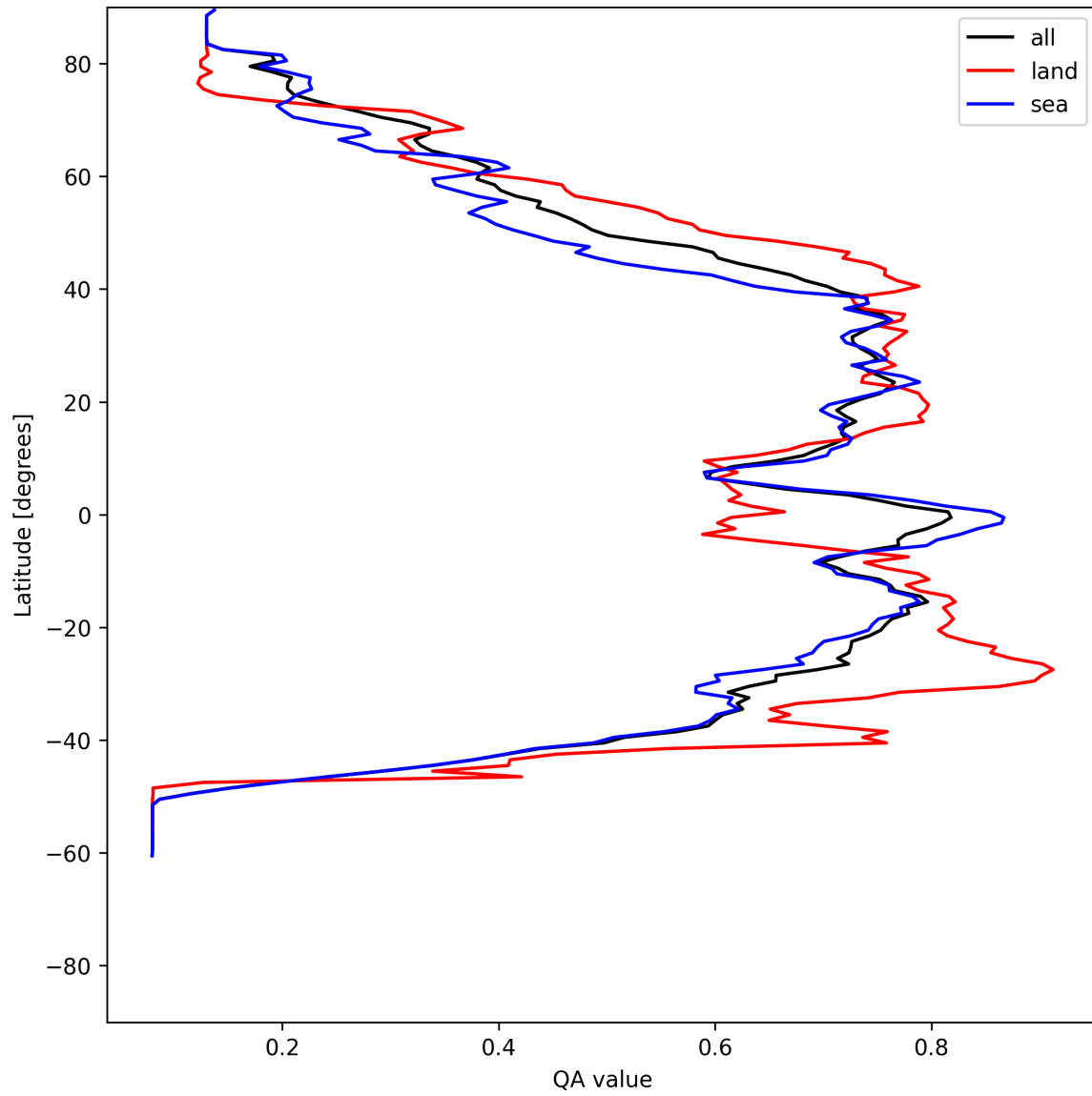
Figure 20: Zonal average of “QA value” for 2025-06-22 to 2025-06-24.
