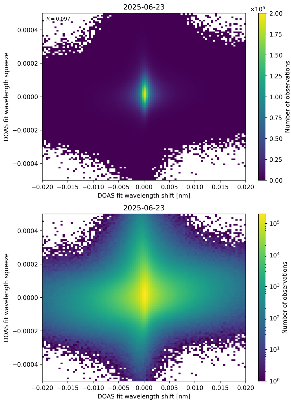
Figure 65: Scatter density plot of “DOAS fit wavelength shift” against “DOAS fit wavelength squeeze” for 2025-06-22 to 2025-06-24.
