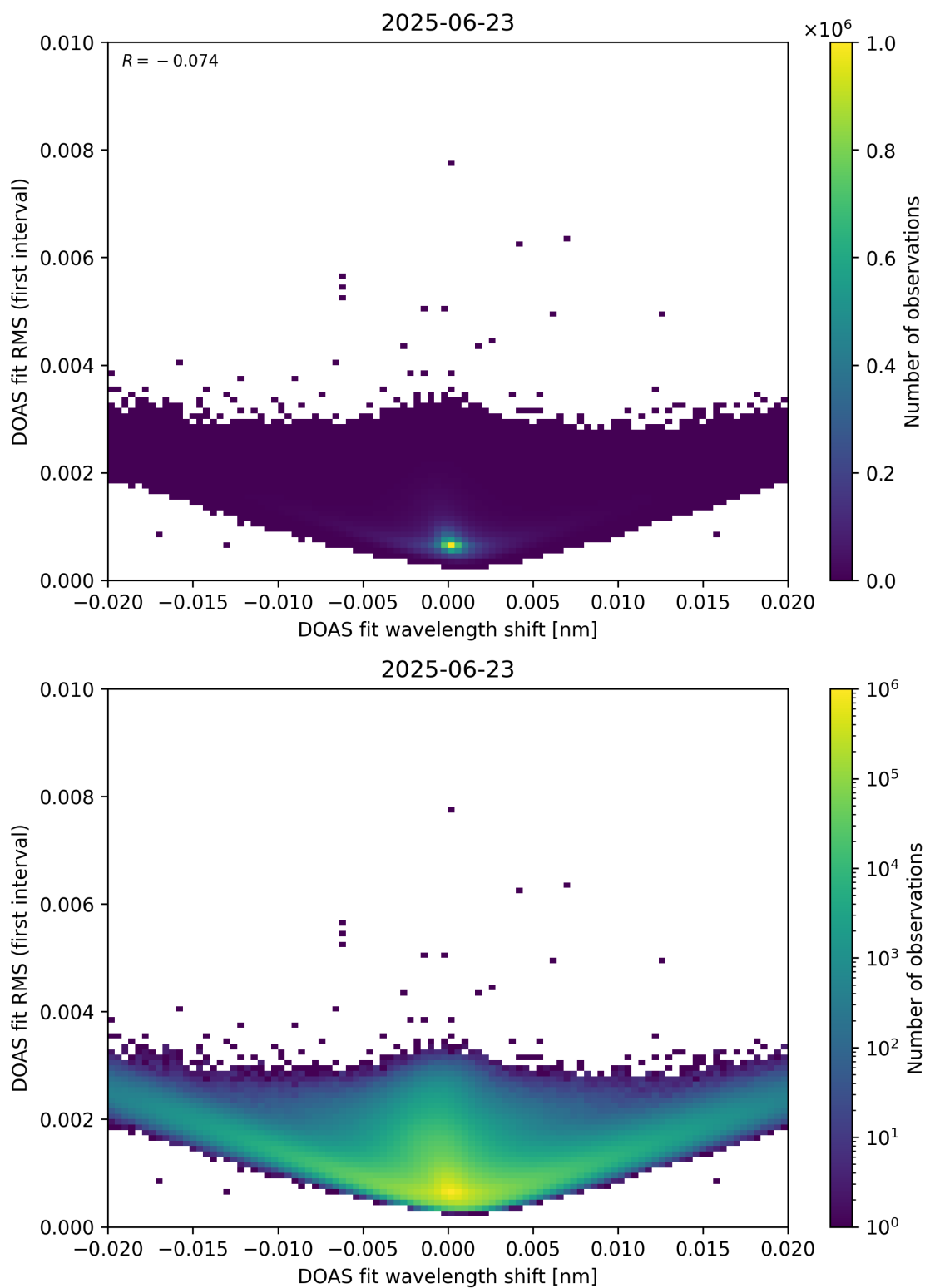
Figure 64: Scatter density plot of “DOAS fit wavelength shift” against “DOAS fit RMS (first interval)” for 2025-06-22 to 2025-06-24.
