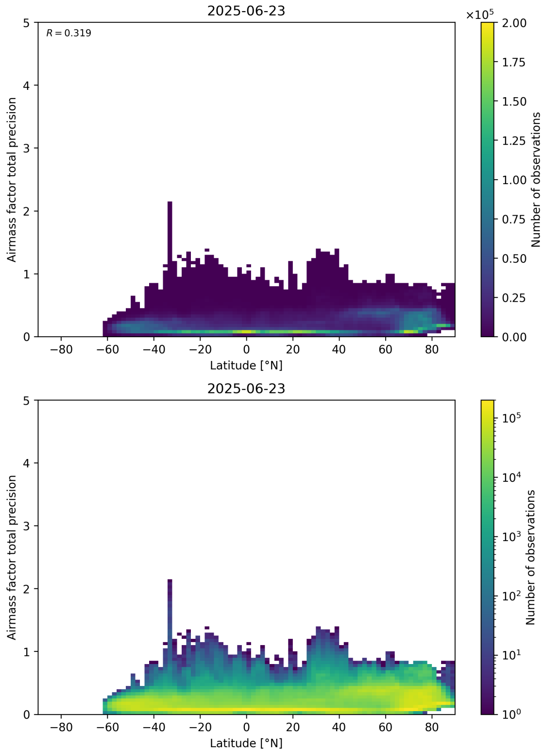
Figure 162: Scatter density plot of “Latitude” against “Airmass factor total precision” for 2025-06-22 to 2025-06-24.
