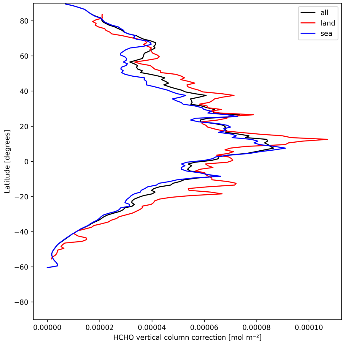
Figure 23: Zonal average of “HCHO vertical column correction” for 2025-06-22 to 2025-06-24.
