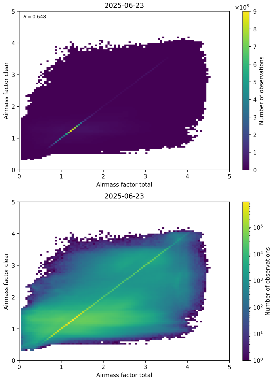
Figure 100: Scatter density plot of “Airmass factor total” against “Airmass factor clear” for 2025-06-22 to 2025-06-24.
