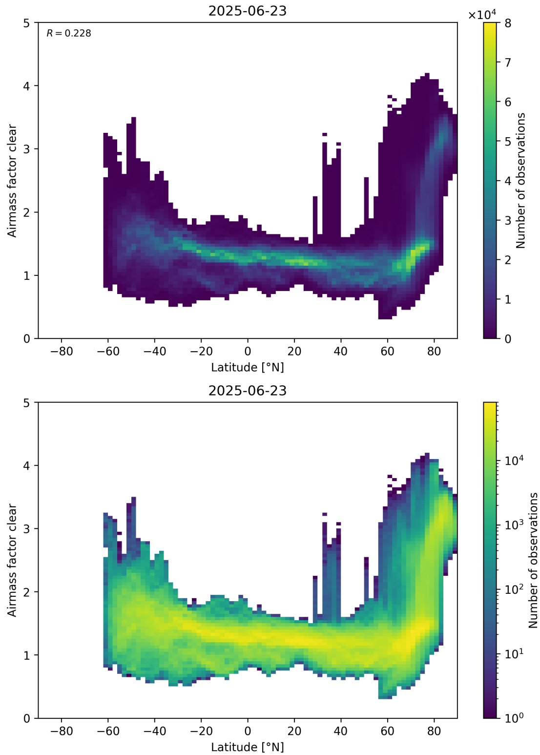
Figure 156: Scatter density plot of “Latitude” against “Airmass factor clear” for 2025-06-22 to 2025-06-24.
