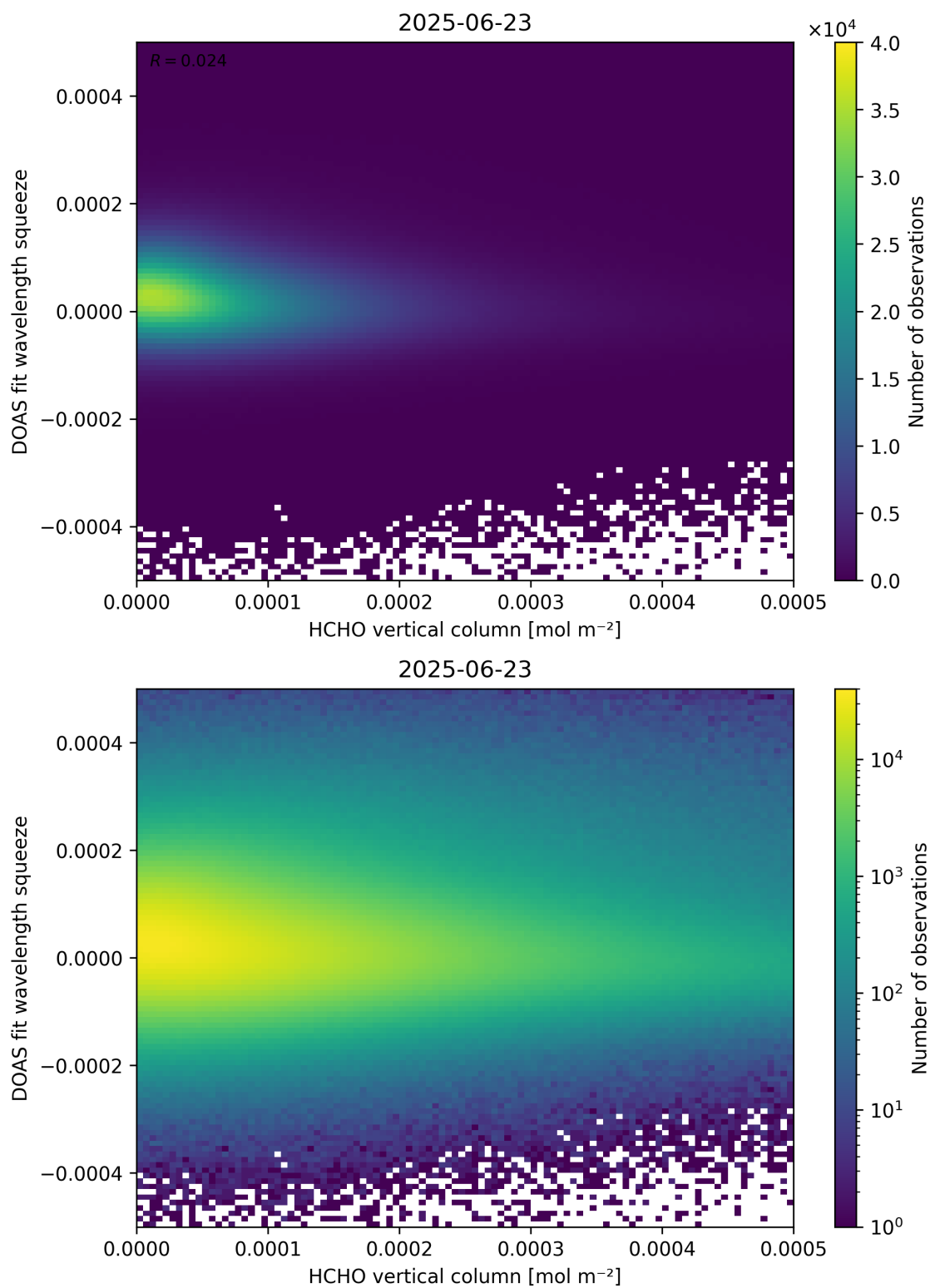
Figure 125: Scatter density plot of “HCHO vertical column” against “DOAS fit wavelength squeeze” for 2025-06-22 to 2025-06-24.
