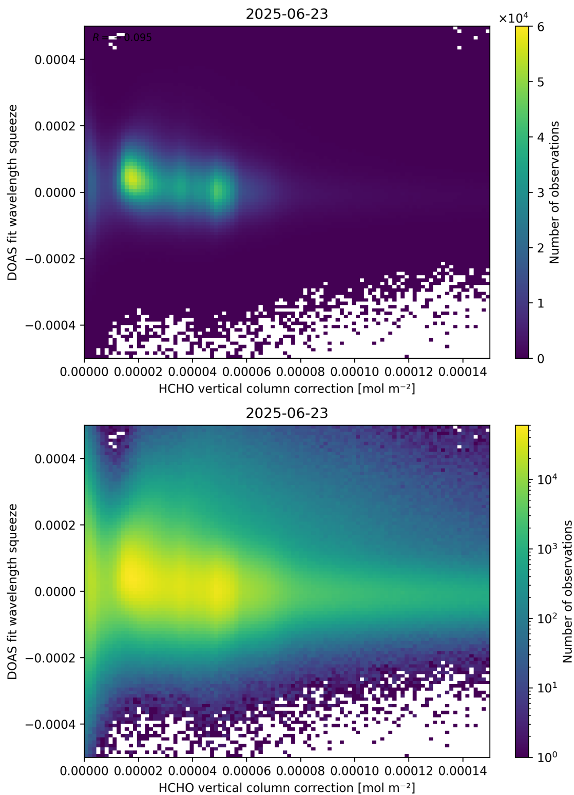
Figure 114: Scatter density plot of “HCHO vertical column correction” against “DOAS fit wavelength squeeze” for 2025-06-22 to 2025-06-24.
