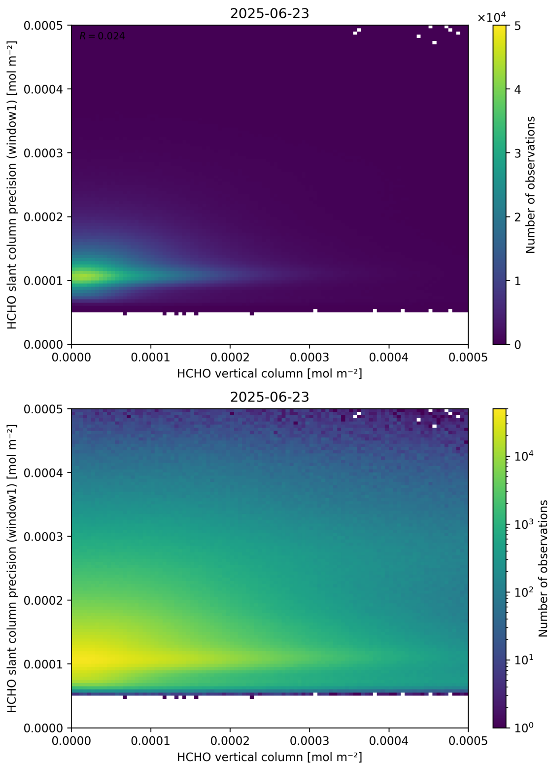
Figure 130: Scatter density plot of “HCHO vertical column” against “HCHO slant column precision (window1)” for 2025-06-22 to 2025-06-24.
