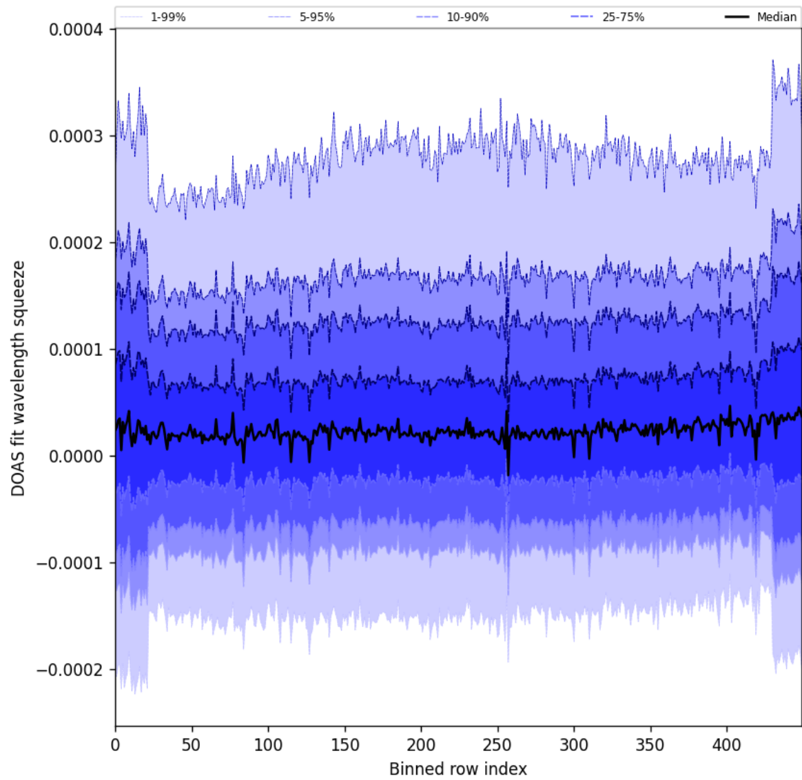
Figure 59: Along track statistics of “DOAS fit wavelength squeeze” for 2025-06-22 to 2025-06-24
