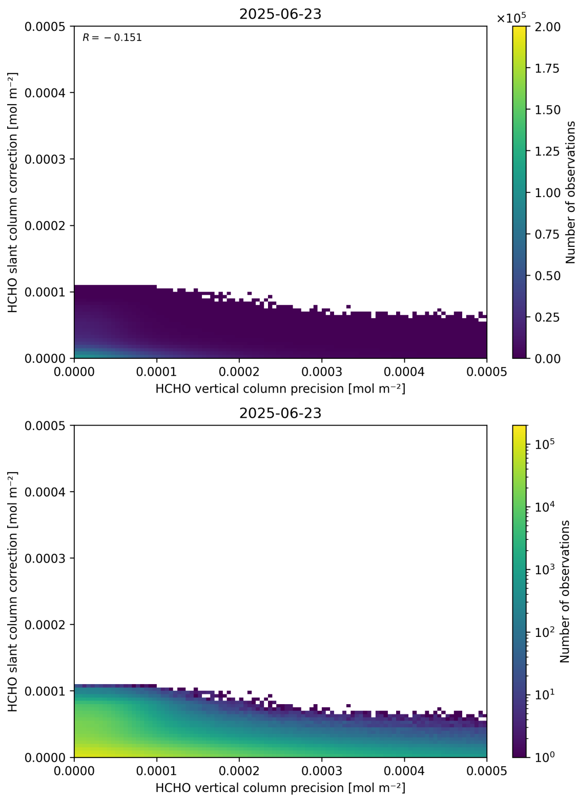
Figure 141: Scatter density plot of “HCHO vertical column precision” against “HCHO slant column correction” for 2025-06-22 to 2025-06-24.
