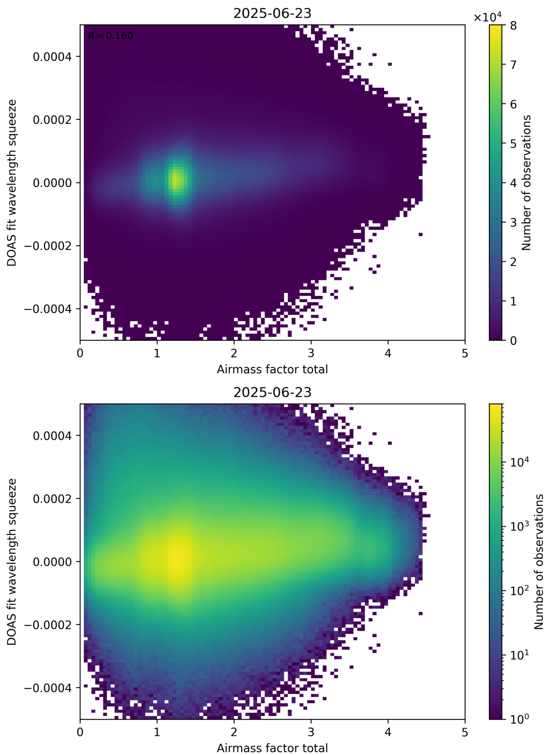
Figure 99: Scatter density plot of “Airmass factor total” against “DOAS fit wavelength squeeze” for 2025-06-22 to 2025-06-24.
