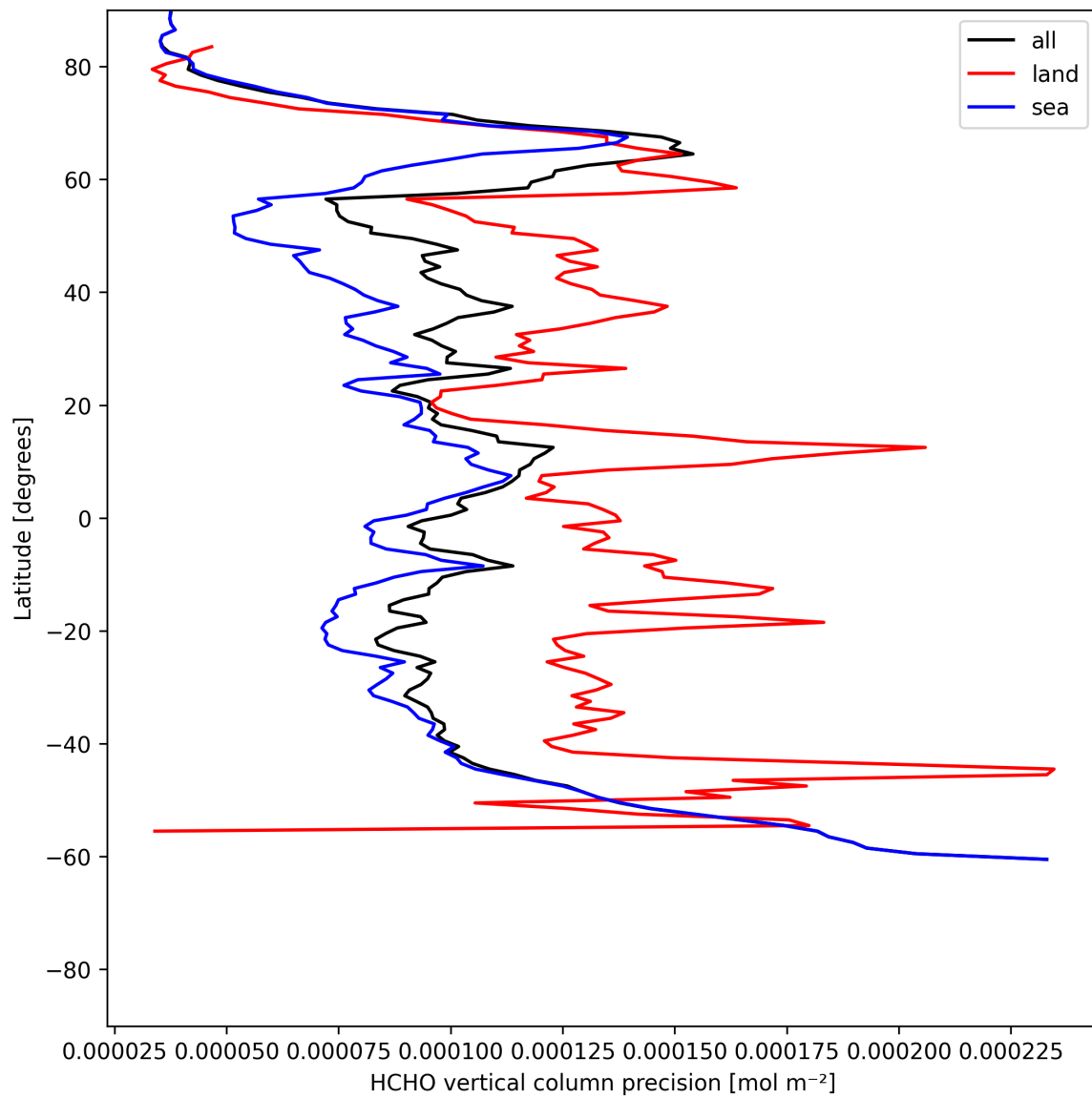
Figure 22: Zonal average of “HCHO vertical column precision” for 2025-06-22 to 2025-06-24.
