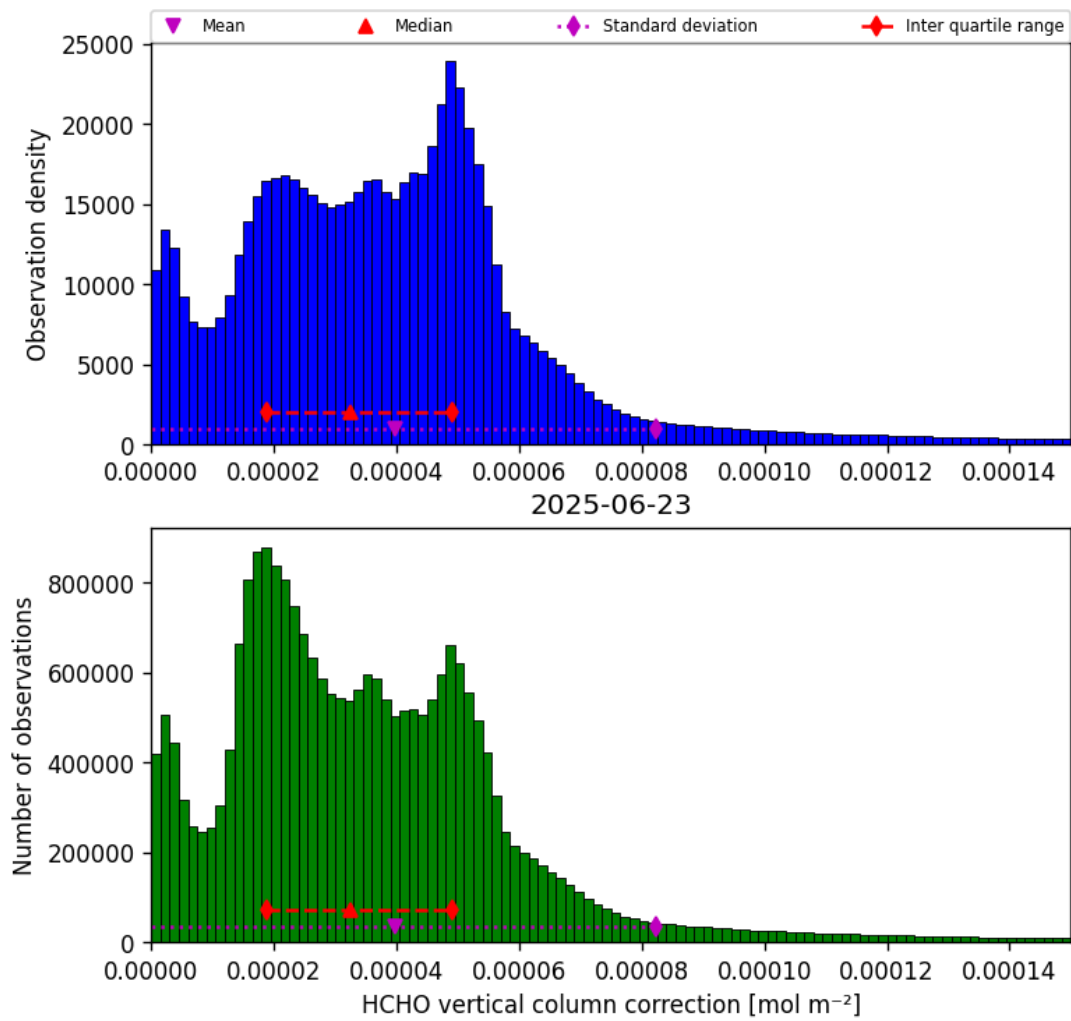
Figure 37: Histogram of “HCHO vertical column correction” for 2025-06-22 to 2025-06-24
