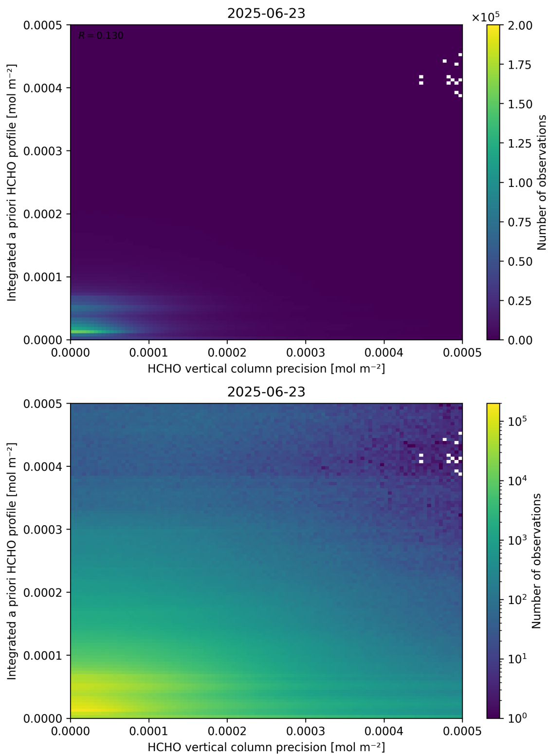
Figure 147: Scatter density plot of “HCHO vertical column precision” against “Integrated a priori HCHO profile” for 2025-06-22 to 2025-06-24.
