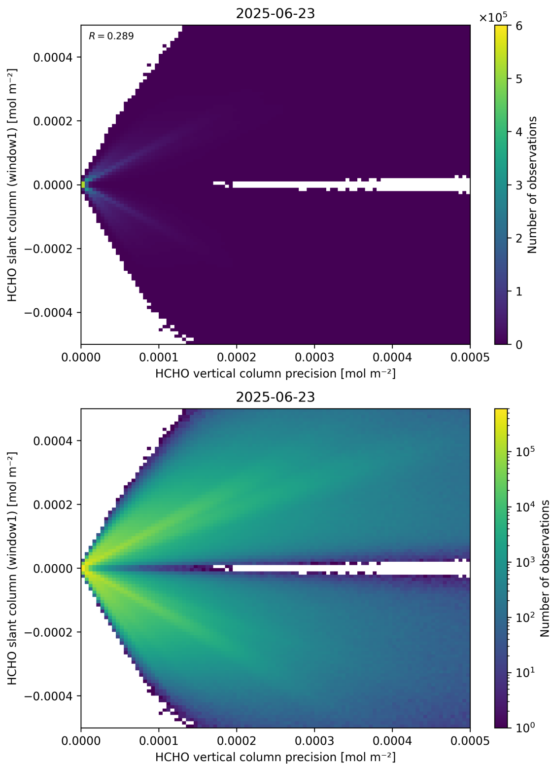
Figure 142: Scatter density plot of “HCHO vertical column precision” against “HCHO slant column (window1)” for 2025-06-22 to 2025-06-24.
