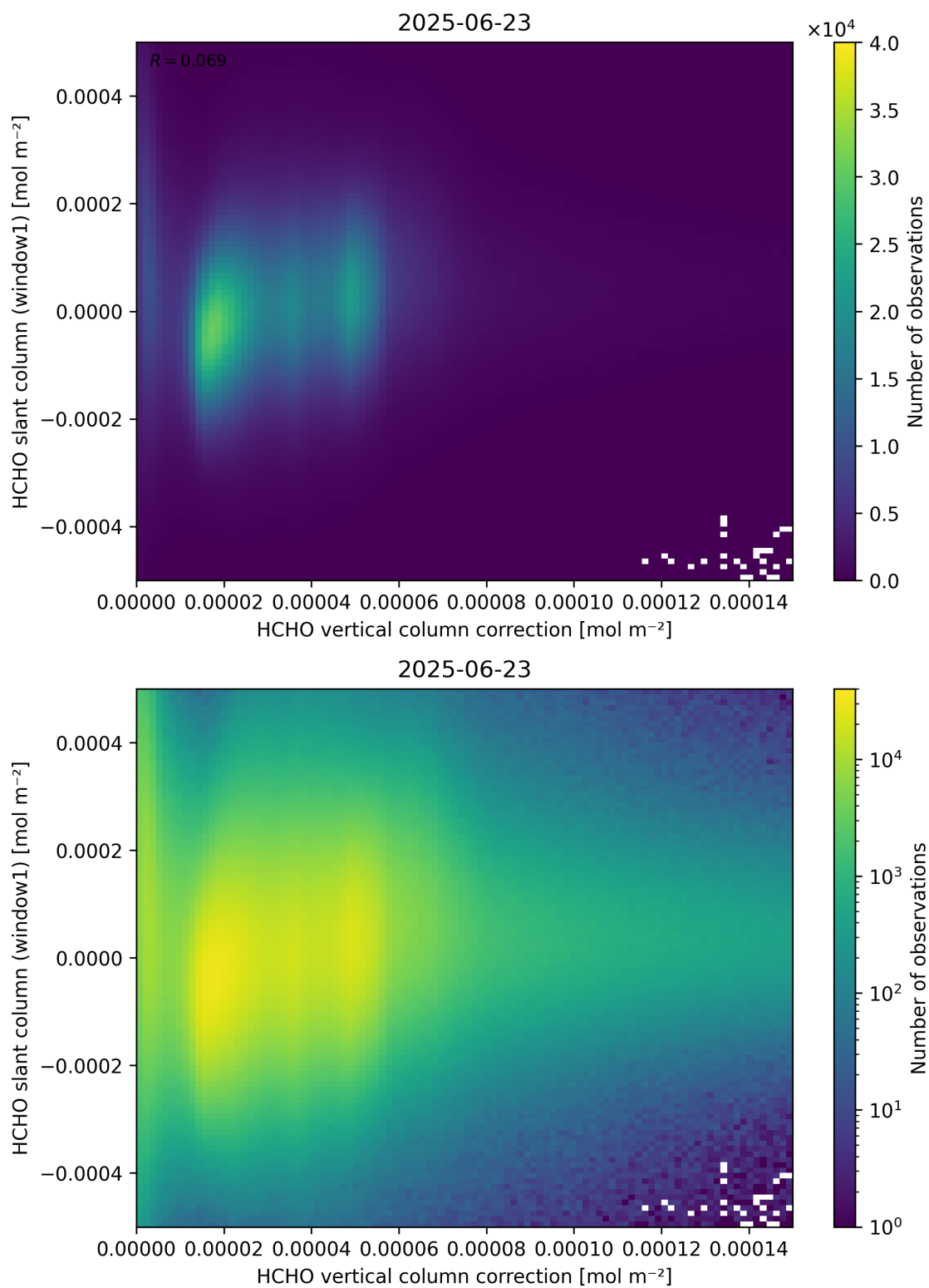
Figure 118: Scatter density plot of “HCHO vertical column correction” against “HCHO slant column (window1)” for 2025-06-22 to 2025-06-24.
