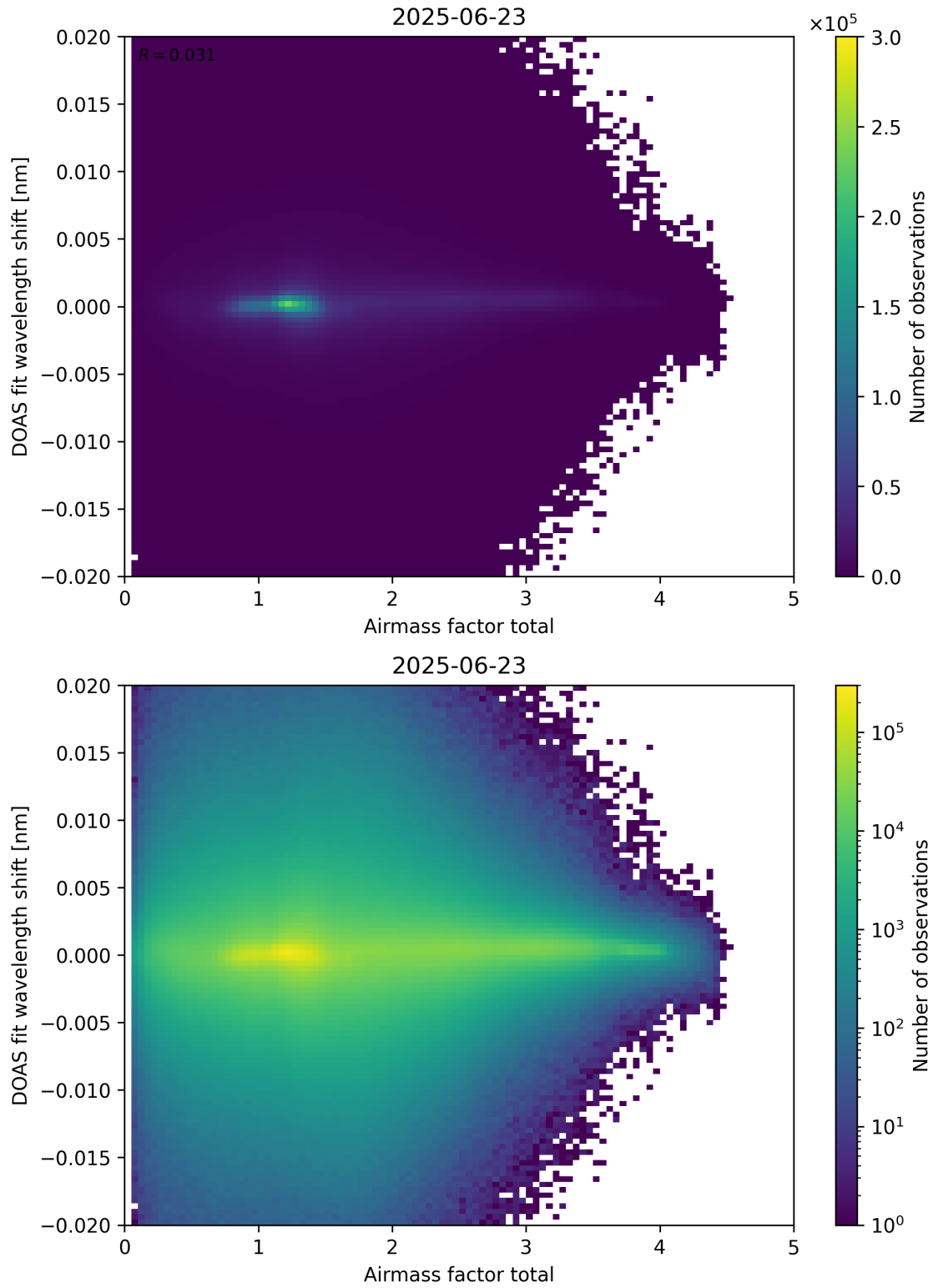
Figure 98: Scatter density plot of “Airmass factor total” against “DOAS fit wavelength shift” for 2025-06-22 to 2025-06-24.
