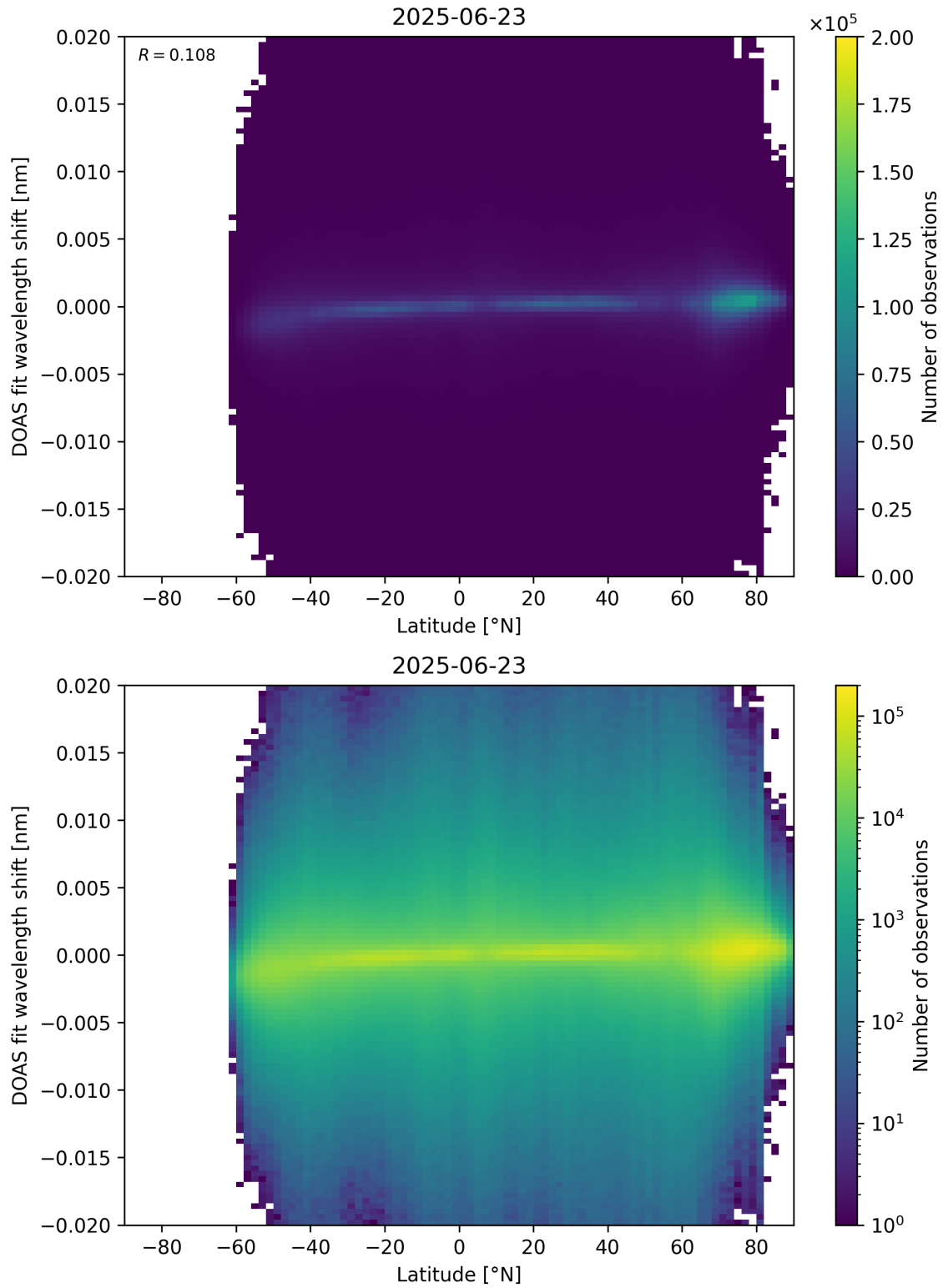
Figure 154: Scatter density plot of “Latitude” against “DOAS fit wavelength shift” for 2025-06-22 to 2025-06-24.
