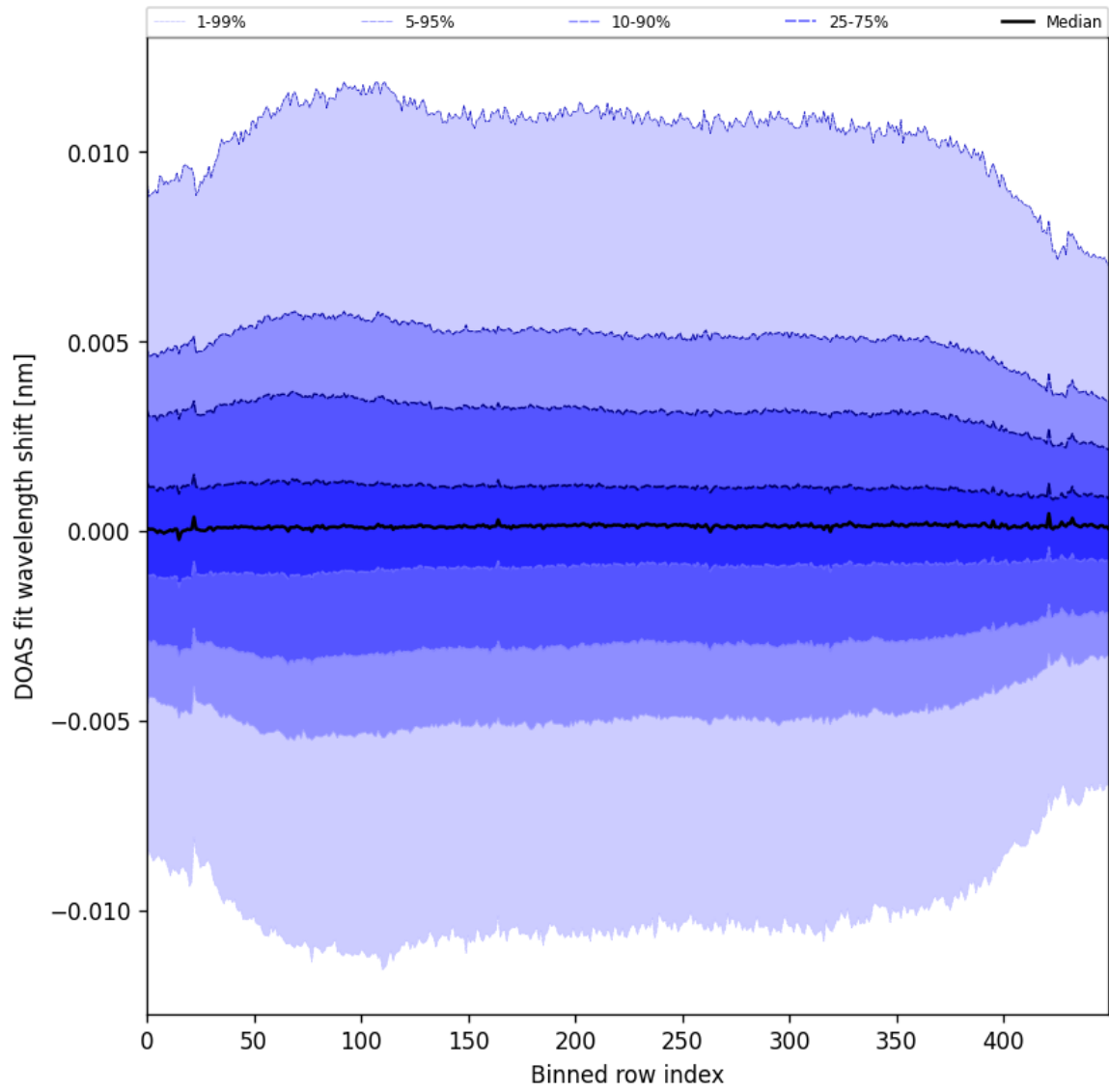
Figure 58: Along track statistics of “DOAS fit wavelength shift” for 2025-06-22 to 2025-06-24
