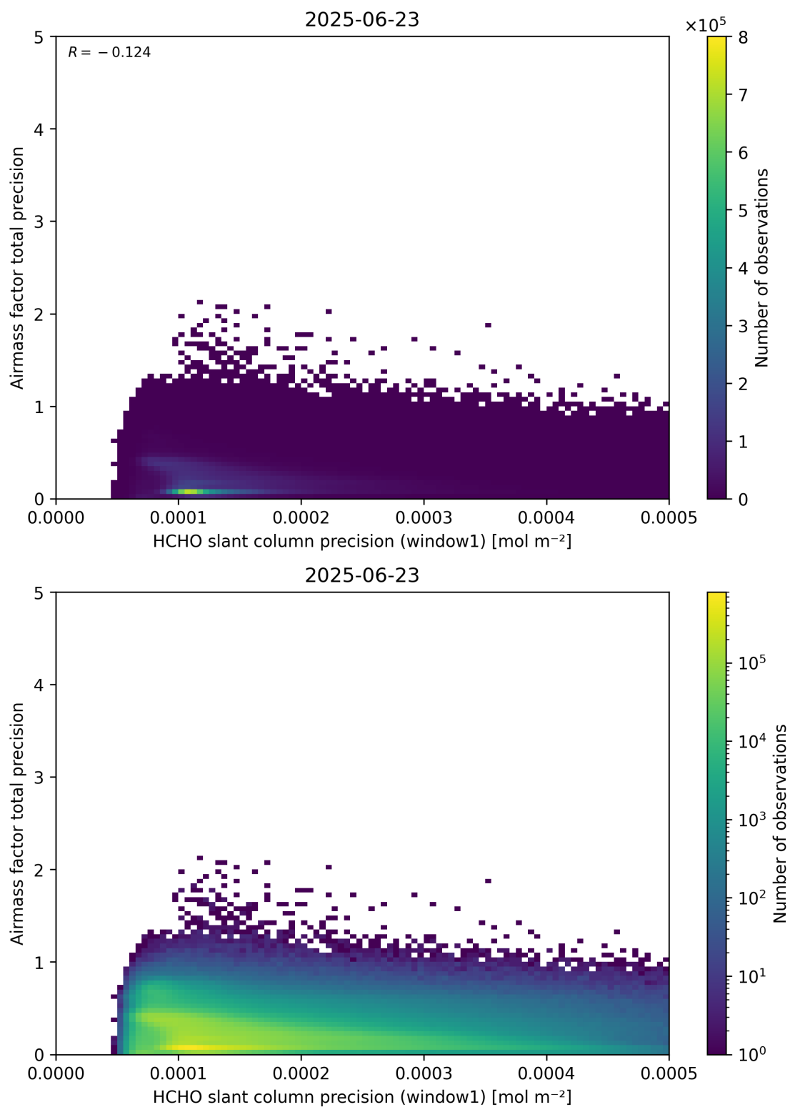
Figure 95: Scatter density plot of “HCHO slant column precision (window1)” against “Airmass factor total precision” for 2025-06-22 to 2025-06-24.
