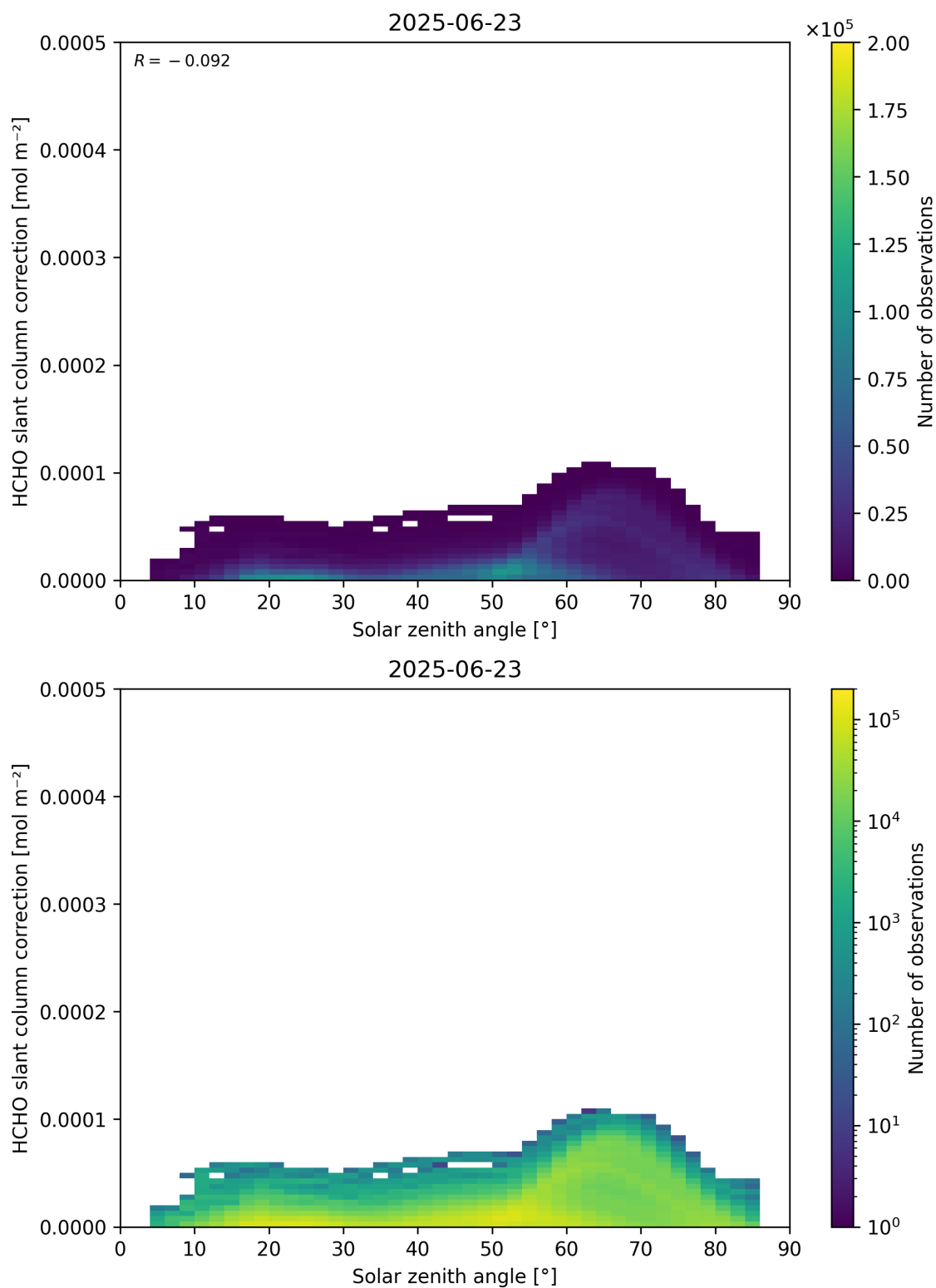
Figure 172: Scatter density plot of “Solar zenith angle” against “HCHO slant column correction” for 2025-06-22 to 2025-06-24.
