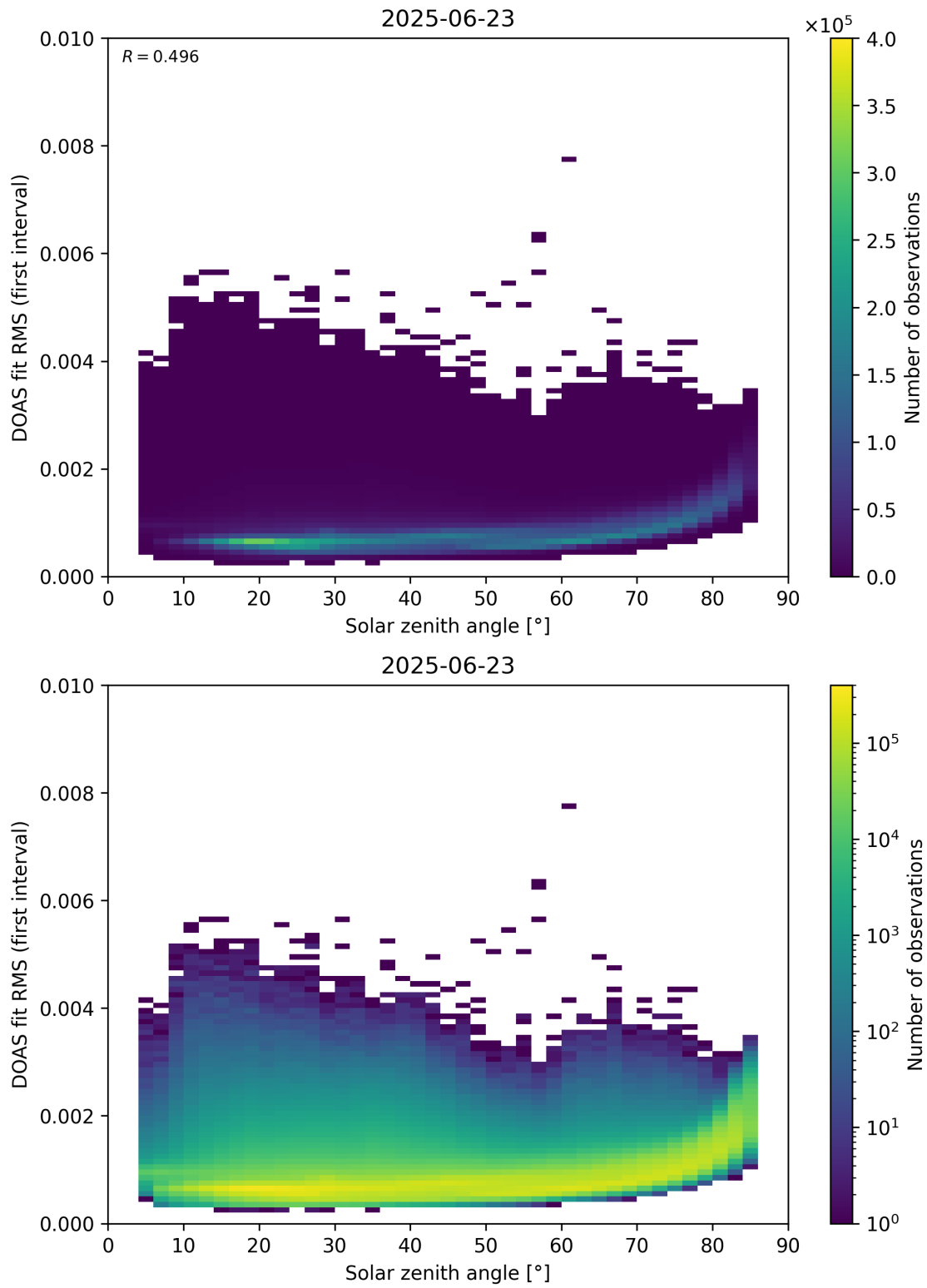
Figure 167: Scatter density plot of “Solar zenith angle” against “DOAS fit RMS (first interval)” for 2025-06-22 to 2025-06-24.
