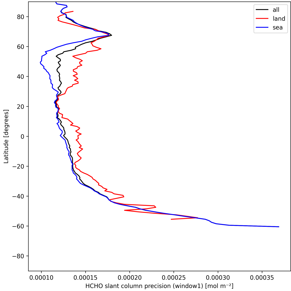
Figure 25: Zonal average of “HCHO slant column precision (window1)” for 2025-06-22 to 2025-06-24.
