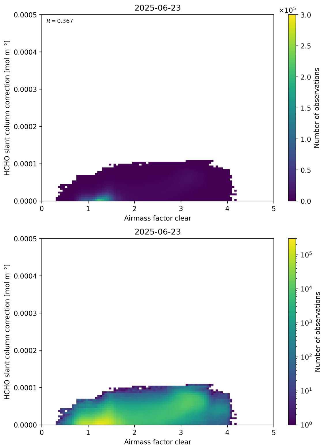
Figure 75: Scatter density plot of “Airmass factor clear” against “HCHO slant column correction” for 2025-06-22 to 2025-06-24.
