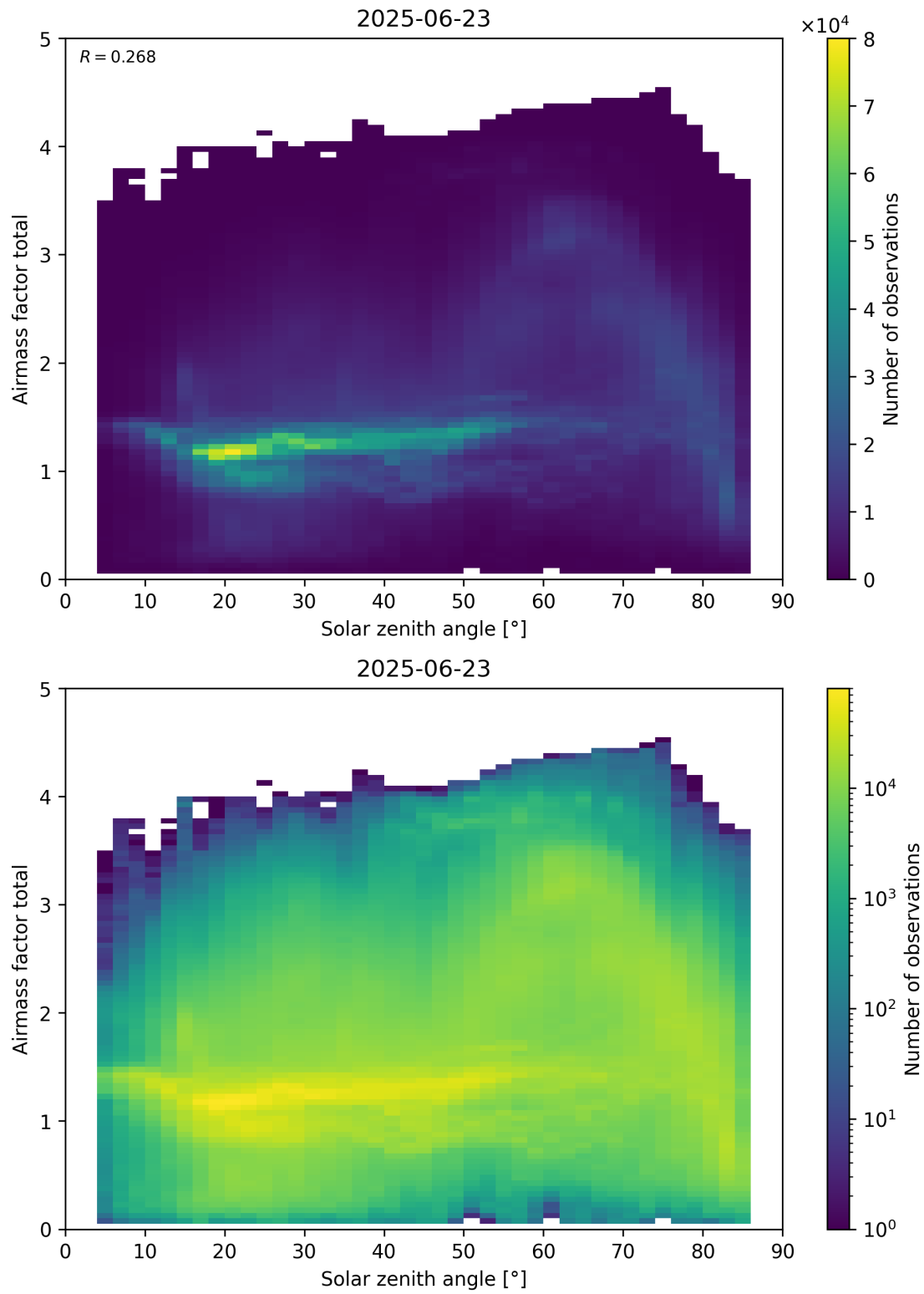
Figure 175: Scatter density plot of “Solar zenith angle” against “Airmass factor total” for 2025-06-22 to 2025-06-24.
