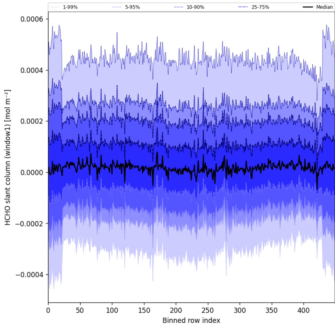
Figure 52: Along track statistics of “HCHO slant column (window1)” for 2025-06-22 to 2025-06-24
