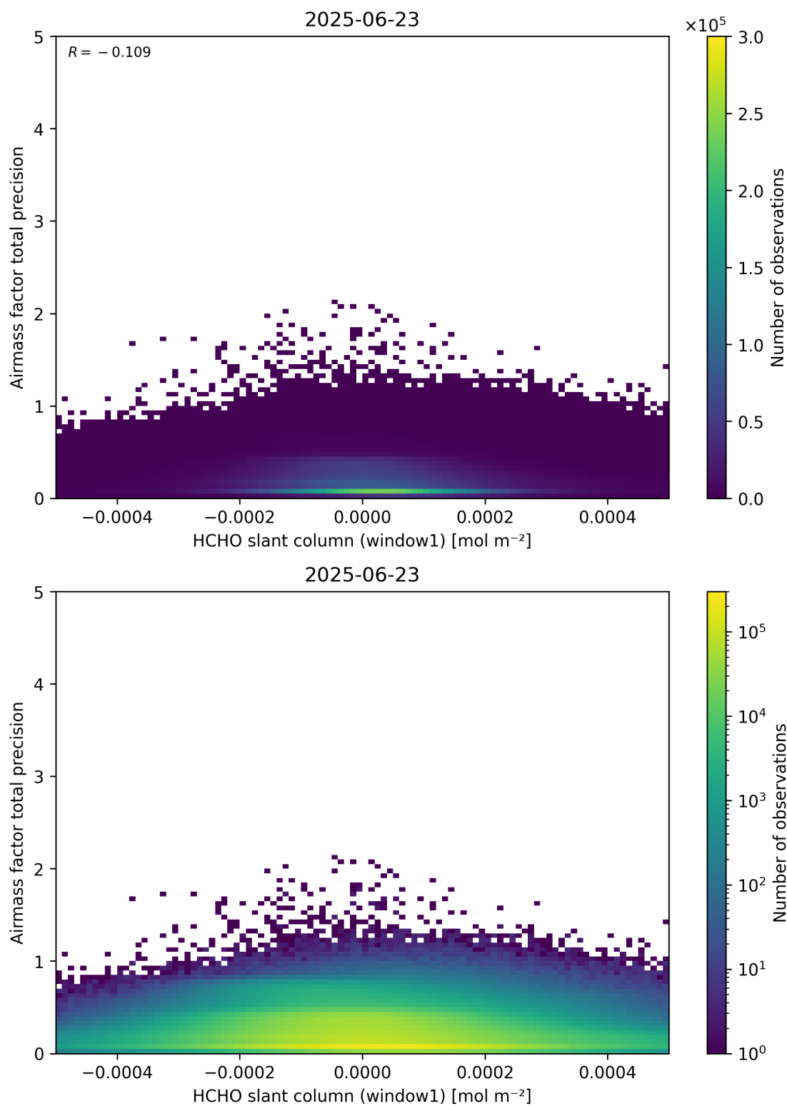
Figure 86: Scatter density plot of “HCHO slant column (window1)” against “Airmass factor total precision” for 2025-06-22 to 2025-06-24.
