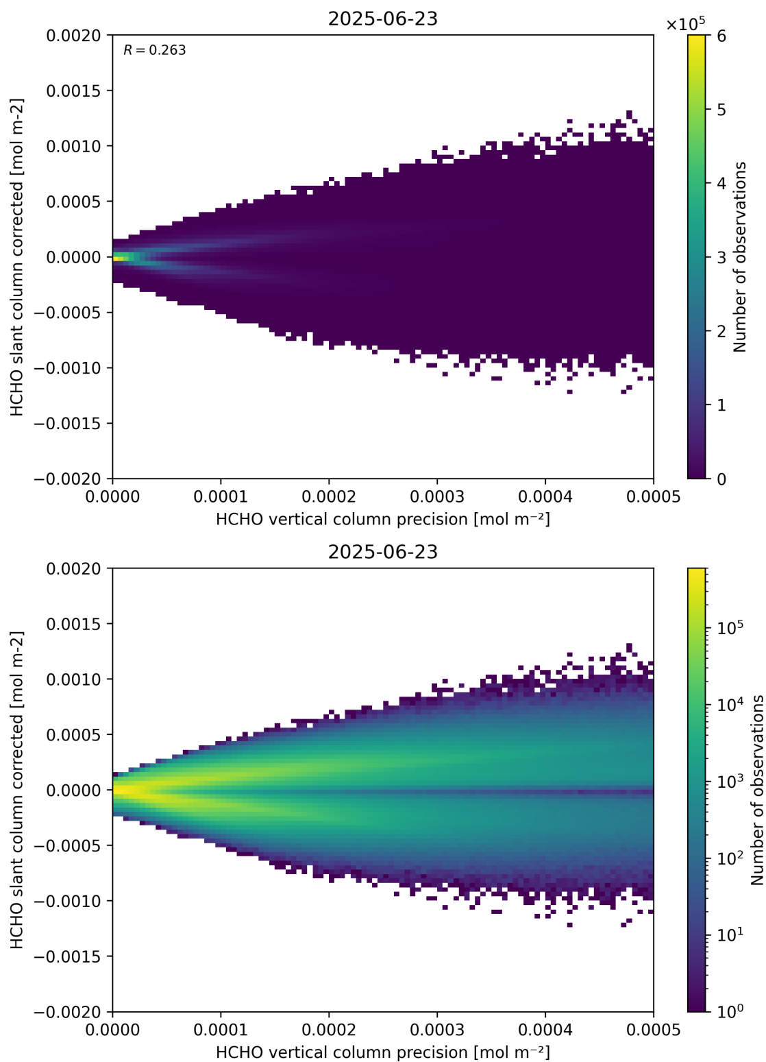
Figure 140: Scatter density plot of “HCHO vertical column precision” against “HCHO slant column corrected” for 2025-06-22 to 2025-06-24.
