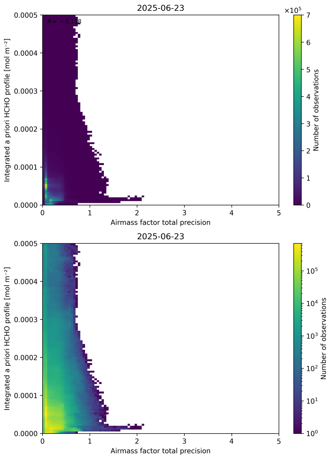
Figure 111: Scatter density plot of “Airmass factor total precision” against “Integrated a priori HCHO profile” for 2025-06-22 to 2025-06-24.
