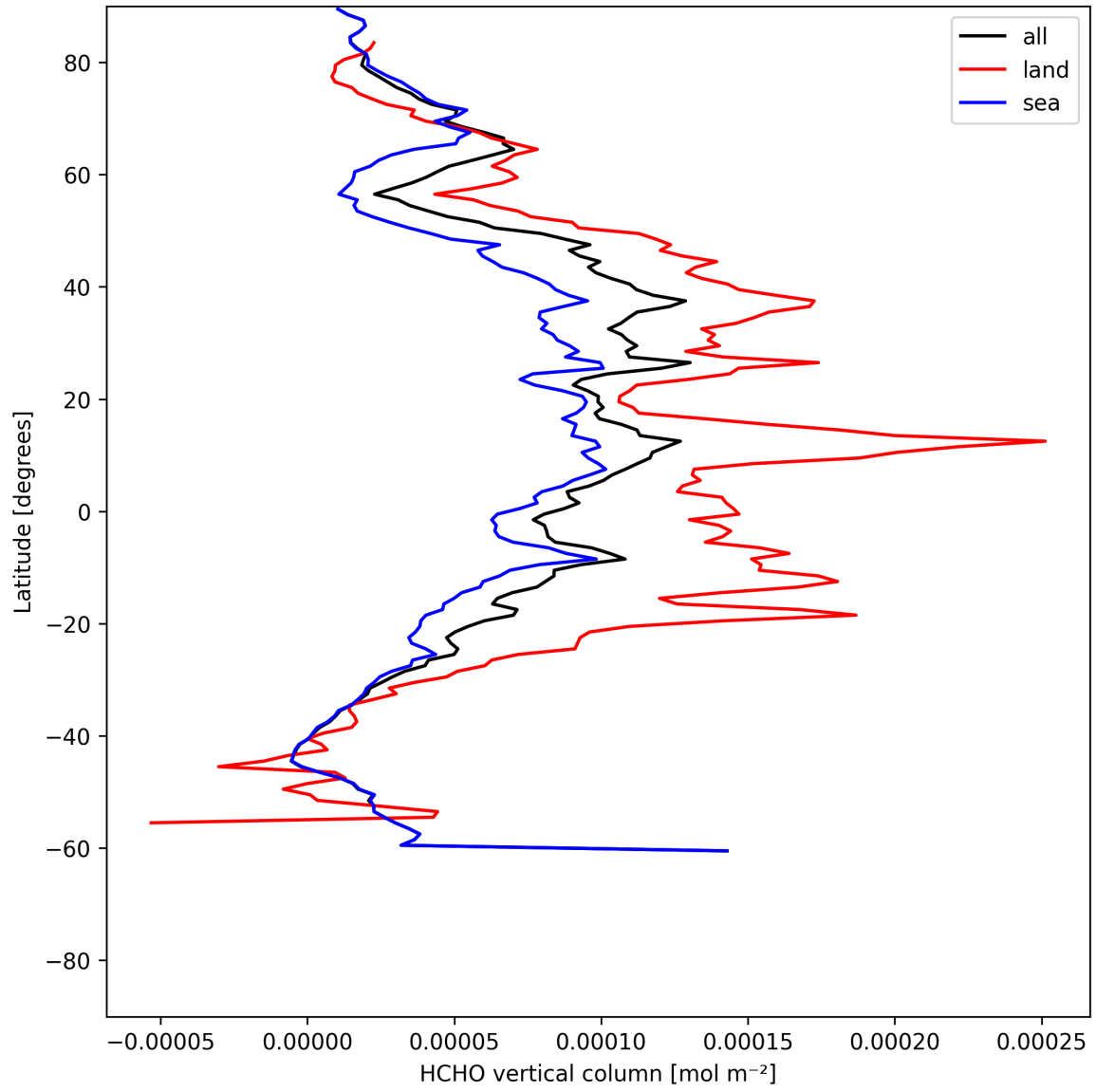
Figure 21: Zonal average of “HCHO vertical column” for 2025-06-22 to 2025-06-24.
