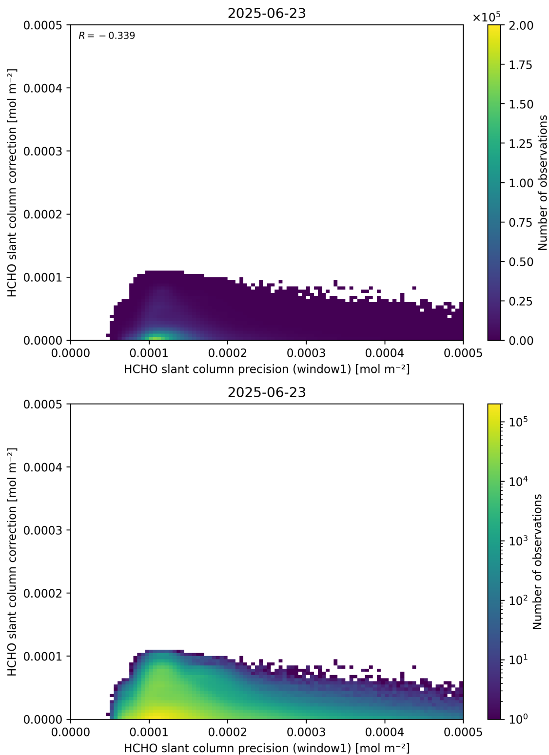
Figure 93: Scatter density plot of “HCHO slant column precision (window1)” against “HCHO slant column correction” for 2025-06-22 to 2025-06-24.
