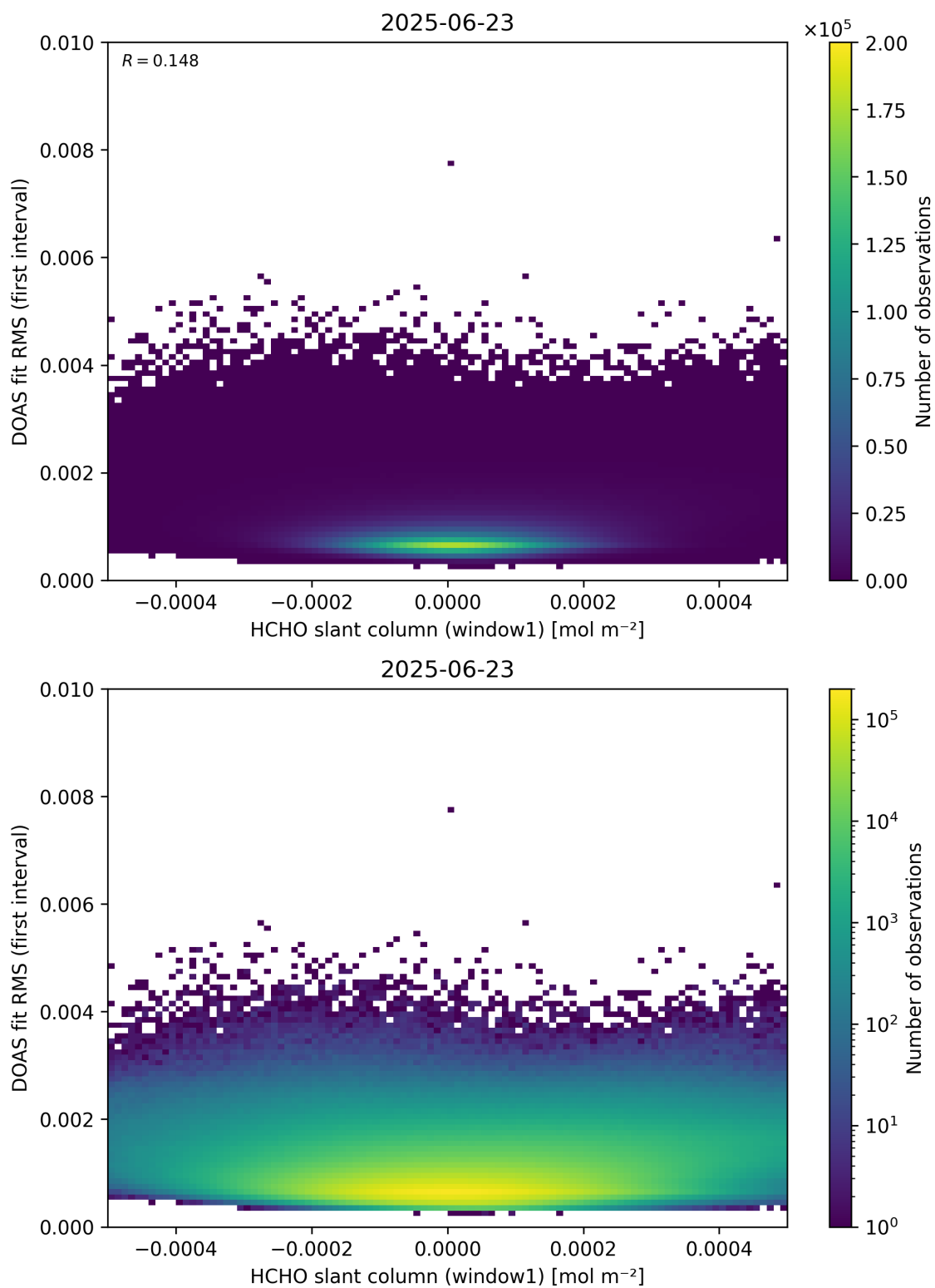
Figure 78: Scatter density plot of “HCHO slant column (window1)” against “DOAS fit RMS (first interval)” for 2025-06-22 to 2025-06-24.
