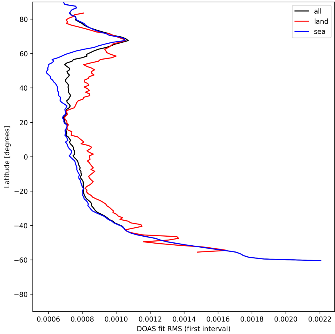
Figure 32: Zonal average of “DOAS fit RMS (first interval)” for 2025-06-22 to 2025-06-24.
