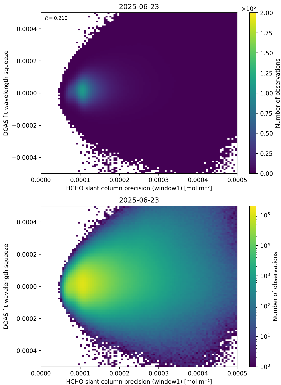
Figure 90: Scatter density plot of “HCHO slant column precision (window1)” against “DOAS fit wavelength squeeze” for 2025-06-22 to 2025-06-24.
