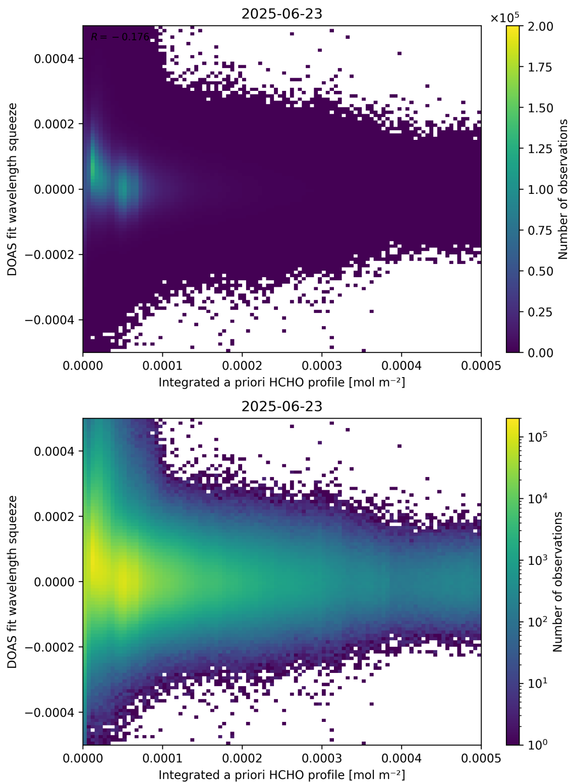
Figure 150: Scatter density plot of “Integrated a priori HCHO profile” against “DOAS fit wavelength squeeze” for 2025-06-22 to 2025-06-24.
