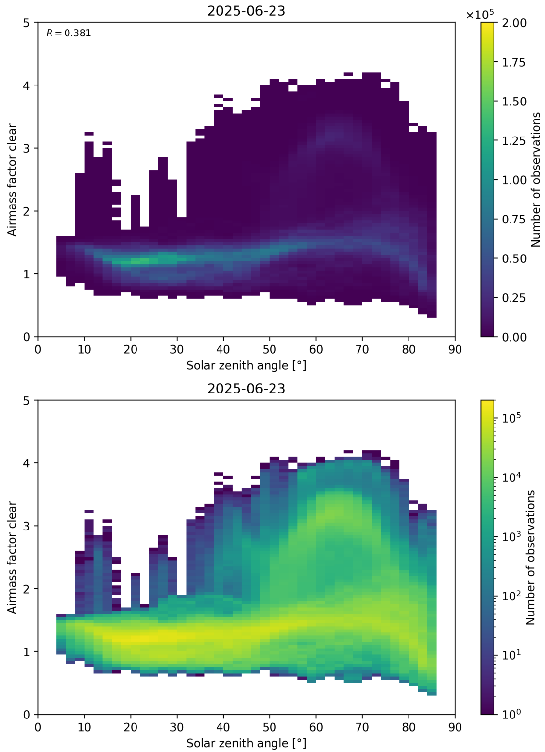
Figure 170: Scatter density plot of “Solar zenith angle” against “Airmass factor clear” for 2025-06-22 to 2025-06-24.
