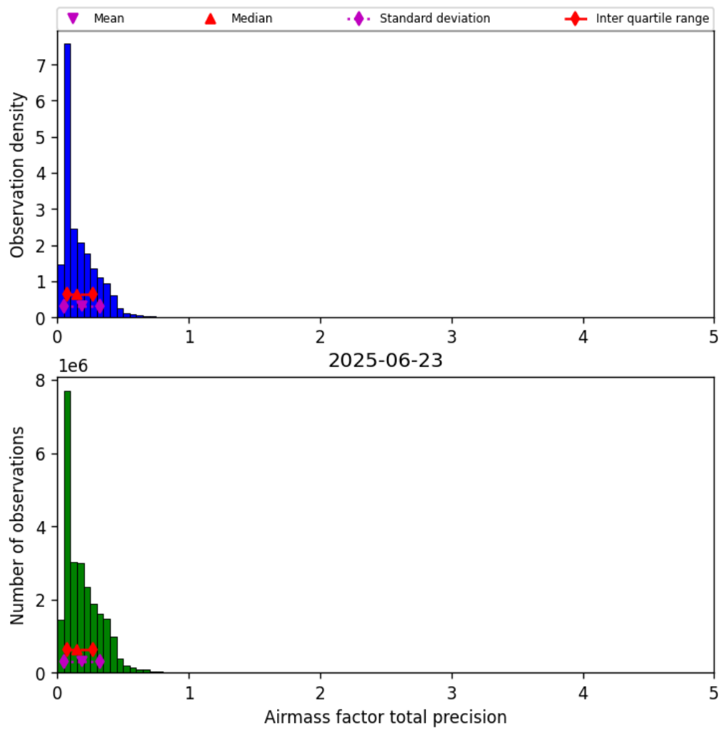
Figure 41: Histogram of “Airmass factor total precision” for 2025-06-22 to 2025-06-24
