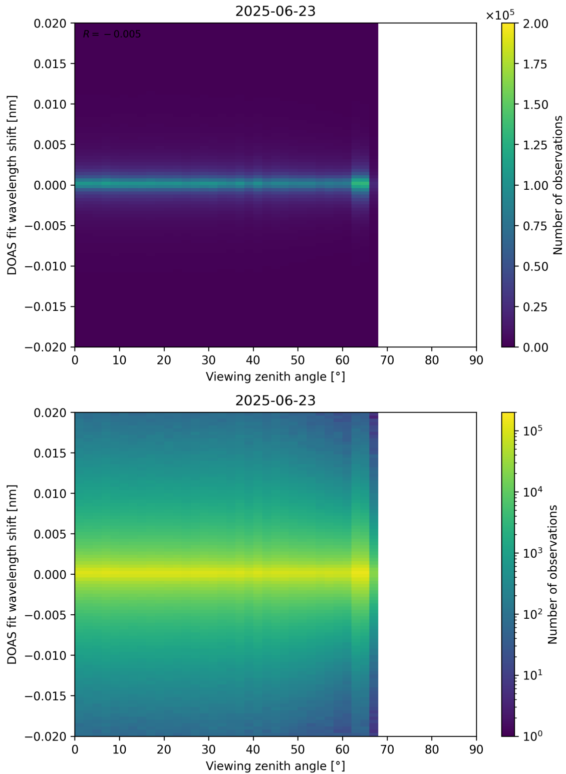
Figure 183: Scatter density plot of “Viewing zenith angle” against “DOAS fit wavelength shift” for 2025-06-22 to 2025-06-24.
