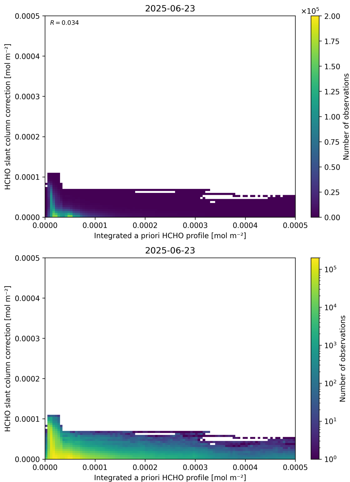
Figure 152: Scatter density plot of “Integrated a priori HCHO profile” against “HCHO slant column correction” for 2025-06-22 to 2025-06-24.
