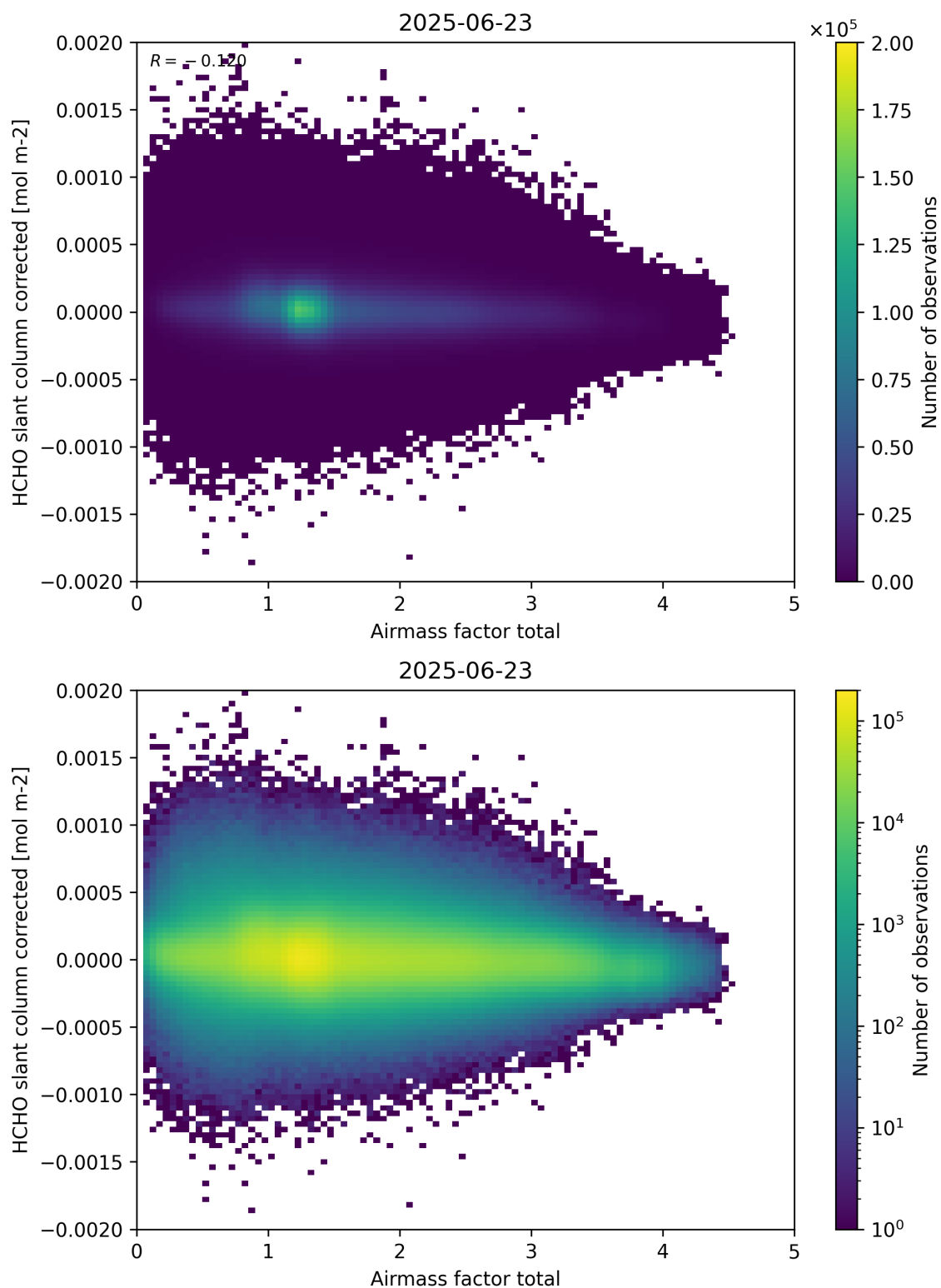
Figure 101: Scatter density plot of “Airmass factor total” against “HCHO slant column corrected” for 2025-06-22 to 2025-06-24.
