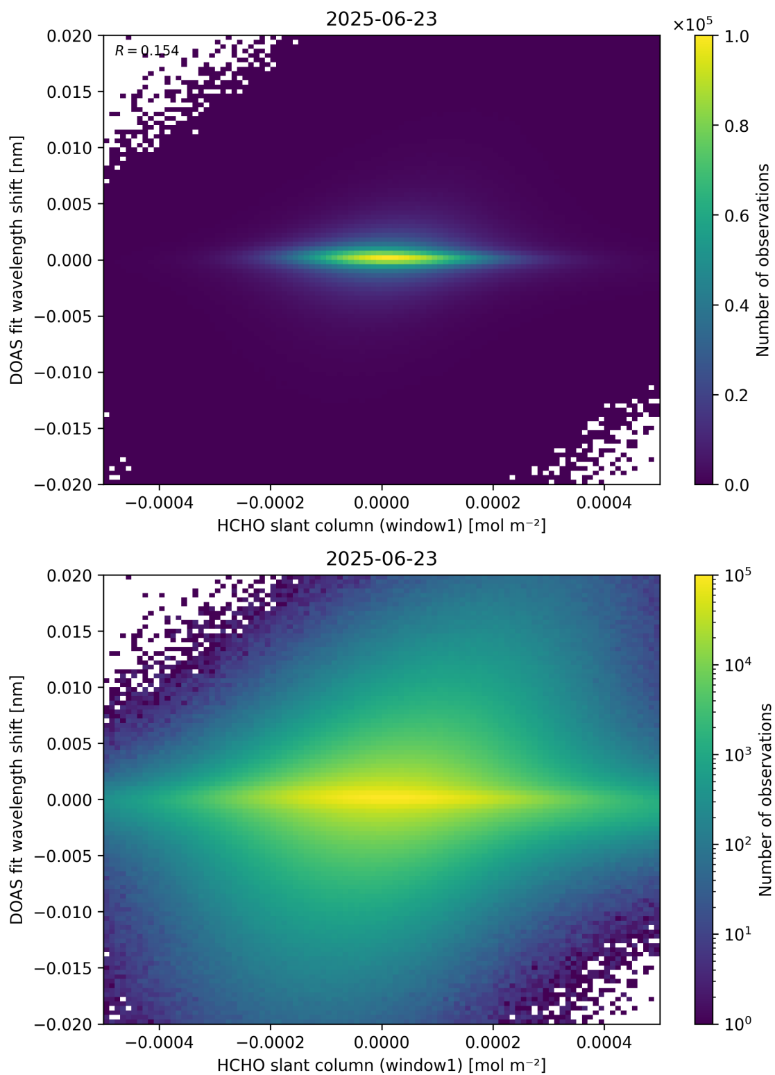
Figure 79: Scatter density plot of “HCHO slant column (window1)” against “DOAS fit wavelength shift” for 2025-06-22 to 2025-06-24.
