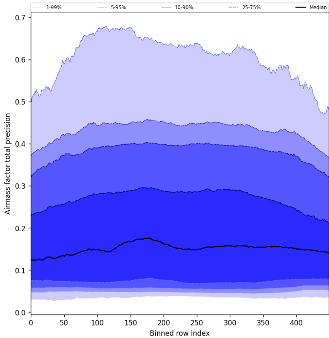
Figure 55: Along track statistics of “Airmass factor total precision” for 2025-06-22 to 2025-06-24
