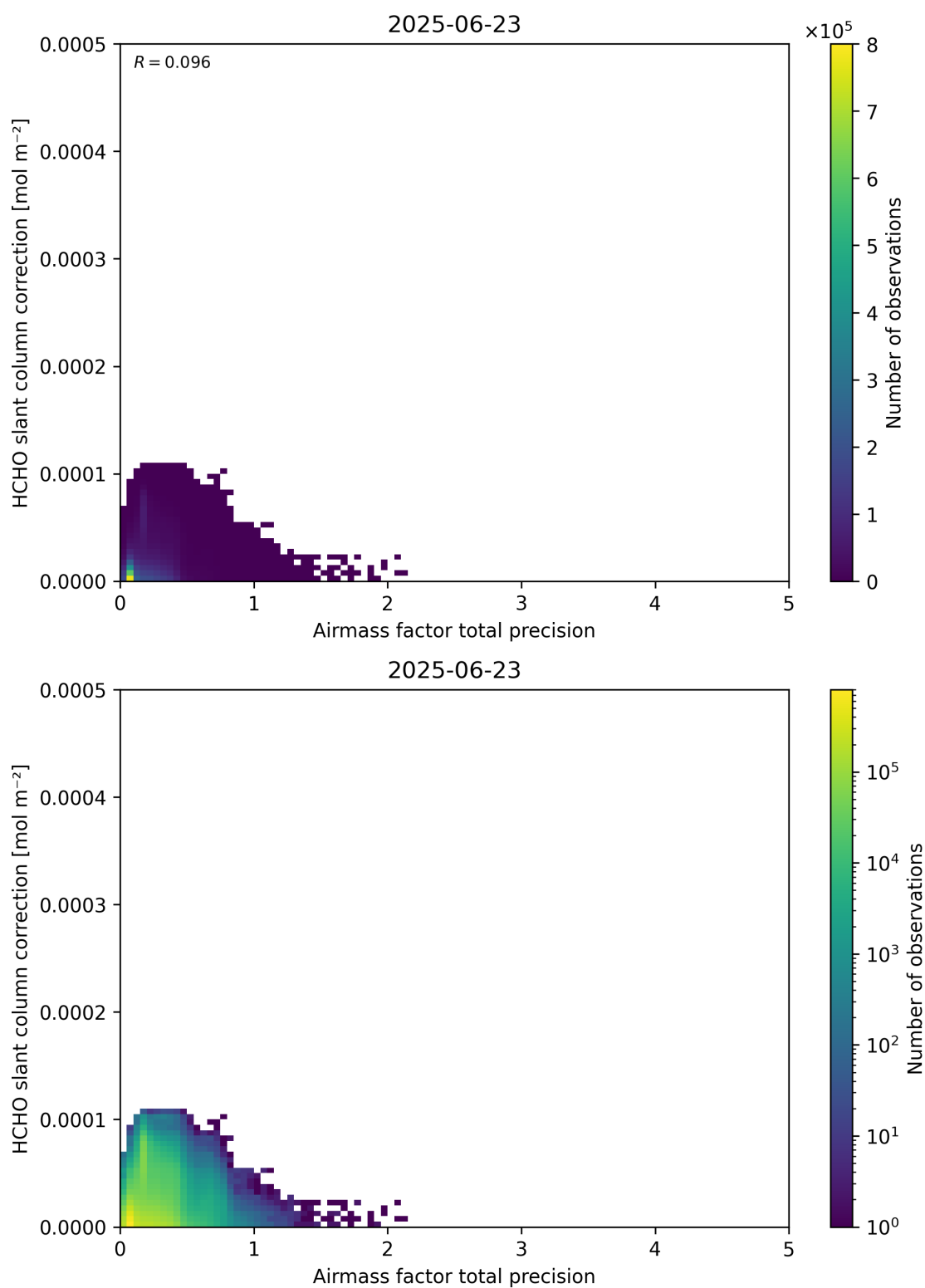
Figure 110: Scatter density plot of “Airmass factor total precision” against “HCHO slant column correction” for 2025-06-22 to 2025-06-24.
