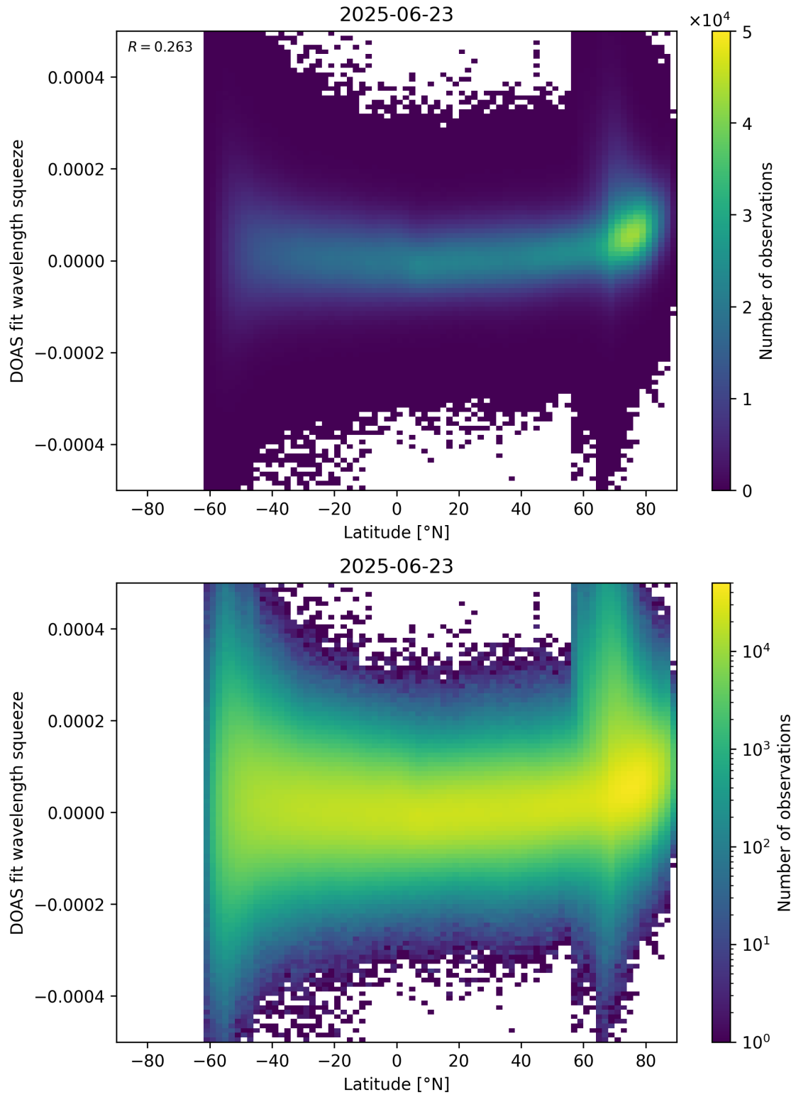
Figure 155: Scatter density plot of “Latitude” against “DOAS fit wavelength squeeze” for 2025-06-22 to 2025-06-24.
