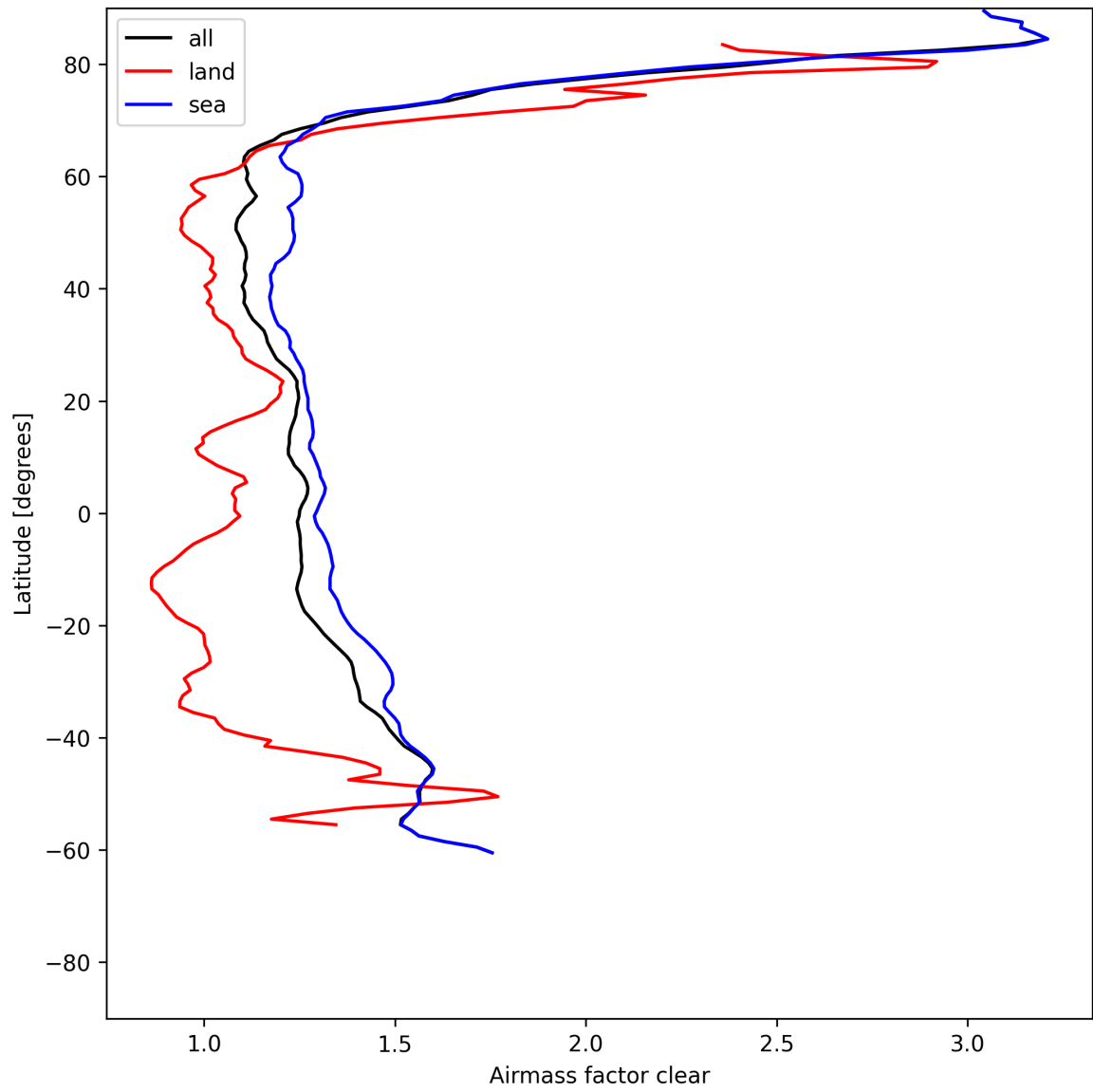
Figure 28: Zonal average of “Airmass factor clear” for 2025-06-22 to 2025-06-24.
