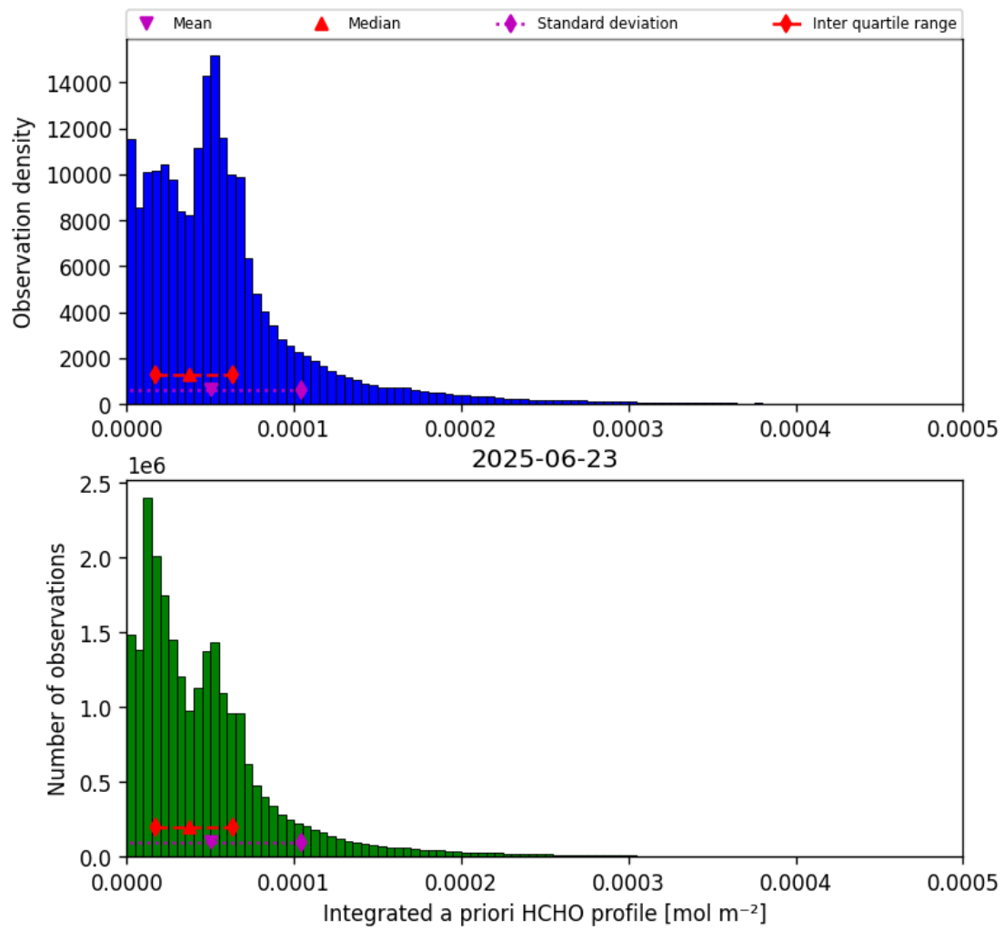
Figure 43: Histogram of “Integrated a priori HCHO profile” for 2025-06-22 to 2025-06-24
