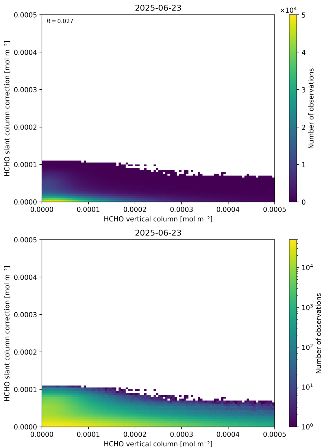
Figure 128: Scatter density plot of “HCHO vertical column” against “HCHO slant column correction” for 2025-06-22 to 2025-06-24.
