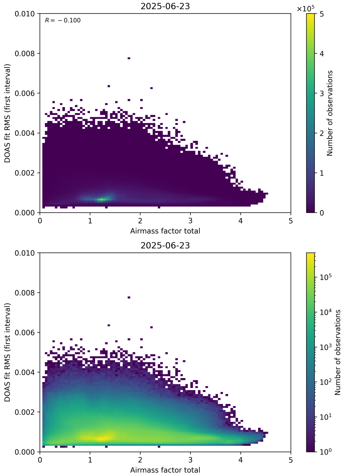
Figure 97: Scatter density plot of “Airmass factor total” against “DOAS fit RMS (first interval)” for 2025-06-22 to 2025-06-24.
