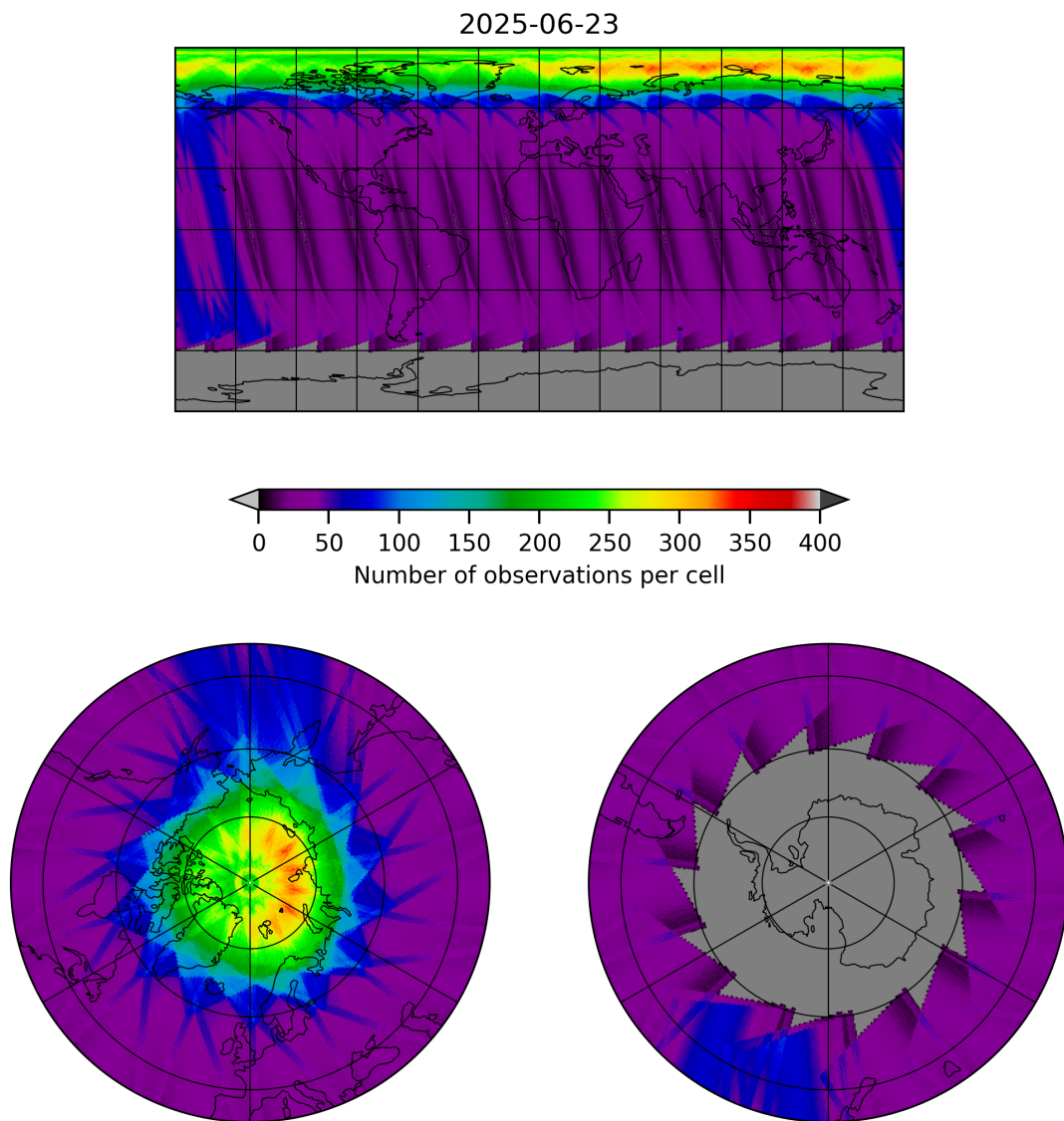
Figure 19: Map of the number of observations for 2025-06-22 to 2025-06-24
