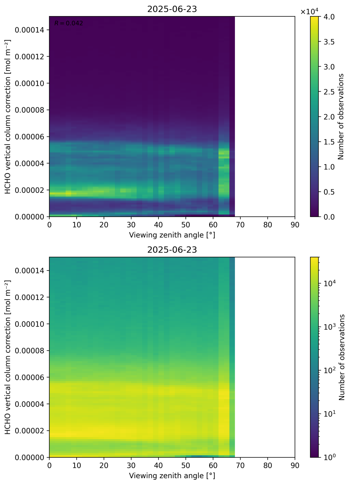
Figure 193: Scatter density plot of “Viewing zenith angle” against “HCHO vertical column correction” for 2025-06-22 to 2025-06-24.
