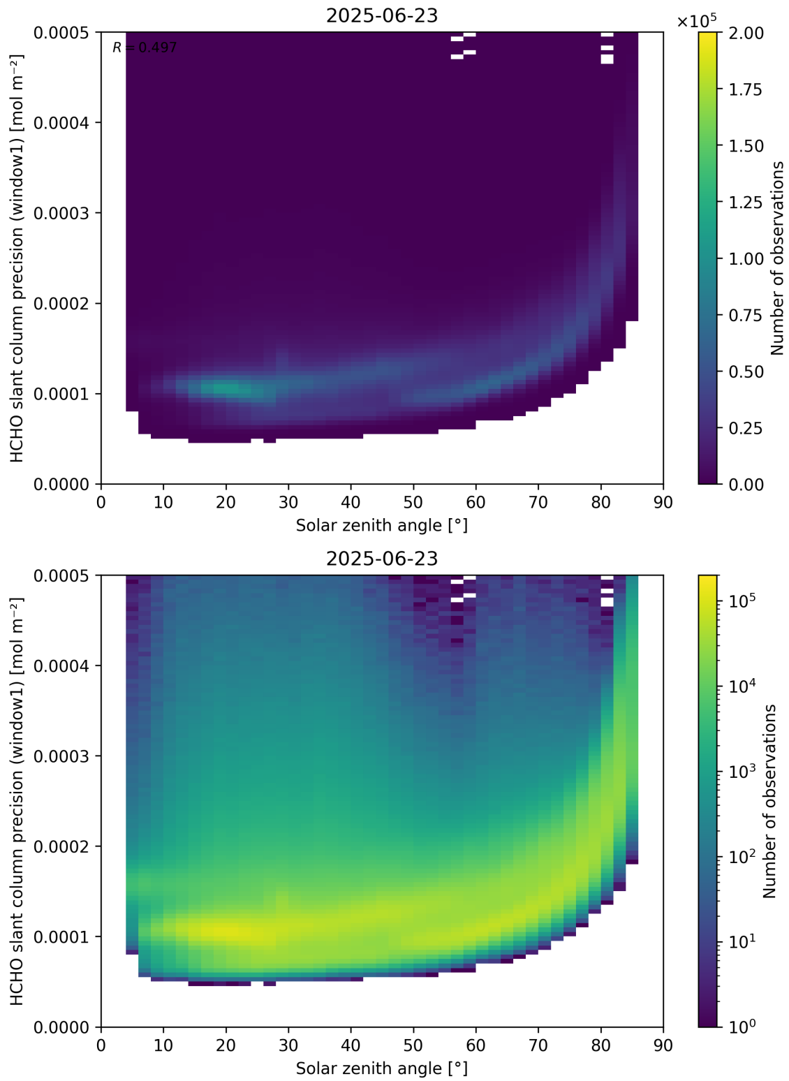
Figure 174: Scatter density plot of “Solar zenith angle” against “HCHO slant column precision (window1)” for 2025-06-22 to 2025-06-24.
