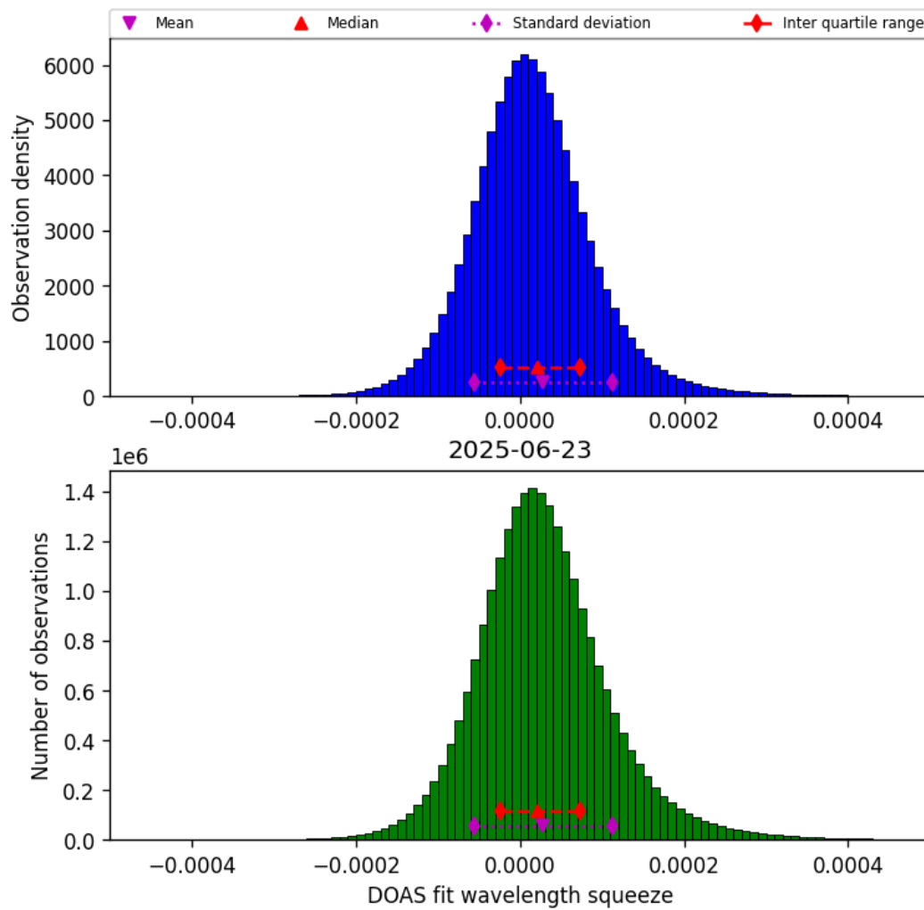
Figure 45: Histogram of “DOAS fit wavelength squeeze” for 2025-06-22 to 2025-06-24
