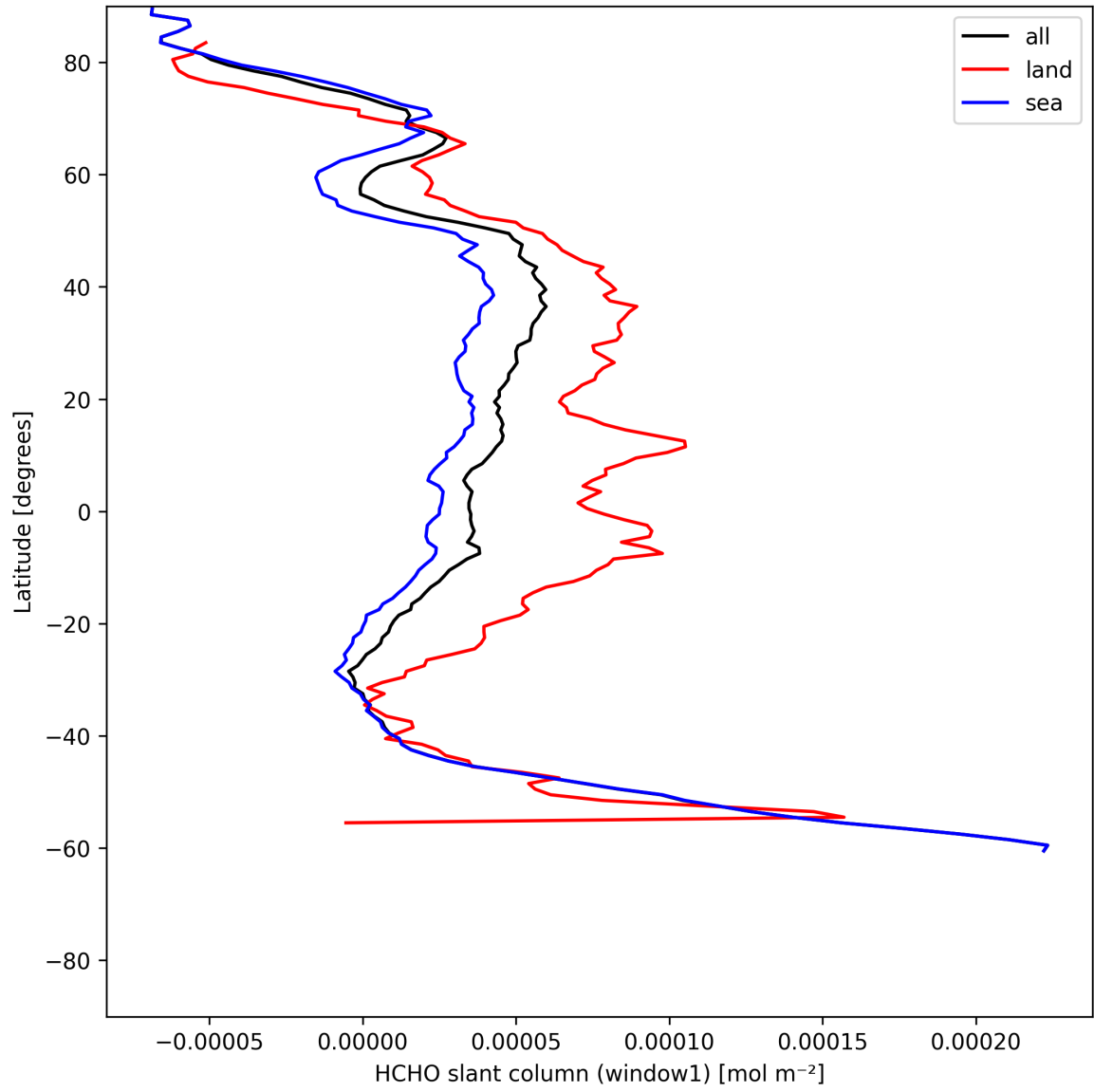
Figure 24: Zonal average of “HCHO slant column (window1)” for 2025-06-22 to 2025-06-24.
