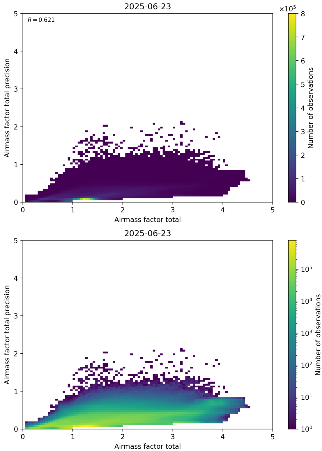
Figure 103: Scatter density plot of “Airmass factor total” against “Airmass factor total precision” for 2025-06-22 to 2025-06-24.
