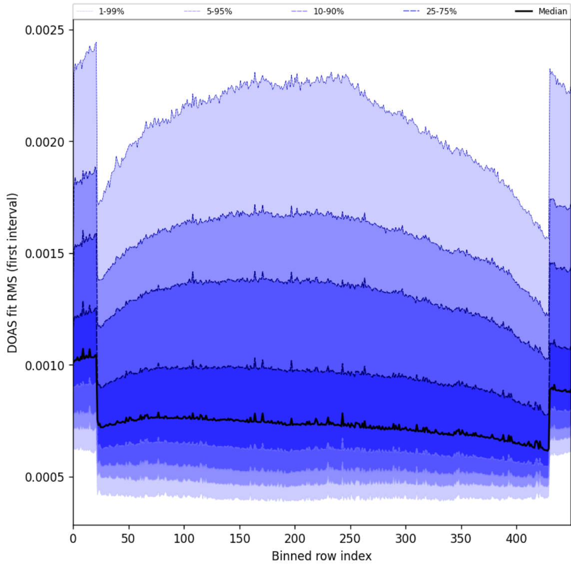
Figure 60: Along track statistics of “DOAS fit RMS (first interval)” for 2025-06-22 to 2025-06-24
