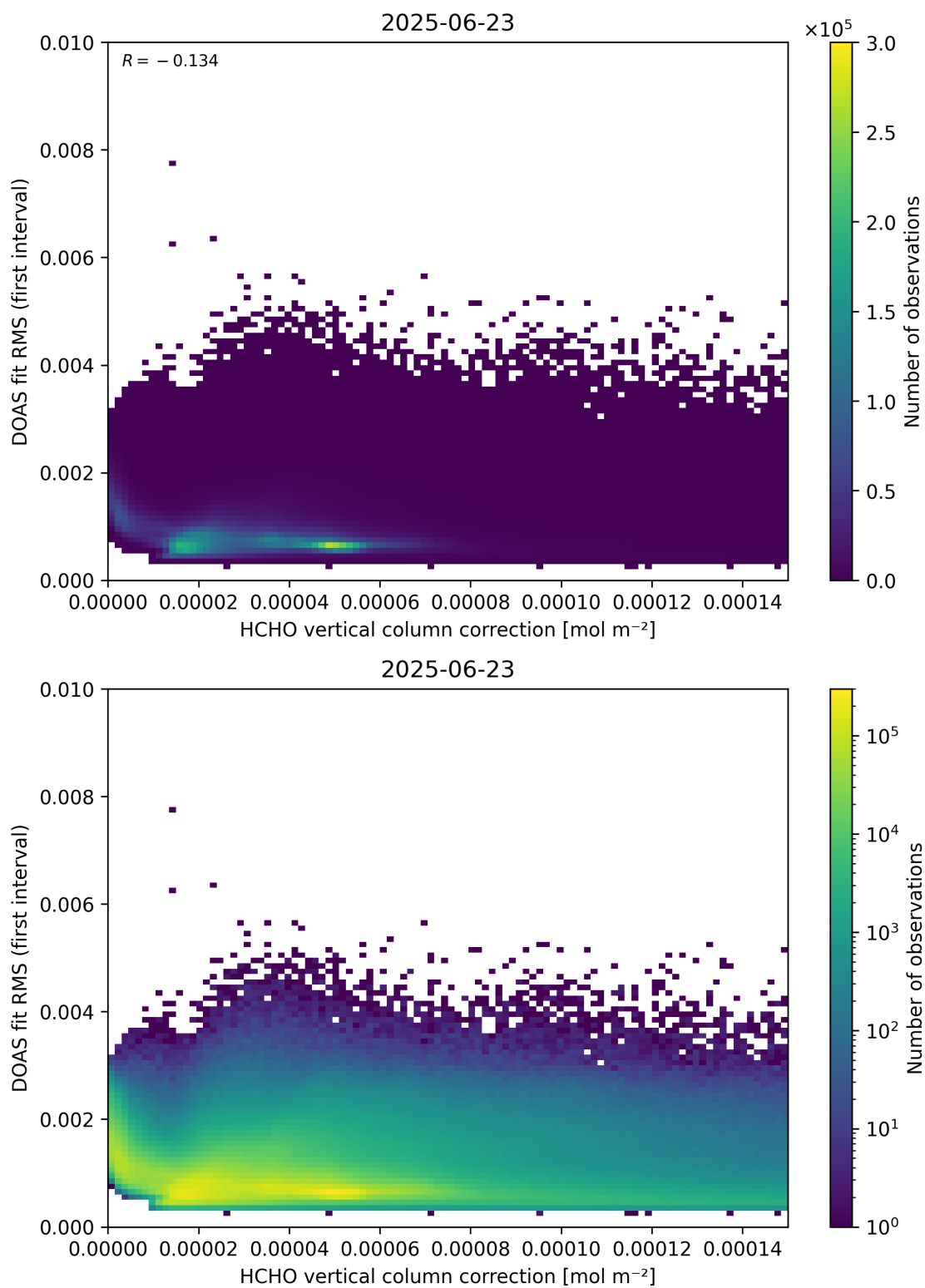
Figure 112: Scatter density plot of “HCHO vertical column correction” against “DOAS fit RMS (first interval)” for 2025-06-22 to 2025-06-24.
