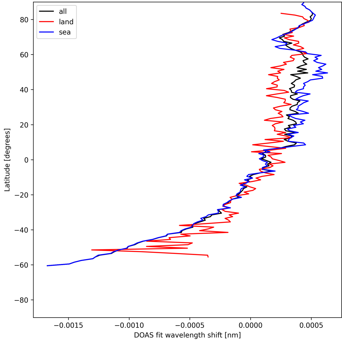
Figure 30: Zonal average of “DOAS fit wavelength shift” for 2025-06-22 to 2025-06-24.
