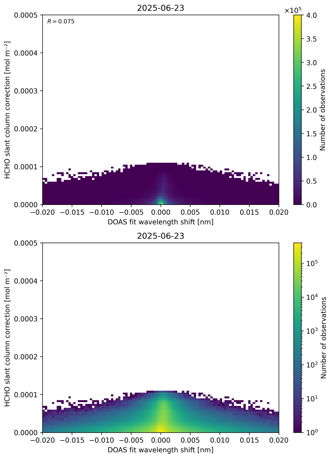
Figure 67: Scatter density plot of “DOAS fit wavelength shift” against “HCHO slant column correction” for 2025-06-22 to 2025-06-24.
