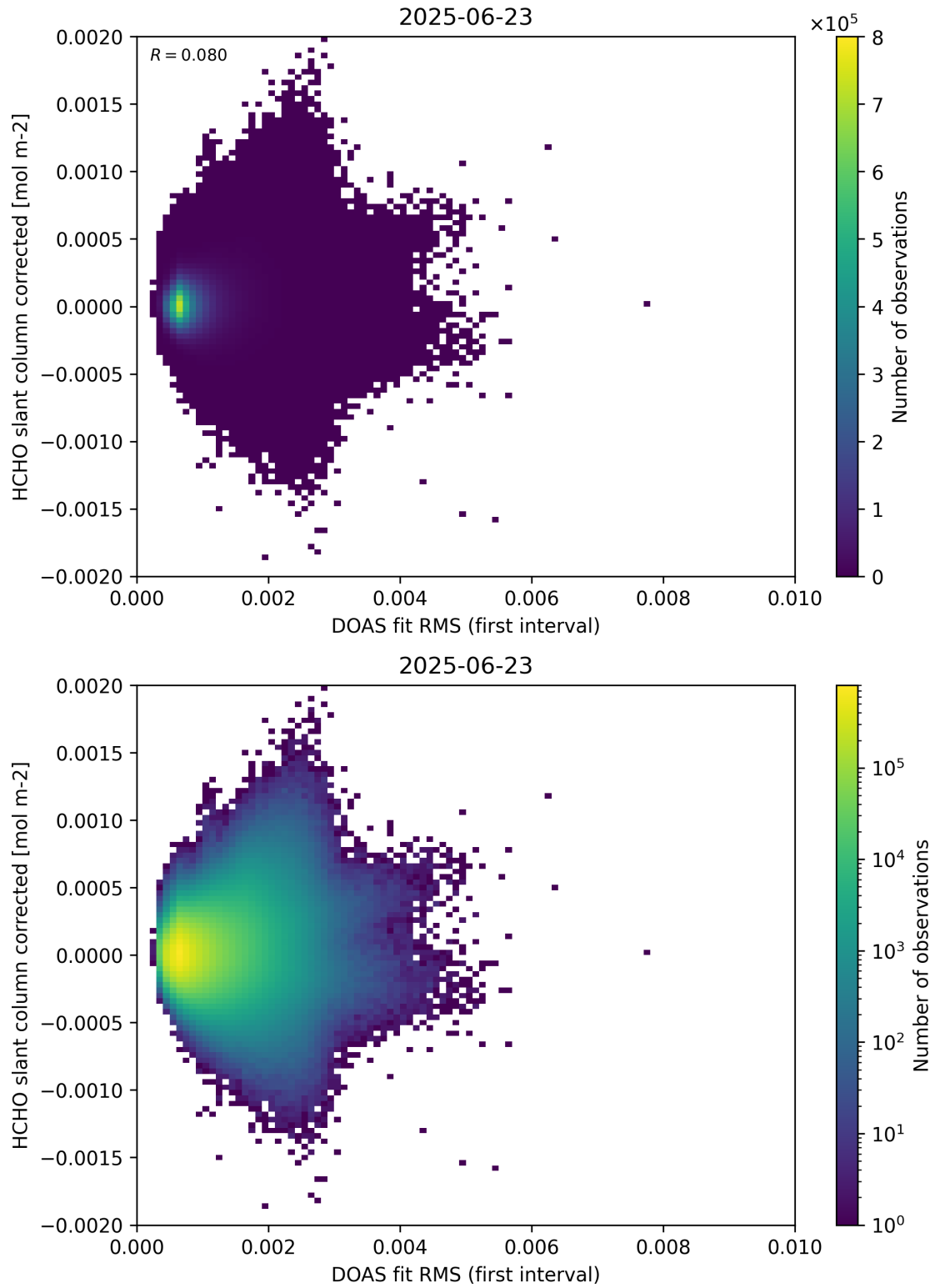
Figure 62: Scatter density plot of “DOAS fit RMS (first interval)” against “HCHO slant column corrected” for 2025-06-22 to 2025-06-24.
