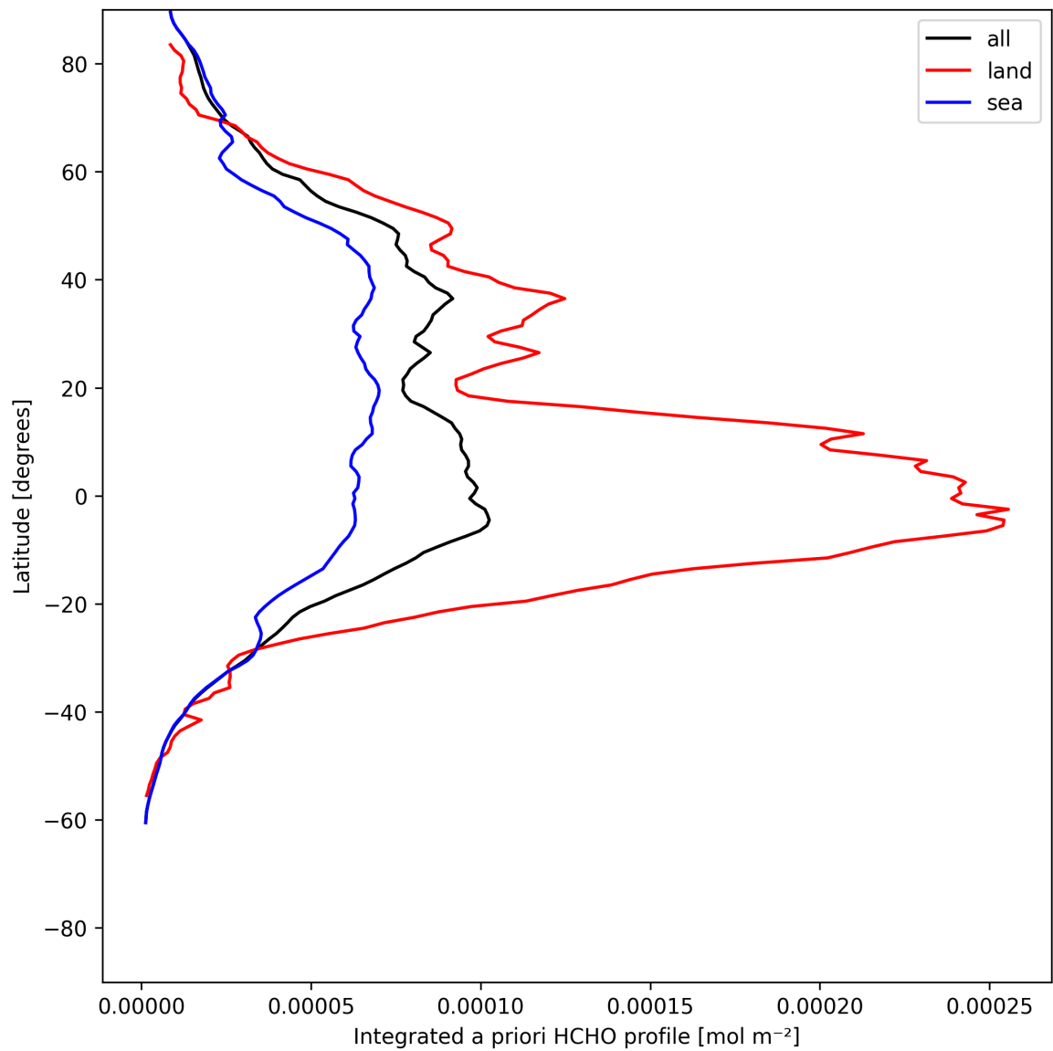
Figure 29: Zonal average of “Integrated a priori HCHO profile” for 2025-06-22 to 2025-06-24.
