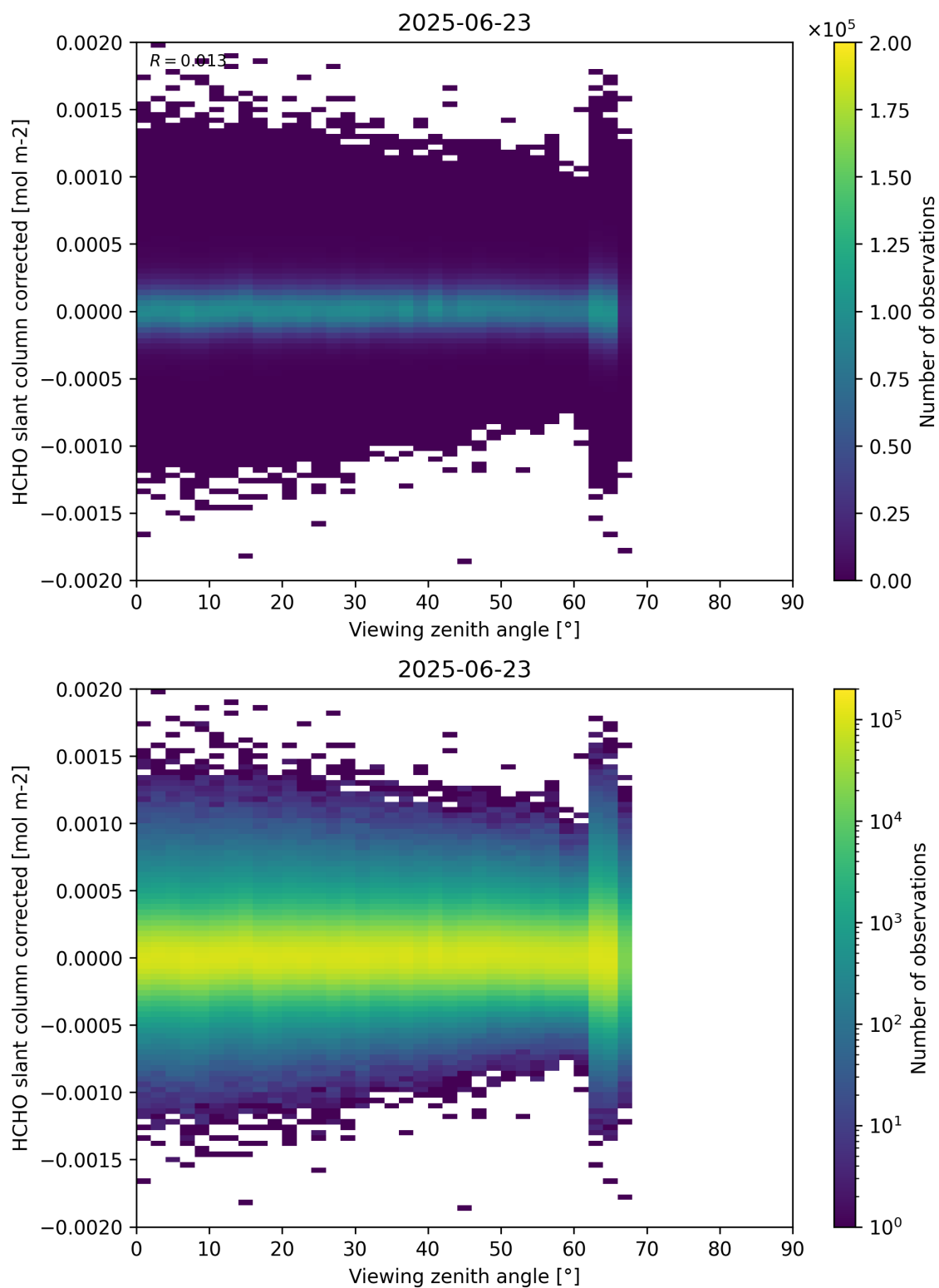
Figure 186: Scatter density plot of “Viewing zenith angle” against “HCHO slant column corrected” for 2025-06-22 to 2025-06-24.
