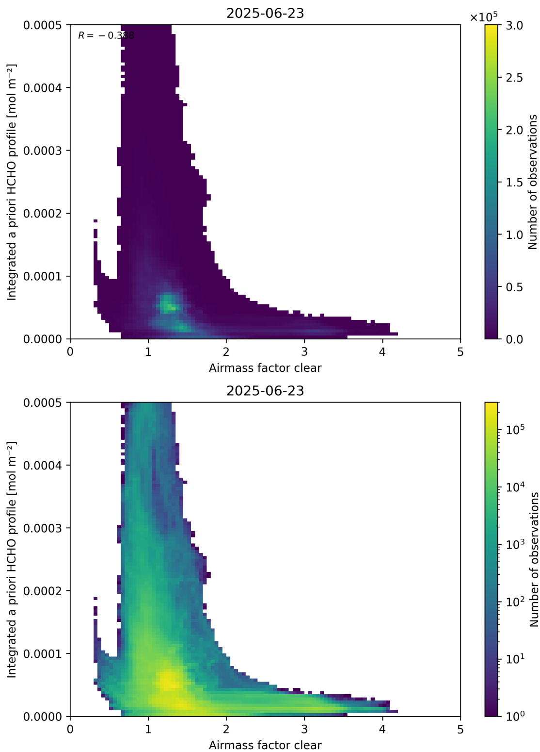
Figure 76: Scatter density plot of “Airmass factor clear” against “Integrated a priori HCHO profile” for 2025-06-22 to 2025-06-24.
