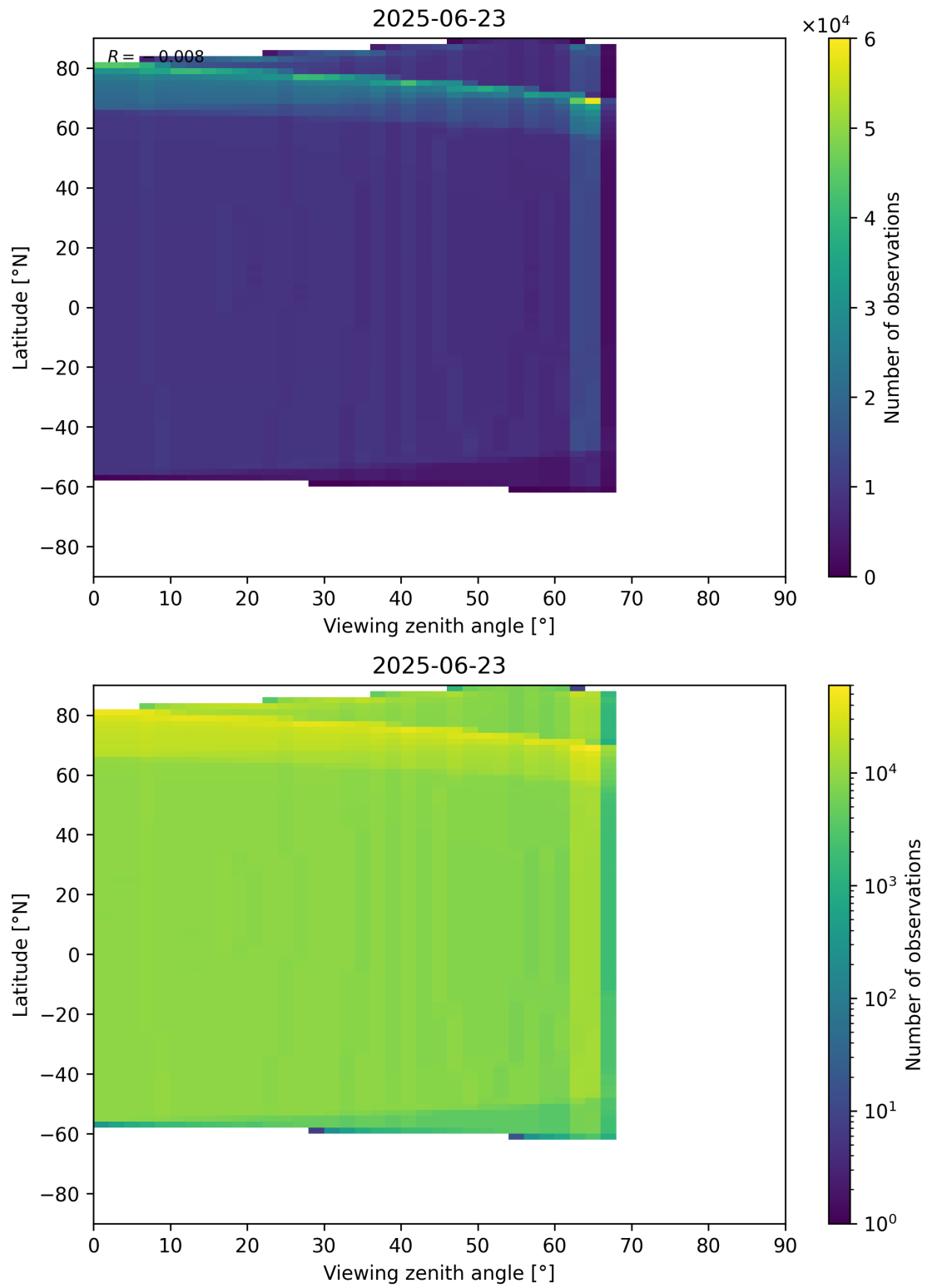
Figure 196: Scatter density plot of “Viewing zenith angle” against “Latitude” for 2025-06-22 to 2025-06-24.
