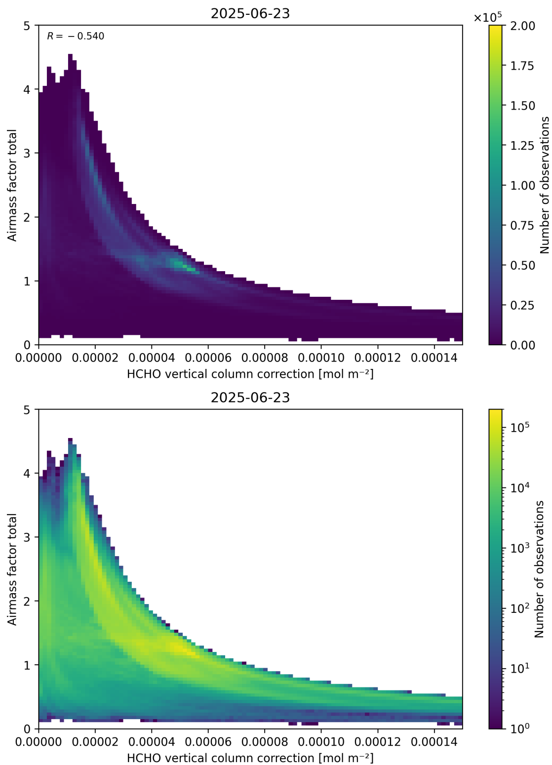
Figure 120: Scatter density plot of “HCHO vertical column correction” against “Airmass factor total” for 2025-06-22 to 2025-06-24.
