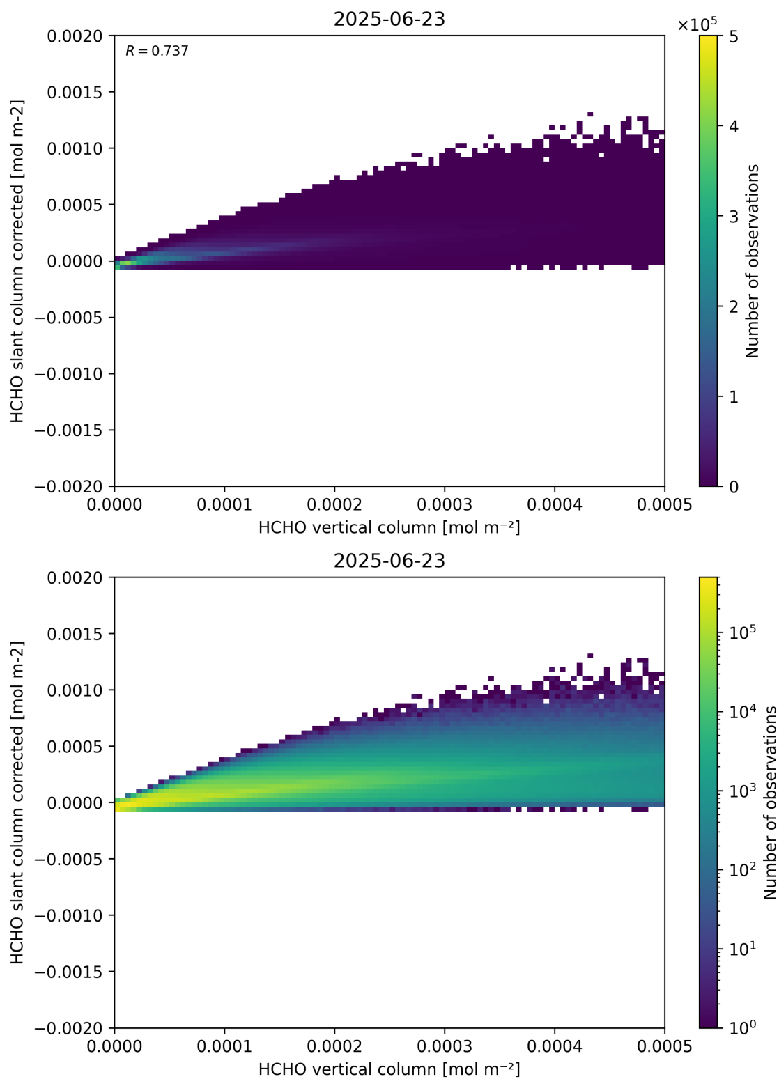
Figure 127: Scatter density plot of “HCHO vertical column” against “HCHO slant column corrected” for 2025-06-22 to 2025-06-24.
