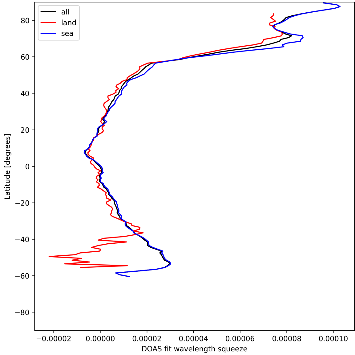
Figure 31: Zonal average of “DOAS fit wavelength squeeze” for 2025-06-22 to 2025-06-24.
