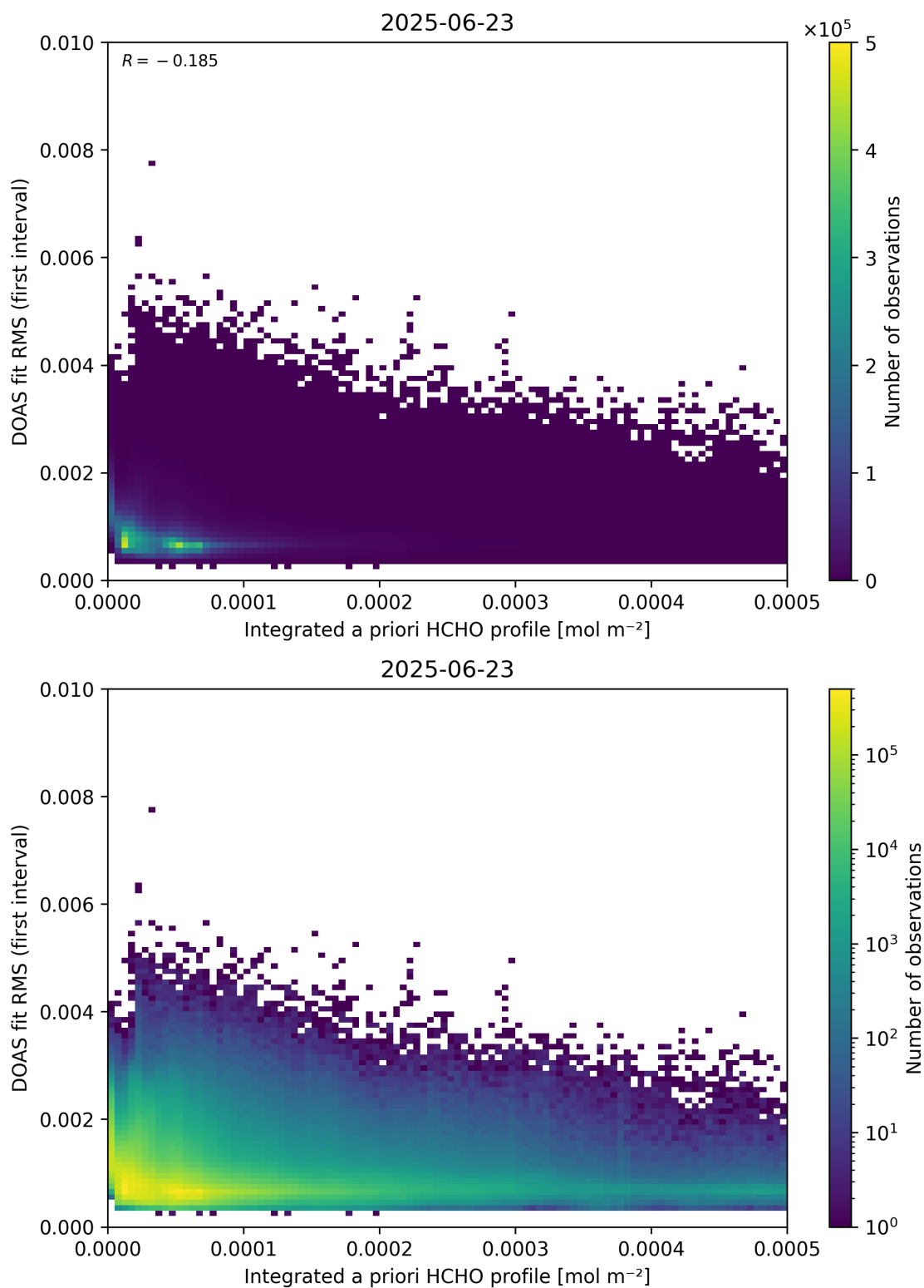
Figure 148: Scatter density plot of “Integrated a priori HCHO profile” against “DOAS fit RMS (first interval)” for 2025-06-22 to 2025-06-24.
