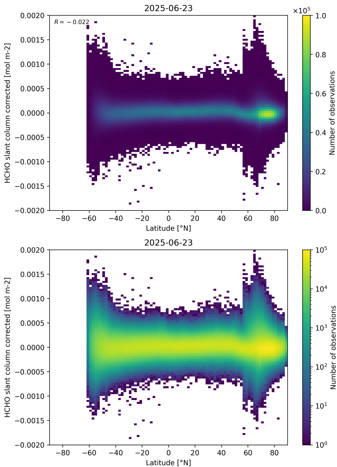
Figure 157: Scatter density plot of “Latitude” against “HCHO slant column corrected” for 2025-06-22 to 2025-06-24.
