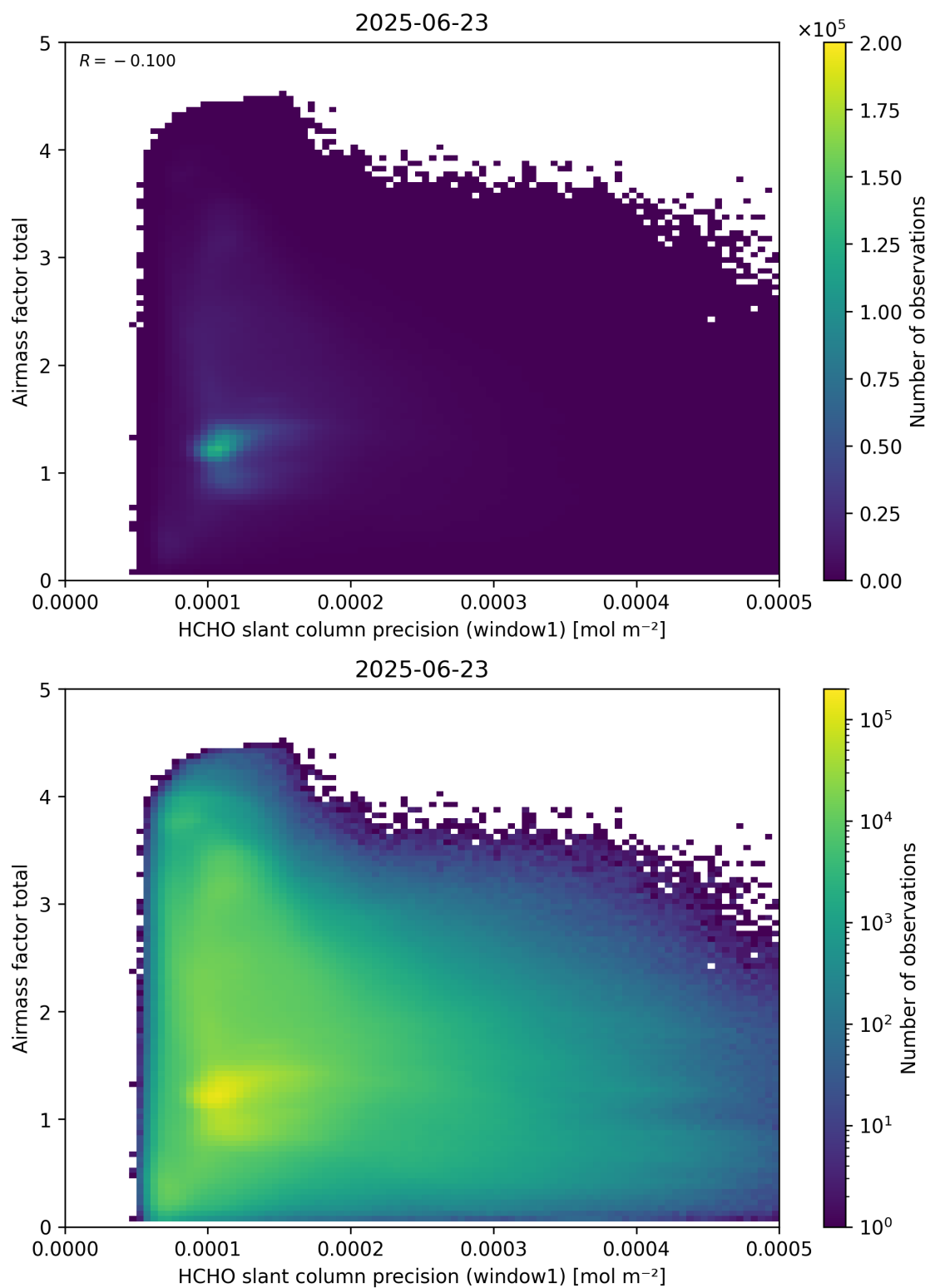
Figure 94: Scatter density plot of “HCHO slant column precision (window1)” against “Airmass factor total” for 2025-06-22 to 2025-06-24.
