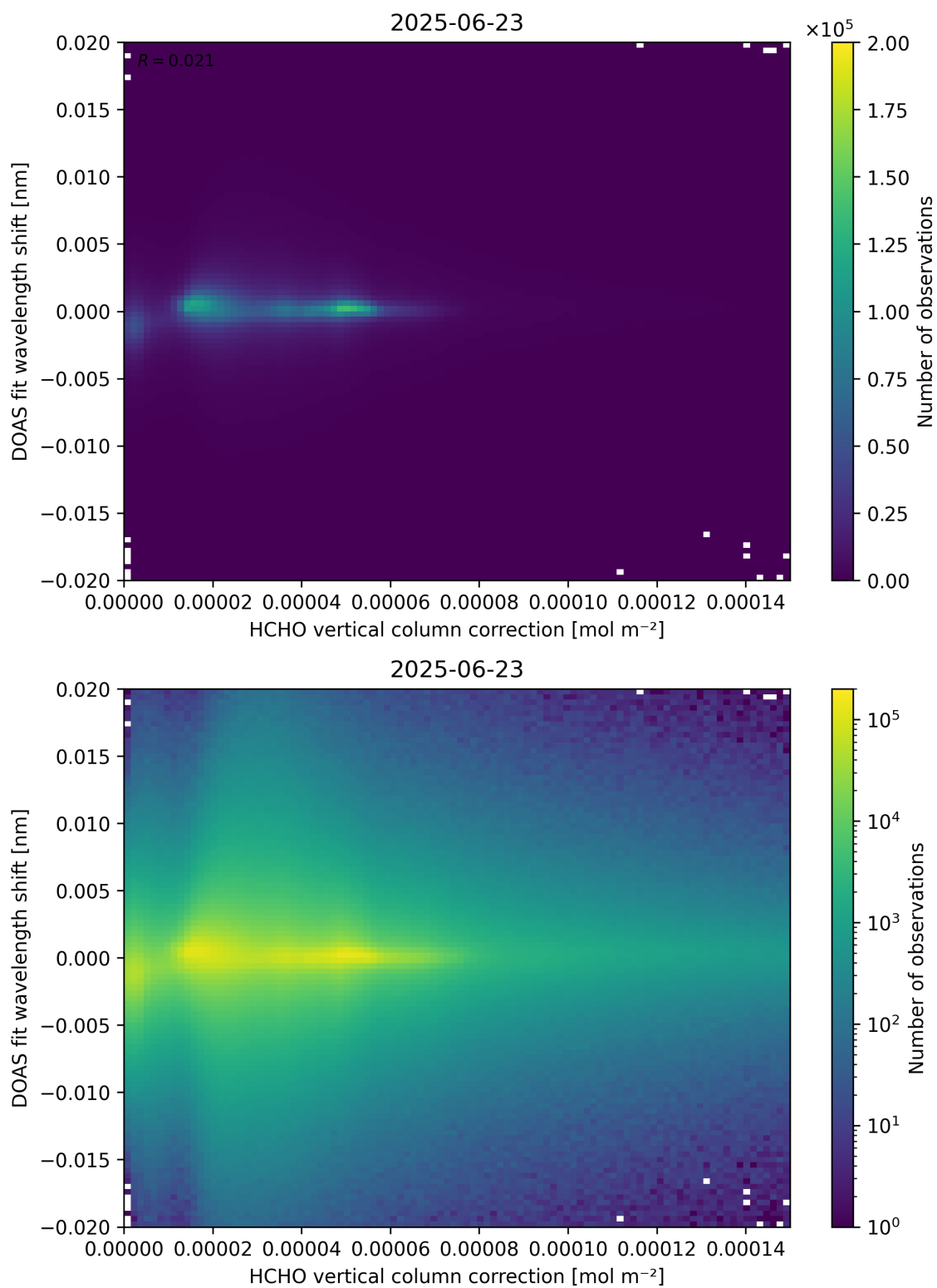
Figure 113: Scatter density plot of “HCHO vertical column correction” against “DOAS fit wavelength shift” for 2025-06-22 to 2025-06-24.
