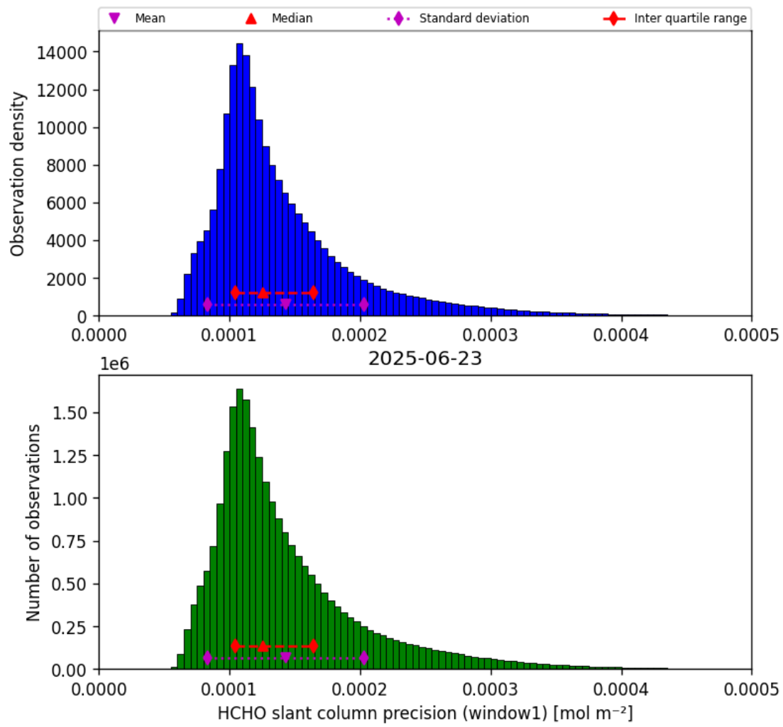
Figure 39: Histogram of “HCHO slant column precision (window1)” for 2025-06-22 to 2025-06-24
