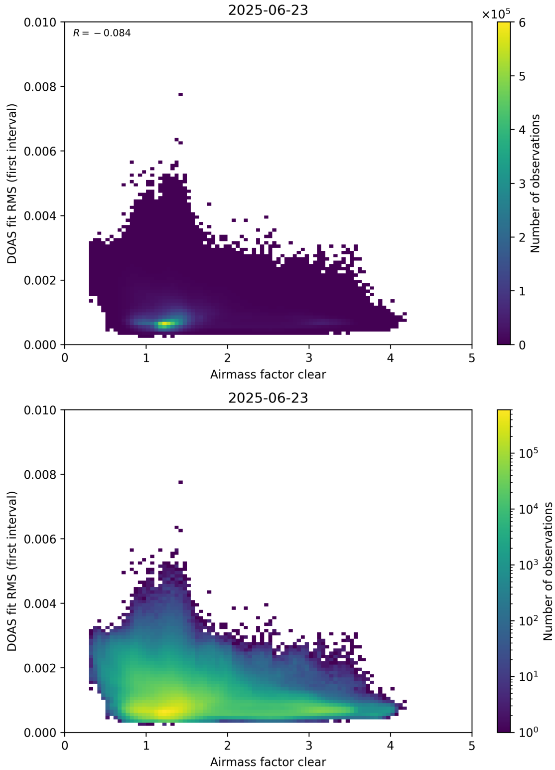
Figure 71: Scatter density plot of “Airmass factor clear” against “DOAS fit RMS (first interval)” for 2025-06-22 to 2025-06-24.
