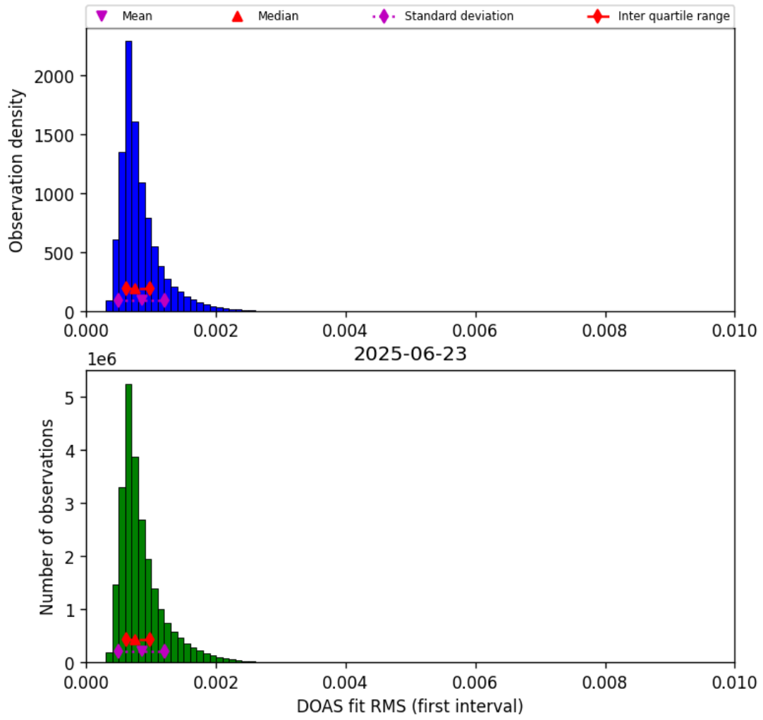
Figure 46: Histogram of “DOAS fit RMS (first interval)” for 2025-06-22 to 2025-06-24
