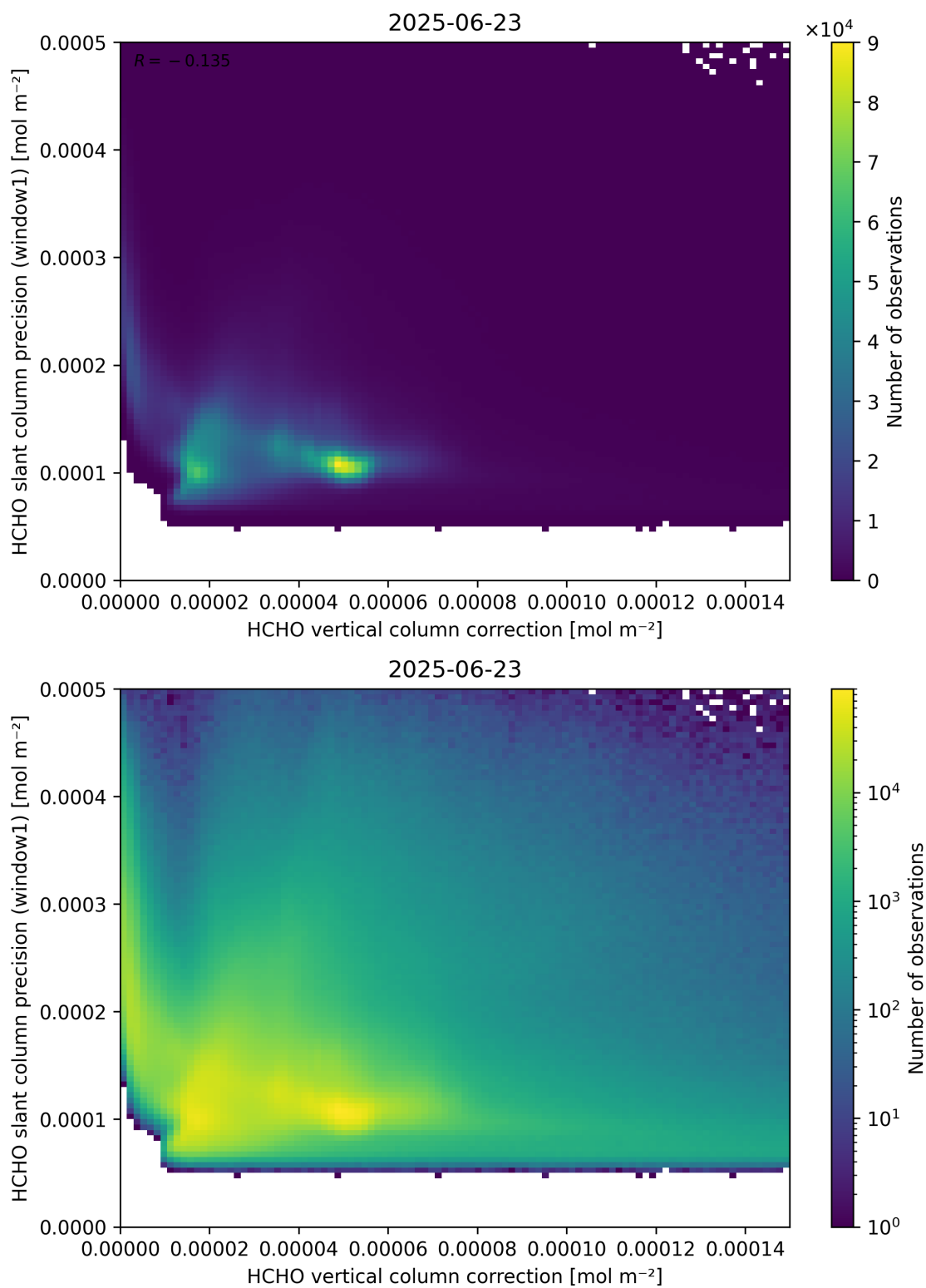
Figure 119: Scatter density plot of “HCHO vertical column correction” against “HCHO slant column precision (window1)” for 2025-06-22 to 2025-06-24.
