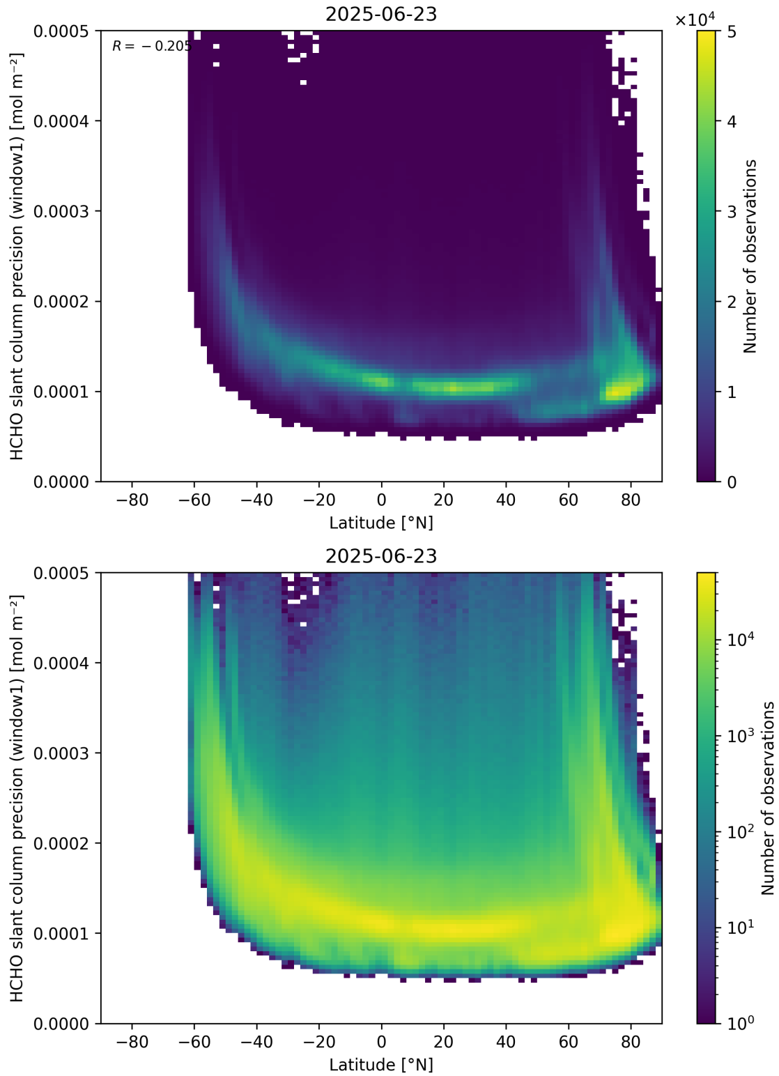
Figure 160: Scatter density plot of “Latitude” against “HCHO slant column precision (window1)” for 2025-06-22 to 2025-06-24.
