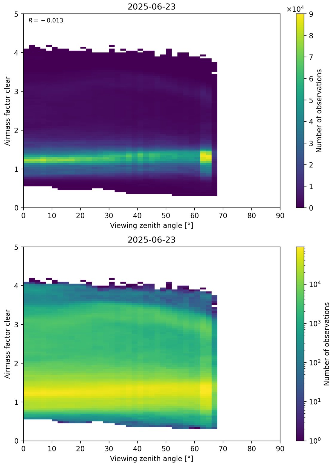
Figure 185: Scatter density plot of “Viewing zenith angle” against “Airmass factor clear” for 2025-06-22 to 2025-06-24.
