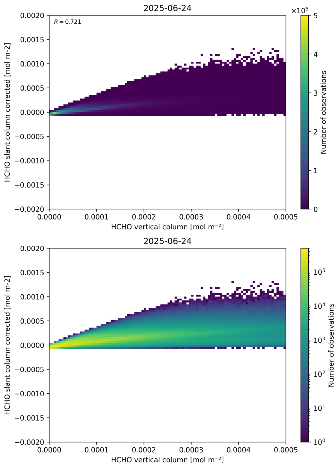
Figure 127: Scatter density plot of “HCHO vertical column” against “HCHO slant column corrected” for 2025-06-23 to 2025-06-25.
