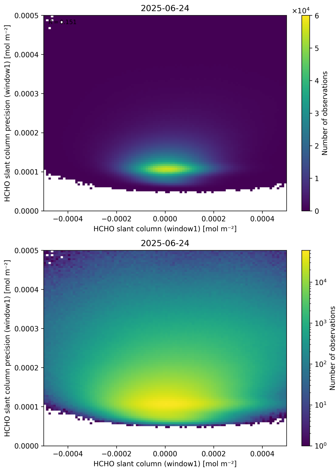
Figure 84: Scatter density plot of “HCHO slant column (window1)” against “HCHO slant column precision (window1)” for 2025-06-23 to 2025-06-25.
