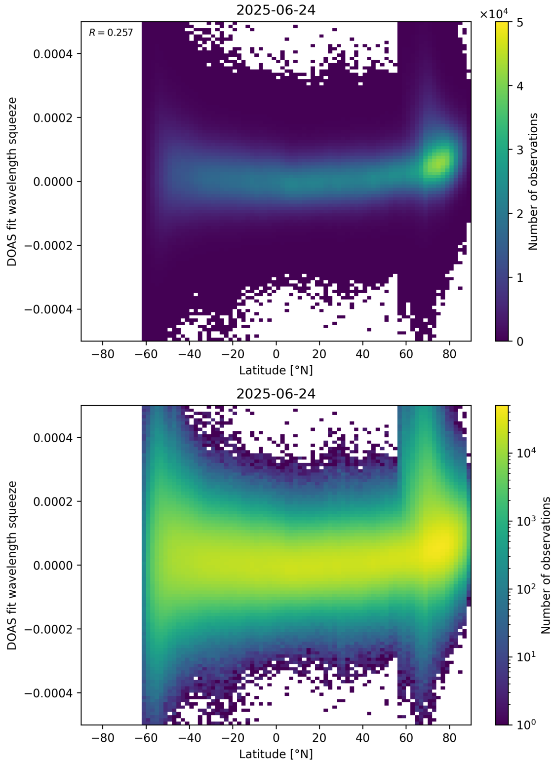
Figure 155: Scatter density plot of “Latitude” against “DOAS fit wavelength squeeze” for 2025-06-23 to 2025-06-25.
