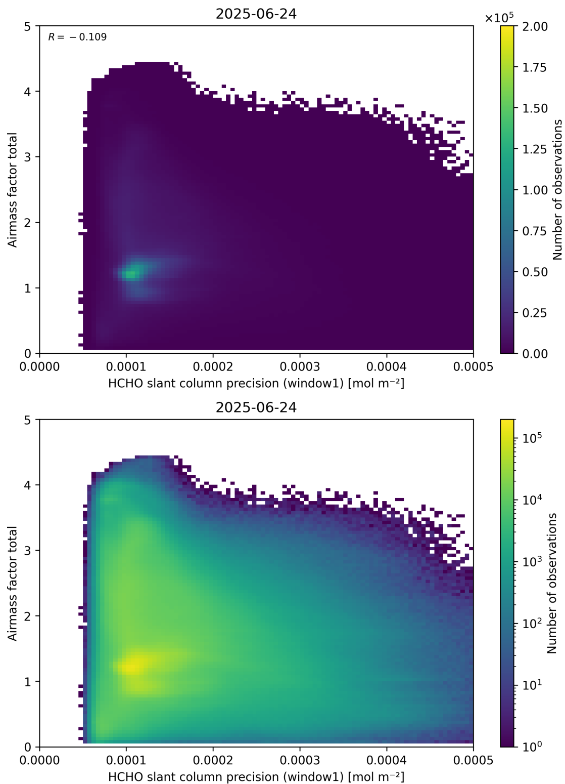
Figure 94: Scatter density plot of “HCHO slant column precision (window1)” against “Airmass factor total” for 2025-06-23 to 2025-06-25.
