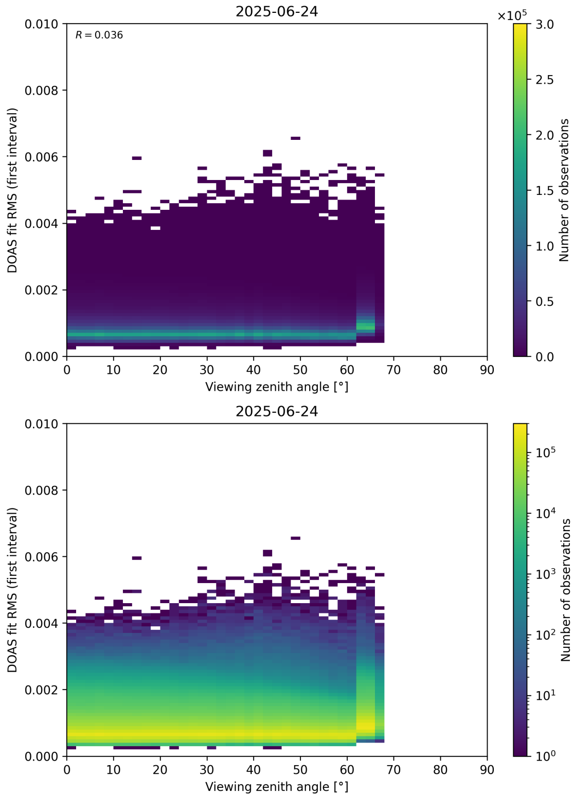
Figure 182: Scatter density plot of “Viewing zenith angle” against “DOAS fit RMS (first interval)” for 2025-06-23 to 2025-06-25.
