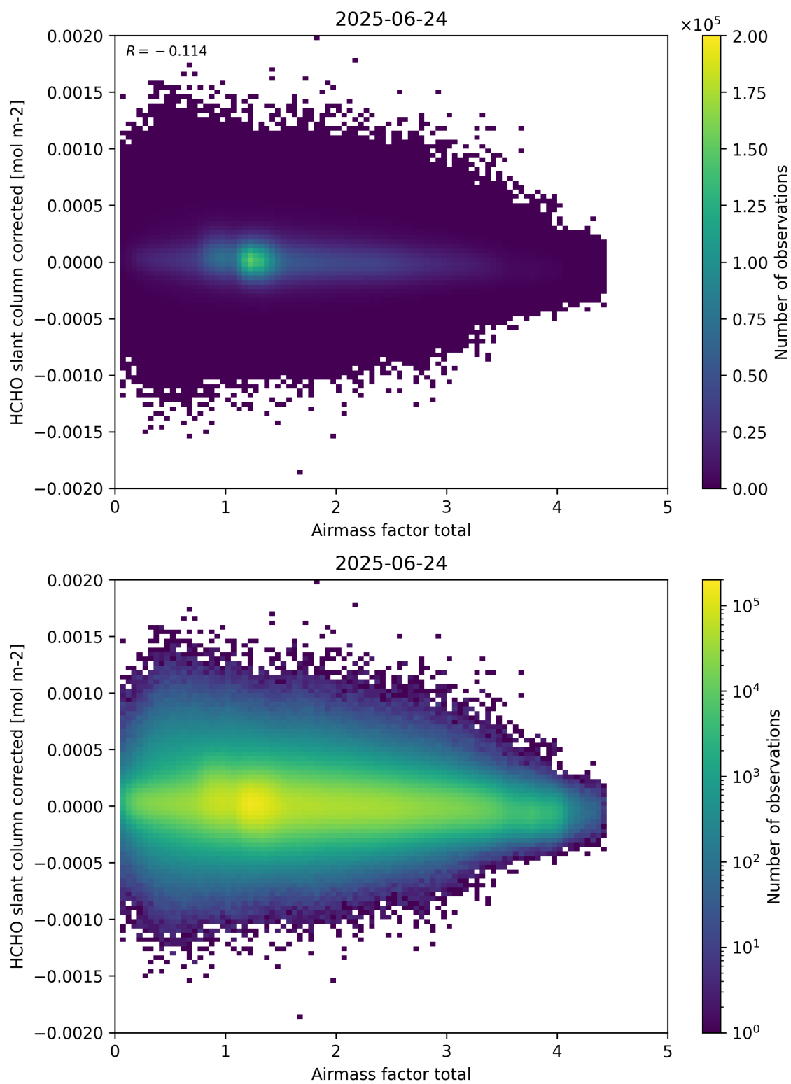
Figure 101: Scatter density plot of “Airmass factor total” against “HCHO slant column corrected” for 2025-06-23 to 2025-06-25.
