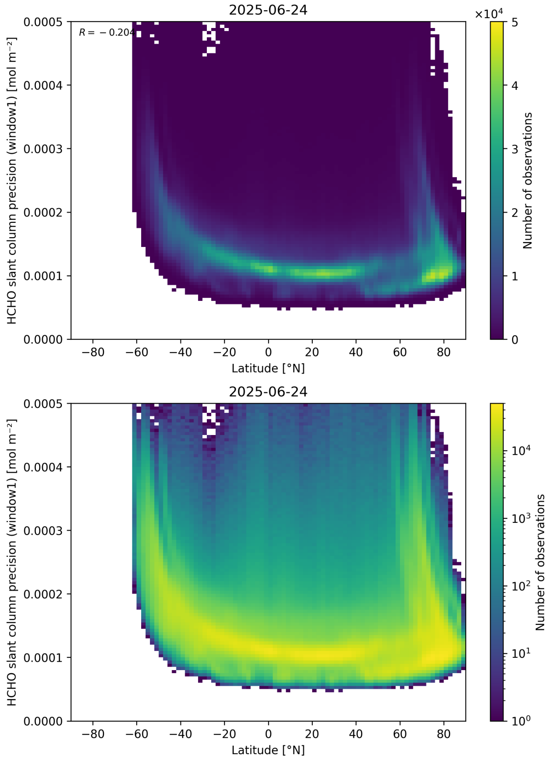
Figure 160: Scatter density plot of “Latitude” against “HCHO slant column precision (window1)” for 2025-06-23 to 2025-06-25.
