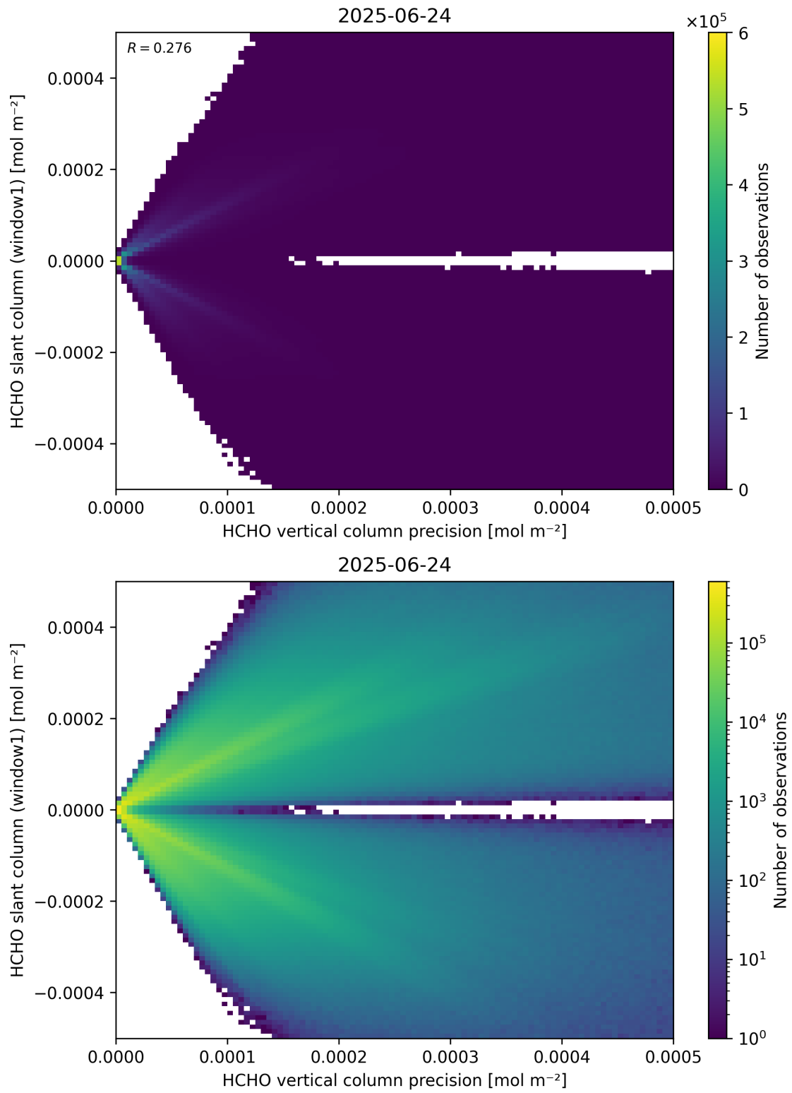
Figure 142: Scatter density plot of “HCHO vertical column precision” against “HCHO slant column (window1)” for 2025-06-23 to 2025-06-25.
