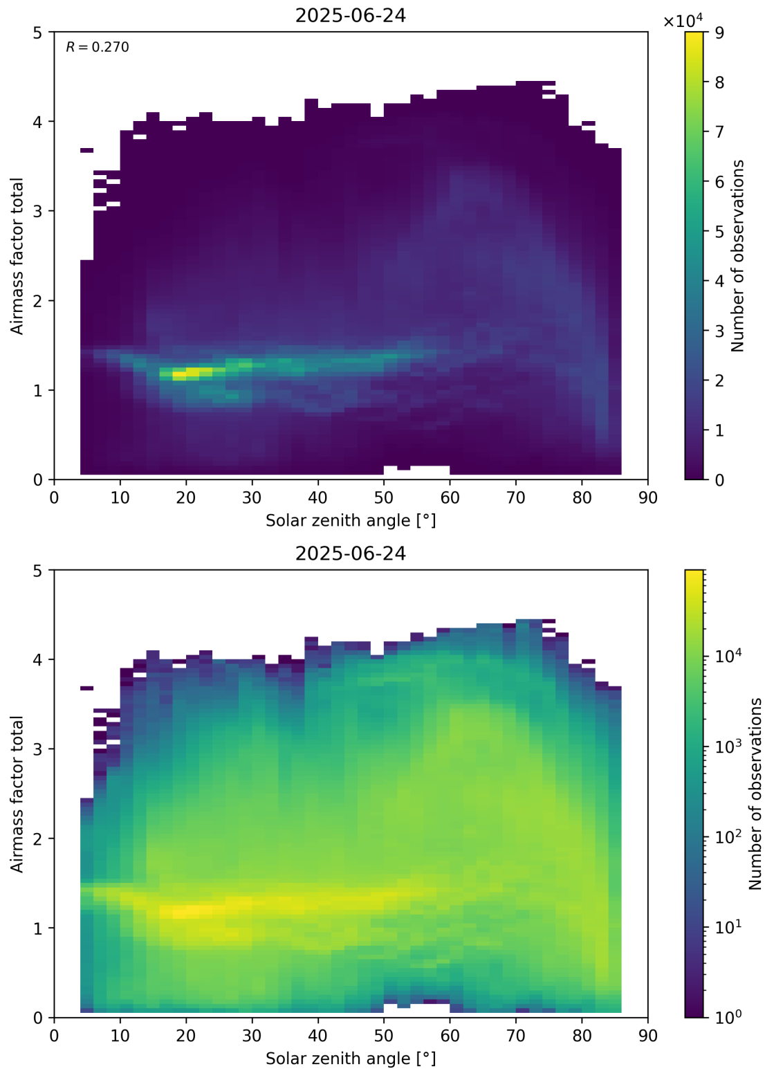
Figure 175: Scatter density plot of “Solar zenith angle” against “Airmass factor total” for 2025-06-23 to 2025-06-25.
