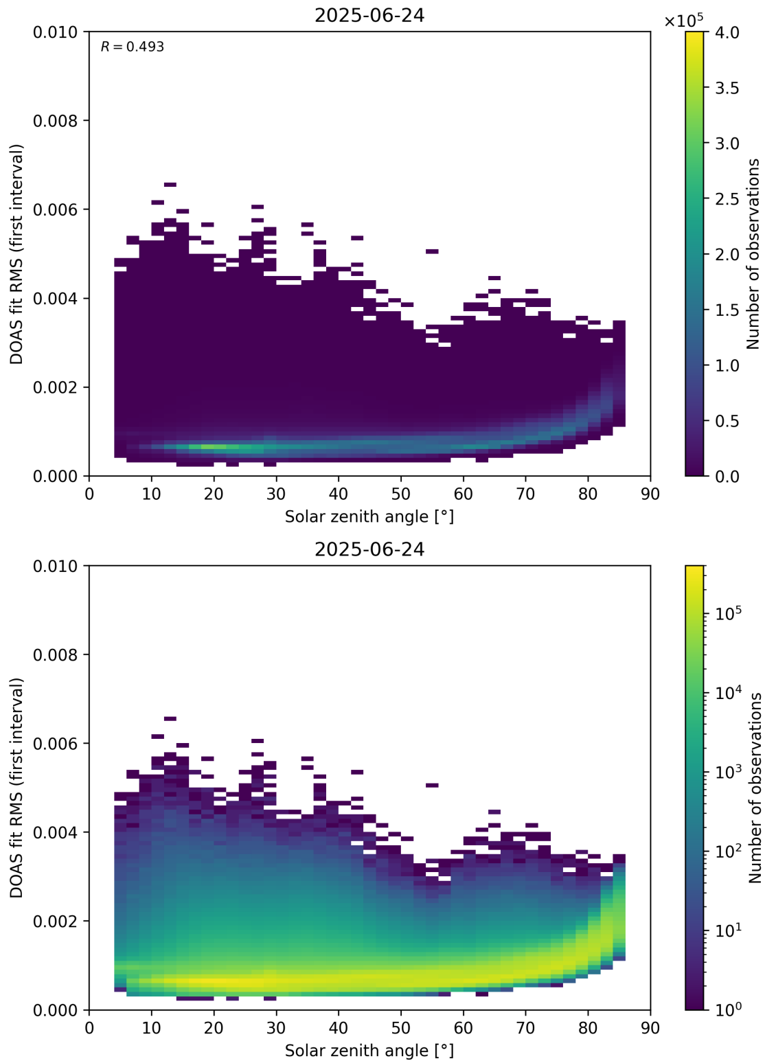
Figure 167: Scatter density plot of “Solar zenith angle” against “DOAS fit RMS (first interval)” for 2025-06-23 to 2025-06-25.
