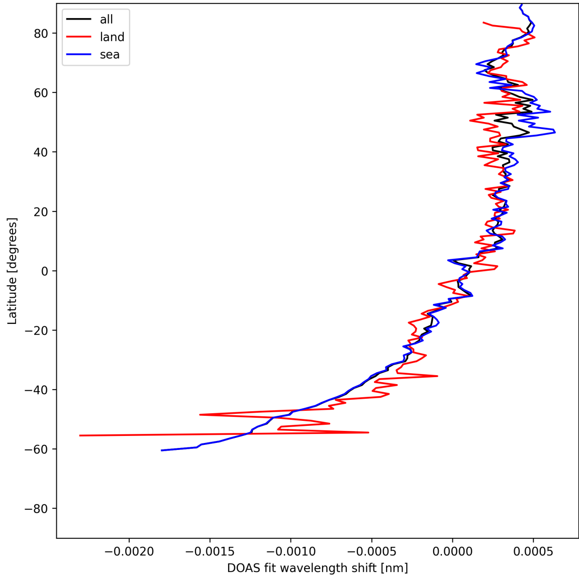
Figure 30: Zonal average of “DOAS fit wavelength shift” for 2025-06-23 to 2025-06-25.
