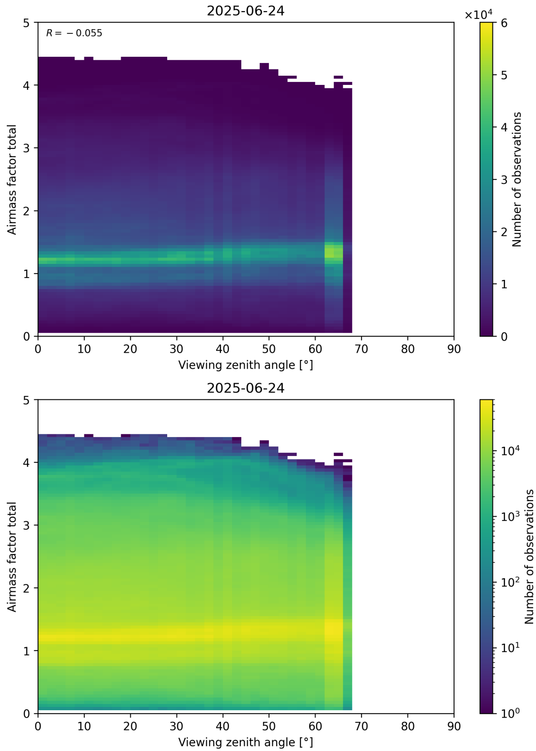
Figure 190: Scatter density plot of “Viewing zenith angle” against “Airmass factor total” for 2025-06-23 to 2025-06-25.
