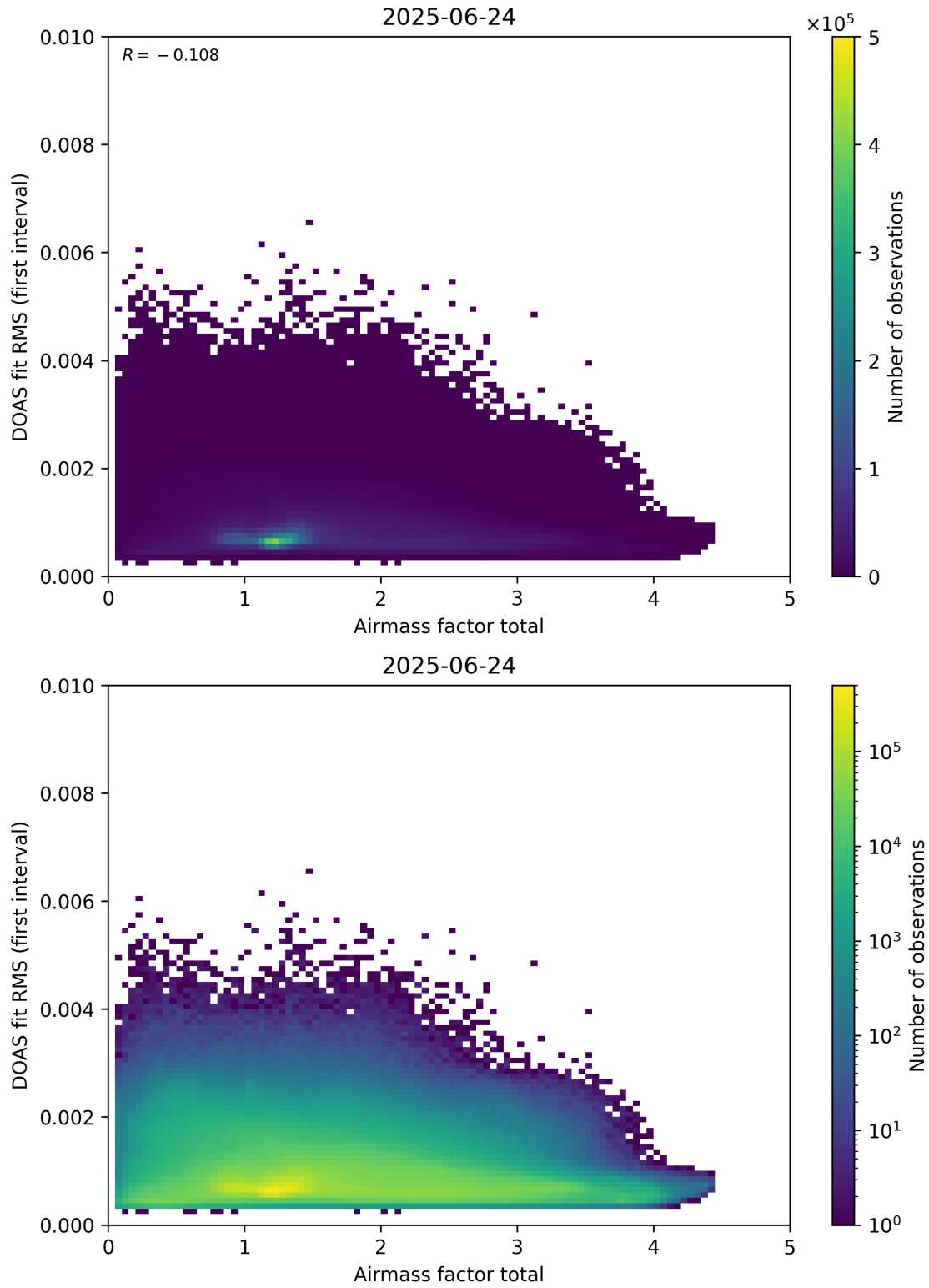
Figure 97: Scatter density plot of “Airmass factor total” against “DOAS fit RMS (first interval)” for 2025-06-23 to 2025-06-25.
