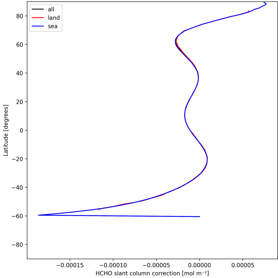
Figure 33: Zonal average of “HCHO slant column correction” for 2025-06-23 to 2025-06-25.
