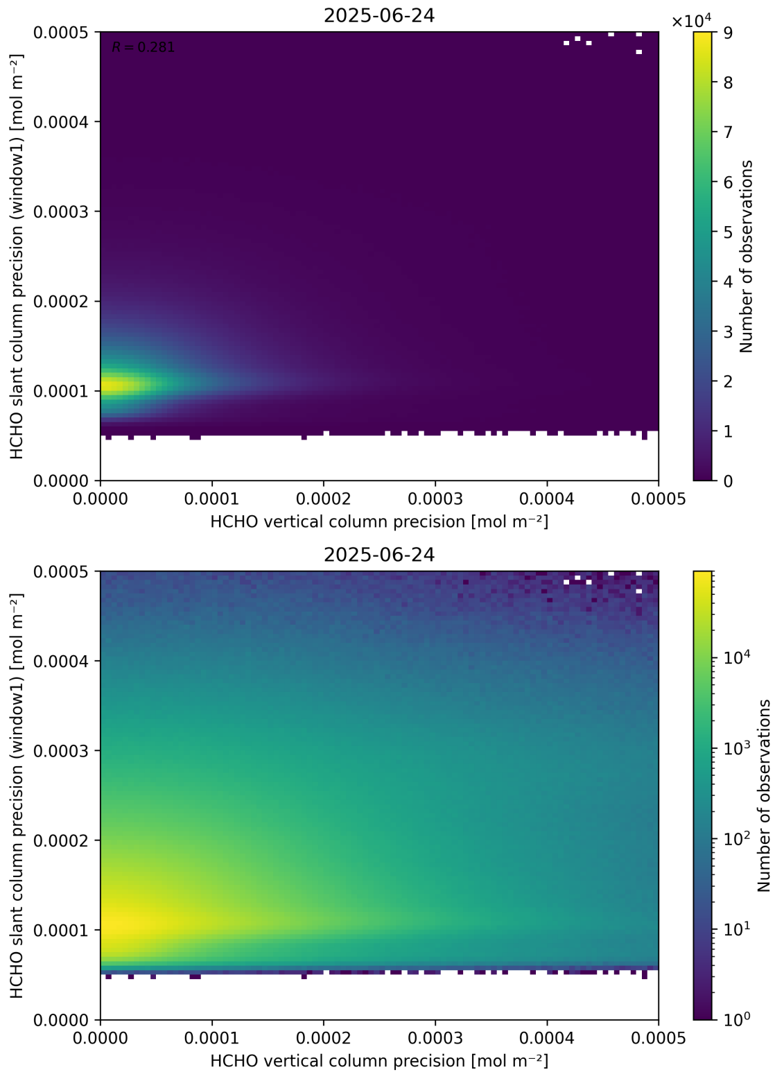
Figure 143: Scatter density plot of “HCHO vertical column precision” against “HCHO slant column precision (window1)” for 2025-06-23 to 2025-06-25.
