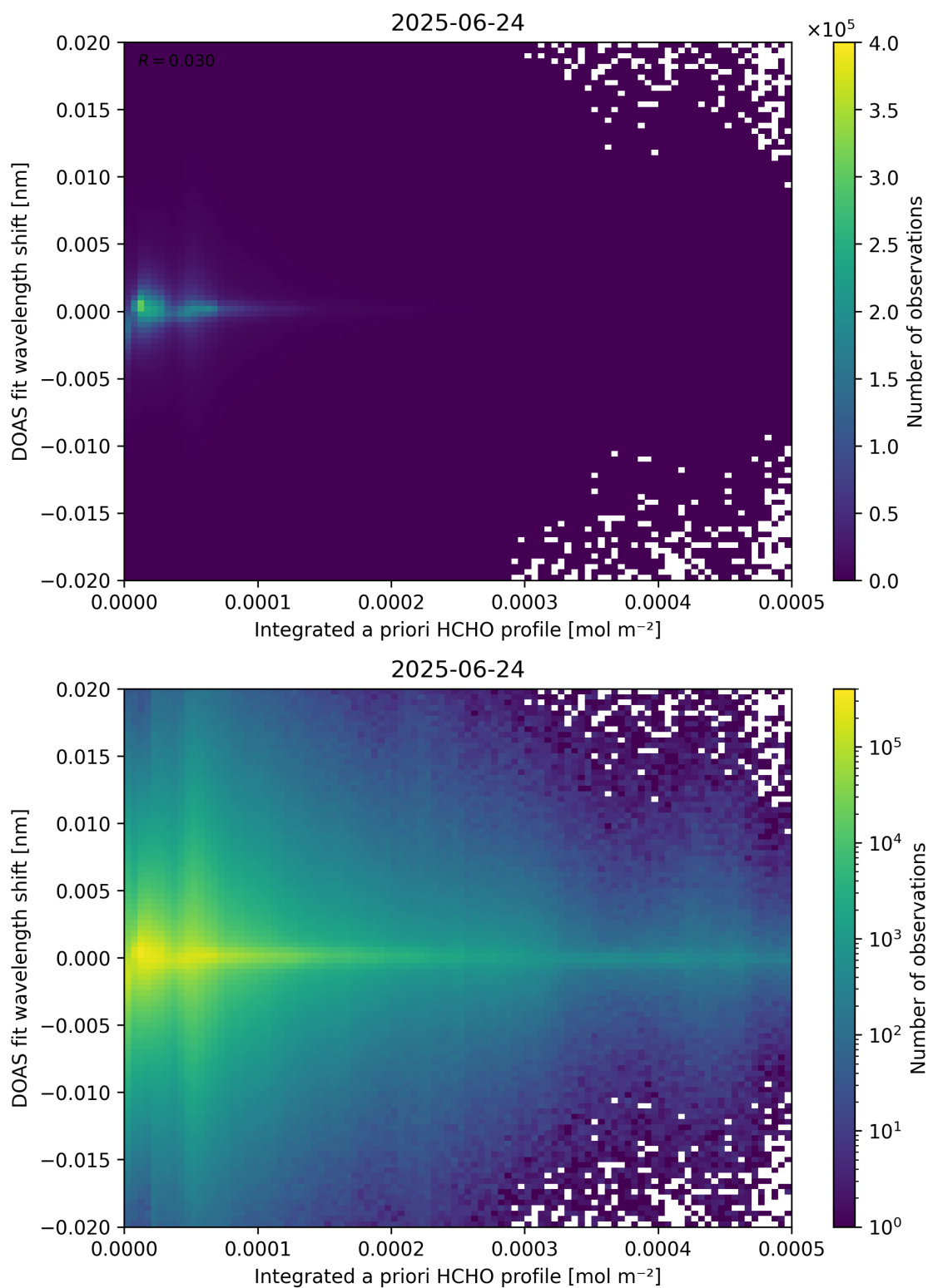
Figure 149: Scatter density plot of “Integrated a priori HCHO profile” against “DOAS fit wavelength shift” for 2025-06-23 to 2025-06-25.
