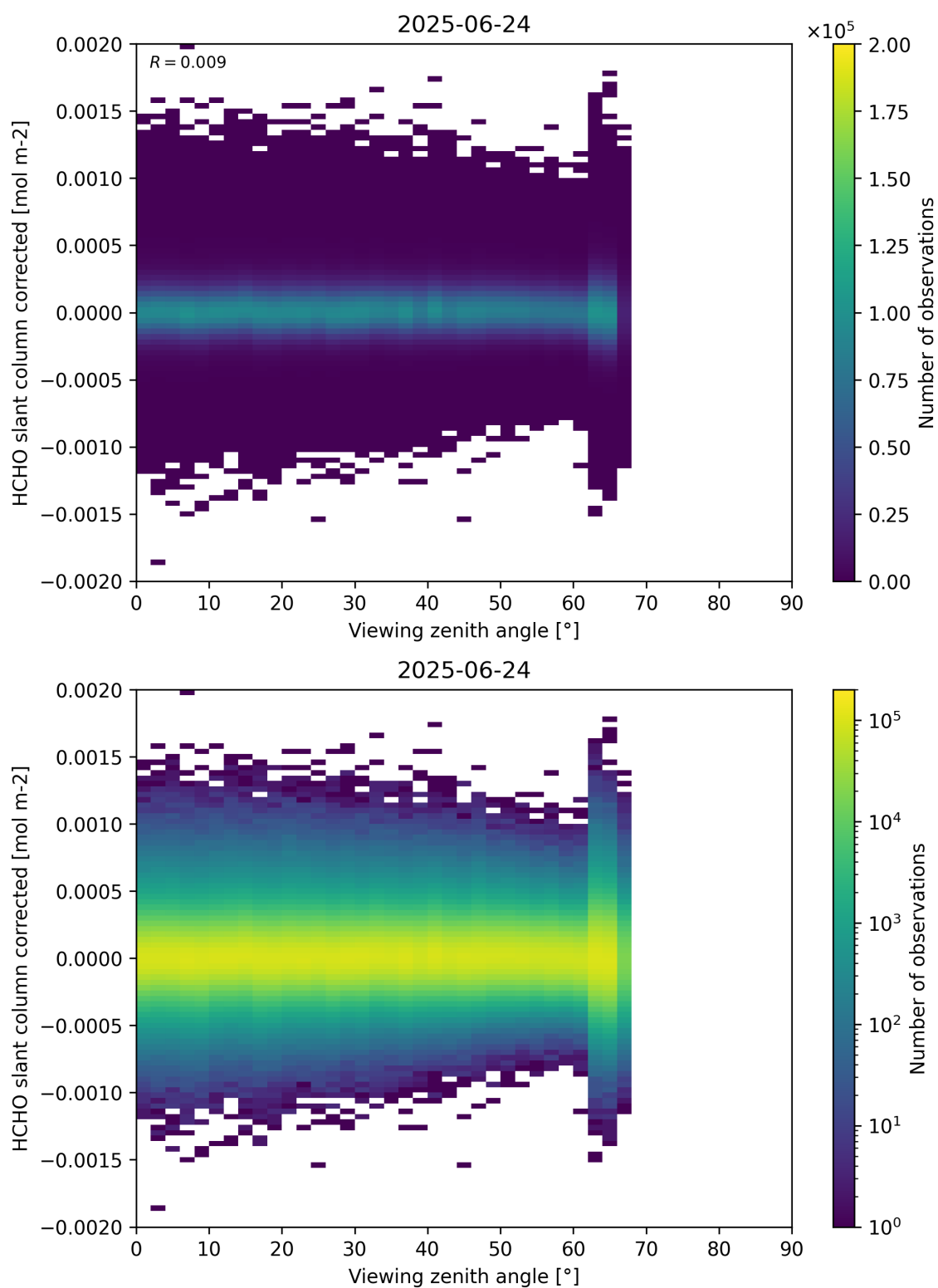
Figure 186: Scatter density plot of “Viewing zenith angle” against “HCHO slant column corrected” for 2025-06-23 to 2025-06-25.
