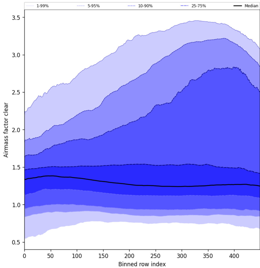
Figure 56: Along track statistics of “Airmass factor clear” for 2025-06-23 to 2025-06-25
