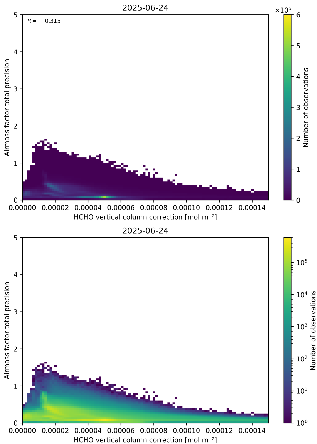
Figure 121: Scatter density plot of “HCHO vertical column correction” against “Airmass factor total precision” for 2025-06-23 to 2025-06-25.
