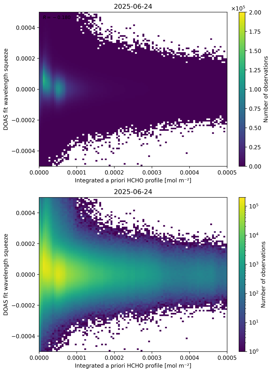
Figure 150: Scatter density plot of “Integrated a priori HCHO profile” against “DOAS fit wavelength squeeze” for 2025-06-23 to 2025-06-25.
