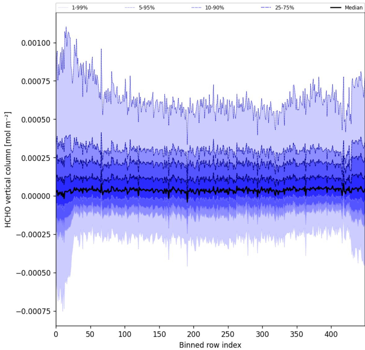
Figure 49: Along track statistics of “HCHO vertical column” for 2025-06-23 to 2025-06-25
