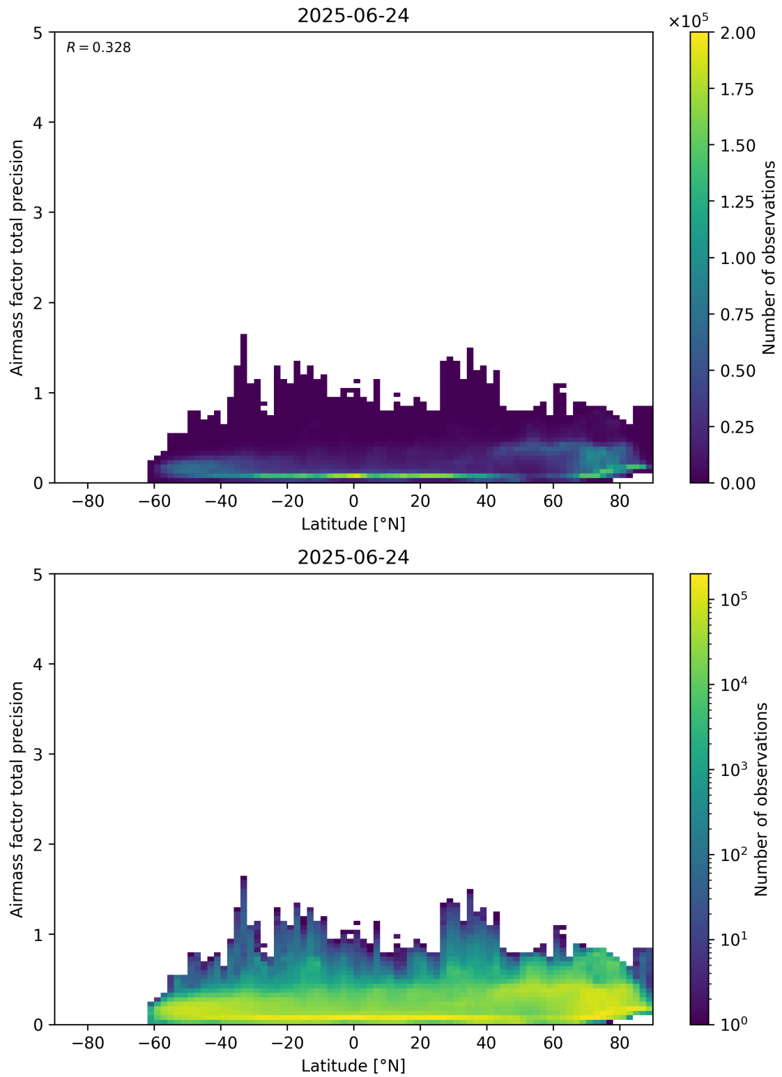
Figure 162: Scatter density plot of “Latitude” against “Airmass factor total precision” for 2025-06-23 to 2025-06-25.
