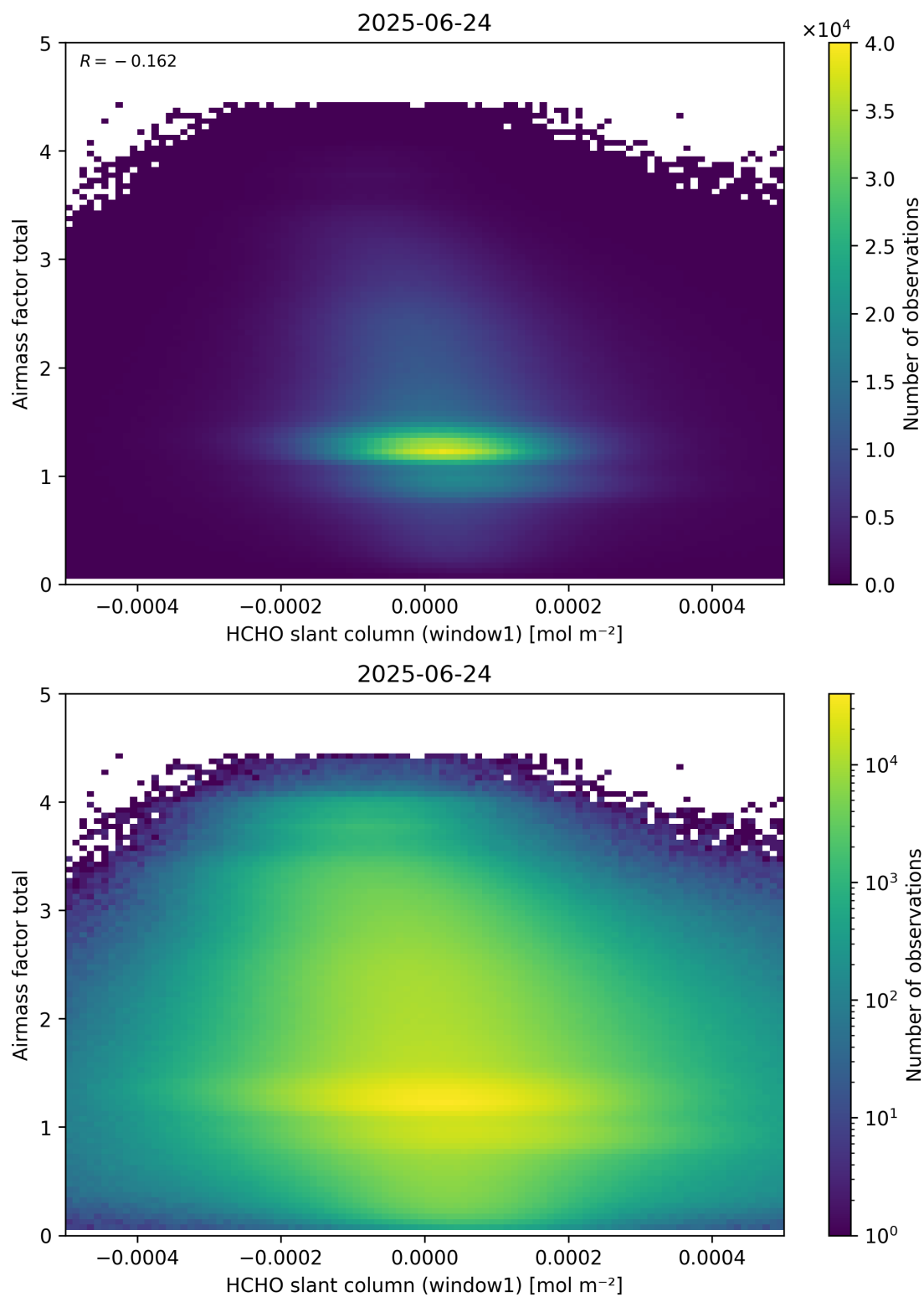
Figure 85: Scatter density plot of “HCHO slant column (window1)” against “Airmass factor total” for 2025-06-23 to 2025-06-25.
