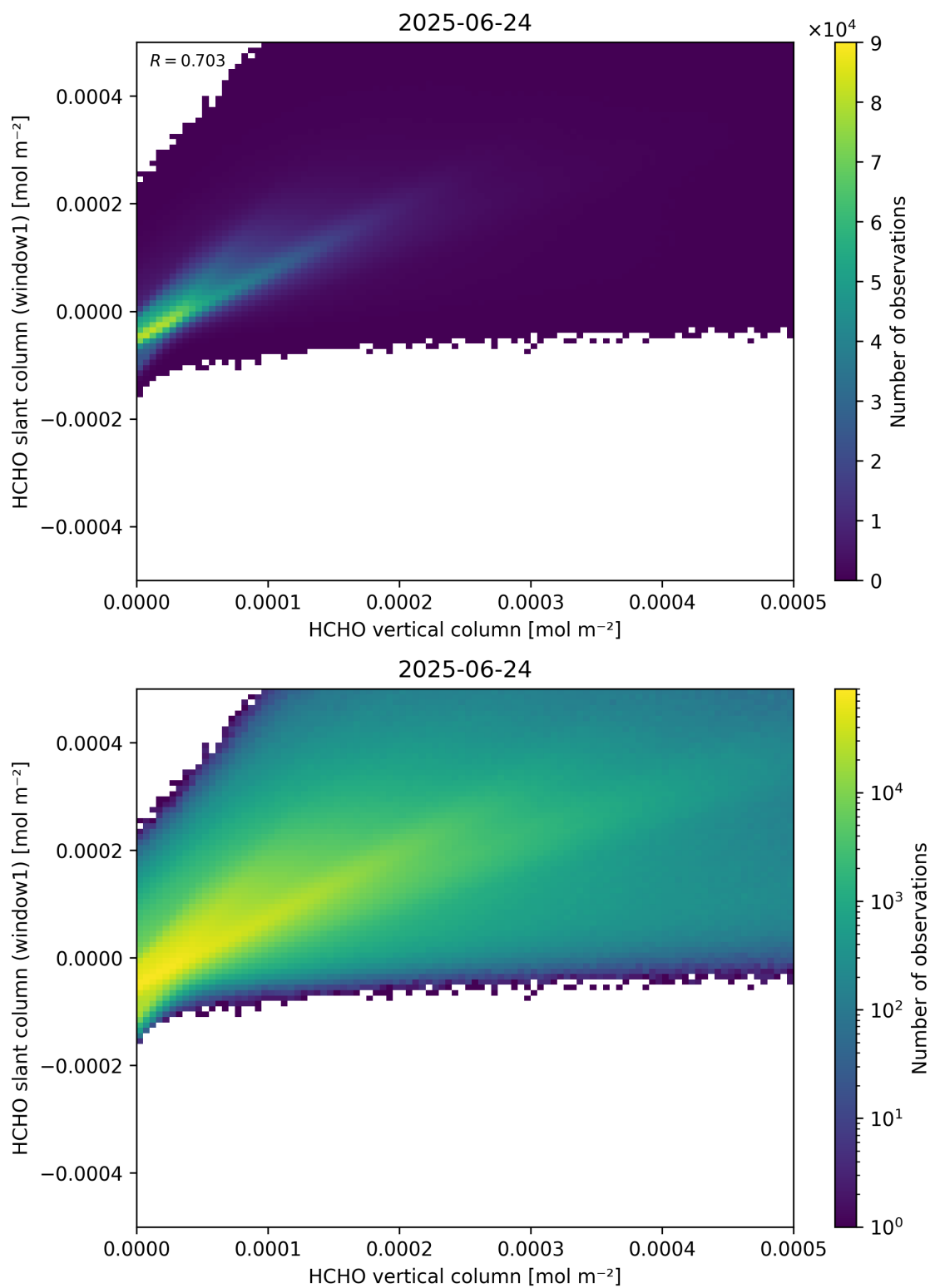
Figure 129: Scatter density plot of “HCHO vertical column” against “HCHO slant column (window1)” for 2025-06-23 to 2025-06-25.
