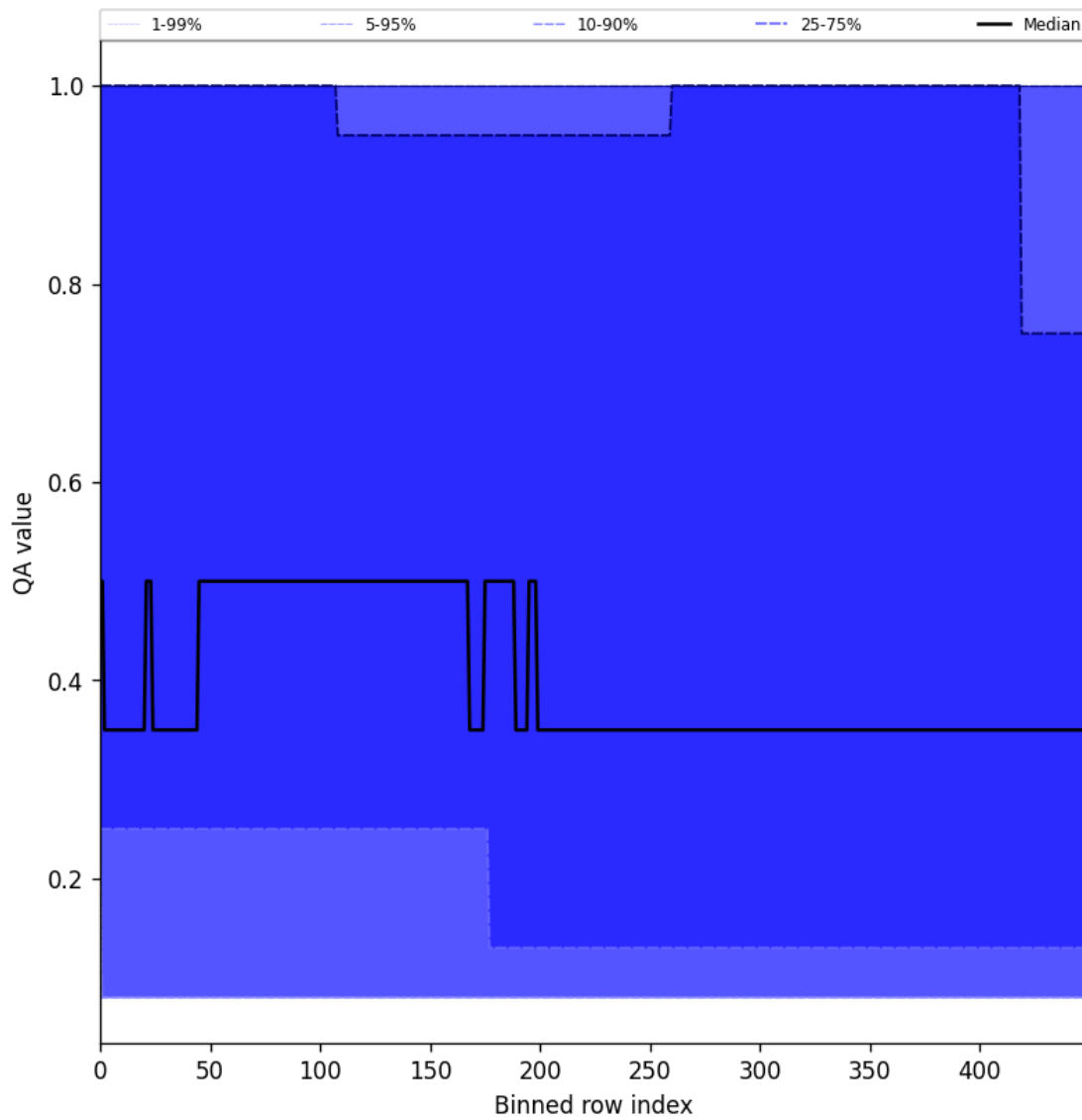
Figure 48: Along track statistics of “QA value” for 2025-06-23 to 2025-06-25
