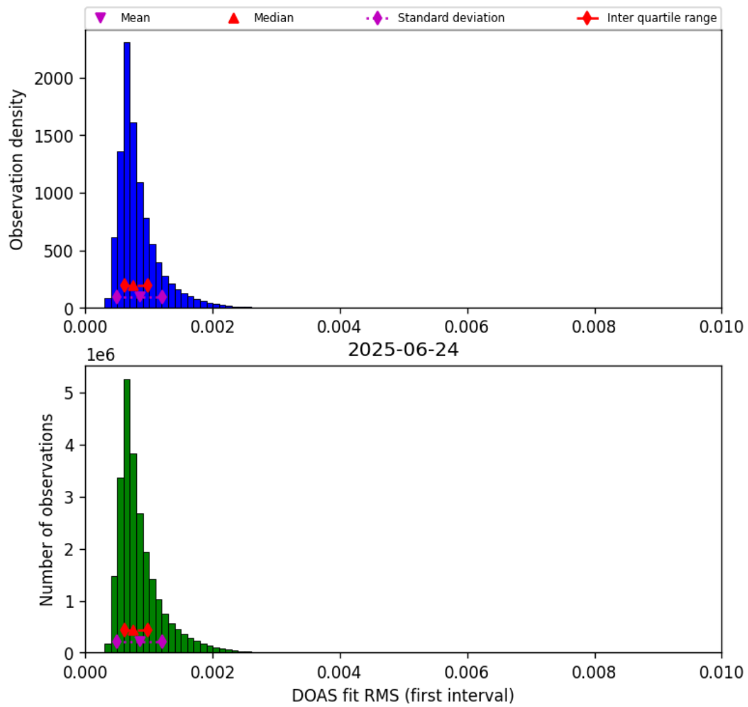
Figure 46: Histogram of “DOAS fit RMS (first interval)” for 2025-06-23 to 2025-06-25
