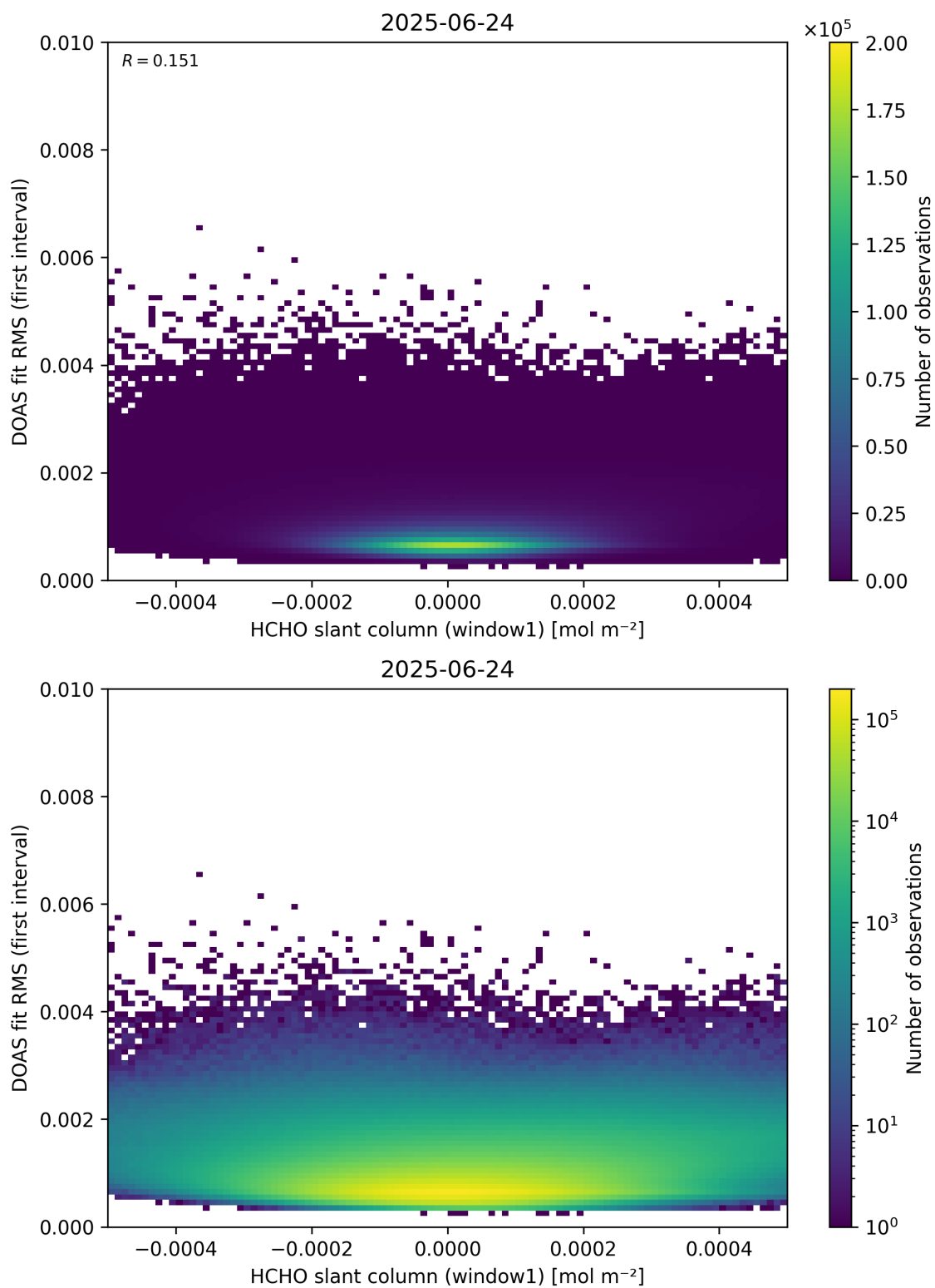
Figure 78: Scatter density plot of “HCHO slant column (window1)” against “DOAS fit RMS (first interval)” for 2025-06-23 to 2025-06-25.
