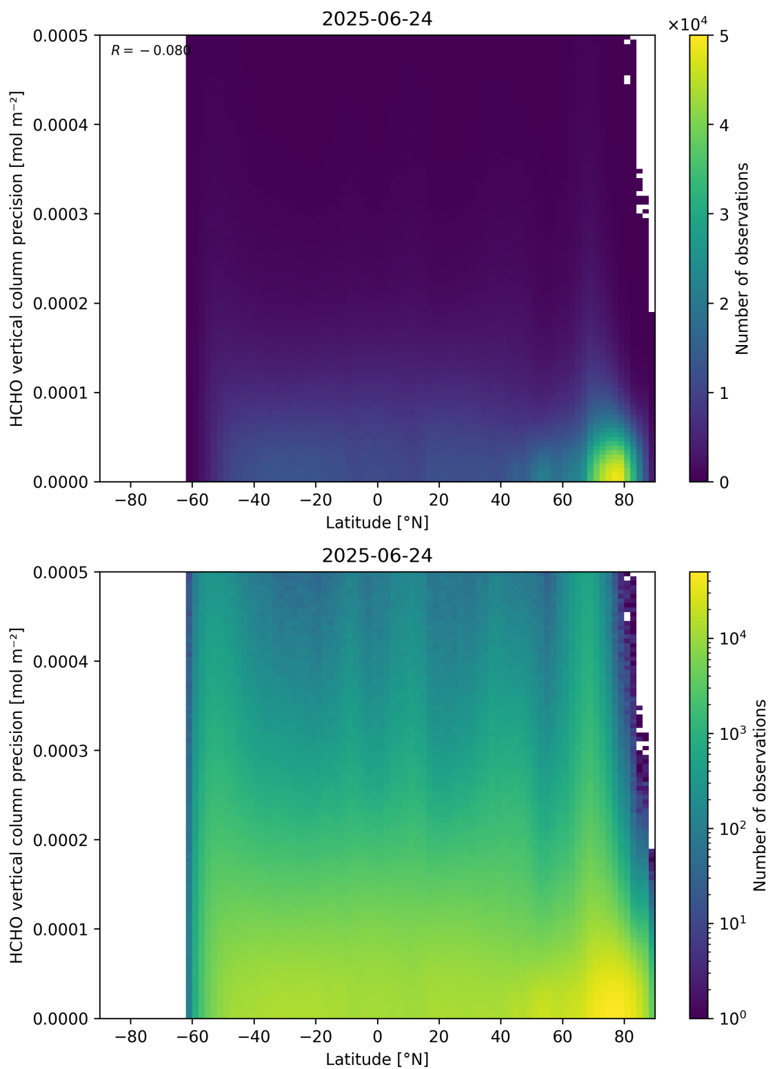
Figure 165: Scatter density plot of “Latitude” against “HCHO vertical column precision” for 2025-06-23 to 2025-06-25.
