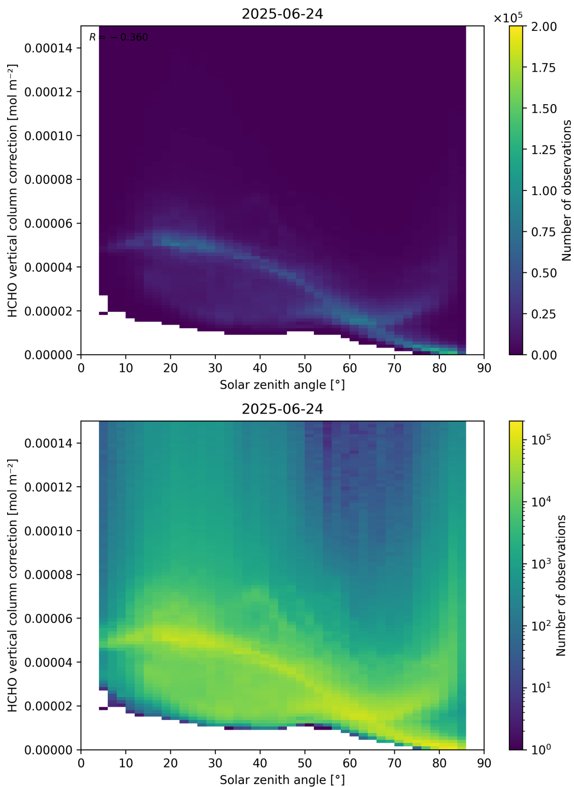
Figure 178: Scatter density plot of “Solar zenith angle” against “HCHO vertical column correction” for 2025-06-23 to 2025-06-25.
