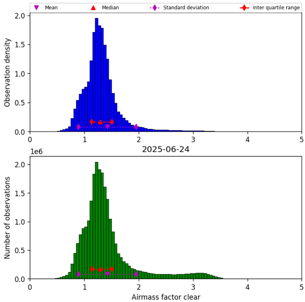
Figure 42: Histogram of “Airmass factor clear” for 2025-06-23 to 2025-06-25
