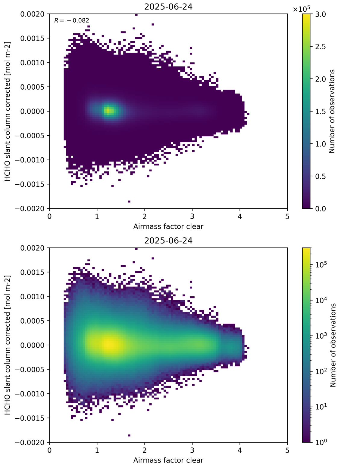
Figure 74: Scatter density plot of “Airmass factor clear” against “HCHO slant column corrected” for 2025-06-23 to 2025-06-25.
