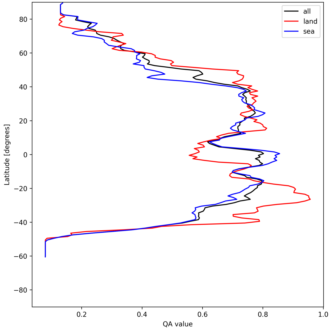
Figure 20: Zonal average of “QA value” for 2025-06-23 to 2025-06-25.
