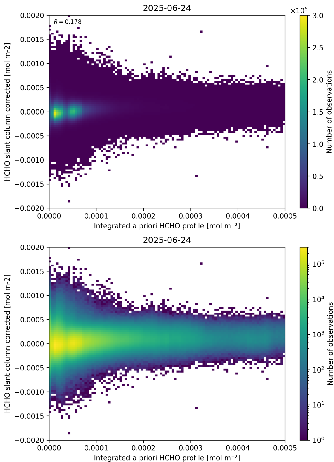
Figure 151: Scatter density plot of “Integrated a priori HCHO profile” against “HCHO slant column corrected” for 2025-06-23 to 2025-06-25.
