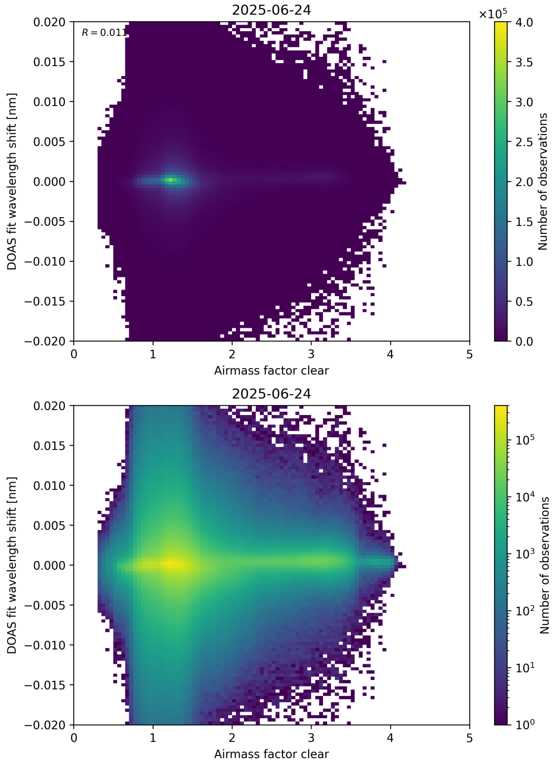
Figure 72: Scatter density plot of “Airmass factor clear” against “DOAS fit wavelength shift” for 2025-06-23 to 2025-06-25.
