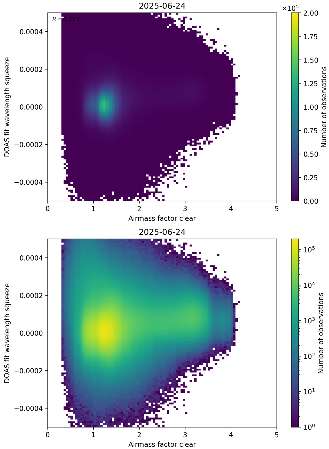
Figure 73: Scatter density plot of “Airmass factor clear” against “DOAS fit wavelength squeeze” for 2025-06-23 to 2025-06-25.
