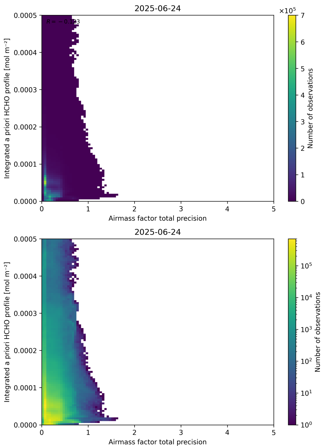
Figure 111: Scatter density plot of “Airmass factor total precision” against “Integrated a priori HCHO profile” for 2025-06-23 to 2025-06-25.
