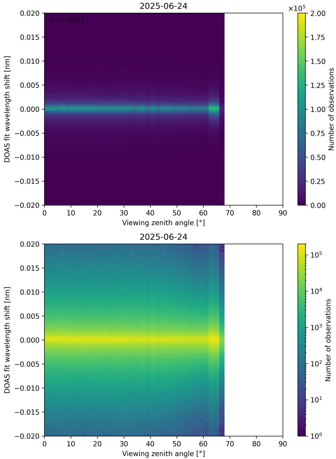
Figure 183: Scatter density plot of “Viewing zenith angle” against “DOAS fit wavelength shift” for 2025-06-23 to 2025-06-25.
