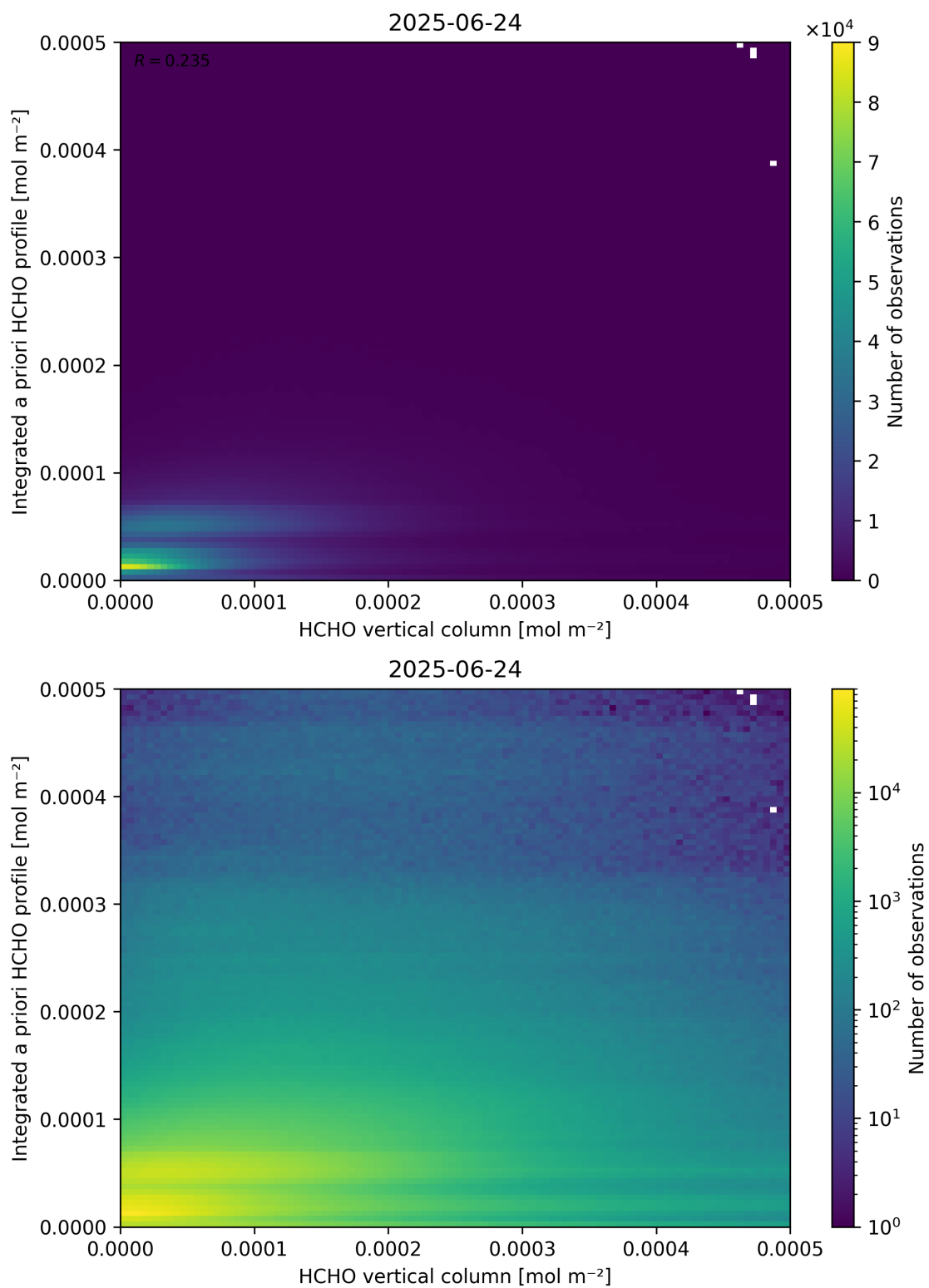
Figure 135: Scatter density plot of “HCHO vertical column” against “Integrated a priori HCHO profile” for 2025-06-23 to 2025-06-25.
