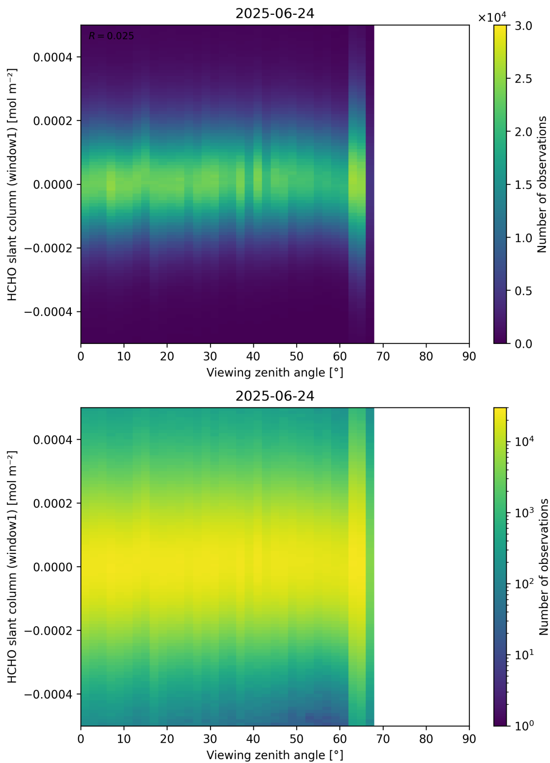
Figure 188: Scatter density plot of “Viewing zenith angle” against “HCHO slant column (window1)” for 2025-06-23 to 2025-06-25.
