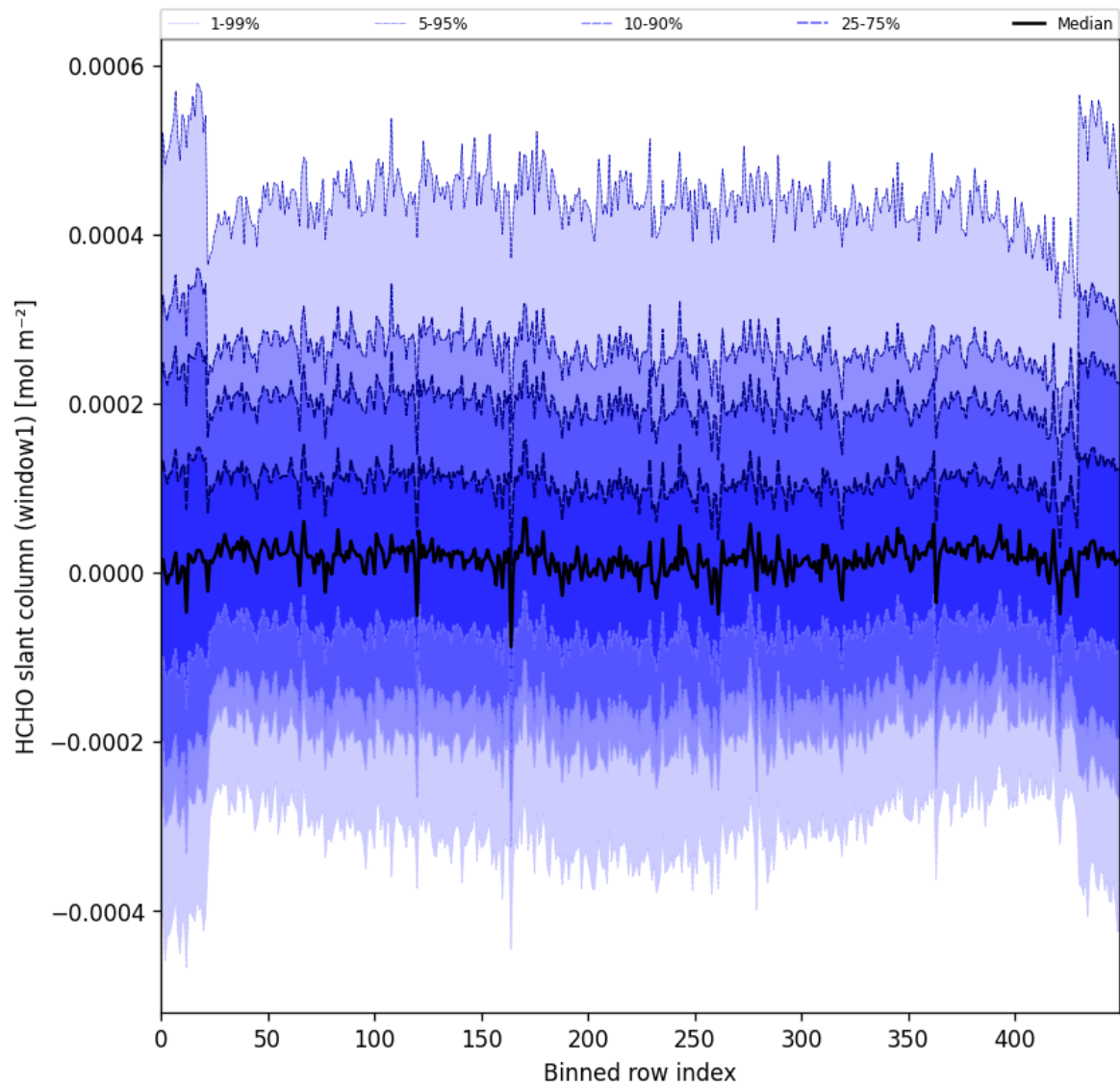
Figure 52: Along track statistics of “HCHO slant column (window1)” for 2025-06-23 to 2025-06-25
