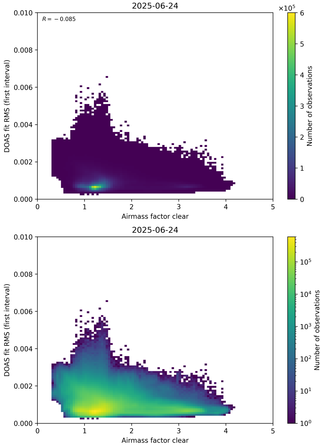
Figure 71: Scatter density plot of “Airmass factor clear” against “DOAS fit RMS (first interval)” for 2025-06-23 to 2025-06-25.
