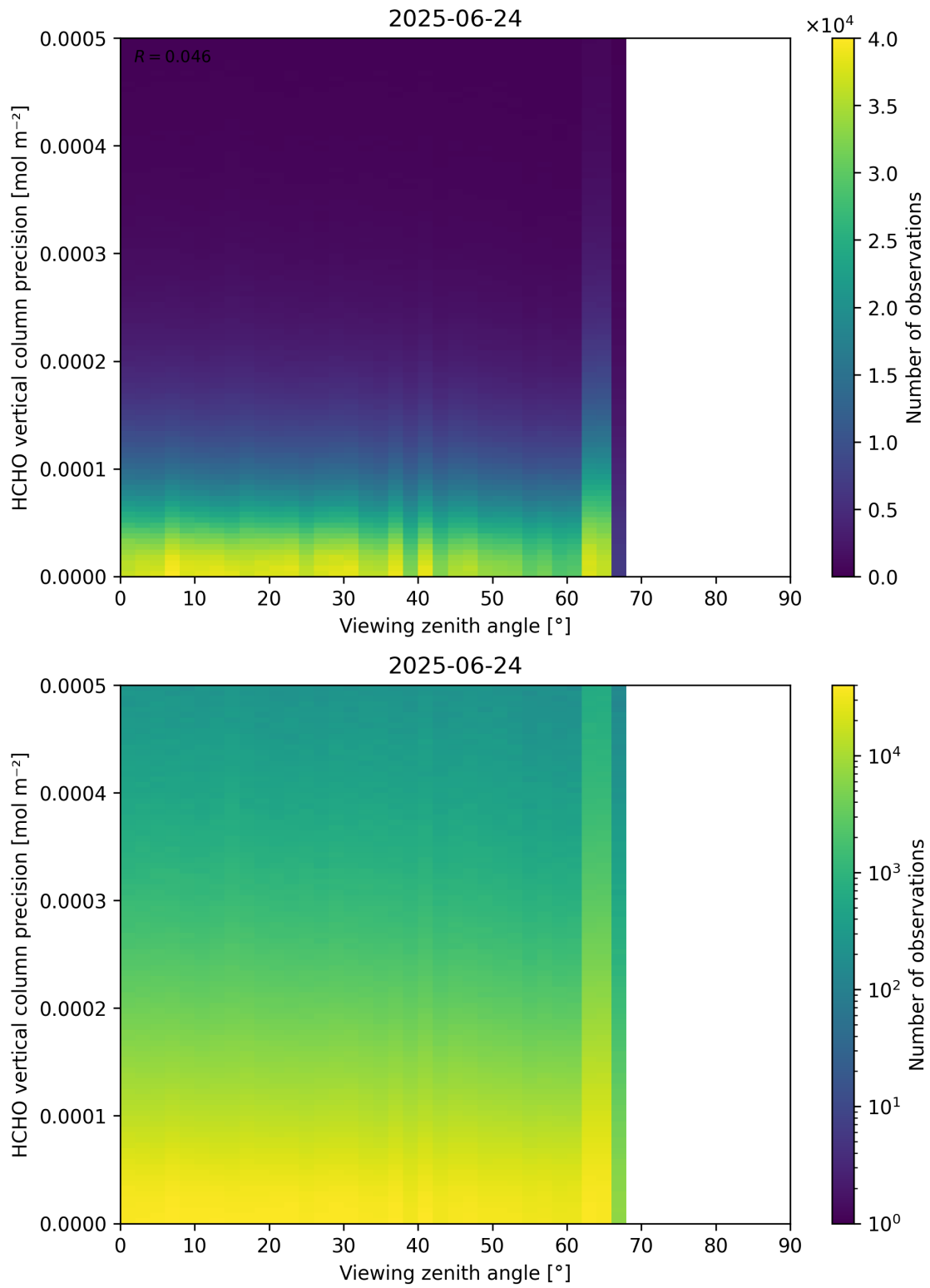
Figure 194: Scatter density plot of “Viewing zenith angle” against “HCHO vertical column precision” for 2025-06-23 to 2025-06-25.
