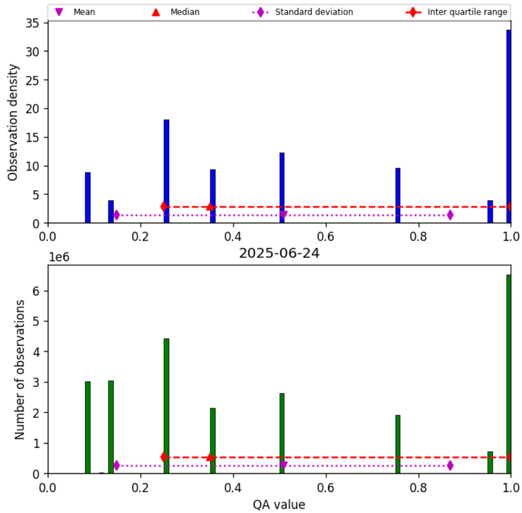
Figure 34: Histogram of “QA value” for 2025-06-23 to 2025-06-25
