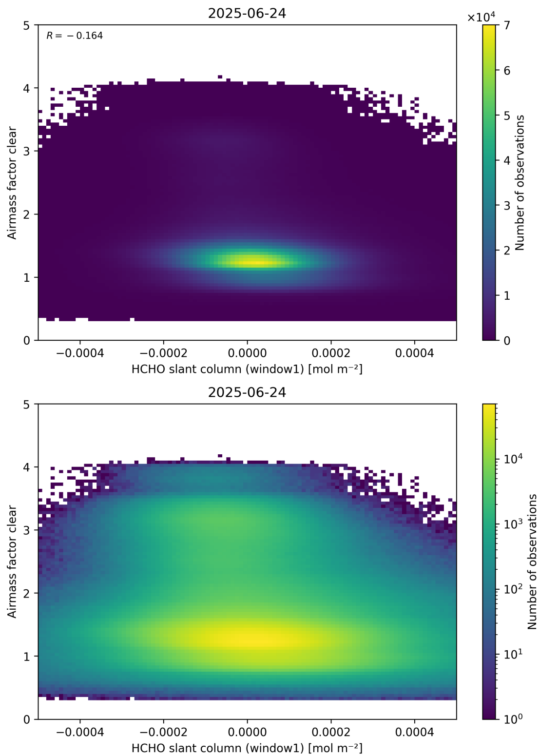
Figure 81: Scatter density plot of “HCHO slant column (window1)” against “Airmass factor clear” for 2025-06-23 to 2025-06-25.
