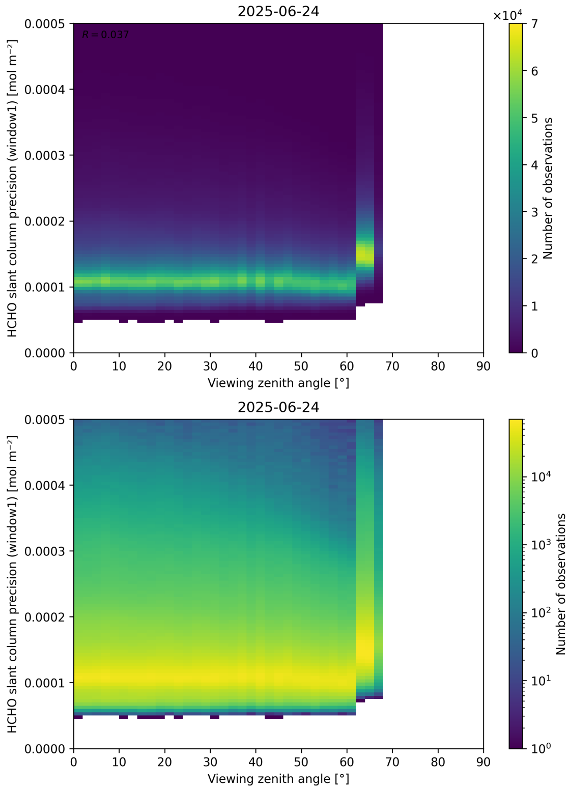
Figure 189: Scatter density plot of “Viewing zenith angle” against “HCHO slant column precision (window1)” for 2025-06-23 to 2025-06-25.
