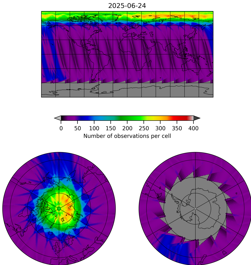
Figure 19: Map of the number of observations for 2025-06-23 to 2025-06-25
