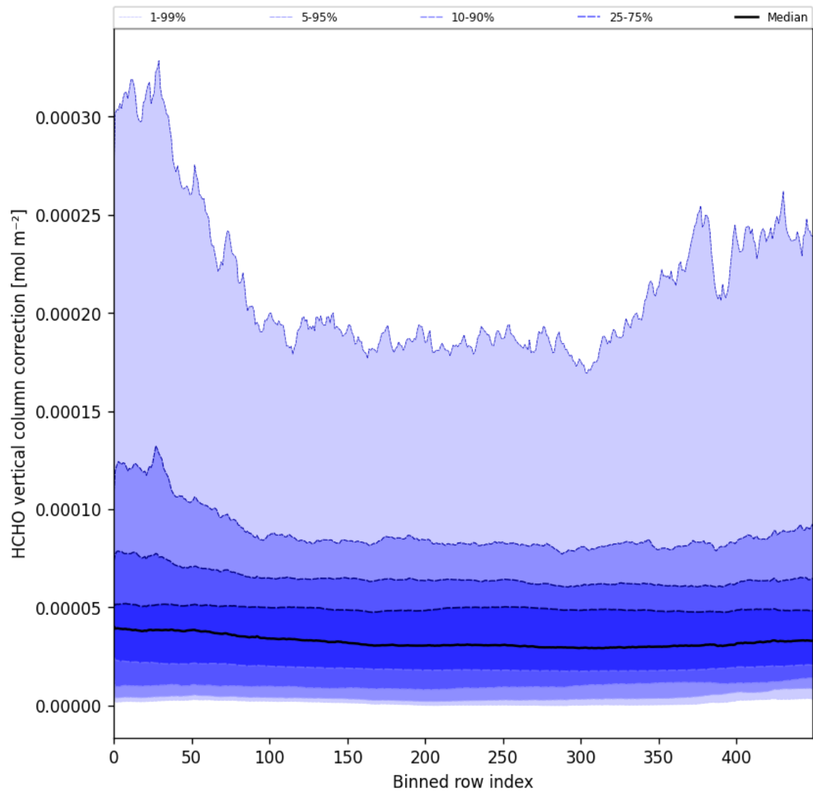
Figure 51: Along track statistics of “HCHO vertical column correction” for 2025-06-23 to 2025-06-25
