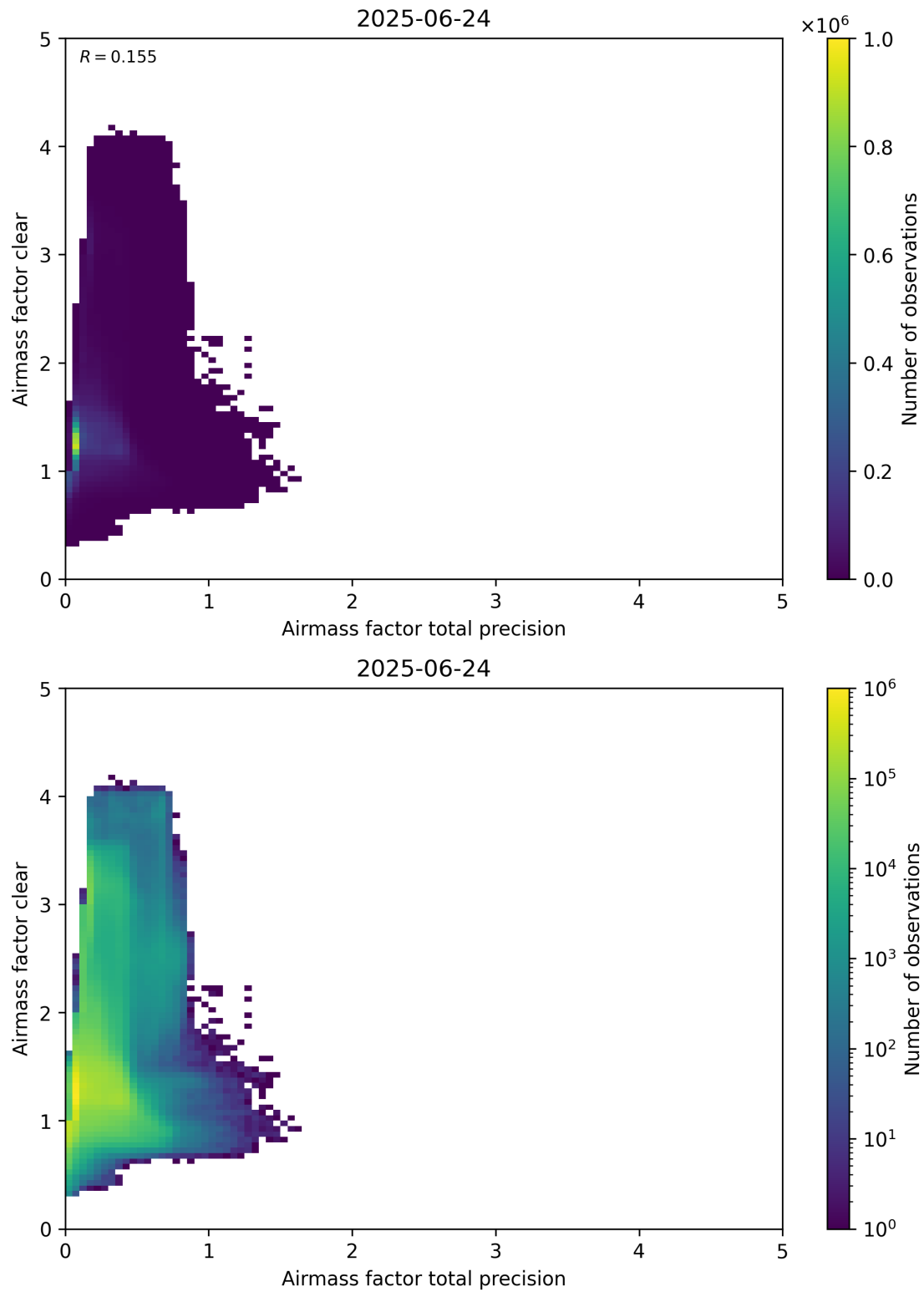
Figure 108: Scatter density plot of “Airmass factor total precision” against “Airmass factor clear” for 2025-06-23 to 2025-06-25.
