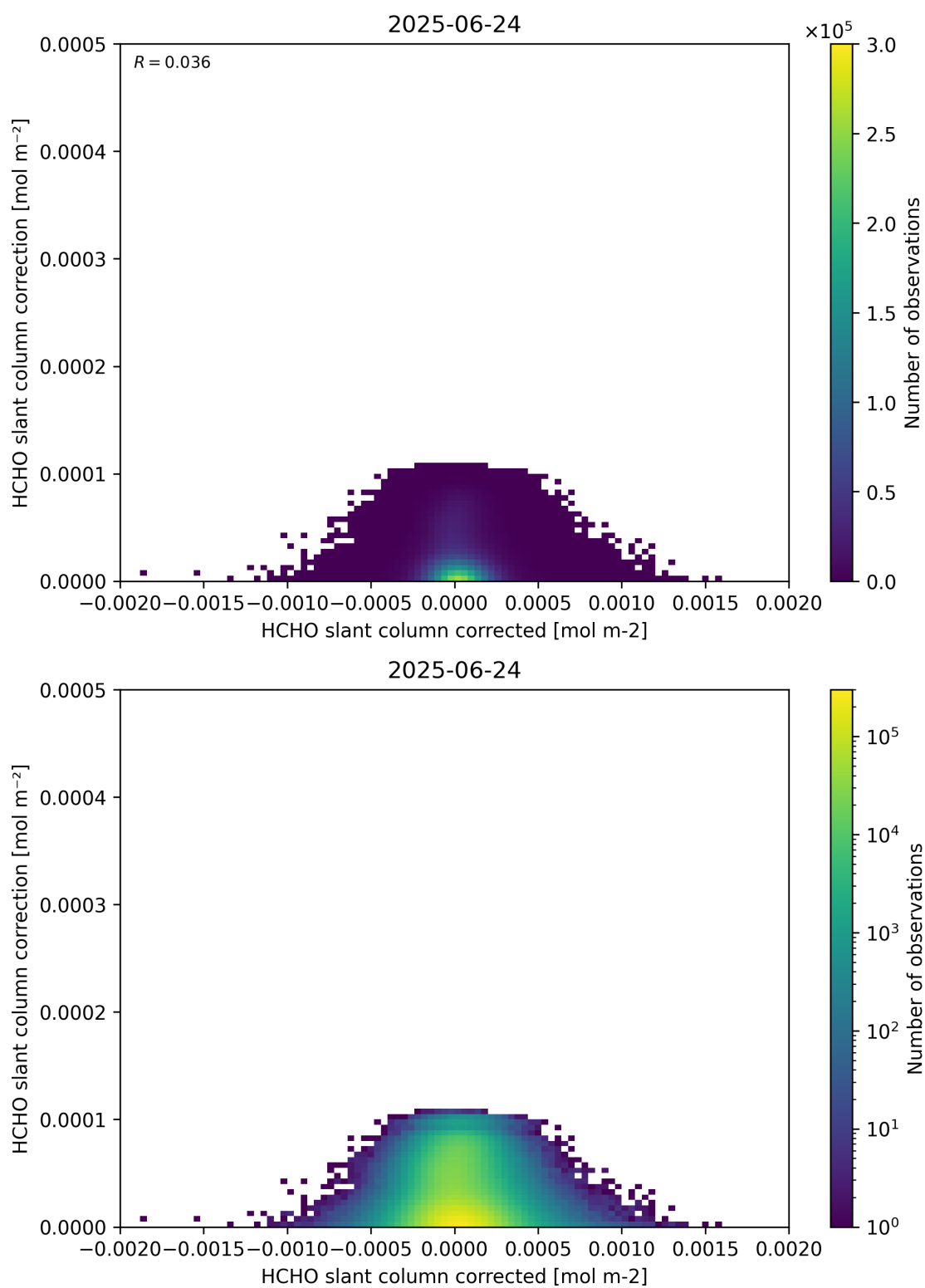
Figure 77: Scatter density plot of “HCHO slant column corrected” against “HCHO slant column correction” for 2025-06-23 to 2025-06-25.
