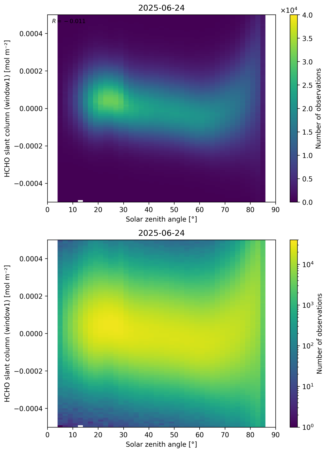
Figure 173: Scatter density plot of “Solar zenith angle” against “HCHO slant column (window1)” for 2025-06-23 to 2025-06-25.
