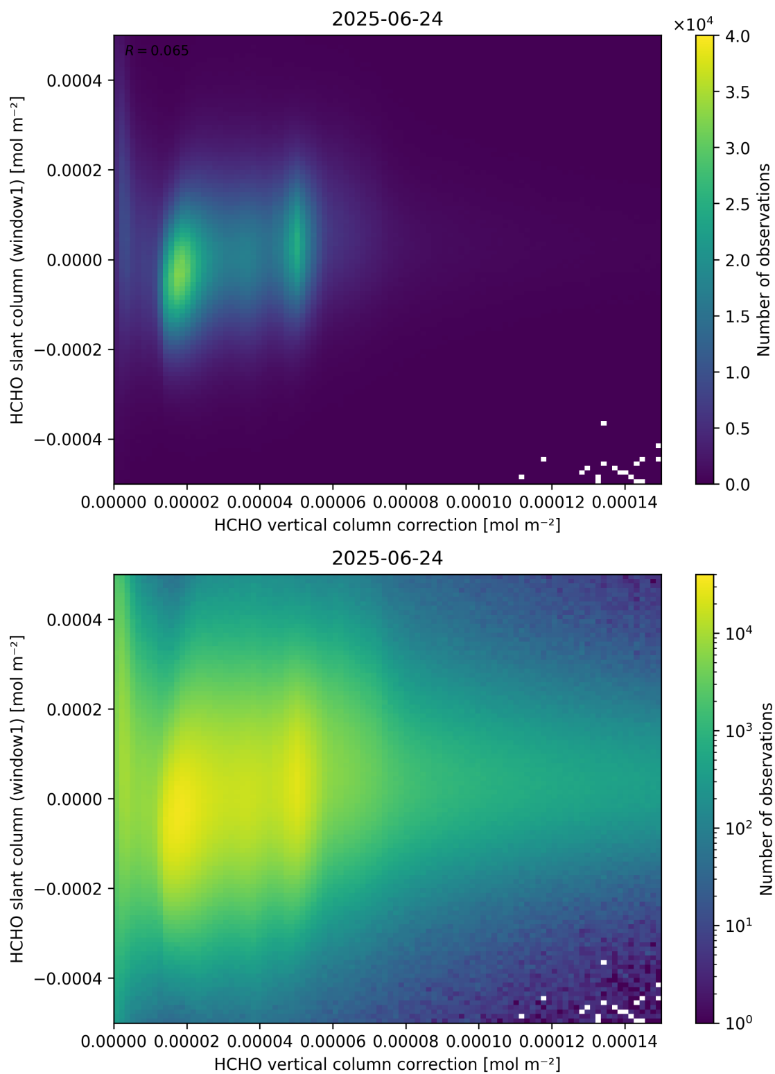
Figure 118: Scatter density plot of “HCHO vertical column correction” against “HCHO slant column (window1)” for 2025-06-23 to 2025-06-25.
