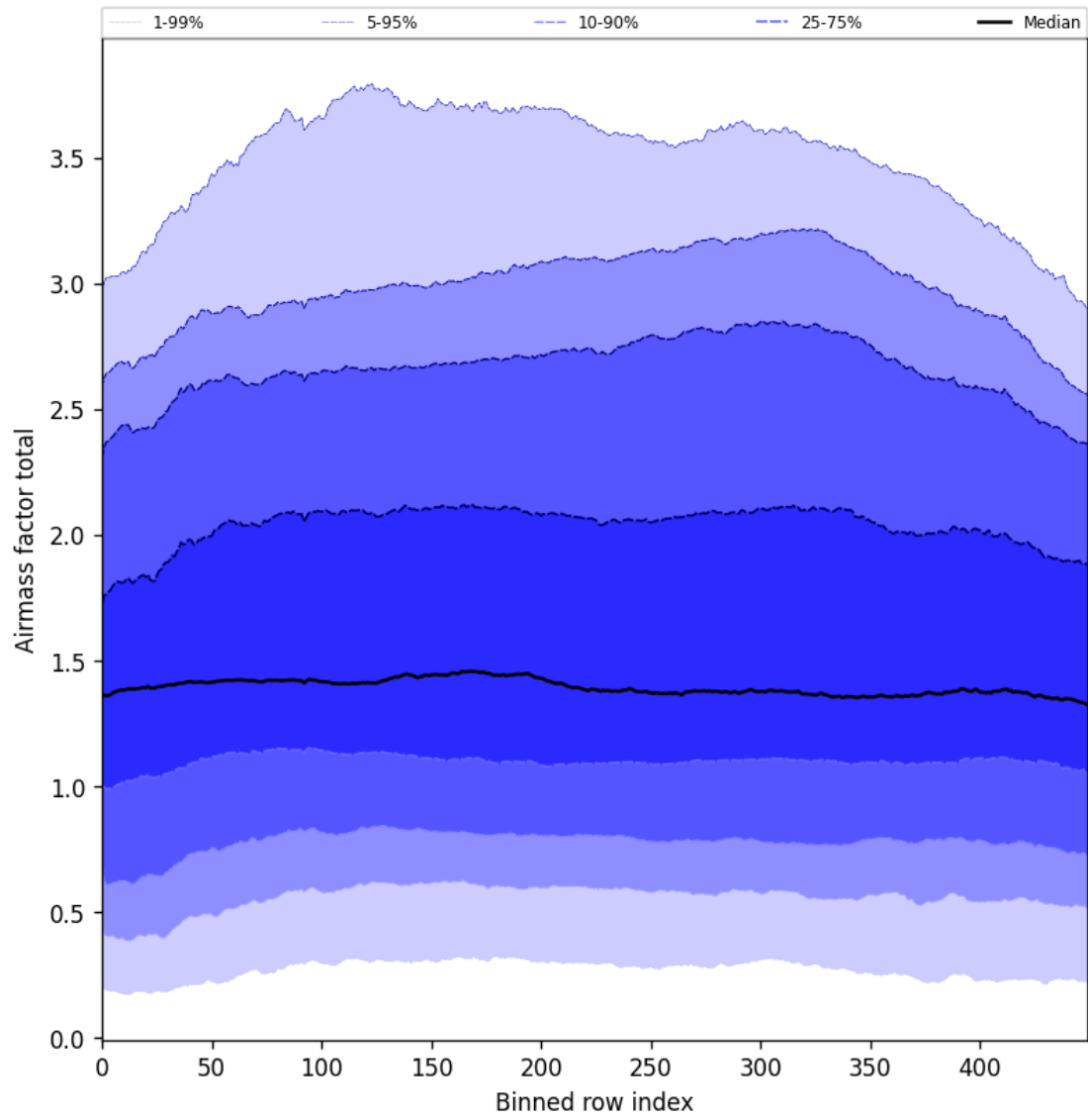
Figure 54: Along track statistics of “Airmass factor total” for 2025-06-23 to 2025-06-25
