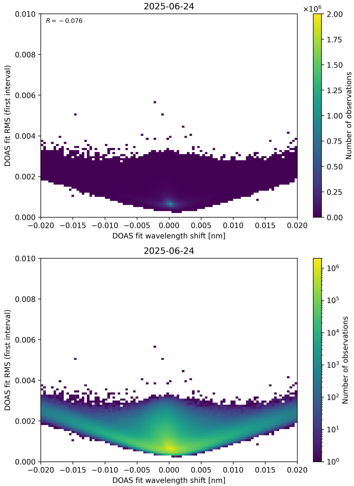
Figure 64: Scatter density plot of “DOAS fit wavelength shift” against “DOAS fit RMS (first interval)” for 2025-06-23 to 2025-06-25.
