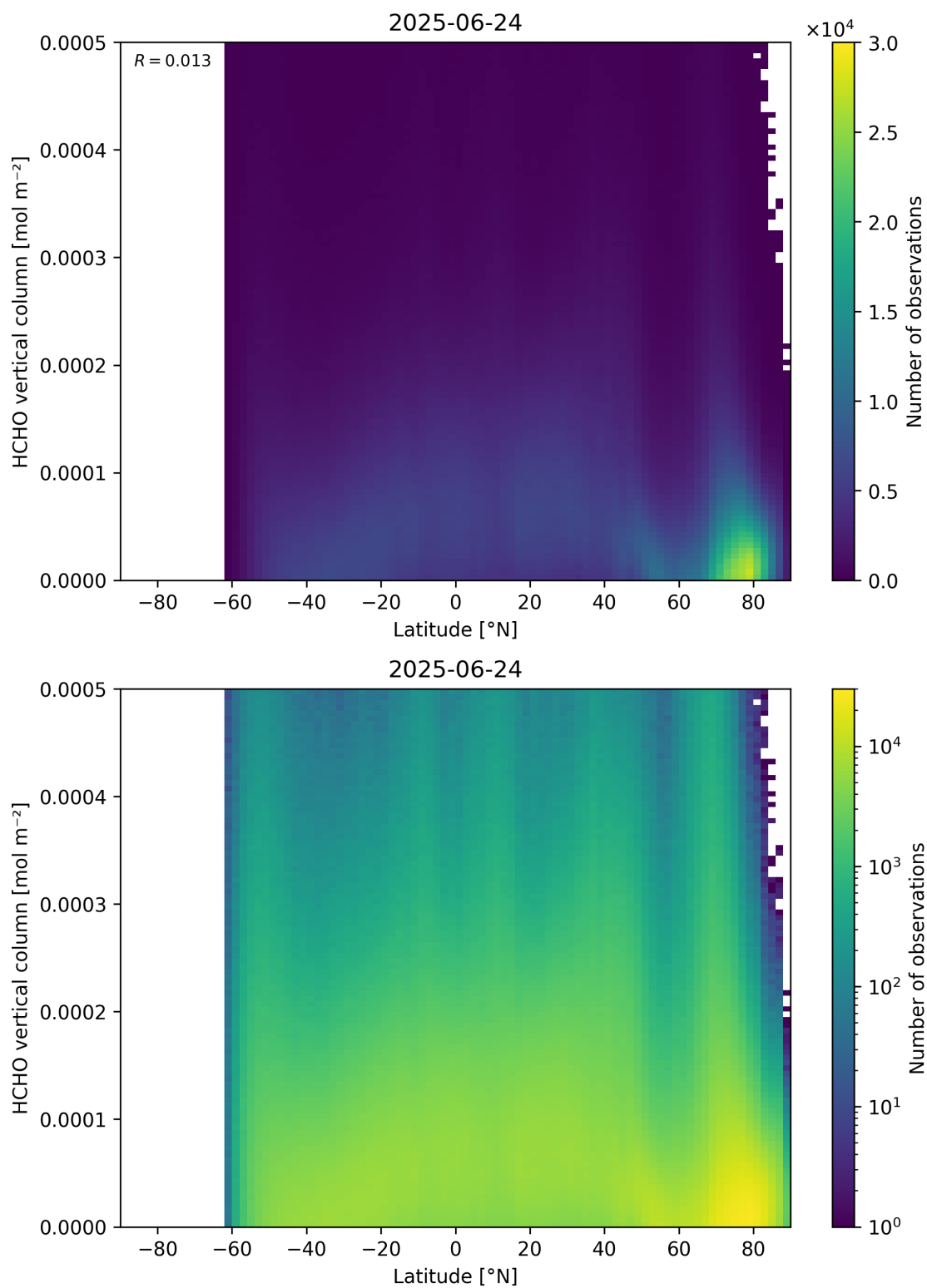
Figure 163: Scatter density plot of “Latitude” against “HCHO vertical column” for 2025-06-23 to 2025-06-25.
