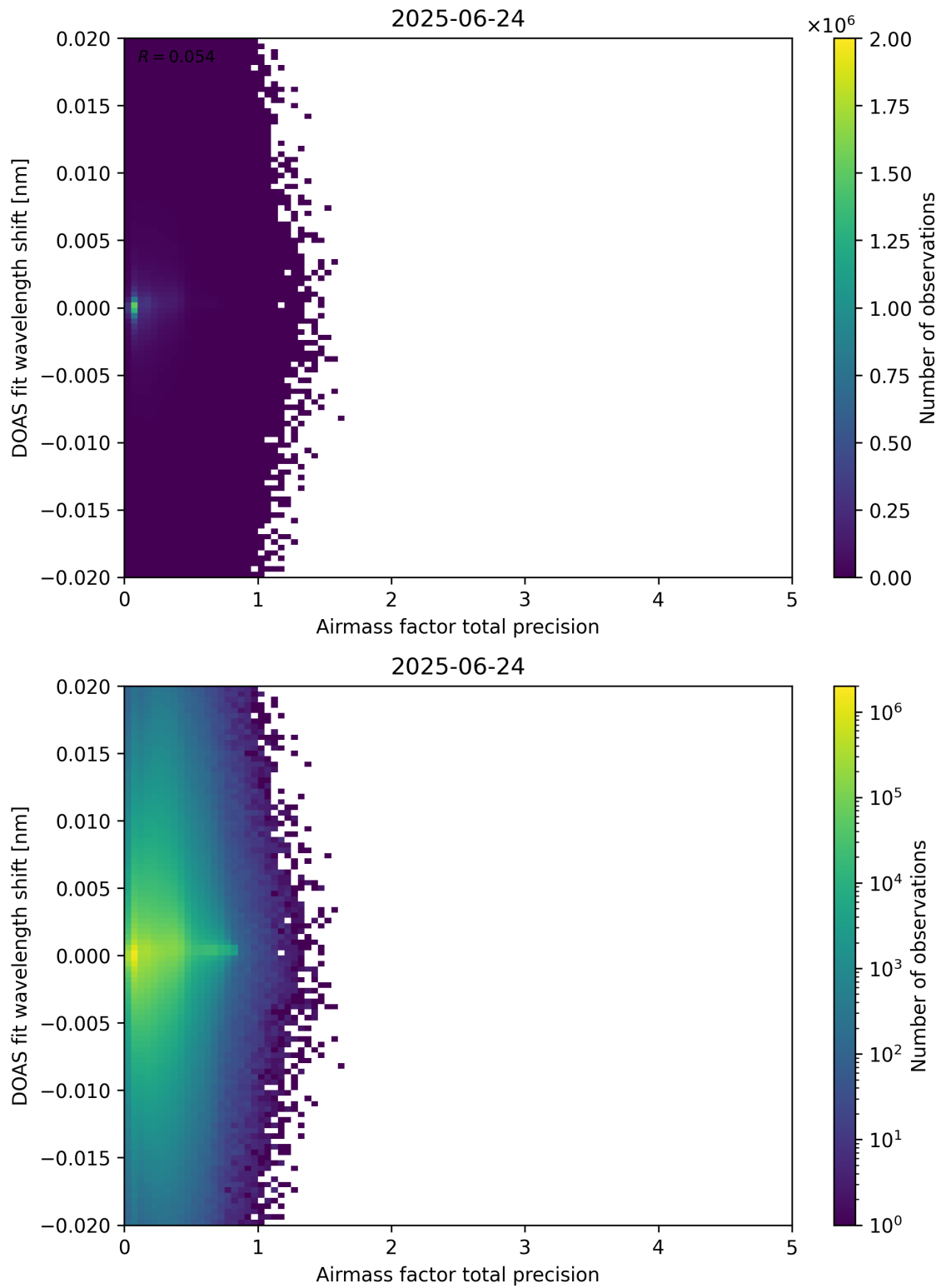
Figure 106: Scatter density plot of “Airmass factor total precision” against “DOAS fit wavelength shift” for 2025-06-23 to 2025-06-25.
