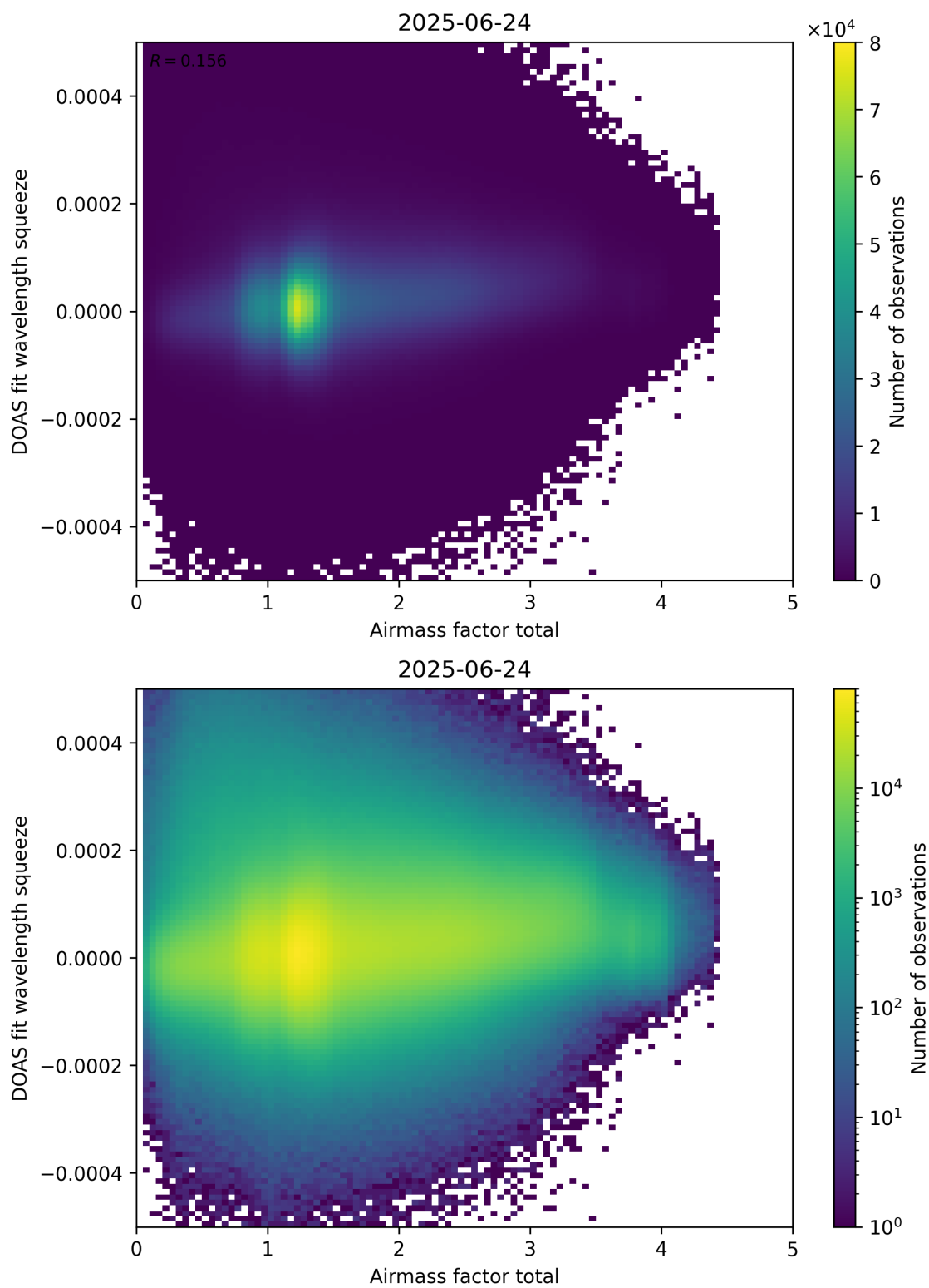
Figure 99: Scatter density plot of “Airmass factor total” against “DOAS fit wavelength squeeze” for 2025-06-23 to 2025-06-25.
