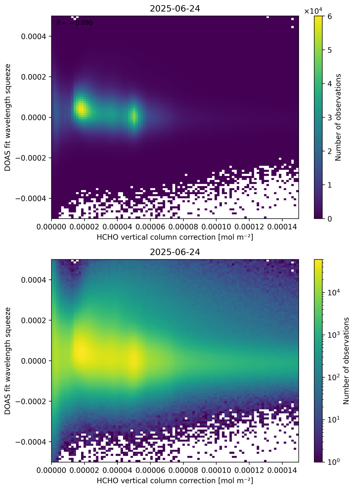
Figure 114: Scatter density plot of “HCHO vertical column correction” against “DOAS fit wavelength squeeze” for 2025-06-23 to 2025-06-25.
