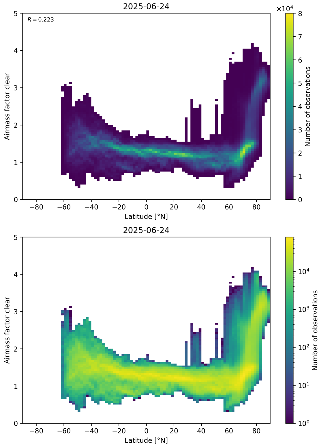
Figure 156: Scatter density plot of “Latitude” against “Airmass factor clear” for 2025-06-23 to 2025-06-25.
