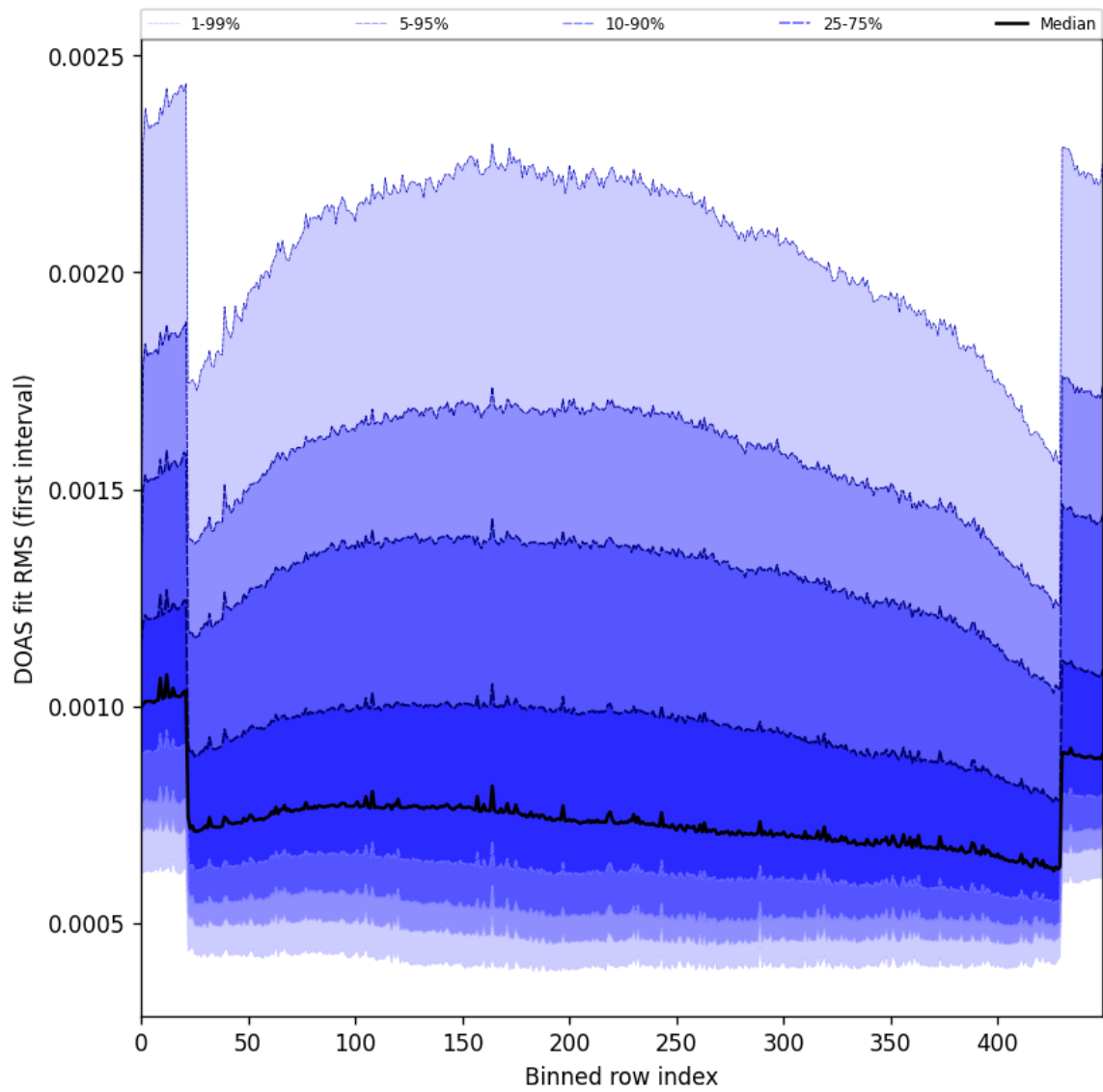
Figure 60: Along track statistics of “DOAS fit RMS (first interval)” for 2025-06-23 to 2025-06-25
