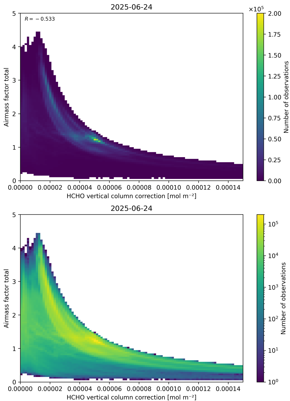
Figure 120: Scatter density plot of “HCHO vertical column correction” against “Airmass factor total” for 2025-06-23 to 2025-06-25.
