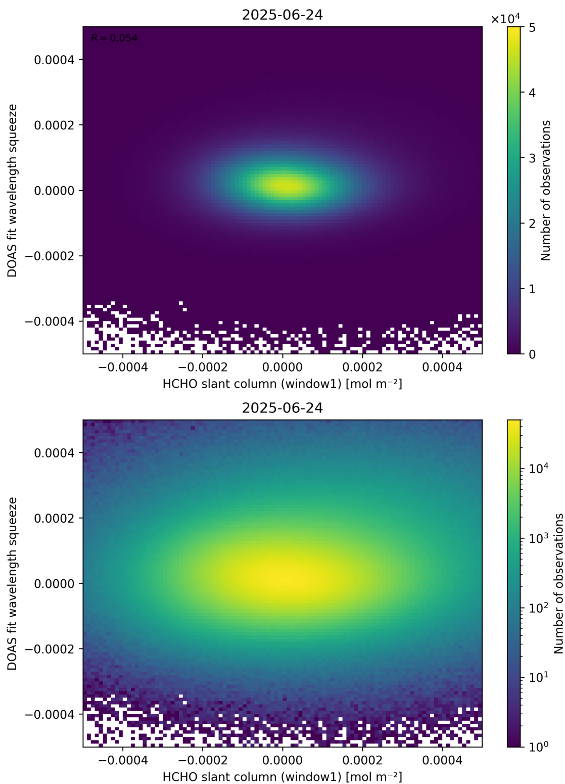
Figure 80: Scatter density plot of “HCHO slant column (window1)” against “DOAS fit wavelength squeeze” for 2025-06-23 to 2025-06-25.
