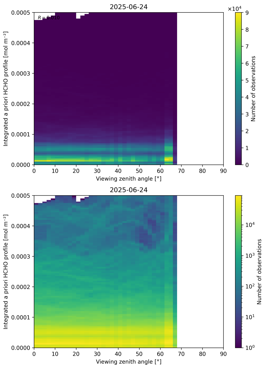
Figure 195: Scatter density plot of “Viewing zenith angle” against “Integrated a priori HCHO profile” for 2025-06-23 to 2025-06-25.
