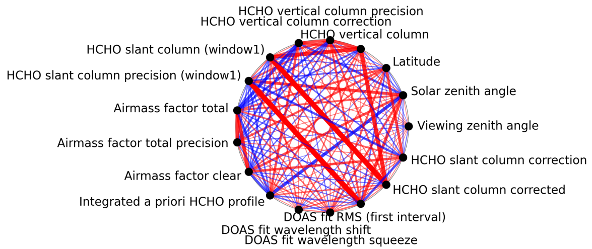
Figure 1: Map of correlation graph for 2025-06-23 to 2025-06-25.
