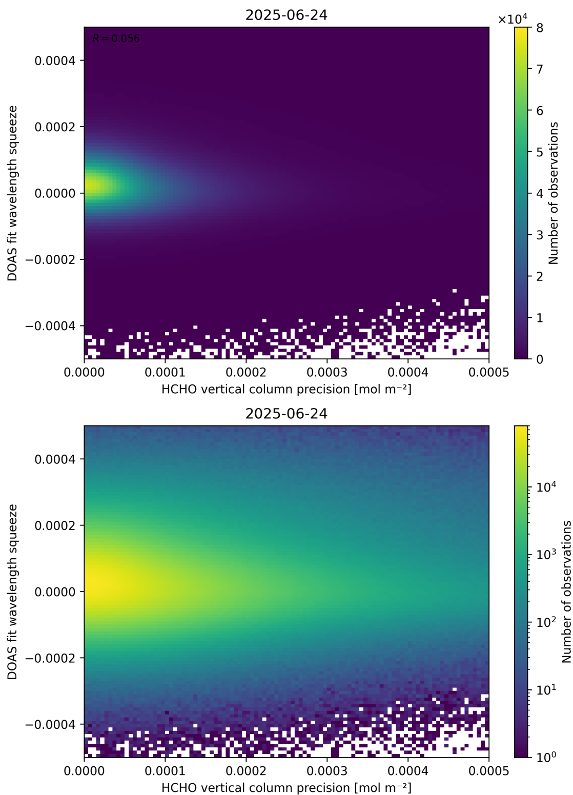
Figure 138: Scatter density plot of “HCHO vertical column precision” against “DOAS fit wavelength squeeze” for 2025-06-23 to 2025-06-25.
