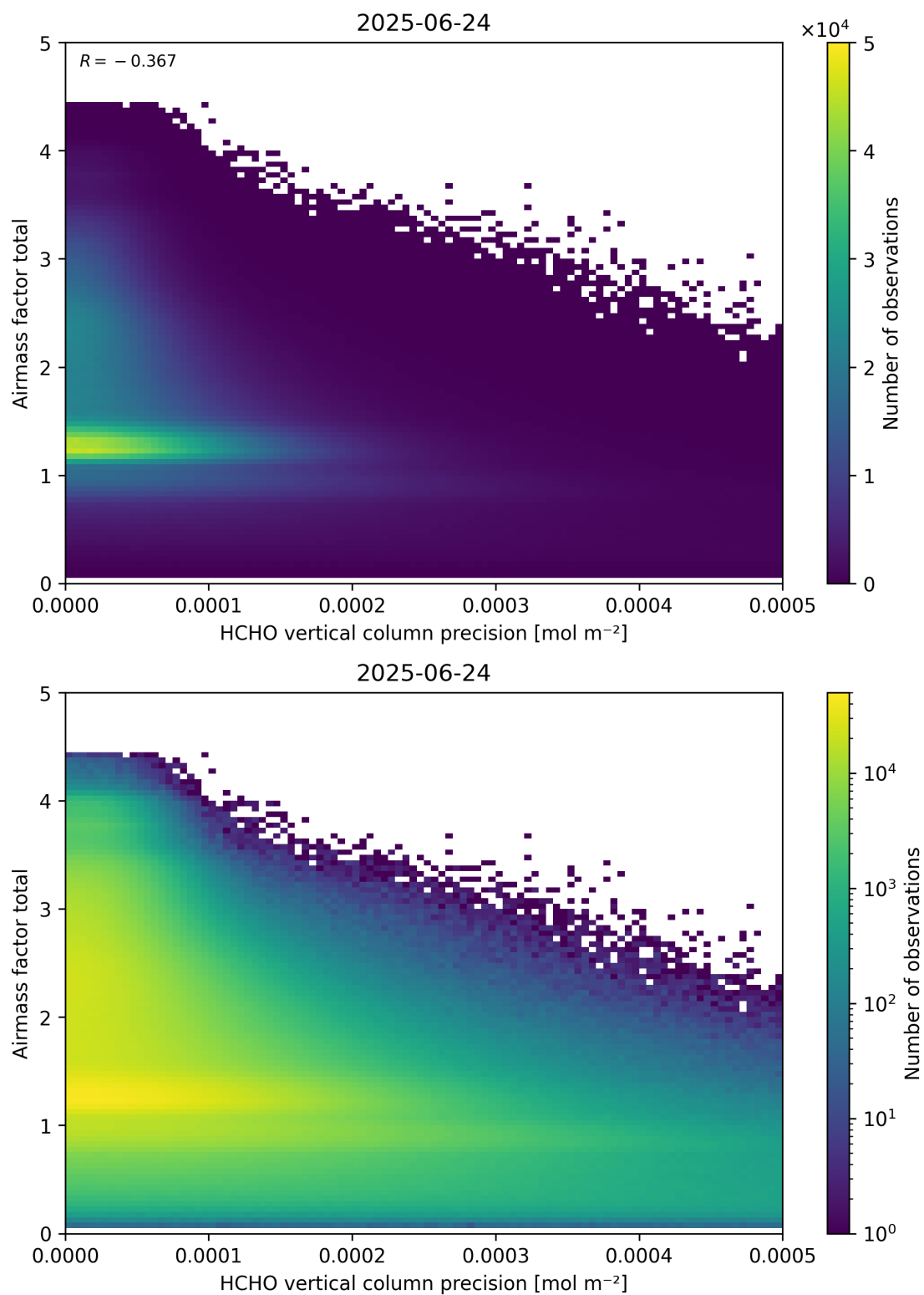
Figure 144: Scatter density plot of “HCHO vertical column precision” against “Airmass factor total” for 2025-06-23 to 2025-06-25.
