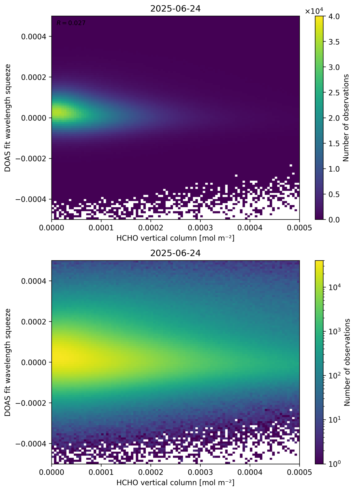
Figure 125: Scatter density plot of “HCHO vertical column” against “DOAS fit wavelength squeeze” for 2025-06-23 to 2025-06-25.
