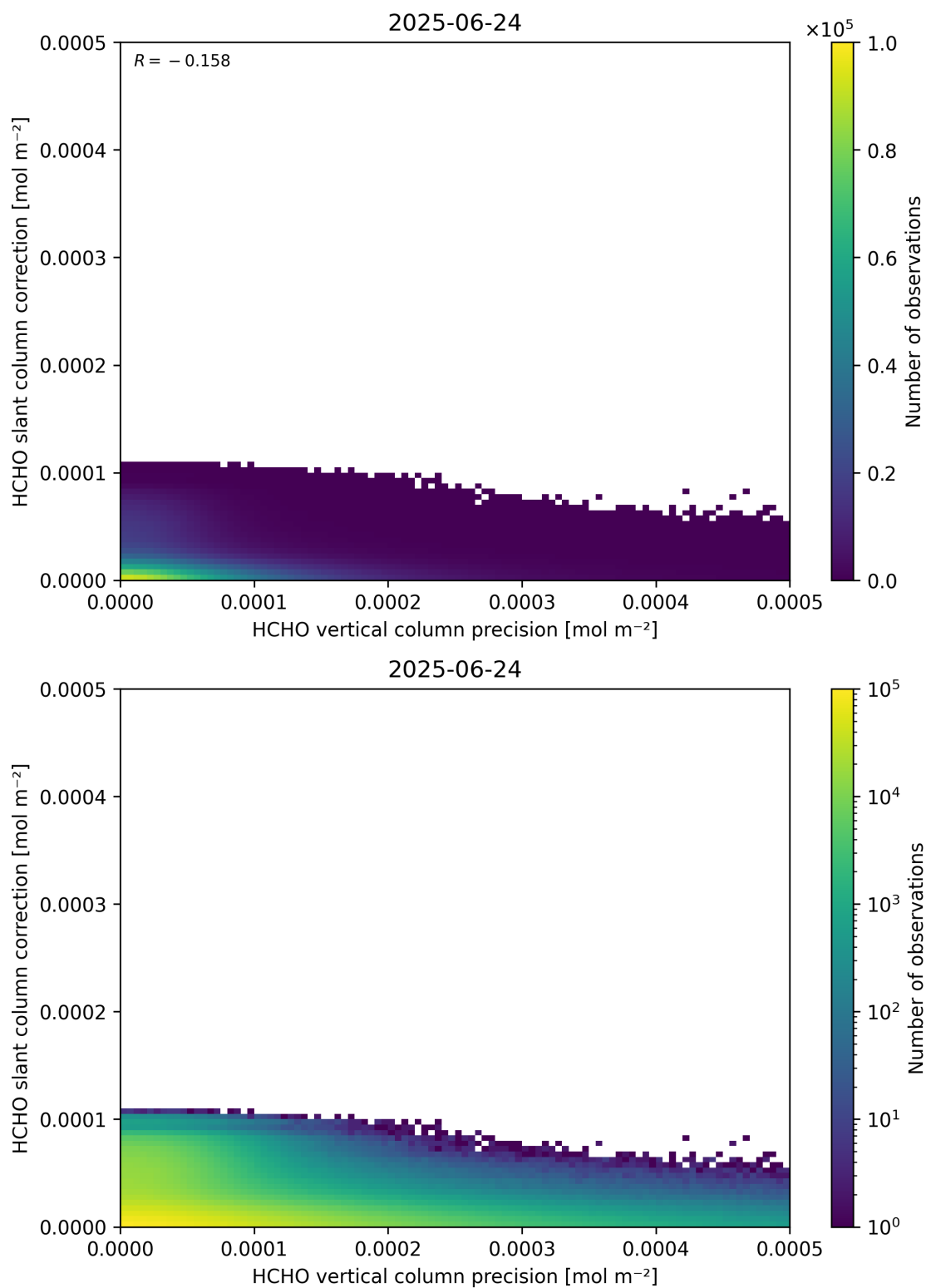
Figure 141: Scatter density plot of “HCHO vertical column precision” against “HCHO slant column correction” for 2025-06-23 to 2025-06-25.
