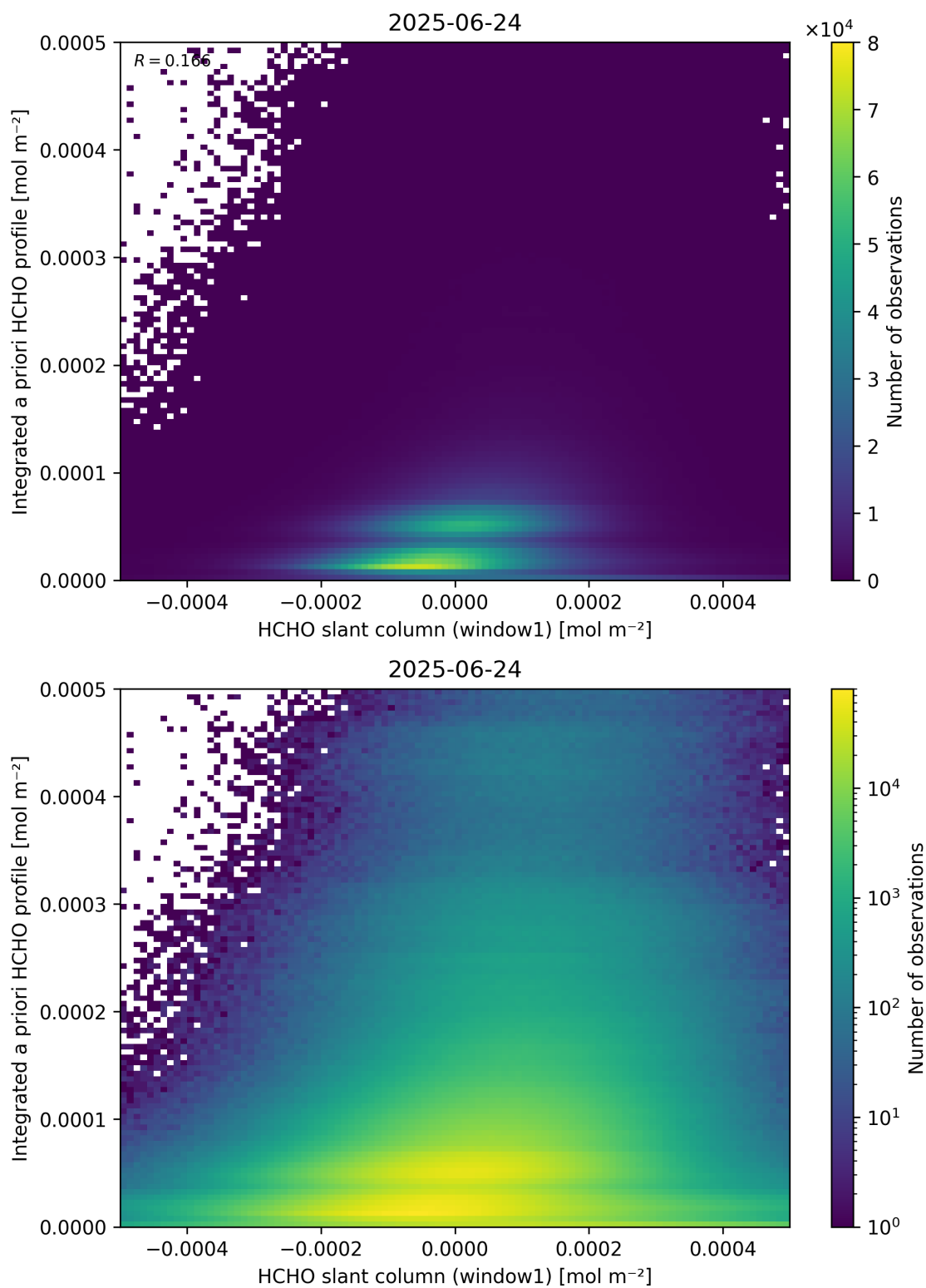
Figure 87: Scatter density plot of “HCHO slant column (window1)” against “Integrated a priori HCHO profile” for 2025-06-23 to 2025-06-25.
