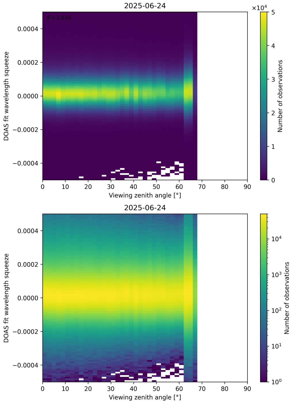
Figure 184: Scatter density plot of “Viewing zenith angle” against “DOAS fit wavelength squeeze” for 2025-06-23 to 2025-06-25.
