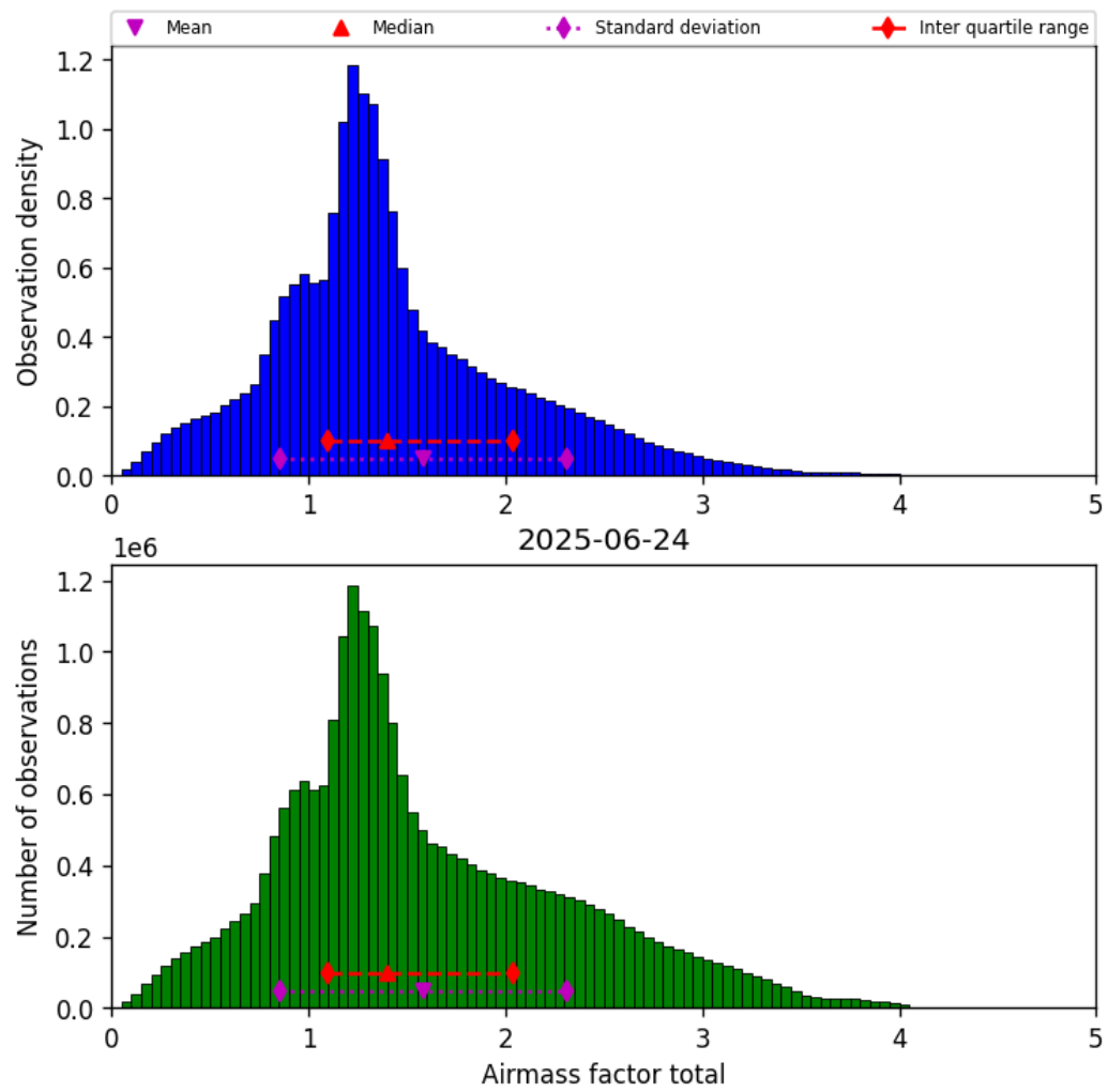
Figure 40: Histogram of “Airmass factor total” for 2025-06-23 to 2025-06-25
