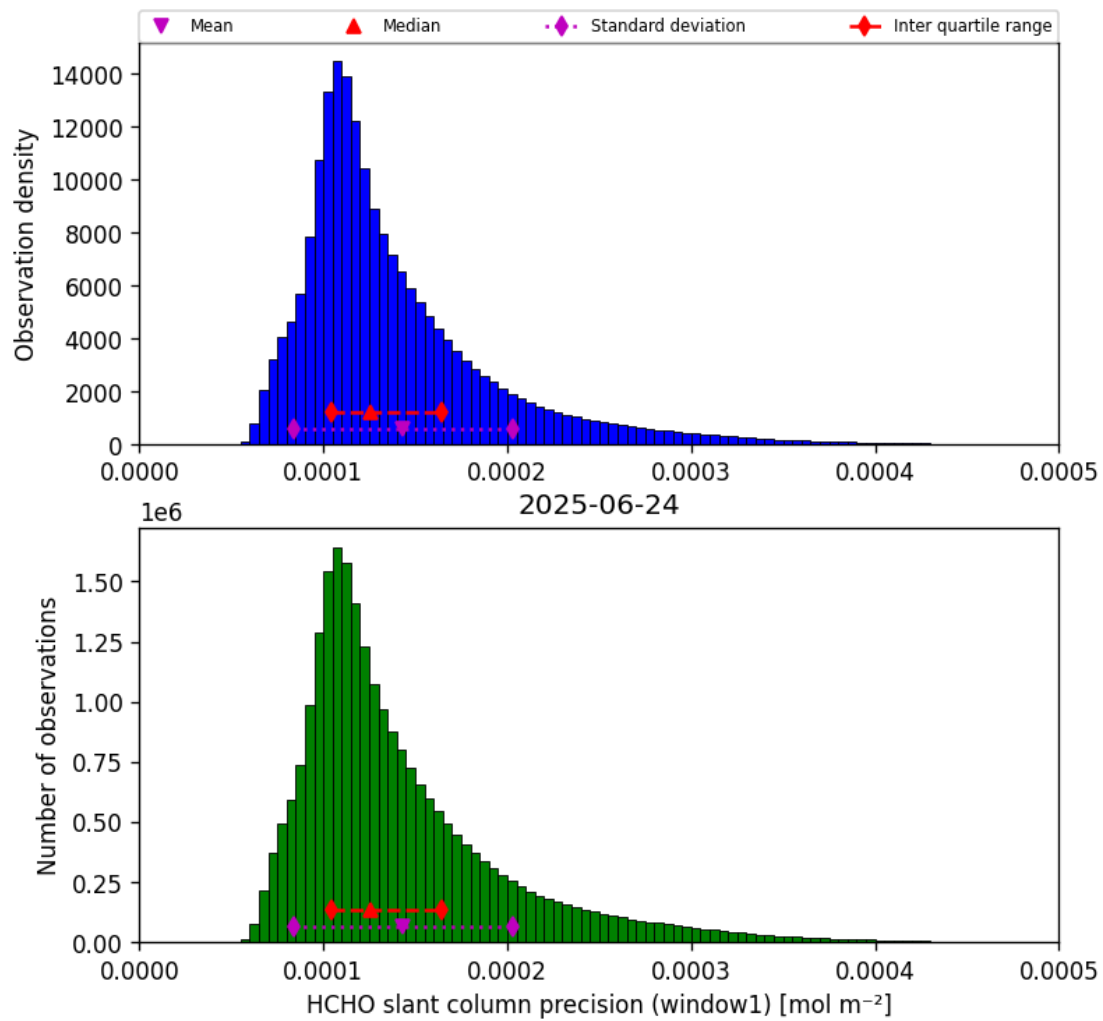
Figure 39: Histogram of “HCHO slant column precision (window1)” for 2025-06-23 to 2025-06-25
