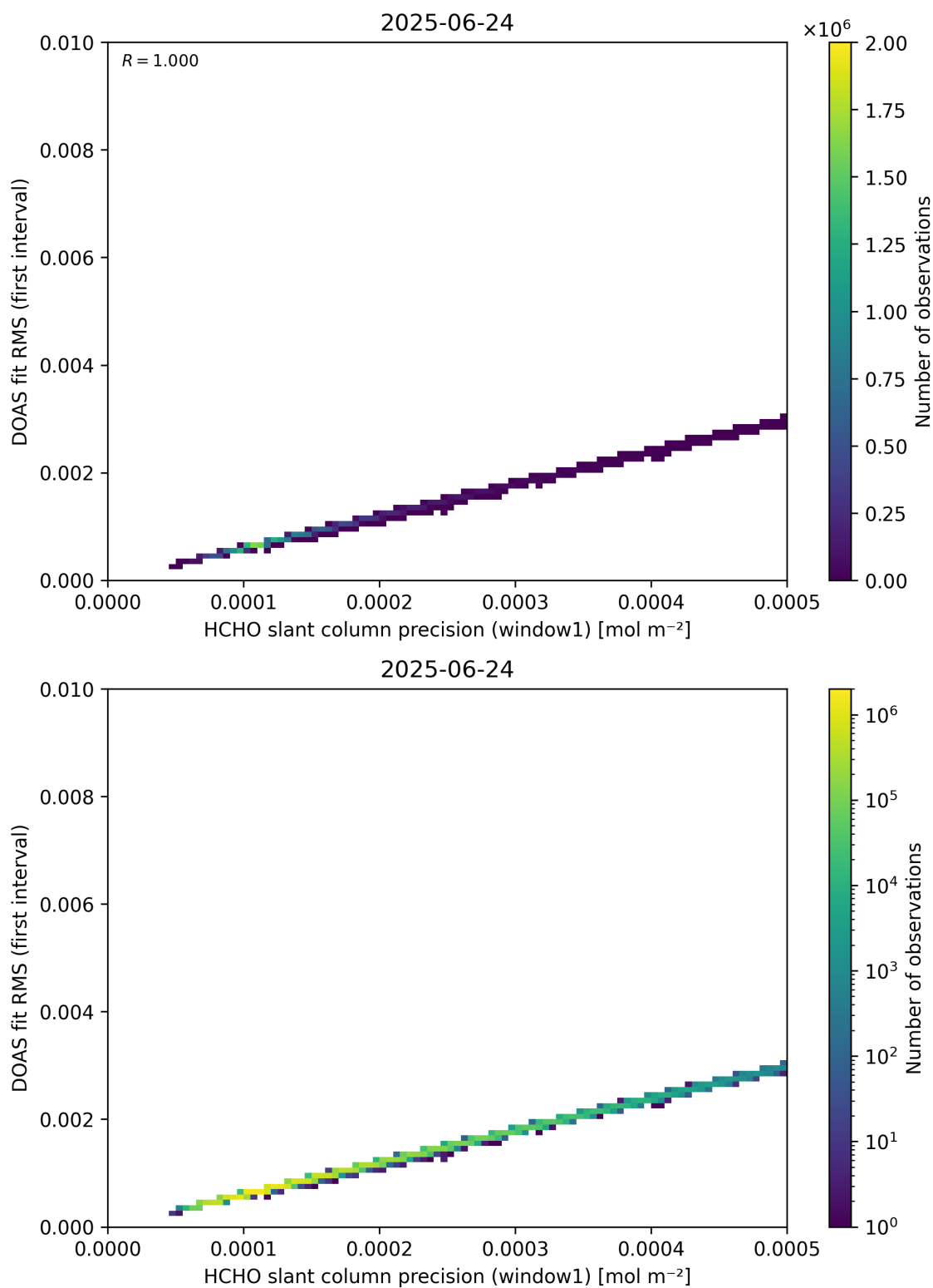
Figure 88: Scatter density plot of “HCHO slant column precision (window1)” against “DOAS fit RMS (first interval)” for 2025-06-23 to 2025-06-25.
