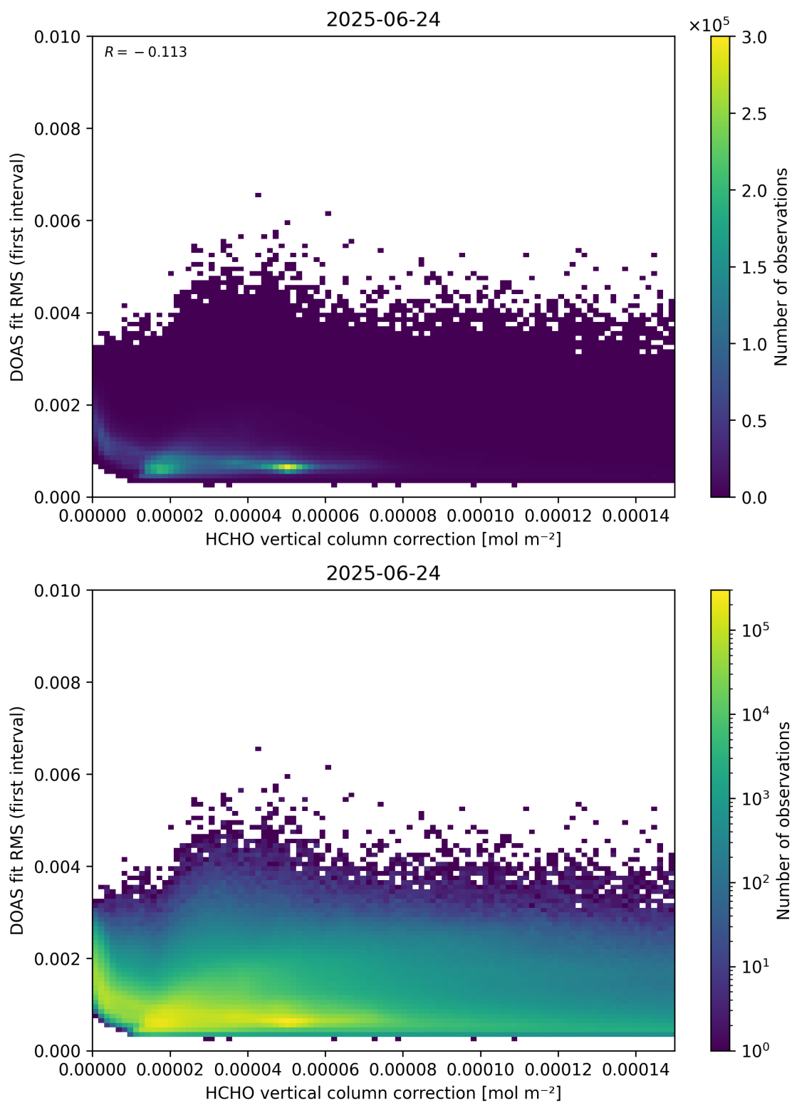
Figure 112: Scatter density plot of “HCHO vertical column correction” against “DOAS fit RMS (first interval)” for 2025-06-23 to 2025-06-25.
