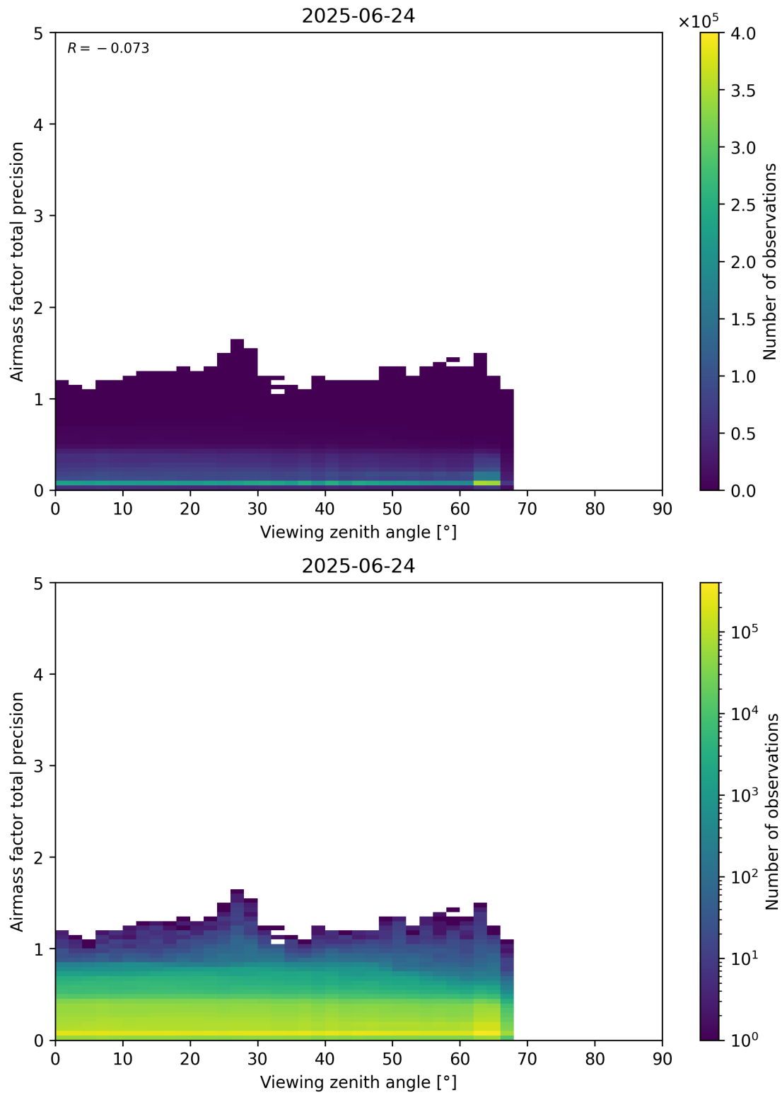
Figure 191: Scatter density plot of “Viewing zenith angle” against “Airmass factor total precision” for 2025-06-23 to 2025-06-25.
