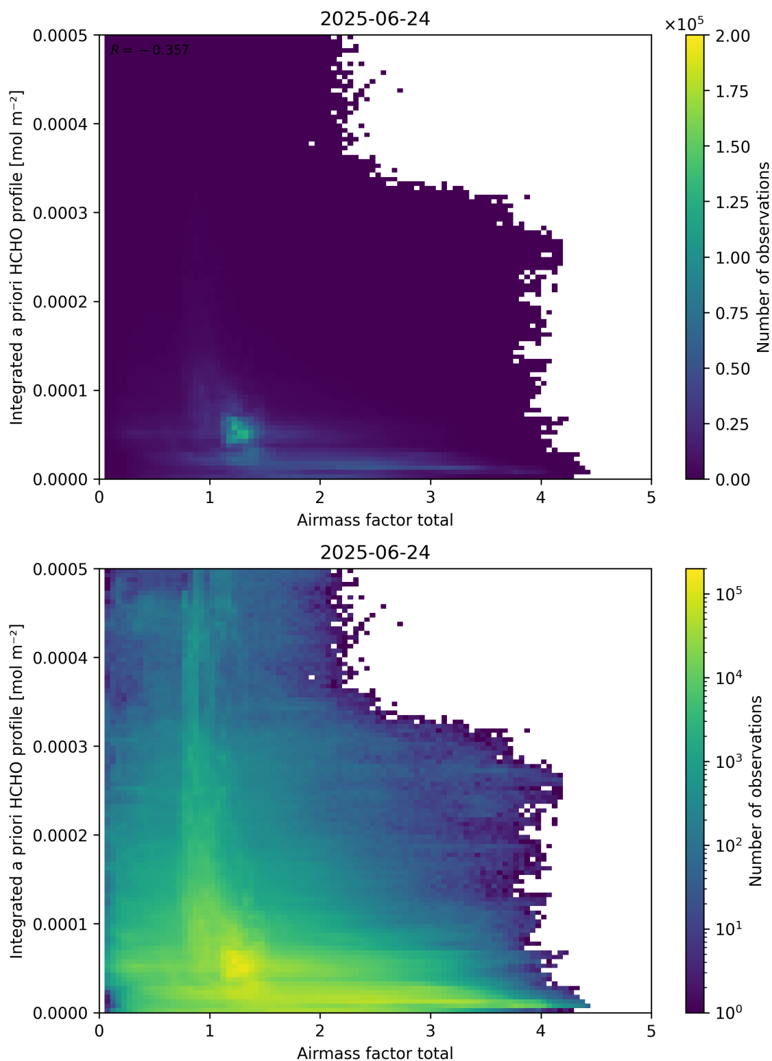
Figure 104: Scatter density plot of “Airmass factor total” against “Integrated a priori HCHO profile” for 2025-06-23 to 2025-06-25.
