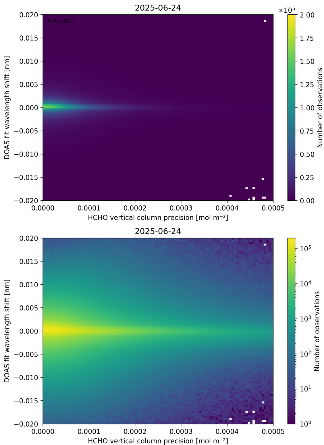
Figure 137: Scatter density plot of “HCHO vertical column precision” against “DOAS fit wavelength shift” for 2025-06-23 to 2025-06-25.
