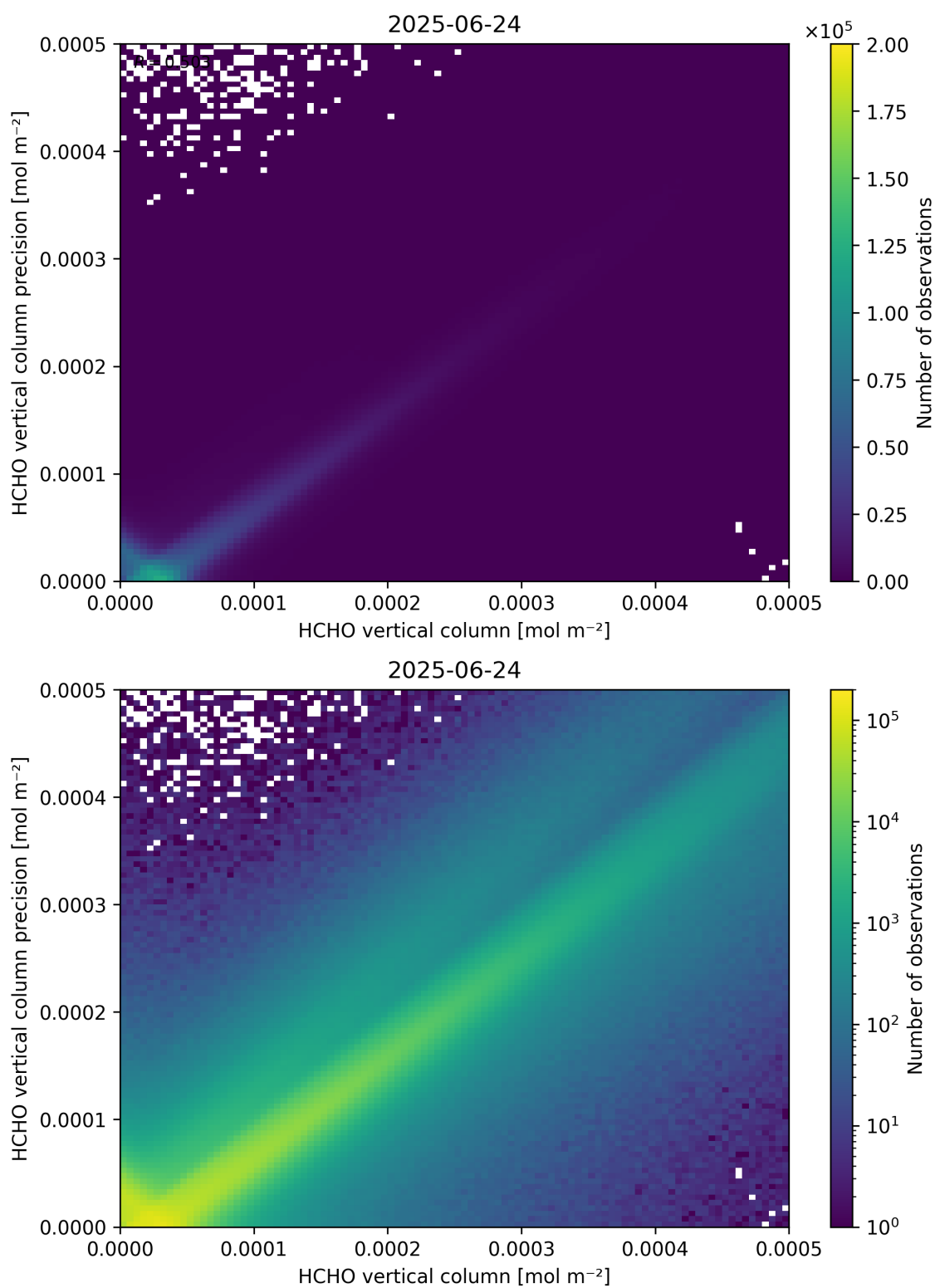
Figure 134: Scatter density plot of “HCHO vertical column” against “HCHO vertical column precision” for 2025-06-23 to 2025-06-25.
