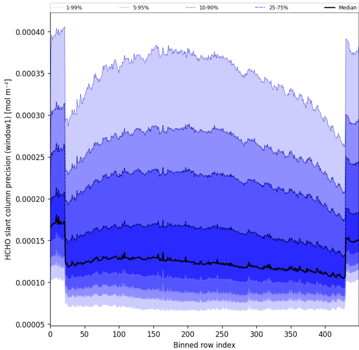
Figure 53: Along track statistics of “HCHO slant column precision (window1)” for 2025-06-23 to 2025-06-25
