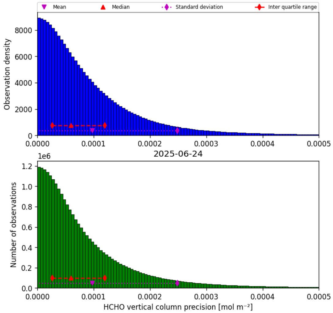
Figure 36: Histogram of “HCHO vertical column precision” for 2025-06-23 to 2025-06-25
