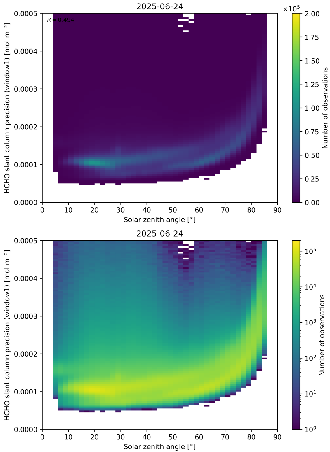
Figure 174: Scatter density plot of “Solar zenith angle” against “HCHO slant column precision (window1)” for 2025-06-23 to 2025-06-25.
