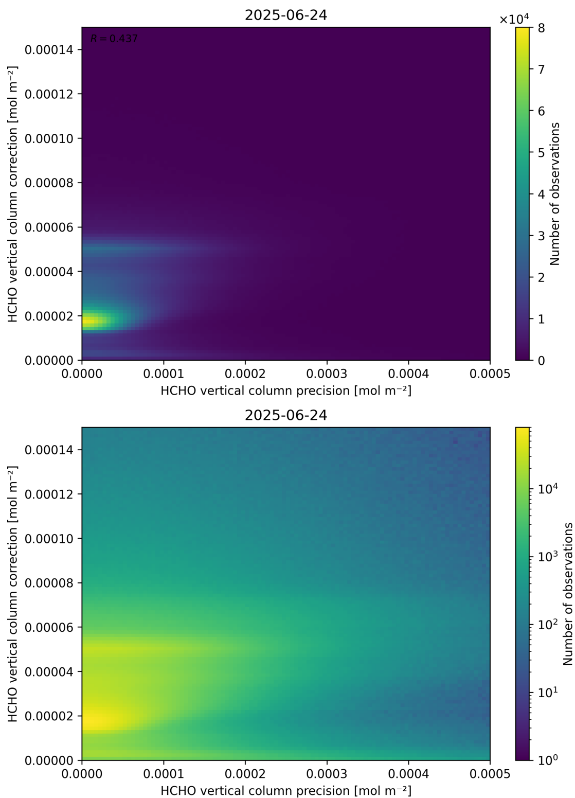
Figure 146: Scatter density plot of “HCHO vertical column precision” against “HCHO vertical column correction” for 2025-06-23 to 2025-06-25.
