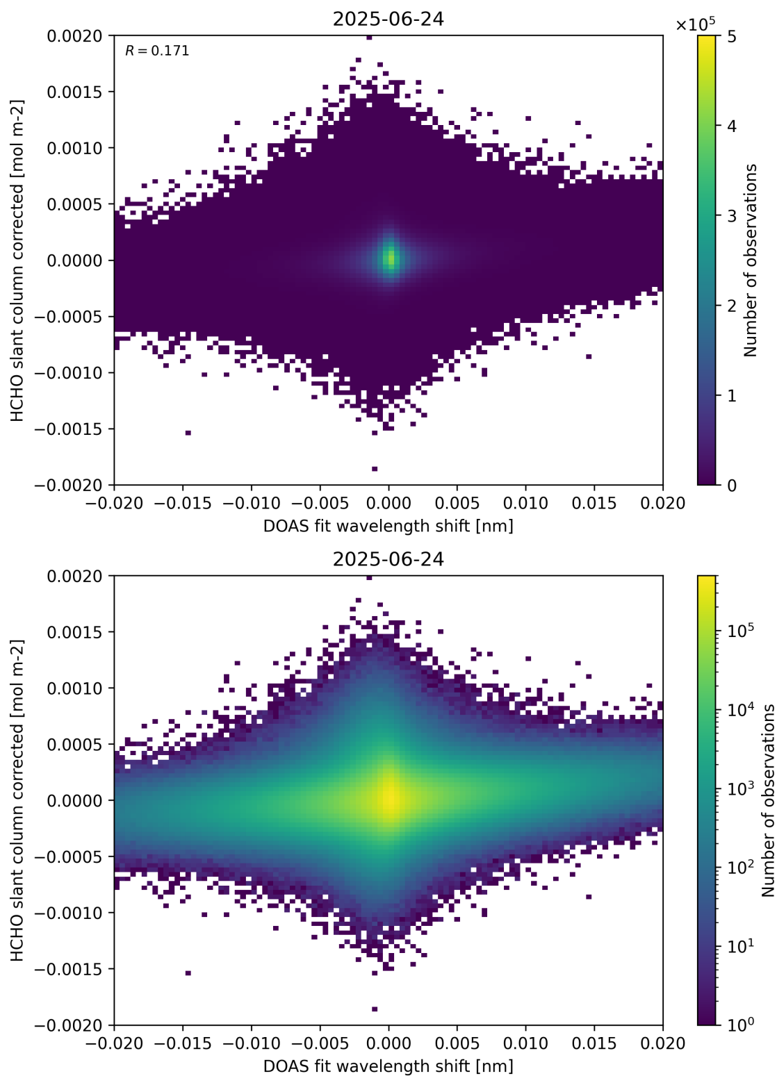
Figure 66: Scatter density plot of “DOAS fit wavelength shift” against “HCHO slant column corrected” for 2025-06-23 to 2025-06-25.
