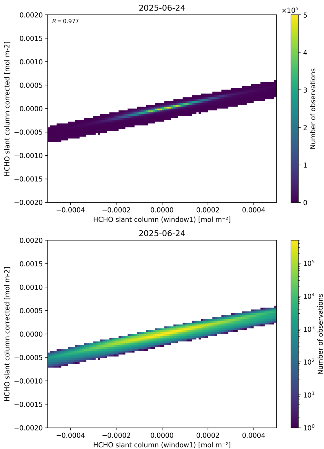
Figure 82: Scatter density plot of “HCHO slant column (window1)” against “HCHO slant column corrected” for 2025-06-23 to 2025-06-25.
