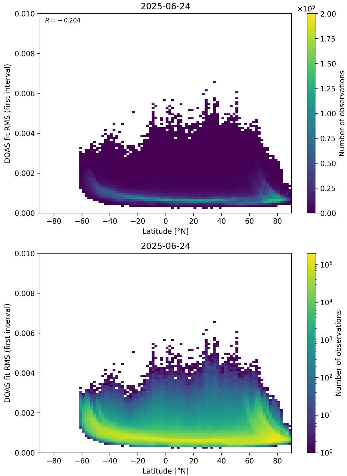
Figure 153: Scatter density plot of “Latitude” against “DOAS fit RMS (first interval)” for 2025-06-23 to 2025-06-25.
