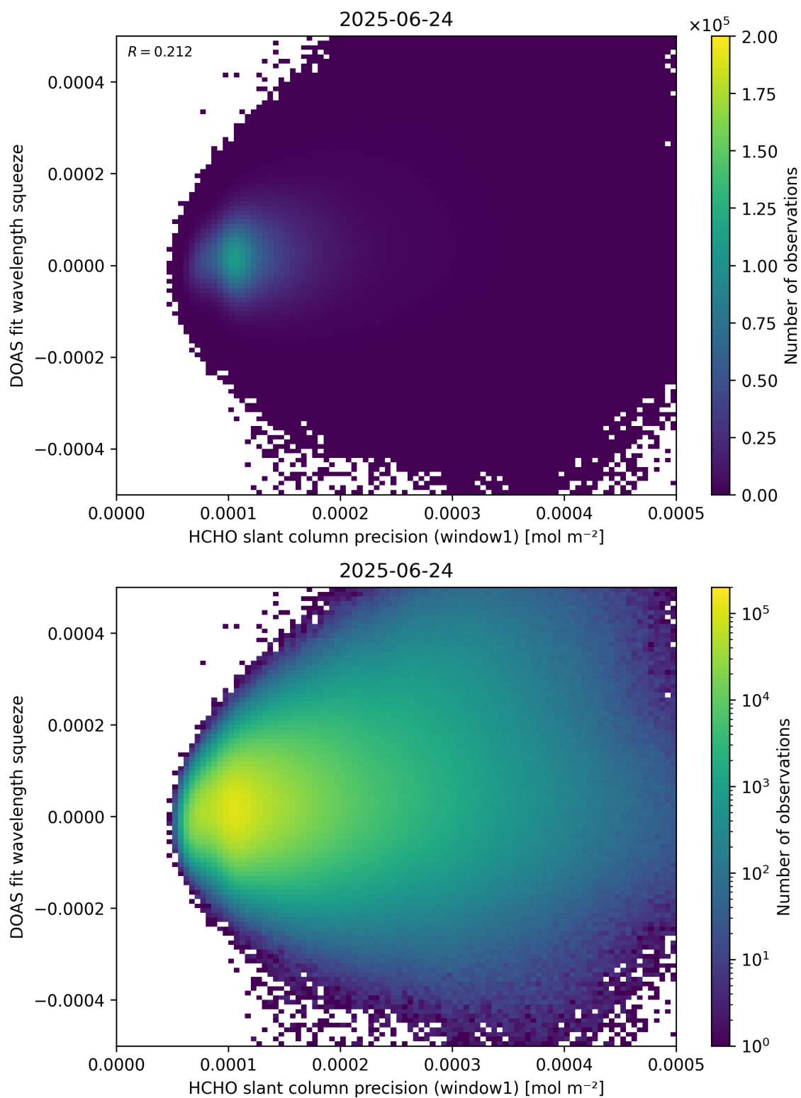
Figure 90: Scatter density plot of “HCHO slant column precision (window1)” against “DOAS fit wavelength squeeze” for 2025-06-23 to 2025-06-25.
