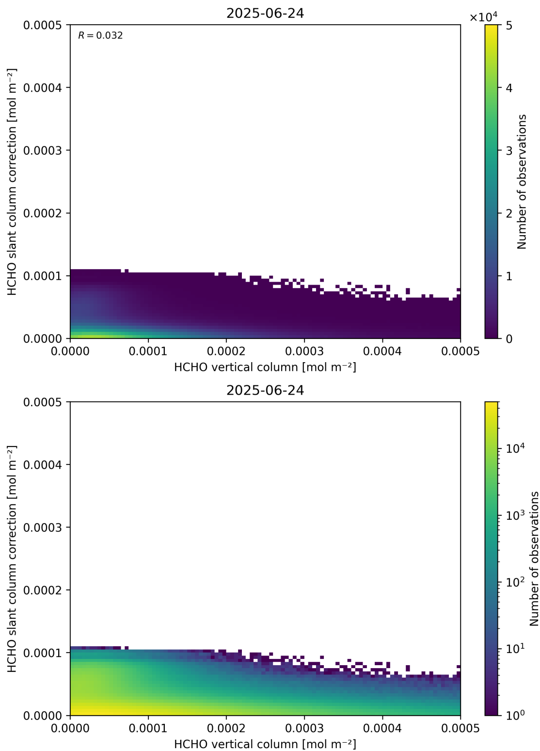
Figure 128: Scatter density plot of “HCHO vertical column” against “HCHO slant column correction” for 2025-06-23 to 2025-06-25.
