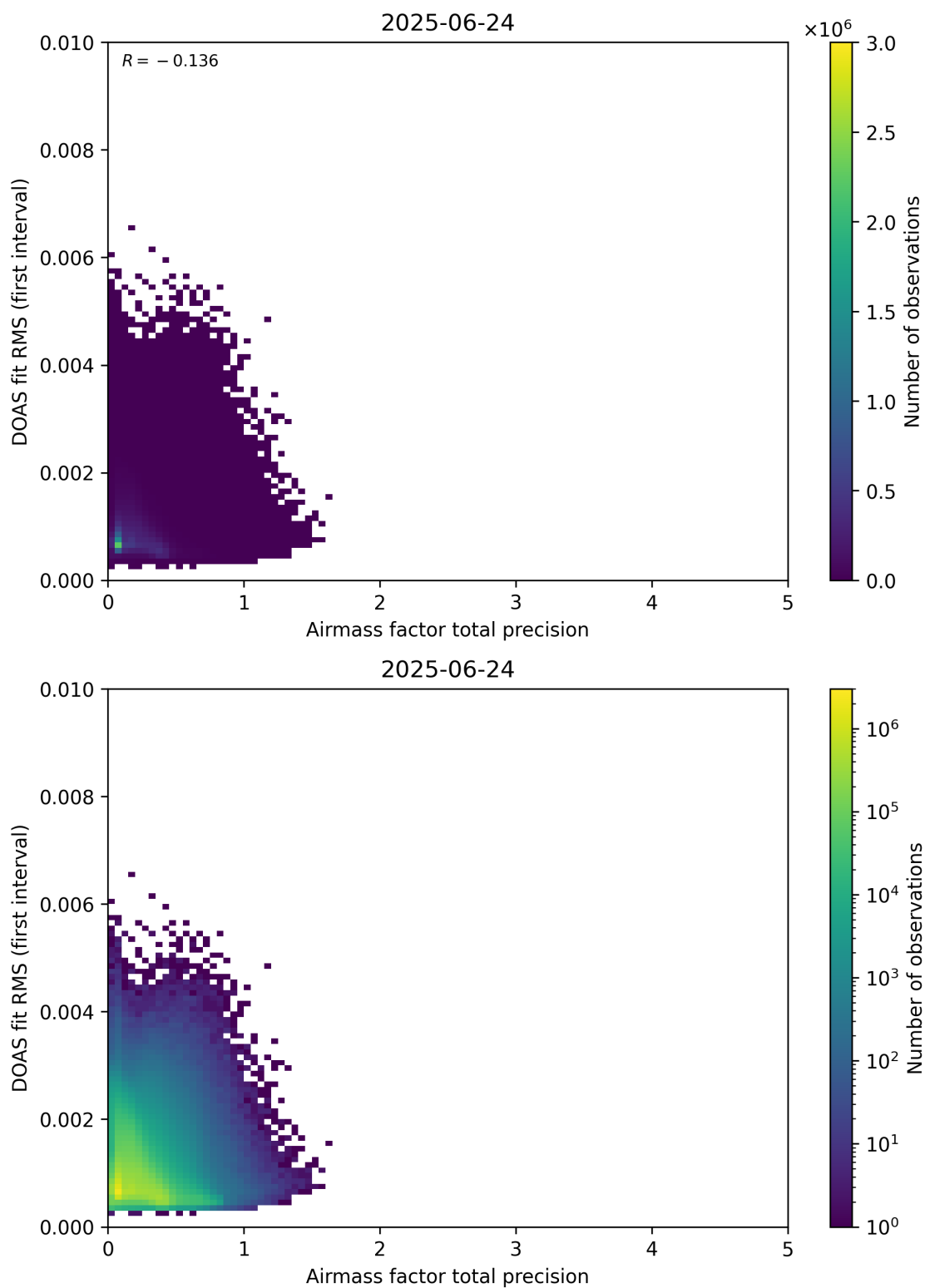
Figure 105: Scatter density plot of “Airmass factor total precision” against “DOAS fit RMS (first interval)” for 2025-06-23 to 2025-06-25.
