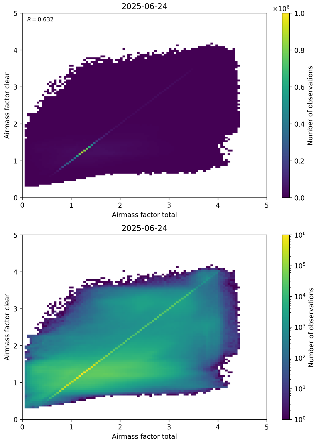
Figure 100: Scatter density plot of “Airmass factor total” against “Airmass factor clear” for 2025-06-23 to 2025-06-25.
