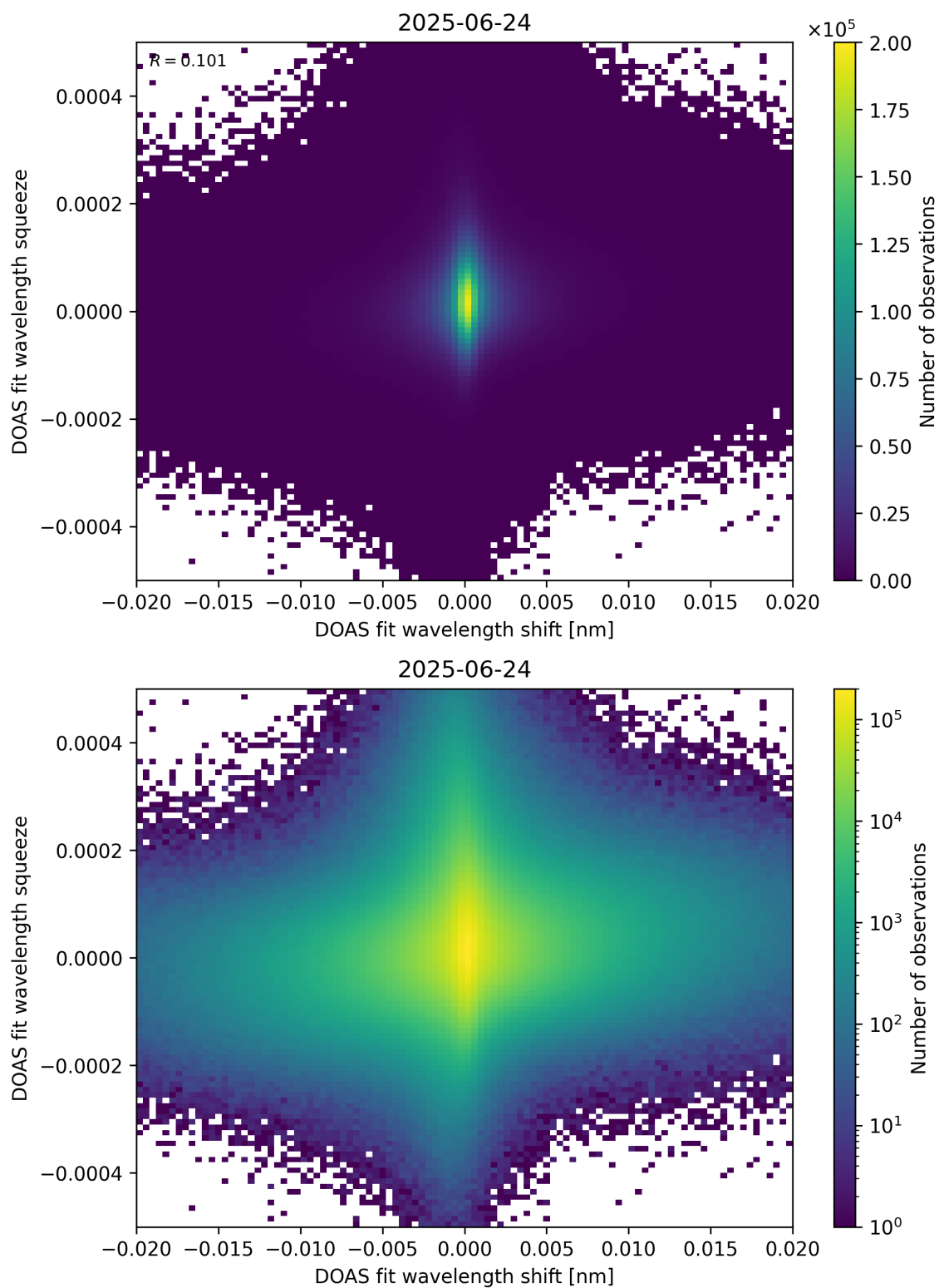
Figure 65: Scatter density plot of “DOAS fit wavelength shift” against “DOAS fit wavelength squeeze” for 2025-06-23 to 2025-06-25.
