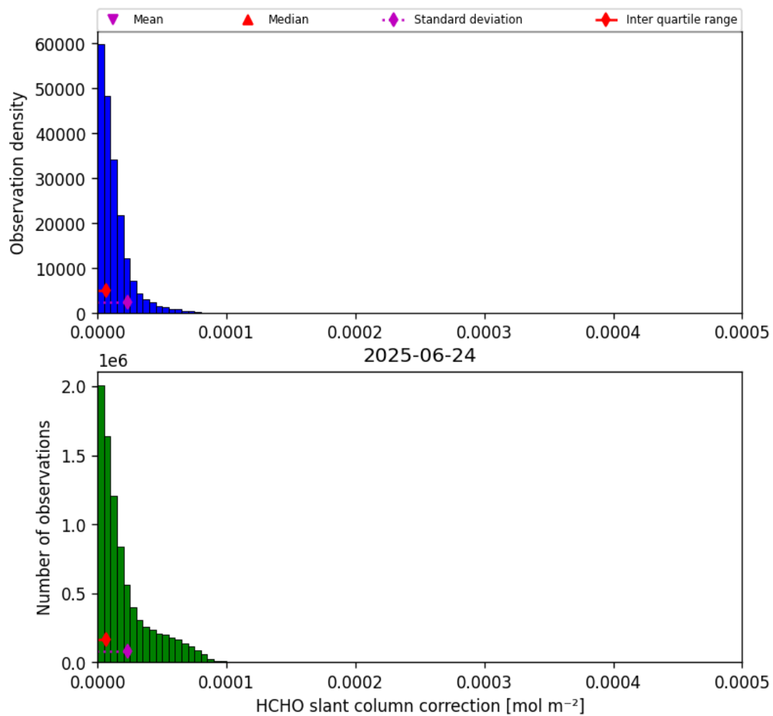
Figure 47: Histogram of “HCHO slant column correction” for 2025-06-23 to 2025-06-25
