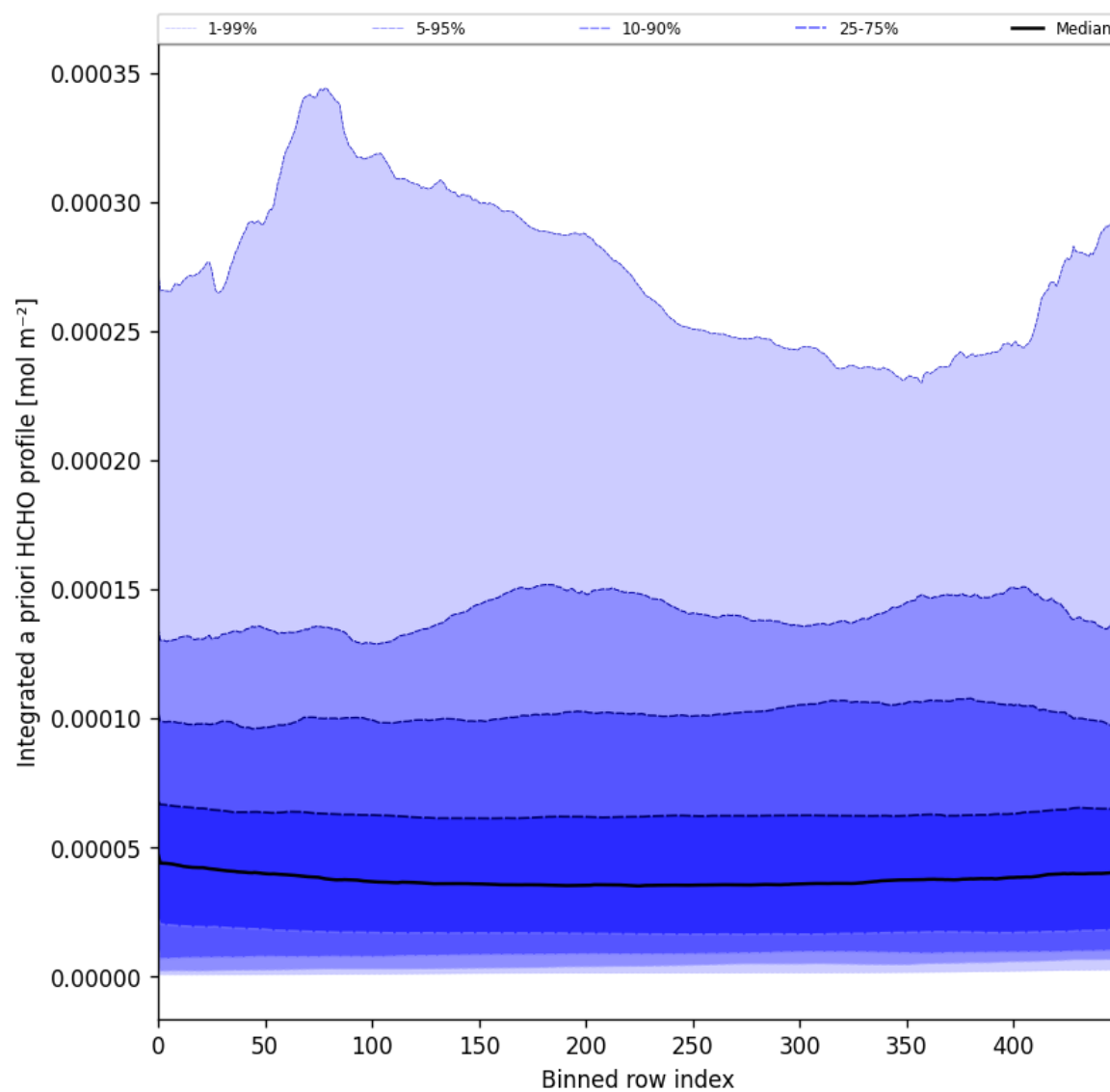
Figure 57: Along track statistics of “Integrated a priori HCHO profile” for 2025-06-23 to 2025-06-25
