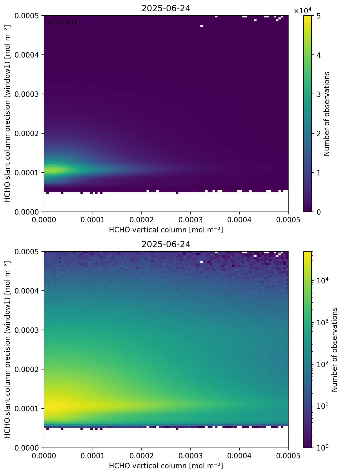
Figure 130: Scatter density plot of “HCHO vertical column” against “HCHO slant column precision (window1)” for 2025-06-23 to 2025-06-25.
