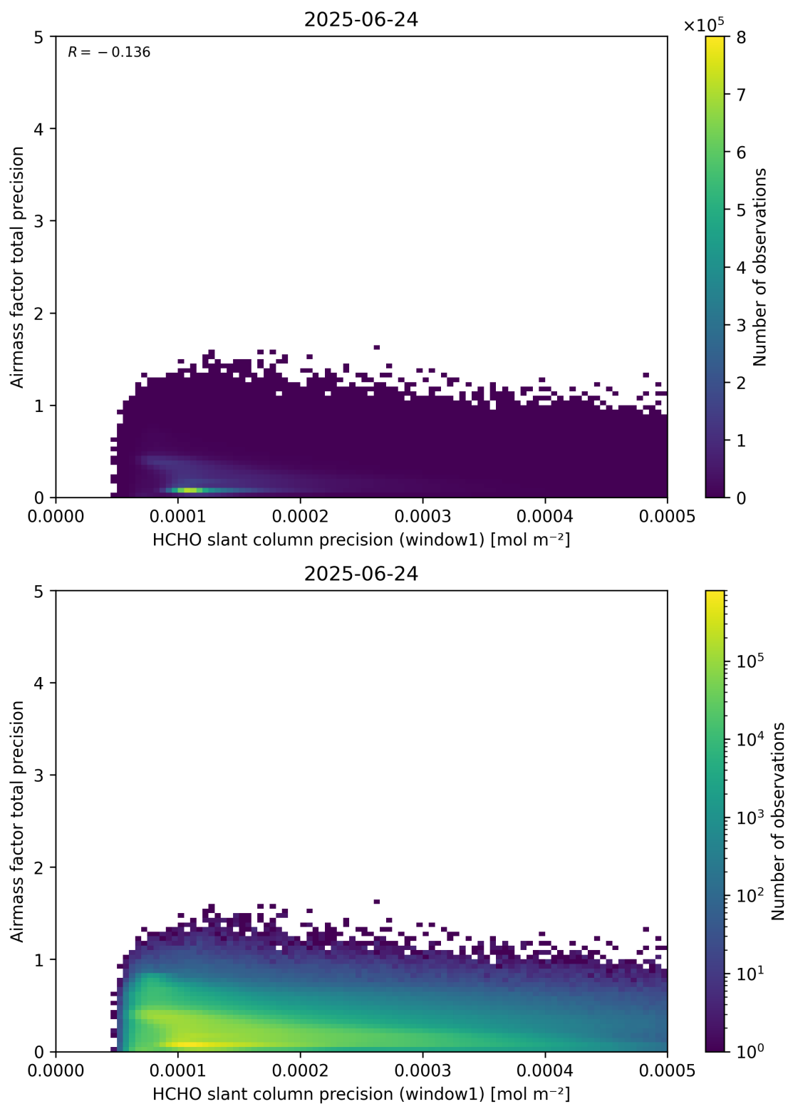
Figure 95: Scatter density plot of “HCHO slant column precision (window1)” against “Airmass factor total precision” for 2025-06-23 to 2025-06-25.
