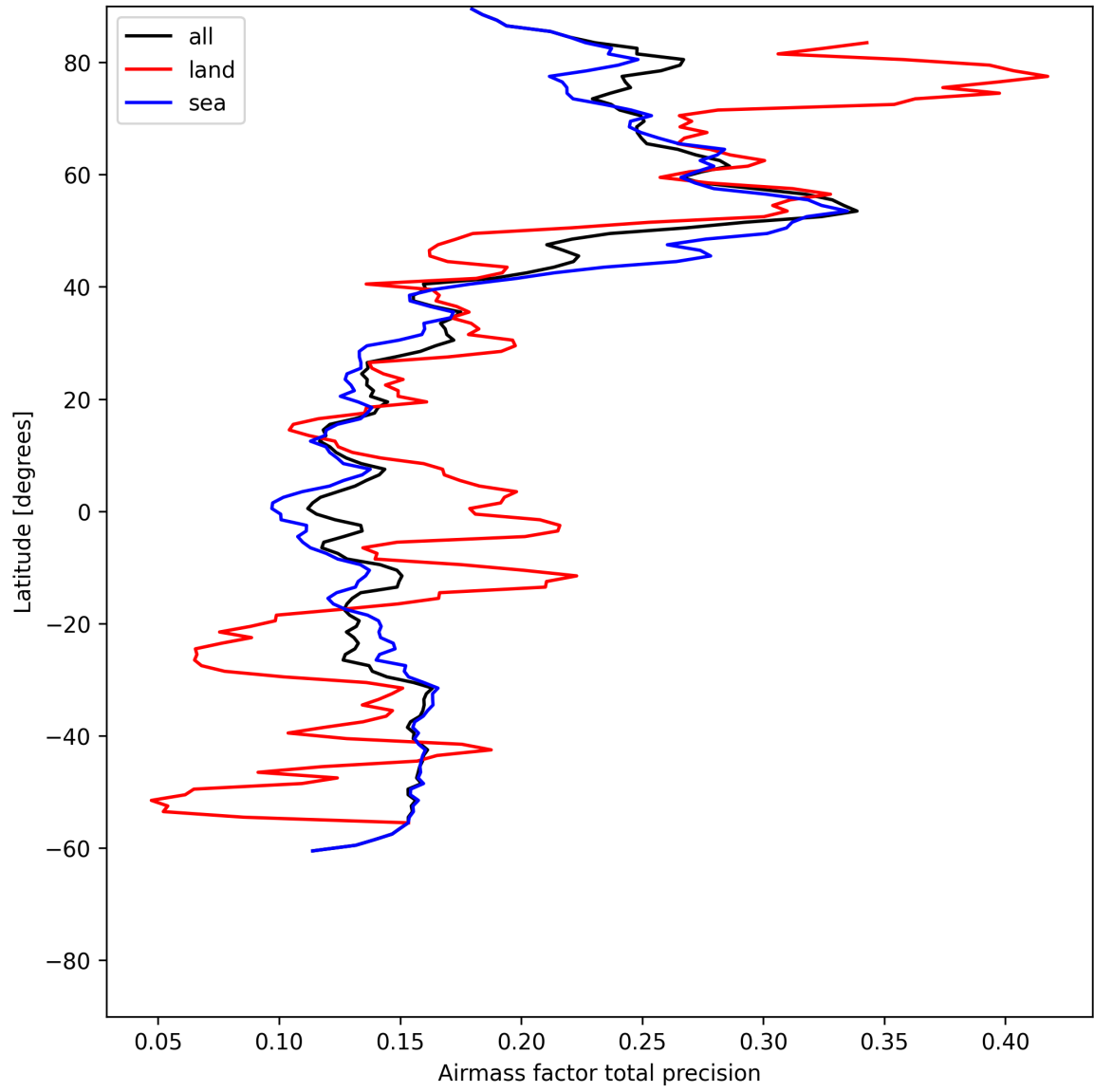
Figure 27: Zonal average of “Airmass factor total precision” for 2025-06-23 to 2025-06-25.
