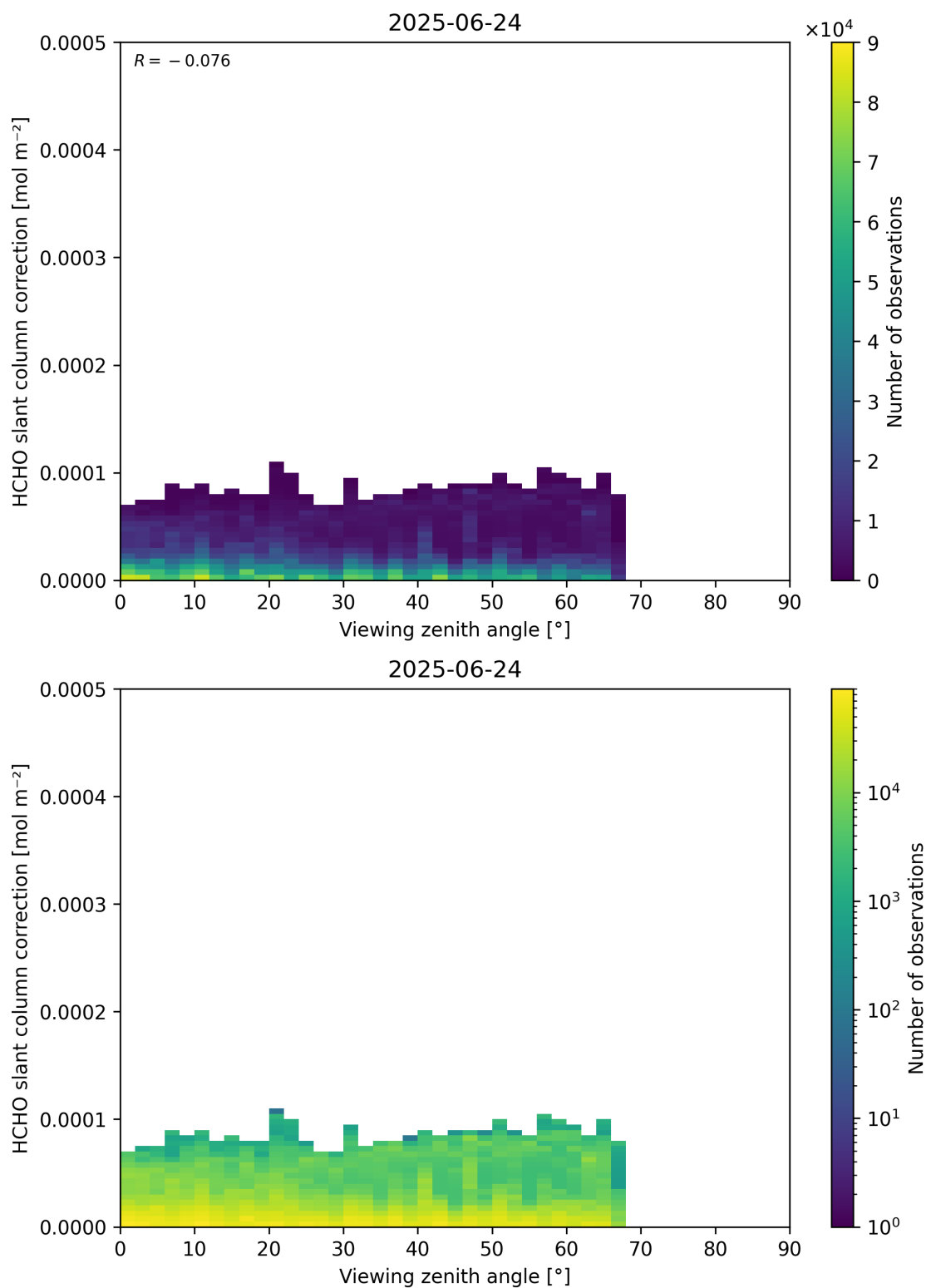
Figure 187: Scatter density plot of “Viewing zenith angle” against “HCHO slant column correction” for 2025-06-23 to 2025-06-25.
