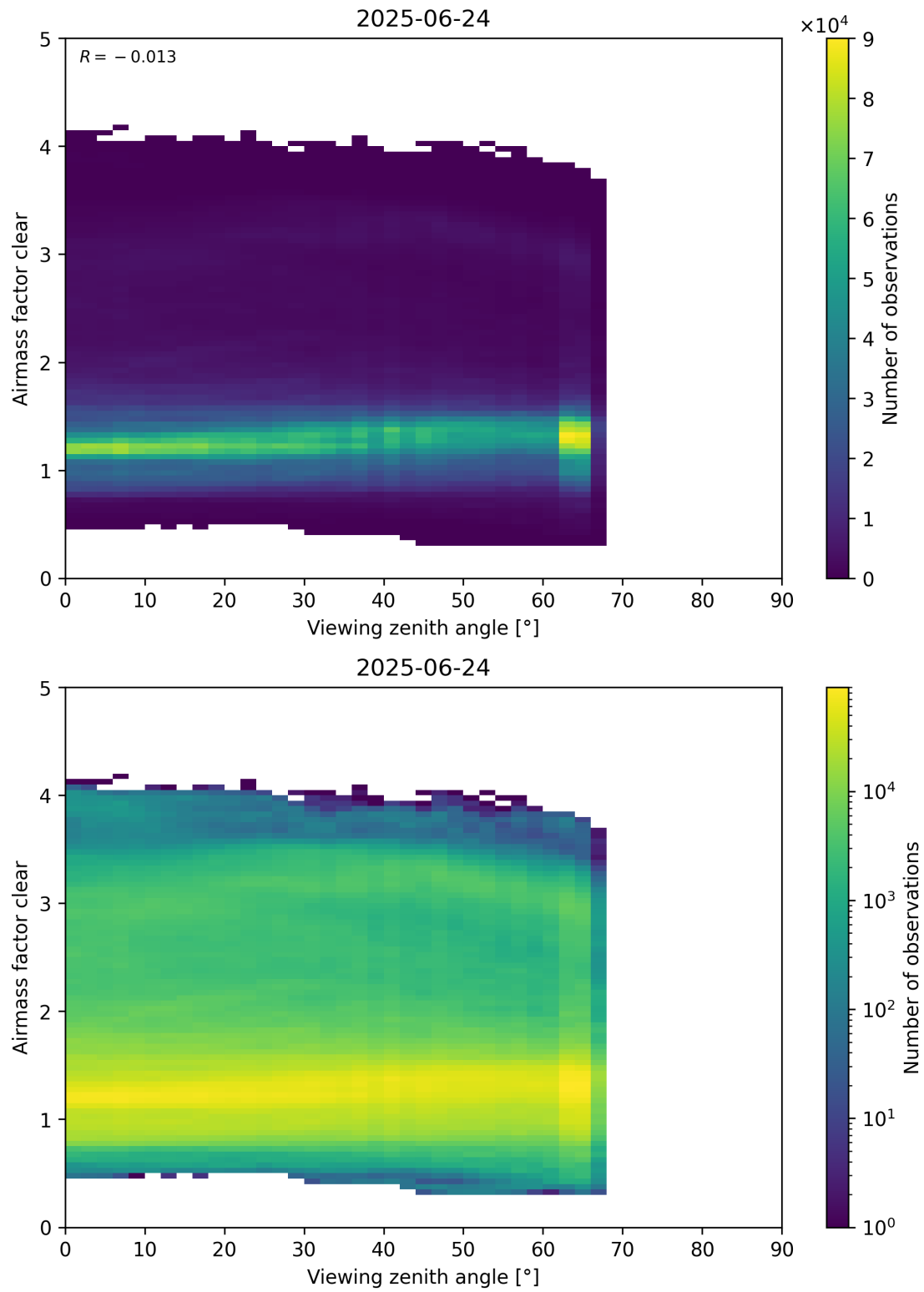
Figure 185: Scatter density plot of “Viewing zenith angle” against “Airmass factor clear” for 2025-06-23 to 2025-06-25.
