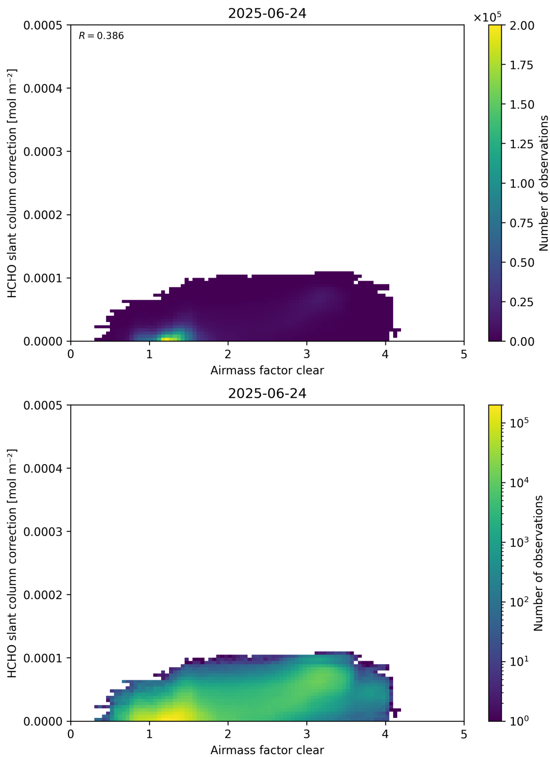
Figure 75: Scatter density plot of “Airmass factor clear” against “HCHO slant column correction” for 2025-06-23 to 2025-06-25.
