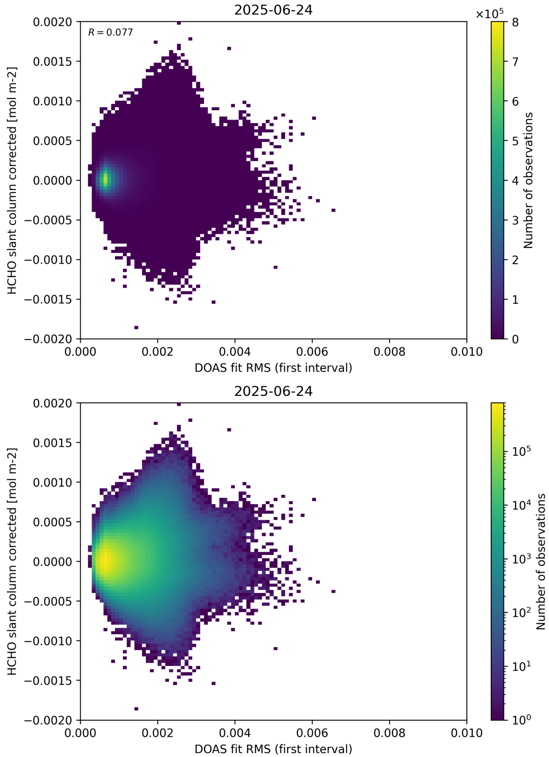
Figure 62: Scatter density plot of “DOAS fit RMS (first interval)” against “HCHO slant column corrected” for 2025-06-23 to 2025-06-25.
