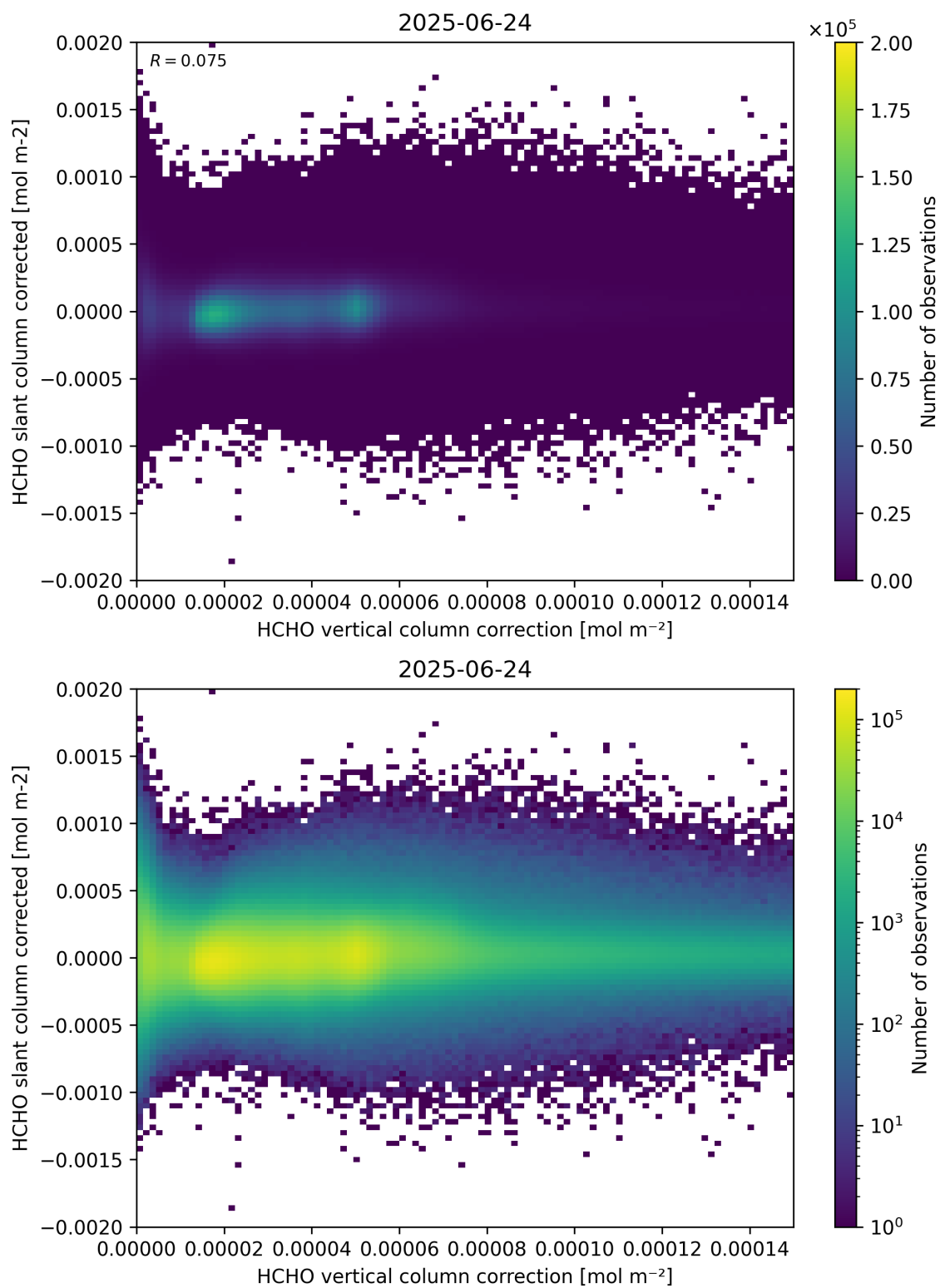
Figure 116: Scatter density plot of “HCHO vertical column correction” against “HCHO slant column corrected” for 2025-06-23 to 2025-06-25.
