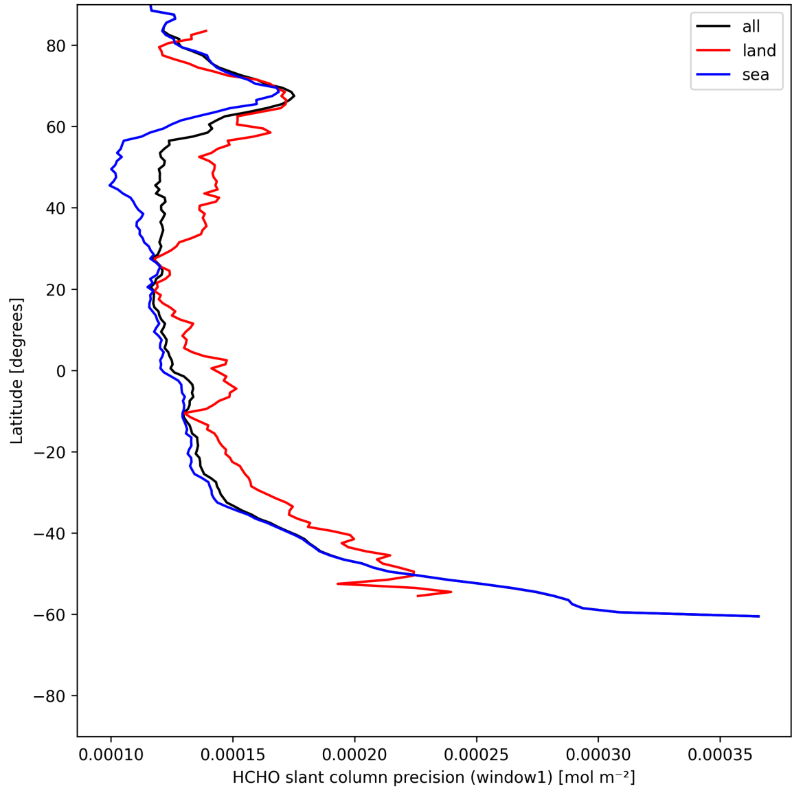
Figure 25: Zonal average of "HCHO slant column precision (window1)" for 2025-06-23 to 2025-06-25.
