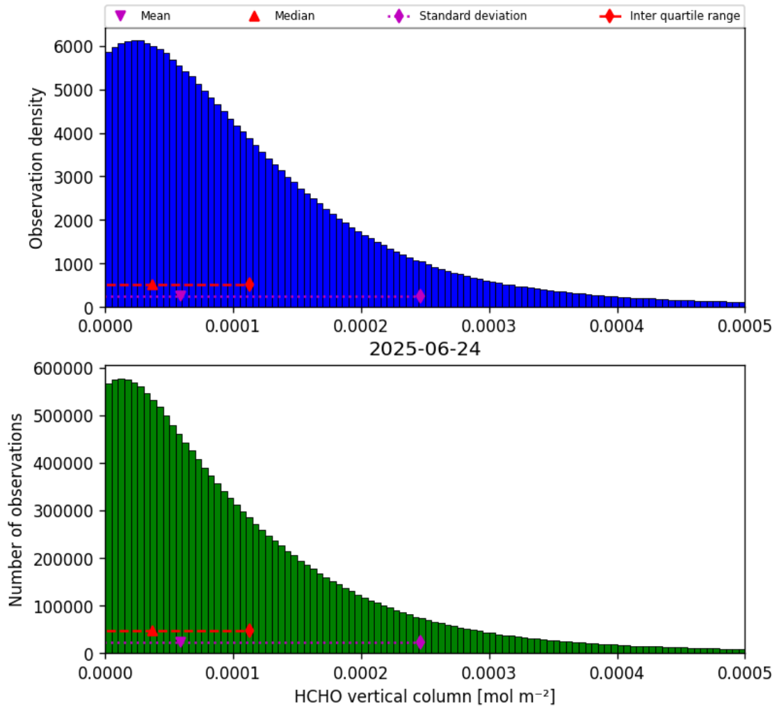
Figure 35: Histogram of “HCHO vertical column” for 2025-06-23 to 2025-06-25
