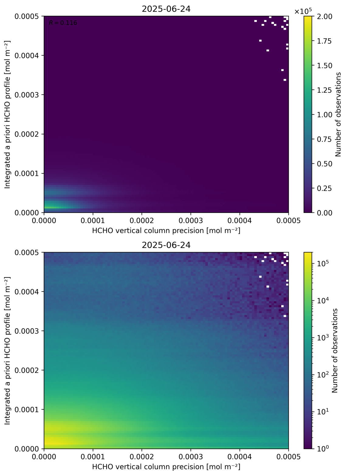
Figure 147: Scatter density plot of “HCHO vertical column precision” against “Integrated a priori HCHO profile” for 2025-06-23 to 2025-06-25.
