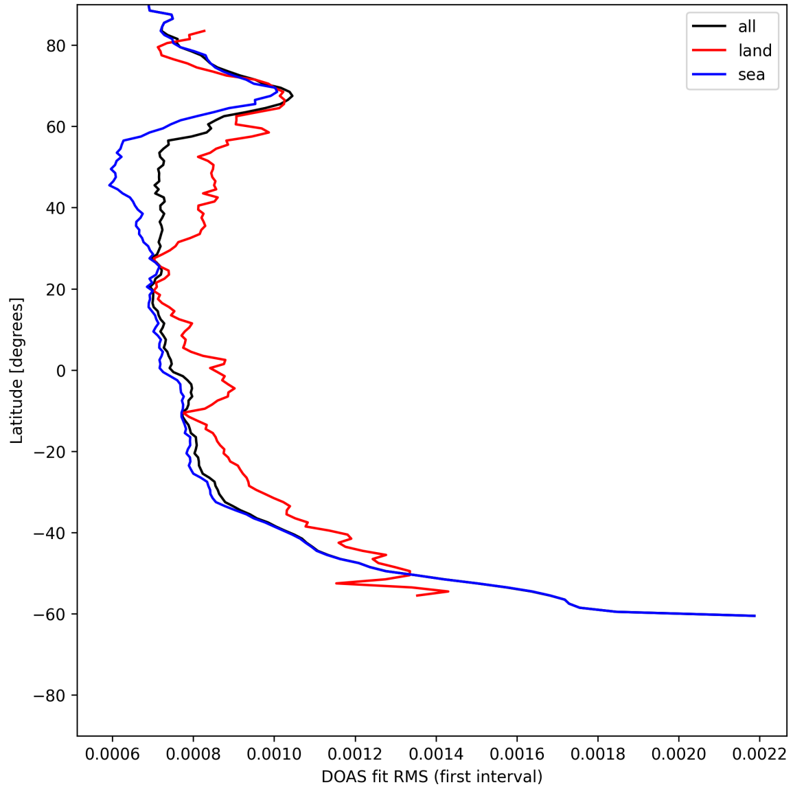
Figure 32: Zonal average of “DOAS fit RMS (first interval)” for 2025-06-23 to 2025-06-25.
