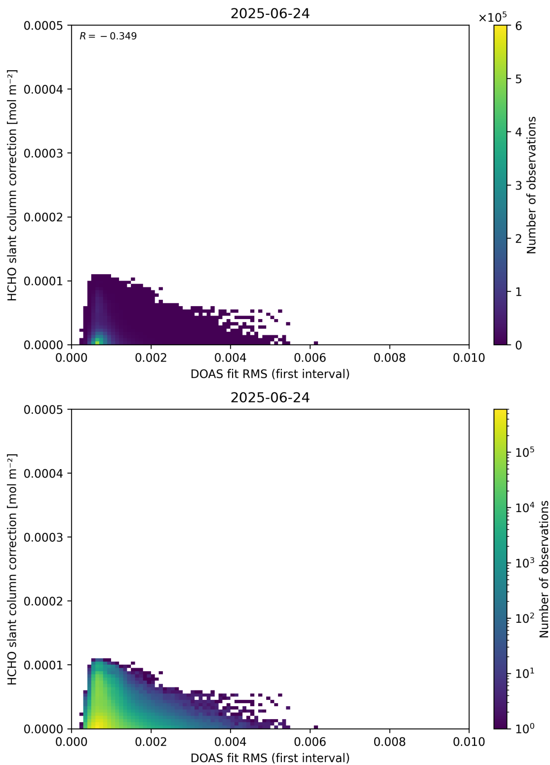
Figure 63: Scatter density plot of “DOAS fit RMS (first interval)” against “HCHO slant column correction” for 2025-06-23 to 2025-06-25.
