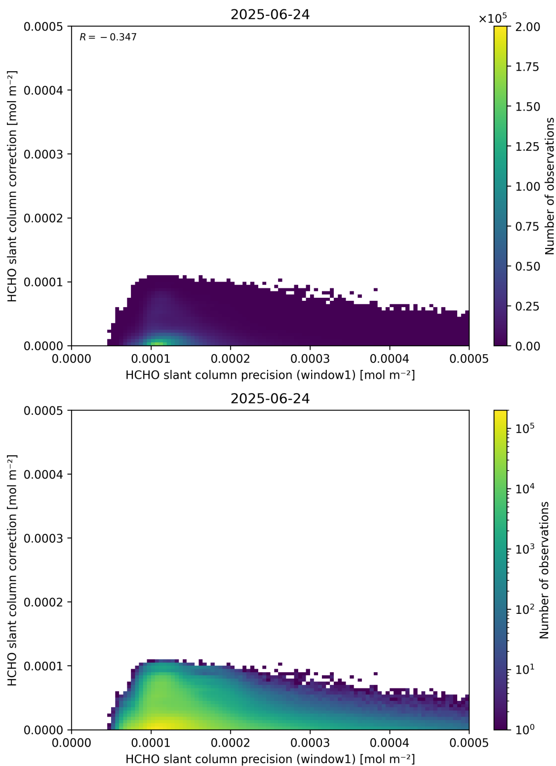
Figure 93: Scatter density plot of “HCHO slant column precision (window1)” against “HCHO slant column correction” for 2025-06-23 to 2025-06-25.
