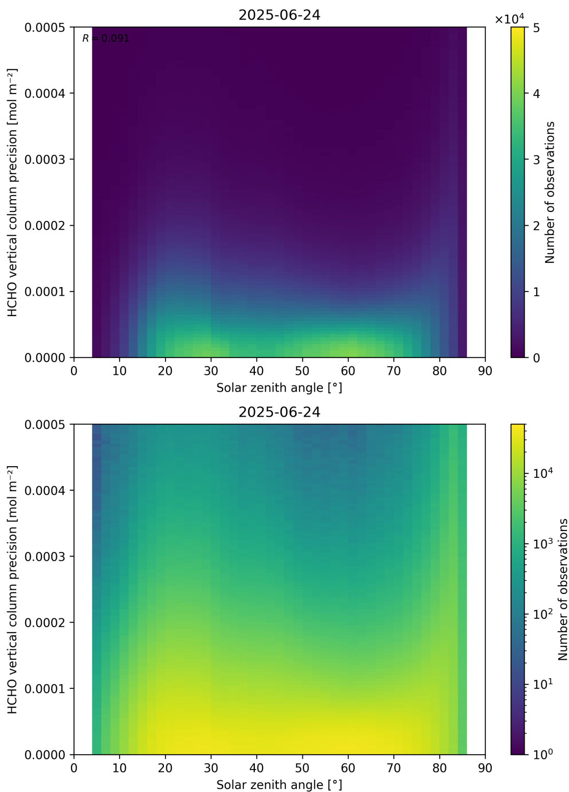
Figure 179: Scatter density plot of “Solar zenith angle” against “HCHO vertical column precision” for 2025-06-23 to 2025-06-25.
