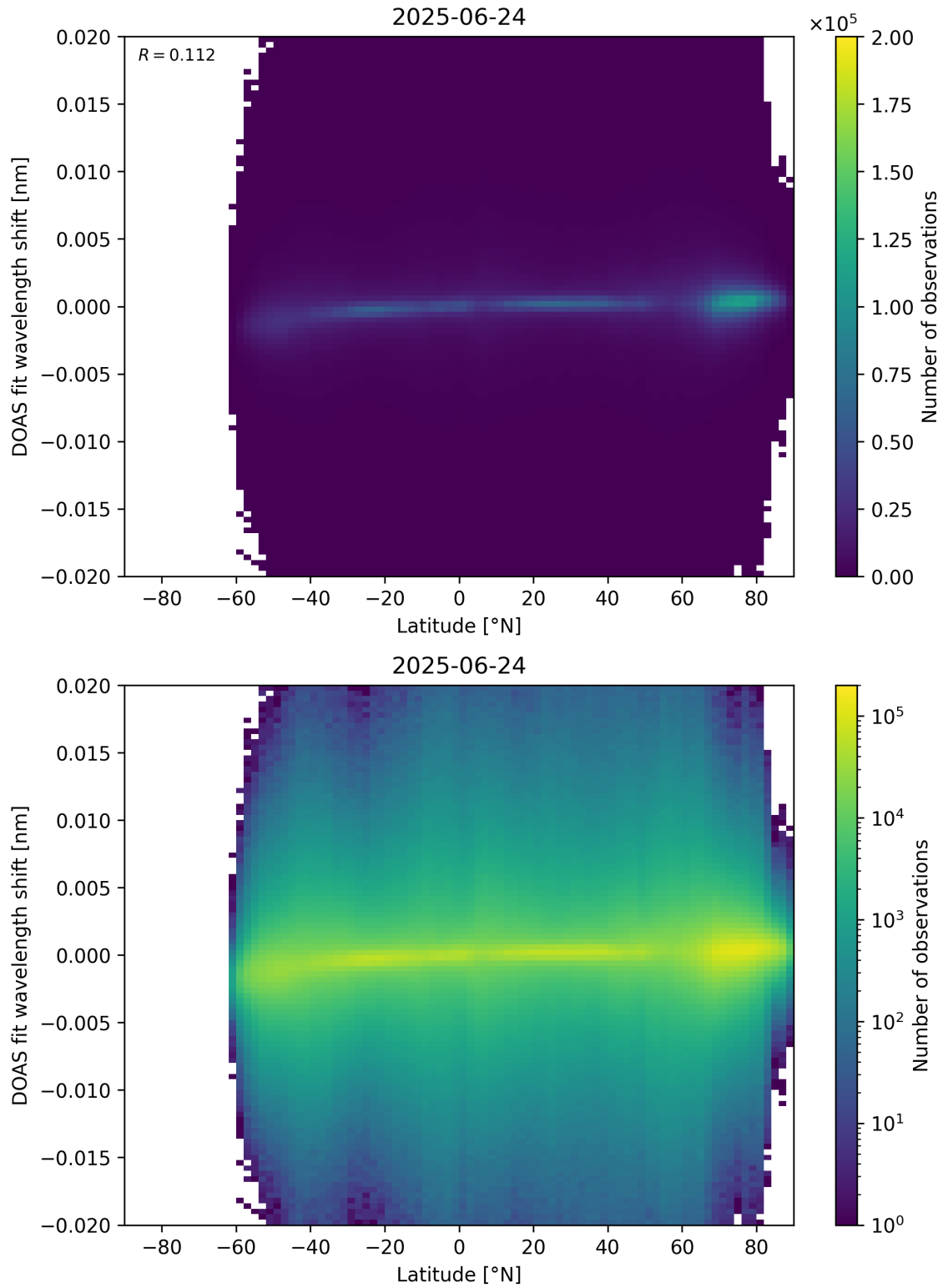
Figure 154: Scatter density plot of “Latitude” against “DOAS fit wavelength shift” for 2025-06-23 to 2025-06-25.
