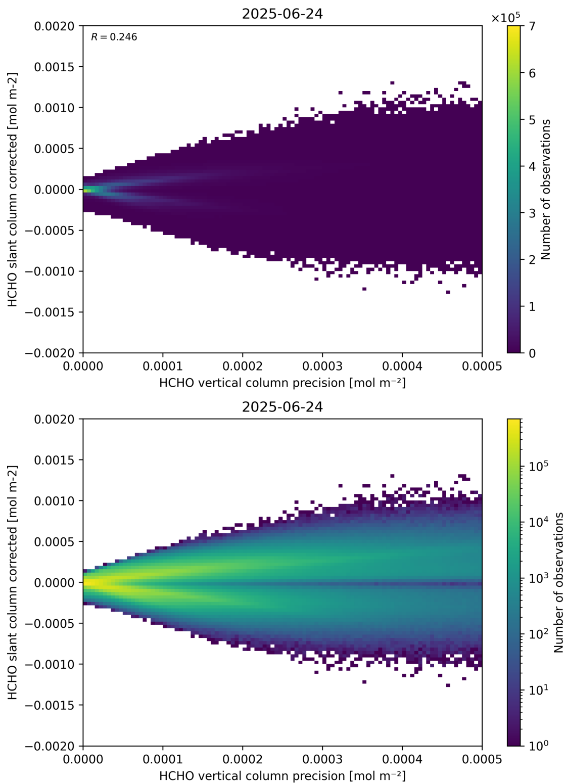
Figure 140: Scatter density plot of “HCHO vertical column precision” against “HCHO slant column corrected” for 2025-06-23 to 2025-06-25.
