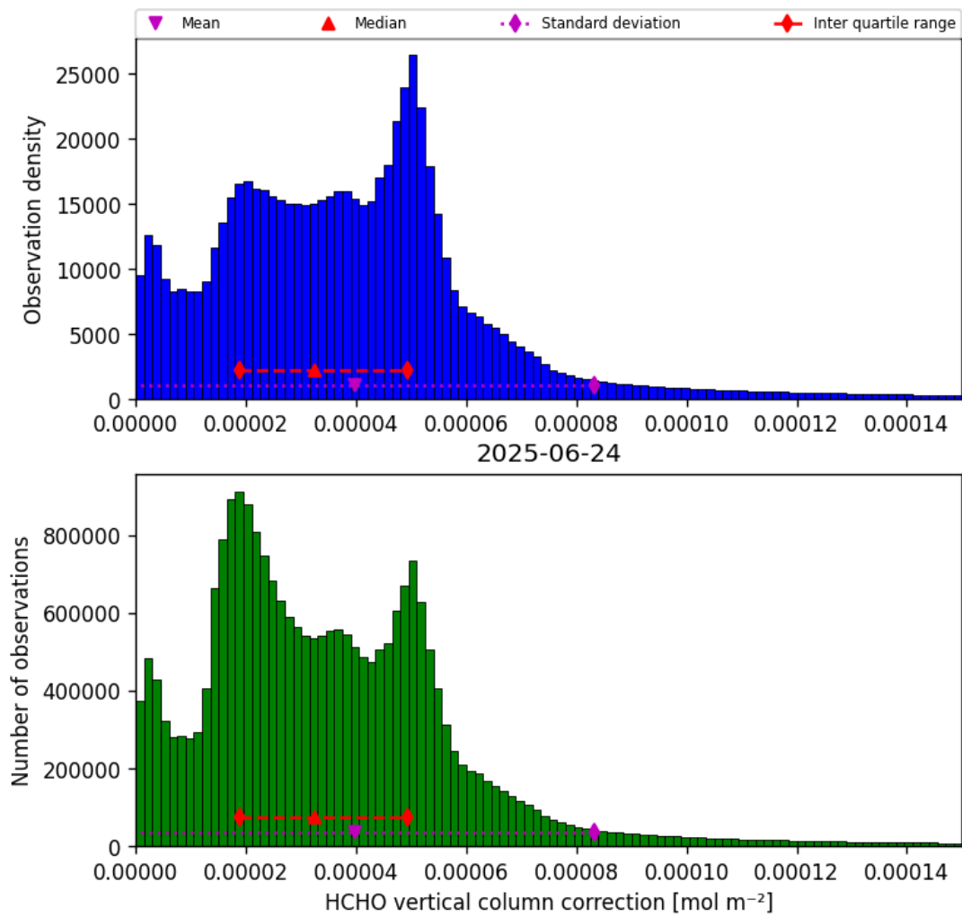
Figure 37: Histogram of “HCHO vertical column correction” for 2025-06-23 to 2025-06-25
