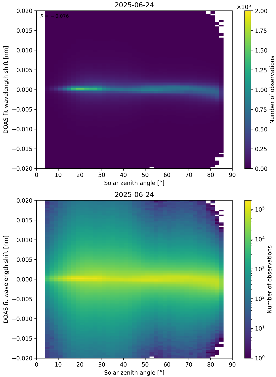
Figure 168: Scatter density plot of “Solar zenith angle” against “DOAS fit wavelength shift” for 2025-06-23 to 2025-06-25.
