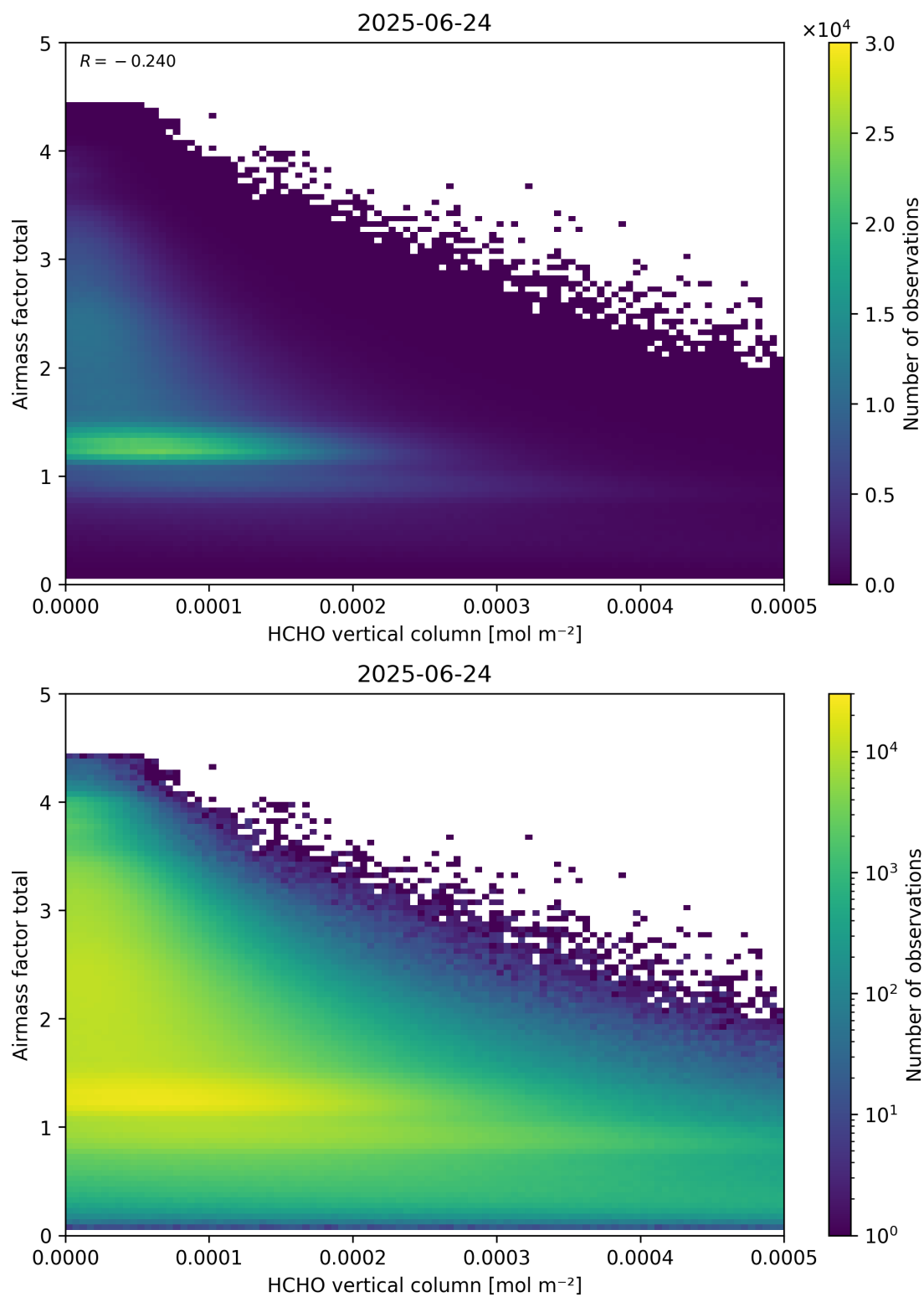
Figure 131: Scatter density plot of “HCHO vertical column” against “Airmass factor total” for 2025-06-23 to 2025-06-25.
