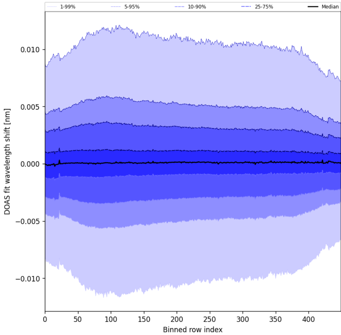
Figure 58: Along track statistics of “DOAS fit wavelength shift” for 2025-06-23 to 2025-06-25
