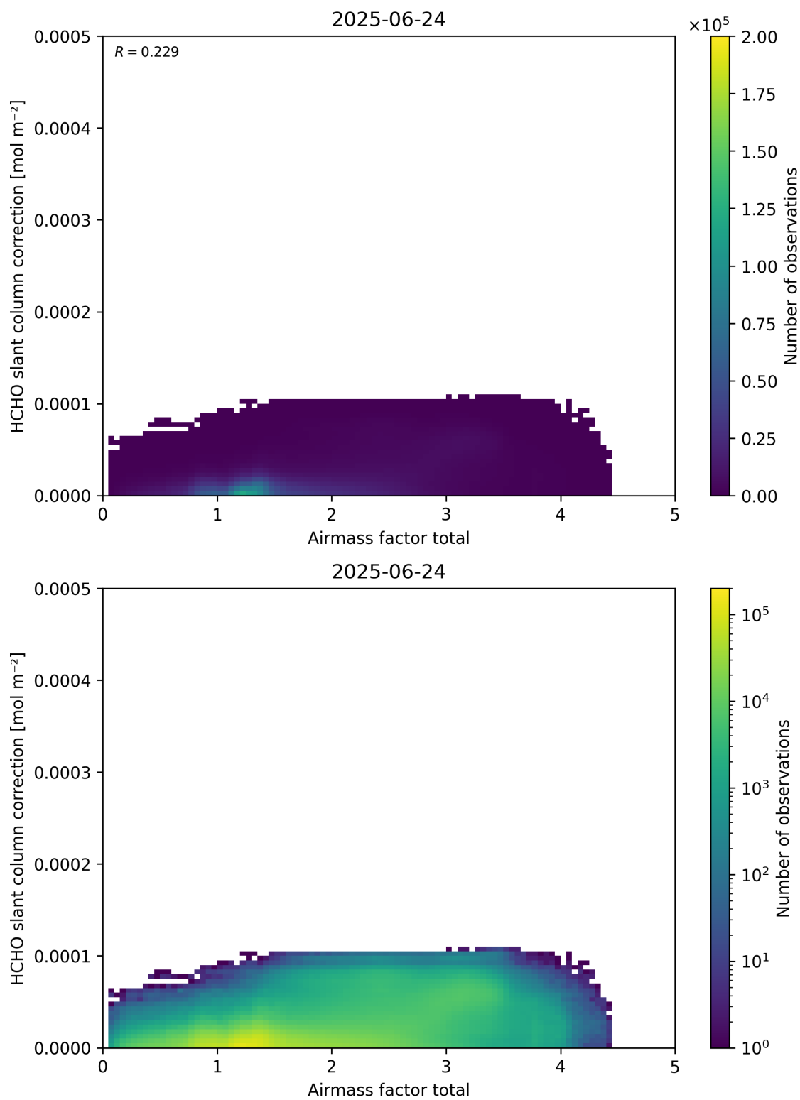
Figure 102: Scatter density plot of “Airmass factor total” against “HCHO slant column correction” for 2025-06-23 to 2025-06-25.
