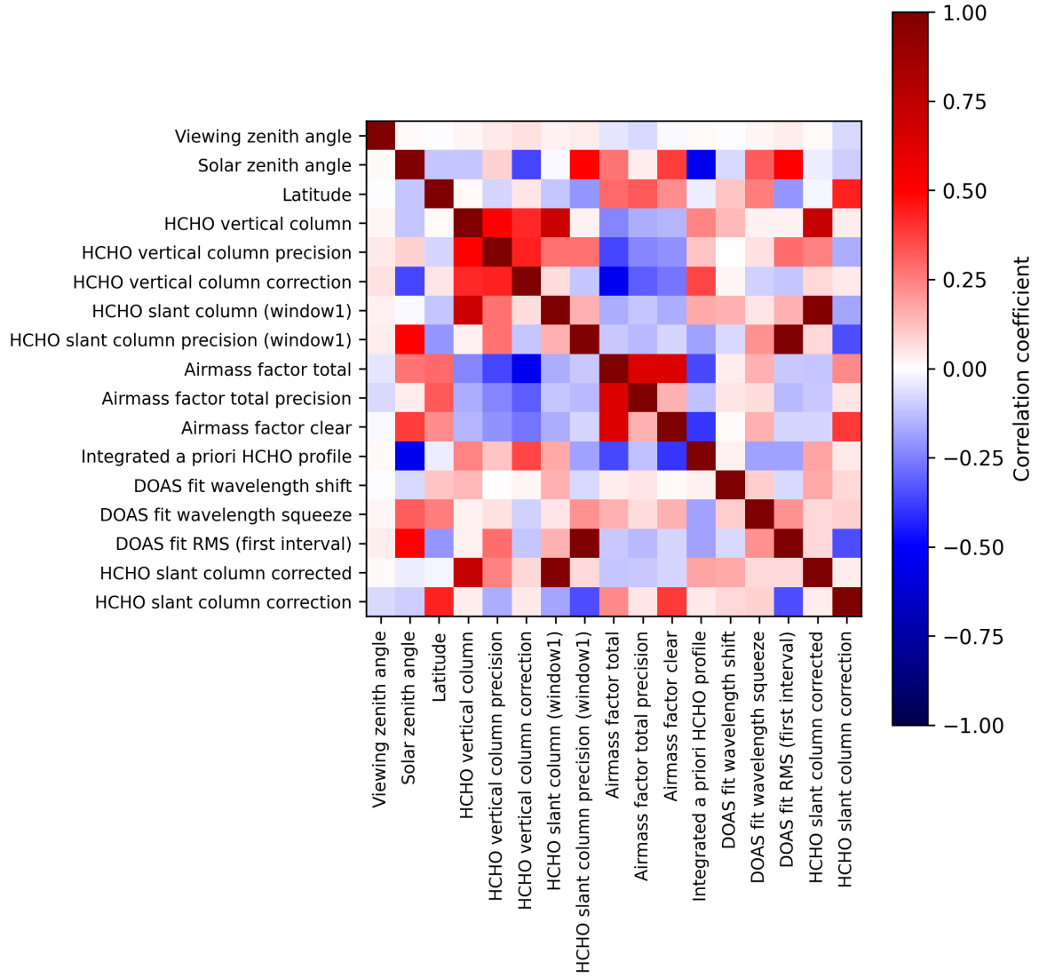
Figure 2: Map of correlation matrix for 2025-06-23 to 2025-06-25.
