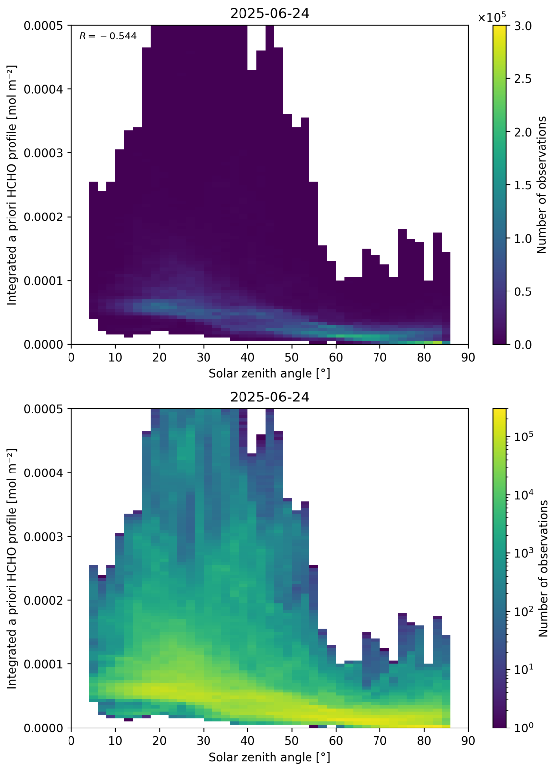
Figure 180: Scatter density plot of “Solar zenith angle” against “Integrated a priori HCHO profile” for 2025-06-23 to 2025-06-25.
