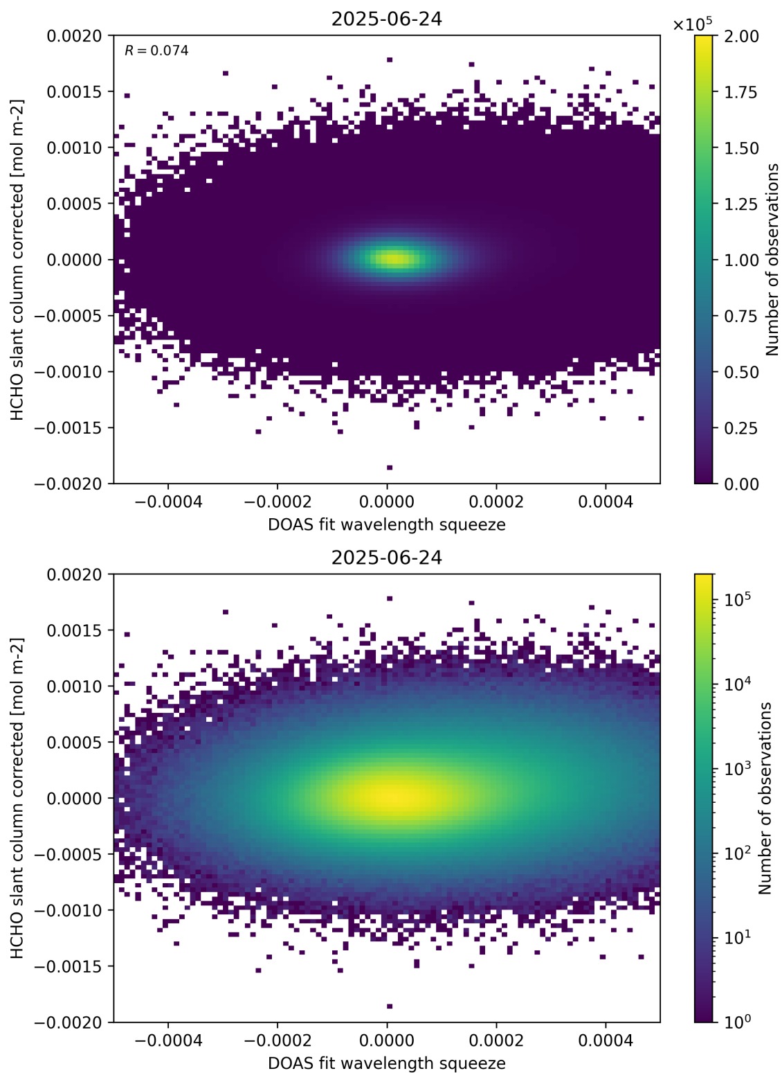
Figure 69: Scatter density plot of “DOAS fit wavelength squeeze” against “HCHO slant column corrected” for 2025-06-23 to 2025-06-25.
