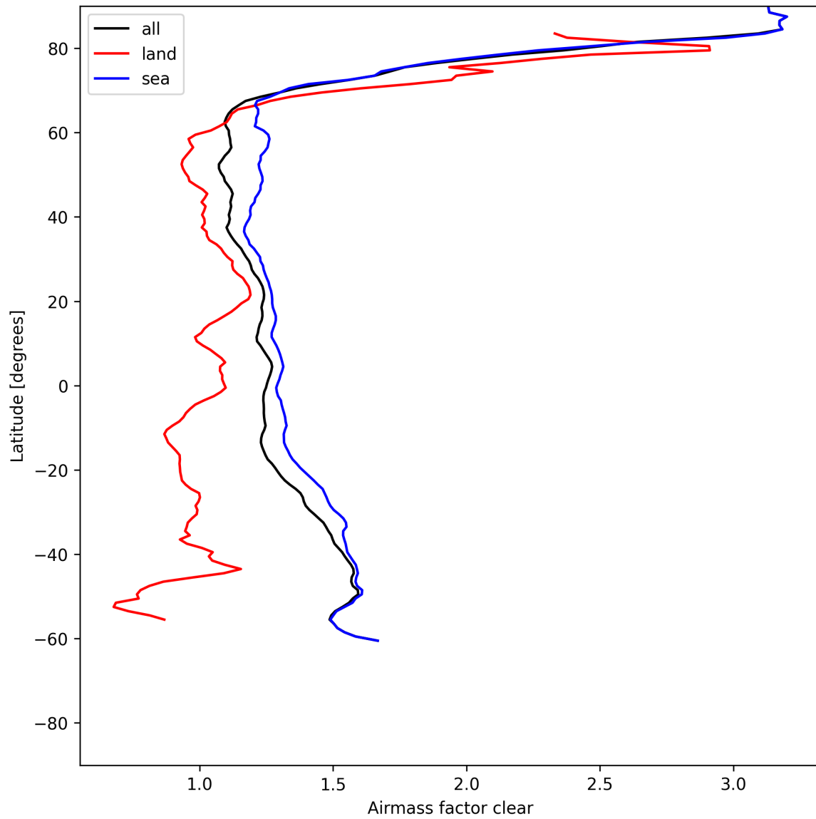
Figure 28: Zonal average of “Airmass factor clear” for 2025-06-23 to 2025-06-25.
