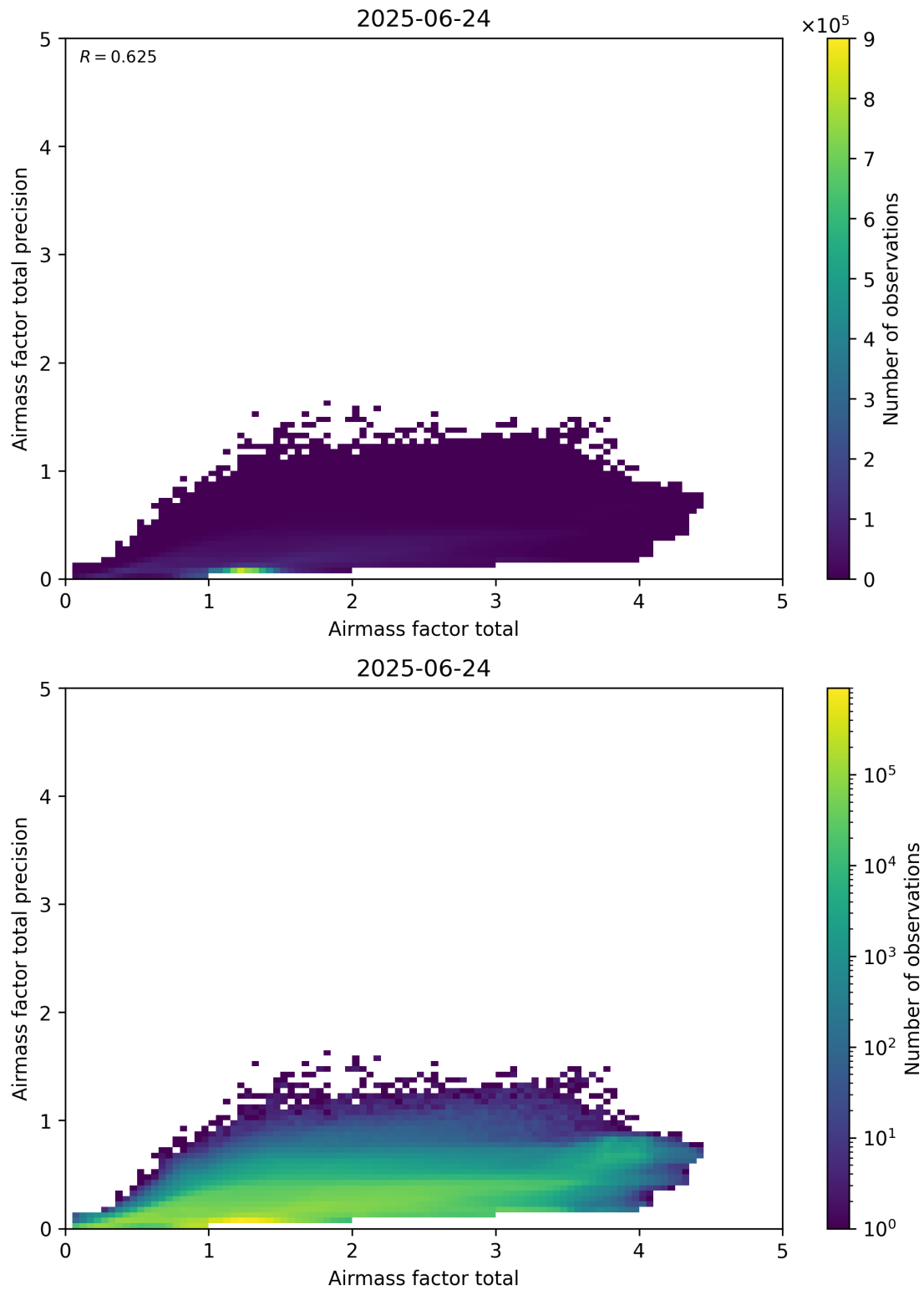
Figure 103: Scatter density plot of “Airmass factor total” against “Airmass factor total precision” for 2025-06-23 to 2025-06-25.
