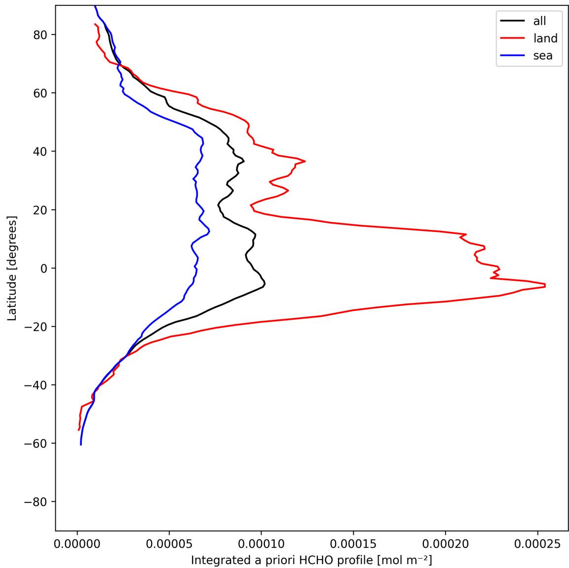
Figure 29: Zonal average of “Integrated a priori HCHO profile” for 2025-06-23 to 2025-06-25.
