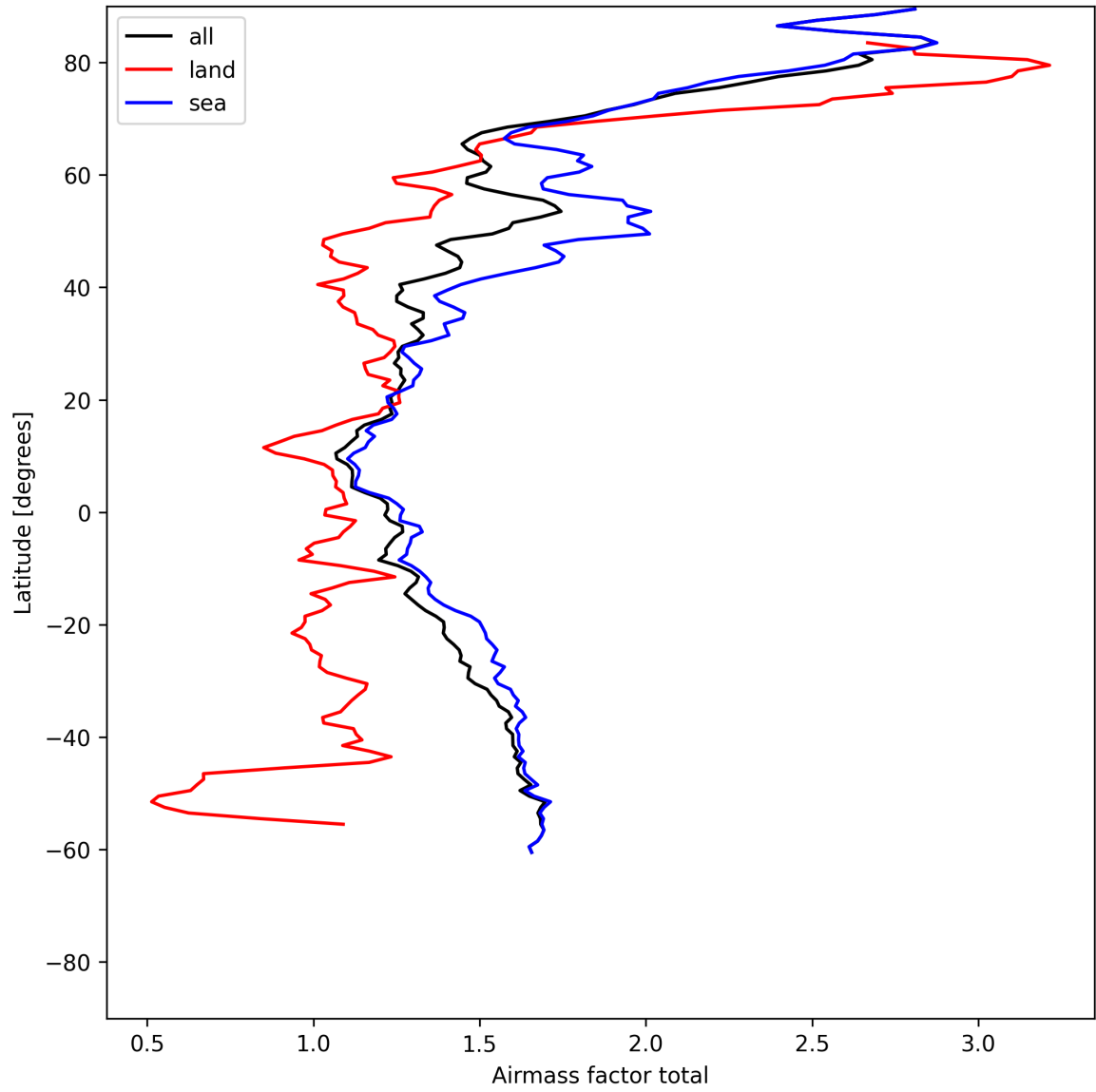
Figure 26: Zonal average of “Airmass factor total” for 2025-06-23 to 2025-06-25.
