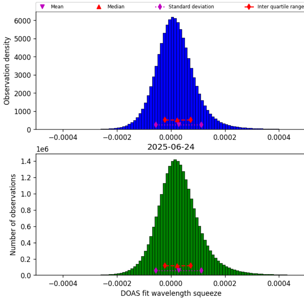
Figure 45: Histogram of “DOAS fit wavelength squeeze” for 2025-06-23 to 2025-06-25
