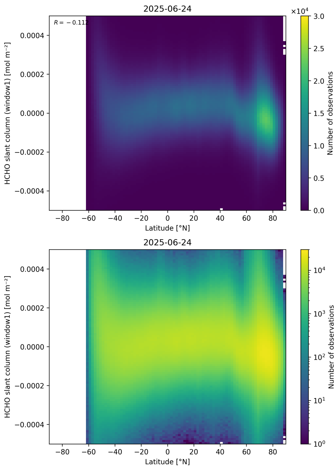
Figure 159: Scatter density plot of “Latitude” against “HCHO slant column (window1)” for 2025-06-23 to 2025-06-25.
