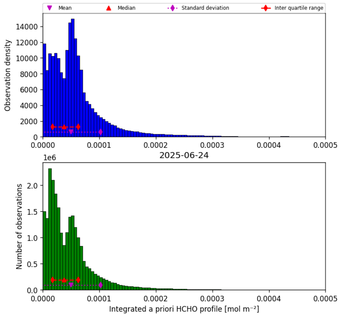
Figure 43: Histogram of “Integrated a priori HCHO profile” for 2025-06-23 to 2025-06-25
