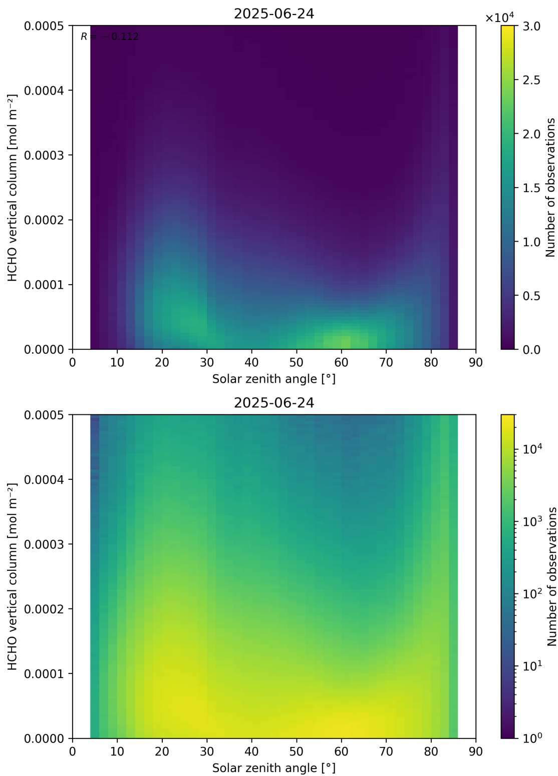
Figure 177: Scatter density plot of “Solar zenith angle” against “HCHO vertical column” for 2025-06-23 to 2025-06-25.
