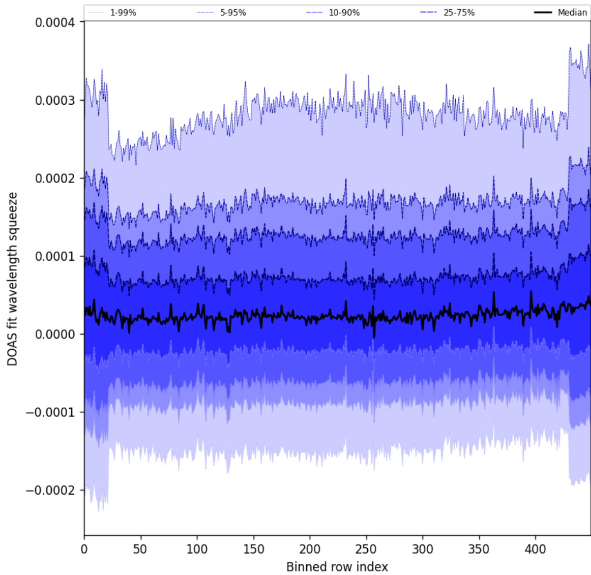
Figure 59: Along track statistics of “DOAS fit wavelength squeeze” for 2025-06-23 to 2025-06-25
