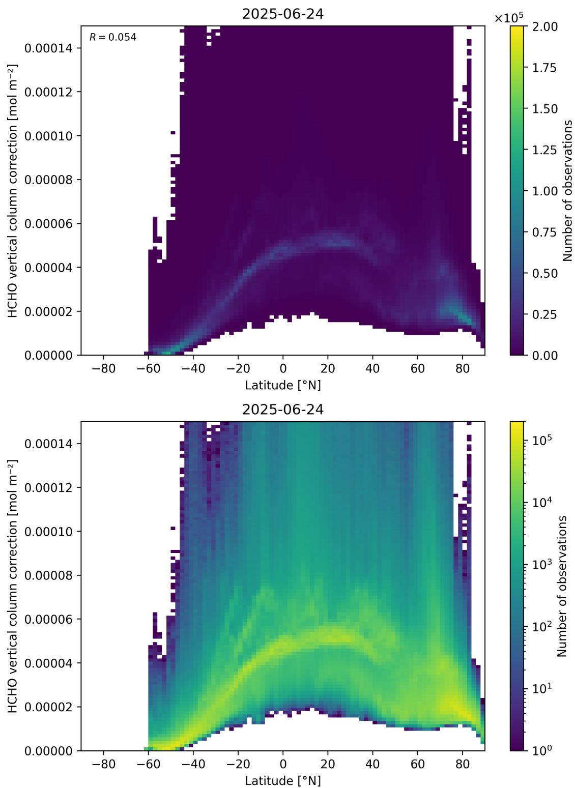
Figure 164: Scatter density plot of “Latitude” against “HCHO vertical column correction” for 2025-06-23 to 2025-06-25.
