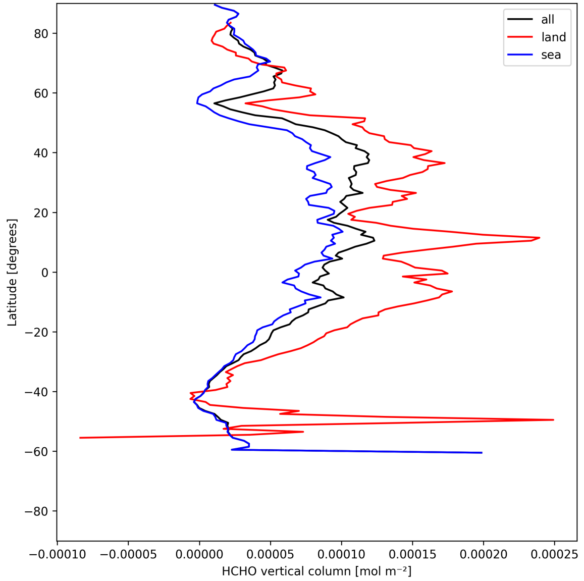
Figure 21: Zonal average of “HCHO vertical column” for 2025-06-23 to 2025-06-25.
