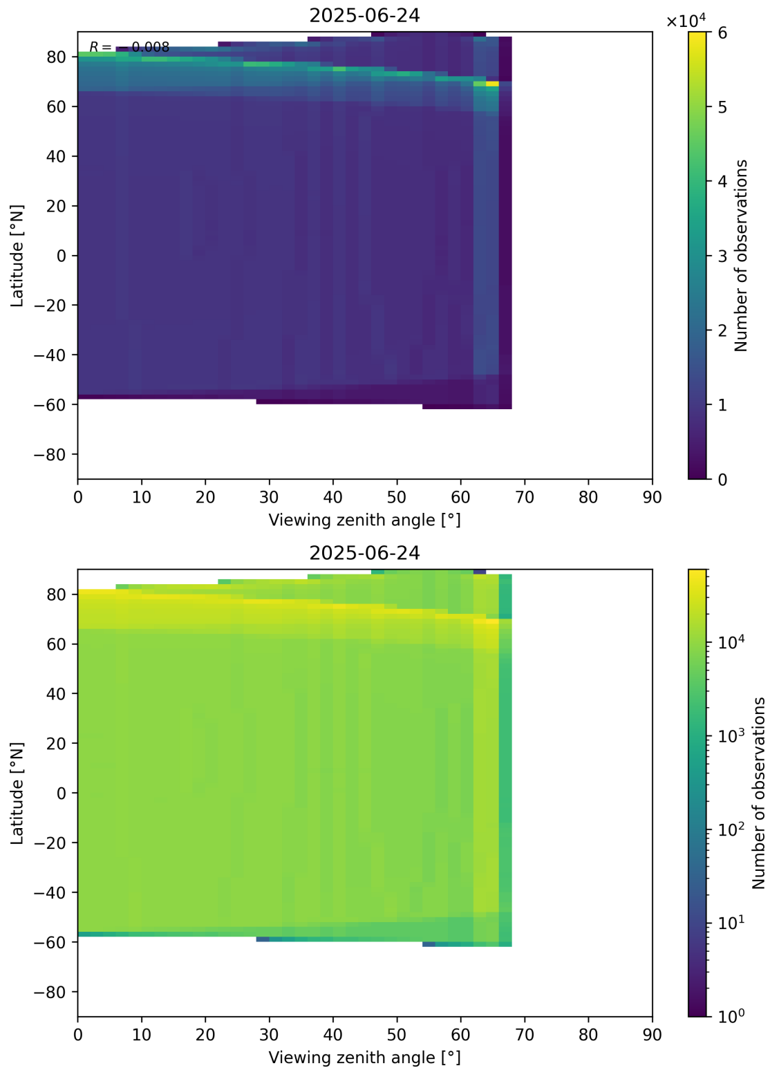
Figure 196: Scatter density plot of “Viewing zenith angle” against “Latitude” for 2025-06-23 to 2025-06-25.
