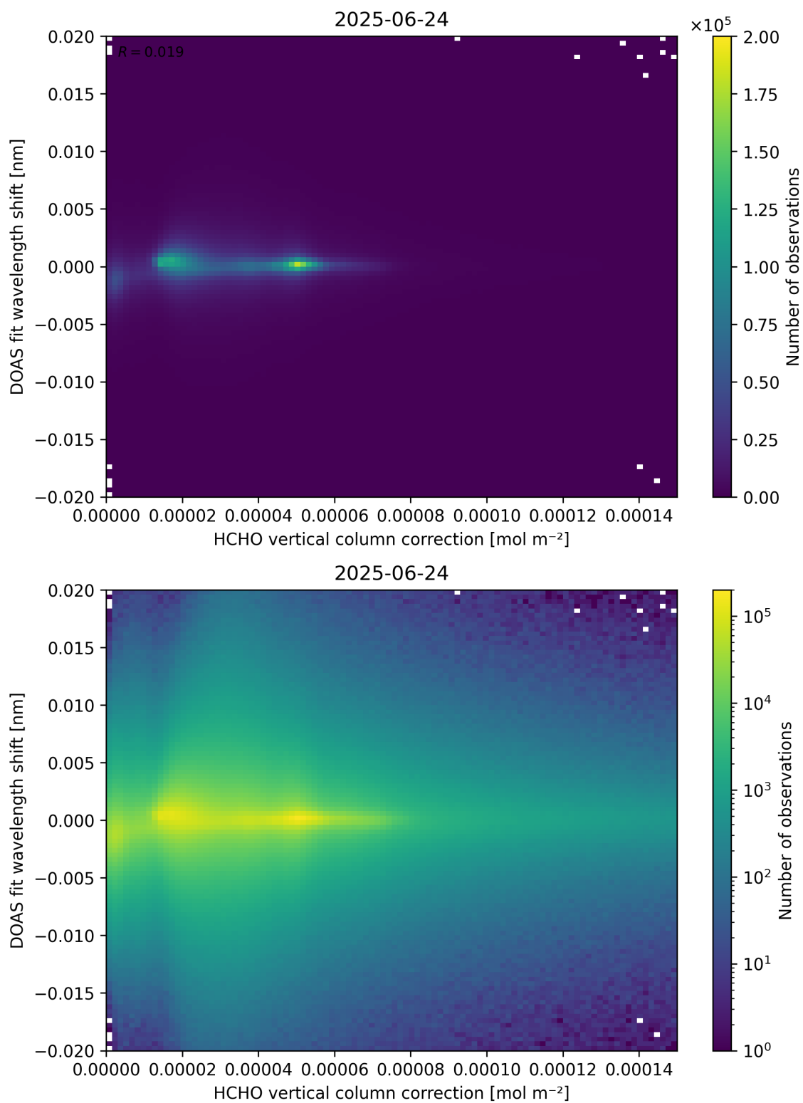
Figure 113: Scatter density plot of “HCHO vertical column correction” against “DOAS fit wavelength shift” for 2025-06-23 to 2025-06-25.
