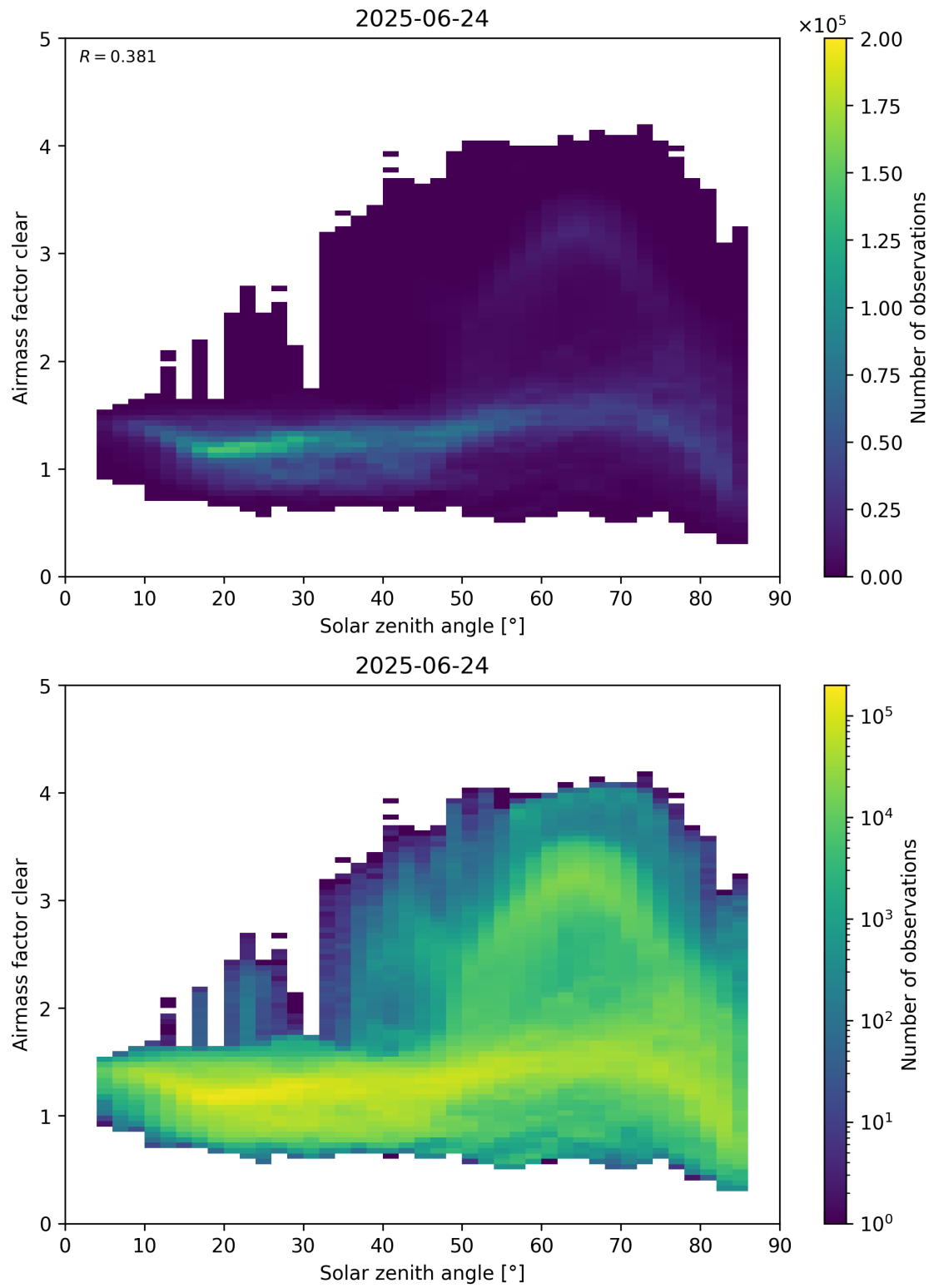
Figure 170: Scatter density plot of “Solar zenith angle” against “Airmass factor clear” for 2025-06-23 to 2025-06-25.
