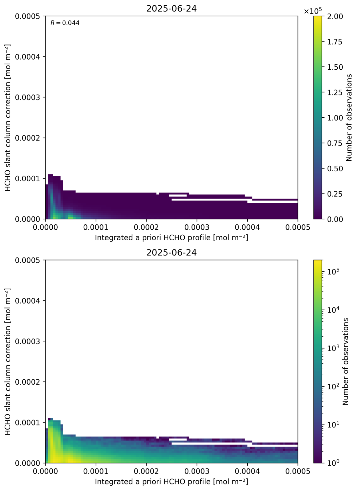
Figure 152: Scatter density plot of “Integrated a priori HCHO profile” against “HCHO slant column correction” for 2025-06-23 to 2025-06-25.
