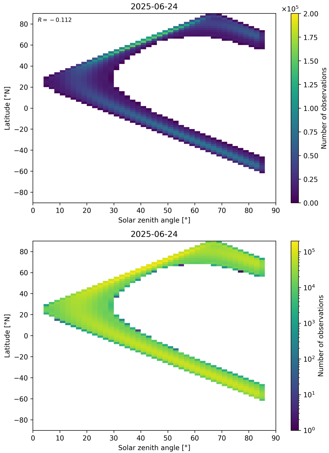
Figure 181: Scatter density plot of “Solar zenith angle” against “Latitude” for 2025-06-23 to 2025-06-25.
