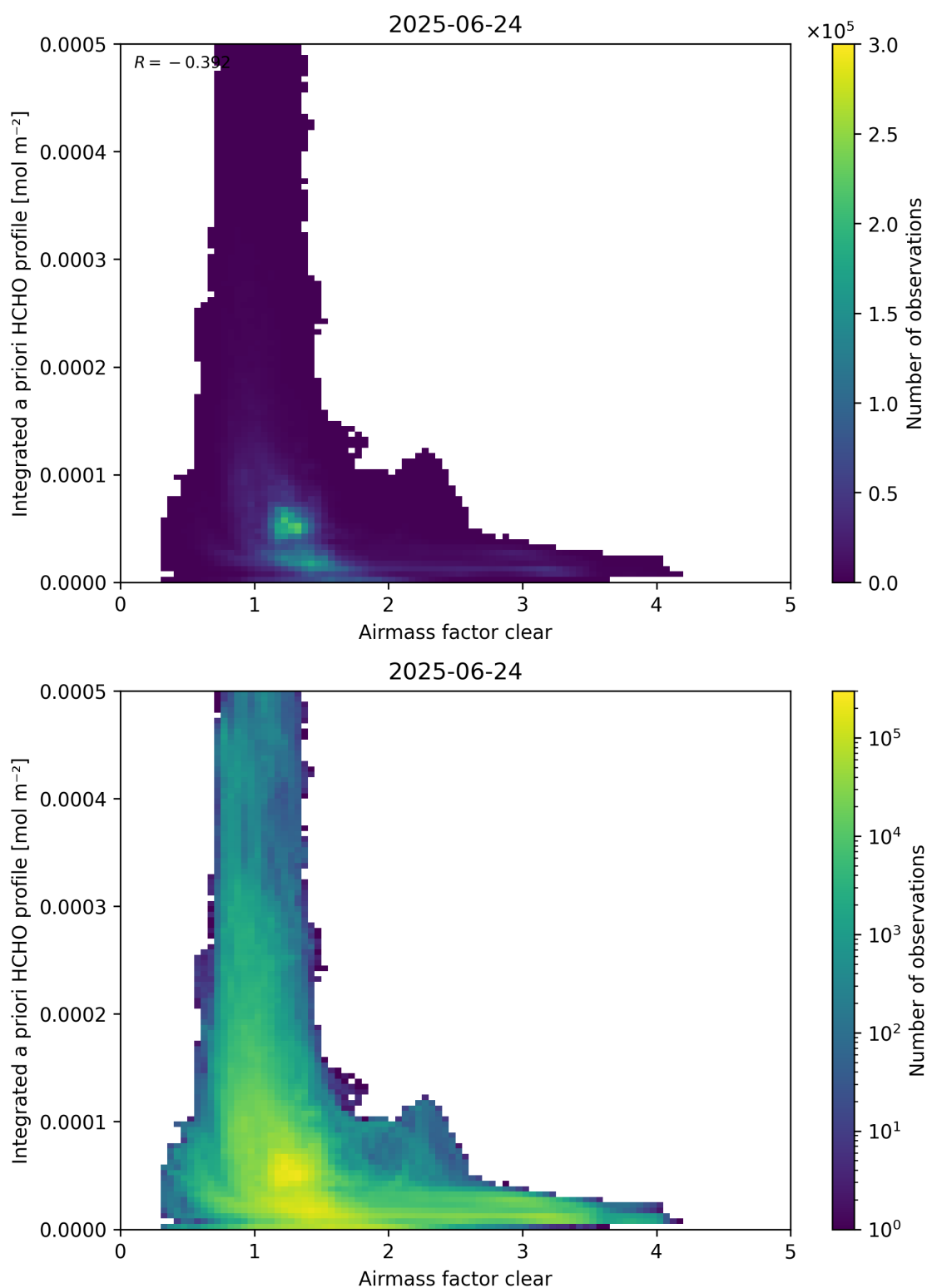
Figure 76: Scatter density plot of “Airmass factor clear” against “Integrated a priori HCHO profile” for 2025-06-23 to 2025-06-25.
