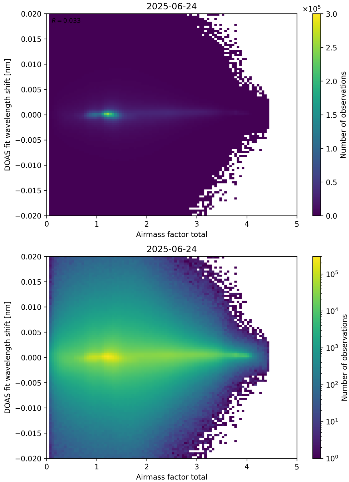
Figure 98: Scatter density plot of “Airmass factor total” against “DOAS fit wavelength shift” for 2025-06-23 to 2025-06-25.
