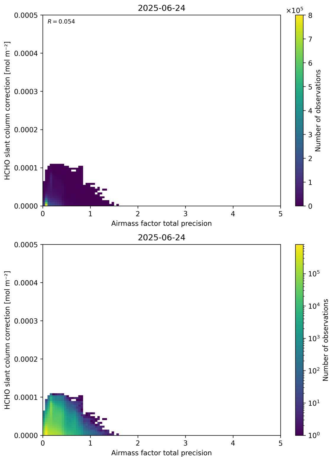
Figure 110: Scatter density plot of “Airmass factor total precision” against “HCHO slant column correction” for 2025-06-23 to 2025-06-25.
