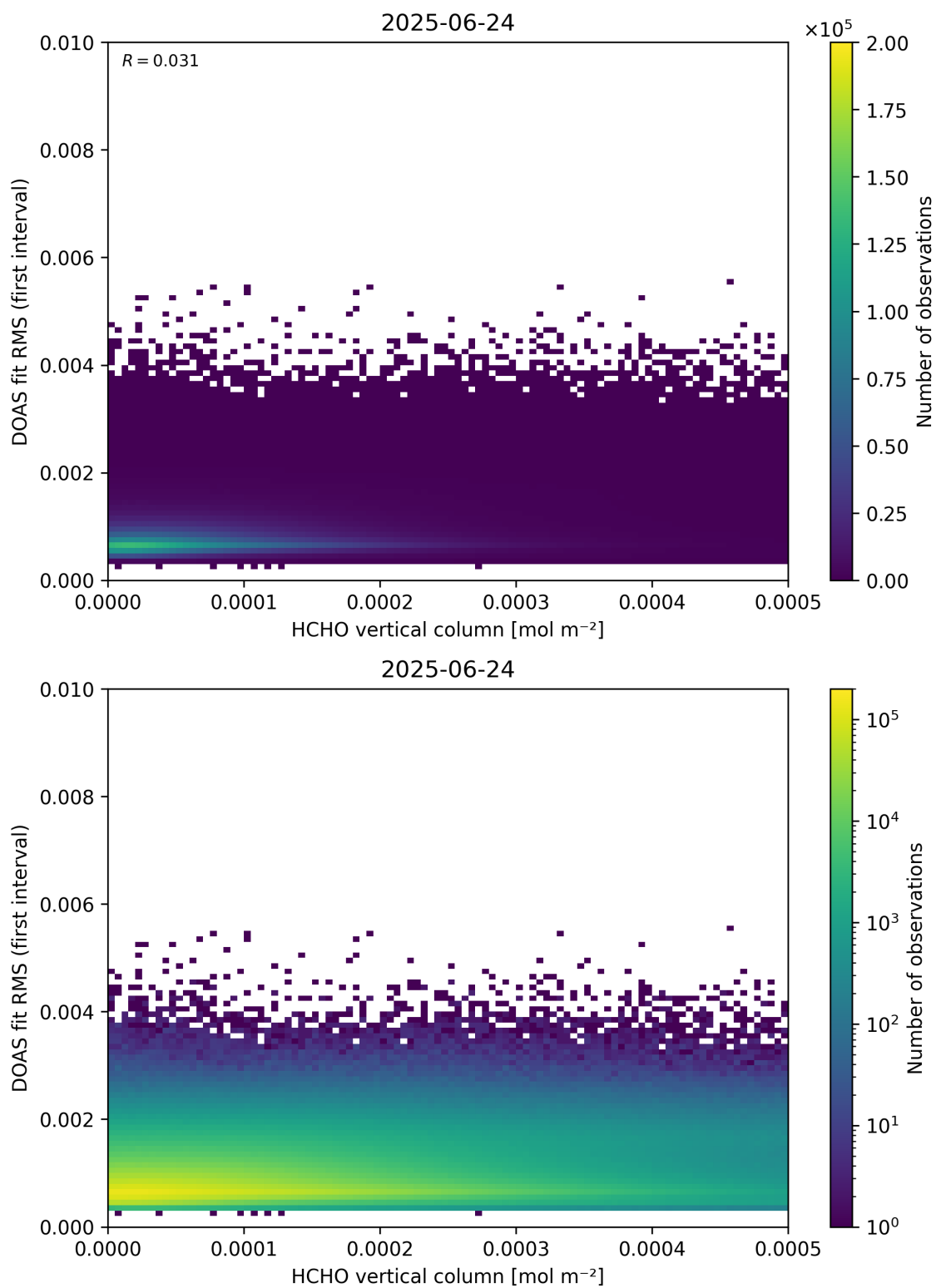
Figure 123: Scatter density plot of “HCHO vertical column” against “DOAS fit RMS (first interval)” for 2025-06-23 to 2025-06-25.
