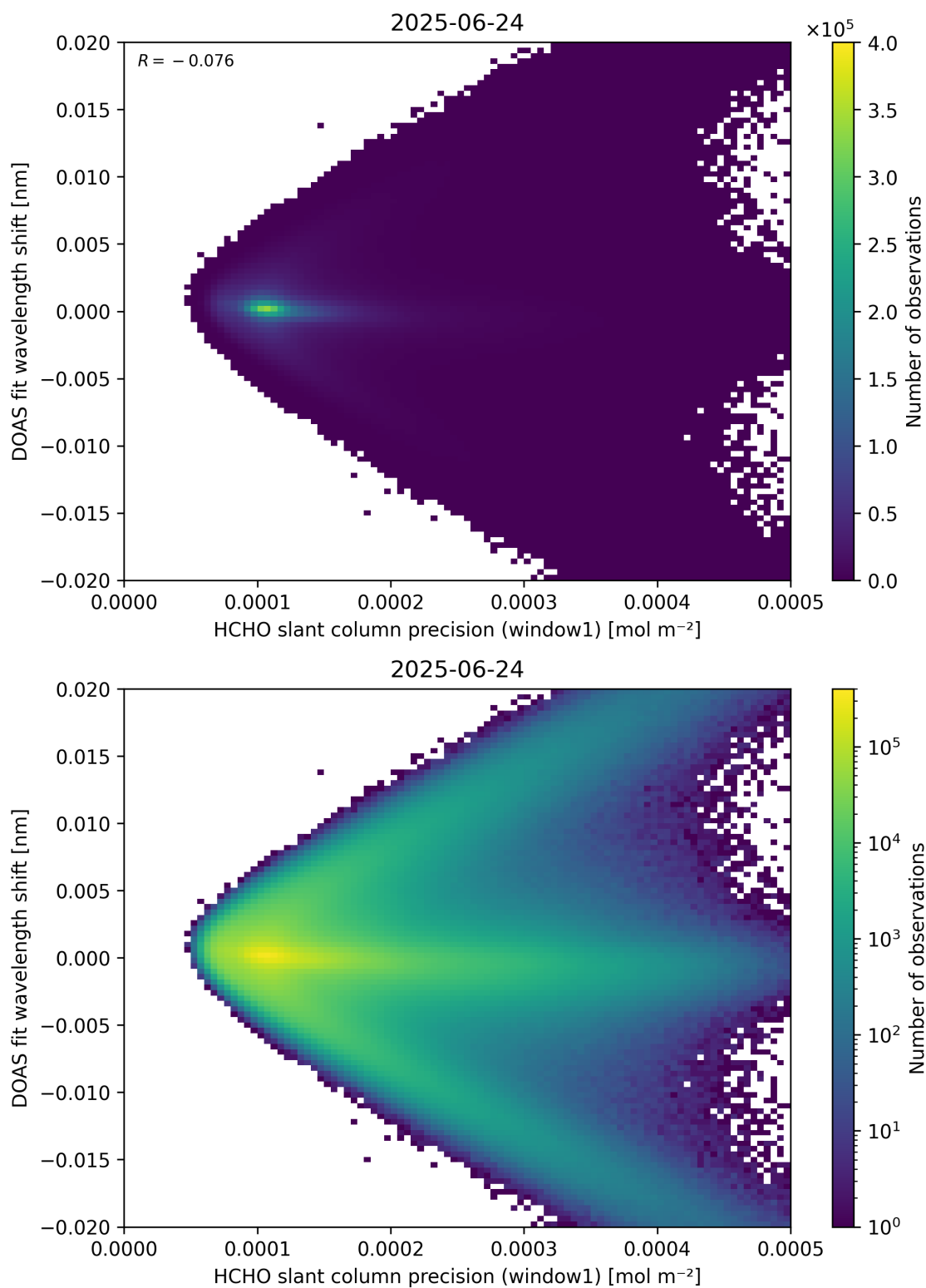
Figure 89: Scatter density plot of “HCHO slant column precision (window1)” against “DOAS fit wavelength shift” for 2025-06-23 to 2025-06-25.
