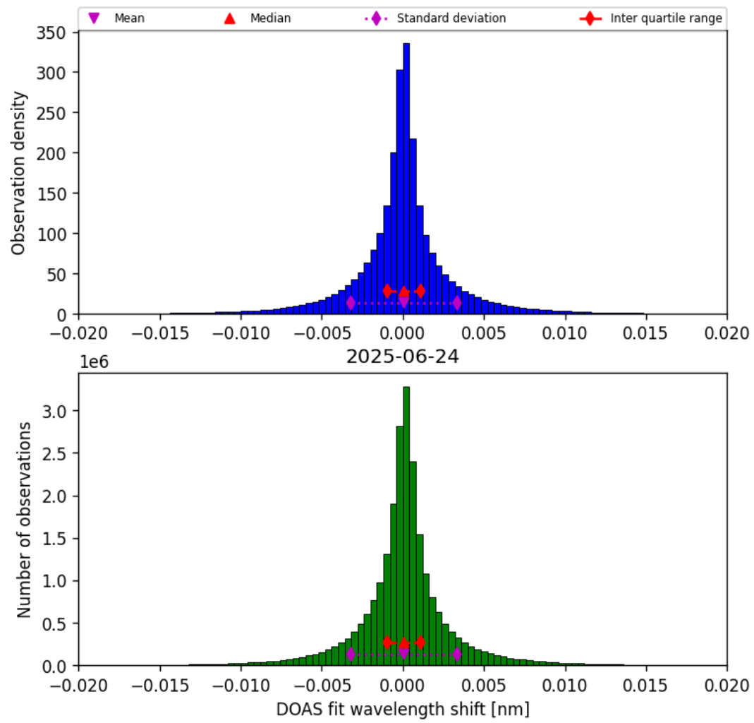
Figure 44: Histogram of “DOAS fit wavelength shift” for 2025-06-23 to 2025-06-25
