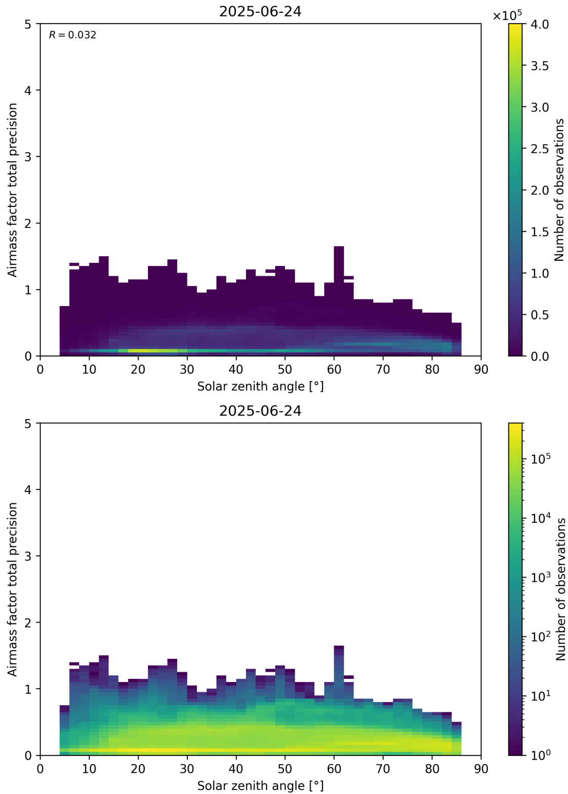
Figure 176: Scatter density plot of “Solar zenith angle” against “Airmass factor total precision” for 2025-06-23 to 2025-06-25.
