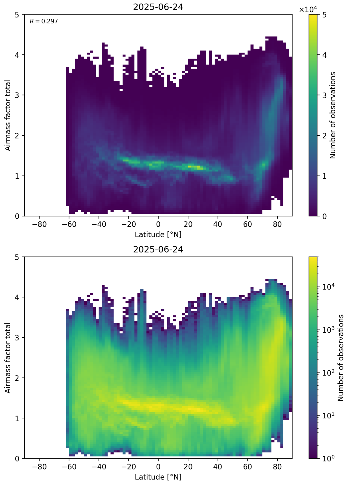
Figure 161: Scatter density plot of “Latitude” against “Airmass factor total” for 2025-06-23 to 2025-06-25.
