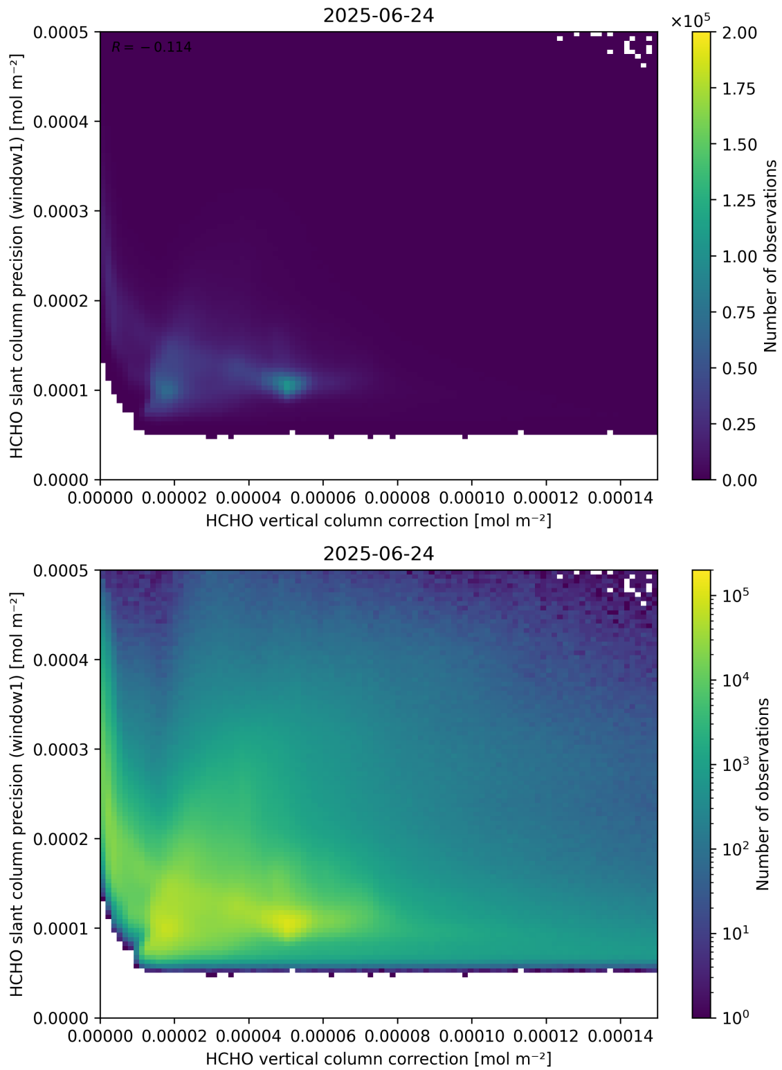
Figure 119: Scatter density plot of “HCHO vertical column correction” against “HCHO slant column precision (window1)” for 2025-06-23 to 2025-06-25.
