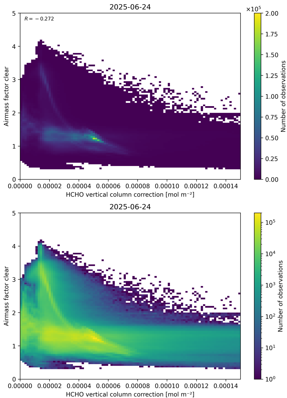
Figure 115: Scatter density plot of “HCHO vertical column correction” against “Airmass factor clear” for 2025-06-23 to 2025-06-25.
