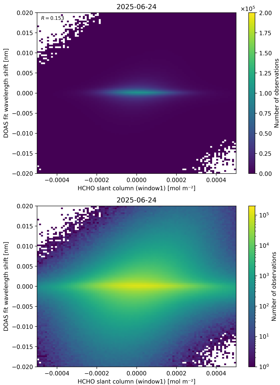
Figure 79: Scatter density plot of “HCHO slant column (window1)” against “DOAS fit wavelength shift” for 2025-06-23 to 2025-06-25.
