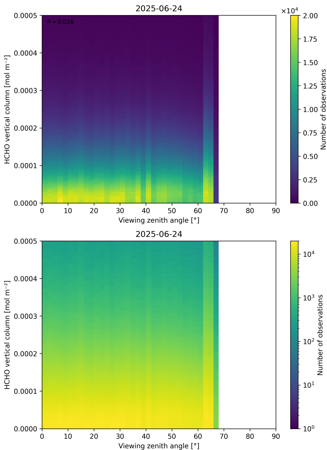
Figure 192: Scatter density plot of “Viewing zenith angle” against “HCHO vertical column” for 2025-06-23 to 2025-06-25.
