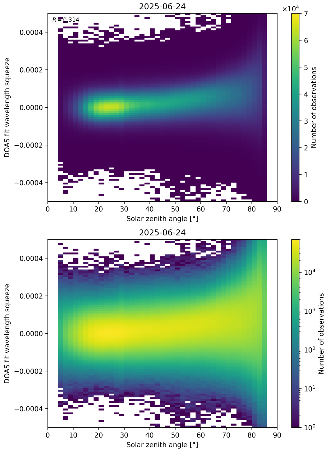
Figure 169: Scatter density plot of “Solar zenith angle” against “DOAS fit wavelength squeeze” for 2025-06-23 to 2025-06-25.
