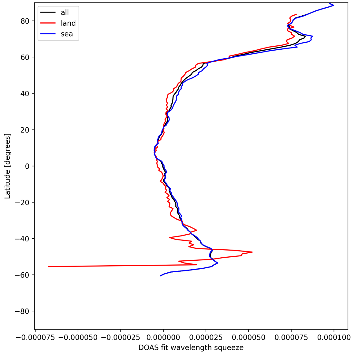
Figure 31: Zonal average of “DOAS fit wavelength squeeze” for 2025-06-23 to 2025-06-25.
