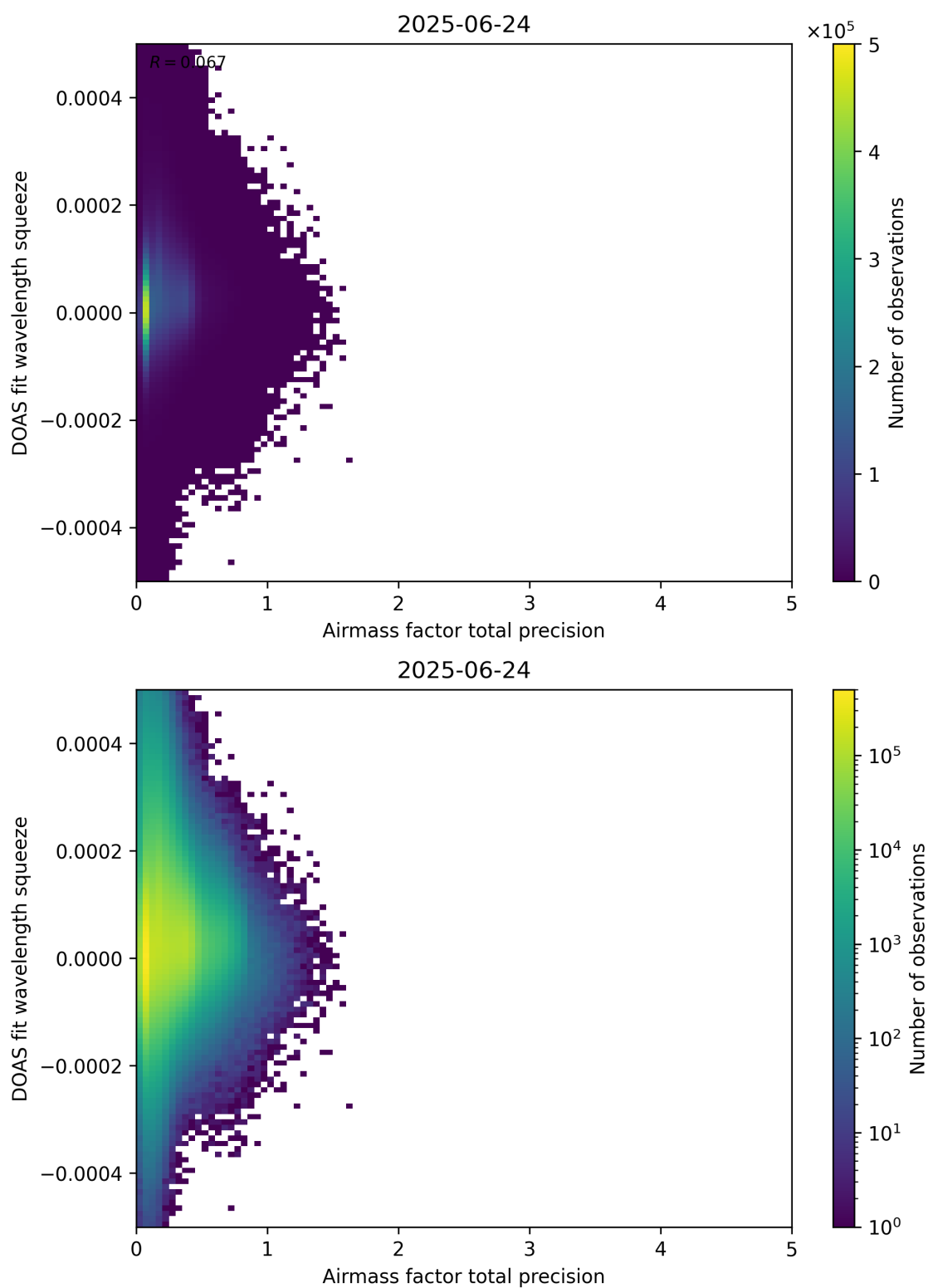
Figure 107: Scatter density plot of “Airmass factor total precision” against “DOAS fit wavelength squeeze” for 2025-06-23 to 2025-06-25.
