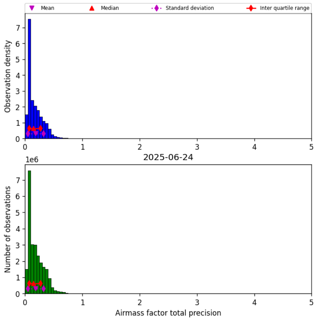
Figure 41: Histogram of “Airmass factor total precision” for 2025-06-23 to 2025-06-25
