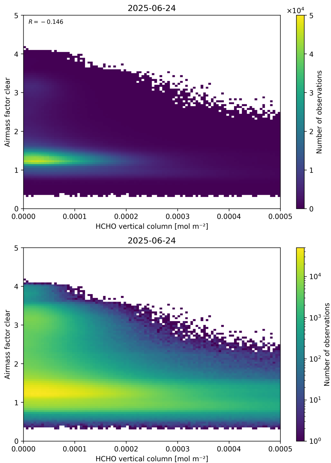
Figure 126: Scatter density plot of “HCHO vertical column” against “Airmass factor clear” for 2025-06-23 to 2025-06-25.
