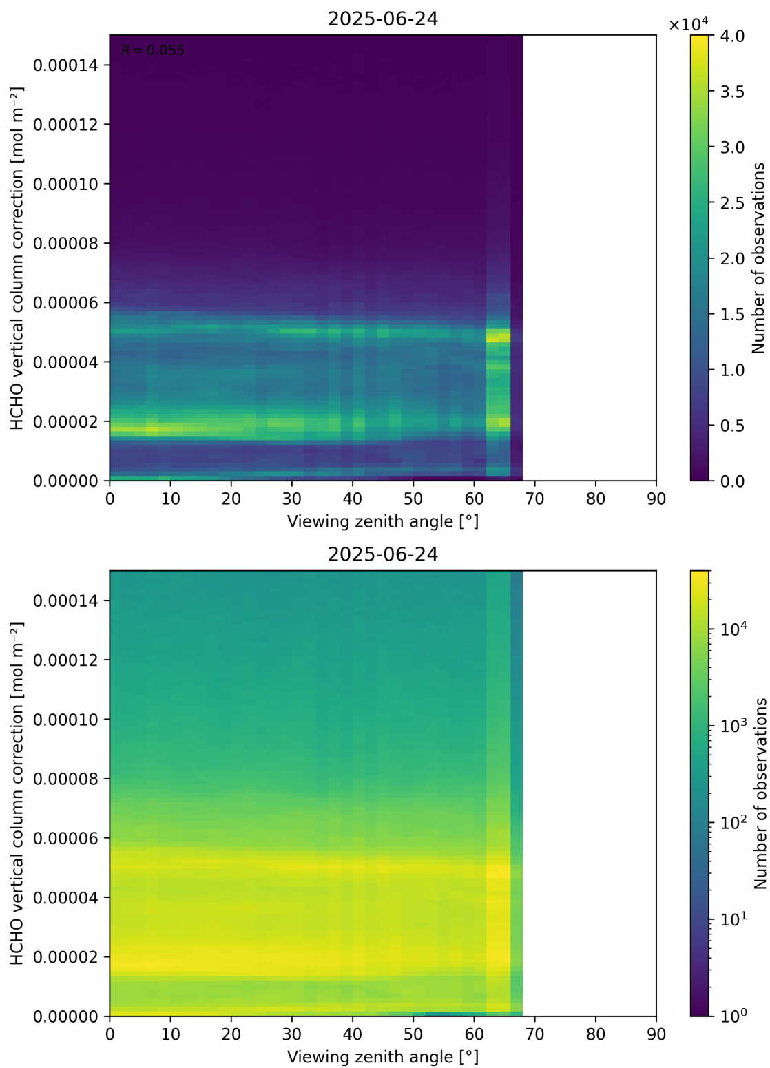
Figure 193: Scatter density plot of “Viewing zenith angle” against “HCHO vertical column correction” for 2025-06-23 to 2025-06-25.
