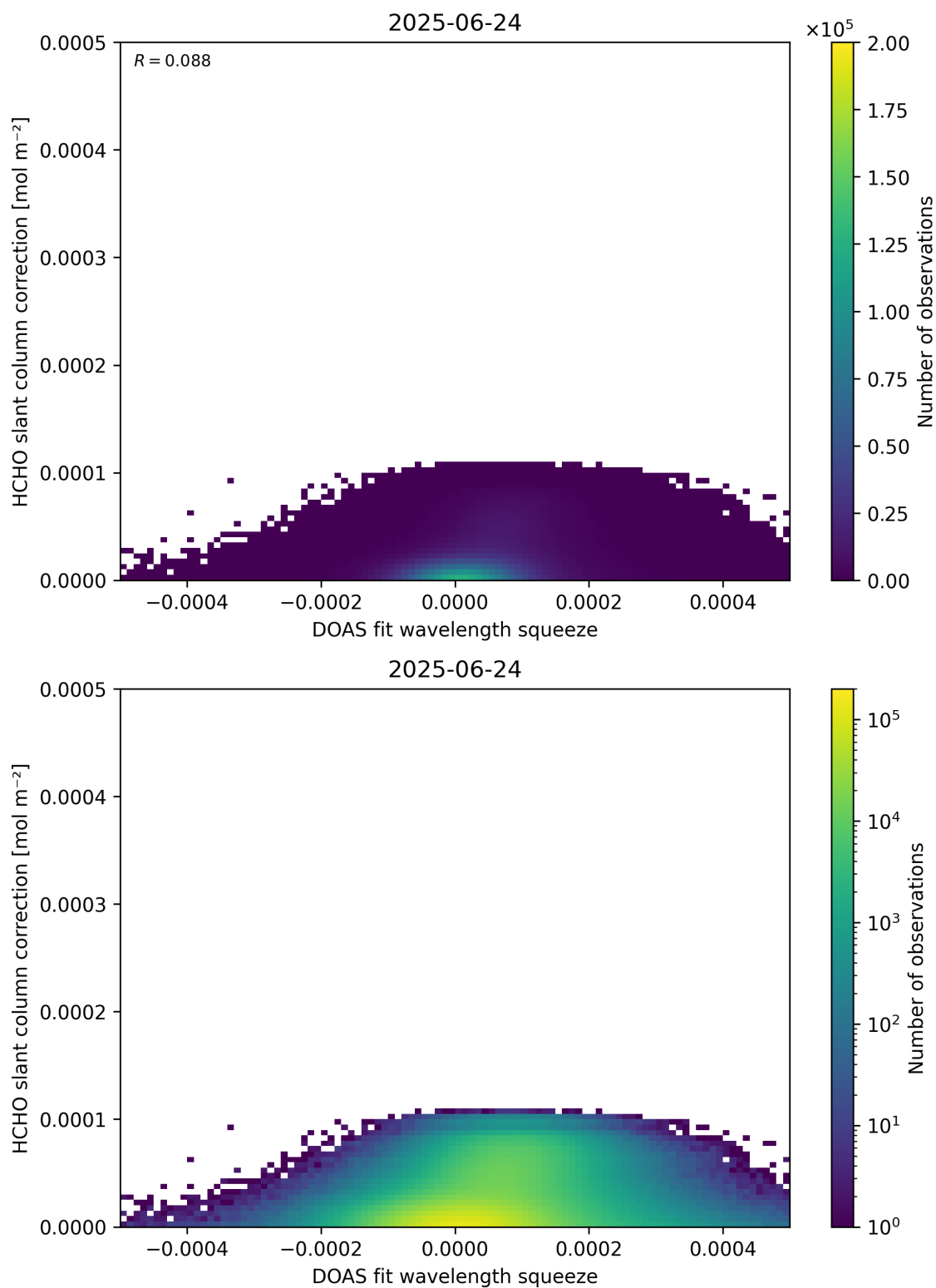
Figure 70: Scatter density plot of “DOAS fit wavelength squeeze” against “HCHO slant column correction” for 2025-06-23 to 2025-06-25.
