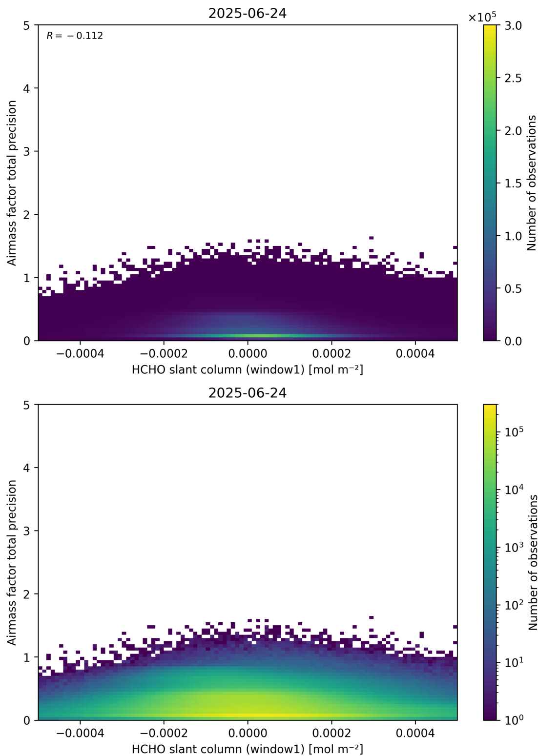
Figure 86: Scatter density plot of “HCHO slant column (window1)” against “Airmass factor total precision” for 2025-06-23 to 2025-06-25.
