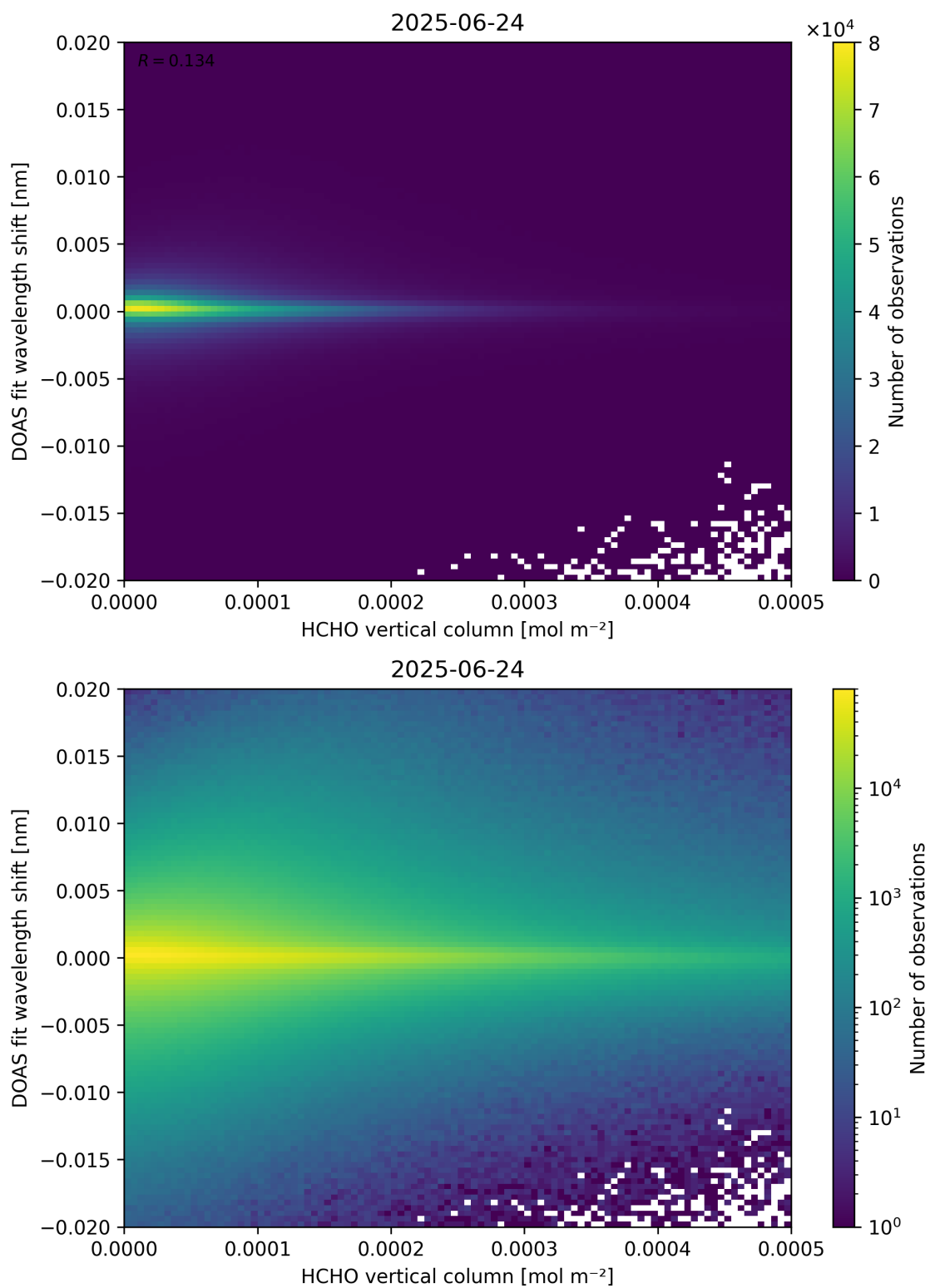
Figure 124: Scatter density plot of “HCHO vertical column” against “DOAS fit wavelength shift” for 2025-06-23 to 2025-06-25.
