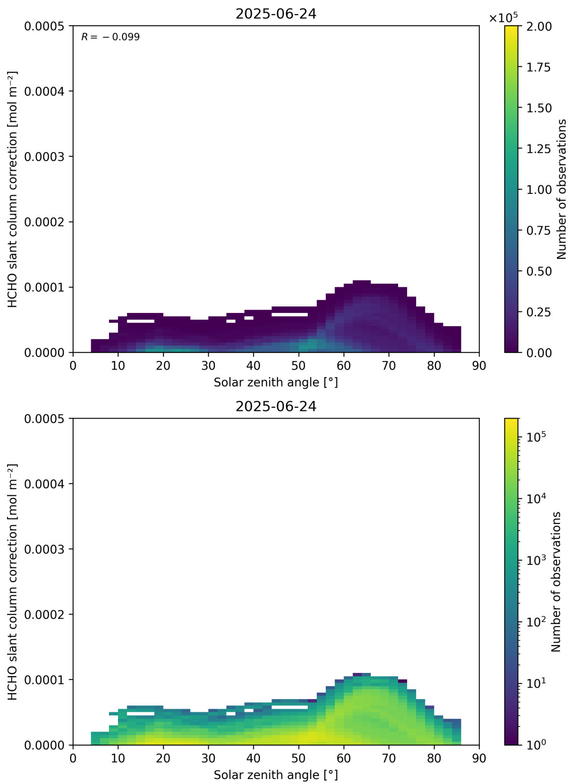
Figure 172: Scatter density plot of “Solar zenith angle” against “HCHO slant column correction” for 2025-06-23 to 2025-06-25.
