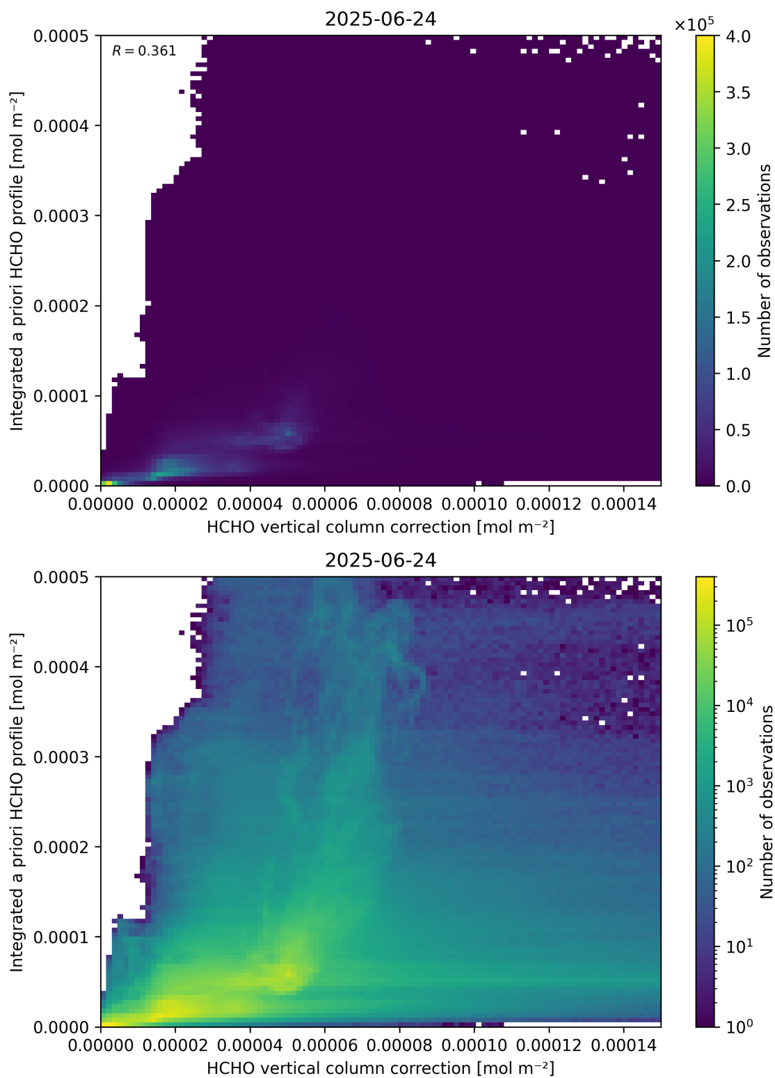
Figure 122: Scatter density plot of “HCHO vertical column correction” against “Integrated a priori HCHO profile” for 2025-06-23 to 2025-06-25.
