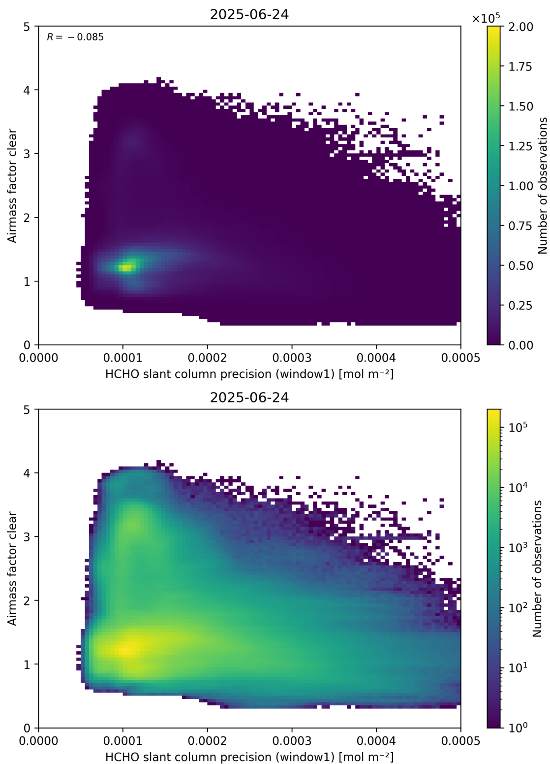
Figure 91: Scatter density plot of “HCHO slant column precision (window1)” against “Airmass factor clear” for 2025-06-23 to 2025-06-25.
