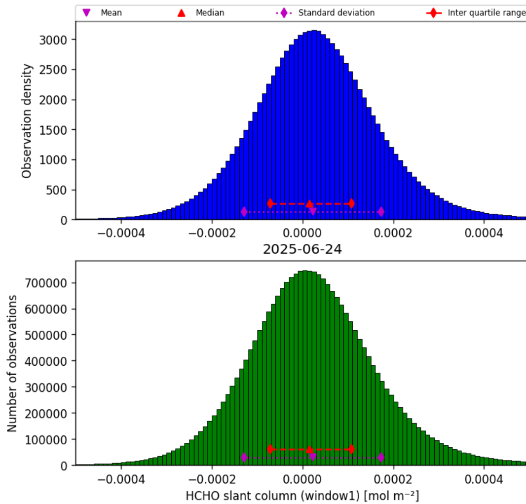
Figure 38: Histogram of “HCHO slant column (window1)” for 2025-06-23 to 2025-06-25
