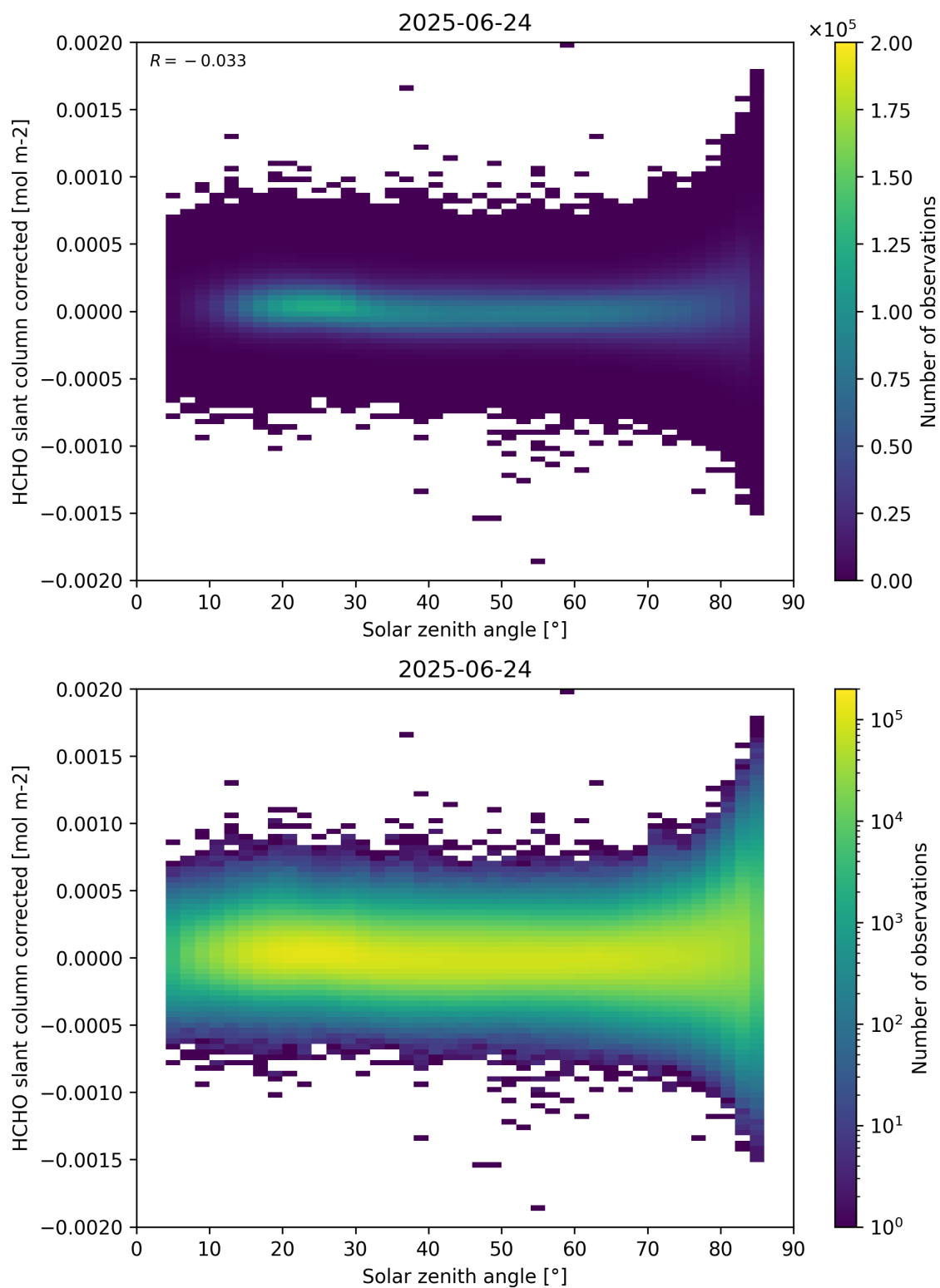
Figure 171: Scatter density plot of “Solar zenith angle” against “HCHO slant column corrected” for 2025-06-23 to 2025-06-25.
