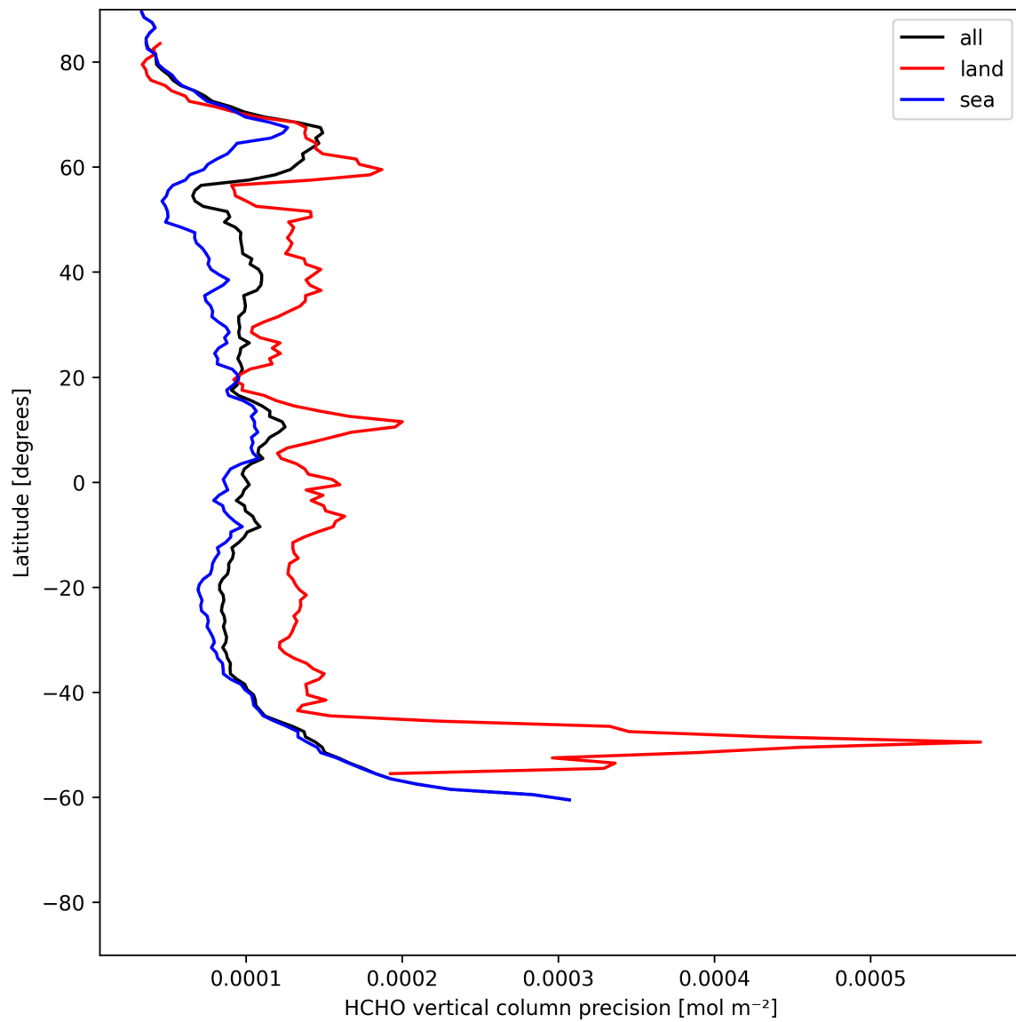
Figure 22: Zonal average of “HCHO vertical column precision” for 2025-06-23 to 2025-06-25.
