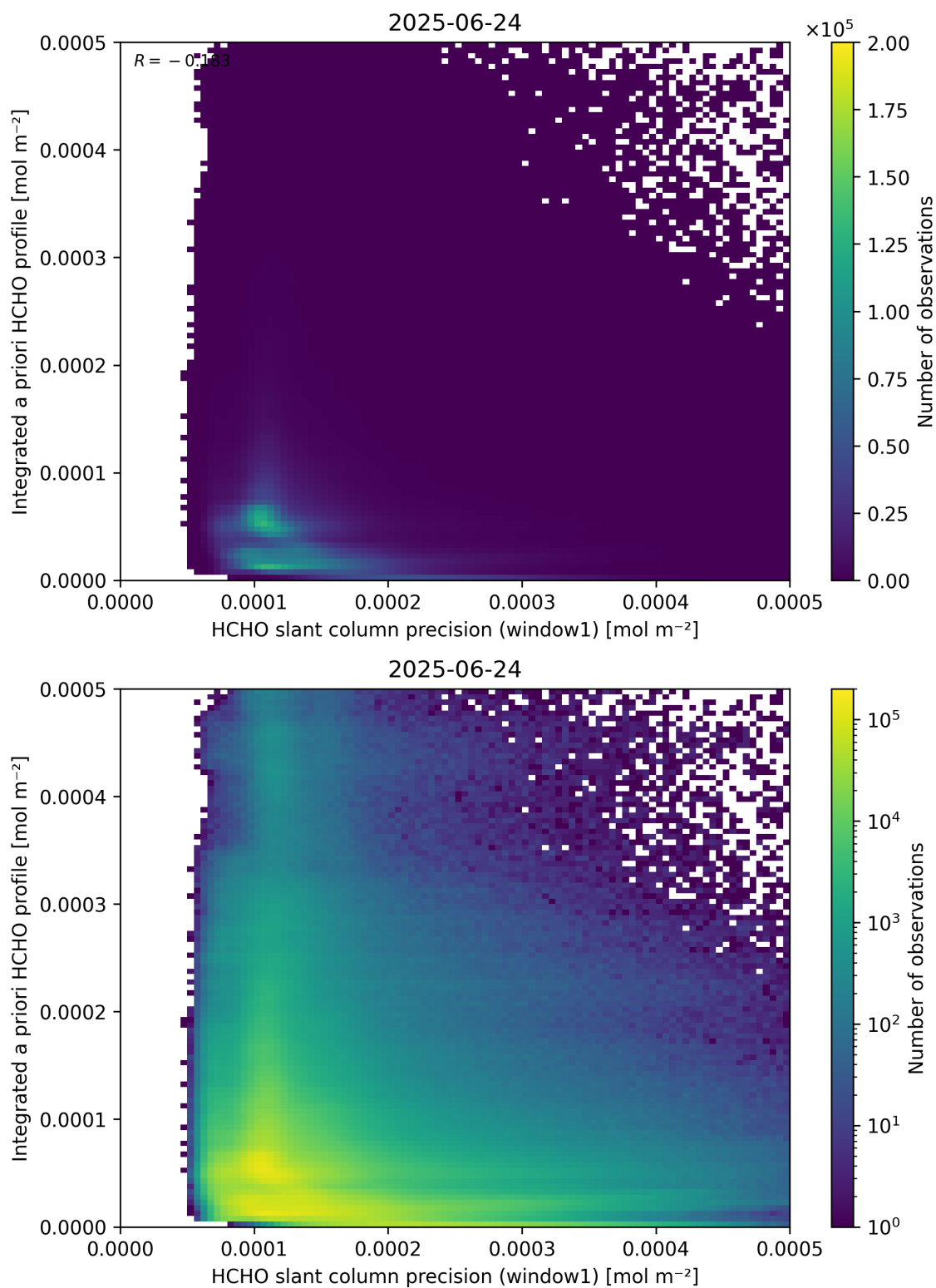
Figure 96: Scatter density plot of “HCHO slant column precision (window1)” against “Integrated a priori HCHO profile” for 2025-06-23 to 2025-06-25.
