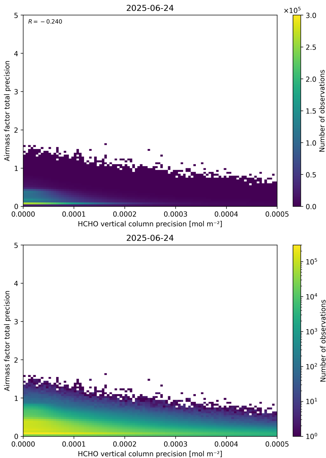
Figure 145: Scatter density plot of “HCHO vertical column precision” against “Airmass factor total precision” for 2025-06-23 to 2025-06-25.
