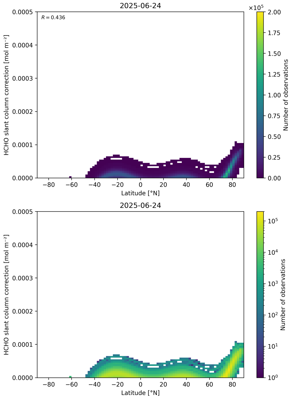
Figure 158: Scatter density plot of “Latitude” against “HCHO slant column correction” for 2025-06-23 to 2025-06-25.
