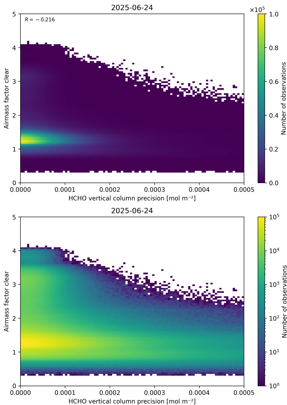
Figure 139: Scatter density plot of “HCHO vertical column precision” against “Airmass factor clear” for 2025-06-23 to 2025-06-25.
