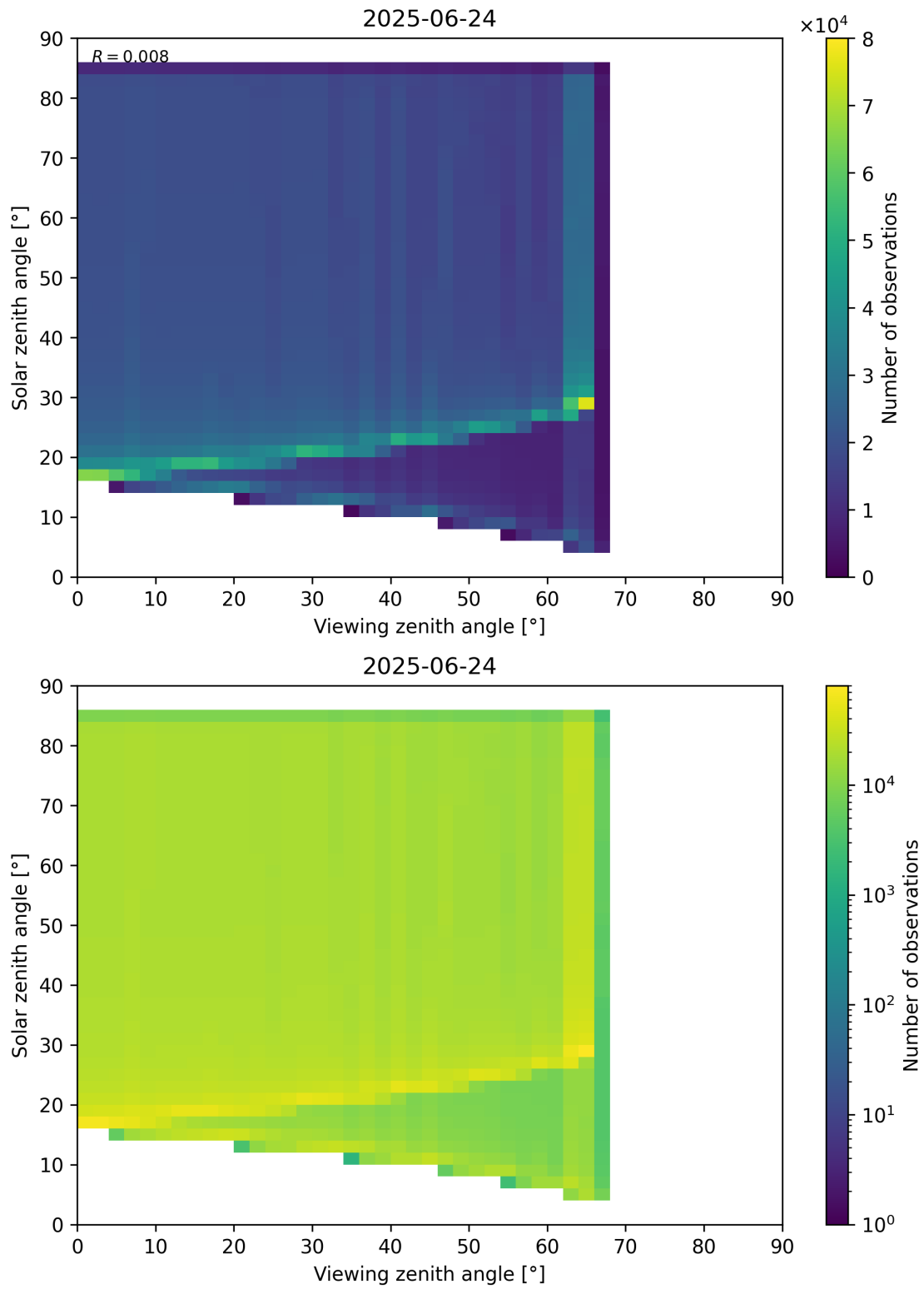
Figure 197: Scatter density plot of “Viewing zenith angle” against “Solar zenith angle” for 2025-06-23 to 2025-06-25.
