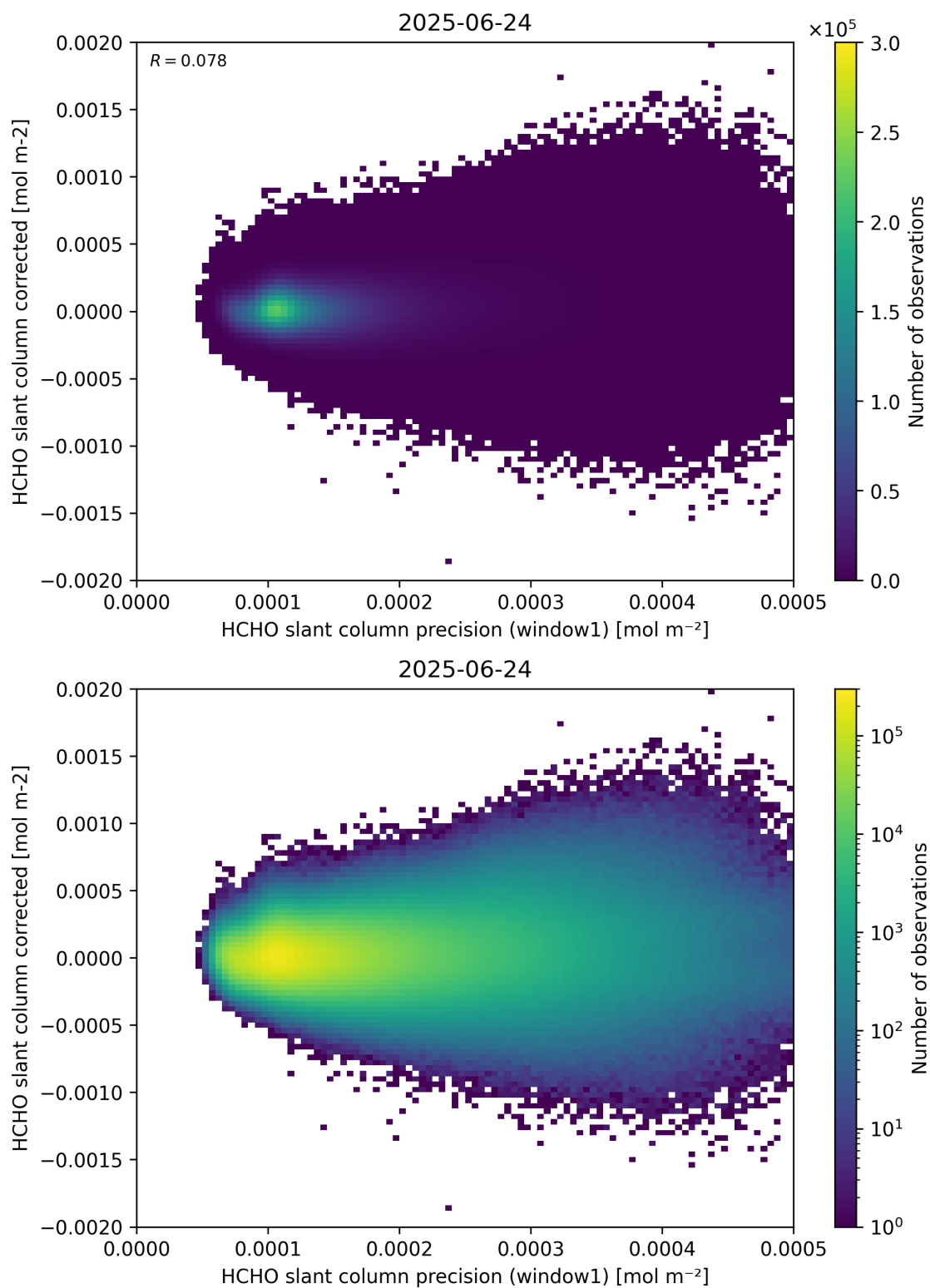
Figure 92: Scatter density plot of “HCHO slant column precision (window1)” against “HCHO slant column corrected” for 2025-06-23 to 2025-06-25.
