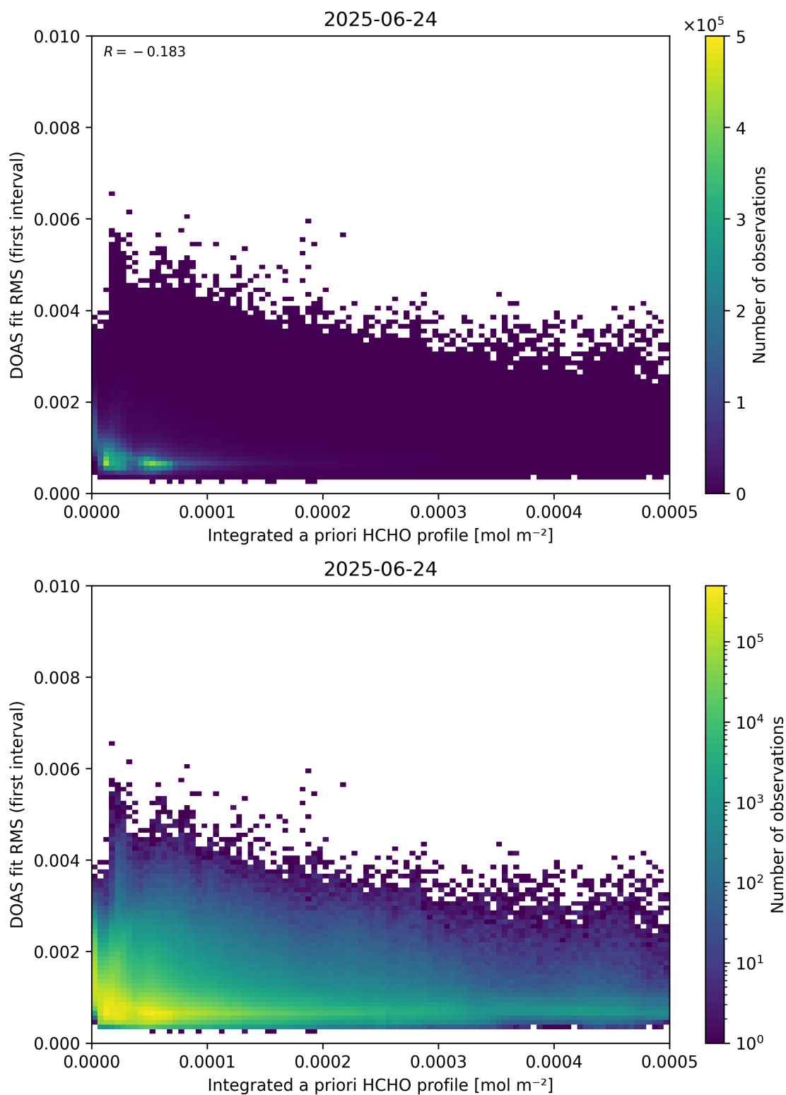
Figure 148: Scatter density plot of “Integrated a priori HCHO profile” against “DOAS fit RMS (first interval)” for 2025-06-23 to 2025-06-25.
