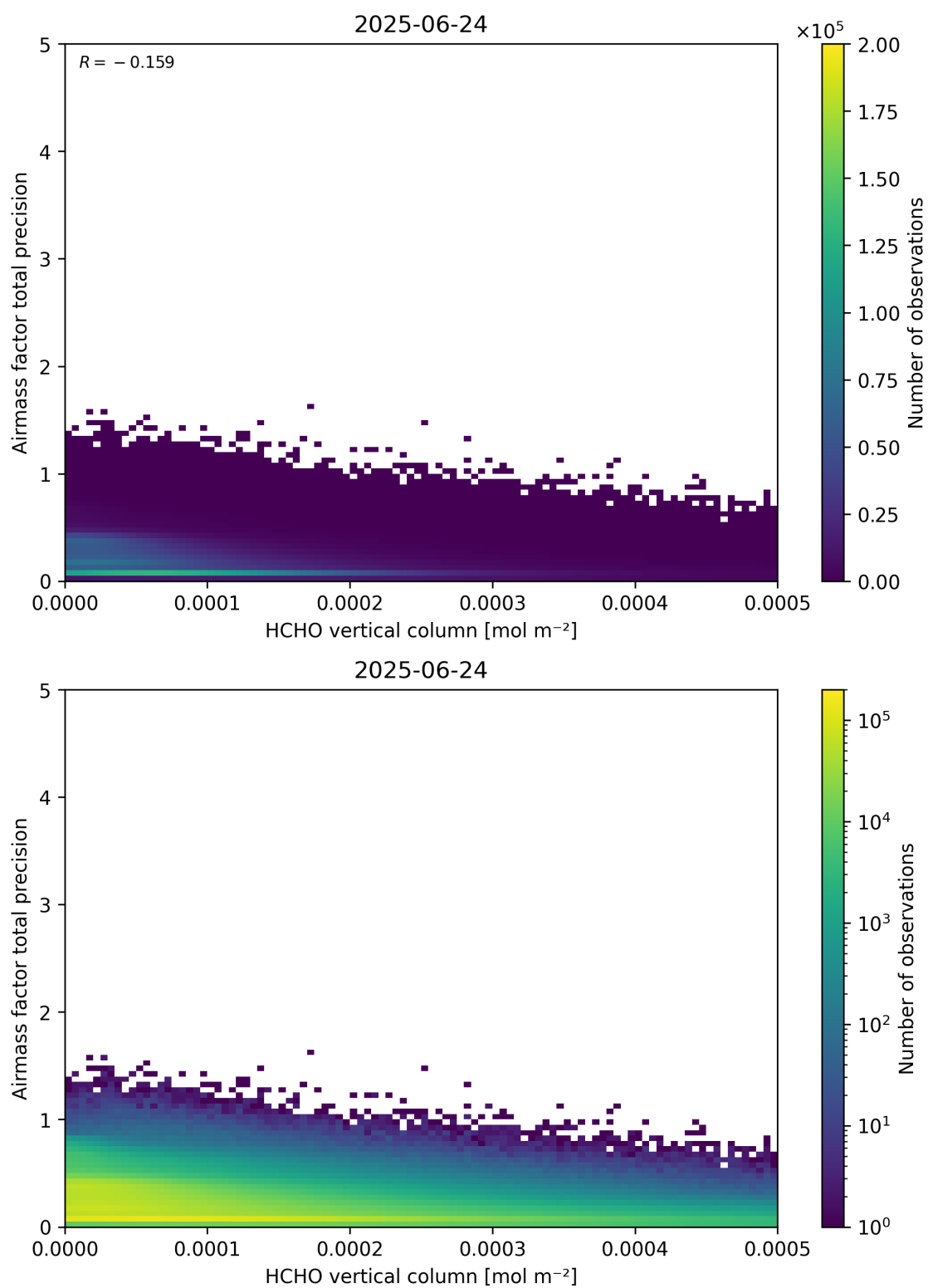
Figure 132: Scatter density plot of “HCHO vertical column” against “Airmass factor total precision” for 2025-06-23 to 2025-06-25.
