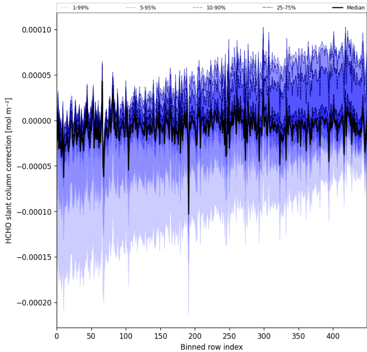
Figure 61: Along track statistics of “HCHO slant column correction” for 2025-06-23 to 2025-06-25
