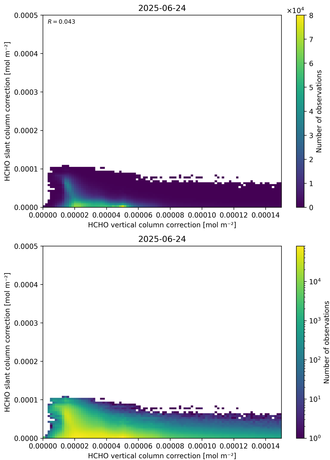
Figure 117: Scatter density plot of “HCHO vertical column correction” against “HCHO slant column correction” for 2025-06-23 to 2025-06-25.
