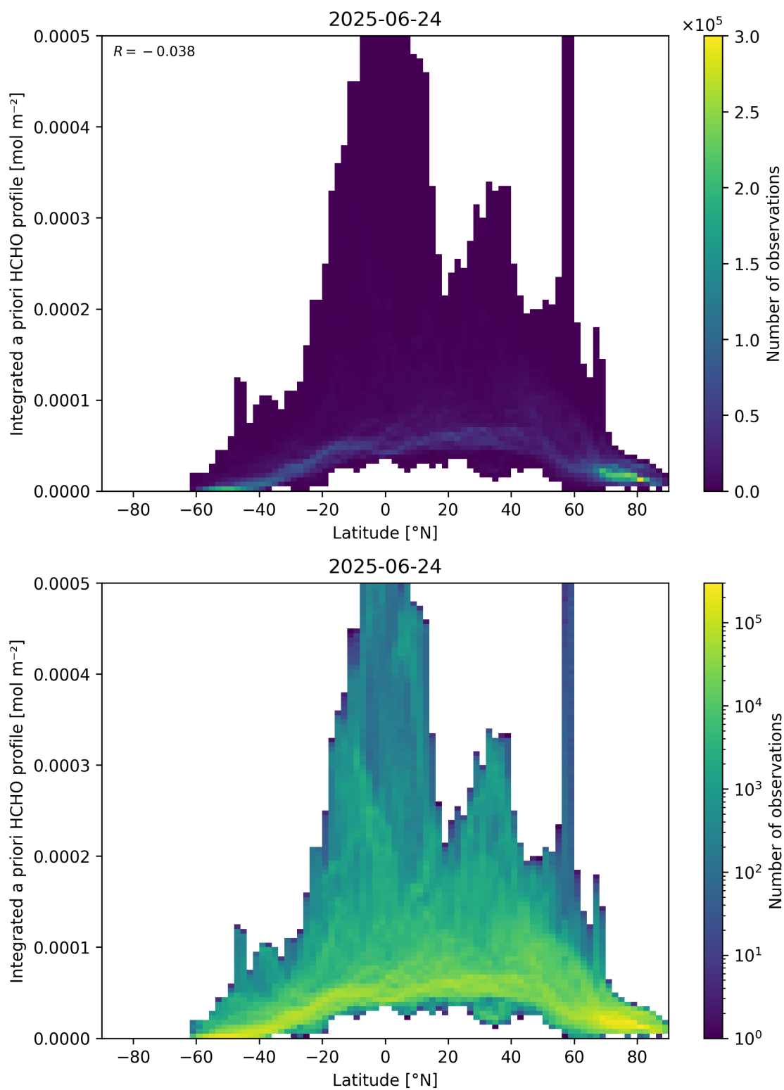
Figure 166: Scatter density plot of “Latitude” against “Integrated a priori HCHO profile” for 2025-06-23 to 2025-06-25.
