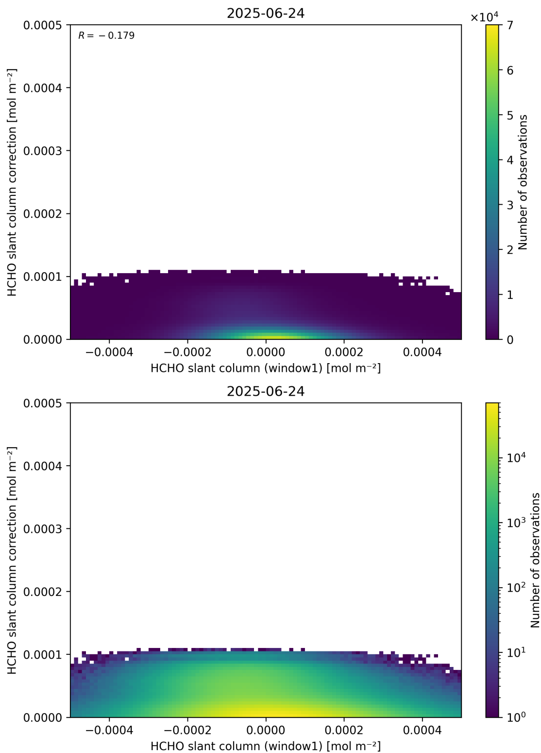
Figure 83: Scatter density plot of “HCHO slant column (window1)” against “HCHO slant column correction” for 2025-06-23 to 2025-06-25.
