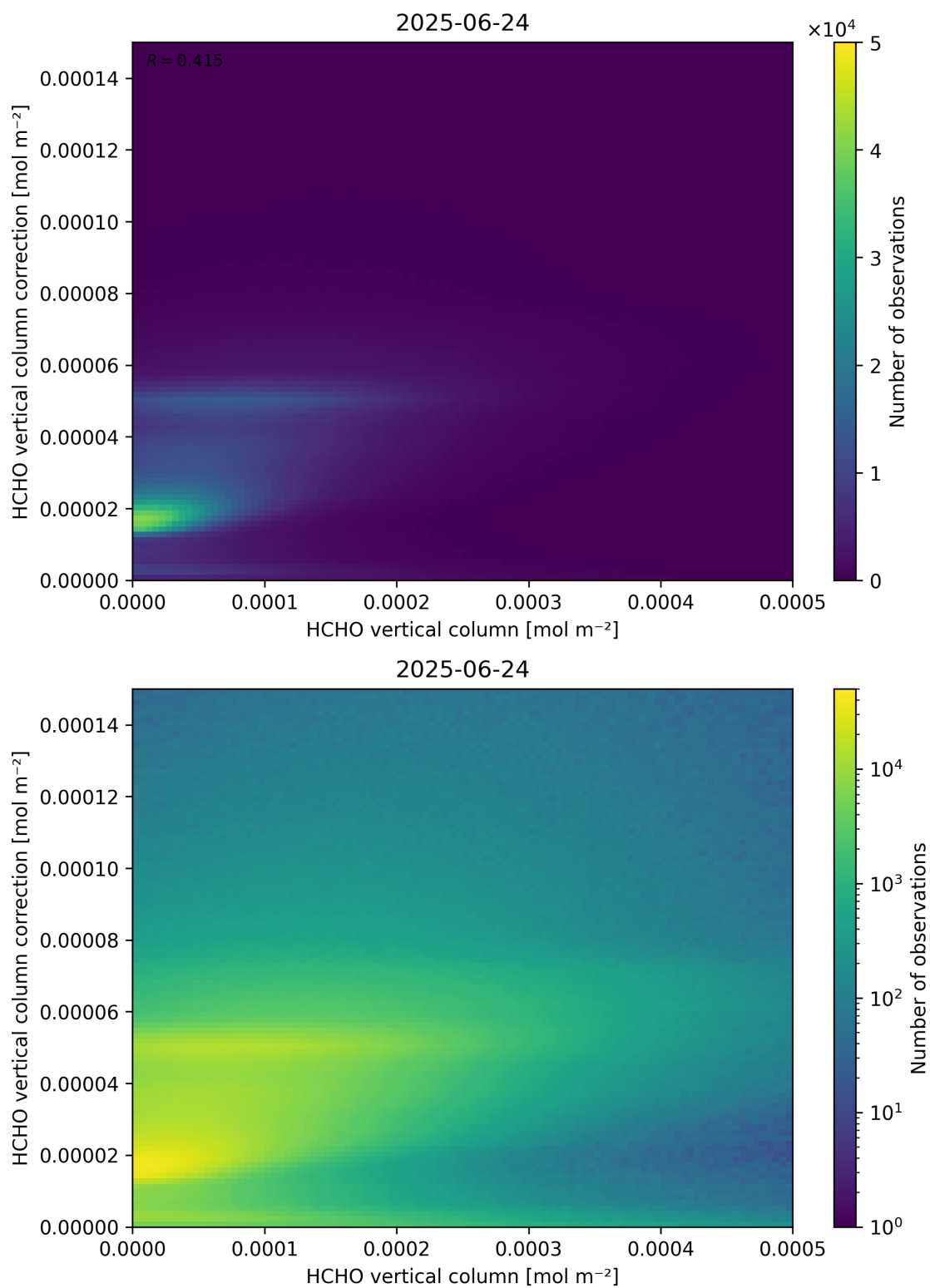
Figure 133: Scatter density plot of “HCHO vertical column” against “HCHO vertical column correction” for 2025-06-23 to 2025-06-25.
