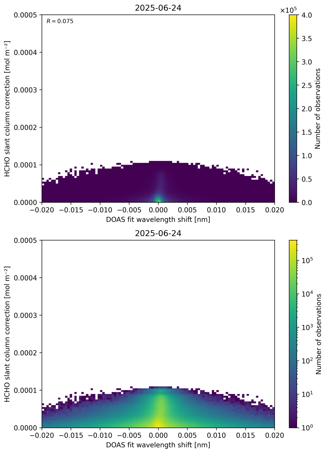
Figure 67: Scatter density plot of “DOAS fit wavelength shift” against “HCHO slant column correction” for 2025-06-23 to 2025-06-25.
