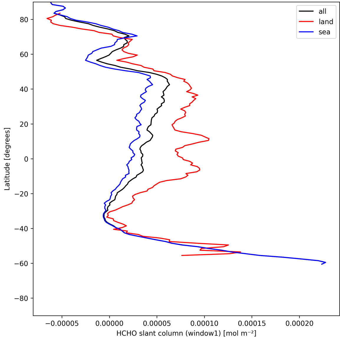
Figure 24: Zonal average of “HCHO slant column (window1)” for 2025-06-23 to 2025-06-25.
