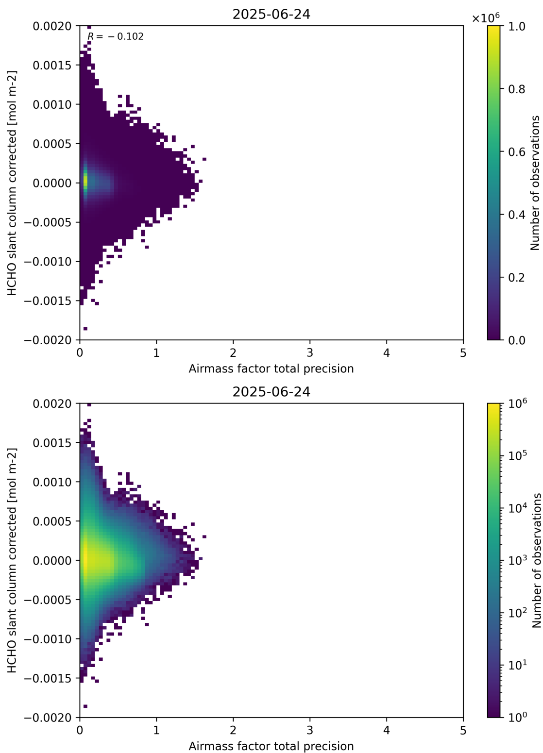
Figure 109: Scatter density plot of “Airmass factor total precision” against “HCHO slant column corrected” for 2025-06-23 to 2025-06-25.
