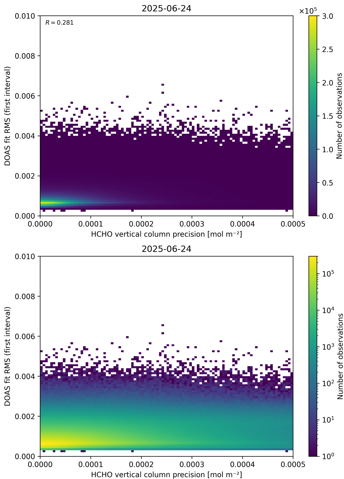
Figure 136: Scatter density plot of “HCHO vertical column precision” against “DOAS fit RMS (first interval)” for 2025-06-23 to 2025-06-25.
