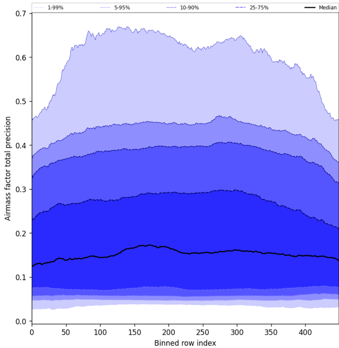
Figure 55: Along track statistics of “Airmass factor total precision” for 2025-06-23 to 2025-06-25
