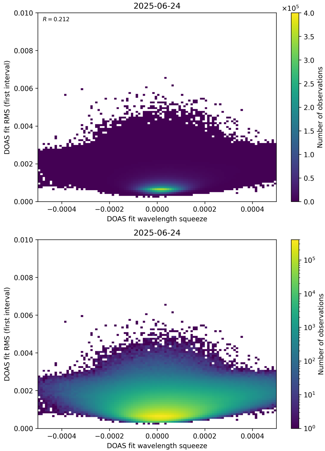
Figure 68: Scatter density plot of “DOAS fit wavelength squeeze” against “DOAS fit RMS (first interval)” for 2025-06-23 to 2025-06-25.
