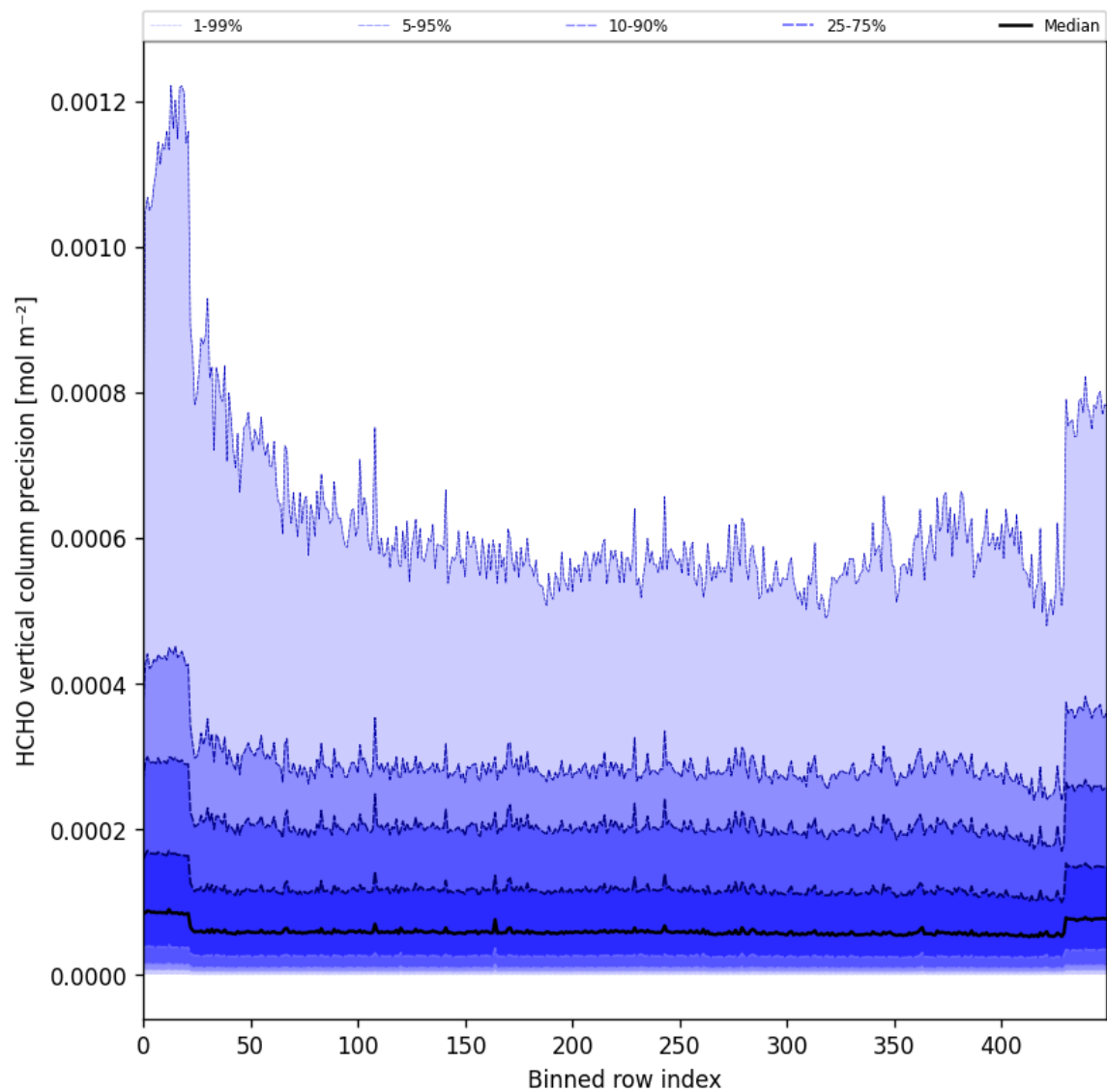
Figure 50: Along track statistics of “HCHO vertical column precision” for 2025-06-23 to 2025-06-25
