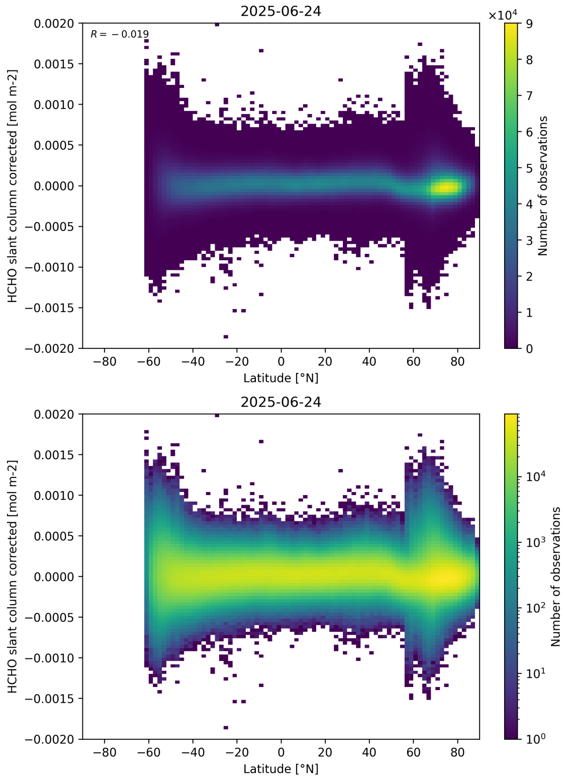
Figure 157: Scatter density plot of “Latitude” against “HCHO slant column corrected” for 2025-06-23 to 2025-06-25.
