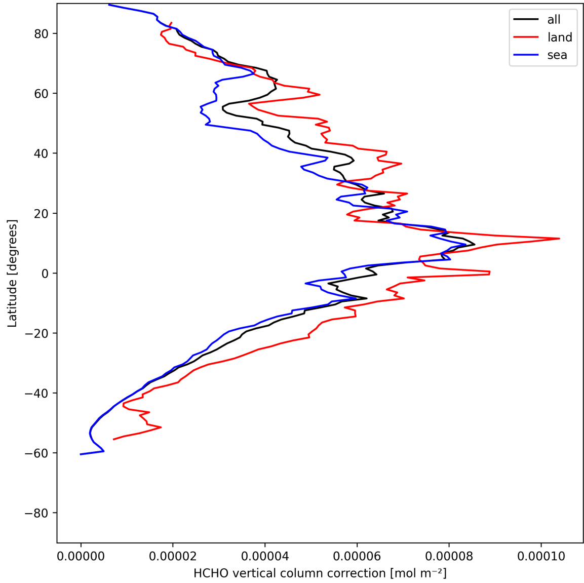
Figure 23: Zonal average of “HCHO vertical column correction” for 2025-06-23 to 2025-06-25.
