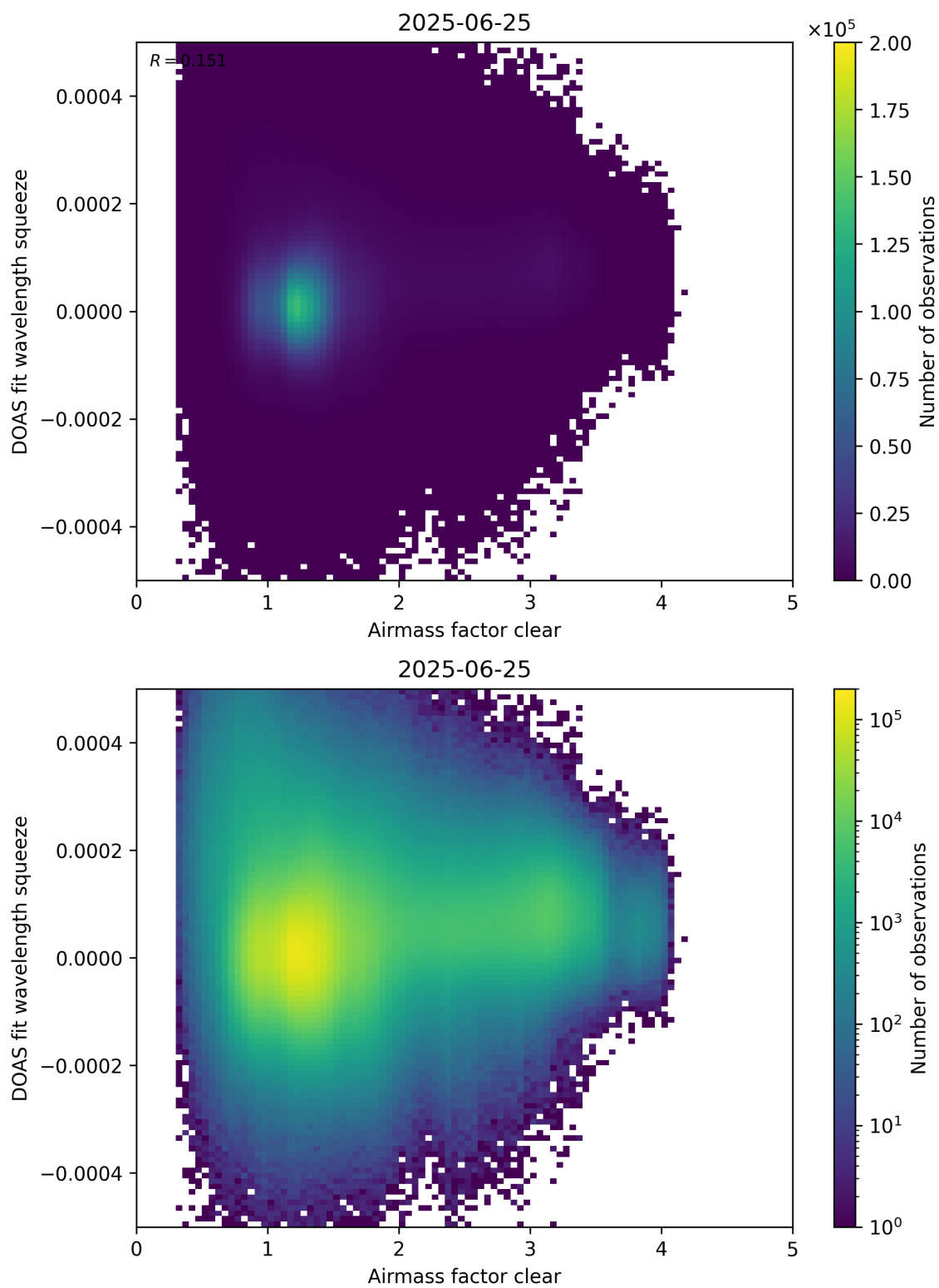
Figure 73: Scatter density plot of “Airmass factor clear” against “DOAS fit wavelength squeeze” for 2025-06-24 to 2025-06-26.
