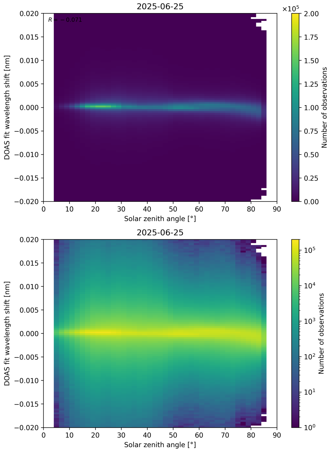
Figure 168: Scatter density plot of “Solar zenith angle” against “DOAS fit wavelength shift” for 2025-06-24 to 2025-06-26.
