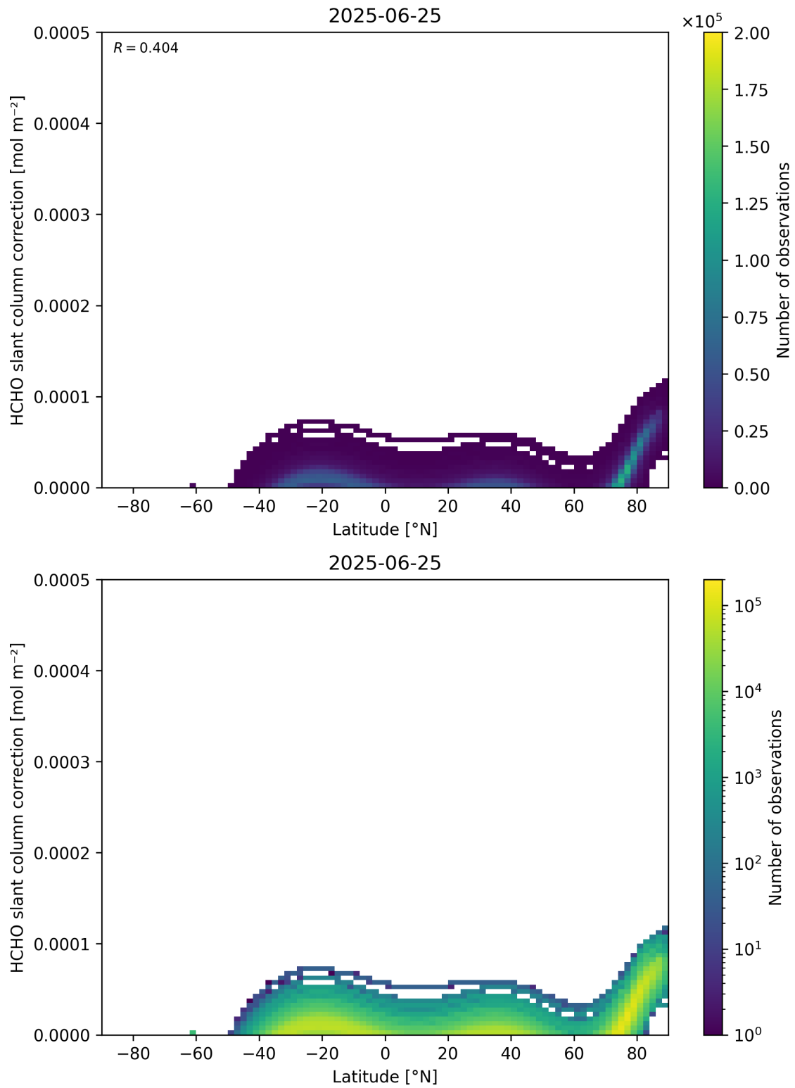
Figure 158: Scatter density plot of “Latitude” against “HCHO slant column correction” for 2025-06-24 to 2025-06-26.
