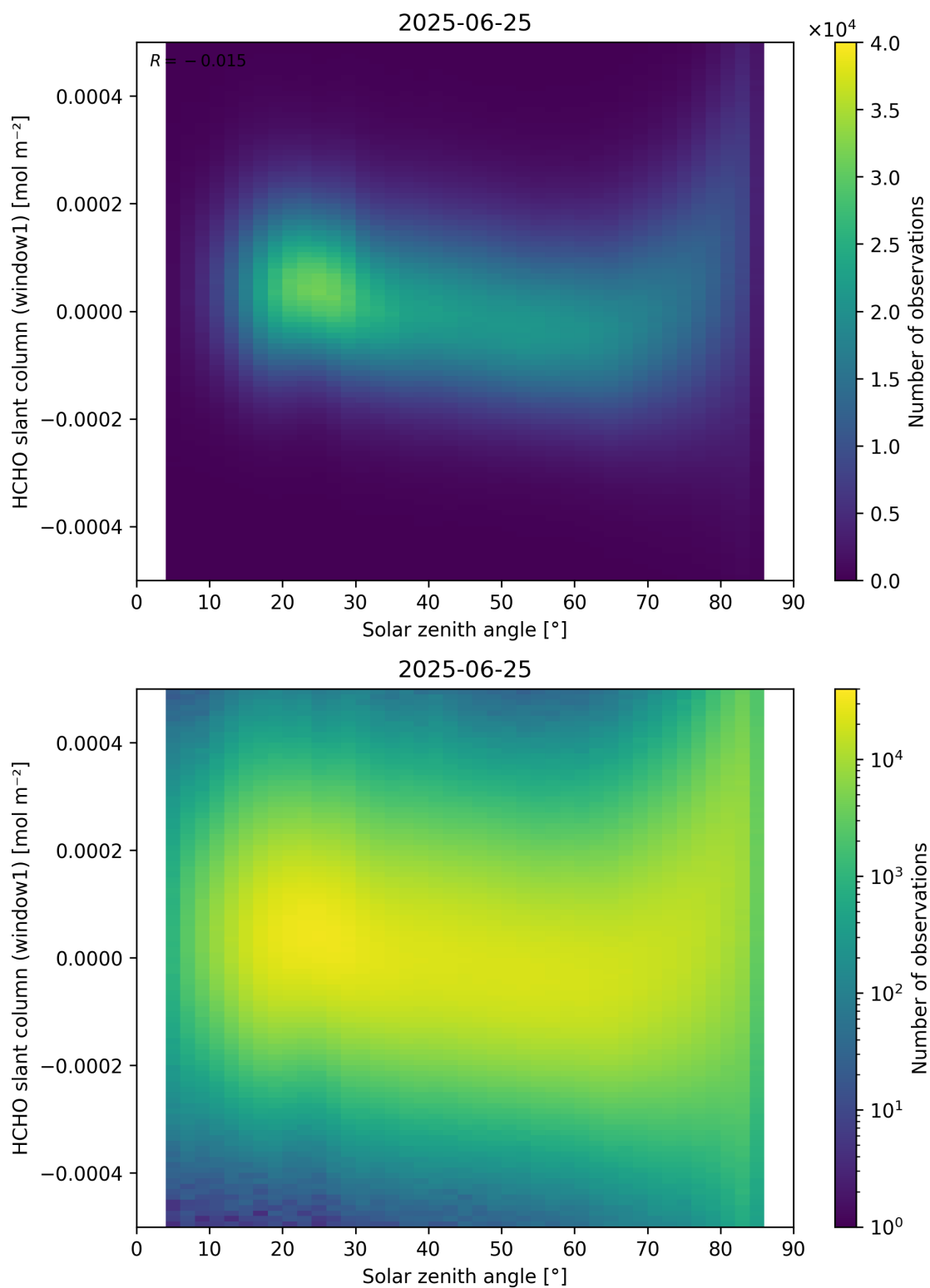
Figure 173: Scatter density plot of “Solar zenith angle” against “HCHO slant column (window1)” for 2025-06-24 to 2025-06-26.
