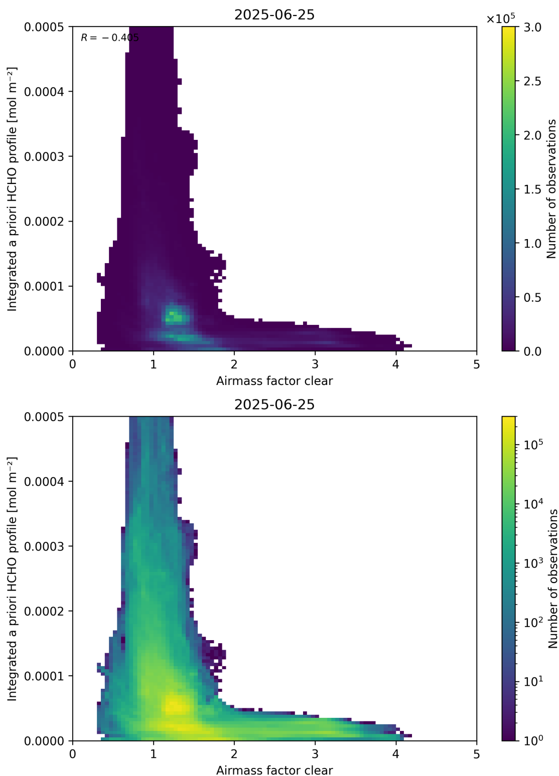
Figure 76: Scatter density plot of “Airmass factor clear” against “Integrated a priori HCHO profile” for 2025-06-24 to 2025-06-26.
