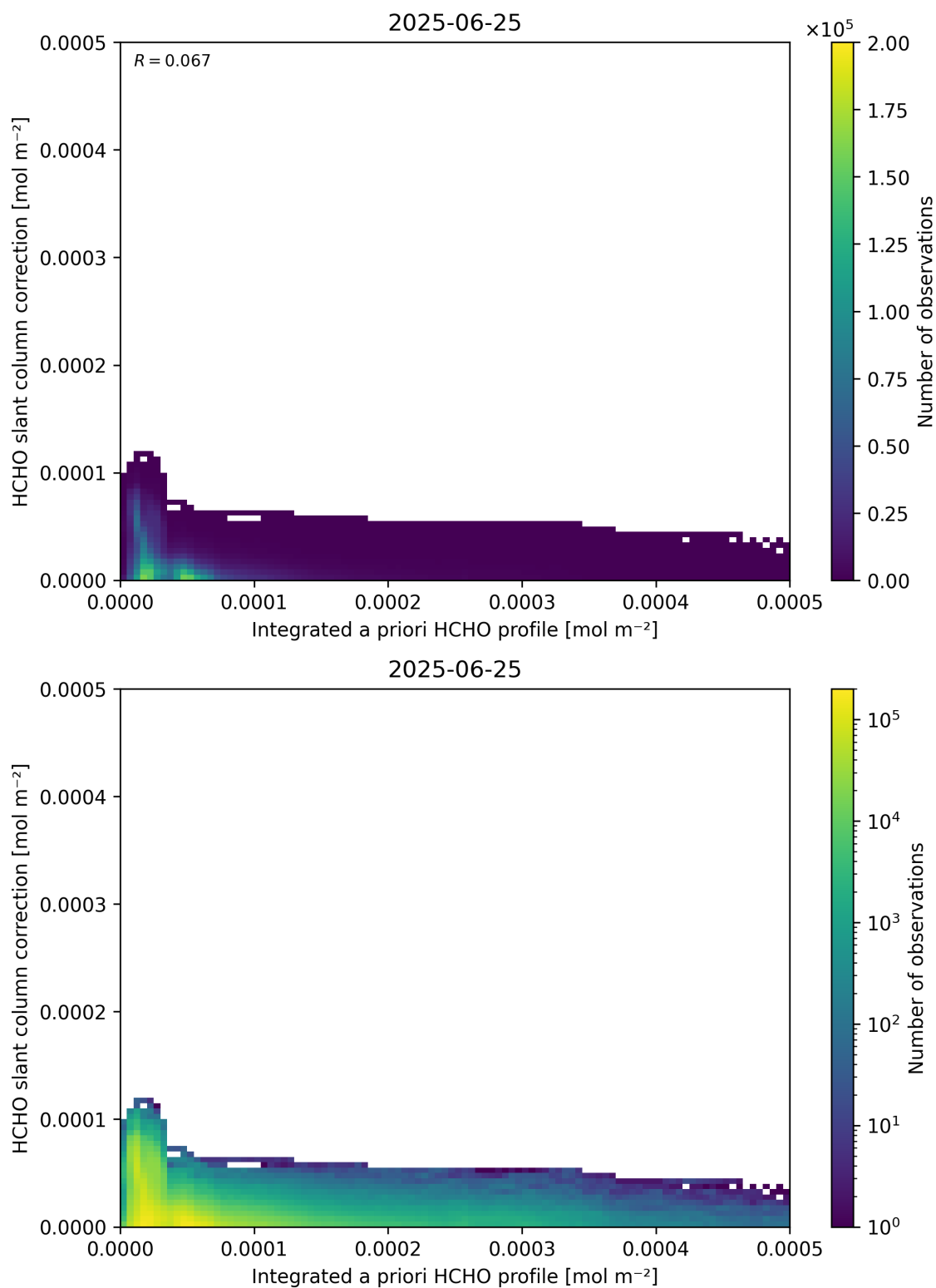
Figure 152: Scatter density plot of “Integrated a priori HCHO profile” against “HCHO slant column correction” for 2025-06-24 to 2025-06-26.
