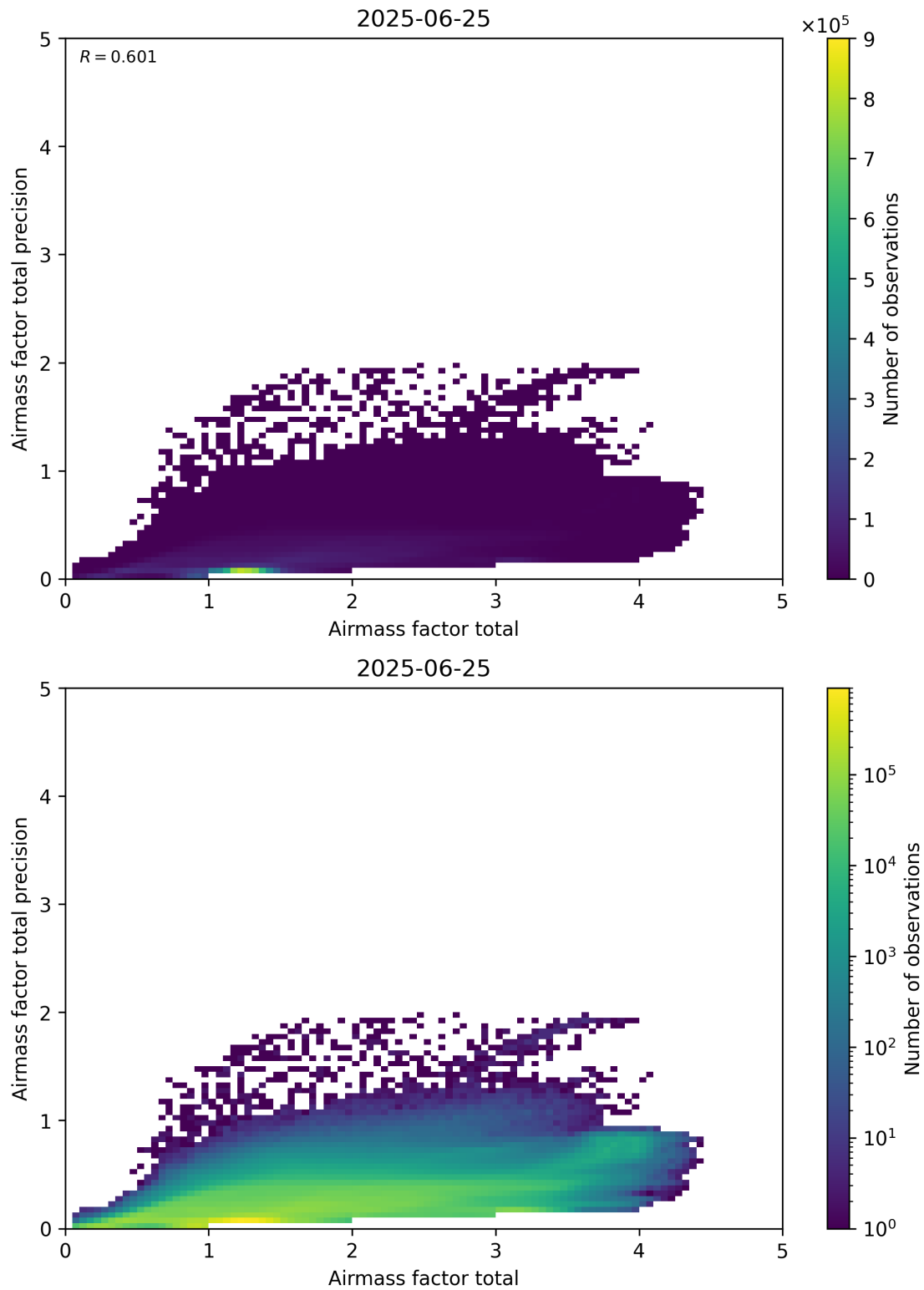
Figure 103: Scatter density plot of “Airmass factor total” against “Airmass factor total precision” for 2025-06-24 to 2025-06-26.
