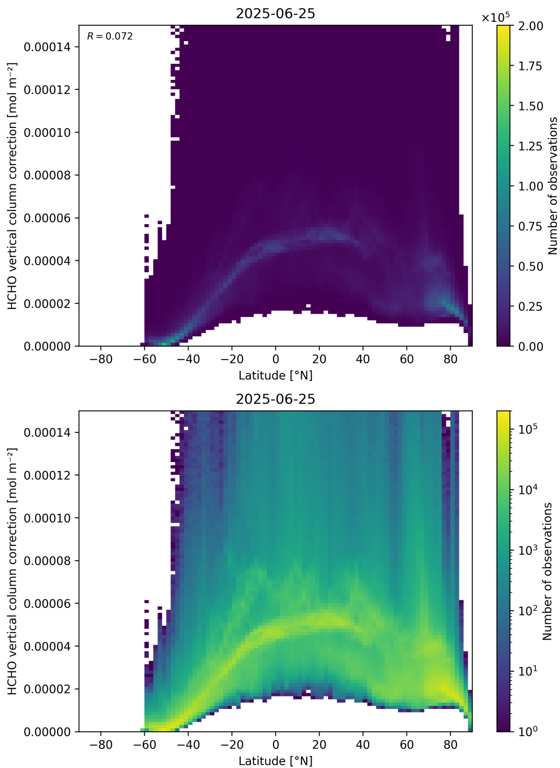
Figure 164: Scatter density plot of “Latitude” against “HCHO vertical column correction” for 2025-06-24 to 2025-06-26.
