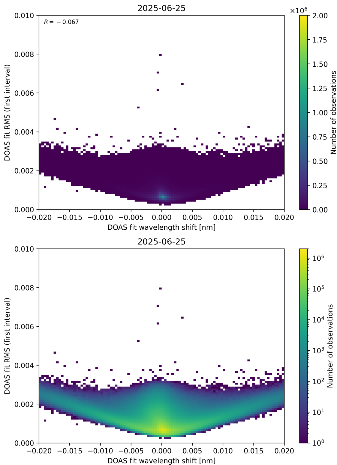
Figure 64: Scatter density plot of “DOAS fit wavelength shift” against “DOAS fit RMS (first interval)” for 2025-06-24 to 2025-06-26.
