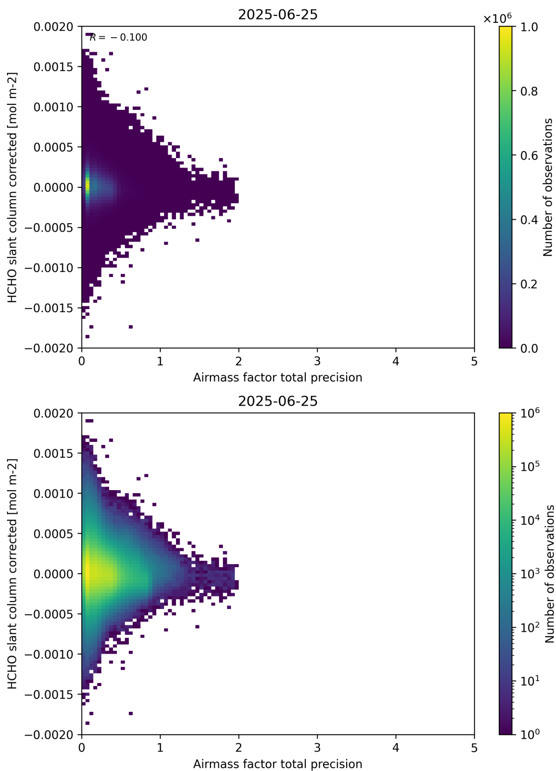
Figure 109: Scatter density plot of “Airmass factor total precision” against “HCHO slant column corrected” for 2025-06-24 to 2025-06-26.
