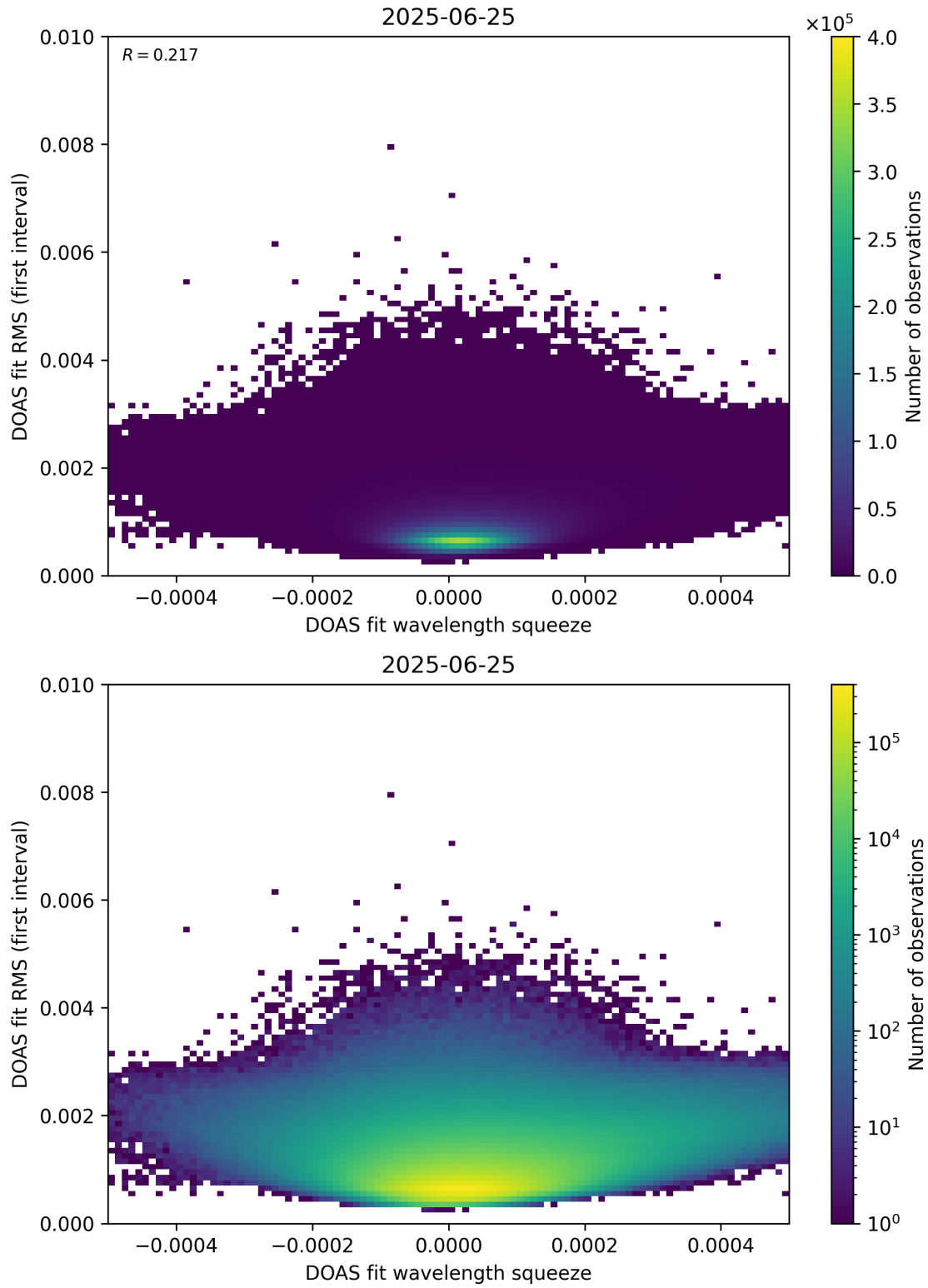
Figure 68: Scatter density plot of “DOAS fit wavelength squeeze” against “DOAS fit RMS (first interval)” for 2025-06-24 to 2025-06-26.
