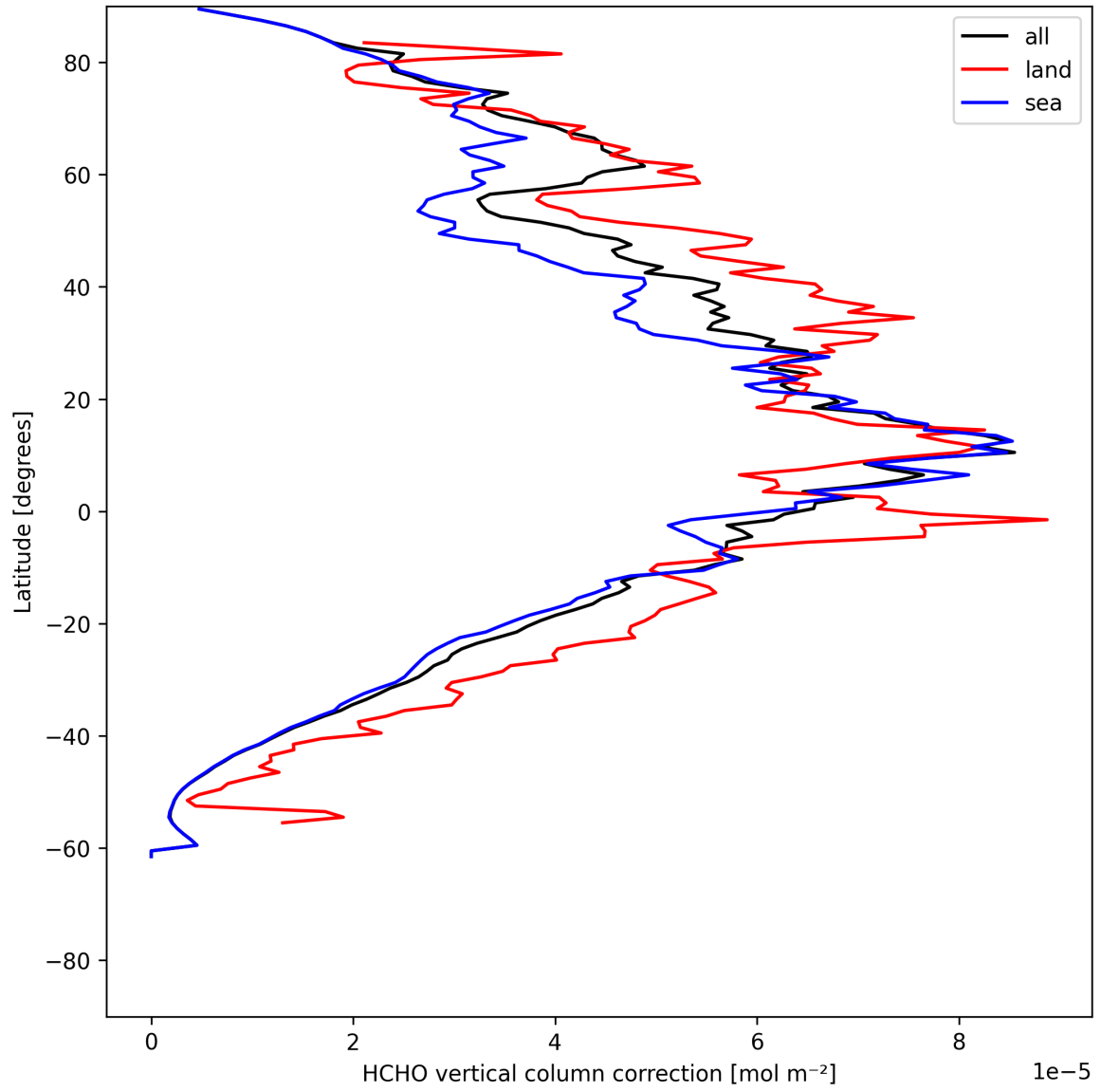
Figure 23: Zonal average of "HCHO vertical column correction" for 2025-06-24 to 2025-06-26.
