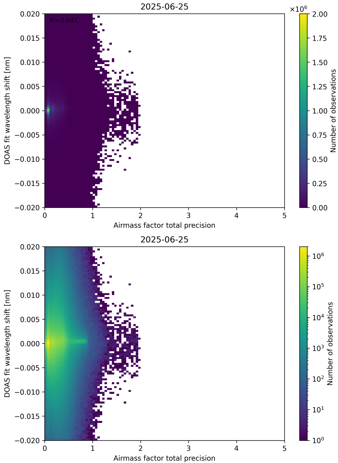
Figure 106: Scatter density plot of “Airmass factor total precision” against “DOAS fit wavelength shift” for 2025-06-24 to 2025-06-26.
