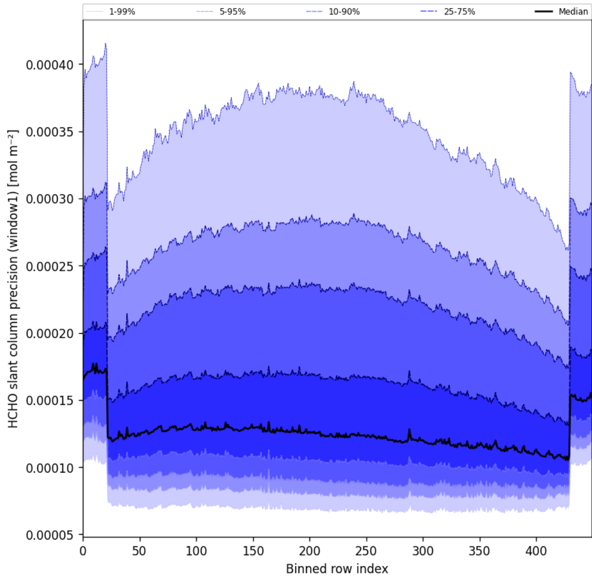
Figure 53: Along track statistics of “HCHO slant column precision (window1)” for 2025-06-24 to 2025-06-26
