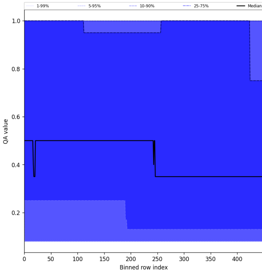
Figure 48: Along track statistics of “QA value” for 2025-06-24 to 2025-06-26
