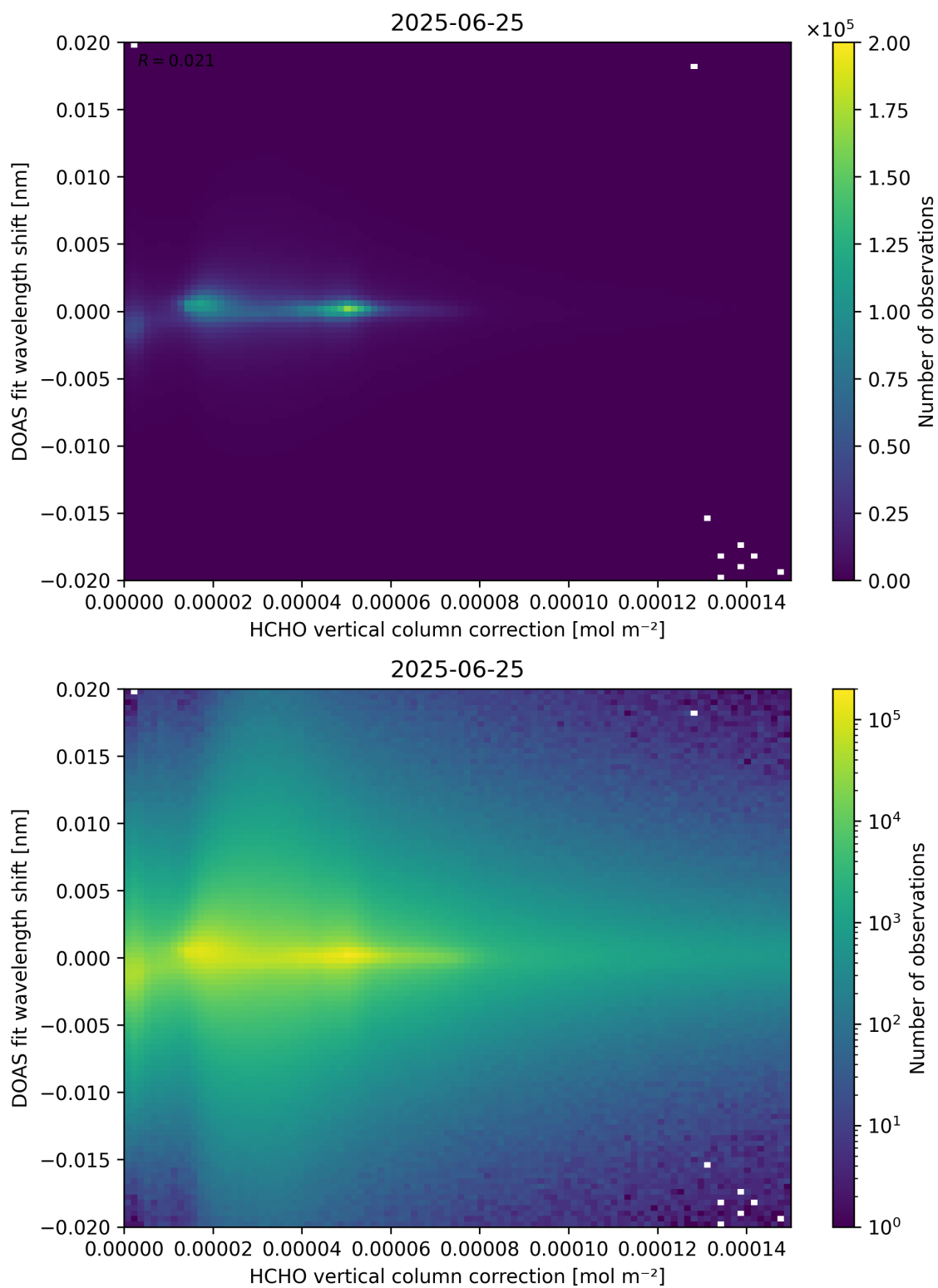
Figure 113: Scatter density plot of “HCHO vertical column correction” against “DOAS fit wavelength shift” for 2025-06-24 to 2025-06-26.
