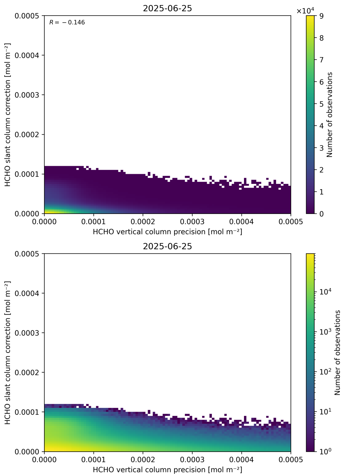
Figure 141: Scatter density plot of “HCHO vertical column precision” against “HCHO slant column correction” for 2025-06-24 to 2025-06-26.
