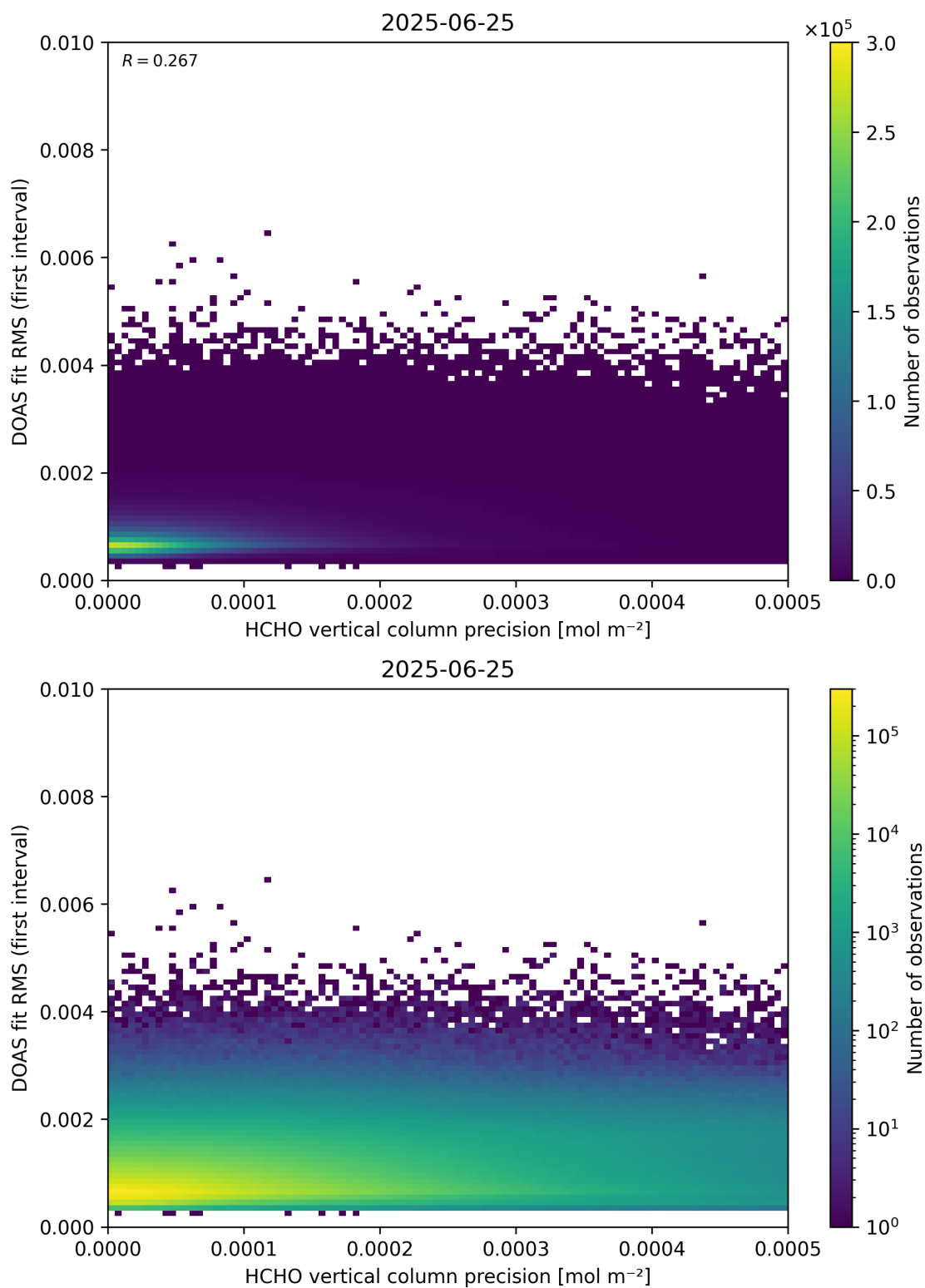
Figure 136: Scatter density plot of “HCHO vertical column precision” against “DOAS fit RMS (first interval)” for 2025-06-24 to 2025-06-26.
