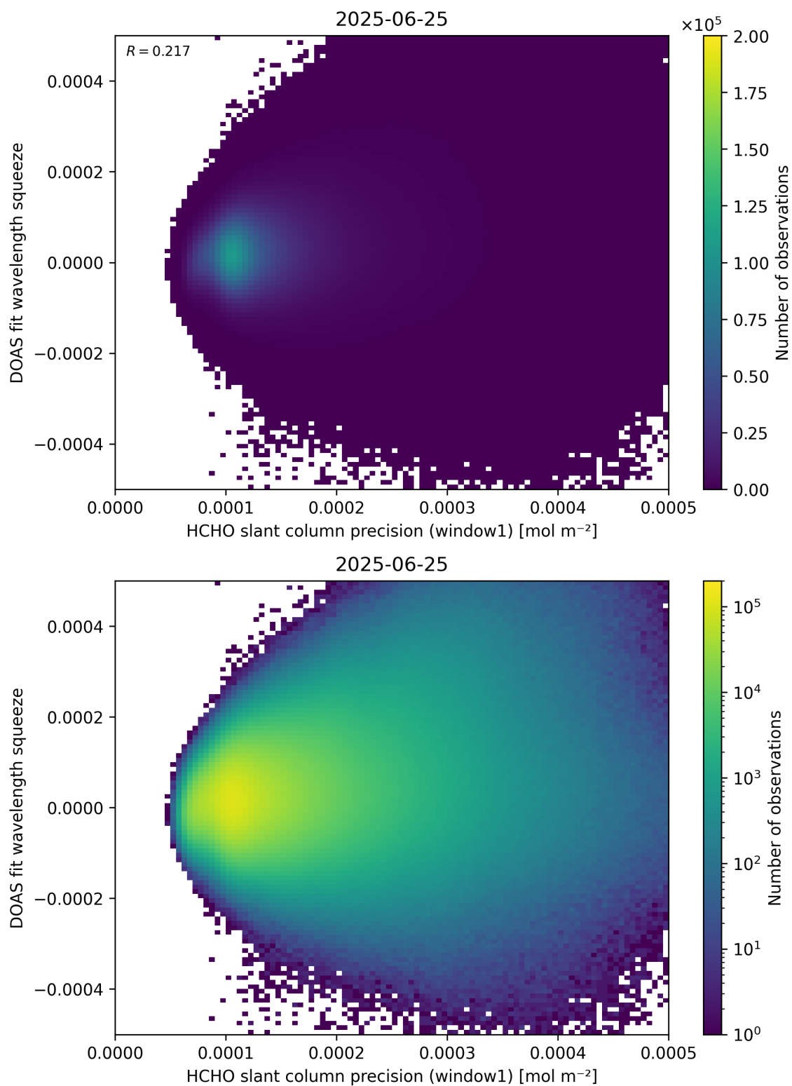
Figure 90: Scatter density plot of “HCHO slant column precision (window1)” against “DOAS fit wavelength squeeze” for 2025-06-24 to 2025-06-26.
