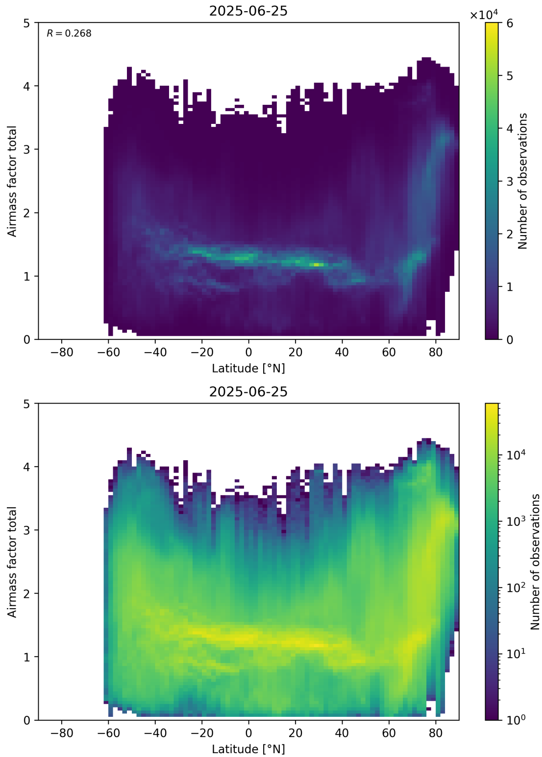
Figure 161: Scatter density plot of “Latitude” against “Airmass factor total” for 2025-06-24 to 2025-06-26.
