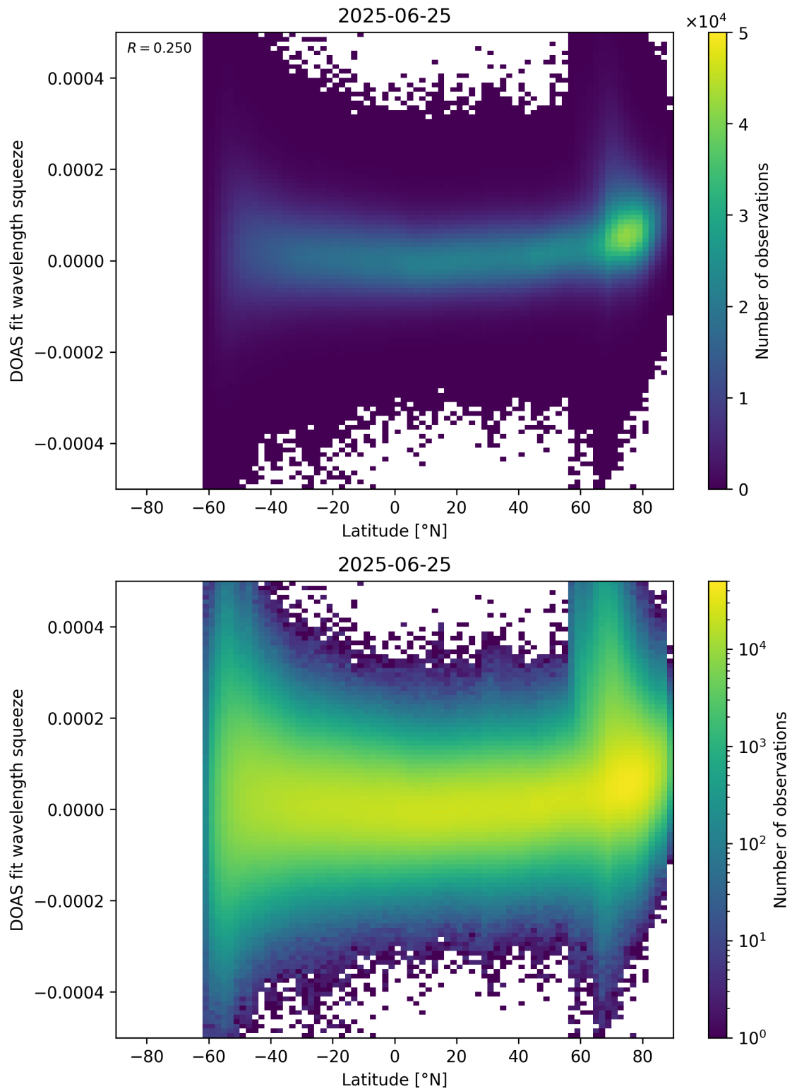
Figure 155: Scatter density plot of “Latitude” against “DOAS fit wavelength squeeze” for 2025-06-24 to 2025-06-26.
