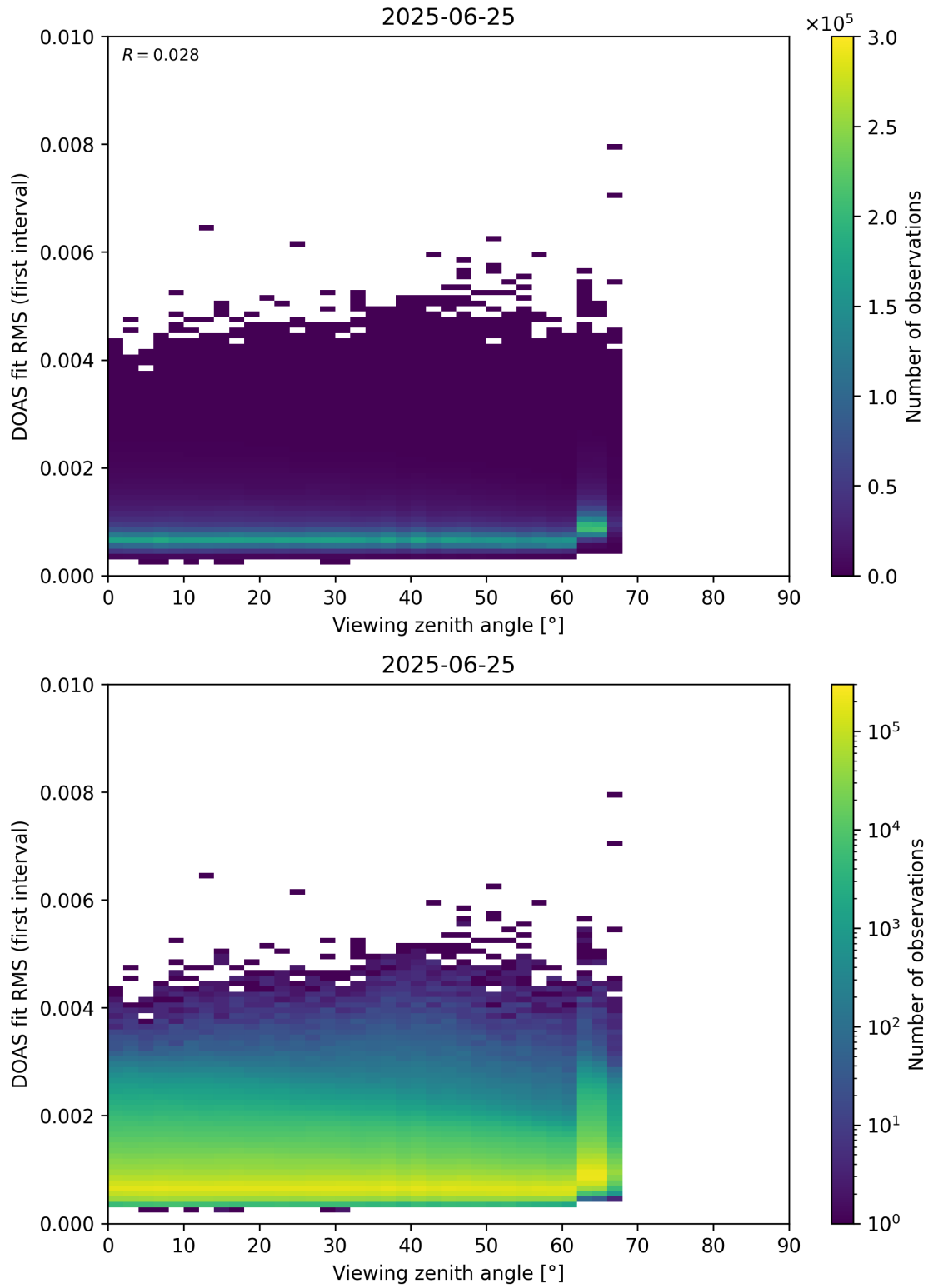
Figure 182: Scatter density plot of “Viewing zenith angle” against “DOAS fit RMS (first interval)” for 2025-06-24 to 2025-06-26.
