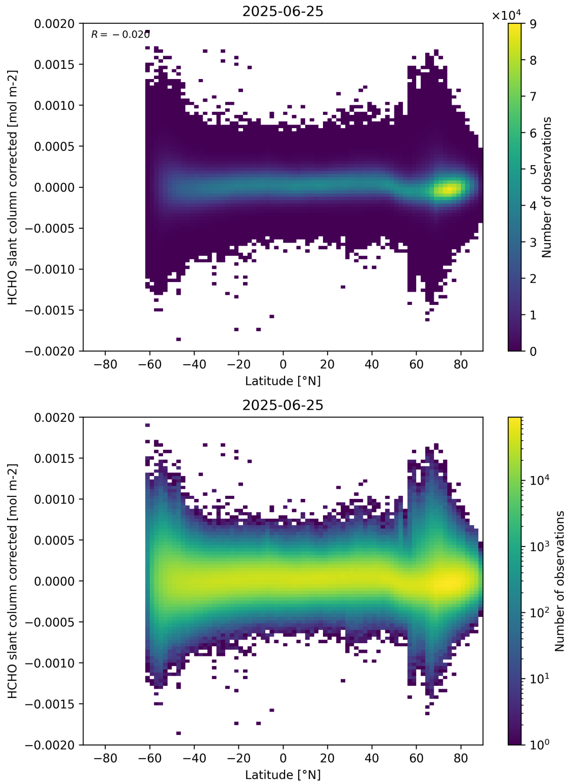
Figure 157: Scatter density plot of “Latitude” against “HCHO slant column corrected” for 2025-06-24 to 2025-06-26.
