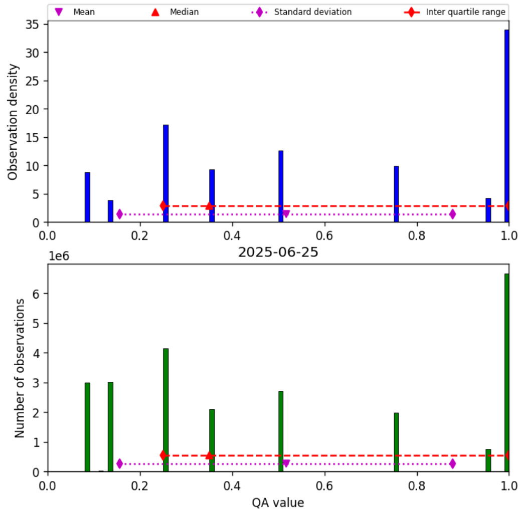
Figure 34: Histogram of “QA value” for 2025-06-24 to 2025-06-26
