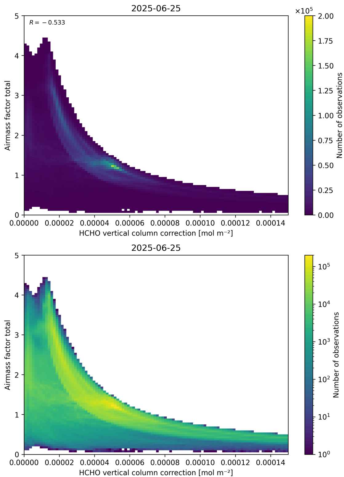
Figure 120: Scatter density plot of “HCHO vertical column correction” against “Airmass factor total” for 2025-06-24 to 2025-06-26.
