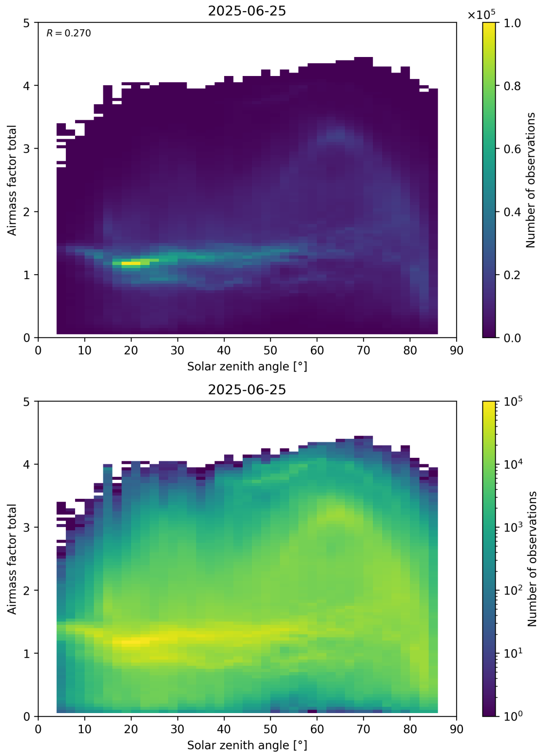
Figure 175: Scatter density plot of “Solar zenith angle” against “Airmass factor total” for 2025-06-24 to 2025-06-26.
