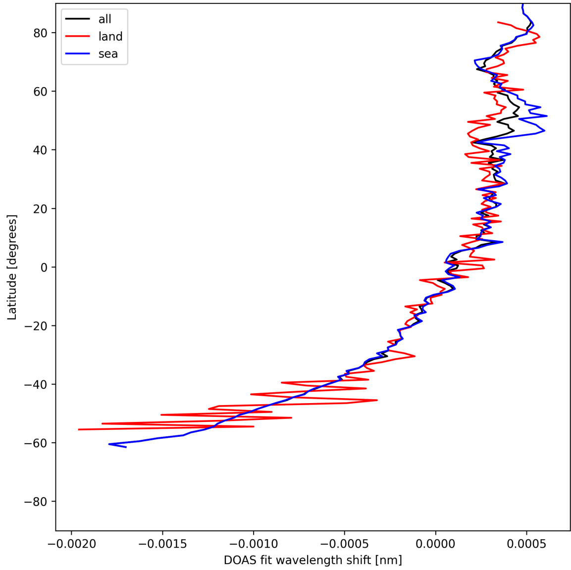
Figure 30: Zonal average of "DOAS fit wavelength shift" for 2025-06-24 to 2025-06-26.
