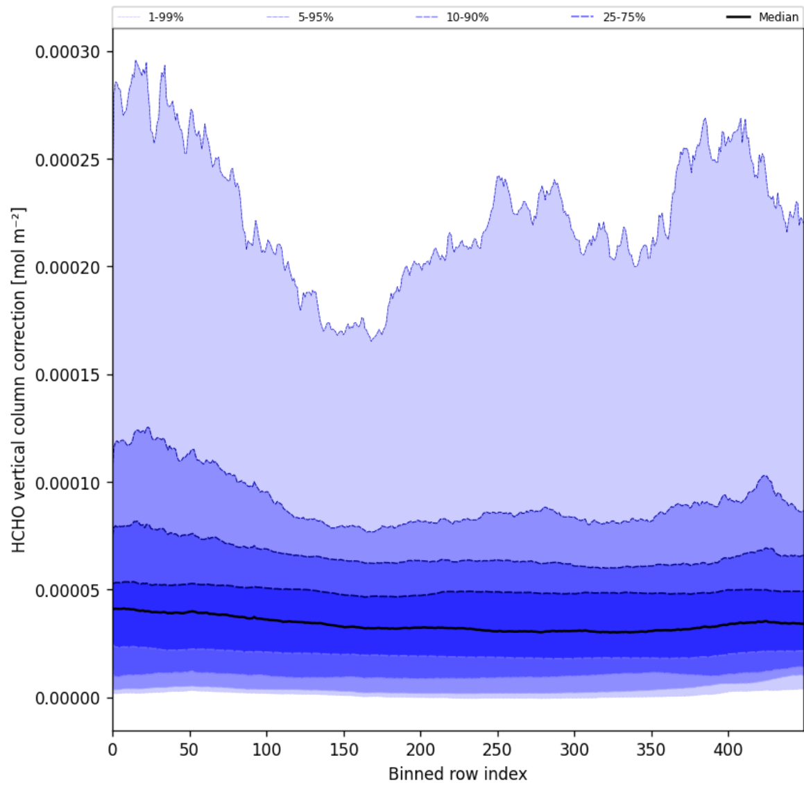
Figure 51: Along track statistics of “HCHO vertical column correction” for 2025-06-24 to 2025-06-26
