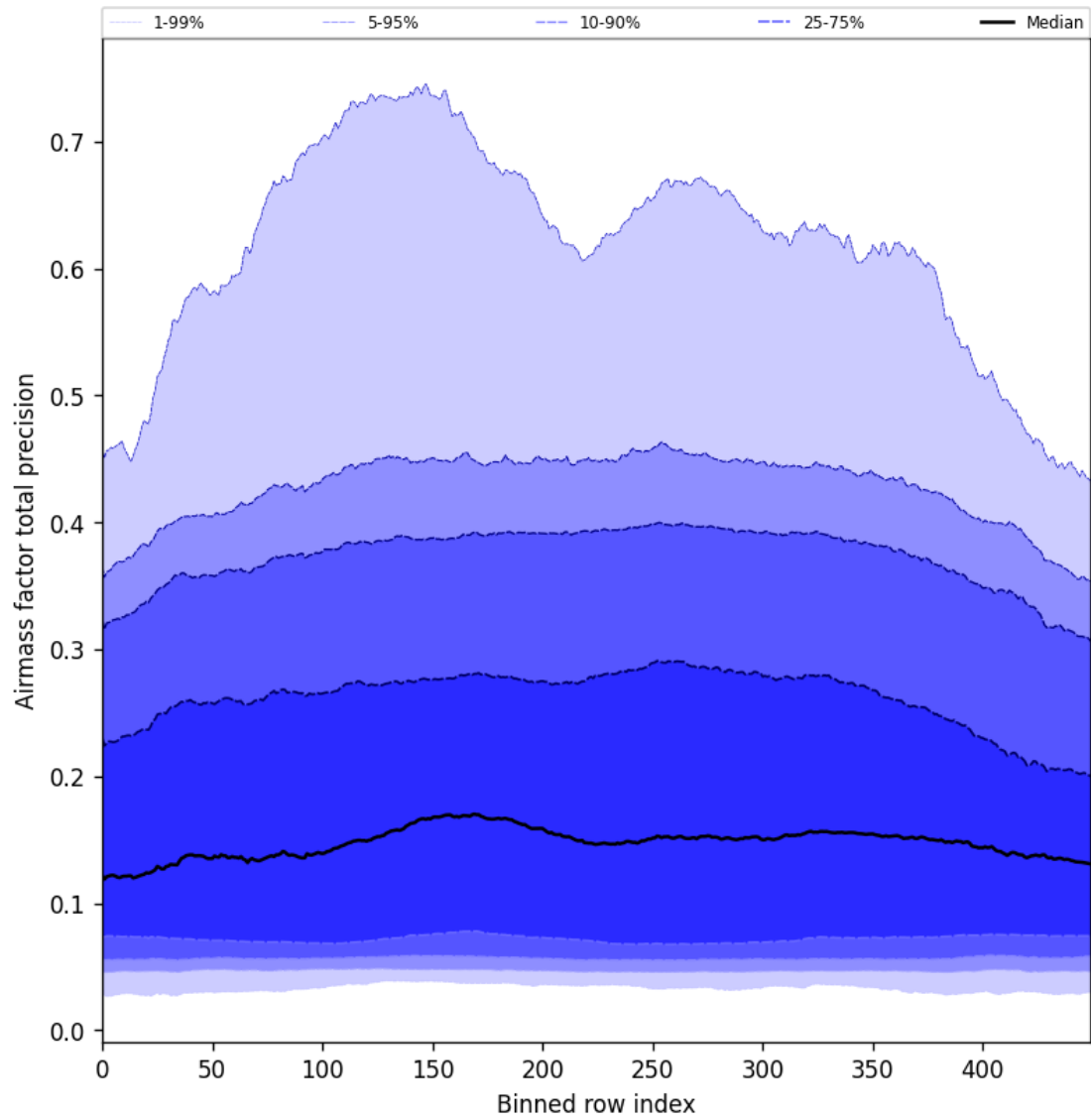
Figure 55: Along track statistics of “Airmass factor total precision” for 2025-06-24 to 2025-06-26
