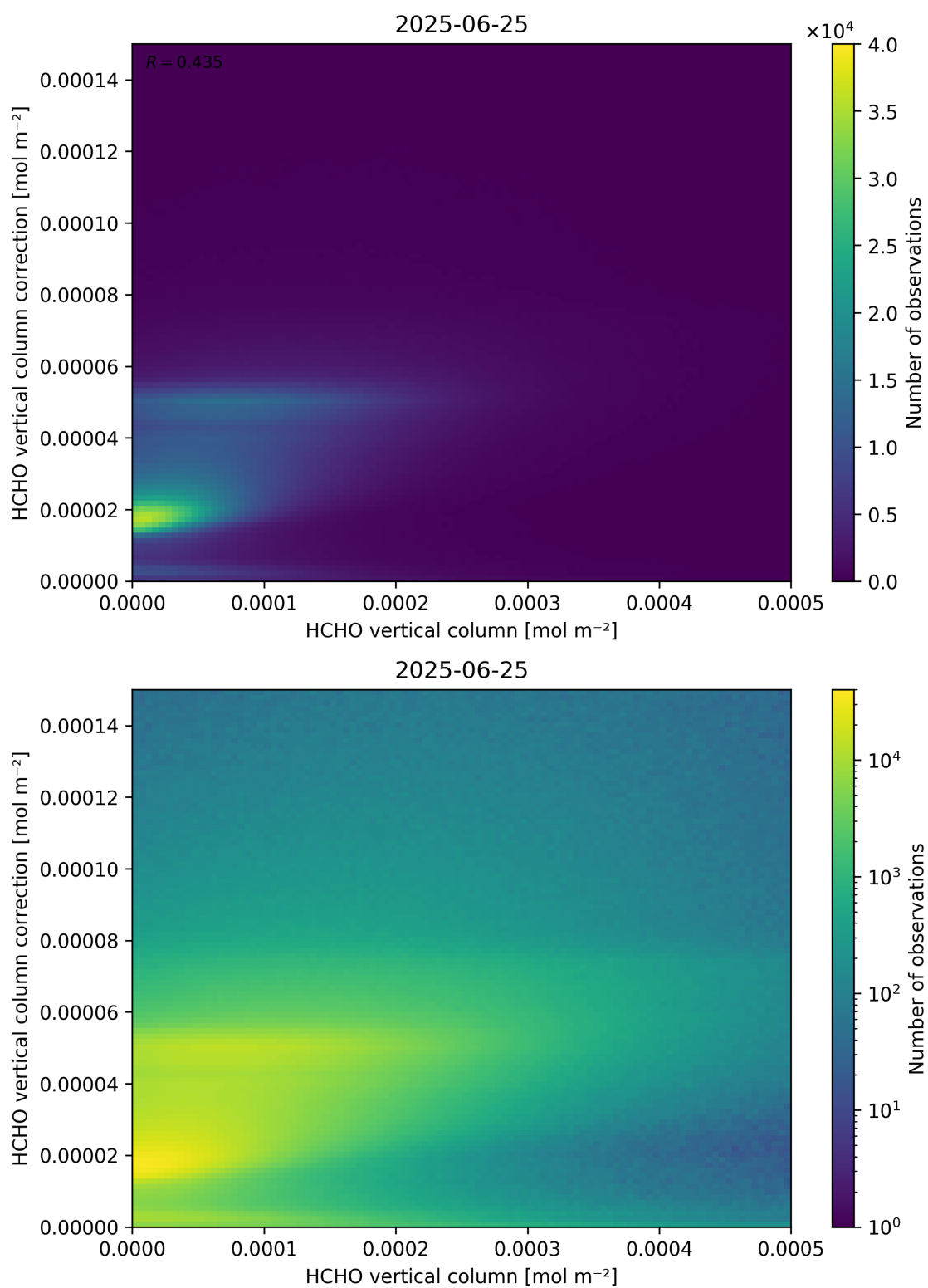
Figure 133: Scatter density plot of “HCHO vertical column” against “HCHO vertical column correction” for 2025-06-24 to 2025-06-26.
