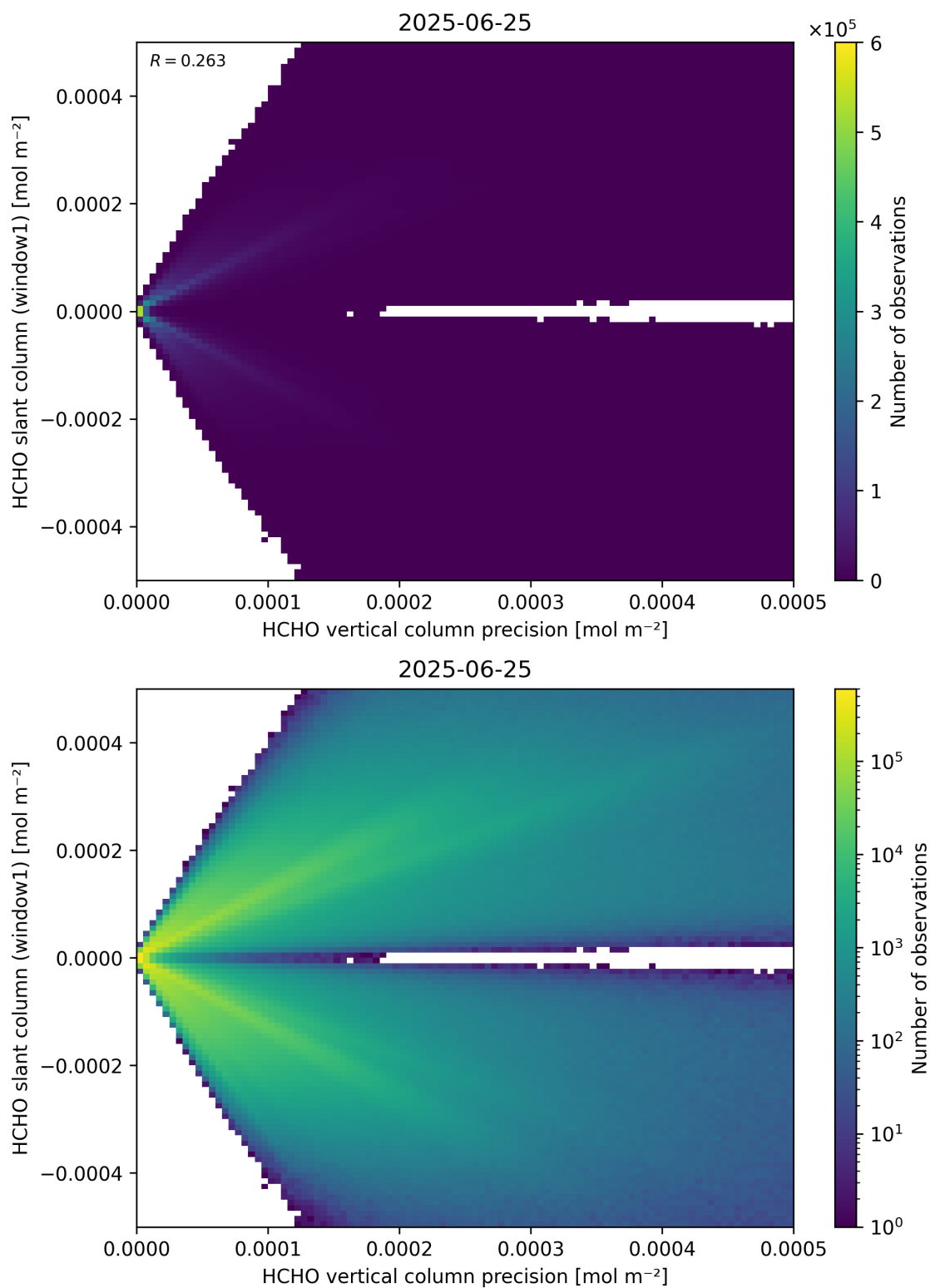
Figure 142: Scatter density plot of “HCHO vertical column precision” against “HCHO slant column (window1)” for 2025-06-24 to 2025-06-26.
