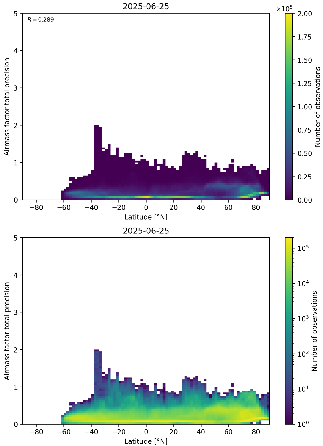
Figure 162: Scatter density plot of “Latitude” against “Airmass factor total precision” for 2025-06-24 to 2025-06-26.
