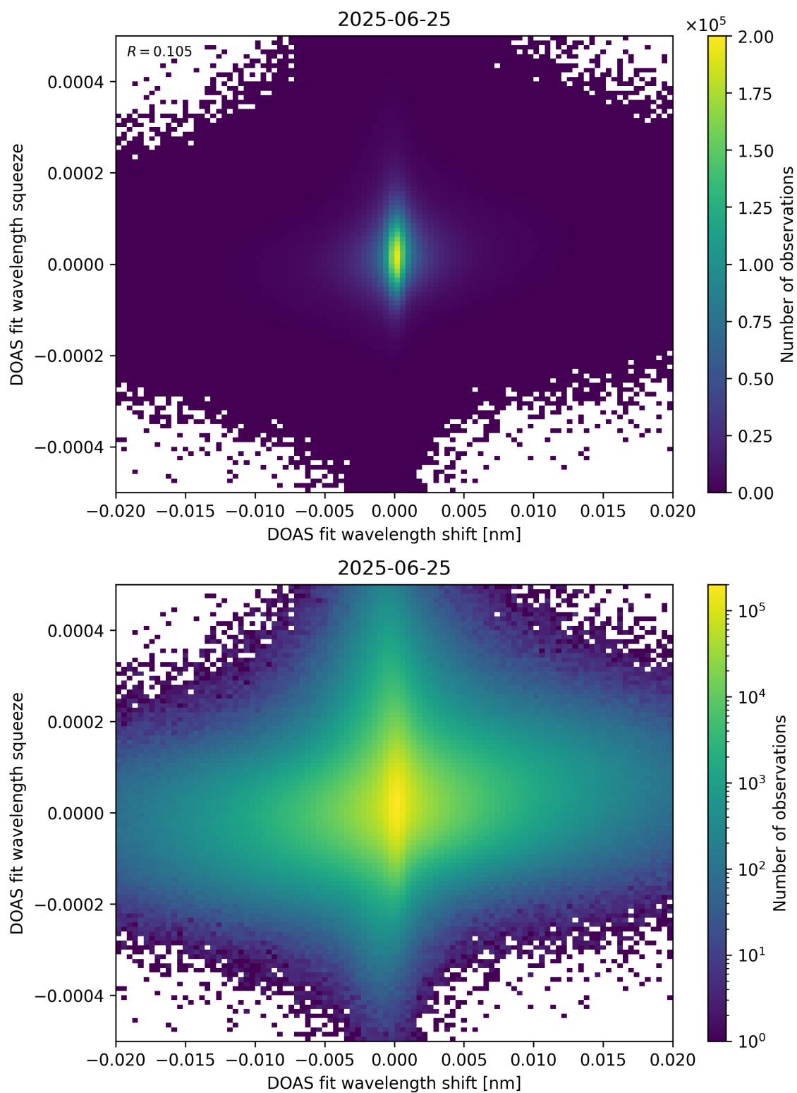
Figure 65: Scatter density plot of “DOAS fit wavelength shift” against “DOAS fit wavelength squeeze” for 2025-06-24 to 2025-06-26.
