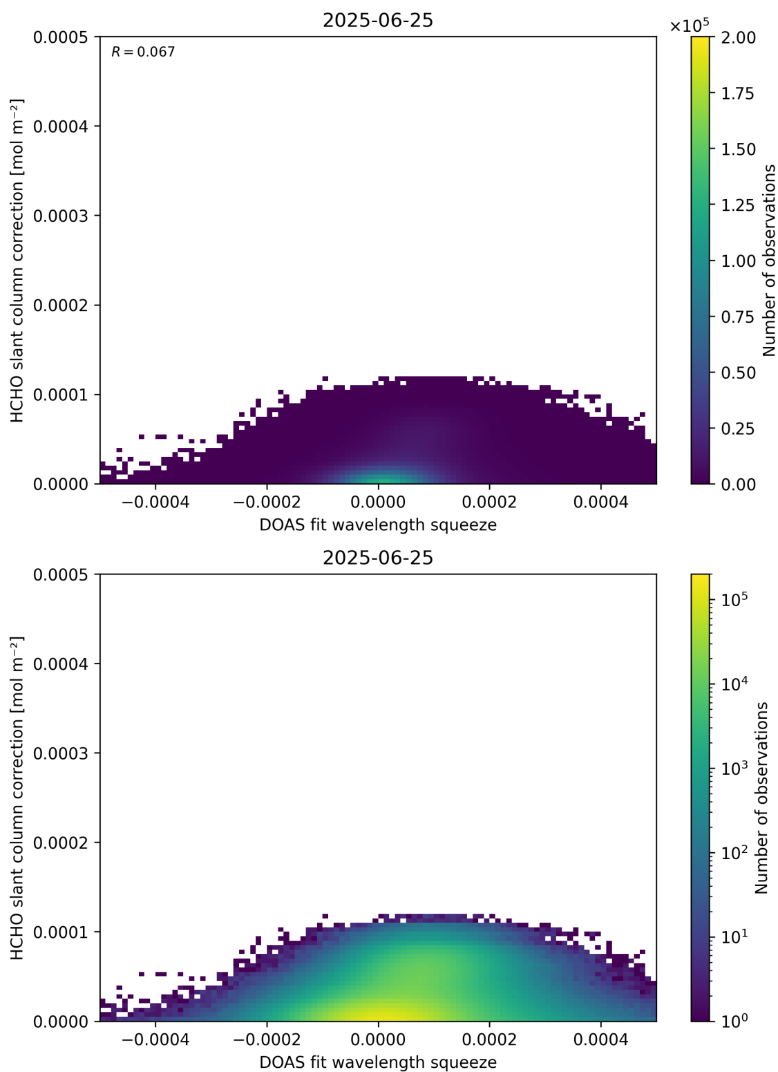
Figure 70: Scatter density plot of “DOAS fit wavelength squeeze” against “HCHO slant column correction” for 2025-06-24 to 2025-06-26.
