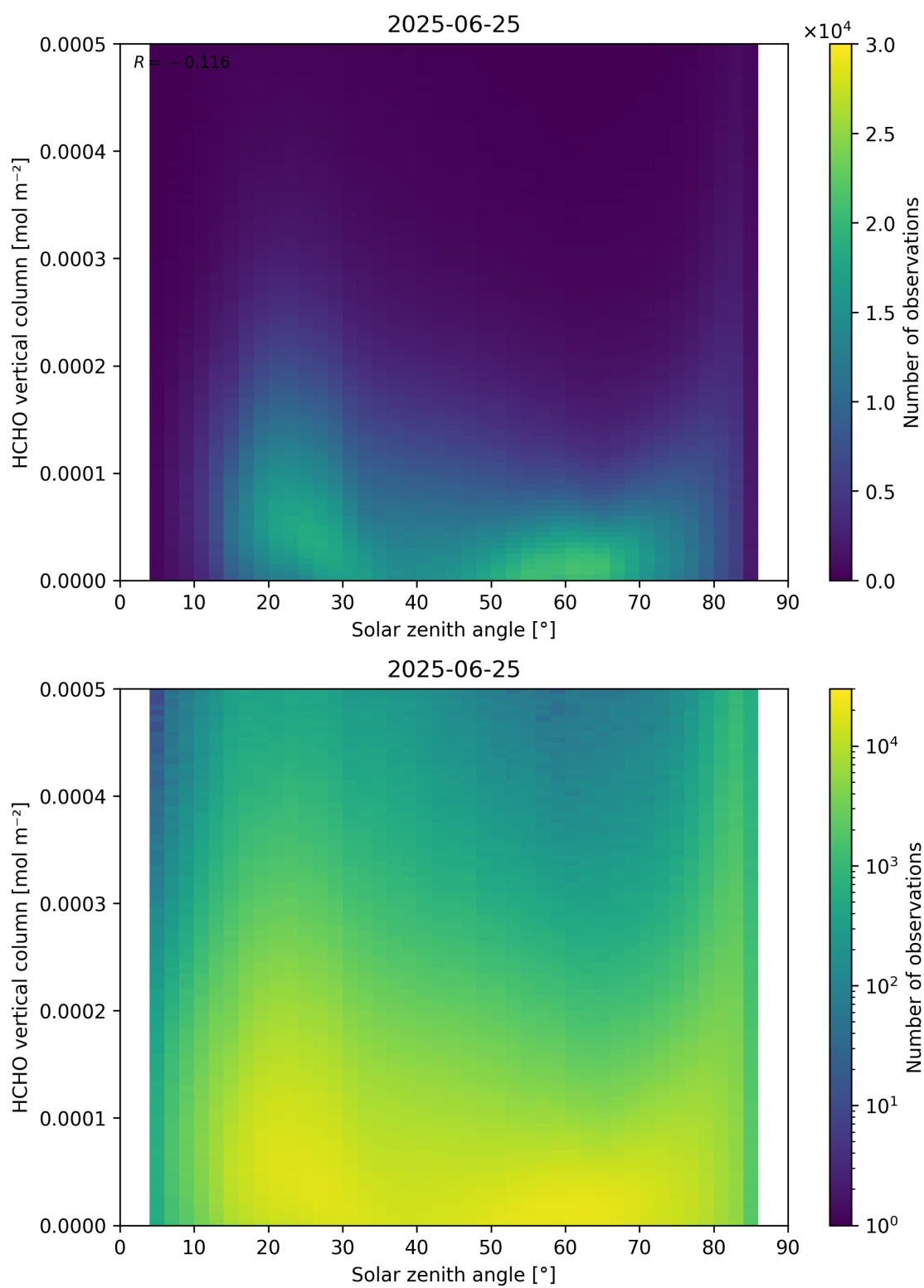
Figure 177: Scatter density plot of “Solar zenith angle” against “HCHO vertical column” for 2025-06-24 to 2025-06-26.
