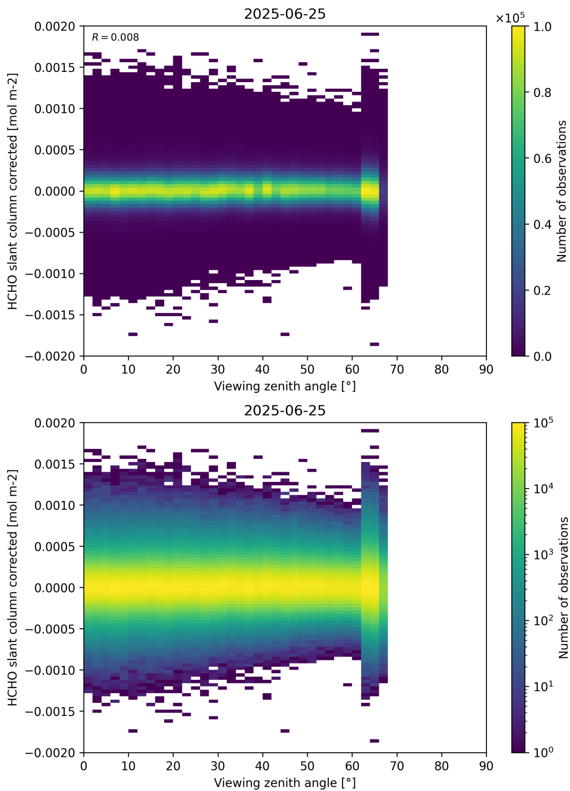
Figure 186: Scatter density plot of “Viewing zenith angle” against “HCHO slant column corrected” for 2025-06-24 to 2025-06-26.
