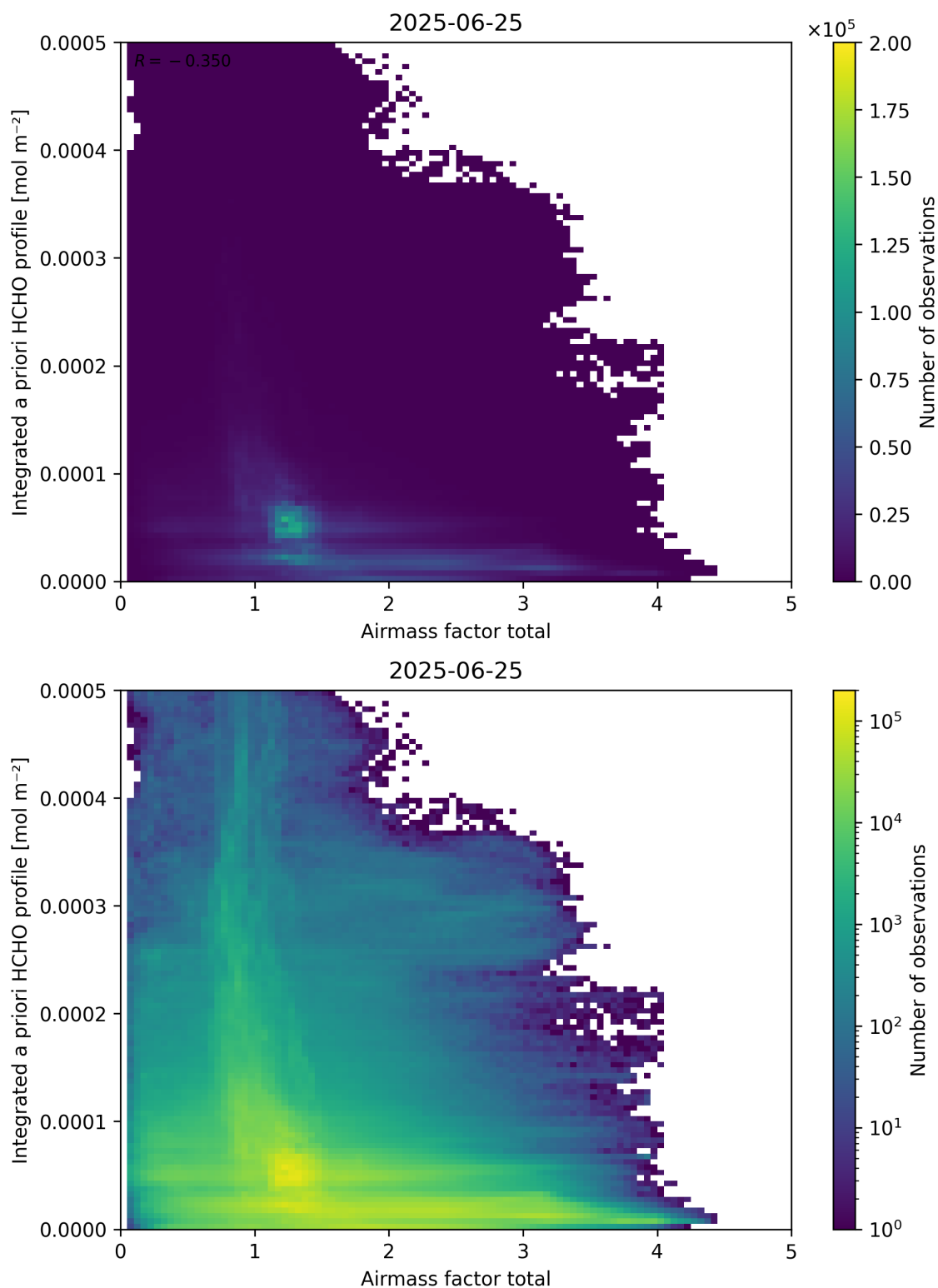
Figure 104: Scatter density plot of “Airmass factor total” against “Integrated a priori HCHO profile” for 2025-06-24 to 2025-06-26.
