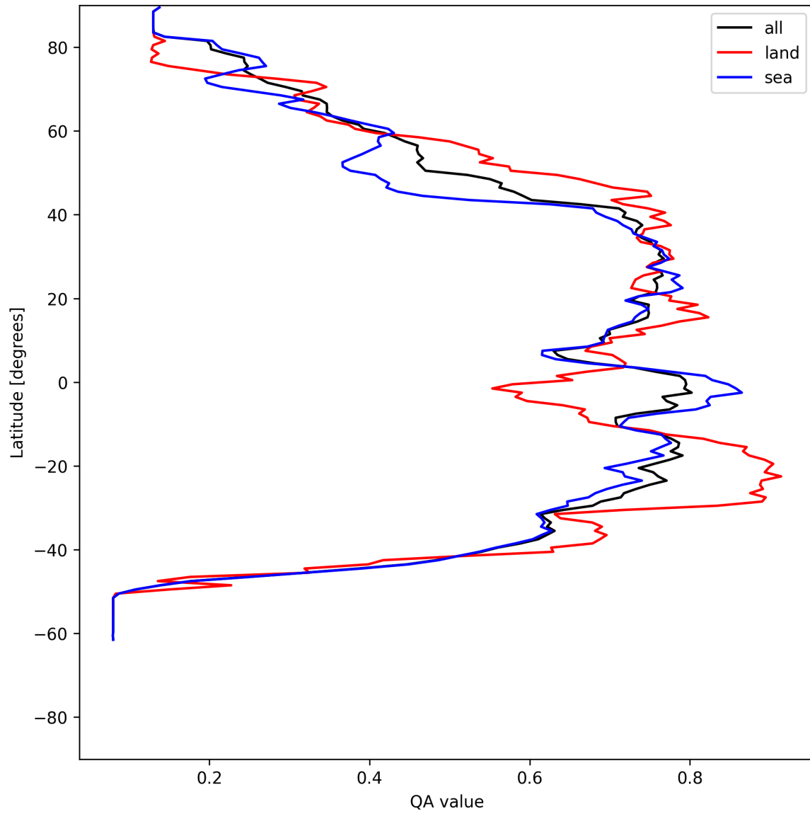
Figure 20: Zonal average of “QA value” for 2025-06-24 to 2025-06-26.
