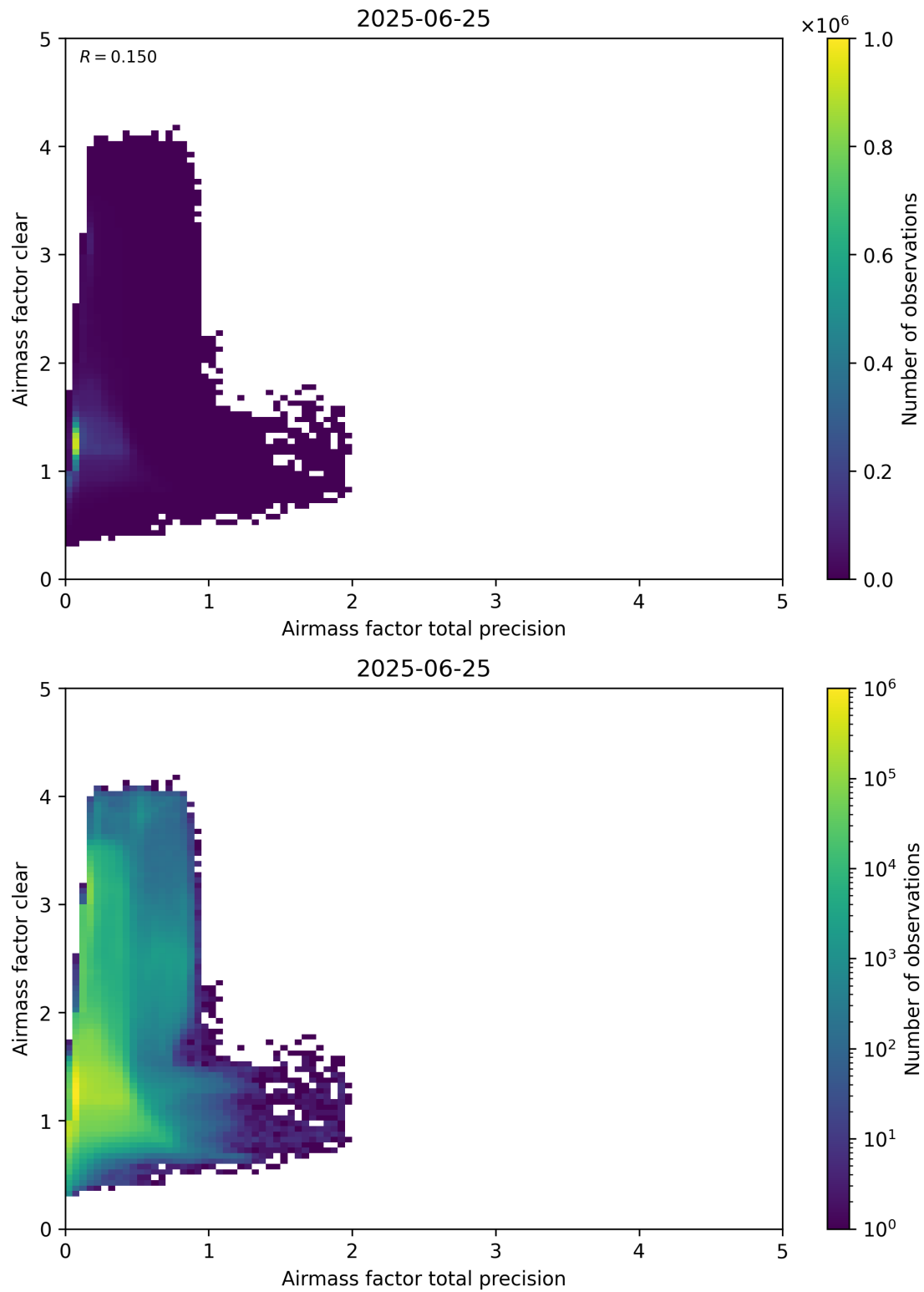
Figure 108: Scatter density plot of “Airmass factor total precision” against “Airmass factor clear” for 2025-06-24 to 2025-06-26.
