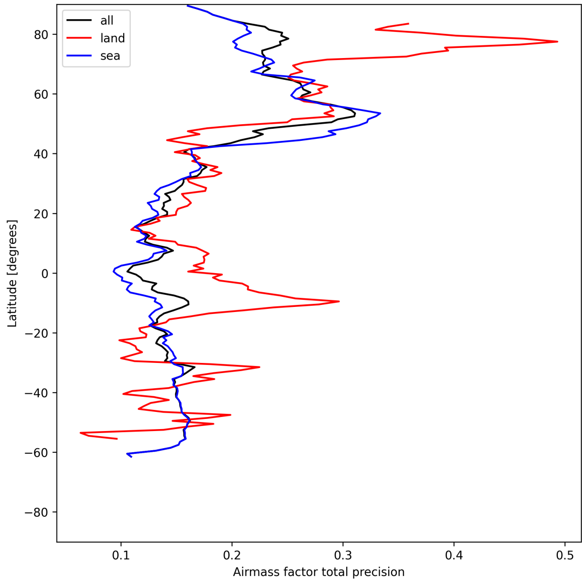
Figure 27: Zonal average of “Airmass factor total precision” for 2025-06-24 to 2025-06-26.
