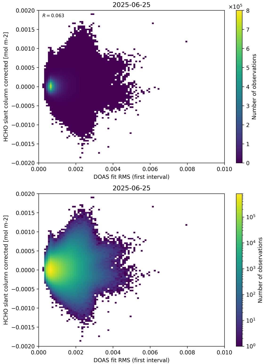
Figure 62: Scatter density plot of “DOAS fit RMS (first interval)” against “HCHO slant column corrected” for 2025-06-24 to 2025-06-26.
