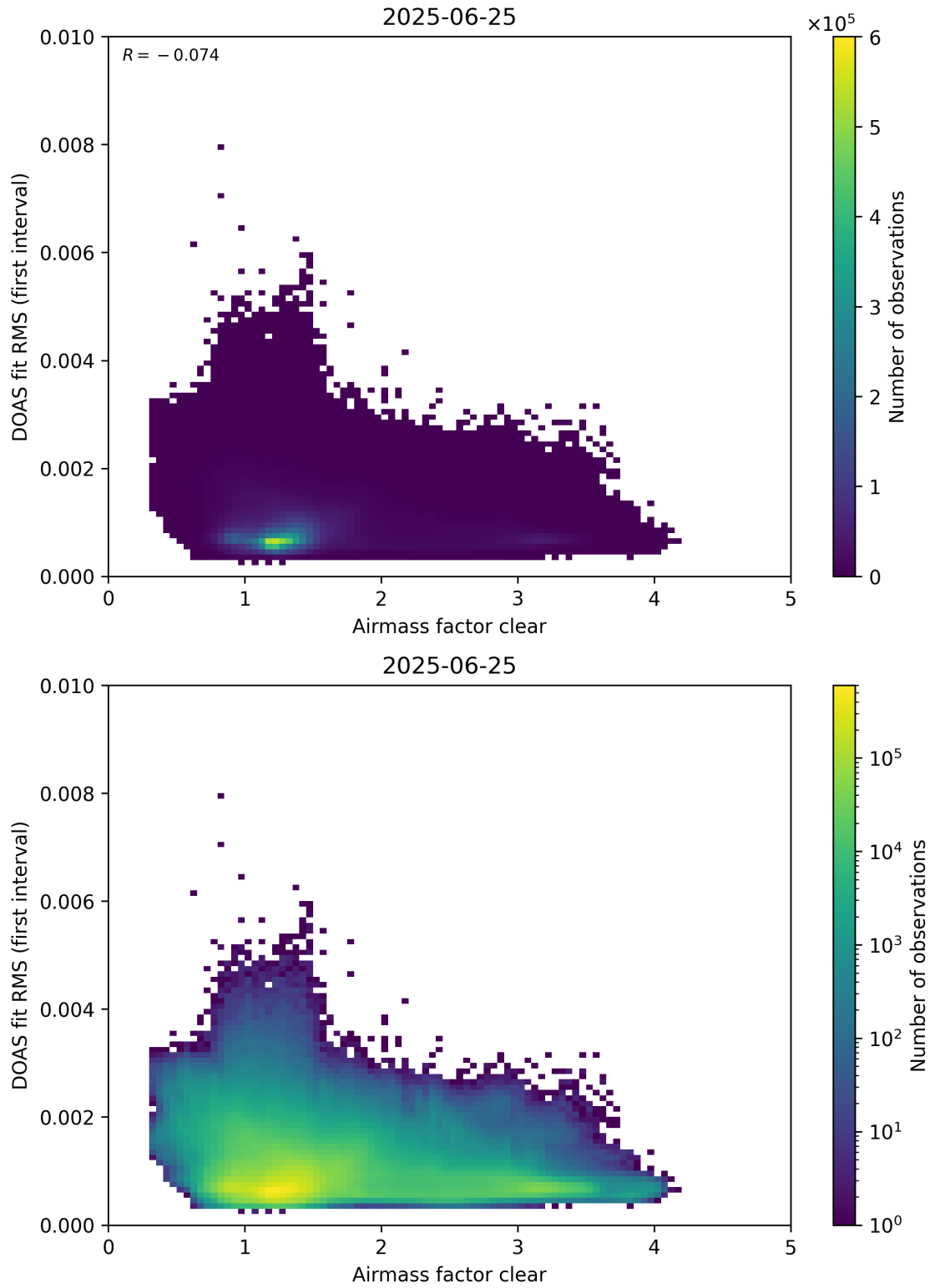
Figure 71: Scatter density plot of “Airmass factor clear” against “DOAS fit RMS (first interval)” for 2025-06-24 to 2025-06-26.
