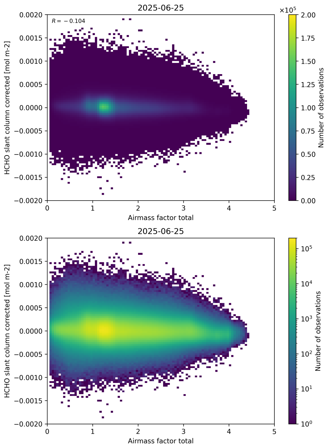
Figure 101: Scatter density plot of “Airmass factor total” against “HCHO slant column corrected” for 2025-06-24 to 2025-06-26.
