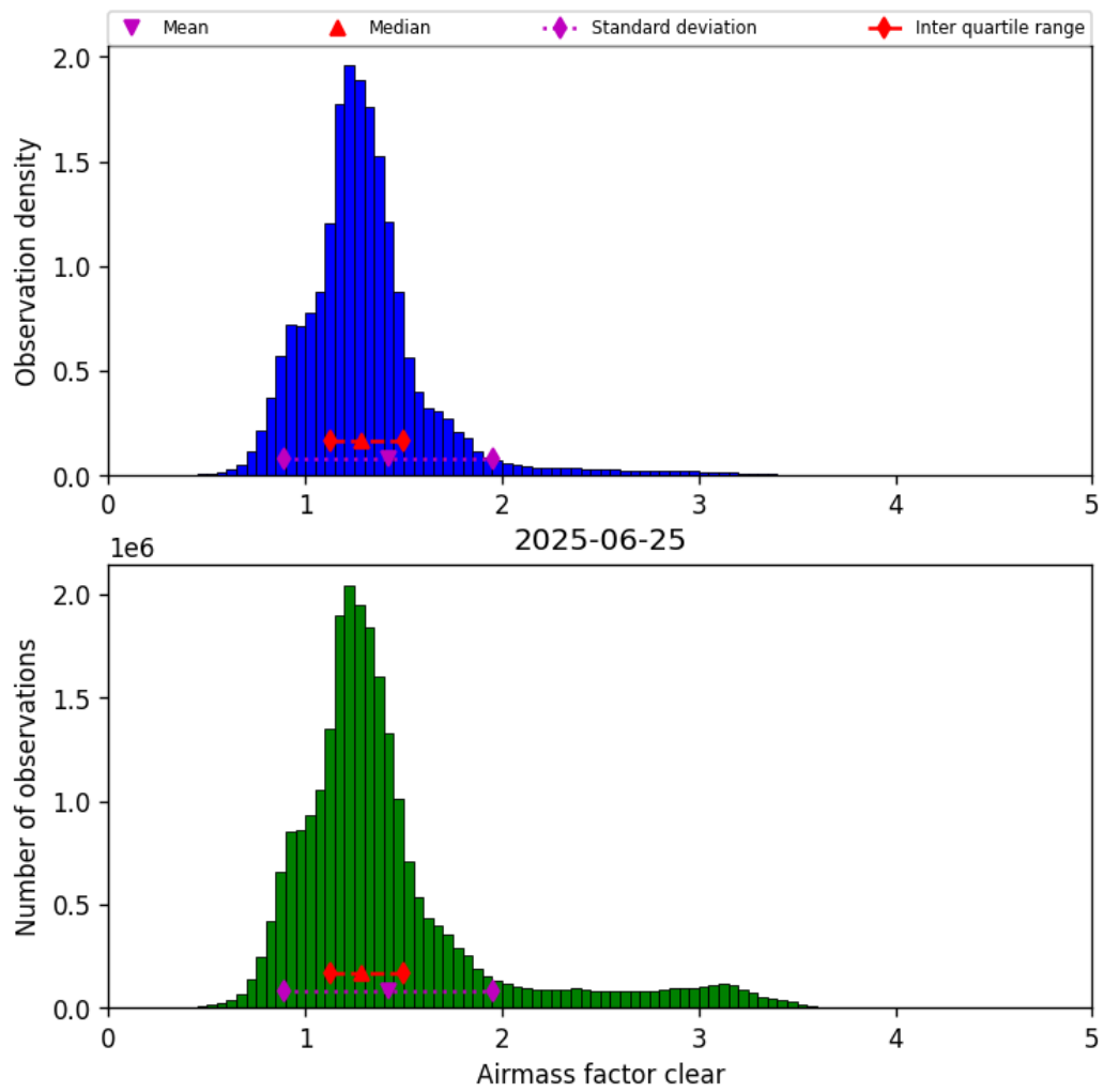
Figure 42: Histogram of “Airmass factor clear” for 2025-06-24 to 2025-06-26
