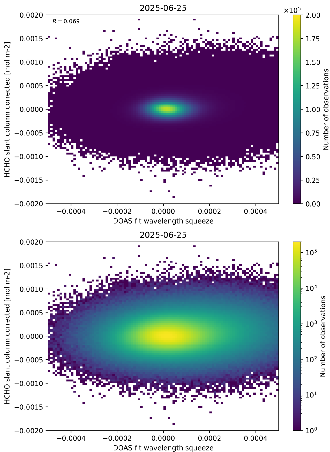
Figure 69: Scatter density plot of “DOAS fit wavelength squeeze” against “HCHO slant column corrected” for 2025-06-24 to 2025-06-26.
