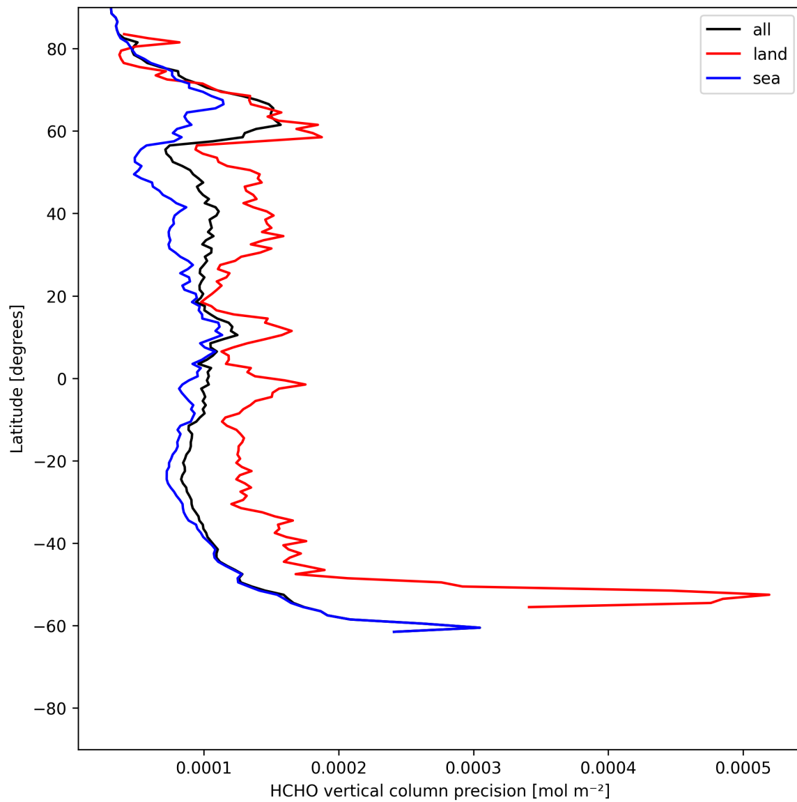
Figure 22: Zonal average of “HCHO vertical column precision” for 2025-06-24 to 2025-06-26.
