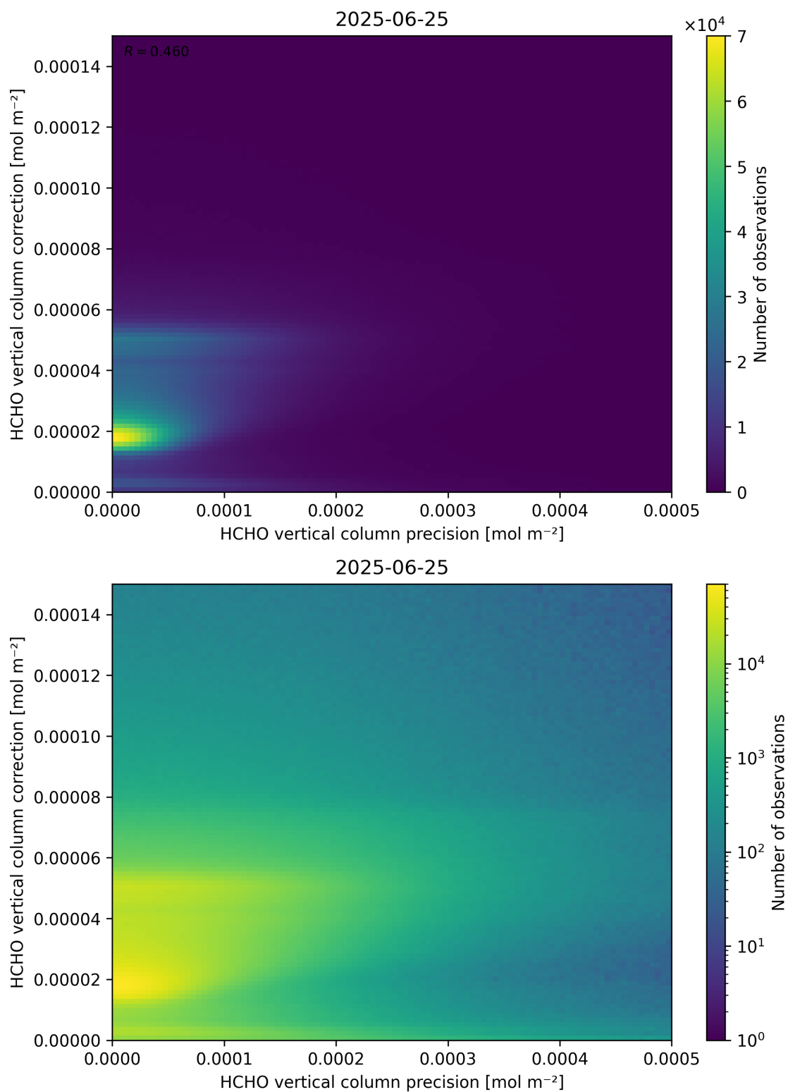
Figure 146: Scatter density plot of “HCHO vertical column precision” against “HCHO vertical column correction” for 2025-06-24 to 2025-06-26.
