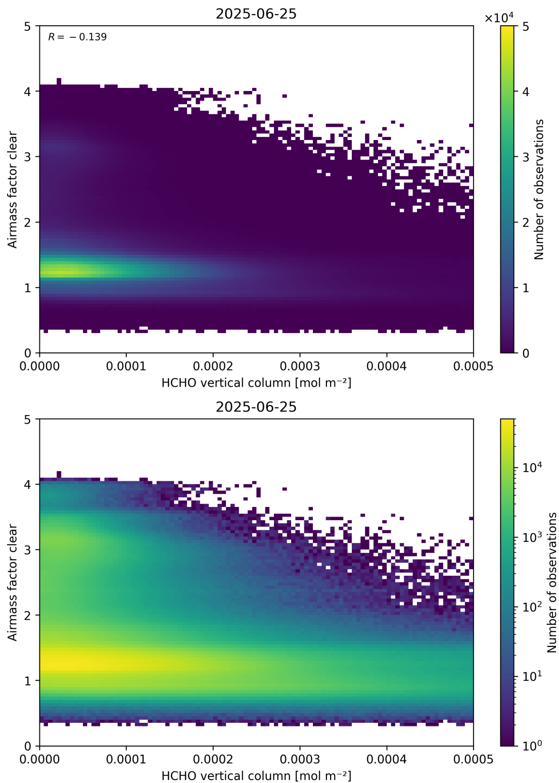
Figure 126: Scatter density plot of “HCHO vertical column” against “Airmass factor clear” for 2025-06-24 to 2025-06-26.
