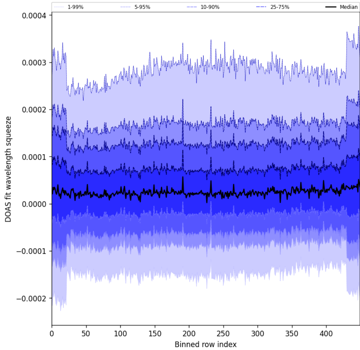
Figure 59: Along track statistics of “DOAS fit wavelength squeeze” for 2025-06-24 to 2025-06-26
