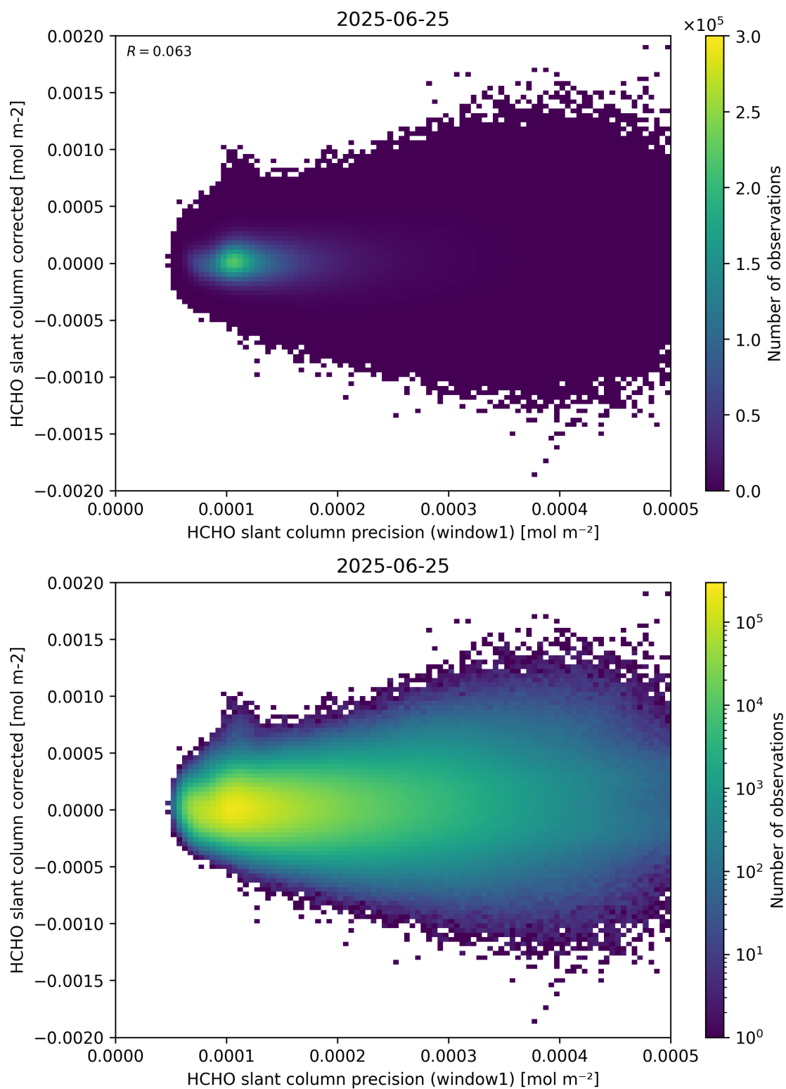
Figure 92: Scatter density plot of “HCHO slant column precision (window1)” against “HCHO slant column corrected” for 2025-06-24 to 2025-06-26.
