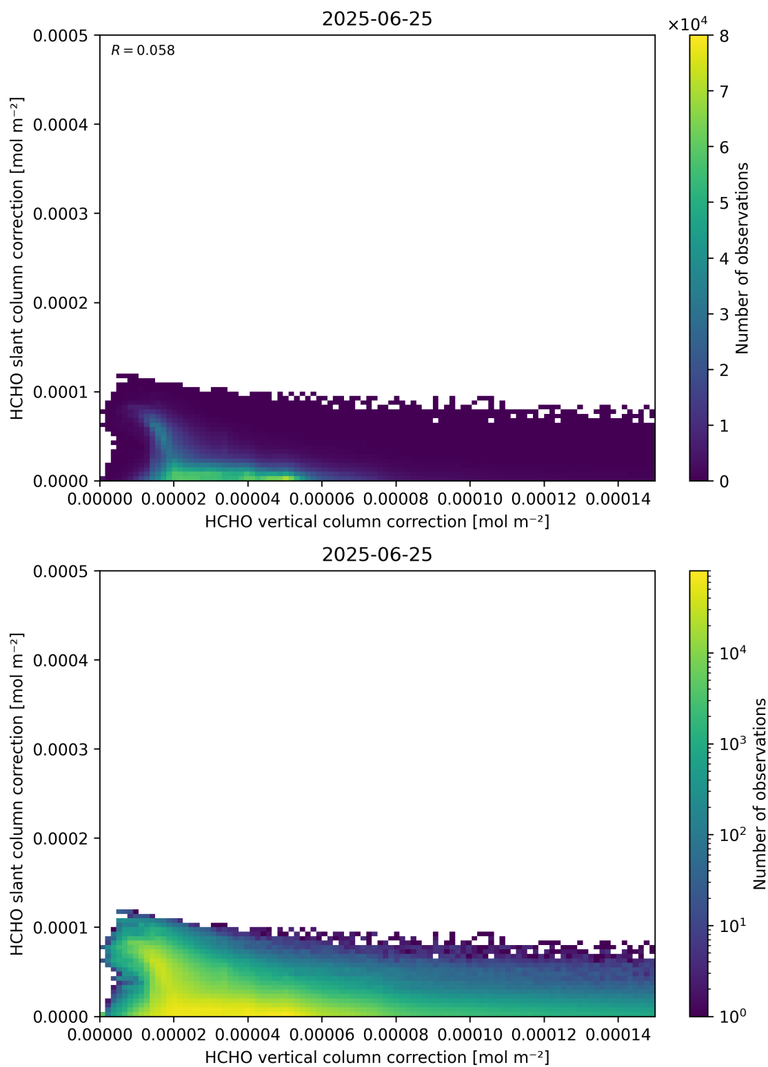
Figure 117: Scatter density plot of “HCHO vertical column correction” against “HCHO slant column correction” for 2025-06-24 to 2025-06-26.
