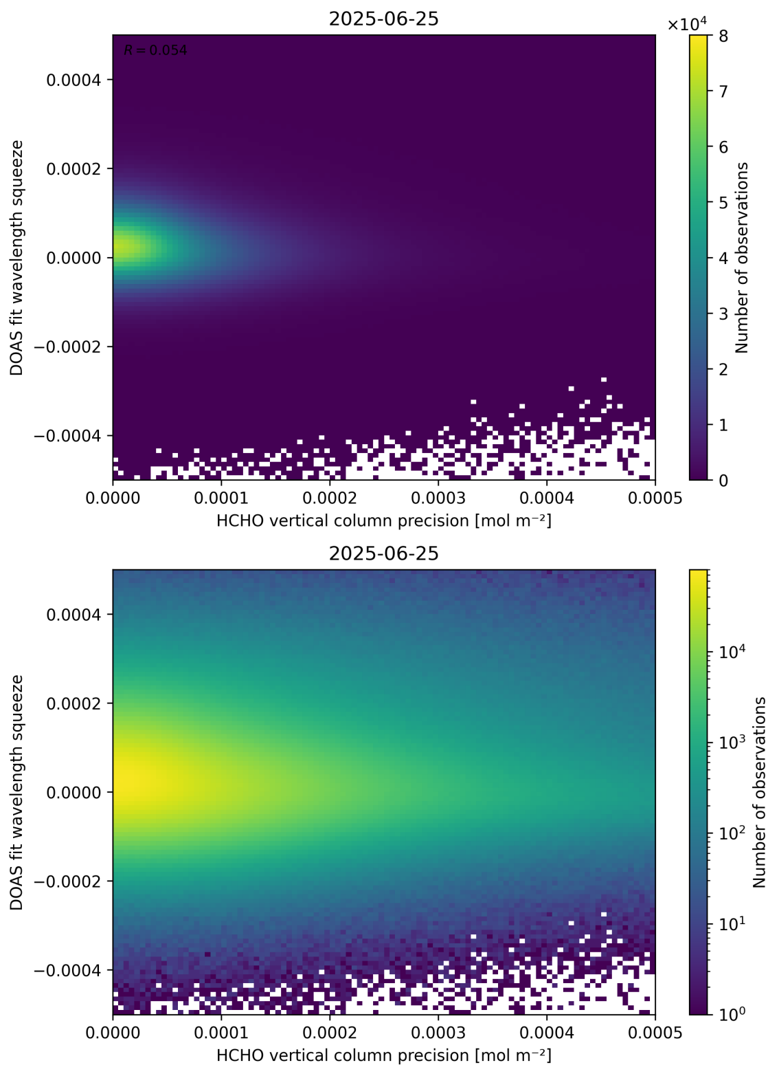
Figure 138: Scatter density plot of “HCHO vertical column precision” against “DOAS fit wavelength squeeze” for 2025-06-24 to 2025-06-26.
