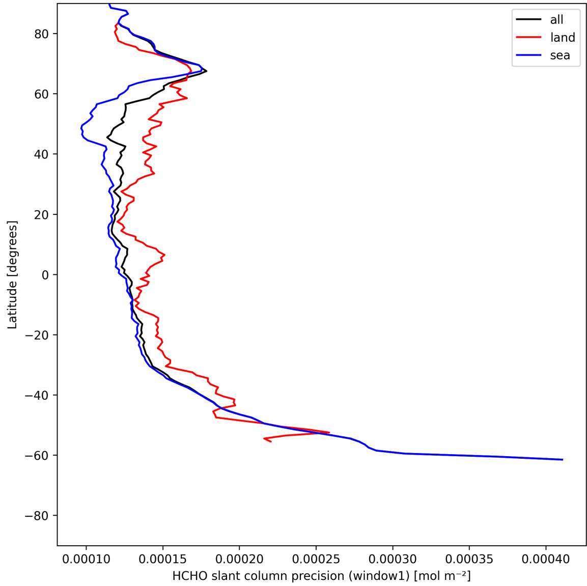
Figure 25: Zonal average of “HCHO slant column precision (window1)” for 2025-06-24 to 2025-06-26.
