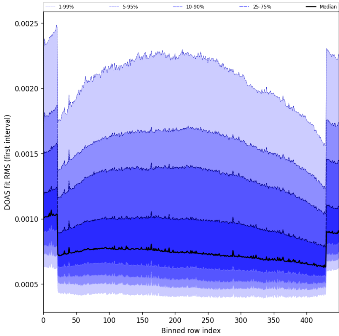
Figure 60: Along track statistics of “DOAS fit RMS (first interval)” for 2025-06-24 to 2025-06-26
