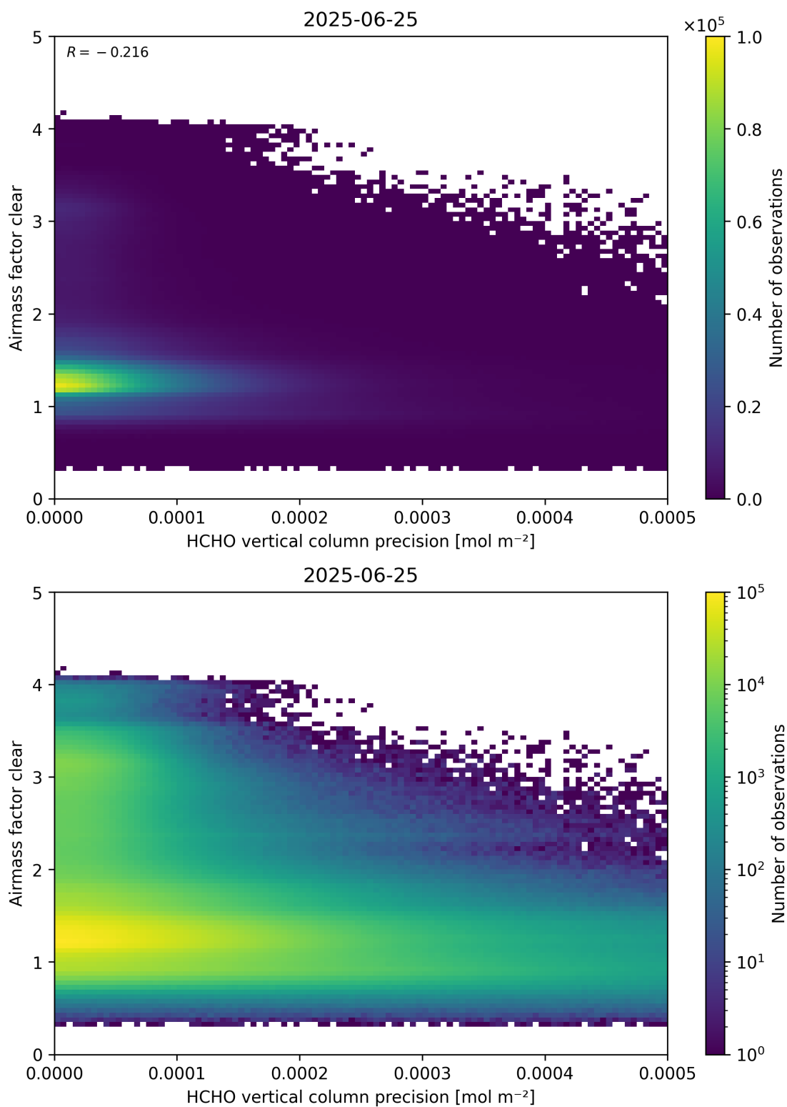
Figure 139: Scatter density plot of “HCHO vertical column precision” against “Airmass factor clear” for 2025-06-24 to 2025-06-26.
