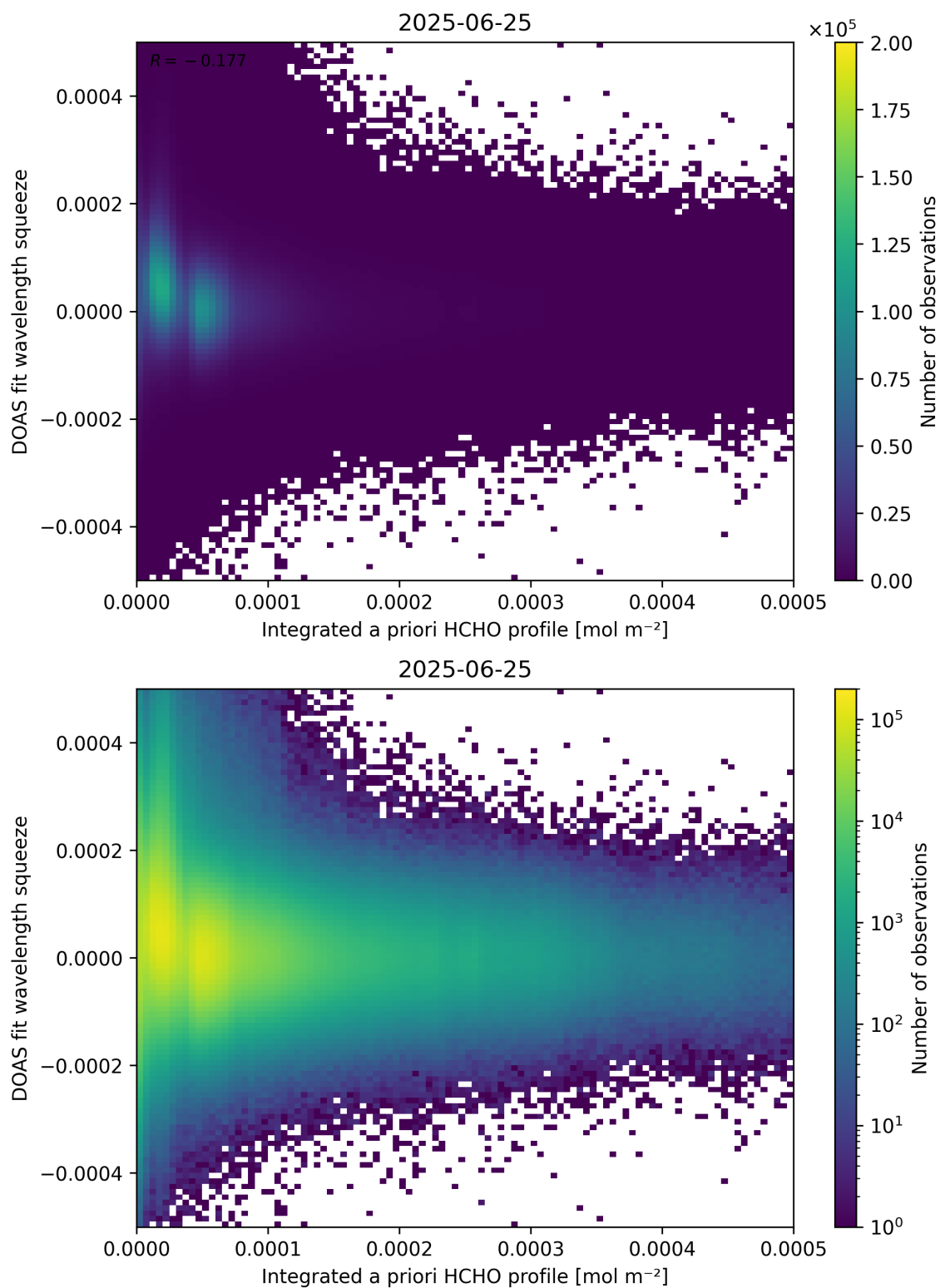
Figure 150: Scatter density plot of “Integrated a priori HCHO profile” against “DOAS fit wavelength squeeze” for 2025-06-24 to 2025-06-26.
