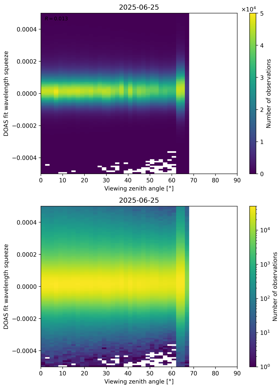
Figure 184: Scatter density plot of “Viewing zenith angle” against “DOAS fit wavelength squeeze” for 2025-06-24 to 2025-06-26.
