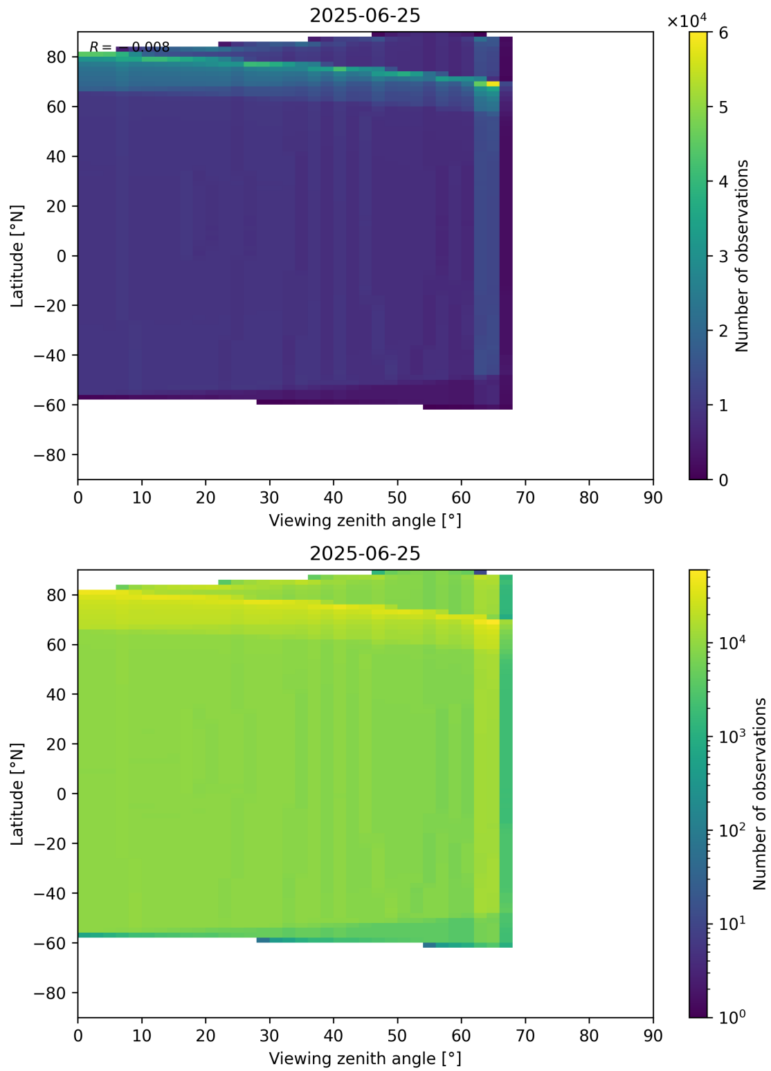
Figure 196: Scatter density plot of “Viewing zenith angle” against “Latitude” for 2025-06-24 to 2025-06-26.
