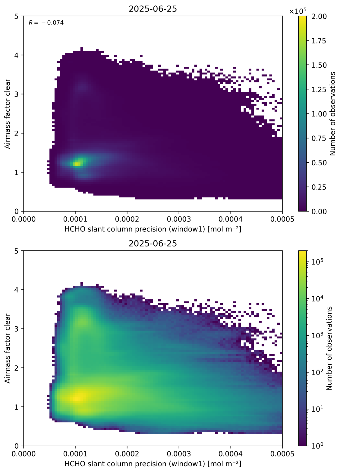
Figure 91: Scatter density plot of “HCHO slant column precision (window1)” against “Airmass factor clear” for 2025-06-24 to 2025-06-26.
