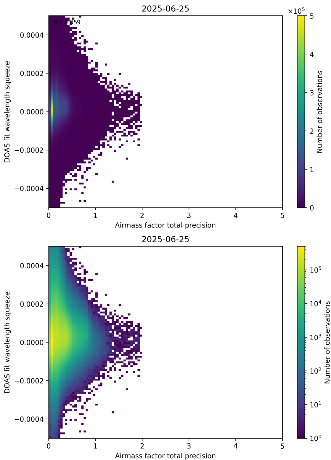
Figure 107: Scatter density plot of “Airmass factor total precision” against “DOAS fit wavelength squeeze” for 2025-06-24 to 2025-06-26.
