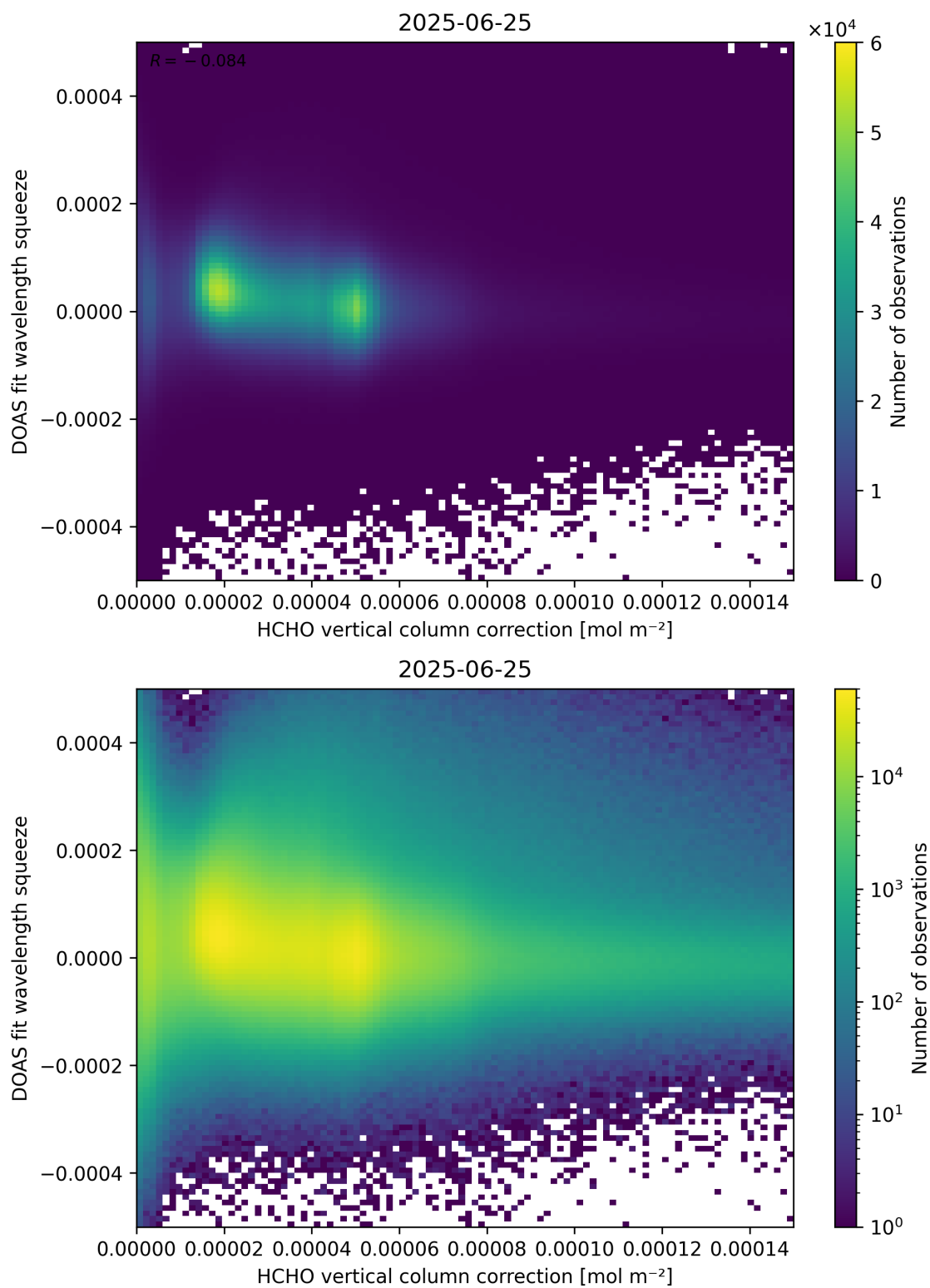
Figure 114: Scatter density plot of “HCHO vertical column correction” against “DOAS fit wavelength squeeze” for 2025-06-24 to 2025-06-26.
