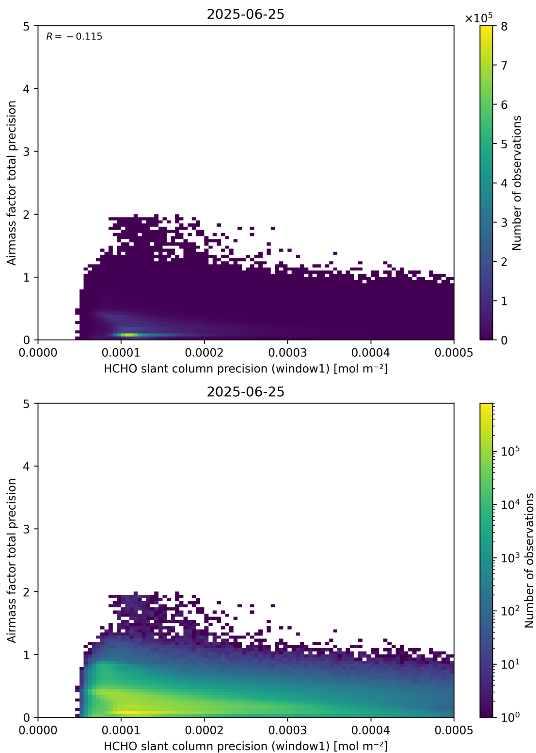
Figure 95: Scatter density plot of “HCHO slant column precision (window1)” against “Airmass factor total precision” for 2025-06-24 to 2025-06-26.
