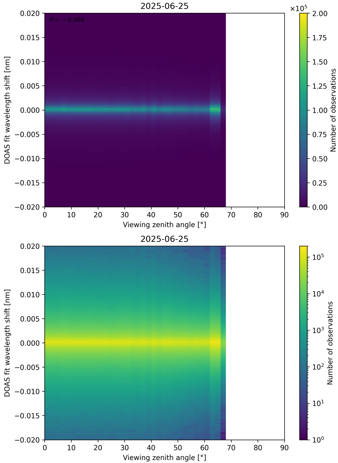
Figure 183: Scatter density plot of “Viewing zenith angle” against “DOAS fit wavelength shift” for 2025-06-24 to 2025-06-26.
