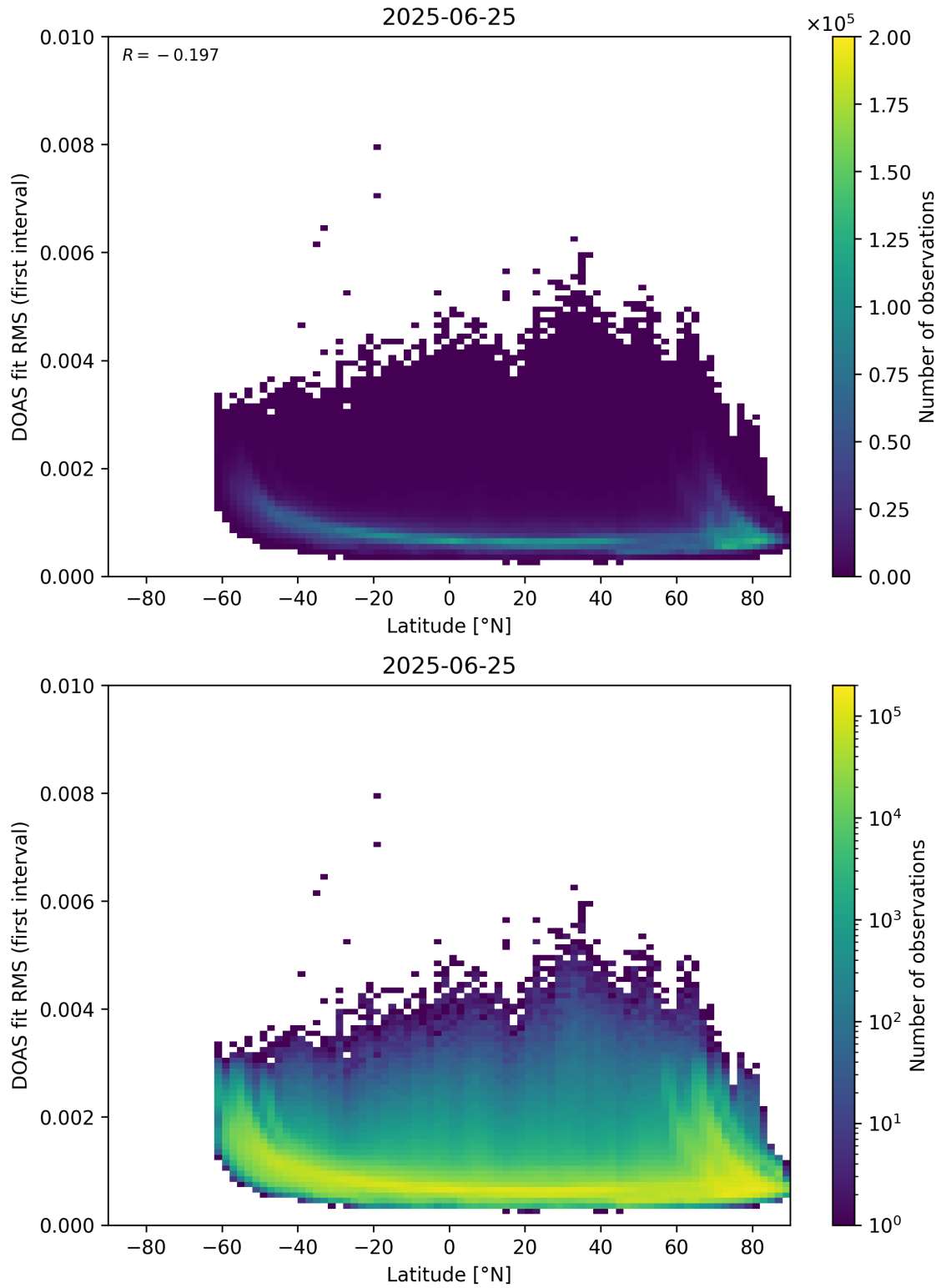
Figure 153: Scatter density plot of “Latitude” against “DOAS fit RMS (first interval)” for 2025-06-24 to 2025-06-26.
