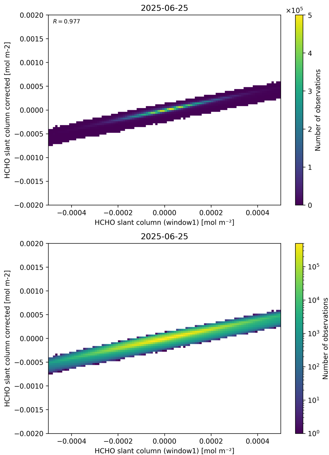
Figure 82: Scatter density plot of “HCHO slant column (window1)” against “HCHO slant column corrected” for 2025-06-24 to 2025-06-26.
