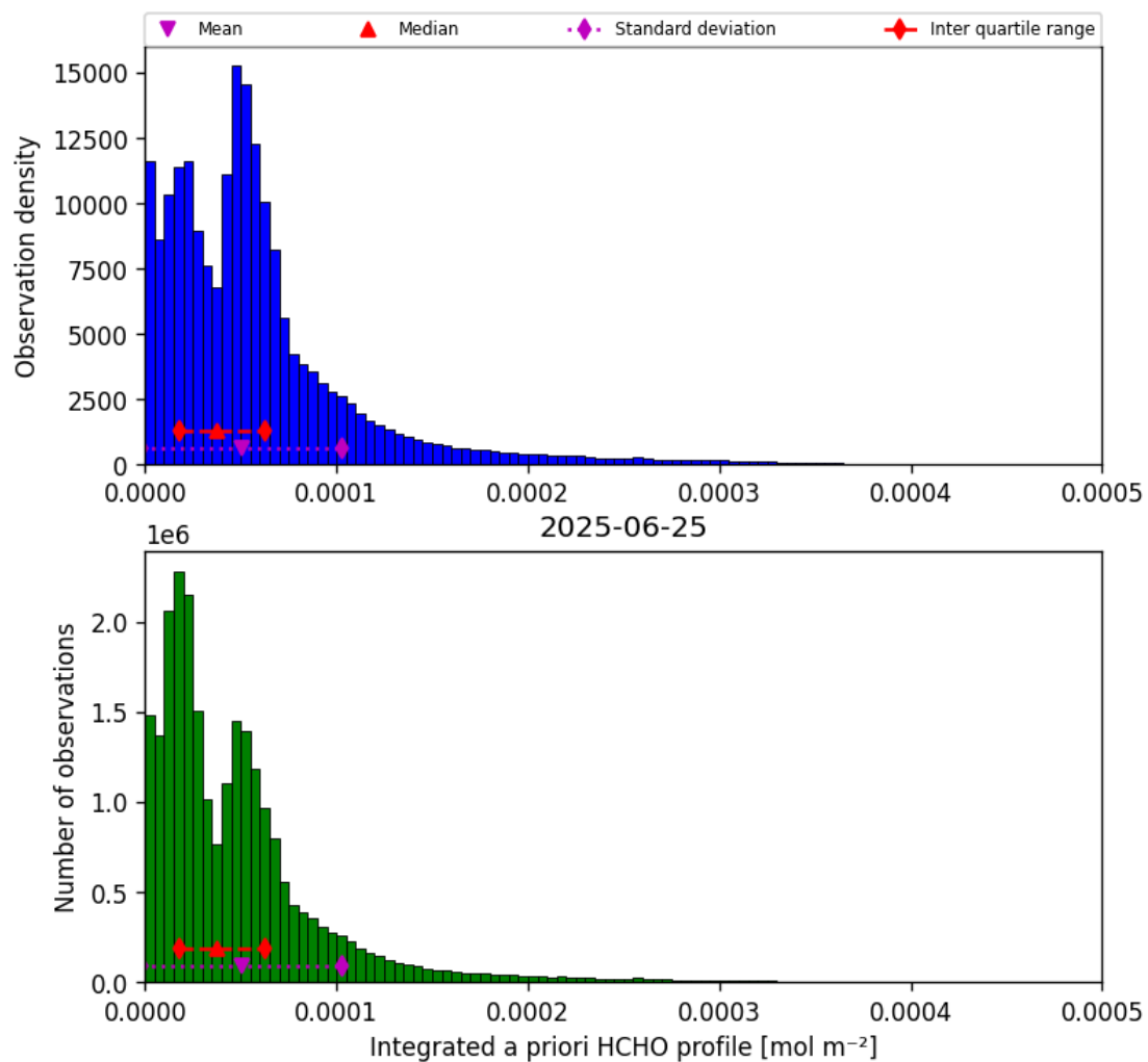
Figure 43: Histogram of “Integrated a priori HCHO profile” for 2025-06-24 to 2025-06-26
