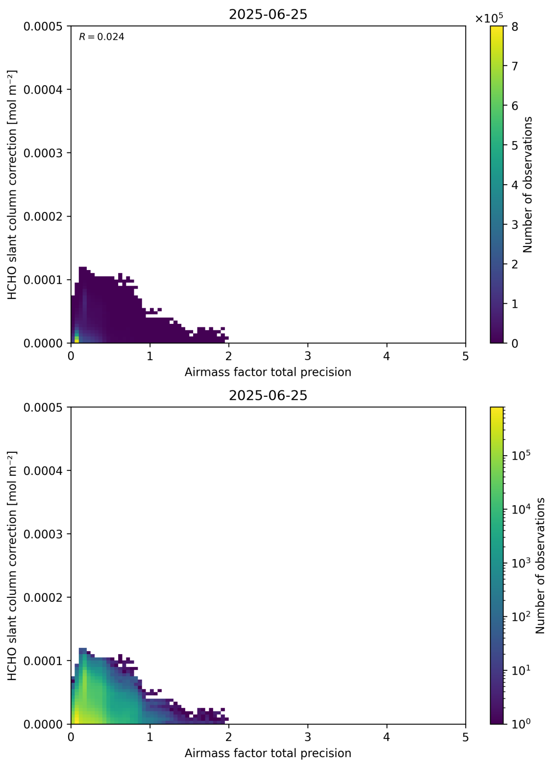
Figure 110: Scatter density plot of “Airmass factor total precision” against “HCHO slant column correction” for 2025-06-24 to 2025-06-26.
