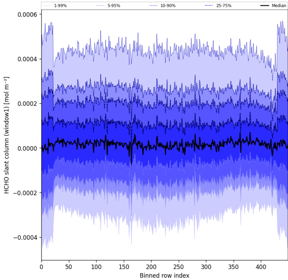
Figure 52: Along track statistics of “HCHO slant column (window1)” for 2025-06-24 to 2025-06-26
