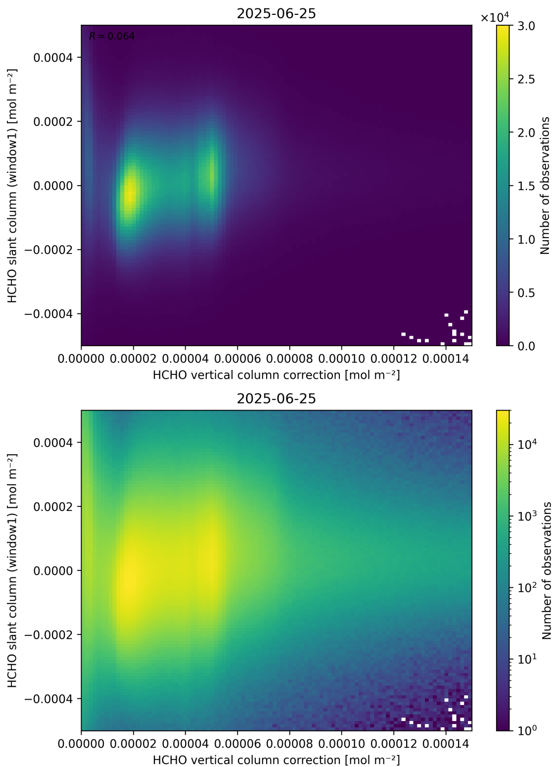
Figure 118: Scatter density plot of “HCHO vertical column correction” against “HCHO slant column (window1)” for 2025-06-24 to 2025-06-26.
