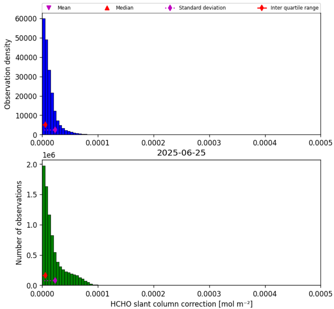
Figure 47: Histogram of “HCHO slant column correction” for 2025-06-24 to 2025-06-26
