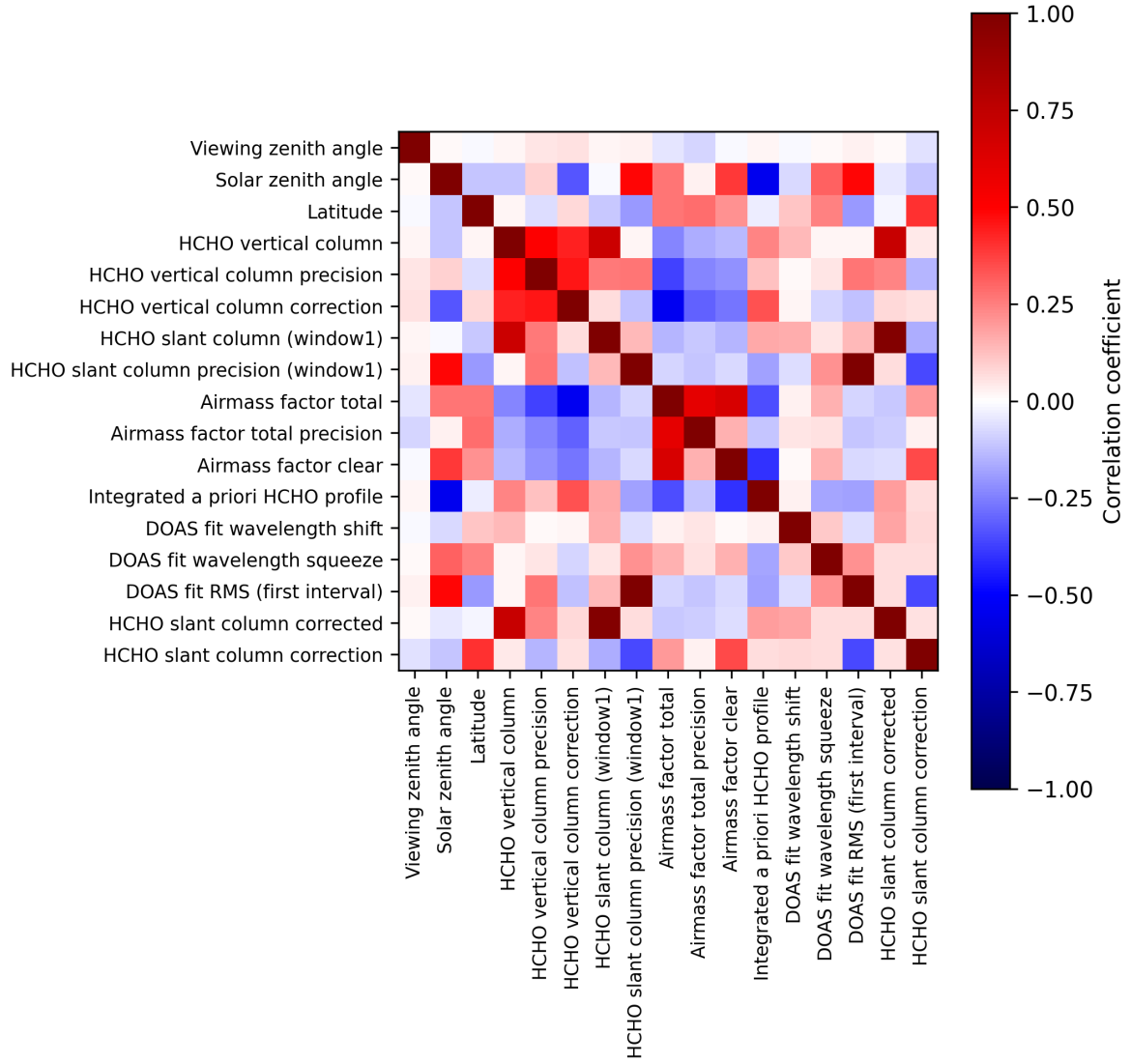
Figure 2: Map of correlation matrix for 2025-06-24 to 2025-06-26.
