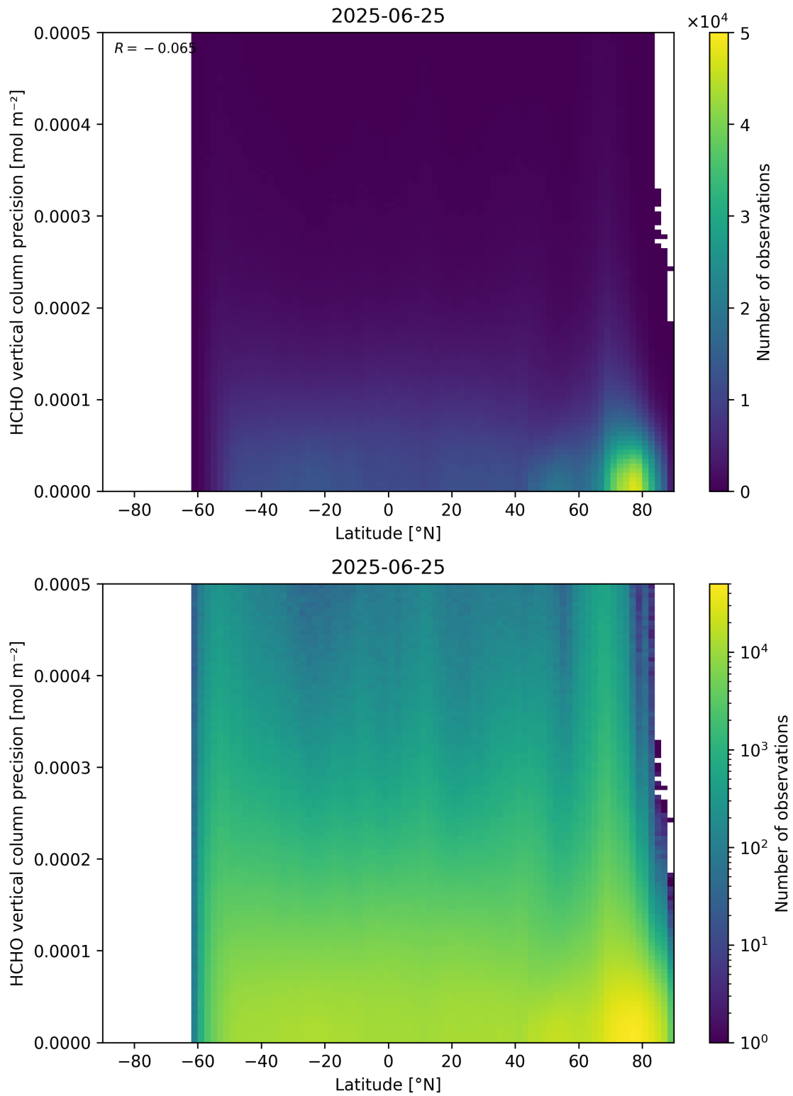
Figure 165: Scatter density plot of “Latitude” against “HCHO vertical column precision” for 2025-06-24 to 2025-06-26.
