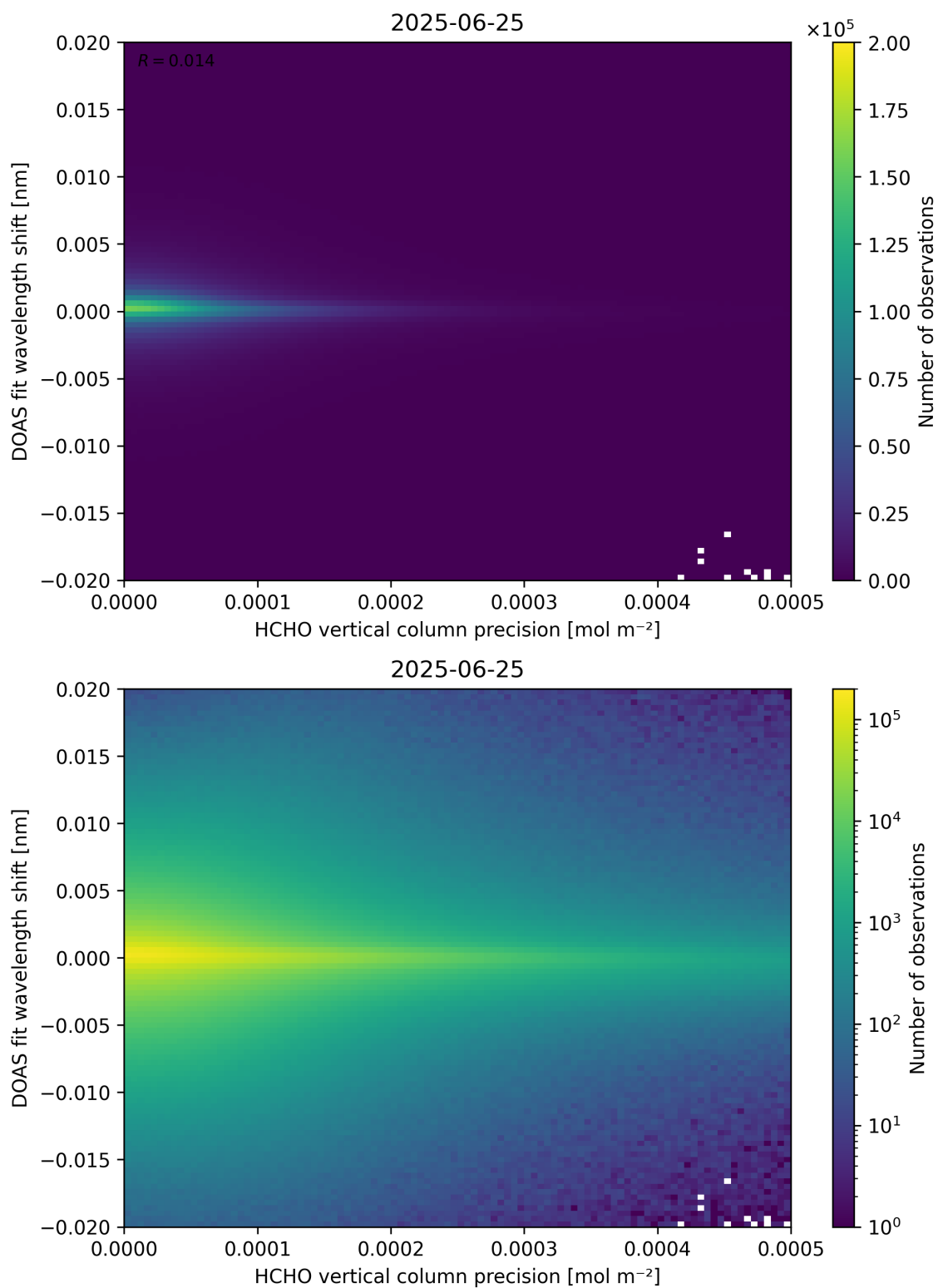
Figure 137: Scatter density plot of “HCHO vertical column precision” against “DOAS fit wavelength shift” for 2025-06-24 to 2025-06-26.
