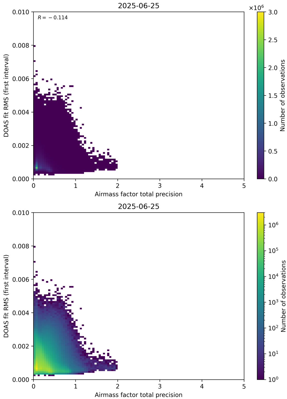
Figure 105: Scatter density plot of “Airmass factor total precision” against “DOAS fit RMS (first interval)” for 2025-06-24 to 2025-06-26.
