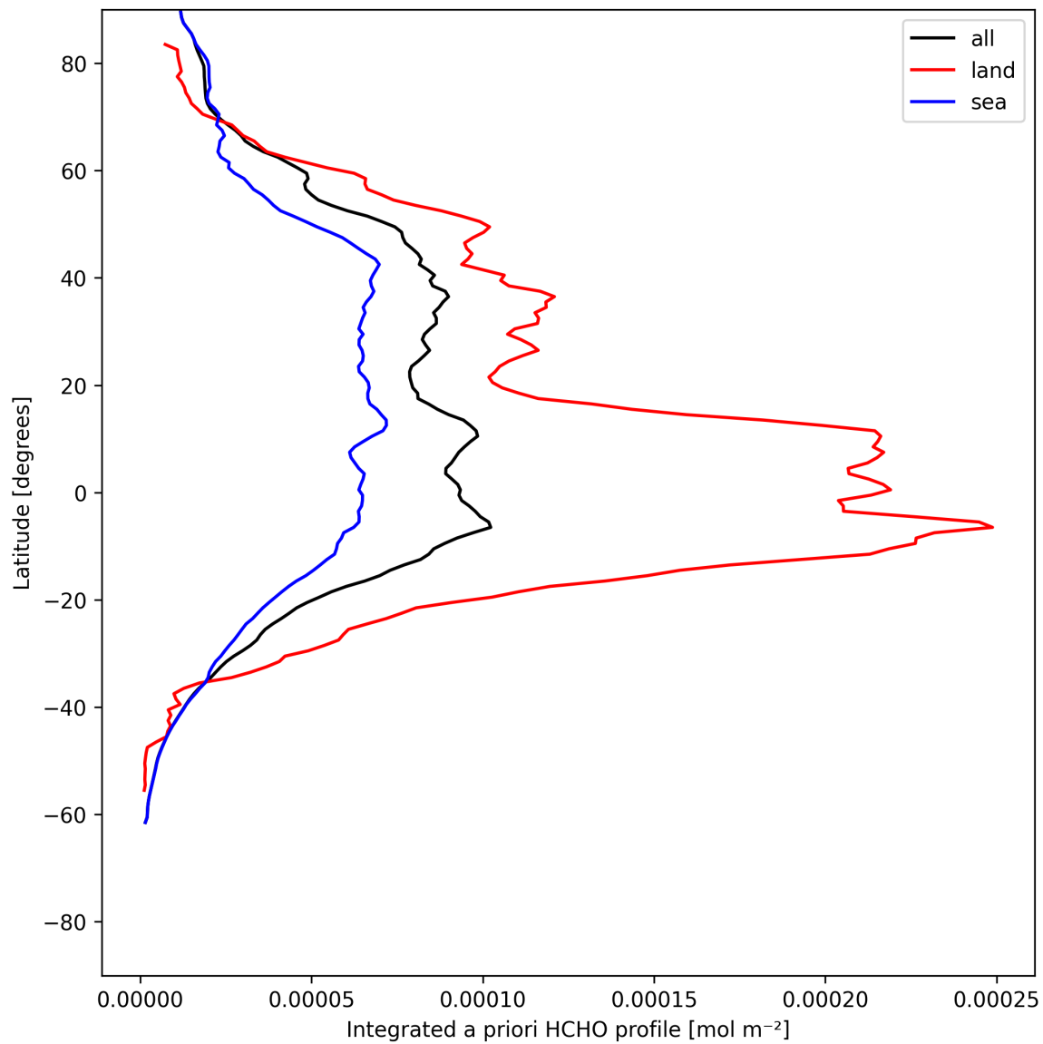
Figure 29: Zonal average of “Integrated a priori HCHO profile” for 2025-06-24 to 2025-06-26.
