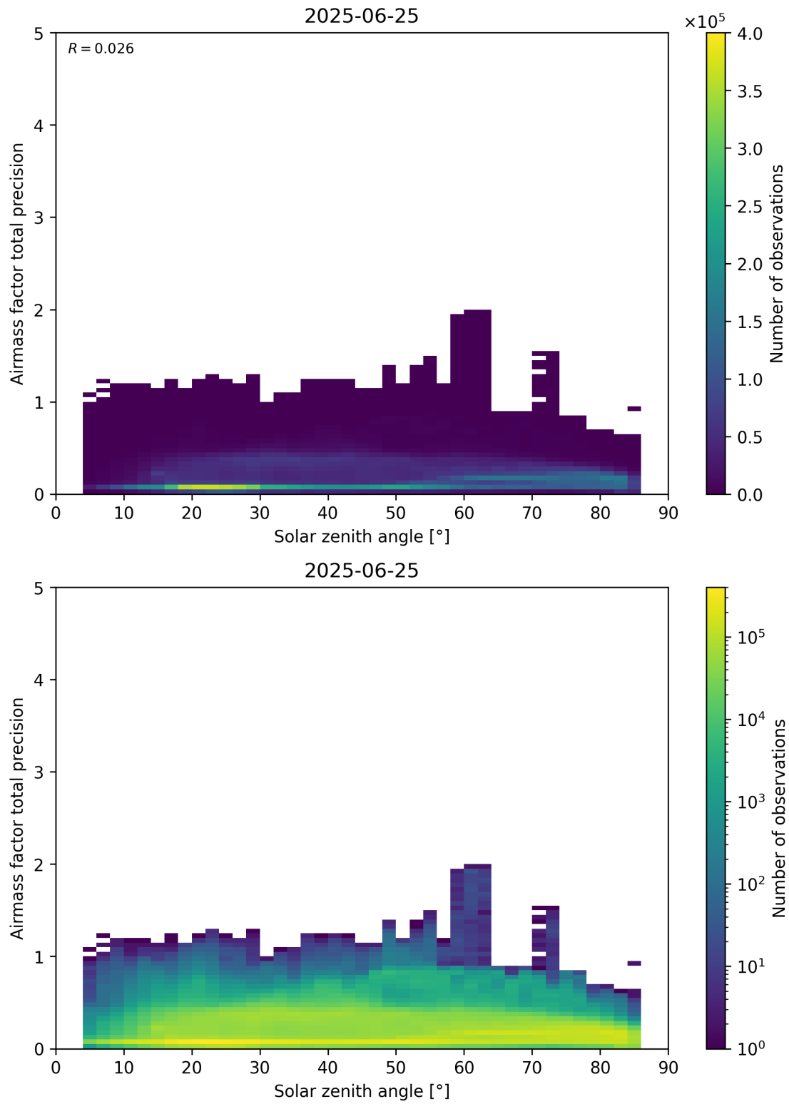
Figure 176: Scatter density plot of “Solar zenith angle” against “Airmass factor total precision” for 2025-06-24 to 2025-06-26.
