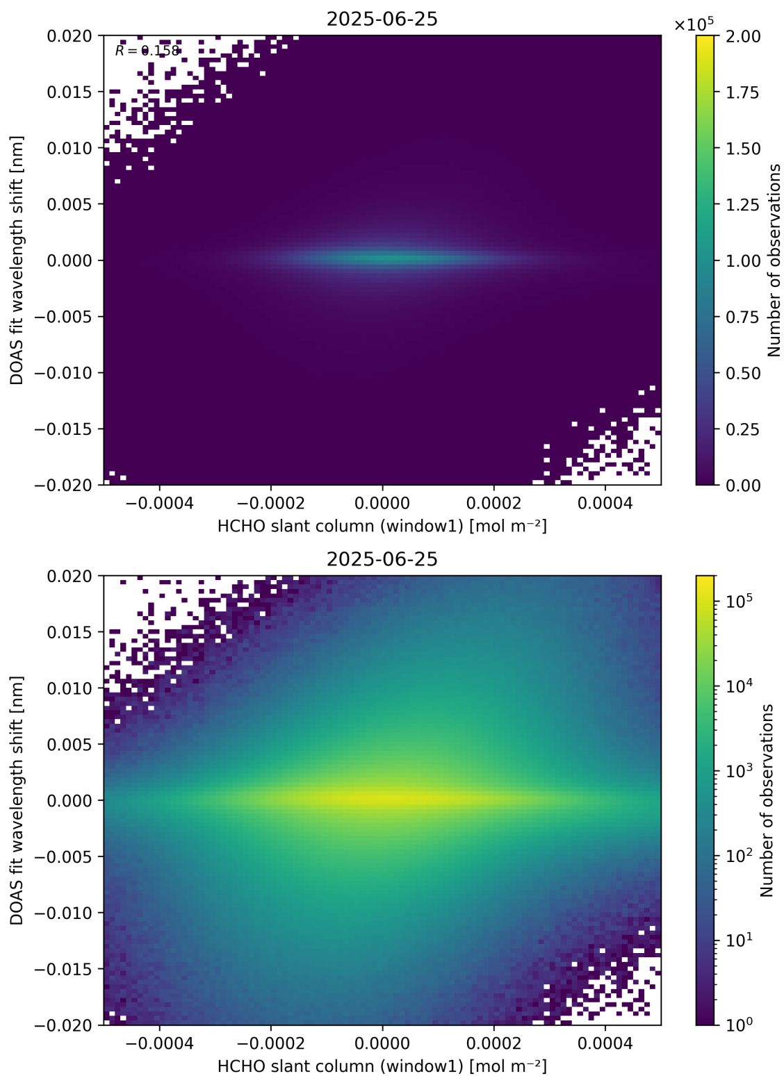
Figure 79: Scatter density plot of “HCHO slant column (window1)” against “DOAS fit wavelength shift” for 2025-06-24 to 2025-06-26.
