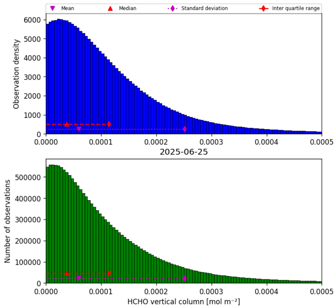
Figure 35: Histogram of “HCHO vertical column” for 2025-06-24 to 2025-06-26
