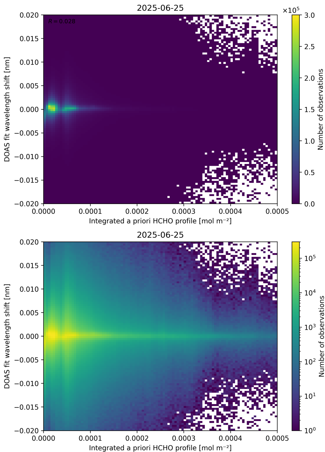
Figure 149: Scatter density plot of “Integrated a priori HCHO profile” against “DOAS fit wavelength shift” for 2025-06-24 to 2025-06-26.
