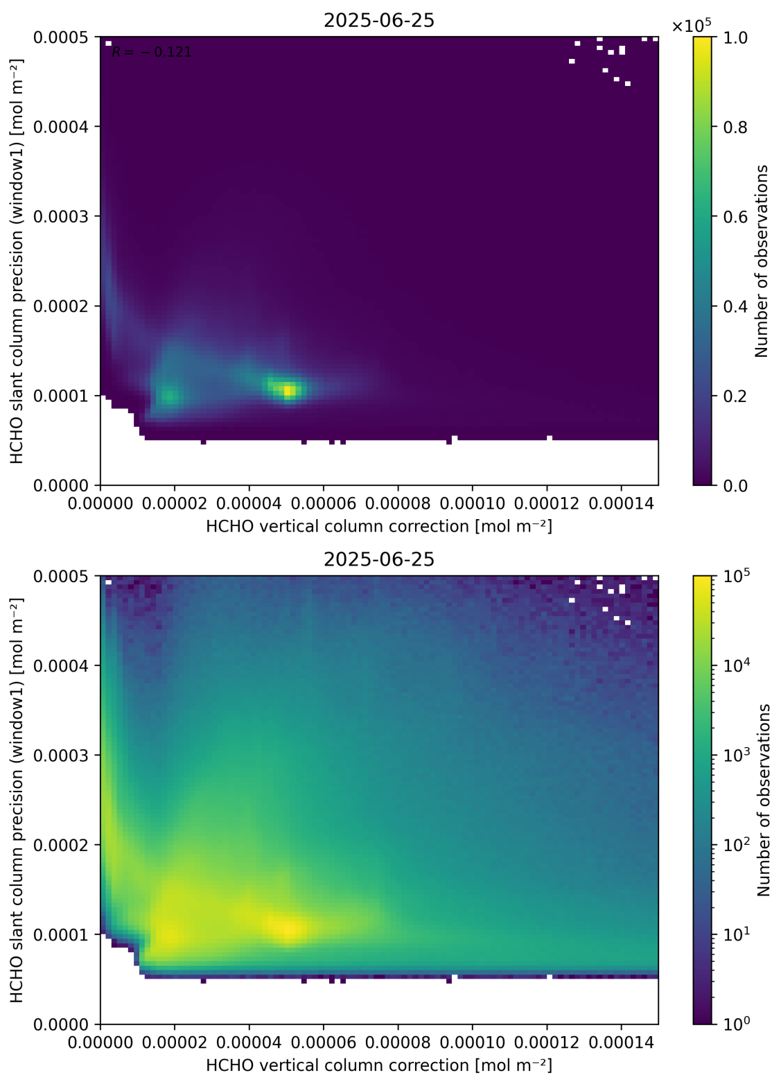
Figure 119: Scatter density plot of “HCHO vertical column correction” against “HCHO slant column precision (window1)” for 2025-06-24 to 2025-06-26.
