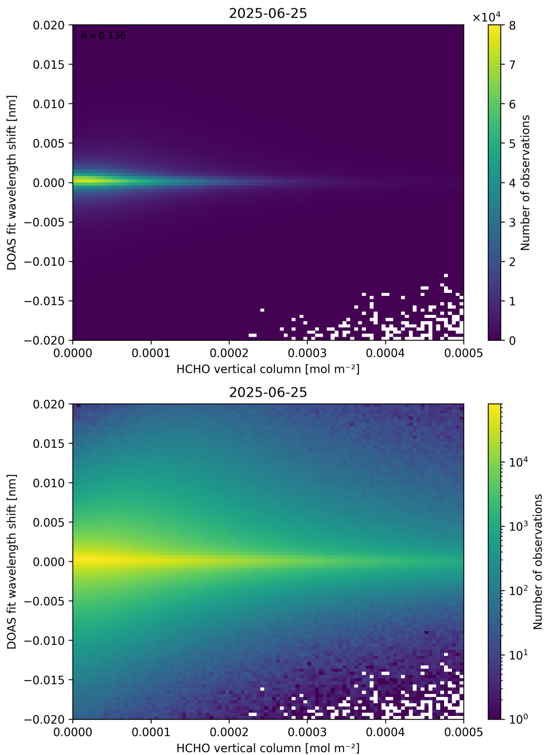
Figure 124: Scatter density plot of “HCHO vertical column” against “DOAS fit wavelength shift” for 2025-06-24 to 2025-06-26.
