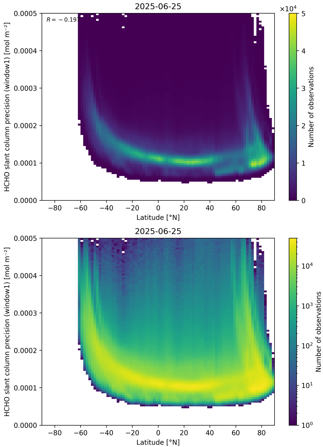
Figure 160: Scatter density plot of “Latitude” against “HCHO slant column precision (window1)” for 2025-06-24 to 2025-06-26.
