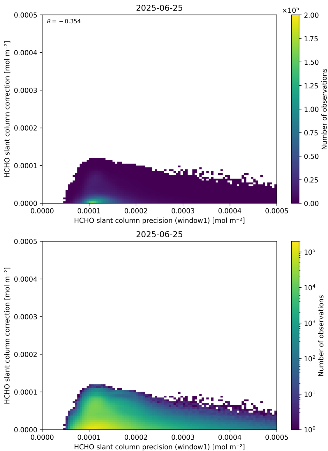
Figure 93: Scatter density plot of “HCHO slant column precision (window1)” against “HCHO slant column correction” for 2025-06-24 to 2025-06-26.
