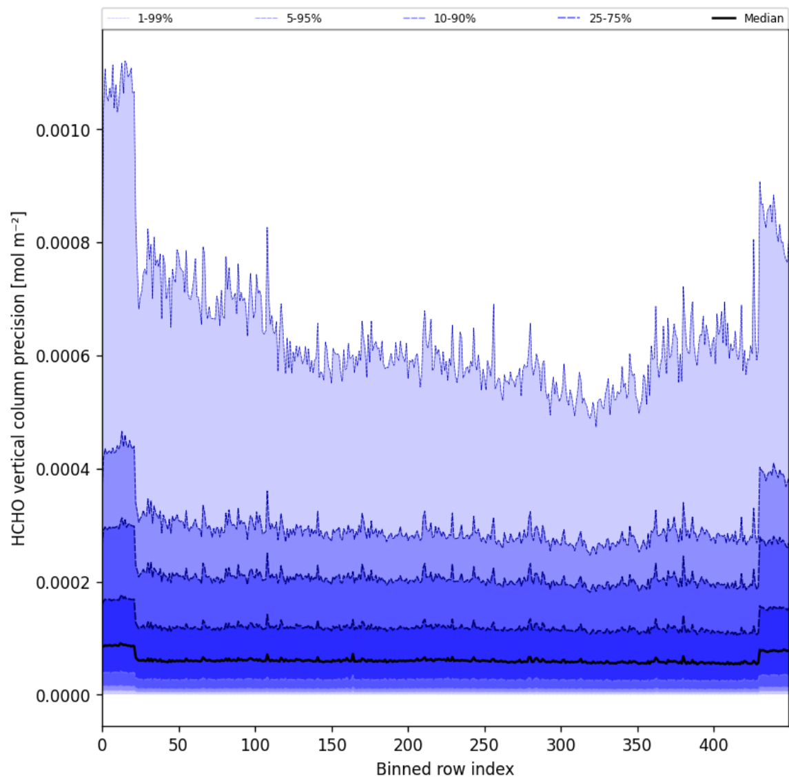
Figure 50: Along track statistics of “HCHO vertical column precision” for 2025-06-24 to 2025-06-26
