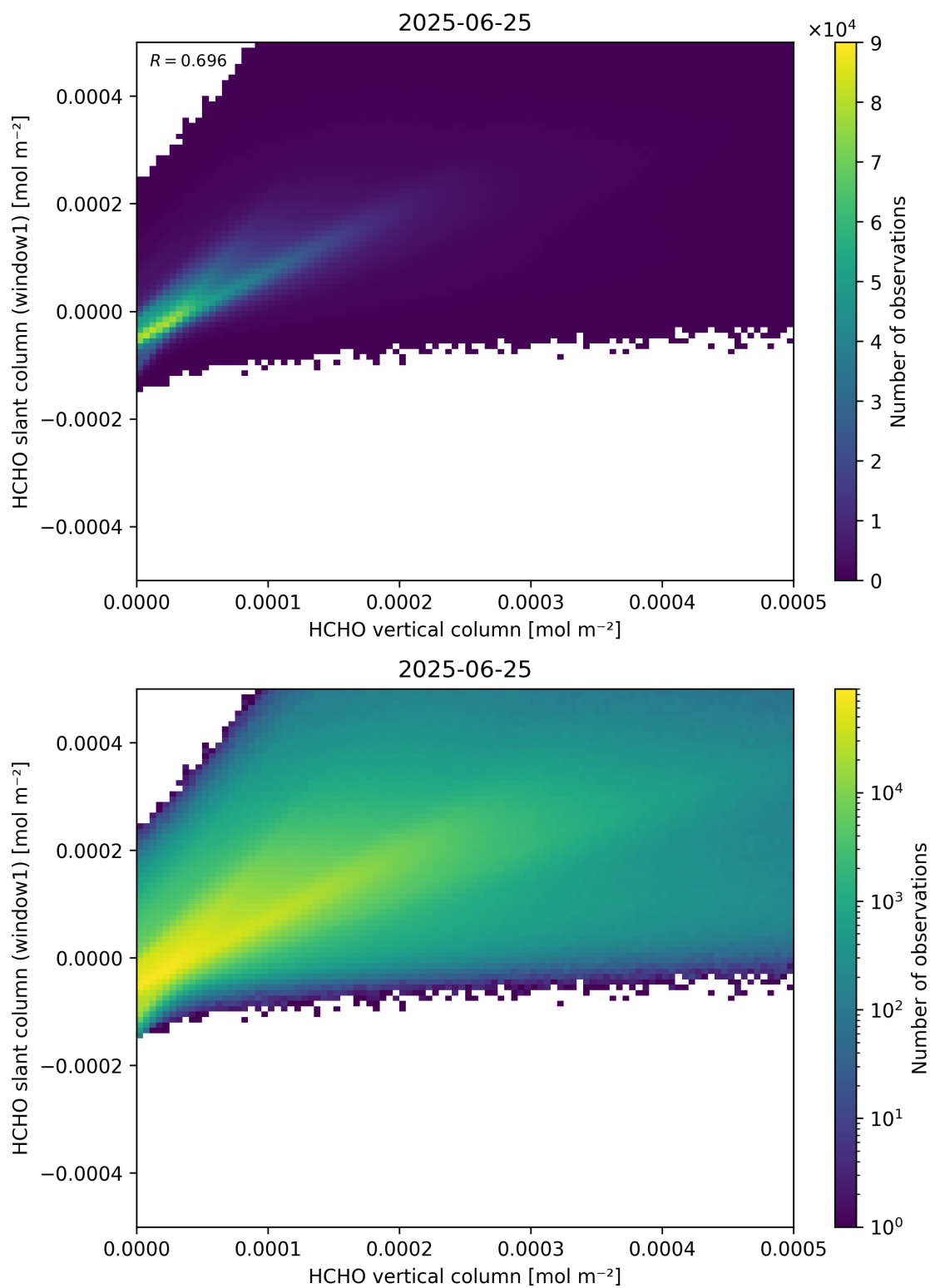
Figure 129: Scatter density plot of “HCHO vertical column” against “HCHO slant column (window1)” for 2025-06-24 to 2025-06-26.
