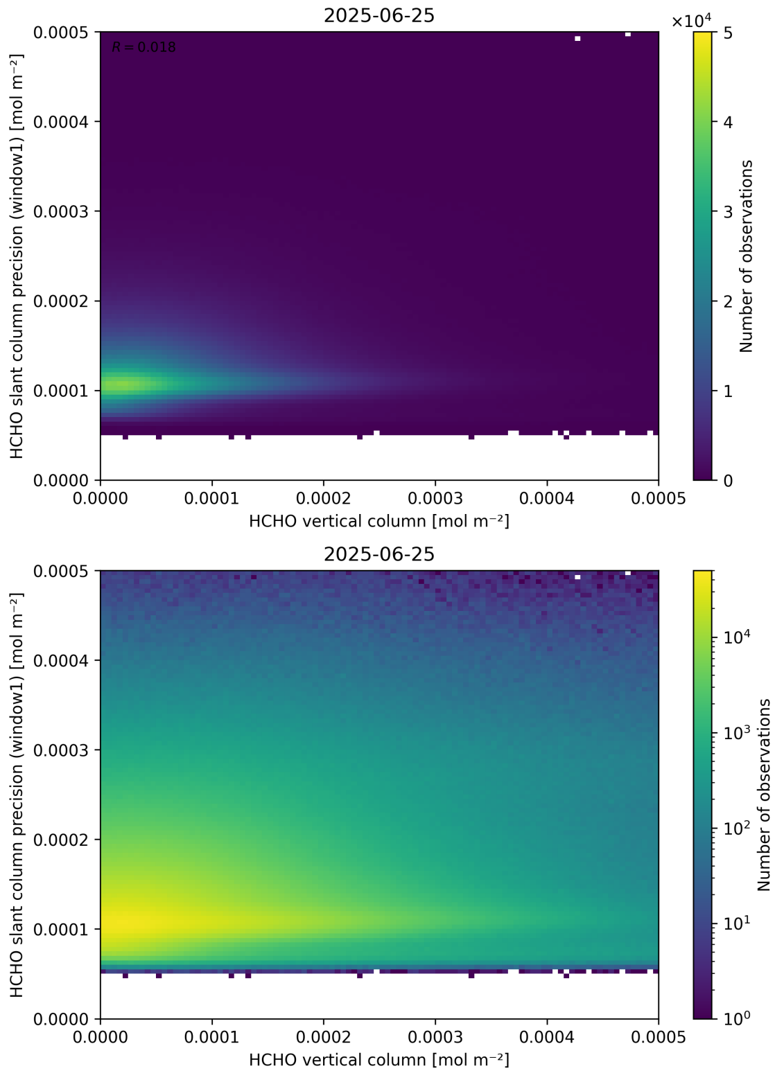
Figure 130: Scatter density plot of “HCHO vertical column” against “HCHO slant column precision (window1)” for 2025-06-24 to 2025-06-26.
