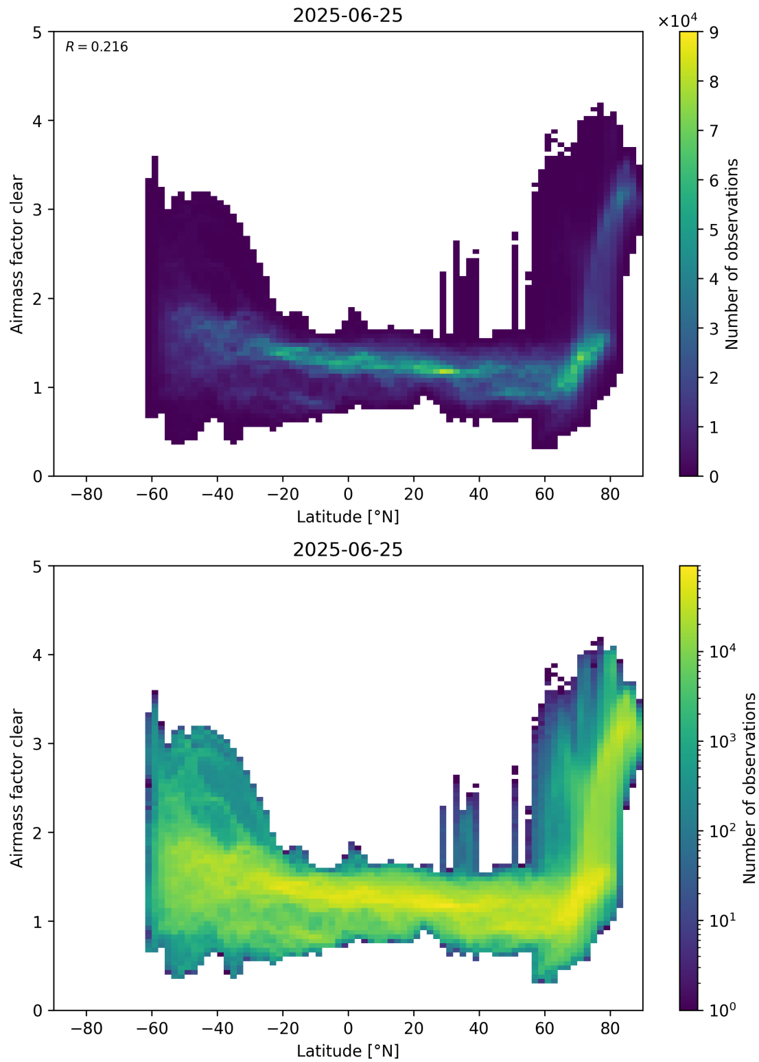
Figure 156: Scatter density plot of “Latitude” against “Airmass factor clear” for 2025-06-24 to 2025-06-26.
