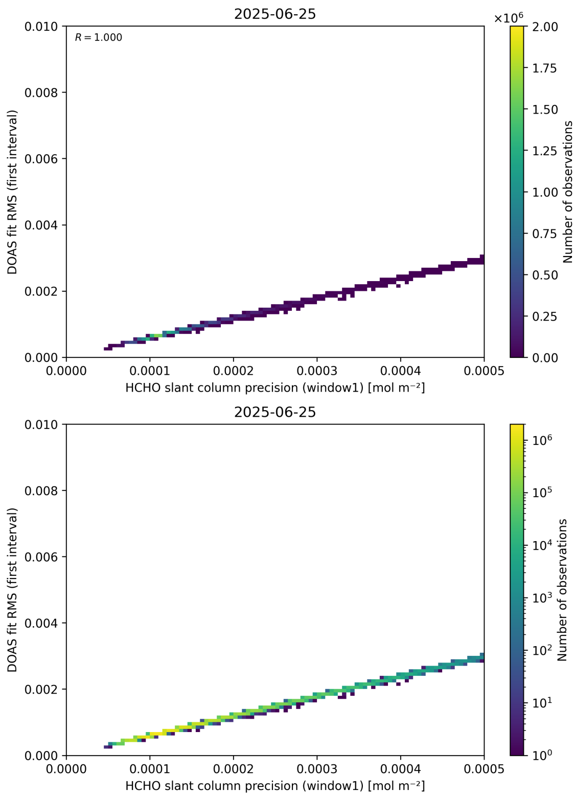
Figure 88: Scatter density plot of “HCHO slant column precision (window1)” against “DOAS fit RMS (first interval)” for 2025-06-24 to 2025-06-26.
