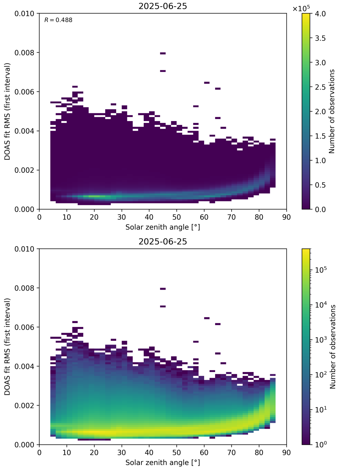
Figure 167: Scatter density plot of “Solar zenith angle” against “DOAS fit RMS (first interval)” for 2025-06-24 to 2025-06-26.
