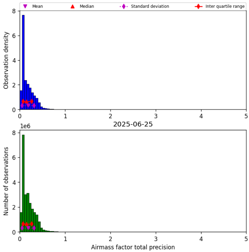
Figure 41: Histogram of “Airmass factor total precision” for 2025-06-24 to 2025-06-26
