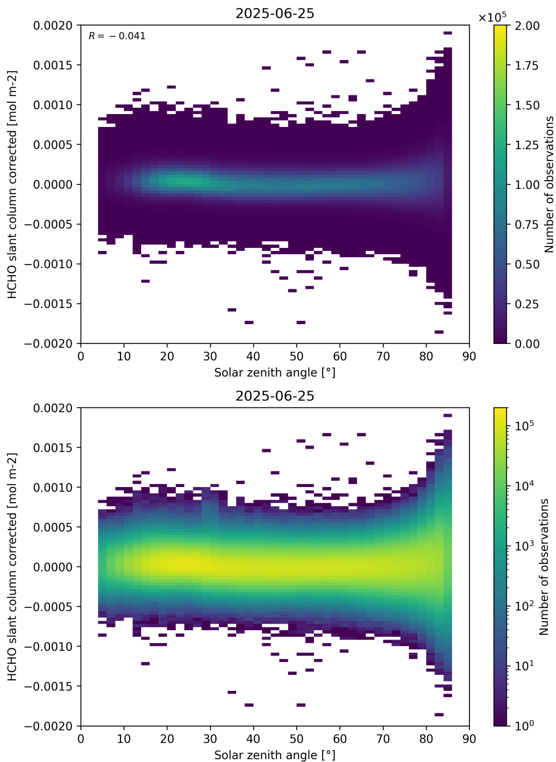
Figure 171: Scatter density plot of “Solar zenith angle” against “HCHO slant column corrected” for 2025-06-24 to 2025-06-26.
