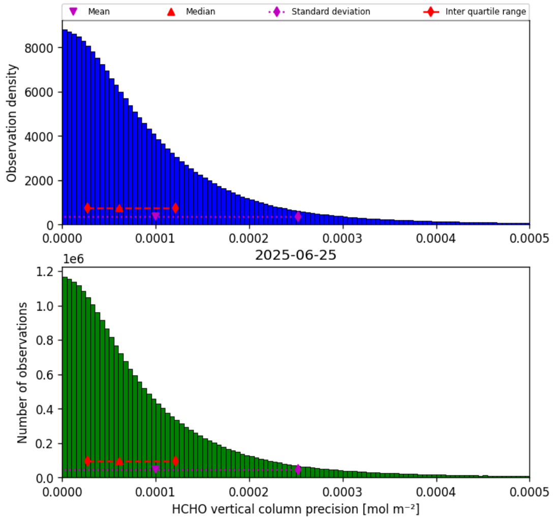
Figure 36: Histogram of “HCHO vertical column precision” for 2025-06-24 to 2025-06-26
