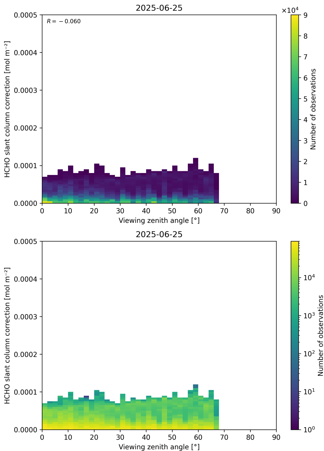
Figure 187: Scatter density plot of “Viewing zenith angle” against “HCHO slant column correction” for 2025-06-24 to 2025-06-26.
