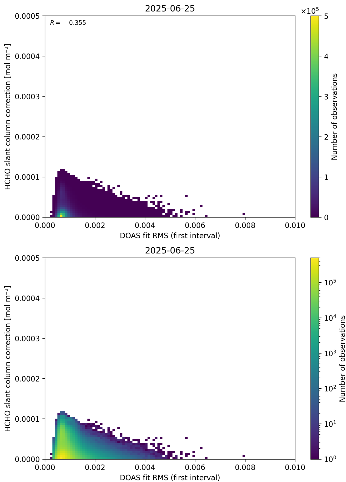
Figure 63: Scatter density plot of “DOAS fit RMS (first interval)” against “HCHO slant column correction” for 2025-06-24 to 2025-06-26.
