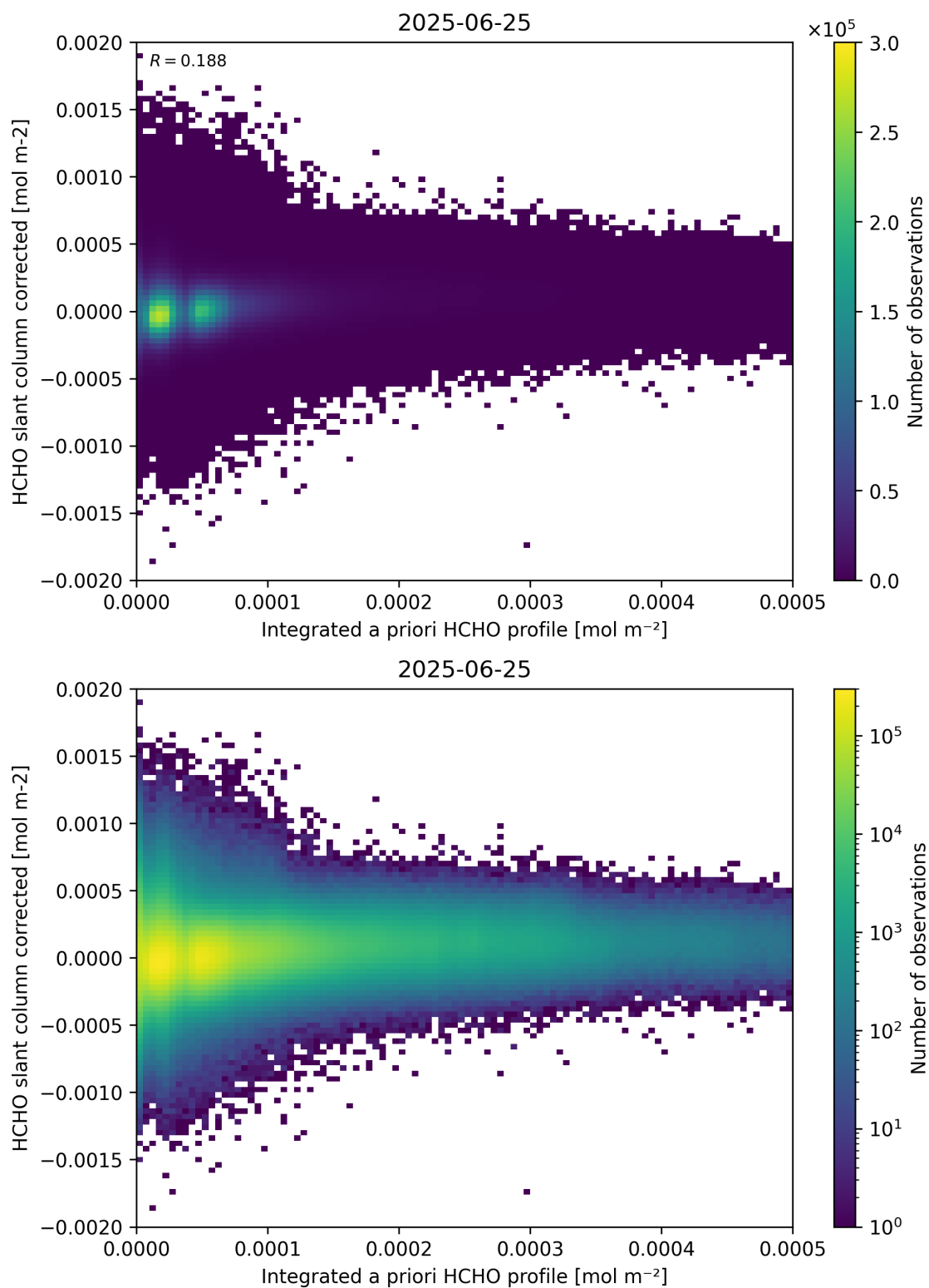
Figure 151: Scatter density plot of “Integrated a priori HCHO profile” against “HCHO slant column corrected” for 2025-06-24 to 2025-06-26.
