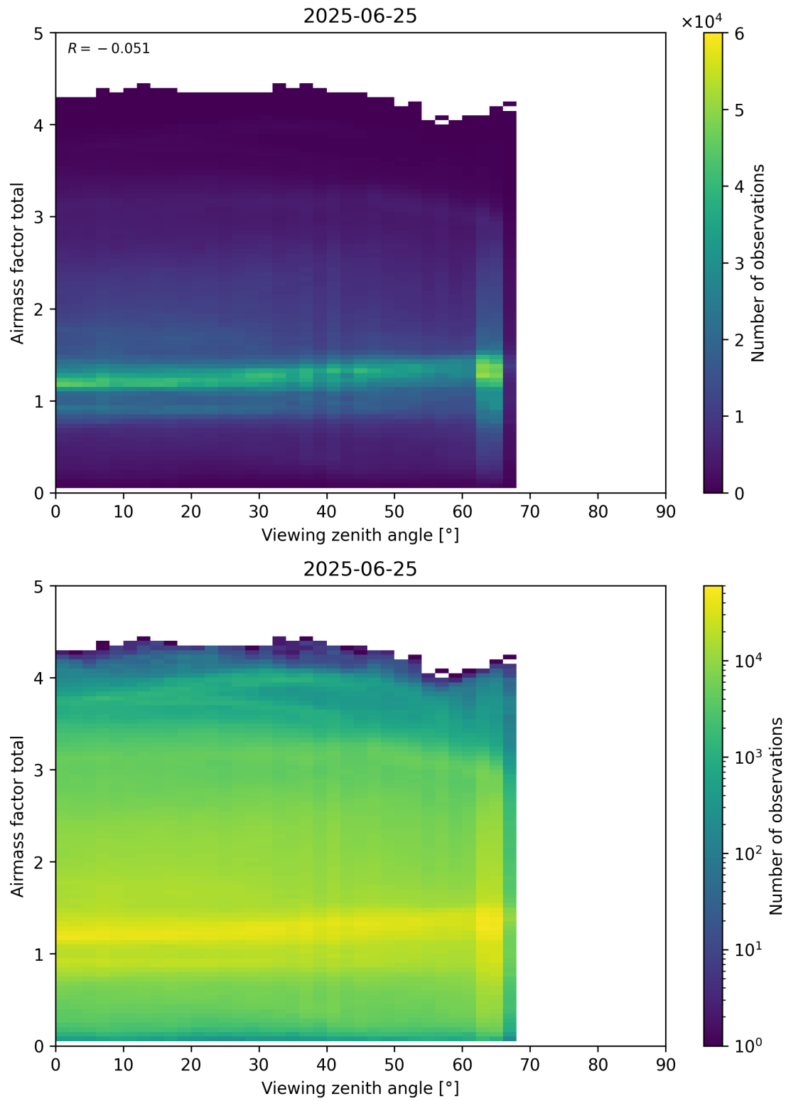
Figure 190: Scatter density plot of “Viewing zenith angle” against “Airmass factor total” for 2025-06-24 to 2025-06-26.
