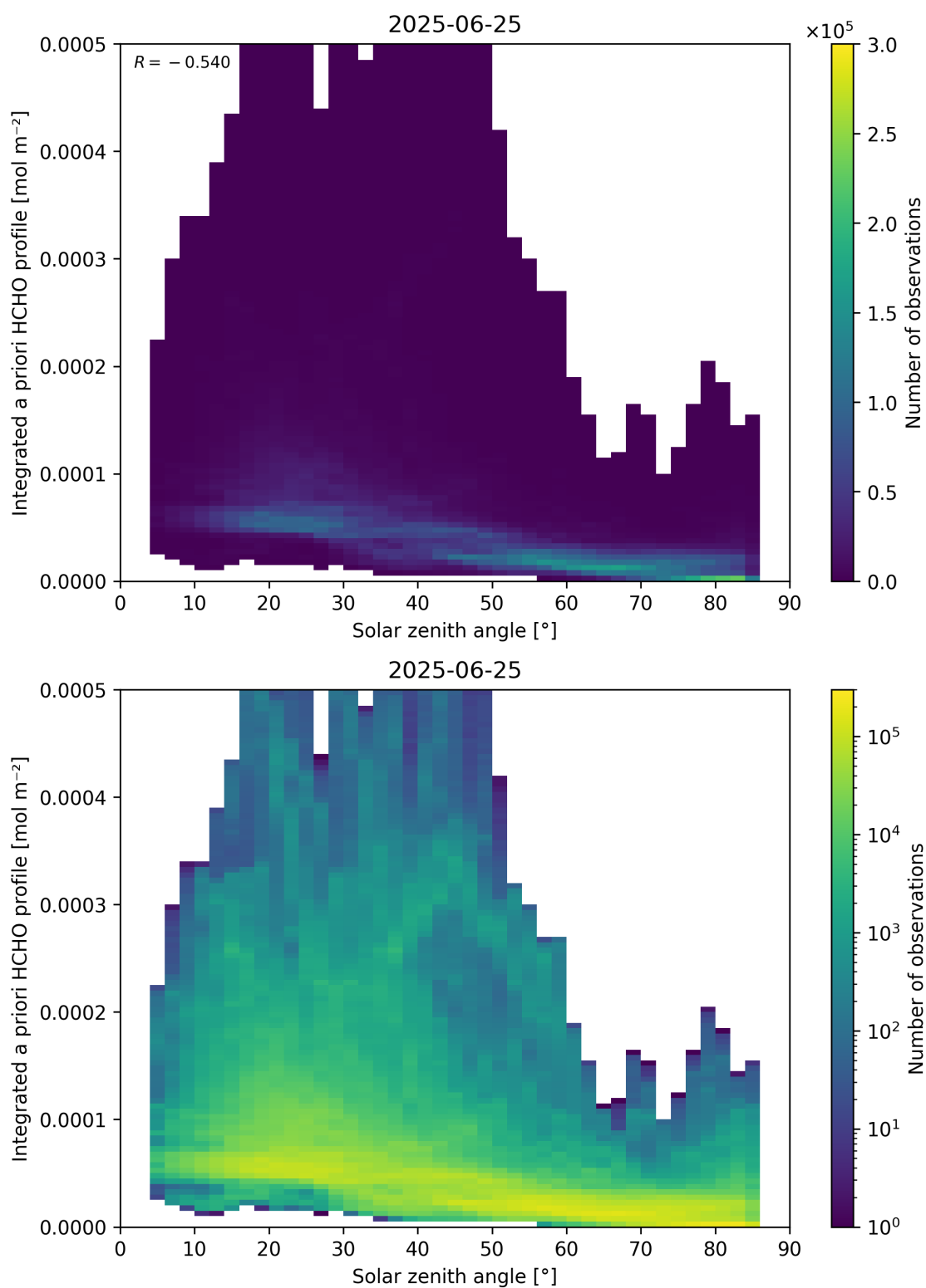
Figure 180: Scatter density plot of “Solar zenith angle” against “Integrated a priori HCHO profile” for 2025-06-24 to 2025-06-26.
