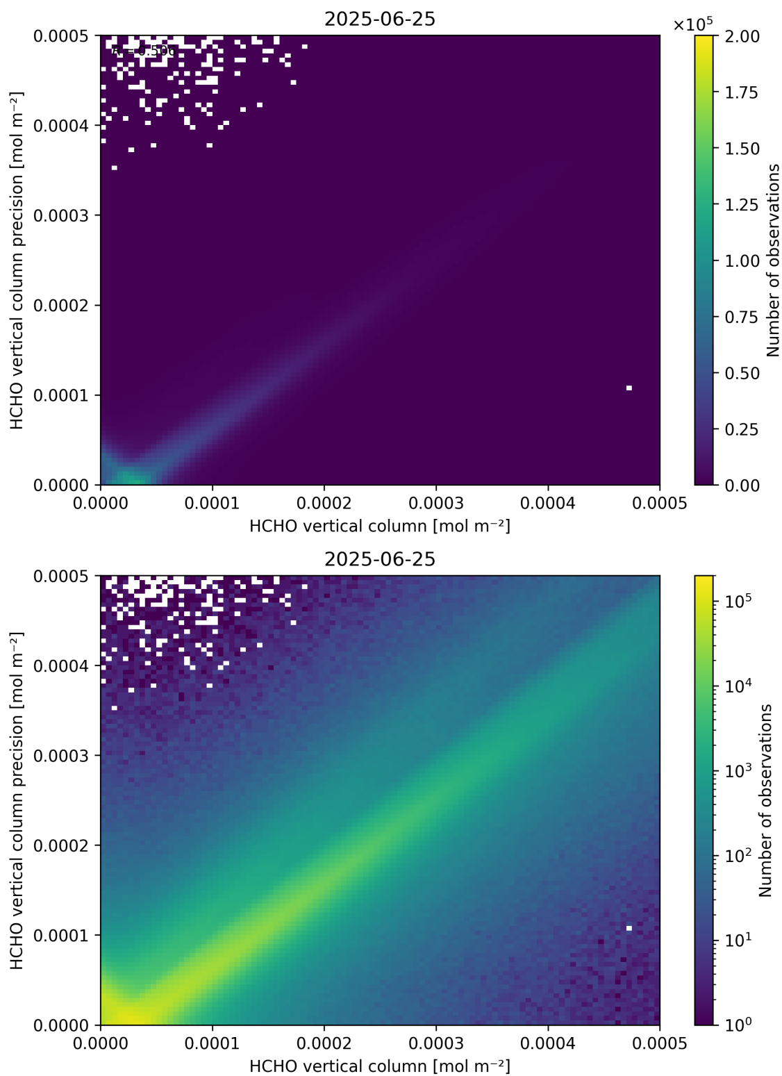
Figure 134: Scatter density plot of “HCHO vertical column” against “HCHO vertical column precision” for 2025-06-24 to 2025-06-26.
