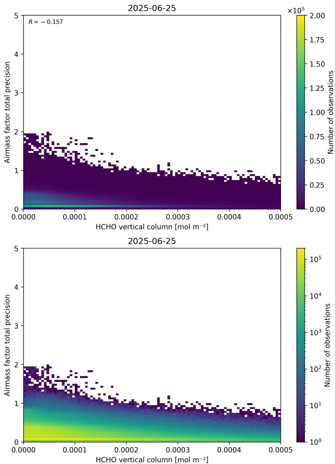
Figure 132: Scatter density plot of “HCHO vertical column” against “Airmass factor total precision” for 2025-06-24 to 2025-06-26.
