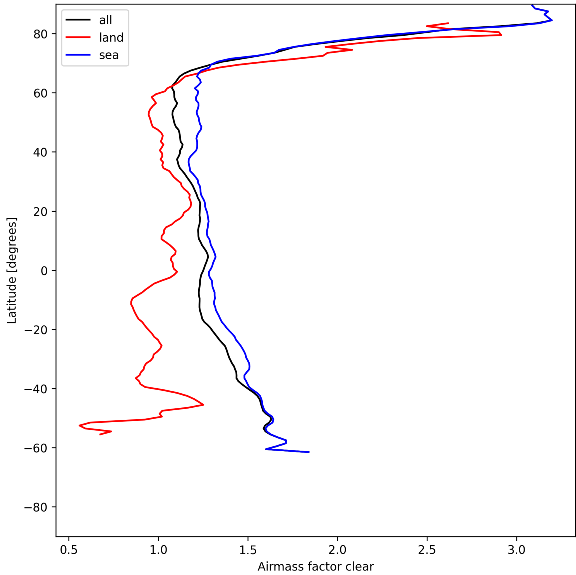
Figure 28: Zonal average of “Airmass factor clear” for 2025-06-24 to 2025-06-26.
