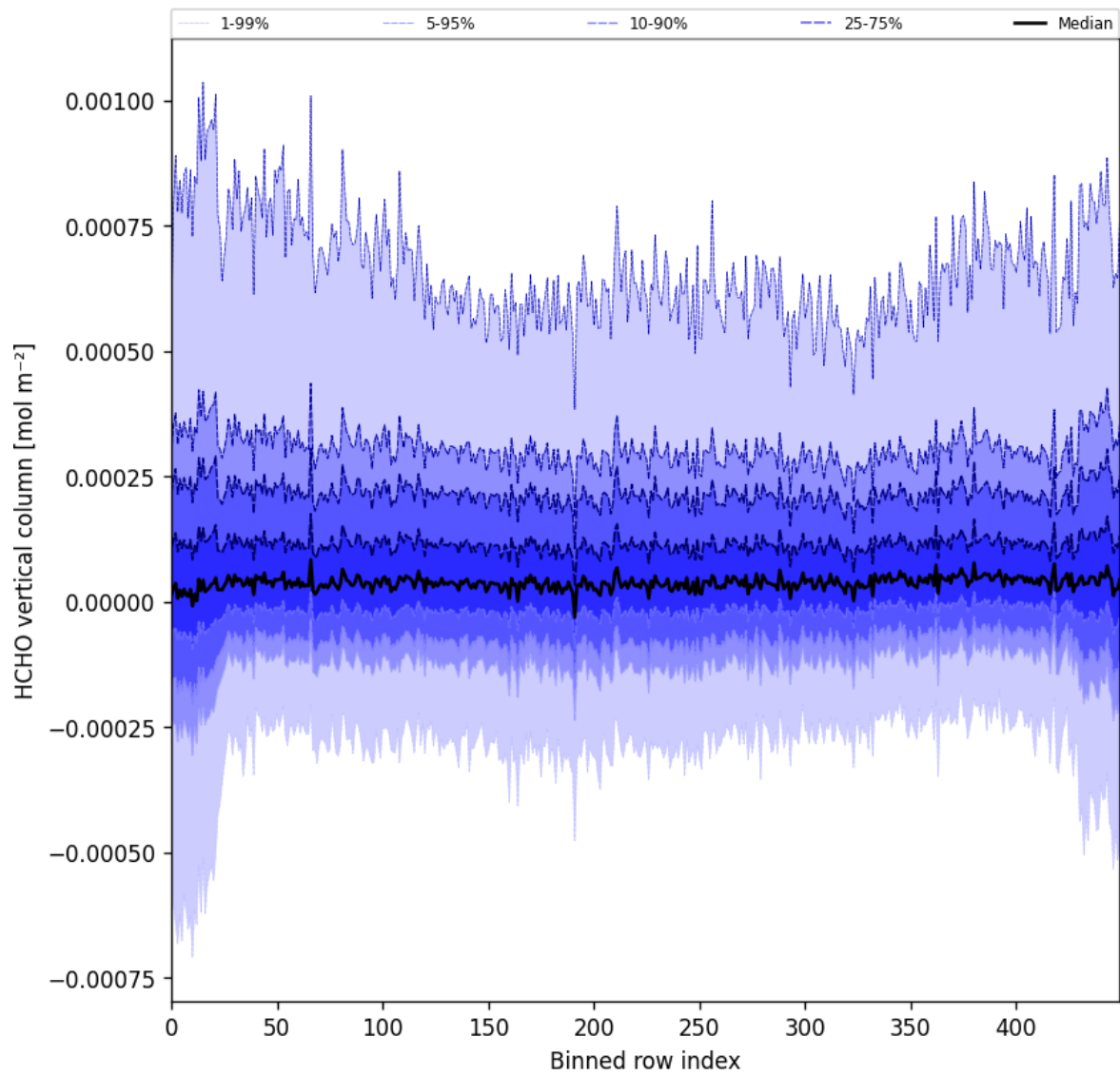
Figure 49: Along track statistics of “HCHO vertical column” for 2025-06-24 to 2025-06-26
