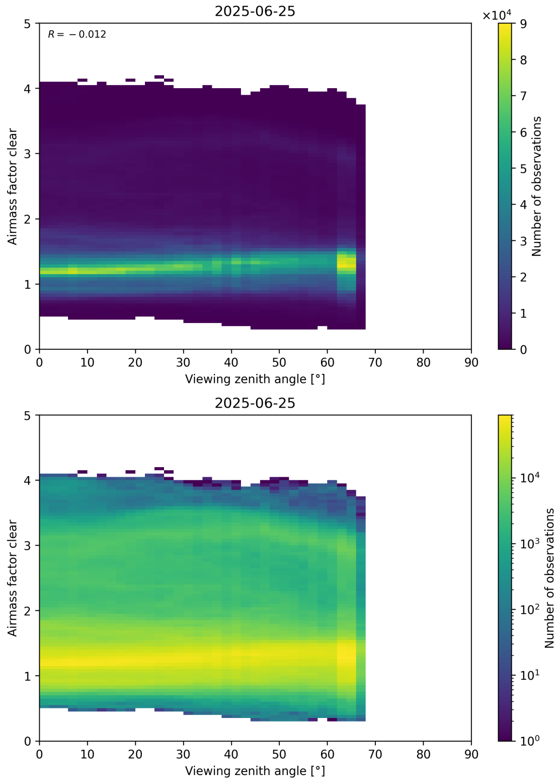
Figure 185: Scatter density plot of “Viewing zenith angle” against “Airmass factor clear” for 2025-06-24 to 2025-06-26.
