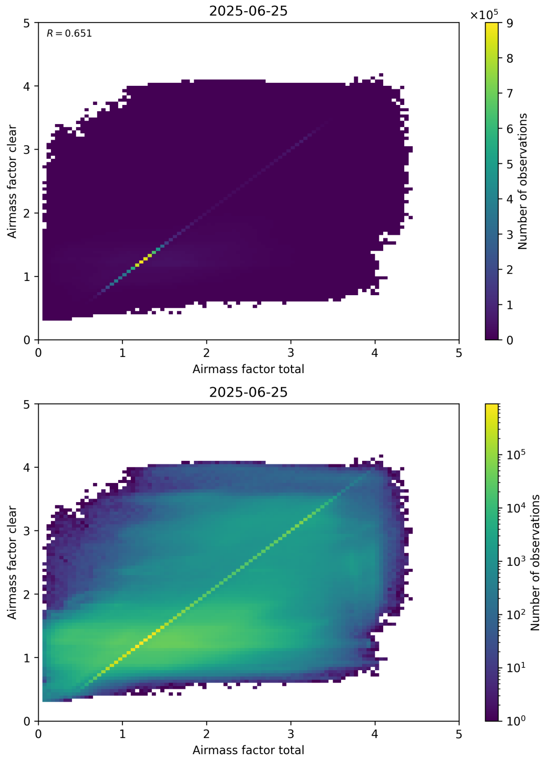
Figure 100: Scatter density plot of “Airmass factor total” against “Airmass factor clear” for 2025-06-24 to 2025-06-26.
