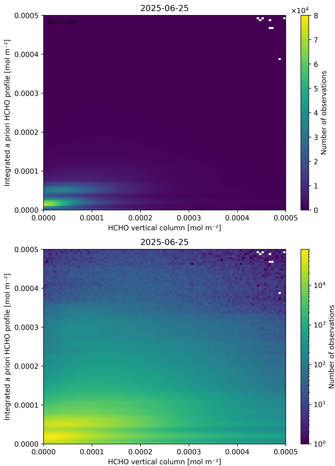
Figure 135: Scatter density plot of “HCHO vertical column” against “Integrated a priori HCHO profile” for 2025-06-24 to 2025-06-26.
