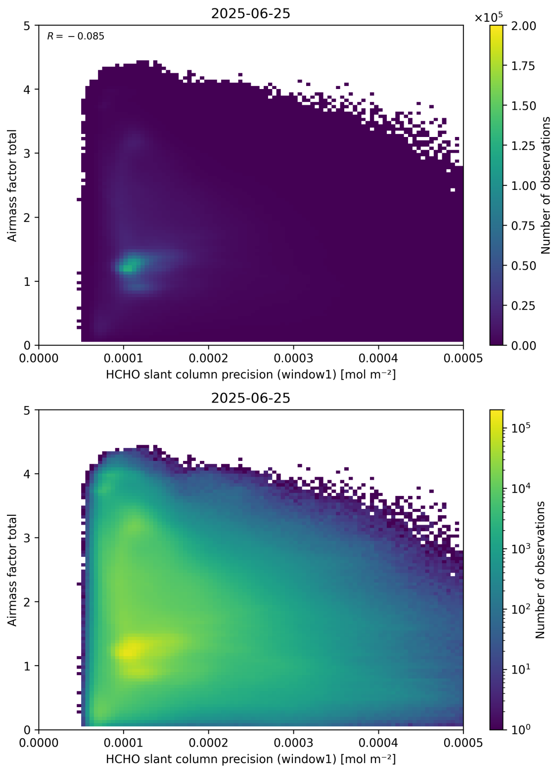
Figure 94: Scatter density plot of “HCHO slant column precision (window1)” against “Airmass factor total” for 2025-06-24 to 2025-06-26.
