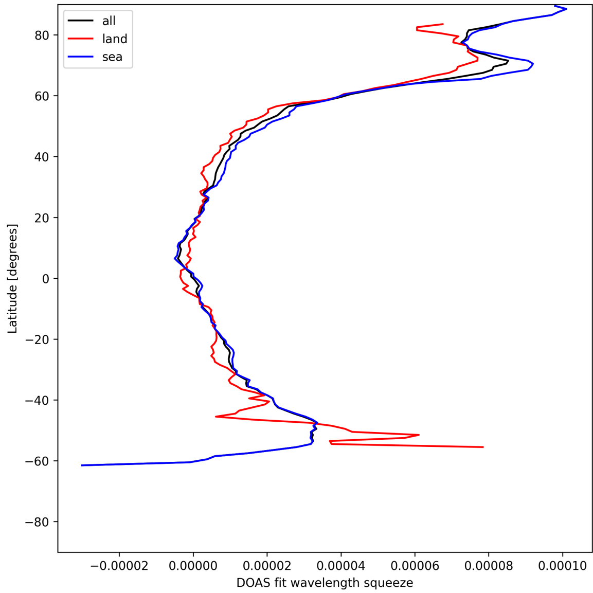
Figure 31: Zonal average of “DOAS fit wavelength squeeze” for 2025-06-24 to 2025-06-26.
