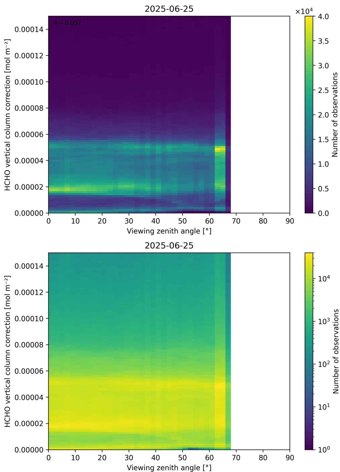
Figure 193: Scatter density plot of “Viewing zenith angle” against “HCHO vertical column correction” for 2025-06-24 to 2025-06-26.
