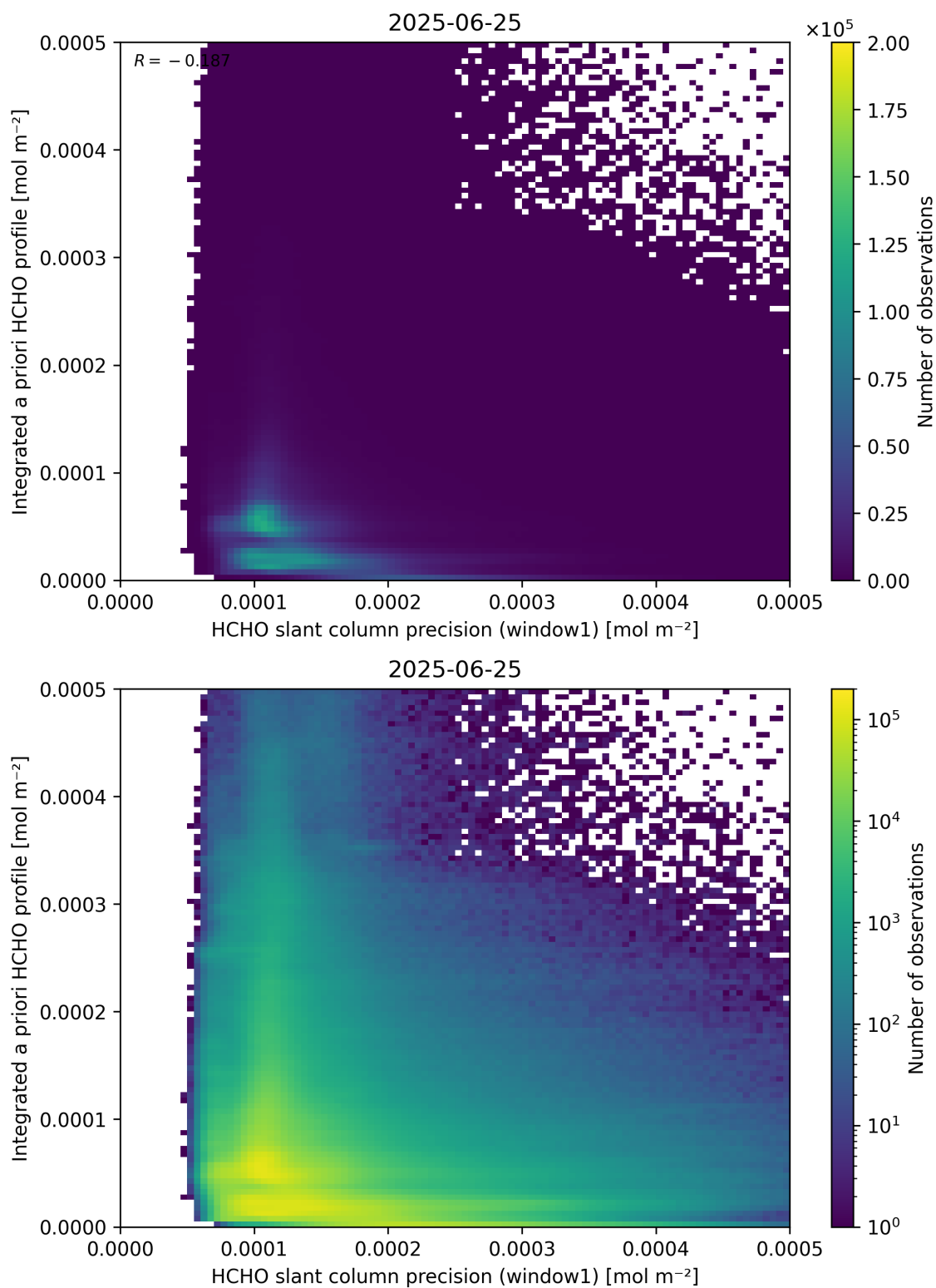
Figure 96: Scatter density plot of “HCHO slant column precision (window1)” against “Integrated a priori HCHO profile” for 2025-06-24 to 2025-06-26.
