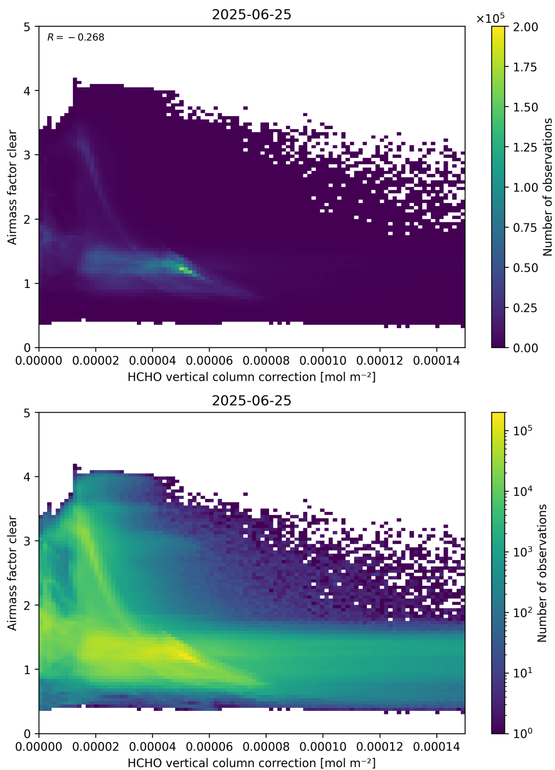
Figure 115: Scatter density plot of “HCHO vertical column correction” against “Airmass factor clear” for 2025-06-24 to 2025-06-26.
