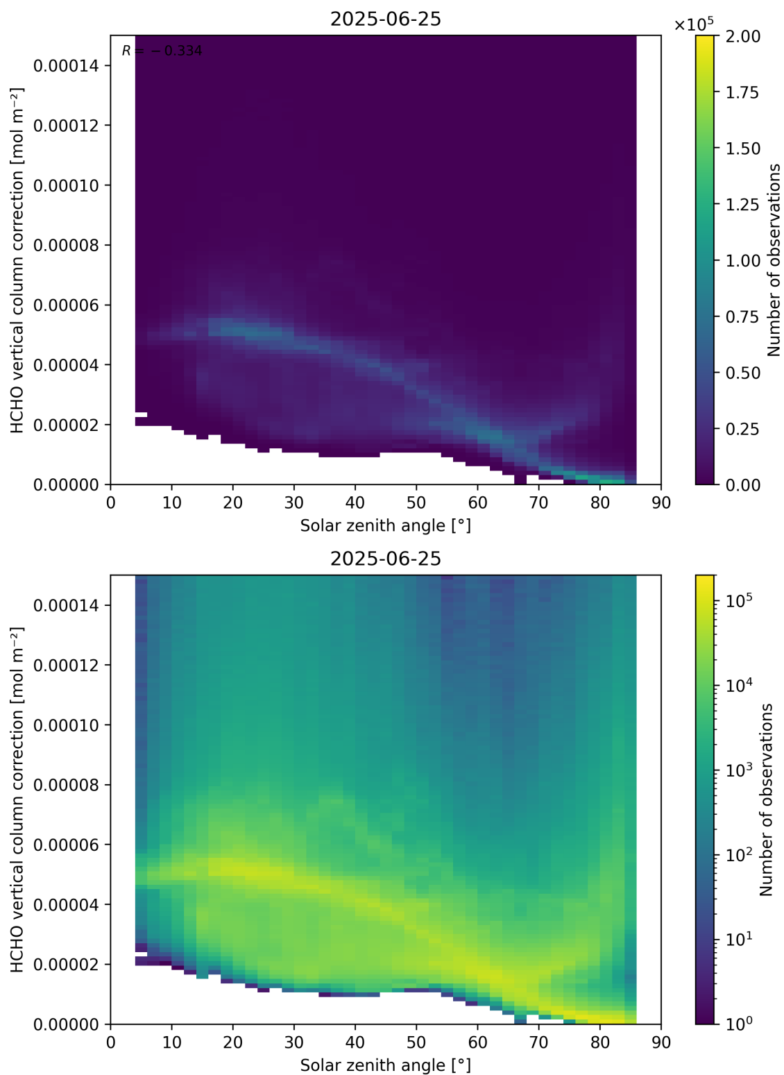
Figure 178: Scatter density plot of “Solar zenith angle” against “HCHO vertical column correction” for 2025-06-24 to 2025-06-26.
