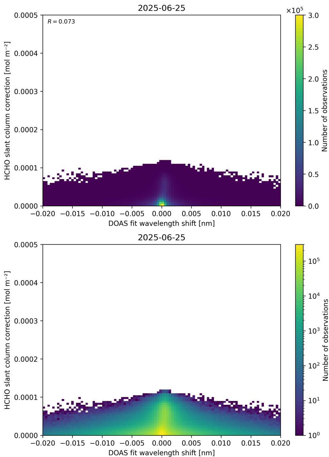
Figure 67: Scatter density plot of “DOAS fit wavelength shift” against “HCHO slant column correction” for 2025-06-24 to 2025-06-26.
