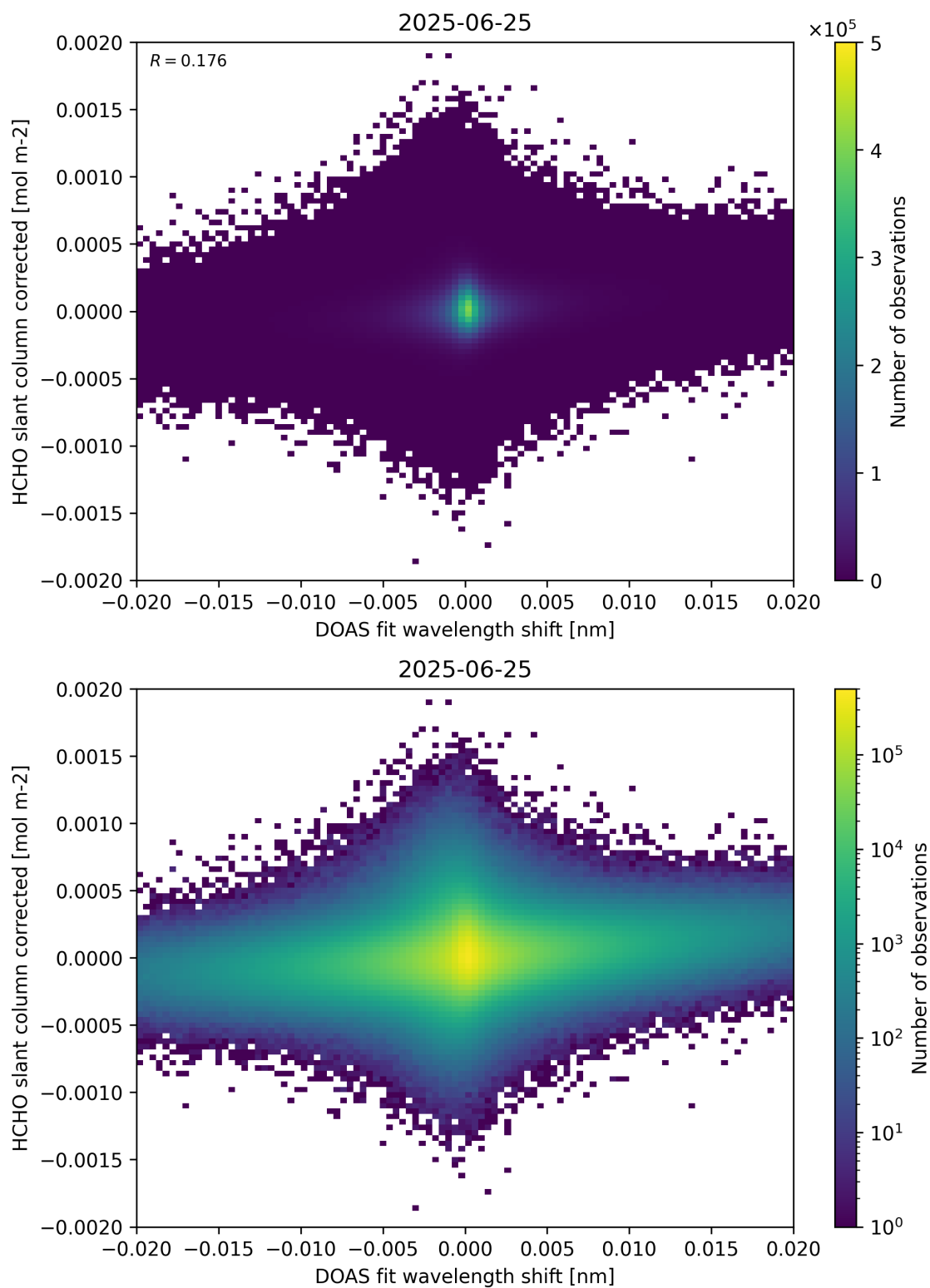
Figure 66: Scatter density plot of “DOAS fit wavelength shift” against “HCHO slant column corrected” for 2025-06-24 to 2025-06-26.
