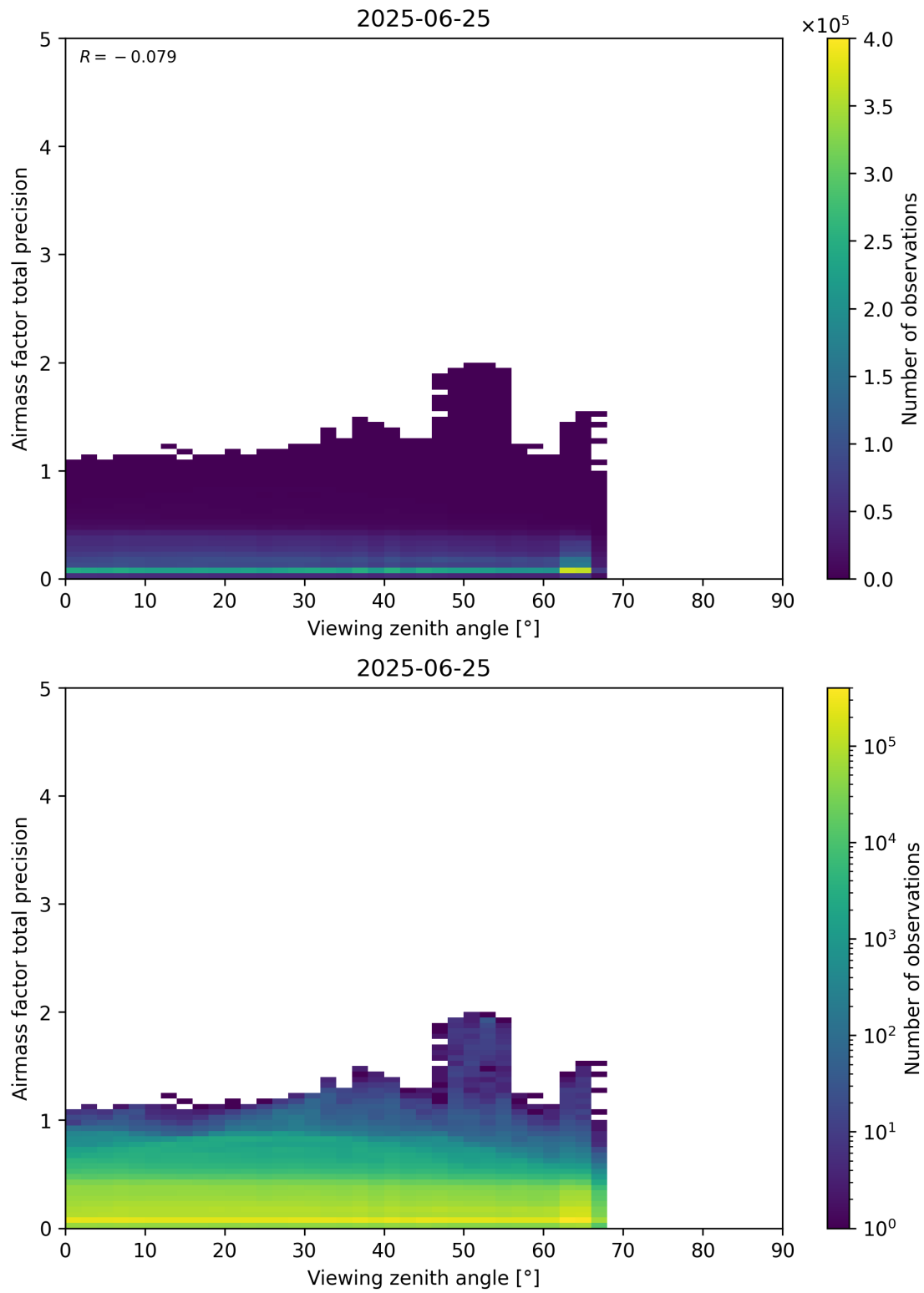
Figure 191: Scatter density plot of “Viewing zenith angle” against “Airmass factor total precision” for 2025-06-24 to 2025-06-26.
