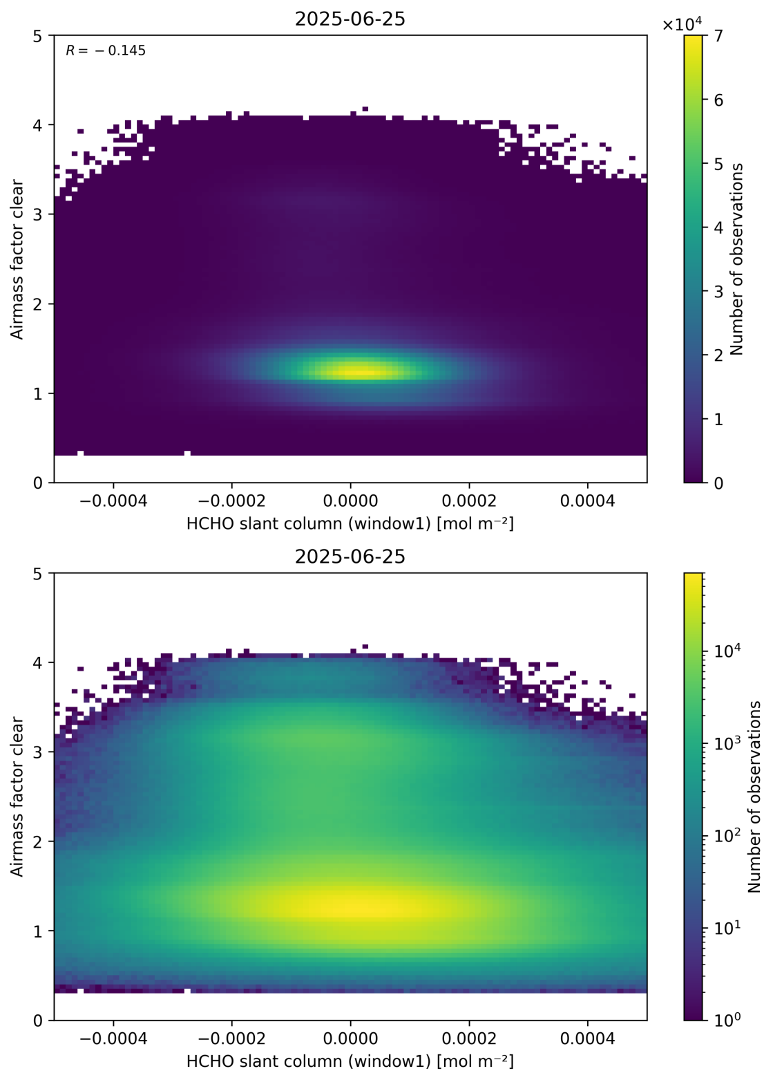
Figure 81: Scatter density plot of “HCHO slant column (window1)” against “Airmass factor clear” for 2025-06-24 to 2025-06-26.
