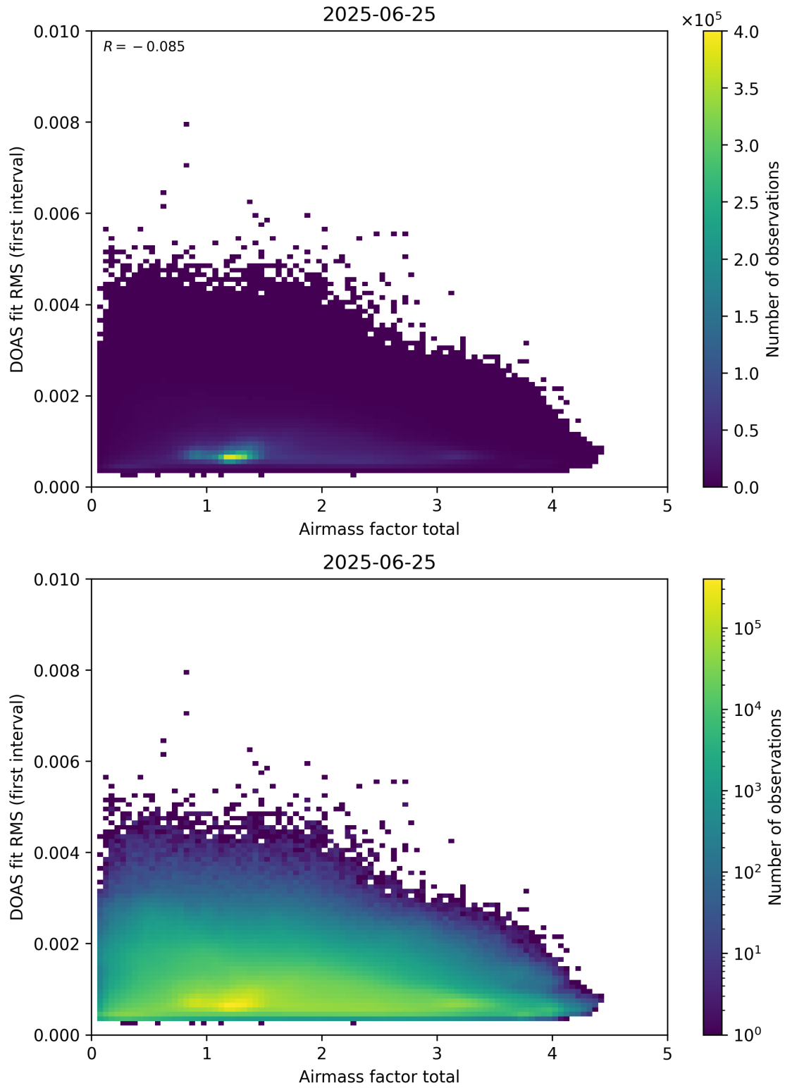
Figure 97: Scatter density plot of “Airmass factor total” against “DOAS fit RMS (first interval)” for 2025-06-24 to 2025-06-26.
