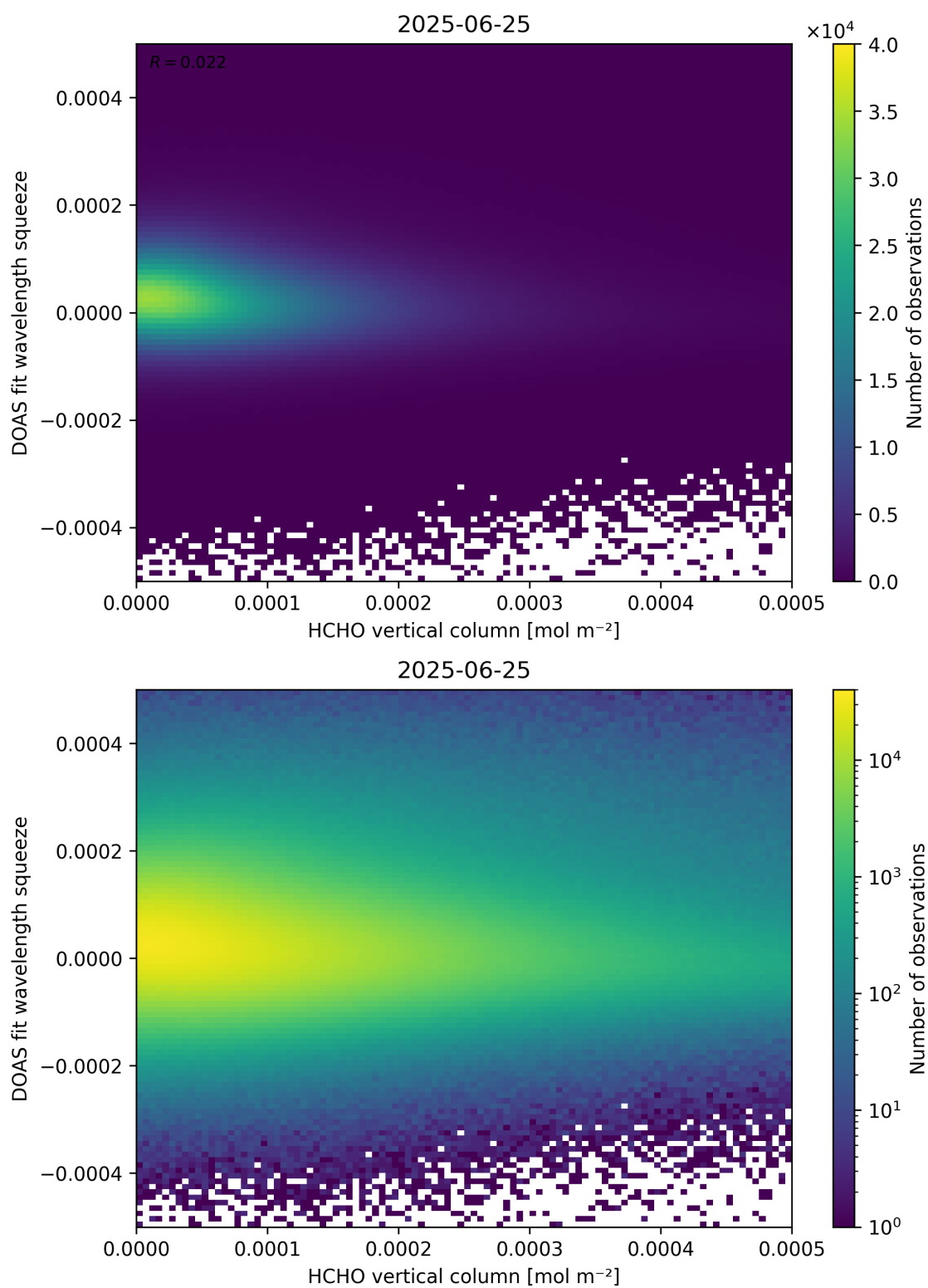
Figure 125: Scatter density plot of “HCHO vertical column” against “DOAS fit wavelength squeeze” for 2025-06-24 to 2025-06-26.
