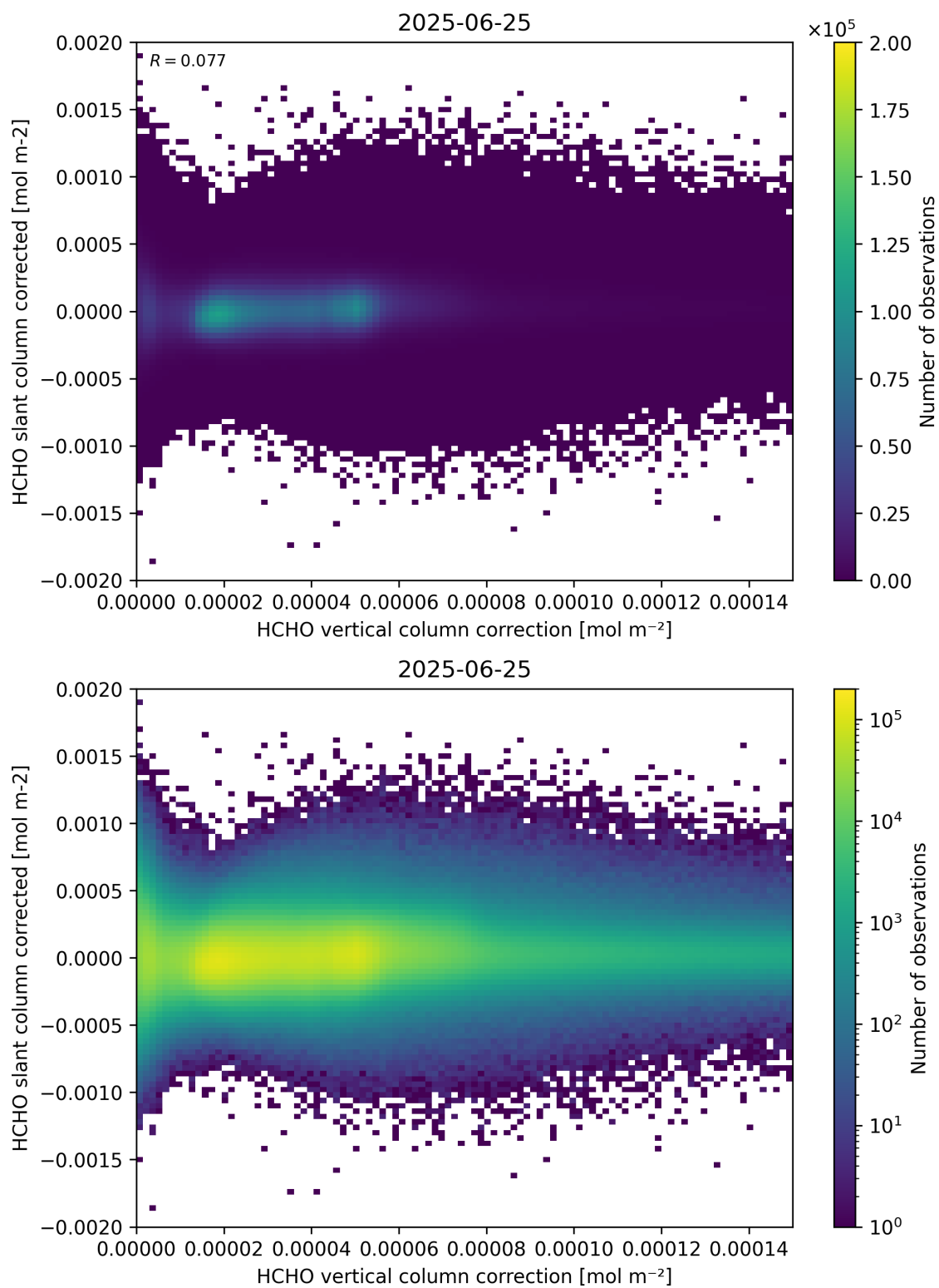
Figure 116: Scatter density plot of “HCHO vertical column correction” against “HCHO slant column corrected” for 2025-06-24 to 2025-06-26.
