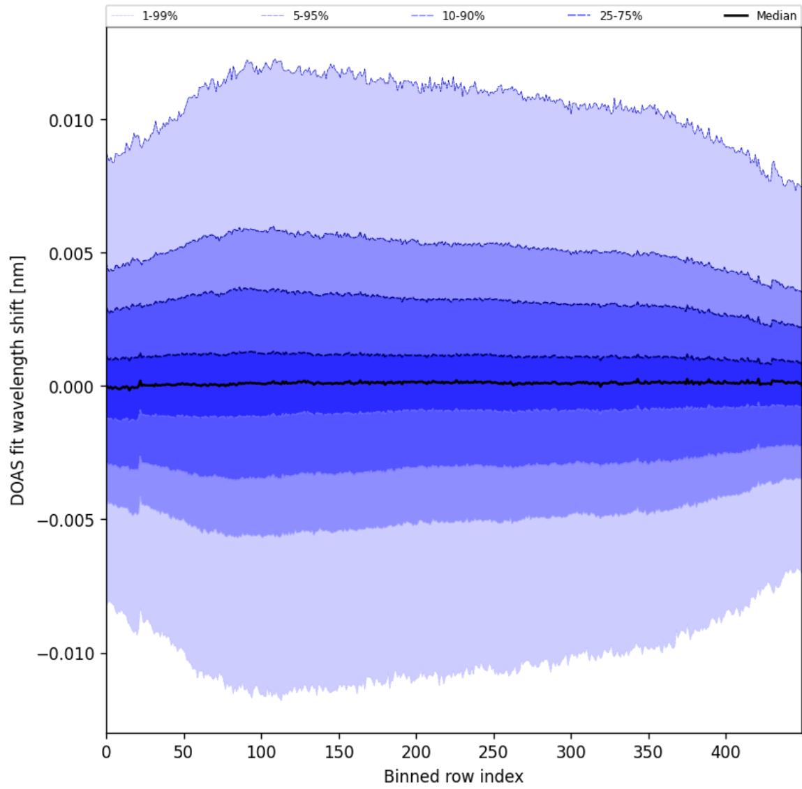
Figure 58: Along track statistics of “DOAS fit wavelength shift” for 2025-06-24 to 2025-06-26
