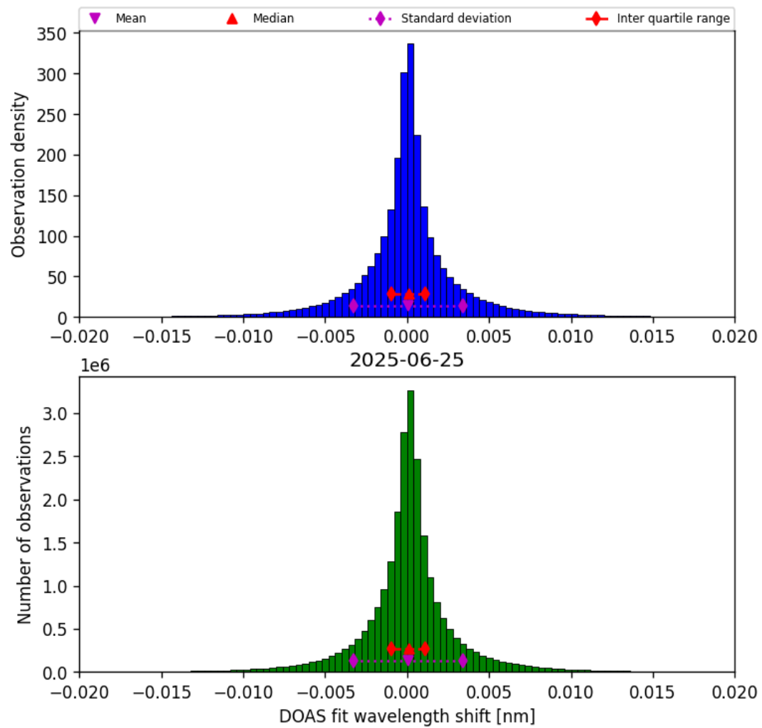
Figure 44: Histogram of “DOAS fit wavelength shift” for 2025-06-24 to 2025-06-26
