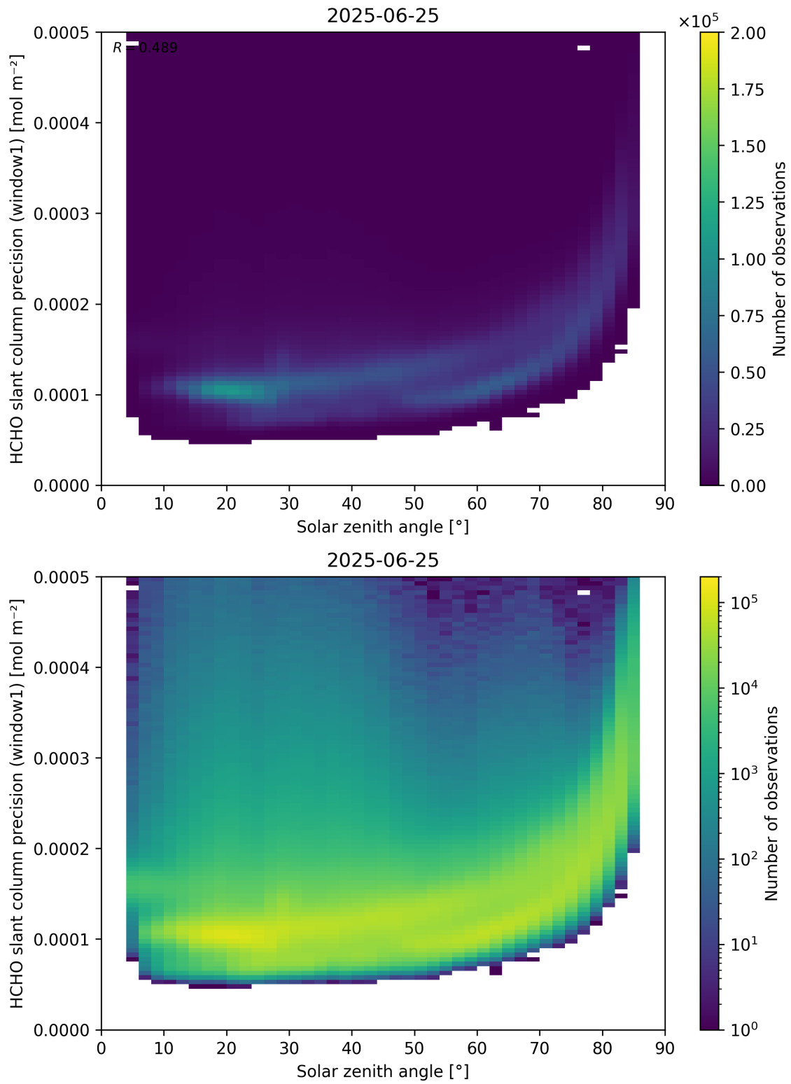
Figure 174: Scatter density plot of “Solar zenith angle” against “HCHO slant column precision (window1)” for 2025-06-24 to 2025-06-26.
