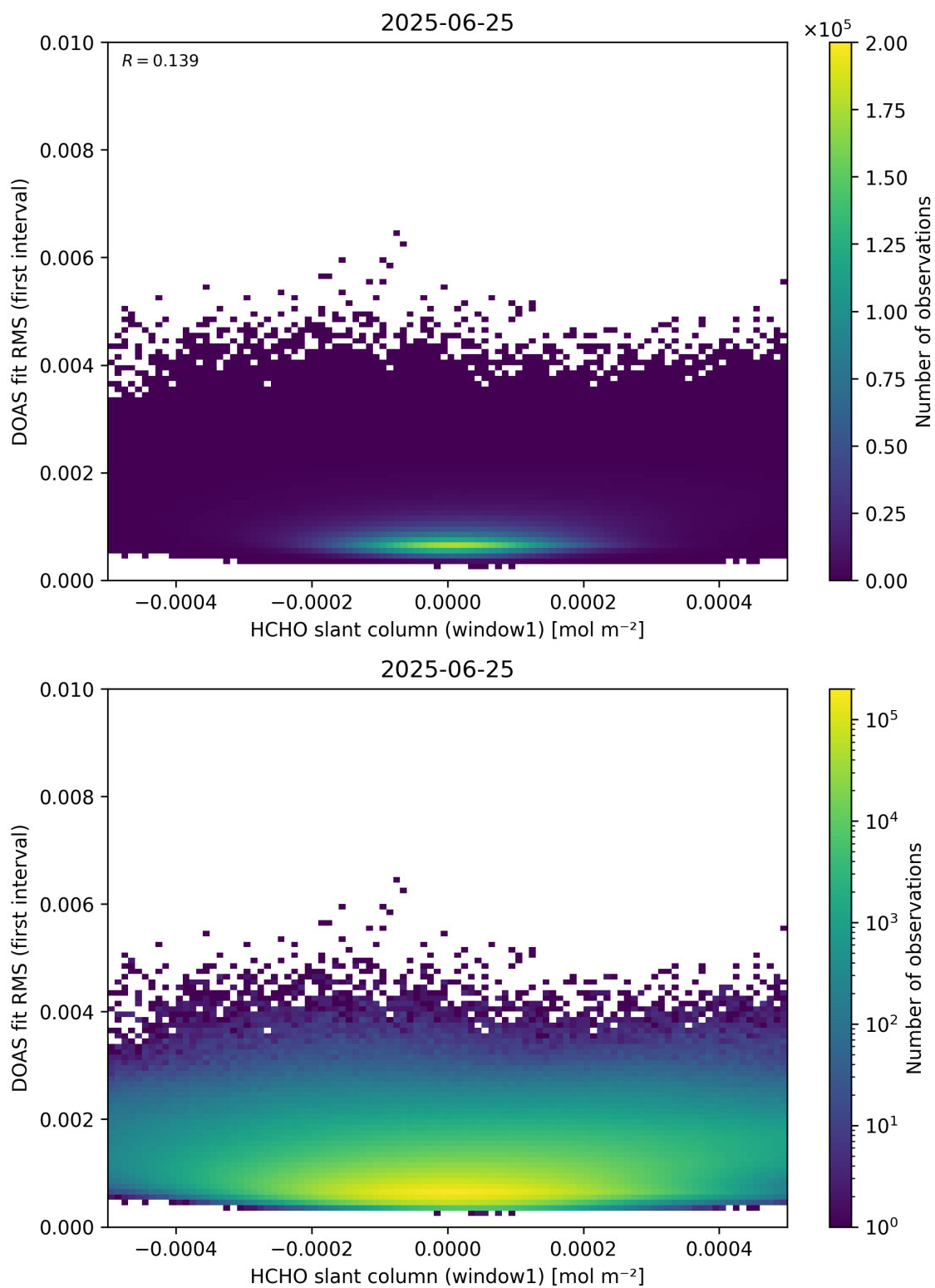
Figure 78: Scatter density plot of “HCHO slant column (window1)” against “DOAS fit RMS (first interval)” for 2025-06-24 to 2025-06-26.
