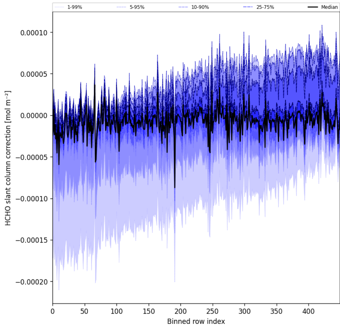
Figure 61: Along track statistics of “HCHO slant column correction” for 2025-06-24 to 2025-06-26
