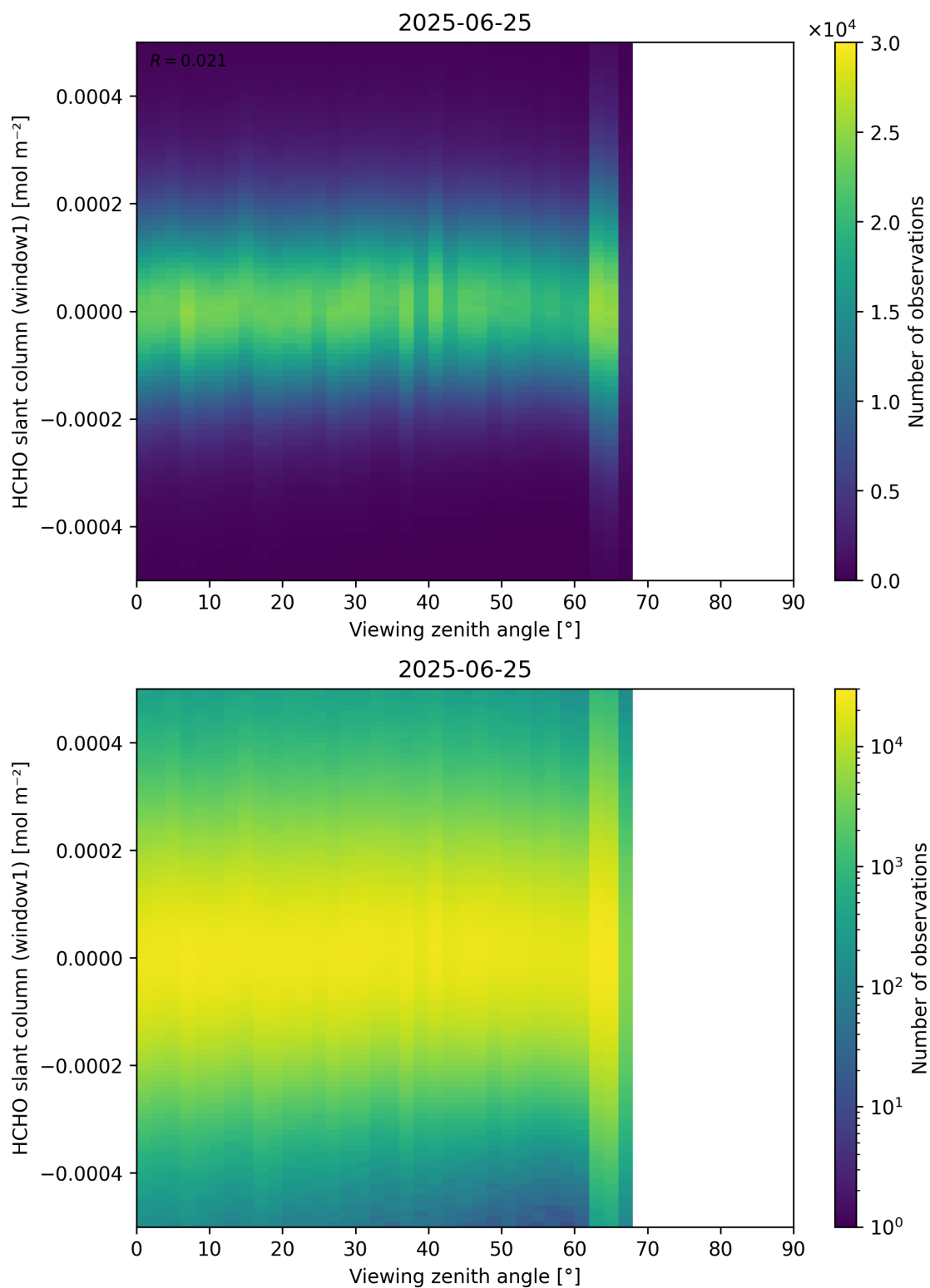
Figure 188: Scatter density plot of “Viewing zenith angle” against “HCHO slant column (window1)” for 2025-06-24 to 2025-06-26.
