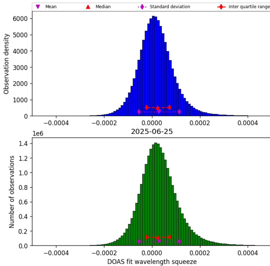
Figure 45: Histogram of “DOAS fit wavelength squeeze” for 2025-06-24 to 2025-06-26
