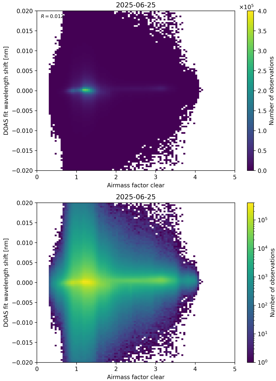
Figure 72: Scatter density plot of “Airmass factor clear” against “DOAS fit wavelength shift” for 2025-06-24 to 2025-06-26.
