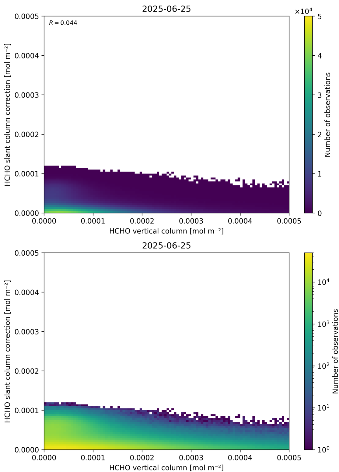
Figure 128: Scatter density plot of “HCHO vertical column” against “HCHO slant column correction” for 2025-06-24 to 2025-06-26.
