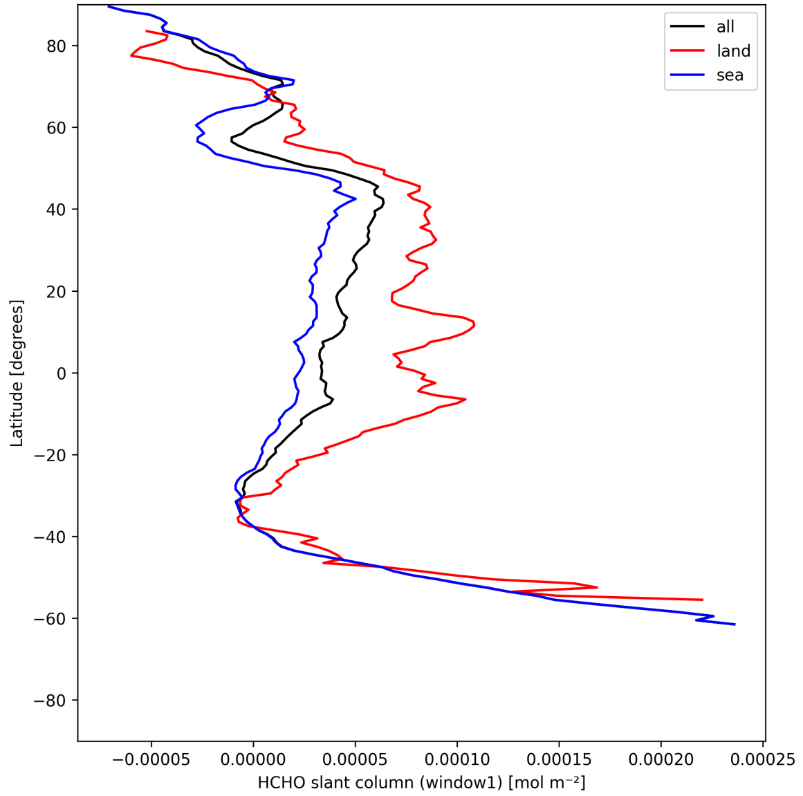
Figure 24: Zonal average of “HCHO slant column (window1)” for 2025-06-24 to 2025-06-26.
