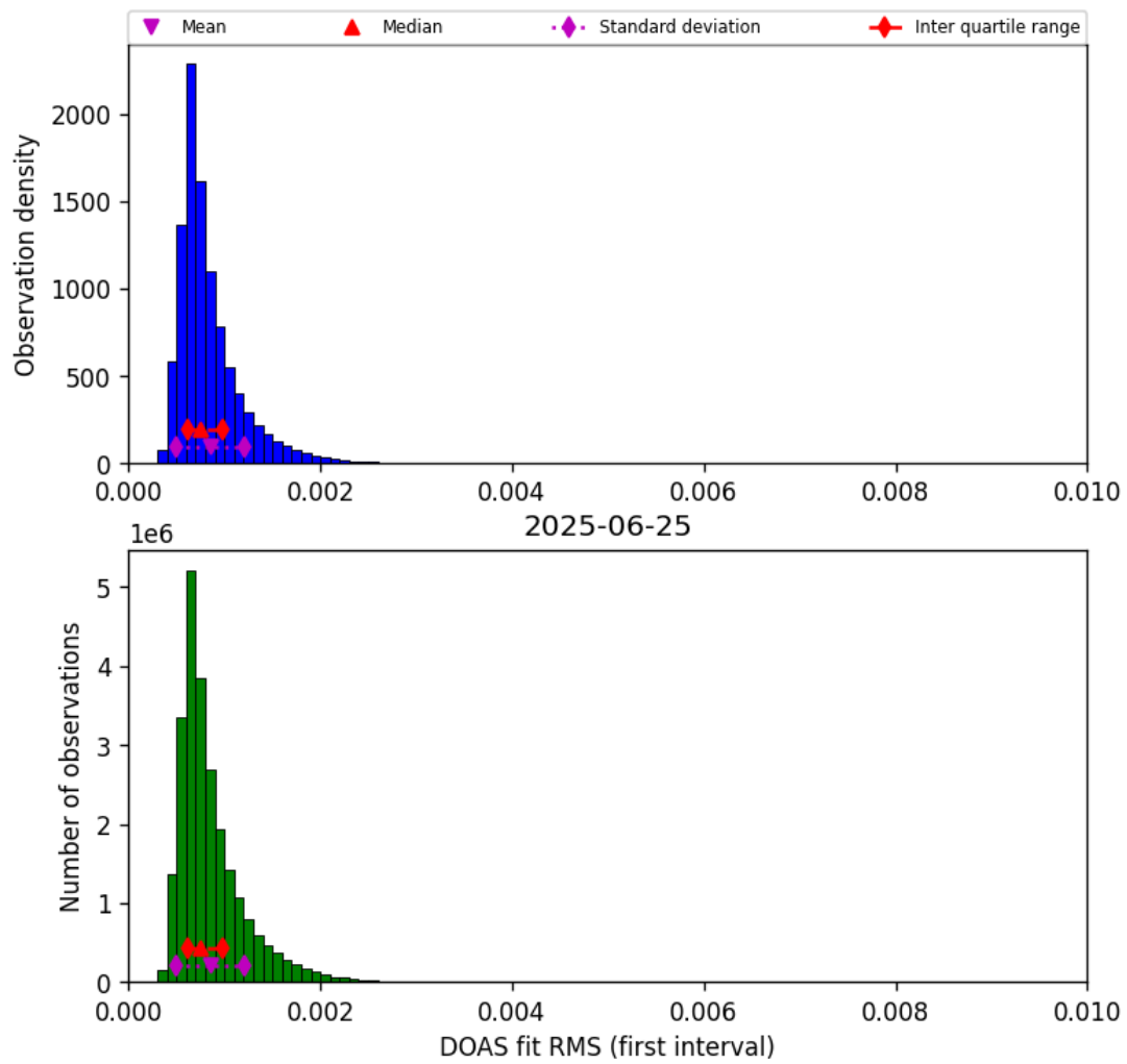
Figure 46: Histogram of “DOAS fit RMS (first interval)” for 2025-06-24 to 2025-06-26
