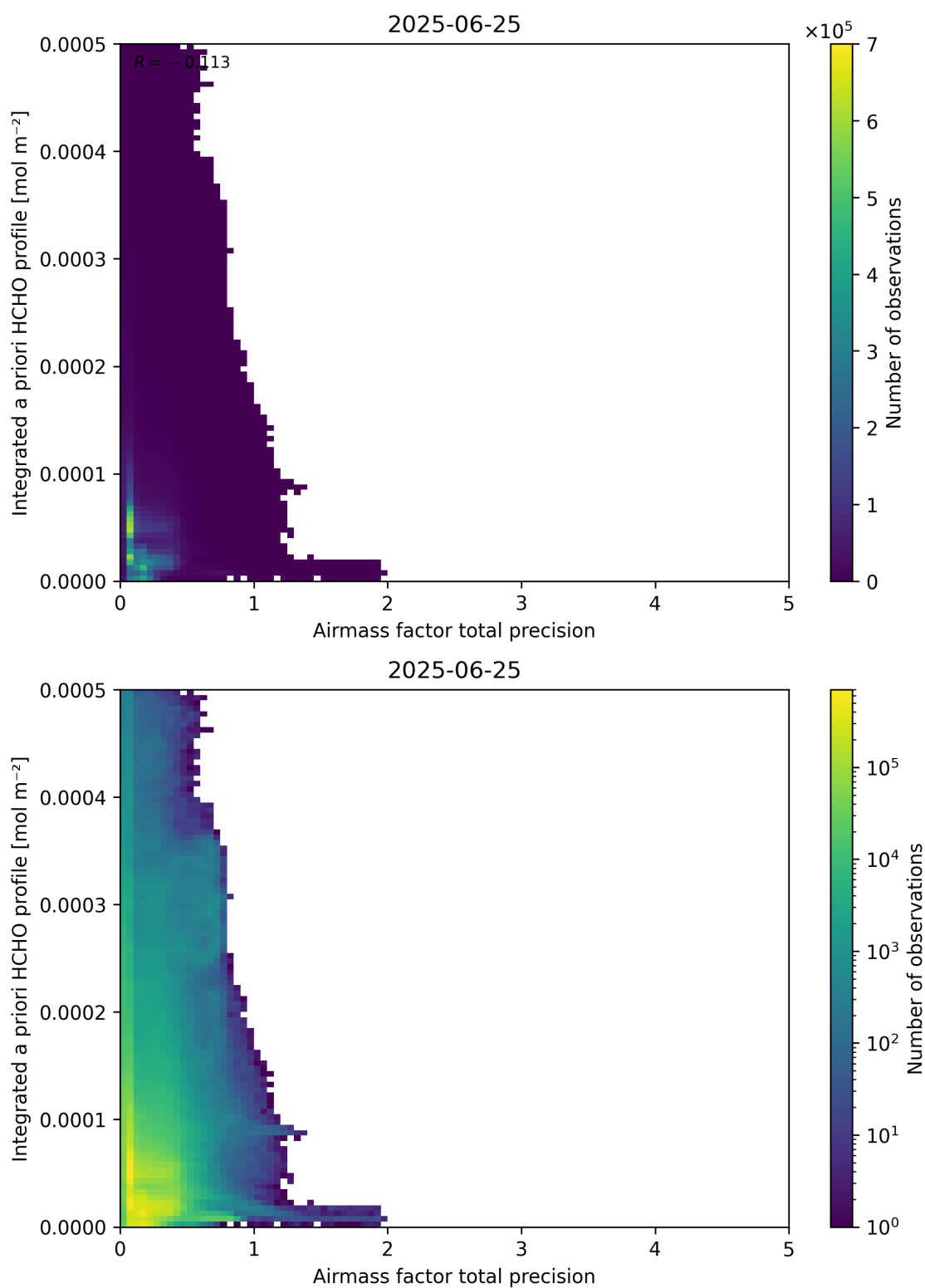
Figure 111: Scatter density plot of “Airmass factor total precision” against “Integrated a priori HCHO profile” for 2025-06-24 to 2025-06-26.
