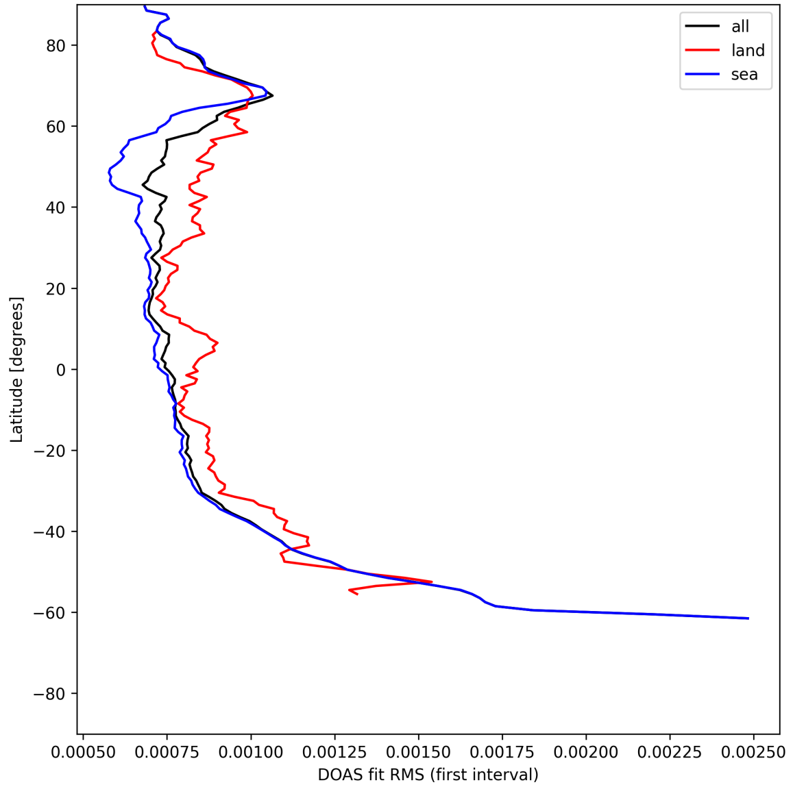
Figure 32: Zonal average of “DOAS fit RMS (first interval)” for 2025-06-24 to 2025-06-26.
