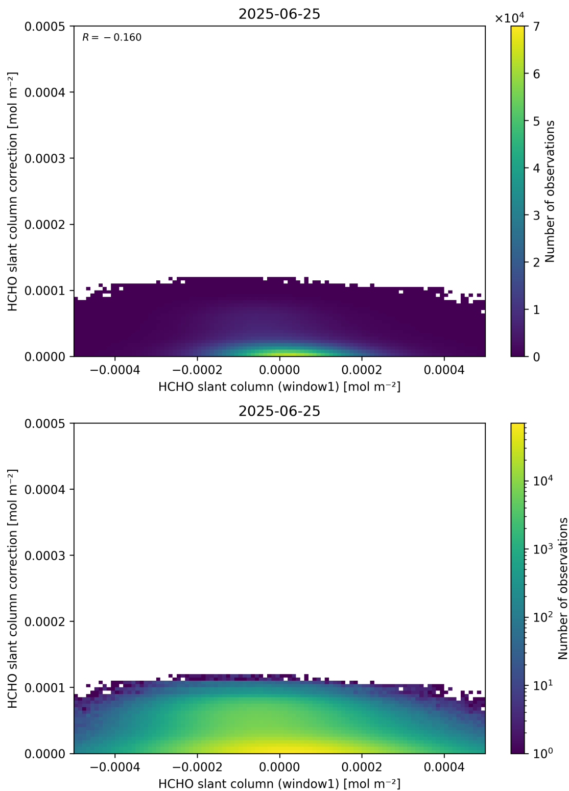
Figure 83: Scatter density plot of “HCHO slant column (window1)” against “HCHO slant column correction” for 2025-06-24 to 2025-06-26.
