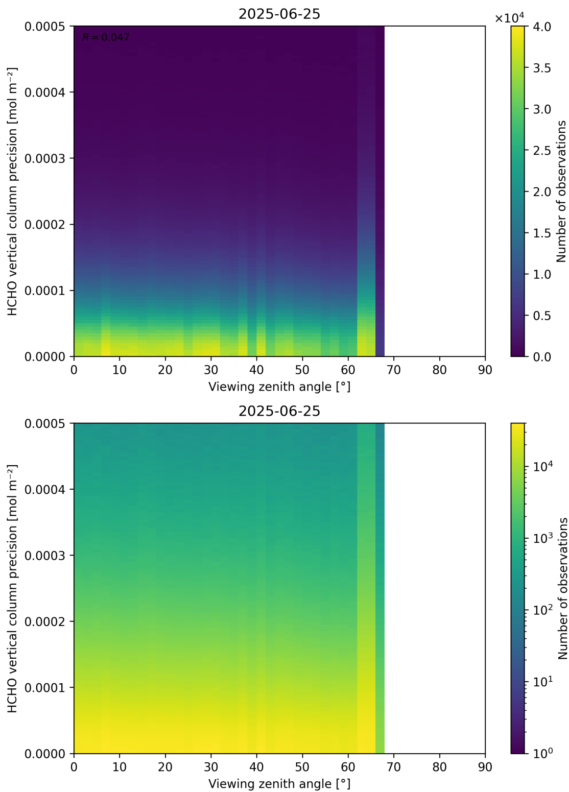
Figure 194: Scatter density plot of “Viewing zenith angle” against “HCHO vertical column precision” for 2025-06-24 to 2025-06-26.
