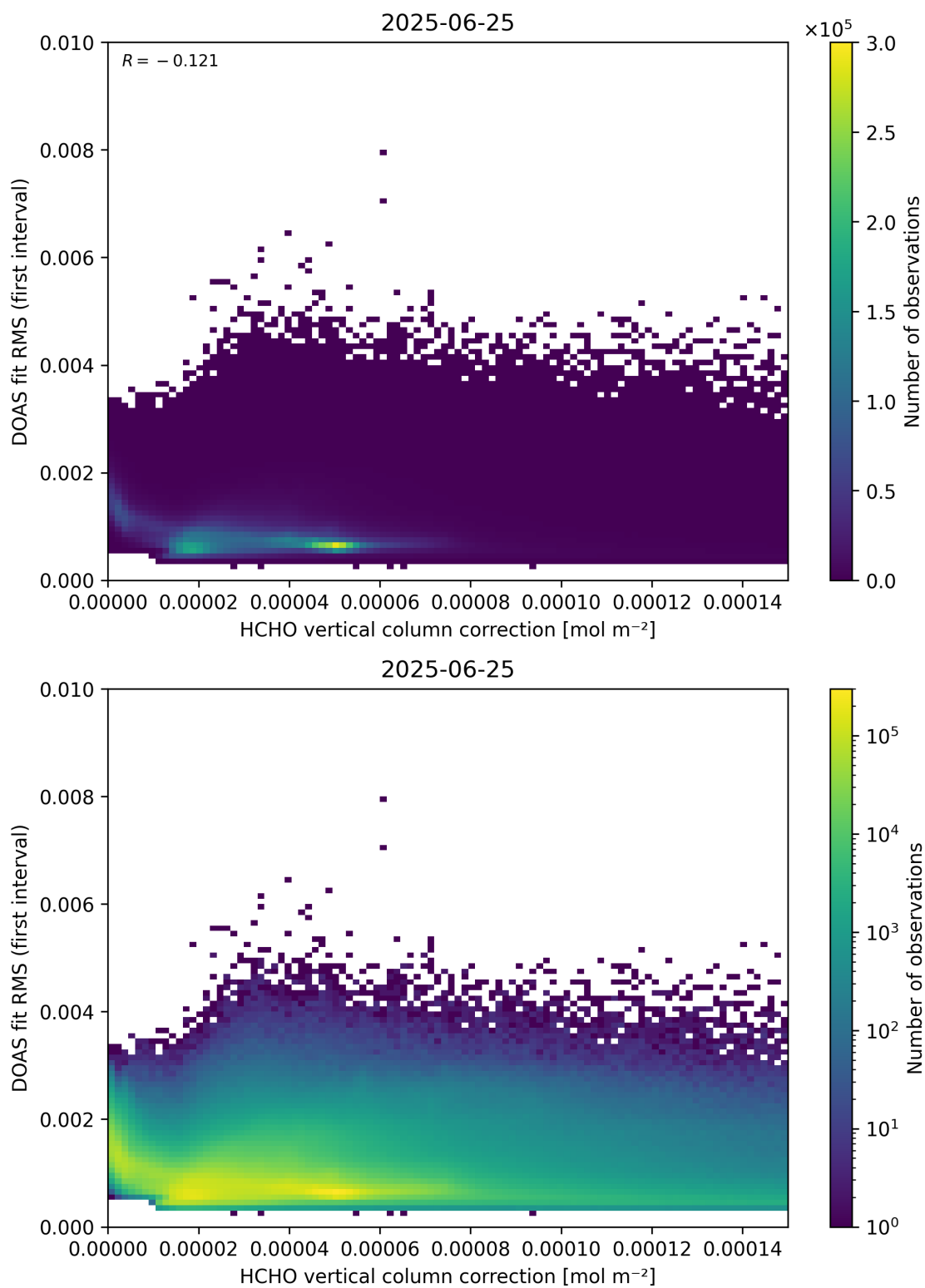
Figure 112: Scatter density plot of “HCHO vertical column correction” against “DOAS fit RMS (first interval)” for 2025-06-24 to 2025-06-26.
