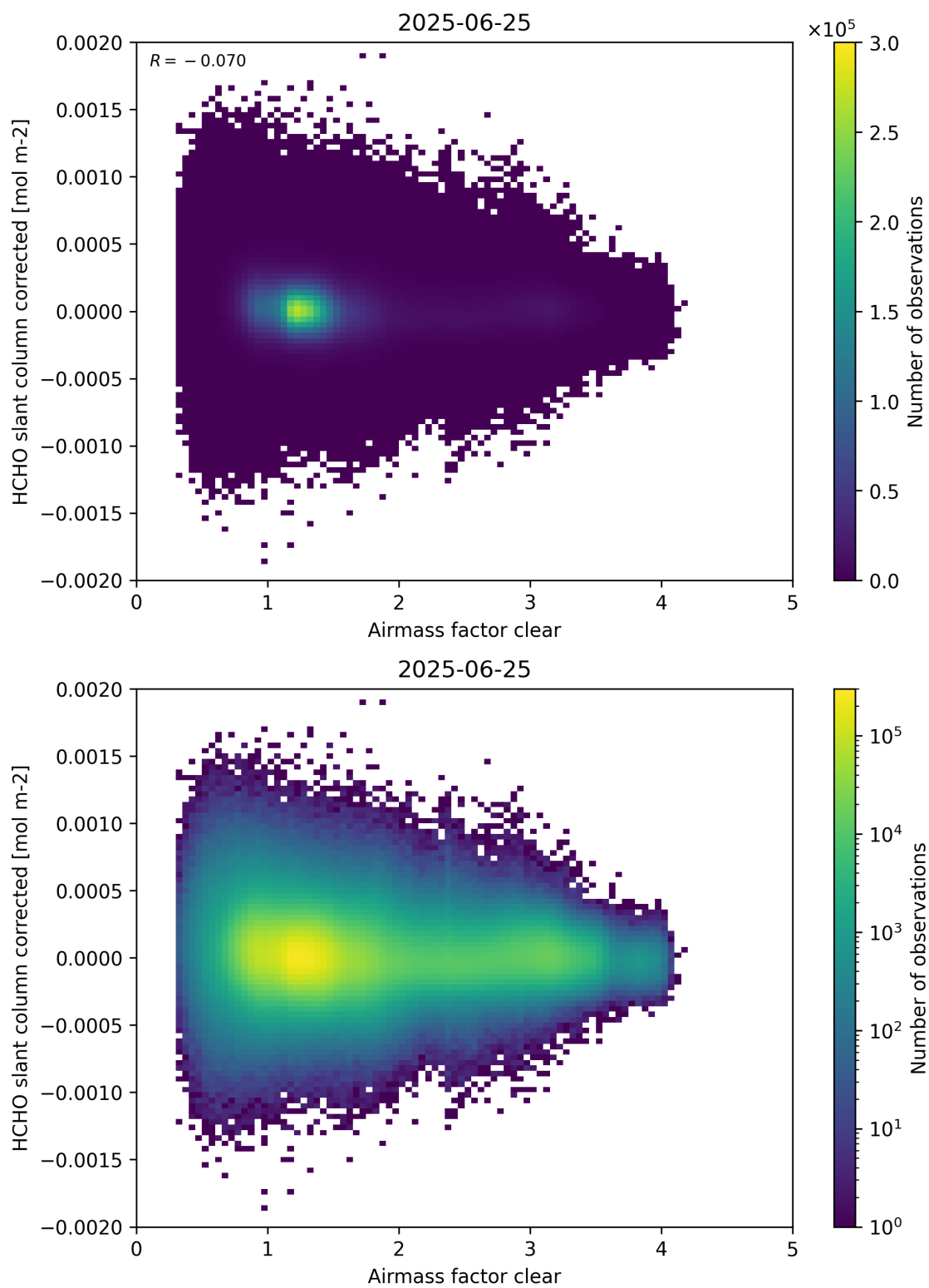
Figure 74: Scatter density plot of “Airmass factor clear” against “HCHO slant column corrected” for 2025-06-24 to 2025-06-26.
