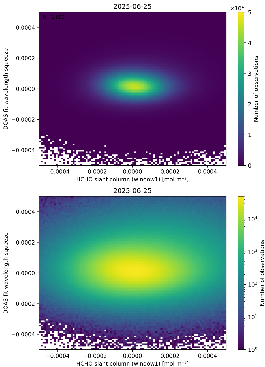
Figure 80: Scatter density plot of “HCHO slant column (window1)” against “DOAS fit wavelength squeeze” for 2025-06-24 to 2025-06-26.
