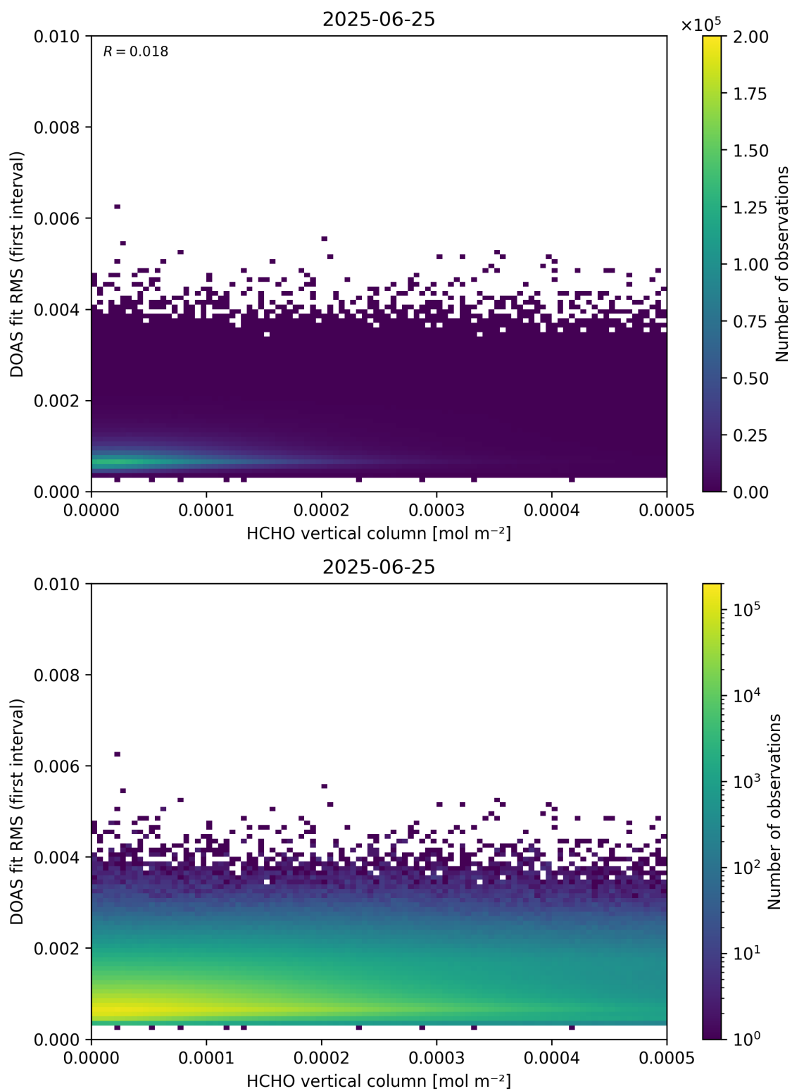
Figure 123: Scatter density plot of “HCHO vertical column” against “DOAS fit RMS (first interval)” for 2025-06-24 to 2025-06-26.
