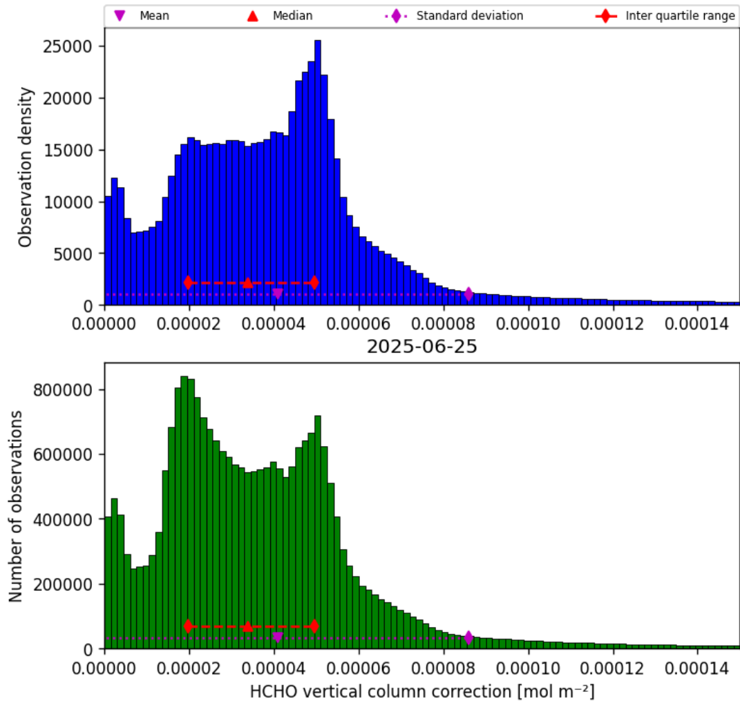
Figure 37: Histogram of “HCHO vertical column correction” for 2025-06-24 to 2025-06-26
