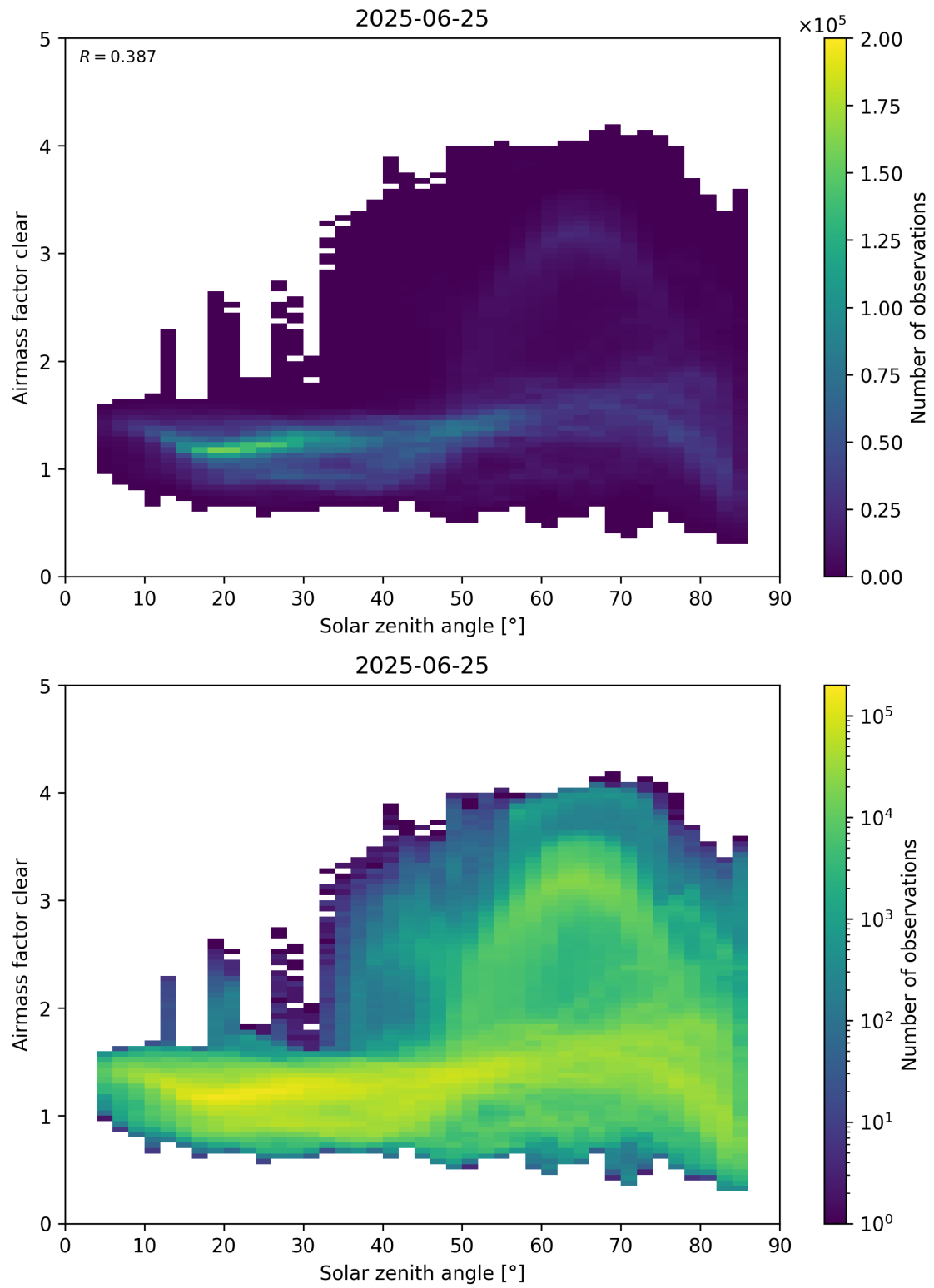
Figure 170: Scatter density plot of “Solar zenith angle” against “Airmass factor clear” for 2025-06-24 to 2025-06-26.
