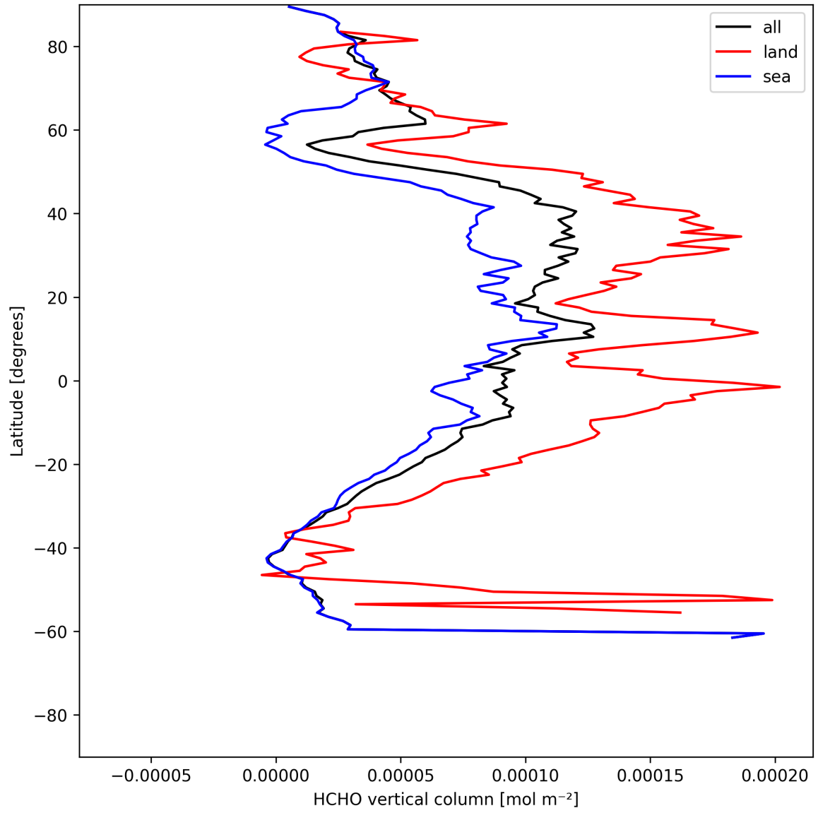
Figure 21: Zonal average of “HCHO vertical column” for 2025-06-24 to 2025-06-26.
