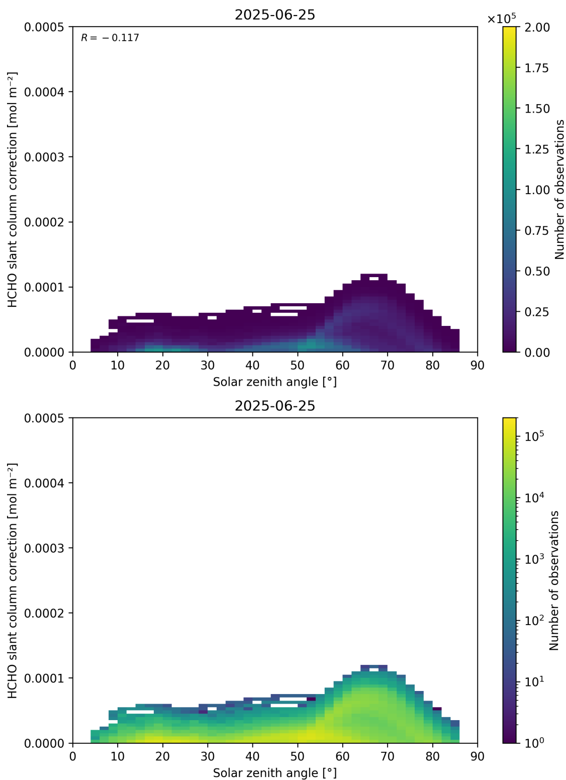
Figure 172: Scatter density plot of “Solar zenith angle” against “HCHO slant column correction” for 2025-06-24 to 2025-06-26.
