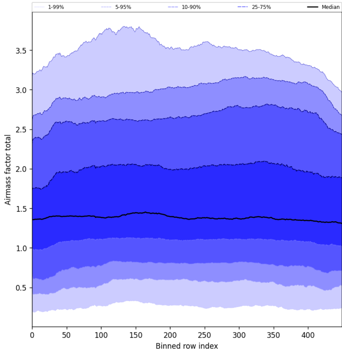
Figure 54: Along track statistics of “Airmass factor total” for 2025-06-24 to 2025-06-26
