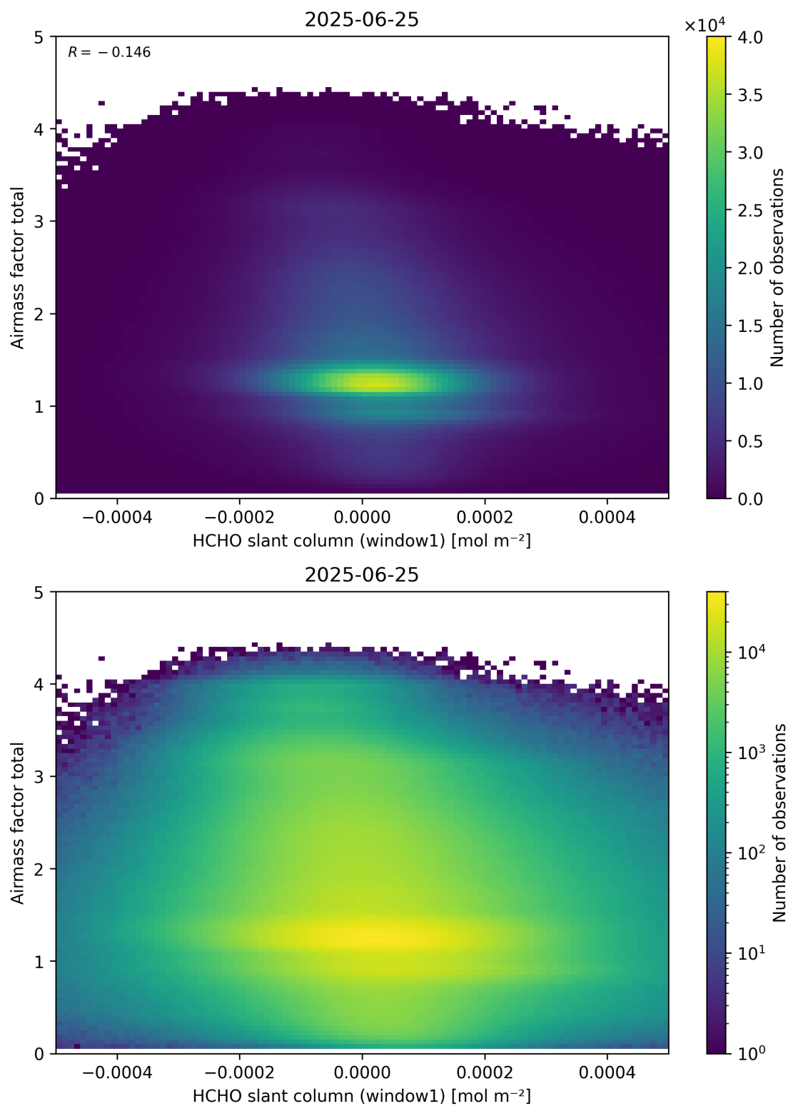
Figure 85: Scatter density plot of “HCHO slant column (window1)” against “Airmass factor total” for 2025-06-24 to 2025-06-26.
