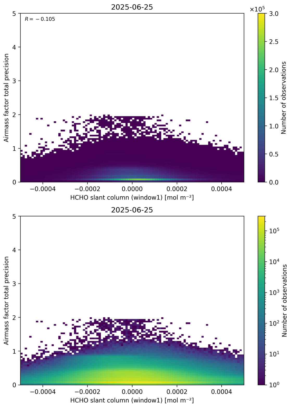
Figure 86: Scatter density plot of “HCHO slant column (window1)” against “Airmass factor total precision” for 2025-06-24 to 2025-06-26.
