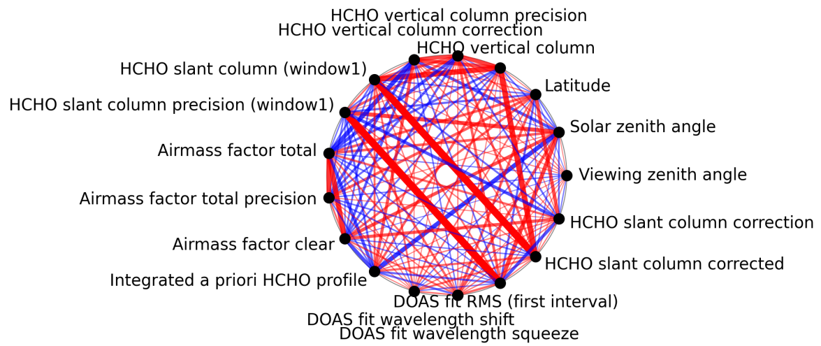
Figure 1: Map of correlation graph for 2025-06-24 to 2025-06-26.
