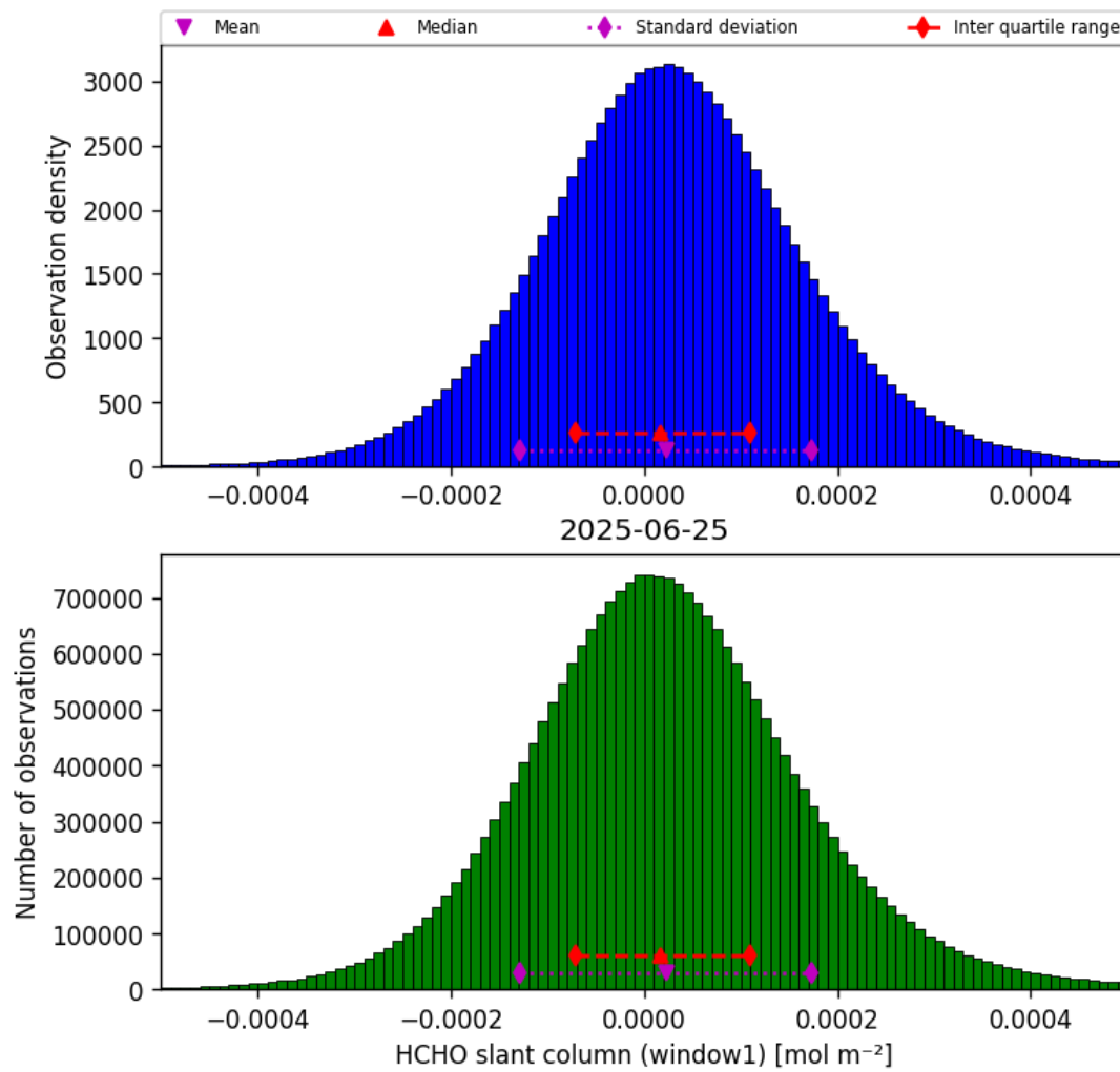
Figure 38: Histogram of “HCHO slant column (window1)” for 2025-06-24 to 2025-06-26
