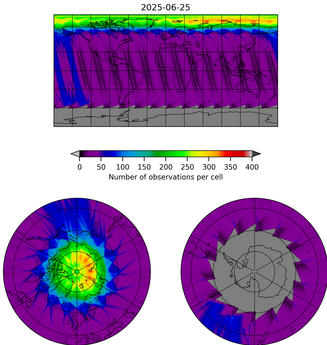
Figure 19: Map of the number of observations for 2025-06-24 to 2025-06-26
