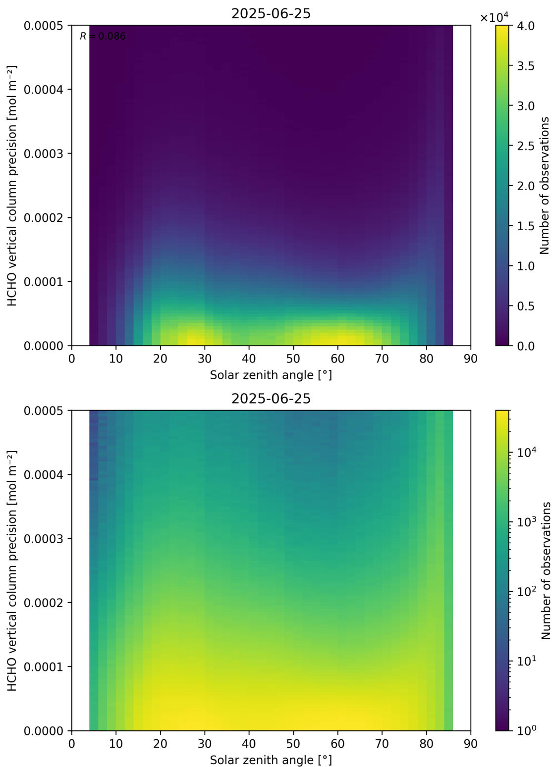
Figure 179: Scatter density plot of “Solar zenith angle” against “HCHO vertical column precision” for 2025-06-24 to 2025-06-26.
