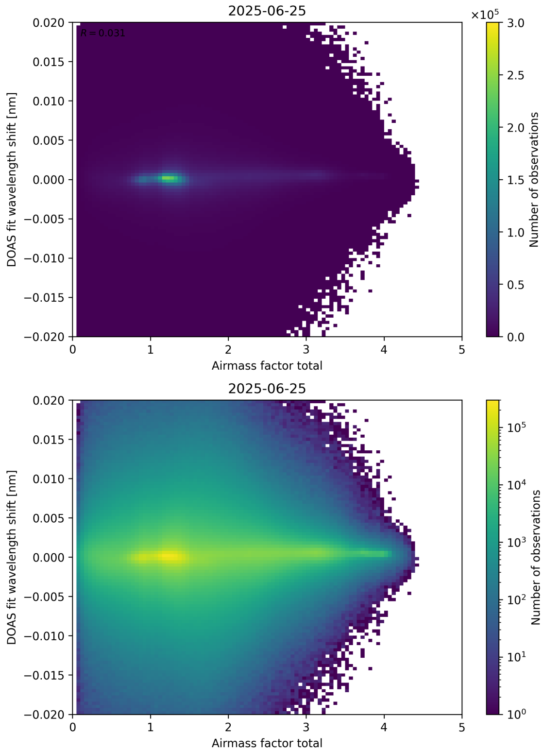
Figure 98: Scatter density plot of “Airmass factor total” against “DOAS fit wavelength shift” for 2025-06-24 to 2025-06-26.
