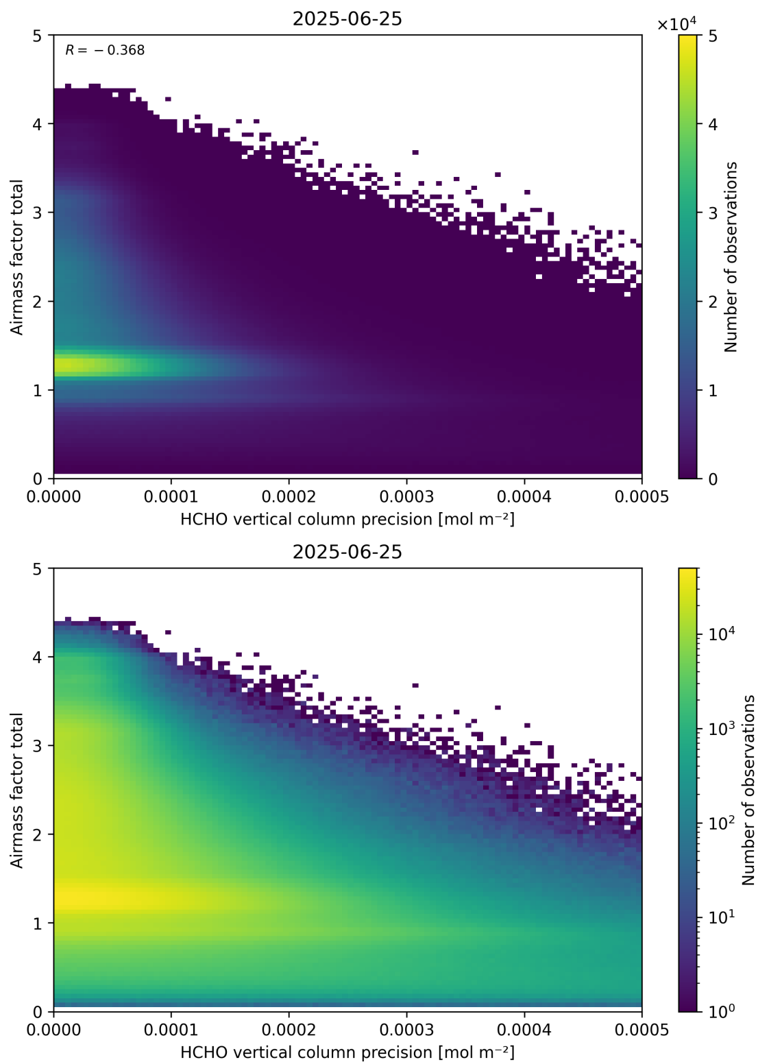
Figure 144: Scatter density plot of “HCHO vertical column precision” against “Airmass factor total” for 2025-06-24 to 2025-06-26.
