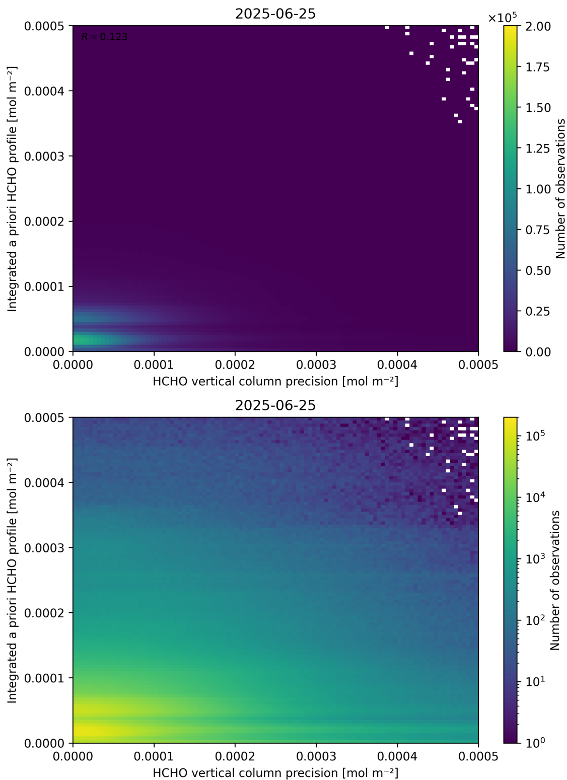
Figure 147: Scatter density plot of “HCHO vertical column precision” against “Integrated a priori HCHO profile” for 2025-06-24 to 2025-06-26.
