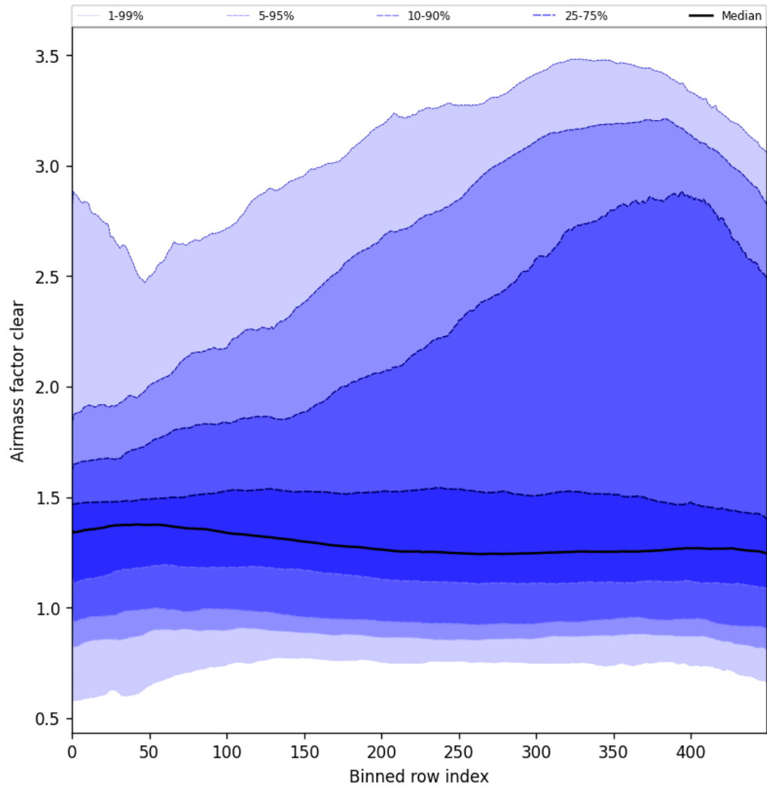
Figure 56: Along track statistics of “Air mass factor clear” for 2025-06-24 to 2025-06-26
