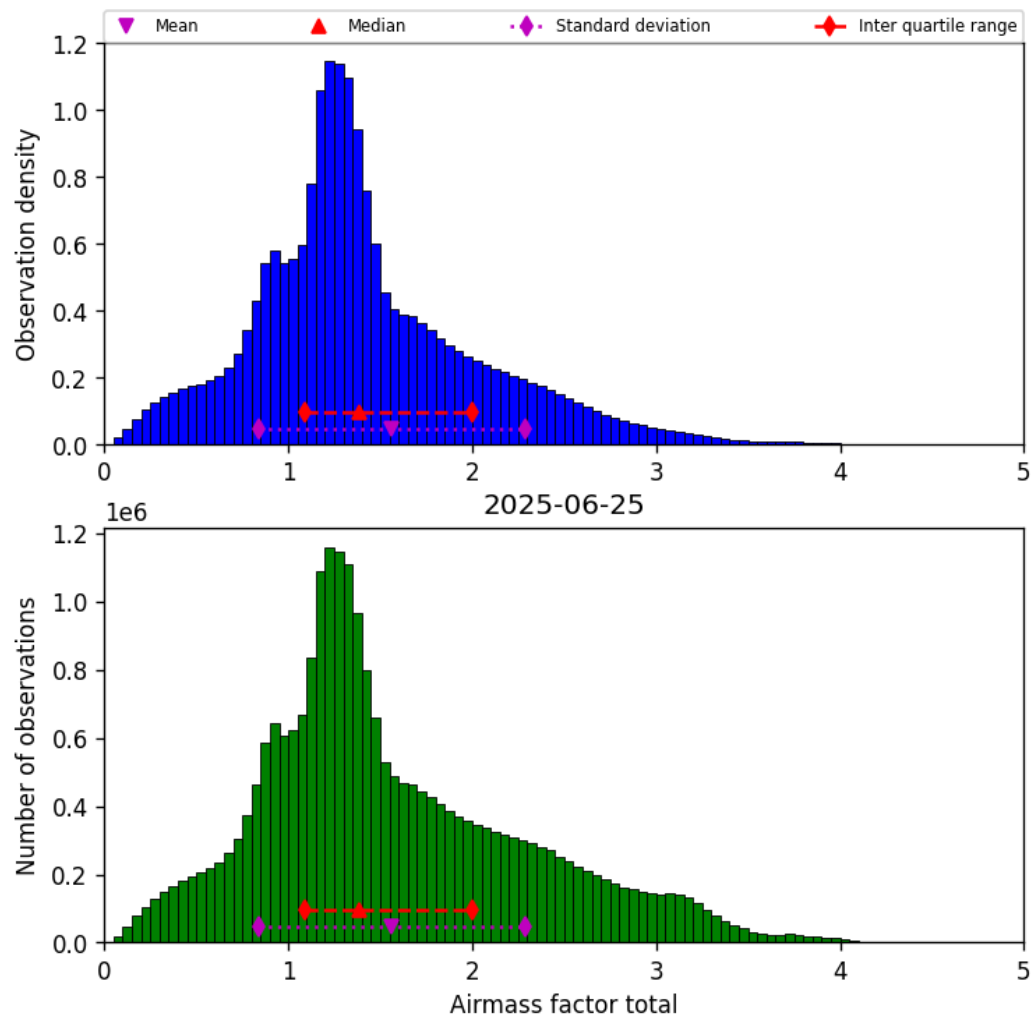
Figure 40: Histogram of “Airmass factor total” for 2025-06-24 to 2025-06-26
