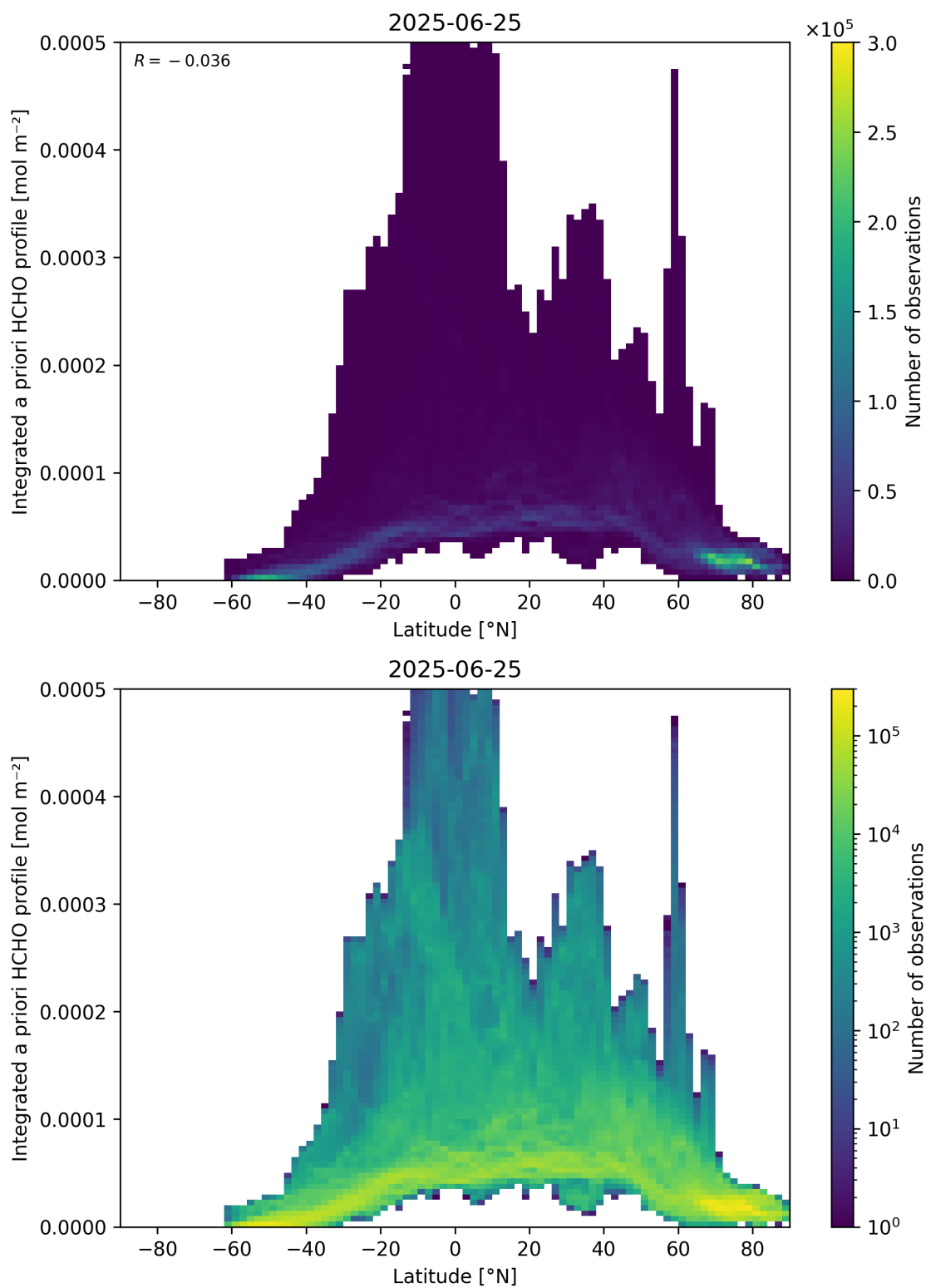
Figure 166: Scatter density plot of “Latitude” against “Integrated a priori HCHO profile” for 2025-06-24 to 2025-06-26.
