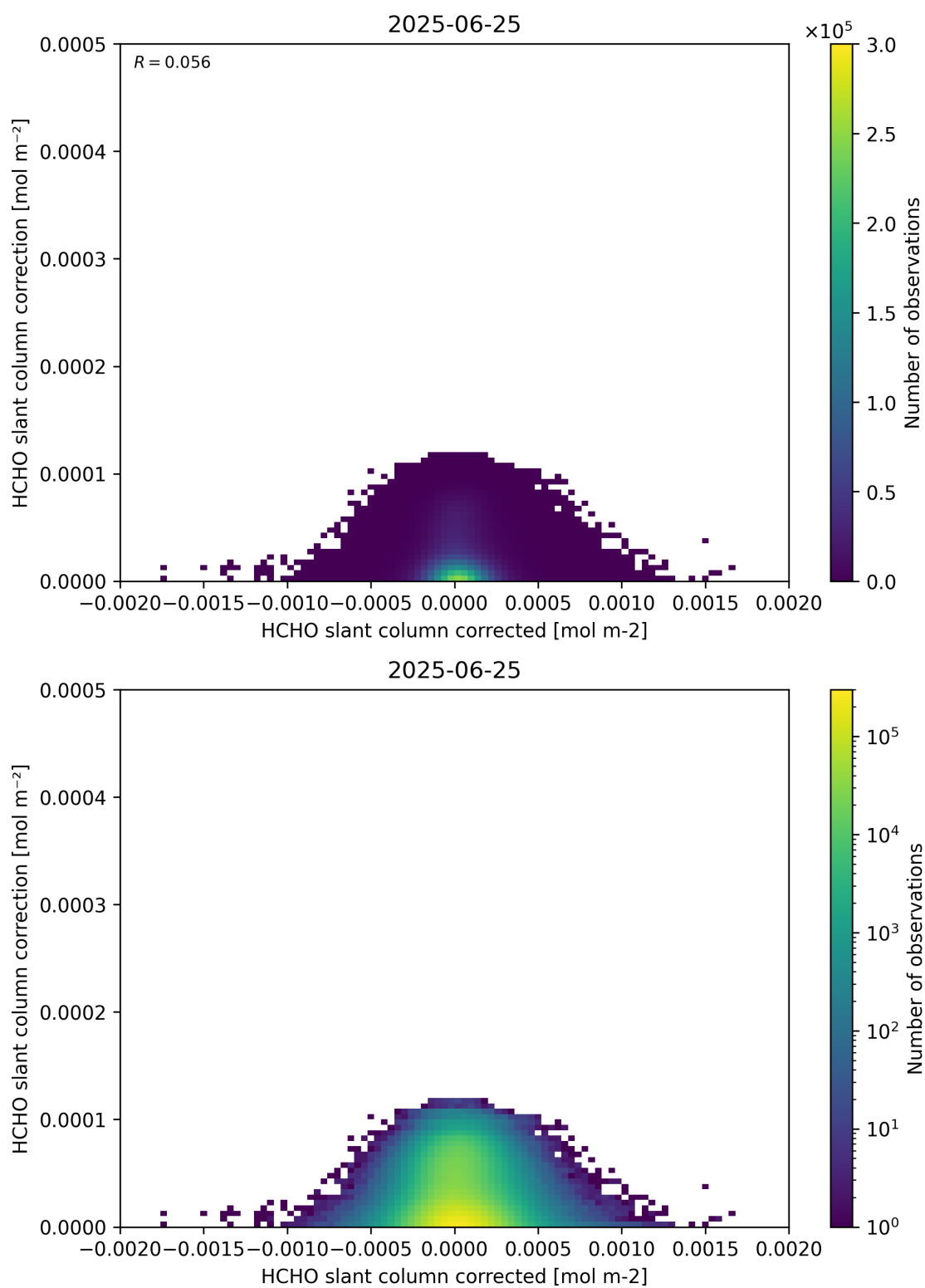
Figure 77: Scatter density plot of “HCHO slant column corrected” against “HCHO slant column correction” for 2025-06-24 to 2025-06-26.
