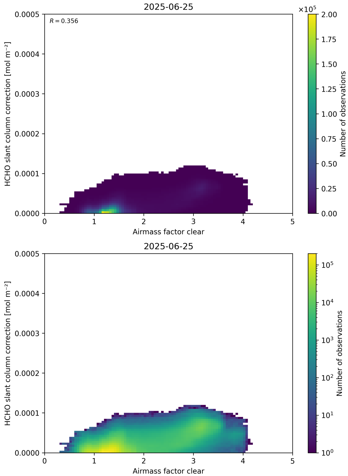
Figure 75: Scatter density plot of “Airmass factor clear” against “HCHO slant column correction” for 2025-06-24 to 2025-06-26.
