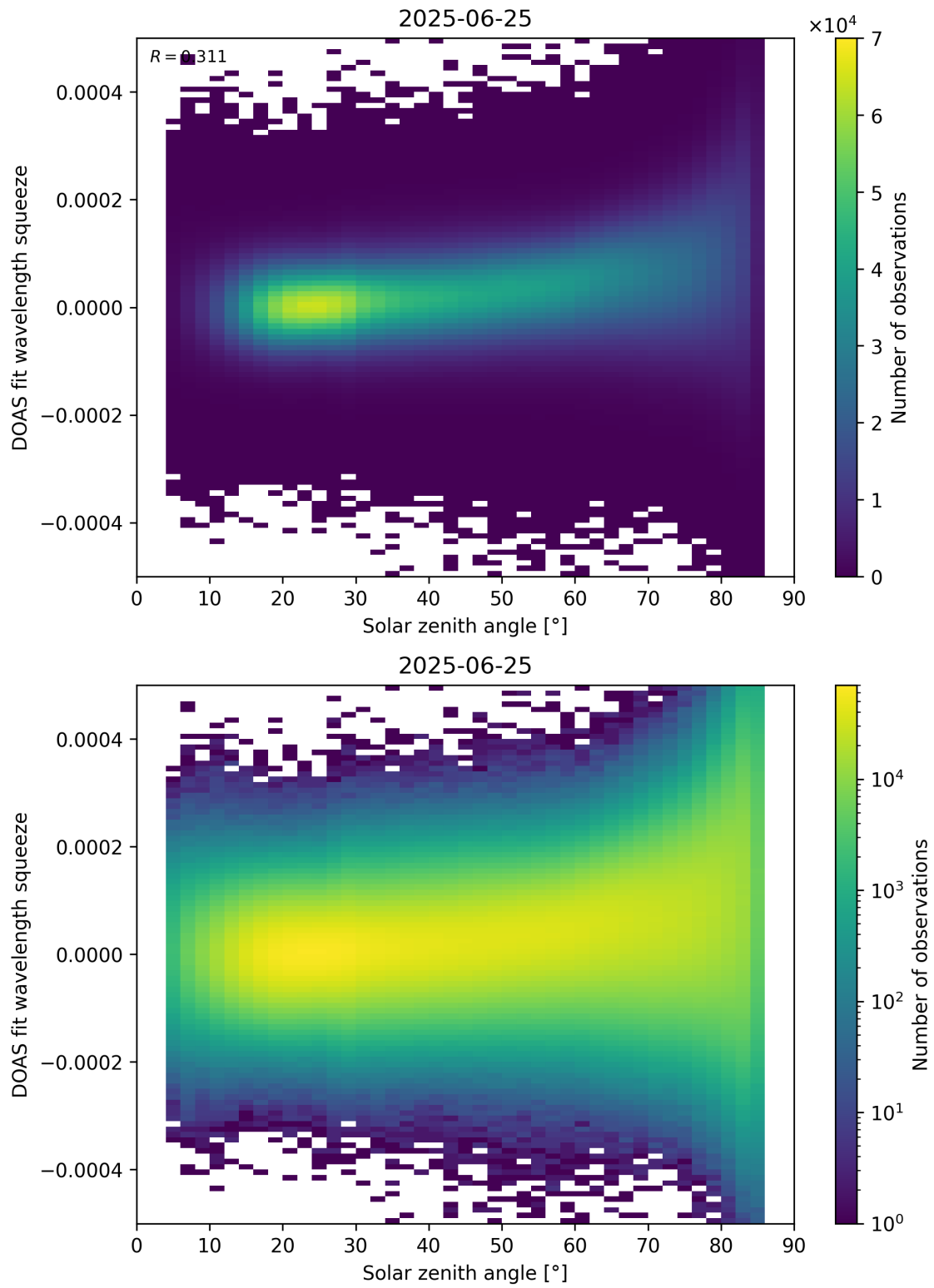
Figure 169: Scatter density plot of “Solar zenith angle” against “DOAS fit wavelength squeeze” for 2025-06-24 to 2025-06-26.
