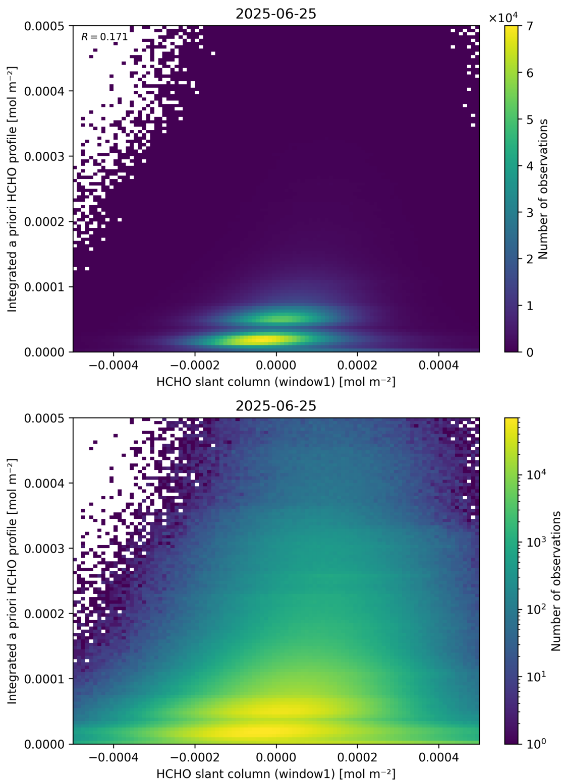
Figure 87: Scatter density plot of “HCHO slant column (window1)” against “Integrated a priori HCHO profile” for 2025-06-24 to 2025-06-26.
