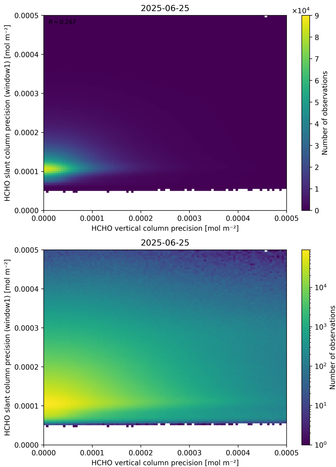
Figure 143: Scatter density plot of “HCHO vertical column precision” against “HCHO slant column precision (window1)” for 2025-06-24 to 2025-06-26.
