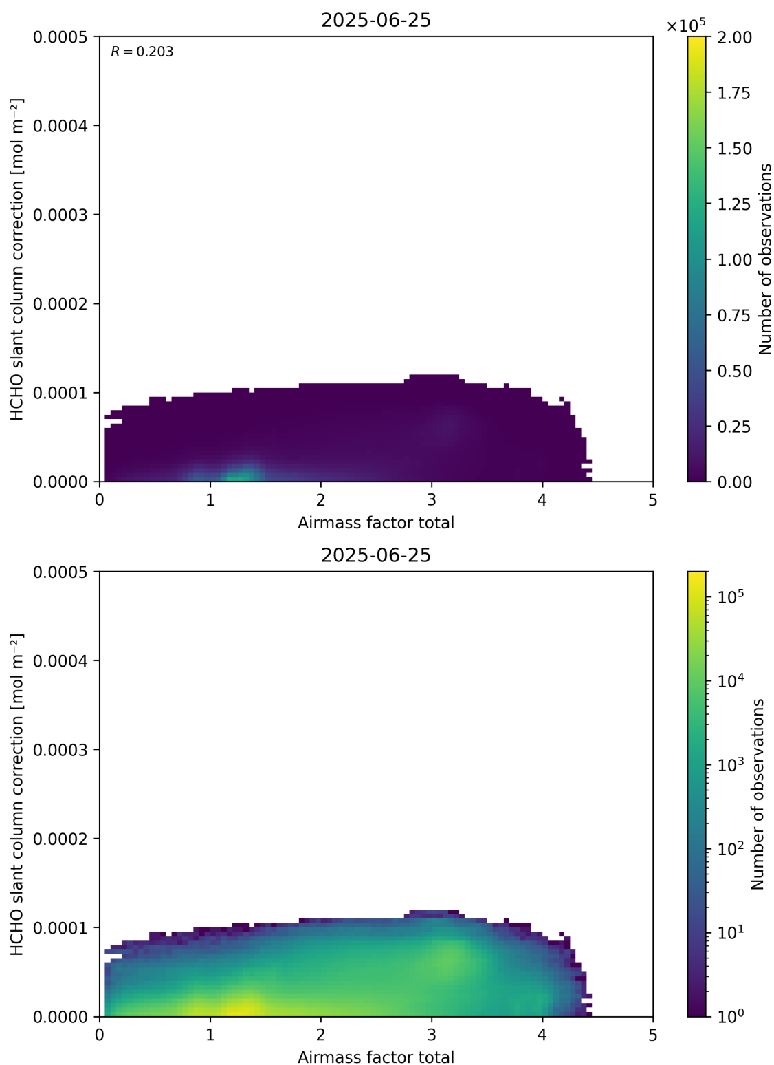
Figure 102: Scatter density plot of “Airmass factor total” against “HCHO slant column correction” for 2025-06-24 to 2025-06-26.
