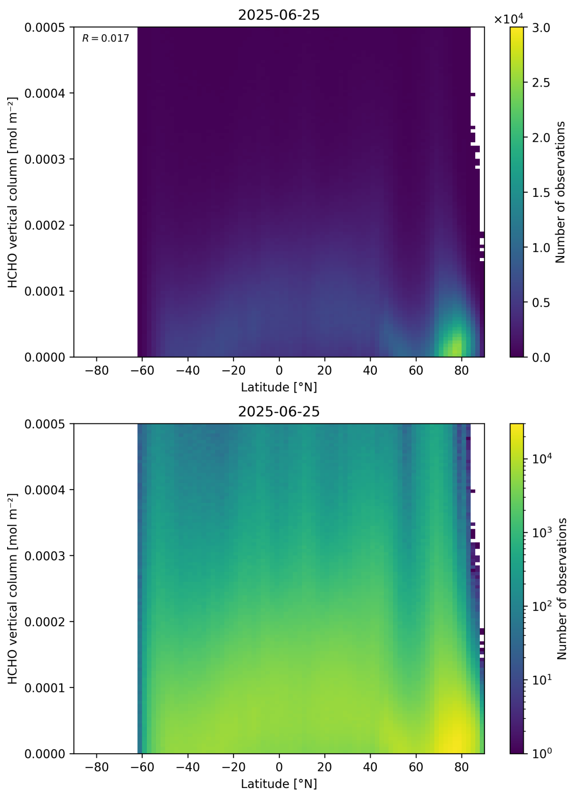
Figure 163: Scatter density plot of “Latitude” against “HCHO vertical column” for 2025-06-24 to 2025-06-26.
