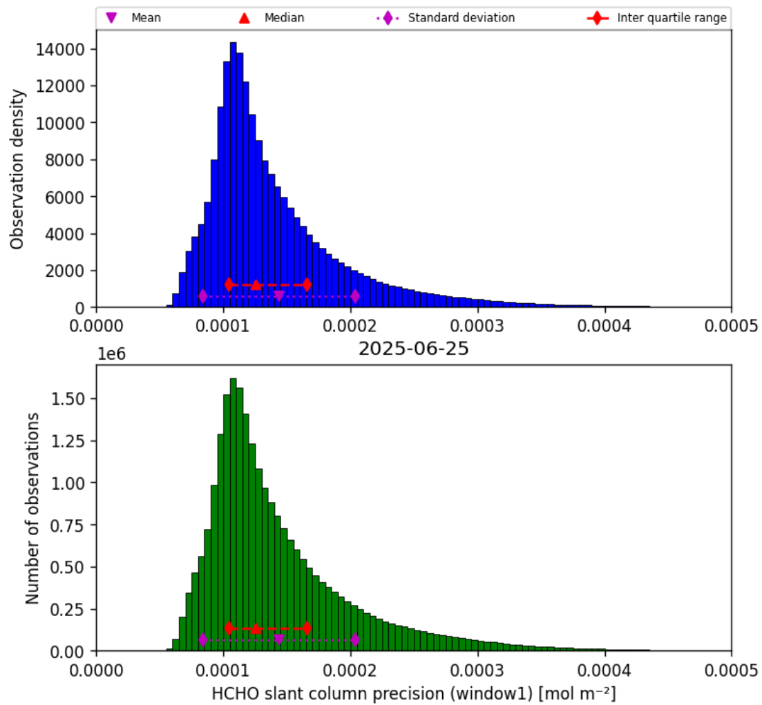
Figure 39: Histogram of “HCHO slant column precision (window1)” for 2025-06-24 to 2025-06-26
