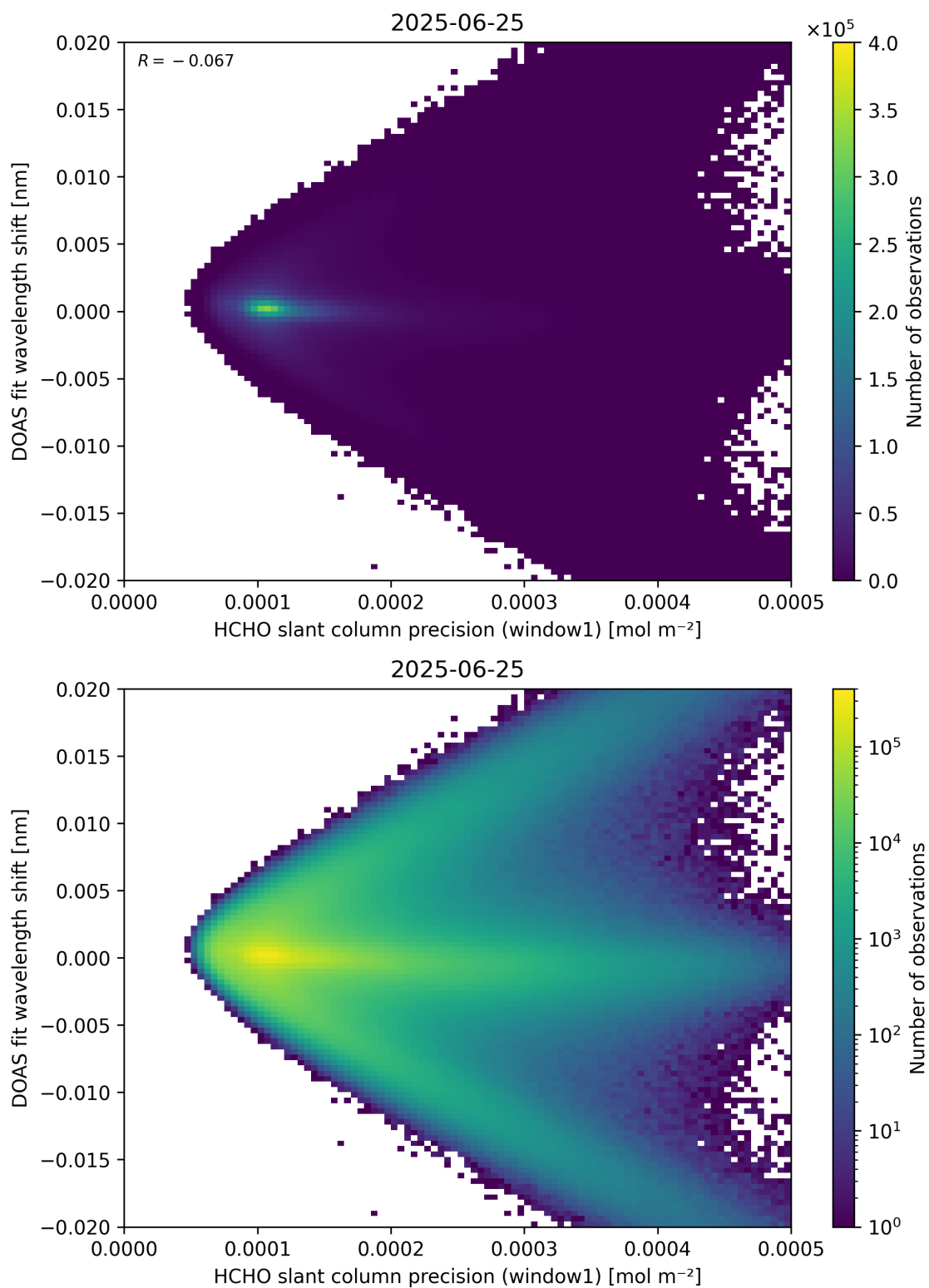
Figure 89: Scatter density plot of “HCHO slant column precision (window1)” against “DOAS fit wavelength shift” for 2025-06-24 to 2025-06-26.
