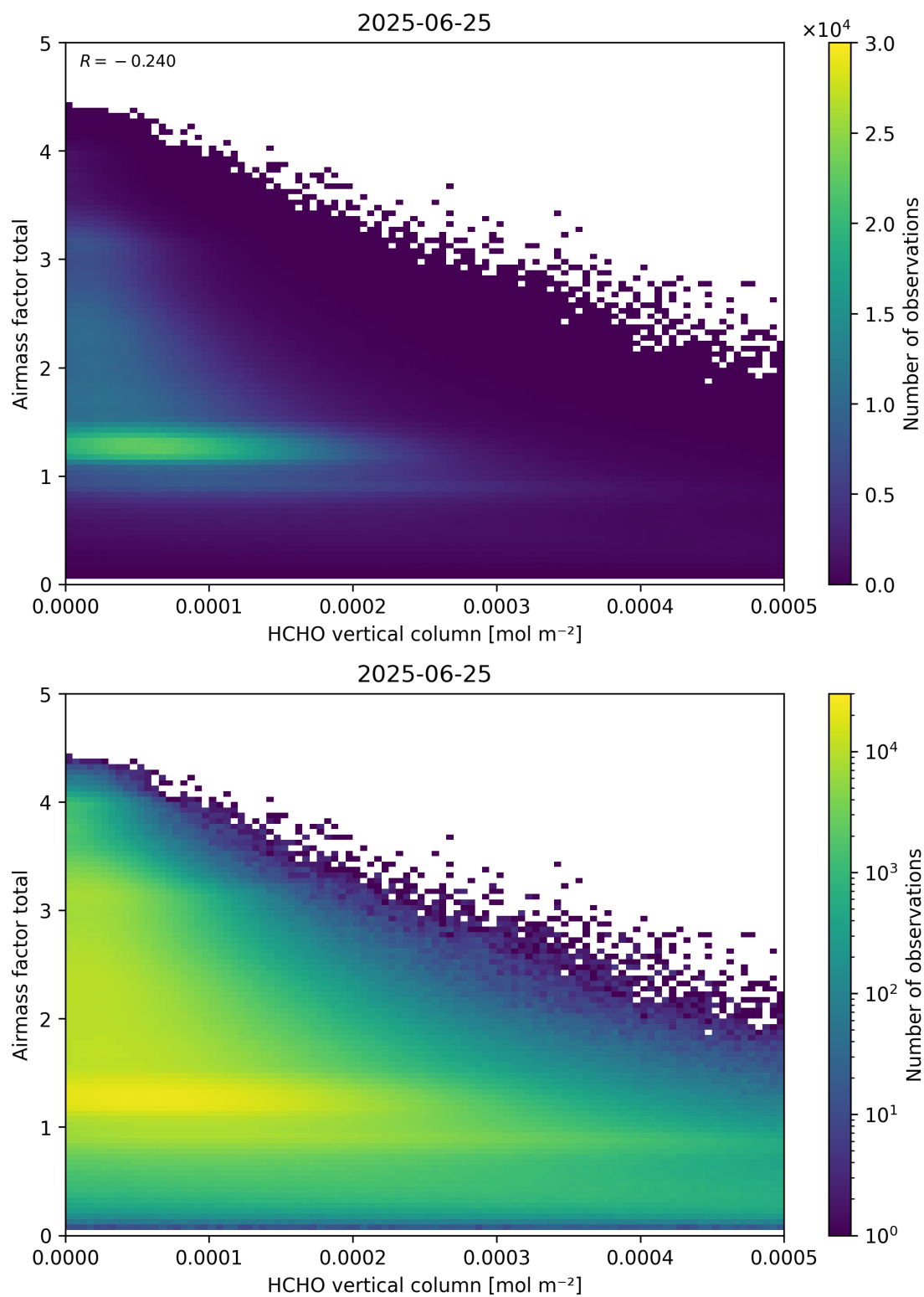
Figure 131: Scatter density plot of “HCHO vertical column” against “Airmass factor total” for 2025-06-24 to 2025-06-26.
