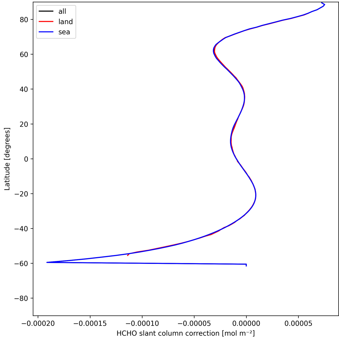
Figure 33: Zonal average of “HCHO slant column correction” for 2025-06-24 to 2025-06-26.
