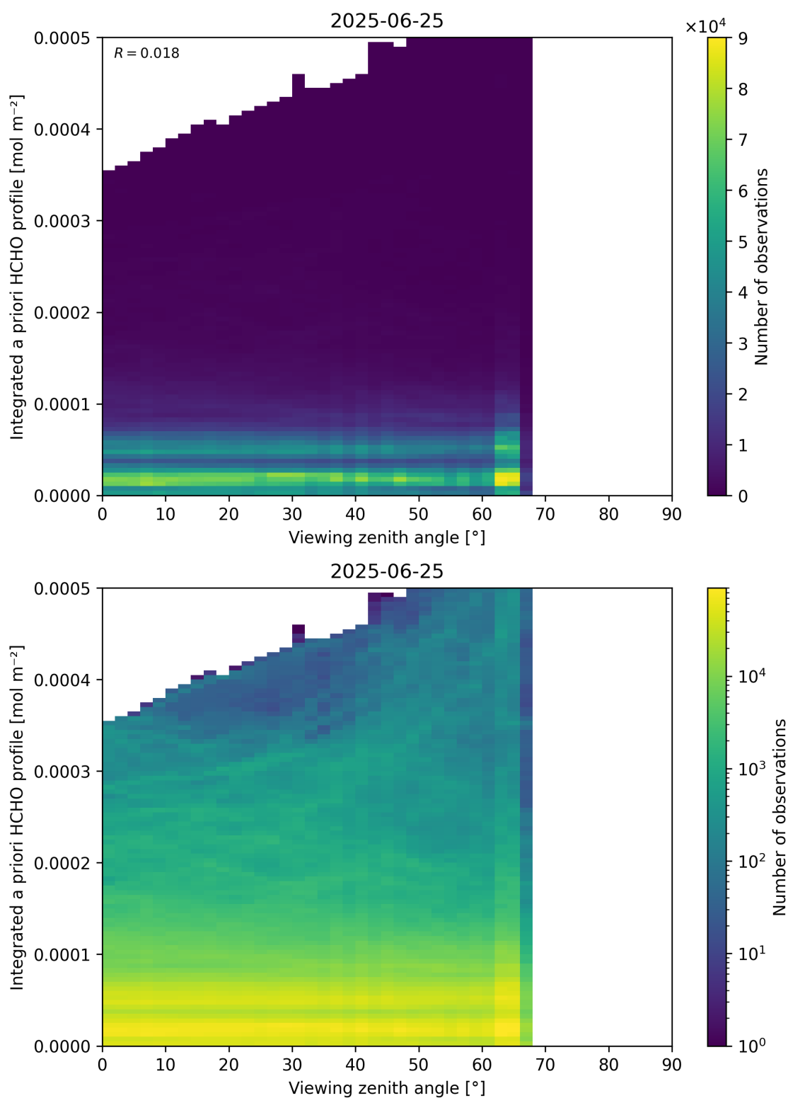
Figure 195: Scatter density plot of “Viewing zenith angle” against “Integrated a priori HCHO profile” for 2025-06-24 to 2025-06-26.
