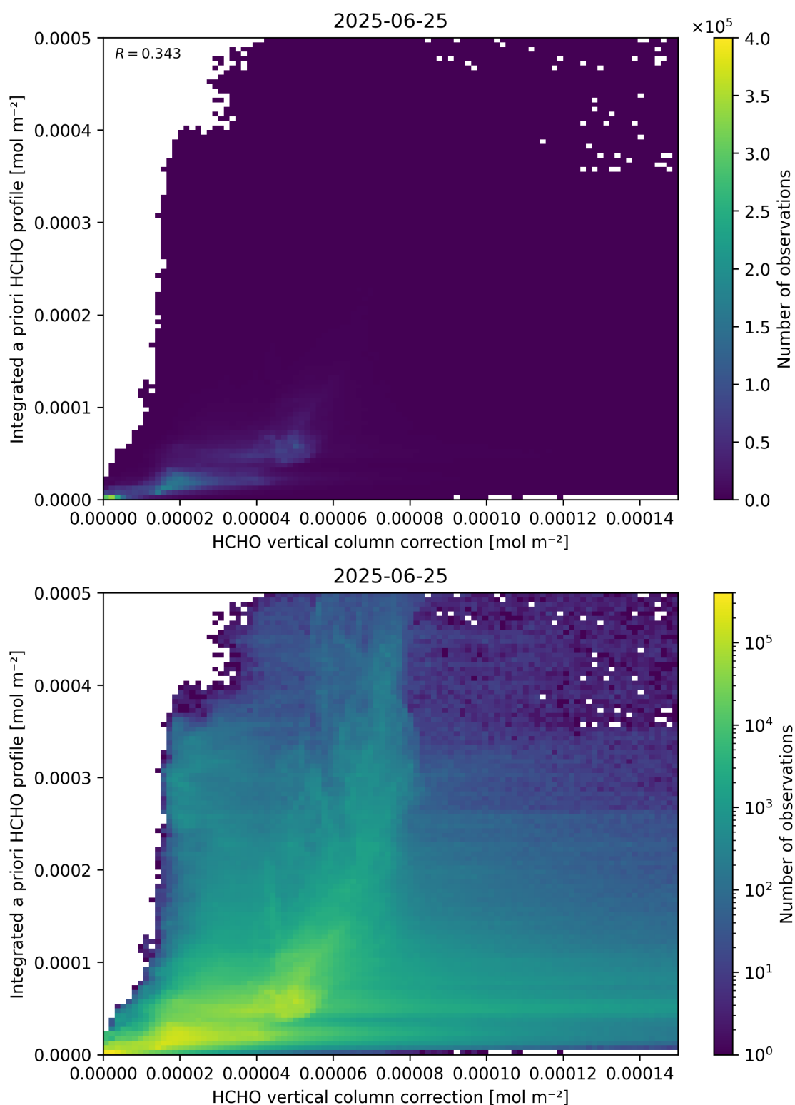
Figure 122: Scatter density plot of “HCHO vertical column correction” against “Integrated a priori HCHO profile” for 2025-06-24 to 2025-06-26.
