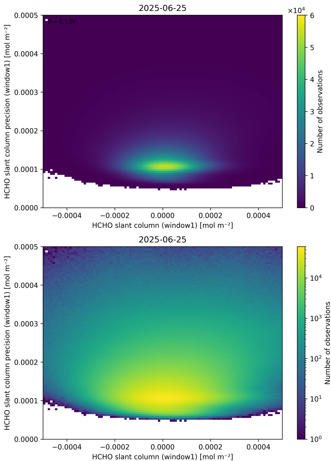
Figure 84: Scatter density plot of “HCHO slant column (window1)” against “HCHO slant column precision (window1)” for 2025-06-24 to 2025-06-26.
