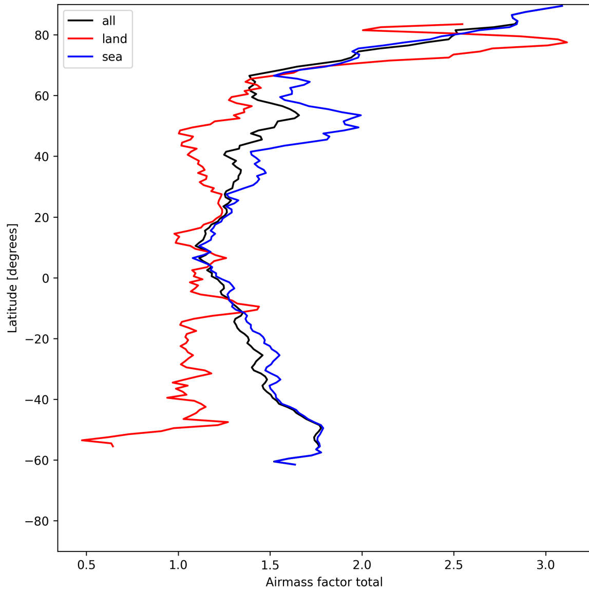
Figure 26: Zonal average of “Airmass factor total” for 2025-06-24 to 2025-06-26.
