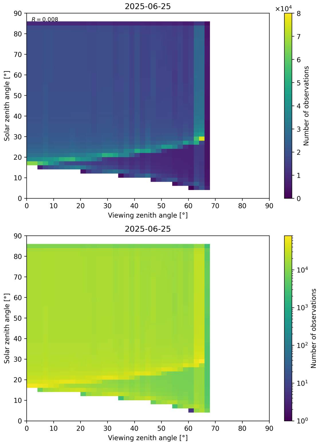
Figure 197: Scatter density plot of “Viewing zenith angle” against “Solar zenith angle” for 2025-06-24 to 2025-06-26.
