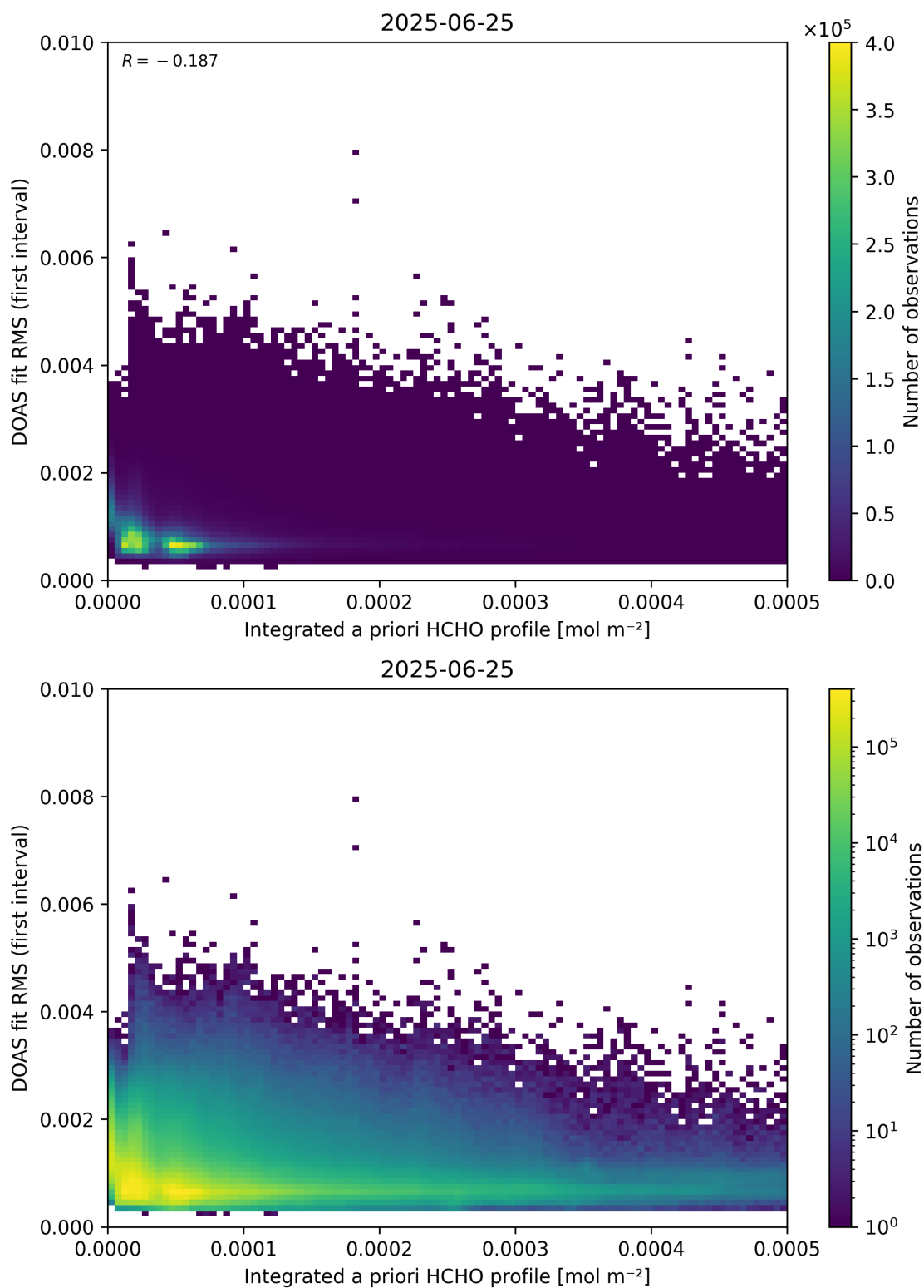
Figure 148: Scatter density plot of “Integrated a priori HCHO profile” against “DOAS fit RMS (first interval)” for 2025-06-24 to 2025-06-26.
