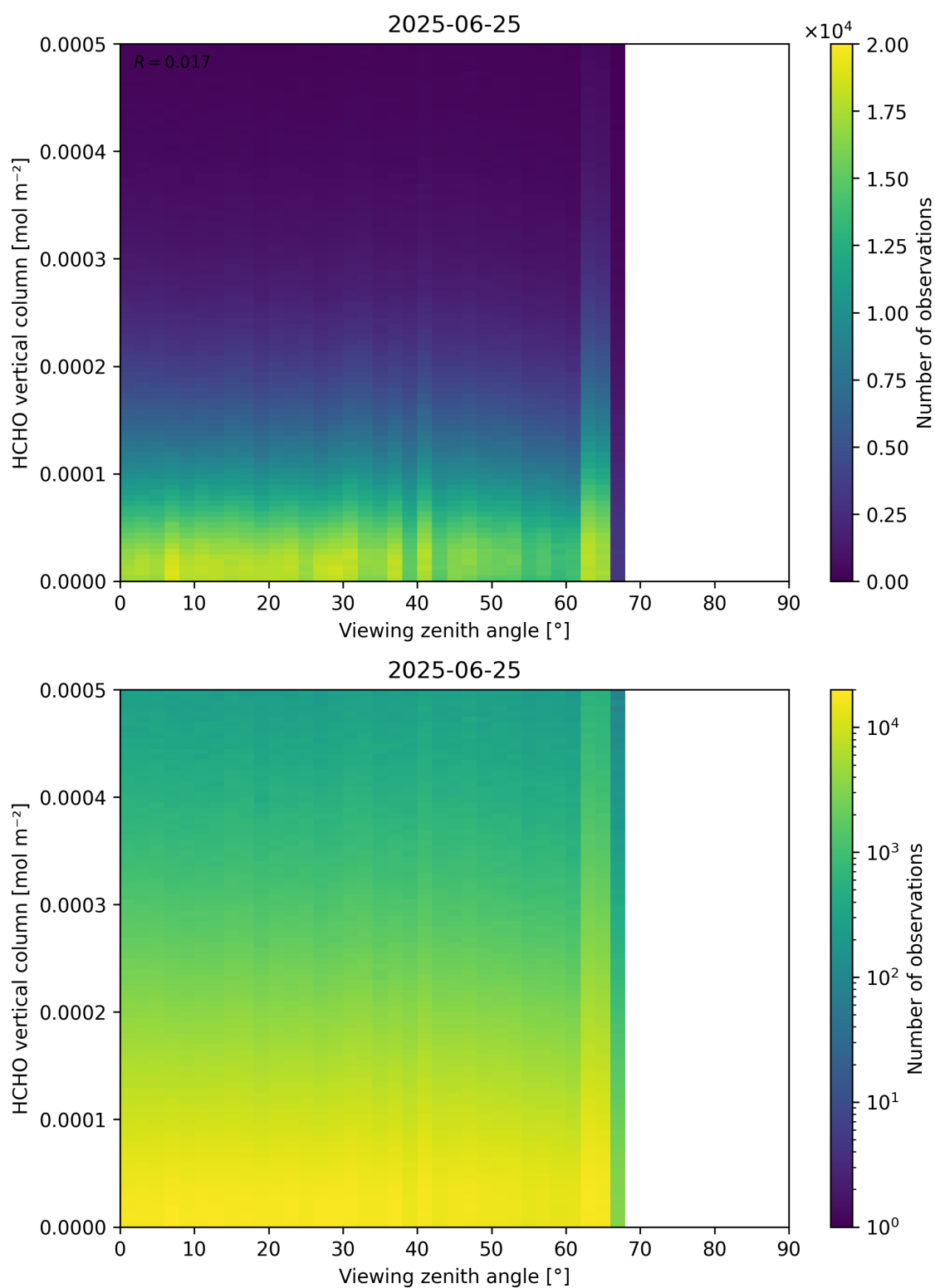
Figure 192: Scatter density plot of “Viewing zenith angle” against “HCHO vertical column” for 2025-06-24 to 2025-06-26.
