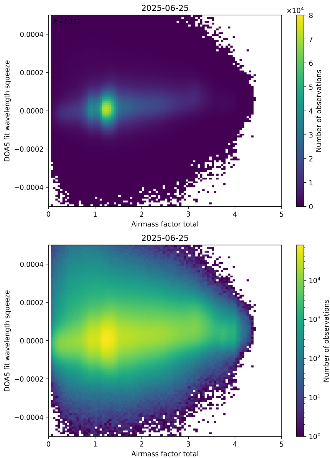
Figure 99: Scatter density plot of “Airmass factor total” against “DOAS fit wavelength squeeze” for 2025-06-24 to 2025-06-26.
