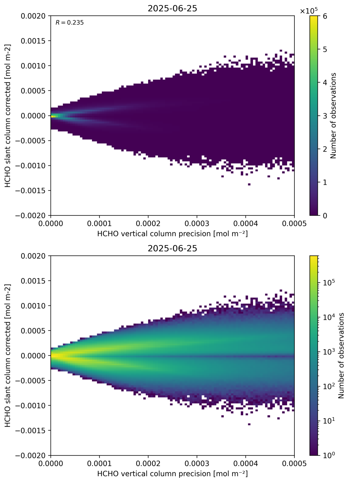
Figure 140: Scatter density plot of “HCHO vertical column precision” against “HCHO slant column corrected” for 2025-06-24 to 2025-06-26.
