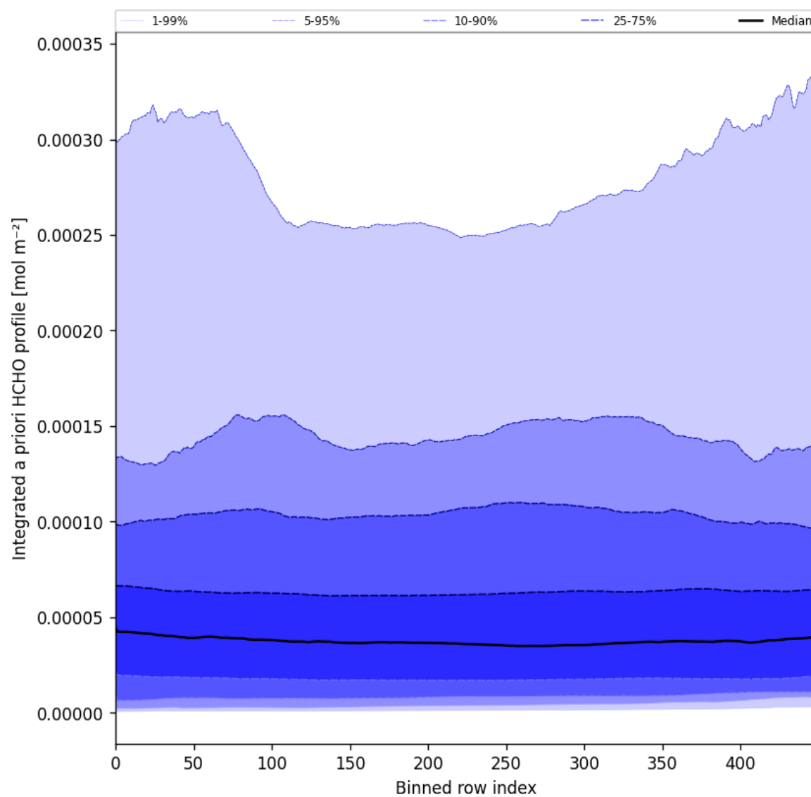
Figure 57: Along track statistics of “Integrated a priori HCHO profile” for 2025-06-24 to 2025-06-26
