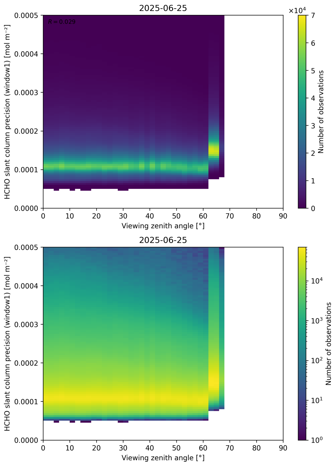
Figure 189: Scatter density plot of “Viewing zenith angle” against “HCHO slant column precision (window1)” for 2025-06-24 to 2025-06-26.
