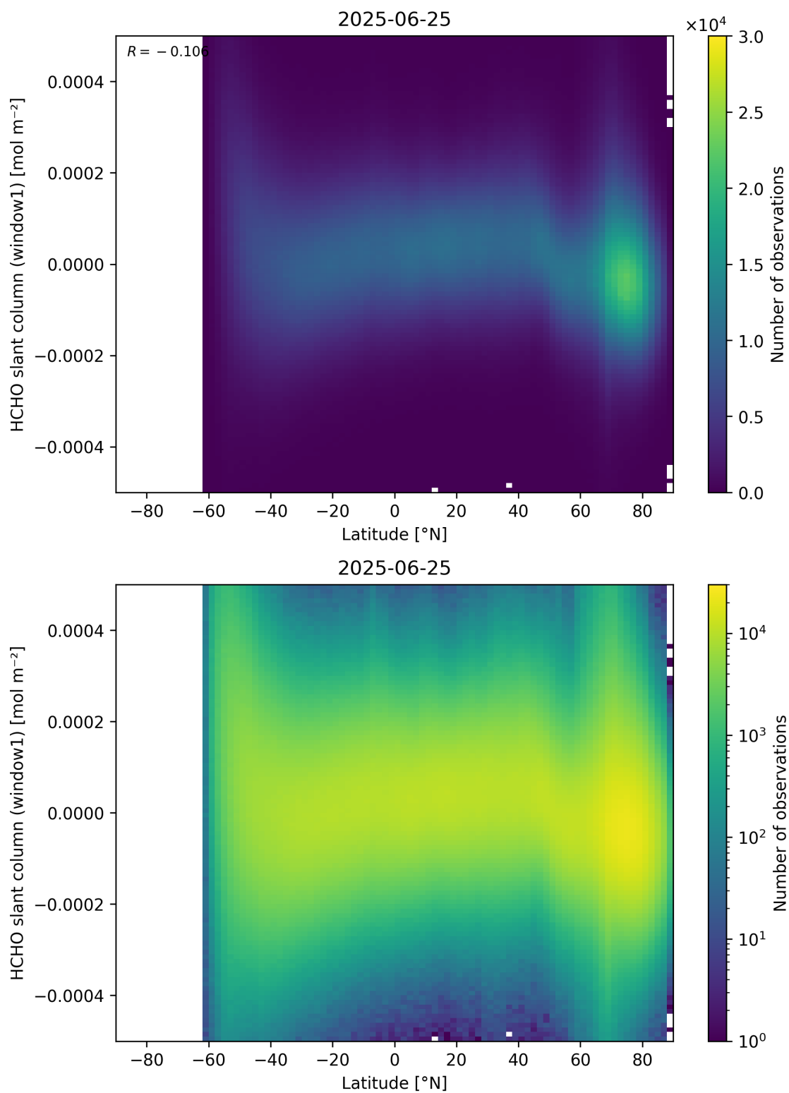
Figure 159: Scatter density plot of “Latitude” against “HCHO slant column (window1)” for 2025-06-24 to 2025-06-26.
