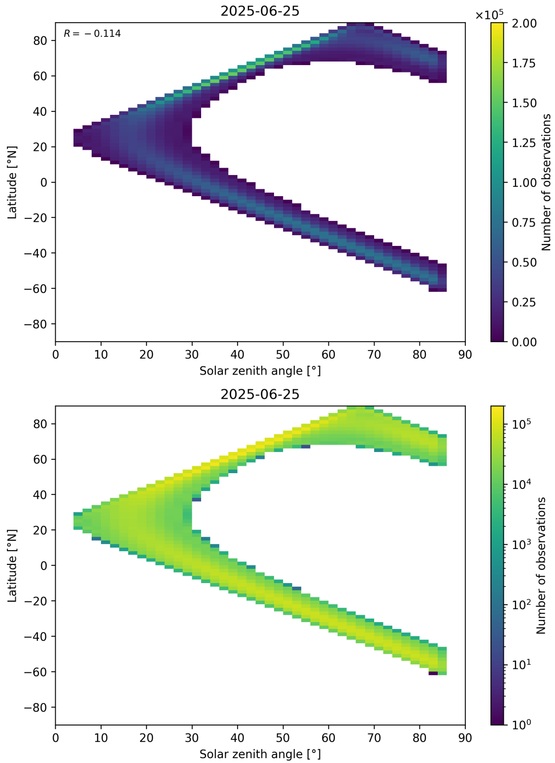
Figure 181: Scatter density plot of “Solar zenith angle” against “Latitude” for 2025-06-24 to 2025-06-26.
