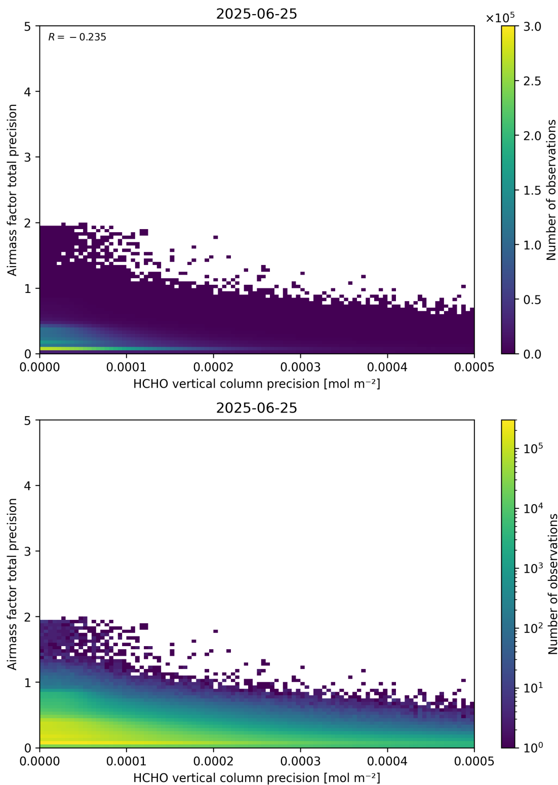
Figure 145: Scatter density plot of “HCHO vertical column precision” against “Airmass factor total precision” for 2025-06-24 to 2025-06-26.
