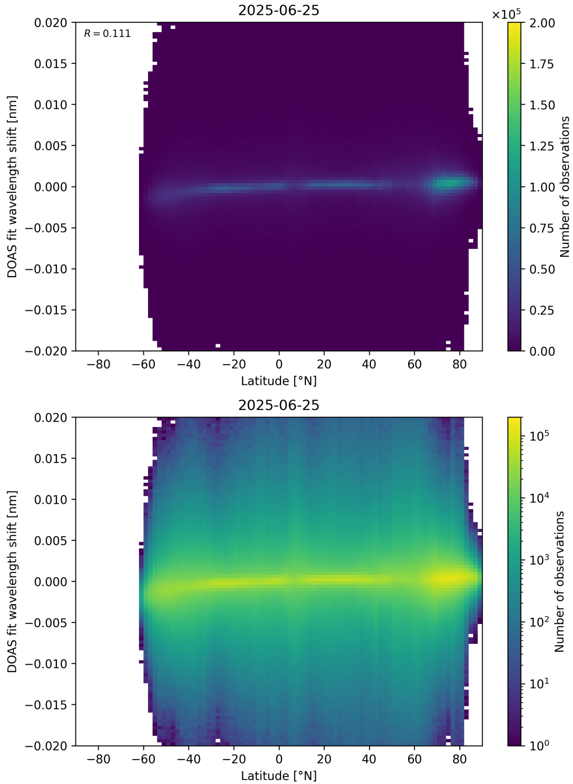
Figure 154: Scatter density plot of “Latitude” against “DOAS fit wavelength shift” for 2025-06-24 to 2025-06-26.
