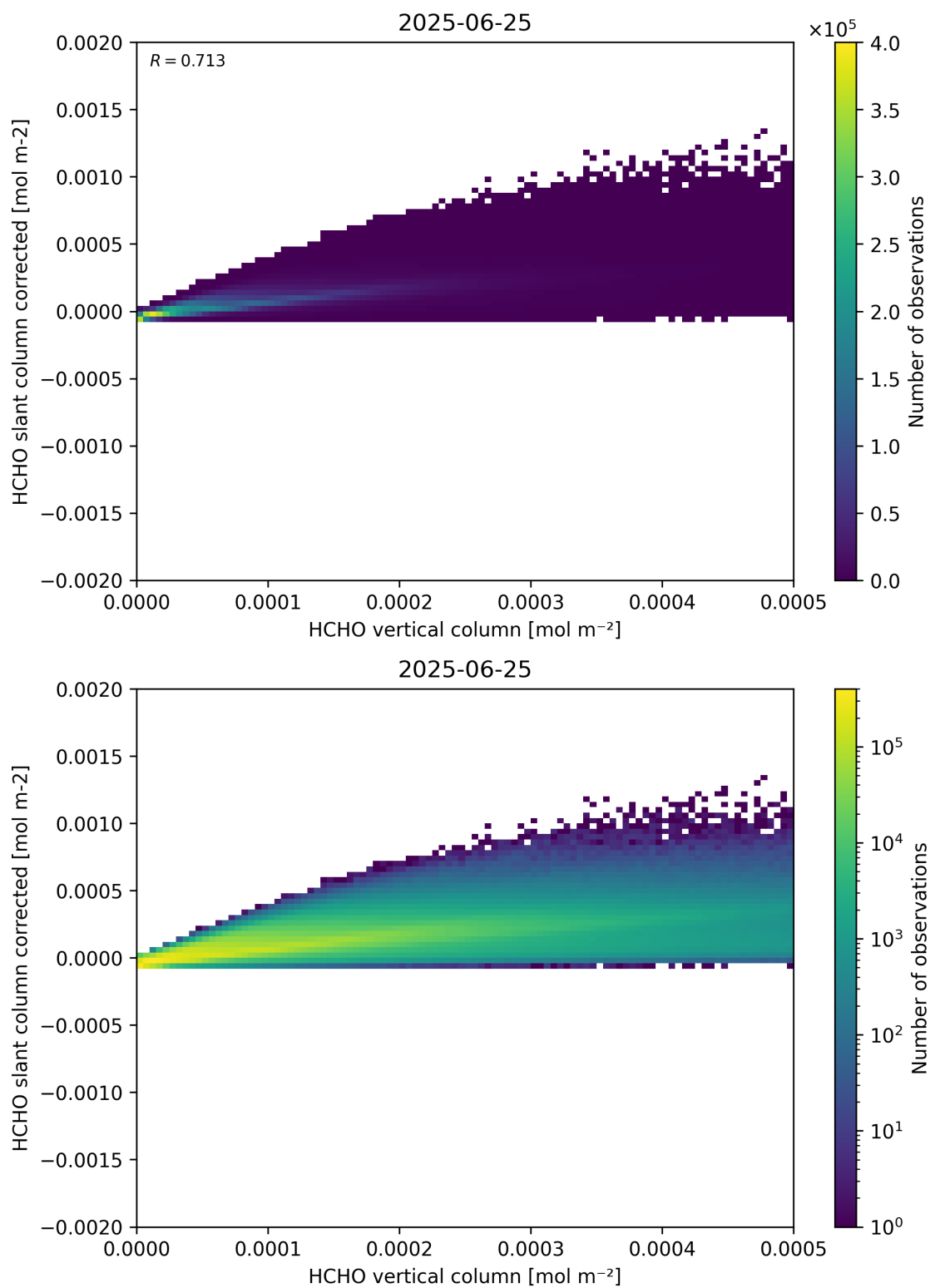
Figure 127: Scatter density plot of “HCHO vertical column” against “HCHO slant column corrected” for 2025-06-24 to 2025-06-26.
