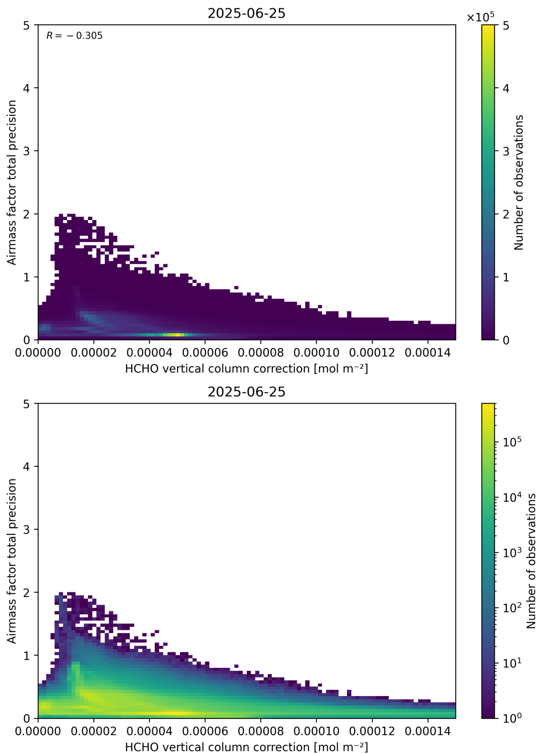
Figure 121: Scatter density plot of “HCHO vertical column correction” against “Airmass factor total precision” for 2025-06-24 to 2025-06-26.
