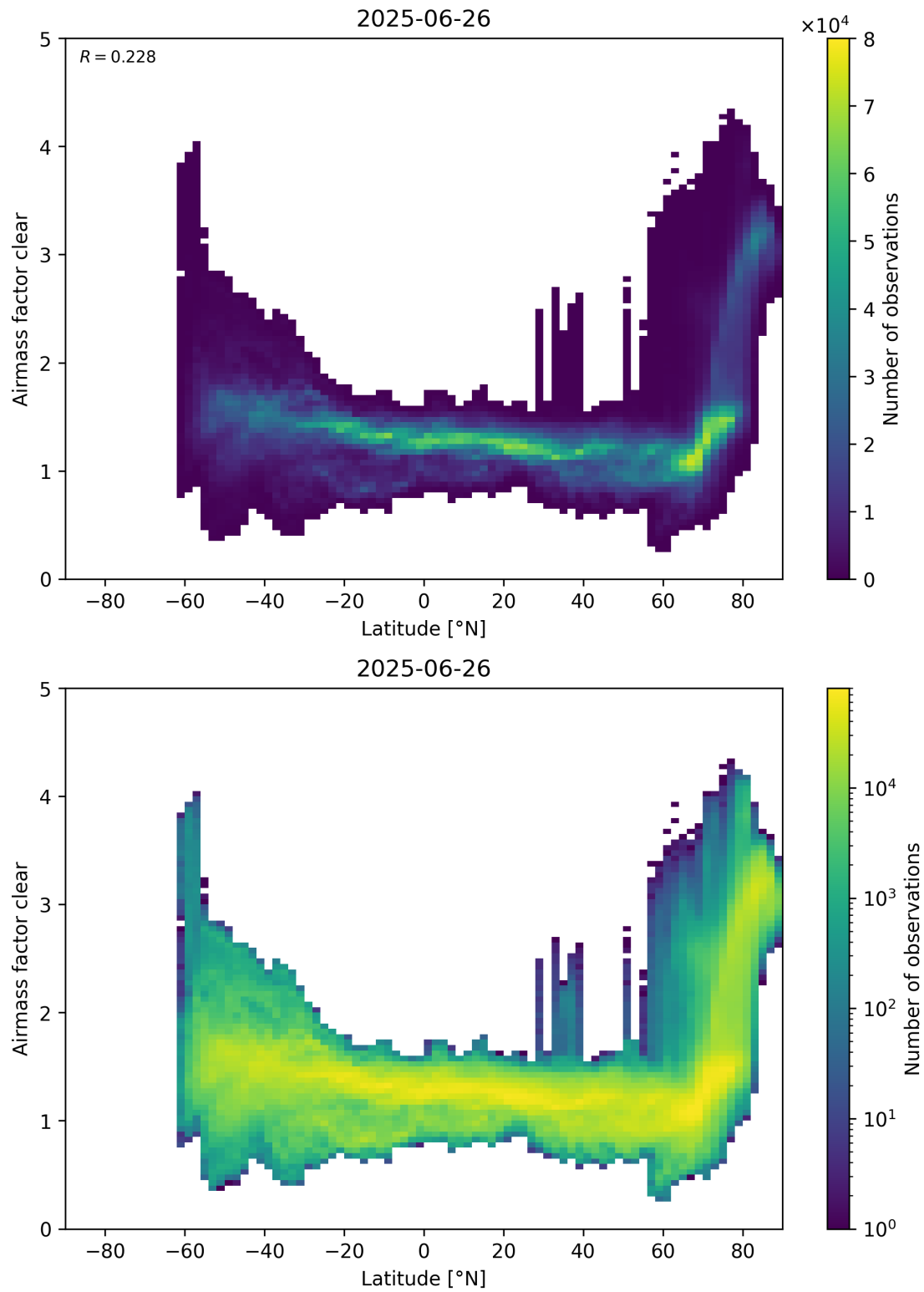
Figure 156: Scatter density plot of “Latitude” against “Airmass factor clear” for 2025-06-25 to 2025-06-27.
