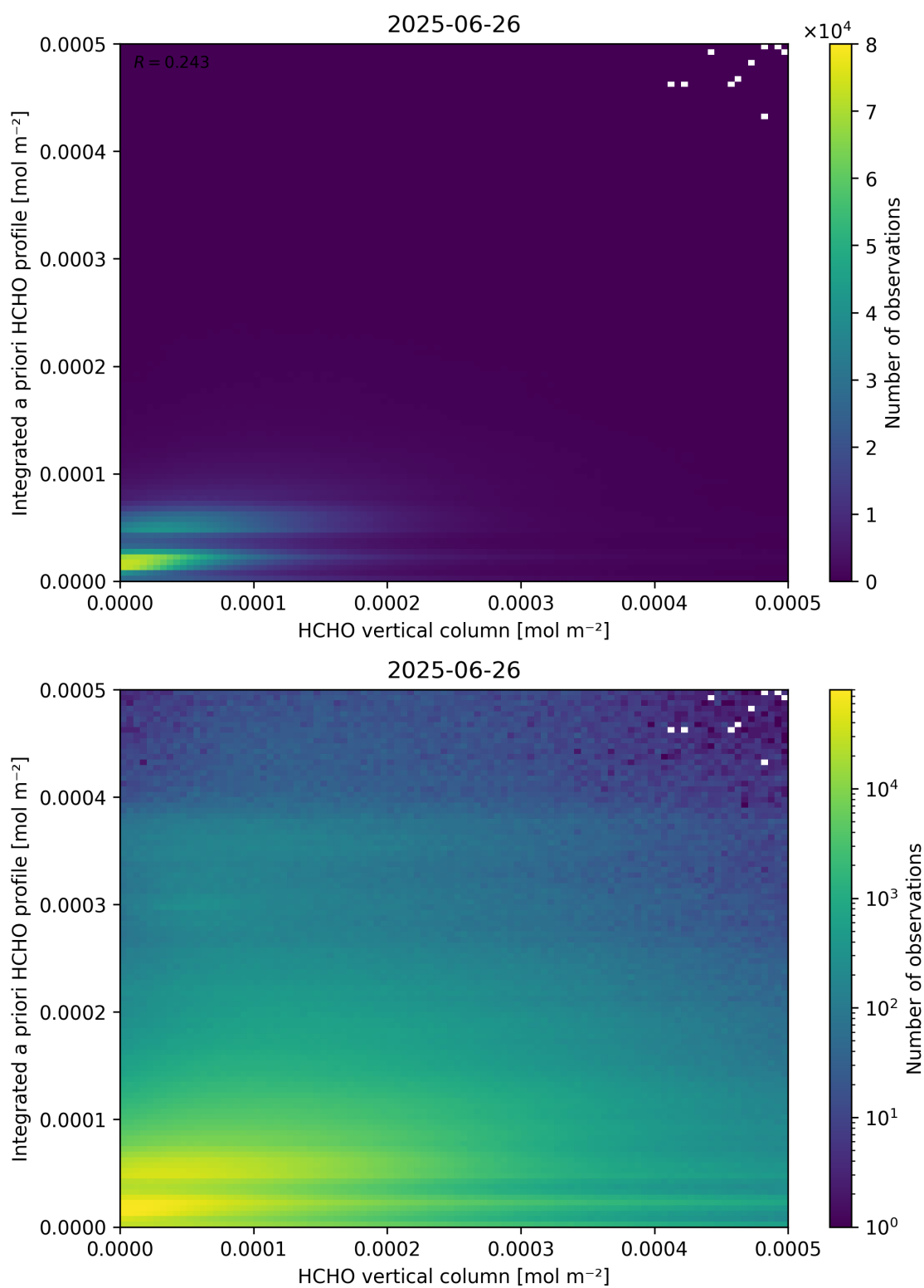
Figure 135: Scatter density plot of “HCHO vertical column” against “Integrated a priori HCHO profile” for 2025-06-25 to 2025-06-27.
