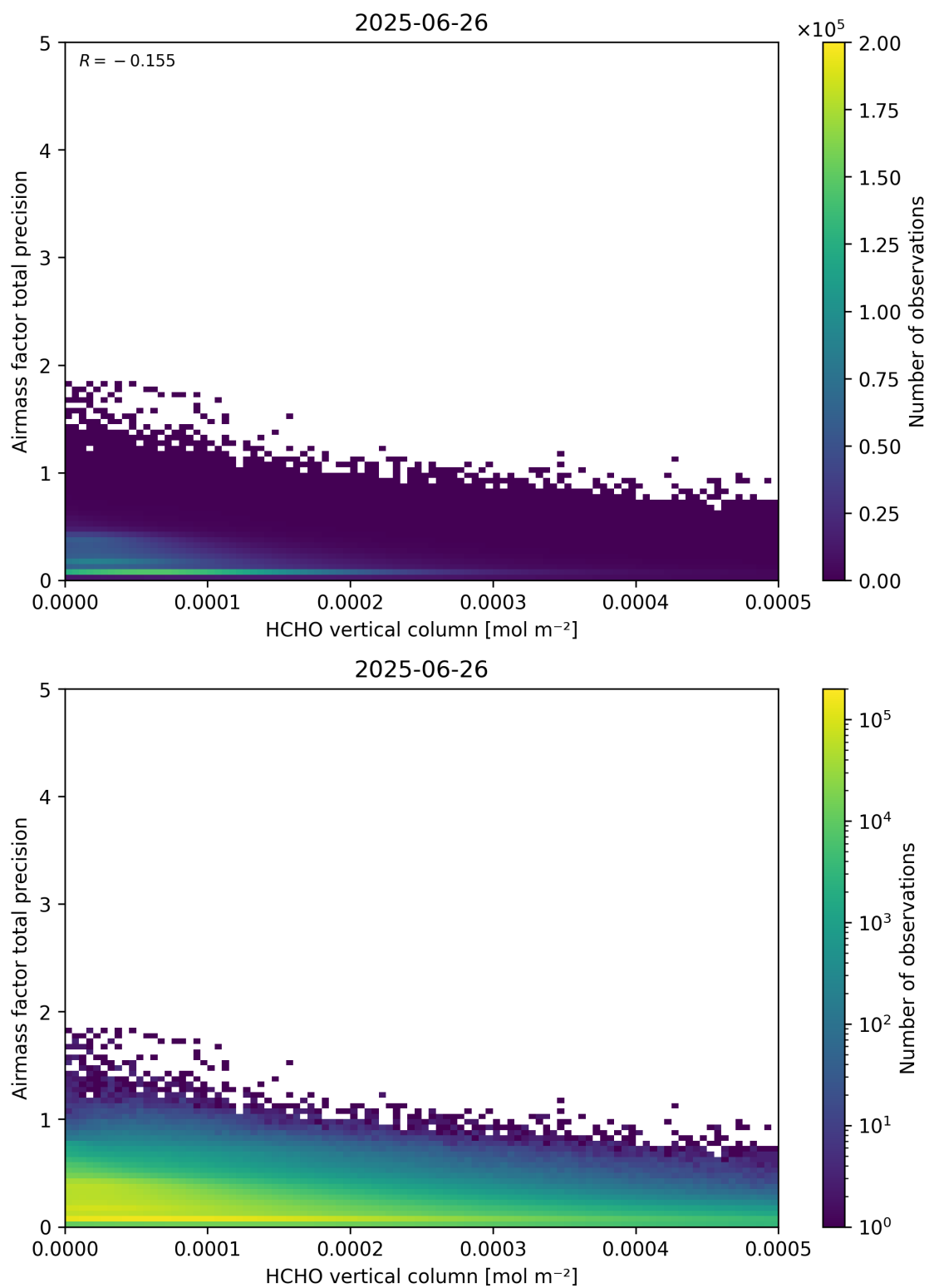
Figure 132: Scatter density plot of “HCHO vertical column” against “Airmass factor total precision” for 2025-06-25 to 2025-06-27.
