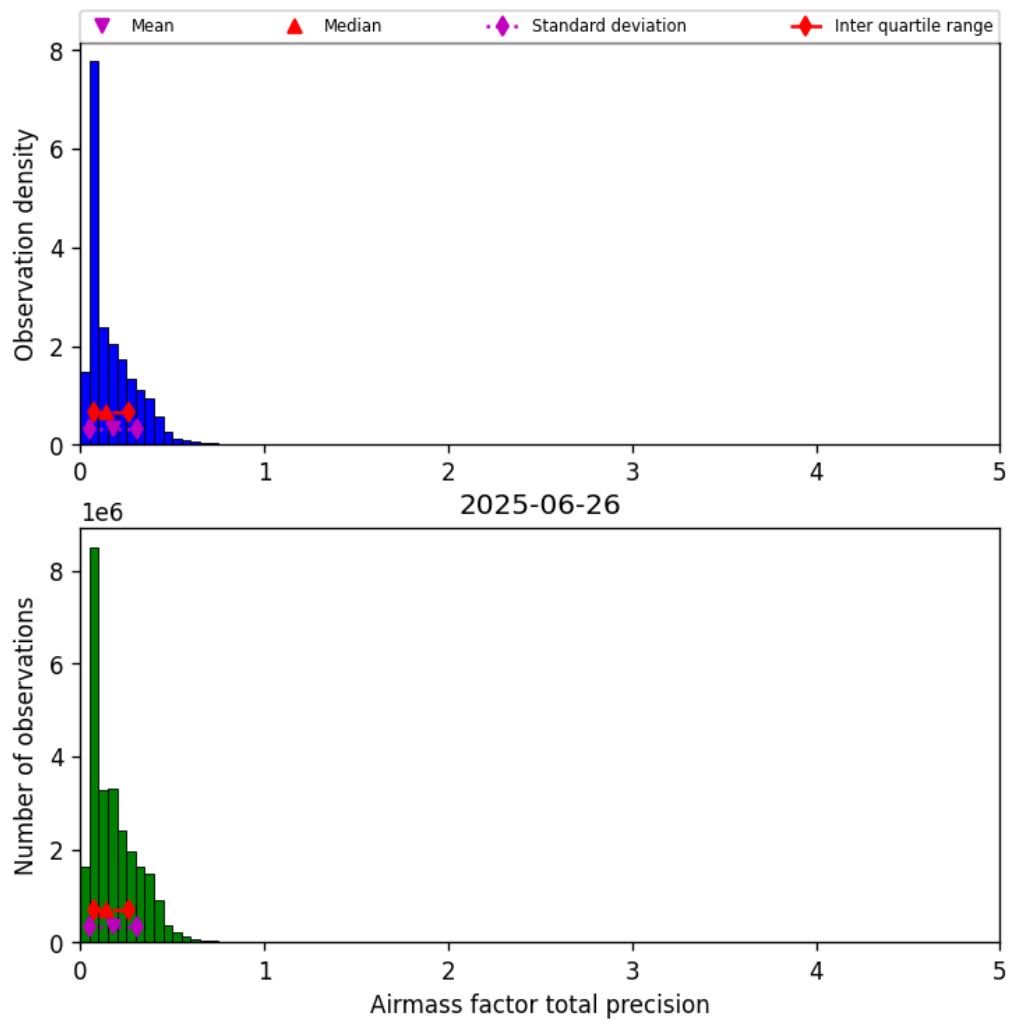
Figure 41: Histogram of “Airmass factor total precision” for 2025-06-25 to 2025-06-27
