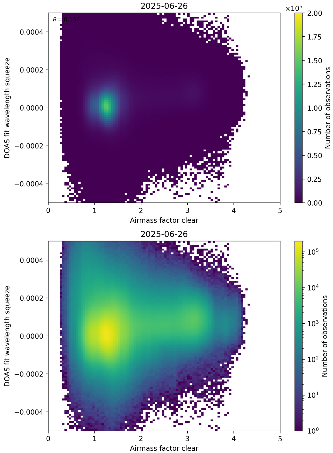
Figure 73: Scatter density plot of “Airmass factor clear” against “DOAS fit wavelength squeeze” for 2025-06-25 to 2025-06-27.
