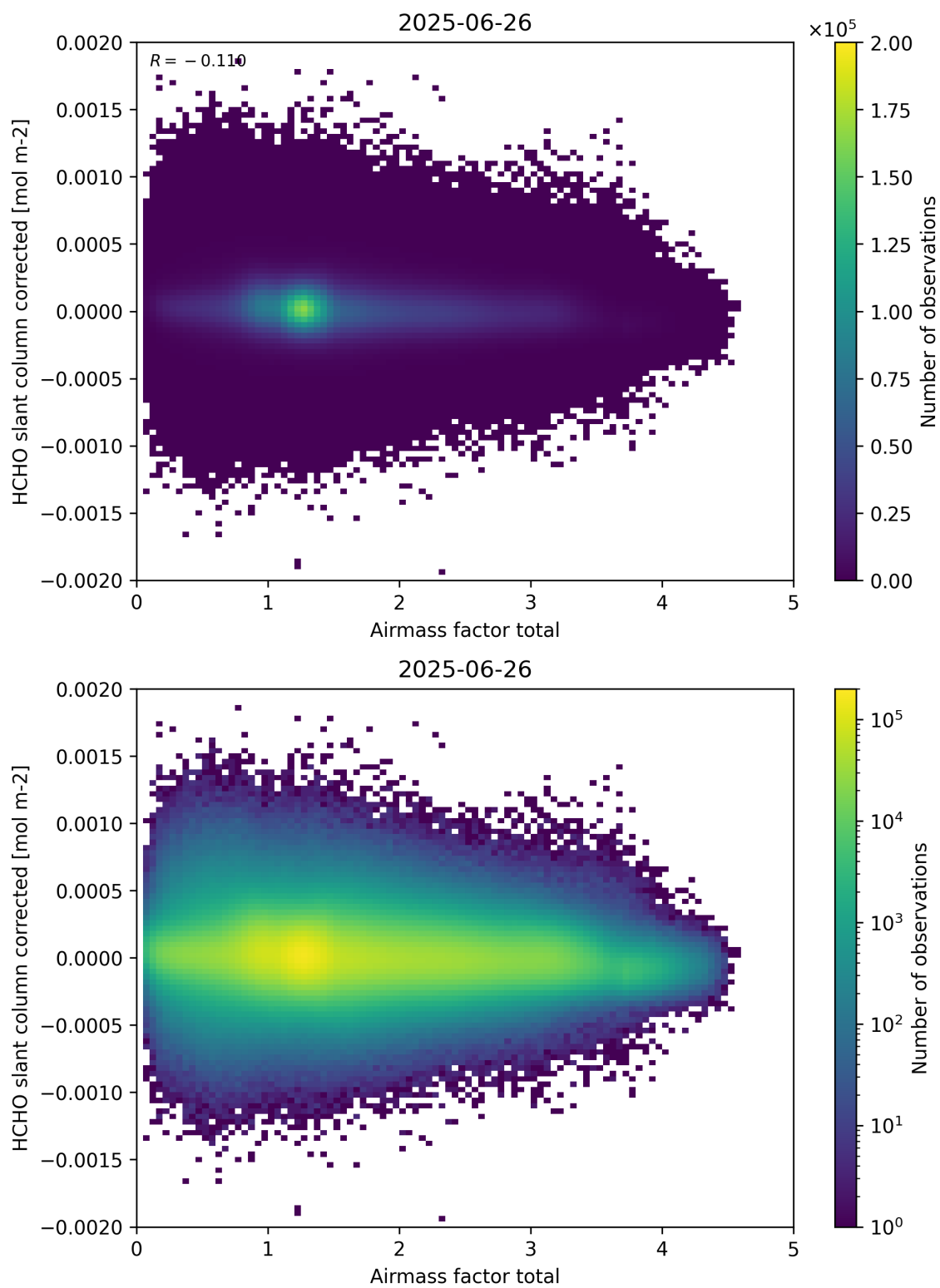
Figure 101: Scatter density plot of “Airmass factor total” against “HCHO slant column corrected” for 2025-06-25 to 2025-06-27.
