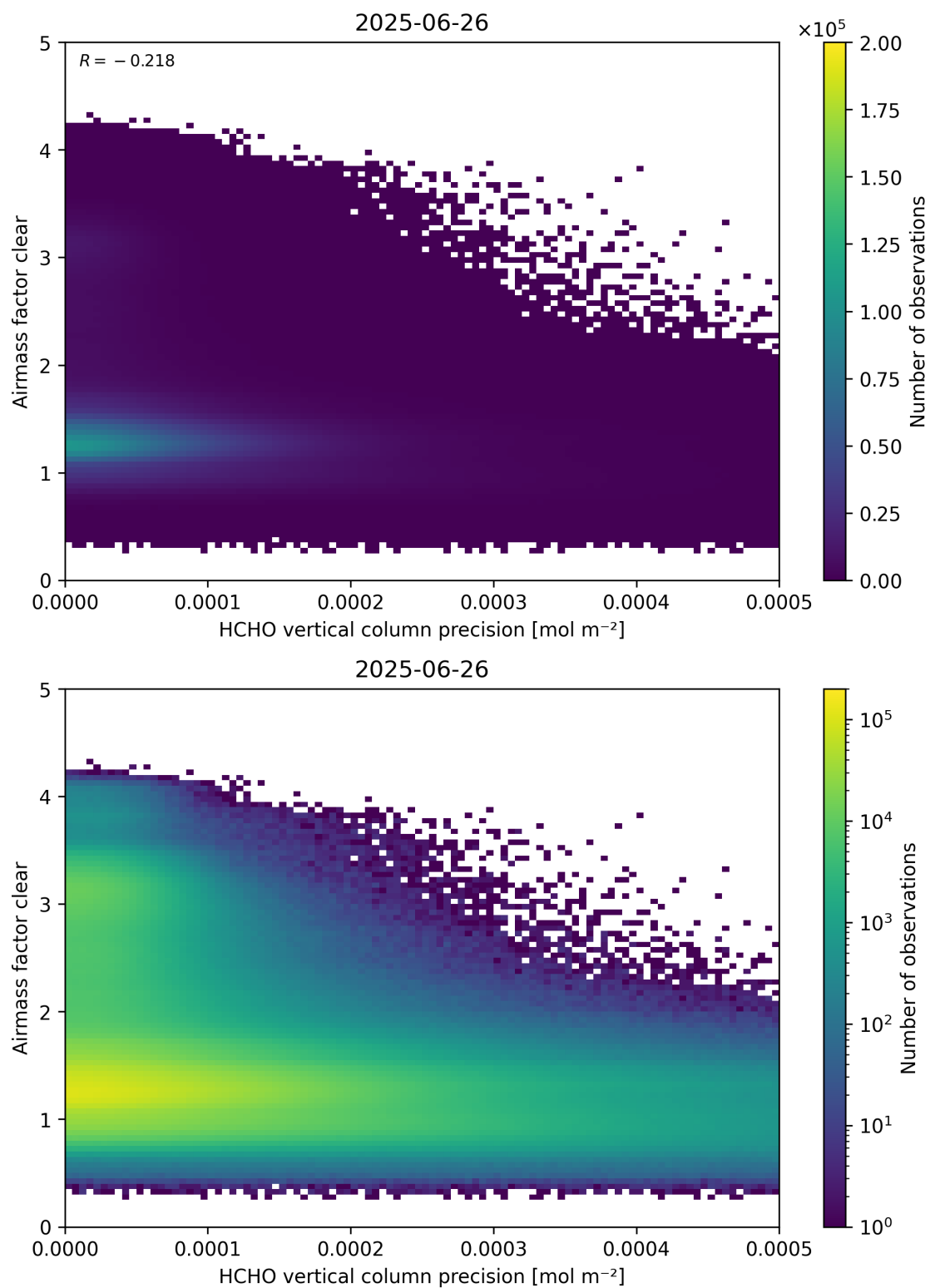
Figure 139: Scatter density plot of “HCHO vertical column precision” against “Airmass factor clear” for 2025-06-25 to 2025-06-27.
