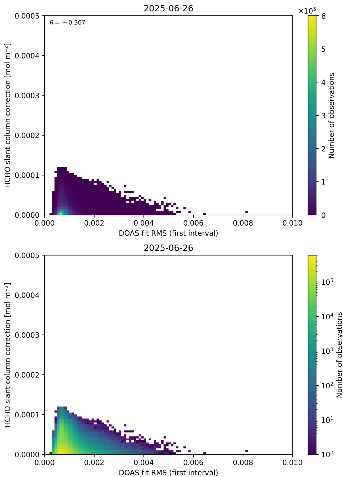
Figure 63: Scatter density plot of “DOAS fit RMS (first interval)” against “HCHO slant column correction” for 2025-06-25 to 2025-06-27.
