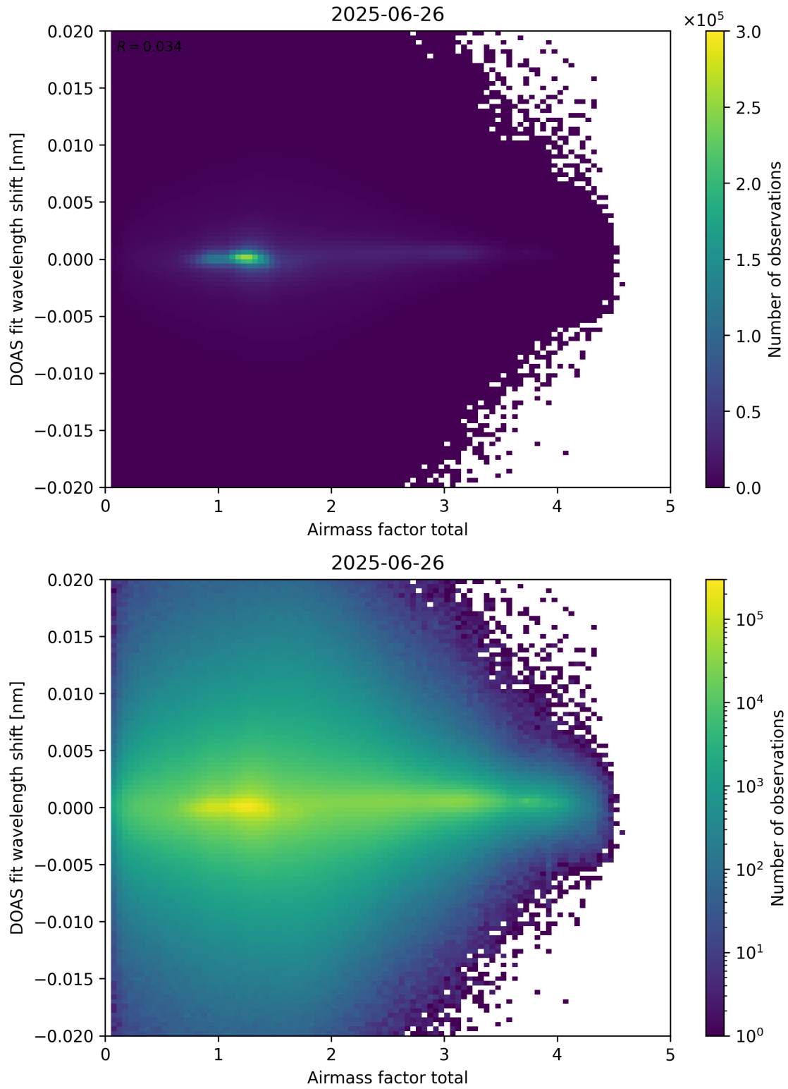
Figure 98: Scatter density plot of “Airmass factor total” against “DOAS fit wavelength shift” for 2025-06-25 to 2025-06-27.
