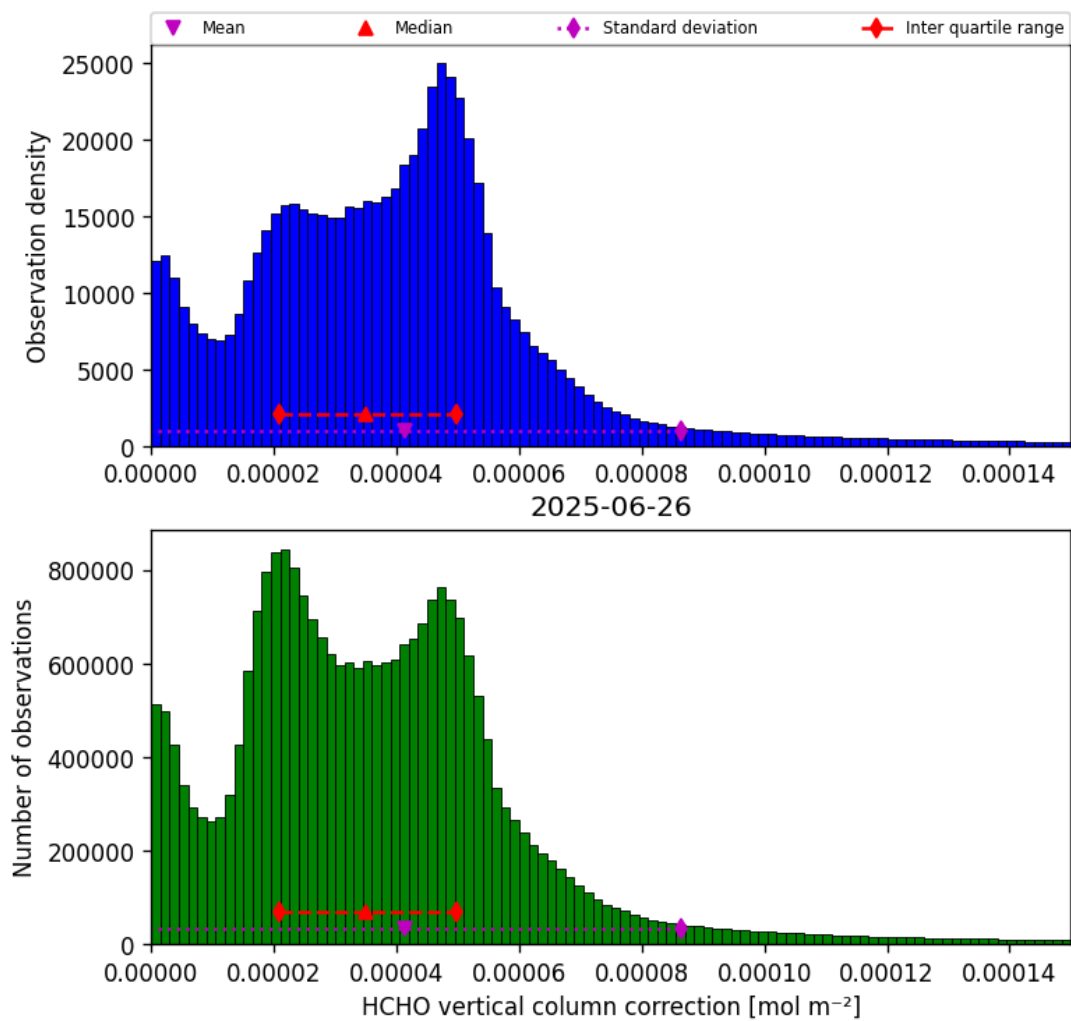
Figure 37: Histogram of “HCHO vertical column correction” for 2025-06-25 to 2025-06-27
