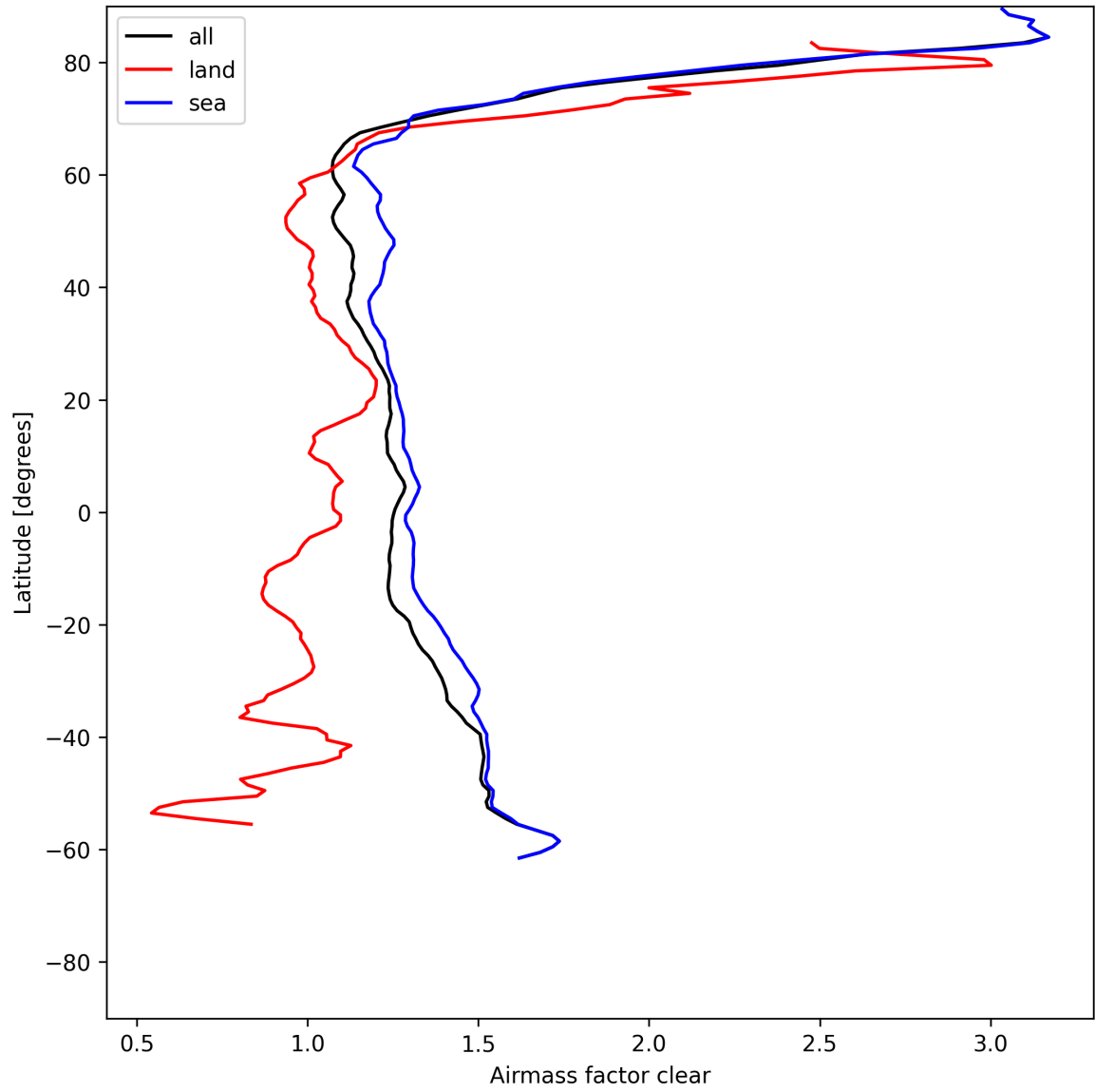
Figure 28: Zonal average of “Airmass factor clear” for 2025-06-25 to 2025-06-27.
