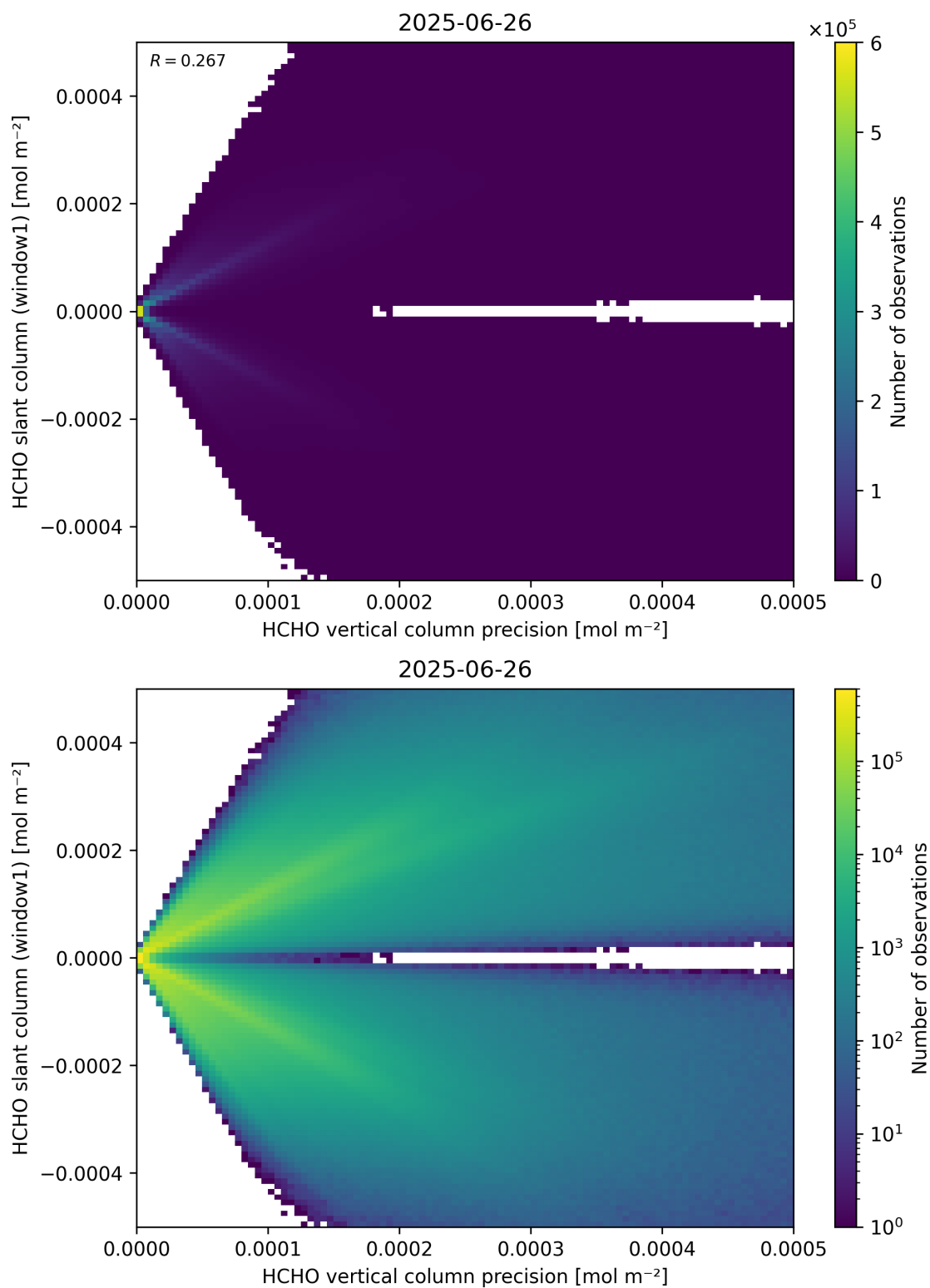
Figure 142: Scatter density plot of “HCHO vertical column precision” against “HCHO slant column (window1)” for 2025-06-25 to 2025-06-27.
