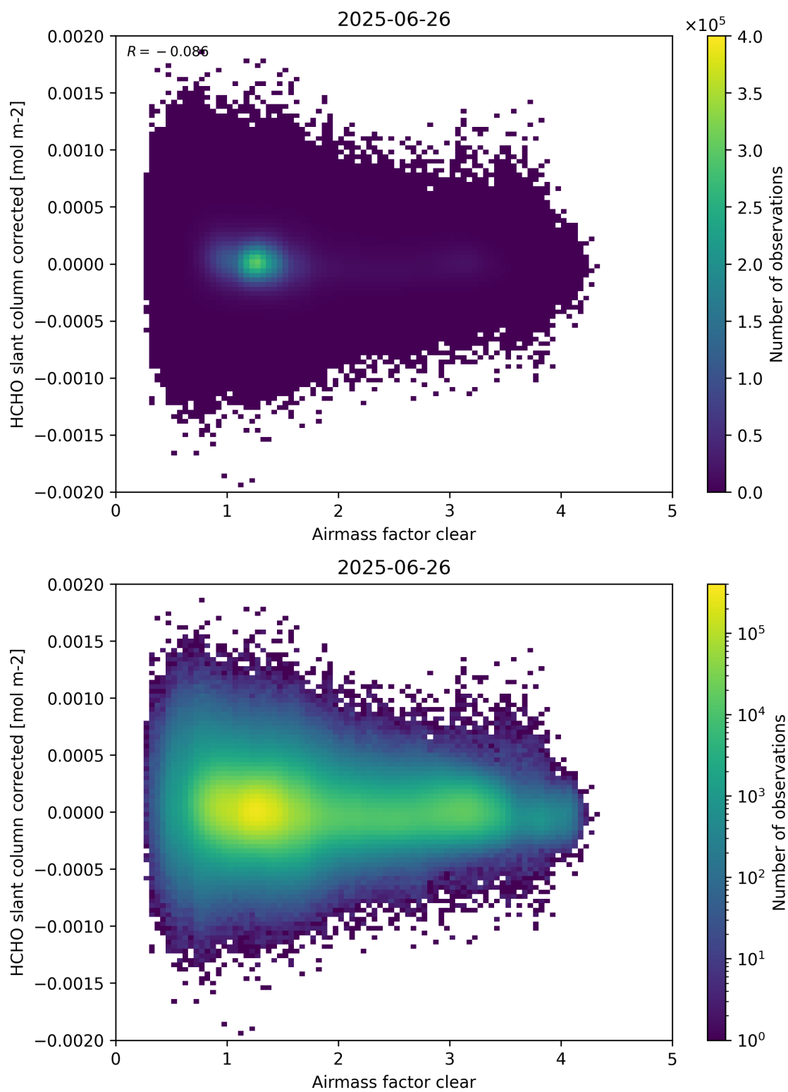
Figure 74: Scatter density plot of “Airmass factor clear” against “HCHO slant column corrected” for 2025-06-25 to 2025-06-27.
