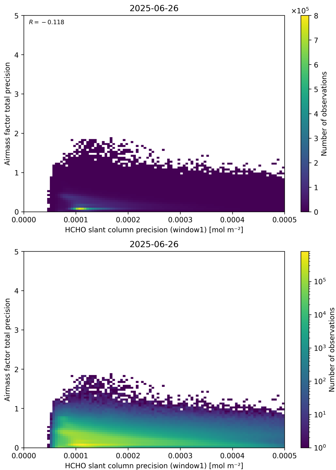
Figure 95: Scatter density plot of “HCHO slant column precision (window1)” against “Airmass factor total precision” for 2025-06-25 to 2025-06-27.
