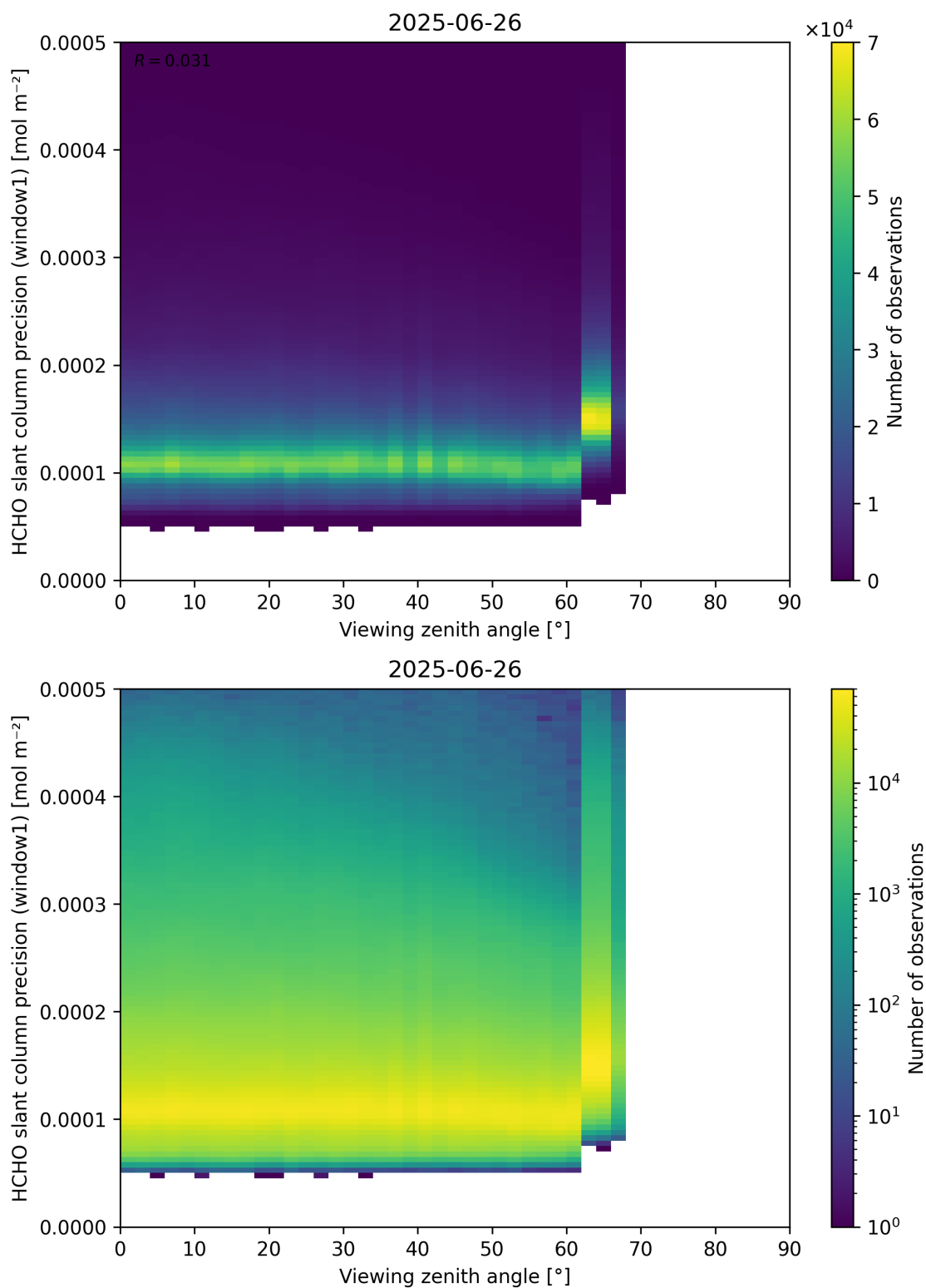
Figure 189: Scatter density plot of “Viewing zenith angle” against “HCHO slant column precision (window1)” for 2025-06-25 to 2025-06-27.
