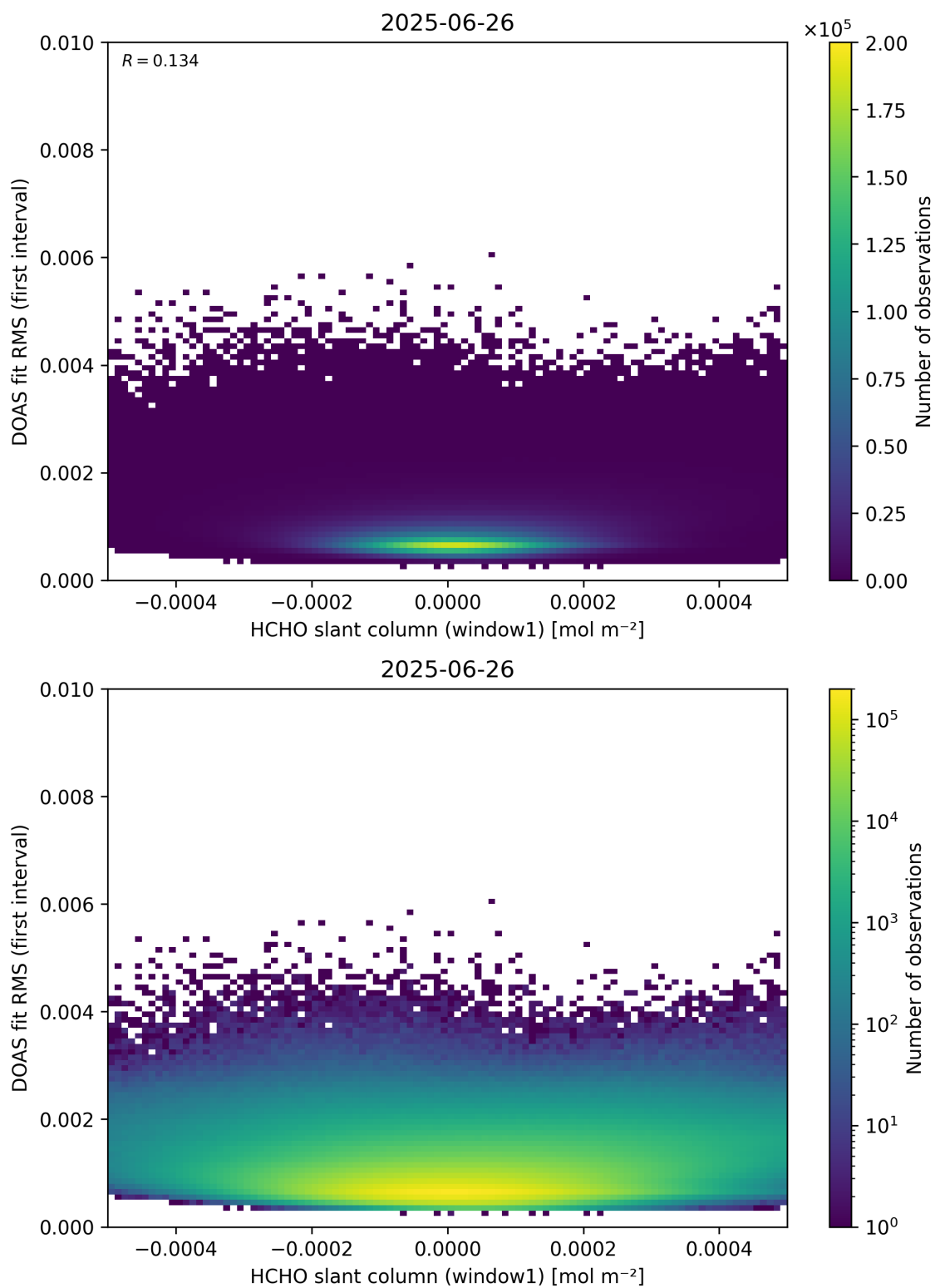
Figure 78: Scatter density plot of “HCHO slant column (window1)” against “DOAS fit RMS (first interval)” for 2025-06-25 to 2025-06-27.
