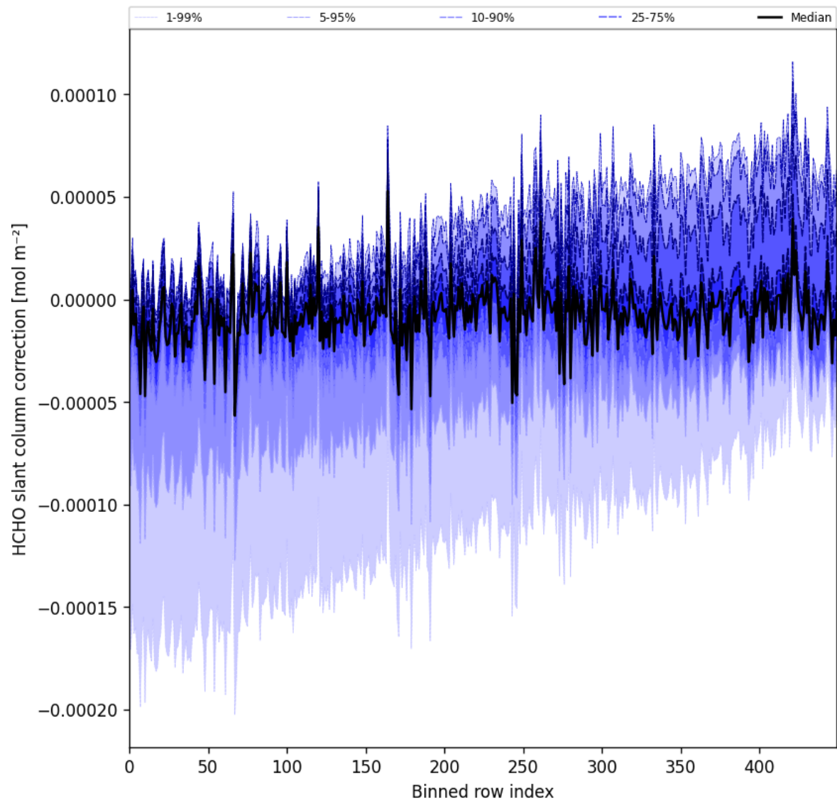
Figure 61: Along track statistics of “HCHO slant column correction” for 2025-06-25 to 2025-06-27
