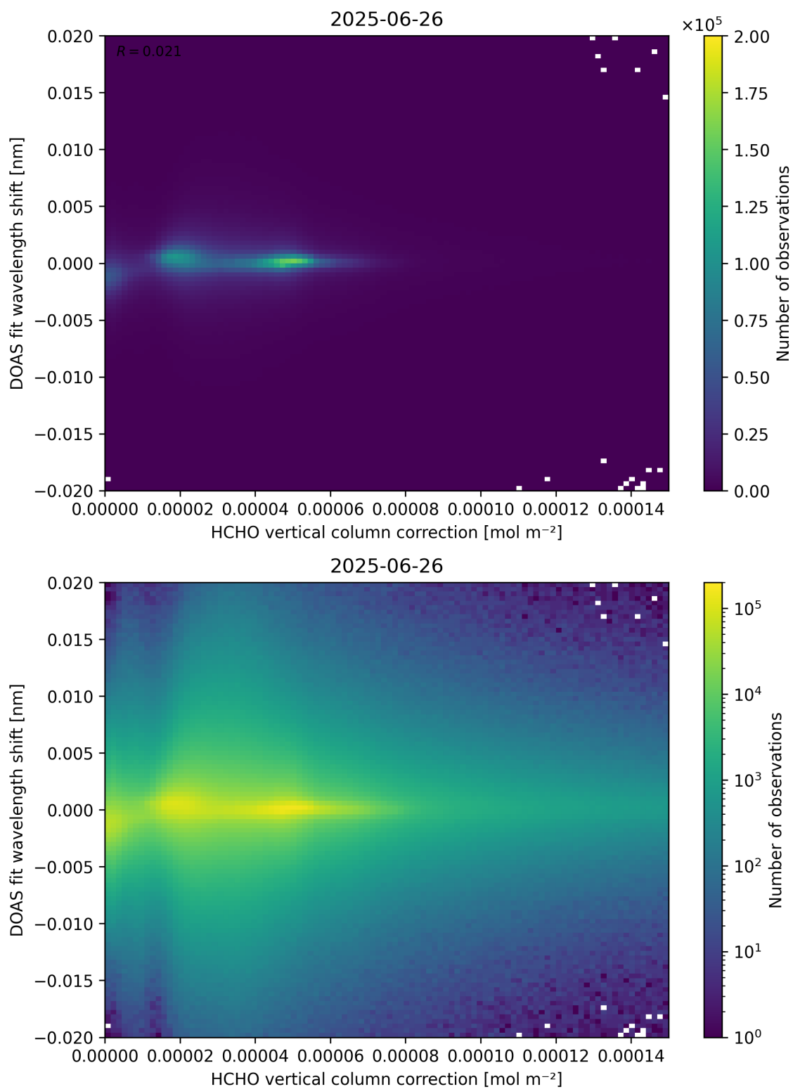
Figure 113: Scatter density plot of “HCHO vertical column correction” against “DOAS fit wavelength shift” for 2025-06-25 to 2025-06-27.
