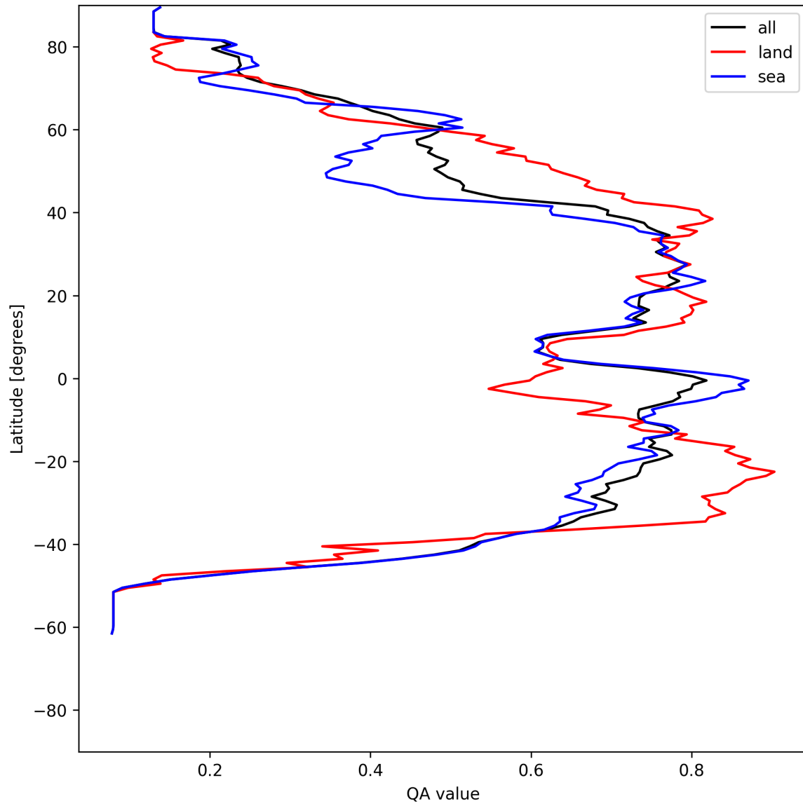
Figure 20: Zonal average of “QA value” for 2025-06-25 to 2025-06-27.
