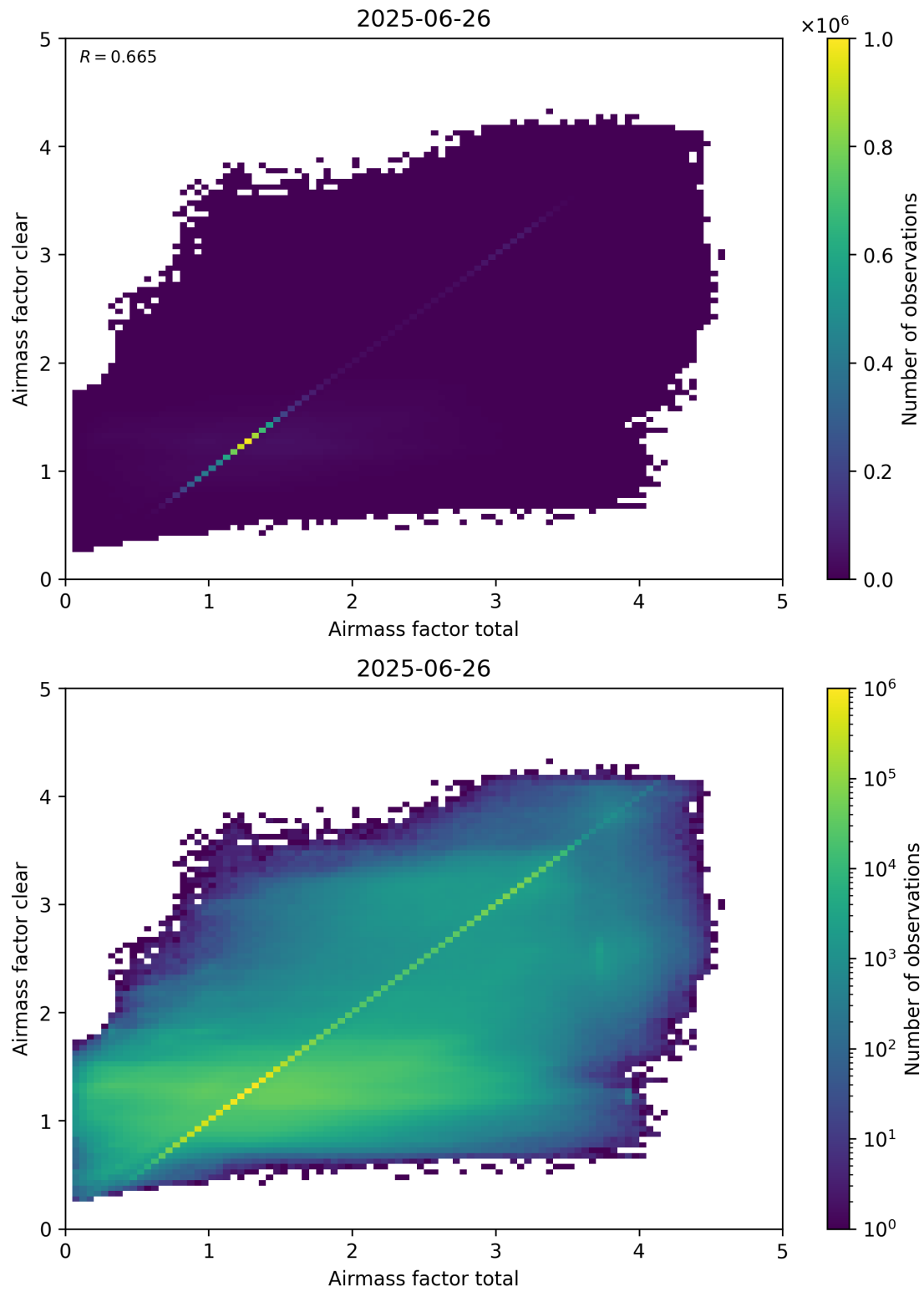
Figure 100: Scatter density plot of “Airmass factor total” against “Airmass factor clear” for 2025-06-25 to 2025-06-27.
