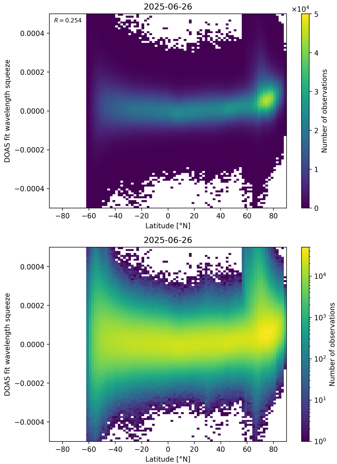
Figure 155: Scatter density plot of “Latitude” against “DOAS fit wavelength squeeze” for 2025-06-25 to 2025-06-27.
