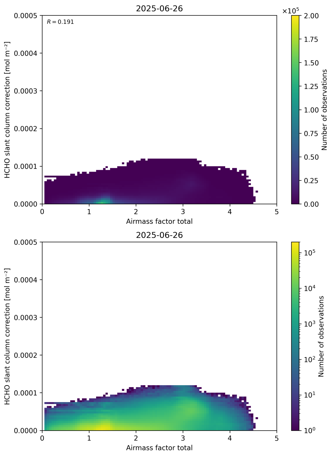
Figure 102: Scatter density plot of “Airmass factor total” against “HCHO slant column correction” for 2025-06-25 to 2025-06-27.
