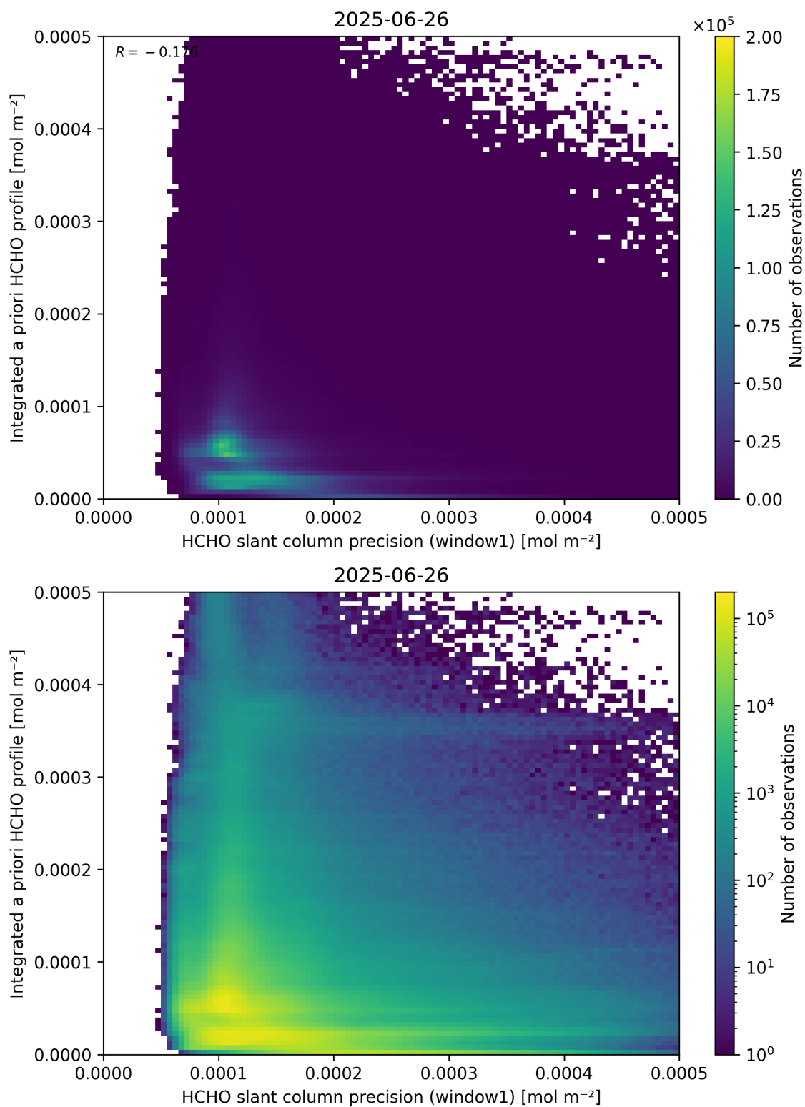
Figure 96: Scatter density plot of “HCHO slant column precision (window1)” against “Integrated a priori HCHO profile” for 2025-06-25 to 2025-06-27.
