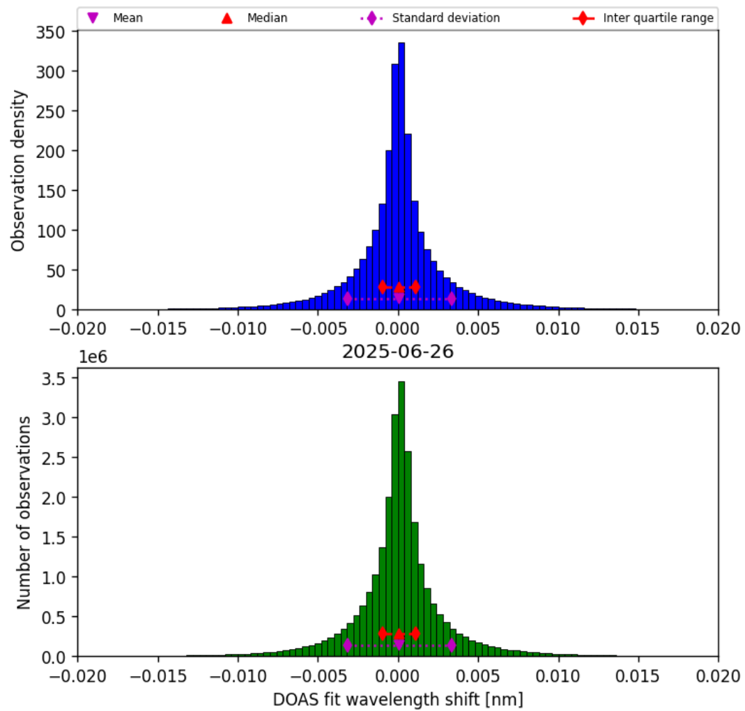
Figure 44: Histogram of “DOAS fit wavelength shift” for 2025-06-25 to 2025-06-27
