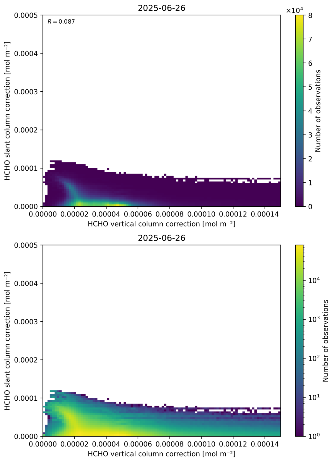
Figure 117: Scatter density plot of “HCHO vertical column correction” against “HCHO slant column correction” for 2025-06-25 to 2025-06-27.
