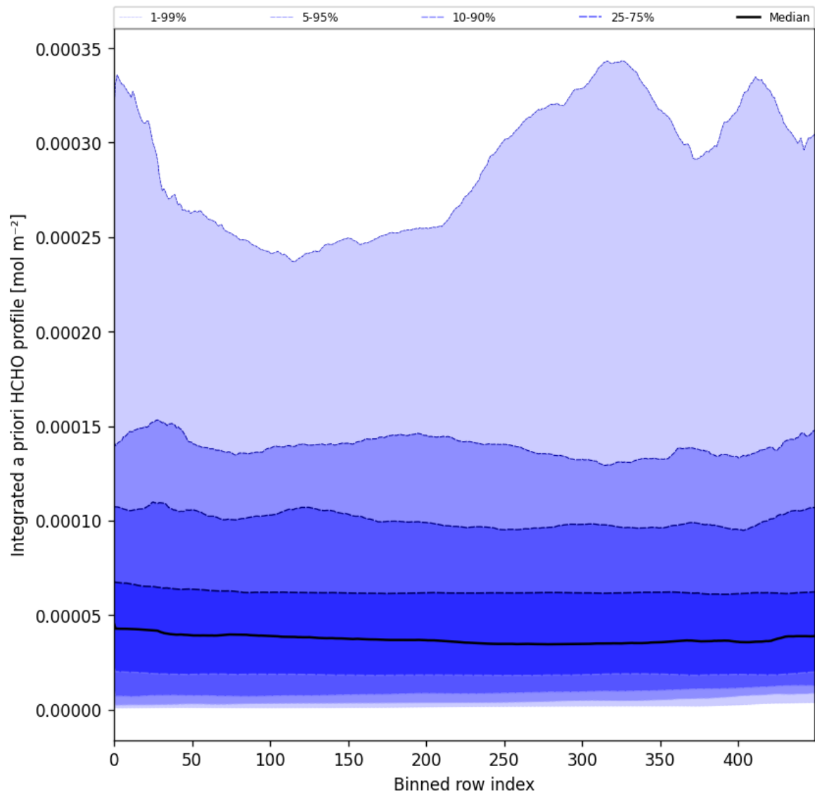
Figure 57: Along track statistics of “Integrated a priori HCHO profile” for 2025-06-25 to 2025-06-27
