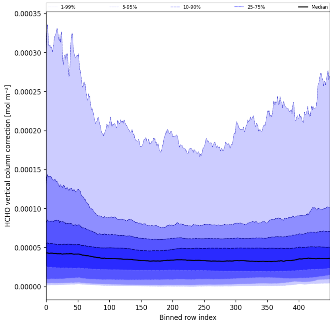
Figure 51: Along track statistics of “HCHO vertical column correction” for 2025-06-25 to 2025-06-27
