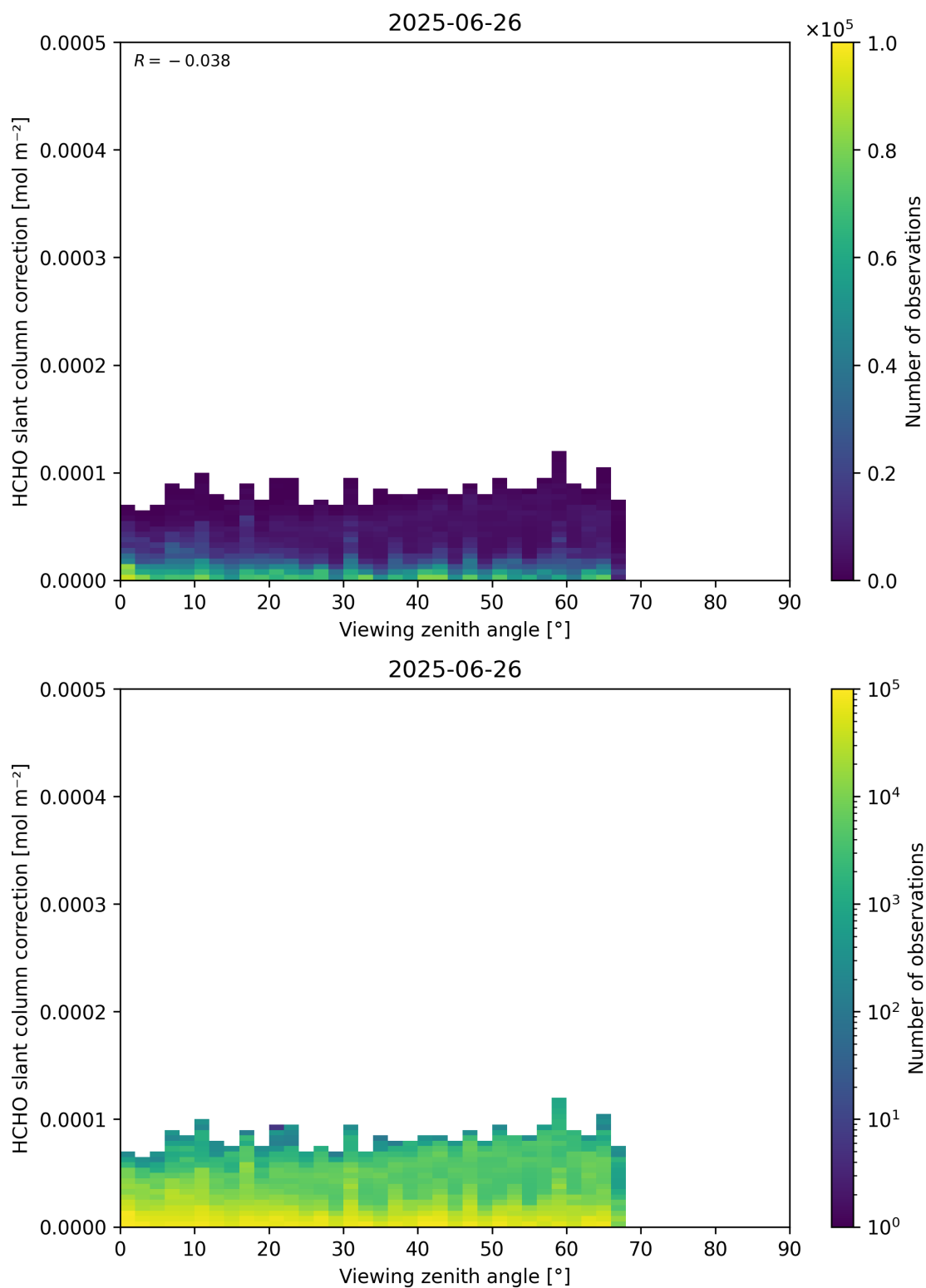
Figure 187: Scatter density plot of “Viewing zenith angle” against “HCHO slant column correction” for 2025-06-25 to 2025-06-27.
