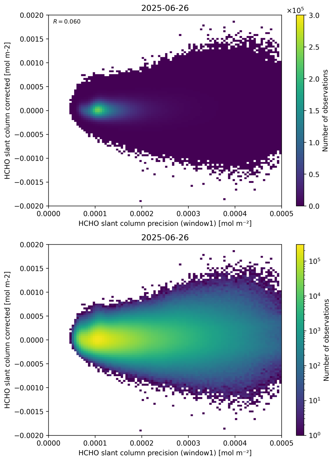
Figure 92: Scatter density plot of “HCHO slant column precision (window1)” against “HCHO slant column corrected” for 2025-06-25 to 2025-06-27.
