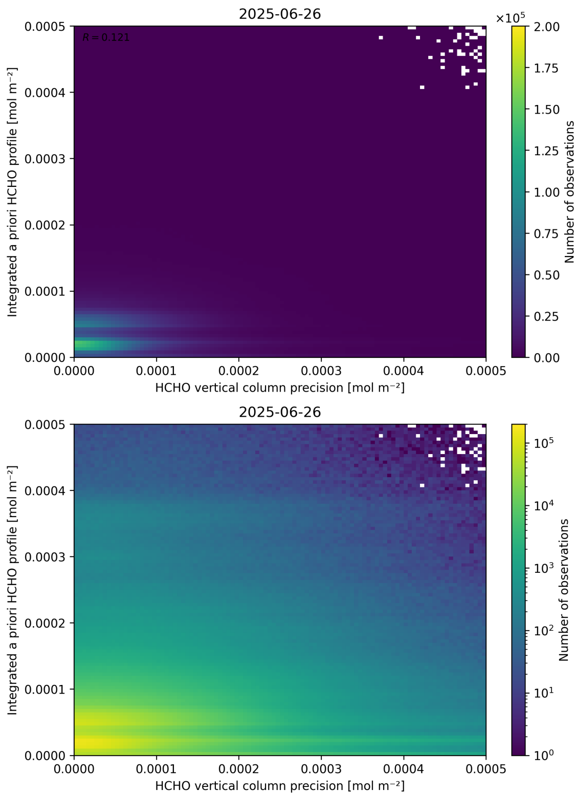
Figure 147: Scatter density plot of “HCHO vertical column precision” against “Integrated a priori HCHO profile” for 2025-06-25 to 2025-06-27.
