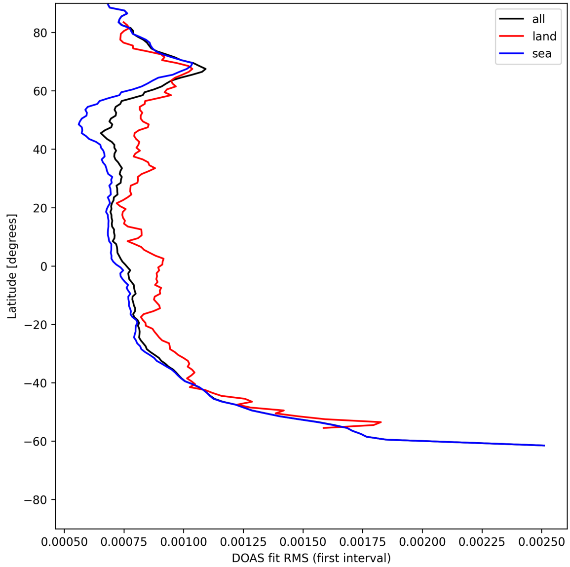
Figure 32: Zonal average of “DOAS fit RMS (first interval)” for 2025-06-25 to 2025-06-27.
