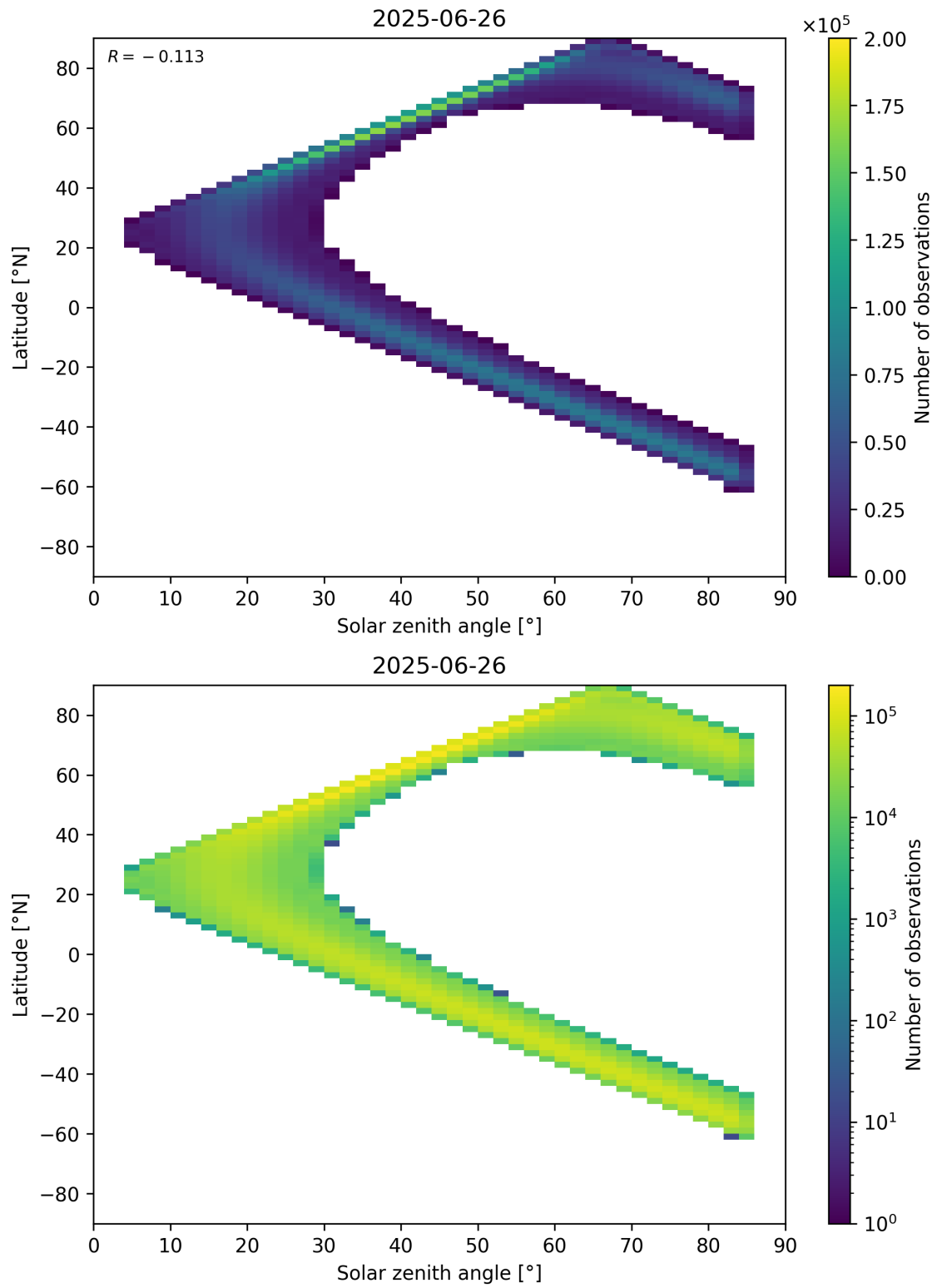
Figure 181: Scatter density plot of “Solar zenith angle” against “Latitude” for 2025-06-25 to 2025-06-27.
