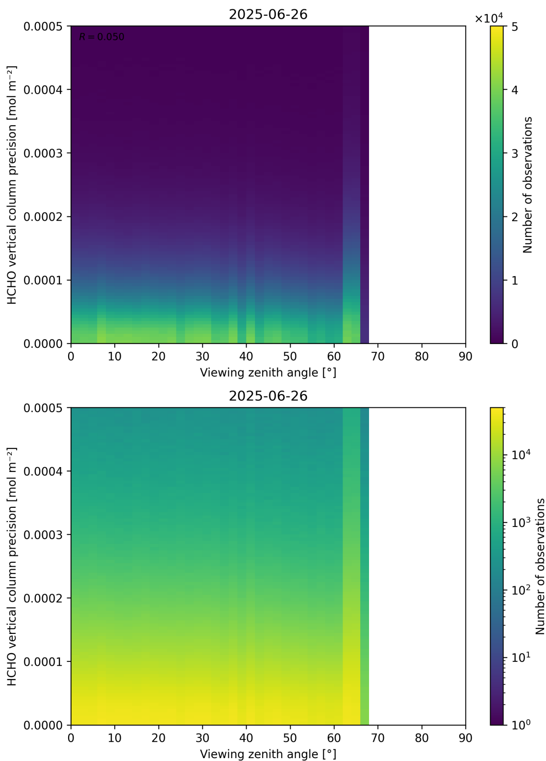
Figure 194: Scatter density plot of “Viewing zenith angle” against “HCHO vertical column precision” for 2025-06-25 to 2025-06-27.
