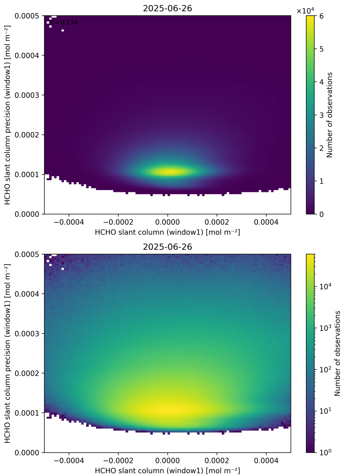
Figure 84: Scatter density plot of “HCHO slant column (window1)” against “HCHO slant column precision (window1)” for 2025-06-25 to 2025-06-27.
