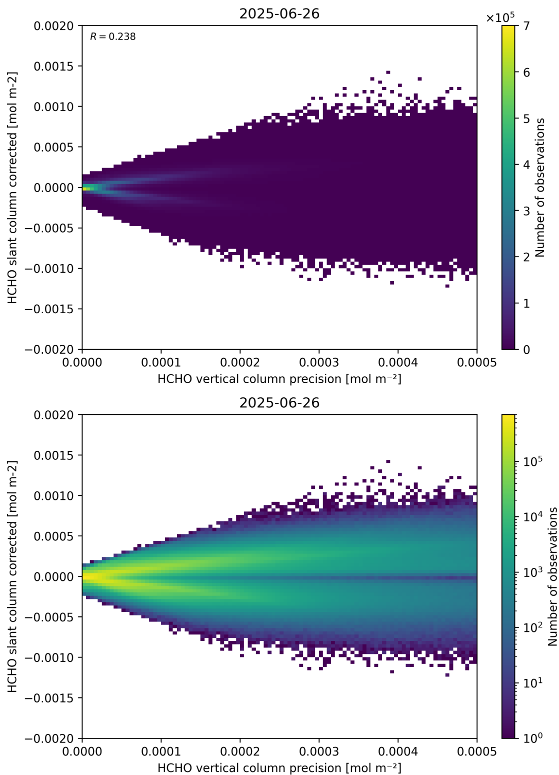
Figure 140: Scatter density plot of “HCHO vertical column precision” against “HCHO slant column corrected” for 2025-06-25 to 2025-06-27.
