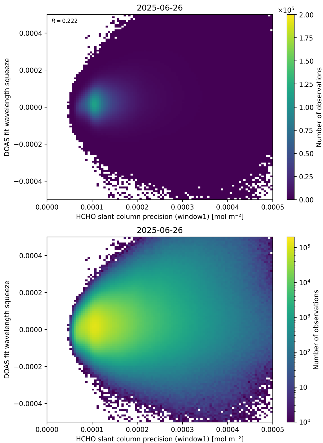
Figure 90: Scatter density plot of “HCHO slant column precision (window1)” against “DOAS fit wavelength squeeze” for 2025-06-25 to 2025-06-27.
