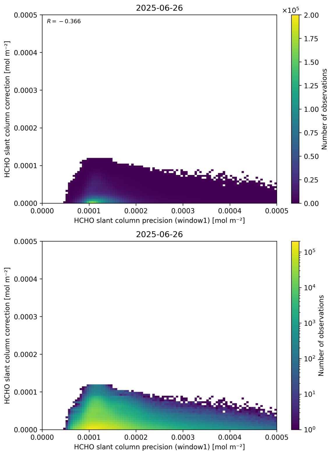
Figure 93: Scatter density plot of “HCHO slant column precision (window1)” against “HCHO slant column correction” for 2025-06-25 to 2025-06-27.
