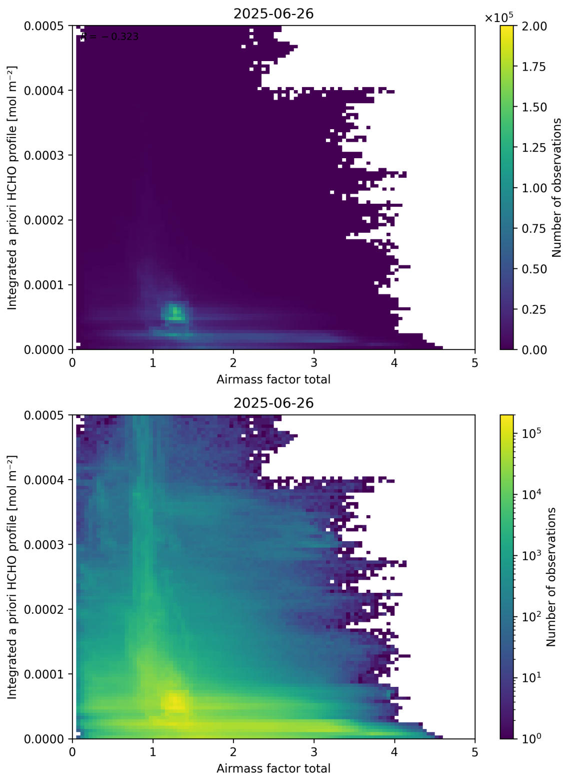
Figure 104: Scatter density plot of “Airmass factor total” against “Integrated a priori HCHO profile” for 2025-06-25 to 2025-06-27.
