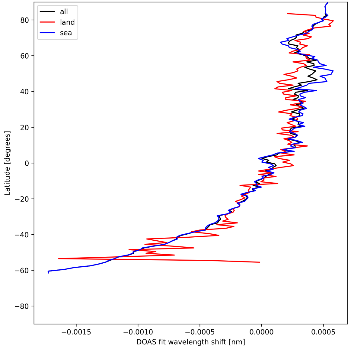
Figure 30: Zonal average of “DOAS fit wavelength shift” for 2025-06-25 to 2025-06-27.
