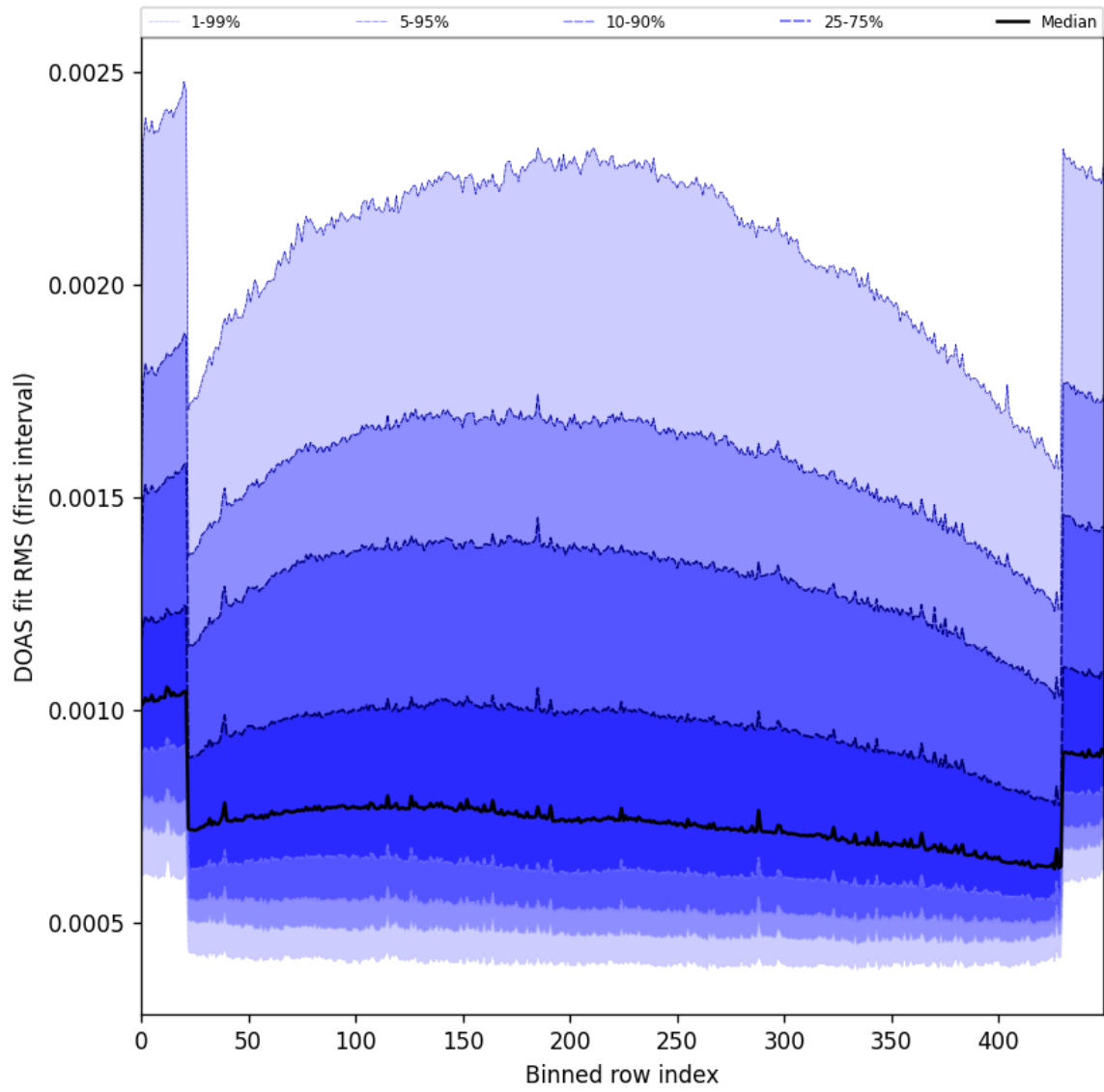
Figure 60: Along track statistics of “DOAS fit RMS (first interval)” for 2025-06-25 to 2025-06-27
