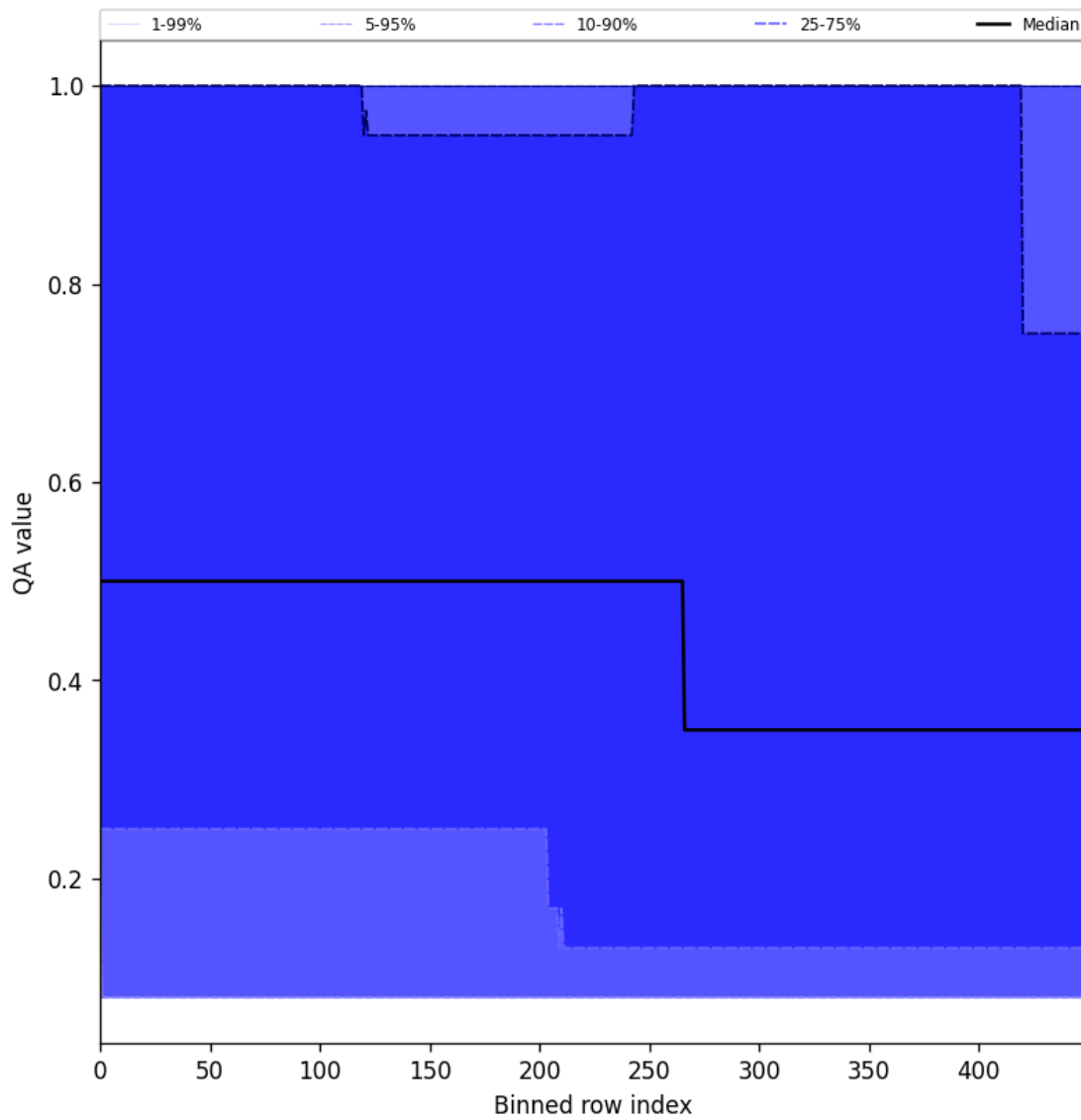
Figure 48: Along track statistics of “QA value” for 2025-06-25 to 2025-06-27
