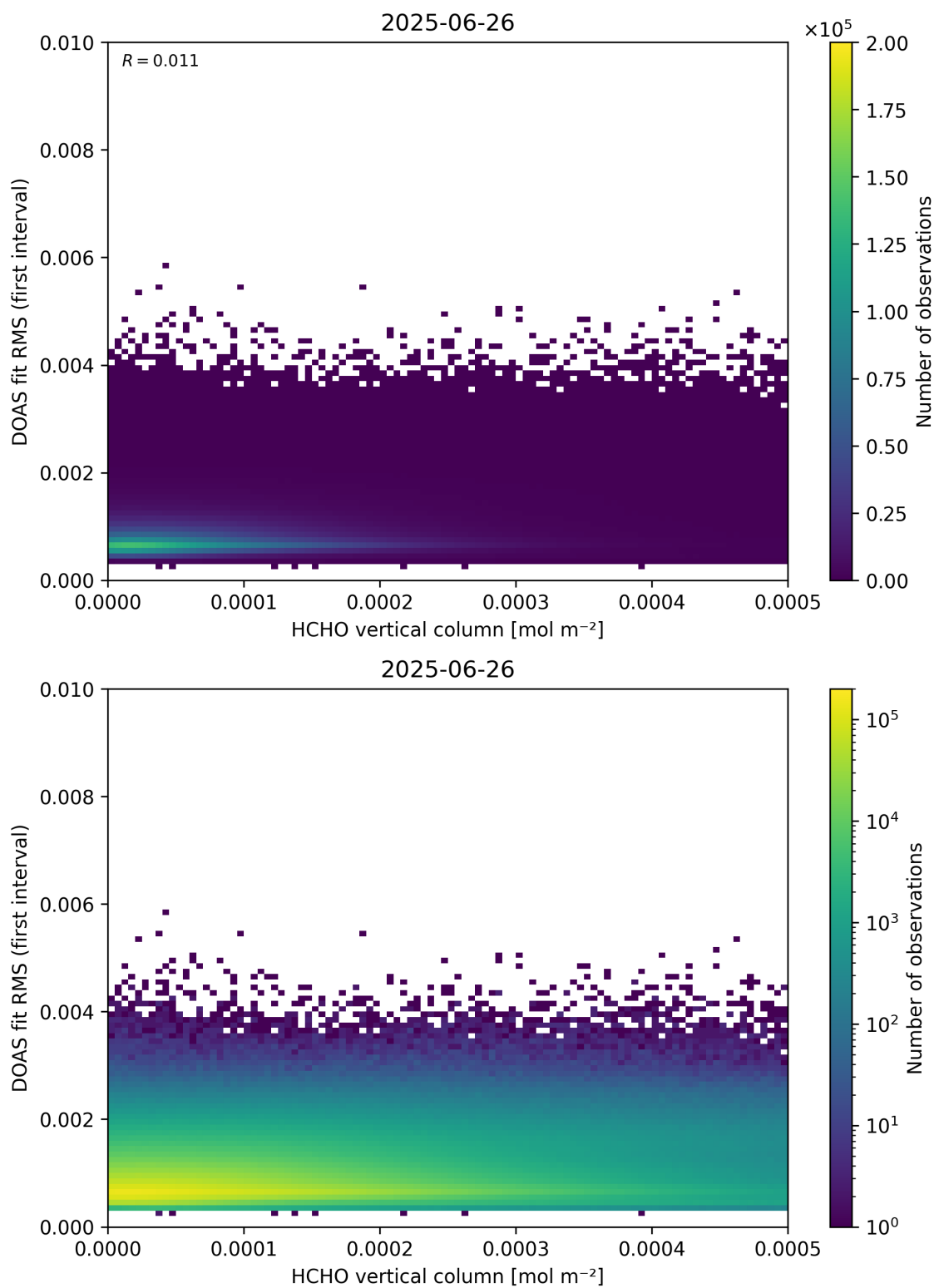
Figure 123: Scatter density plot of “HCHO vertical column” against “DOAS fit RMS (first interval)” for 2025-06-25 to 2025-06-27.
