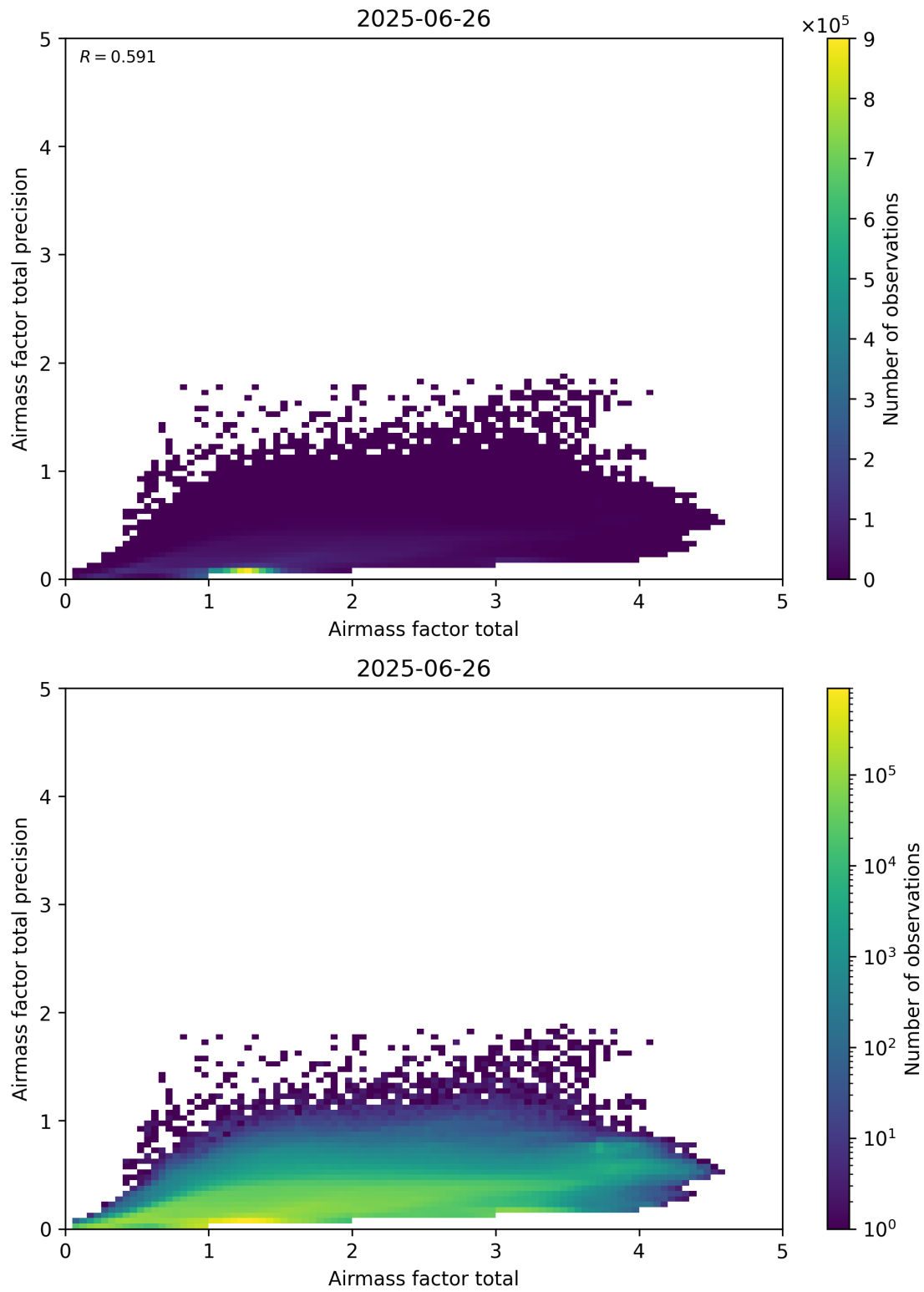
Figure 103: Scatter density plot of “Airmass factor total” against “Airmass factor total precision” for 2025-06-25 to 2025-06-27.
