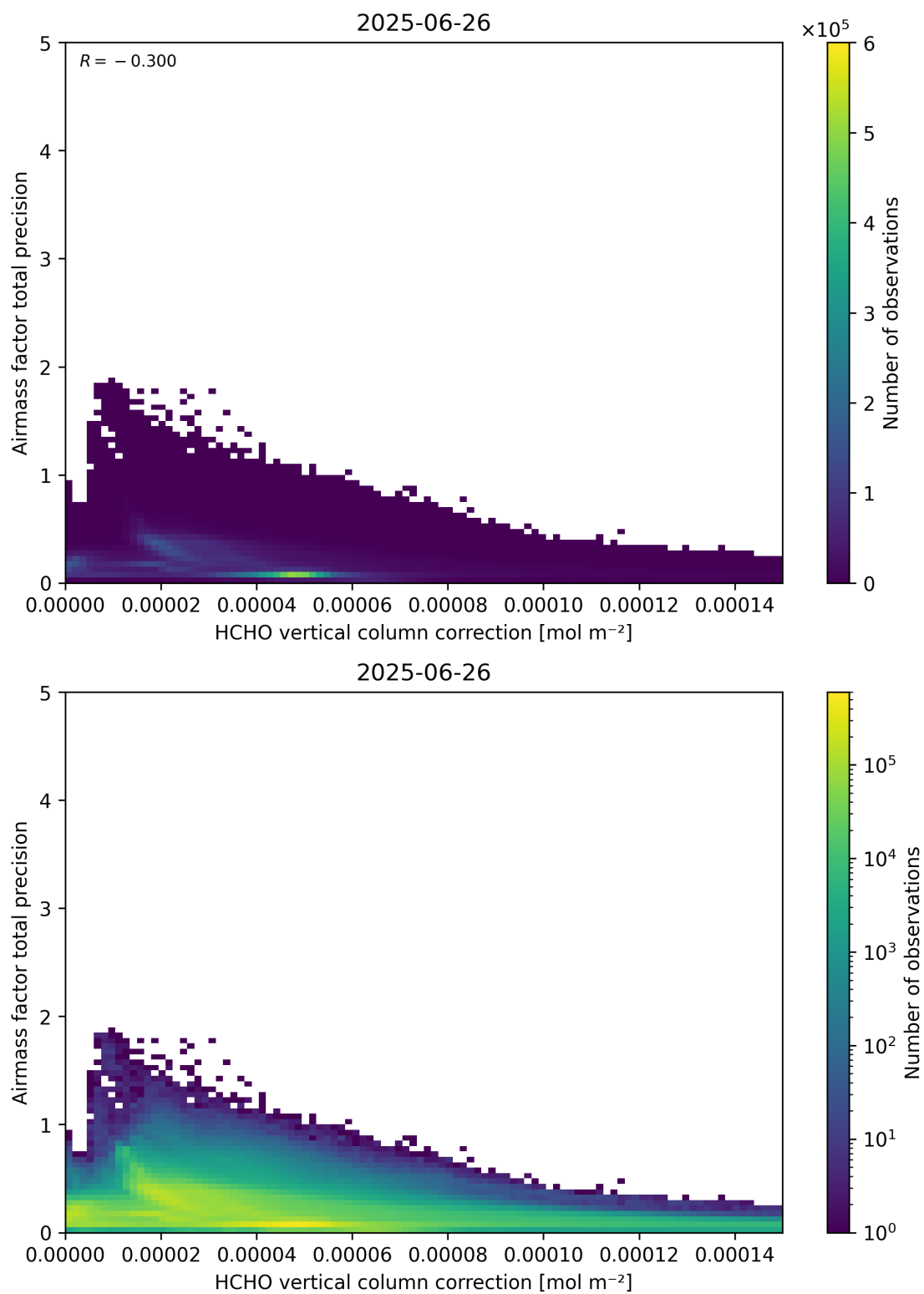
Figure 121: Scatter density plot of “HCHO vertical column correction” against “Airmass factor total precision” for 2025-06-25 to 2025-06-27.
