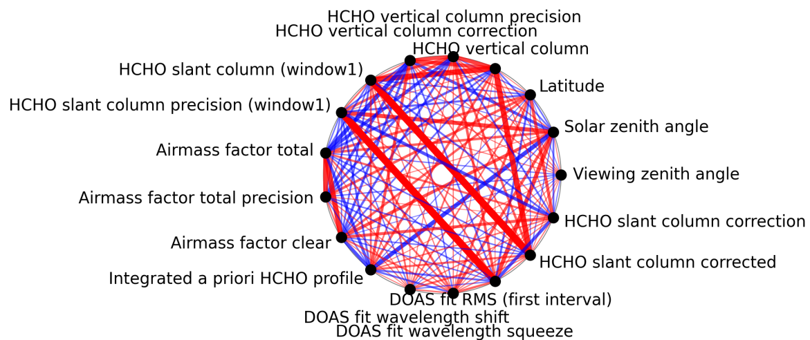
Figure 1: Map of correlation graph for 2025-06-25 to 2025-06-27.
