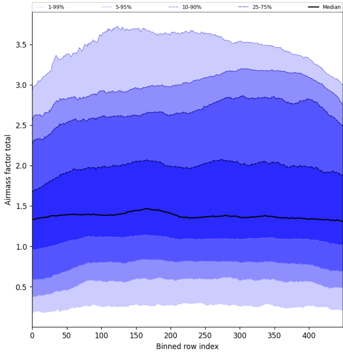
Figure 54: Along track statistics of “Airmass factor total” for 2025-06-25 to 2025-06-27
