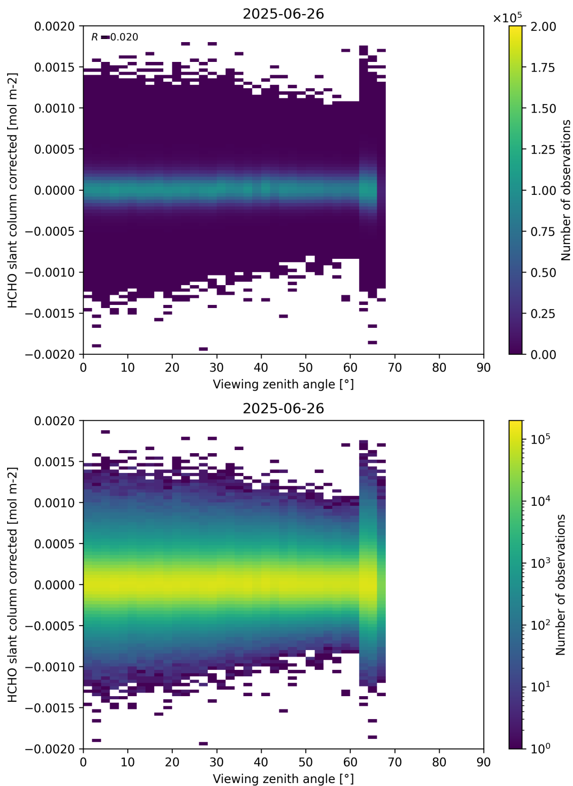
Figure 186: Scatter density plot of “Viewing zenith angle” against “HCHO slant column corrected” for 2025-06-25 to 2025-06-27.
