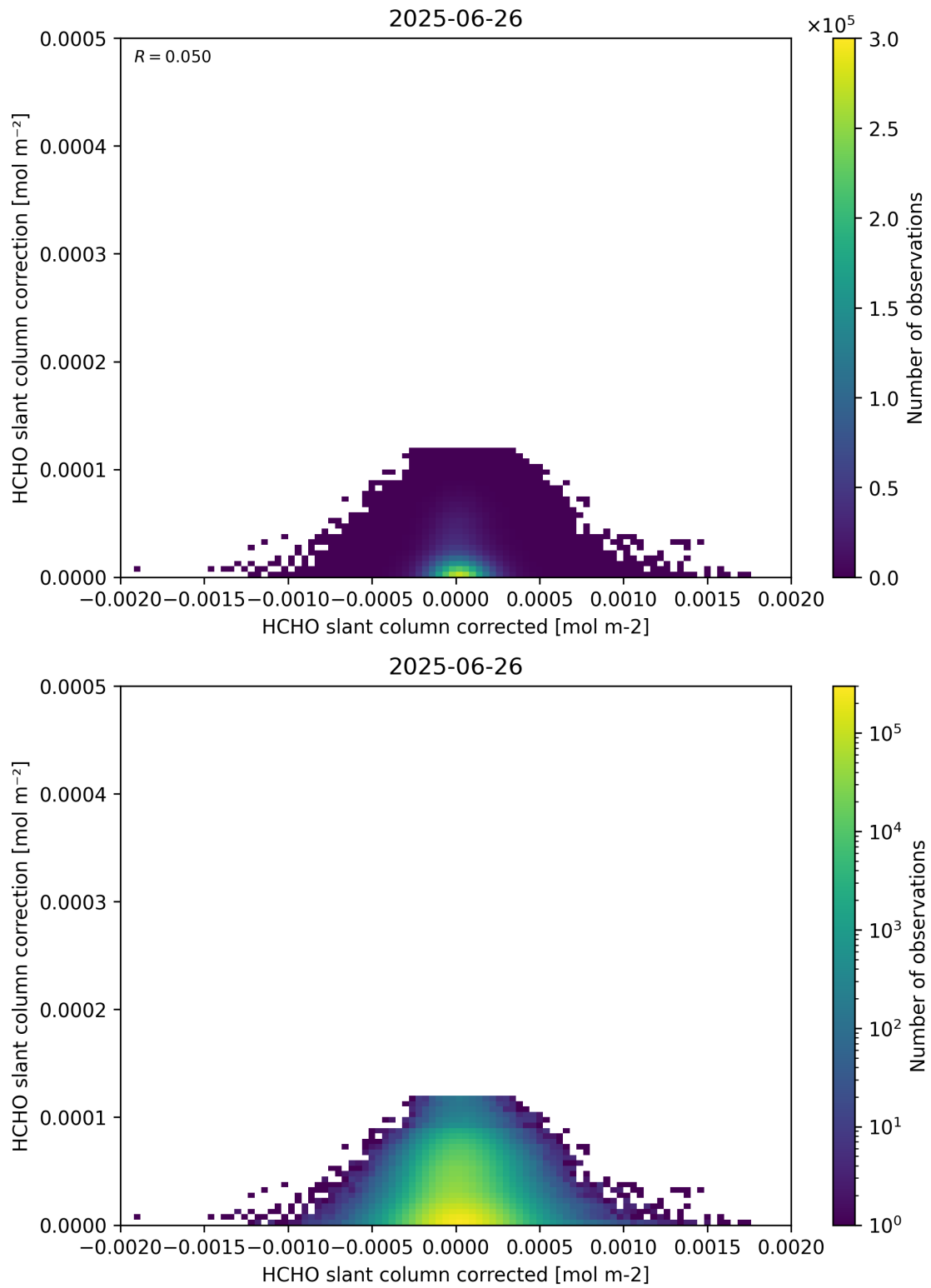
Figure 77: Scatter density plot of “HCHO slant column corrected” against “HCHO slant column correction” for 2025-06-25 to 2025-06-27.
