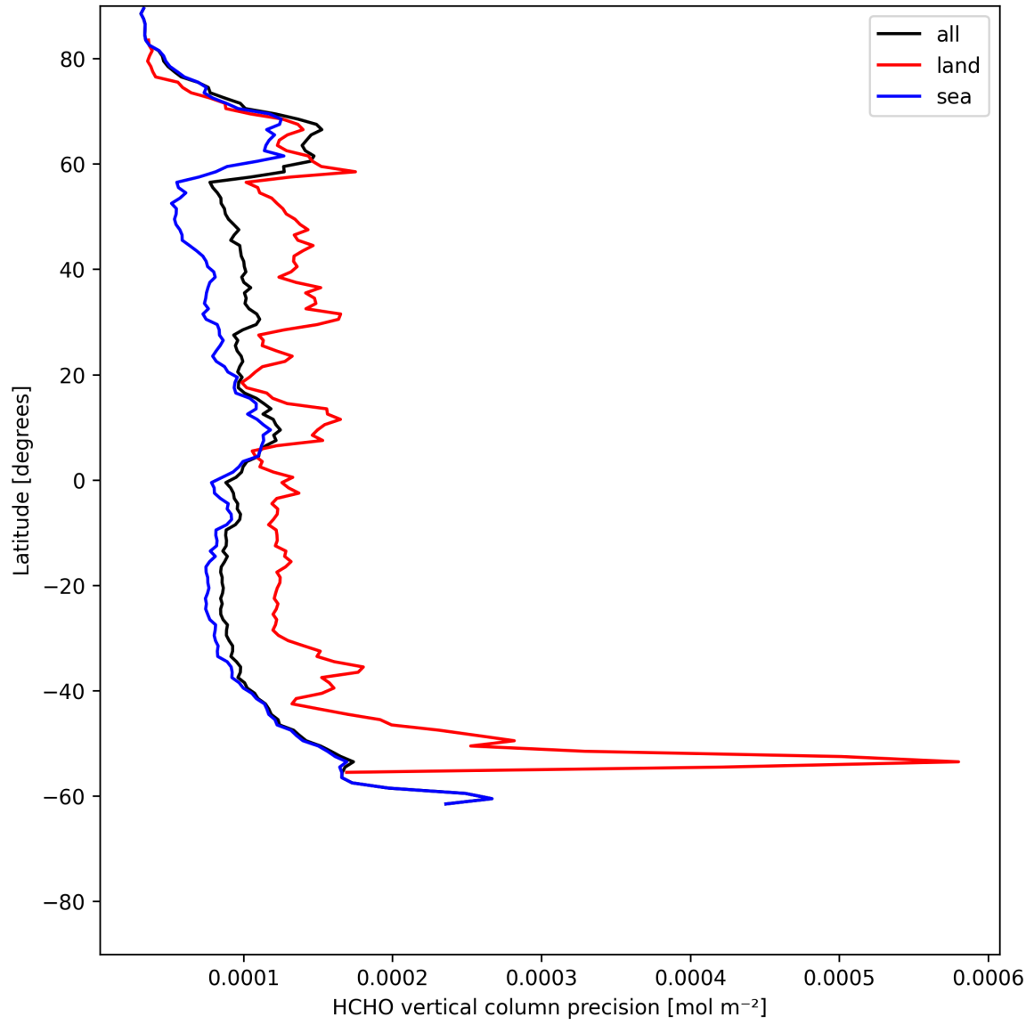
Figure 22: Zonal average of “HCHO vertical column precision” for 2025-06-25 to 2025-06-27.
