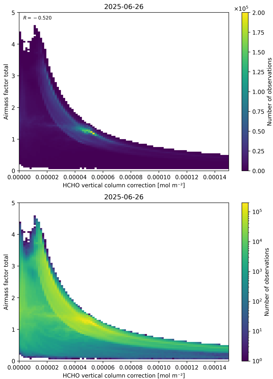
Figure 120: Scatter density plot of “HCHO vertical column correction” against “Airmass factor total” for 2025-06-25 to 2025-06-27.
