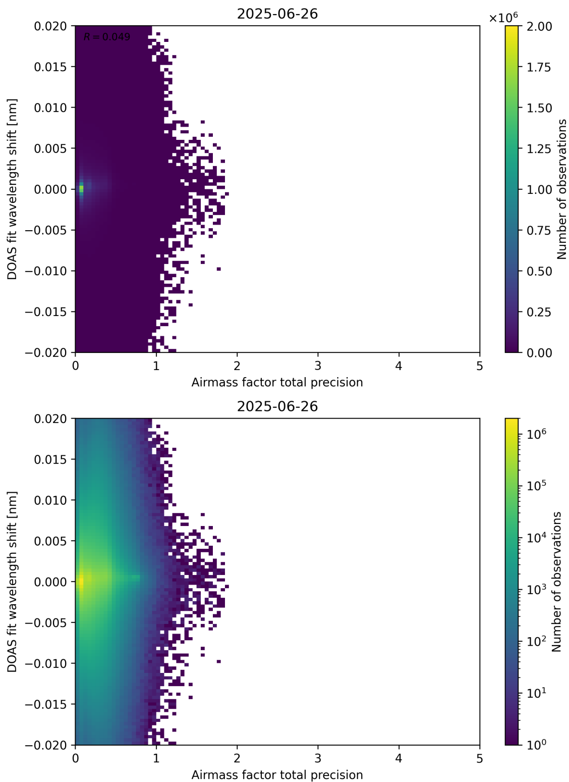
Figure 106: Scatter density plot of “Airmass factor total precision” against “DOAS fit wavelength shift” for 2025-06-25 to 2025-06-27.
