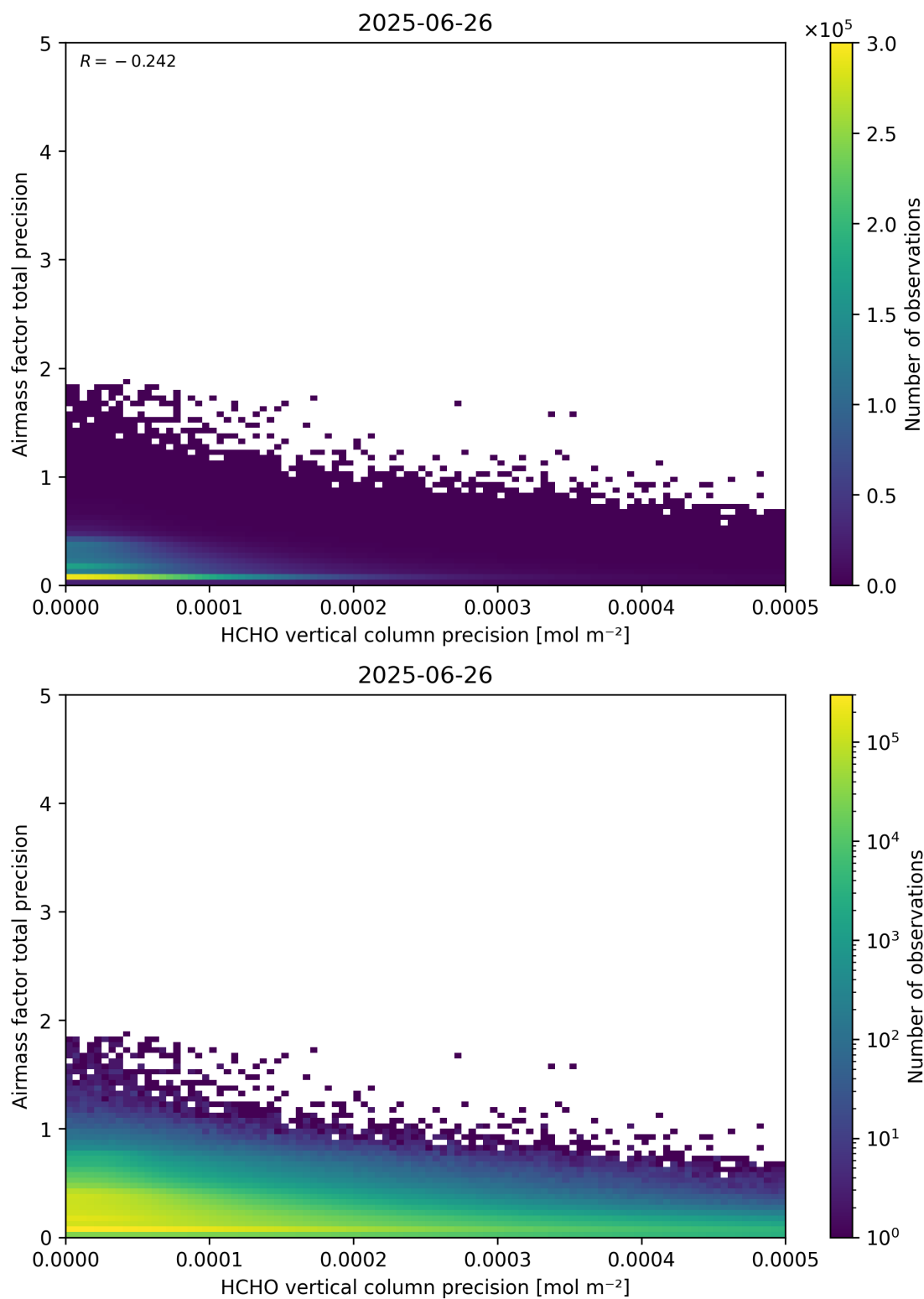
Figure 145: Scatter density plot of “HCHO vertical column precision” against “Airmass factor total precision” for 2025-06-25 to 2025-06-27.
