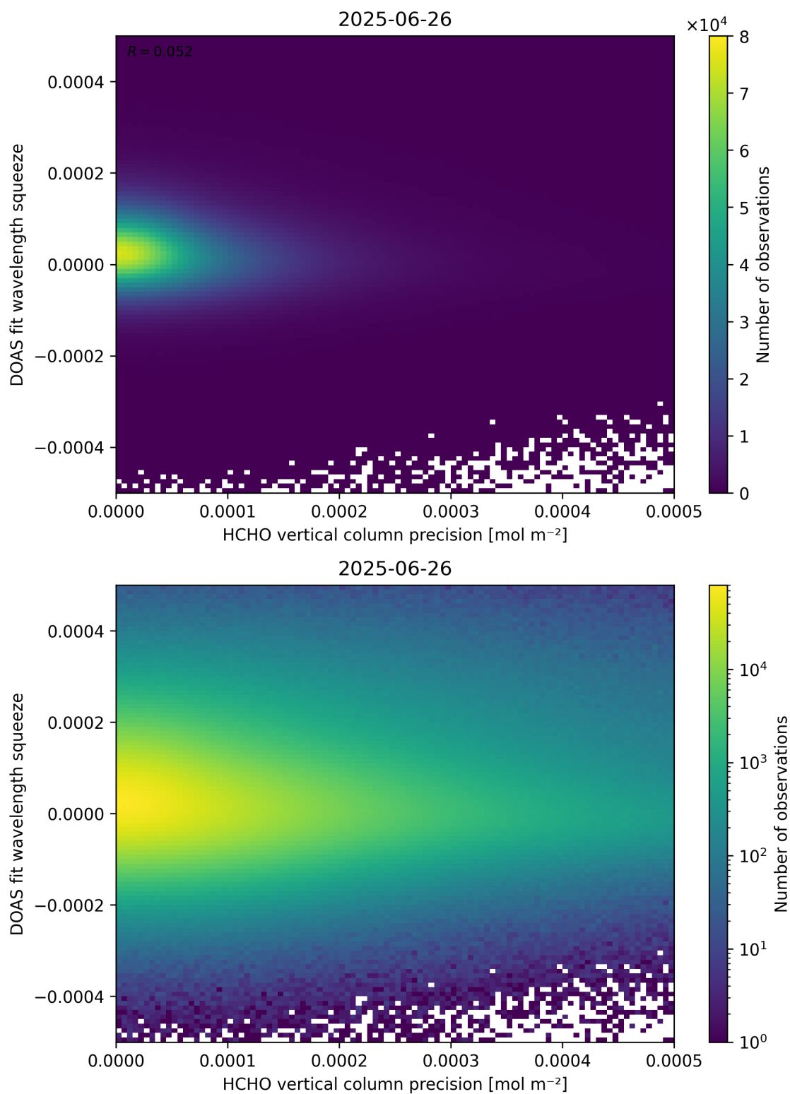
Figure 138: Scatter density plot of “HCHO vertical column precision” against “DOAS fit wavelength squeeze” for 2025-06-25 to 2025-06-27.
