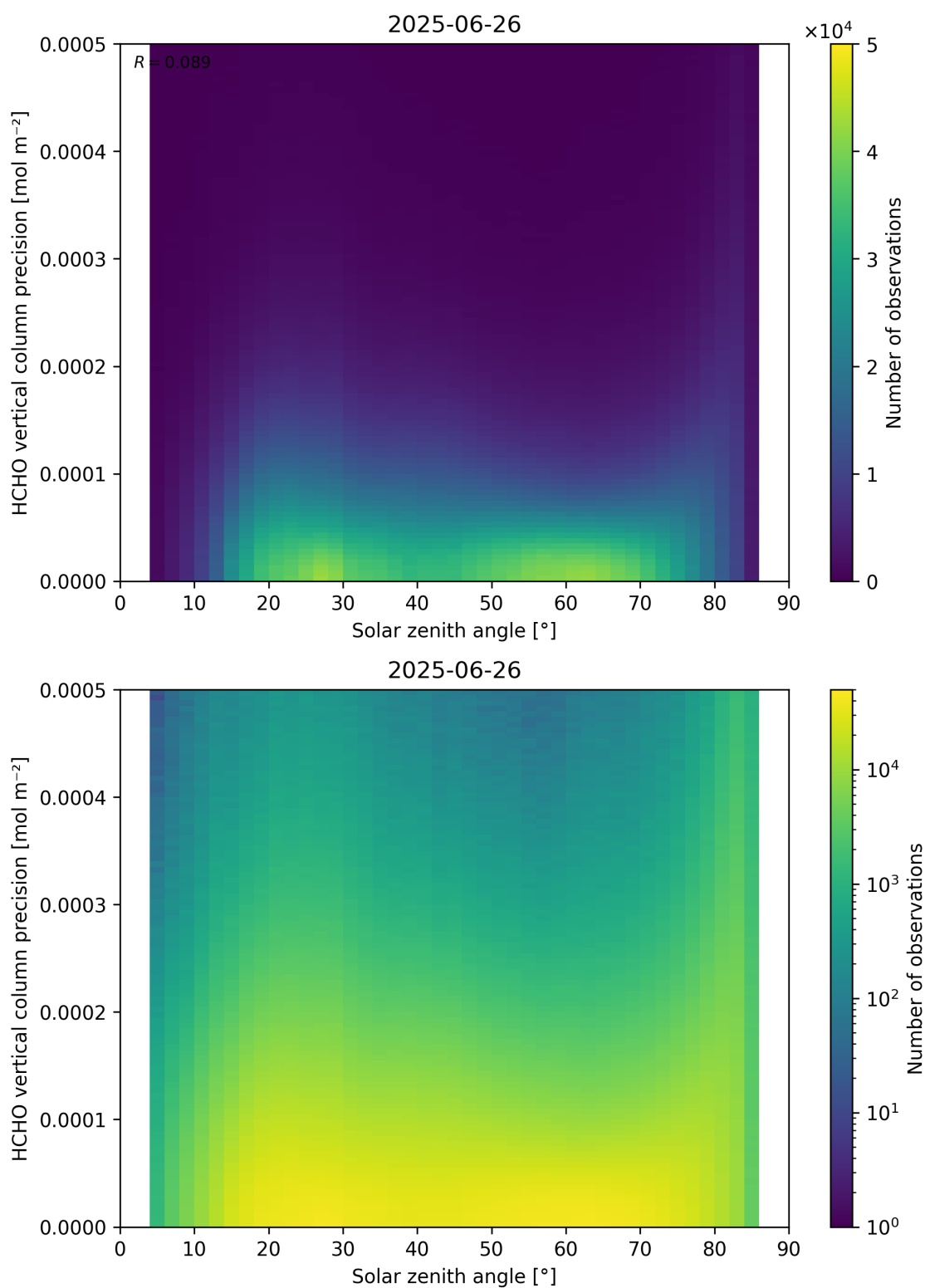
Figure 179: Scatter density plot of “Solar zenith angle” against “HCHO vertical column precision” for 2025-06-25 to 2025-06-27.
