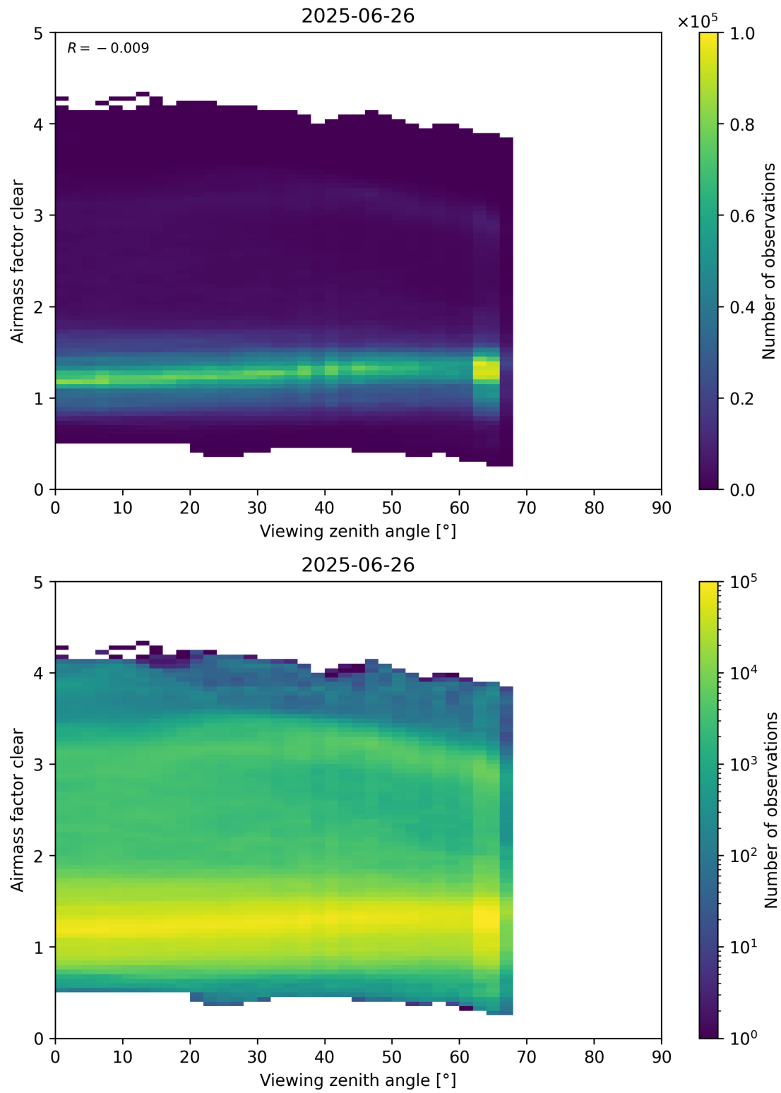
Figure 185: Scatter density plot of “Viewing zenith angle” against “Airmass factor clear” for 2025-06-25 to 2025-06-27.
