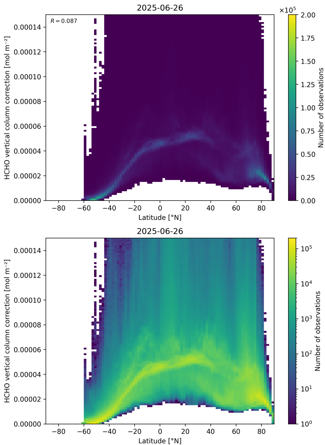
Figure 164: Scatter density plot of “Latitude” against “HCHO vertical column correction” for 2025-06-25 to 2025-06-27.
