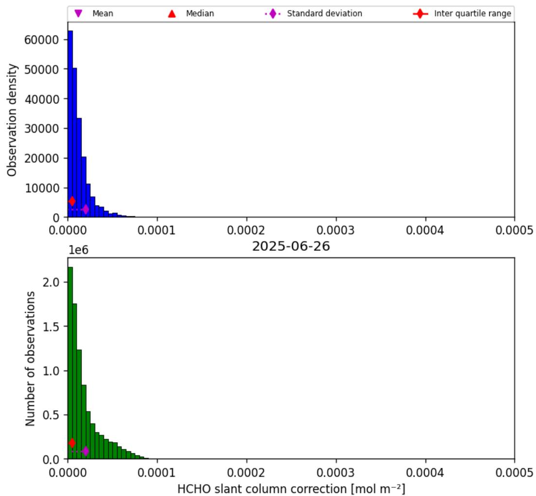
Figure 47: Histogram of “HCHO slant column correction” for 2025-06-25 to 2025-06-27
