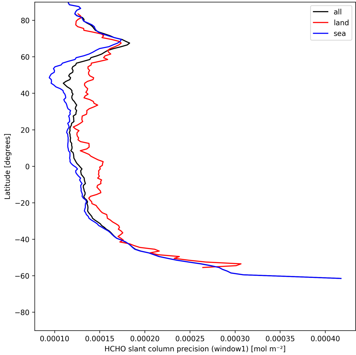
Figure 25: Zonal average of “HCHO slant column precision (window1)” for 2025-06-25 to 2025-06-27.
