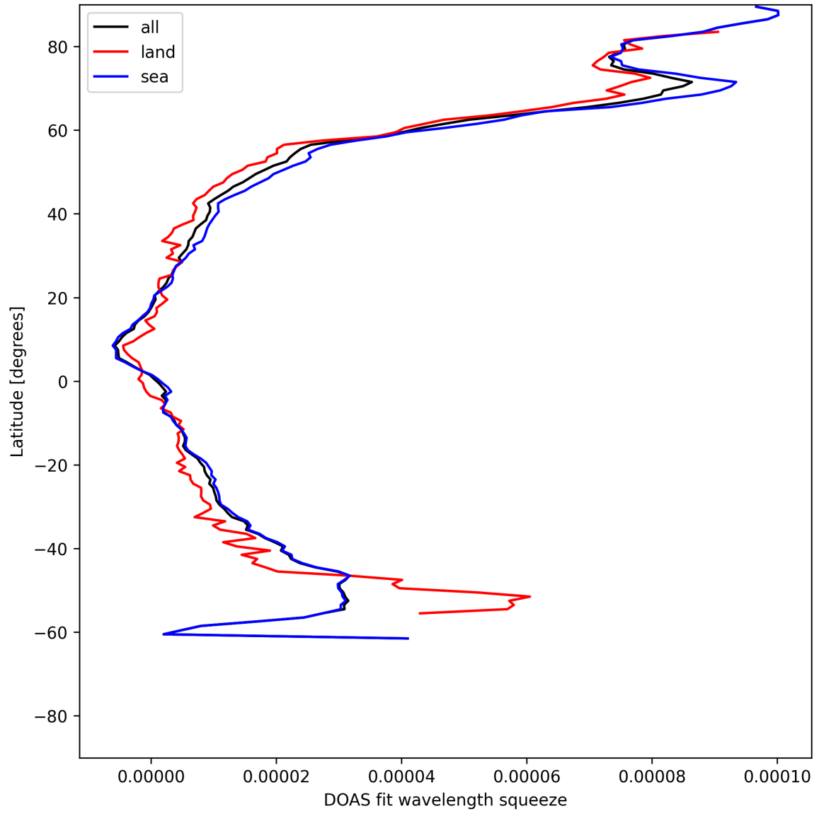
Figure 31: Zonal average of “DOAS fit wavelength squeeze” for 2025-06-25 to 2025-06-27.
