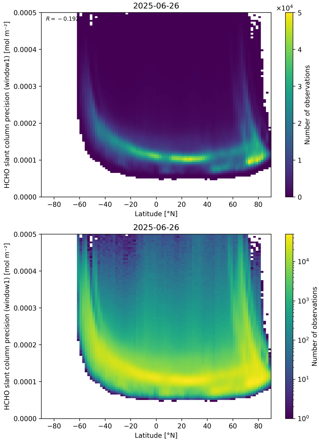
Figure 160: Scatter density plot of “Latitude” against “HCHO slant column precision (window1)” for 2025-06-25 to 2025-06-27.
