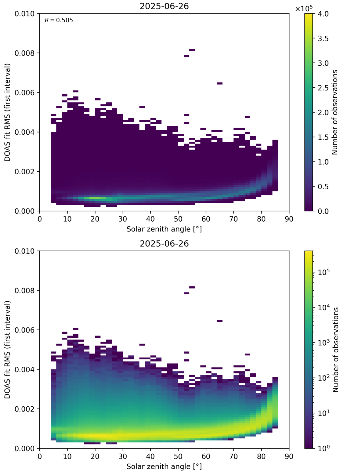
Figure 167: Scatter density plot of “Solar zenith angle” against “DOAS fit RMS (first interval)” for 2025-06-25 to 2025-06-27.
