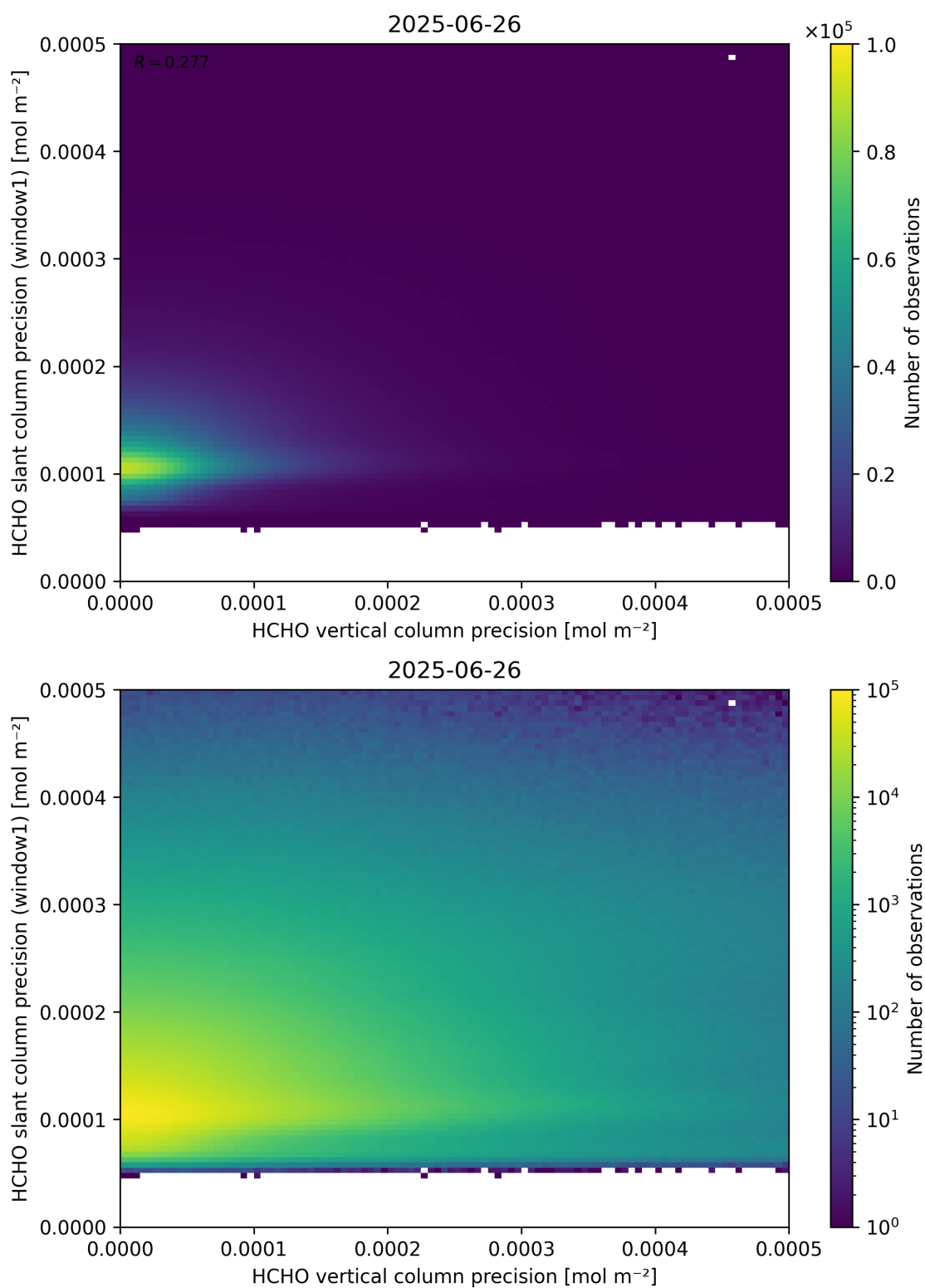
Figure 143: Scatter density plot of “HCHO vertical column precision” against “HCHO slant column precision (window1)” for 2025-06-25 to 2025-06-27.
