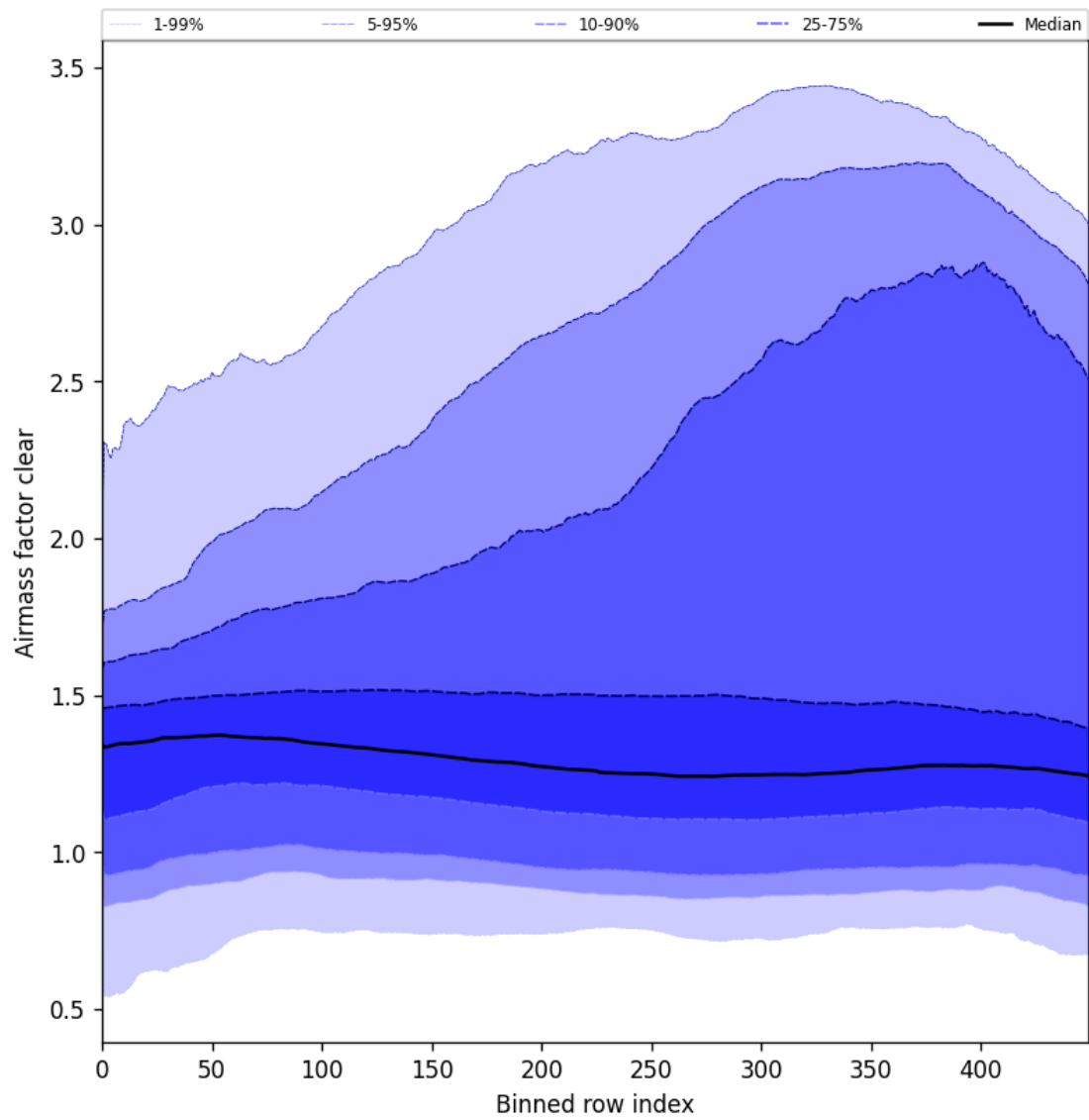
Figure 56: Along track statistics of “Airmass factor clear” for 2025-06-25 to 2025-06-27
