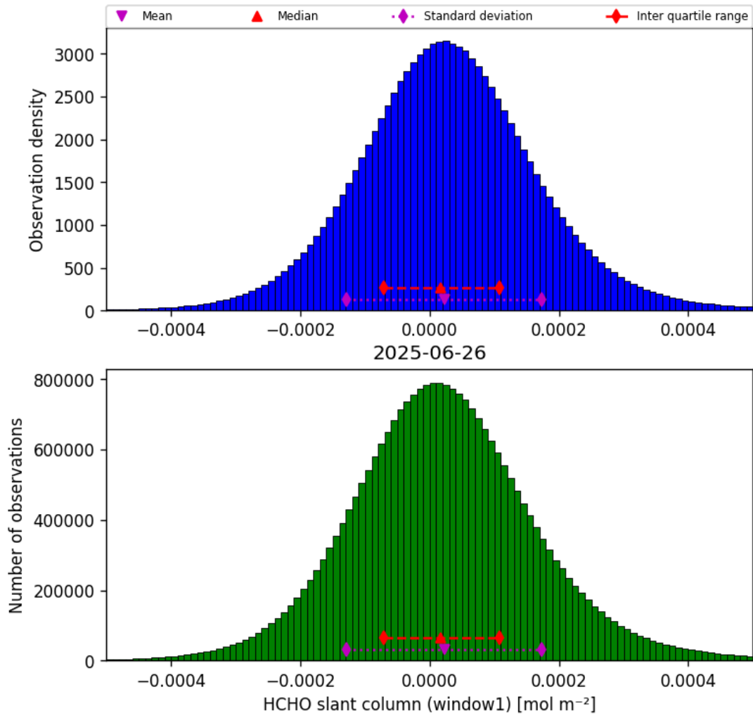
Figure 38: Histogram of “HCHO slant column (window1)” for 2025-06-25 to 2025-06-27
