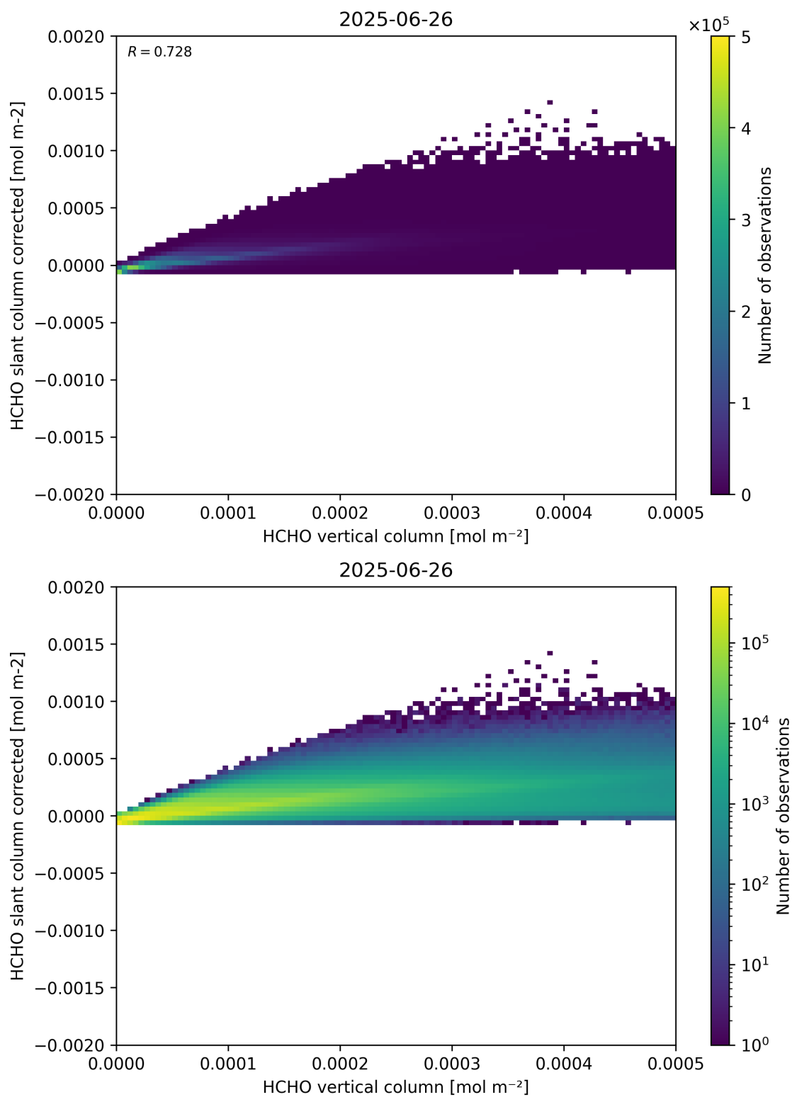
Figure 127: Scatter density plot of “HCHO vertical column” against “HCHO slant column corrected” for 2025-06-25 to 2025-06-27.
