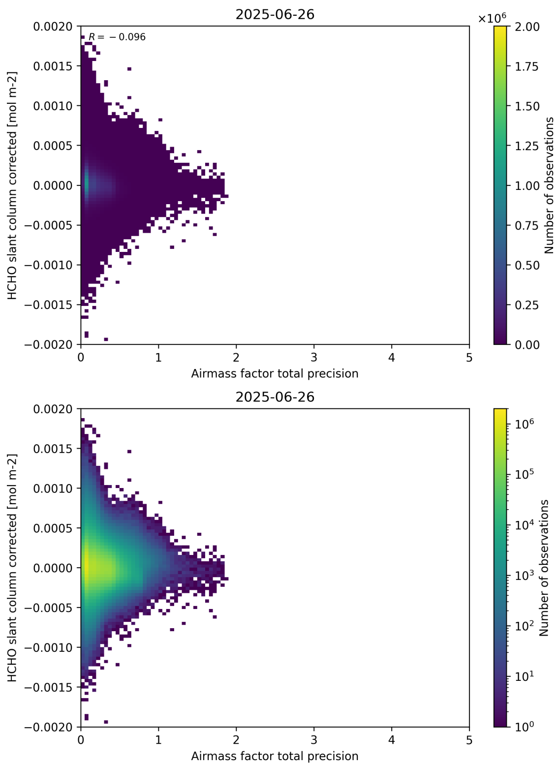
Figure 109: Scatter density plot of “Airmass factor total precision” against “HCHO slant column corrected” for 2025-06-25 to 2025-06-27.
