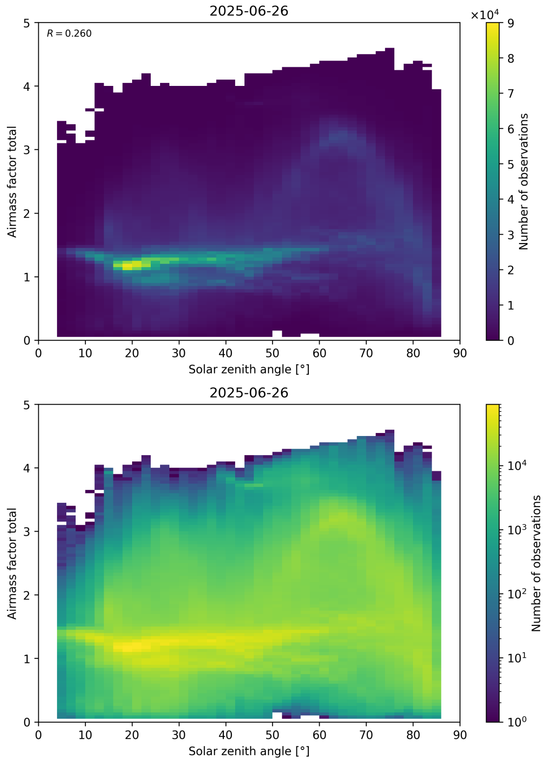
Figure 175: Scatter density plot of “Solar zenith angle” against “Airmass factor total” for 2025-06-25 to 2025-06-27.
