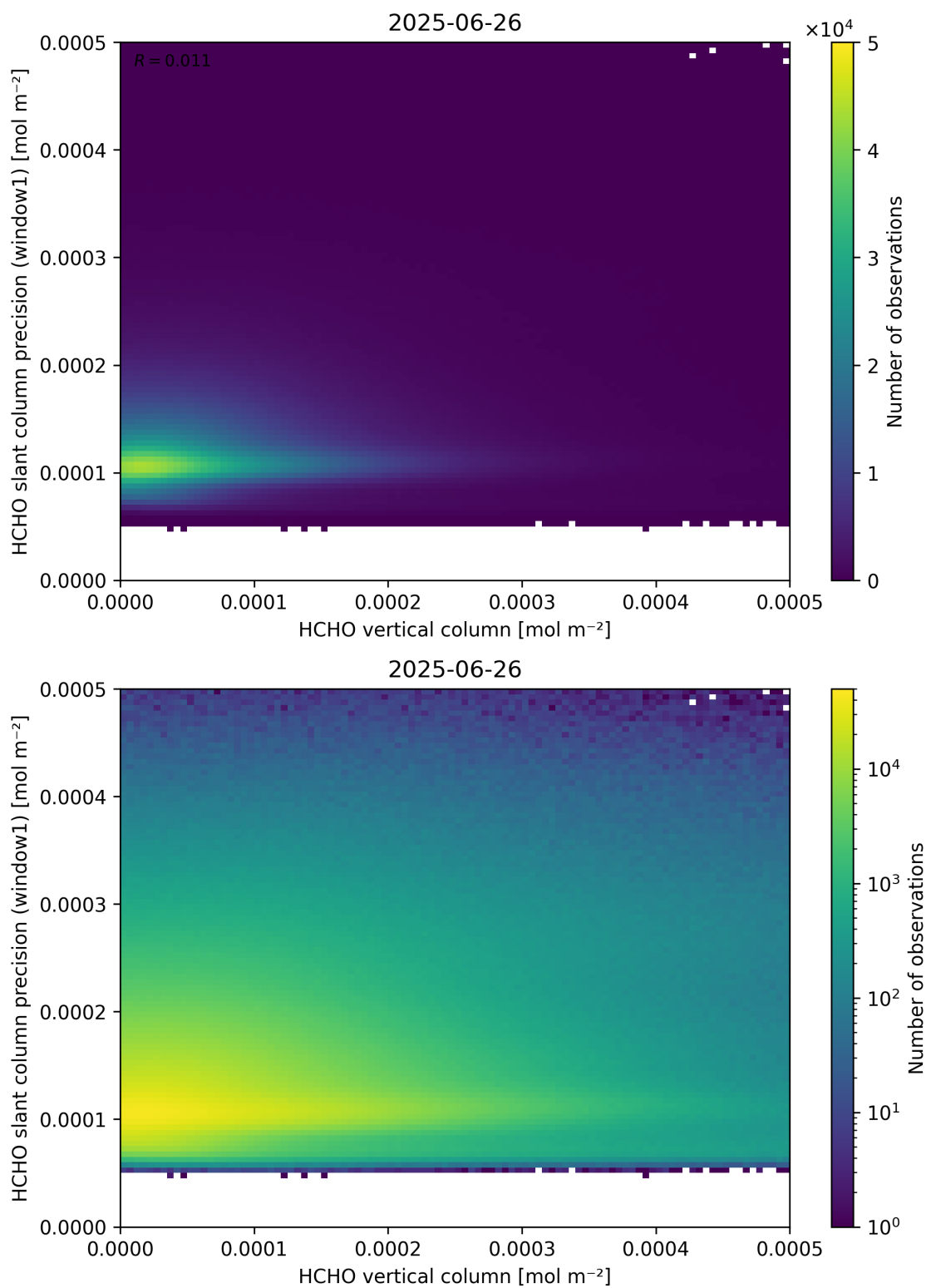
Figure 130: Scatter density plot of “HCHO vertical column” against “HCHO slant column precision (window1)” for 2025-06-25 to 2025-06-27.
