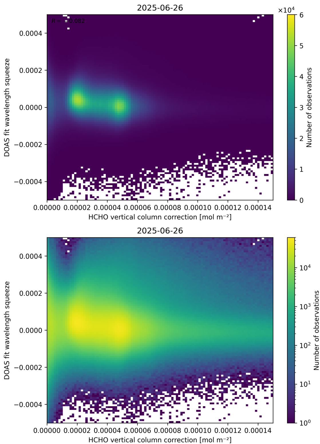
Figure 114: Scatter density plot of “HCHO vertical column correction” against “DOAS fit wavelength squeeze” for 2025-06-25 to 2025-06-27.
