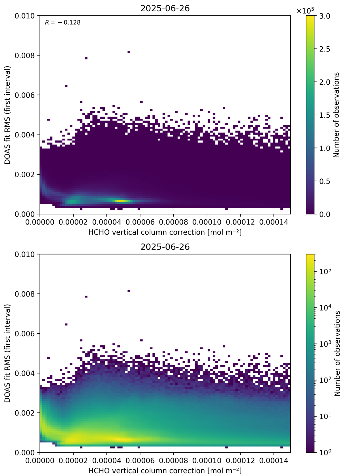
Figure 112: Scatter density plot of “HCHO vertical column correction” against “DOAS fit RMS (first interval)” for 2025-06-25 to 2025-06-27.
