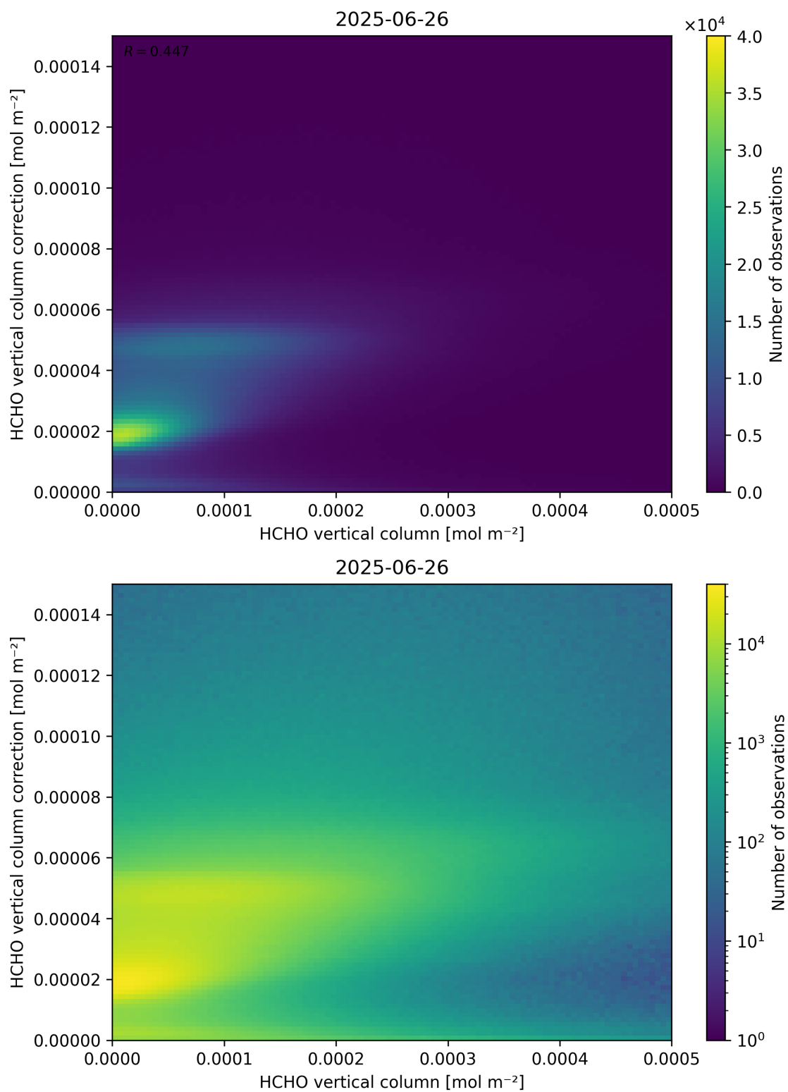
Figure 133: Scatter density plot of “HCHO vertical column” against “HCHO vertical column correction” for 2025-06-25 to 2025-06-27.
