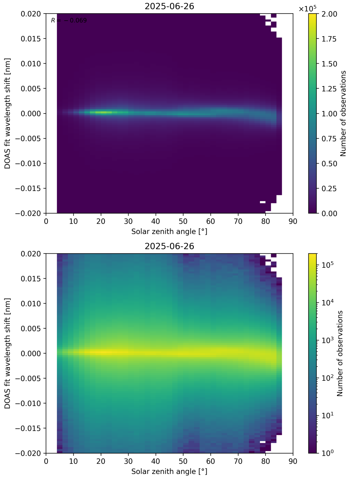
Figure 168: Scatter density plot of “Solar zenith angle” against “DOAS fit wavelength shift” for 2025-06-25 to 2025-06-27.
