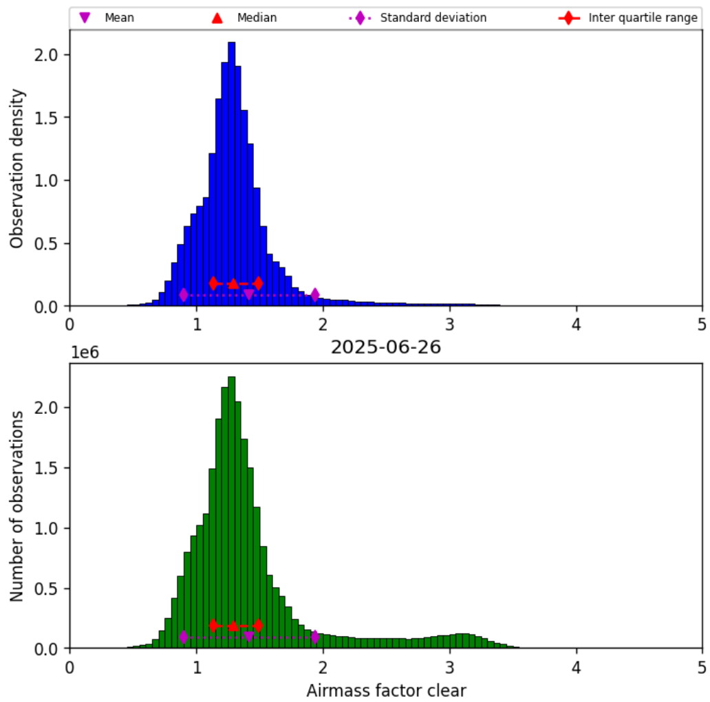
Figure 42: Histogram of “Airmass factor clear” for 2025-06-25 to 2025-06-27
