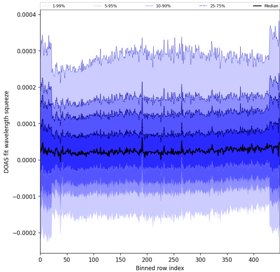
Figure 59: Along track statistics of “DOAS fit wavelength squeeze” for 2025-06-25 to 2025-06-27
