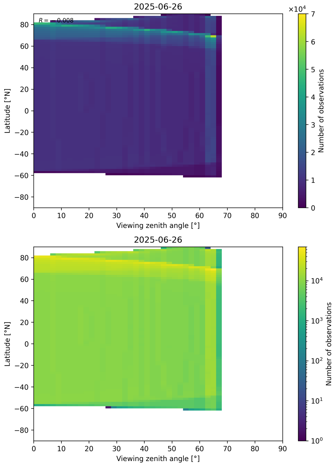
Figure 196: Scatter density plot of “Viewing zenith angle” against “Latitude” for 2025-06-25 to 2025-06-27.
