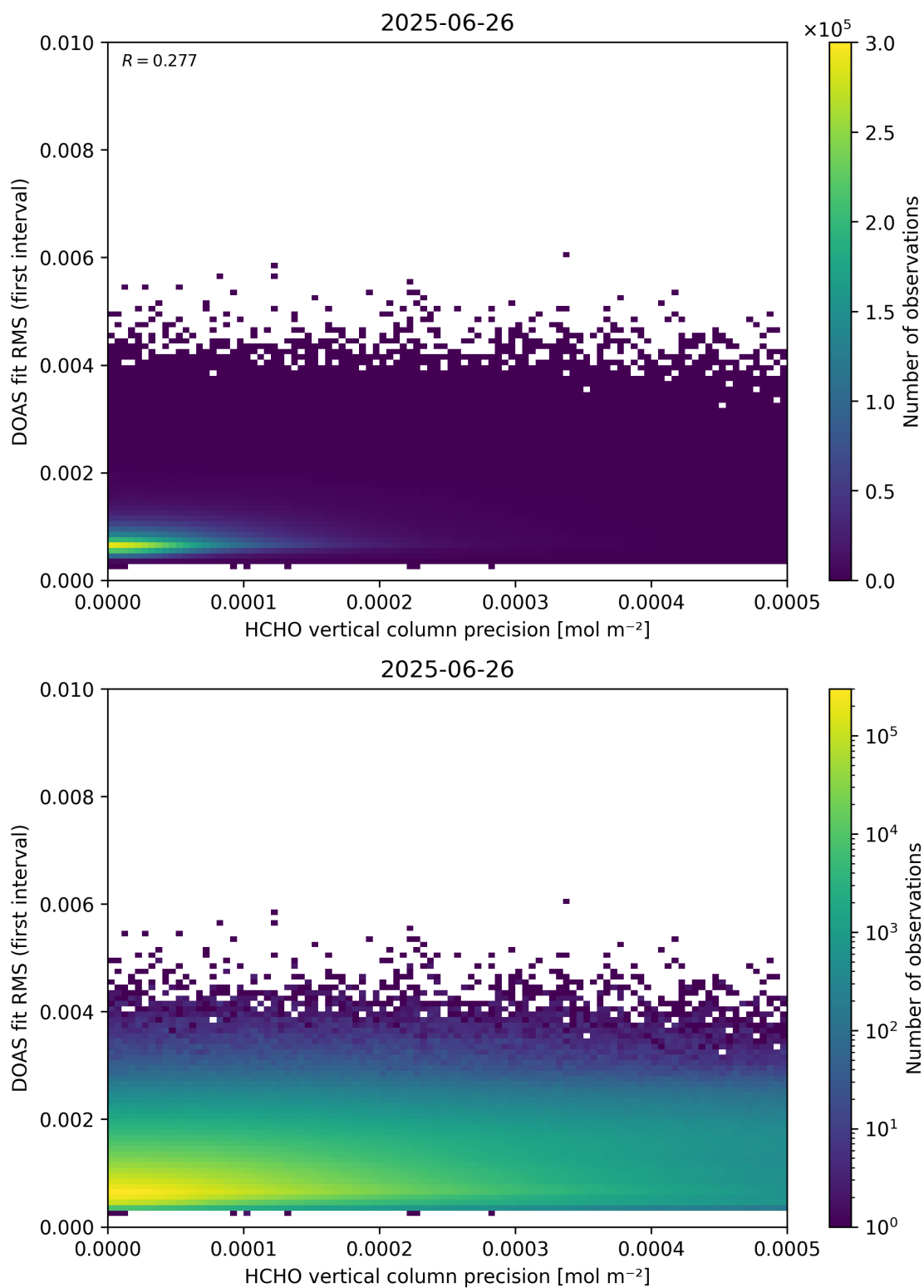
Figure 136: Scatter density plot of “HCHO vertical column precision” against “DOAS fit RMS (first interval)” for 2025-06-25 to 2025-06-27.
