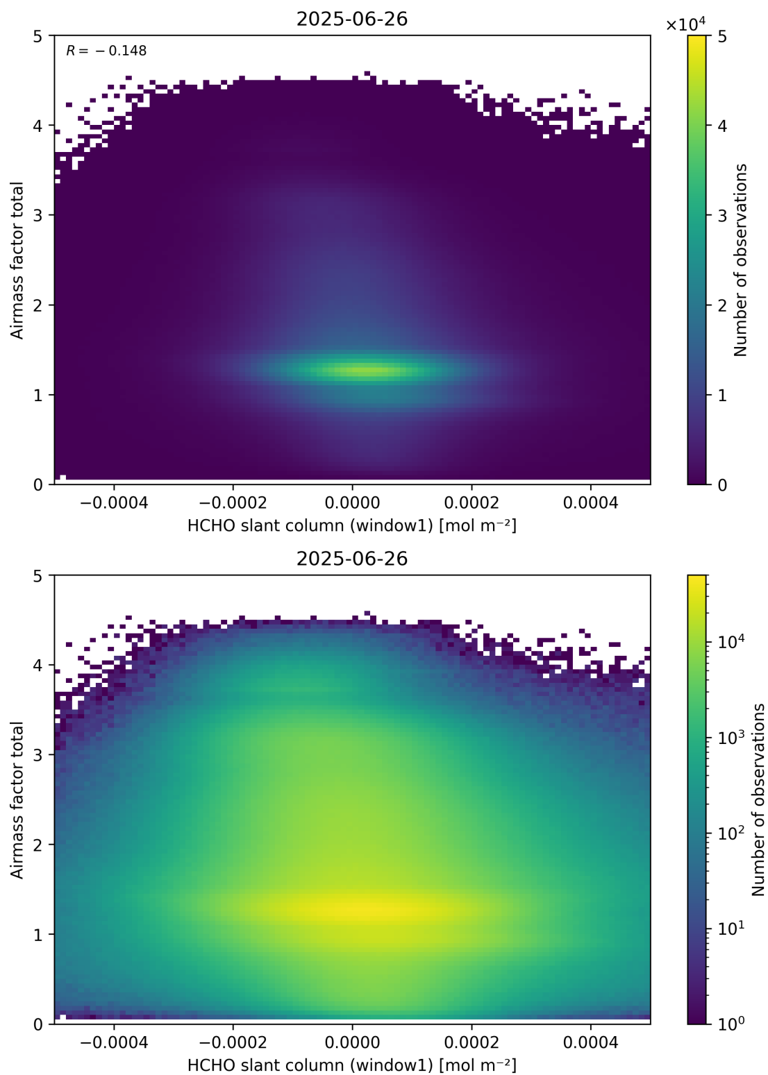
Figure 85: Scatter density plot of “HCHO slant column (window1)” against “Airmass factor total” for 2025-06-25 to 2025-06-27.
