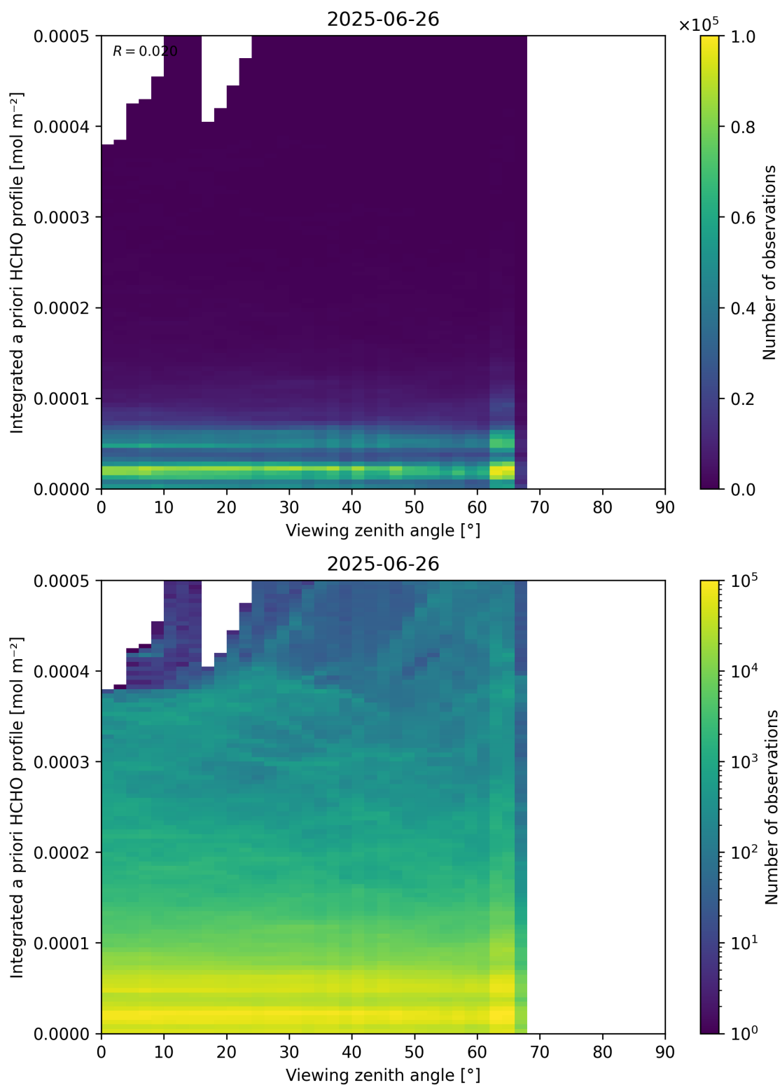
Figure 195: Scatter density plot of “Viewing zenith angle” against “Integrated a priori HCHO profile” for 2025-06-25 to 2025-06-27.
