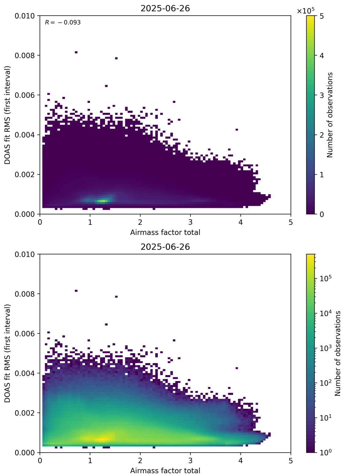
Figure 97: Scatter density plot of “Airmass factor total” against “DOAS fit RMS (first interval)” for 2025-06-25 to 2025-06-27.
