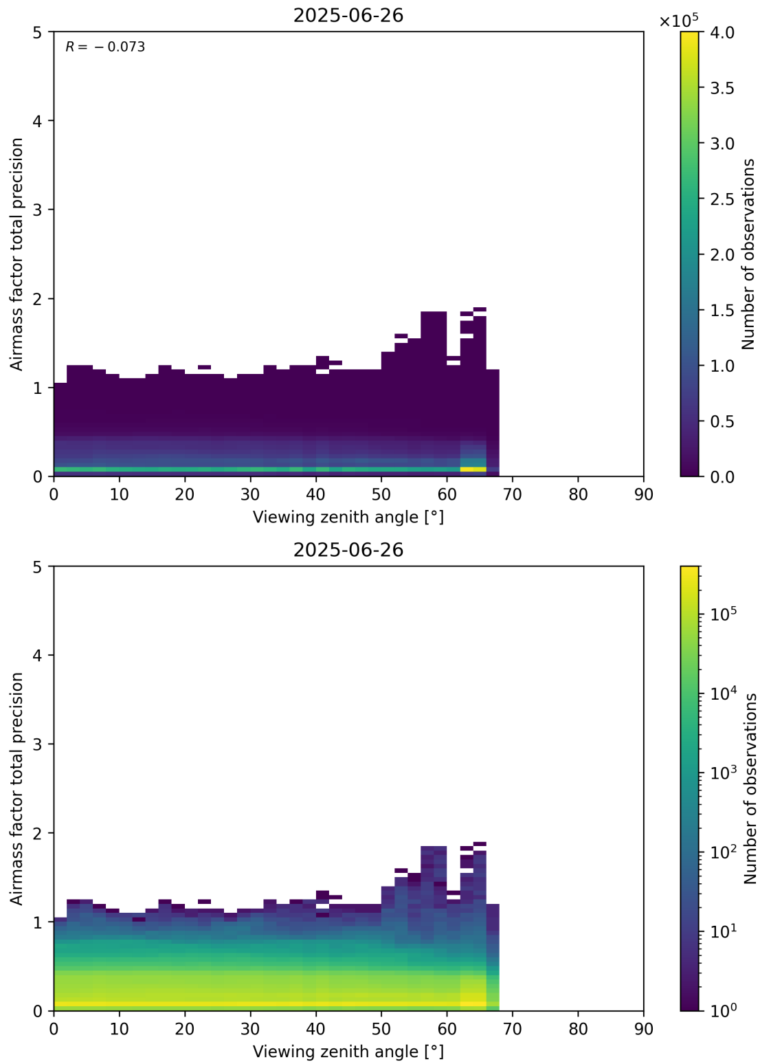
Figure 191: Scatter density plot of “Viewing zenith angle” against “Airmass factor total precision” for 2025-06-25 to 2025-06-27.
