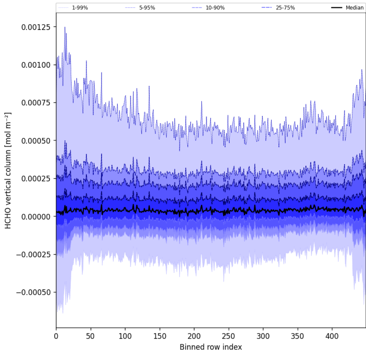
Figure 49: Along track statistics of “HCHO vertical column” for 2025-06-25 to 2025-06-27
