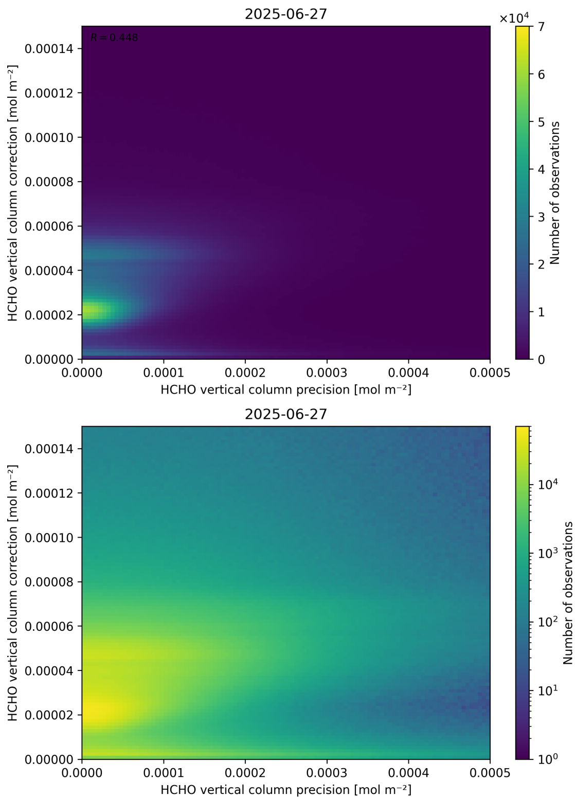
Figure 146: Scatter density plot of “HCHO vertical column precision” against “HCHO vertical column correction” for 2025-06-27 to 2025-06-28.
