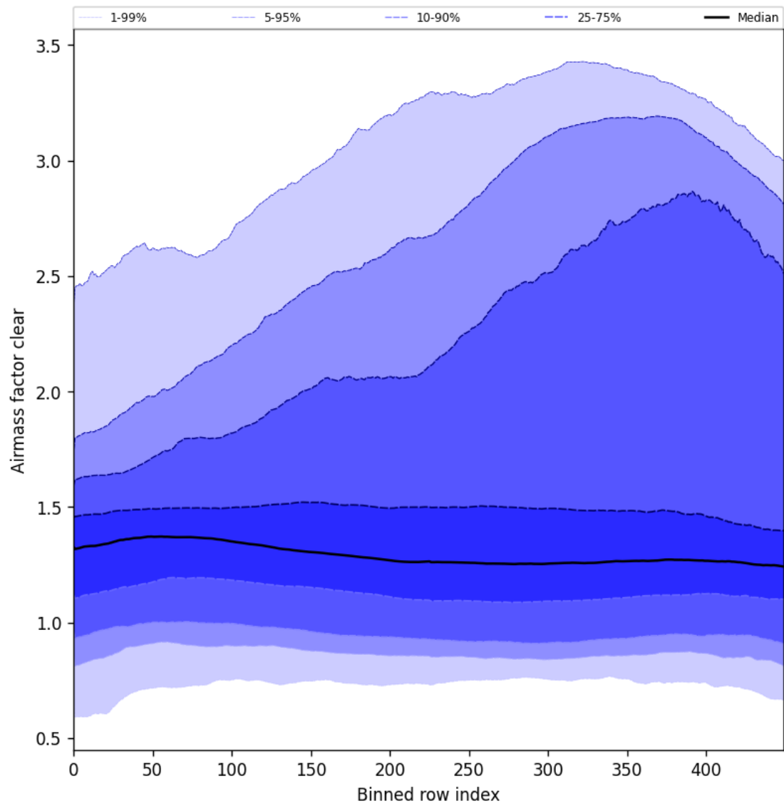
Figure 56: Along track statistics of “Airmass factor clear” for 2025-06-27 to 2025-06-28
