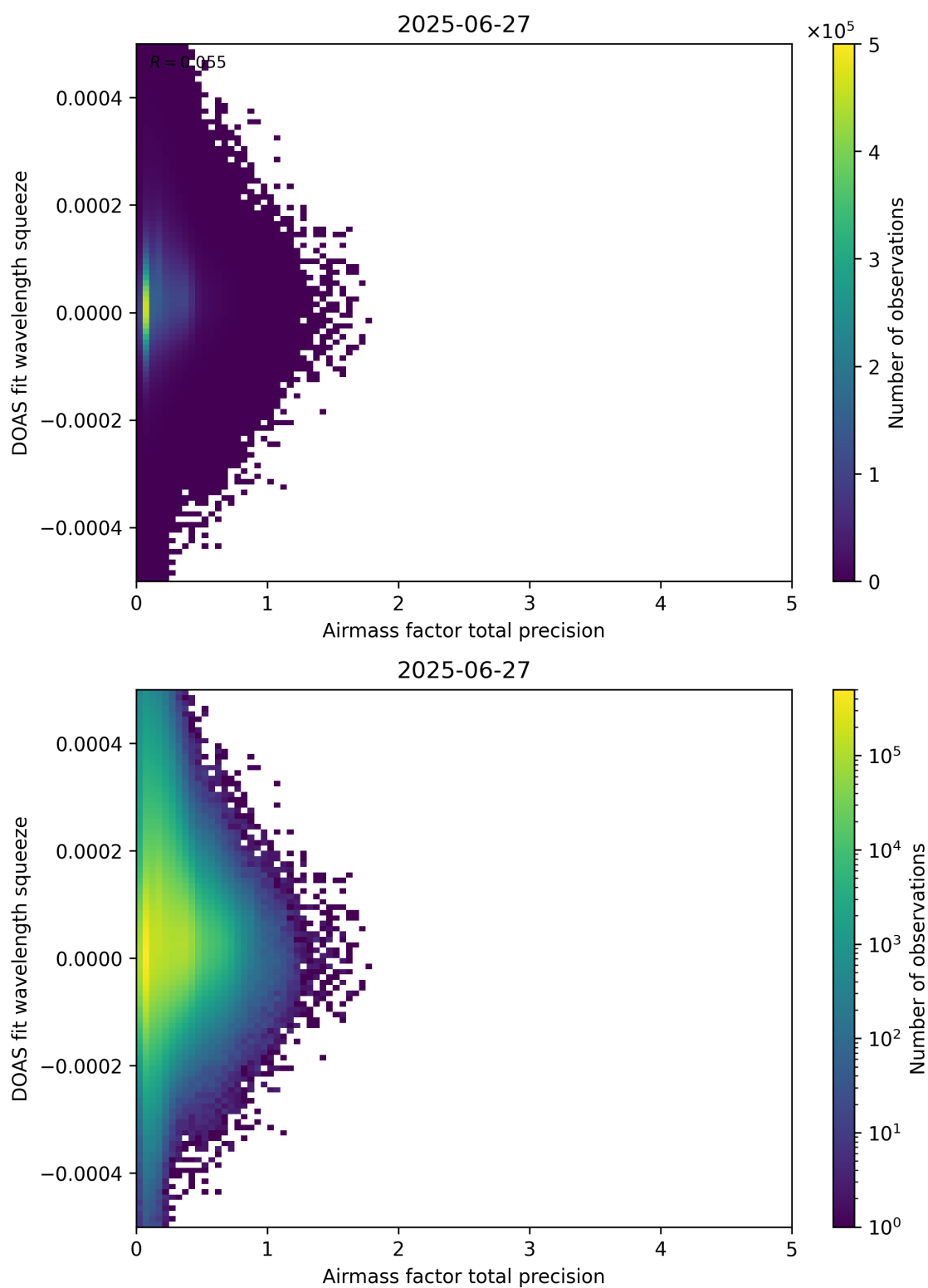
Figure 107: Scatter density plot of “Airmass factor total precision” against “DOAS fit wavelength squeeze” for 2025-06-27 to 2025-06-28.
