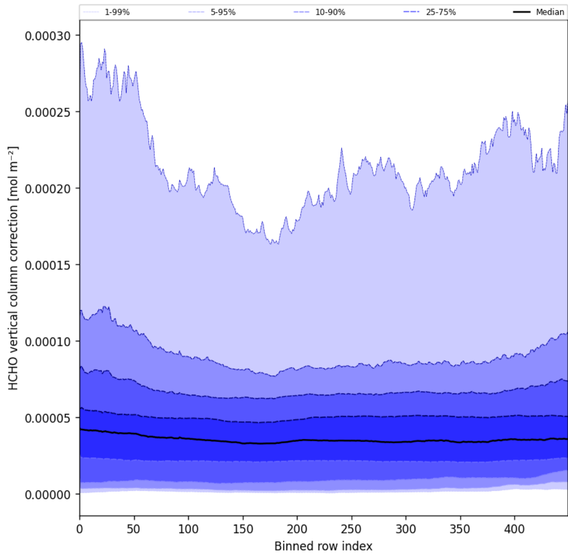
Figure 51: Along track statistics of “HCHO vertical column correction” for 2025-06-27 to 2025-06-28
