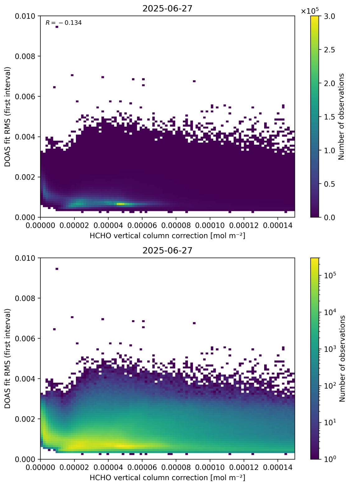
Figure 112: Scatter density plot of “HCHO vertical column correction” against “DOAS fit RMS (first interval)” for 2025-06-27 to 2025-06-28.
