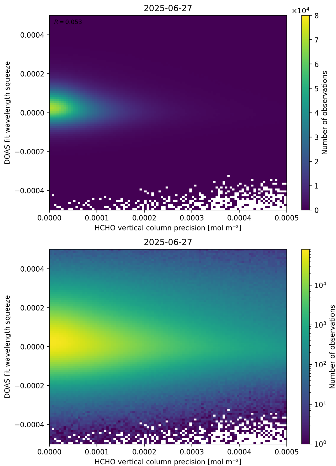
Figure 138: Scatter density plot of “HCHO vertical column precision” against “DOAS fit wavelength squeeze” for 2025-06-27 to 2025-06-28.
