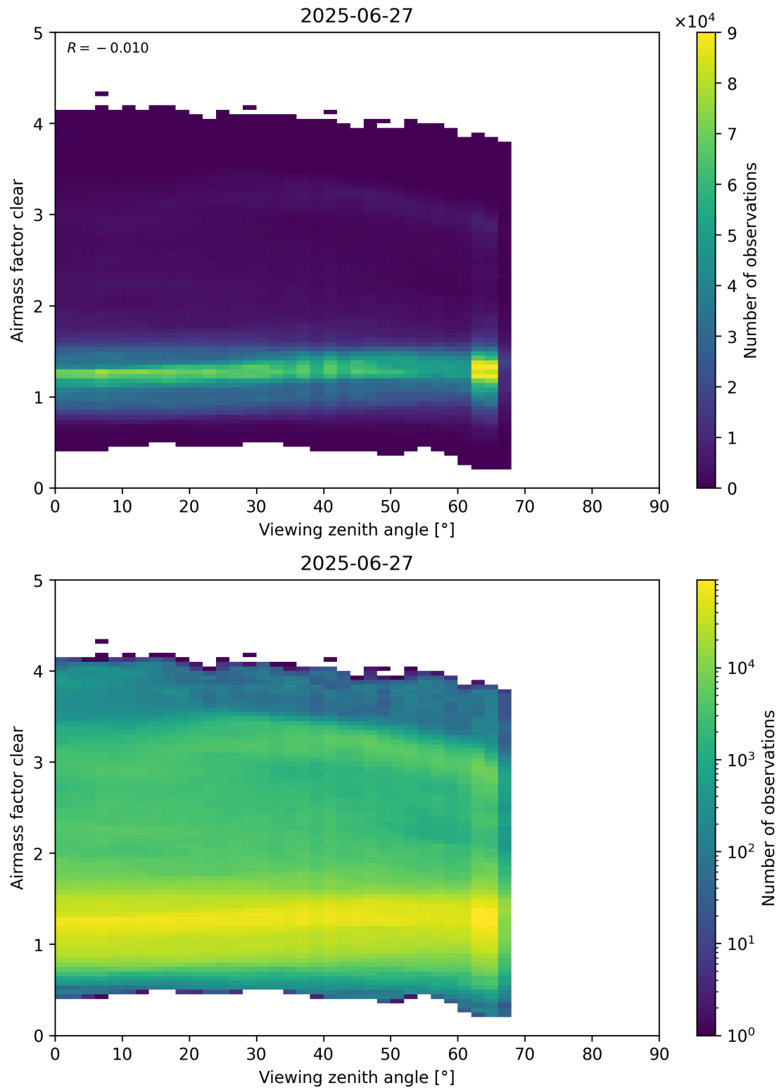
Figure 185: Scatter density plot of “Viewing zenith angle” against “Airmass factor clear” for 2025-06-27 to 2025-06-28.
