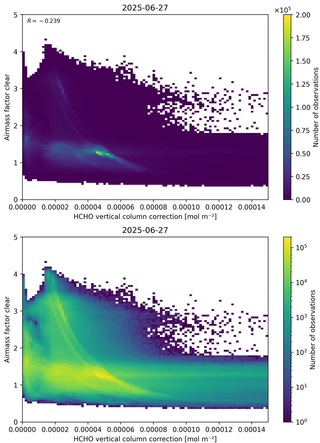
Figure 115: Scatter density plot of “HCHO vertical column correction” against “Airmass factor clear” for 2025-06-27 to 2025-06-28.
