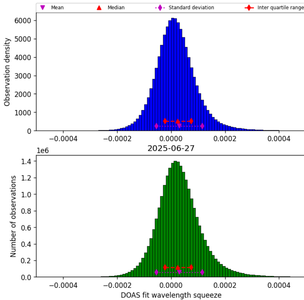
Figure 45: Histogram of “DOAS fit wavelength squeeze” for 2025-06-27 to 2025-06-28
