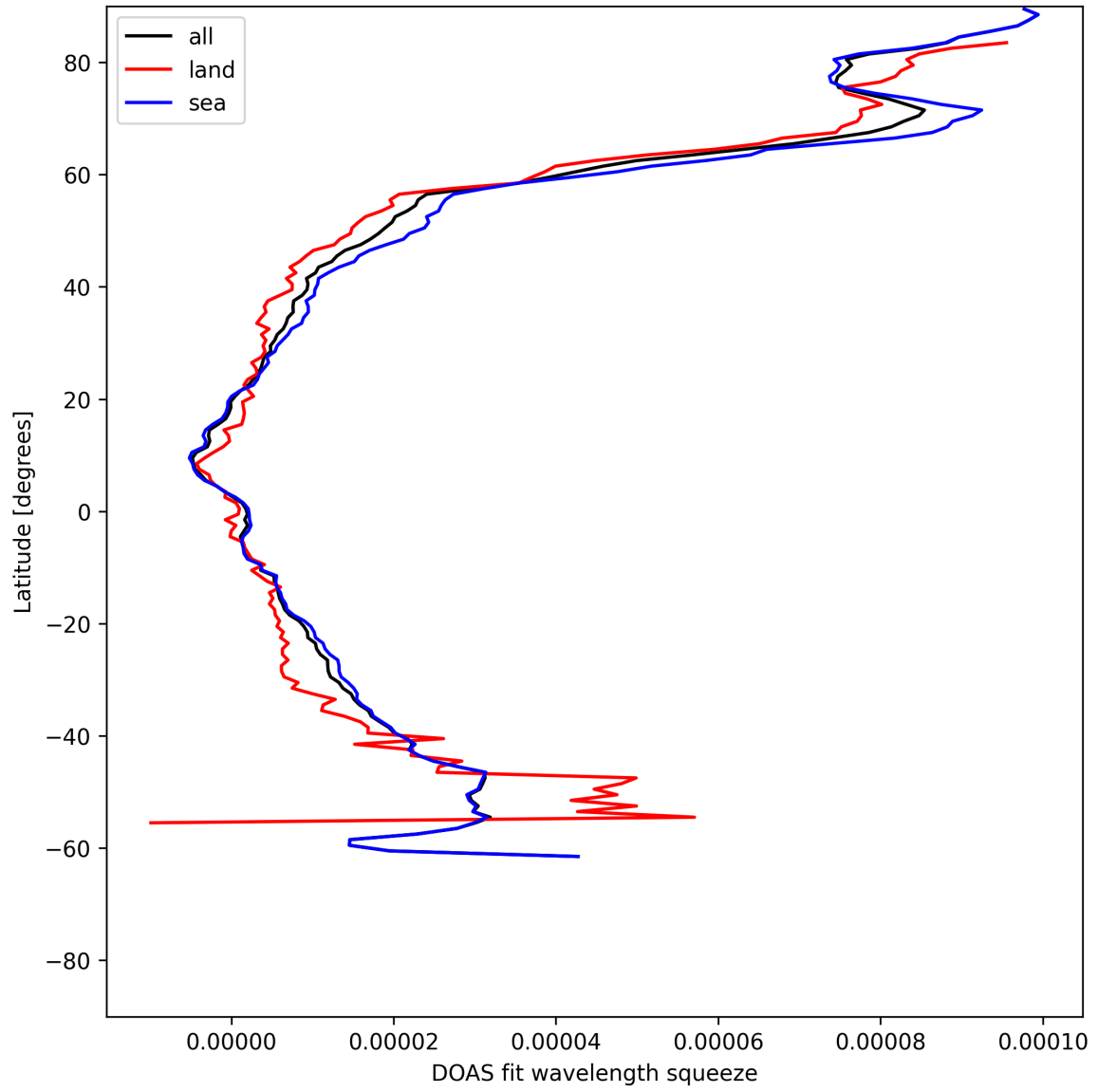
Figure 31: Zonal average of “DOAS fit wavelength squeeze” for 2025-06-27 to 2025-06-28.
