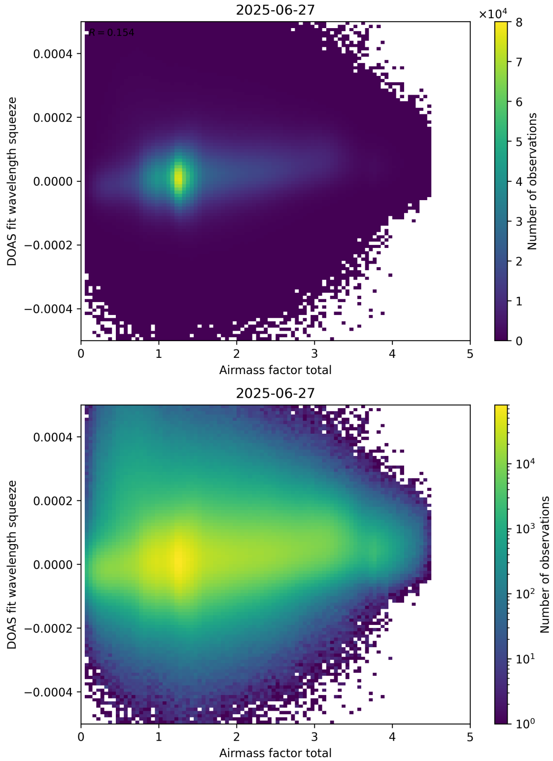
Figure 99: Scatter density plot of “Airmass factor total” against “DOAS fit wavelength squeeze” for 2025-06-27 to 2025-06-28.
