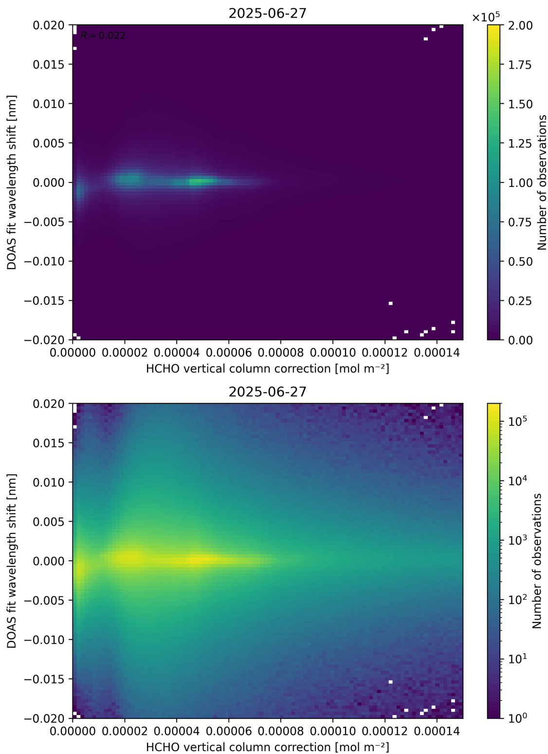
Figure 113: Scatter density plot of “HCHO vertical column correction” against “DOAS fit wavelength shift” for 2025-06-27 to 2025-06-28.
