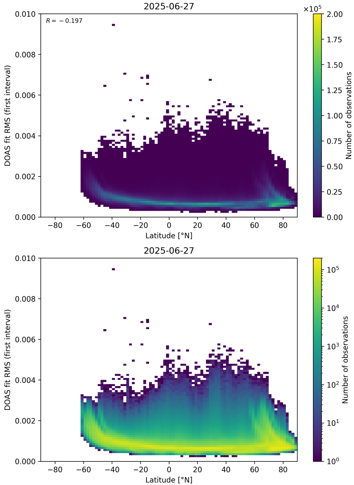
Figure 153: Scatter density plot of “Latitude” against “DOAS fit RMS (first interval)” for 2025-06-27 to 2025-06-28.
