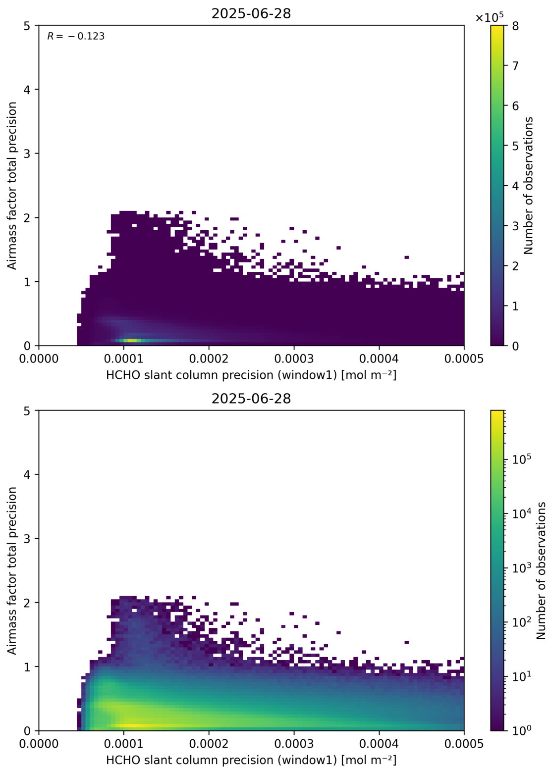
Figure 95: Scatter density plot of “HCHO slant column precision (window1)” against “Airmass factor total precision” for 2025-06-27 to 2025-06-29.
