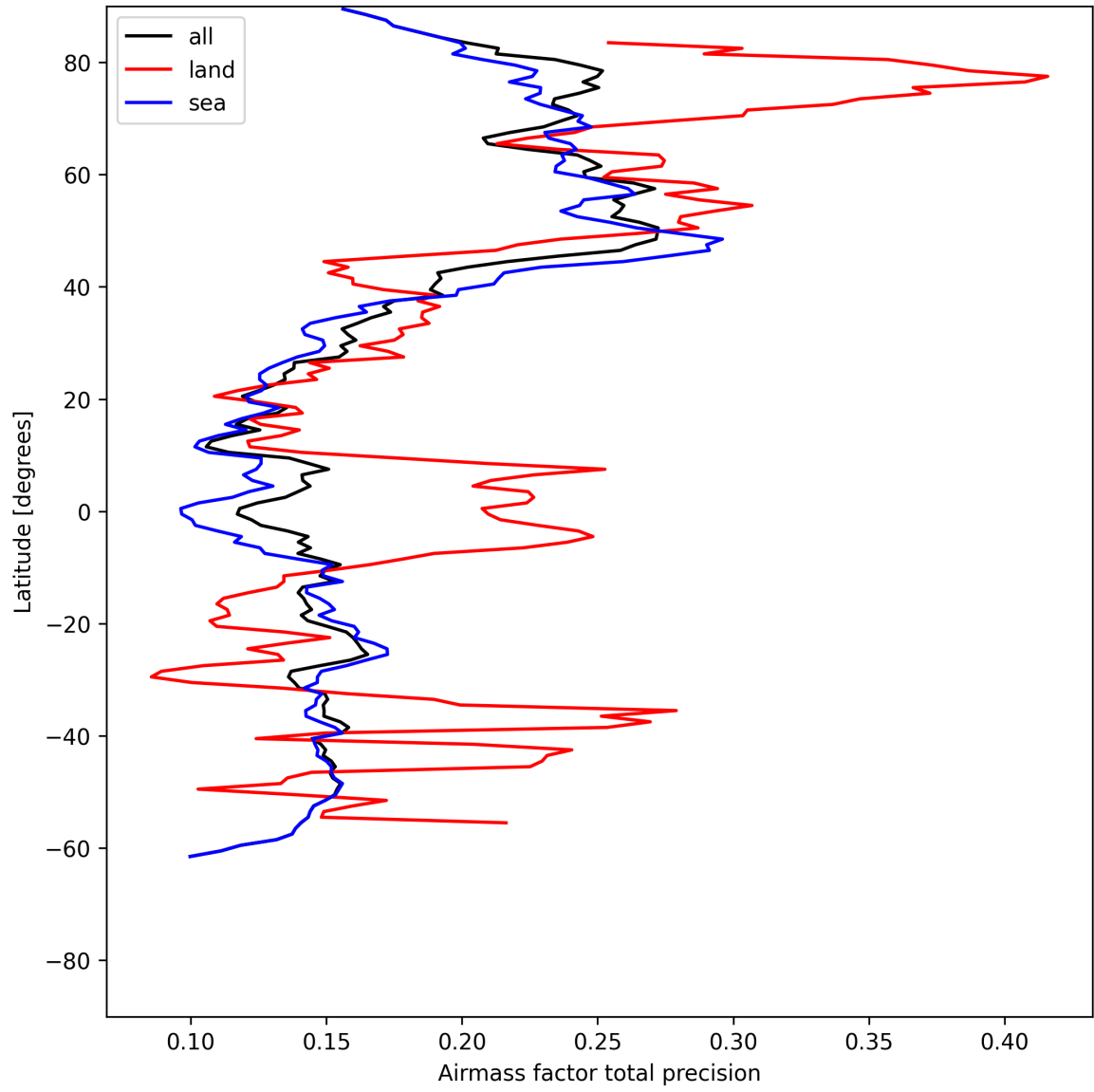
Figure 27: Zonal average of “Airmass factor total precision” for 2025-06-27 to 2025-06-29.
