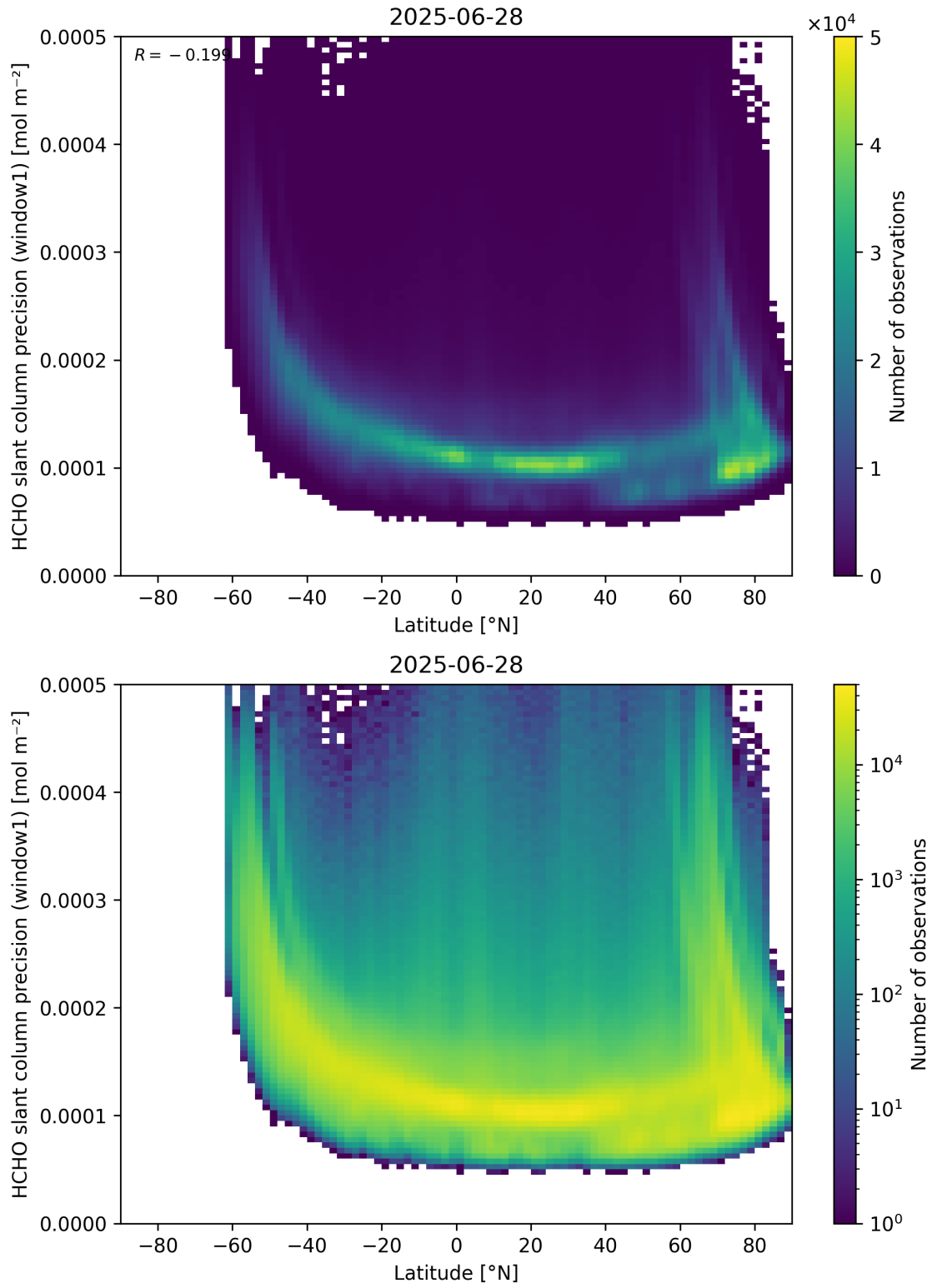
Figure 160: Scatter density plot of “Latitude” against “HCHO slant column precision (window1)” for 2025-06-27 to 2025-06-29.
