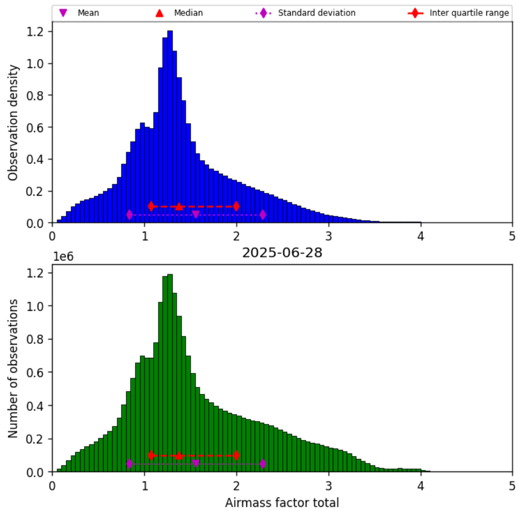
Figure 40: Histogram of “Airmass factor total” for 2025-06-27 to 2025-06-29
