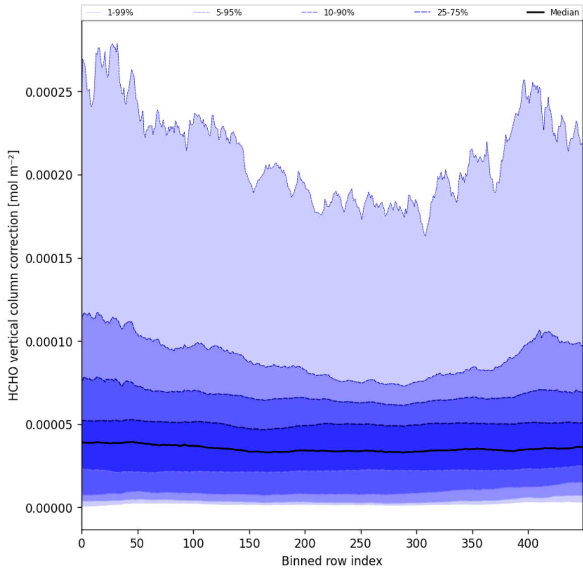
Figure 51: Along track statistics of “HCHO vertical column correction” for 2025-06-27 to 2025-06-29
