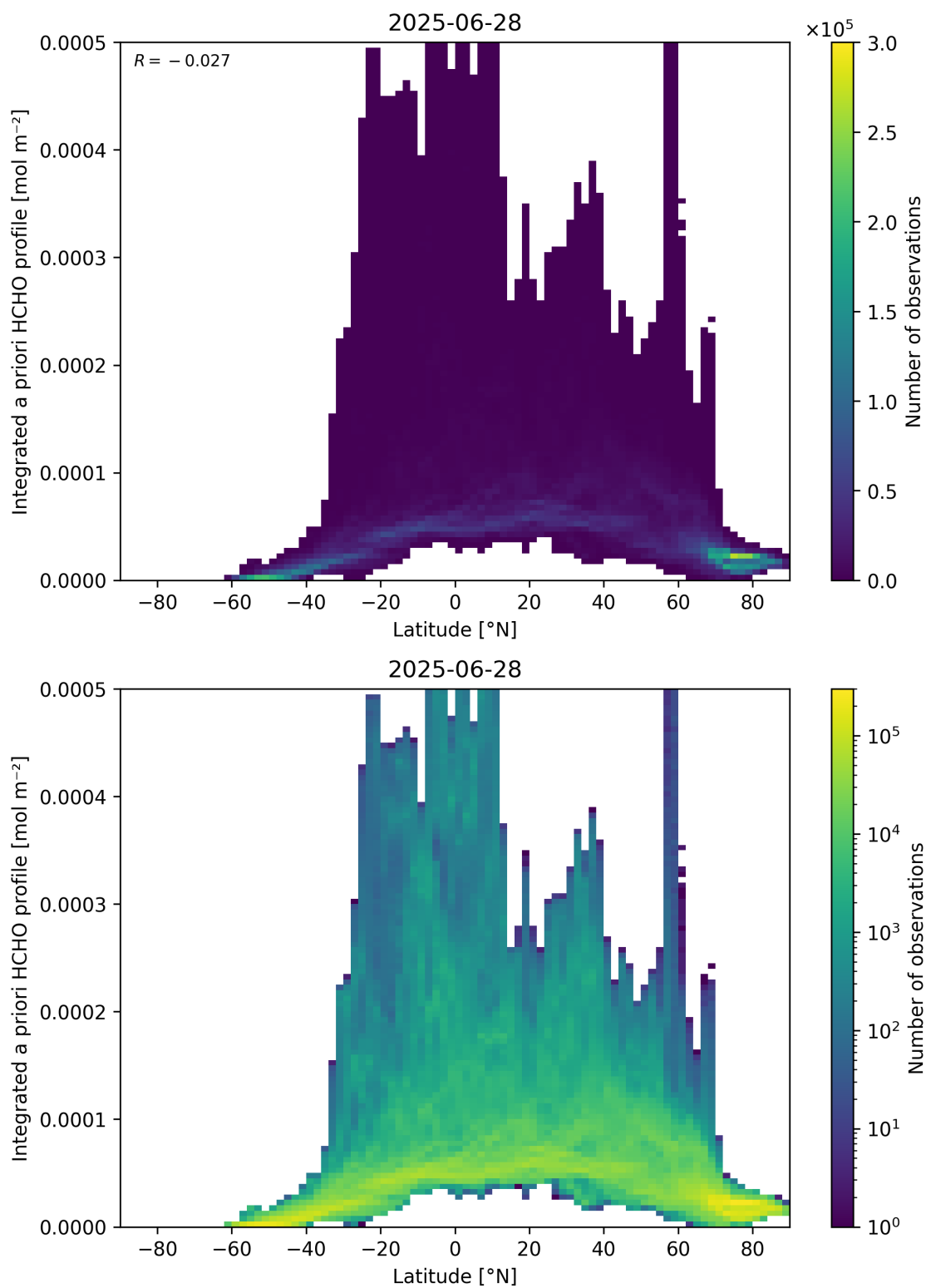
Figure 166: Scatter density plot of “Latitude” against “Integrated a priori HCHO profile” for 2025-06-27 to 2025-06-29.
