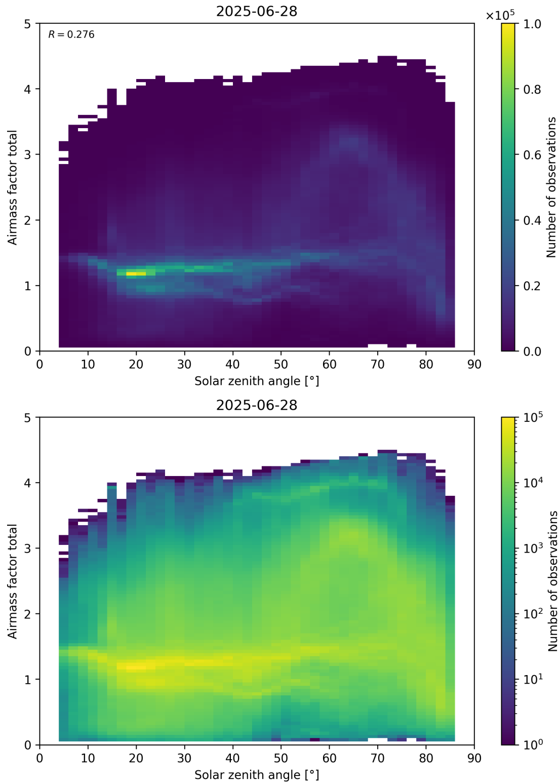
Figure 175: Scatter density plot of “Solar zenith angle” against “Airmass factor total” for 2025-06-27 to 2025-06-29.
