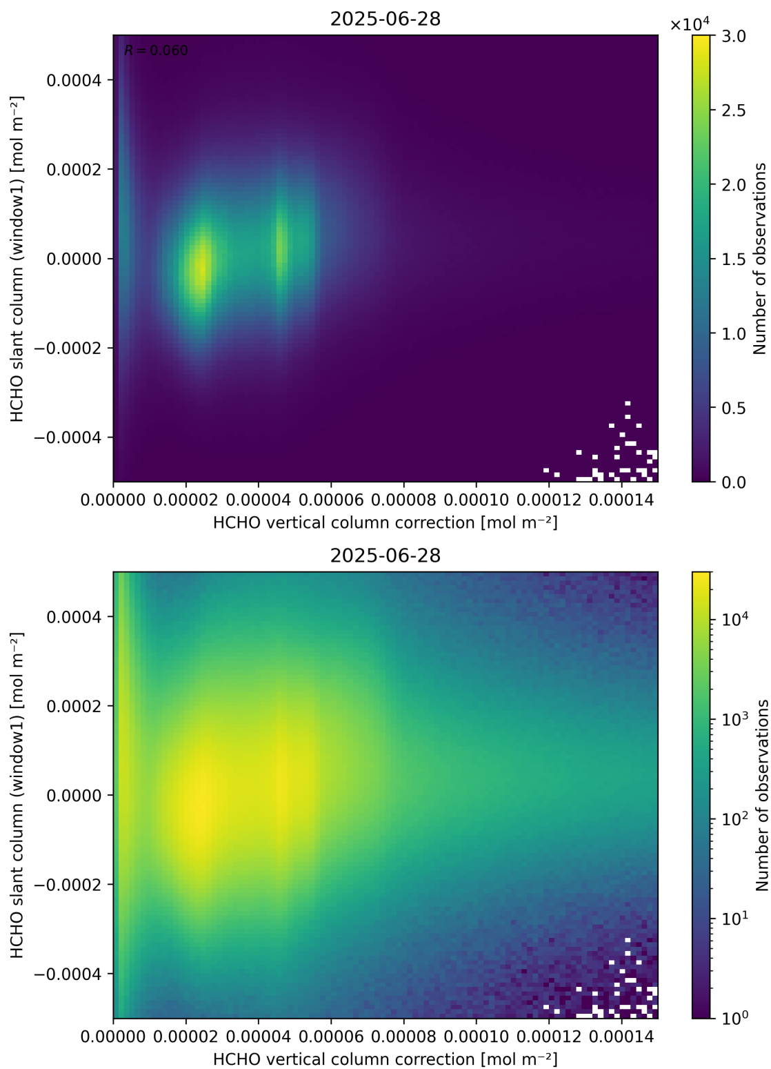
Figure 118: Scatter density plot of “HCHO vertical column correction” against “HCHO slant column (window1)” for 2025-06-27 to 2025-06-29.
