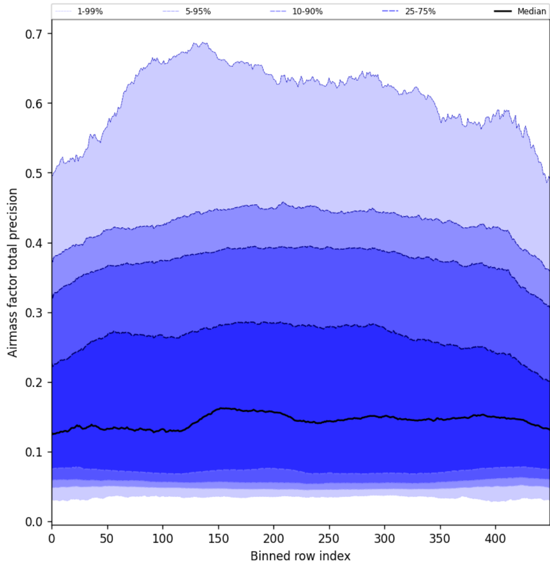
Figure 55: Along track statistics of “Airmass factor total precision” for 2025-06-27 to 2025-06-29
