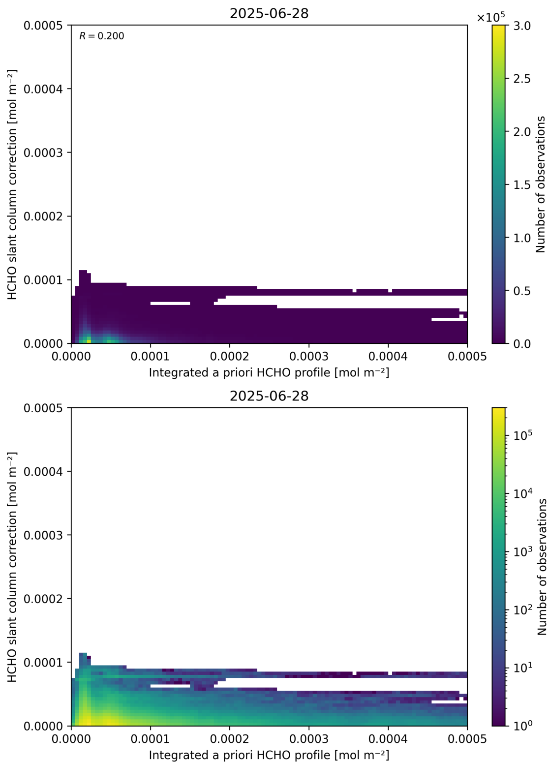
Figure 152: Scatter density plot of “Integrated a priori HCHO profile” against “HCHO slant column correction” for 2025-06-27 to 2025-06-29.
