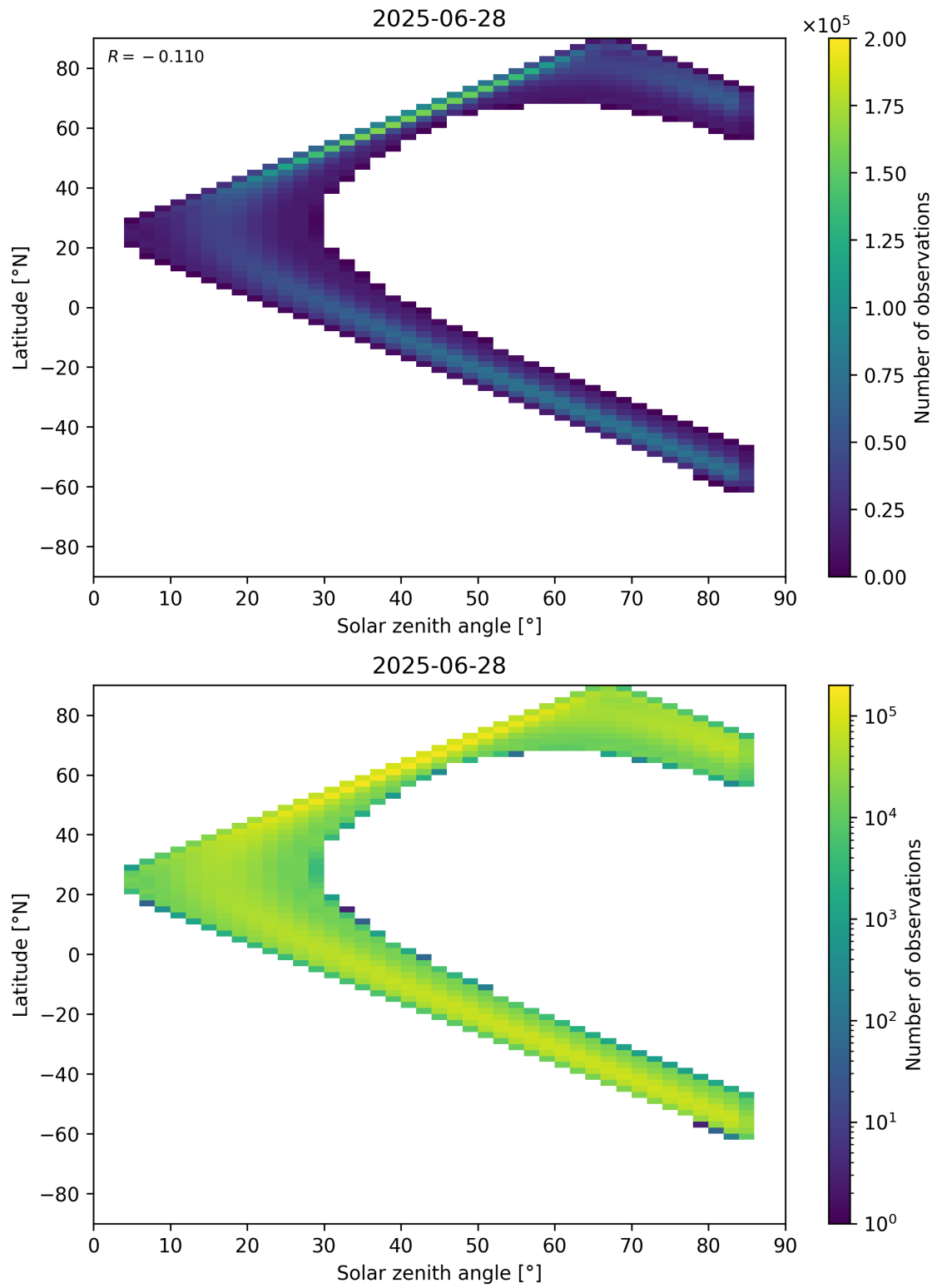
Figure 181: Scatter density plot of “Solar zenith angle” against “Latitude” for 2025-06-27 to 2025-06-29.
