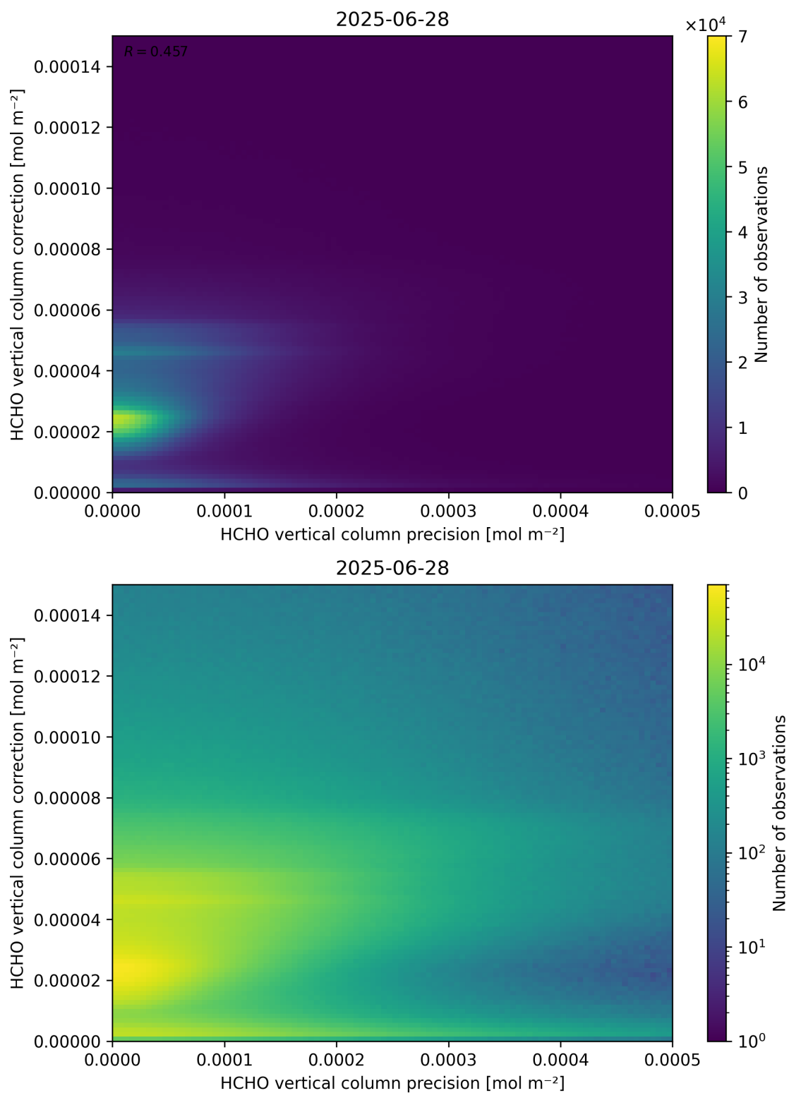
Figure 146: Scatter density plot of “HCHO vertical column precision” against “HCHO vertical column correction” for 2025-06-27 to 2025-06-29.
