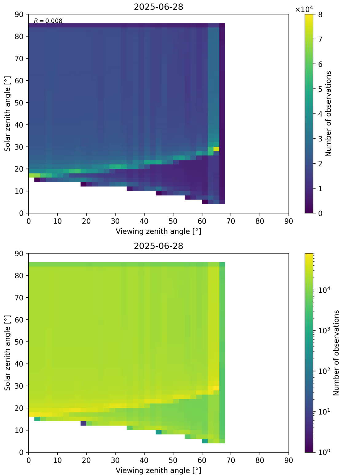
Figure 197: Scatter density plot of “Viewing zenith angle” against “Solar zenith angle” for 2025-06-27 to 2025-06-29.
