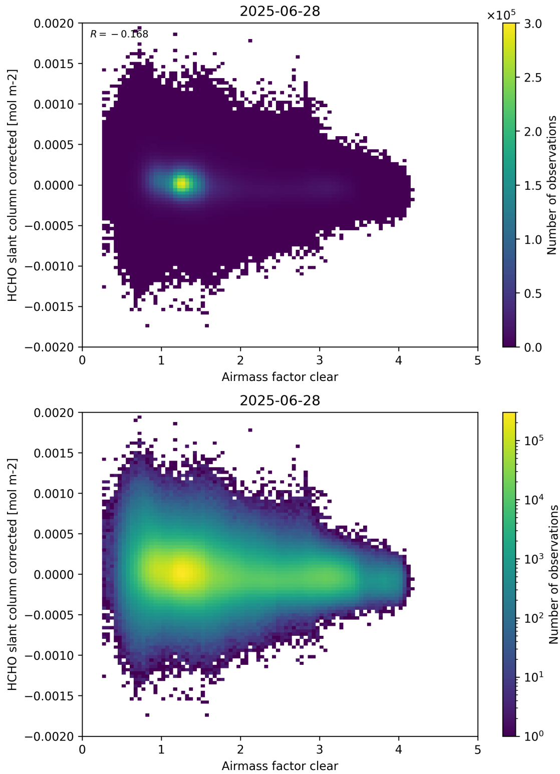
Figure 74: Scatter density plot of “Airmass factor clear” against “HCHO slant column corrected” for 2025-06-27 to 2025-06-29.
