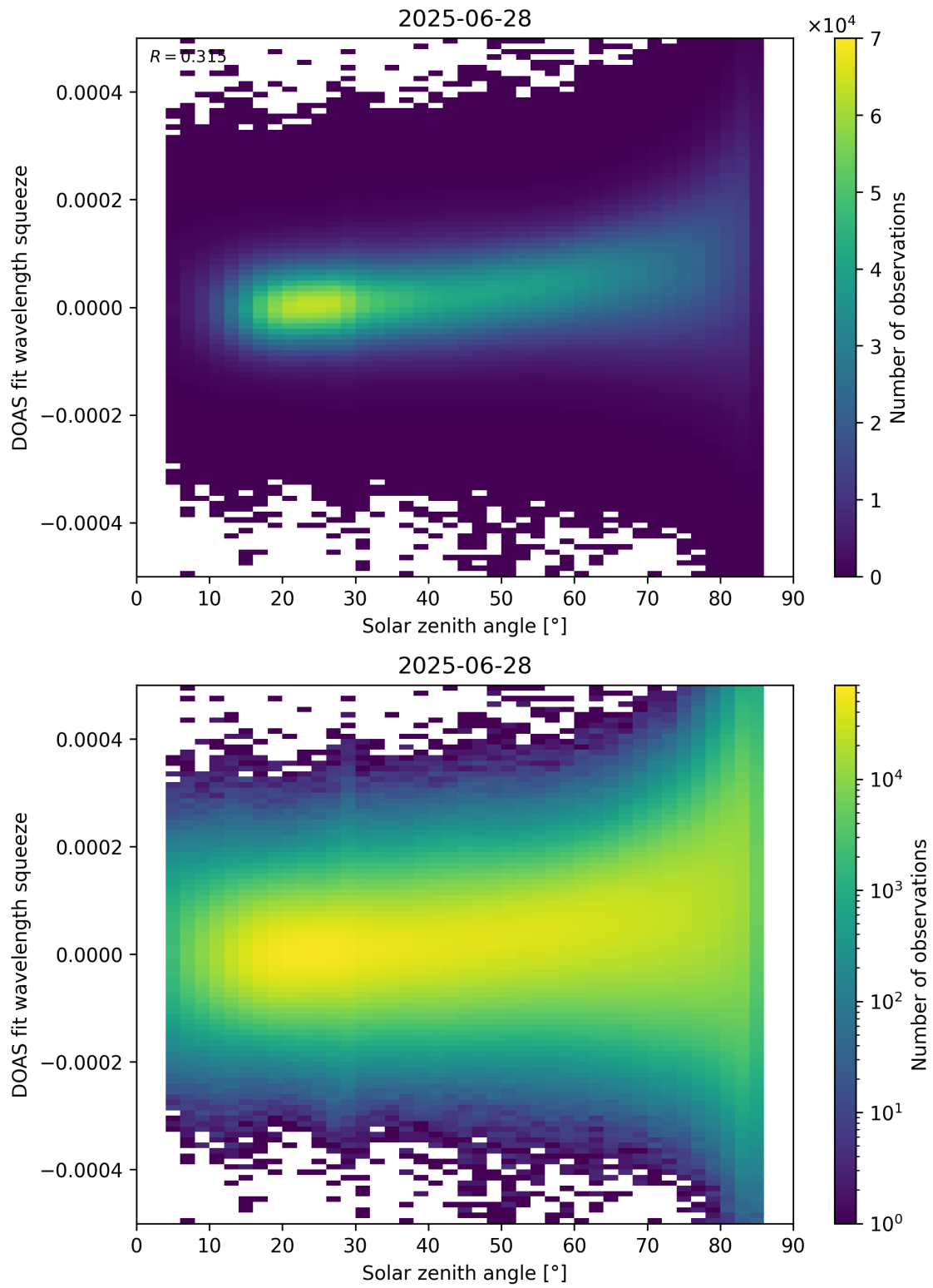
Figure 169: Scatter density plot of “Solar zenith angle” against “DOAS fit wavelength squeeze” for 2025-06-27 to 2025-06-29.
