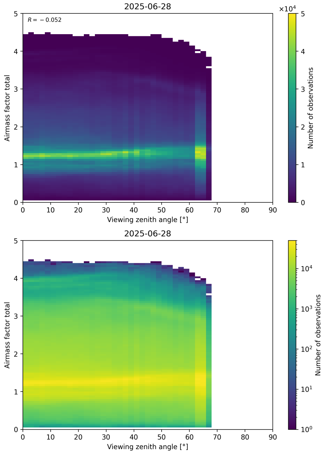
Figure 190: Scatter density plot of “Viewing zenith angle” against “Airmass factor total” for 2025-06-27 to 2025-06-29.
