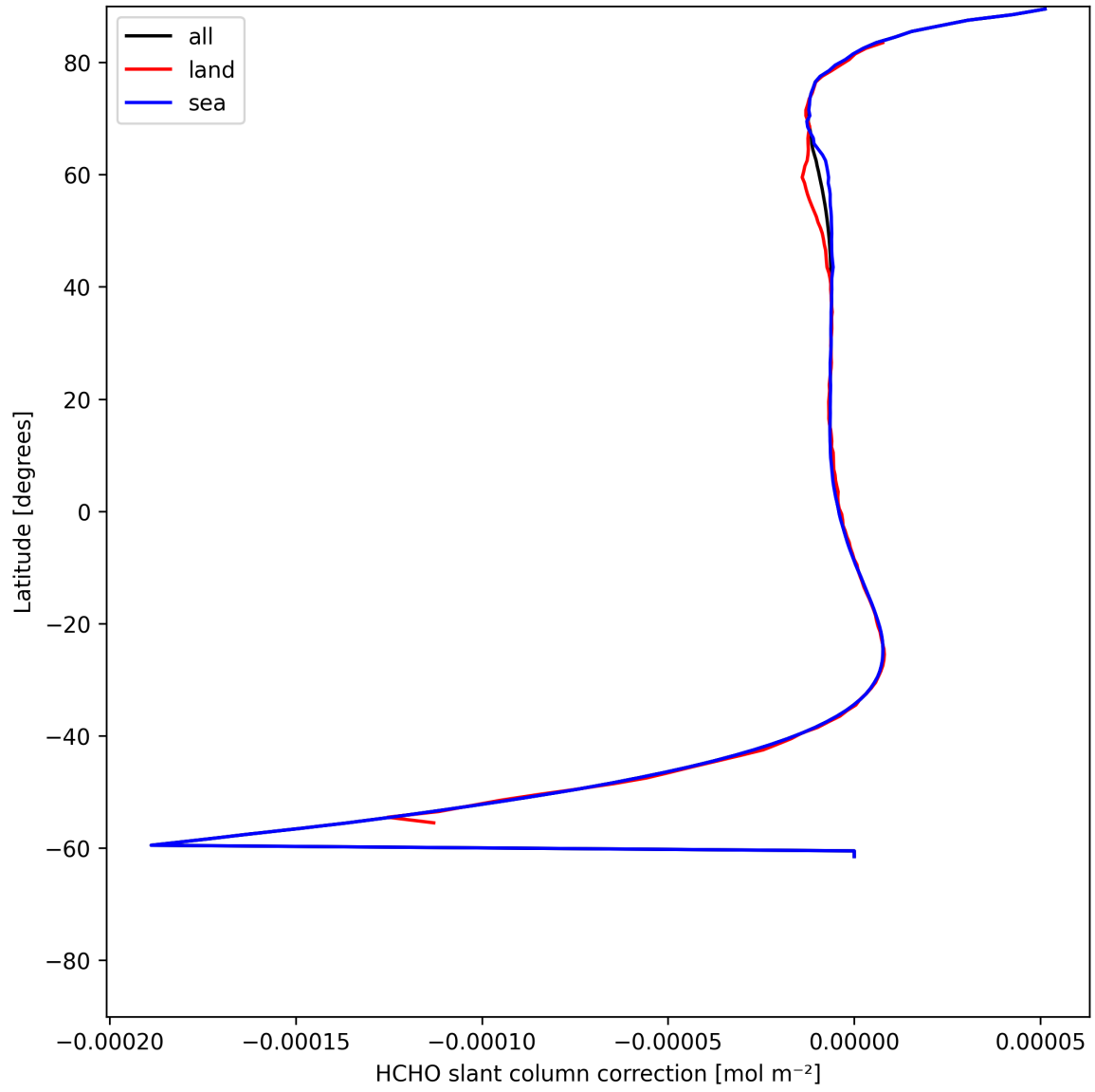
Figure 33: Zonal average of “HCHO slant column correction” for 2025-06-27 to 2025-06-29.
