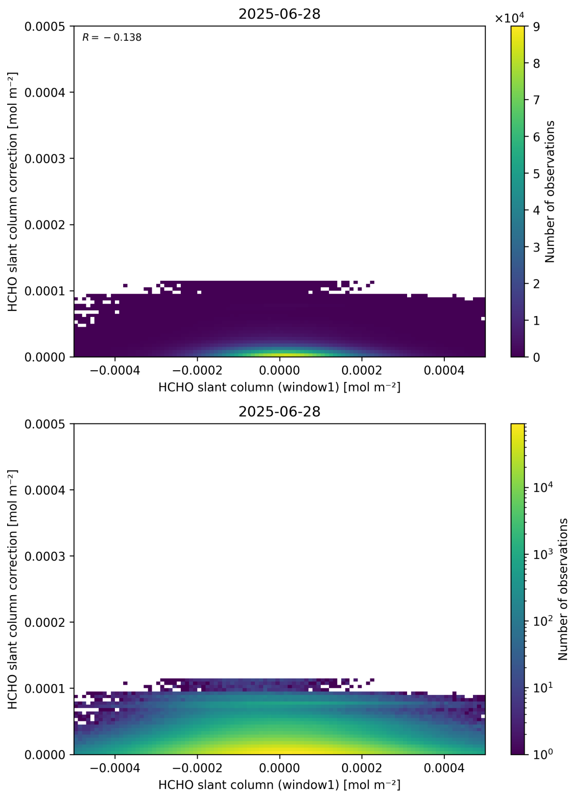
Figure 83: Scatter density plot of “HCHO slant column (window1)” against “HCHO slant column correction” for 2025-06-27 to 2025-06-29.
