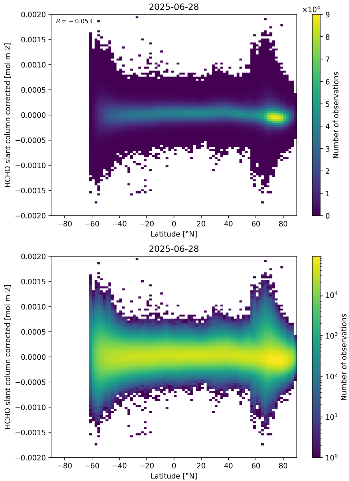
Figure 157: Scatter density plot of “Latitude” against “HCHO slant column corrected” for 2025-06-27 to 2025-06-29.
