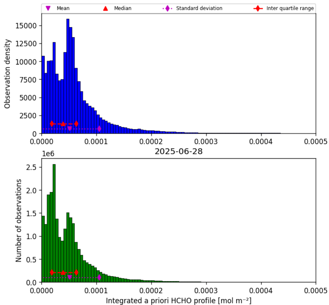
Figure 43: Histogram of “Integrated a priori HCHO profile” for 2025-06-27 to 2025-06-29
