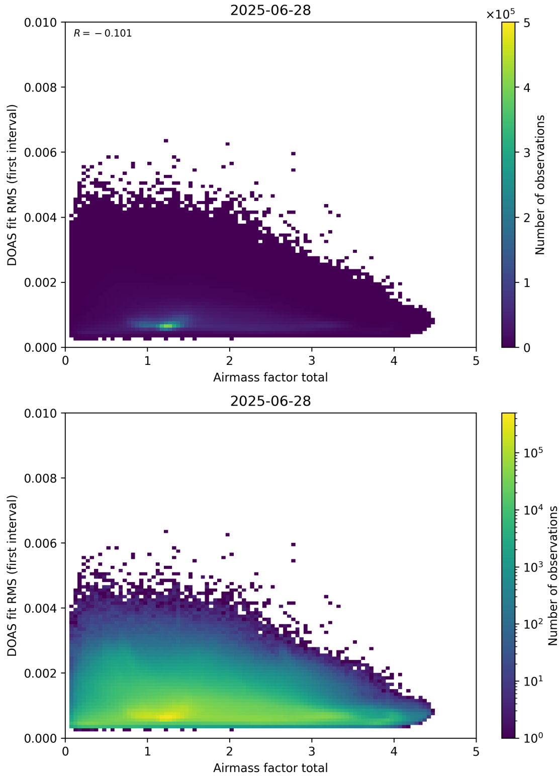
Figure 97: Scatter density plot of “Airmass factor total” against “DOAS fit RMS (first interval)” for 2025-06-27 to 2025-06-29.
