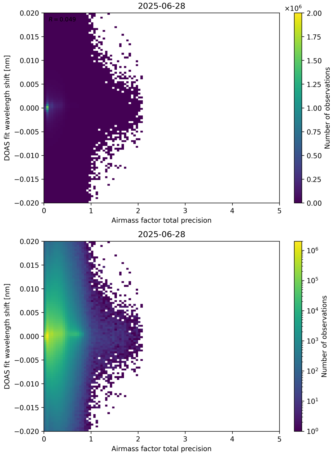
Figure 106: Scatter density plot of “Airmass factor total precision” against “DOAS fit wavelength shift” for 2025-06-27 to 2025-06-29.
