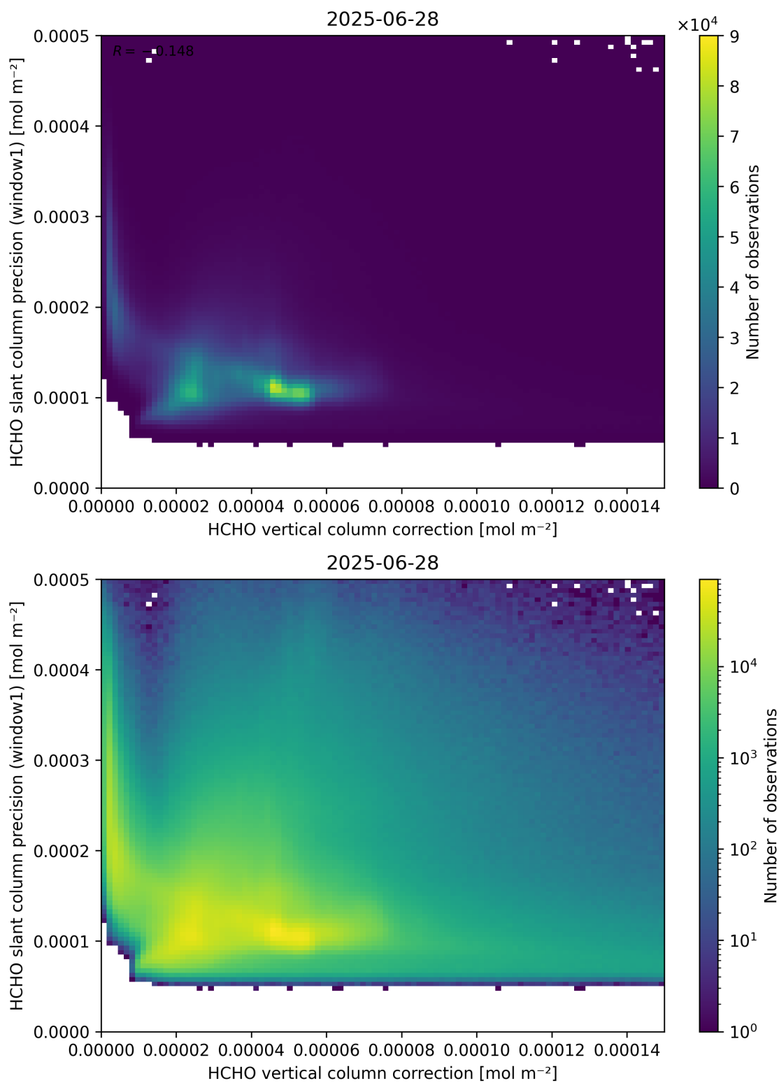
Figure 119: Scatter density plot of “HCHO vertical column correction” against “HCHO slant column precision (window1)” for 2025-06-27 to 2025-06-29.
