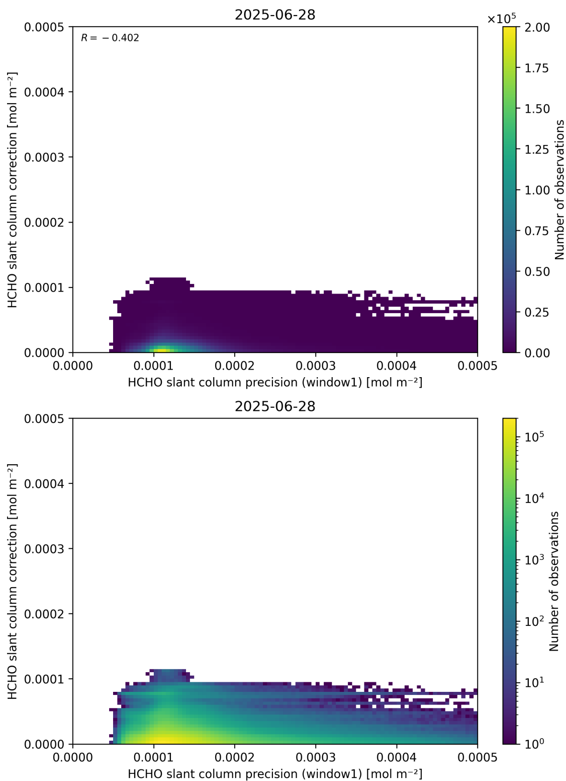
Figure 93: Scatter density plot of “HCHO slant column precision (window1)” against “HCHO slant column correction” for 2025-06-27 to 2025-06-29.
