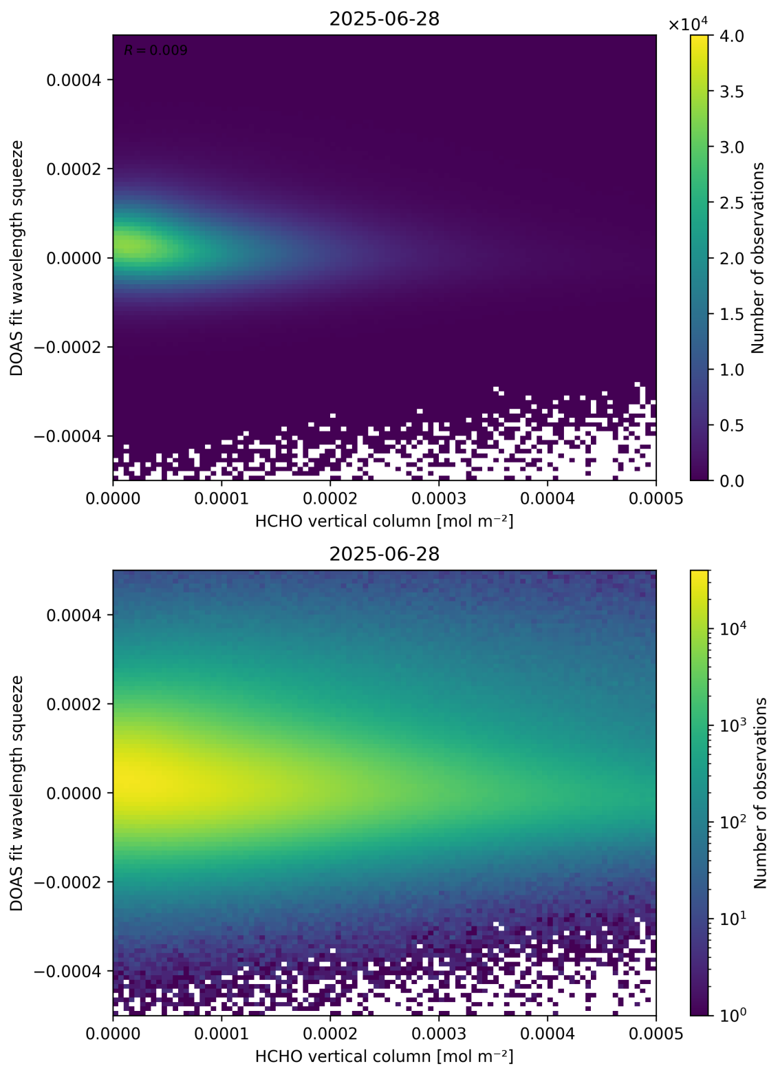
Figure 125: Scatter density plot of “HCHO vertical column” against “DOAS fit wavelength squeeze” for 2025-06-27 to 2025-06-29.
