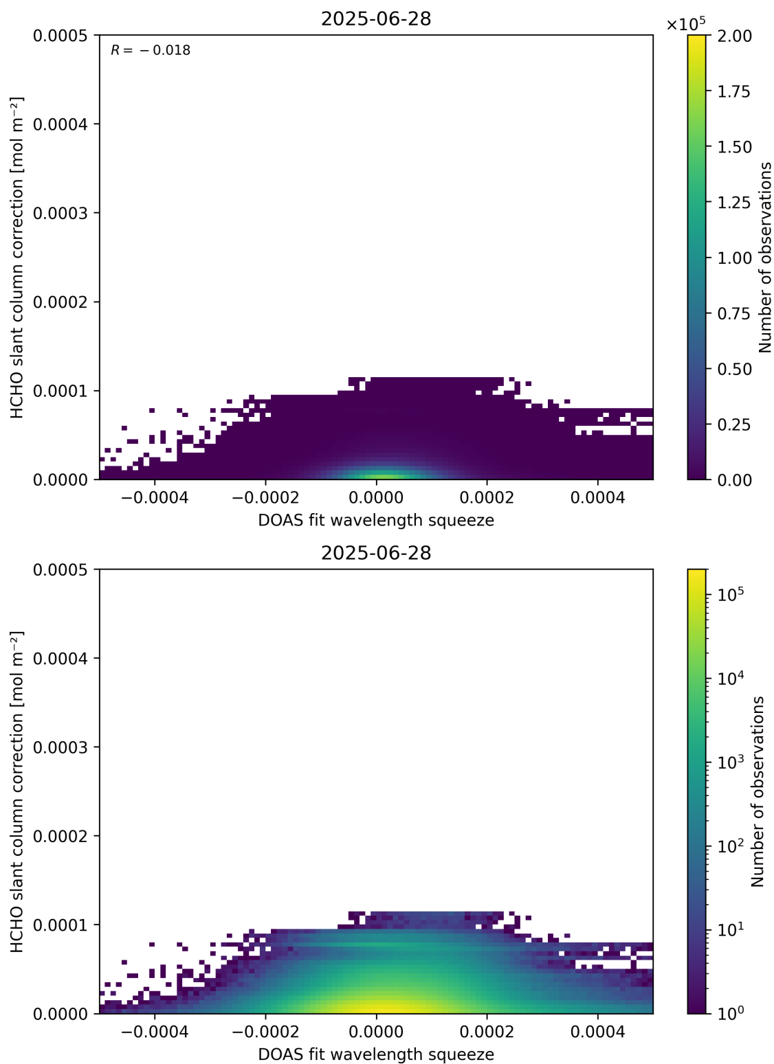
Figure 70: Scatter density plot of “DOAS fit wavelength squeeze” against “HCHO slant column correction” for 2025-06-27 to 2025-06-29.
