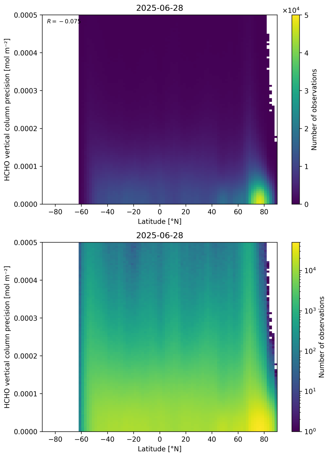
Figure 165: Scatter density plot of “Latitude” against “HCHO vertical column precision” for 2025-06-27 to 2025-06-29.
