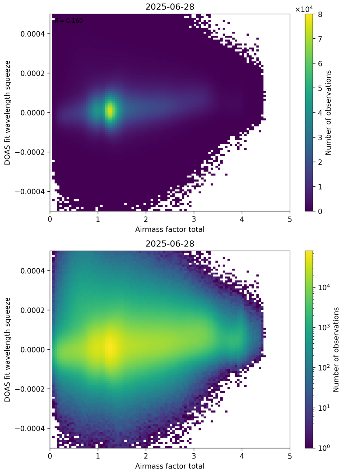
Figure 99: Scatter density plot of “Airmass factor total” against “DOAS fit wavelength squeeze” for 2025-06-27 to 2025-06-29.
