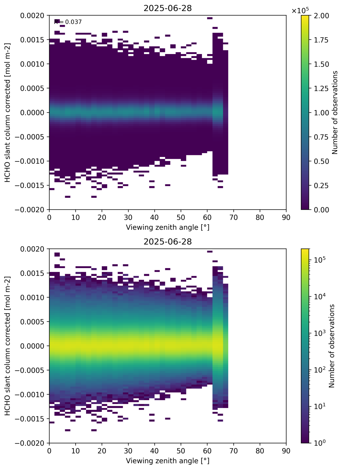
Figure 186: Scatter density plot of “Viewing zenith angle” against “HCHO slant column corrected” for 2025-06-27 to 2025-06-29.
