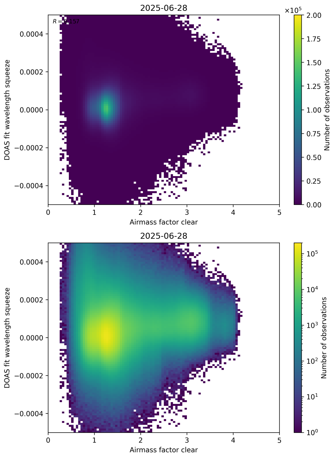
Figure 73: Scatter density plot of “Airmass factor clear” against “DOAS fit wavelength squeeze” for 2025-06-27 to 2025-06-29.
