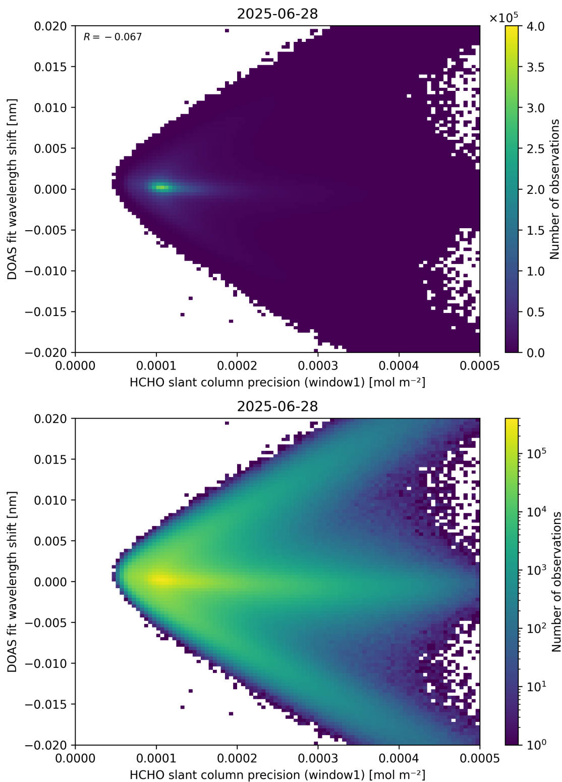
Figure 89: Scatter density plot of “HCHO slant column precision (window1)” against “DOAS fit wavelength shift” for 2025-06-27 to 2025-06-29.
