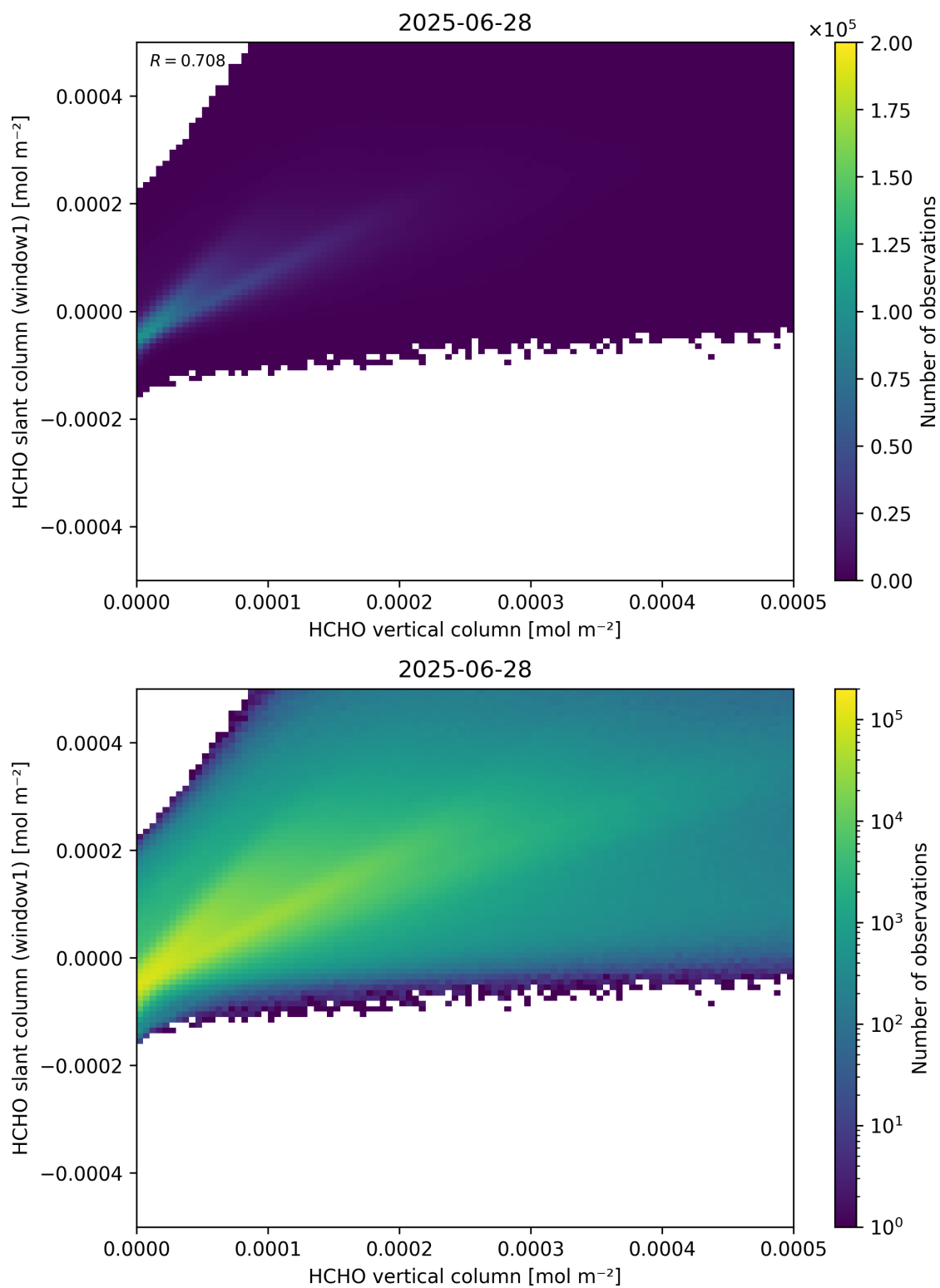
Figure 129: Scatter density plot of “HCHO vertical column” against “HCHO slant column (window1)” for 2025-06-27 to 2025-06-29.
