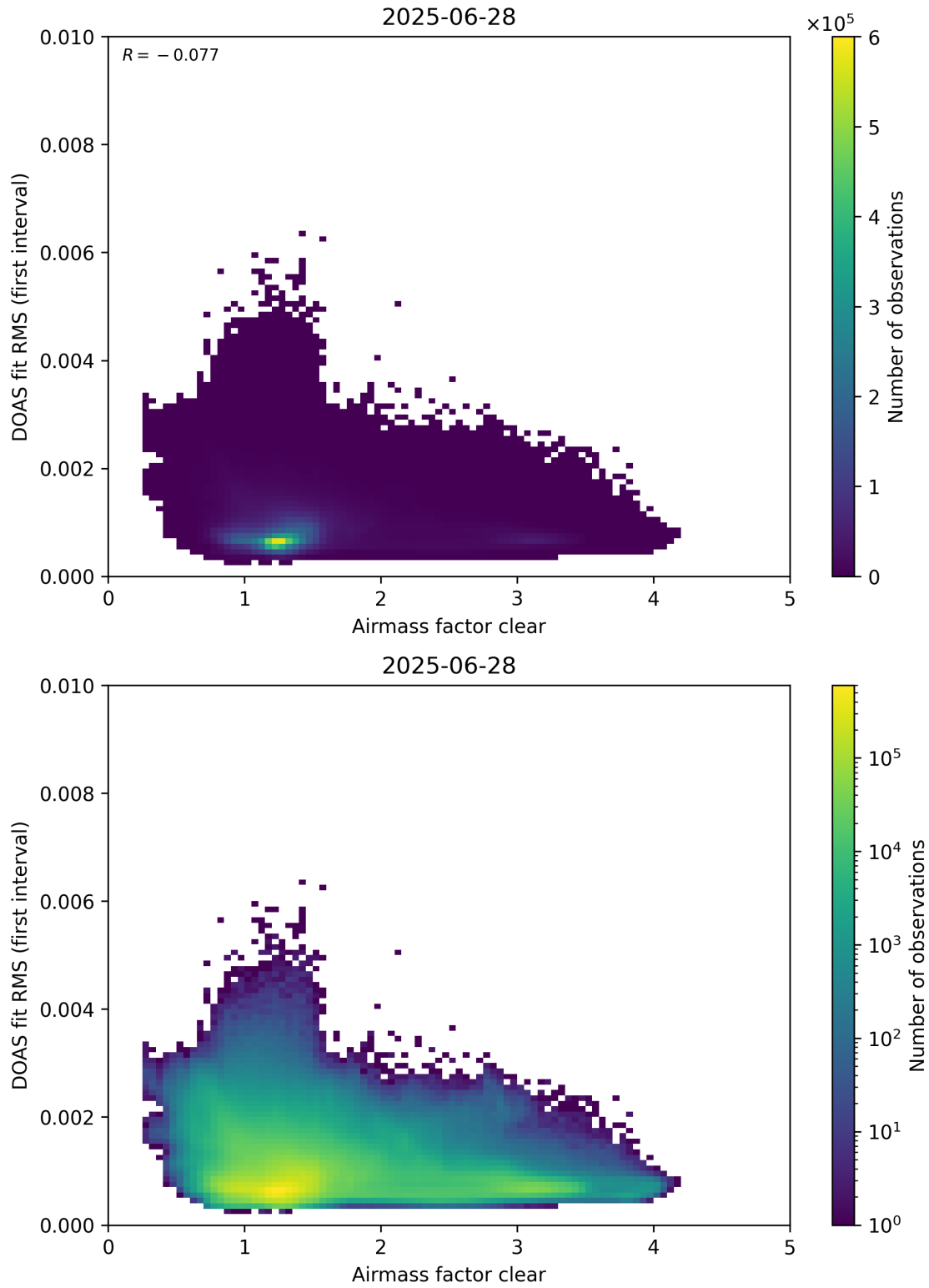
Figure 71: Scatter density plot of “Airmass factor clear” against “DOAS fit RMS (first interval)” for 2025-06-27 to 2025-06-29.
