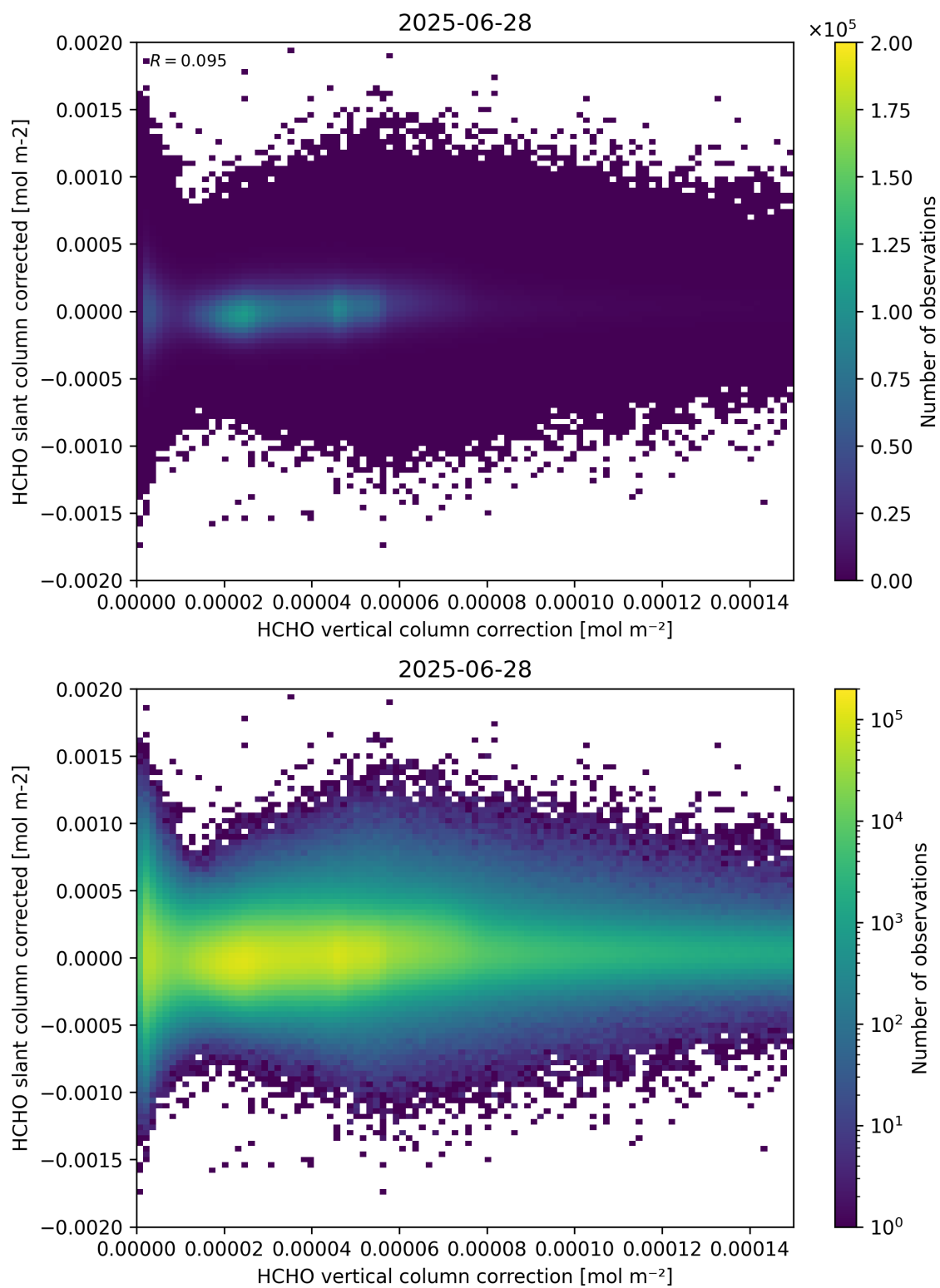
Figure 116: Scatter density plot of “HCHO vertical column correction” against “HCHO slant column corrected” for 2025-06-27 to 2025-06-29.
