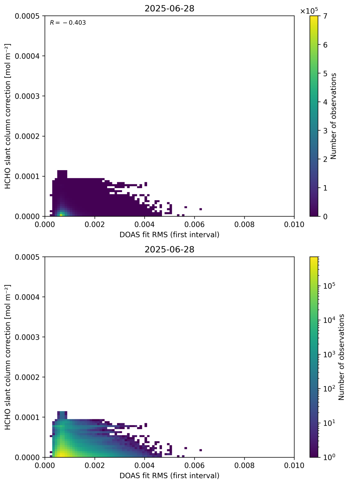
Figure 63: Scatter density plot of “DOAS fit RMS (first interval)” against “HCHO slant column correction” for 2025-06-27 to 2025-06-29.
