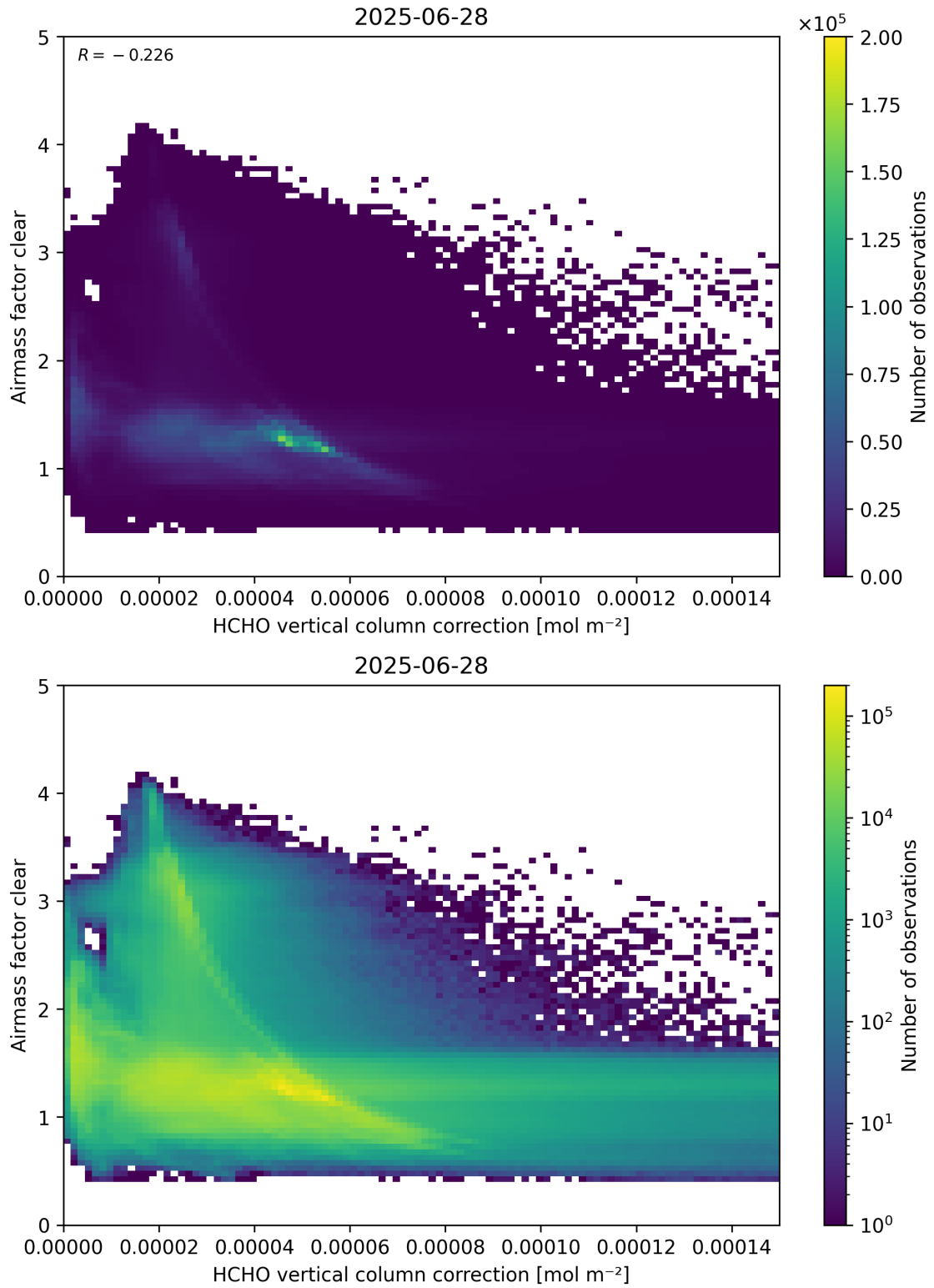
Figure 115: Scatter density plot of “HCHO vertical column correction” against “Airmass factor clear” for 2025-06-27 to 2025-06-29.
