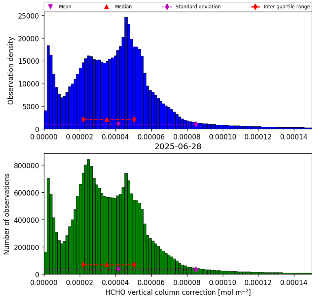
Figure 37: Histogram of “HCHO vertical column correction” for 2025-06-27 to 2025-06-29
