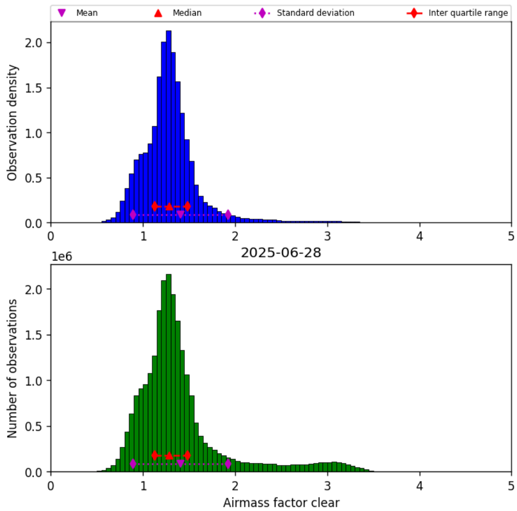
Figure 42: Histogram of “Airmass factor clear” for 2025-06-27 to 2025-06-29
