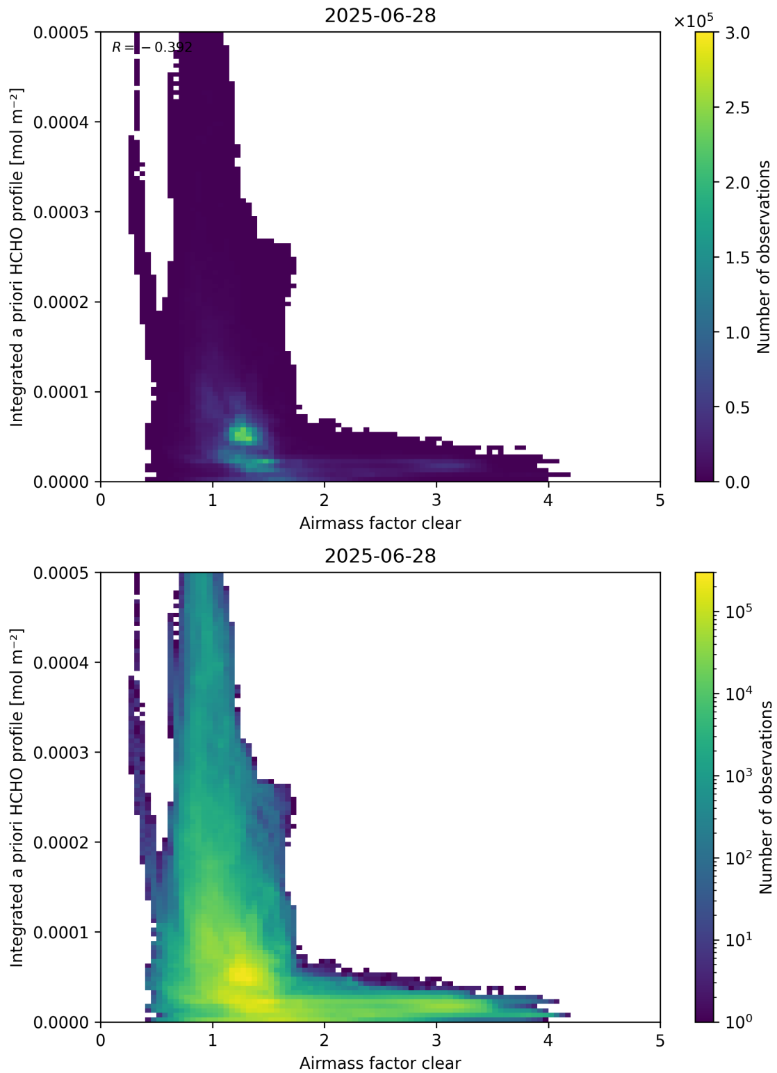
Figure 76: Scatter density plot of “Airmass factor clear” against “Integrated a priori HCHO profile” for 2025-06-27 to 2025-06-29.
