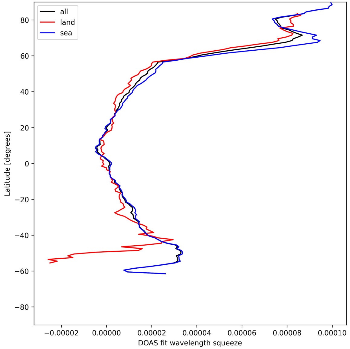
Figure 31: Zonal average of “DOAS fit wavelength squeeze” for 2025-06-27 to 2025-06-29.
