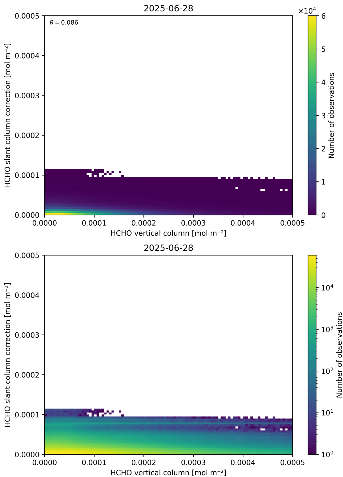
Figure 128: Scatter density plot of “HCHO vertical column” against “HCHO slant column correction” for 2025-06-27 to 2025-06-29.
