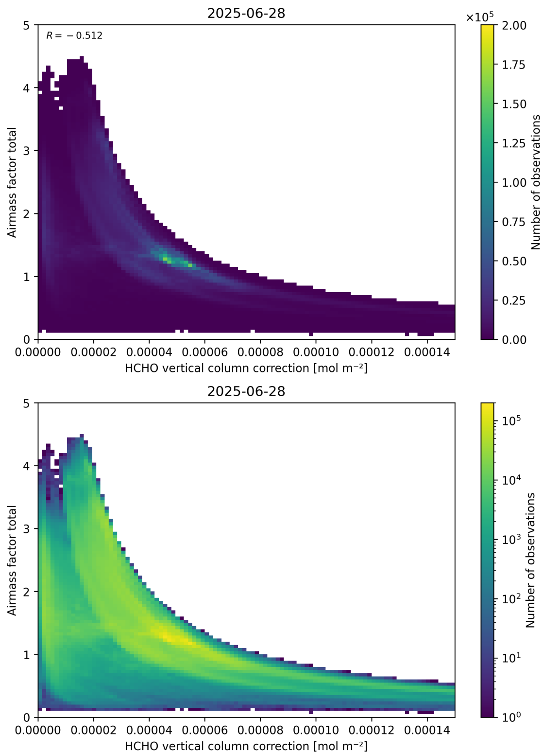
Figure 120: Scatter density plot of “HCHO vertical column correction” against “Airmass factor total” for 2025-06-27 to 2025-06-29.
