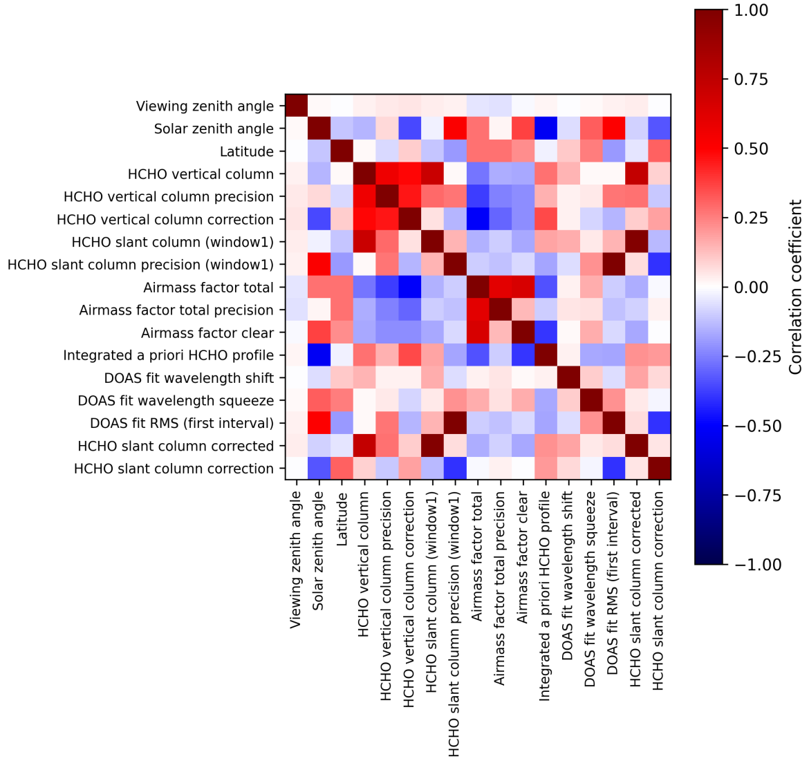
Figure 2: Map of correlation matrix for 2025-06-27 to 2025-06-29.
