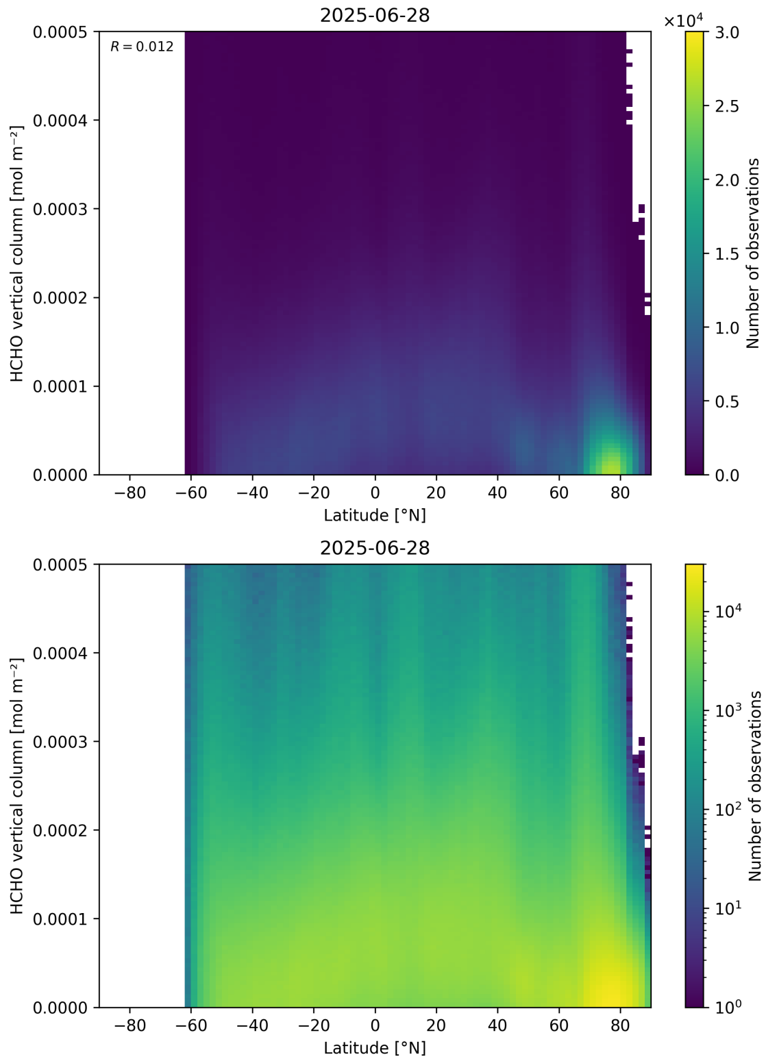
Figure 163: Scatter density plot of “Latitude” against “HCHO vertical column” for 2025-06-27 to 2025-06-29.
