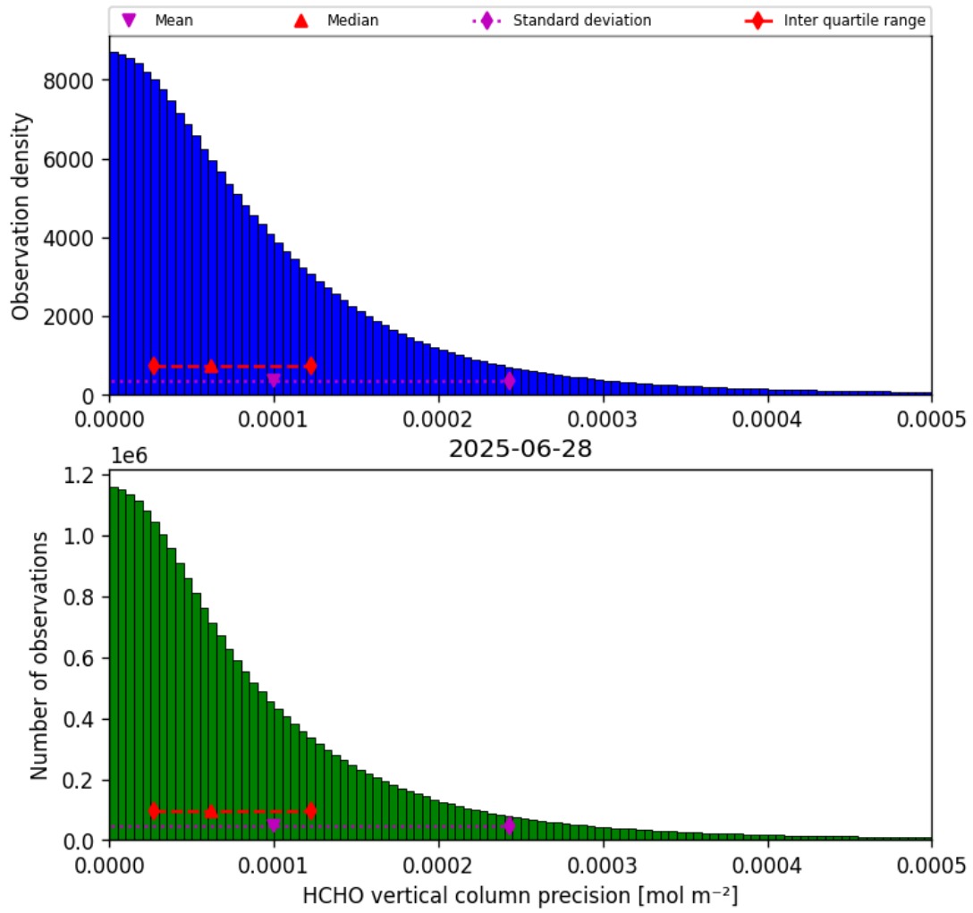
Figure 36: Histogram of “HCHO vertical column precision” for 2025-06-27 to 2025-06-29
