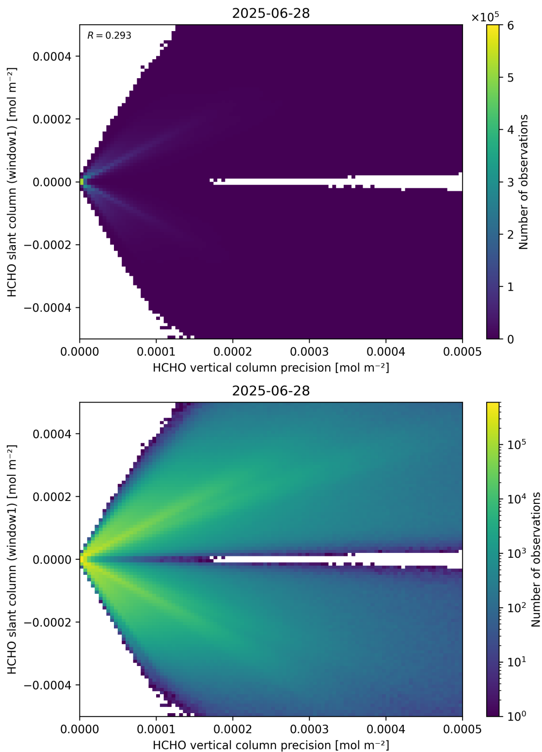
Figure 142: Scatter density plot of “HCHO vertical column precision” against “HCHO slant column (window1)” for 2025-06-27 to 2025-06-29.
