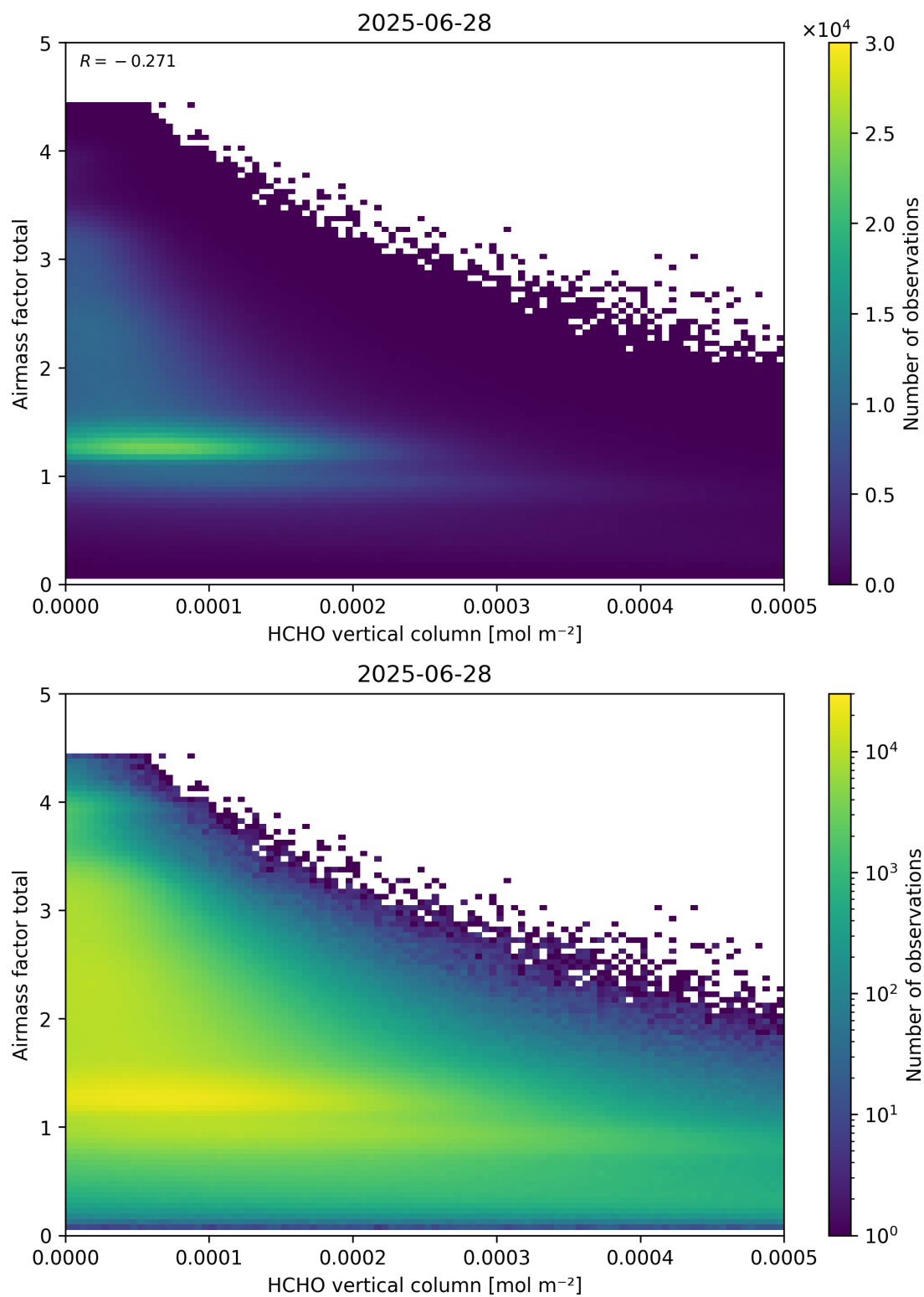
Figure 131: Scatter density plot of “HCHO vertical column” against “Airmass factor total” for 2025-06-27 to 2025-06-29.
