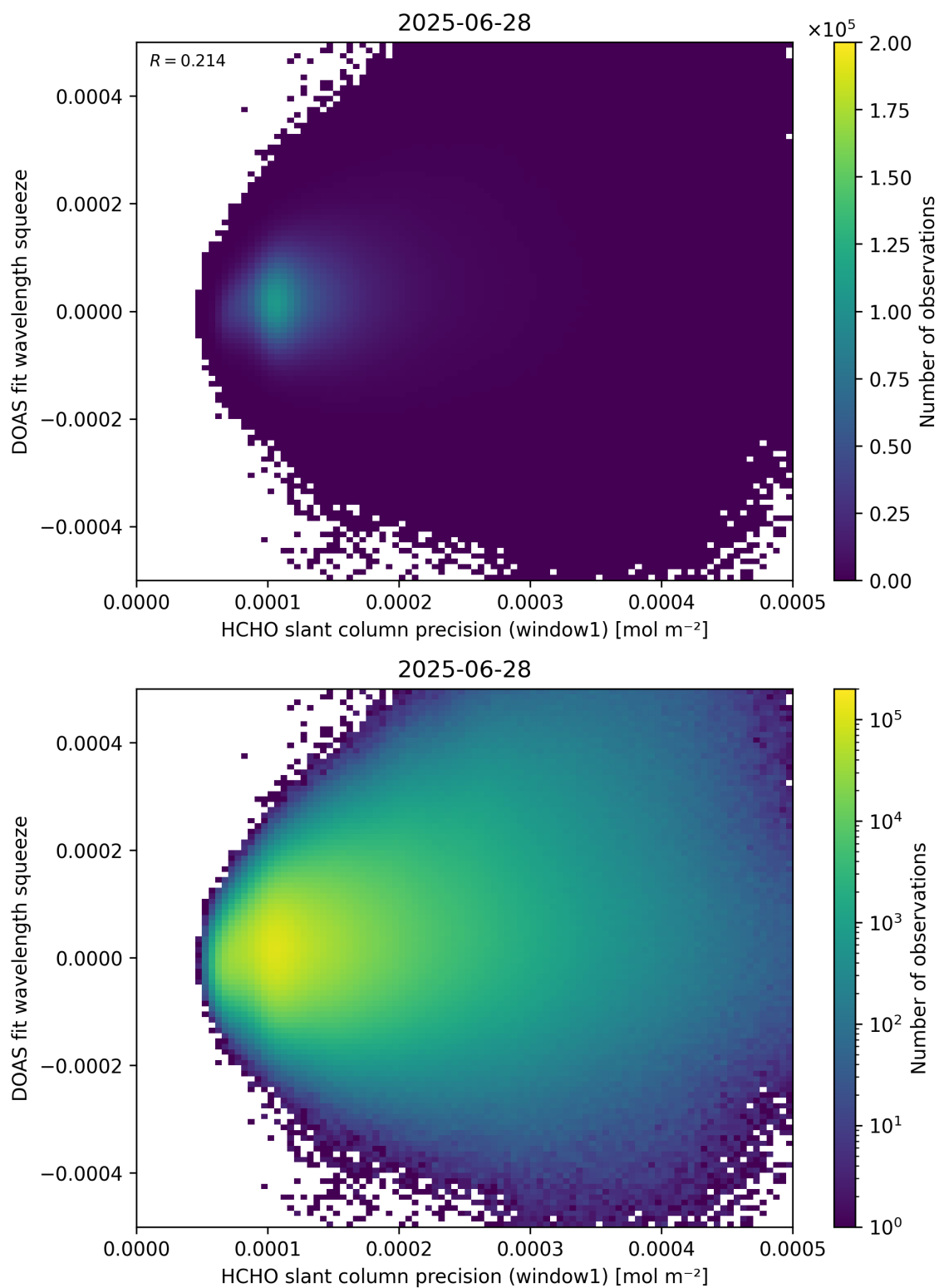
Figure 90: Scatter density plot of “HCHO slant column precision (window1)” against “DOAS fit wavelength squeeze” for 2025-06-27 to 2025-06-29.
