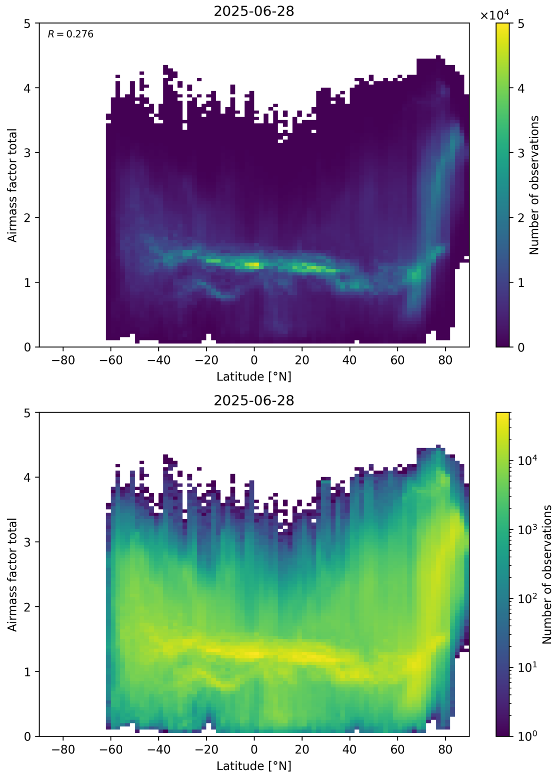
Figure 161: Scatter density plot of “Latitude” against “Airmass factor total” for 2025-06-27 to 2025-06-29.
