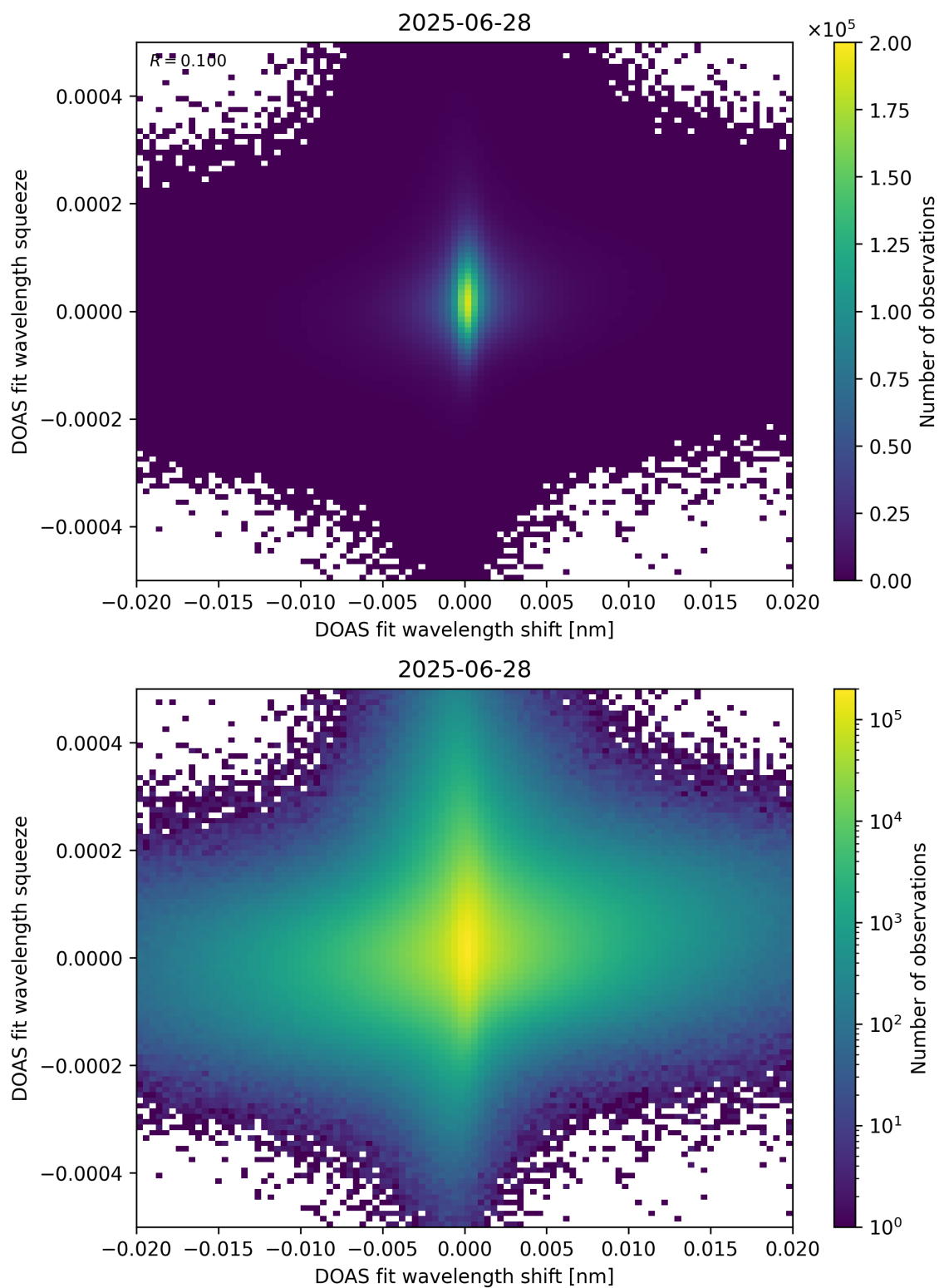
Figure 65: Scatter density plot of “DOAS fit wavelength shift” against “DOAS fit wavelength squeeze” for 2025-06-27 to 2025-06-29.
