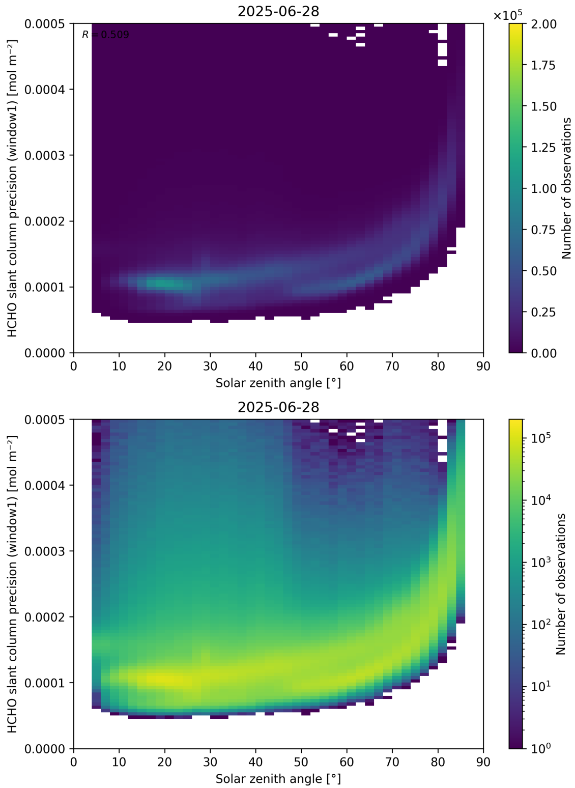
Figure 174: Scatter density plot of “Solar zenith angle” against “HCHO slant column precision (window1)” for 2025-06-27 to 2025-06-29.
