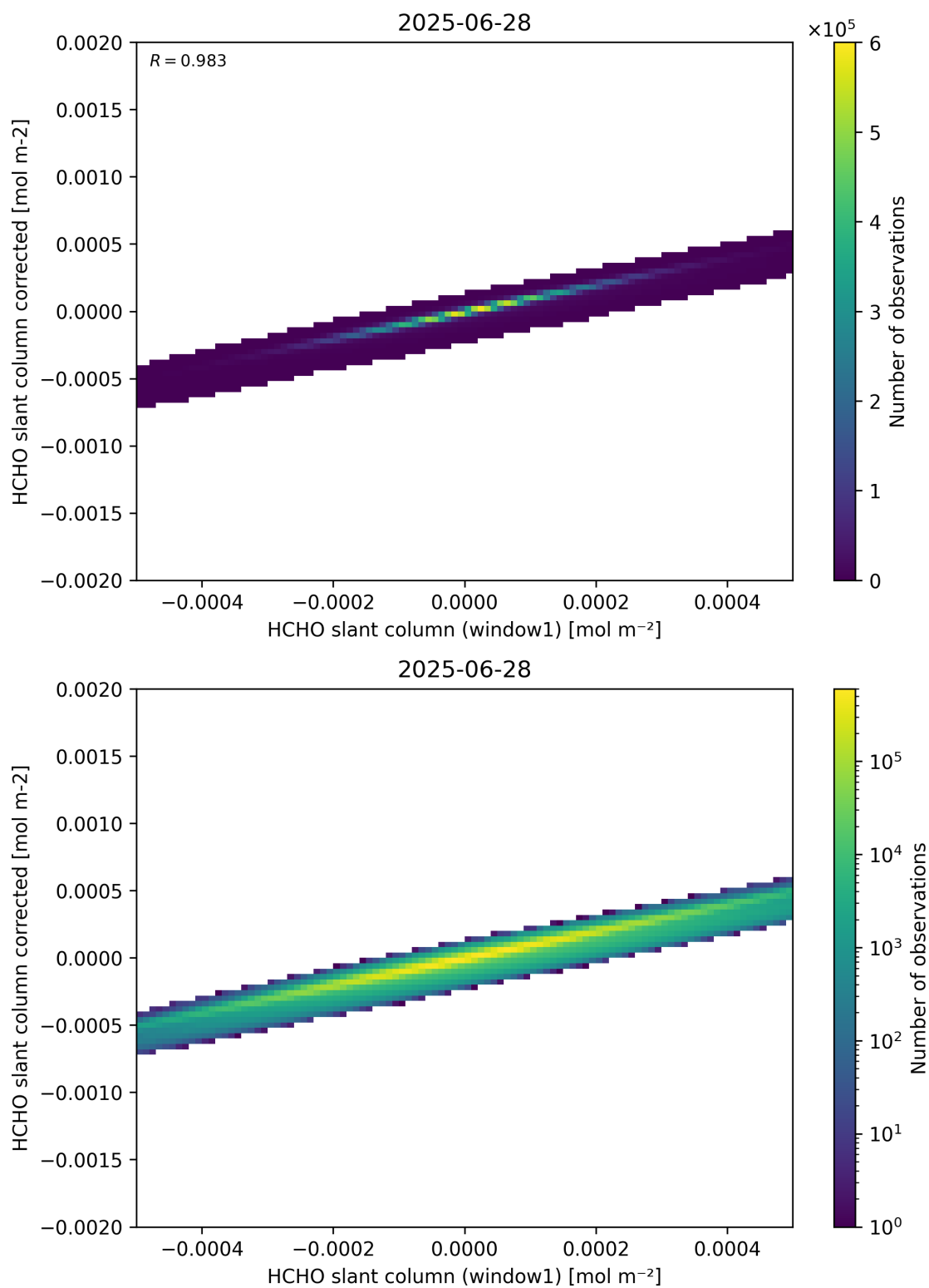
Figure 82: Scatter density plot of “HCHO slant column (window1)” against “HCHO slant column corrected” for 2025-06-27 to 2025-06-29.
