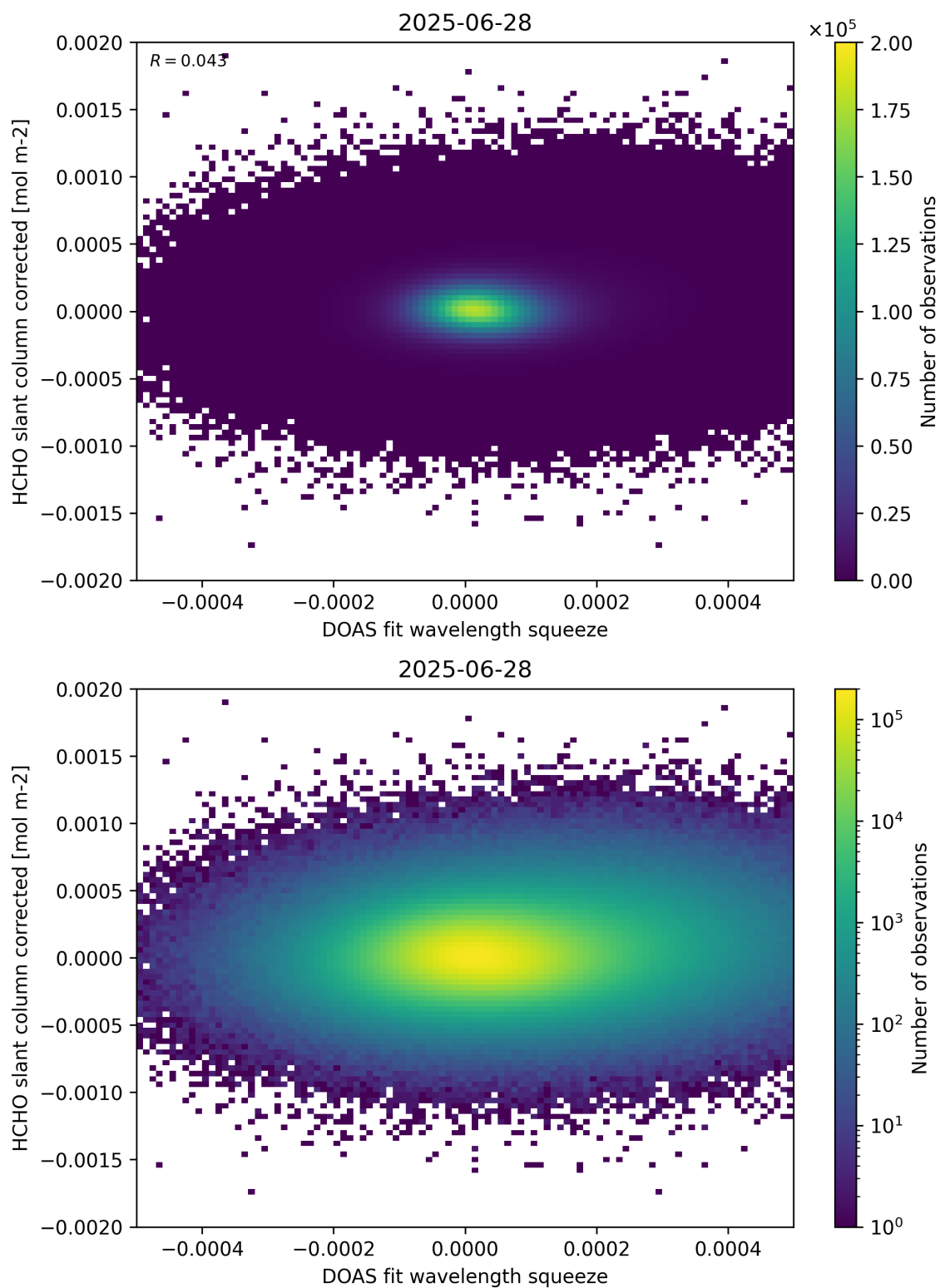
Figure 69: Scatter density plot of “DOAS fit wavelength squeeze” against “HCHO slant column corrected” for 2025-06-27 to 2025-06-29.
