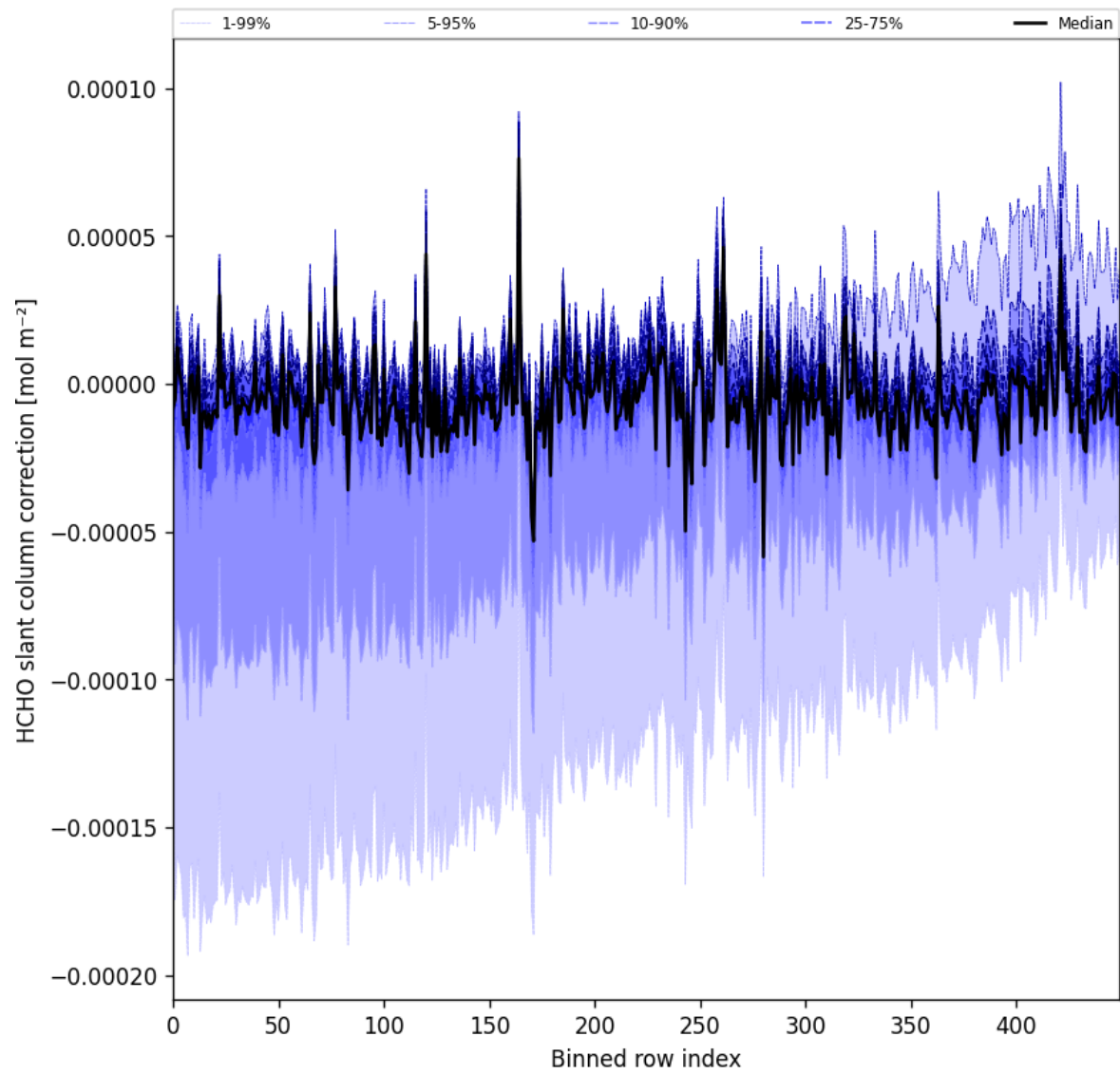
Figure 61: Along track statistics of “HCHO slant column correction” for 2025-06-27 to 2025-06-29
