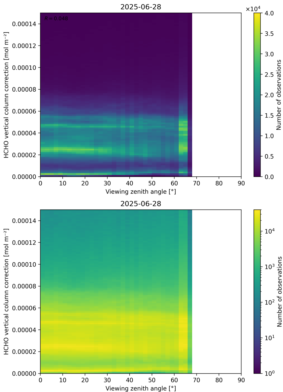
Figure 193: Scatter density plot of “Viewing zenith angle” against “HCHO vertical column correction” for 2025-06-27 to 2025-06-29.
