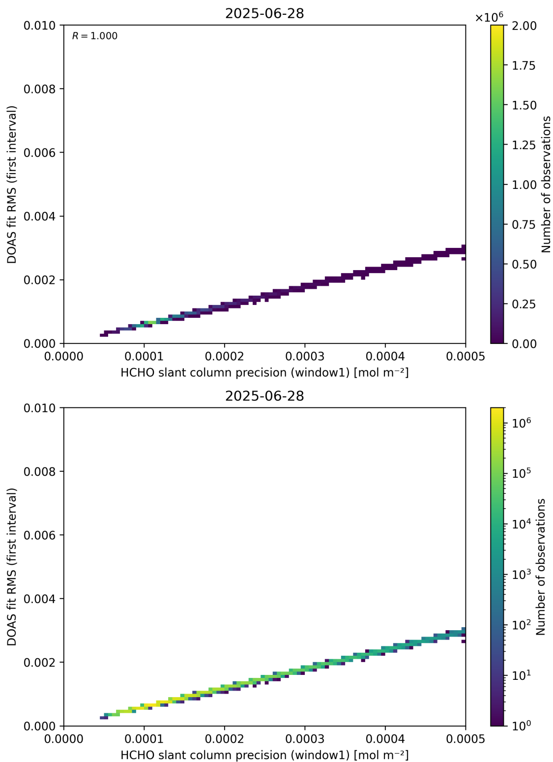
Figure 88: Scatter density plot of “HCHO slant column precision (window1)” against “DOAS fit RMS (first interval)” for 2025-06-27 to 2025-06-29.
