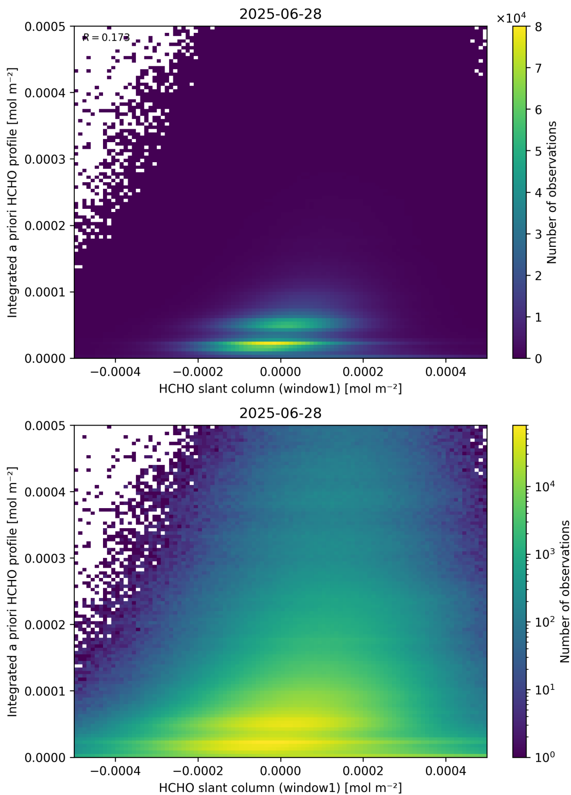
Figure 87: Scatter density plot of “HCHO slant column (window1)” against “Integrated a priori HCHO profile” for 2025-06-27 to 2025-06-29.
