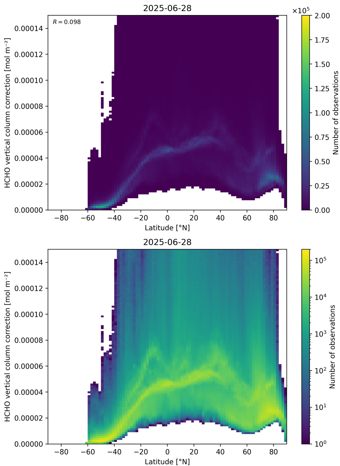
Figure 164: Scatter density plot of “Latitude” against “HCHO vertical column correction” for 2025-06-27 to 2025-06-29.
