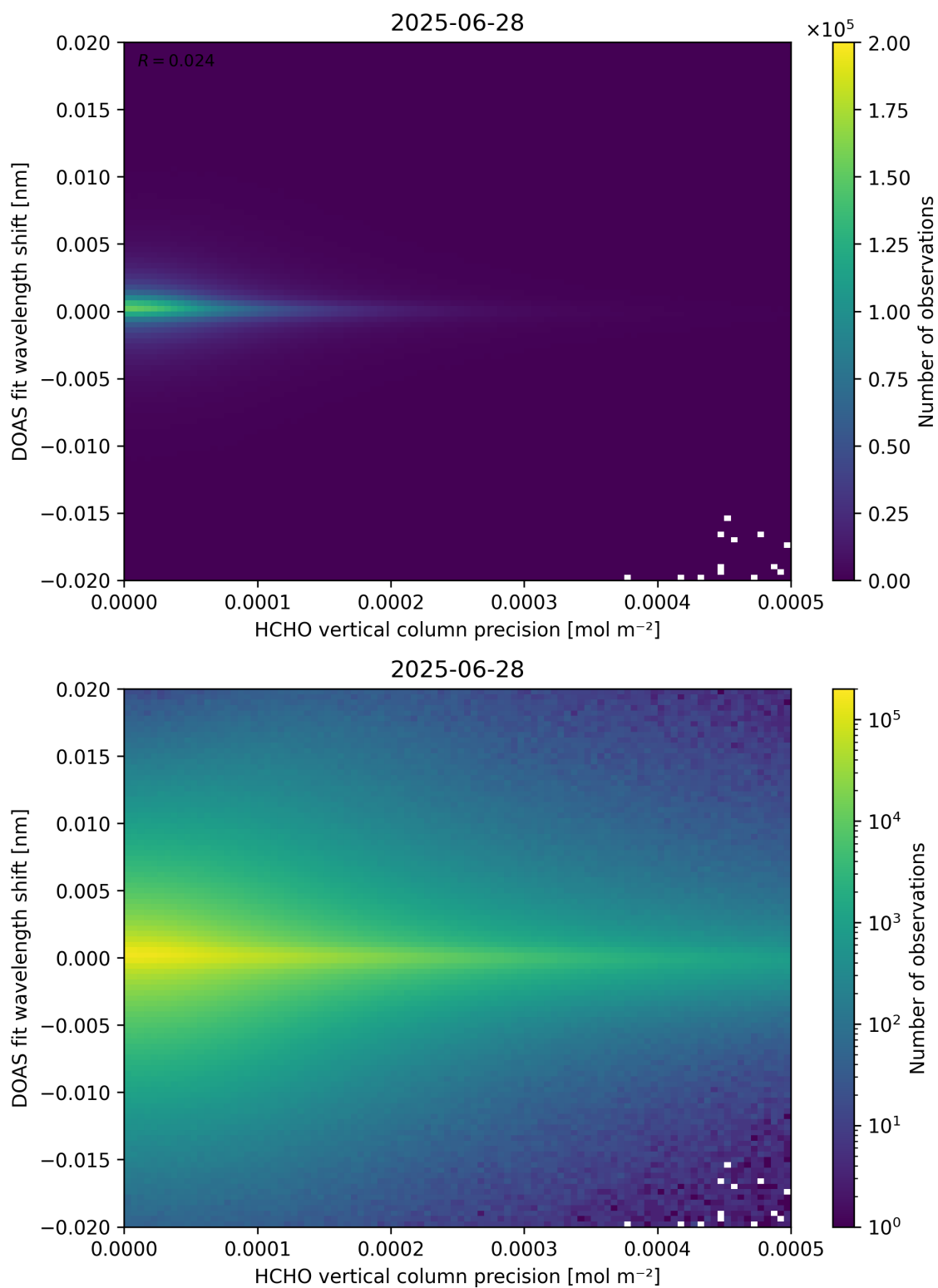
Figure 137: Scatter density plot of “HCHO vertical column precision” against “DOAS fit wavelength shift” for 2025-06-27 to 2025-06-29.
