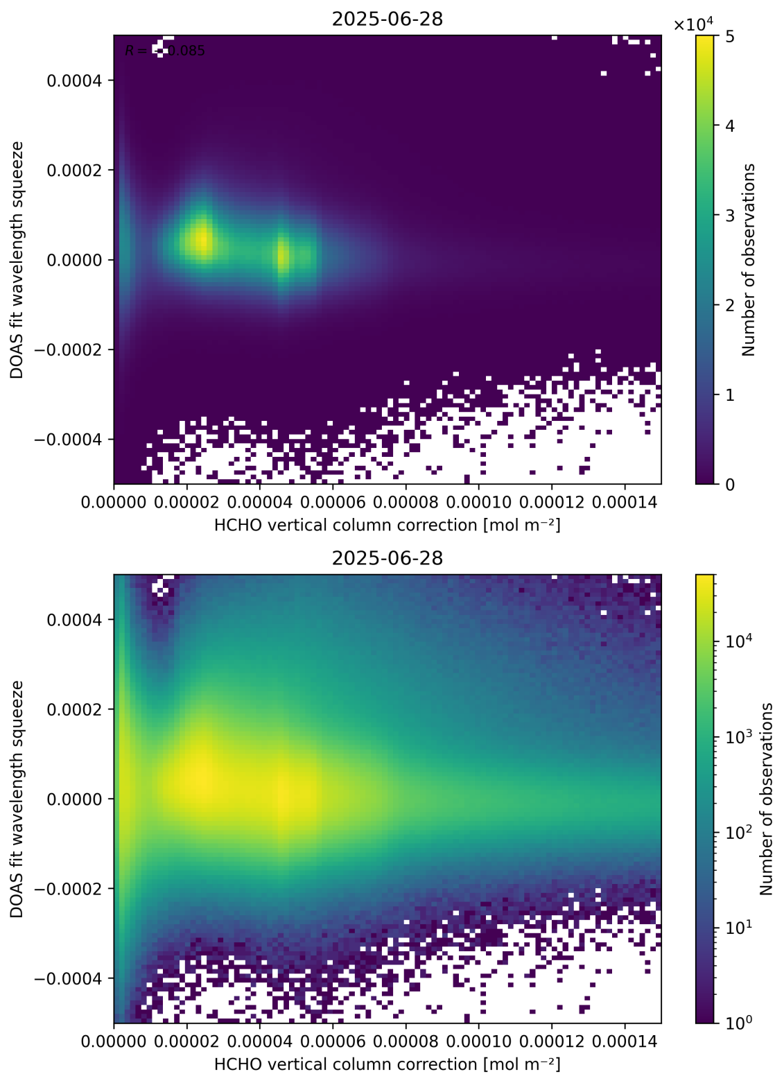
Figure 114: Scatter density plot of “HCHO vertical column correction” against “DOAS fit wavelength squeeze” for 2025-06-27 to 2025-06-29.
