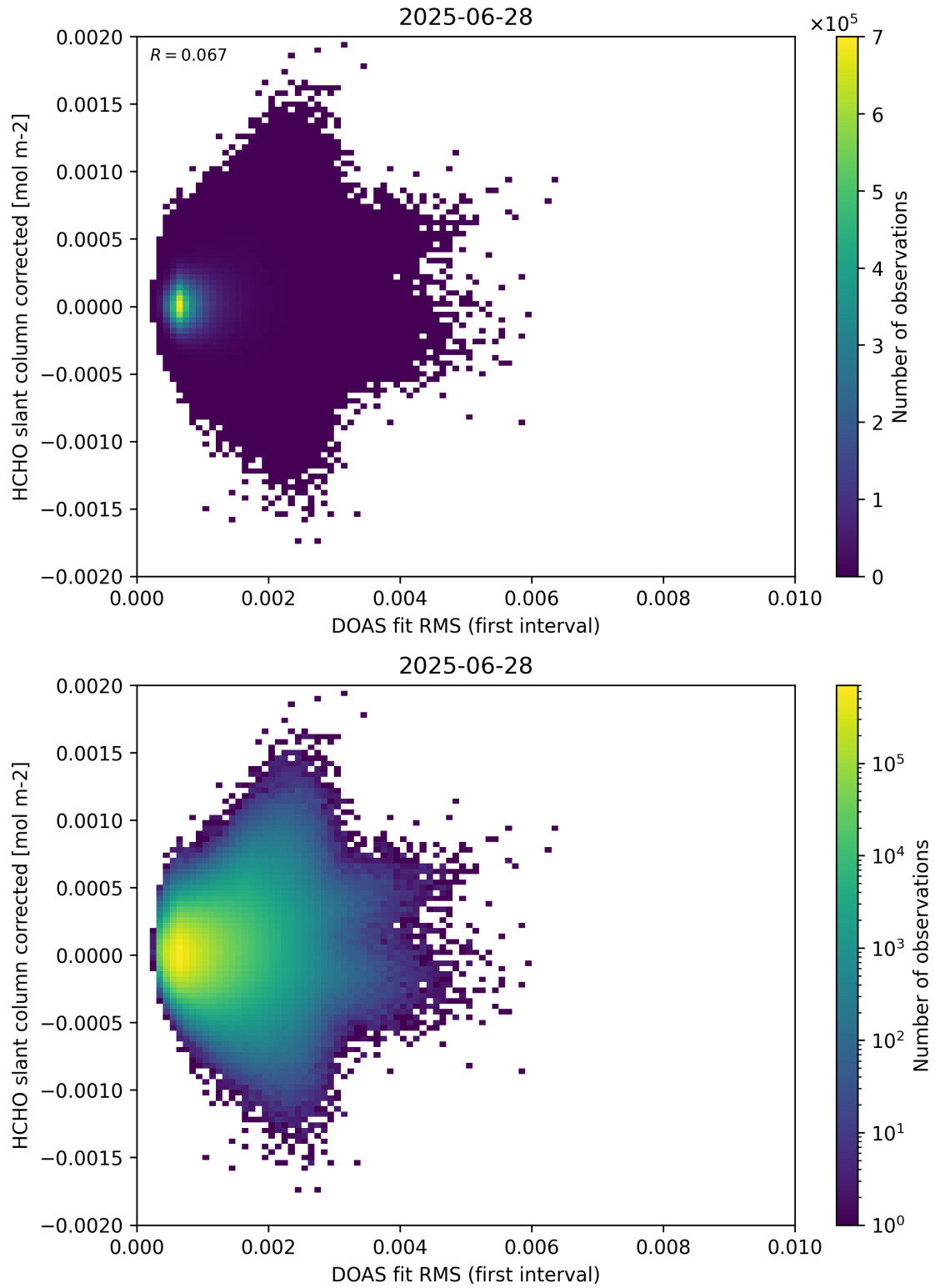
Figure 62: Scatter density plot of “DOAS fit RMS (first interval)” against “HCHO slant column corrected” for 2025-06-27 to 2025-06-29.
