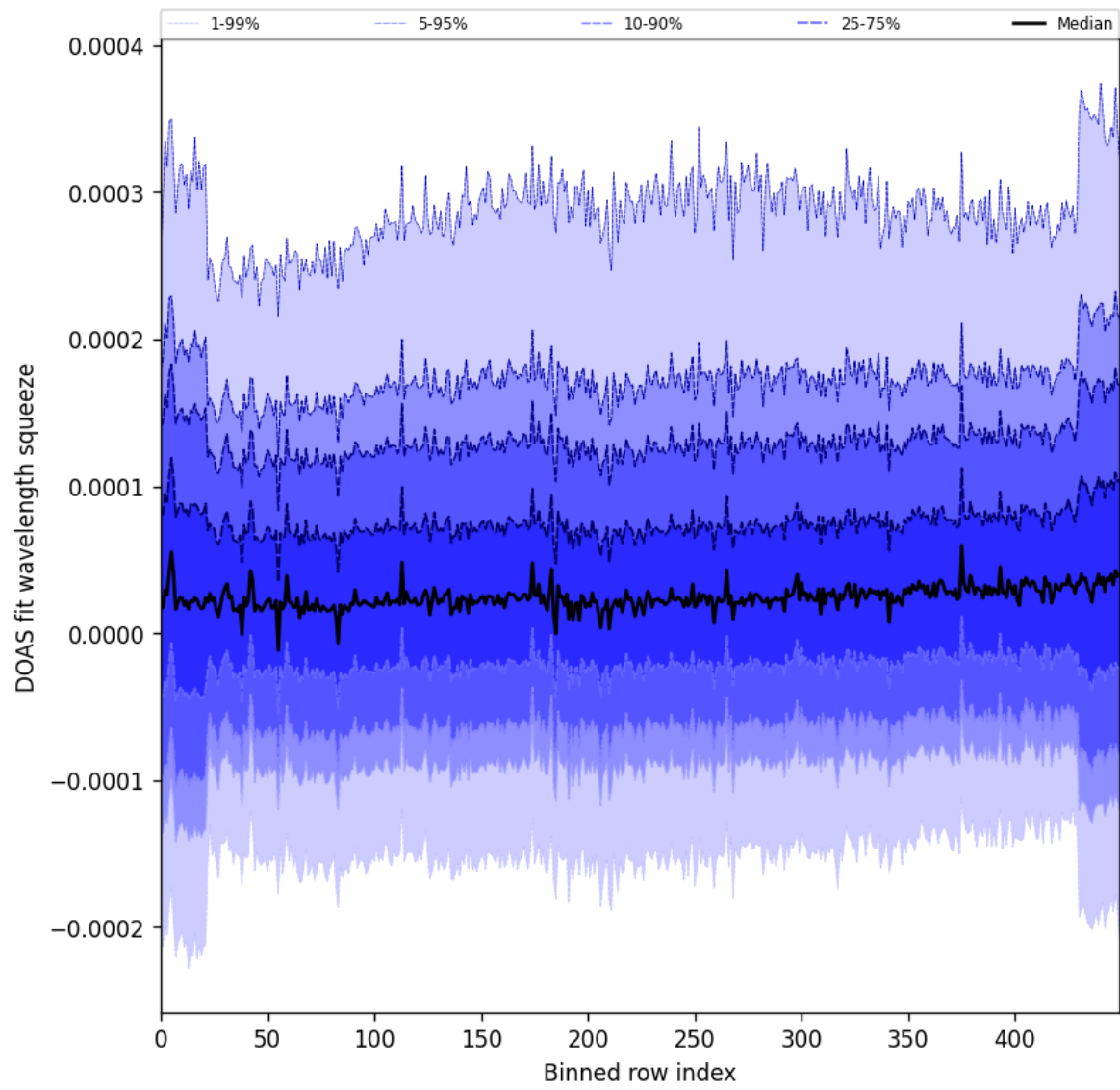
Figure 59: Along track statistics of “DOAS fit wavelength squeeze” for 2025-06-27 to 2025-06-29
