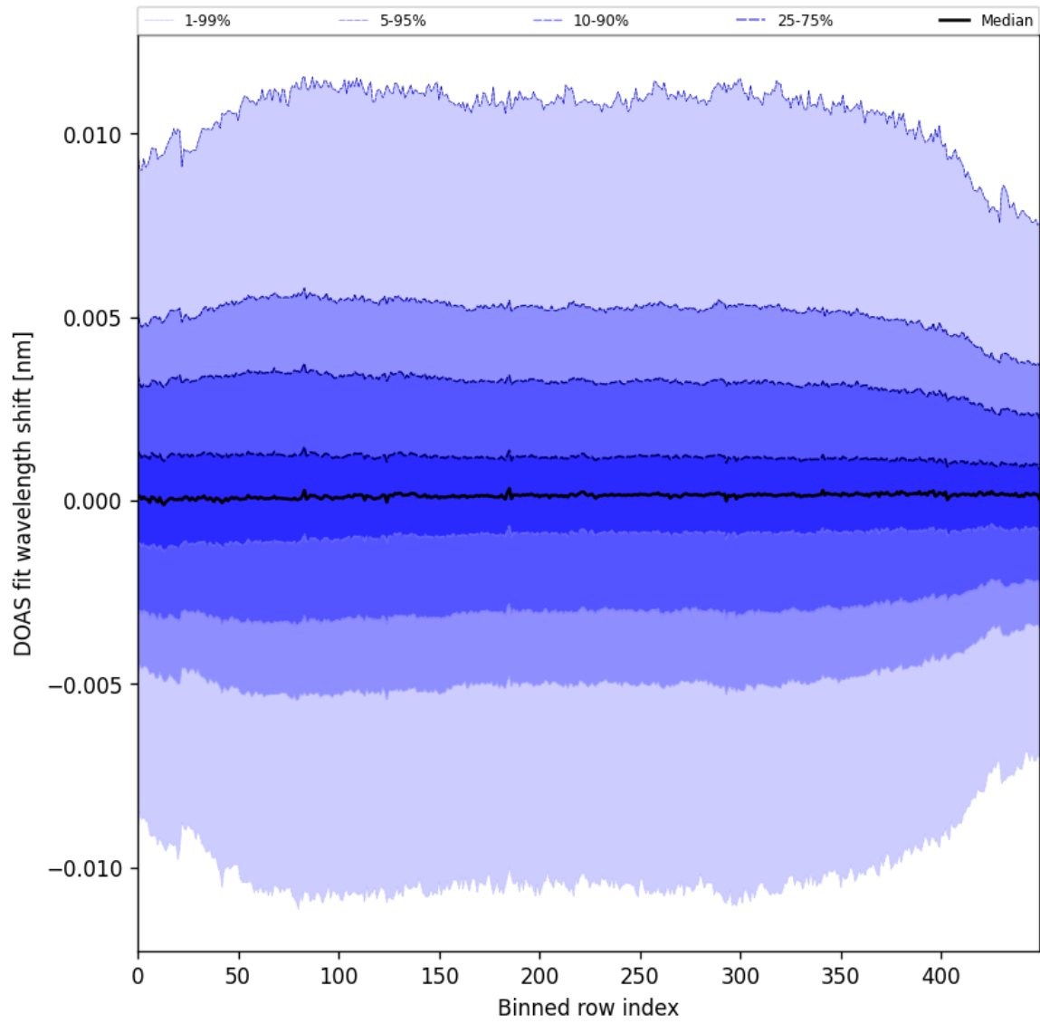
Figure 58: Along track statistics of “DOAS fit wavelength shift” for 2025-06-27 to 2025-06-29
