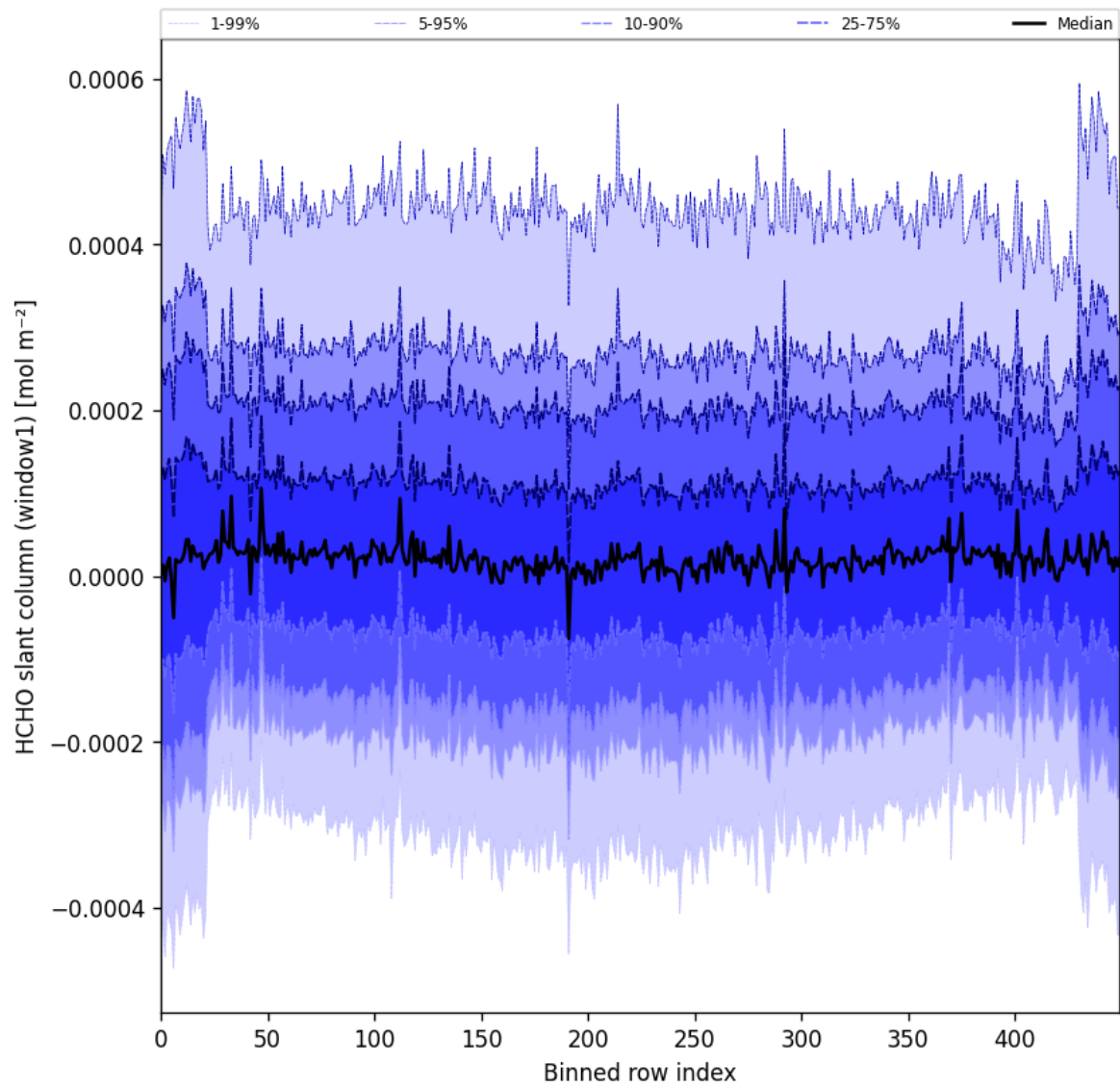
Figure 52: Along track statistics of “HCHO slant column (window1)” for 2025-06-27 to 2025-06-29
