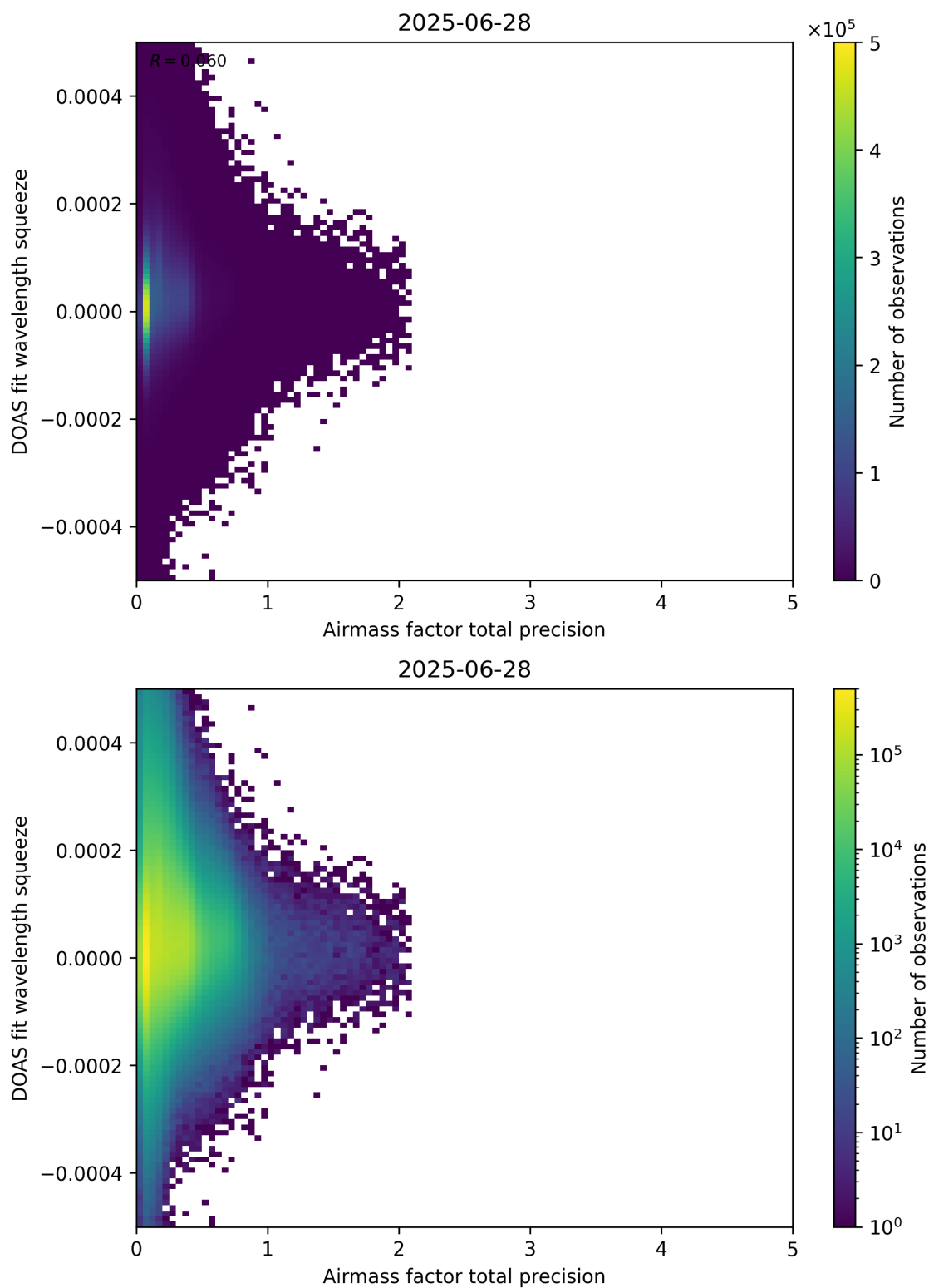
Figure 107: Scatter density plot of “Airmass factor total precision” against “DOAS fit wavelength squeeze” for 2025-06-27 to 2025-06-29.
