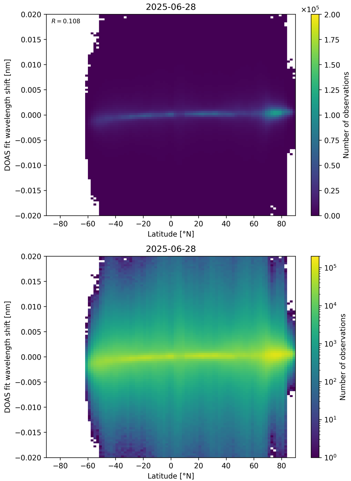
Figure 154: Scatter density plot of “Latitude” against “DOAS fit wavelength shift” for 2025-06-27 to 2025-06-29.
