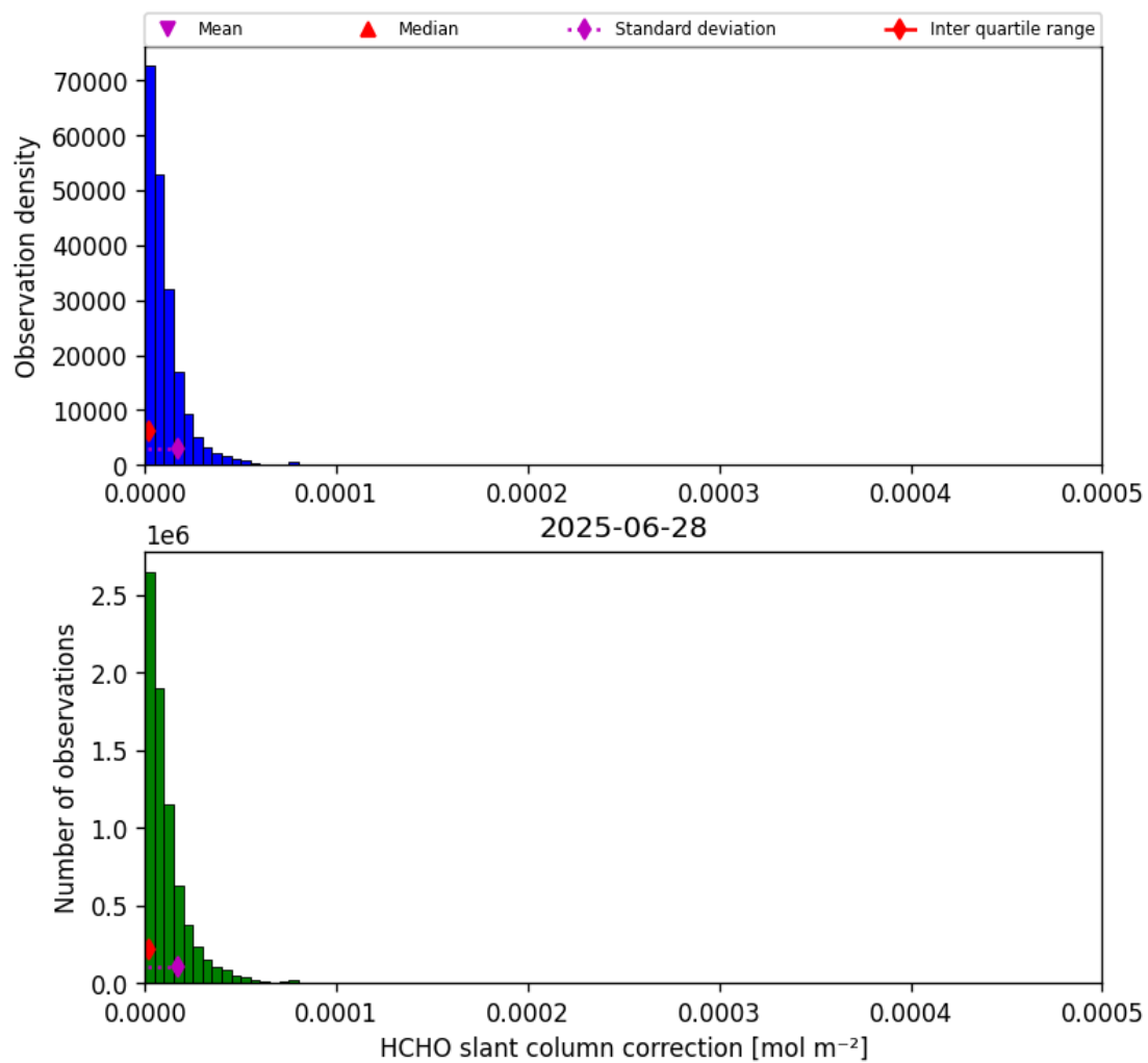
Figure 47: Histogram of “HCHO slant column correction” for 2025-06-27 to 2025-06-29
