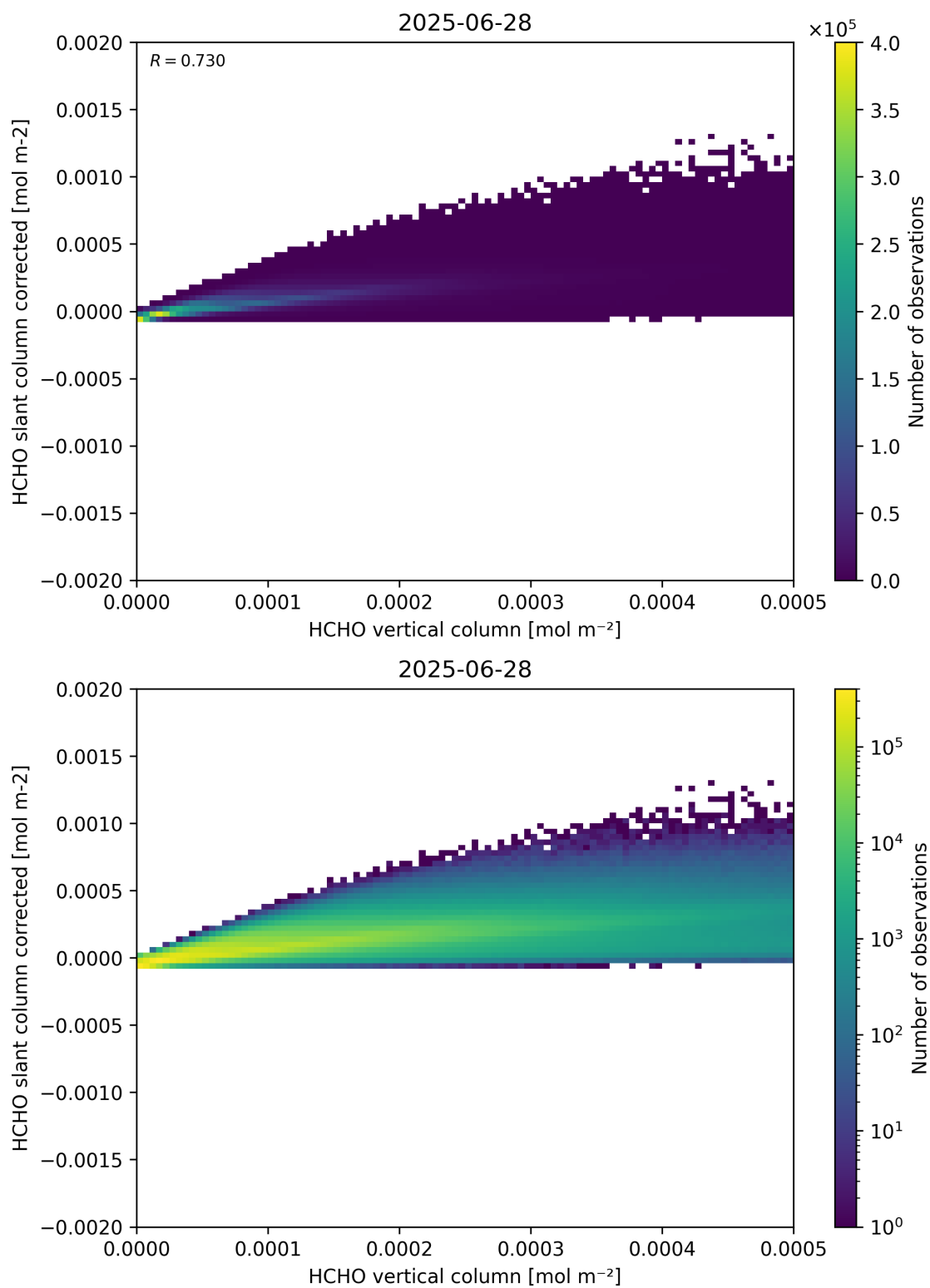
Figure 127: Scatter density plot of “HCHO vertical column” against “HCHO slant column corrected” for 2025-06-27 to 2025-06-29.
