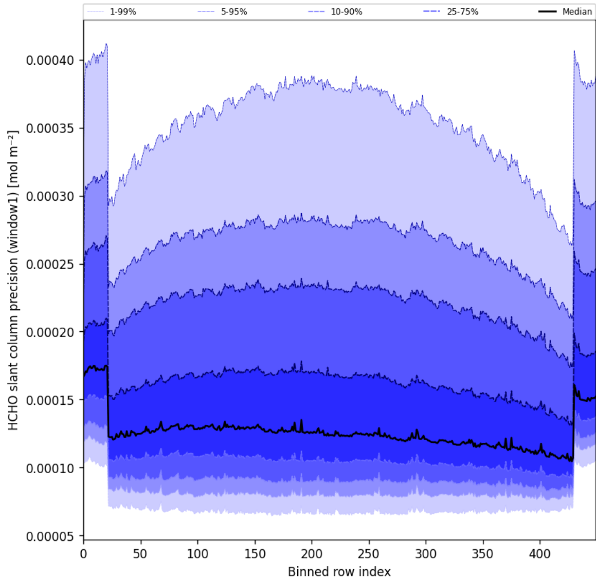
Figure 53: Along track statistics of “HCHO slant column precision (window1)” for 2025-06-27 to 2025-06-29
