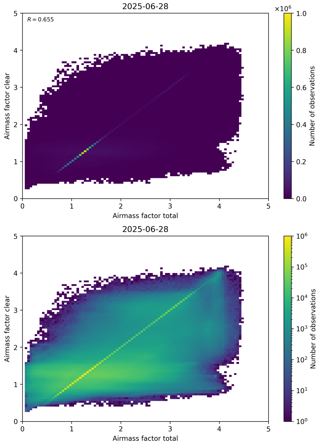
Figure 100: Scatter density plot of “Airmass factor total” against “Airmass factor clear” for 2025-06-27 to 2025-06-29.
