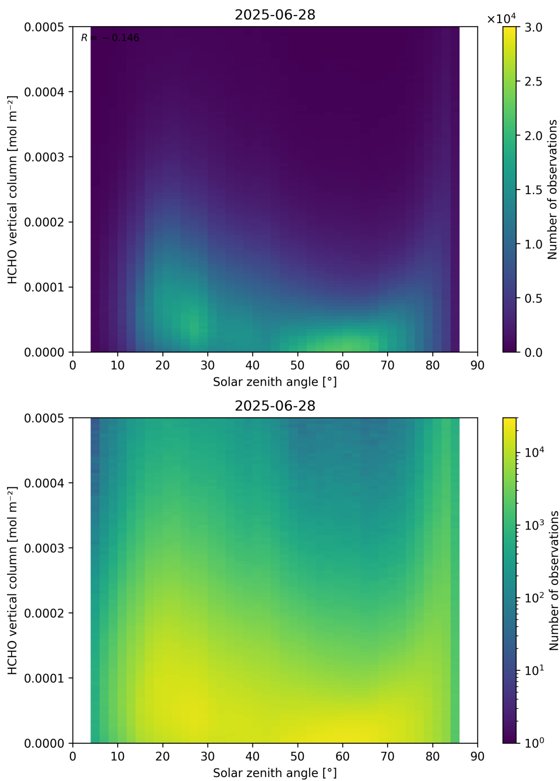
Figure 177: Scatter density plot of “Solar zenith angle” against “HCHO vertical column” for 2025-06-27 to 2025-06-29.
