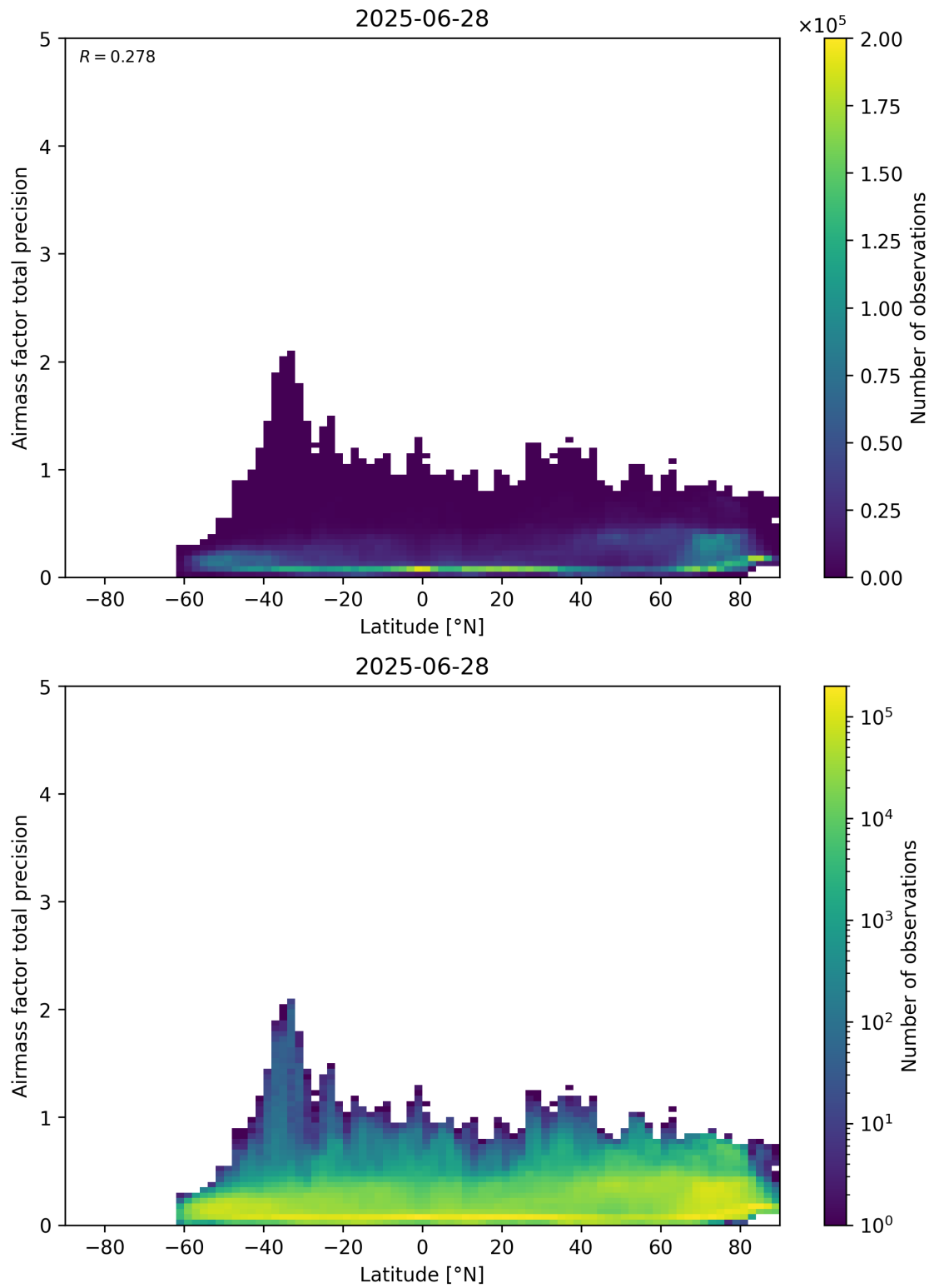
Figure 162: Scatter density plot of “Latitude” against “Airmass factor total precision” for 2025-06-27 to 2025-06-29.
