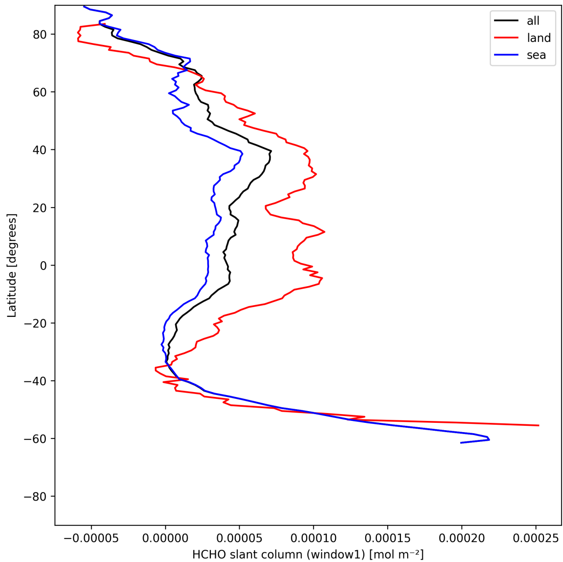
Figure 24: Zonal average of “HCHO slant column (window1)” for 2025-06-27 to 2025-06-29.
