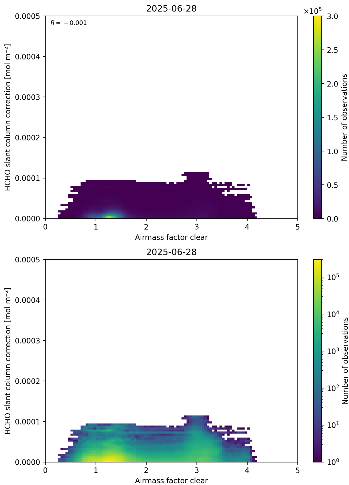
Figure 75: Scatter density plot of “Airmass factor clear” against “HCHO slant column correction” for 2025-06-27 to 2025-06-29.
