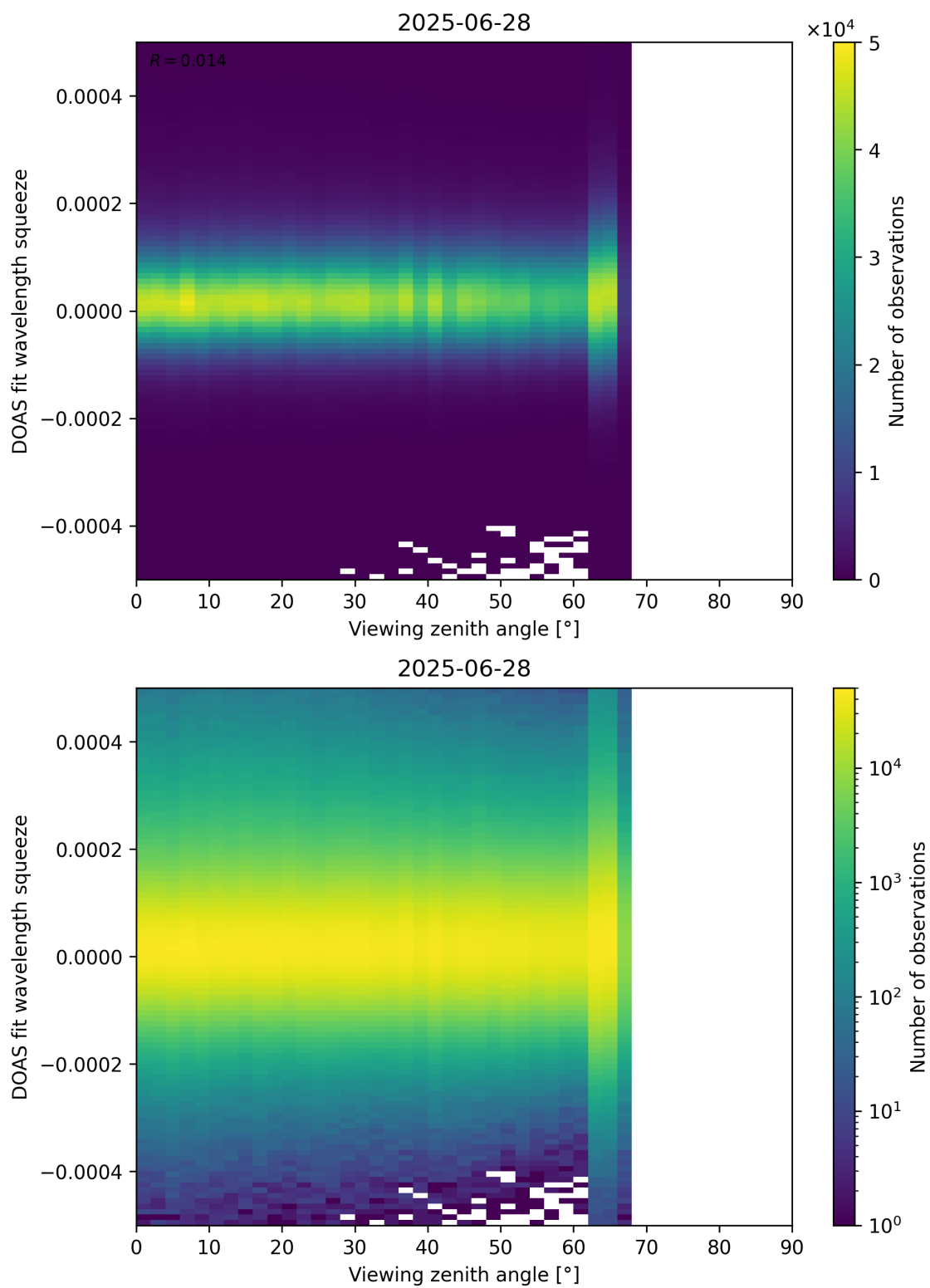
Figure 184: Scatter density plot of “Viewing zenith angle” against “DOAS fit wavelength squeeze” for 2025-06-27 to 2025-06-29.
