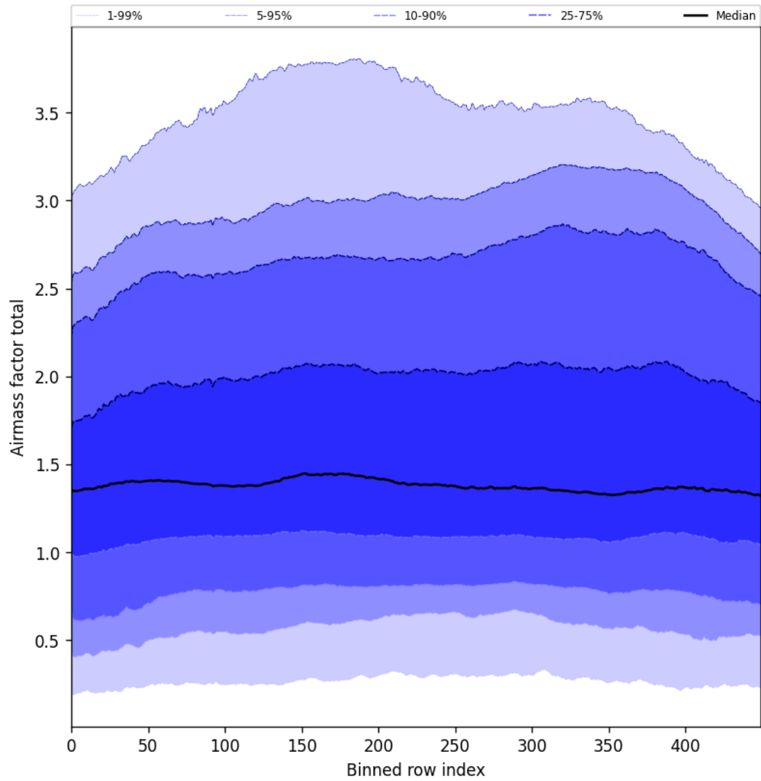
Figure 54: Along track statistics of “Airmass factor total” for 2025-06-27 to 2025-06-29
