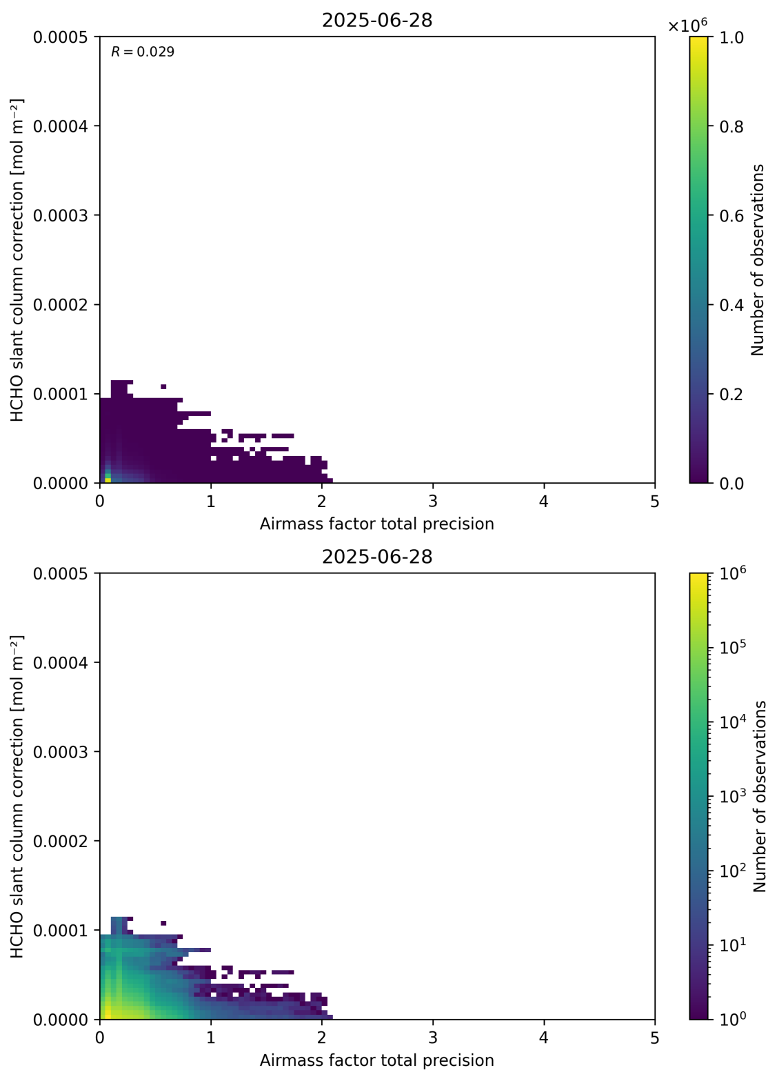
Figure 110: Scatter density plot of “Airmass factor total precision” against “HCHO slant column correction” for 2025-06-27 to 2025-06-29.
