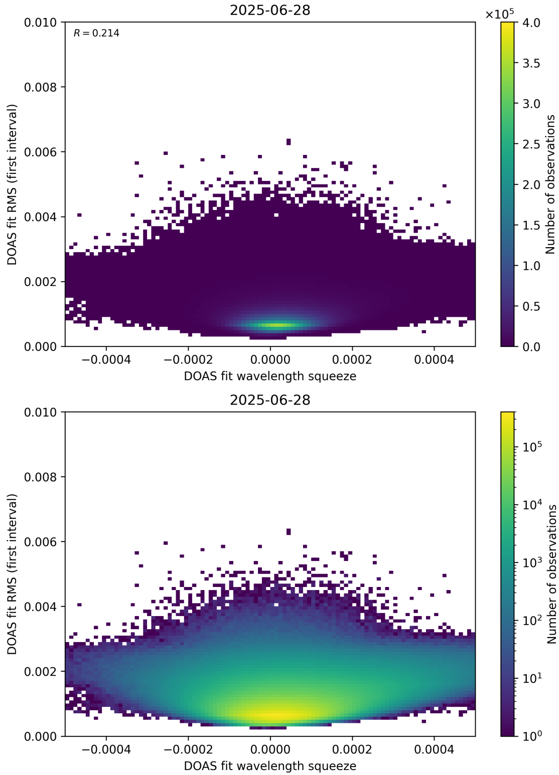
Figure 68: Scatter density plot of “DOAS fit wavelength squeeze” against “DOAS fit RMS (first interval)” for 2025-06-27 to 2025-06-29.
