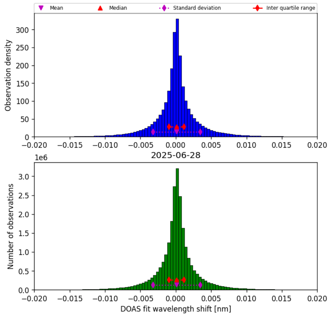
Figure 44: Histogram of “DOAS fit wavelength shift” for 2025-06-27 to 2025-06-29
