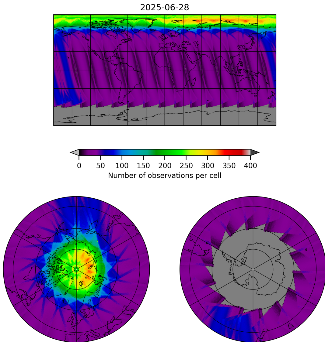
Figure 19: Map of the number of observations for 2025-06-27 to 2025-06-29
