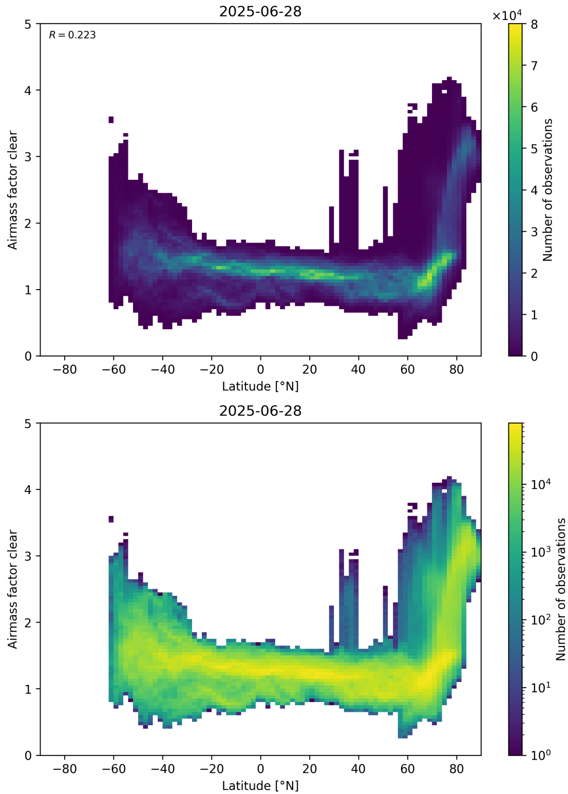
Figure 156: Scatter density plot of “Latitude” against “Airmass factor clear” for 2025-06-27 to 2025-06-29.
