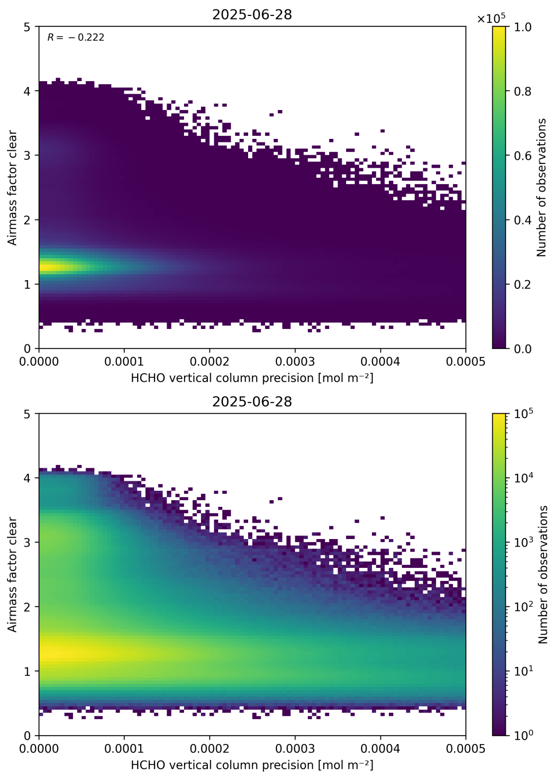
Figure 139: Scatter density plot of “HCHO vertical column precision” against “Airmass factor clear” for 2025-06-27 to 2025-06-29.
