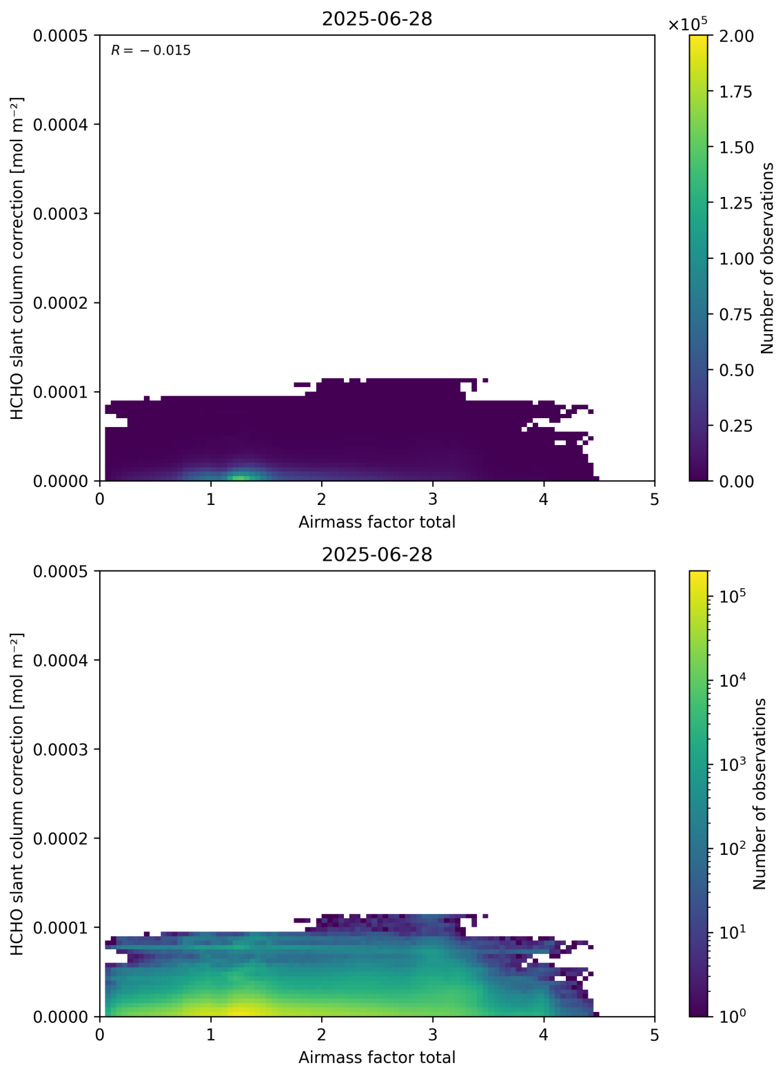
Figure 102: Scatter density plot of “Airmass factor total” against “HCHO slant column correction” for 2025-06-27 to 2025-06-29.
