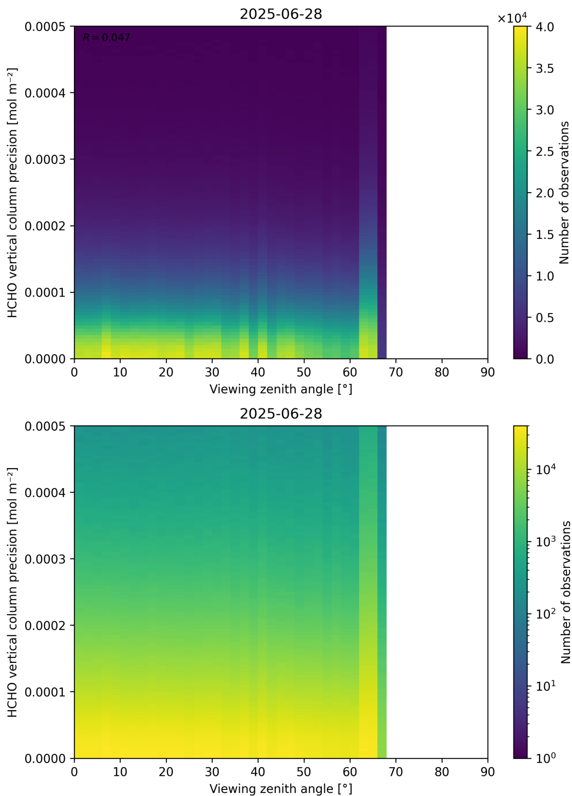
Figure 194: Scatter density plot of “Viewing zenith angle” against “HCHO vertical column precision” for 2025-06-27 to 2025-06-29.
