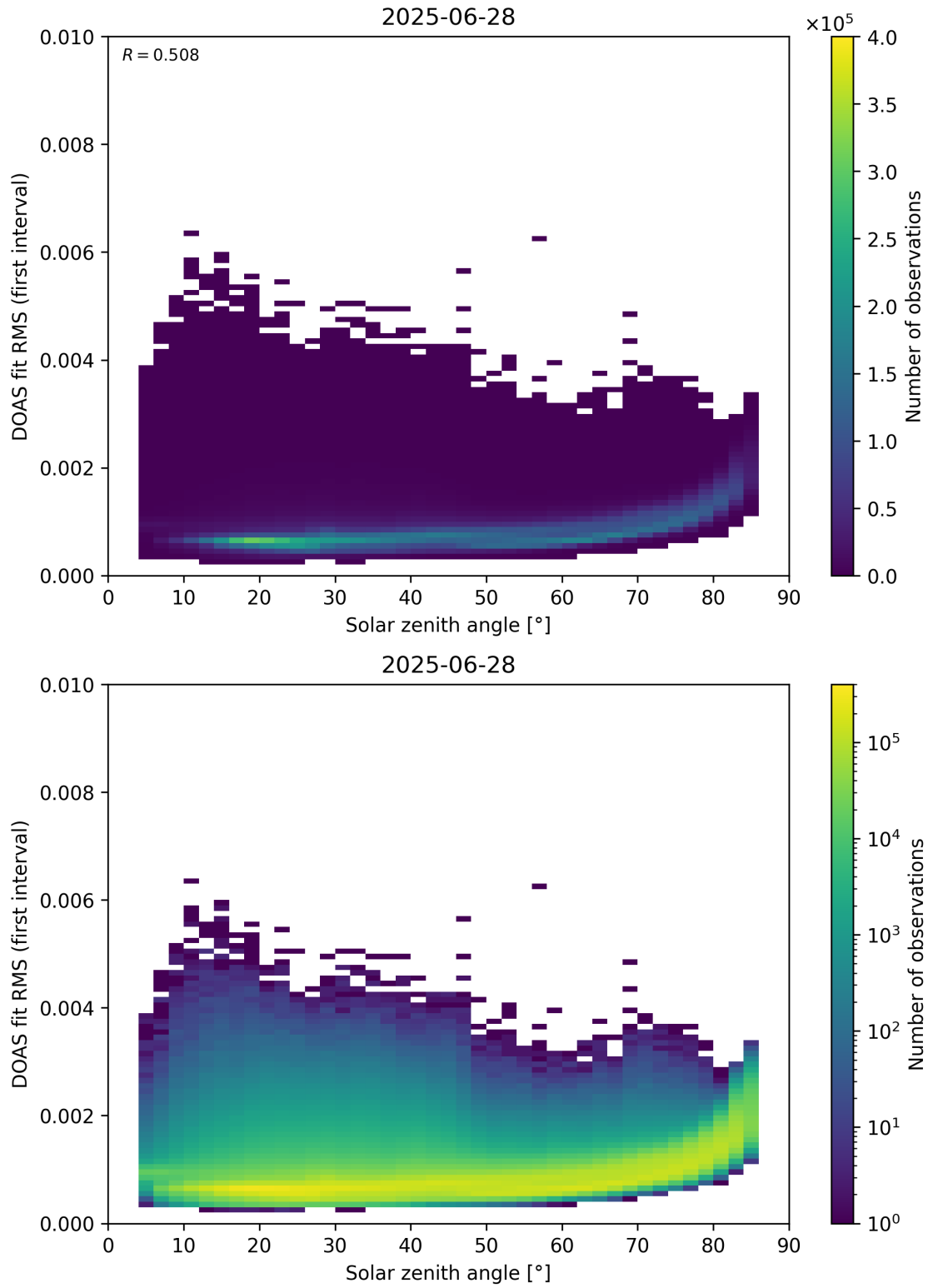
Figure 167: Scatter density plot of “Solar zenith angle” against “DOAS fit RMS (first interval)” for 2025-06-27 to 2025-06-29.
