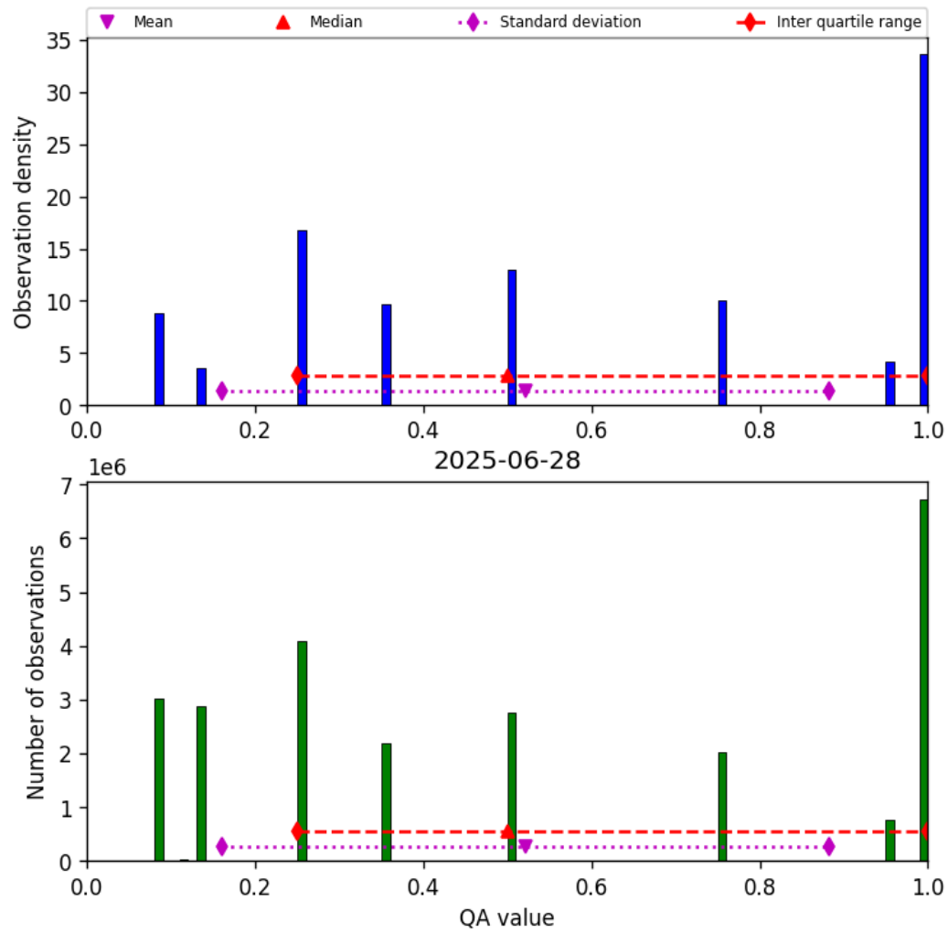
Figure 34: Histogram of “QA value” for 2025-06-27 to 2025-06-29
