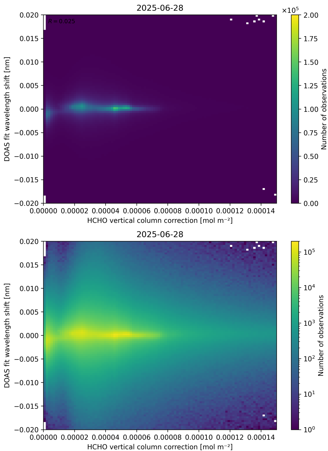
Figure 113: Scatter density plot of “HCHO vertical column correction” against “DOAS fit wavelength shift” for 2025-06-27 to 2025-06-29.
