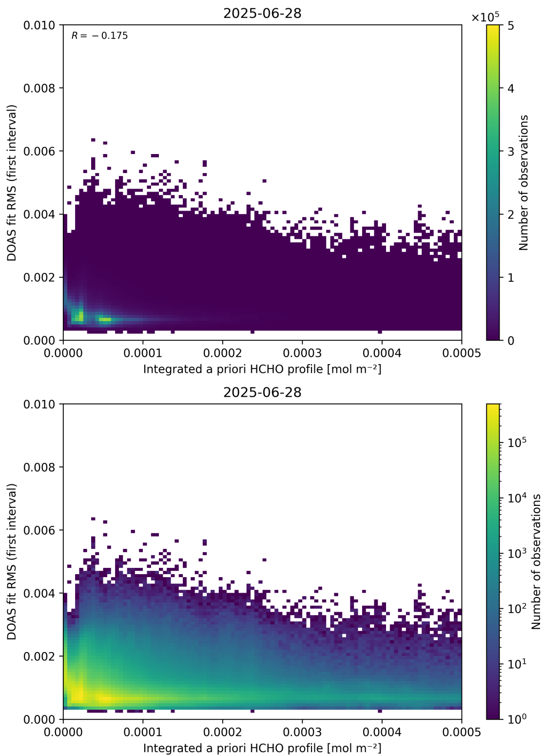
Figure 148: Scatter density plot of “Integrated a priori HCHO profile” against “DOAS fit RMS (first interval)” for 2025-06-27 to 2025-06-29.
