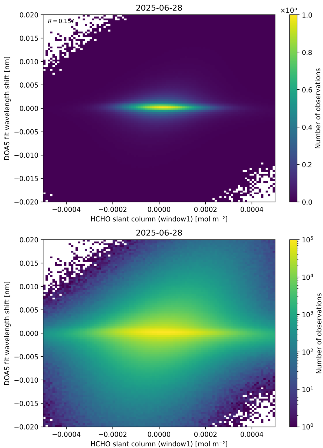
Figure 79: Scatter density plot of “HCHO slant column (window1)” against “DOAS fit wavelength shift” for 2025-06-27 to 2025-06-29.
