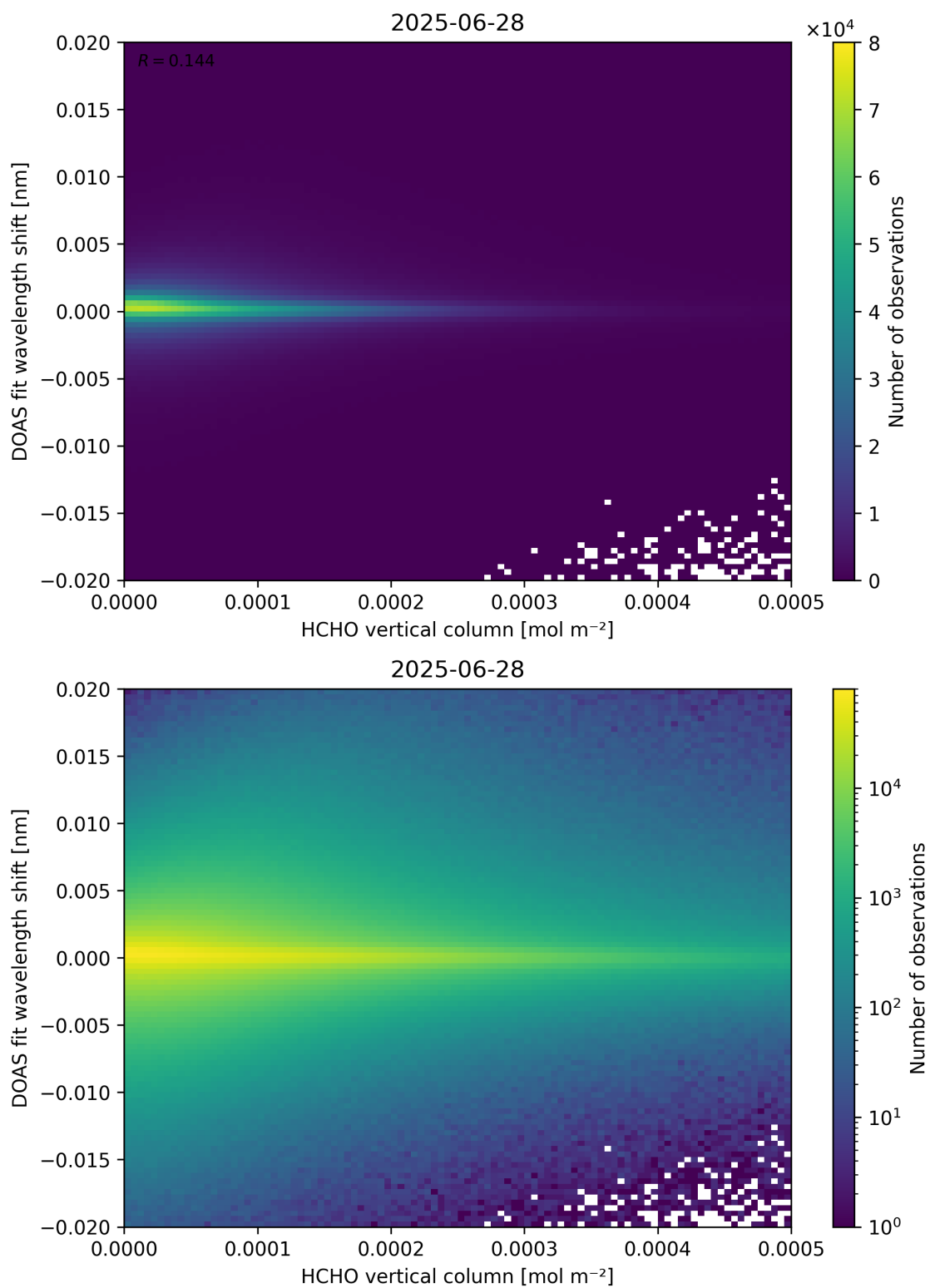
Figure 124: Scatter density plot of “HCHO vertical column” against “DOAS fit wavelength shift” for 2025-06-27 to 2025-06-29.
