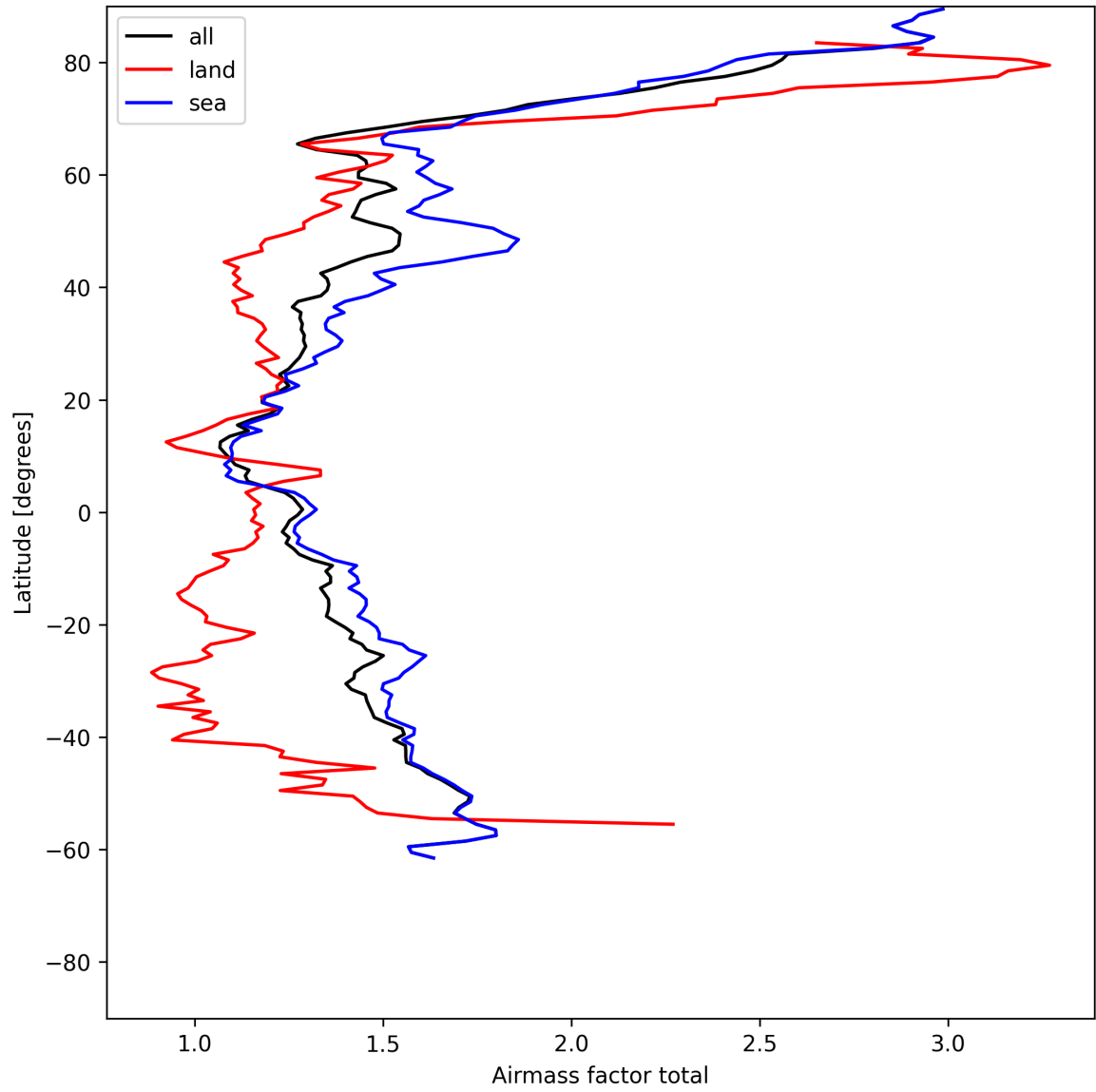
Figure 26: Zonal average of “Airmass factor total” for 2025-06-27 to 2025-06-29.
