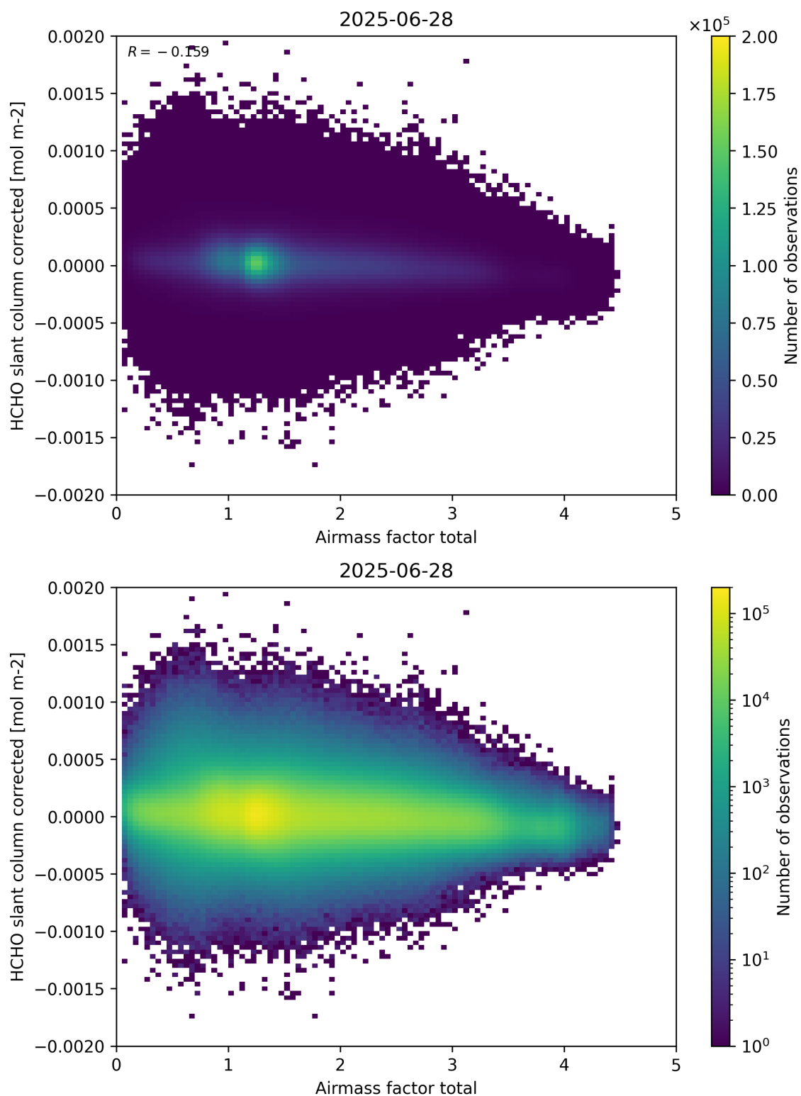
Figure 101: Scatter density plot of “Airmass factor total” against “HCHO slant column corrected” for 2025-06-27 to 2025-06-29.
