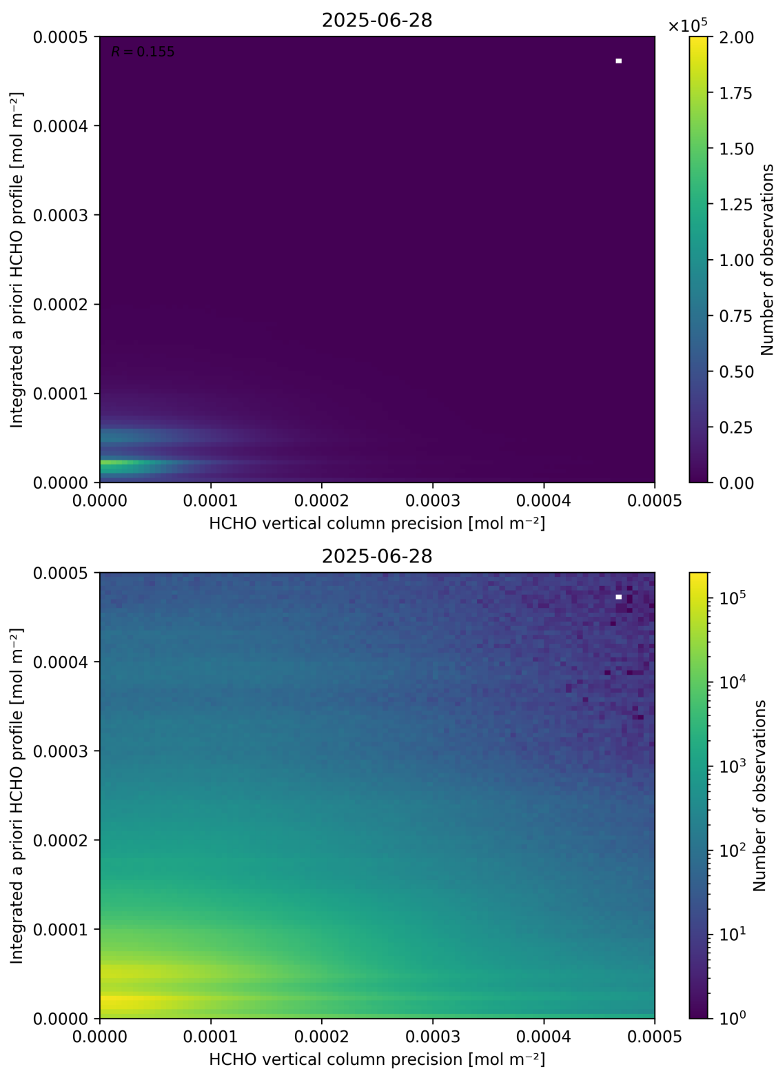
Figure 147: Scatter density plot of “HCHO vertical column precision” against “Integrated a priori HCHO profile” for 2025-06-27 to 2025-06-29.
