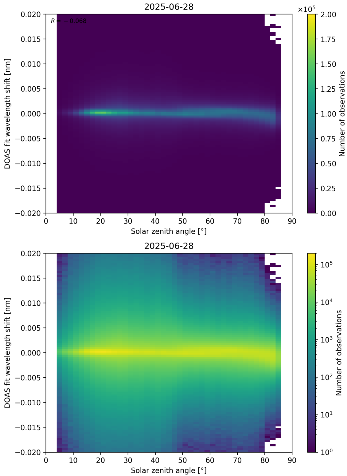
Figure 168: Scatter density plot of “Solar zenith angle” against “DOAS fit wavelength shift” for 2025-06-27 to 2025-06-29.
