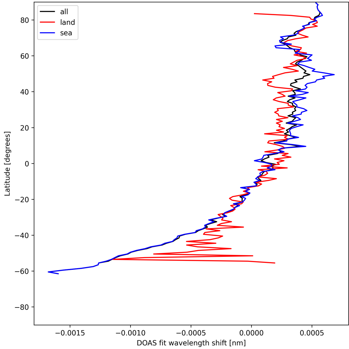
Figure 30: Zonal average of “DOAS fit wavelength shift” for 2025-06-27 to 2025-06-29.
