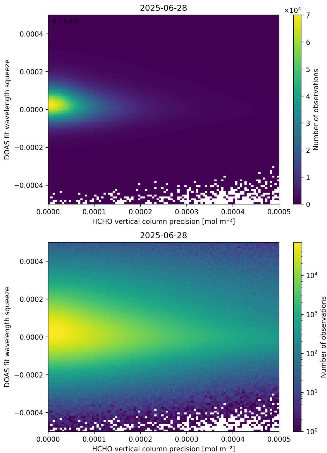
Figure 138: Scatter density plot of “HCHO vertical column precision” against “DOAS fit wavelength squeeze” for 2025-06-27 to 2025-06-29.
