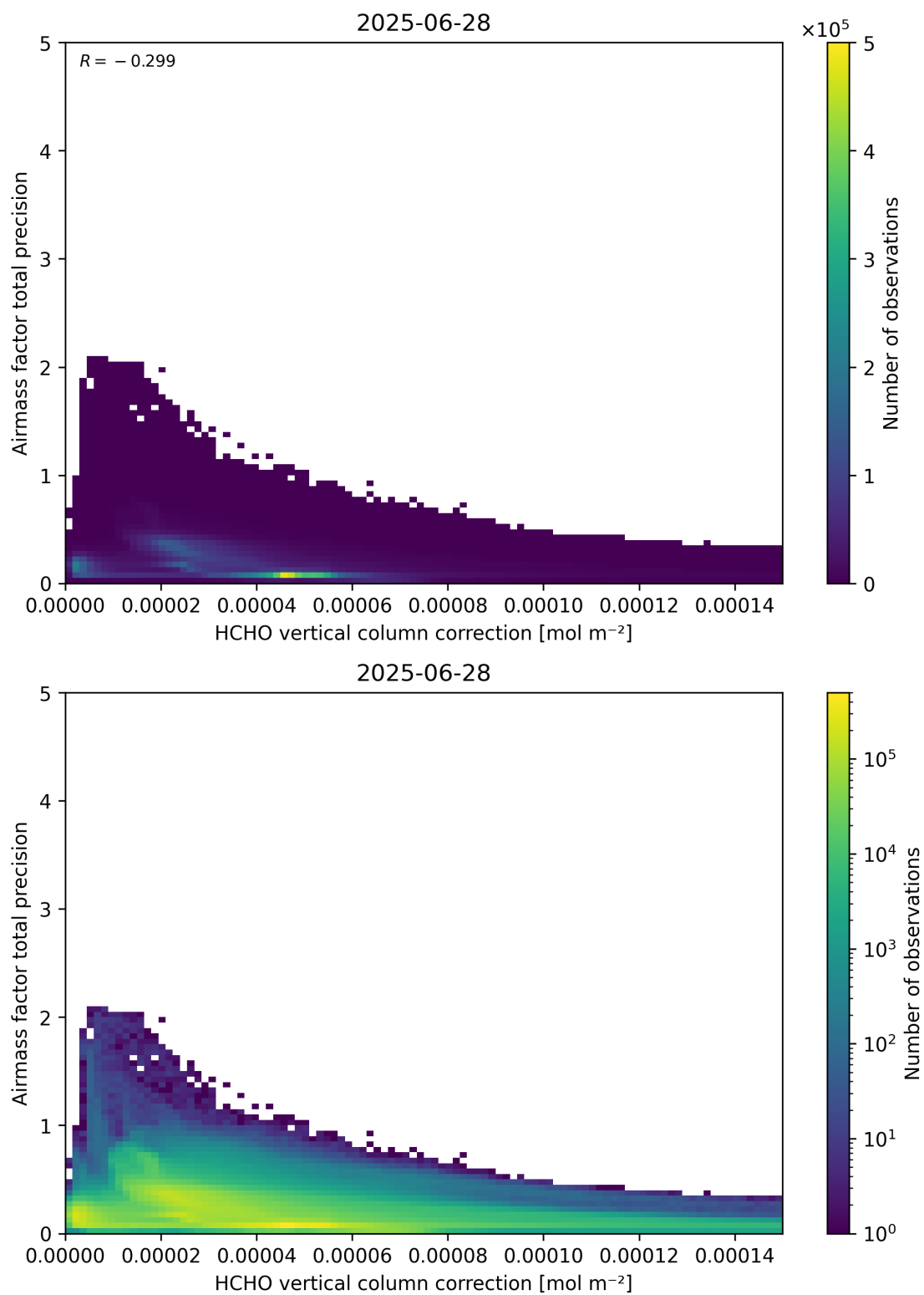
Figure 121: Scatter density plot of “HCHO vertical column correction” against “Airmass factor total precision” for 2025-06-27 to 2025-06-29.
