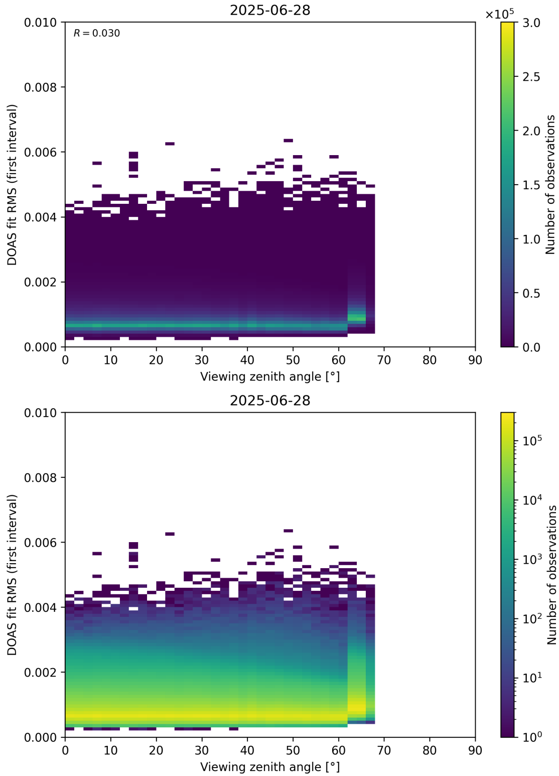
Figure 182: Scatter density plot of “Viewing zenith angle” against “DOAS fit RMS (first interval)” for 2025-06-27 to 2025-06-29.
