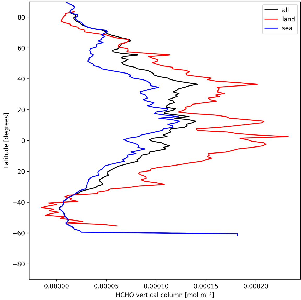
Figure 21: Zonal average of “HCHO vertical column” for 2025-06-27 to 2025-06-29.
