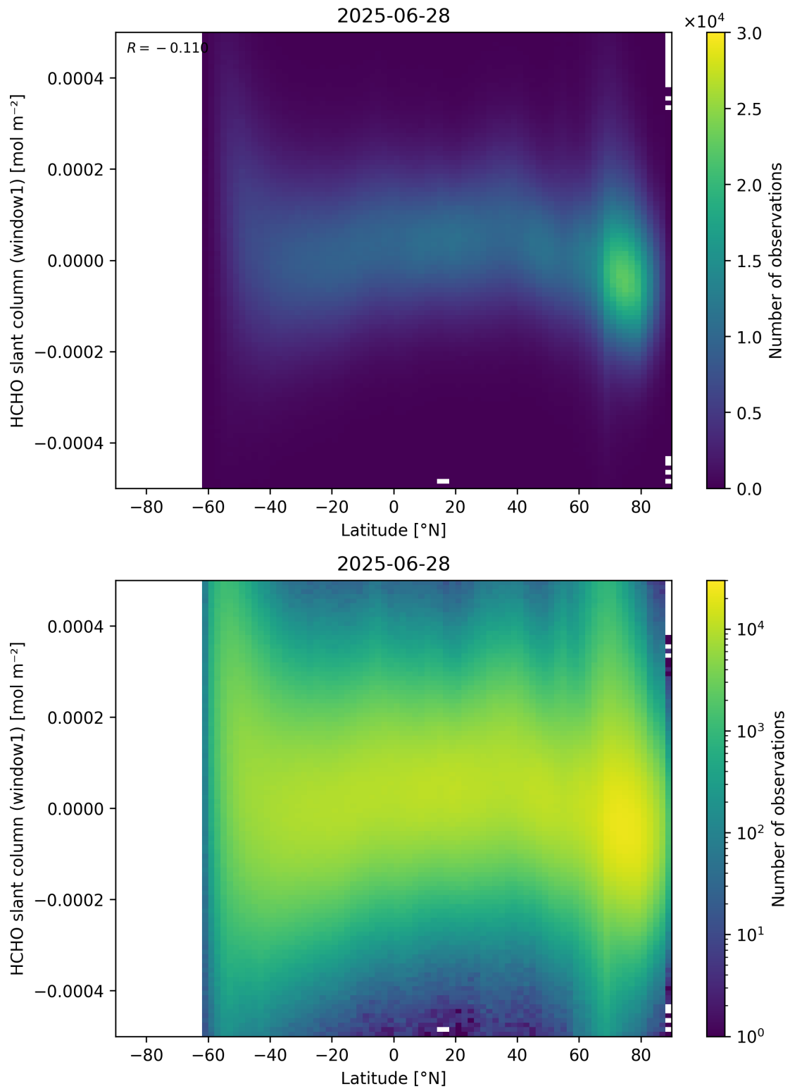
Figure 159: Scatter density plot of “Latitude” against “HCHO slant column (window1)” for 2025-06-27 to 2025-06-29.
