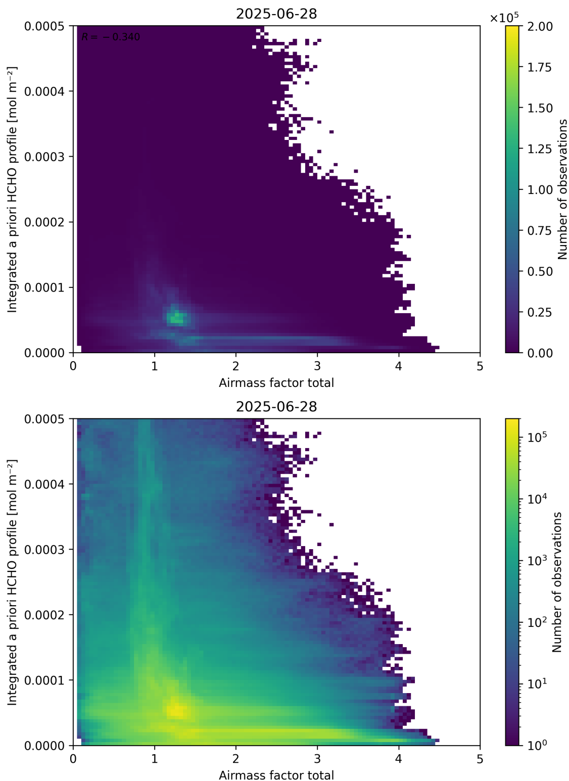
Figure 104: Scatter density plot of “Airmass factor total” against “Integrated a priori HCHO profile” for 2025-06-27 to 2025-06-29.
