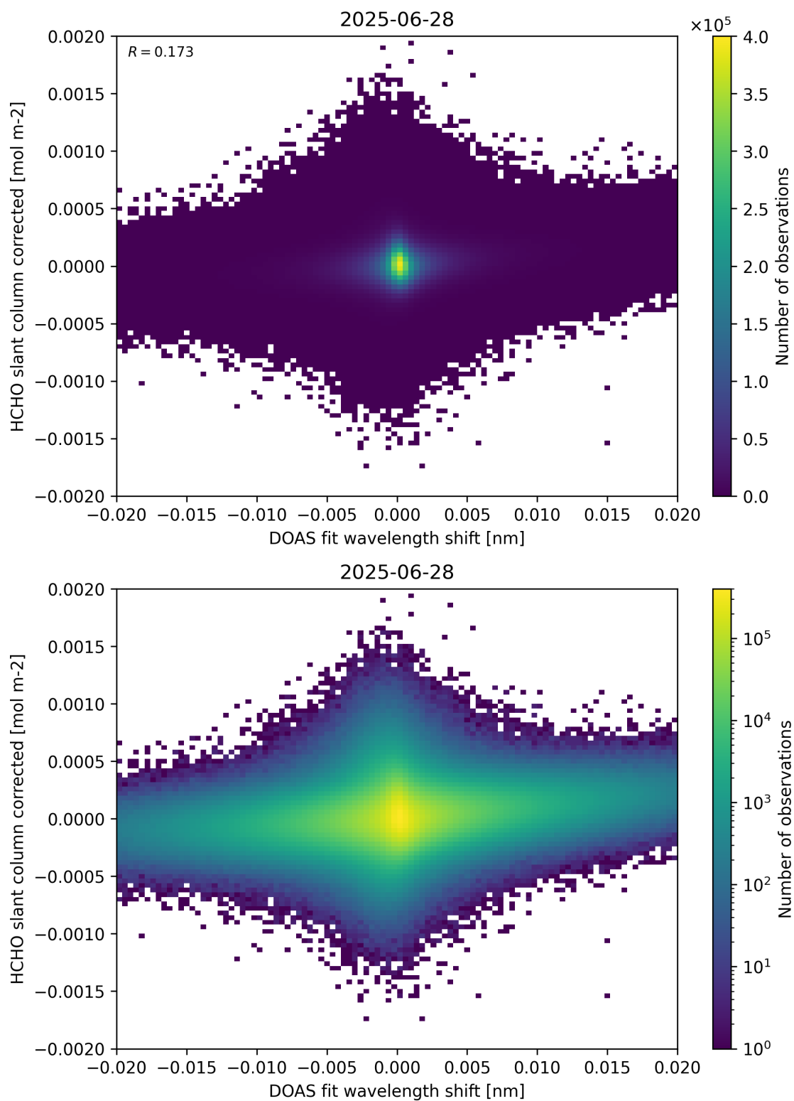
Figure 66: Scatter density plot of “DOAS fit wavelength shift” against “HCHO slant column corrected” for 2025-06-27 to 2025-06-29.
