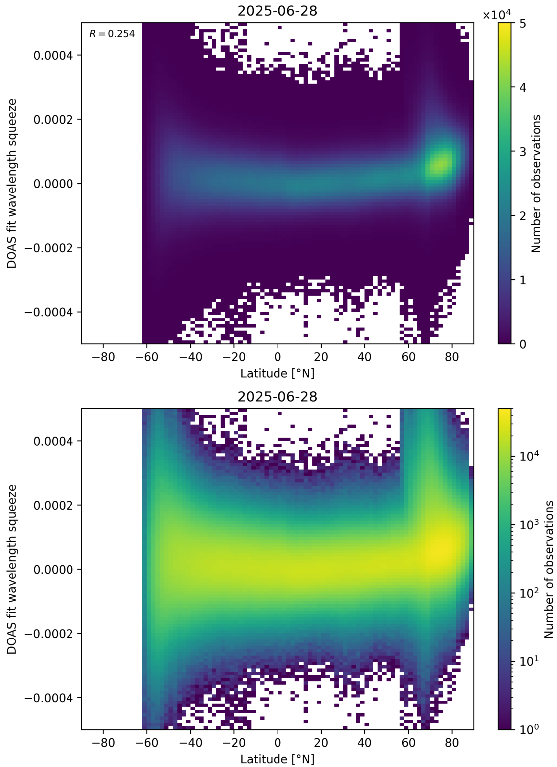
Figure 155: Scatter density plot of “Latitude” against “DOAS fit wavelength squeeze” for 2025-06-27 to 2025-06-29.
