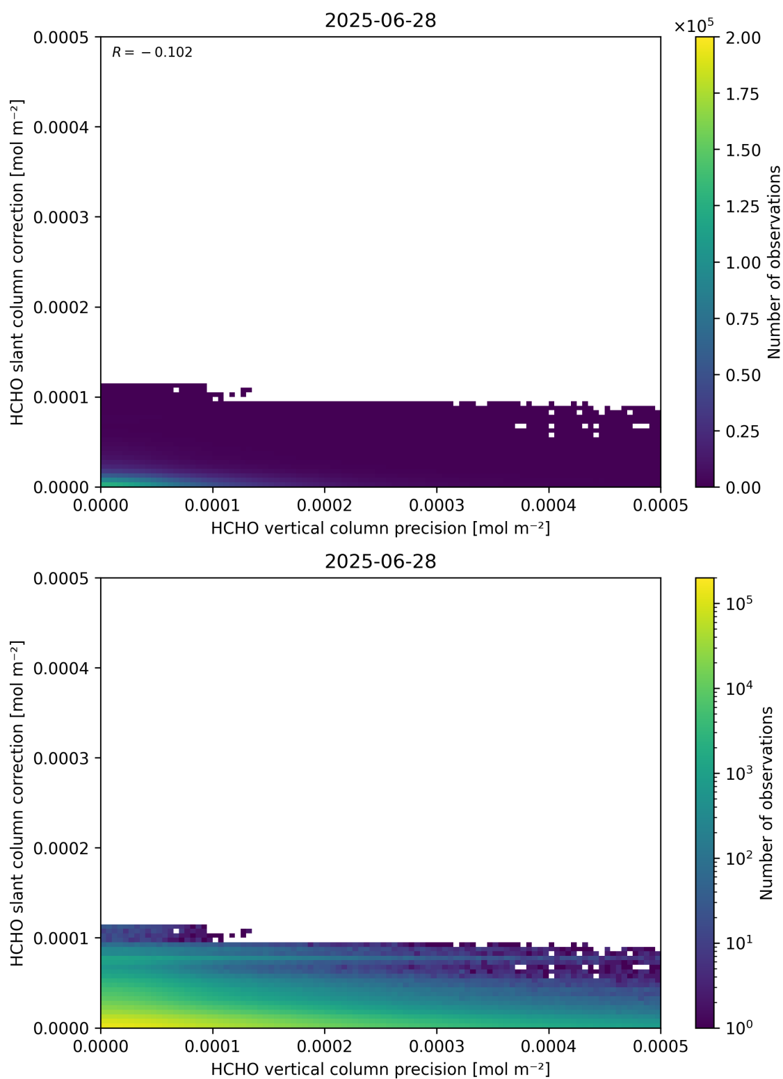
Figure 141: Scatter density plot of “HCHO vertical column precision” against “HCHO slant column correction” for 2025-06-27 to 2025-06-29.
