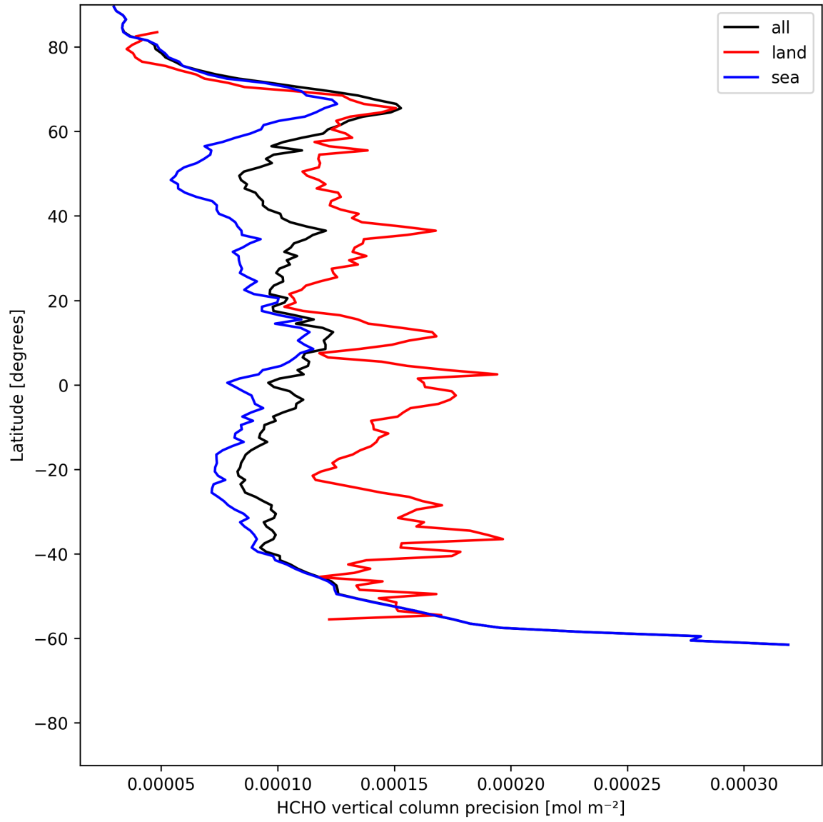
Figure 22: Zonal average of “HCHO vertical column precision” for 2025-06-27 to 2025-06-29.
