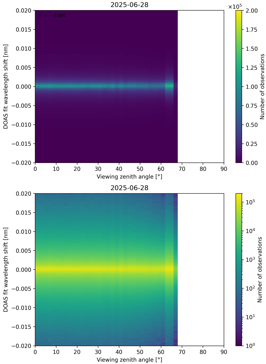
Figure 183: Scatter density plot of “Viewing zenith angle” against “DOAS fit wavelength shift” for 2025-06-27 to 2025-06-29.
