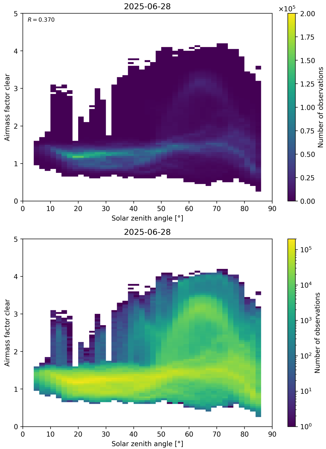
Figure 170: Scatter density plot of “Solar zenith angle” against “Airmass factor clear” for 2025-06-27 to 2025-06-29.
