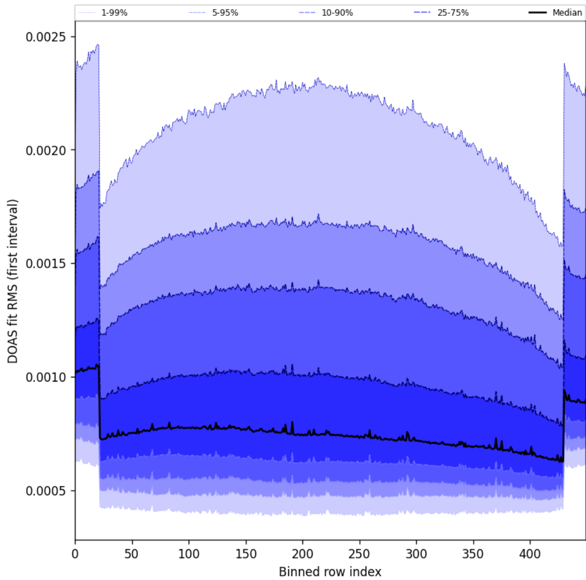
Figure 60: Along track statistics of “DOAS fit RMS (first interval)” for 2025-06-27 to 2025-06-29
