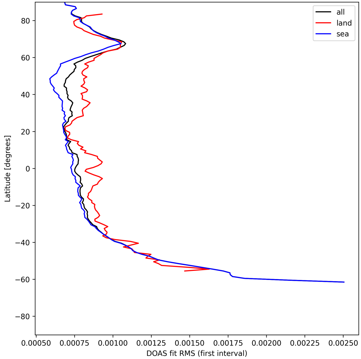
Figure 32: Zonal average of "DOAS fit RMS (first interval)" for 2025-06-27 to 2025-06-29.
