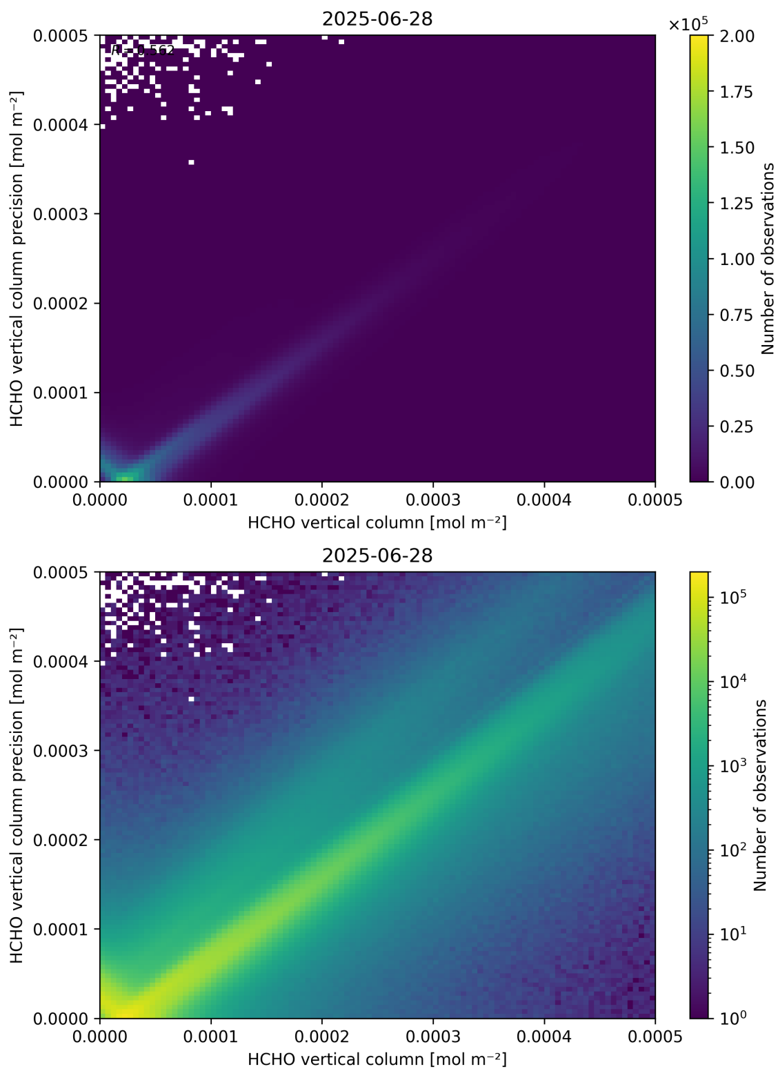
Figure 134: Scatter density plot of “HCHO vertical column” against “HCHO vertical column precision” for 2025-06-27 to 2025-06-29.
