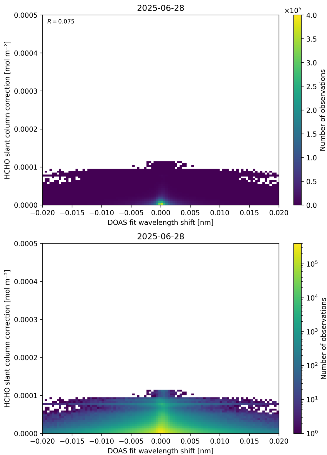
Figure 67: Scatter density plot of “DOAS fit wavelength shift” against “HCHO slant column correction” for 2025-06-27 to 2025-06-29.
