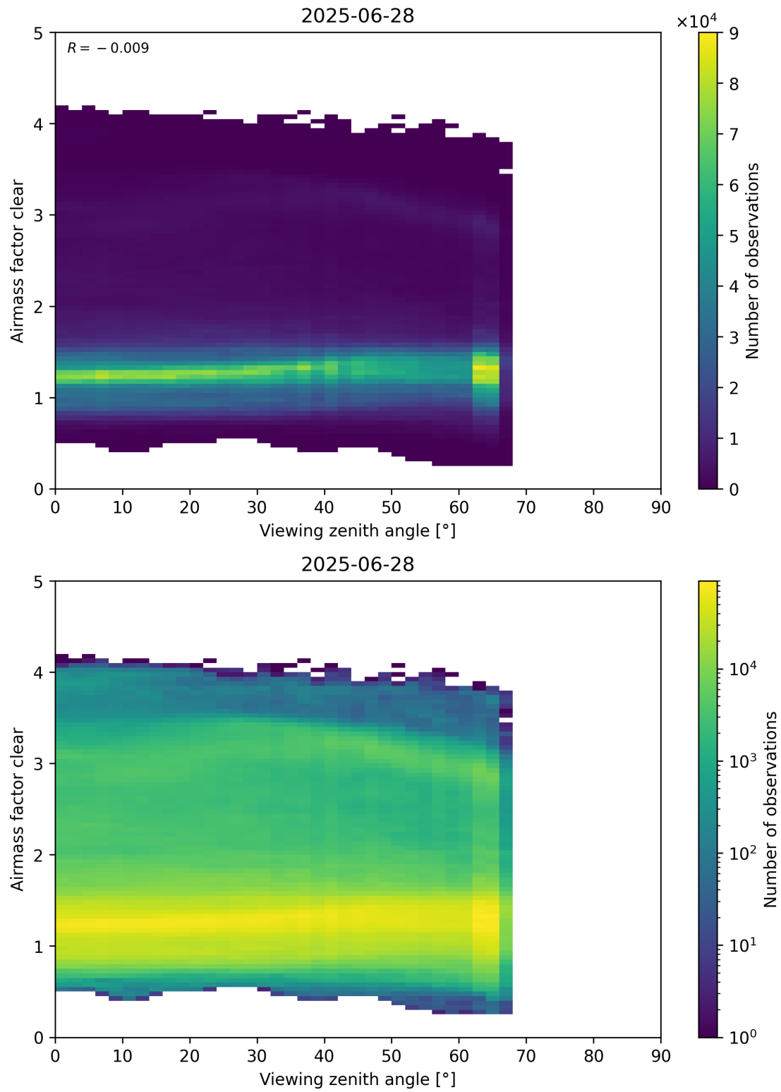
Figure 185: Scatter density plot of “Viewing zenith angle” against “Airmass factor clear” for 2025-06-27 to 2025-06-29.
