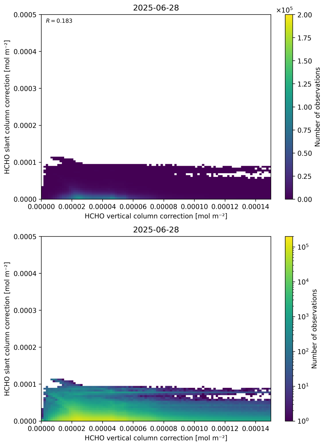
Figure 117: Scatter density plot of “HCHO vertical column correction” against “HCHO slant column correction” for 2025-06-27 to 2025-06-29.
