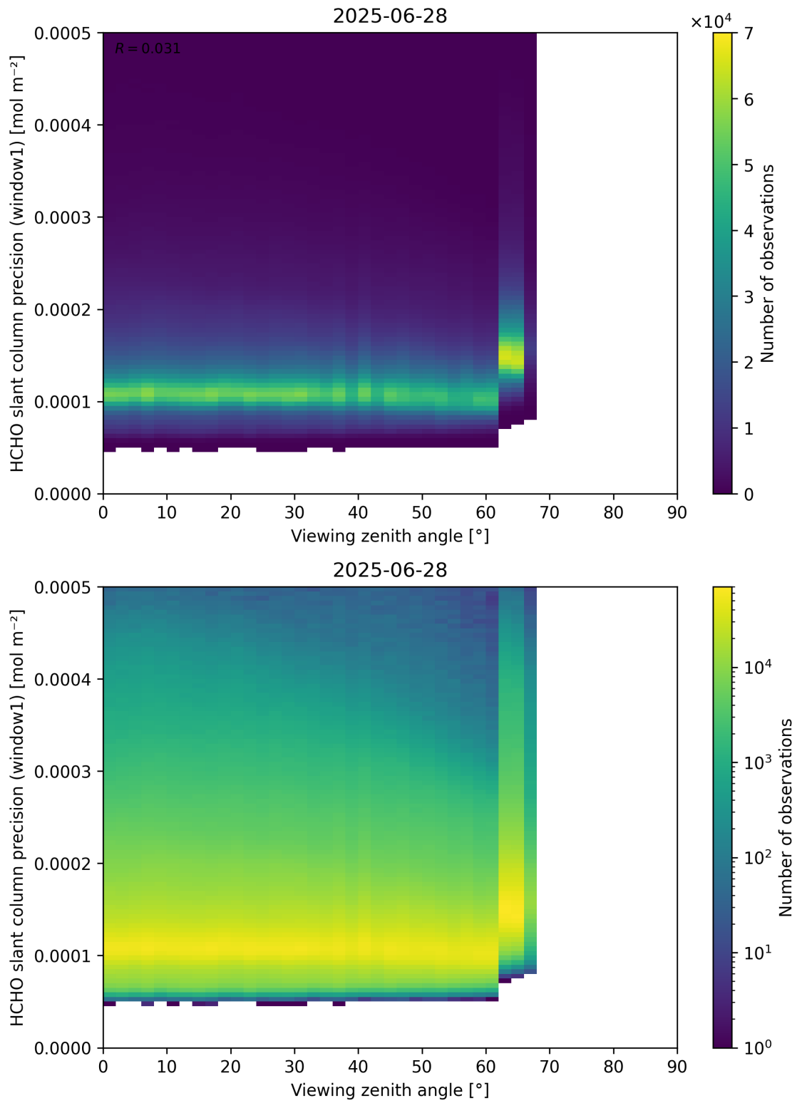
Figure 189: Scatter density plot of “Viewing zenith angle” against “HCHO slant column precision (window1)” for 2025-06-27 to 2025-06-29.
