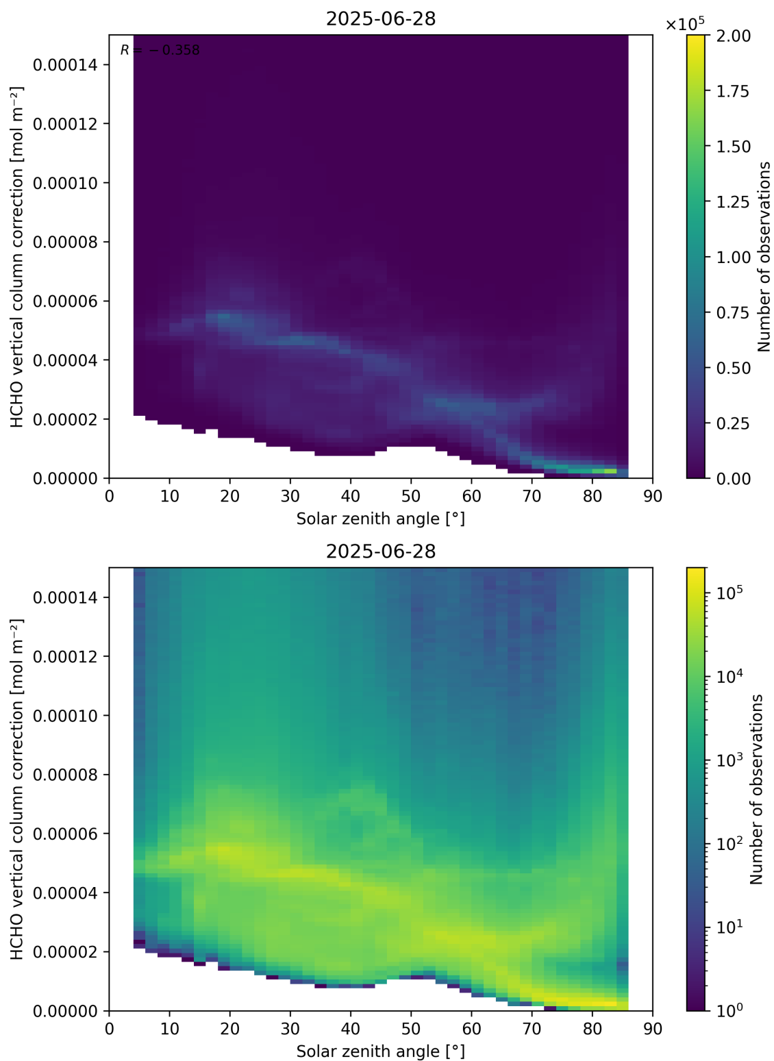
Figure 178: Scatter density plot of “Solar zenith angle” against “HCHO vertical column correction” for 2025-06-27 to 2025-06-29.
