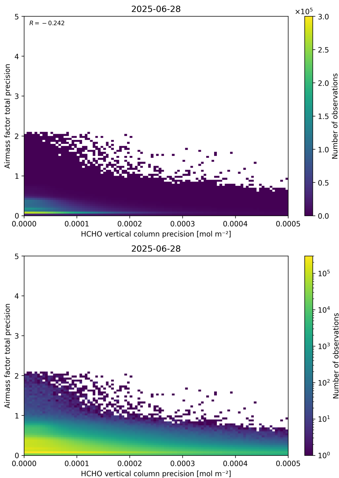
Figure 145: Scatter density plot of “HCHO vertical column precision” against “Airmass factor total precision” for 2025-06-27 to 2025-06-29.
