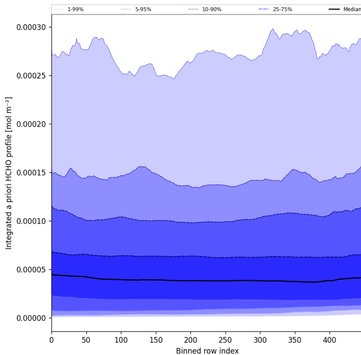
Figure 57: Along track statistics of “Integrated a priori HCHO profile” for 2025-06-27 to 2025-06-29
