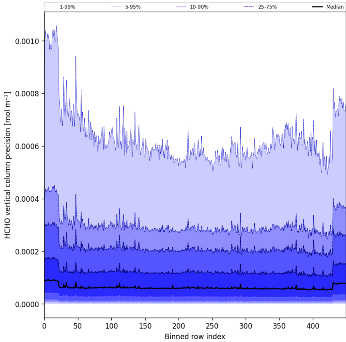
Figure 50: Along track statistics of “HCHO vertical column precision” for 2025-06-27 to 2025-06-29
