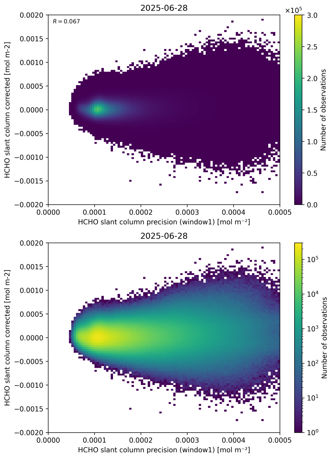
Figure 92: Scatter density plot of “HCHO slant column precision (window1)” against “HCHO slant column corrected” for 2025-06-27 to 2025-06-29.
