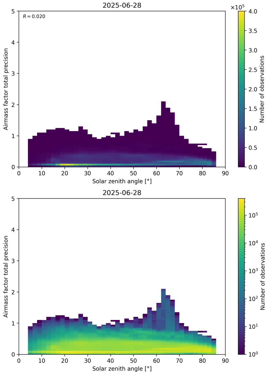
Figure 176: Scatter density plot of “Solar zenith angle” against “Airmass factor total precision” for 2025-06-27 to 2025-06-29.
