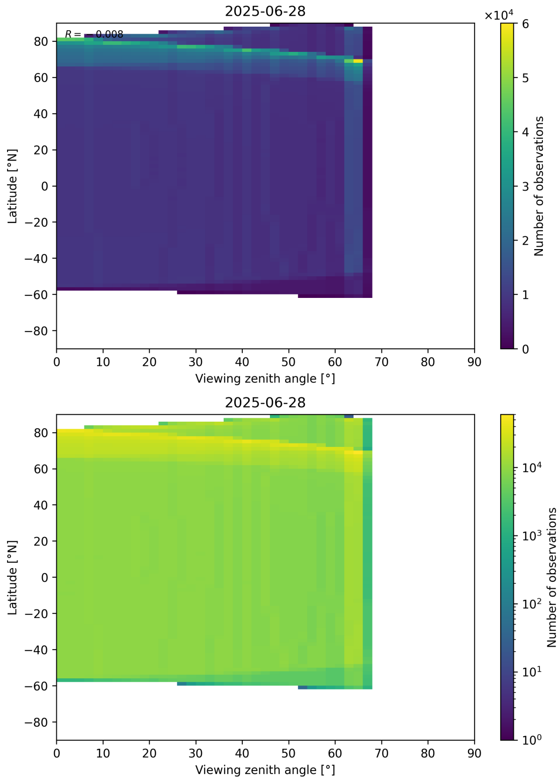
Figure 196: Scatter density plot of “Viewing zenith angle” against “Latitude” for 2025-06-27 to 2025-06-29.
