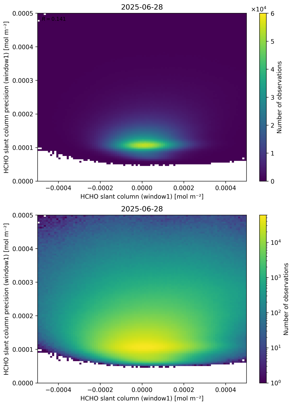
Figure 84: Scatter density plot of “HCHO slant column (window1)” against “HCHO slant column precision (window1)” for 2025-06-27 to 2025-06-29.
