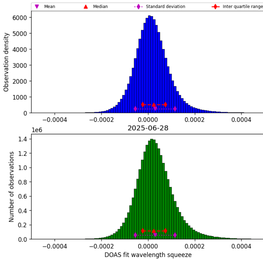
Figure 45: Histogram of “DOAS fit wavelength squeeze” for 2025-06-27 to 2025-06-29
