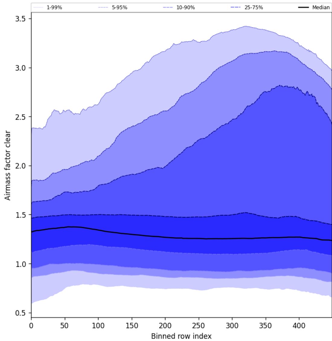
Figure 56: Along track statistics of “Air mass factor clear” for 2025-06-27 to 2025-06-29
