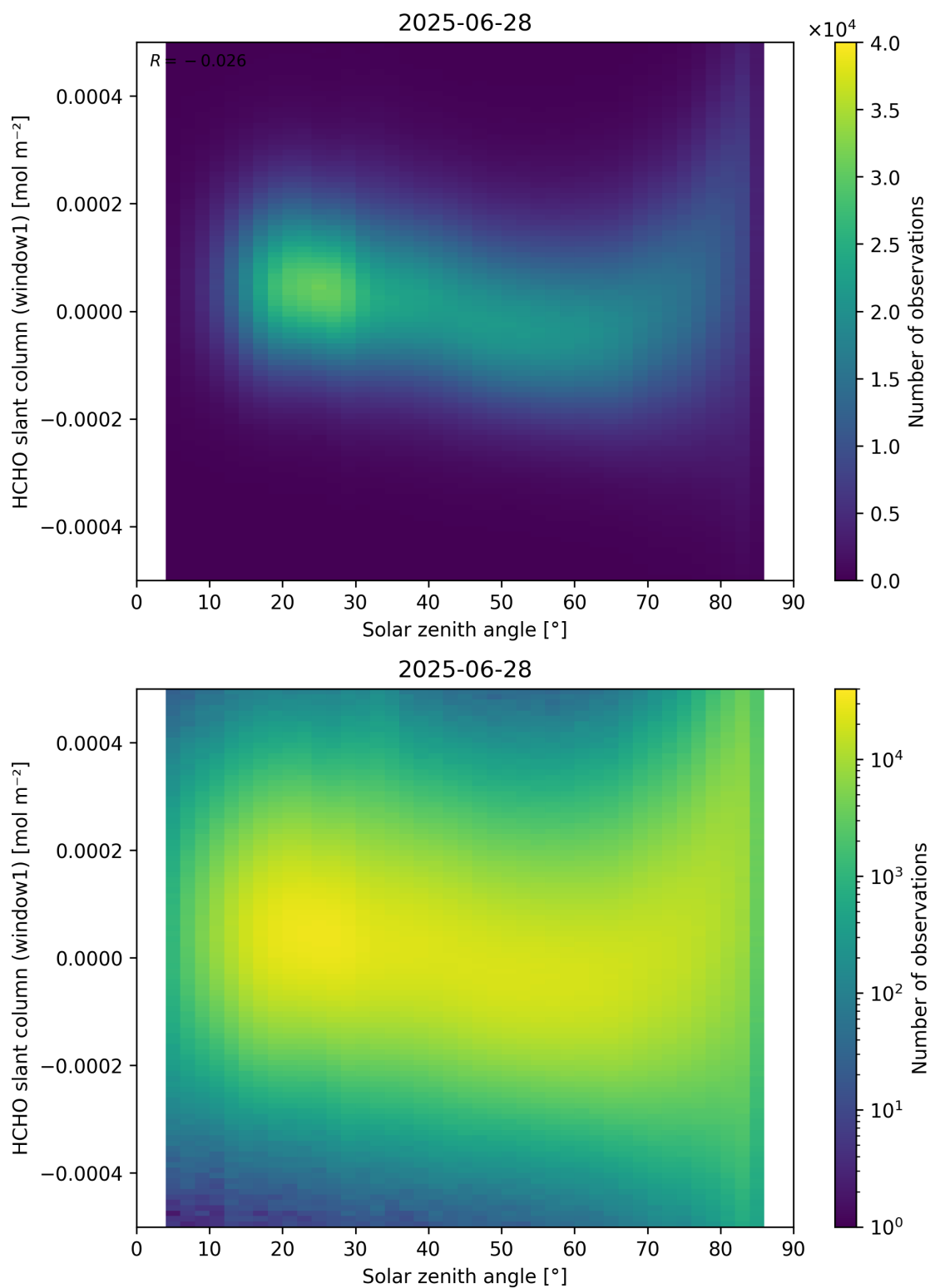
Figure 173: Scatter density plot of “Solar zenith angle” against “HCHO slant column (window1)” for 2025-06-27 to 2025-06-29.
