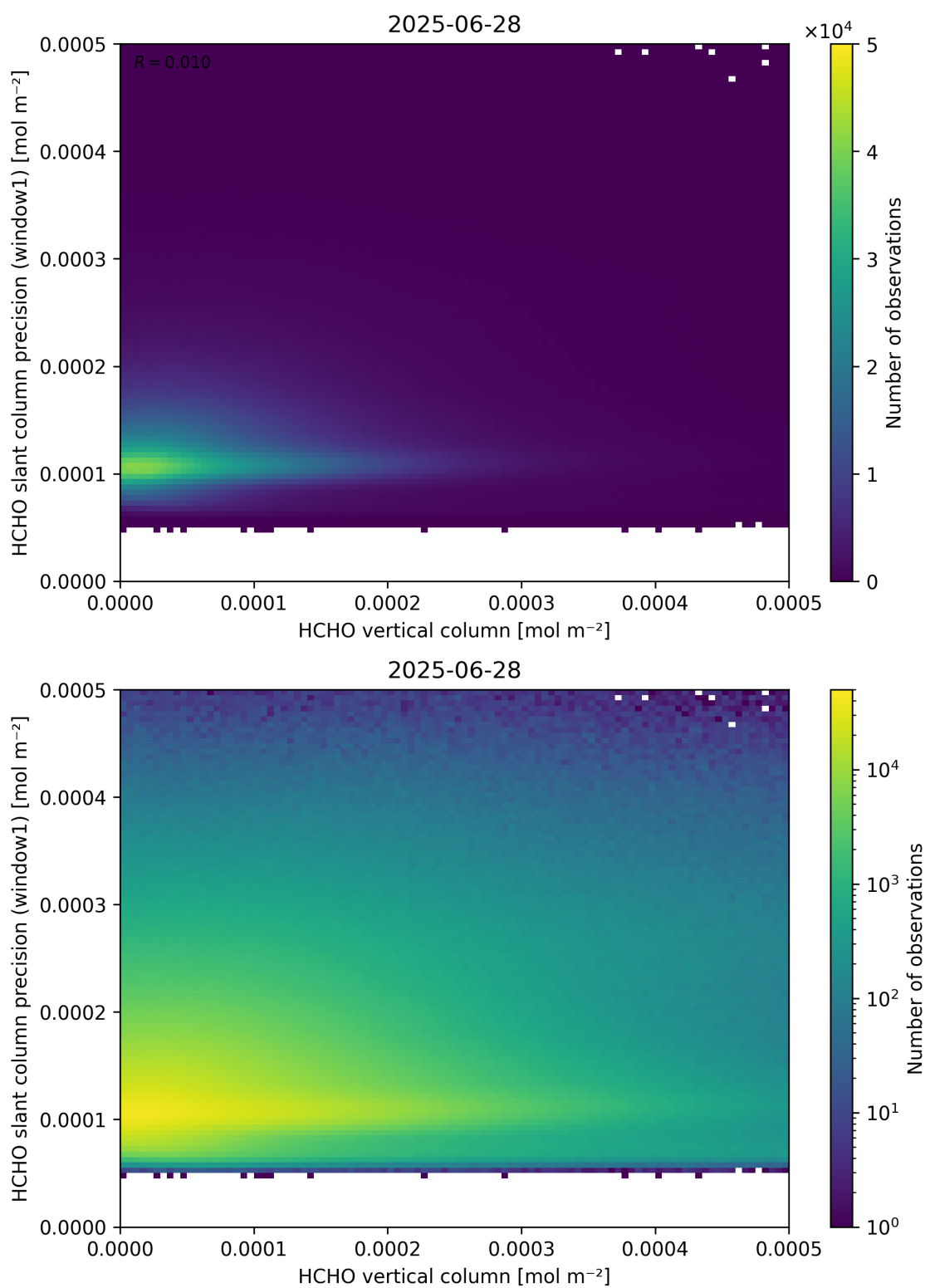
Figure 130: Scatter density plot of “HCHO vertical column” against “HCHO slant column precision (window1)” for 2025-06-27 to 2025-06-29.
