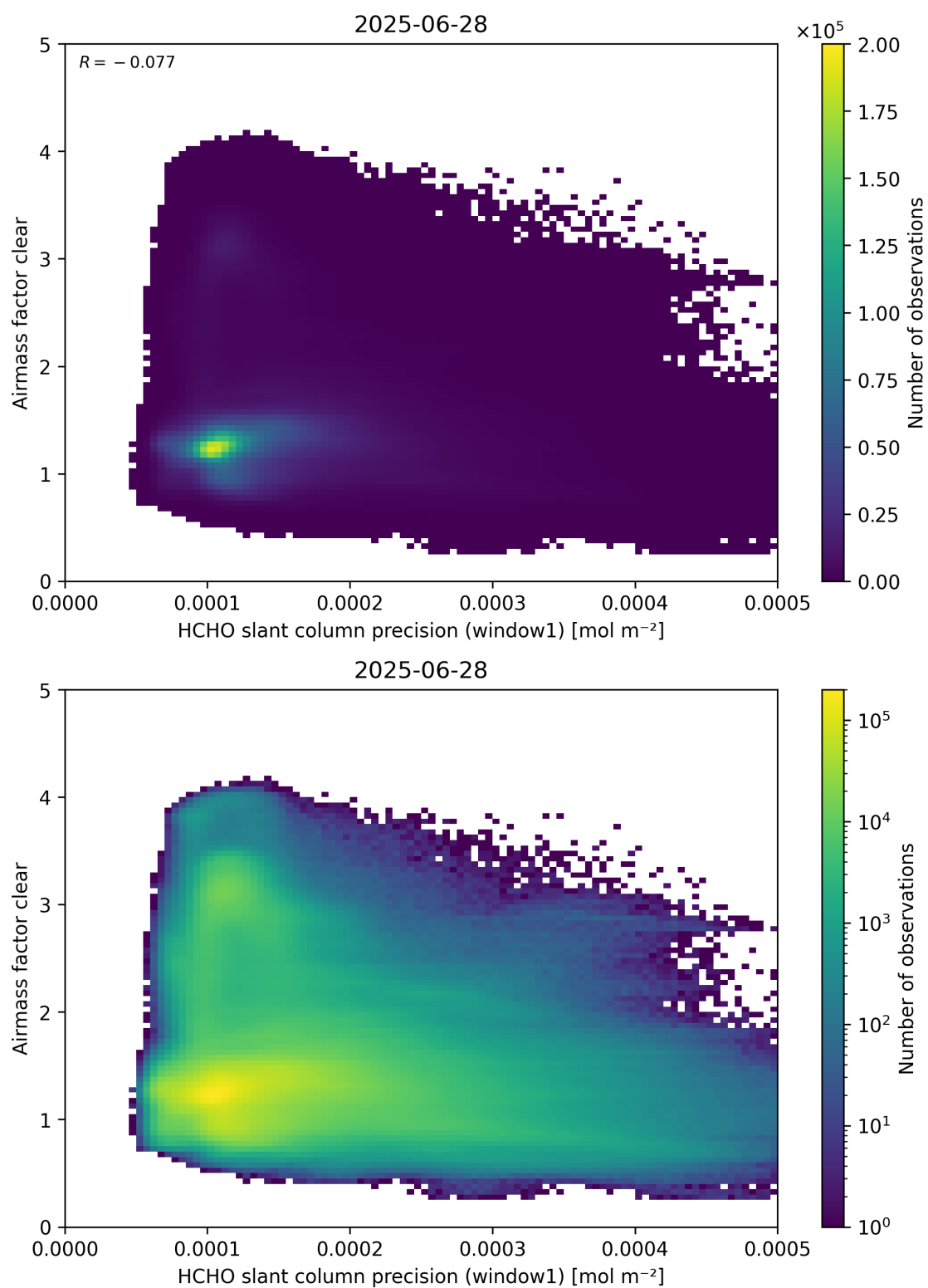
Figure 91: Scatter density plot of “HCHO slant column precision (window1)” against “Airmass factor clear” for 2025-06-27 to 2025-06-29.
