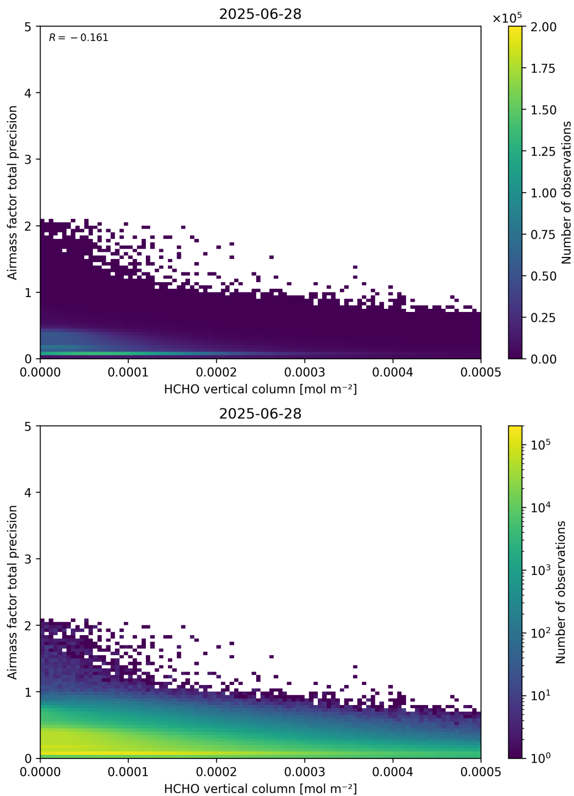
Figure 132: Scatter density plot of “HCHO vertical column” against “Airmass factor total precision” for 2025-06-27 to 2025-06-29.
