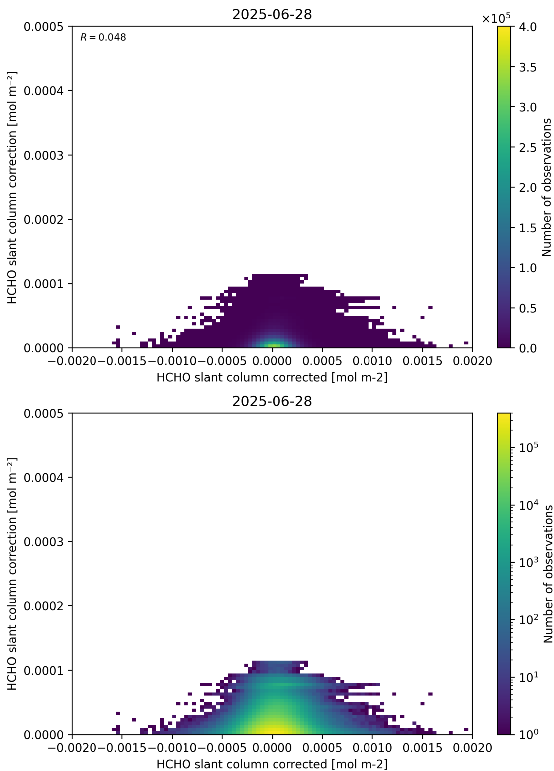
Figure 77: Scatter density plot of “HCHO slant column corrected” against “HCHO slant column correction” for 2025-06-27 to 2025-06-29.
