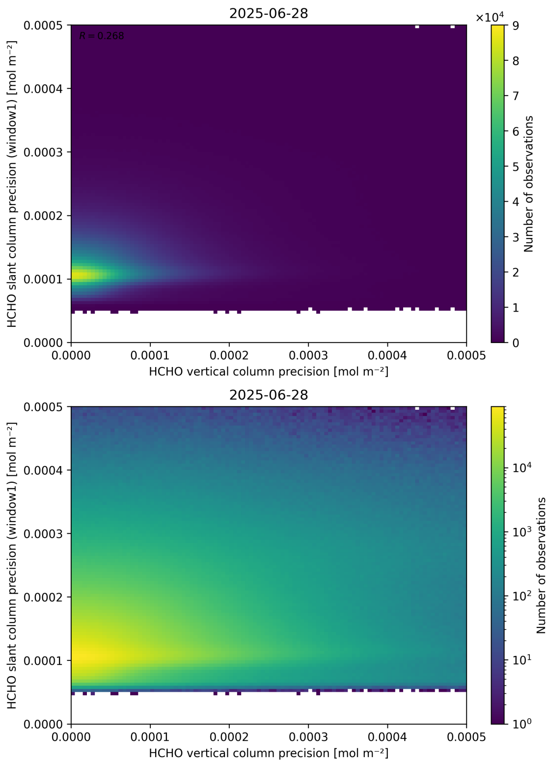
Figure 143: Scatter density plot of “HCHO vertical column precision” against “HCHO slant column precision (window1)” for 2025-06-27 to 2025-06-29.
