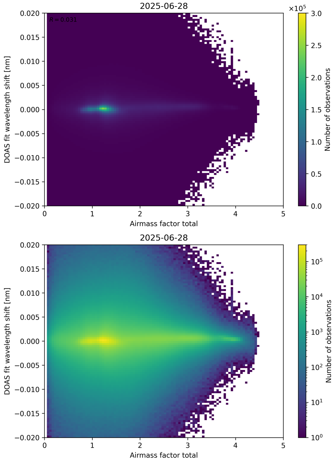
Figure 98: Scatter density plot of “Airmass factor total” against “DOAS fit wavelength shift” for 2025-06-27 to 2025-06-29.
