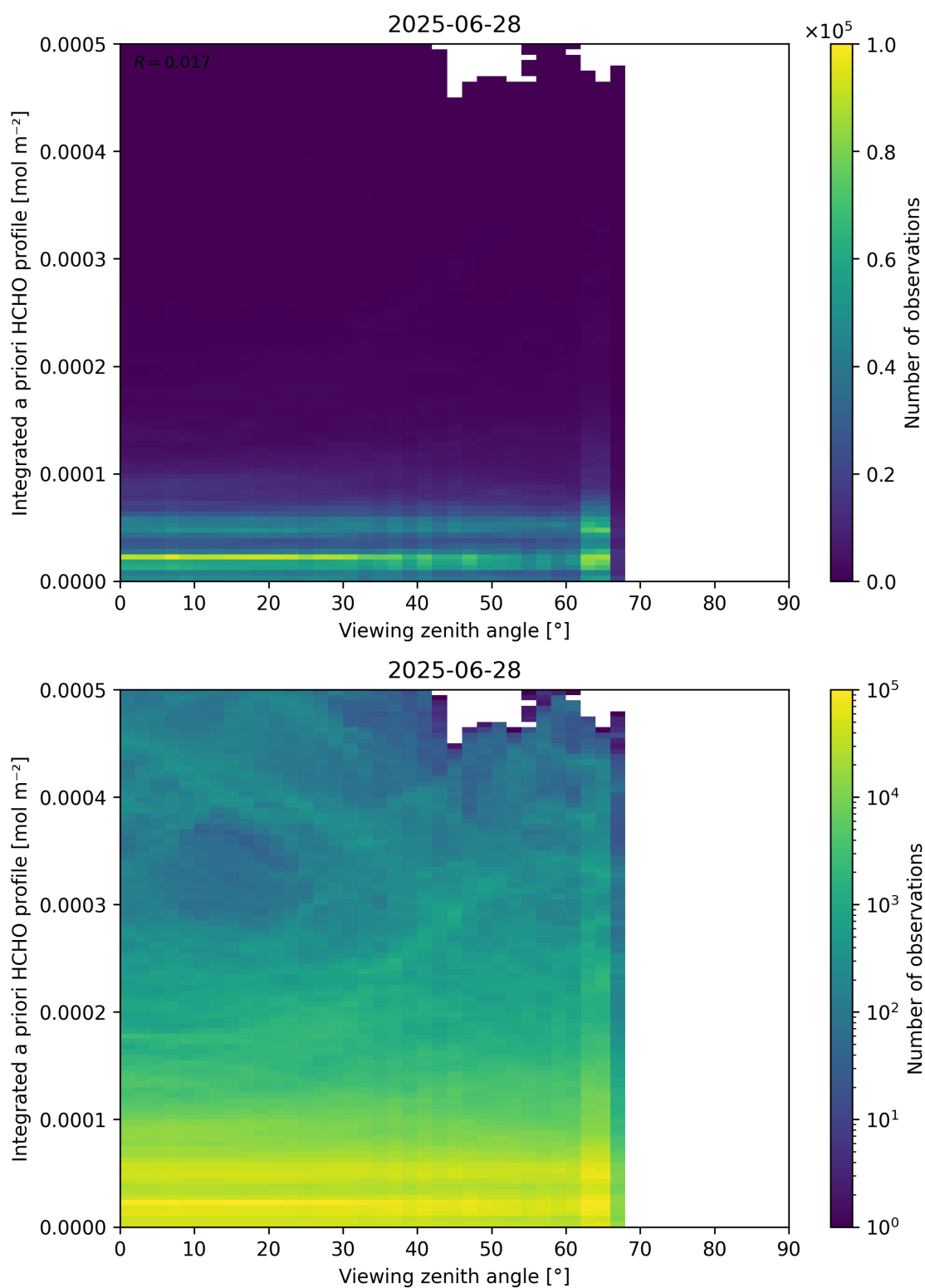
Figure 195: Scatter density plot of “Viewing zenith angle” against “Integrated a priori HCHO profile” for 2025-06-27 to 2025-06-29.
