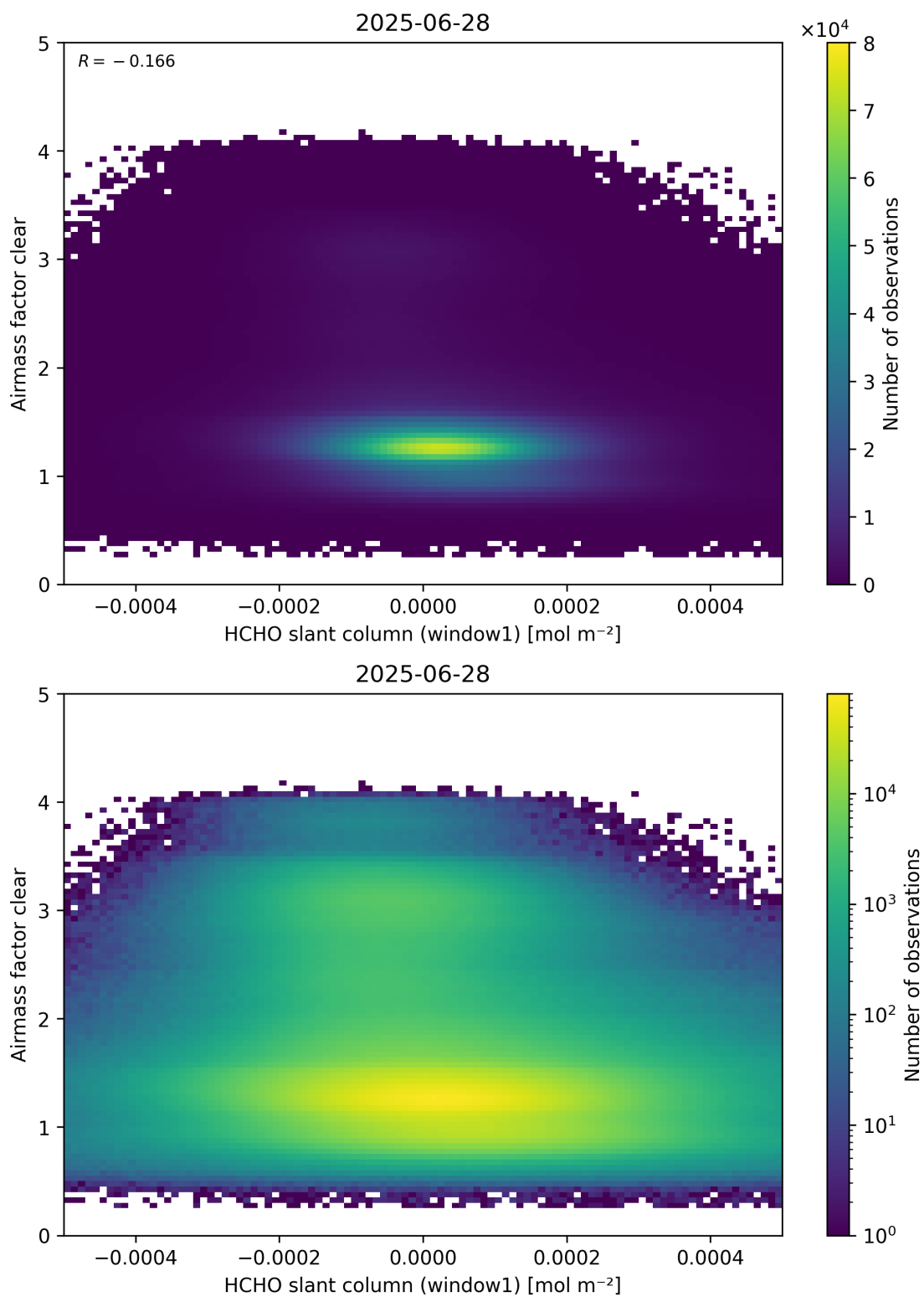
Figure 81: Scatter density plot of “HCHO slant column (window1)” against “Airmass factor clear” for 2025-06-27 to 2025-06-29.
