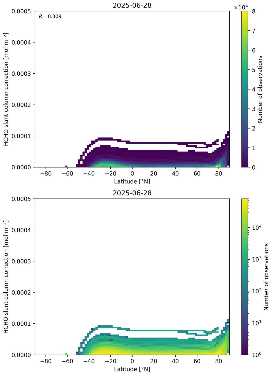
Figure 158: Scatter density plot of “Latitude” against “HCHO slant column correction” for 2025-06-27 to 2025-06-29.
