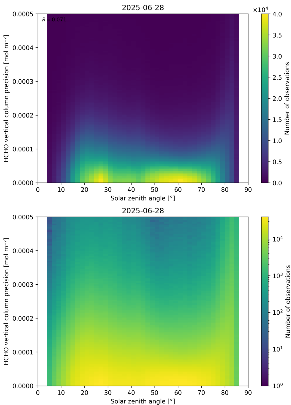
Figure 179: Scatter density plot of “Solar zenith angle” against “HCHO vertical column precision” for 2025-06-27 to 2025-06-29.
