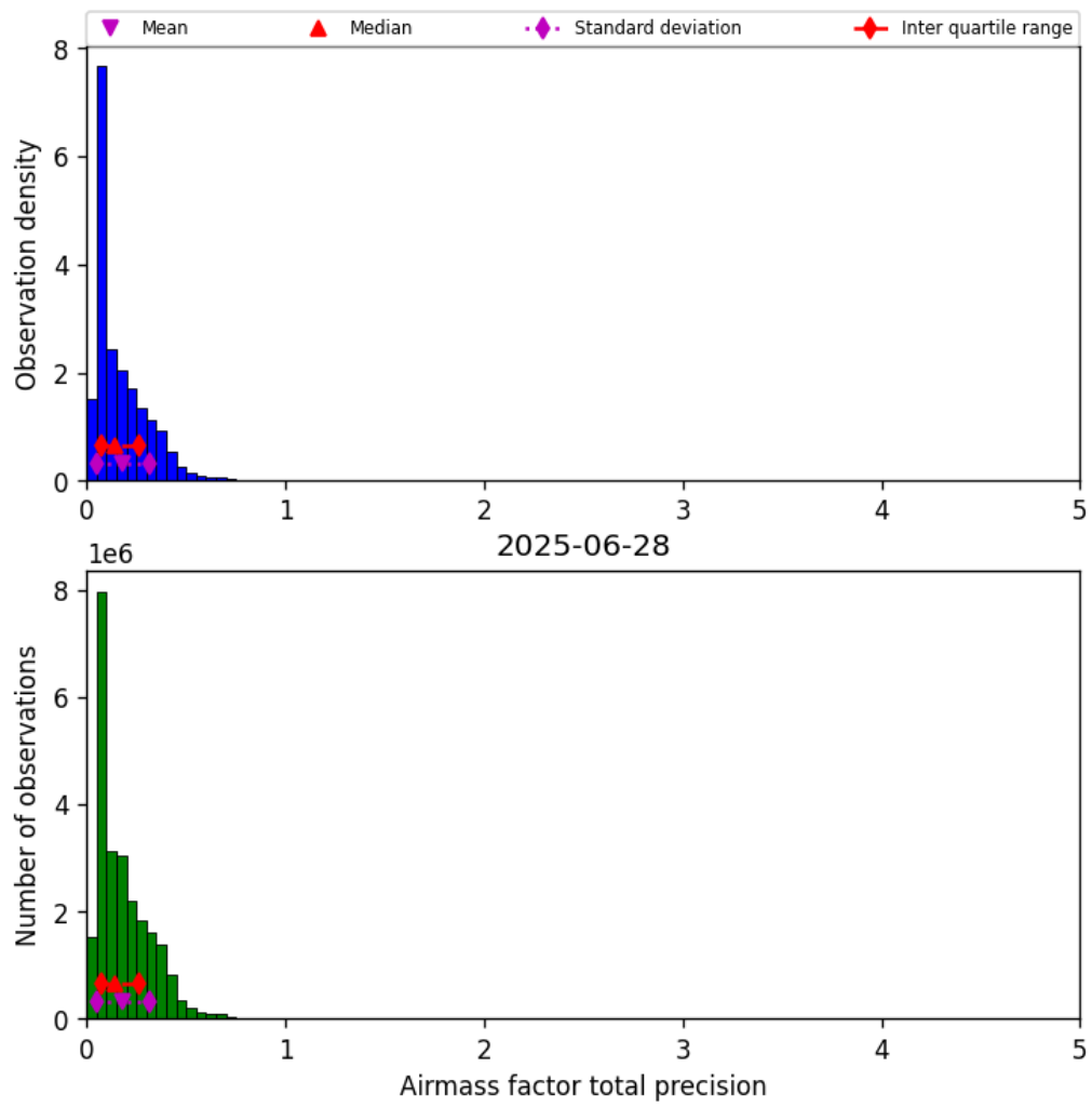
Figure 41: Histogram of “Airmass factor total precision” for 2025-06-27 to 2025-06-29
