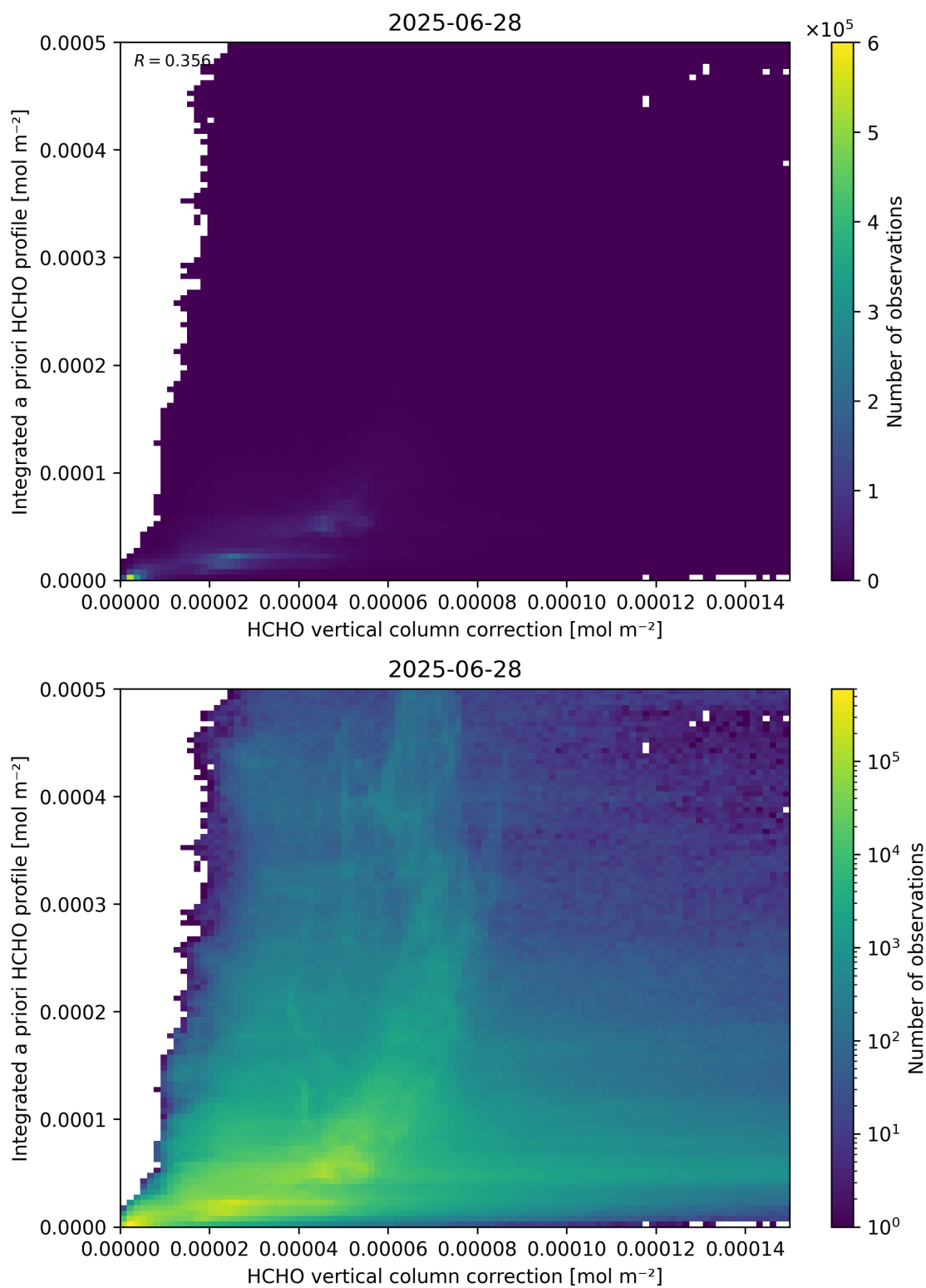
Figure 122: Scatter density plot of “HCHO vertical column correction” against “Integrated a priori HCHO profile” for 2025-06-27 to 2025-06-29.
