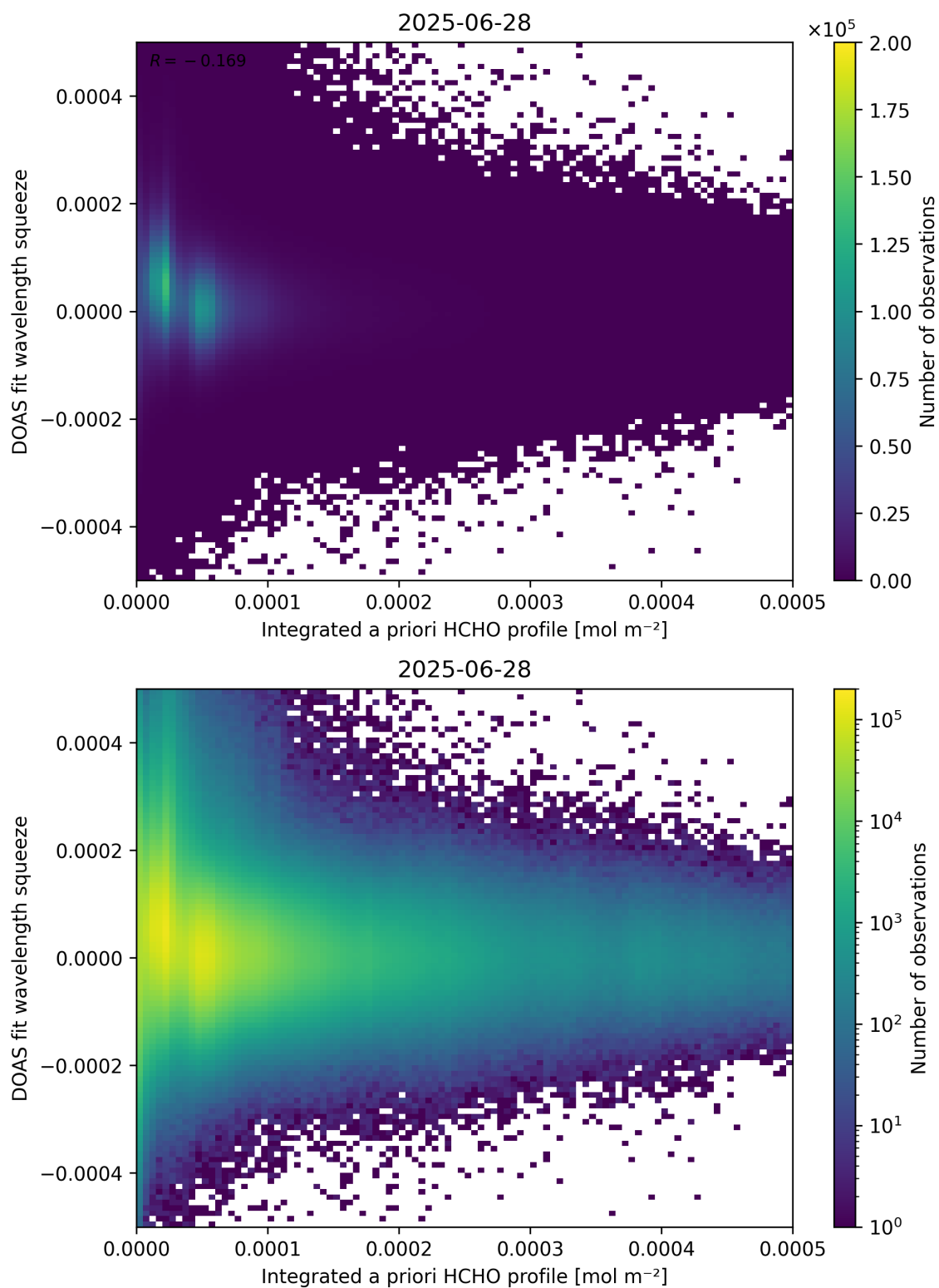
Figure 150: Scatter density plot of “Integrated a priori HCHO profile” against “DOAS fit wavelength squeeze” for 2025-06-27 to 2025-06-29.
