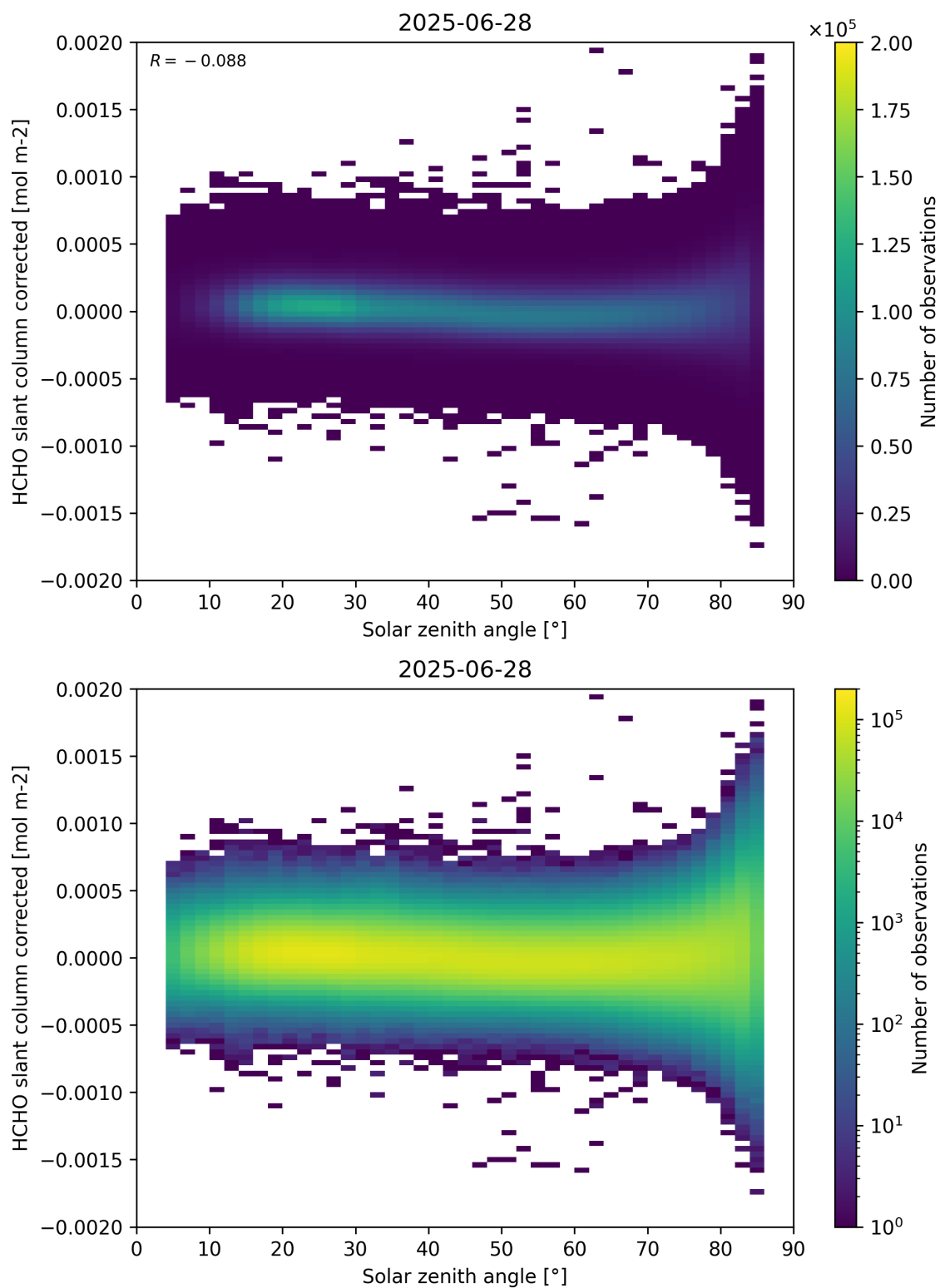
Figure 171: Scatter density plot of “Solar zenith angle” against “HCHO slant column corrected” for 2025-06-27 to 2025-06-29.
