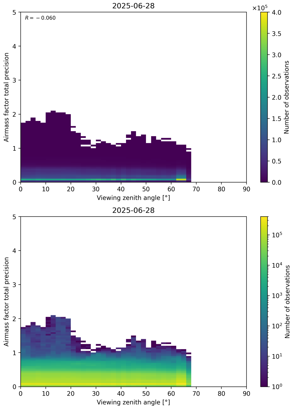
Figure 191: Scatter density plot of “Viewing zenith angle” against “Airmass factor total precision” for 2025-06-27 to 2025-06-29.
