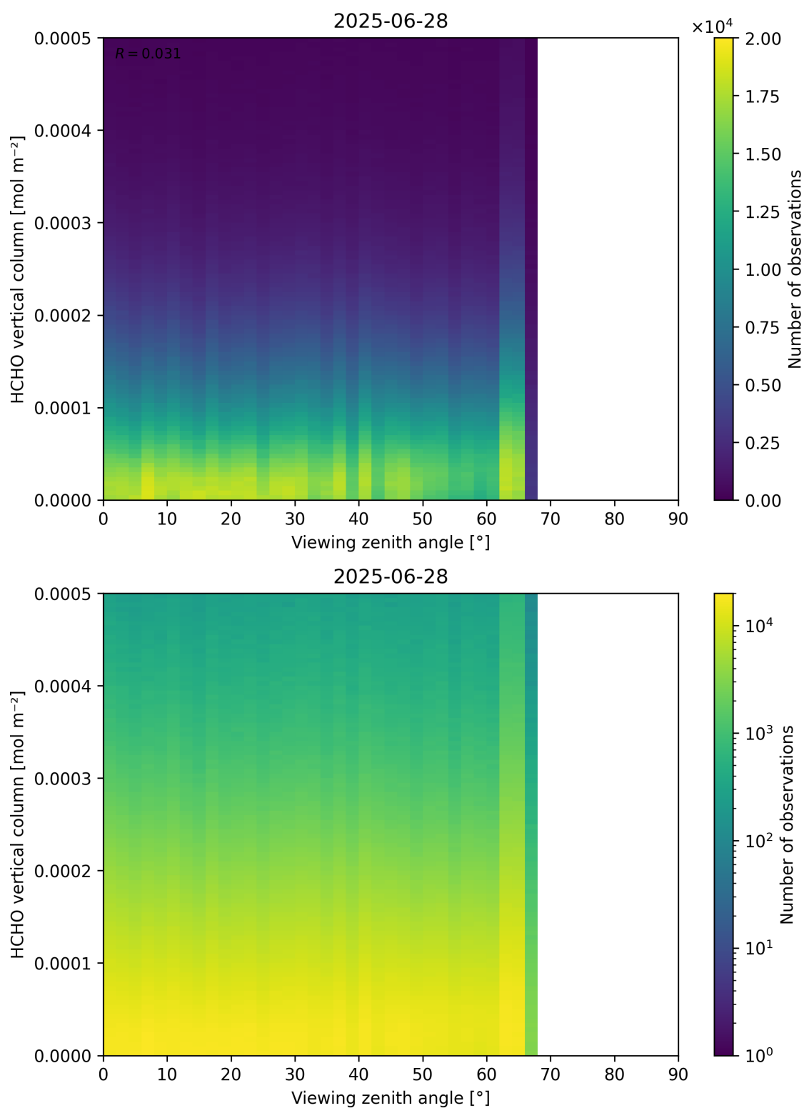
Figure 192: Scatter density plot of “Viewing zenith angle” against “HCHO vertical column” for 2025-06-27 to 2025-06-29.
