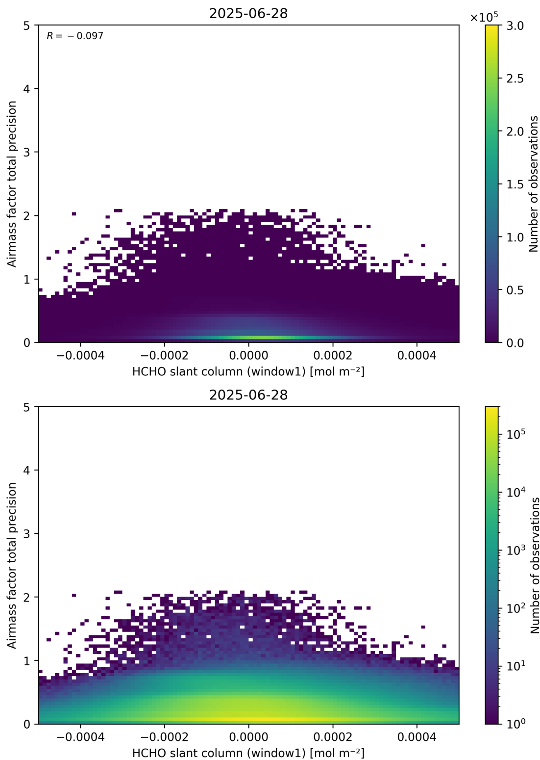
Figure 86: Scatter density plot of “HCHO slant column (window1)” against “Airmass factor total precision” for 2025-06-27 to 2025-06-29.
