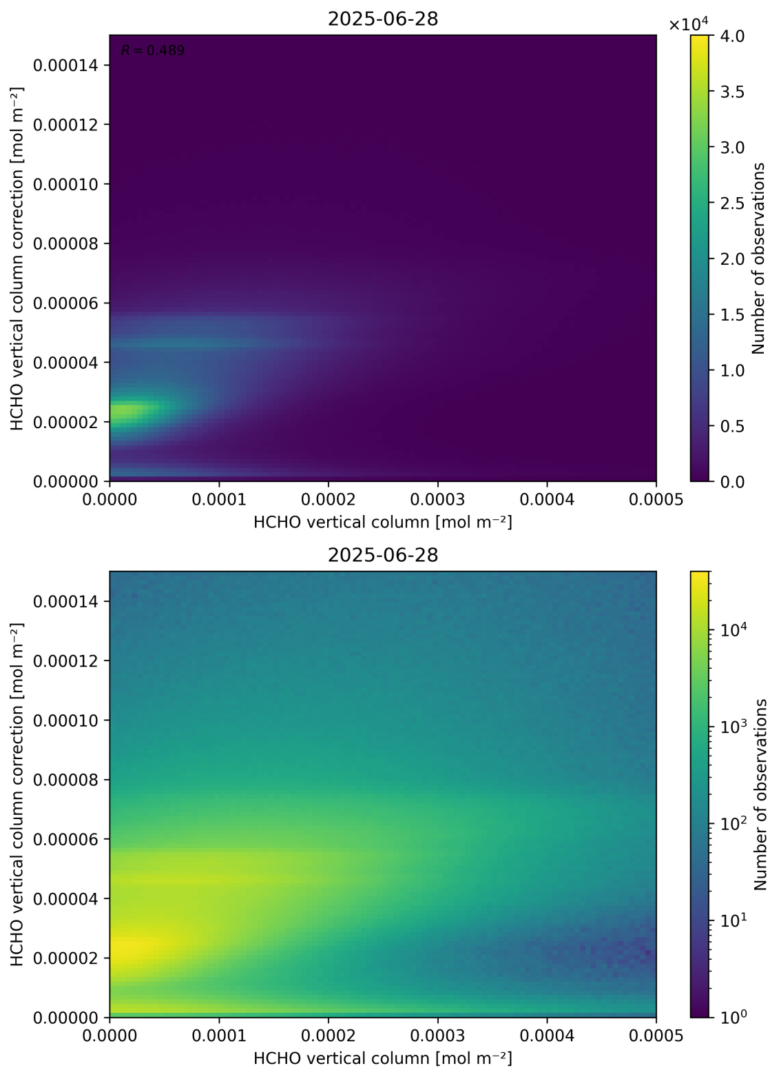
Figure 133: Scatter density plot of “HCHO vertical column” against “HCHO vertical column correction” for 2025-06-27 to 2025-06-29.
