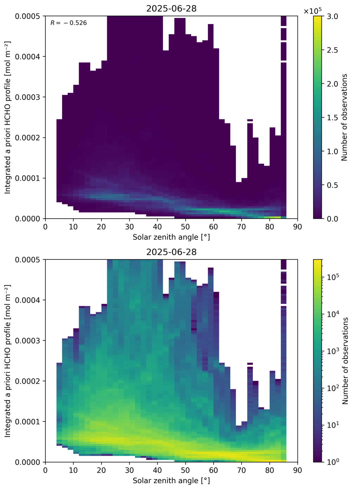
Figure 180: Scatter density plot of “Solar zenith angle” against “Integrated a priori HCHO profile” for 2025-06-27 to 2025-06-29.
