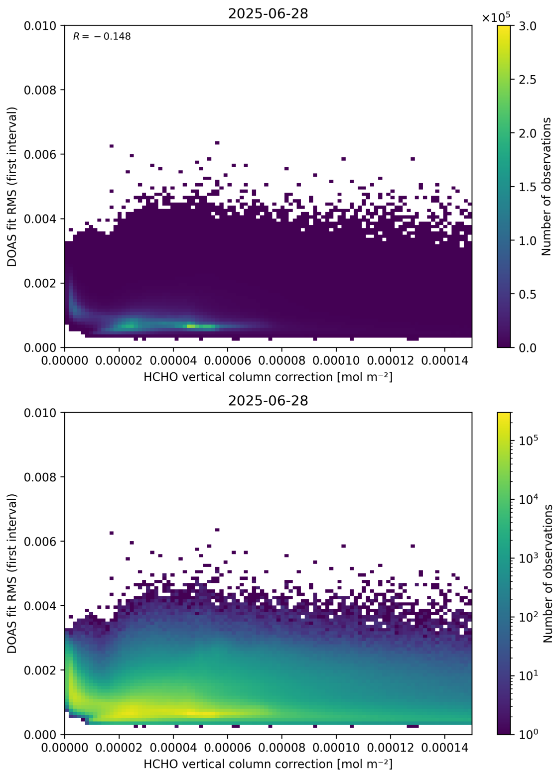
Figure 112: Scatter density plot of “HCHO vertical column correction” against “DOAS fit RMS (first interval)” for 2025-06-27 to 2025-06-29.
