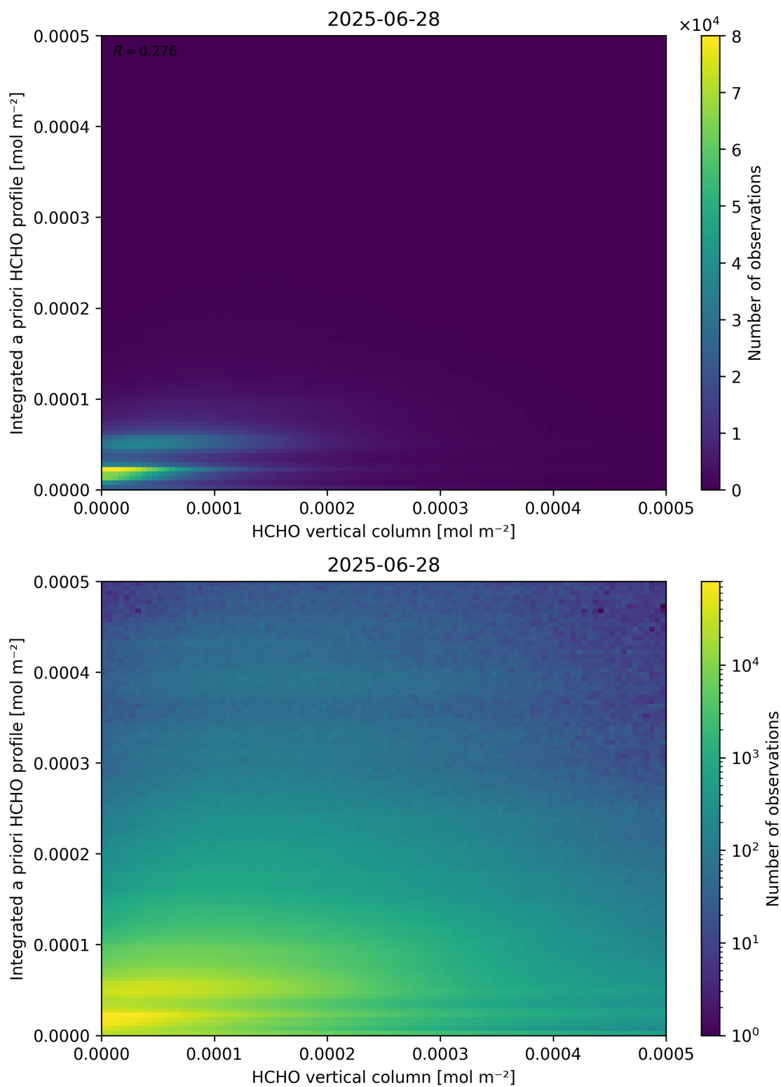
Figure 135: Scatter density plot of “HCHO vertical column” against “Integrated a priori HCHO profile” for 2025-06-27 to 2025-06-29.
