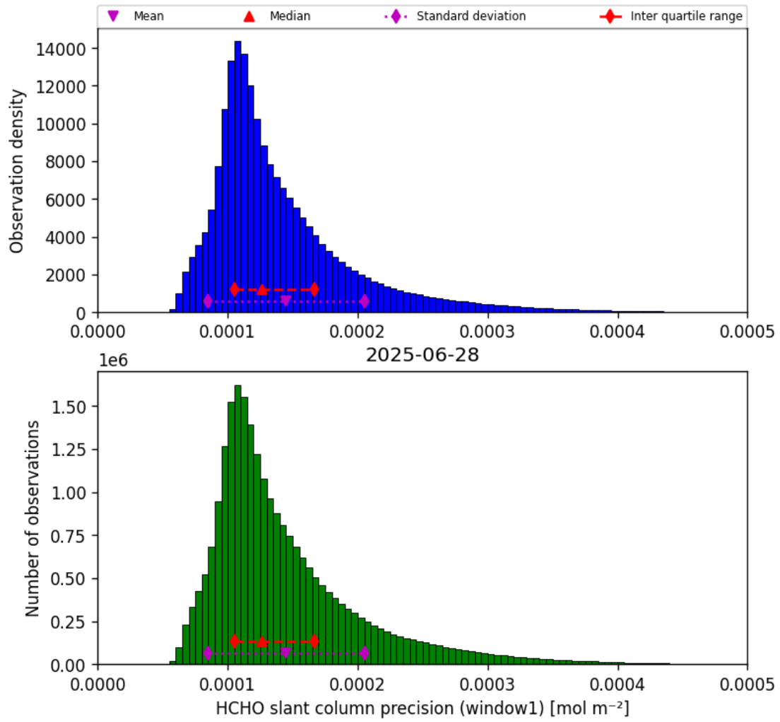
Figure 39: Histogram of “HCHO slant column precision (window1)” for 2025-06-27 to 2025-06-29
