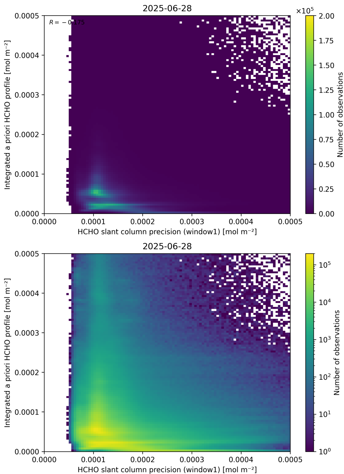
Figure 96: Scatter density plot of “HCHO slant column precision (window1)” against “Integrated a priori HCHO profile” for 2025-06-27 to 2025-06-29.
