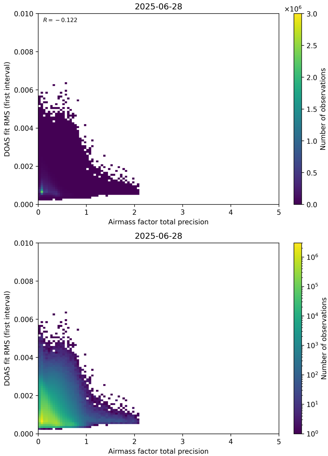
Figure 105: Scatter density plot of “Airmass factor total precision” against “DOAS fit RMS (first interval)” for 2025-06-27 to 2025-06-29.
