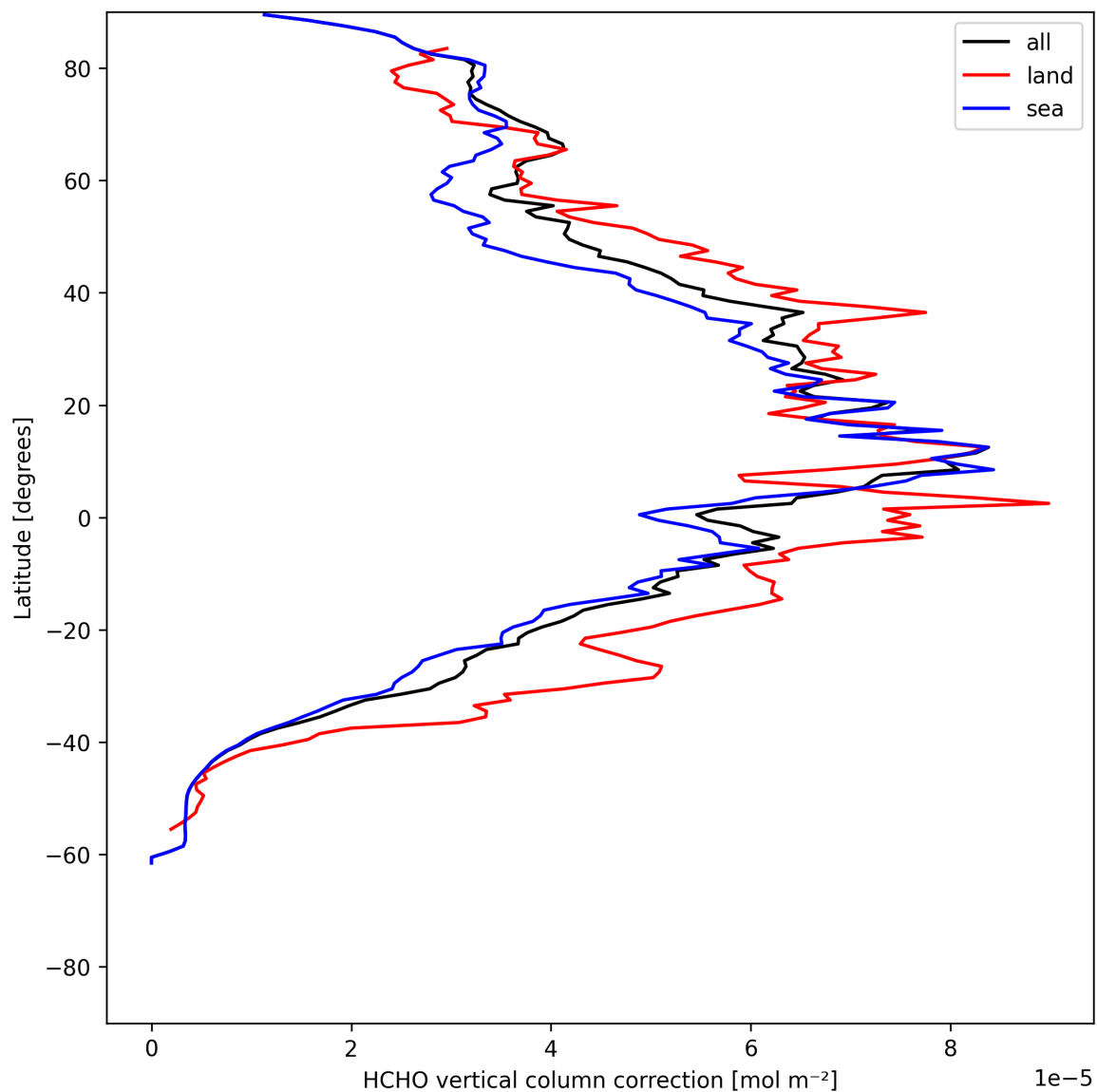
Figure 23: Zonal average of “HCHO vertical column correction” for 2025-06-27 to 2025-06-29.
