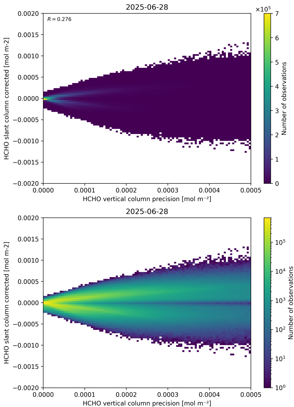
Figure 140: Scatter density plot of “HCHO vertical column precision” against “HCHO slant column corrected” for 2025-06-27 to 2025-06-29.
