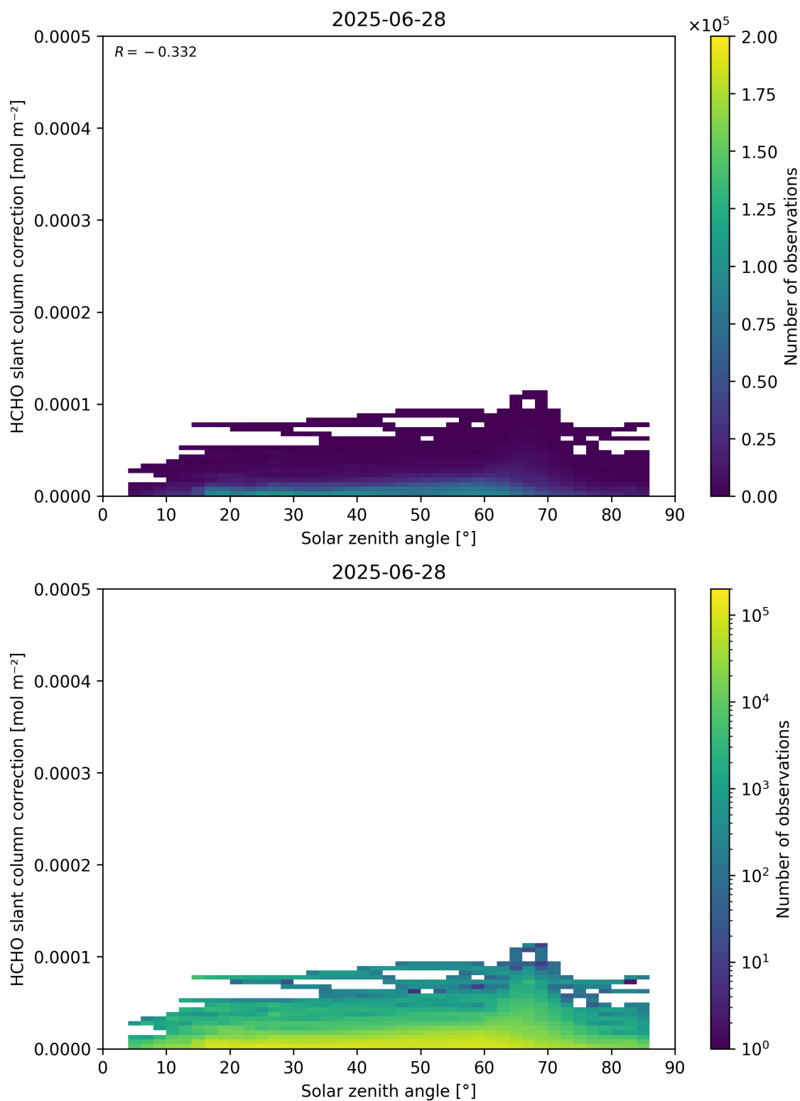
Figure 172: Scatter density plot of “Solar zenith angle” against “HCHO slant column correction” for 2025-06-27 to 2025-06-29.
