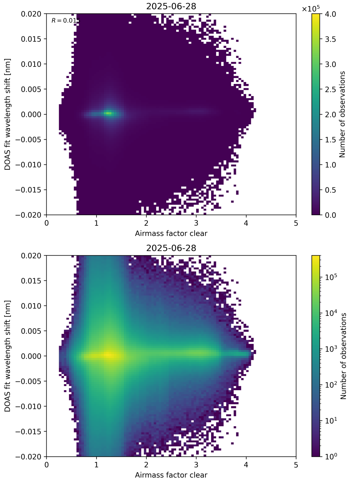
Figure 72: Scatter density plot of “Airmass factor clear” against “DOAS fit wavelength shift” for 2025-06-27 to 2025-06-29.
