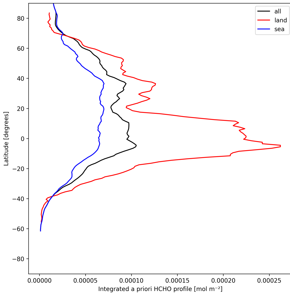
Figure 29: Zonal average of “Integrated a priori HCHO profile” for 2025-06-27 to 2025-06-29.
