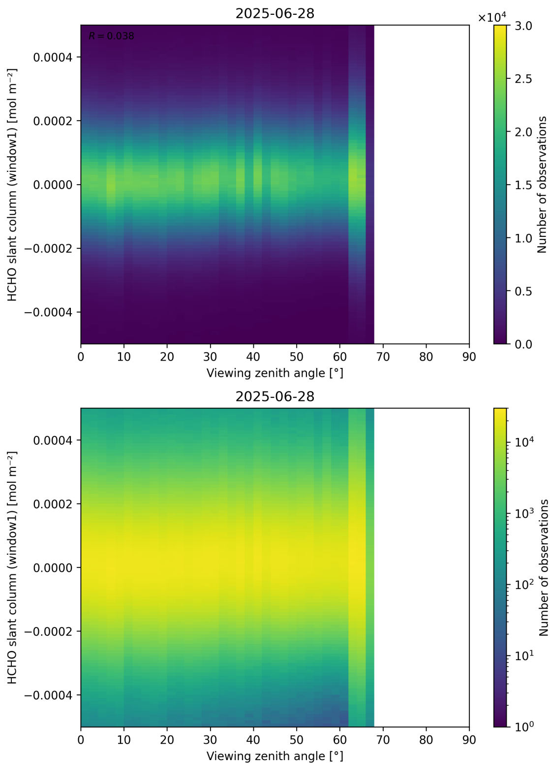
Figure 188: Scatter density plot of “Viewing zenith angle” against “HCHO slant column (window1)” for 2025-06-27 to 2025-06-29.
