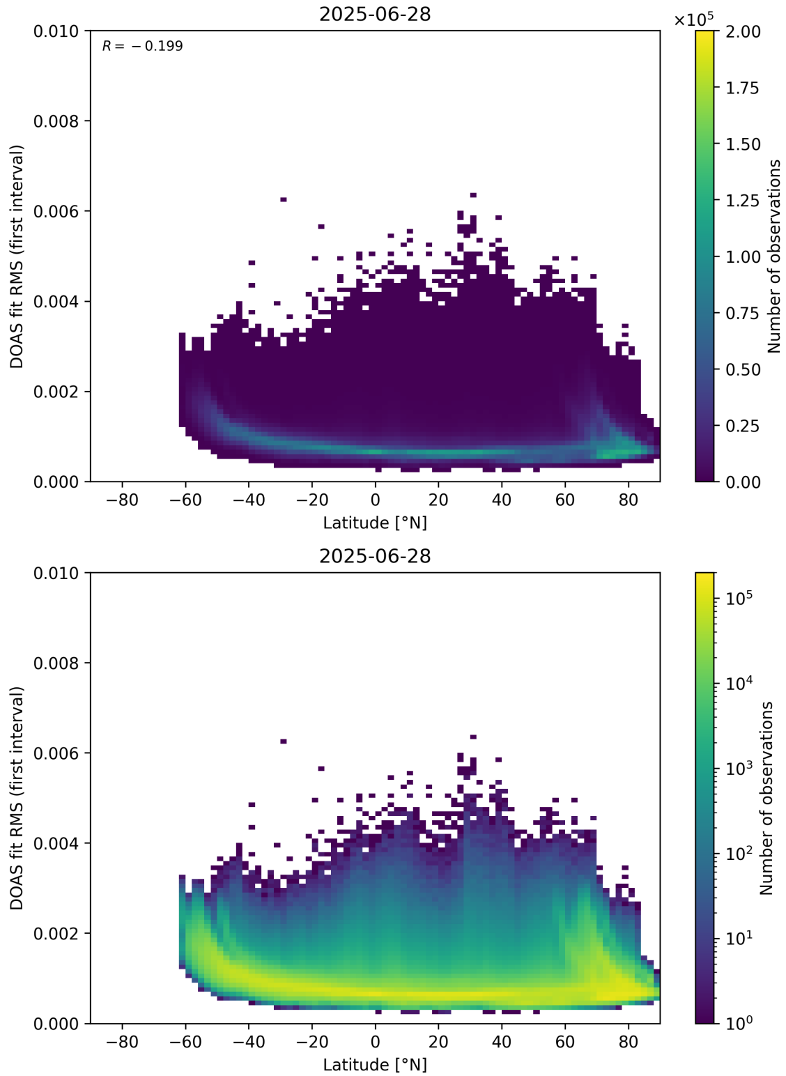
Figure 153: Scatter density plot of “Latitude” against “DOAS fit RMS (first interval)” for 2025-06-27 to 2025-06-29.
