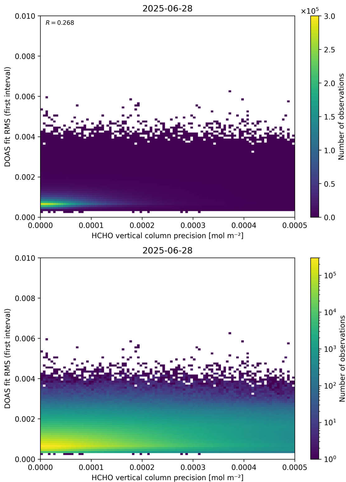
Figure 136: Scatter density plot of “HCHO vertical column precision” against “DOAS fit RMS (first interval)” for 2025-06-27 to 2025-06-29.
