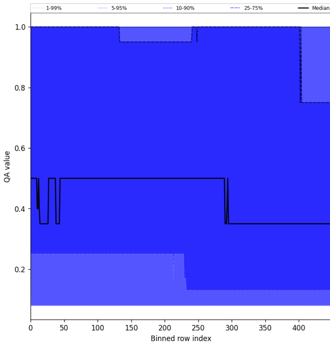
Figure 48: Along track statistics of “QA value” for 2025-06-27 to 2025-06-29
