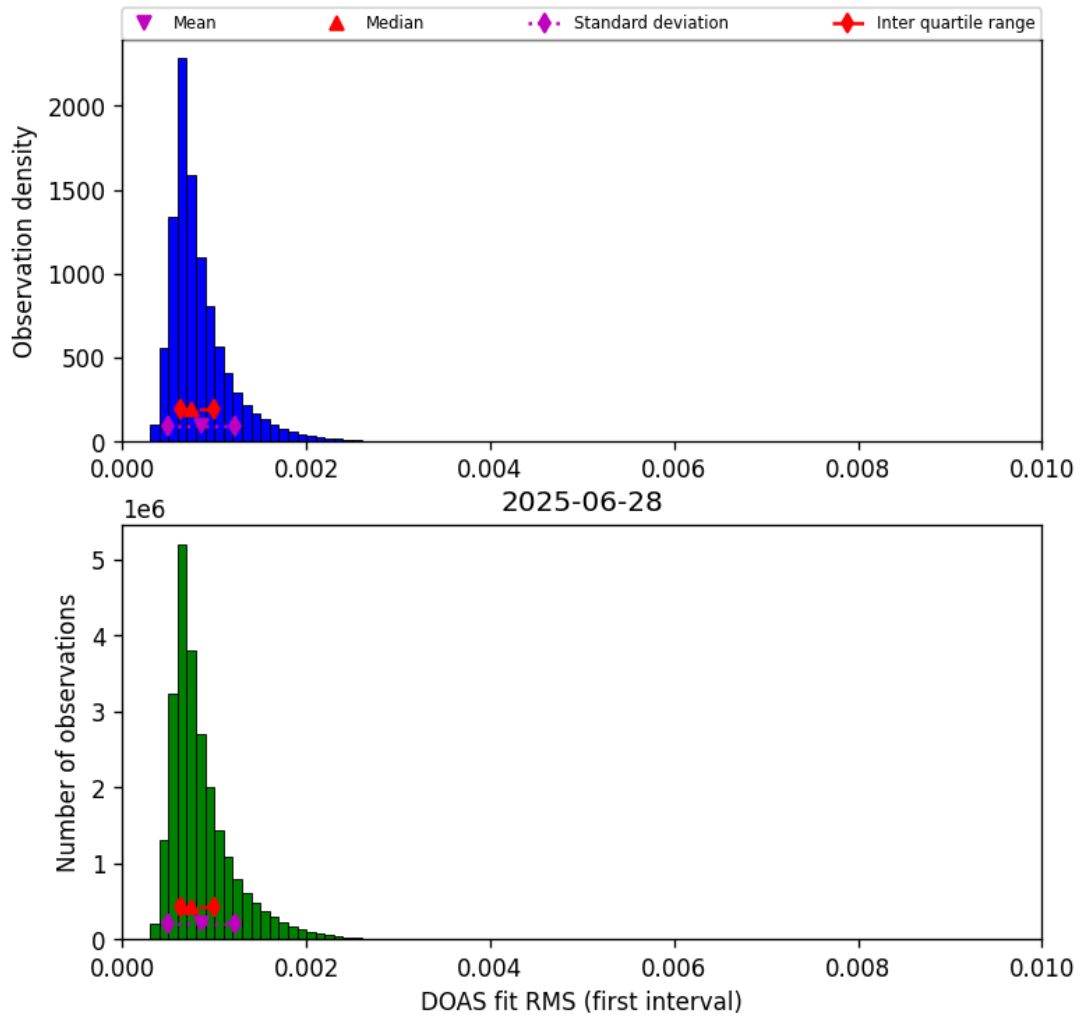
Figure 46: Histogram of “DOAS fit RMS (first interval)” for 2025-06-27 to 2025-06-29
