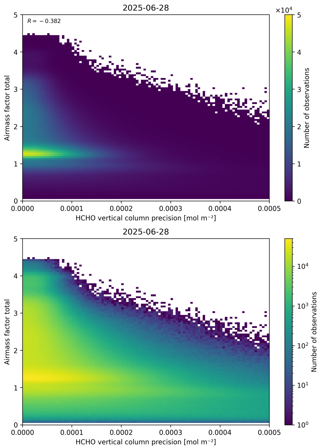
Figure 144: Scatter density plot of “HCHO vertical column precision” against “Airmass factor total” for 2025-06-27 to 2025-06-29.
