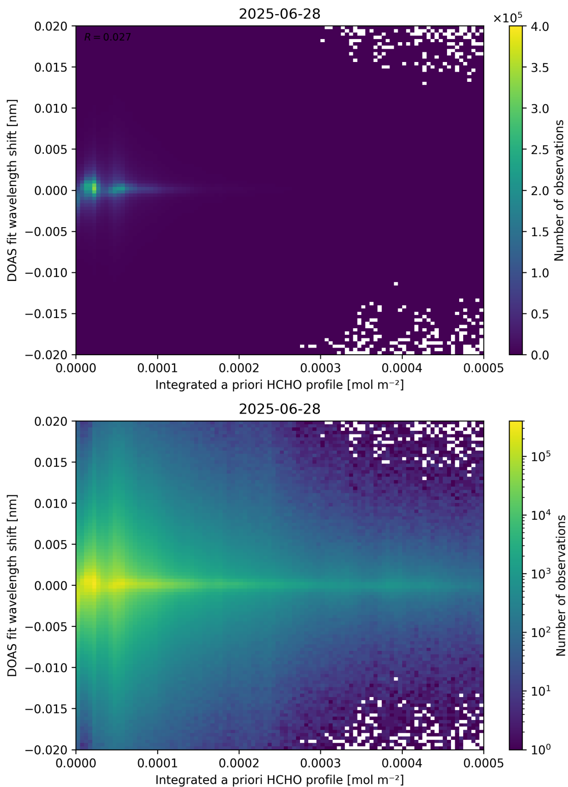
Figure 149: Scatter density plot of “Integrated a priori HCHO profile” against “DOAS fit wavelength shift” for 2025-06-27 to 2025-06-29.
