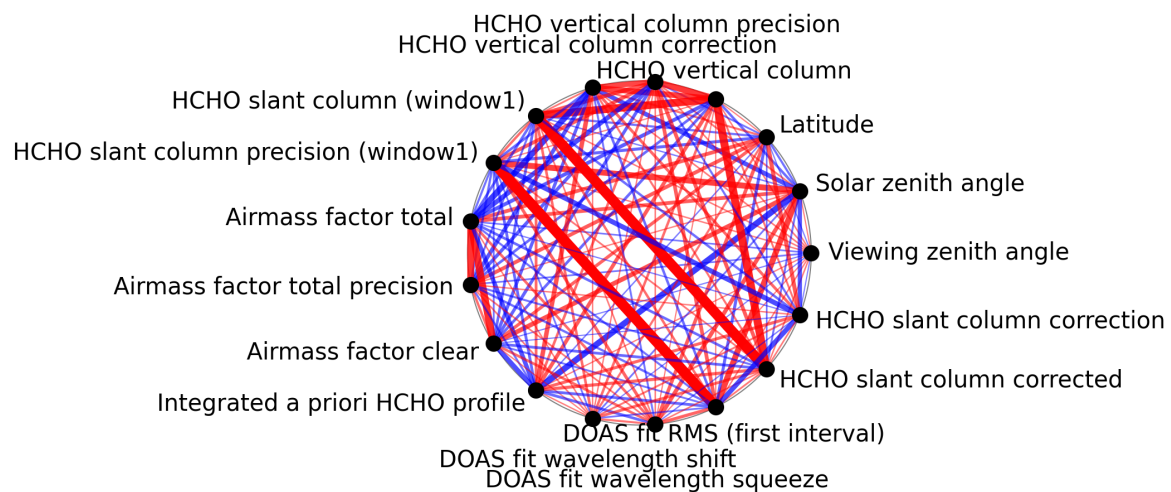
Figure 1: Map of correlation graph for 2025-06-27 to 2025-06-29.
