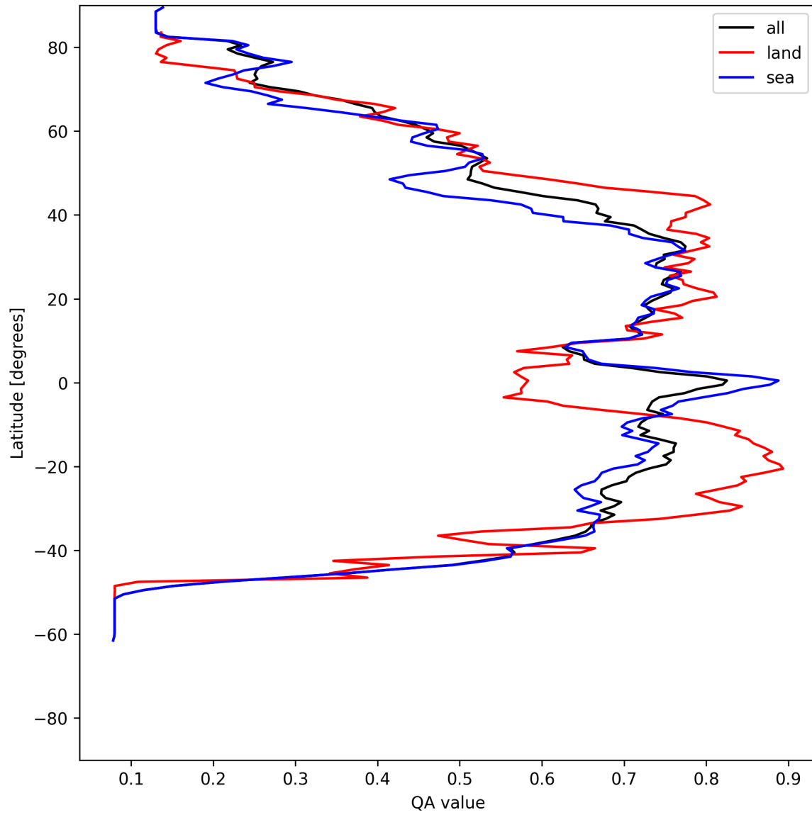
Figure 20: Zonal average of “QA value” for 2025-06-27 to 2025-06-29.
