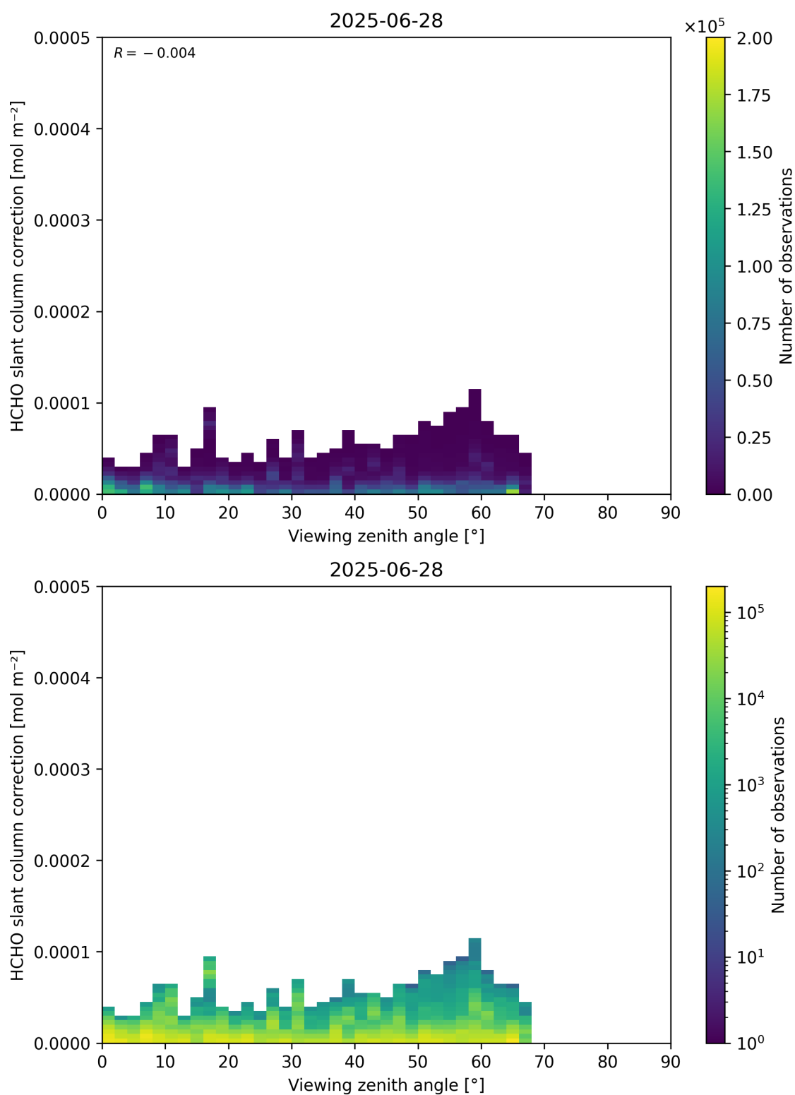
Figure 187: Scatter density plot of “Viewing zenith angle” against “HCHO slant column correction” for 2025-06-27 to 2025-06-29.
