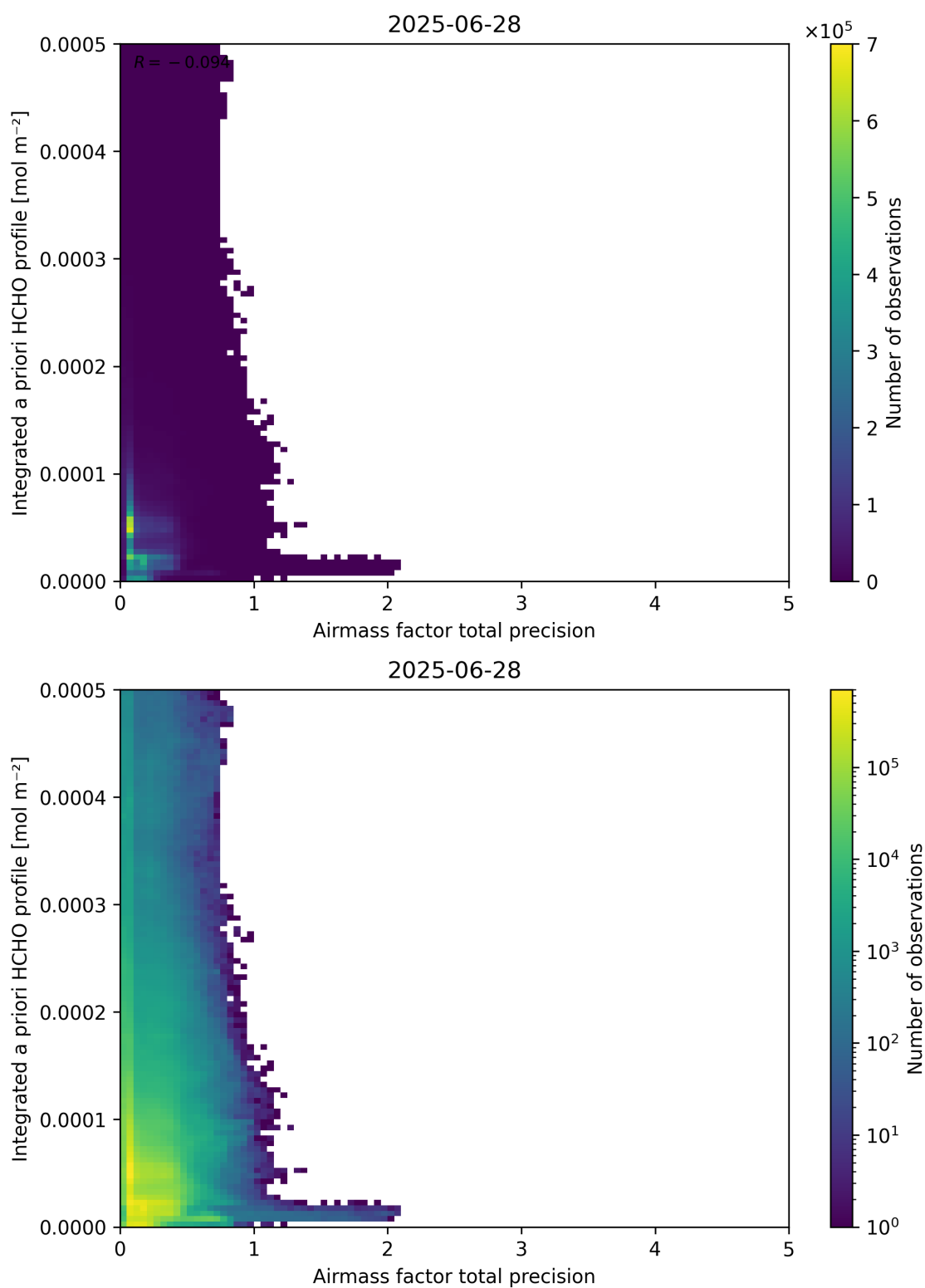
Figure 111: Scatter density plot of “Airmass factor total precision” against “Integrated a priori HCHO profile” for 2025-06-27 to 2025-06-29.
