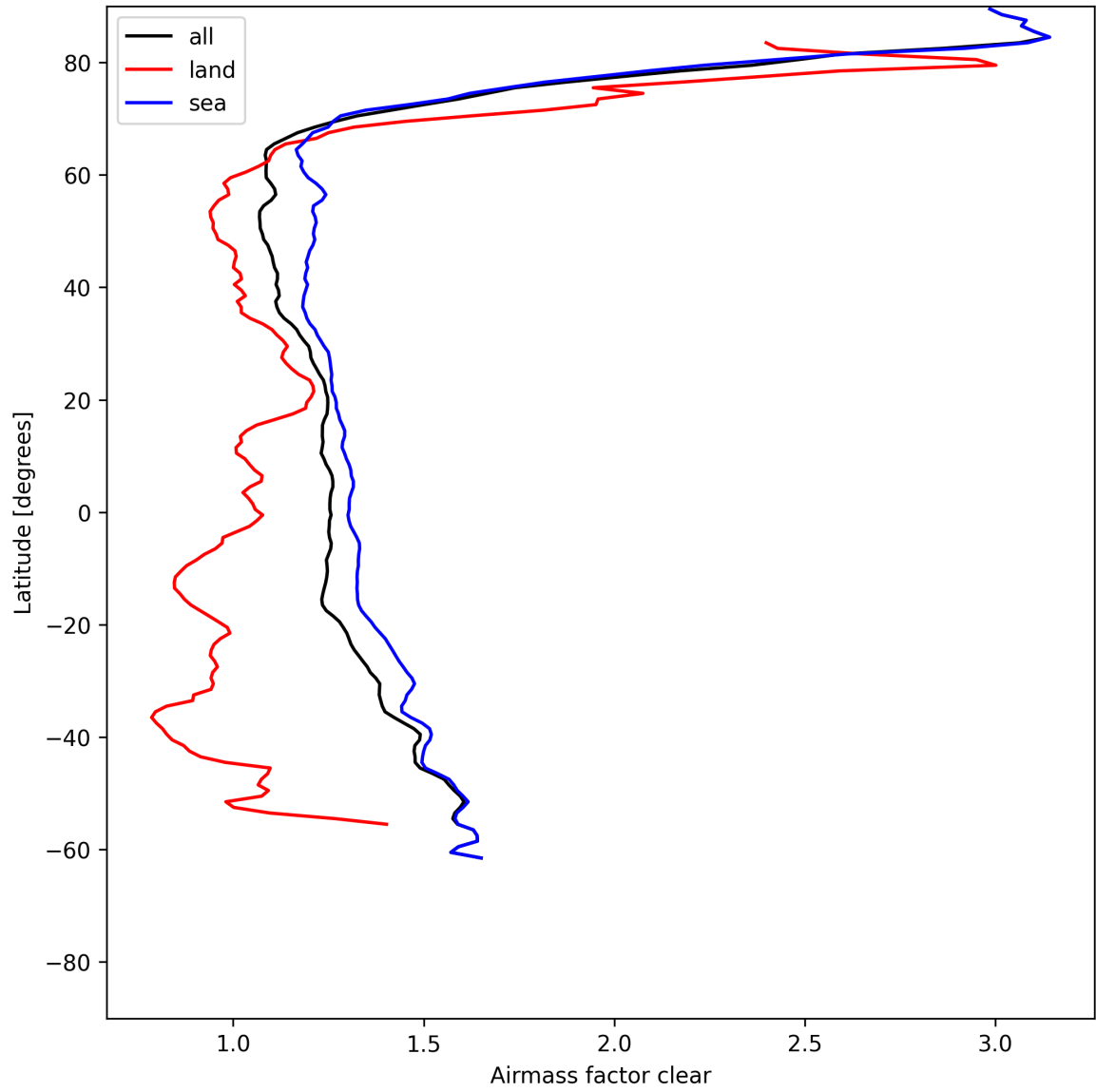
Figure 28: Zonal average of “Airmass factor clear” for 2025-06-27 to 2025-06-29.
