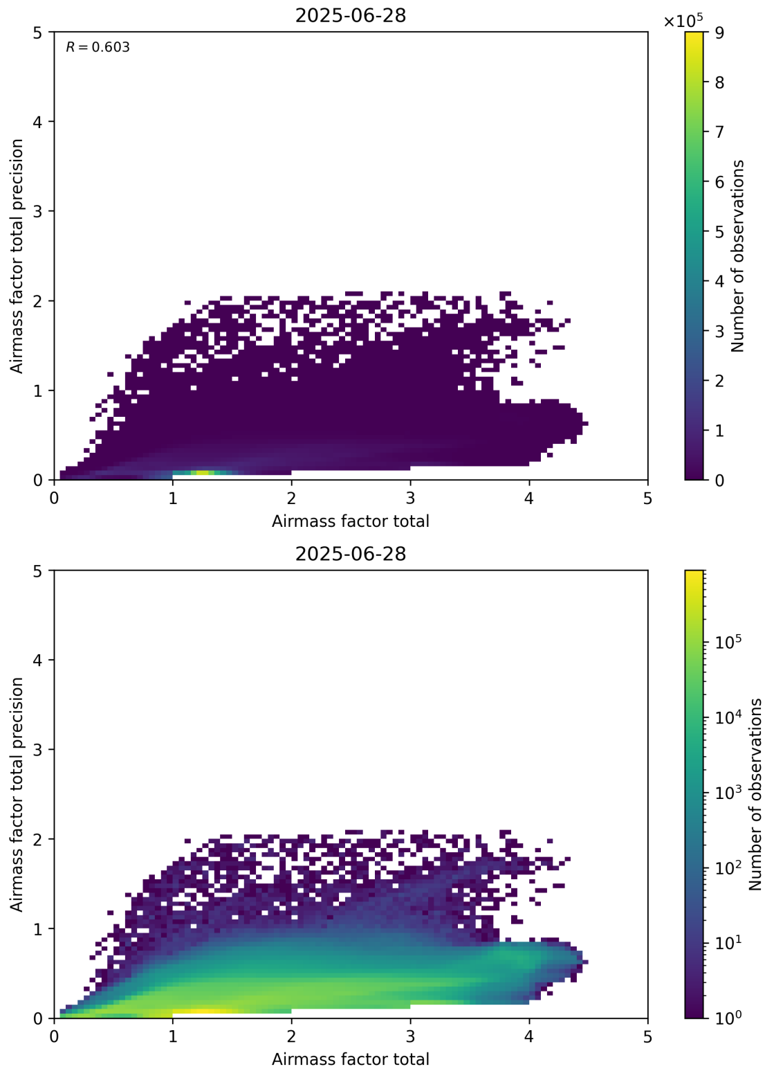
Figure 103: Scatter density plot of “Airmass factor total” against “Airmass factor total precision” for 2025-06-27 to 2025-06-29.
