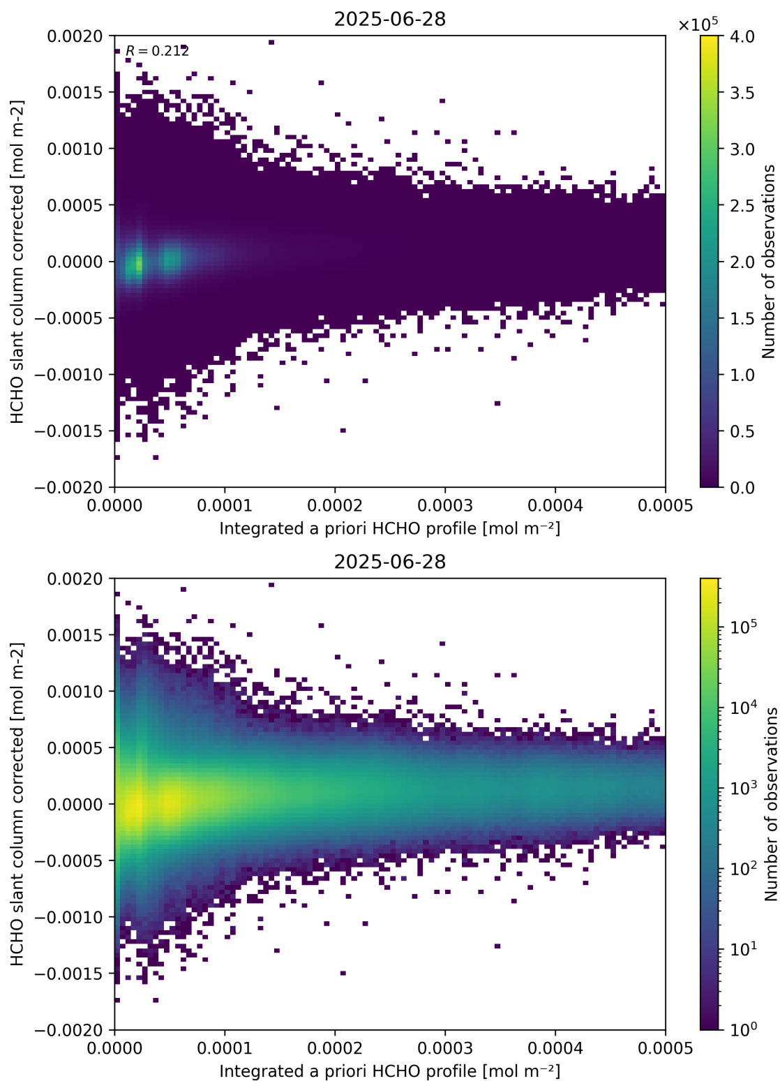
Figure 151: Scatter density plot of “Integrated a priori HCHO profile” against “HCHO slant column corrected” for 2025-06-27 to 2025-06-29.
