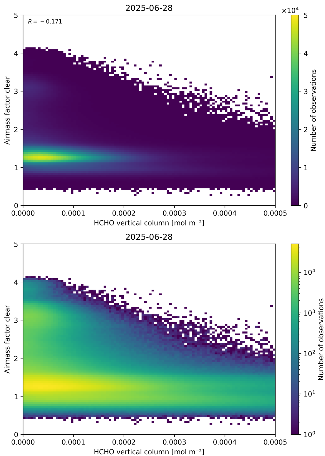
Figure 126: Scatter density plot of “HCHO vertical column” against “Airmass factor clear” for 2025-06-27 to 2025-06-29.
