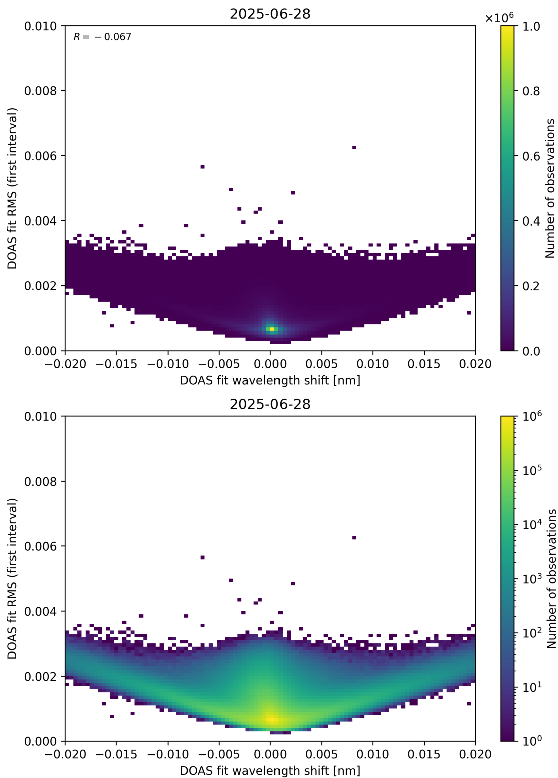
Figure 64: Scatter density plot of “DOAS fit wavelength shift” against “DOAS fit RMS (first interval)” for 2025-06-27 to 2025-06-29.
