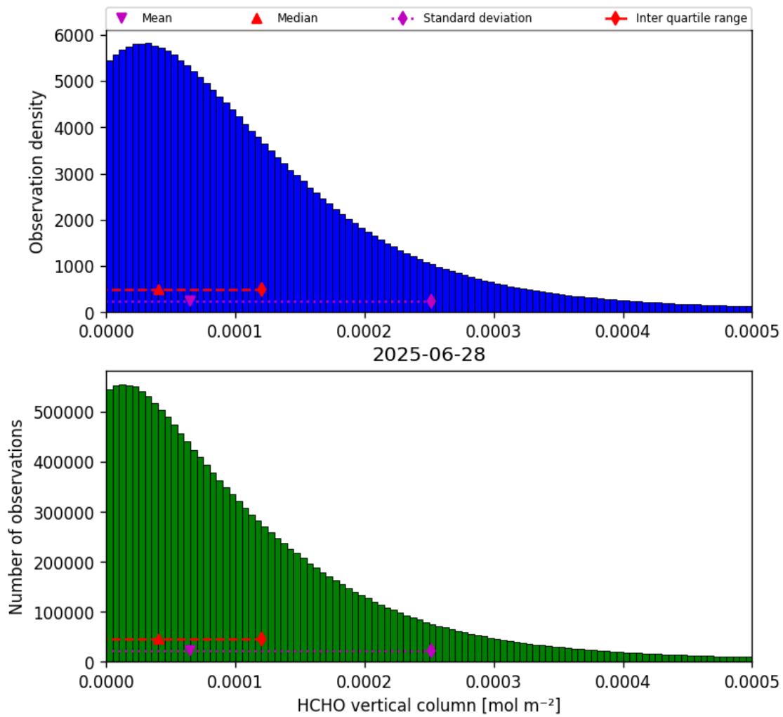
Figure 35: Histogram of “HCHO vertical column” for 2025-06-27 to 2025-06-29
