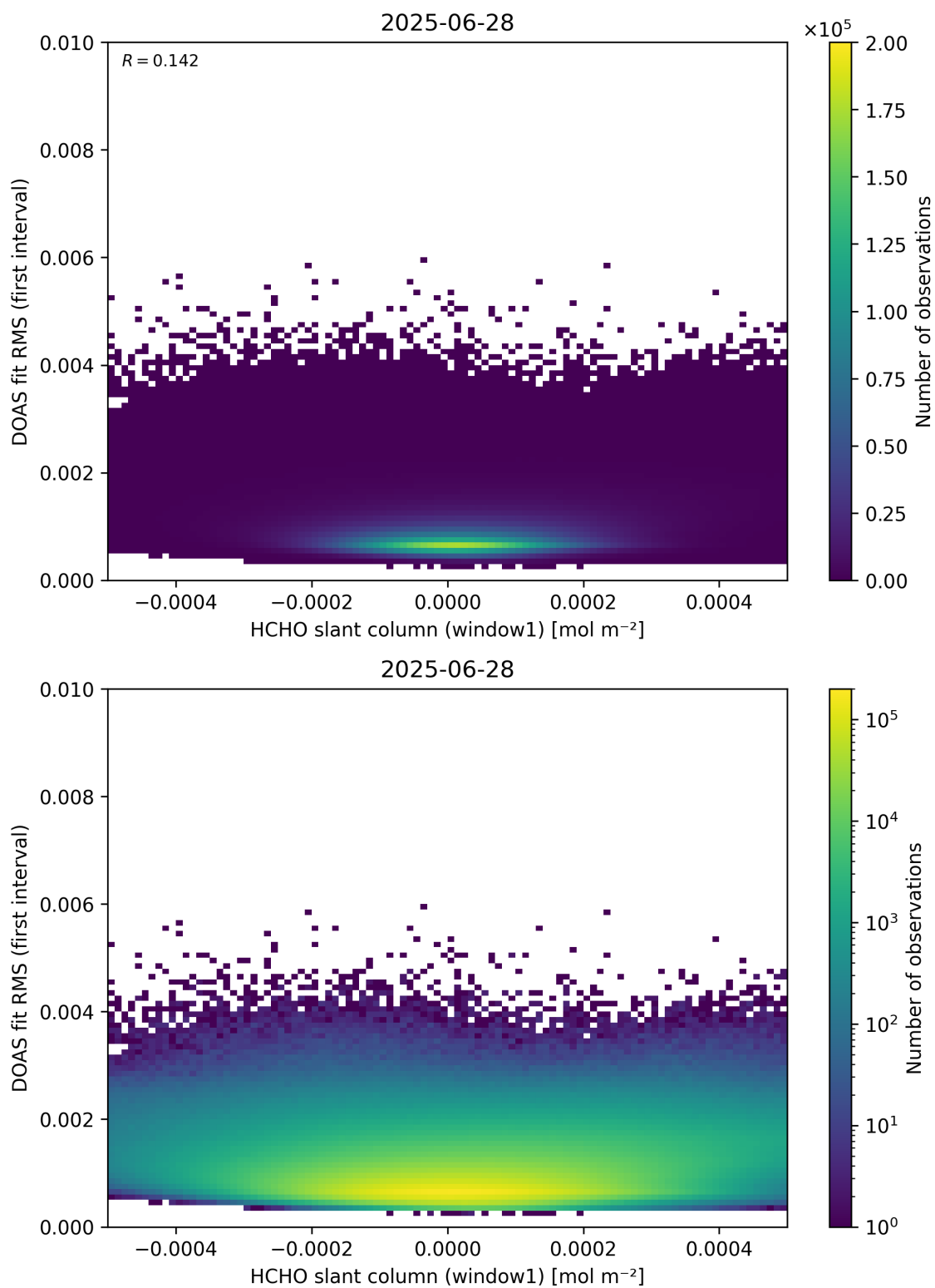
Figure 78: Scatter density plot of “HCHO slant column (window1)” against “DOAS fit RMS (first interval)” for 2025-06-27 to 2025-06-29.
