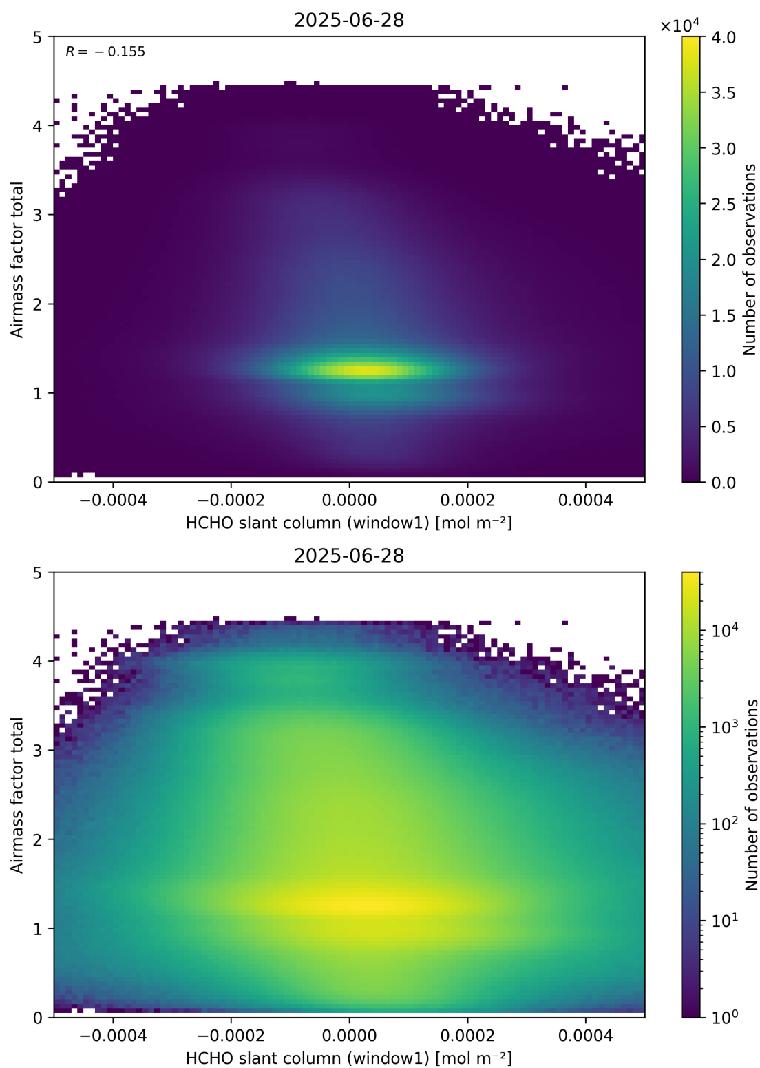
Figure 85: Scatter density plot of “HCHO slant column (window1)” against “Airmass factor total” for 2025-06-27 to 2025-06-29.
