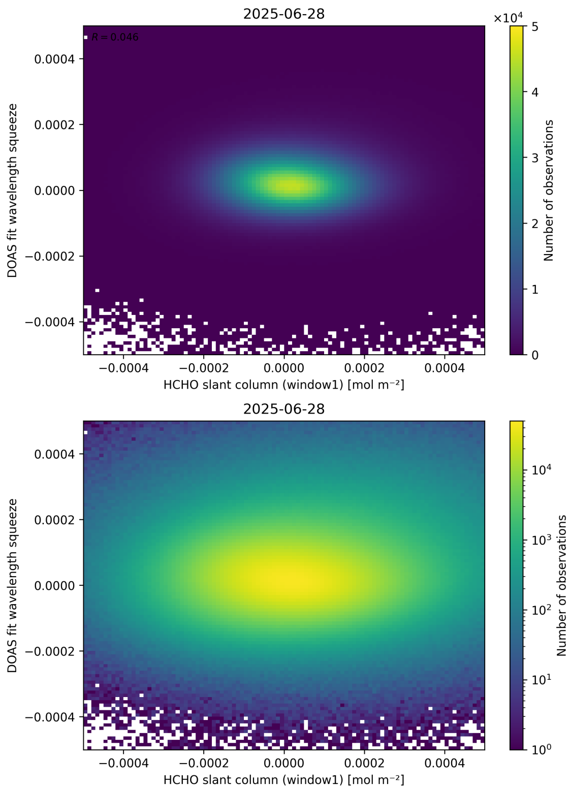
Figure 80: Scatter density plot of “HCHO slant column (window1)” against “DOAS fit wavelength squeeze” for 2025-06-27 to 2025-06-29.
