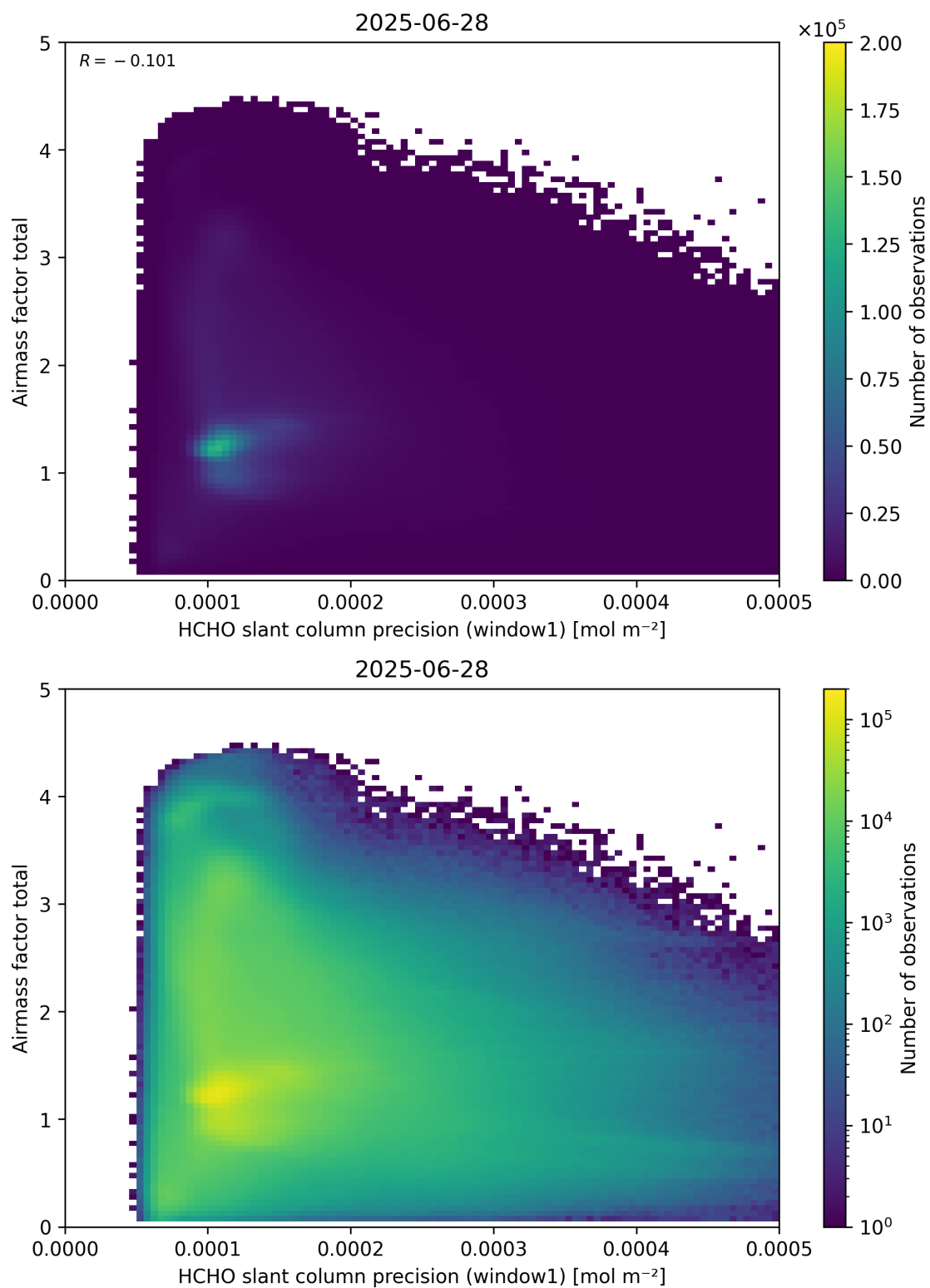
Figure 94: Scatter density plot of “HCHO slant column precision (window1)” against “Airmass factor total” for 2025-06-27 to 2025-06-29.
