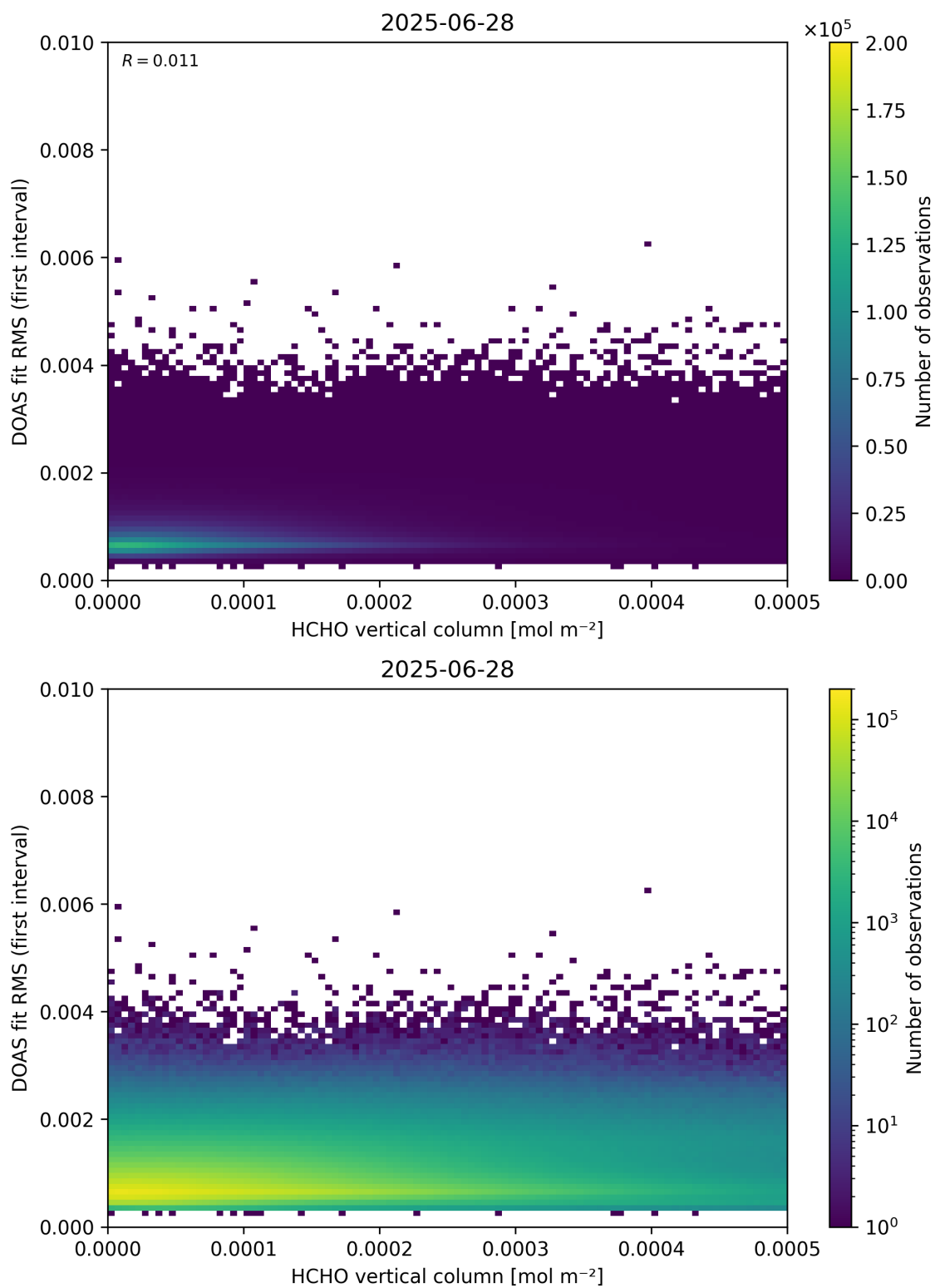
Figure 123: Scatter density plot of “HCHO vertical column” against “DOAS fit RMS (first interval)” for 2025-06-27 to 2025-06-29.
