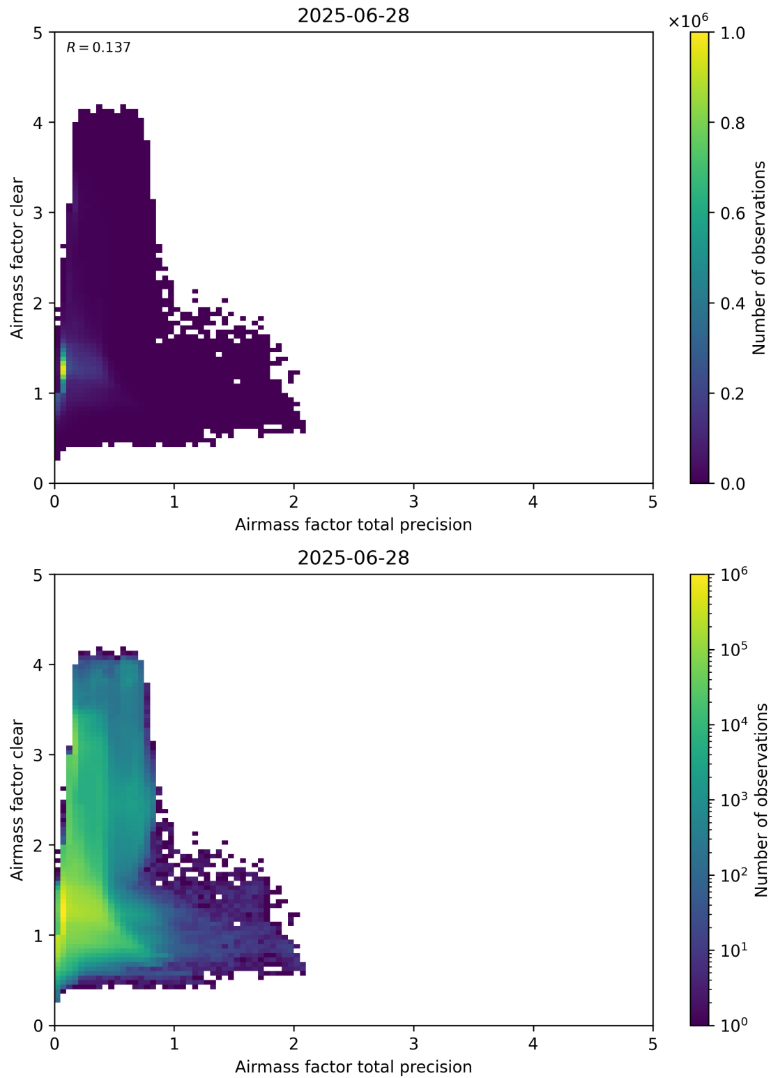
Figure 108: Scatter density plot of “Airmass factor total precision” against “Airmass factor clear” for 2025-06-27 to 2025-06-29.
