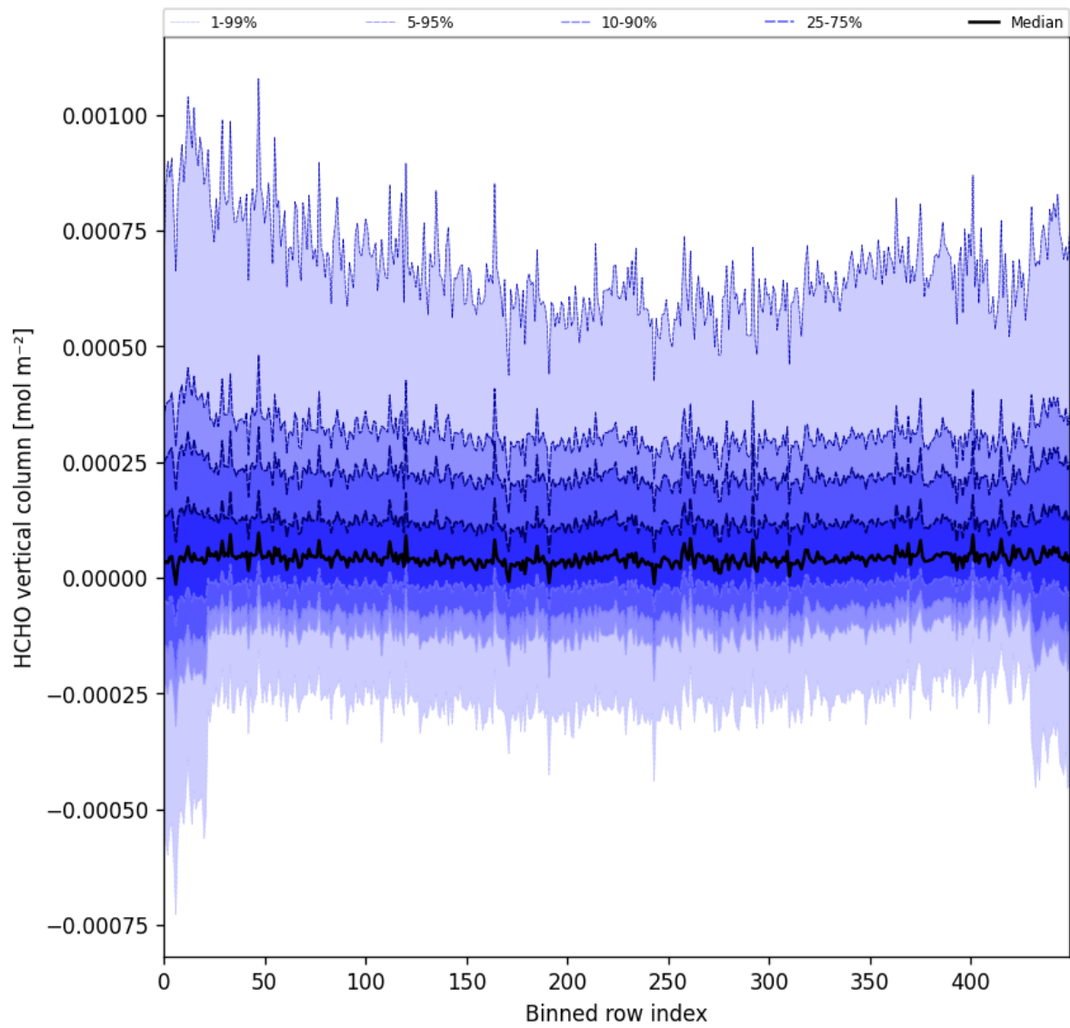
Figure 49: Along track statistics of “HCHO vertical column” for 2025-06-27 to 2025-06-29
