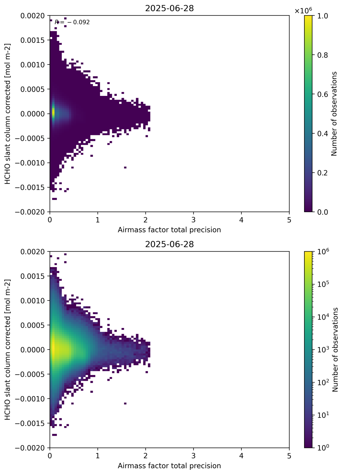
Figure 109: Scatter density plot of “Airmass factor total precision” against “HCHO slant column corrected” for 2025-06-27 to 2025-06-29.
