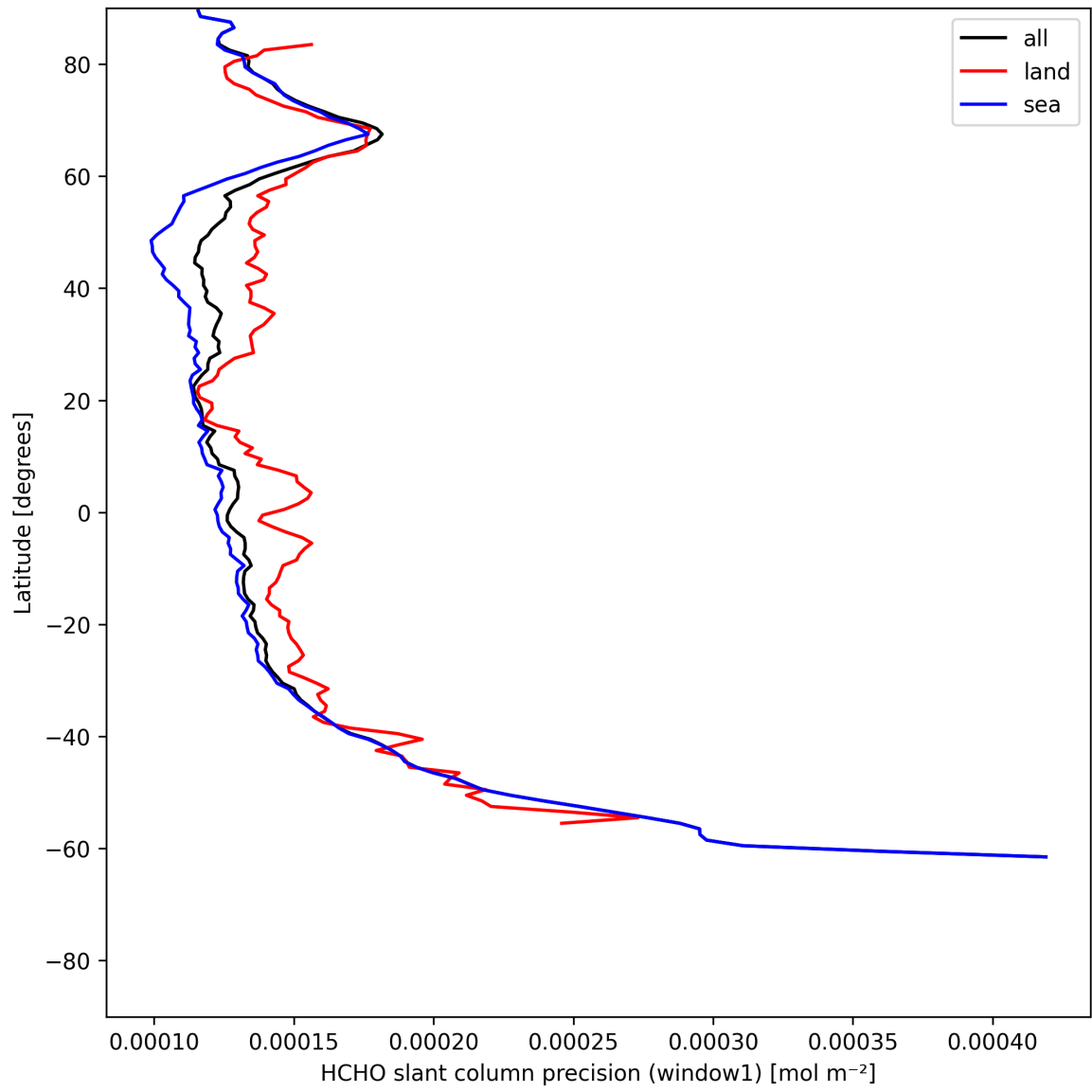
Figure 25: Zonal average of “HCHO slant column precision (window1)” for 2025-06-27 to 2025-06-29.
