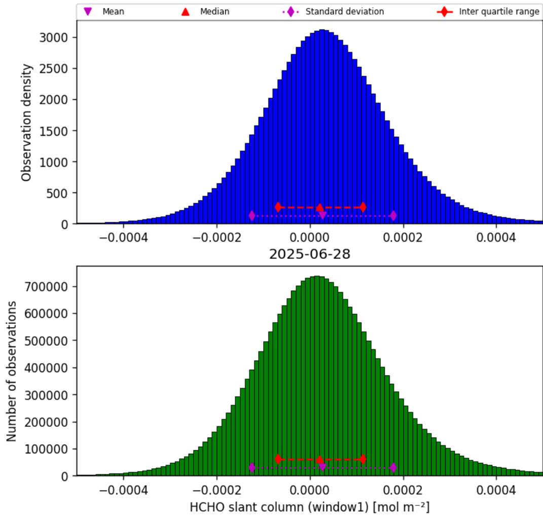
Figure 38: Histogram of “HCHO slant column (window1)” for 2025-06-27 to 2025-06-29
