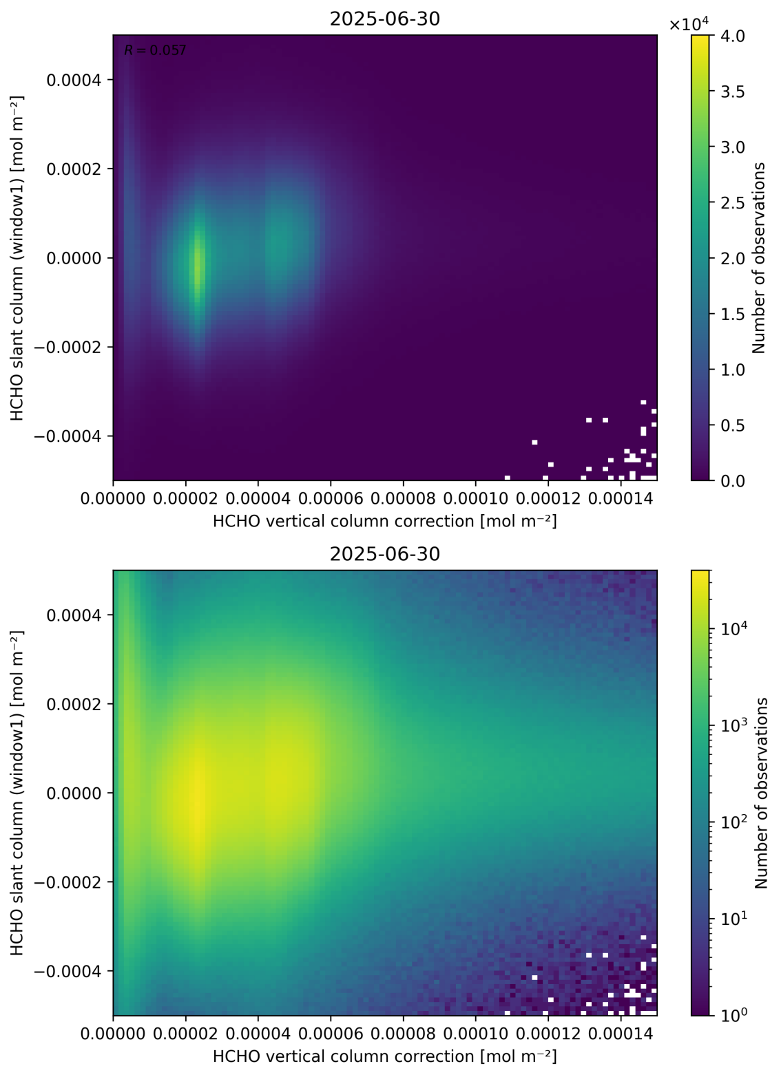
Figure 118: Scatter density plot of “HCHO vertical column correction” against “HCHO slant column (window1)” for 2025-06-29 to 2025-07-01.
