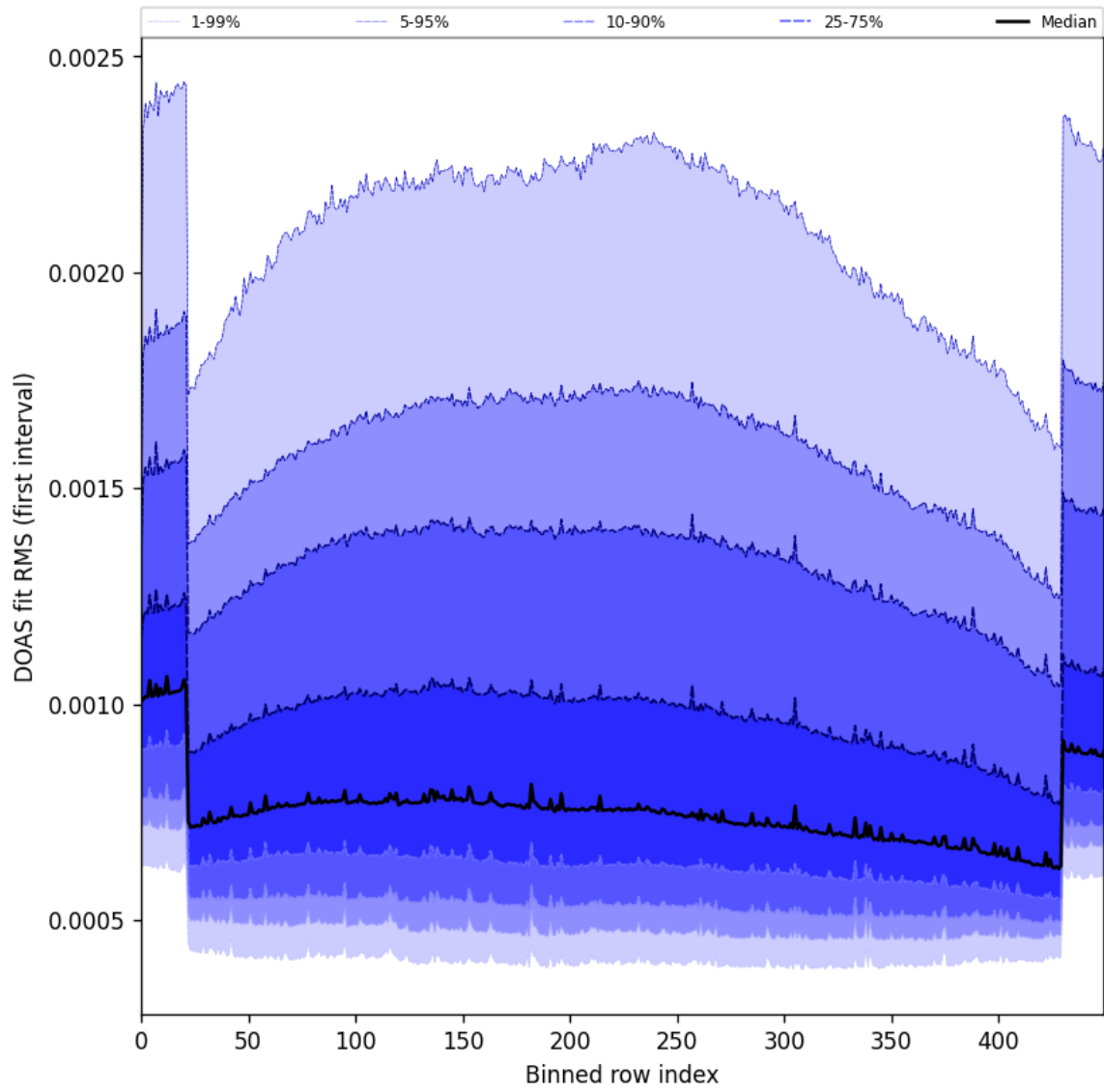
Figure 60: Along track statistics of “DOAS fit RMS (first interval)” for 2025-06-29 to 2025-07-01
