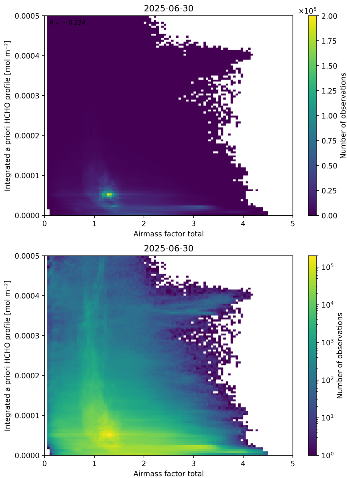
Figure 104: Scatter density plot of “Airmass factor total” against “Integrated a priori HCHO profile” for 2025-06-29 to 2025-07-01.
