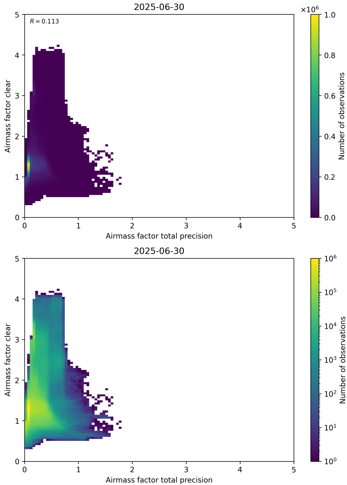
Figure 108: Scatter density plot of “Airmass factor total precision” against “Airmass factor clear” for 2025-06-29 to 2025-07-01.
