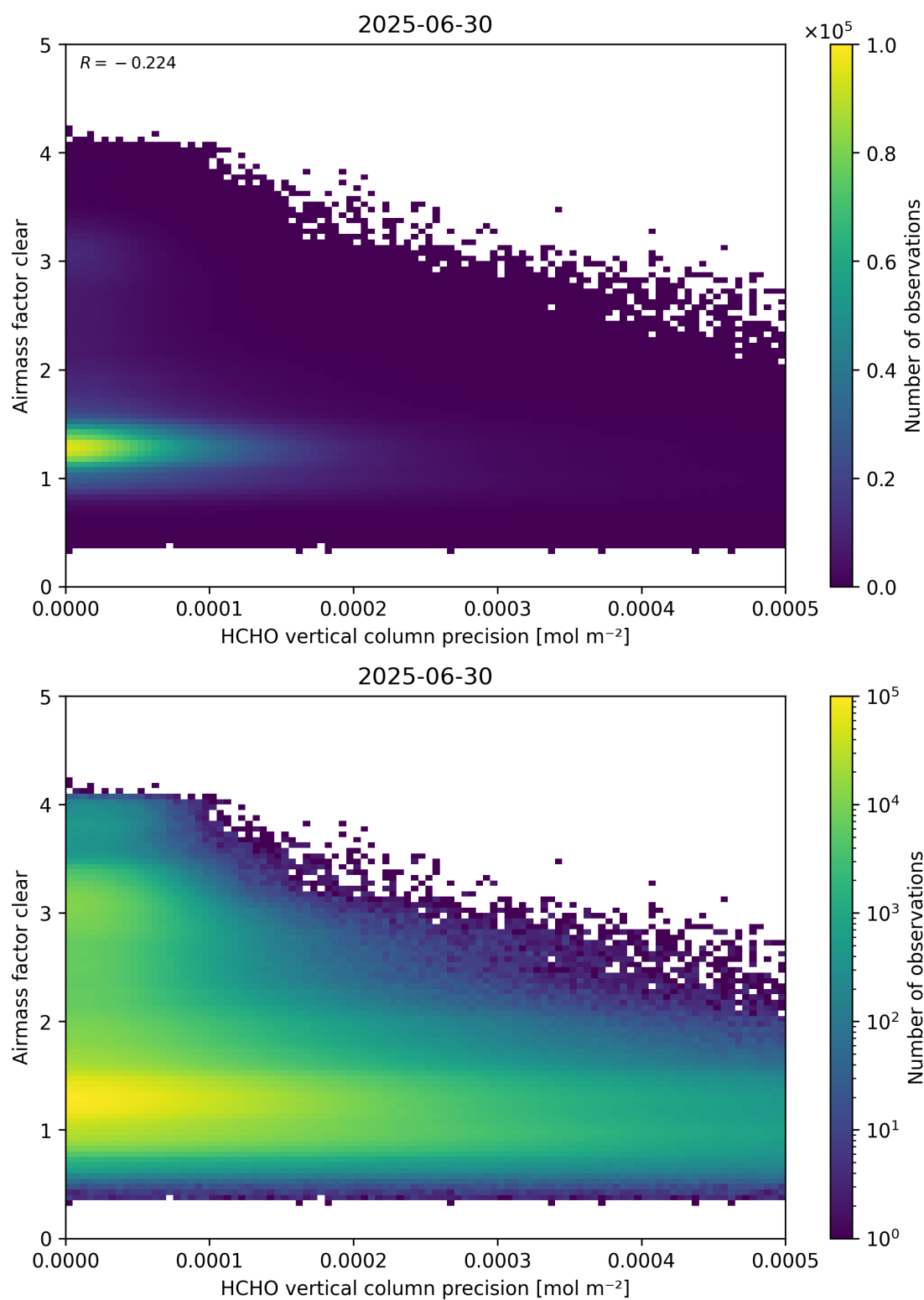
Figure 139: Scatter density plot of “HCHO vertical column precision” against “Airmass factor clear” for 2025-06-29 to 2025-07-01.
