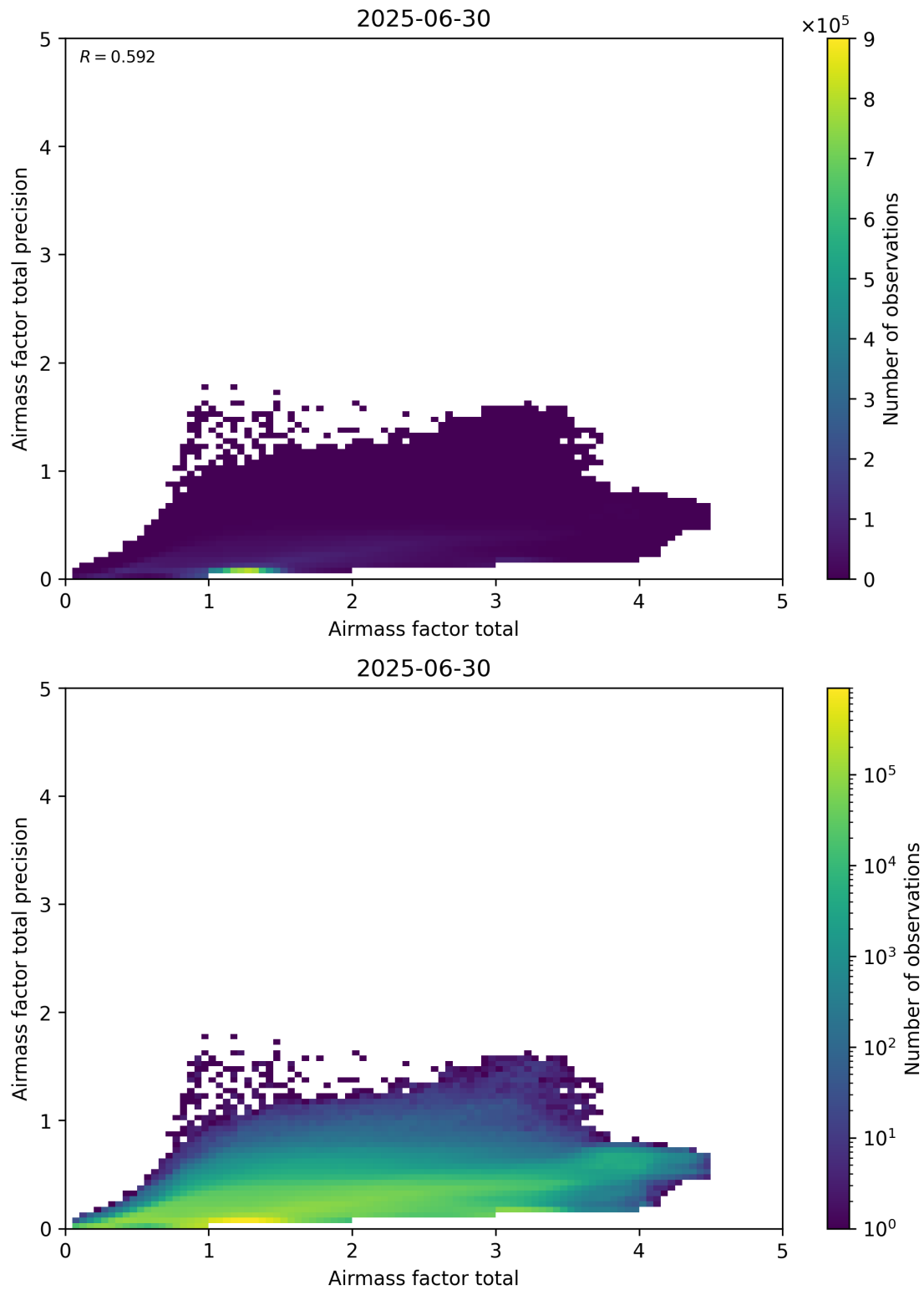
Figure 103: Scatter density plot of “Airmass factor total” against “Airmass factor total precision” for 2025-06-29 to 2025-07-01.
