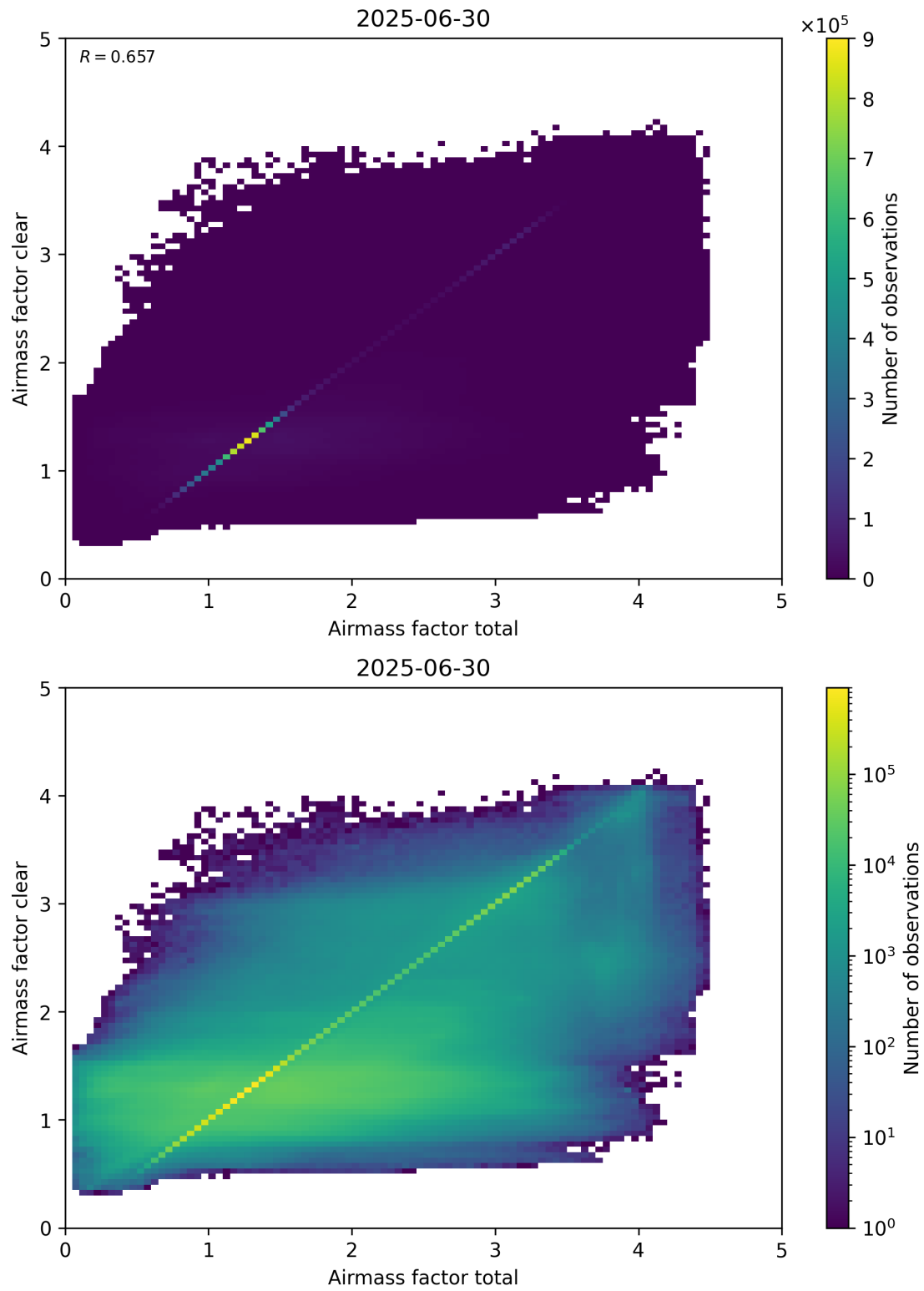
Figure 100: Scatter density plot of “Airmass factor total” against “Airmass factor clear” for 2025-06-29 to 2025-07-01.
