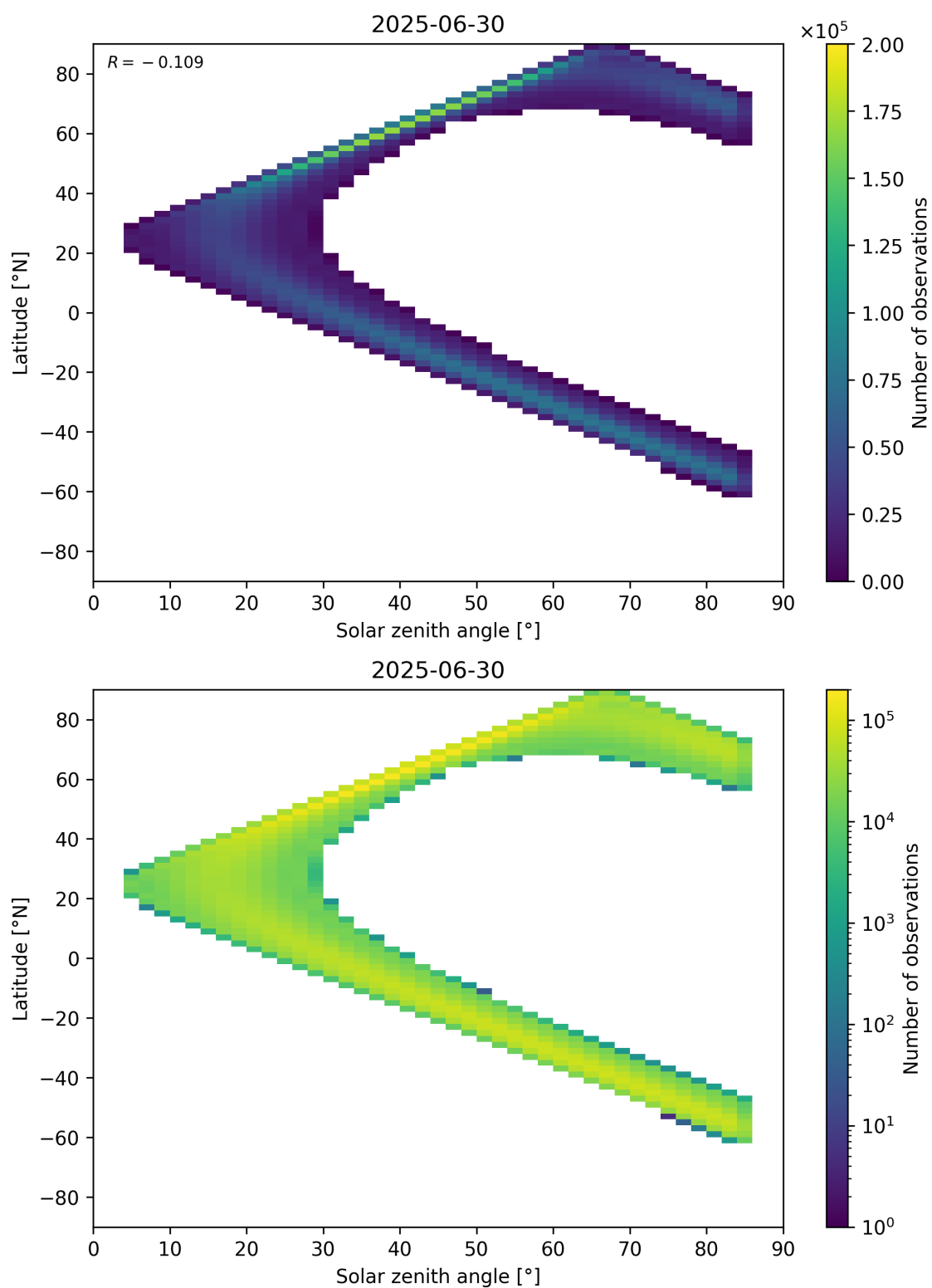
Figure 181: Scatter density plot of “Solar zenith angle” against “Latitude” for 2025-06-29 to 2025-07-01.
