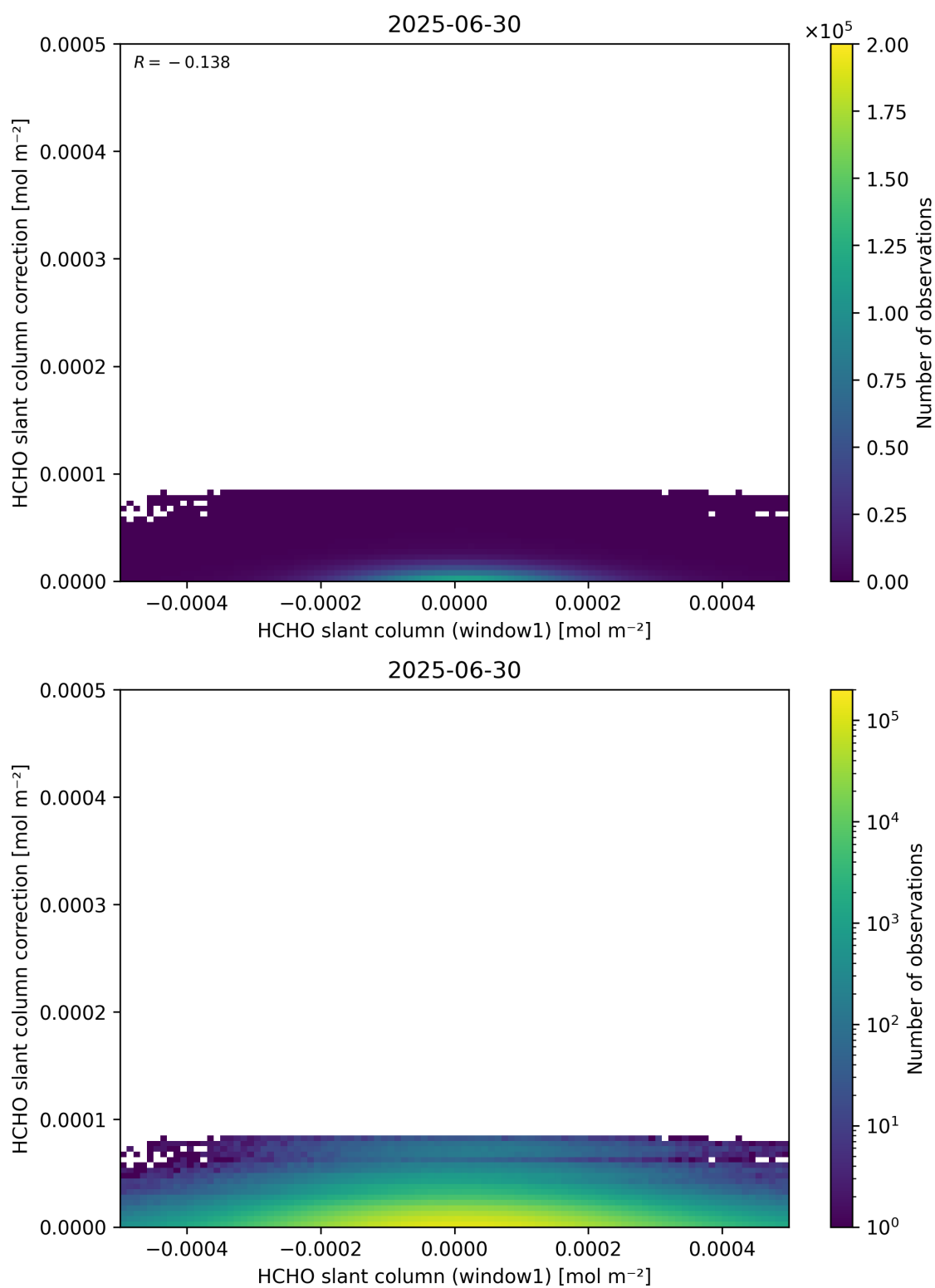
Figure 83: Scatter density plot of “HCHO slant column (window1)” against “HCHO slant column correction” for 2025-06-29 to 2025-07-01.
