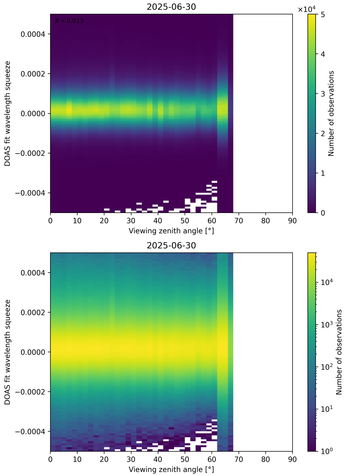
Figure 184: Scatter density plot of “Viewing zenith angle” against “DOAS fit wavelength squeeze” for 2025-06-29 to 2025-07-01.
