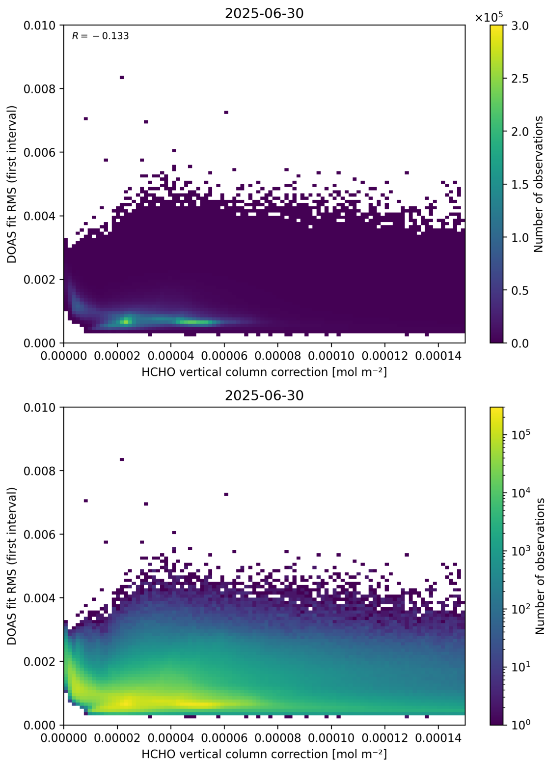
Figure 112: Scatter density plot of “HCHO vertical column correction” against “DOAS fit RMS (first interval)” for 2025-06-29 to 2025-07-01.
