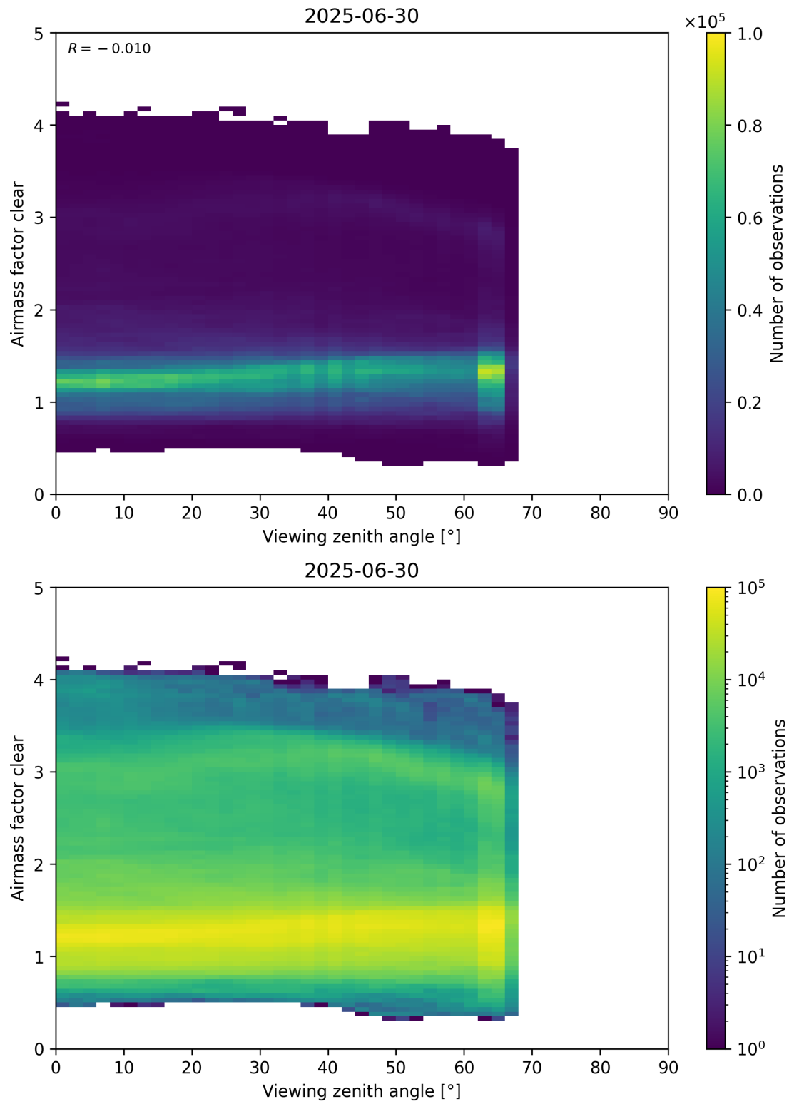
Figure 185: Scatter density plot of “Viewing zenith angle” against “Airmass factor clear” for 2025-06-29 to 2025-07-01.
