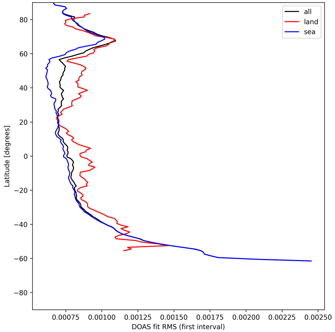
Figure 32: Zonal average of "DOAS fit RMS (first interval)" for 2025-06-29 to 2025-07-01.
