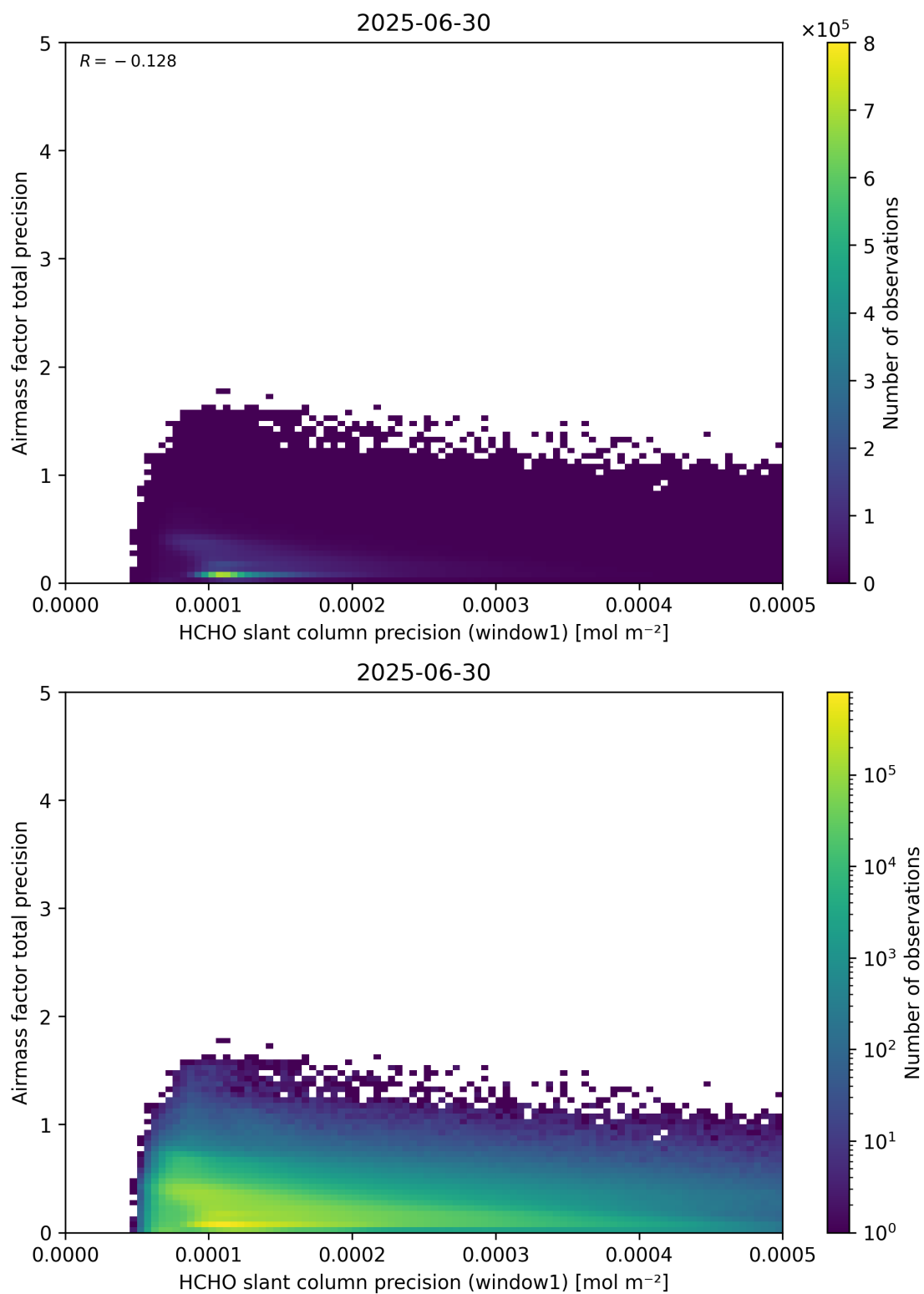
Figure 95: Scatter density plot of “HCHO slant column precision (window1)” against “Airmass factor total precision” for 2025-06-29 to 2025-07-01.
