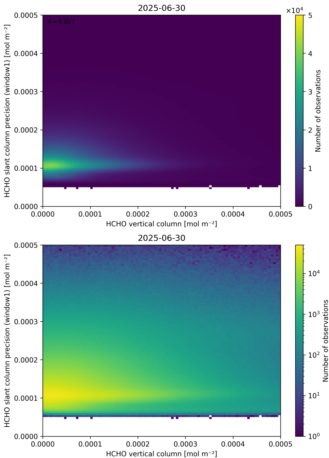
Figure 130: Scatter density plot of “HCHO vertical column” against “HCHO slant column precision (window1)” for 2025-06-29 to 2025-07-01.
