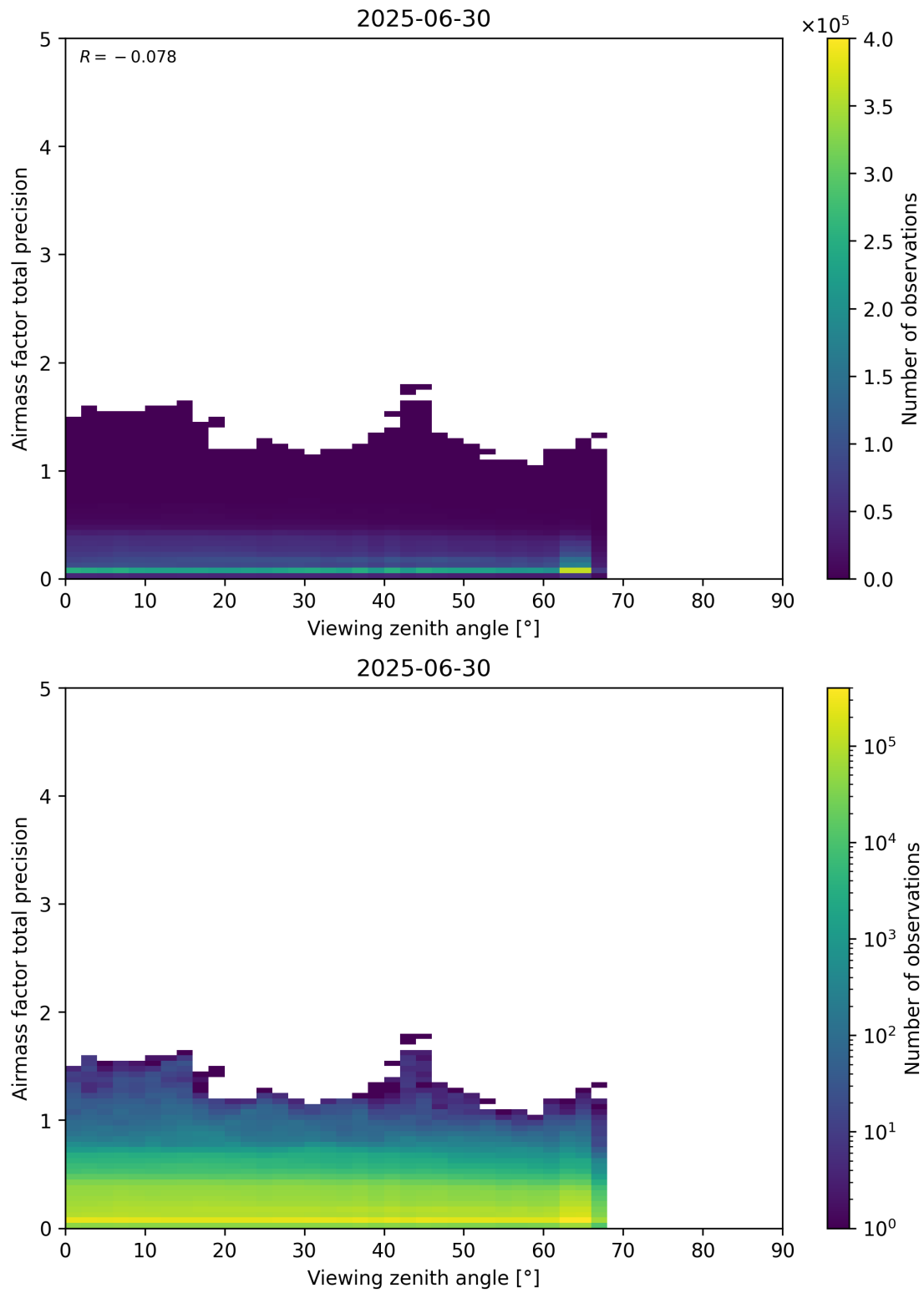
Figure 191: Scatter density plot of “Viewing zenith angle” against “Airmass factor total precision” for 2025-06-29 to 2025-07-01.
