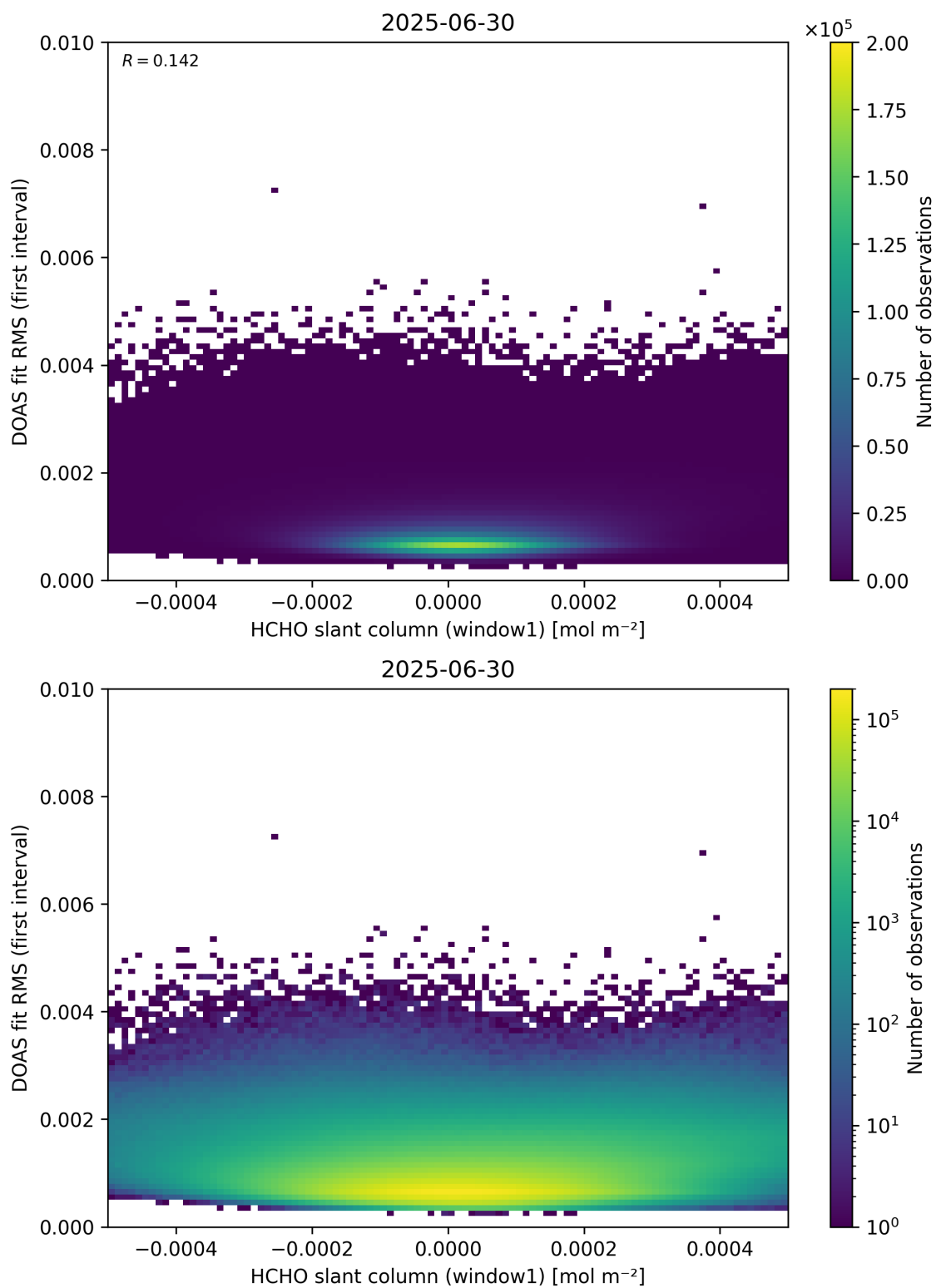
Figure 78: Scatter density plot of “HCHO slant column (window1)” against “DOAS fit RMS (first interval)” for 2025-06-29 to 2025-07-01.
