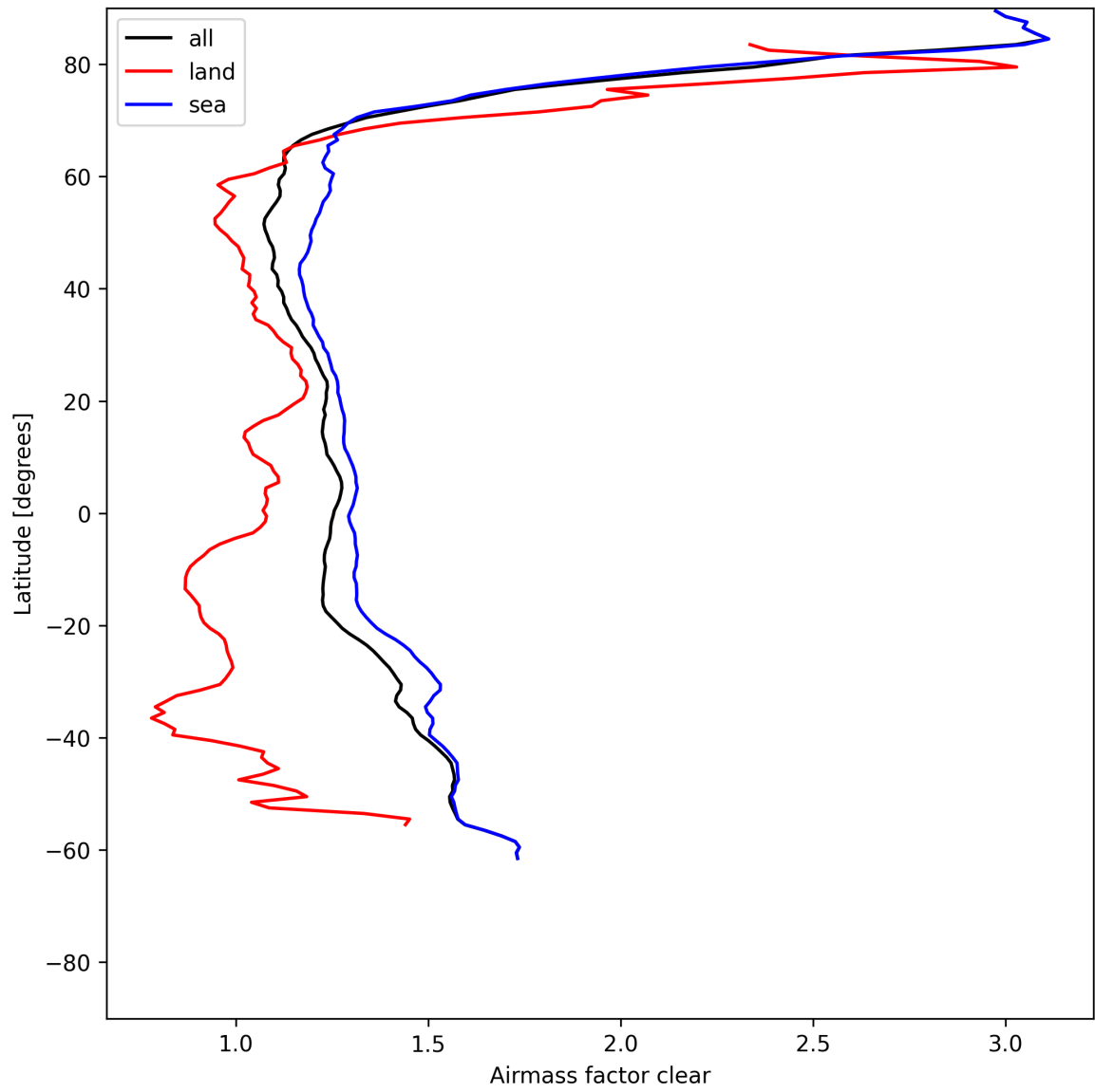
Figure 28: Zonal average of “Airmass factor clear” for 2025-06-29 to 2025-07-01.
