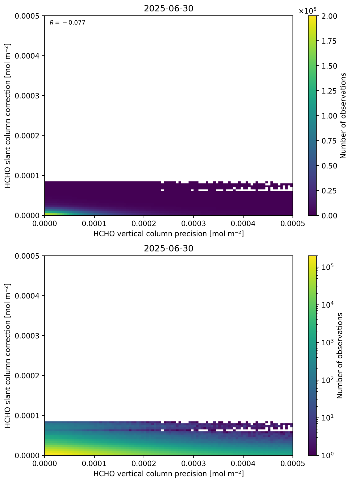
Figure 141: Scatter density plot of “HCHO vertical column precision” against “HCHO slant column correction” for 2025-06-29 to 2025-07-01.
