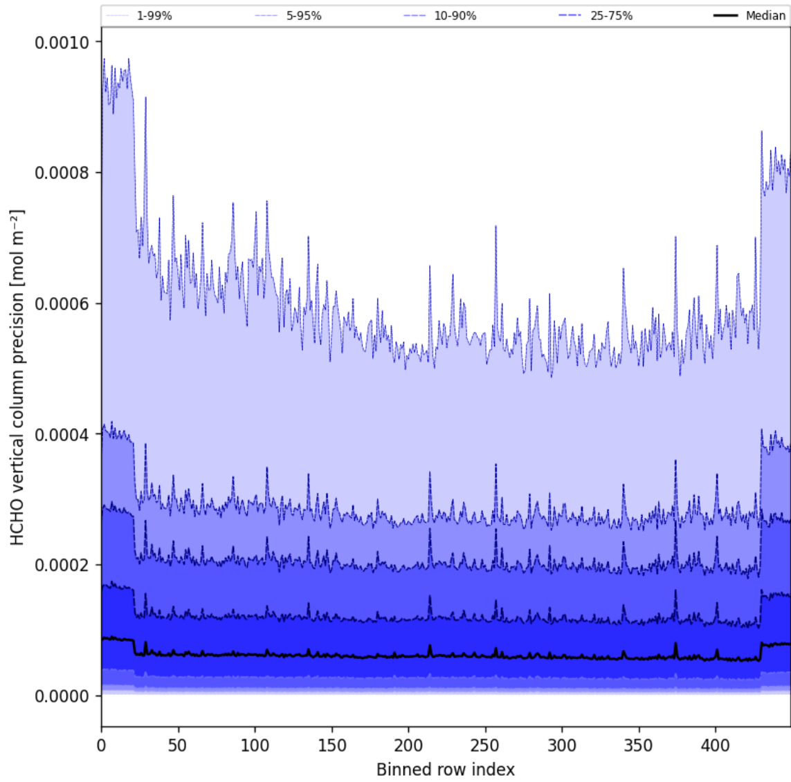
Figure 50: Along track statistics of “HCHO vertical column precision” for 2025-06-29 to 2025-07-01
