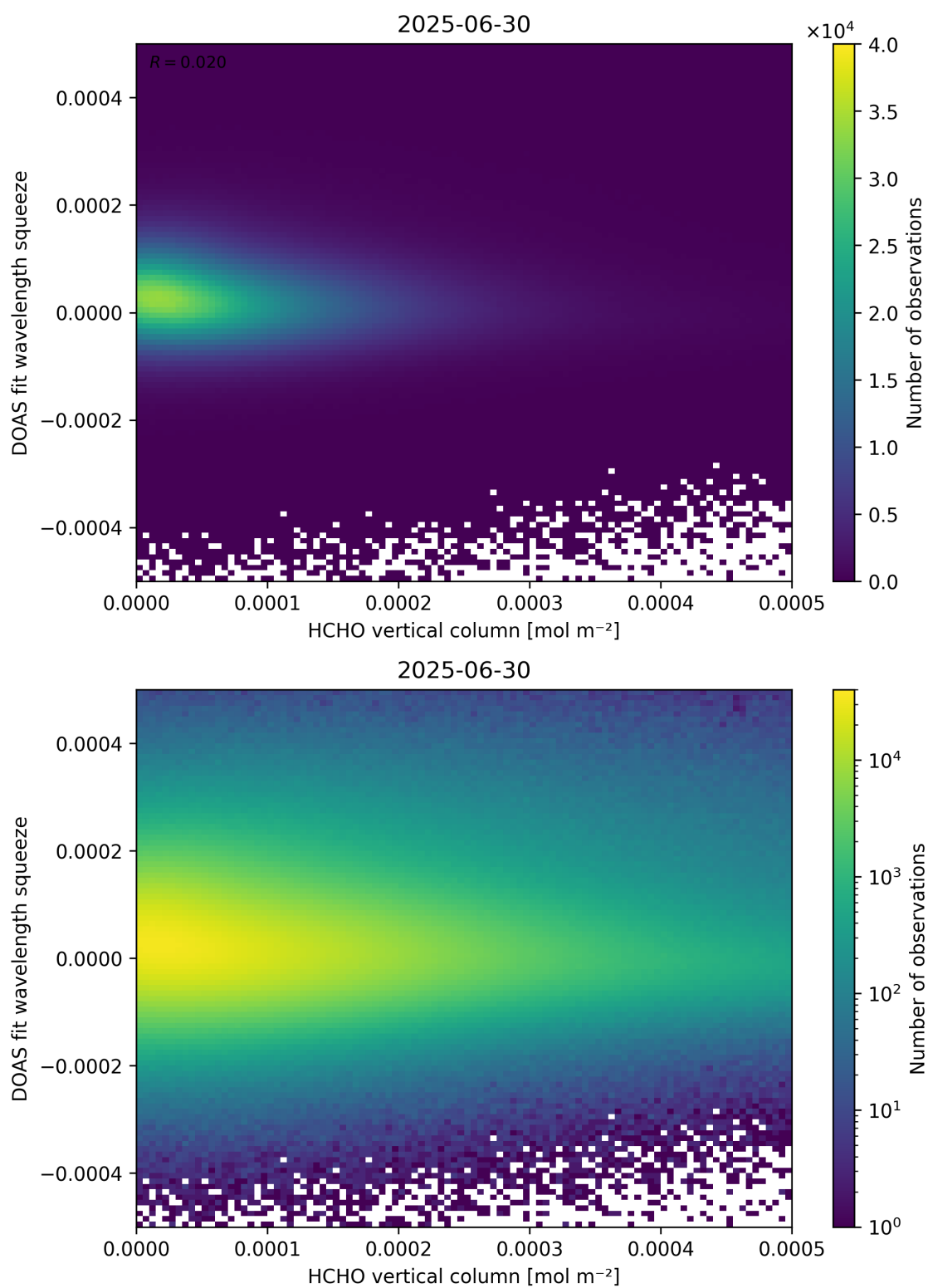
Figure 125: Scatter density plot of “HCHO vertical column” against “DOAS fit wavelength squeeze” for 2025-06-29 to 2025-07-01.
