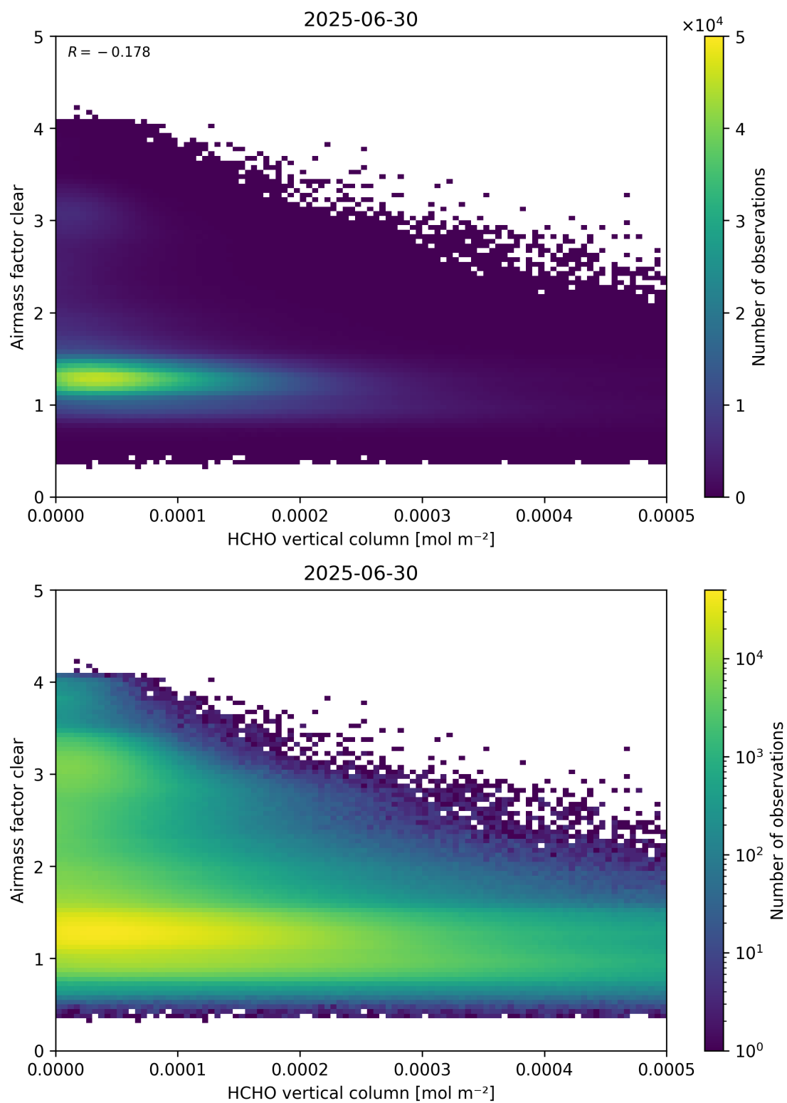
Figure 126: Scatter density plot of “HCHO vertical column” against “Airmass factor clear” for 2025-06-29 to 2025-07-01.
