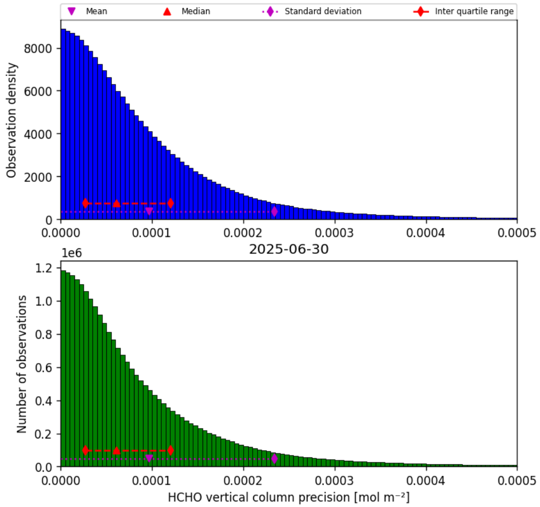
Figure 36: Histogram of “HCHO vertical column precision” for 2025-06-29 to 2025-07-01
