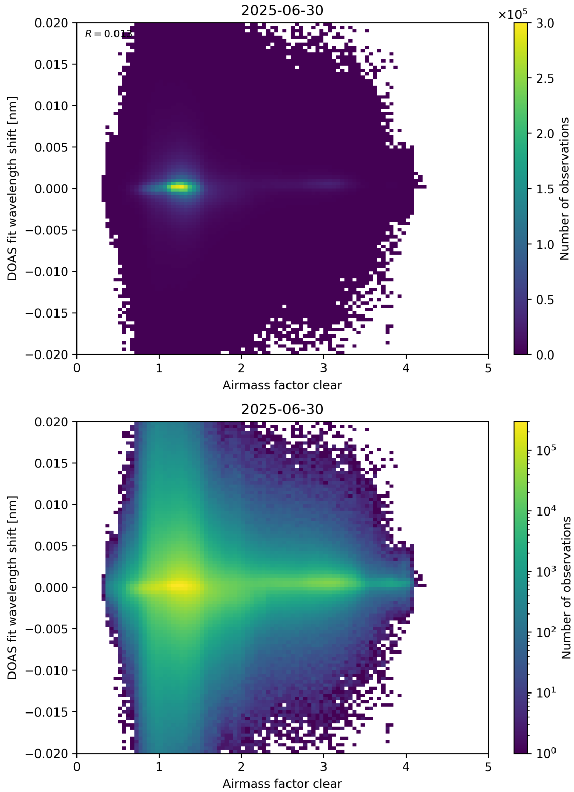
Figure 72: Scatter density plot of “Airmass factor clear” against “DOAS fit wavelength shift” for 2025-06-29 to 2025-07-01.
