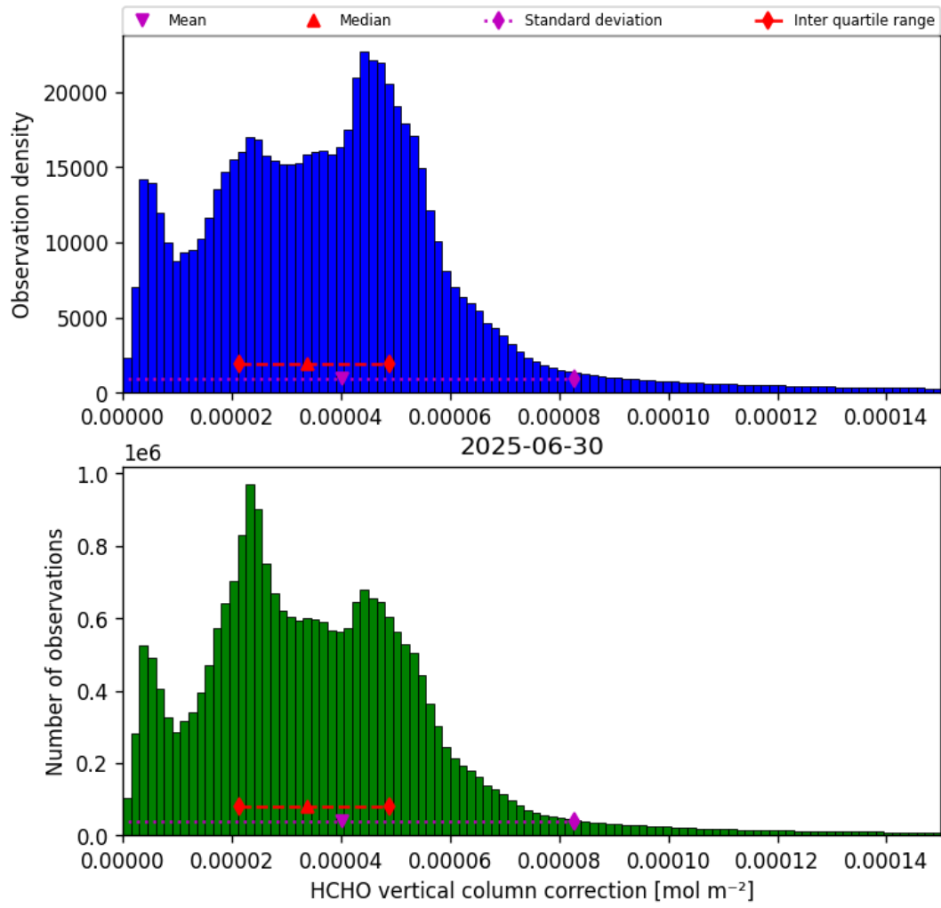
Figure 37: Histogram of “HCHO vertical column correction” for 2025-06-29 to 2025-07-01
