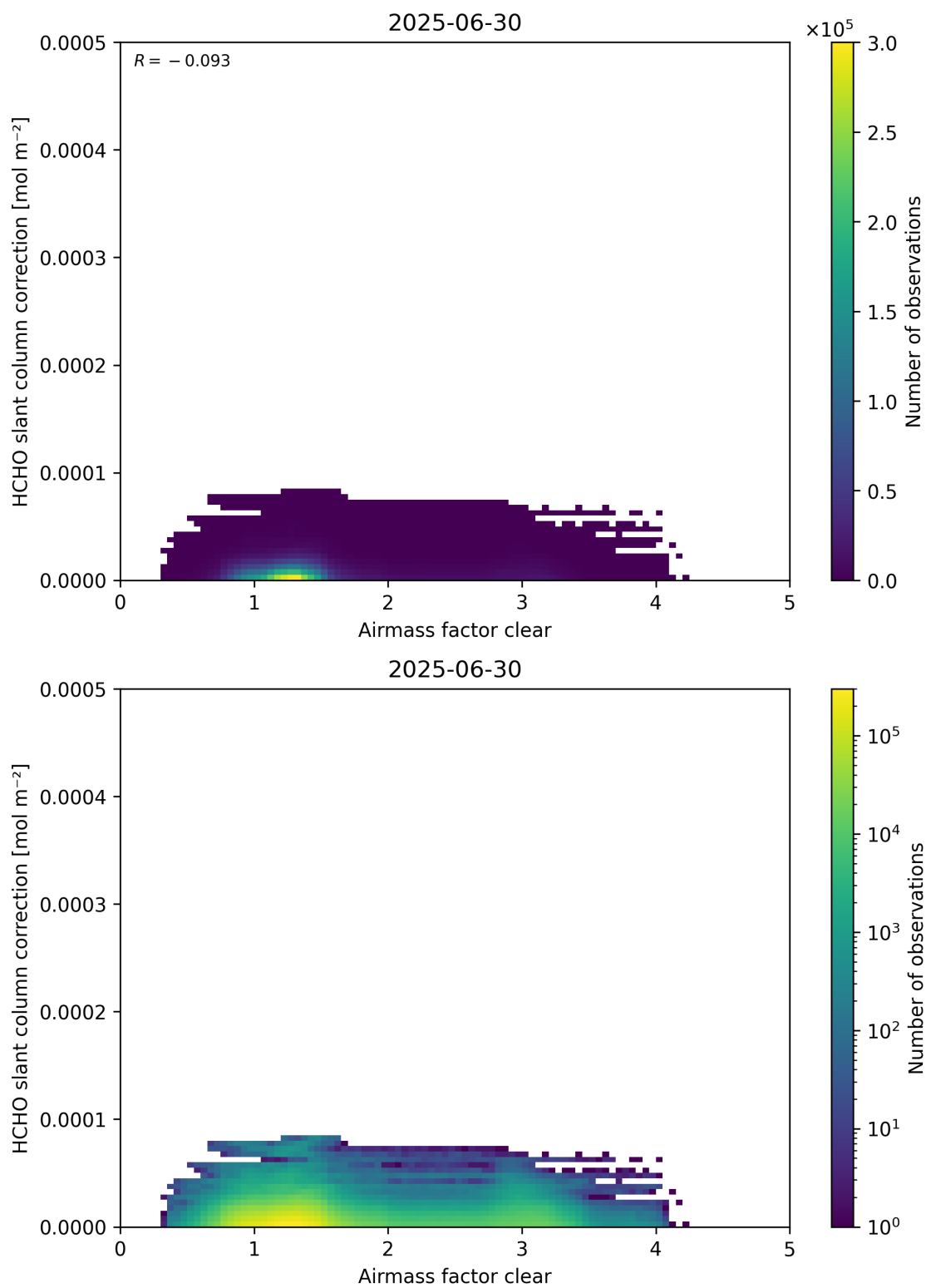
Figure 75: Scatter density plot of “Airmass factor clear” against “HCHO slant column correction” for 2025-06-29 to 2025-07-01.
