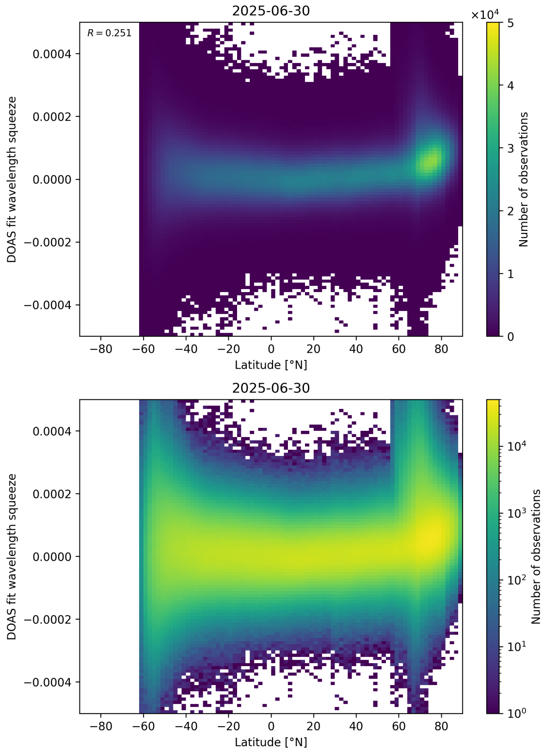
Figure 155: Scatter density plot of “Latitude” against “DOAS fit wavelength squeeze” for 2025-06-29 to 2025-07-01.
