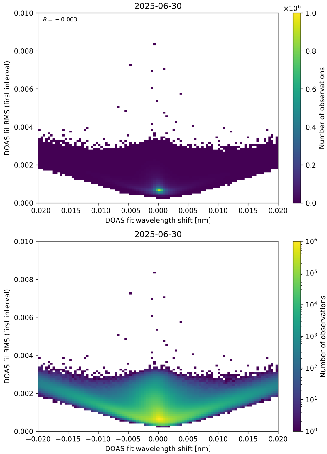
Figure 64: Scatter density plot of “DOAS fit wavelength shift” against “DOAS fit RMS (first interval)” for 2025-06-29 to 2025-07-01.
