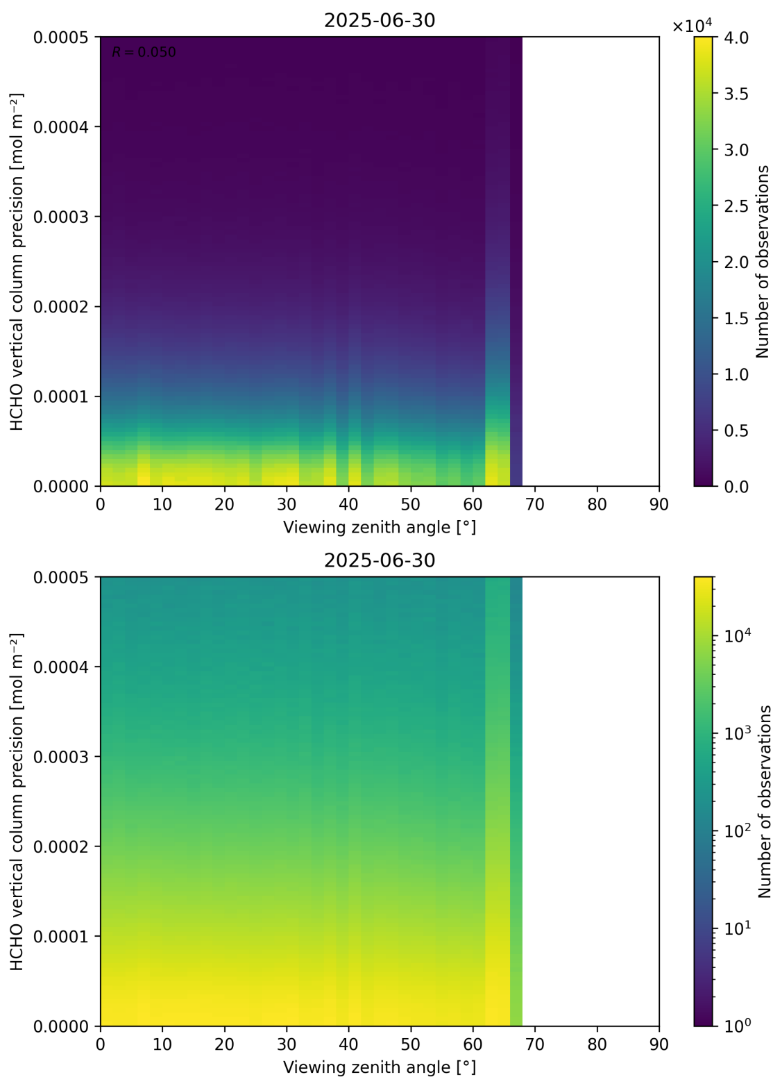
Figure 194: Scatter density plot of “Viewing zenith angle” against “HCHO vertical column precision” for 2025-06-29 to 2025-07-01.
