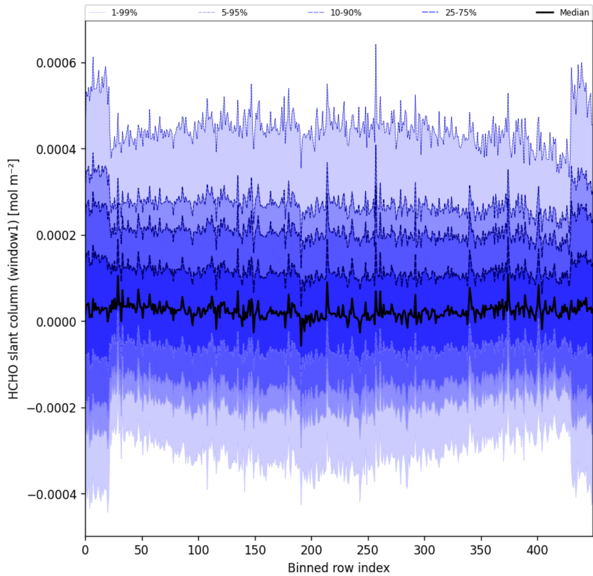
Figure 52: Along track statistics of “HCHO slant column (window1)” for 2025-06-29 to 2025-07-01
