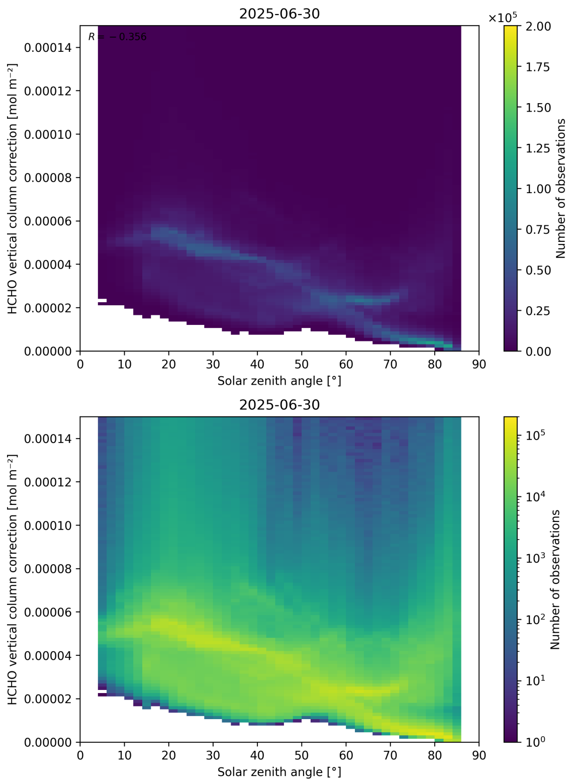
Figure 178: Scatter density plot of “Solar zenith angle” against “HCHO vertical column correction” for 2025-06-29 to 2025-07-01.
