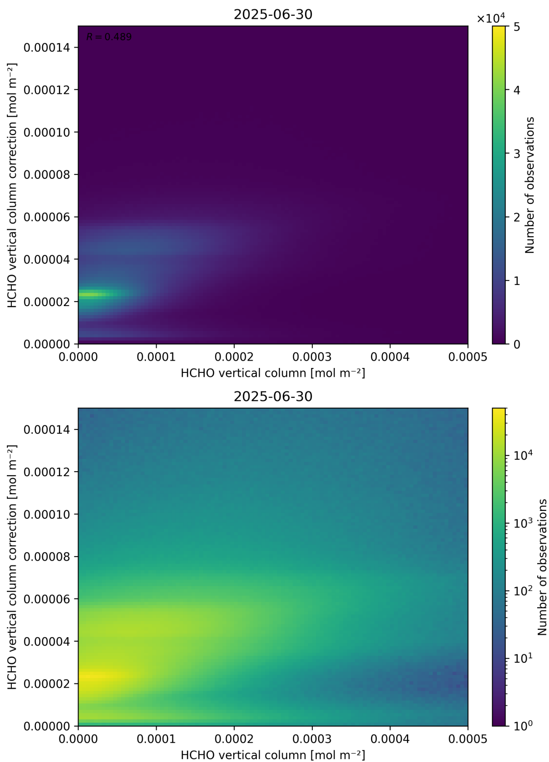
Figure 133: Scatter density plot of “HCHO vertical column” against “HCHO vertical column correction” for 2025-06-29 to 2025-07-01.
