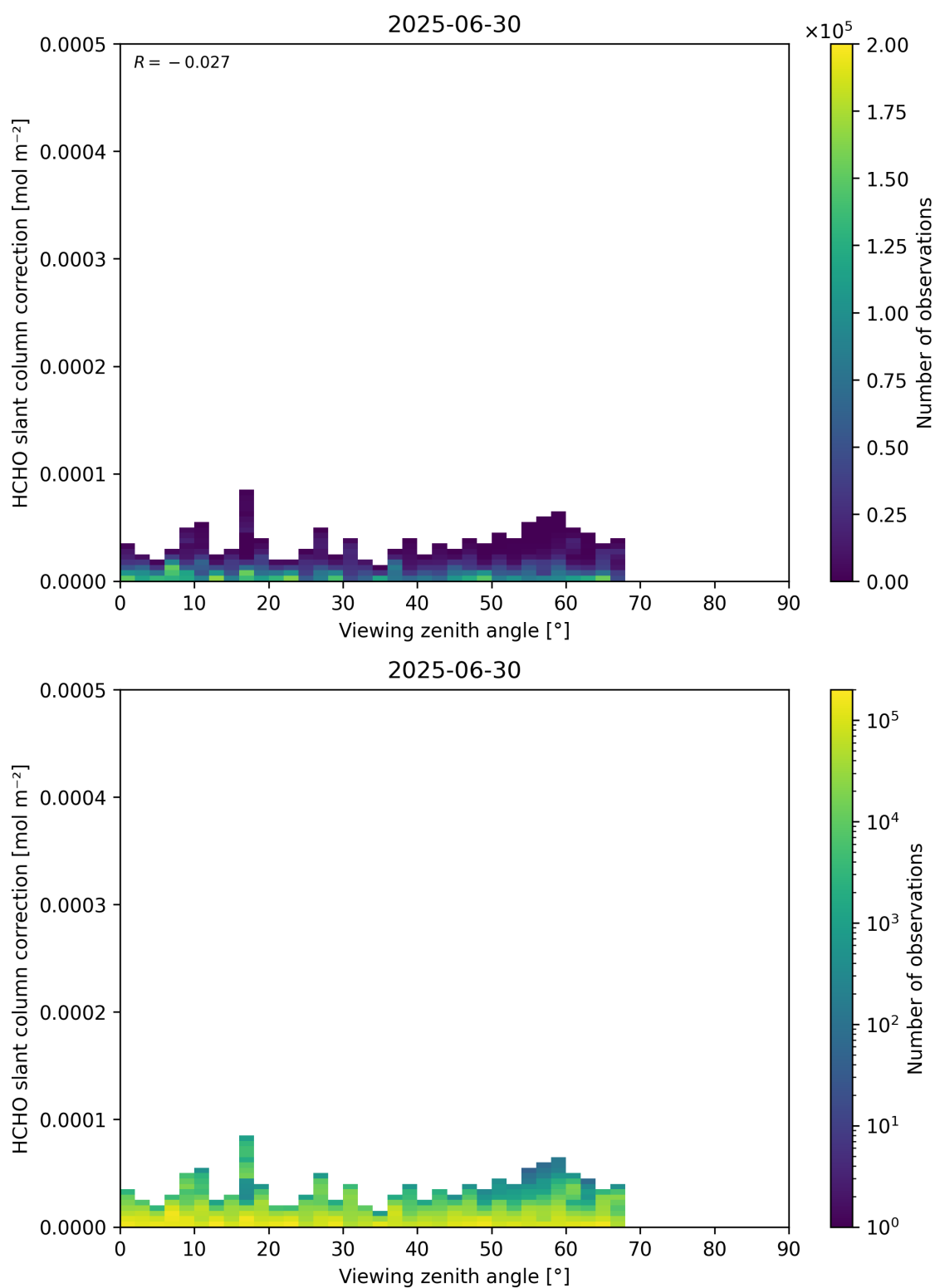
Figure 187: Scatter density plot of “Viewing zenith angle” against “HCHO slant column correction” for 2025-06-29 to 2025-07-01.
