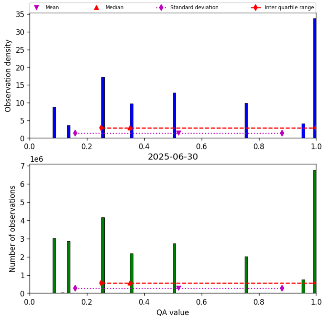
Figure 34: Histogram of “QA value” for 2025-06-29 to 2025-07-01
