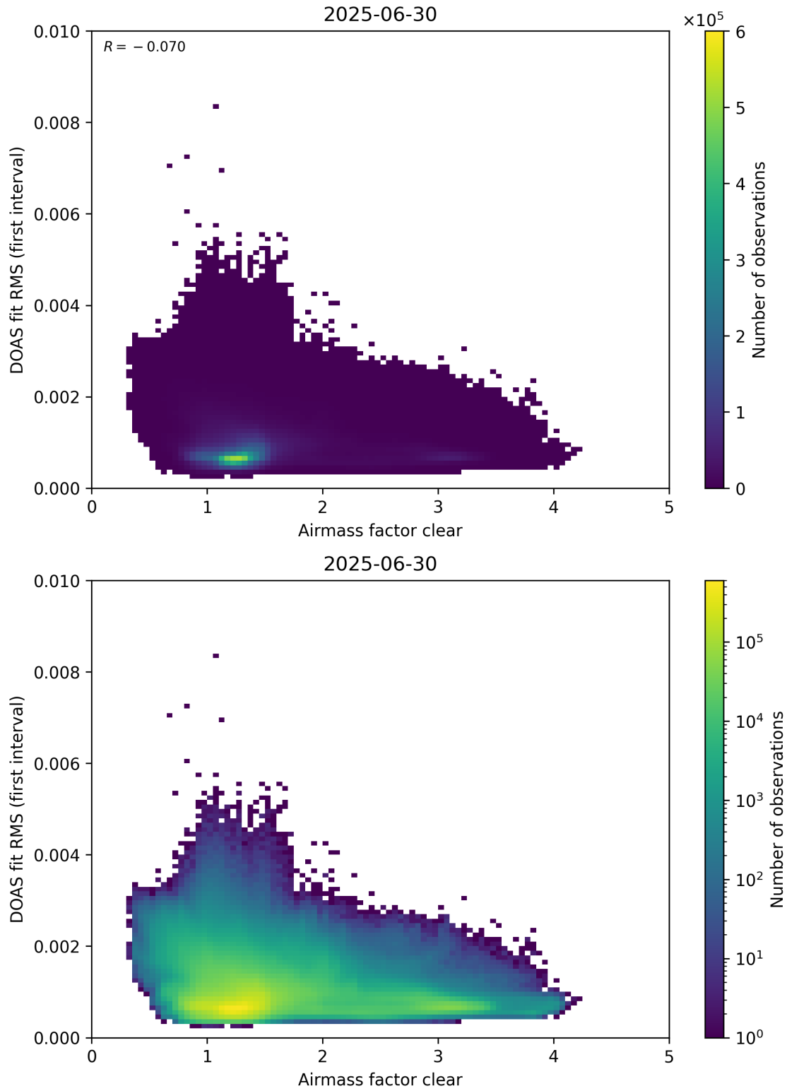
Figure 71: Scatter density plot of “Airmass factor clear” against “DOAS fit RMS (first interval)” for 2025-06-29 to 2025-07-01.
