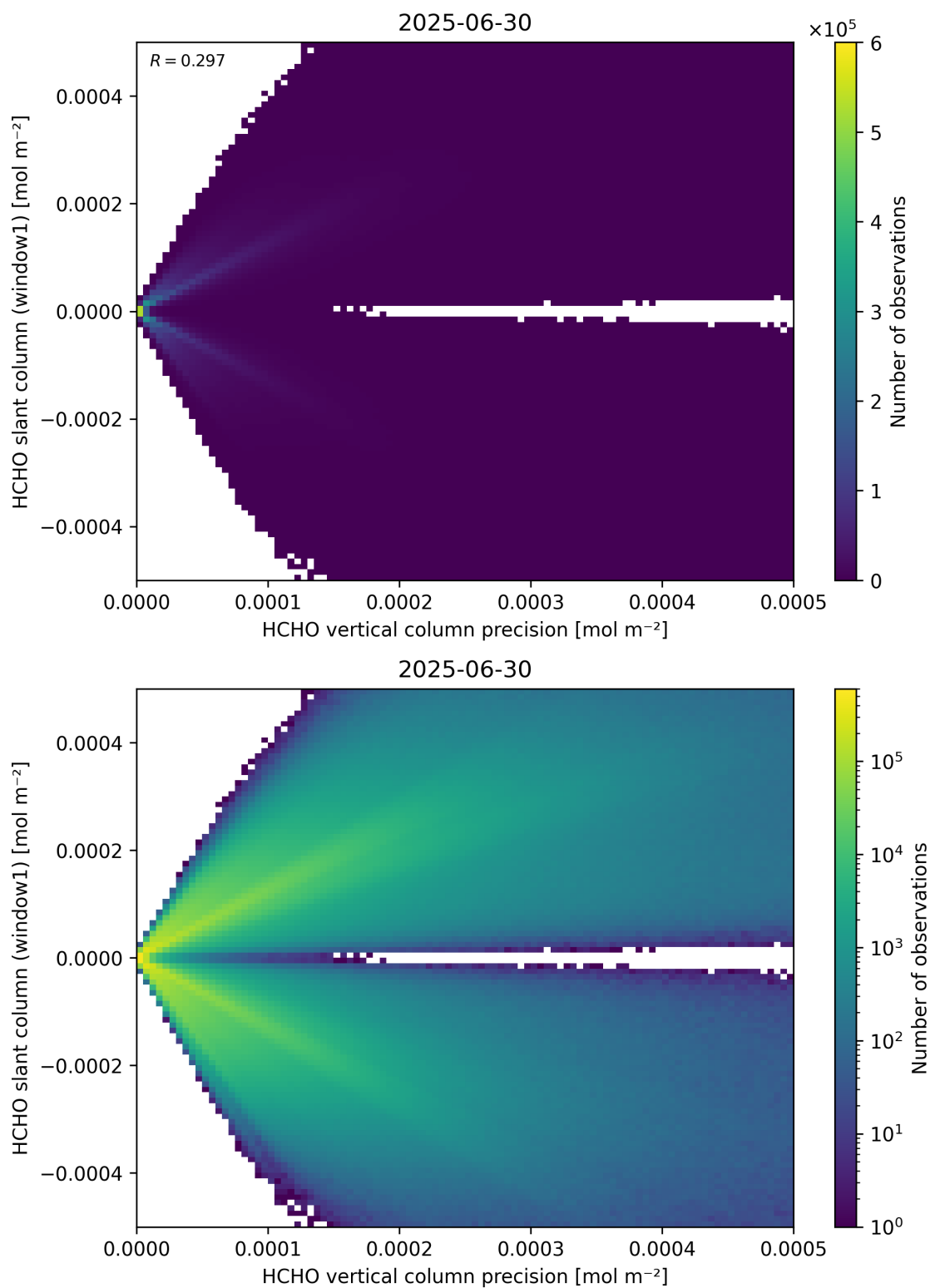
Figure 142: Scatter density plot of “HCHO vertical column precision” against “HCHO slant column (window1)” for 2025-06-29 to 2025-07-01.
