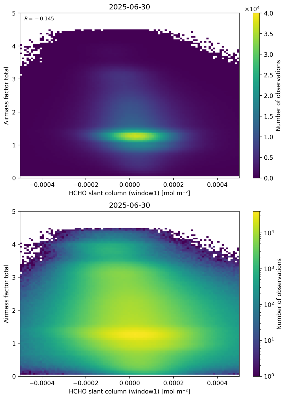
Figure 85: Scatter density plot of “HCHO slant column (window1)” against “Airmass factor total” for 2025-06-29 to 2025-07-01.
