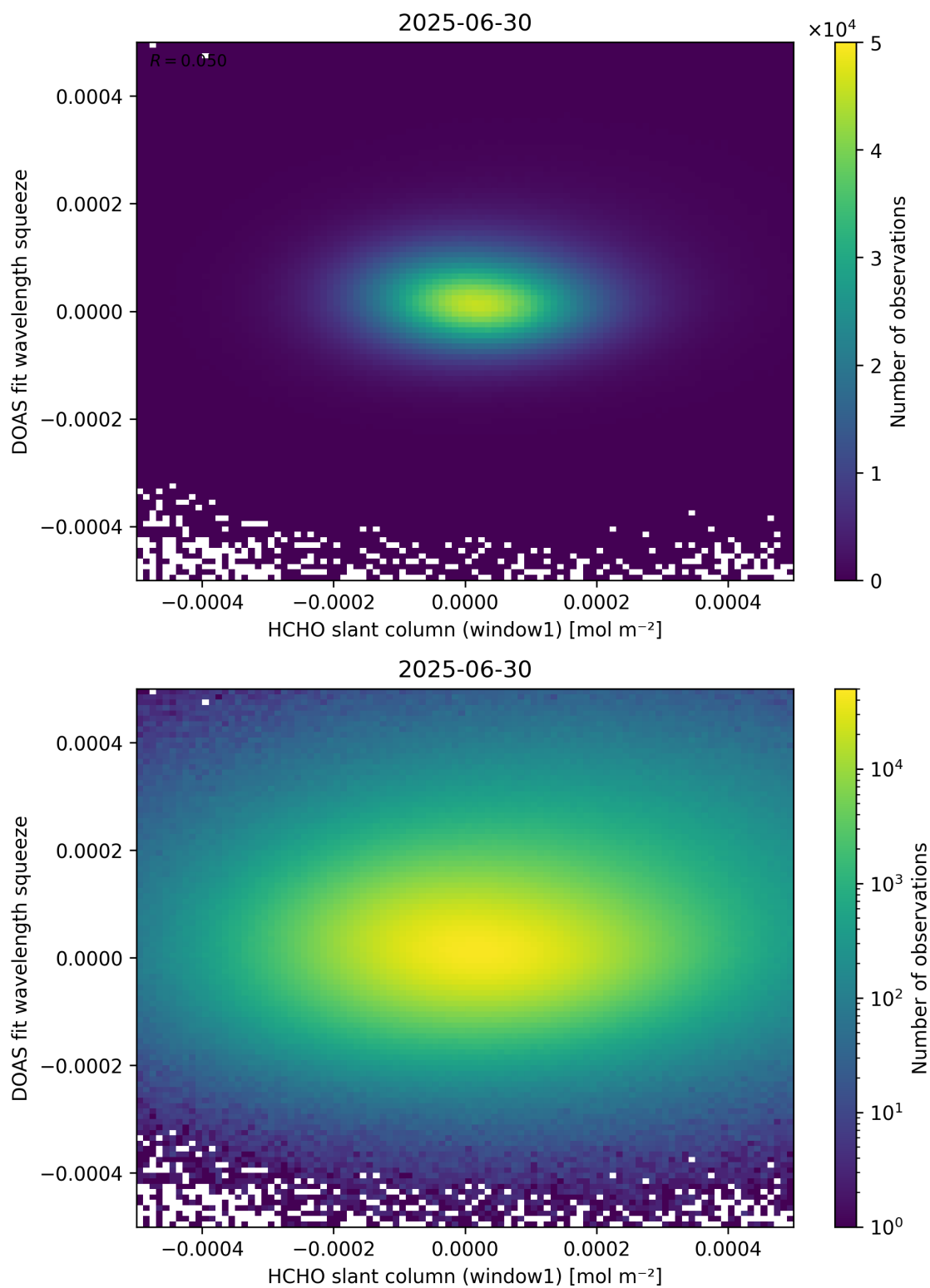
Figure 80: Scatter density plot of “HCHO slant column (window1)” against “DOAS fit wavelength squeeze” for 2025-06-29 to 2025-07-01.
