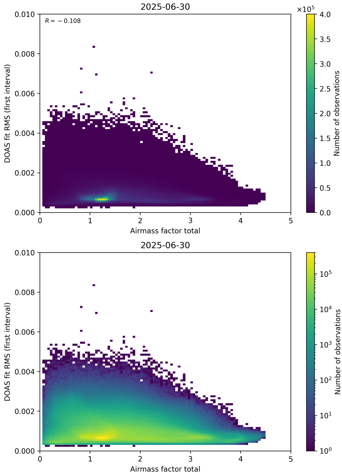
Figure 97: Scatter density plot of “Airmass factor total” against “DOAS fit RMS (first interval)” for 2025-06-29 to 2025-07-01.
