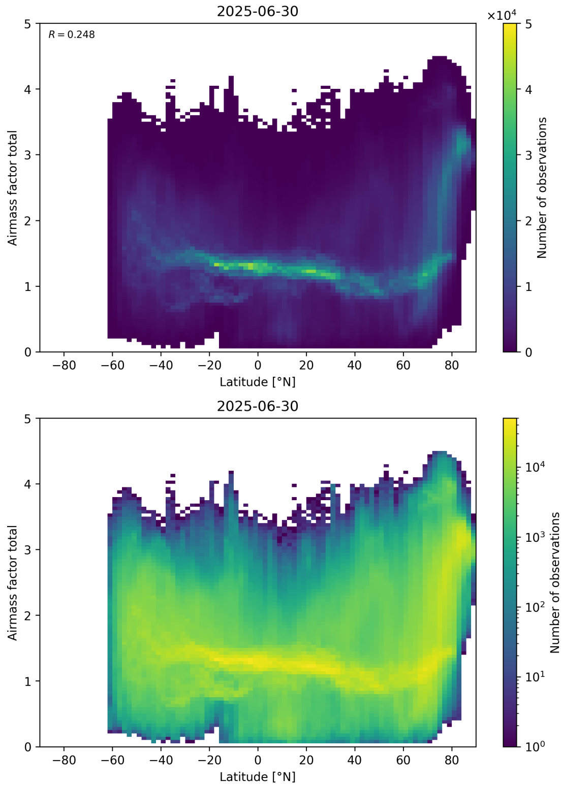
Figure 161: Scatter density plot of “Latitude” against “Airmass factor total” for 2025-06-29 to 2025-07-01.
