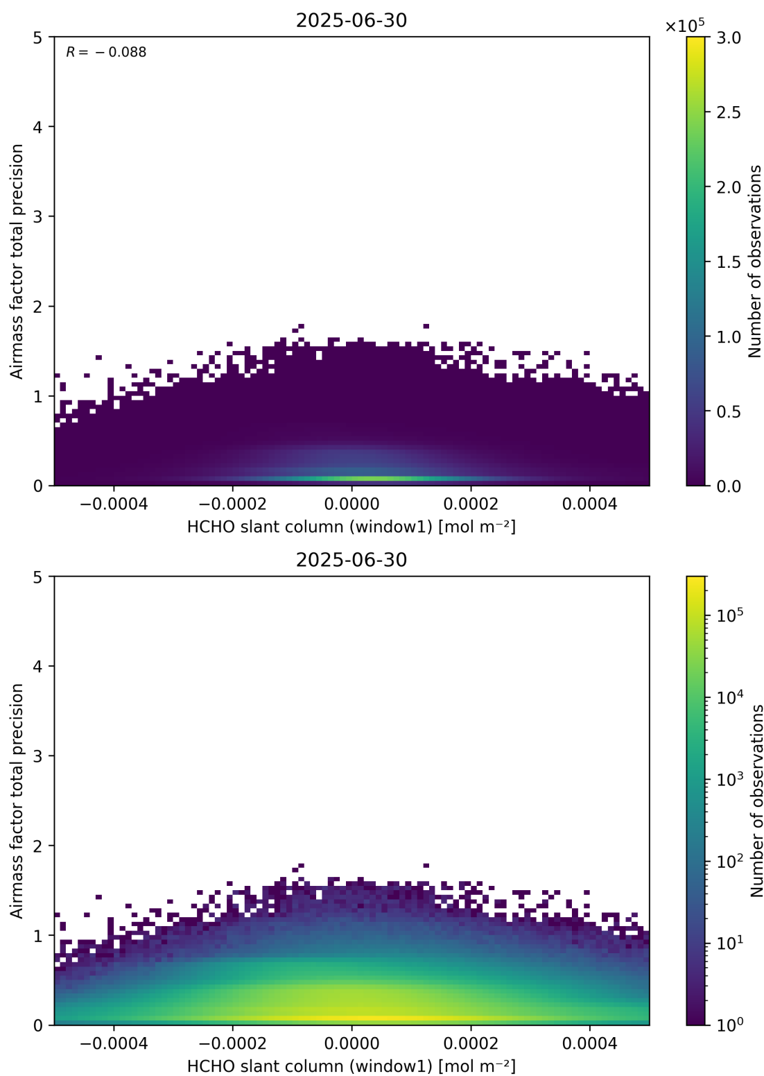
Figure 86: Scatter density plot of “HCHO slant column (window1)” against “Airmass factor total precision” for 2025-06-29 to 2025-07-01.
