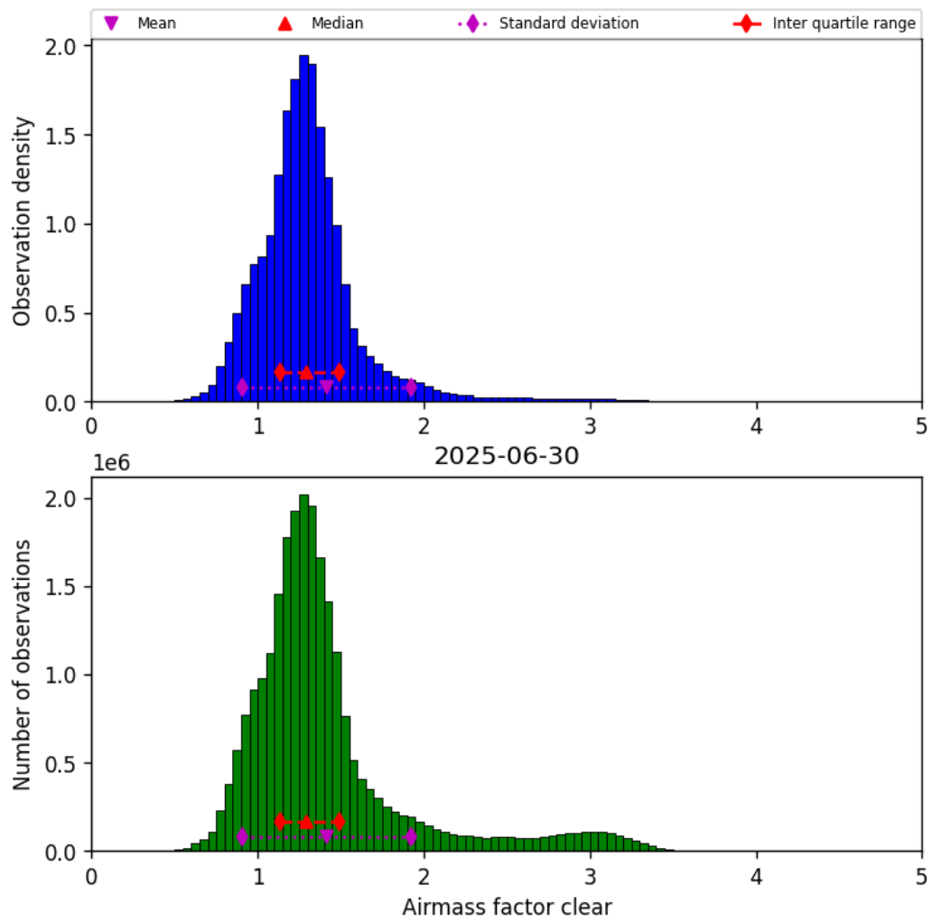
Figure 42: Histogram of “Airmass factor clear” for 2025-06-29 to 2025-07-01
