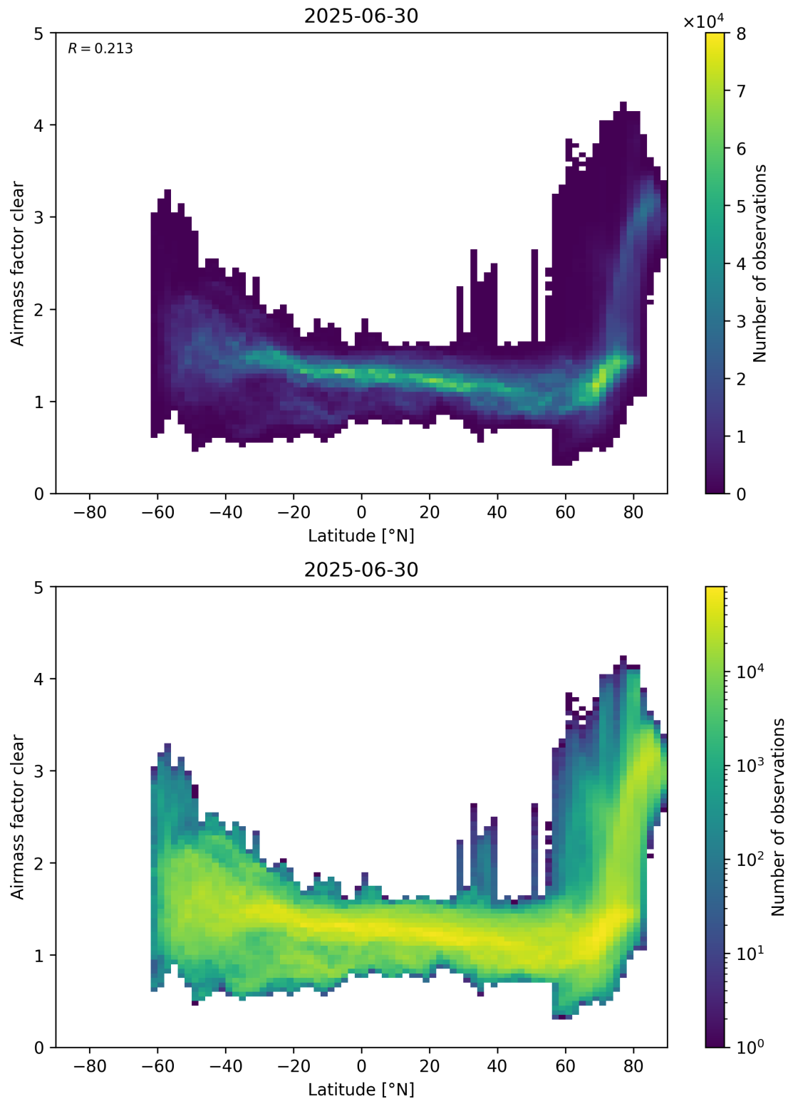
Figure 156: Scatter density plot of “Latitude” against “Airmass factor clear” for 2025-06-29 to 2025-07-01.
