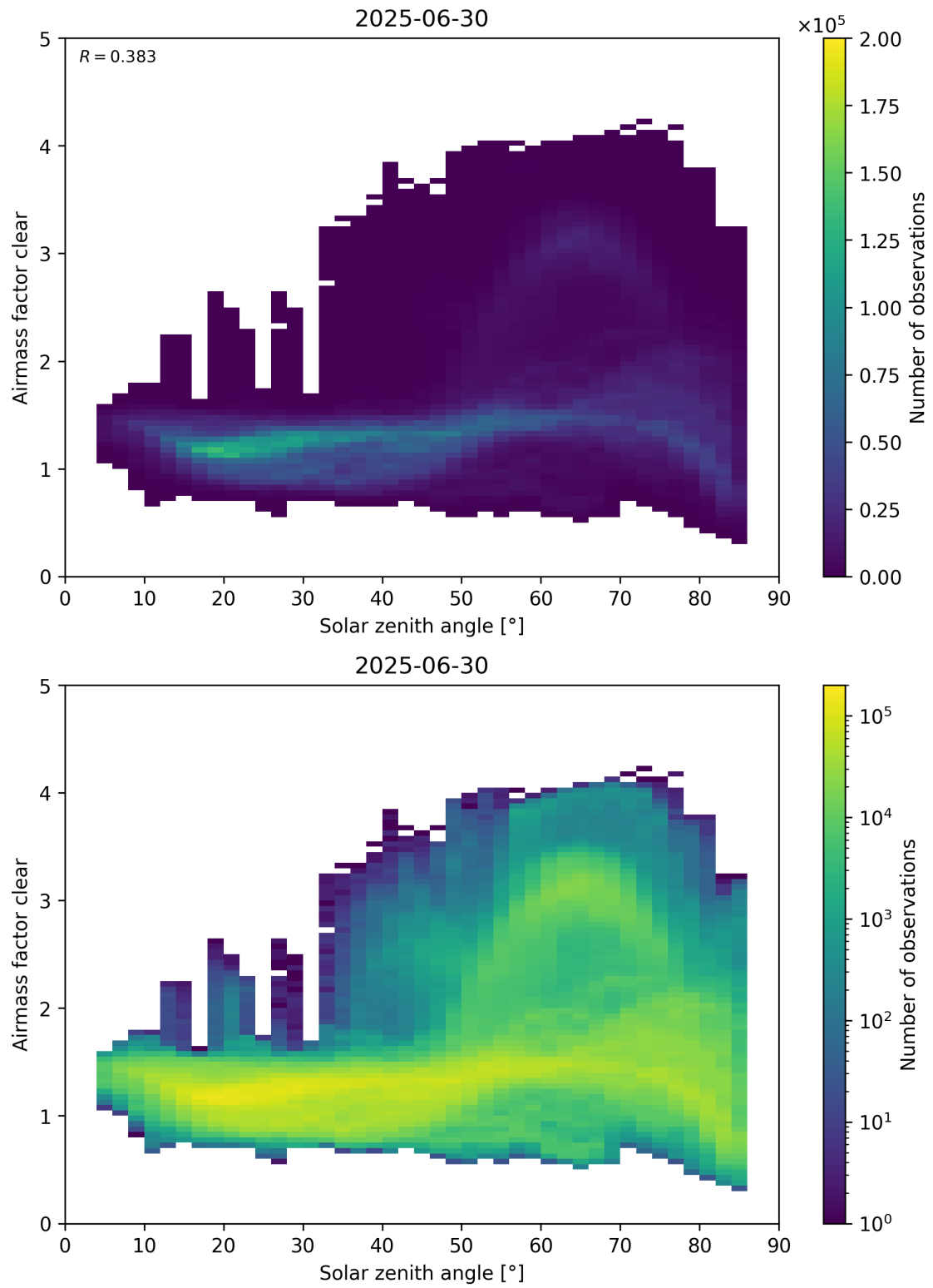
Figure 170: Scatter density plot of “Solar zenith angle” against “Airmass factor clear” for 2025-06-29 to 2025-07-01.
