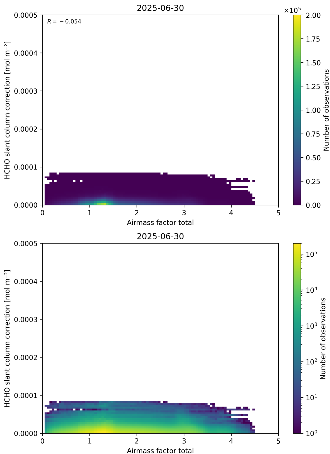
Figure 102: Scatter density plot of “Airmass factor total” against “HCHO slant column correction” for 2025-06-29 to 2025-07-01.
