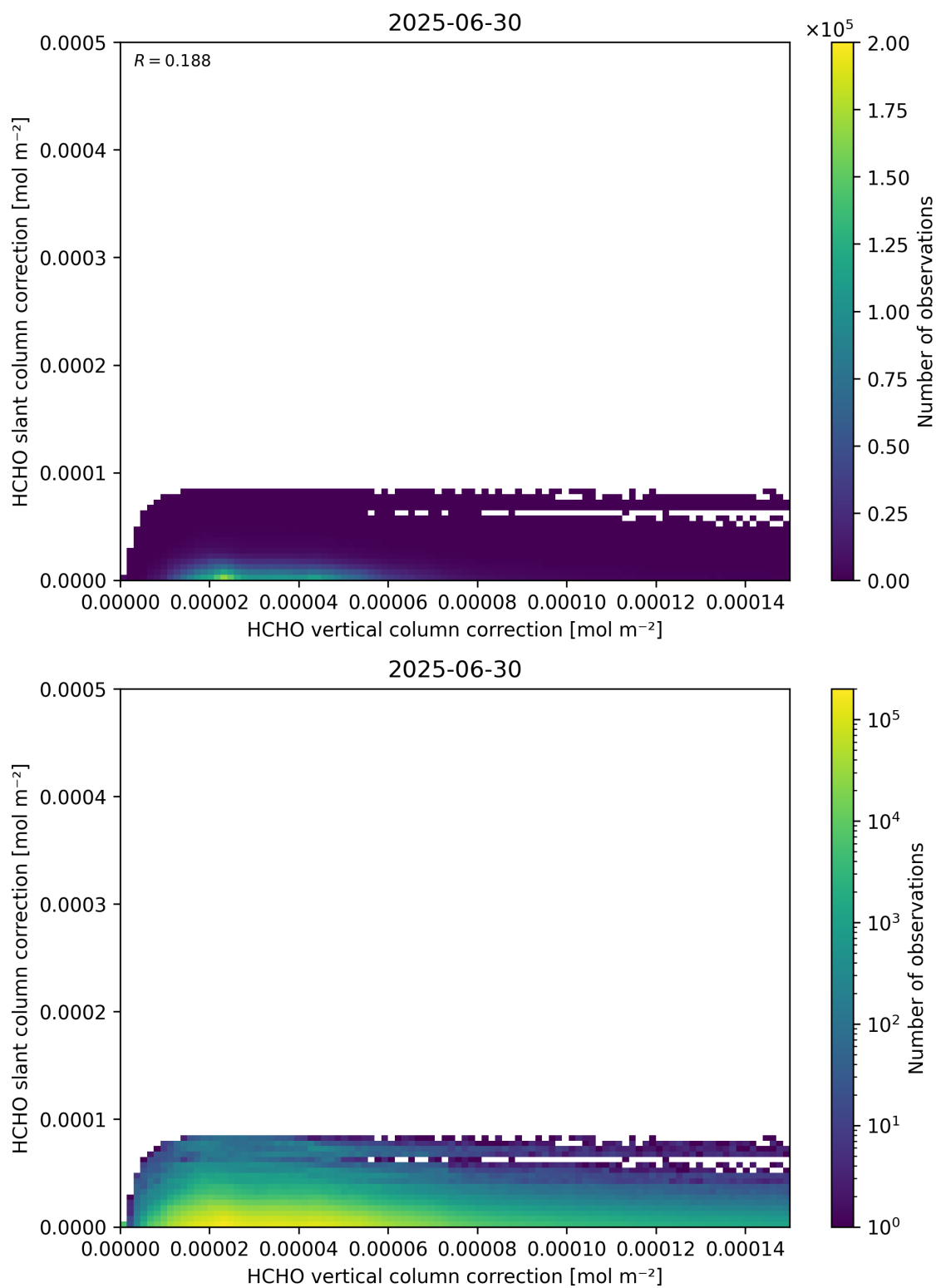
Figure 117: Scatter density plot of “HCHO vertical column correction” against “HCHO slant column correction” for 2025-06-29 to 2025-07-01.
