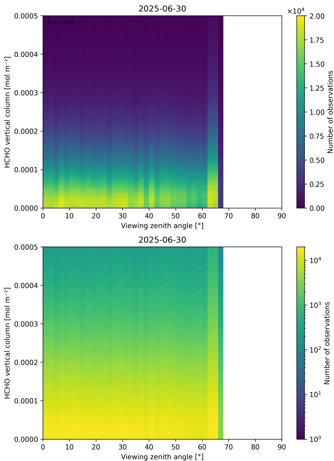
Figure 192: Scatter density plot of “Viewing zenith angle” against “HCHO vertical column” for 2025-06-29 to 2025-07-01.
