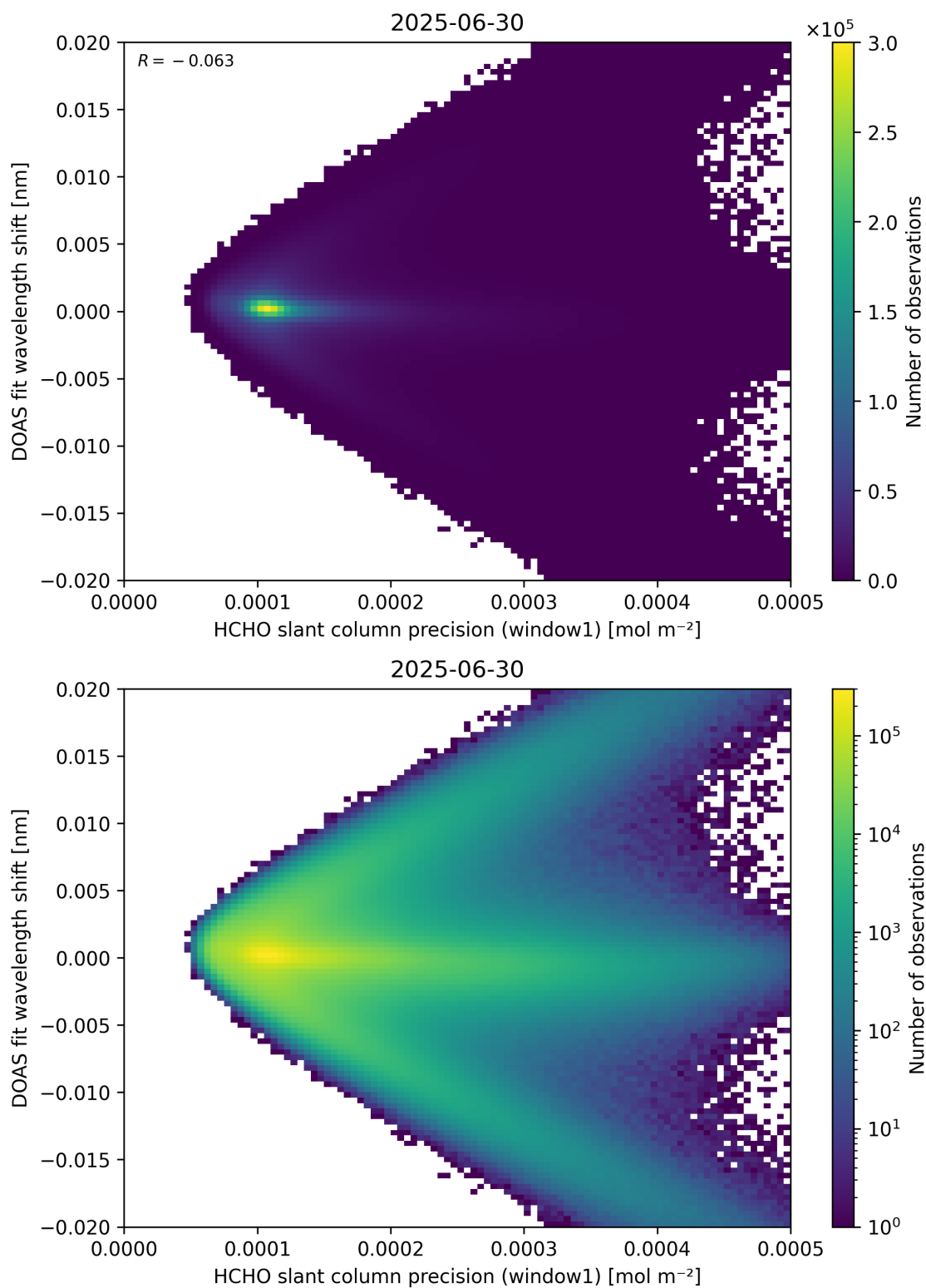
Figure 89: Scatter density plot of “HCHO slant column precision (window1)” against “DOAS fit wavelength shift” for 2025-06-29 to 2025-07-01.
