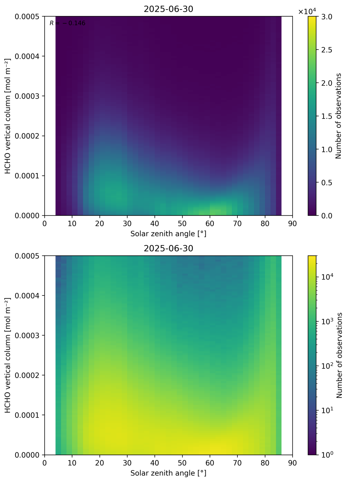
Figure 177: Scatter density plot of “Solar zenith angle” against “HCHO vertical column” for 2025-06-29 to 2025-07-01.
