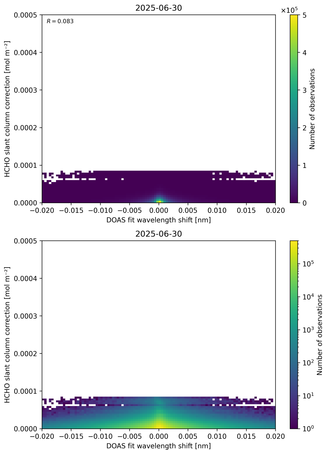
Figure 67: Scatter density plot of “DOAS fit wavelength shift” against “HCHO slant column correction” for 2025-06-29 to 2025-07-01.
