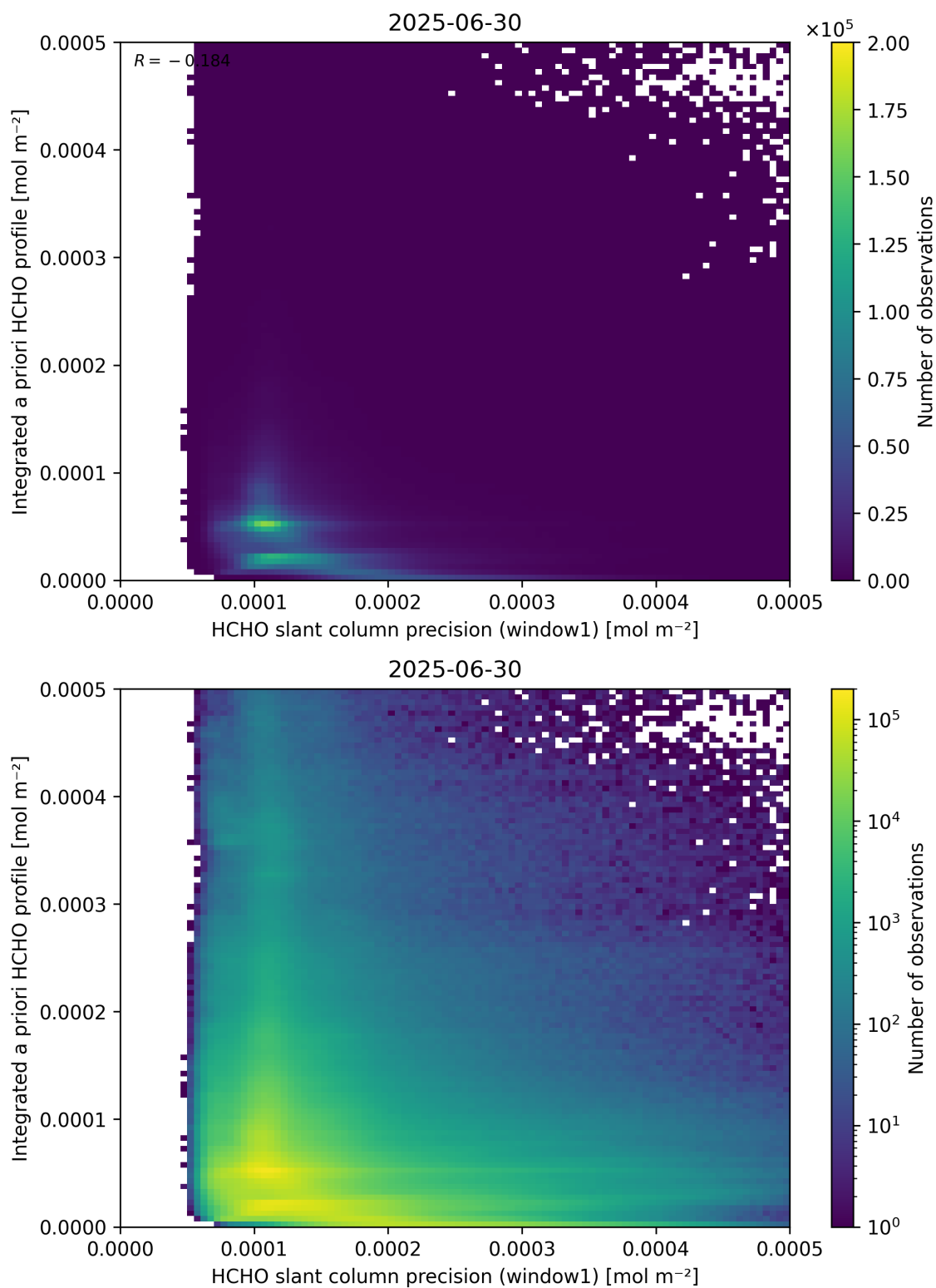
Figure 96: Scatter density plot of “HCHO slant column precision (window1)” against “Integrated a priori HCHO profile” for 2025-06-29 to 2025-07-01.
