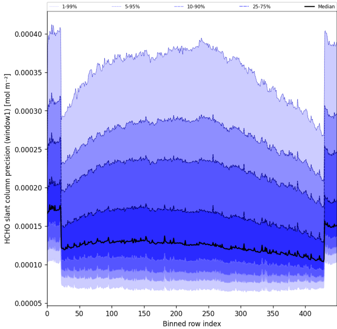
Figure 53: Along track statistics of “HCHO slant column precision (window1)” for 2025-06-29 to 2025-07-01
