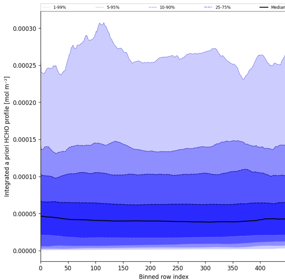
Figure 57: Along track statistics of “Integrated a priori HCHO profile” for 2025-06-29 to 2025-07-01
