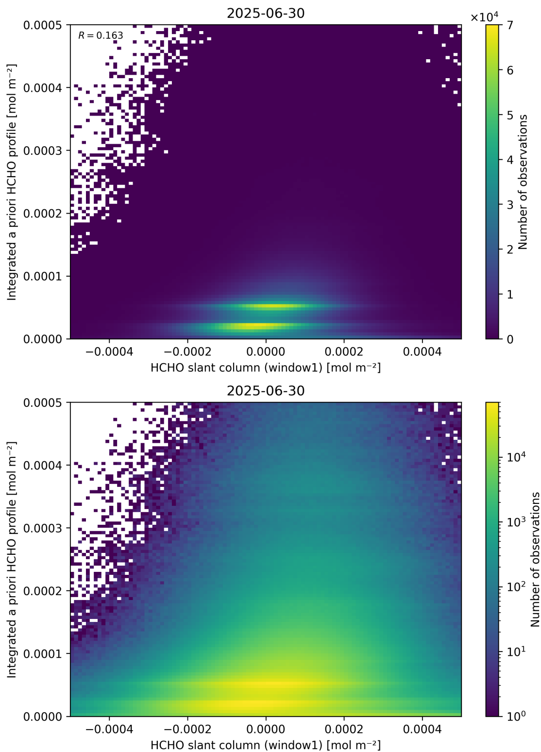
Figure 87: Scatter density plot of “HCHO slant column (window1)” against “Integrated a priori HCHO profile” for 2025-06-29 to 2025-07-01.
