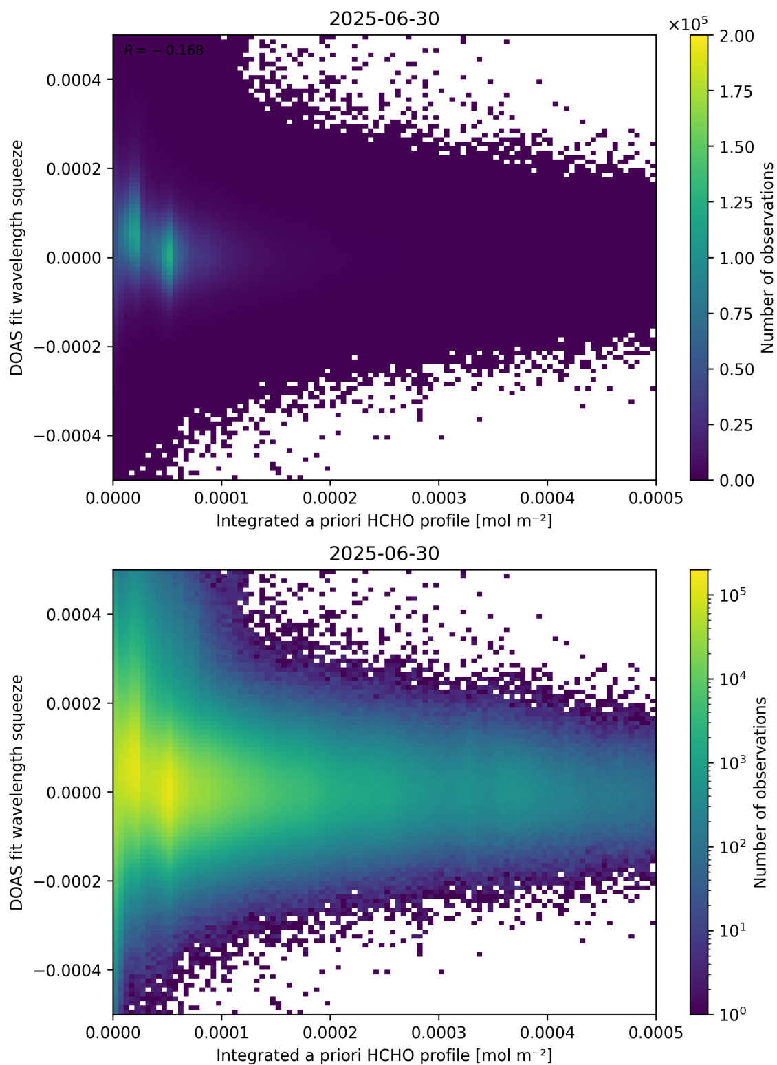
Figure 150: Scatter density plot of “Integrated a priori HCHO profile” against “DOAS fit wavelength squeeze” for 2025-06-29 to 2025-07-01.
