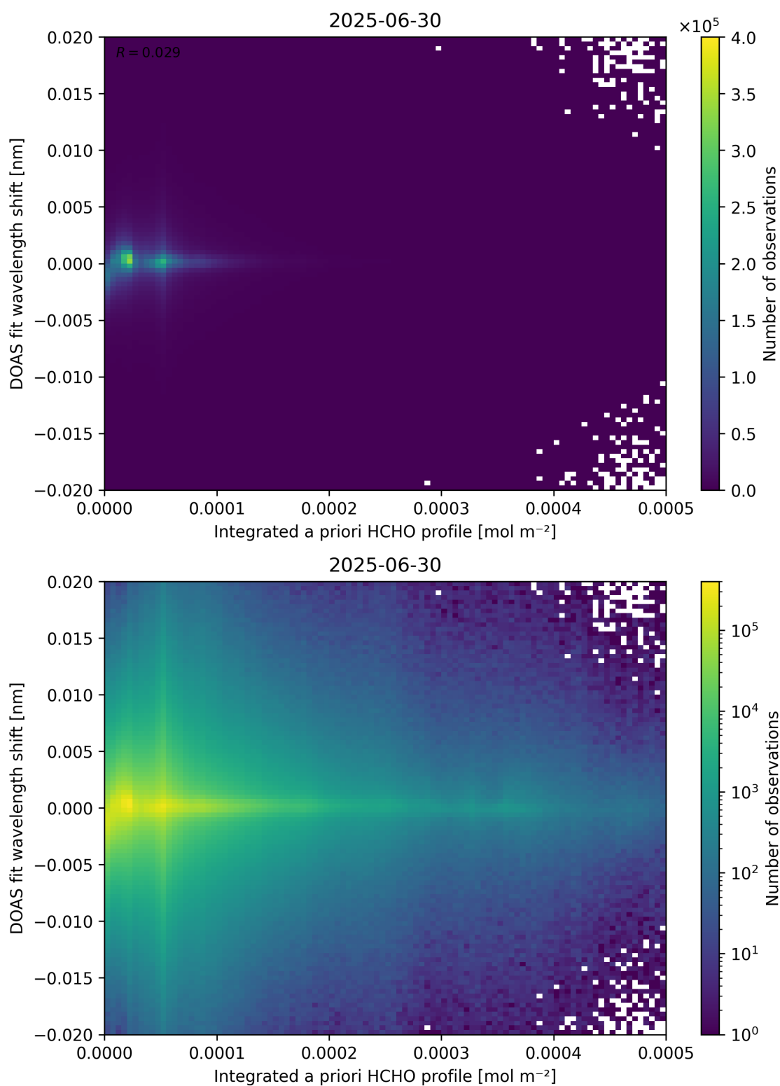
Figure 149: Scatter density plot of “Integrated a priori HCHO profile” against “DOAS fit wavelength shift” for 2025-06-29 to 2025-07-01.
