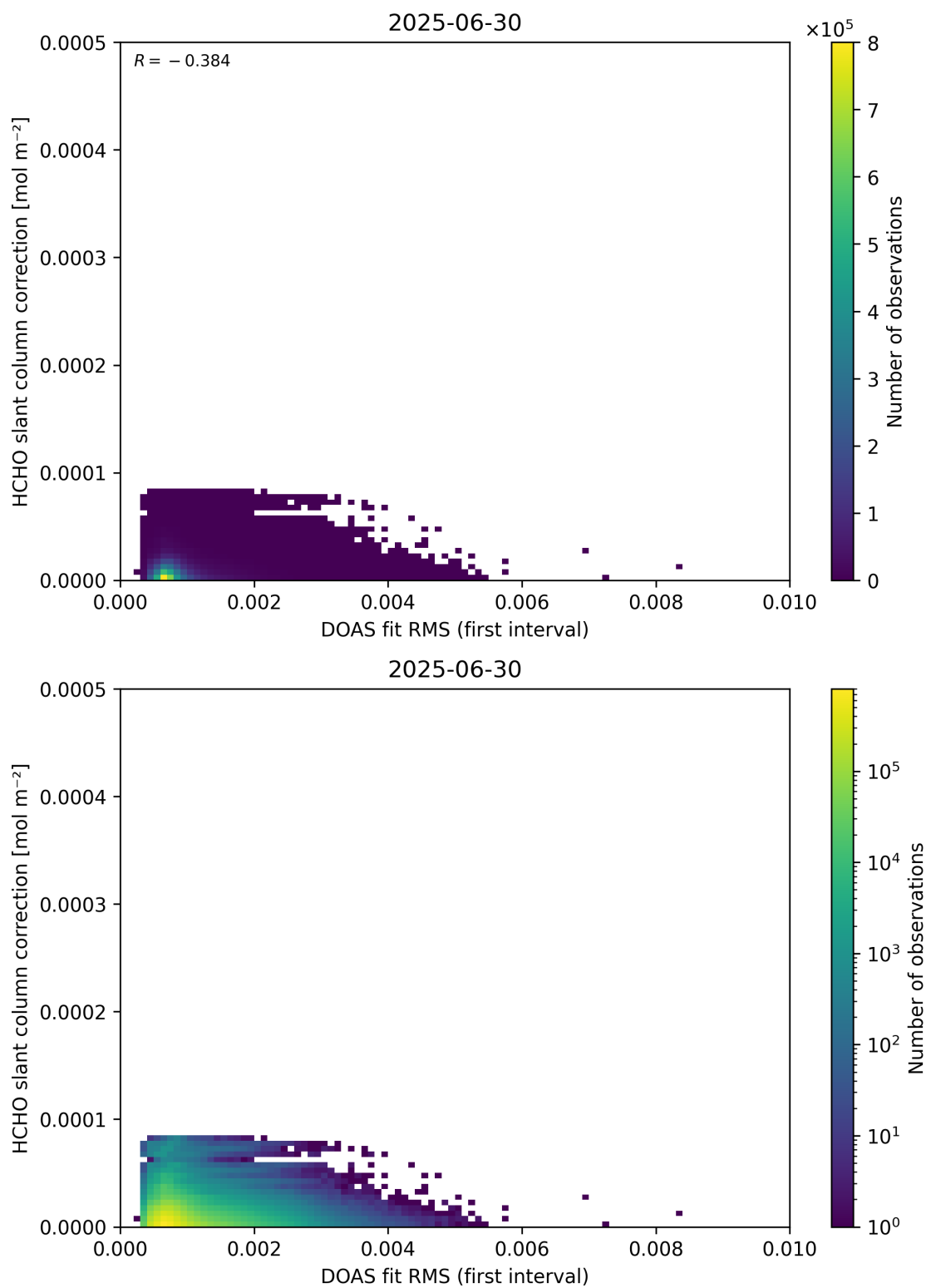
Figure 63: Scatter density plot of “DOAS fit RMS (first interval)” against “HCHO slant column correction” for 2025-06-29 to 2025-07-01.
