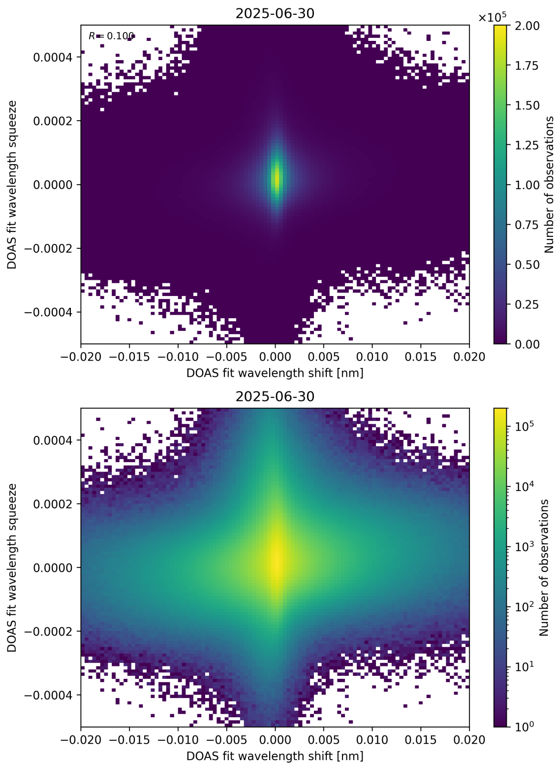
Figure 65: Scatter density plot of “DOAS fit wavelength shift” against “DOAS fit wavelength squeeze” for 2025-06-29 to 2025-07-01.
