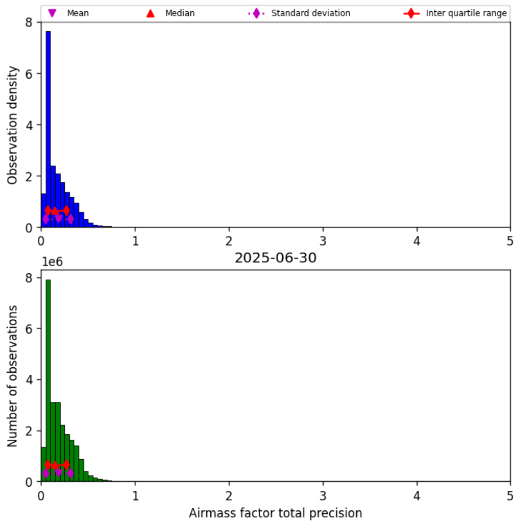
Figure 41: Histogram of “Airmass factor total precision” for 2025-06-29 to 2025-07-01
