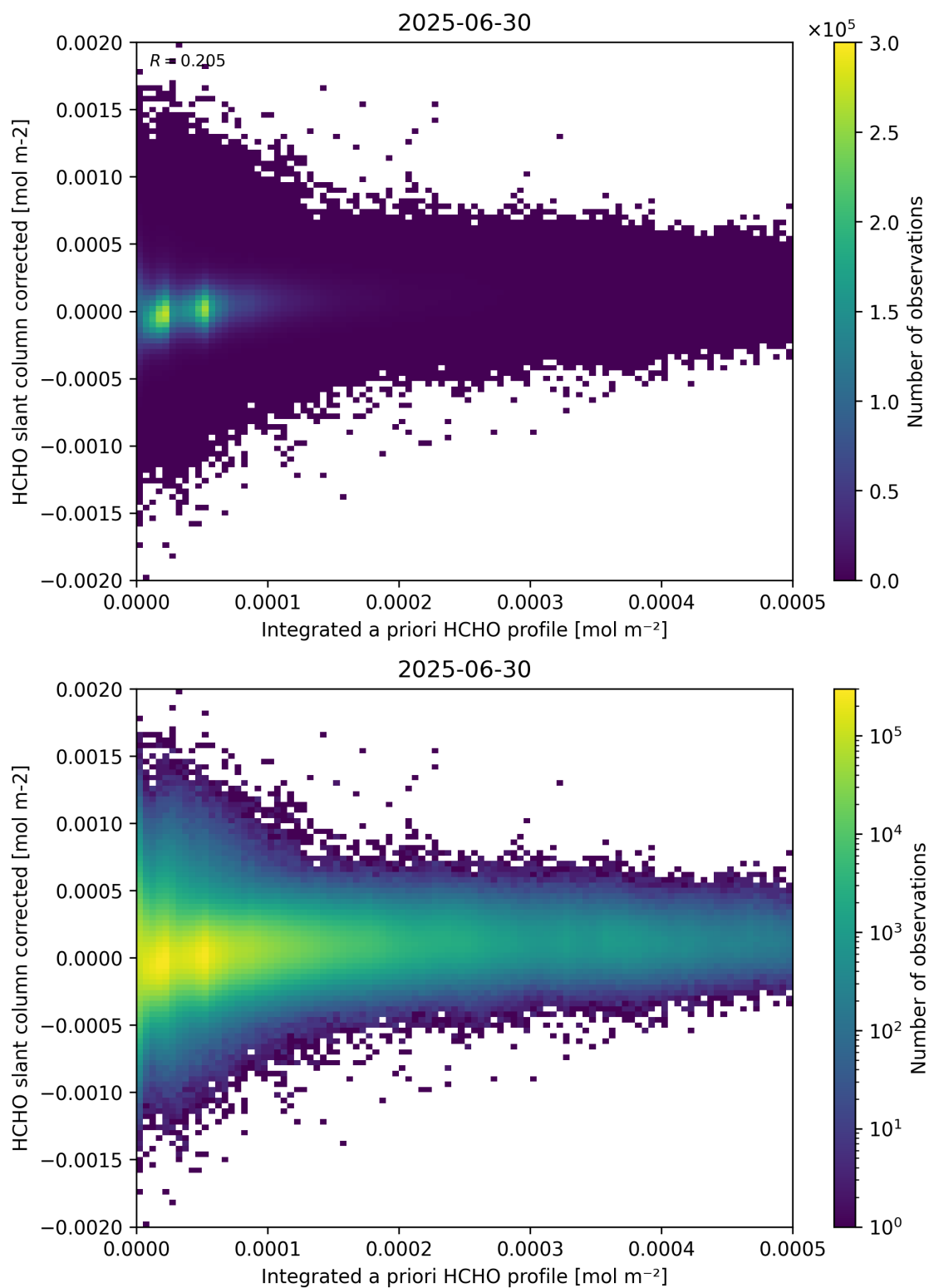
Figure 151: Scatter density plot of “Integrated a priori HCHO profile” against “HCHO slant column corrected” for 2025-06-29 to 2025-07-01.
