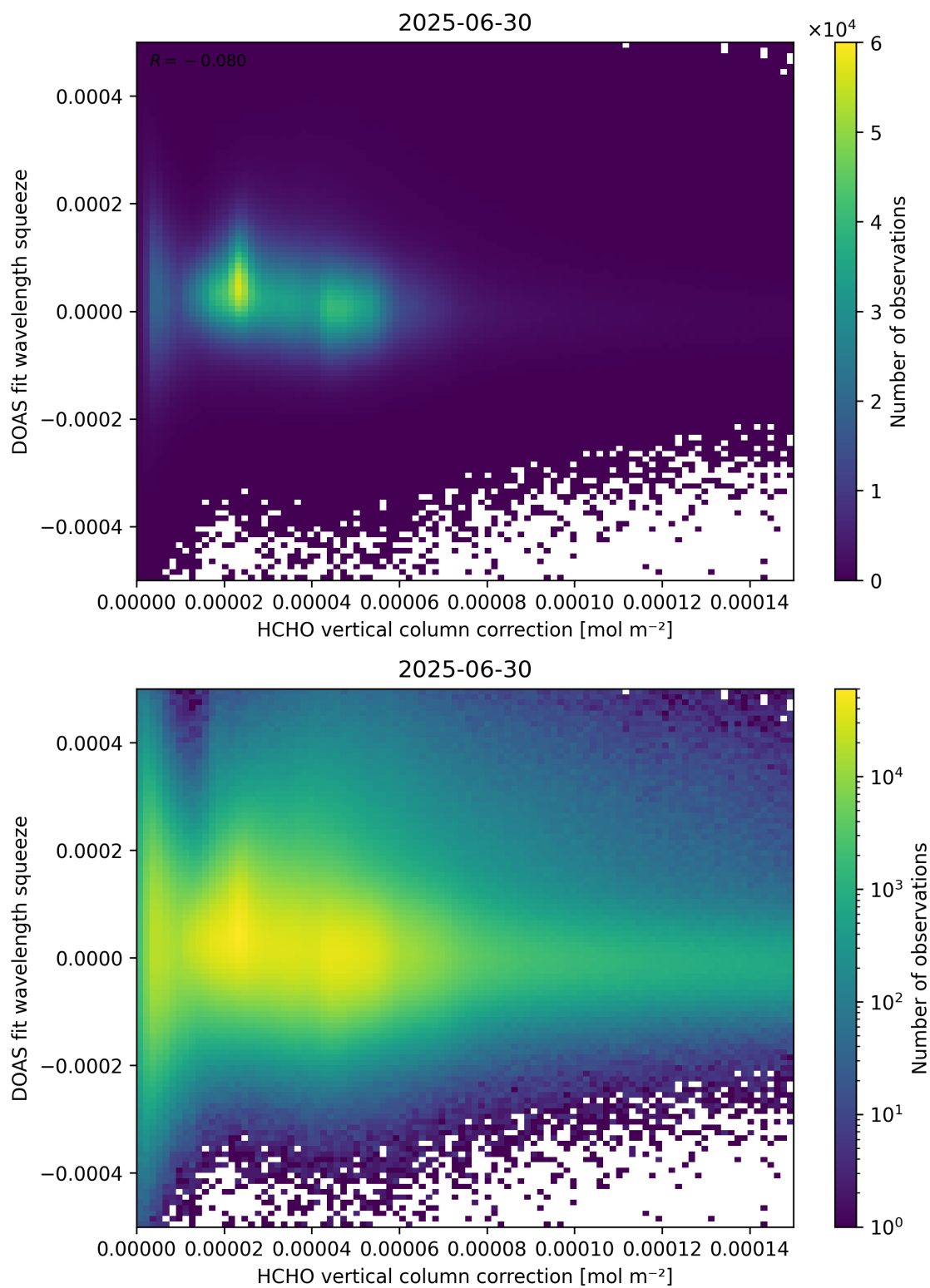
Figure 114: Scatter density plot of “HCHO vertical column correction” against “DOAS fit wavelength squeeze” for 2025-06-29 to 2025-07-01.
