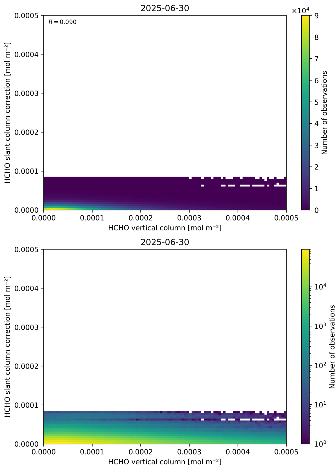
Figure 128: Scatter density plot of “HCHO vertical column” against “HCHO slant column correction” for 2025-06-29 to 2025-07-01.
