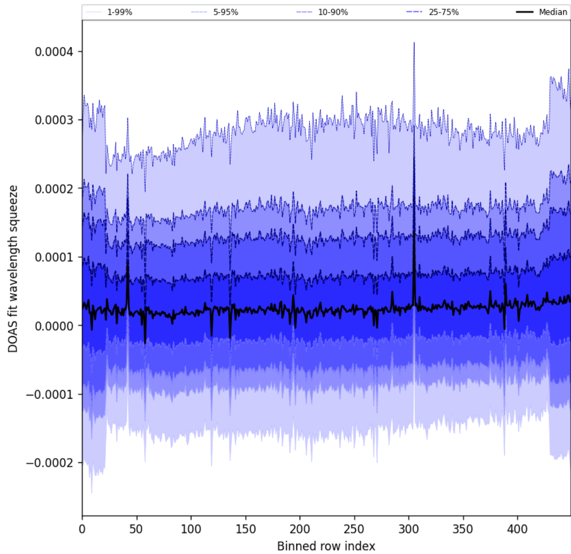
Figure 59: Along track statistics of “DOAS fit wavelength squeeze” for 2025-06-29 to 2025-07-01
