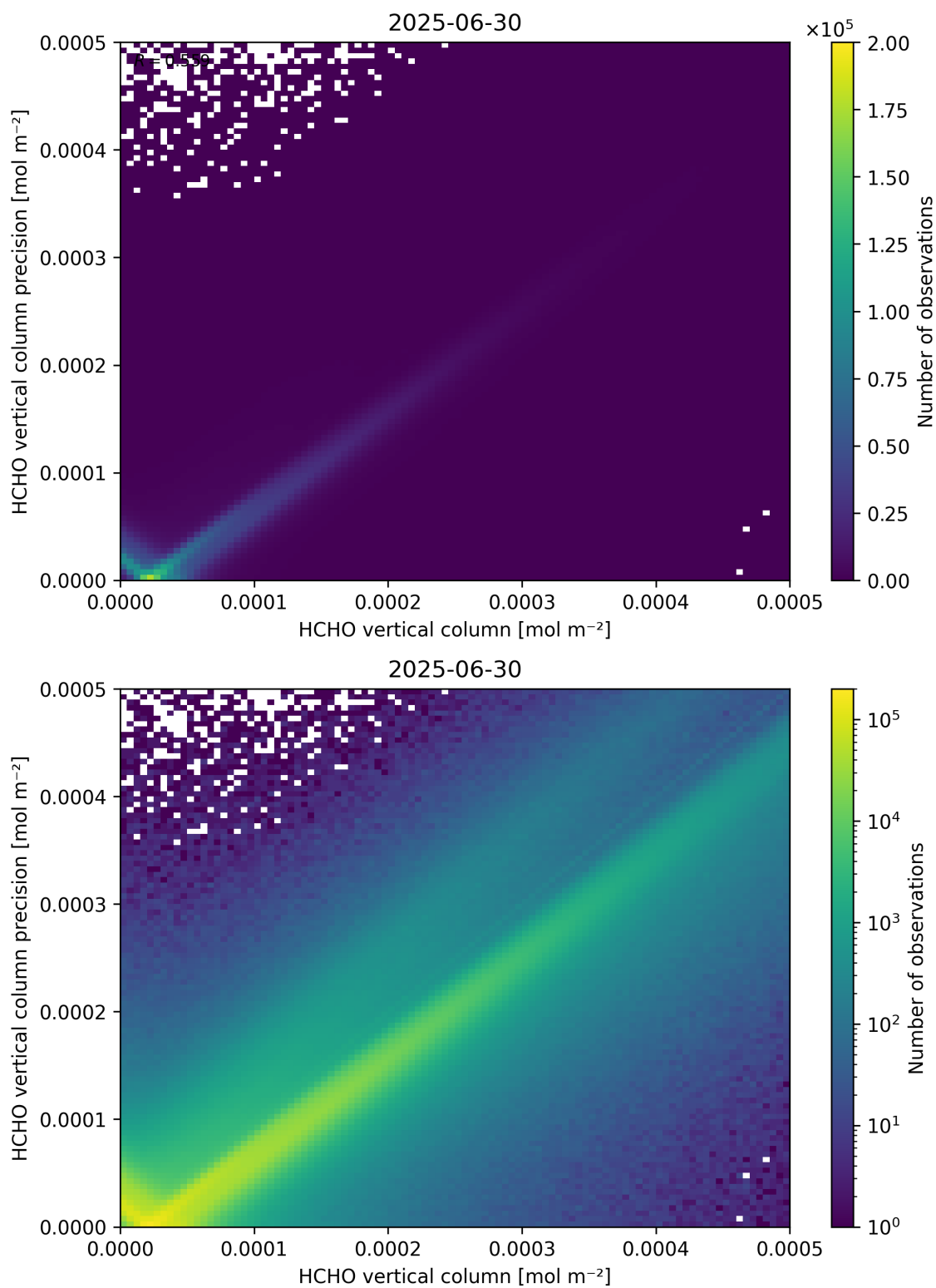
Figure 134: Scatter density plot of “HCHO vertical column” against “HCHO vertical column precision” for 2025-06-29 to 2025-07-01.
