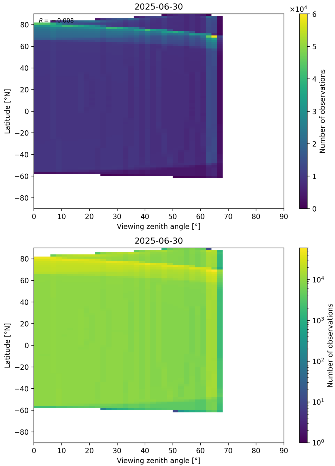
Figure 196: Scatter density plot of “Viewing zenith angle” against “Latitude” for 2025-06-29 to 2025-07-01.
