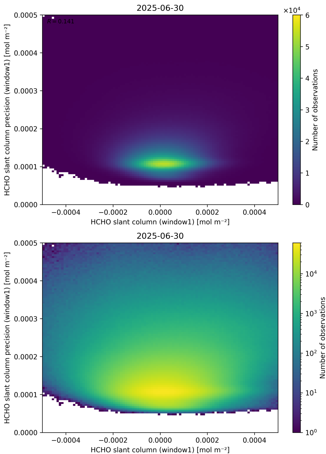
Figure 84: Scatter density plot of “HCHO slant column (window1)” against “HCHO slant column precision (window1)” for 2025-06-29 to 2025-07-01.
