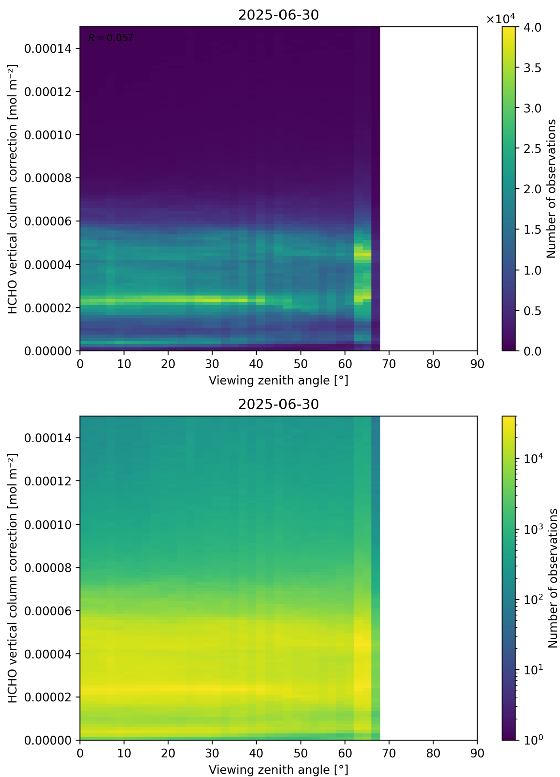
Figure 193: Scatter density plot of “Viewing zenith angle” against “HCHO vertical column correction” for 2025-06-29 to 2025-07-01.
