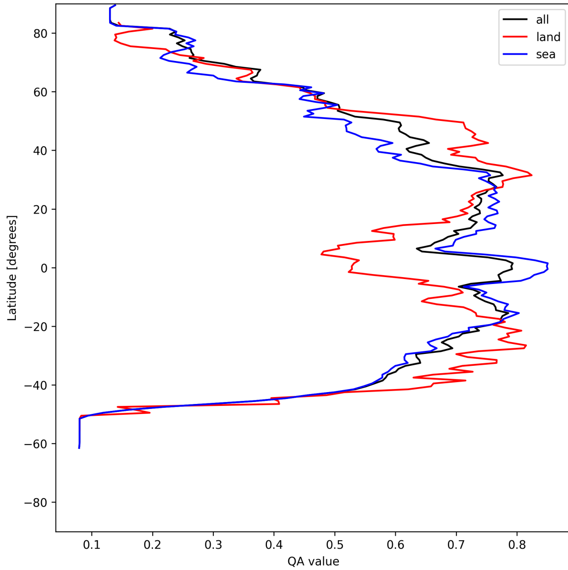
Figure 20: Zonal average of “QA value” for 2025-06-29 to 2025-07-01.
