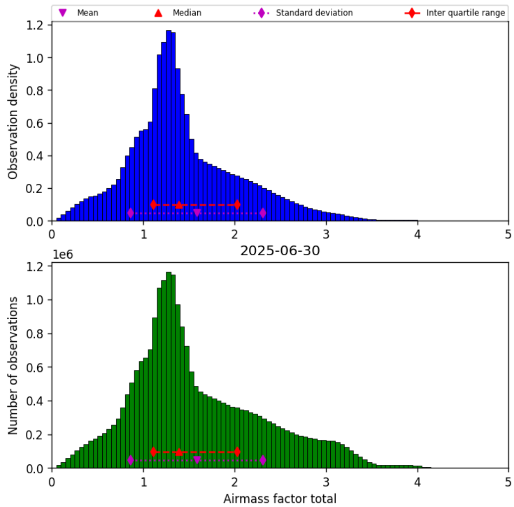
Figure 40: Histogram of “Airmass factor total” for 2025-06-29 to 2025-07-01
