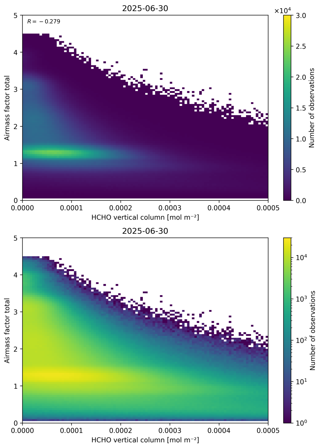
Figure 131: Scatter density plot of “HCHO vertical column” against “Airmass factor total” for 2025-06-29 to 2025-07-01.
