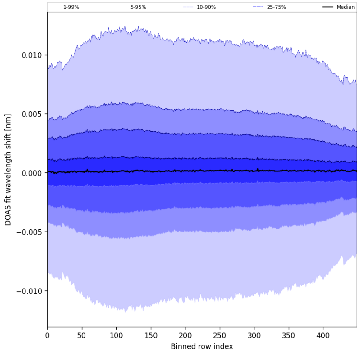
Figure 58: Along track statistics of “DOAS fit wavelength shift” for 2025-06-29 to 2025-07-01
