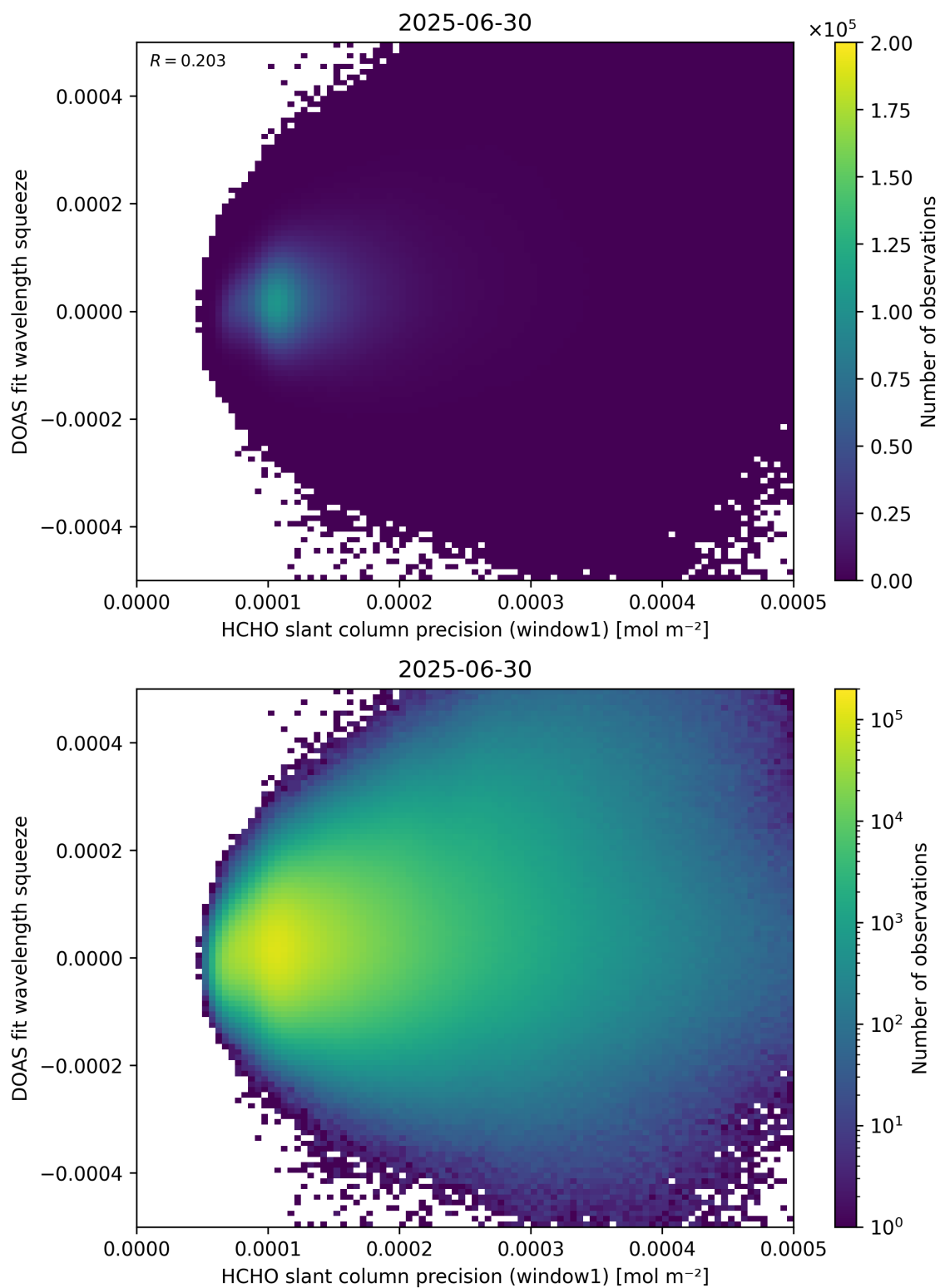
Figure 90: Scatter density plot of “HCHO slant column precision (window1)” against “DOAS fit wavelength squeeze” for 2025-06-29 to 2025-07-01.
