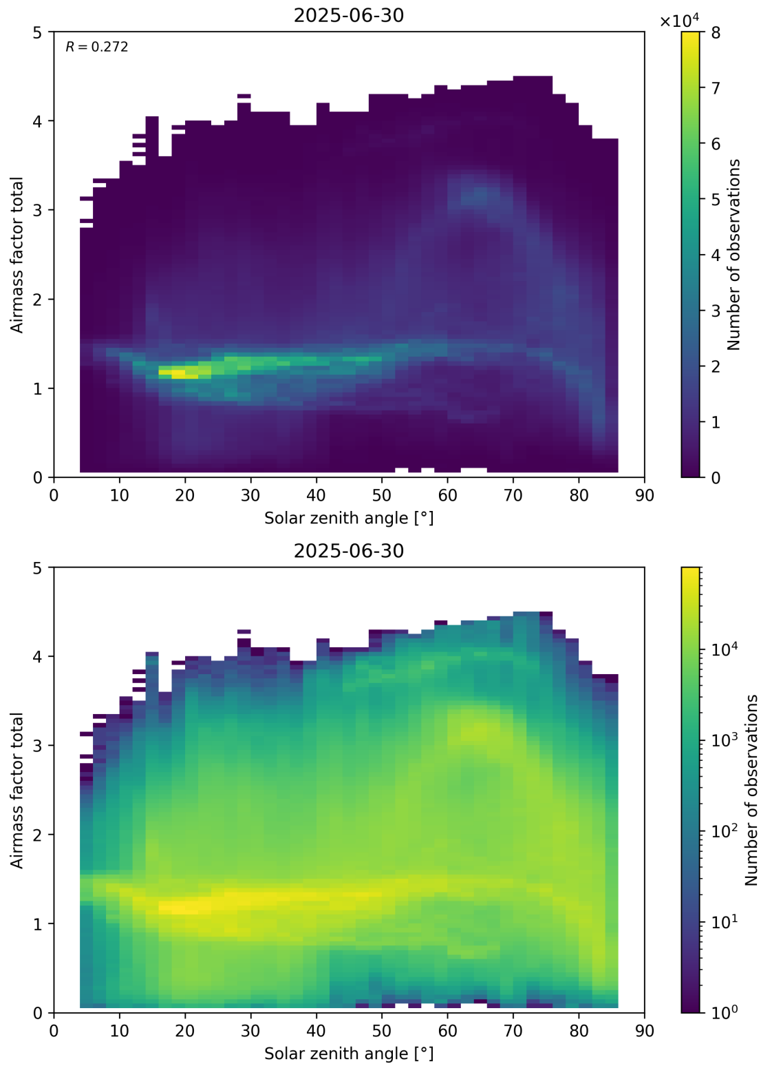
Figure 175: Scatter density plot of “Solar zenith angle” against “Airmass factor total” for 2025-06-29 to 2025-07-01.
