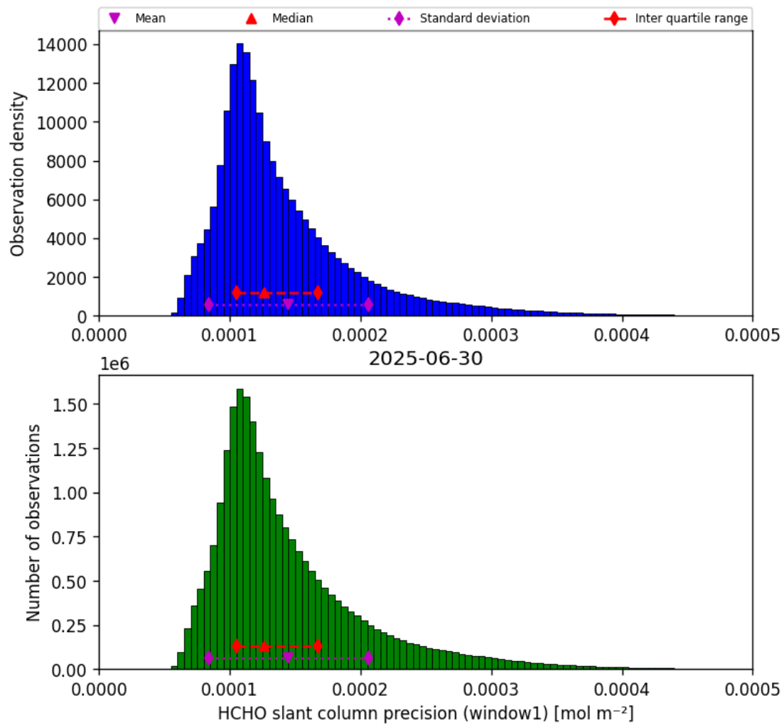
Figure 39: Histogram of “HCHO slant column precision (window1)” for 2025-06-29 to 2025-07-01
