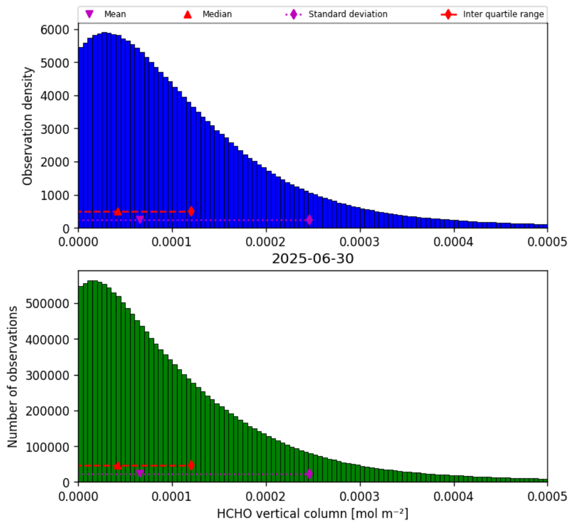
Figure 35: Histogram of “HCHO vertical column” for 2025-06-29 to 2025-07-01
