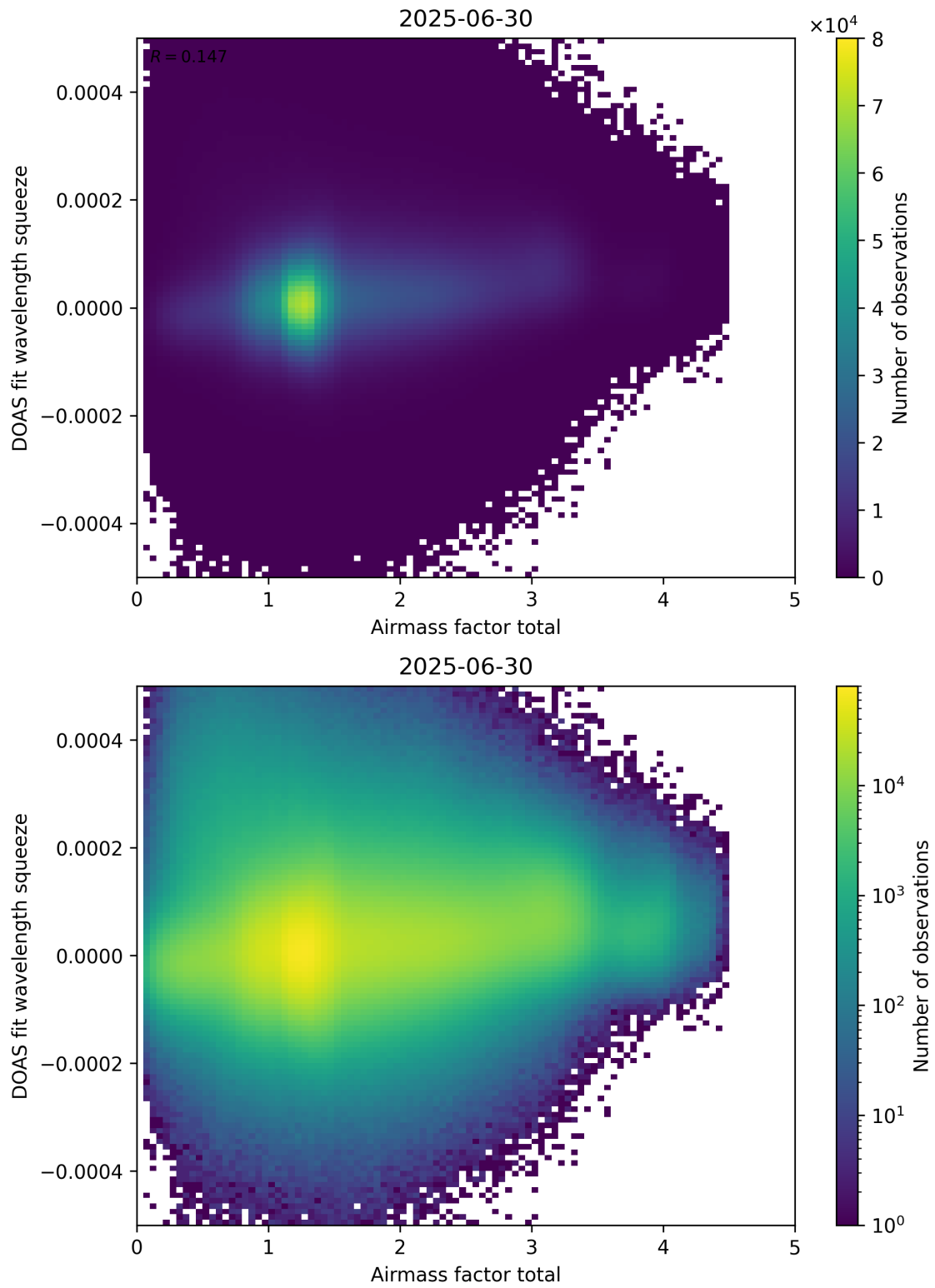
Figure 99: Scatter density plot of “Airmass factor total” against “DOAS fit wavelength squeeze” for 2025-06-29 to 2025-07-01.
