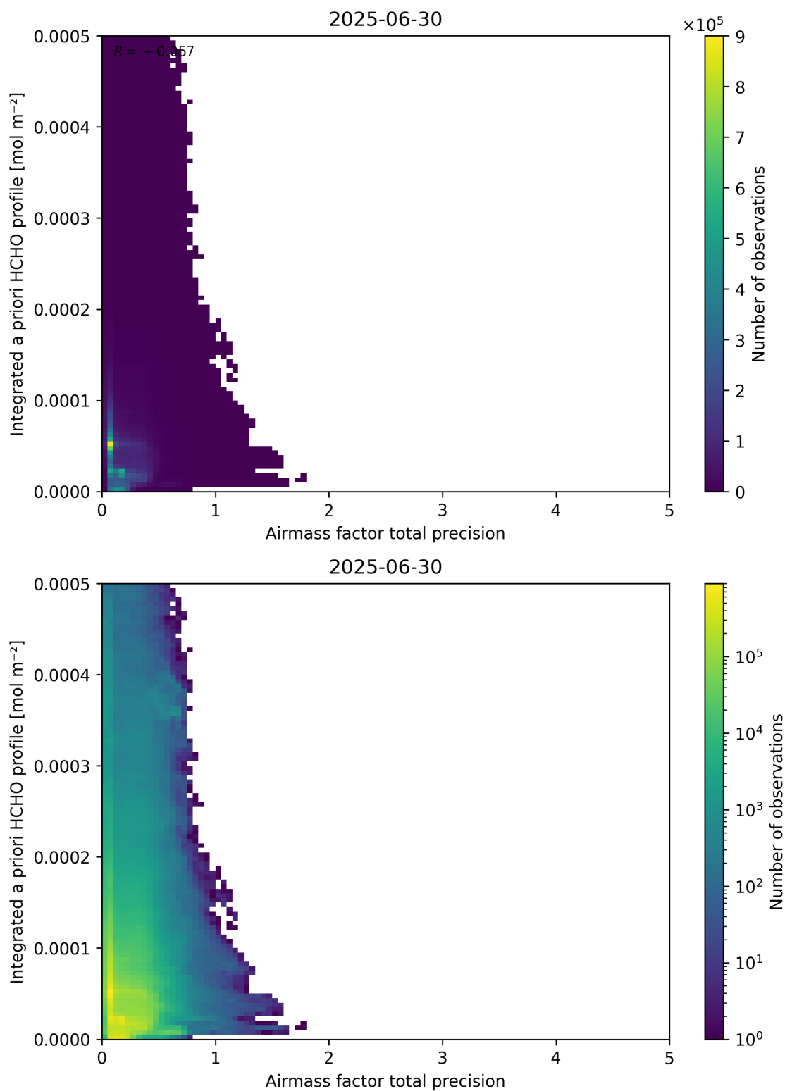
Figure 111: Scatter density plot of “Airmass factor total precision” against “Integrated a priori HCHO profile” for 2025-06-29 to 2025-07-01.
