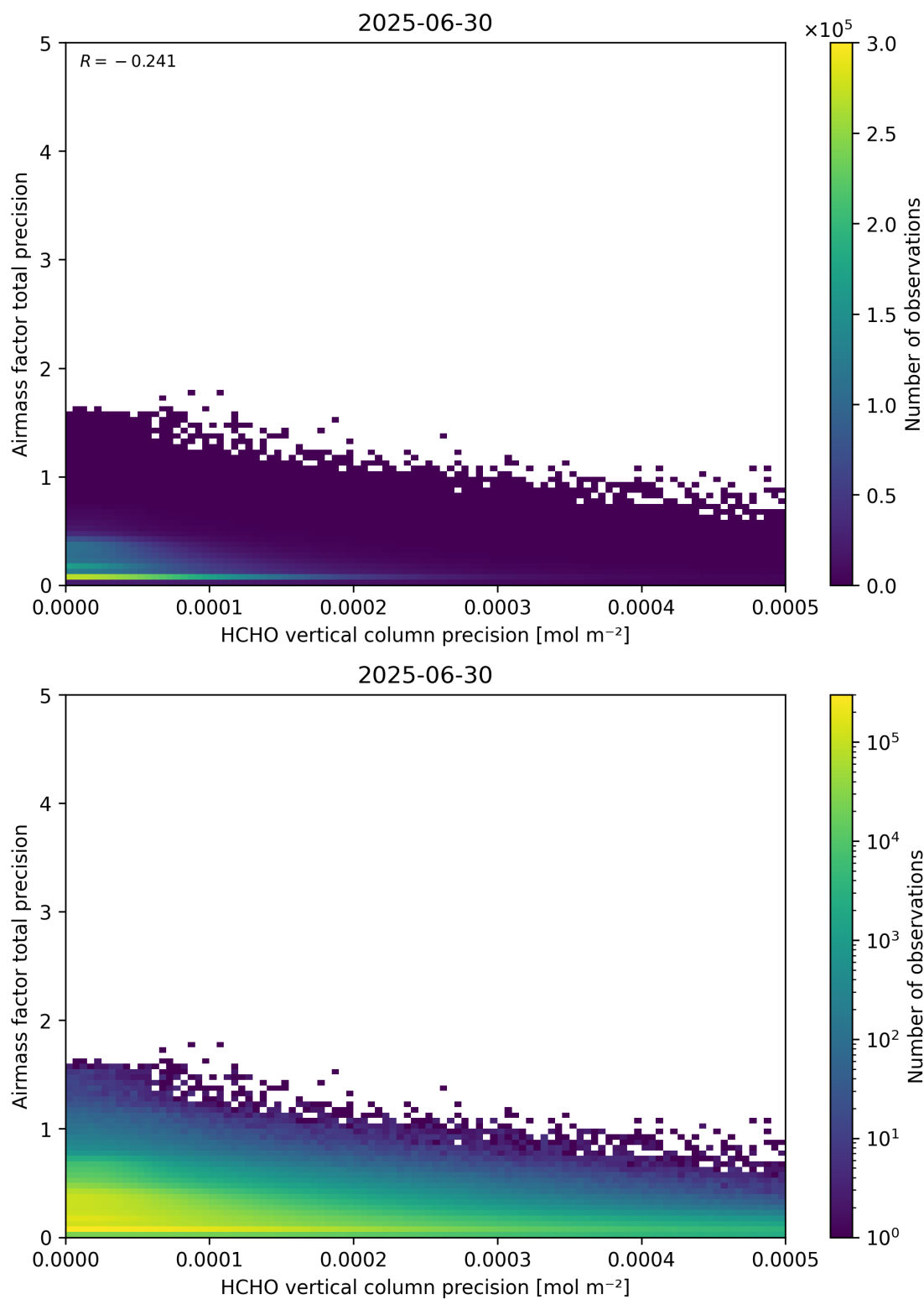
Figure 145: Scatter density plot of “HCHO vertical column precision” against “Airmass factor total precision” for 2025-06-29 to 2025-07-01.
