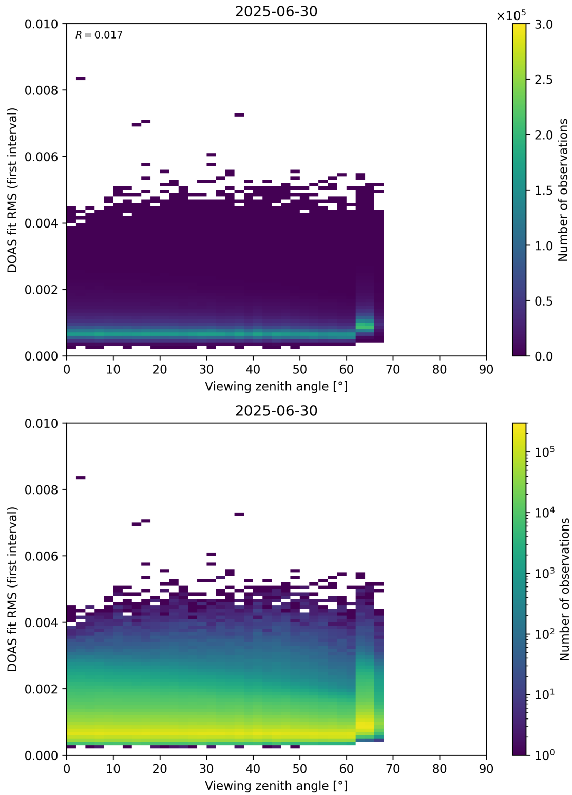
Figure 182: Scatter density plot of “Viewing zenith angle” against “DOAS fit RMS (first interval)” for 2025-06-29 to 2025-07-01.
