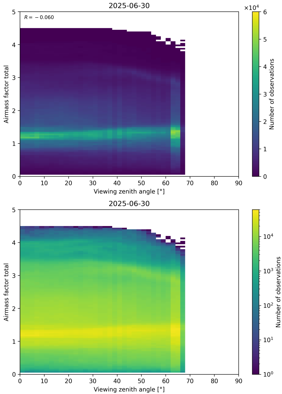
Figure 190: Scatter density plot of “Viewing zenith angle” against “Airmass factor total” for 2025-06-29 to 2025-07-01.
