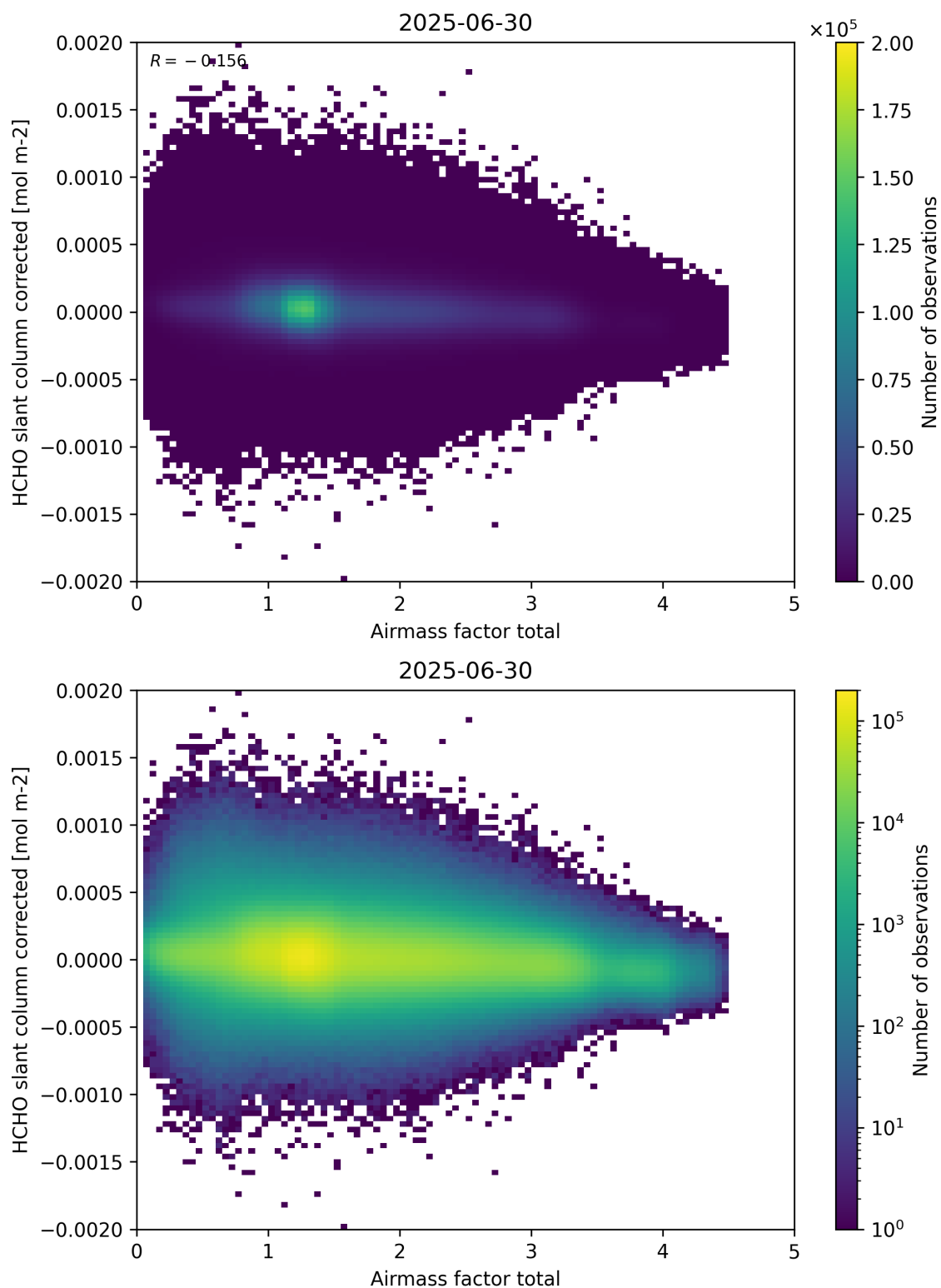
Figure 101: Scatter density plot of “Airmass factor total” against “HCHO slant column corrected” for 2025-06-29 to 2025-07-01.
