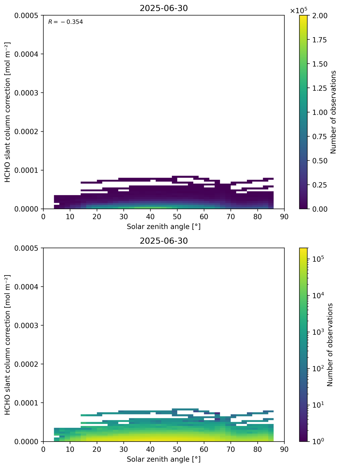
Figure 172: Scatter density plot of “Solar zenith angle” against “HCHO slant column correction” for 2025-06-29 to 2025-07-01.
