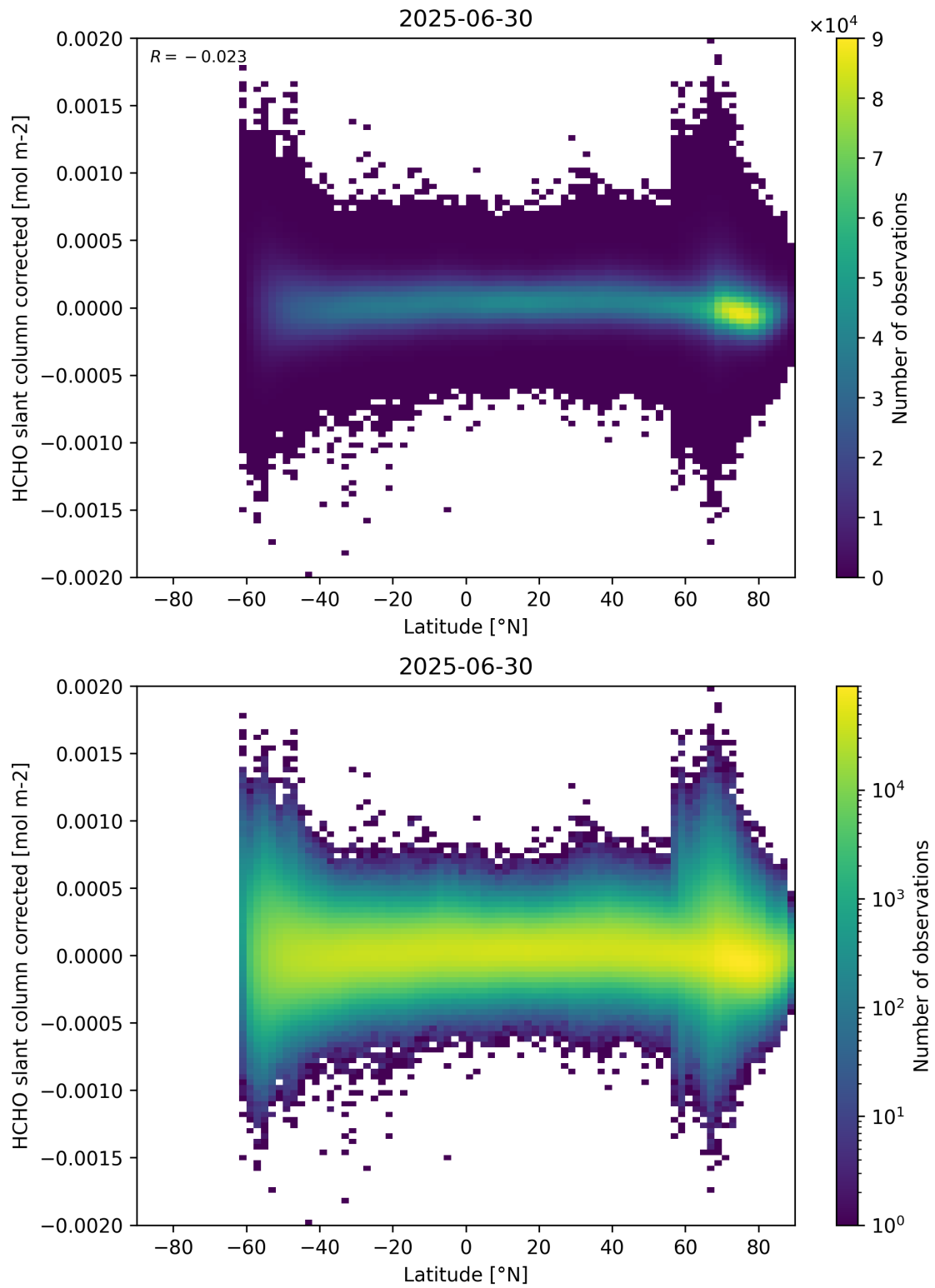
Figure 157: Scatter density plot of “Latitude” against “HCHO slant column corrected” for 2025-06-29 to 2025-07-01.
