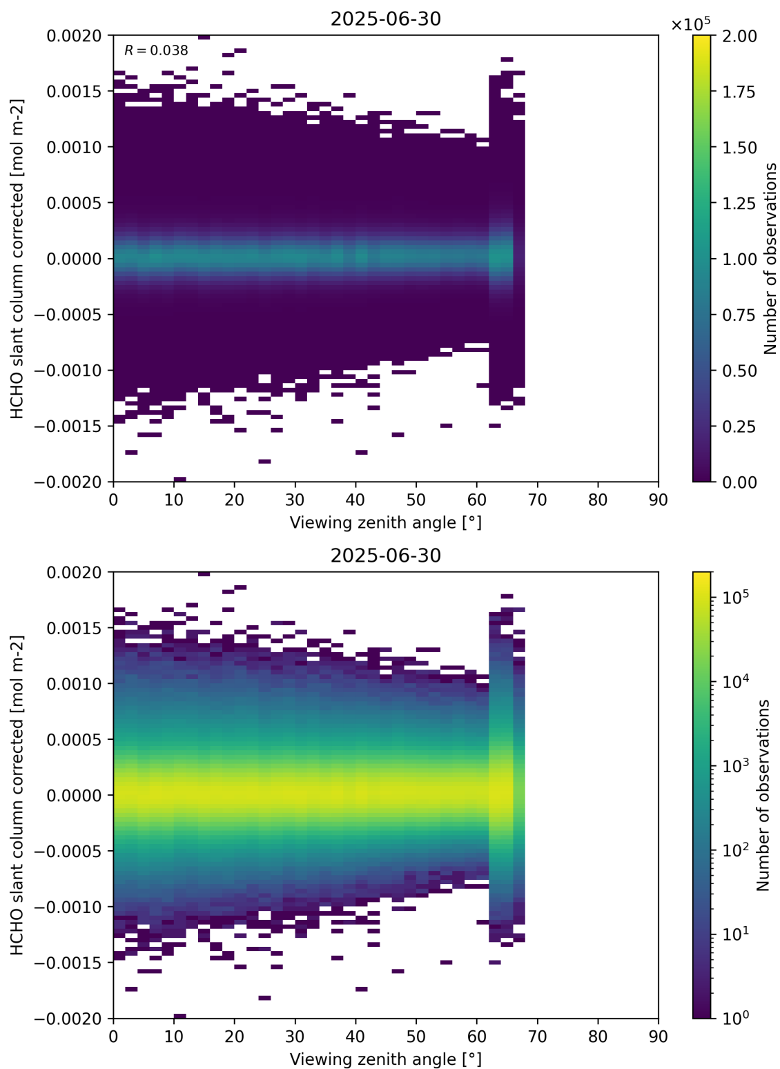
Figure 186: Scatter density plot of “Viewing zenith angle” against “HCHO slant column corrected” for 2025-06-29 to 2025-07-01.
