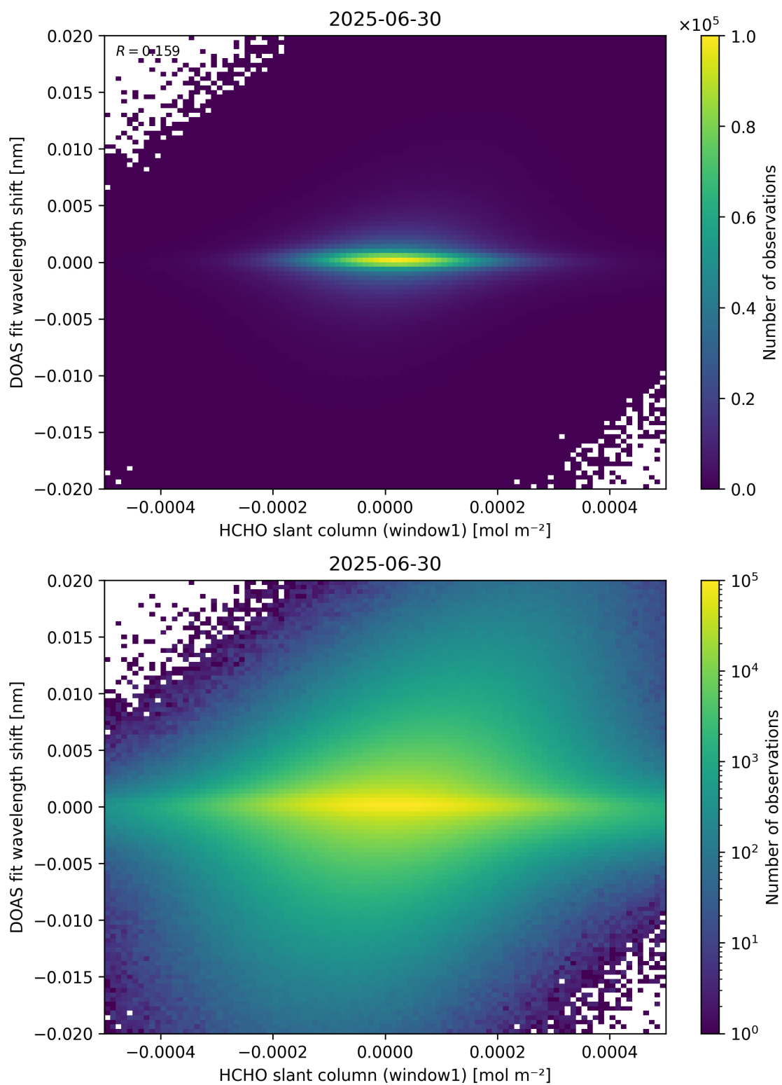
Figure 79: Scatter density plot of “HCHO slant column (window1)” against “DOAS fit wavelength shift” for 2025-06-29 to 2025-07-01.
