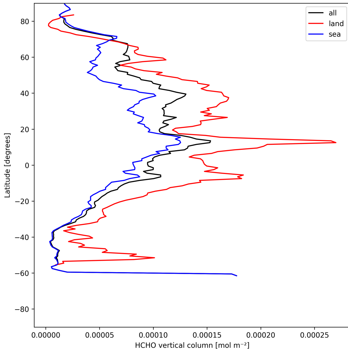
Figure 21: Zonal average of “HCHO vertical column” for 2025-06-29 to 2025-07-01.
