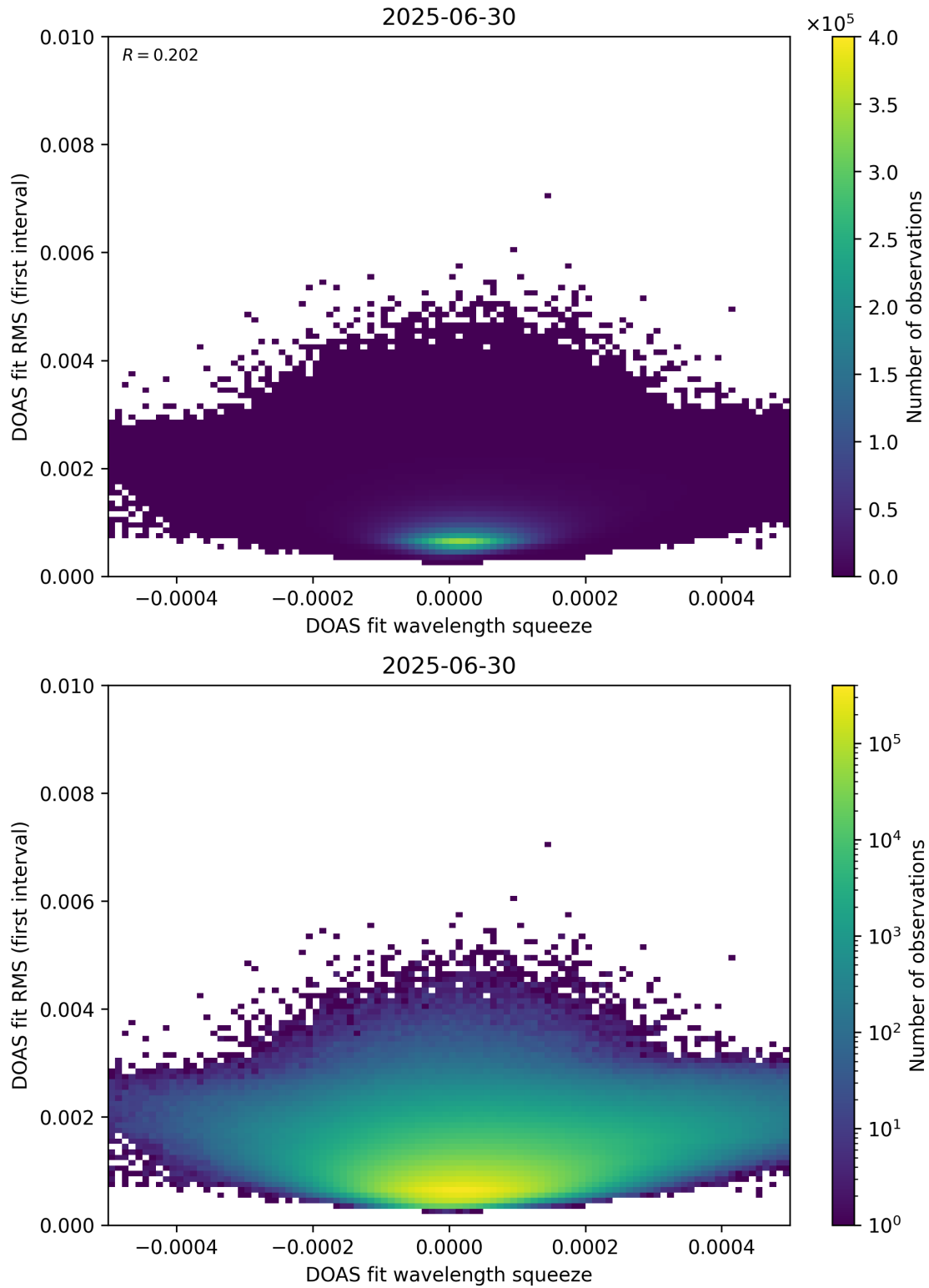
Figure 68: Scatter density plot of “DOAS fit wavelength squeeze” against “DOAS fit RMS (first interval)” for 2025-06-29 to 2025-07-01.
