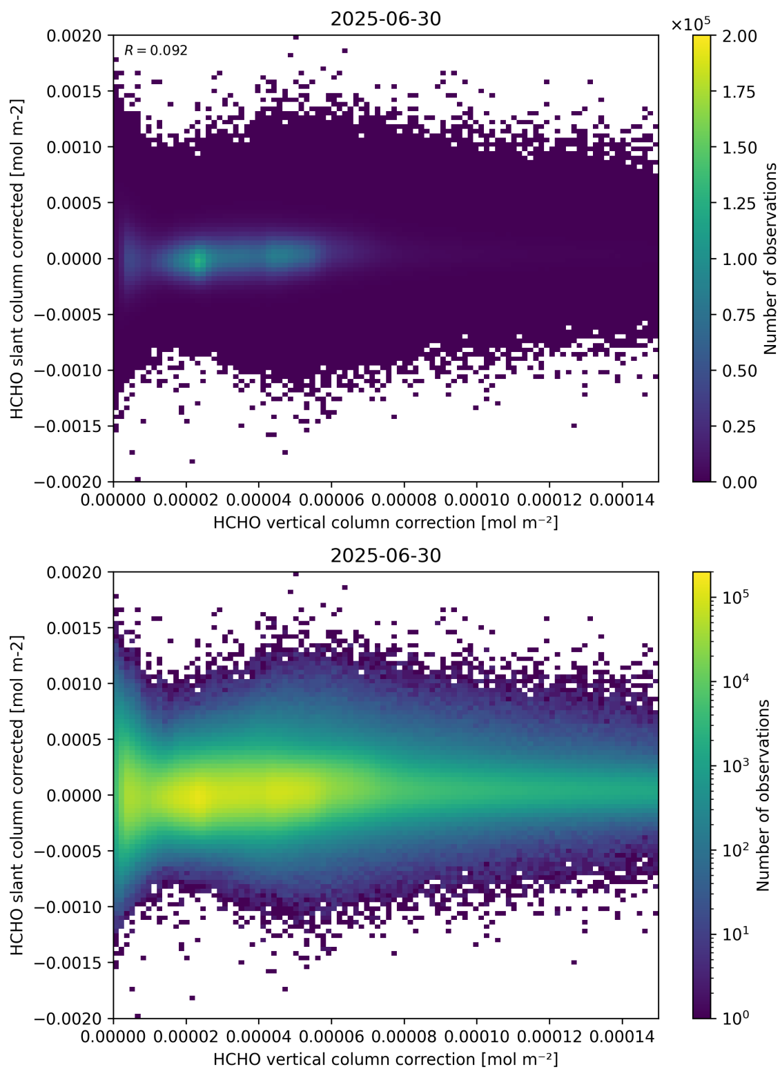
Figure 116: Scatter density plot of “HCHO vertical column correction” against “HCHO slant column corrected” for 2025-06-29 to 2025-07-01.
