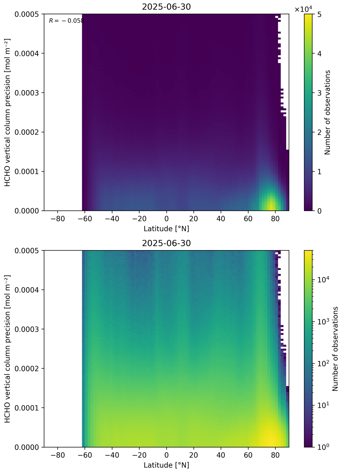
Figure 165: Scatter density plot of “Latitude” against “HCHO vertical column precision” for 2025-06-29 to 2025-07-01.
