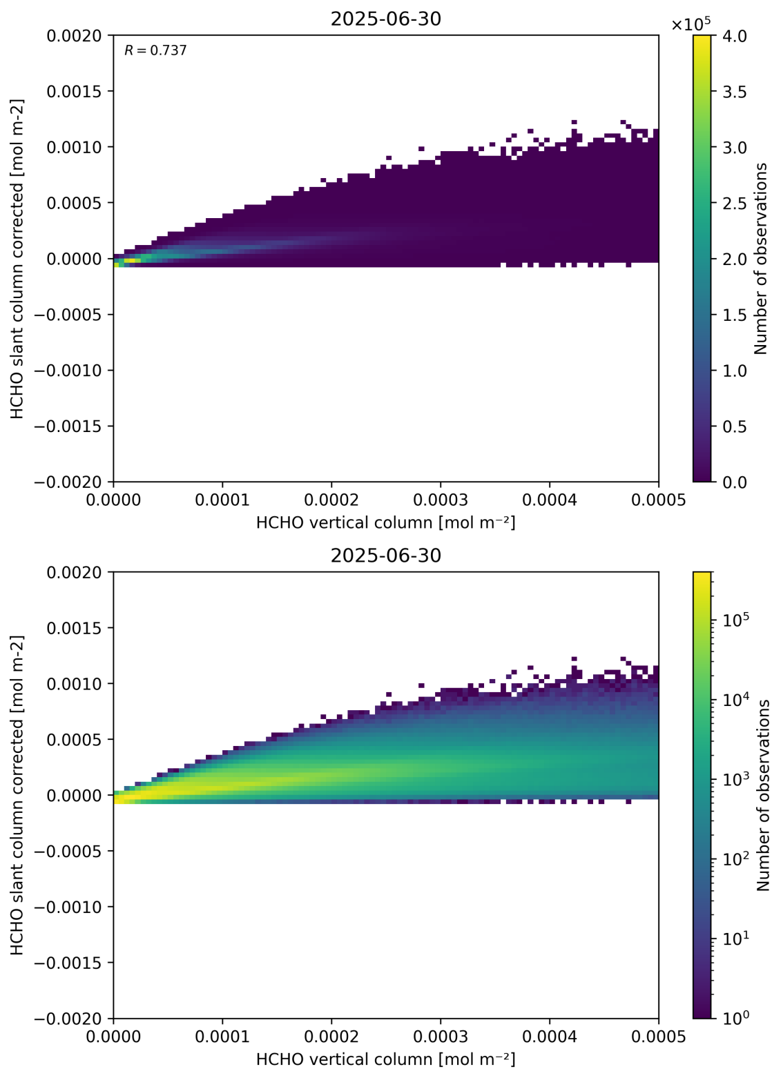
Figure 127: Scatter density plot of “HCHO vertical column” against “HCHO slant column corrected” for 2025-06-29 to 2025-07-01.
