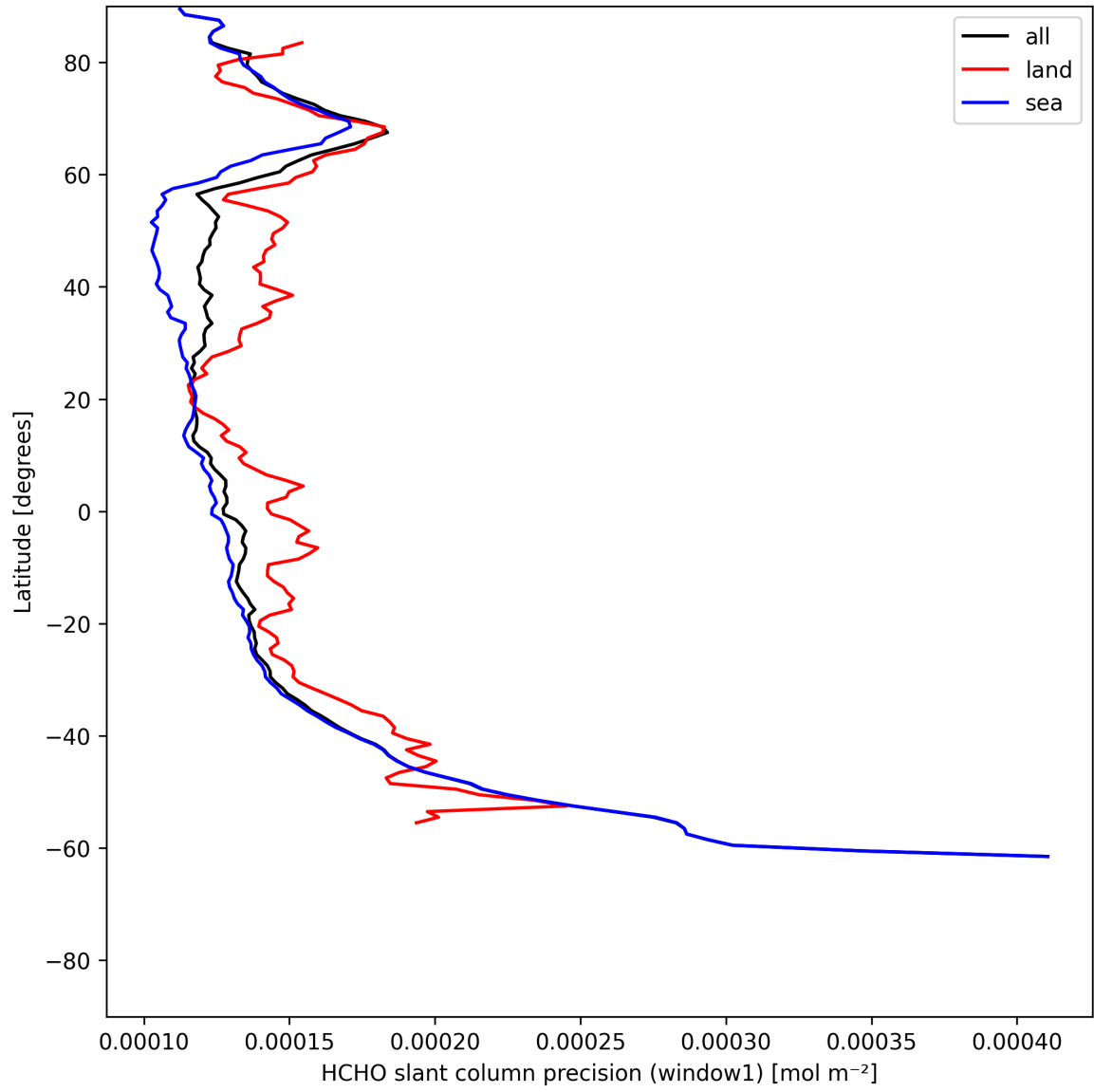
Figure 25: Zonal average of “HCHO slant column precision (window1)” for 2025-06-29 to 2025-07-01.
