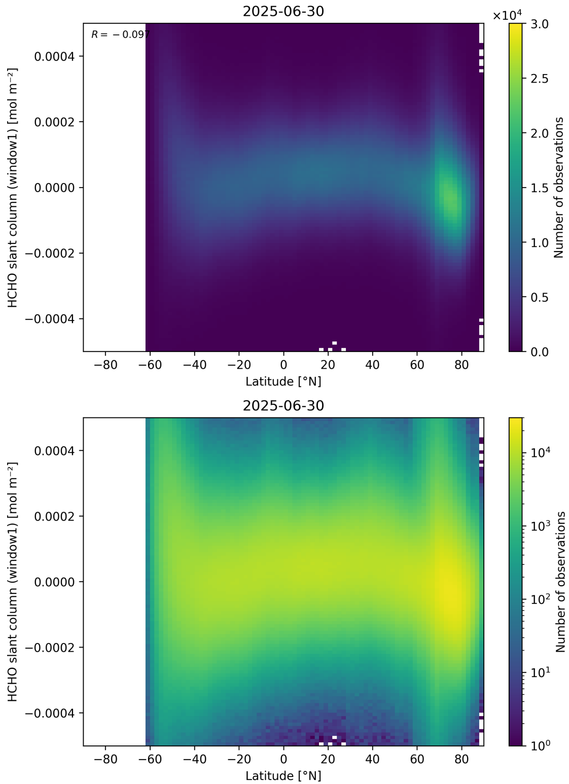
Figure 159: Scatter density plot of “Latitude” against “HCHO slant column (window1)” for 2025-06-29 to 2025-07-01.
