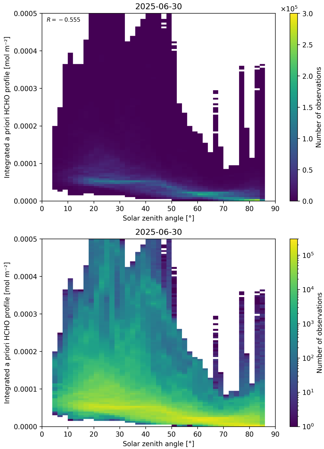
Figure 180: Scatter density plot of “Solar zenith angle” against “Integrated a priori HCHO profile” for 2025-06-29 to 2025-07-01.
