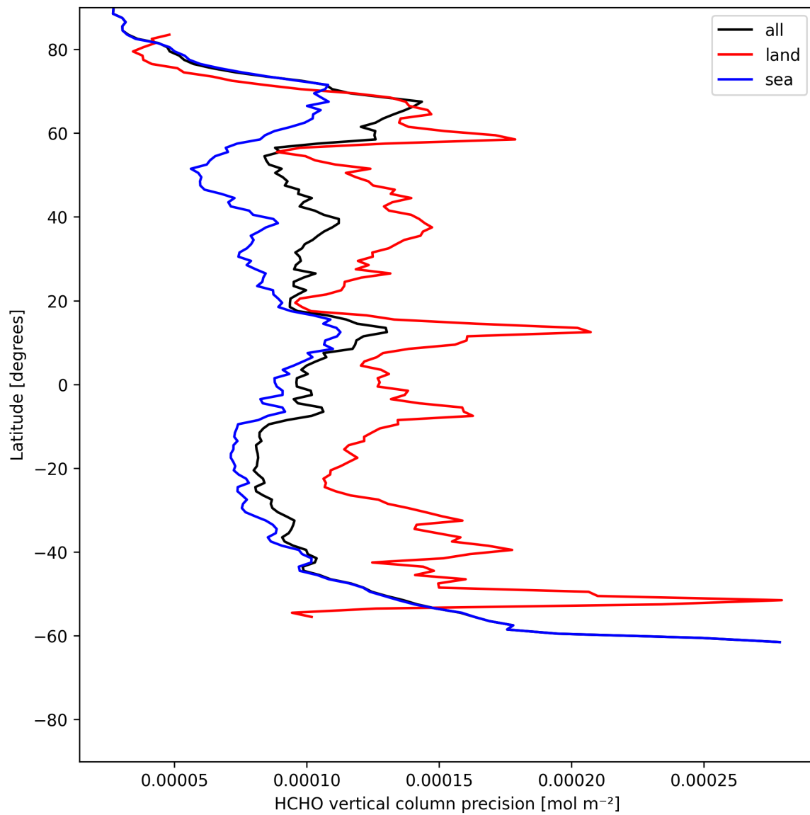
Figure 22: Zonal average of “HCHO vertical column precision” for 2025-06-29 to 2025-07-01.
