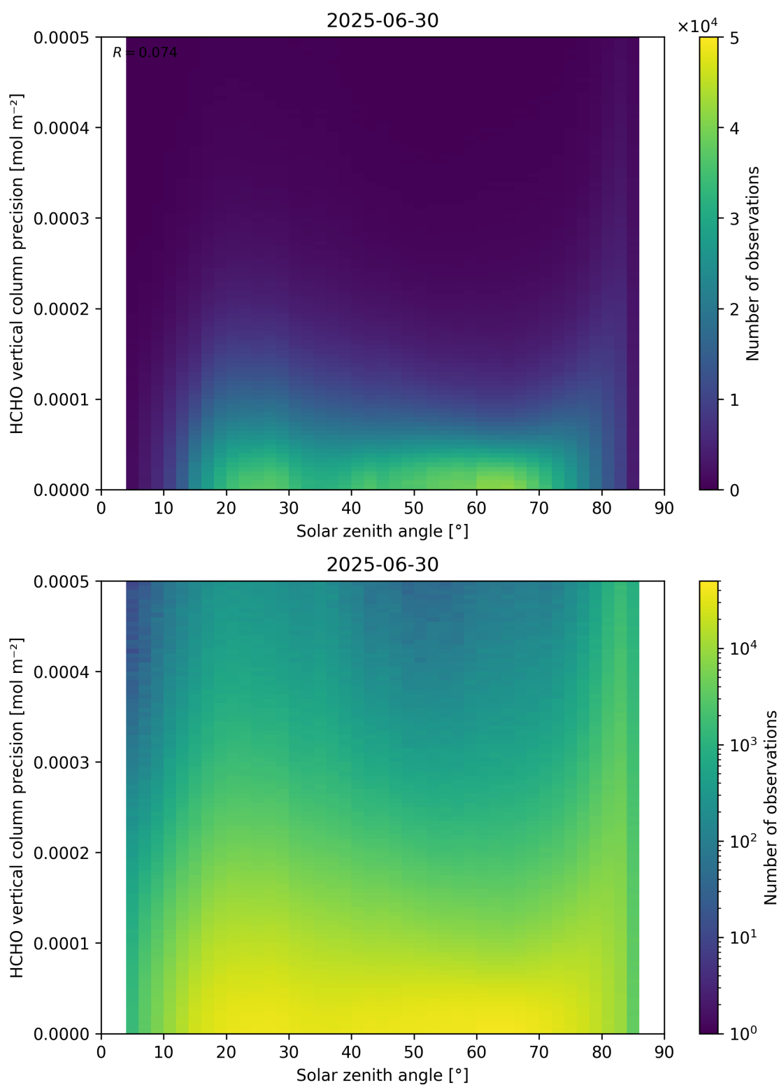
Figure 179: Scatter density plot of “Solar zenith angle” against “HCHO vertical column precision” for 2025-06-29 to 2025-07-01.
