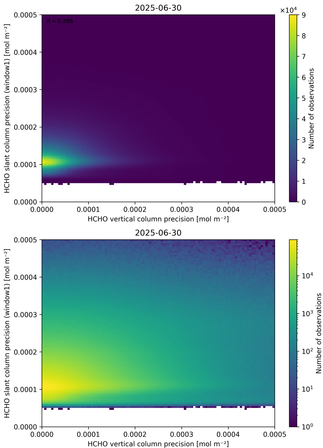
Figure 143: Scatter density plot of “HCHO vertical column precision” against “HCHO slant column precision (window1)” for 2025-06-29 to 2025-07-01.
