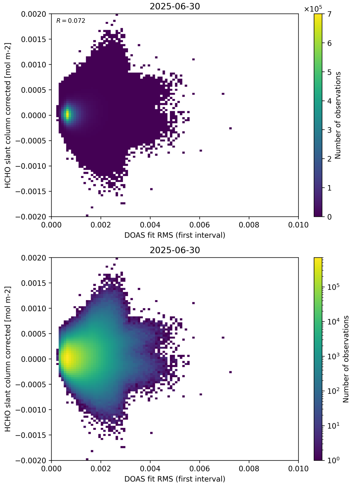
Figure 62: Scatter density plot of “DOAS fit RMS (first interval)” against “HCHO slant column corrected” for 2025-06-29 to 2025-07-01.
