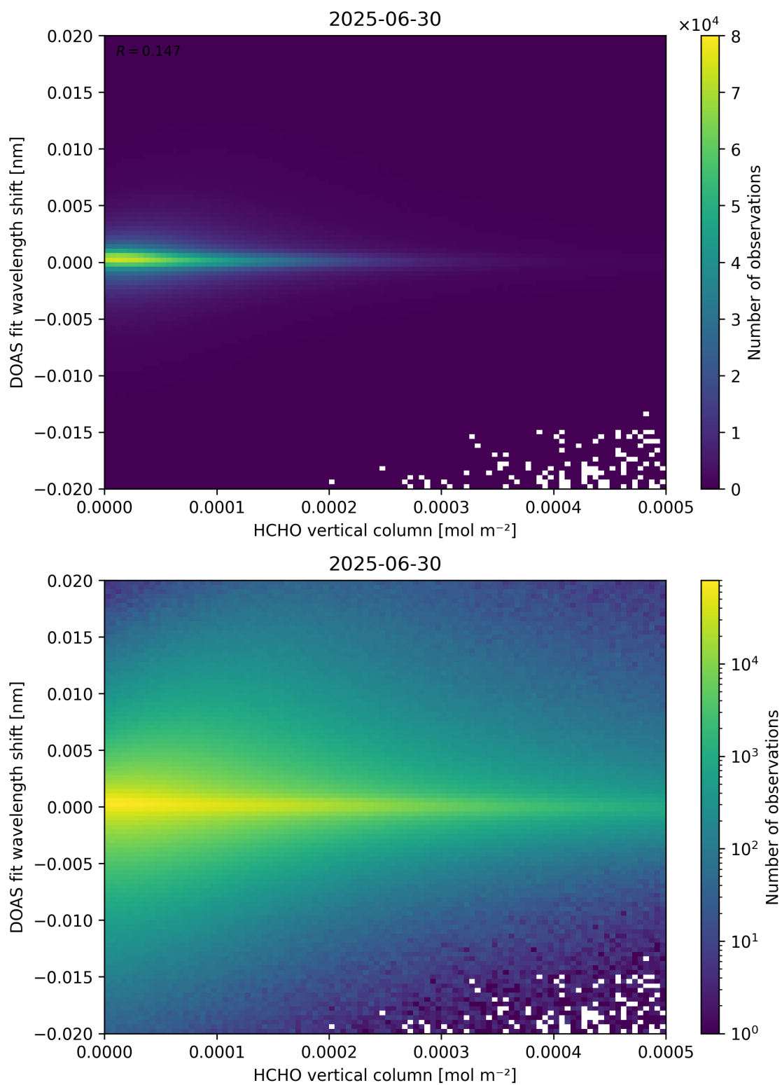
Figure 124: Scatter density plot of “HCHO vertical column” against “DOAS fit wavelength shift” for 2025-06-29 to 2025-07-01.
