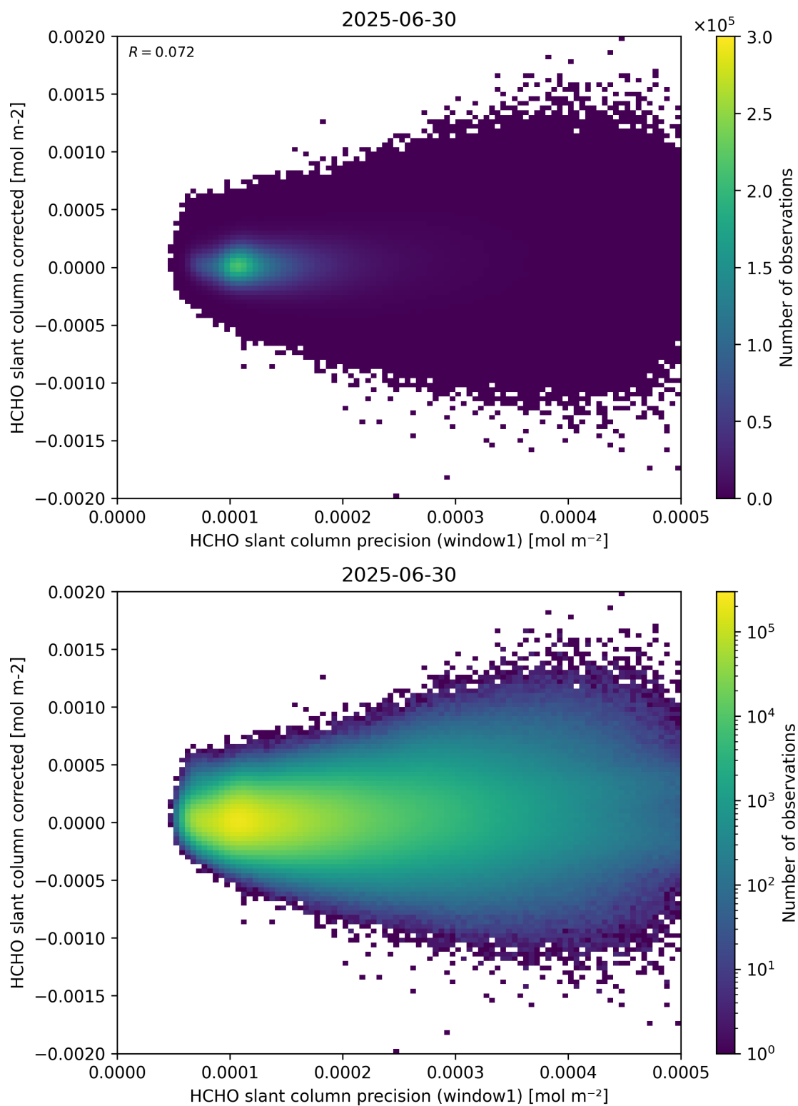
Figure 92: Scatter density plot of “HCHO slant column precision (window1)” against “HCHO slant column corrected” for 2025-06-29 to 2025-07-01.
