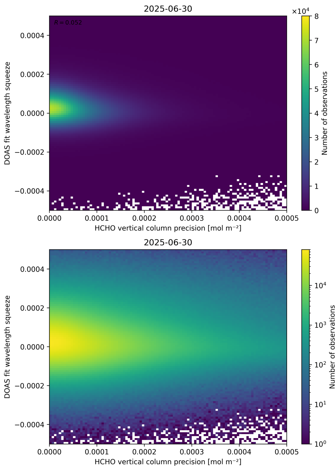
Figure 138: Scatter density plot of “HCHO vertical column precision” against “DOAS fit wavelength squeeze” for 2025-06-29 to 2025-07-01.
