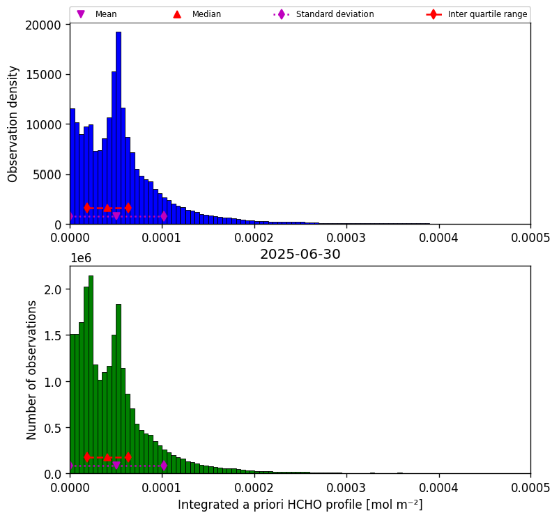
Figure 43: Histogram of “Integrated a priori HCHO profile” for 2025-06-29 to 2025-07-01
