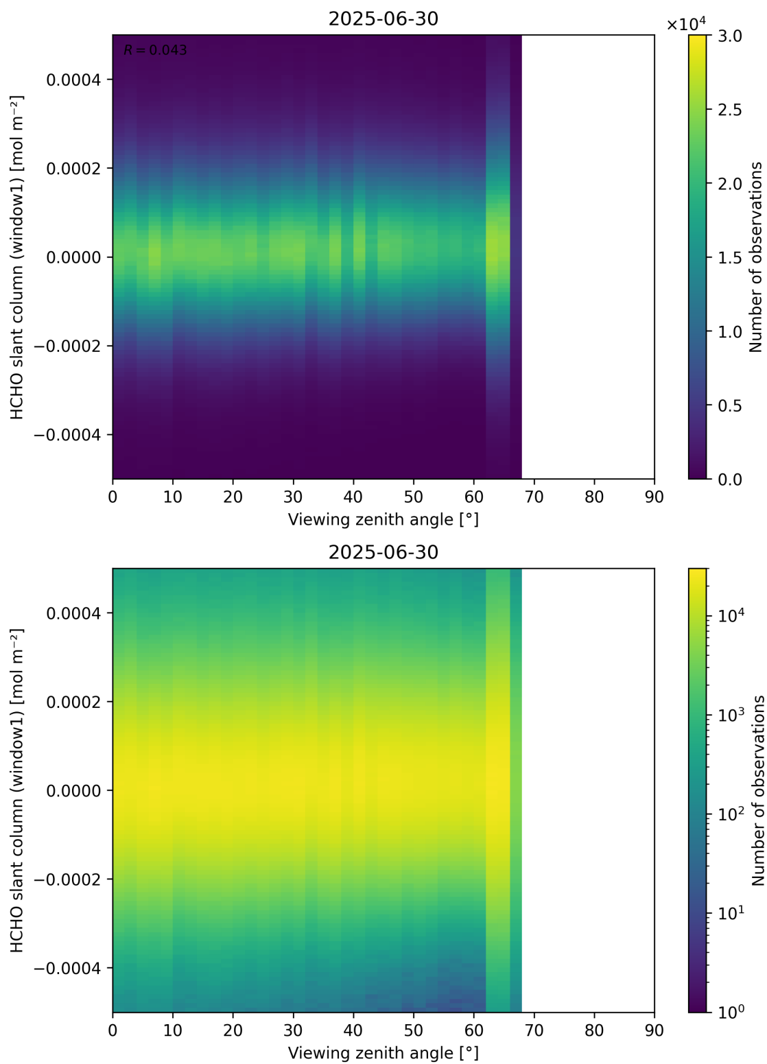
Figure 188: Scatter density plot of “Viewing zenith angle” against “HCHO slant column (window1)” for 2025-06-29 to 2025-07-01.
