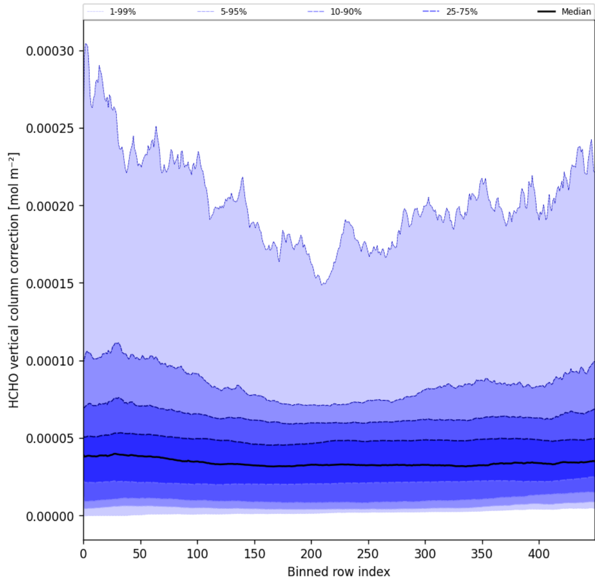
Figure 51: Along track statistics of “HCHO vertical column correction” for 2025-06-29 to 2025-07-01
