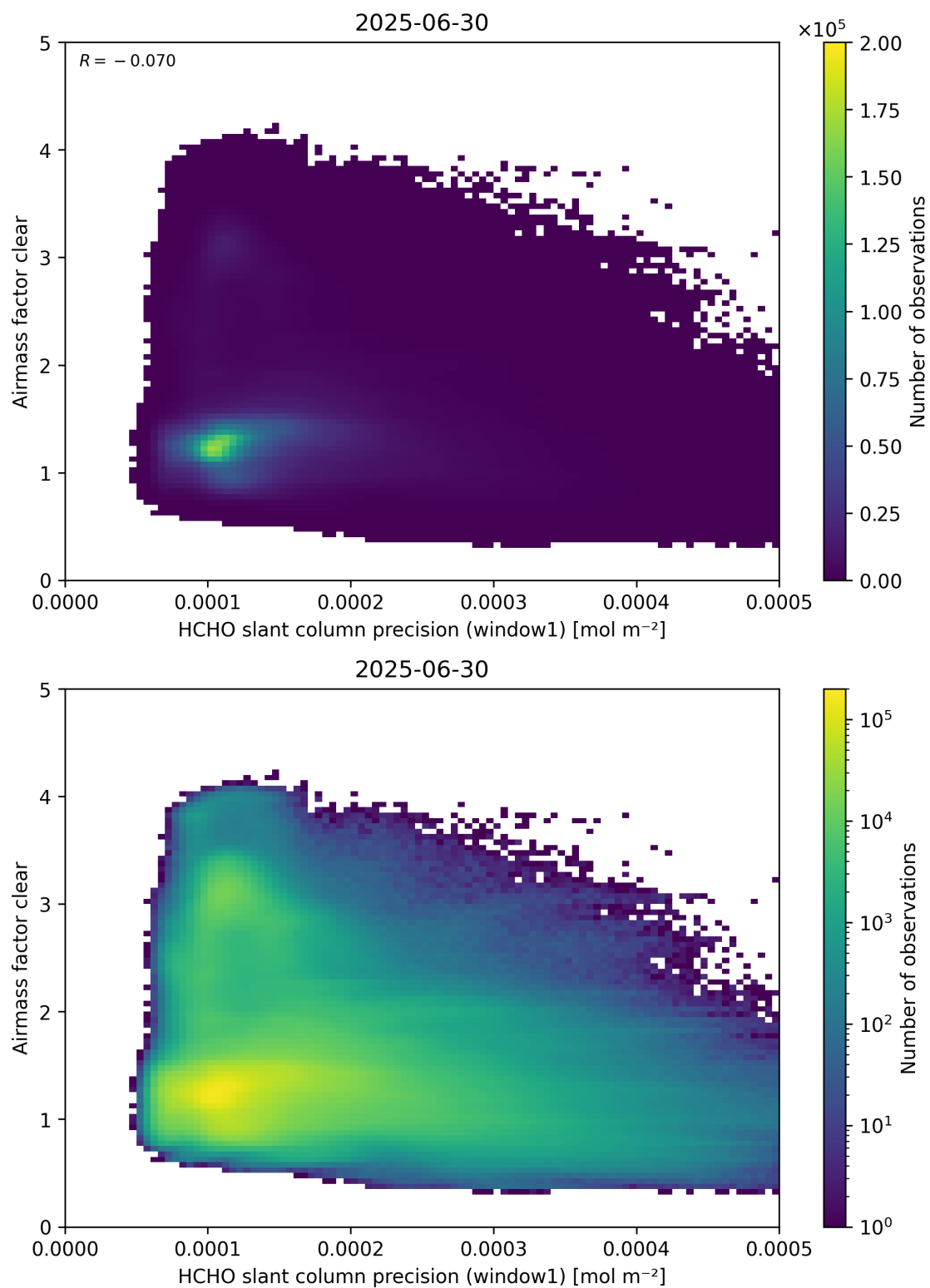
Figure 91: Scatter density plot of “HCHO slant column precision (window1)” against “Airmass factor clear” for 2025-06-29 to 2025-07-01.
