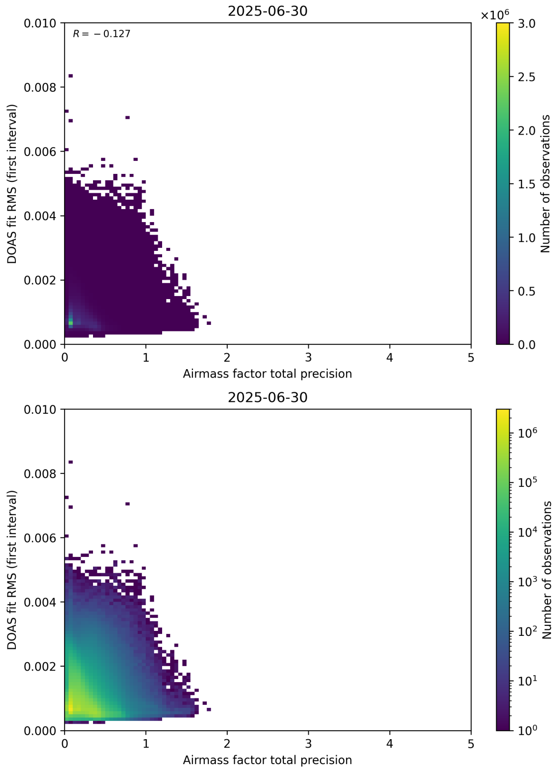
Figure 105: Scatter density plot of “Airmass factor total precision” against “DOAS fit RMS (first interval)” for 2025-06-29 to 2025-07-01.
