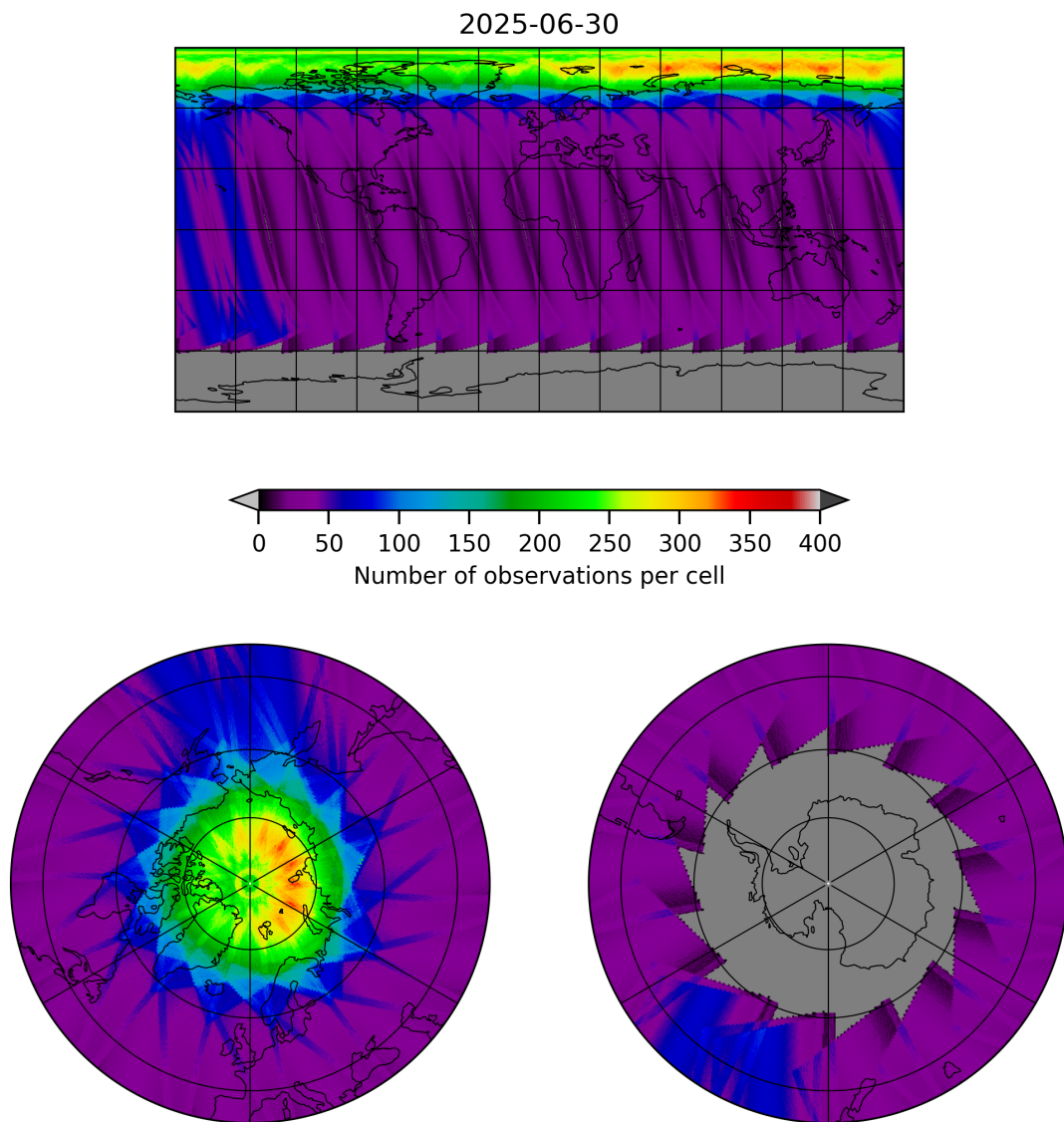
Figure 19: Map of the number of observations for 2025-06-29 to 2025-07-01
