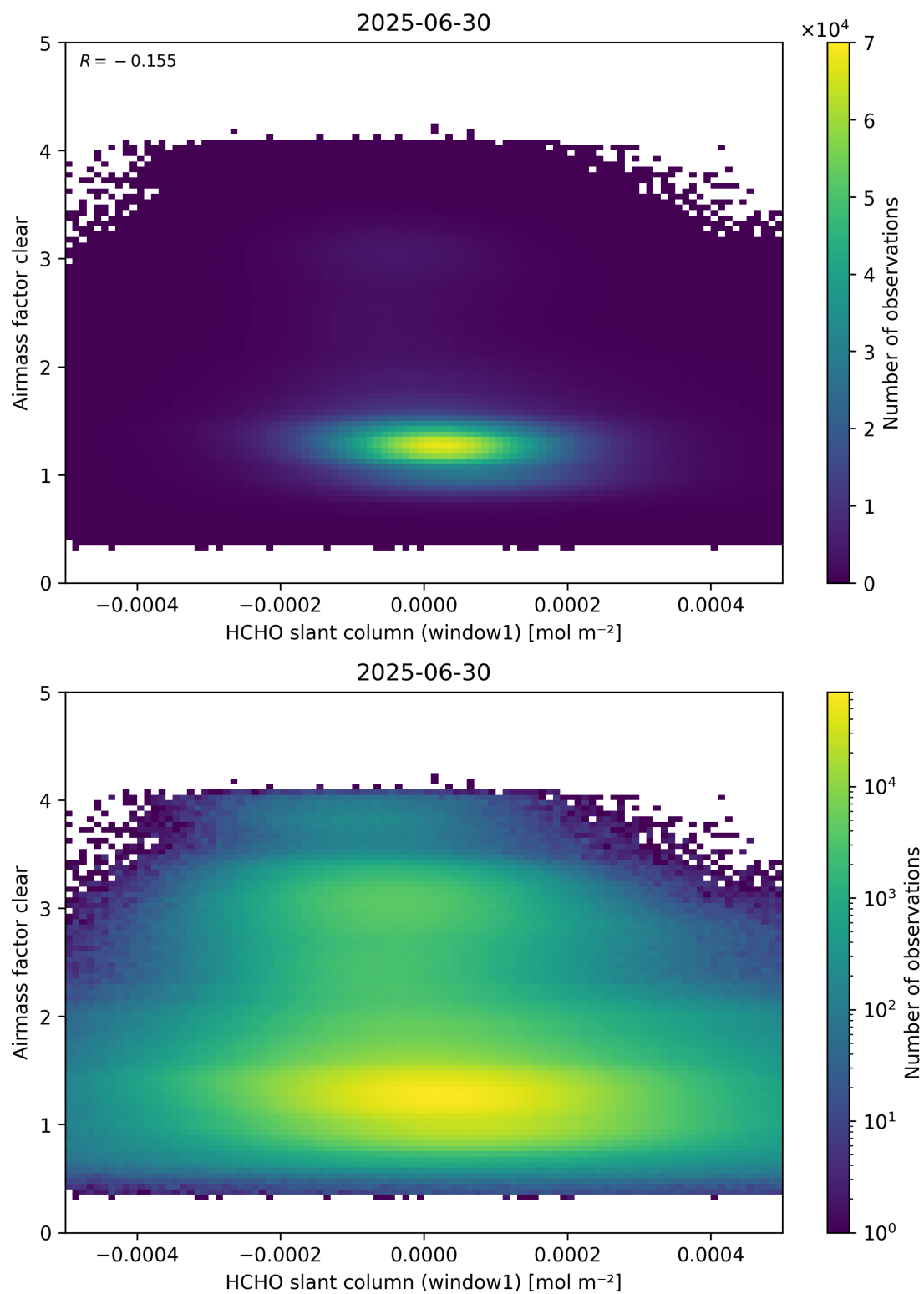
Figure 81: Scatter density plot of “HCHO slant column (window1)” against “Airmass factor clear” for 2025-06-29 to 2025-07-01.
