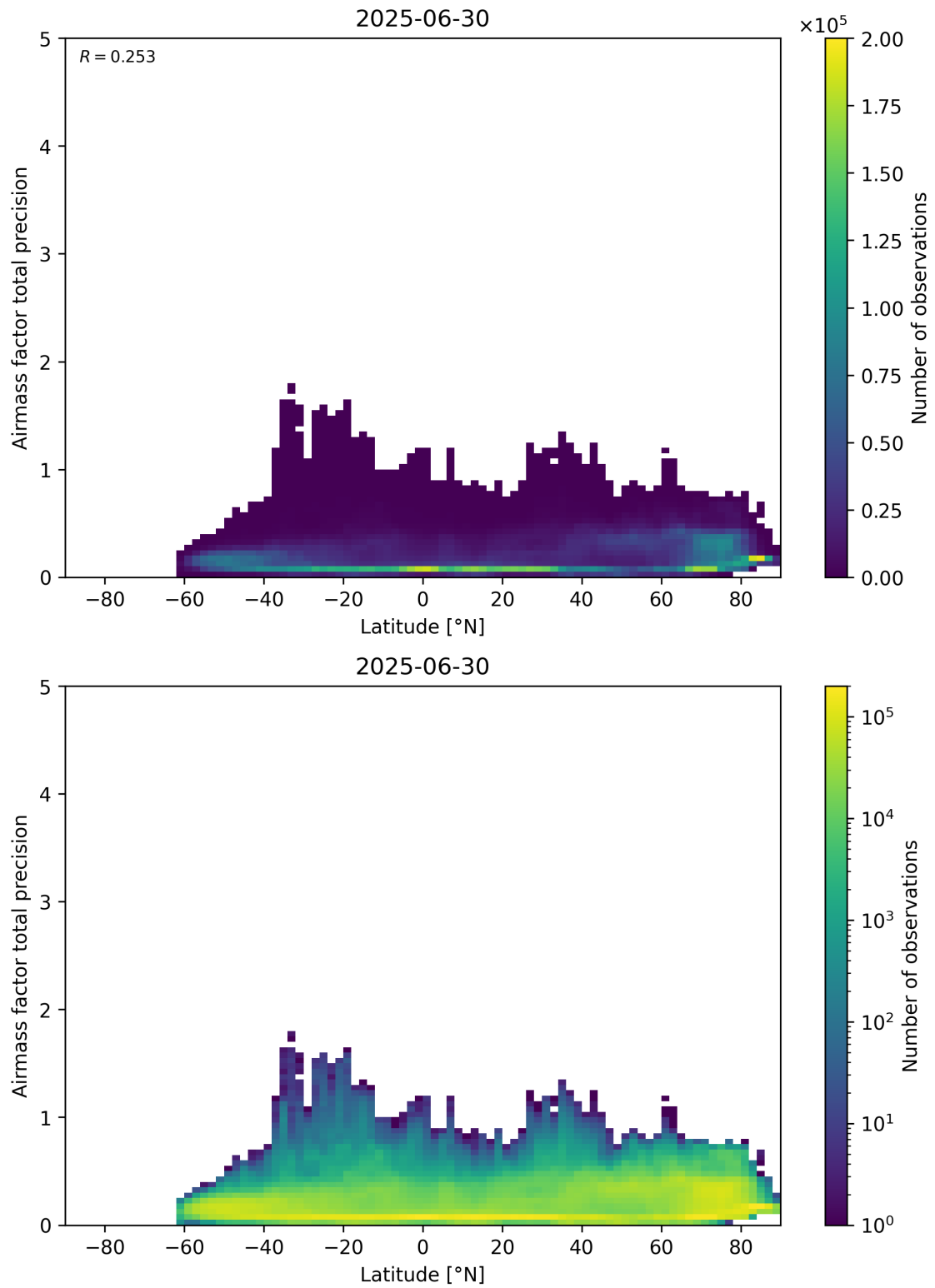
Figure 162: Scatter density plot of “Latitude” against “Airmass factor total precision” for 2025-06-29 to 2025-07-01.
