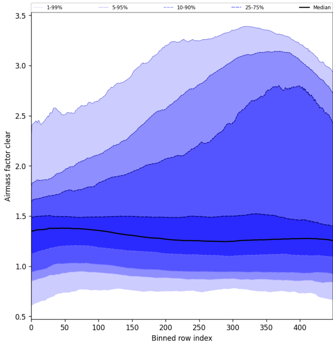
Figure 56: Along track statistics of “Air mass factor clear” for 2025-06-29 to 2025-07-01
