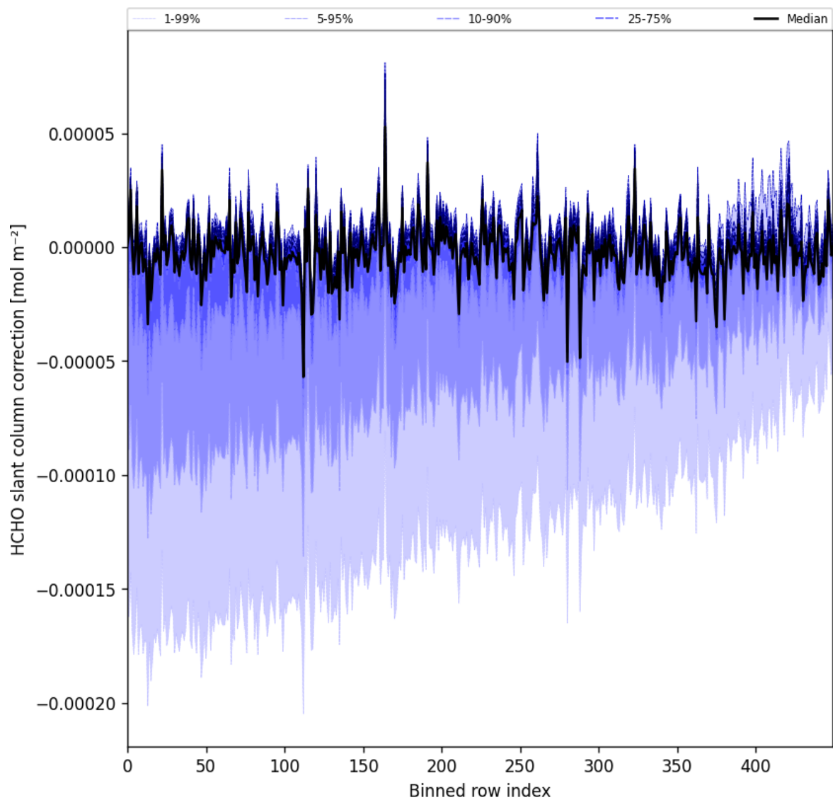
Figure 61: Along track statistics of “HCHO slant column correction” for 2025-06-29 to 2025-07-01
