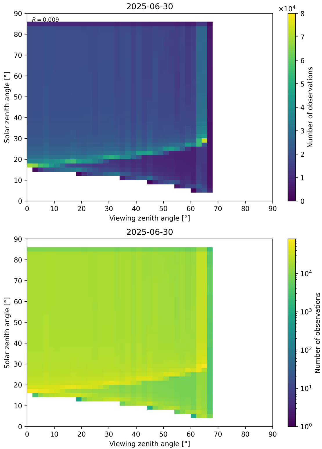
Figure 197: Scatter density plot of “Viewing zenith angle” against “Solar zenith angle” for 2025-06-29 to 2025-07-01.
