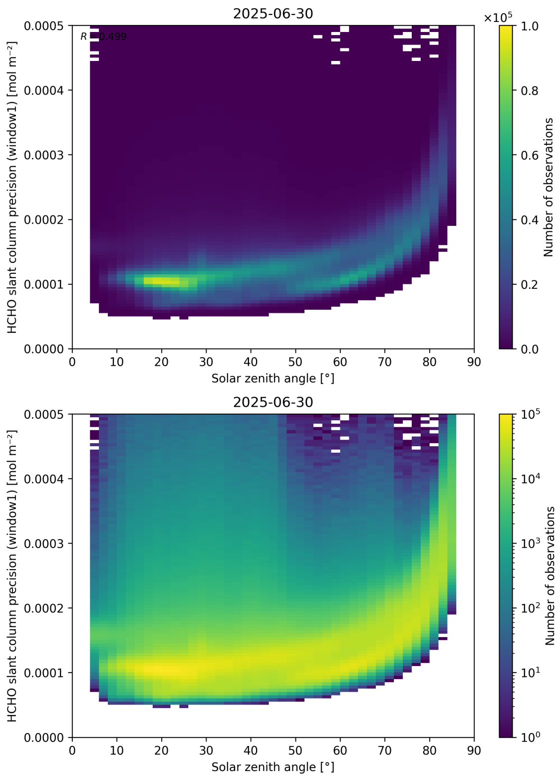
Figure 174: Scatter density plot of “Solar zenith angle” against “HCHO slant column precision (window1)” for 2025-06-29 to 2025-07-01.
