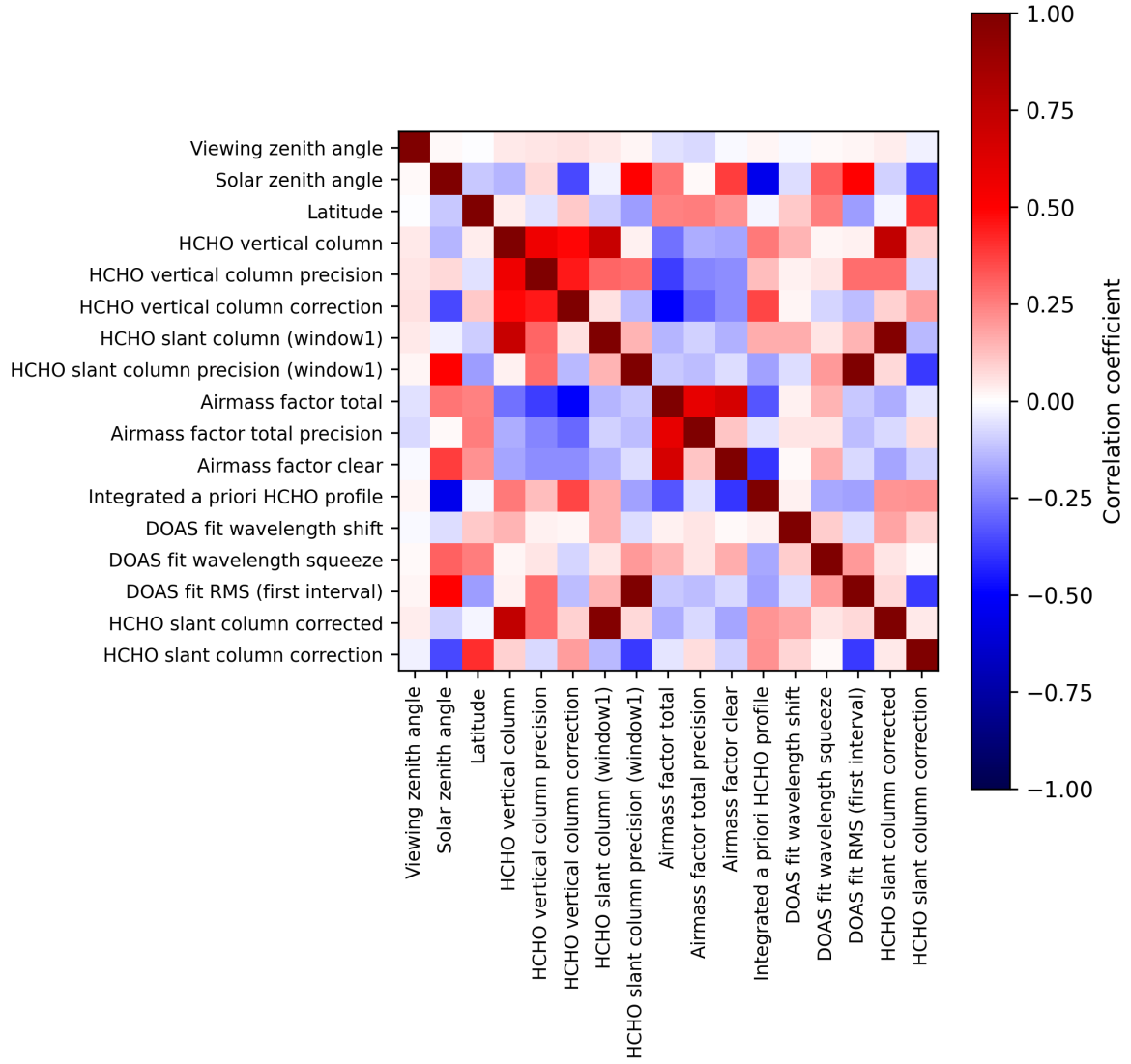
Figure 2: Map of correlation matrix for 2025-06-29 to 2025-07-01.
