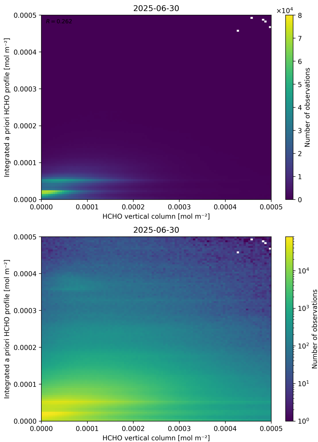
Figure 135: Scatter density plot of “HCHO vertical column” against “Integrated a priori HCHO profile” for 2025-06-29 to 2025-07-01.
