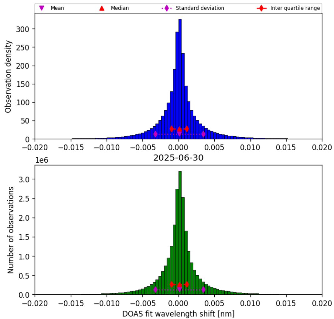
Figure 44: Histogram of “DOAS fit wavelength shift” for 2025-06-29 to 2025-07-01
