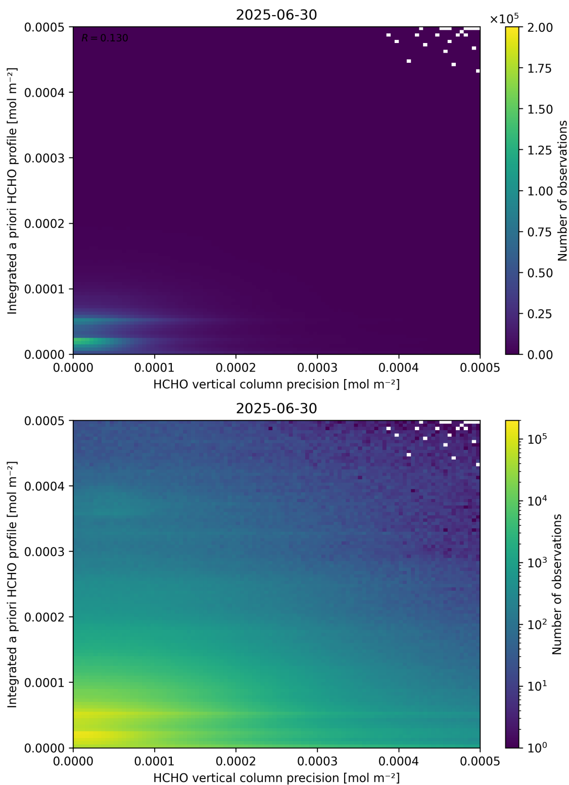
Figure 147: Scatter density plot of “HCHO vertical column precision” against “Integrated a priori HCHO profile” for 2025-06-29 to 2025-07-01.
