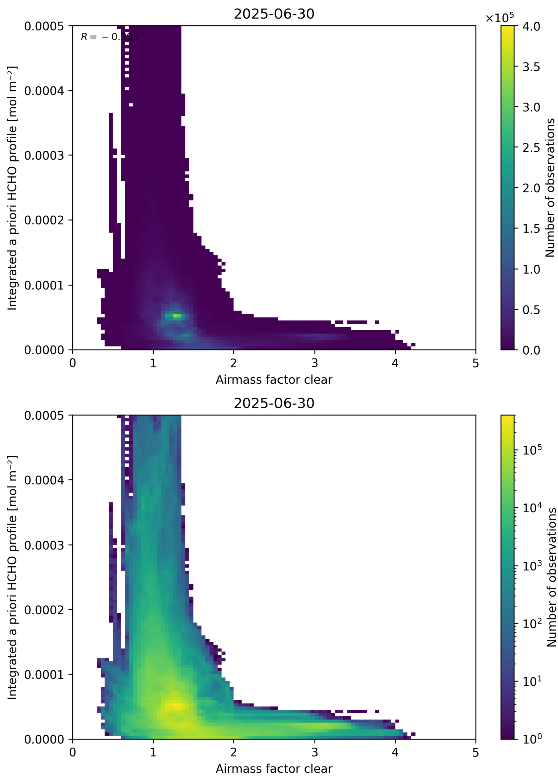
Figure 76: Scatter density plot of “Airmass factor clear” against “Integrated a priori HCHO profile” for 2025-06-29 to 2025-07-01.
