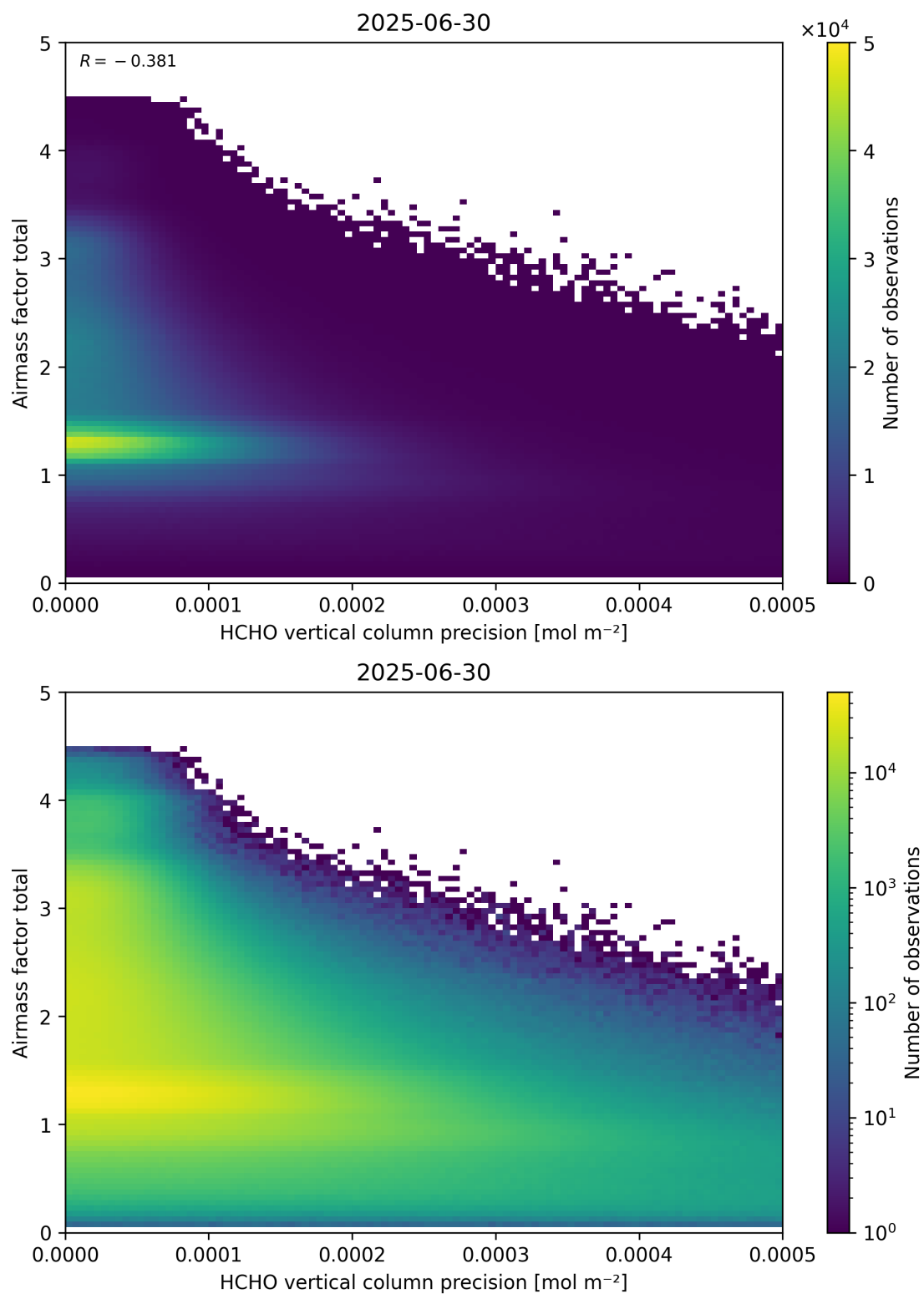
Figure 144: Scatter density plot of “HCHO vertical column precision” against “Airmass factor total” for 2025-06-29 to 2025-07-01.
