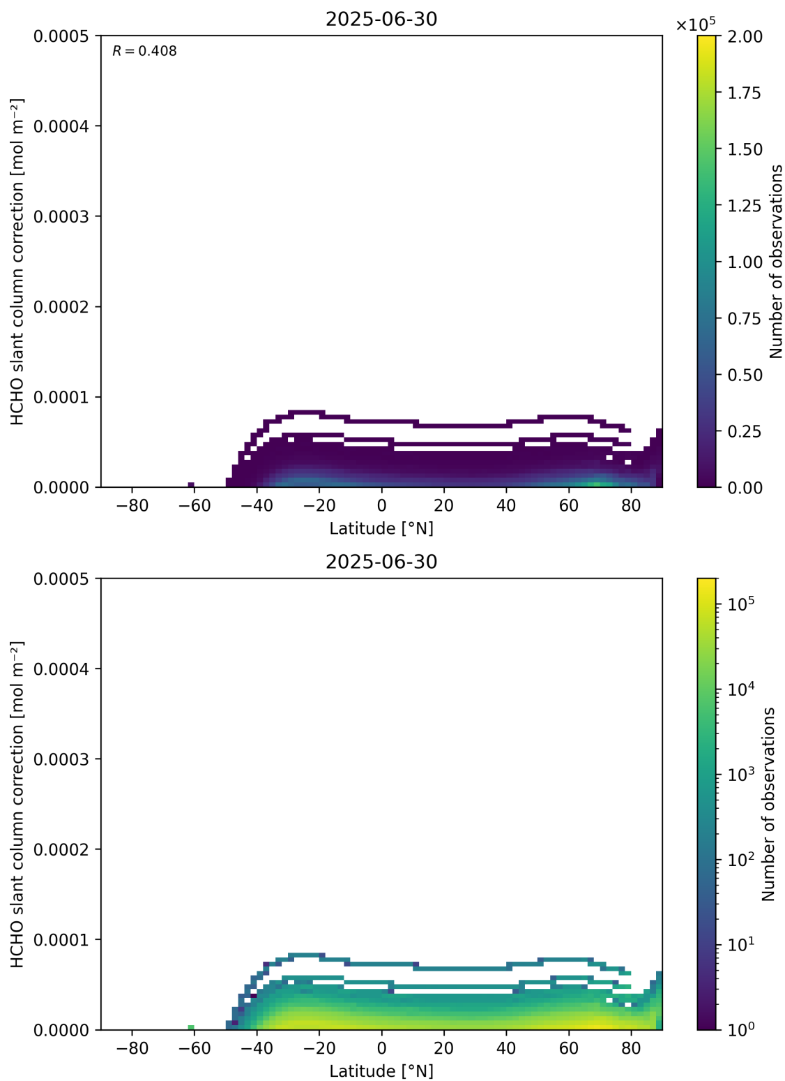
Figure 158: Scatter density plot of “Latitude” against “HCHO slant column correction” for 2025-06-29 to 2025-07-01.
