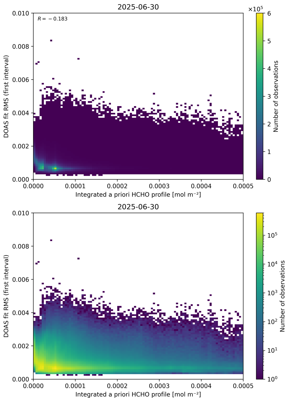
Figure 148: Scatter density plot of “Integrated a priori HCHO profile” against “DOAS fit RMS (first interval)” for 2025-06-29 to 2025-07-01.
