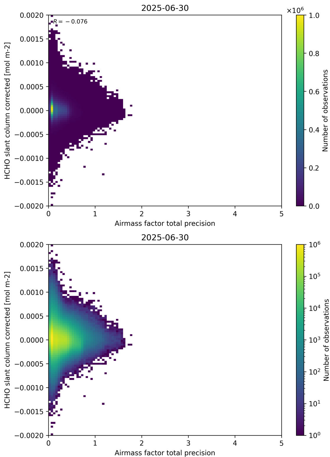
Figure 109: Scatter density plot of “Airmass factor total precision” against “HCHO slant column corrected” for 2025-06-29 to 2025-07-01.
