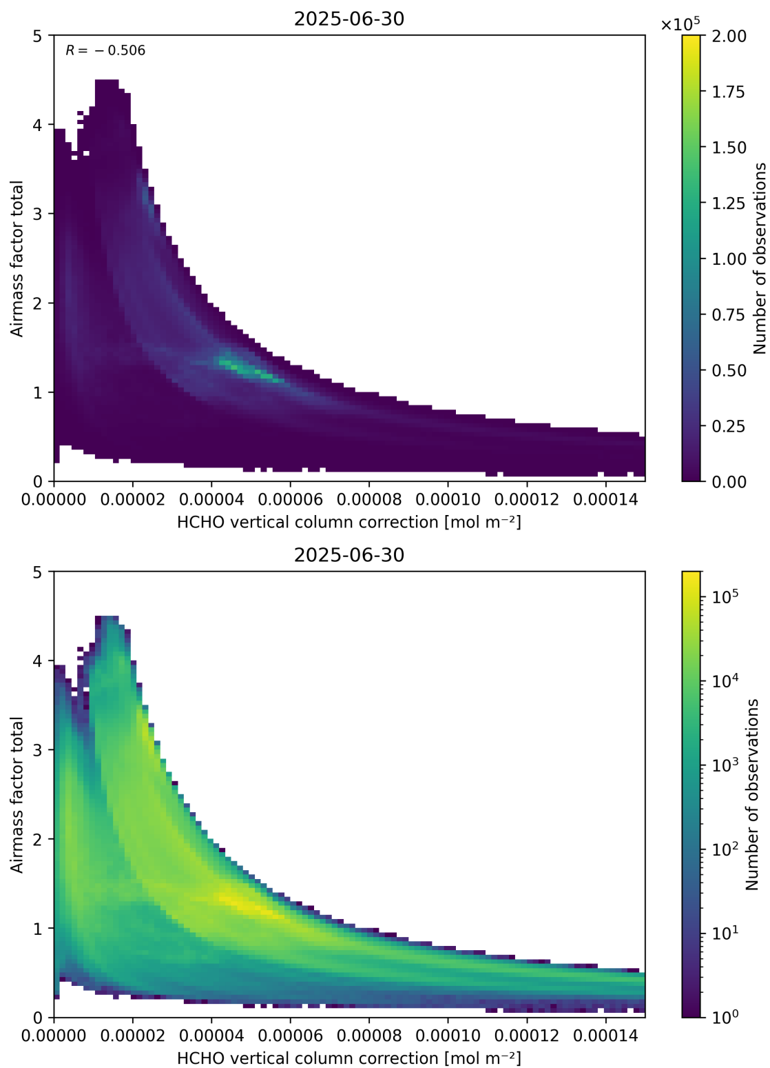
Figure 120: Scatter density plot of “HCHO vertical column correction” against “Airmass factor total” for 2025-06-29 to 2025-07-01.
