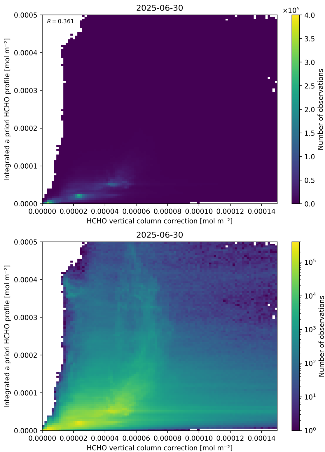
Figure 122: Scatter density plot of “HCHO vertical column correction” against “Integrated a priori HCHO profile” for 2025-06-29 to 2025-07-01.
