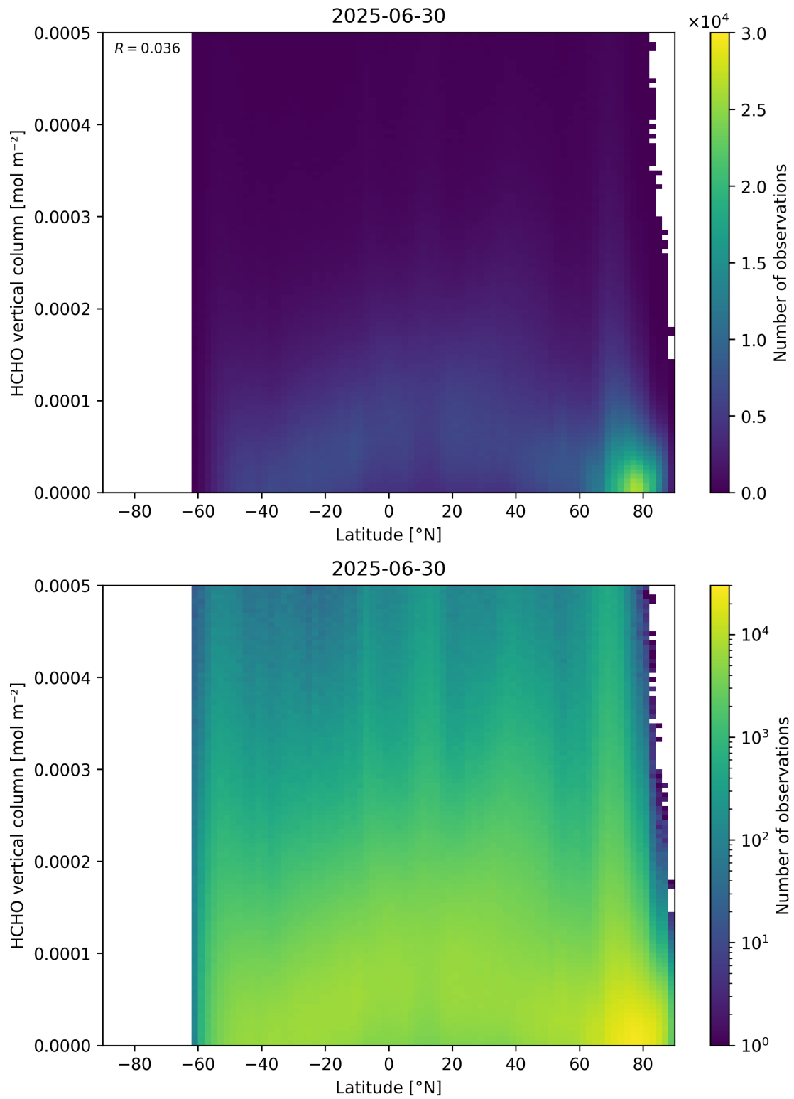
Figure 163: Scatter density plot of “Latitude” against “HCHO vertical column” for 2025-06-29 to 2025-07-01.
