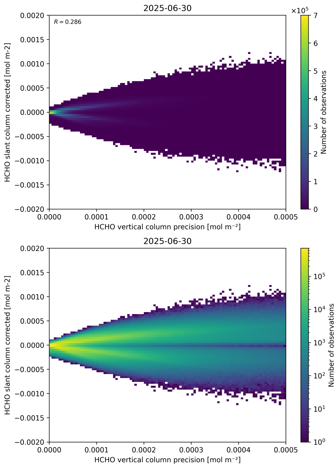
Figure 140: Scatter density plot of “HCHO vertical column precision” against “HCHO slant column corrected” for 2025-06-29 to 2025-07-01.
