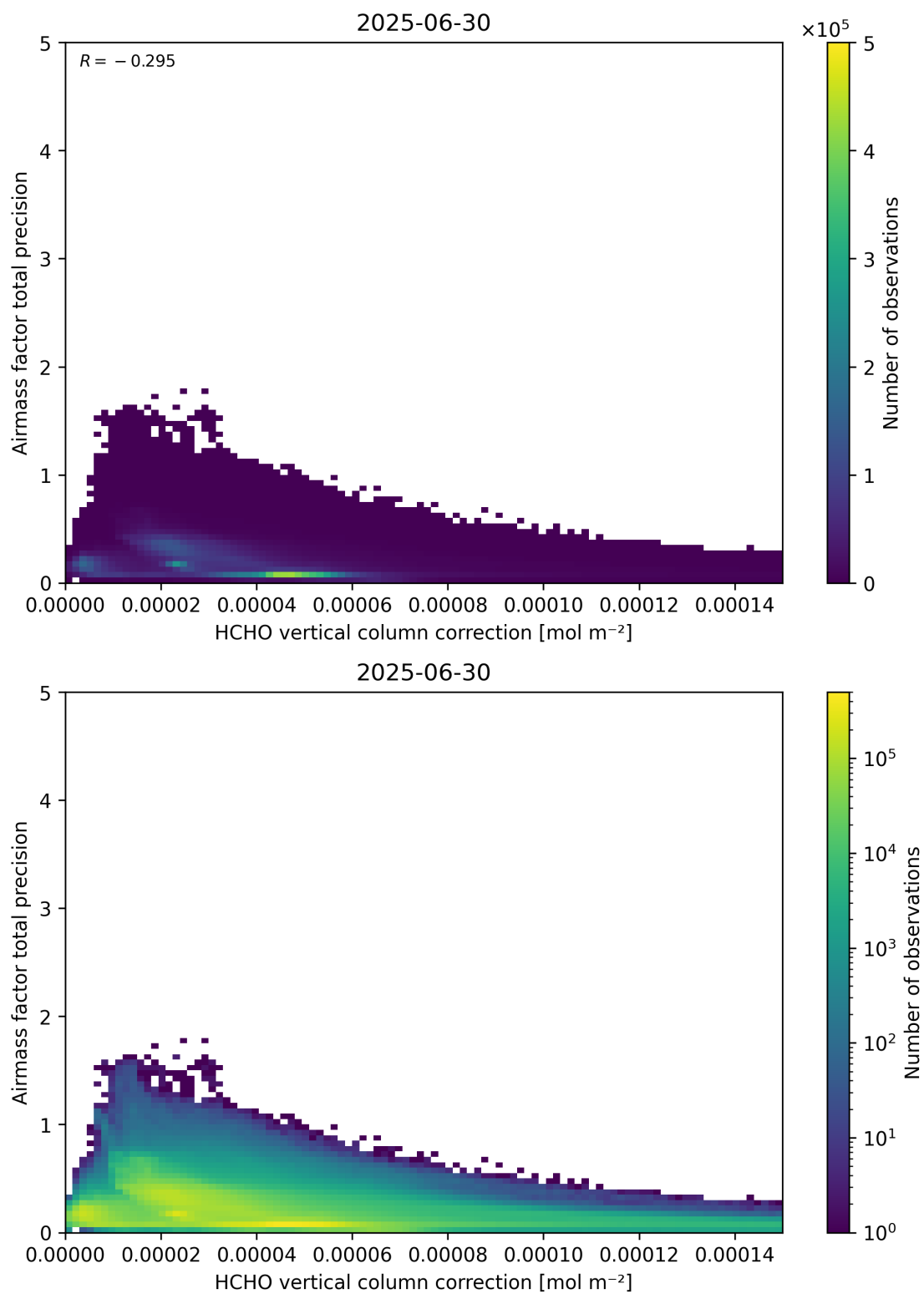
Figure 121: Scatter density plot of “HCHO vertical column correction” against “Airmass factor total precision” for 2025-06-29 to 2025-07-01.
