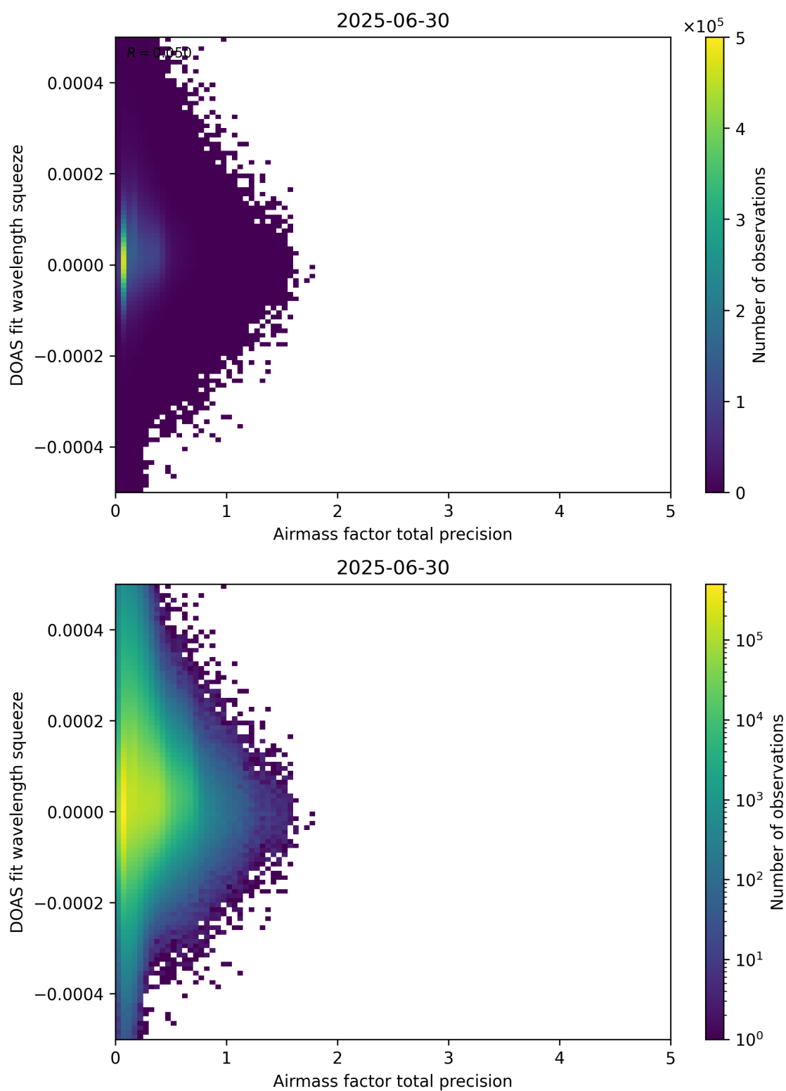
Figure 107: Scatter density plot of “Airmass factor total precision” against “DOAS fit wavelength squeeze” for 2025-06-29 to 2025-07-01.
