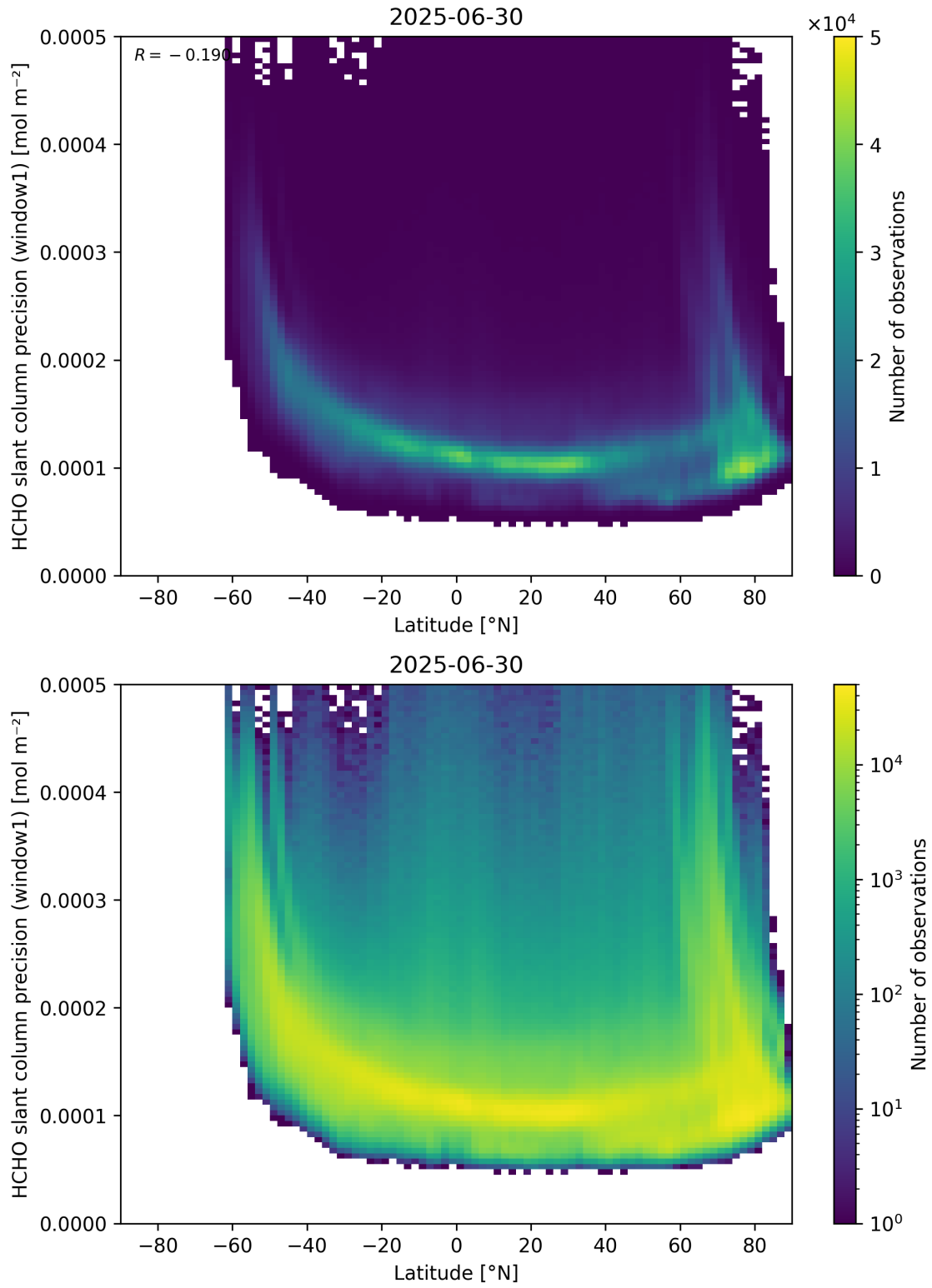
Figure 160: Scatter density plot of “Latitude” against “HCHO slant column precision (window1)” for 2025-06-29 to 2025-07-01.
