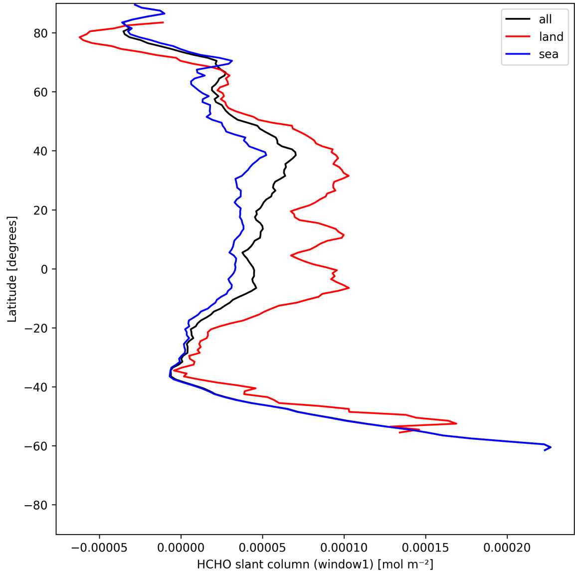
Figure 24: Zonal average of “HCHO slant column (window1)” for 2025-06-29 to 2025-07-01.
