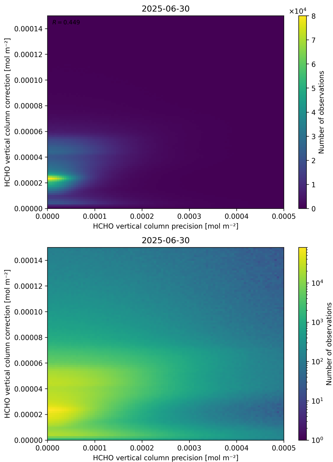
Figure 146: Scatter density plot of “HCHO vertical column precision” against “HCHO vertical column correction” for 2025-06-29 to 2025-07-01.
