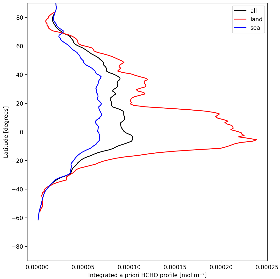
Figure 29: Zonal average of “Integrated a priori HCHO profile” for 2025-06-29 to 2025-07-01.
