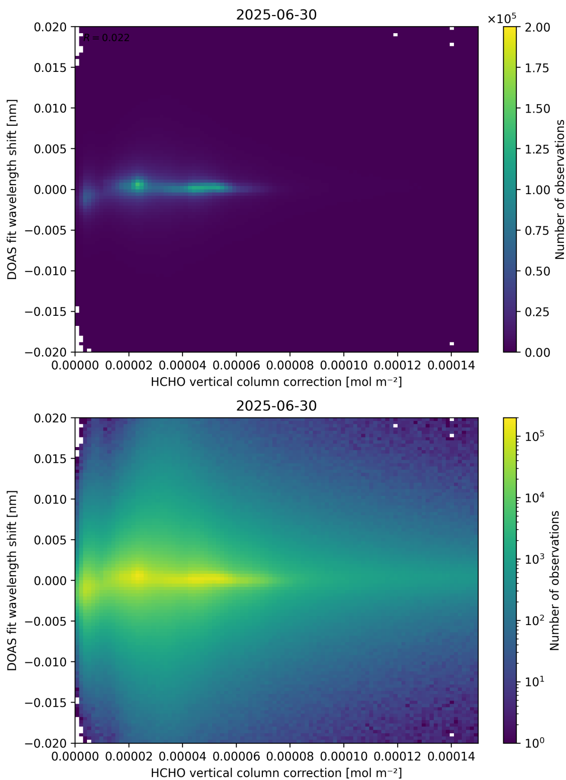
Figure 113: Scatter density plot of “HCHO vertical column correction” against “DOAS fit wavelength shift” for 2025-06-29 to 2025-07-01.
