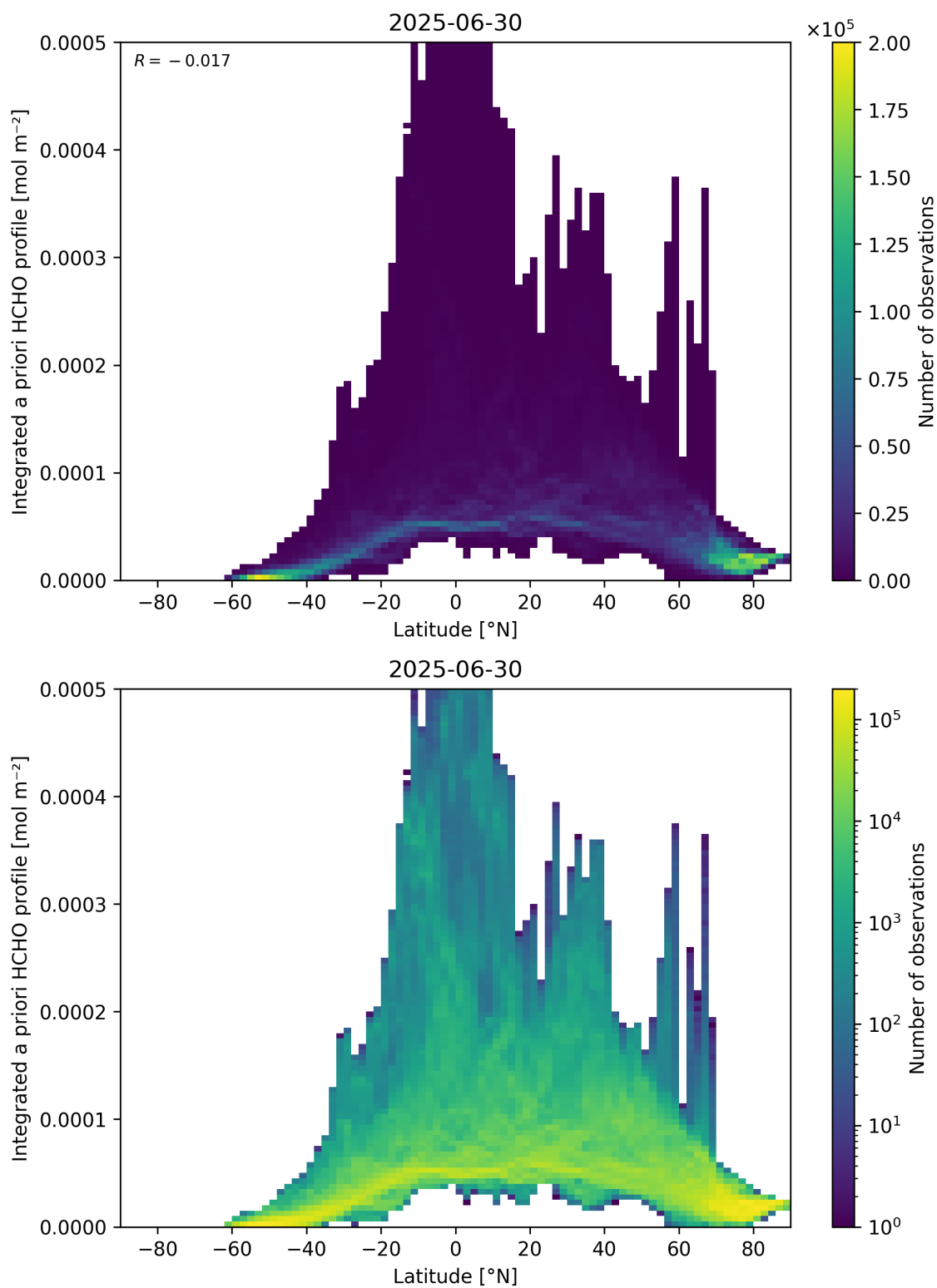
Figure 166: Scatter density plot of “Latitude” against “Integrated a priori HCHO profile” for 2025-06-29 to 2025-07-01.
