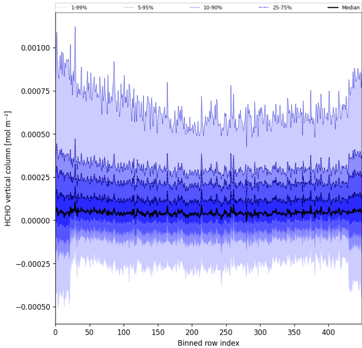
Figure 49: Along track statistics of “HCHO vertical column” for 2025-06-29 to 2025-07-01
