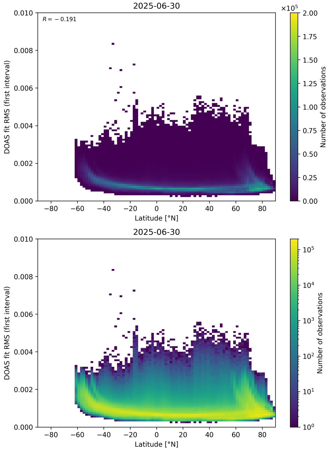
Figure 153: Scatter density plot of “Latitude” against “DOAS fit RMS (first interval)” for 2025-06-29 to 2025-07-01.
