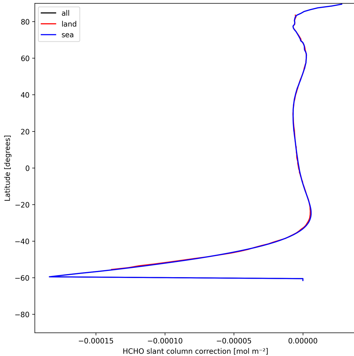
Figure 33: Zonal average of “HCHO slant column correction” for 2025-06-29 to 2025-07-01.
