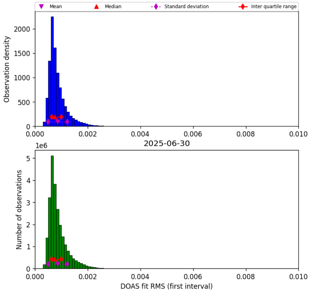
Figure 46: Histogram of “DOAS fit RMS (first interval)” for 2025-06-29 to 2025-07-01
