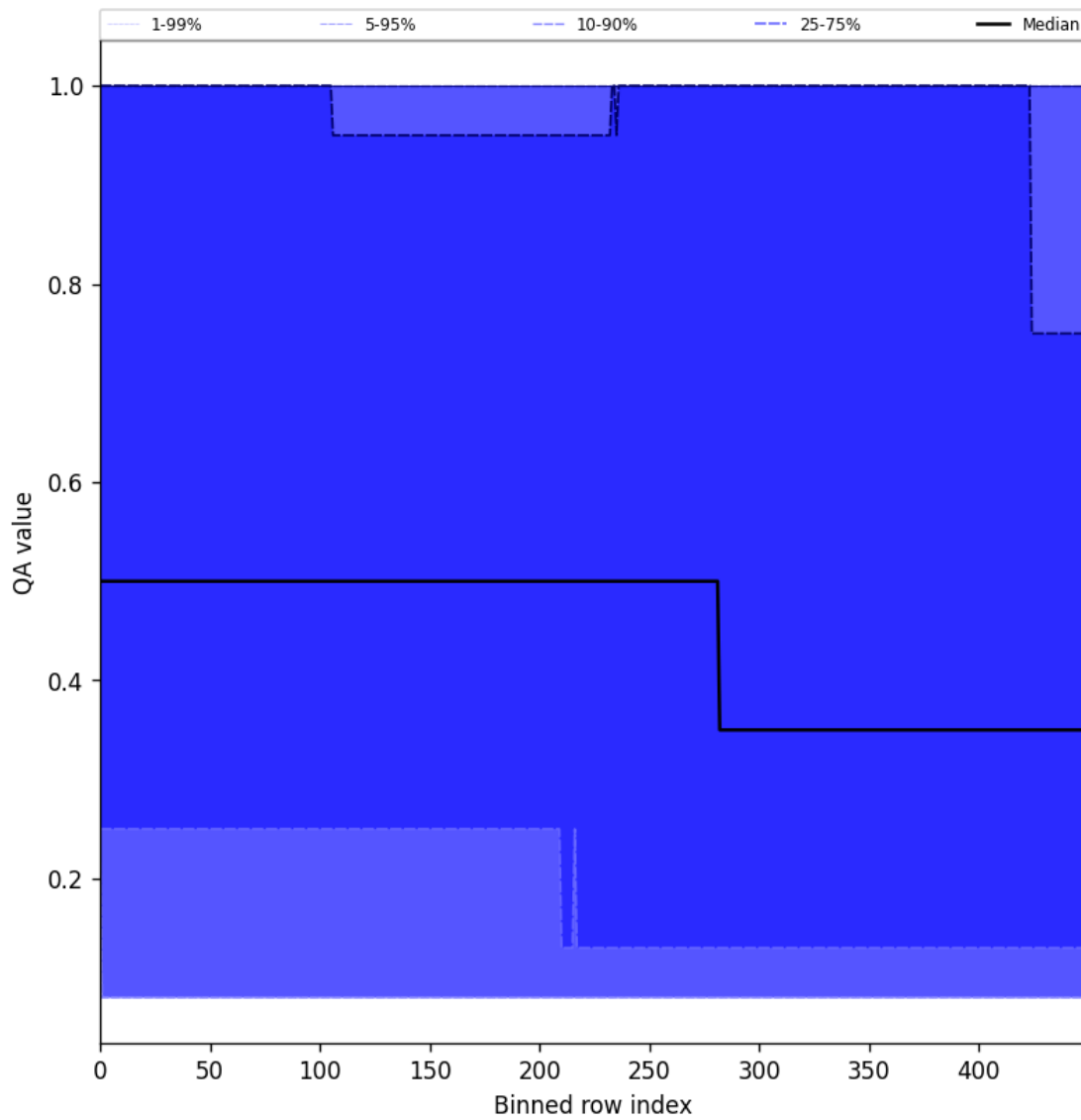
Figure 48: Along track statistics of “QA value” for 2025-06-29 to 2025-07-01
