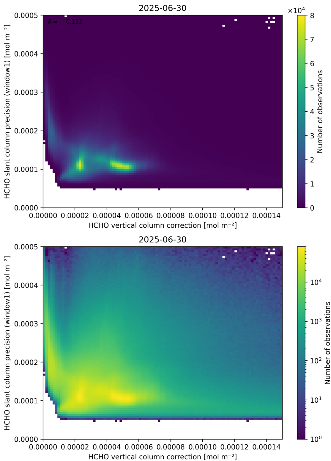
Figure 119: Scatter density plot of “HCHO vertical column correction” against “HCHO slant column precision (window1)” for 2025-06-29 to 2025-07-01.
