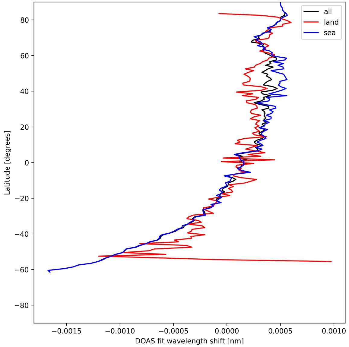
Figure 30: Zonal average of “DOAS fit wavelength shift” for 2025-06-29 to 2025-07-01.
