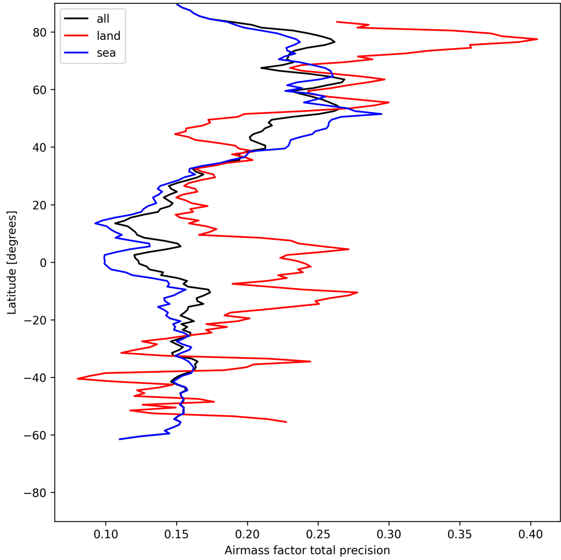
Figure 27: Zonal average of “Airmass factor total precision” for 2025-06-29 to 2025-07-01.
