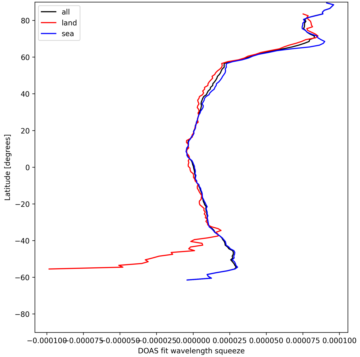
Figure 31: Zonal average of “DOAS fit wavelength squeeze” for 2025-06-29 to 2025-07-01.
