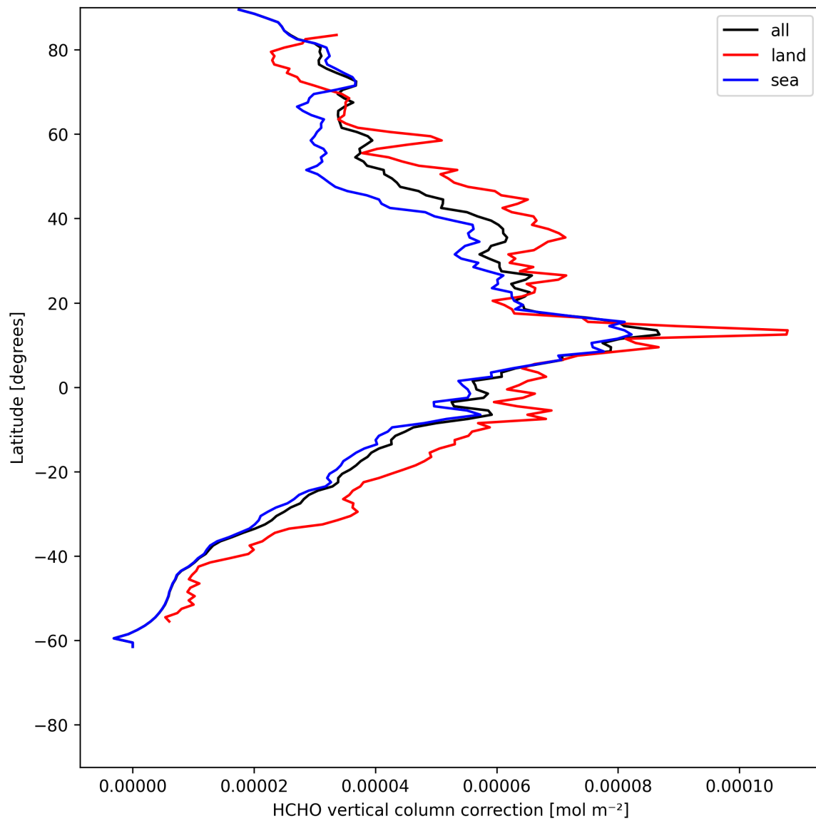
Figure 23: Zonal average of “HCHO vertical column correction” for 2025-06-29 to 2025-07-01.
