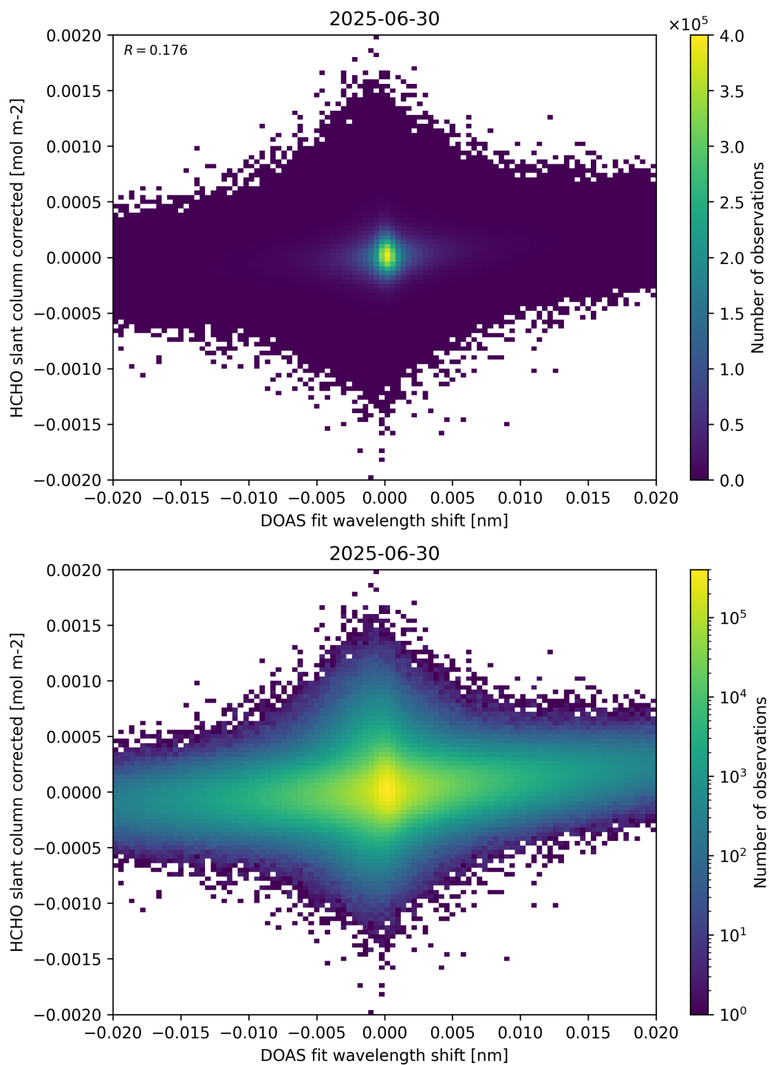
Figure 66: Scatter density plot of “DOAS fit wavelength shift” against “HCHO slant column corrected” for 2025-06-29 to 2025-07-01.
