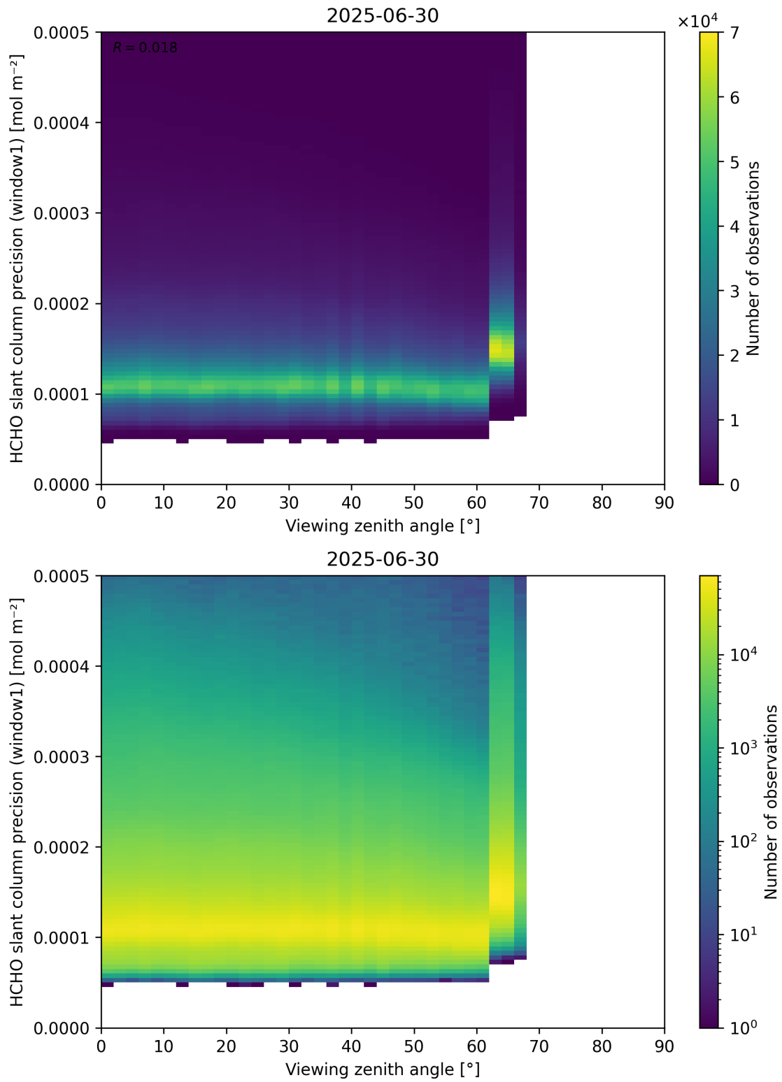
Figure 189: Scatter density plot of “Viewing zenith angle” against “HCHO slant column precision (window1)” for 2025-06-29 to 2025-07-01.
