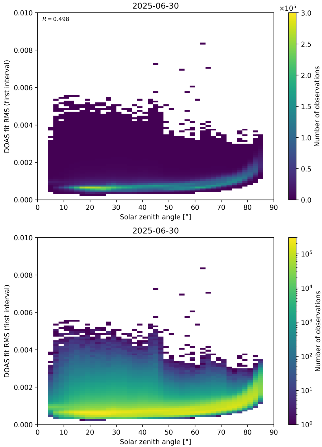
Figure 167: Scatter density plot of “Solar zenith angle” against “DOAS fit RMS (first interval)” for 2025-06-29 to 2025-07-01.
