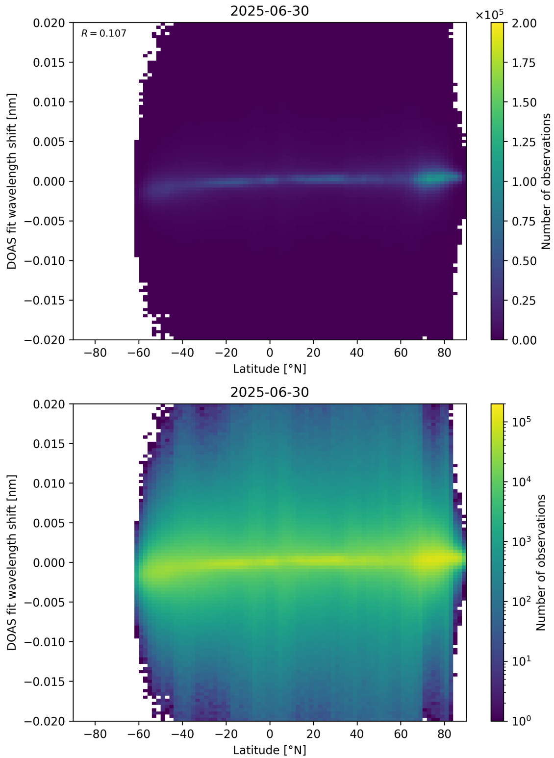
Figure 154: Scatter density plot of “Latitude” against “DOAS fit wavelength shift” for 2025-06-29 to 2025-07-01.
