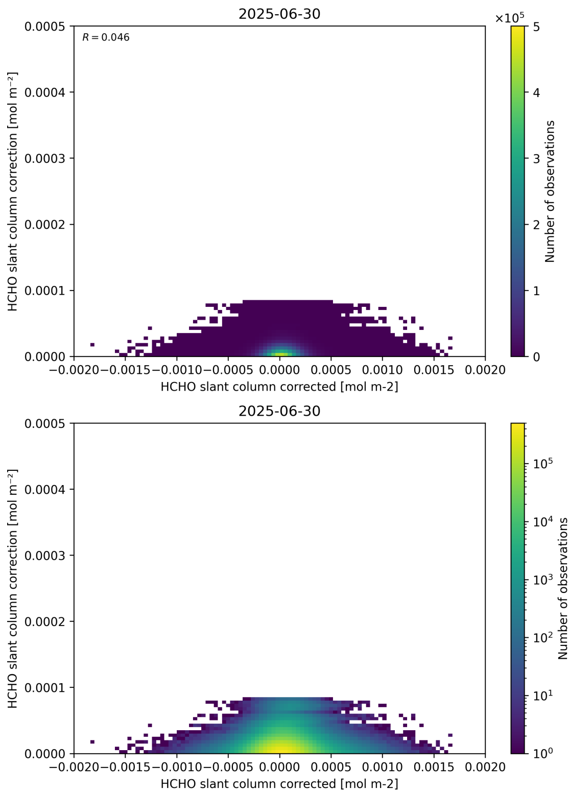
Figure 77: Scatter density plot of “HCHO slant column corrected” against “HCHO slant column correction” for 2025-06-29 to 2025-07-01.
