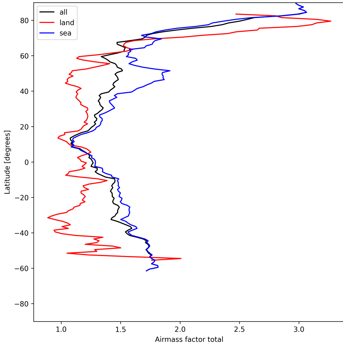
Figure 26: Zonal average of “Airmass factor total” for 2025-06-29 to 2025-07-01.
