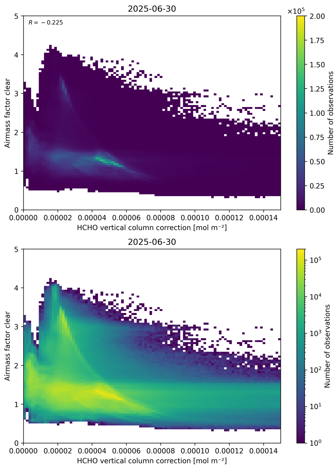
Figure 115: Scatter density plot of “HCHO vertical column correction” against “Airmass factor clear” for 2025-06-29 to 2025-07-01.
