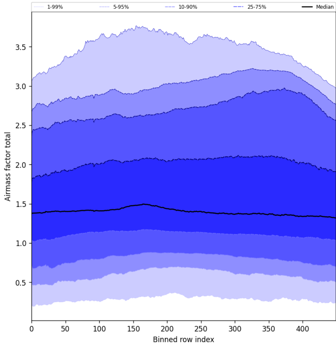
Figure 54: Along track statistics of “Airmass factor total” for 2025-06-29 to 2025-07-01
