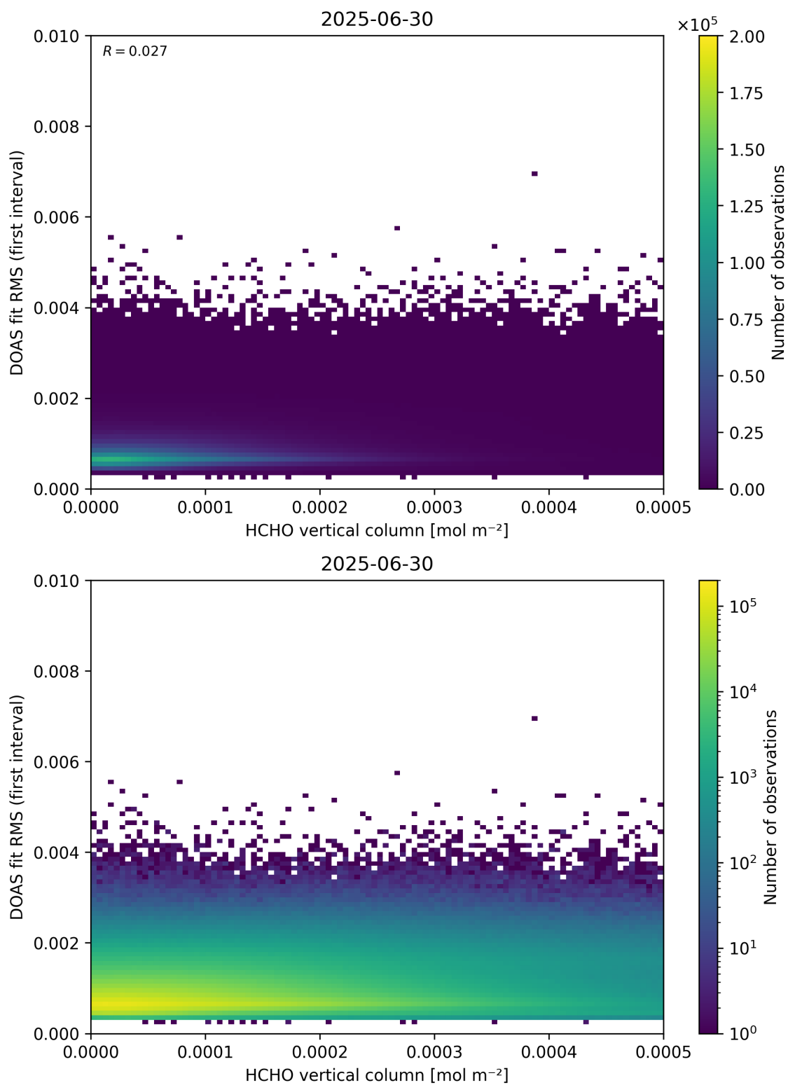
Figure 123: Scatter density plot of “HCHO vertical column” against “DOAS fit RMS (first interval)” for 2025-06-29 to 2025-07-01.
