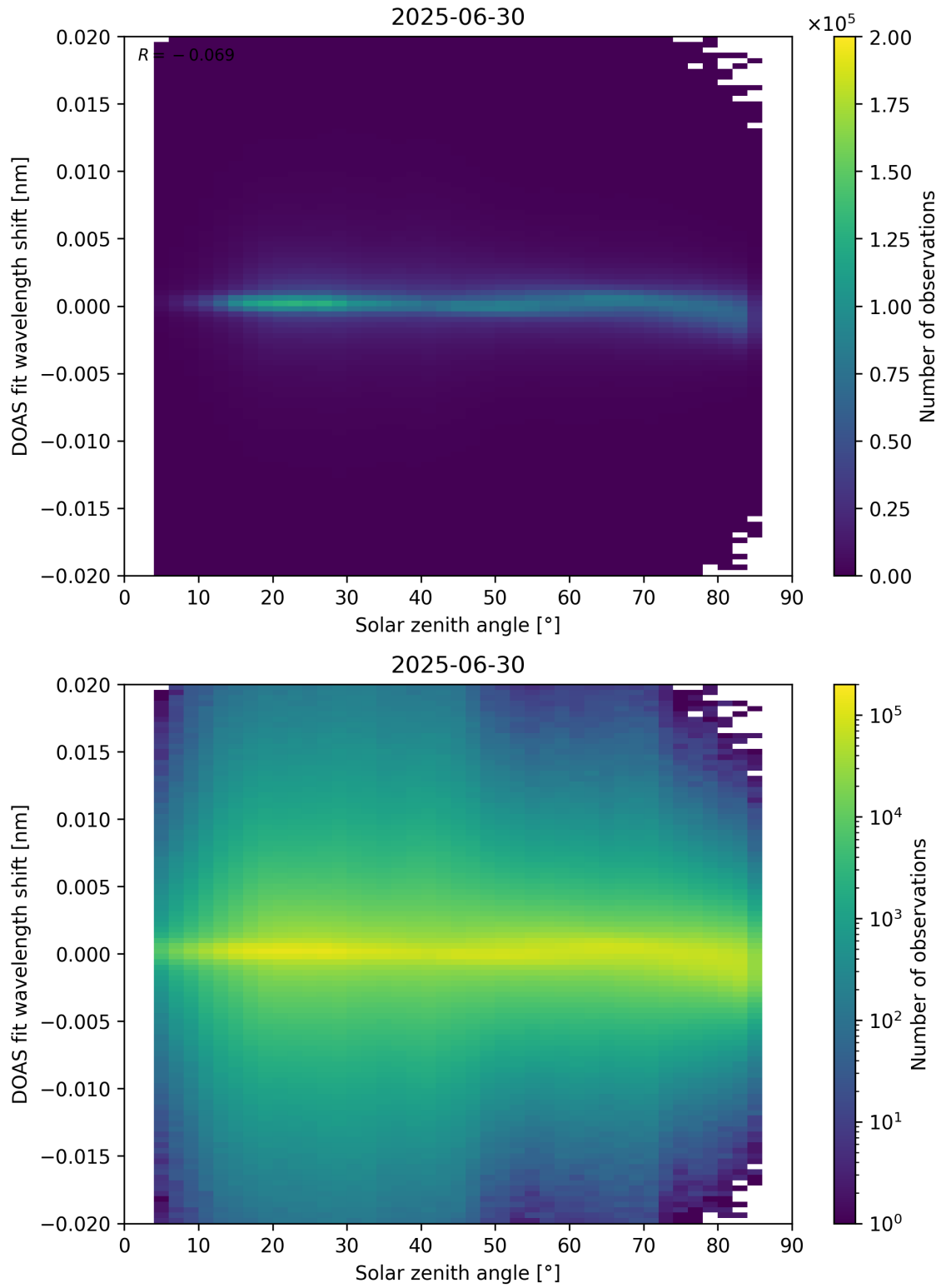
Figure 168: Scatter density plot of “Solar zenith angle” against “DOAS fit wavelength shift” for 2025-06-29 to 2025-07-01.
