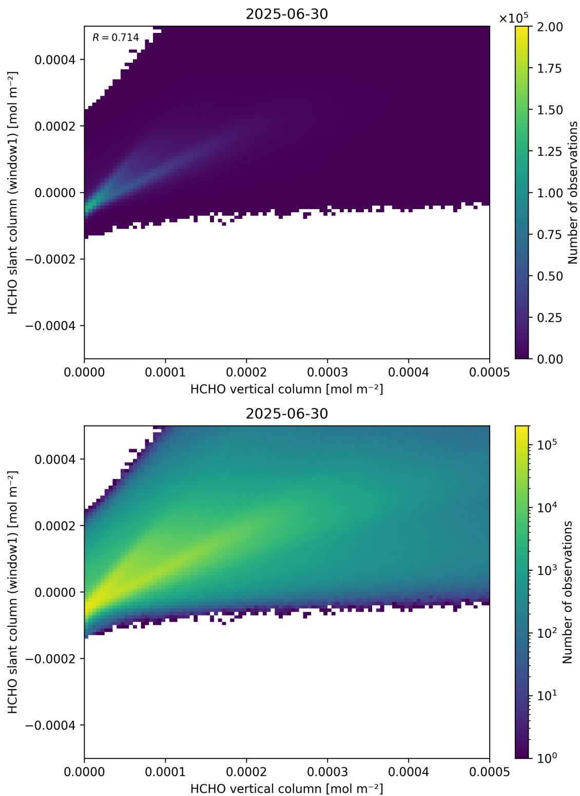
Figure 129: Scatter density plot of “HCHO vertical column” against “HCHO slant column (window1)” for 2025-06-29 to 2025-07-01.
