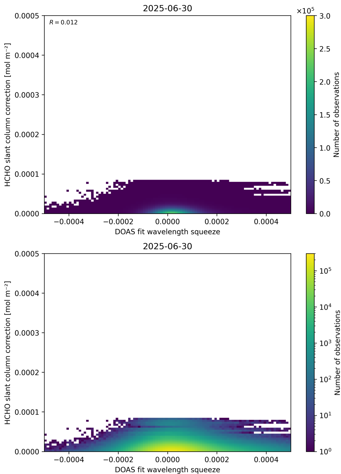
Figure 70: Scatter density plot of “DOAS fit wavelength squeeze” against “HCHO slant column correction” for 2025-06-29 to 2025-07-01.
