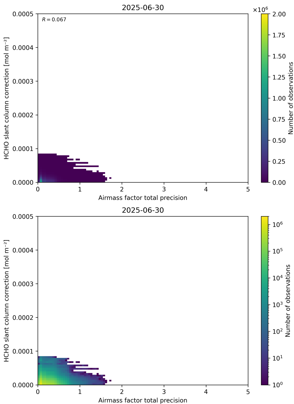
Figure 110: Scatter density plot of “Airmass factor total precision” against “HCHO slant column correction” for 2025-06-29 to 2025-07-01.
