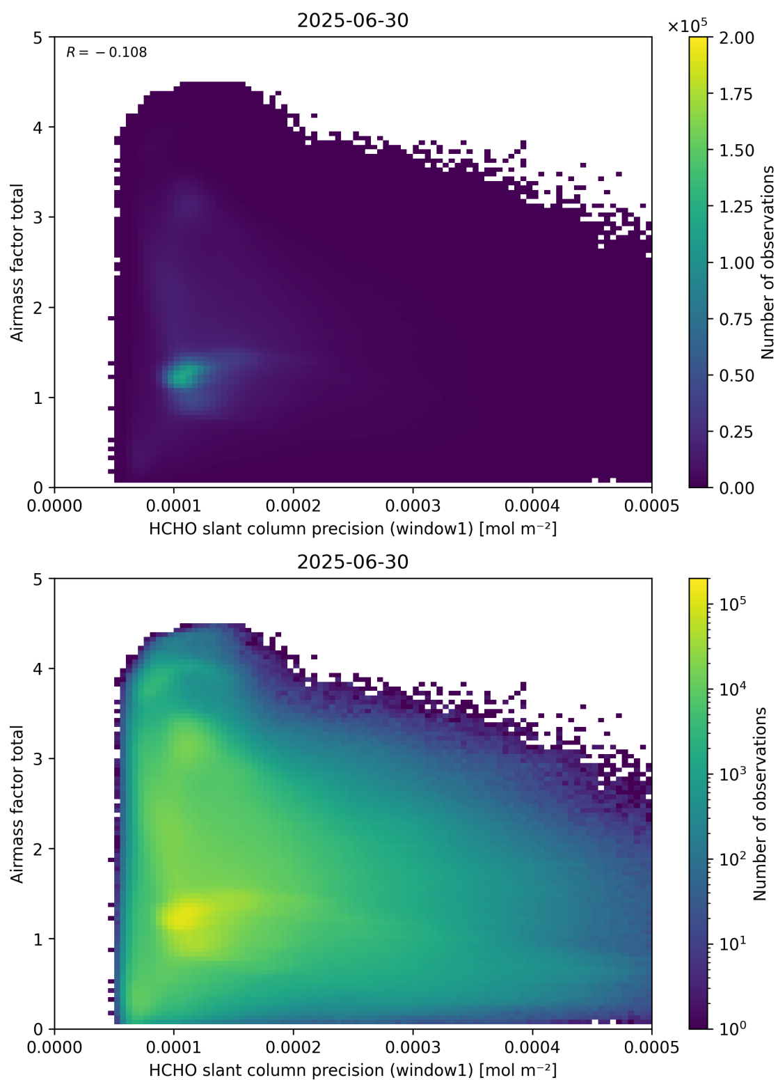
Figure 94: Scatter density plot of “HCHO slant column precision (window1)” against “Airmass factor total” for 2025-06-29 to 2025-07-01.
