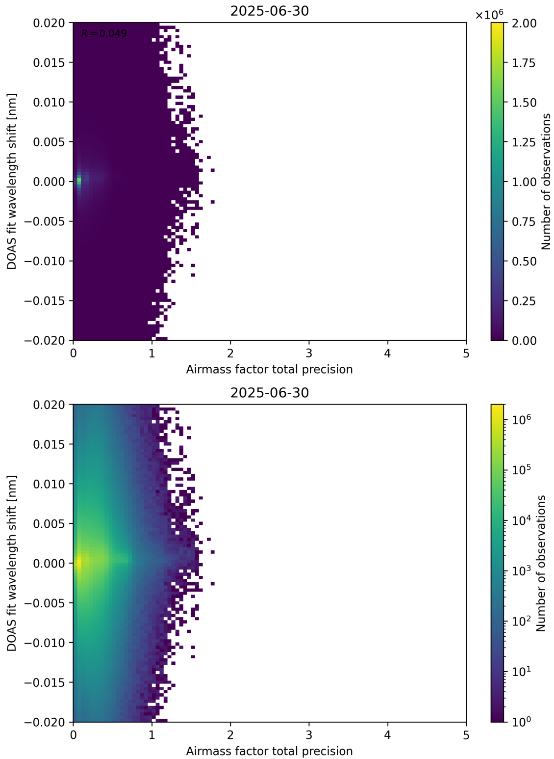
Figure 106: Scatter density plot of “Airmass factor total precision” against “DOAS fit wavelength shift” for 2025-06-29 to 2025-07-01.
