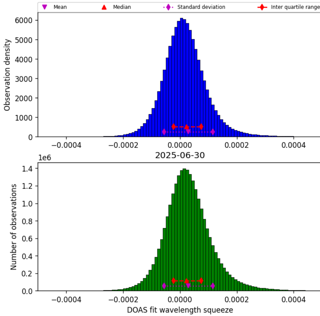
Figure 45: Histogram of “DOAS fit wavelength squeeze” for 2025-06-29 to 2025-07-01
