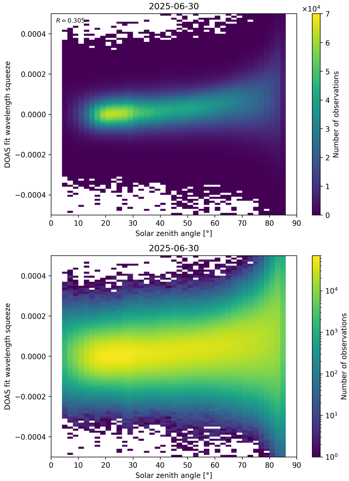
Figure 169: Scatter density plot of “Solar zenith angle” against “DOAS fit wavelength squeeze” for 2025-06-29 to 2025-07-01.
