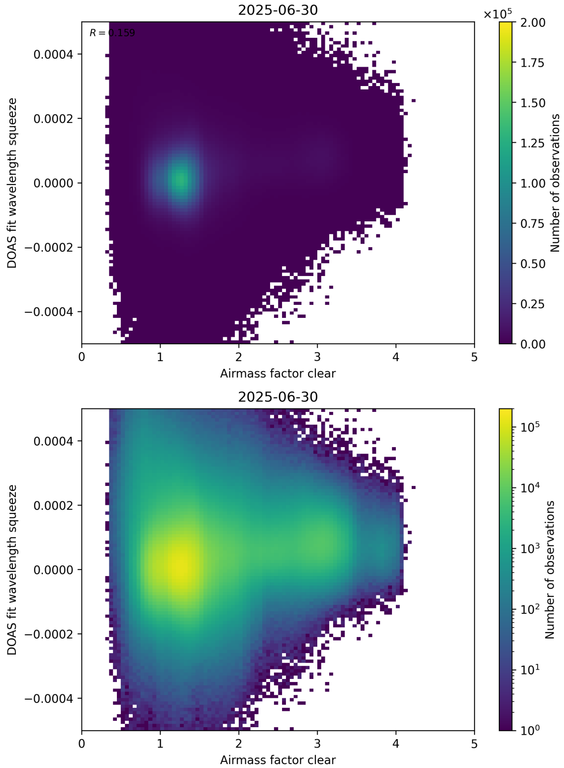
Figure 73: Scatter density plot of “Airmass factor clear” against “DOAS fit wavelength squeeze” for 2025-06-29 to 2025-07-01.
