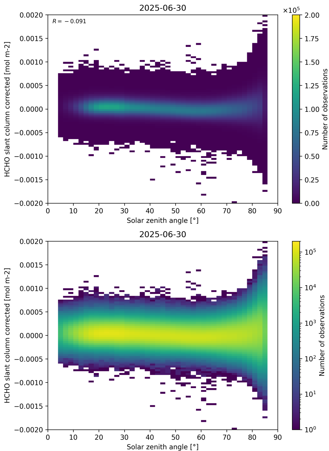
Figure 171: Scatter density plot of “Solar zenith angle” against “HCHO slant column corrected” for 2025-06-29 to 2025-07-01.
