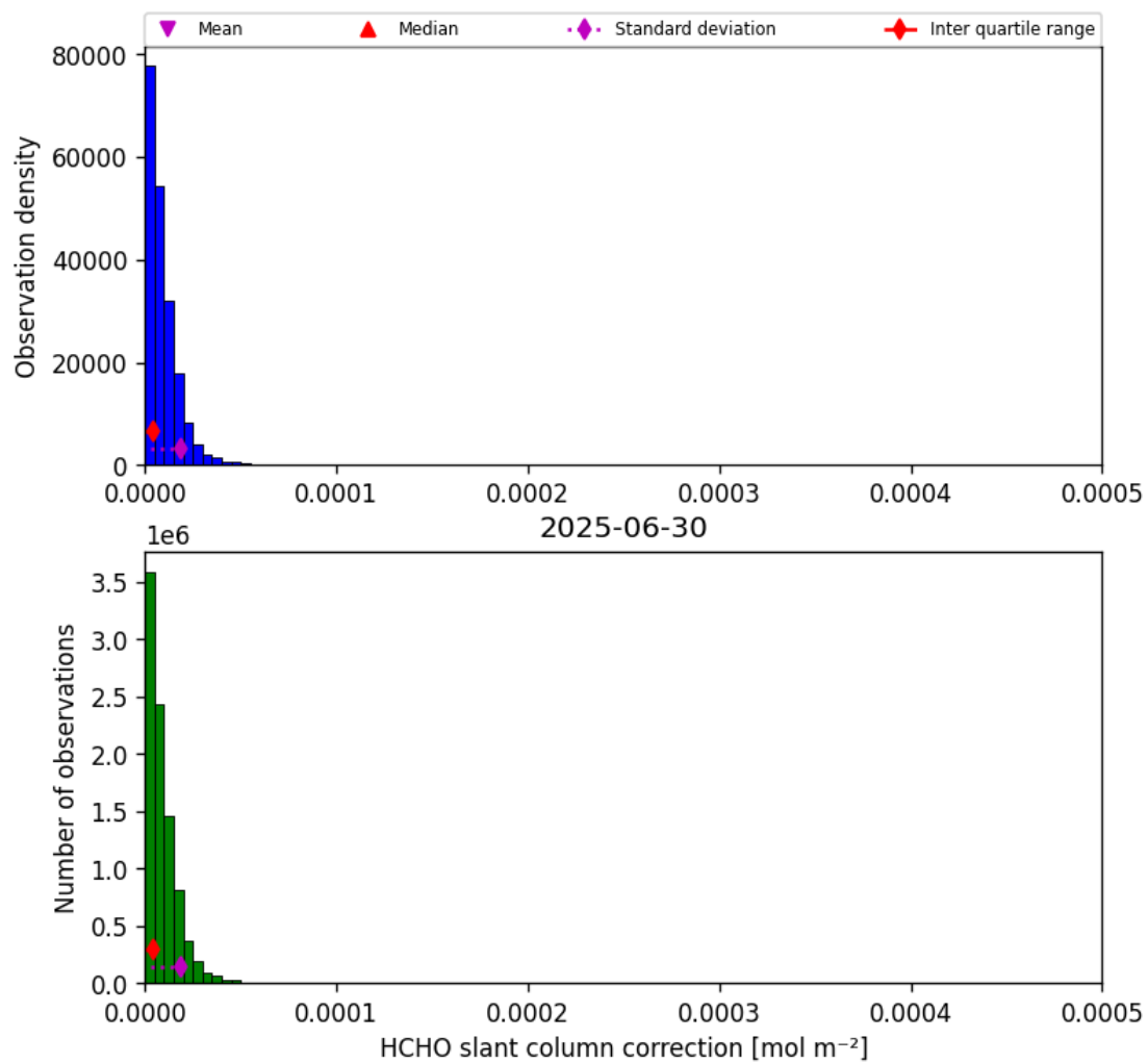
Figure 47: Histogram of “HCHO slant column correction” for 2025-06-29 to 2025-07-01
