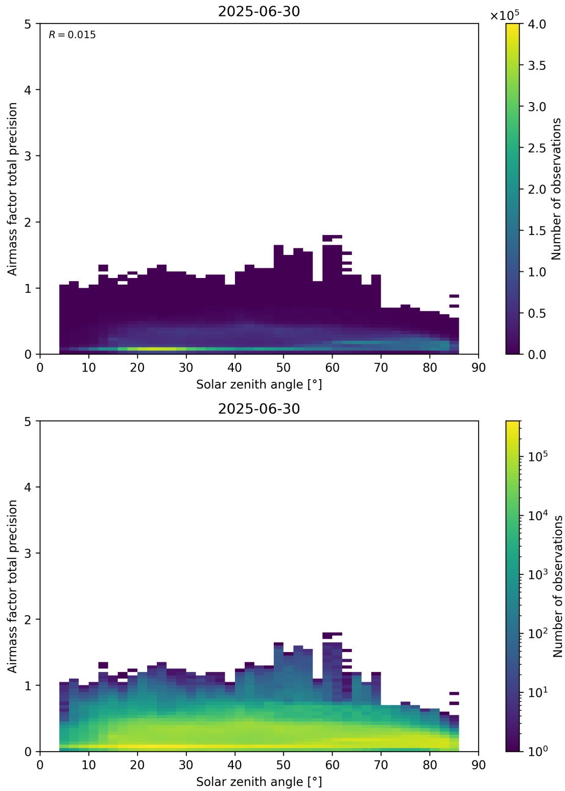
Figure 176: Scatter density plot of “Solar zenith angle” against “Airmass factor total precision” for 2025-06-29 to 2025-07-01.
