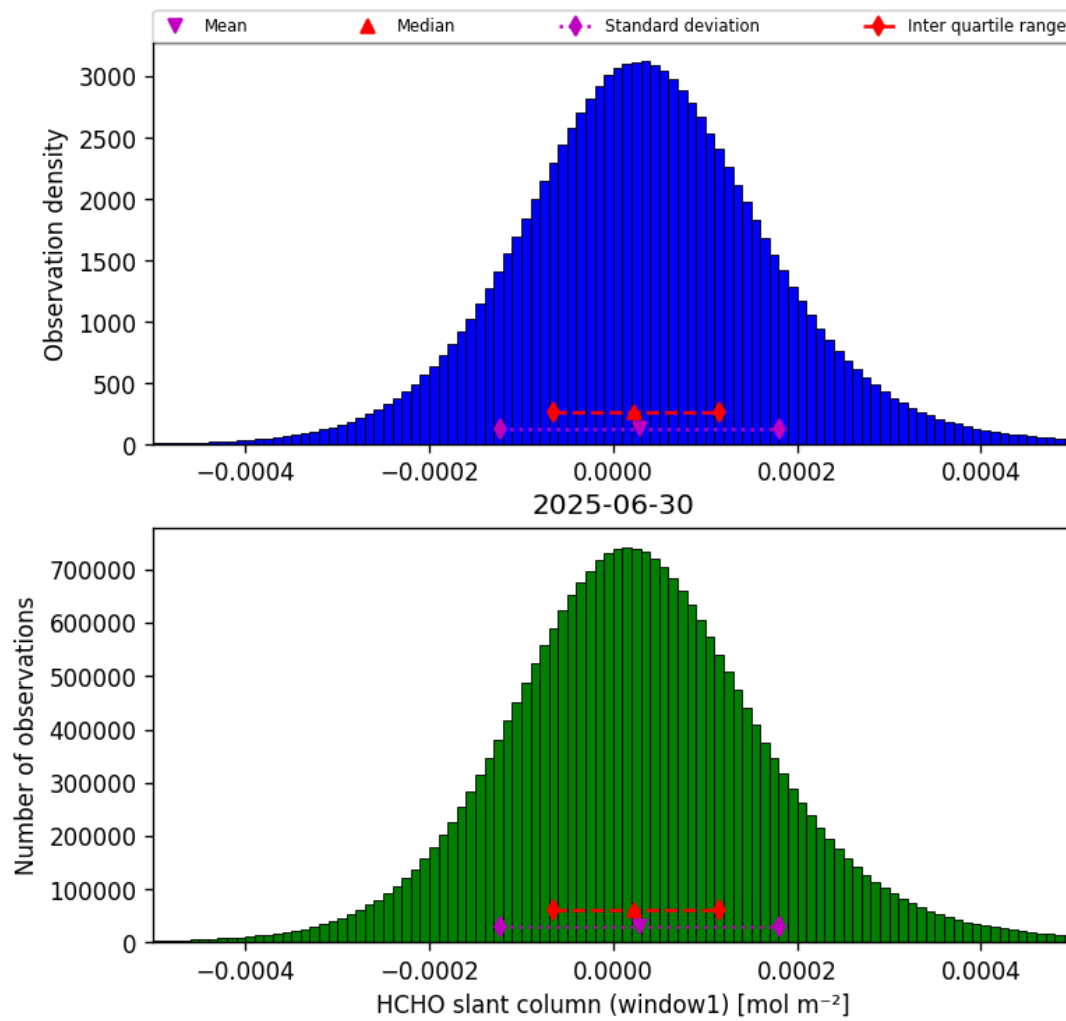
Figure 38: Histogram of “HCHO slant column (window1)” for 2025-06-29 to 2025-07-01
