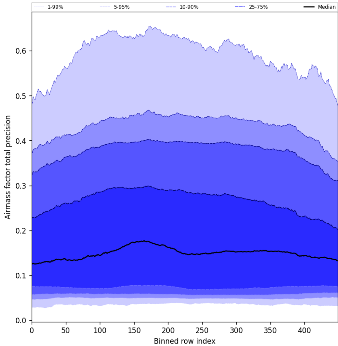
Figure 55: Along track statistics of “Airmass factor total precision” for 2025-06-29 to 2025-07-01
