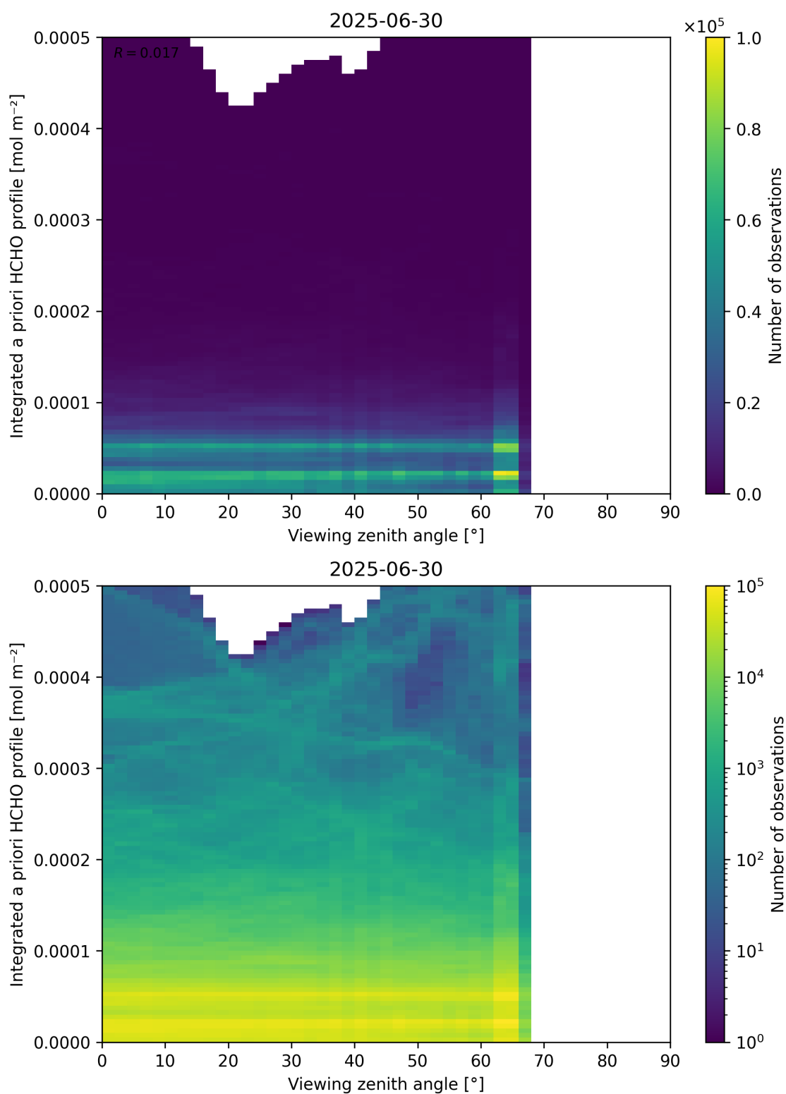
Figure 195: Scatter density plot of “Viewing zenith angle” against “Integrated a priori HCHO profile” for 2025-06-29 to 2025-07-01.
