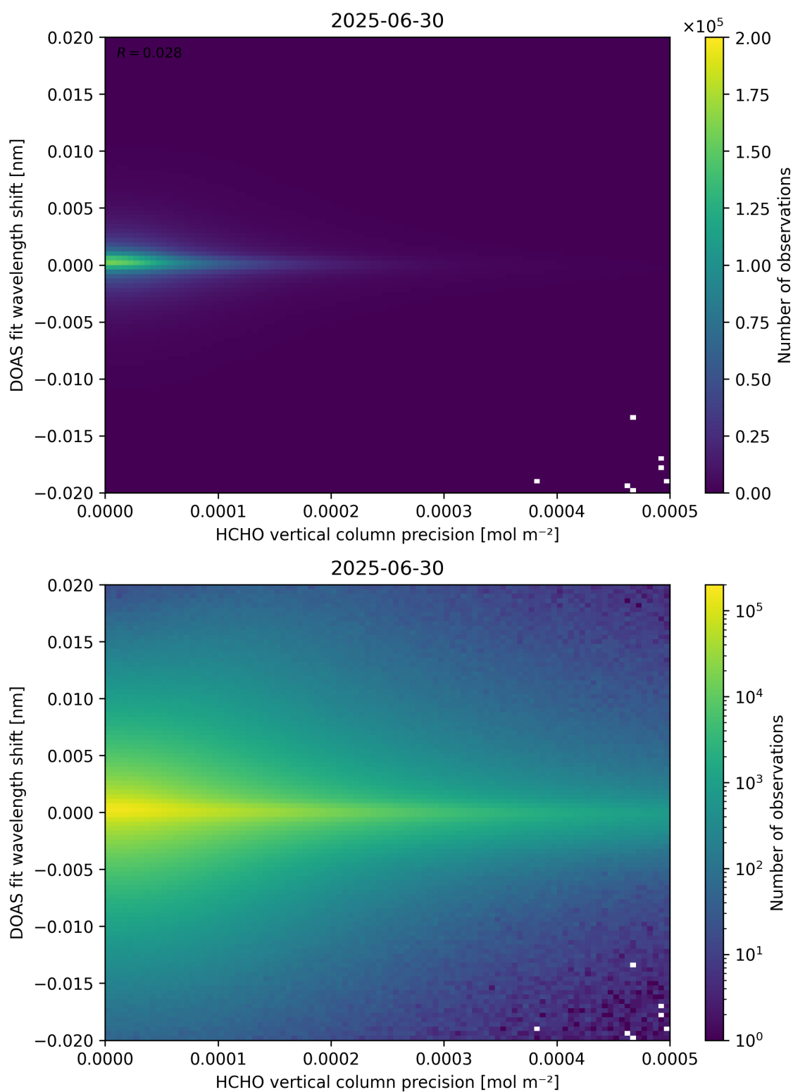
Figure 137: Scatter density plot of “HCHO vertical column precision” against “DOAS fit wavelength shift” for 2025-06-29 to 2025-07-01.
