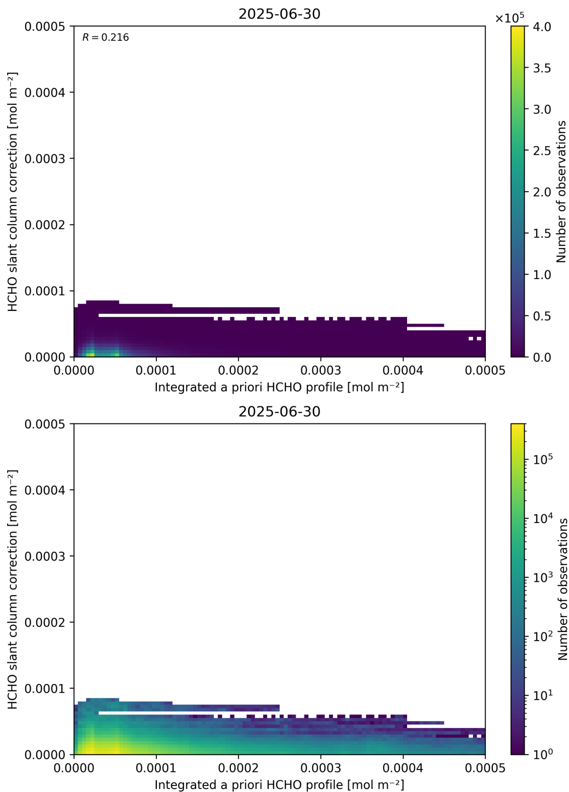
Figure 152: Scatter density plot of “Integrated a priori HCHO profile” against “HCHO slant column correction” for 2025-06-29 to 2025-07-01.
