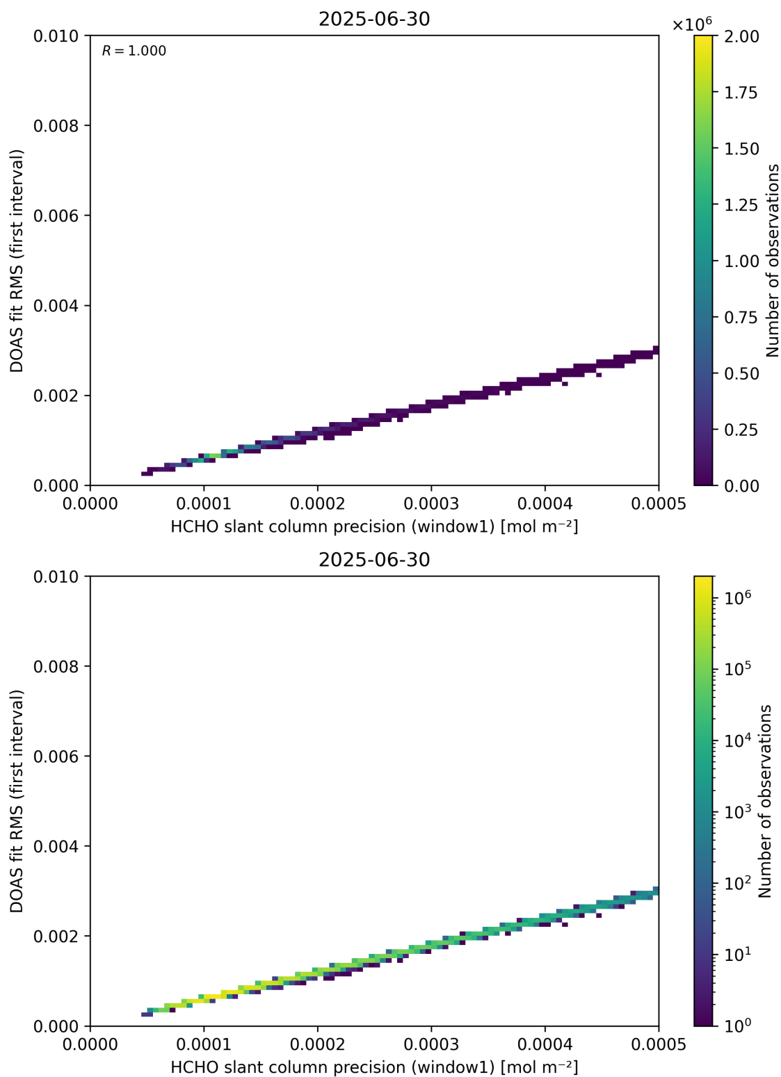
Figure 88: Scatter density plot of “HCHO slant column precision (window1)” against “DOAS fit RMS (first interval)” for 2025-06-29 to 2025-07-01.
