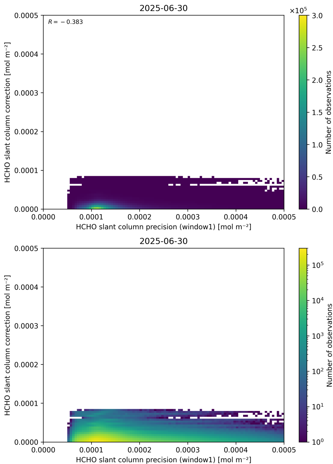
Figure 93: Scatter density plot of “HCHO slant column precision (window1)” against “HCHO slant column correction” for 2025-06-29 to 2025-07-01.
