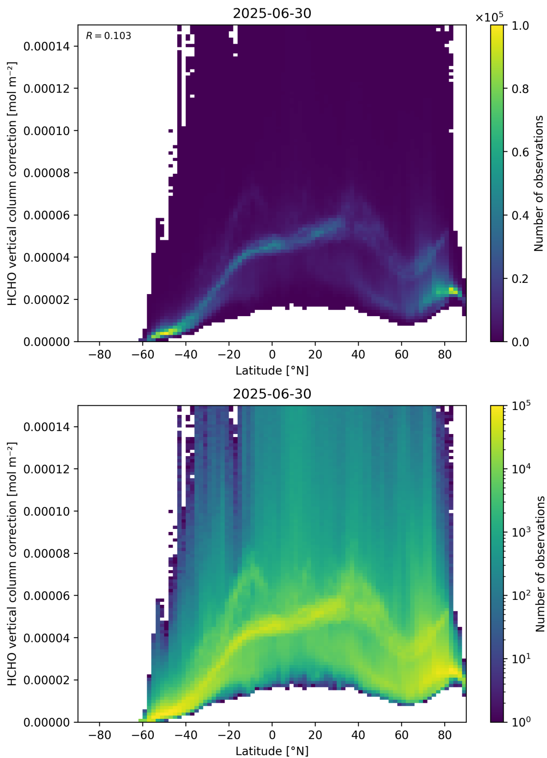
Figure 164: Scatter density plot of “Latitude” against “HCHO vertical column correction” for 2025-06-29 to 2025-07-01.
