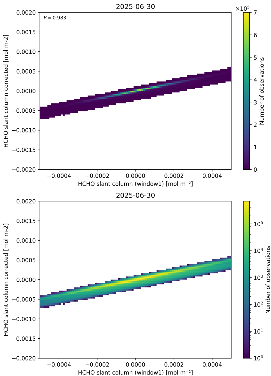
Figure 82: Scatter density plot of “HCHO slant column (window1)” against “HCHO slant column corrected” for 2025-06-29 to 2025-07-01.
