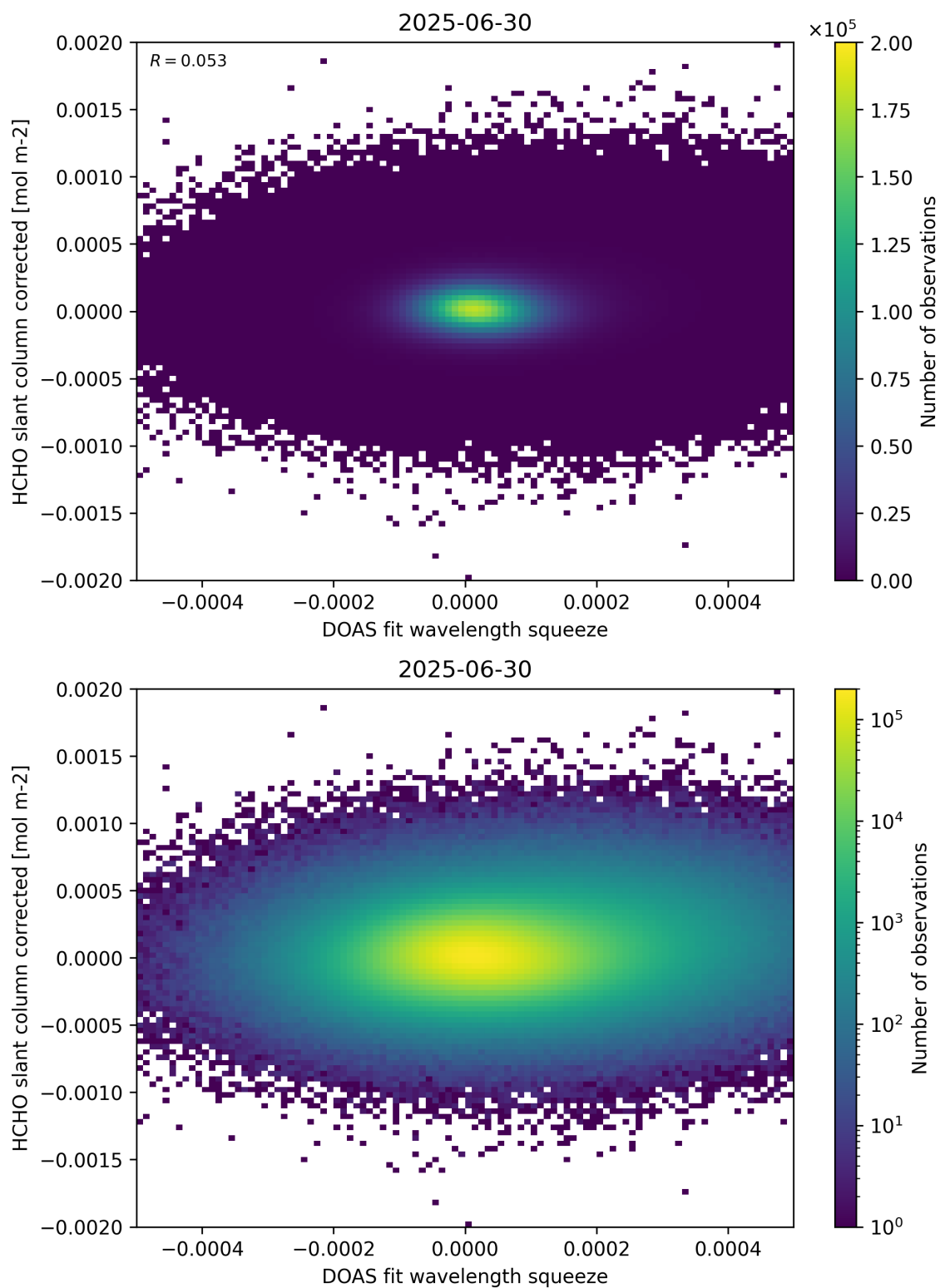
Figure 69: Scatter density plot of “DOAS fit wavelength squeeze” against “HCHO slant column corrected” for 2025-06-29 to 2025-07-01.
