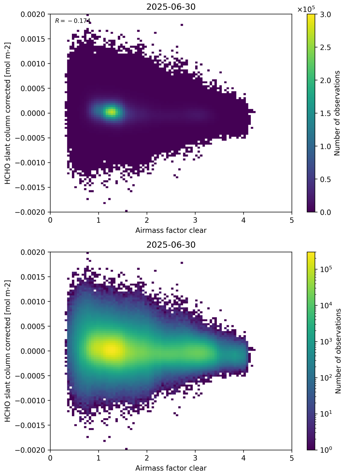
Figure 74: Scatter density plot of “Airmass factor clear” against “HCHO slant column corrected” for 2025-06-29 to 2025-07-01.
