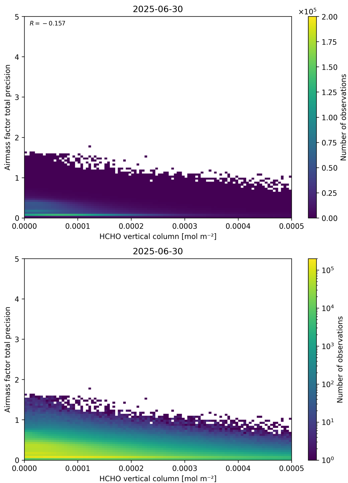
Figure 132: Scatter density plot of “HCHO vertical column” against “Airmass factor total precision” for 2025-06-29 to 2025-07-01.
