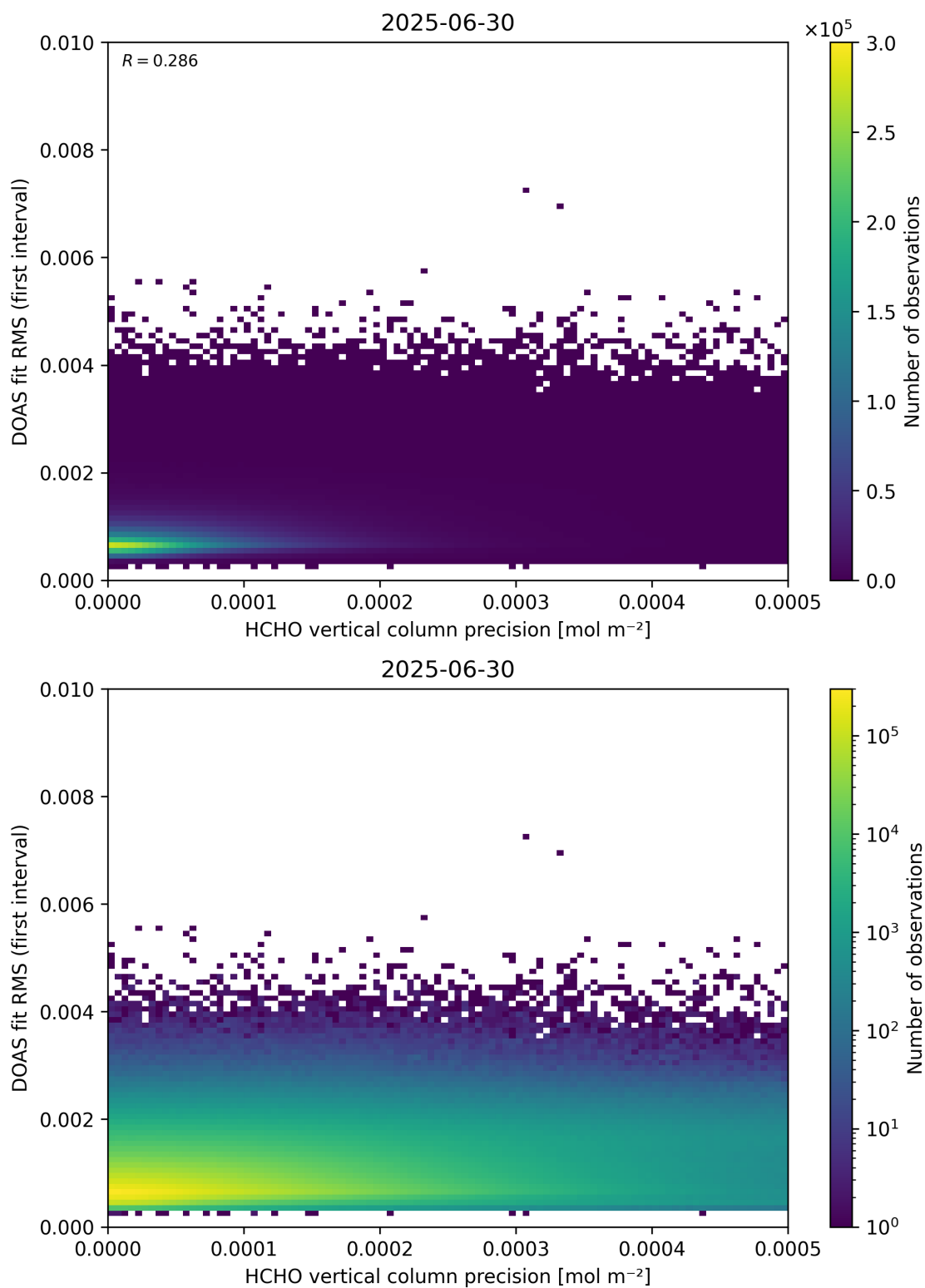
Figure 136: Scatter density plot of “HCHO vertical column precision” against “DOAS fit RMS (first interval)” for 2025-06-29 to 2025-07-01.
