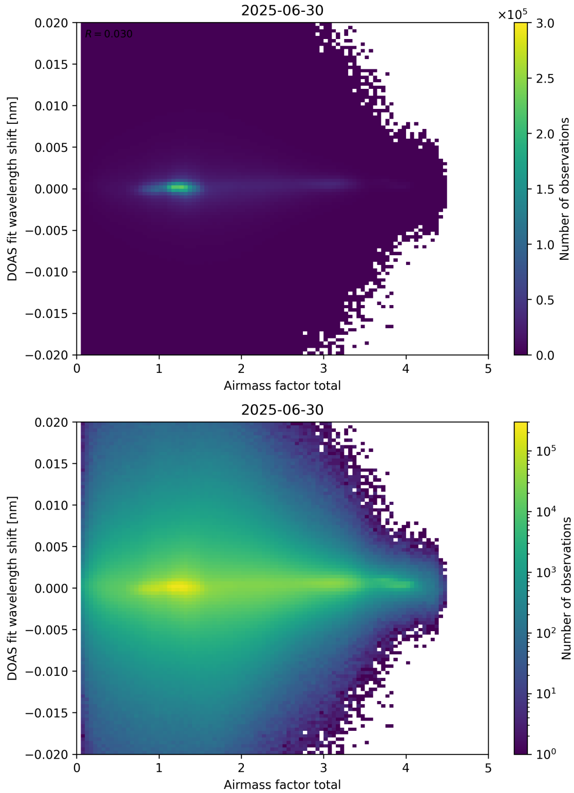
Figure 98: Scatter density plot of “Airmass factor total” against “DOAS fit wavelength shift” for 2025-06-29 to 2025-07-01.
