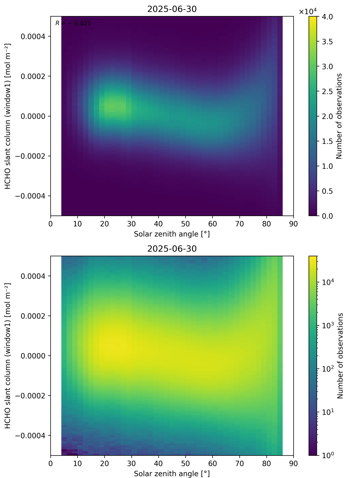
Figure 173: Scatter density plot of “Solar zenith angle” against “HCHO slant column (window1)” for 2025-06-29 to 2025-07-01.
