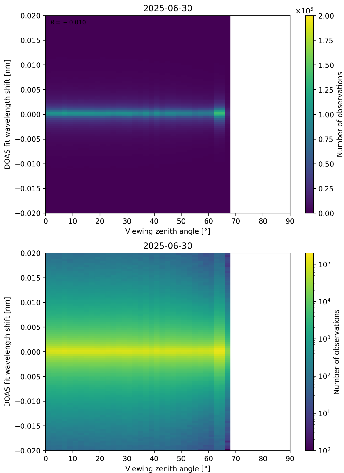
Figure 183: Scatter density plot of “Viewing zenith angle” against “DOAS fit wavelength shift” for 2025-06-29 to 2025-07-01.
