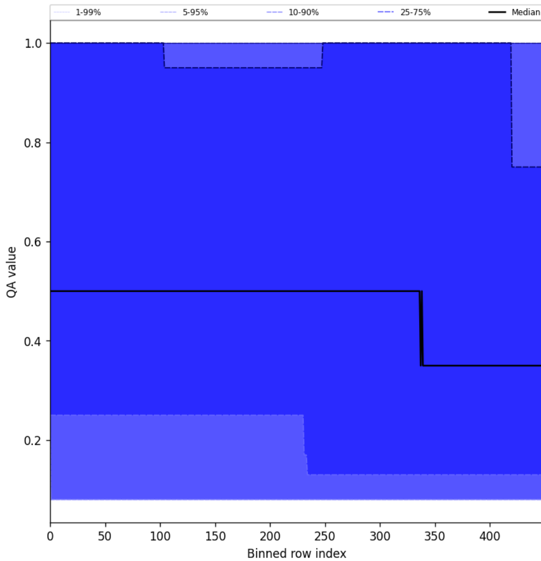
Figure 48: Along track statistics of “QA value” for 2025-06-30 to 2025-07-02
