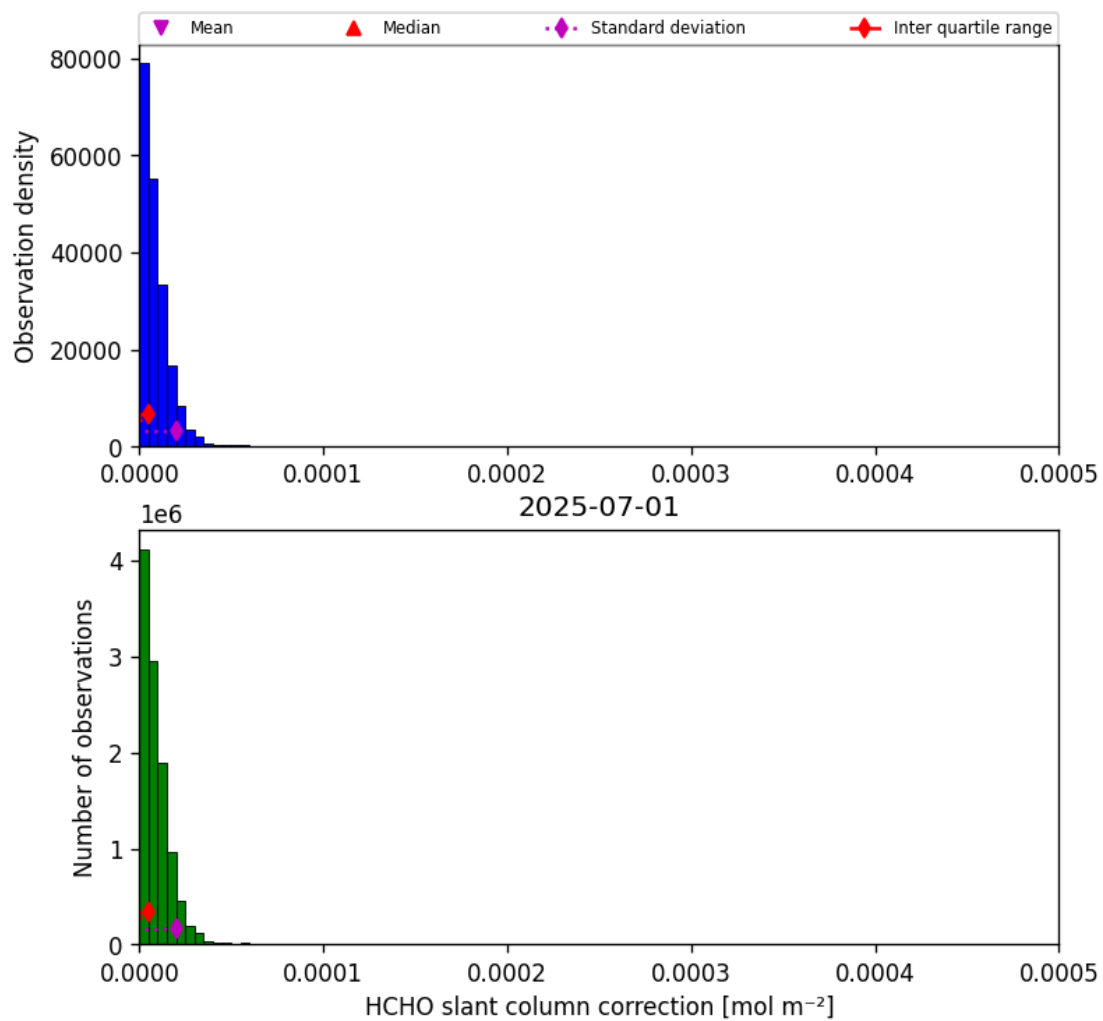
Figure 47: Histogram of “HCHO slant column correction” for 2025-06-30 to 2025-07-02
