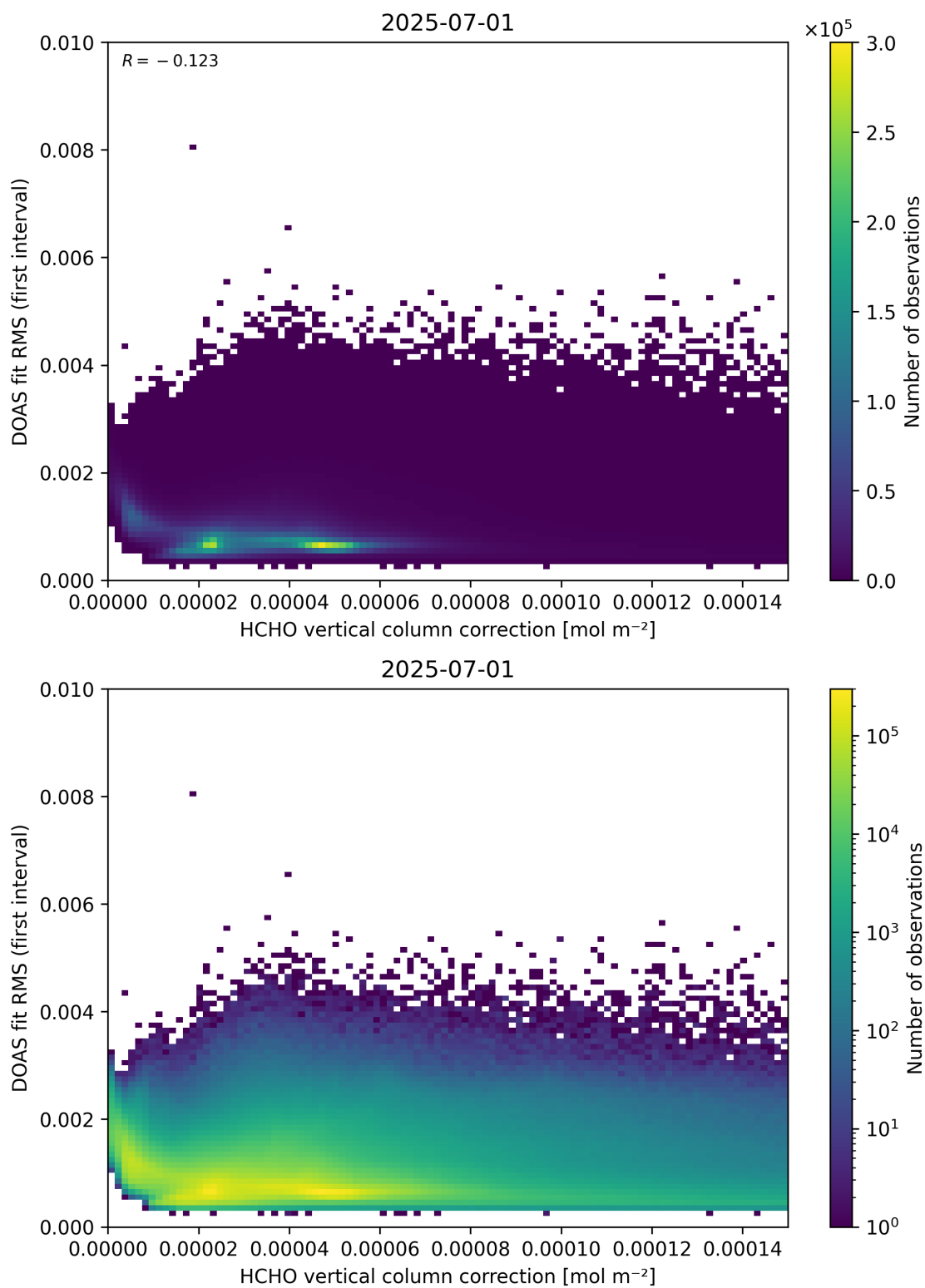
Figure 112: Scatter density plot of “HCHO vertical column correction” against “DOAS fit RMS (first interval)” for 2025-06-30 to 2025-07-02.
