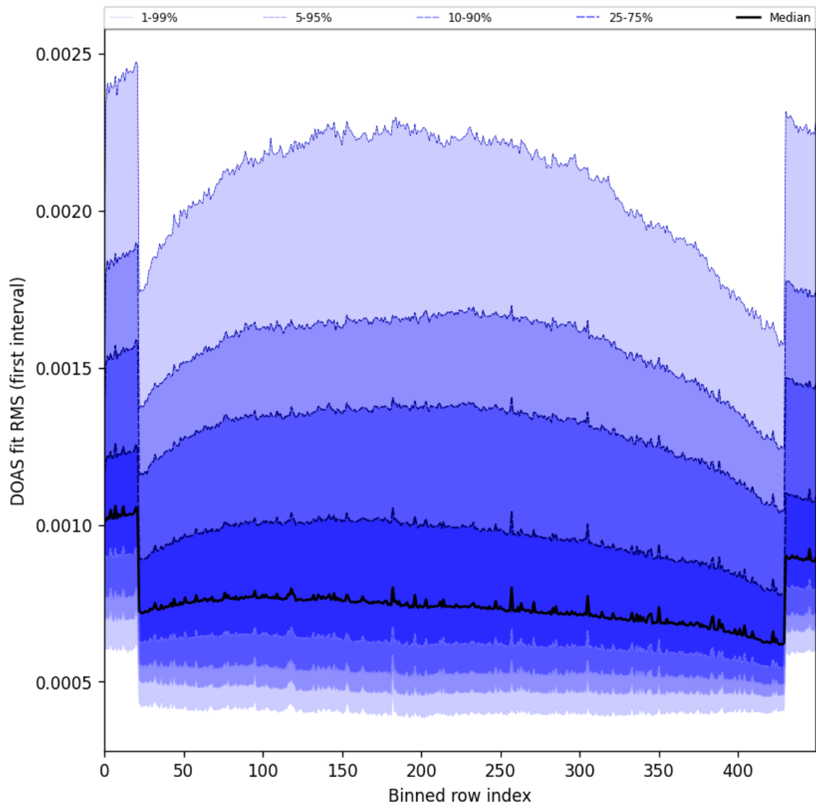
Figure 60: Along track statistics of “DOAS fit RMS (first interval)” for 2025-06-30 to 2025-07-02
