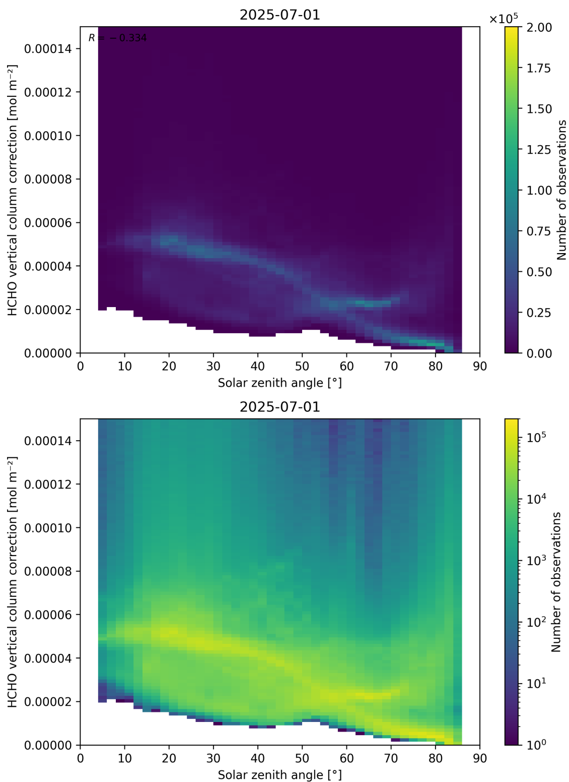
Figure 178: Scatter density plot of “Solar zenith angle” against “HCHO vertical column correction” for 2025-06-30 to 2025-07-02.
