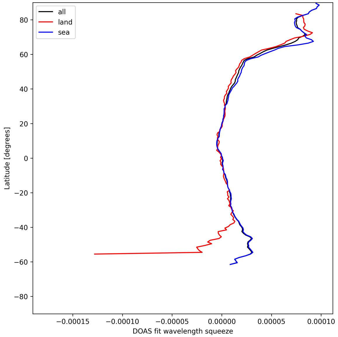
Figure 31: Zonal average of “DOAS fit wavelength squeeze” for 2025-06-30 to 2025-07-02.
