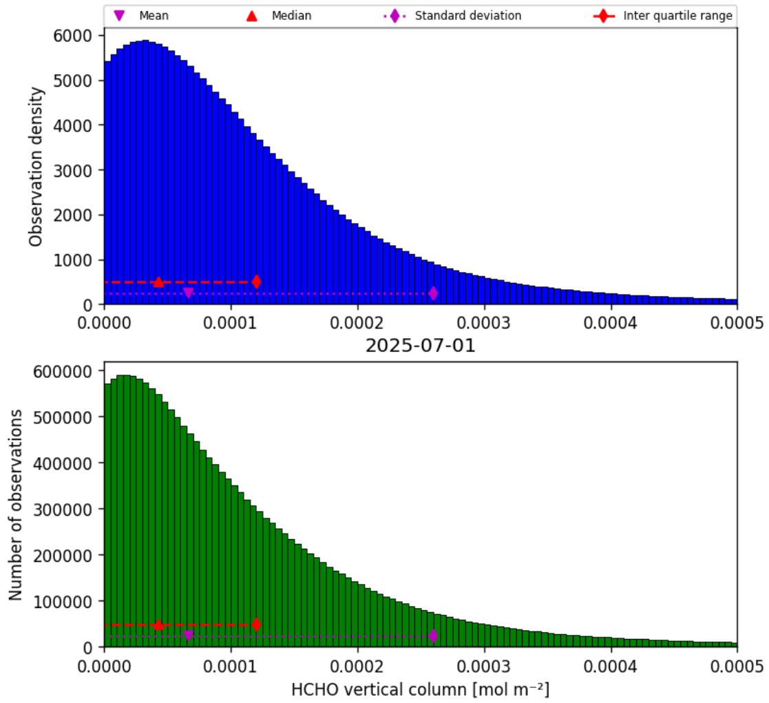
Figure 35: Histogram of “HCHO vertical column” for 2025-06-30 to 2025-07-02
