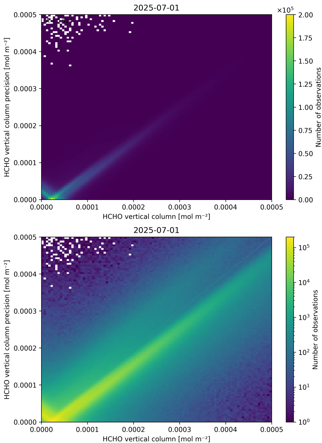
Figure 134: Scatter density plot of “HCHO vertical column” against “HCHO vertical column precision” for 2025-06-30 to 2025-07-02.
