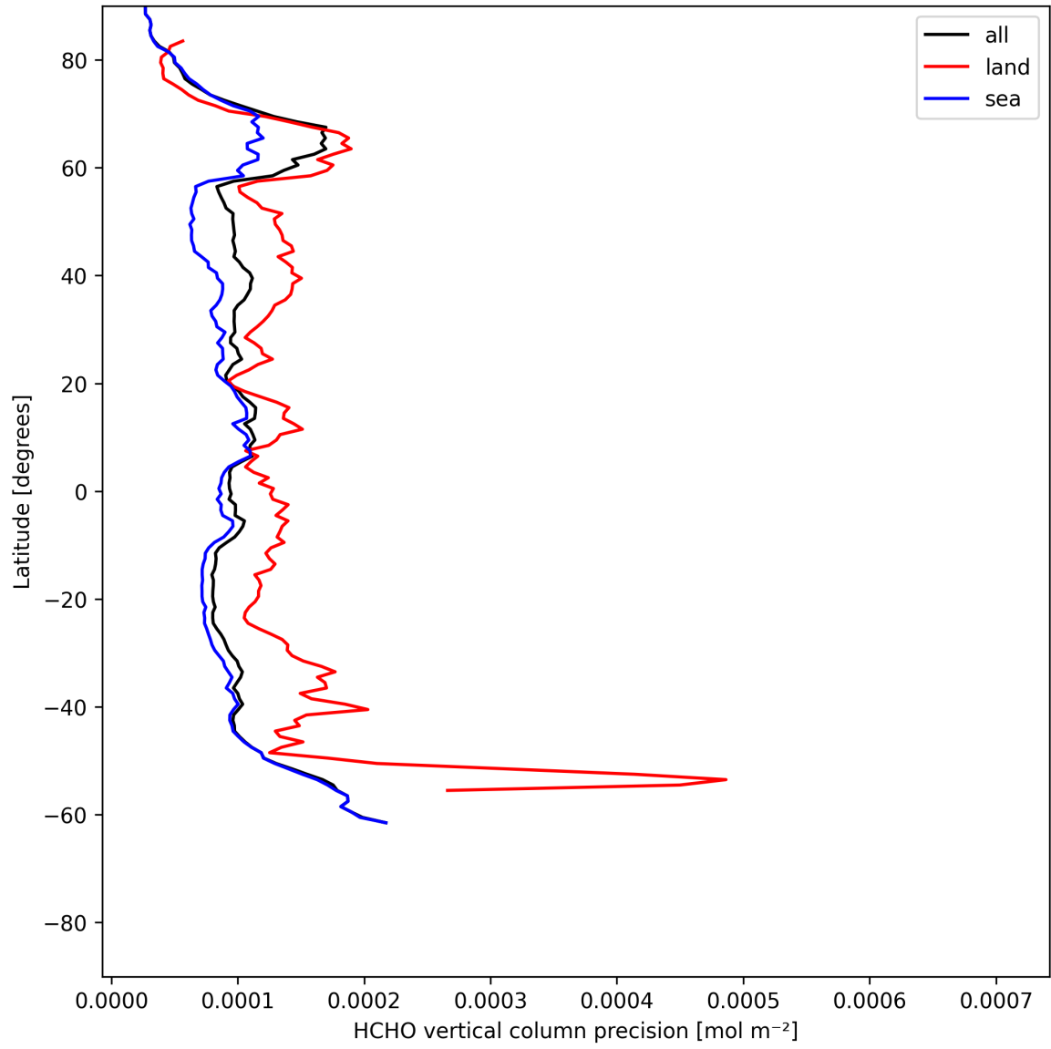
Figure 22: Zonal average of “HCHO vertical column precision” for 2025-06-30 to 2025-07-02.
