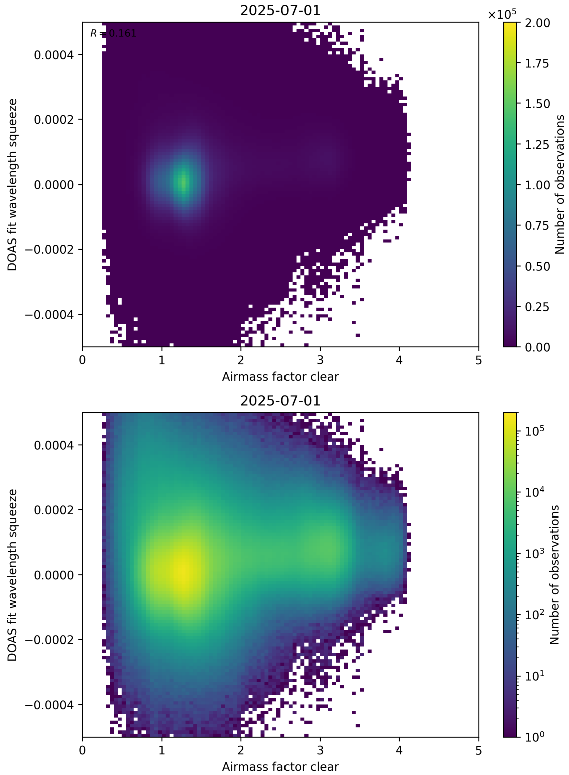
Figure 73: Scatter density plot of “Airmass factor clear” against “DOAS fit wavelength squeeze” for 2025-06-30 to 2025-07-02.
