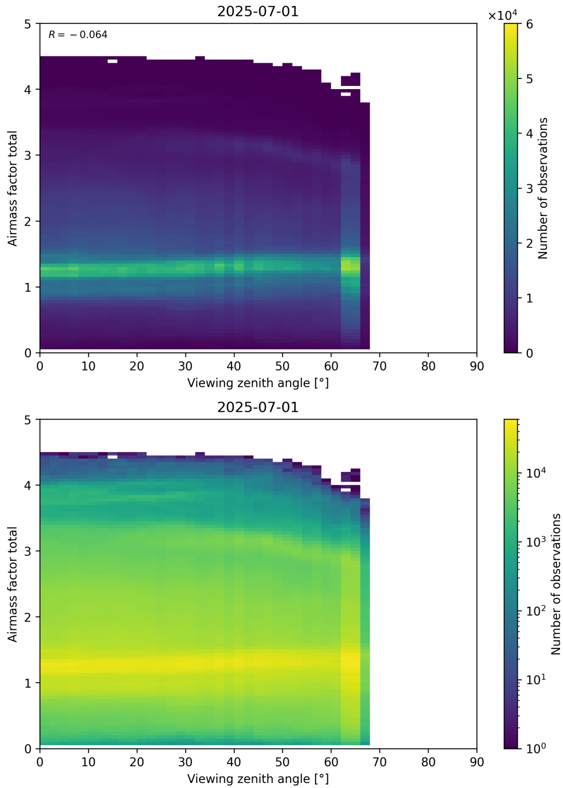
Figure 190: Scatter density plot of “Viewing zenith angle” against “Airmass factor total” for 2025-06-30 to 2025-07-02.
