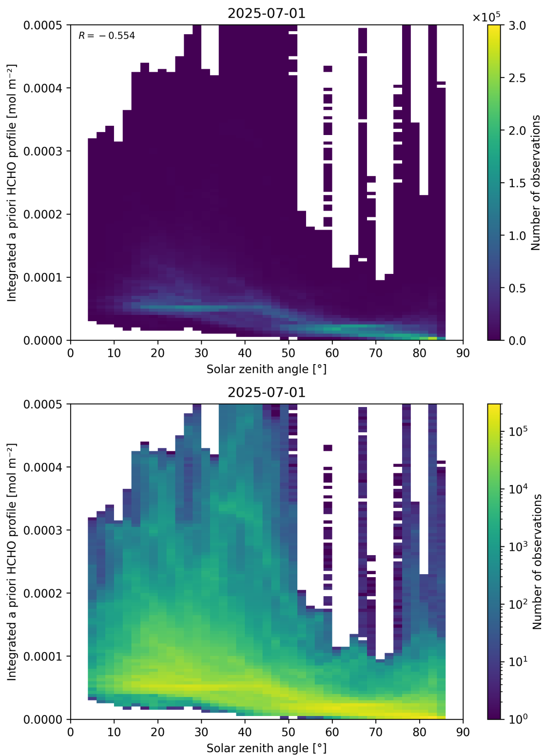
Figure 180: Scatter density plot of “Solar zenith angle” against “Integrated a priori HCHO profile” for 2025-06-30 to 2025-07-02.
