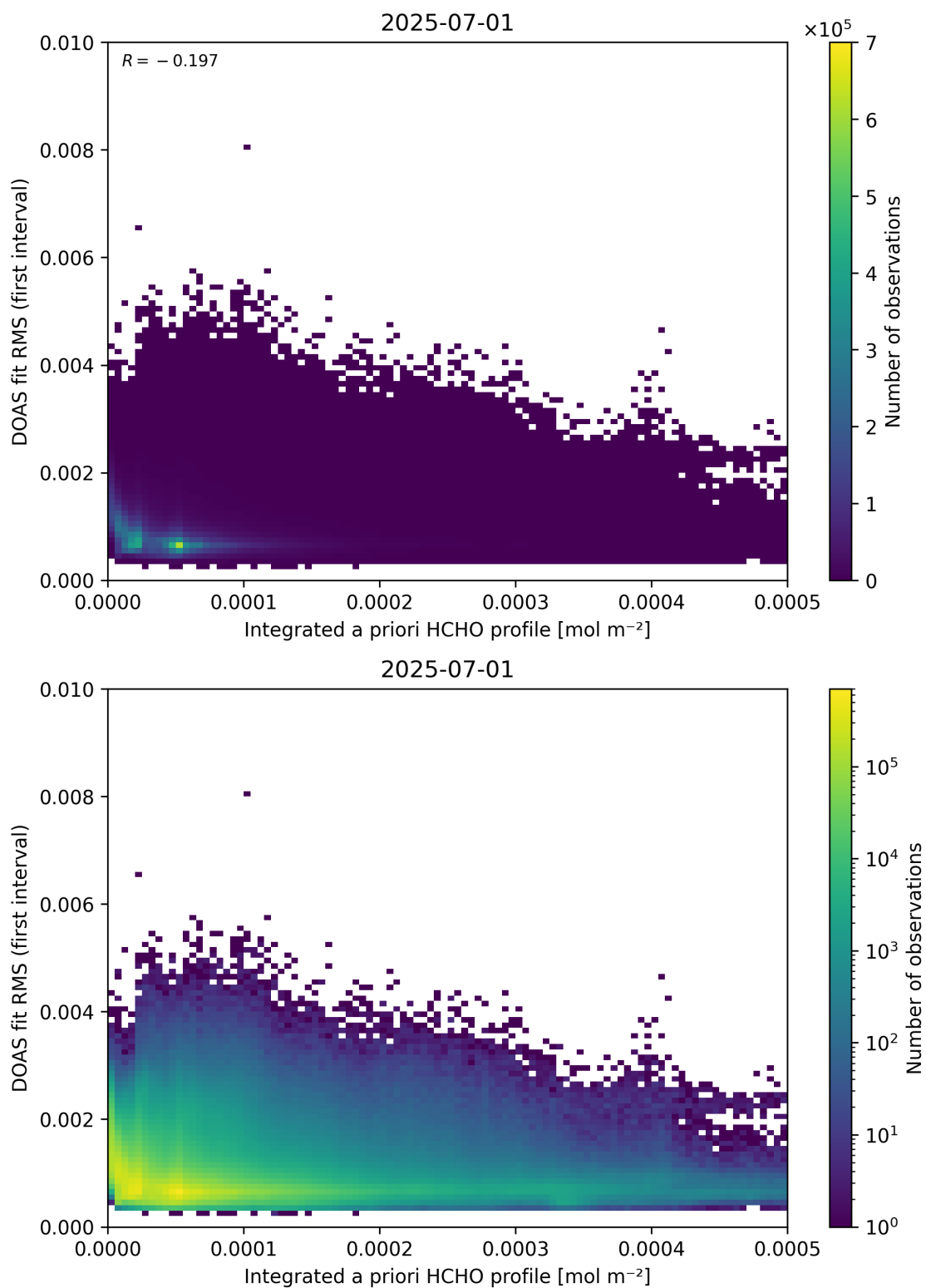
Figure 148: Scatter density plot of “Integrated a priori HCHO profile” against “DOAS fit RMS (first interval)” for 2025-06-30 to 2025-07-02.
