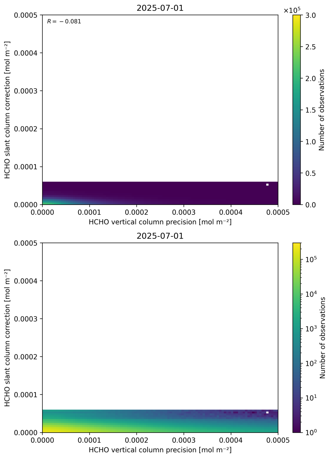
Figure 141: Scatter density plot of “HCHO vertical column precision” against “HCHO slant column correction” for 2025-06-30 to 2025-07-02.
