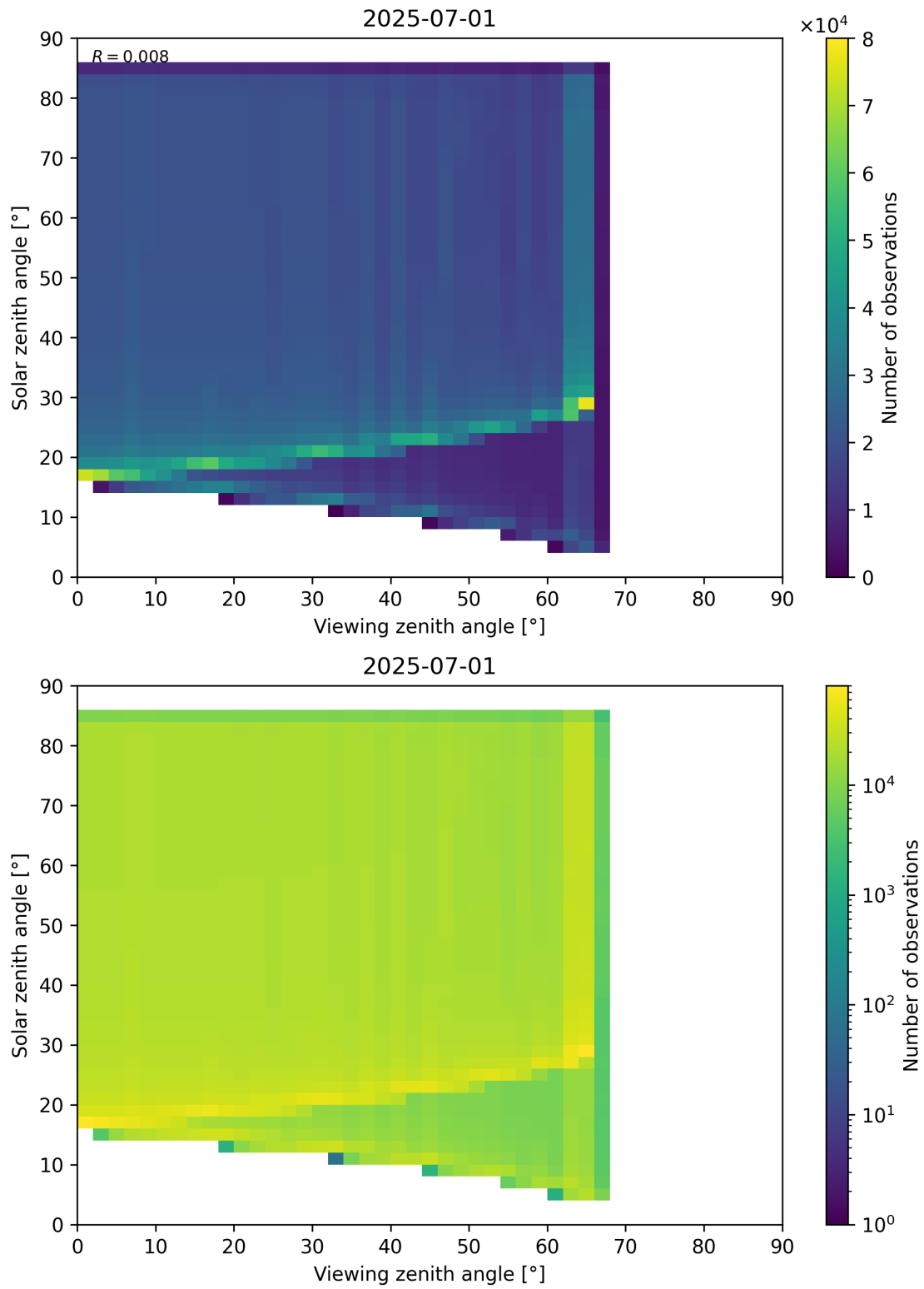
Figure 197: Scatter density plot of “Viewing zenith angle” against “Solar zenith angle” for 2025-06-30 to 2025-07-02.
