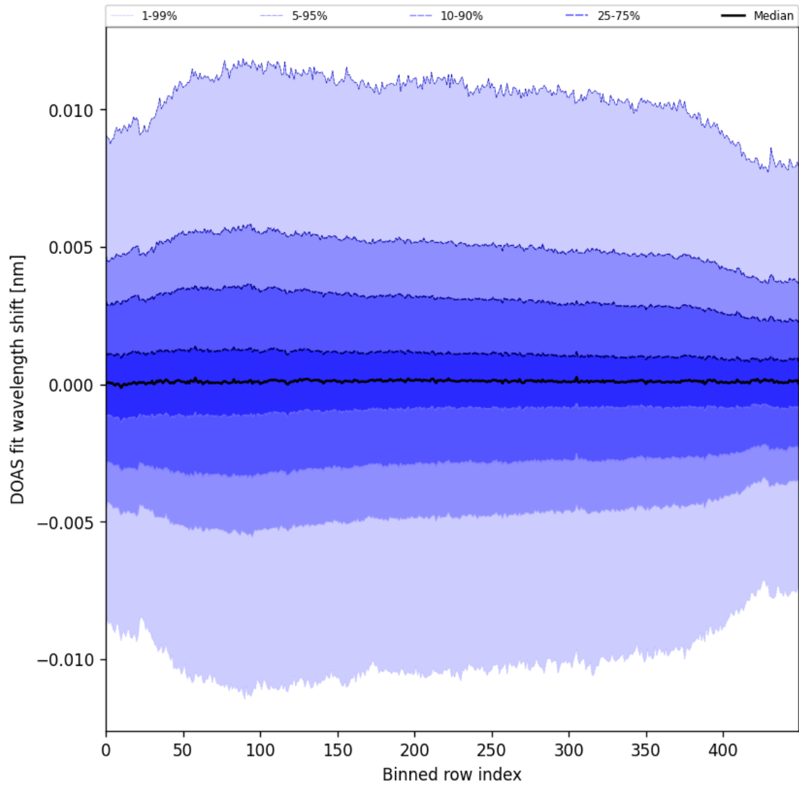
Figure 58: Along track statistics of “DOAS fit wavelength shift” for 2025-06-30 to 2025-07-02
