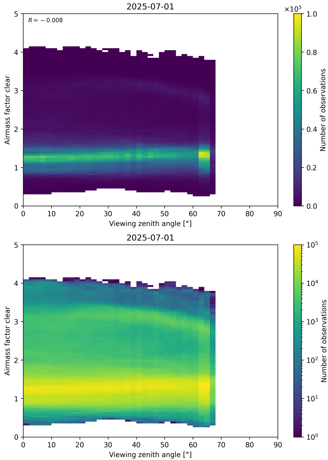
Figure 185: Scatter density plot of “Viewing zenith angle” against “Airmass factor clear” for 2025-06-30 to 2025-07-02.
