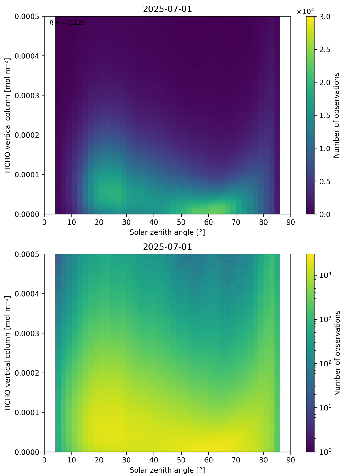
Figure 177: Scatter density plot of “Solar zenith angle” against “HCHO vertical column” for 2025-06-30 to 2025-07-02.
