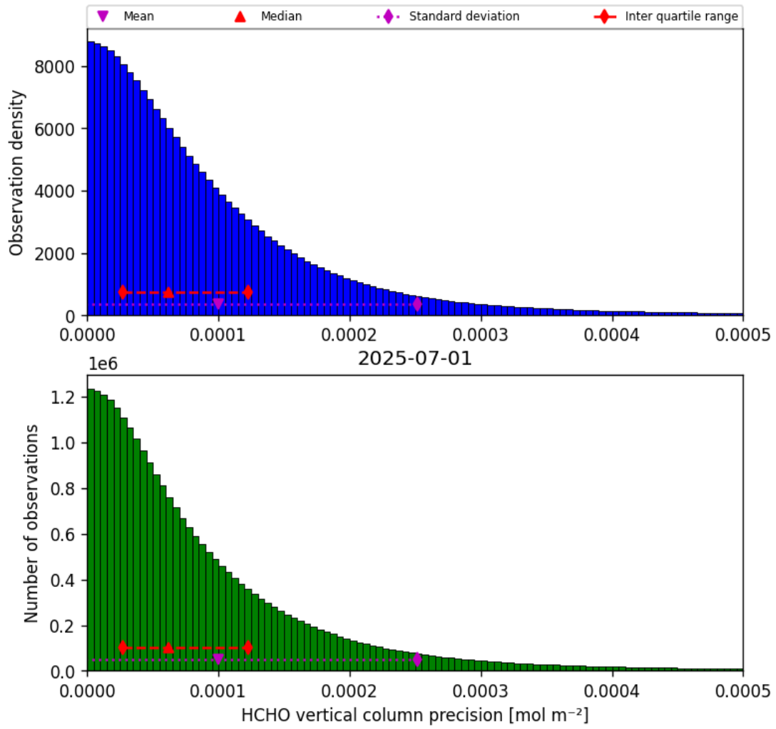
Figure 36: Histogram of “HCHO vertical column precision” for 2025-06-30 to 2025-07-02
