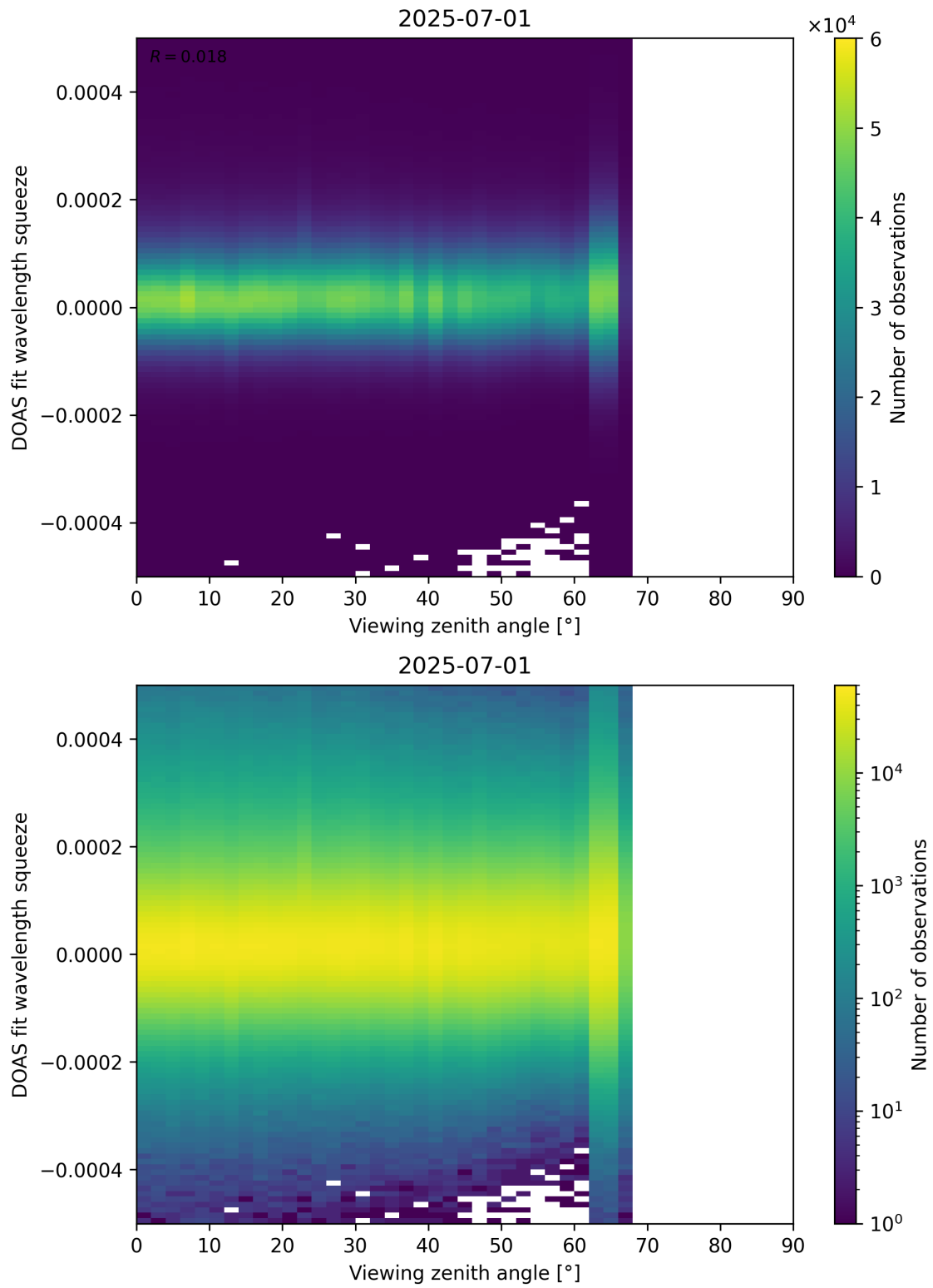
Figure 184: Scatter density plot of “Viewing zenith angle” against “DOAS fit wavelength squeeze” for 2025-06-30 to 2025-07-02.
