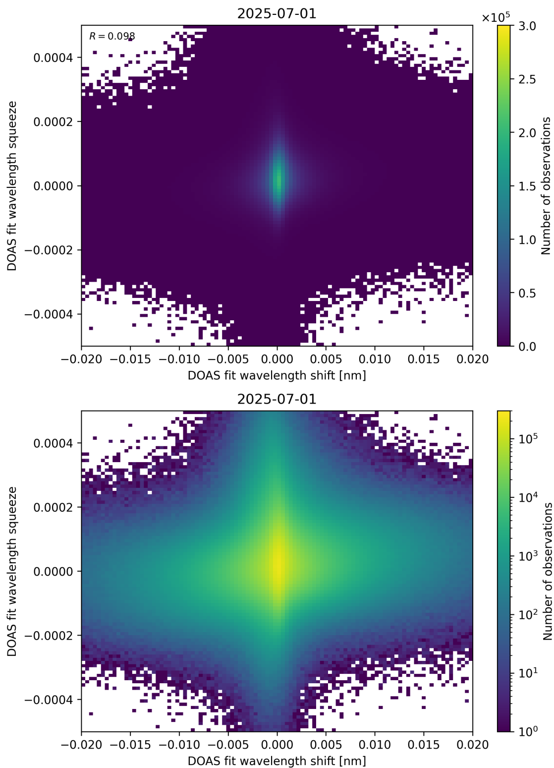
Figure 65: Scatter density plot of “DOAS fit wavelength shift” against “DOAS fit wavelength squeeze” for 2025-06-30 to 2025-07-02.
