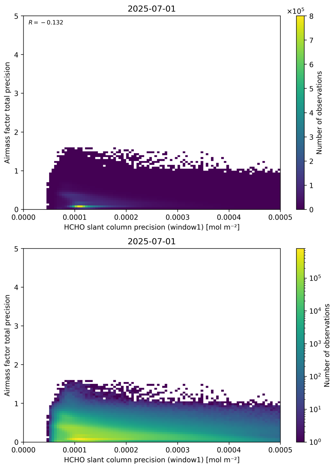
Figure 95: Scatter density plot of “HCHO slant column precision (window1)” against “Airmass factor total precision” for 2025-06-30 to 2025-07-02.
