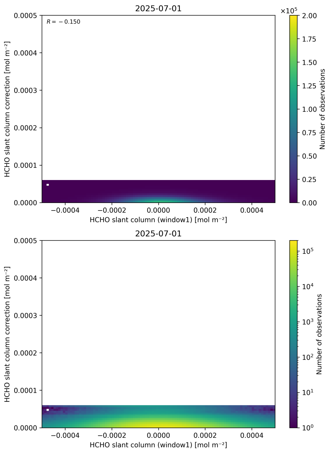
Figure 83: Scatter density plot of “HCHO slant column (window1)” against “HCHO slant column correction” for 2025-06-30 to 2025-07-02.
