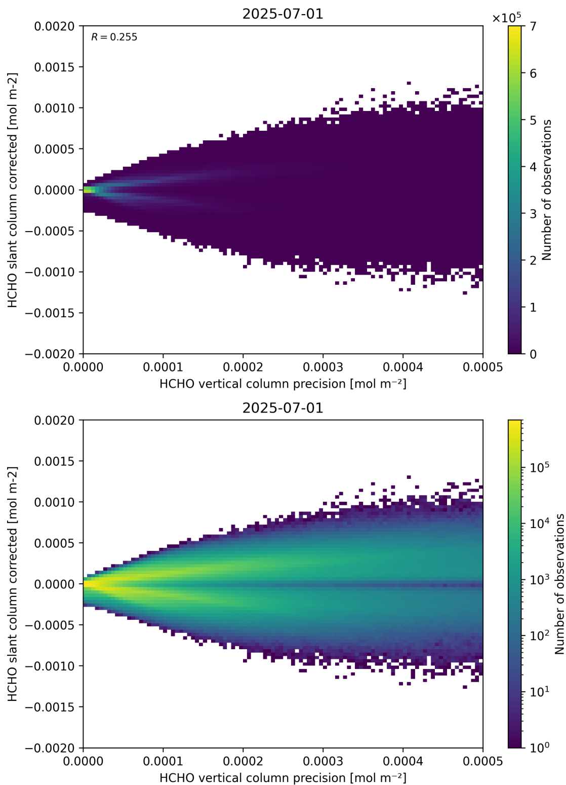
Figure 140: Scatter density plot of “HCHO vertical column precision” against “HCHO slant column corrected” for 2025-06-30 to 2025-07-02.
