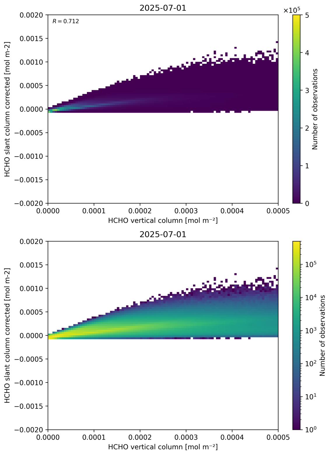
Figure 127: Scatter density plot of “HCHO vertical column” against “HCHO slant column corrected” for 2025-06-30 to 2025-07-02.
