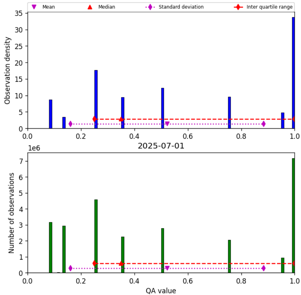
Figure 34: Histogram of “QA value” for 2025-06-30 to 2025-07-02
