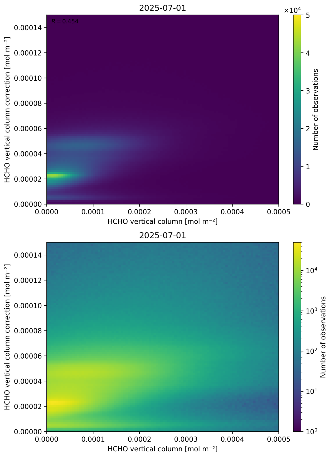
Figure 133: Scatter density plot of “HCHO vertical column” against “HCHO vertical column correction” for 2025-06-30 to 2025-07-02.
