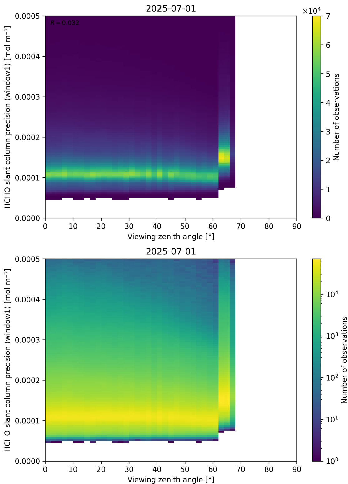
Figure 189: Scatter density plot of “Viewing zenith angle” against “HCHO slant column precision (window1)” for 2025-06-30 to 2025-07-02.
