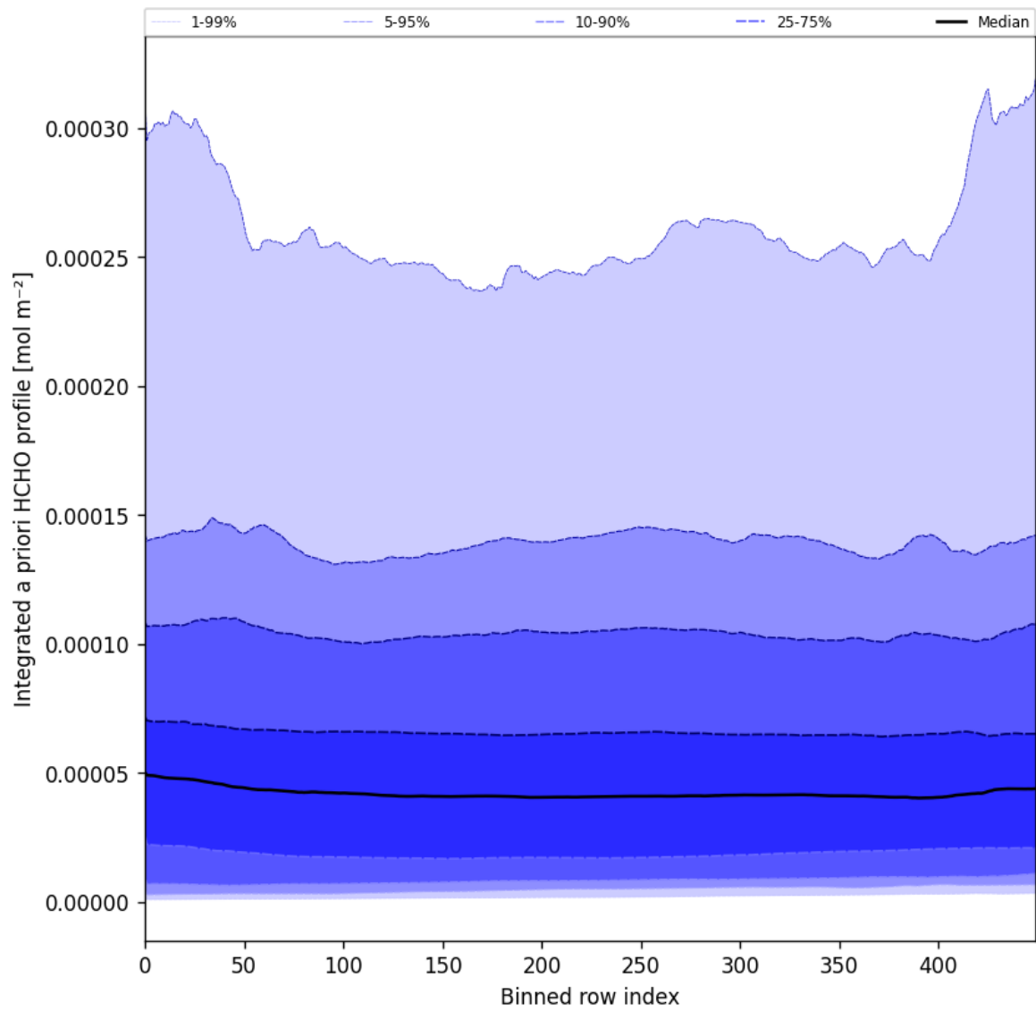
Figure 57: Along track statistics of "Integrated a priori HCHO profile" for 2025-06-30 to 2025-07-02
