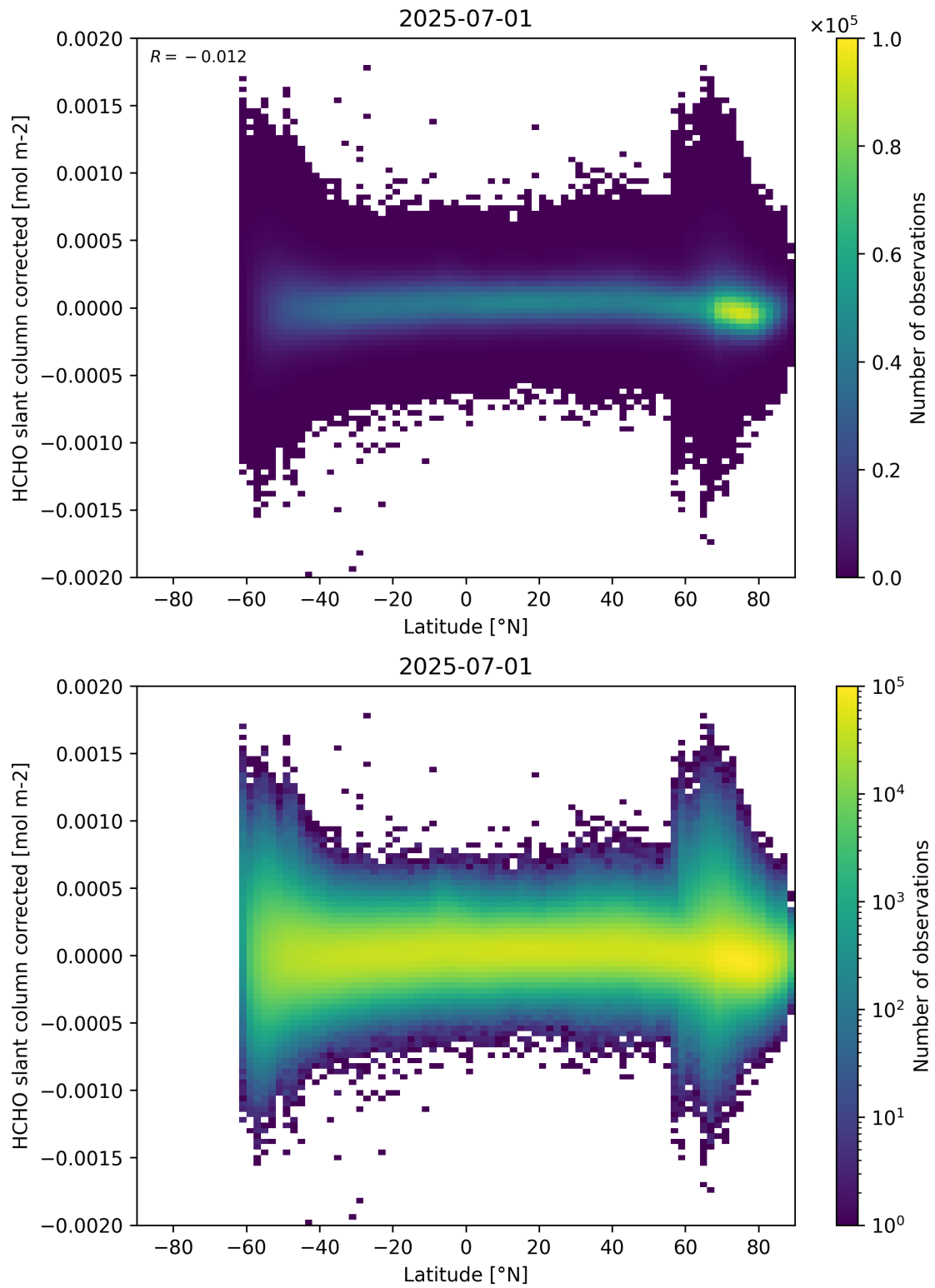
Figure 157: Scatter density plot of “Latitude” against “HCHO slant column corrected” for 2025-06-30 to 2025-07-02.
