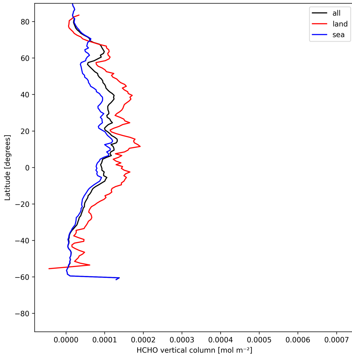
Figure 21: Zonal average of “HCHO vertical column” for 2025-06-30 to 2025-07-02.
