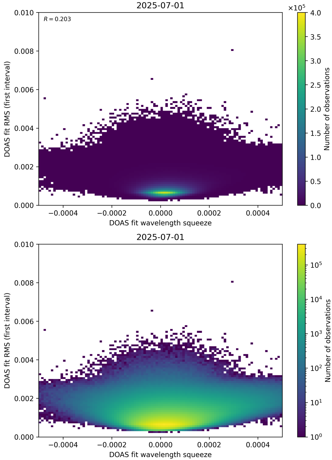
Figure 68: Scatter density plot of “DOAS fit wavelength squeeze” against “DOAS fit RMS (first interval)” for 2025-06-30 to 2025-07-02.
