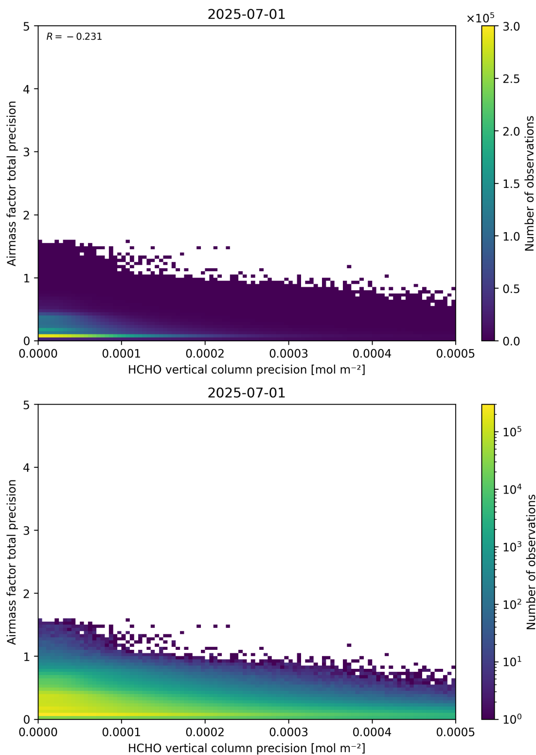
Figure 145: Scatter density plot of “HCHO vertical column precision” against “Airmass factor total precision” for 2025-06-30 to 2025-07-02.
