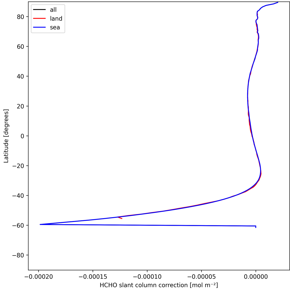
Figure 33: Zonal average of “HCHO slant column correction” for 2025-06-30 to 2025-07-02.
