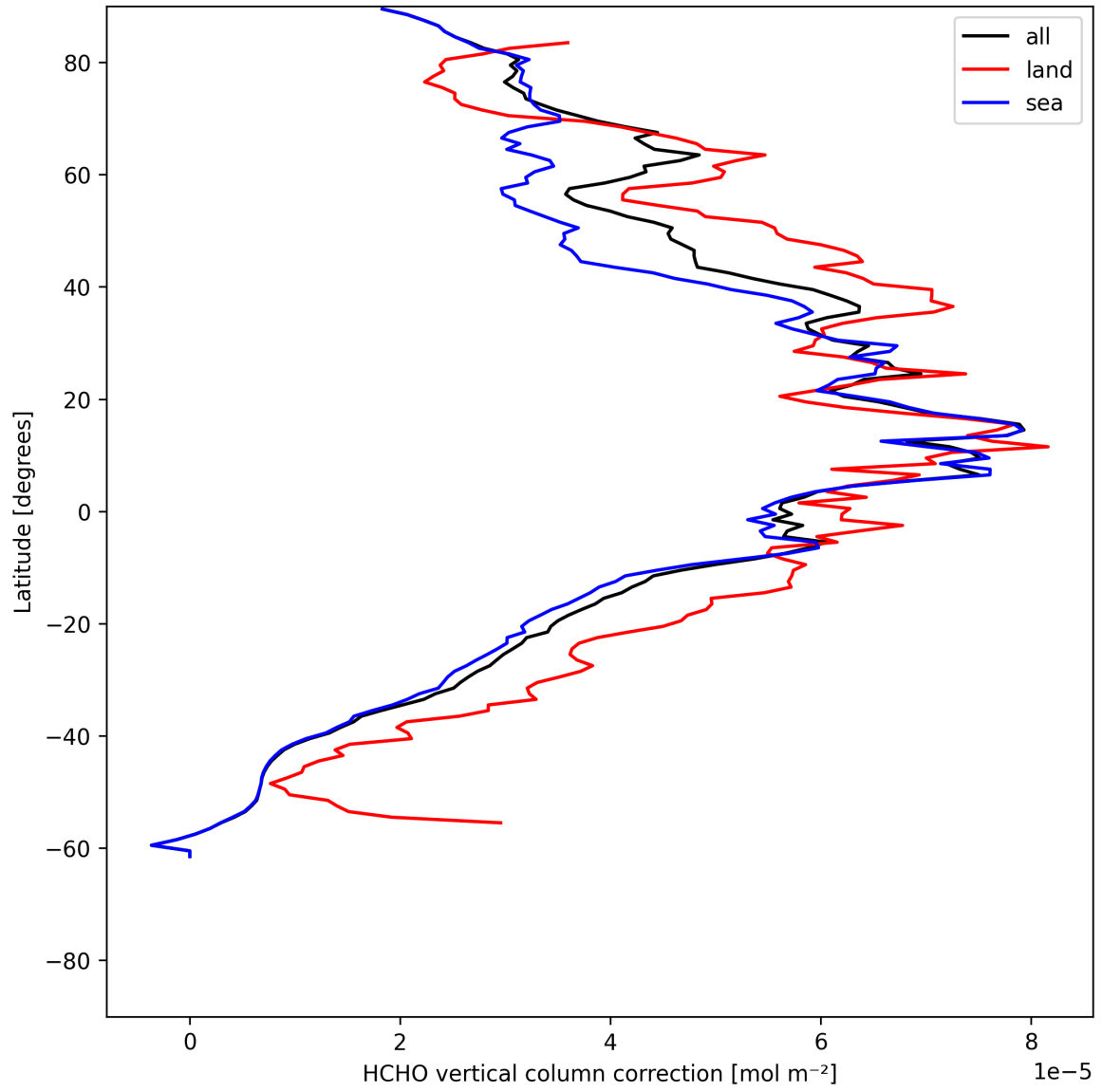
Figure 23: Zonal average of “HCHO vertical column correction” for 2025-06-30 to 2025-07-02.
