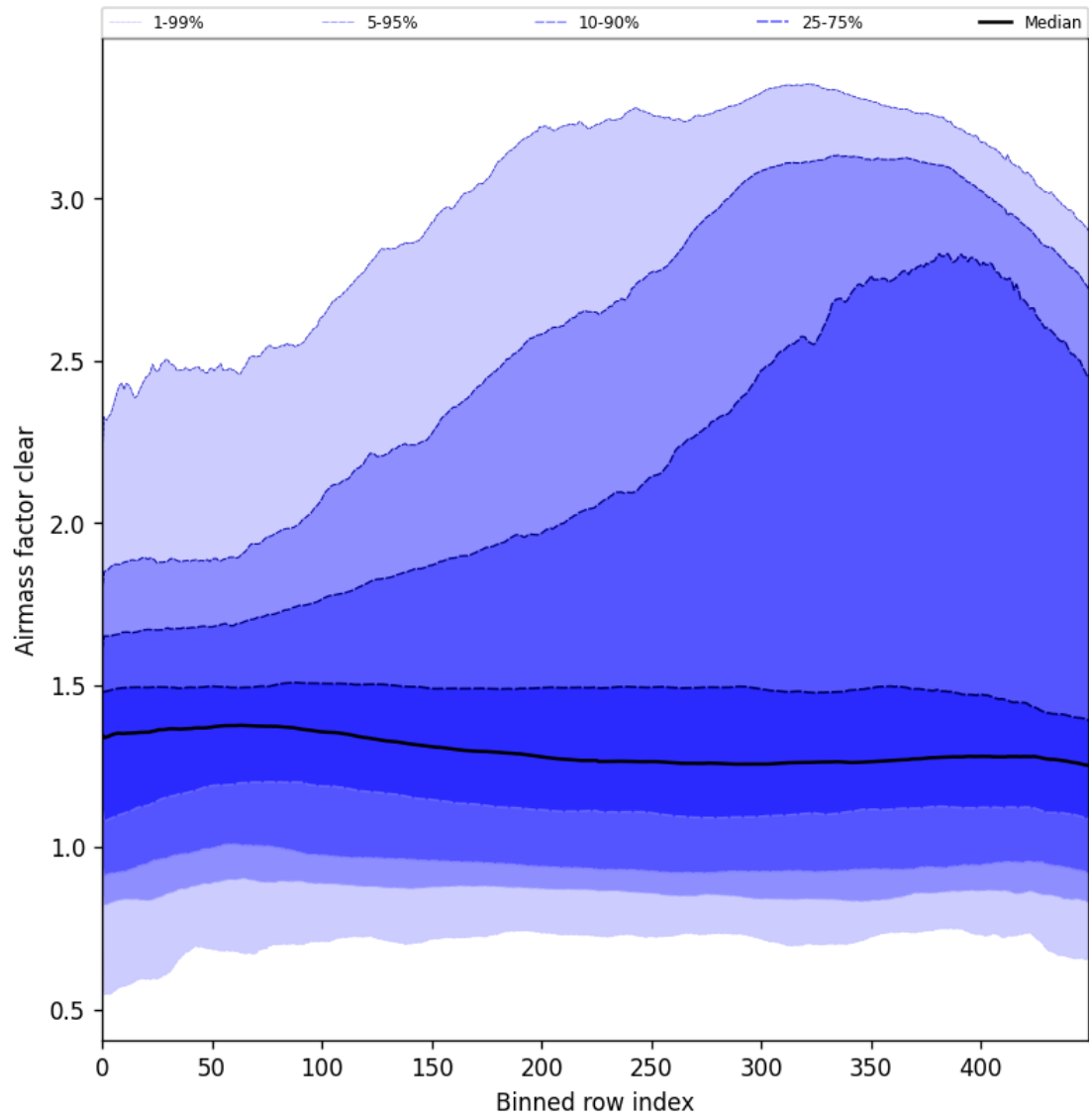
Figure 56: Along track statistics of “Airmass factor clear” for 2025-06-30 to 2025-07-02
