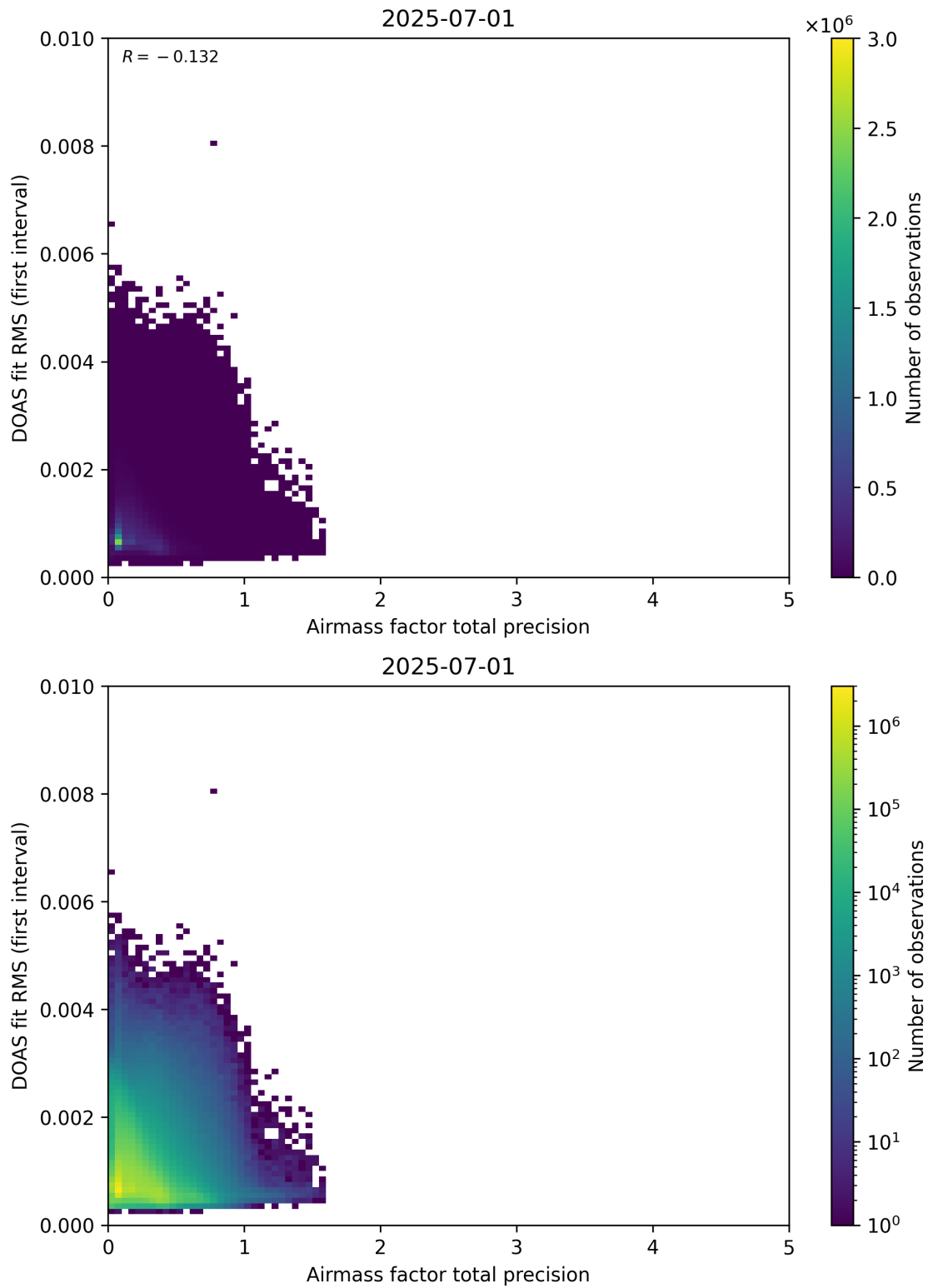
Figure 105: Scatter density plot of “Airmass factor total precision” against “DOAS fit RMS (first interval)” for 2025-06-30 to 2025-07-02.
