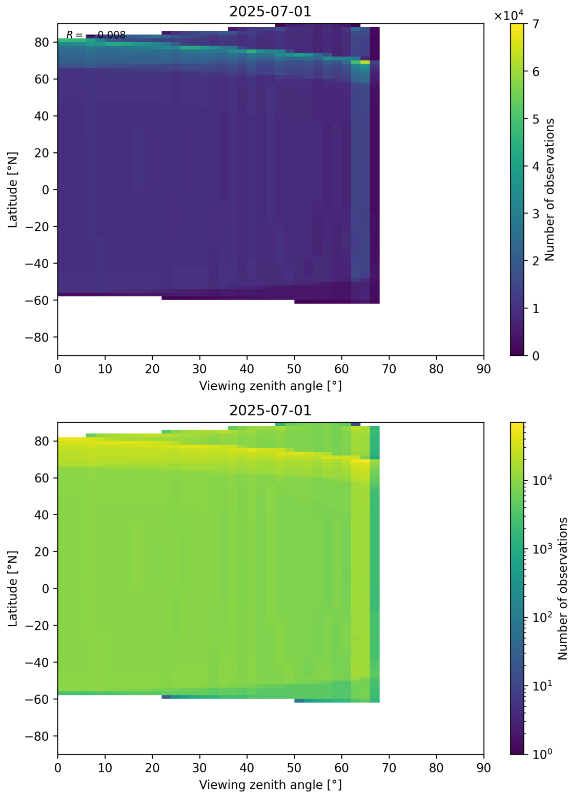
Figure 196: Scatter density plot of “Viewing zenith angle” against “Latitude” for 2025-06-30 to 2025-07-02.
