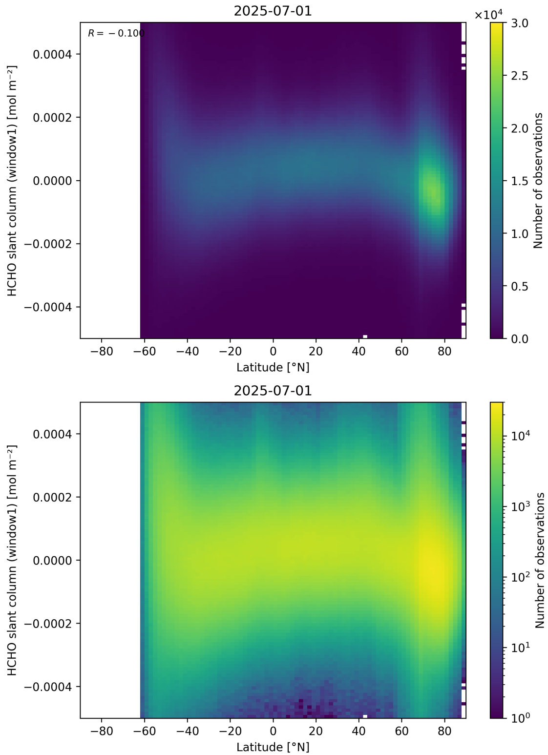
Figure 159: Scatter density plot of “Latitude” against “HCHO slant column (window1)” for 2025-06-30 to 2025-07-02.
