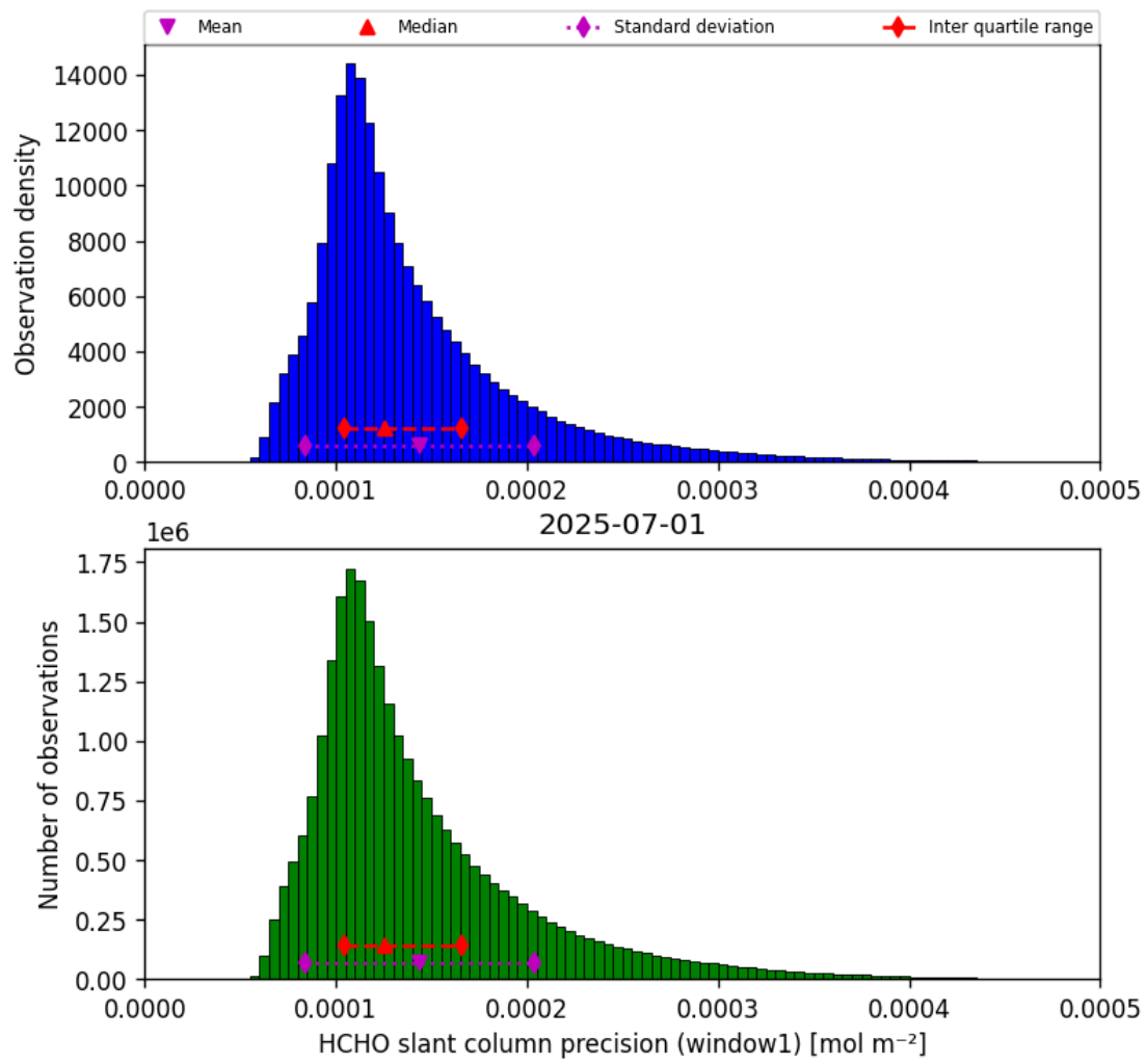
Figure 39: Histogram of “HCHO slant column precision (window1)” for 2025-06-30 to 2025-07-02
