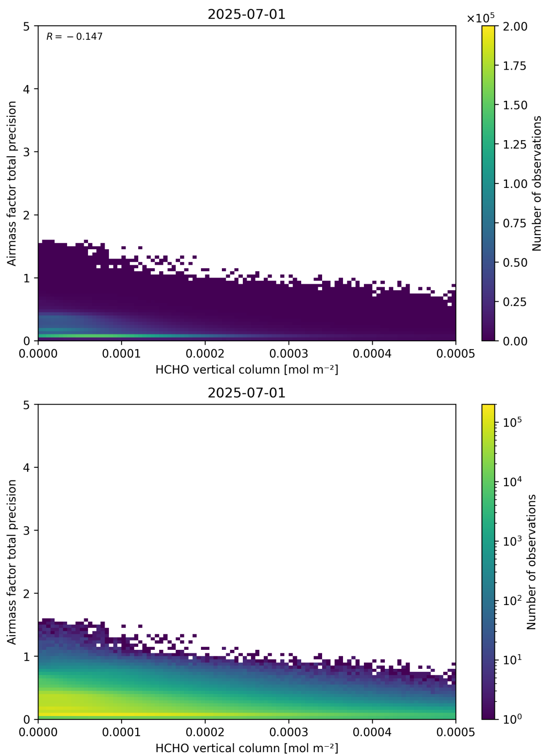
Figure 132: Scatter density plot of “HCHO vertical column” against “Airmass factor total precision” for 2025-06-30 to 2025-07-02.
