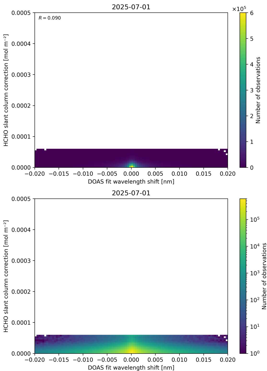
Figure 67: Scatter density plot of “DOAS fit wavelength shift” against “HCHO slant column correction” for 2025-06-30 to 2025-07-02.
