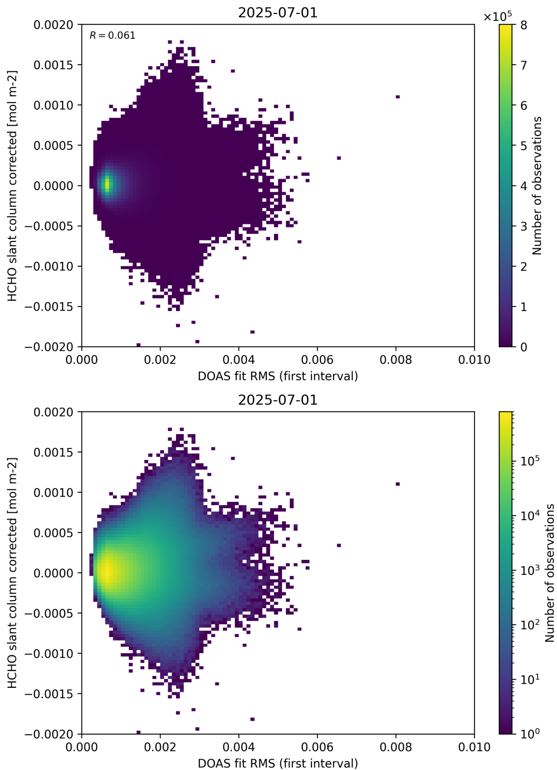
Figure 62: Scatter density plot of “DOAS fit RMS (first interval)” against “HCHO slant column corrected” for 2025-06-30 to 2025-07-02.
