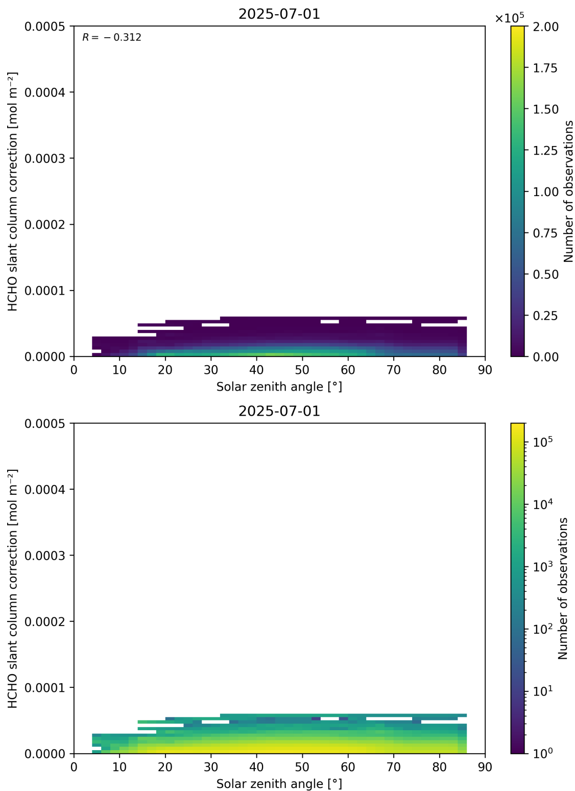
Figure 172: Scatter density plot of “Solar zenith angle” against “HCHO slant column correction” for 2025-06-30 to 2025-07-02.
