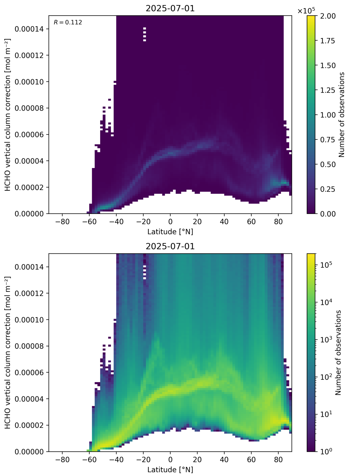
Figure 164: Scatter density plot of “Latitude” against “HCHO vertical column correction” for 2025-06-30 to 2025-07-02.
