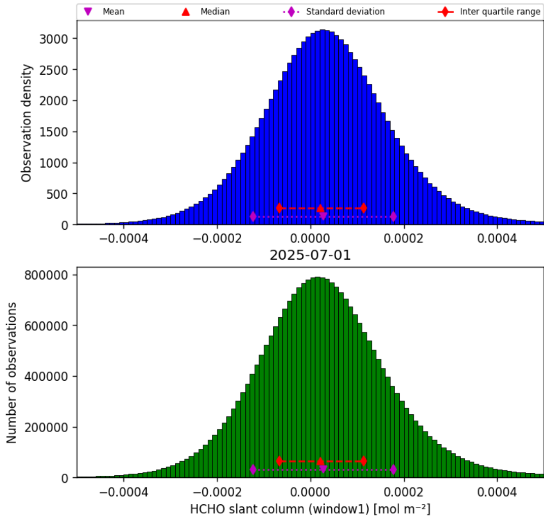
Figure 38: Histogram of “HCHO slant column (window1)” for 2025-06-30 to 2025-07-02
