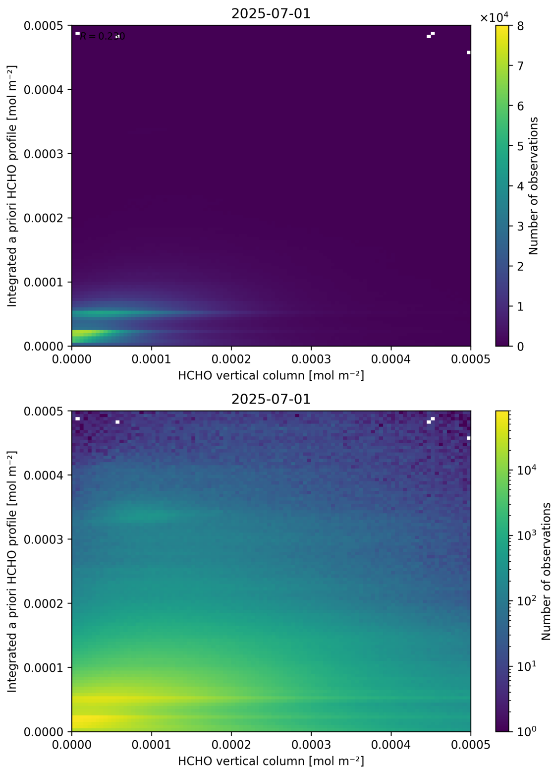
Figure 135: Scatter density plot of “HCHO vertical column” against “Integrated a priori HCHO profile” for 2025-06-30 to 2025-07-02.
