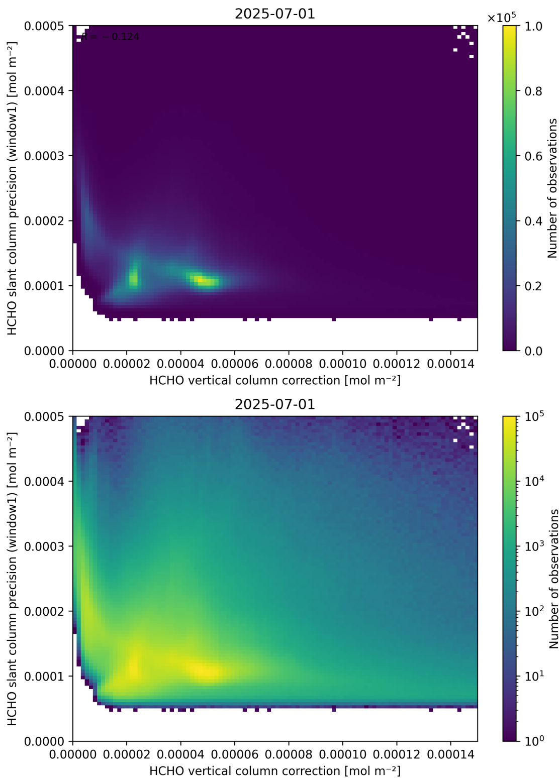
Figure 119: Scatter density plot of “HCHO vertical column correction” against “HCHO slant column precision (window1)” for 2025-06-30 to 2025-07-02.
