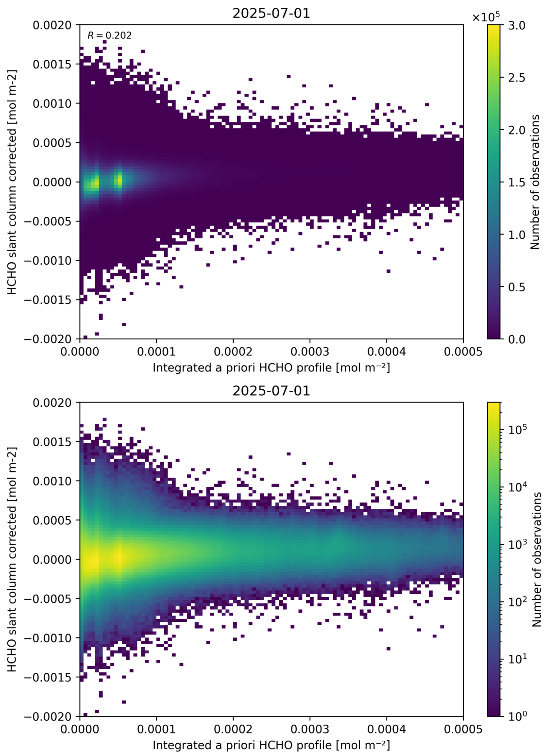
Figure 151: Scatter density plot of “Integrated a priori HCHO profile” against “HCHO slant column corrected” for 2025-06-30 to 2025-07-02.
