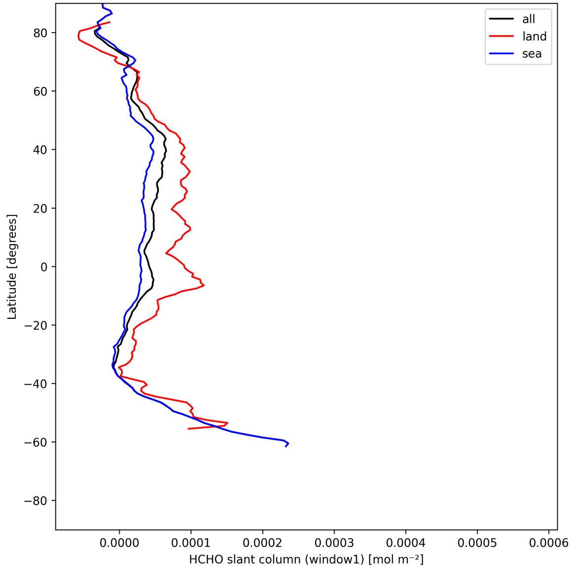
Figure 24: Zonal average of “HCHO slant column (window1)” for 2025-06-30 to 2025-07-02.
