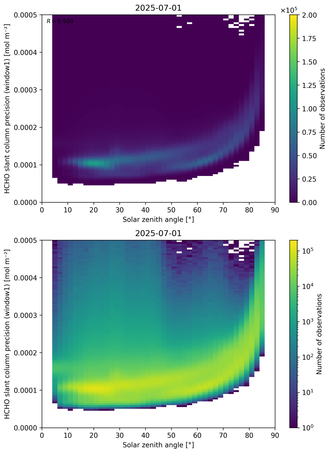
Figure 174: Scatter density plot of “Solar zenith angle” against “HCHO slant column precision (window1)” for 2025-06-30 to 2025-07-02.
