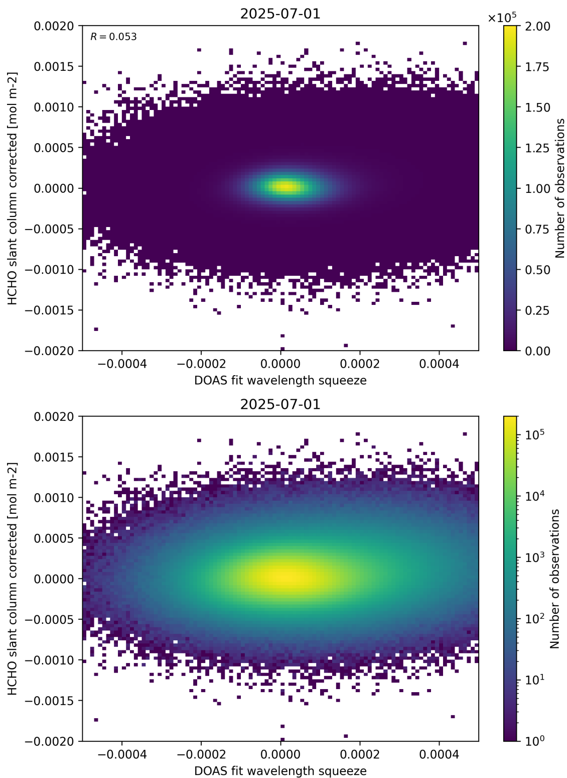
Figure 69: Scatter density plot of “DOAS fit wavelength squeeze” against “HCHO slant column corrected” for 2025-06-30 to 2025-07-02.
