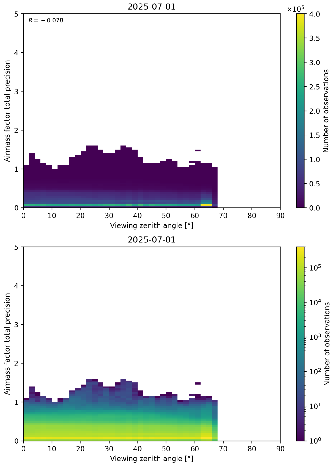
Figure 191: Scatter density plot of “Viewing zenith angle” against “Airmass factor total precision” for 2025-06-30 to 2025-07-02.
