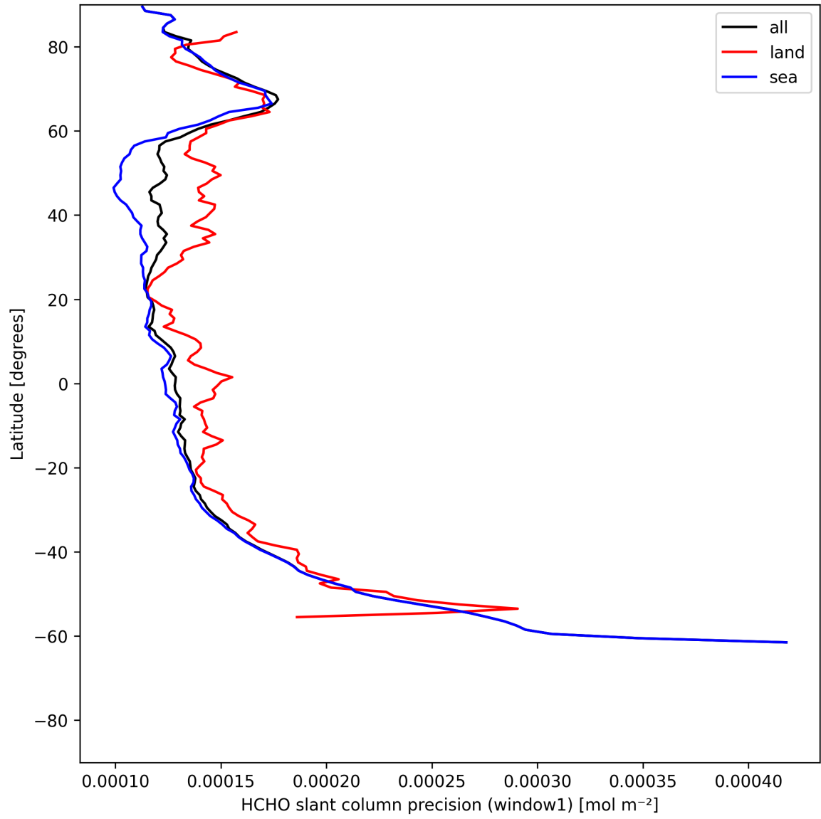
Figure 25: Zonal average of "HCHO slant column precision (window1)" for 2025-06-30 to 2025-07-02.
