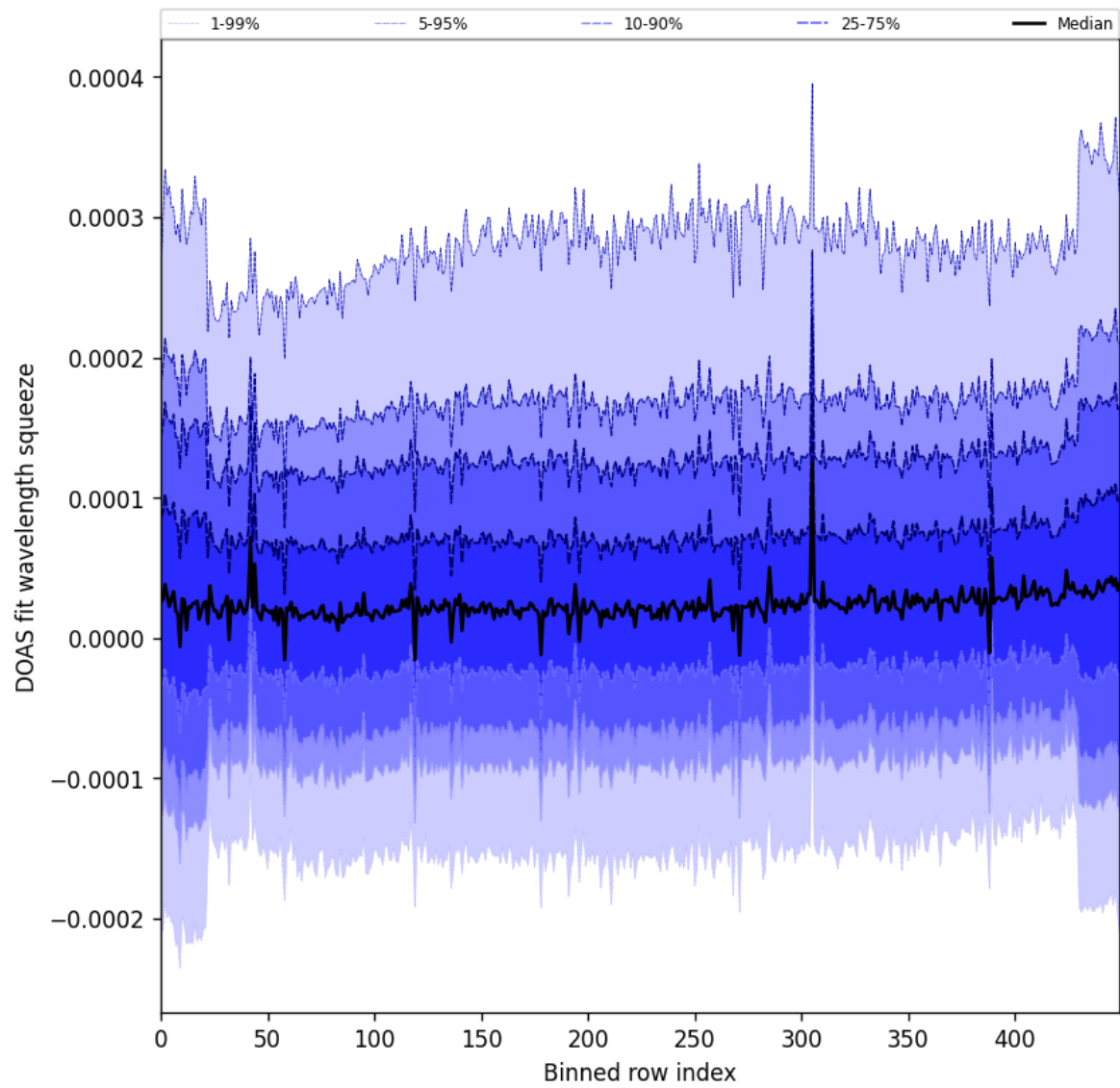
Figure 59: Along track statistics of “DOAS fit wavelength squeeze” for 2025-06-30 to 2025-07-02
