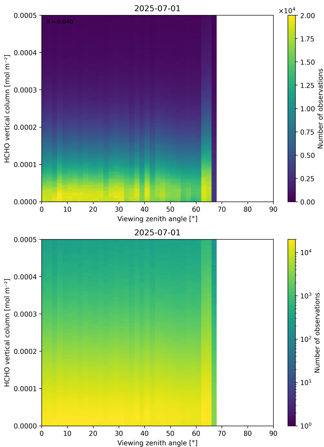
Figure 192: Scatter density plot of “Viewing zenith angle” against “HCHO vertical column” for 2025-06-30 to 2025-07-02.
