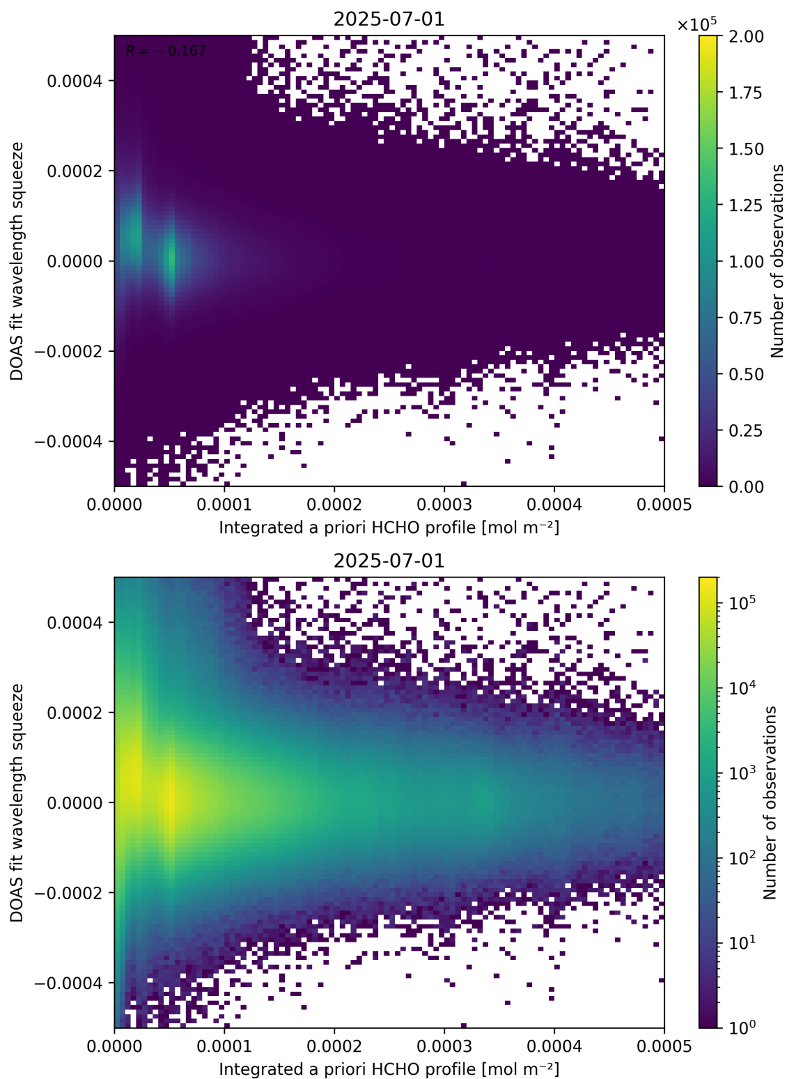
Figure 150: Scatter density plot of “Integrated a priori HCHO profile” against “DOAS fit wavelength squeeze” for 2025-06-30 to 2025-07-02.
