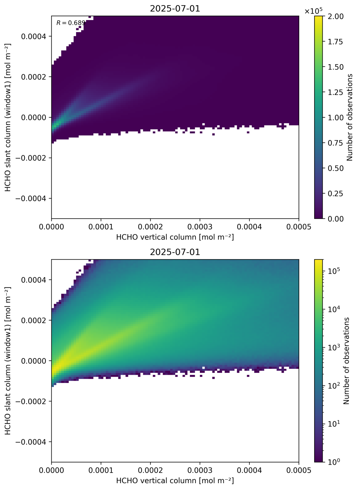
Figure 129: Scatter density plot of “HCHO vertical column” against “HCHO slant column (window1)” for 2025-06-30 to 2025-07-02.
