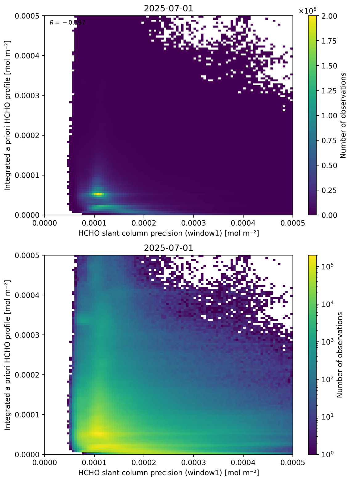
Figure 96: Scatter density plot of “HCHO slant column precision (window1)” against “Integrated a priori HCHO profile” for 2025-06-30 to 2025-07-02.
