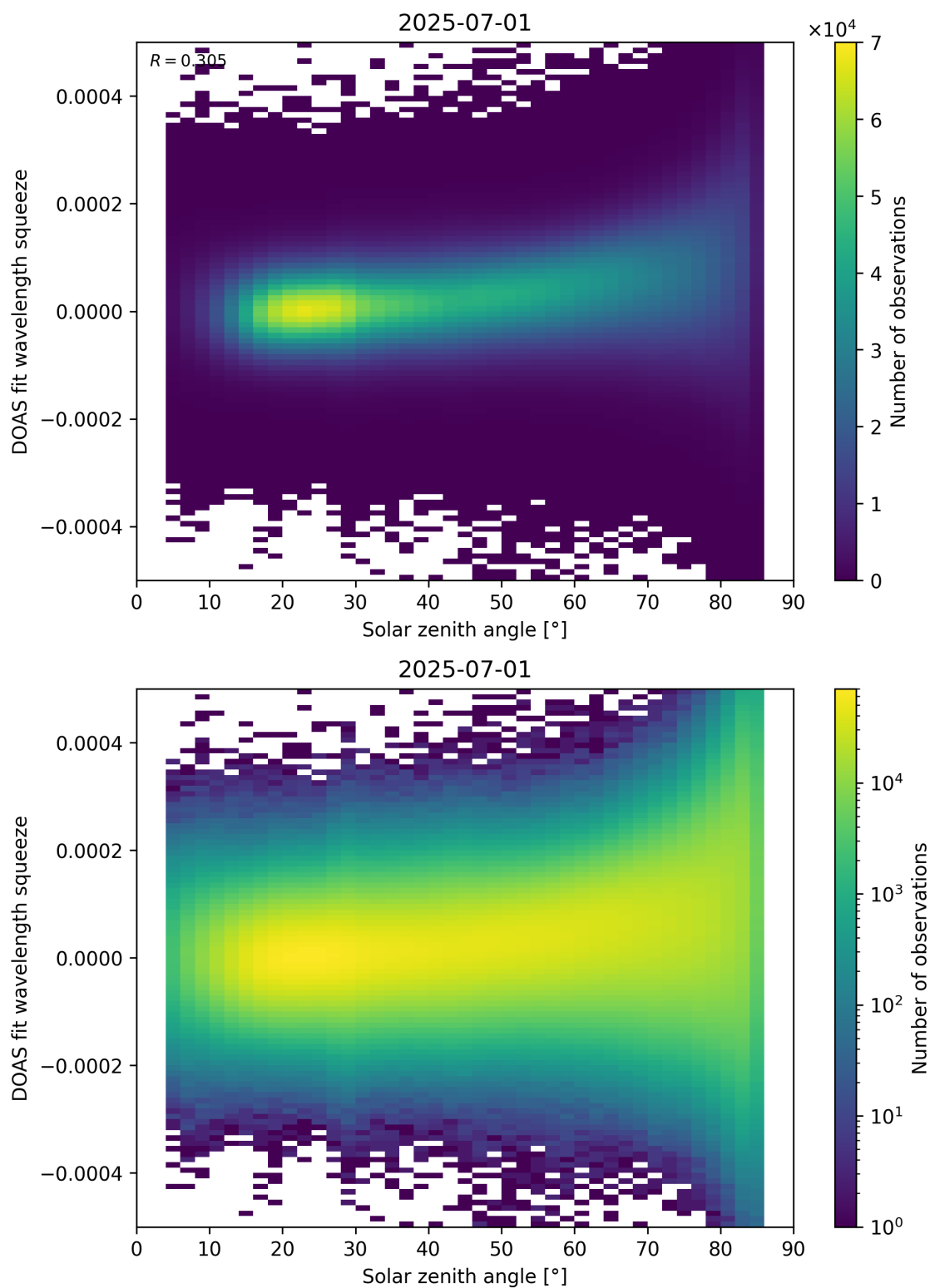
Figure 169: Scatter density plot of “Solar zenith angle” against “DOAS fit wavelength squeeze” for 2025-06-30 to 2025-07-02.
