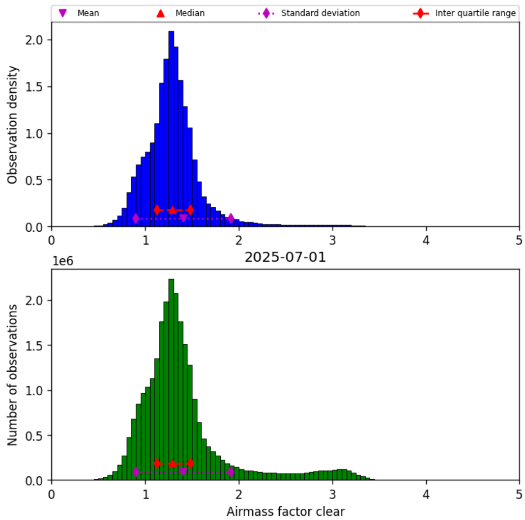
Figure 42: Histogram of “Airmass factor clear” for 2025-06-30 to 2025-07-02
