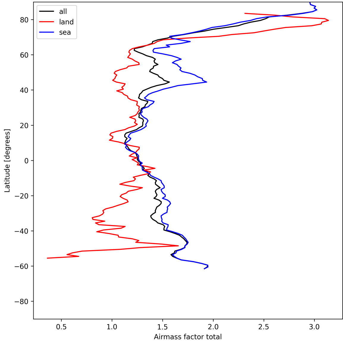
Figure 26: Zonal average of “Airmass factor total” for 2025-06-30 to 2025-07-02.
