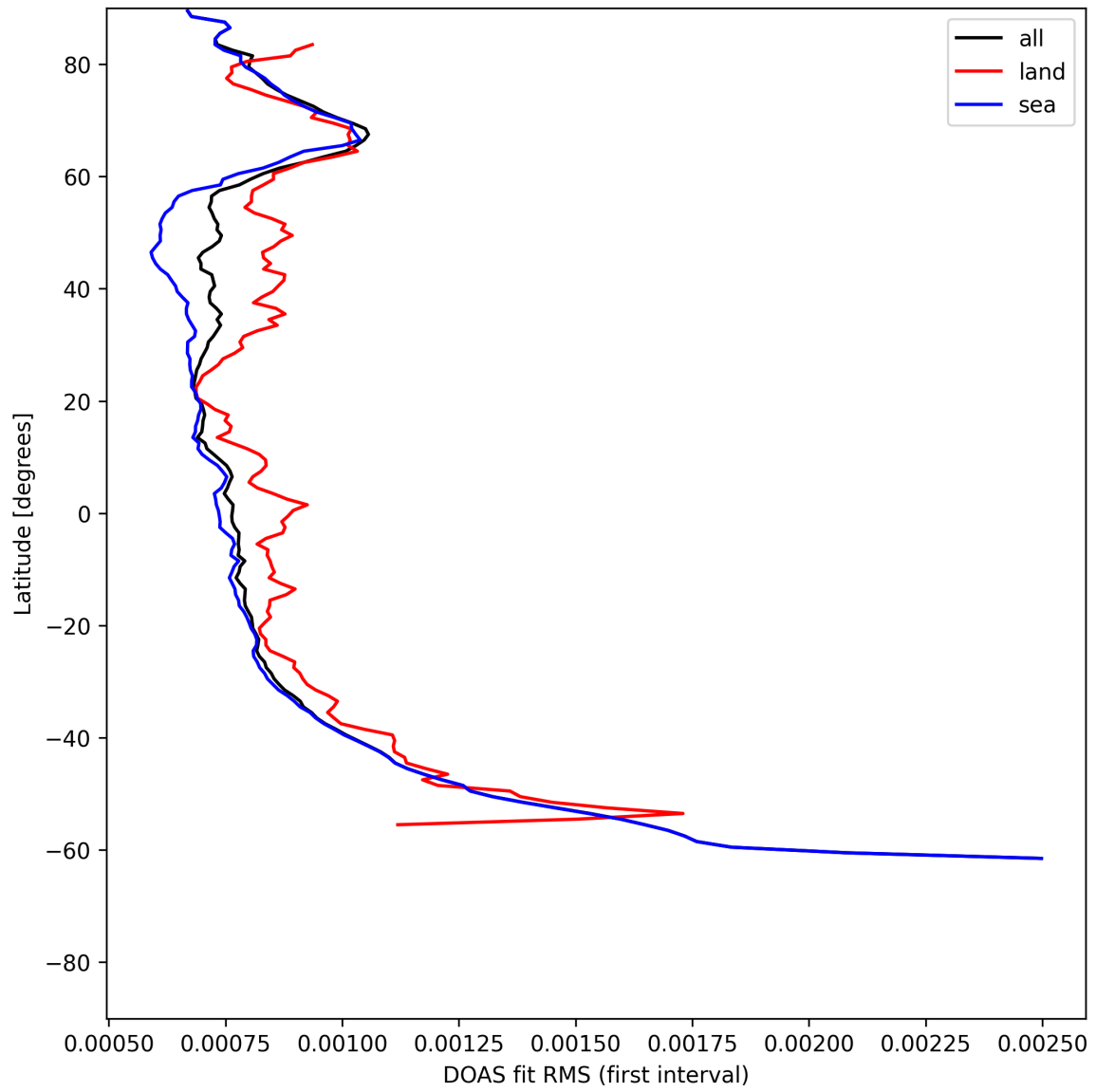
Figure 32: Zonal average of “DOAS fit RMS (first interval)” for 2025-06-30 to 2025-07-02.
