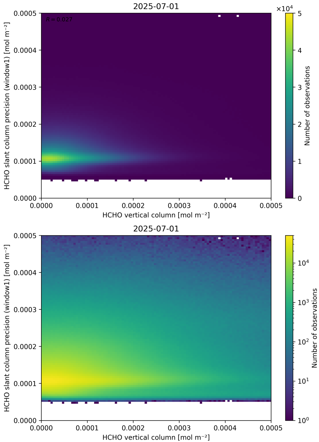
Figure 130: Scatter density plot of “HCHO vertical column” against “HCHO slant column precision (window1)” for 2025-06-30 to 2025-07-02.
