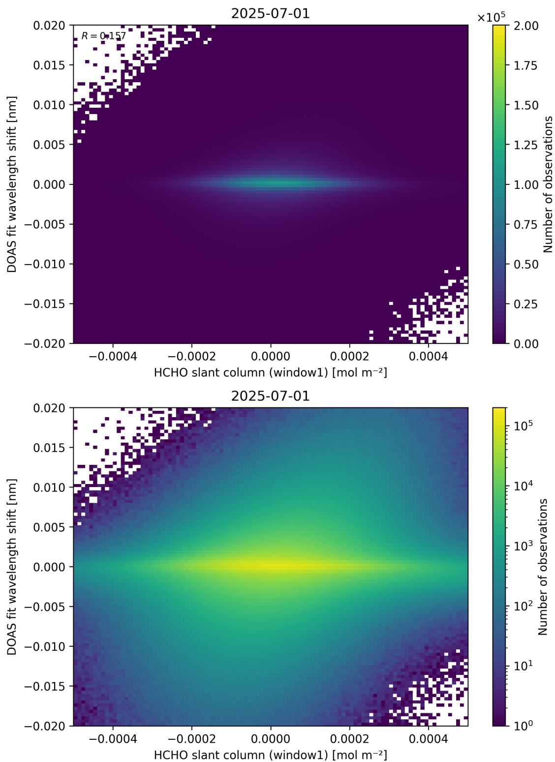
Figure 79: Scatter density plot of “HCHO slant column (window1)” against “DOAS fit wavelength shift” for 2025-06-30 to 2025-07-02.
