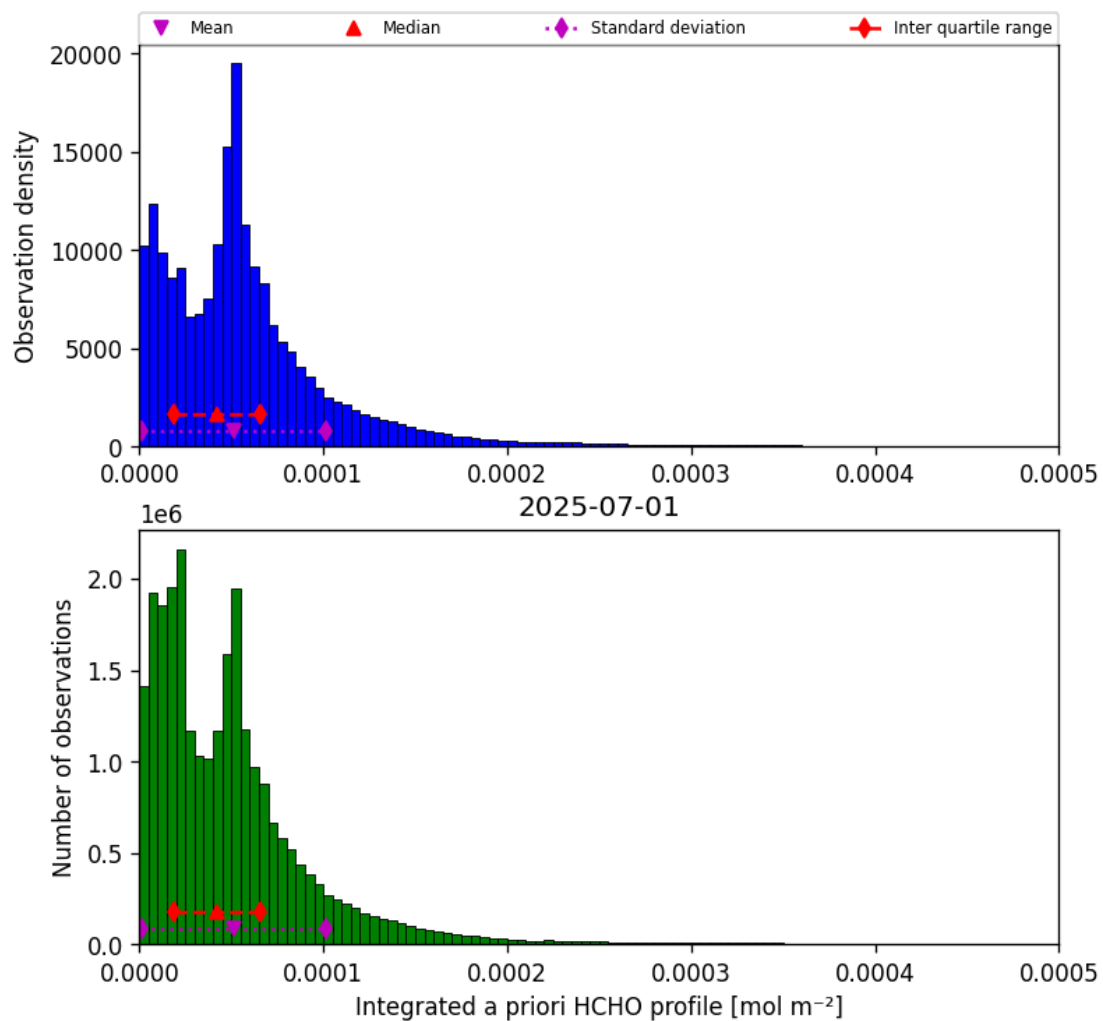
Figure 43: Histogram of “Integrated a priori HCHO profile” for 2025-06-30 to 2025-07-02
