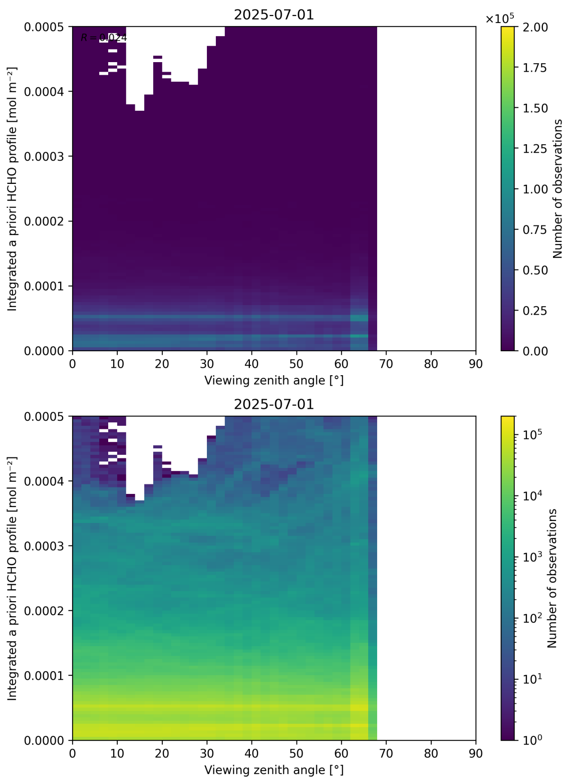
Figure 195: Scatter density plot of “Viewing zenith angle” against “Integrated a priori HCHO profile” for 2025-06-30 to 2025-07-02.
