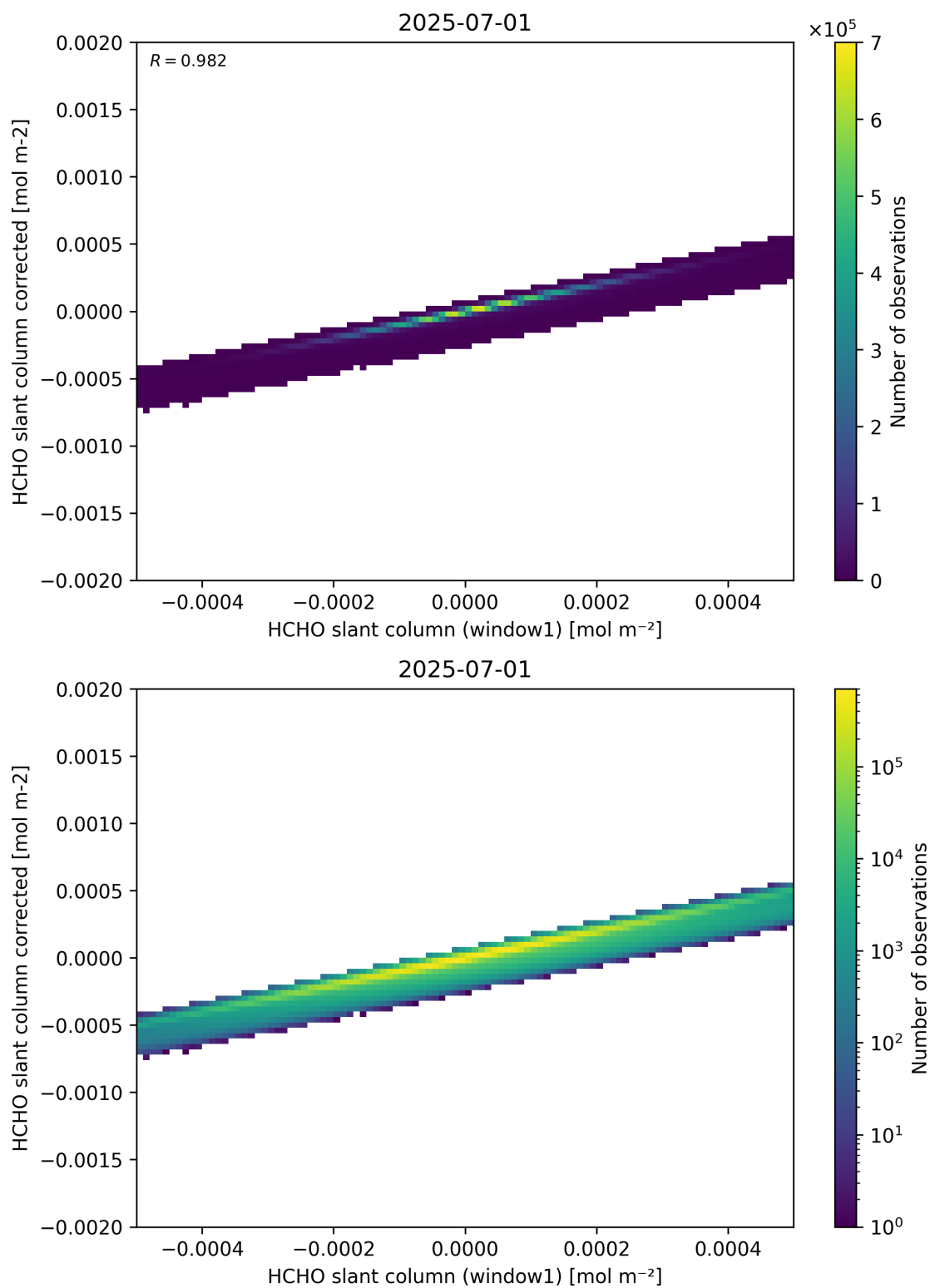
Figure 82: Scatter density plot of “HCHO slant column (window1)” against “HCHO slant column corrected” for 2025-06-30 to 2025-07-02.
