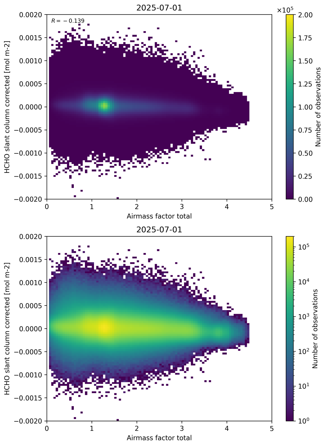
Figure 101: Scatter density plot of “Airmass factor total” against “HCHO slant column corrected” for 2025-06-30 to 2025-07-02.
