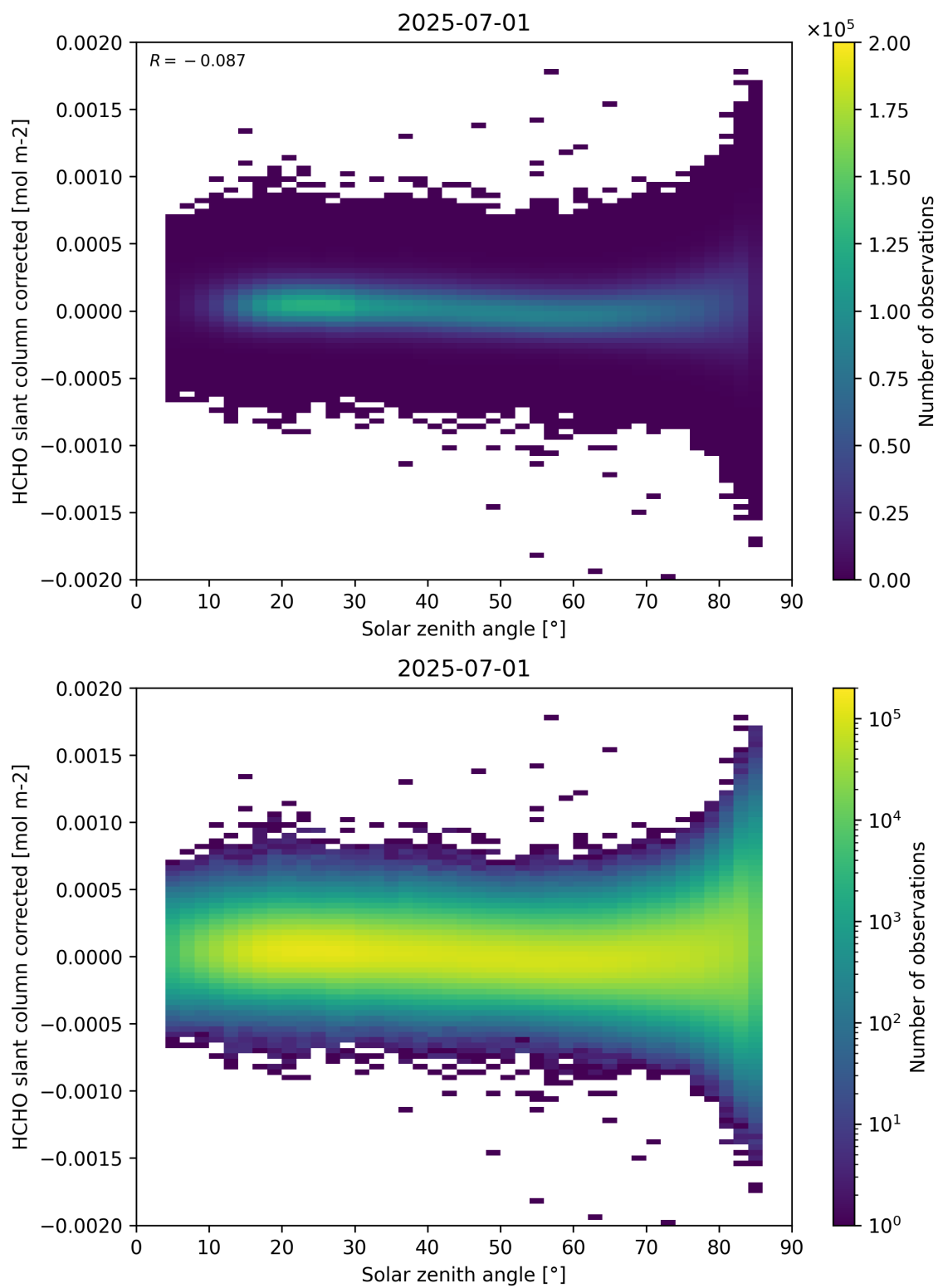
Figure 171: Scatter density plot of “Solar zenith angle” against “HCHO slant column corrected” for 2025-06-30 to 2025-07-02.
