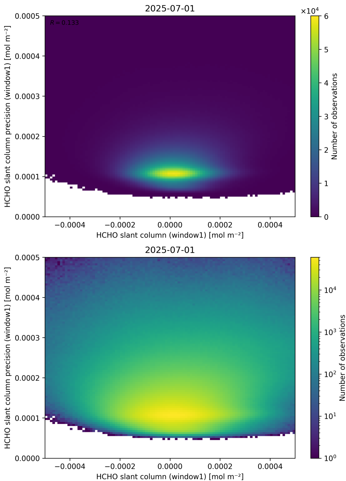
Figure 84: Scatter density plot of “HCHO slant column (window1)” against “HCHO slant column precision (window1)” for 2025-06-30 to 2025-07-02.
