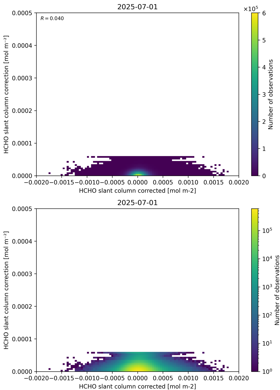
Figure 77: Scatter density plot of “HCHO slant column corrected” against “HCHO slant column correction” for 2025-06-30 to 2025-07-02.
