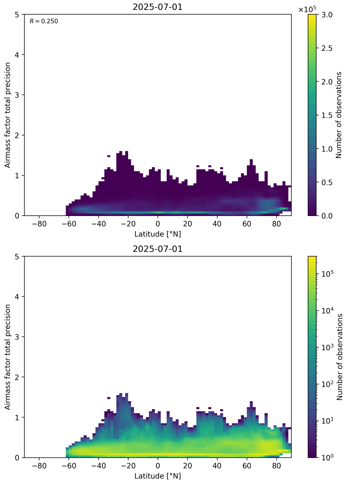
Figure 162: Scatter density plot of “Latitude” against “Airmass factor total precision” for 2025-06-30 to 2025-07-02.
