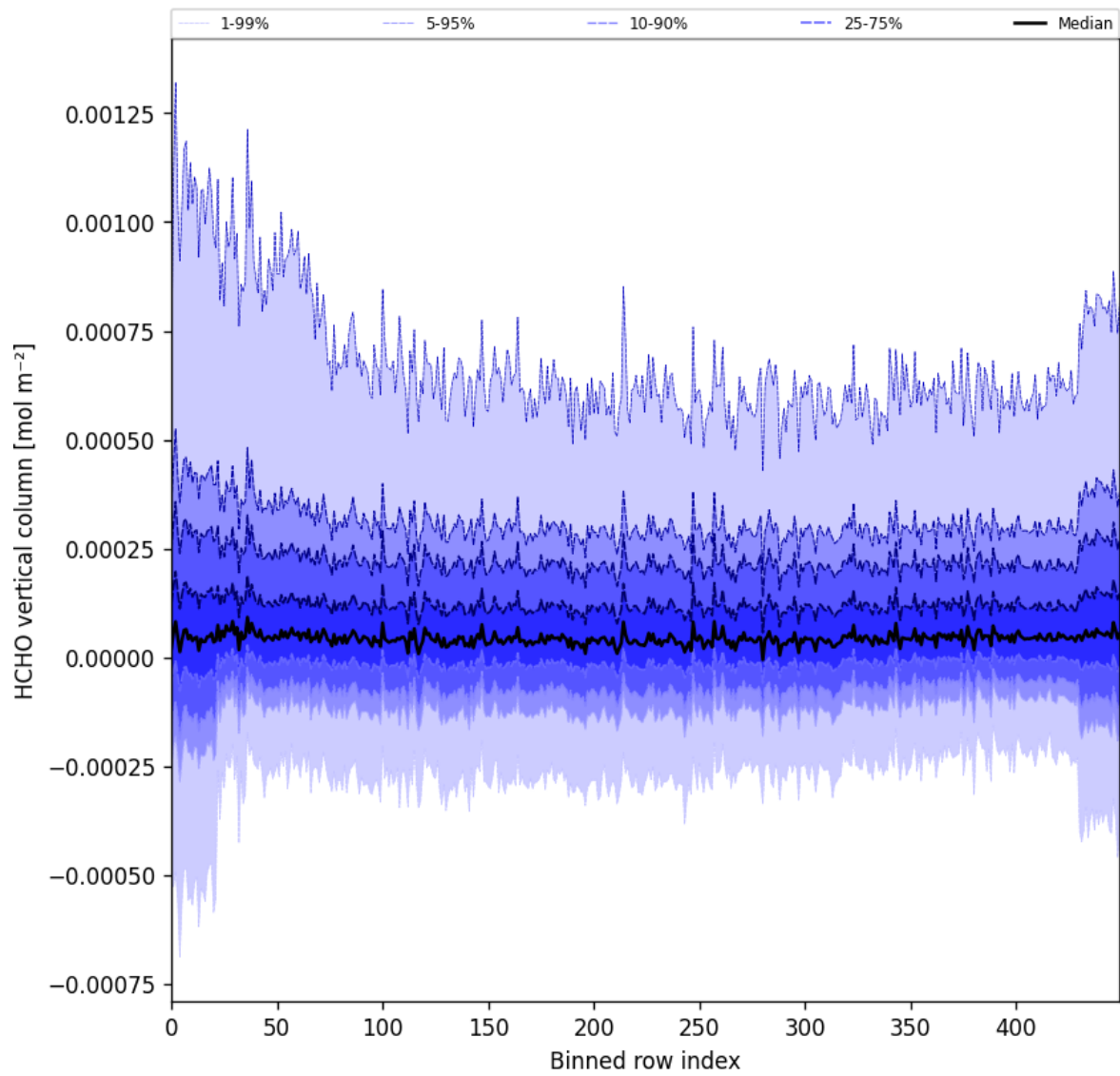
Figure 49: Along track statistics of “HCHO vertical column” for 2025-06-30 to 2025-07-02
