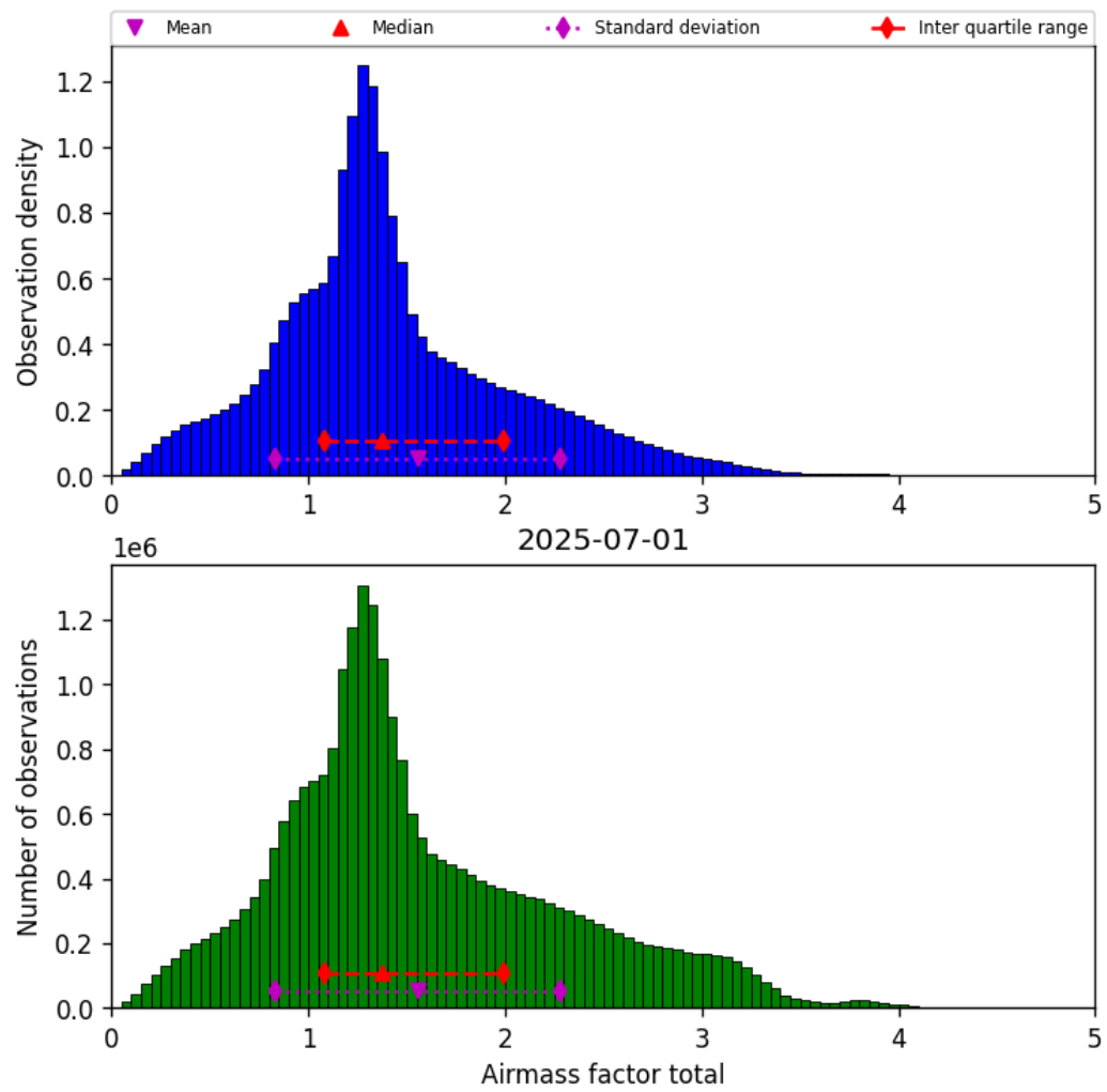
Figure 40: Histogram of “Airmass factor total” for 2025-06-30 to 2025-07-02
