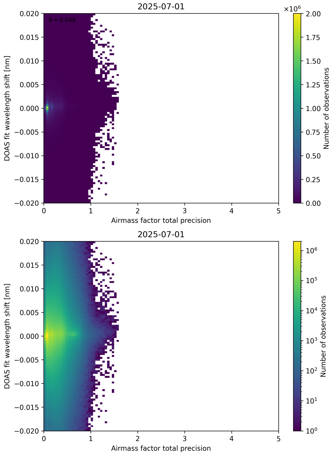
Figure 106: Scatter density plot of “Airmass factor total precision” against “DOAS fit wavelength shift” for 2025-06-30 to 2025-07-02.
