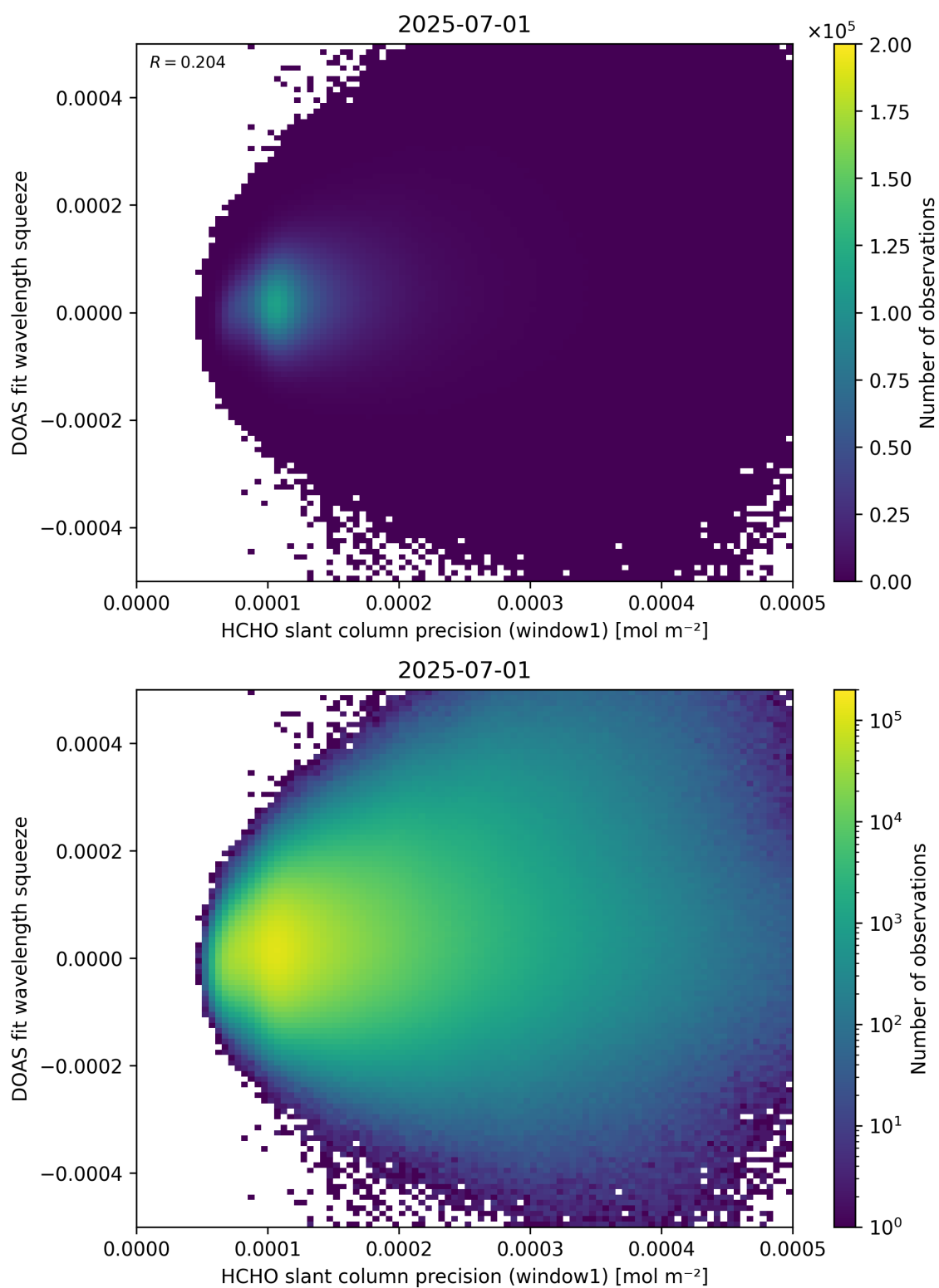
Figure 90: Scatter density plot of “HCHO slant column precision (window1)” against “DOAS fit wavelength squeeze” for 2025-06-30 to 2025-07-02.
