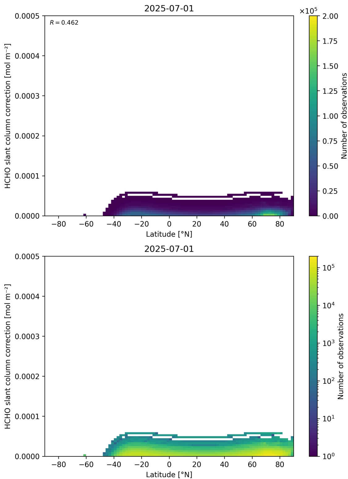
Figure 158: Scatter density plot of “Latitude” against “HCHO slant column correction” for 2025-06-30 to 2025-07-02.
