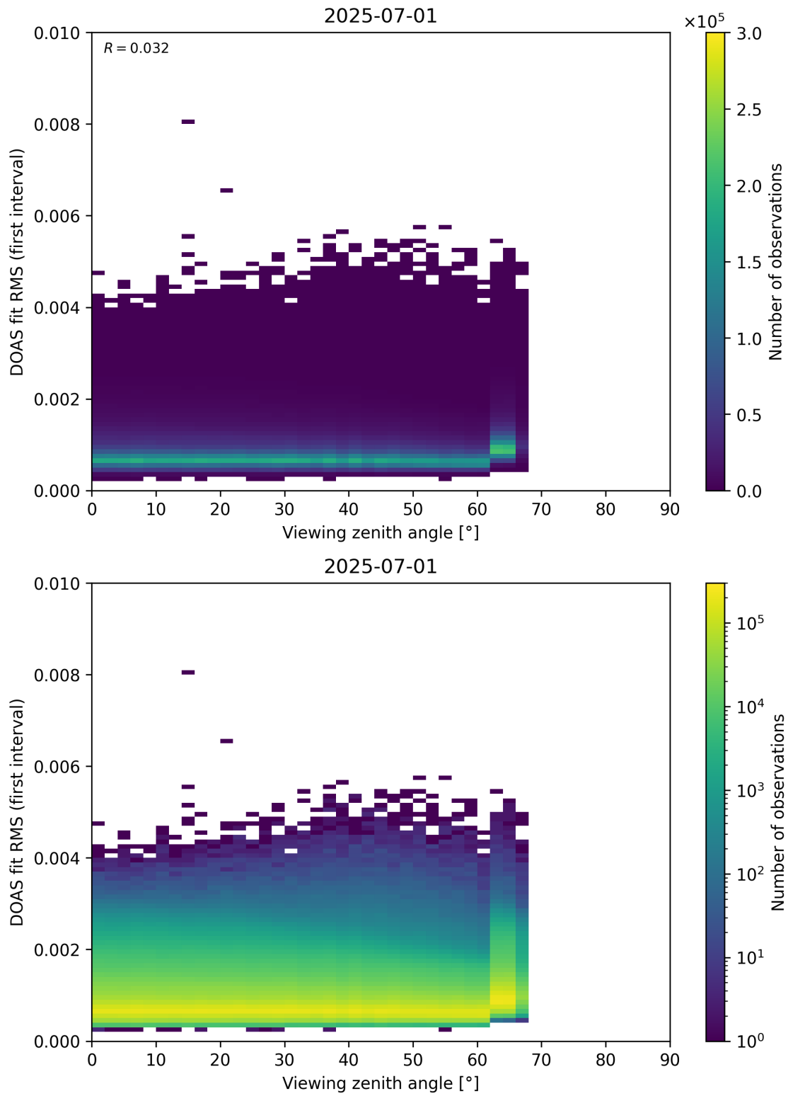
Figure 182: Scatter density plot of “Viewing zenith angle” against “DOAS fit RMS (first interval)” for 2025-06-30 to 2025-07-02.
