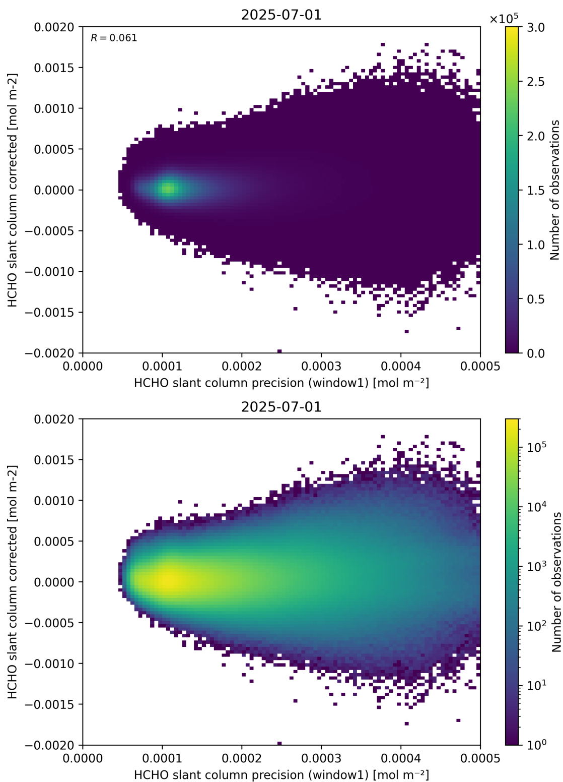
Figure 92: Scatter density plot of “HCHO slant column precision (window1)” against “HCHO slant column corrected” for 2025-06-30 to 2025-07-02.
