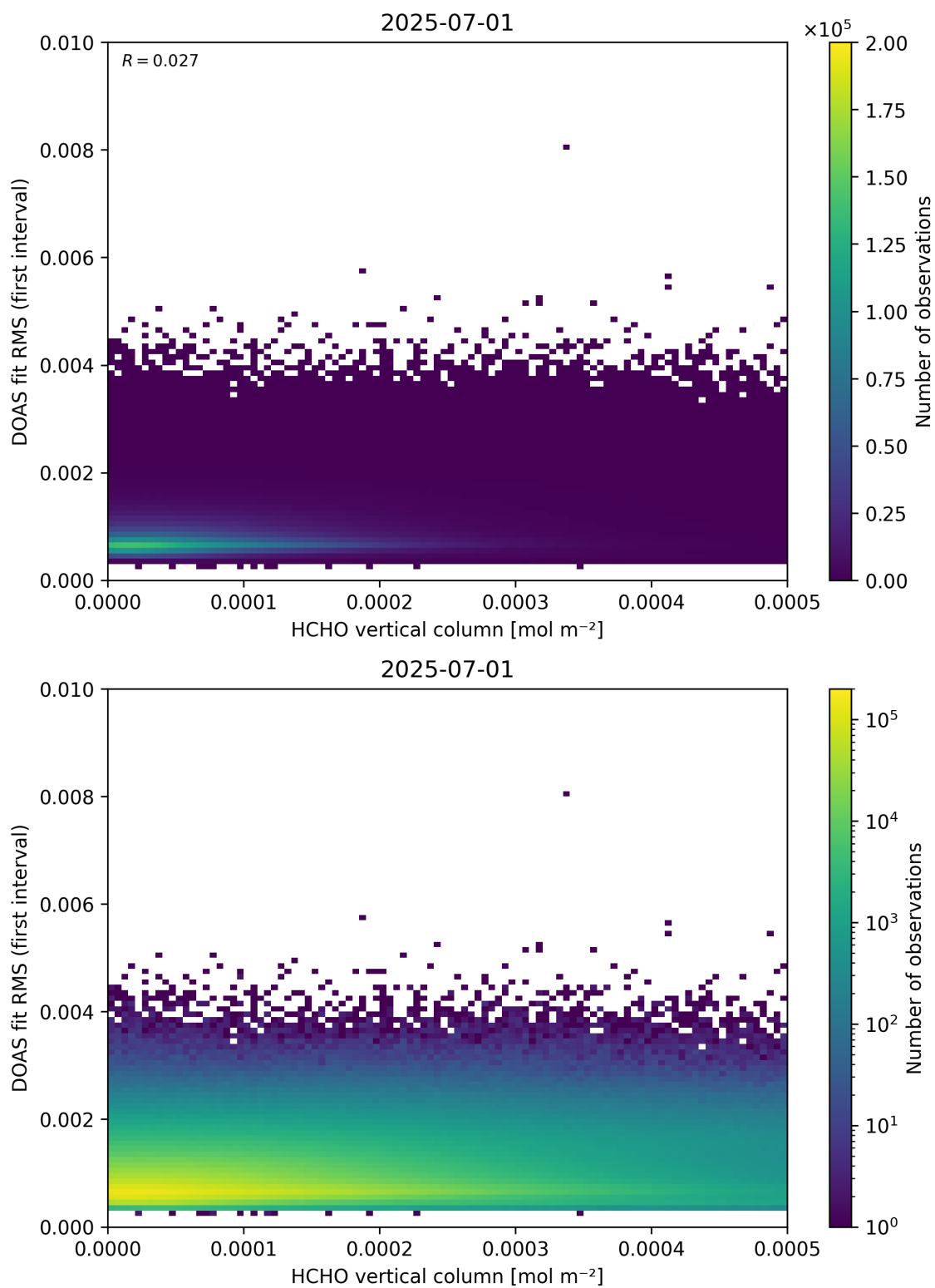
Figure 123: Scatter density plot of “HCHO vertical column” against “DOAS fit RMS (first interval)” for 2025-06-30 to 2025-07-02.
