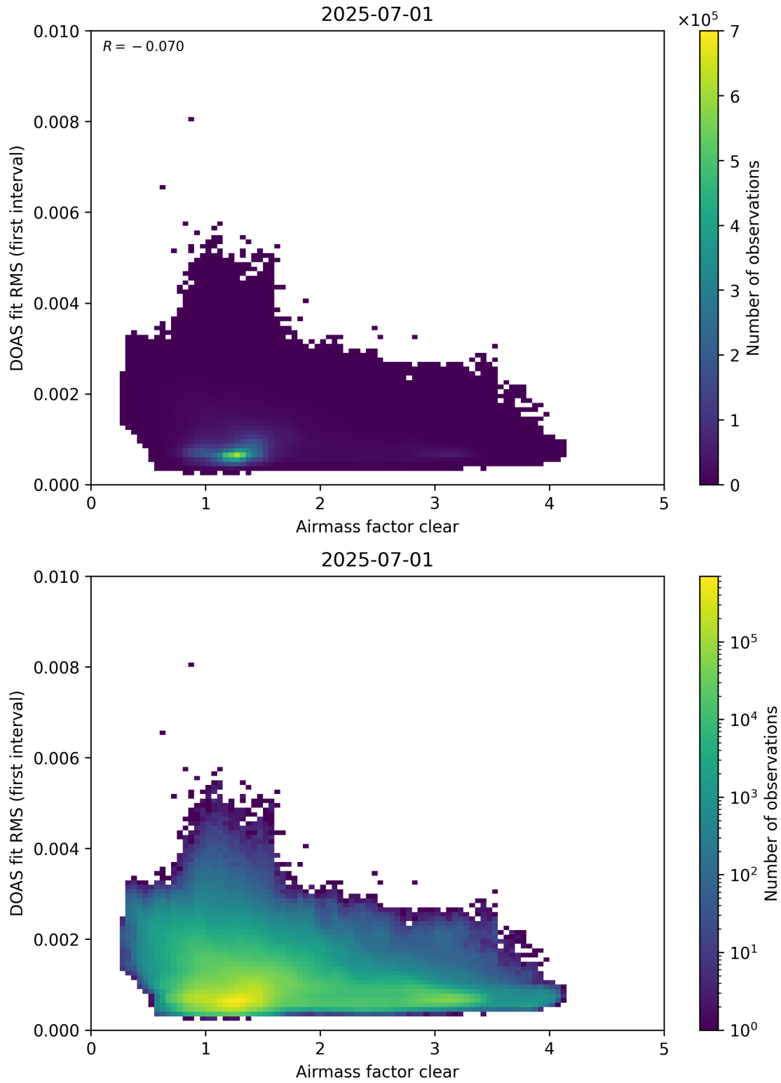
Figure 71: Scatter density plot of “Airmass factor clear” against “DOAS fit RMS (first interval)” for 2025-06-30 to 2025-07-02.
