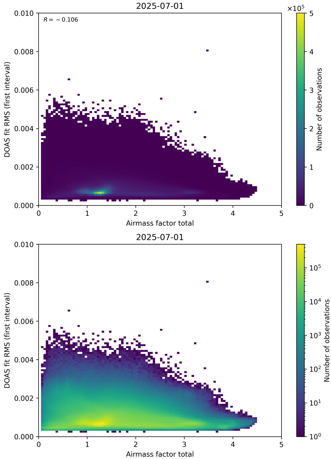
Figure 97: Scatter density plot of “Airmass factor total” against “DOAS fit RMS (first interval)” for 2025-06-30 to 2025-07-02.
