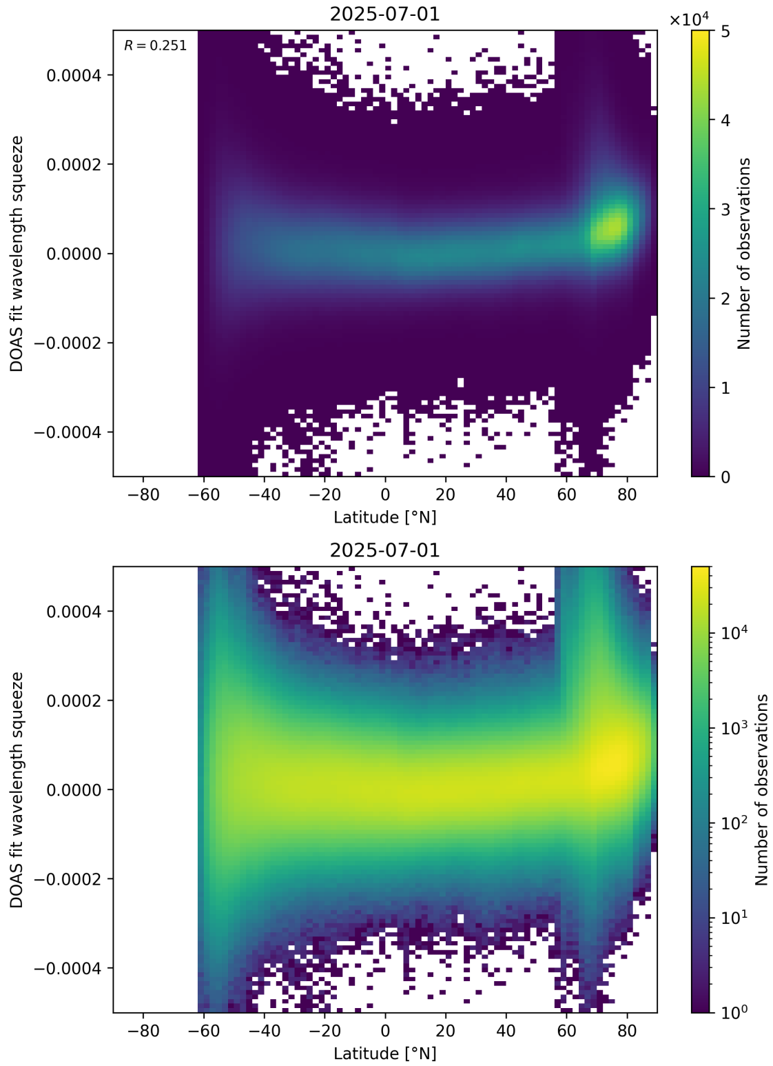
Figure 155: Scatter density plot of “Latitude” against “DOAS fit wavelength squeeze” for 2025-06-30 to 2025-07-02.
