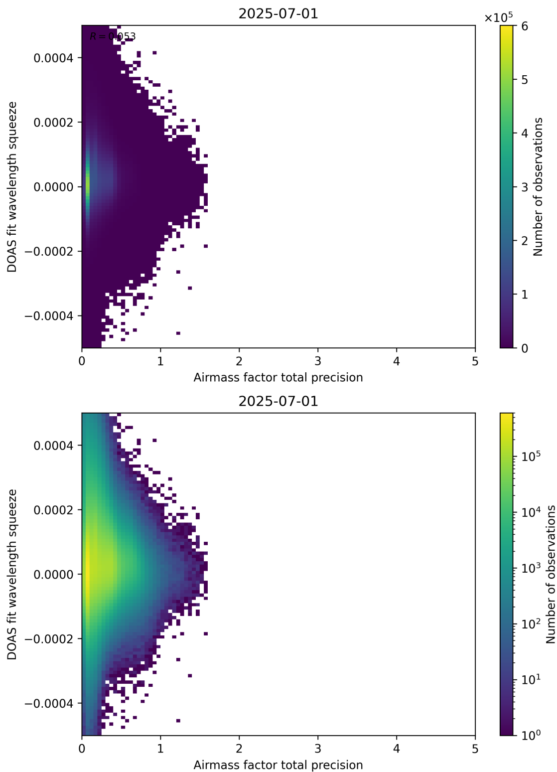
Figure 107: Scatter density plot of “Airmass factor total precision” against “DOAS fit wavelength squeeze” for 2025-06-30 to 2025-07-02.
