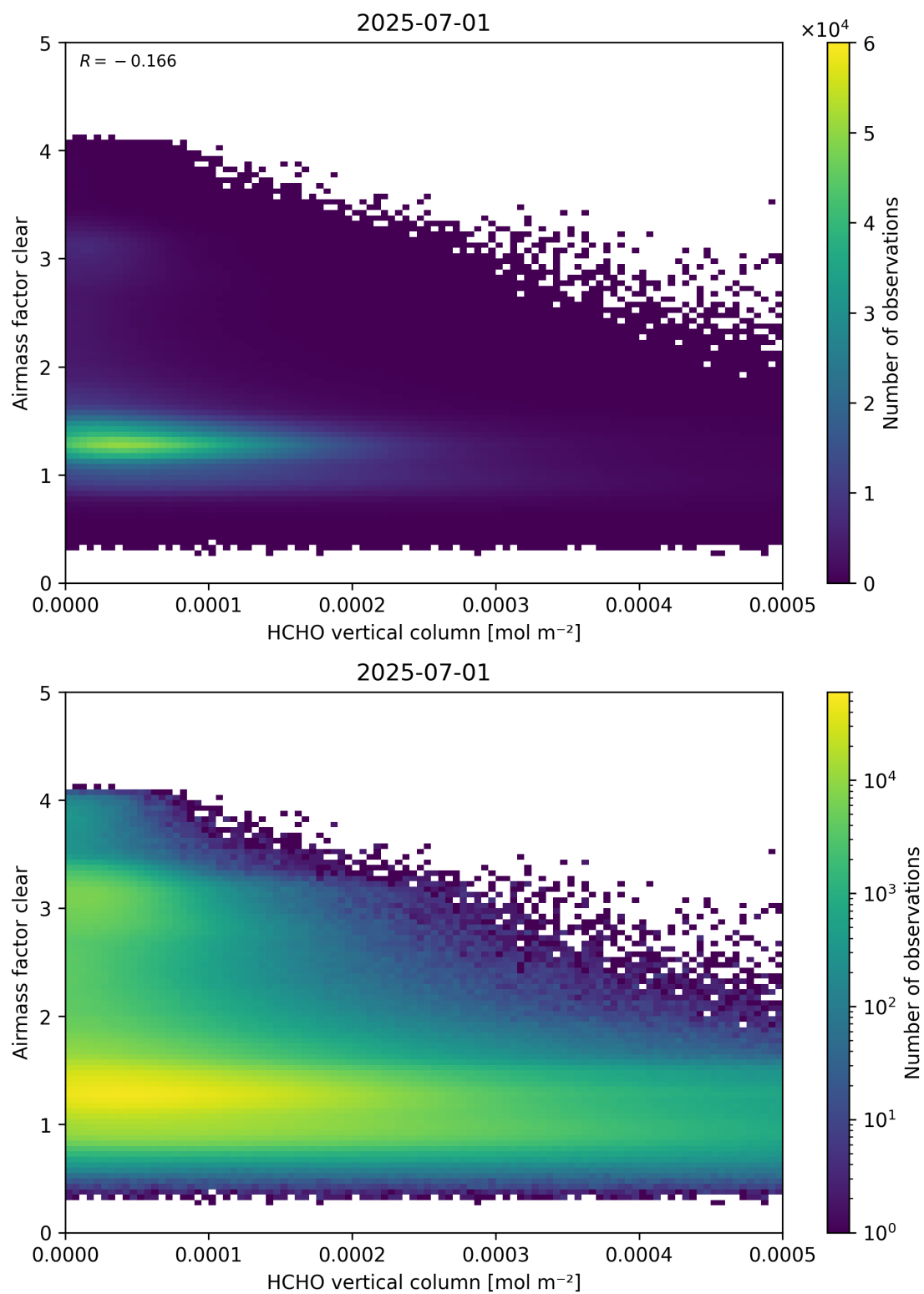
Figure 126: Scatter density plot of “HCHO vertical column” against “Airmass factor clear” for 2025-06-30 to 2025-07-02.
