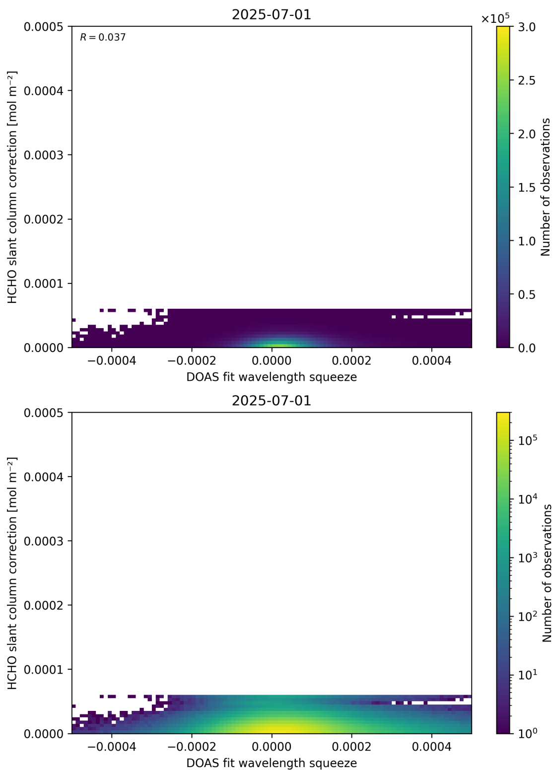
Figure 70: Scatter density plot of “DOAS fit wavelength squeeze” against “HCHO slant column correction” for 2025-06-30 to 2025-07-02.
