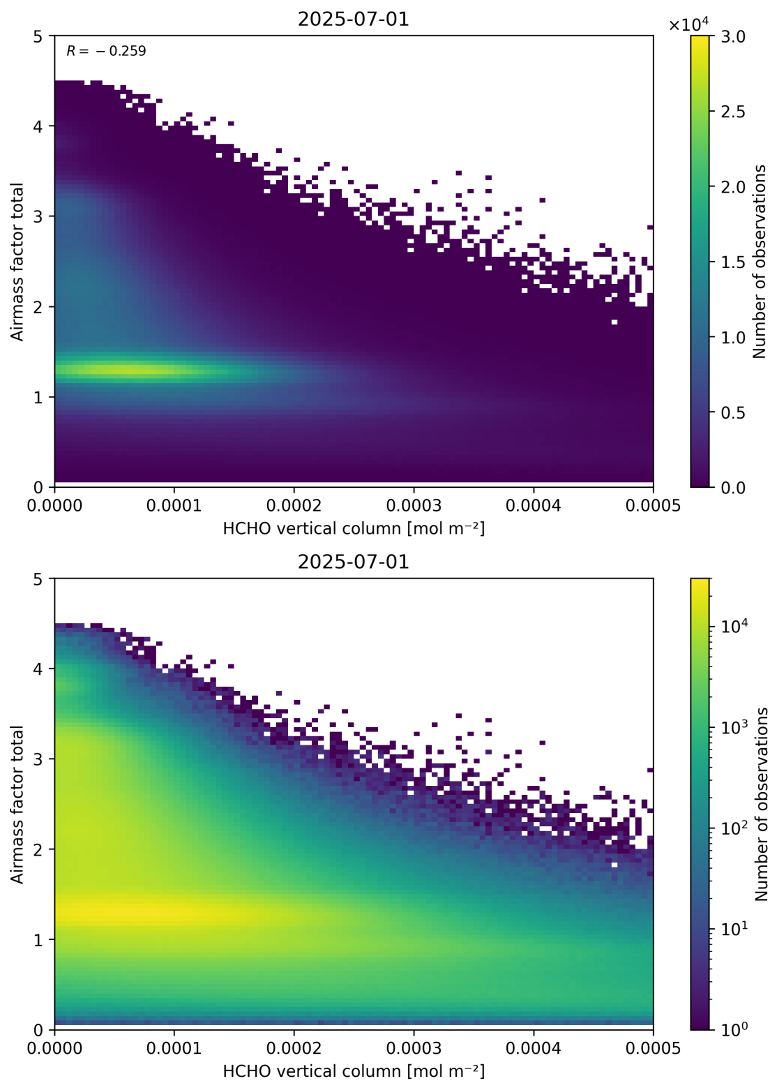
Figure 131: Scatter density plot of “HCHO vertical column” against “Airmass factor total” for 2025-06-30 to 2025-07-02.
