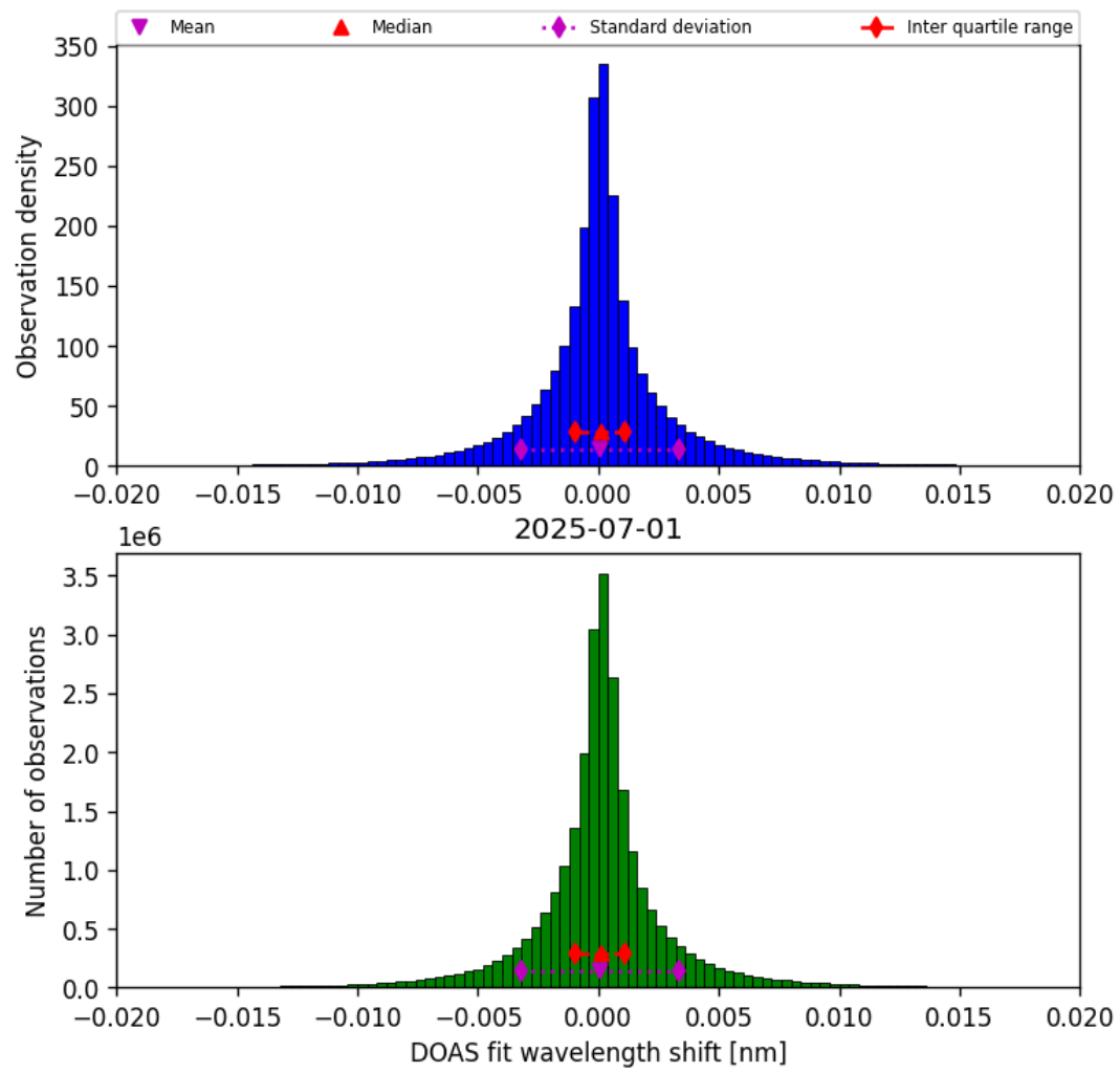
Figure 44: Histogram of “DOAS fit wavelength shift” for 2025-06-30 to 2025-07-02
