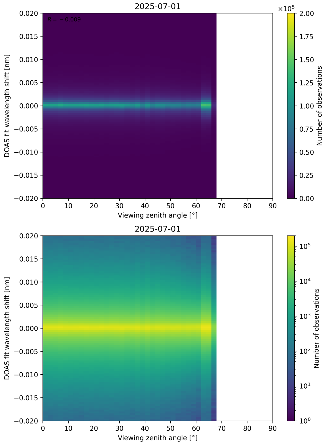
Figure 183: Scatter density plot of “Viewing zenith angle” against “DOAS fit wavelength shift” for 2025-06-30 to 2025-07-02.
