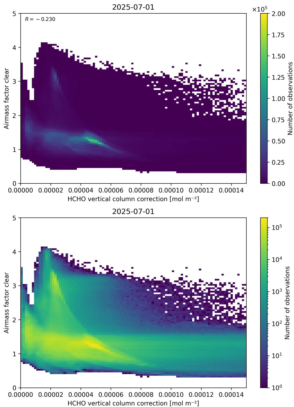
Figure 115: Scatter density plot of “HCHO vertical column correction” against “Airmass factor clear” for 2025-06-30 to 2025-07-02.
