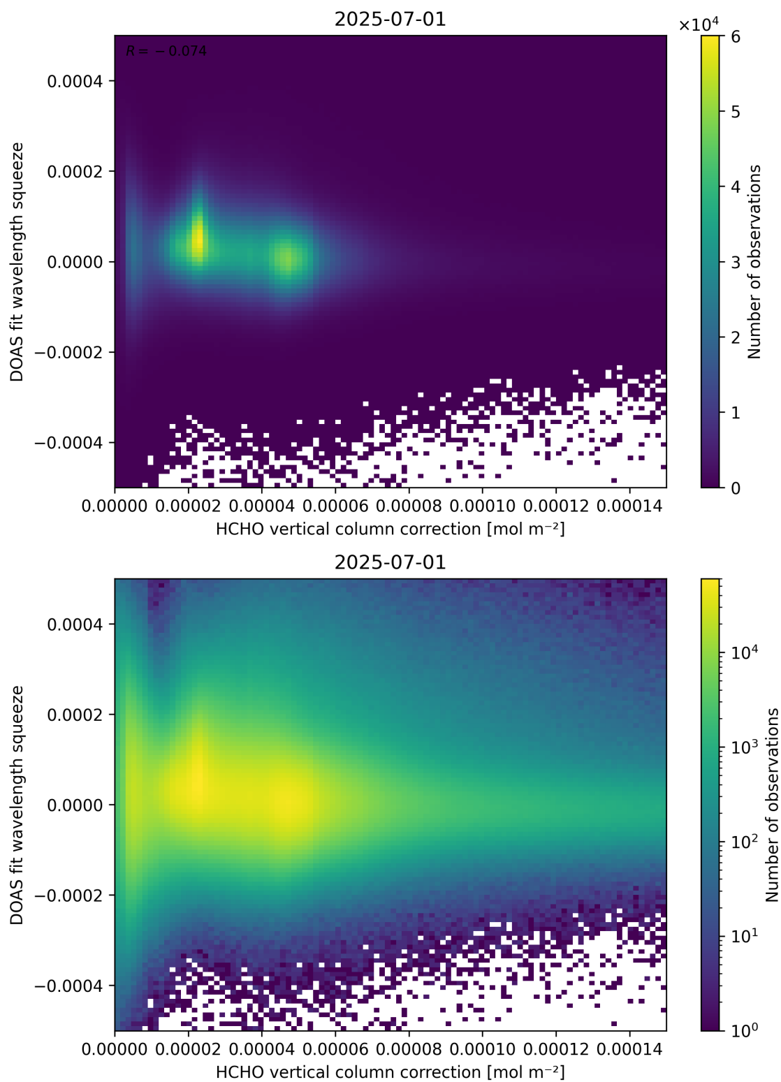
Figure 114: Scatter density plot of “HCHO vertical column correction” against “DOAS fit wavelength squeeze” for 2025-06-30 to 2025-07-02.
