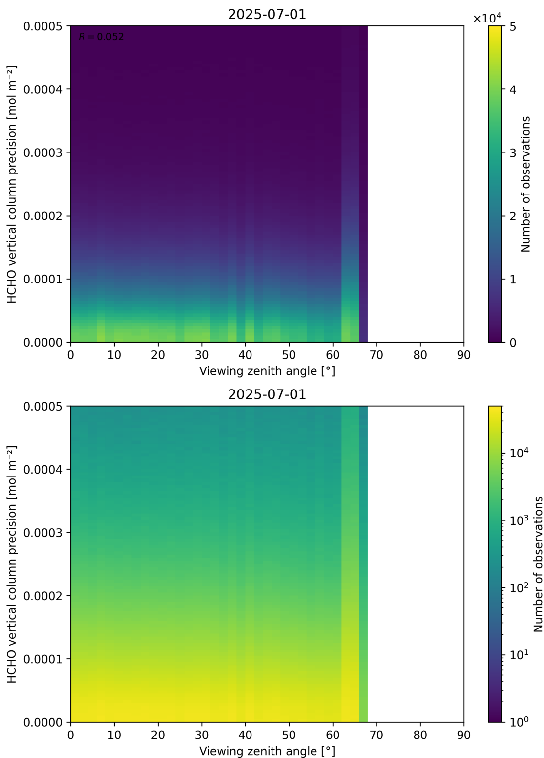
Figure 194: Scatter density plot of “Viewing zenith angle” against “HCHO vertical column precision” for 2025-06-30 to 2025-07-02.
