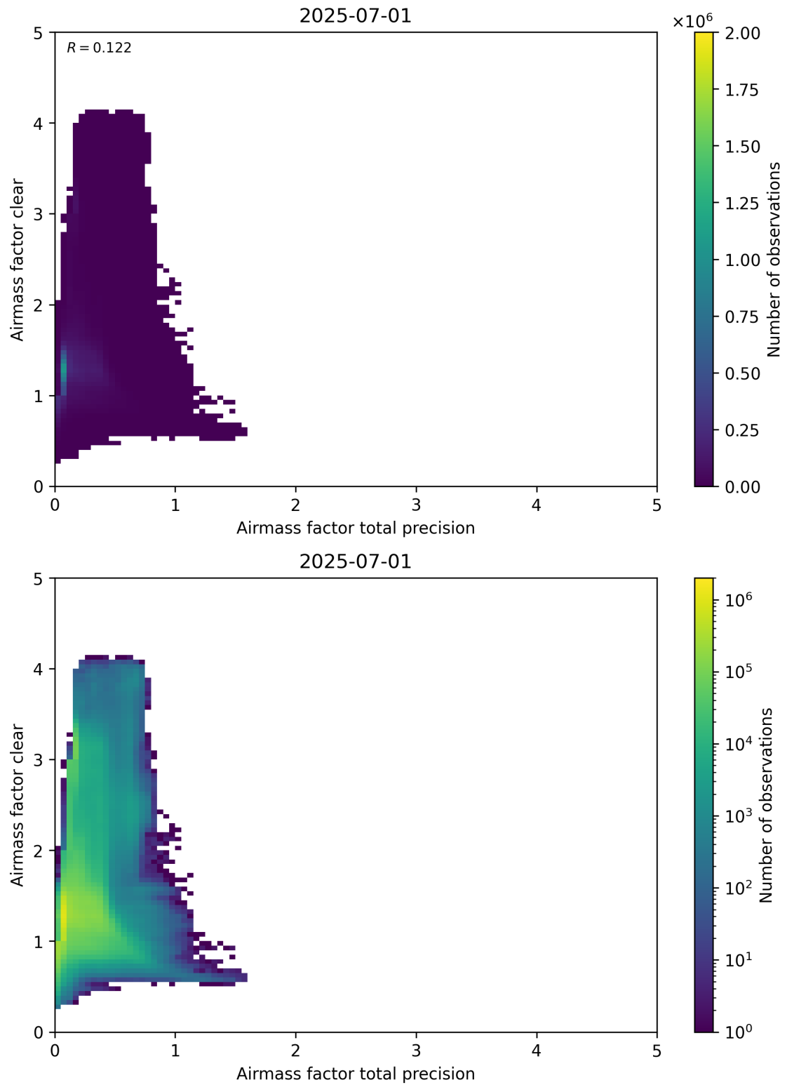
Figure 108: Scatter density plot of “Airmass factor total precision” against “Airmass factor clear” for 2025-06-30 to 2025-07-02.
