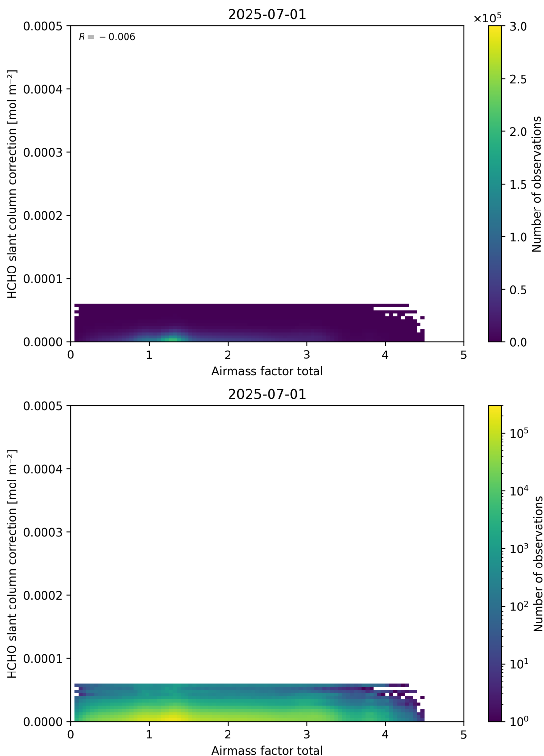
Figure 102: Scatter density plot of “Airmass factor total” against “HCHO slant column correction” for 2025-06-30 to 2025-07-02.
