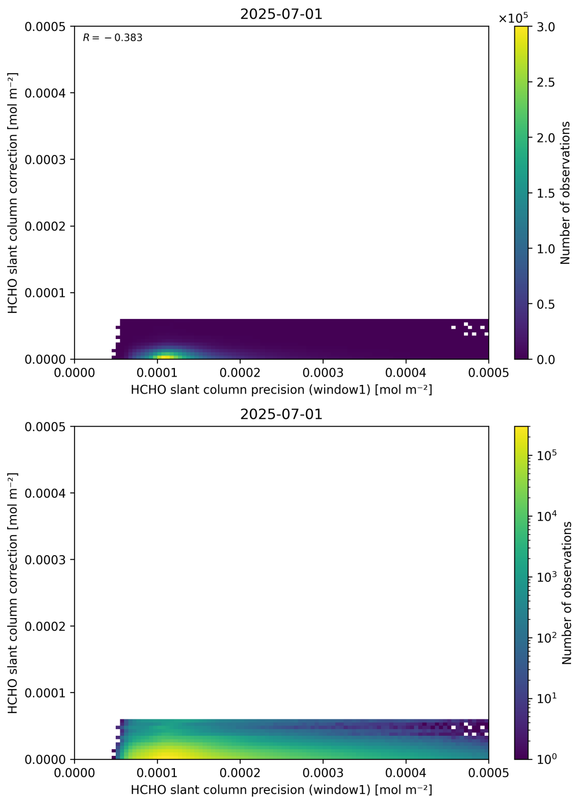
Figure 93: Scatter density plot of “HCHO slant column precision (window1)” against “HCHO slant column correction” for 2025-06-30 to 2025-07-02.
