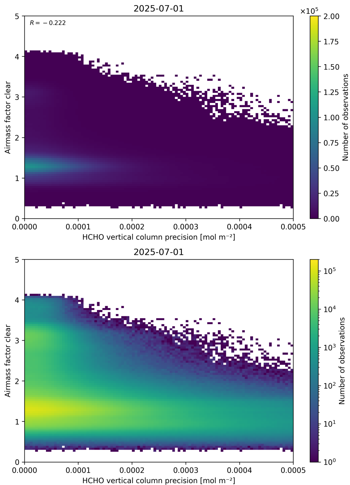
Figure 139: Scatter density plot of “HCHO vertical column precision” against “Airmass factor clear” for 2025-06-30 to 2025-07-02.
