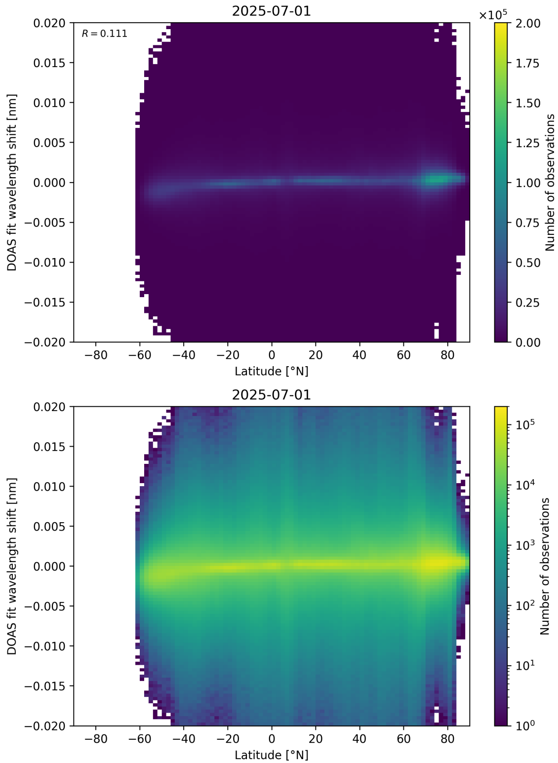
Figure 154: Scatter density plot of “Latitude” against “DOAS fit wavelength shift” for 2025-06-30 to 2025-07-02.
