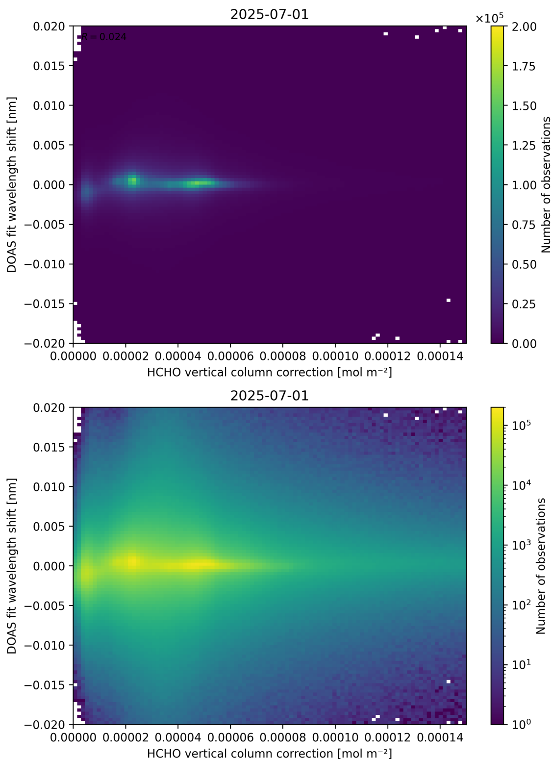
Figure 113: Scatter density plot of “HCHO vertical column correction” against “DOAS fit wavelength shift” for 2025-06-30 to 2025-07-02.
