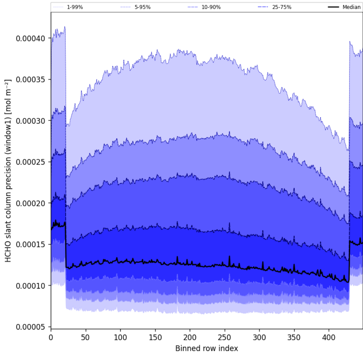
Figure 53: Along track statistics of “HCHO slant column precision (window1)” for 2025-06-30 to 2025-07-02
