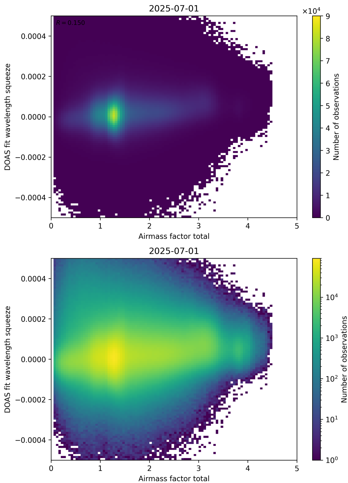
Figure 99: Scatter density plot of “Airmass factor total” against “DOAS fit wavelength squeeze” for 2025-06-30 to 2025-07-02.
