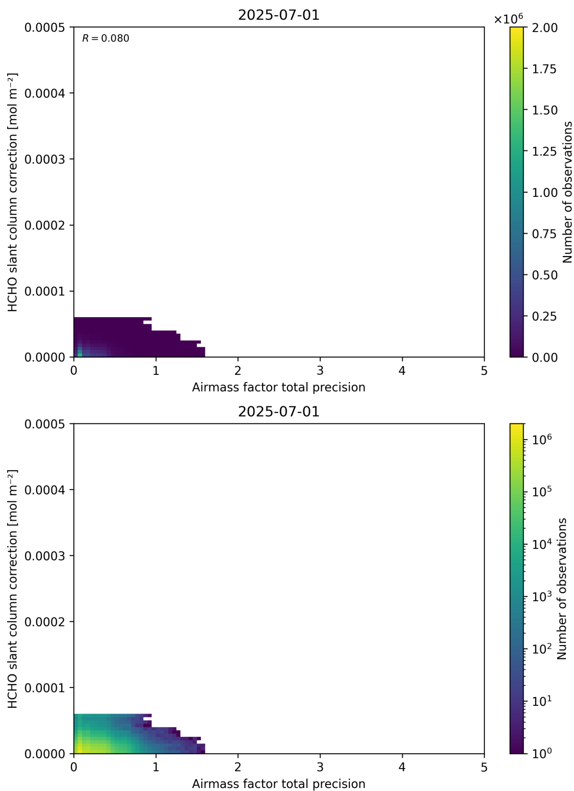
Figure 110: Scatter density plot of “Airmass factor total precision” against “HCHO slant column correction” for 2025-06-30 to 2025-07-02.
