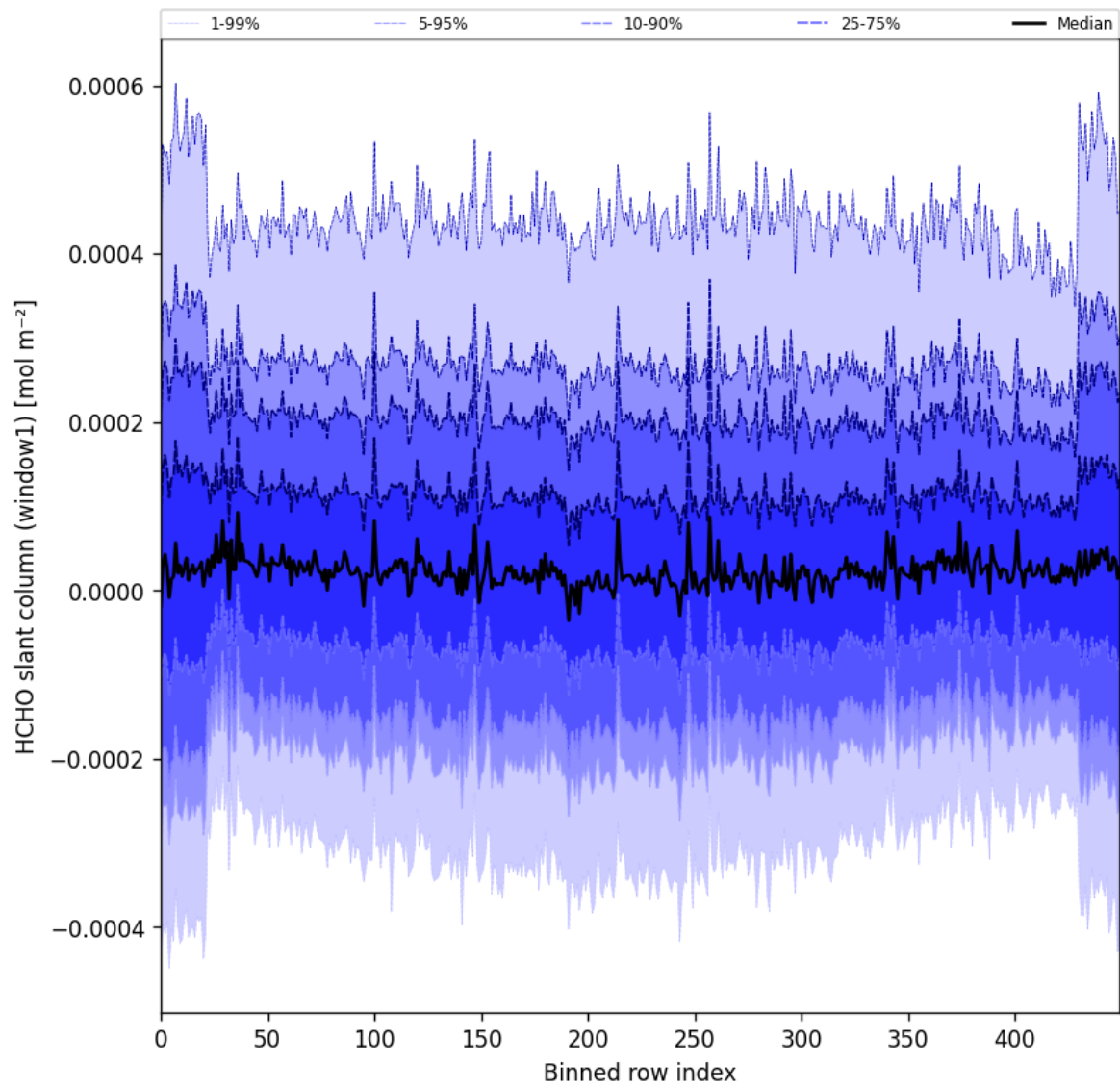
Figure 52: Along track statistics of “HCHO slant column (window1)” for 2025-06-30 to 2025-07-02
