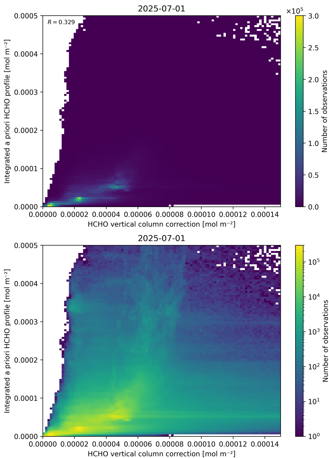
Figure 122: Scatter density plot of “HCHO vertical column correction” against “Integrated a priori HCHO profile” for 2025-06-30 to 2025-07-02.
