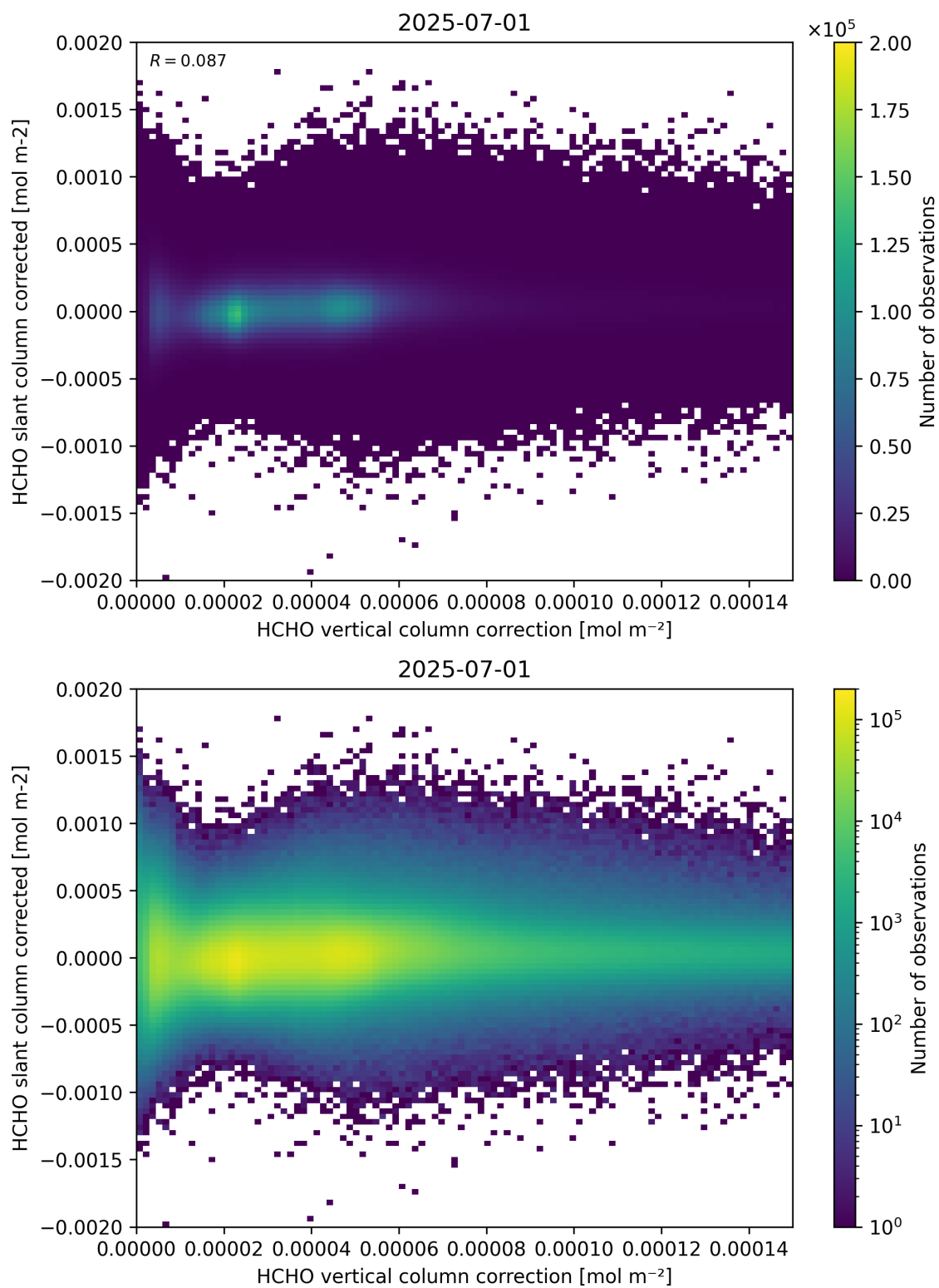
Figure 116: Scatter density plot of “HCHO vertical column correction” against “HCHO slant column corrected” for 2025-06-30 to 2025-07-02.
