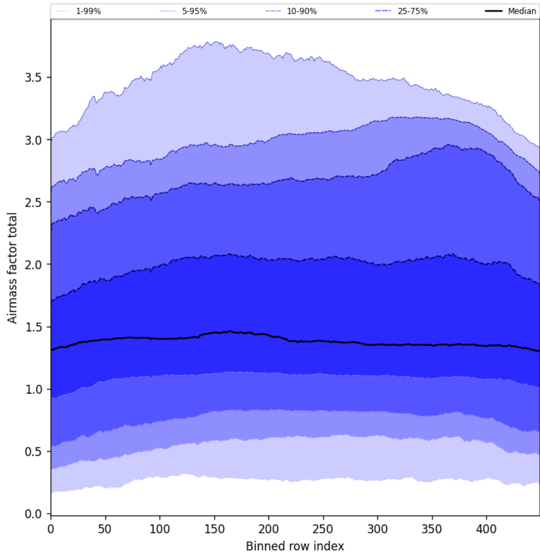
Figure 54: Along track statistics of “Airmass factor total” for 2025-06-30 to 2025-07-02
