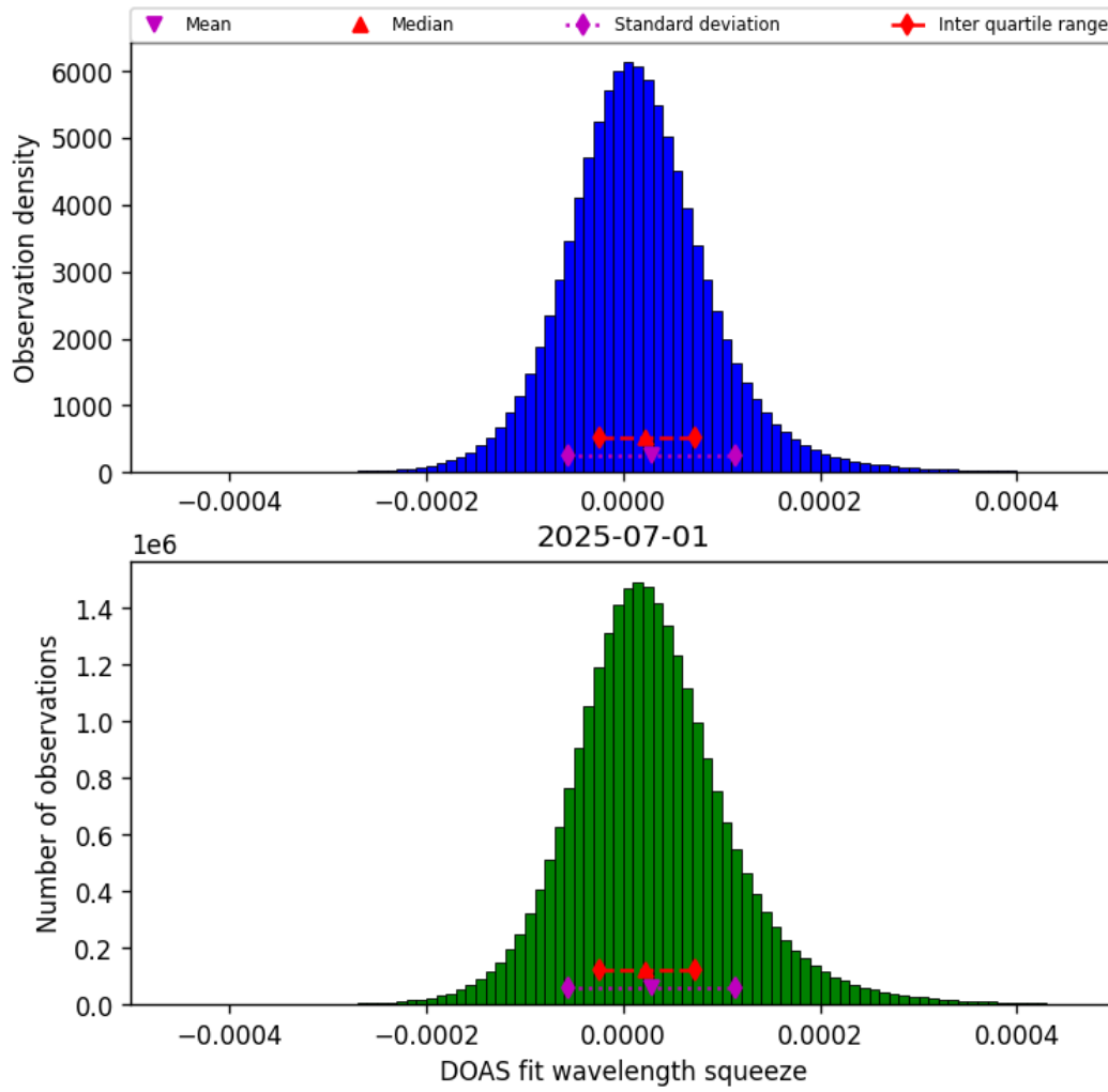
Figure 45: Histogram of “DOAS fit wavelength squeeze” for 2025-06-30 to 2025-07-02
