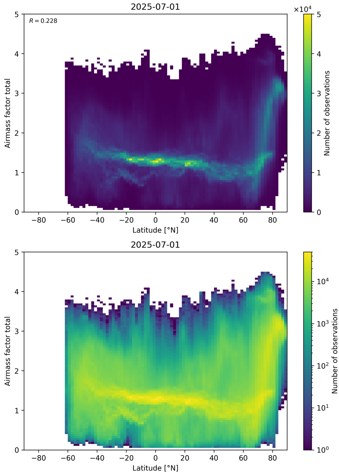
Figure 161: Scatter density plot of “Latitude” against “Airmass factor total” for 2025-06-30 to 2025-07-02.
