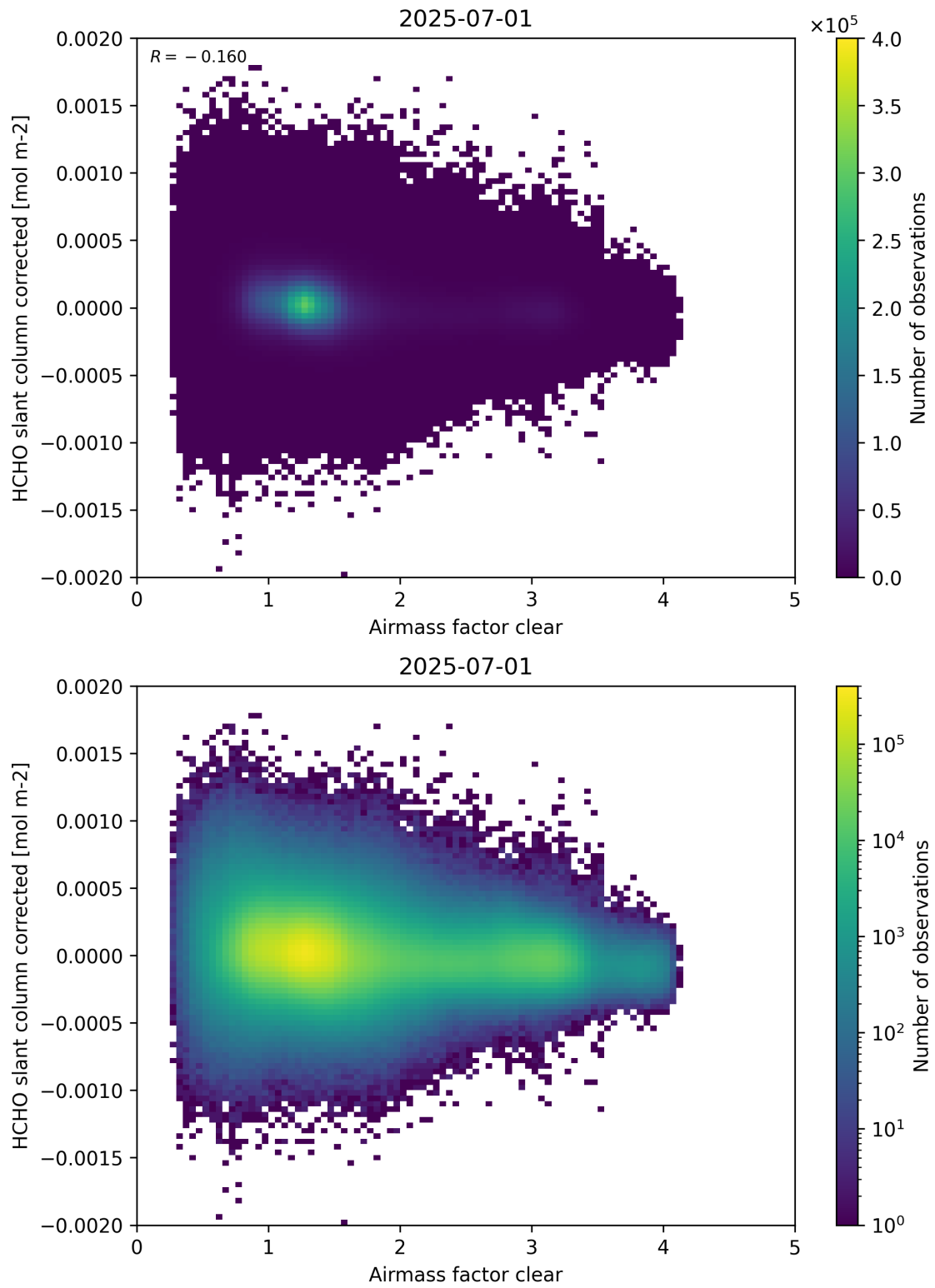
Figure 74: Scatter density plot of “Airmass factor clear” against “HCHO slant column corrected” for 2025-06-30 to 2025-07-02.
