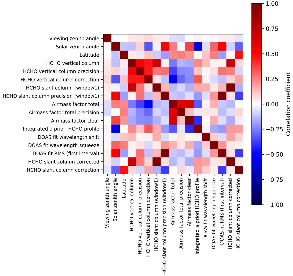
Figure 2: Map of correlation matrix for 2025-06-30 to 2025-07-02.
