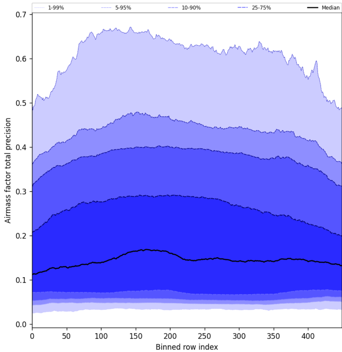
Figure 55: Along track statistics of “Airmass factor total precision” for 2025-06-30 to 2025-07-02
