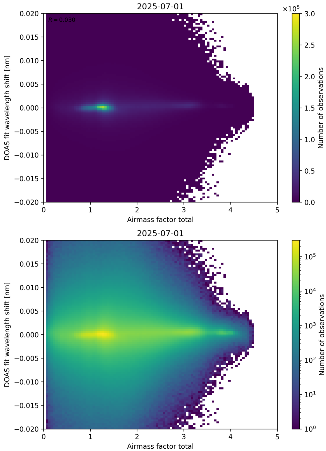
Figure 98: Scatter density plot of “Airmass factor total” against “DOAS fit wavelength shift” for 2025-06-30 to 2025-07-02.
