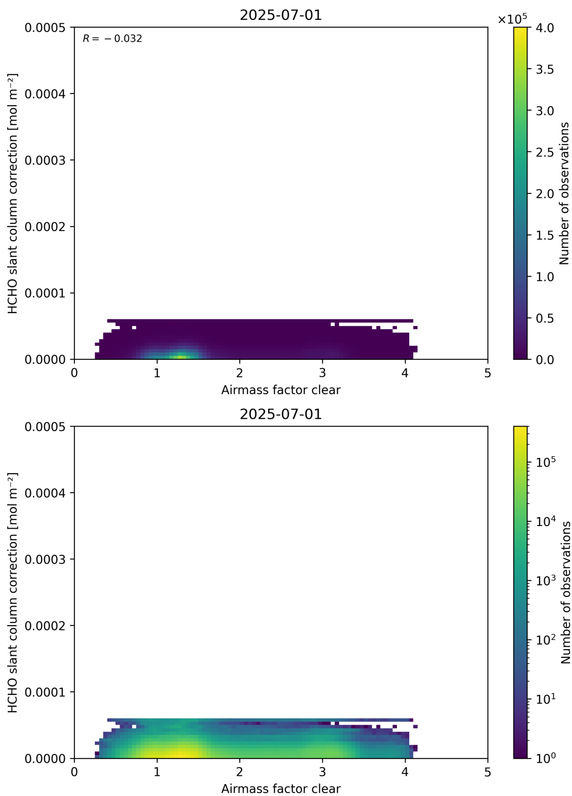
Figure 75: Scatter density plot of “Airmass factor clear” against “HCHO slant column correction” for 2025-06-30 to 2025-07-02.
