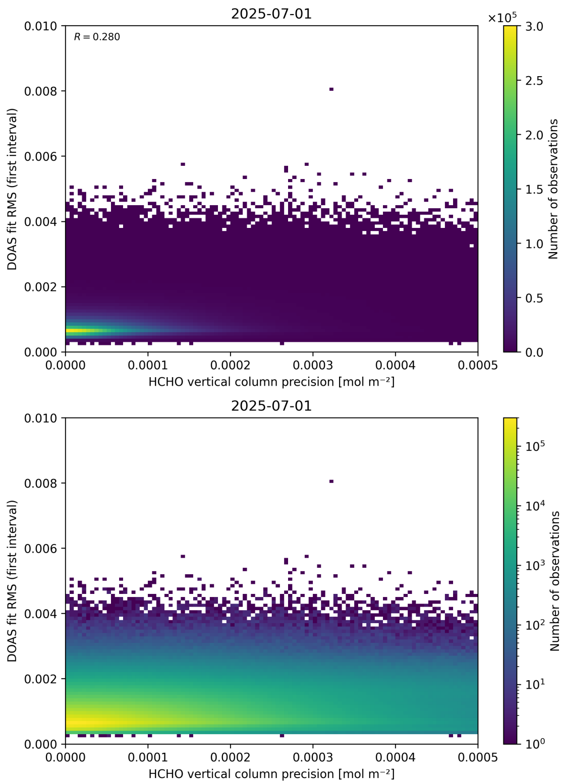
Figure 136: Scatter density plot of “HCHO vertical column precision” against “DOAS fit RMS (first interval)” for 2025-06-30 to 2025-07-02.
