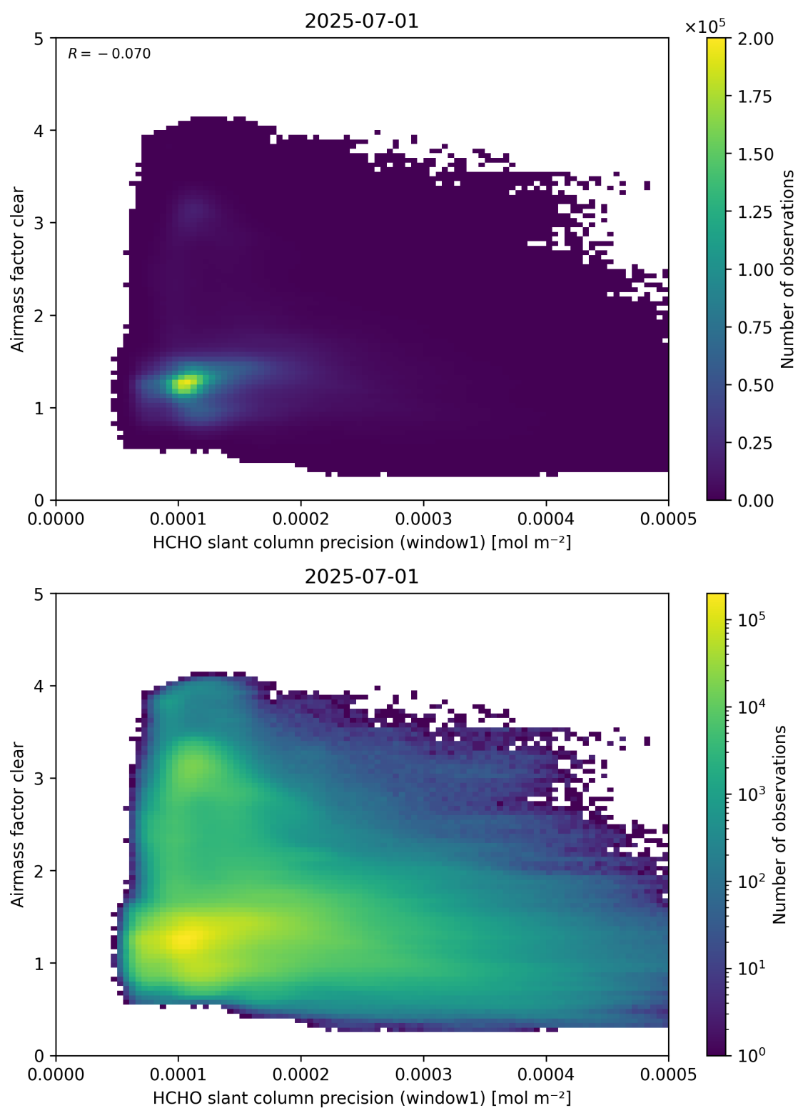
Figure 91: Scatter density plot of “HCHO slant column precision (window1)” against “Airmass factor clear” for 2025-06-30 to 2025-07-02.
