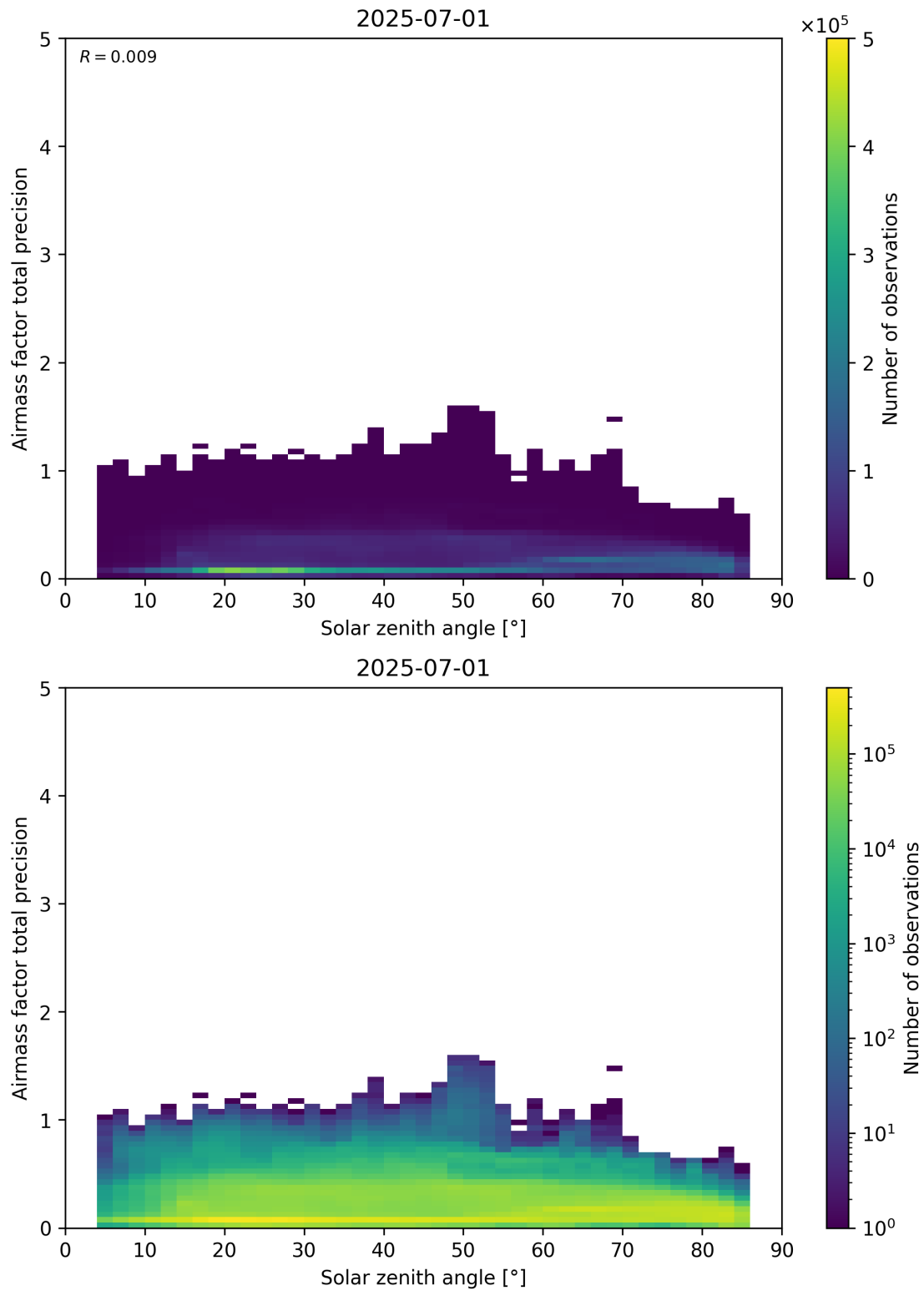
Figure 176: Scatter density plot of “Solar zenith angle” against “Airmass factor total precision” for 2025-06-30 to 2025-07-02.
