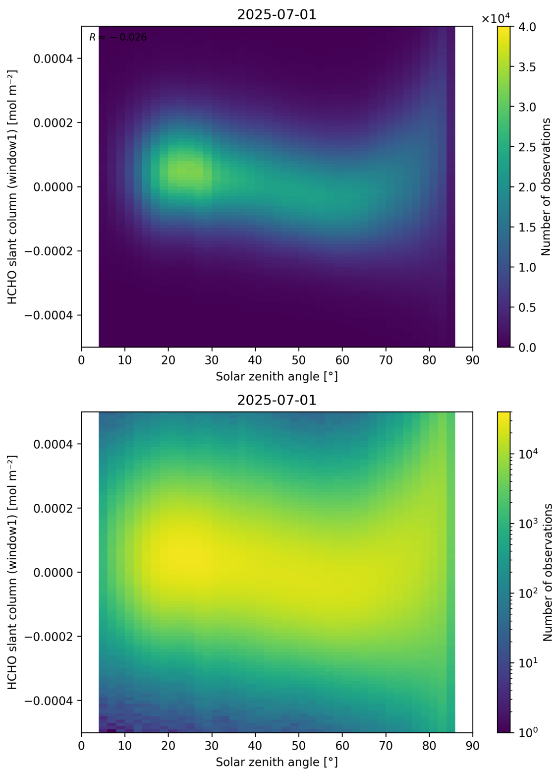
Figure 173: Scatter density plot of “Solar zenith angle” against “HCHO slant column (window1)” for 2025-06-30 to 2025-07-02.
