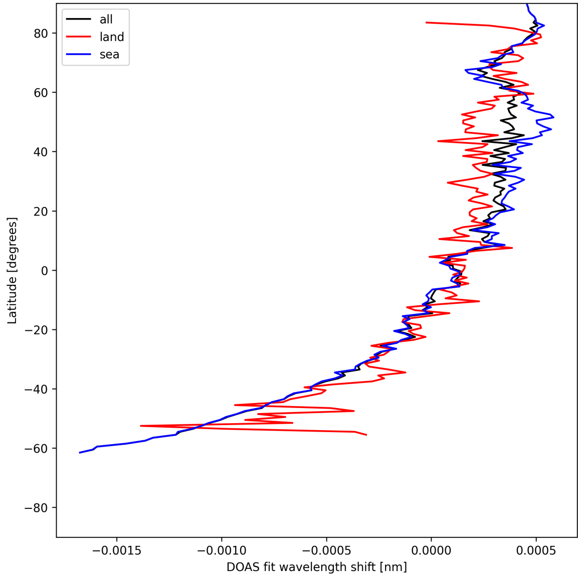
Figure 30: Zonal average of “DOAS fit wavelength shift” for 2025-06-30 to 2025-07-02.
