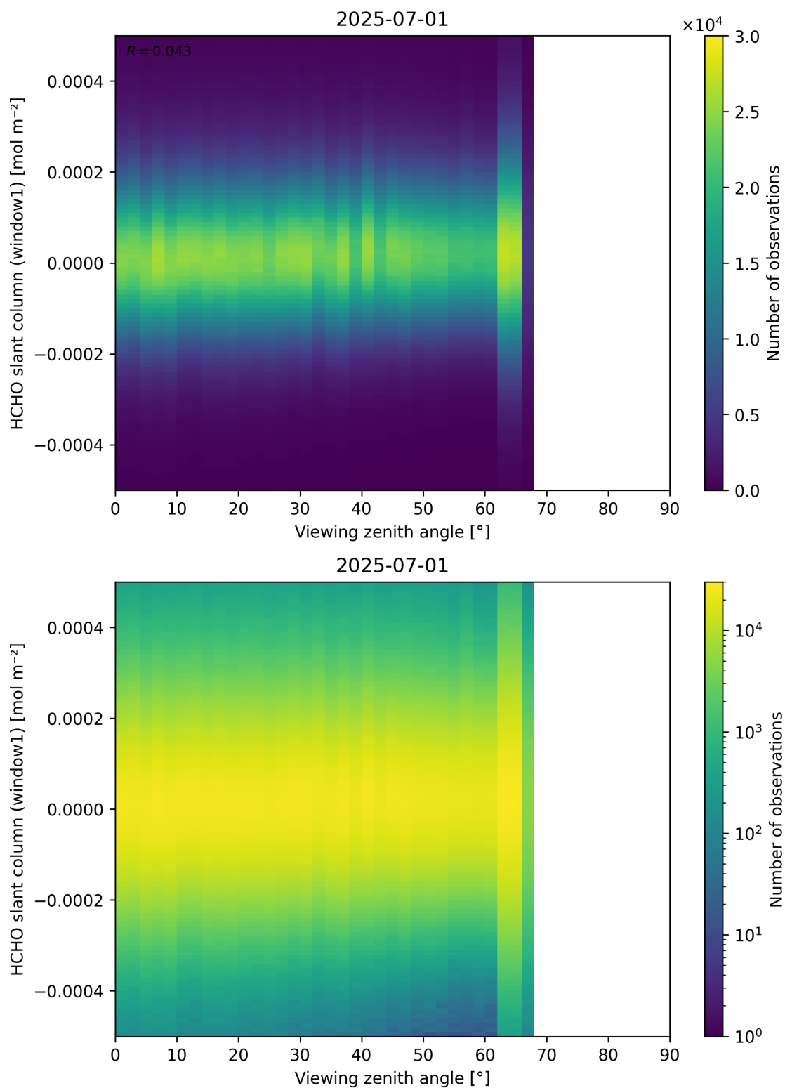
Figure 188: Scatter density plot of “Viewing zenith angle” against “HCHO slant column (window1)” for 2025-06-30 to 2025-07-02.
