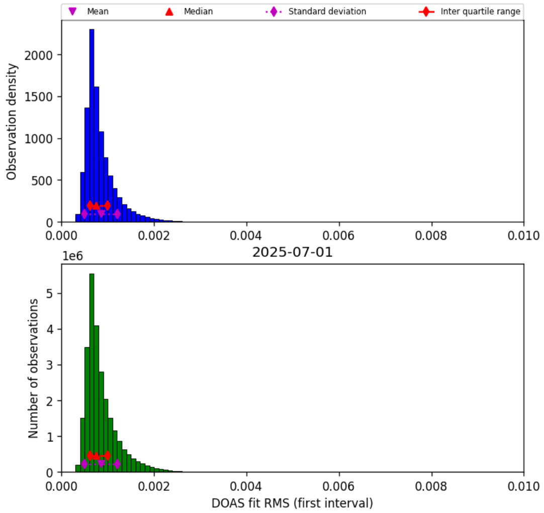
Figure 46: Histogram of “DOAS fit RMS (first interval)” for 2025-06-30 to 2025-07-02
