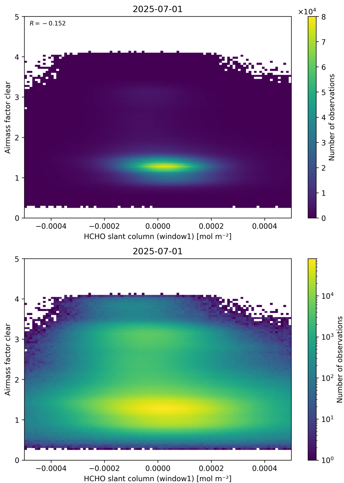
Figure 81: Scatter density plot of “HCHO slant column (window1)” against “Airmass factor clear” for 2025-06-30 to 2025-07-02.
