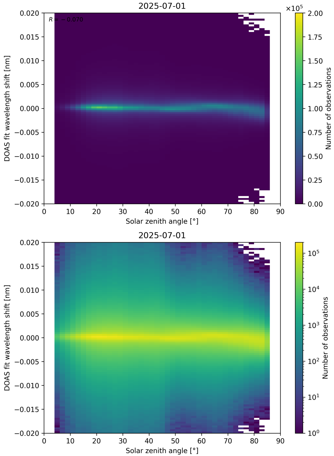
Figure 168: Scatter density plot of “Solar zenith angle” against “DOAS fit wavelength shift” for 2025-06-30 to 2025-07-02.
