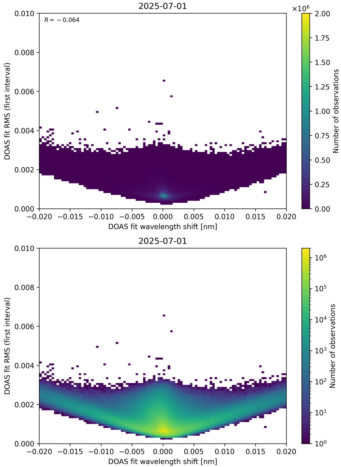
Figure 64: Scatter density plot of “DOAS fit wavelength shift” against “DOAS fit RMS (first interval)” for 2025-06-30 to 2025-07-02.
