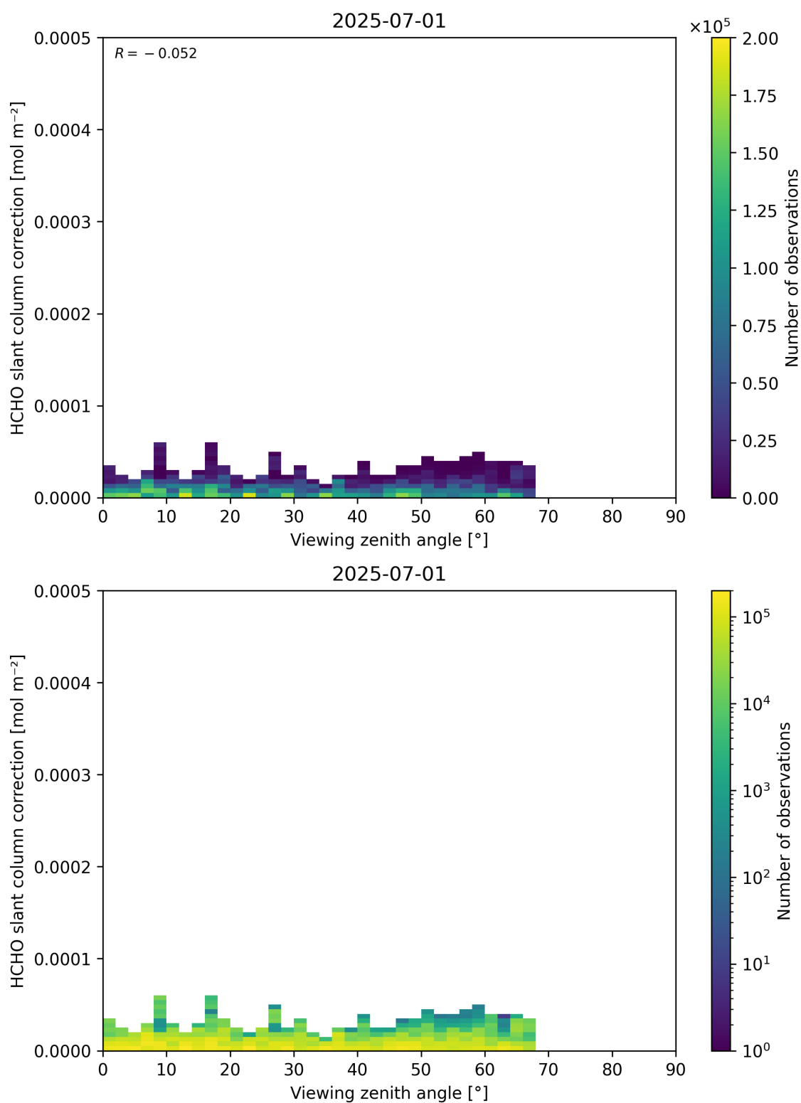
Figure 187: Scatter density plot of “Viewing zenith angle” against “HCHO slant column correction” for 2025-06-30 to 2025-07-02.
