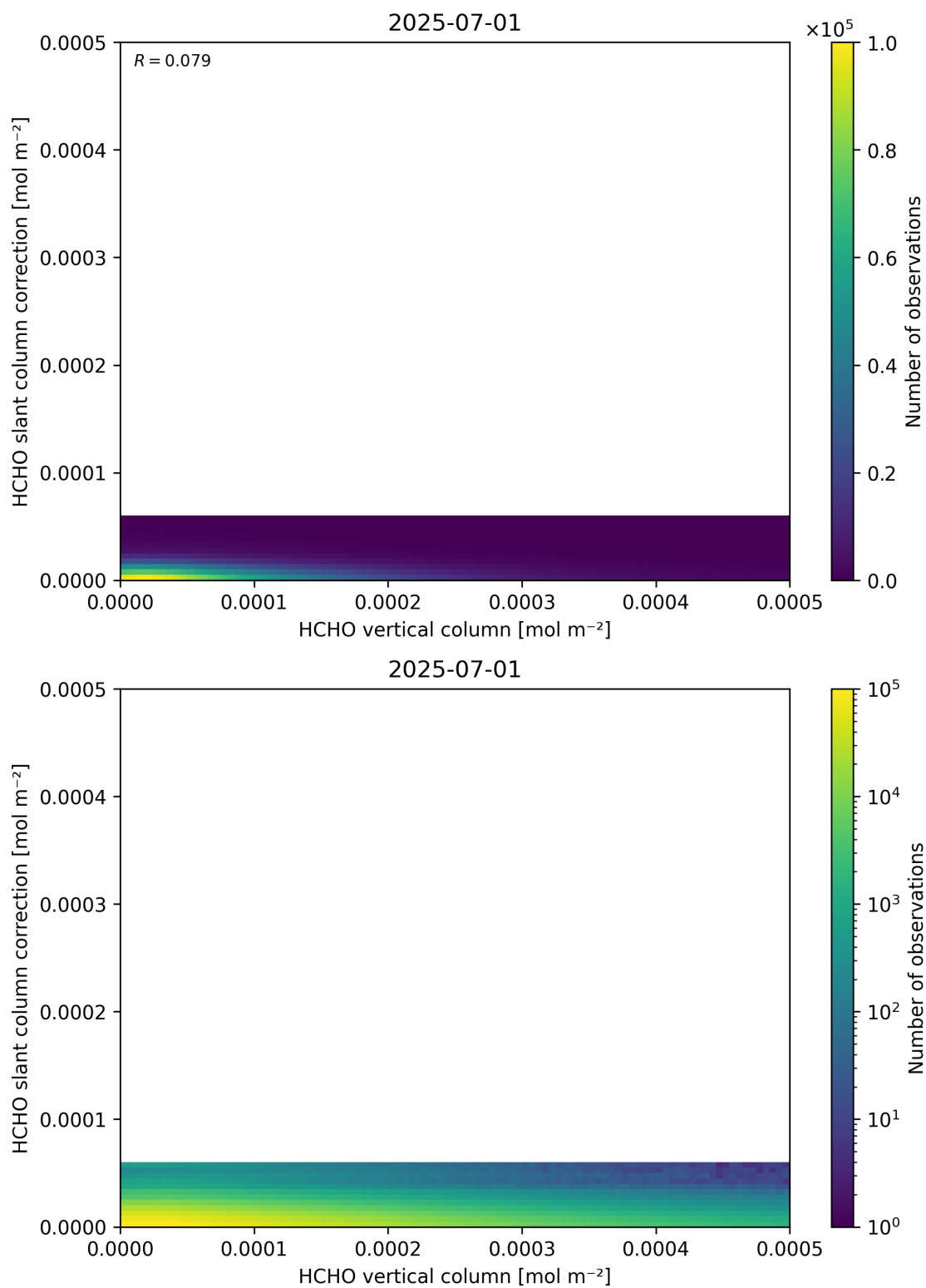
Figure 128: Scatter density plot of “HCHO vertical column” against “HCHO slant column correction” for 2025-06-30 to 2025-07-02.
