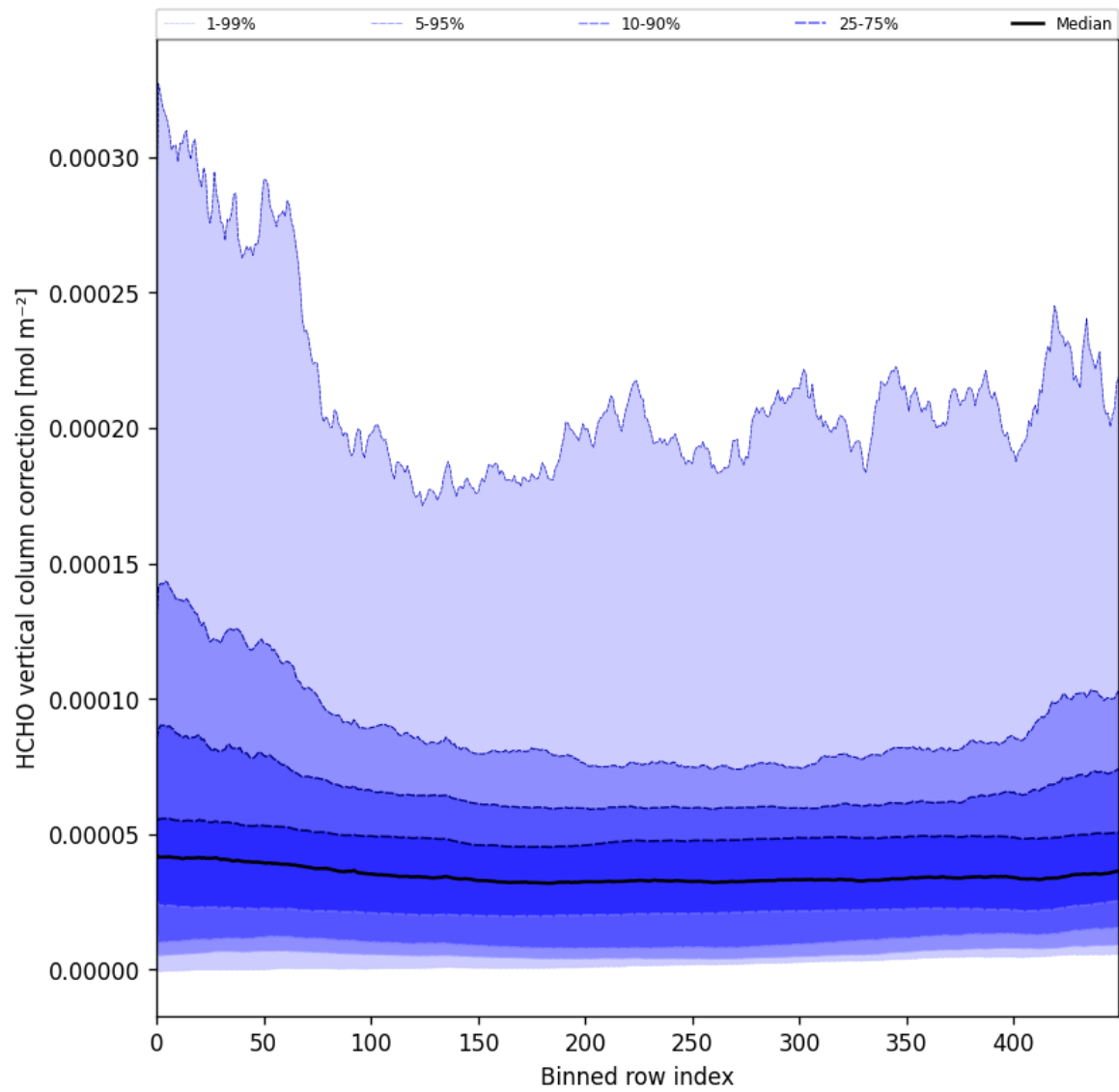
Figure 51: Along track statistics of “HCHO vertical column correction” for 2025-06-30 to 2025-07-02
