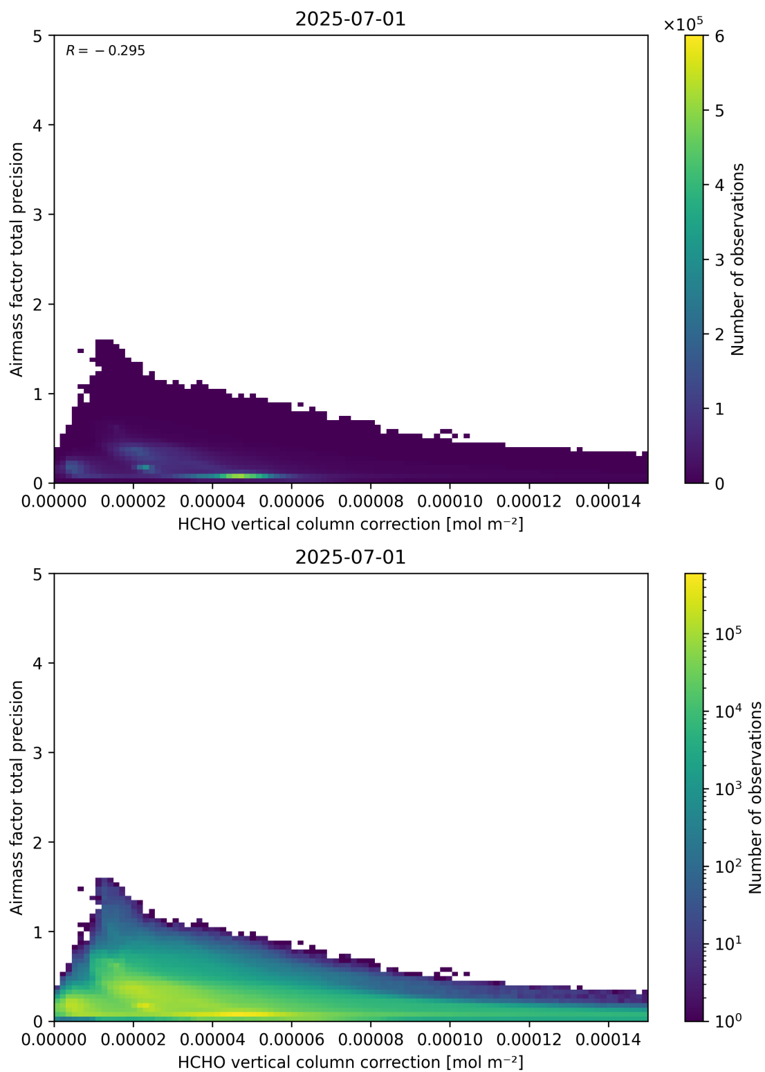
Figure 121: Scatter density plot of “HCHO vertical column correction” against “Airmass factor total precision” for 2025-06-30 to 2025-07-02.
