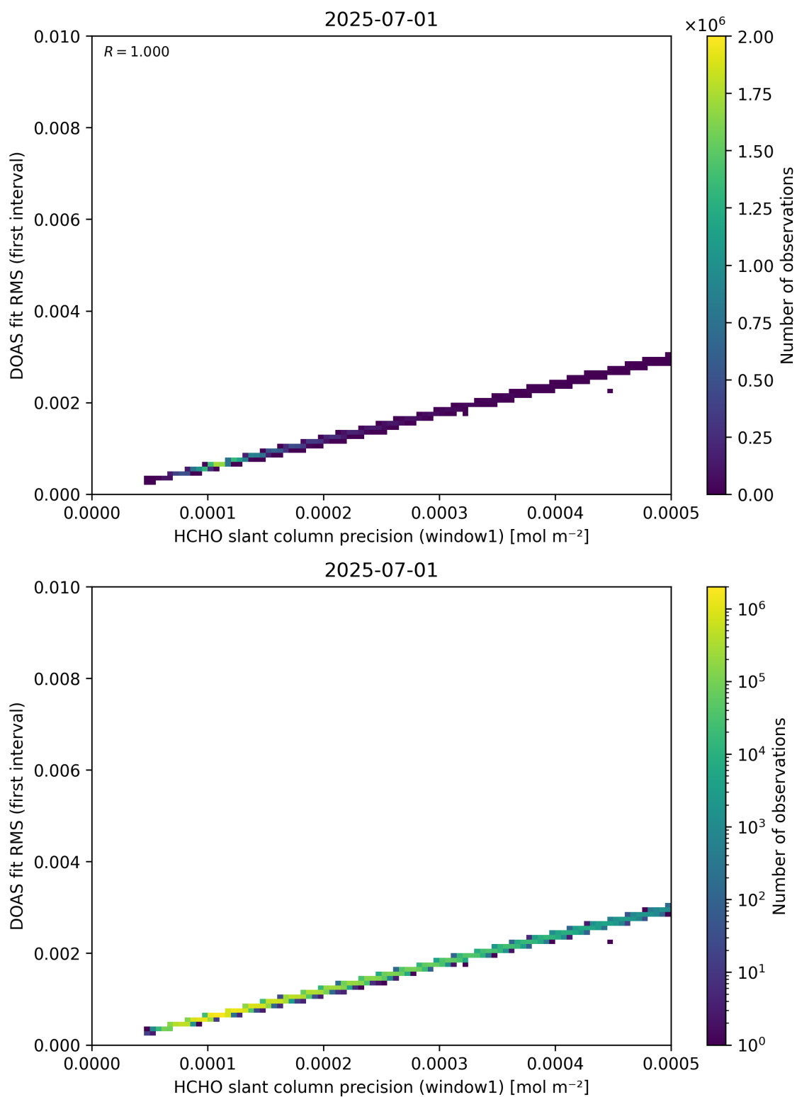
Figure 88: Scatter density plot of “HCHO slant column precision (window1)” against “DOAS fit RMS (first interval)” for 2025-06-30 to 2025-07-02.
