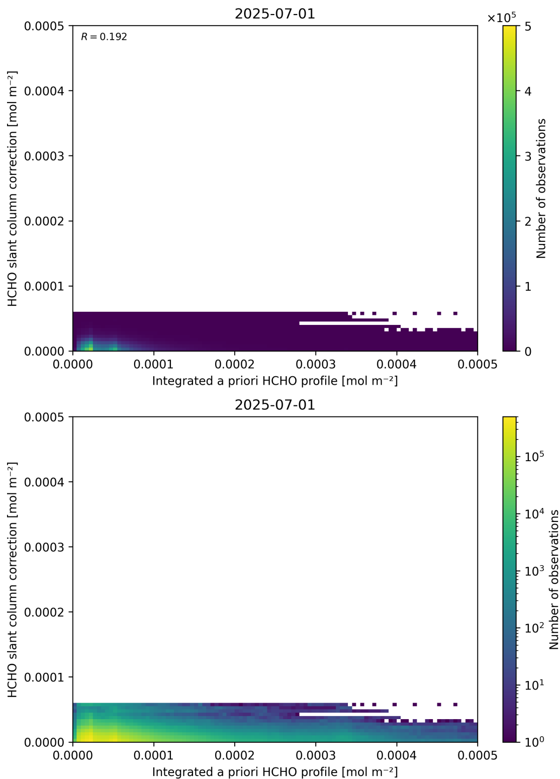
Figure 152: Scatter density plot of “Integrated a priori HCHO profile” against “HCHO slant column correction” for 2025-06-30 to 2025-07-02.
