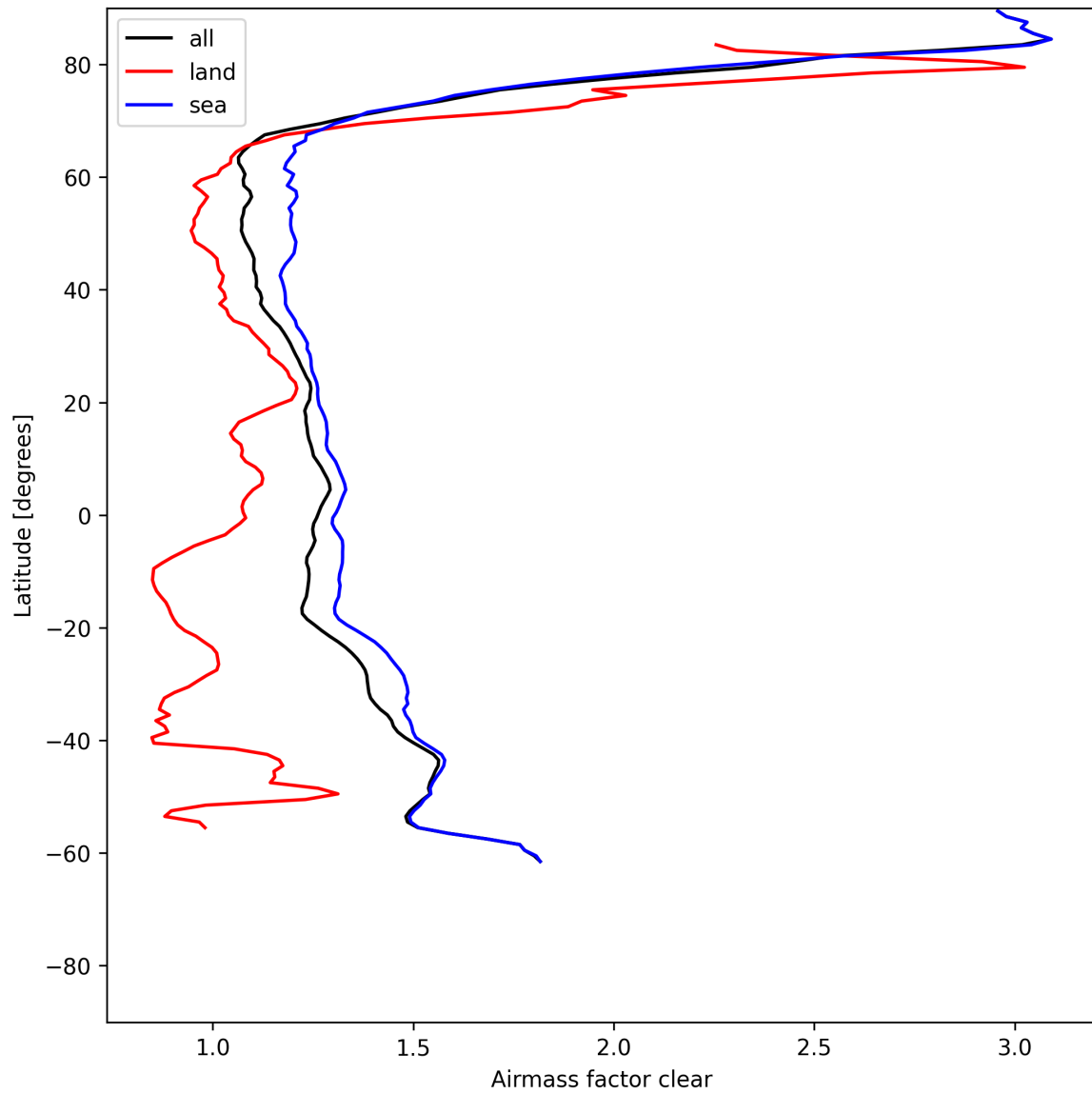
Figure 28: Zonal average of “Airmass factor clear” for 2025-06-30 to 2025-07-02.
