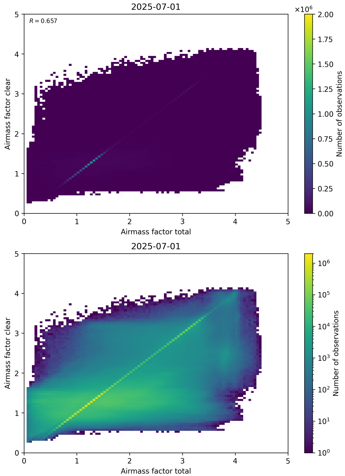
Figure 100: Scatter density plot of “Airmass factor total” against “Airmass factor clear” for 2025-06-30 to 2025-07-02.
