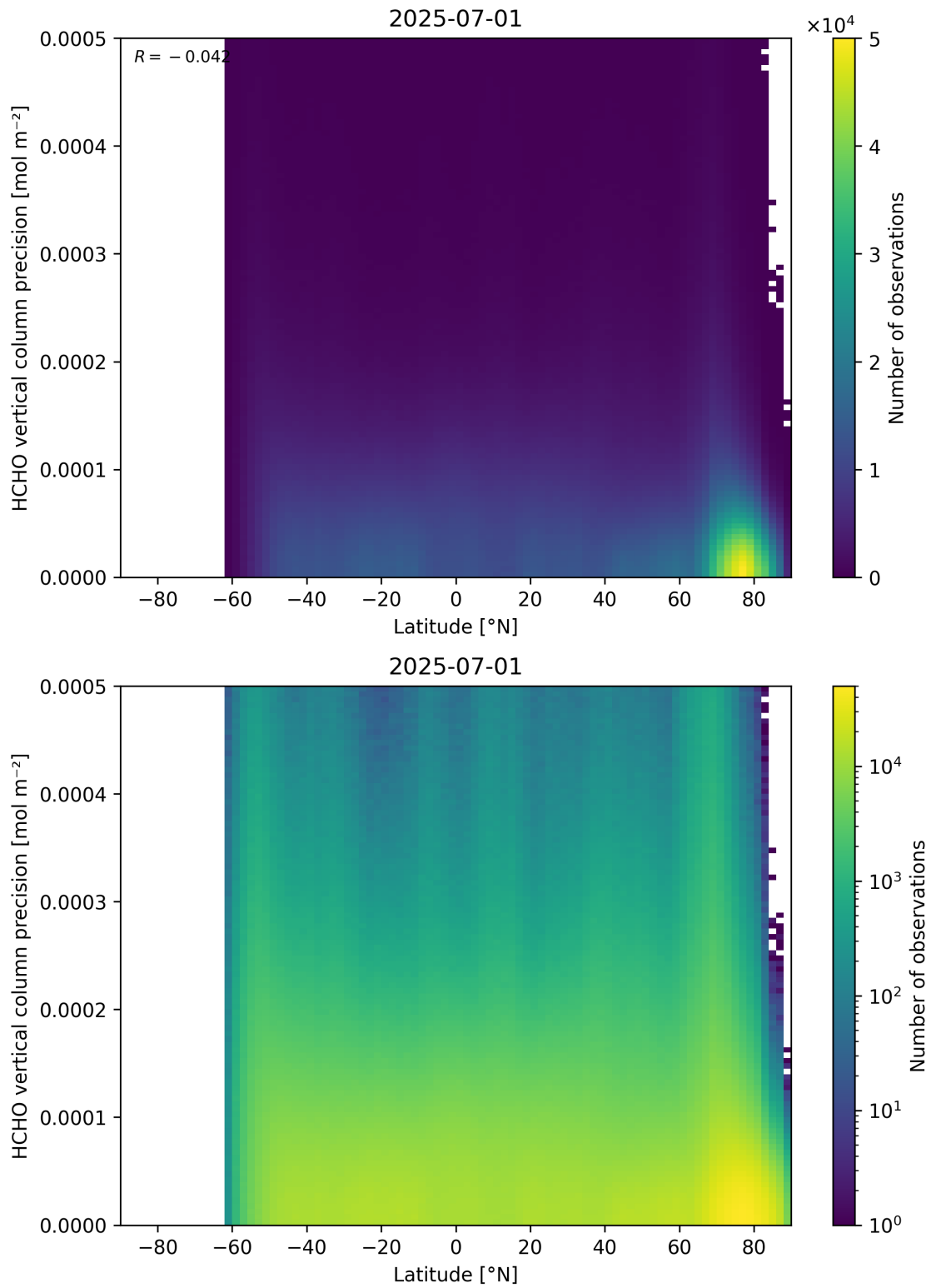
Figure 165: Scatter density plot of “Latitude” against “HCHO vertical column precision” for 2025-06-30 to 2025-07-02.
