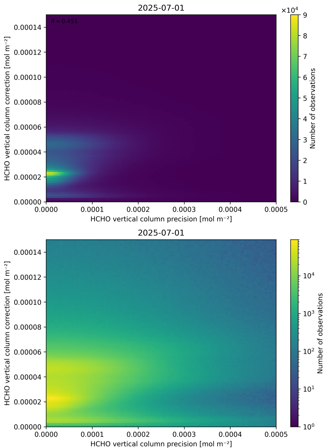
Figure 146: Scatter density plot of “HCHO vertical column precision” against “HCHO vertical column correction” for 2025-06-30 to 2025-07-02.
