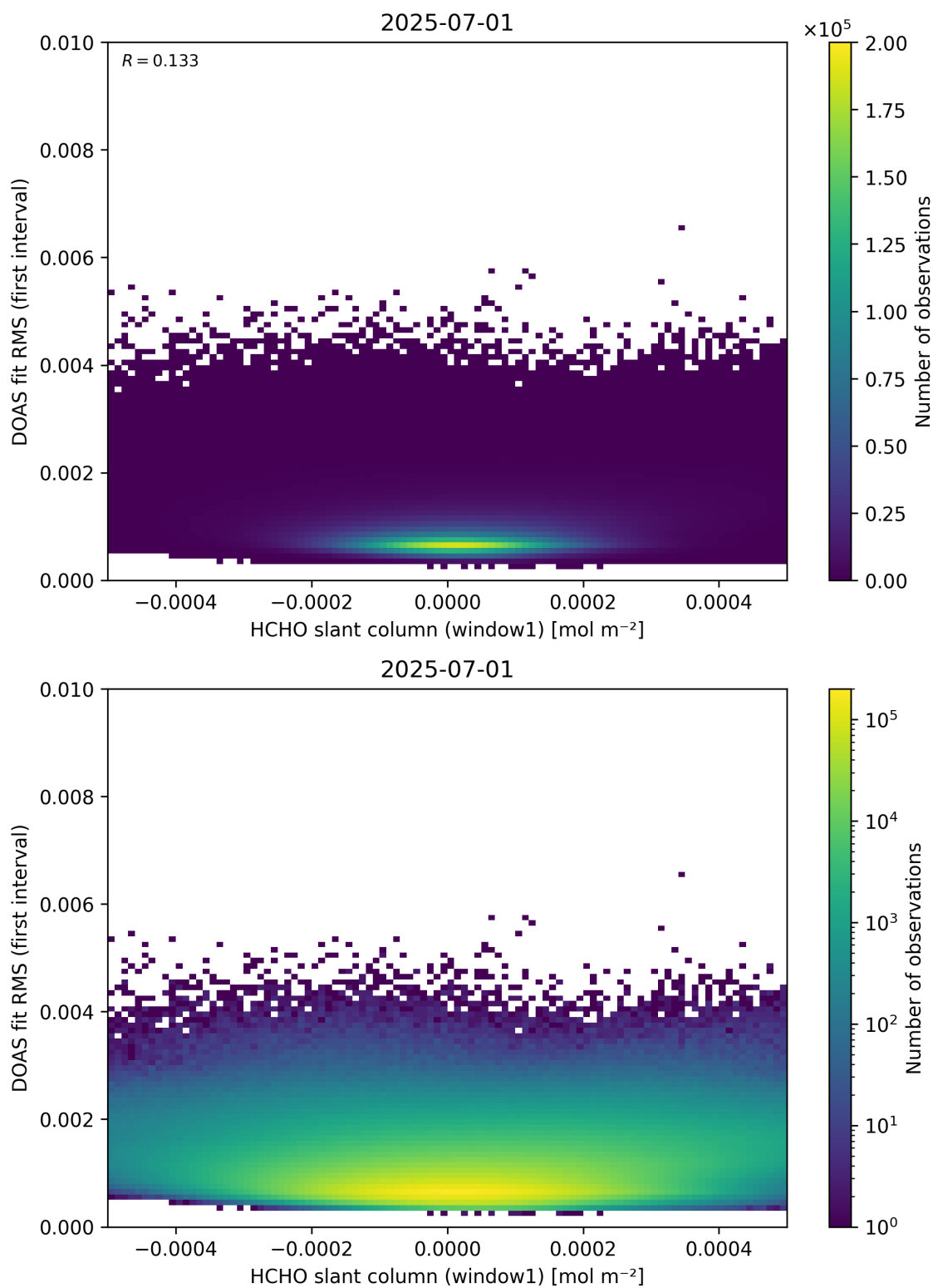
Figure 78: Scatter density plot of “HCHO slant column (window1)” against “DOAS fit RMS (first interval)” for 2025-06-30 to 2025-07-02.
