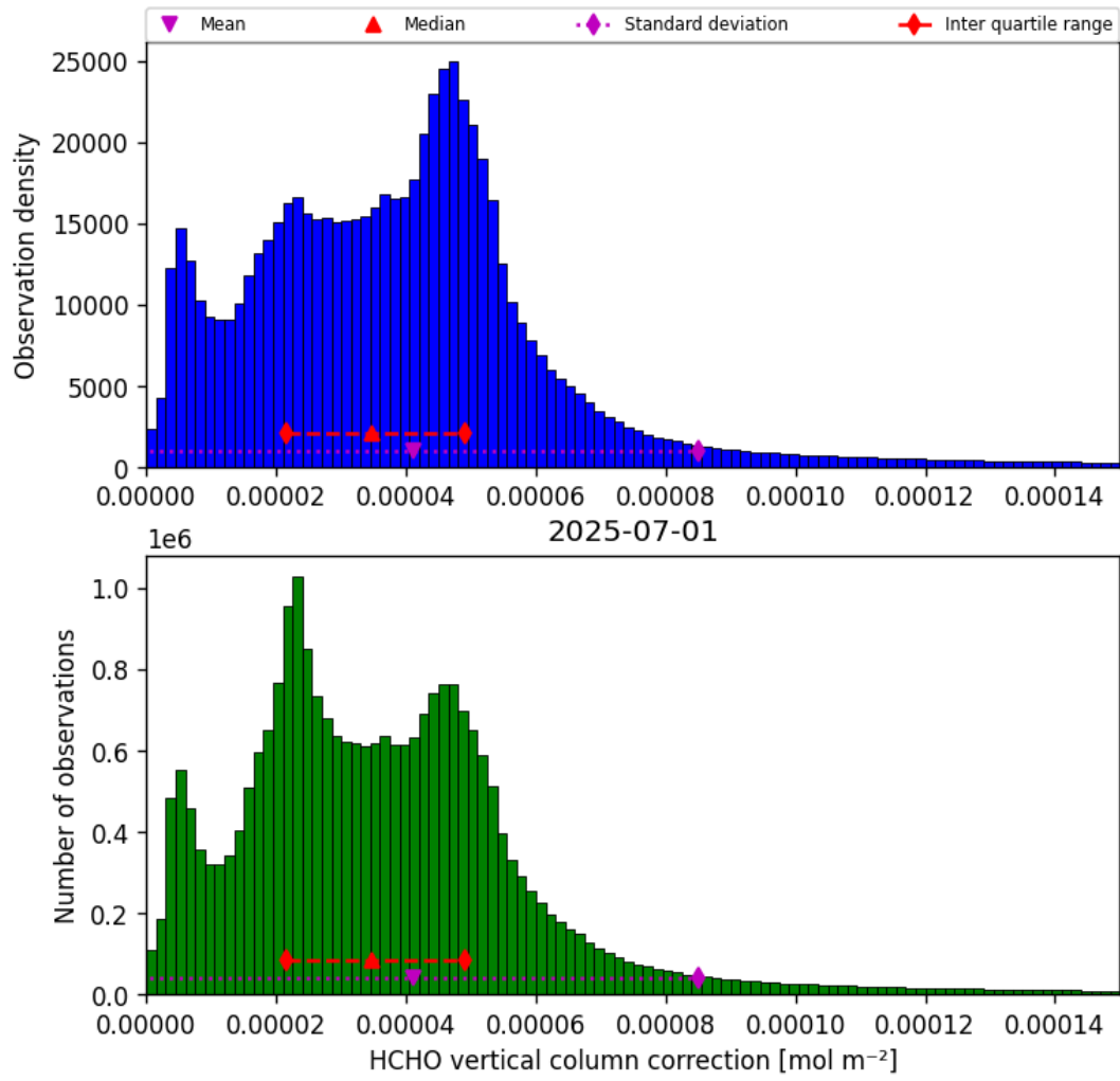
Figure 37: Histogram of “HCHO vertical column correction” for 2025-06-30 to 2025-07-02
