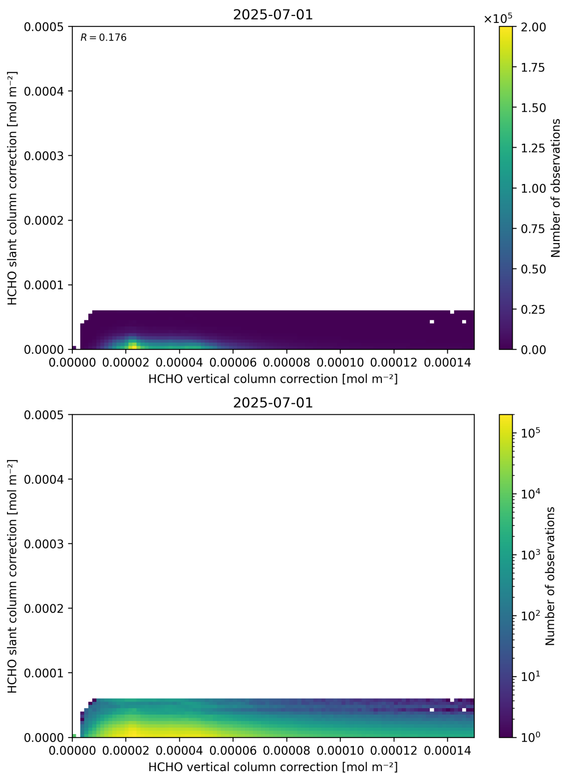
Figure 117: Scatter density plot of “HCHO vertical column correction” against “HCHO slant column correction” for 2025-06-30 to 2025-07-02.
