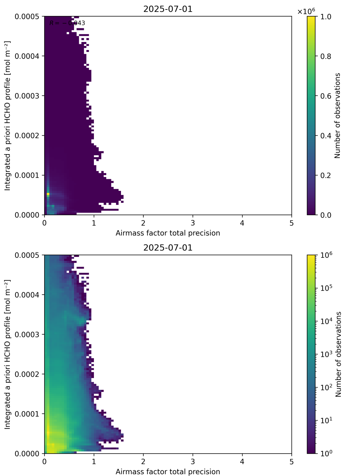
Figure 111: Scatter density plot of “Airmass factor total precision” against “Integrated a priori HCHO profile” for 2025-06-30 to 2025-07-02.
