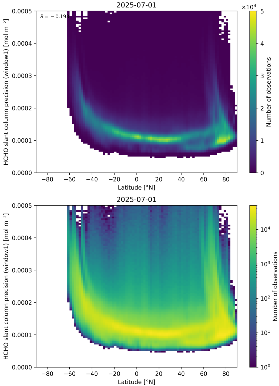
Figure 160: Scatter density plot of “Latitude” against “HCHO slant column precision (window1)” for 2025-06-30 to 2025-07-02.
