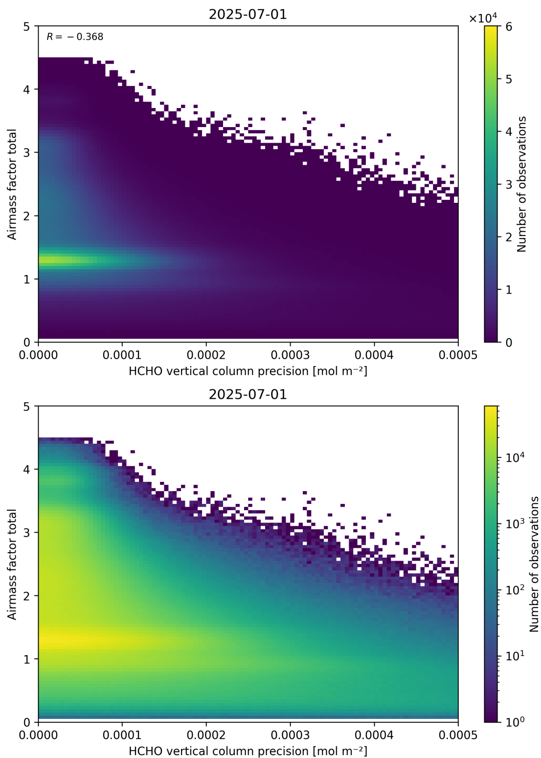
Figure 144: Scatter density plot of “HCHO vertical column precision” against “Airmass factor total” for 2025-06-30 to 2025-07-02.
