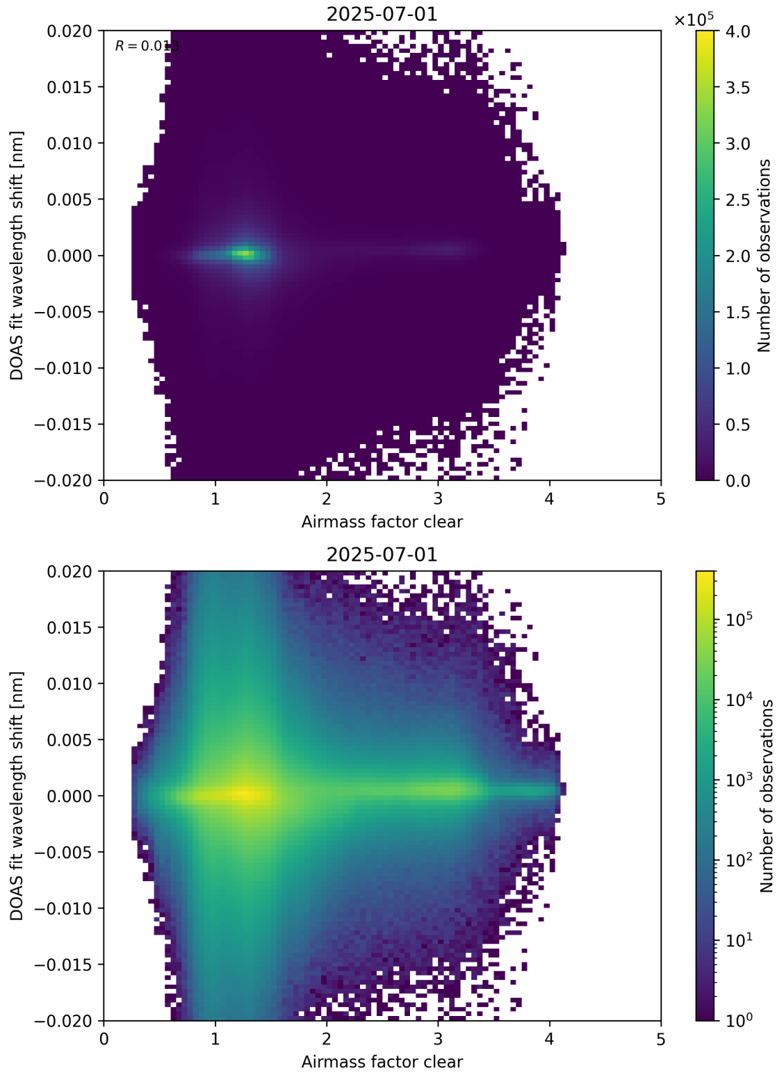
Figure 72: Scatter density plot of “Airmass factor clear” against “DOAS fit wavelength shift” for 2025-06-30 to 2025-07-02.
