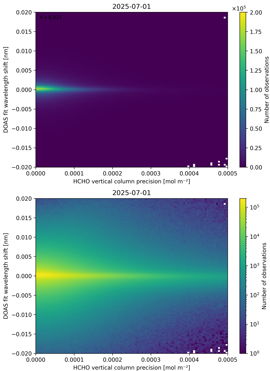
Figure 137: Scatter density plot of “HCHO vertical column precision” against “DOAS fit wavelength shift” for 2025-06-30 to 2025-07-02.
