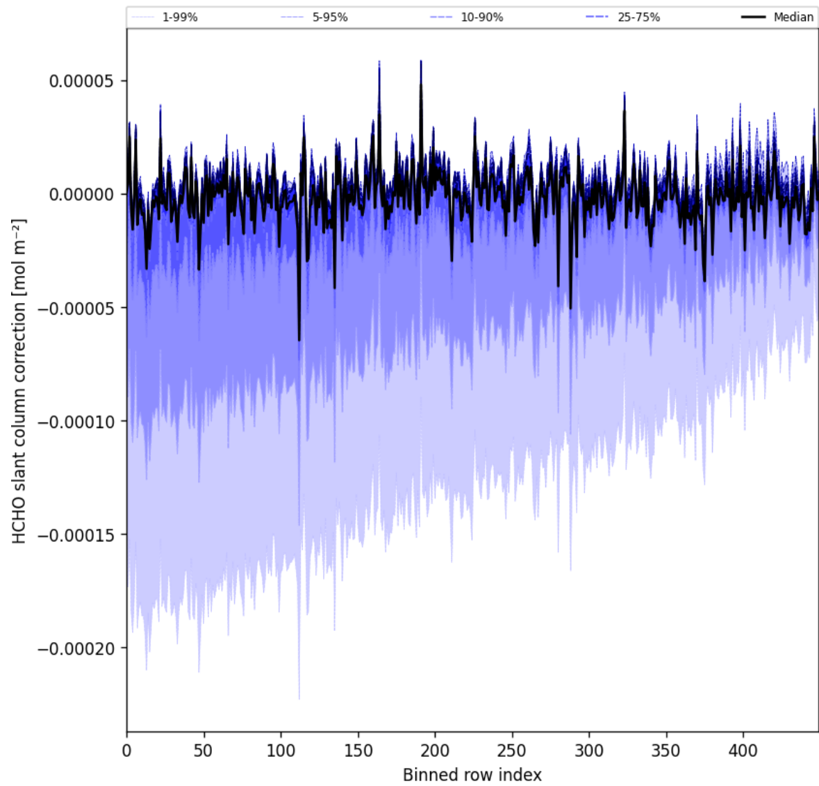
Figure 61: Along track statistics of “HCHO slant column correction” for 2025-06-30 to 2025-07-02
