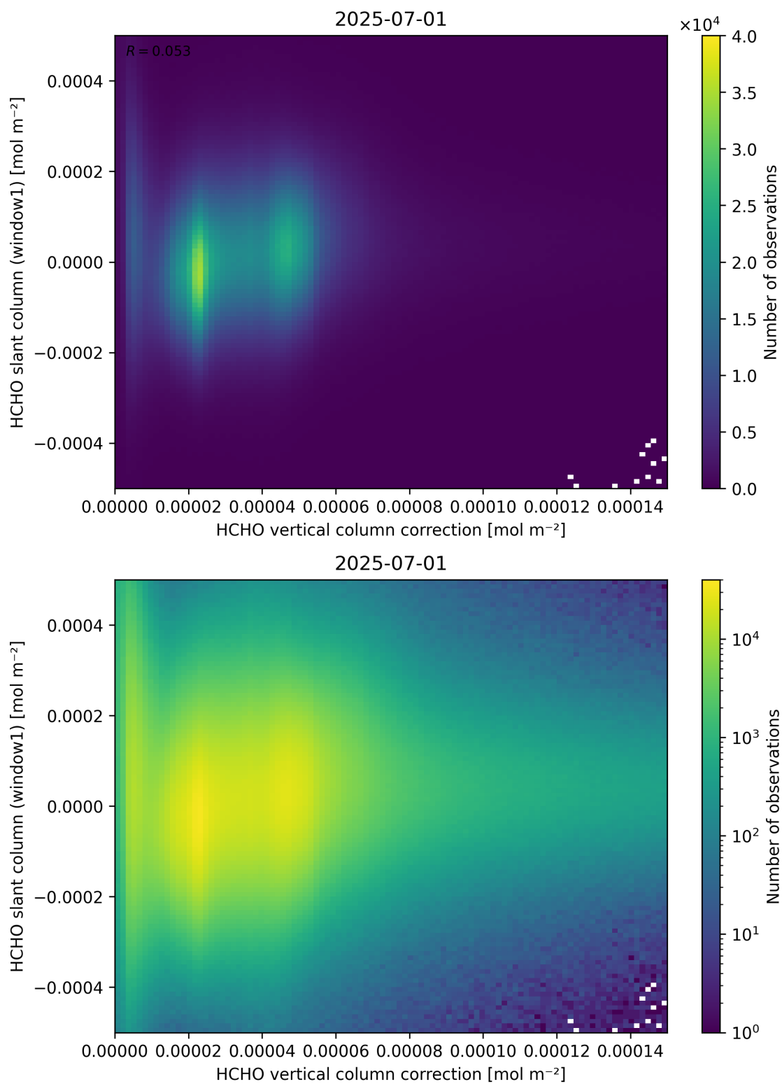
Figure 118: Scatter density plot of “HCHO vertical column correction” against “HCHO slant column (window1)” for 2025-06-30 to 2025-07-02.
