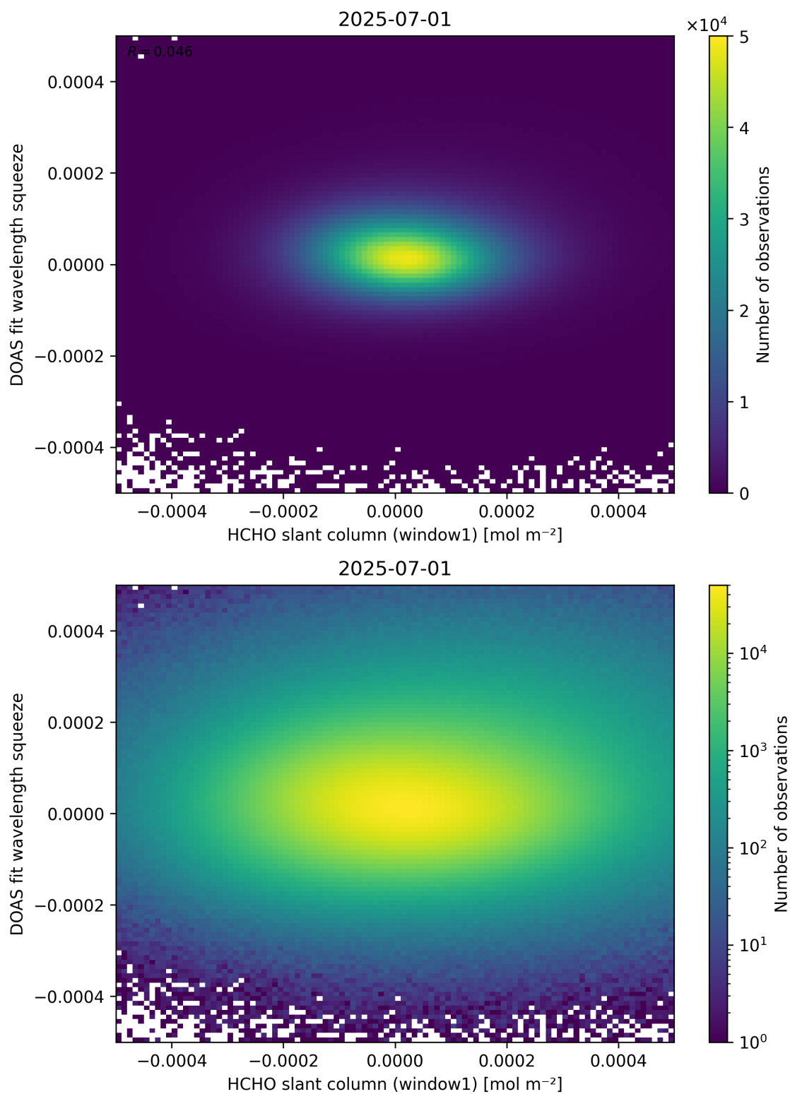
Figure 80: Scatter density plot of “HCHO slant column (window1)” against “DOAS fit wavelength squeeze” for 2025-06-30 to 2025-07-02.
