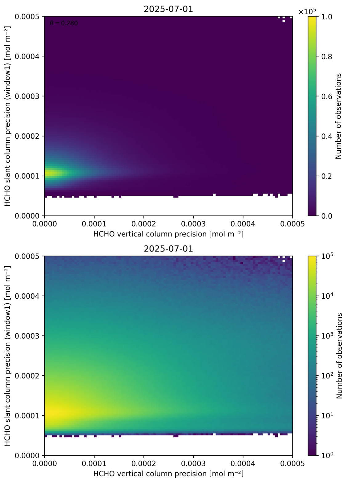
Figure 143: Scatter density plot of “HCHO vertical column precision” against “HCHO slant column precision (window1)” for 2025-06-30 to 2025-07-02.
