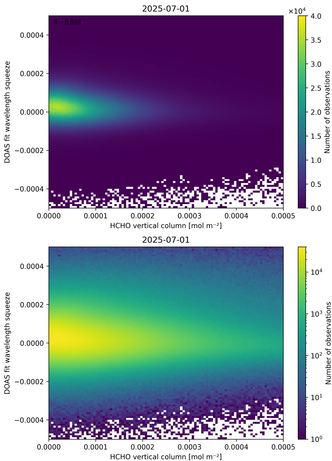
Figure 125: Scatter density plot of “HCHO vertical column” against “DOAS fit wavelength squeeze” for 2025-06-30 to 2025-07-02.
