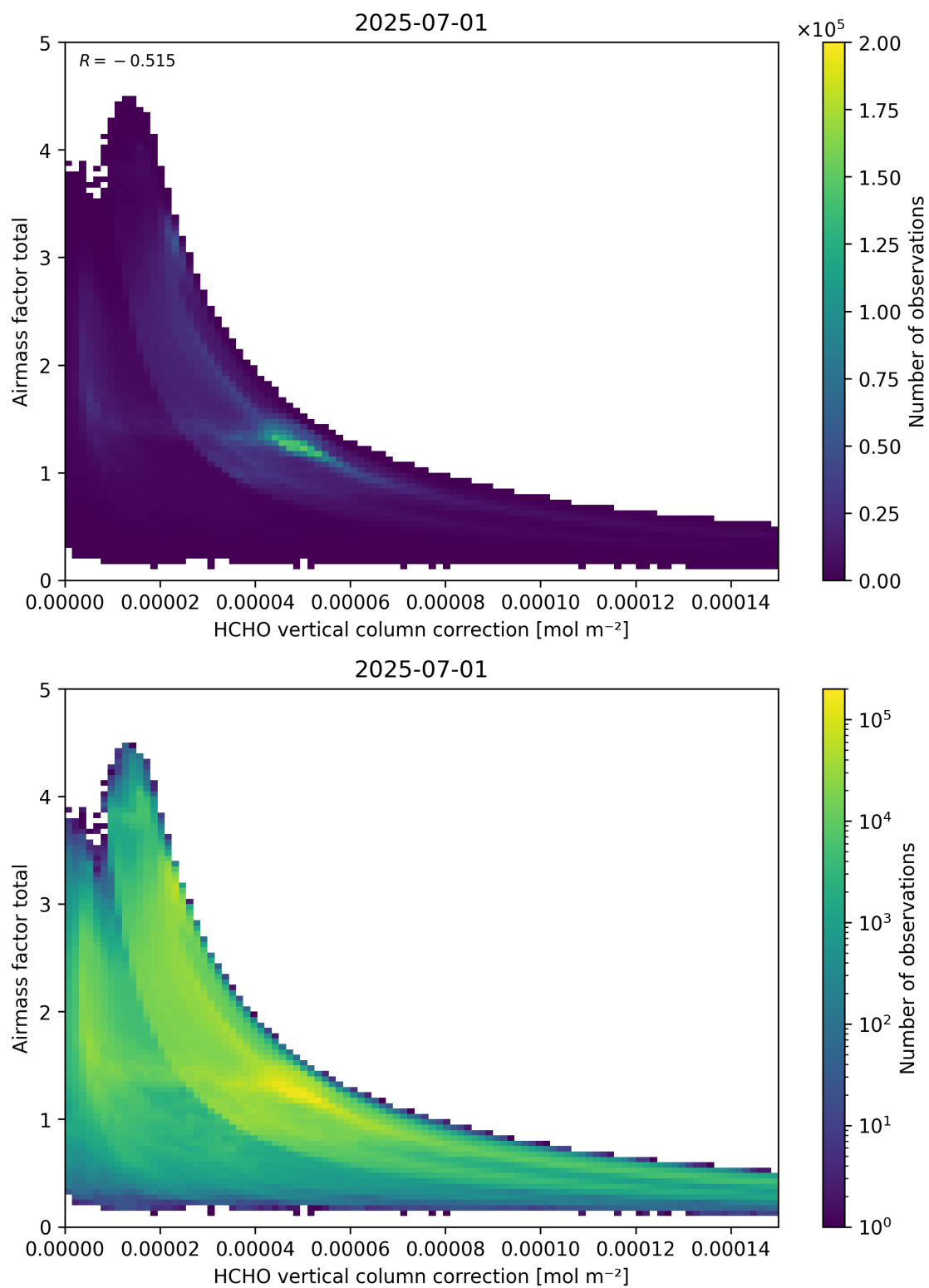
Figure 120: Scatter density plot of “HCHO vertical column correction” against “Airmass factor total” for 2025-06-30 to 2025-07-02.
