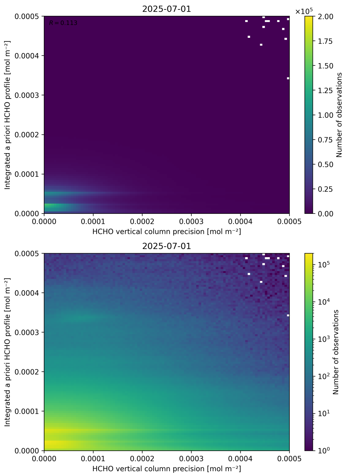
Figure 147: Scatter density plot of “HCHO vertical column precision” against “Integrated a priori HCHO profile” for 2025-06-30 to 2025-07-02.
