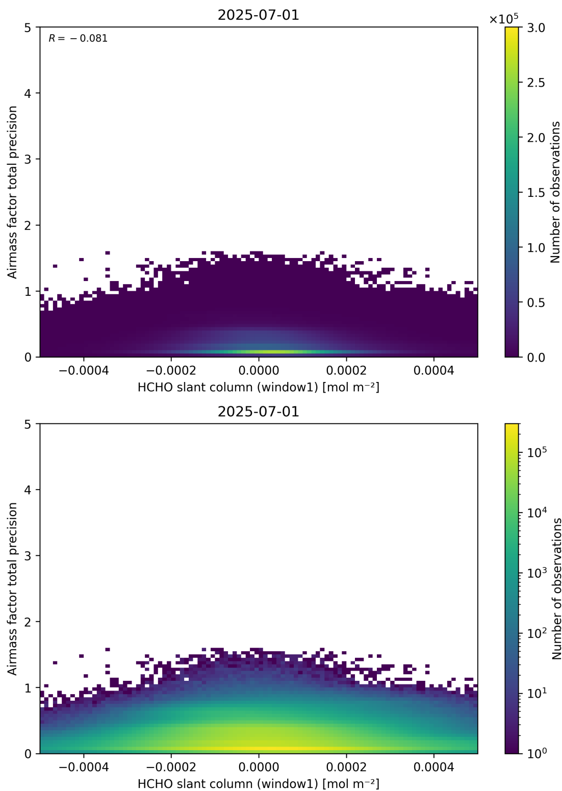
Figure 86: Scatter density plot of “HCHO slant column (window1)” against “Airmass factor total precision” for 2025-06-30 to 2025-07-02.
