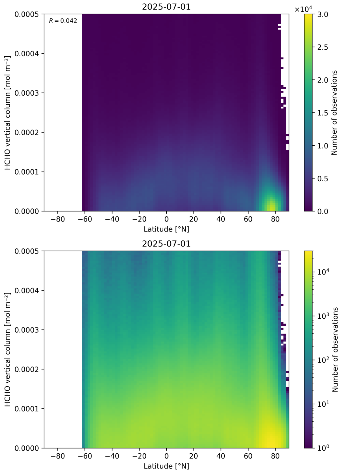
Figure 163: Scatter density plot of “Latitude” against “HCHO vertical column” for 2025-06-30 to 2025-07-02.
