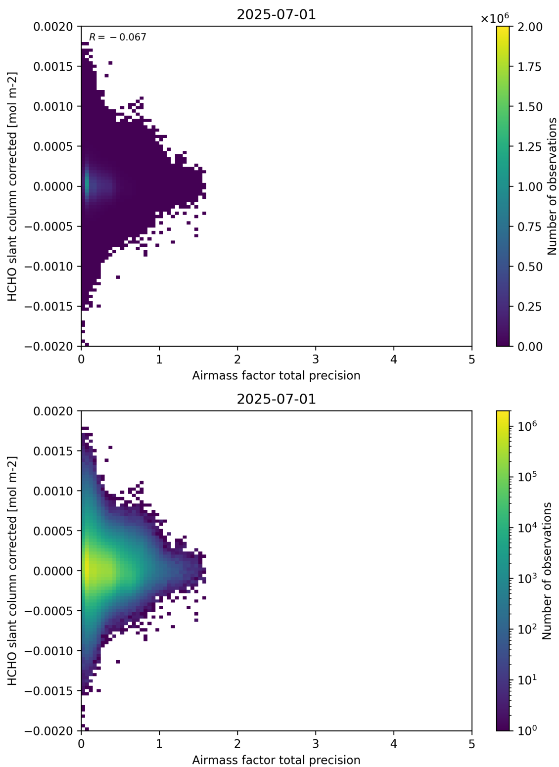
Figure 109: Scatter density plot of “Airmass factor total precision” against “HCHO slant column corrected” for 2025-06-30 to 2025-07-02.
