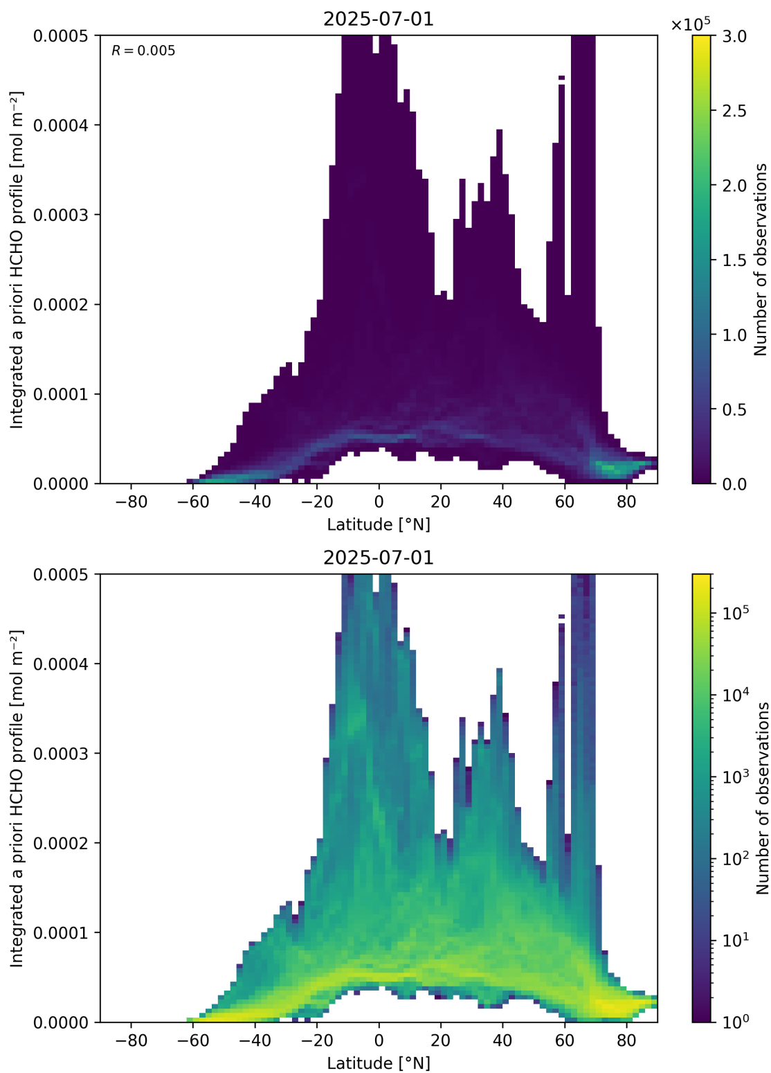
Figure 166: Scatter density plot of “Latitude” against “Integrated a priori HCHO profile” for 2025-06-30 to 2025-07-02.
