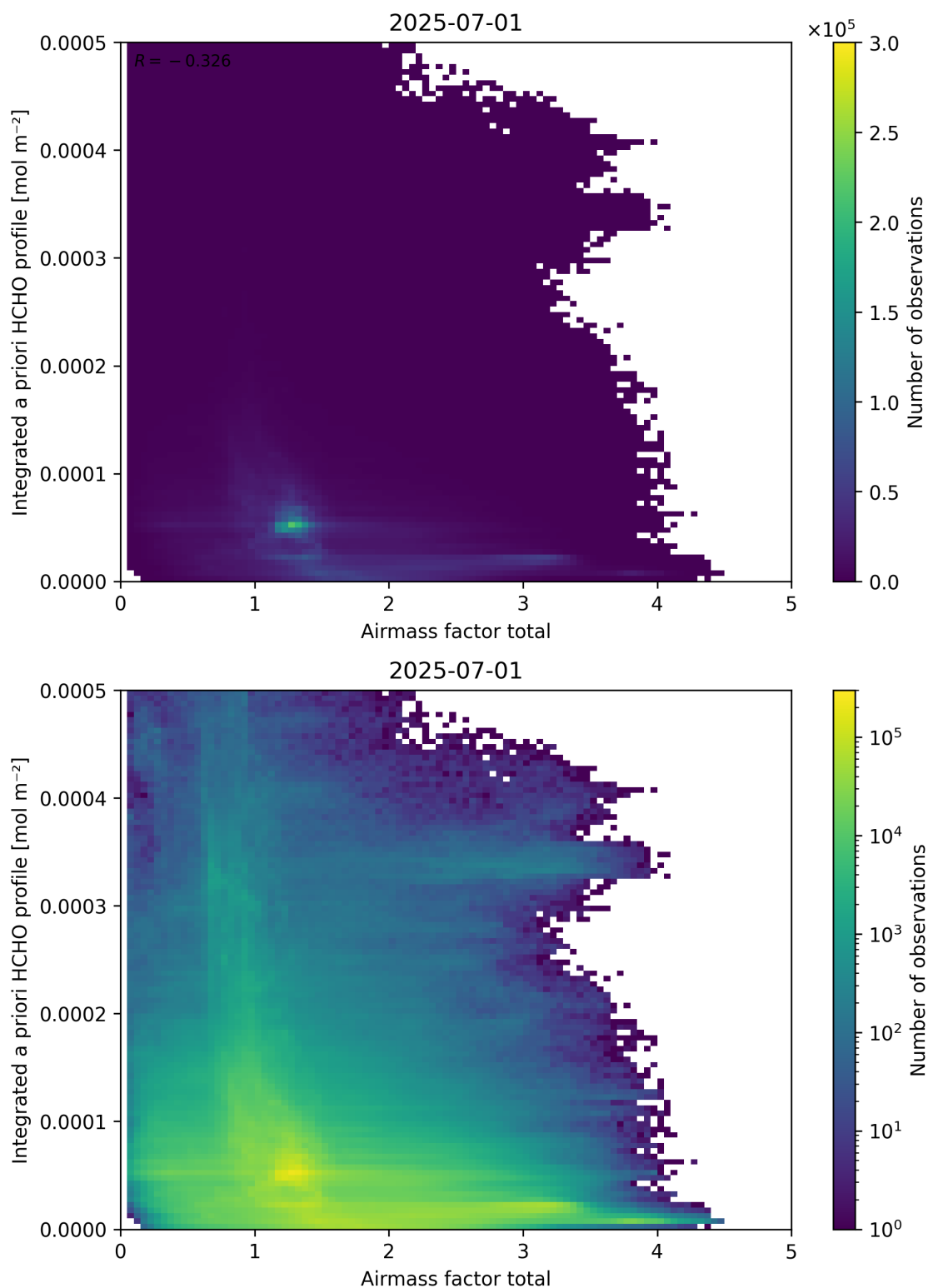
Figure 104: Scatter density plot of “Airmass factor total” against “Integrated a priori HCHO profile” for 2025-06-30 to 2025-07-02.
