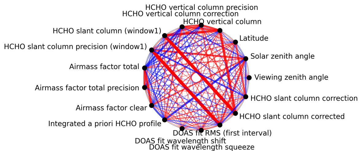
Figure 1: Map of correlation graph for 2025-06-30 to 2025-07-02.
