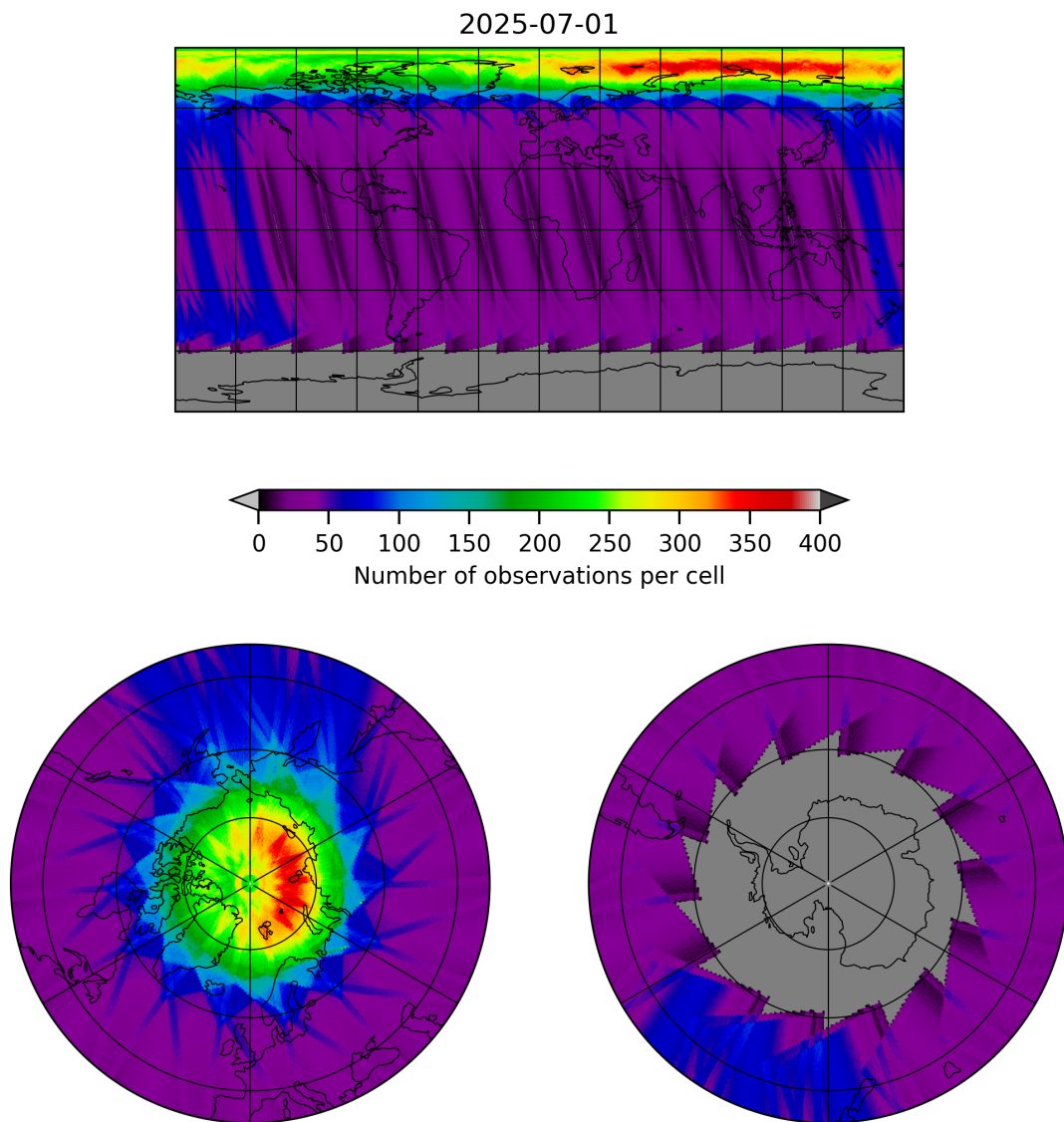
Figure 19: Map of the number of observations for 2025-06-30 to 2025-07-02
