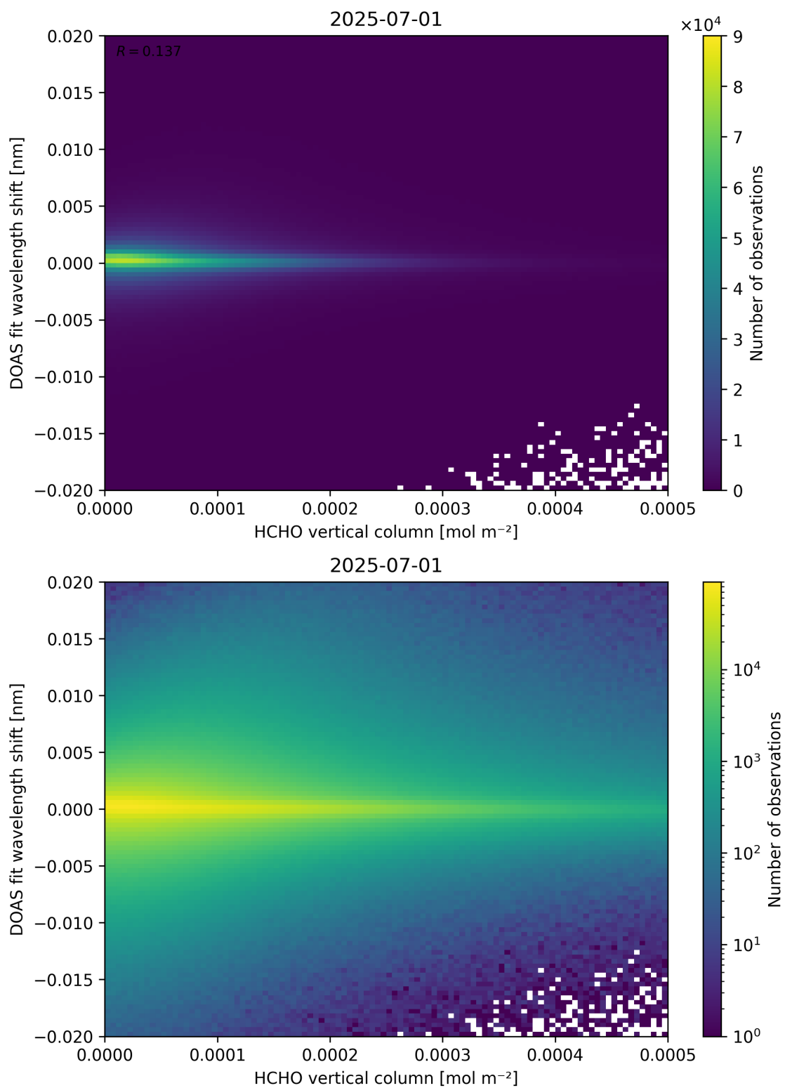
Figure 124: Scatter density plot of “HCHO vertical column” against “DOAS fit wavelength shift” for 2025-06-30 to 2025-07-02.
