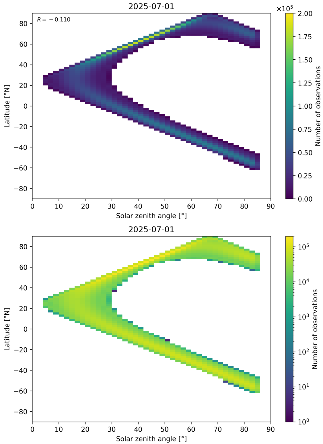
Figure 181: Scatter density plot of “Solar zenith angle” against “Latitude” for 2025-06-30 to 2025-07-02.
