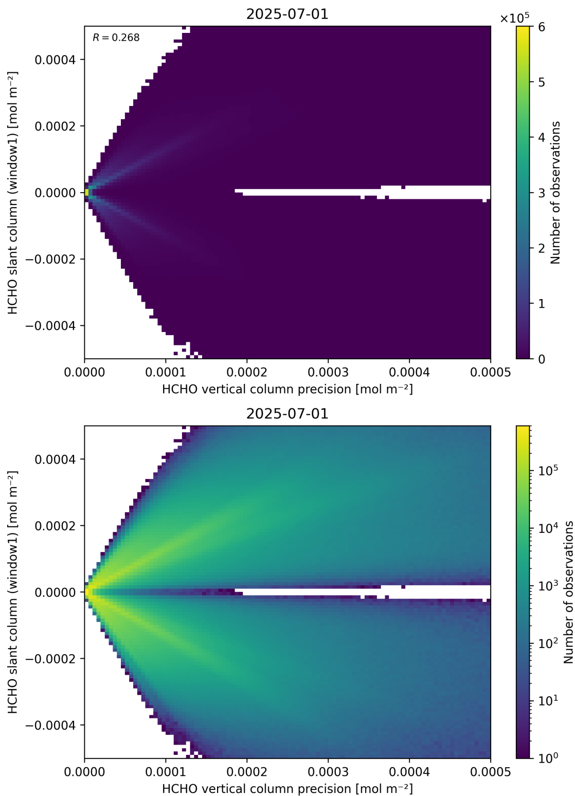
Figure 142: Scatter density plot of “HCHO vertical column precision” against “HCHO slant column (window1)” for 2025-06-30 to 2025-07-02.
