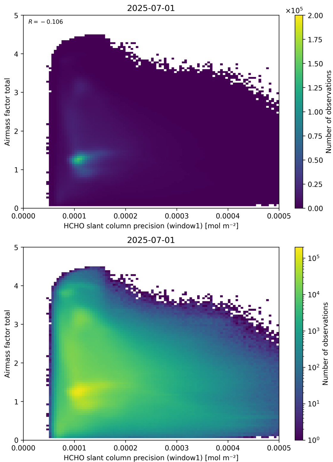
Figure 94: Scatter density plot of “HCHO slant column precision (window1)” against “Airmass factor total” for 2025-06-30 to 2025-07-02.
