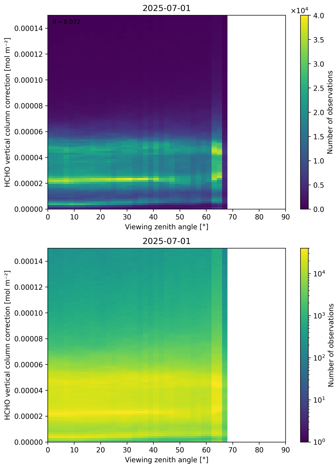
Figure 193: Scatter density plot of “Viewing zenith angle” against “HCHO vertical column correction” for 2025-06-30 to 2025-07-02.
