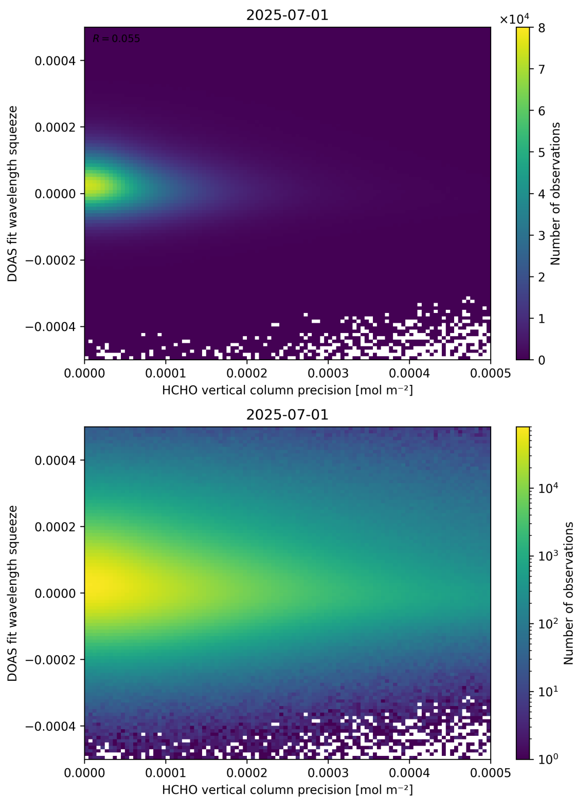
Figure 138: Scatter density plot of “HCHO vertical column precision” against “DOAS fit wavelength squeeze” for 2025-06-30 to 2025-07-02.
