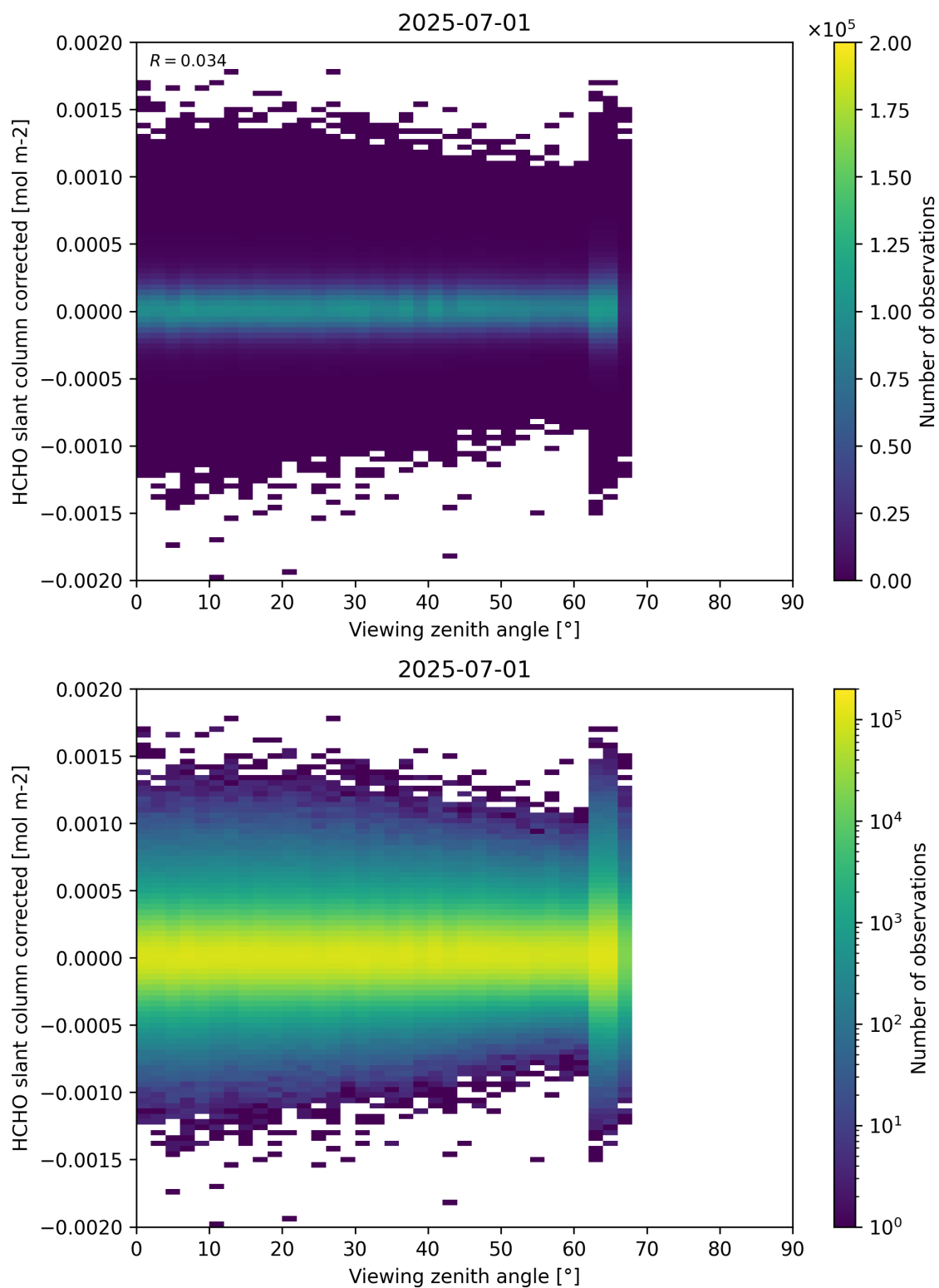
Figure 186: Scatter density plot of “Viewing zenith angle” against “HCHO slant column corrected” for 2025-06-30 to 2025-07-02.
