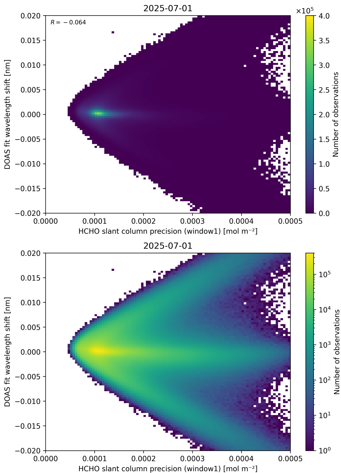
Figure 89: Scatter density plot of “HCHO slant column precision (window1)” against “DOAS fit wavelength shift” for 2025-06-30 to 2025-07-02.
