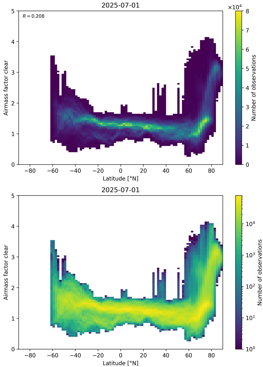
Figure 156: Scatter density plot of “Latitude” against “Airmass factor clear” for 2025-06-30 to 2025-07-02.
