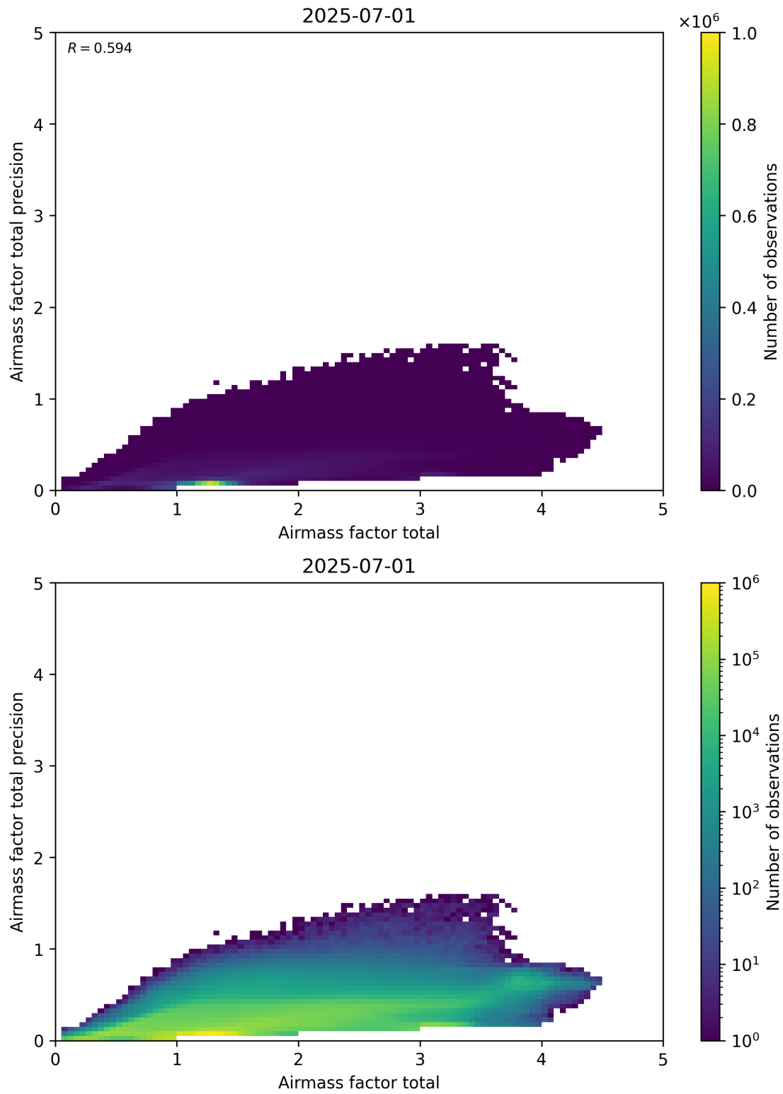
Figure 103: Scatter density plot of “Airmass factor total” against “Airmass factor total precision” for 2025-06-30 to 2025-07-02.
