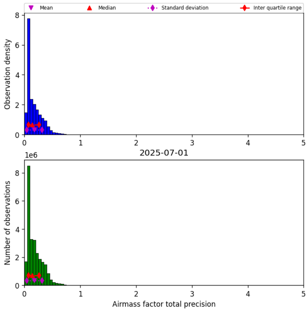
Figure 41: Histogram of “Airmass factor total precision” for 2025-06-30 to 2025-07-02
