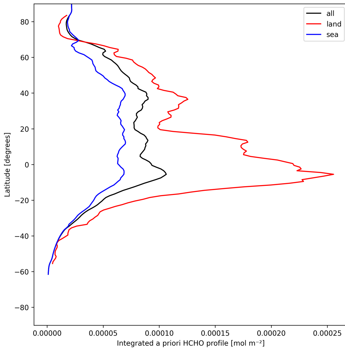
Figure 29: Zonal average of “Integrated a priori HCHO profile” for 2025-06-30 to 2025-07-02.
