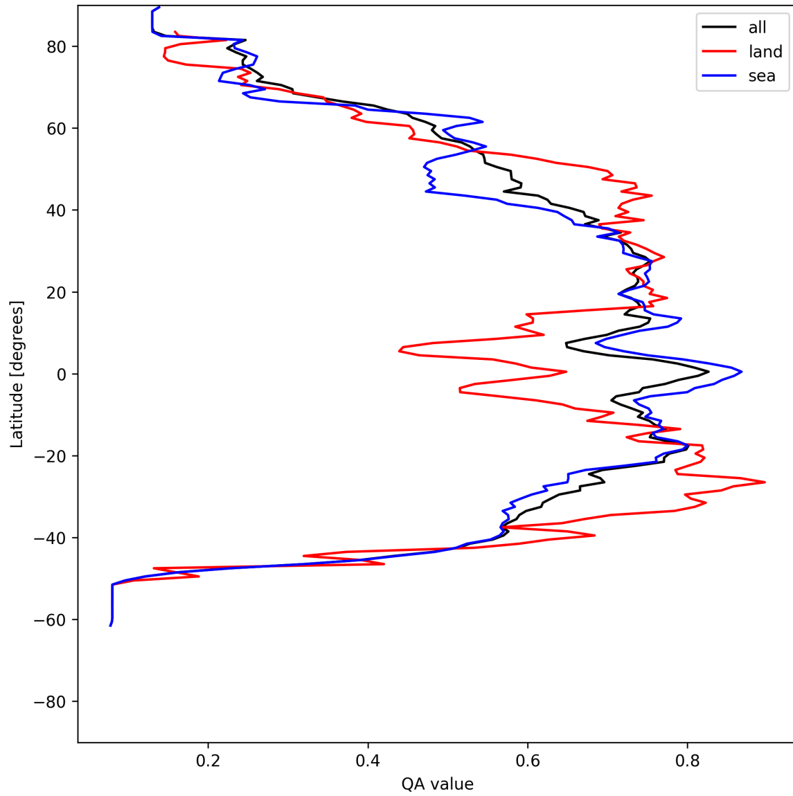
Figure 20: Zonal average of “QA value” for 2025-06-30 to 2025-07-02.
