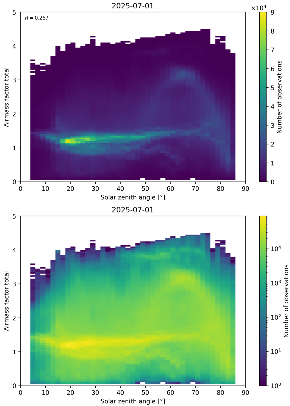
Figure 175: Scatter density plot of “Solar zenith angle” against “Airmass factor total” for 2025-06-30 to 2025-07-02.
