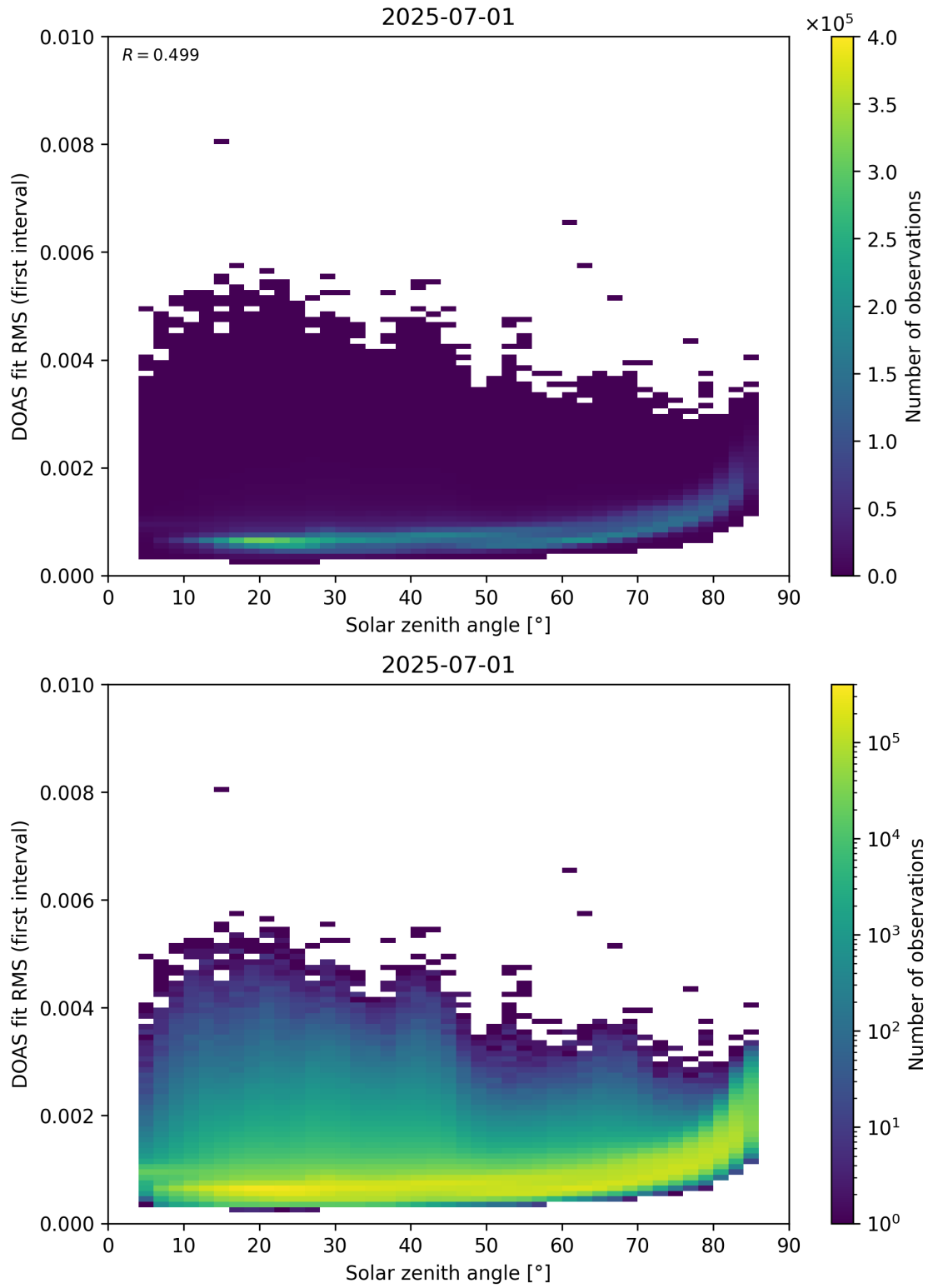
Figure 167: Scatter density plot of “Solar zenith angle” against “DOAS fit RMS (first interval)” for 2025-06-30 to 2025-07-02.
