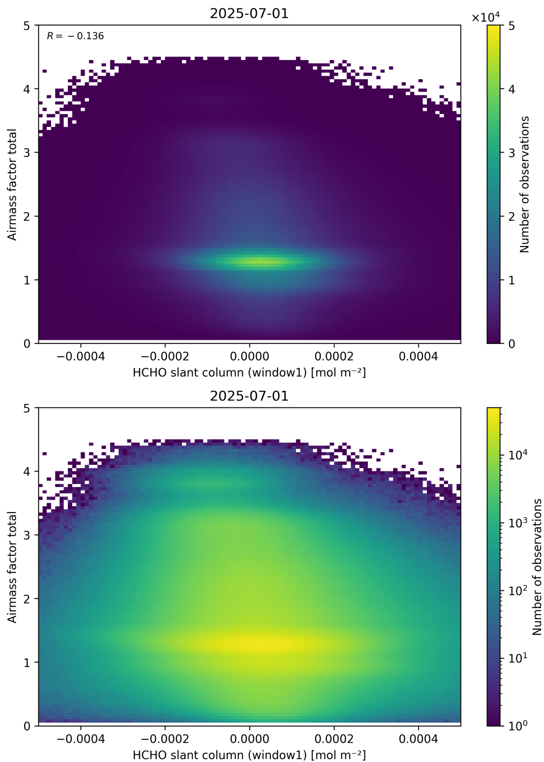
Figure 85: Scatter density plot of “HCHO slant column (window1)” against “Airmass factor total” for 2025-06-30 to 2025-07-02.
