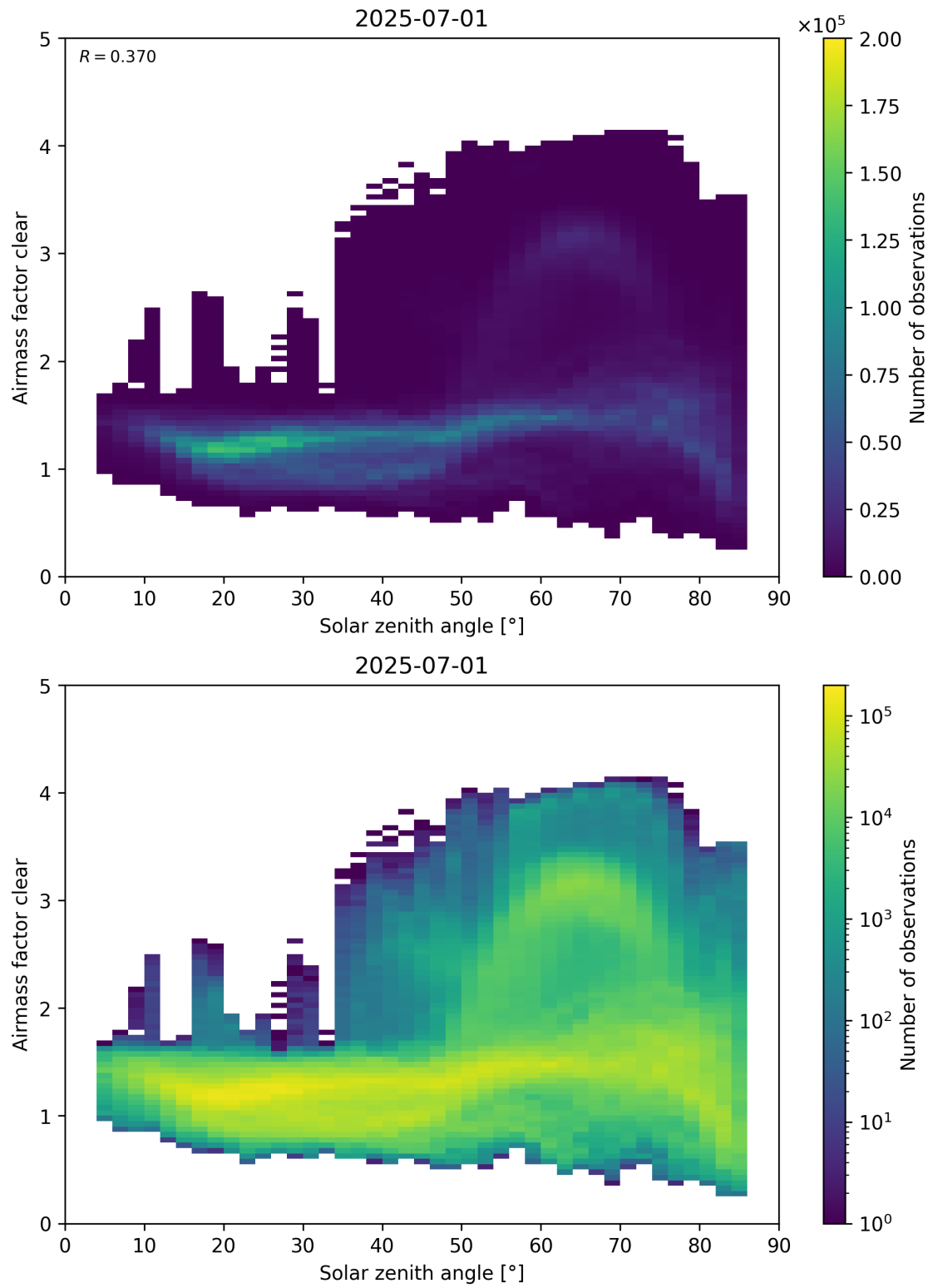
Figure 170: Scatter density plot of “Solar zenith angle” against “Airmass factor clear” for 2025-06-30 to 2025-07-02.
