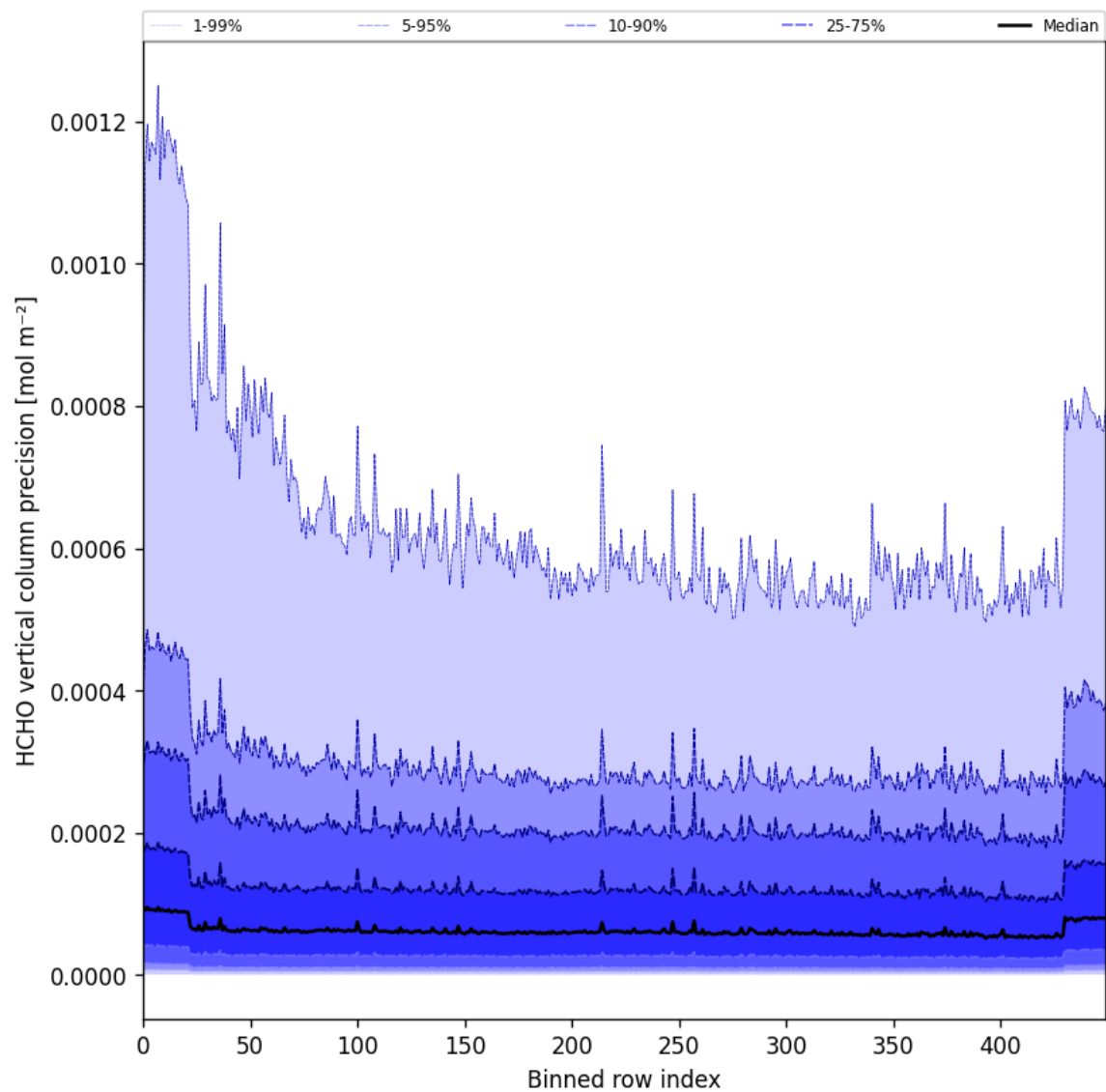
Figure 50: Along track statistics of “HCHO vertical column precision” for 2025-06-30 to 2025-07-02
