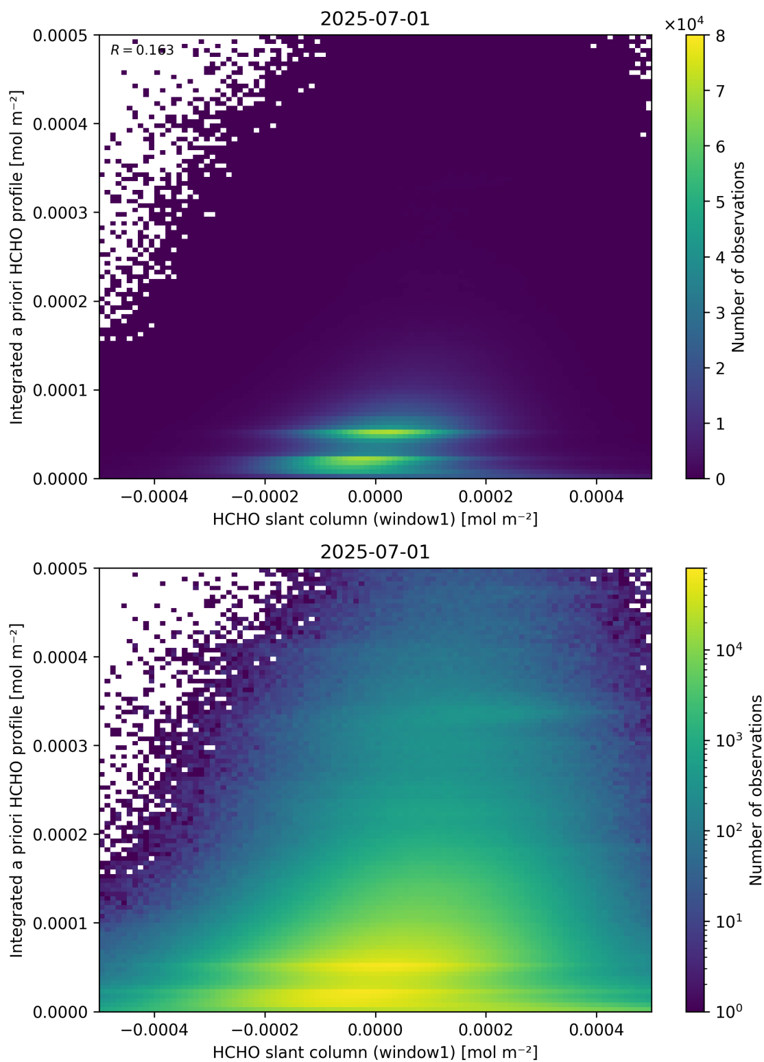
Figure 87: Scatter density plot of “HCHO slant column (window1)” against “Integrated a priori HCHO profile” for 2025-06-30 to 2025-07-02.
