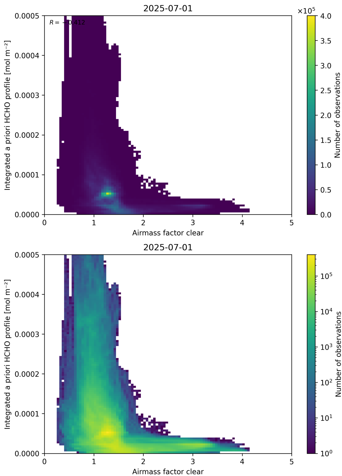
Figure 76: Scatter density plot of “Airmass factor clear” against “Integrated a priori HCHO profile” for 2025-06-30 to 2025-07-02.
