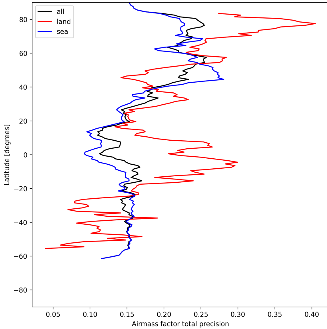
Figure 27: Zonal average of “Airmass factor total precision” for 2025-06-30 to 2025-07-02.
