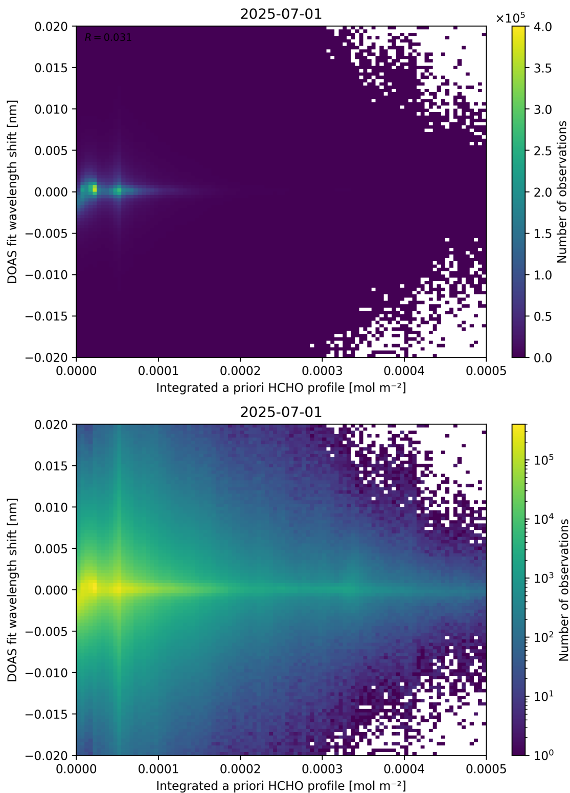
Figure 149: Scatter density plot of “Integrated a priori HCHO profile” against “DOAS fit wavelength shift” for 2025-06-30 to 2025-07-02.
