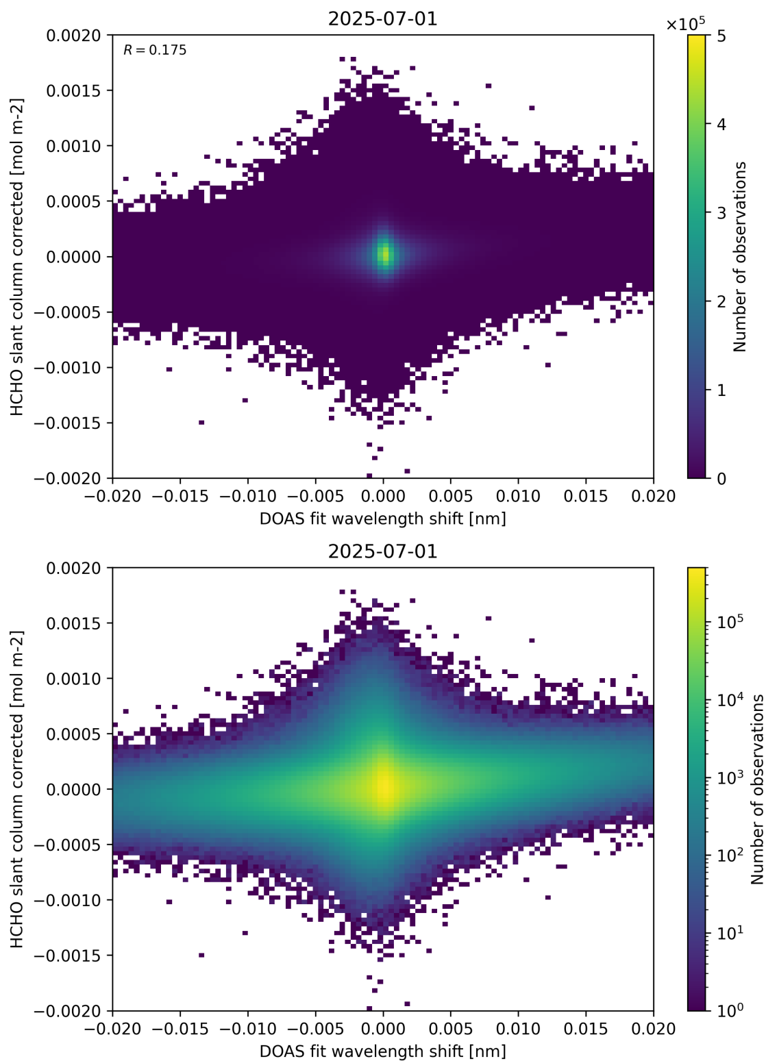
Figure 66: Scatter density plot of “DOAS fit wavelength shift” against “HCHO slant column corrected” for 2025-06-30 to 2025-07-02.
