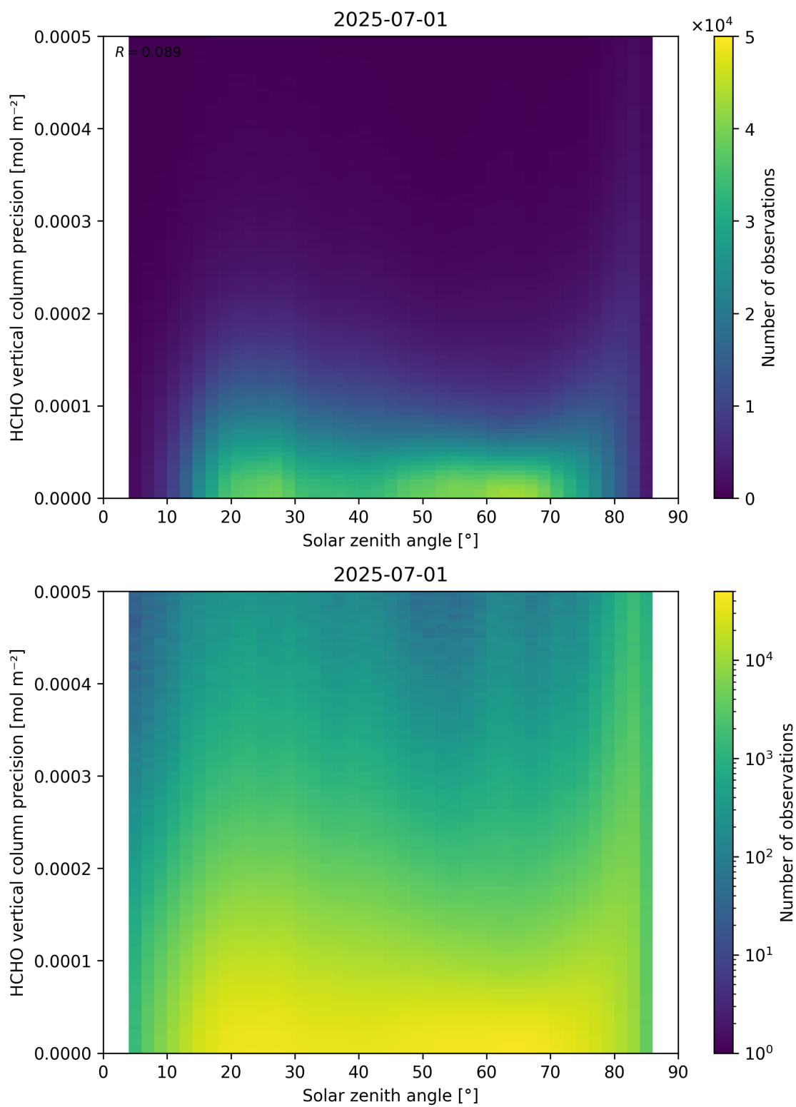
Figure 179: Scatter density plot of “Solar zenith angle” against “HCHO vertical column precision” for 2025-06-30 to 2025-07-02.
