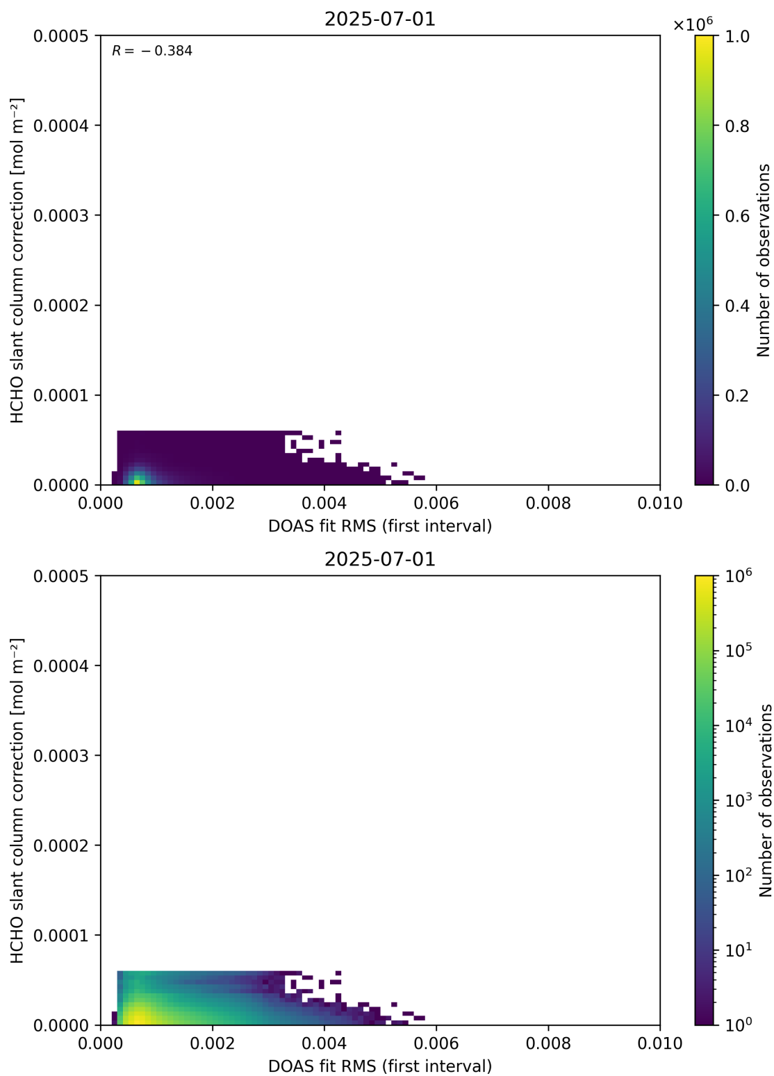
Figure 63: Scatter density plot of “DOAS fit RMS (first interval)” against “HCHO slant column correction” for 2025-06-30 to 2025-07-02.
