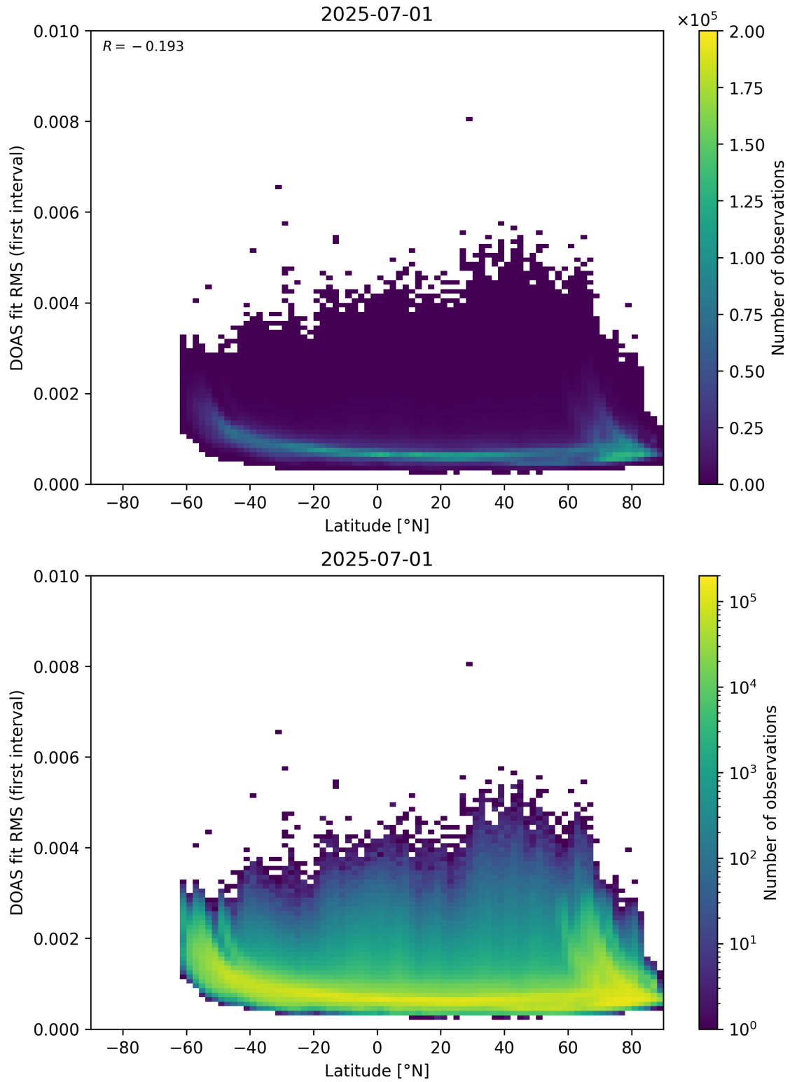
Figure 153: Scatter density plot of “Latitude” against “DOAS fit RMS (first interval)” for 2025-06-30 to 2025-07-02.
