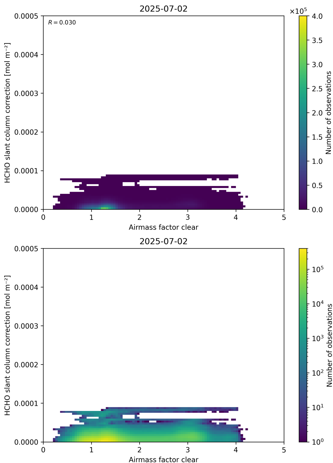
Figure 75: Scatter density plot of “Air mass factor clear” against “HCHO slant column correction” for 2025-07-02 to 2025-07-03.
