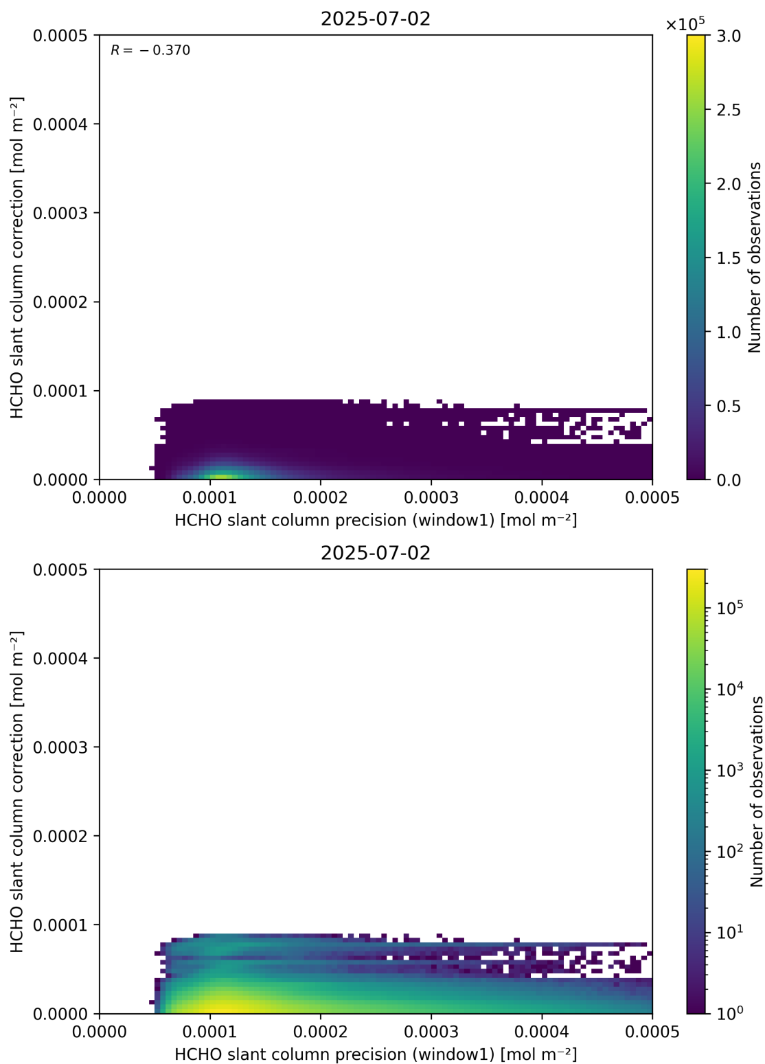
Figure 93: Scatter density plot of “HCHO slant column precision (window1)” against “HCHO slant column correction” for 2025-07-02 to 2025-07-03.
