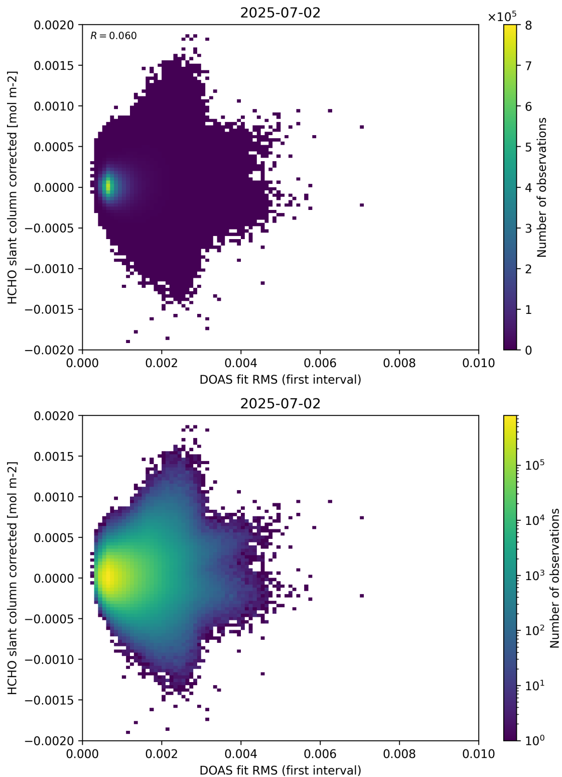
Figure 62: Scatter density plot of “DOAS fit RMS (first interval)” against “HCHO slant column corrected” for 2025-07-02 to 2025-07-03.
