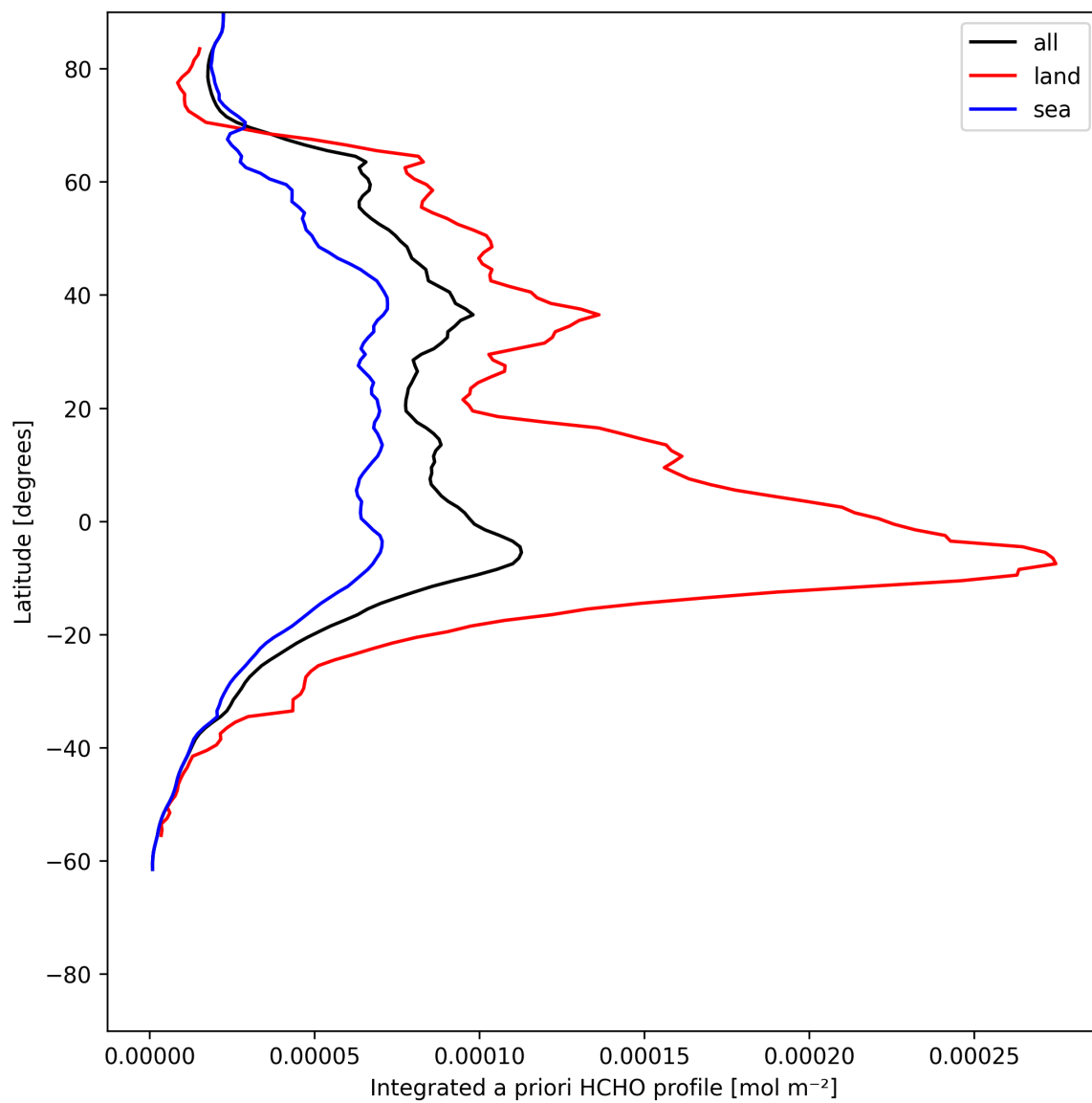
Figure 29: Zonal average of “Integrated a priori HCHO profile” for 2025-07-02 to 2025-07-03.
