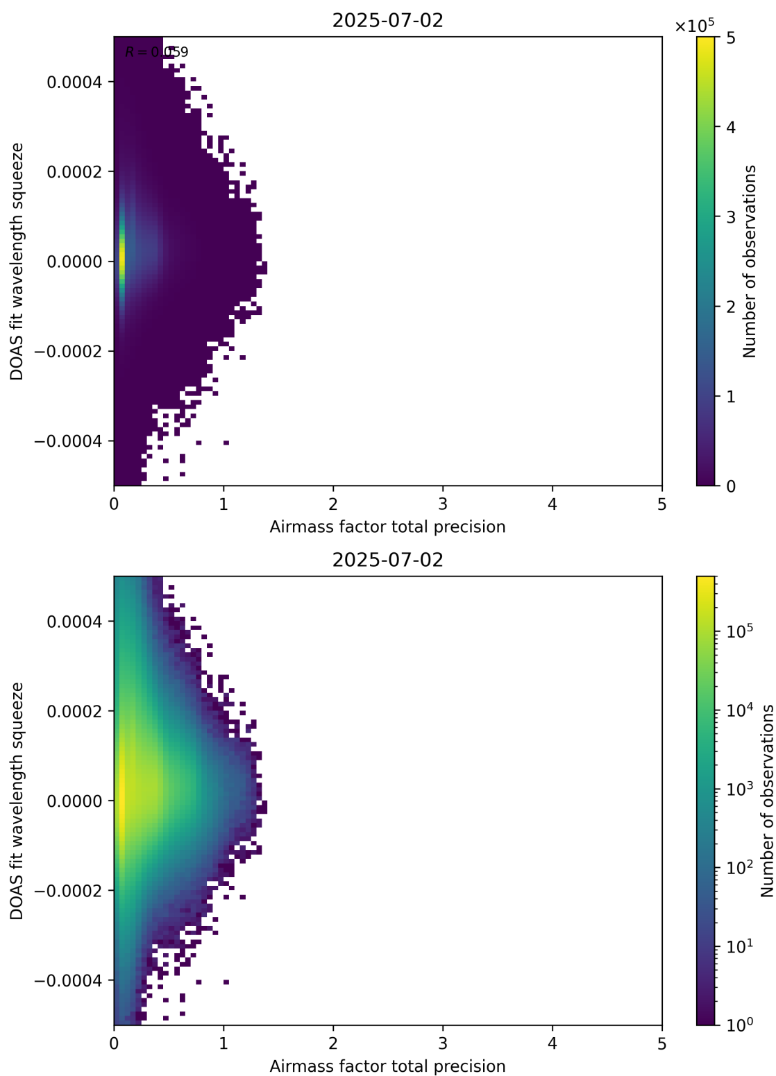
Figure 107: Scatter density plot of “Airmass factor total precision” against “DOAS fit wavelength squeeze” for 2025-07-02 to 2025-07-03.
