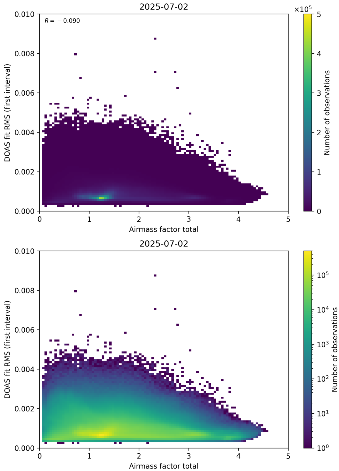
Figure 97: Scatter density plot of “Airmass factor total” against “DOAS fit RMS (first interval)” for 2025-07-02 to 2025-07-03.
