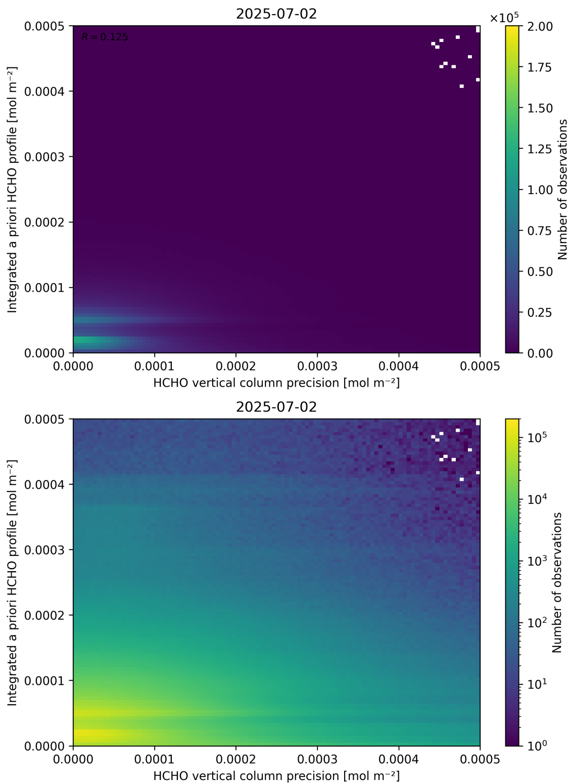
Figure 147: Scatter density plot of “HCHO vertical column precision” against “Integrated a priori HCHO profile” for 2025-07-02 to 2025-07-03.
