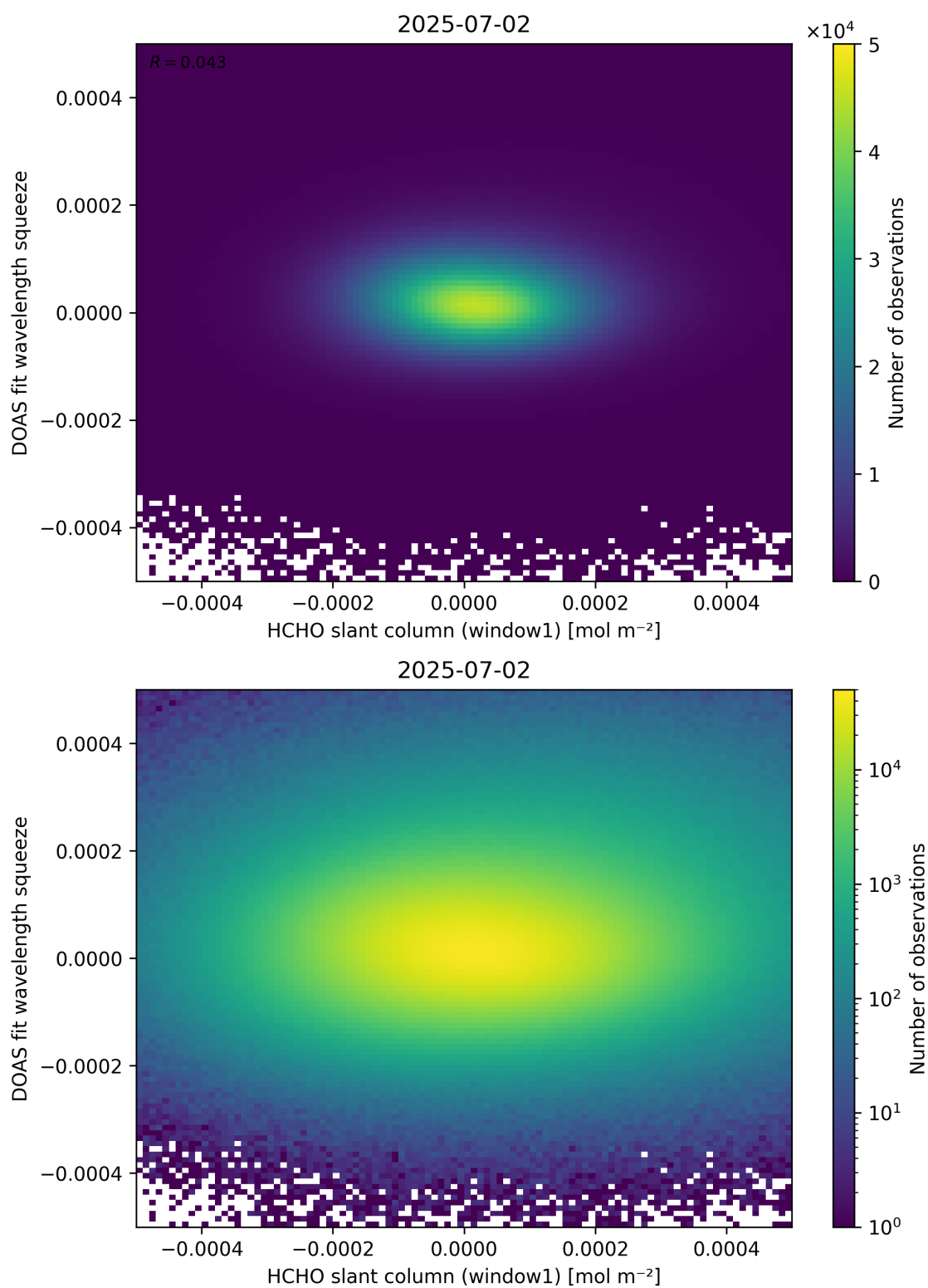
Figure 80: Scatter density plot of “HCHO slant column (window1)” against “DOAS fit wavelength squeeze” for 2025-07-02 to 2025-07-03.
