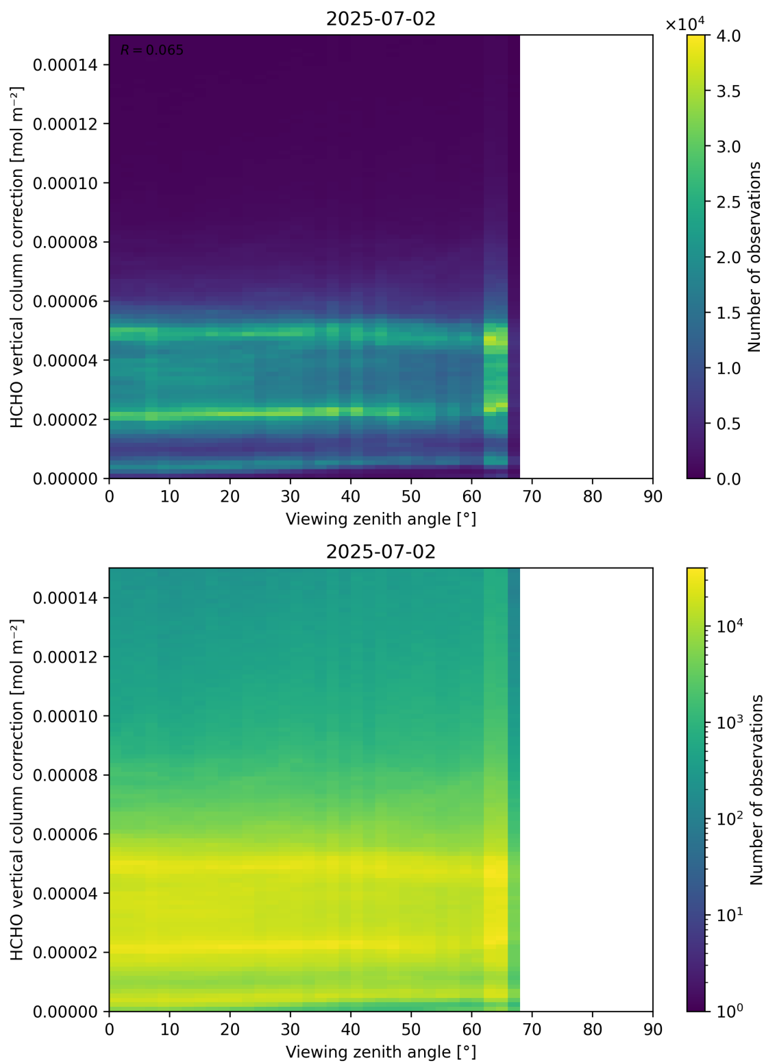
Figure 193: Scatter density plot of “Viewing zenith angle” against “HCHO vertical column correction” for 2025-07-02 to 2025-07-03.
