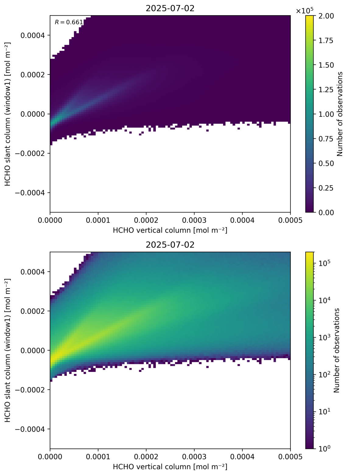
Figure 129: Scatter density plot of “HCHO vertical column” against “HCHO slant column (window1)” for 2025-07-02 to 2025-07-03.
