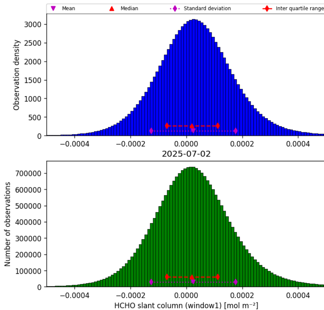
Figure 38: Histogram of “HCHO slant column (window1)” for 2025-07-02 to 2025-07-03
