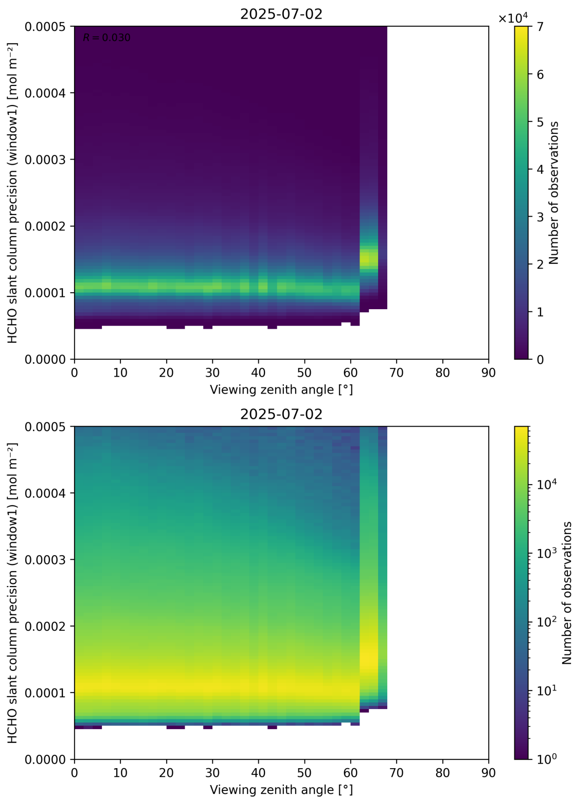
Figure 189: Scatter density plot of “Viewing zenith angle” against “HCHO slant column precision (window1)” for 2025-07-02 to 2025-07-03.
