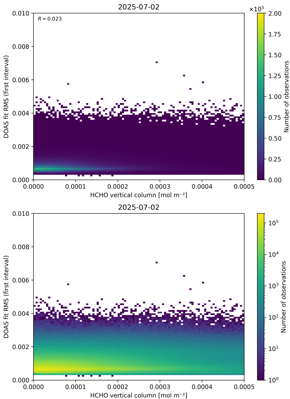
Figure 123: Scatter density plot of “HCHO vertical column” against “DOAS fit RMS (first interval)” for 2025-07-02 to 2025-07-03.
