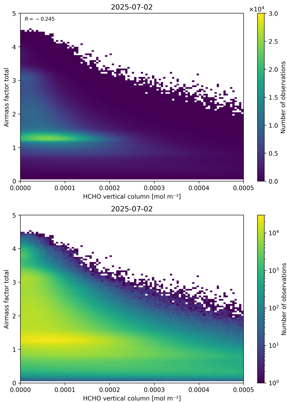
Figure 131: Scatter density plot of “HCHO vertical column” against “Airmass factor total” for 2025-07-02 to 2025-07-03.
