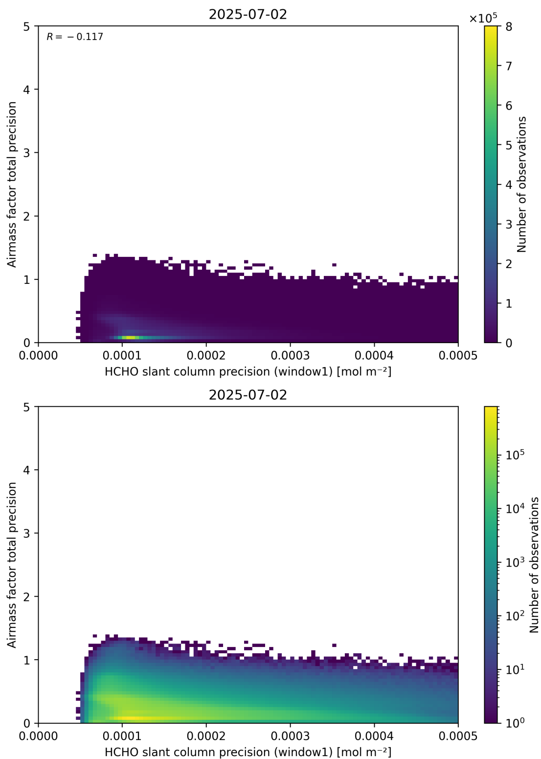
Figure 95: Scatter density plot of “HCHO slant column precision (window1)” against “Airmass factor total precision” for 2025-07-02 to 2025-07-03.
