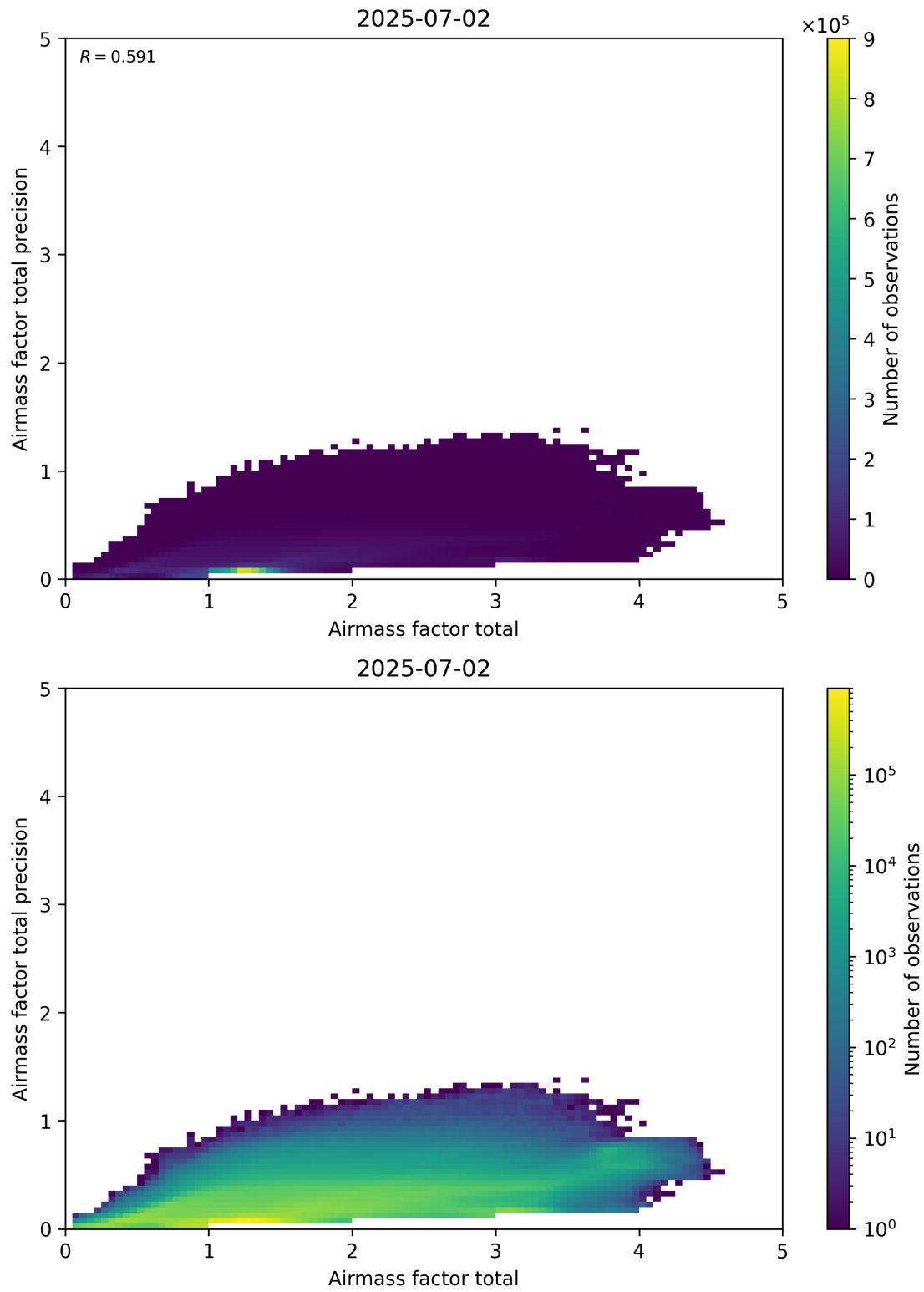
Figure 103: Scatter density plot of “Airmass factor total” against “Airmass factor total precision” for 2025-07-02 to 2025-07-03.
