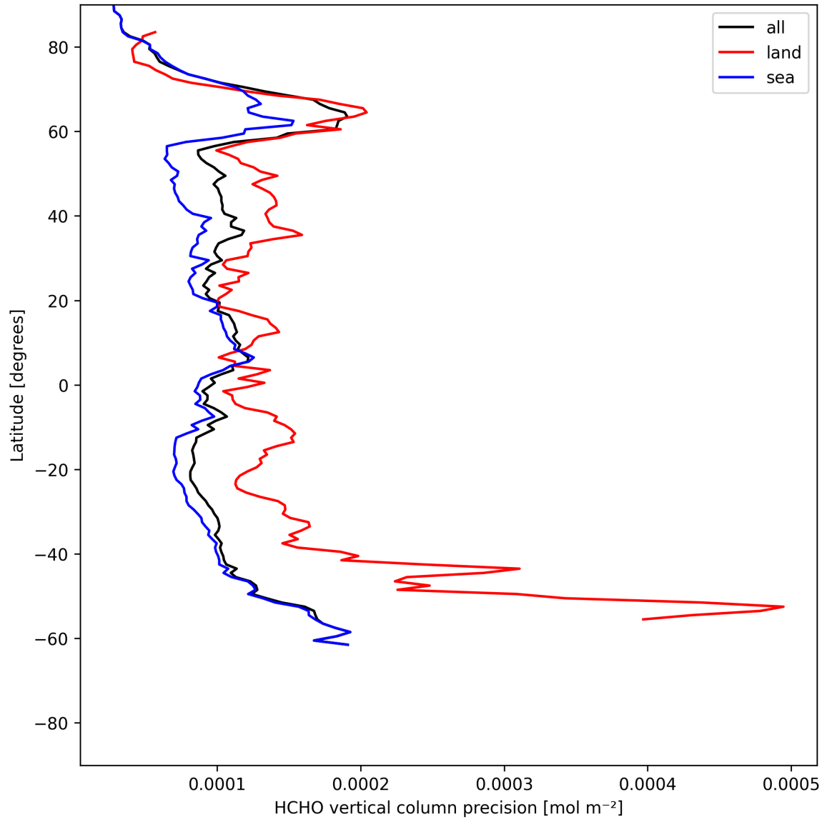
Figure 22: Zonal average of “HCHO vertical column precision” for 2025-07-02 to 2025-07-03.
