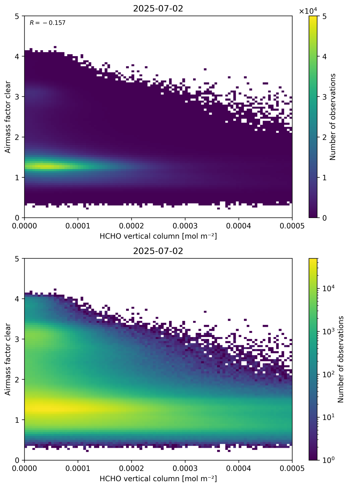
Figure 126: Scatter density plot of “HCHO vertical column” against “Airmass factor clear” for 2025-07-02 to 2025-07-03.
