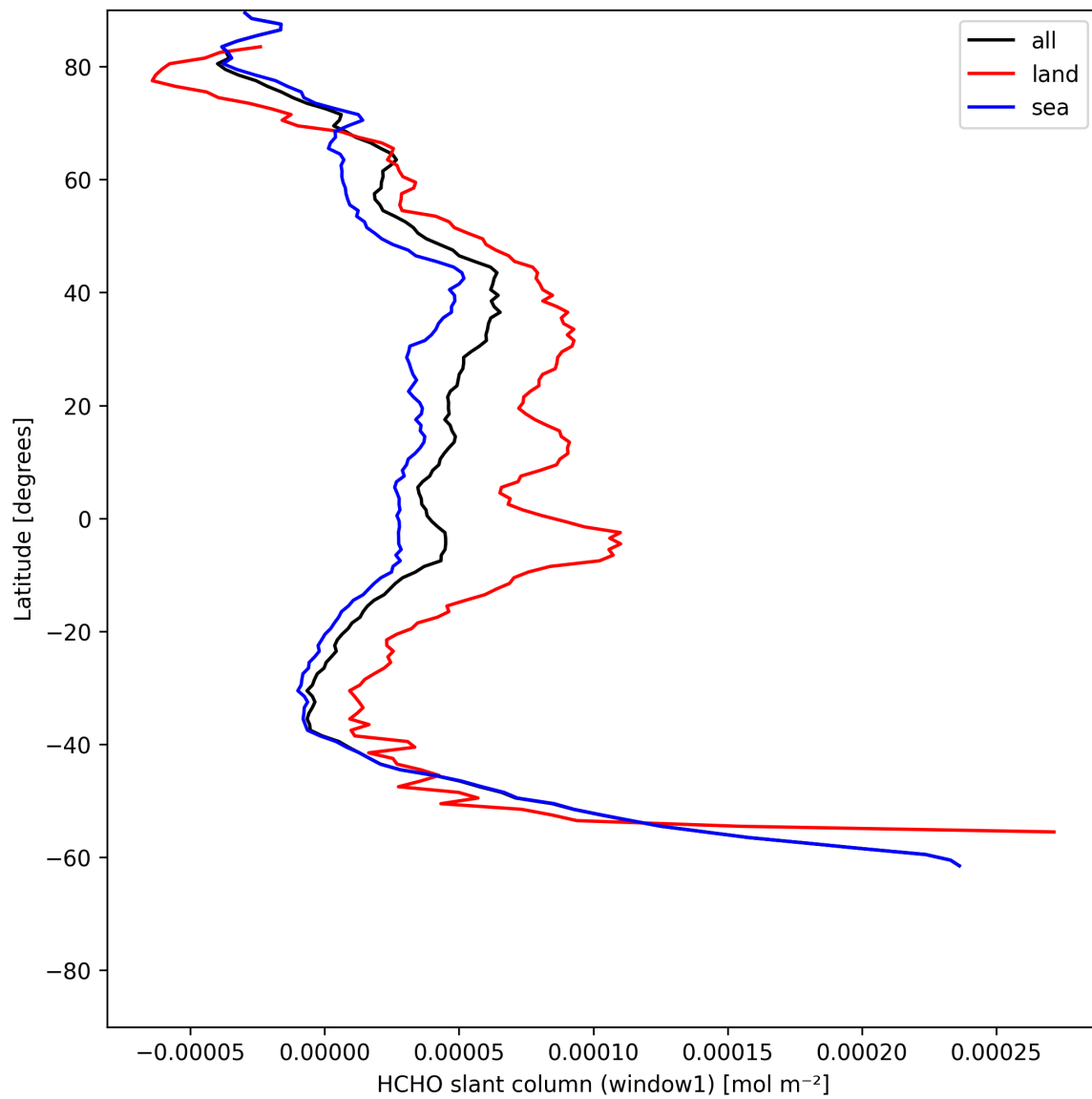
Figure 24: Zonal average of “HCHO slant column (window1)” for 2025-07-02 to 2025-07-03.
