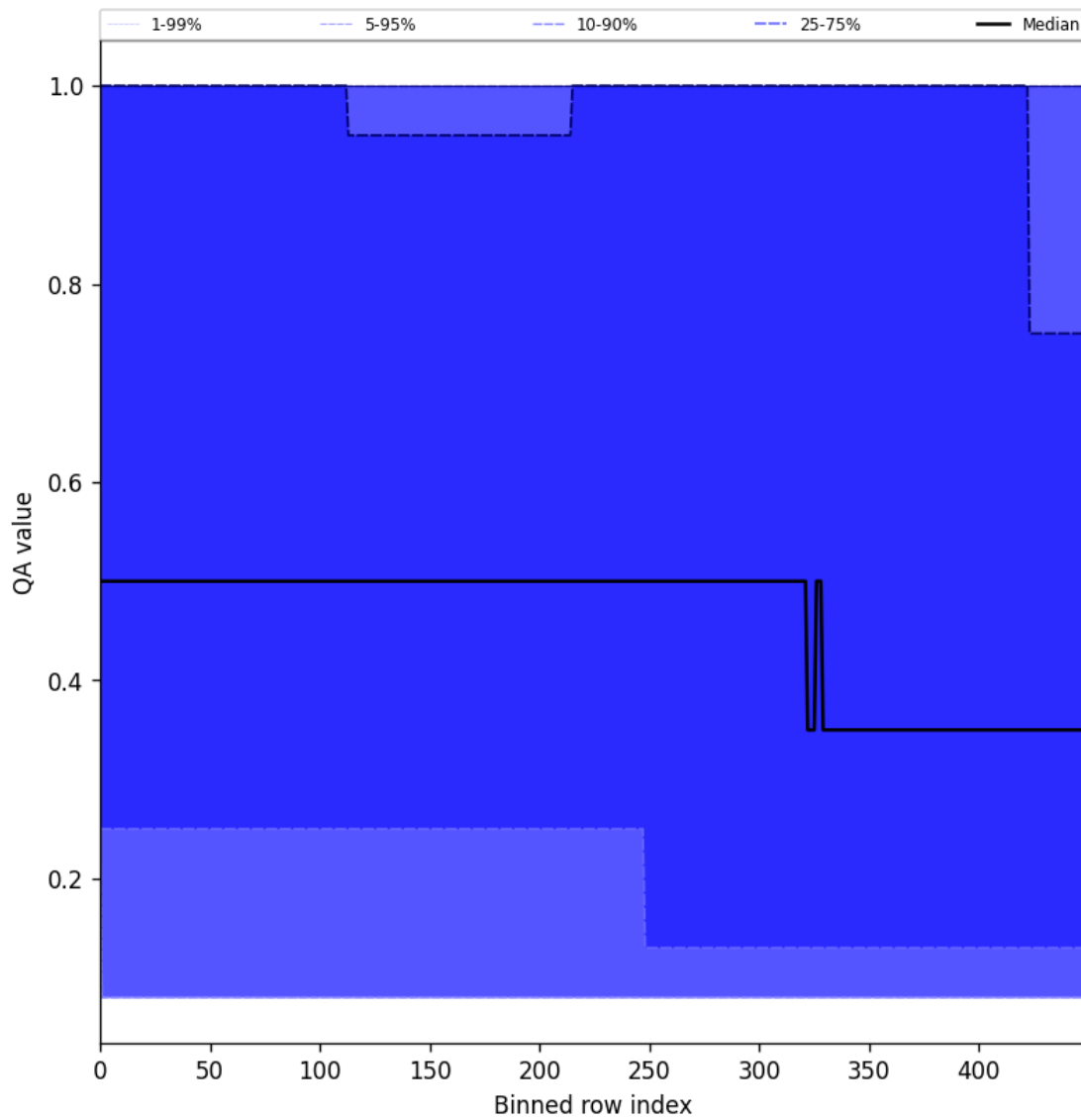
Figure 48: Along track statistics of “QA value” for 2025-07-02 to 2025-07-03
