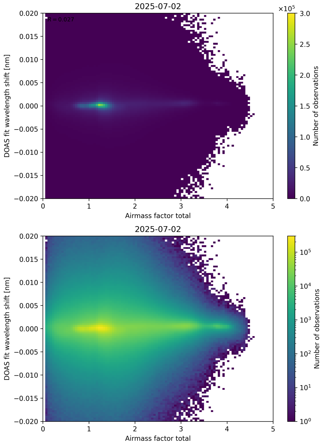
Figure 98: Scatter density plot of “Airmass factor total” against “DOAS fit wavelength shift” for 2025-07-02 to 2025-07-03.
