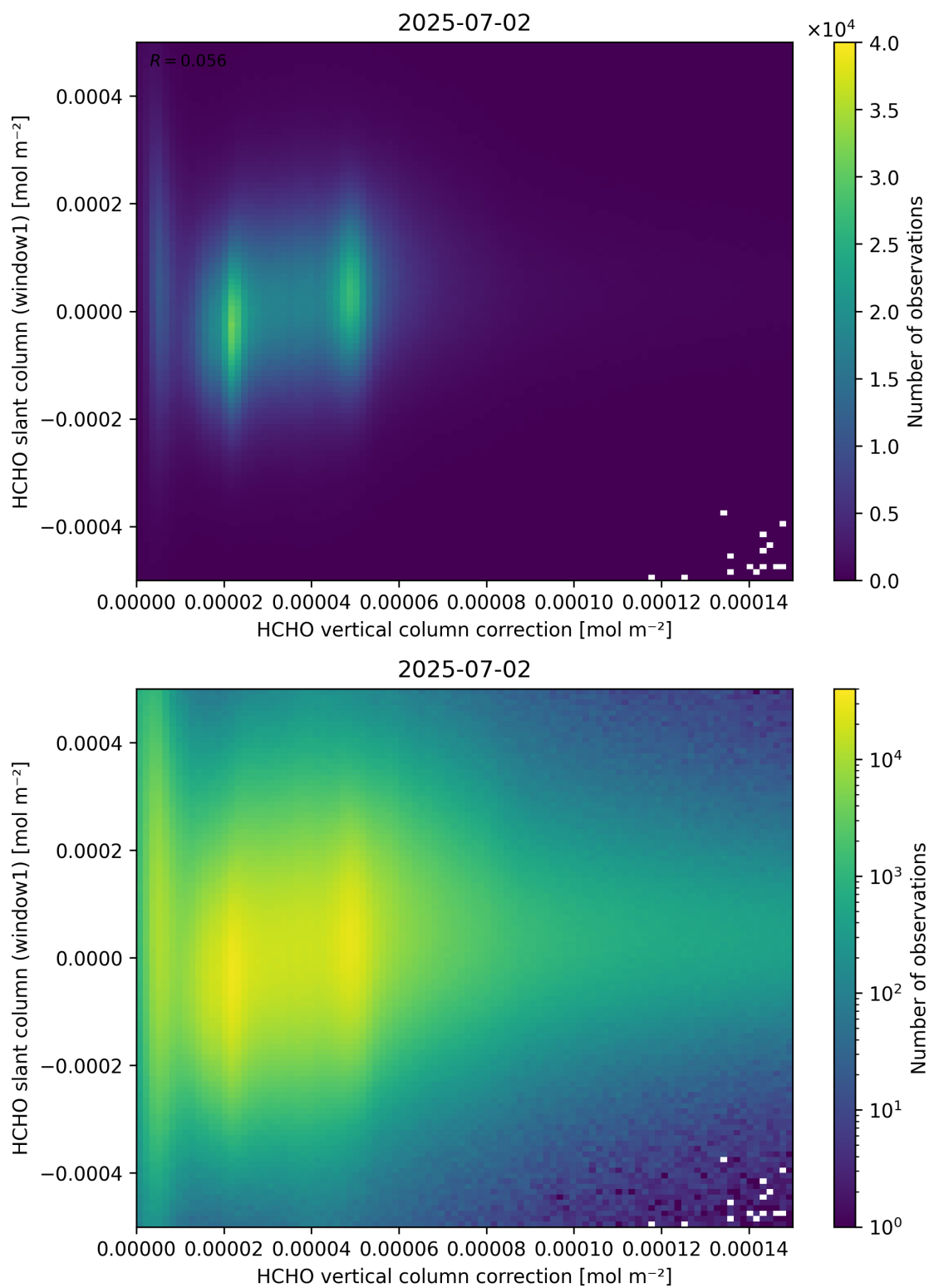
Figure 118: Scatter density plot of “HCHO vertical column correction” against “HCHO slant column (window1)” for 2025-07-02 to 2025-07-03.
