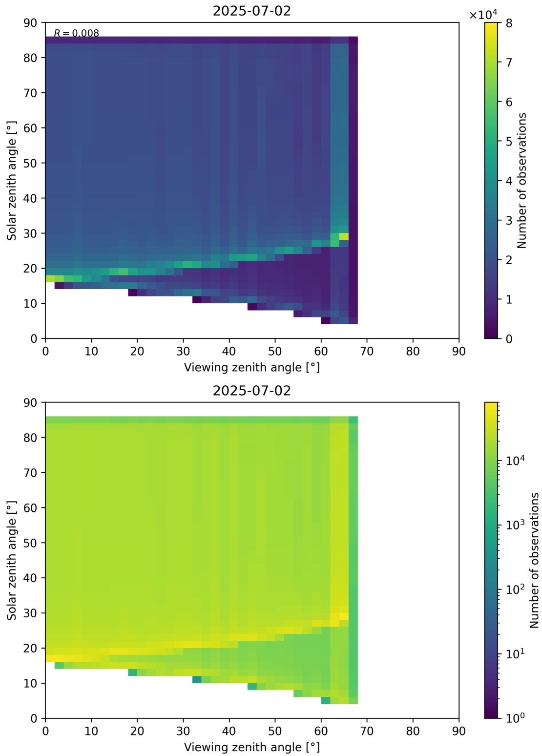
Figure 197: Scatter density plot of “Viewing zenith angle” against “Solar zenith angle” for 2025-07-02 to 2025-07-03.
