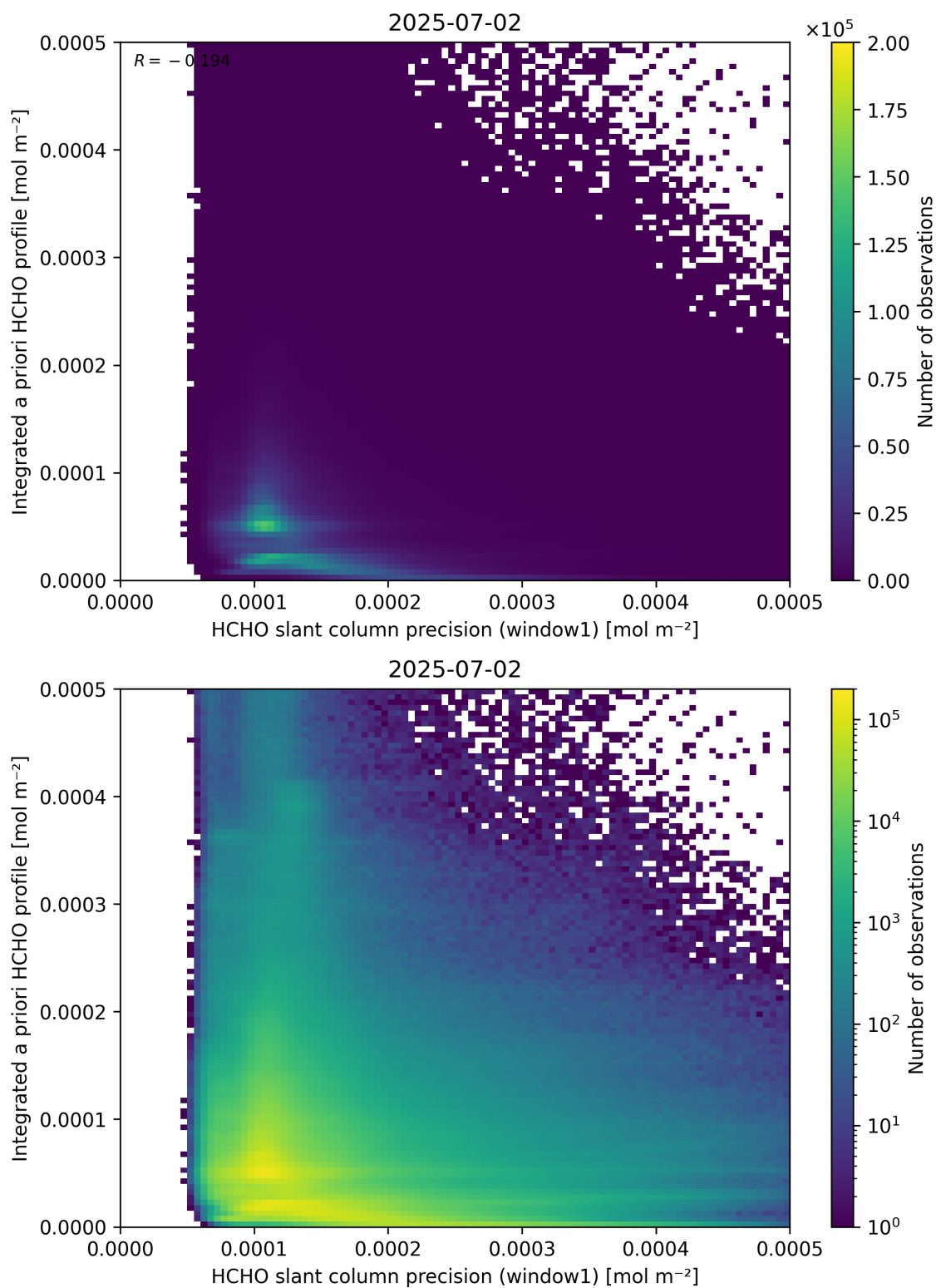
Figure 96: Scatter density plot of “HCHO slant column precision (window1)” against “Integrated a priori HCHO profile” for 2025-07-02 to 2025-07-03.
