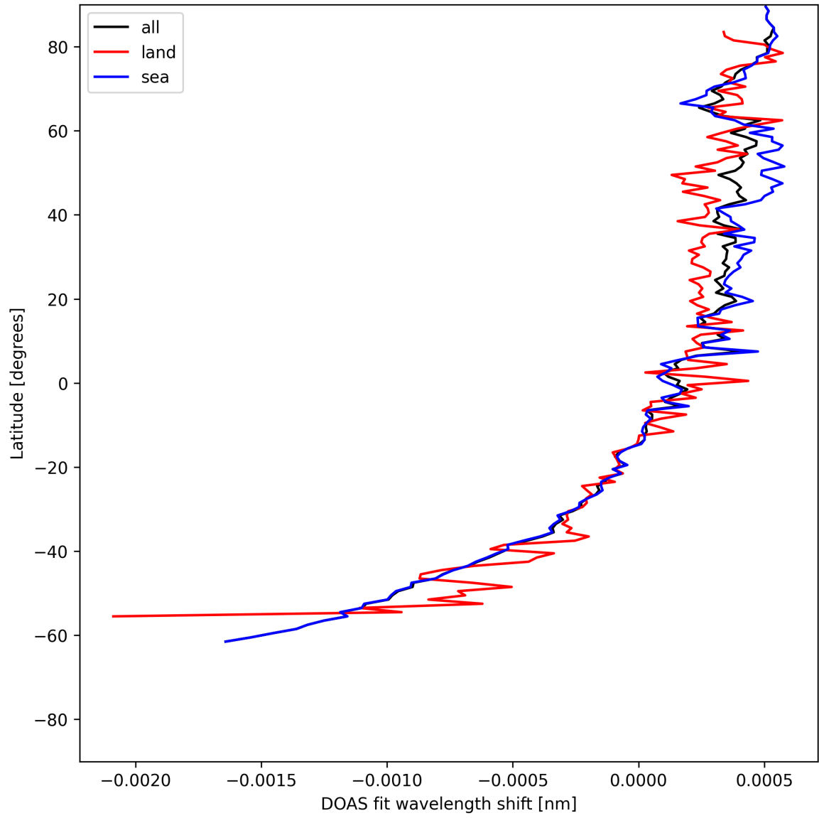
Figure 30: Zonal average of “DOAS fit wavelength shift” for 2025-07-02 to 2025-07-03.
