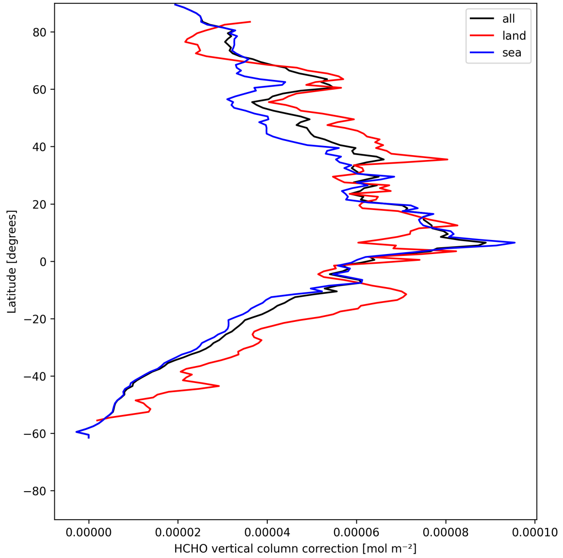
Figure 23: Zonal average of “HCHO vertical column correction” for 2025-07-02 to 2025-07-03.
