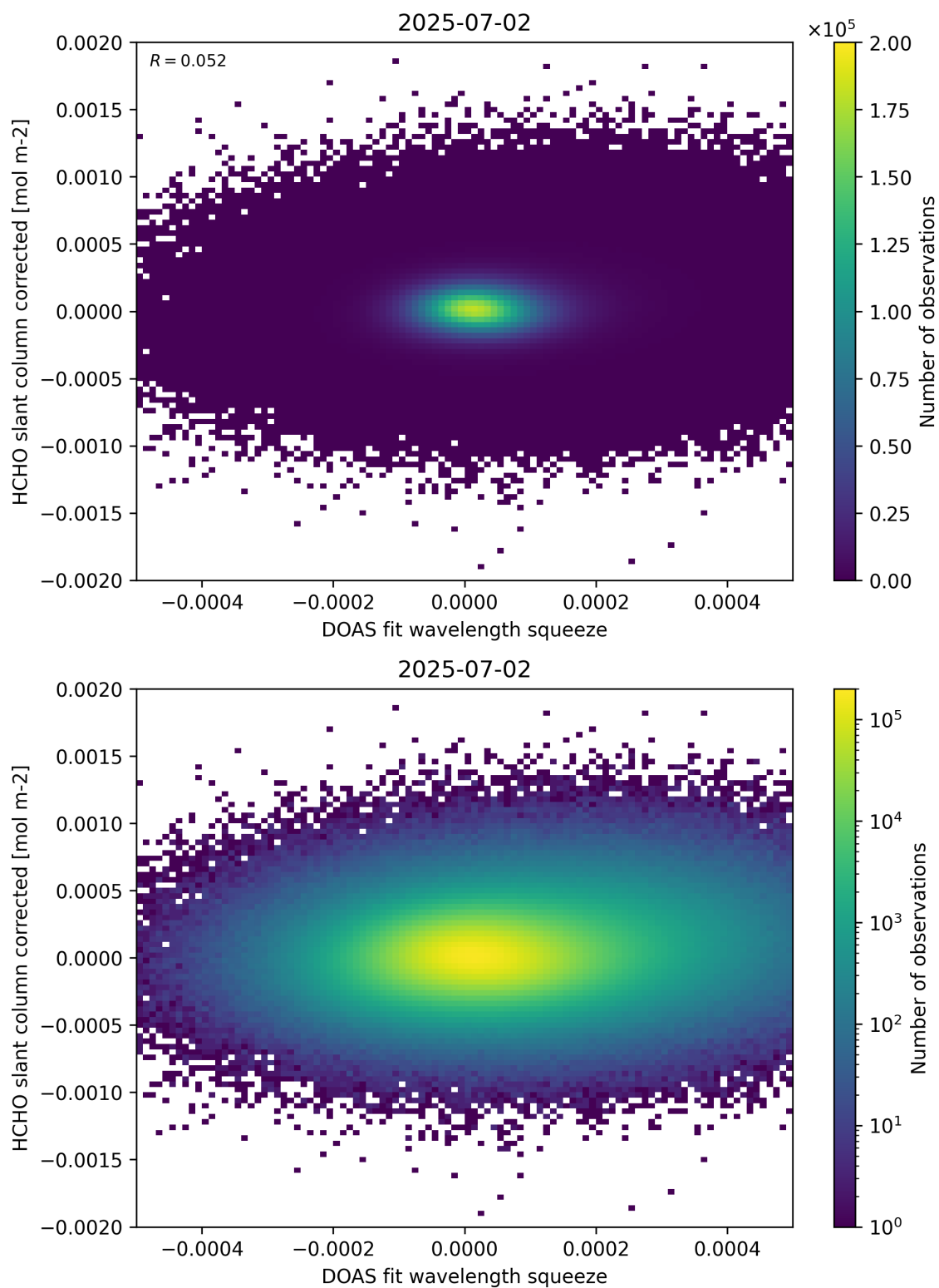
Figure 69: Scatter density plot of “DOAS fit wavelength squeeze” against “HCHO slant column corrected” for 2025-07-02 to 2025-07-03.
