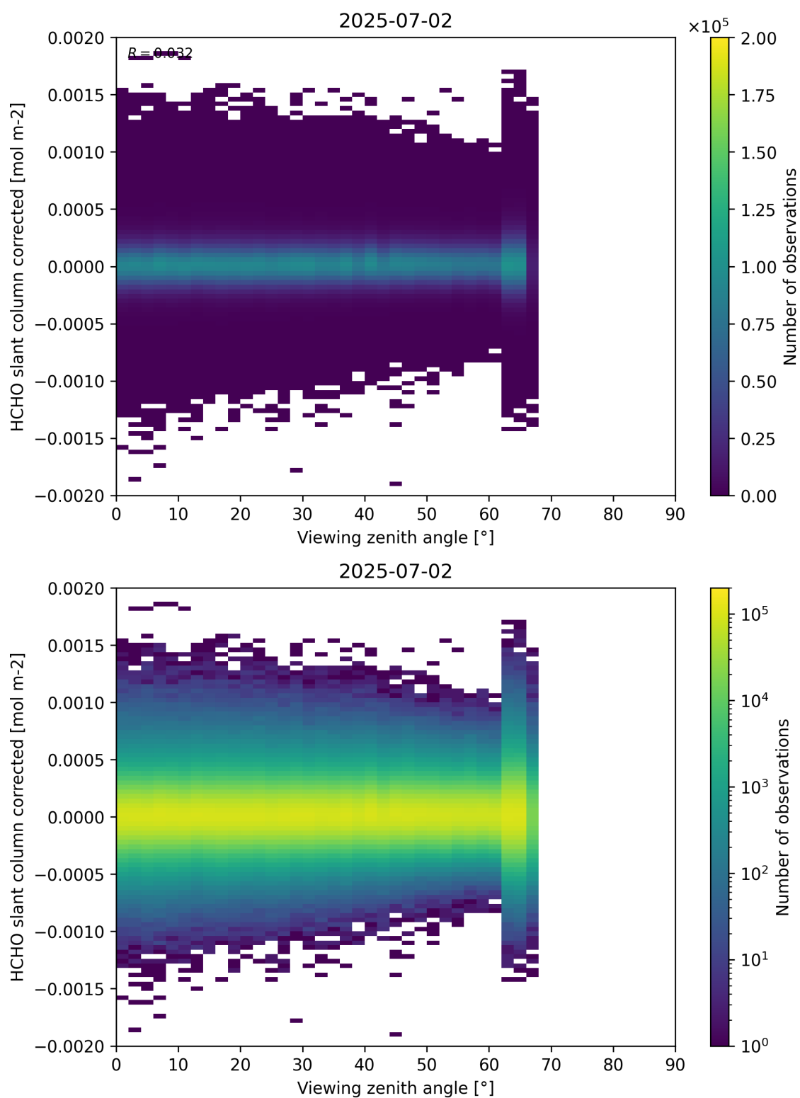
Figure 186: Scatter density plot of “Viewing zenith angle” against “HCHO slant column corrected” for 2025-07-02 to 2025-07-03.
