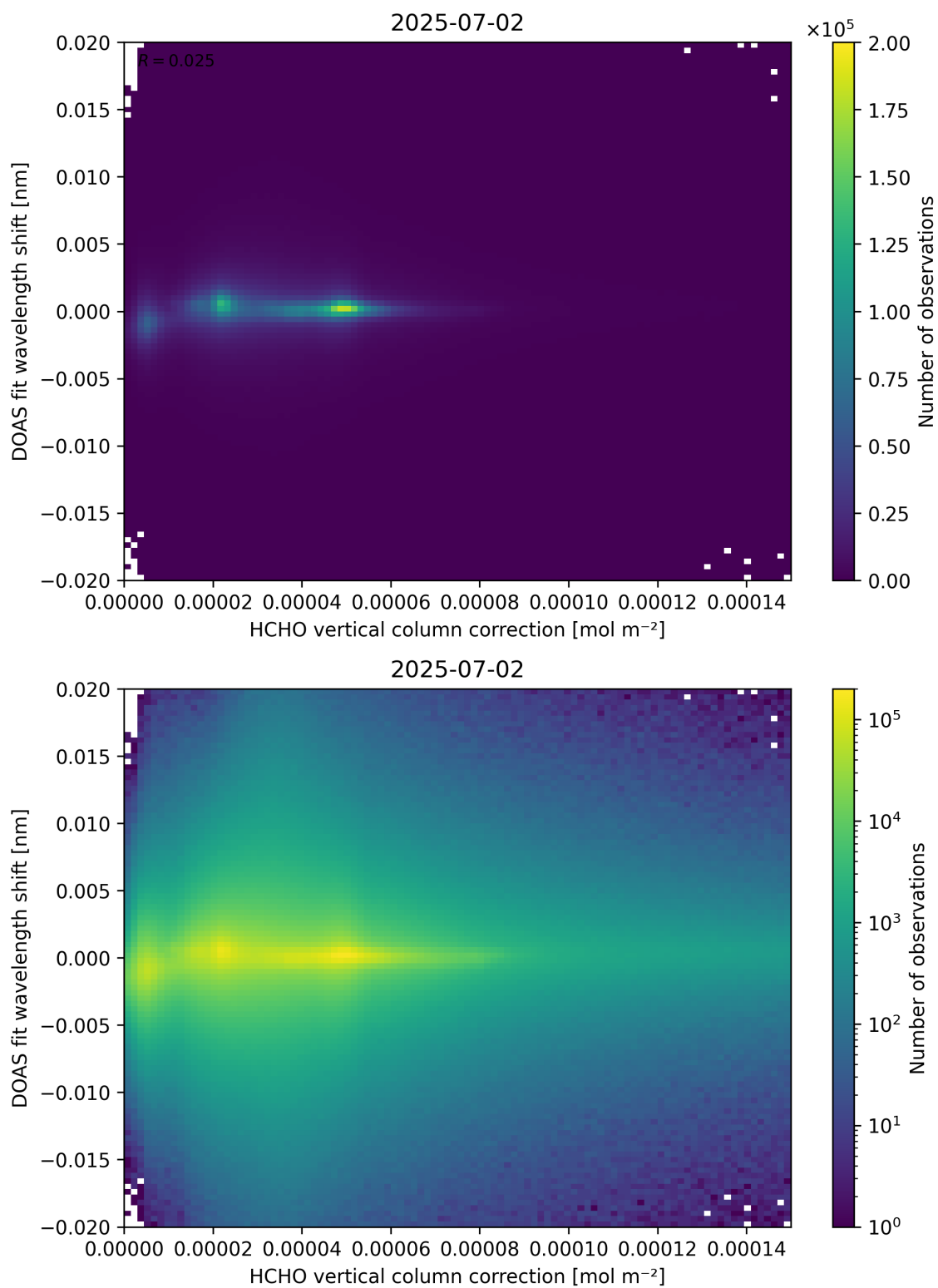
Figure 113: Scatter density plot of “HCHO vertical column correction” against “DOAS fit wavelength shift” for 2025-07-02 to 2025-07-03.
