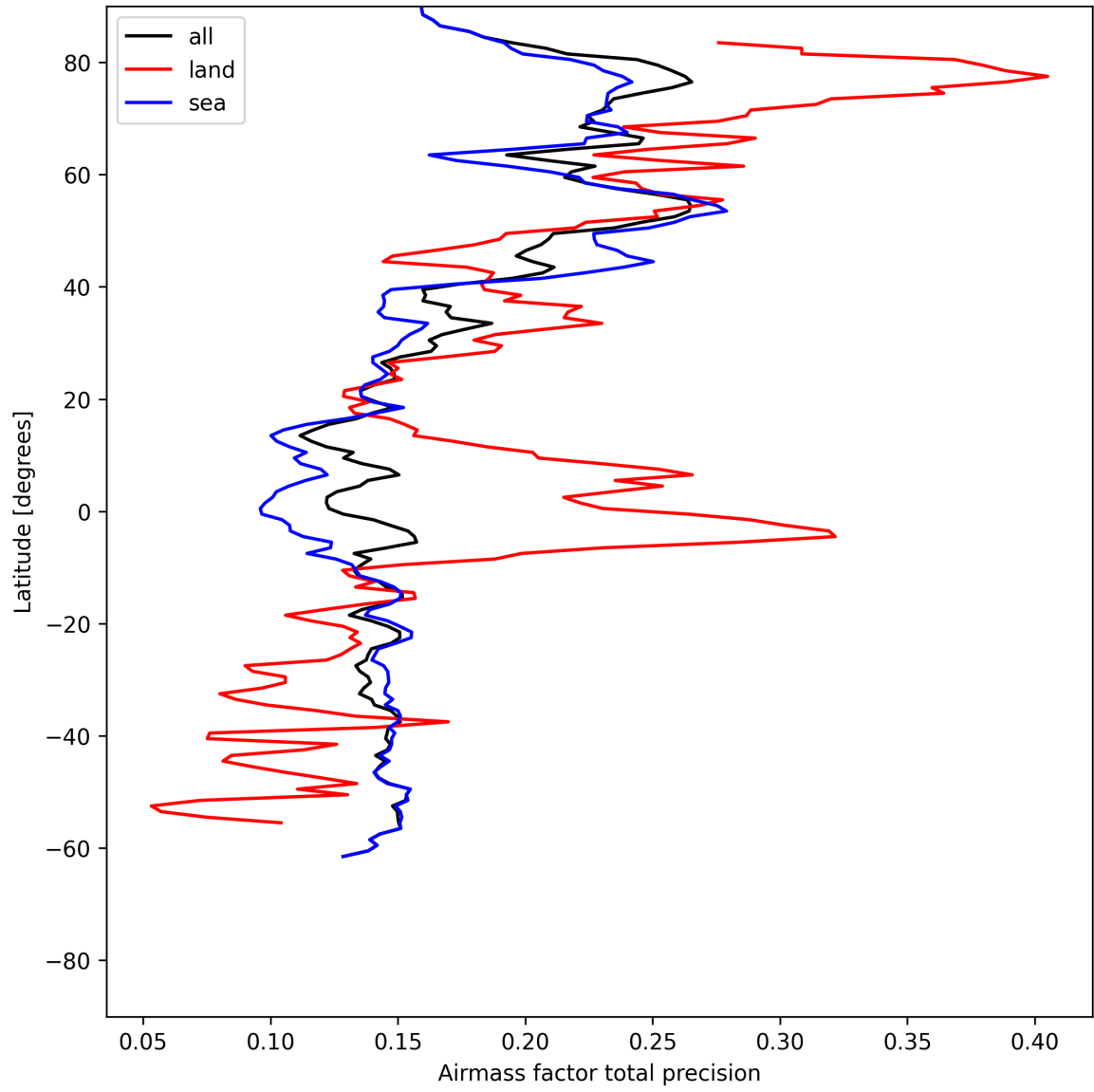
Figure 27: Zonal average of “Airmass factor total precision” for 2025-07-02 to 2025-07-03.
