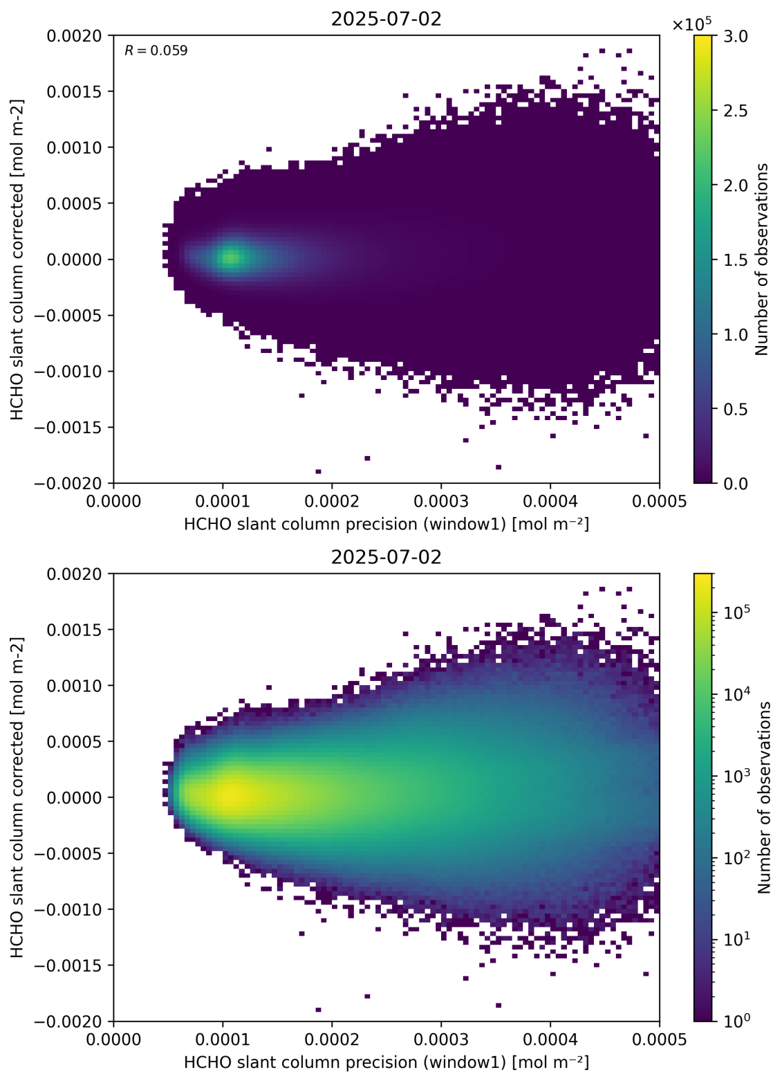
Figure 92: Scatter density plot of “HCHO slant column precision (window1)” against “HCHO slant column corrected” for 2025-07-02 to 2025-07-03.
