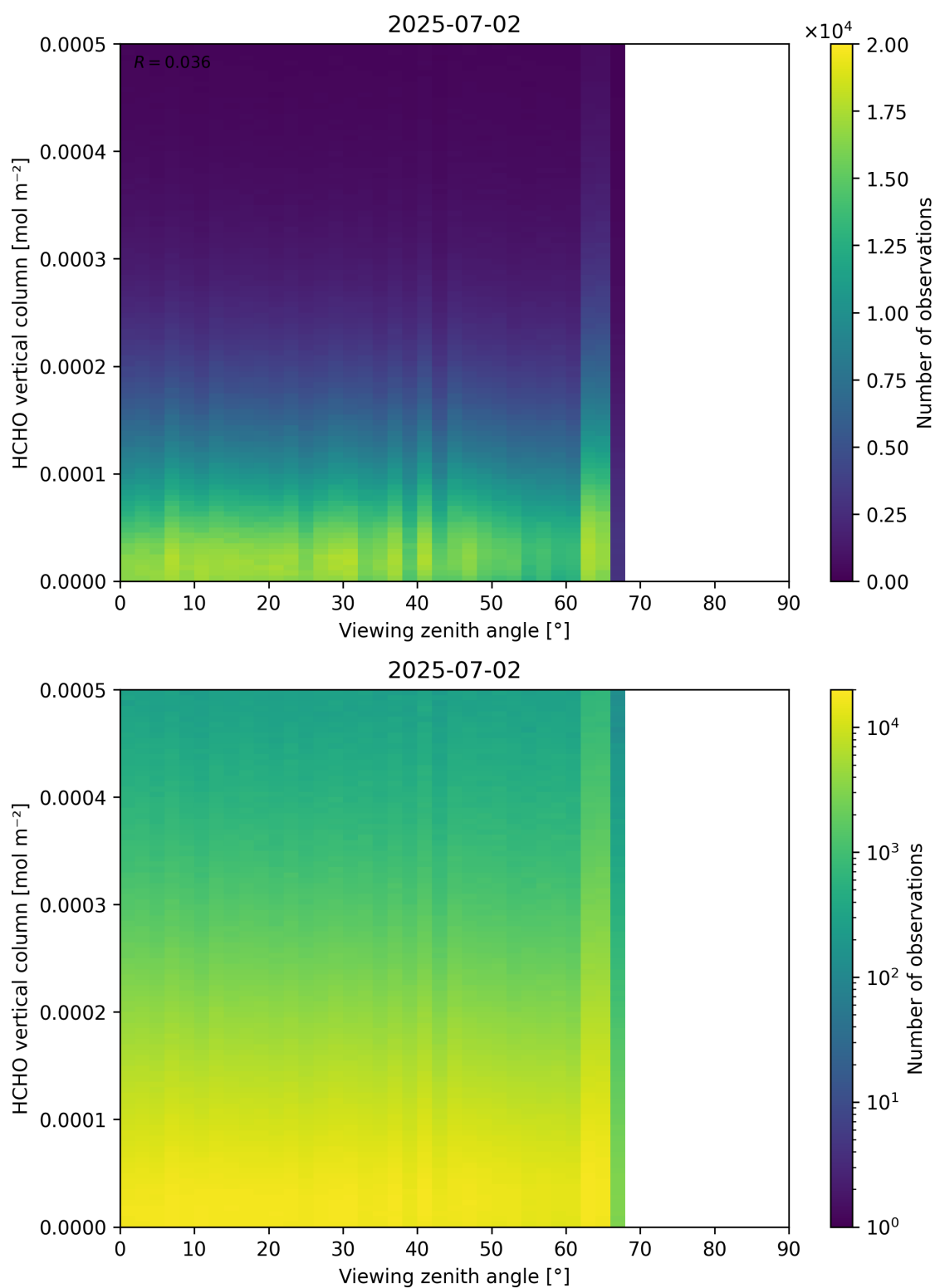
Figure 192: Scatter density plot of “Viewing zenith angle” against “HCHO vertical column” for 2025-07-02 to 2025-07-03.
