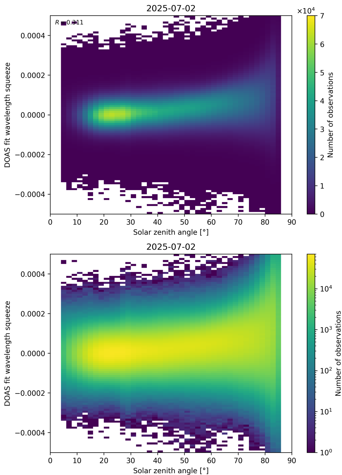
Figure 169: Scatter density plot of “Solar zenith angle” against “DOAS fit wavelength squeeze” for 2025-07-02 to 2025-07-03.
