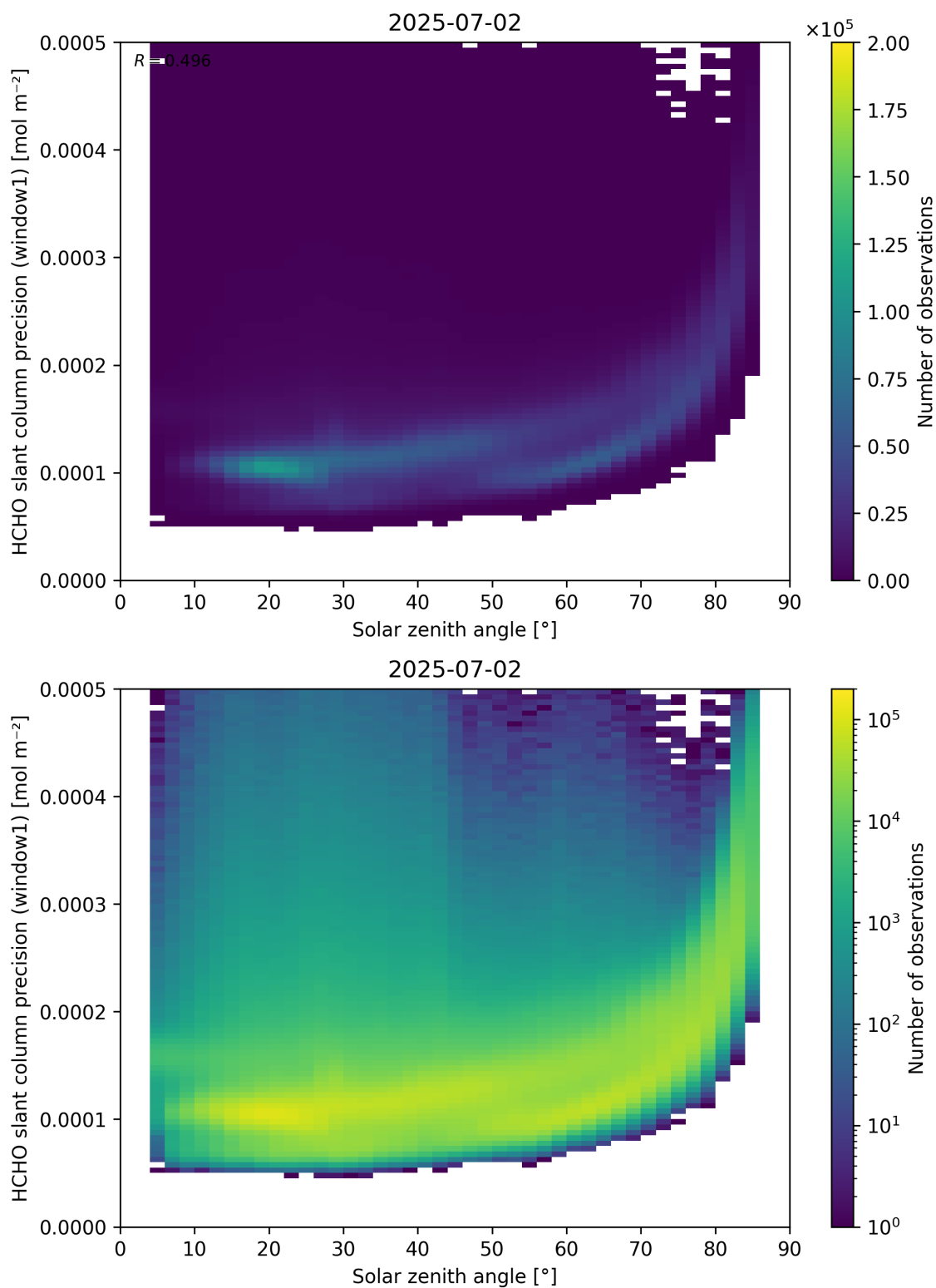
Figure 174: Scatter density plot of “Solar zenith angle” against “HCHO slant column precision (window1)” for 2025-07-02 to 2025-07-03.
