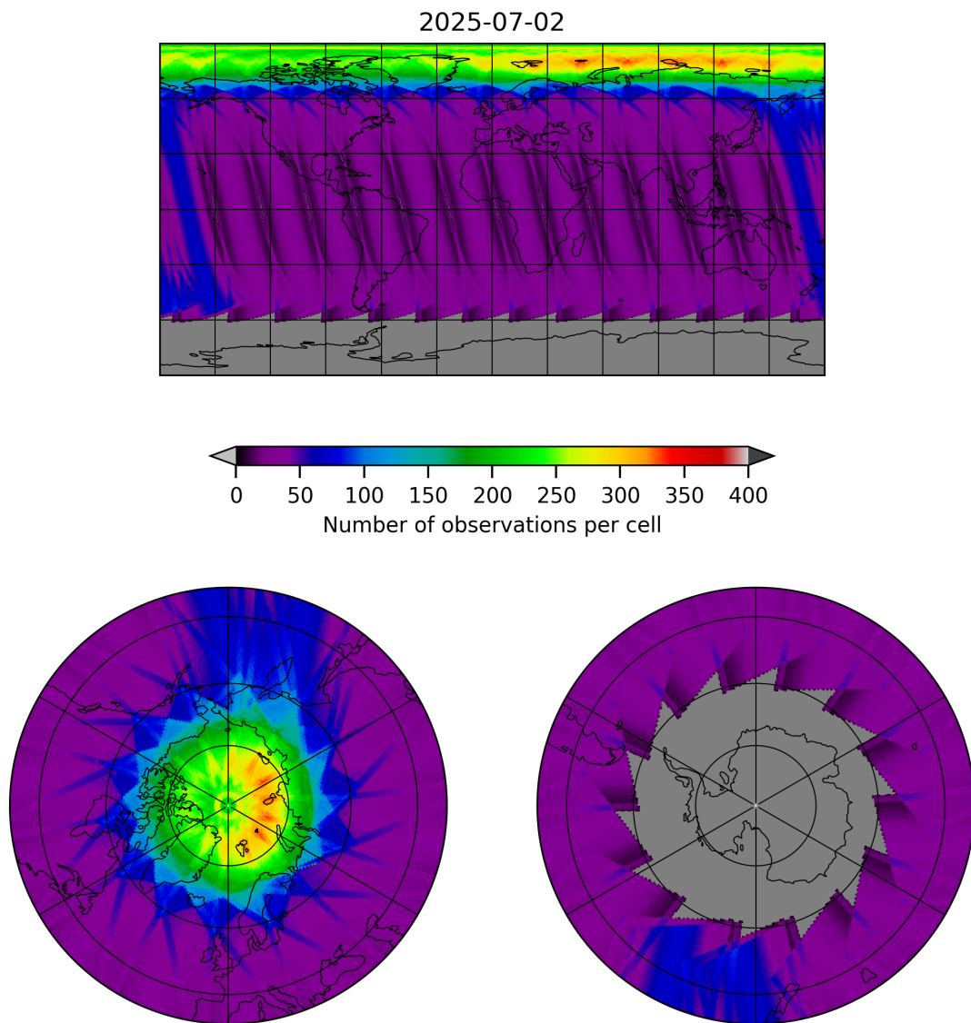
Figure 19: Map of the number of observations for 2025-07-02 to 2025-07-03
