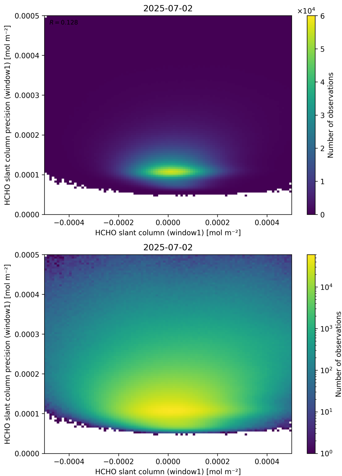
Figure 84: Scatter density plot of “HCHO slant column (window1)” against “HCHO slant column precision (window1)” for 2025-07-02 to 2025-07-03.
