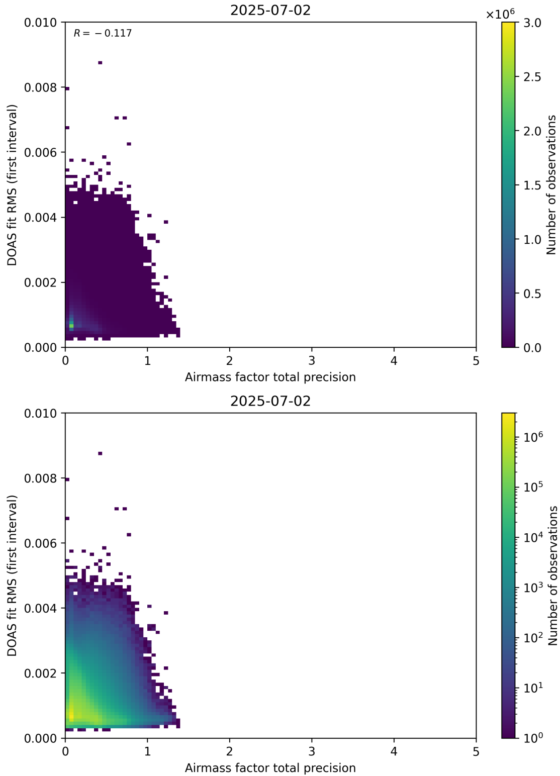
Figure 105: Scatter density plot of “Airmass factor total precision” against “DOAS fit RMS (first interval)” for 2025-07-02 to 2025-07-03.
