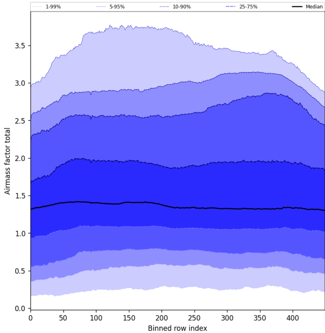
Figure 54: Along track statistics of “Airmass factor total” for 2025-07-02 to 2025-07-03
