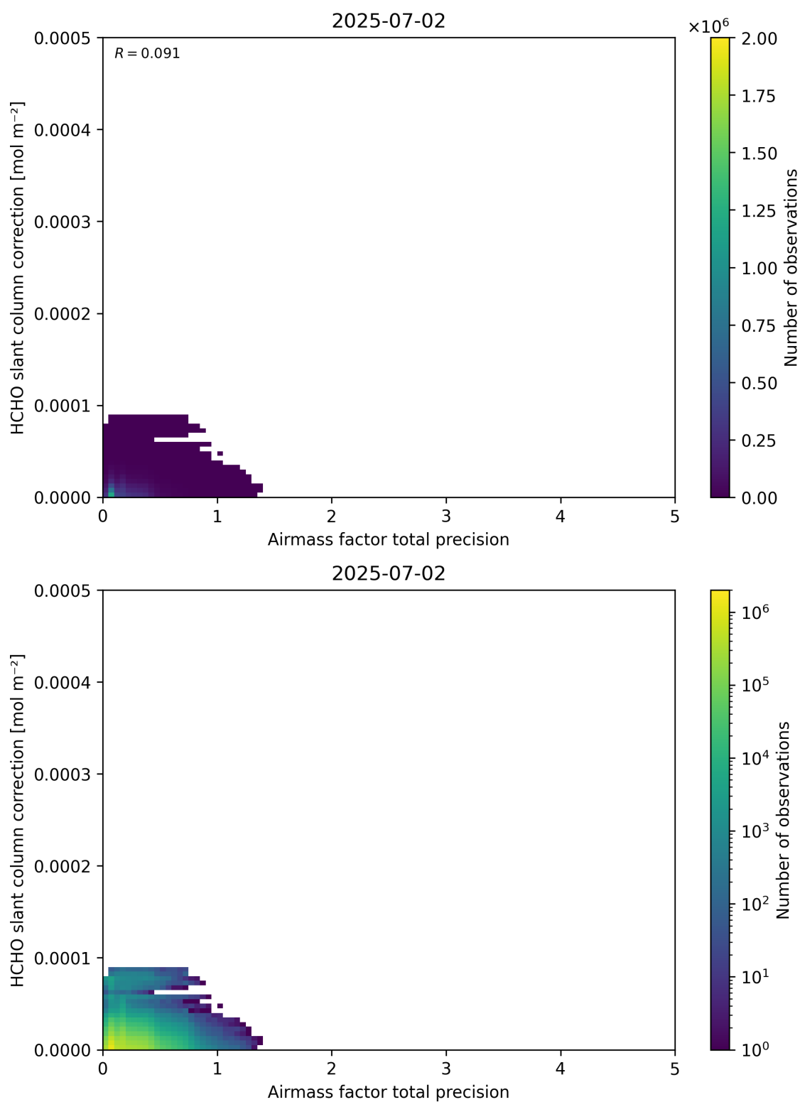
Figure 110: Scatter density plot of “Airmass factor total precision” against “HCHO slant column correction” for 2025-07-02 to 2025-07-03.
