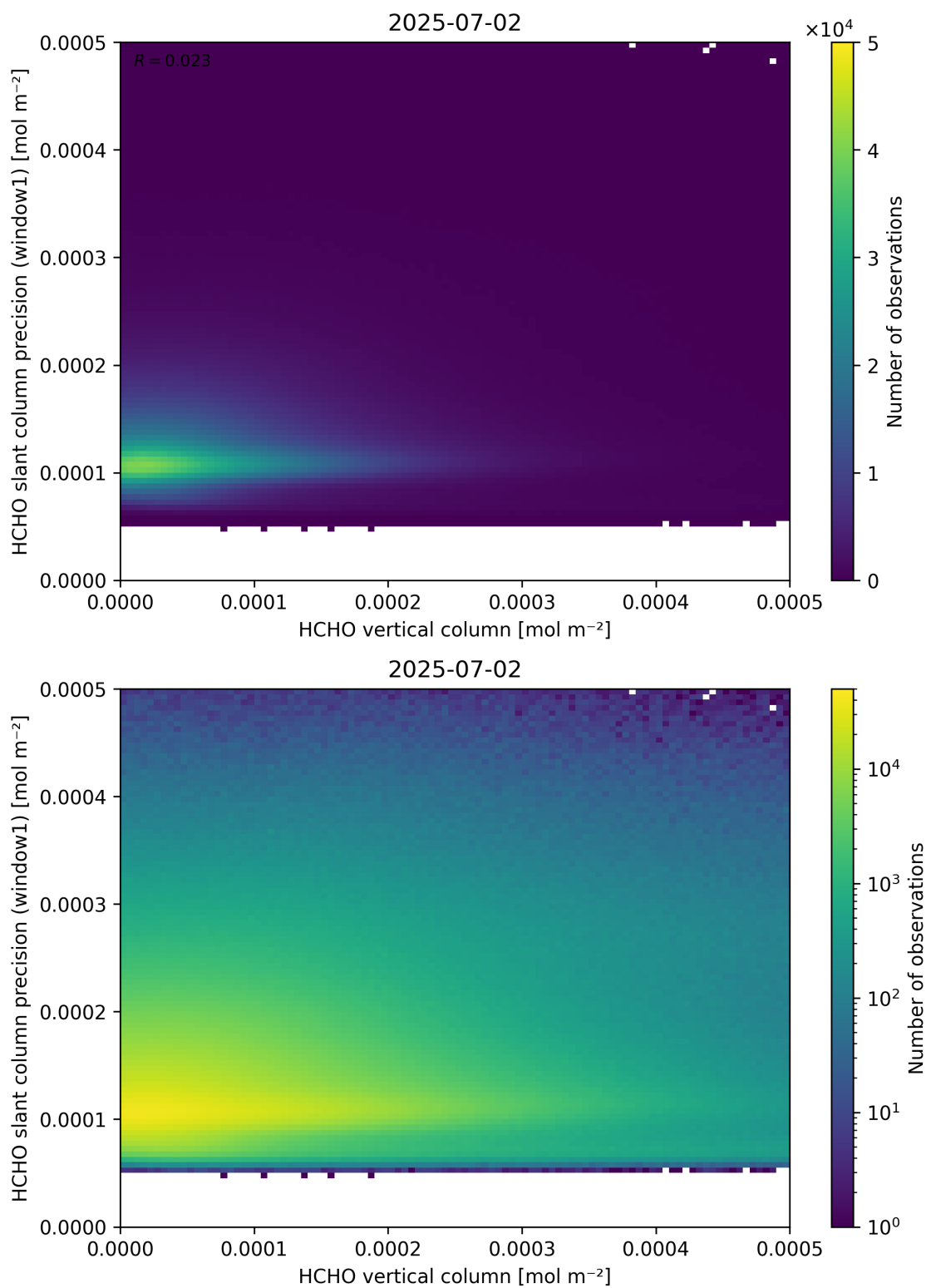
Figure 130: Scatter density plot of “HCHO vertical column” against “HCHO slant column precision (window1)” for 2025-07-02 to 2025-07-03.
