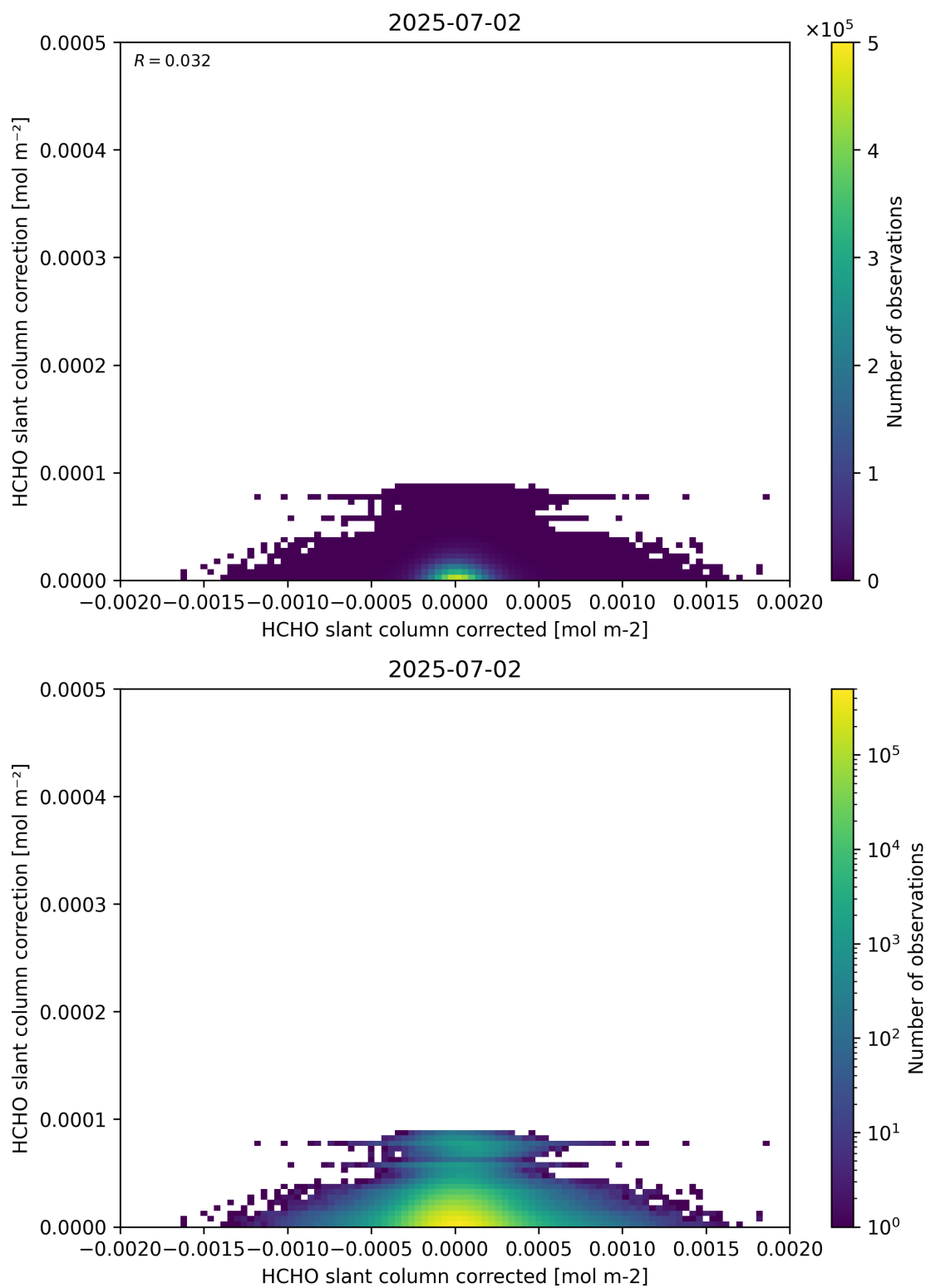
Figure 77: Scatter density plot of “HCHO slant column corrected” against “HCHO slant column correction” for 2025-07-02 to 2025-07-03.
