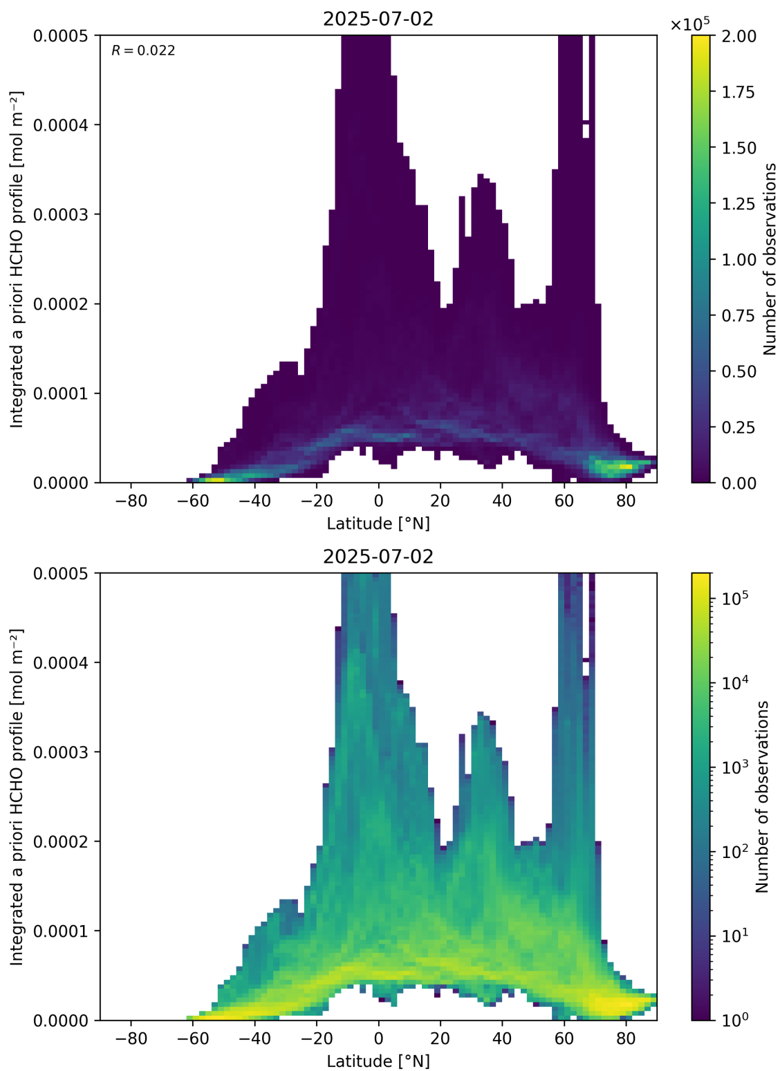
Figure 166: Scatter density plot of “Latitude” against “Integrated a priori HCHO profile” for 2025-07-02 to 2025-07-03.
