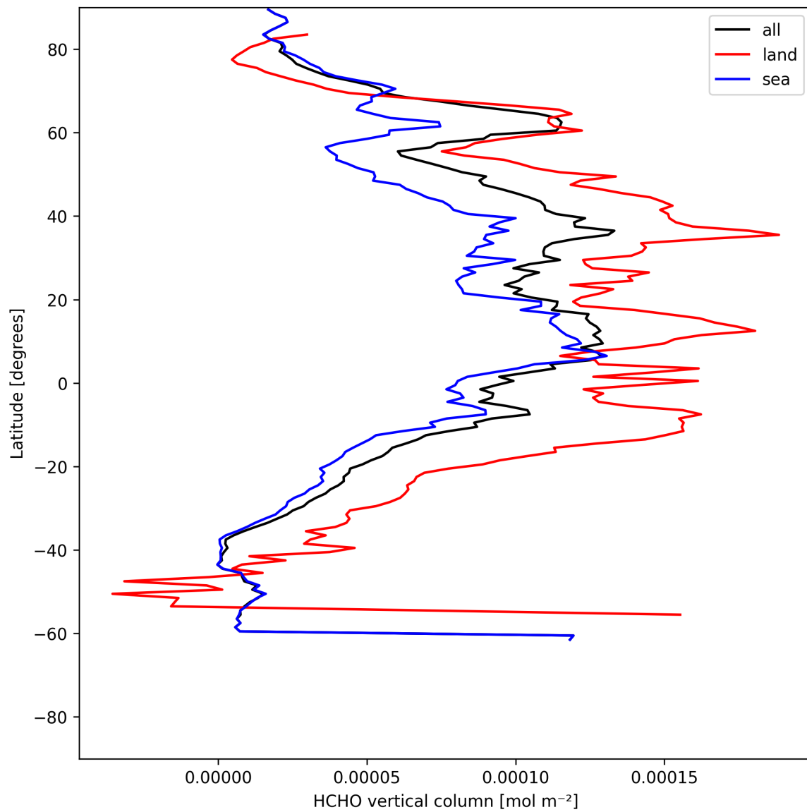
Figure 21: Zonal average of “HCHO vertical column” for 2025-07-02 to 2025-07-03.
