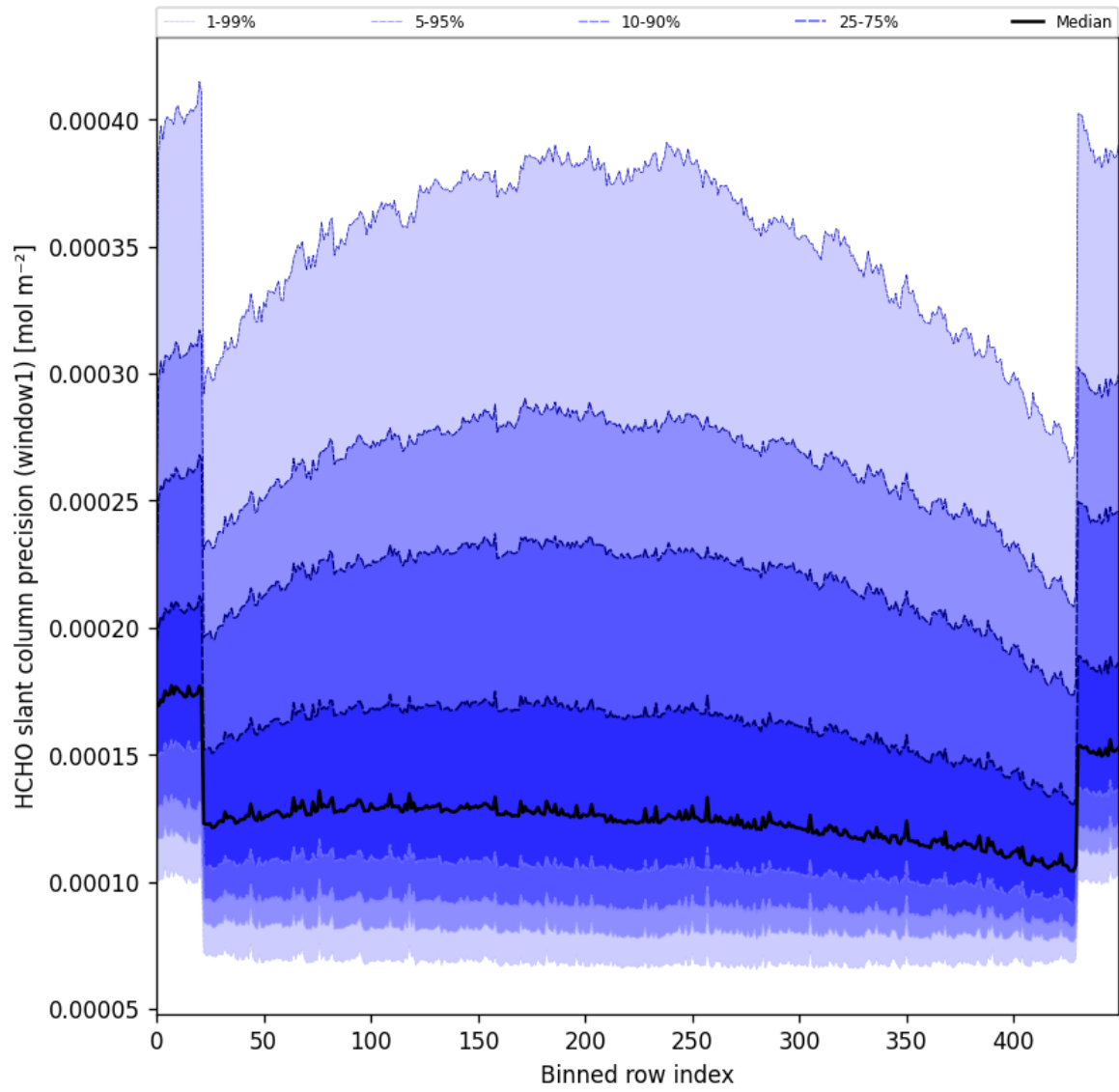
Figure 53: Along track statistics of “HCHO slant column precision (window1)” for 2025-07-02 to 2025-07-03
