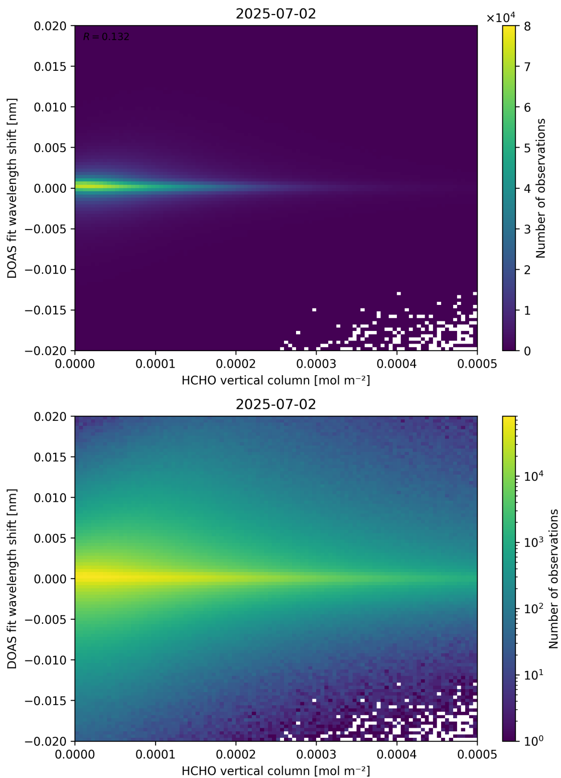
Figure 124: Scatter density plot of “HCHO vertical column” against “DOAS fit wavelength shift” for 2025-07-02 to 2025-07-03.
