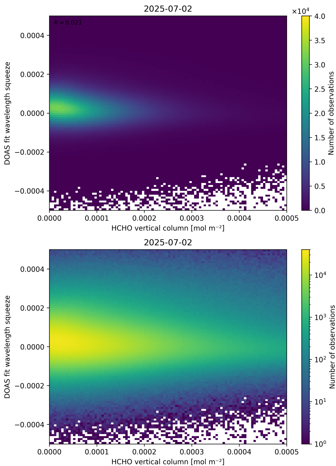
Figure 125: Scatter density plot of “HCHO vertical column” against “DOAS fit wavelength squeeze” for 2025-07-02 to 2025-07-03.
