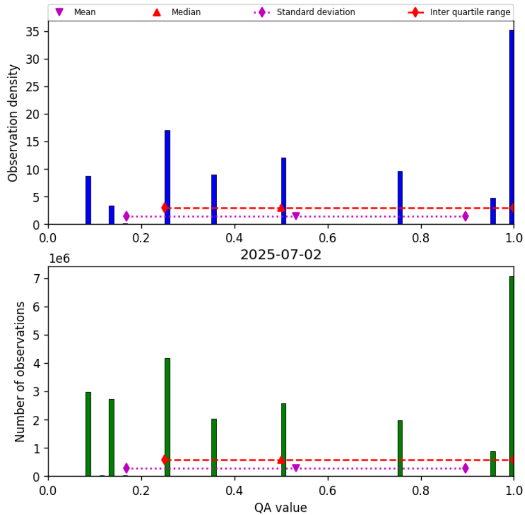
Figure 34: Histogram of “QA value” for 2025-07-02 to 2025-07-03
