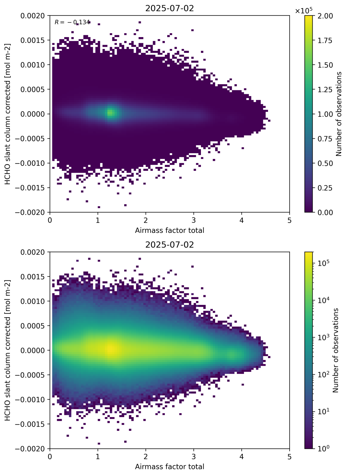
Figure 101: Scatter density plot of “Airmass factor total” against “HCHO slant column corrected” for 2025-07-02 to 2025-07-03.
