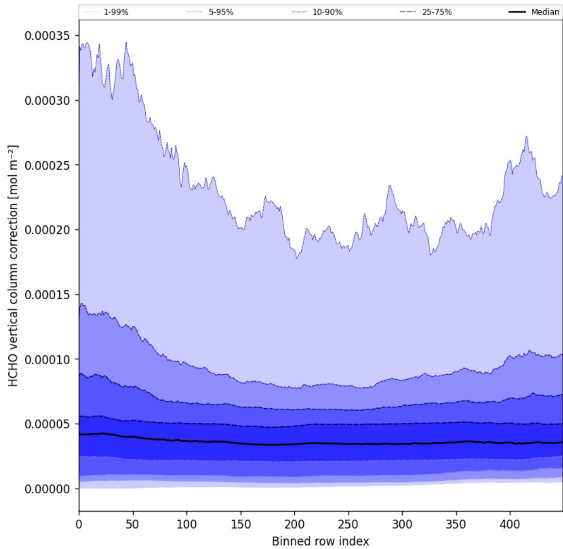
Figure 51: Along track statistics of “HCHO vertical column correction” for 2025-07-02 to 2025-07-03
