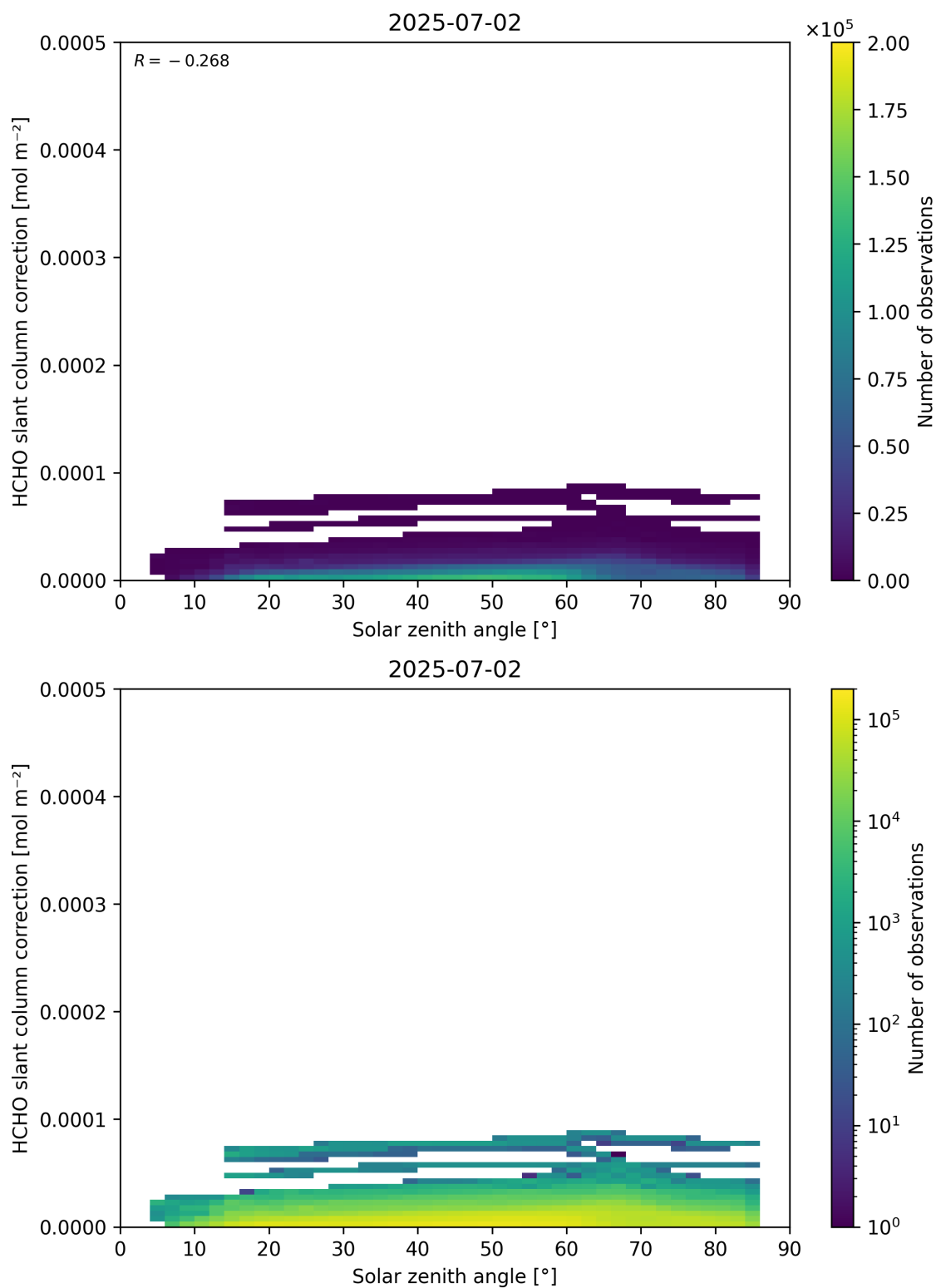
Figure 172: Scatter density plot of “Solar zenith angle” against “HCHO slant column correction” for 2025-07-02 to 2025-07-03.
