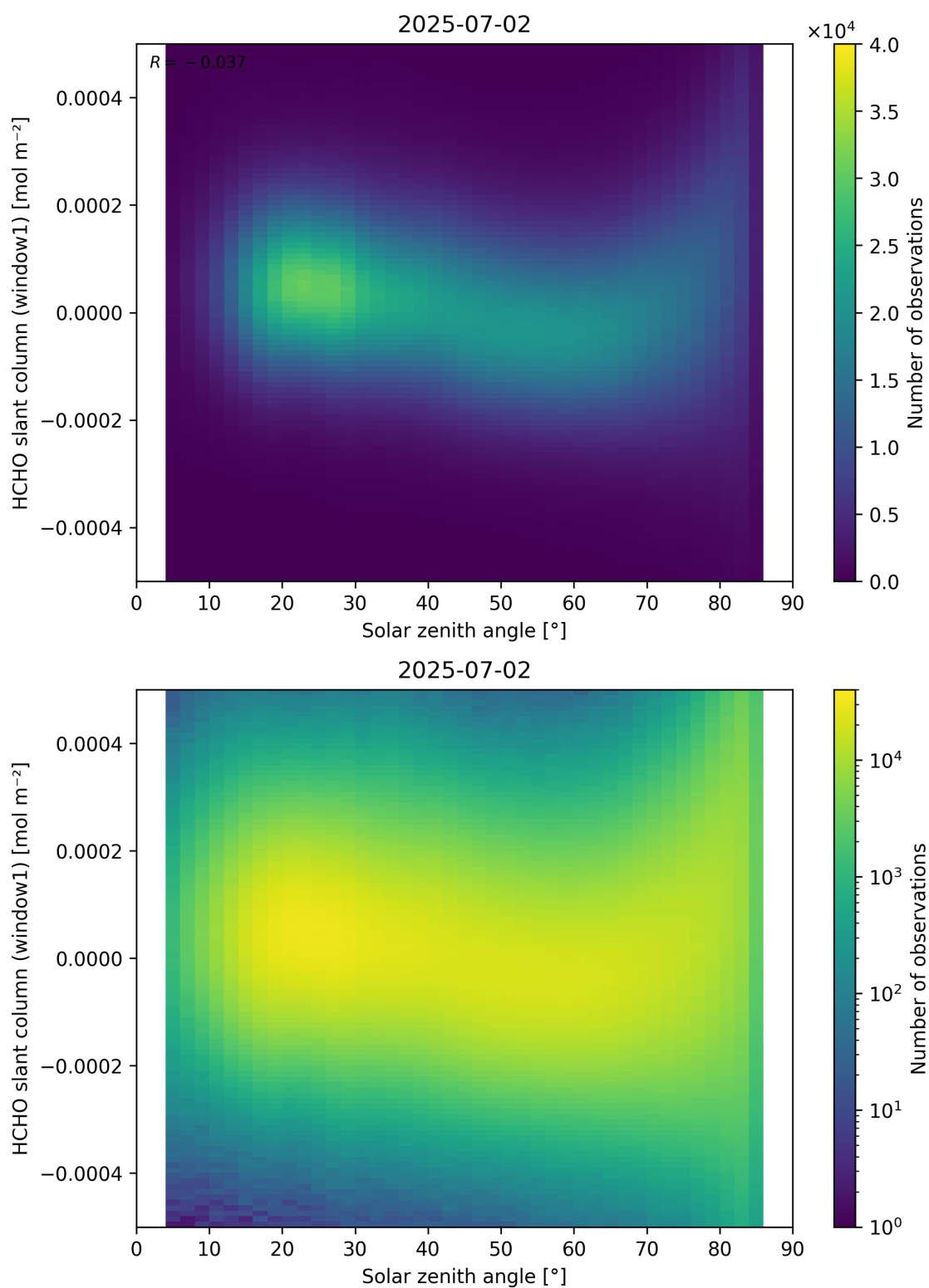
Figure 173: Scatter density plot of “Solar zenith angle” against “HCHO slant column (window1)” for 2025-07-02 to 2025-07-03.
