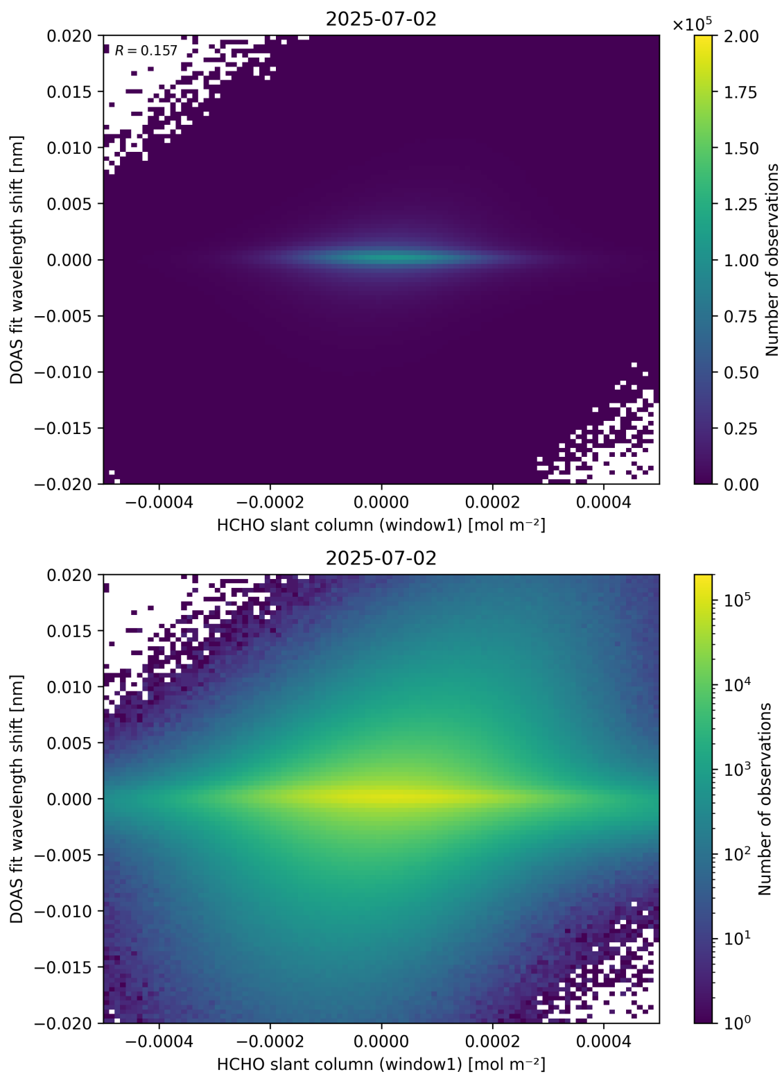
Figure 79: Scatter density plot of “HCHO slant column (window1)” against “DOAS fit wavelength shift” for 2025-07-02 to 2025-07-03.
