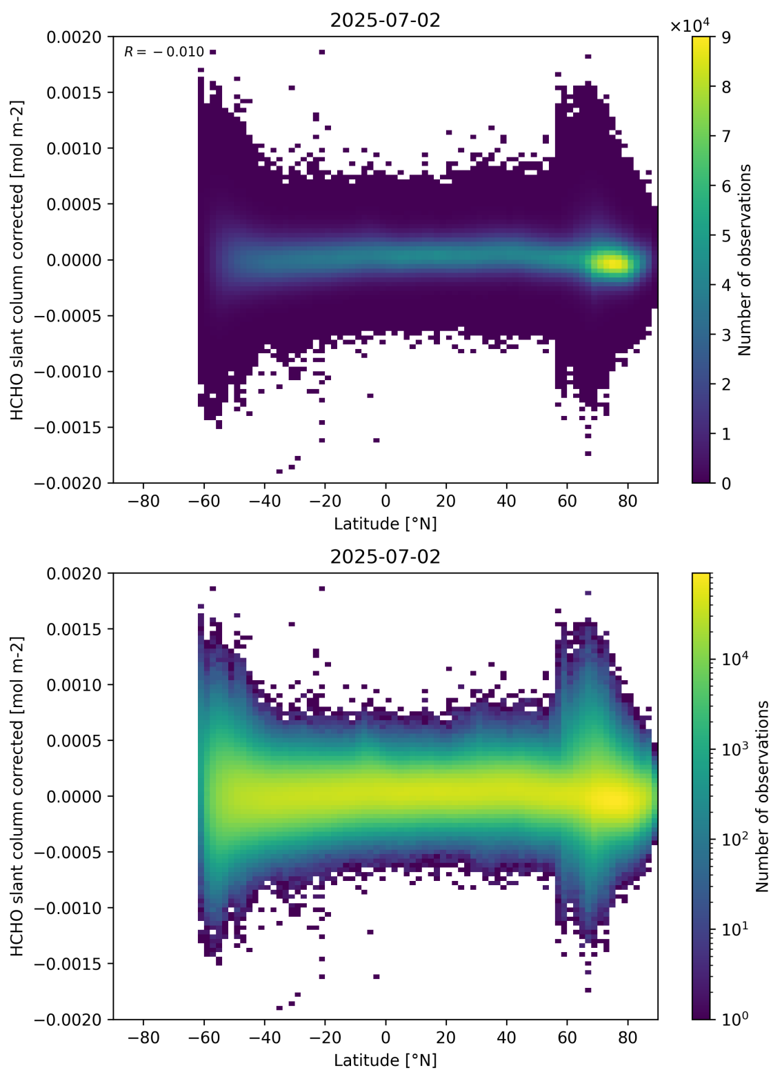
Figure 157: Scatter density plot of “Latitude” against “HCHO slant column corrected” for 2025-07-02 to 2025-07-03.
