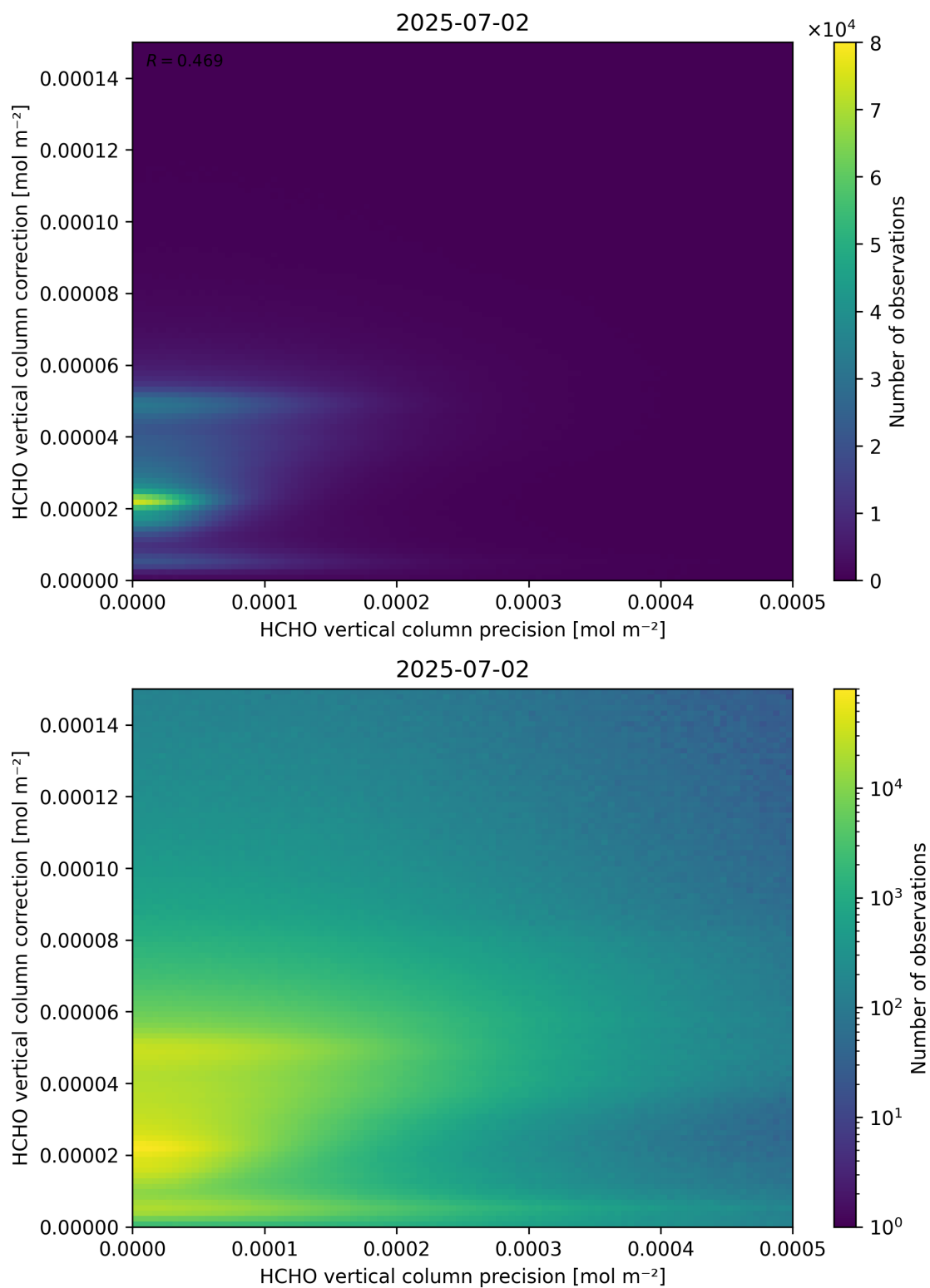
Figure 146: Scatter density plot of “HCHO vertical column precision” against “HCHO vertical column correction” for 2025-07-02 to 2025-07-03.
