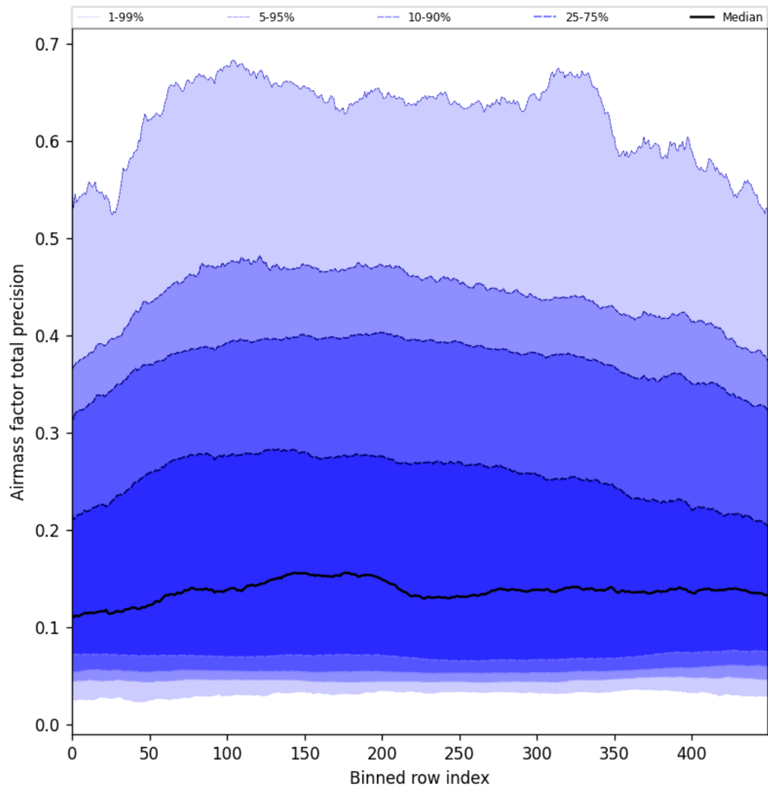
Figure 55: Along track statistics of “Airmass factor total precision” for 2025-07-02 to 2025-07-03
