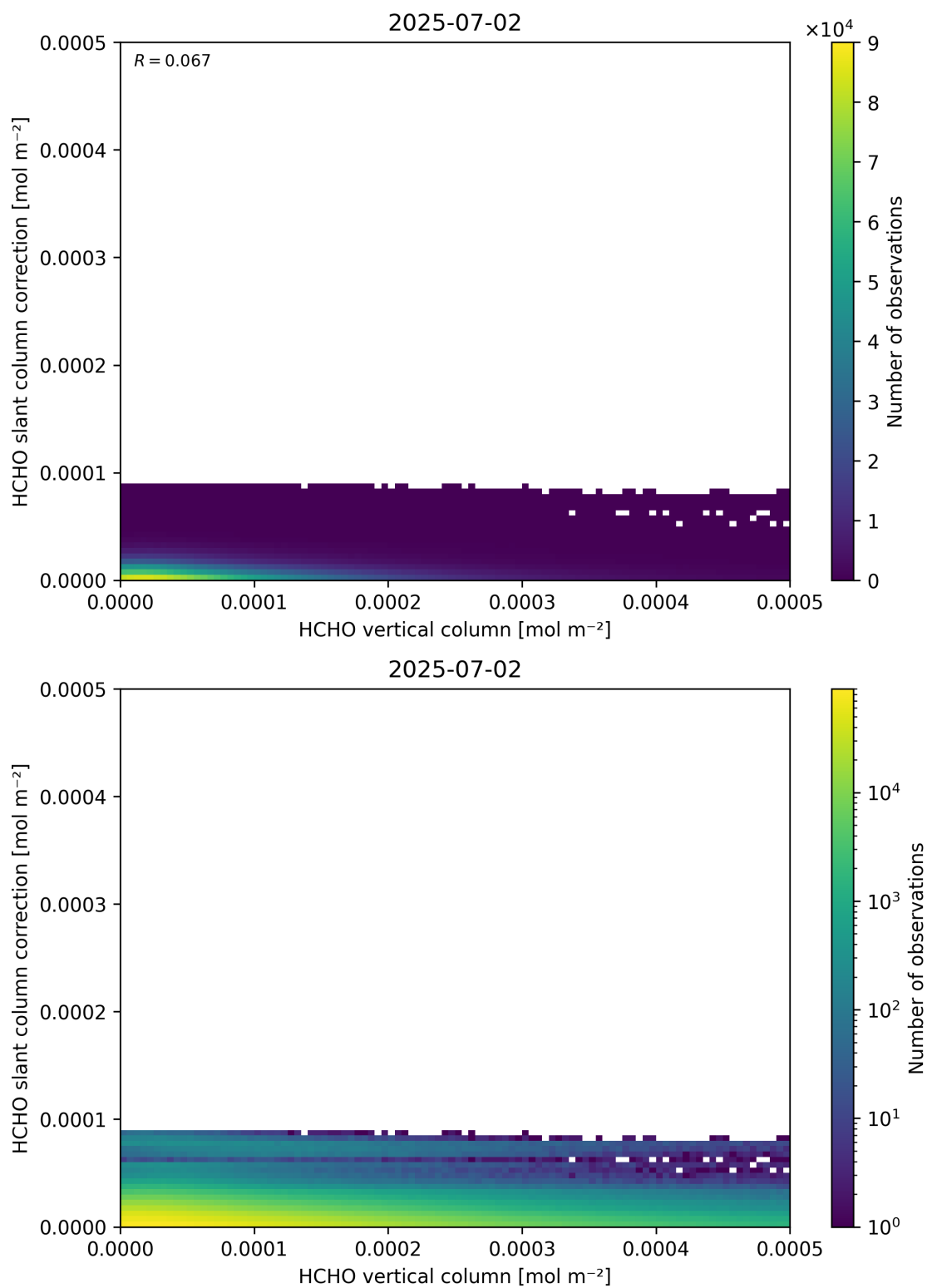
Figure 128: Scatter density plot of “HCHO vertical column” against “HCHO slant column correction” for 2025-07-02 to 2025-07-03.
