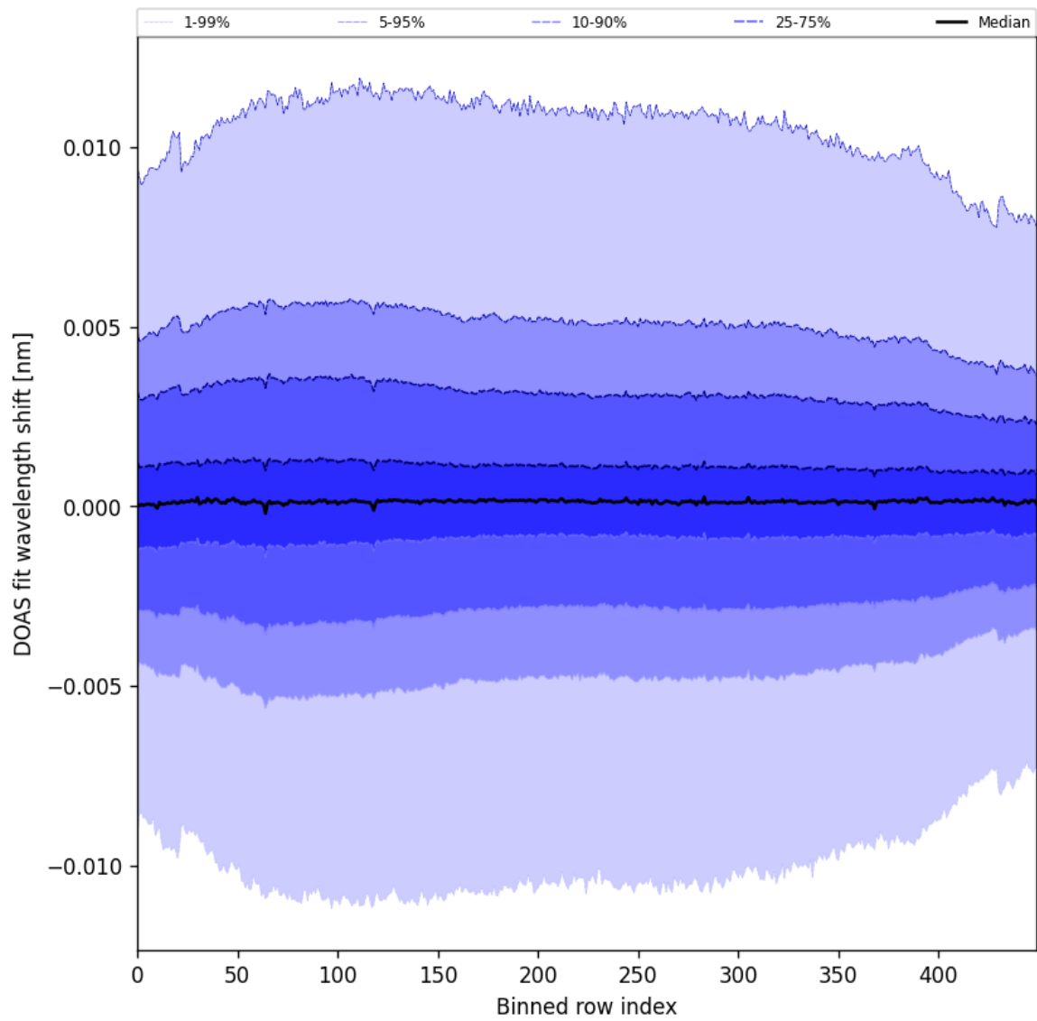
Figure 58: Along track statistics of “DOAS fit wavelength shift” for 2025-07-02 to 2025-07-03
