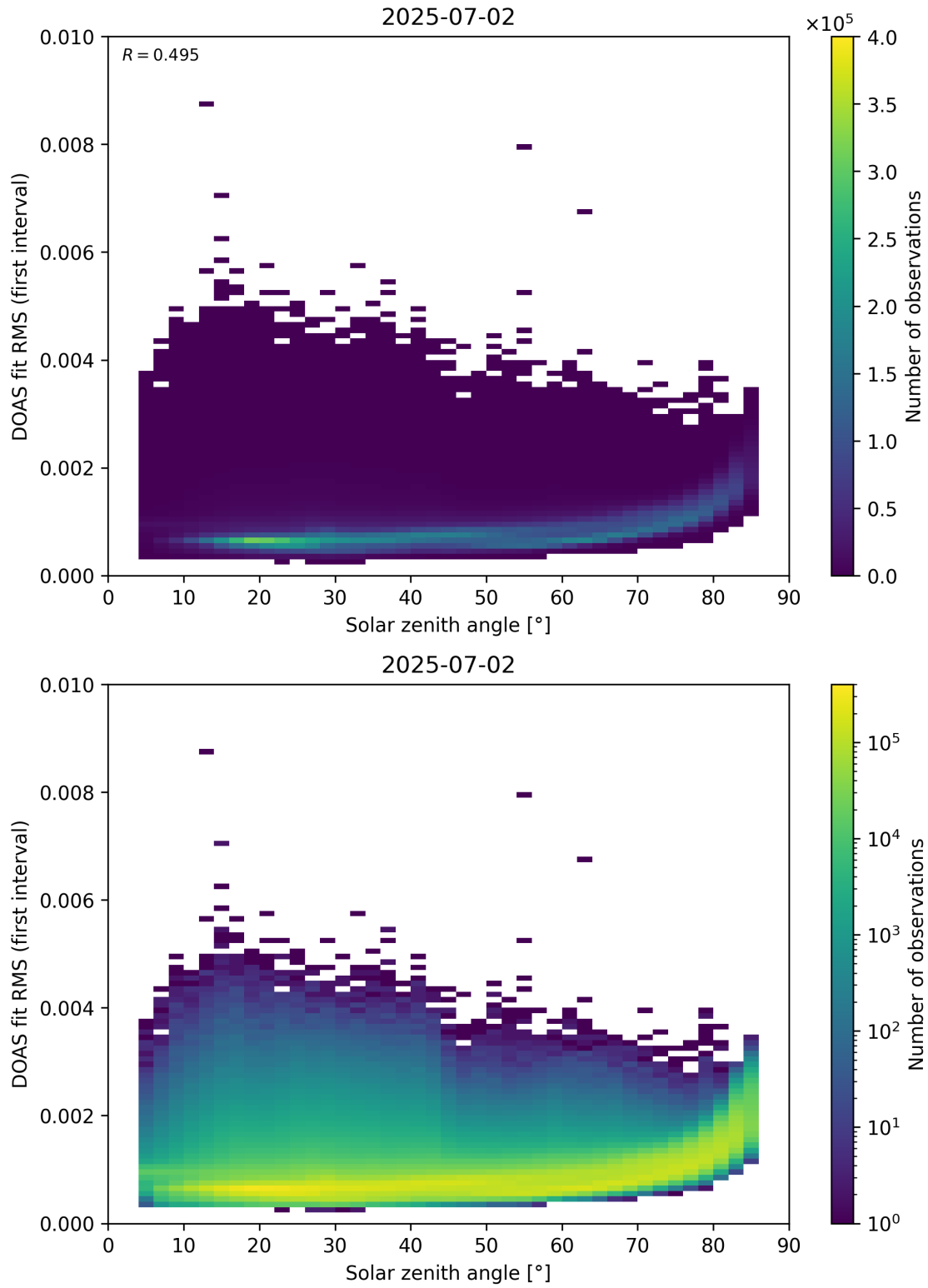
Figure 167: Scatter density plot of “Solar zenith angle” against “DOAS fit RMS (first interval)” for 2025-07-02 to 2025-07-03.
