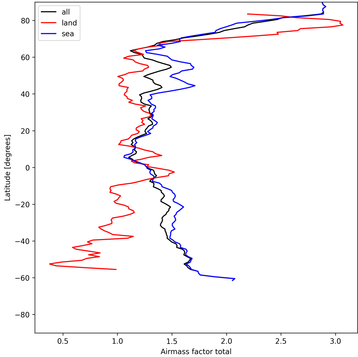
Figure 26: Zonal average of “Airmass factor total” for 2025-07-02 to 2025-07-03.
