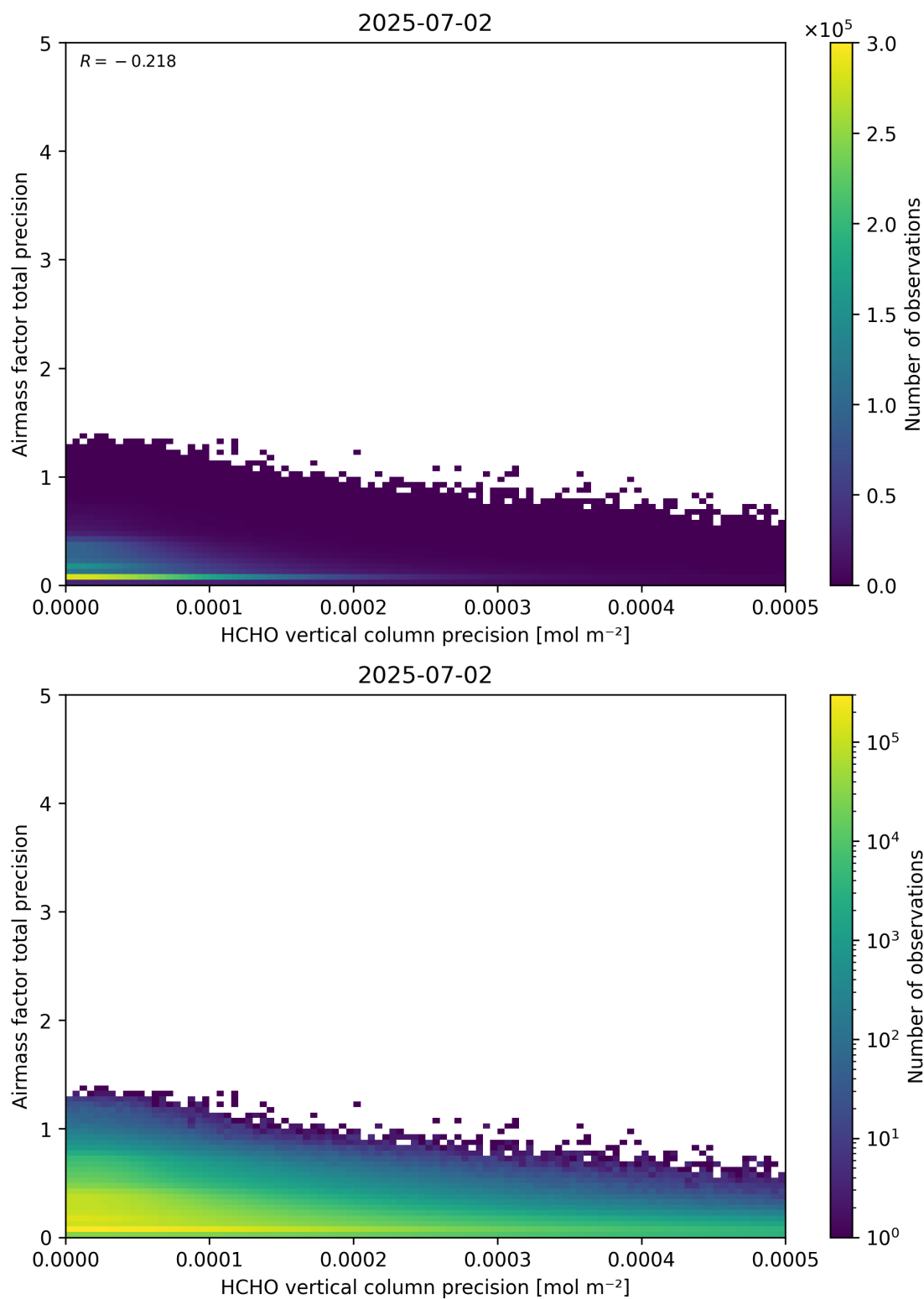
Figure 145: Scatter density plot of “HCHO vertical column precision” against “Airmass factor total precision” for 2025-07-02 to 2025-07-03.
