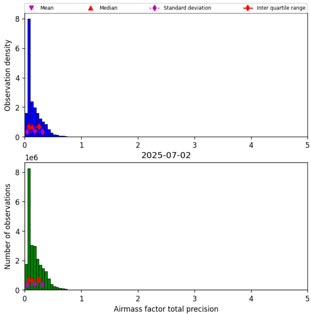
Figure 41: Histogram of “Airmass factor total precision” for 2025-07-02 to 2025-07-03
