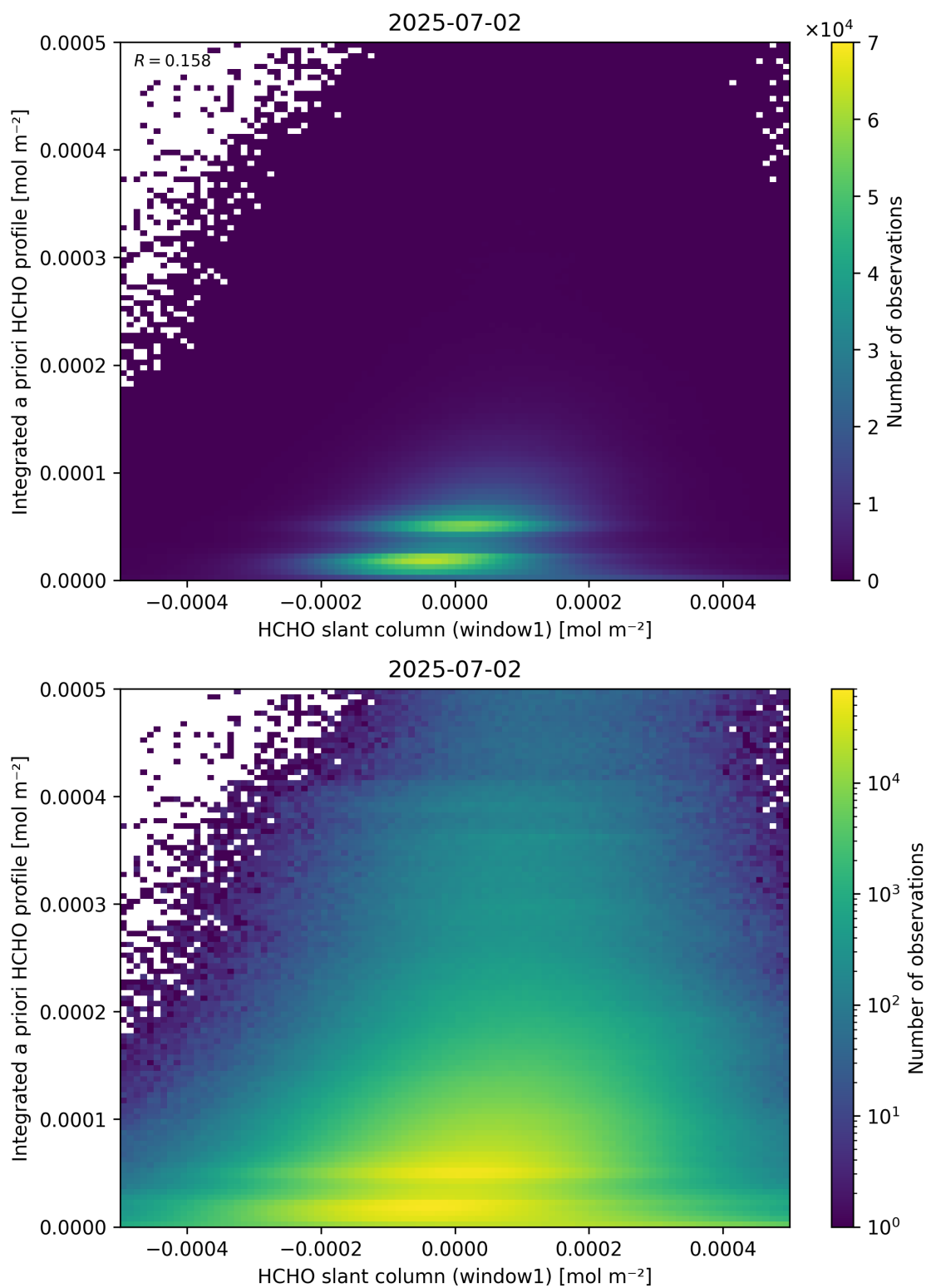
Figure 87: Scatter density plot of “HCHO slant column (window1)” against “Integrated a priori HCHO profile” for 2025-07-02 to 2025-07-03.
