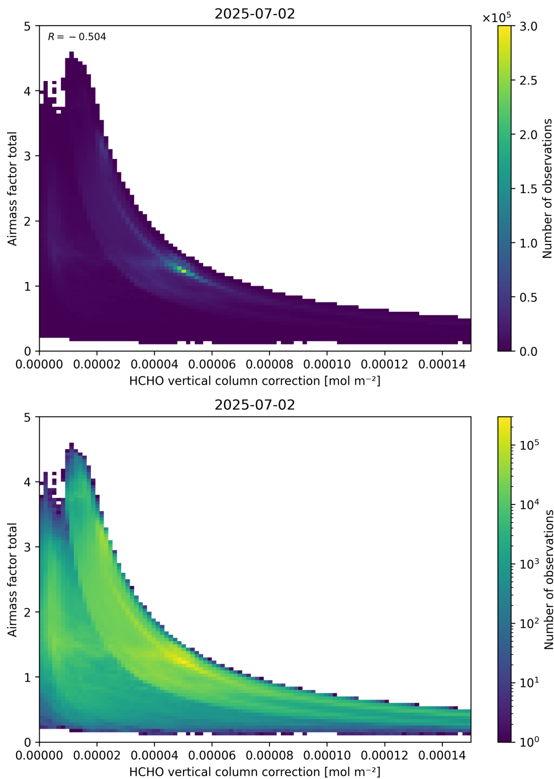
Figure 120: Scatter density plot of “HCHO vertical column correction” against “Airmass factor total” for 2025-07-02 to 2025-07-03.
