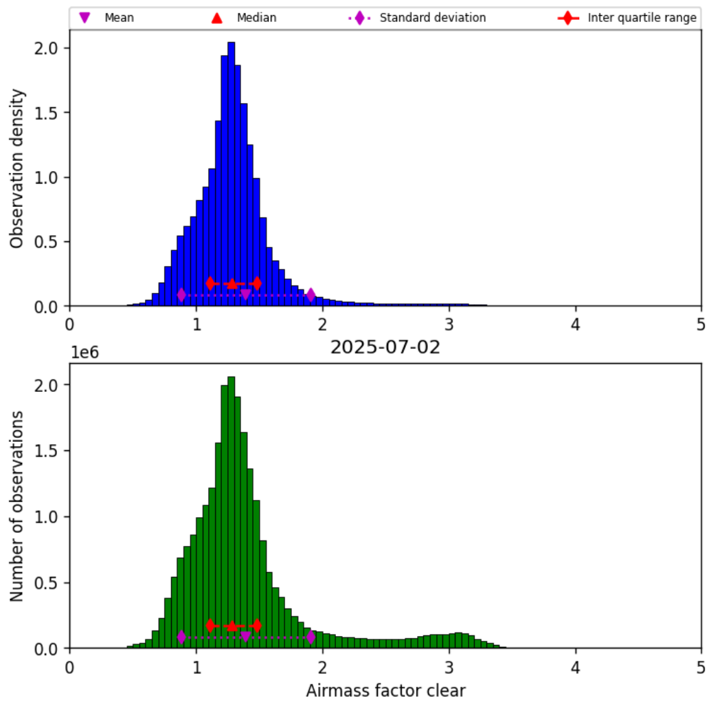
Figure 42: Histogram of “Airmass factor clear” for 2025-07-02 to 2025-07-03
