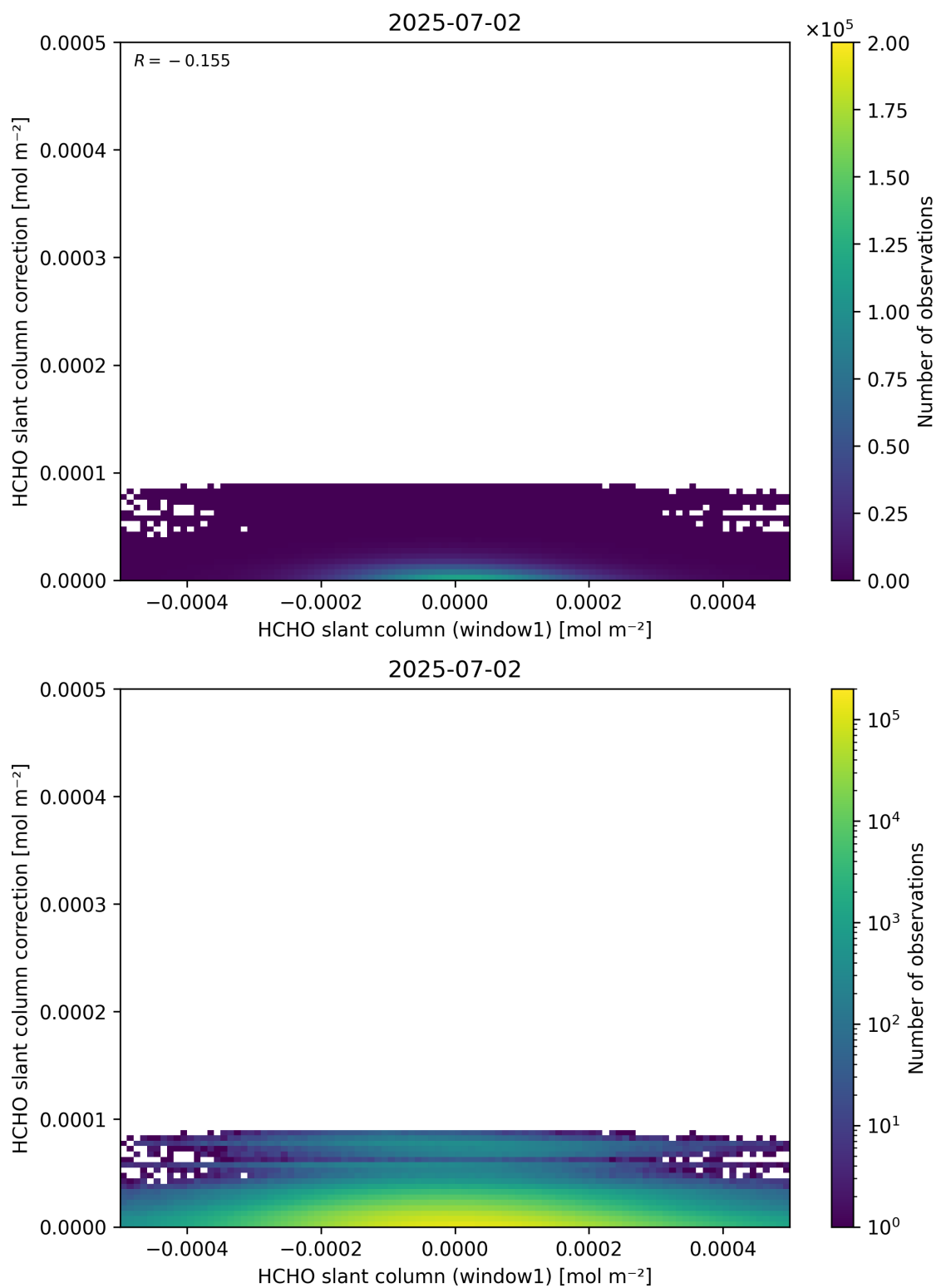
Figure 83: Scatter density plot of “HCHO slant column (window1)” against “HCHO slant column correction” for 2025-07-02 to 2025-07-03.
