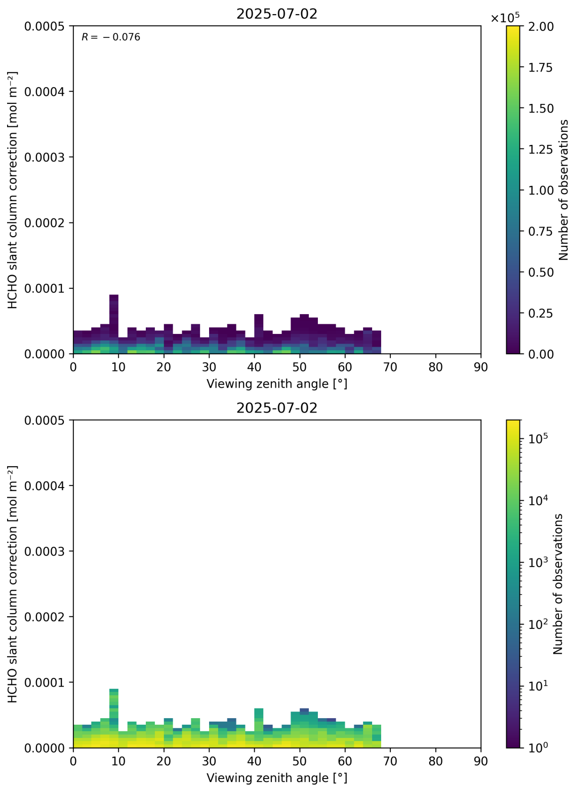
Figure 187: Scatter density plot of “Viewing zenith angle” against “HCHO slant column correction” for 2025-07-02 to 2025-07-03.
