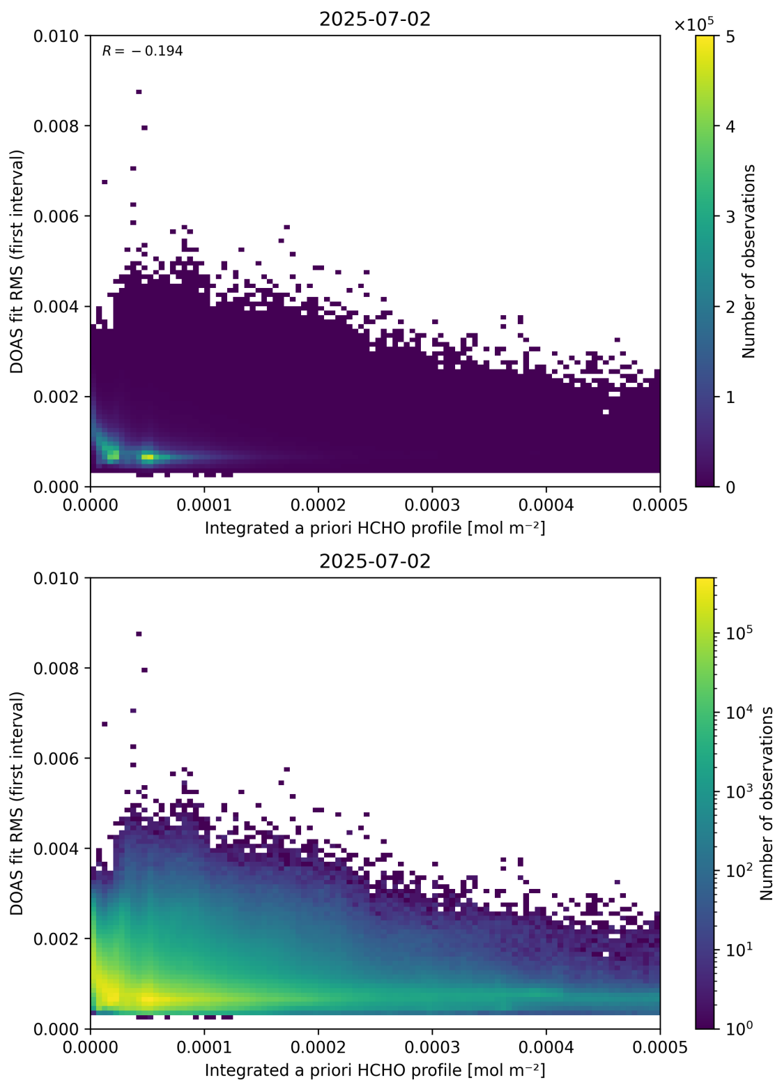
Figure 148: Scatter density plot of “Integrated a priori HCHO profile” against “DOAS fit RMS (first interval)” for 2025-07-02 to 2025-07-03.
