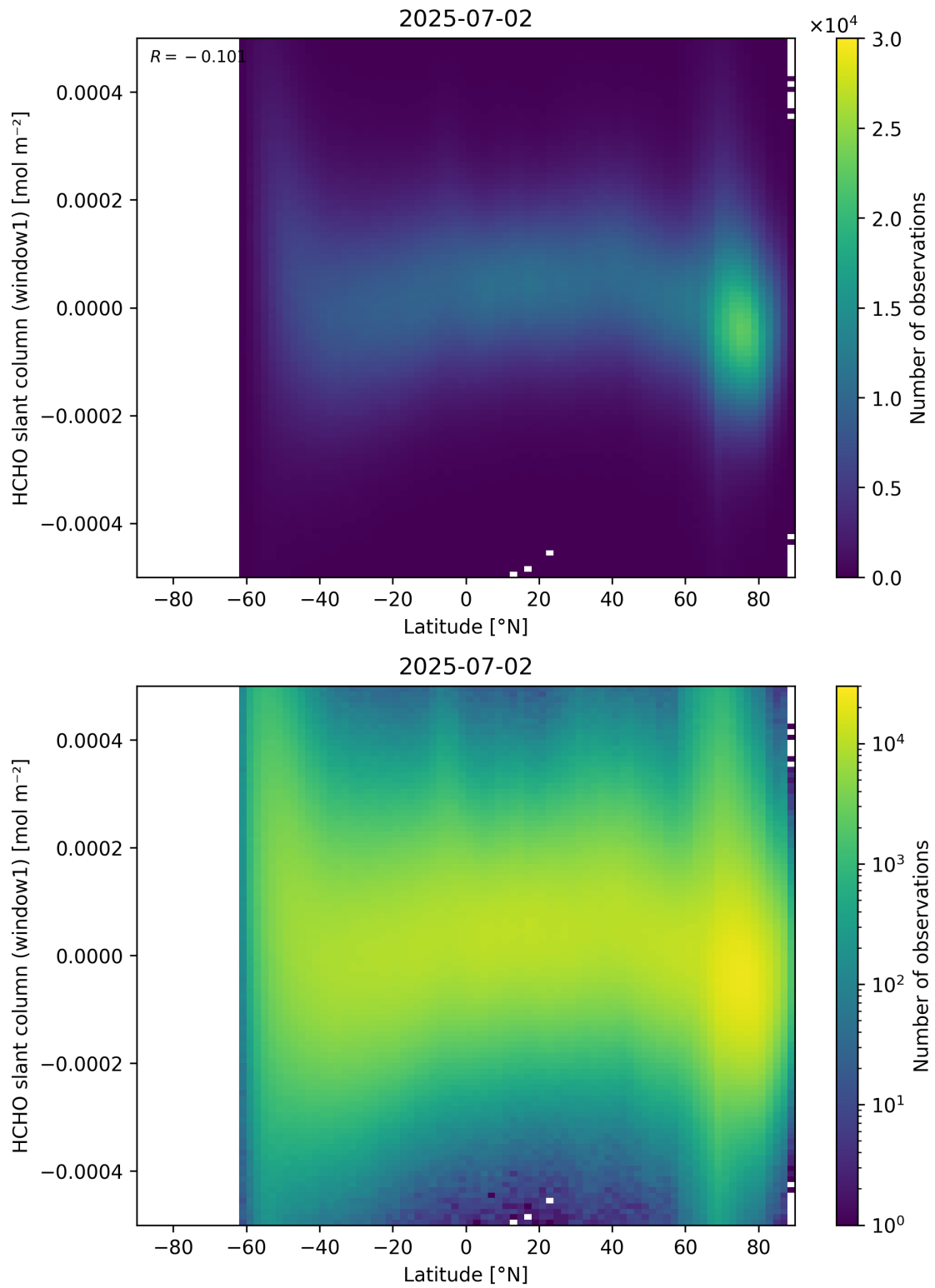
Figure 159: Scatter density plot of “Latitude” against “HCHO slant column (window1)” for 2025-07-02 to 2025-07-03.
