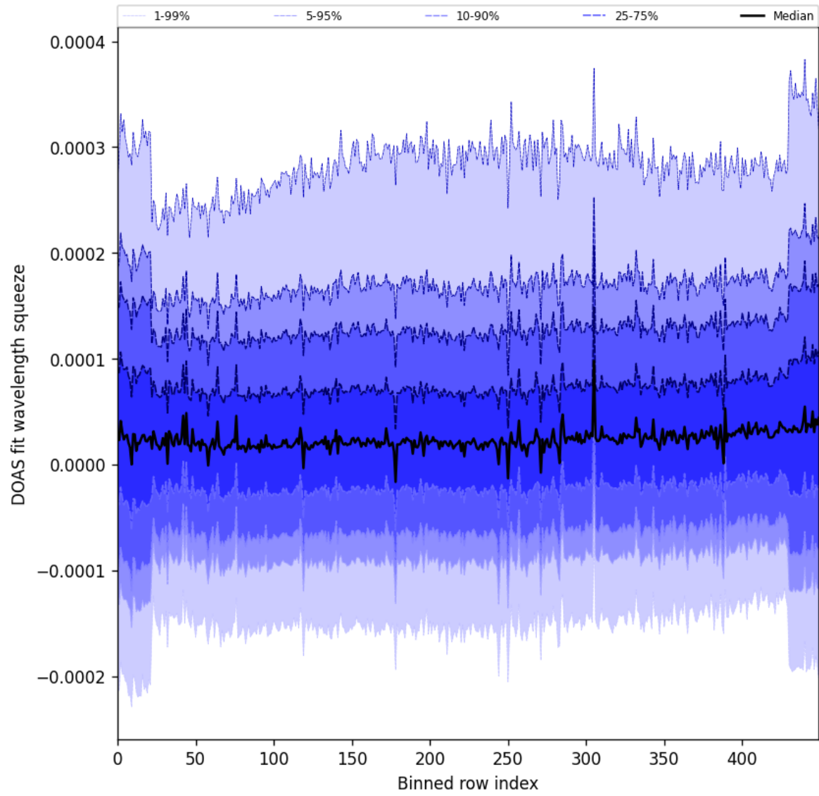
Figure 59: Along track statistics of “DOAS fit wavelength squeeze” for 2025-07-02 to 2025-07-03
