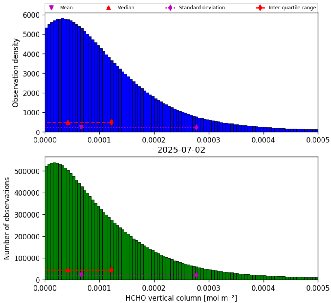
Figure 35: Histogram of “HCHO vertical column” for 2025-07-02 to 2025-07-03
