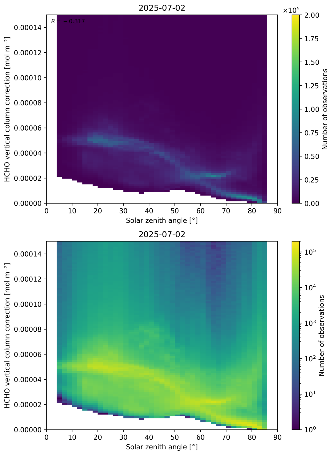
Figure 178: Scatter density plot of “Solar zenith angle” against “HCHO vertical column correction” for 2025-07-02 to 2025-07-03.
