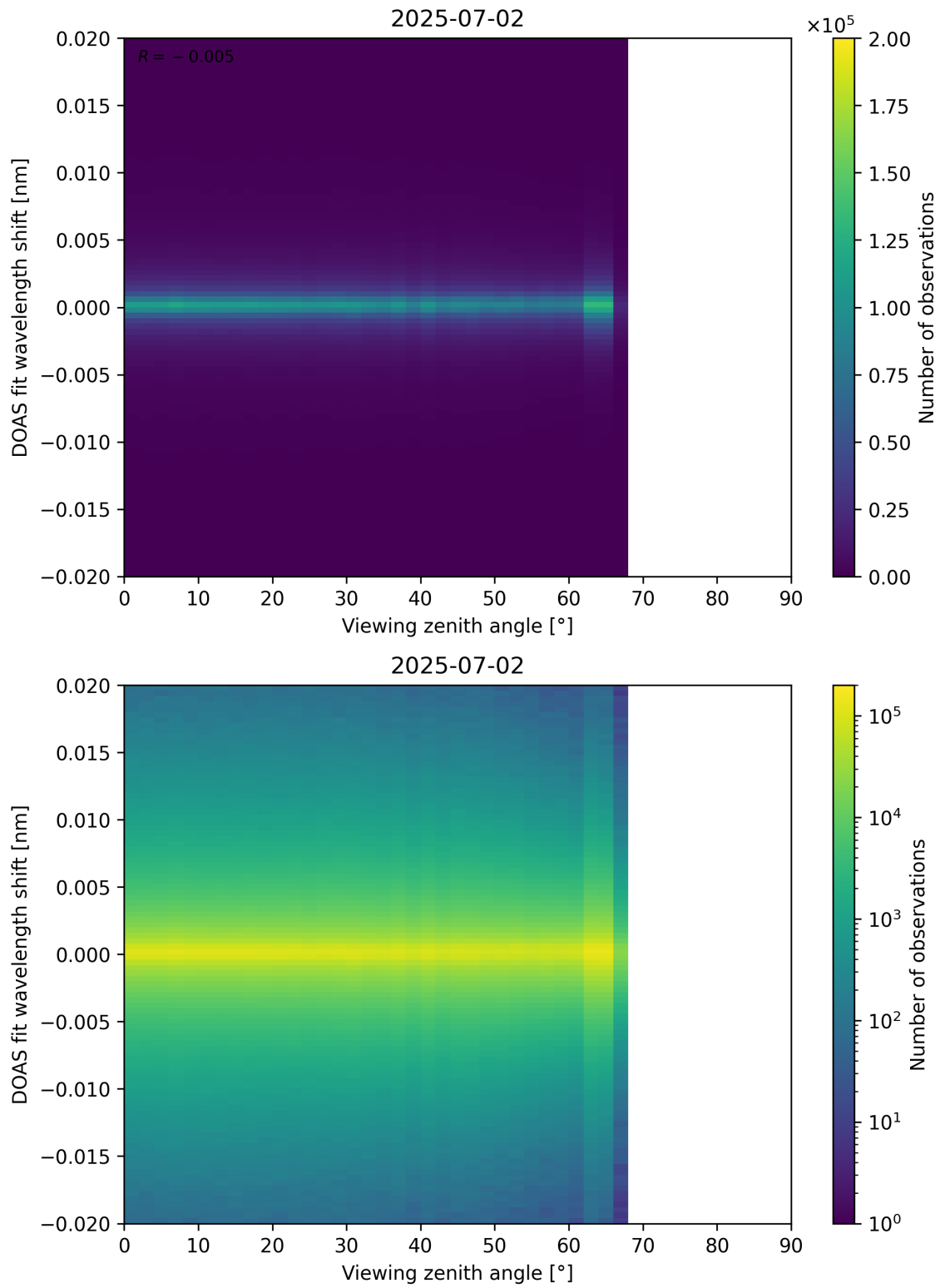
Figure 183: Scatter density plot of “Viewing zenith angle” against “DOAS fit wavelength shift” for 2025-07-02 to 2025-07-03.
