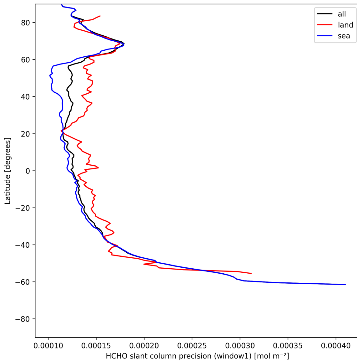
Figure 25: Zonal average of "HCHO slant column precision (window1)" for 2025-07-02 to 2025-07-03.
