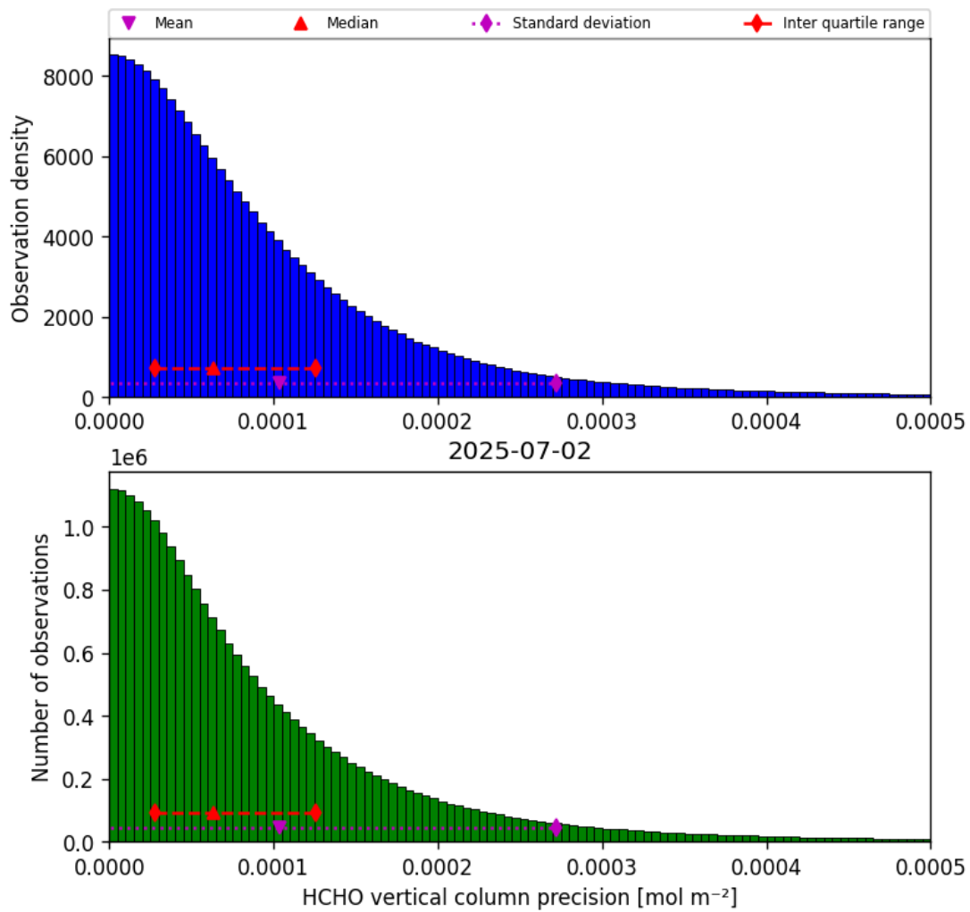
Figure 36: Histogram of “HCHO vertical column precision” for 2025-07-02 to 2025-07-03
