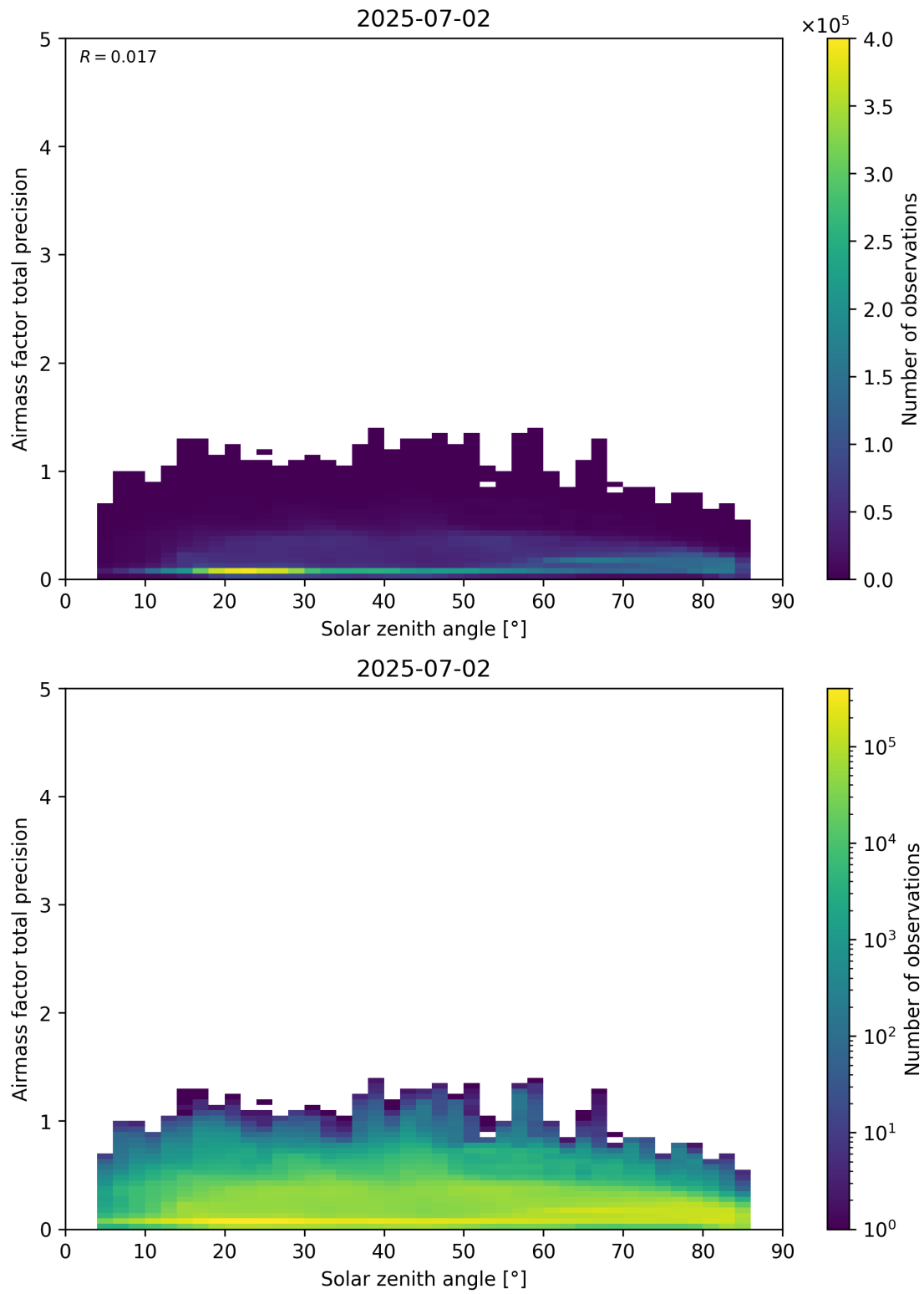
Figure 176: Scatter density plot of “Solar zenith angle” against “Airmass factor total precision” for 2025-07-02 to 2025-07-03.
