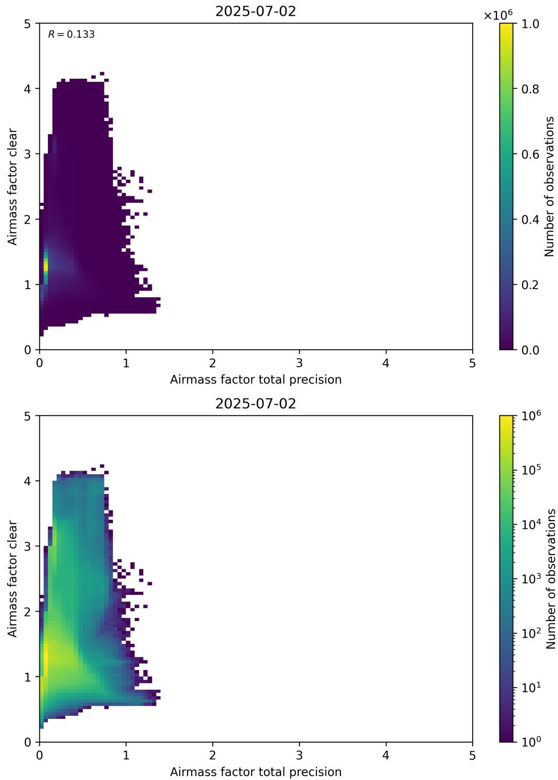
Figure 108: Scatter density plot of “Airmass factor total precision” against “Airmass factor clear” for 2025-07-02 to 2025-07-03.
