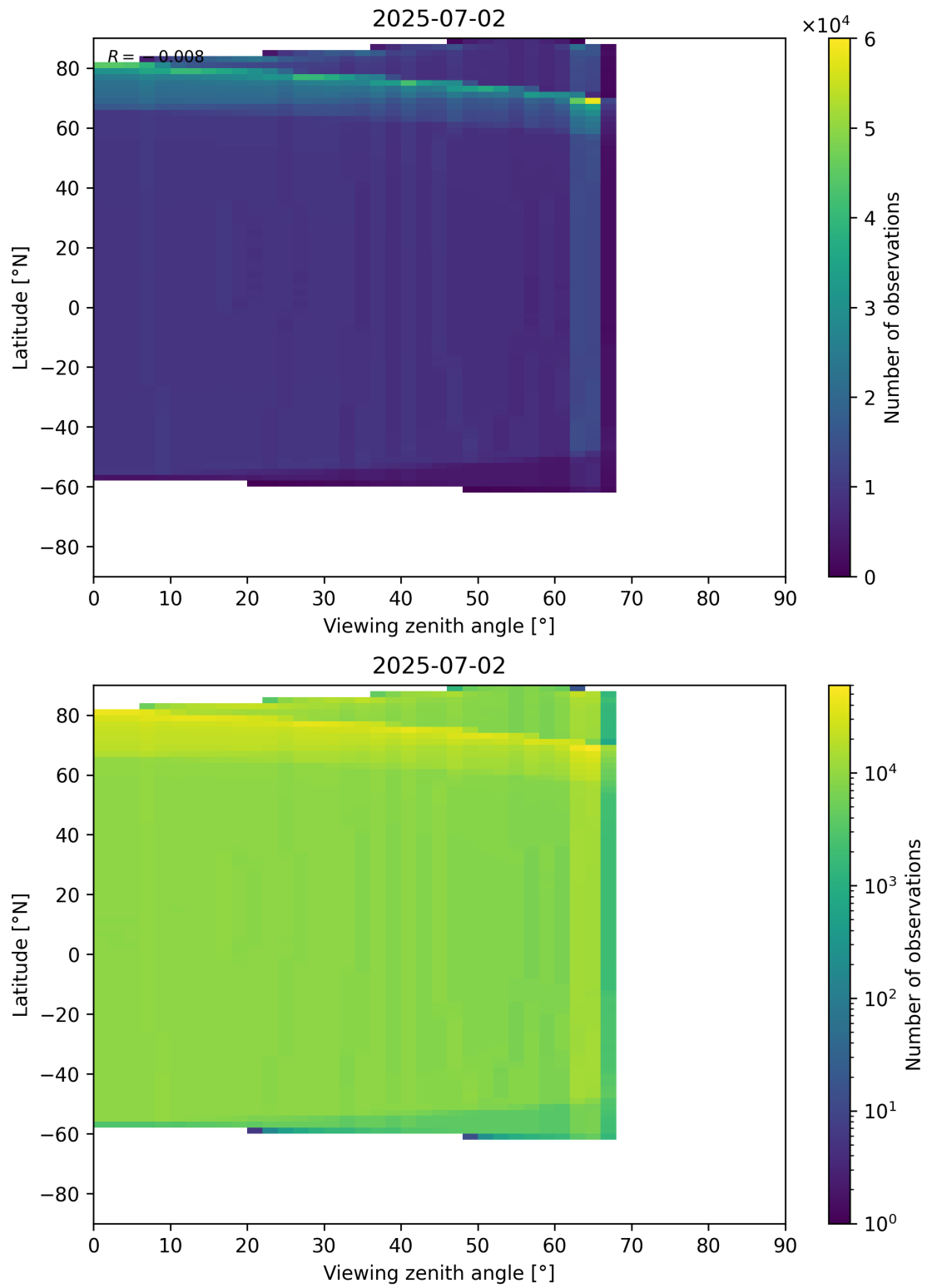
Figure 196: Scatter density plot of “Viewing zenith angle” against “Latitude” for 2025-07-02 to 2025-07-03.
