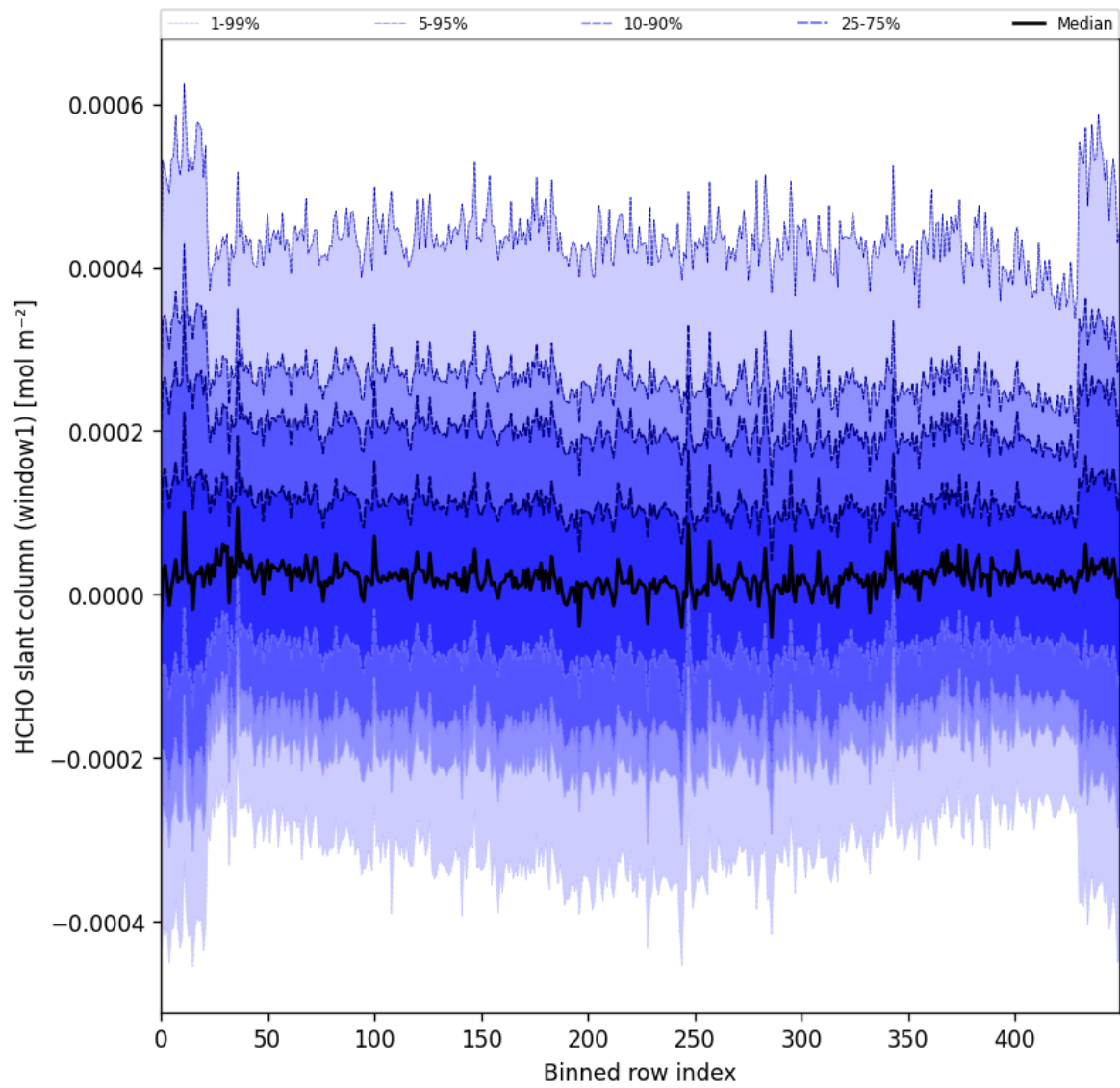
Figure 52: Along track statistics of “HCHO slant column (window1)” for 2025-07-02 to 2025-07-03
