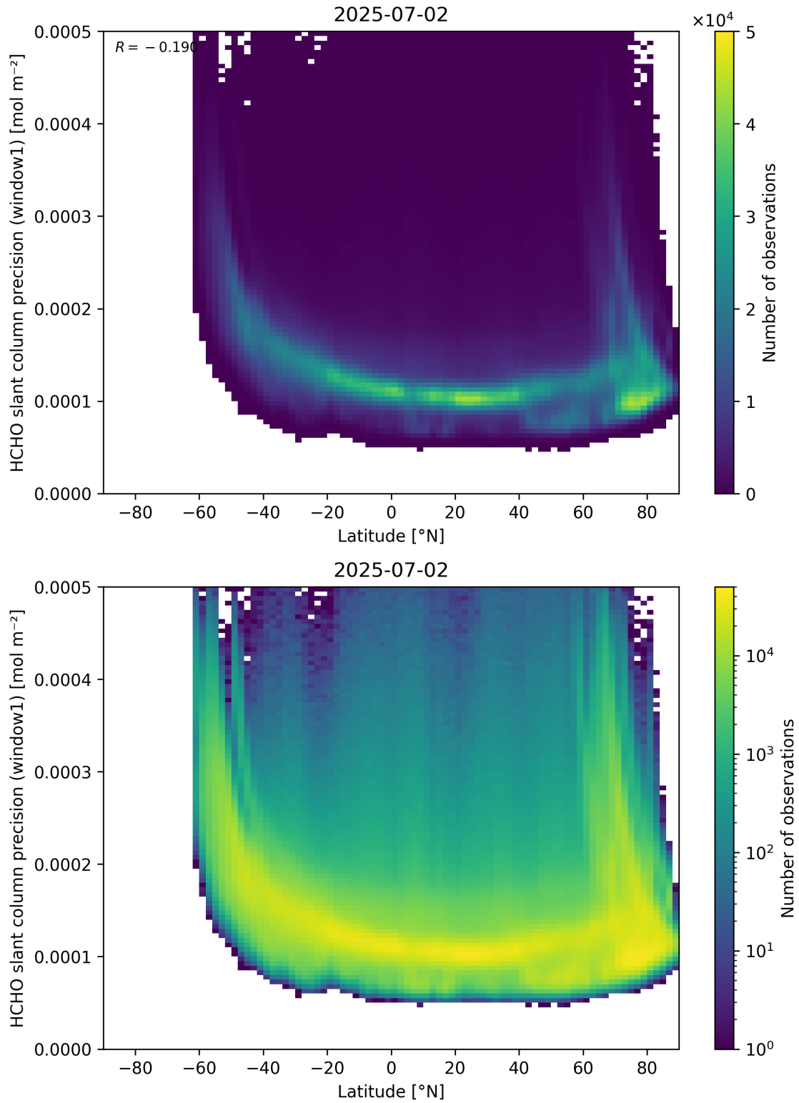
Figure 160: Scatter density plot of “Latitude” against “HCHO slant column precision (window1)” for 2025-07-02 to 2025-07-03.
