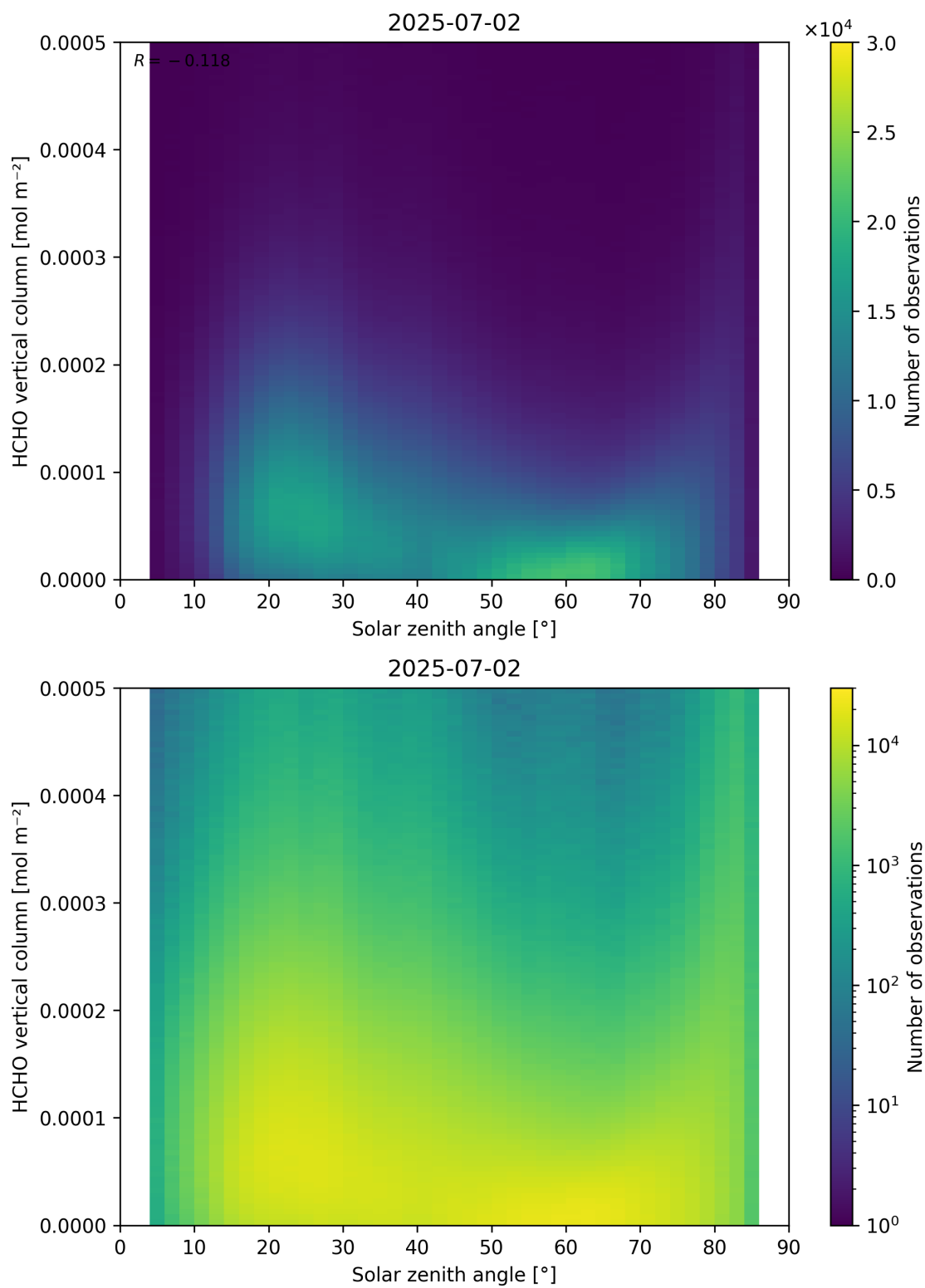
Figure 177: Scatter density plot of “Solar zenith angle” against “HCHO vertical column” for 2025-07-02 to 2025-07-03.
