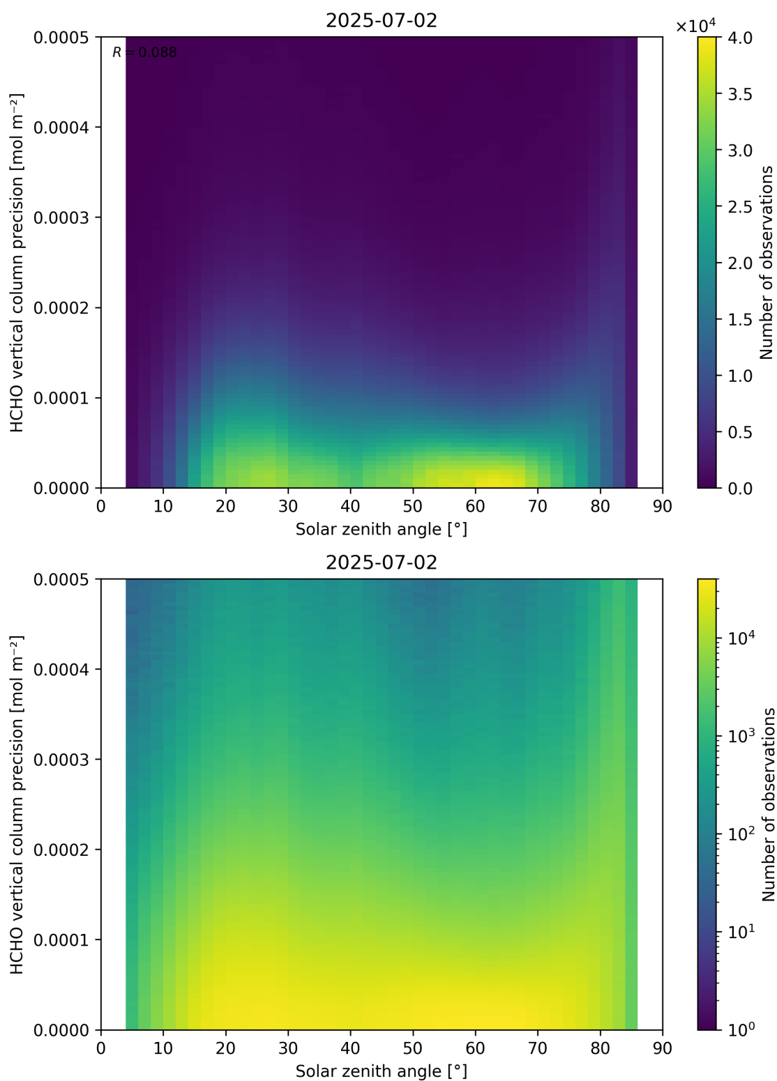
Figure 179: Scatter density plot of “Solar zenith angle” against “HCHO vertical column precision” for 2025-07-02 to 2025-07-03.
