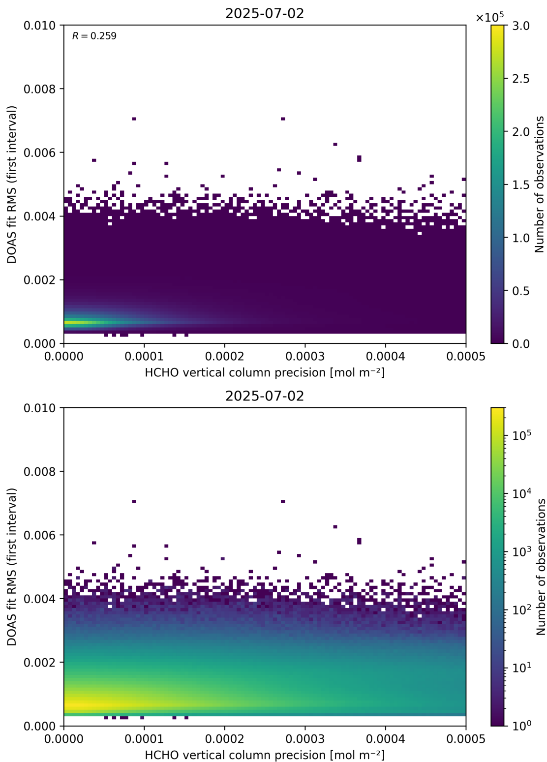
Figure 136: Scatter density plot of “HCHO vertical column precision” against “DOAS fit RMS (first interval)” for 2025-07-02 to 2025-07-03.
