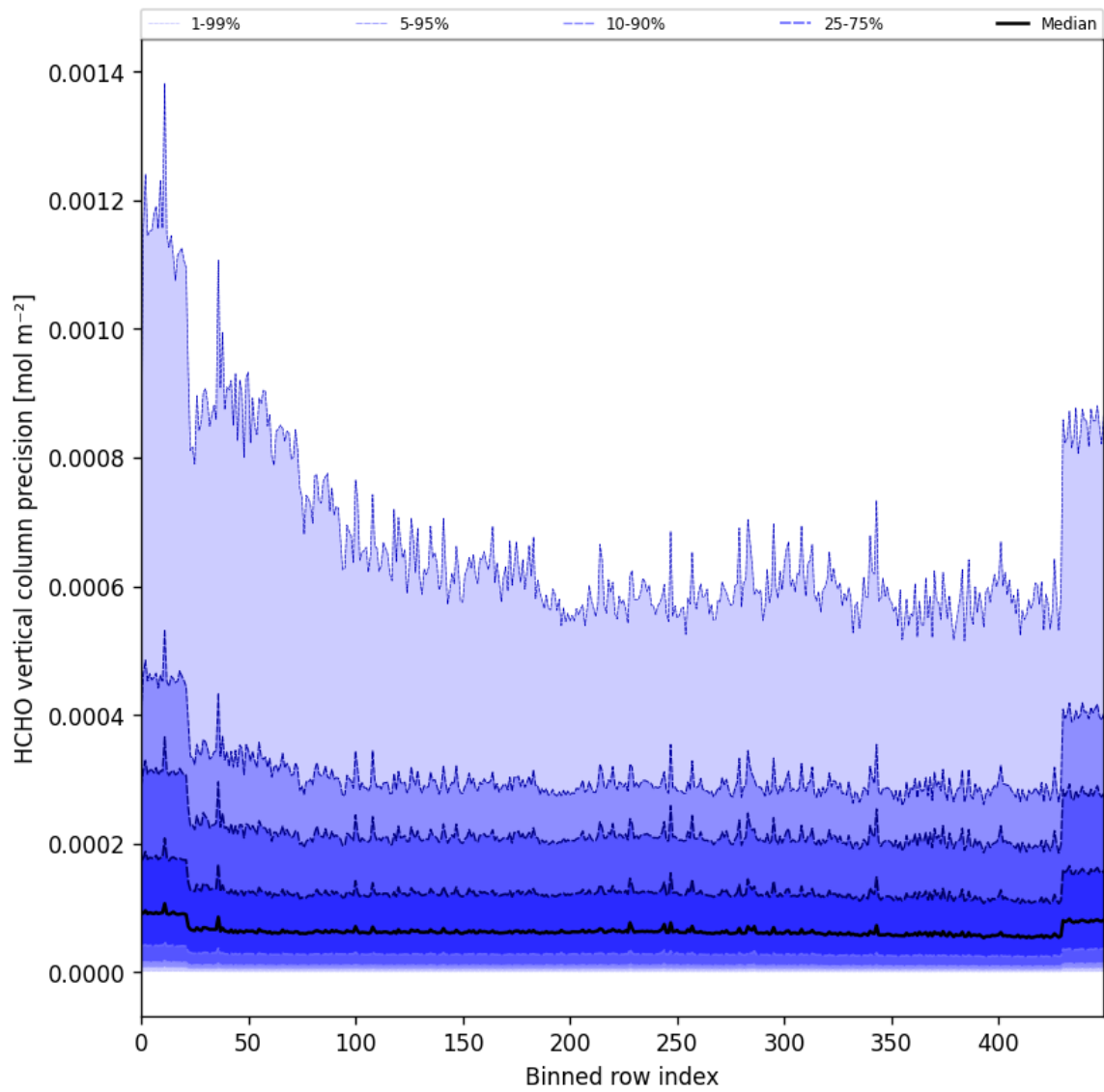
Figure 50: Along track statistics of “HCHO vertical column precision” for 2025-07-02 to 2025-07-03
