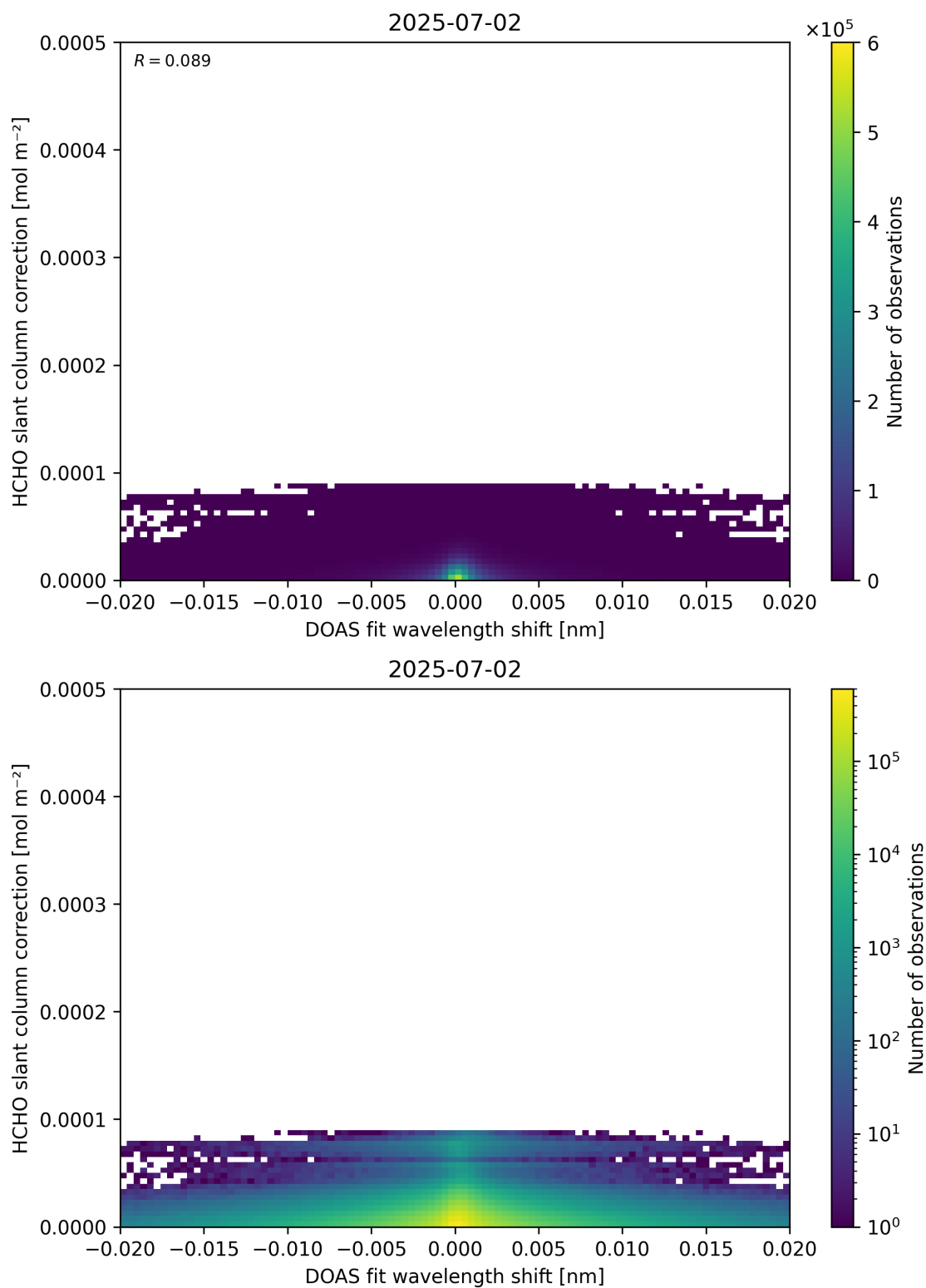
Figure 67: Scatter density plot of “DOAS fit wavelength shift” against “HCHO slant column correction” for 2025-07-02 to 2025-07-03.
