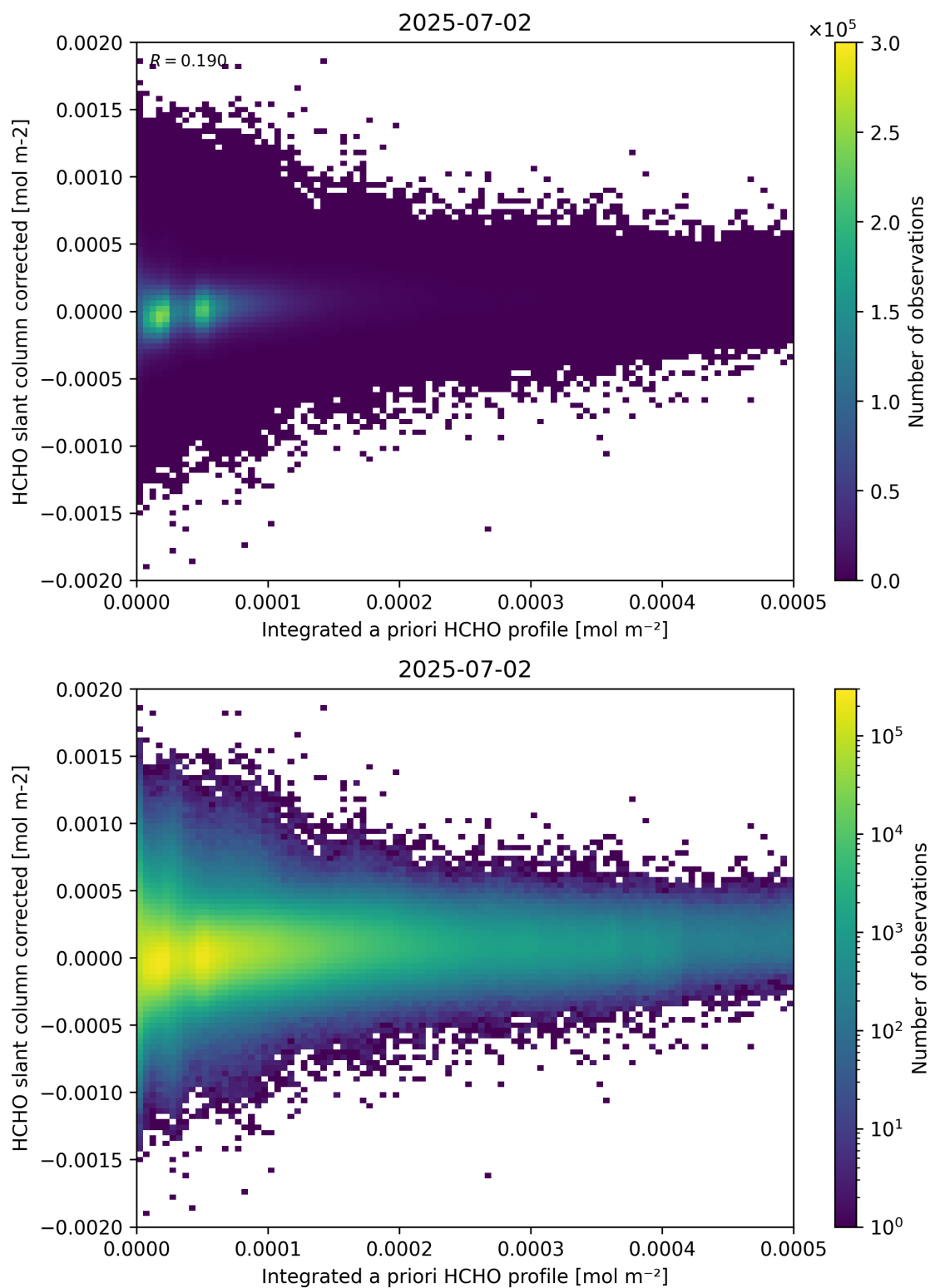
Figure 151: Scatter density plot of “Integrated a priori HCHO profile” against “HCHO slant column corrected” for 2025-07-02 to 2025-07-03.
