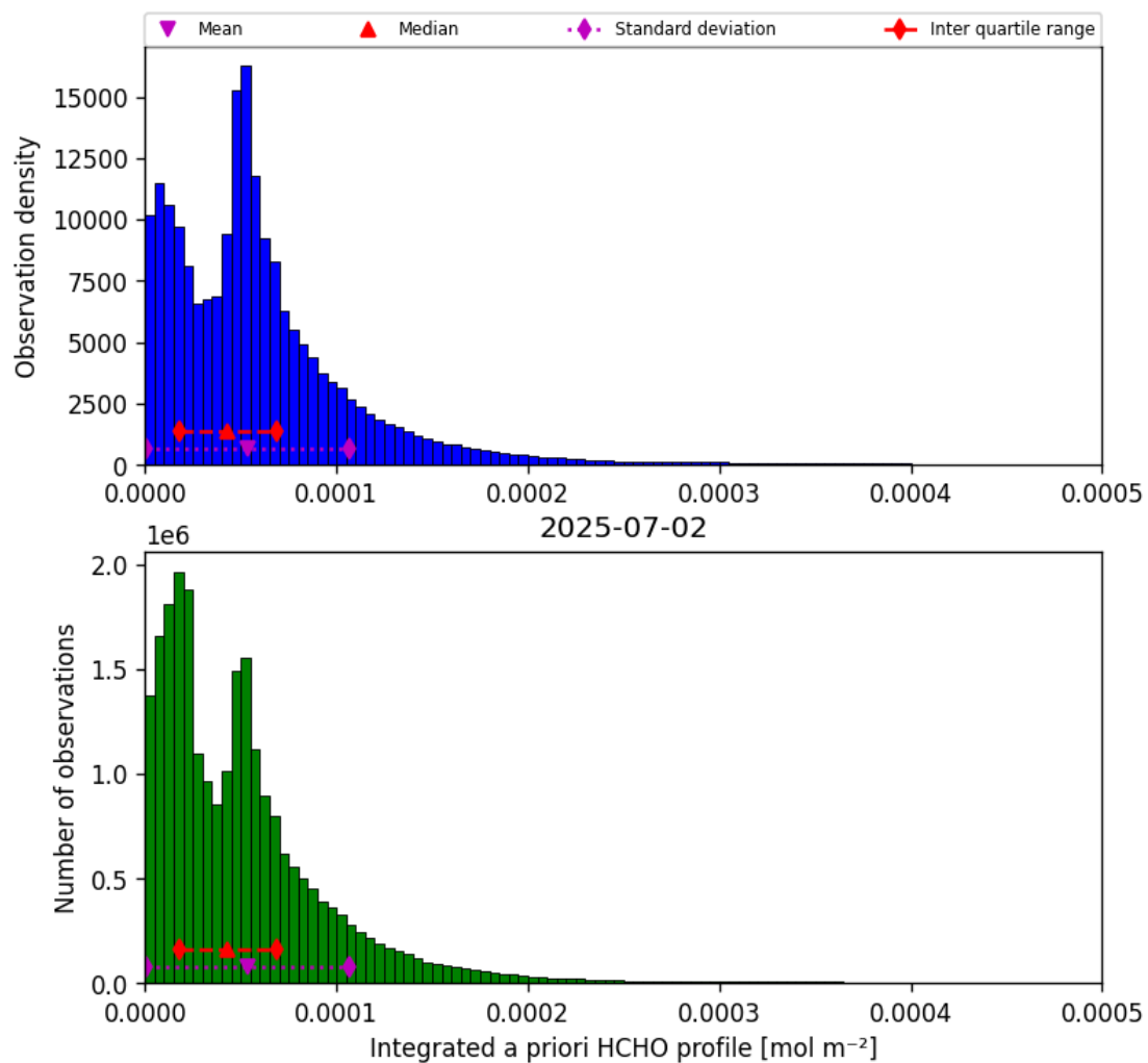
Figure 43: Histogram of “Integrated a priori HCHO profile” for 2025-07-02 to 2025-07-03
