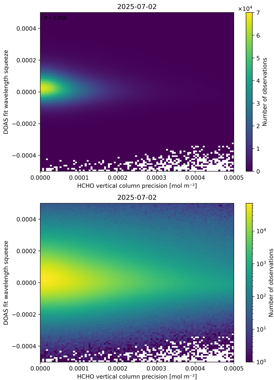
Figure 138: Scatter density plot of “HCHO vertical column precision” against “DOAS fit wavelength squeeze” for 2025-07-02 to 2025-07-03.
