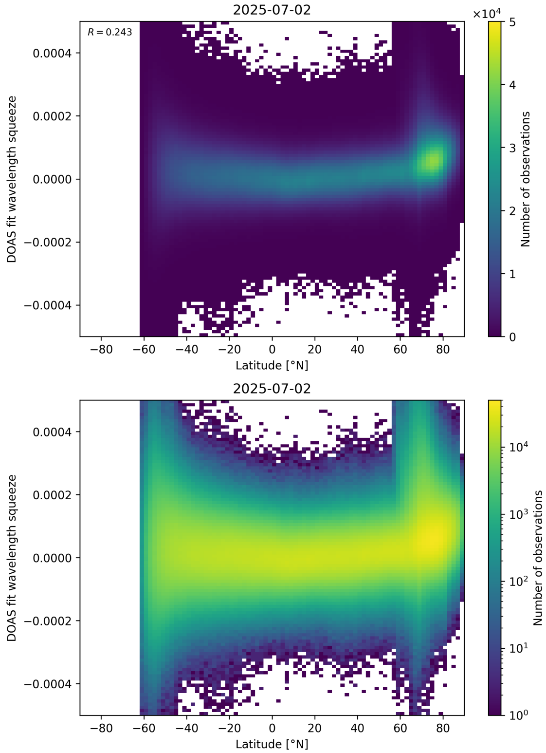
Figure 155: Scatter density plot of “Latitude” against “DOAS fit wavelength squeeze” for 2025-07-02 to 2025-07-03.
