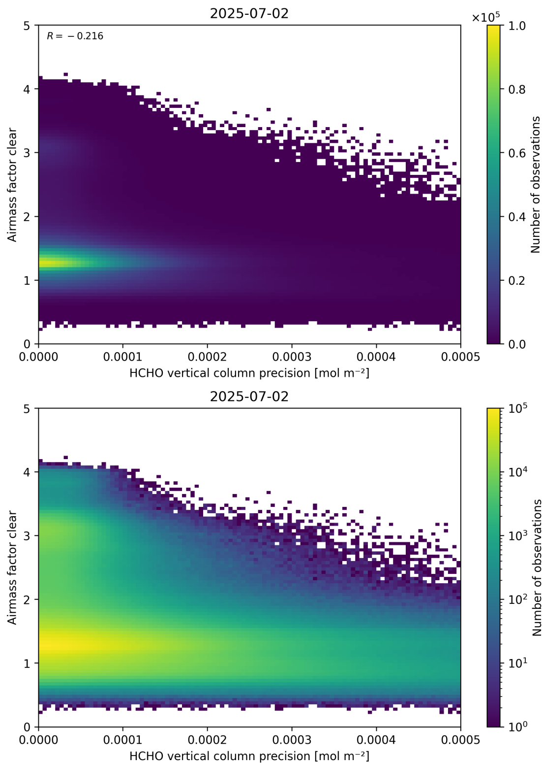
Figure 139: Scatter density plot of “HCHO vertical column precision” against “Airmass factor clear” for 2025-07-02 to 2025-07-03.
