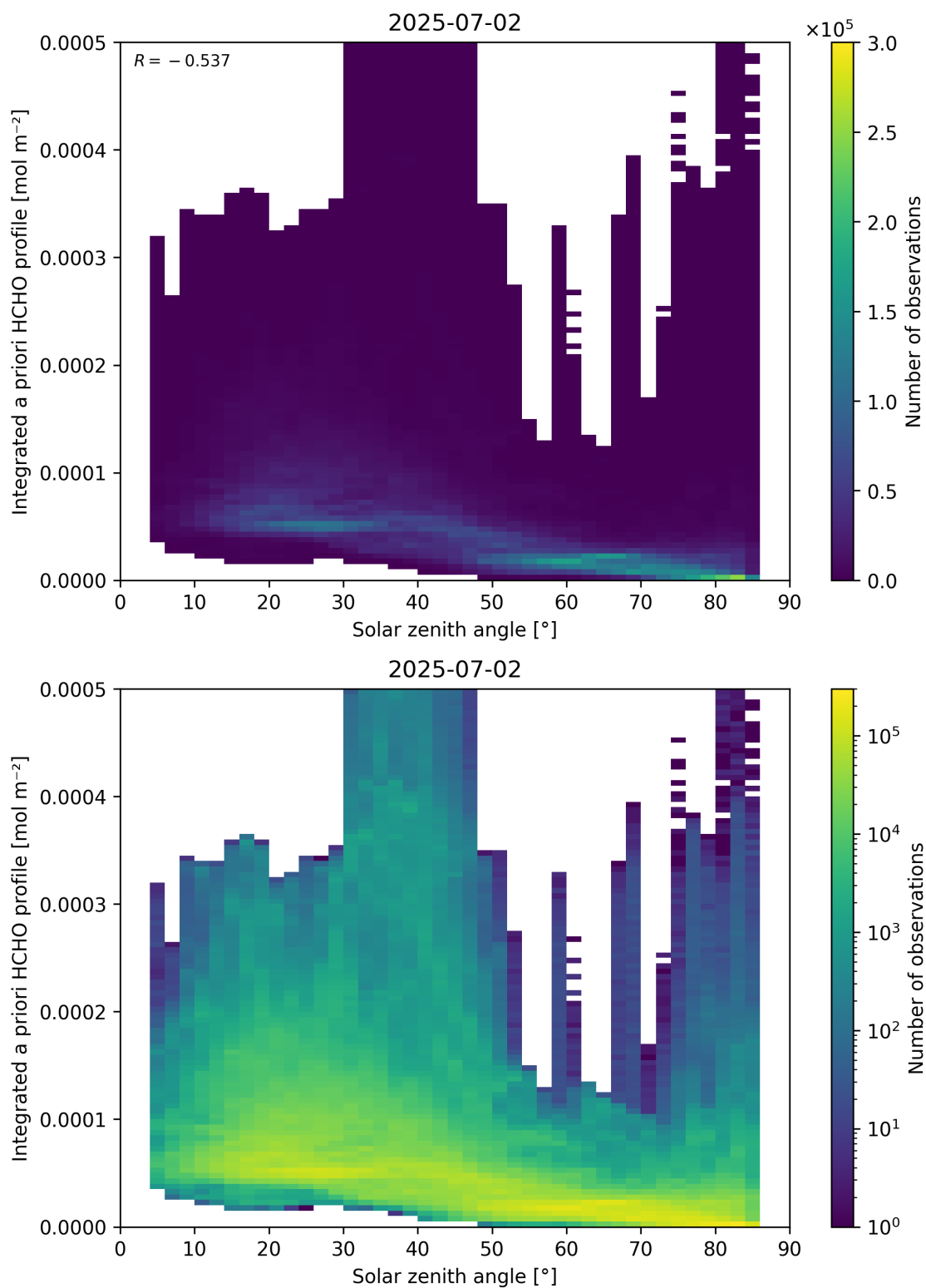
Figure 180: Scatter density plot of “Solar zenith angle” against “Integrated a priori HCHO profile” for 2025-07-02 to 2025-07-03.
