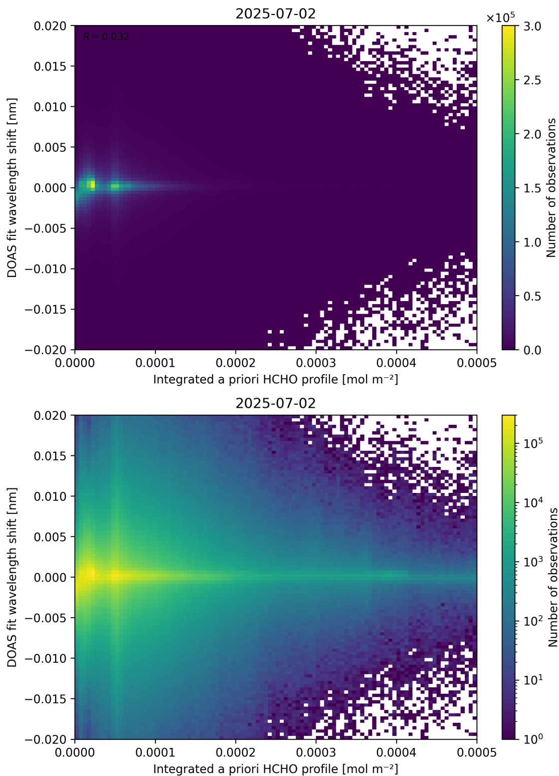
Figure 149: Scatter density plot of “Integrated a priori HCHO profile” against “DOAS fit wavelength shift” for 2025-07-02 to 2025-07-03.
