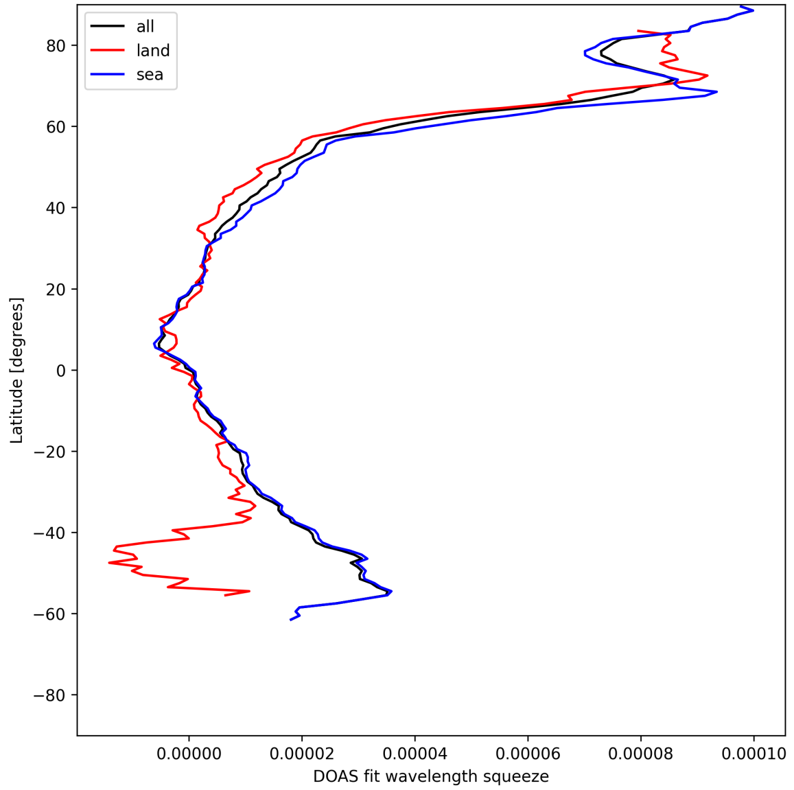
Figure 31: Zonal average of “DOAS fit wavelength squeeze” for 2025-07-02 to 2025-07-03.
