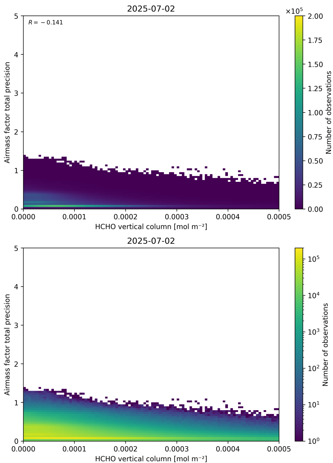
Figure 132: Scatter density plot of “HCHO vertical column” against “Airmass factor total precision” for 2025-07-02 to 2025-07-03.
