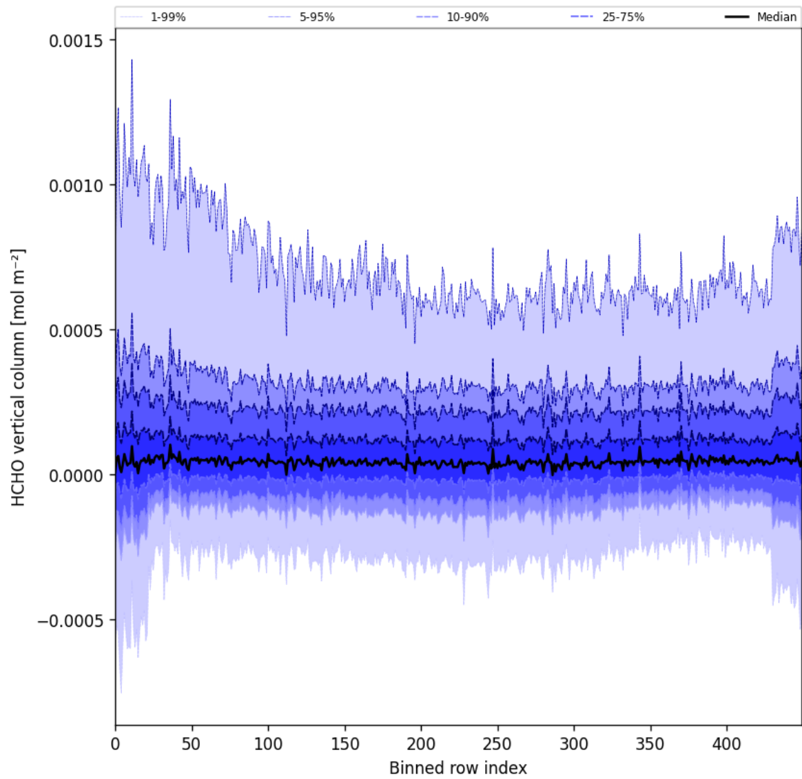
Figure 49: Along track statistics of “HCHO vertical column” for 2025-07-02 to 2025-07-03
