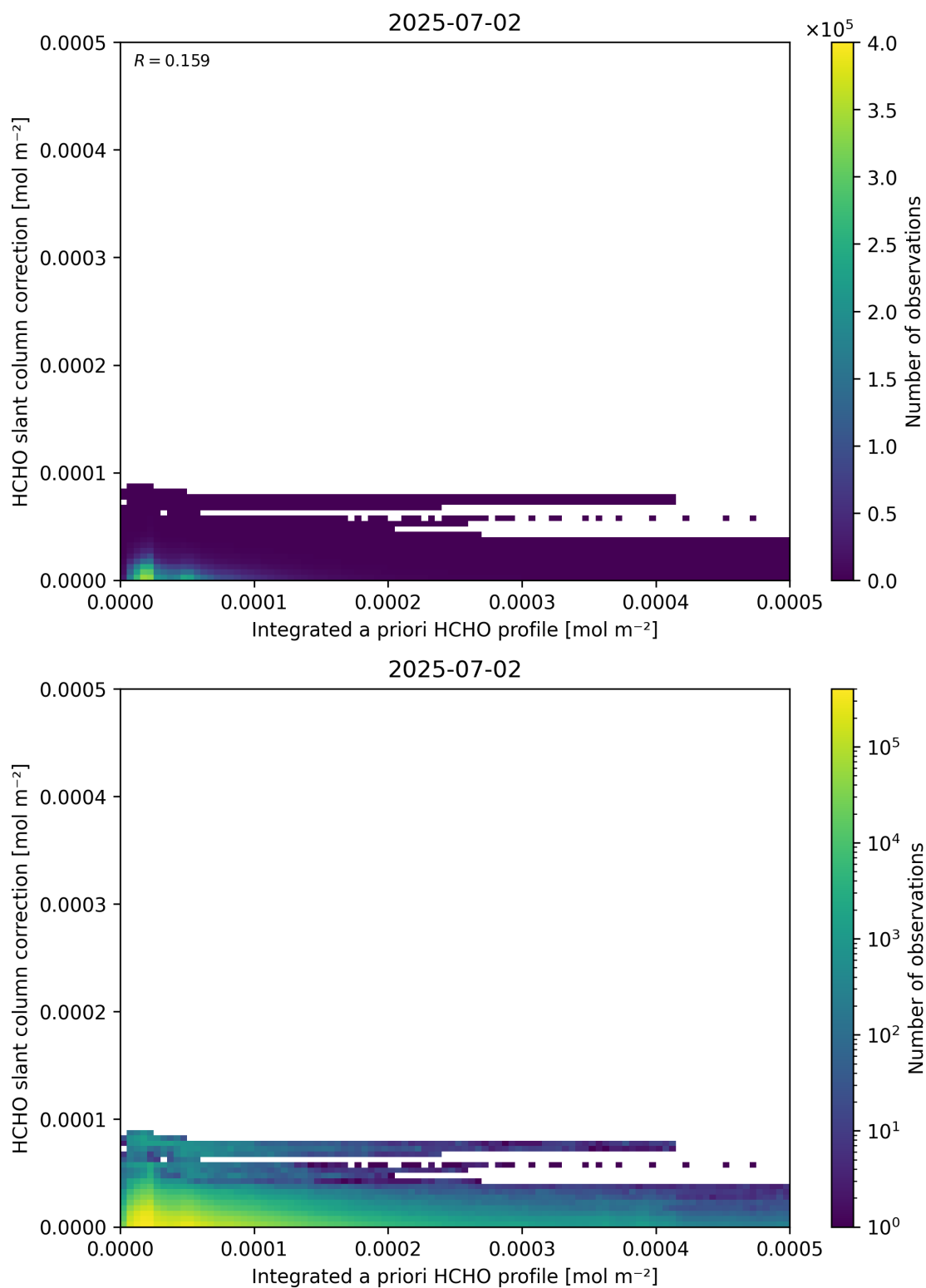
Figure 152: Scatter density plot of “Integrated a priori HCHO profile” against “HCHO slant column correction” for 2025-07-02 to 2025-07-03.
