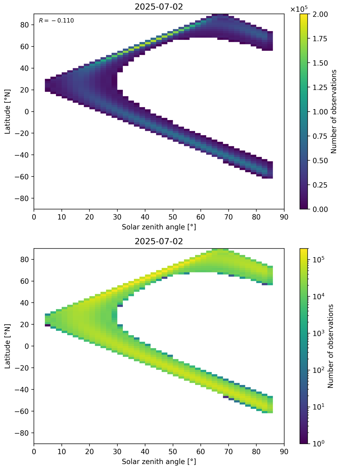
Figure 181: Scatter density plot of “Solar zenith angle” against “Latitude” for 2025-07-02 to 2025-07-03.
