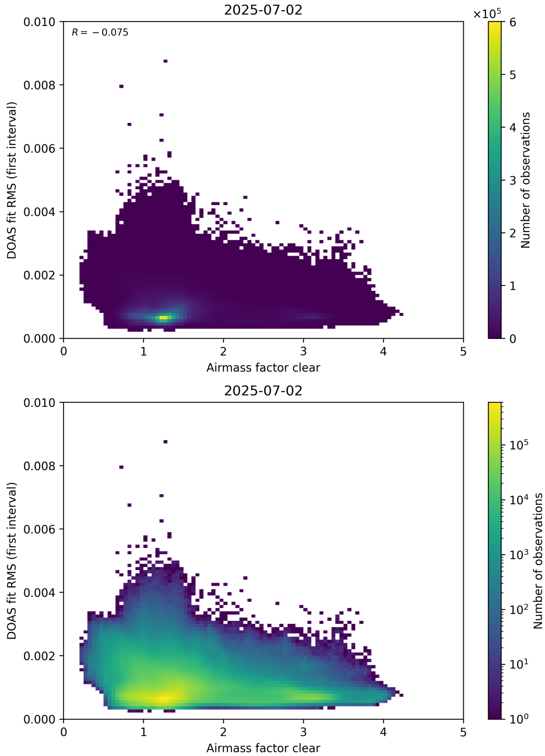
Figure 71: Scatter density plot of “Airmass factor clear” against “DOAS fit RMS (first interval)” for 2025-07-02 to 2025-07-03.
