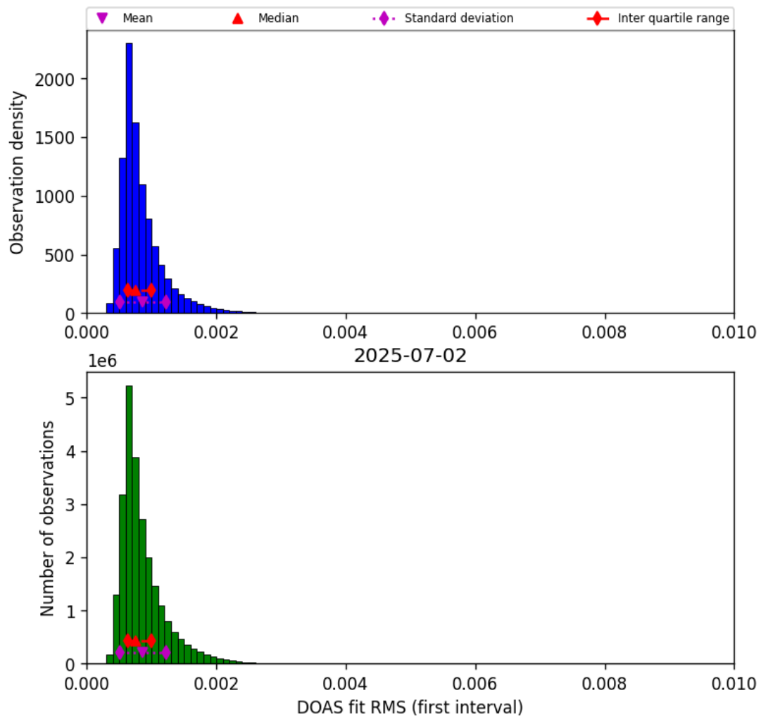
Figure 46: Histogram of "DOAS fit RMS (first interval)" for 2025-07-02 to 2025-07-03
