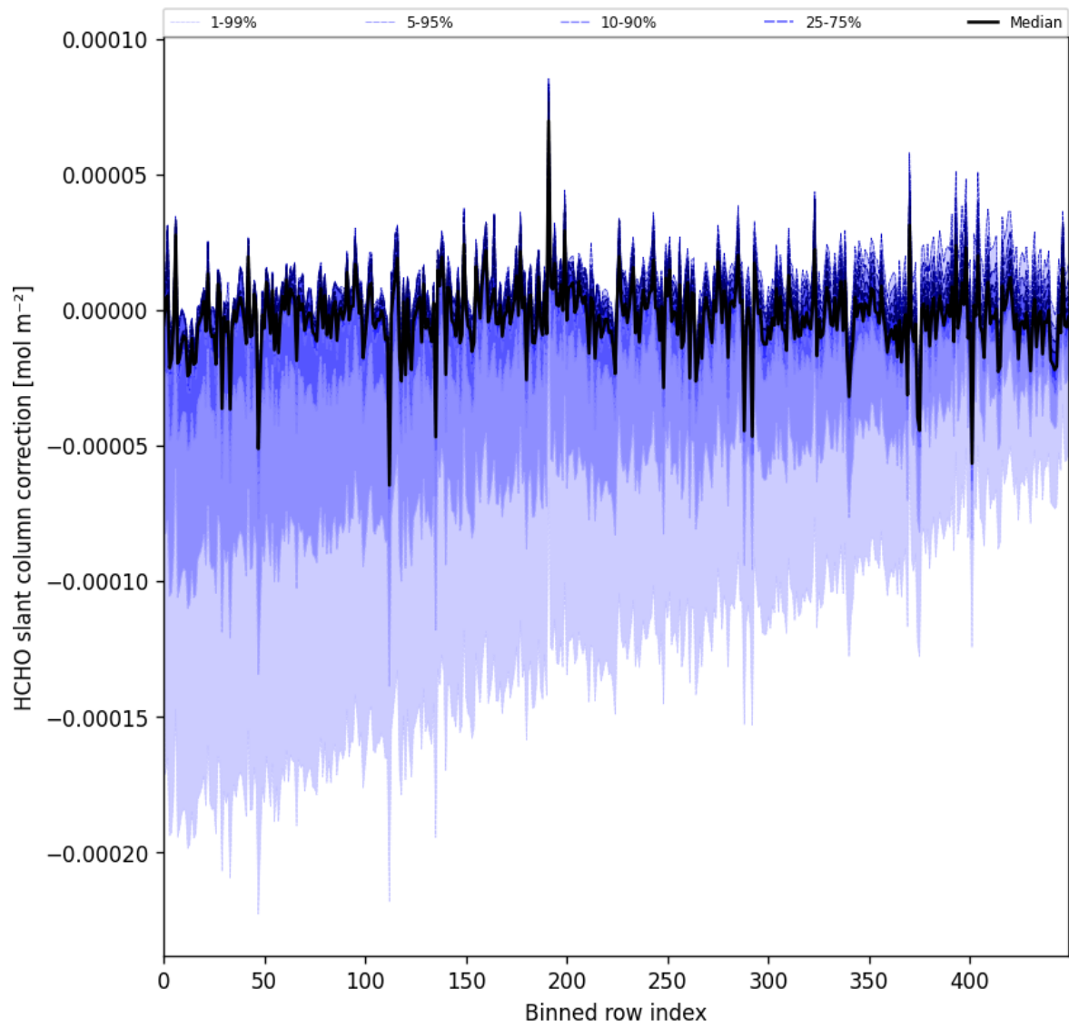
Figure 61: Along track statistics of “HCHO slant column correction” for 2025-07-02 to 2025-07-03
