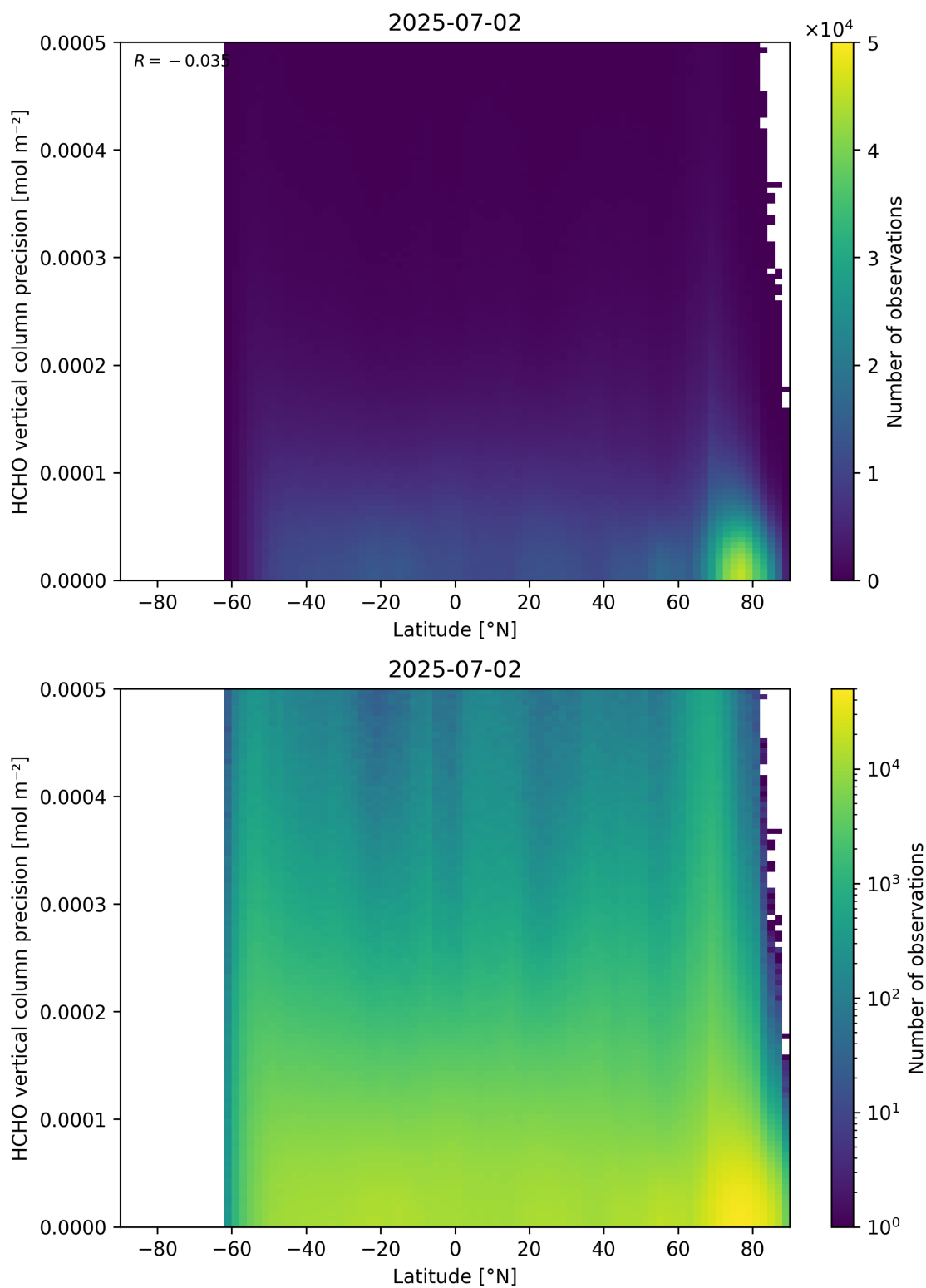
Figure 165: Scatter density plot of “Latitude” against “HCHO vertical column precision” for 2025-07-02 to 2025-07-03.
