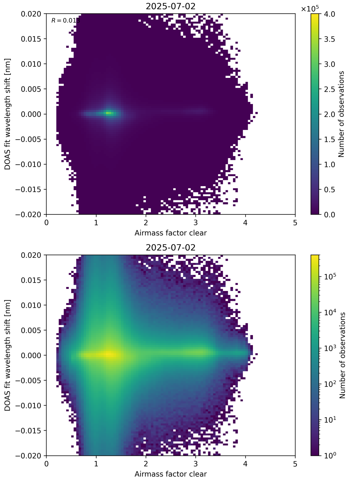
Figure 72: Scatter density plot of “Airmass factor clear” against “DOAS fit wavelength shift” for 2025-07-02 to 2025-07-03.
