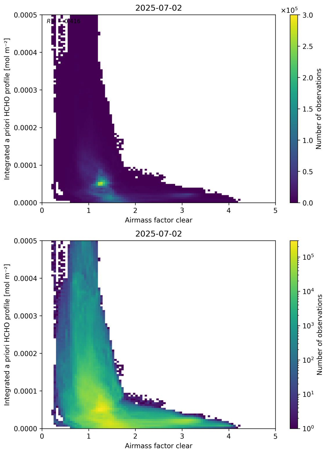
Figure 76: Scatter density plot of “Airmass factor clear” against “Integrated a priori HCHO profile” for 2025-07-02 to 2025-07-03.
