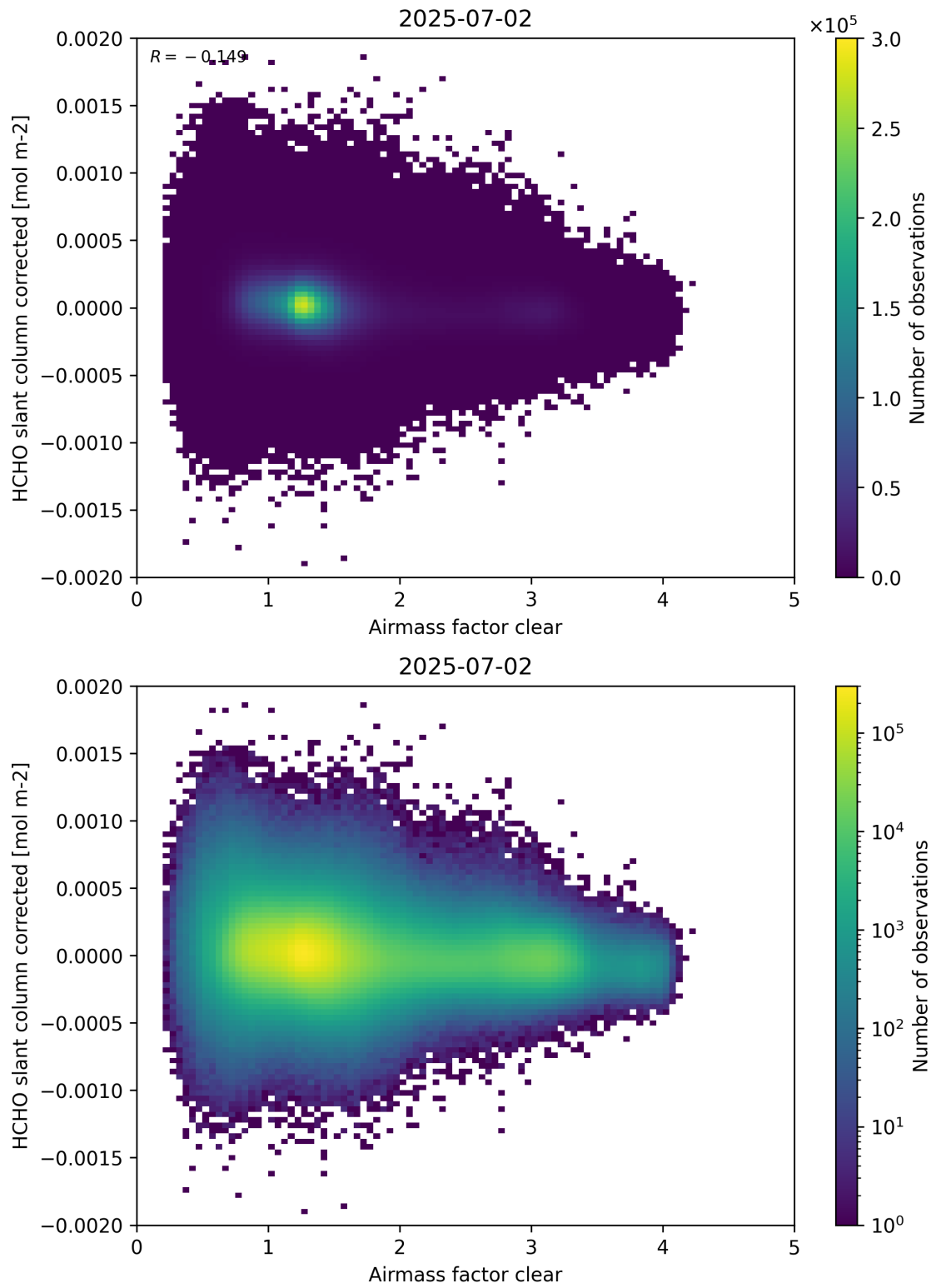
Figure 74: Scatter density plot of “Airmass factor clear” against “HCHO slant column corrected” for 2025-07-02 to 2025-07-03.
