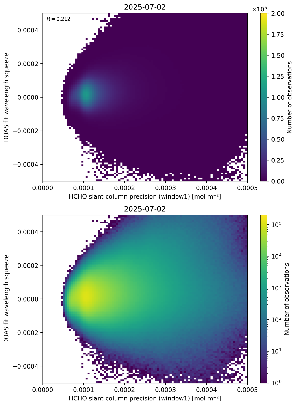
Figure 90: Scatter density plot of “HCHO slant column precision (window1)” against “DOAS fit wavelength squeeze” for 2025-07-02 to 2025-07-03.
