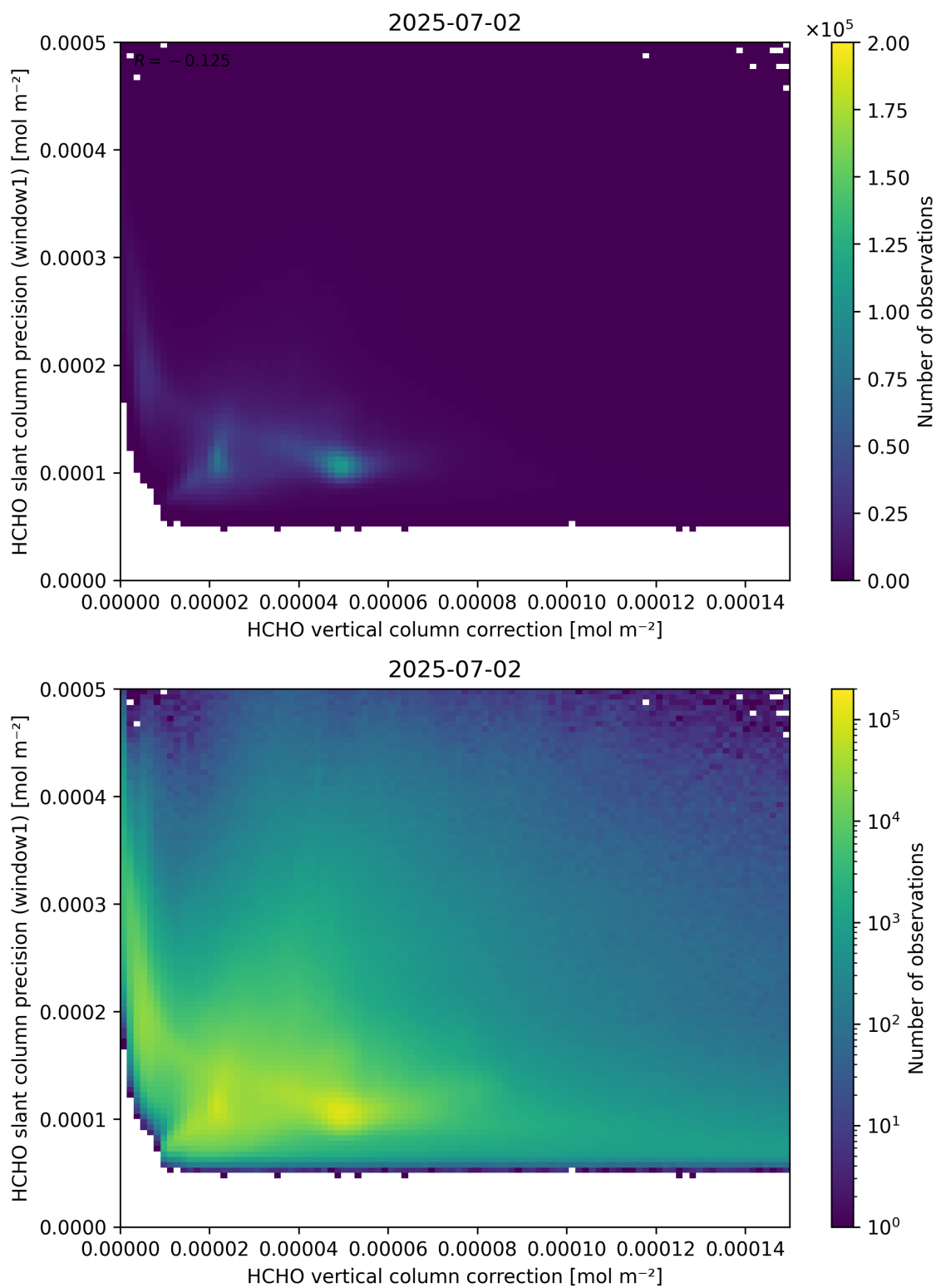
Figure 119: Scatter density plot of “HCHO vertical column correction” against “HCHO slant column precision (window1)” for 2025-07-02 to 2025-07-03.
