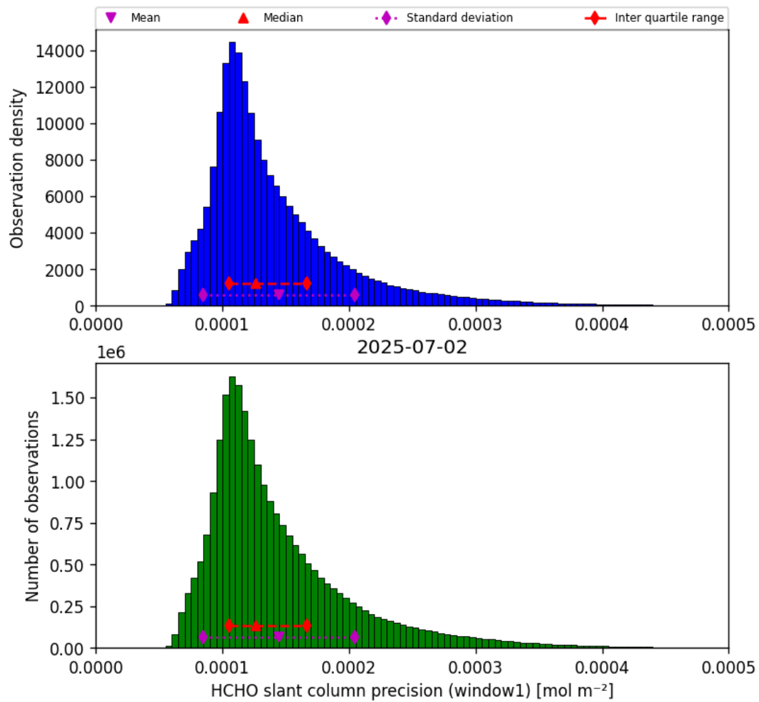
Figure 39: Histogram of “HCHO slant column precision (window1)” for 2025-07-02 to 2025-07-03
