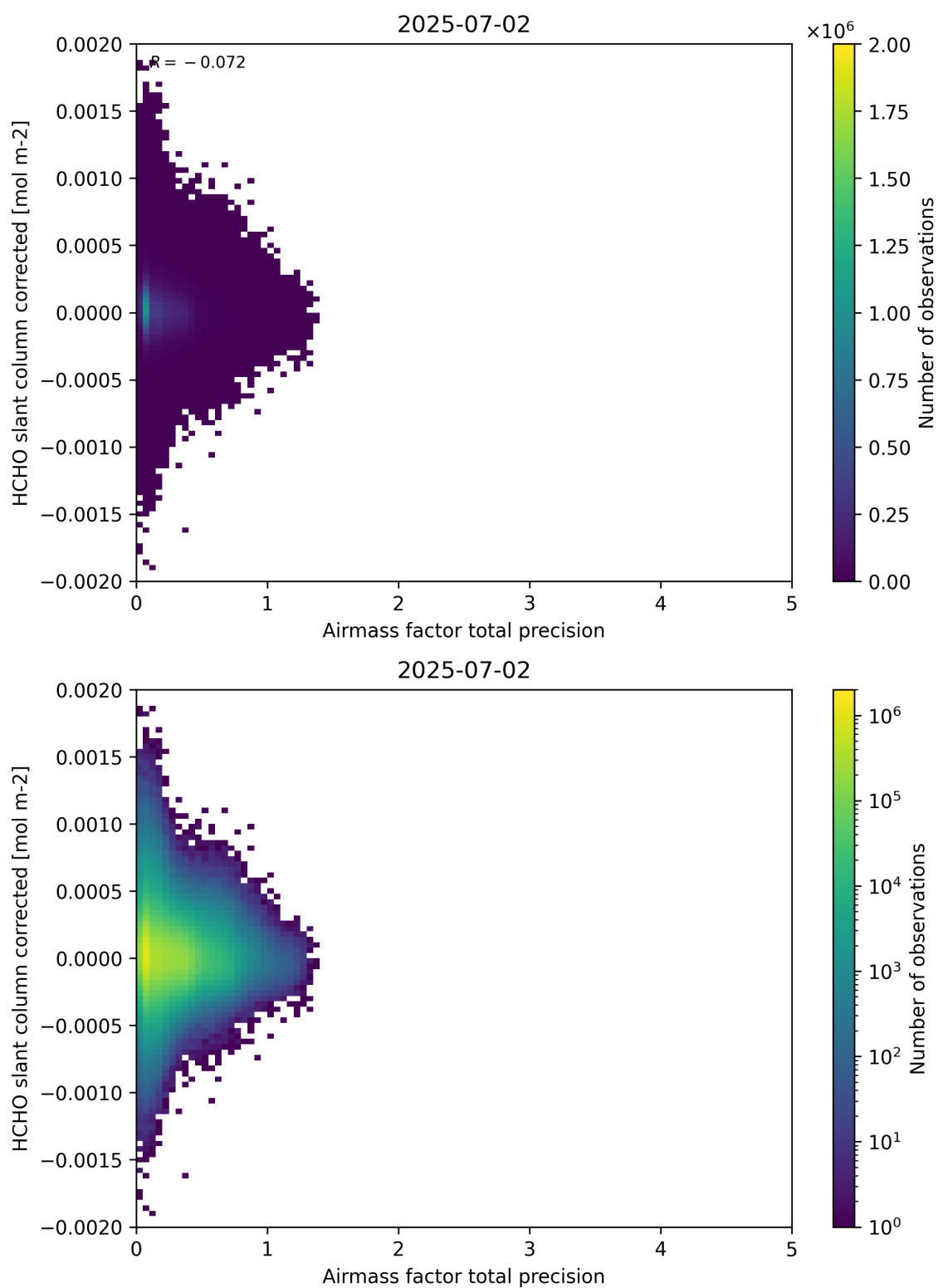
Figure 109: Scatter density plot of “Airmass factor total precision” against “HCHO slant column corrected” for 2025-07-02 to 2025-07-03.
