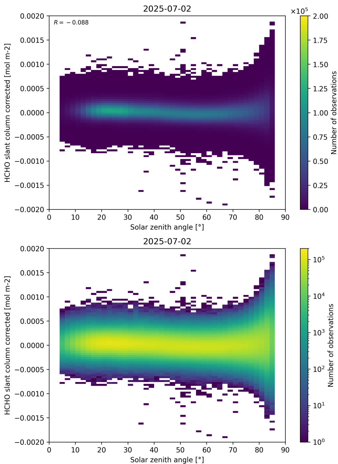
Figure 171: Scatter density plot of “Solar zenith angle” against “HCHO slant column corrected” for 2025-07-02 to 2025-07-03.
