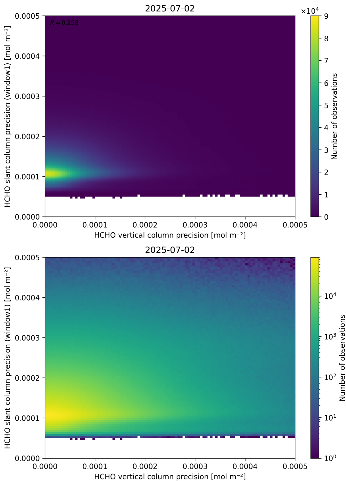
Figure 143: Scatter density plot of “HCHO vertical column precision” against “HCHO slant column precision (window1)” for 2025-07-02 to 2025-07-03.
