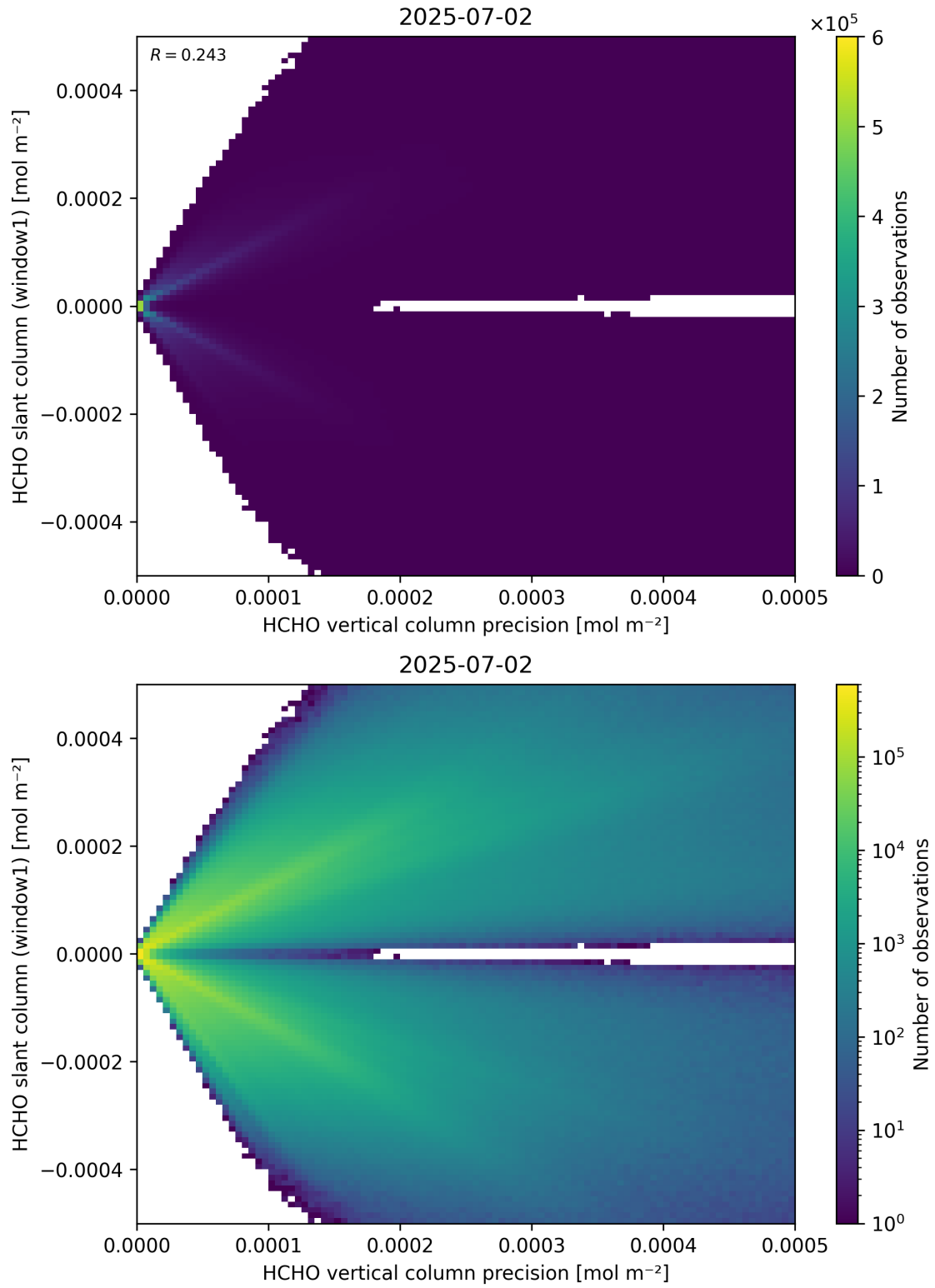
Figure 142: Scatter density plot of “HCHO vertical column precision” against “HCHO slant column (window1)” for 2025-07-02 to 2025-07-03.
