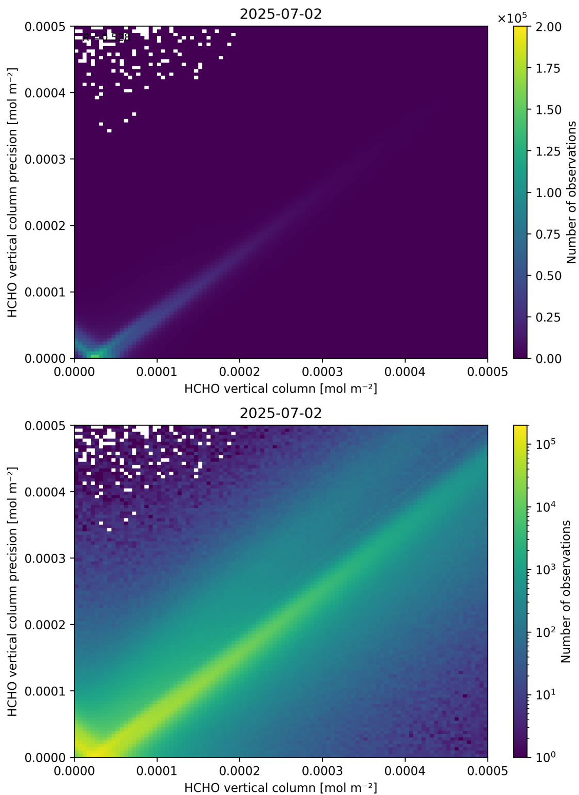
Figure 134: Scatter density plot of “HCHO vertical column” against “HCHO vertical column precision” for 2025-07-02 to 2025-07-03.
