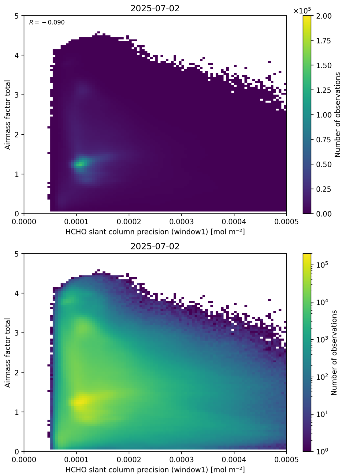
Figure 94: Scatter density plot of “HCHO slant column precision (window1)” against “Airmass factor total” for 2025-07-02 to 2025-07-03.
