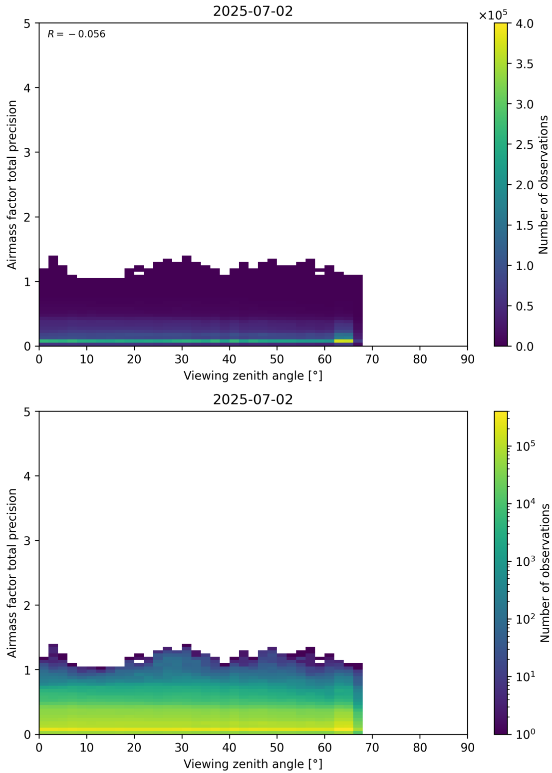
Figure 191: Scatter density plot of “Viewing zenith angle” against “Airmass factor total precision” for 2025-07-02 to 2025-07-03.
