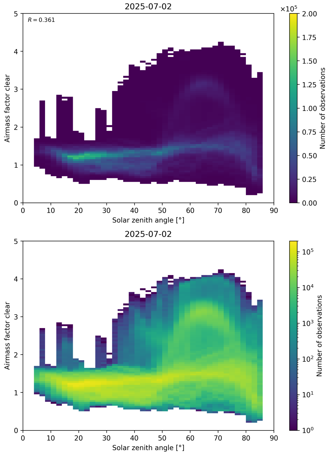
Figure 170: Scatter density plot of “Solar zenith angle” against “Airmass factor clear” for 2025-07-02 to 2025-07-03.
