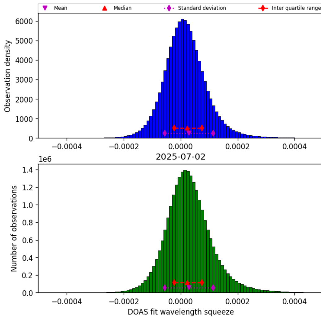
Figure 45: Histogram of “DOAS fit wavelength squeeze” for 2025-07-02 to 2025-07-03
