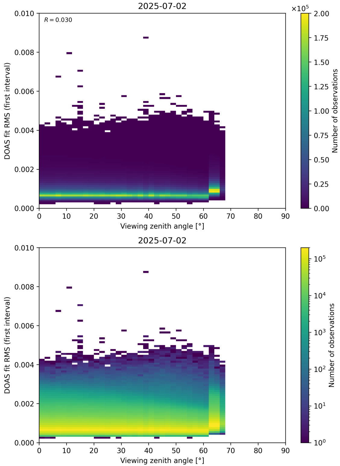
Figure 182: Scatter density plot of “Viewing zenith angle” against “DOAS fit RMS (first interval)” for 2025-07-02 to 2025-07-03.
