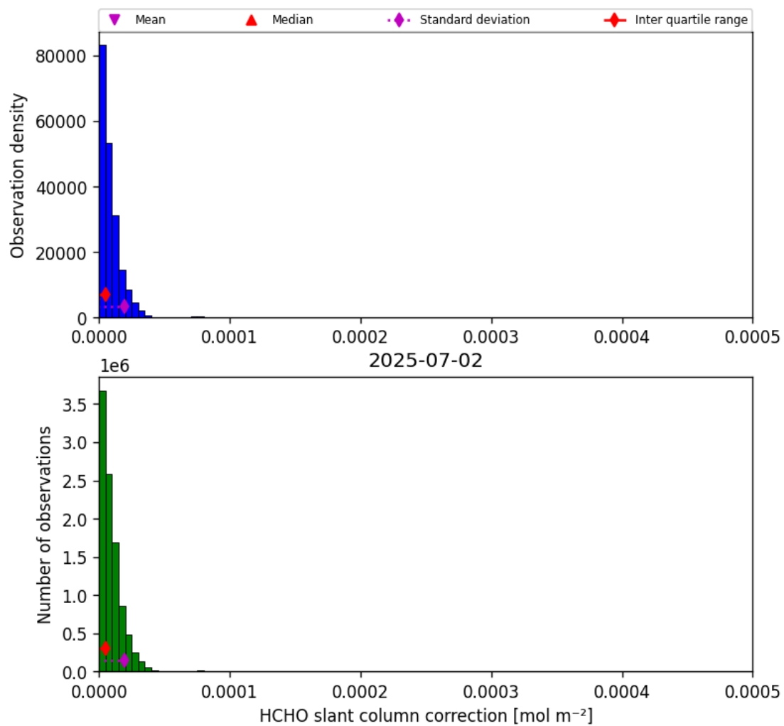
Figure 47: Histogram of “HCHO slant column correction” for 2025-07-02 to 2025-07-03
