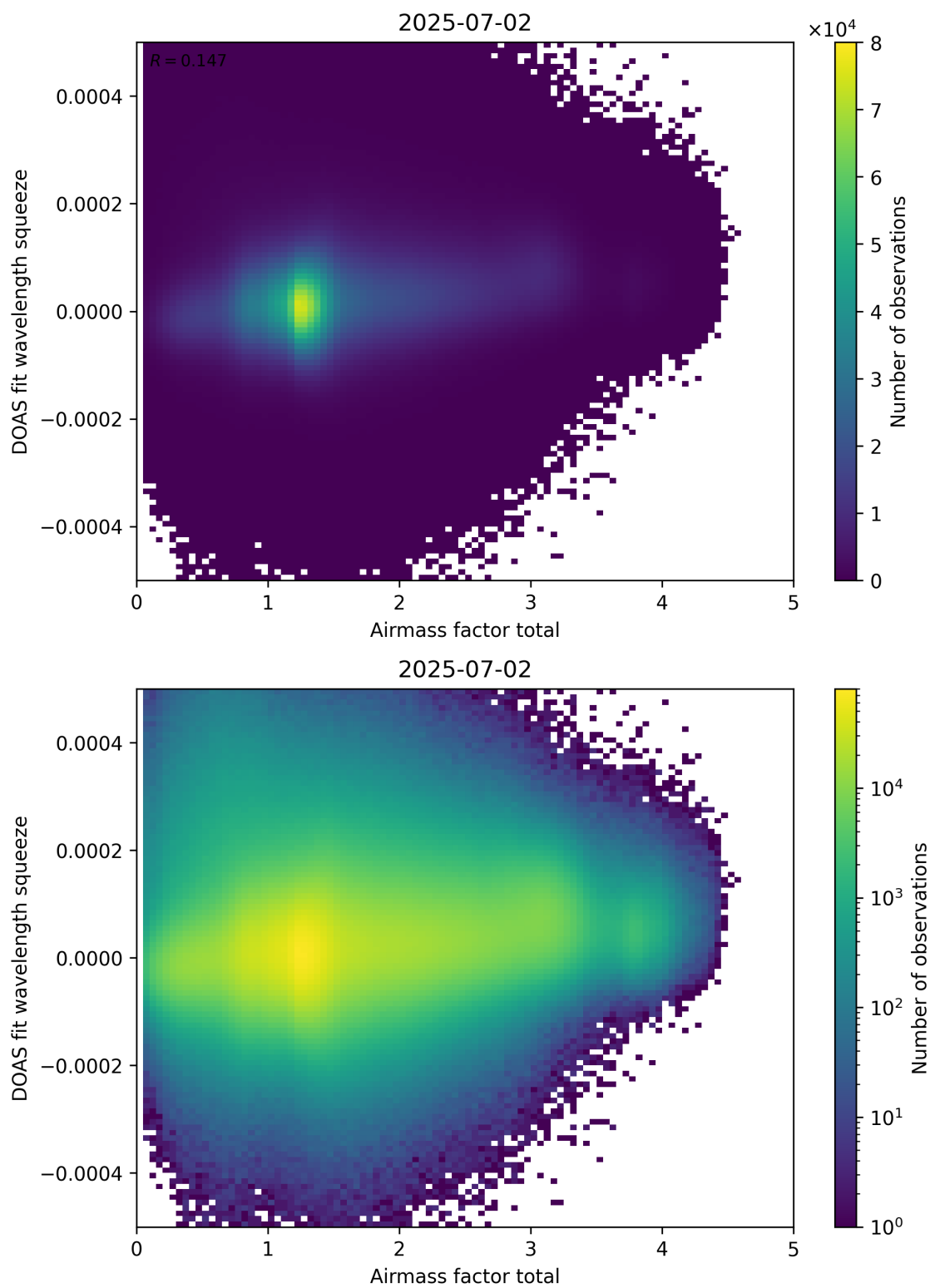
Figure 99: Scatter density plot of “Airmass factor total” against “DOAS fit wavelength squeeze” for 2025-07-02 to 2025-07-03.
