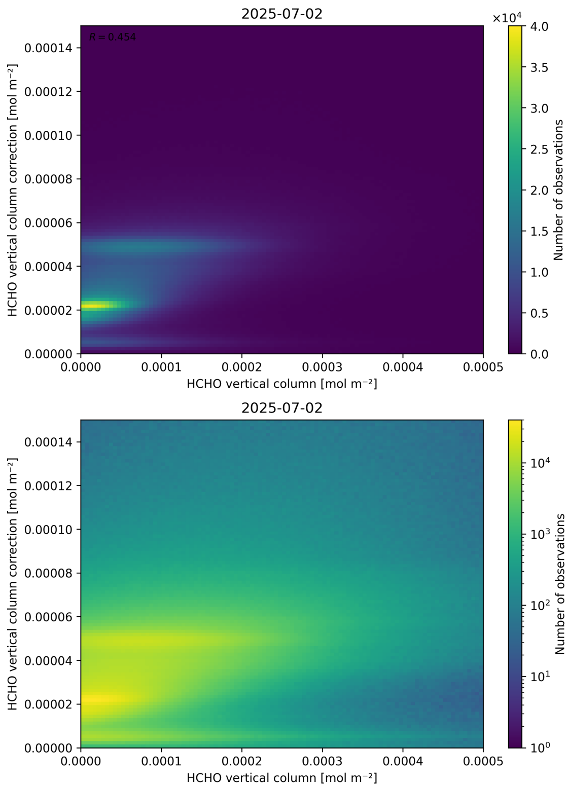
Figure 133: Scatter density plot of “HCHO vertical column” against “HCHO vertical column correction” for 2025-07-02 to 2025-07-03.
