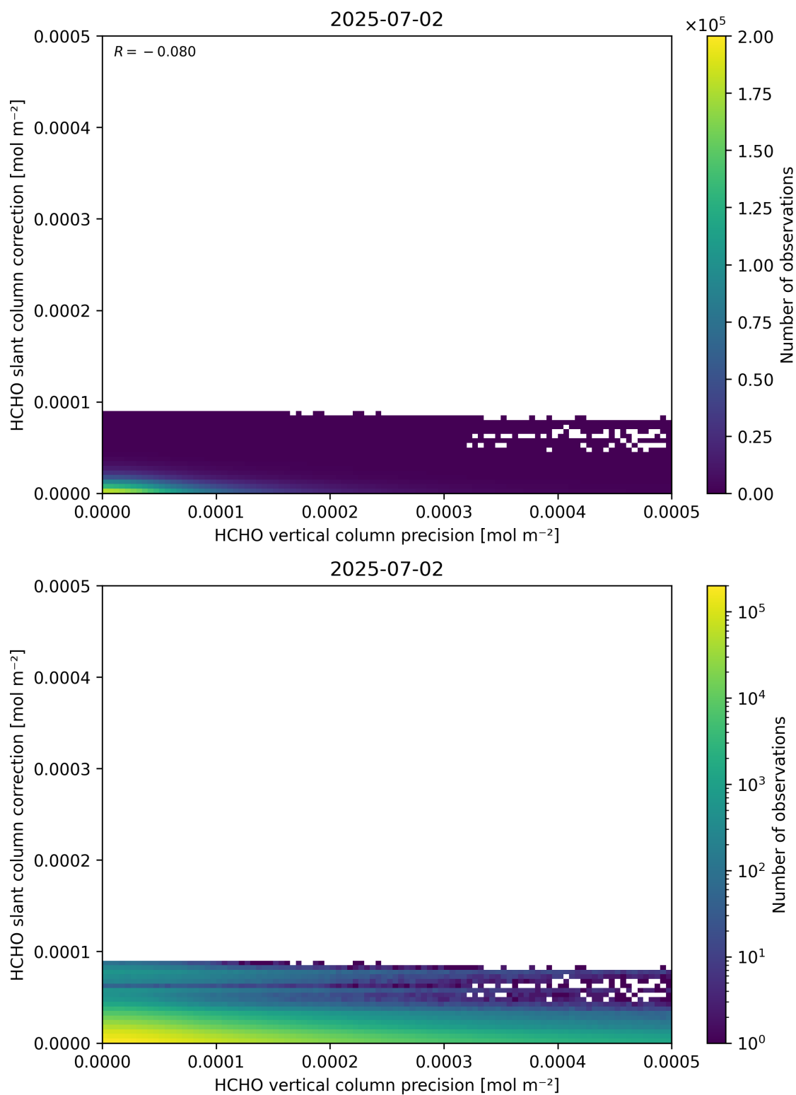
Figure 141: Scatter density plot of “HCHO vertical column precision” against “HCHO slant column correction” for 2025-07-02 to 2025-07-03.
