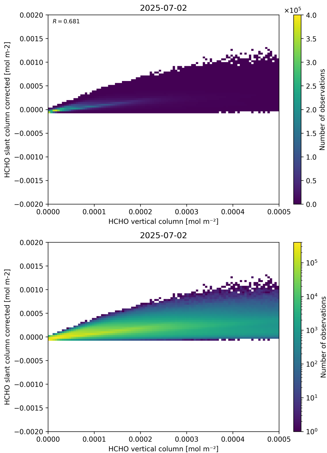
Figure 127: Scatter density plot of “HCHO vertical column” against “HCHO slant column corrected” for 2025-07-02 to 2025-07-03.
