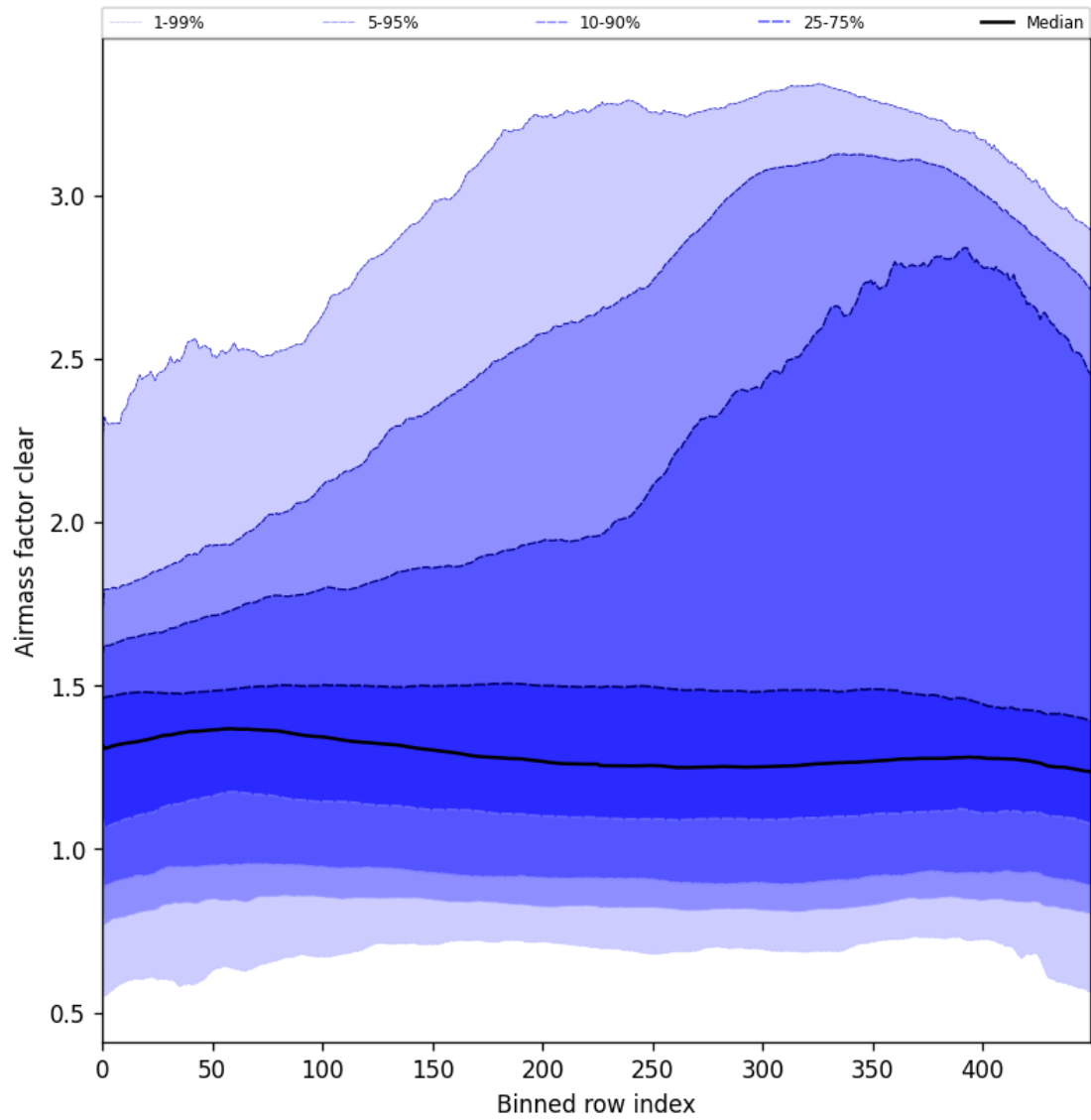
Figure 56: Along track statistics of “Airmass factor clear” for 2025-07-02 to 2025-07-03
