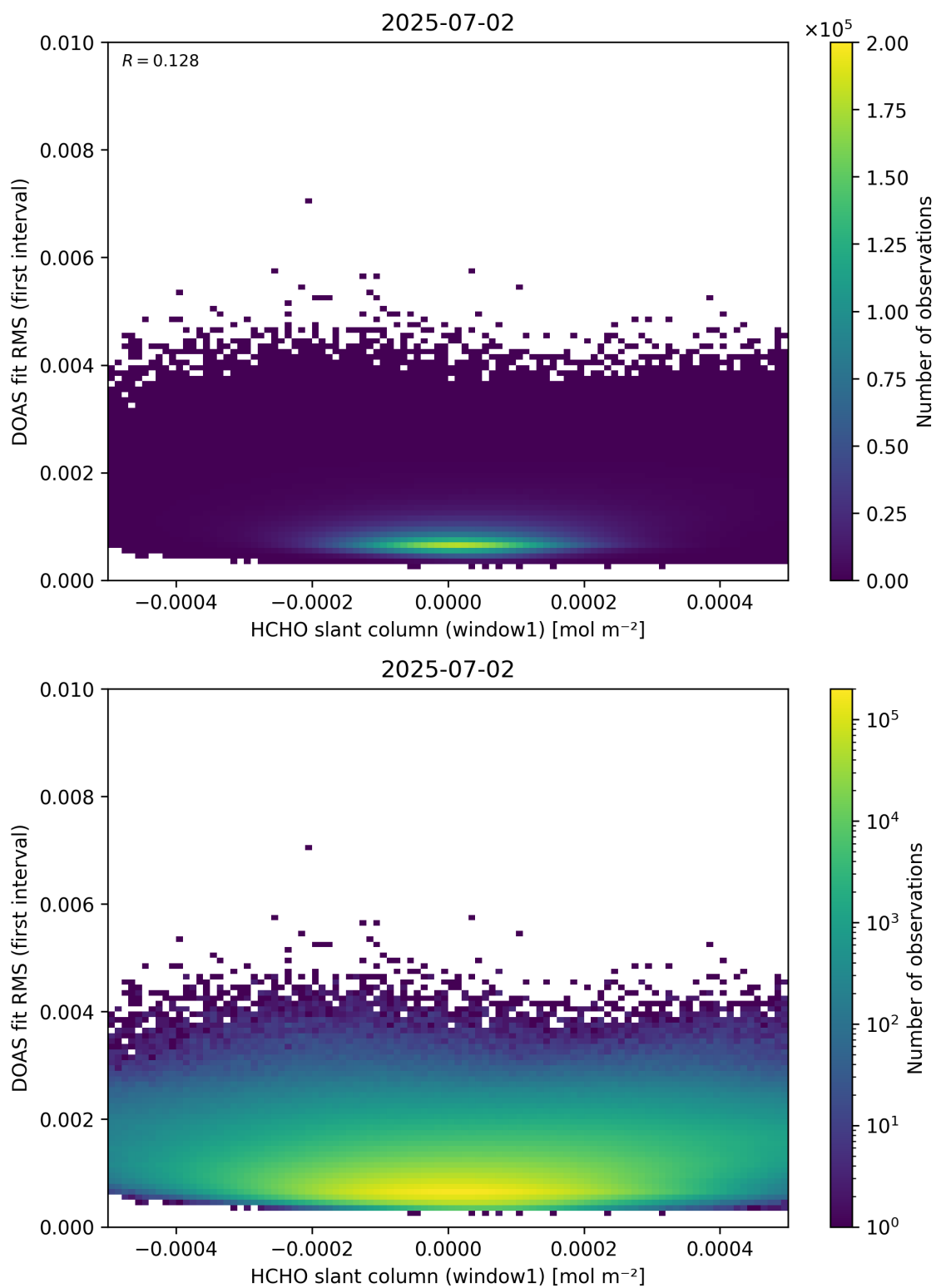
Figure 78: Scatter density plot of “HCHO slant column (window1)” against “DOAS fit RMS (first interval)” for 2025-07-02 to 2025-07-03.
