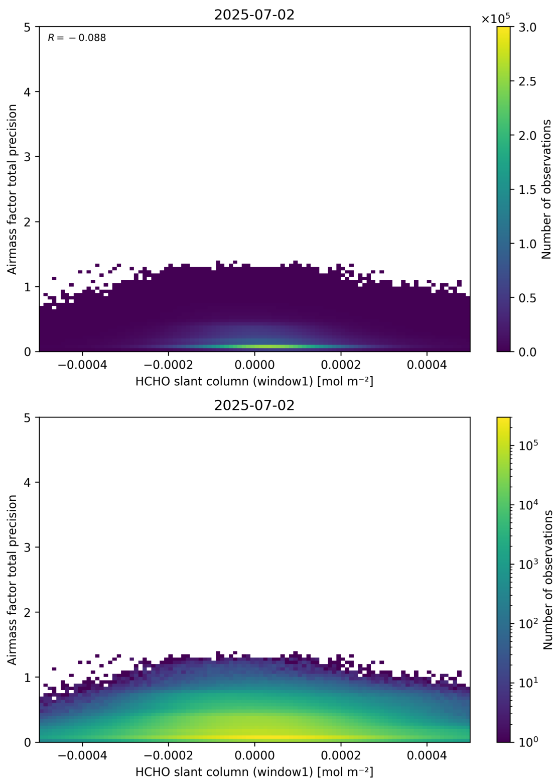
Figure 86: Scatter density plot of “HCHO slant column (window1)” against “Airmass factor total precision” for 2025-07-02 to 2025-07-03.
