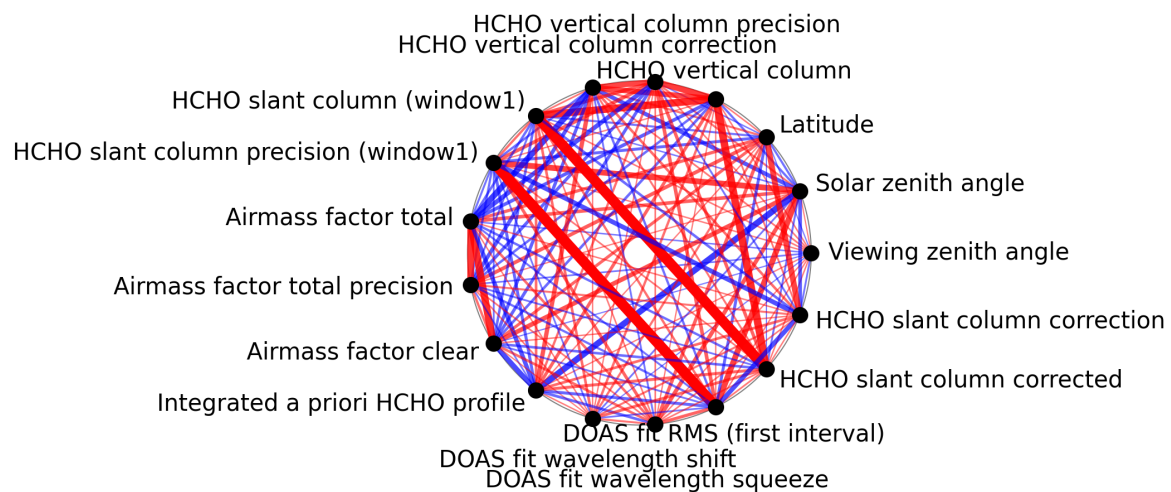
Figure 1: Map of correlation graph for 2025-07-02 to 2025-07-03.
