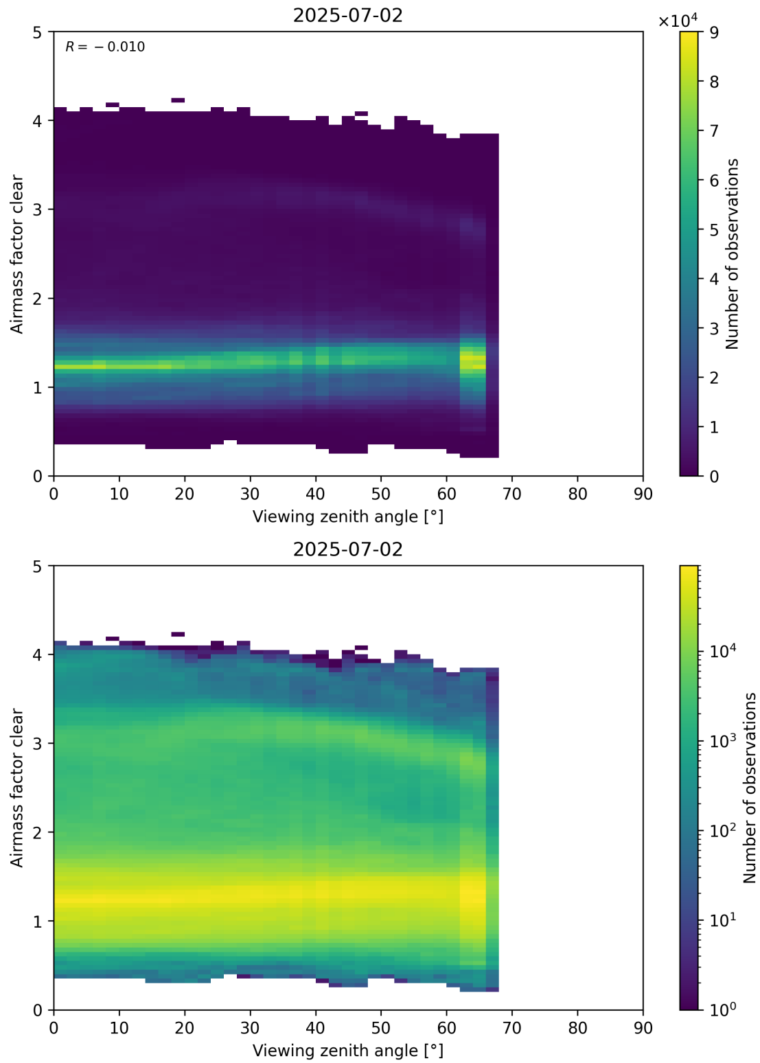
Figure 185: Scatter density plot of “Viewing zenith angle” against “Airmass factor clear” for 2025-07-02 to 2025-07-03.
