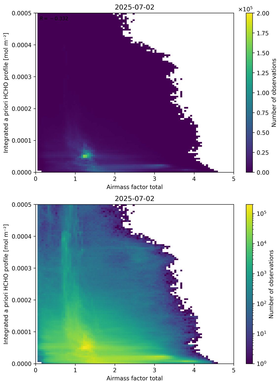
Figure 104: Scatter density plot of “Airmass factor total” against “Integrated a priori HCHO profile” for 2025-07-02 to 2025-07-03.
