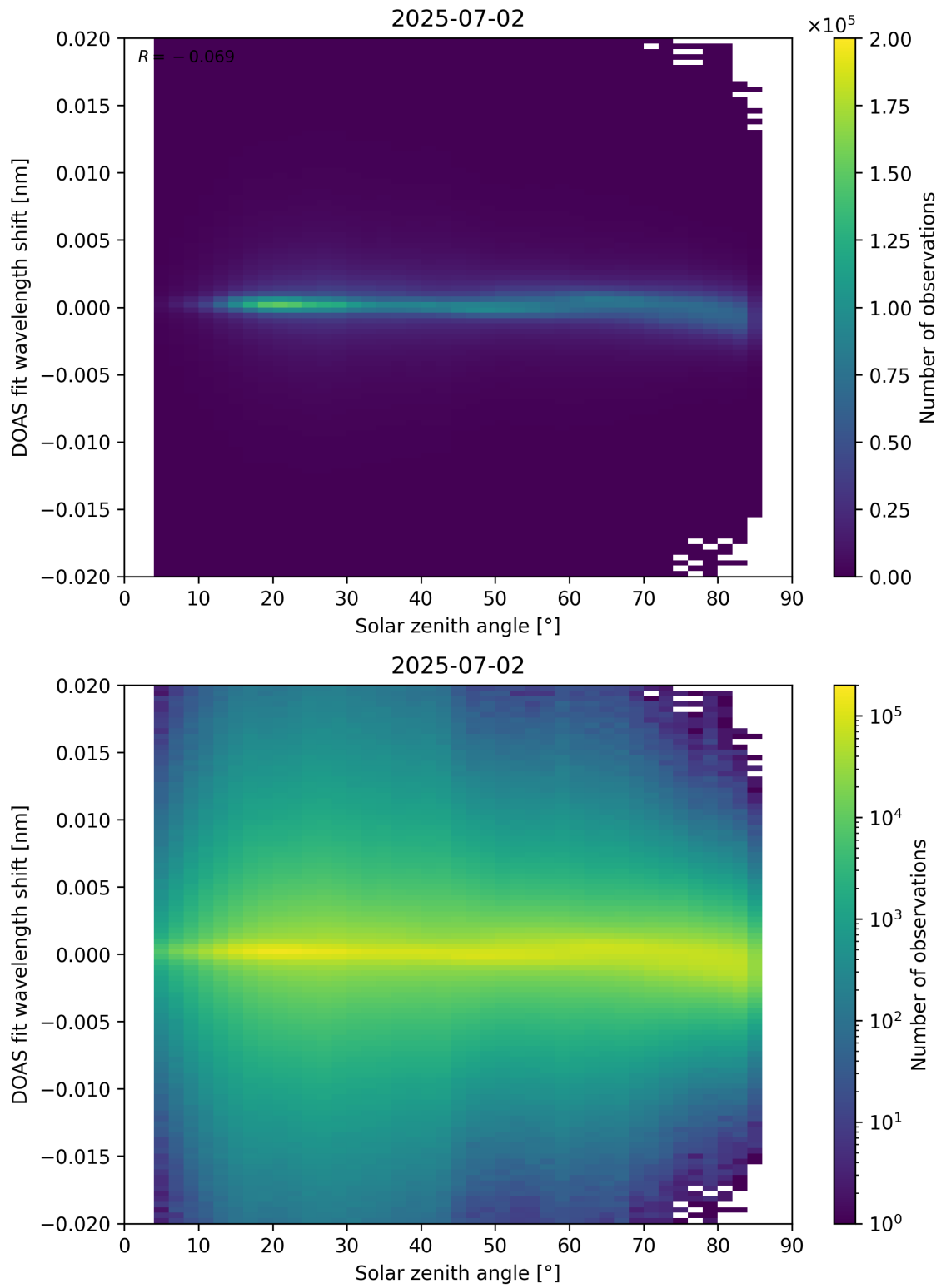
Figure 168: Scatter density plot of “Solar zenith angle” against “DOAS fit wavelength shift” for 2025-07-02 to 2025-07-03.
