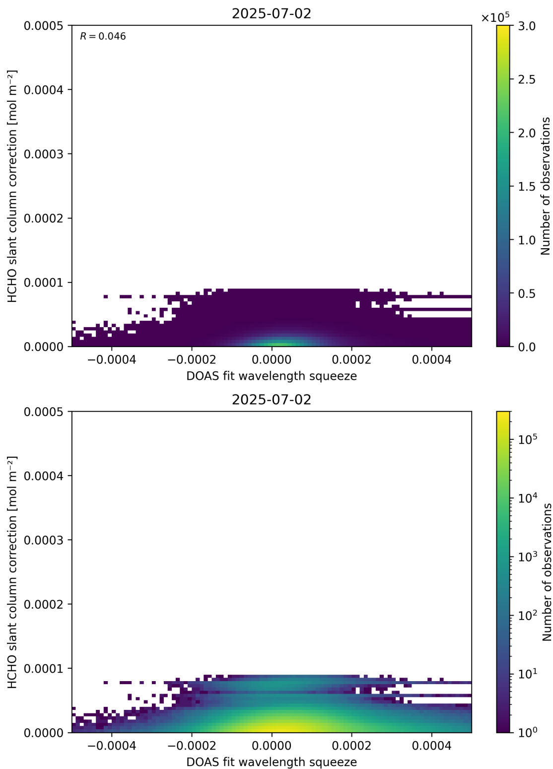
Figure 70: Scatter density plot of “DOAS fit wavelength squeeze” against “HCHO slant column correction” for 2025-07-02 to 2025-07-03.
