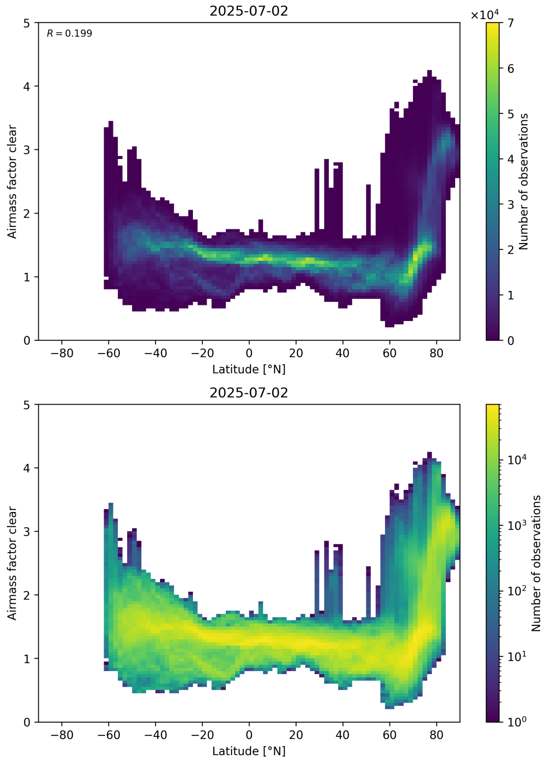
Figure 156: Scatter density plot of “Latitude” against “Airmass factor clear” for 2025-07-02 to 2025-07-03.
