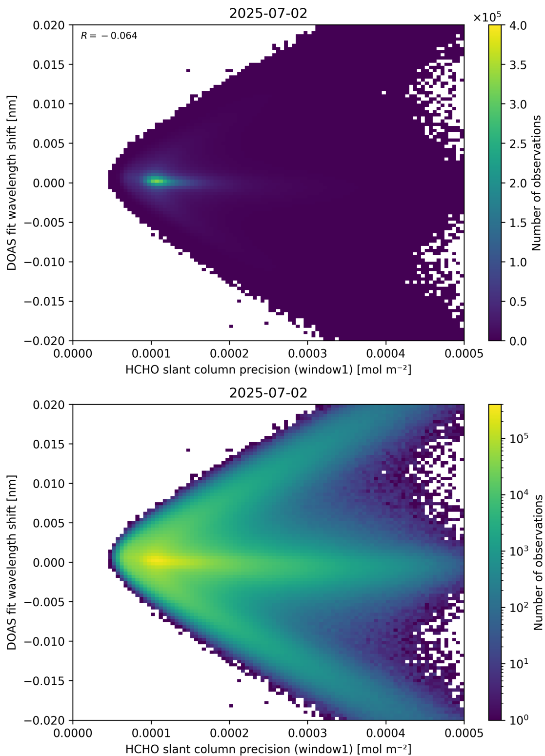
Figure 89: Scatter density plot of “HCHO slant column precision (window1)” against “DOAS fit wavelength shift” for 2025-07-02 to 2025-07-03.
