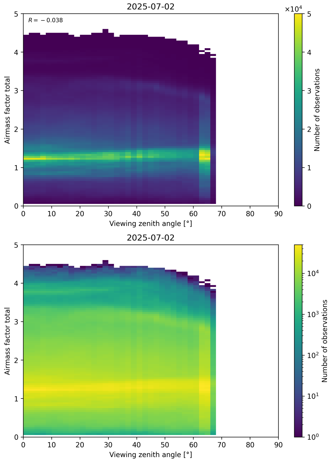
Figure 190: Scatter density plot of “Viewing zenith angle” against “Airmass factor total” for 2025-07-02 to 2025-07-03.
