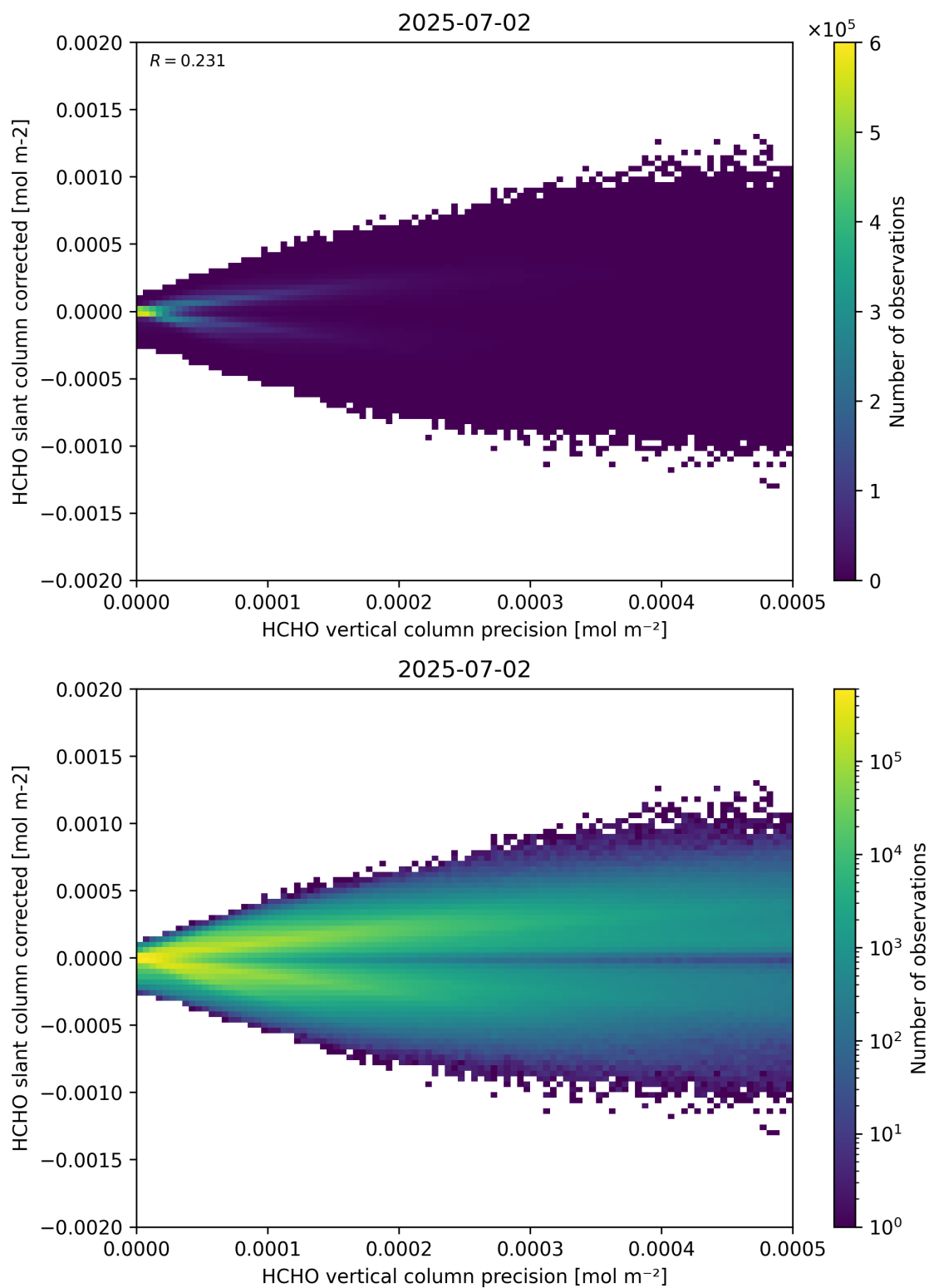
Figure 140: Scatter density plot of “HCHO vertical column precision” against “HCHO slant column corrected” for 2025-07-02 to 2025-07-03.
