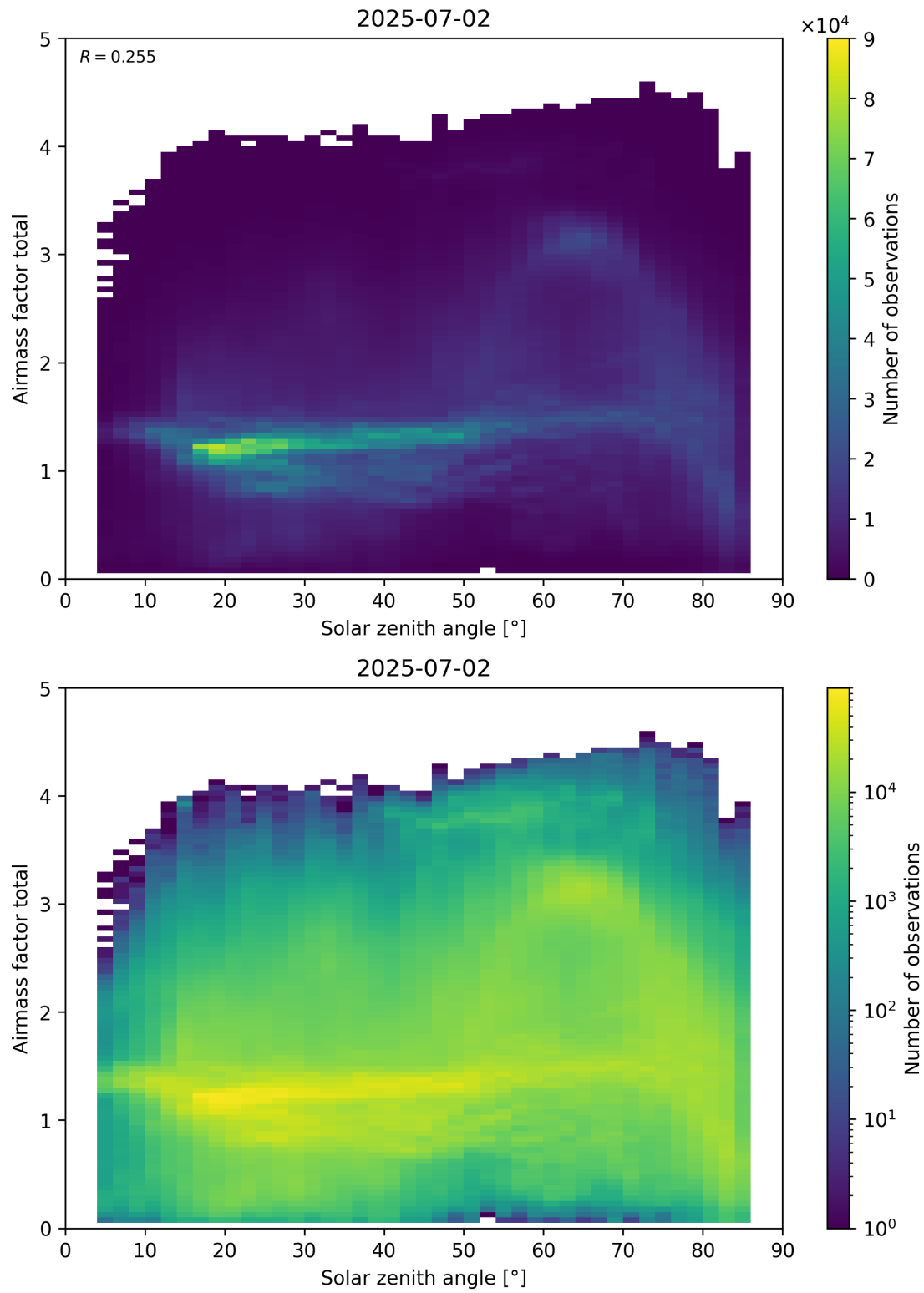
Figure 175: Scatter density plot of “Solar zenith angle” against “Airmass factor total” for 2025-07-02 to 2025-07-03.
