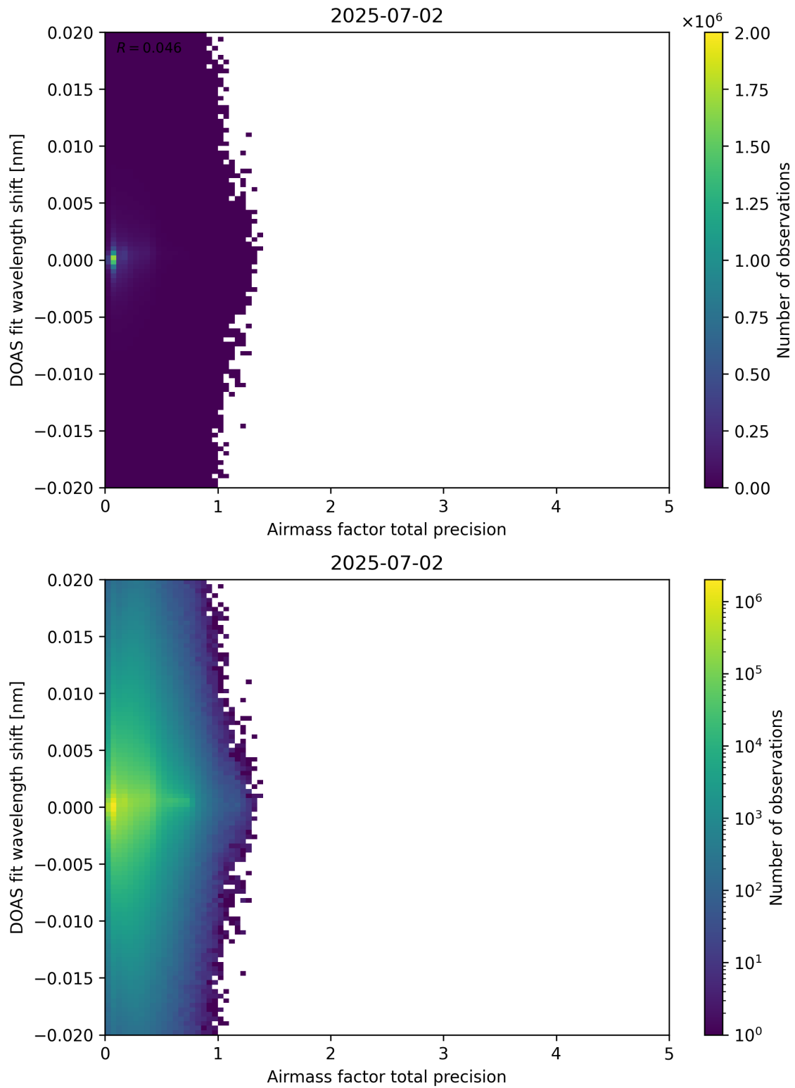
Figure 106: Scatter density plot of “Airmass factor total precision” against “DOAS fit wavelength shift” for 2025-07-02 to 2025-07-03.
