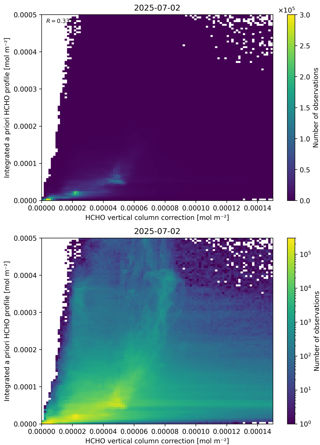
Figure 122: Scatter density plot of “HCHO vertical column correction” against “Integrated a priori HCHO profile” for 2025-07-02 to 2025-07-03.
