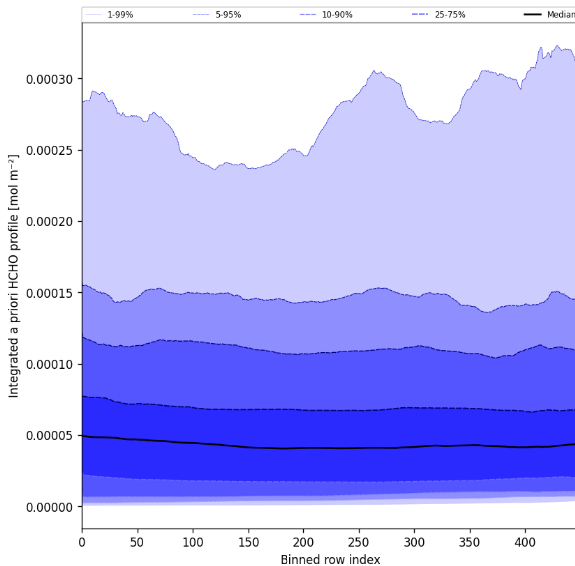
Figure 57: Along track statistics of "Integrated a priori HCHO profile" for 2025-07-02 to 2025-07-03
