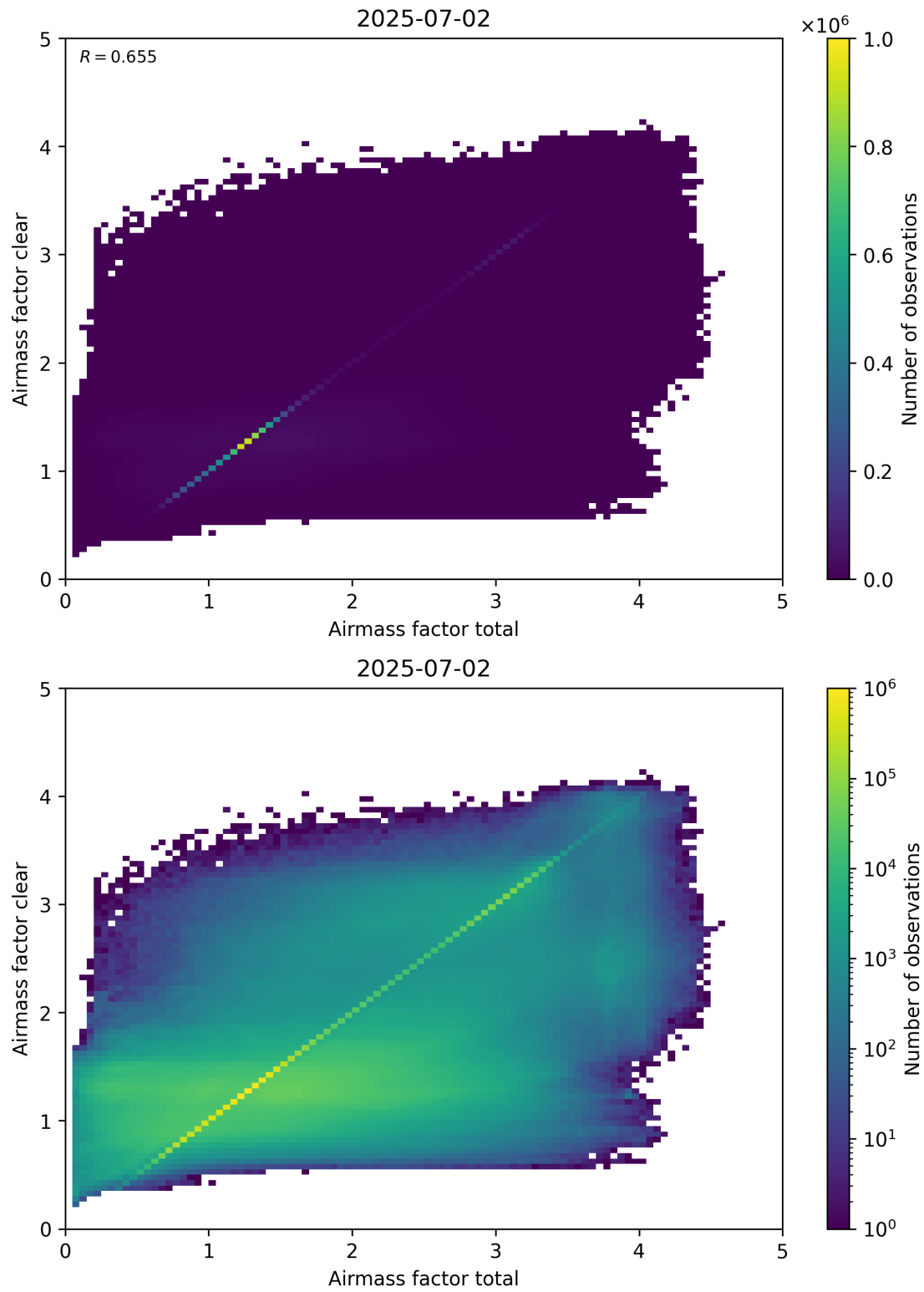
Figure 100: Scatter density plot of “Airmass factor total” against “Airmass factor clear” for 2025-07-02 to 2025-07-03.
