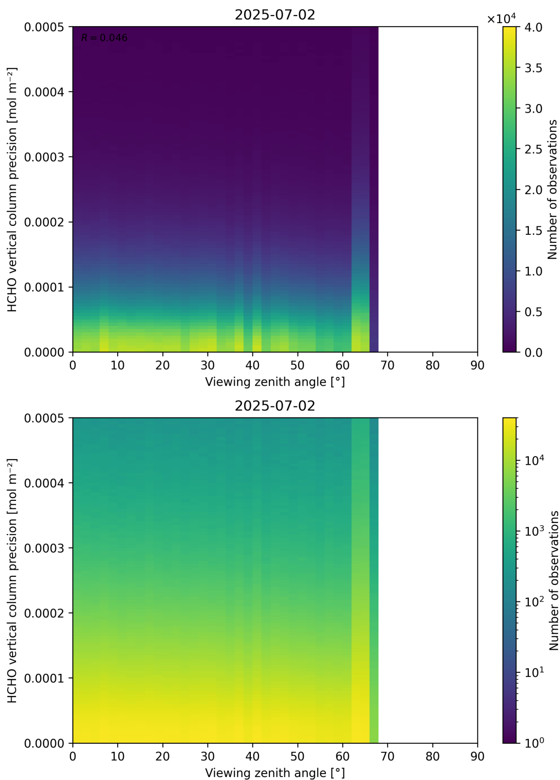
Figure 194: Scatter density plot of “Viewing zenith angle” against “HCHO vertical column precision” for 2025-07-02 to 2025-07-03.
