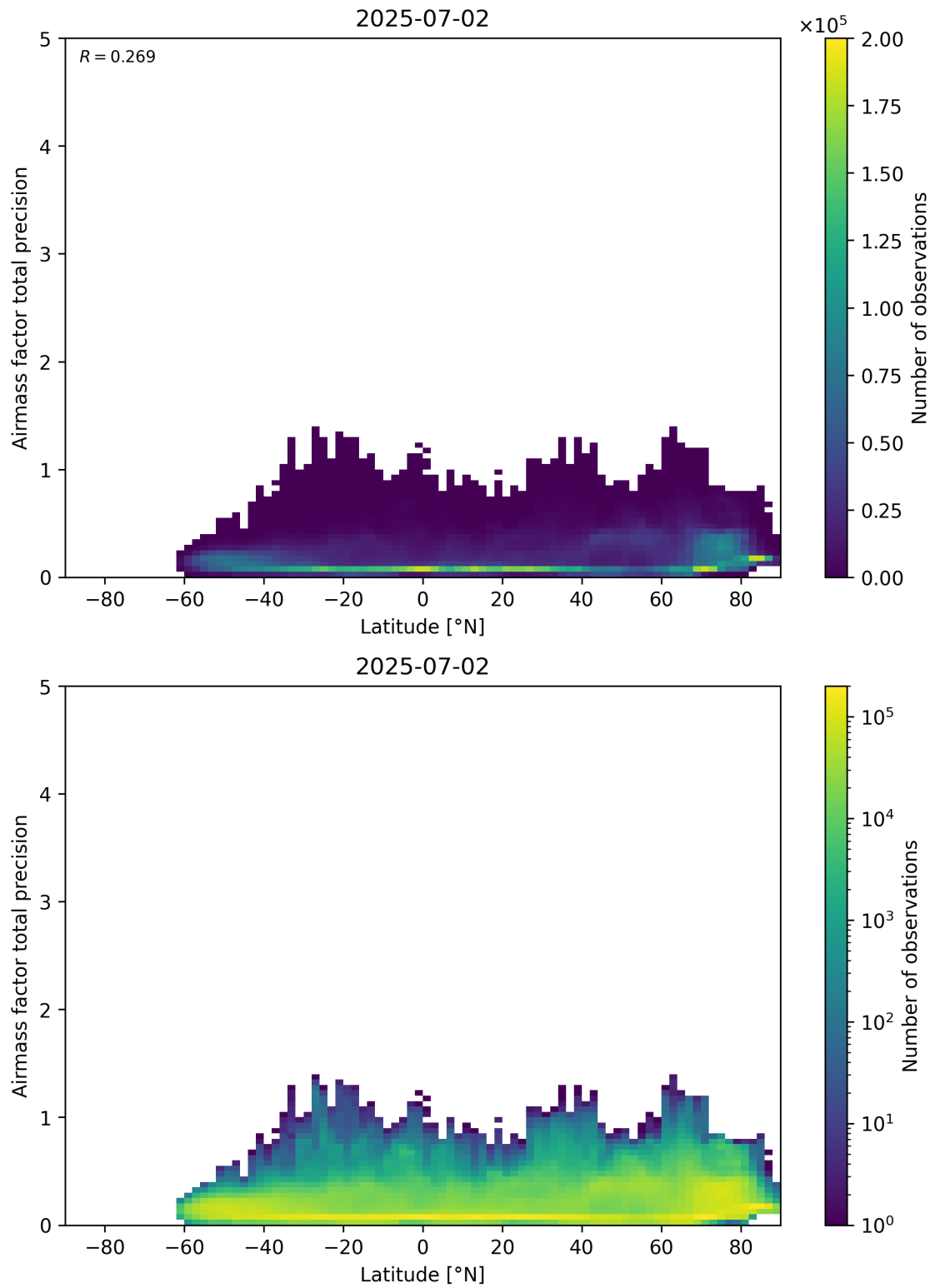
Figure 162: Scatter density plot of “Latitude” against “Airmass factor total precision” for 2025-07-02 to 2025-07-03.
