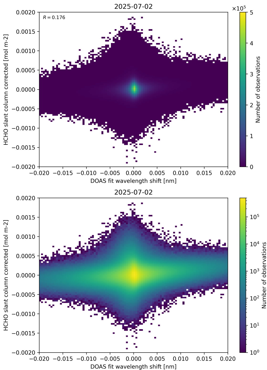
Figure 66: Scatter density plot of “DOAS fit wavelength shift” against “HCHO slant column corrected” for 2025-07-02 to 2025-07-03.
