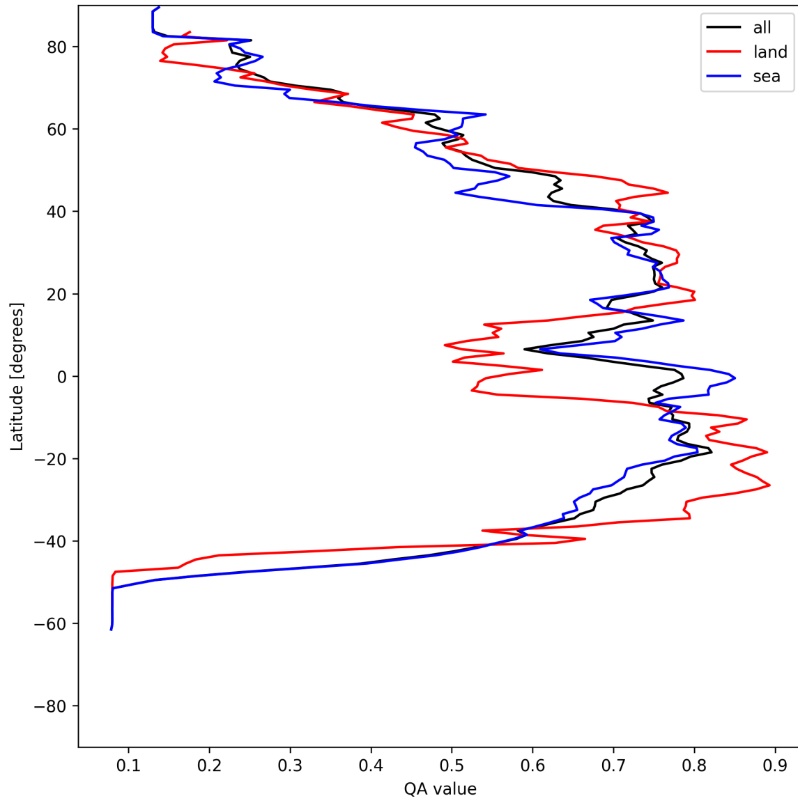
Figure 20: Zonal average of “QA value” for 2025-07-02 to 2025-07-03.
