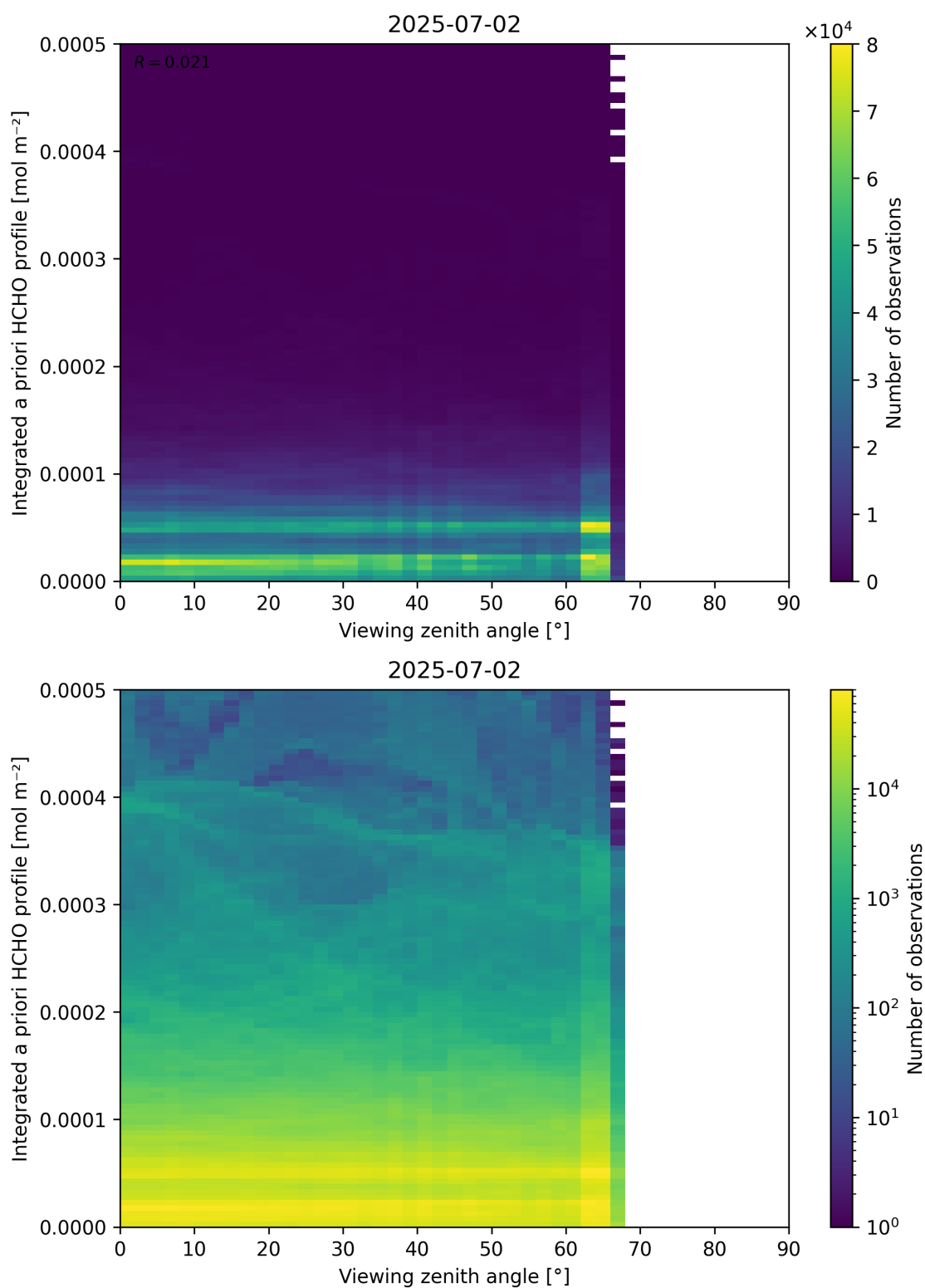
Figure 195: Scatter density plot of “Viewing zenith angle” against “Integrated a priori HCHO profile” for 2025-07-02 to 2025-07-03.
