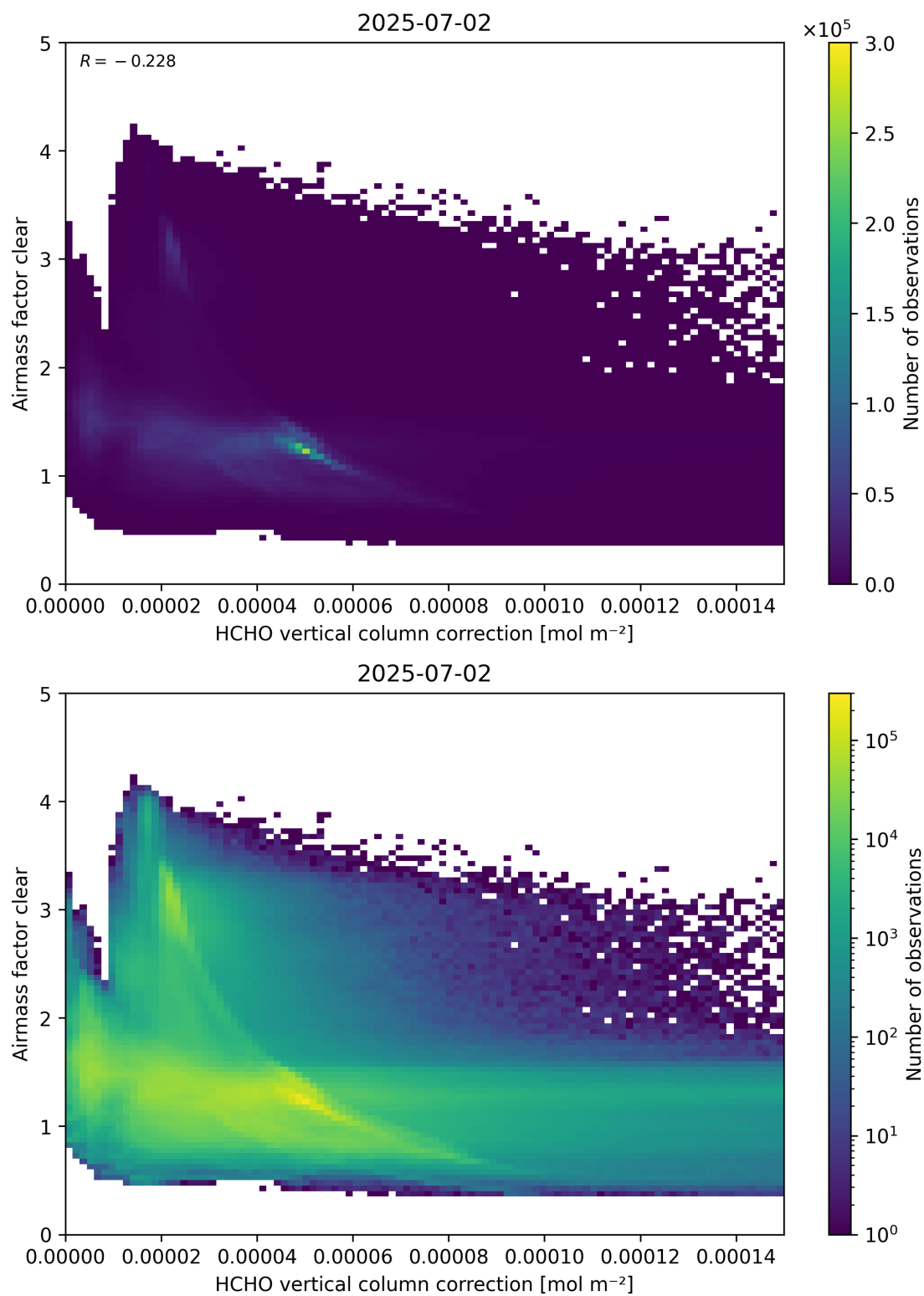
Figure 115: Scatter density plot of “HCHO vertical column correction” against “Airmass factor clear” for 2025-07-02 to 2025-07-03.
