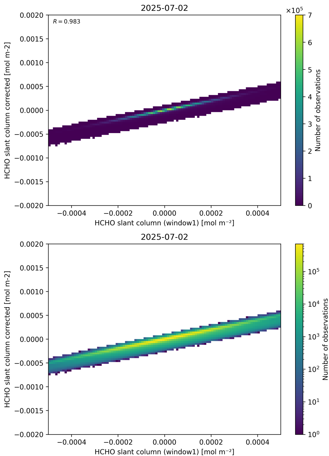
Figure 82: Scatter density plot of “HCHO slant column (window1)” against “HCHO slant column corrected” for 2025-07-02 to 2025-07-03.
