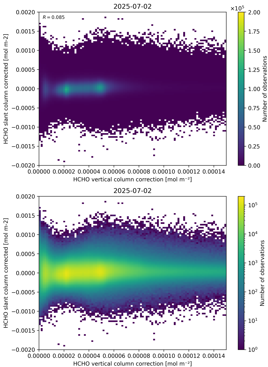
Figure 116: Scatter density plot of “HCHO vertical column correction” against “HCHO slant column corrected” for 2025-07-02 to 2025-07-03.
