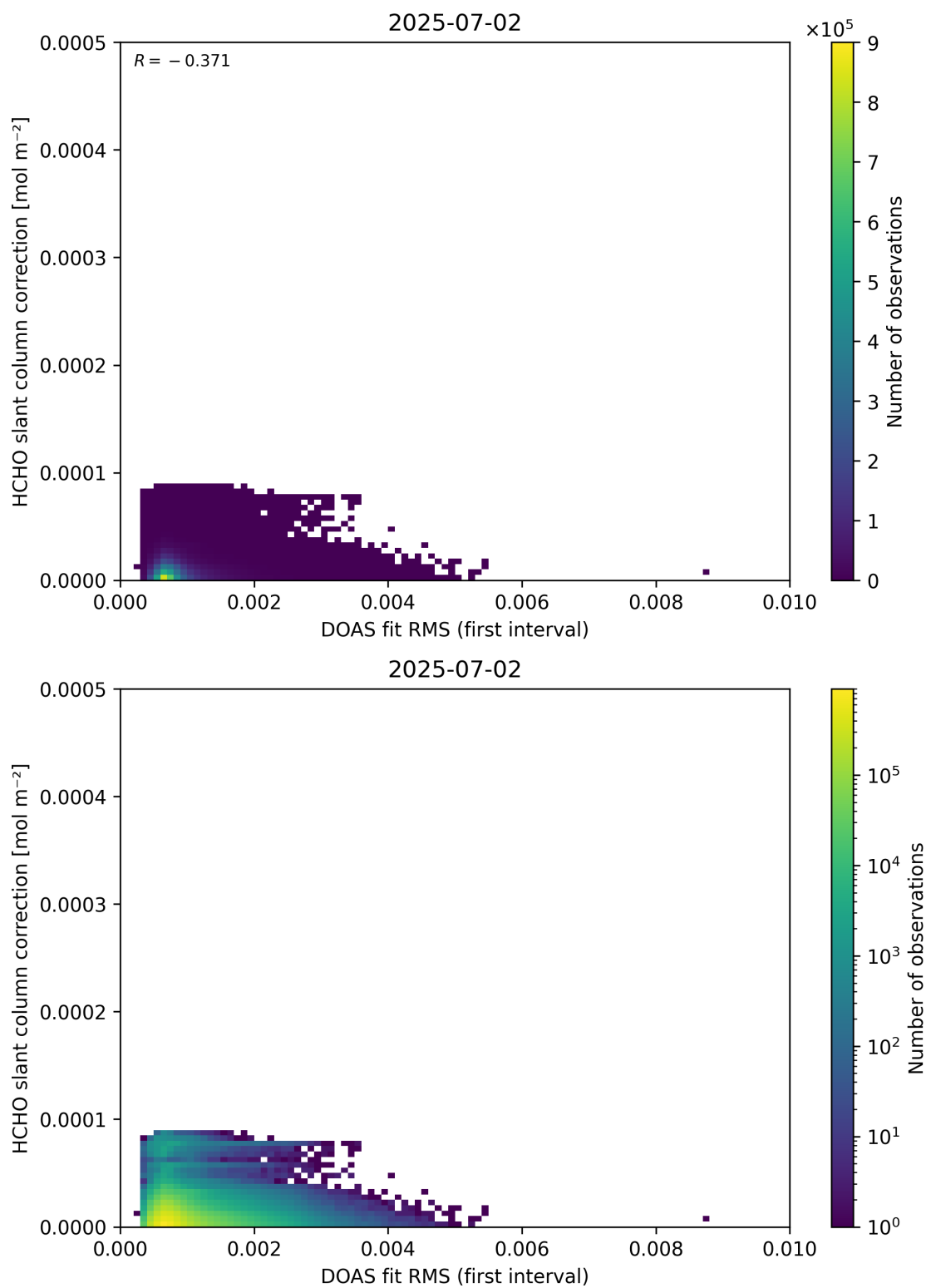
Figure 63: Scatter density plot of “DOAS fit RMS (first interval)” against “HCHO slant column correction” for 2025-07-02 to 2025-07-03.
