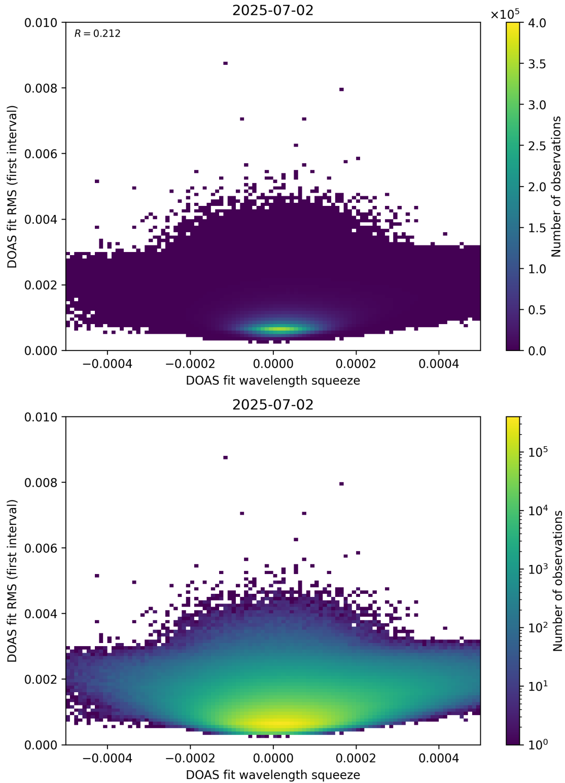
Figure 68: Scatter density plot of “DOAS fit wavelength squeeze” against “DOAS fit RMS (first interval)” for 2025-07-02 to 2025-07-03.
