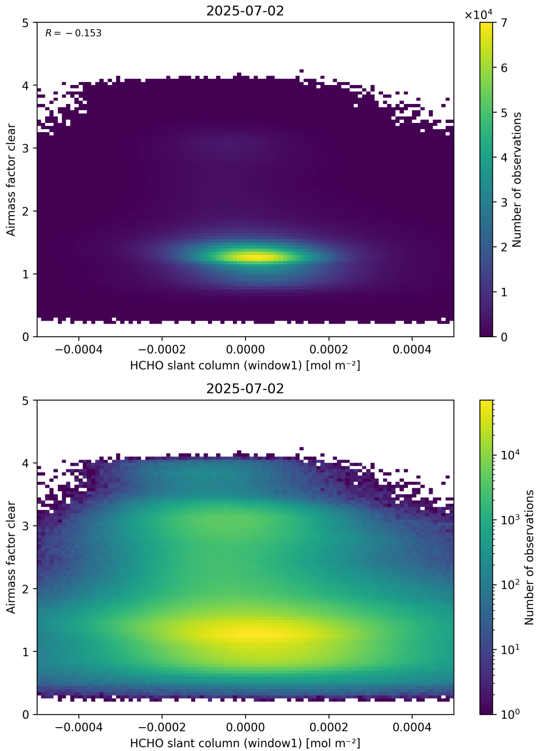
Figure 81: Scatter density plot of “HCHO slant column (window1)” against “Airmass factor clear” for 2025-07-02 to 2025-07-03.
