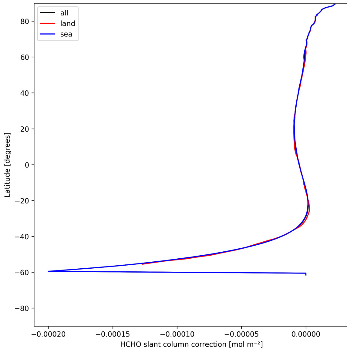
Figure 33: Zonal average of “HCHO slant column correction” for 2025-07-02 to 2025-07-03.
