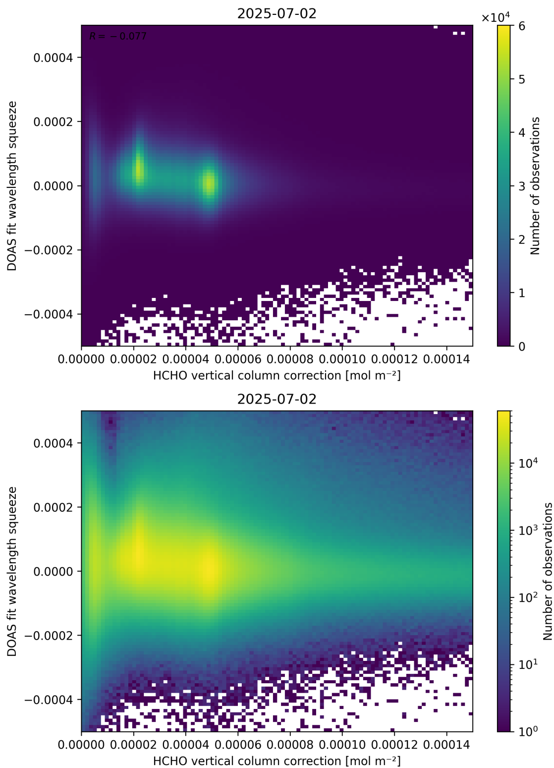
Figure 114: Scatter density plot of “HCHO vertical column correction” against “DOAS fit wavelength squeeze” for 2025-07-02 to 2025-07-03.
