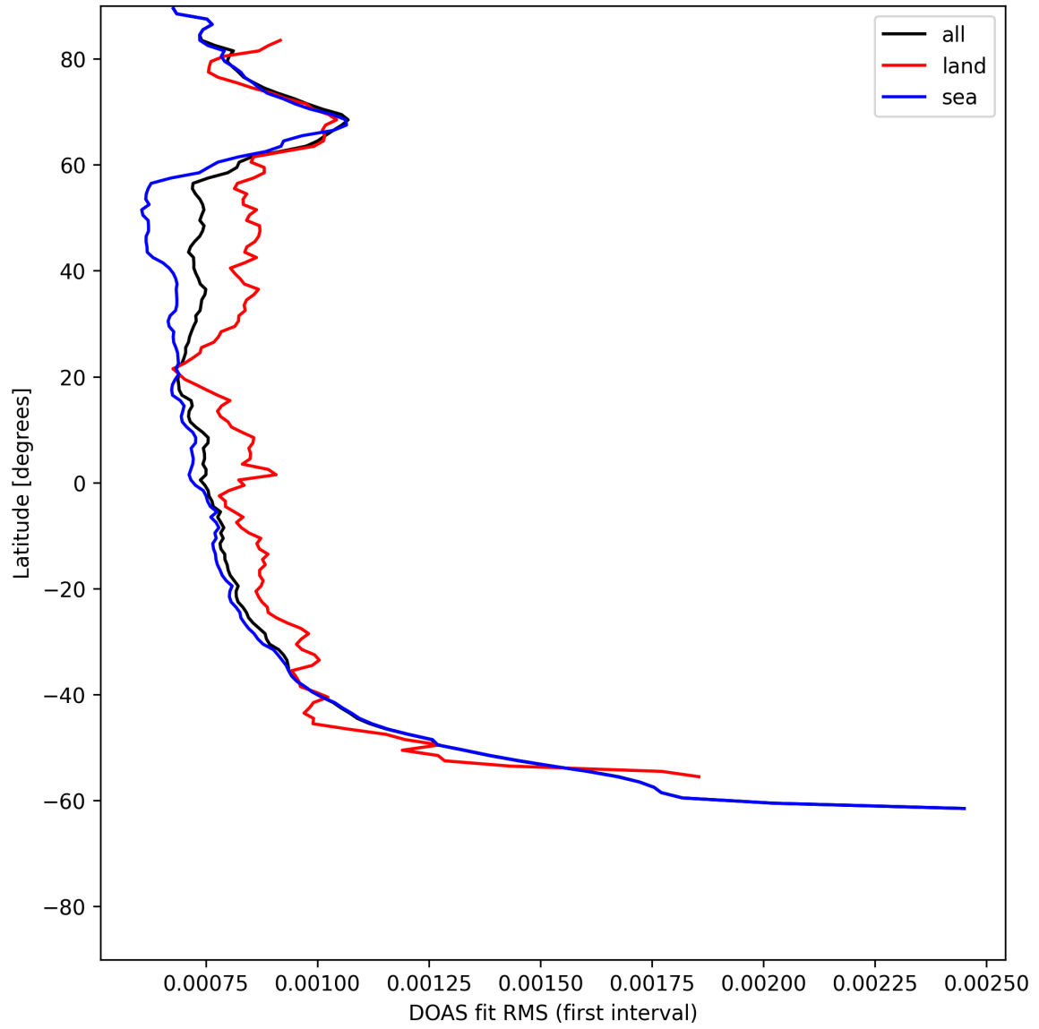
Figure 32: Zonal average of “DOAS fit RMS (first interval)” for 2025-07-02 to 2025-07-03.
