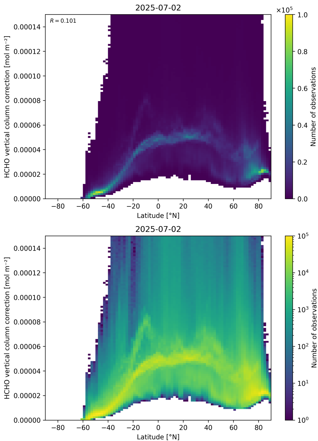
Figure 164: Scatter density plot of “Latitude” against “HCHO vertical column correction” for 2025-07-02 to 2025-07-03.
