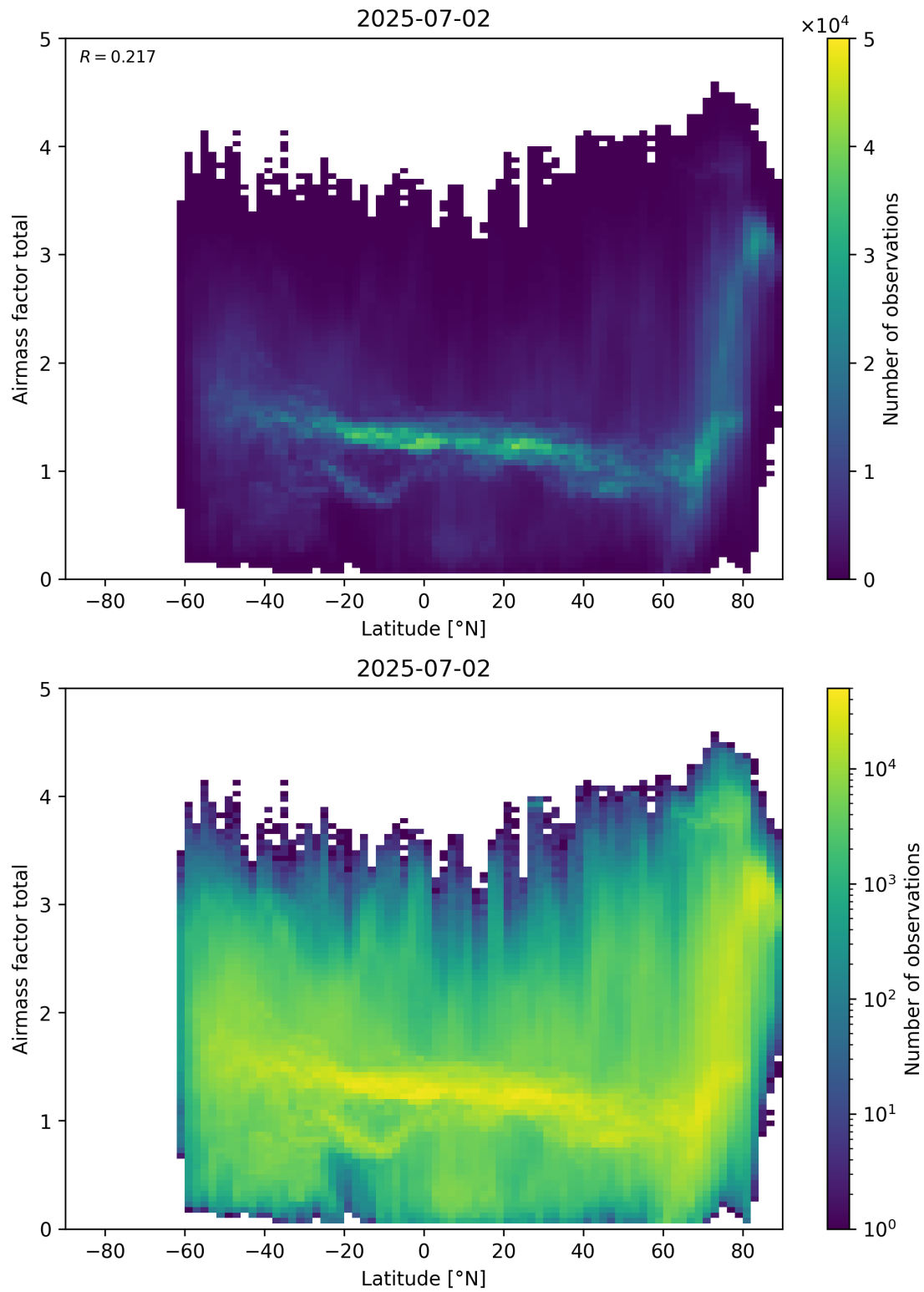
Figure 161: Scatter density plot of “Latitude” against “Airmass factor total” for 2025-07-02 to 2025-07-03.
