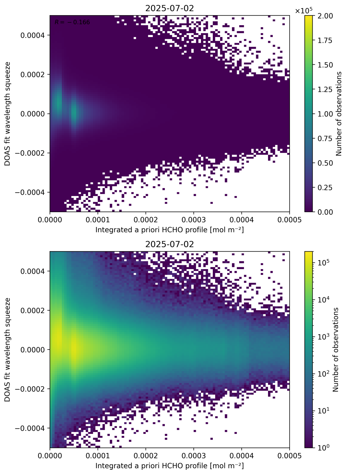
Figure 150: Scatter density plot of “Integrated a priori HCHO profile” against “DOAS fit wavelength squeeze” for 2025-07-02 to 2025-07-03.
