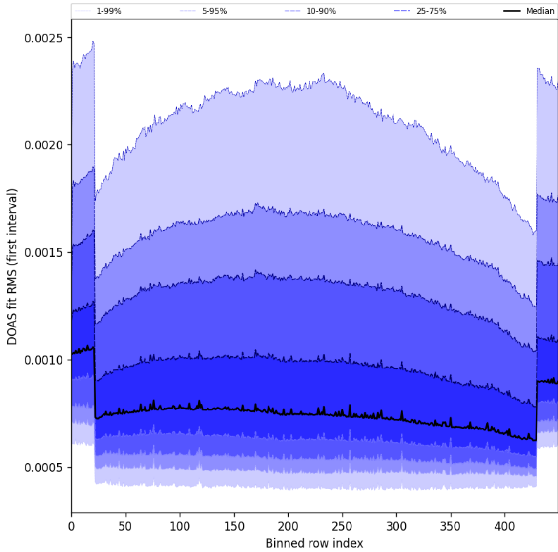
Figure 60: Along track statistics of “DOAS fit RMS (first interval)” for 2025-07-02 to 2025-07-03
