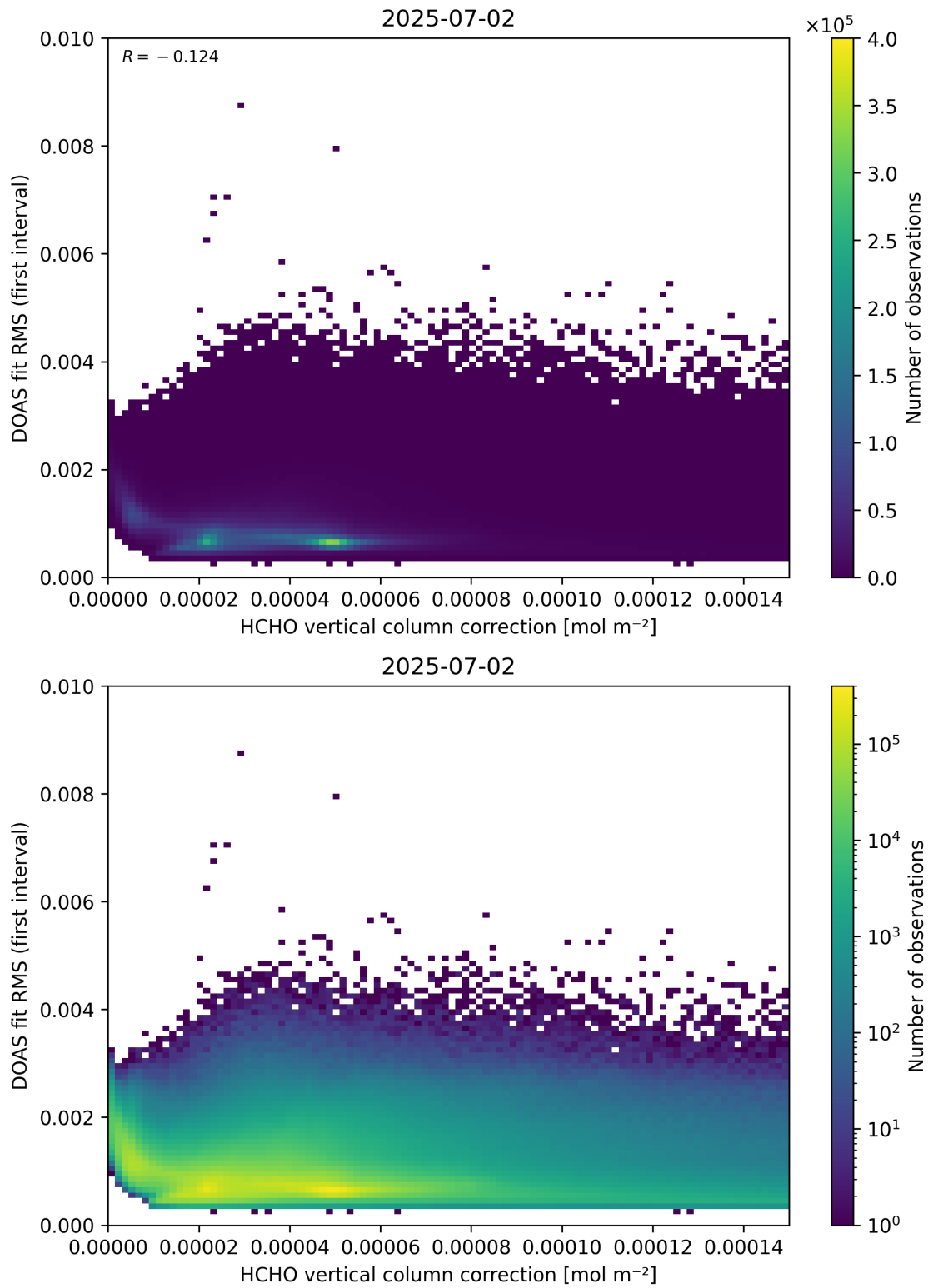
Figure 112: Scatter density plot of “HCHO vertical column correction” against “DOAS fit RMS (first interval)” for 2025-07-02 to 2025-07-03.
