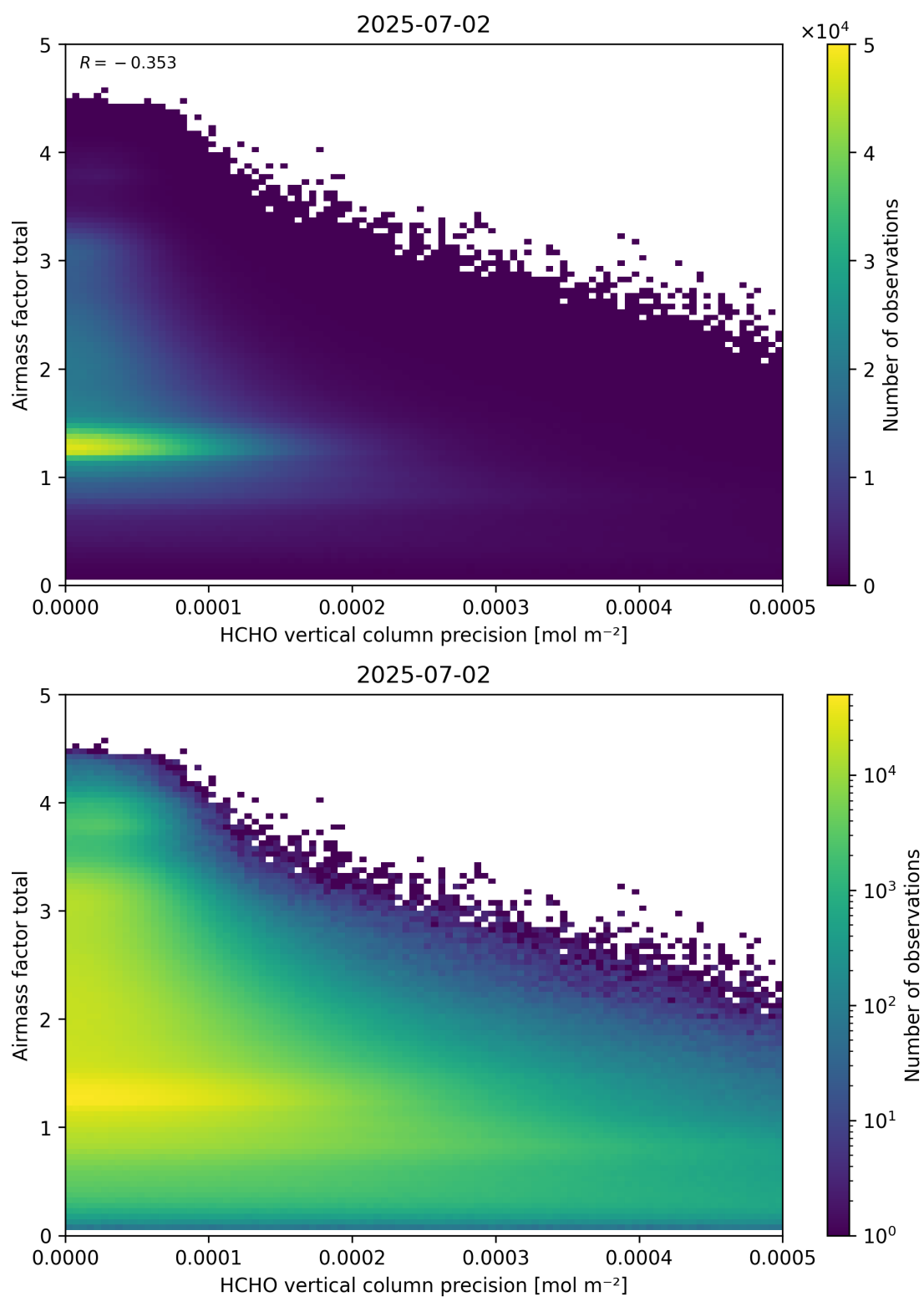
Figure 144: Scatter density plot of “HCHO vertical column precision” against “Airmass factor total” for 2025-07-02 to 2025-07-03.
