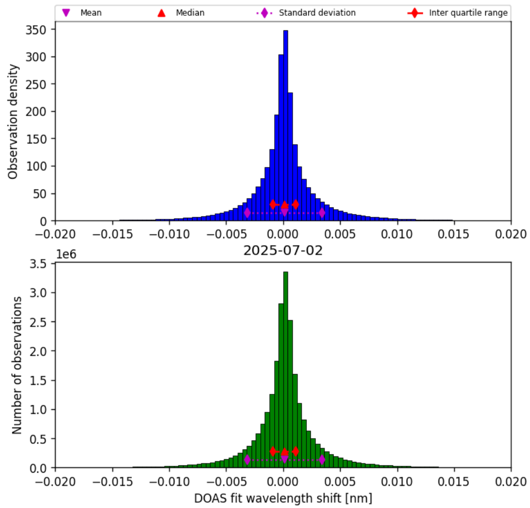
Figure 44: Histogram of “DOAS fit wavelength shift” for 2025-07-02 to 2025-07-03
