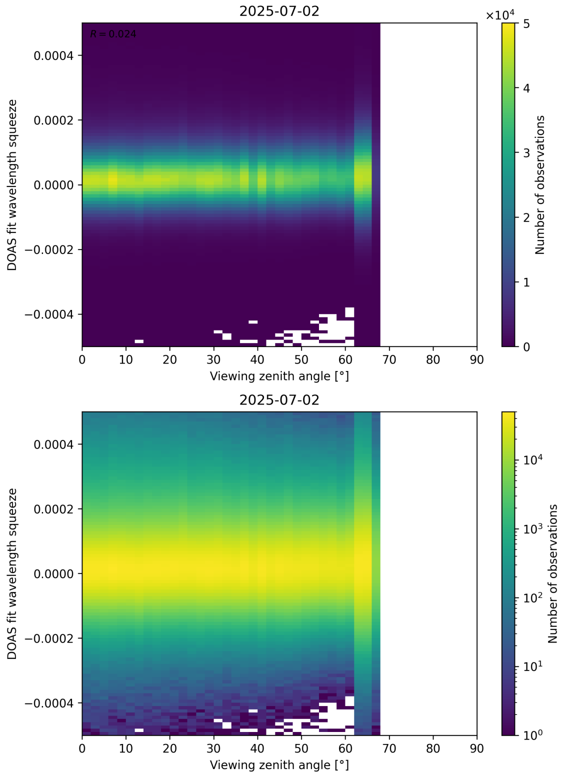
Figure 184: Scatter density plot of “Viewing zenith angle” against “DOAS fit wavelength squeeze” for 2025-07-02 to 2025-07-03.
