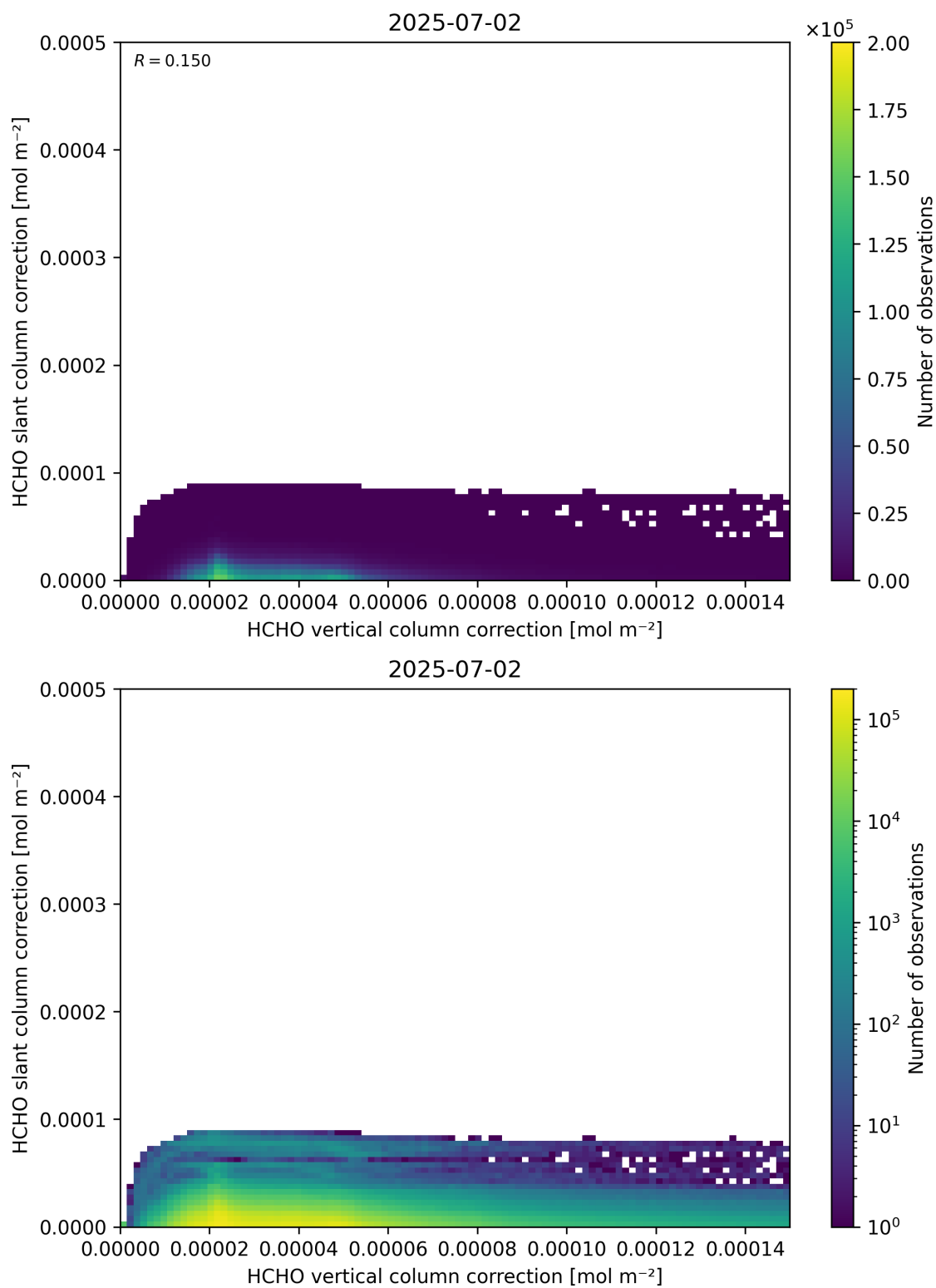
Figure 117: Scatter density plot of “HCHO vertical column correction” against “HCHO slant column correction” for 2025-07-02 to 2025-07-03.
