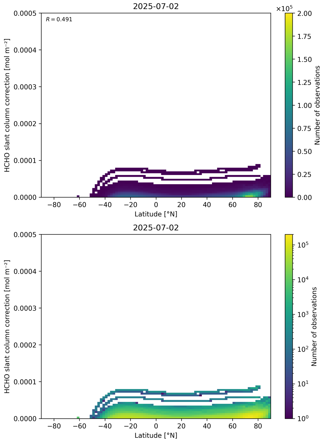
Figure 158: Scatter density plot of “Latitude” against “HCHO slant column correction” for 2025-07-02 to 2025-07-03.
