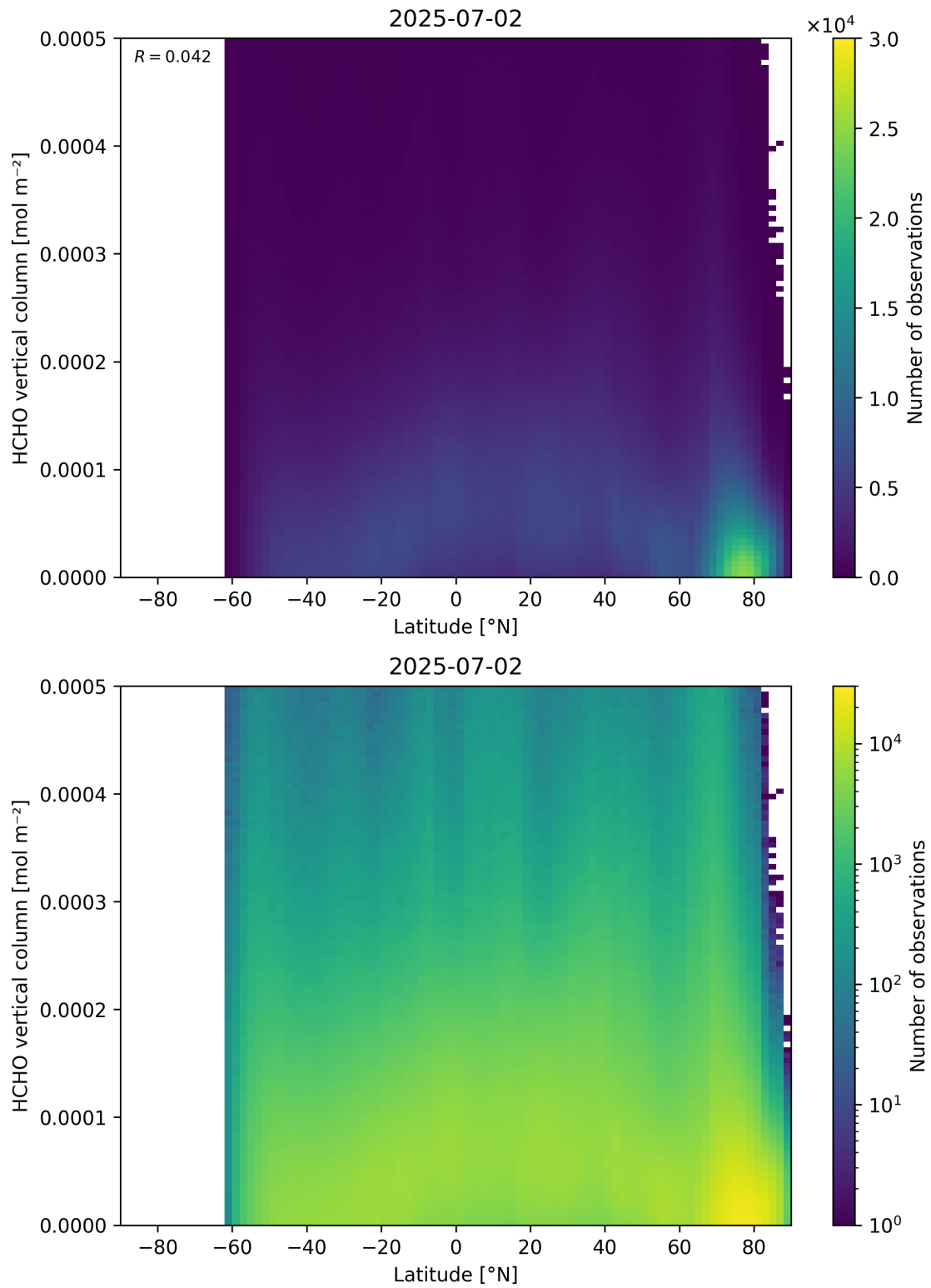
Figure 163: Scatter density plot of “Latitude” against “HCHO vertical column” for 2025-07-02 to 2025-07-03.
