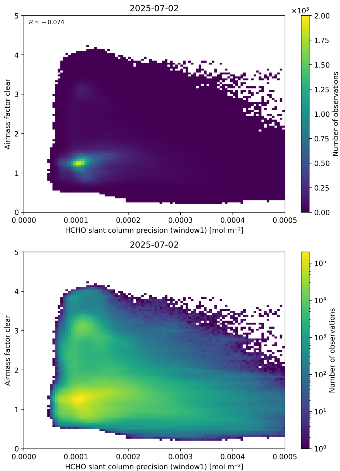
Figure 91: Scatter density plot of “HCHO slant column precision (window1)” against “Airmass factor clear” for 2025-07-02 to 2025-07-03.
