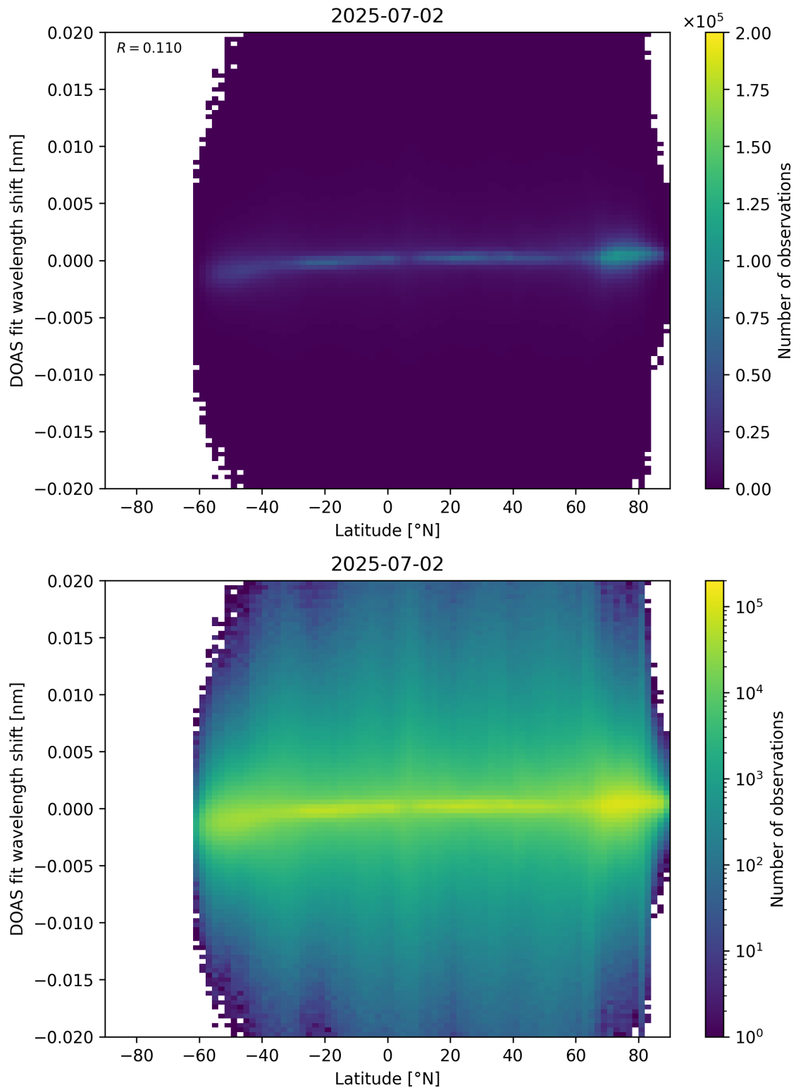
Figure 154: Scatter density plot of “Latitude” against “DOAS fit wavelength shift” for 2025-07-02 to 2025-07-03.
