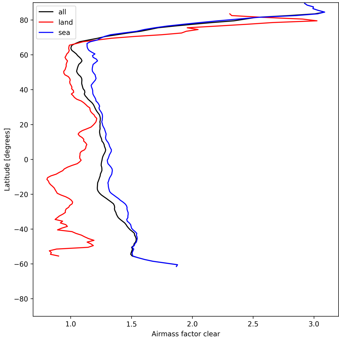
Figure 28: Zonal average of “Airmass factor clear” for 2025-07-02 to 2025-07-03.
