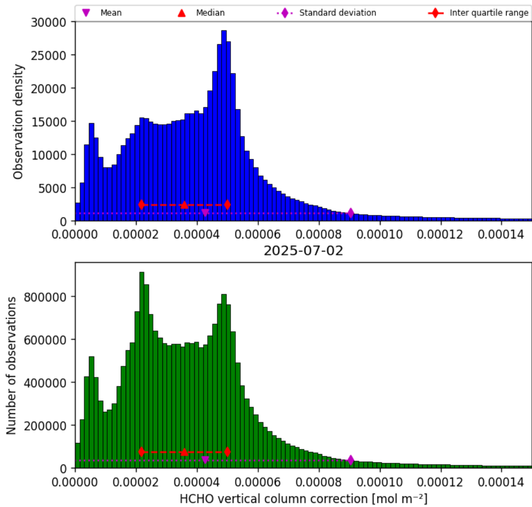
Figure 37: Histogram of “HCHO vertical column correction” for 2025-07-02 to 2025-07-03
