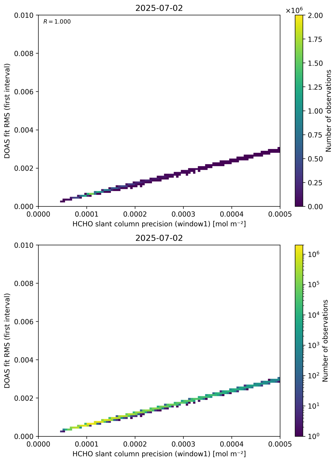
Figure 88: Scatter density plot of “HCHO slant column precision (window1)” against “DOAS fit RMS (first interval)” for 2025-07-02 to 2025-07-03.
