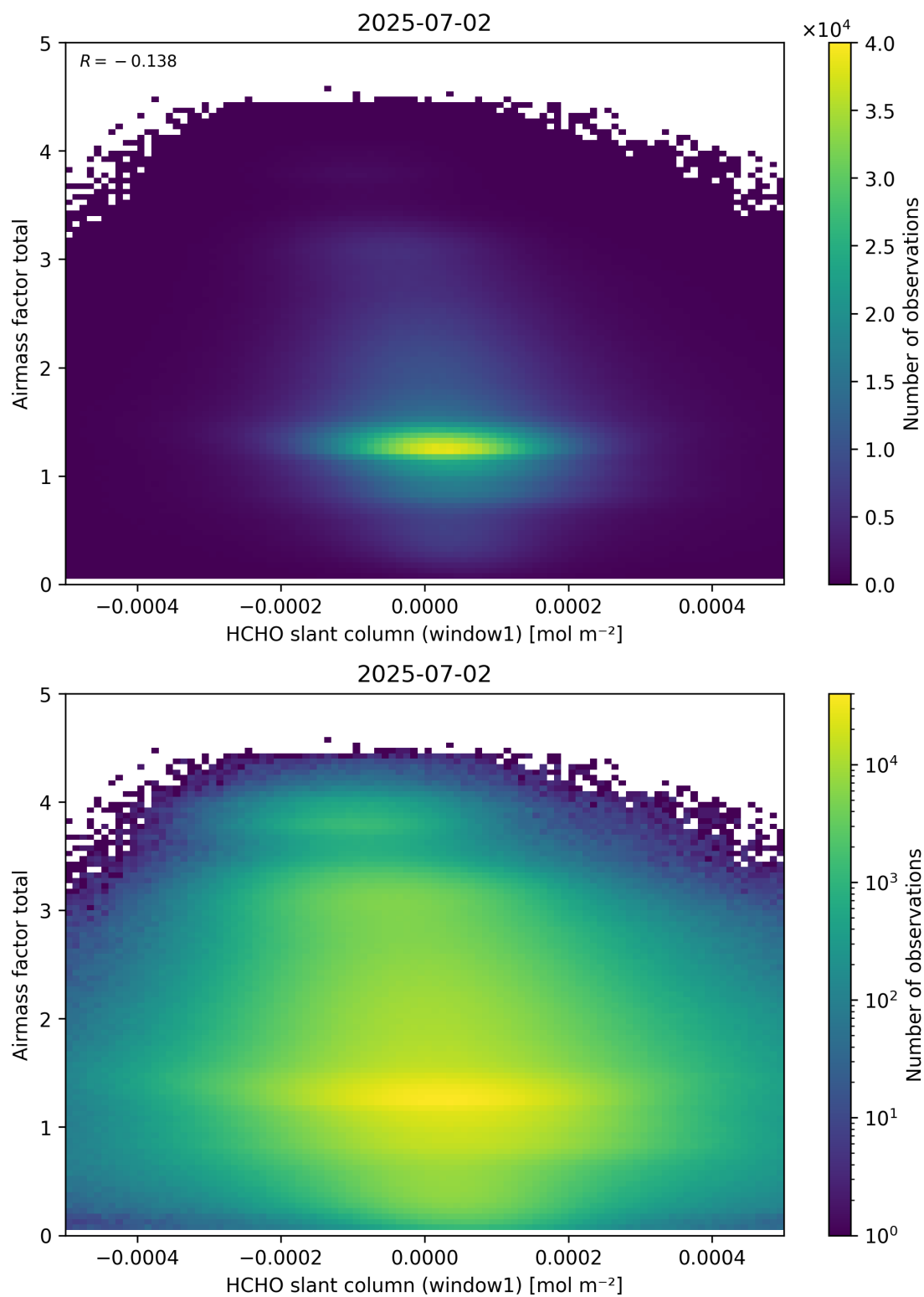
Figure 85: Scatter density plot of “HCHO slant column (window1)” against “Airmass factor total” for 2025-07-02 to 2025-07-03.
