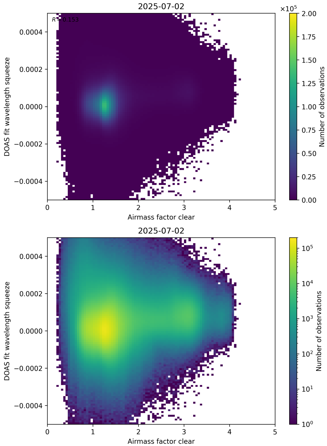
Figure 73: Scatter density plot of “Airmass factor clear” against “DOAS fit wavelength squeeze” for 2025-07-02 to 2025-07-03.
