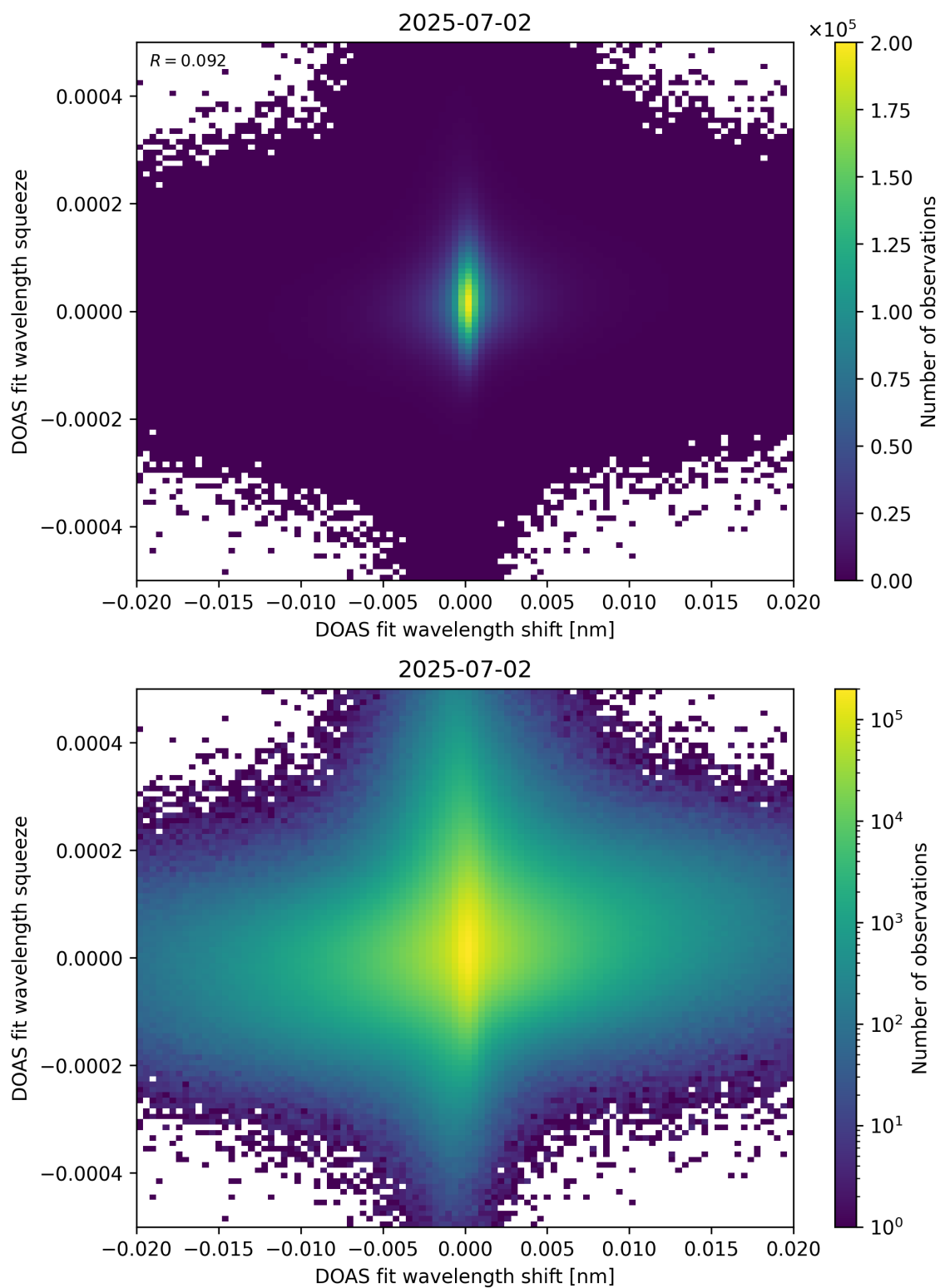
Figure 65: Scatter density plot of “DOAS fit wavelength shift” against “DOAS fit wavelength squeeze” for 2025-07-02 to 2025-07-03.
