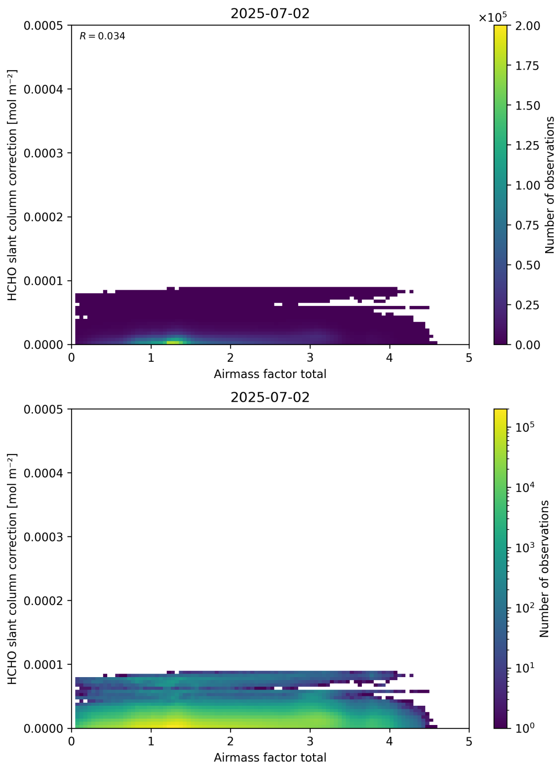
Figure 102: Scatter density plot of “Airmass factor total” against “HCHO slant column correction” for 2025-07-02 to 2025-07-03.
