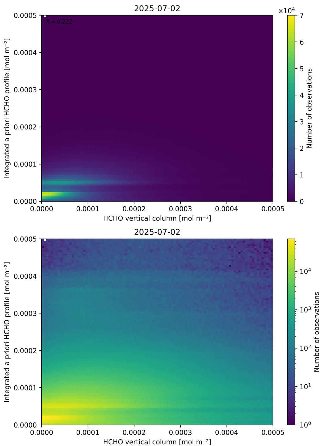
Figure 135: Scatter density plot of “HCHO vertical column” against “Integrated a priori HCHO profile” for 2025-07-02 to 2025-07-03.
