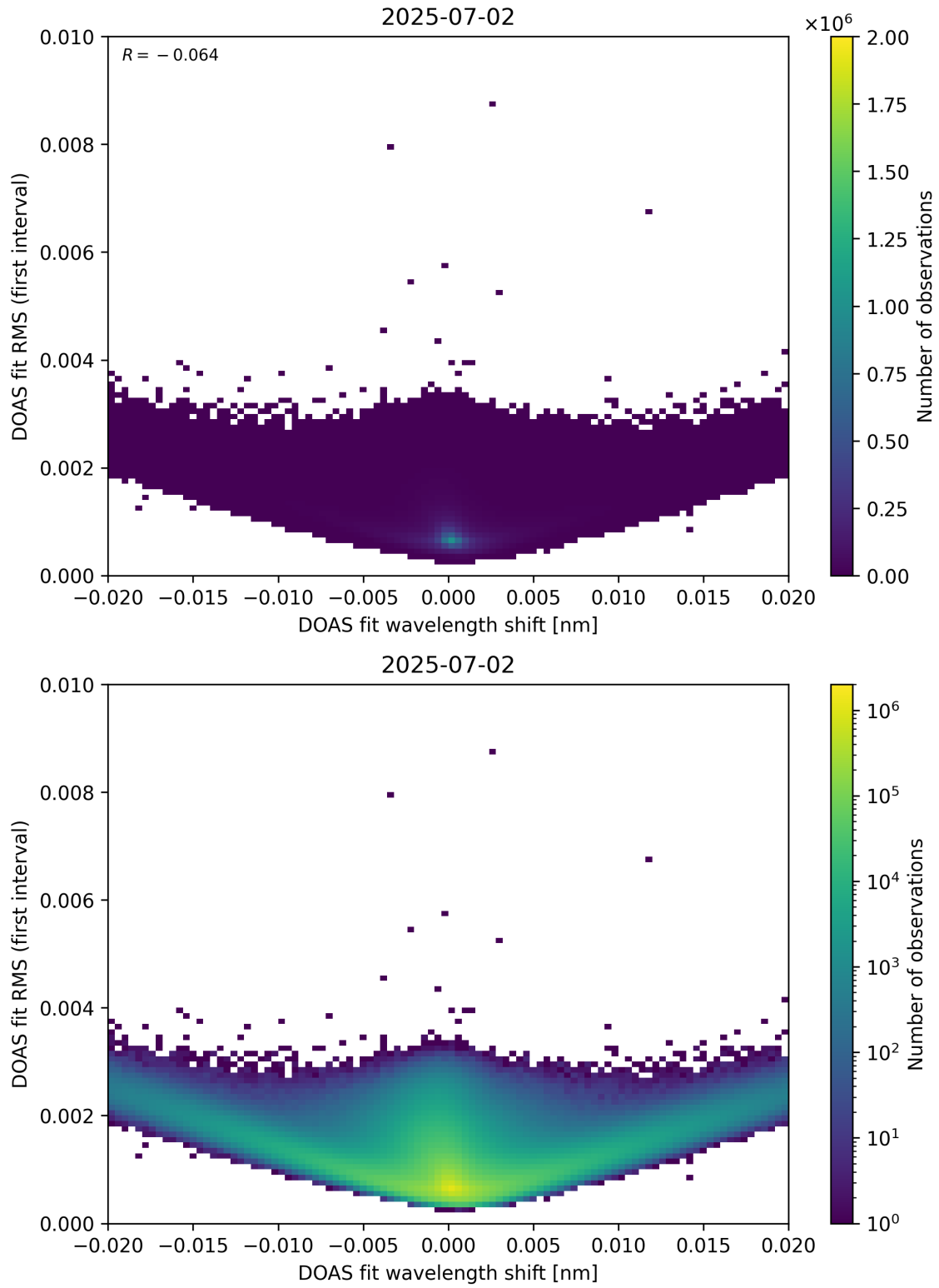
Figure 64: Scatter density plot of “DOAS fit wavelength shift” against “DOAS fit RMS (first interval)” for 2025-07-02 to 2025-07-03.
