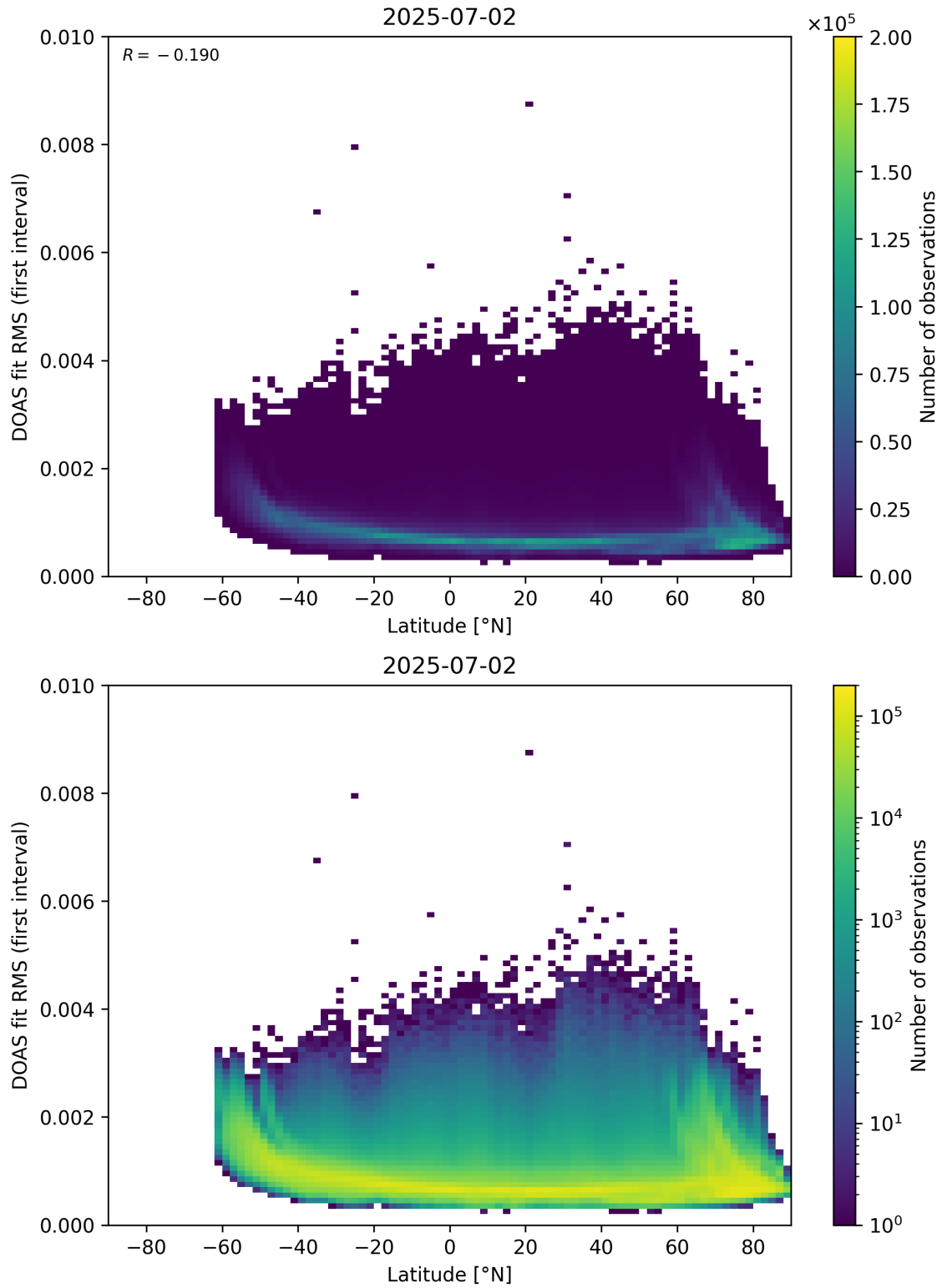
Figure 153: Scatter density plot of “Latitude” against “DOAS fit RMS (first interval)” for 2025-07-02 to 2025-07-03.
