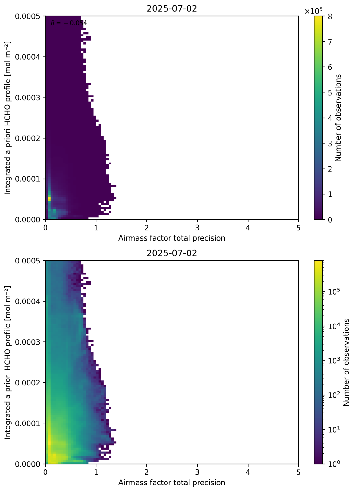
Figure 111: Scatter density plot of “Airmass factor total precision” against “Integrated a priori HCHO profile” for 2025-07-02 to 2025-07-03.
