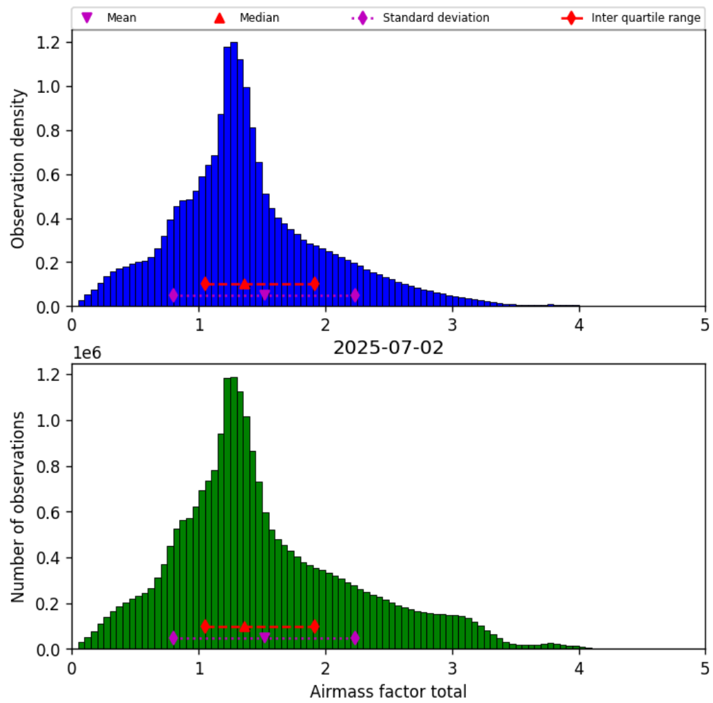
Figure 40: Histogram of “Airmass factor total” for 2025-07-02 to 2025-07-03
