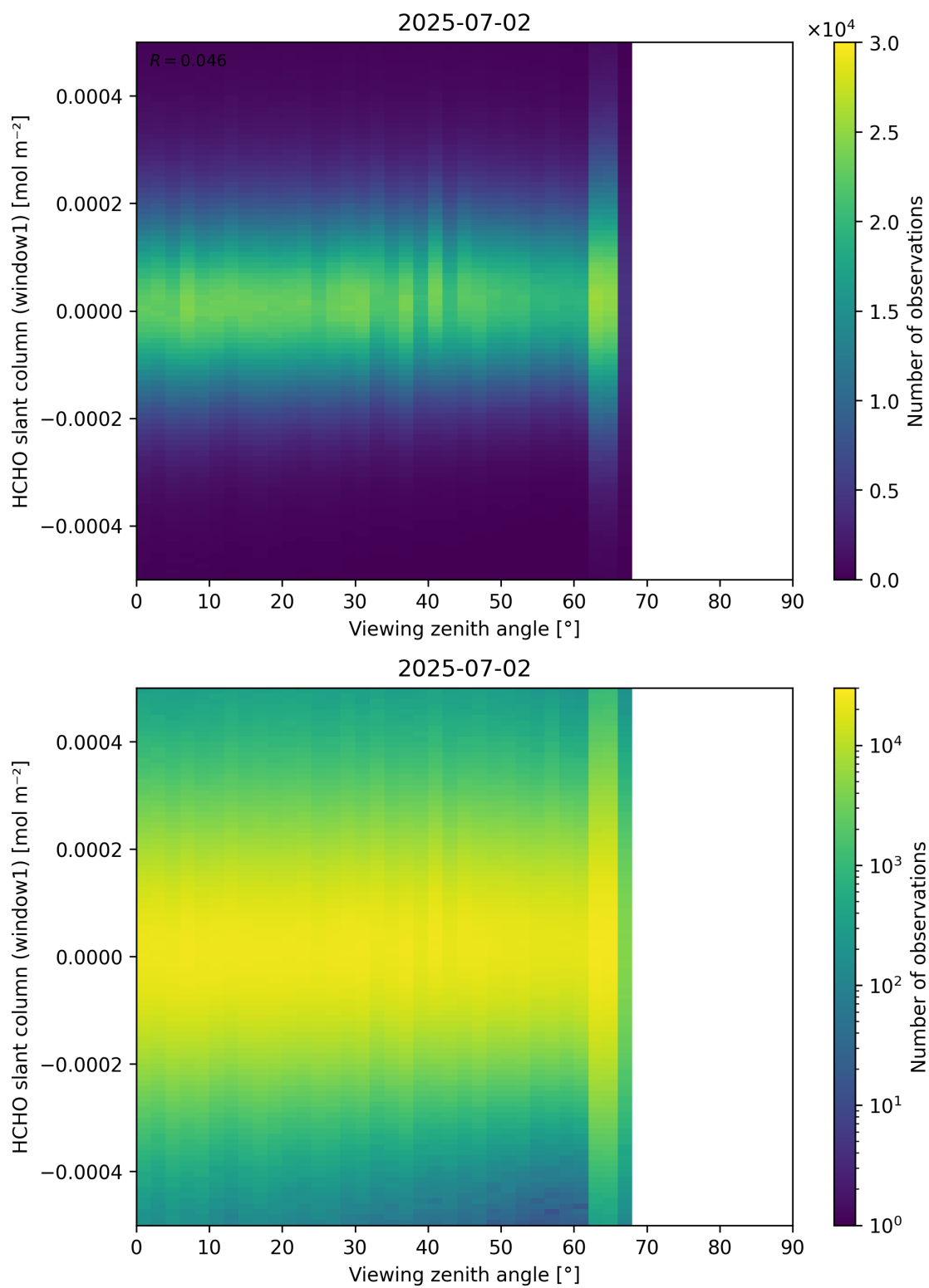
Figure 188: Scatter density plot of “Viewing zenith angle” against “HCHO slant column (window1)” for 2025-07-02 to 2025-07-03.
