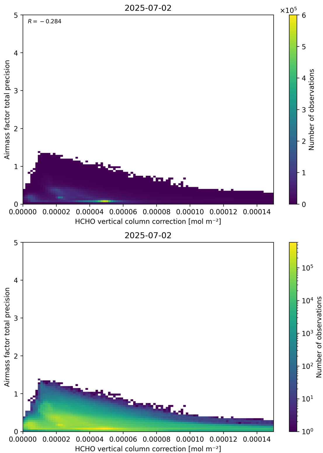
Figure 121: Scatter density plot of “HCHO vertical column correction” against “Airmass factor total precision” for 2025-07-02 to 2025-07-03.
