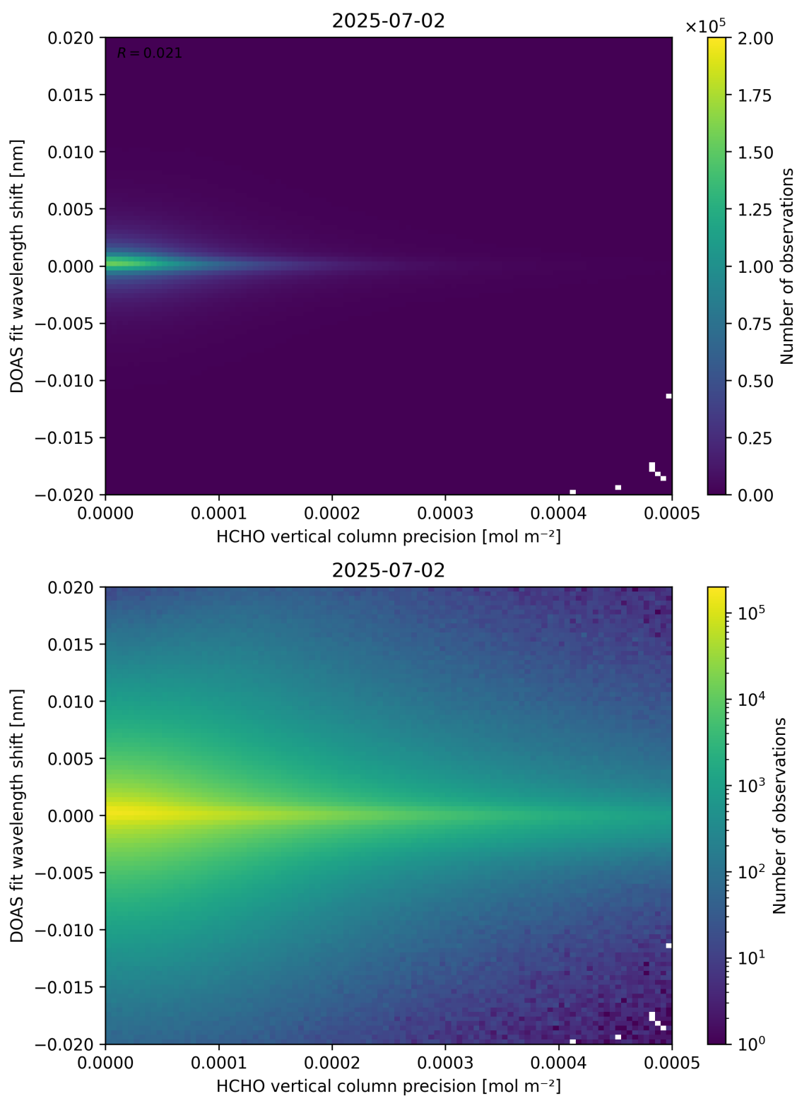
Figure 137: Scatter density plot of “HCHO vertical column precision” against “DOAS fit wavelength shift” for 2025-07-02 to 2025-07-03.
