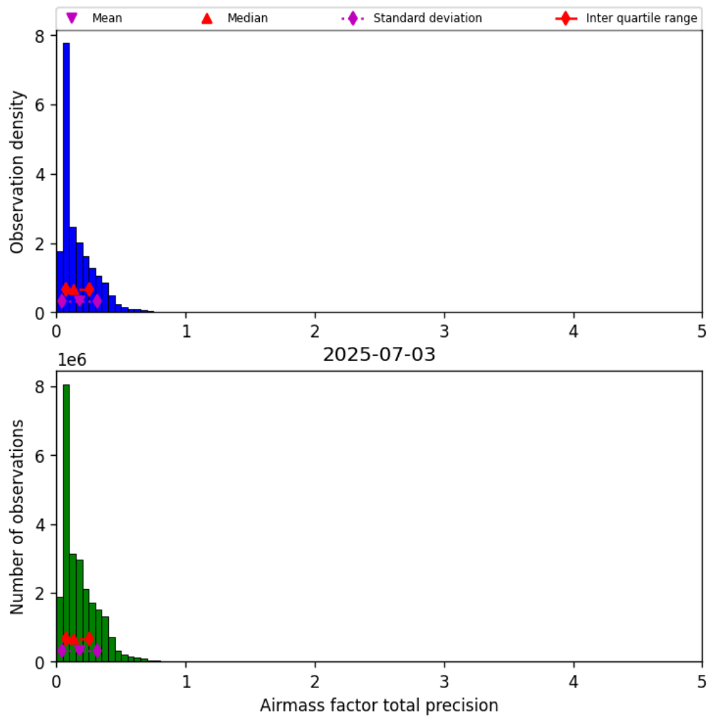
Figure 41: Histogram of “Airmass factor total precision” for 2025-07-03 to 2025-07-04
