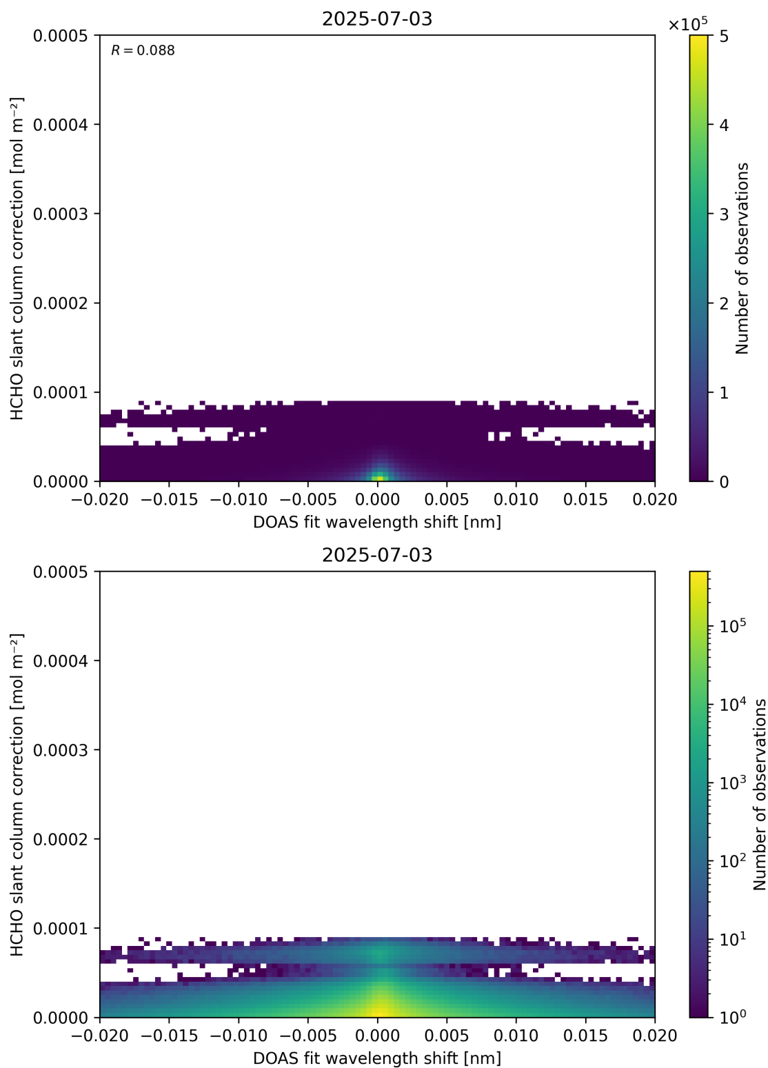
Figure 67: Scatter density plot of “DOAS fit wavelength shift” against “HCHO slant column correction” for 2025-07-03 to 2025-07-04.
