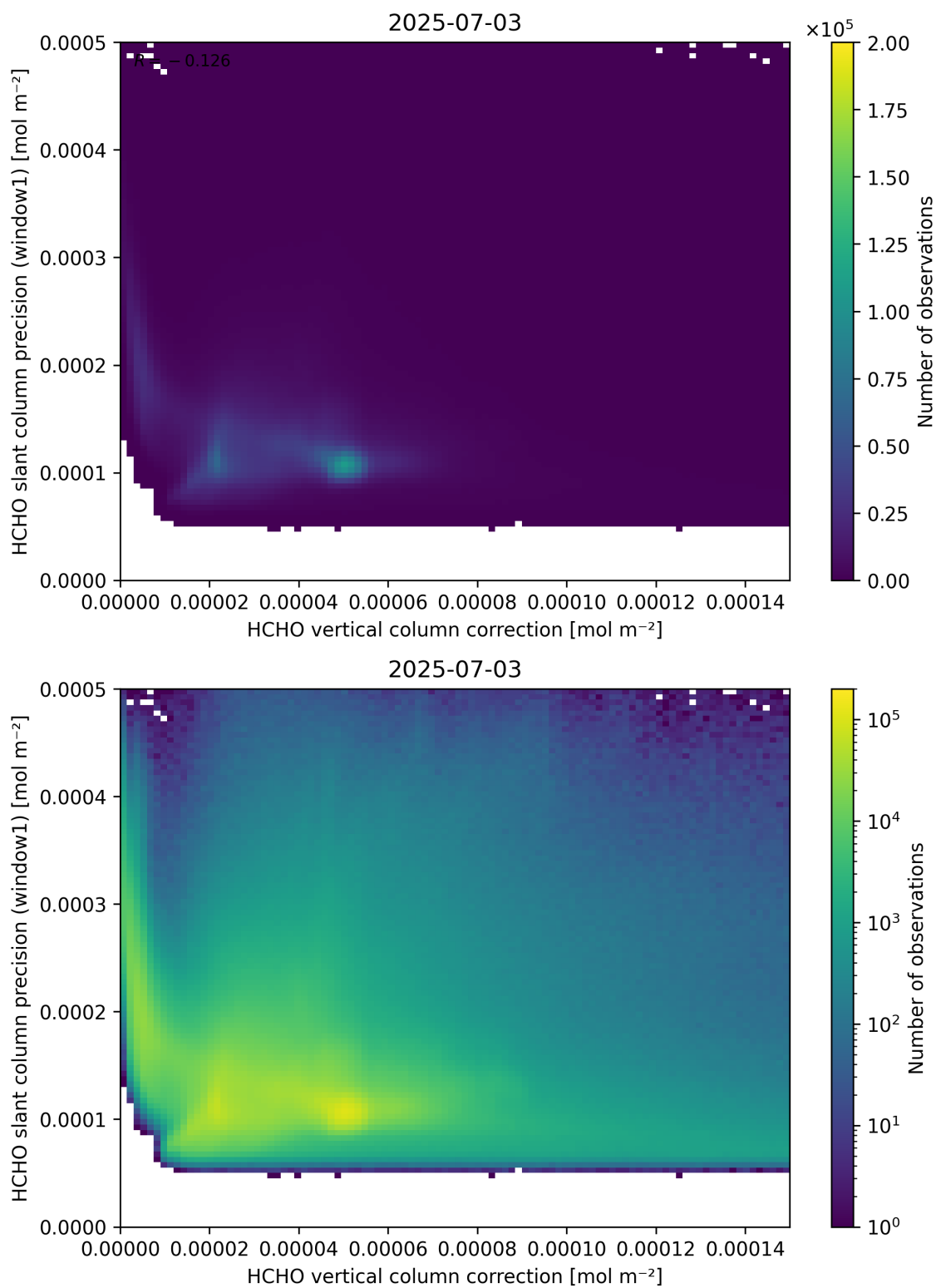
Figure 119: Scatter density plot of “HCHO vertical column correction” against “HCHO slant column precision (window1)” for 2025-07-03 to 2025-07-04.
