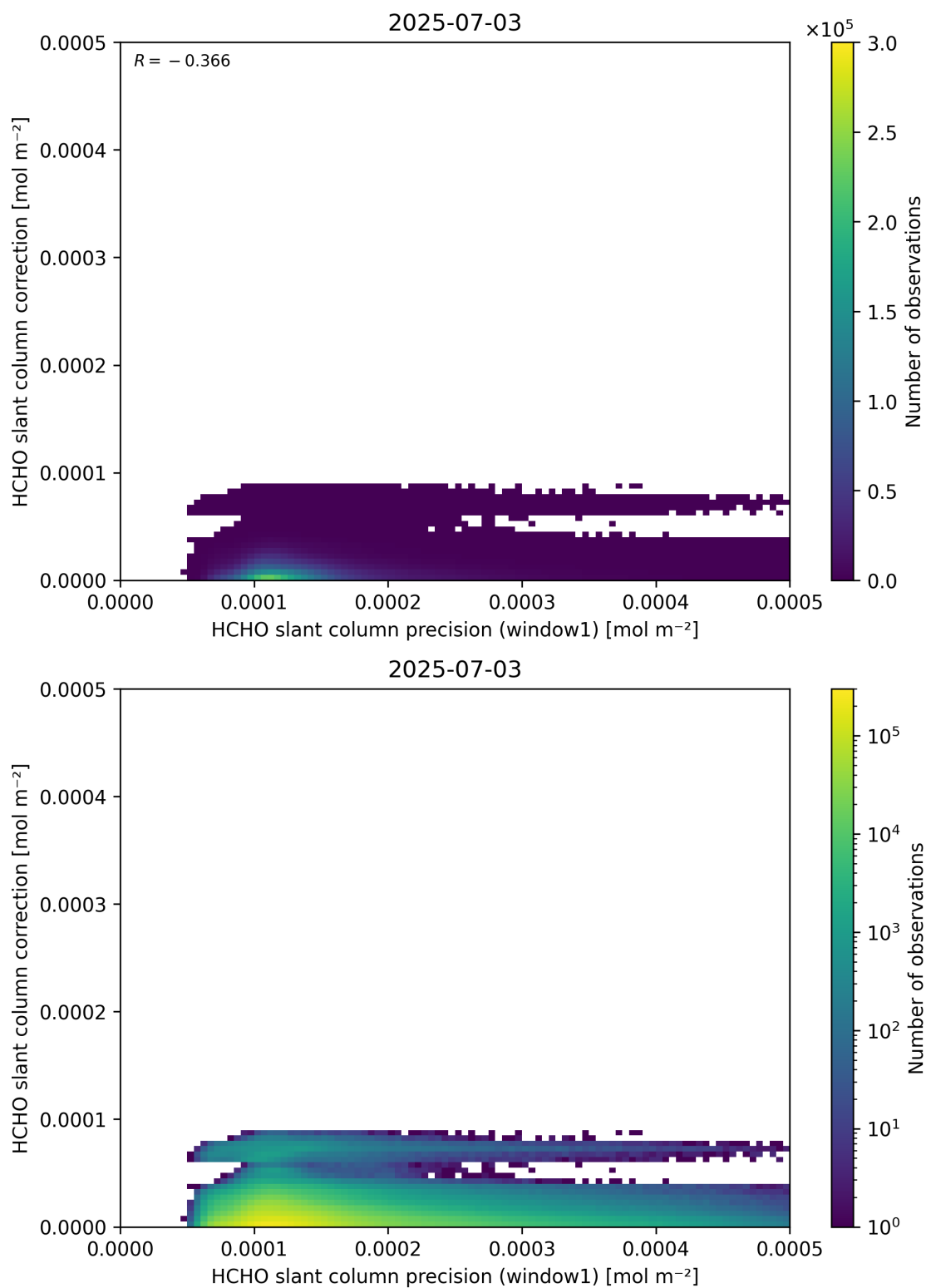
Figure 93: Scatter density plot of “HCHO slant column precision (window1)” against “HCHO slant column correction” for 2025-07-03 to 2025-07-04.
