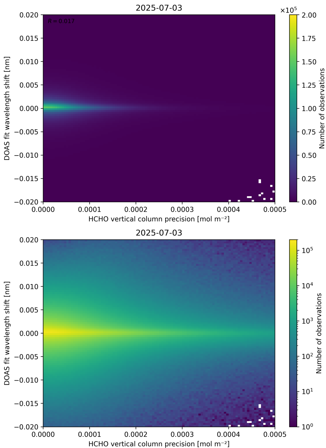
Figure 137: Scatter density plot of “HCHO vertical column precision” against “DOAS fit wavelength shift” for 2025-07-03 to 2025-07-04.
