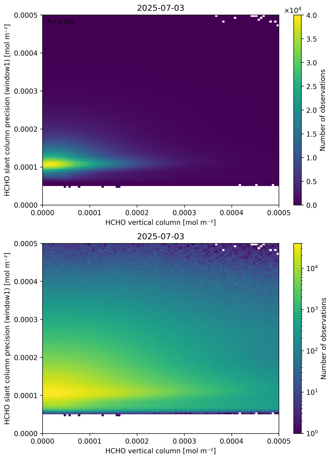
Figure 130: Scatter density plot of “HCHO vertical column” against “HCHO slant column precision (window1)” for 2025-07-03 to 2025-07-04.
