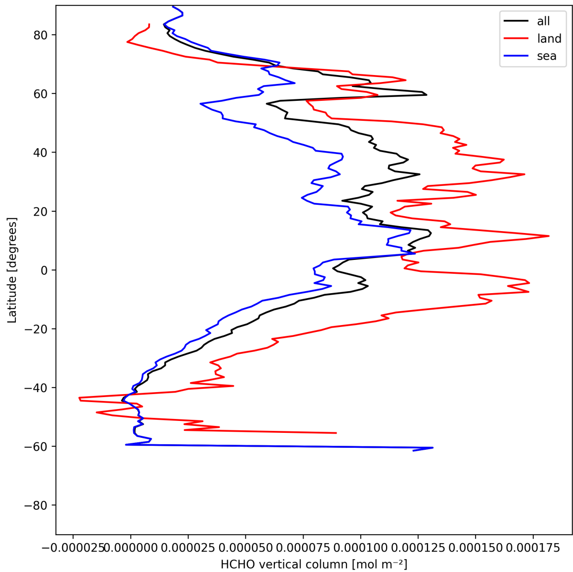
Figure 21: Zonal average of “HCHO vertical column” for 2025-07-03 to 2025-07-04.
