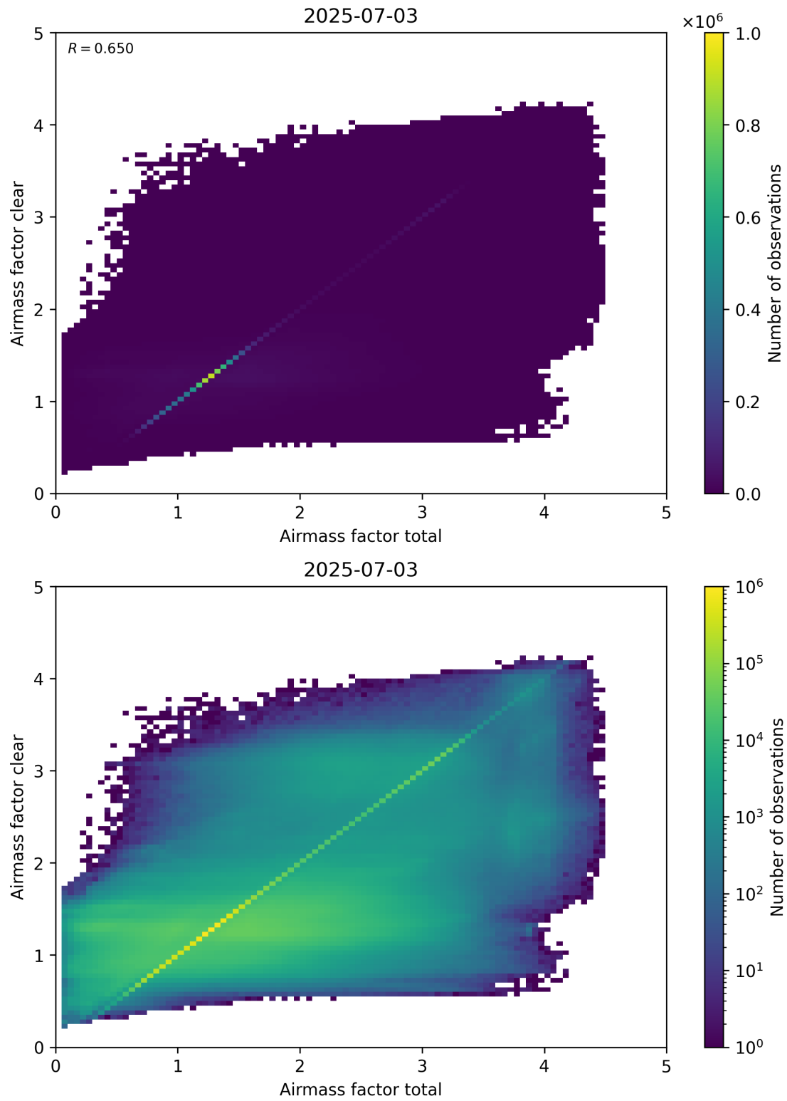
Figure 100: Scatter density plot of “Airmass factor total” against “Airmass factor clear” for 2025-07-03 to 2025-07-04.
