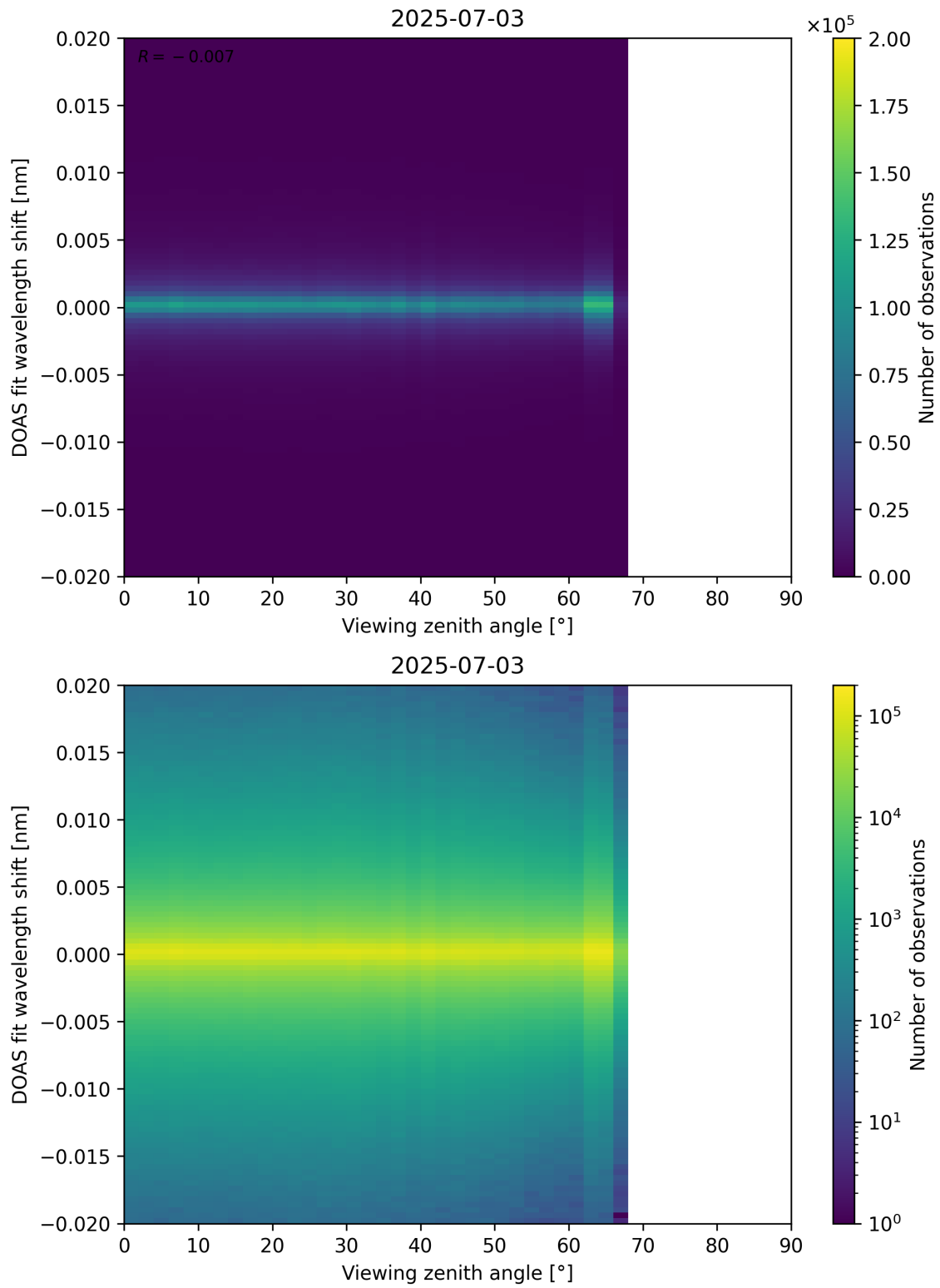
Figure 183: Scatter density plot of “Viewing zenith angle” against “DOAS fit wavelength shift” for 2025-07-03 to 2025-07-04.
