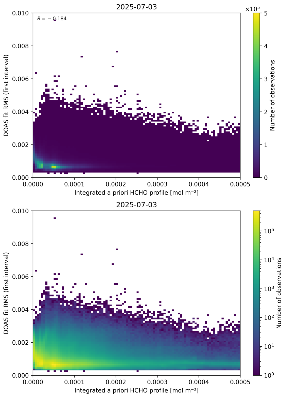
Figure 148: Scatter density plot of “Integrated a priori HCHO profile” against “DOAS fit RMS (first interval)” for 2025-07-03 to 2025-07-04.
