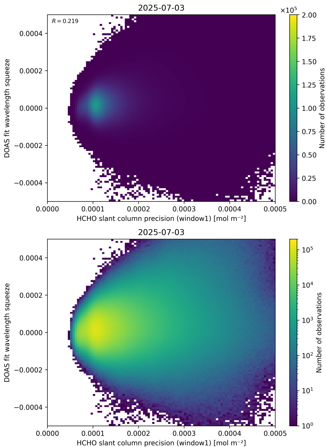
Figure 90: Scatter density plot of “HCHO slant column precision (window1)” against “DOAS fit wavelength squeeze” for 2025-07-03 to 2025-07-04.
