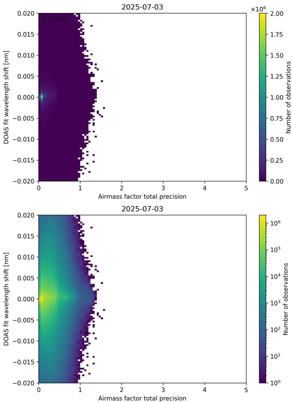
Figure 106: Scatter density plot of “Airmass factor total precision” against “DOAS fit wavelength shift” for 2025-07-03 to 2025-07-04.
