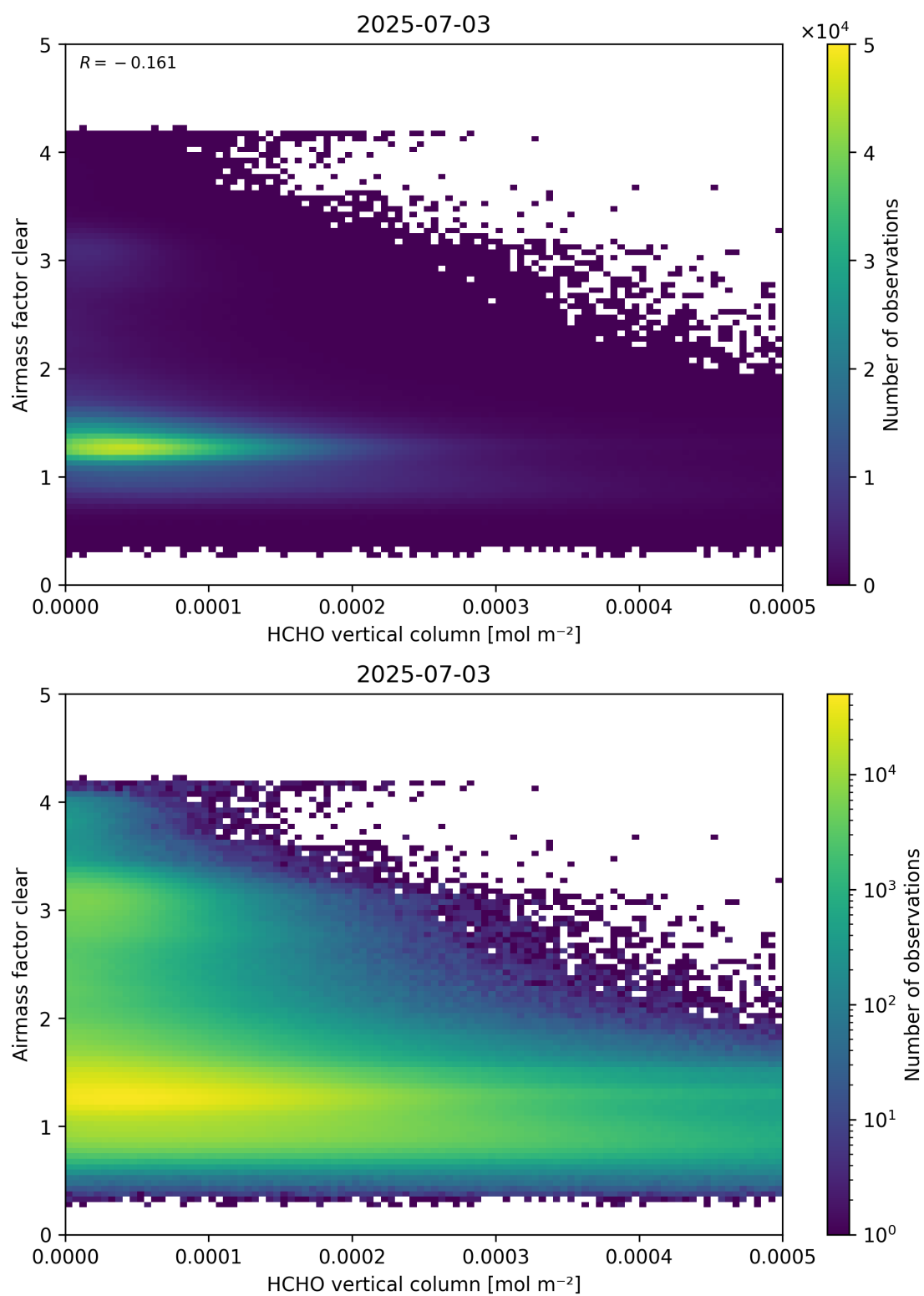
Figure 126: Scatter density plot of “HCHO vertical column” against “Airmass factor clear” for 2025-07-03 to 2025-07-04.
