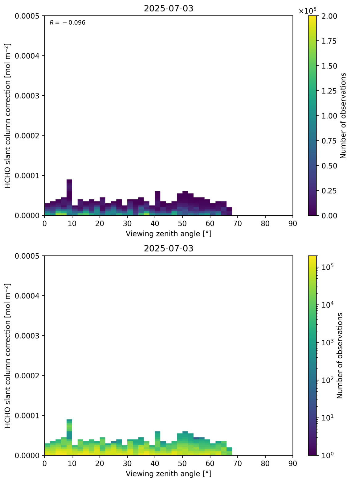
Figure 187: Scatter density plot of “Viewing zenith angle” against “HCHO slant column correction” for 2025-07-03 to 2025-07-04.
