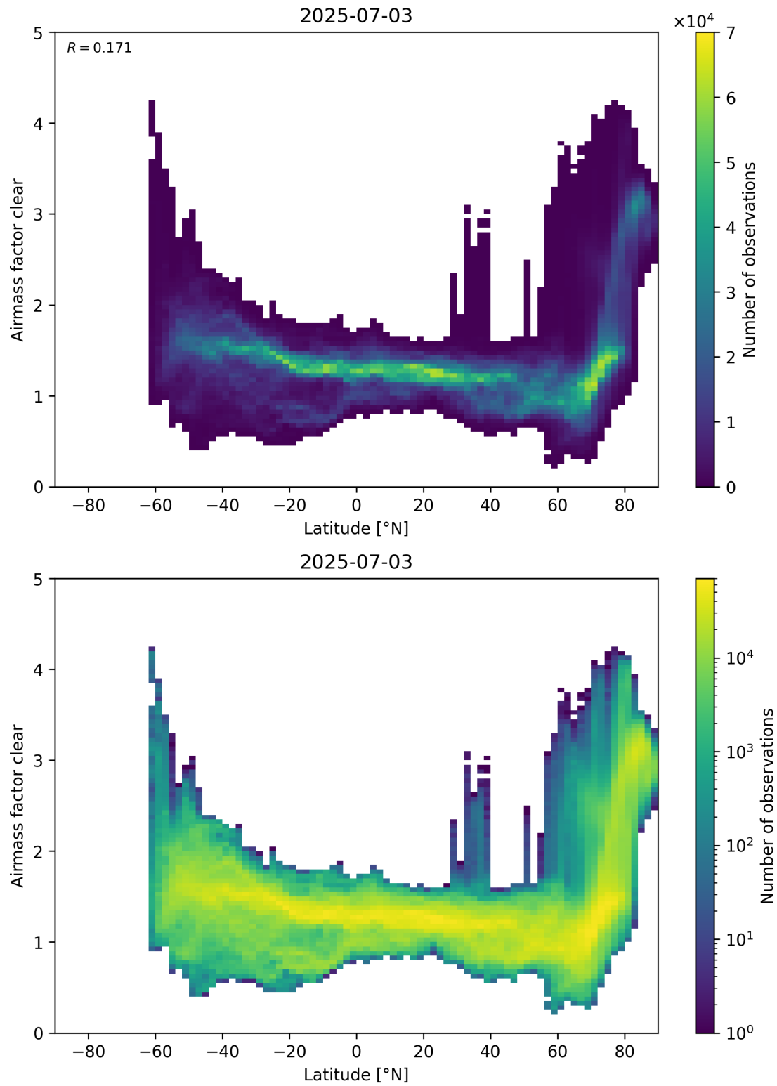
Figure 156: Scatter density plot of “Latitude” against “Airmass factor clear” for 2025-07-03 to 2025-07-04.
