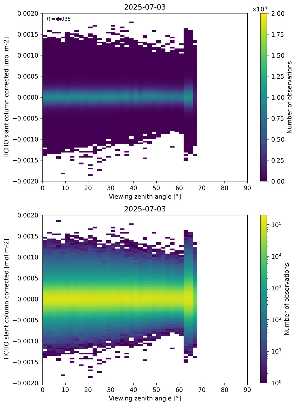
Figure 186: Scatter density plot of “Viewing zenith angle” against “HCHO slant column corrected” for 2025-07-03 to 2025-07-04.
