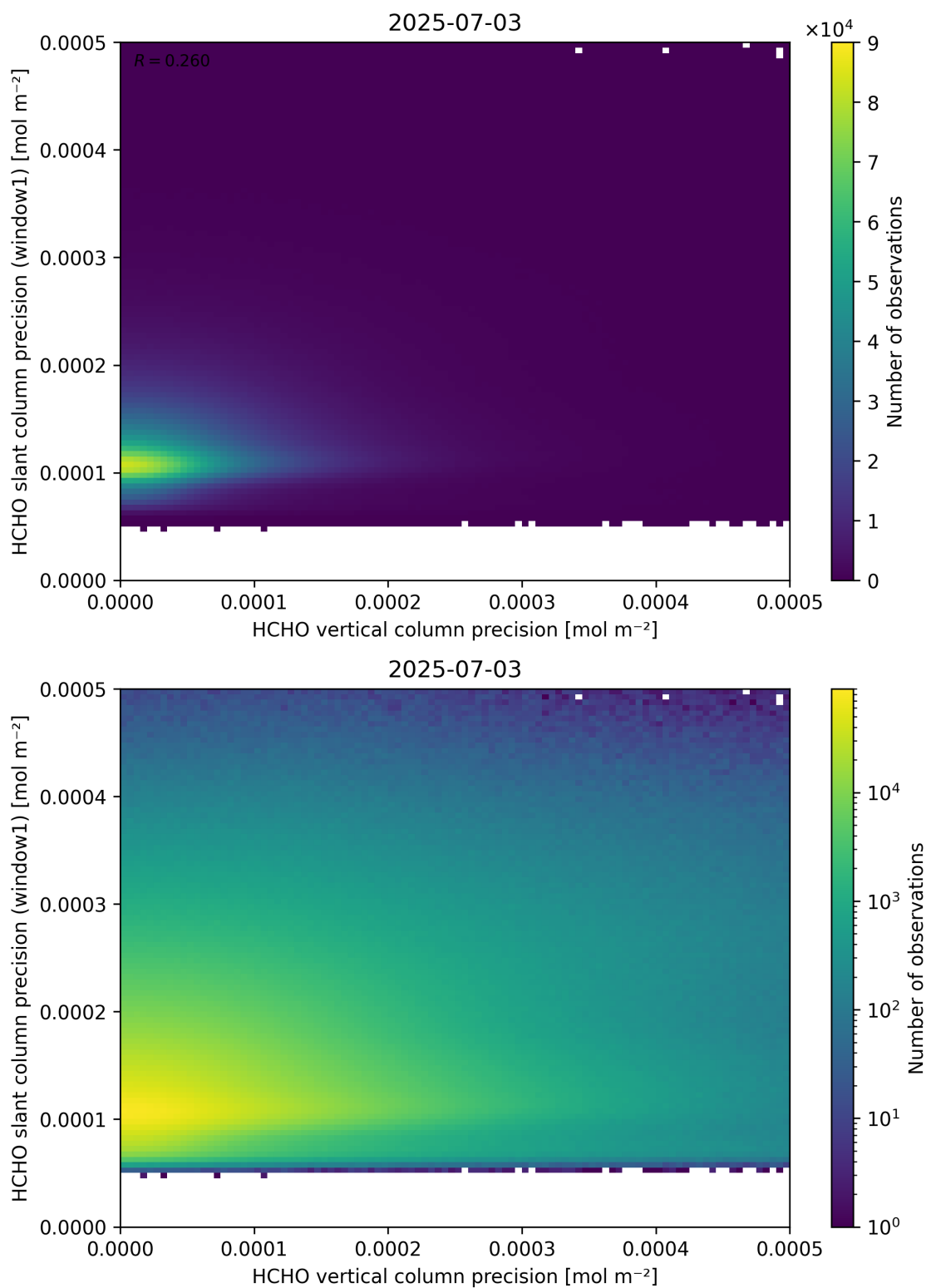
Figure 143: Scatter density plot of “HCHO vertical column precision” against “HCHO slant column precision (window1)” for 2025-07-03 to 2025-07-04.
