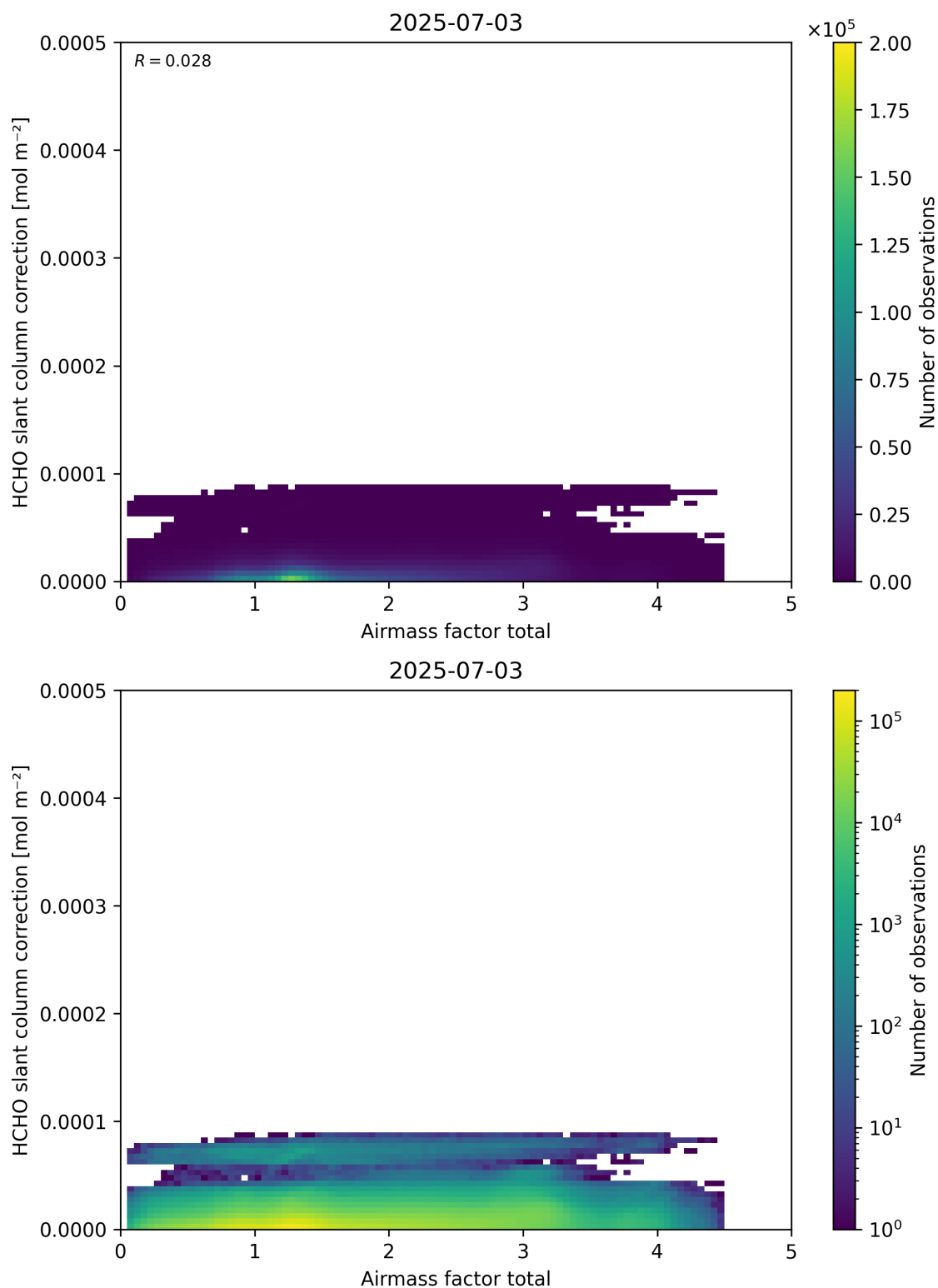
Figure 102: Scatter density plot of “Airmass factor total” against “HCHO slant column correction” for 2025-07-03 to 2025-07-04.
