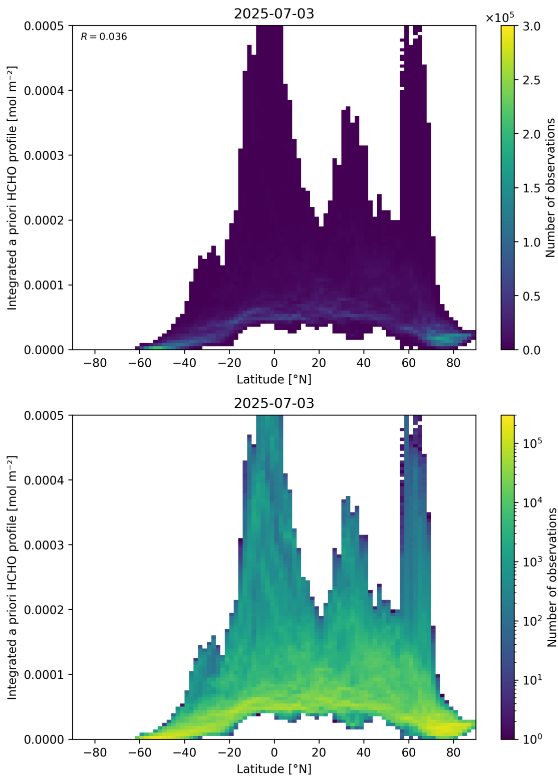
Figure 166: Scatter density plot of “Latitude” against “Integrated a priori HCHO profile” for 2025-07-03 to 2025-07-04.
