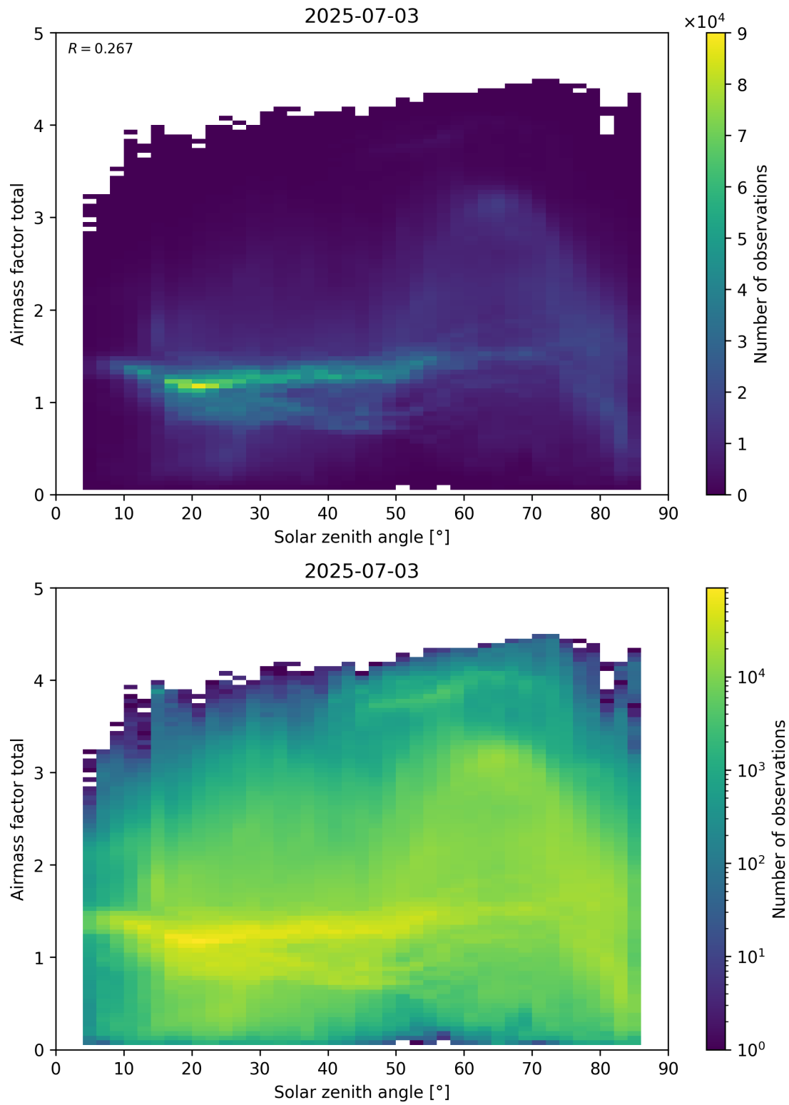
Figure 175: Scatter density plot of “Solar zenith angle” against “Airmass factor total” for 2025-07-03 to 2025-07-04.
