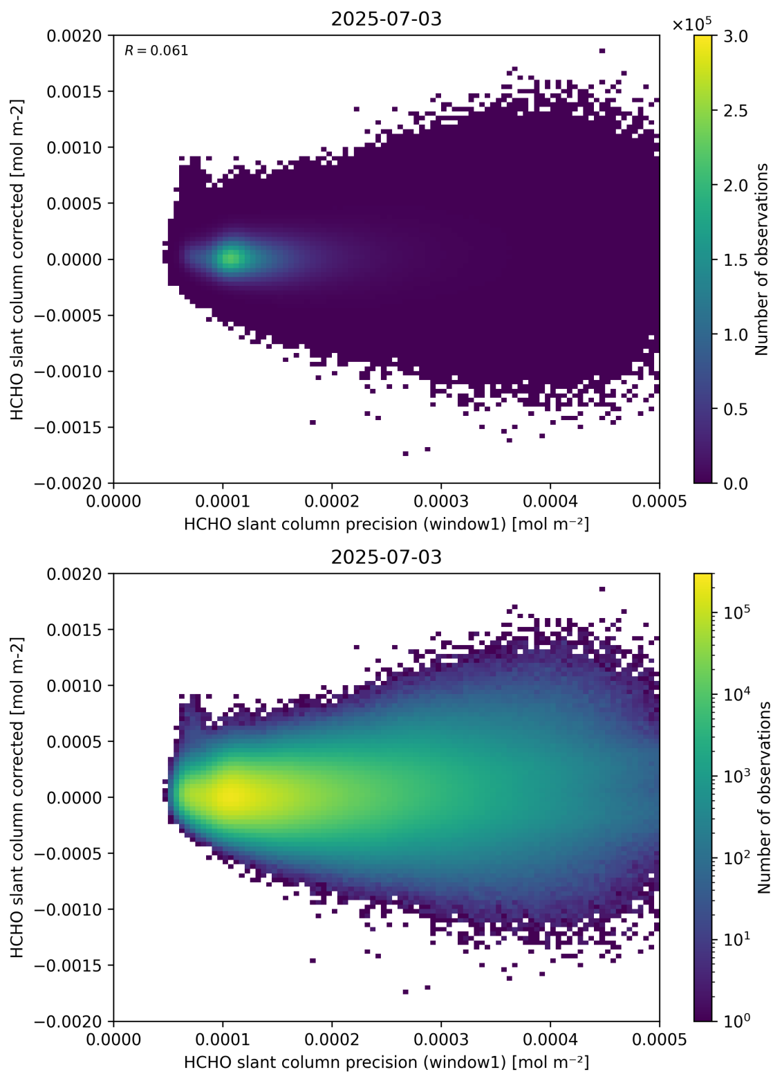
Figure 92: Scatter density plot of “HCHO slant column precision (window1)” against “HCHO slant column corrected” for 2025-07-03 to 2025-07-04.
