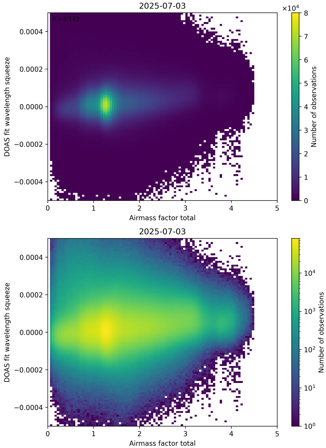
Figure 99: Scatter density plot of “Airmass factor total” against “DOAS fit wavelength squeeze” for 2025-07-03 to 2025-07-04.
