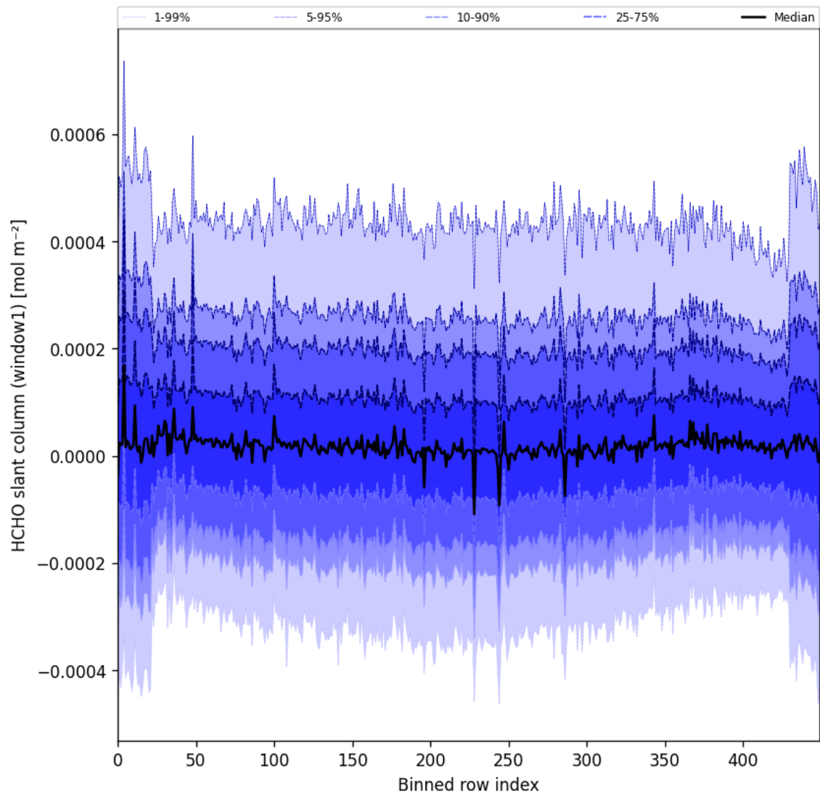
Figure 52: Along track statistics of “HCHO slant column (window1)” for 2025-07-03 to 2025-07-04
