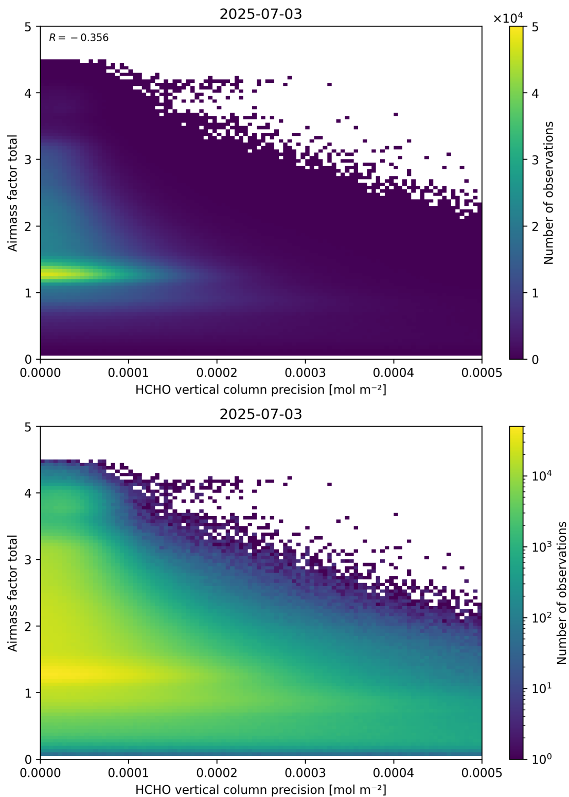
Figure 144: Scatter density plot of “HCHO vertical column precision” against “Airmass factor total” for 2025-07-03 to 2025-07-04.
