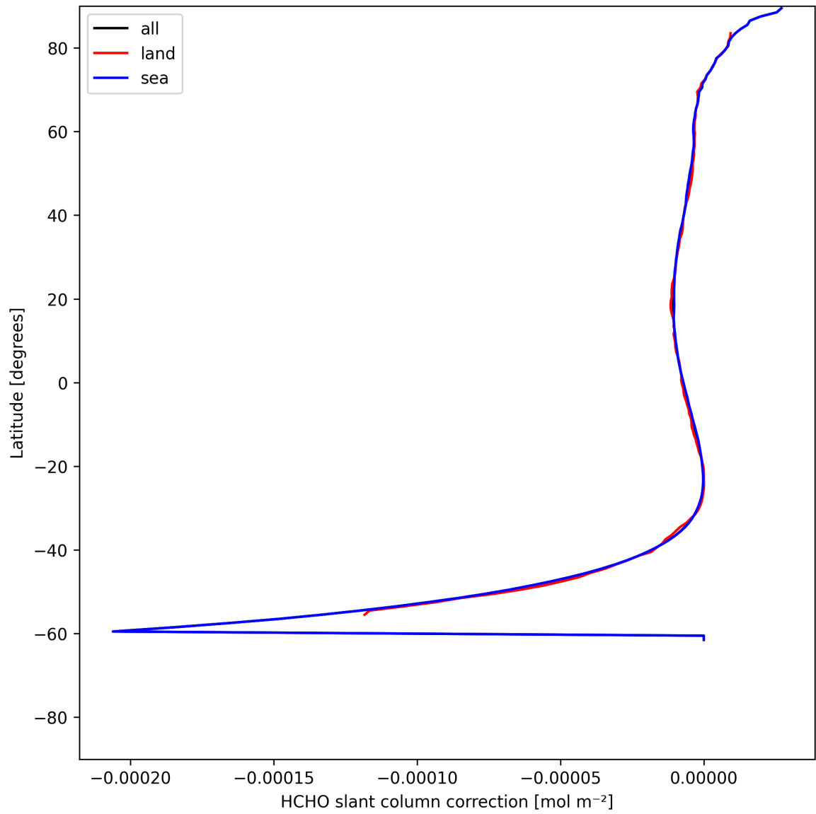
Figure 33: Zonal average of “HCHO slant column correction” for 2025-07-03 to 2025-07-04.
