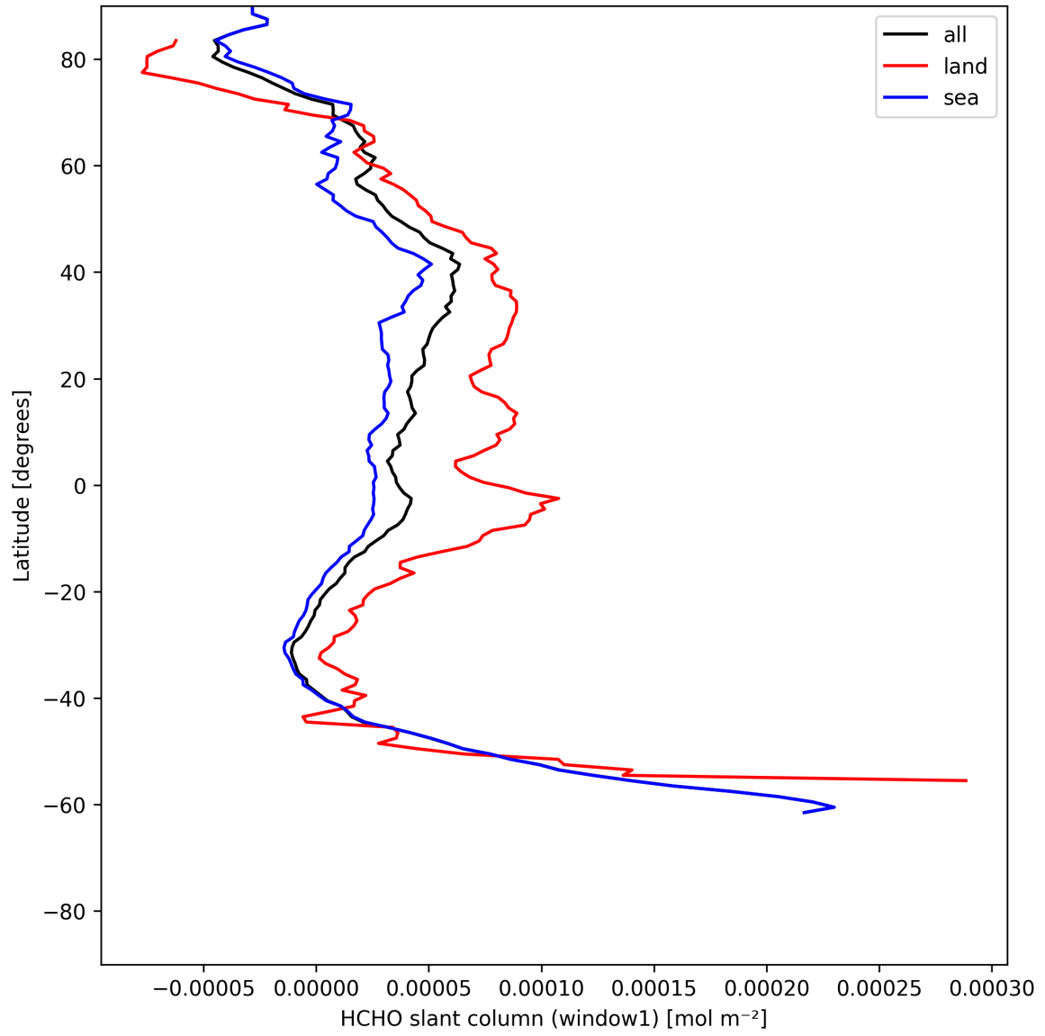
Figure 24: Zonal average of “HCHO slant column (window1)” for 2025-07-03 to 2025-07-04.
