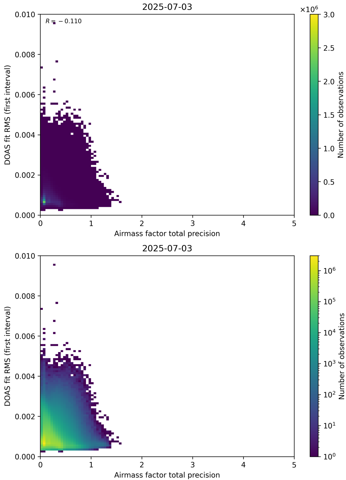
Figure 105: Scatter density plot of “Airmass factor total precision” against “DOAS fit RMS (first interval)” for 2025-07-03 to 2025-07-04.
