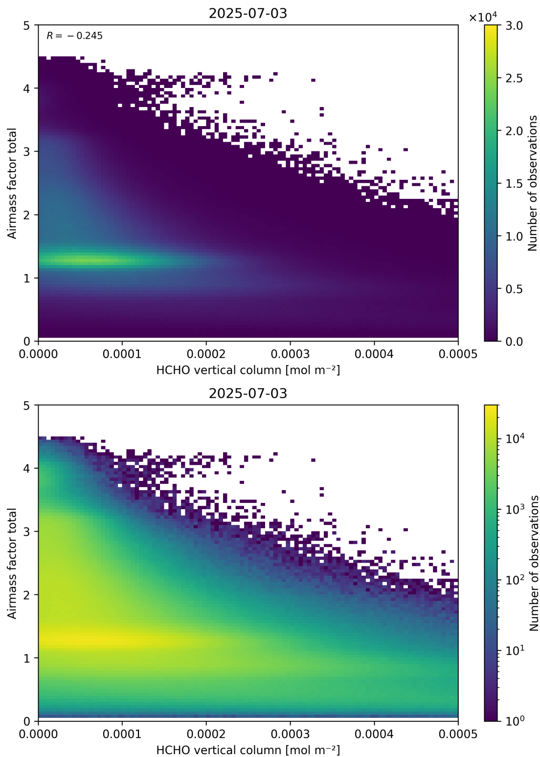
Figure 131: Scatter density plot of “HCHO vertical column” against “Airmass factor total” for 2025-07-03 to 2025-07-04.
