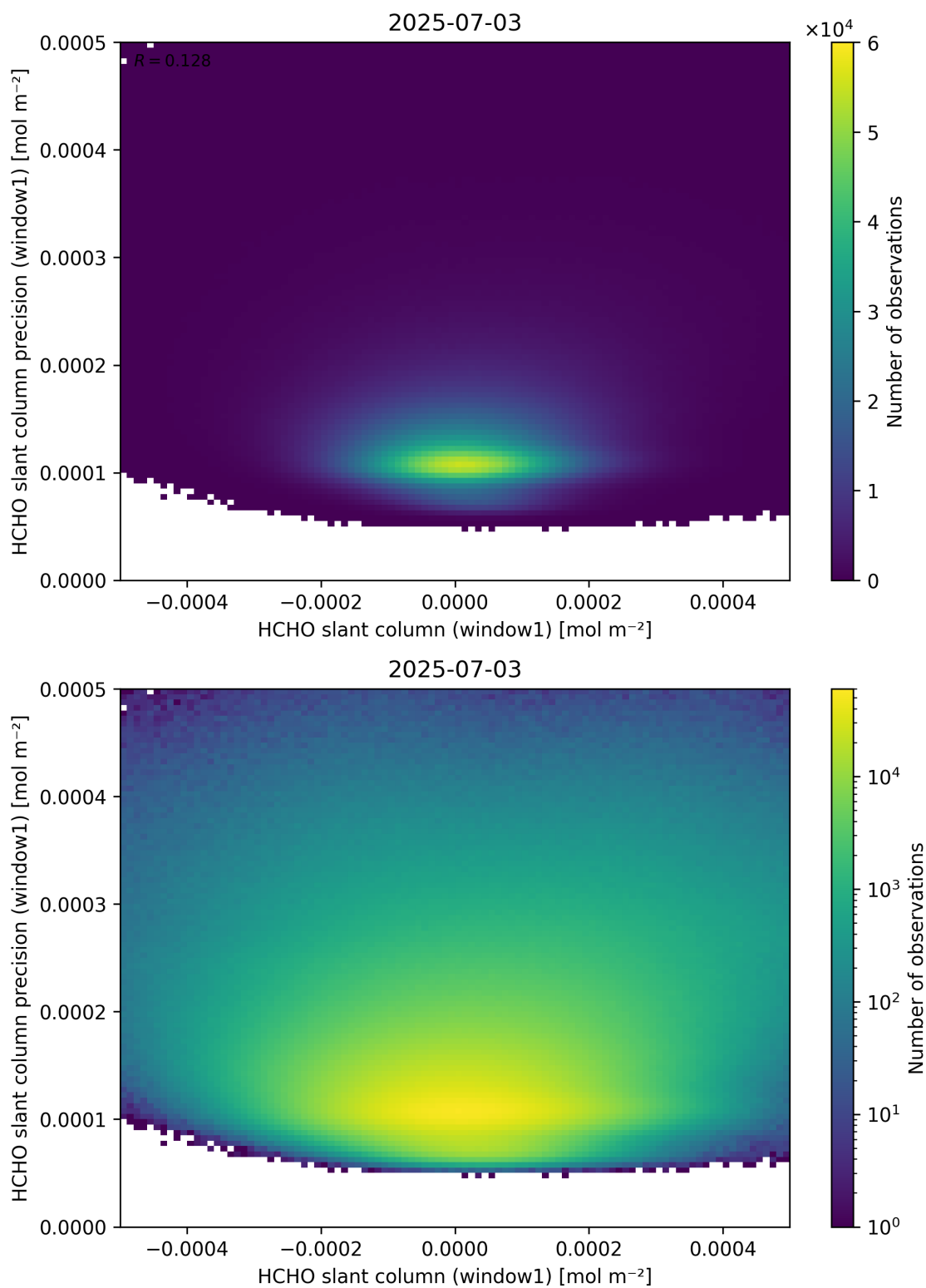
Figure 84: Scatter density plot of “HCHO slant column (window1)” against “HCHO slant column precision (window1)” for 2025-07-03 to 2025-07-04.
