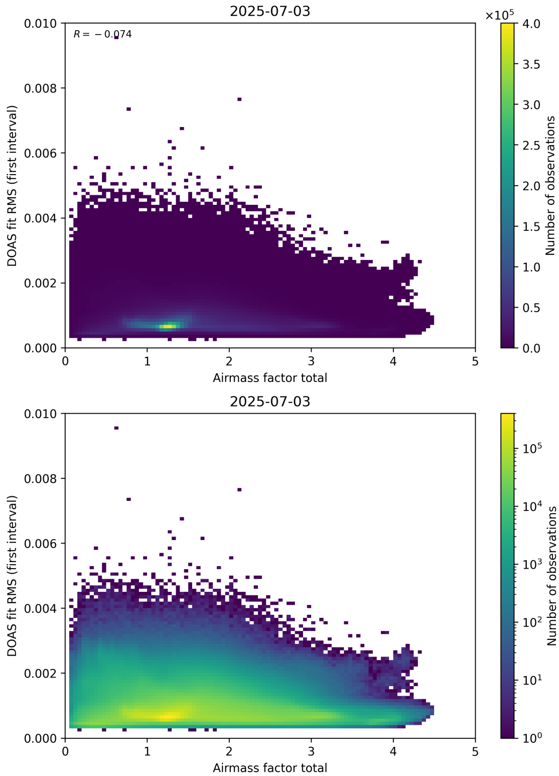
Figure 97: Scatter density plot of “Airmass factor total” against “DOAS fit RMS (first interval)” for 2025-07-03 to 2025-07-04.
