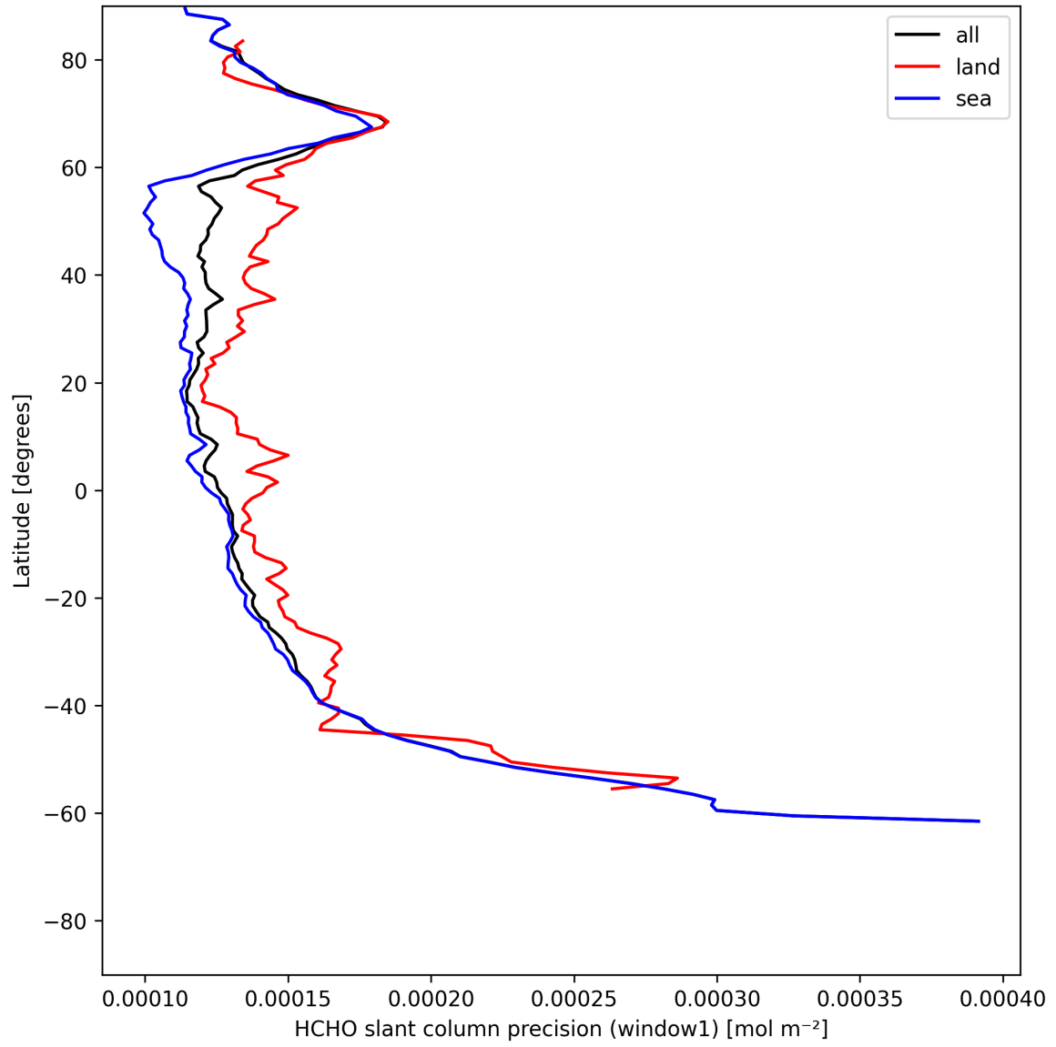
Figure 25: Zonal average of “HCHO slant column precision (window1)” for 2025-07-03 to 2025-07-04.
