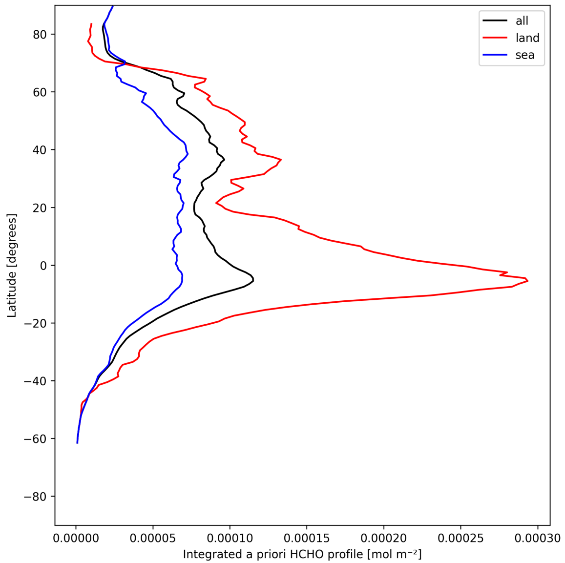
Figure 29: Zonal average of “Integrated a priori HCHO profile” for 2025-07-03 to 2025-07-04.
