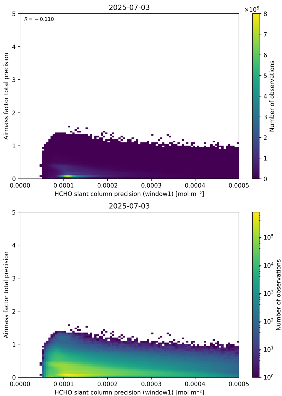
Figure 95: Scatter density plot of “HCHO slant column precision (window1)” against “Airmass factor total precision” for 2025-07-03 to 2025-07-04.
