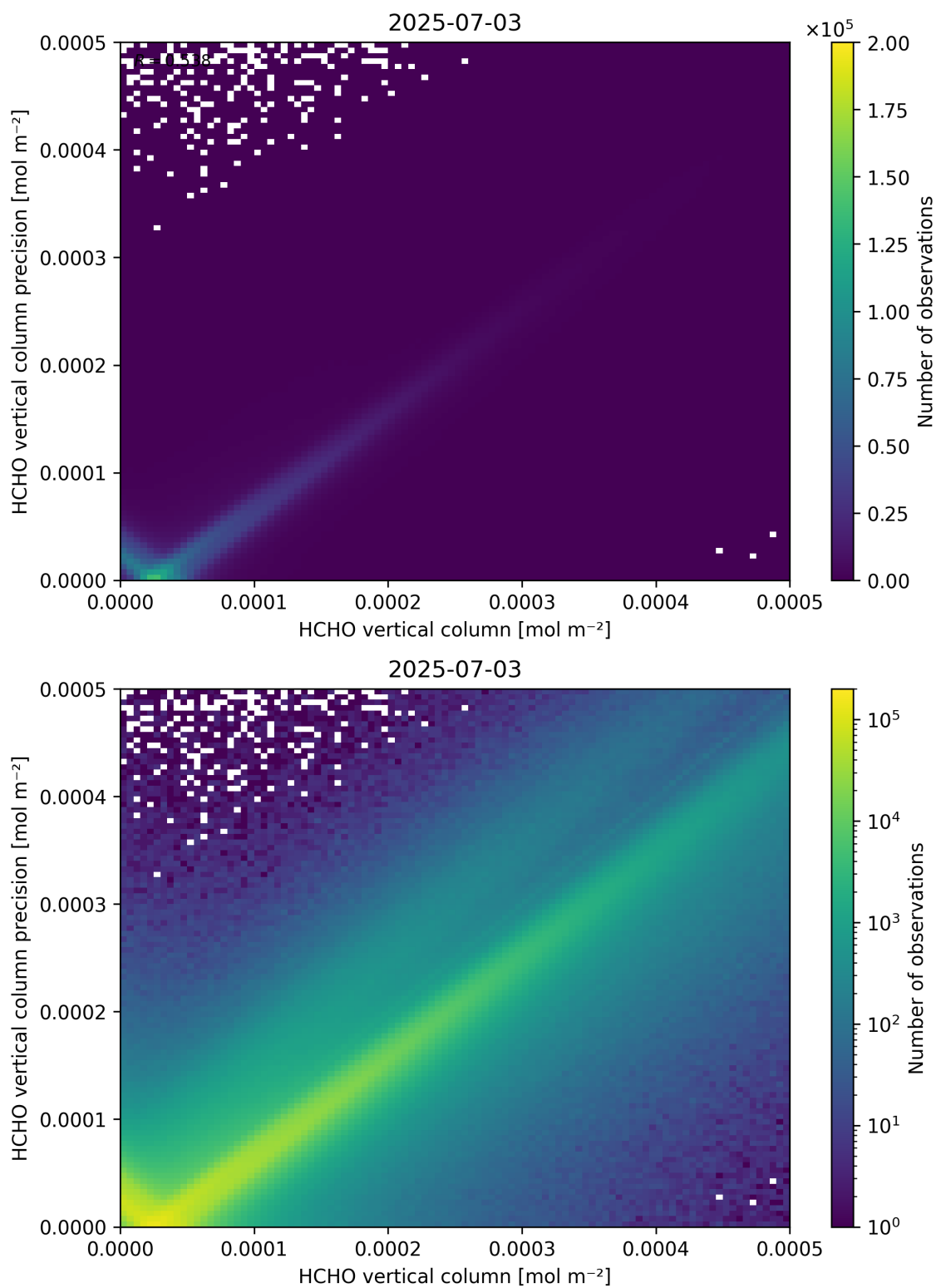
Figure 134: Scatter density plot of “HCHO vertical column” against “HCHO vertical column precision” for 2025-07-03 to 2025-07-04.
