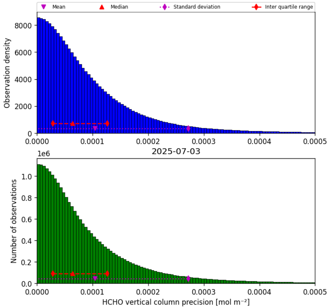
Figure 36: Histogram of “HCHO vertical column precision” for 2025-07-03 to 2025-07-04
