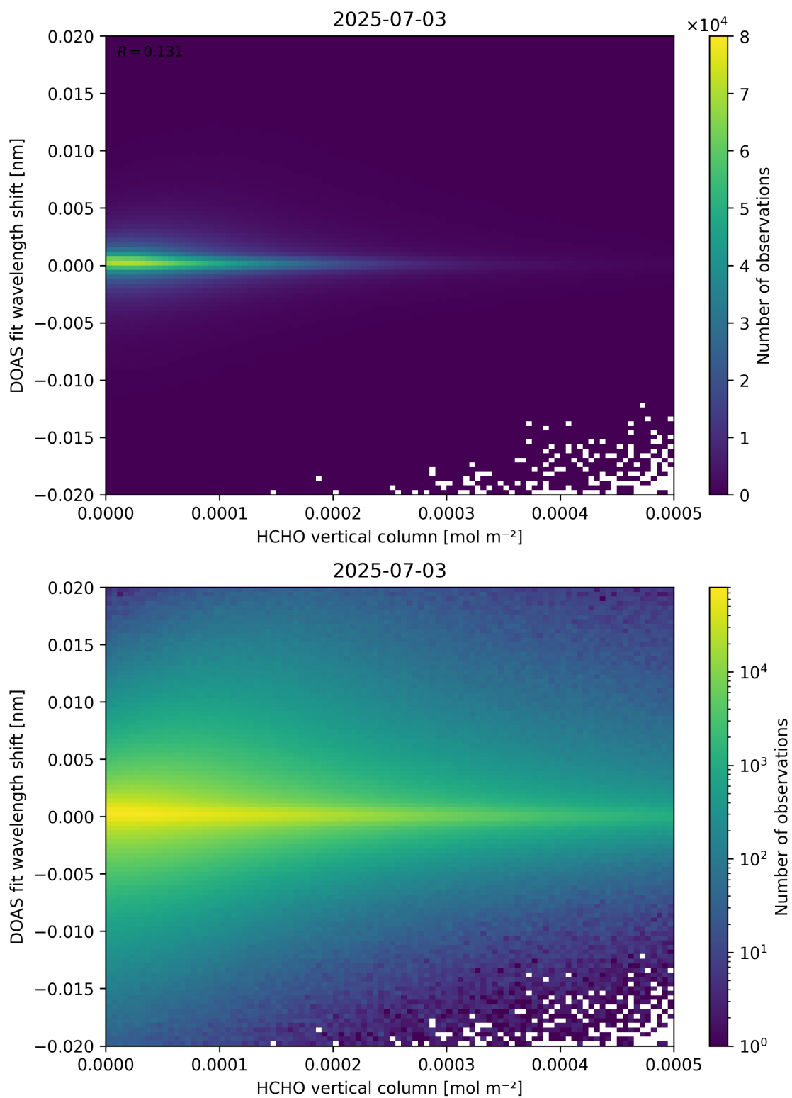
Figure 124: Scatter density plot of “HCHO vertical column” against “DOAS fit wavelength shift” for 2025-07-03 to 2025-07-04.
