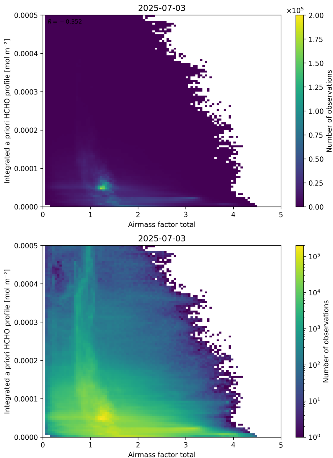
Figure 104: Scatter density plot of “Airmass factor total” against “Integrated a priori HCHO profile” for 2025-07-03 to 2025-07-04.
