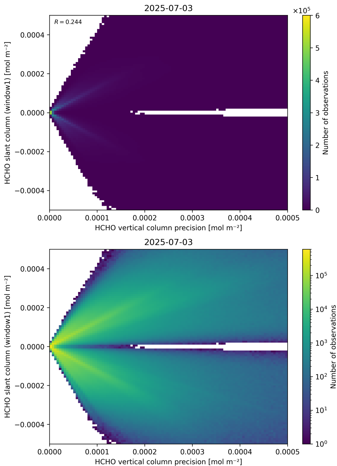
Figure 142: Scatter density plot of “HCHO vertical column precision” against “HCHO slant column (window1)” for 2025-07-03 to 2025-07-04.
