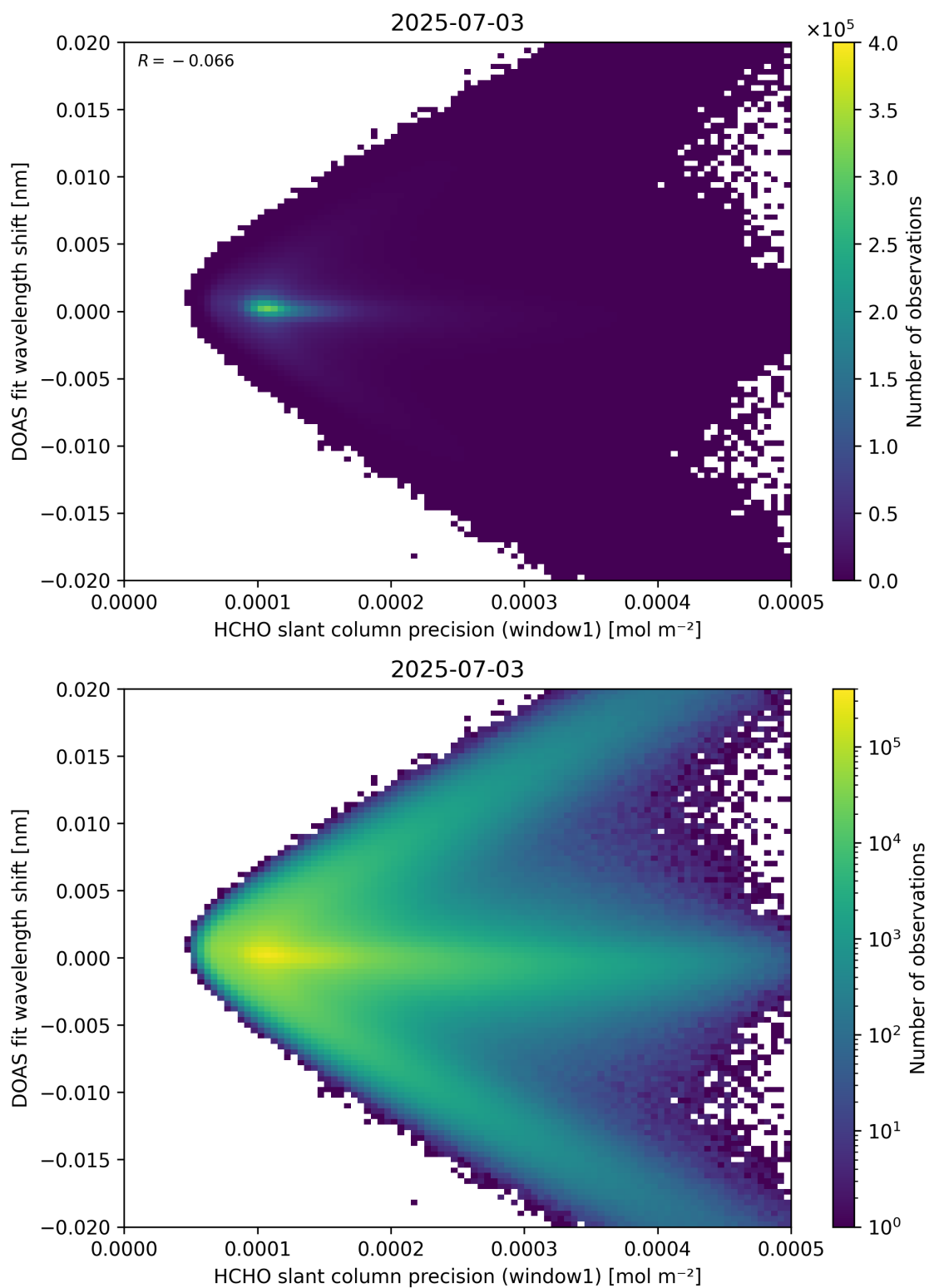
Figure 89: Scatter density plot of “HCHO slant column precision (window1)” against “DOAS fit wavelength shift” for 2025-07-03 to 2025-07-04.
