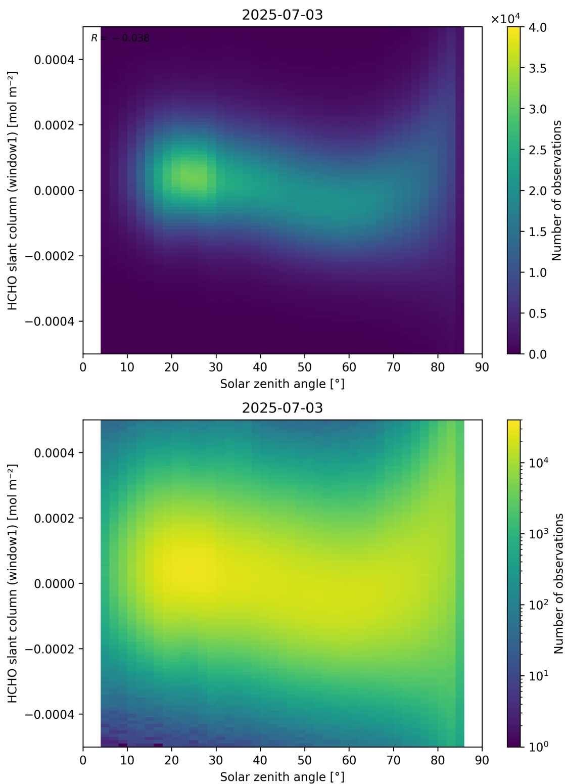
Figure 173: Scatter density plot of “Solar zenith angle” against “HCHO slant column (window1)” for 2025-07-03 to 2025-07-04.
