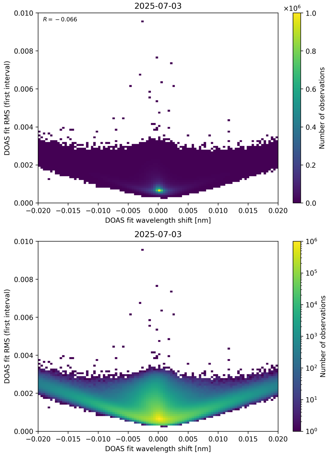
Figure 64: Scatter density plot of “DOAS fit wavelength shift” against “DOAS fit RMS (first interval)” for 2025-07-03 to 2025-07-04.
