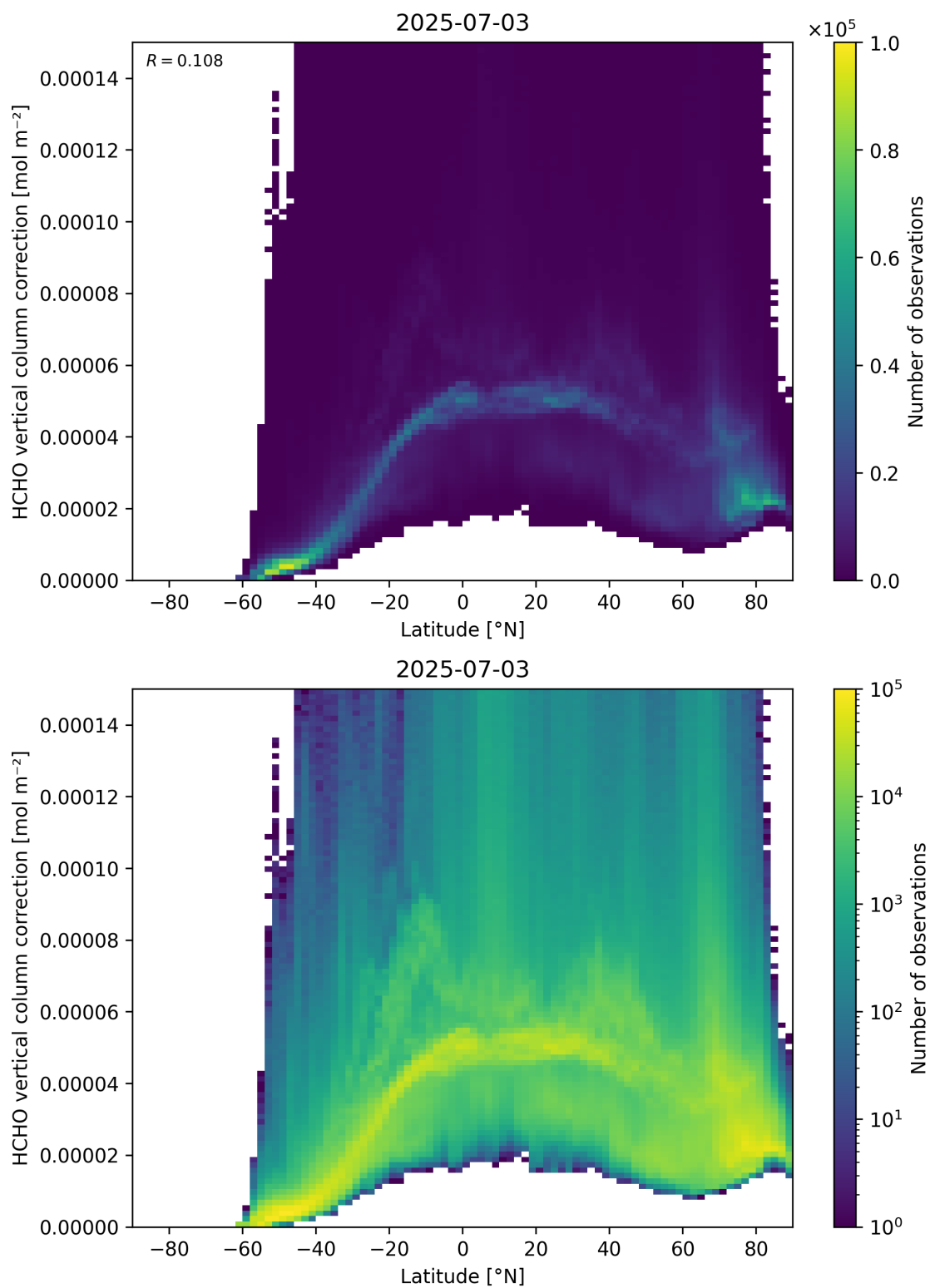
Figure 164: Scatter density plot of “Latitude” against “HCHO vertical column correction” for 2025-07-03 to 2025-07-04.
