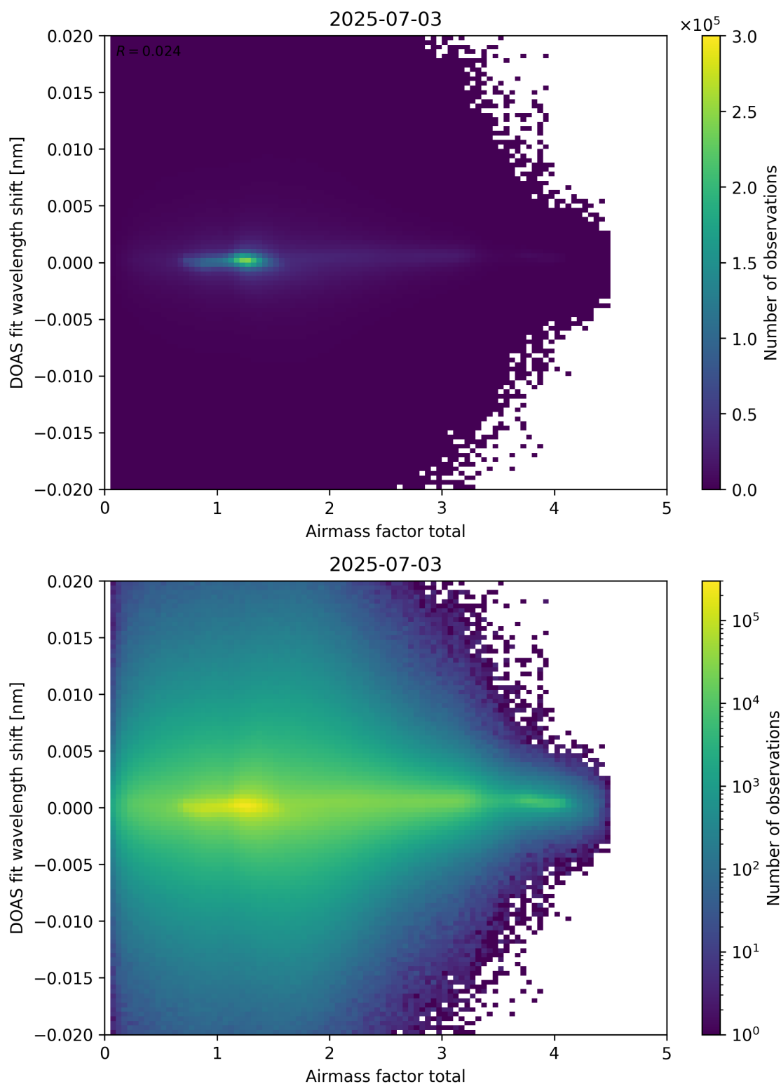
Figure 98: Scatter density plot of “Airmass factor total” against “DOAS fit wavelength shift” for 2025-07-03 to 2025-07-04.
