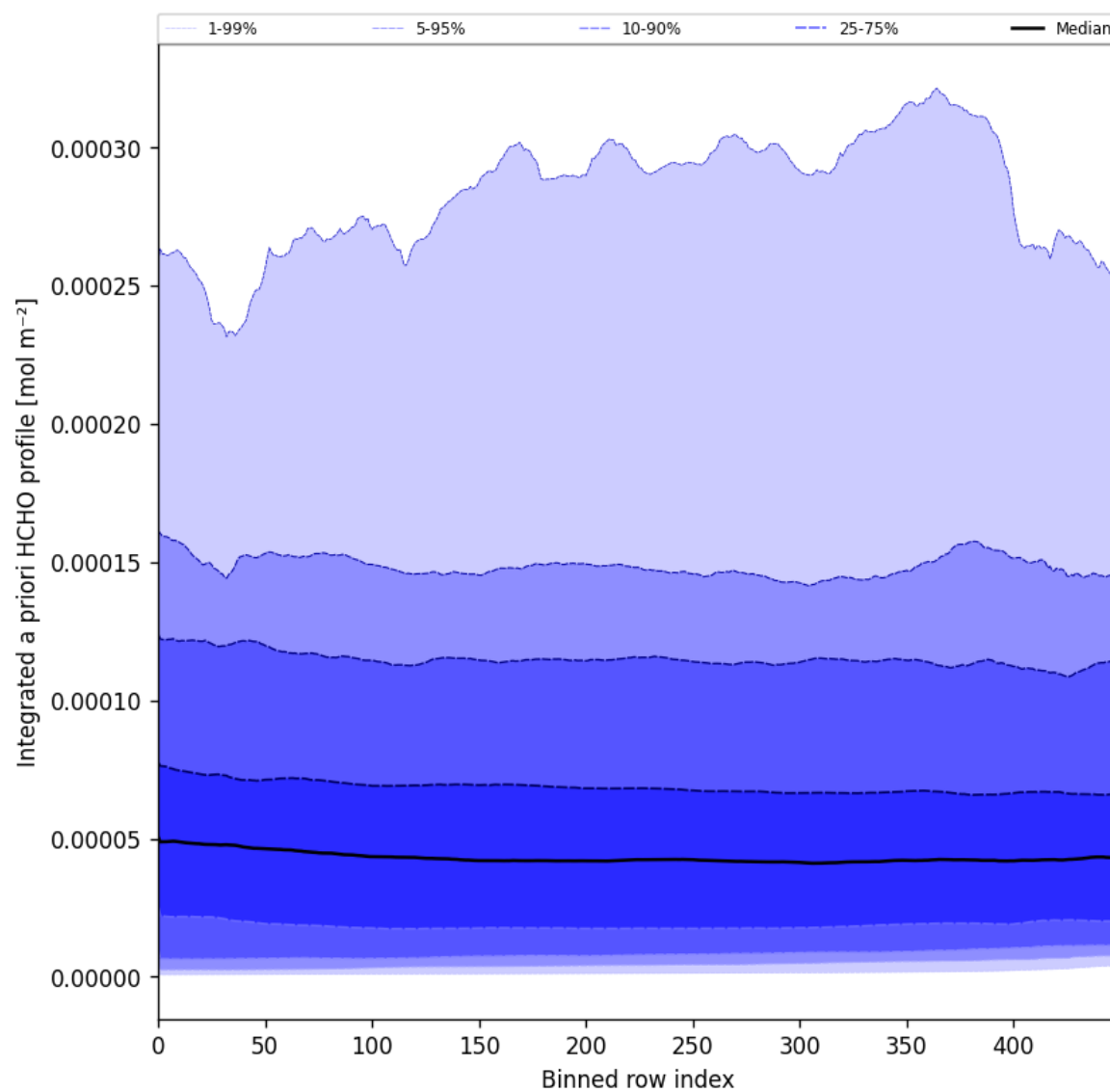
Figure 57: Along track statistics of “Integrated a priori HCHO profile” for 2025-07-03 to 2025-07-04
