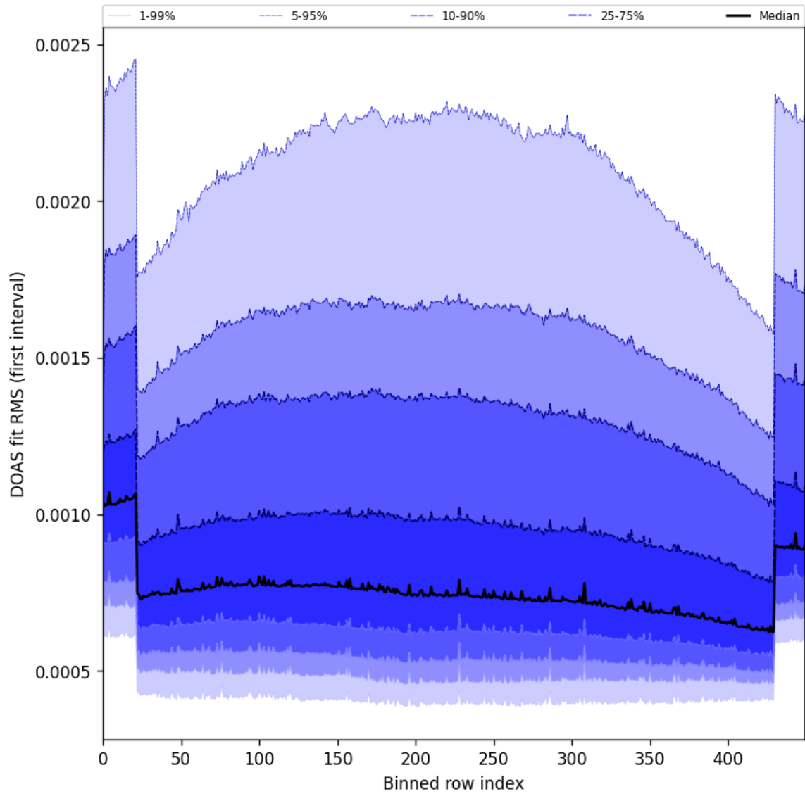
Figure 60: Along track statistics of “DOAS fit RMS (first interval)” for 2025-07-03 to 2025-07-04
