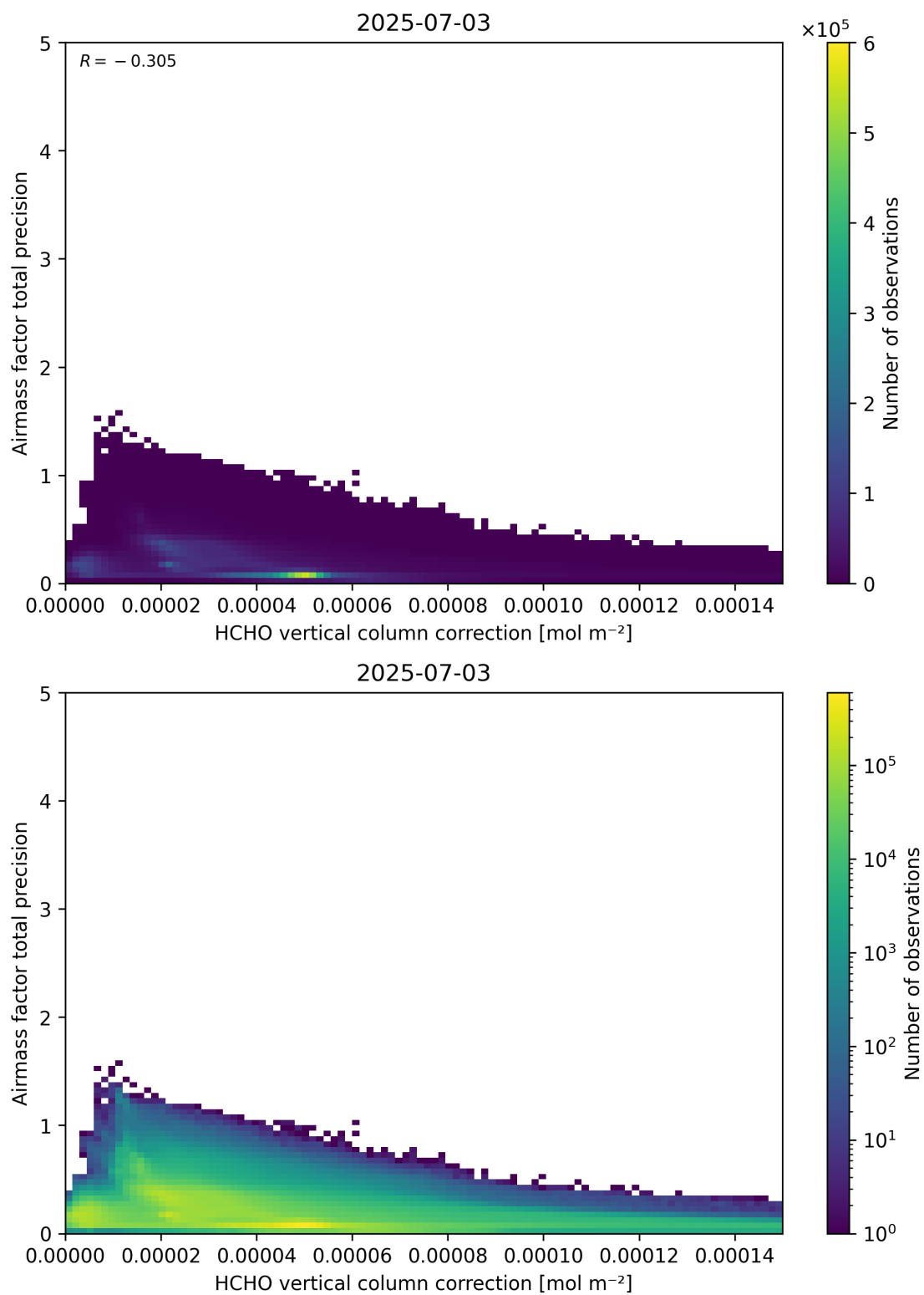
Figure 121: Scatter density plot of “HCHO vertical column correction” against “Airmass factor total precision” for 2025-07-03 to 2025-07-04.
