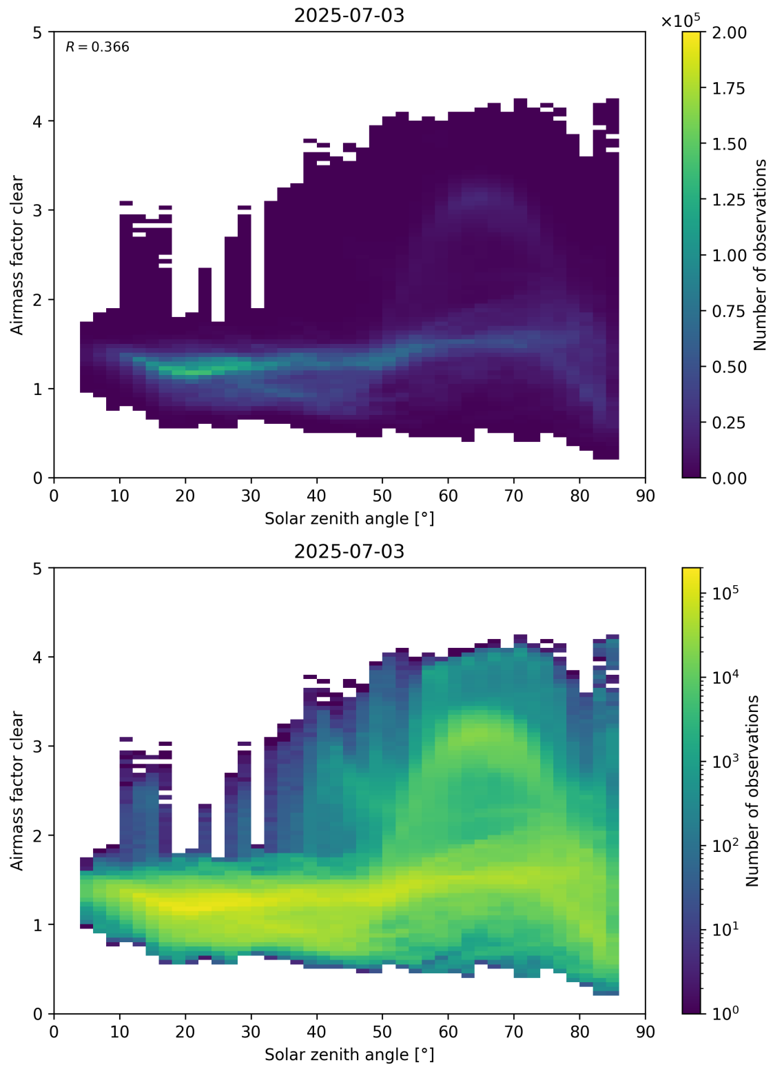
Figure 170: Scatter density plot of “Solar zenith angle” against “Airmass factor clear” for 2025-07-03 to 2025-07-04.
