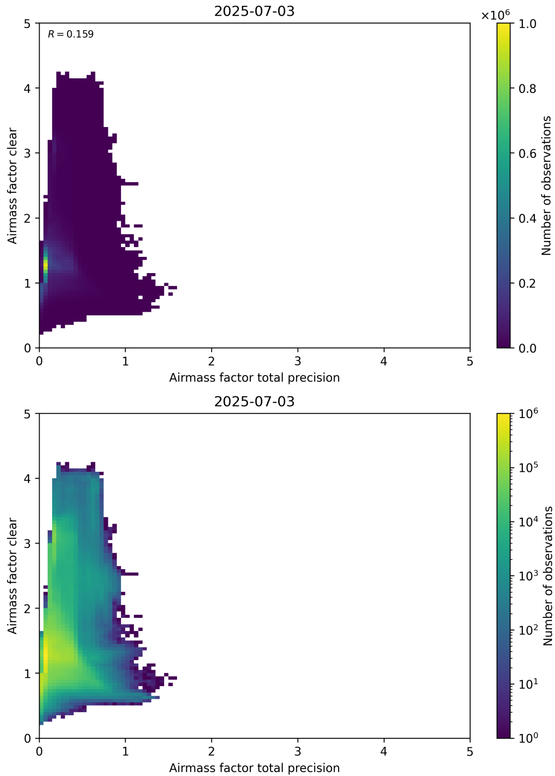
Figure 108: Scatter density plot of “Airmass factor total precision” against “Airmass factor clear” for 2025-07-03 to 2025-07-04.
