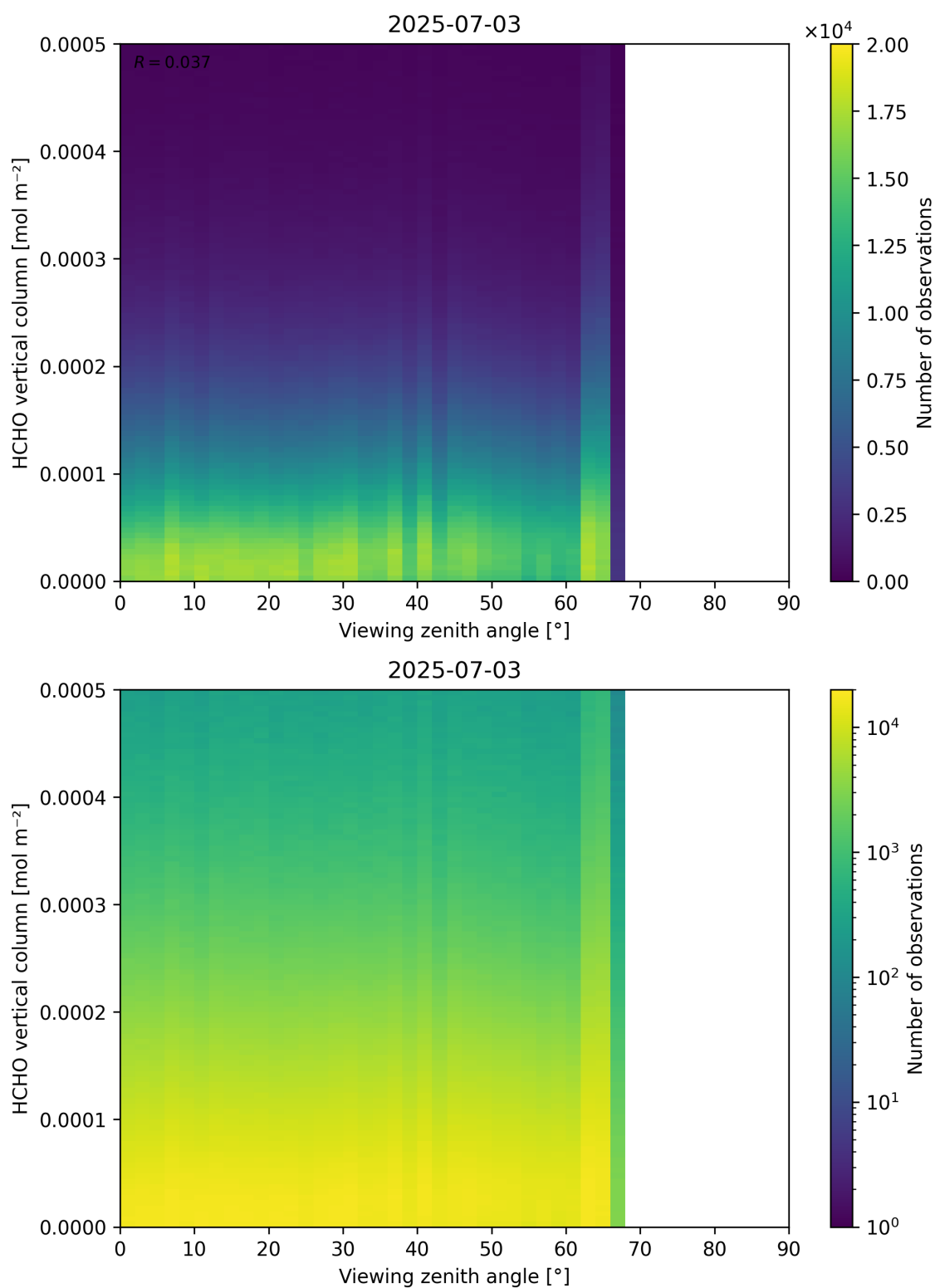
Figure 192: Scatter density plot of “Viewing zenith angle” against “HCHO vertical column” for 2025-07-03 to 2025-07-04.
