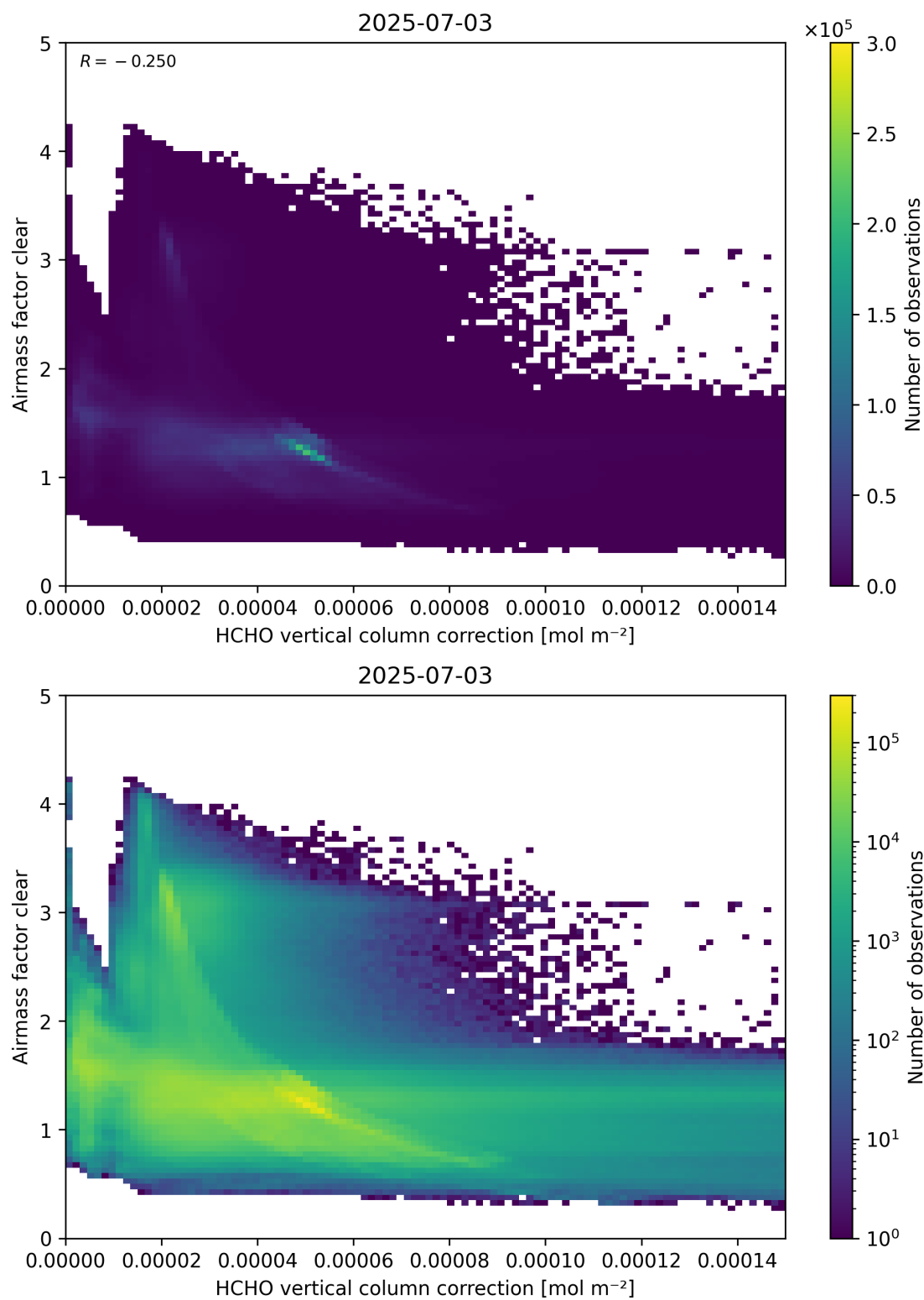
Figure 115: Scatter density plot of “HCHO vertical column correction” against “Airmass factor clear” for 2025-07-03 to 2025-07-04.
