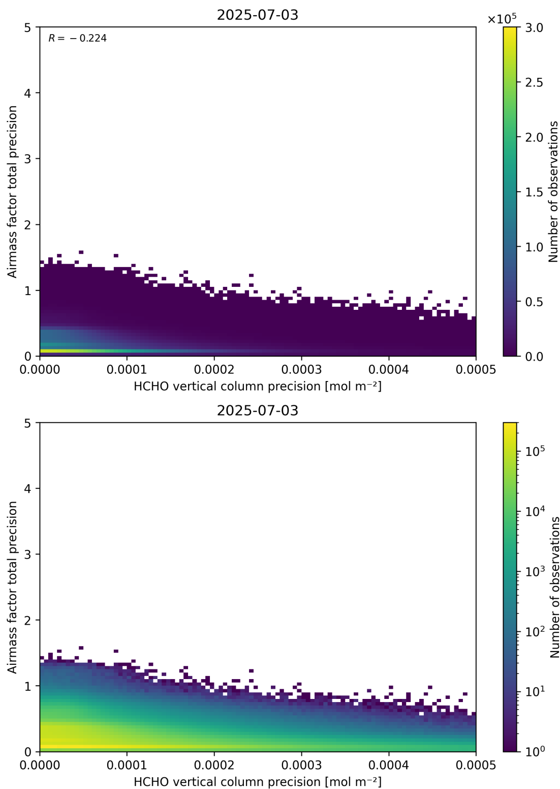
Figure 145: Scatter density plot of “HCHO vertical column precision” against “Airmass factor total precision” for 2025-07-03 to 2025-07-04.
