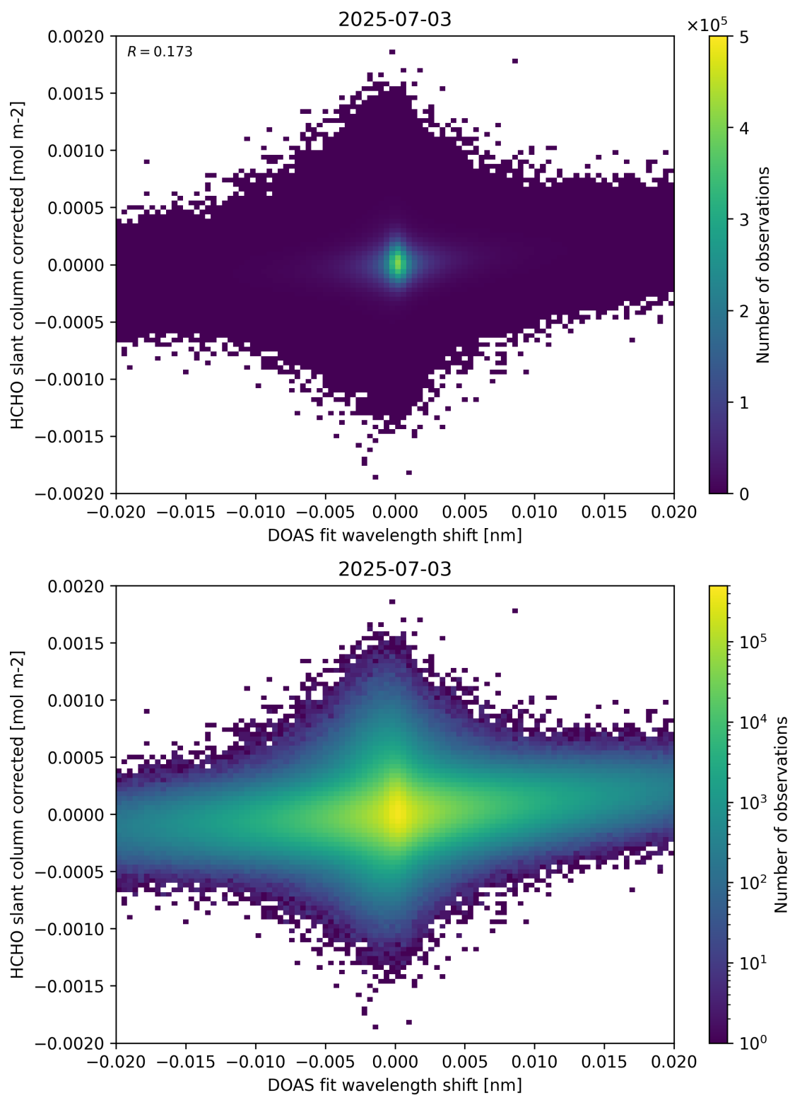
Figure 66: Scatter density plot of “DOAS fit wavelength shift” against “HCHO slant column corrected” for 2025-07-03 to 2025-07-04.
