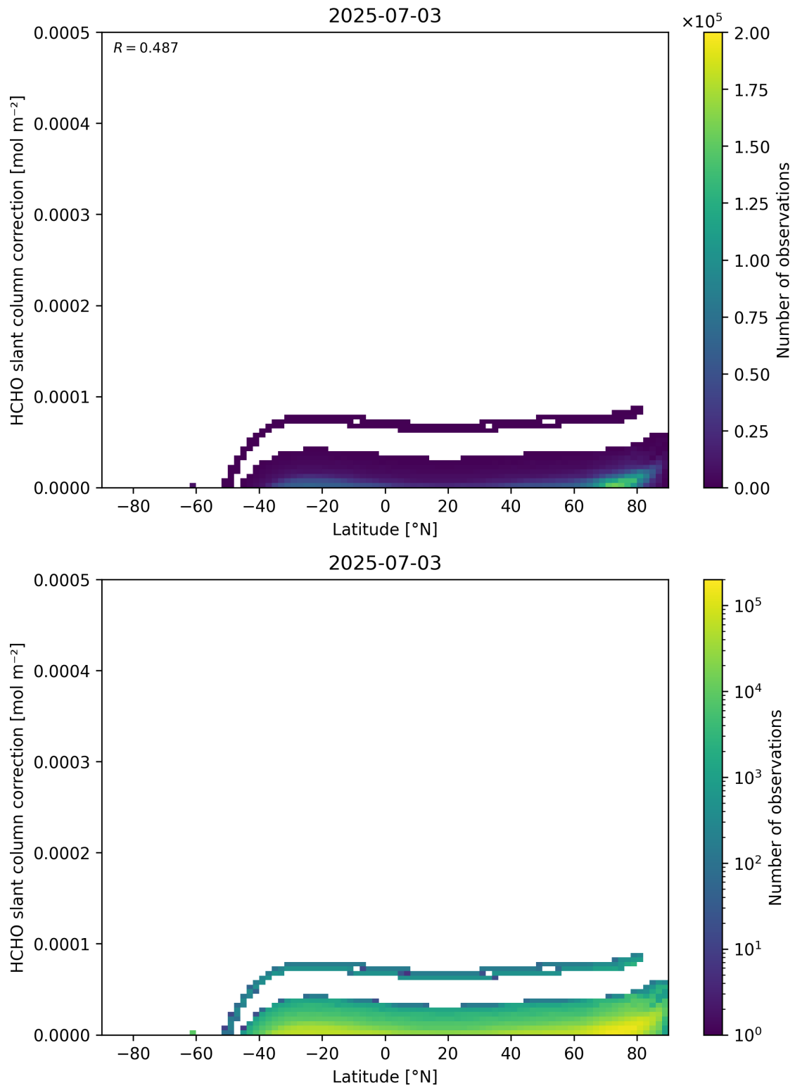
Figure 158: Scatter density plot of “Latitude” against “HCHO slant column correction” for 2025-07-03 to 2025-07-04.
