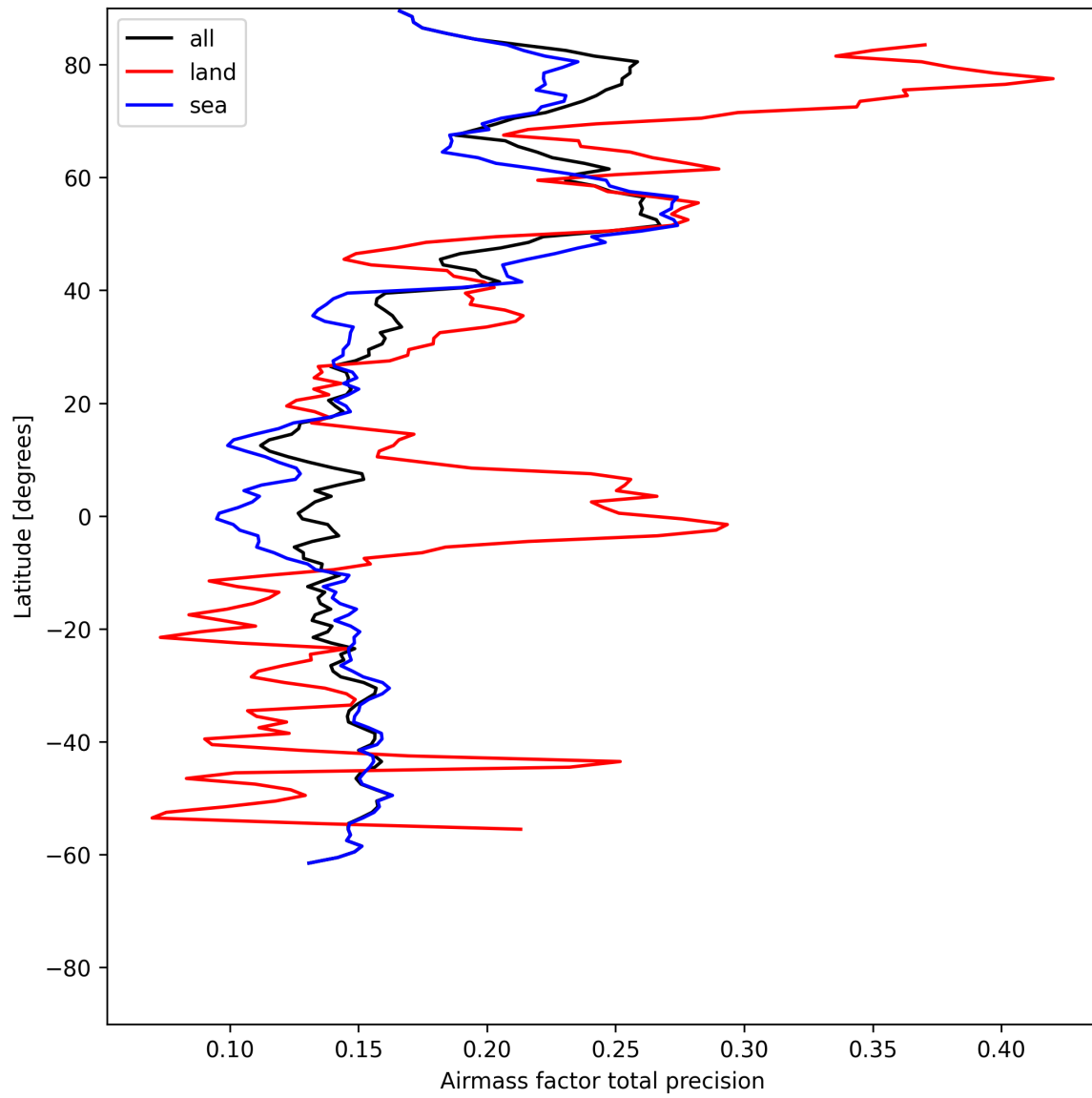
Figure 27: Zonal average of “Airmass factor total precision” for 2025-07-03 to 2025-07-04.
