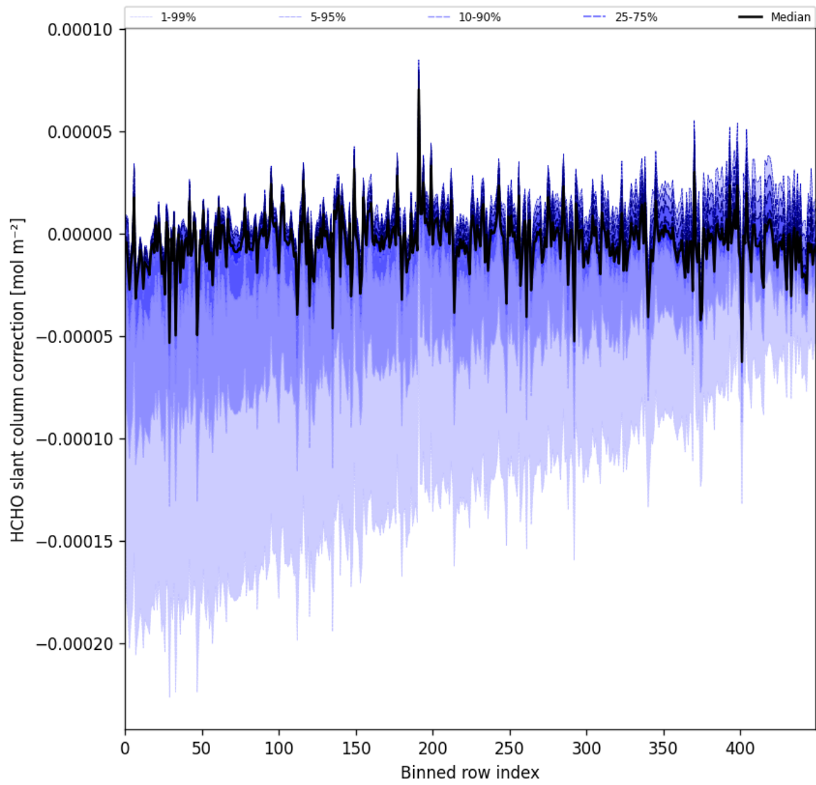
Figure 61: Along track statistics of “HCHO slant column correction” for 2025-07-03 to 2025-07-04
