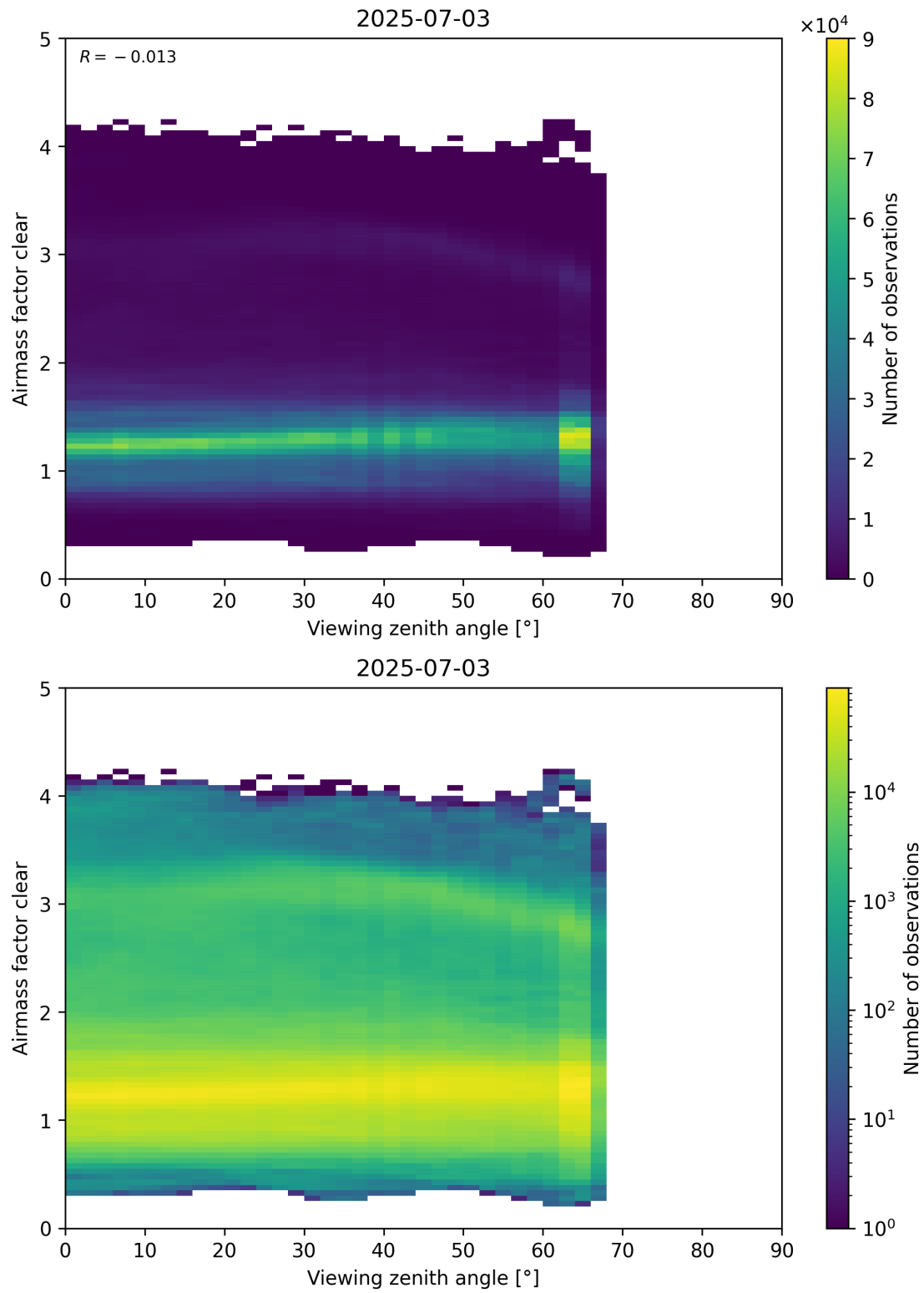
Figure 185: Scatter density plot of “Viewing zenith angle” against “Airmass factor clear” for 2025-07-03 to 2025-07-04.
