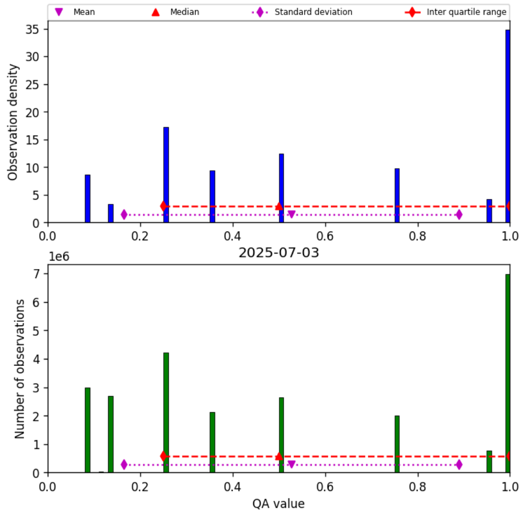
Figure 34: Histogram of “QA value” for 2025-07-03 to 2025-07-04
