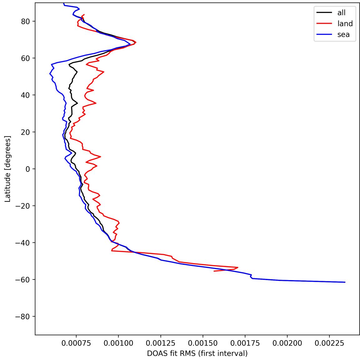
Figure 32: Zonal average of "DOAS fit RMS (first interval)" for 2025-07-03 to 2025-07-04.
