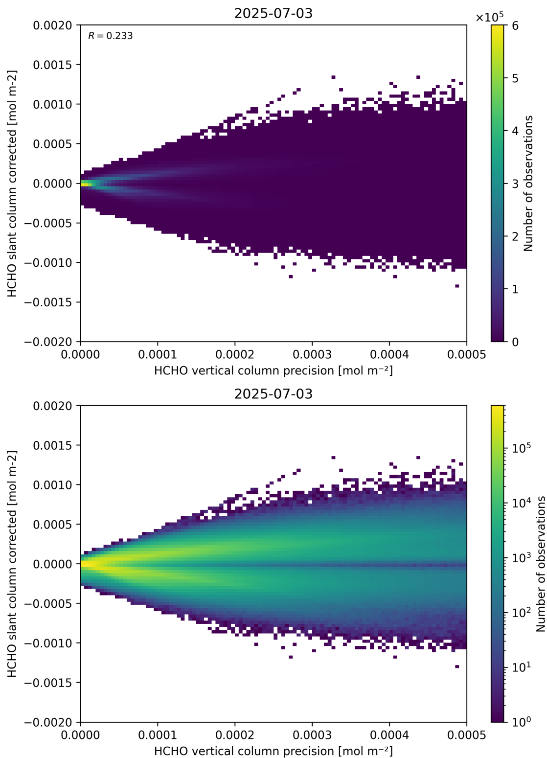
Figure 140: Scatter density plot of “HCHO vertical column precision” against “HCHO slant column corrected” for 2025-07-03 to 2025-07-04.
