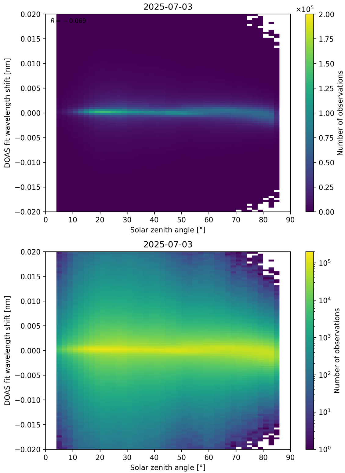
Figure 168: Scatter density plot of “Solar zenith angle” against “DOAS fit wavelength shift” for 2025-07-03 to 2025-07-04.
