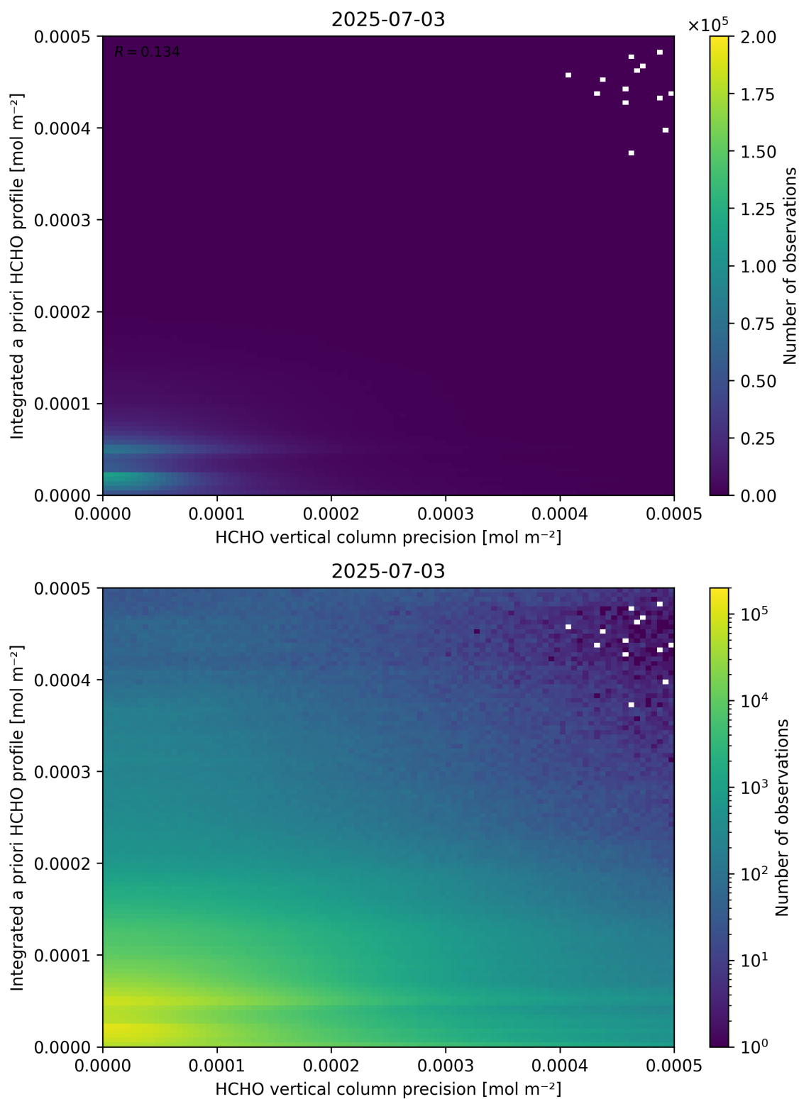
Figure 147: Scatter density plot of “HCHO vertical column precision” against “Integrated a priori HCHO profile” for 2025-07-03 to 2025-07-04.
