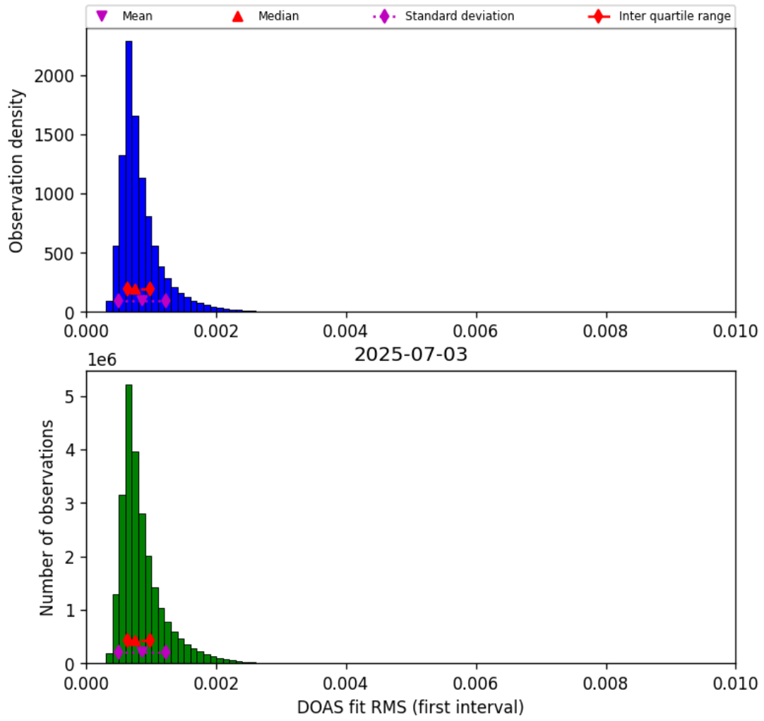
Figure 46: Histogram of “DOAS fit RMS (first interval)” for 2025-07-03 to 2025-07-04
