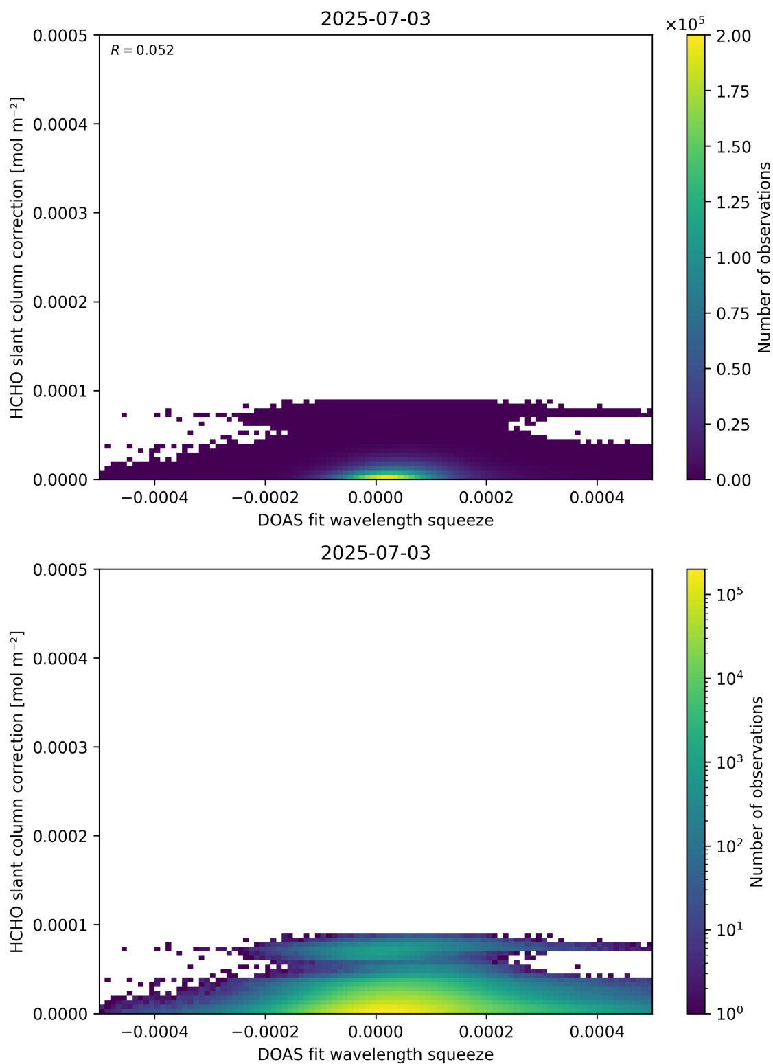
Figure 70: Scatter density plot of “DOAS fit wavelength squeeze” against “HCHO slant column correction” for 2025-07-03 to 2025-07-04.
