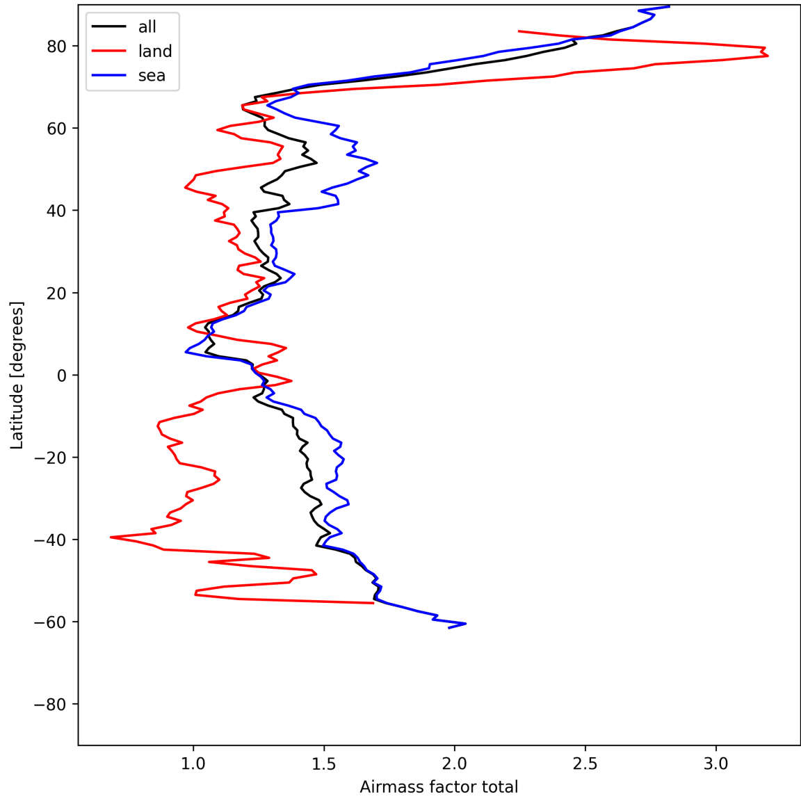
Figure 26: Zonal average of “Airmass factor total” for 2025-07-03 to 2025-07-04.
