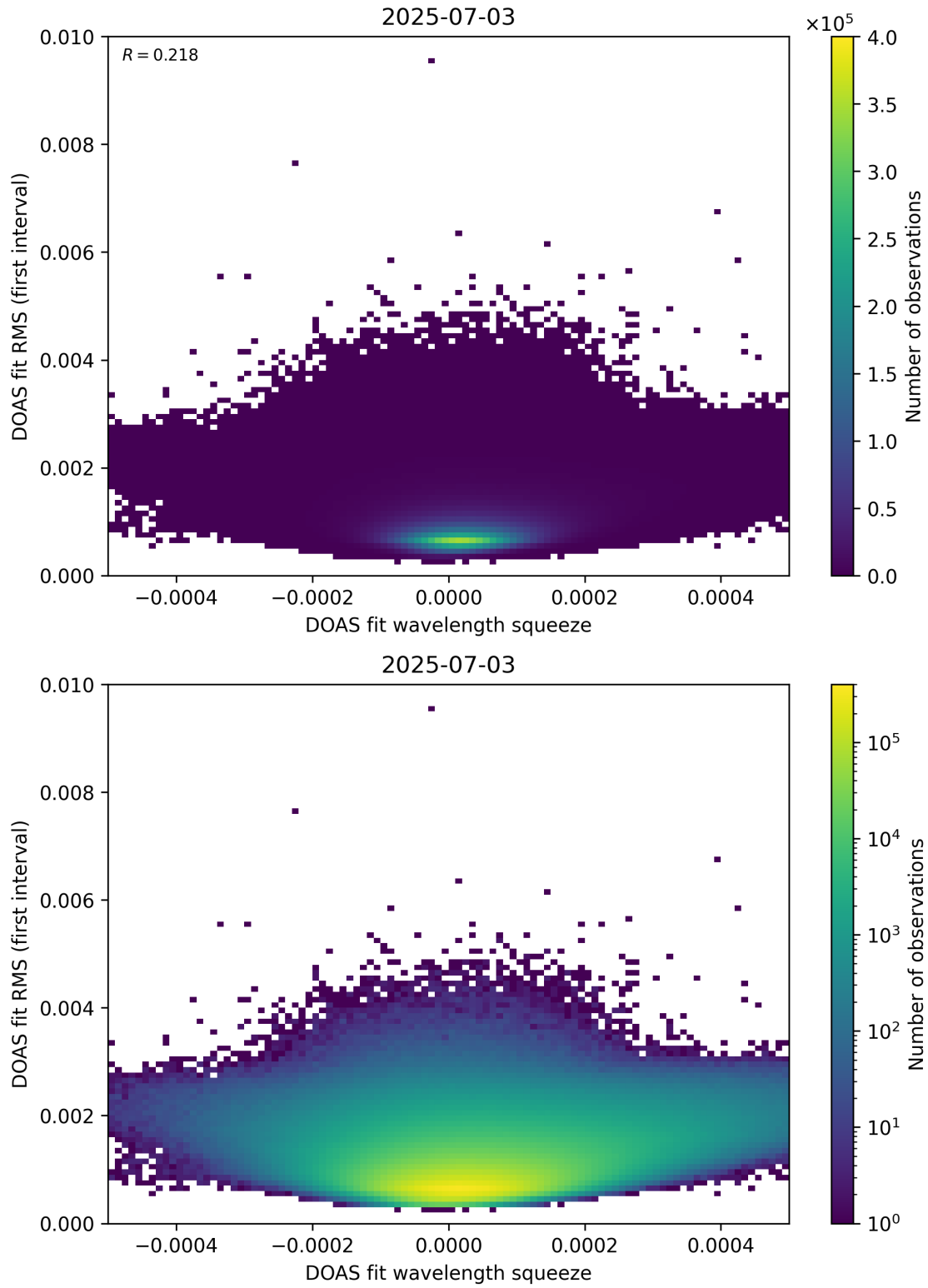
Figure 68: Scatter density plot of “DOAS fit wavelength squeeze” against “DOAS fit RMS (first interval)” for 2025-07-03 to 2025-07-04.
