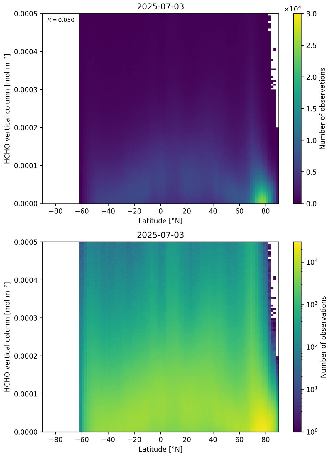
Figure 163: Scatter density plot of “Latitude” against “HCHO vertical column” for 2025-07-03 to 2025-07-04.
