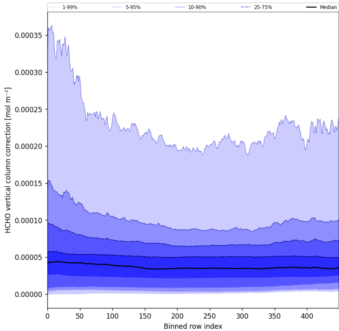
Figure 51: Along track statistics of “HCHO vertical column correction” for 2025-07-03 to 2025-07-04
