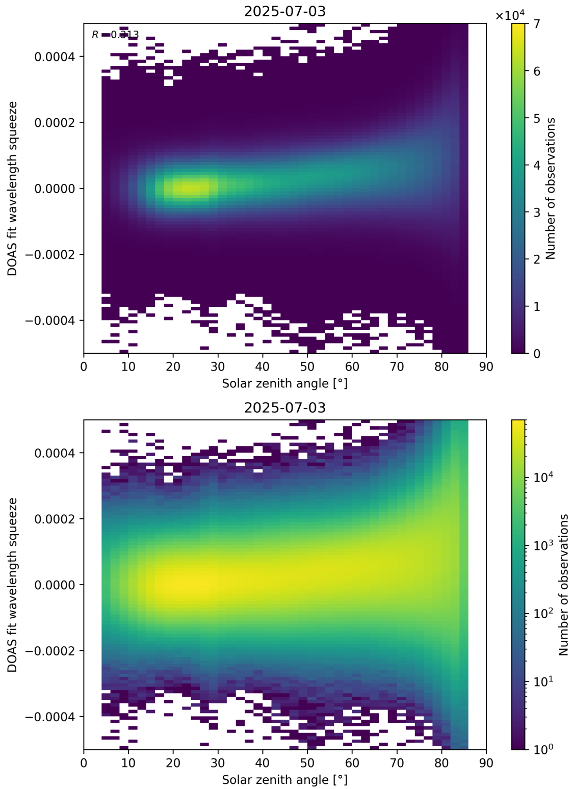
Figure 169: Scatter density plot of “Solar zenith angle” against “DOAS fit wavelength squeeze” for 2025-07-03 to 2025-07-04.
