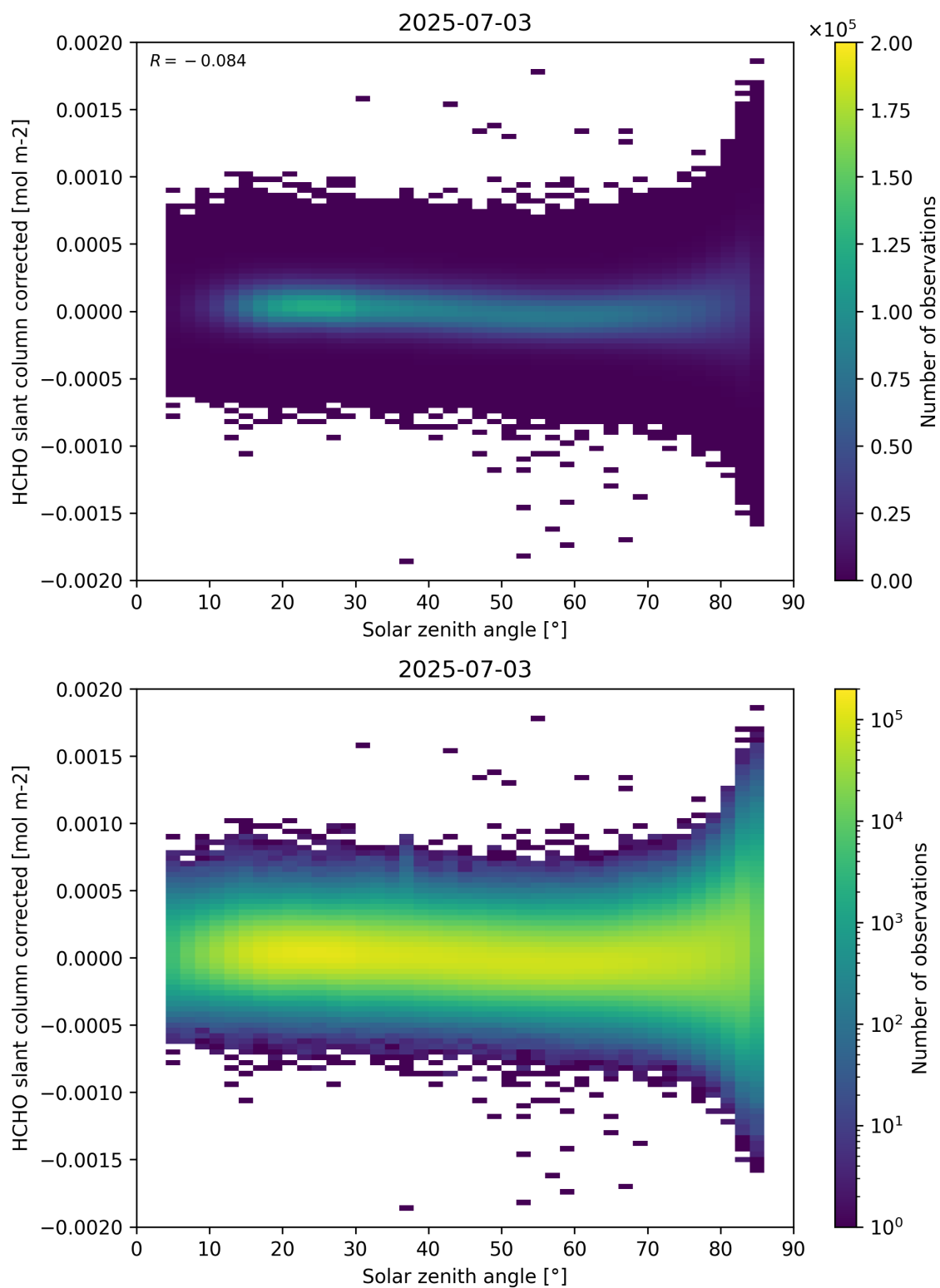
Figure 171: Scatter density plot of “Solar zenith angle” against “HCHO slant column corrected” for 2025-07-03 to 2025-07-04.
