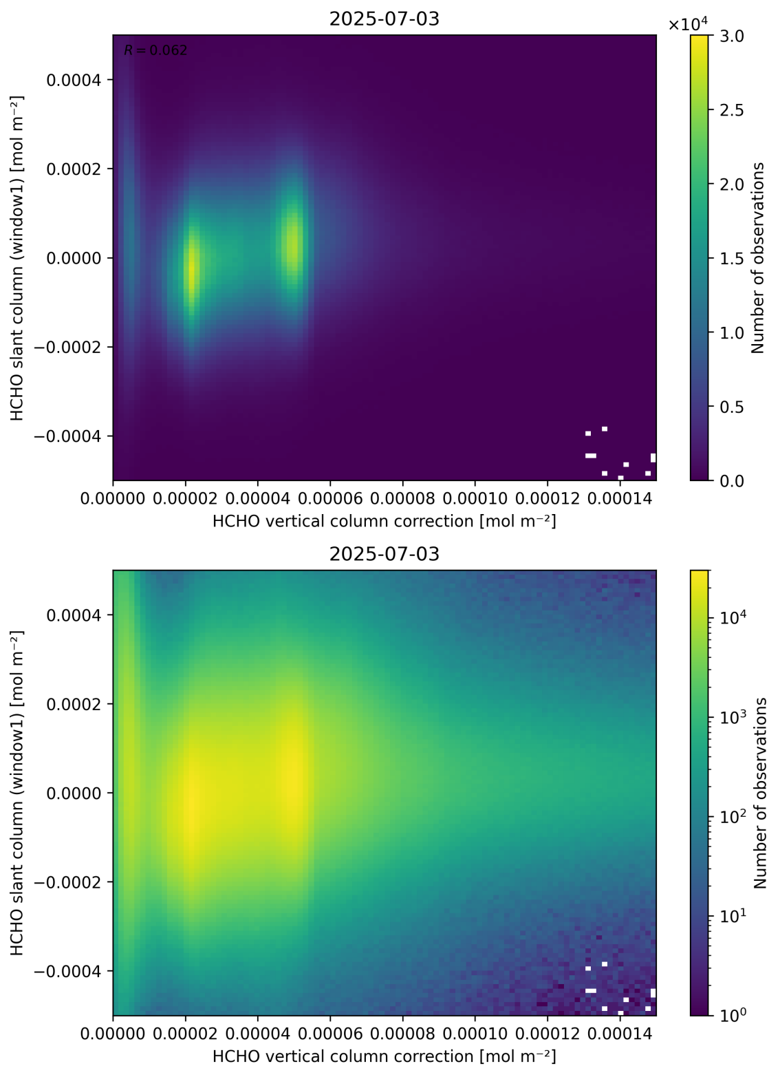
Figure 118: Scatter density plot of “HCHO vertical column correction” against “HCHO slant column (window1)” for 2025-07-03 to 2025-07-04.
