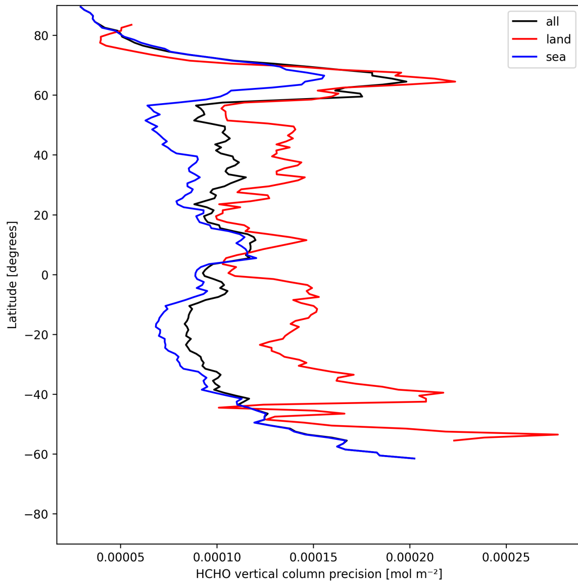
Figure 22: Zonal average of “HCHO vertical column precision” for 2025-07-03 to 2025-07-04.
