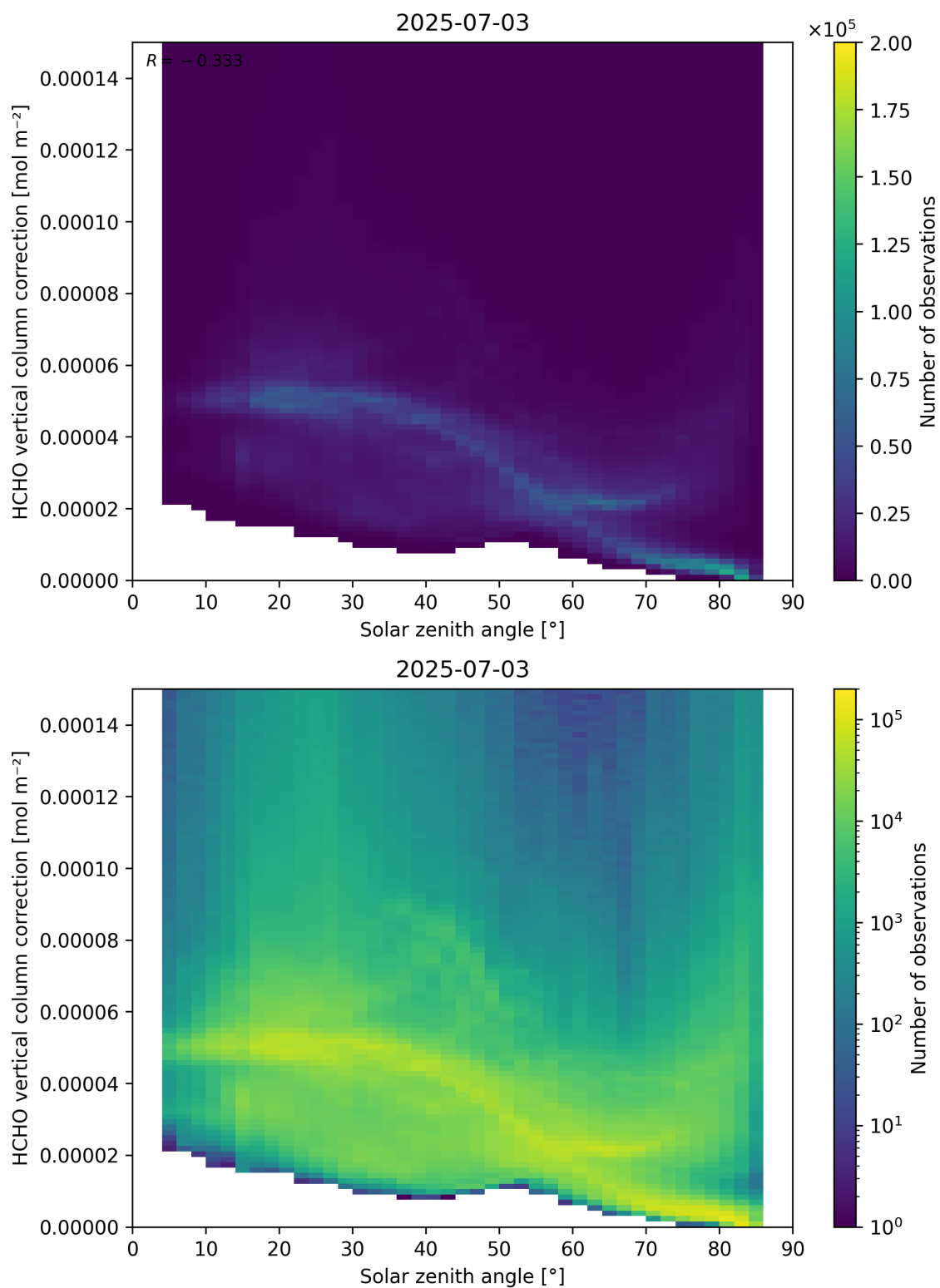
Figure 178: Scatter density plot of “Solar zenith angle” against “HCHO vertical column correction” for 2025-07-03 to 2025-07-04.
