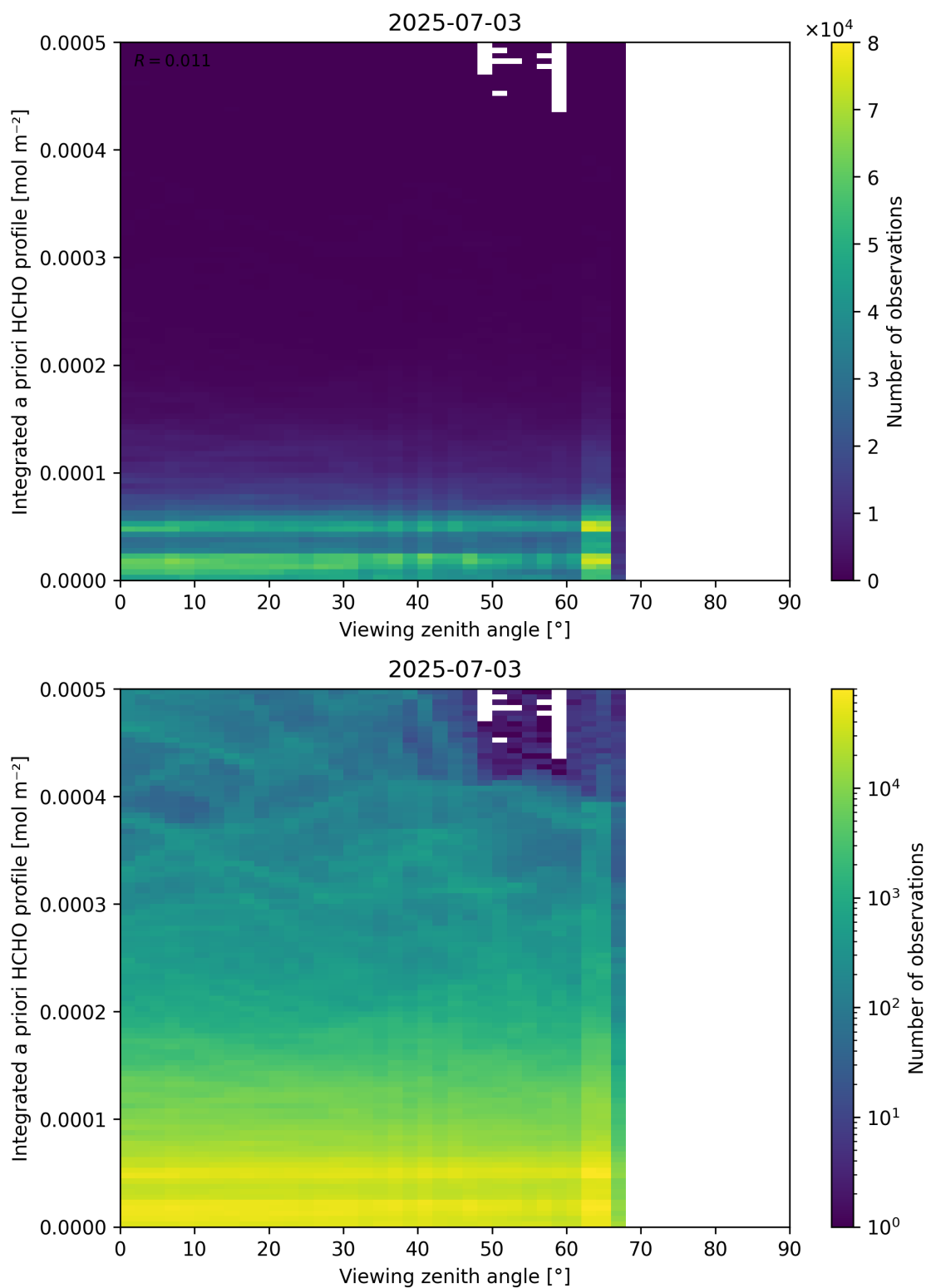
Figure 195: Scatter density plot of “Viewing zenith angle” against “Integrated a priori HCHO profile” for 2025-07-03 to 2025-07-04.
