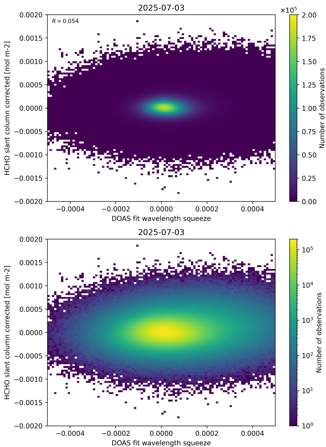
Figure 69: Scatter density plot of “DOAS fit wavelength squeeze” against “HCHO slant column corrected” for 2025-07-03 to 2025-07-04.
