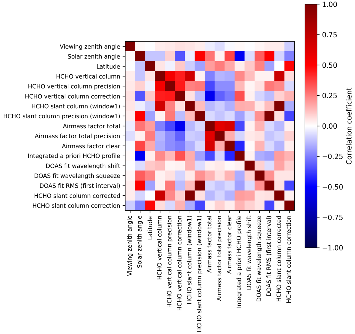
Figure 2: Map of correlation matrix for 2025-07-03 to 2025-07-04.
