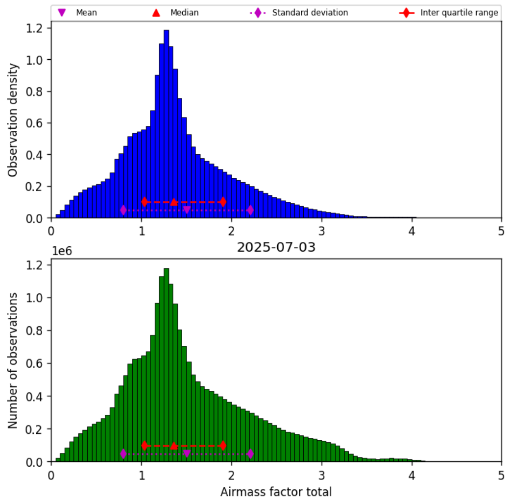
Figure 40: Histogram of “Airmass factor total” for 2025-07-03 to 2025-07-04
