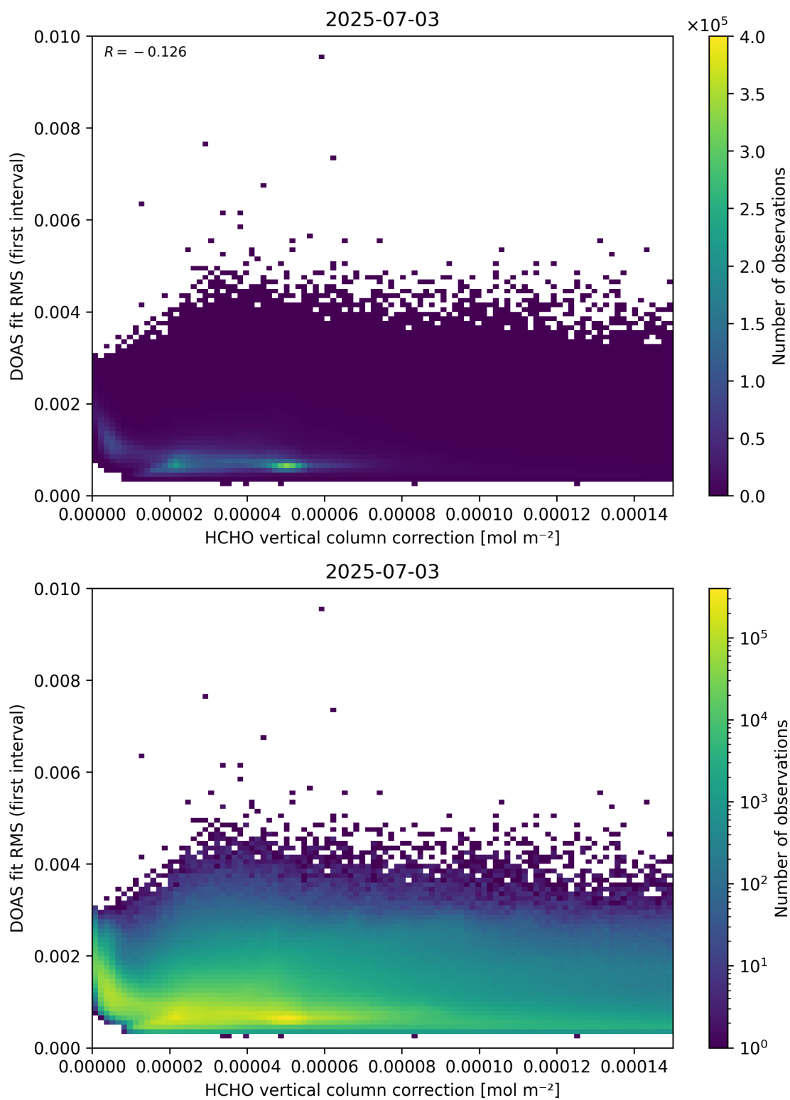
Figure 112: Scatter density plot of “HCHO vertical column correction” against “DOAS fit RMS (first interval)” for 2025-07-03 to 2025-07-04.
