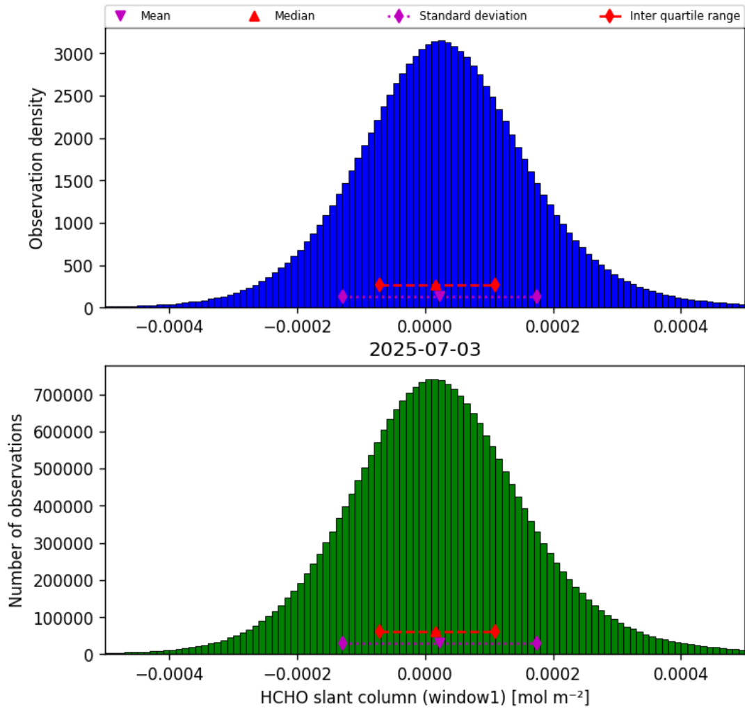
Figure 38: Histogram of “HCHO slant column (window1)” for 2025-07-03 to 2025-07-04
