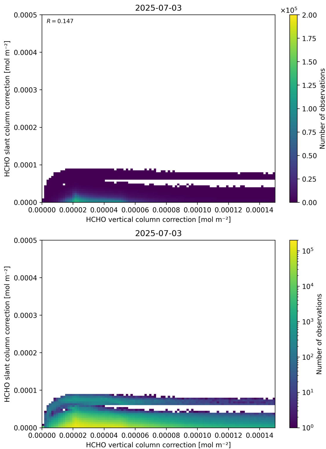
Figure 117: Scatter density plot of “HCHO vertical column correction” against “HCHO slant column correction” for 2025-07-03 to 2025-07-04.
