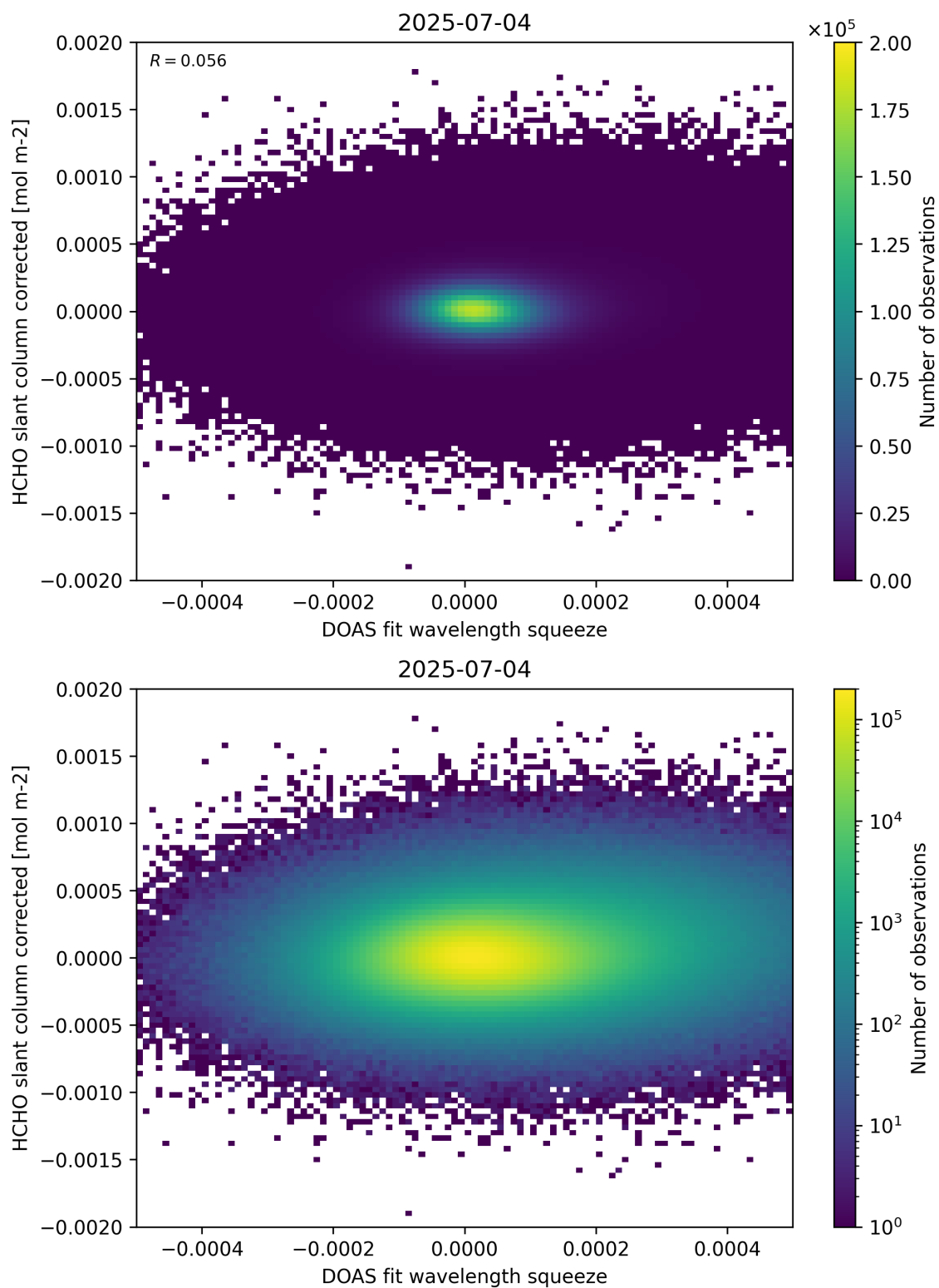
Figure 69: Scatter density plot of “DOAS fit wavelength squeeze” against “HCHO slant column corrected” for 2025-07-03 to 2025-07-05.
