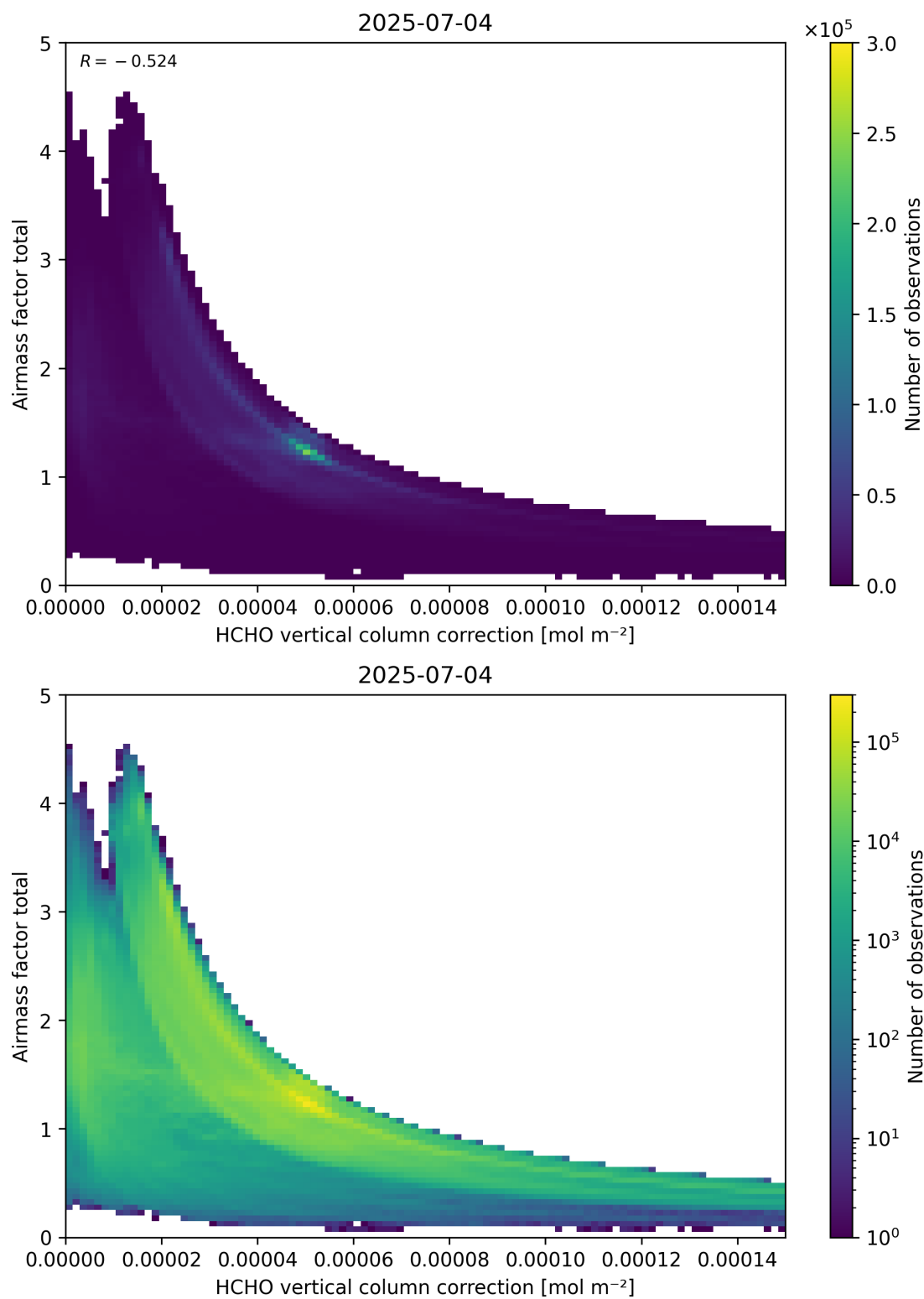
Figure 120: Scatter density plot of “HCHO vertical column correction” against “Airmass factor total” for 2025-07-03 to 2025-07-05.
