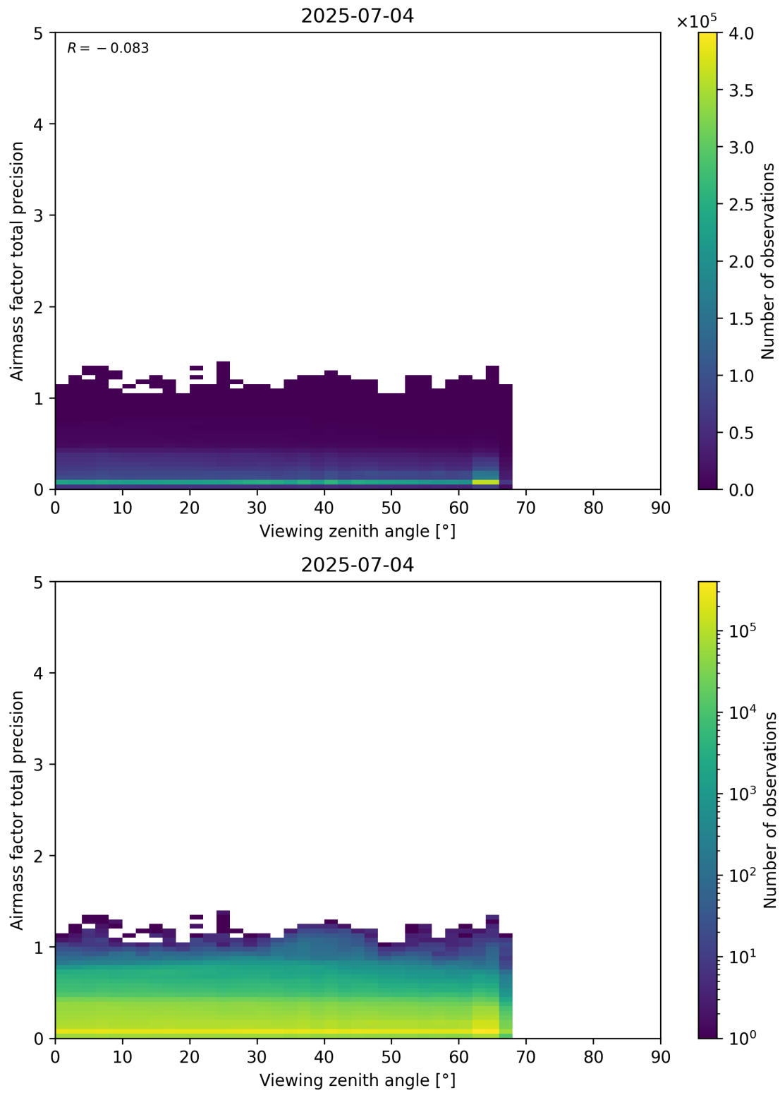
Figure 191: Scatter density plot of “Viewing zenith angle” against “Airmass factor total precision” for 2025-07-03 to 2025-07-05.
