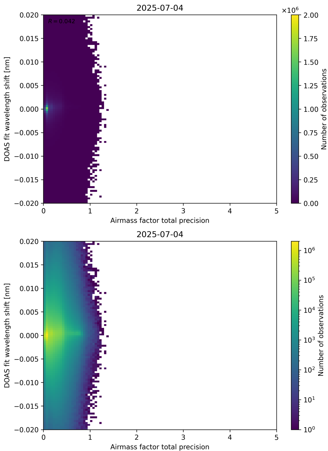
Figure 106: Scatter density plot of “Airmass factor total precision” against “DOAS fit wavelength shift” for 2025-07-03 to 2025-07-05.
