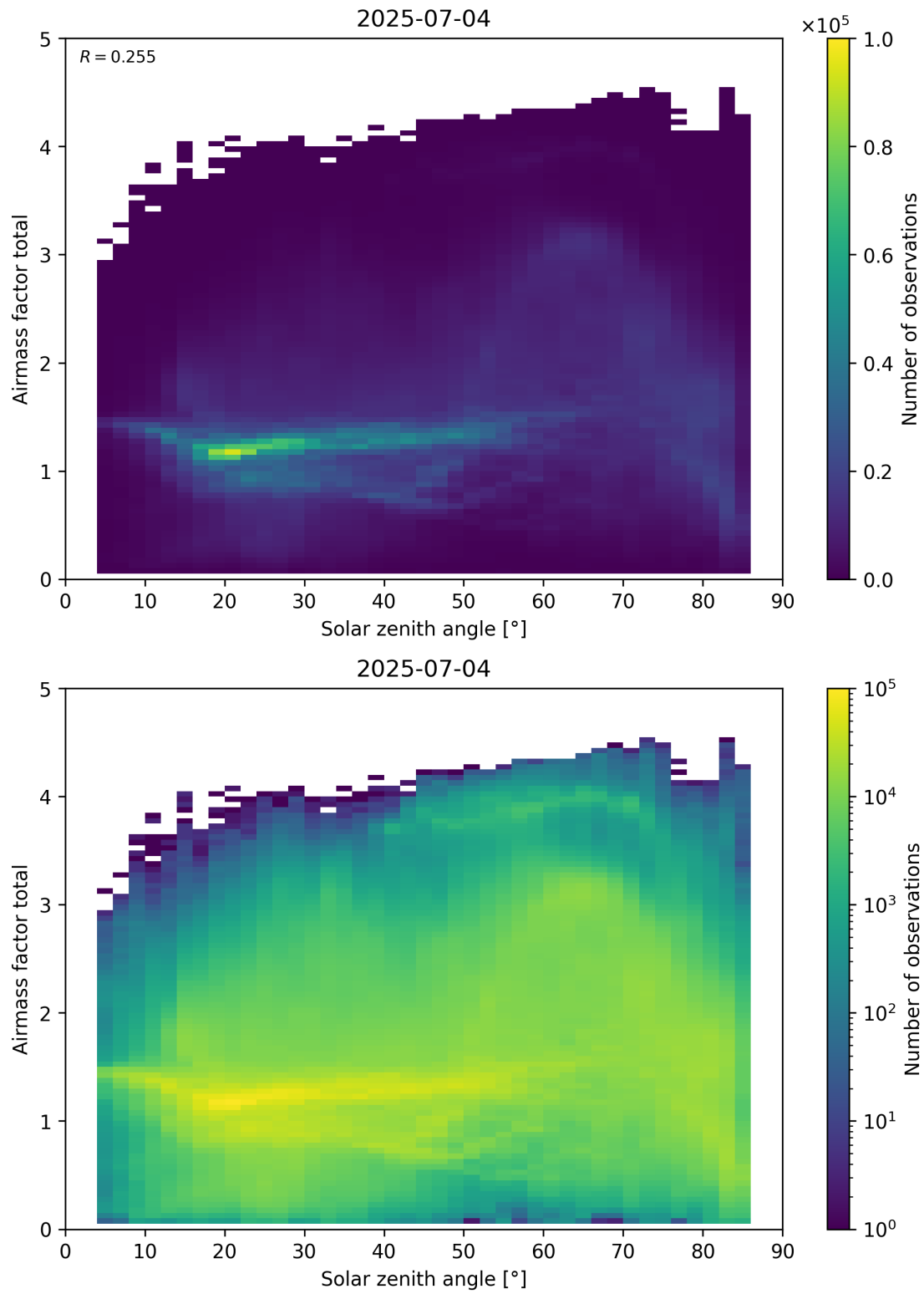
Figure 175: Scatter density plot of “Solar zenith angle” against “Airmass factor total” for 2025-07-03 to 2025-07-05.
