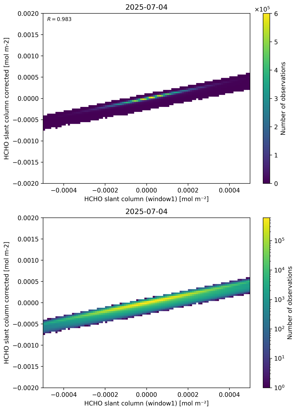
Figure 82: Scatter density plot of “HCHO slant column (window1)” against “HCHO slant column corrected” for 2025-07-03 to 2025-07-05.
