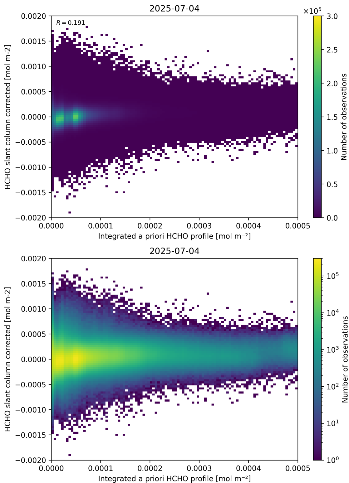
Figure 151: Scatter density plot of “Integrated a priori HCHO profile” against “HCHO slant column corrected” for 2025-07-03 to 2025-07-05.
