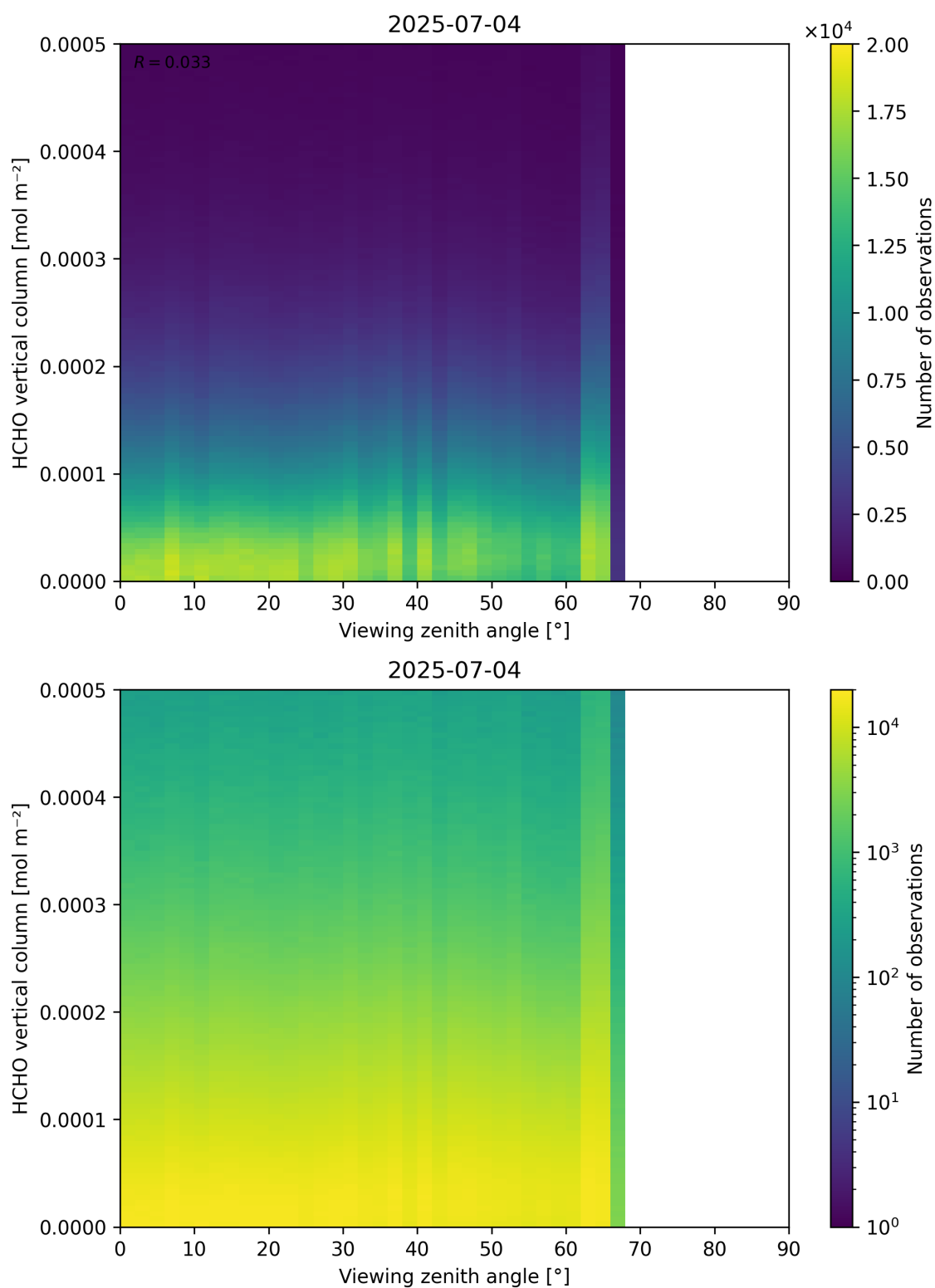
Figure 192: Scatter density plot of “Viewing zenith angle” against “HCHO vertical column” for 2025-07-03 to 2025-07-05.
