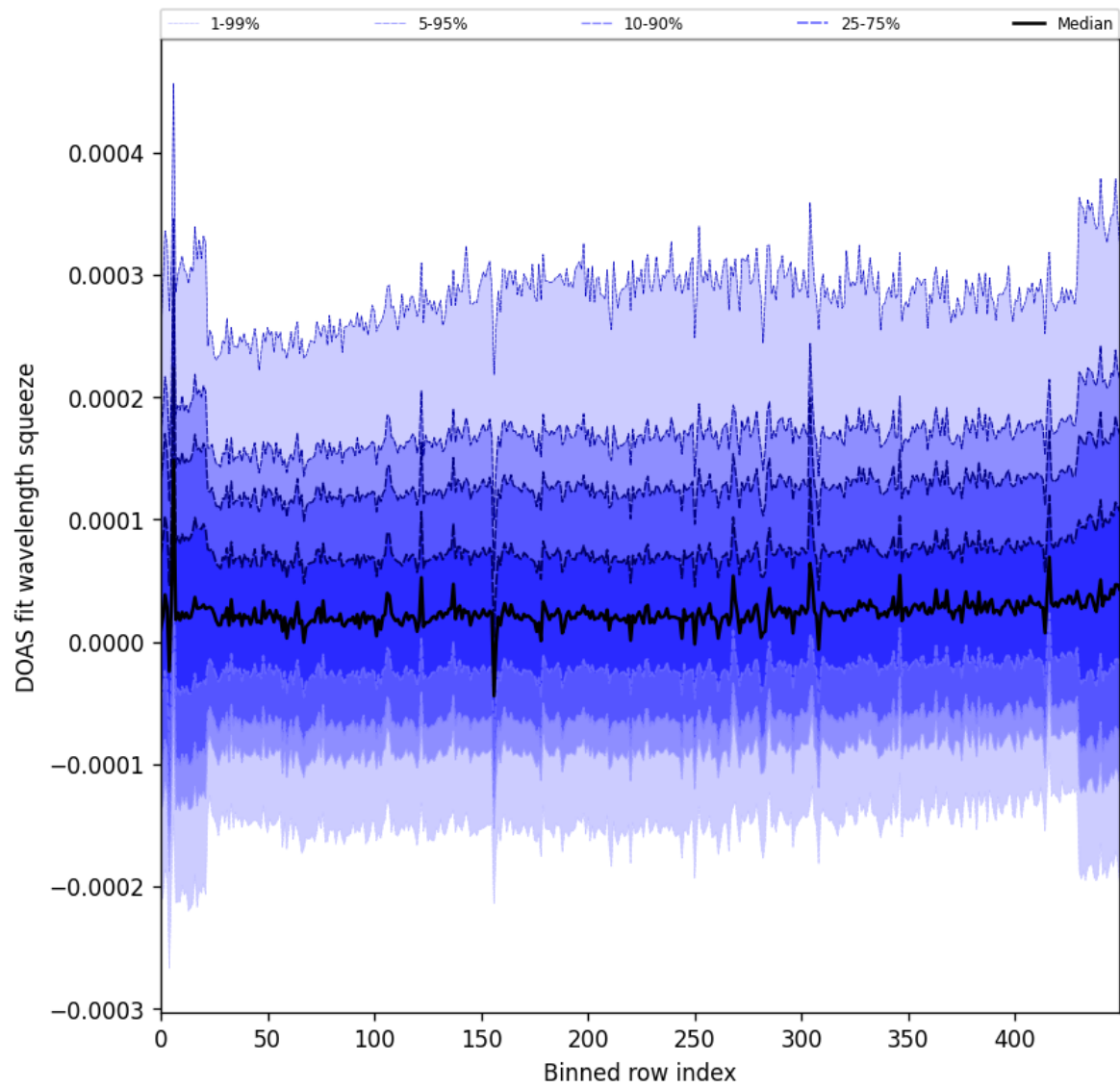
Figure 59: Along track statistics of “DOAS fit wavelength squeeze” for 2025-07-03 to 2025-07-05
