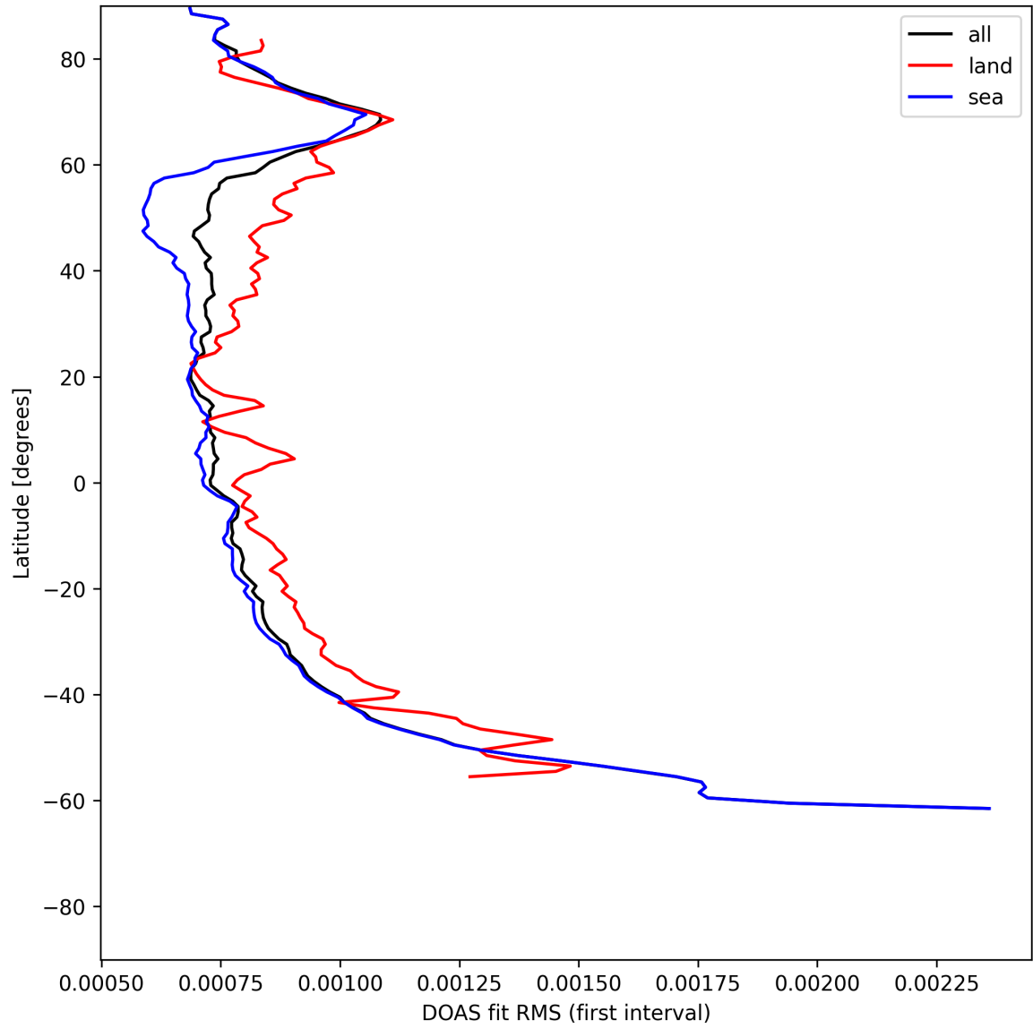
Figure 32: Zonal average of “DOAS fit RMS (first interval)” for 2025-07-03 to 2025-07-05.
