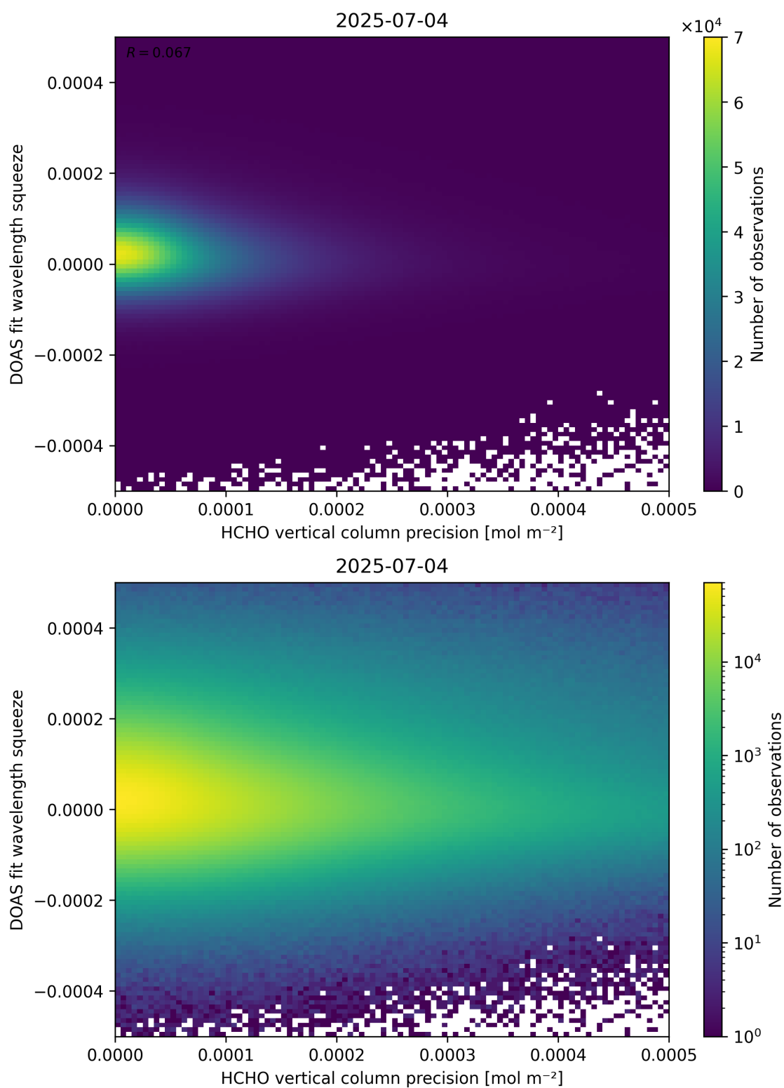
Figure 138: Scatter density plot of “HCHO vertical column precision” against “DOAS fit wavelength squeeze” for 2025-07-03 to 2025-07-05.
