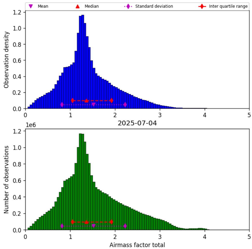
Figure 40: Histogram of “Airmass factor total” for 2025-07-03 to 2025-07-05
