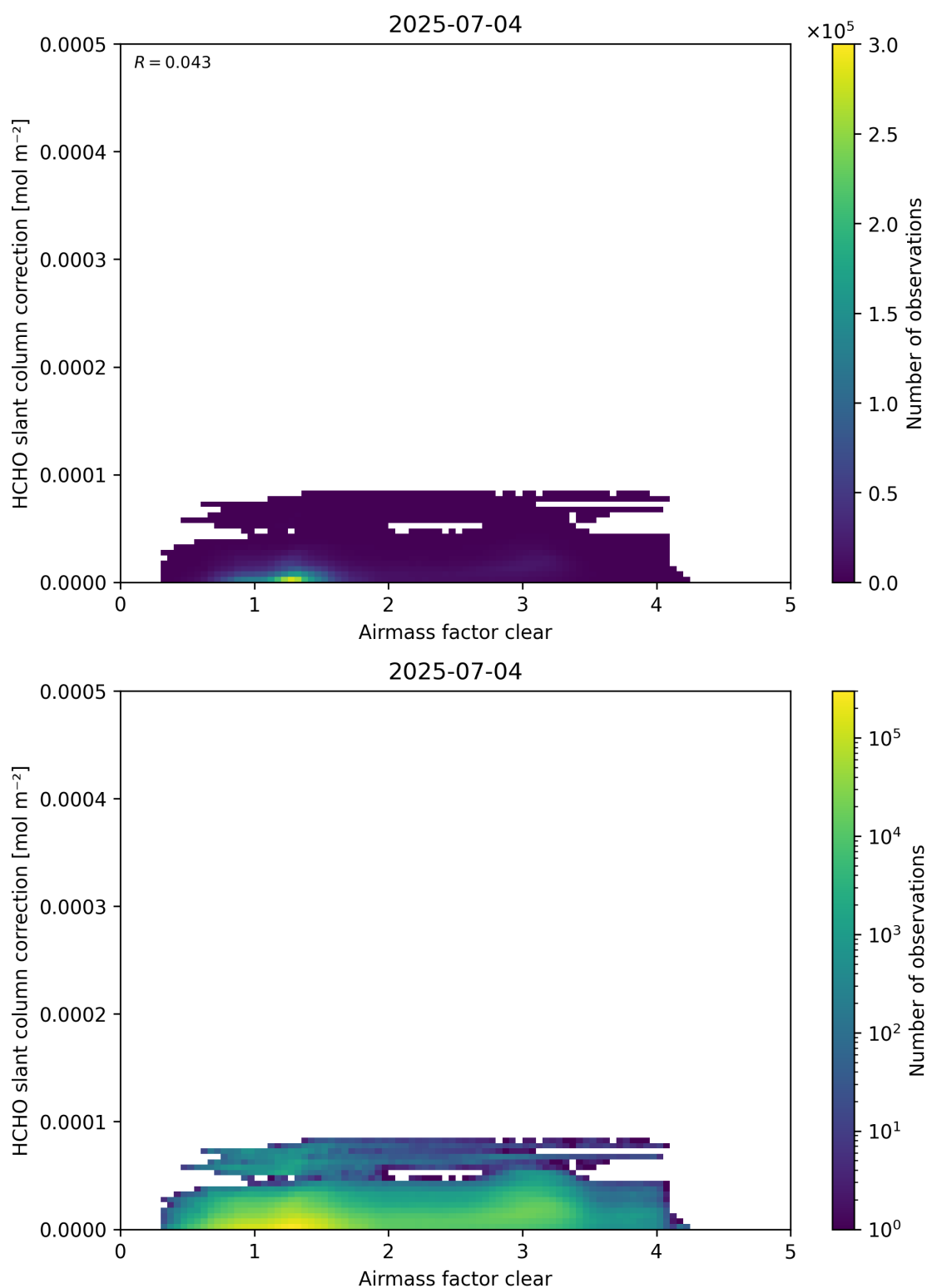
Figure 75: Scatter density plot of “Airmass factor clear” against “HCHO slant column correction” for 2025-07-03 to 2025-07-05.
