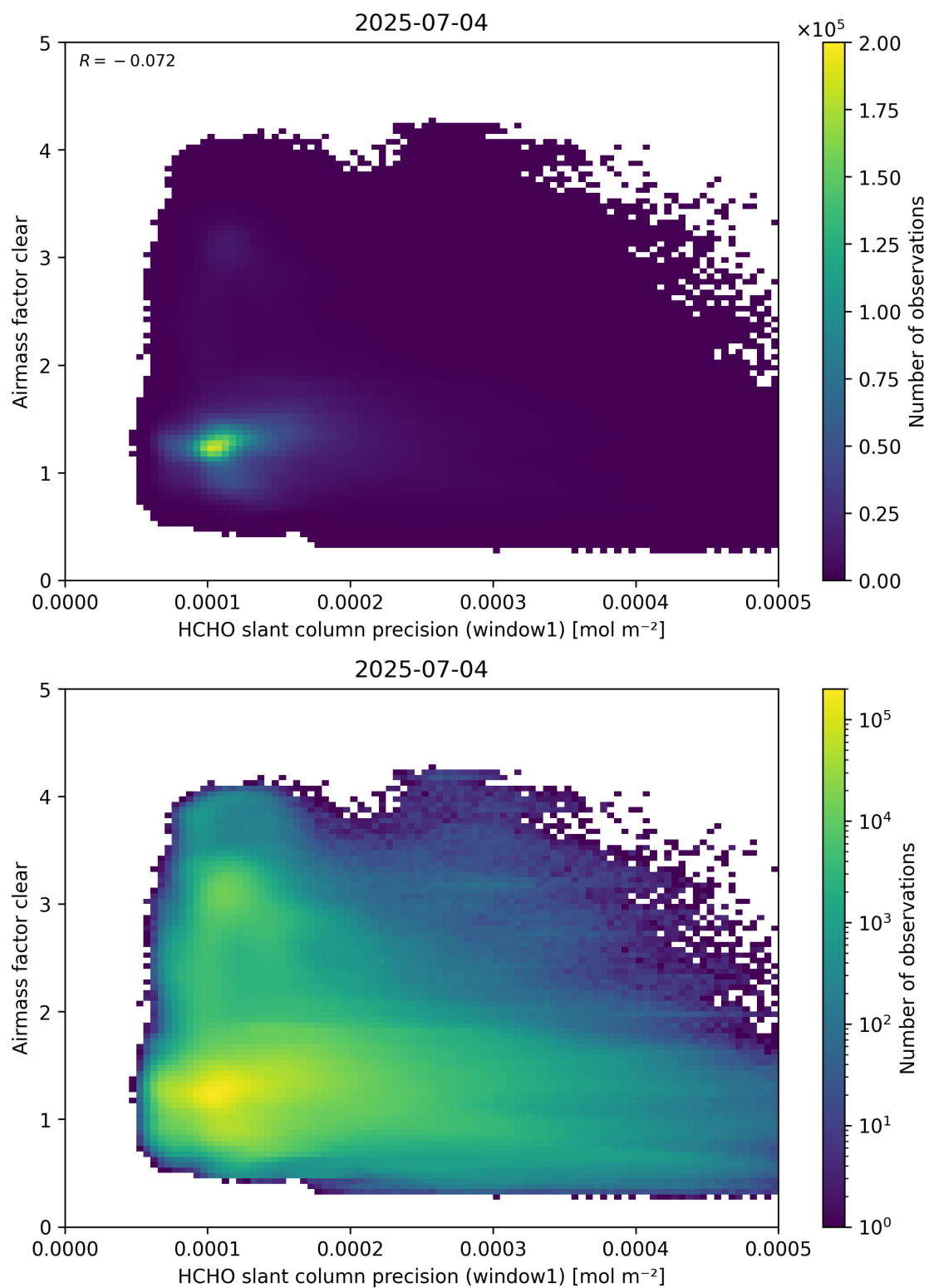
Figure 91: Scatter density plot of “HCHO slant column precision (window1)” against “Airmass factor clear” for 2025-07-03 to 2025-07-05.
