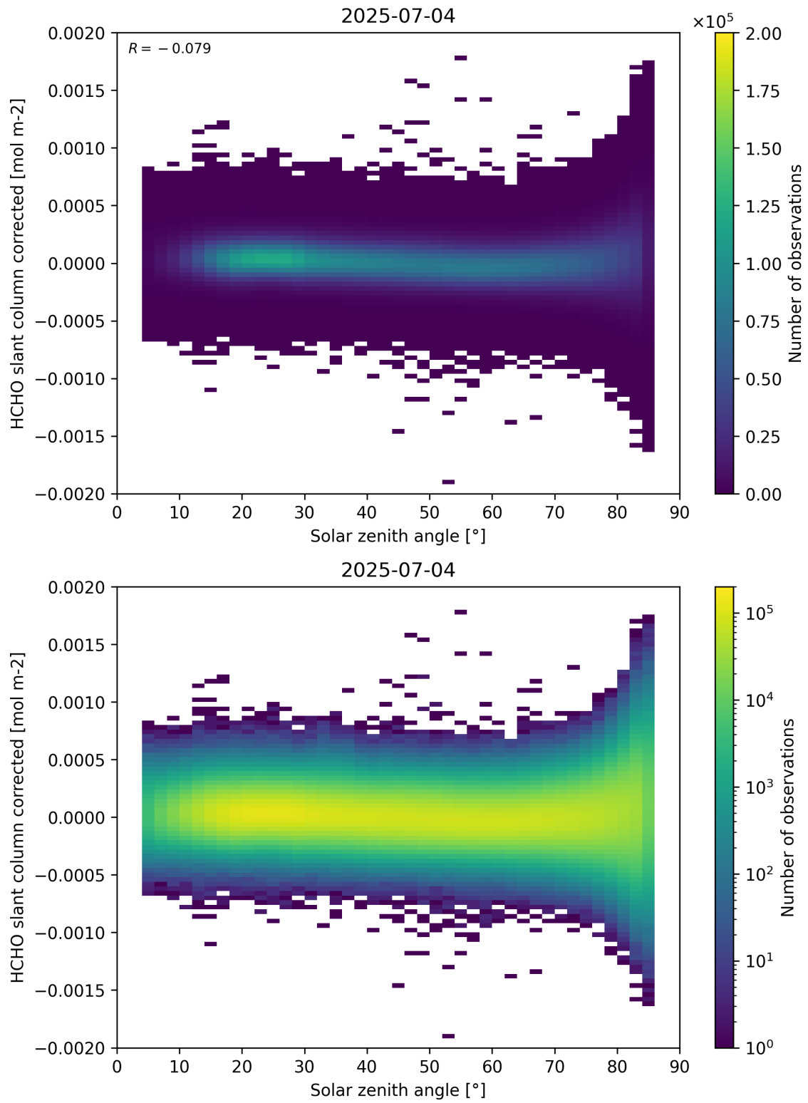
Figure 171: Scatter density plot of “Solar zenith angle” against “HCHO slant column corrected” for 2025-07-03 to 2025-07-05.
