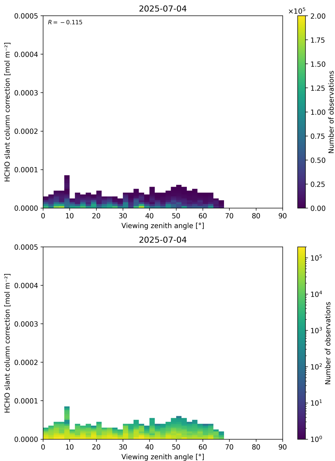
Figure 187: Scatter density plot of “Viewing zenith angle” against “HCHO slant column correction” for 2025-07-03 to 2025-07-05.
