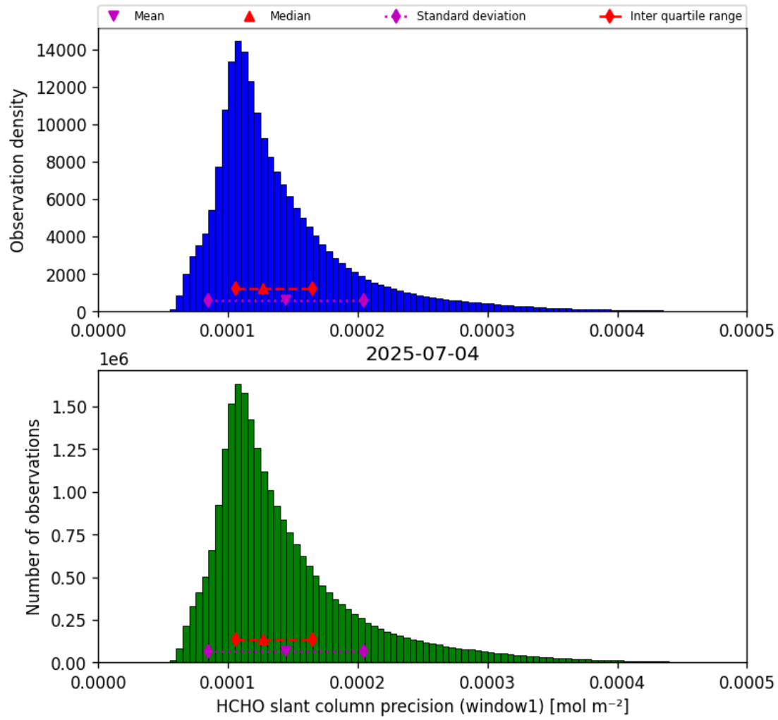
Figure 39: Histogram of “HCHO slant column precision (window1)” for 2025-07-03 to 2025-07-05
