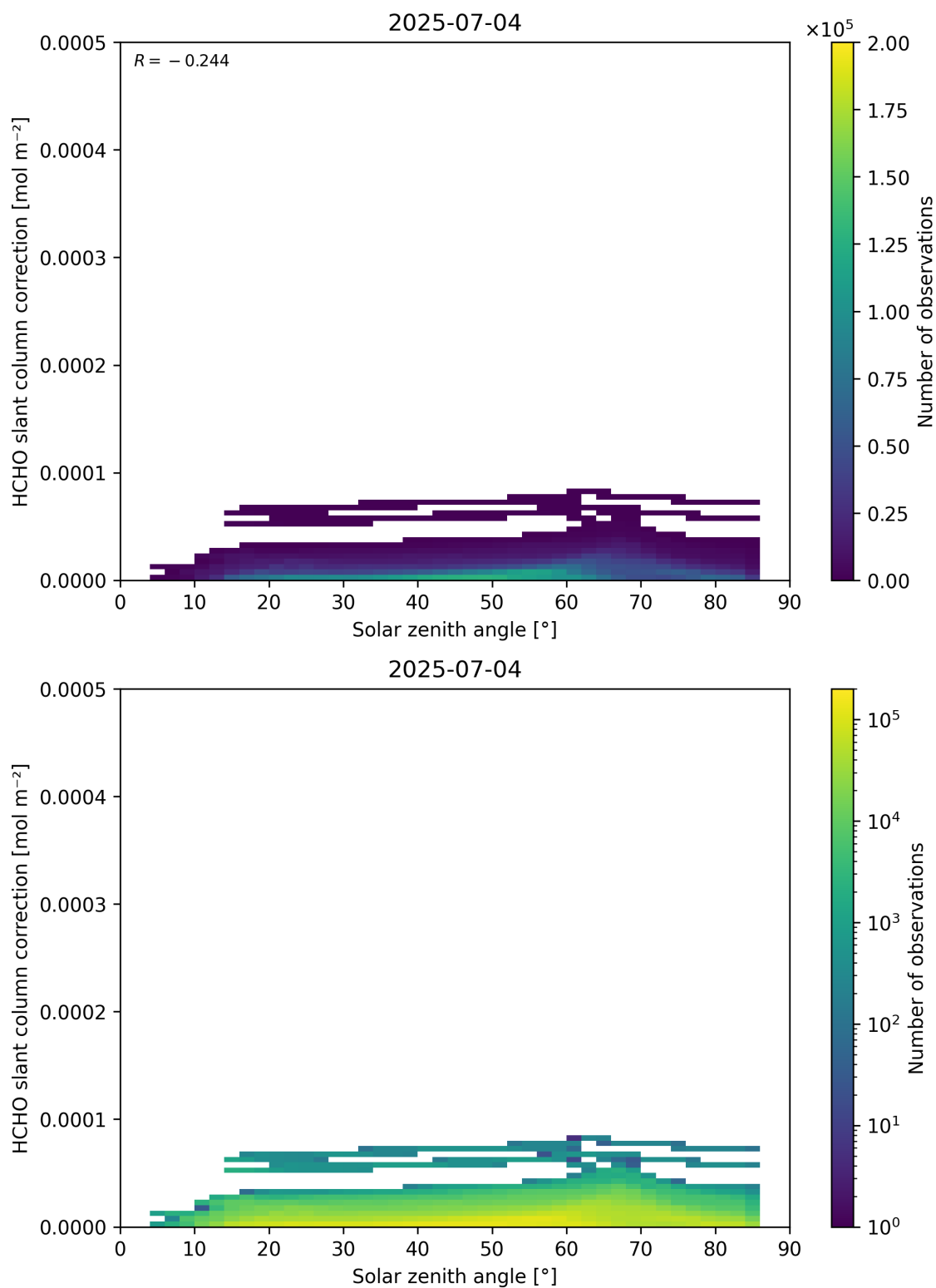
Figure 172: Scatter density plot of “Solar zenith angle” against “HCHO slant column correction” for 2025-07-03 to 2025-07-05.
