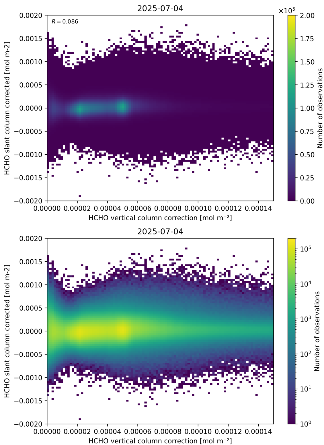
Figure 116: Scatter density plot of “HCHO vertical column correction” against “HCHO slant column corrected” for 2025-07-03 to 2025-07-05.
