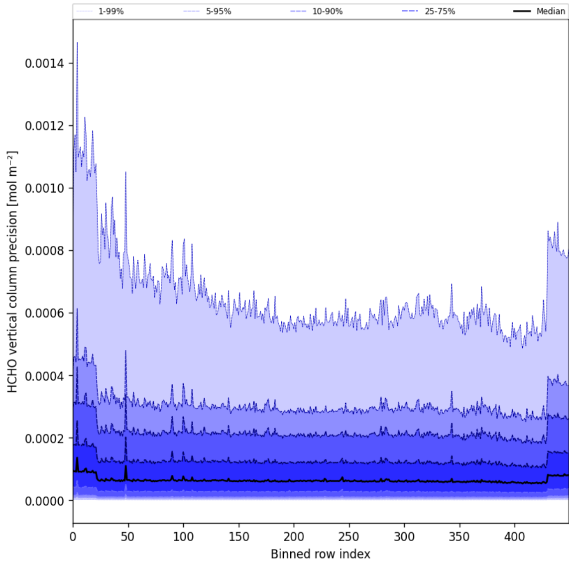
Figure 50: Along track statistics of “HCHO vertical column precision” for 2025-07-03 to 2025-07-05
