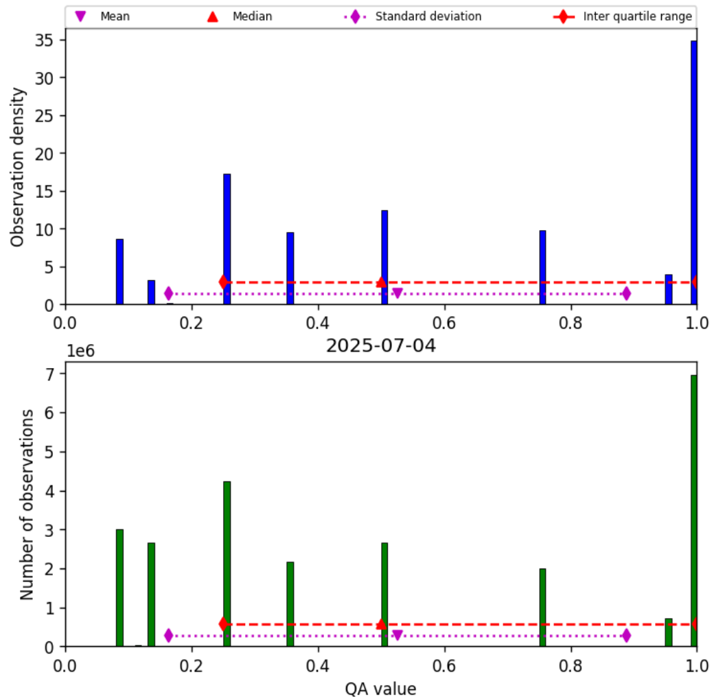
Figure 34: Histogram of “QA value” for 2025-07-03 to 2025-07-05
