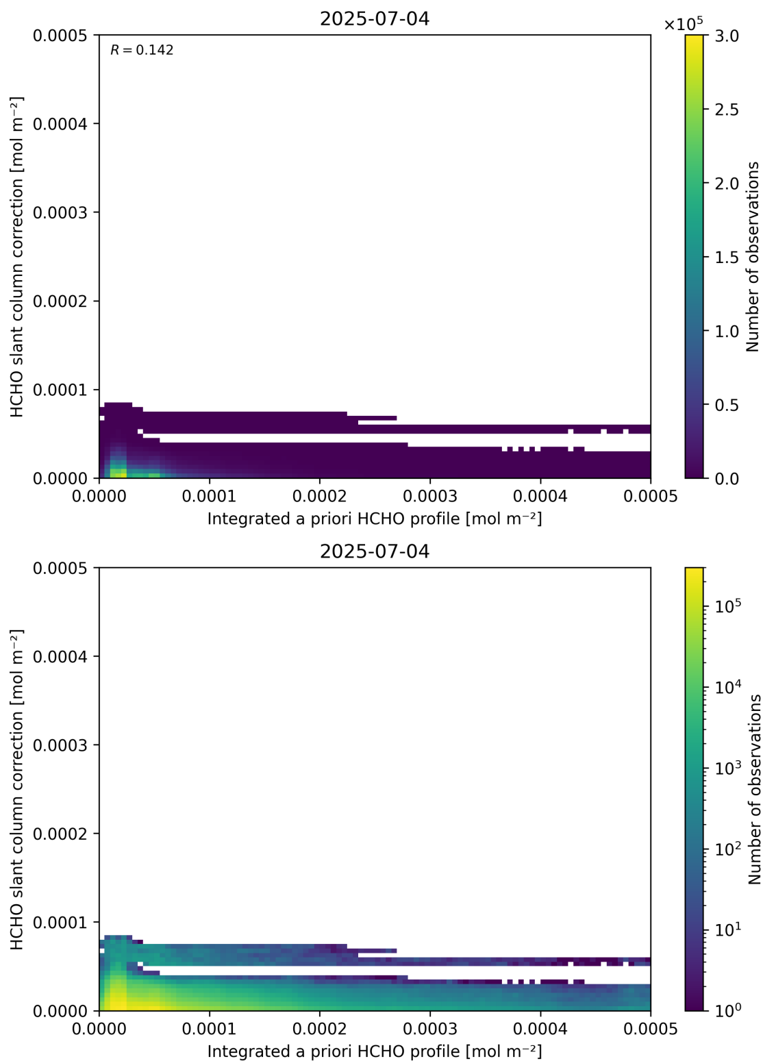
Figure 152: Scatter density plot of “Integrated a priori HCHO profile” against “HCHO slant column correction” for 2025-07-03 to 2025-07-05.
