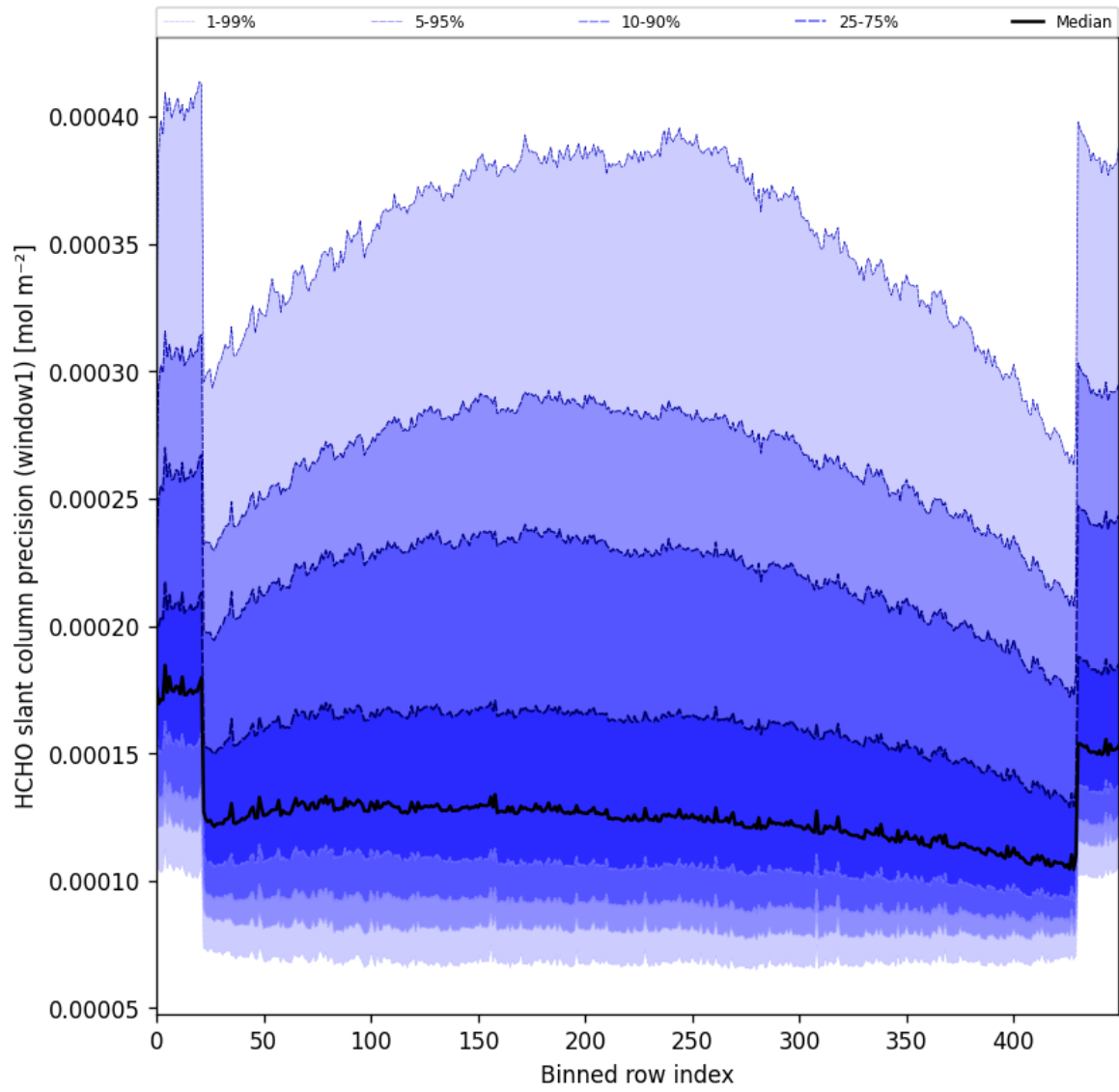
Figure 53: Along track statistics of “HCHO slant column precision (window1)” for 2025-07-03 to 2025-07-05
