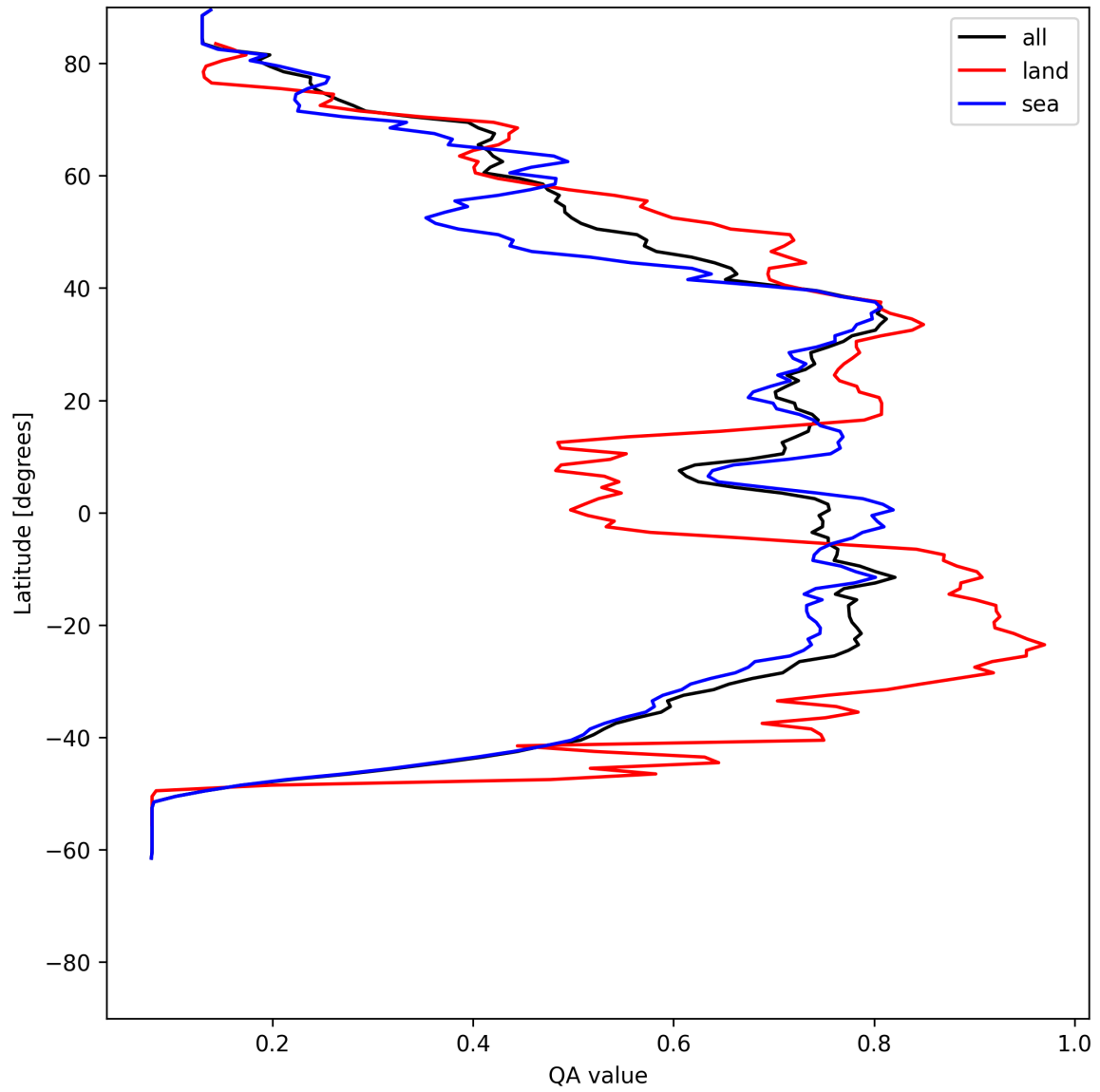
Figure 20: Zonal average of “QA value” for 2025-07-03 to 2025-07-05.
