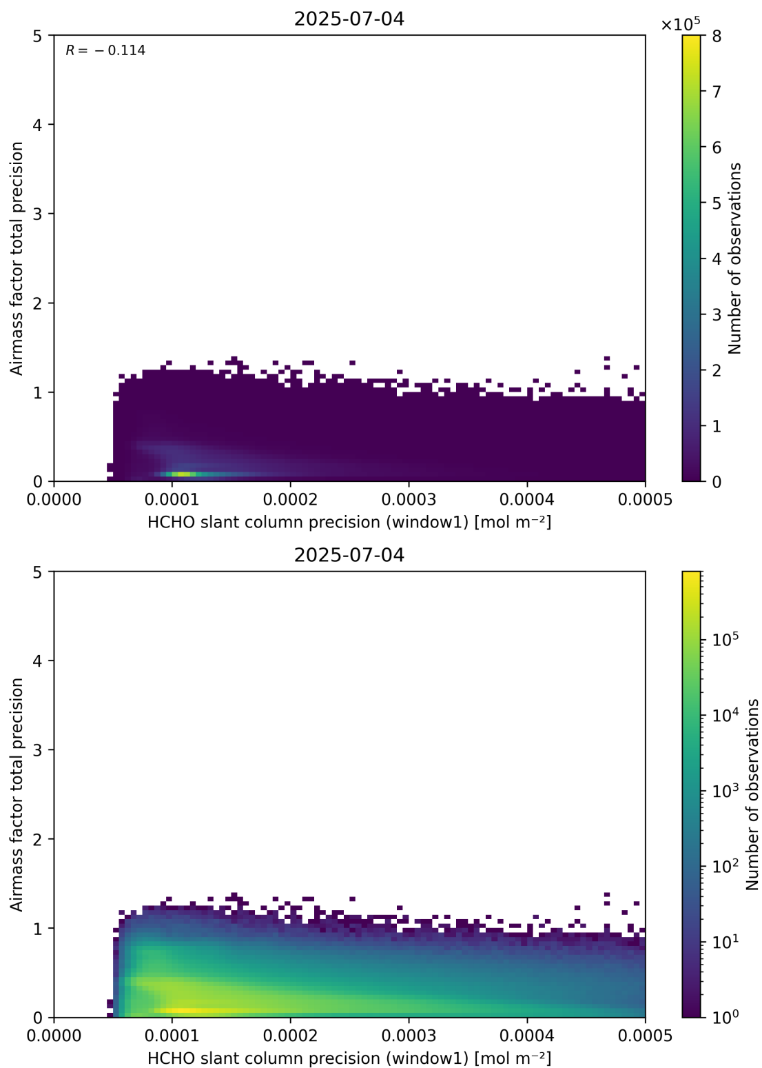
Figure 95: Scatter density plot of “HCHO slant column precision (window1)” against “Airmass factor total precision” for 2025-07-03 to 2025-07-05.
