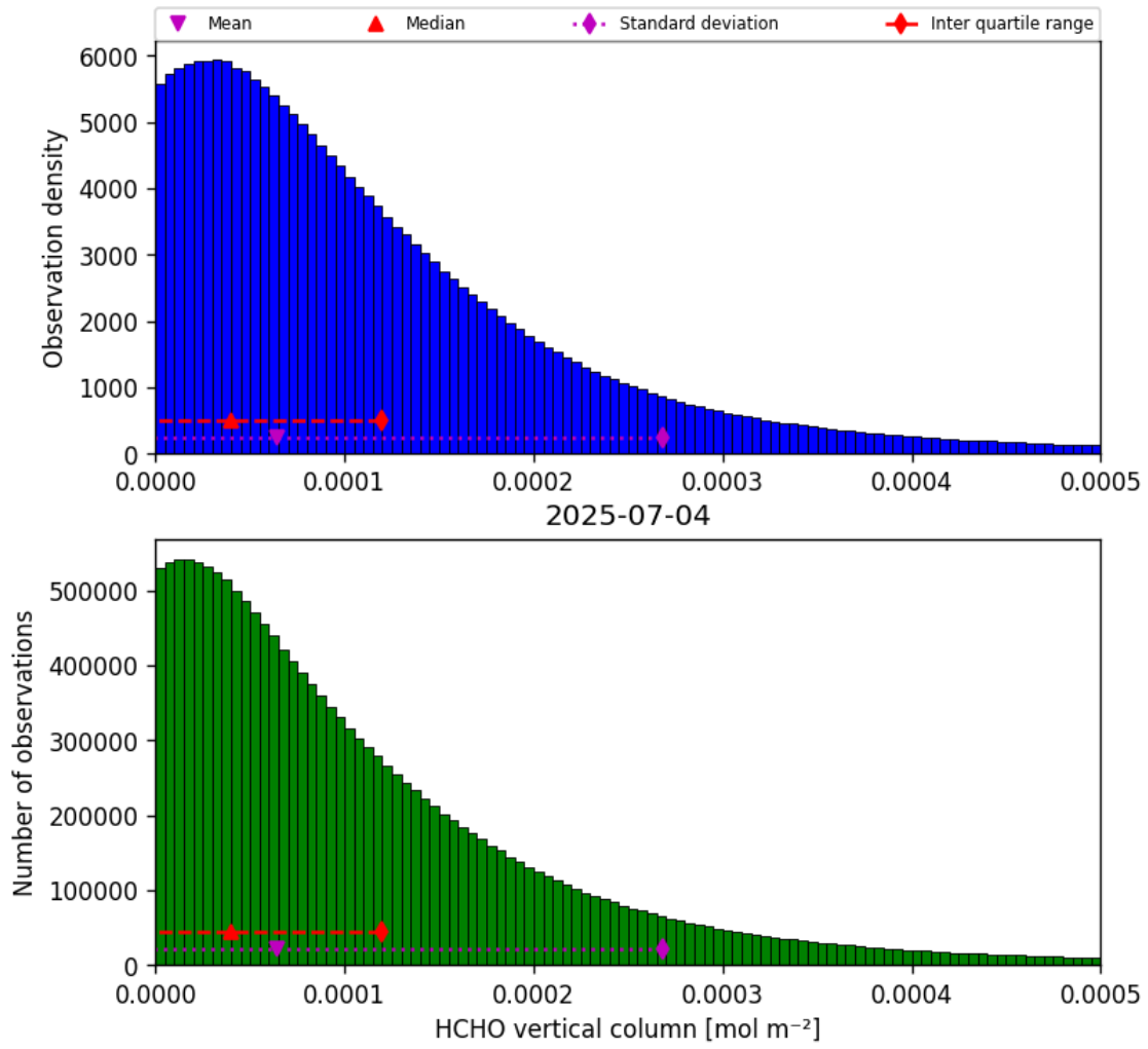
Figure 35: Histogram of “HCHO vertical column” for 2025-07-03 to 2025-07-05
