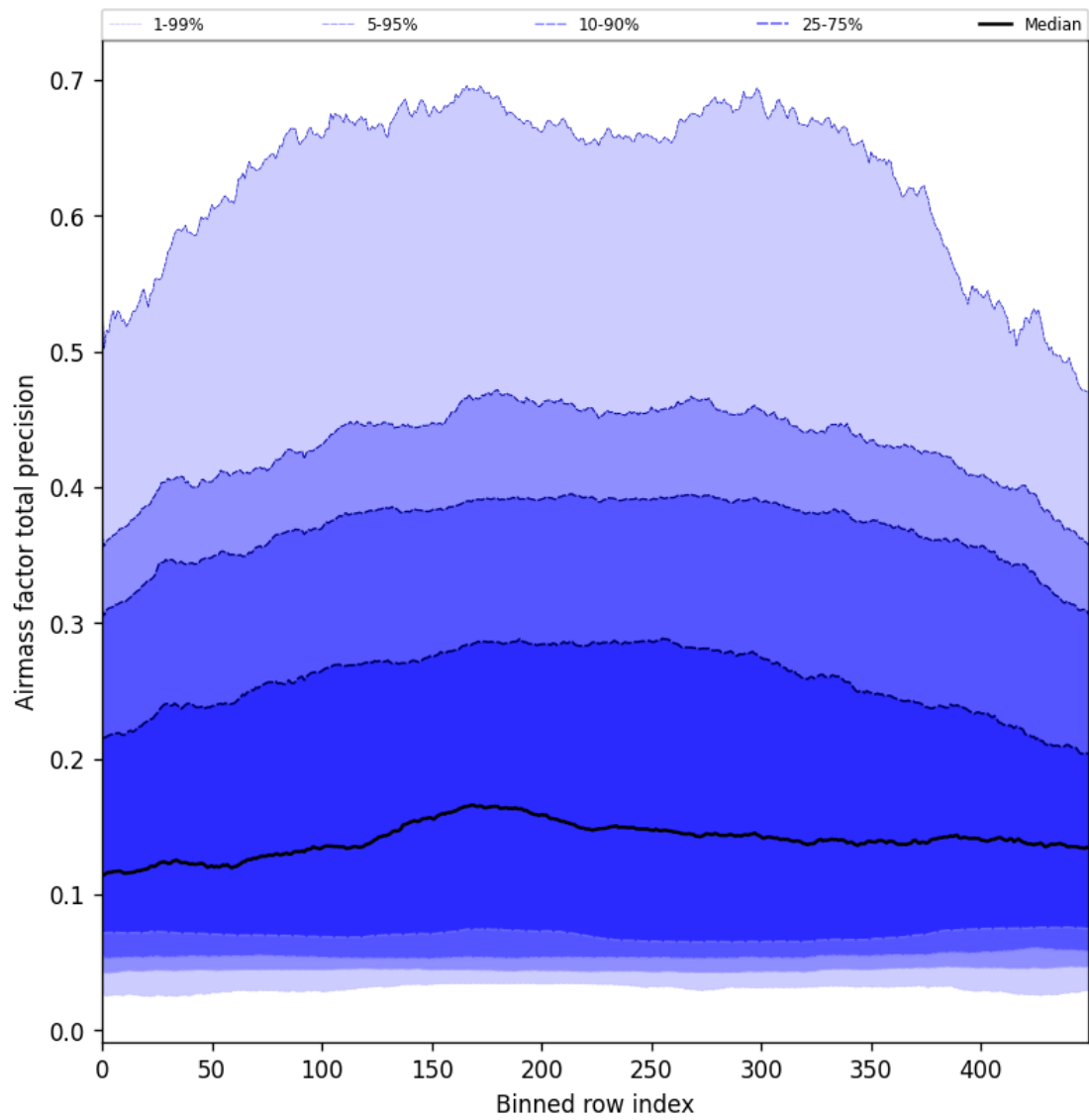
Figure 55: Along track statistics of “Airmass factor total precision” for 2025-07-03 to 2025-07-05
