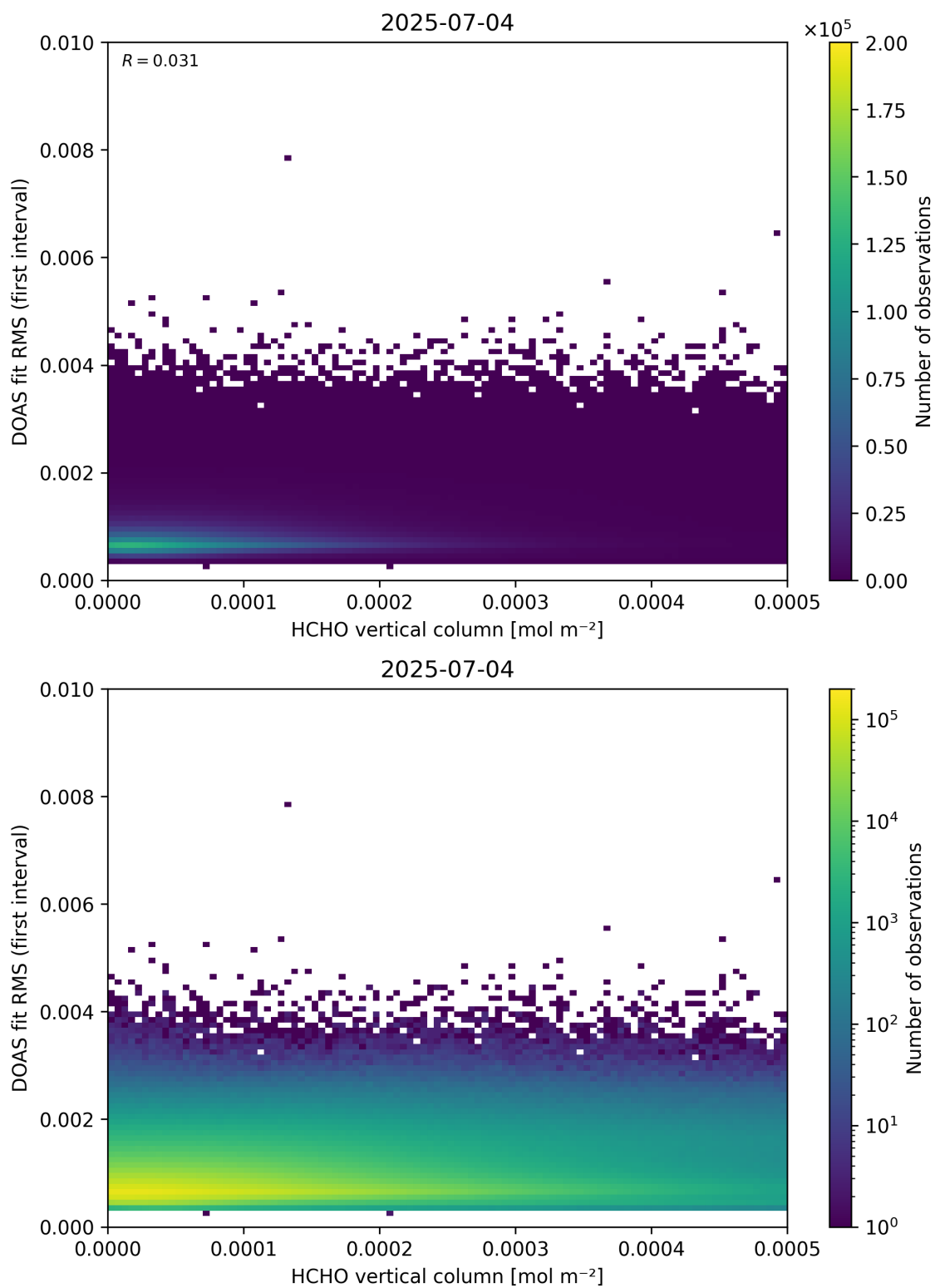
Figure 123: Scatter density plot of “HCHO vertical column” against “DOAS fit RMS (first interval)” for 2025-07-03 to 2025-07-05.
