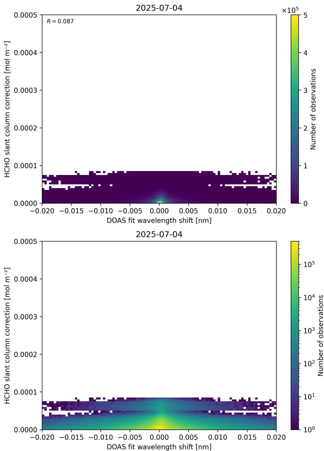
Figure 67: Scatter density plot of “DOAS fit wavelength shift” against “HCHO slant column correction” for 2025-07-03 to 2025-07-05.
