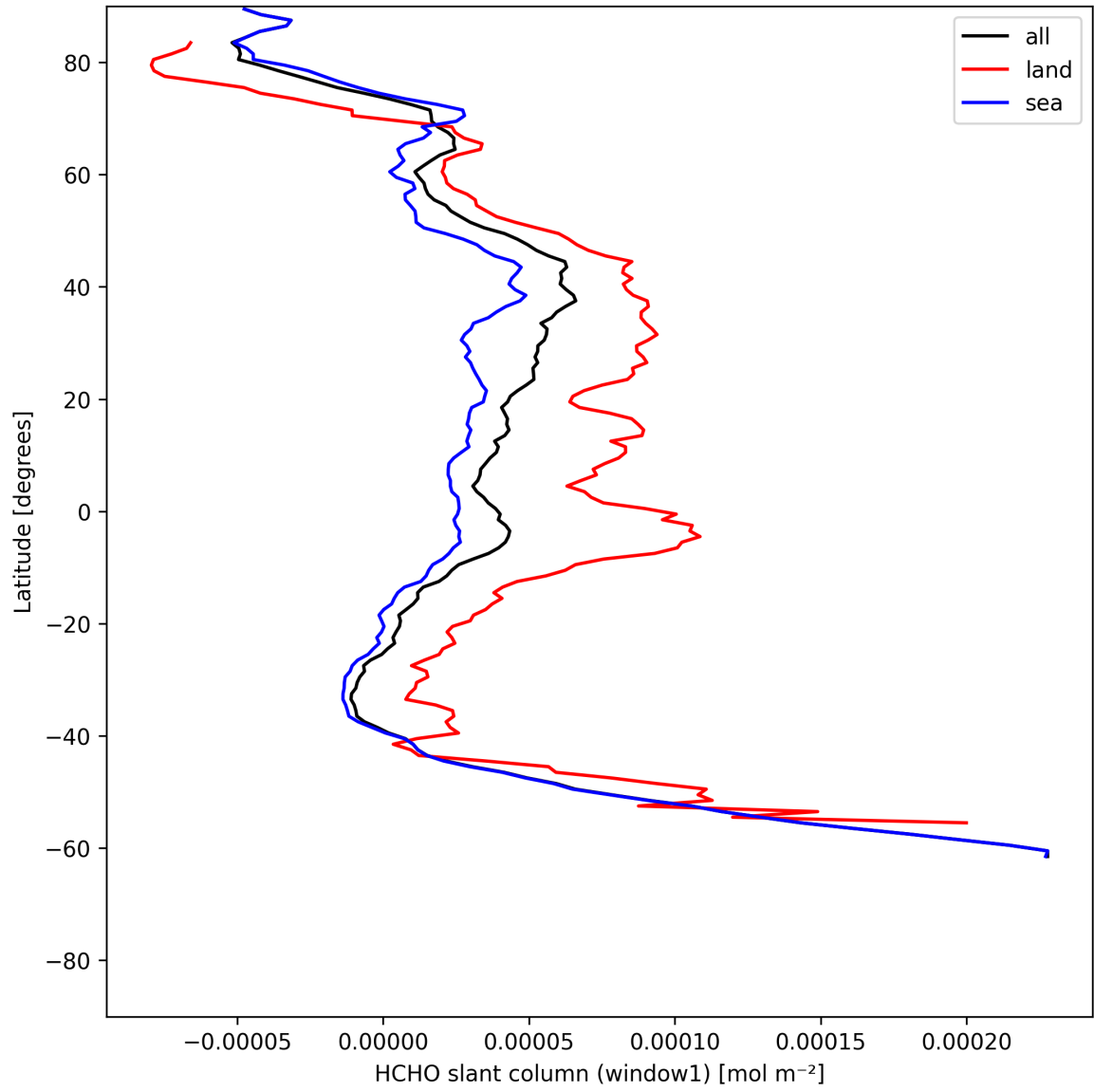
Figure 24: Zonal average of “HCHO slant column (window1)” for 2025-07-03 to 2025-07-05.
