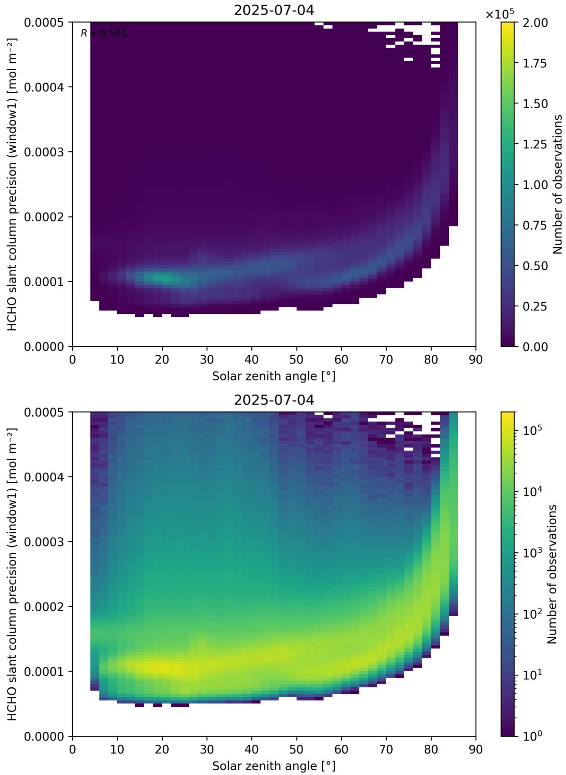
Figure 174: Scatter density plot of “Solar zenith angle” against “HCHO slant column precision (window1)” for 2025-07-03 to 2025-07-05.
