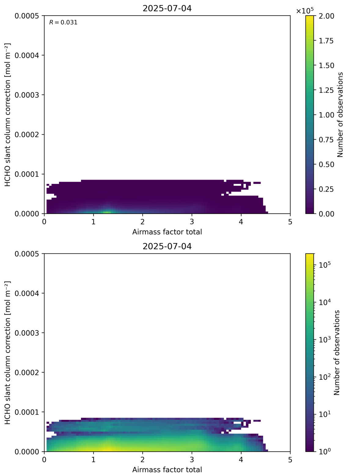
Figure 102: Scatter density plot of “Airmass factor total” against “HCHO slant column correction” for 2025-07-03 to 2025-07-05.
