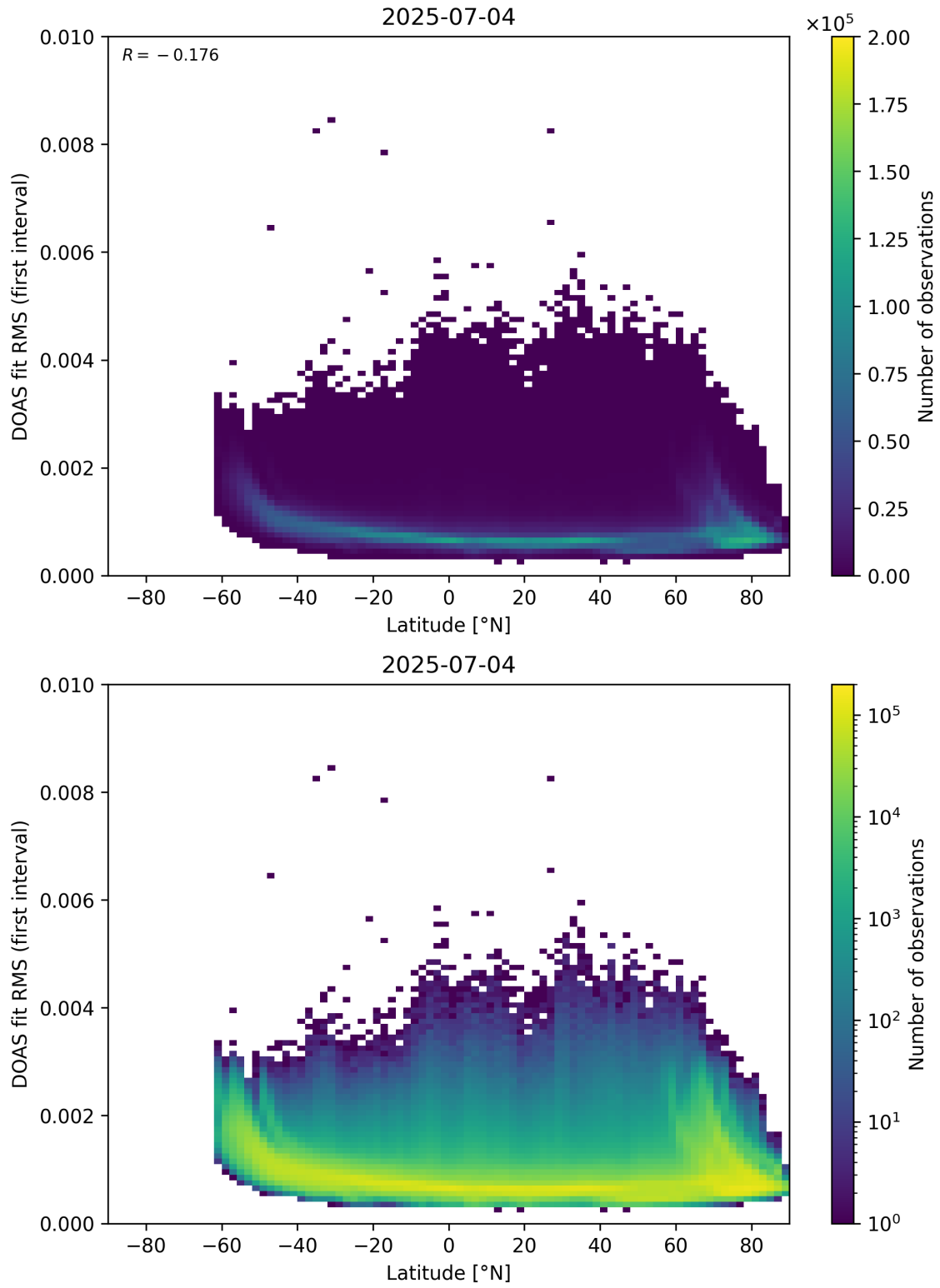
Figure 153: Scatter density plot of “Latitude” against “DOAS fit RMS (first interval)” for 2025-07-03 to 2025-07-05.
