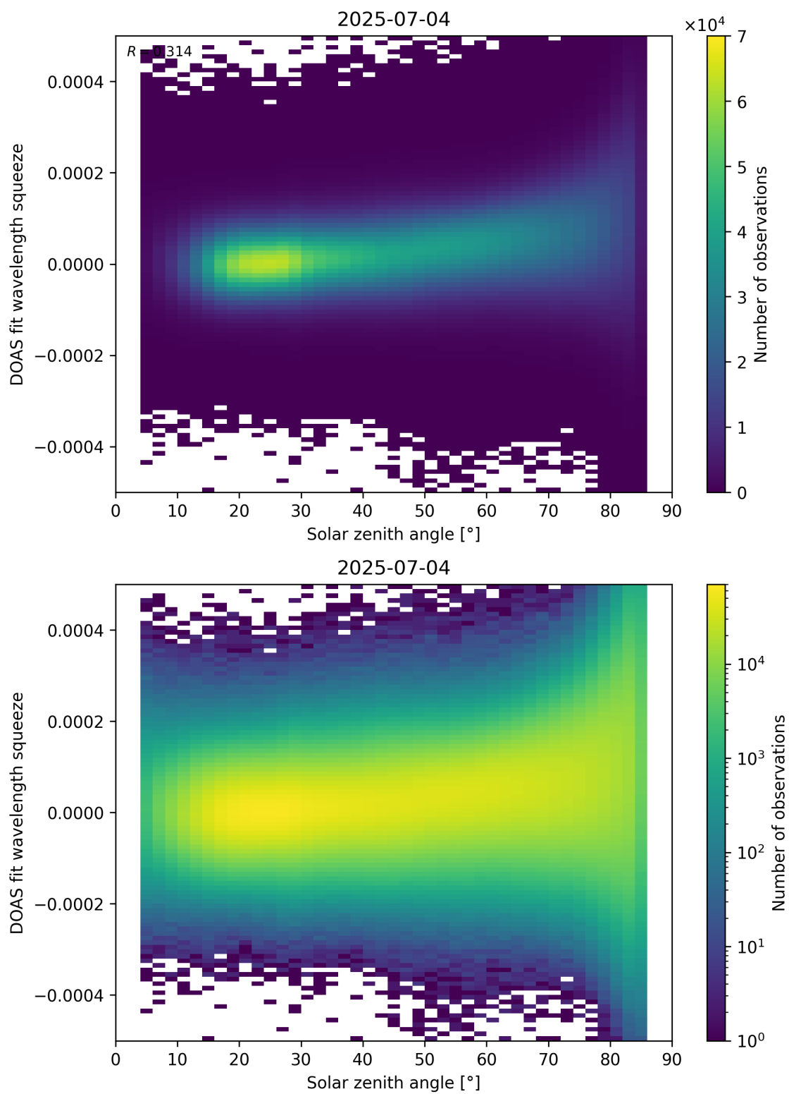
Figure 169: Scatter density plot of “Solar zenith angle” against “DOAS fit wavelength squeeze” for 2025-07-03 to 2025-07-05.
