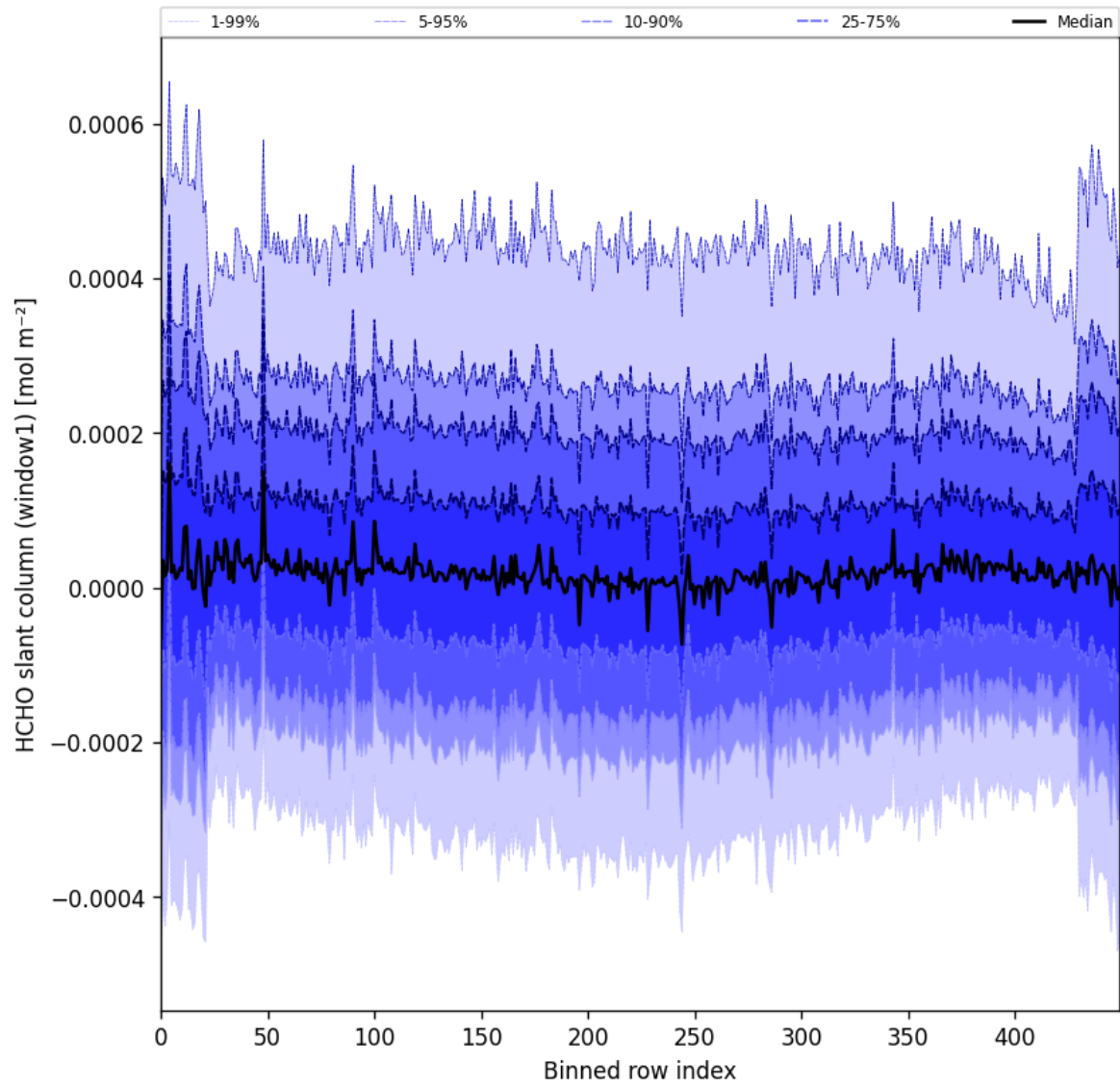
Figure 52: Along track statistics of “HCHO slant column (window1)” for 2025-07-03 to 2025-07-05
