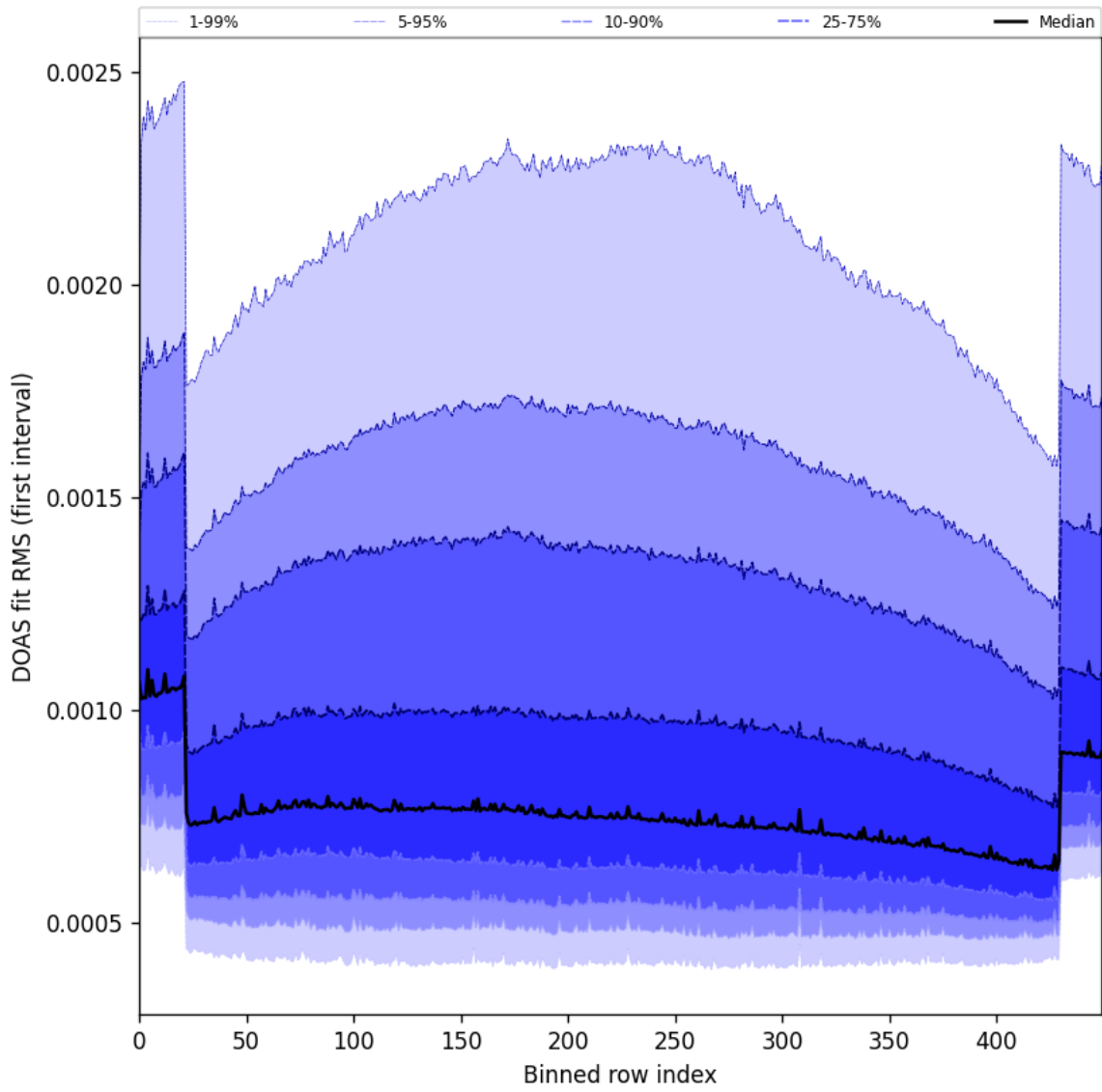
Figure 60: Along track statistics of “DOAS fit RMS (first interval)” for 2025-07-03 to 2025-07-05
