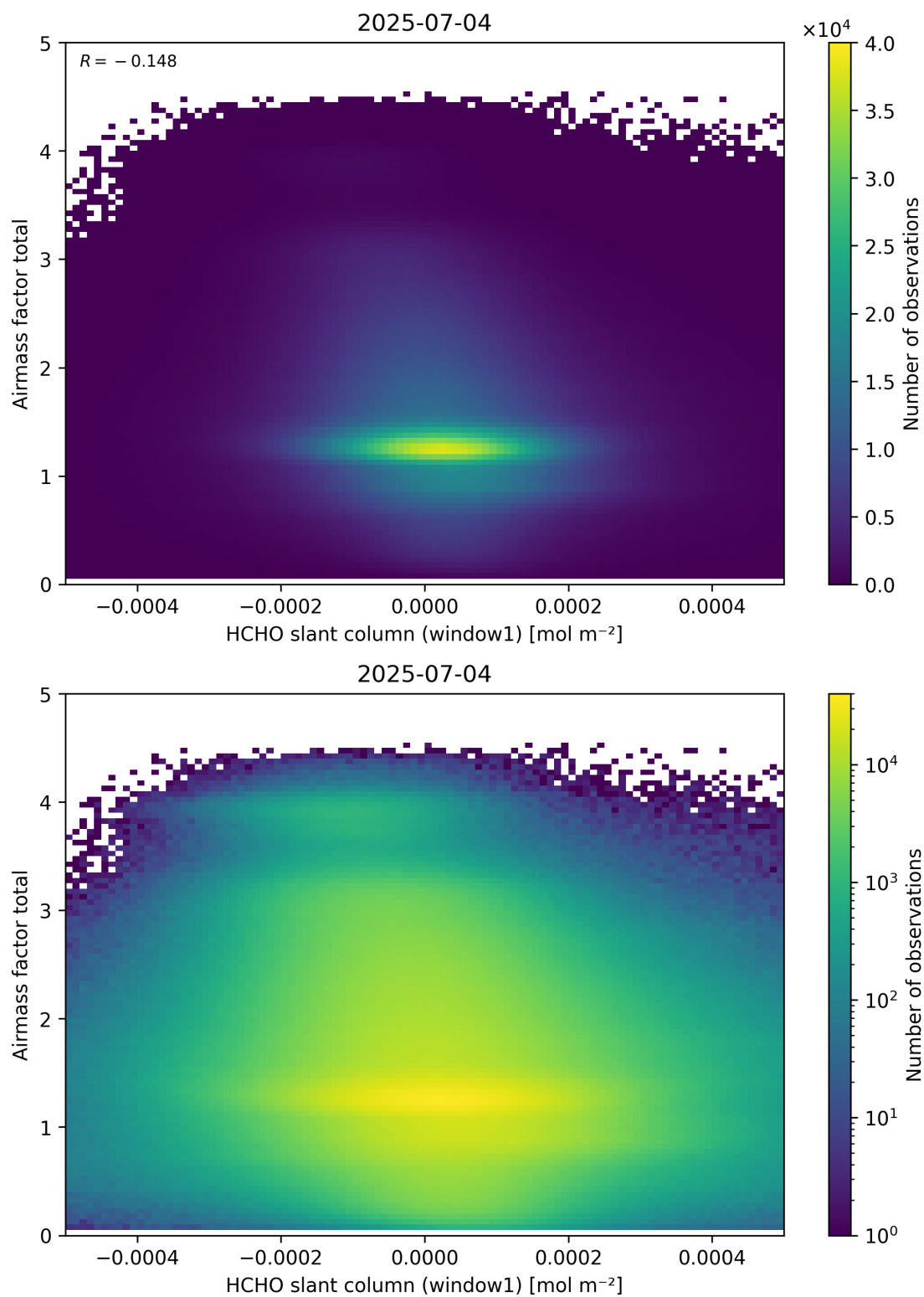
Figure 85: Scatter density plot of “HCHO slant column (window1)” against “Airmass factor total” for 2025-07-03 to 2025-07-05.
