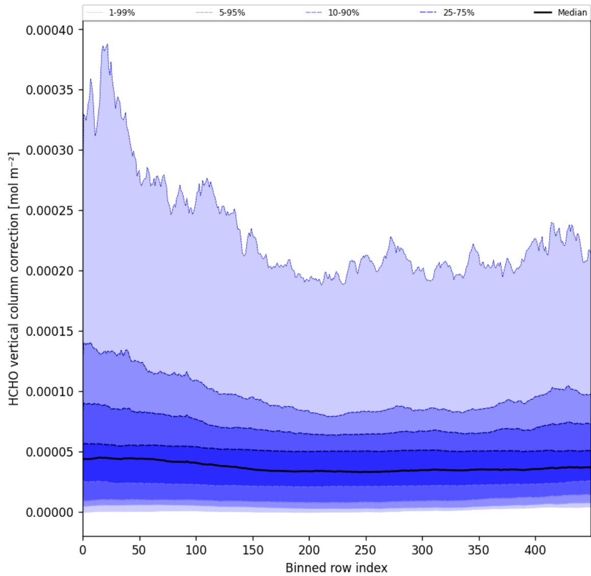
Figure 51: Along track statistics of “HCHO vertical column correction” for 2025-07-03 to 2025-07-05
