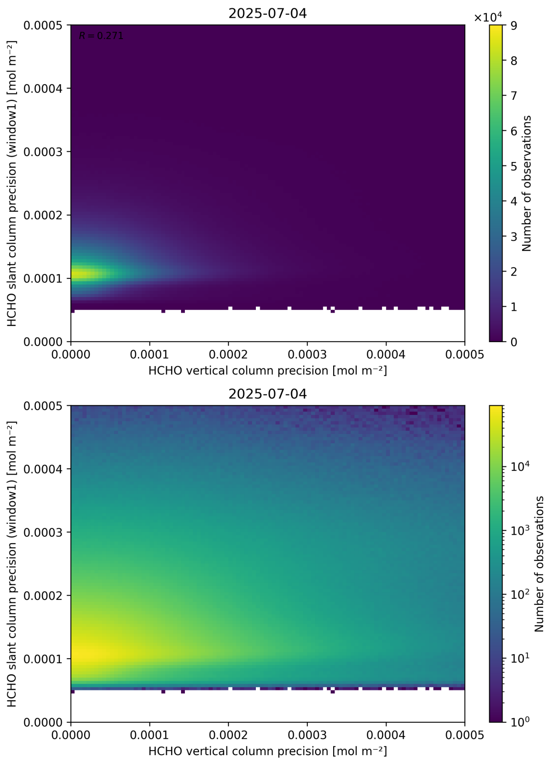
Figure 143: Scatter density plot of “HCHO vertical column precision” against “HCHO slant column precision (window1)” for 2025-07-03 to 2025-07-05.
