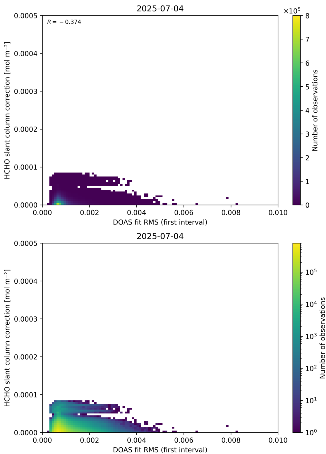
Figure 63: Scatter density plot of “DOAS fit RMS (first interval)” against “HCHO slant column correction” for 2025-07-03 to 2025-07-05.
