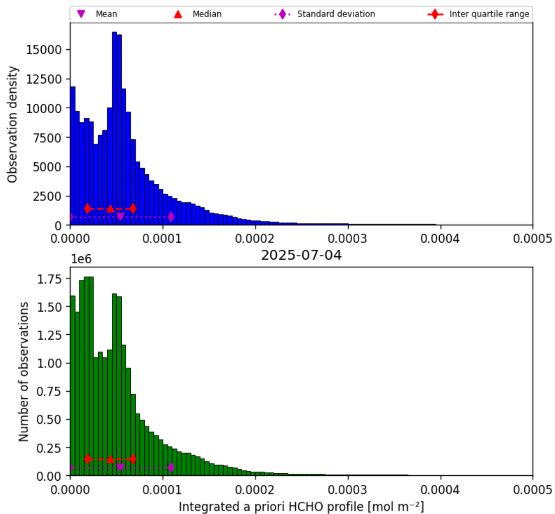
Figure 43: Histogram of “Integrated a priori HCHO profile” for 2025-07-03 to 2025-07-05
