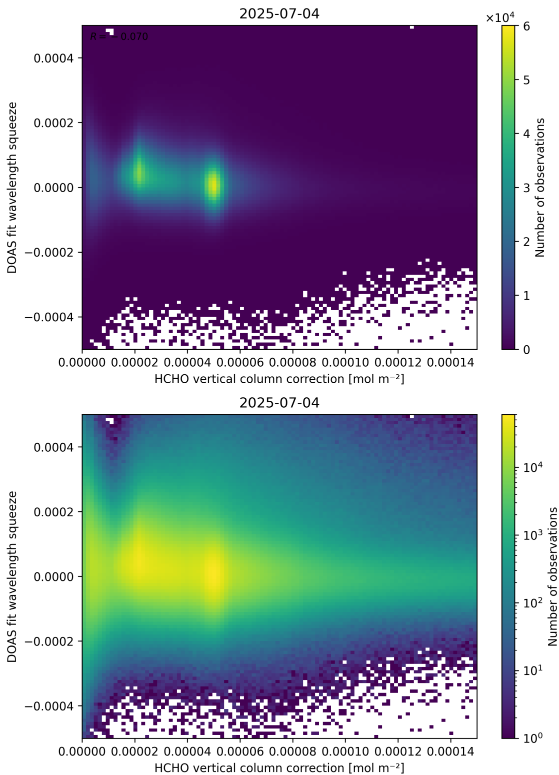
Figure 114: Scatter density plot of “HCHO vertical column correction” against “DOAS fit wavelength squeeze” for 2025-07-03 to 2025-07-05.
