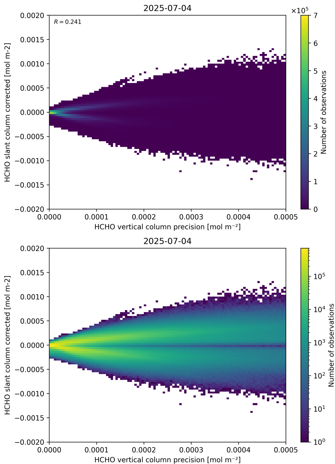
Figure 140: Scatter density plot of “HCHO vertical column precision” against “HCHO slant column corrected” for 2025-07-03 to 2025-07-05.
