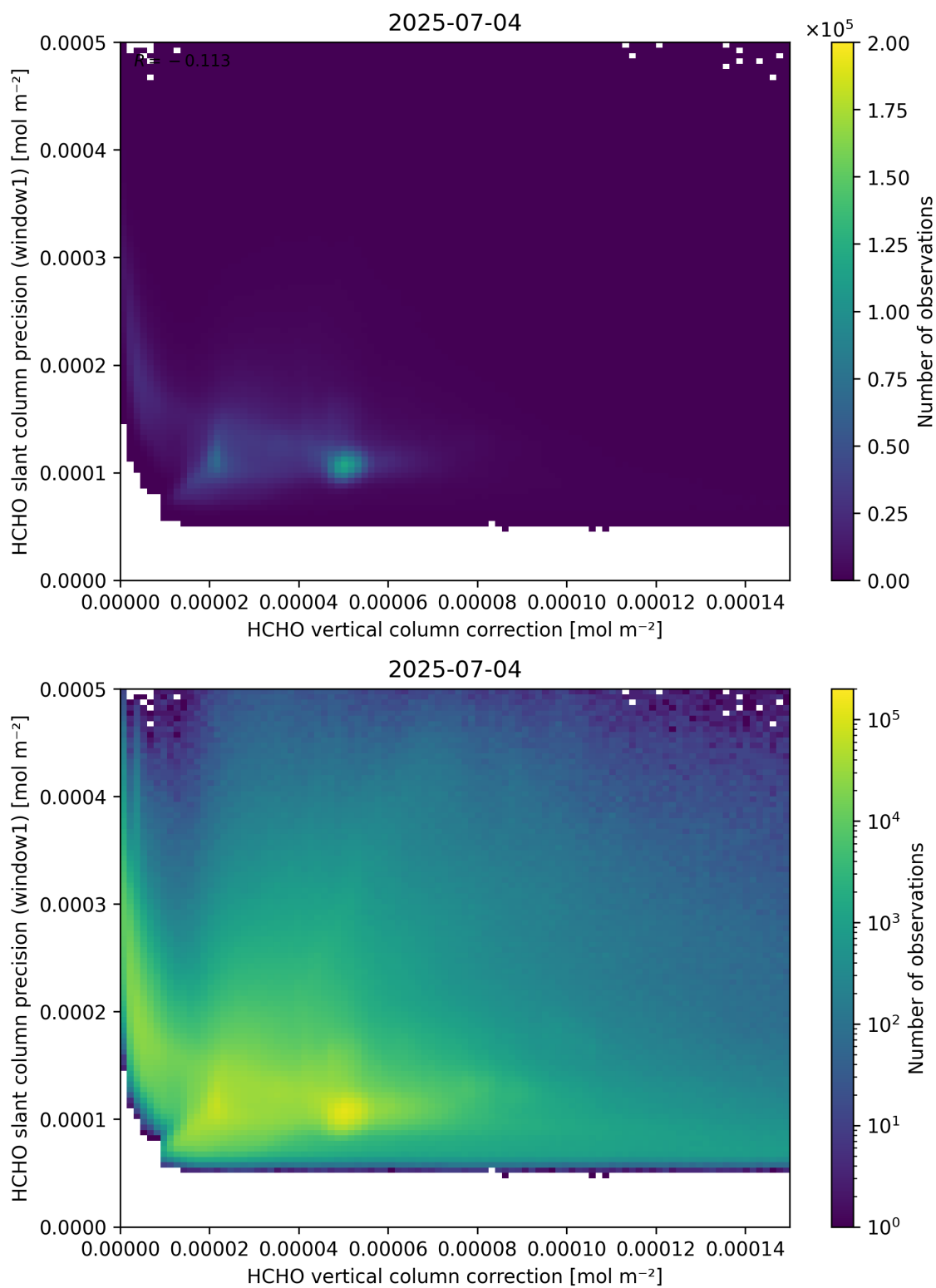
Figure 119: Scatter density plot of “HCHO vertical column correction” against “HCHO slant column precision (window1)” for 2025-07-03 to 2025-07-05.
