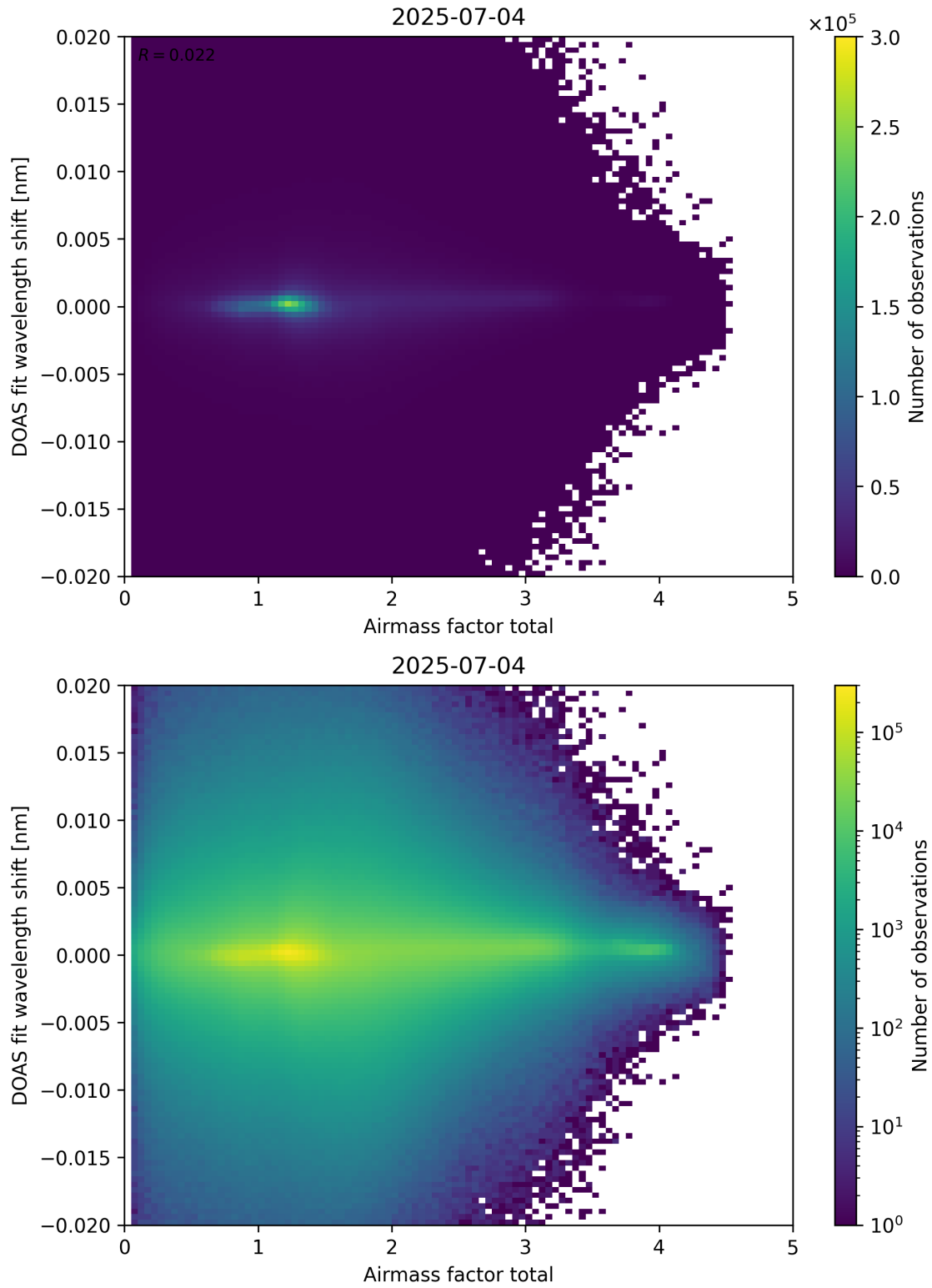
Figure 98: Scatter density plot of “Airmass factor total” against “DOAS fit wavelength shift” for 2025-07-03 to 2025-07-05.
