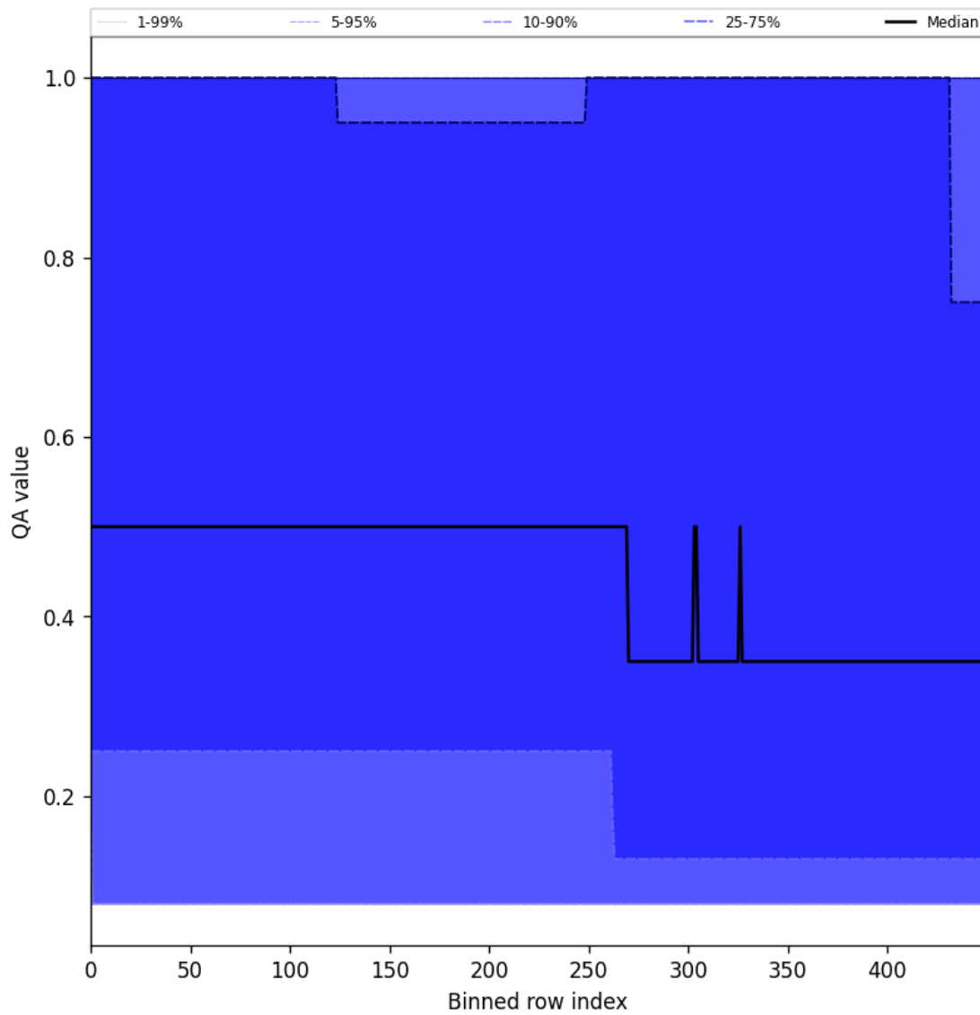
Figure 48: Along track statistics of "QA value" for 2025-07-03 to 2025-07-05
