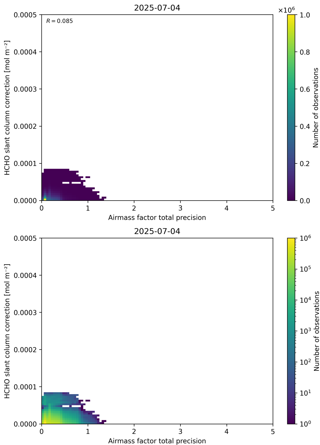
Figure 110: Scatter density plot of “Airmass factor total precision” against “HCHO slant column correction” for 2025-07-03 to 2025-07-05.
