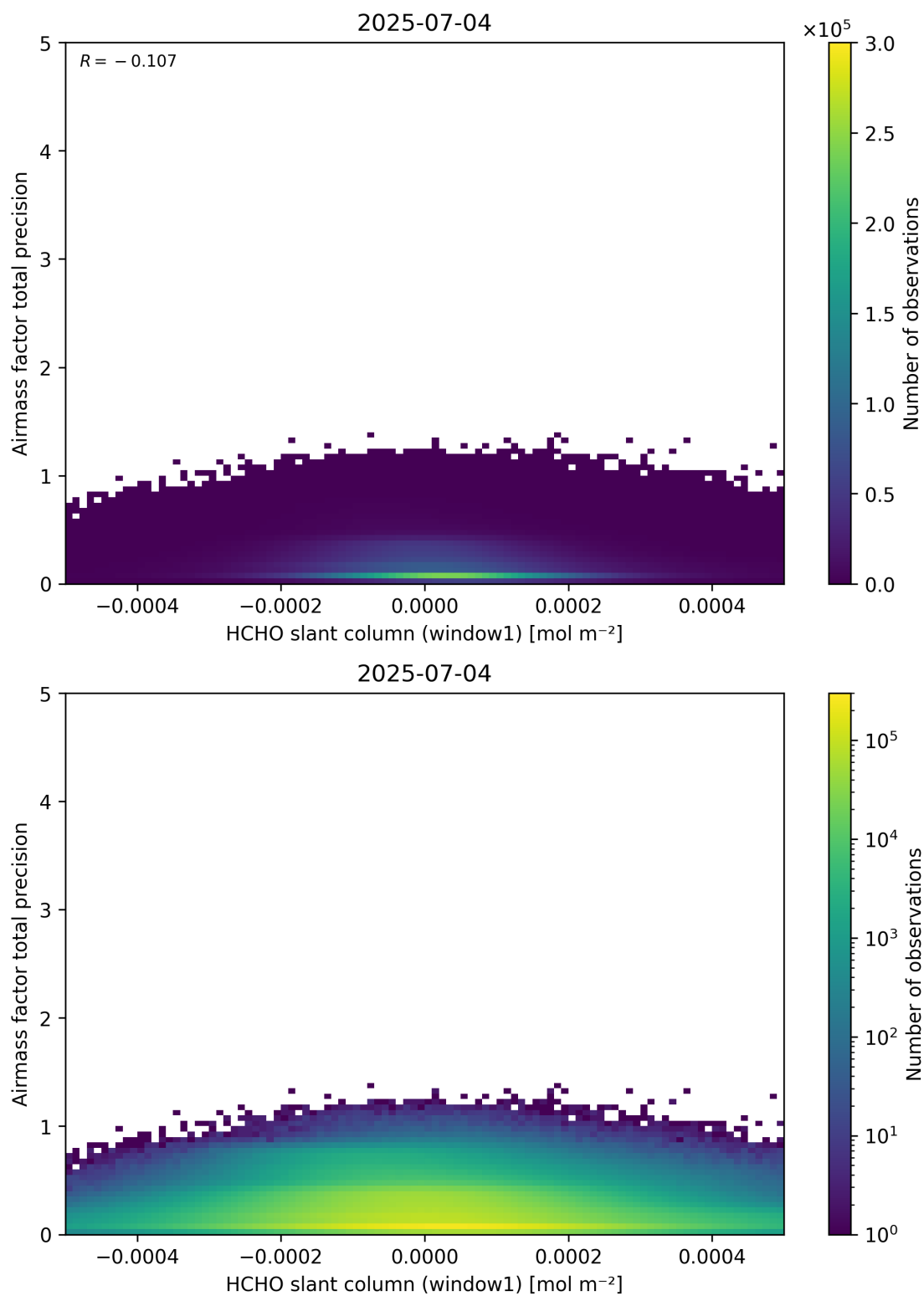
Figure 86: Scatter density plot of “HCHO slant column (window1)” against “Airmass factor total precision” for 2025-07-03 to 2025-07-05.
