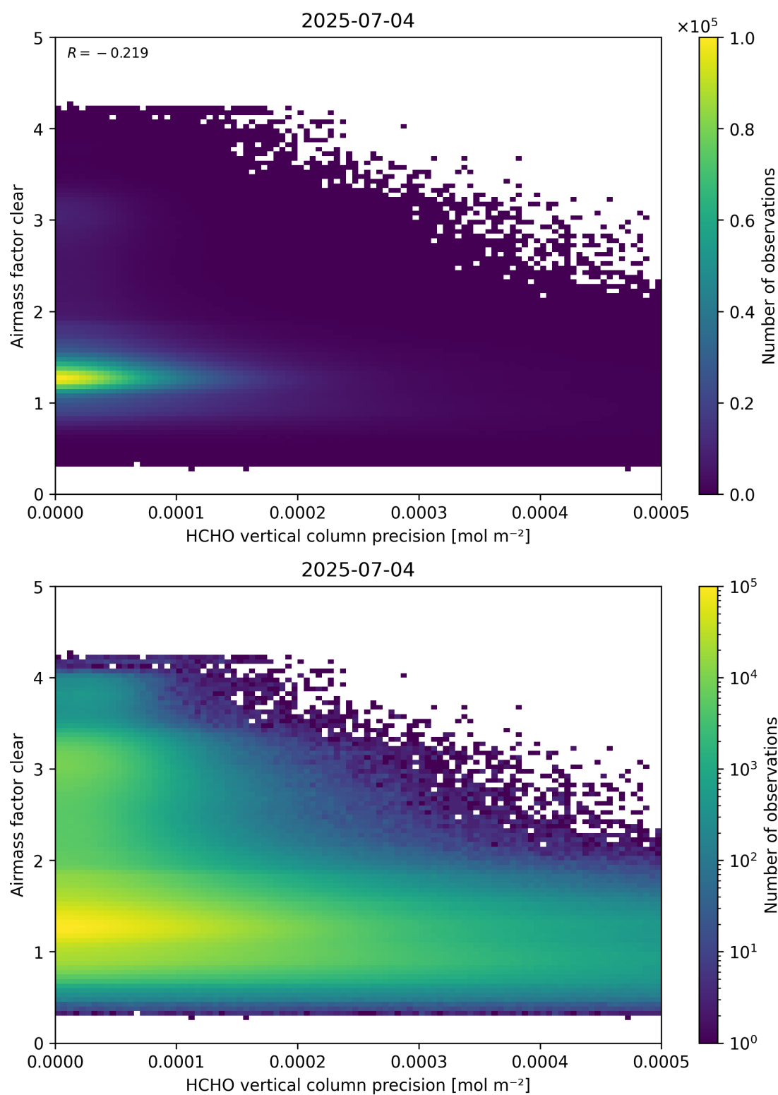
Figure 139: Scatter density plot of “HCHO vertical column precision” against “Airmass factor clear” for 2025-07-03 to 2025-07-05.
