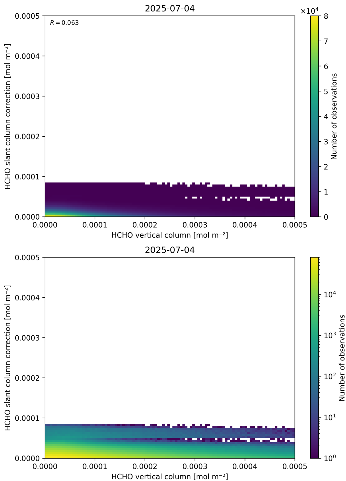
Figure 128: Scatter density plot of “HCHO vertical column” against “HCHO slant column correction” for 2025-07-03 to 2025-07-05.
