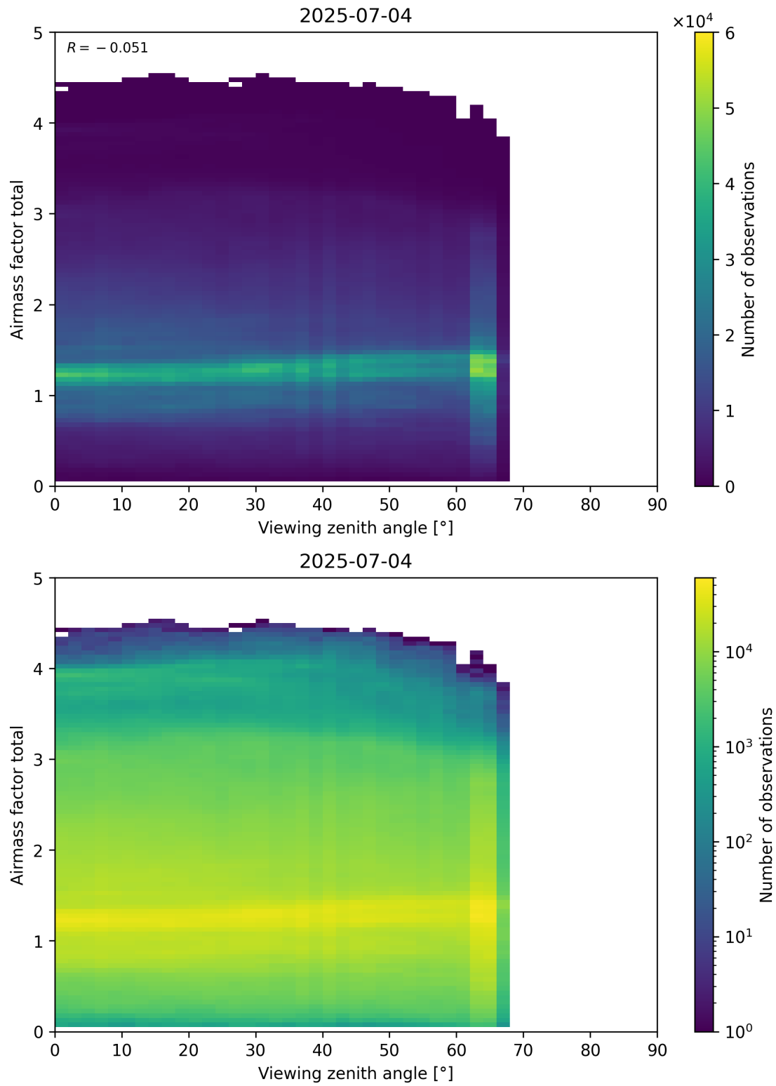
Figure 190: Scatter density plot of “Viewing zenith angle” against “Airmass factor total” for 2025-07-03 to 2025-07-05.
