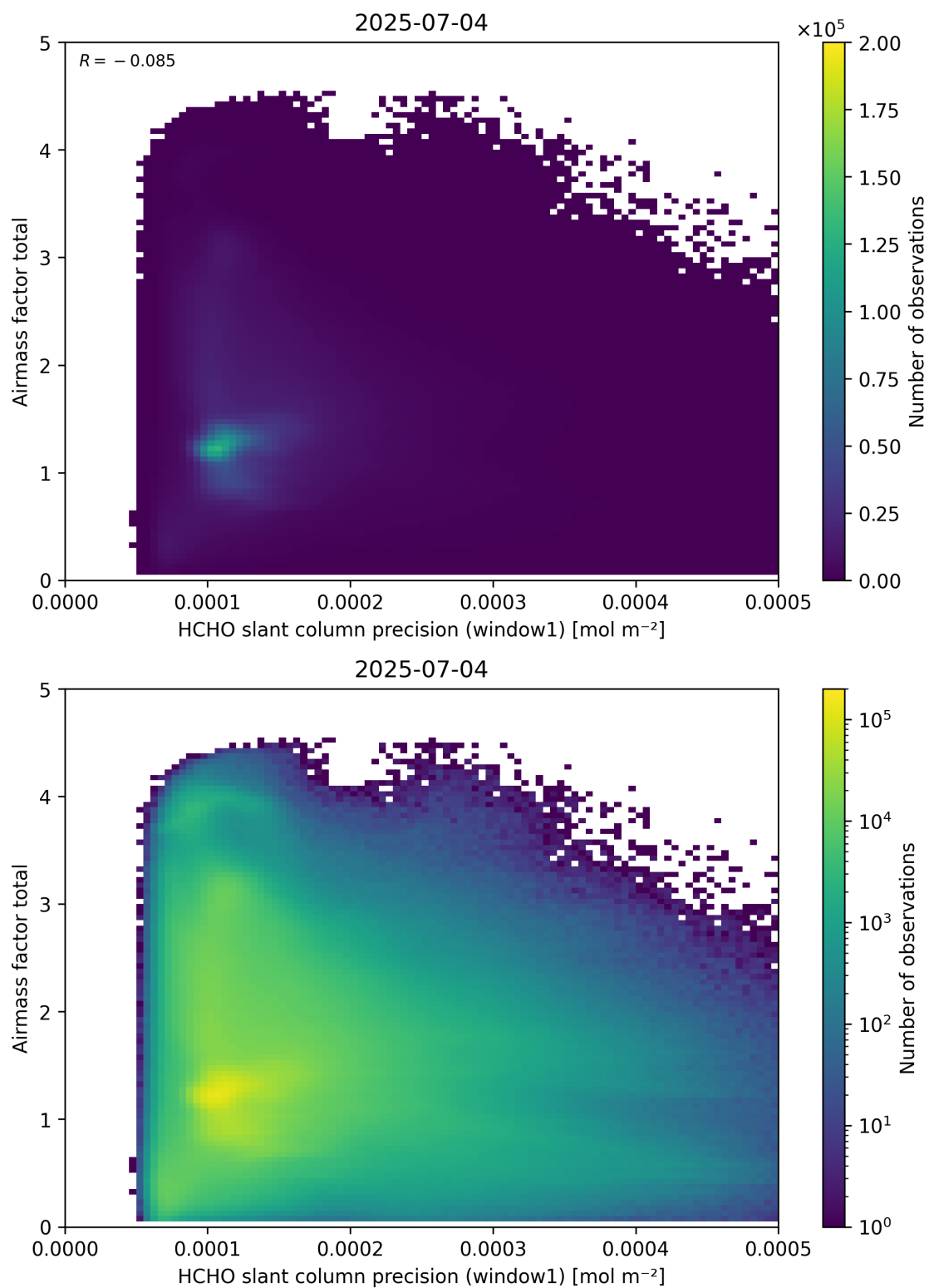
Figure 94: Scatter density plot of “HCHO slant column precision (window1)” against “Airmass factor total” for 2025-07-03 to 2025-07-05.
