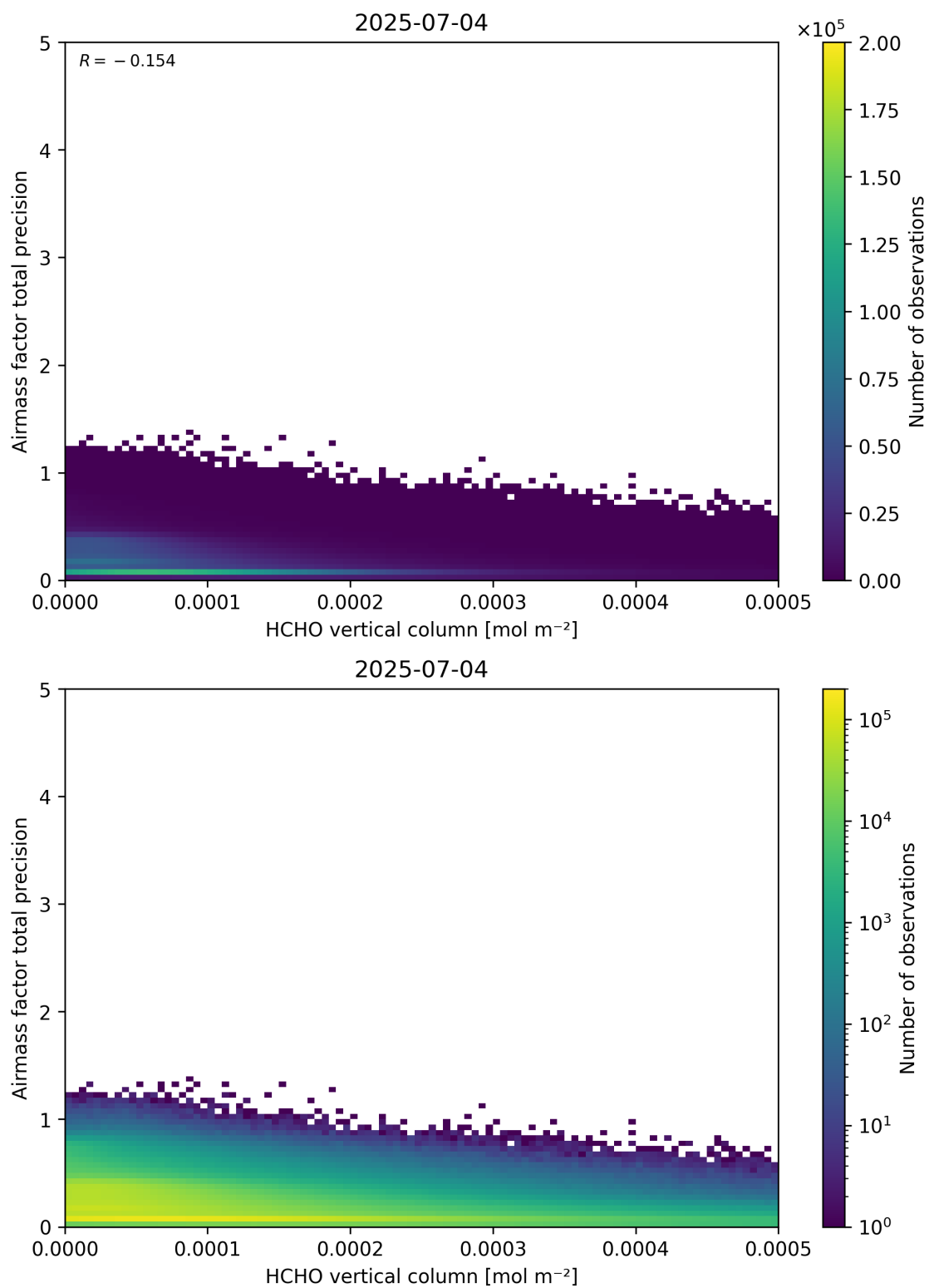
Figure 132: Scatter density plot of “HCHO vertical column” against “Airmass factor total precision” for 2025-07-03 to 2025-07-05.
