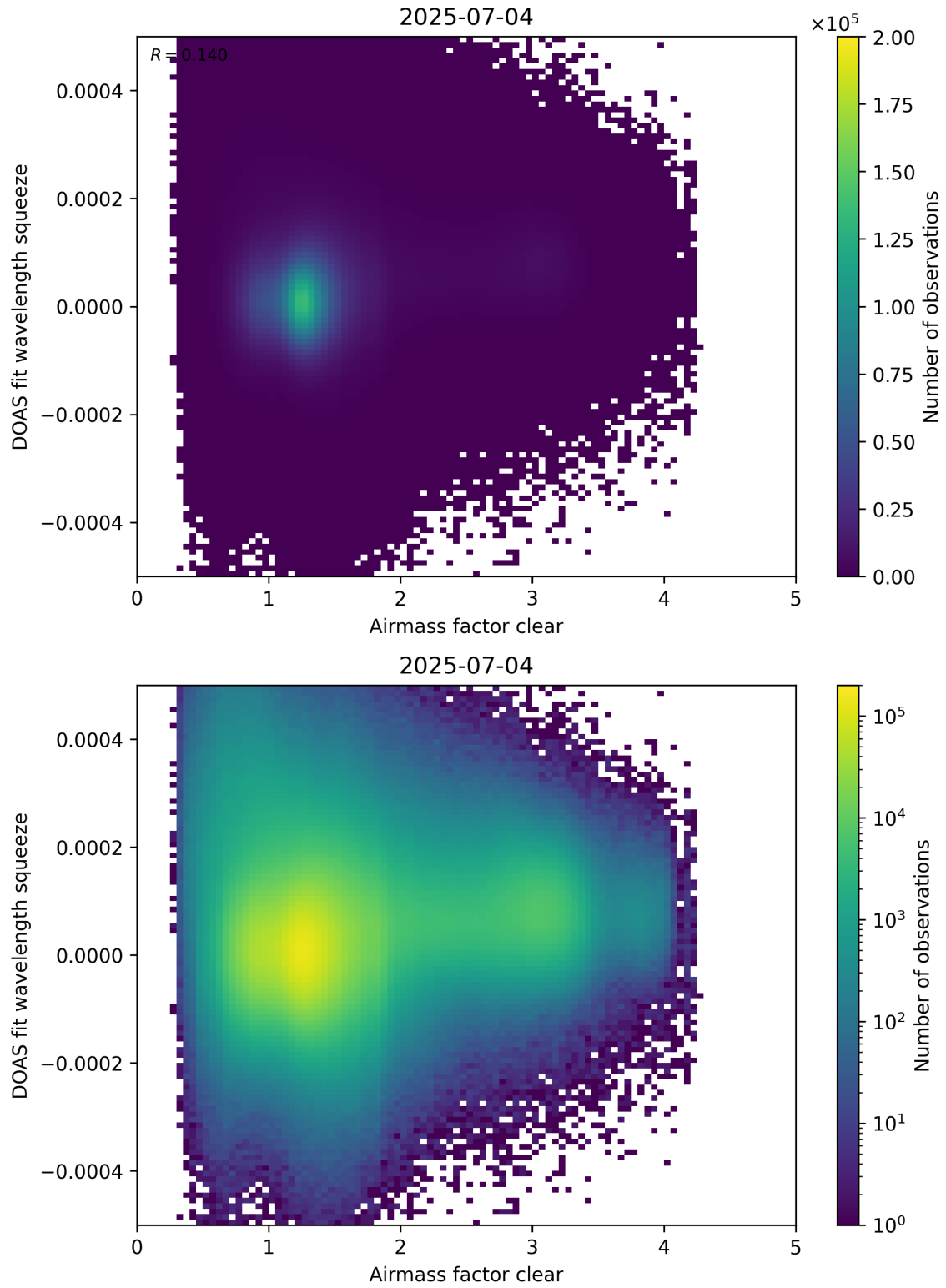
Figure 73: Scatter density plot of “Airmass factor clear” against “DOAS fit wavelength squeeze” for 2025-07-03 to 2025-07-05.
