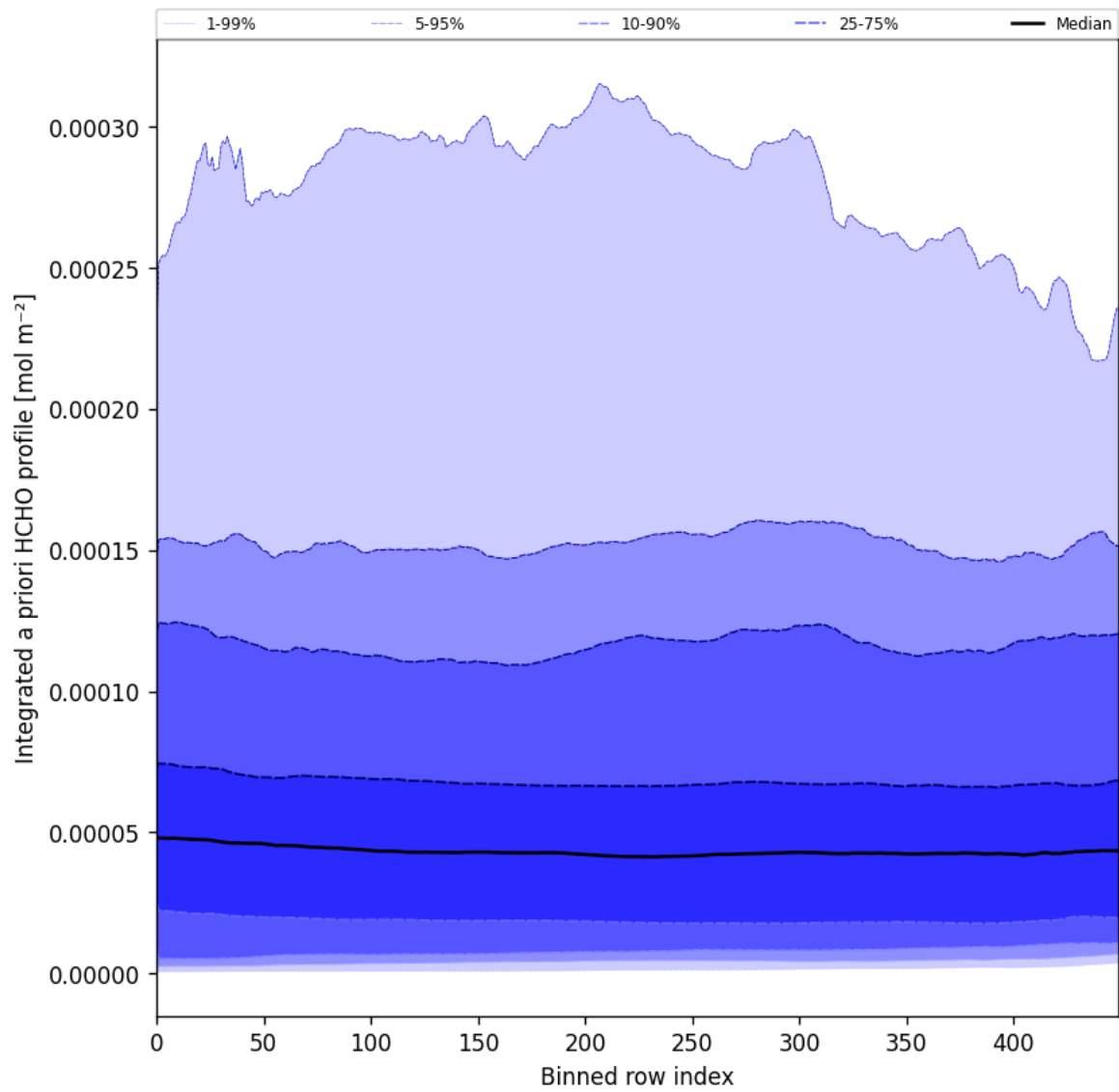
Figure 57: Along track statistics of “Integrated a priori HCHO profile” for 2025-07-03 to 2025-07-05
