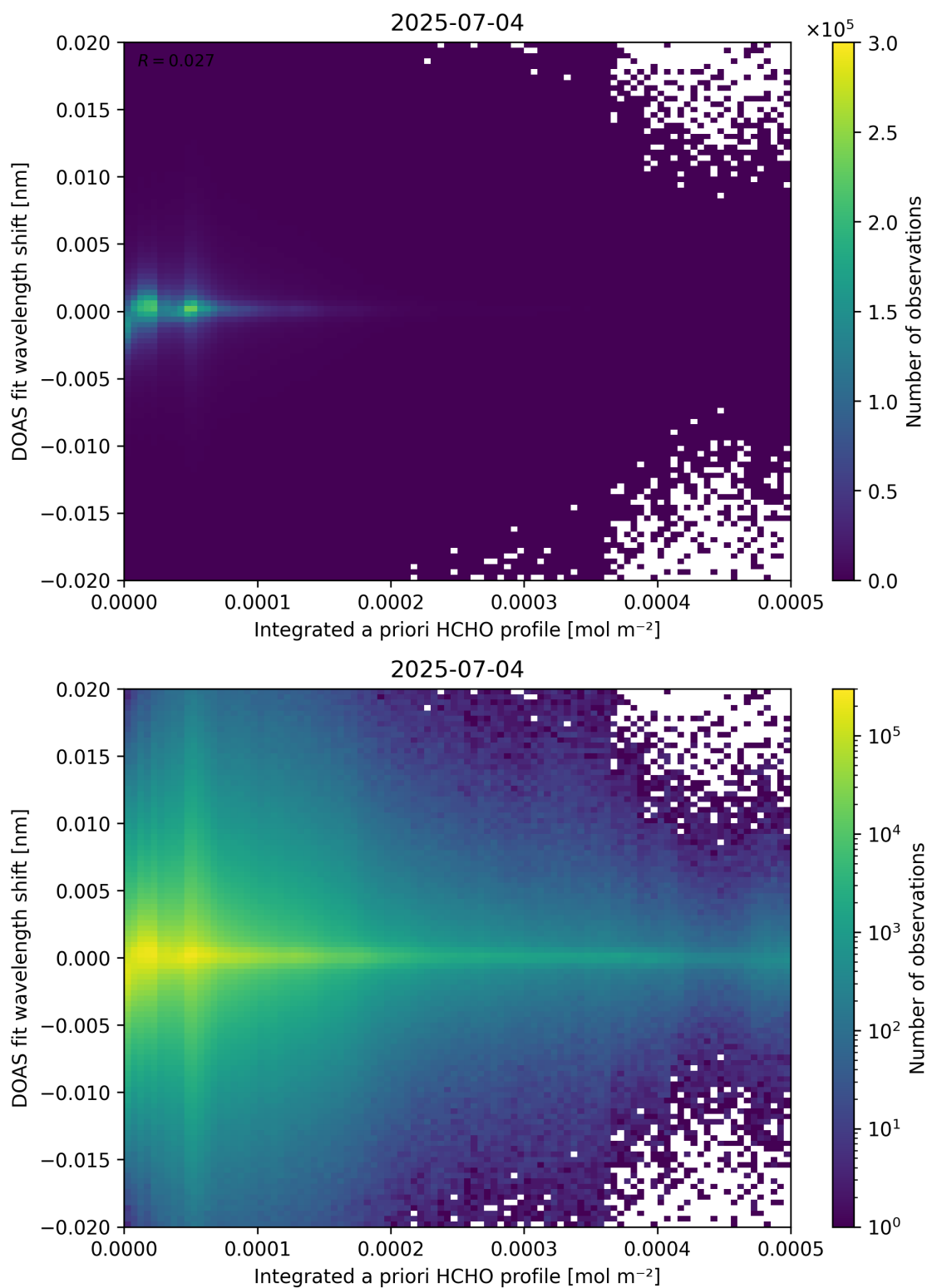
Figure 149: Scatter density plot of “Integrated a priori HCHO profile” against “DOAS fit wavelength shift” for 2025-07-03 to 2025-07-05.
