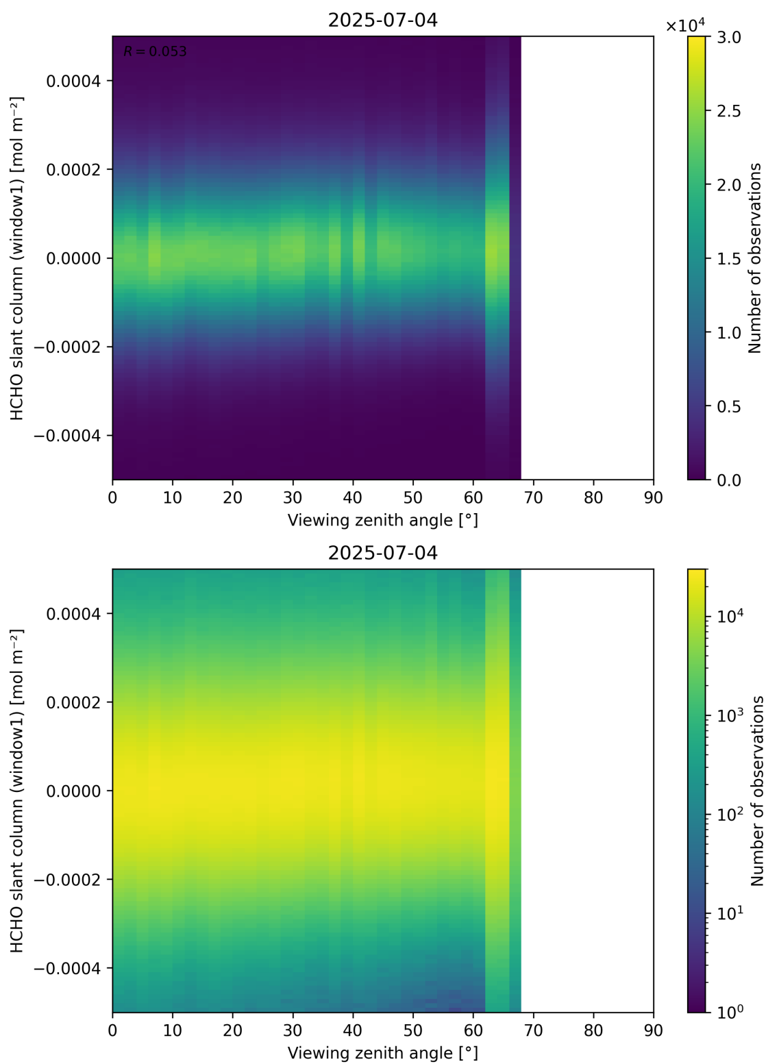
Figure 188: Scatter density plot of “Viewing zenith angle” against “HCHO slant column (window1)” for 2025-07-03 to 2025-07-05.
