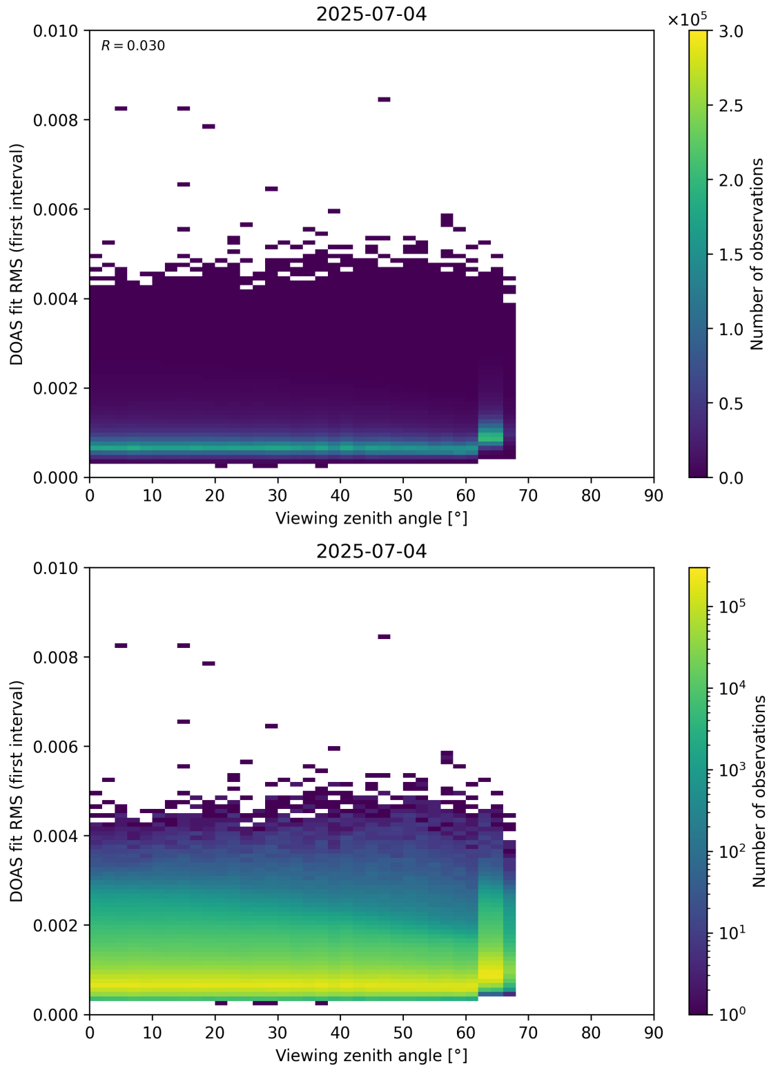
Figure 182: Scatter density plot of “Viewing zenith angle” against “DOAS fit RMS (first interval)” for 2025-07-03 to 2025-07-05.
