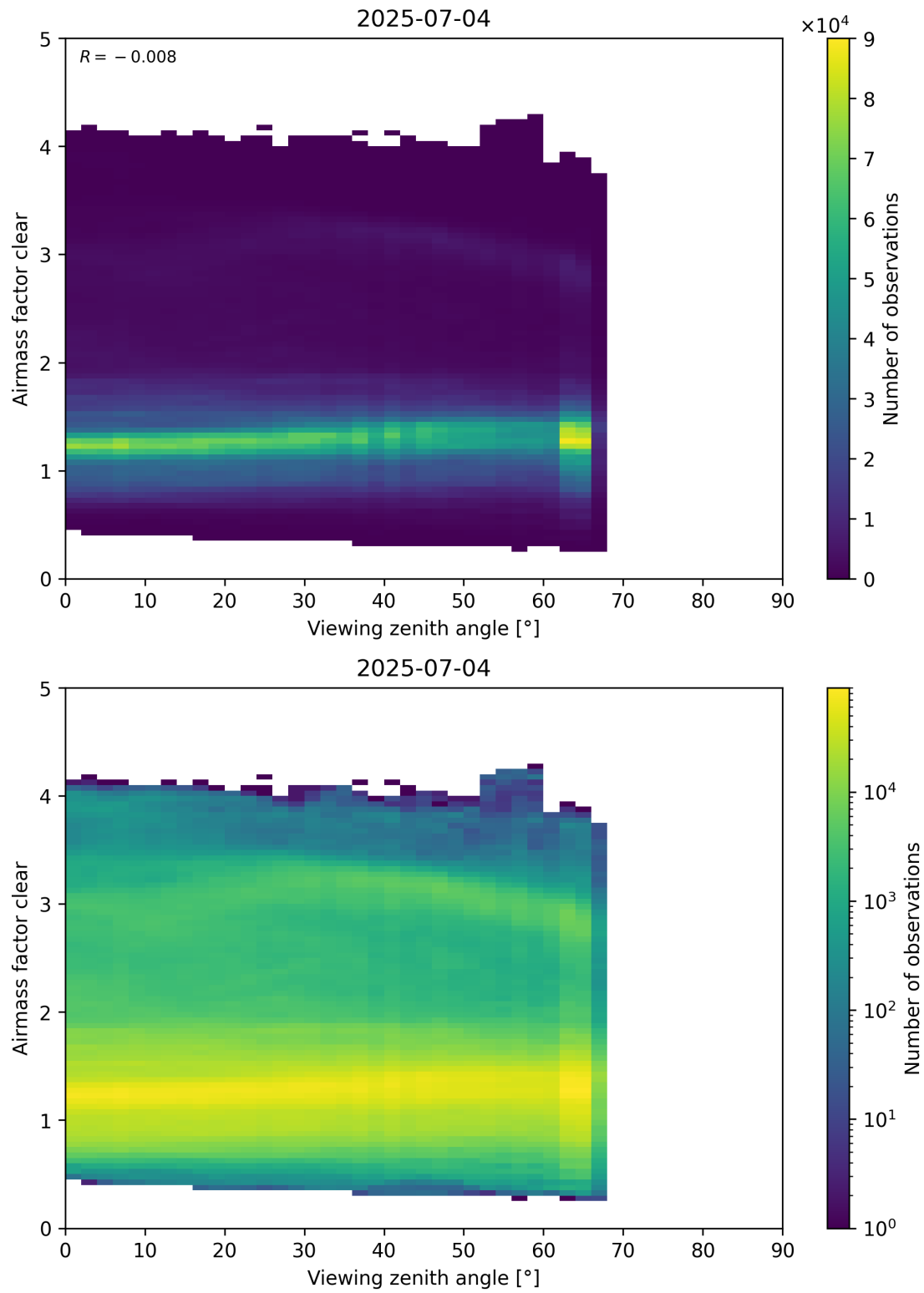
Figure 185: Scatter density plot of “Viewing zenith angle” against “Airmass factor clear” for 2025-07-03 to 2025-07-05.
