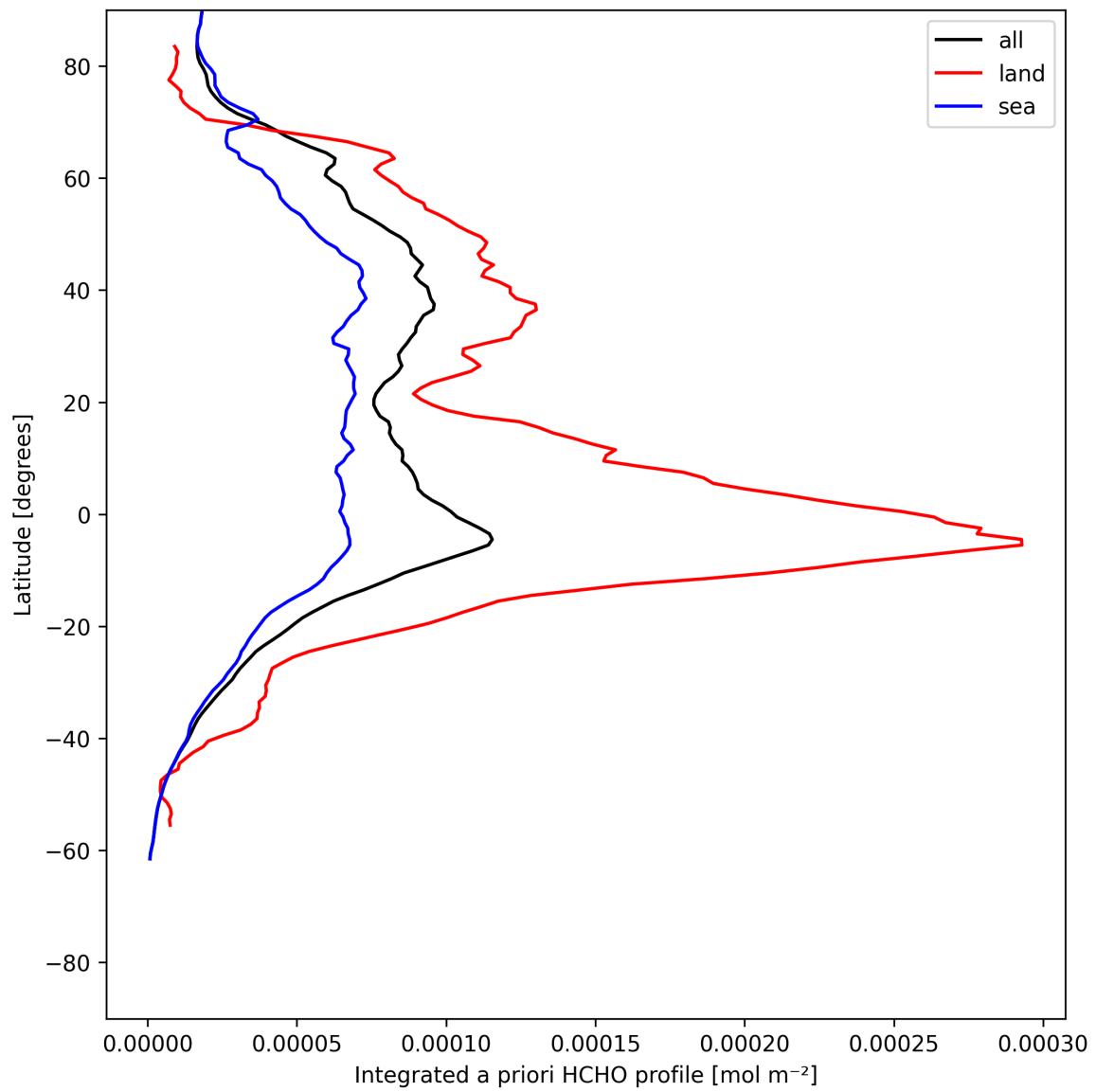
Figure 29: Zonal average of “Integrated a priori HCHO profile” for 2025-07-03 to 2025-07-05.
