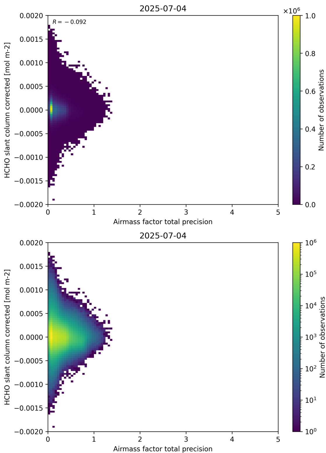
Figure 109: Scatter density plot of “Airmass factor total precision” against “HCHO slant column corrected” for 2025-07-03 to 2025-07-05.
