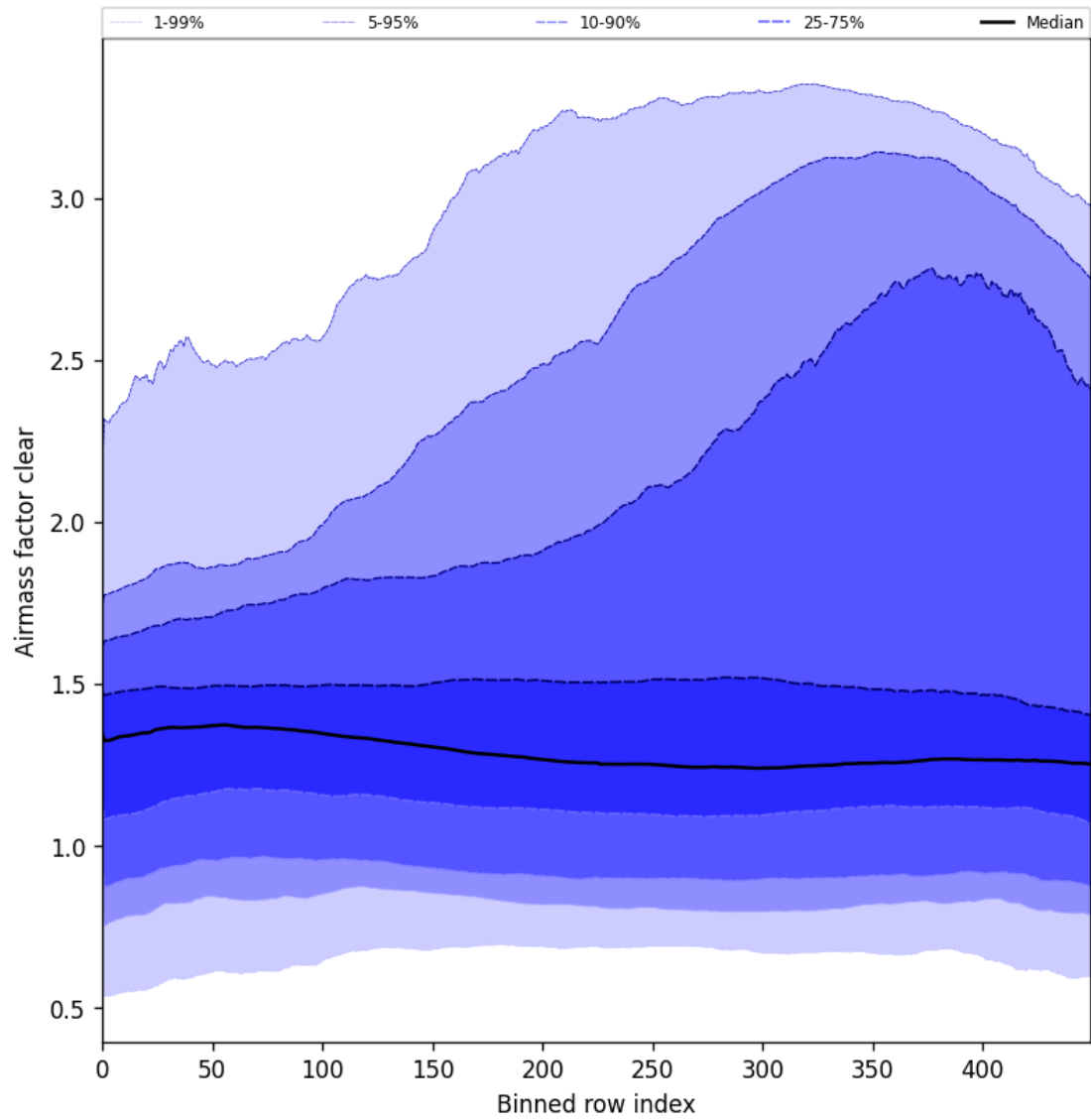
Figure 56: Along track statistics of “Airmass factor clear” for 2025-07-03 to 2025-07-05
