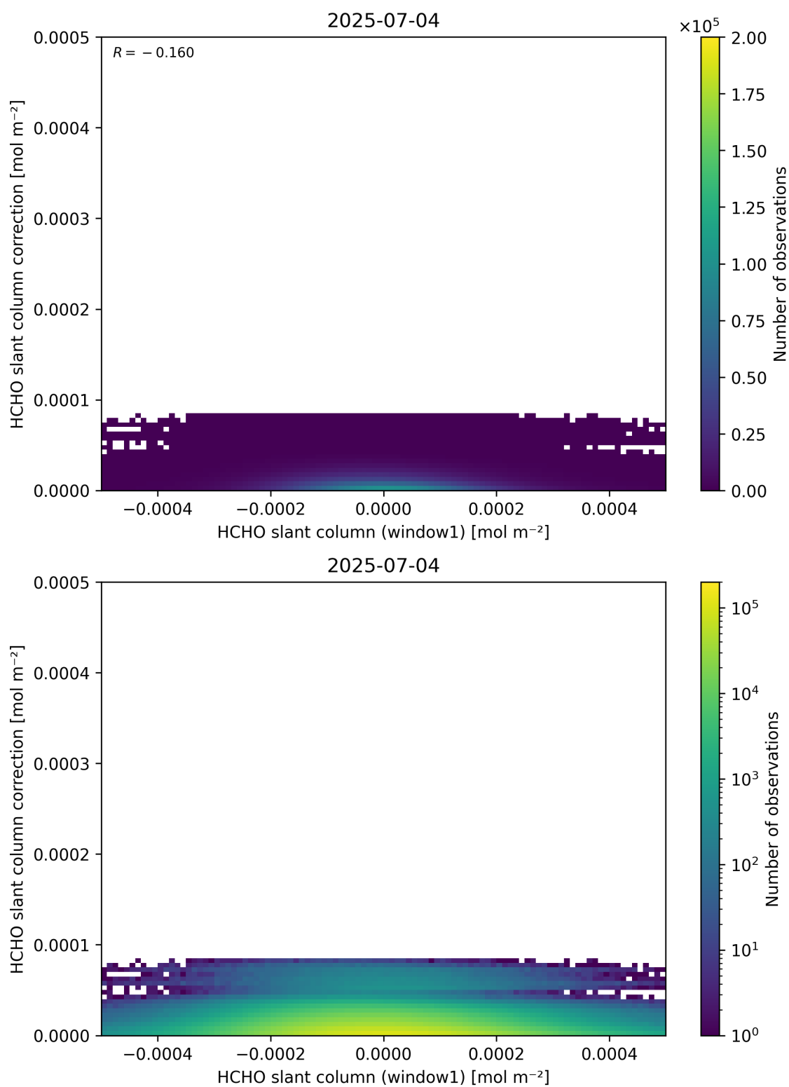
Figure 83: Scatter density plot of “HCHO slant column (window1)” against “HCHO slant column correction” for 2025-07-03 to 2025-07-05.
