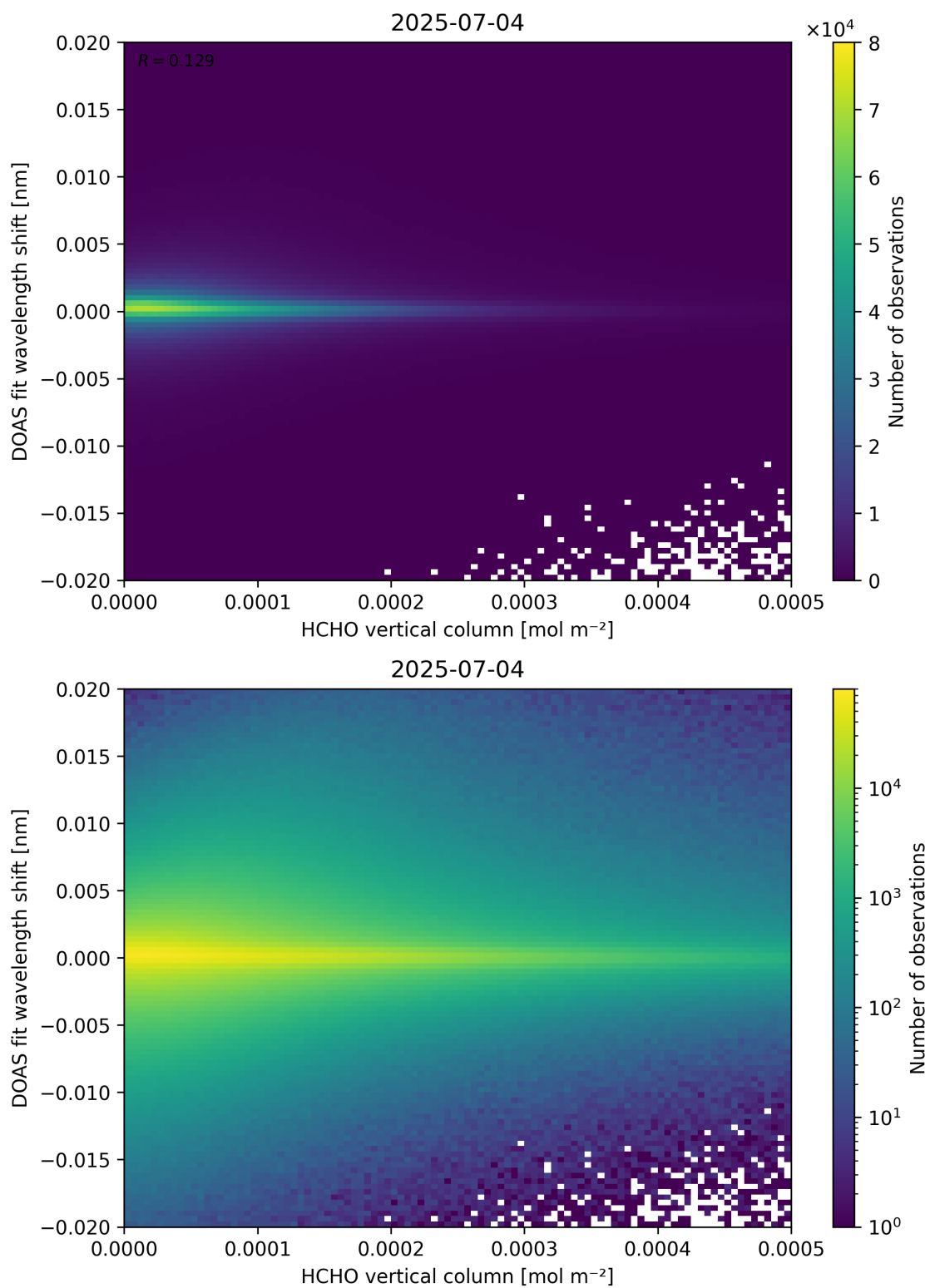
Figure 124: Scatter density plot of “HCHO vertical column” against “DOAS fit wavelength shift” for 2025-07-03 to 2025-07-05.
