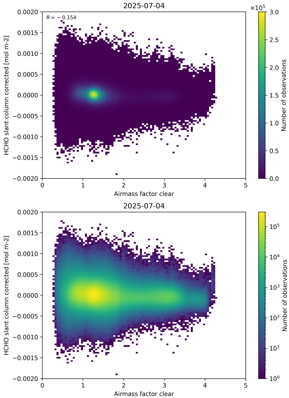
Figure 74: Scatter density plot of “Airmass factor clear” against “HCHO slant column corrected” for 2025-07-03 to 2025-07-05.
