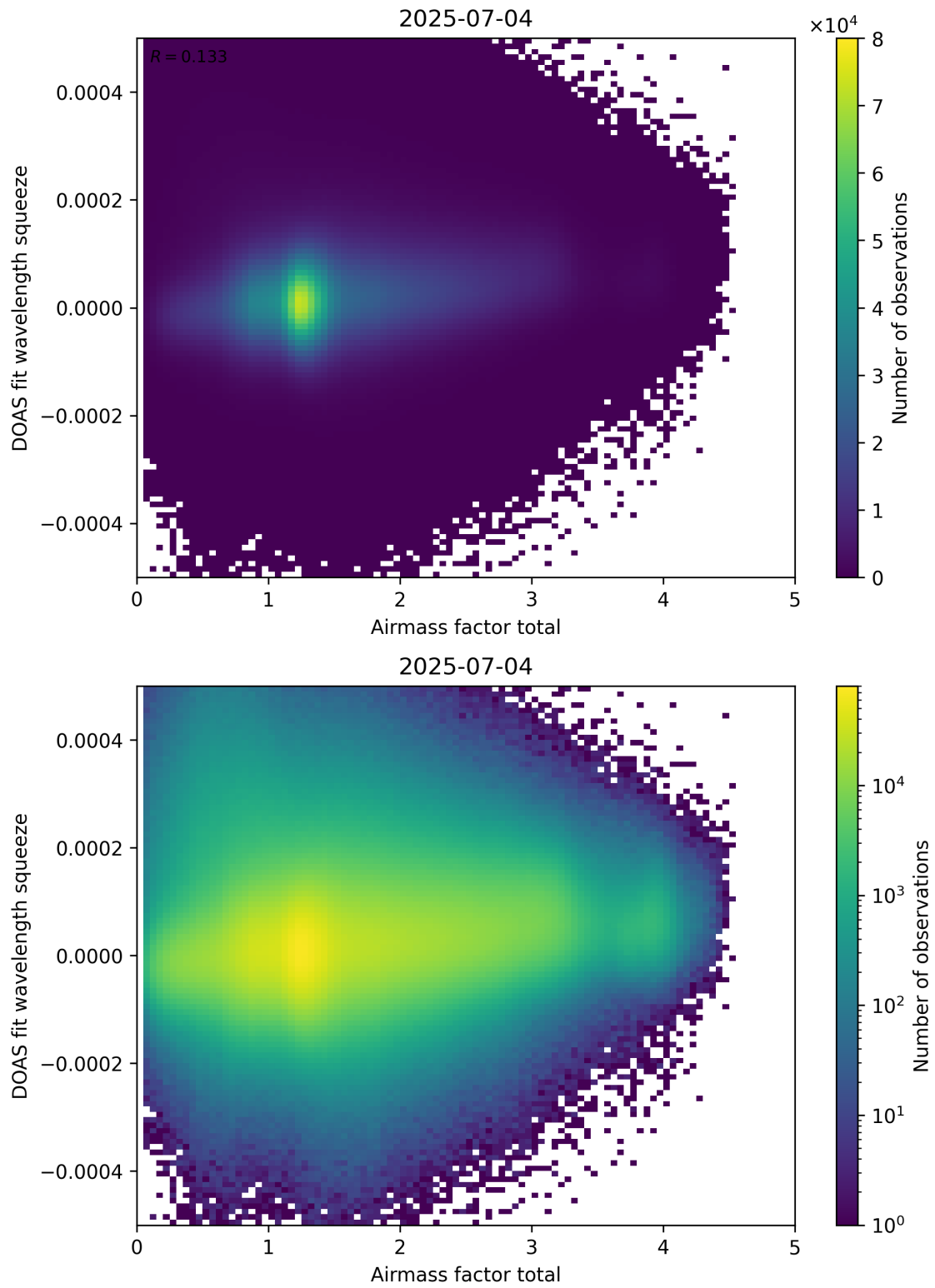
Figure 99: Scatter density plot of “Airmass factor total” against “DOAS fit wavelength squeeze” for 2025-07-03 to 2025-07-05.
