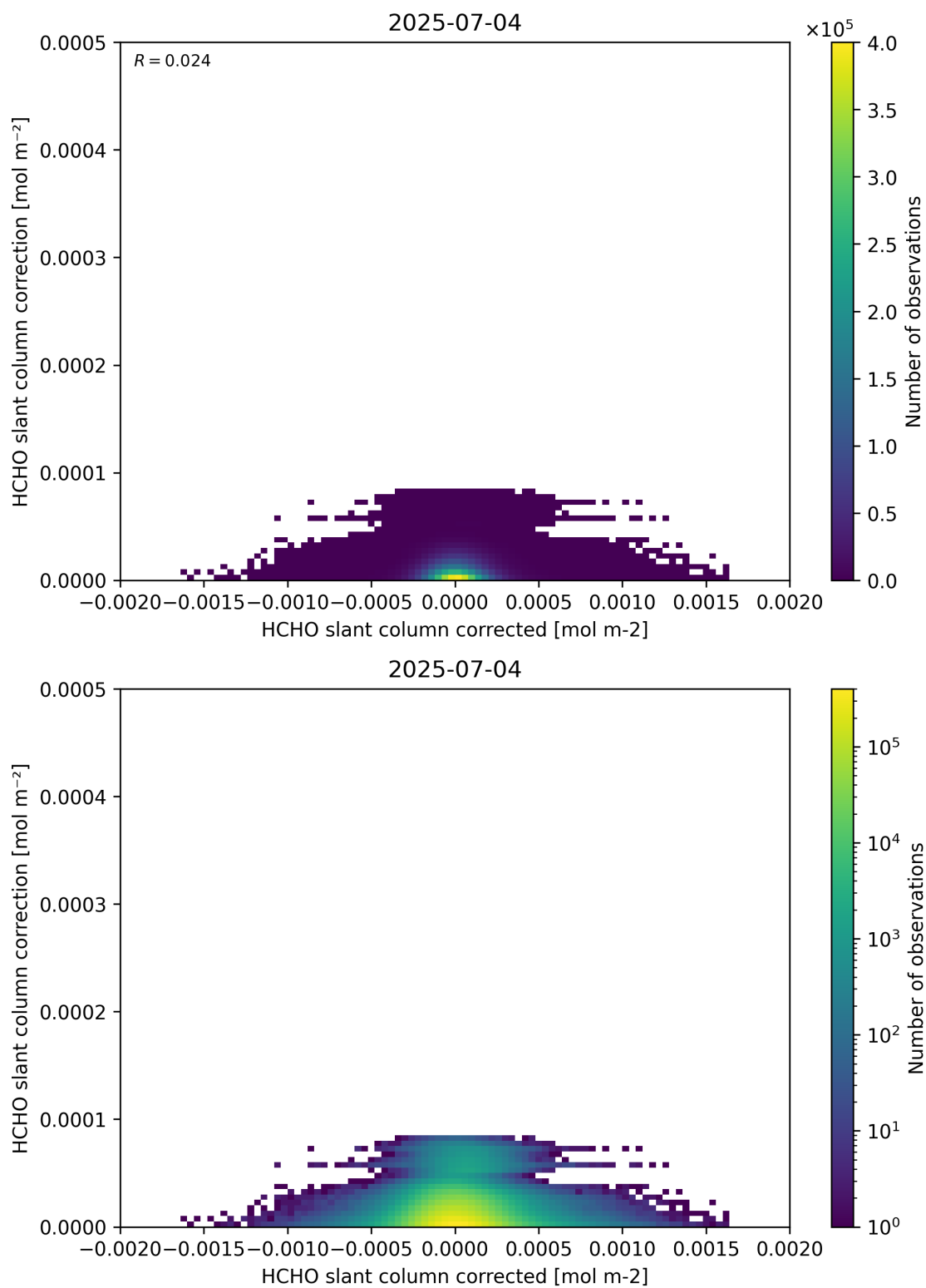
Figure 77: Scatter density plot of “HCHO slant column corrected” against “HCHO slant column correction” for 2025-07-03 to 2025-07-05.
