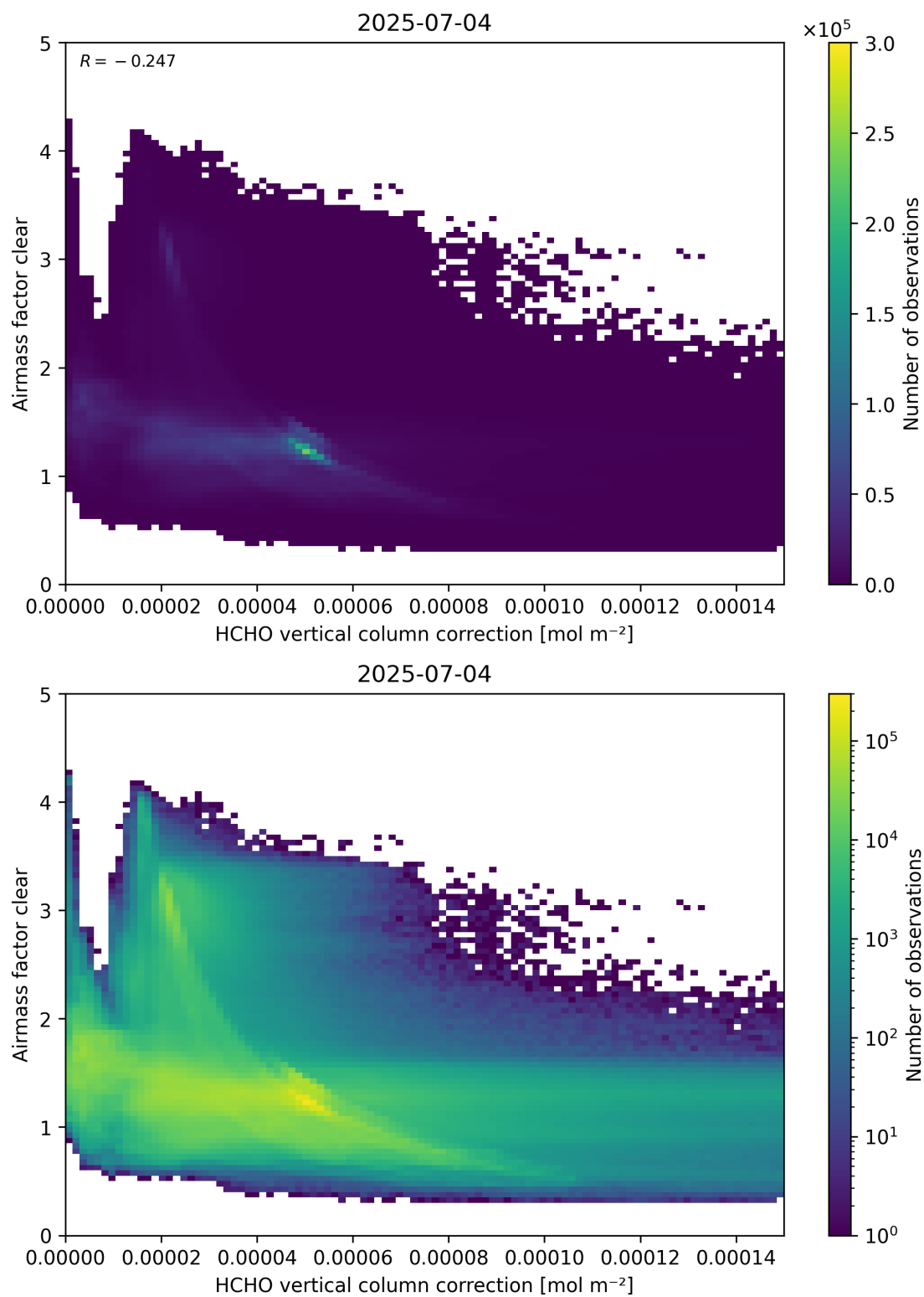
Figure 115: Scatter density plot of “HCHO vertical column correction” against “Airmass factor clear” for 2025-07-03 to 2025-07-05.
