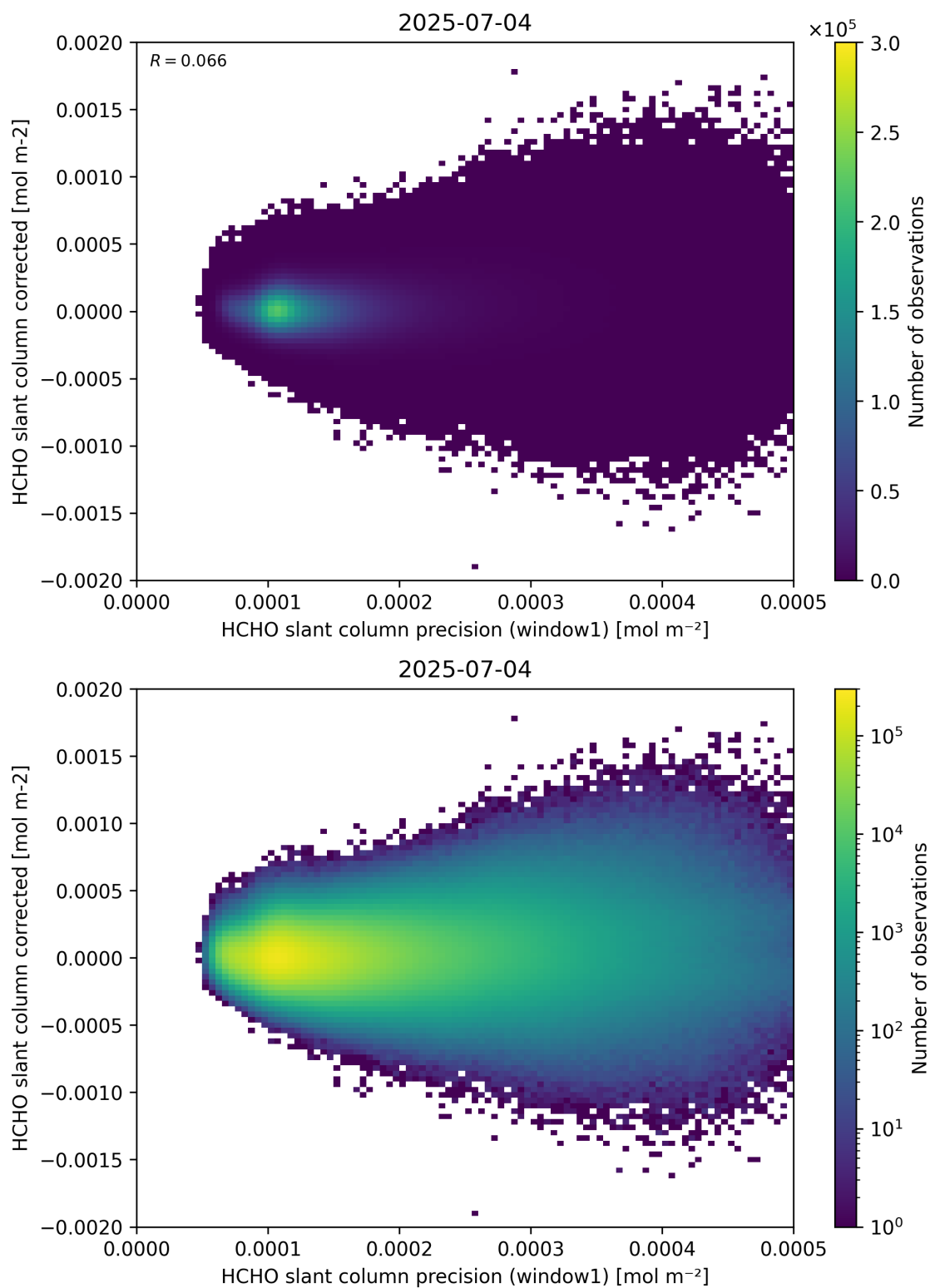
Figure 92: Scatter density plot of “HCHO slant column precision (window1)” against “HCHO slant column corrected” for 2025-07-03 to 2025-07-05.
