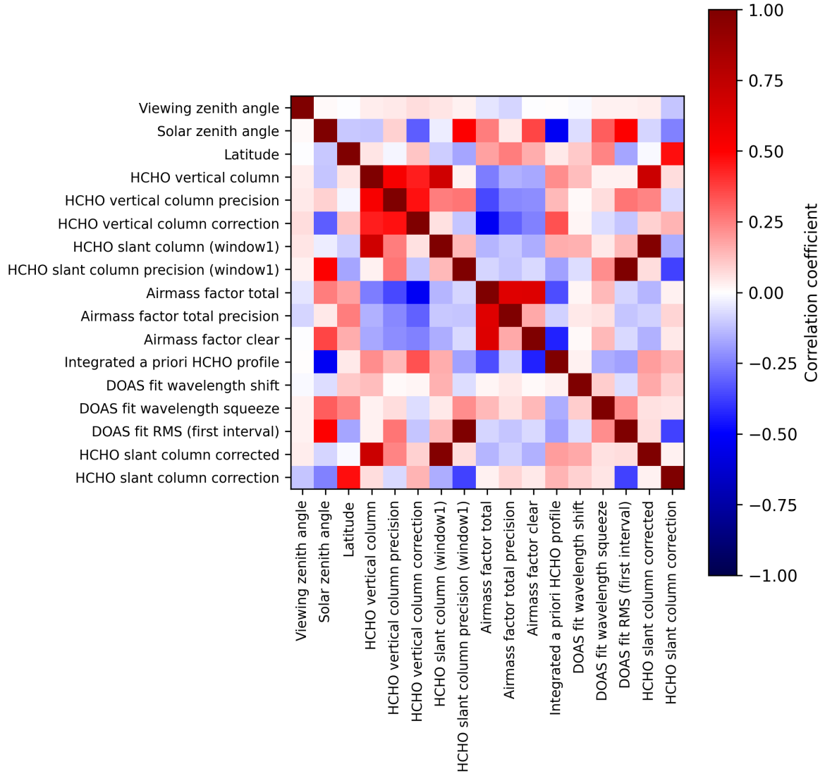
Figure 2: Map of correlation matrix for 2025-07-03 to 2025-07-05.
