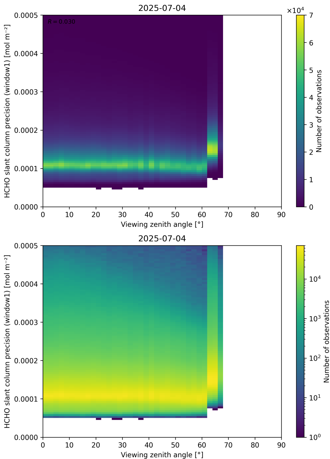
Figure 189: Scatter density plot of “Viewing zenith angle” against “HCHO slant column precision (window1)” for 2025-07-03 to 2025-07-05.
