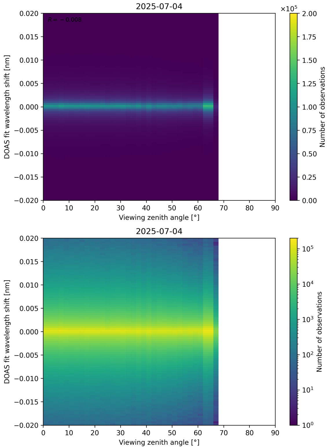
Figure 183: Scatter density plot of “Viewing zenith angle” against “DOAS fit wavelength shift” for 2025-07-03 to 2025-07-05.
