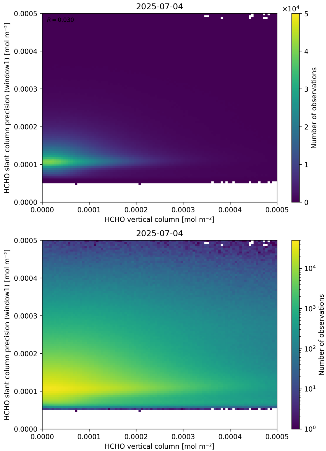
Figure 130: Scatter density plot of “HCHO vertical column” against “HCHO slant column precision (window1)” for 2025-07-03 to 2025-07-05.
