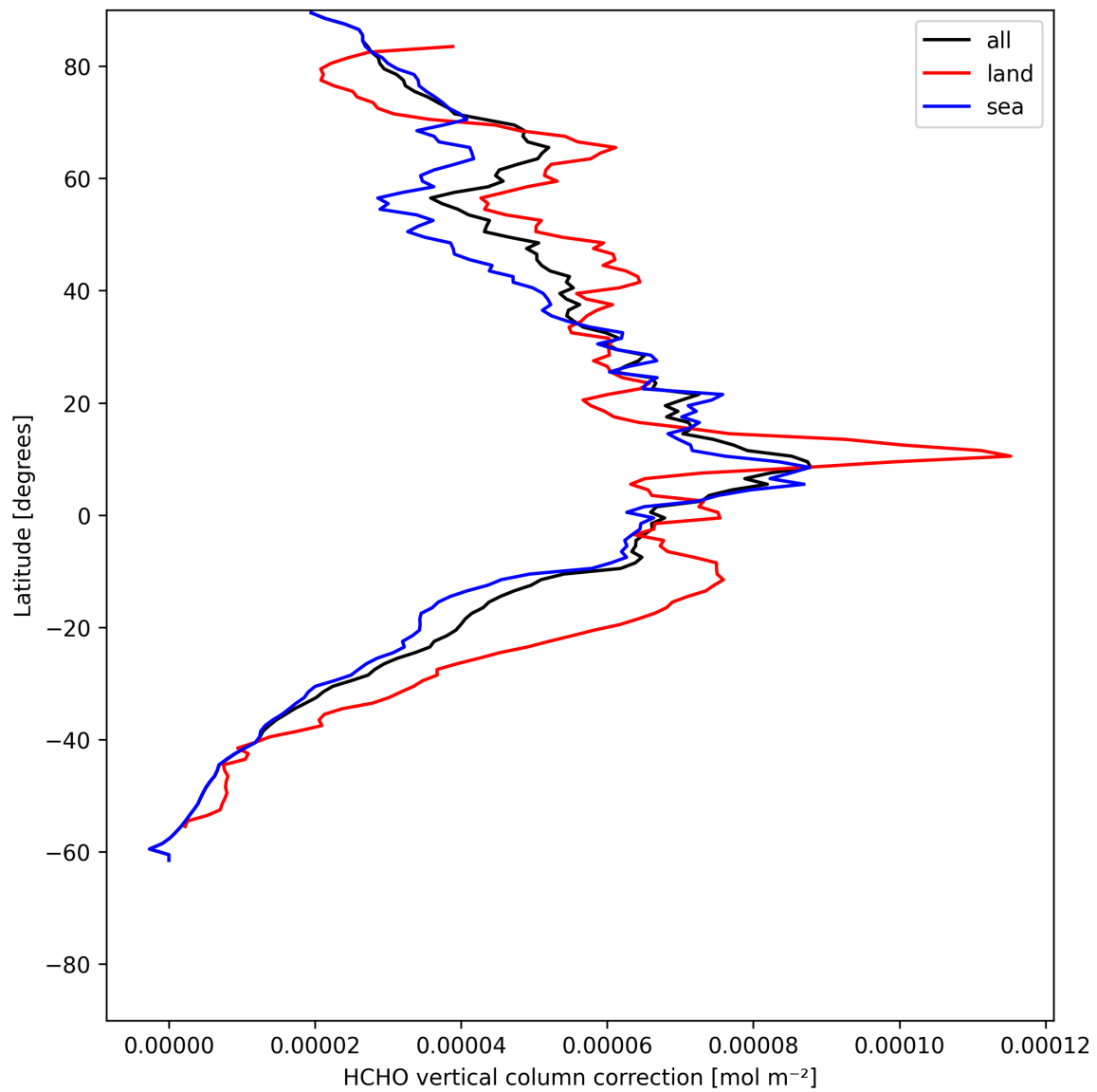
Figure 23: Zonal average of “HCHO vertical column correction” for 2025-07-03 to 2025-07-05.
