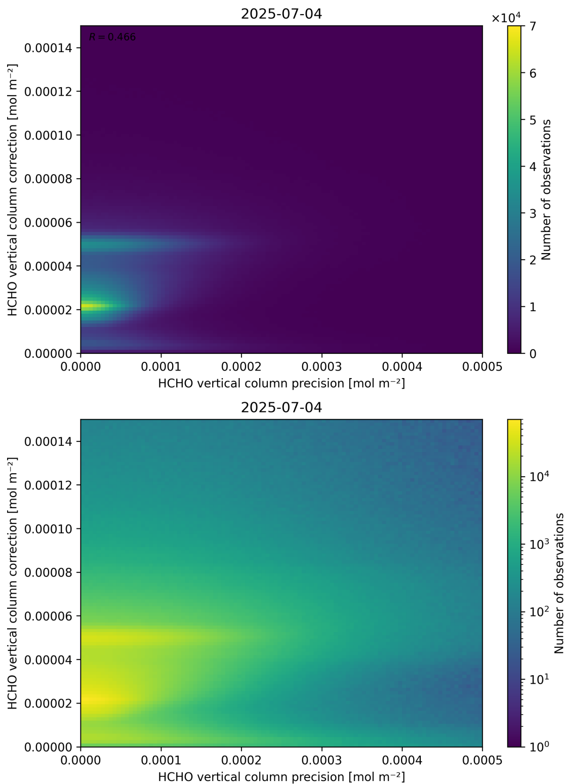
Figure 146: Scatter density plot of “HCHO vertical column precision” against “HCHO vertical column correction” for 2025-07-03 to 2025-07-05.
