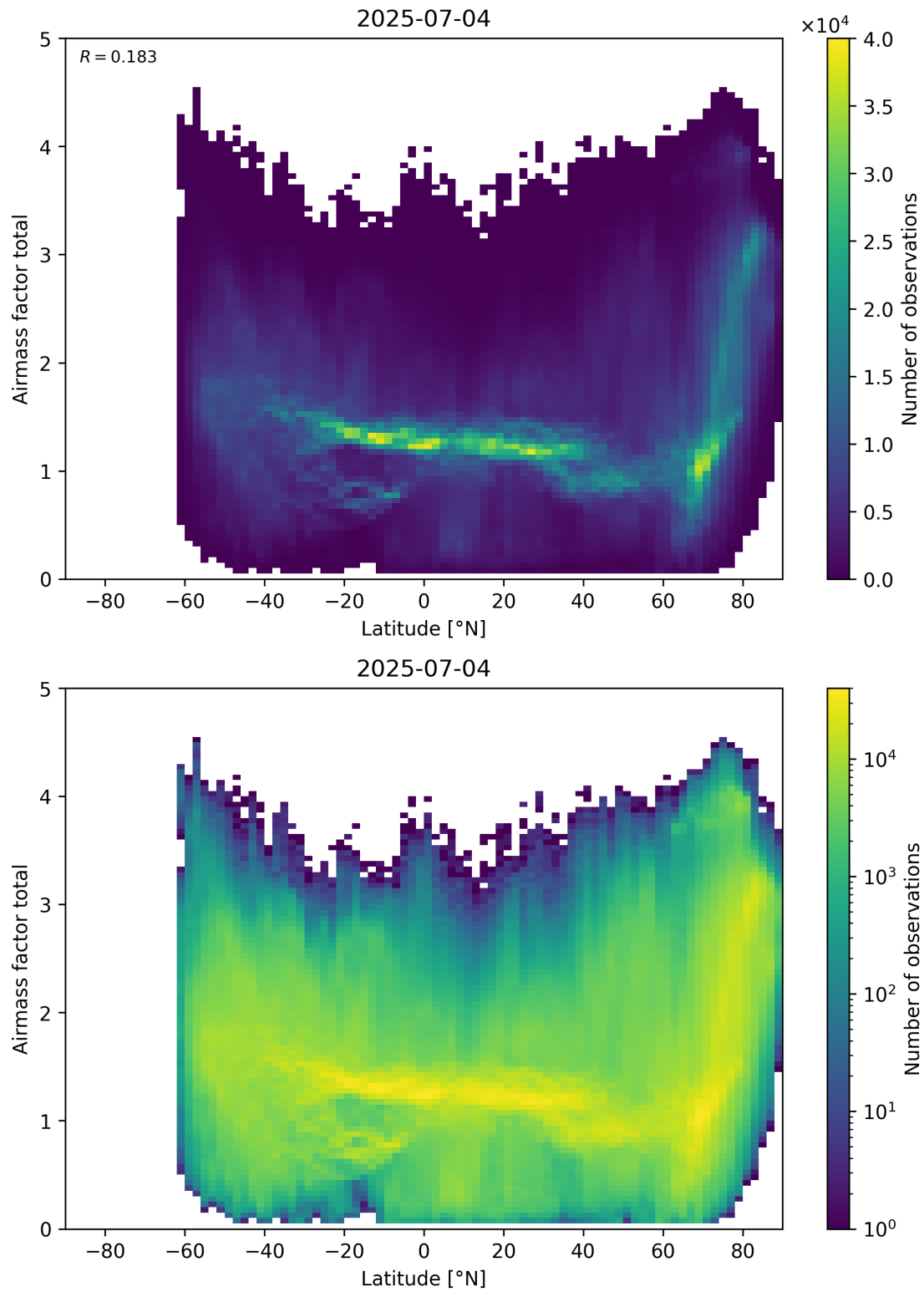
Figure 161: Scatter density plot of “Latitude” against “Airmass factor total” for 2025-07-03 to 2025-07-05.
