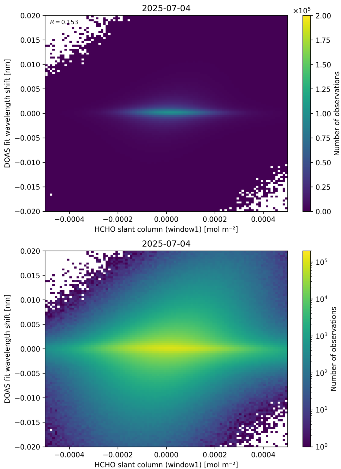
Figure 79: Scatter density plot of “HCHO slant column (window1)” against “DOAS fit wavelength shift” for 2025-07-03 to 2025-07-05.
