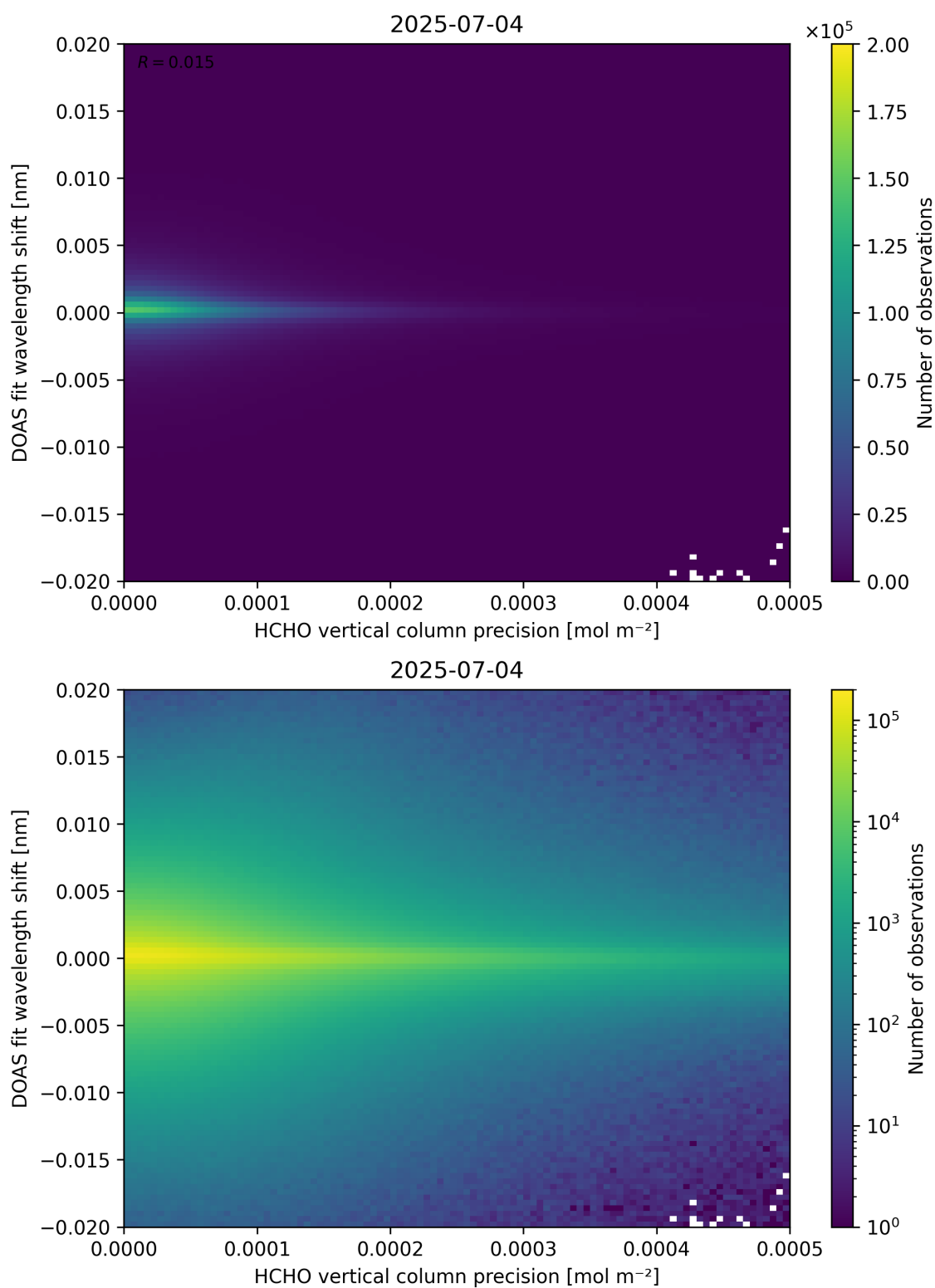
Figure 137: Scatter density plot of “HCHO vertical column precision” against “DOAS fit wavelength shift” for 2025-07-03 to 2025-07-05.
