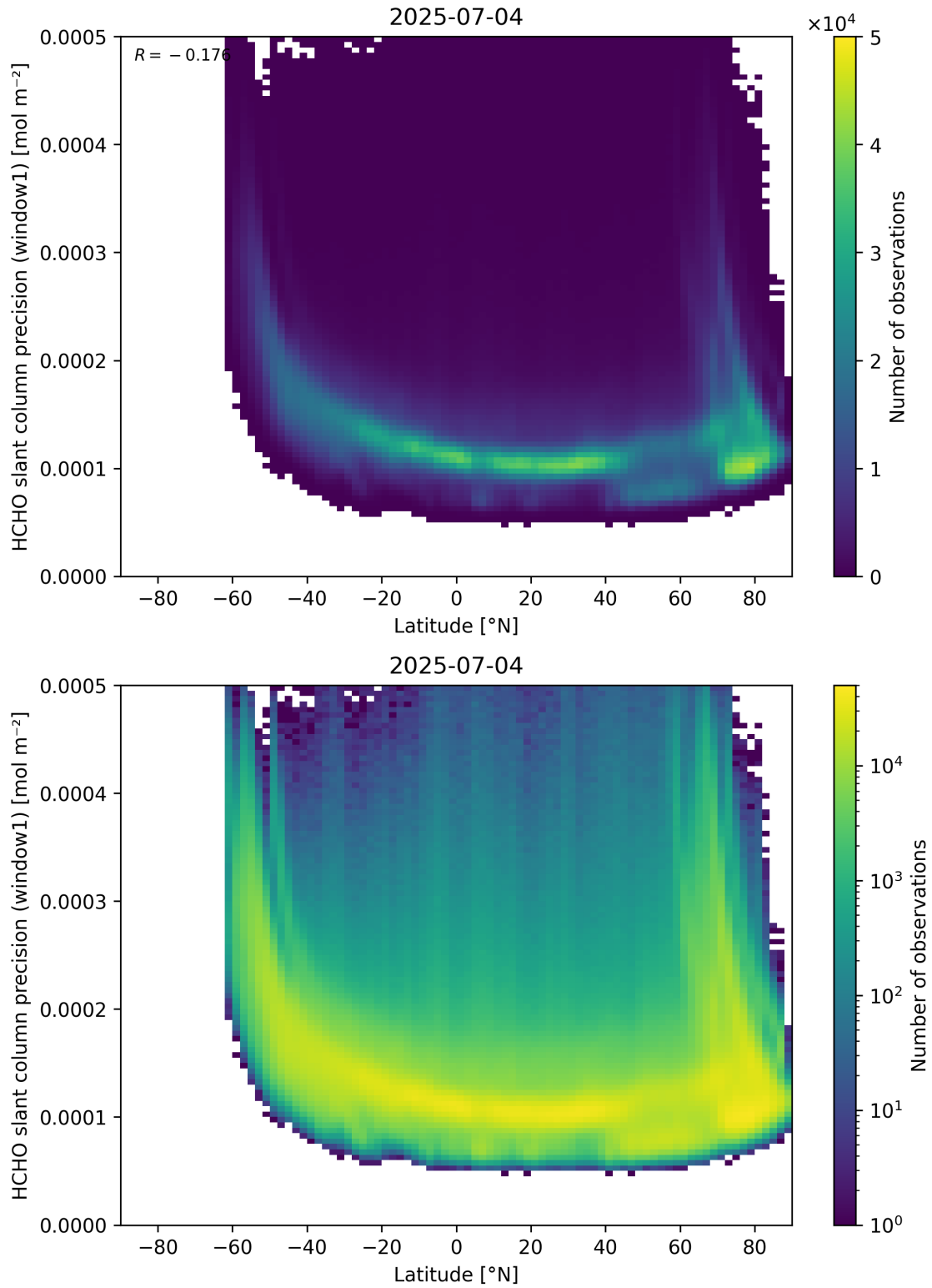
Figure 160: Scatter density plot of “Latitude” against “HCHO slant column precision (window1)” for 2025-07-03 to 2025-07-05.
