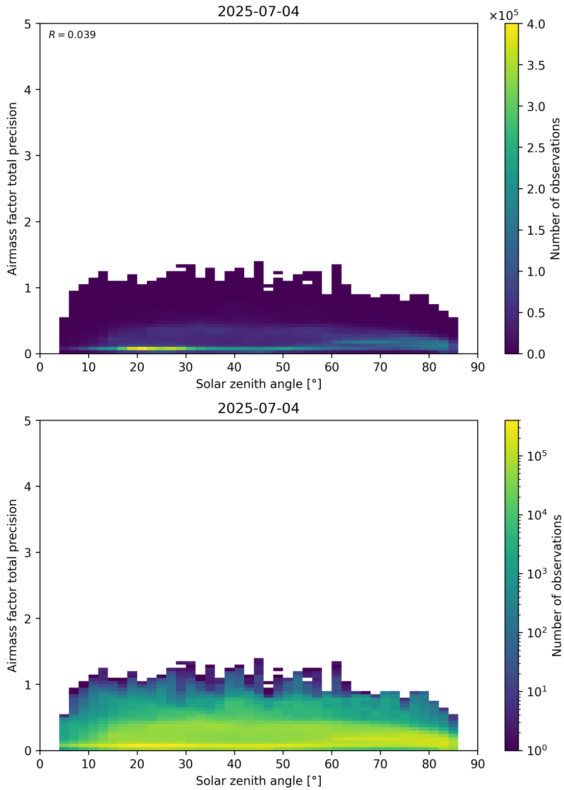
Figure 176: Scatter density plot of “Solar zenith angle” against “Airmass factor total precision” for 2025-07-03 to 2025-07-05.
