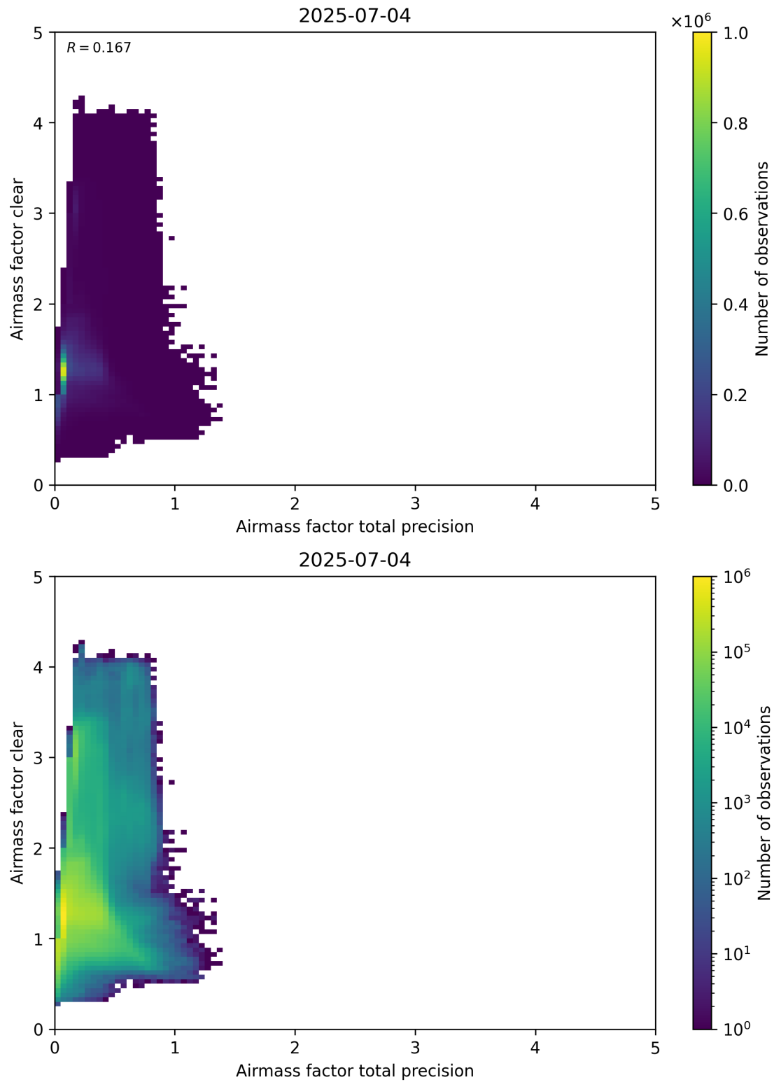
Figure 108: Scatter density plot of “Airmass factor total precision” against “Airmass factor clear” for 2025-07-03 to 2025-07-05.
