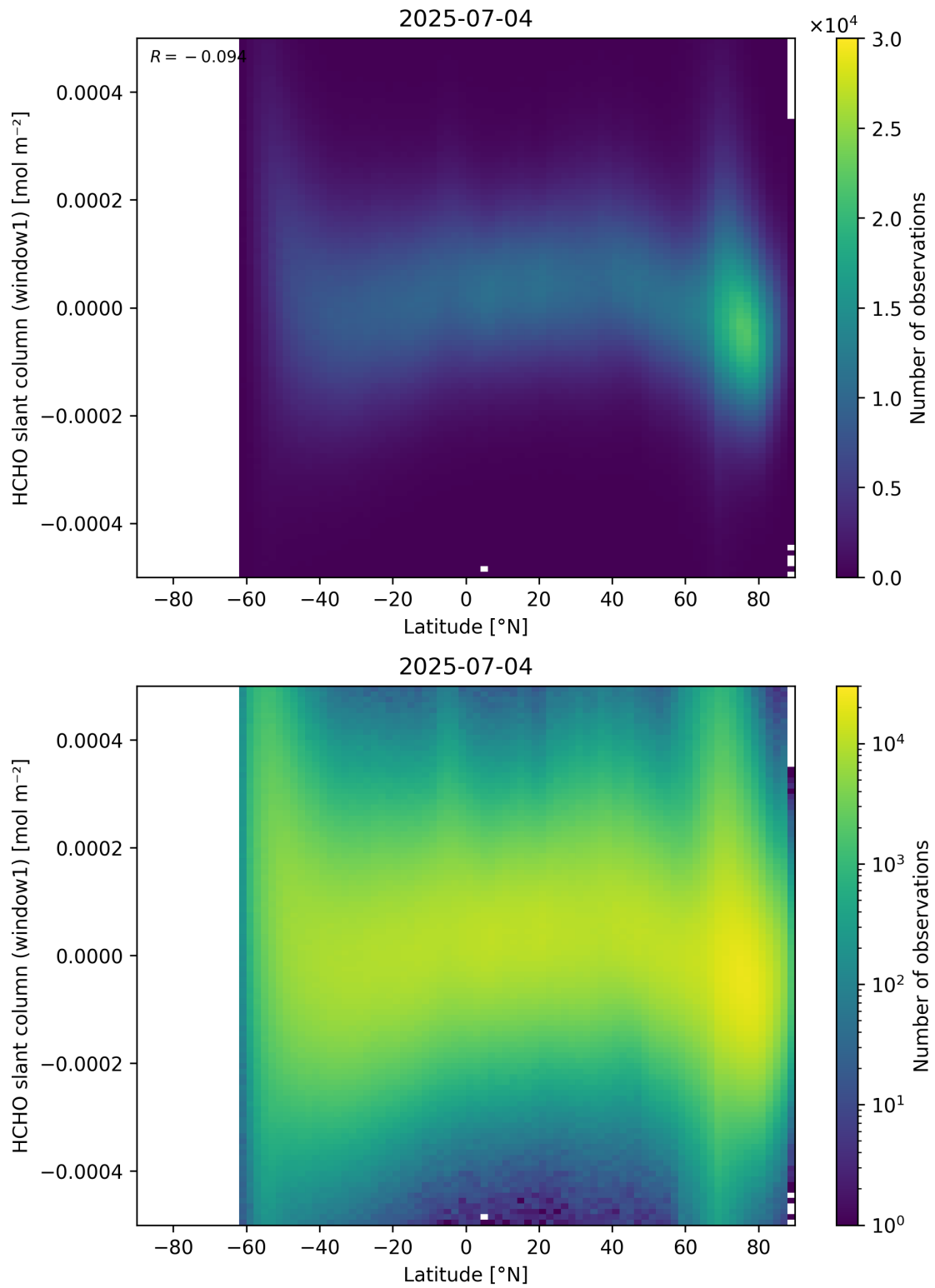
Figure 159: Scatter density plot of “Latitude” against “HCHO slant column (window1)” for 2025-07-03 to 2025-07-05.
