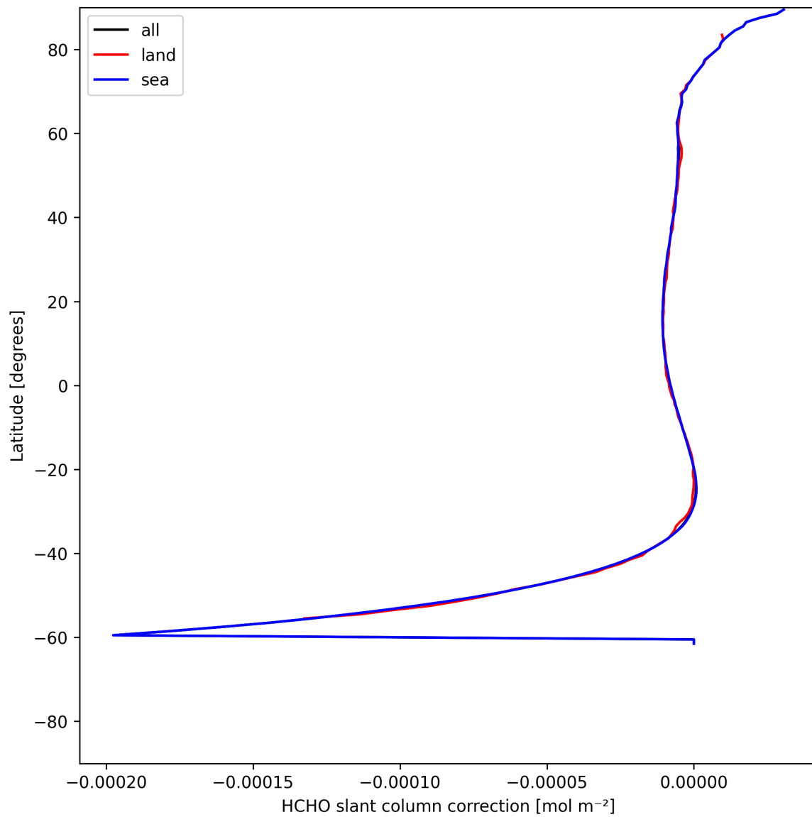
Figure 33: Zonal average of “HCHO slant column correction” for 2025-07-03 to 2025-07-05.
