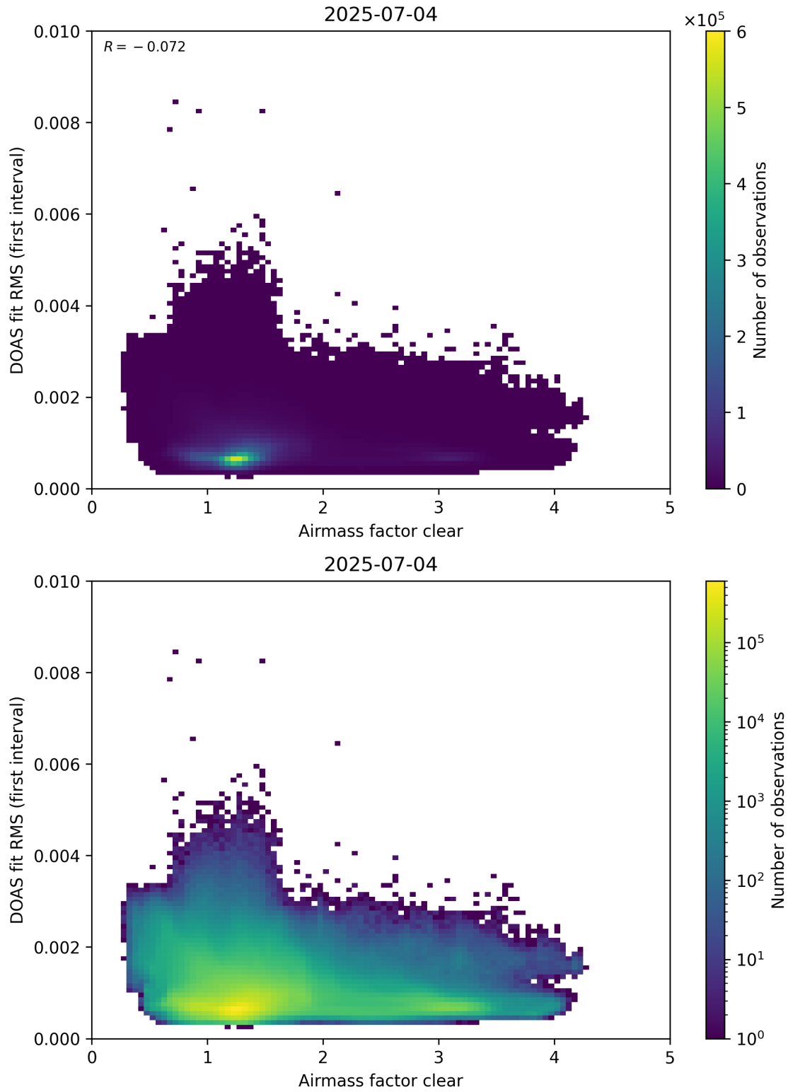
Figure 71: Scatter density plot of “Airmass factor clear” against “DOAS fit RMS (first interval)” for 2025-07-03 to 2025-07-05.
