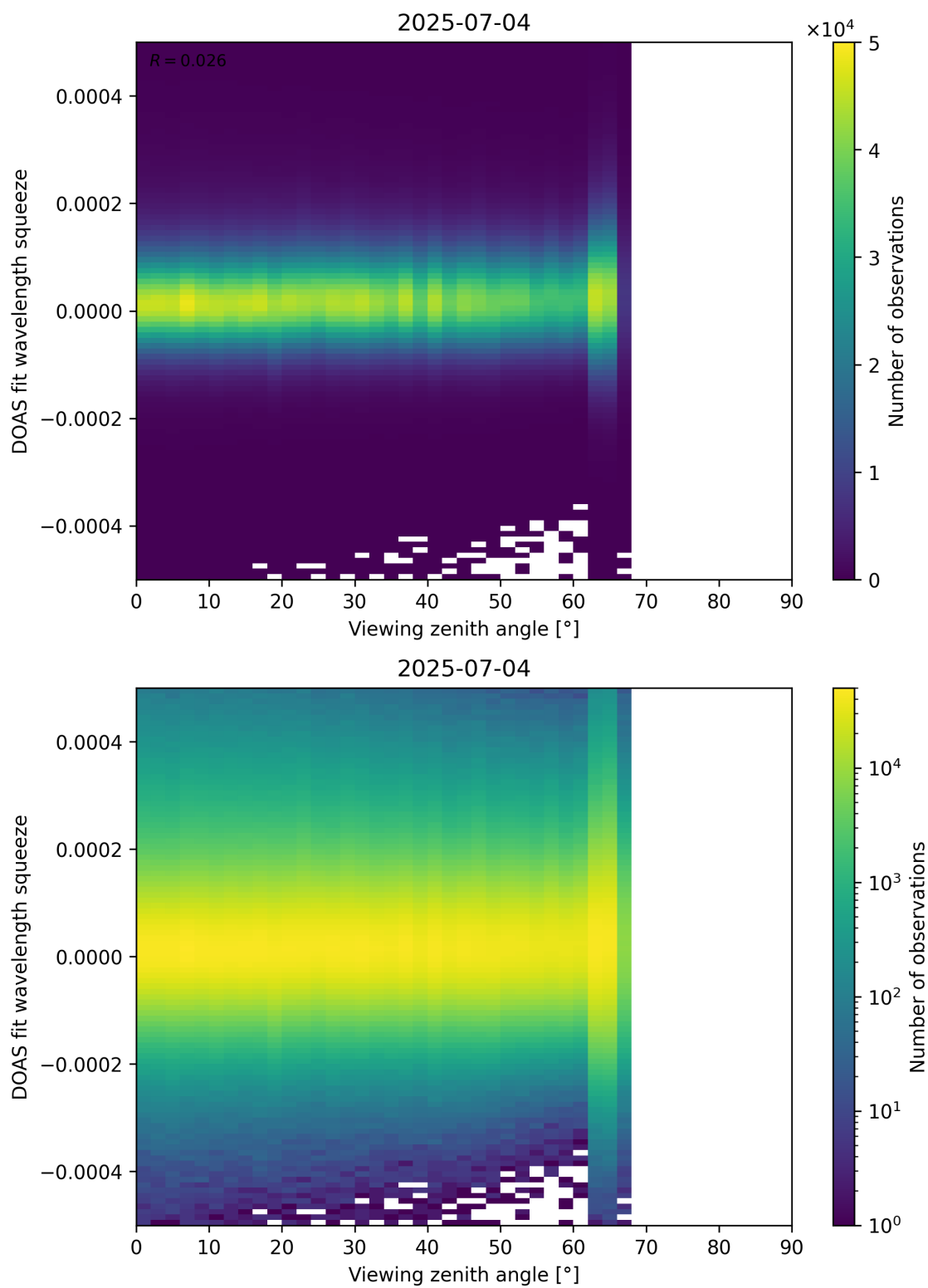
Figure 184: Scatter density plot of “Viewing zenith angle” against “DOAS fit wavelength squeeze” for 2025-07-03 to 2025-07-05.
