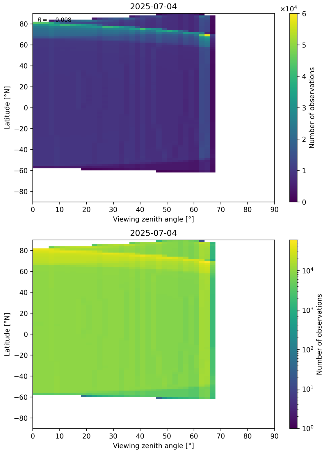
Figure 196: Scatter density plot of “Viewing zenith angle” against “Latitude” for 2025-07-03 to 2025-07-05.
