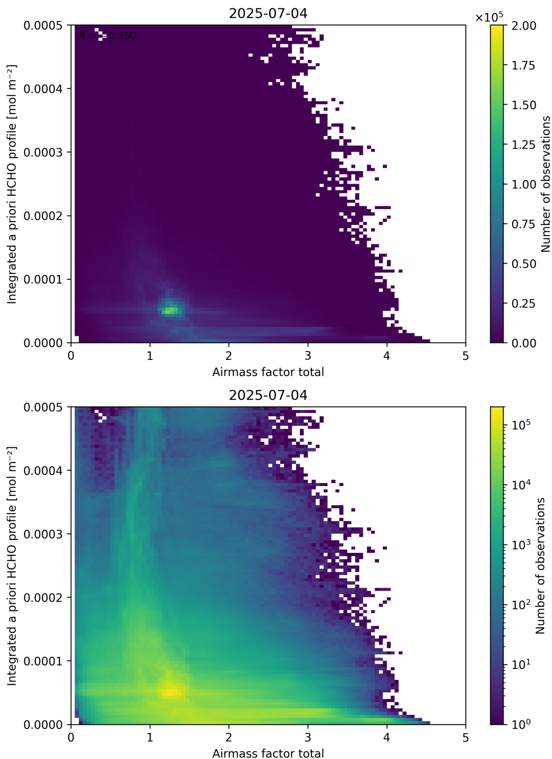
Figure 104: Scatter density plot of “Airmass factor total” against “Integrated a priori HCHO profile” for 2025-07-03 to 2025-07-05.
