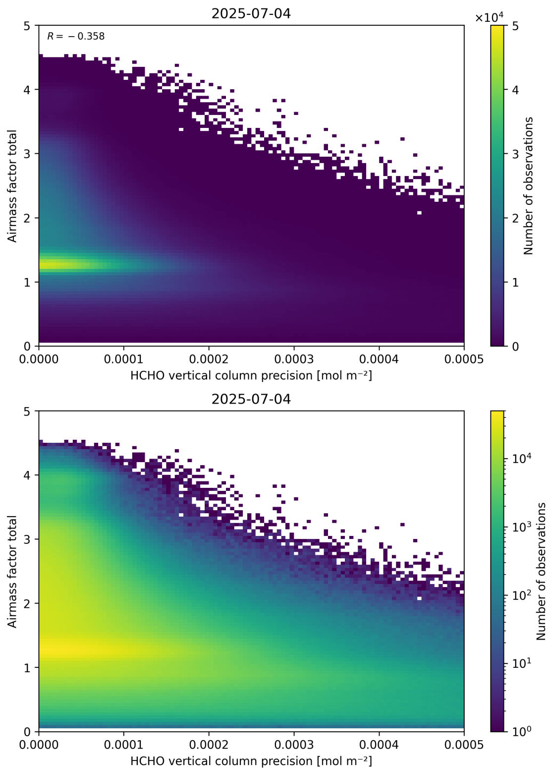
Figure 144: Scatter density plot of “HCHO vertical column precision” against “Airmass factor total” for 2025-07-03 to 2025-07-05.
