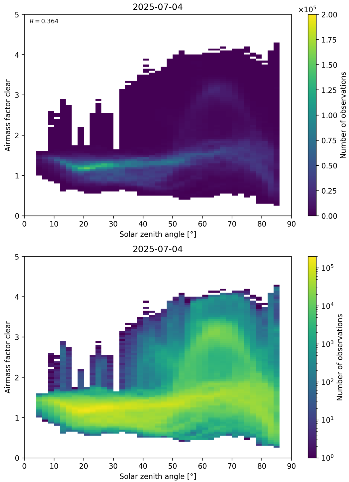
Figure 170: Scatter density plot of “Solar zenith angle” against “Airmass factor clear” for 2025-07-03 to 2025-07-05.
