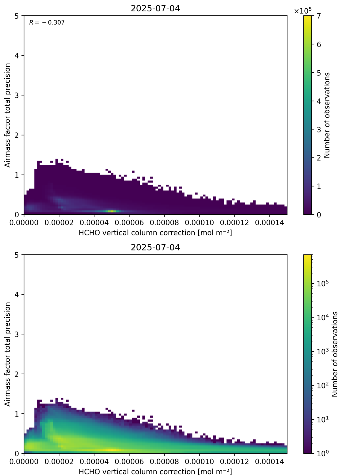
Figure 121: Scatter density plot of “HCHO vertical column correction” against “Airmass factor total precision” for 2025-07-03 to 2025-07-05.
