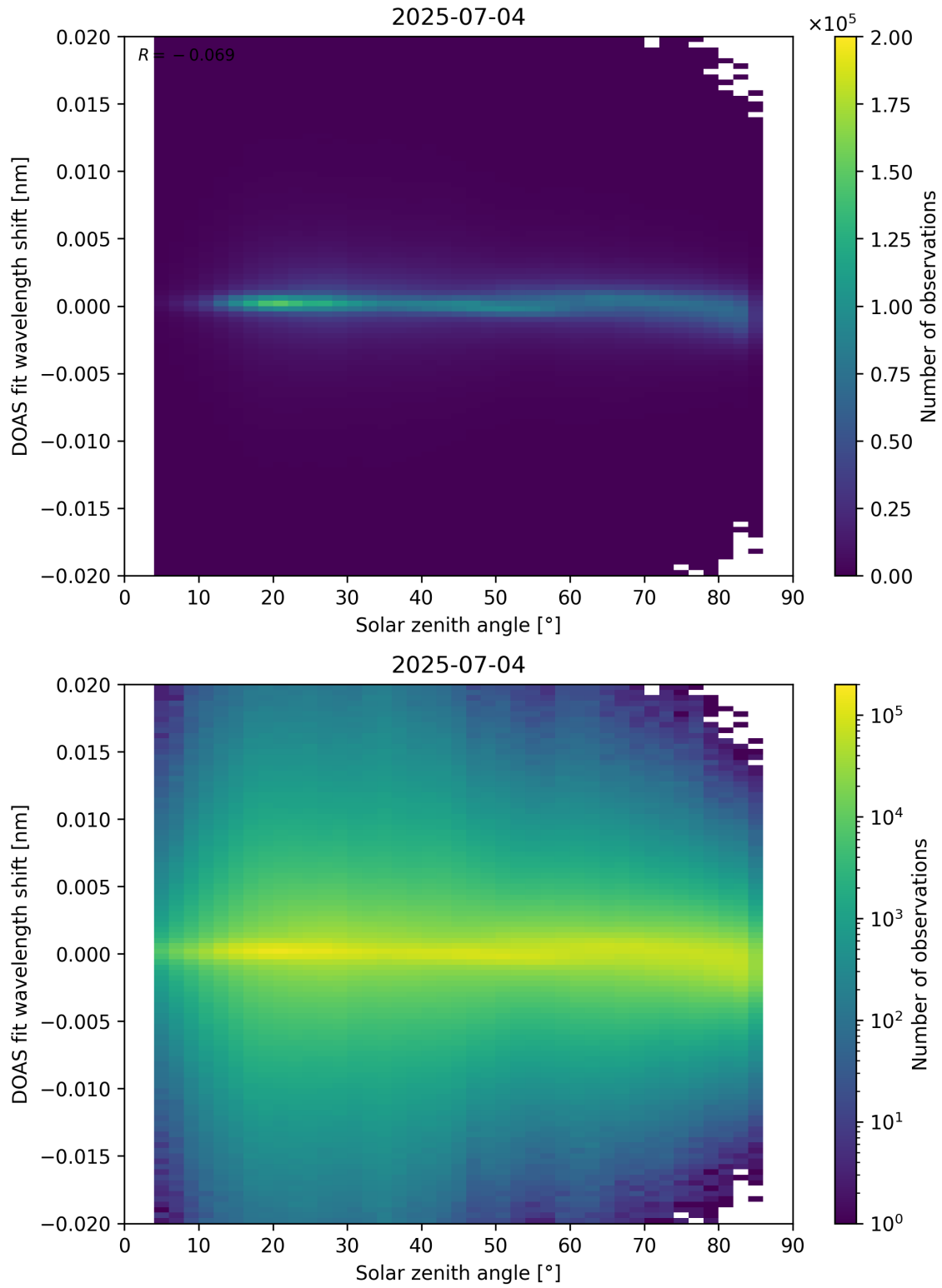
Figure 168: Scatter density plot of “Solar zenith angle” against “DOAS fit wavelength shift” for 2025-07-03 to 2025-07-05.
