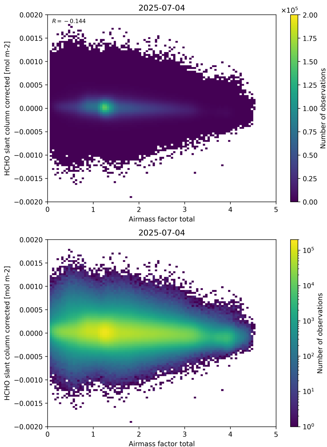
Figure 101: Scatter density plot of “Airmass factor total” against “HCHO slant column corrected” for 2025-07-03 to 2025-07-05.
