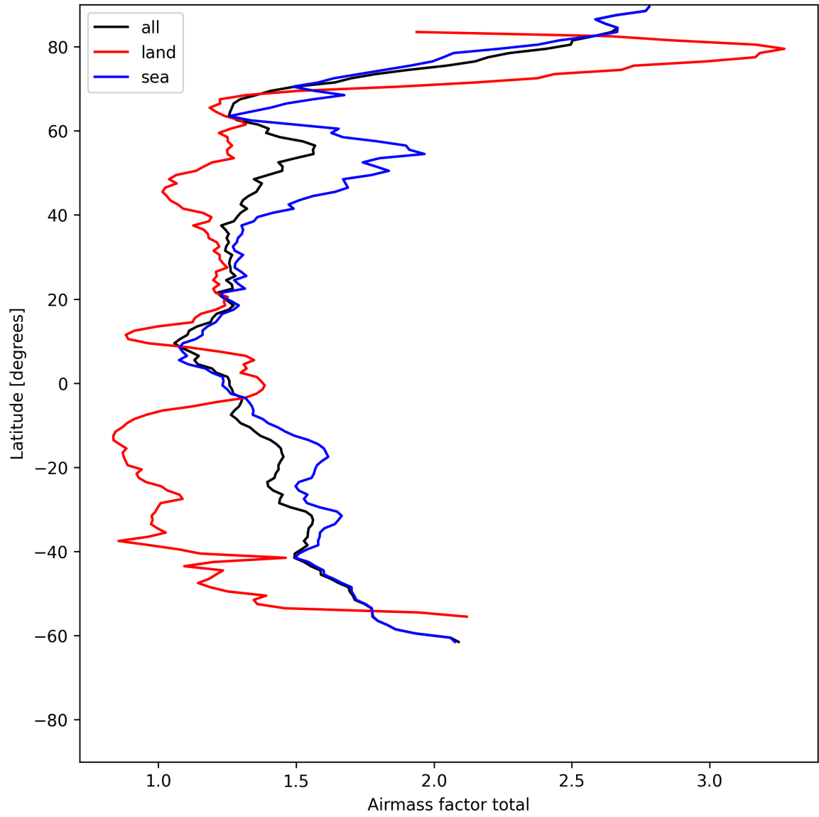
Figure 26: Zonal average of “Airmass factor total” for 2025-07-03 to 2025-07-05.
