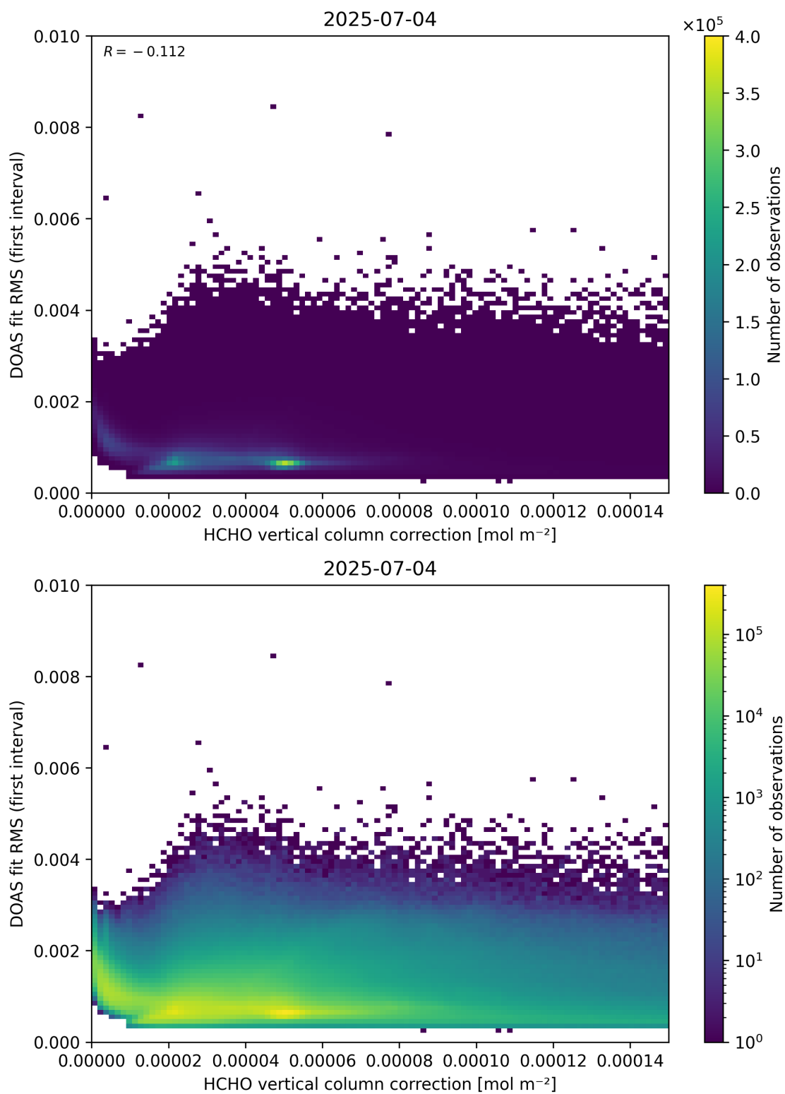
Figure 112: Scatter density plot of “HCHO vertical column correction” against “DOAS fit RMS (first interval)” for 2025-07-03 to 2025-07-05.
