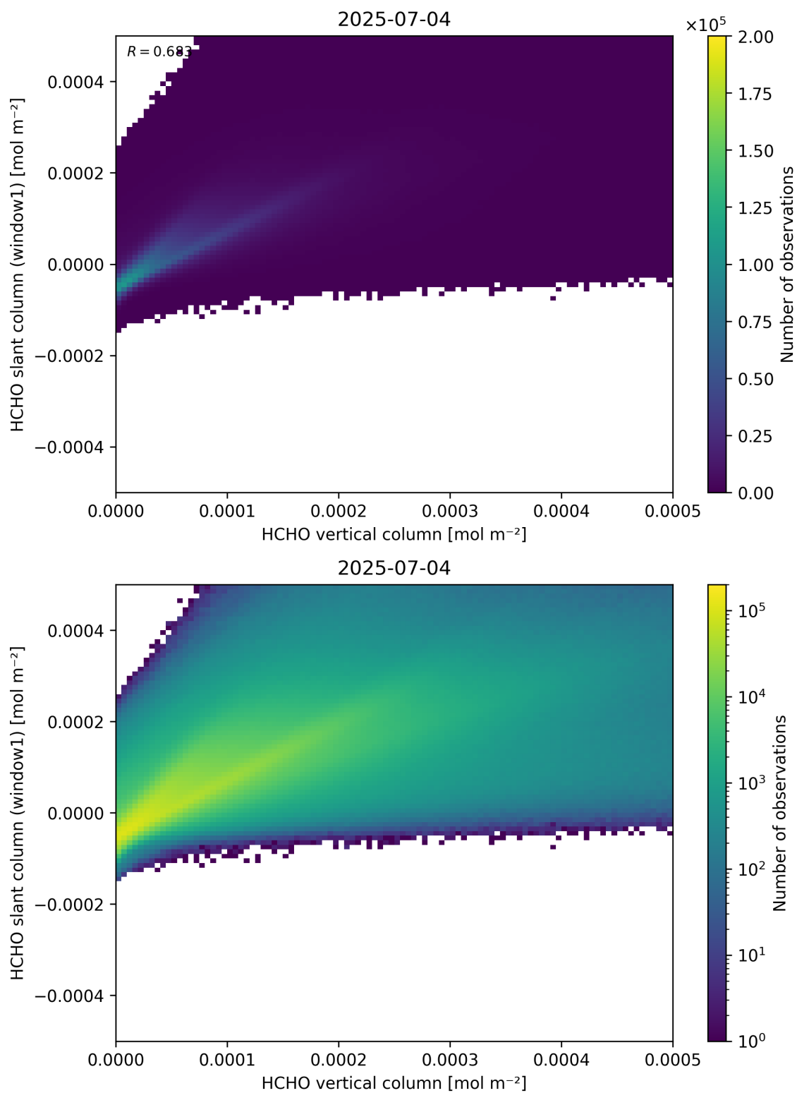
Figure 129: Scatter density plot of “HCHO vertical column” against “HCHO slant column (window1)” for 2025-07-03 to 2025-07-05.
