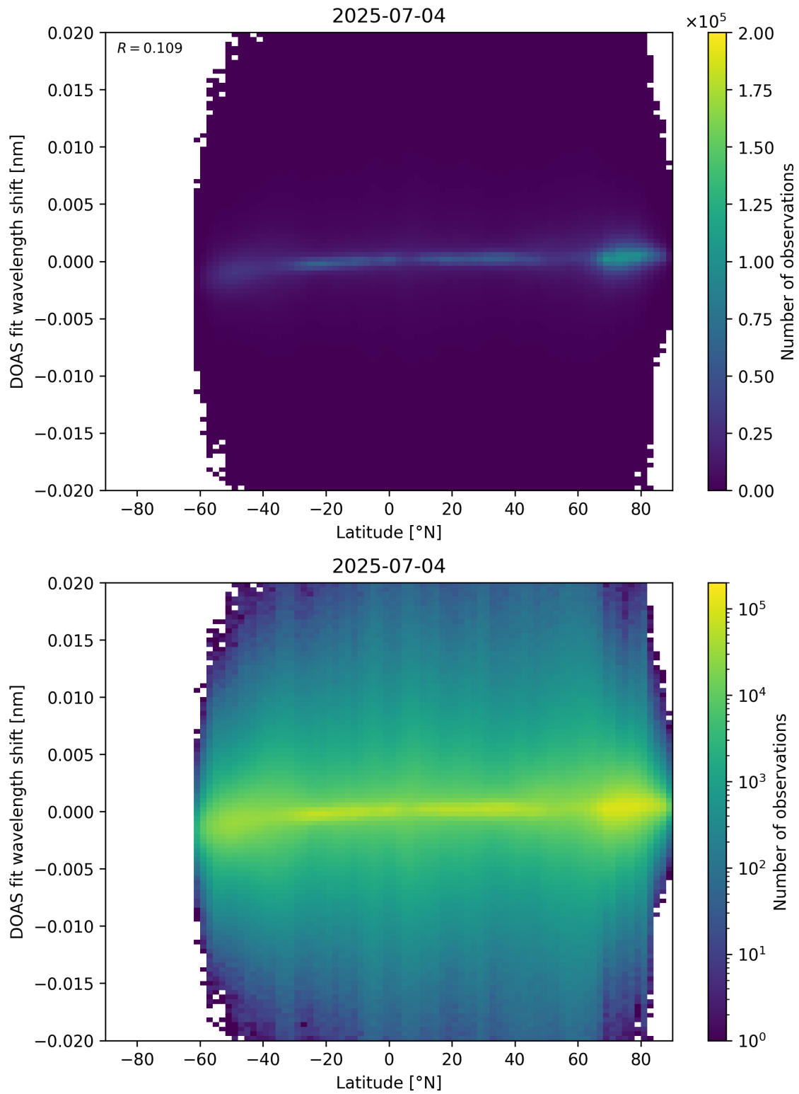
Figure 154: Scatter density plot of “Latitude” against “DOAS fit wavelength shift” for 2025-07-03 to 2025-07-05.
