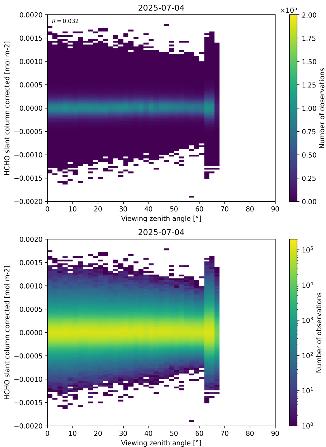
Figure 186: Scatter density plot of “Viewing zenith angle” against “HCHO slant column corrected” for 2025-07-03 to 2025-07-05.
