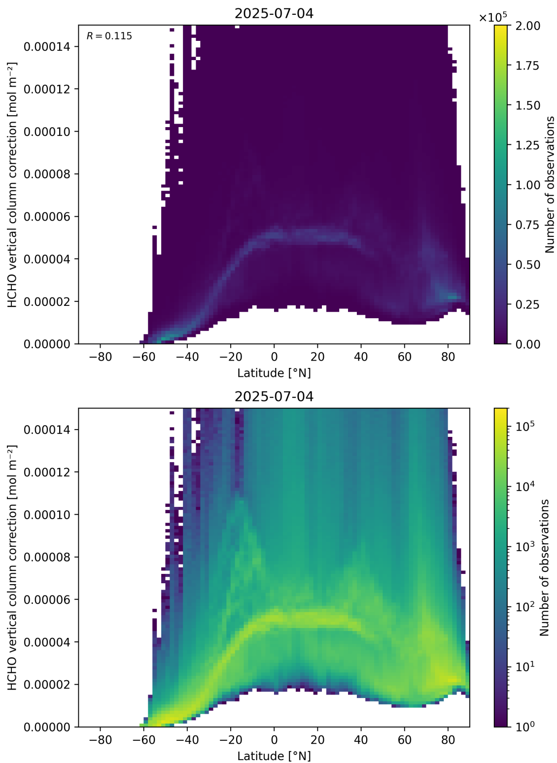
Figure 164: Scatter density plot of “Latitude” against “HCHO vertical column correction” for 2025-07-03 to 2025-07-05.
