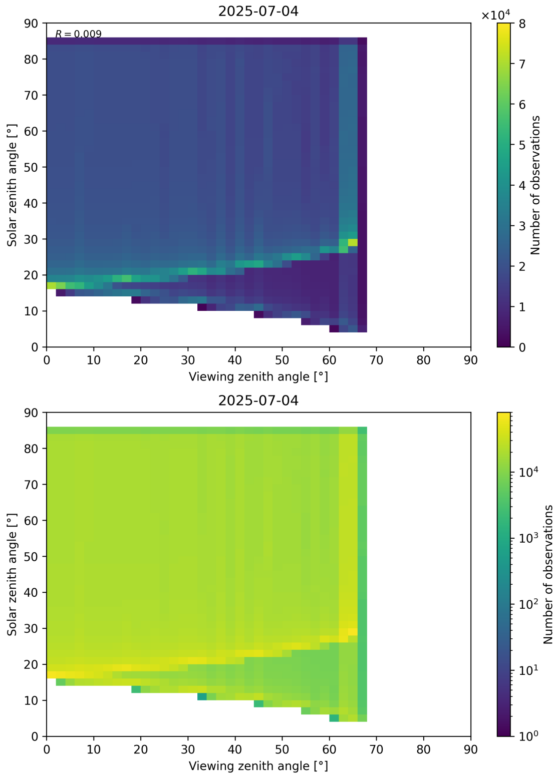
Figure 197: Scatter density plot of “Viewing zenith angle” against “Solar zenith angle” for 2025-07-03 to 2025-07-05.
