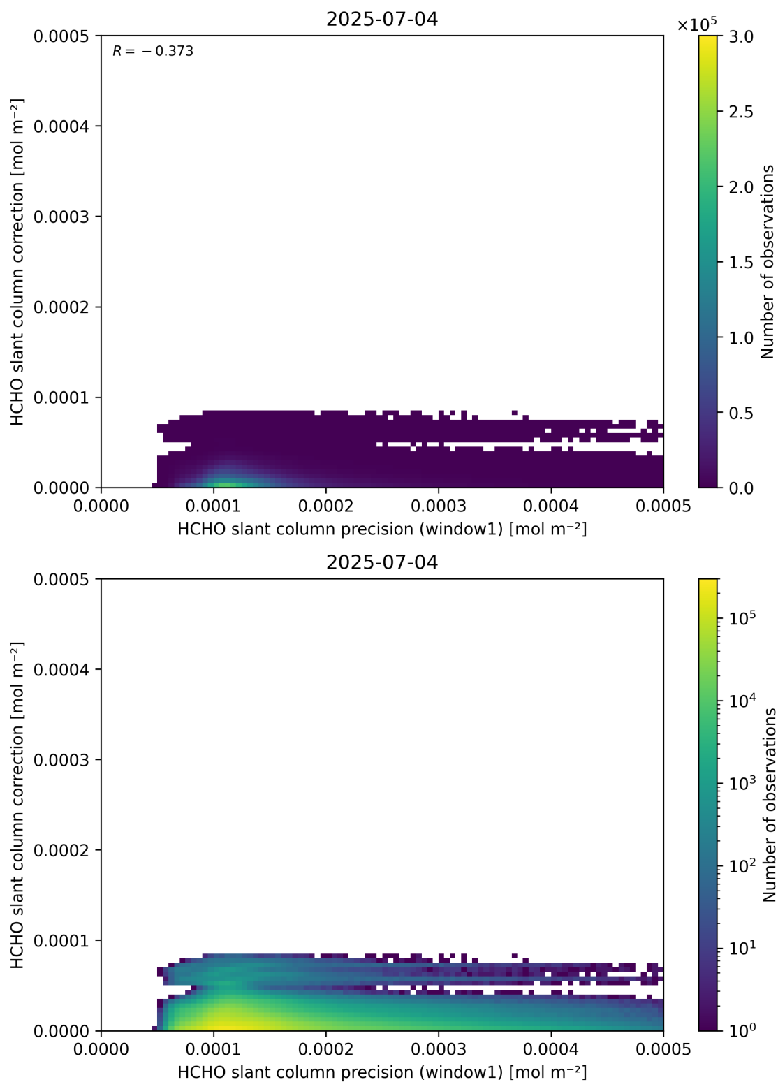
Figure 93: Scatter density plot of “HCHO slant column precision (window1)” against “HCHO slant column correction” for 2025-07-03 to 2025-07-05.
