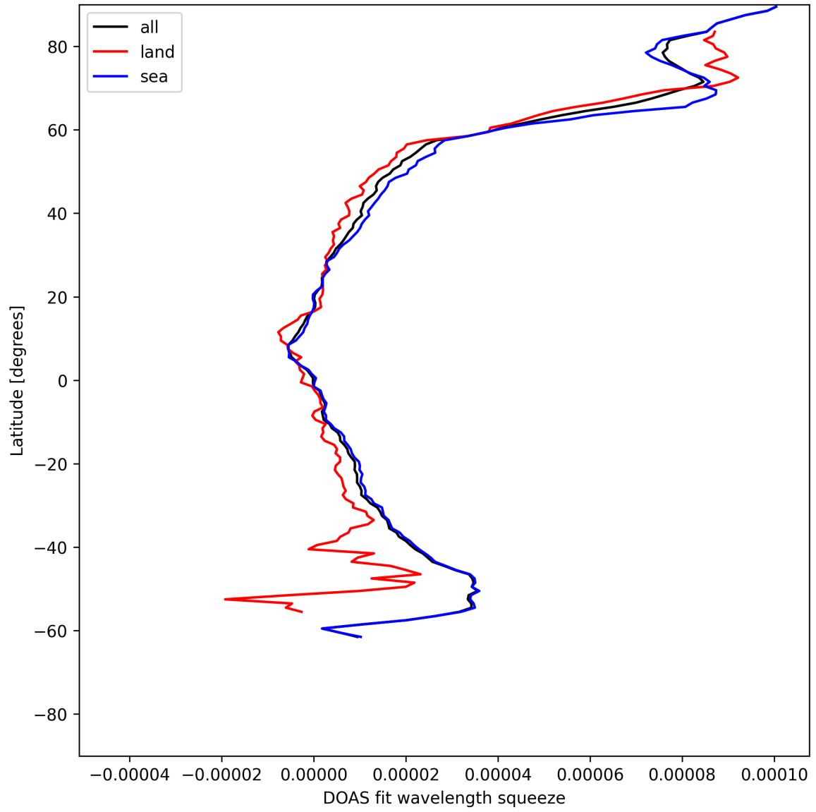
Figure 31: Zonal average of “DOAS fit wavelength squeeze” for 2025-07-03 to 2025-07-05.
