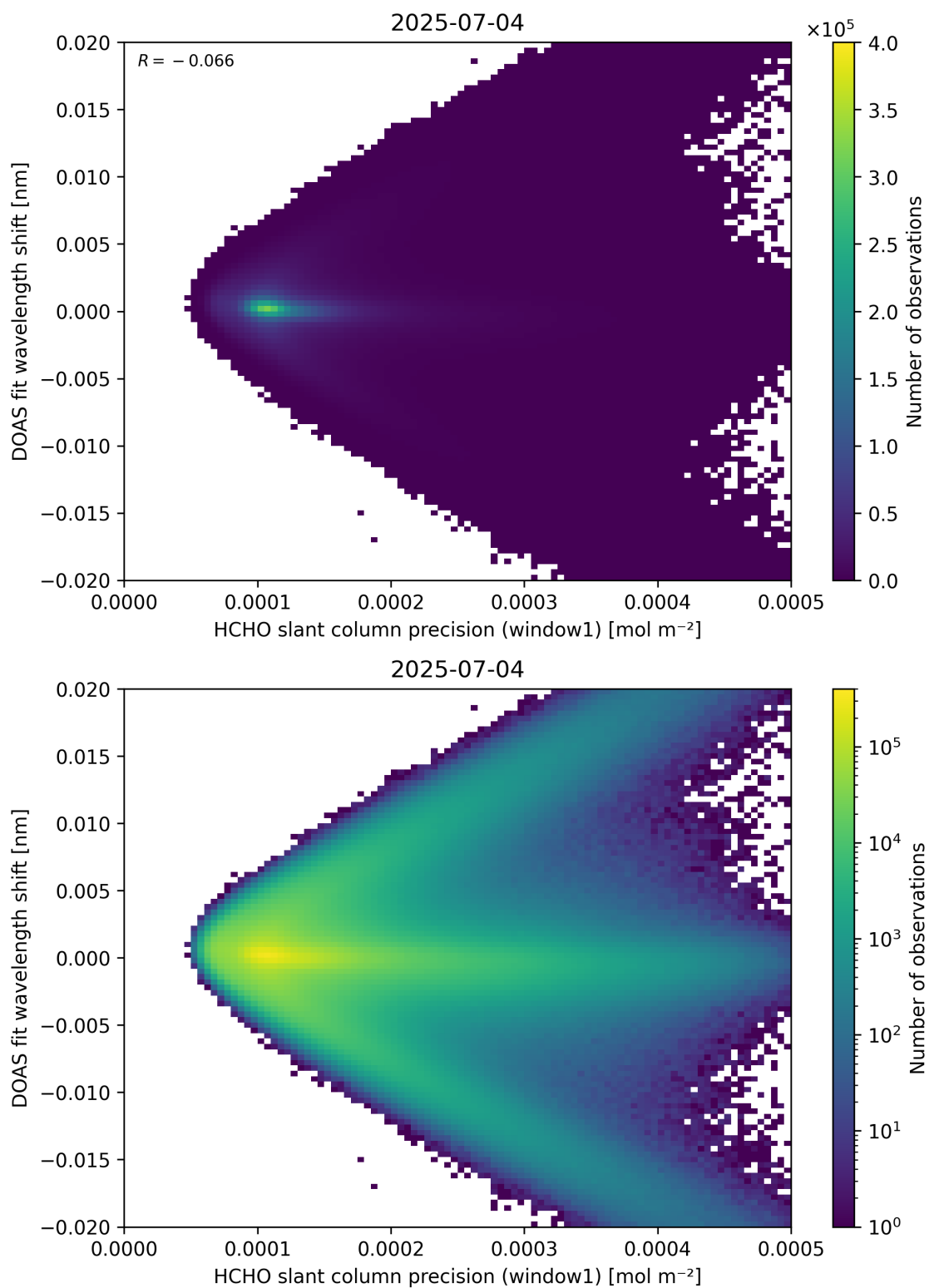
Figure 89: Scatter density plot of “HCHO slant column precision (window1)” against “DOAS fit wavelength shift” for 2025-07-03 to 2025-07-05.
