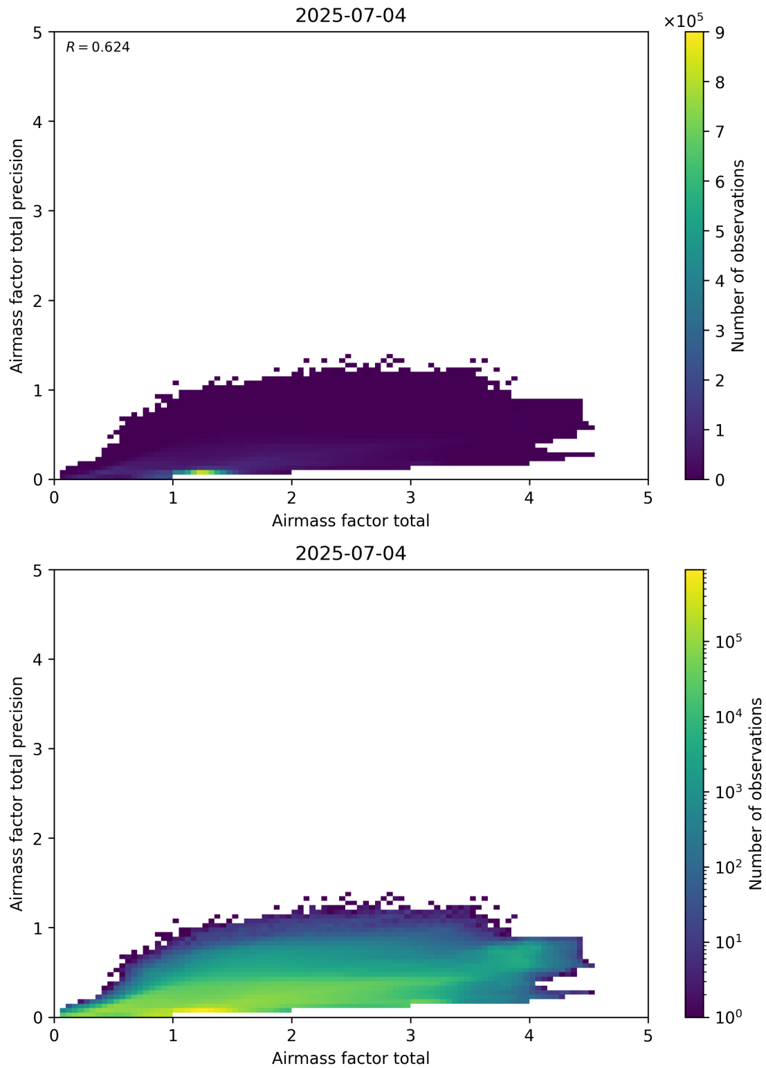
Figure 103: Scatter density plot of “Airmass factor total” against “Airmass factor total precision” for 2025-07-03 to 2025-07-05.
