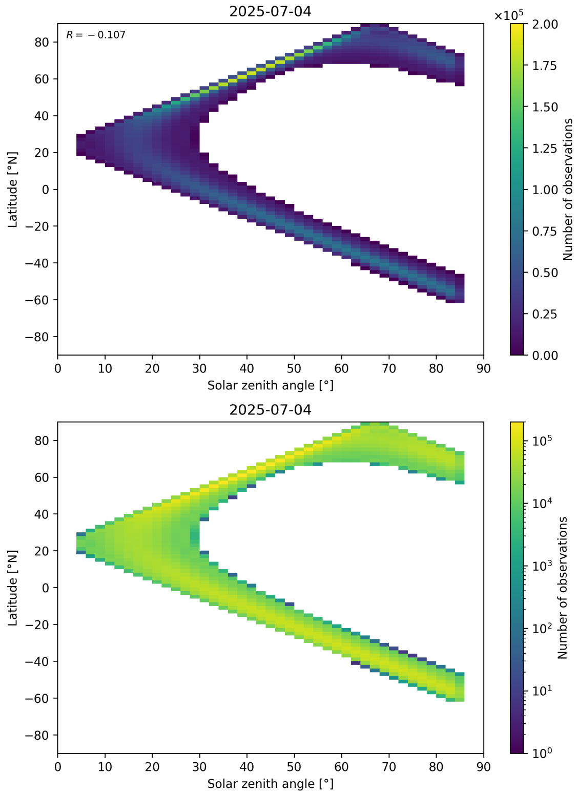
Figure 181: Scatter density plot of “Solar zenith angle” against “Latitude” for 2025-07-03 to 2025-07-05.
