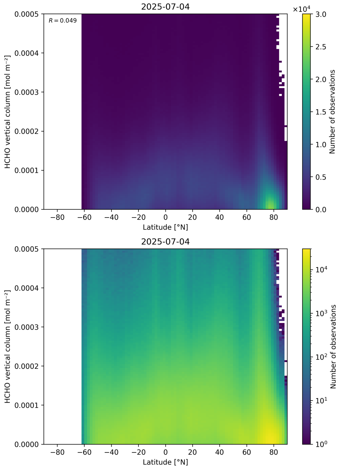
Figure 163: Scatter density plot of “Latitude” against “HCHO vertical column” for 2025-07-03 to 2025-07-05.
