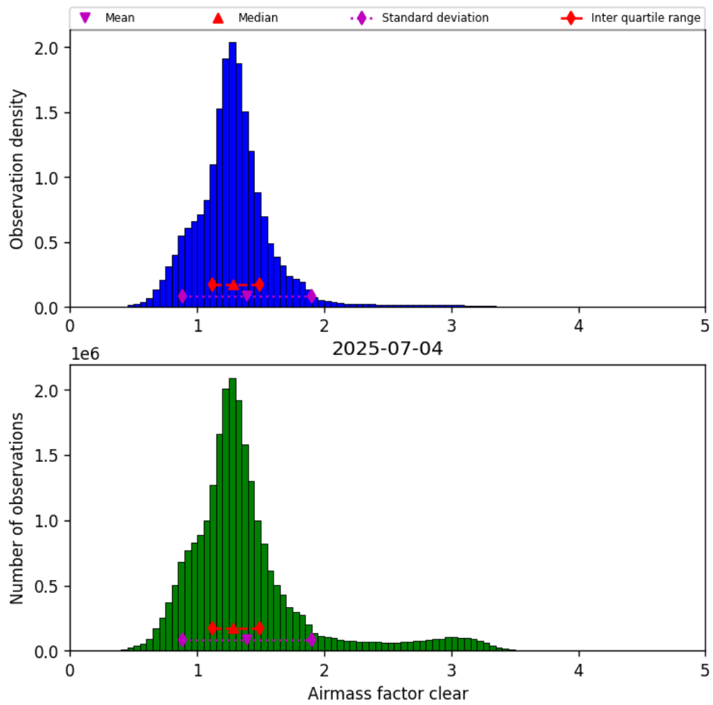
Figure 42: Histogram of “Airmass factor clear” for 2025-07-03 to 2025-07-05
