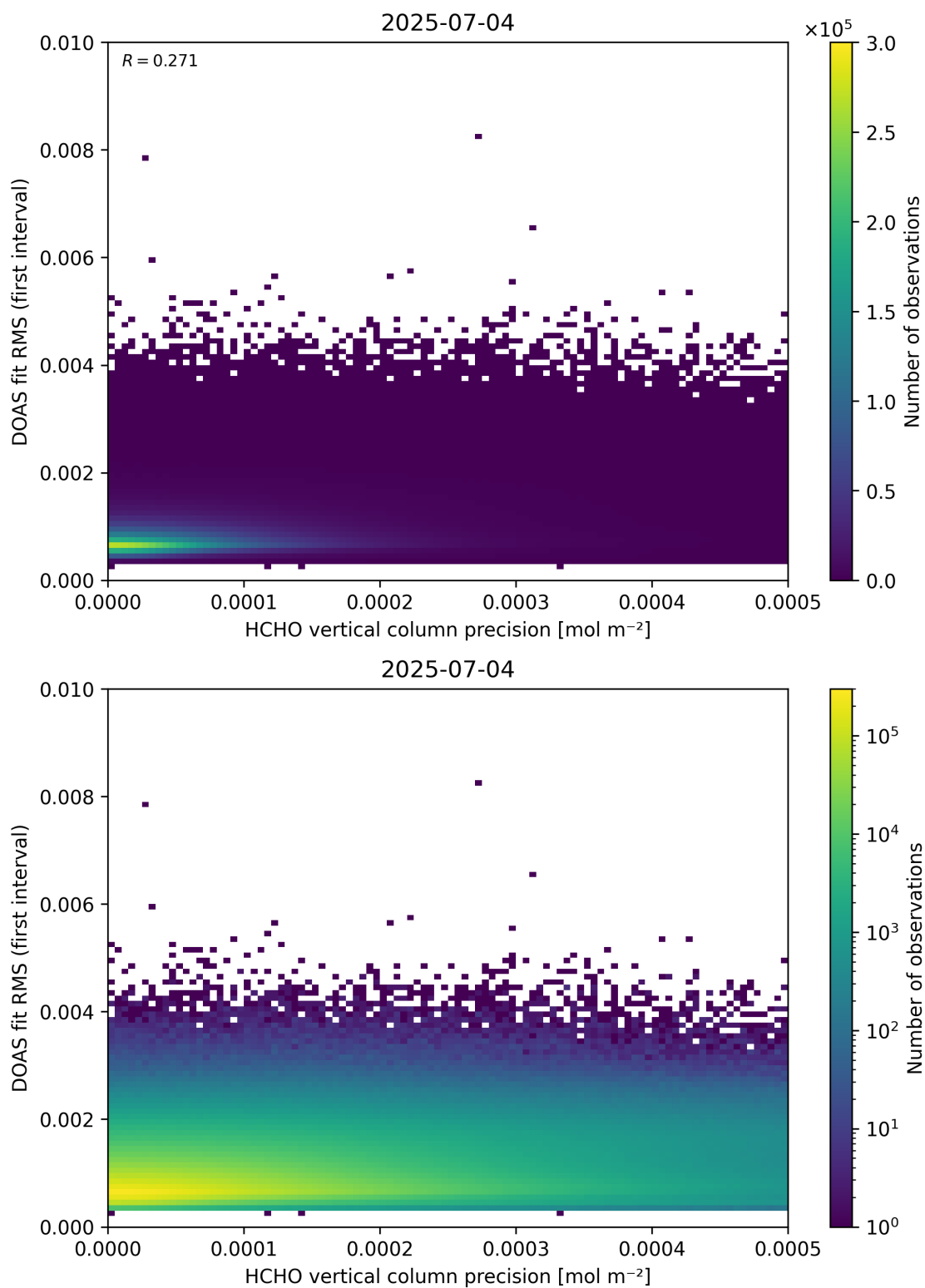
Figure 136: Scatter density plot of “HCHO vertical column precision” against “DOAS fit RMS (first interval)” for 2025-07-03 to 2025-07-05.
