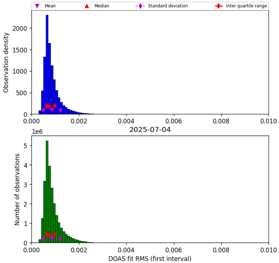
Figure 46: Histogram of “DOAS fit RMS (first interval)” for 2025-07-03 to 2025-07-05
