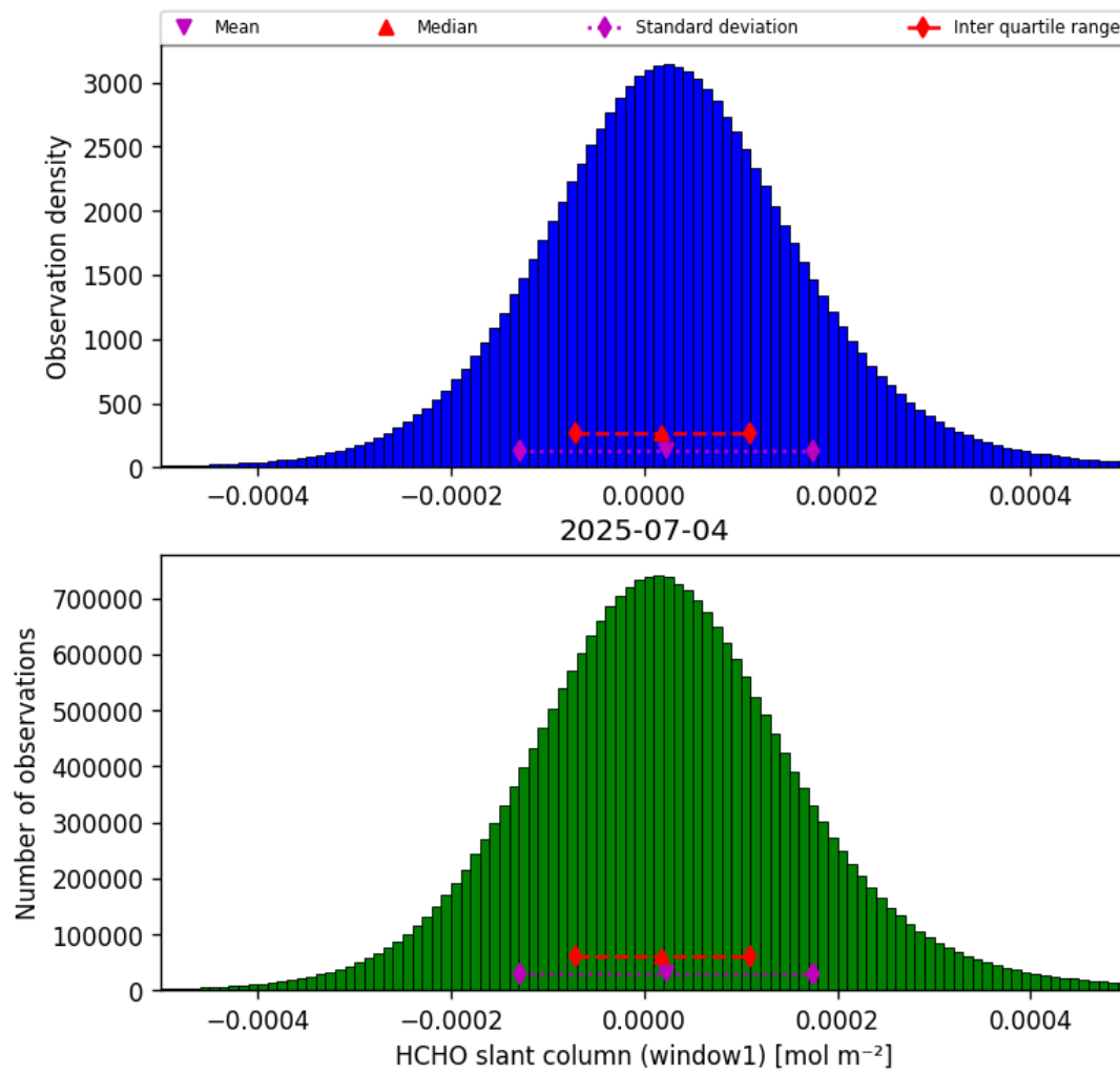
Figure 38: Histogram of “HCHO slant column (window1)” for 2025-07-03 to 2025-07-05
