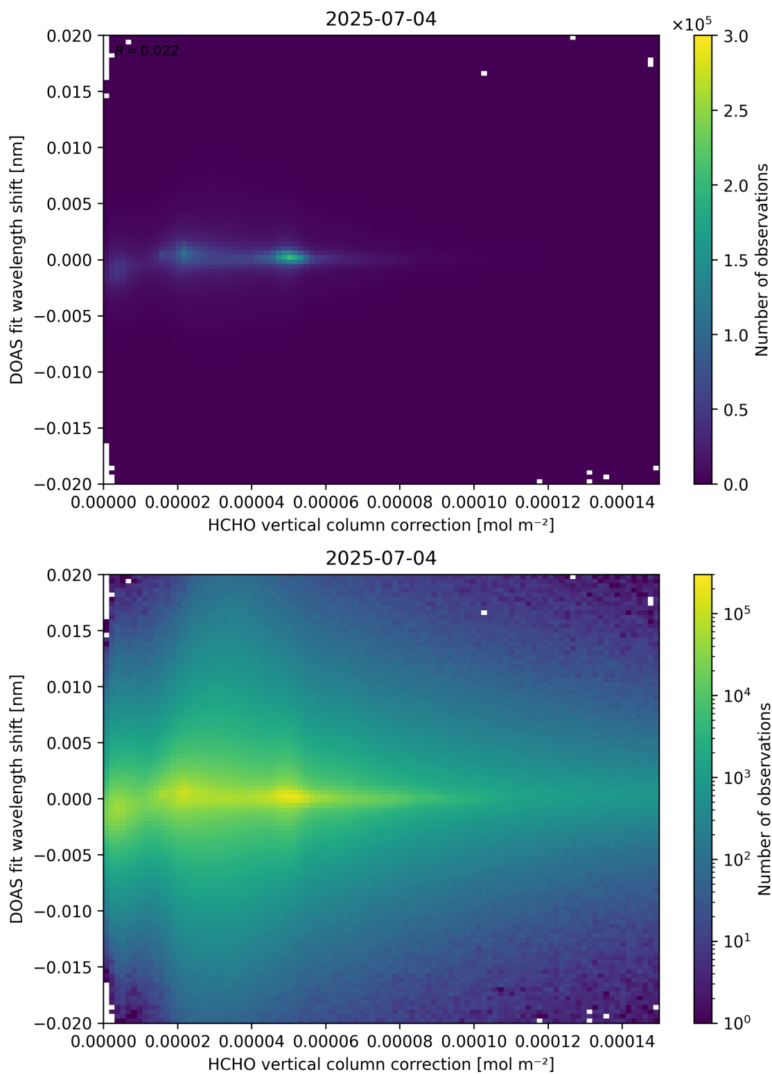
Figure 113: Scatter density plot of “HCHO vertical column correction” against “DOAS fit wavelength shift” for 2025-07-03 to 2025-07-05.
