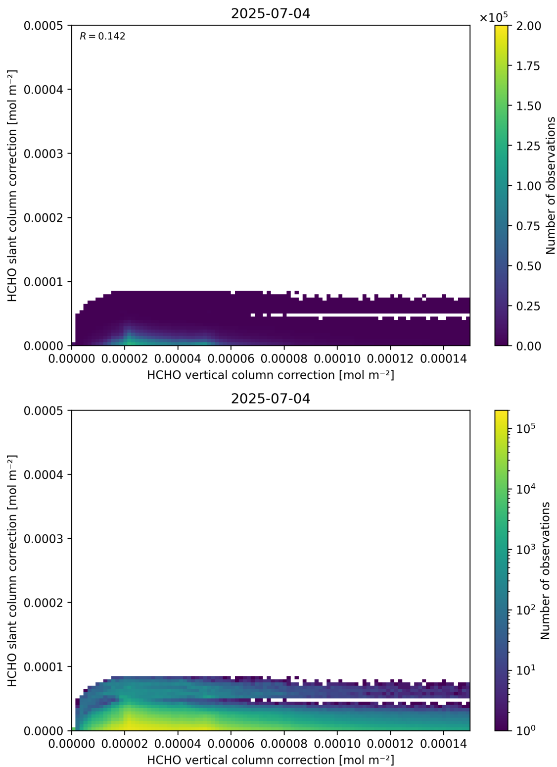
Figure 117: Scatter density plot of “HCHO vertical column correction” against “HCHO slant column correction” for 2025-07-03 to 2025-07-05.
