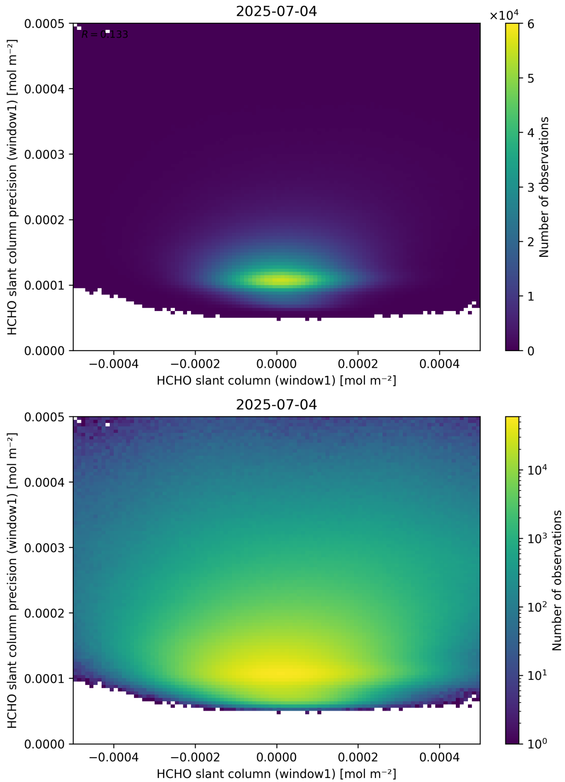
Figure 84: Scatter density plot of “HCHO slant column (window1)” against “HCHO slant column precision (window1)” for 2025-07-03 to 2025-07-05.
