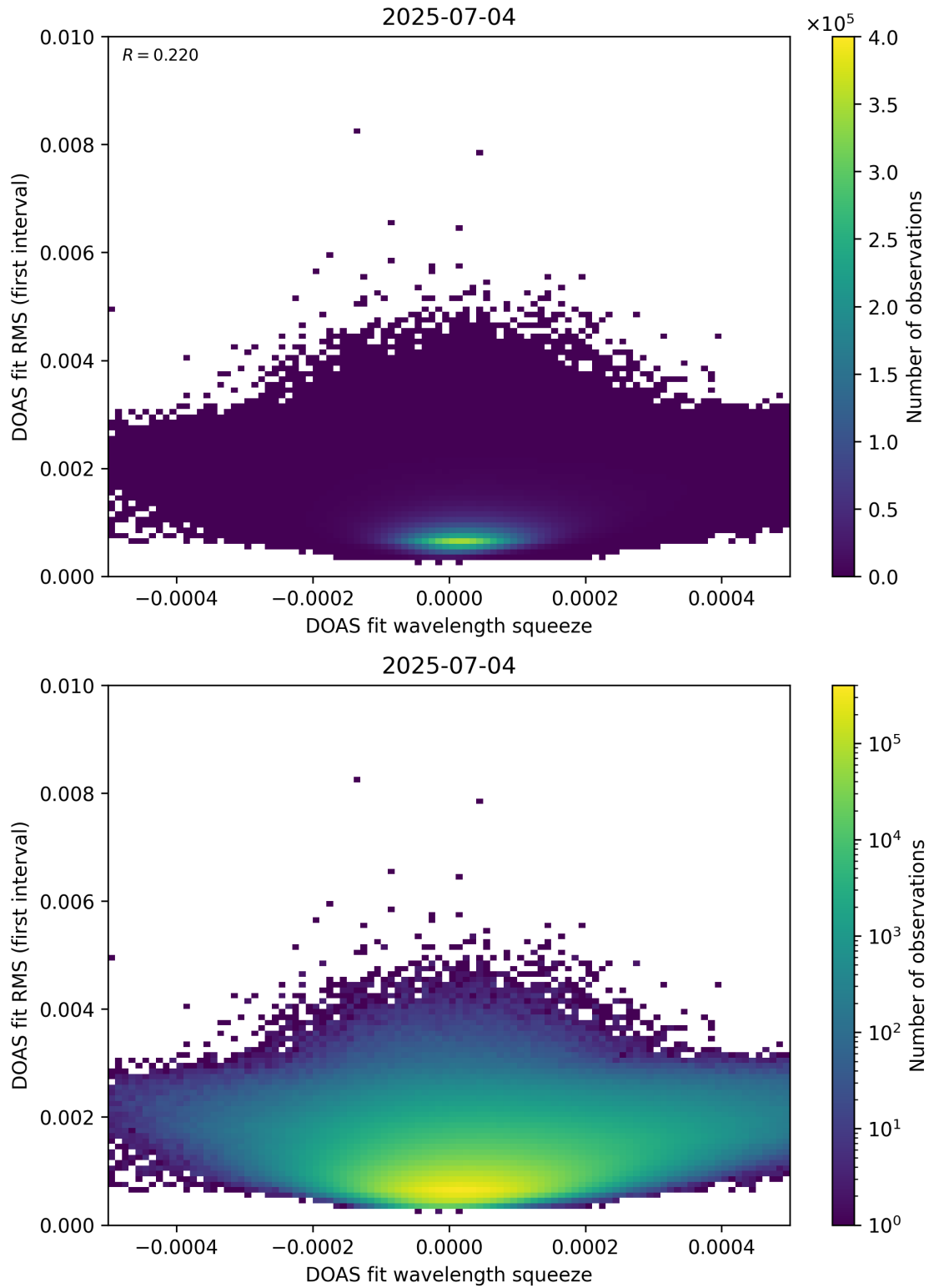
Figure 68: Scatter density plot of “DOAS fit wavelength squeeze” against “DOAS fit RMS (first interval)” for 2025-07-03 to 2025-07-05.
