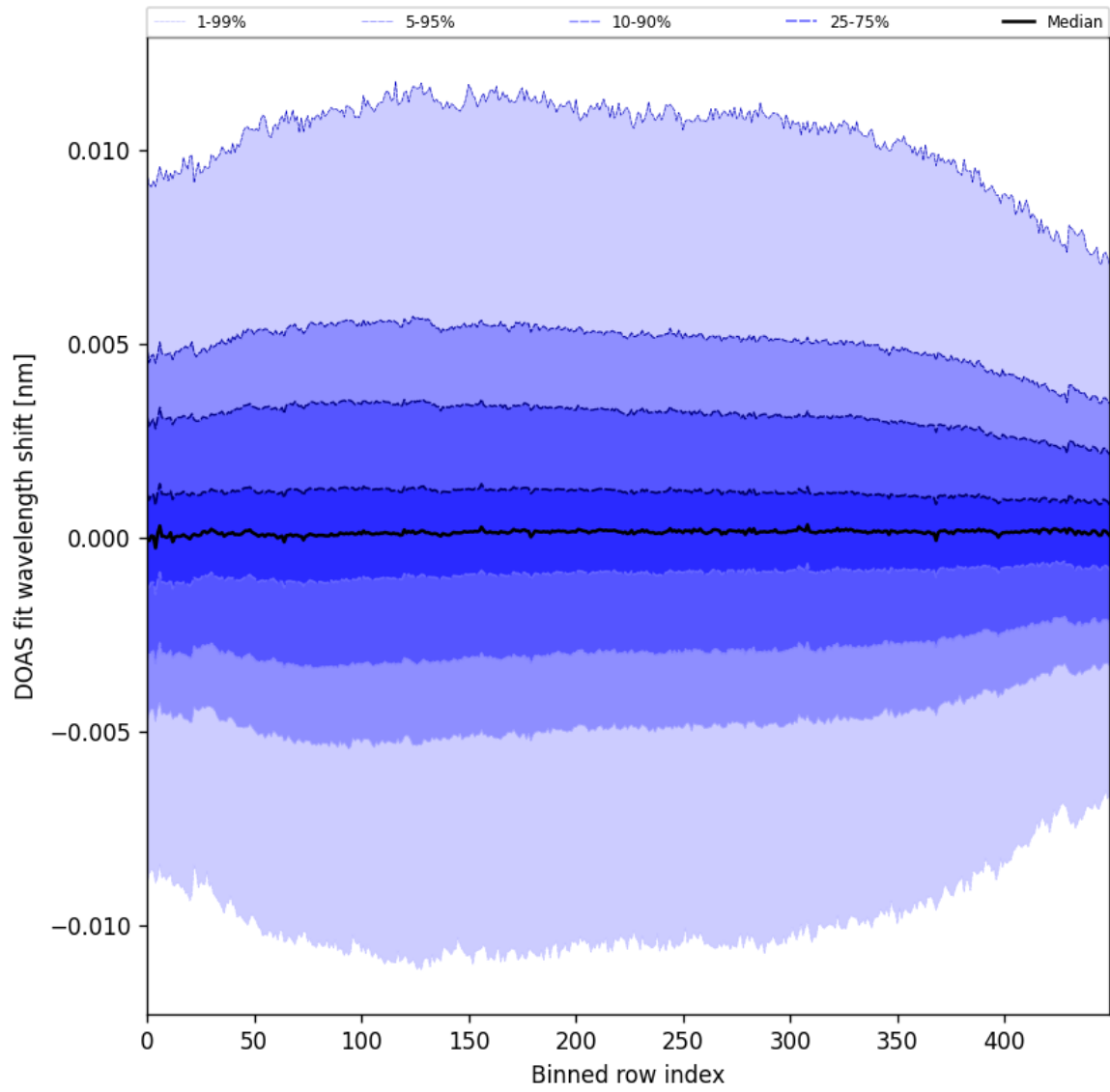
Figure 58: Along track statistics of “DOAS fit wavelength shift” for 2025-07-03 to 2025-07-05
