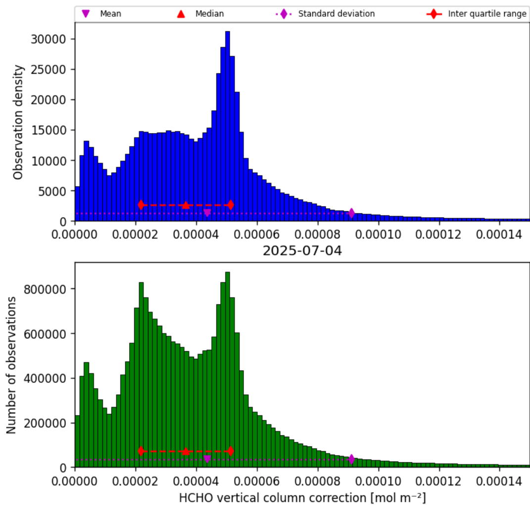
Figure 37: Histogram of “HCHO vertical column correction” for 2025-07-03 to 2025-07-05
