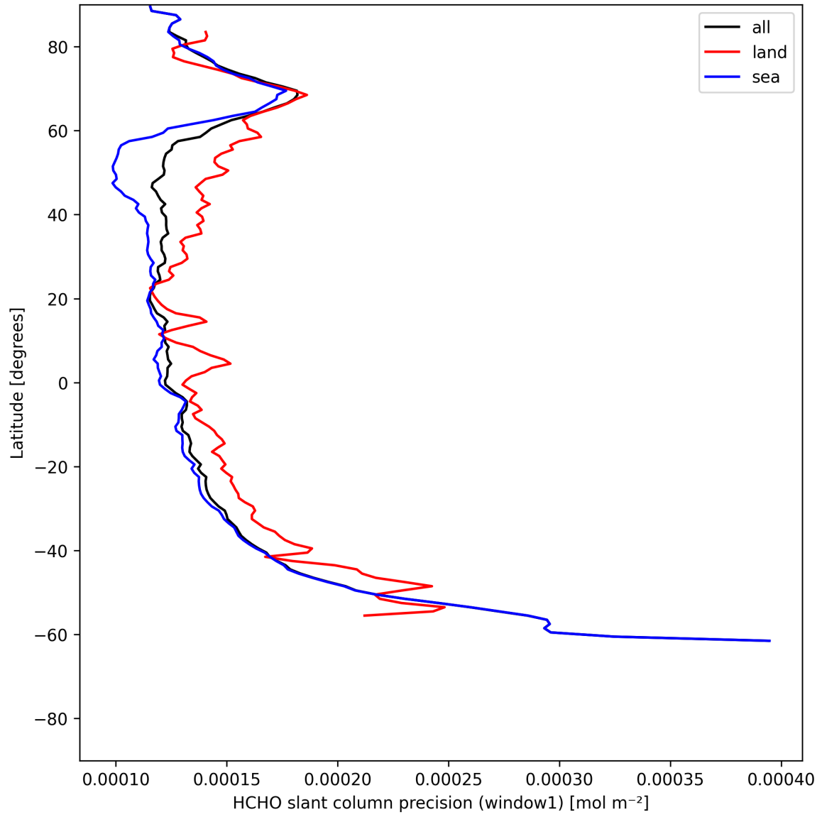
Figure 25: Zonal average of “HCHO slant column precision (window1)” for 2025-07-03 to 2025-07-05.
