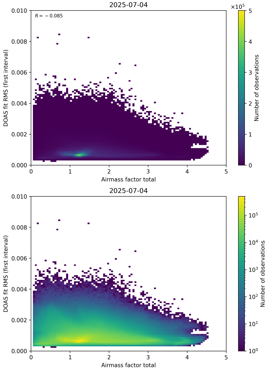
Figure 97: Scatter density plot of “Airmass factor total” against “DOAS fit RMS (first interval)” for 2025-07-03 to 2025-07-05.
