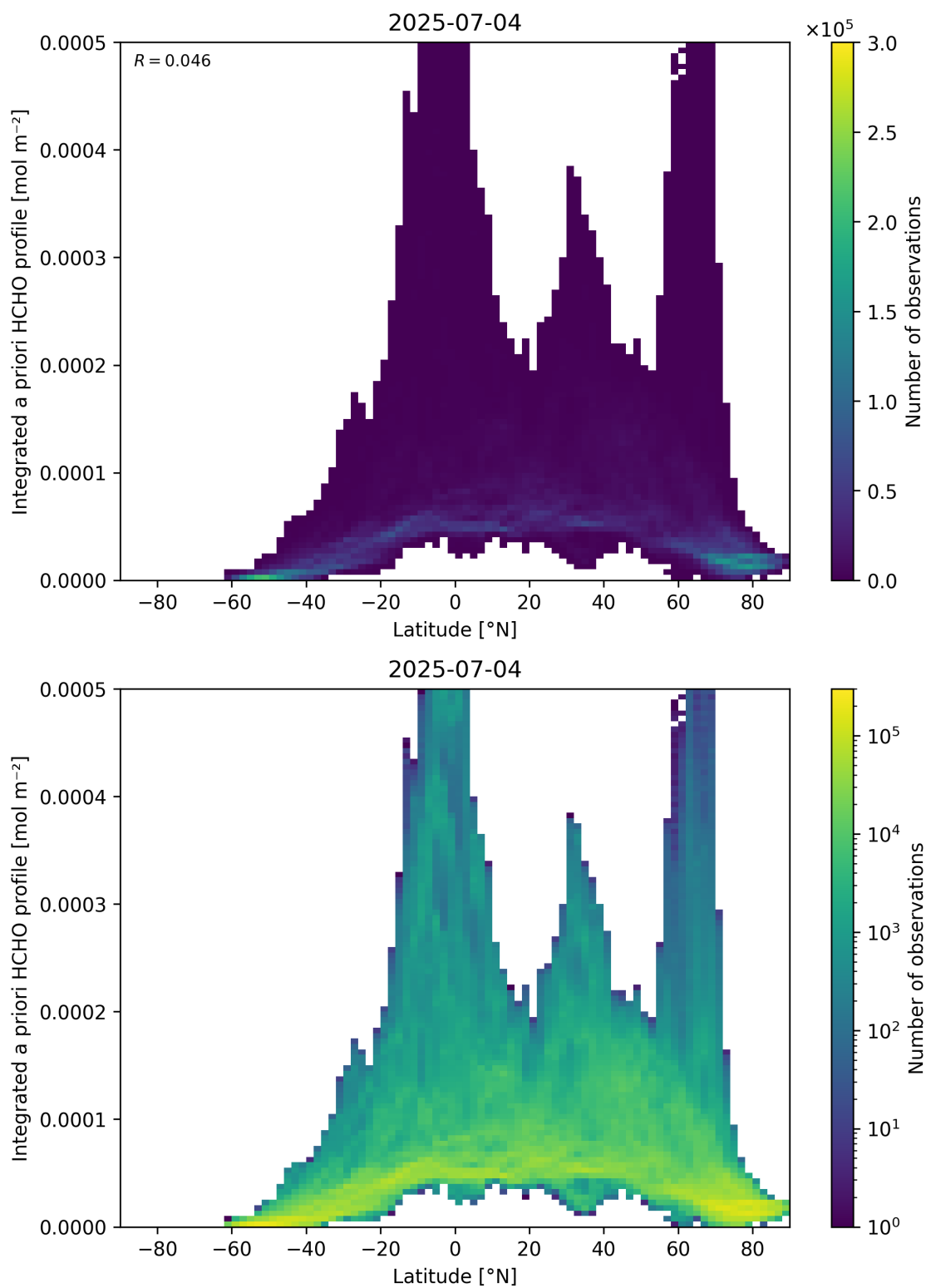
Figure 166: Scatter density plot of “Latitude” against “Integrated a priori HCHO profile” for 2025-07-03 to 2025-07-05.
