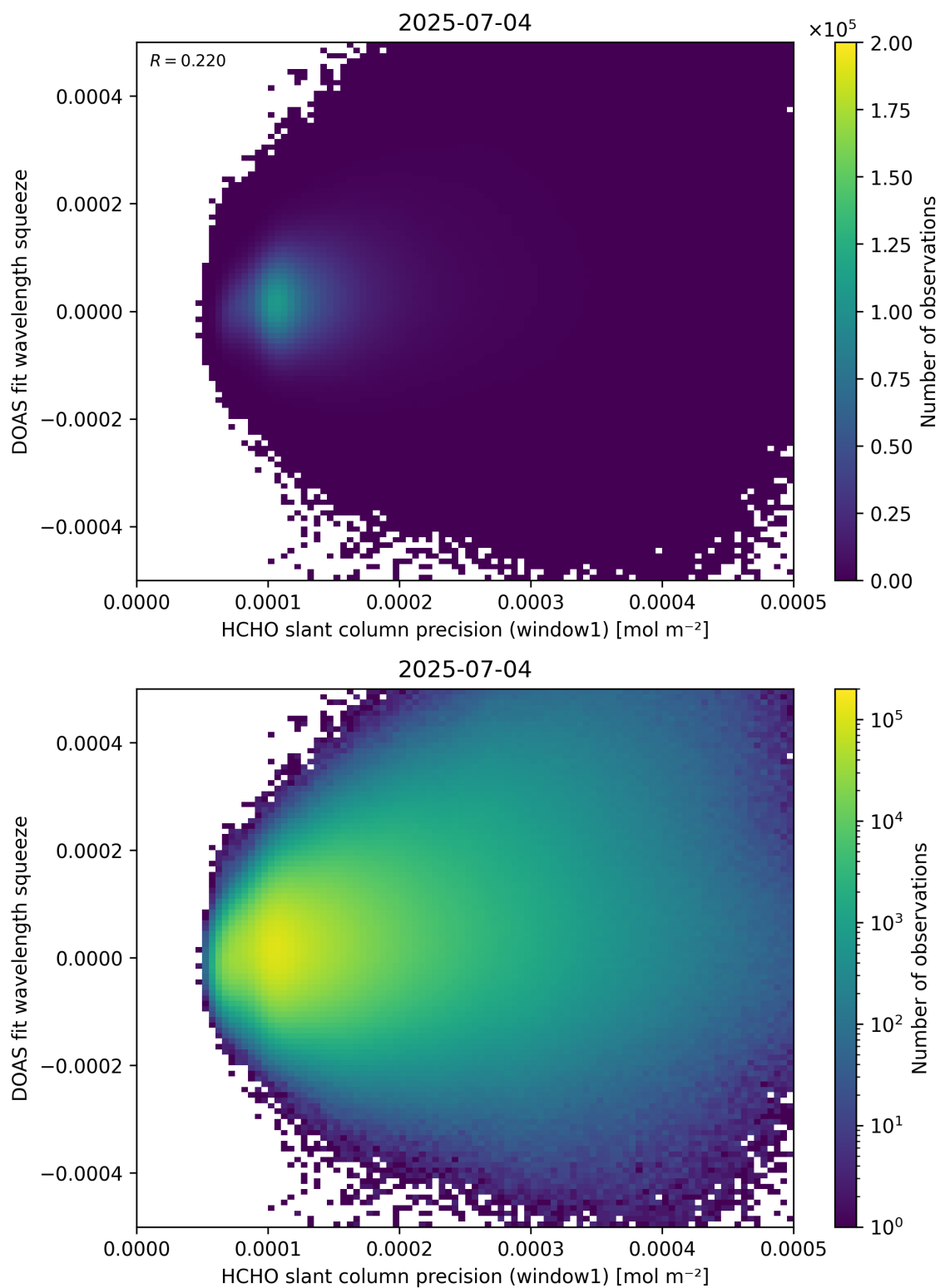
Figure 90: Scatter density plot of “HCHO slant column precision (window1)” against “DOAS fit wavelength squeeze” for 2025-07-03 to 2025-07-05.
