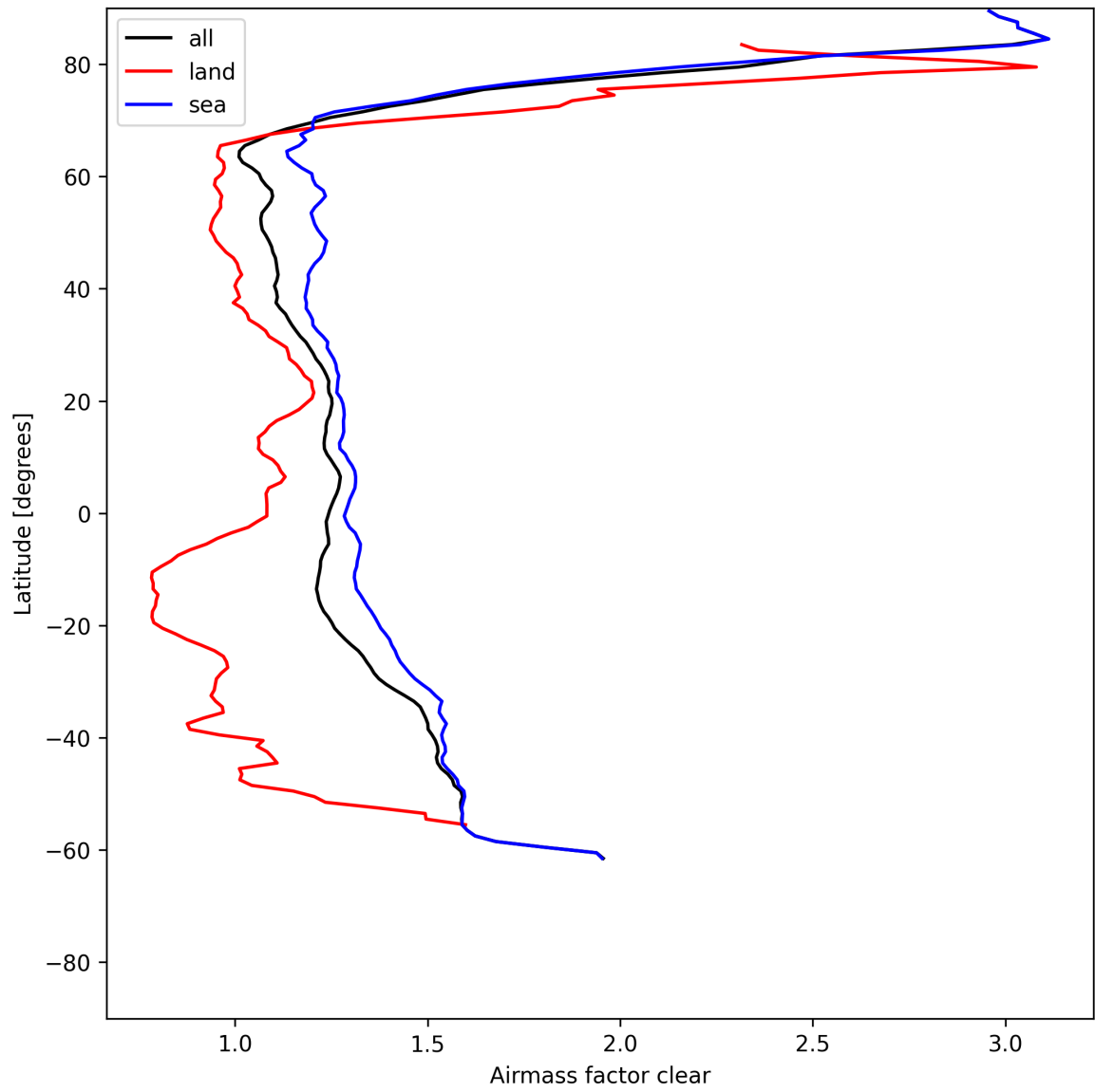
Figure 28: Zonal average of “Airmass factor clear” for 2025-07-03 to 2025-07-05.
