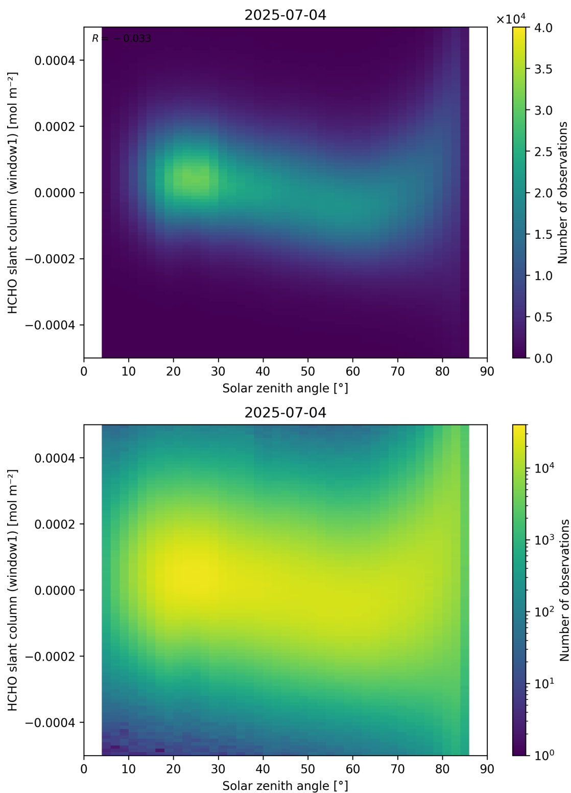
Figure 173: Scatter density plot of “Solar zenith angle” against “HCHO slant column (window1)” for 2025-07-03 to 2025-07-05.
