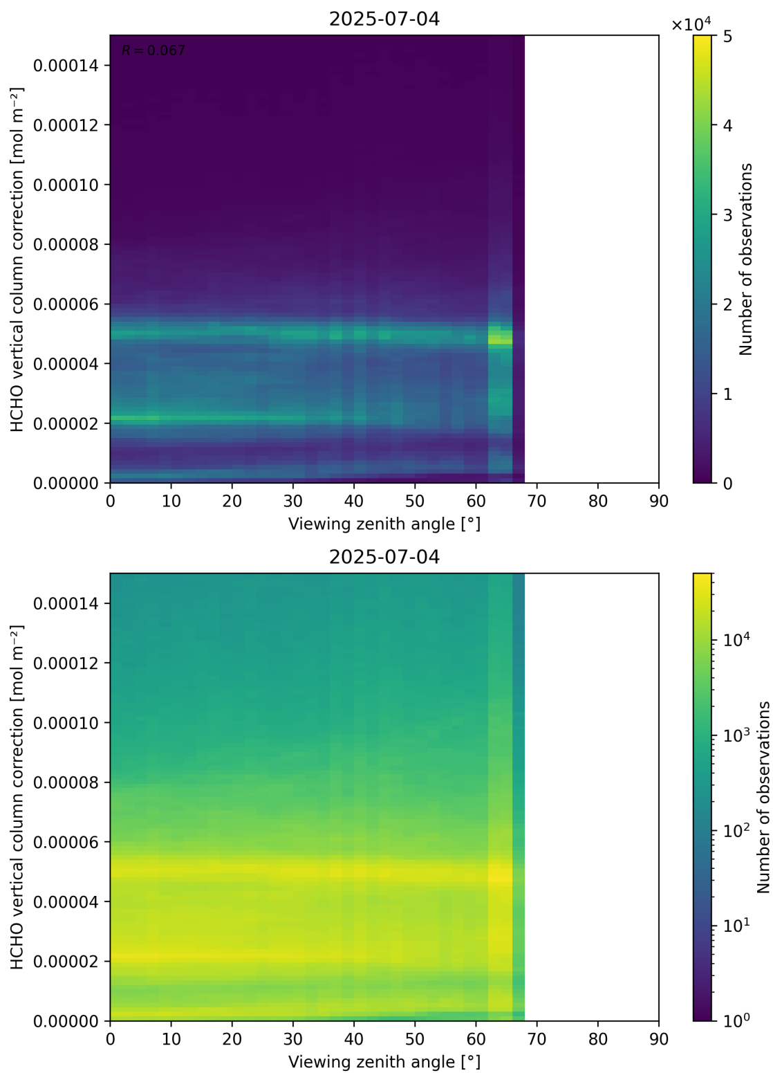
Figure 193: Scatter density plot of “Viewing zenith angle” against “HCHO vertical column correction” for 2025-07-03 to 2025-07-05.
