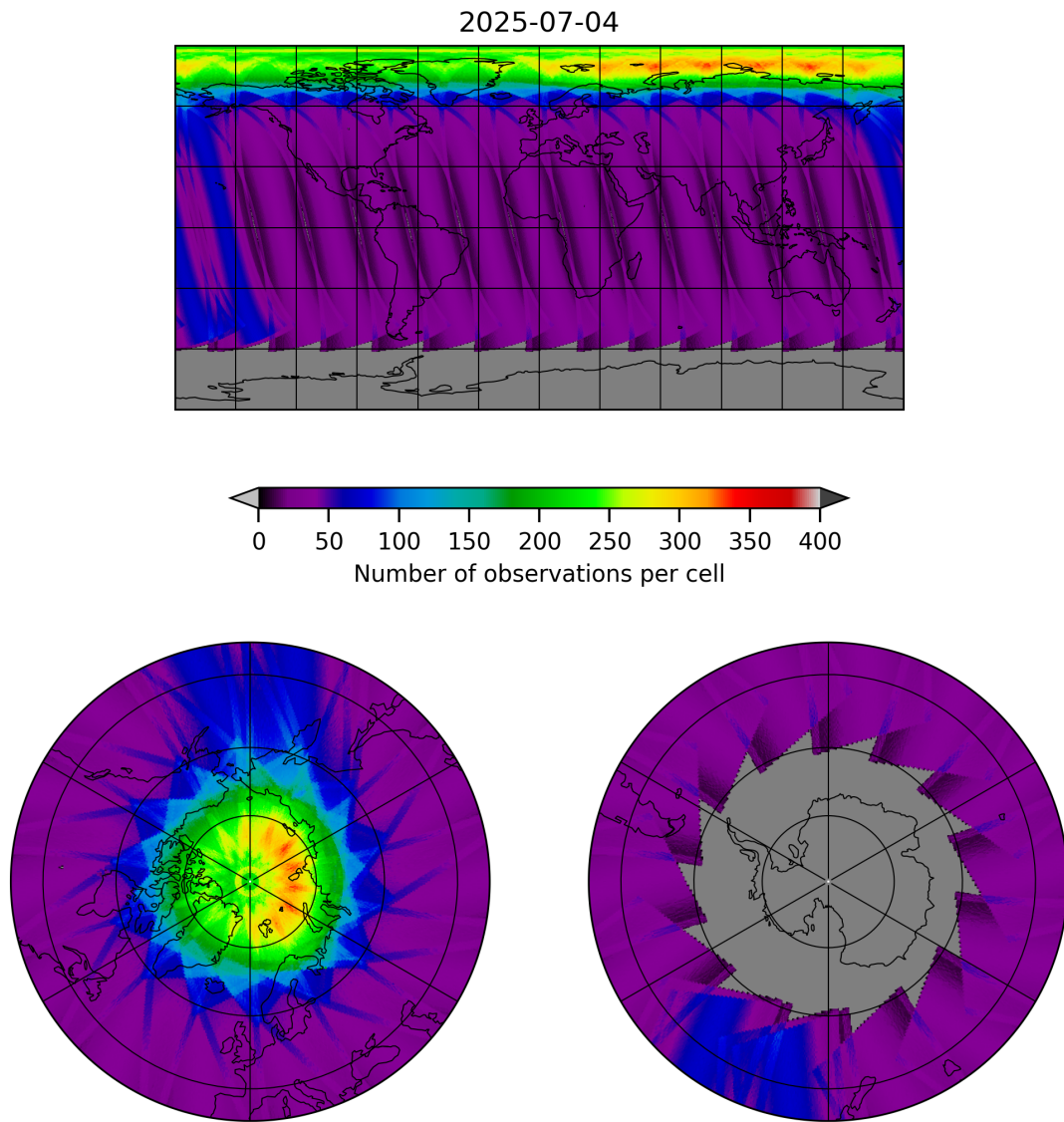
Figure 19: Map of the number of observations for 2025-07-03 to 2025-07-05
