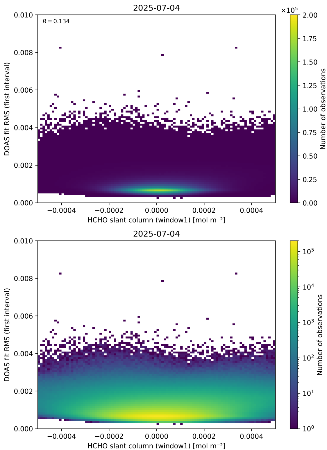
Figure 78: Scatter density plot of “HCHO slant column (window1)” against “DOAS fit RMS (first interval)” for 2025-07-03 to 2025-07-05.
