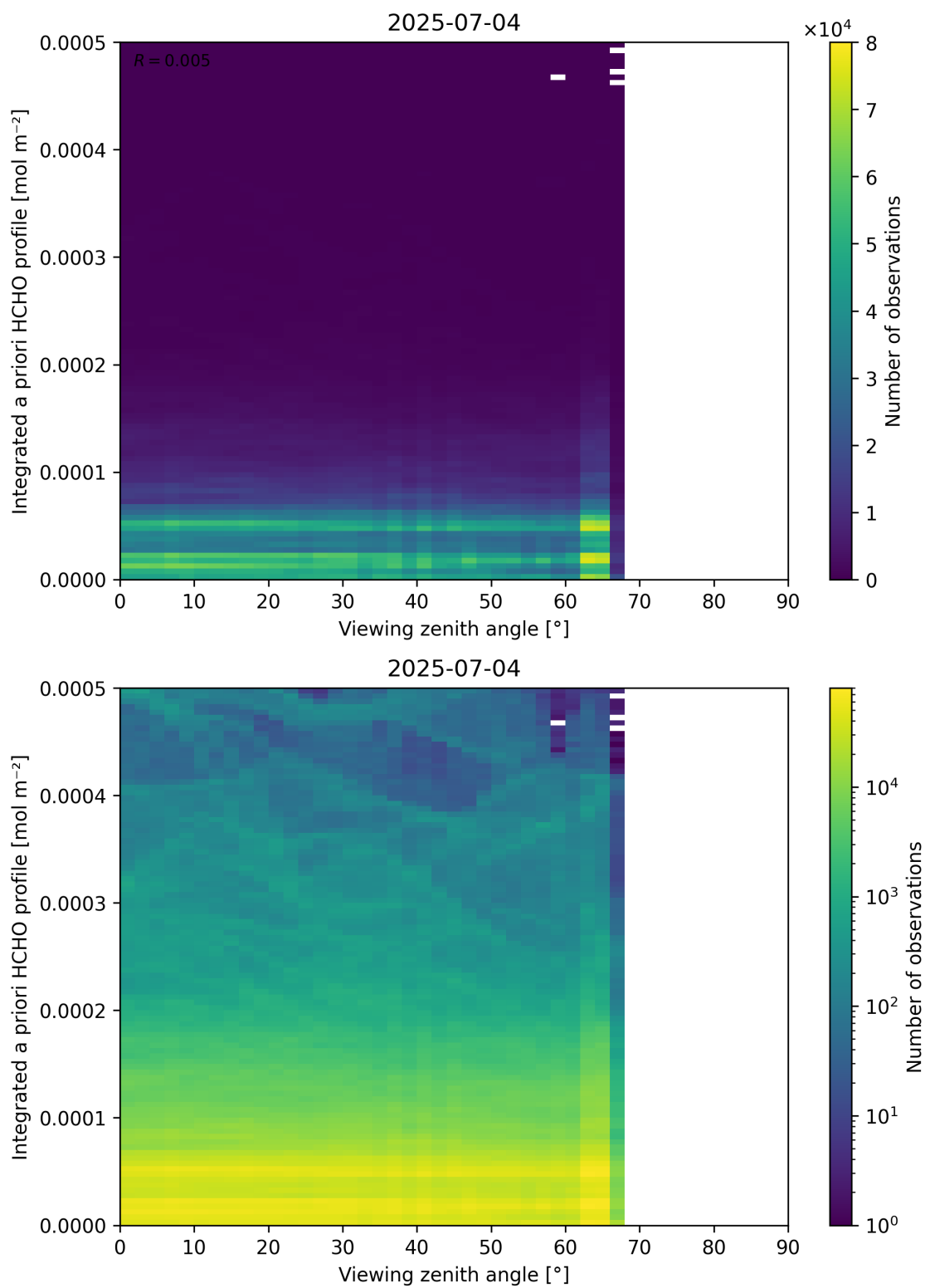
Figure 195: Scatter density plot of “Viewing zenith angle” against “Integrated a priori HCHO profile” for 2025-07-03 to 2025-07-05.
