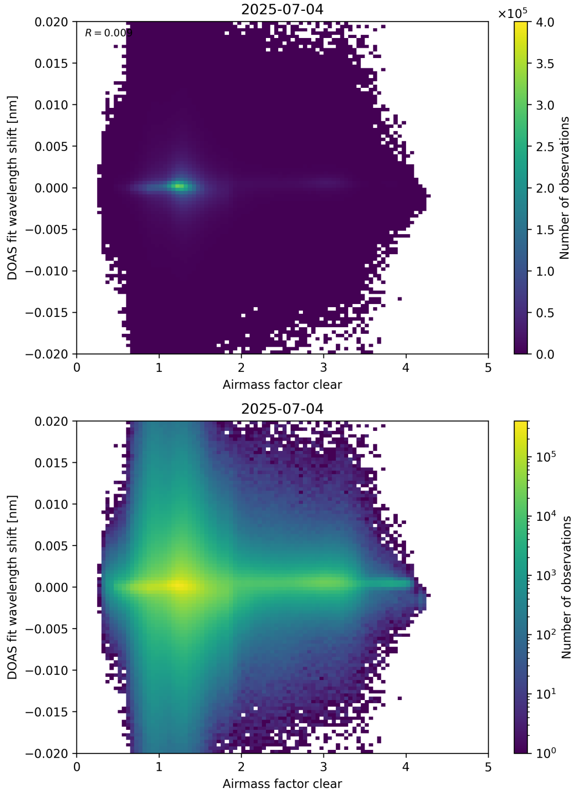
Figure 72: Scatter density plot of “Airmass factor clear” against “DOAS fit wavelength shift” for 2025-07-03 to 2025-07-05.
