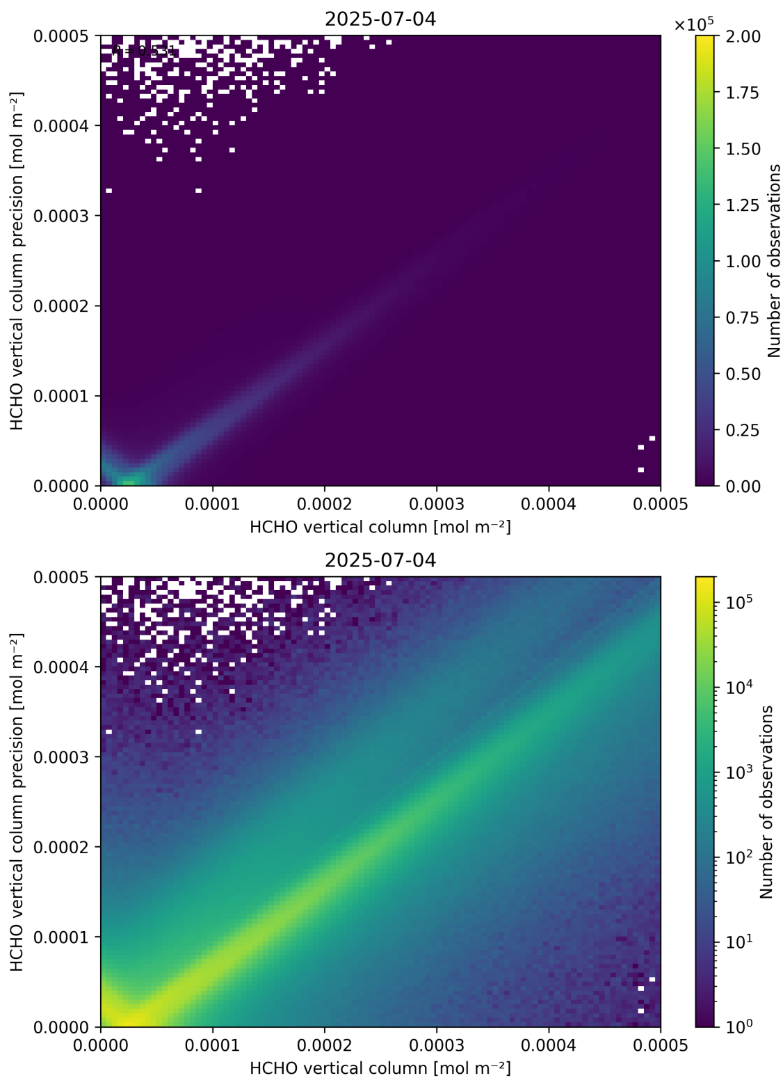
Figure 134: Scatter density plot of “HCHO vertical column” against “HCHO vertical column precision” for 2025-07-03 to 2025-07-05.
