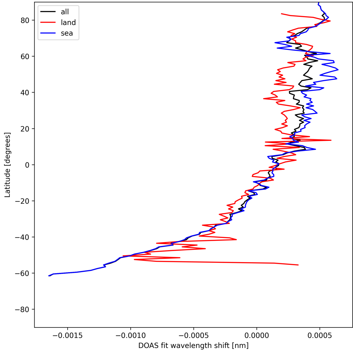
Figure 30: Zonal average of “DOAS fit wavelength shift” for 2025-07-03 to 2025-07-05.
