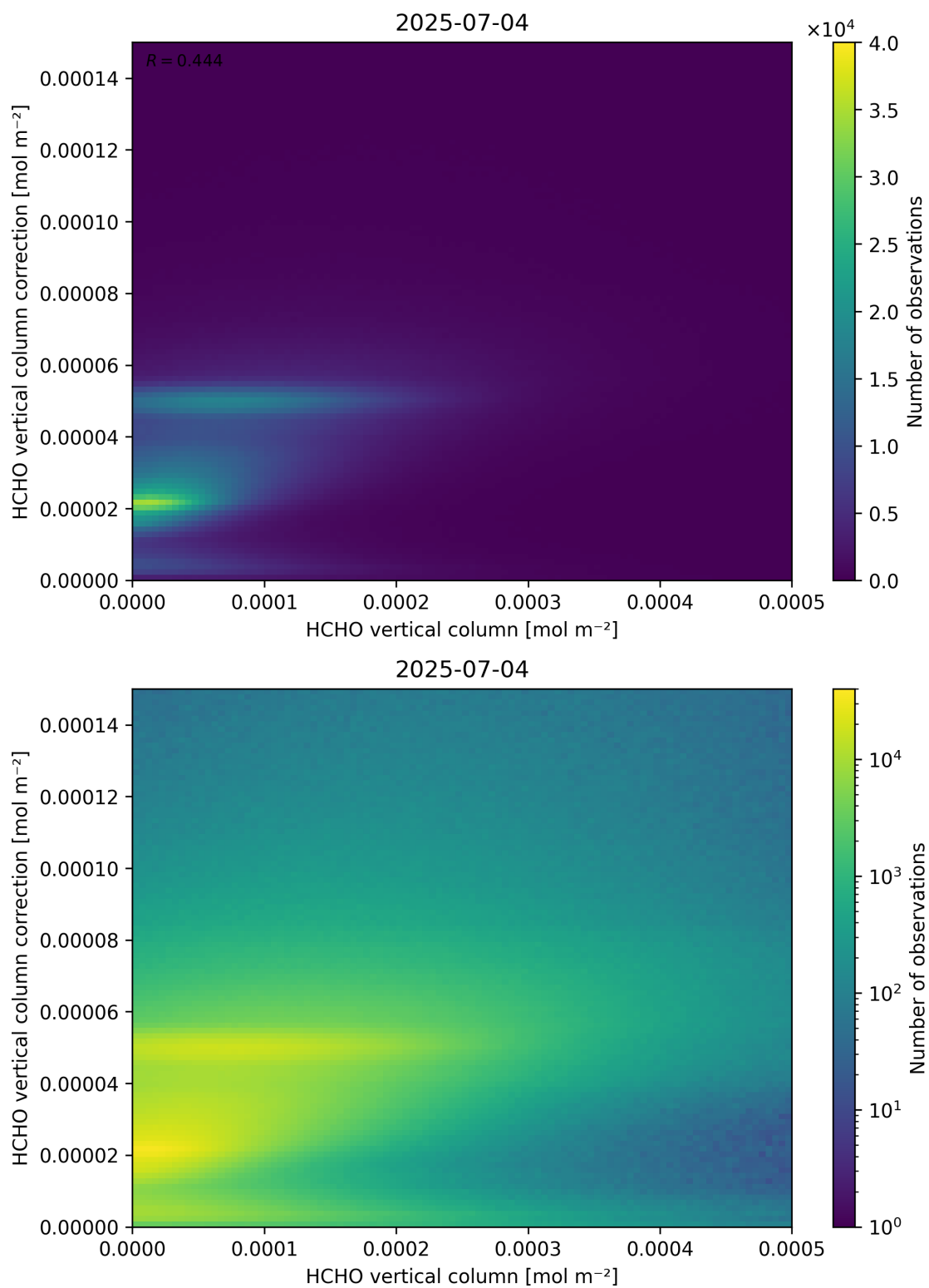
Figure 133: Scatter density plot of “HCHO vertical column” against “HCHO vertical column correction” for 2025-07-03 to 2025-07-05.
