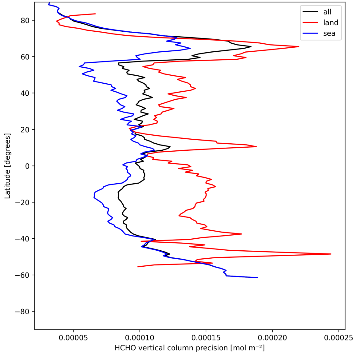
Figure 22: Zonal average of “HCHO vertical column precision” for 2025-07-03 to 2025-07-05.
