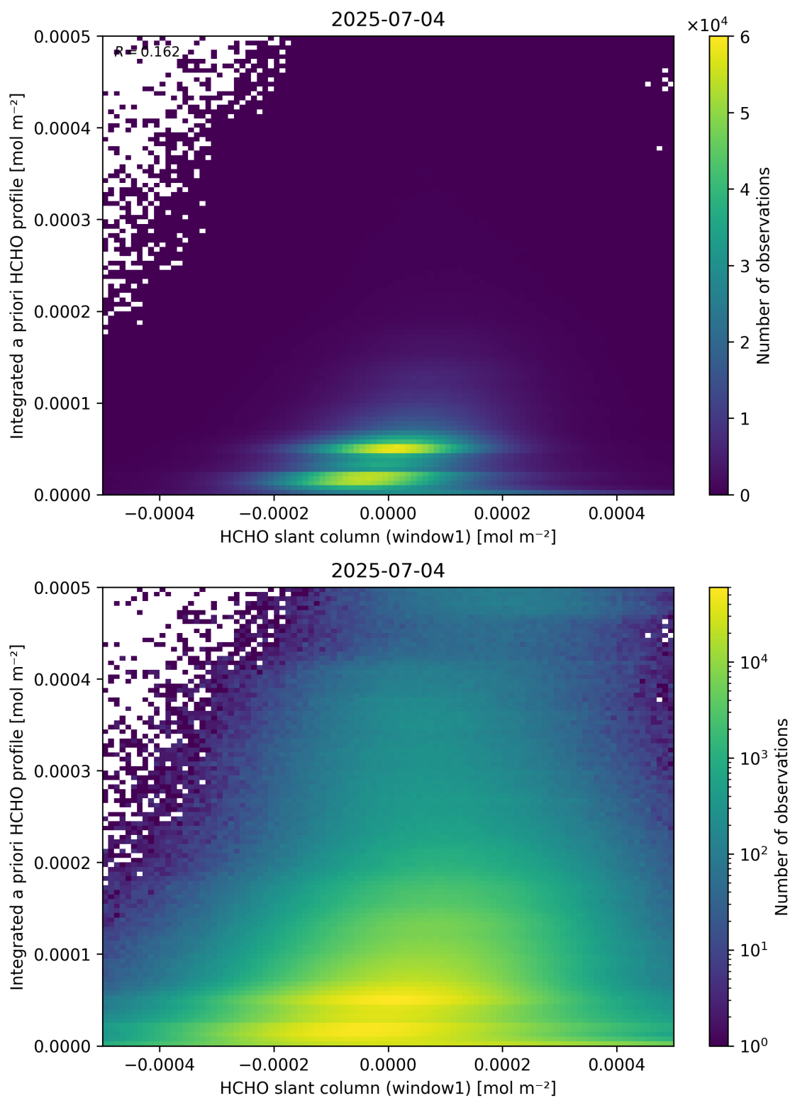
Figure 87: Scatter density plot of “HCHO slant column (window1)” against “Integrated a priori HCHO profile” for 2025-07-03 to 2025-07-05.
