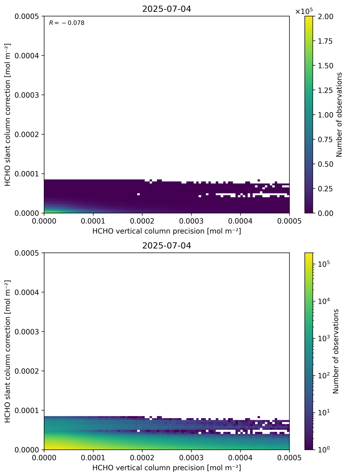
Figure 141: Scatter density plot of “HCHO vertical column precision” against “HCHO slant column correction” for 2025-07-03 to 2025-07-05.
