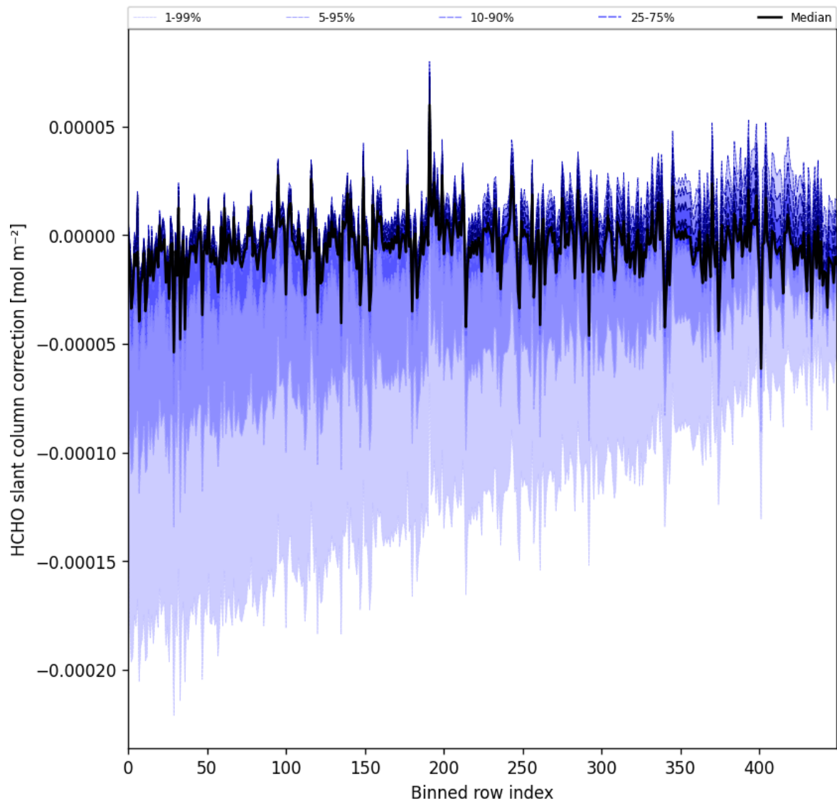
Figure 61: Along track statistics of “HCHO slant column correction” for 2025-07-03 to 2025-07-05
