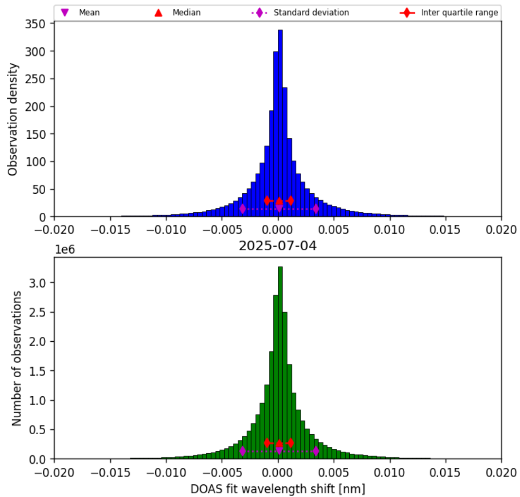
Figure 44: Histogram of “DOAS fit wavelength shift” for 2025-07-03 to 2025-07-05
