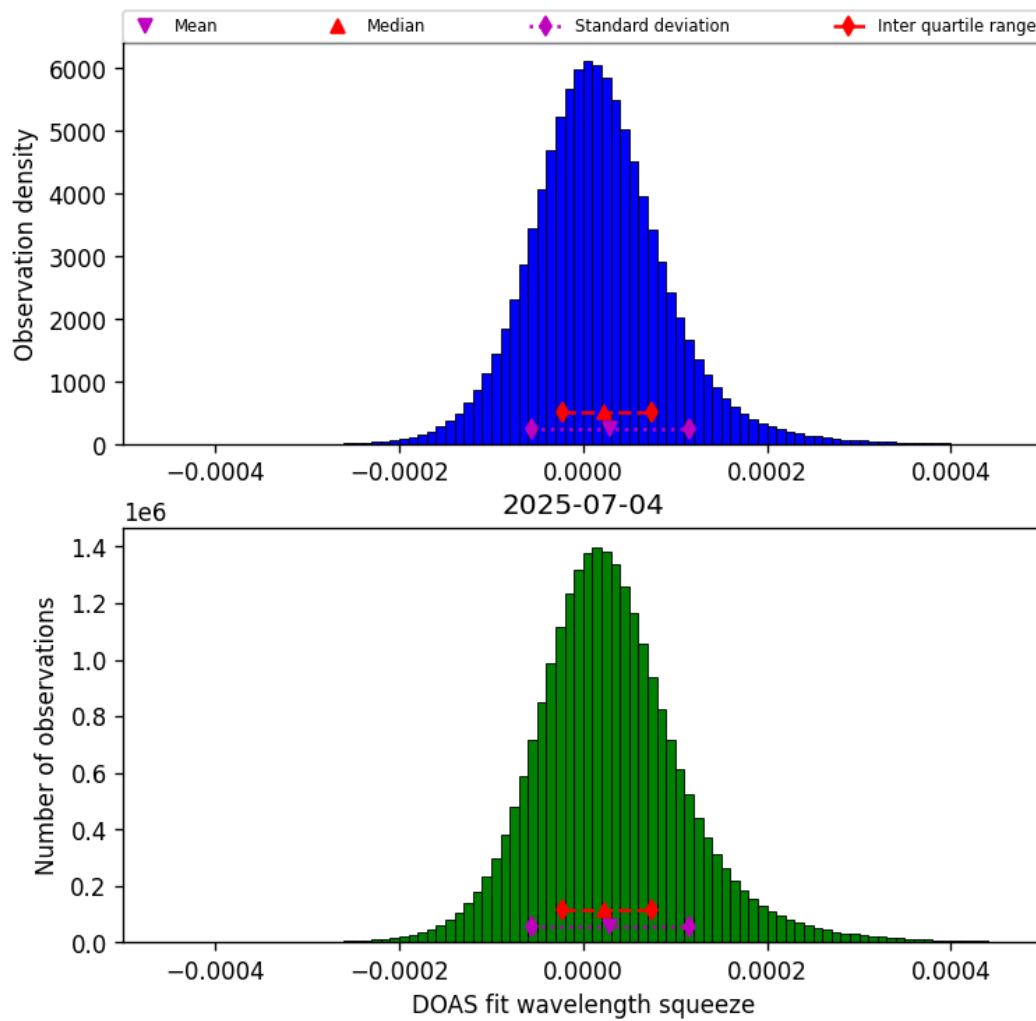
Figure 45: Histogram of “DOAS fit wavelength squeeze” for 2025-07-03 to 2025-07-05
