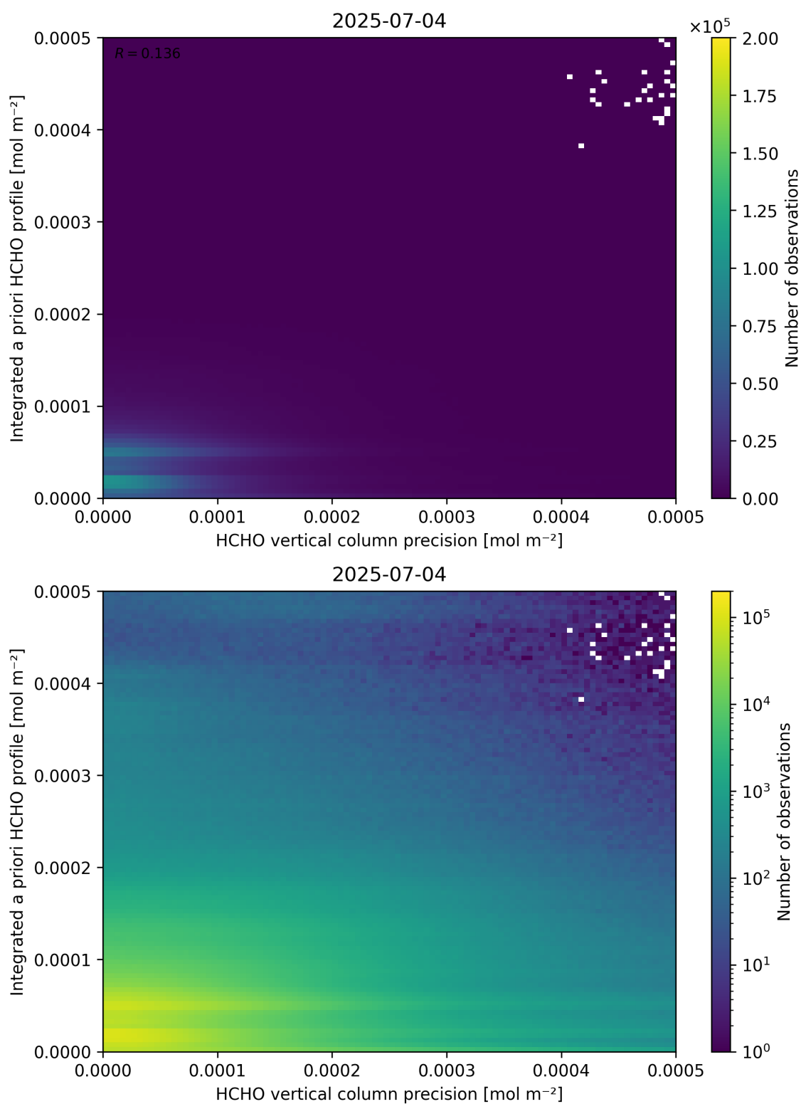
Figure 147: Scatter density plot of “HCHO vertical column precision” against “Integrated a priori HCHO profile” for 2025-07-03 to 2025-07-05.
