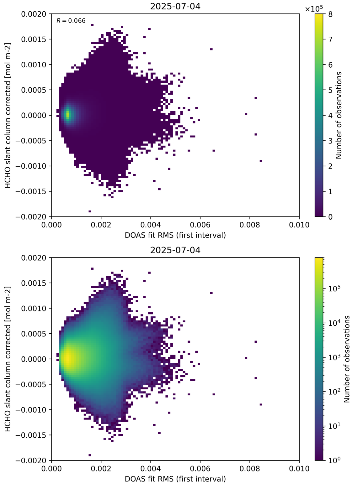
Figure 62: Scatter density plot of “DOAS fit RMS (first interval)” against “HCHO slant column corrected” for 2025-07-03 to 2025-07-05.
