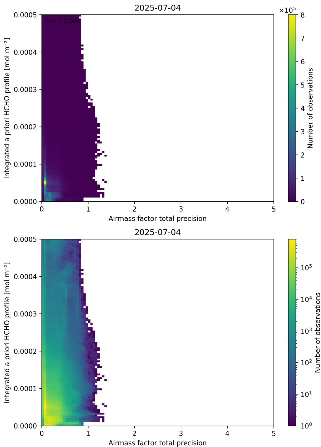
Figure 111: Scatter density plot of “Airmass factor total precision” against “Integrated a priori HCHO profile” for 2025-07-03 to 2025-07-05.
