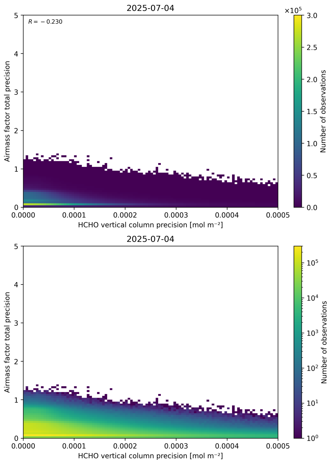
Figure 145: Scatter density plot of “HCHO vertical column precision” against “Airmass factor total precision” for 2025-07-03 to 2025-07-05.
