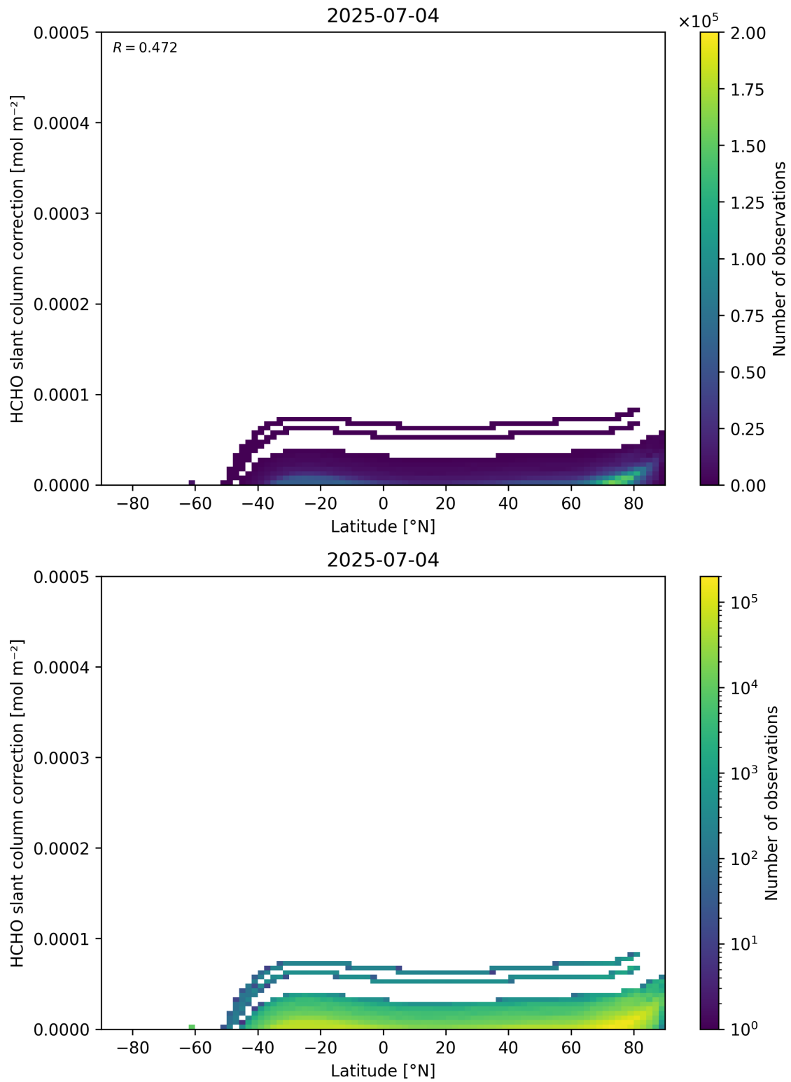
Figure 158: Scatter density plot of “Latitude” against “HCHO slant column correction” for 2025-07-03 to 2025-07-05.
