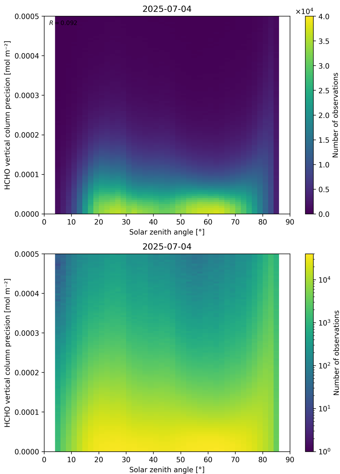
Figure 179: Scatter density plot of “Solar zenith angle” against “HCHO vertical column precision” for 2025-07-03 to 2025-07-05.
