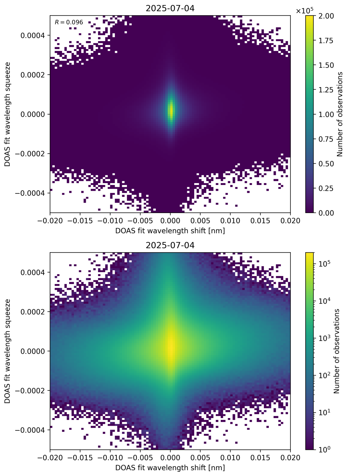
Figure 65: Scatter density plot of “DOAS fit wavelength shift” against “DOAS fit wavelength squeeze” for 2025-07-03 to 2025-07-05.
