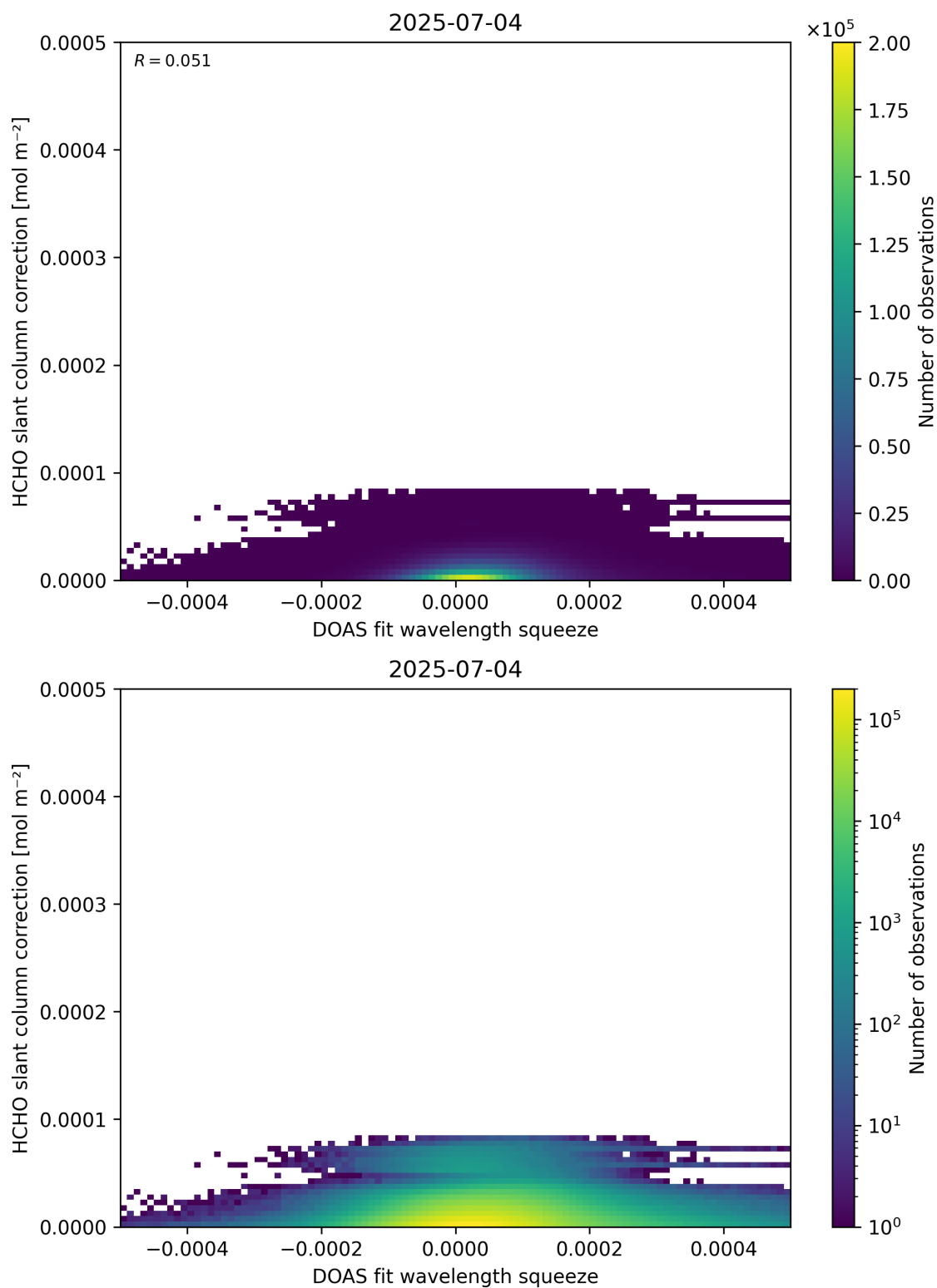
Figure 70: Scatter density plot of “DOAS fit wavelength squeeze” against “HCHO slant column correction” for 2025-07-03 to 2025-07-05.
