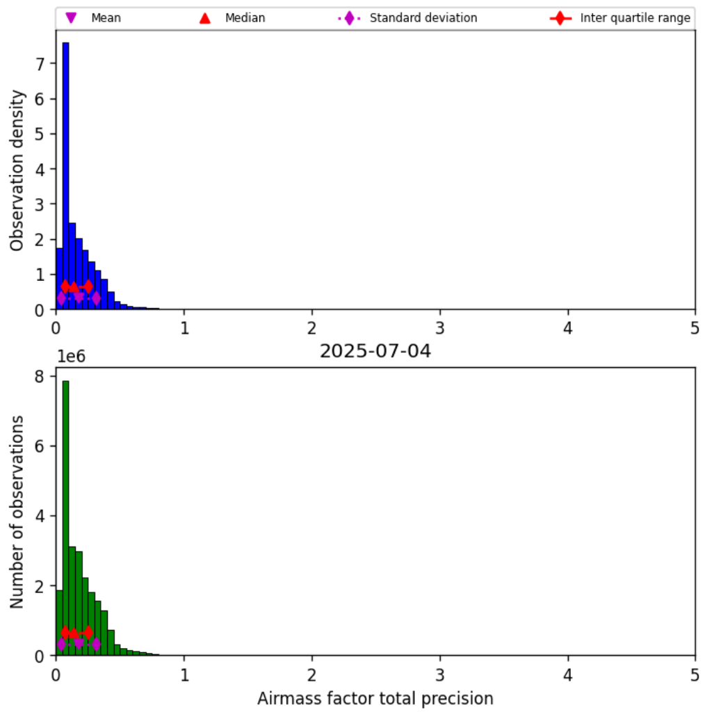
Figure 41: Histogram of “Airmass factor total precision” for 2025-07-03 to 2025-07-05
