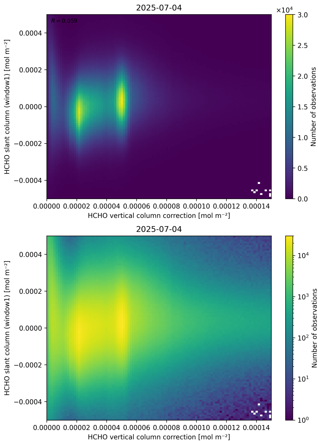
Figure 118: Scatter density plot of “HCHO vertical column correction” against “HCHO slant column (window1)” for 2025-07-03 to 2025-07-05.
