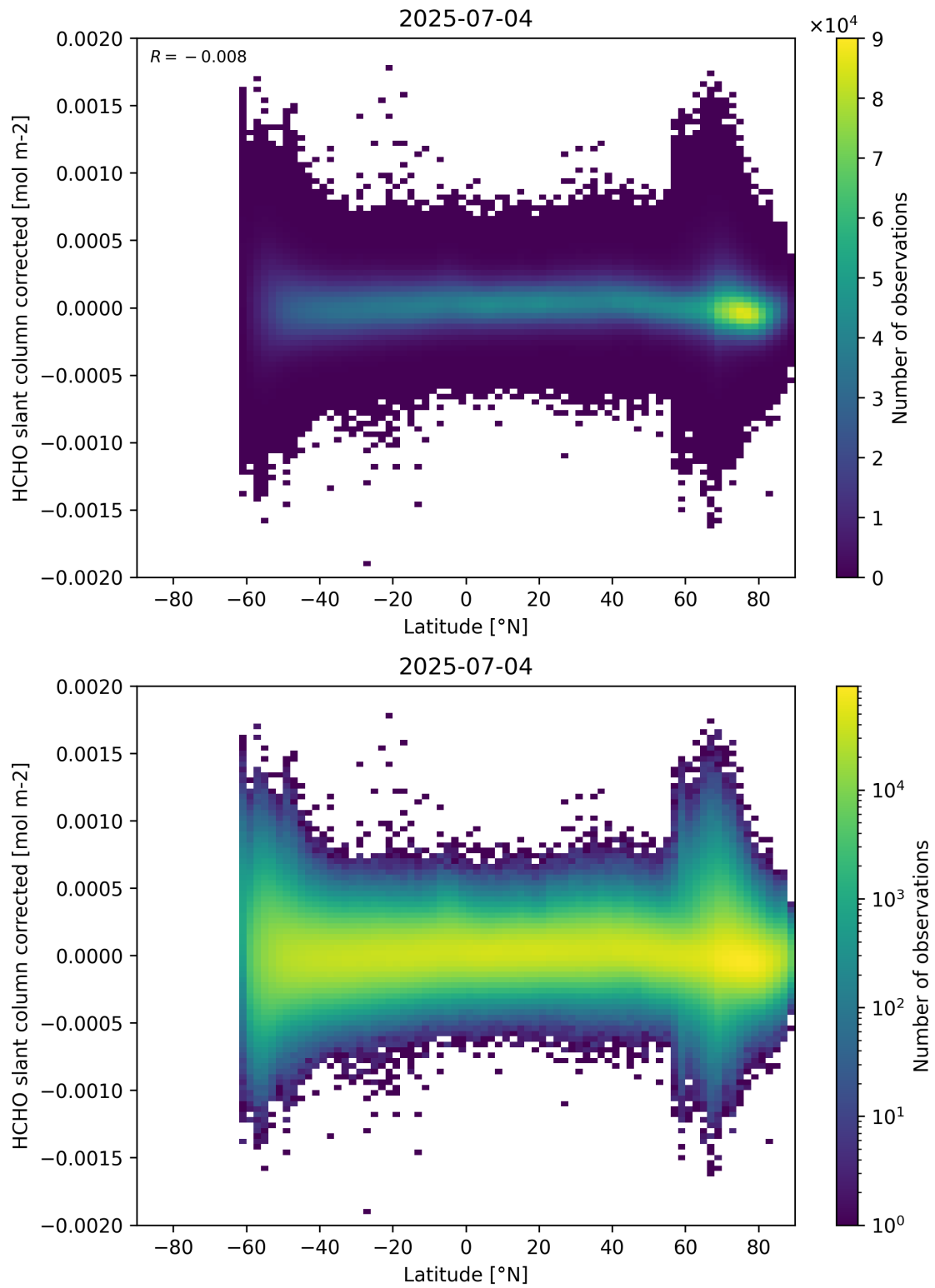
Figure 157: Scatter density plot of “Latitude” against “HCHO slant column corrected” for 2025-07-03 to 2025-07-05.
