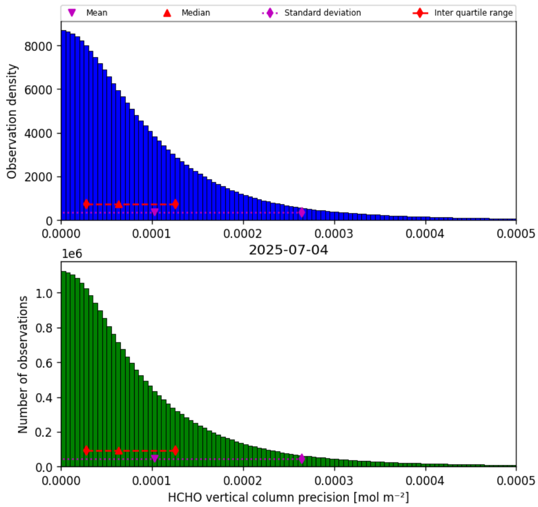
Figure 36: Histogram of “HCHO vertical column precision” for 2025-07-03 to 2025-07-05
