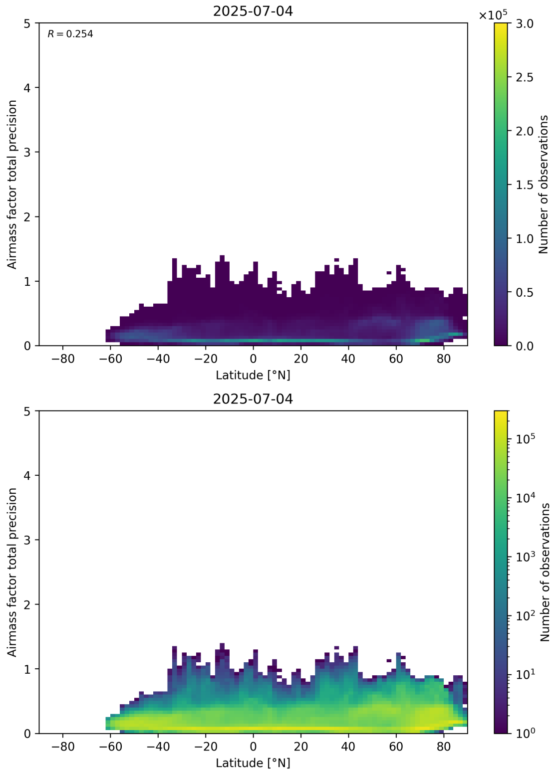
Figure 162: Scatter density plot of “Latitude” against “Airmass factor total precision” for 2025-07-03 to 2025-07-05.
