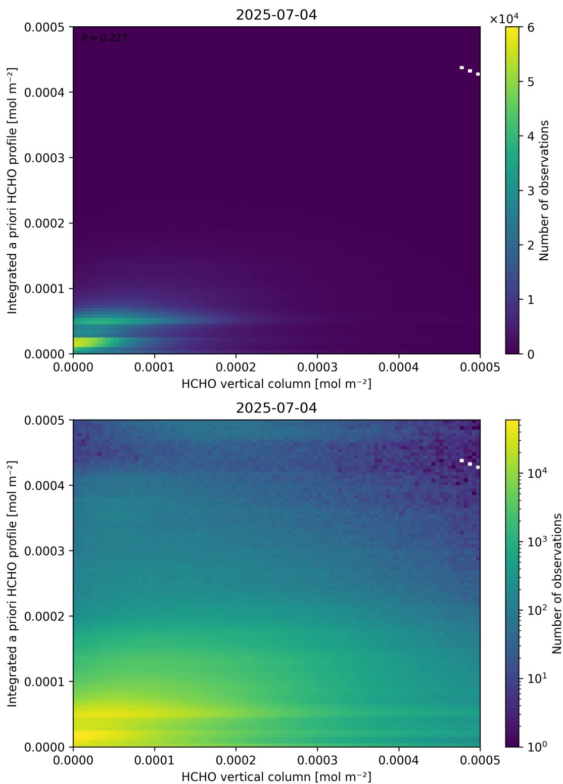
Figure 135: Scatter density plot of “HCHO vertical column” against “Integrated a priori HCHO profile” for 2025-07-03 to 2025-07-05.
