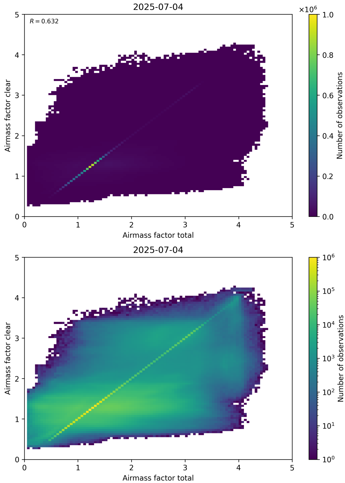
Figure 100: Scatter density plot of “Airmass factor total” against “Airmass factor clear” for 2025-07-03 to 2025-07-05.
