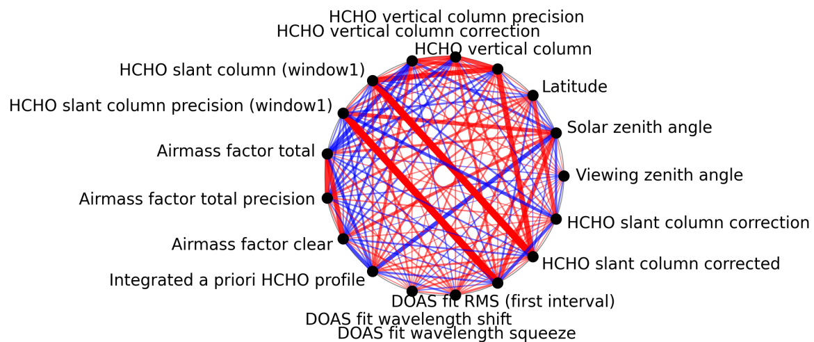
Figure 1: Map of correlation graph for 2025-07-03 to 2025-07-05.
