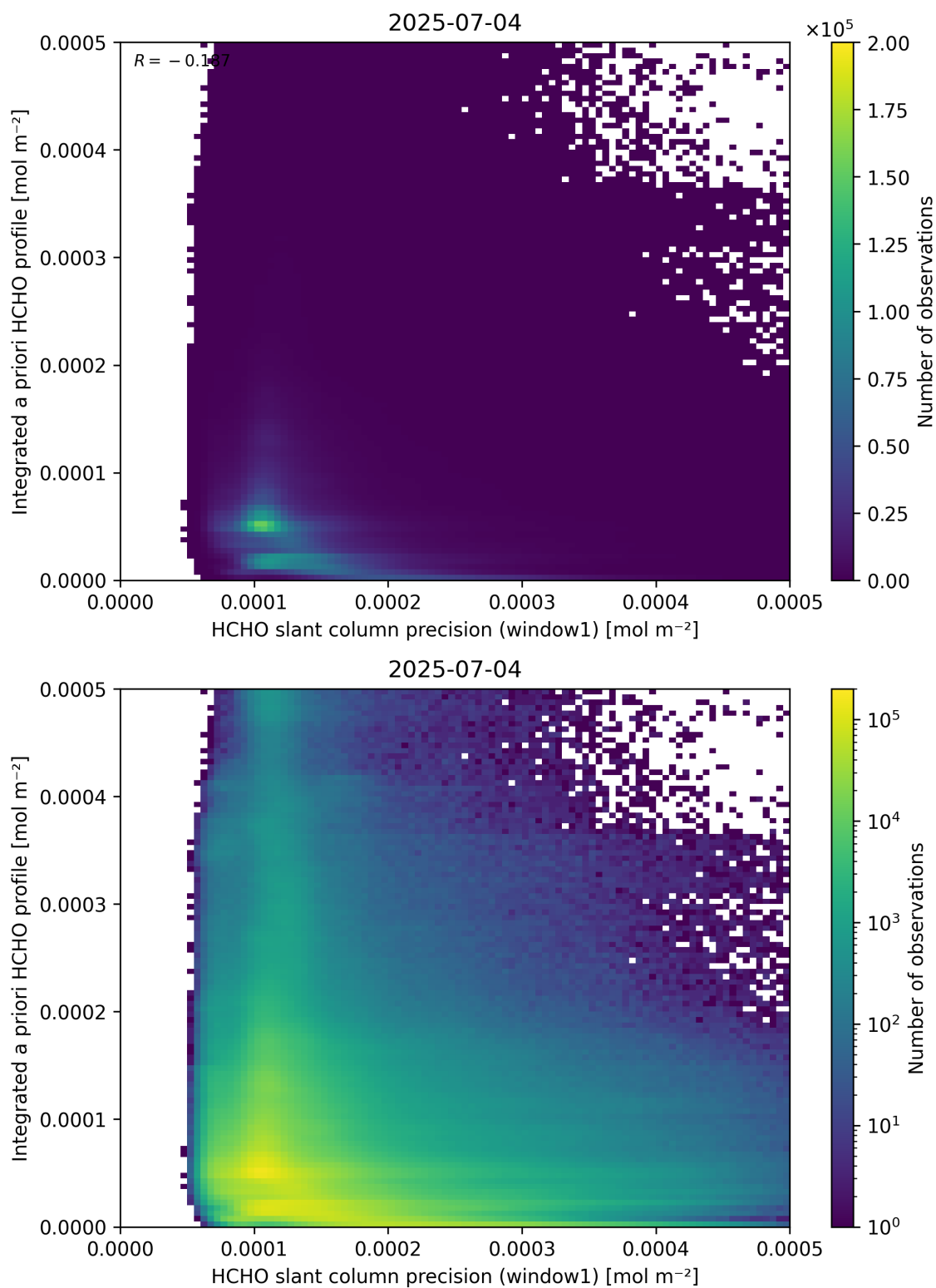
Figure 96: Scatter density plot of “HCHO slant column precision (window1)” against “Integrated a priori HCHO profile” for 2025-07-03 to 2025-07-05.
