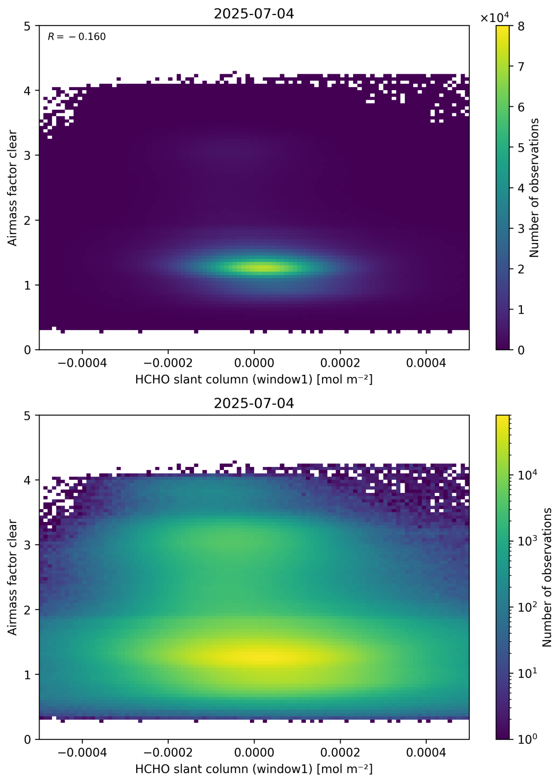
Figure 81: Scatter density plot of “HCHO slant column (window1)” against “Airmass factor clear” for 2025-07-03 to 2025-07-05.
