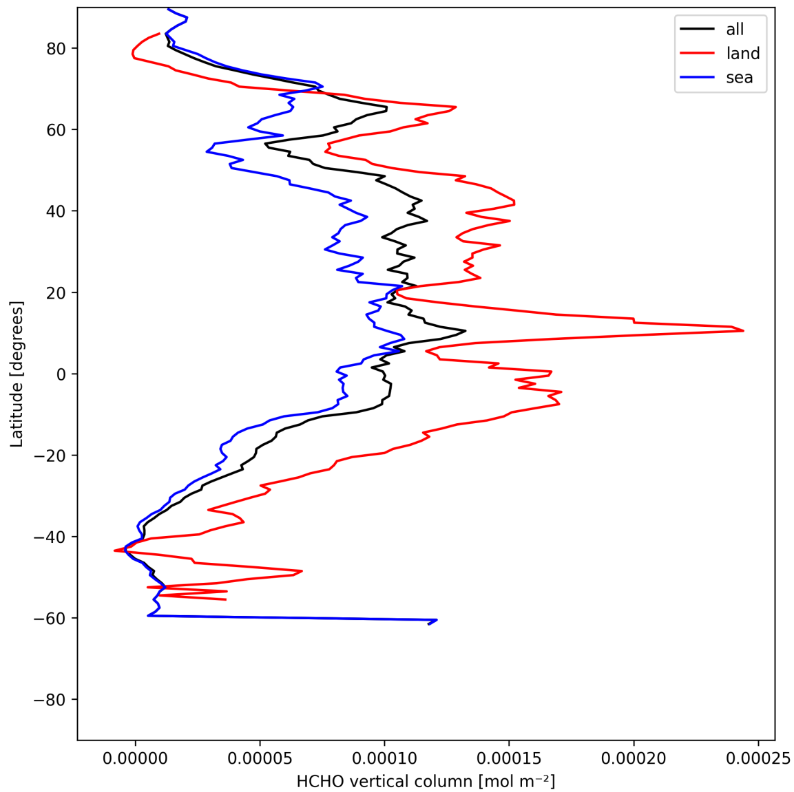
Figure 21: Zonal average of “HCHO vertical column” for 2025-07-03 to 2025-07-05.
