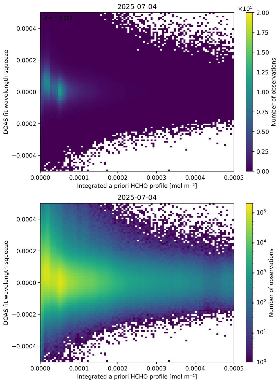
Figure 150: Scatter density plot of “Integrated a priori HCHO profile” against “DOAS fit wavelength squeeze” for 2025-07-03 to 2025-07-05.
