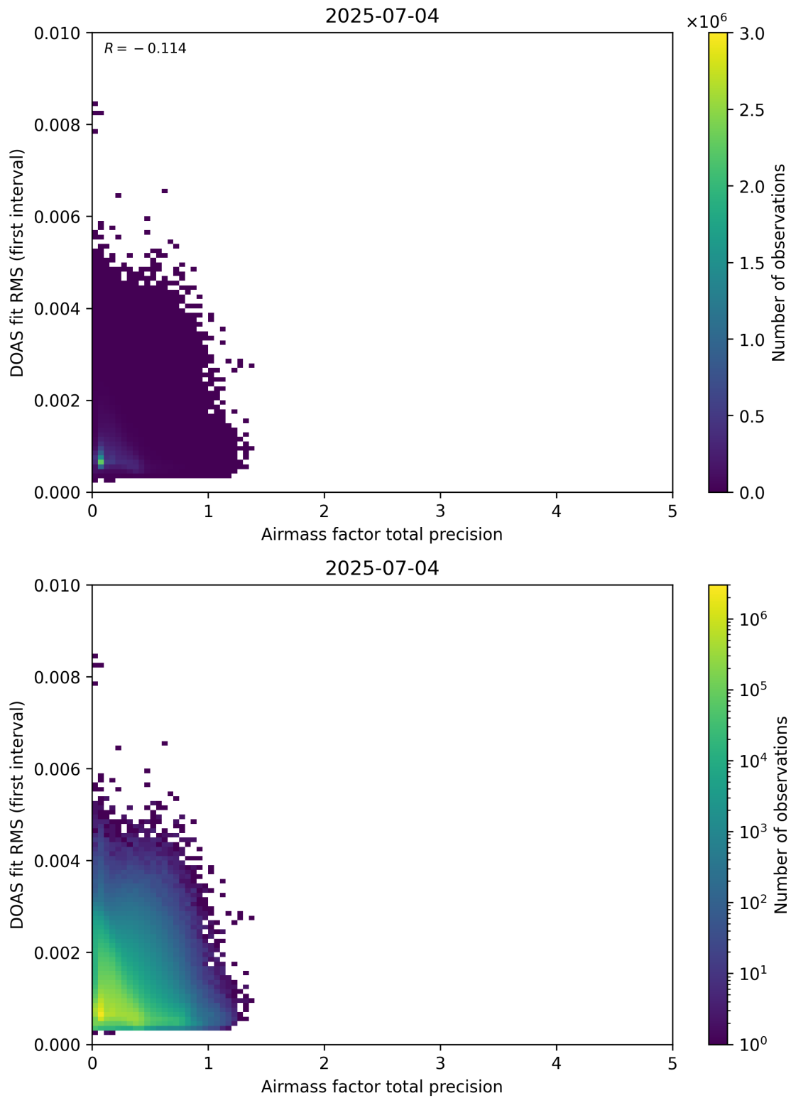
Figure 105: Scatter density plot of “Airmass factor total precision” against “DOAS fit RMS (first interval)” for 2025-07-03 to 2025-07-05.
