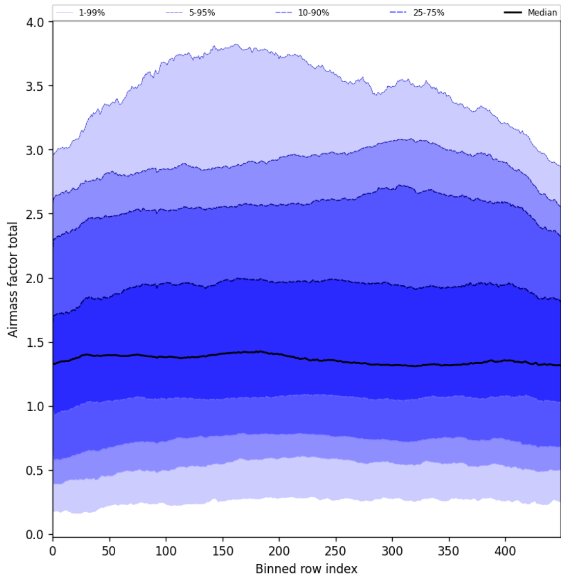
Figure 54: Along track statistics of “Airmass factor total” for 2025-07-03 to 2025-07-05
