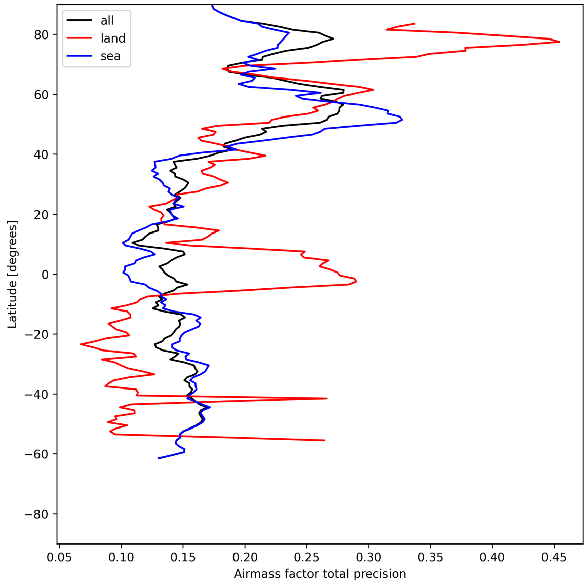
Figure 27: Zonal average of “Airmass factor total precision” for 2025-07-03 to 2025-07-05.
