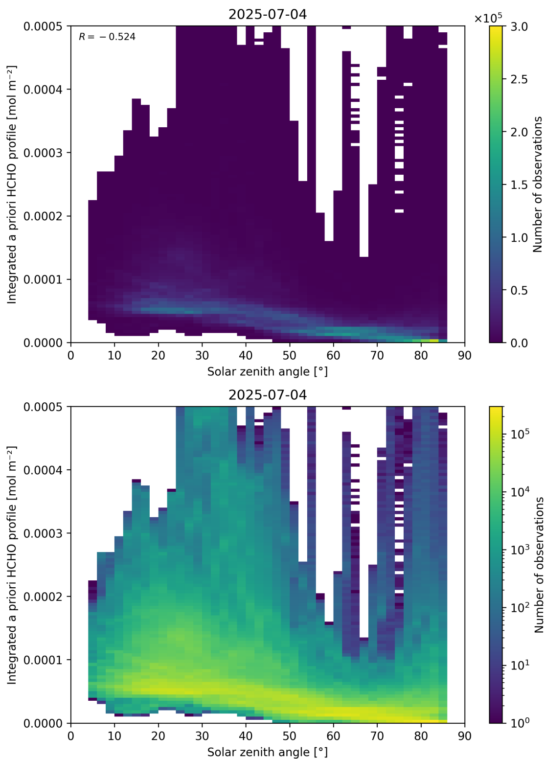
Figure 180: Scatter density plot of “Solar zenith angle” against “Integrated a priori HCHO profile” for 2025-07-03 to 2025-07-05.
