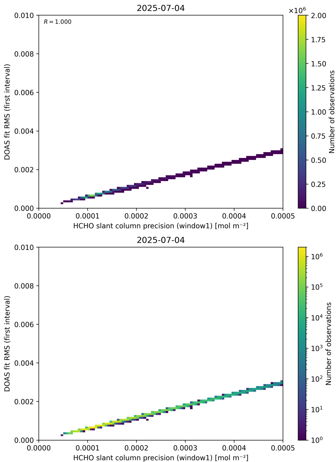
Figure 88: Scatter density plot of “HCHO slant column precision (window1)” against “DOAS fit RMS (first interval)” for 2025-07-03 to 2025-07-05.
