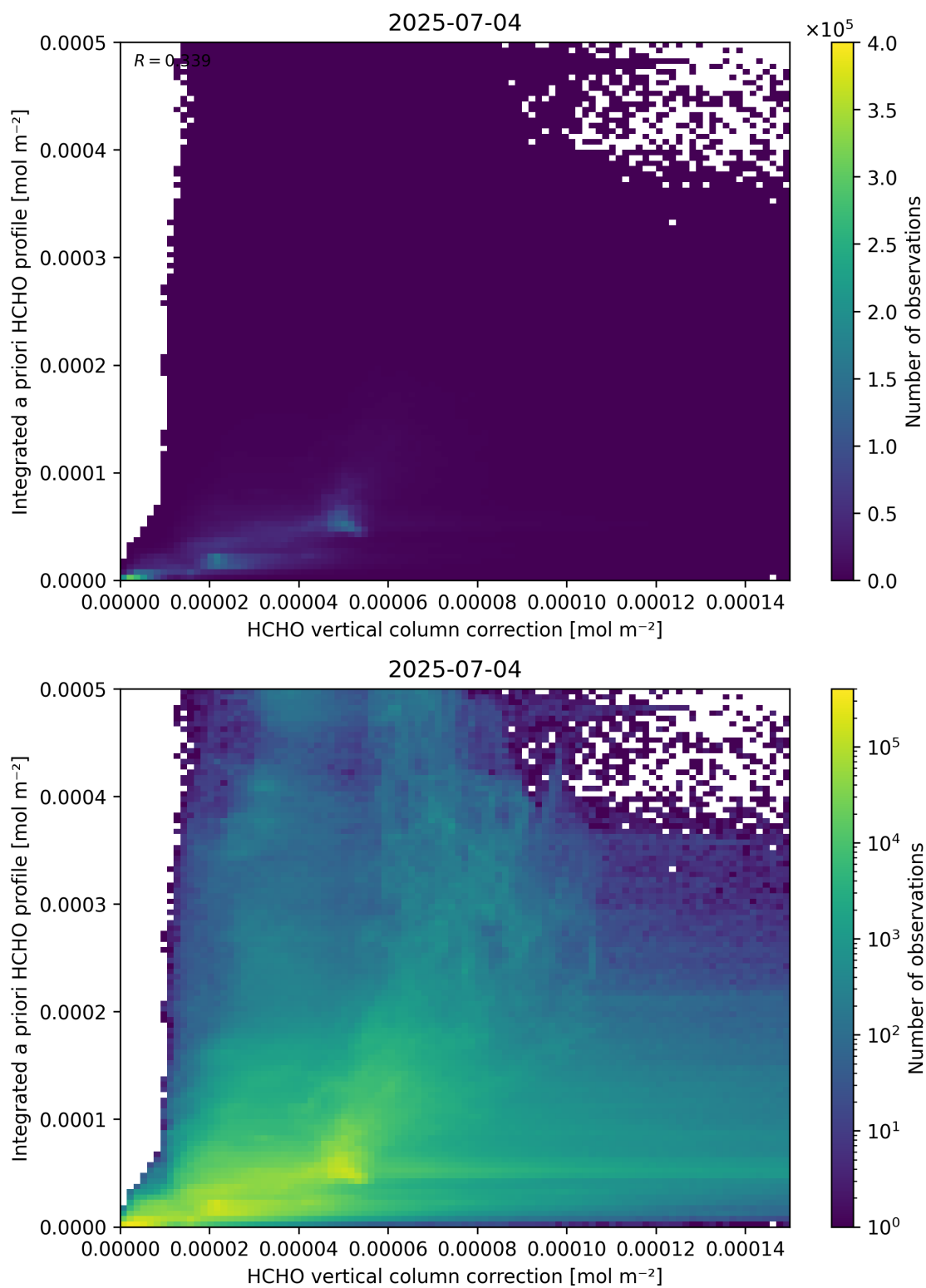
Figure 122: Scatter density plot of “HCHO vertical column correction” against “Integrated a priori HCHO profile” for 2025-07-03 to 2025-07-05.
