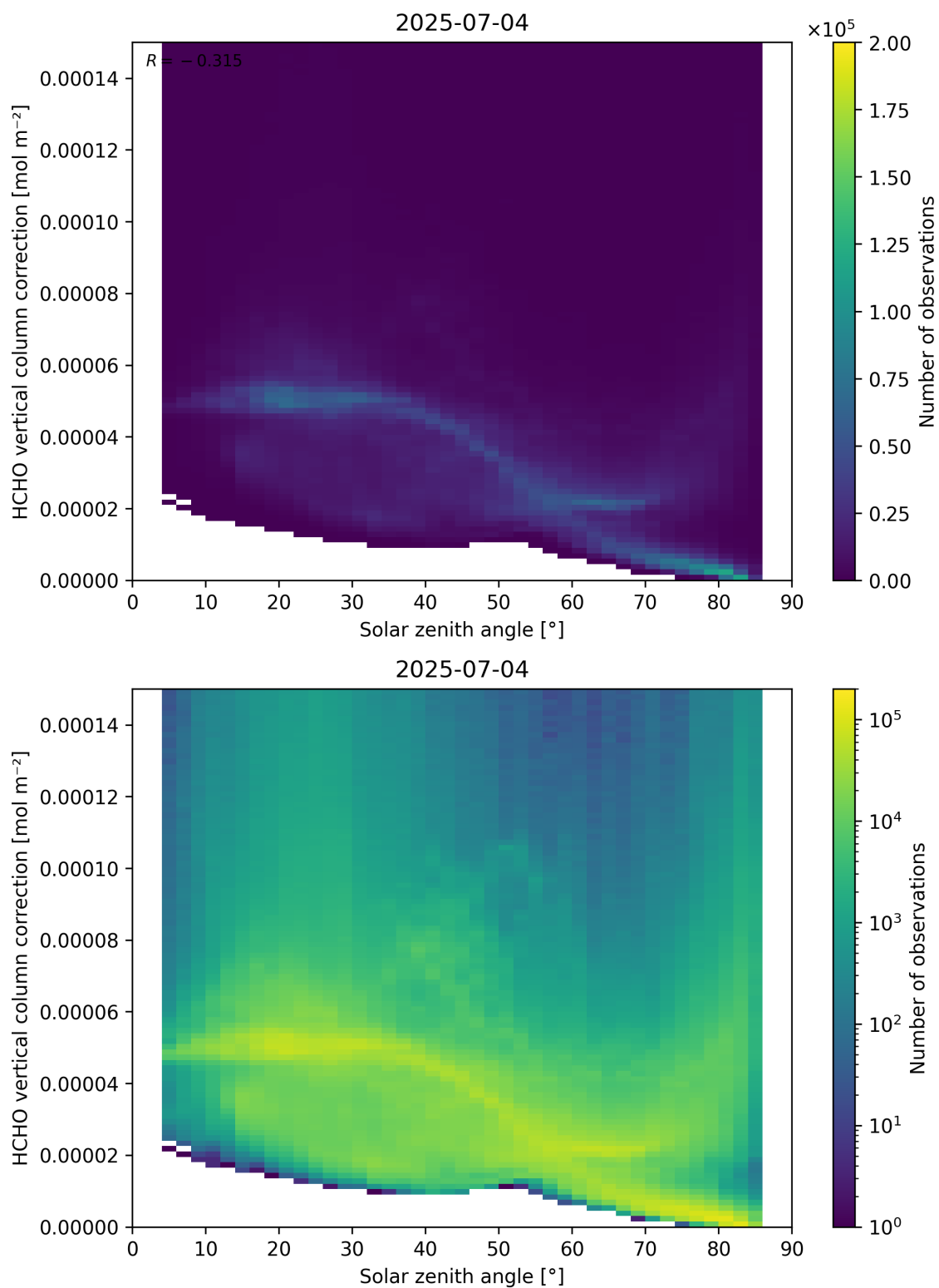
Figure 178: Scatter density plot of “Solar zenith angle” against “HCHO vertical column correction” for 2025-07-03 to 2025-07-05.
