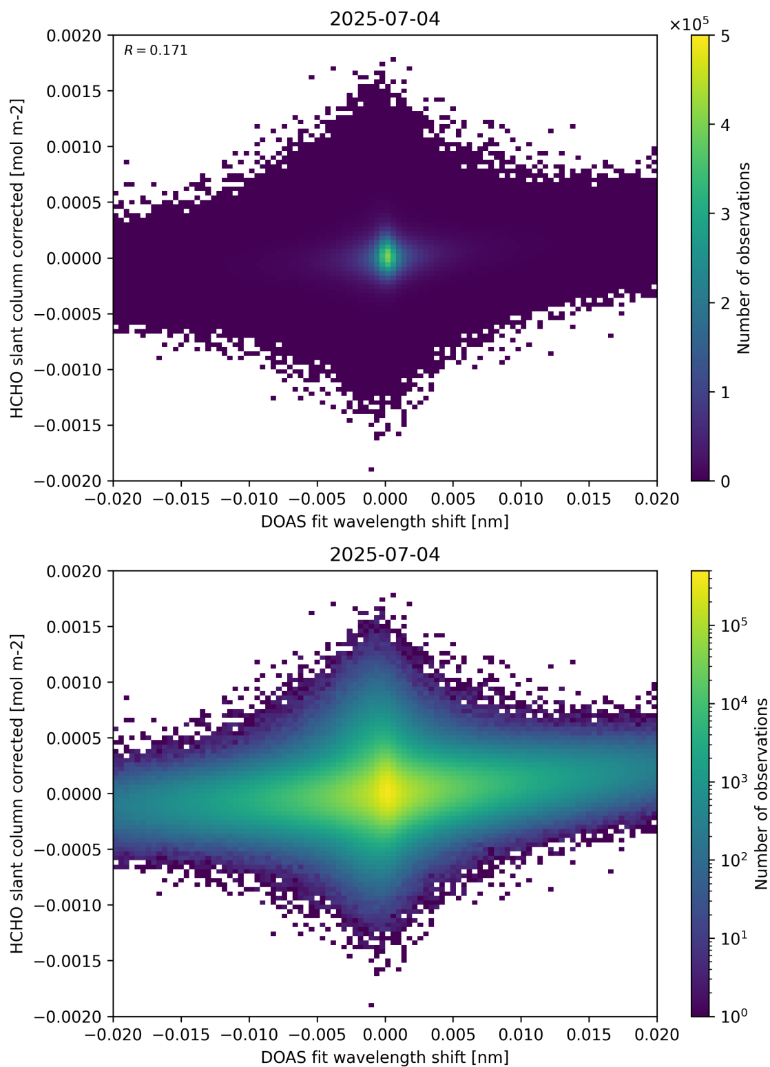
Figure 66: Scatter density plot of “DOAS fit wavelength shift” against “HCHO slant column corrected” for 2025-07-03 to 2025-07-05.
