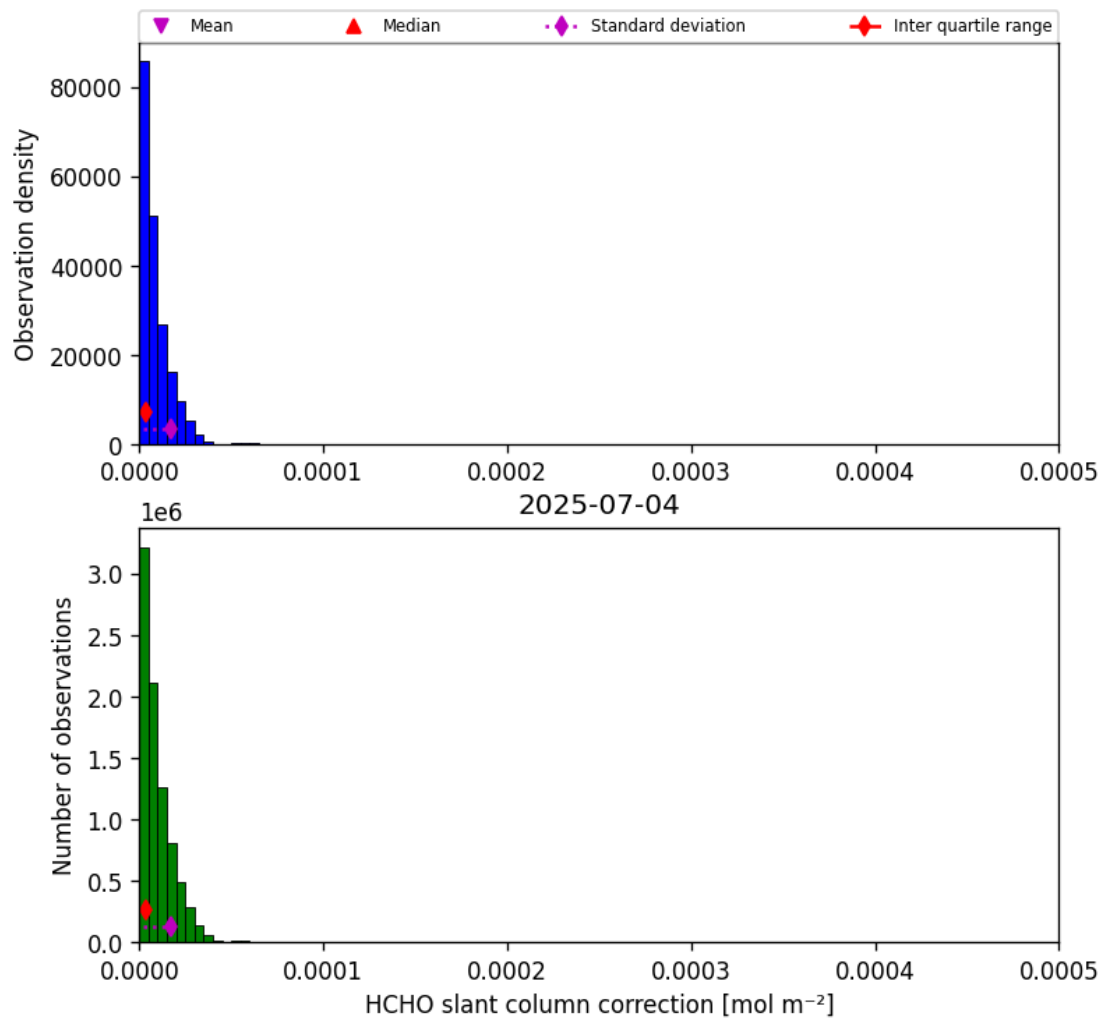
Figure 47: Histogram of “HCHO slant column correction” for 2025-07-03 to 2025-07-05
