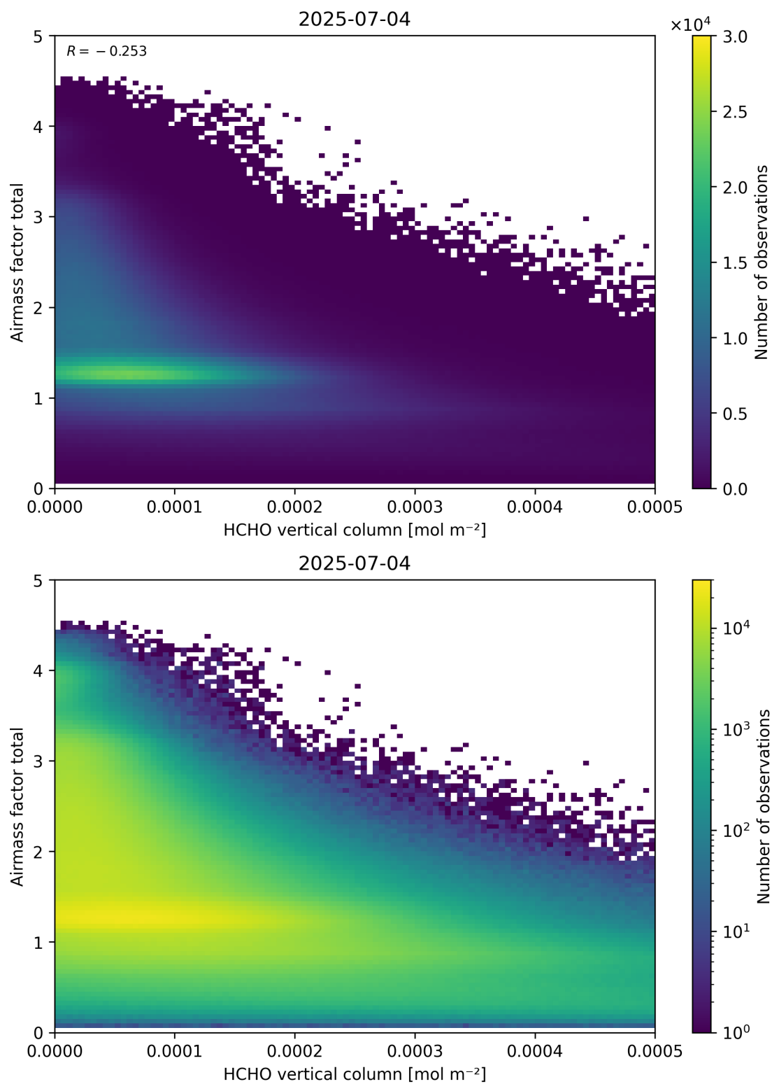
Figure 131: Scatter density plot of “HCHO vertical column” against “Airmass factor total” for 2025-07-03 to 2025-07-05.
