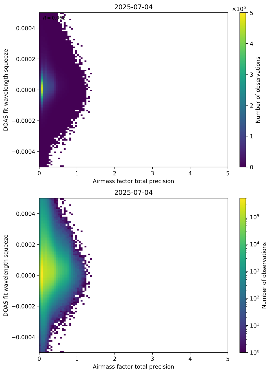
Figure 107: Scatter density plot of “Airmass factor total precision” against “DOAS fit wavelength squeeze” for 2025-07-03 to 2025-07-05.
