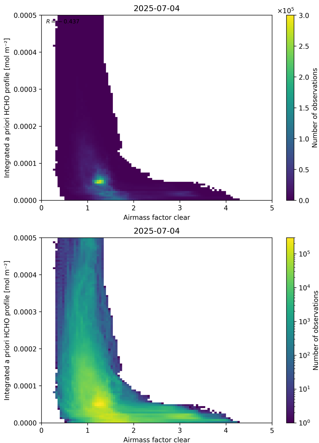
Figure 76: Scatter density plot of “Airmass factor clear” against “Integrated a priori HCHO profile” for 2025-07-03 to 2025-07-05.
