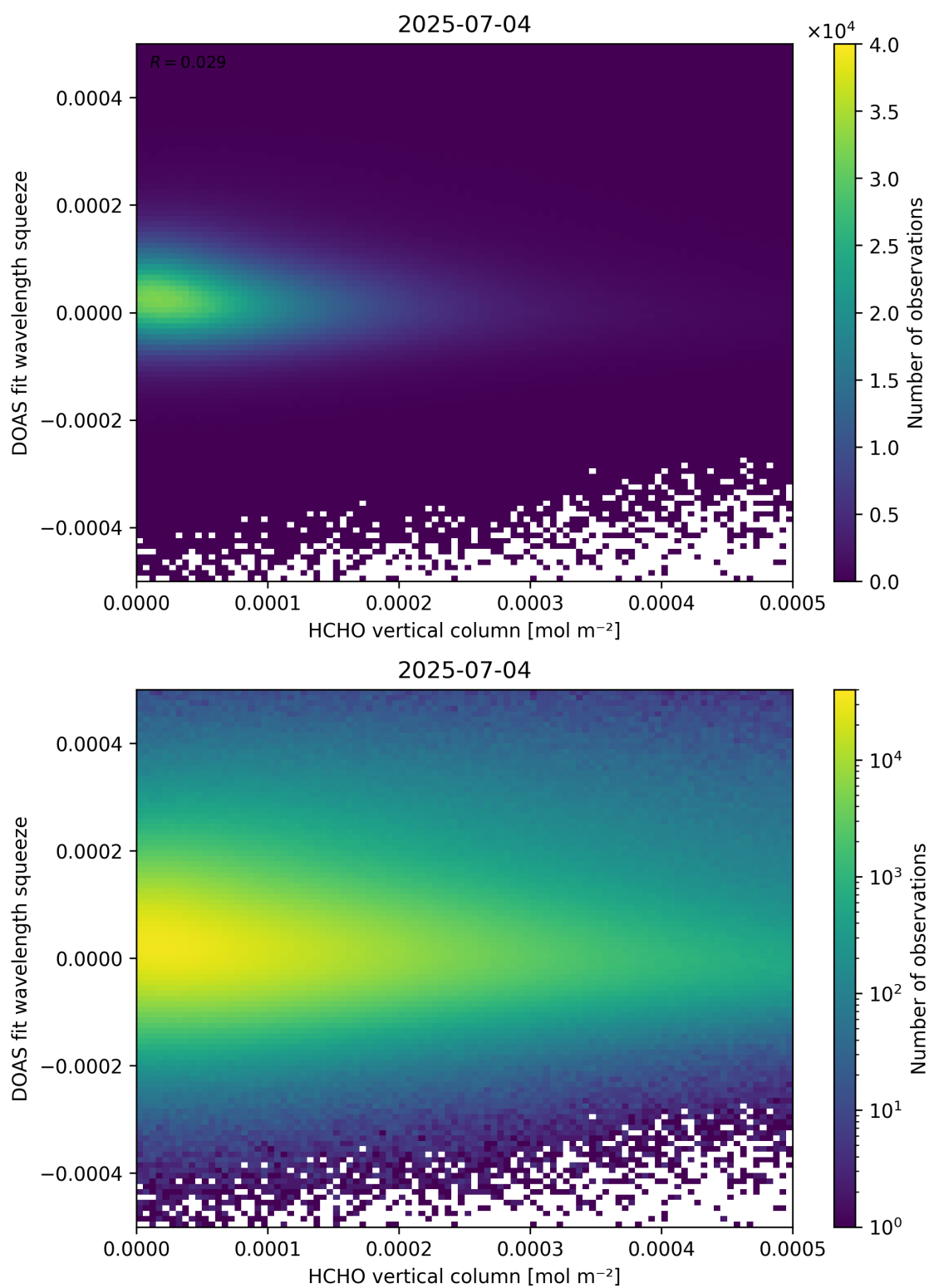
Figure 125: Scatter density plot of “HCHO vertical column” against “DOAS fit wavelength squeeze” for 2025-07-03 to 2025-07-05.
