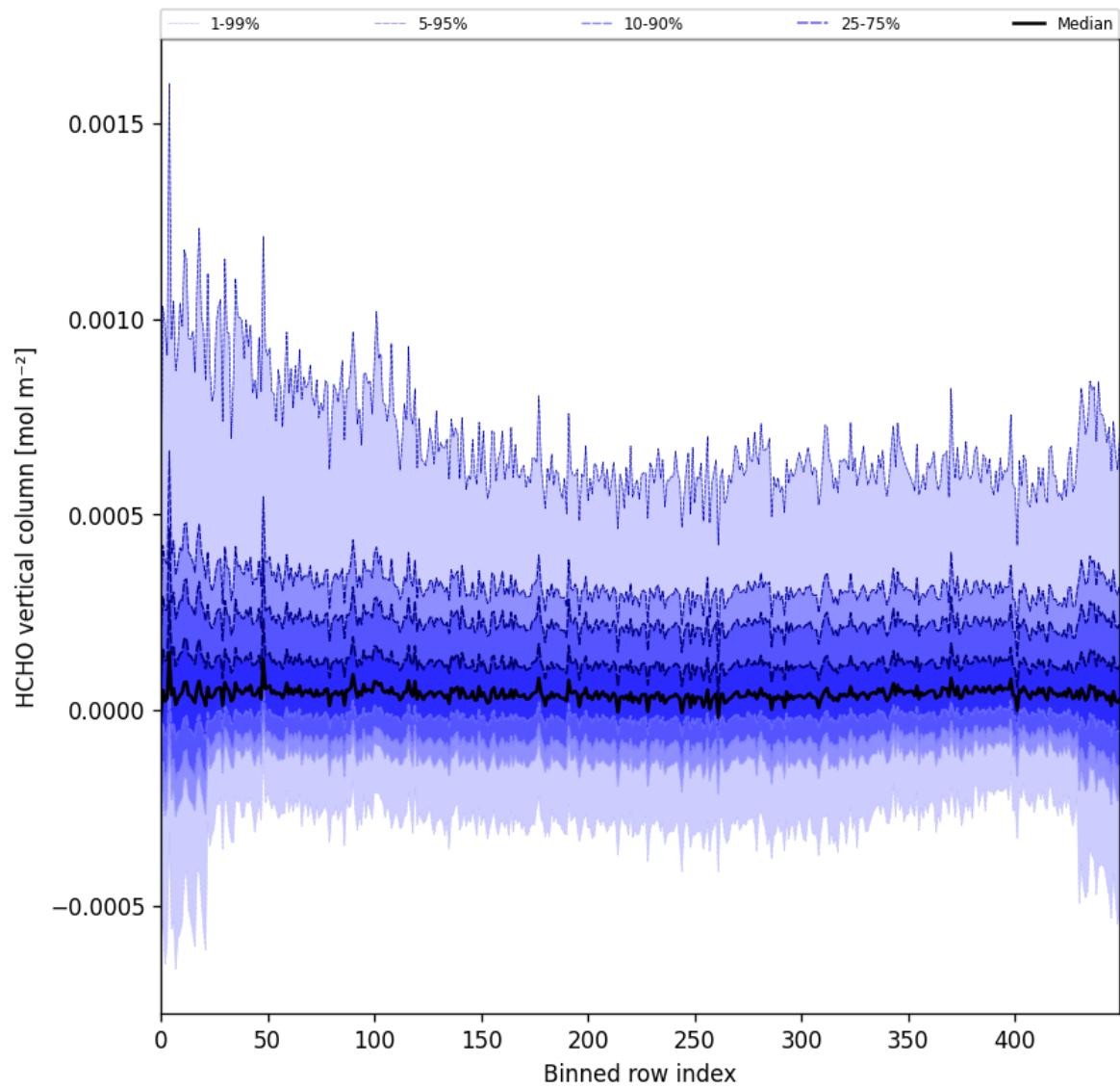
Figure 49: Along track statistics of “HCHO vertical column” for 2025-07-03 to 2025-07-05
