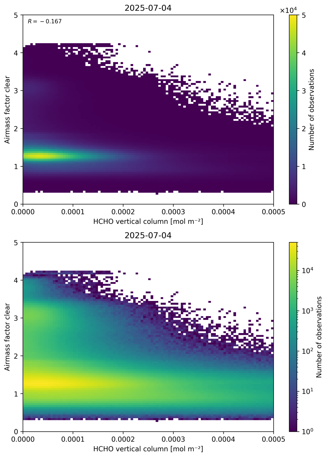
Figure 126: Scatter density plot of “HCHO vertical column” against “Airmass factor clear” for 2025-07-03 to 2025-07-05.
