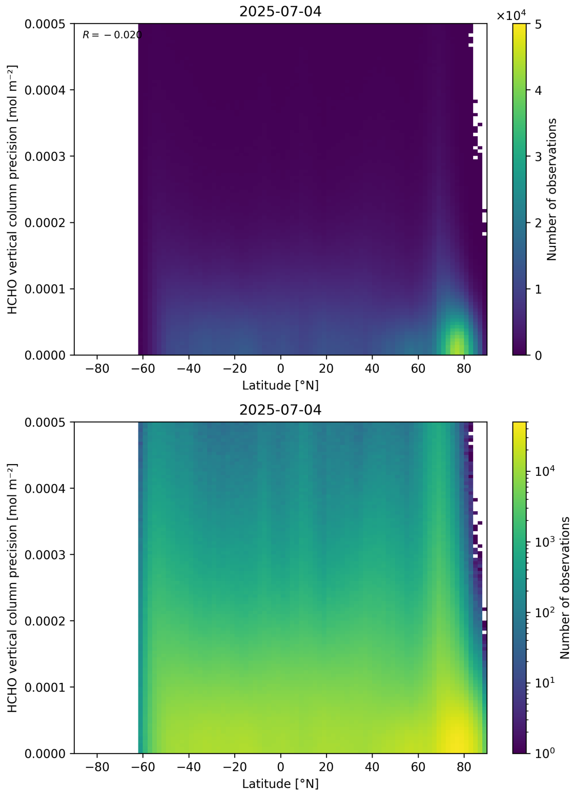
Figure 165: Scatter density plot of “Latitude” against “HCHO vertical column precision” for 2025-07-03 to 2025-07-05.
