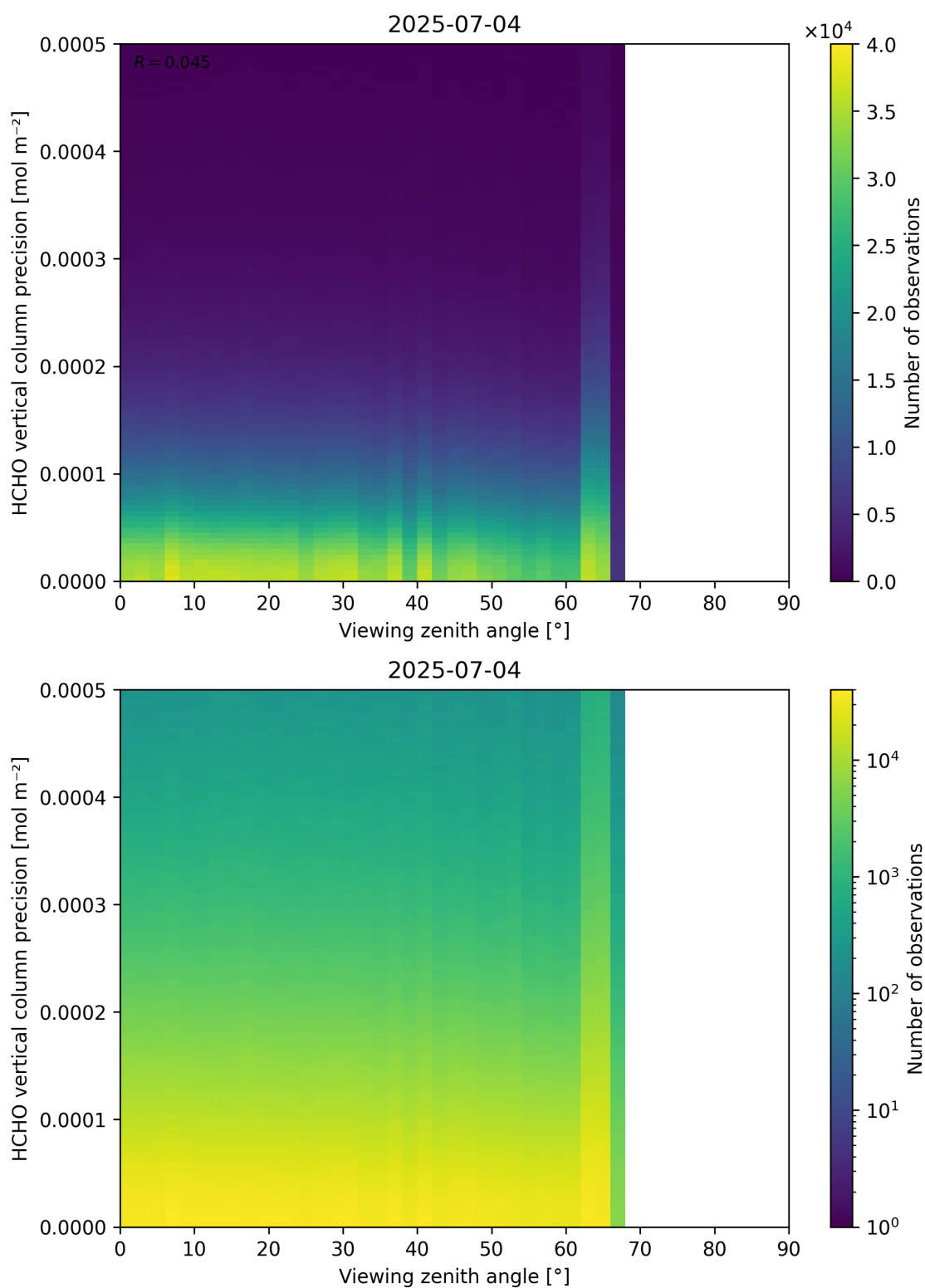
Figure 194: Scatter density plot of “Viewing zenith angle” against “HCHO vertical column precision” for 2025-07-03 to 2025-07-05.
