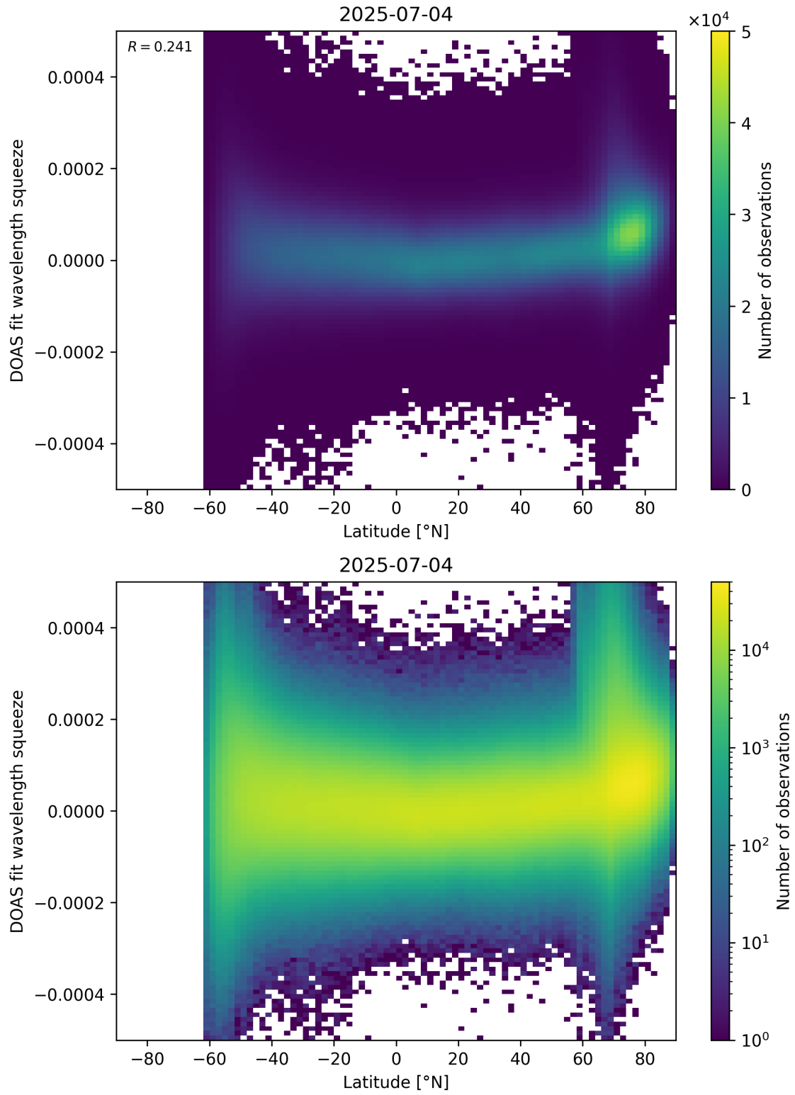
Figure 155: Scatter density plot of “Latitude” against “DOAS fit wavelength squeeze” for 2025-07-03 to 2025-07-05.
