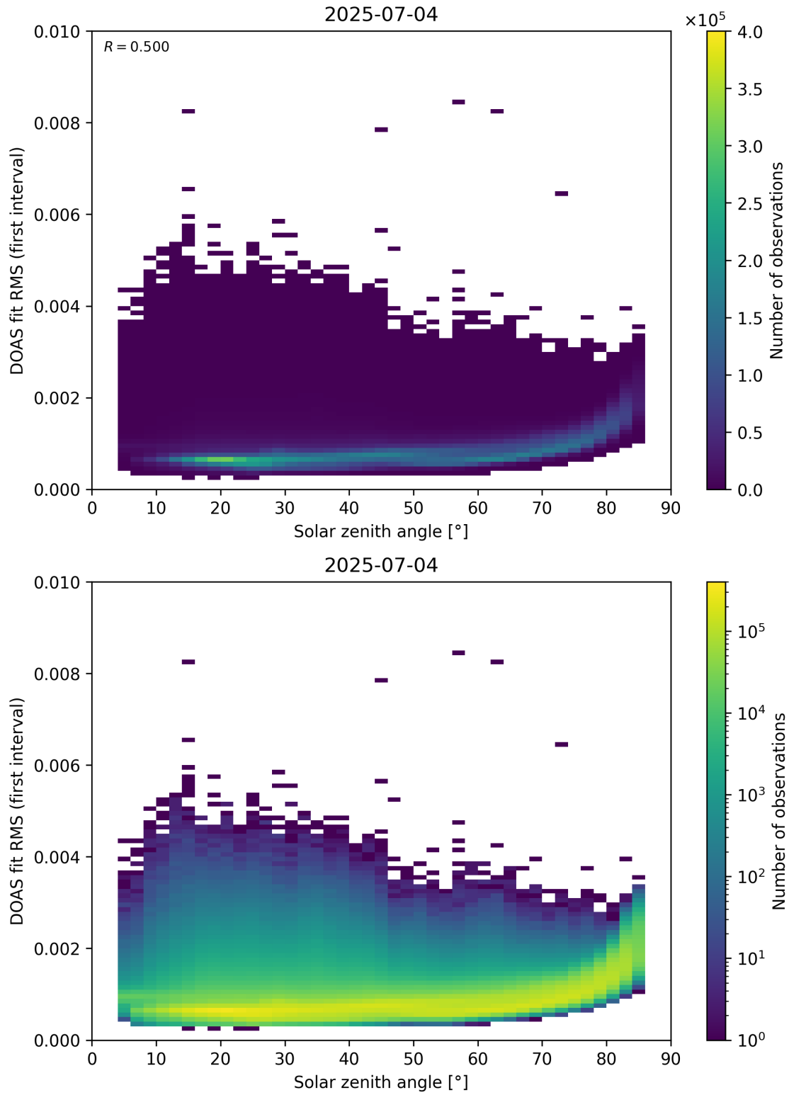
Figure 167: Scatter density plot of “Solar zenith angle” against “DOAS fit RMS (first interval)” for 2025-07-03 to 2025-07-05.
