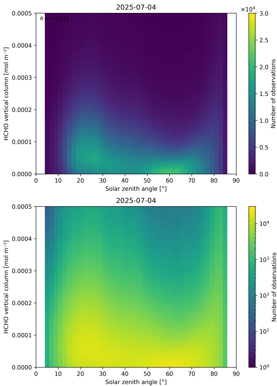
Figure 177: Scatter density plot of “Solar zenith angle” against “HCHO vertical column” for 2025-07-03 to 2025-07-05.
