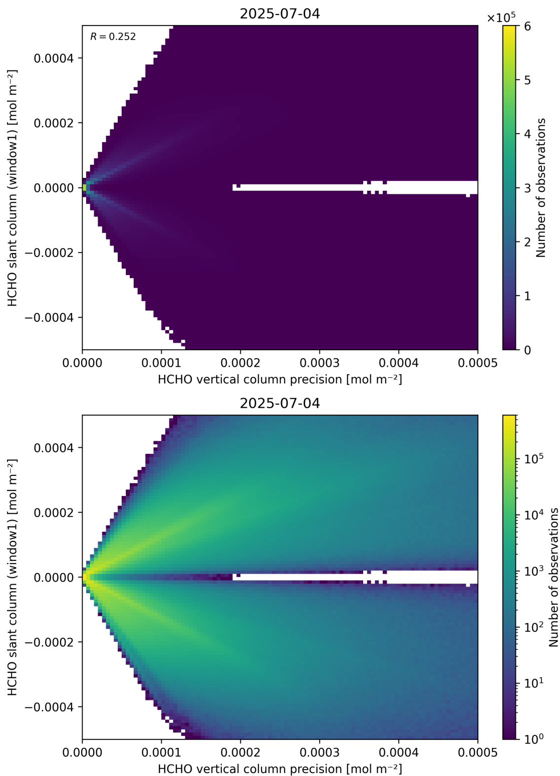
Figure 142: Scatter density plot of “HCHO vertical column precision” against “HCHO slant column (window1)” for 2025-07-03 to 2025-07-05.
