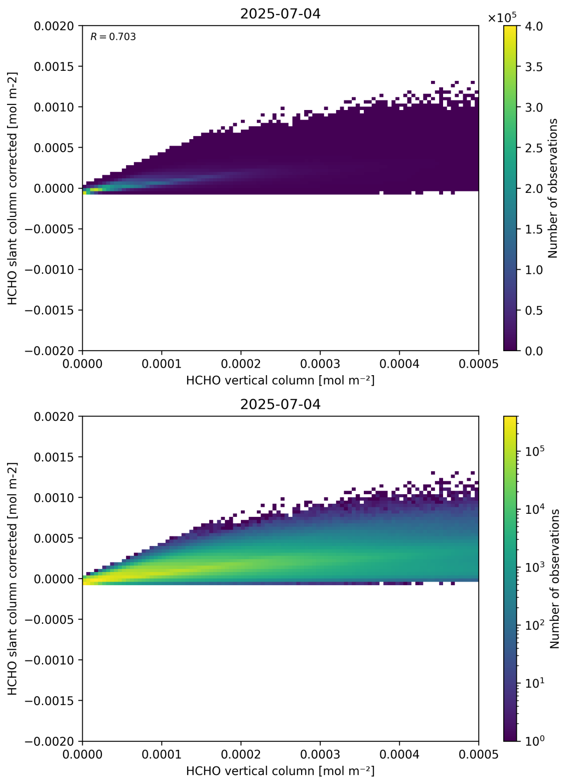
Figure 127: Scatter density plot of “HCHO vertical column” against “HCHO slant column corrected” for 2025-07-03 to 2025-07-05.
