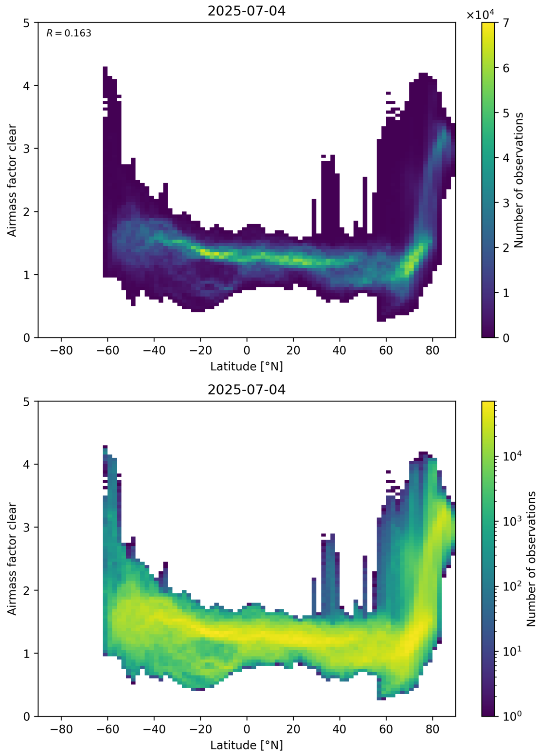
Figure 156: Scatter density plot of “Latitude” against “Airmass factor clear” for 2025-07-03 to 2025-07-05.
