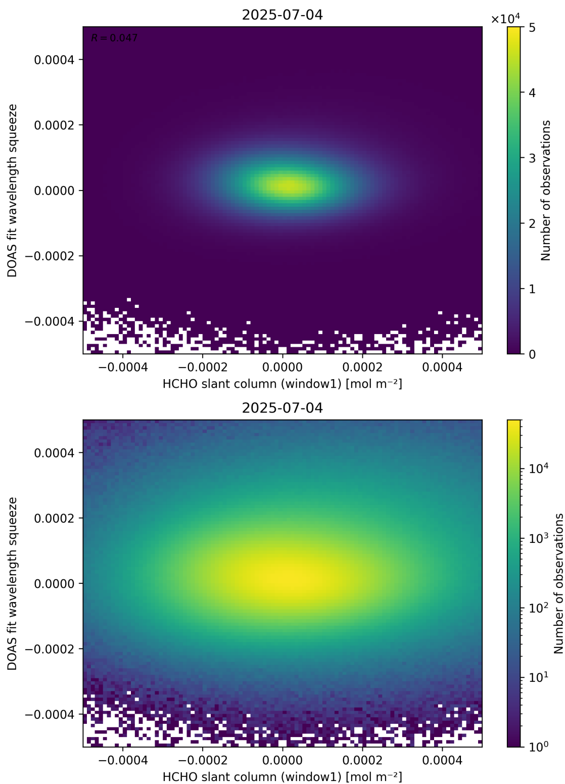
Figure 80: Scatter density plot of “HCHO slant column (window1)” against “DOAS fit wavelength squeeze” for 2025-07-03 to 2025-07-05.
