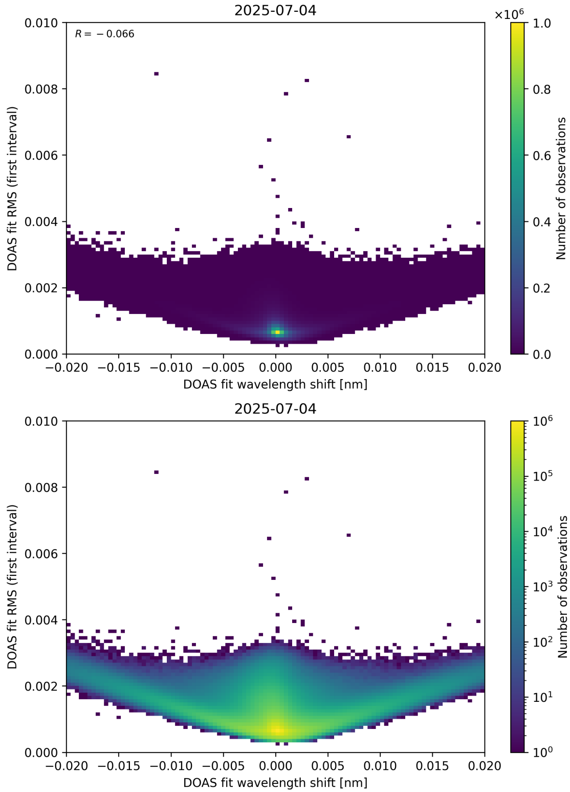
Figure 64: Scatter density plot of “DOAS fit wavelength shift” against “DOAS fit RMS (first interval)” for 2025-07-03 to 2025-07-05.
