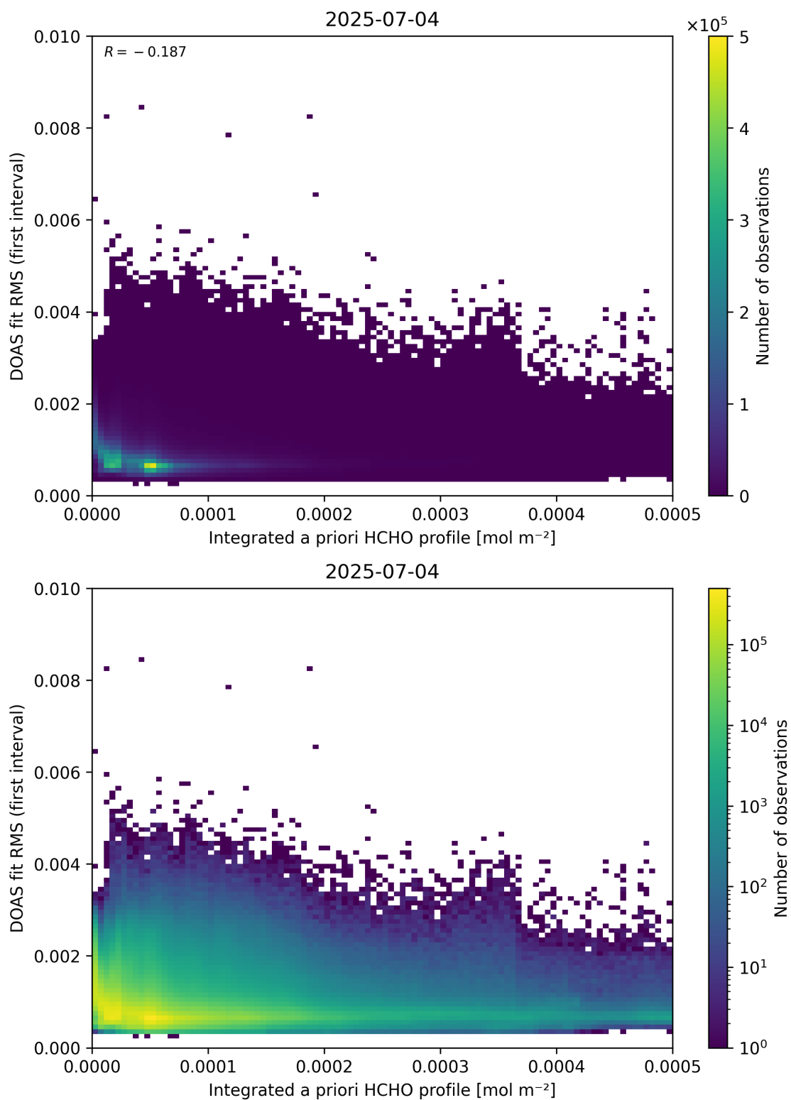
Figure 148: Scatter density plot of “Integrated a priori HCHO profile” against “DOAS fit RMS (first interval)” for 2025-07-03 to 2025-07-05.
