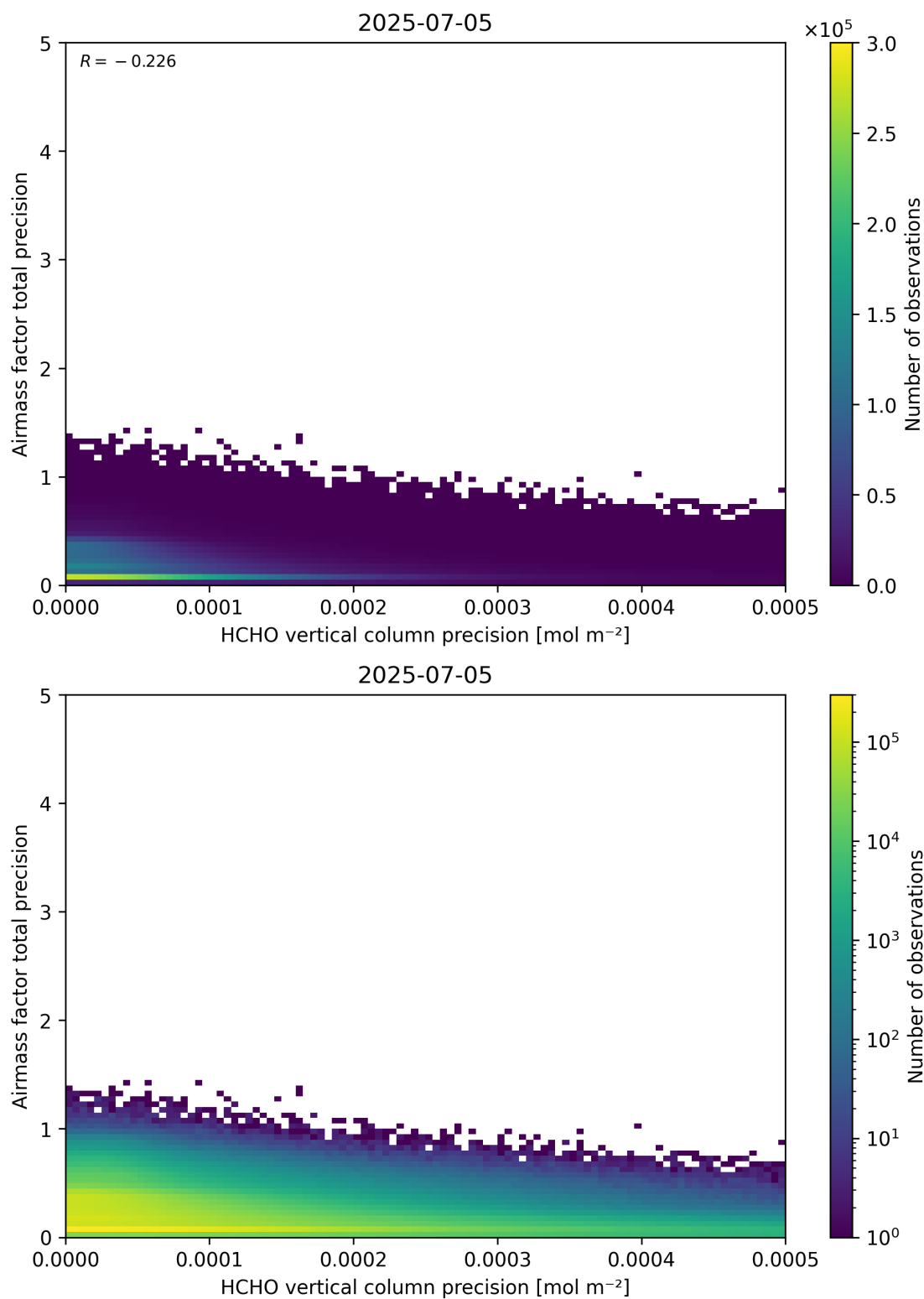
Figure 145: Scatter density plot of “HCHO vertical column precision” against “Airmass factor total precision” for 2025-07-04 to 2025-07-06.
