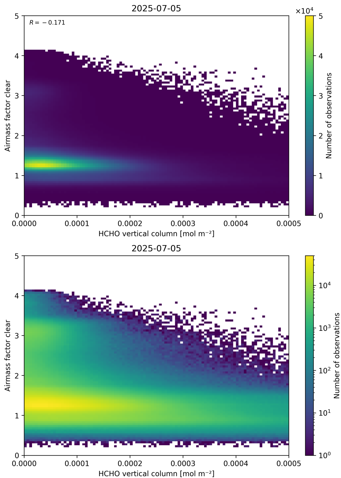
Figure 126: Scatter density plot of “HCHO vertical column” against “Airmass factor clear” for 2025-07-04 to 2025-07-06.
