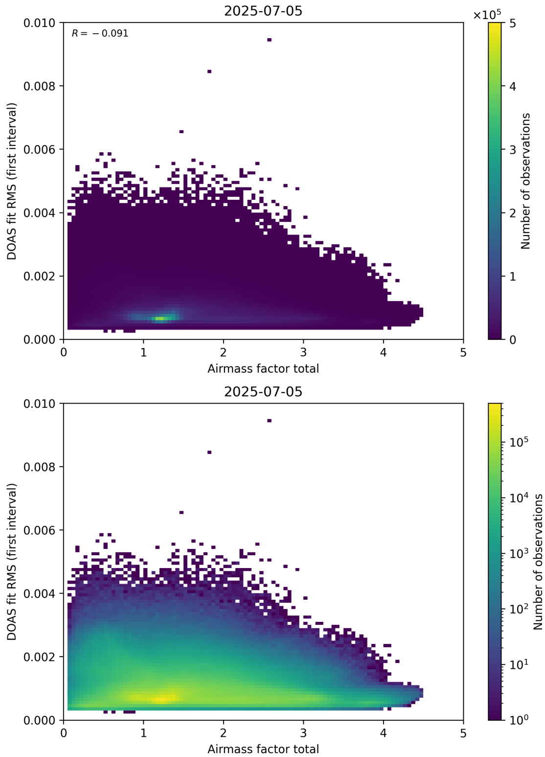
Figure 97: Scatter density plot of “Airmass factor total” against “DOAS fit RMS (first interval)” for 2025-07-04 to 2025-07-06.
