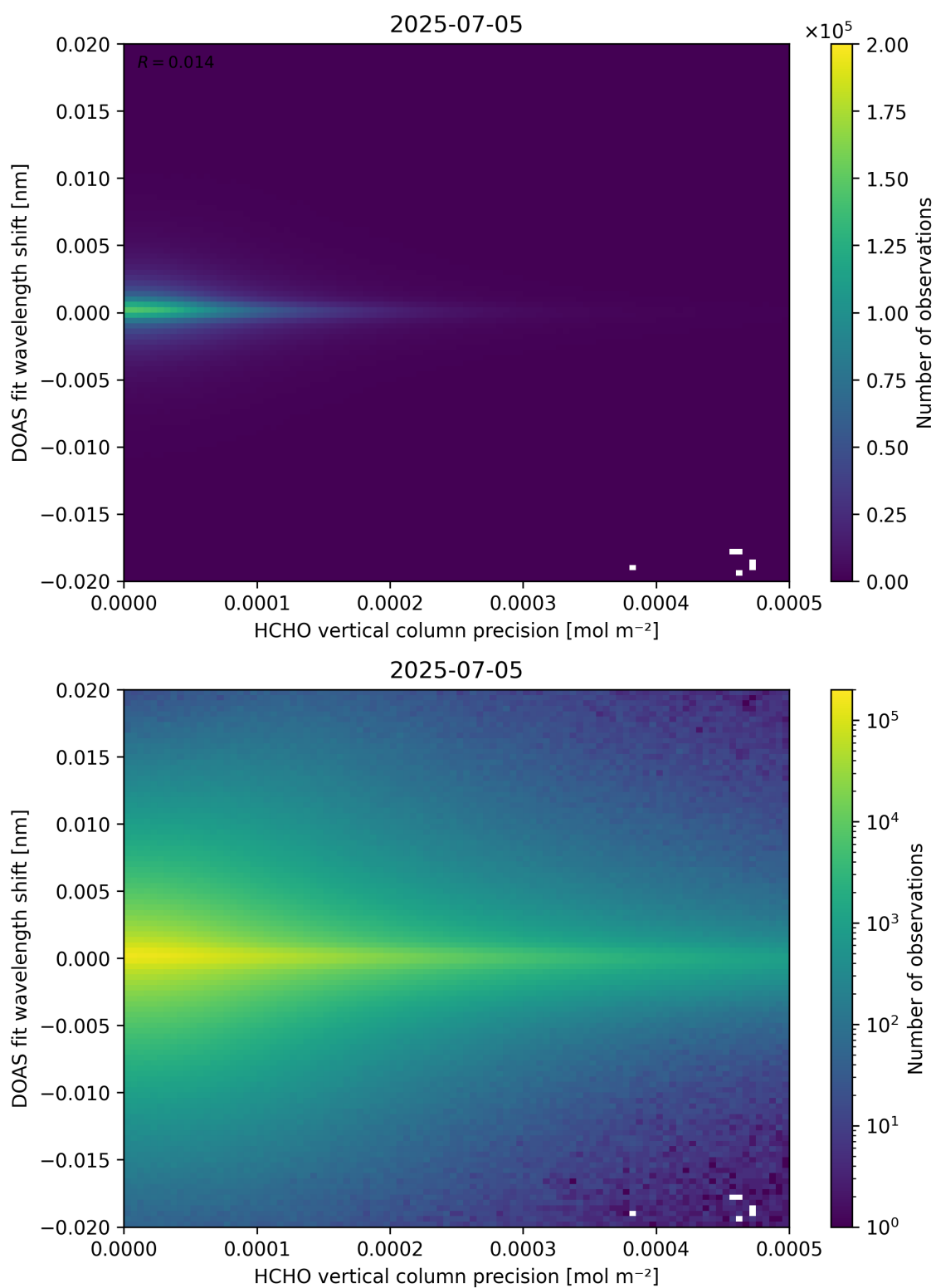
Figure 137: Scatter density plot of “HCHO vertical column precision” against “DOAS fit wavelength shift” for 2025-07-04 to 2025-07-06.
