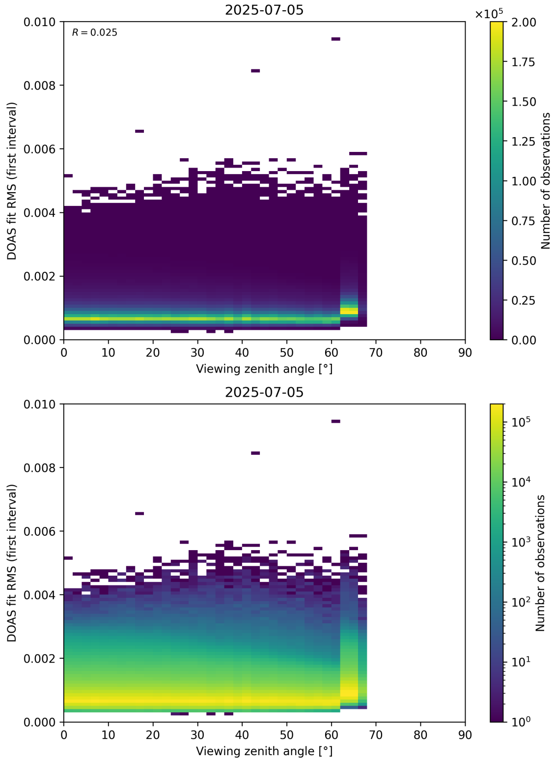
Figure 182: Scatter density plot of “Viewing zenith angle” against “DOAS fit RMS (first interval)” for 2025-07-04 to 2025-07-06.
