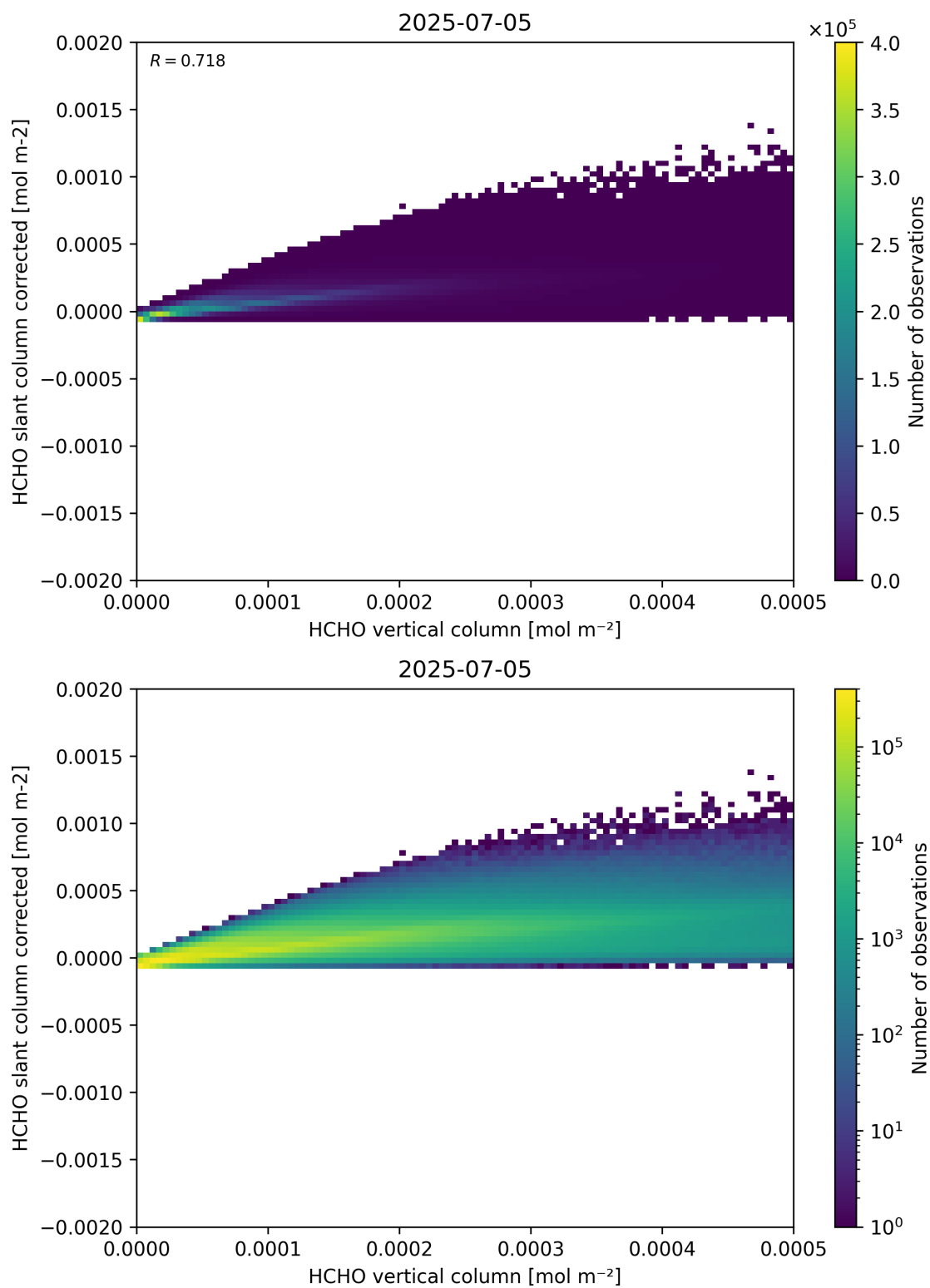
Figure 127: Scatter density plot of “HCHO vertical column” against “HCHO slant column corrected” for 2025-07-04 to 2025-07-06.
