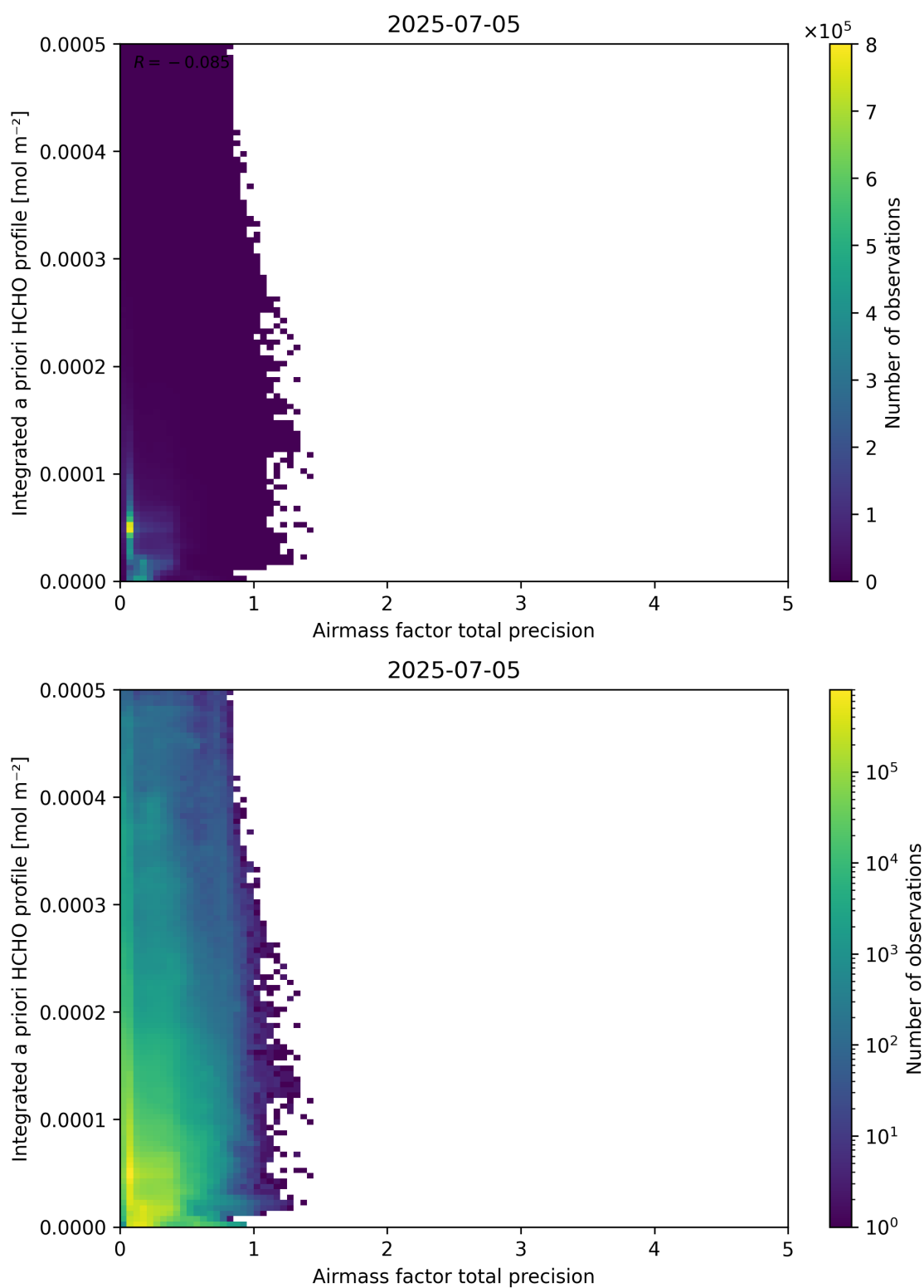
Figure 111: Scatter density plot of “Airmass factor total precision” against “Integrated a priori HCHO profile” for 2025-07-04 to 2025-07-06.
