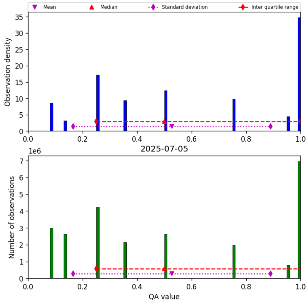
Figure 34: Histogram of “QA value” for 2025-07-04 to 2025-07-06
