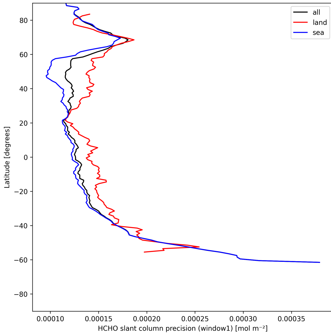
Figure 25: Zonal average of “HCHO slant column precision (window1)” for 2025-07-04 to 2025-07-06.
