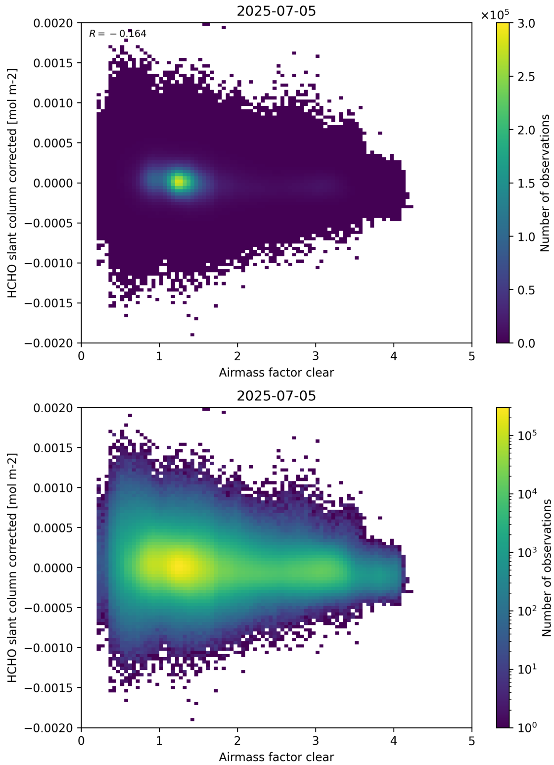
Figure 74: Scatter density plot of “Airmass factor clear” against “HCHO slant column corrected” for 2025-07-04 to 2025-07-06.
