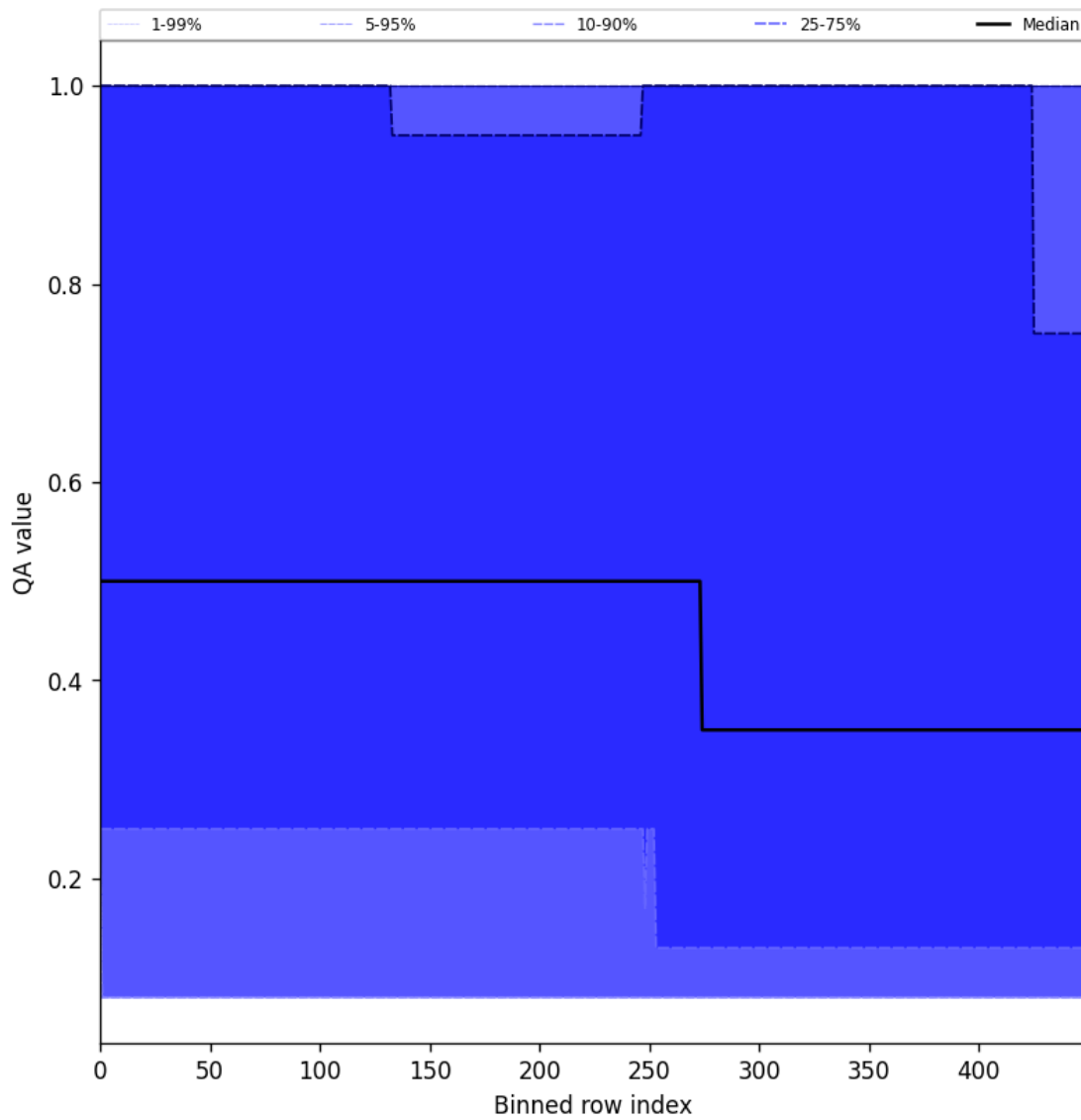
Figure 48: Along track statistics of “QA value” for 2025-07-04 to 2025-07-06
