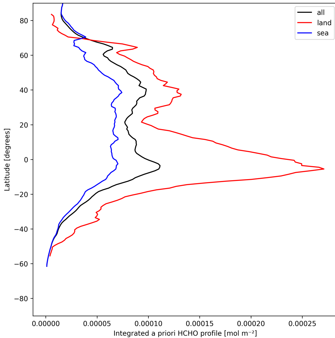
Figure 29: Zonal average of “Integrated a priori HCHO profile” for 2025-07-04 to 2025-07-06.
