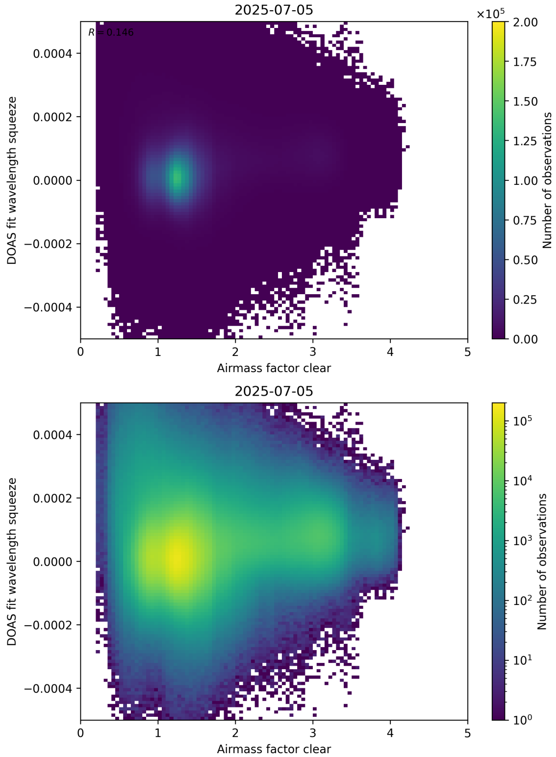
Figure 73: Scatter density plot of “Airmass factor clear” against “DOAS fit wavelength squeeze” for 2025-07-04 to 2025-07-06.
