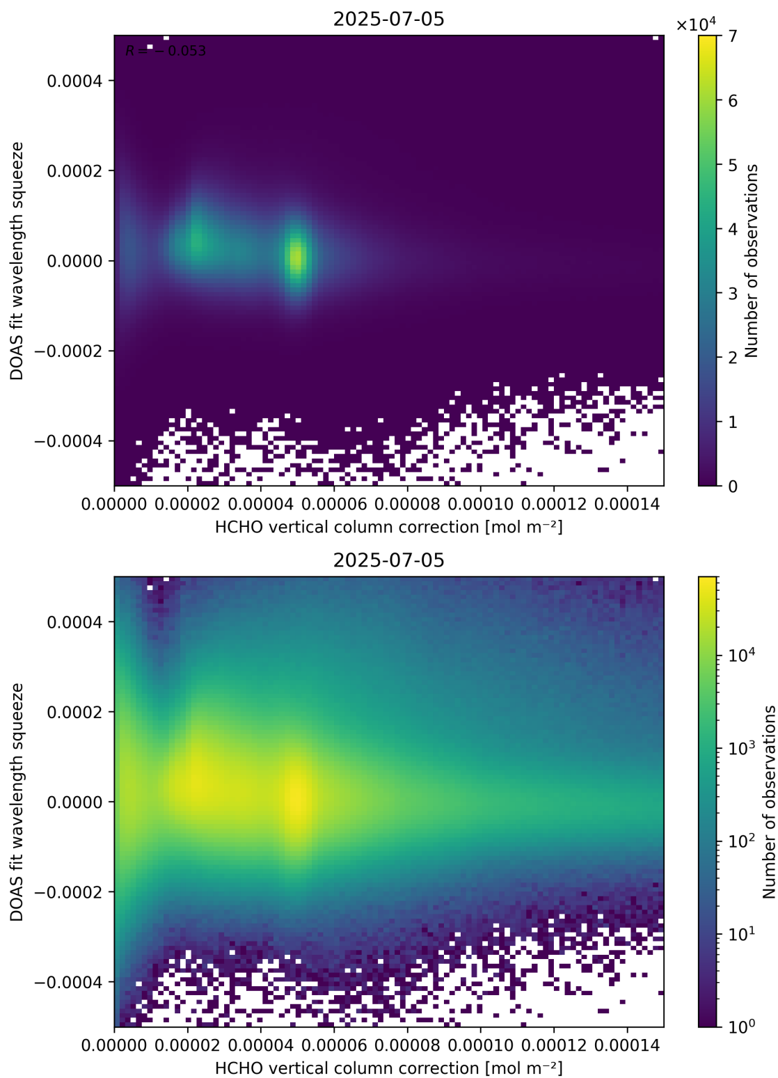
Figure 114: Scatter density plot of “HCHO vertical column correction” against “DOAS fit wavelength squeeze” for 2025-07-04 to 2025-07-06.
