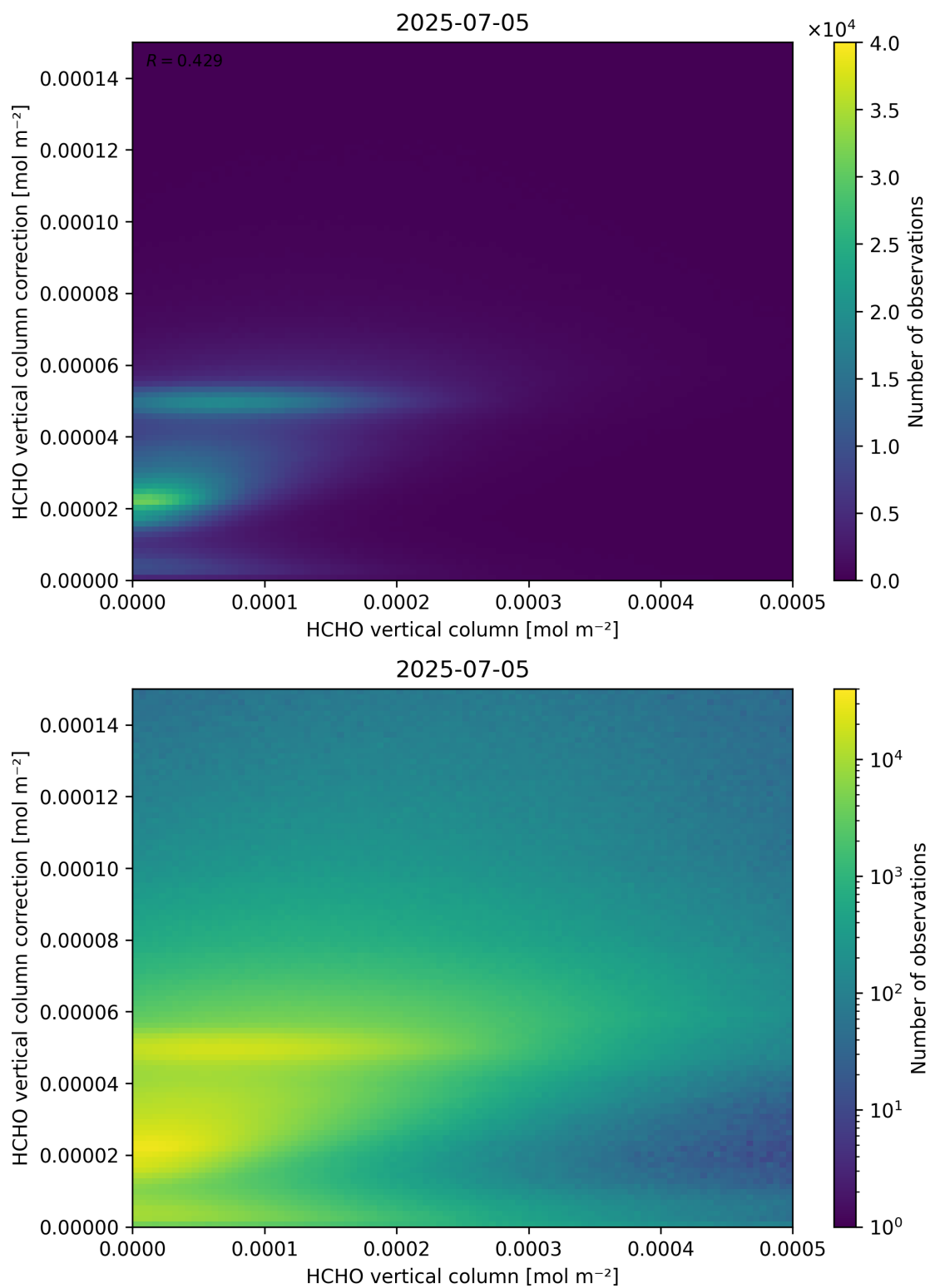
Figure 133: Scatter density plot of “HCHO vertical column” against “HCHO vertical column correction” for 2025-07-04 to 2025-07-06.
