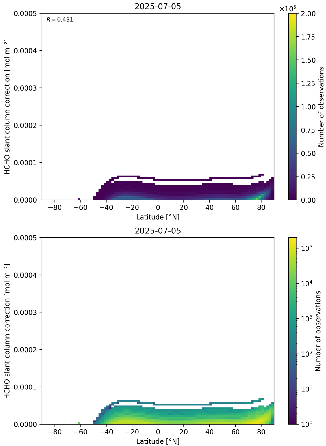
Figure 158: Scatter density plot of “Latitude” against “HCHO slant column correction” for 2025-07-04 to 2025-07-06.
