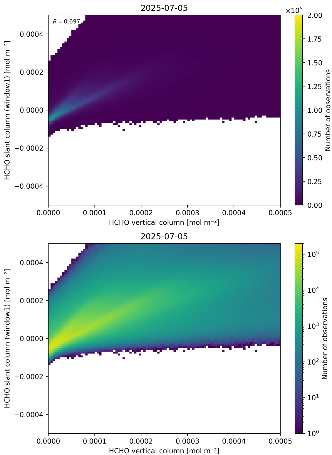
Figure 129: Scatter density plot of “HCHO vertical column” against “HCHO slant column (window1)” for 2025-07-04 to 2025-07-06.
