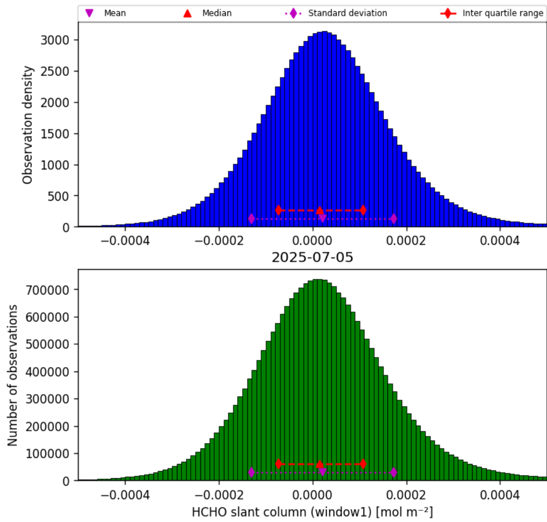
Figure 38: Histogram of “HCHO slant column (window1)” for 2025-07-04 to 2025-07-06
