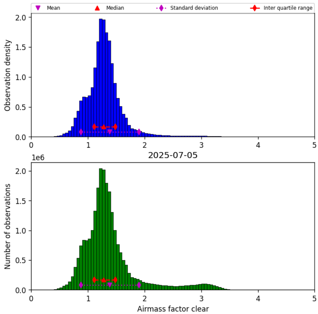
Figure 42: Histogram of “Airmass factor clear” for 2025-07-04 to 2025-07-06
