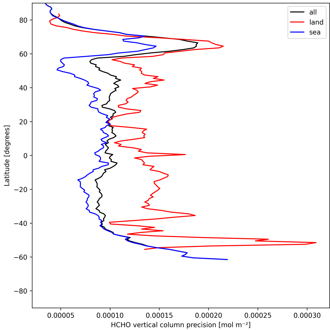
Figure 22: Zonal average of “HCHO vertical column precision” for 2025-07-04 to 2025-07-06.
