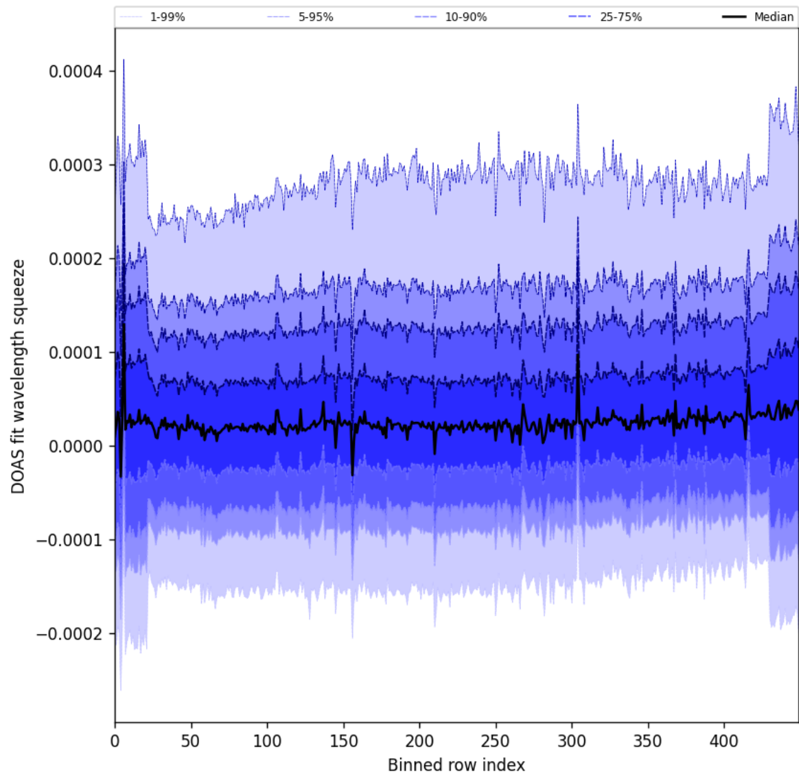
Figure 59: Along track statistics of “DOAS fit wavelength squeeze” for 2025-07-04 to 2025-07-06
