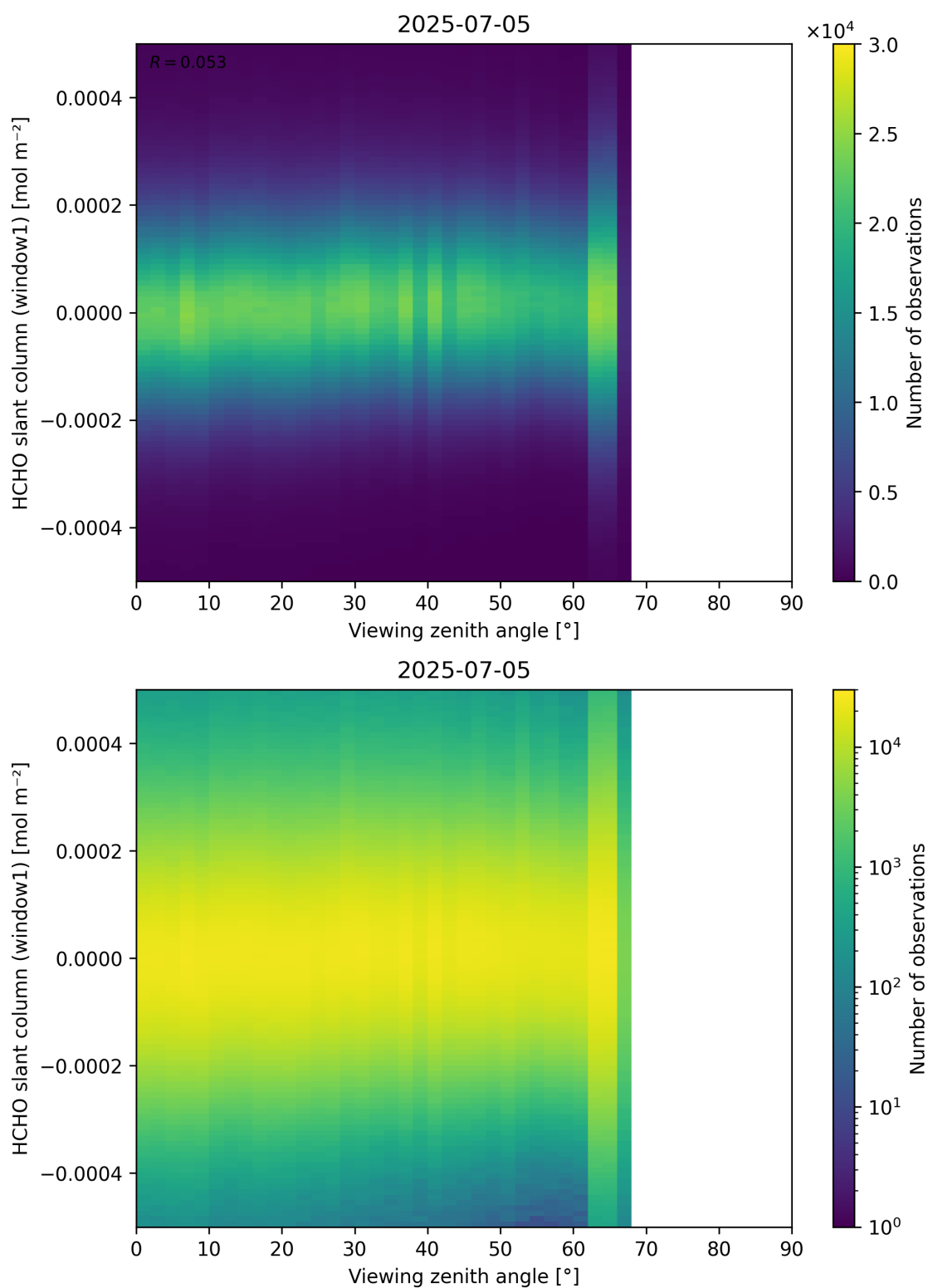
Figure 188: Scatter density plot of “Viewing zenith angle” against “HCHO slant column (window1)” for 2025-07-04 to 2025-07-06.
