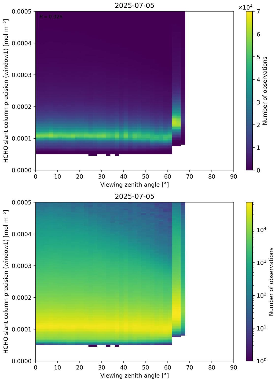
Figure 189: Scatter density plot of “Viewing zenith angle” against “HCHO slant column precision (window1)” for 2025-07-04 to 2025-07-06.
