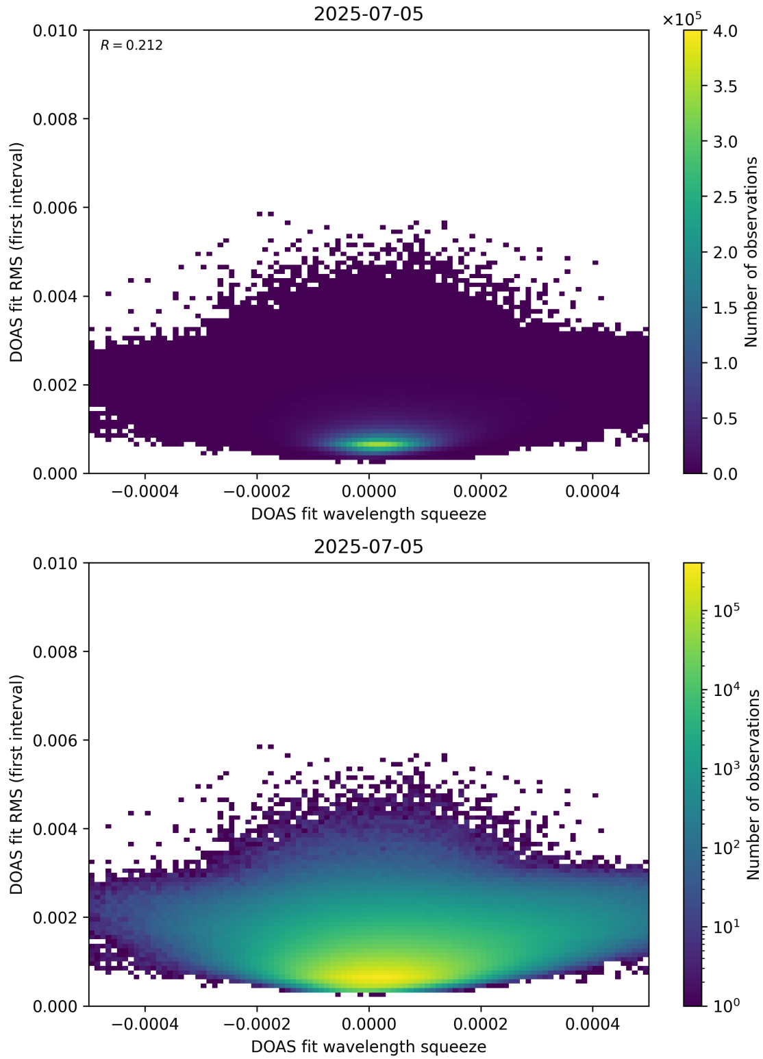
Figure 68: Scatter density plot of “DOAS fit wavelength squeeze” against “DOAS fit RMS (first interval)” for 2025-07-04 to 2025-07-06.
