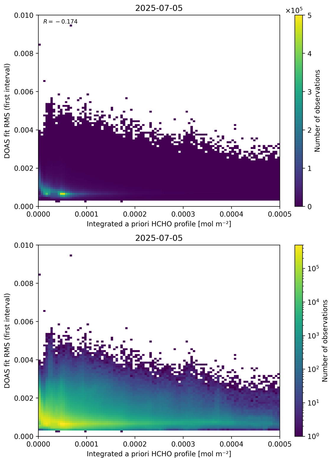
Figure 148: Scatter density plot of “Integrated a priori HCHO profile” against “DOAS fit RMS (first interval)” for 2025-07-04 to 2025-07-06.
