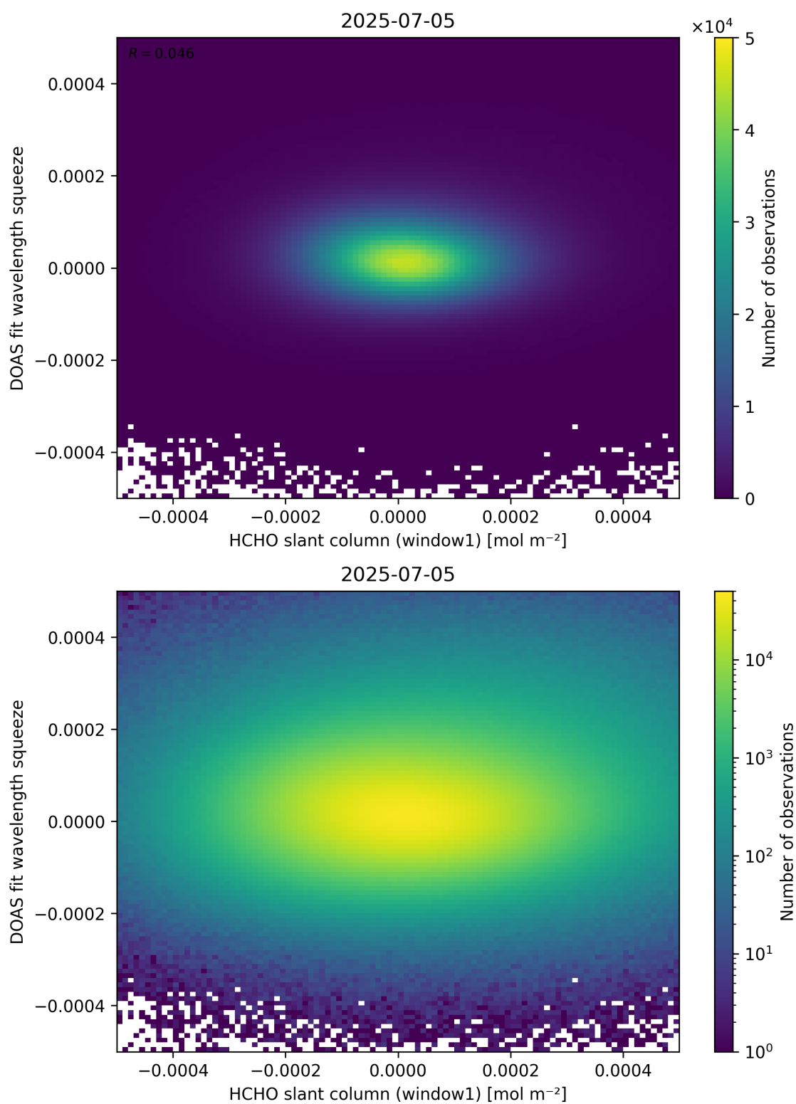
Figure 80: Scatter density plot of “HCHO slant column (window1)” against “DOAS fit wavelength squeeze” for 2025-07-04 to 2025-07-06.
