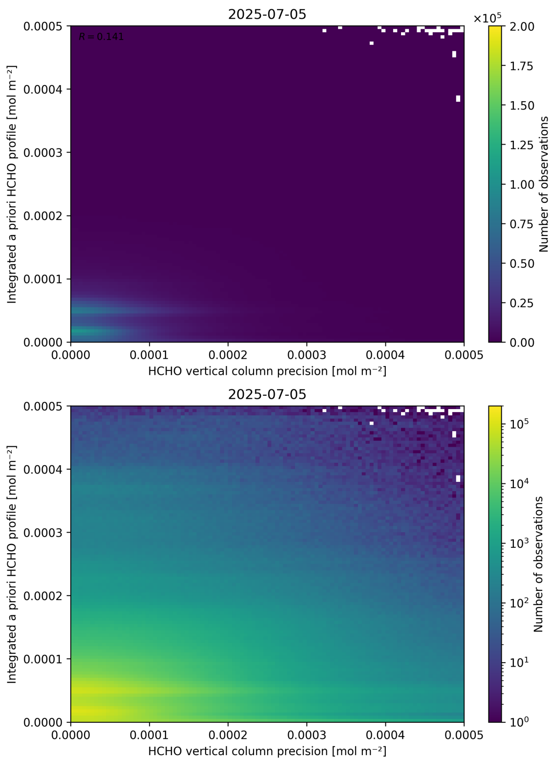
Figure 147: Scatter density plot of “HCHO vertical column precision” against “Integrated a priori HCHO profile” for 2025-07-04 to 2025-07-06.
