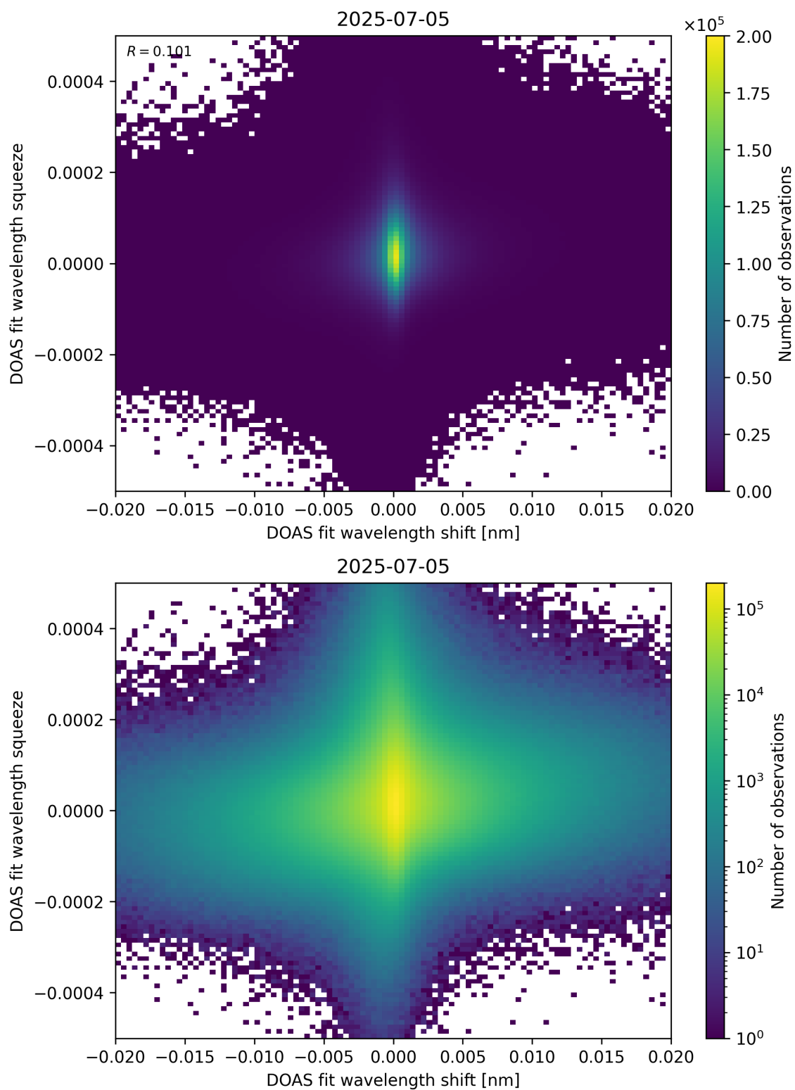
Figure 65: Scatter density plot of “DOAS fit wavelength shift” against “DOAS fit wavelength squeeze” for 2025-07-04 to 2025-07-06.
