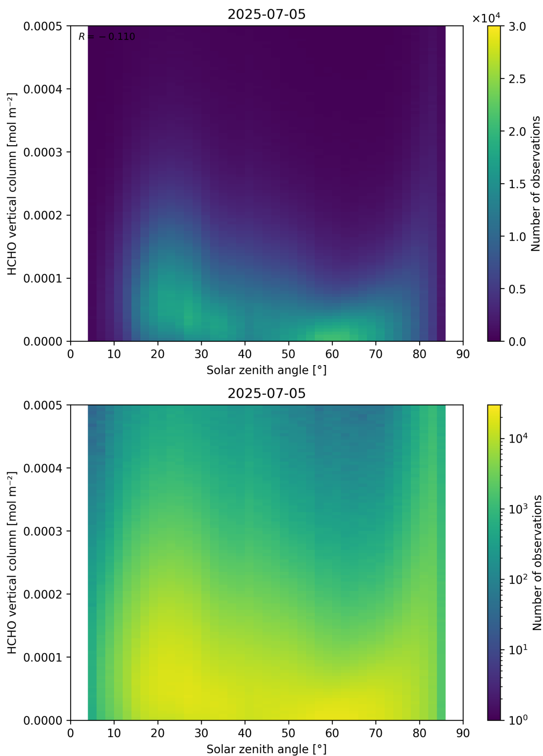
Figure 177: Scatter density plot of “Solar zenith angle” against “HCHO vertical column” for 2025-07-04 to 2025-07-06.
