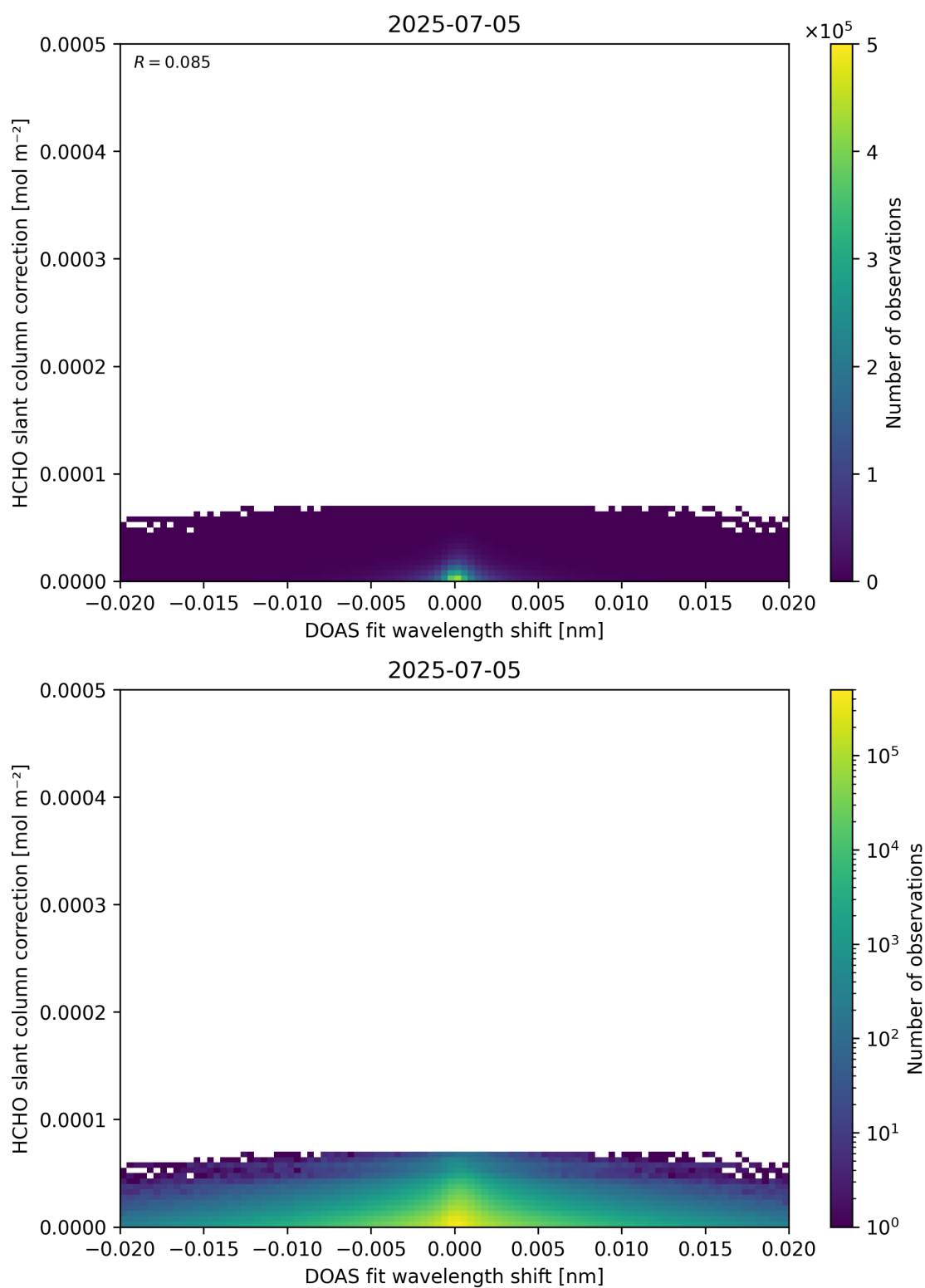
Figure 67: Scatter density plot of “DOAS fit wavelength shift” against “HCHO slant column correction” for 2025-07-04 to 2025-07-06.
