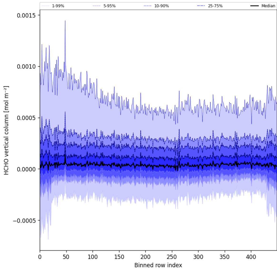
Figure 49: Along track statistics of “HCHO vertical column” for 2025-07-04 to 2025-07-06
