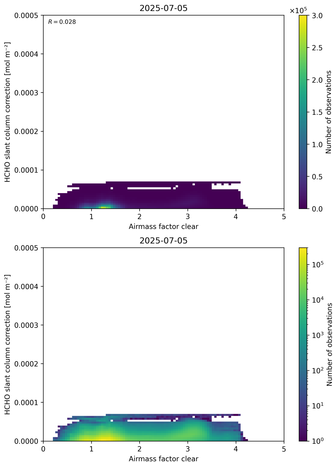
Figure 75: Scatter density plot of “Airmass factor clear” against “HCHO slant column correction” for 2025-07-04 to 2025-07-06.
