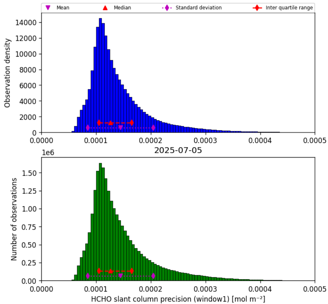
Figure 39: Histogram of “HCHO slant column precision (window1)” for 2025-07-04 to 2025-07-06
