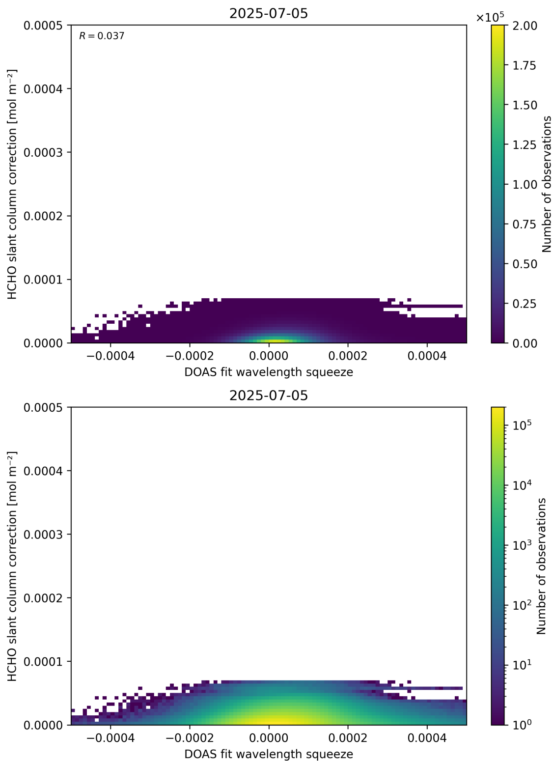
Figure 70: Scatter density plot of “DOAS fit wavelength squeeze” against “HCHO slant column correction” for 2025-07-04 to 2025-07-06.
