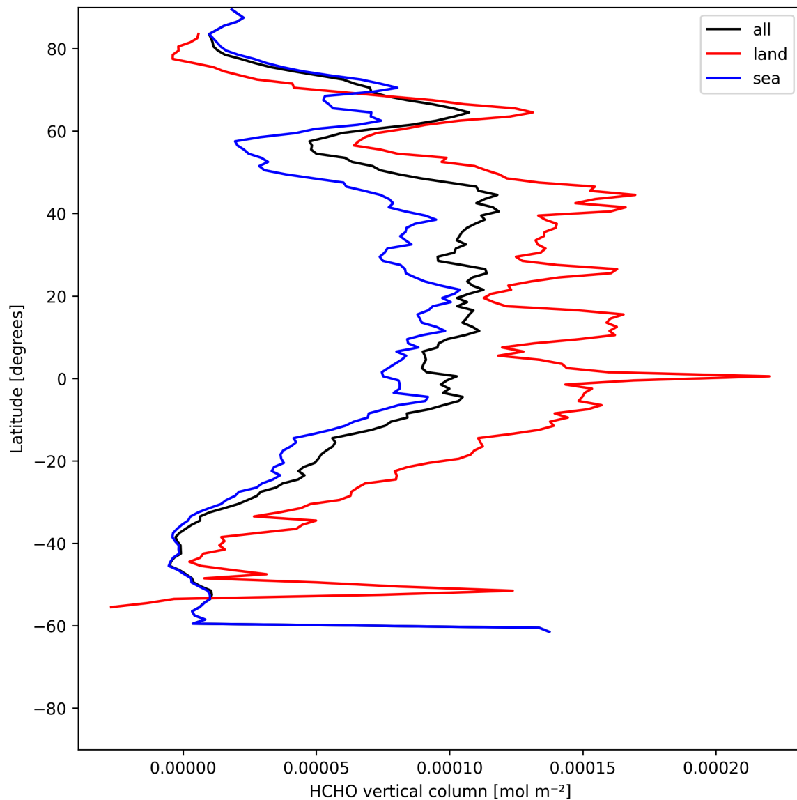
Figure 21: Zonal average of “HCHO vertical column” for 2025-07-04 to 2025-07-06.
