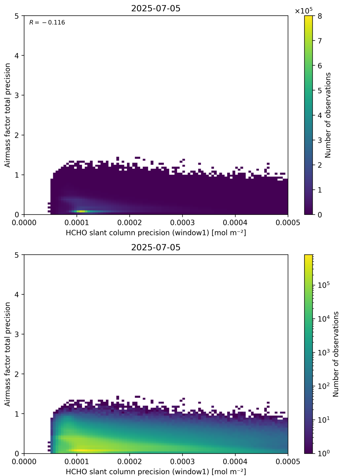
Figure 95: Scatter density plot of “HCHO slant column precision (window1)” against “Airmass factor total precision” for 2025-07-04 to 2025-07-06.
