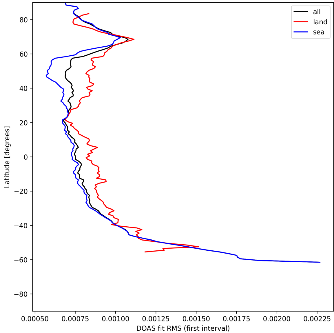
Figure 32: Zonal average of “DOAS fit RMS (first interval)” for 2025-07-04 to 2025-07-06.
