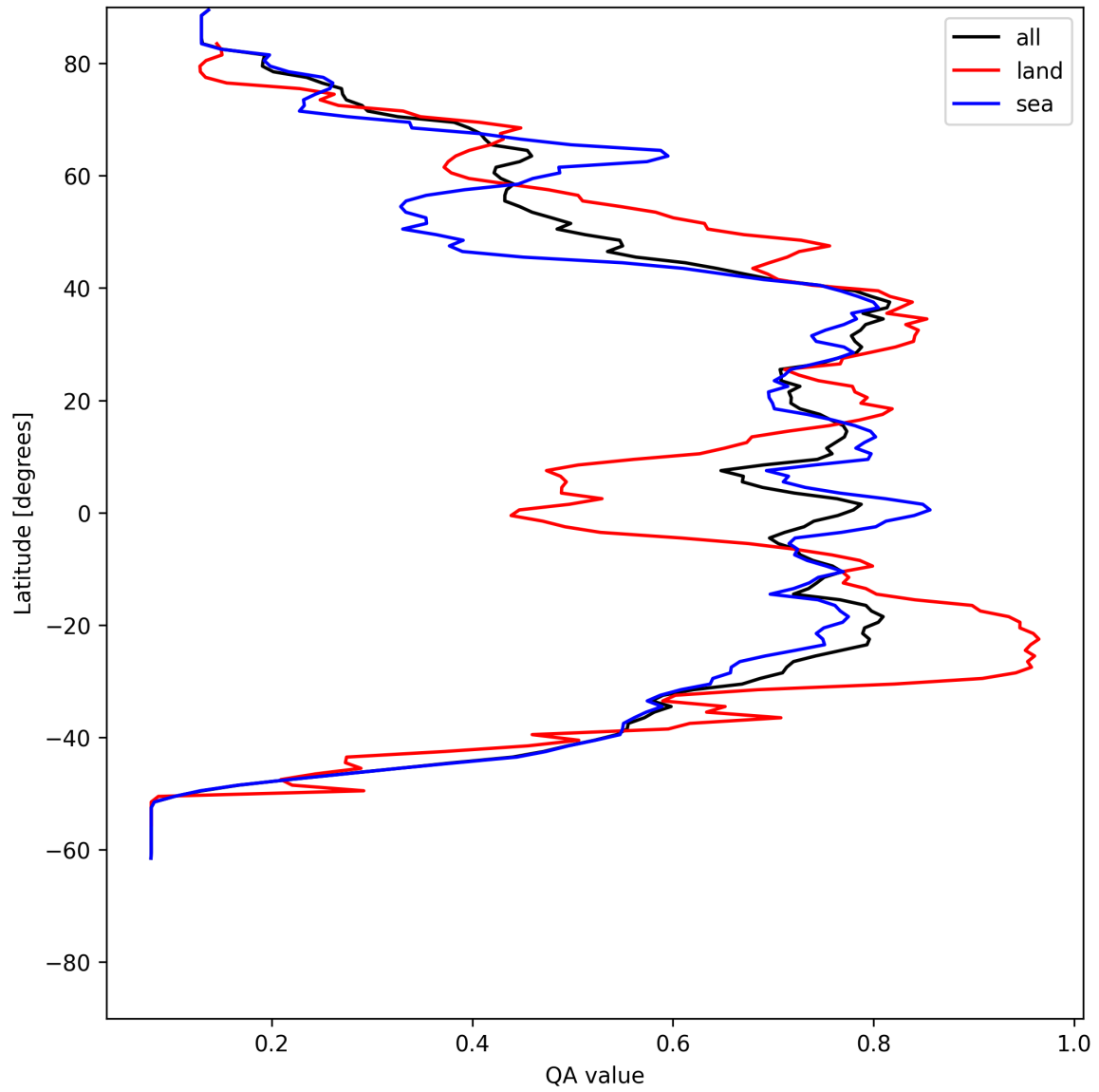
Figure 20: Zonal average of “QA value” for 2025-07-04 to 2025-07-06.
