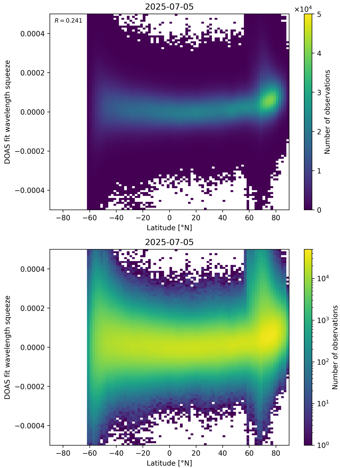
Figure 155: Scatter density plot of “Latitude” against “DOAS fit wavelength squeeze” for 2025-07-04 to 2025-07-06.
