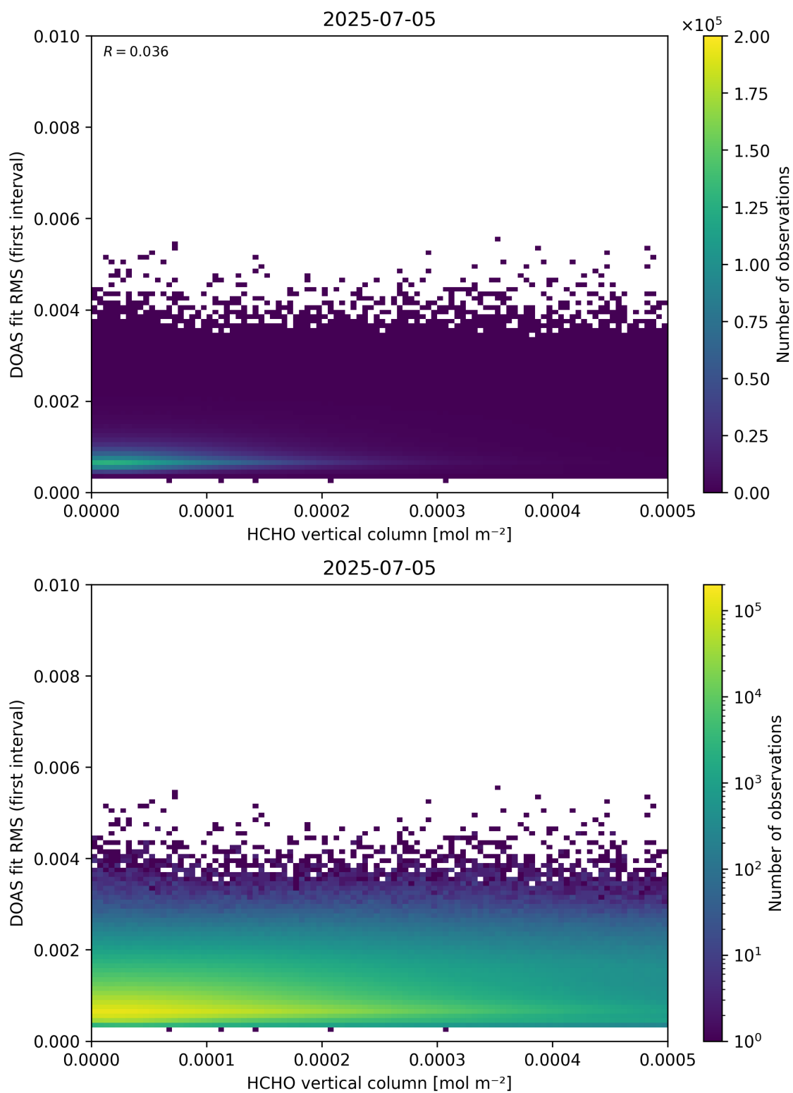
Figure 123: Scatter density plot of “HCHO vertical column” against “DOAS fit RMS (first interval)” for 2025-07-04 to 2025-07-06.
