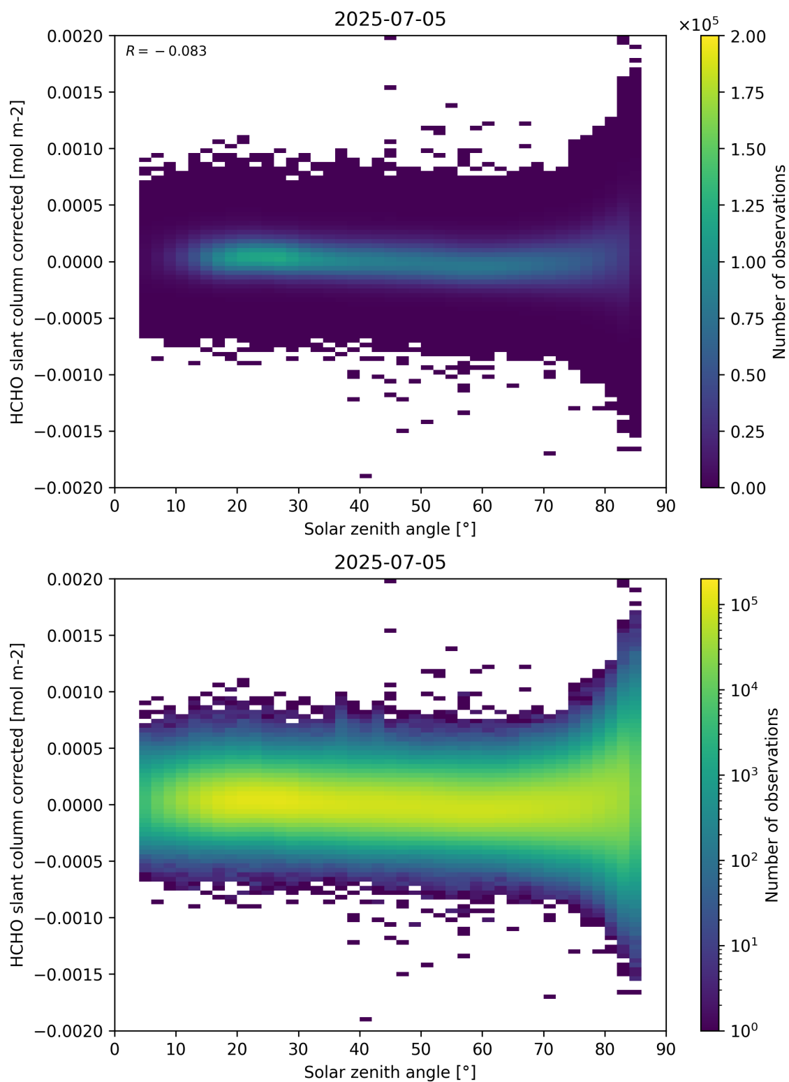
Figure 171: Scatter density plot of “Solar zenith angle” against “HCHO slant column corrected” for 2025-07-04 to 2025-07-06.
