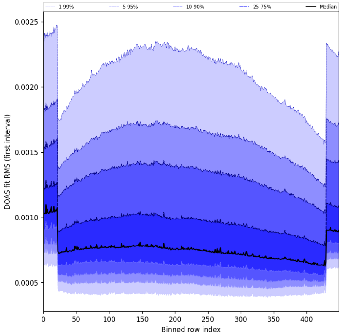
Figure 60: Along track statistics of “DOAS fit RMS (first interval)” for 2025-07-04 to 2025-07-06
