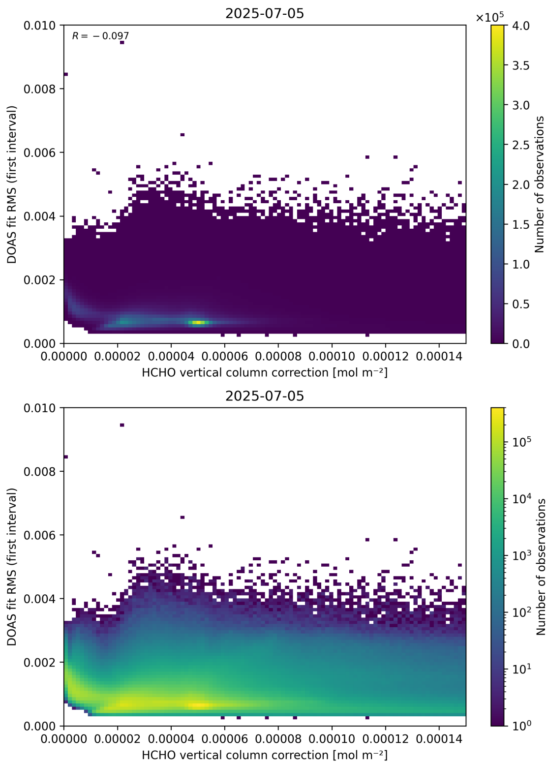
Figure 112: Scatter density plot of “HCHO vertical column correction” against “DOAS fit RMS (first interval)” for 2025-07-04 to 2025-07-06.
