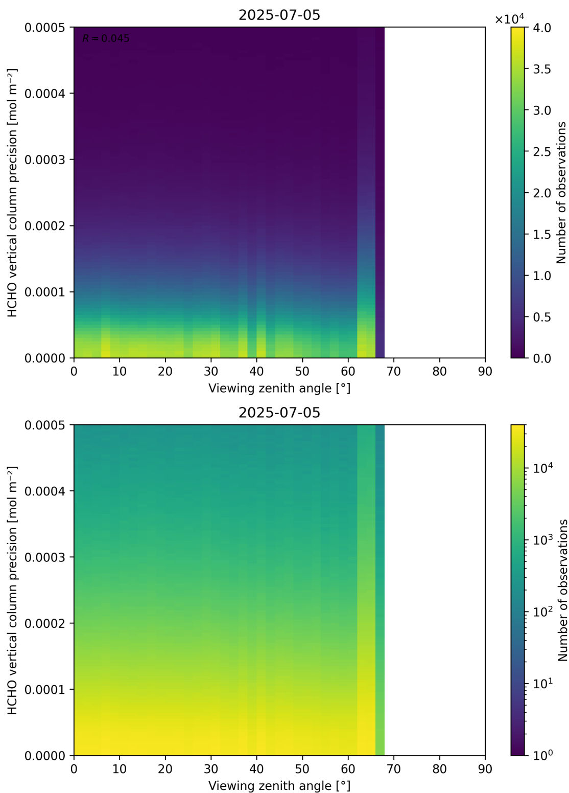
Figure 194: Scatter density plot of “Viewing zenith angle” against “HCHO vertical column precision” for 2025-07-04 to 2025-07-06.
