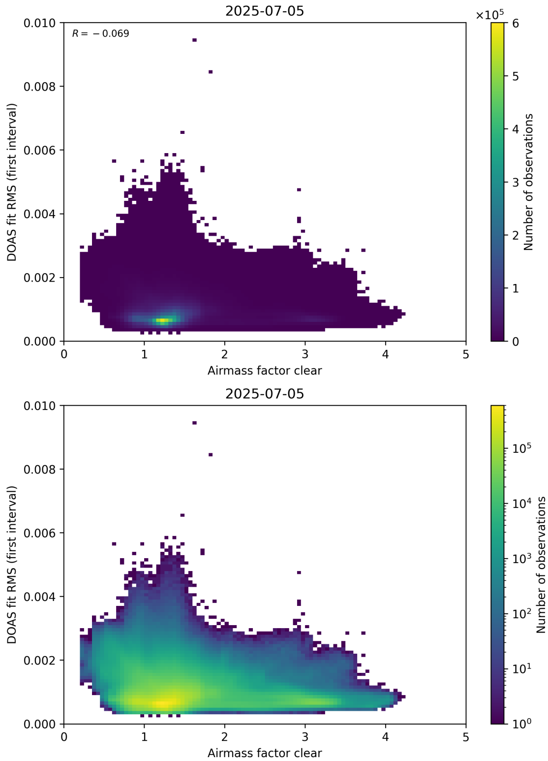
Figure 71: Scatter density plot of “Airmass factor clear” against “DOAS fit RMS (first interval)” for 2025-07-04 to 2025-07-06.
