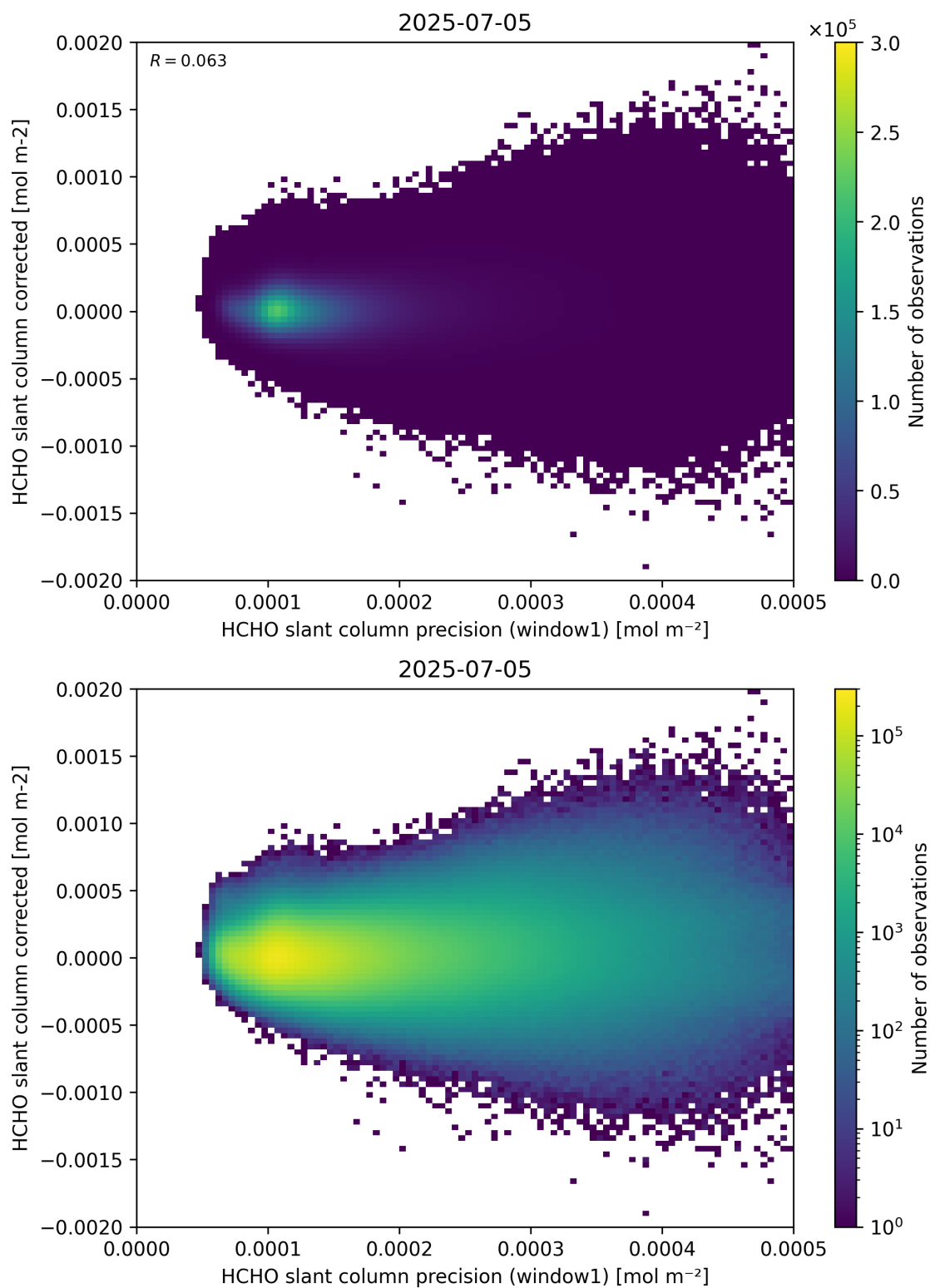
Figure 92: Scatter density plot of “HCHO slant column precision (window1)” against “HCHO slant column corrected” for 2025-07-04 to 2025-07-06.
