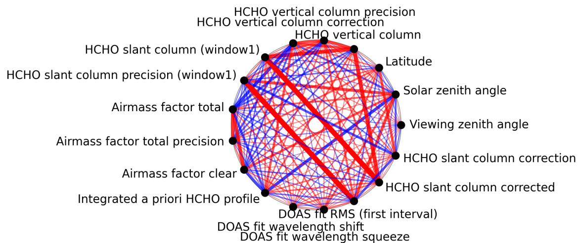
Figure 1: Map of correlation graph for 2025-07-04 to 2025-07-06.
