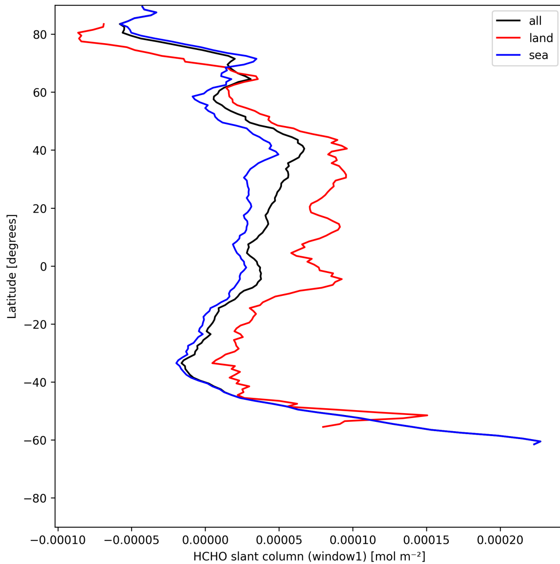
Figure 24: Zonal average of “HCHO slant column (window1)” for 2025-07-04 to 2025-07-06.
