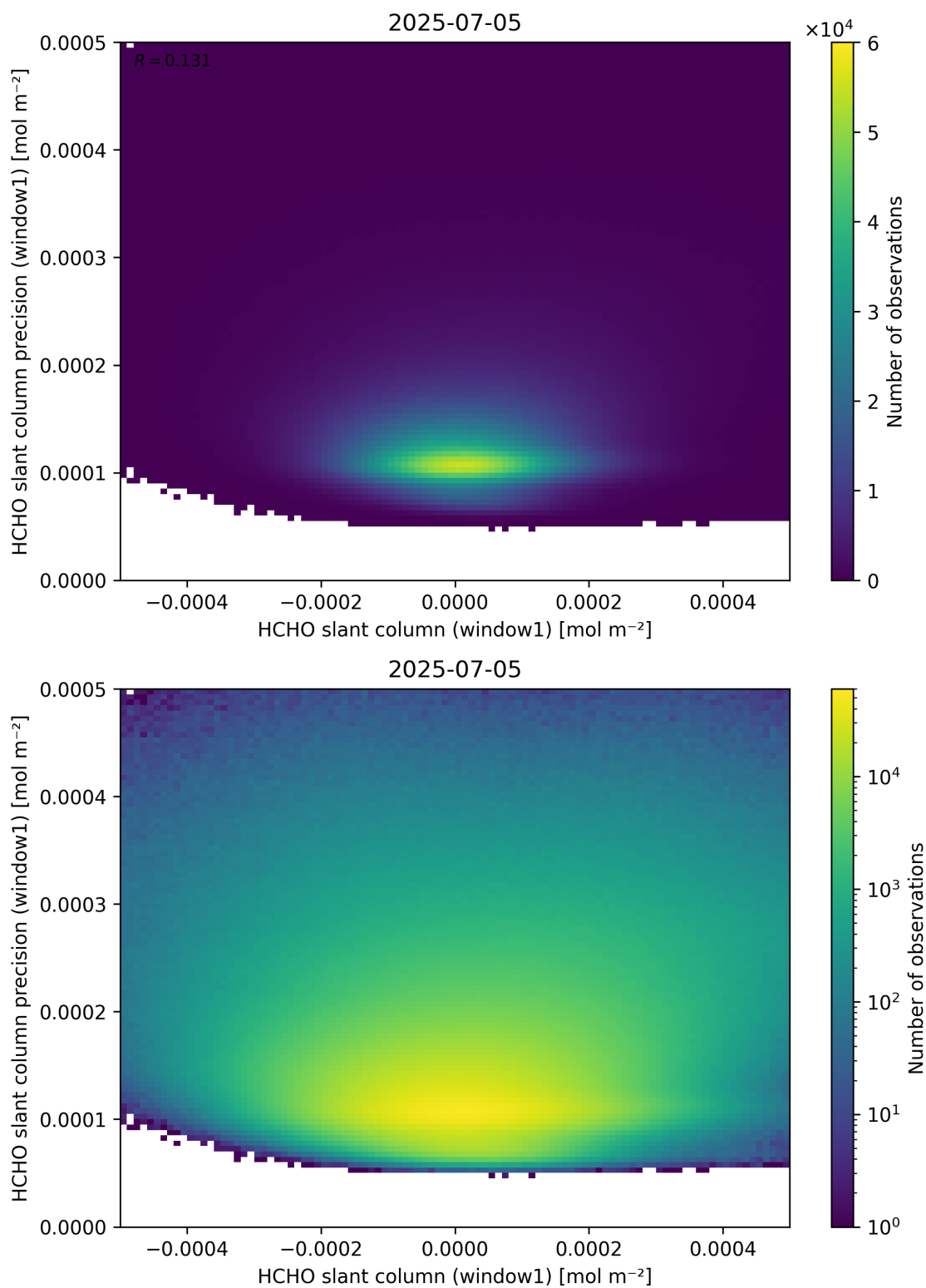
Figure 84: Scatter density plot of “HCHO slant column (window1)” against “HCHO slant column precision (window1)” for 2025-07-04 to 2025-07-06.
