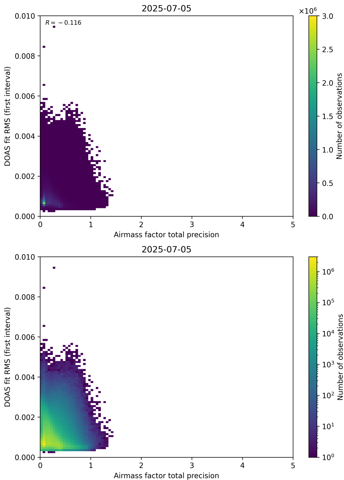
Figure 105: Scatter density plot of “Airmass factor total precision” against “DOAS fit RMS (first interval)” for 2025-07-04 to 2025-07-06.
