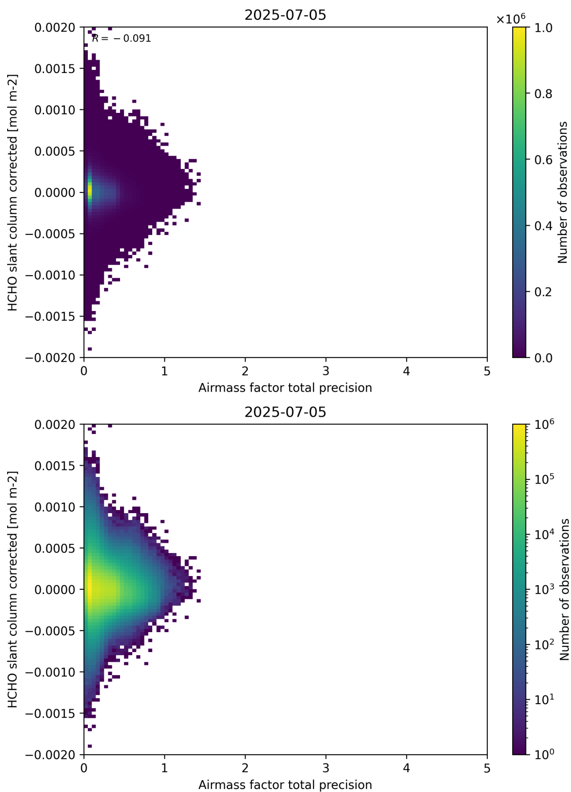
Figure 109: Scatter density plot of “Airmass factor total precision” against “HCHO slant column corrected” for 2025-07-04 to 2025-07-06.
