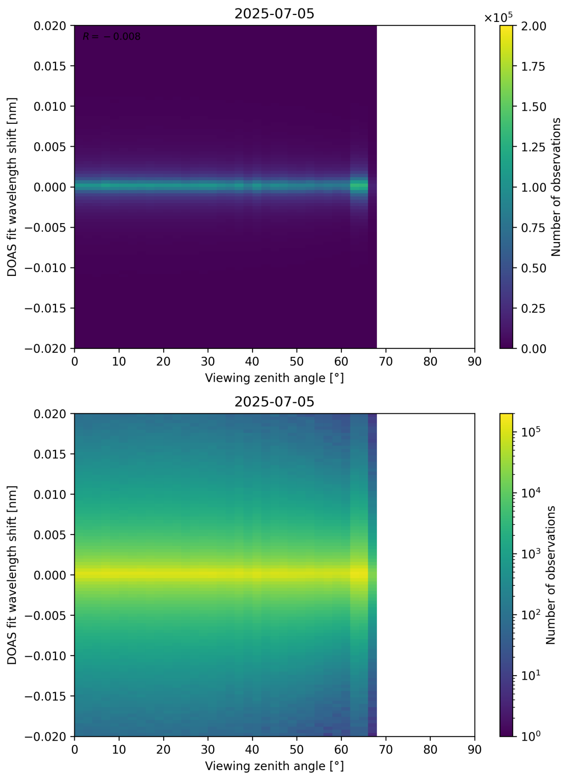
Figure 183: Scatter density plot of “Viewing zenith angle” against “DOAS fit wavelength shift” for 2025-07-04 to 2025-07-06.
