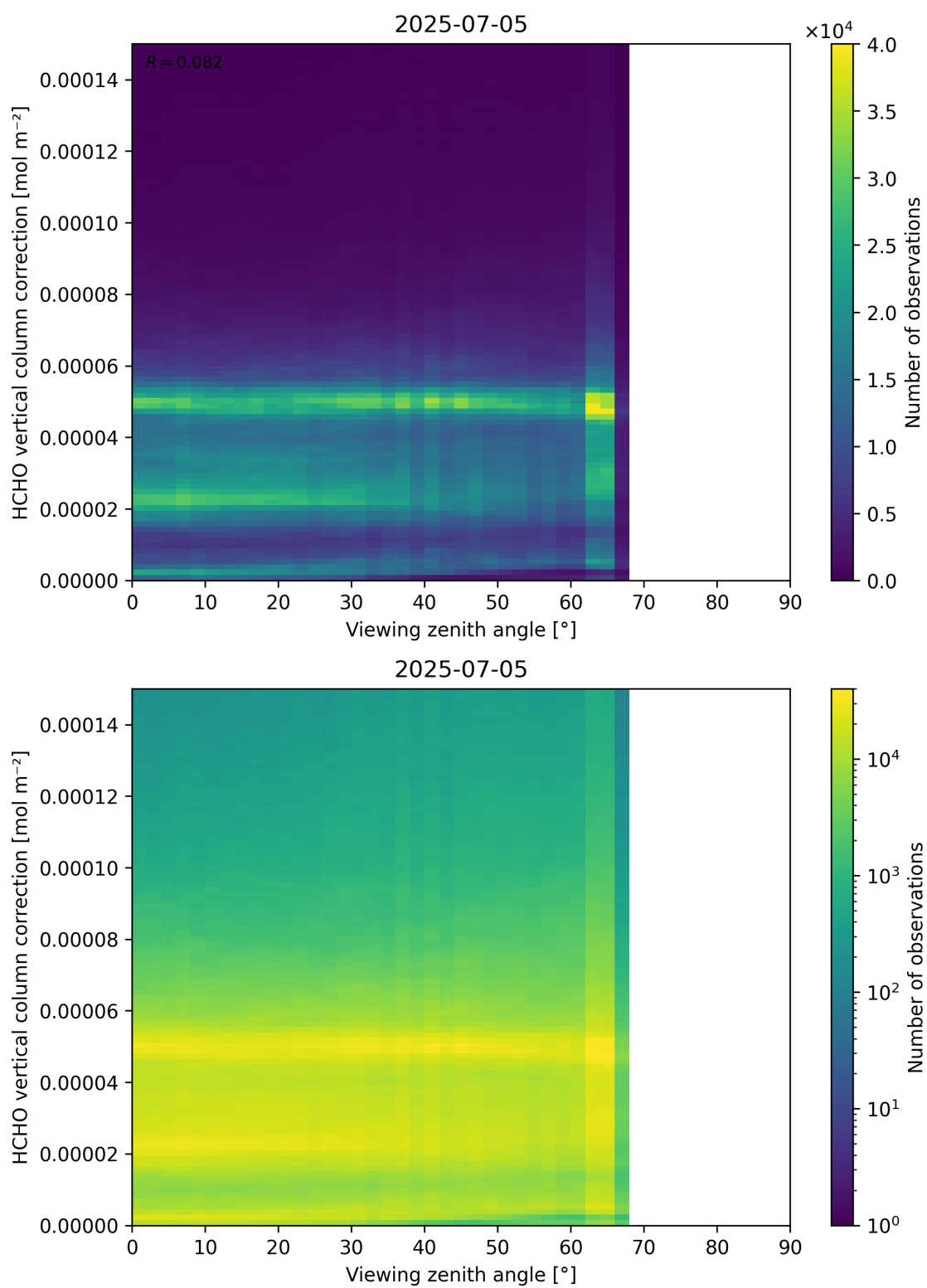
Figure 193: Scatter density plot of “Viewing zenith angle” against “HCHO vertical column correction” for 2025-07-04 to 2025-07-06.
