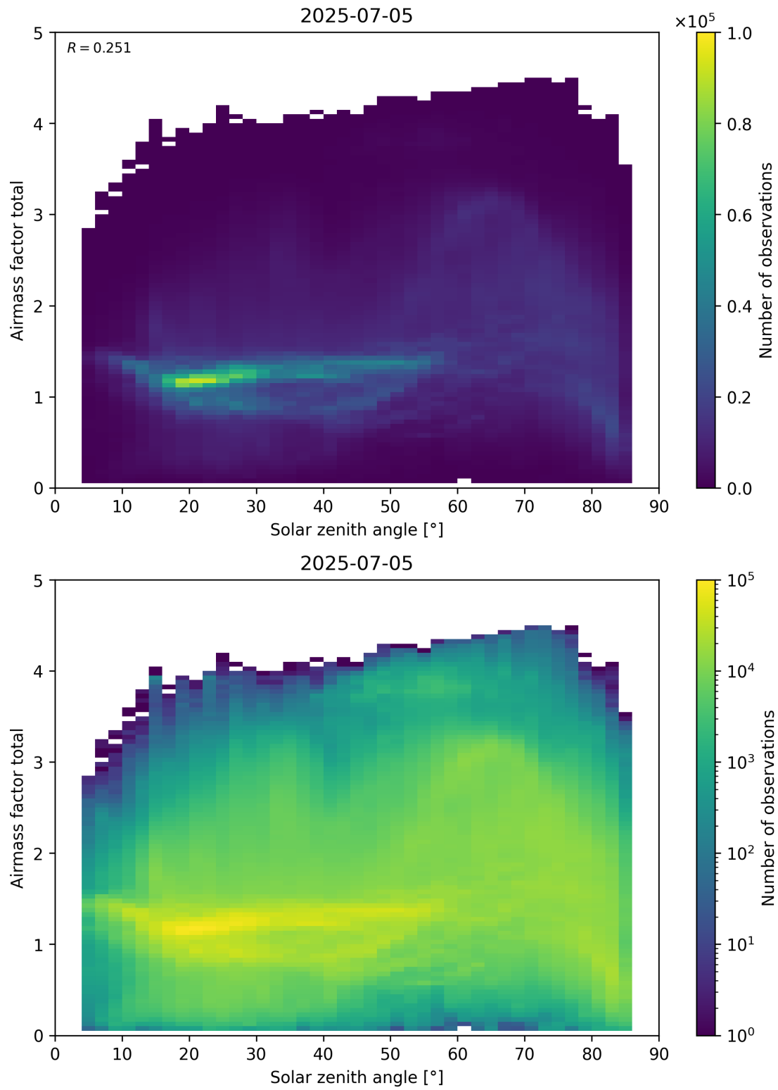
Figure 175: Scatter density plot of “Solar zenith angle” against “Airmass factor total” for 2025-07-04 to 2025-07-06.
