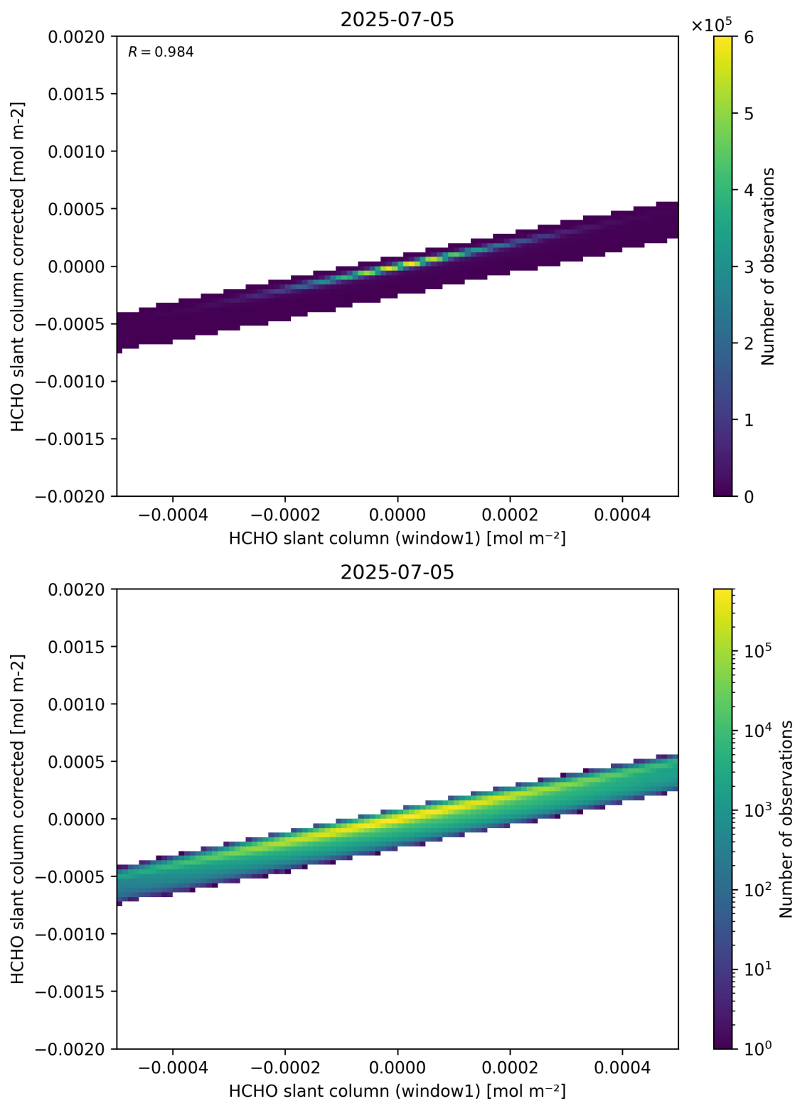
Figure 82: Scatter density plot of “HCHO slant column (window1)” against “HCHO slant column corrected” for 2025-07-04 to 2025-07-06.
