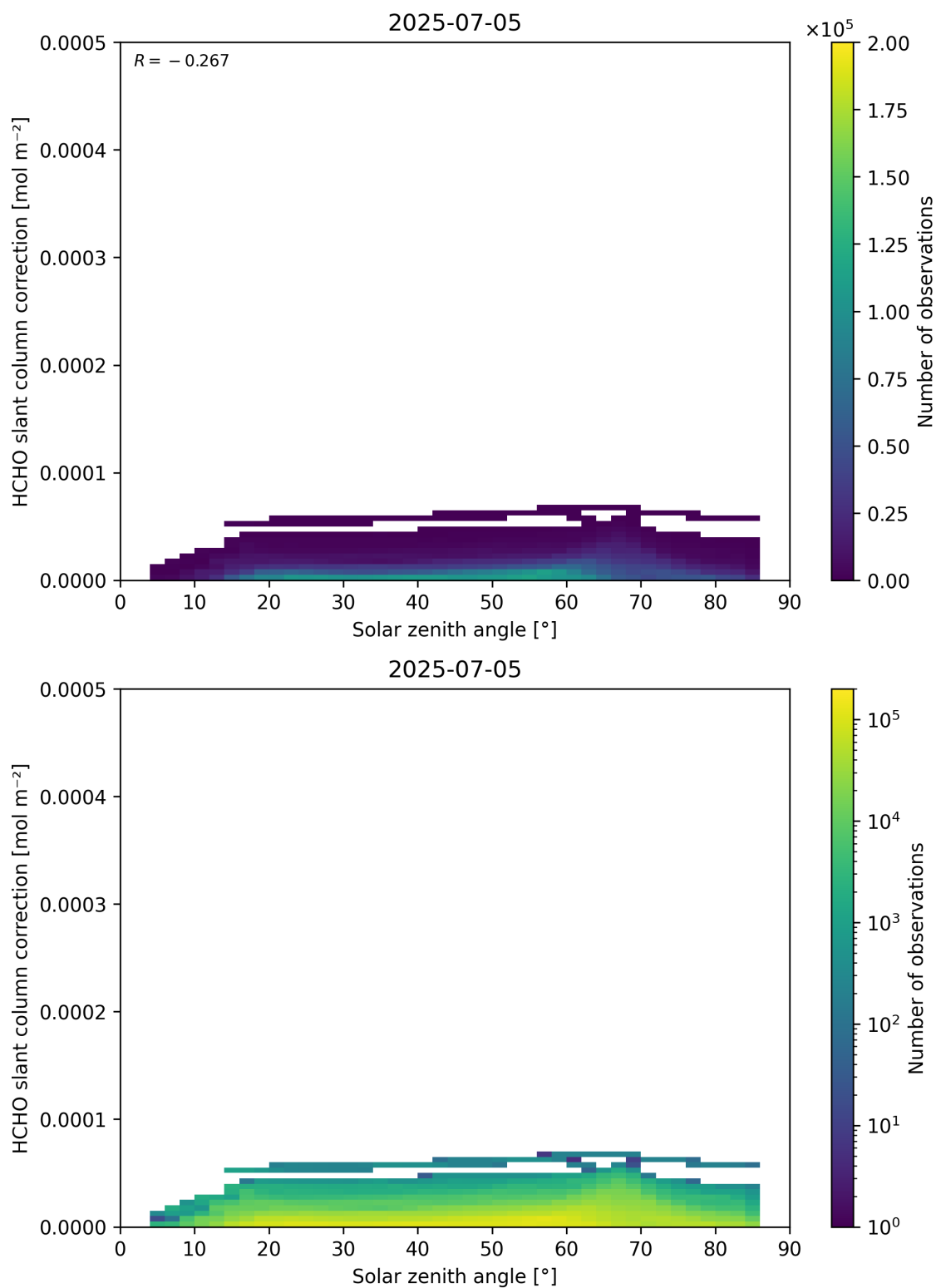
Figure 172: Scatter density plot of “Solar zenith angle” against “HCHO slant column correction” for 2025-07-04 to 2025-07-06.
