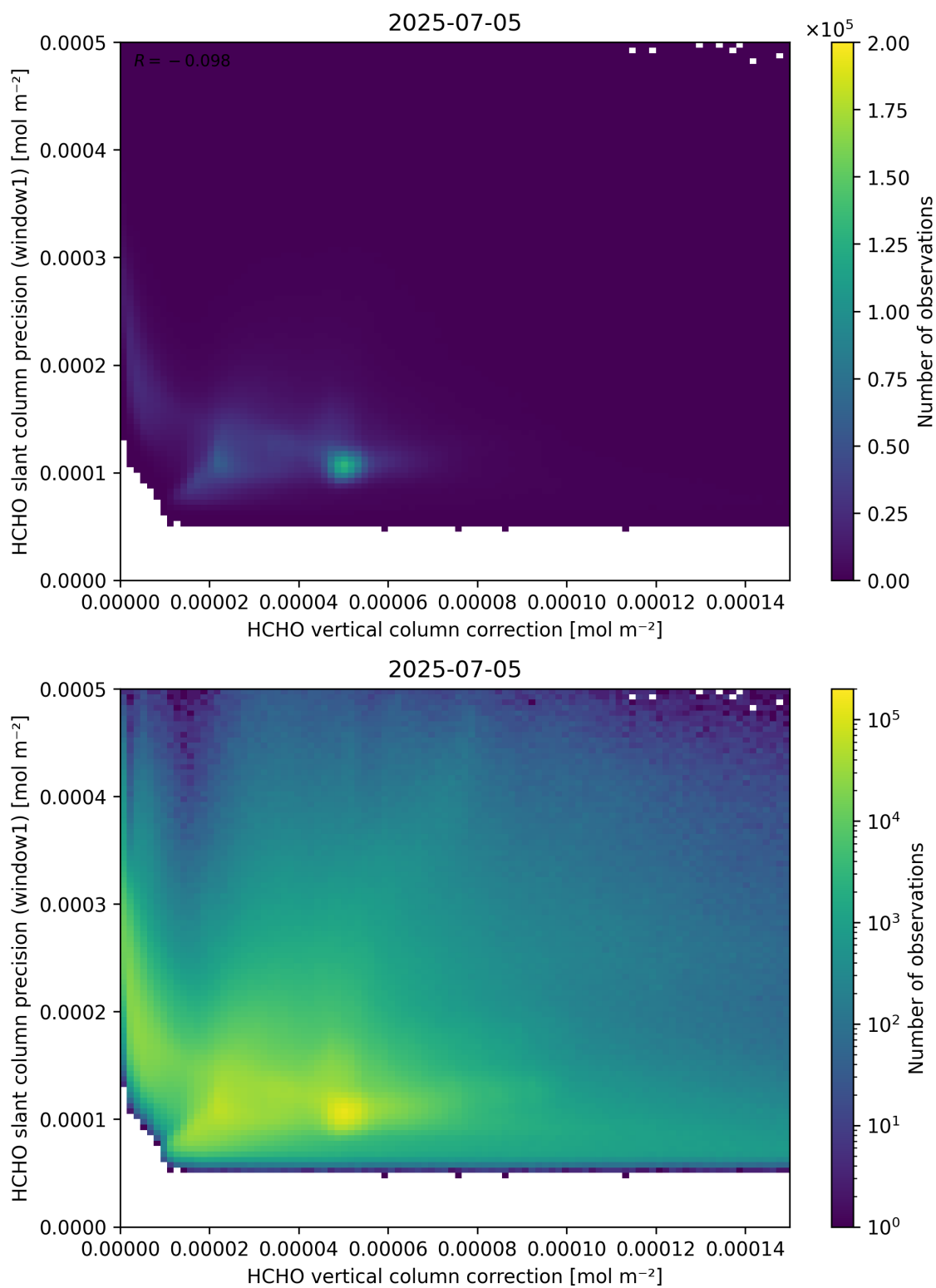
Figure 119: Scatter density plot of “HCHO vertical column correction” against “HCHO slant column precision (window1)” for 2025-07-04 to 2025-07-06.
