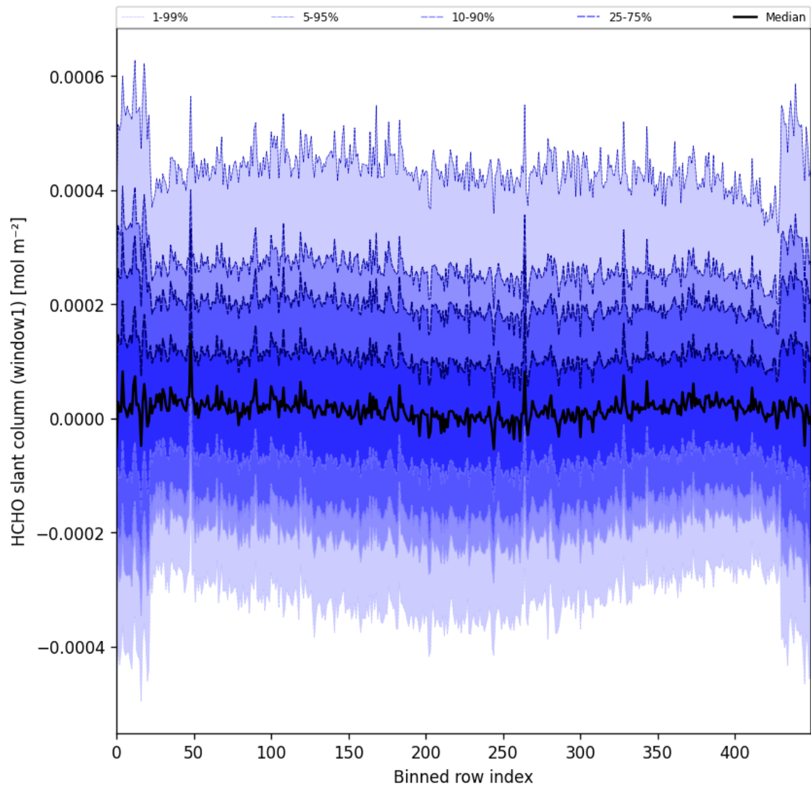
Figure 52: Along track statistics of “HCHO slant column (window1)” for 2025-07-04 to 2025-07-06
