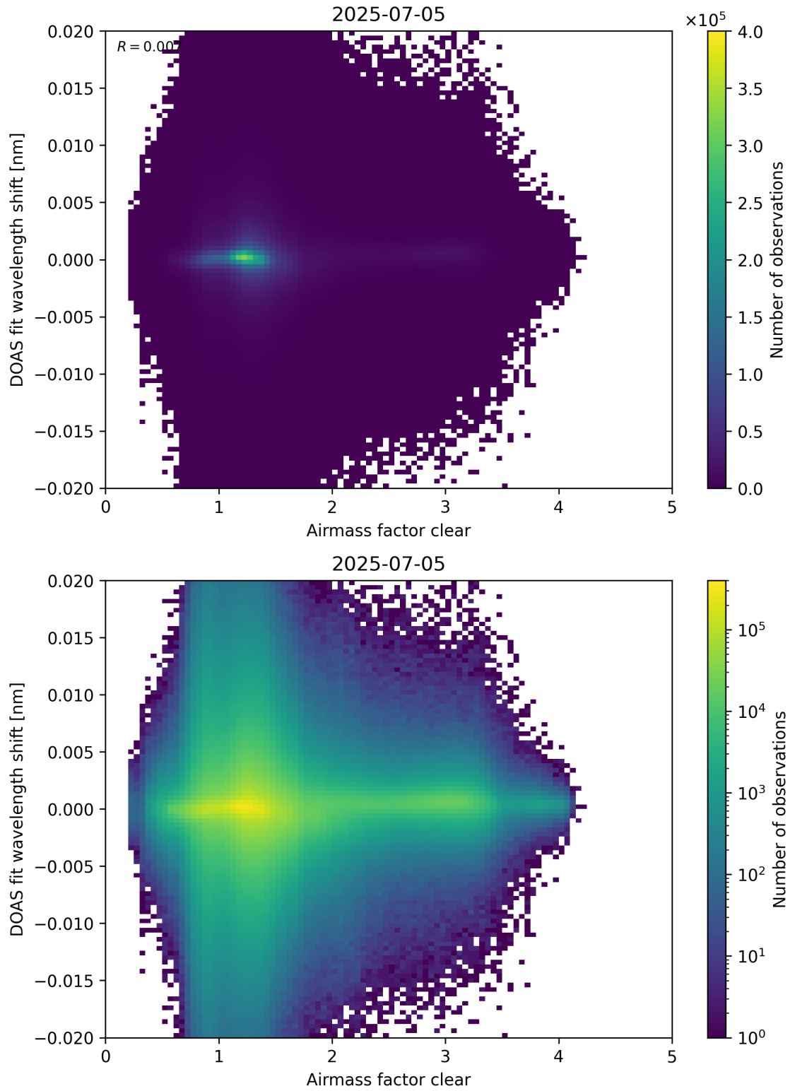
Figure 72: Scatter density plot of “Airmass factor clear” against “DOAS fit wavelength shift” for 2025-07-04 to 2025-07-06.
