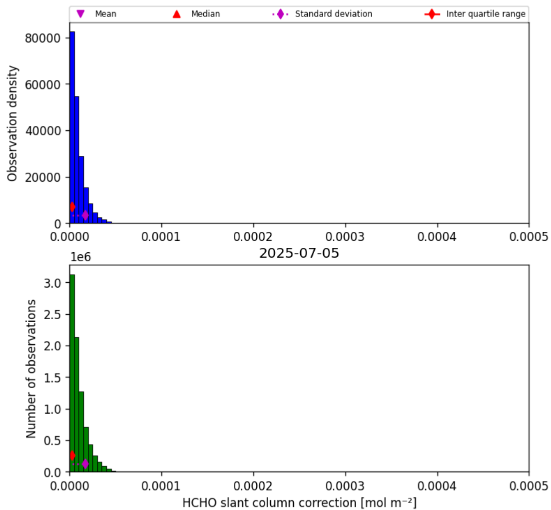
Figure 47: Histogram of “HCHO slant column correction” for 2025-07-04 to 2025-07-06
