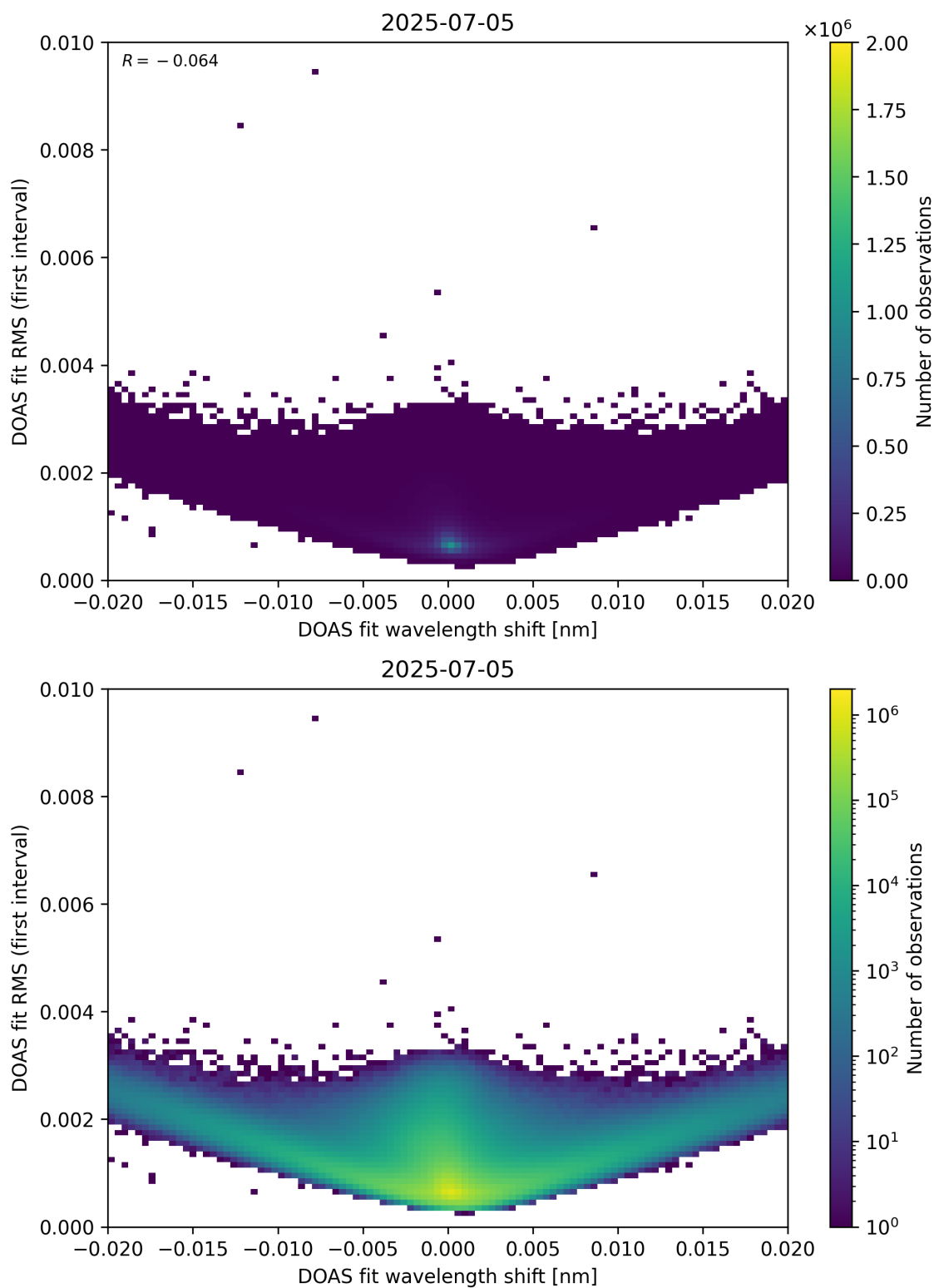
Figure 64: Scatter density plot of “DOAS fit wavelength shift” against “DOAS fit RMS (first interval)” for 2025-07-04 to 2025-07-06.
