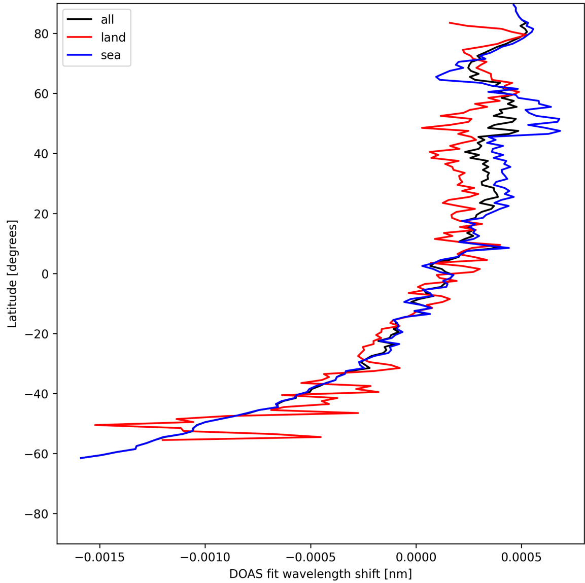
Figure 30: Zonal average of “DOAS fit wavelength shift” for 2025-07-04 to 2025-07-06.
