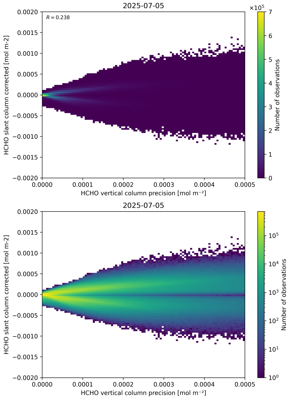
Figure 140: Scatter density plot of “HCHO vertical column precision” against “HCHO slant column corrected” for 2025-07-04 to 2025-07-06.
