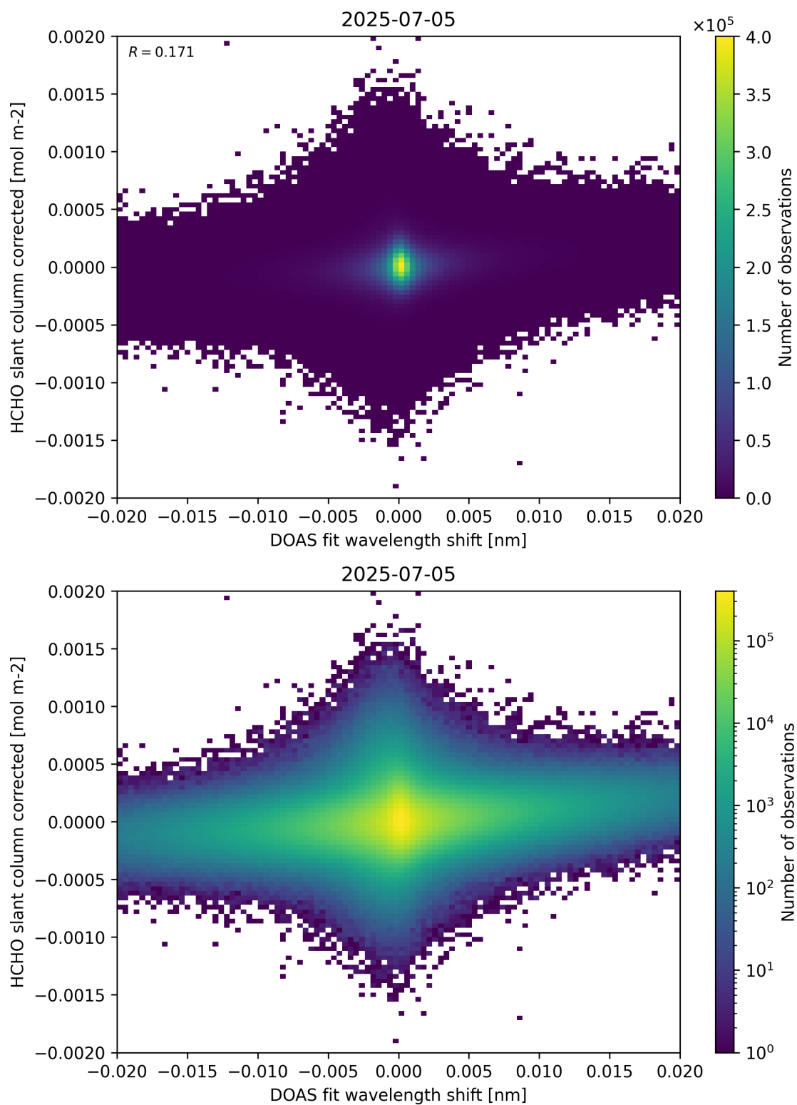
Figure 66: Scatter density plot of “DOAS fit wavelength shift” against “HCHO slant column corrected” for 2025-07-04 to 2025-07-06.
