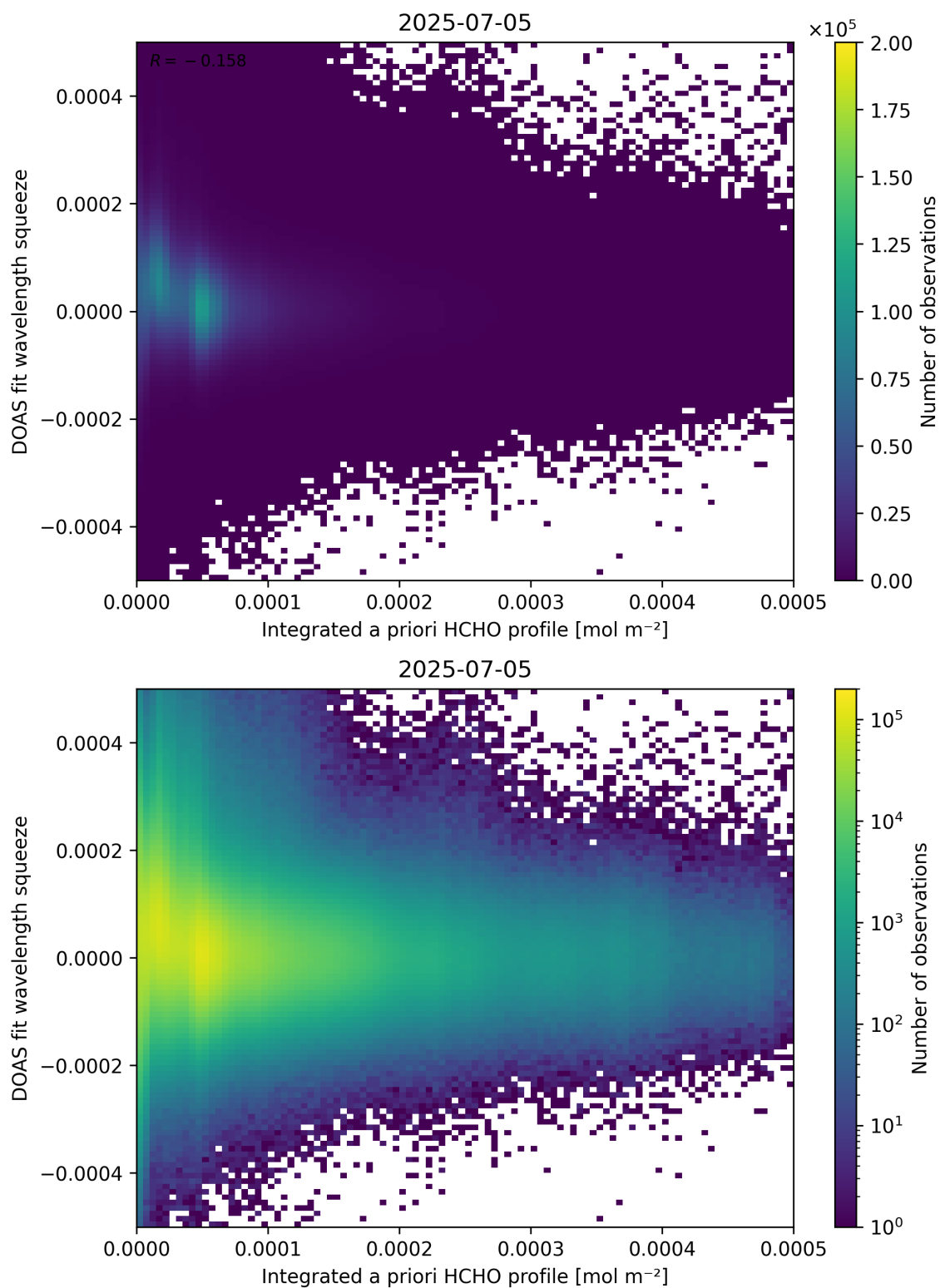
Figure 150: Scatter density plot of “Integrated a priori HCHO profile” against “DOAS fit wavelength squeeze” for 2025-07-04 to 2025-07-06.
