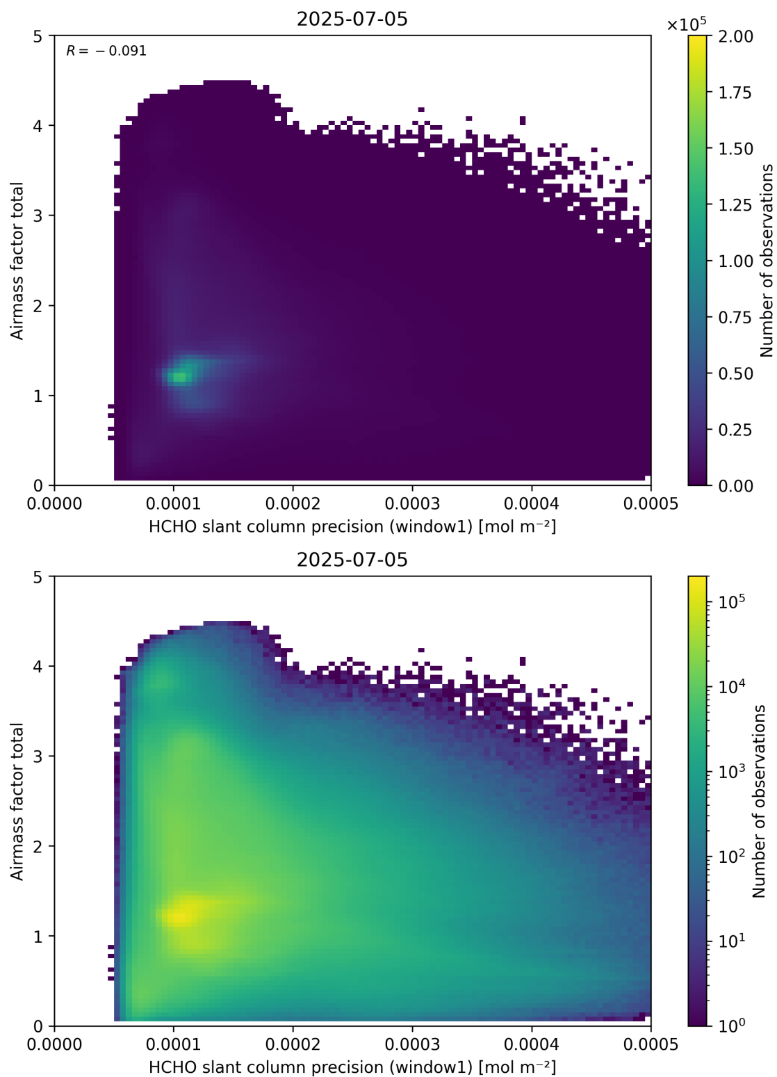
Figure 94: Scatter density plot of “HCHO slant column precision (window1)” against “Airmass factor total” for 2025-07-04 to 2025-07-06.
