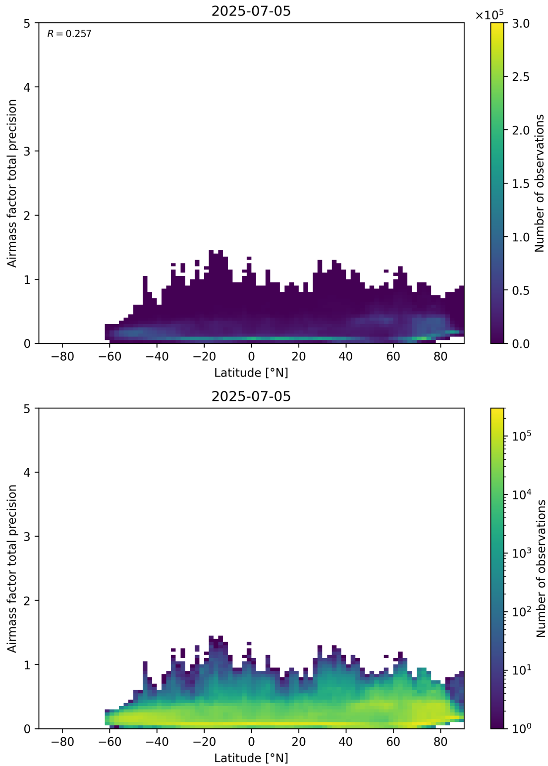
Figure 162: Scatter density plot of “Latitude” against “Airmass factor total precision” for 2025-07-04 to 2025-07-06.
