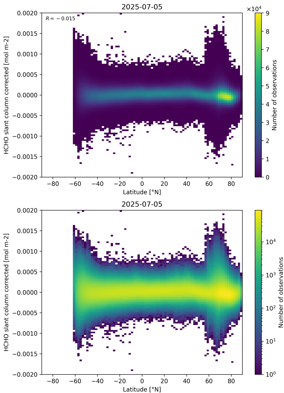
Figure 157: Scatter density plot of “Latitude” against “HCHO slant column corrected” for 2025-07-04 to 2025-07-06.
