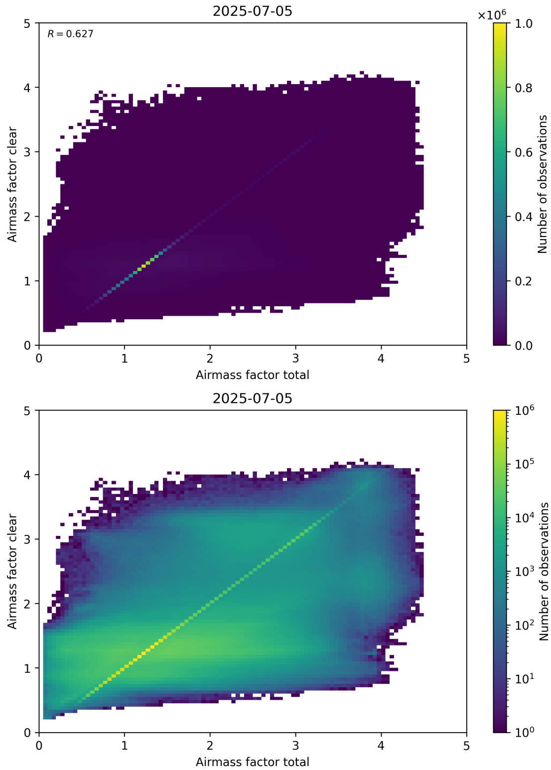
Figure 100: Scatter density plot of “Airmass factor total” against “Airmass factor clear” for 2025-07-04 to 2025-07-06.
