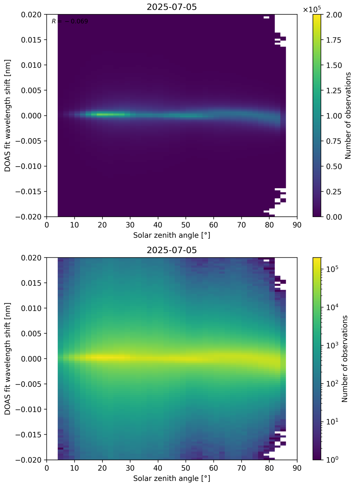
Figure 168: Scatter density plot of “Solar zenith angle” against “DOAS fit wavelength shift” for 2025-07-04 to 2025-07-06.
