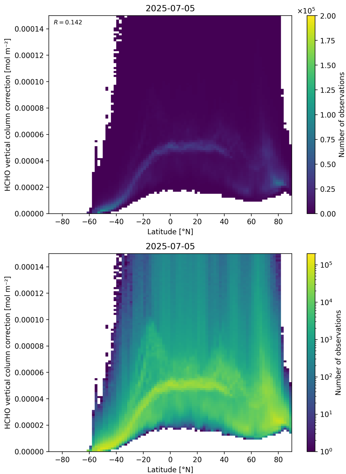
Figure 164: Scatter density plot of “Latitude” against “HCHO vertical column correction” for 2025-07-04 to 2025-07-06.
