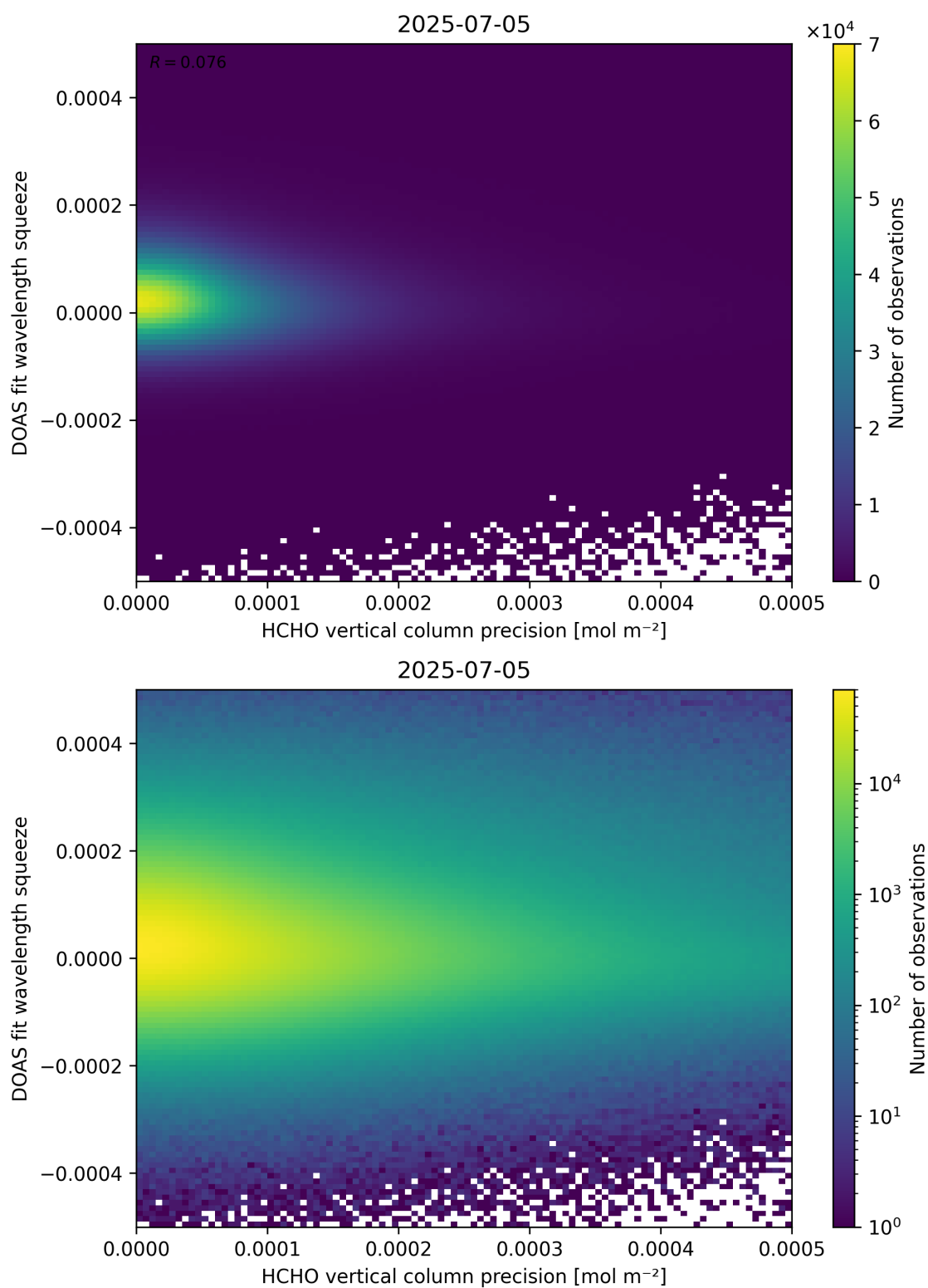
Figure 138: Scatter density plot of “HCHO vertical column precision” against “DOAS fit wavelength squeeze” for 2025-07-04 to 2025-07-06.
