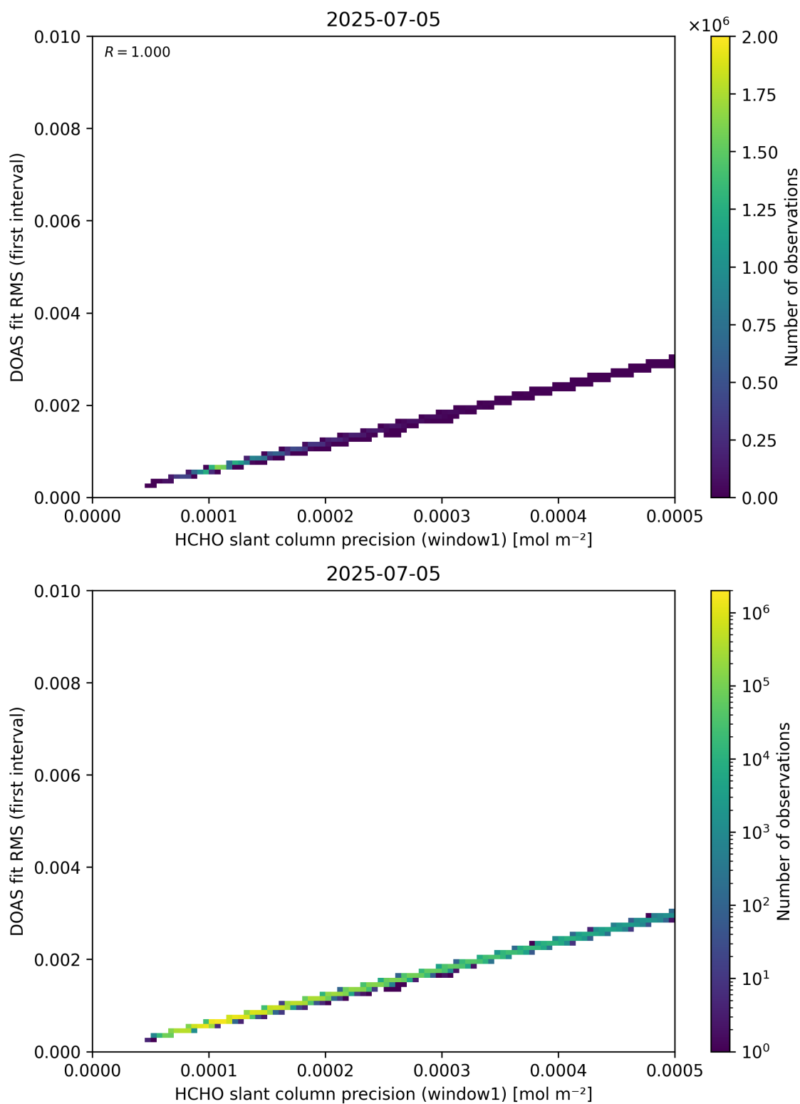
Figure 88: Scatter density plot of “HCHO slant column precision (window1)” against “DOAS fit RMS (first interval)” for 2025-07-04 to 2025-07-06.
