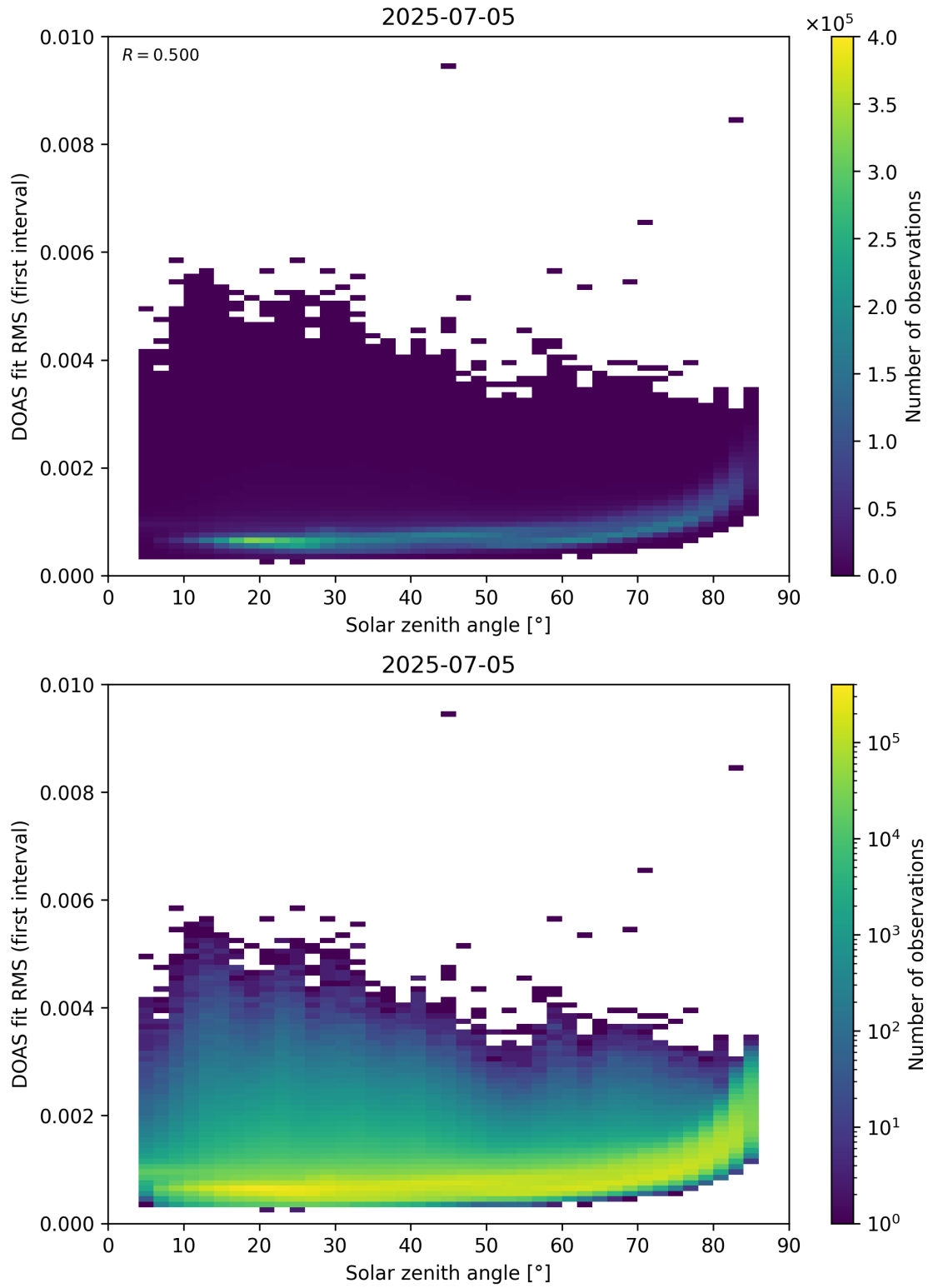
Figure 167: Scatter density plot of “Solar zenith angle” against “DOAS fit RMS (first interval)” for 2025-07-04 to 2025-07-06.
