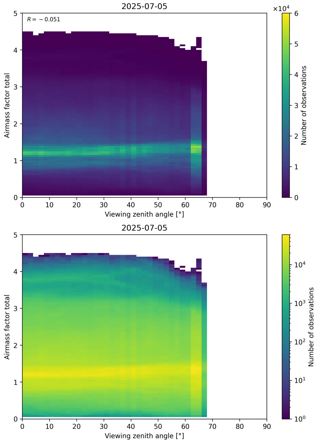
Figure 190: Scatter density plot of “Viewing zenith angle” against “Airmass factor total” for 2025-07-04 to 2025-07-06.
