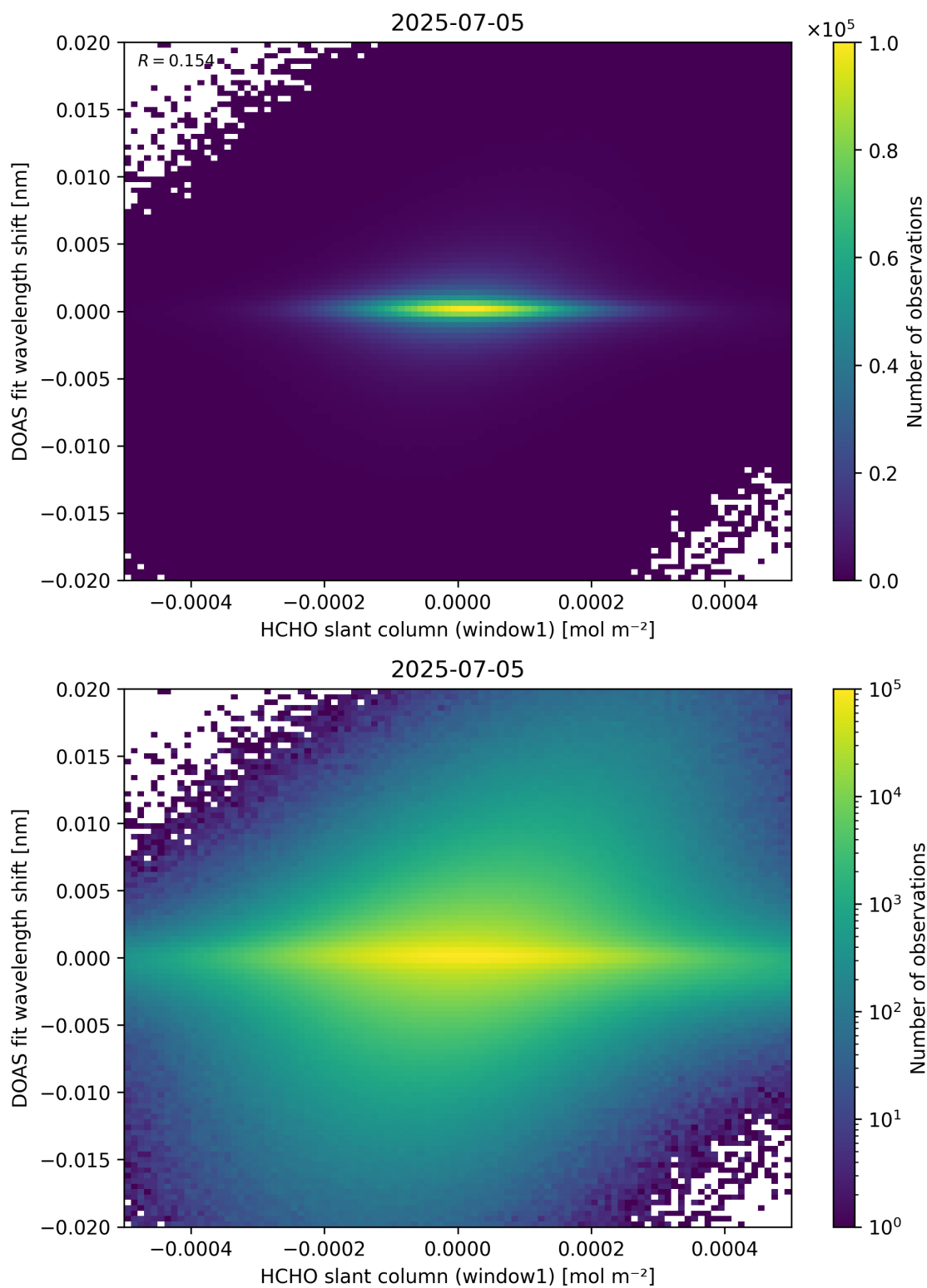
Figure 79: Scatter density plot of “HCHO slant column (window1)” against “DOAS fit wavelength shift” for 2025-07-04 to 2025-07-06.
