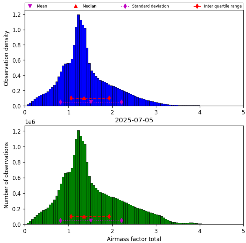
Figure 40: Histogram of “Airmass factor total” for 2025-07-04 to 2025-07-06
