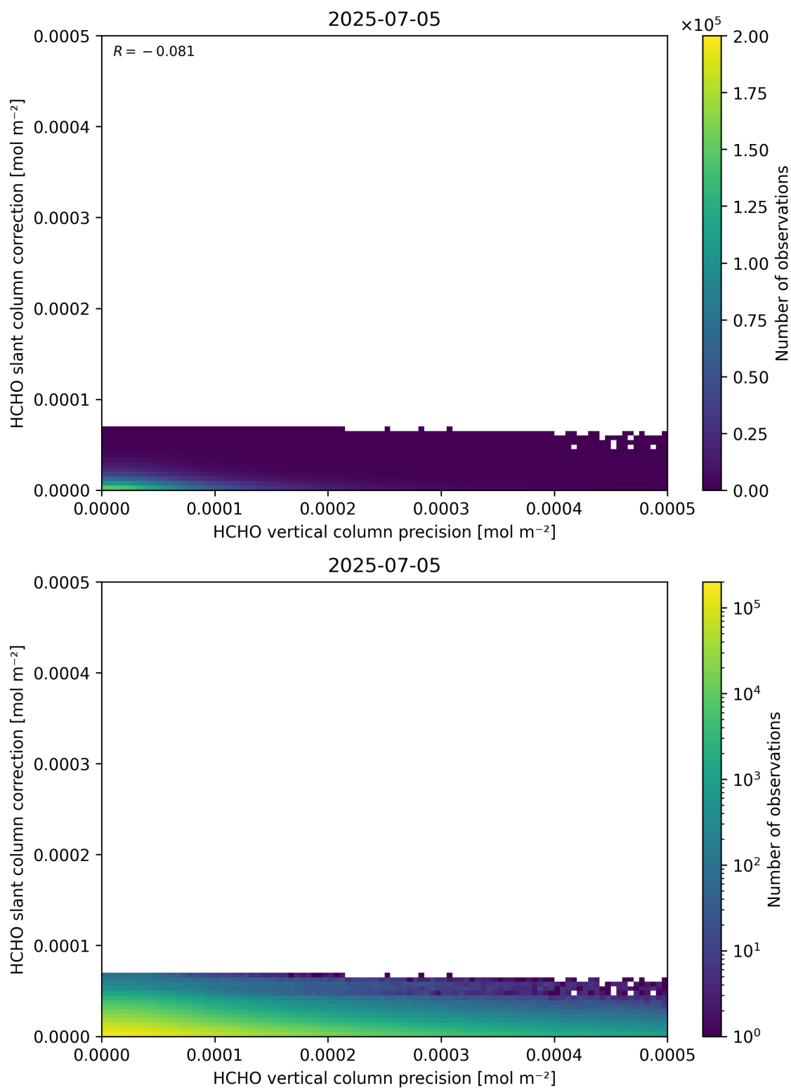
Figure 141: Scatter density plot of “HCHO vertical column precision” against “HCHO slant column correction” for 2025-07-04 to 2025-07-06.
