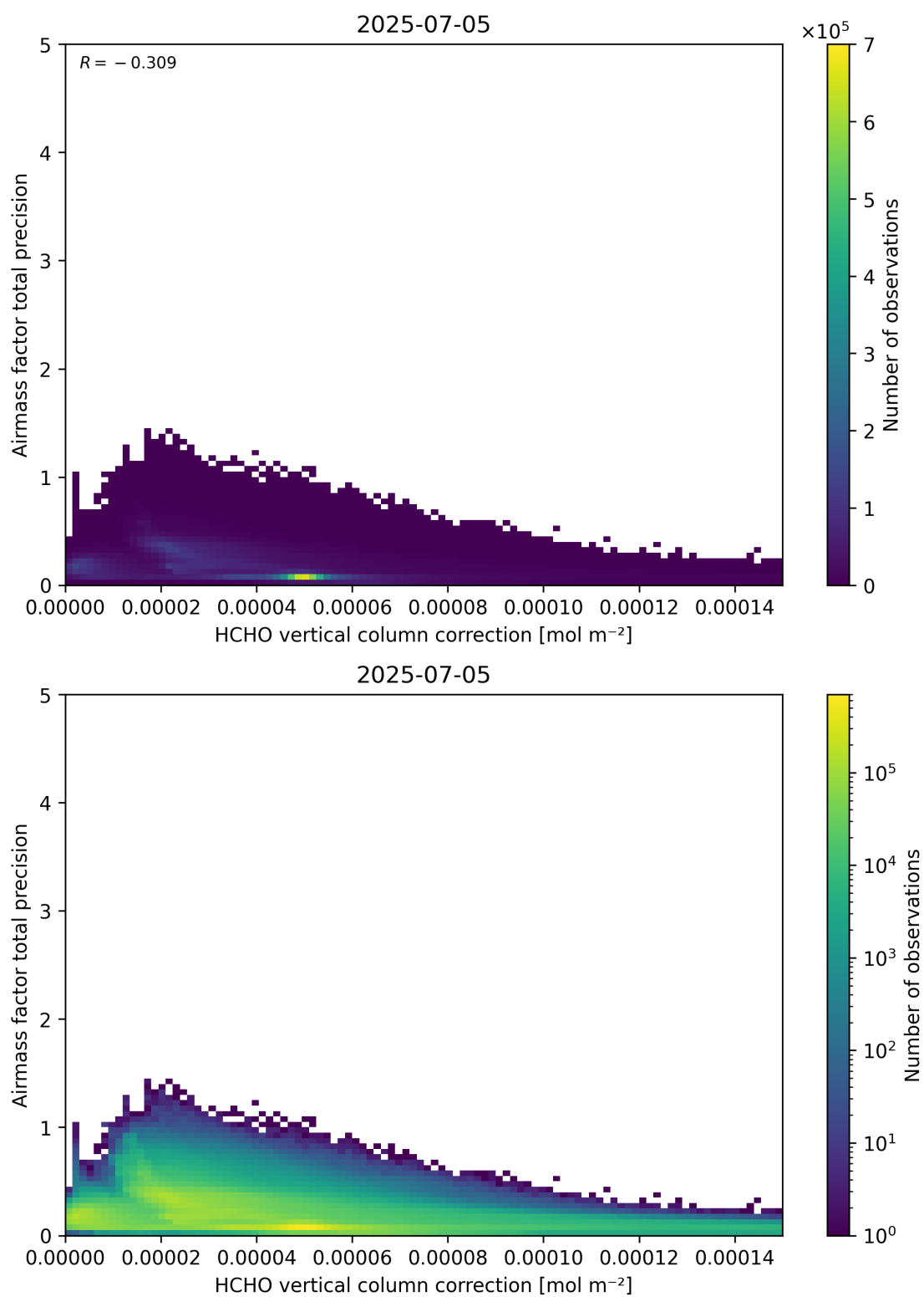
Figure 121: Scatter density plot of “HCHO vertical column correction” against “Airmass factor total precision” for 2025-07-04 to 2025-07-06.
