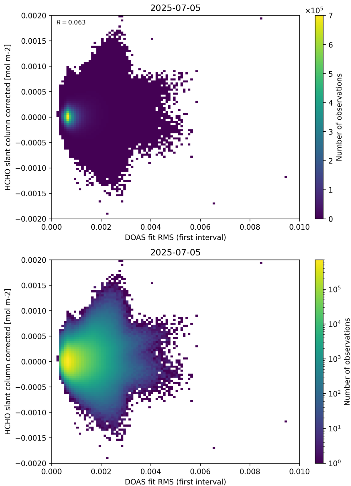
Figure 62: Scatter density plot of “DOAS fit RMS (first interval)” against “HCHO slant column corrected” for 2025-07-04 to 2025-07-06.
