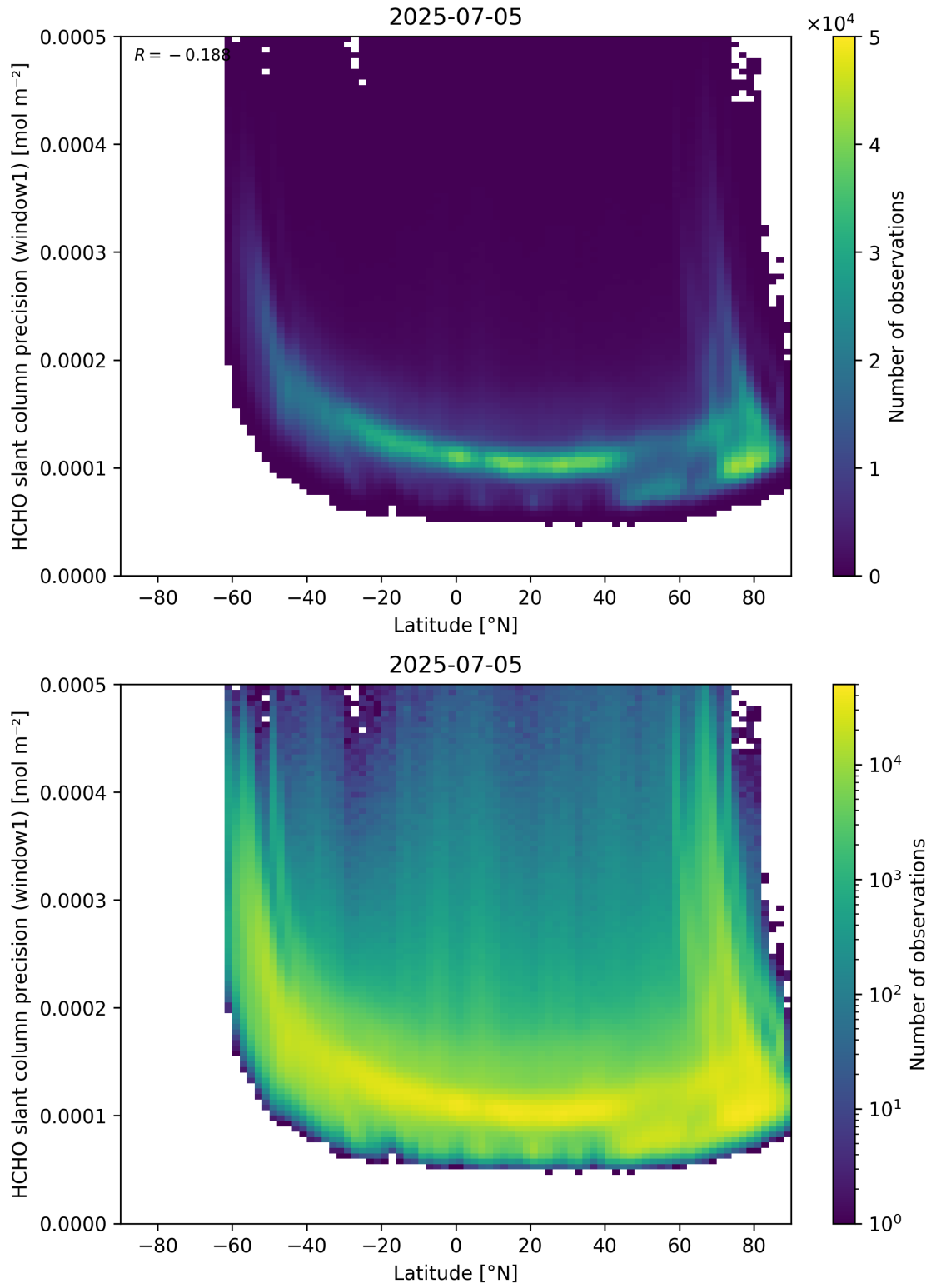
Figure 160: Scatter density plot of “Latitude” against “HCHO slant column precision (window1)” for 2025-07-04 to 2025-07-06.
