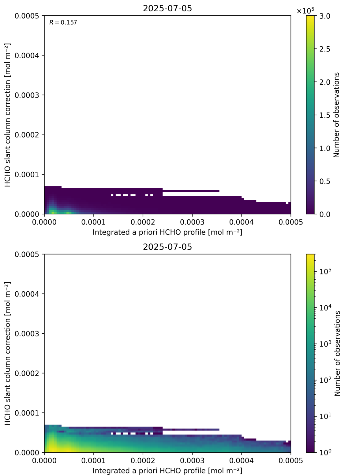
Figure 152: Scatter density plot of “Integrated a priori HCHO profile” against “HCHO slant column correction” for 2025-07-04 to 2025-07-06.
