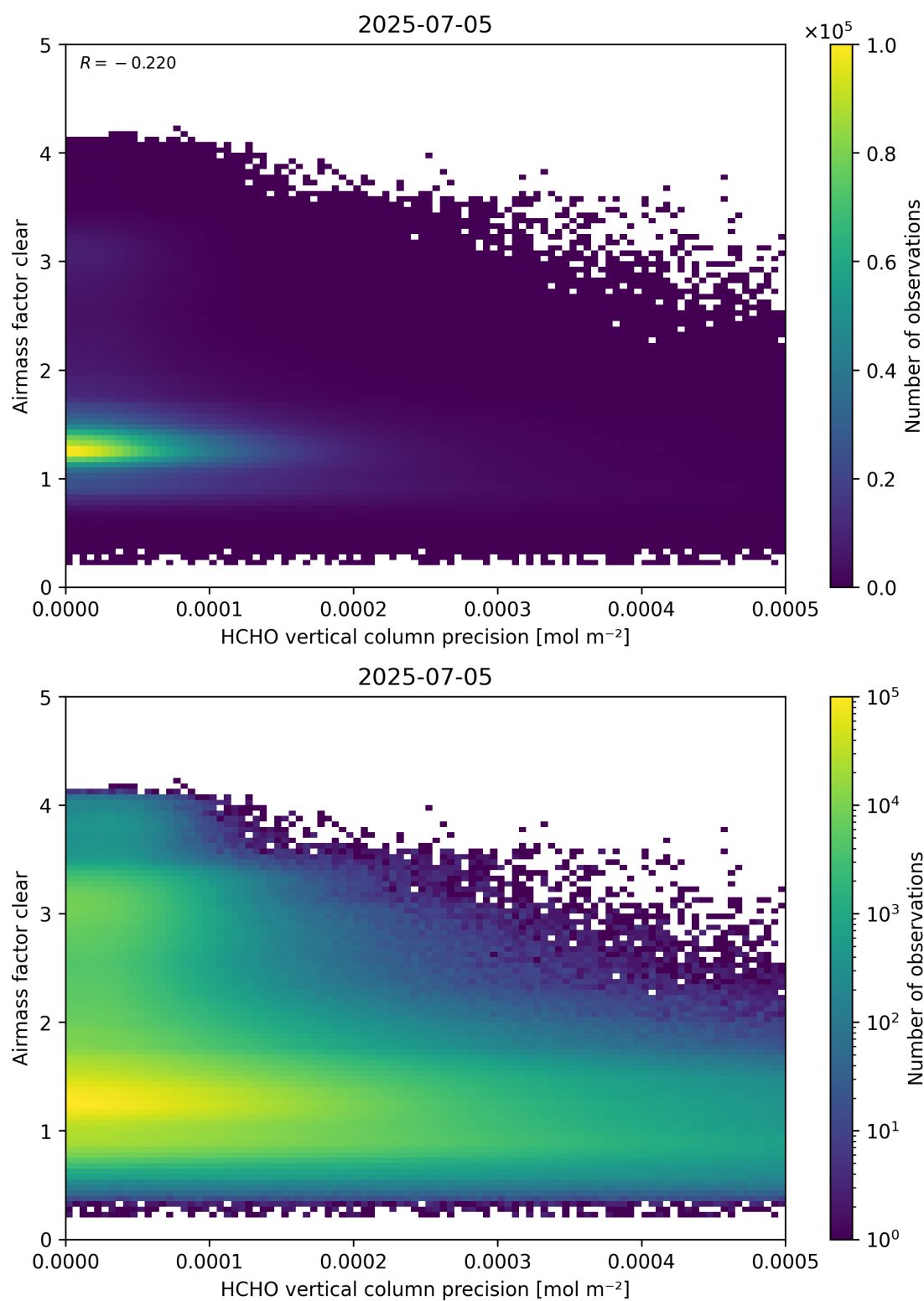
Figure 139: Scatter density plot of “HCHO vertical column precision” against “Airmass factor clear” for 2025-07-04 to 2025-07-06.
