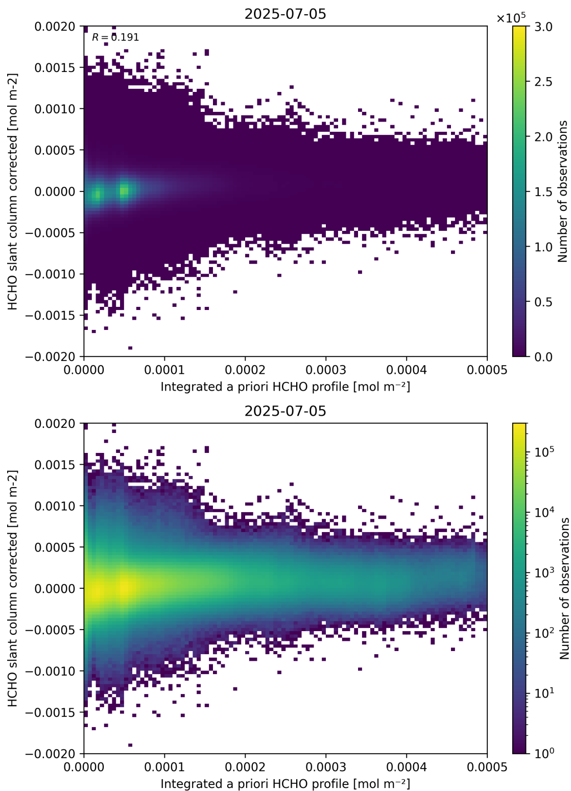
Figure 151: Scatter density plot of “Integrated a priori HCHO profile” against “HCHO slant column corrected” for 2025-07-04 to 2025-07-06.
