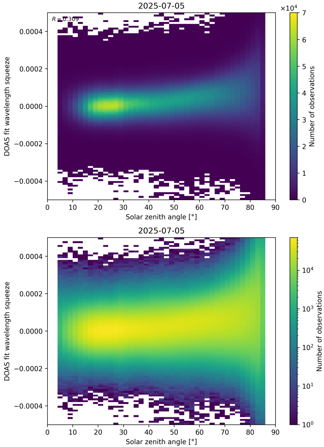
Figure 169: Scatter density plot of “Solar zenith angle” against “DOAS fit wavelength squeeze” for 2025-07-04 to 2025-07-06.
