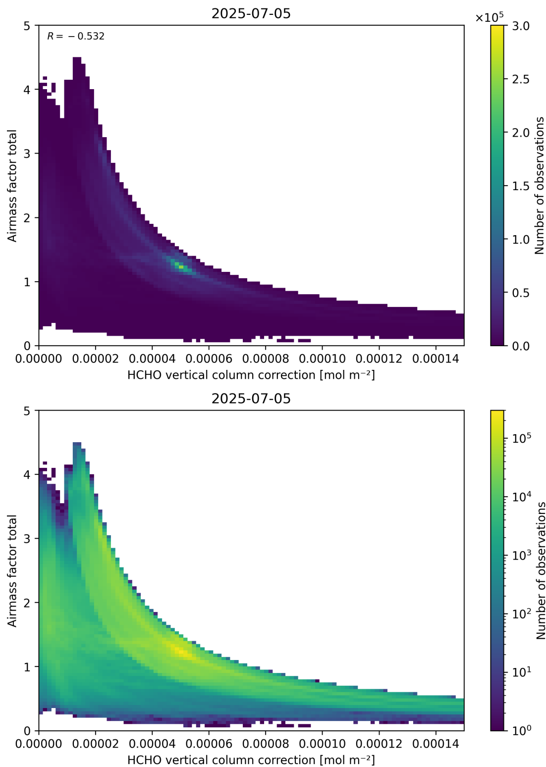
Figure 120: Scatter density plot of “HCHO vertical column correction” against “Airmass factor total” for 2025-07-04 to 2025-07-06.
