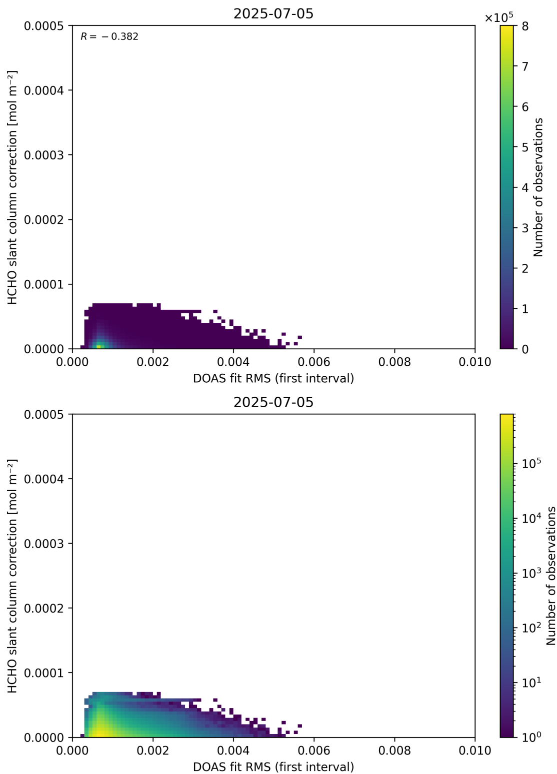
Figure 63: Scatter density plot of “DOAS fit RMS (first interval)” against “HCHO slant column correction” for 2025-07-04 to 2025-07-06.
