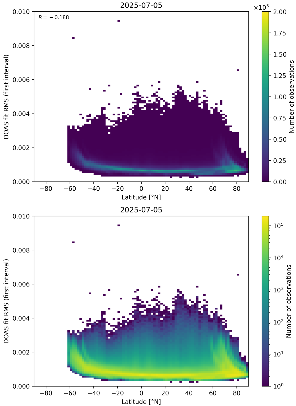
Figure 153: Scatter density plot of “Latitude” against “DOAS fit RMS (first interval)” for 2025-07-04 to 2025-07-06.
