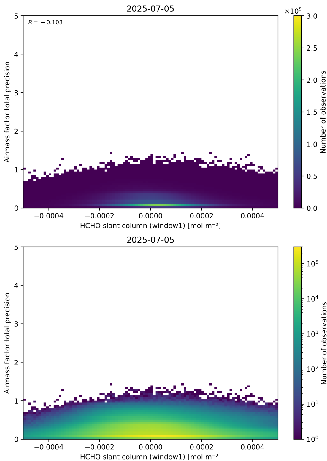
Figure 86: Scatter density plot of “HCHO slant column (window1)” against “Airmass factor total precision” for 2025-07-04 to 2025-07-06.
