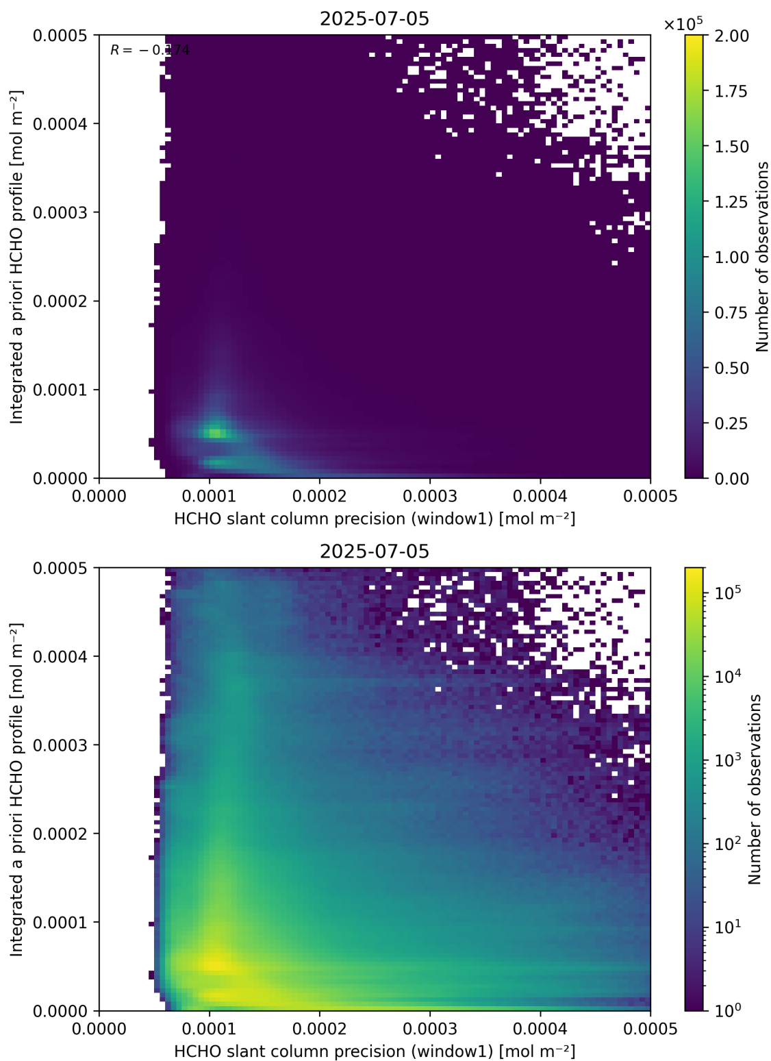
Figure 96: Scatter density plot of “HCHO slant column precision (window1)” against “Integrated a priori HCHO profile” for 2025-07-04 to 2025-07-06.
