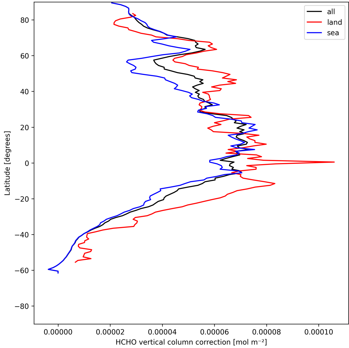
Figure 23: Zonal average of “HCHO vertical column correction” for 2025-07-04 to 2025-07-06.
