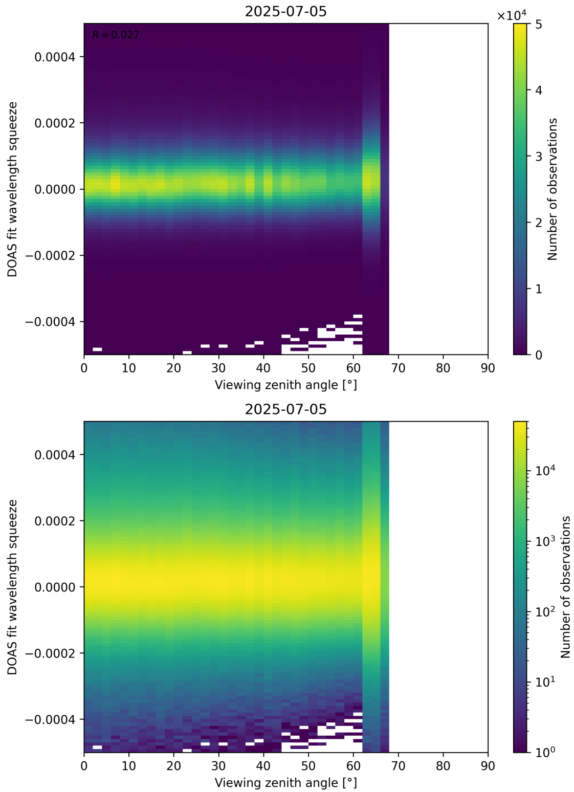
Figure 184: Scatter density plot of “Viewing zenith angle” against “DOAS fit wavelength squeeze” for 2025-07-04 to 2025-07-06.
