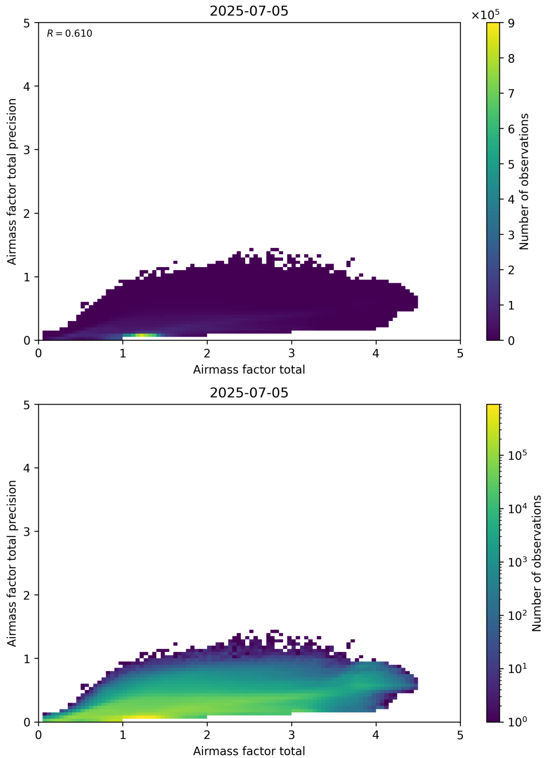
Figure 103: Scatter density plot of “Airmass factor total” against “Airmass factor total precision” for 2025-07-04 to 2025-07-06.
