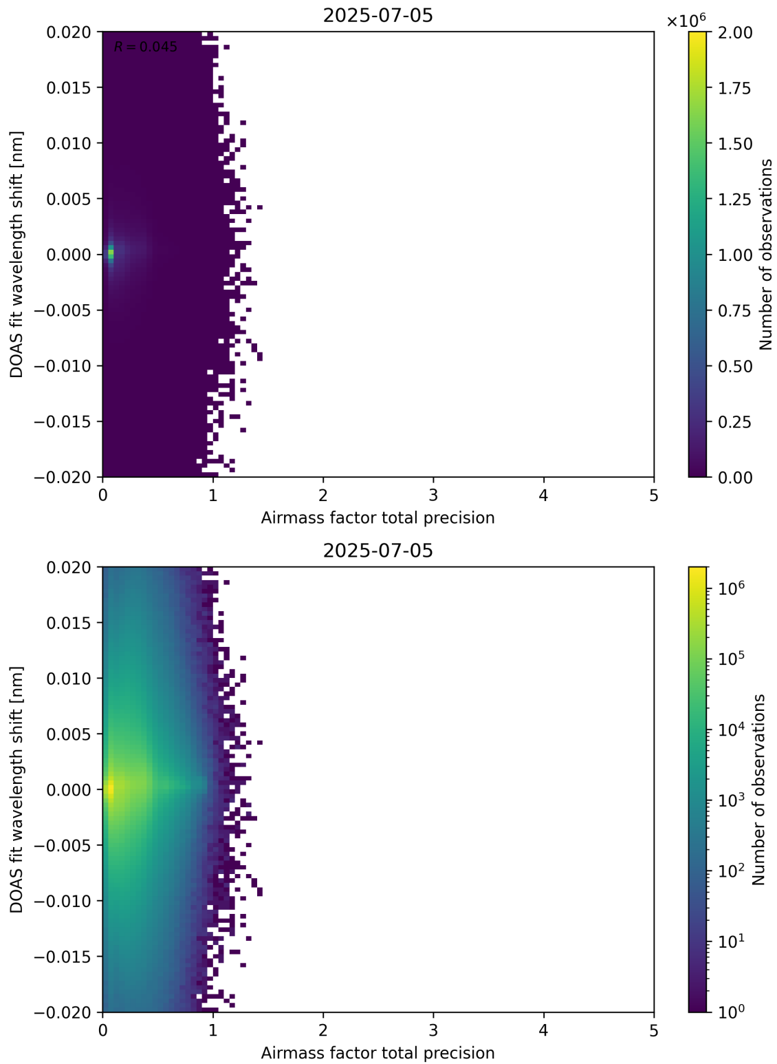
Figure 106: Scatter density plot of “Airmass factor total precision” against “DOAS fit wavelength shift” for 2025-07-04 to 2025-07-06.
