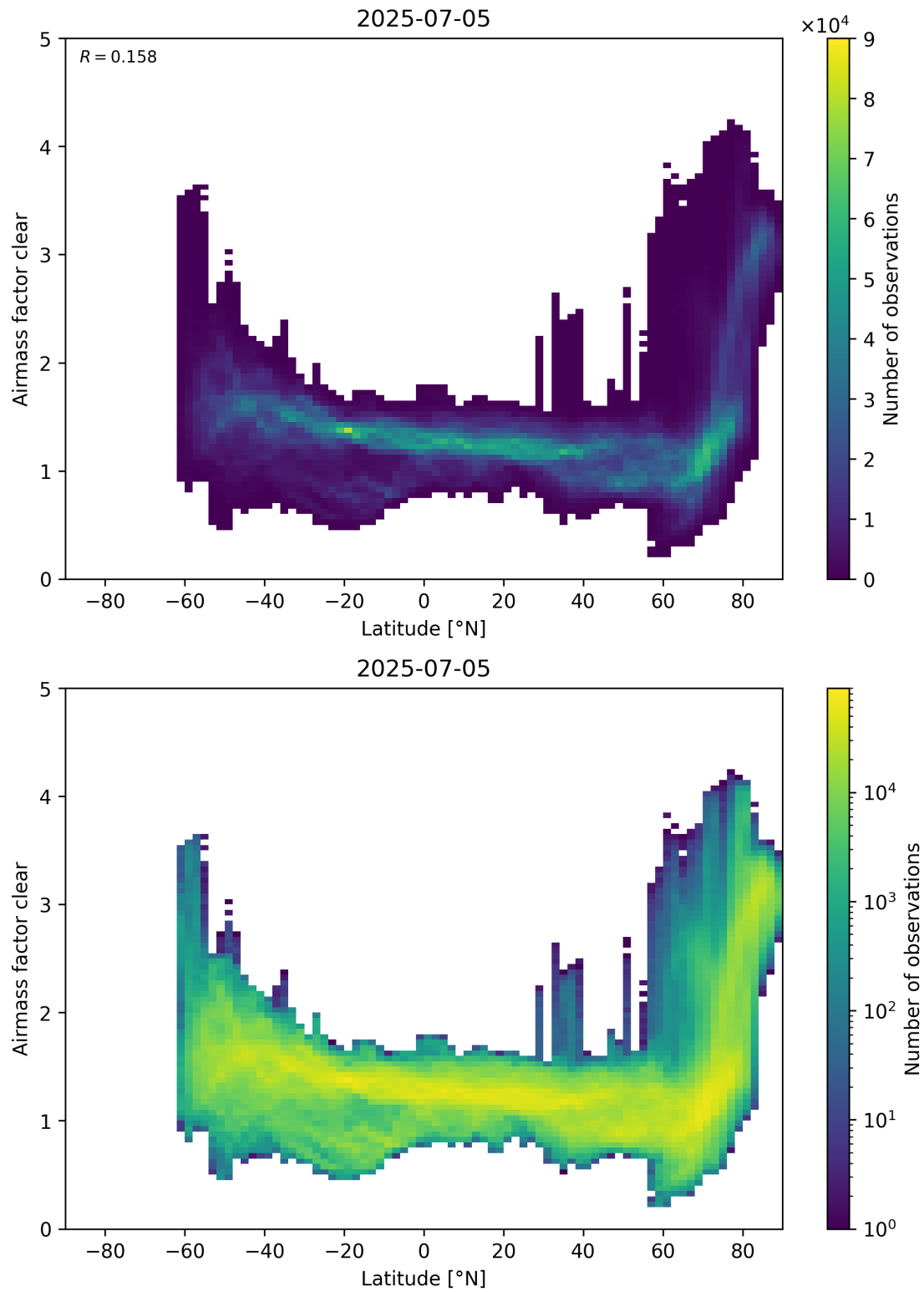
Figure 156: Scatter density plot of “Latitude” against “Airmass factor clear” for 2025-07-04 to 2025-07-06.
