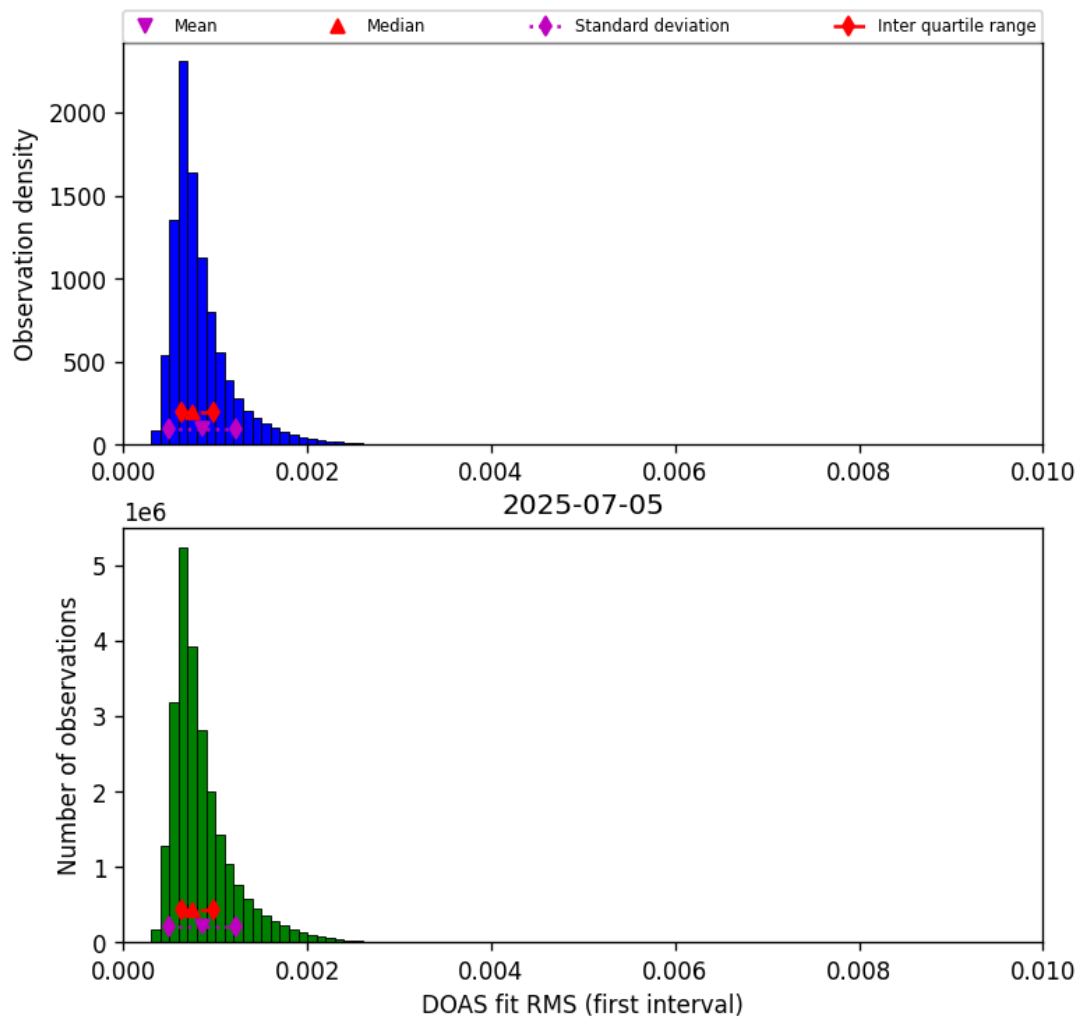
Figure 46: Histogram of “DOAS fit RMS (first interval)” for 2025-07-04 to 2025-07-06
