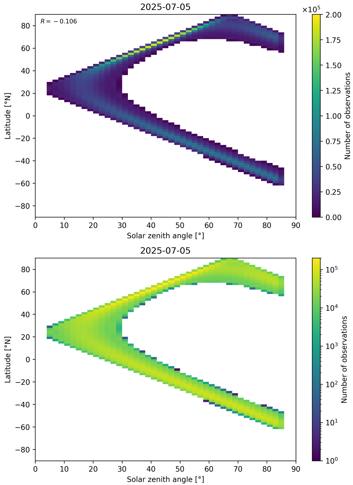
Figure 181: Scatter density plot of “Solar zenith angle” against “Latitude” for 2025-07-04 to 2025-07-06.
