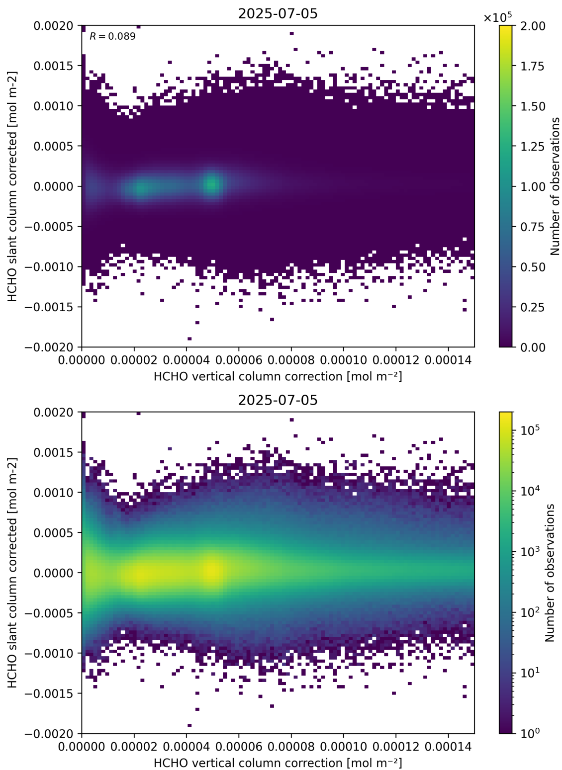
Figure 116: Scatter density plot of “HCHO vertical column correction” against “HCHO slant column corrected” for 2025-07-04 to 2025-07-06.
