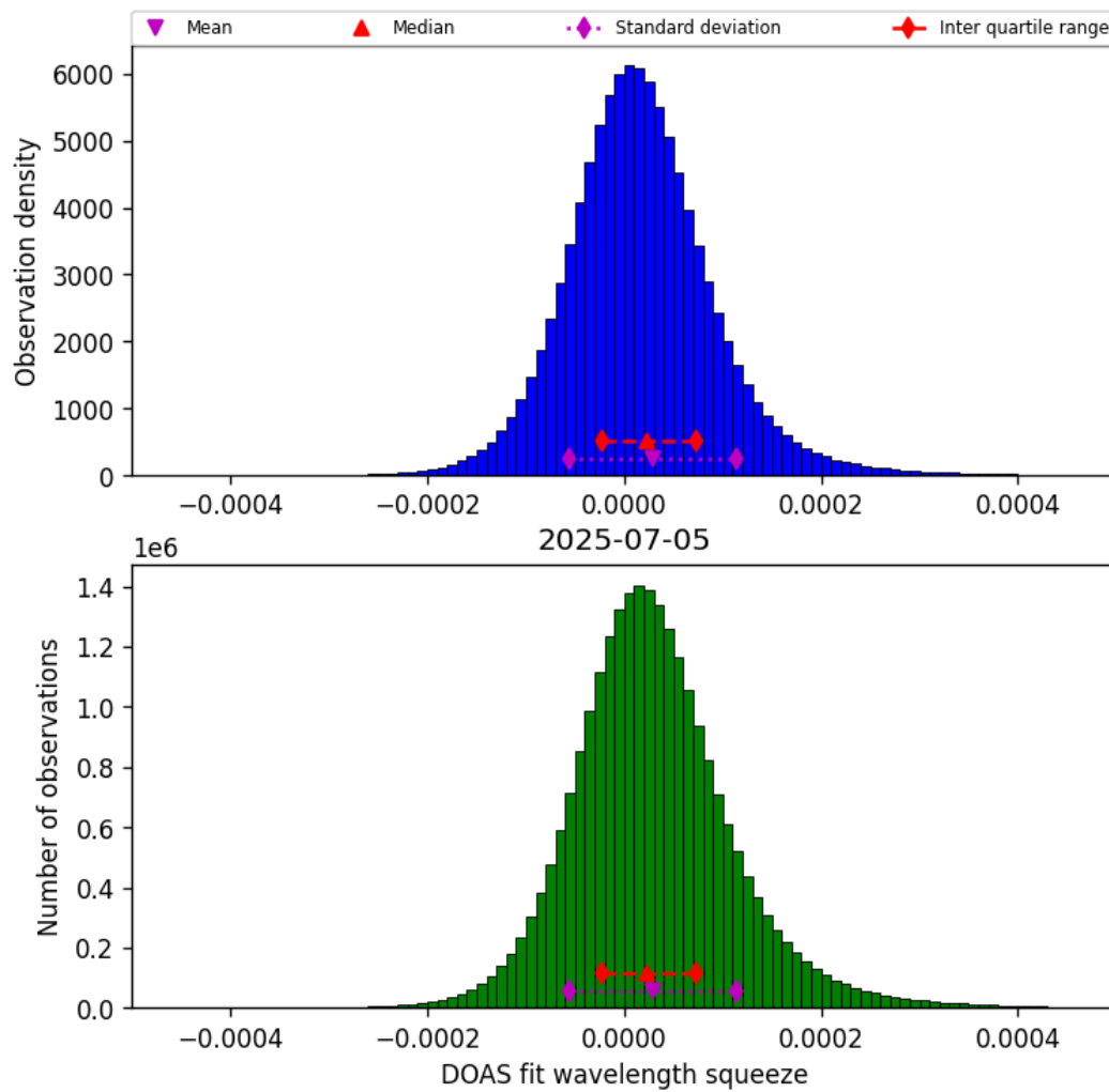
Figure 45: Histogram of “DOAS fit wavelength squeeze” for 2025-07-04 to 2025-07-06
