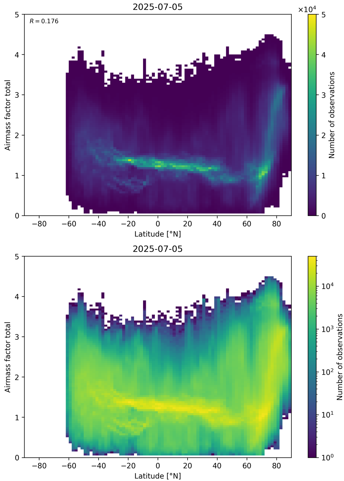
Figure 161: Scatter density plot of “Latitude” against “Airmass factor total” for 2025-07-04 to 2025-07-06.
