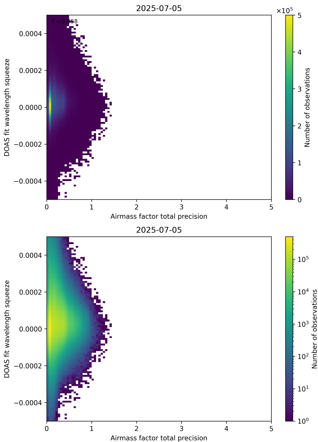
Figure 107: Scatter density plot of “Airmass factor total precision” against “DOAS fit wavelength squeeze” for 2025-07-04 to 2025-07-06.
