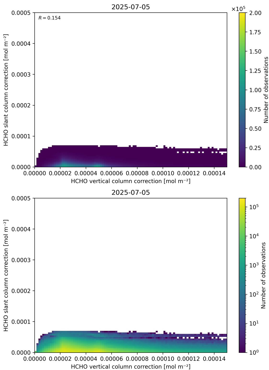
Figure 117: Scatter density plot of “HCHO vertical column correction” against “HCHO slant column correction” for 2025-07-04 to 2025-07-06.
