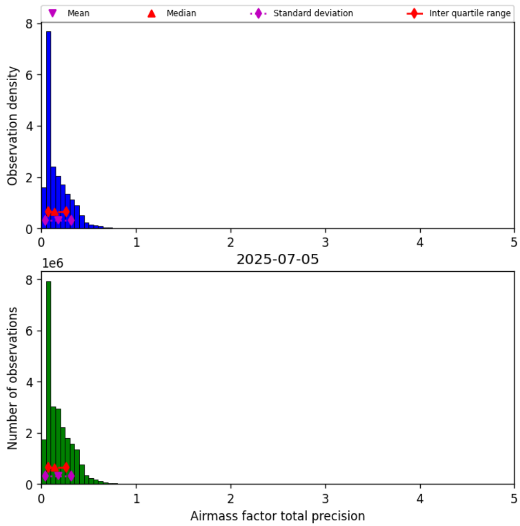
Figure 41: Histogram of “Airmass factor total precision” for 2025-07-04 to 2025-07-06
