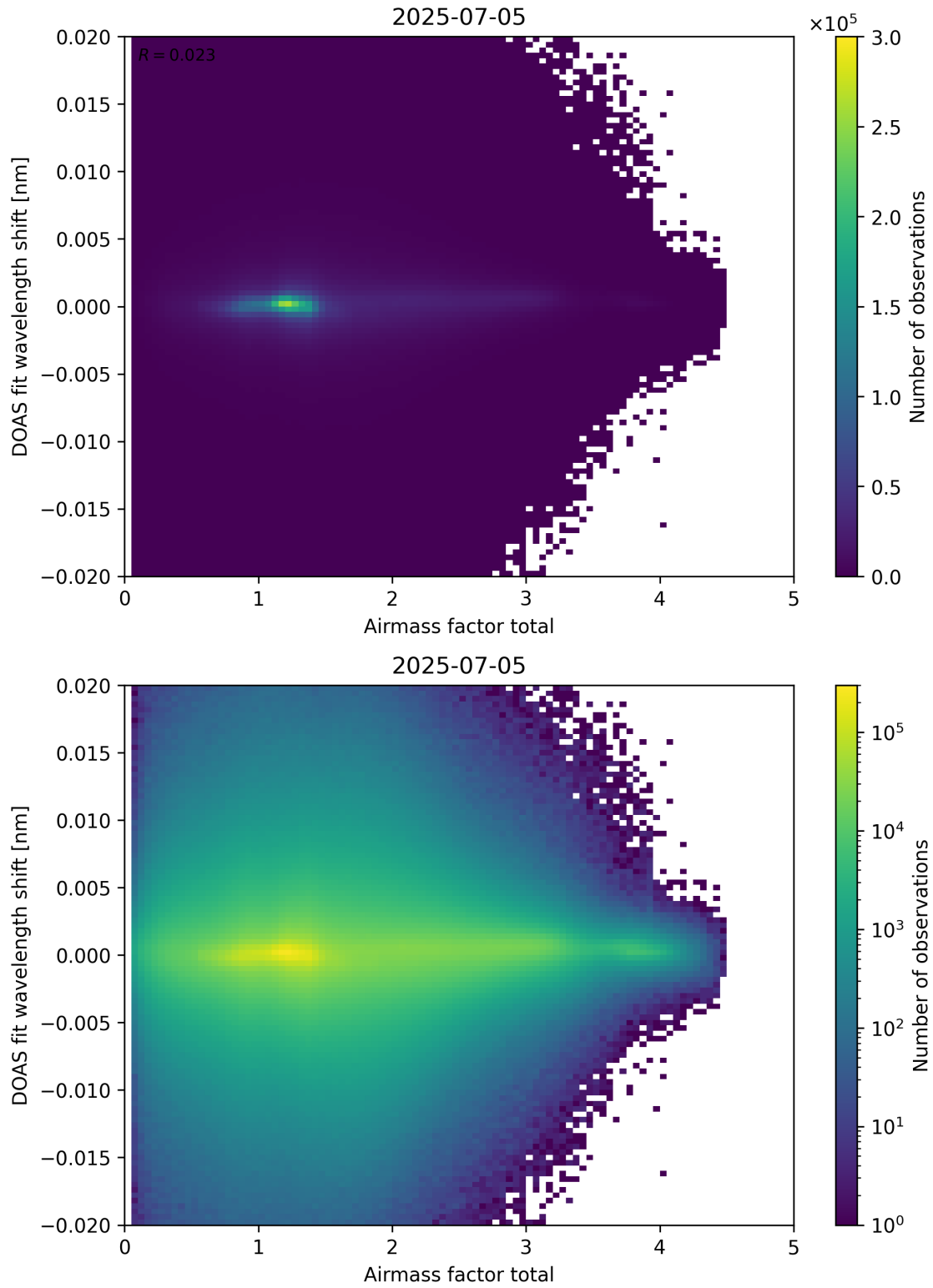
Figure 98: Scatter density plot of “Airmass factor total” against “DOAS fit wavelength shift” for 2025-07-04 to 2025-07-06.
