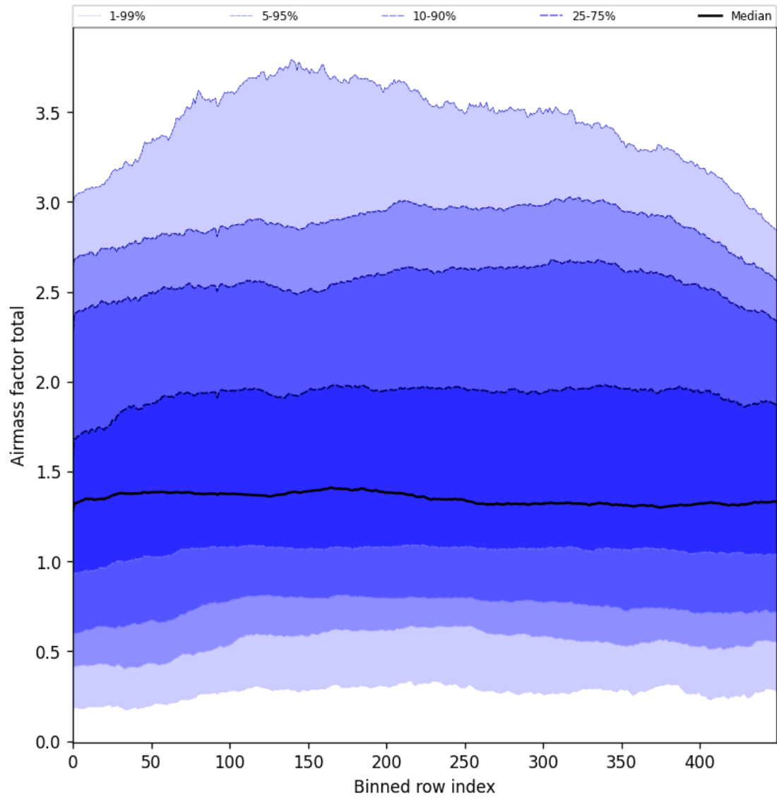
Figure 54: Along track statistics of “Airmass factor total” for 2025-07-04 to 2025-07-06
