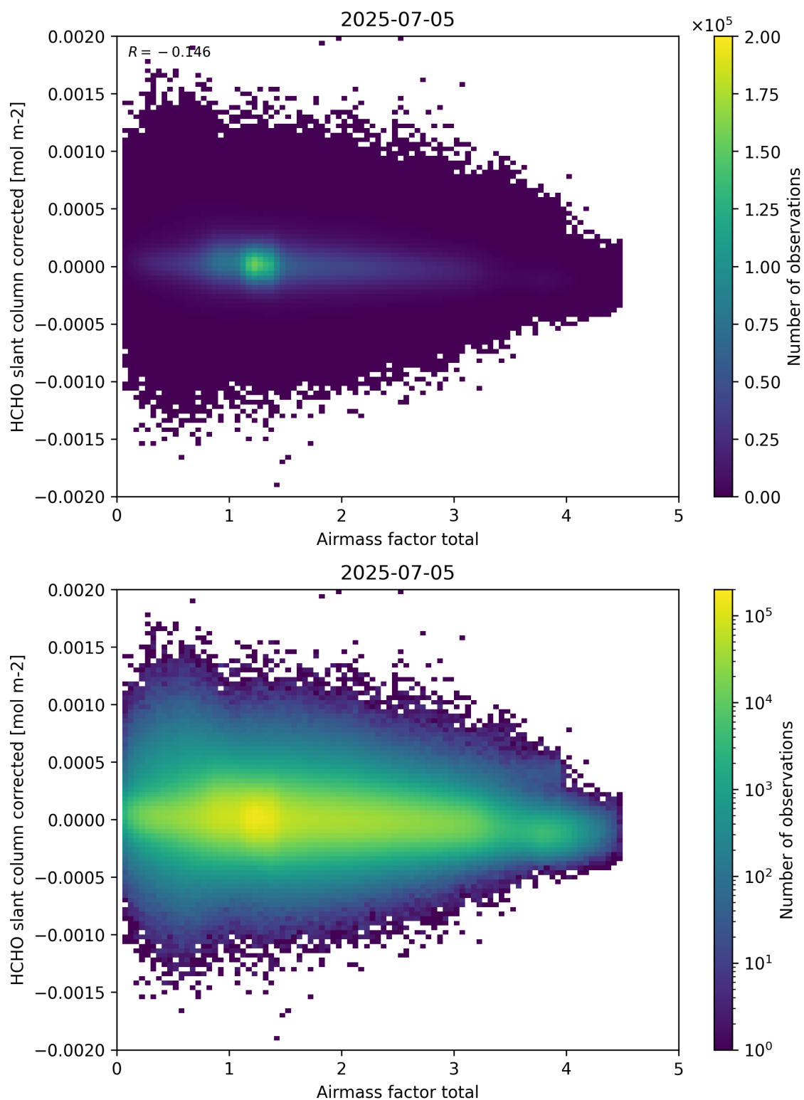
Figure 101: Scatter density plot of “Airmass factor total” against “HCHO slant column corrected” for 2025-07-04 to 2025-07-06.
