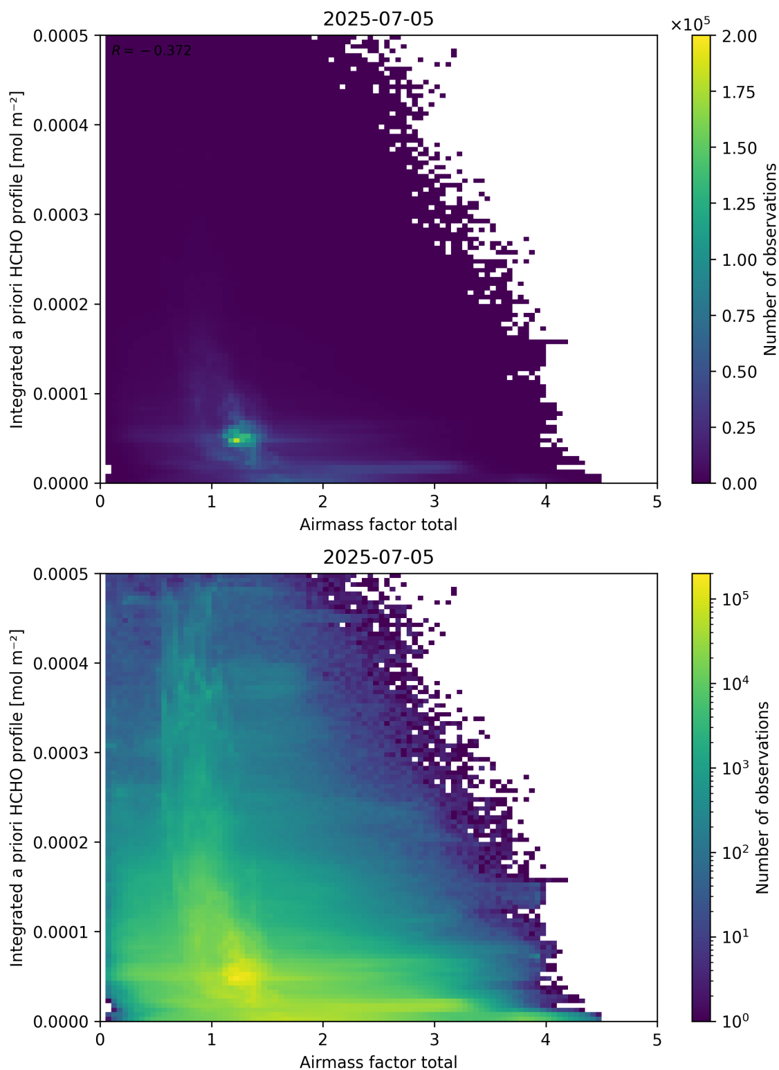
Figure 104: Scatter density plot of “Airmass factor total” against “Integrated a priori HCHO profile” for 2025-07-04 to 2025-07-06.
