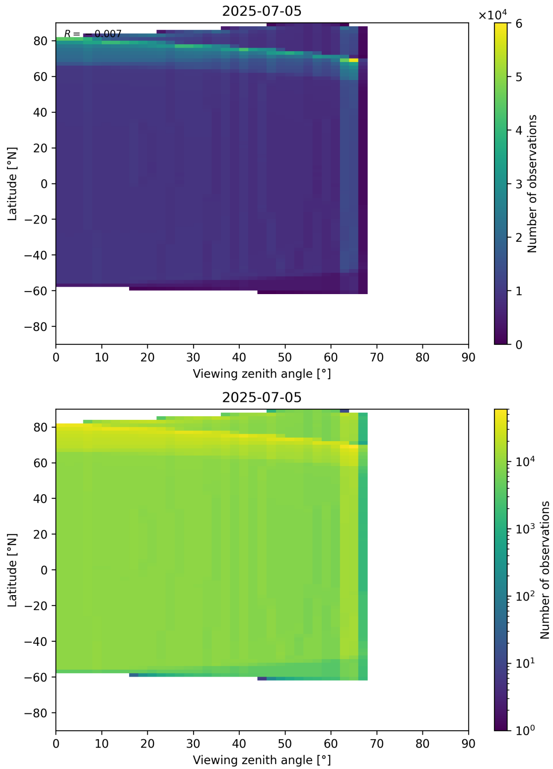
Figure 196: Scatter density plot of “Viewing zenith angle” against “Latitude” for 2025-07-04 to 2025-07-06.
