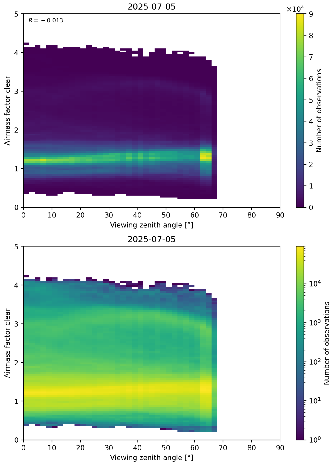
Figure 185: Scatter density plot of “Viewing zenith angle” against “Airmass factor clear” for 2025-07-04 to 2025-07-06.
