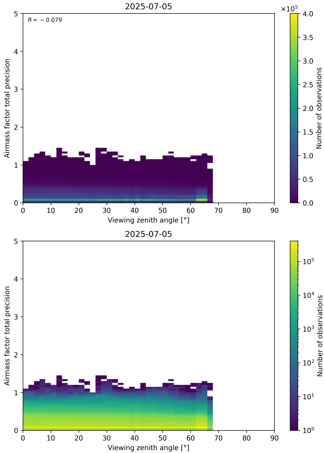
Figure 191: Scatter density plot of “Viewing zenith angle” against “Airmass factor total precision” for 2025-07-04 to 2025-07-06.
