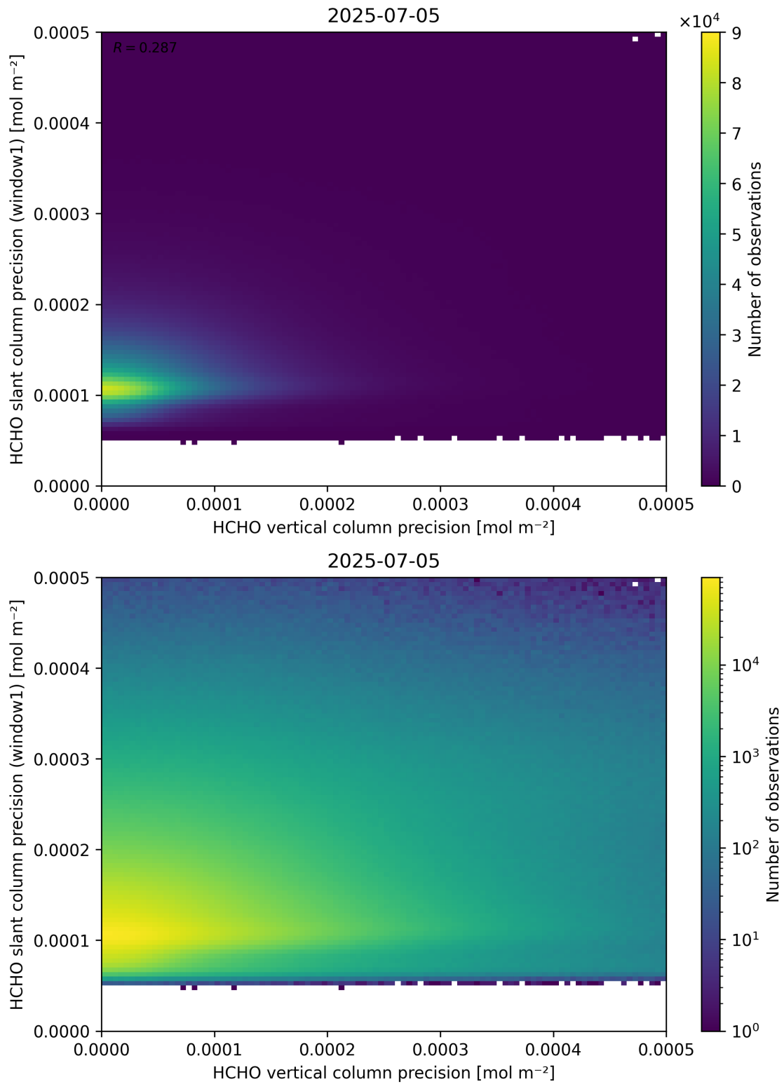
Figure 143: Scatter density plot of “HCHO vertical column precision” against “HCHO slant column precision (window1)” for 2025-07-04 to 2025-07-06.
