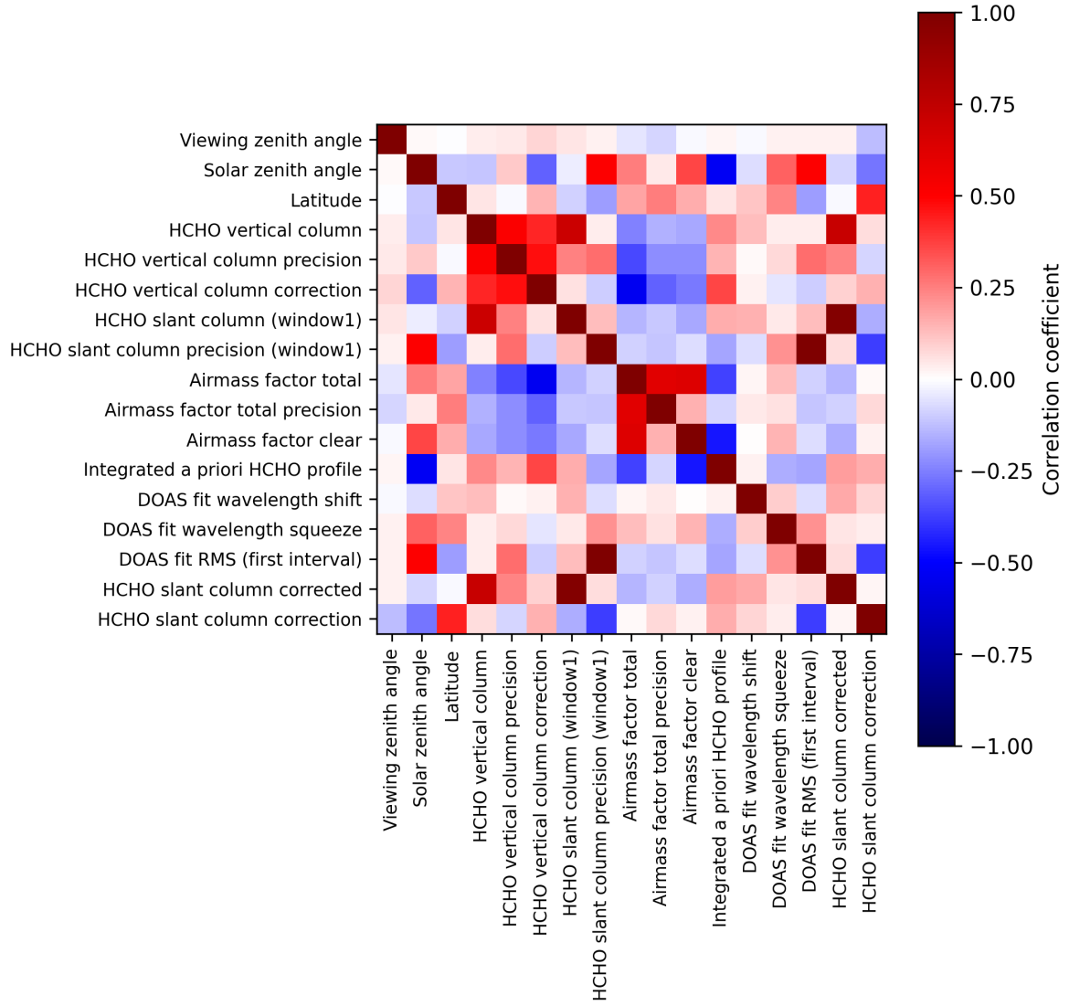
Figure 2: Map of correlation matrix for 2025-07-04 to 2025-07-06.
