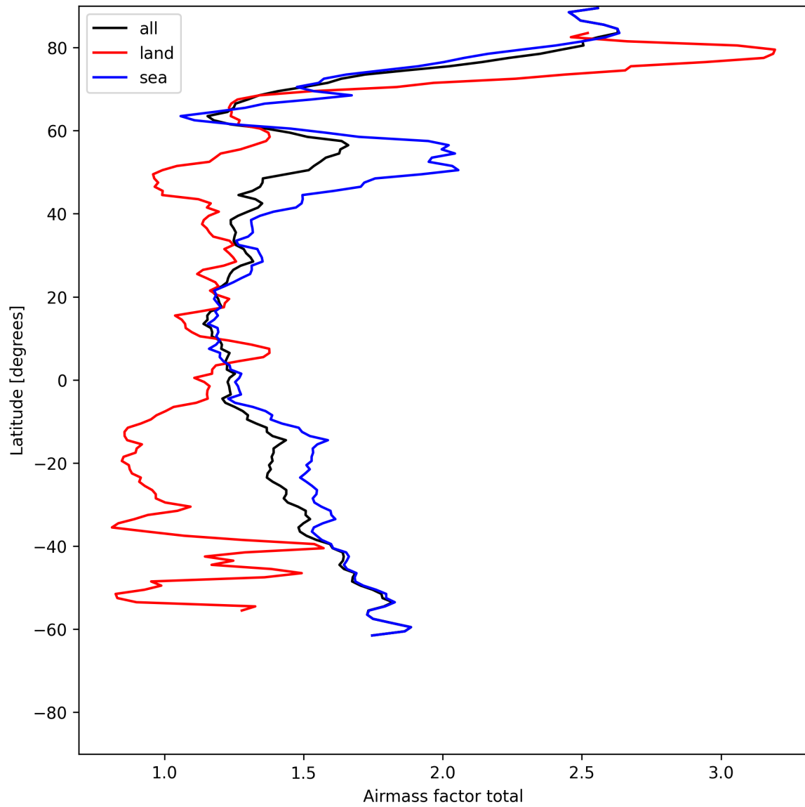
Figure 26: Zonal average of “Airmass factor total” for 2025-07-04 to 2025-07-06.
