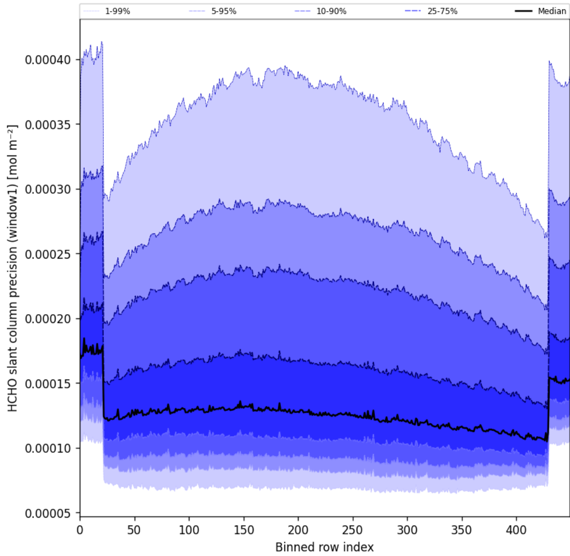
Figure 53: Along track statistics of “HCHO slant column precision (window1)” for 2025-07-04 to 2025-07-06
