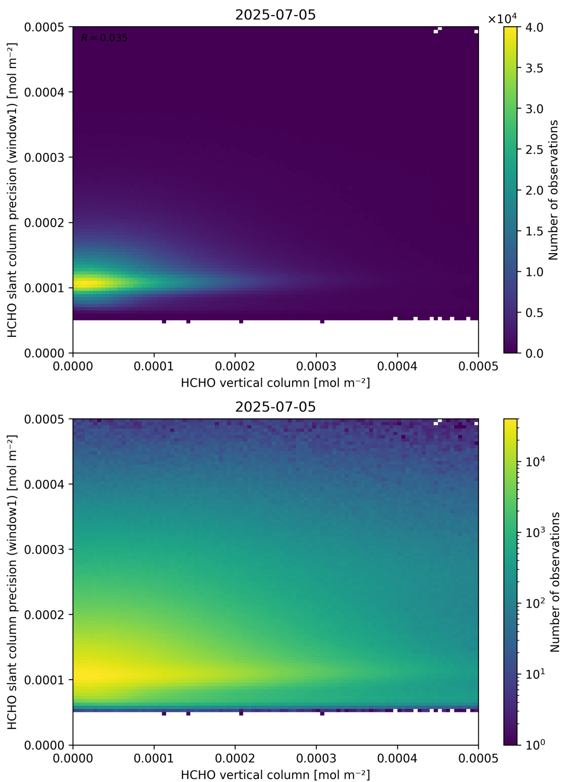
Figure 130: Scatter density plot of “HCHO vertical column” against “HCHO slant column precision (window1)” for 2025-07-04 to 2025-07-06.
