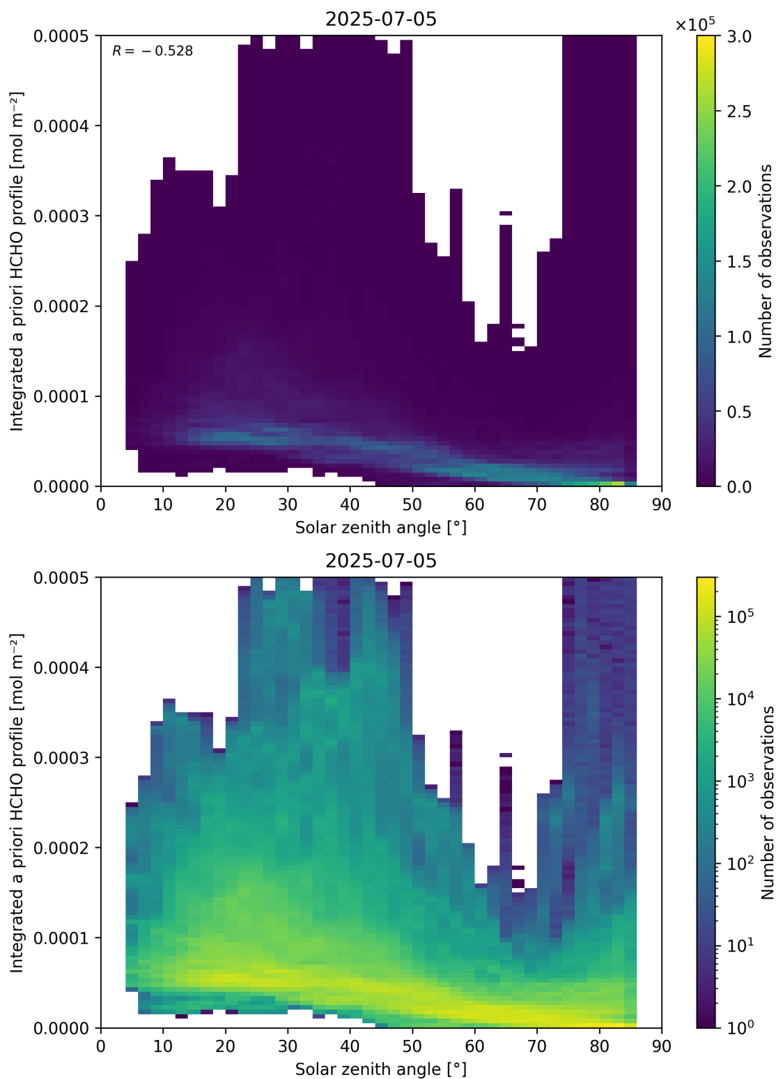
Figure 180: Scatter density plot of “Solar zenith angle” against “Integrated a priori HCHO profile” for 2025-07-04 to 2025-07-06.
