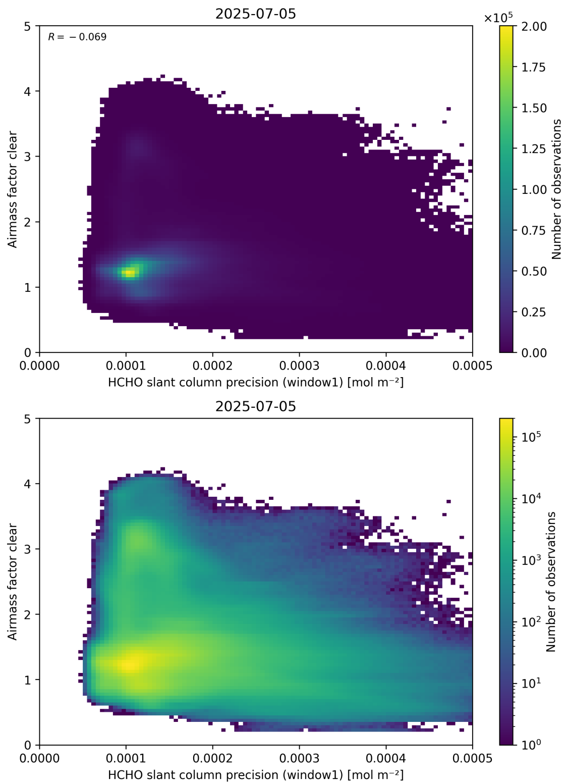
Figure 91: Scatter density plot of “HCHO slant column precision (window1)” against “Airmass factor clear” for 2025-07-04 to 2025-07-06.
