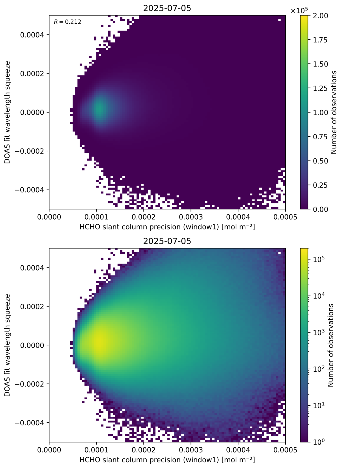
Figure 90: Scatter density plot of “HCHO slant column precision (window1)” against “DOAS fit wavelength squeeze” for 2025-07-04 to 2025-07-06.
