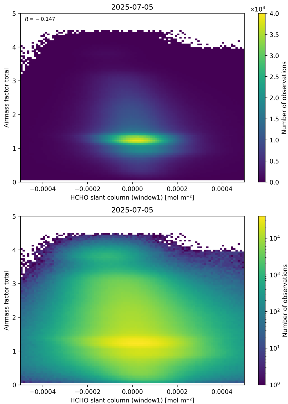
Figure 85: Scatter density plot of “HCHO slant column (window1)” against “Airmass factor total” for 2025-07-04 to 2025-07-06.
