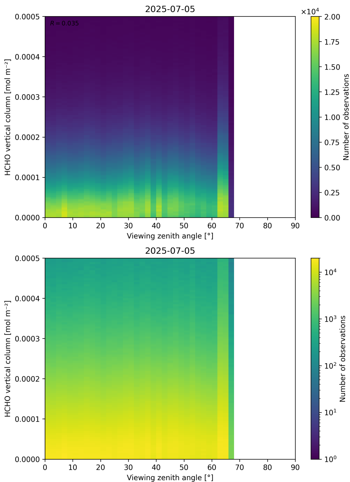
Figure 192: Scatter density plot of “Viewing zenith angle” against “HCHO vertical column” for 2025-07-04 to 2025-07-06.
