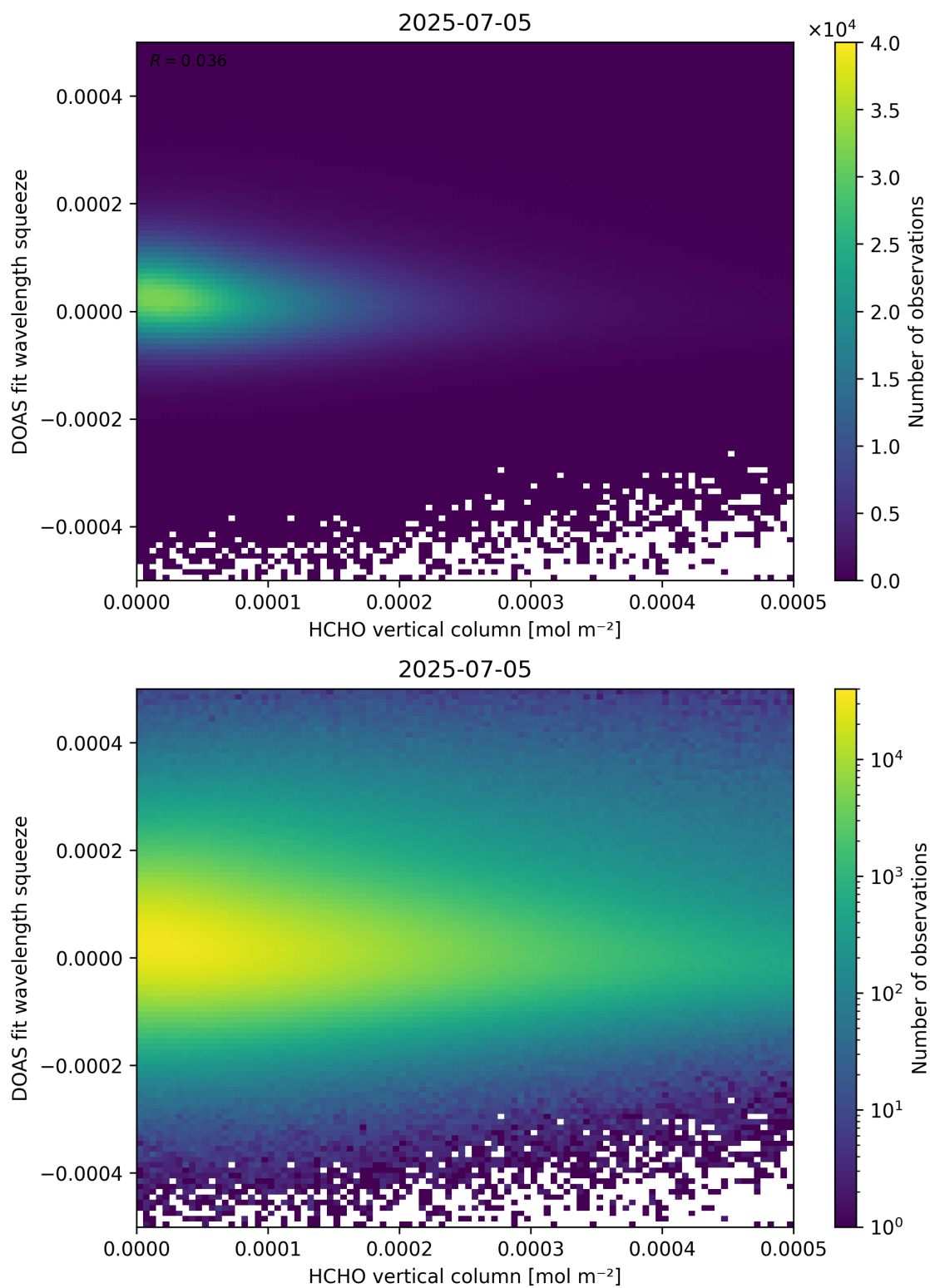
Figure 125: Scatter density plot of “HCHO vertical column” against “DOAS fit wavelength squeeze” for 2025-07-04 to 2025-07-06.
