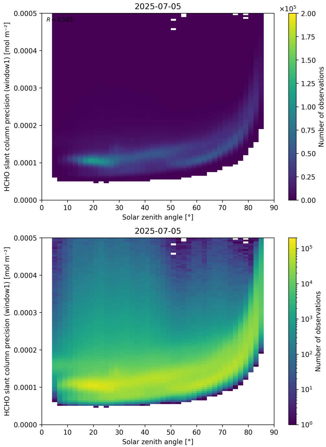
Figure 174: Scatter density plot of “Solar zenith angle” against “HCHO slant column precision (window1)” for 2025-07-04 to 2025-07-06.
