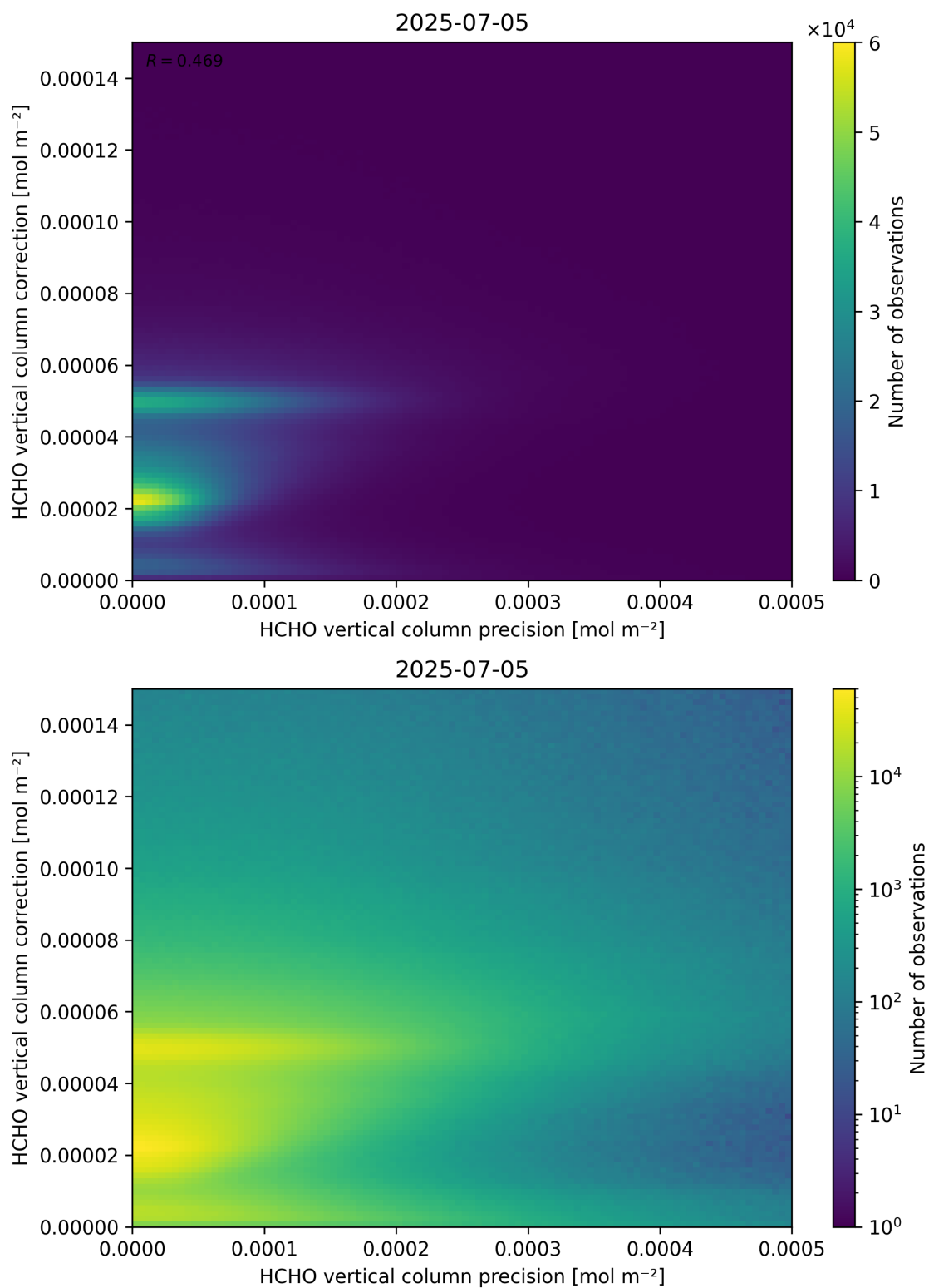
Figure 146: Scatter density plot of “HCHO vertical column precision” against “HCHO vertical column correction” for 2025-07-04 to 2025-07-06.
