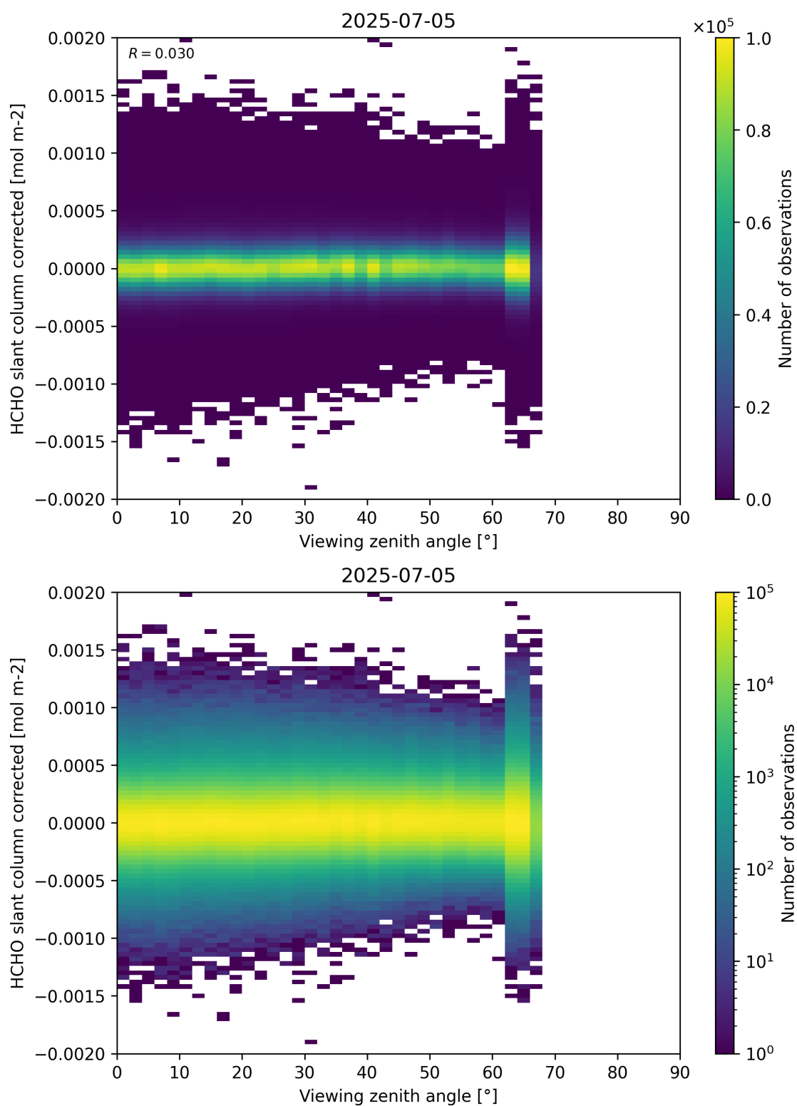
Figure 186: Scatter density plot of “Viewing zenith angle” against “HCHO slant column corrected” for 2025-07-04 to 2025-07-06.
