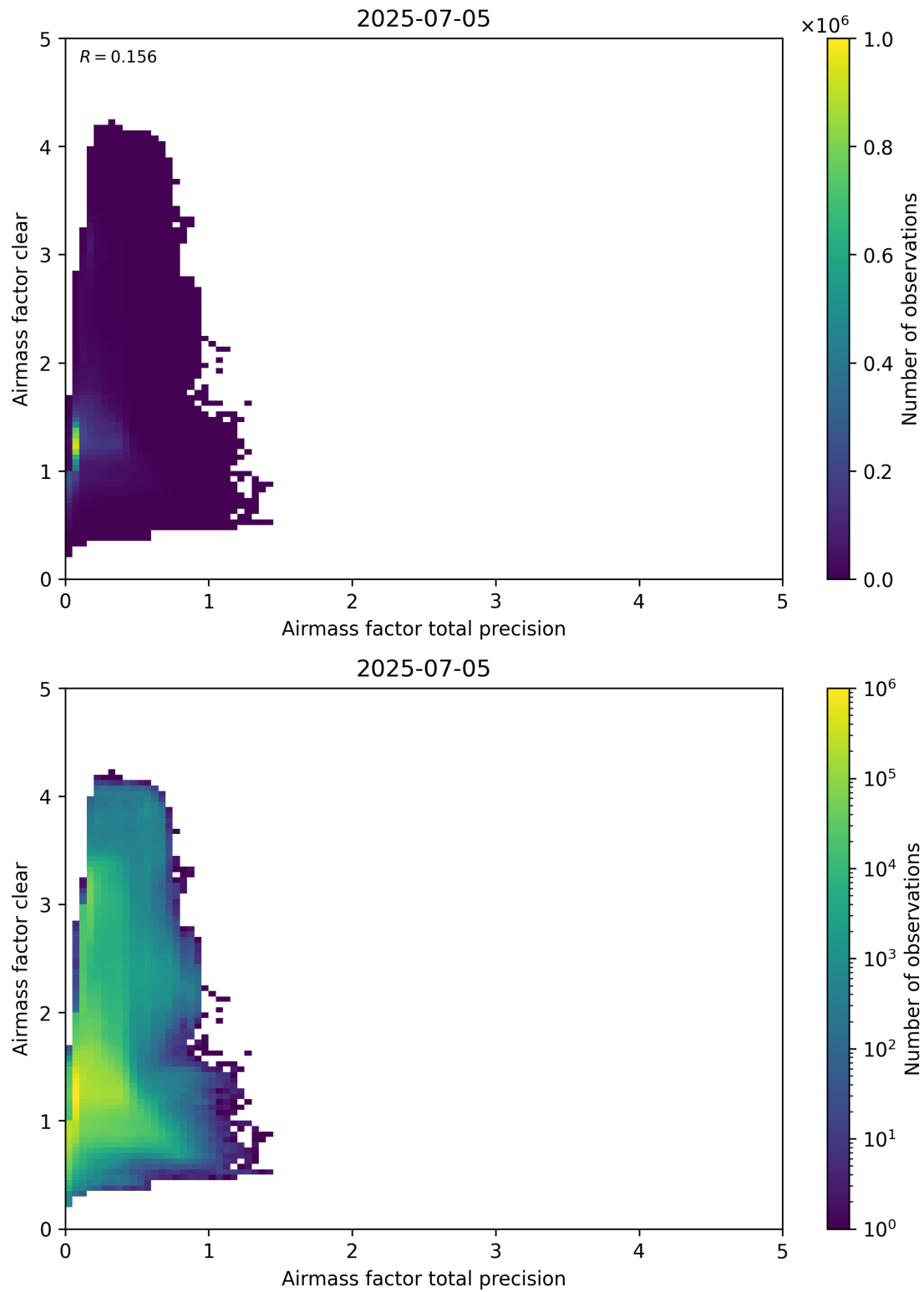
Figure 108: Scatter density plot of “Airmass factor total precision” against “Airmass factor clear” for 2025-07-04 to 2025-07-06.
