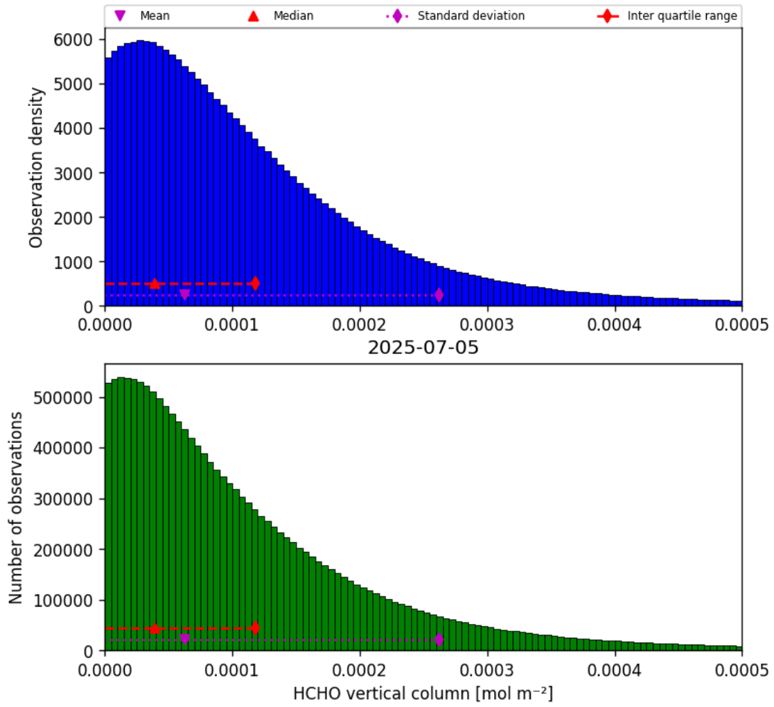
Figure 35: Histogram of “HCHO vertical column” for 2025-07-04 to 2025-07-06
