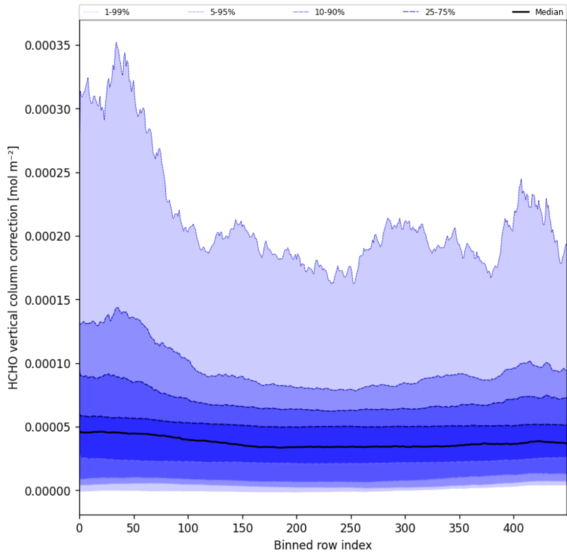
Figure 51: Along track statistics of “HCHO vertical column correction” for 2025-07-04 to 2025-07-06
