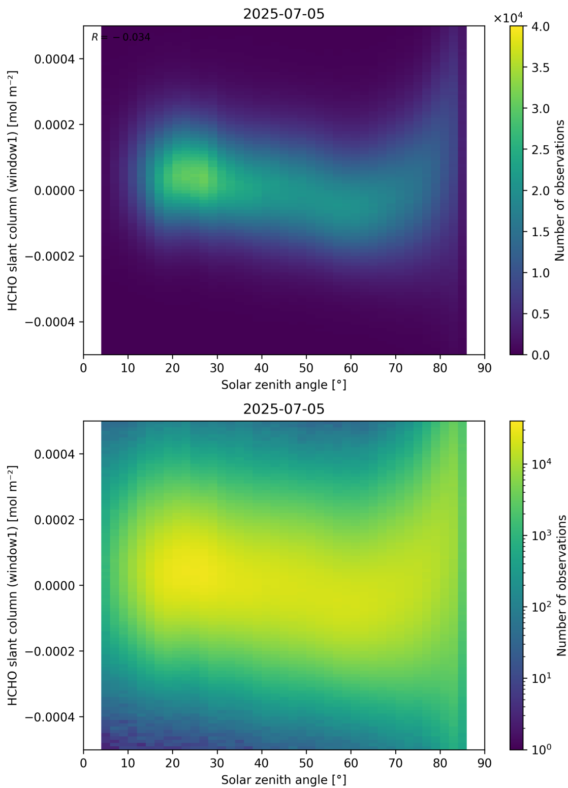
Figure 173: Scatter density plot of “Solar zenith angle” against “HCHO slant column (window1)” for 2025-07-04 to 2025-07-06.
