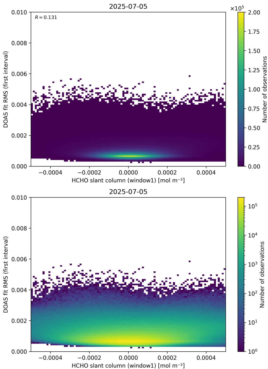
Figure 78: Scatter density plot of “HCHO slant column (window1)” against “DOAS fit RMS (first interval)” for 2025-07-04 to 2025-07-06.
