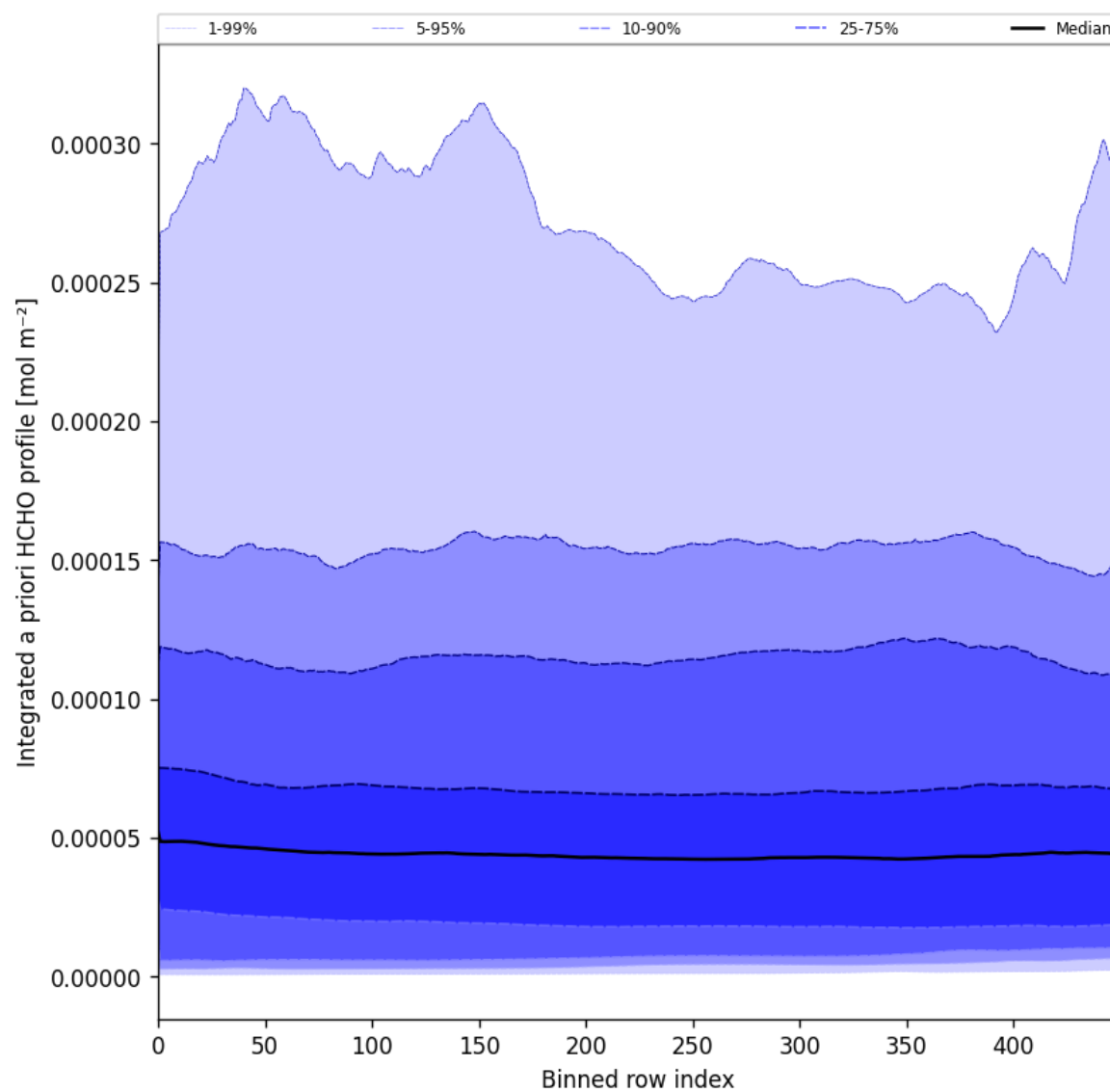
Figure 57: Along track statistics of "Integrated a priori HCHO profile" for 2025-07-04 to 2025-07-06
