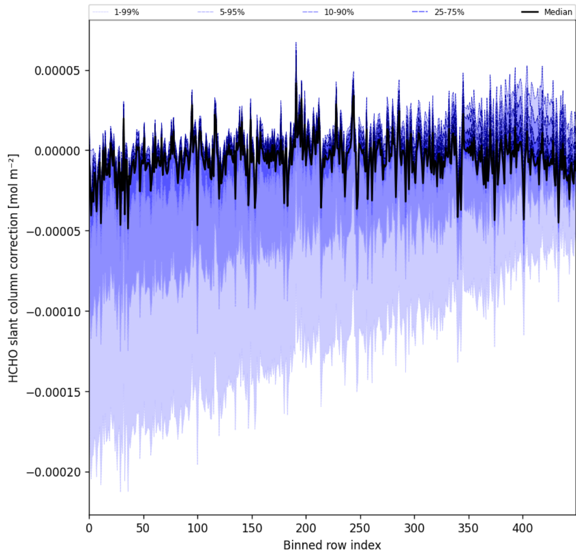
Figure 61: Along track statistics of “HCHO slant column correction” for 2025-07-04 to 2025-07-06
