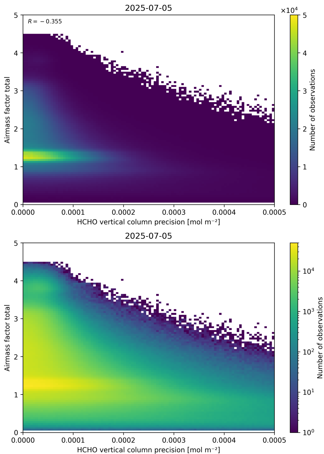
Figure 144: Scatter density plot of “HCHO vertical column precision” against “Airmass factor total” for 2025-07-04 to 2025-07-06.
