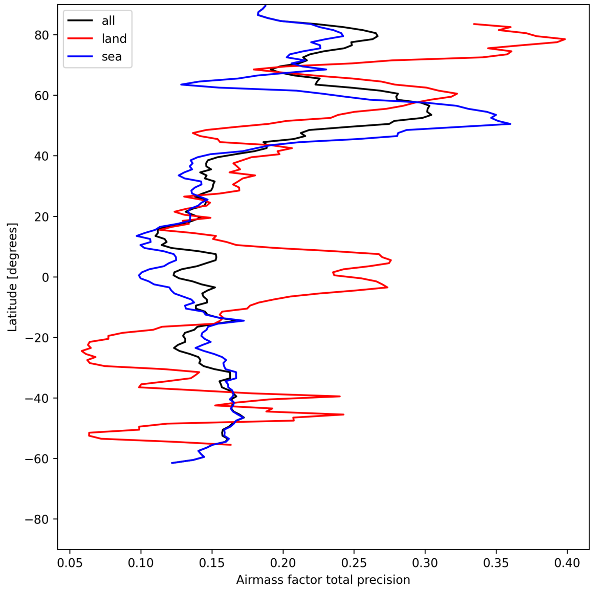
Figure 27: Zonal average of “Airmass factor total precision” for 2025-07-04 to 2025-07-06.
