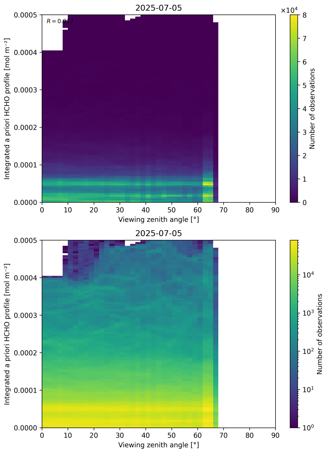
Figure 195: Scatter density plot of “Viewing zenith angle” against “Integrated a priori HCHO profile” for 2025-07-04 to 2025-07-06.
