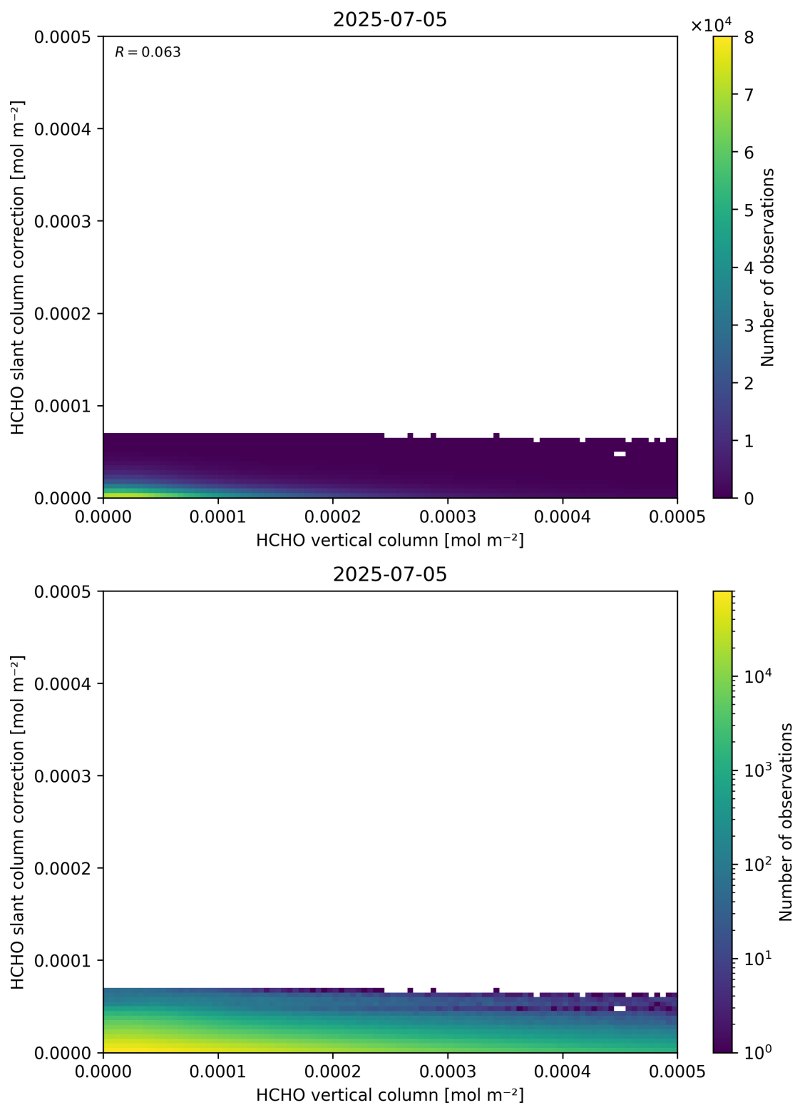
Figure 128: Scatter density plot of “HCHO vertical column” against “HCHO slant column correction” for 2025-07-04 to 2025-07-06.
