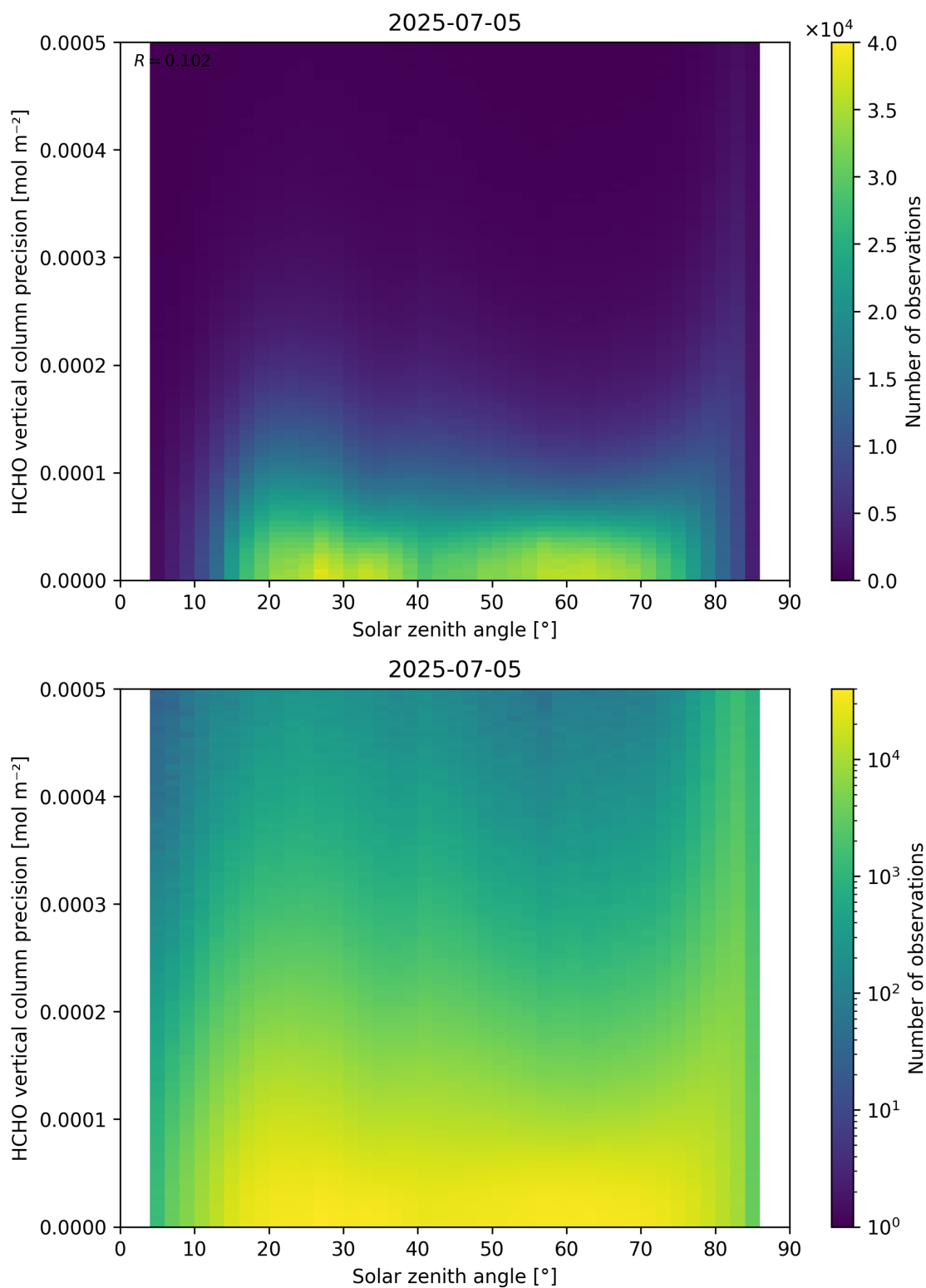
Figure 179: Scatter density plot of “Solar zenith angle” against “HCHO vertical column precision” for 2025-07-04 to 2025-07-06.
