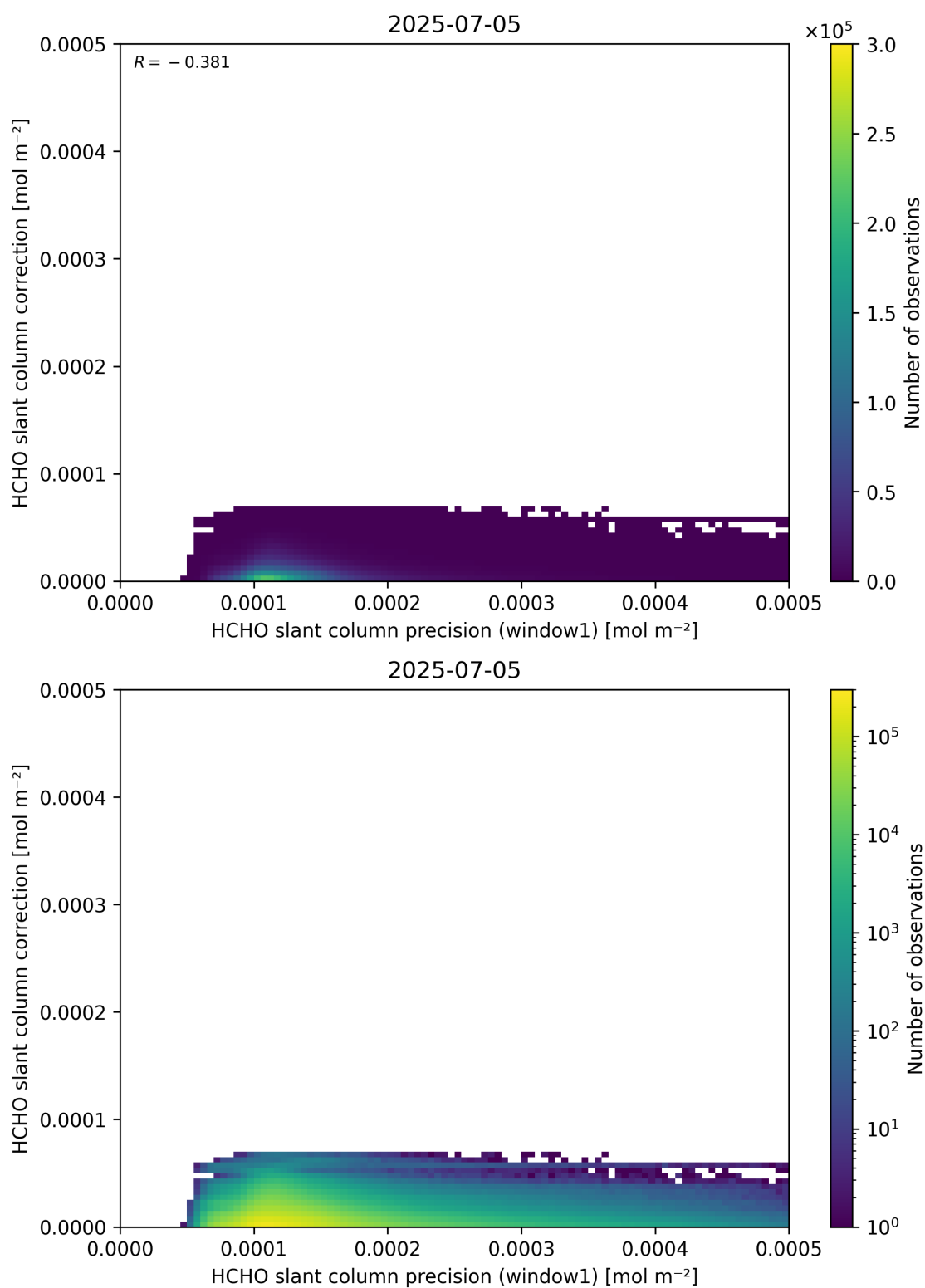
Figure 93: Scatter density plot of “HCHO slant column precision (window1)” against “HCHO slant column correction” for 2025-07-04 to 2025-07-06.
