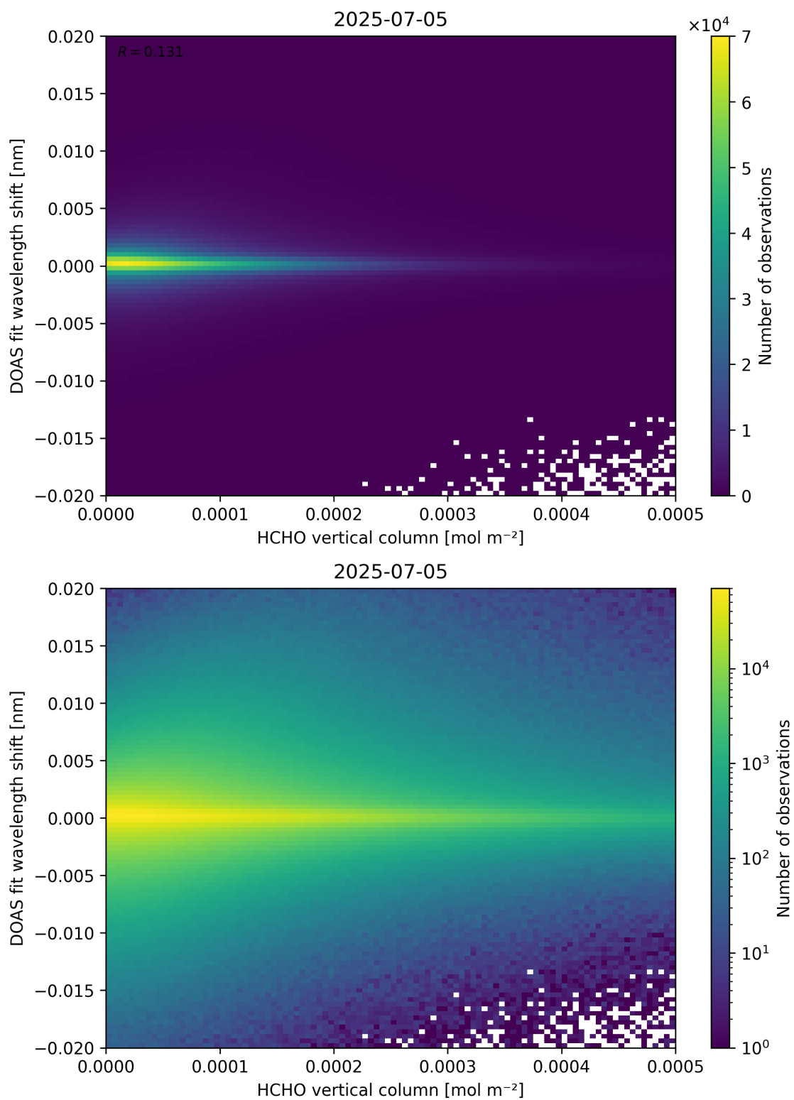
Figure 124: Scatter density plot of “HCHO vertical column” against “DOAS fit wavelength shift” for 2025-07-04 to 2025-07-06.
