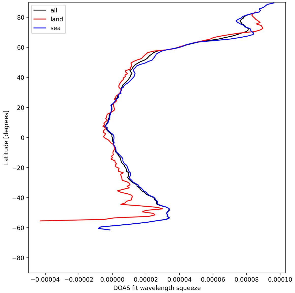
Figure 31: Zonal average of “DOAS fit wavelength squeeze” for 2025-07-04 to 2025-07-06.
