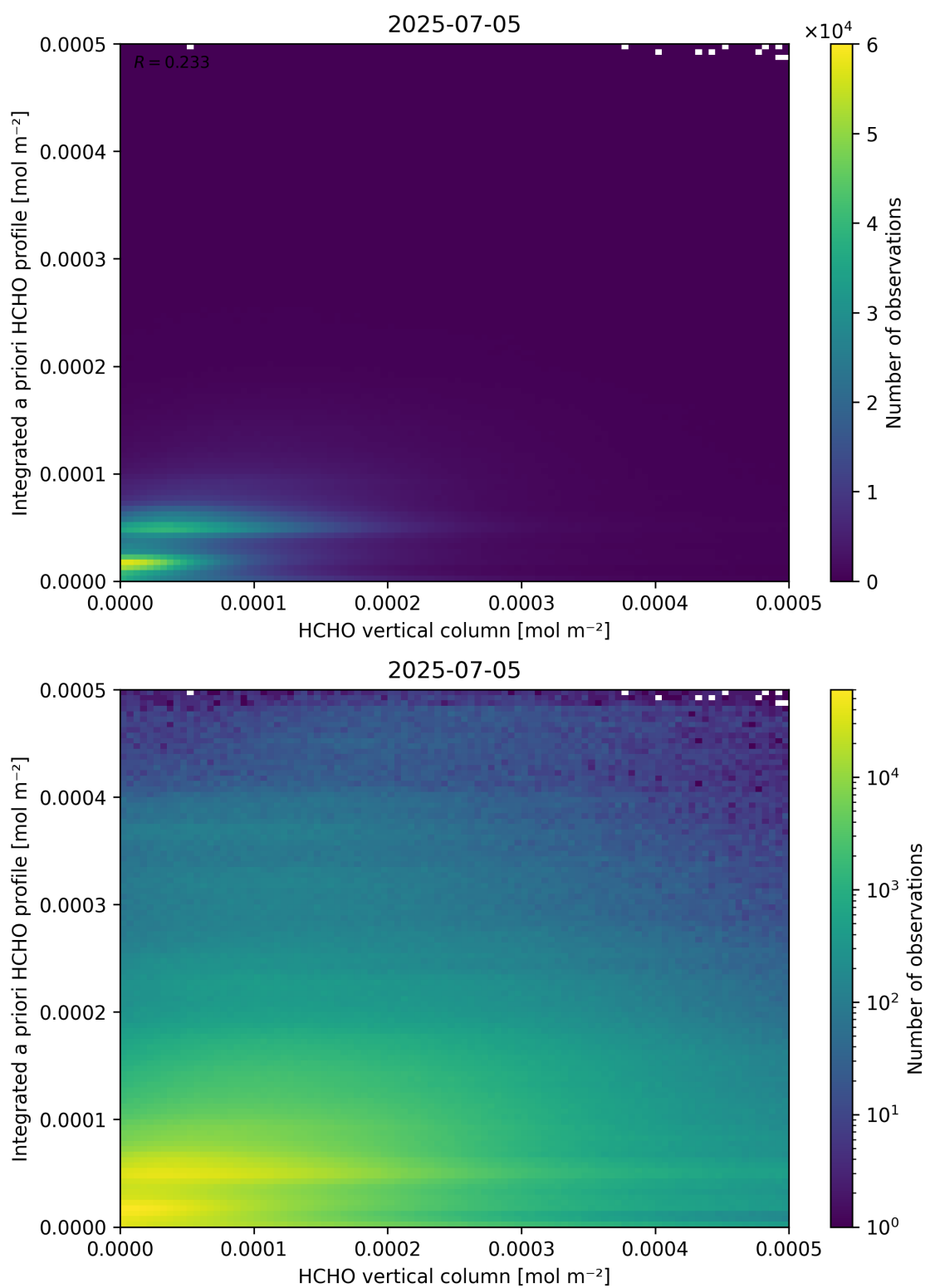
Figure 135: Scatter density plot of “HCHO vertical column” against “Integrated a priori HCHO profile” for 2025-07-04 to 2025-07-06.
