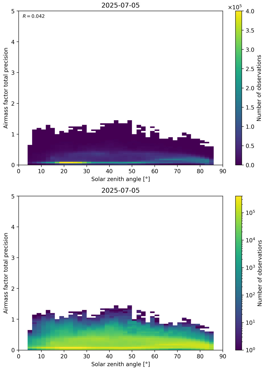
Figure 176: Scatter density plot of “Solar zenith angle” against “Airmass factor total precision” for 2025-07-04 to 2025-07-06.
