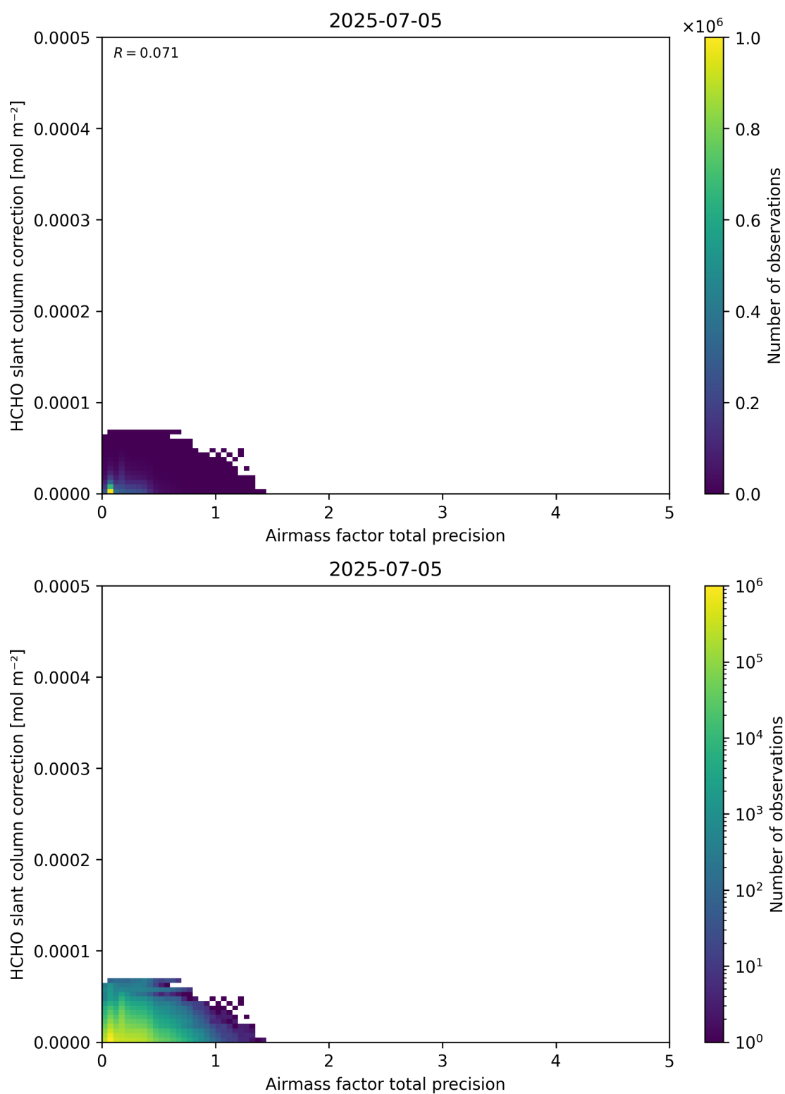
Figure 110: Scatter density plot of “Airmass factor total precision” against “HCHO slant column correction” for 2025-07-04 to 2025-07-06.
