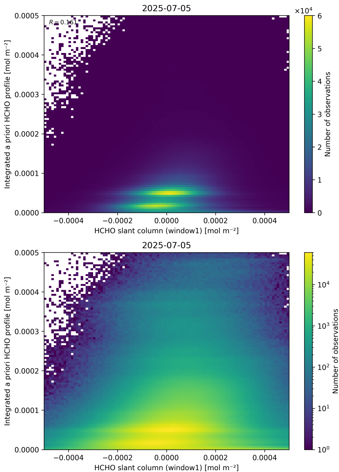
Figure 87: Scatter density plot of “HCHO slant column (window1)” against “Integrated a priori HCHO profile” for 2025-07-04 to 2025-07-06.
