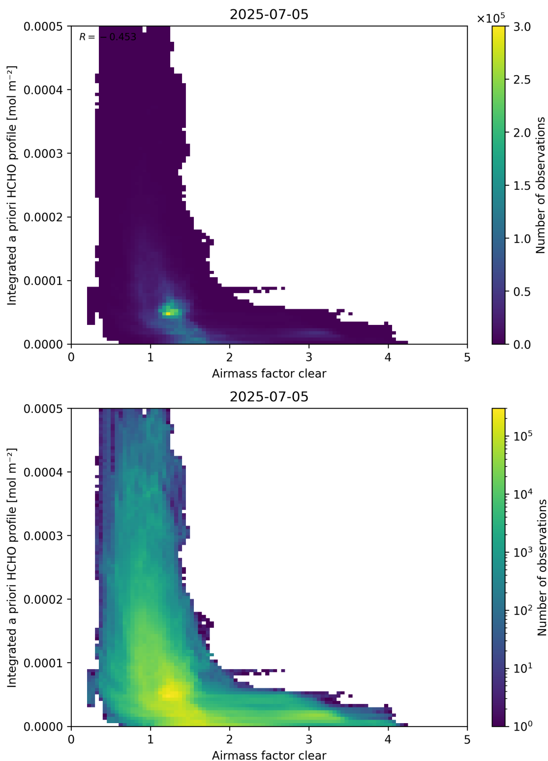
Figure 76: Scatter density plot of “Airmass factor clear” against “Integrated a priori HCHO profile” for 2025-07-04 to 2025-07-06.
