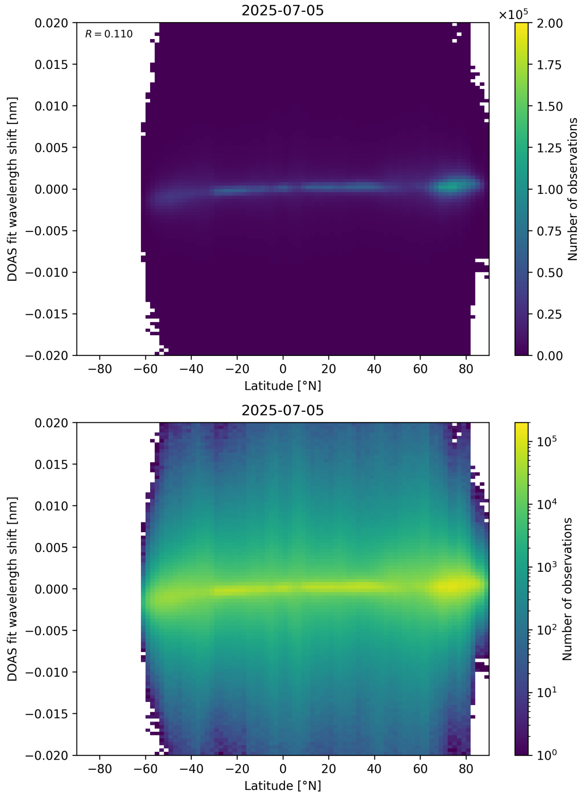
Figure 154: Scatter density plot of “Latitude” against “DOAS fit wavelength shift” for 2025-07-04 to 2025-07-06.
