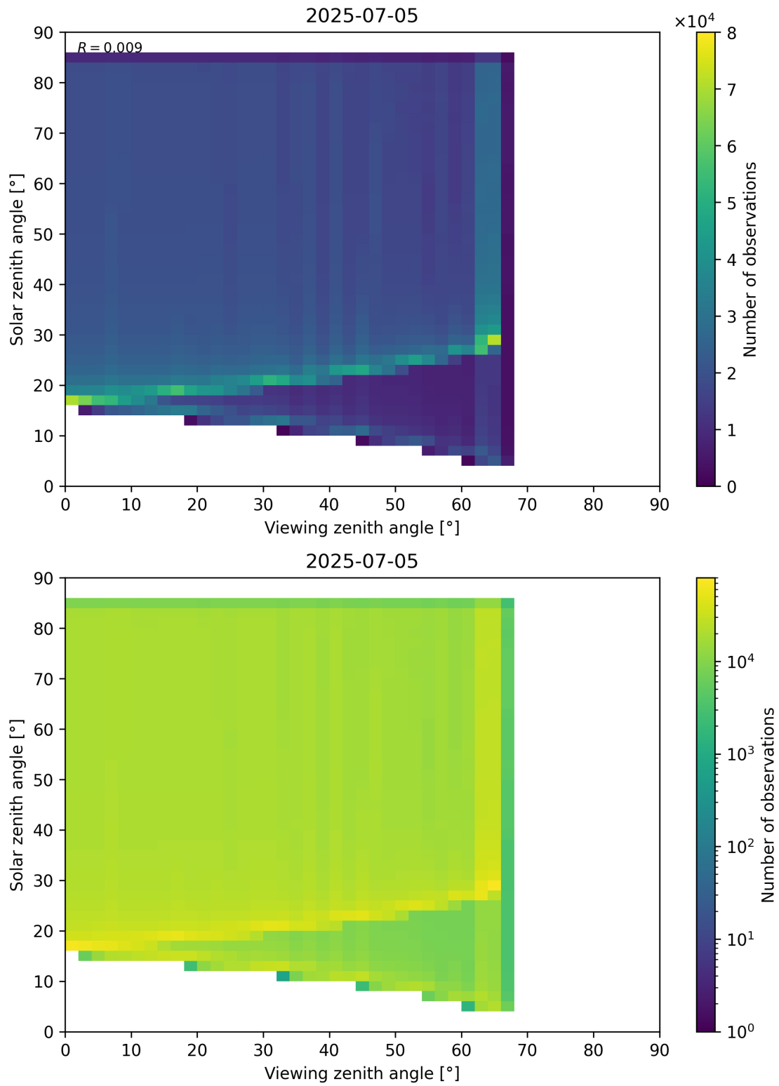
Figure 197: Scatter density plot of “Viewing zenith angle” against “Solar zenith angle” for 2025-07-04 to 2025-07-06.
