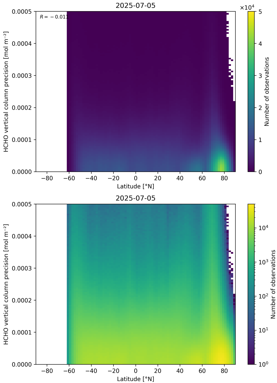
Figure 165: Scatter density plot of “Latitude” against “HCHO vertical column precision” for 2025-07-04 to 2025-07-06.
