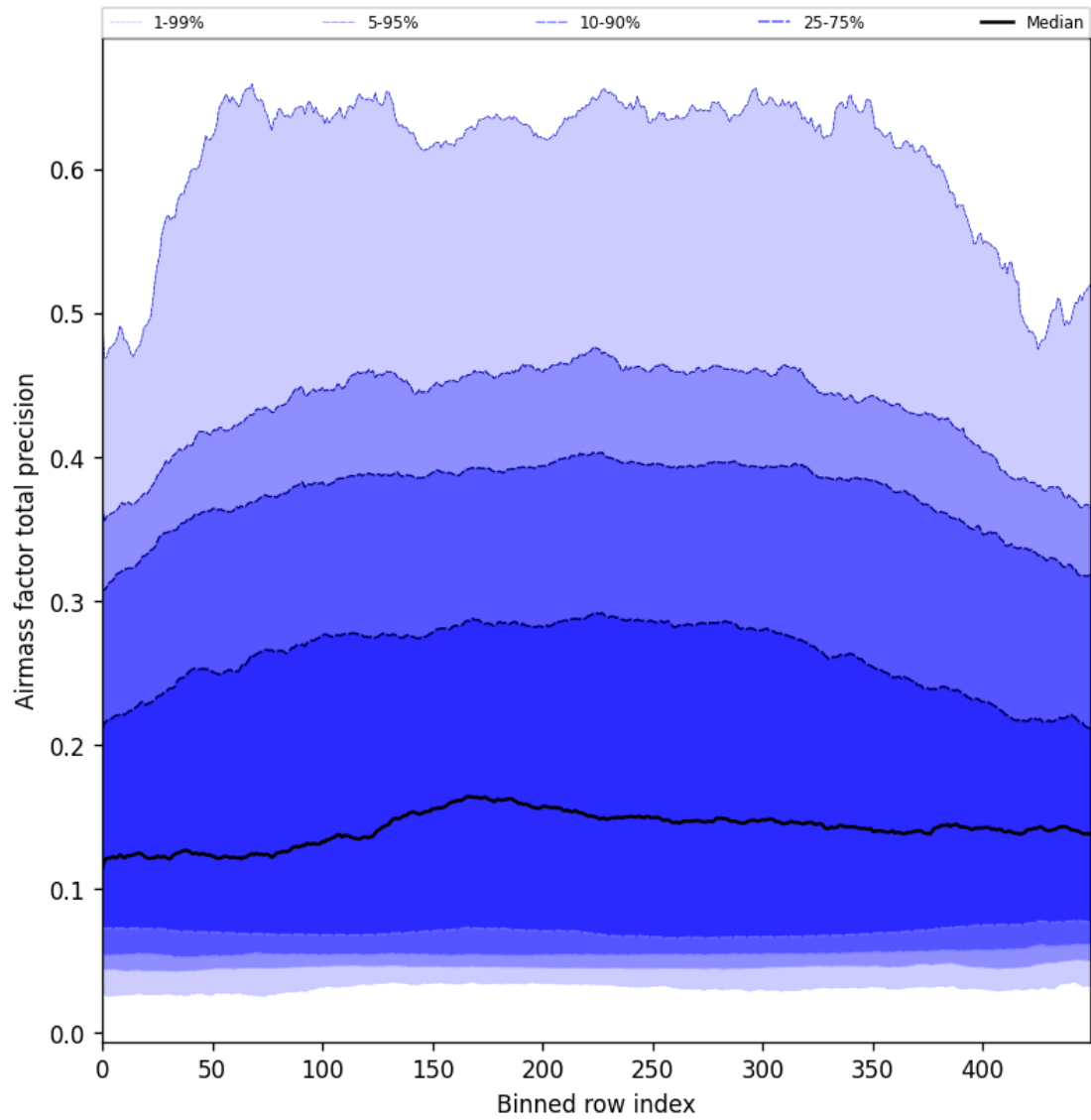
Figure 55: Along track statistics of “Airmass factor total precision” for 2025-07-04 to 2025-07-06
