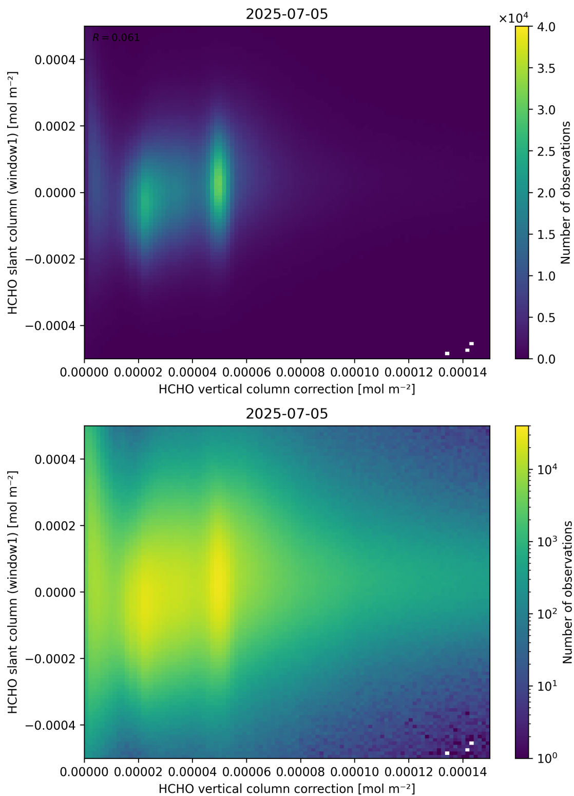
Figure 118: Scatter density plot of “HCHO vertical column correction” against “HCHO slant column (window1)” for 2025-07-04 to 2025-07-06.
