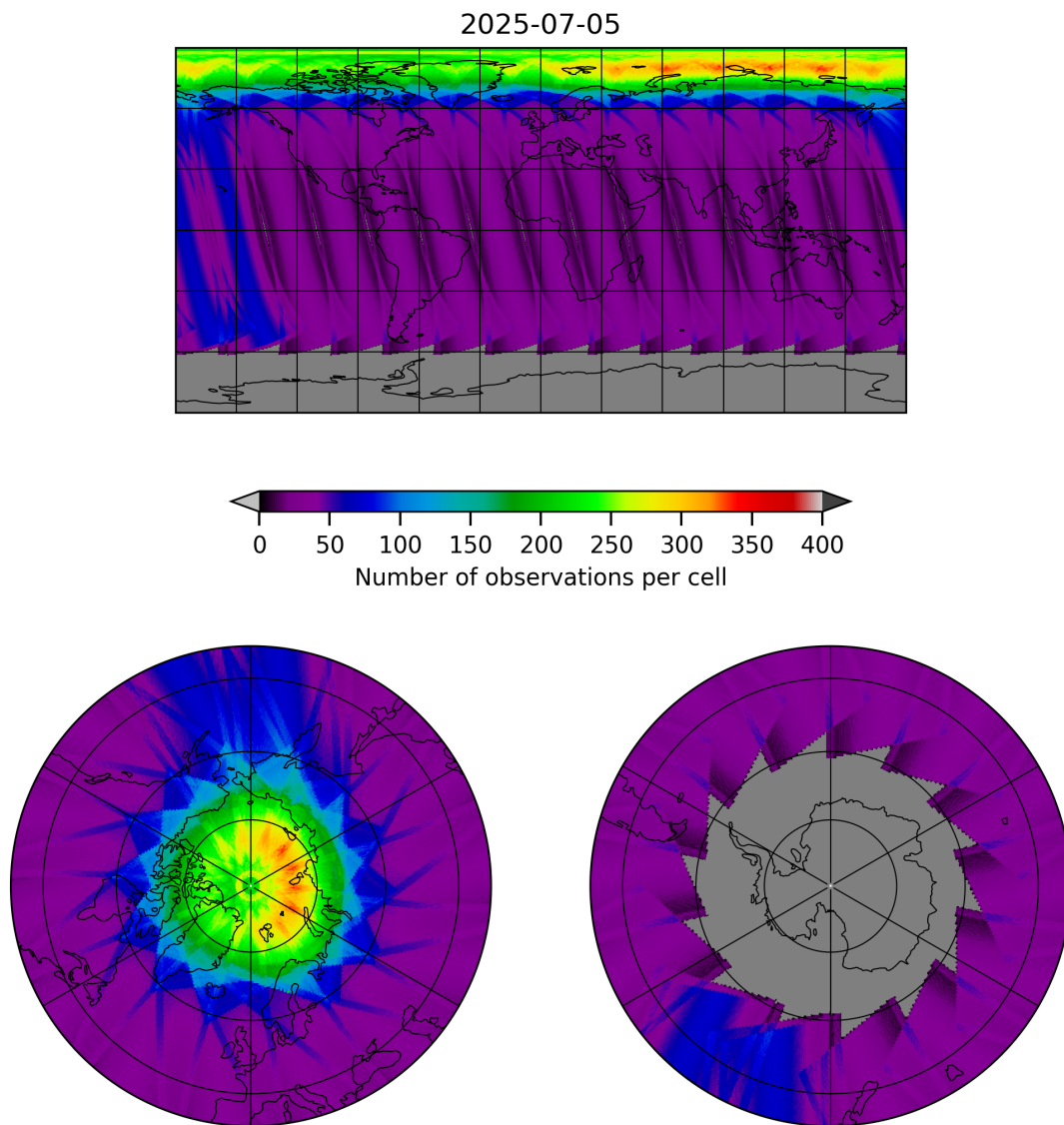
Figure 19: Map of the number of observations for 2025-07-04 to 2025-07-06
