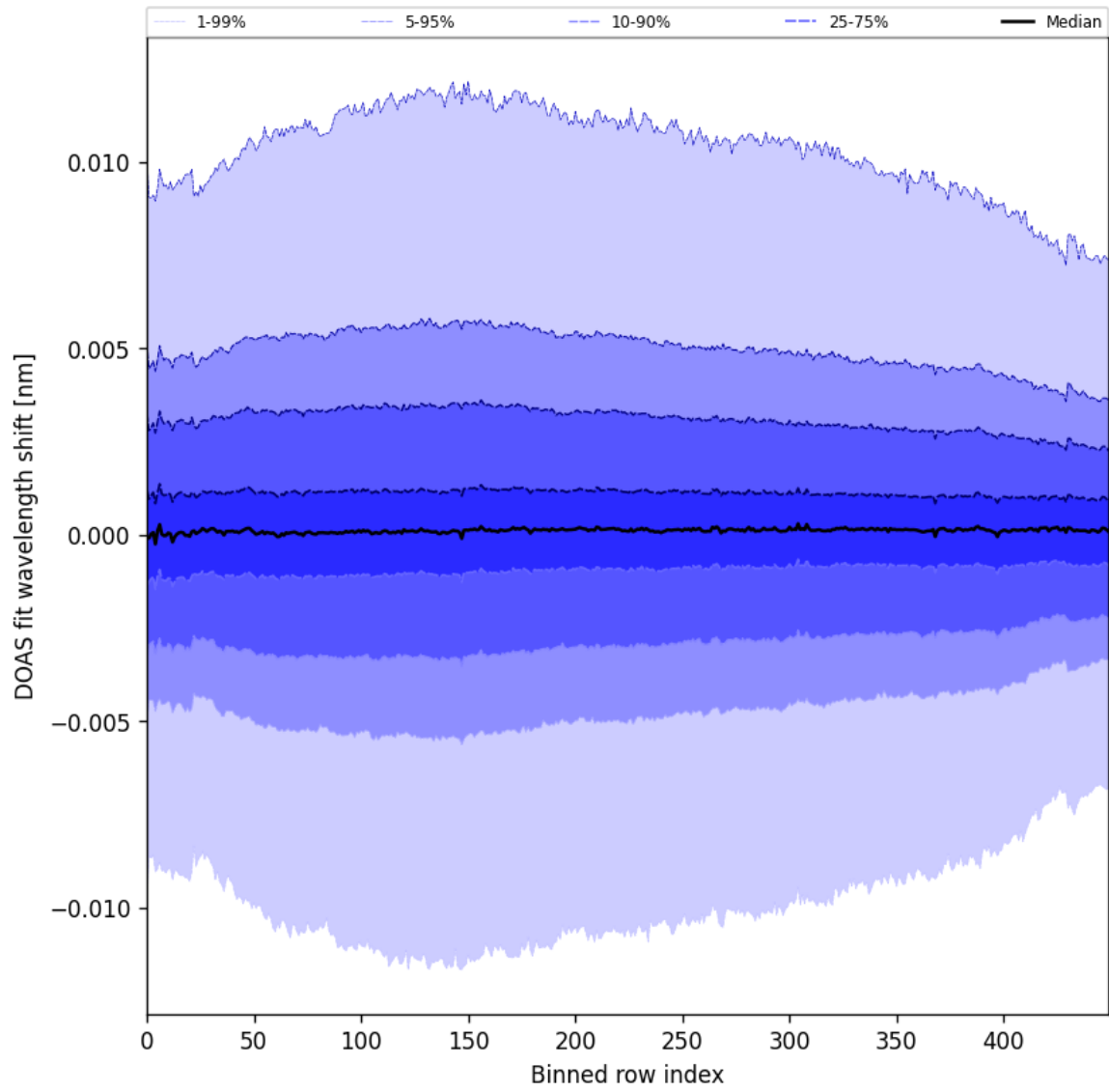
Figure 58: Along track statistics of “DOAS fit wavelength shift” for 2025-07-04 to 2025-07-06
