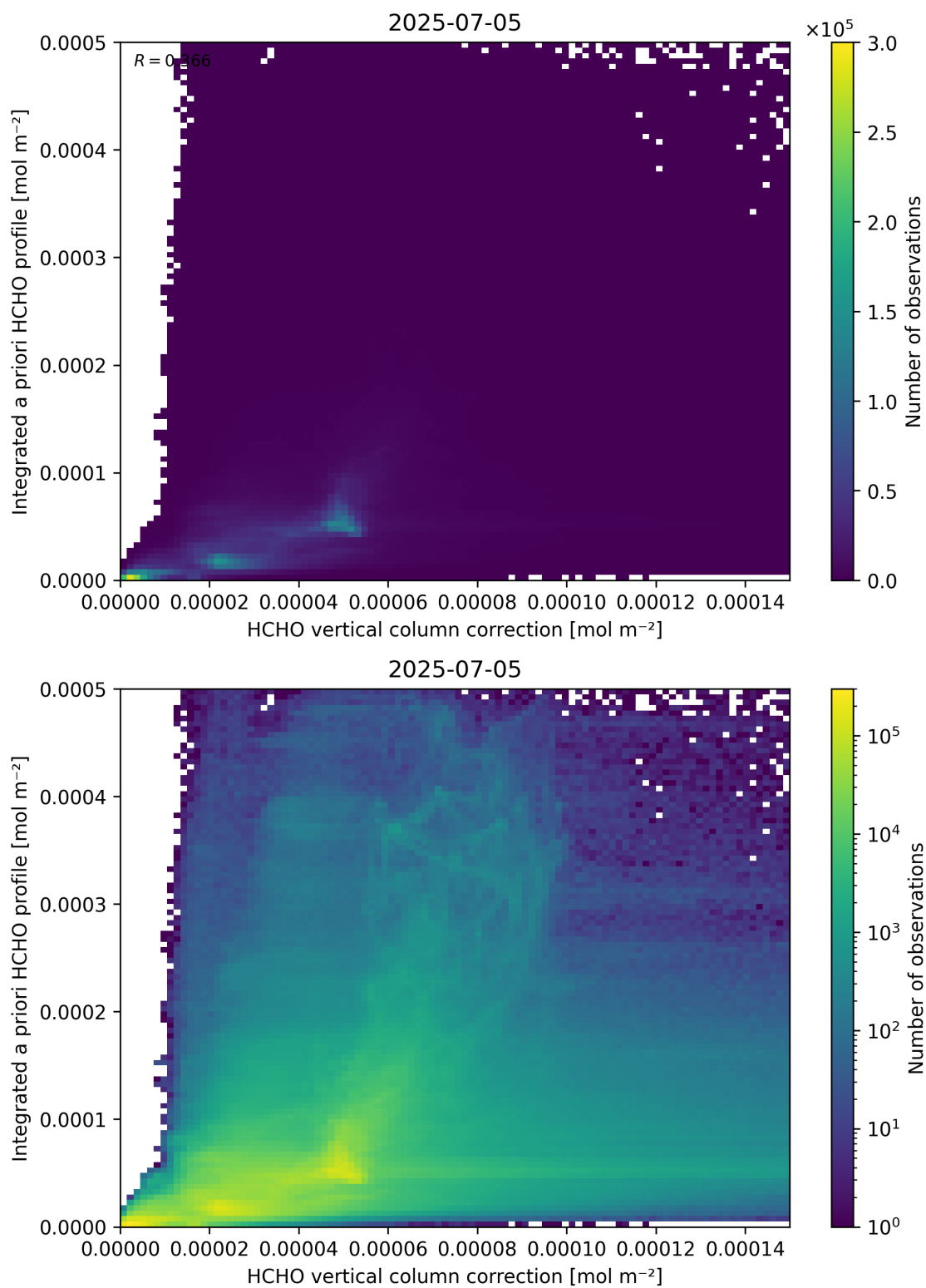
Figure 122: Scatter density plot of “HCHO vertical column correction” against “Integrated a priori HCHO profile” for 2025-07-04 to 2025-07-06.
