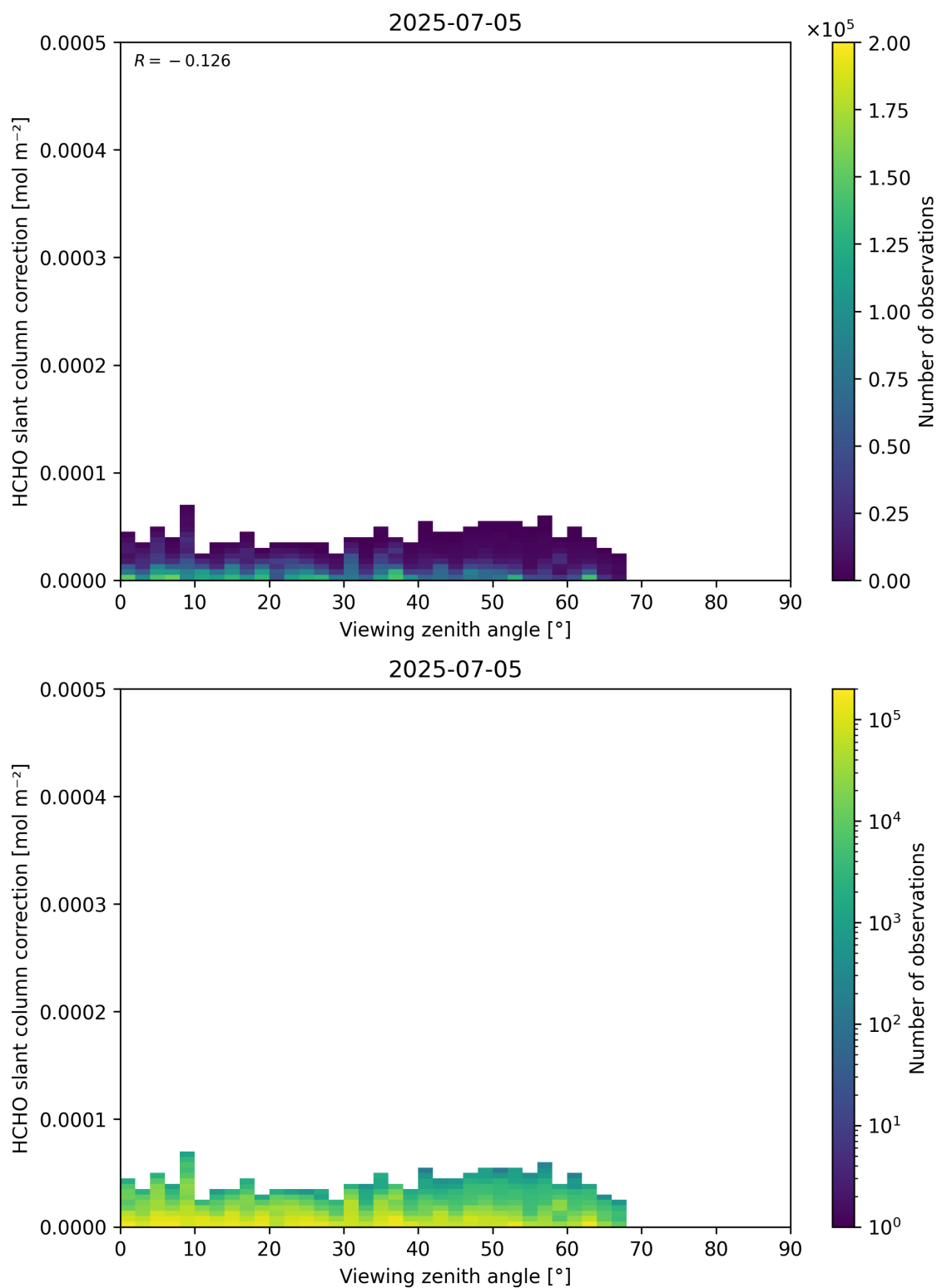
Figure 187: Scatter density plot of “Viewing zenith angle” against “HCHO slant column correction” for 2025-07-04 to 2025-07-06.
