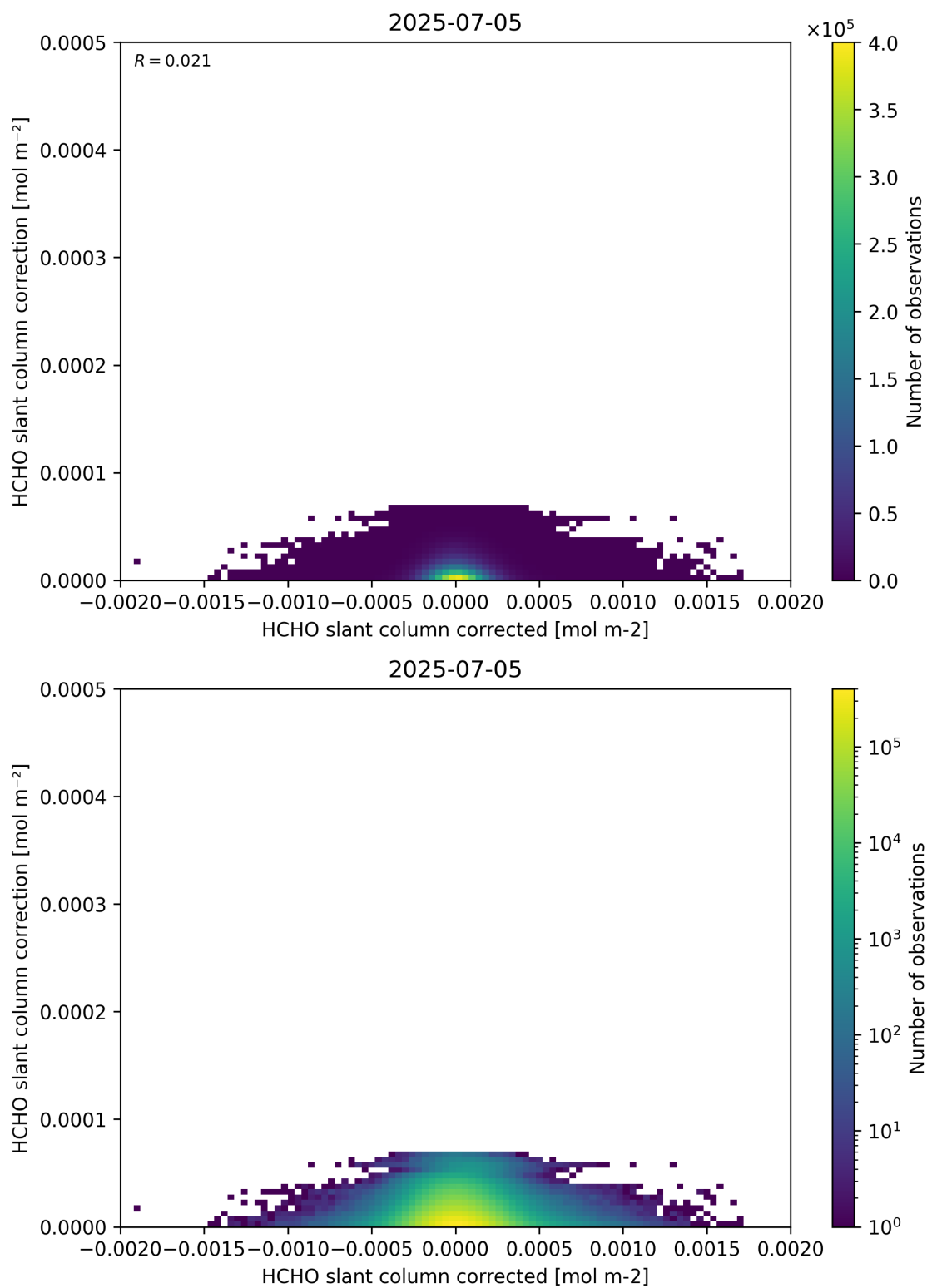
Figure 77: Scatter density plot of “HCHO slant column corrected” against “HCHO slant column correction” for 2025-07-04 to 2025-07-06.
