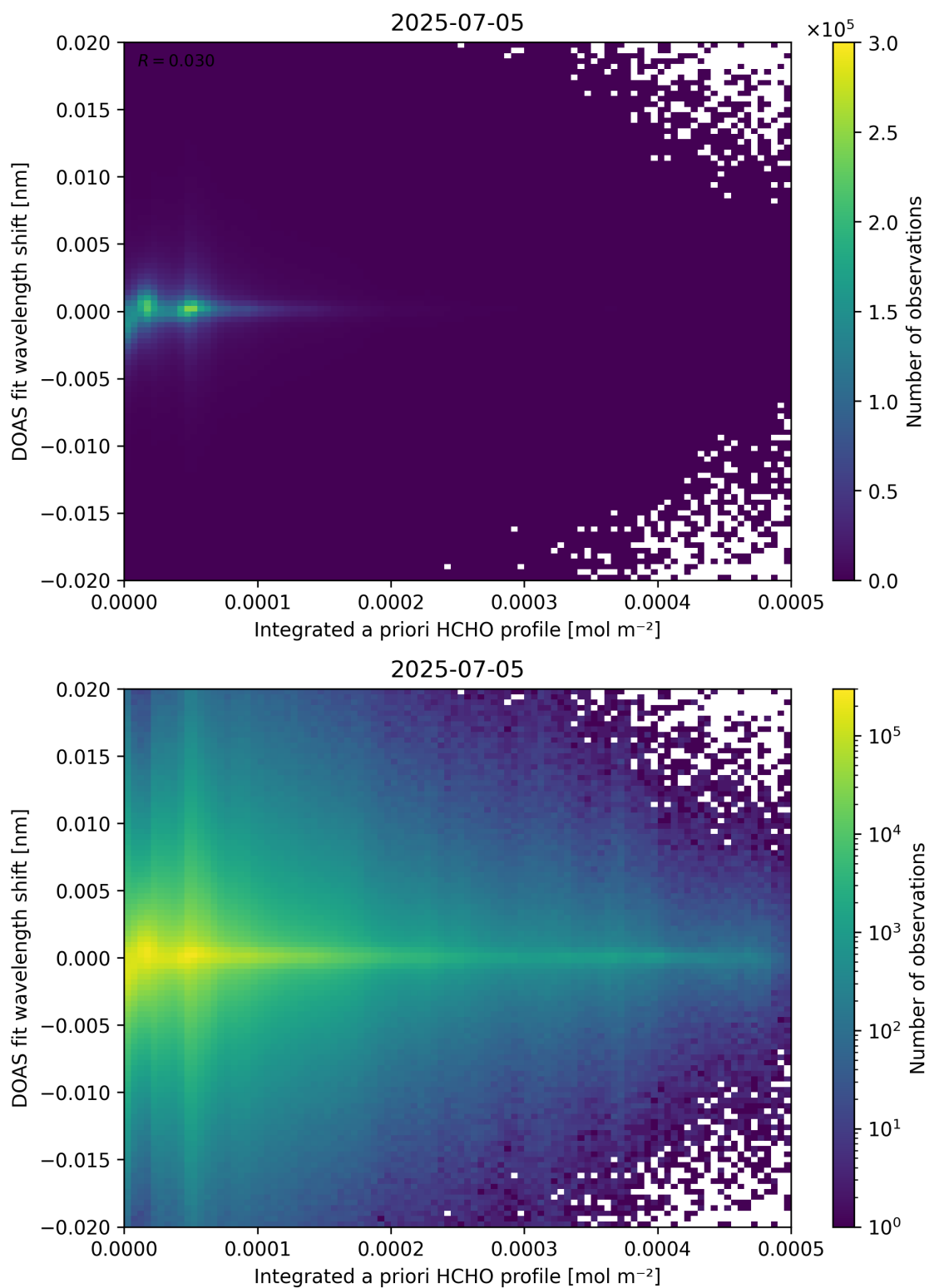
Figure 149: Scatter density plot of “Integrated a priori HCHO profile” against “DOAS fit wavelength shift” for 2025-07-04 to 2025-07-06.
