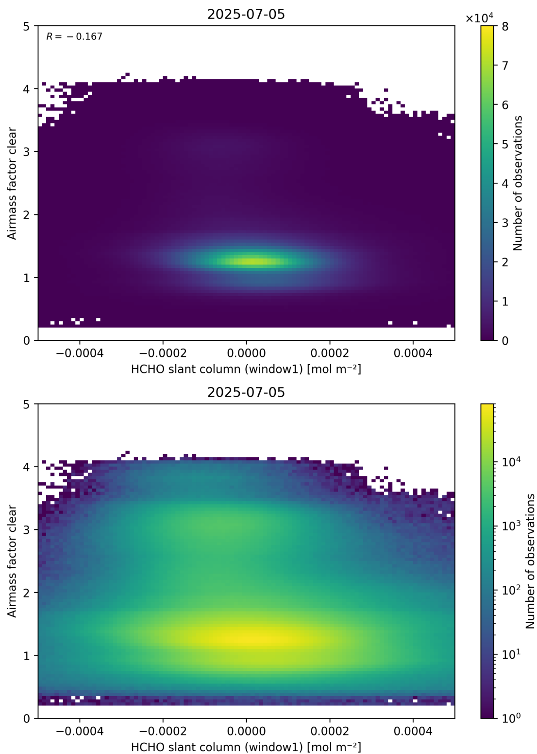
Figure 81: Scatter density plot of “HCHO slant column (window1)” against “Airmass factor clear” for 2025-07-04 to 2025-07-06.
