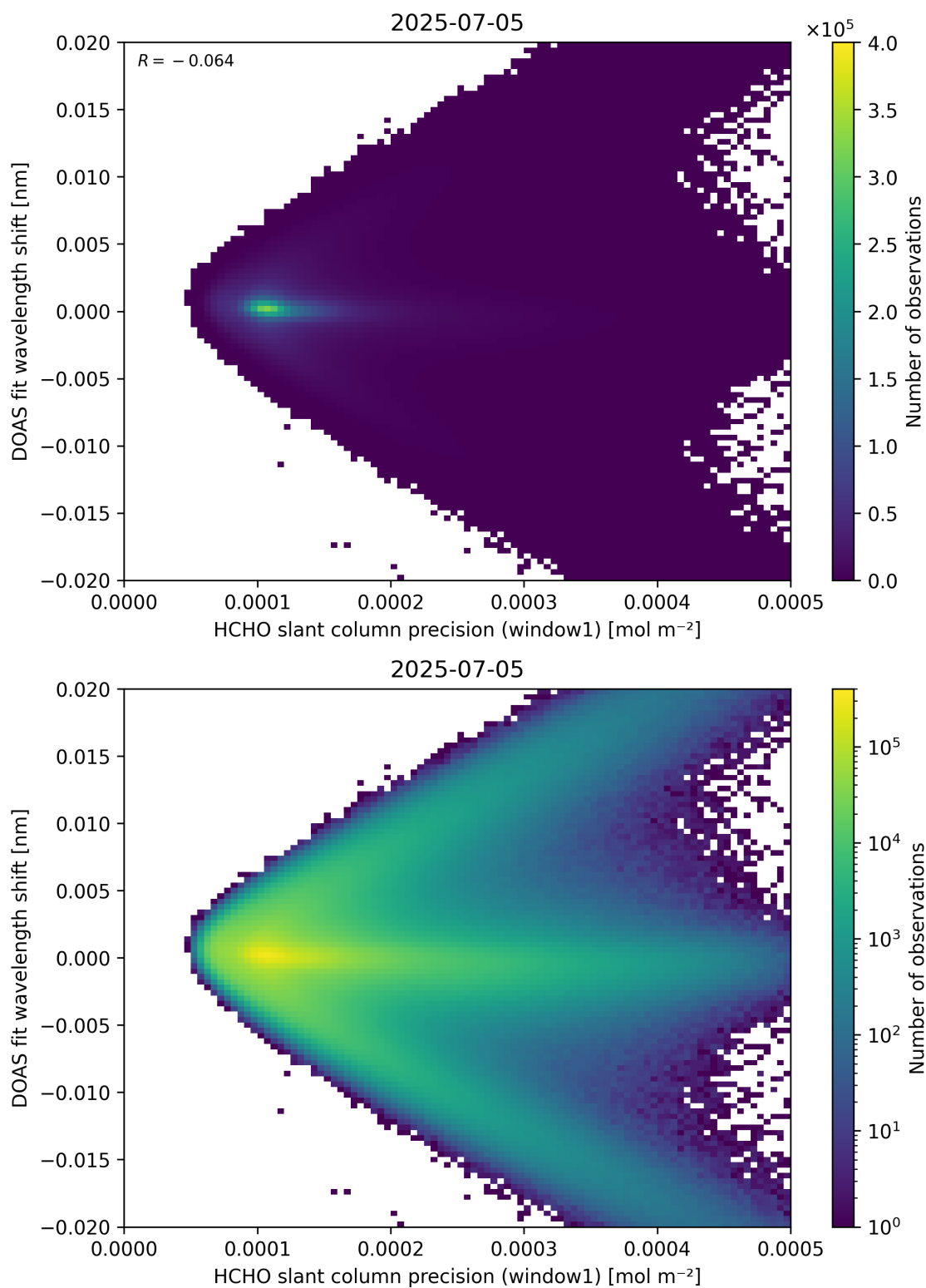
Figure 89: Scatter density plot of “HCHO slant column precision (window1)” against “DOAS fit wavelength shift” for 2025-07-04 to 2025-07-06.
