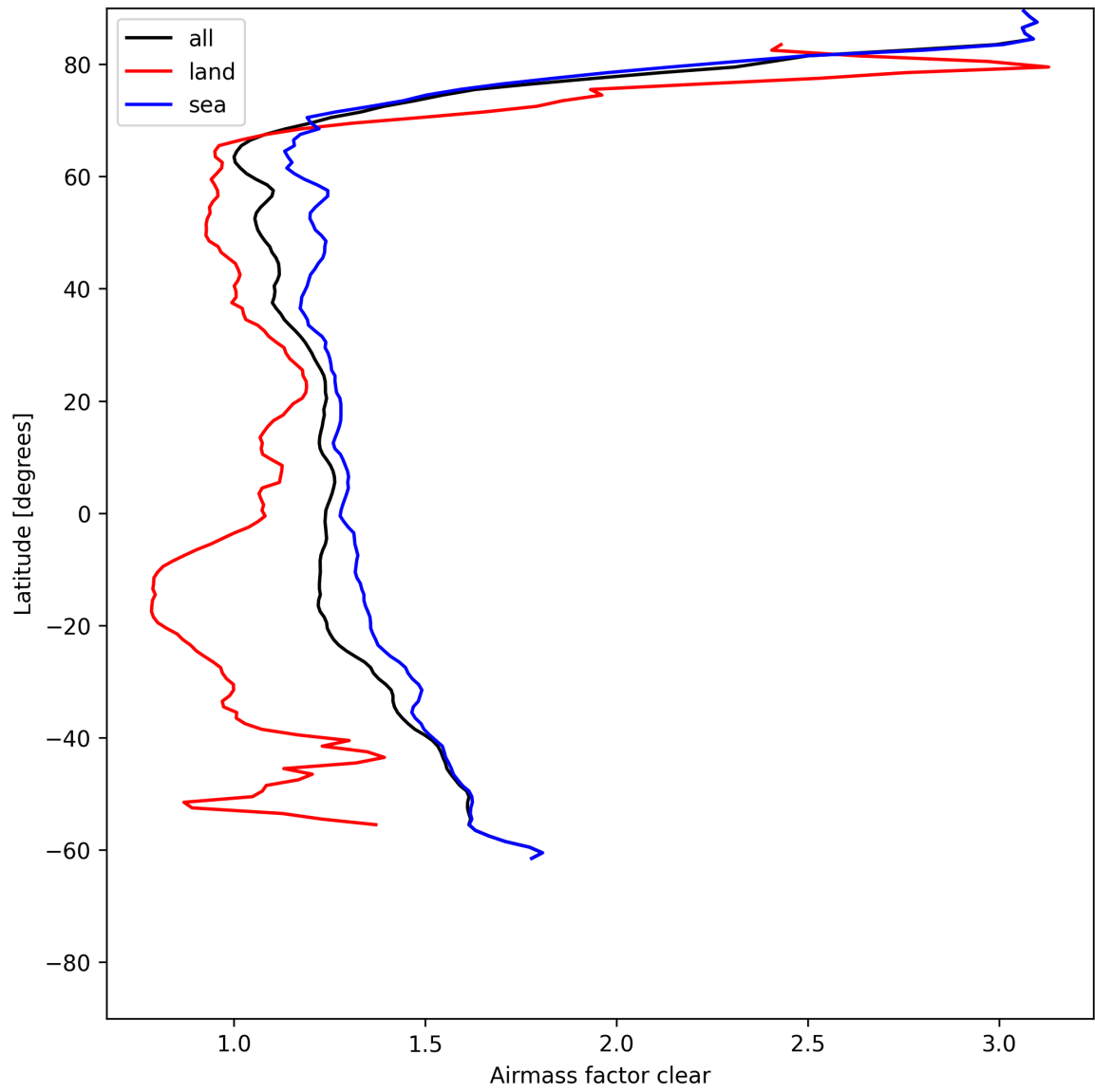
Figure 28: Zonal average of “Airmass factor clear” for 2025-07-04 to 2025-07-06.
