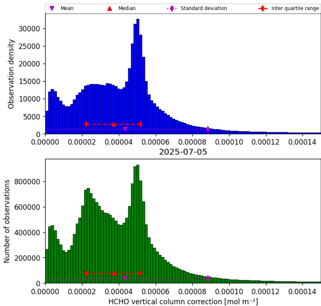
Figure 37: Histogram of “HCHO vertical column correction” for 2025-07-04 to 2025-07-06
