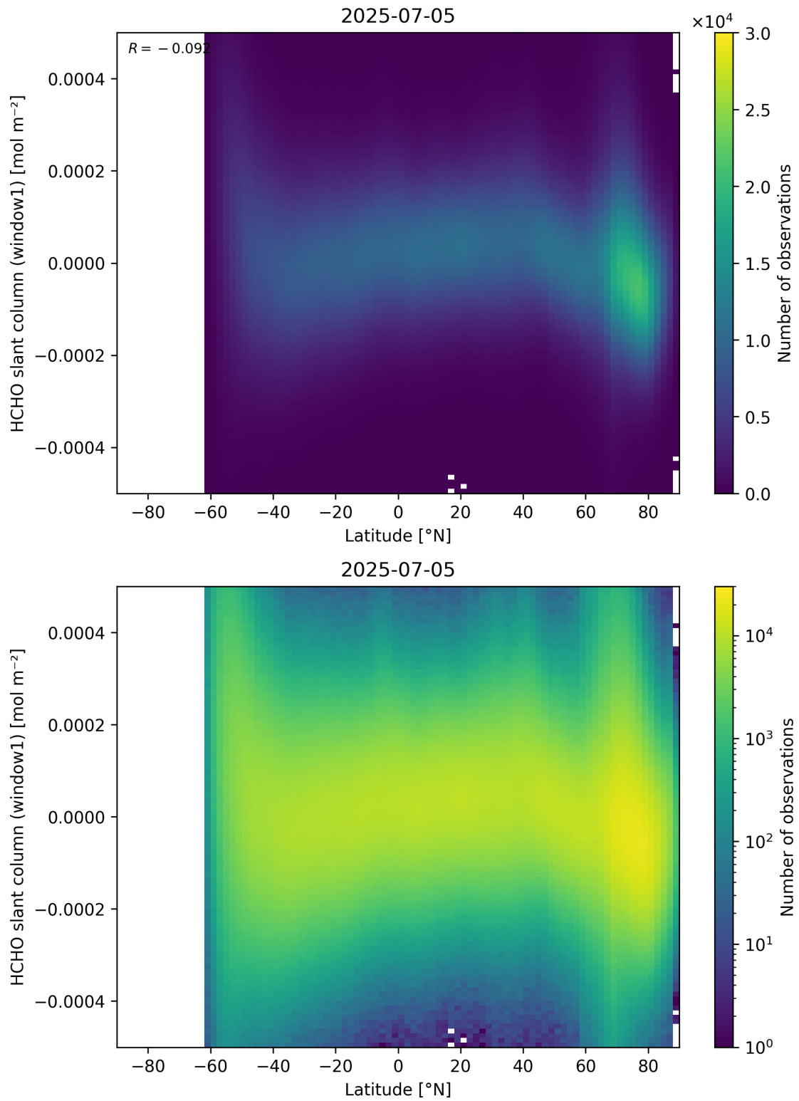
Figure 159: Scatter density plot of “Latitude” against “HCHO slant column (window1)” for 2025-07-04 to 2025-07-06.
