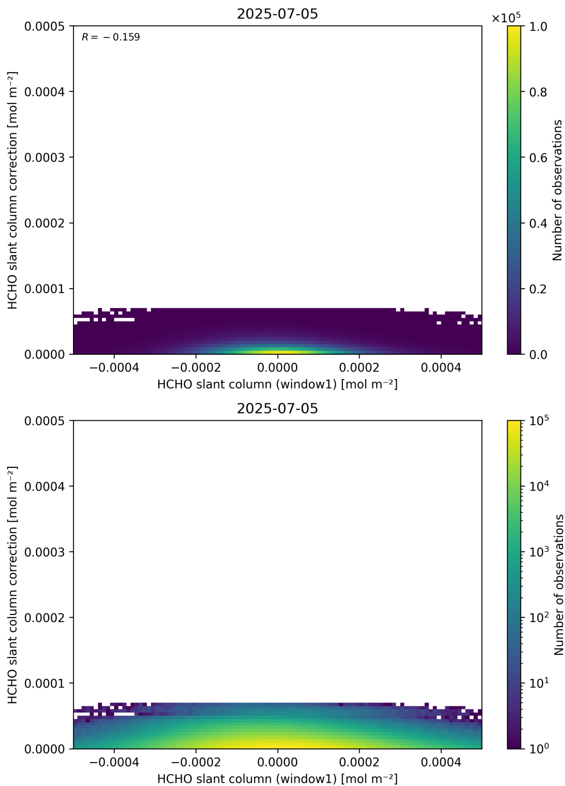
Figure 83: Scatter density plot of “HCHO slant column (window1)” against “HCHO slant column correction” for 2025-07-04 to 2025-07-06.
