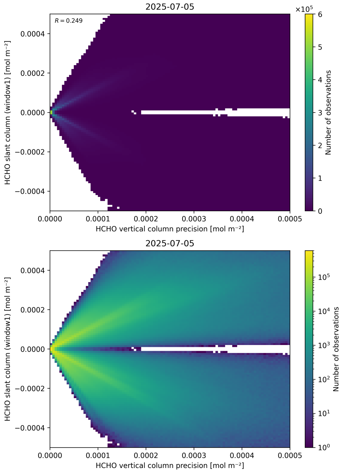
Figure 142: Scatter density plot of “HCHO vertical column precision” against “HCHO slant column (window1)” for 2025-07-04 to 2025-07-06.
