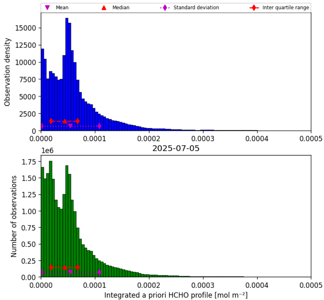
Figure 43: Histogram of “Integrated a priori HCHO profile” for 2025-07-04 to 2025-07-06
