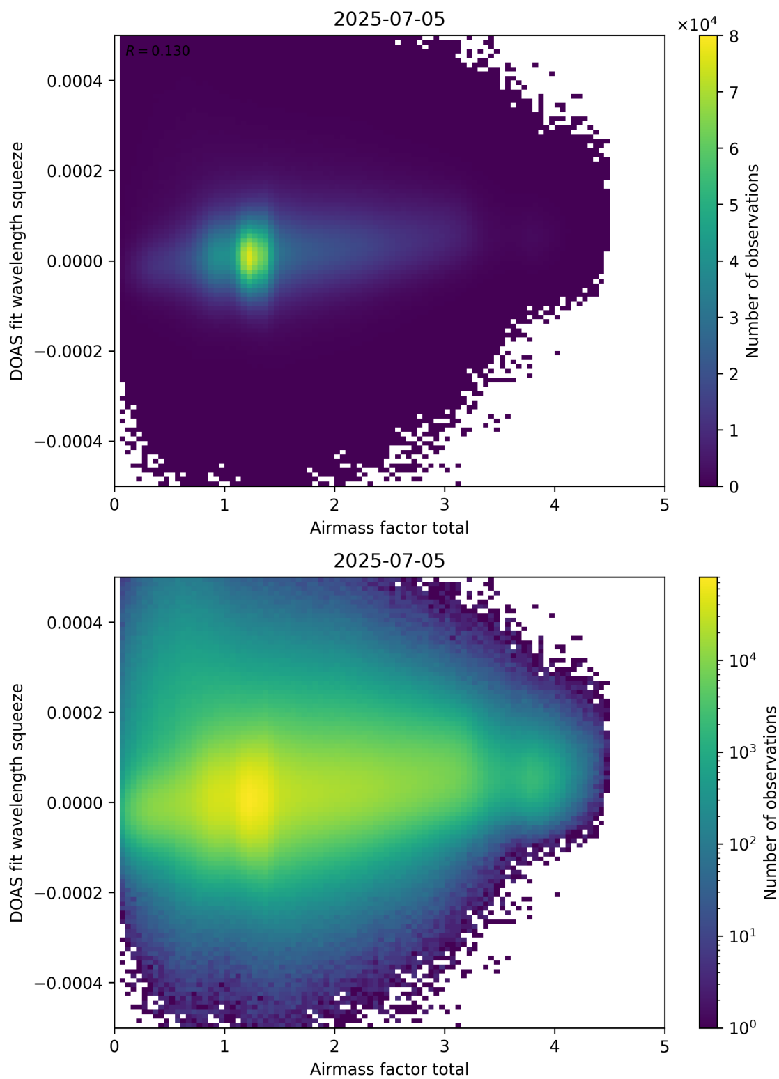
Figure 99: Scatter density plot of “Airmass factor total” against “DOAS fit wavelength squeeze” for 2025-07-04 to 2025-07-06.
