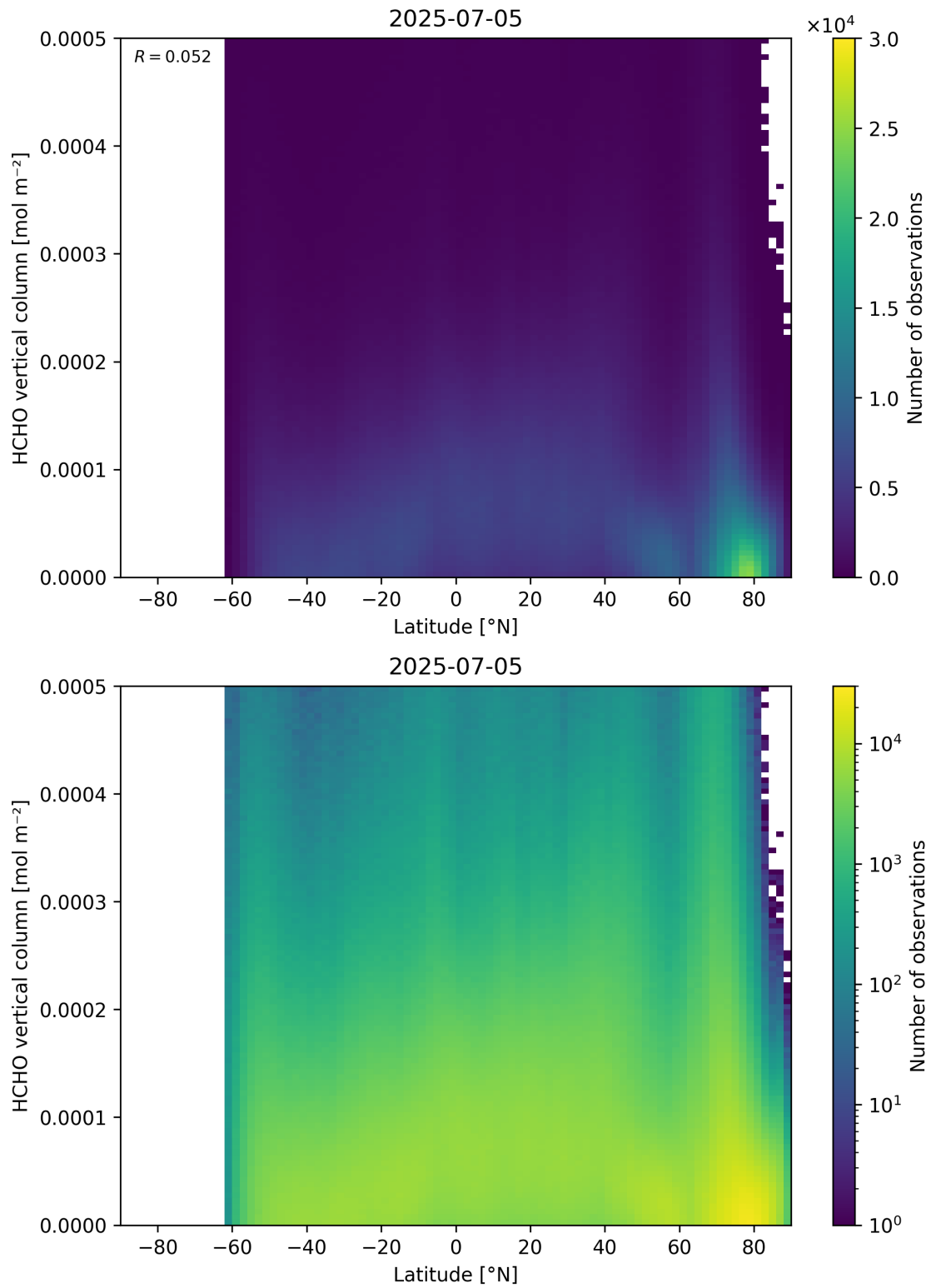
Figure 163: Scatter density plot of “Latitude” against “HCHO vertical column” for 2025-07-04 to 2025-07-06.
