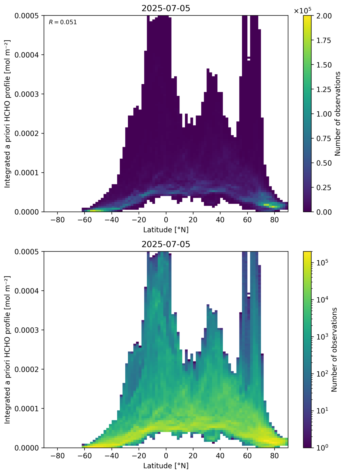
Figure 166: Scatter density plot of “Latitude” against “Integrated a priori HCHO profile” for 2025-07-04 to 2025-07-06.
