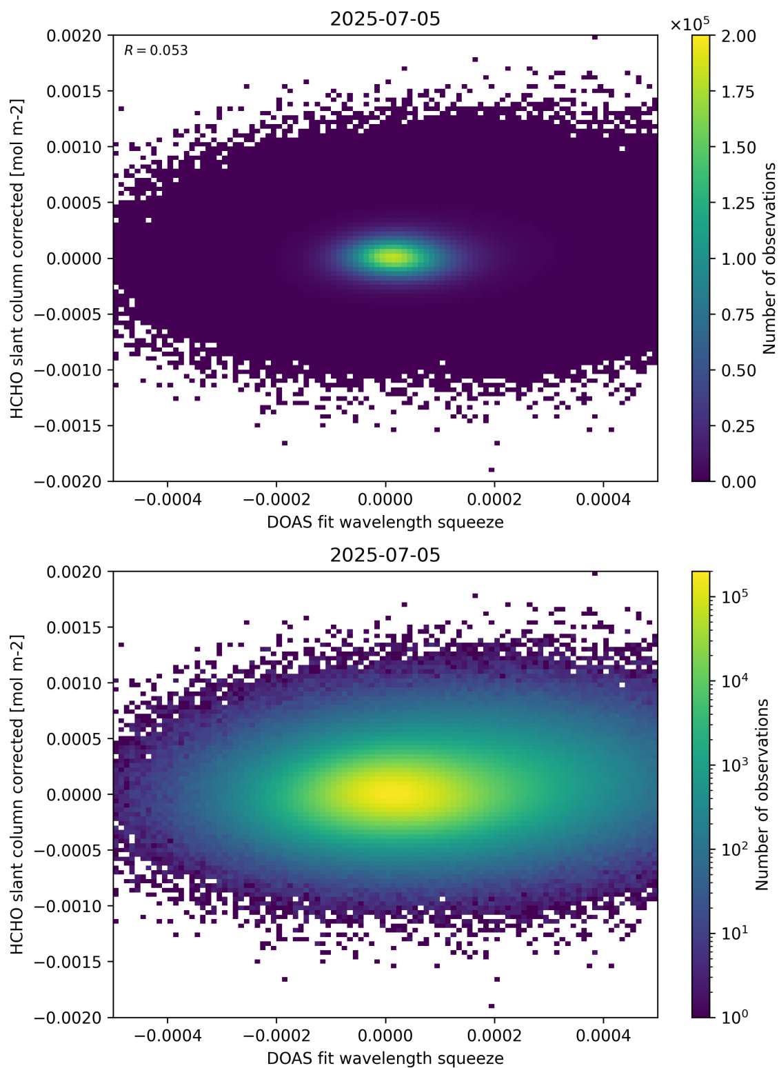
Figure 69: Scatter density plot of “DOAS fit wavelength squeeze” against “HCHO slant column corrected” for 2025-07-04 to 2025-07-06.
