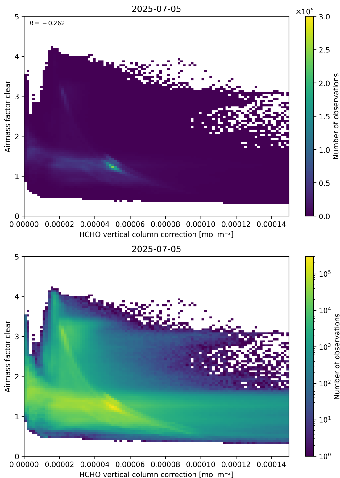
Figure 115: Scatter density plot of “HCHO vertical column correction” against “Airmass factor clear” for 2025-07-04 to 2025-07-06.
