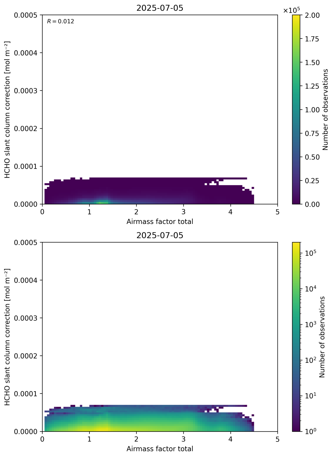
Figure 102: Scatter density plot of “Airmass factor total” against “HCHO slant column correction” for 2025-07-04 to 2025-07-06.
