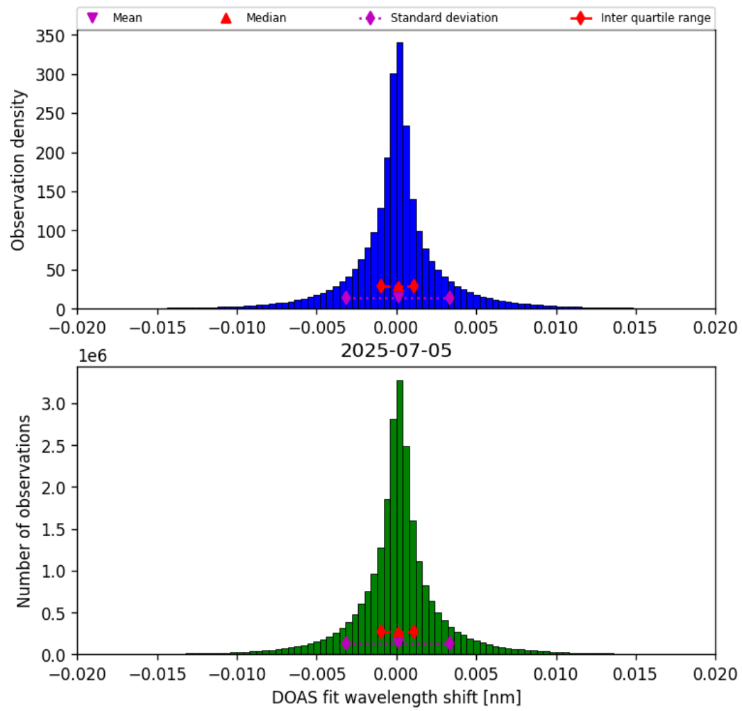
Figure 44: Histogram of “DOAS fit wavelength shift” for 2025-07-04 to 2025-07-06
