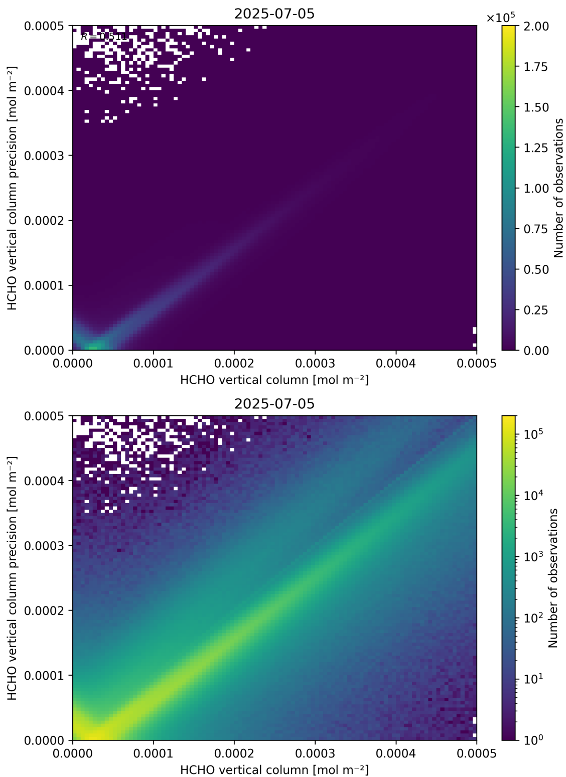
Figure 134: Scatter density plot of “HCHO vertical column” against “HCHO vertical column precision” for 2025-07-04 to 2025-07-06.
