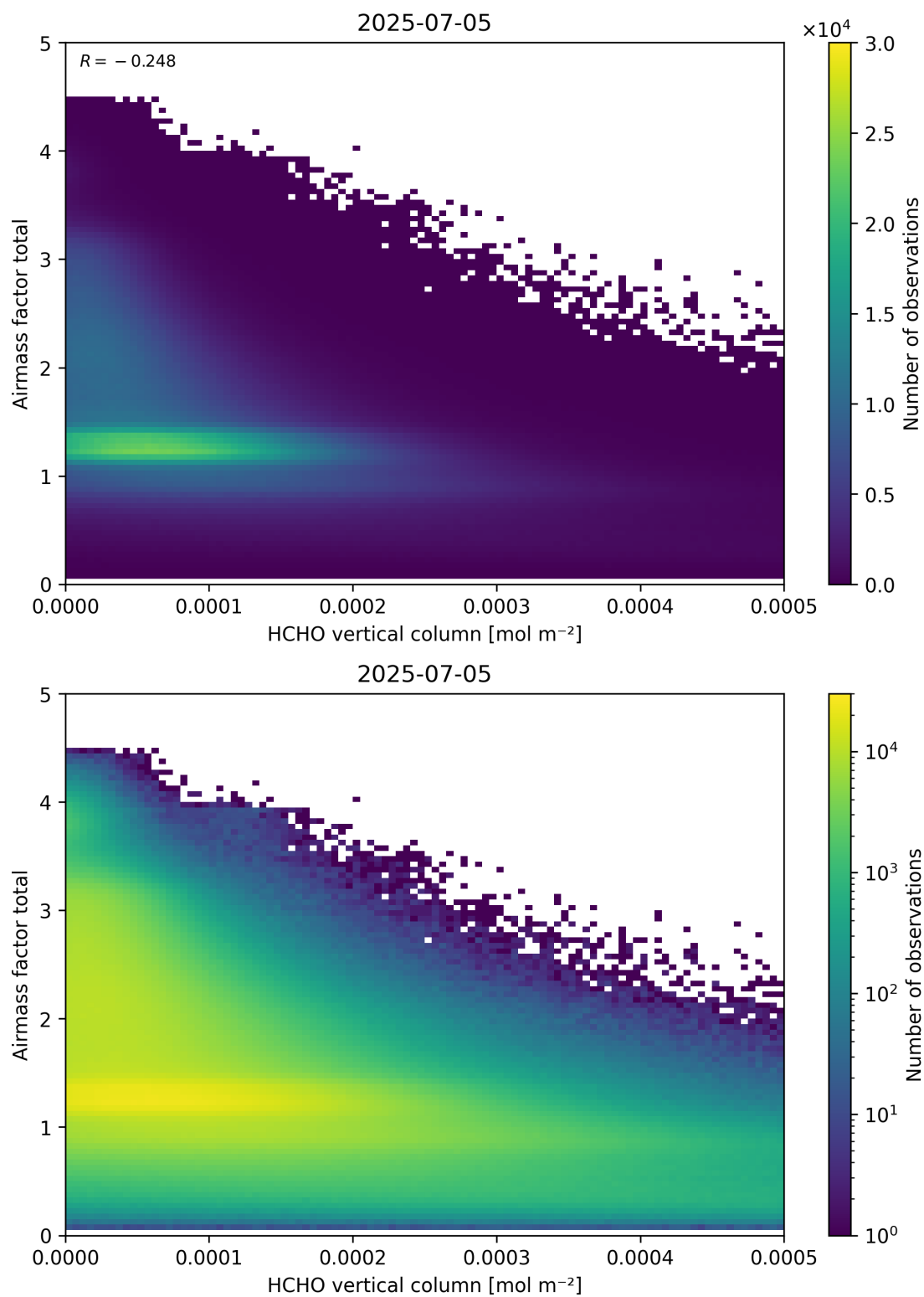
Figure 131: Scatter density plot of “HCHO vertical column” against “Airmass factor total” for 2025-07-04 to 2025-07-06.
