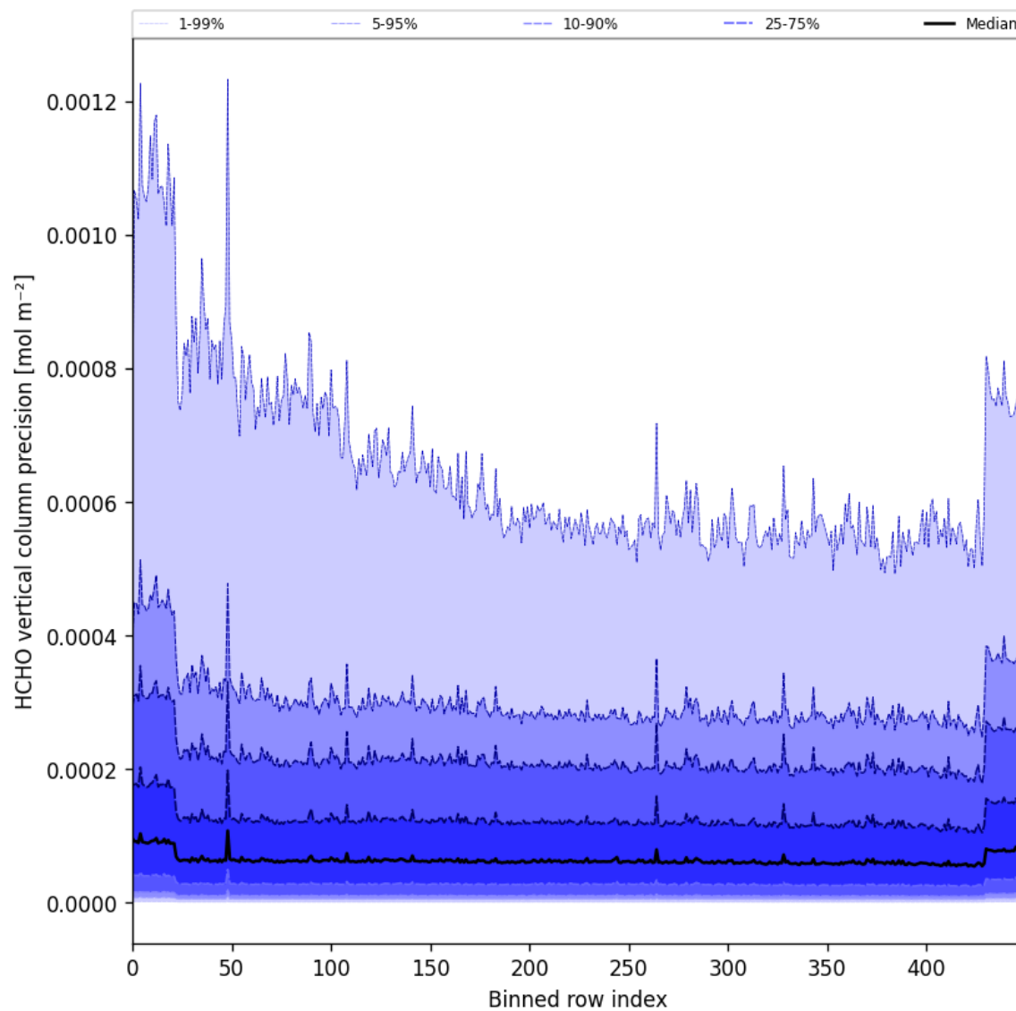
Figure 50: Along track statistics of “HCHO vertical column precision” for 2025-07-04 to 2025-07-06
