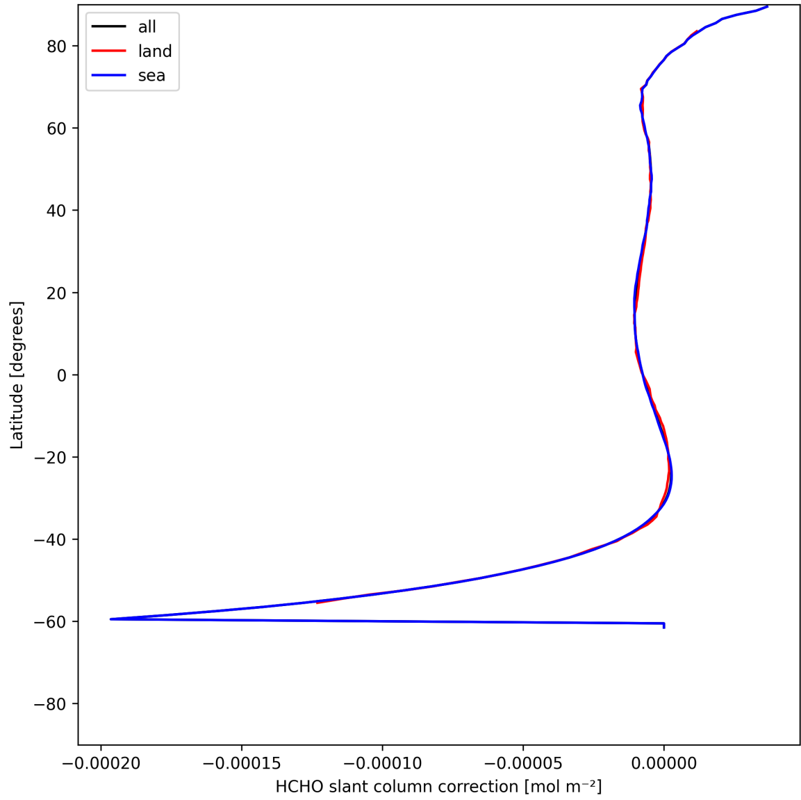
Figure 33: Zonal average of “HCHO slant column correction” for 2025-07-04 to 2025-07-06.
