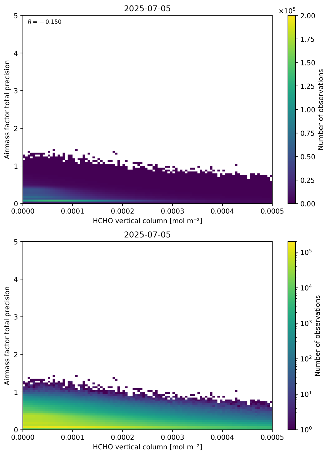
Figure 132: Scatter density plot of “HCHO vertical column” against “Airmass factor total precision” for 2025-07-04 to 2025-07-06.
