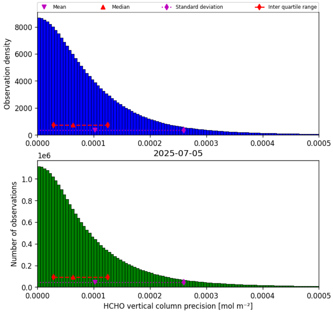
Figure 36: Histogram of “HCHO vertical column precision” for 2025-07-04 to 2025-07-06
