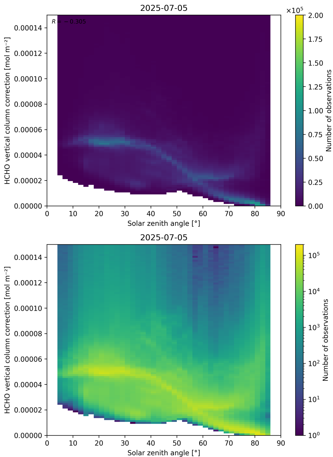
Figure 178: Scatter density plot of “Solar zenith angle” against “HCHO vertical column correction” for 2025-07-04 to 2025-07-06.
