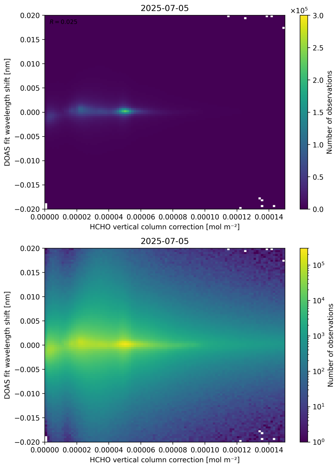
Figure 113: Scatter density plot of “HCHO vertical column correction” against “DOAS fit wavelength shift” for 2025-07-04 to 2025-07-06.
