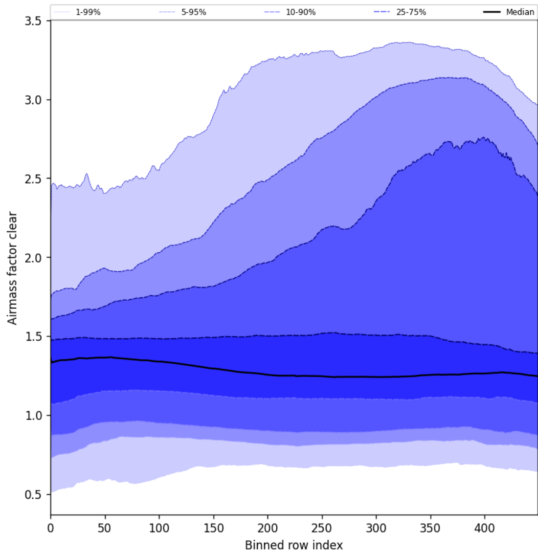
Figure 56: Along track statistics of “Air mass factor clear” for 2025-07-04 to 2025-07-06
