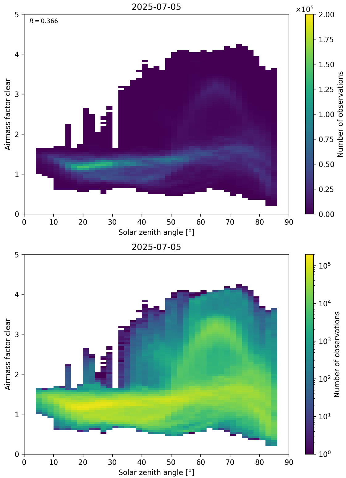
Figure 170: Scatter density plot of “Solar zenith angle” against “Airmass factor clear” for 2025-07-04 to 2025-07-06.
