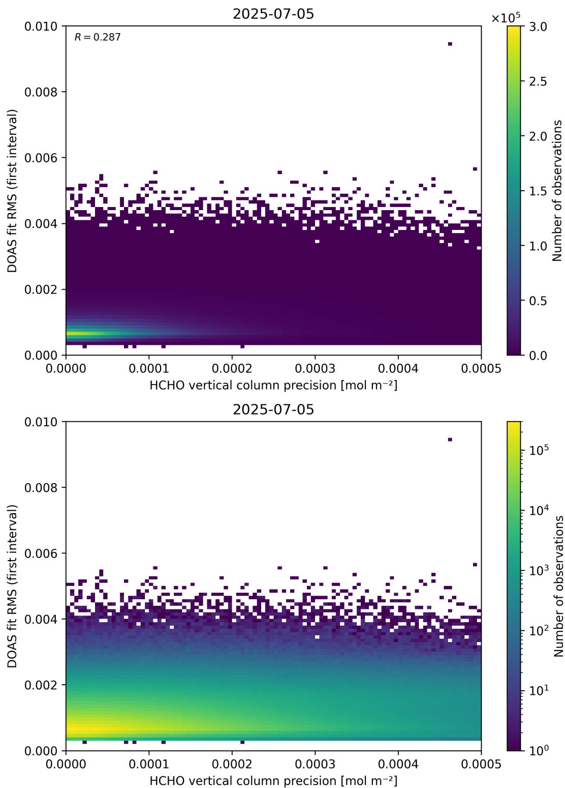
Figure 136: Scatter density plot of “HCHO vertical column precision” against “DOAS fit RMS (first interval)” for 2025-07-04 to 2025-07-06.
