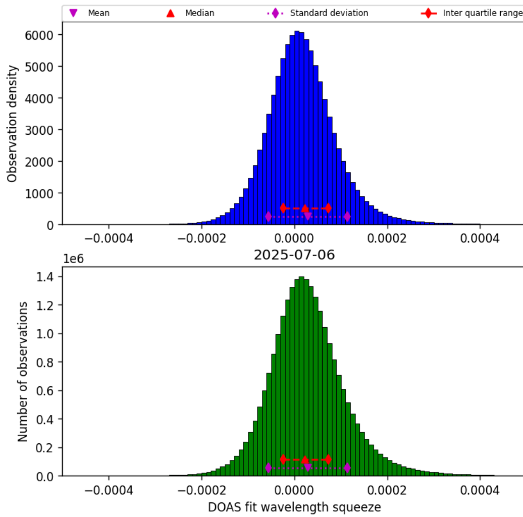
Figure 45: Histogram of “DOAS fit wavelength squeeze” for 2025-07-05 to 2025-07-07
