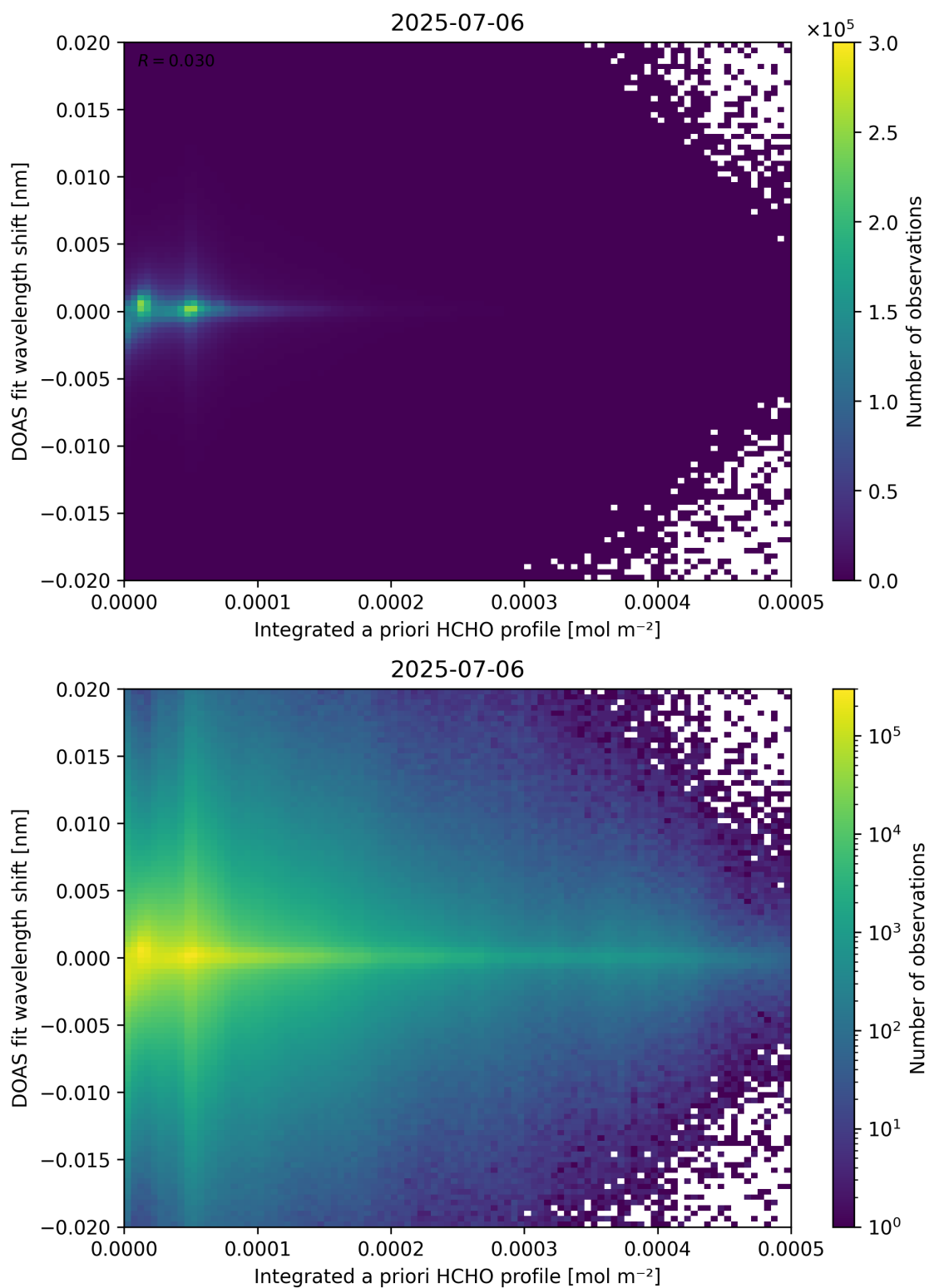
Figure 149: Scatter density plot of “Integrated a priori HCHO profile” against “DOAS fit wavelength shift” for 2025-07-05 to 2025-07-07.
