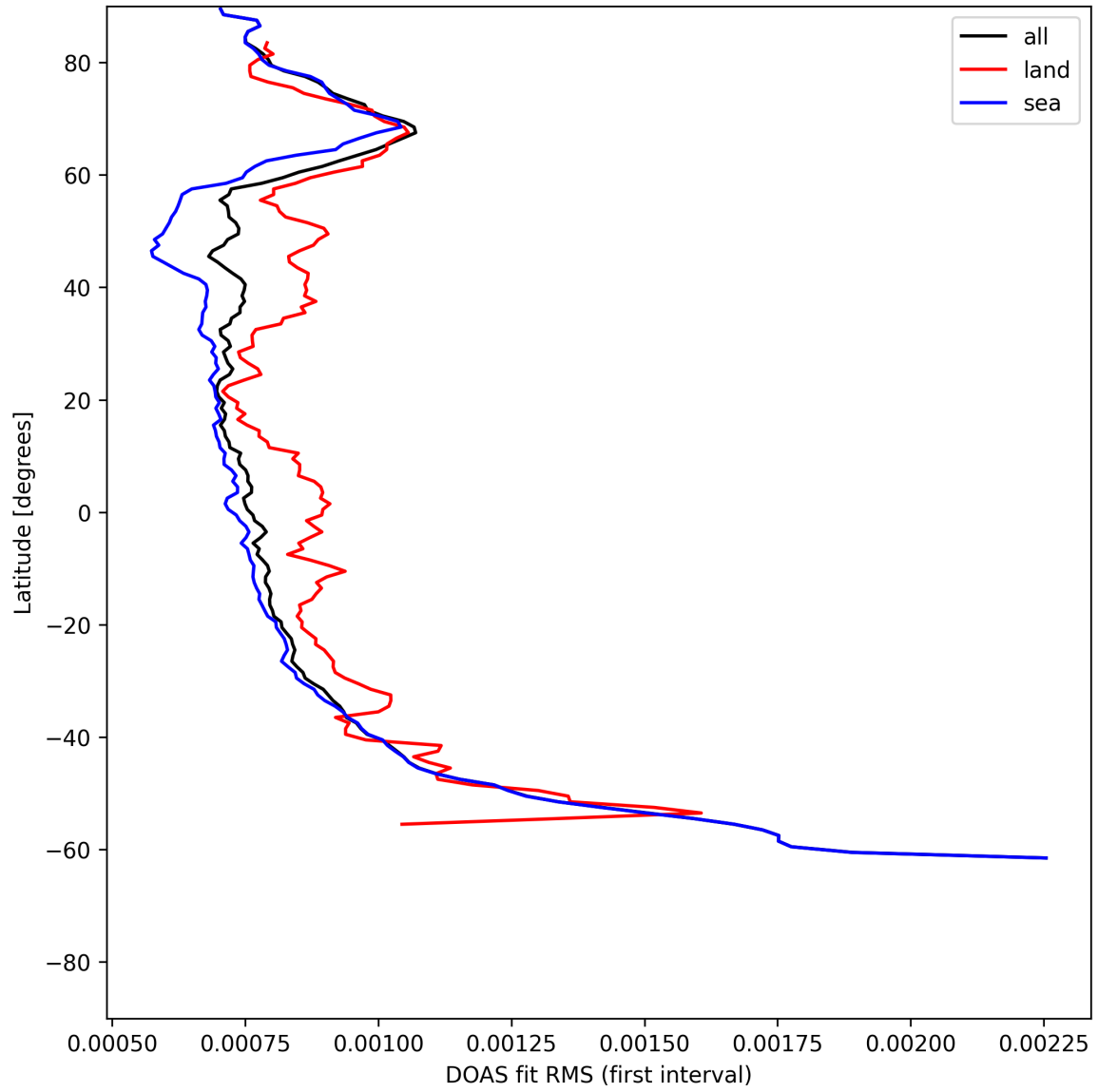
Figure 32: Zonal average of "DOAS fit RMS (first interval)" for 2025-07-05 to 2025-07-07.
