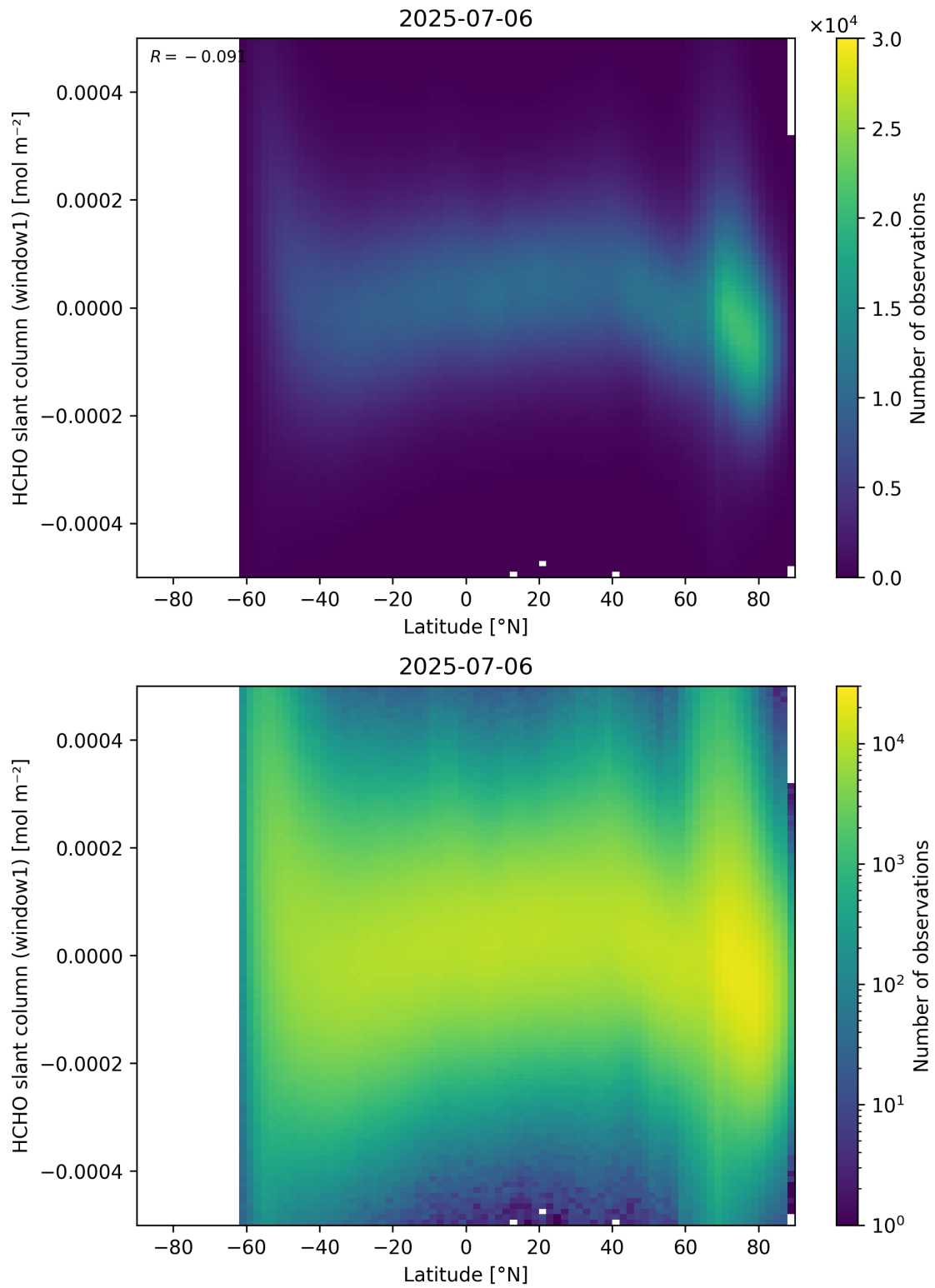
Figure 159: Scatter density plot of “Latitude” against “HCHO slant column (window1)” for 2025-07-05 to 2025-07-07.
