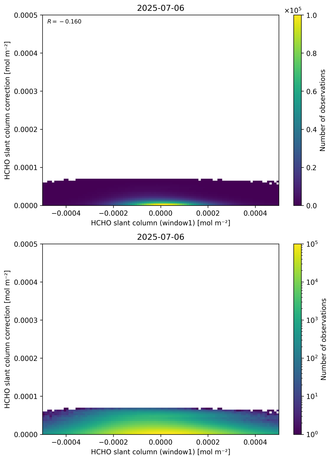
Figure 83: Scatter density plot of “HCHO slant column (window1)” against “HCHO slant column correction” for 2025-07-05 to 2025-07-07.
