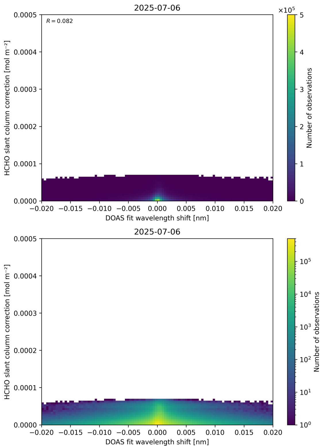
Figure 67: Scatter density plot of “DOAS fit wavelength shift” against “HCHO slant column correction” for 2025-07-05 to 2025-07-07.
