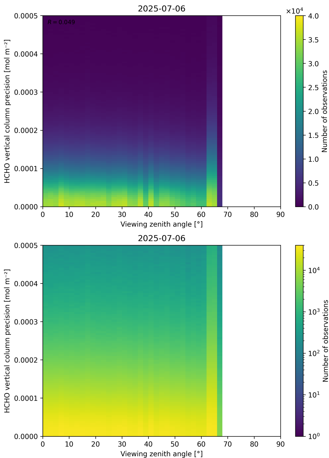
Figure 194: Scatter density plot of “Viewing zenith angle” against “HCHO vertical column precision” for 2025-07-05 to 2025-07-07.
