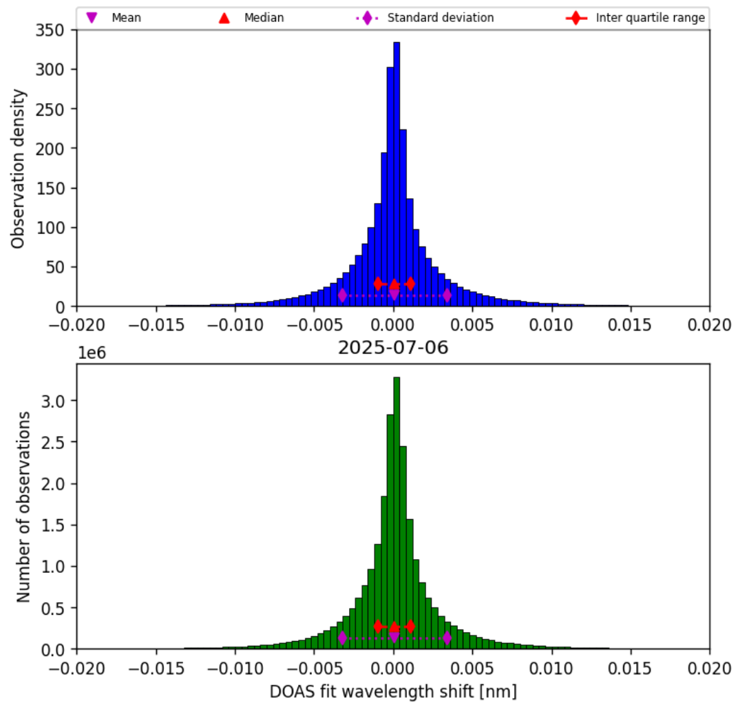
Figure 44: Histogram of “DOAS fit wavelength shift” for 2025-07-05 to 2025-07-07
