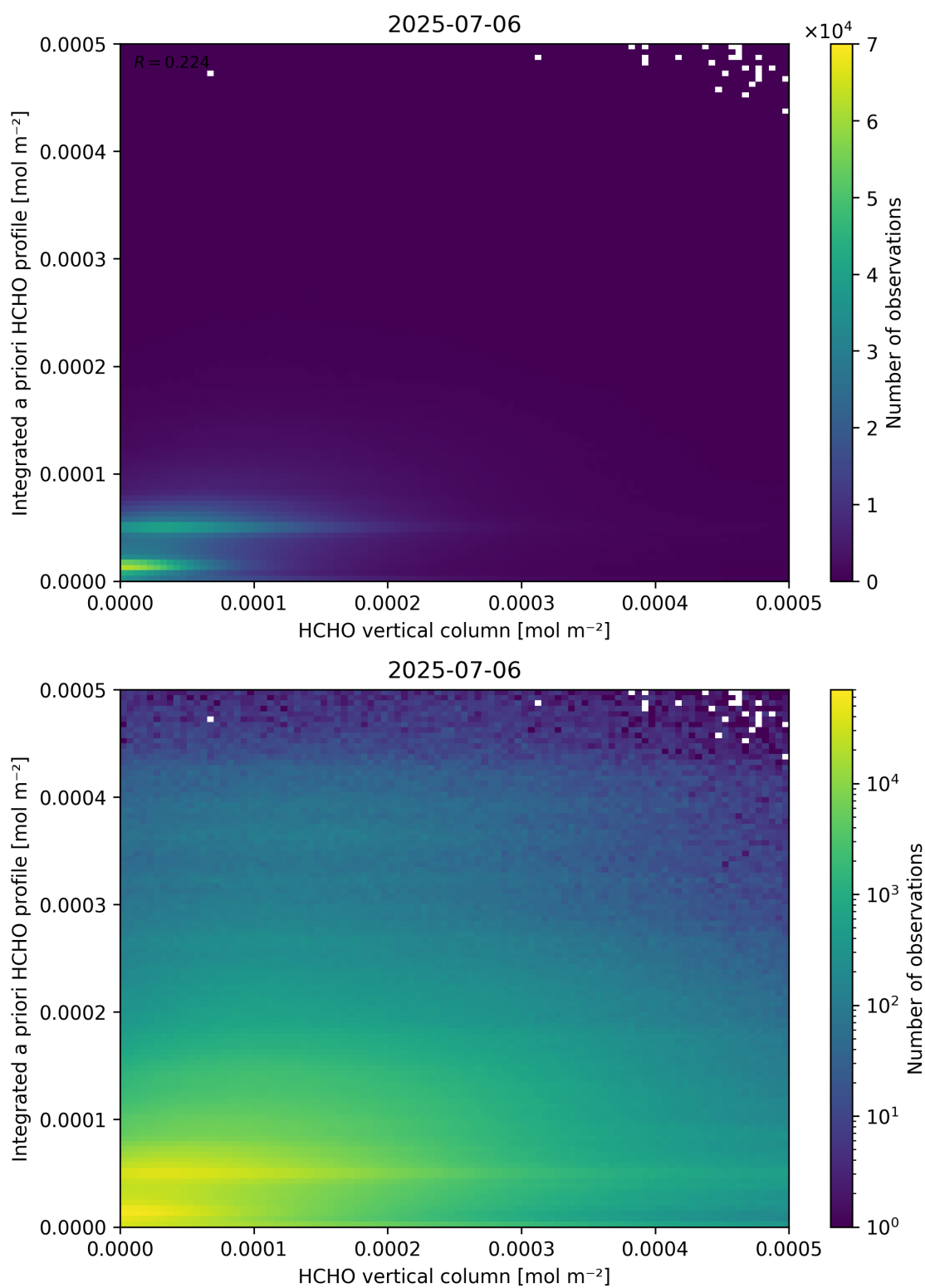
Figure 135: Scatter density plot of “HCHO vertical column” against “Integrated a priori HCHO profile” for 2025-07-05 to 2025-07-07.
