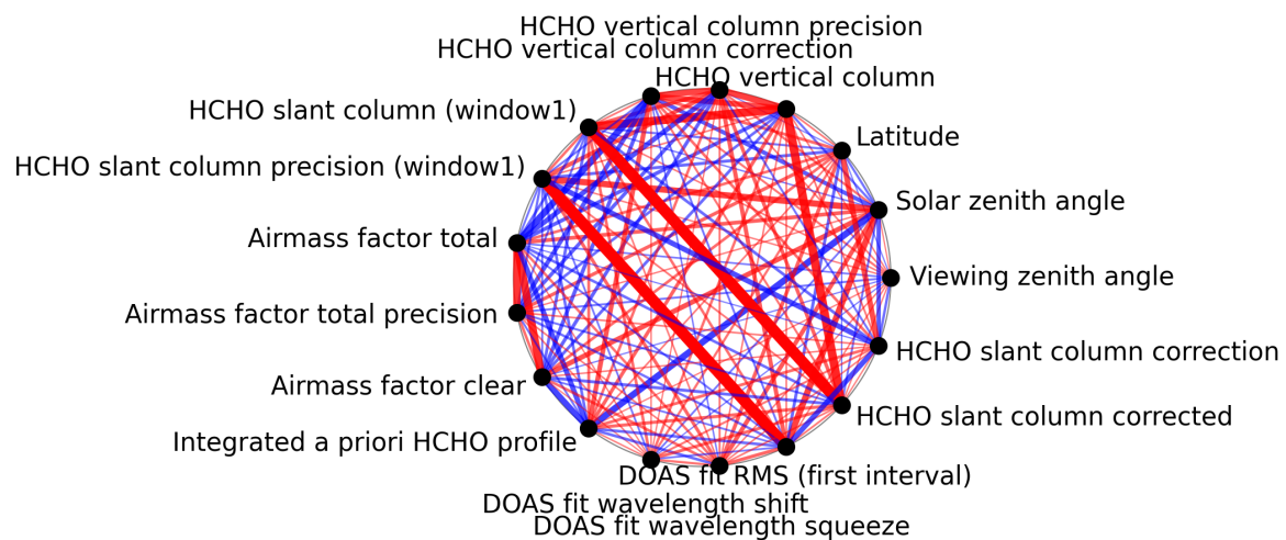
Figure 1: Map of correlation graph for 2025-07-05 to 2025-07-07.
