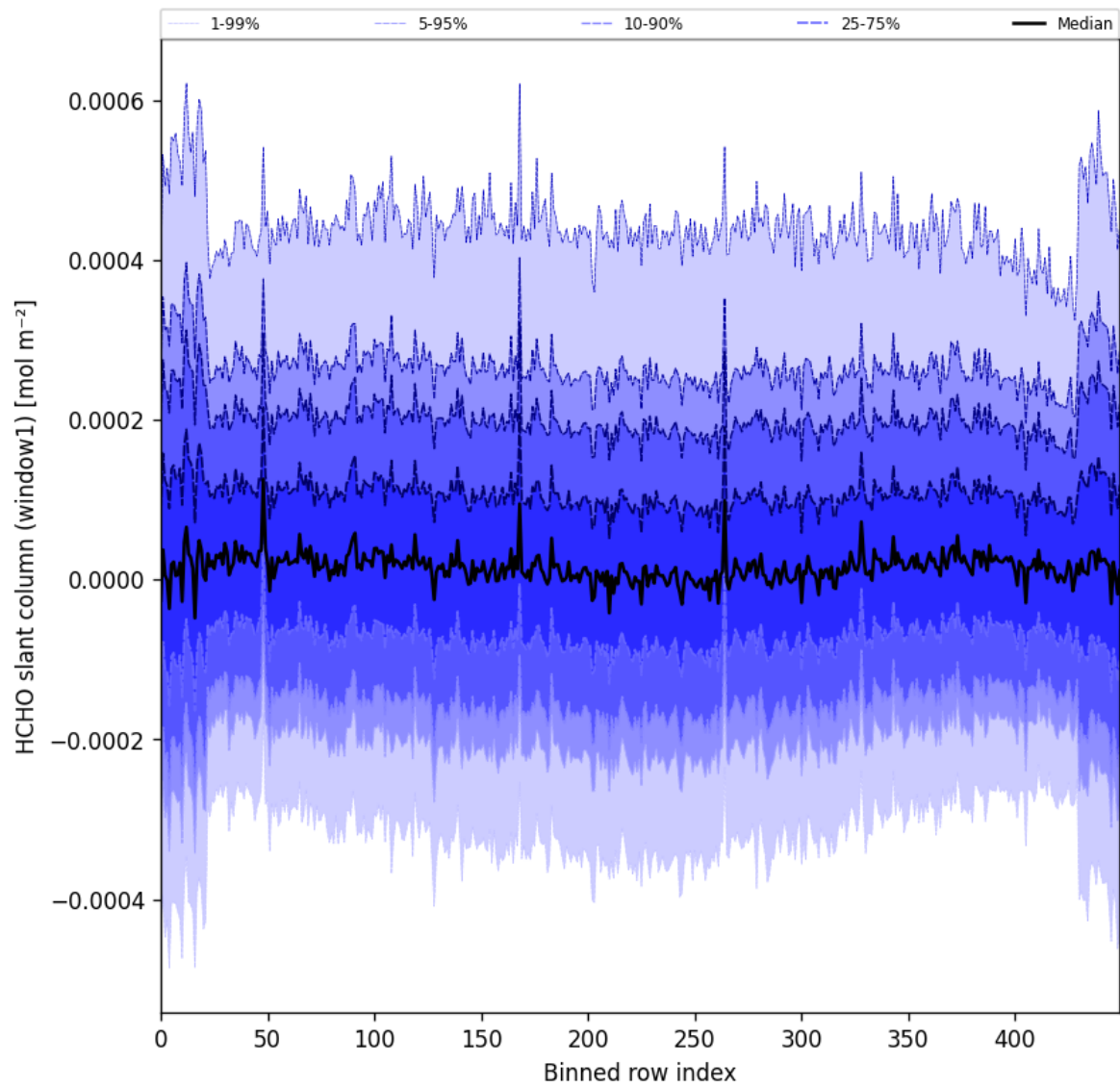
Figure 52: Along track statistics of “HCHO slant column (window1)” for 2025-07-05 to 2025-07-07
