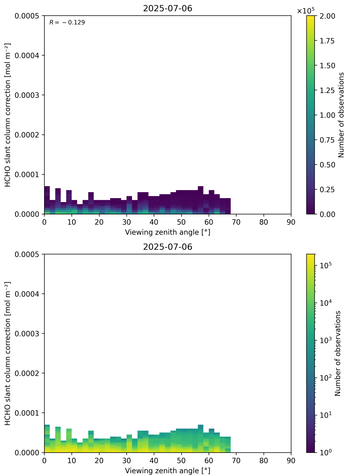
Figure 187: Scatter density plot of “Viewing zenith angle” against “HCHO slant column correction” for 2025-07-05 to 2025-07-07.
