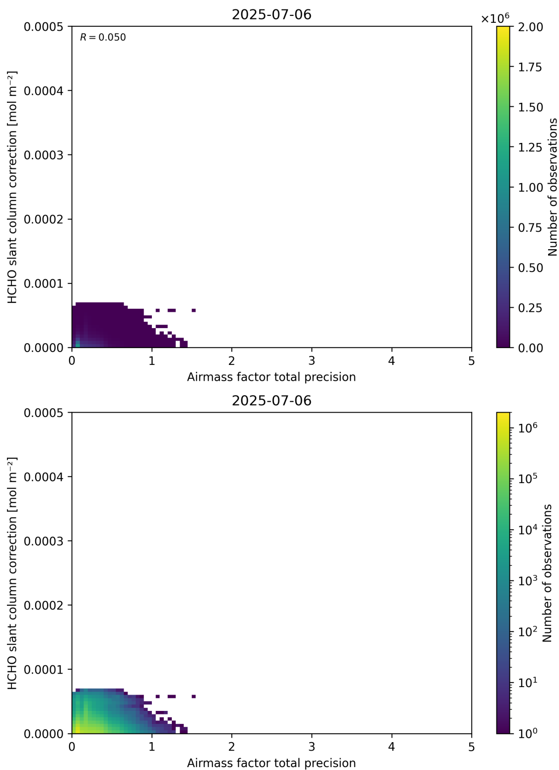
Figure 110: Scatter density plot of “Airmass factor total precision” against “HCHO slant column correction” for 2025-07-05 to 2025-07-07.
