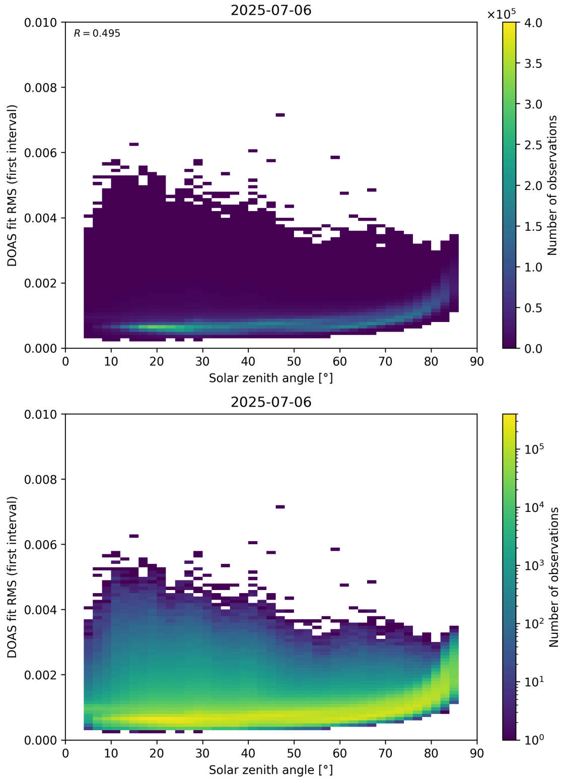
Figure 167: Scatter density plot of “Solar zenith angle” against “DOAS fit RMS (first interval)” for 2025-07-05 to 2025-07-07.
