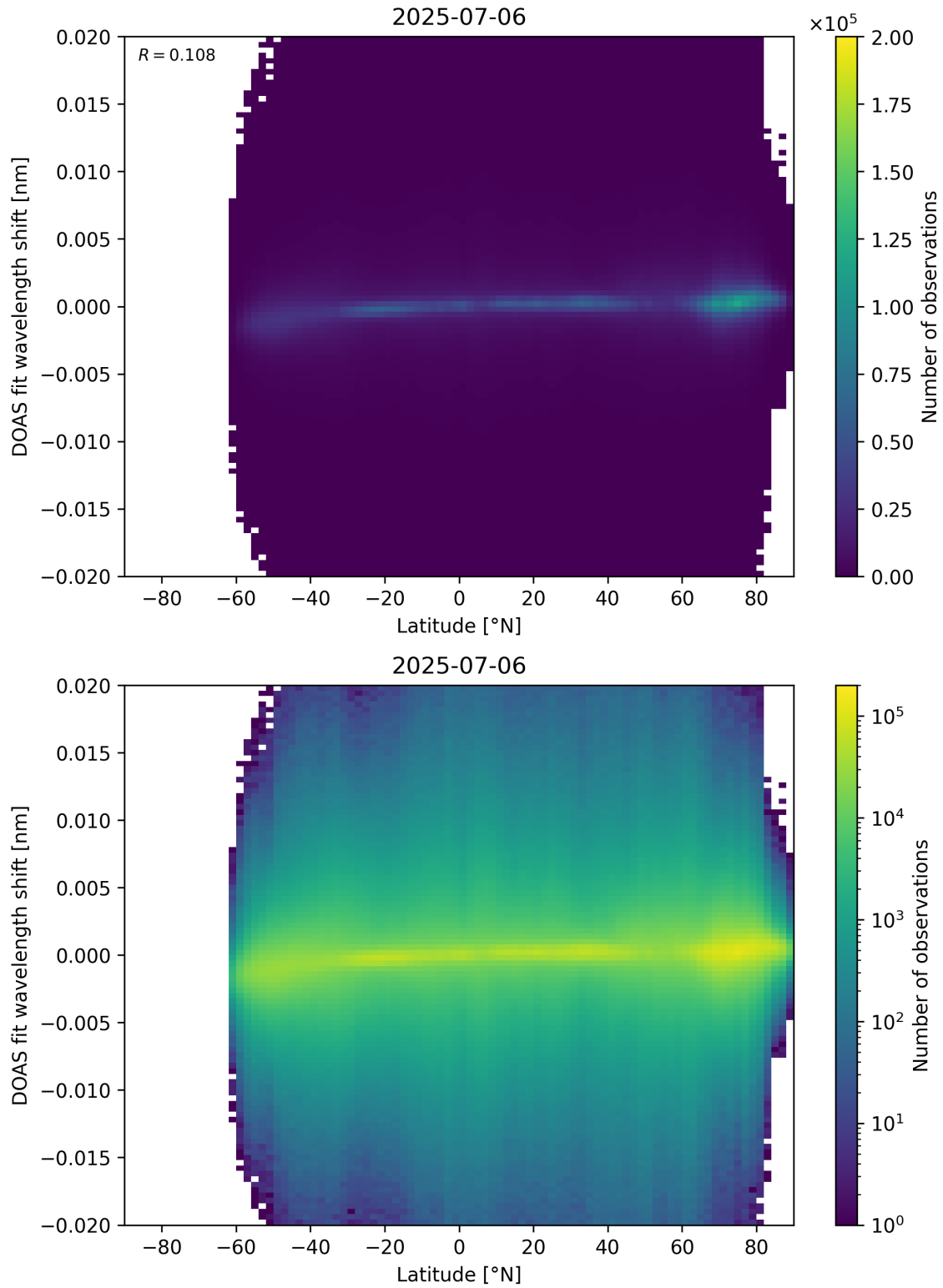
Figure 154: Scatter density plot of “Latitude” against “DOAS fit wavelength shift” for 2025-07-05 to 2025-07-07.
