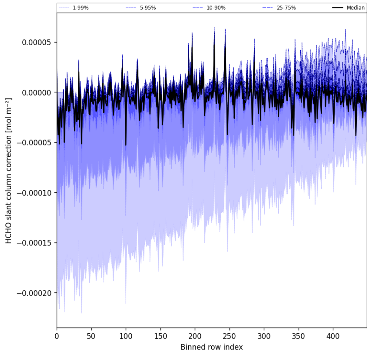
Figure 61: Along track statistics of “HCHO slant column correction” for 2025-07-05 to 2025-07-07
