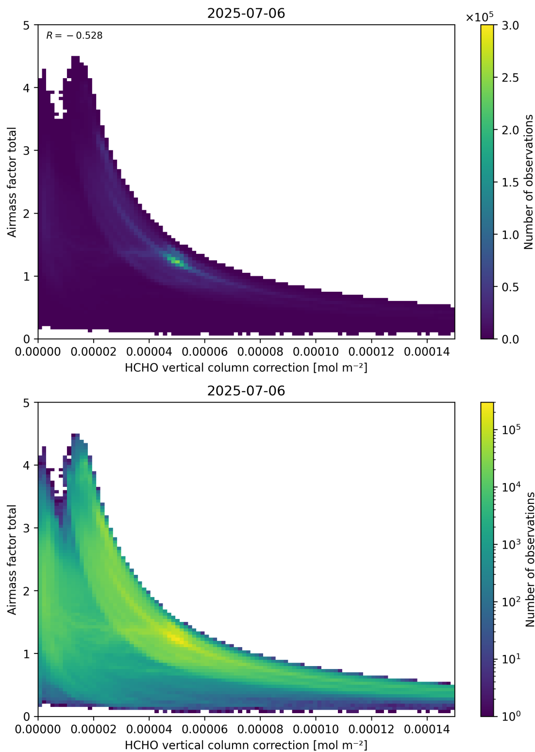
Figure 120: Scatter density plot of “HCHO vertical column correction” against “Airmass factor total” for 2025-07-05 to 2025-07-07.
