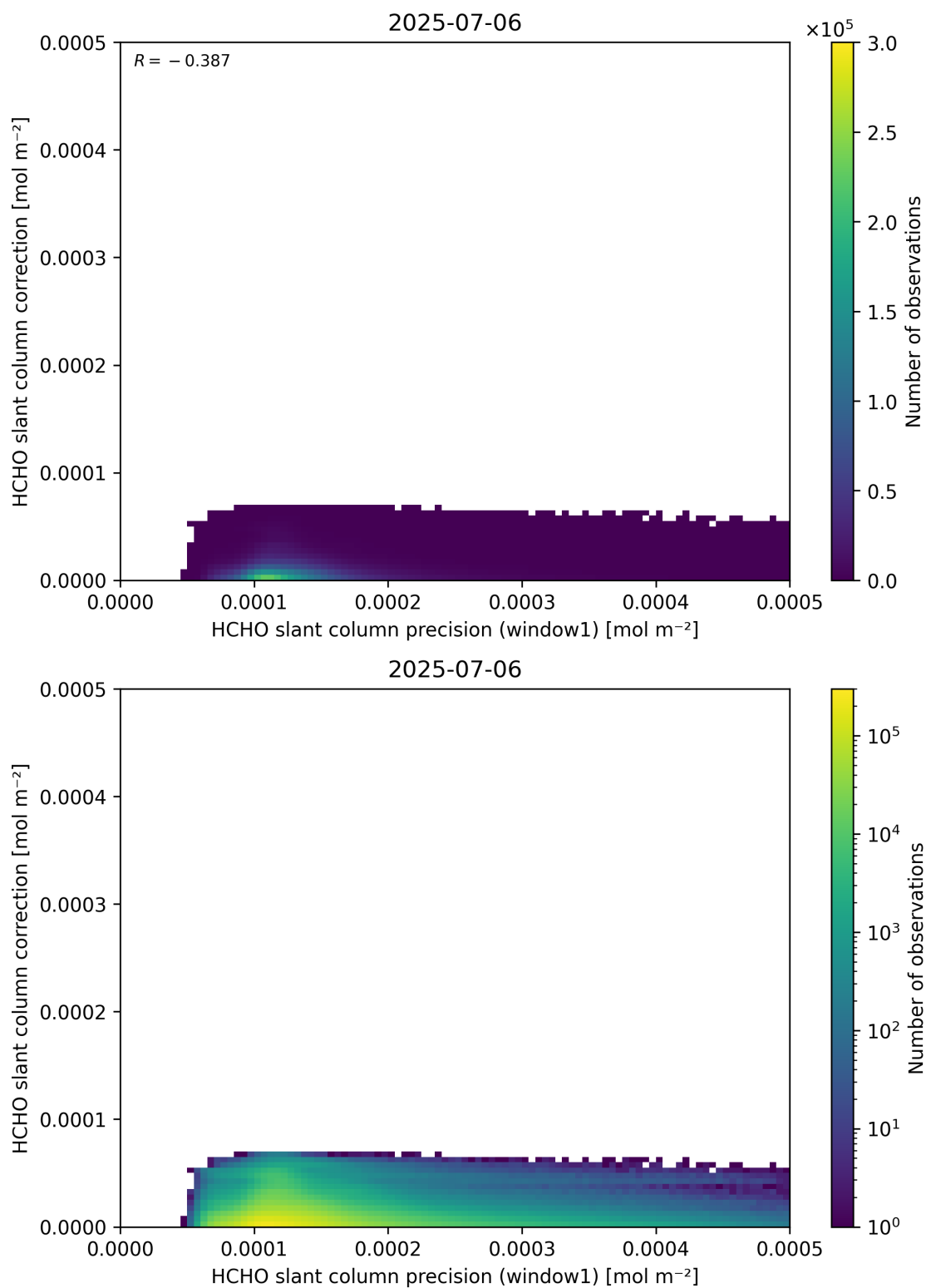
Figure 93: Scatter density plot of “HCHO slant column precision (window1)” against “HCHO slant column correction” for 2025-07-05 to 2025-07-07.
