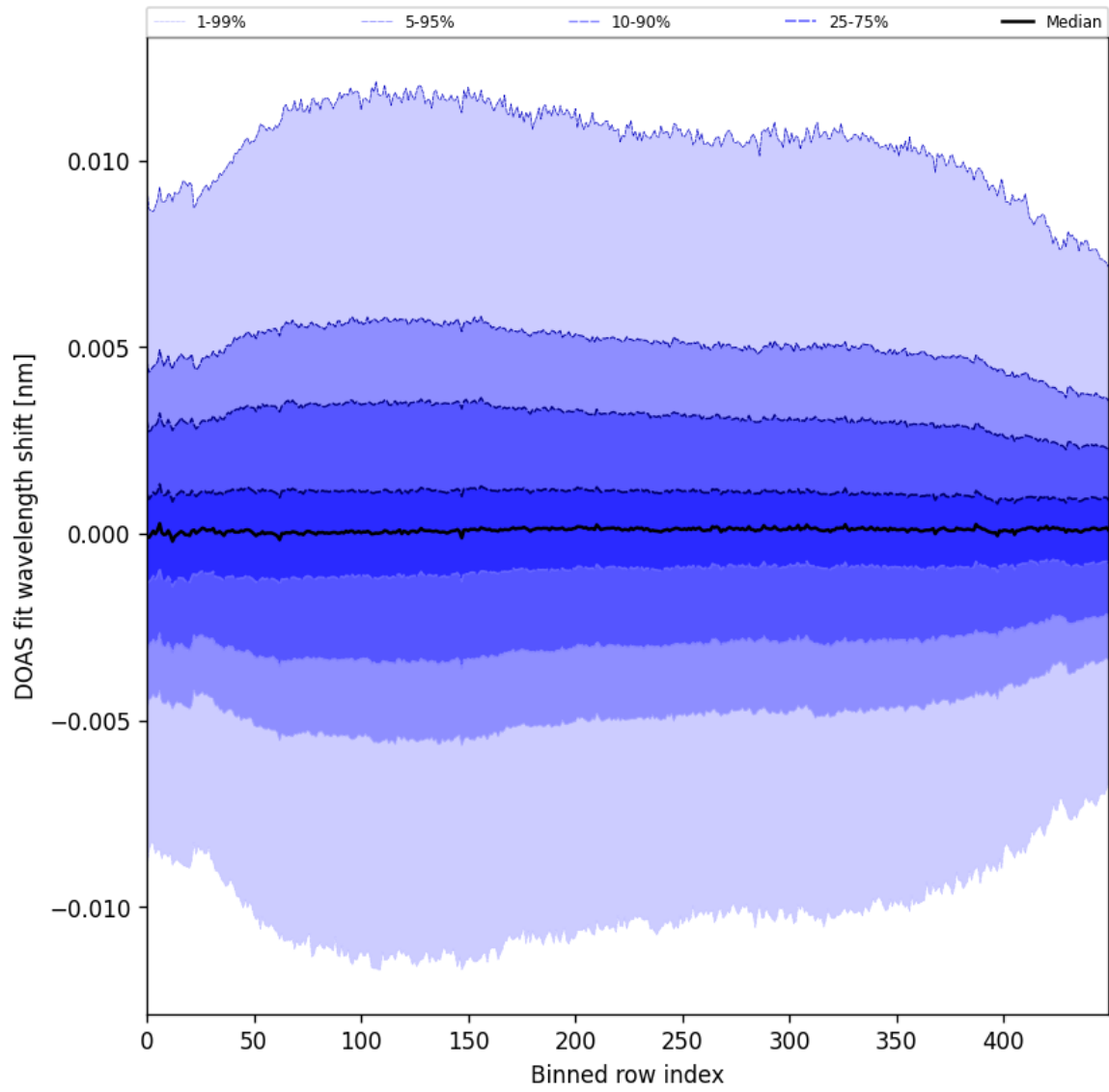
Figure 58: Along track statistics of “DOAS fit wavelength shift” for 2025-07-05 to 2025-07-07
