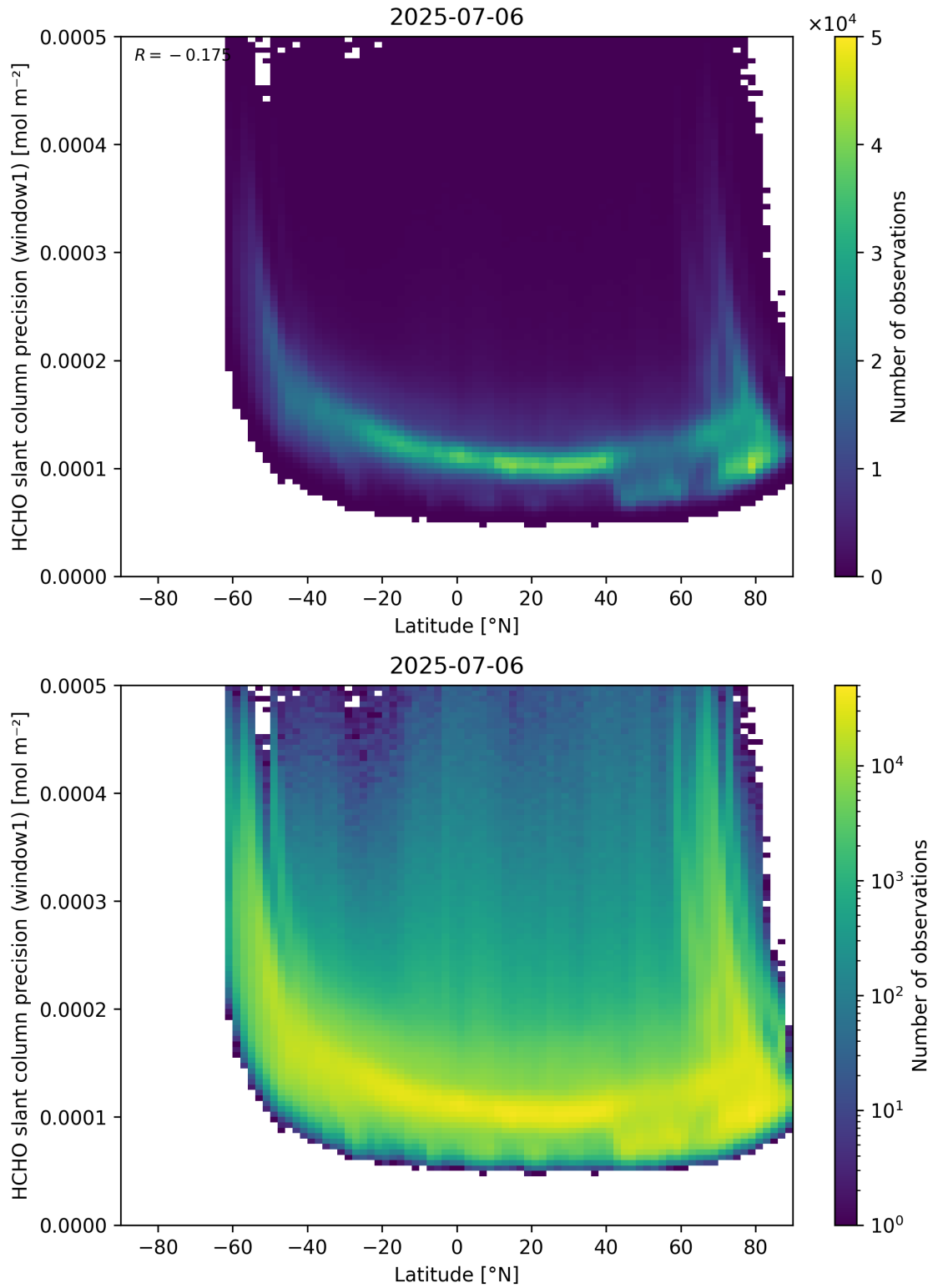
Figure 160: Scatter density plot of “Latitude” against “HCHO slant column precision (window1)” for 2025-07-05 to 2025-07-07.
