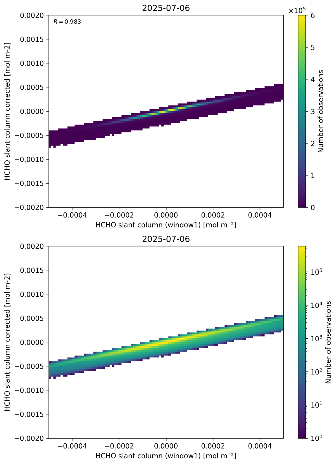
Figure 82: Scatter density plot of “HCHO slant column (window1)” against “HCHO slant column corrected” for 2025-07-05 to 2025-07-07.
