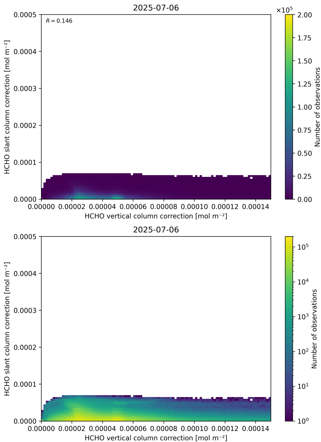
Figure 117: Scatter density plot of “HCHO vertical column correction” against “HCHO slant column correction” for 2025-07-05 to 2025-07-07.
