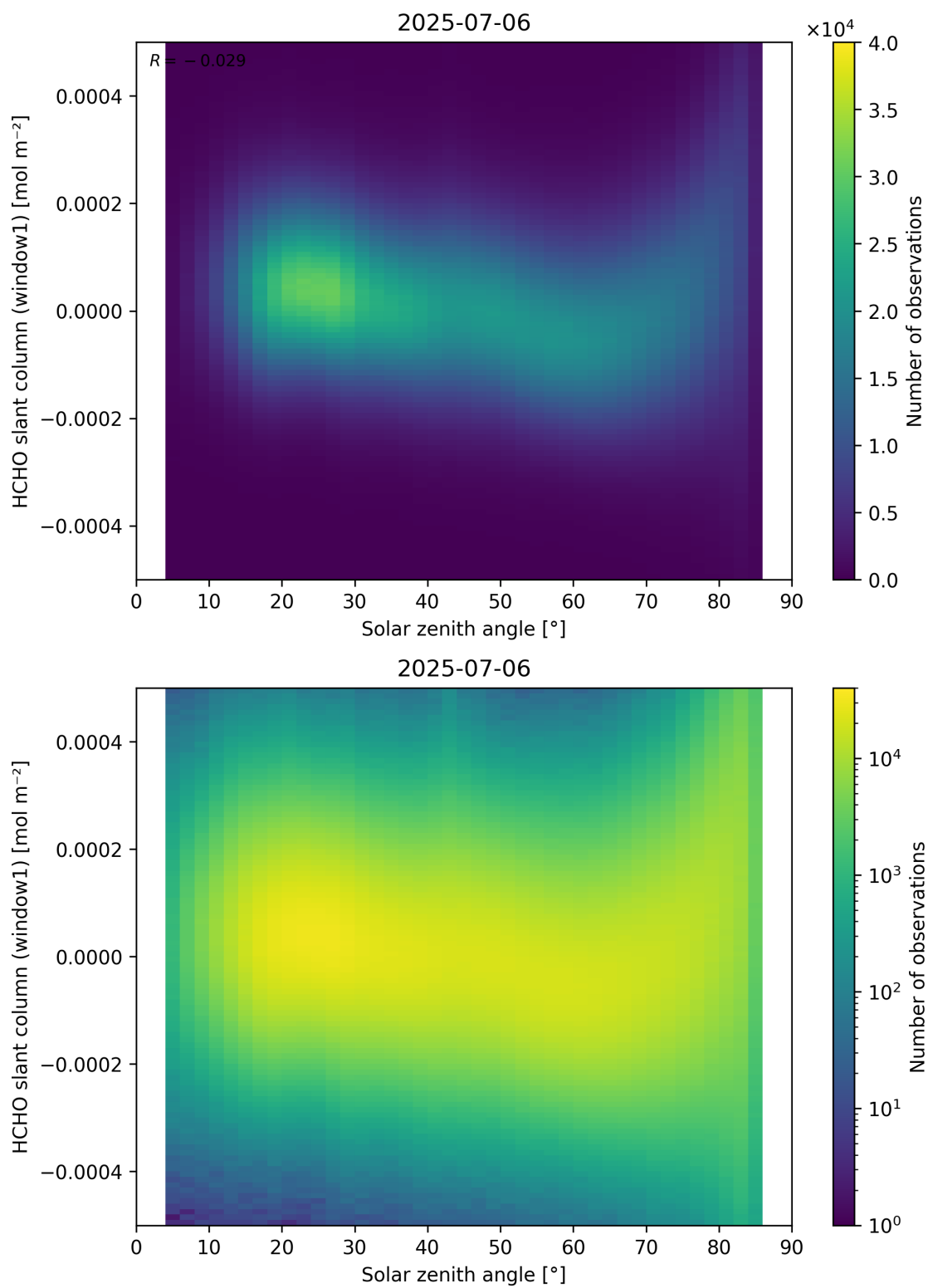
Figure 173: Scatter density plot of “Solar zenith angle” against “HCHO slant column (window1)” for 2025-07-05 to 2025-07-07.
