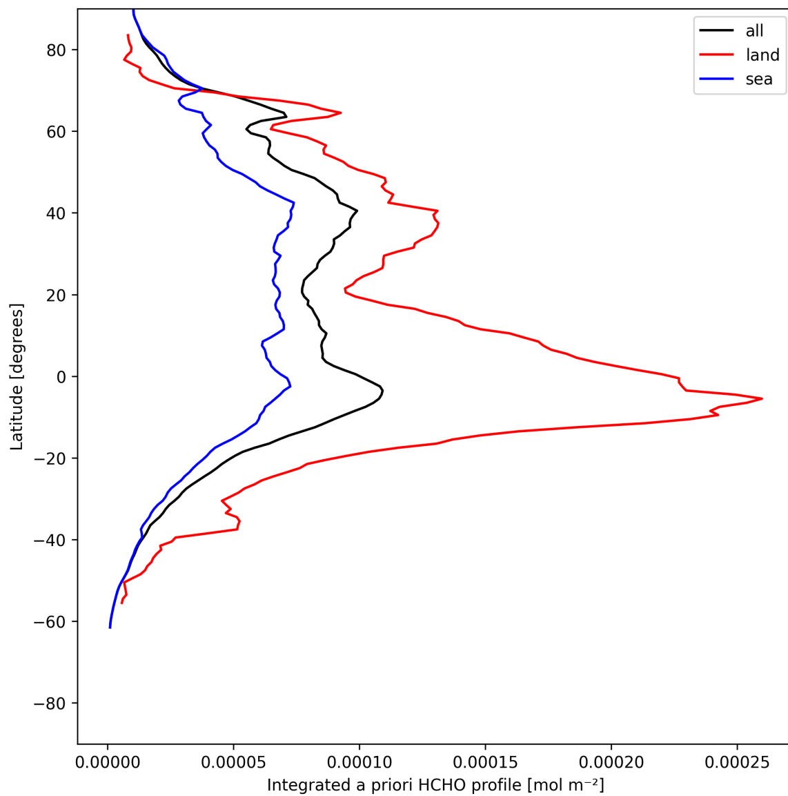
Figure 29: Zonal average of “Integrated a priori HCHO profile” for 2025-07-05 to 2025-07-07.
