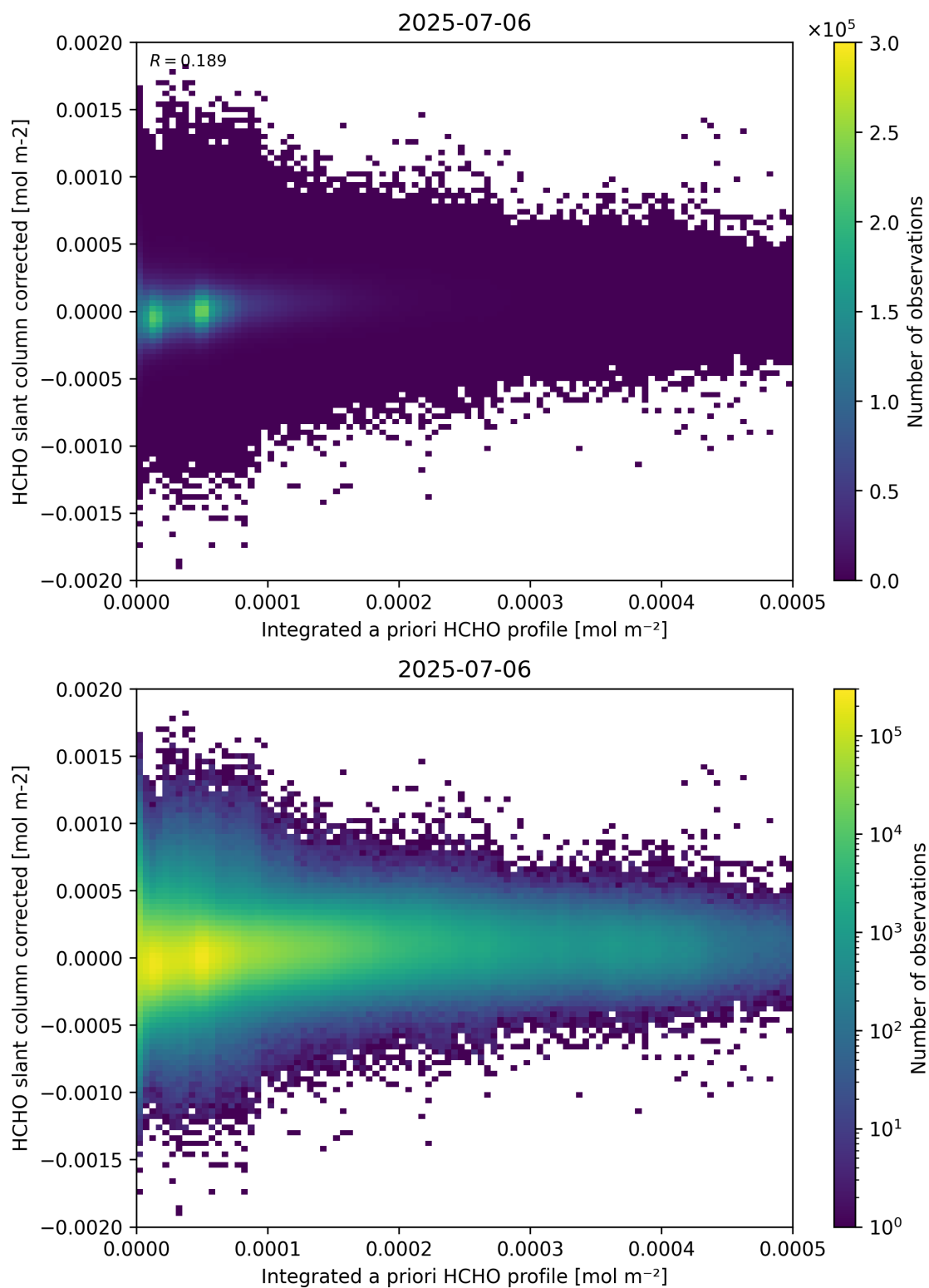
Figure 151: Scatter density plot of “Integrated a priori HCHO profile” against “HCHO slant column corrected” for 2025-07-05 to 2025-07-07.
