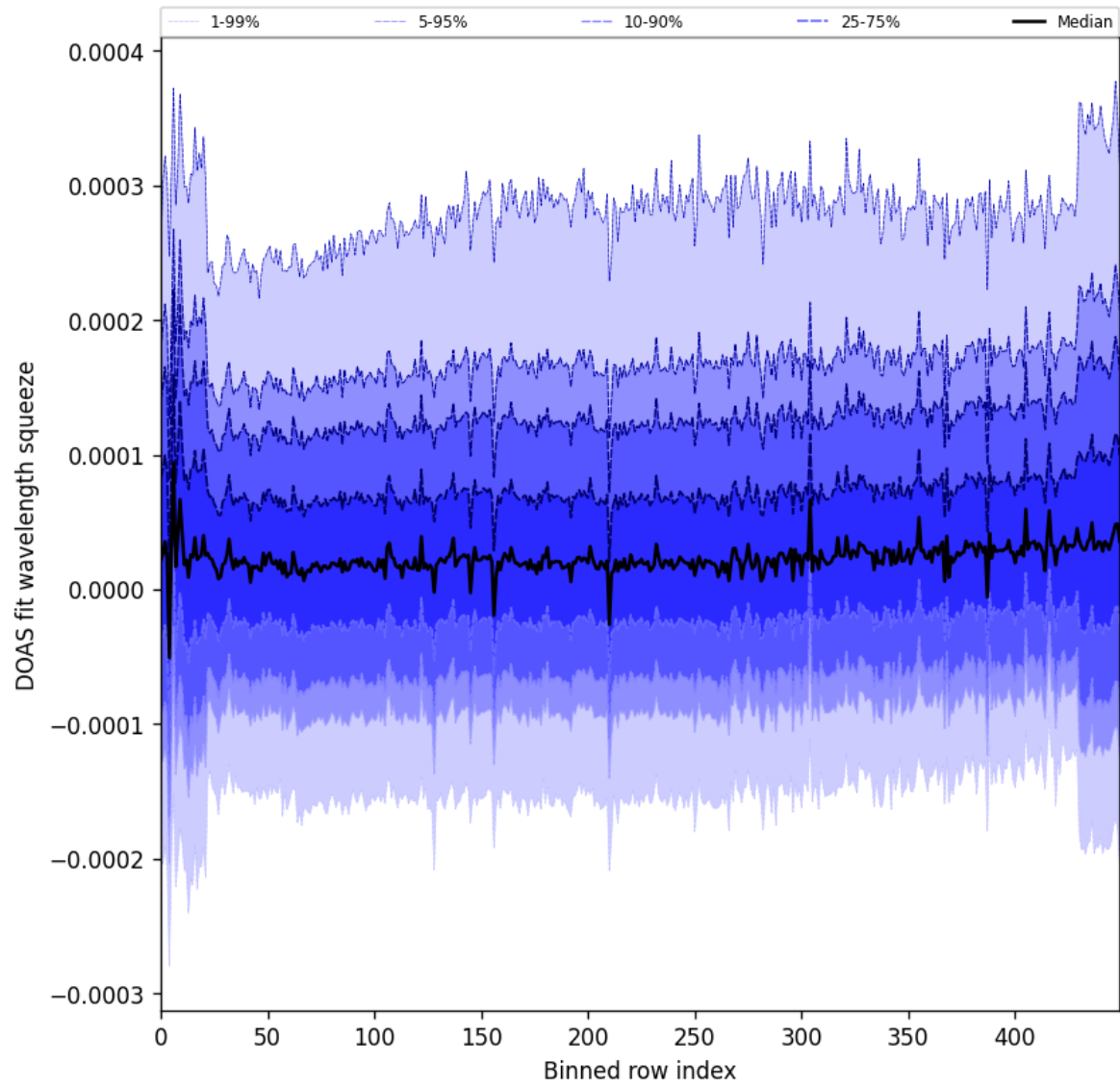
Figure 59: Along track statistics of “DOAS fit wavelength squeeze” for 2025-07-05 to 2025-07-07
