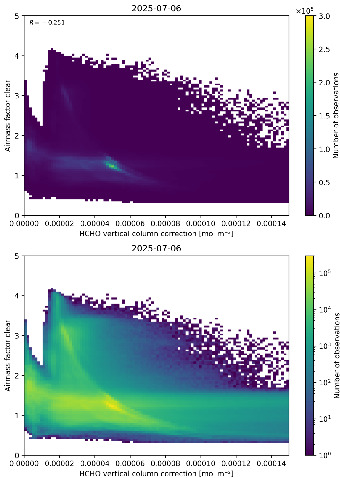
Figure 115: Scatter density plot of “HCHO vertical column correction” against “Airmass factor clear” for 2025-07-05 to 2025-07-07.
