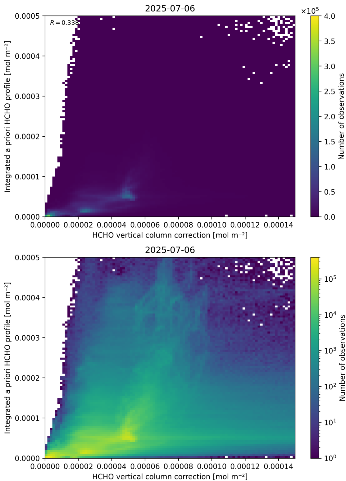
Figure 122: Scatter density plot of “HCHO vertical column correction” against “Integrated a priori HCHO profile” for 2025-07-05 to 2025-07-07.
