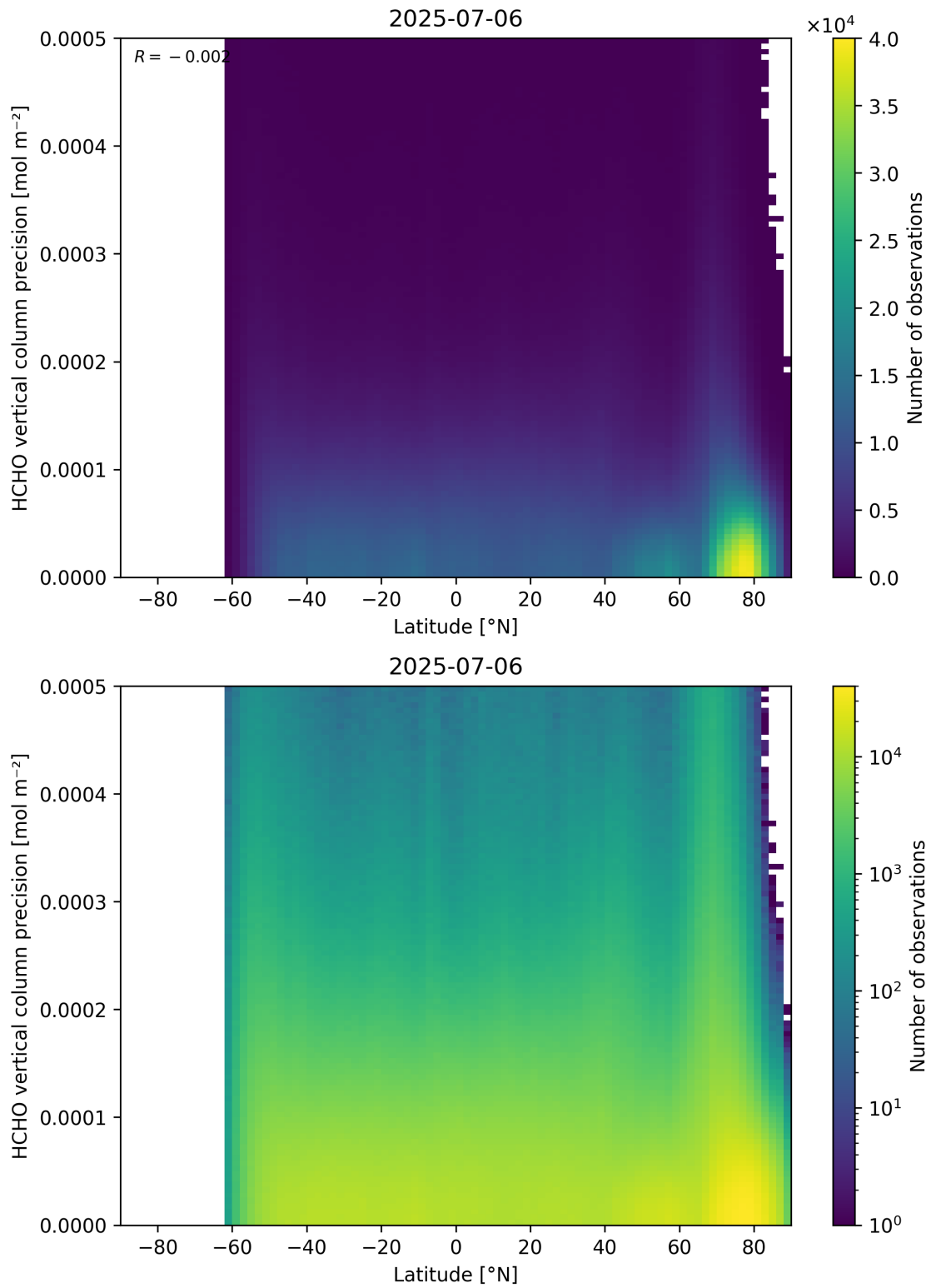
Figure 165: Scatter density plot of “Latitude” against “HCHO vertical column precision” for 2025-07-05 to 2025-07-07.
