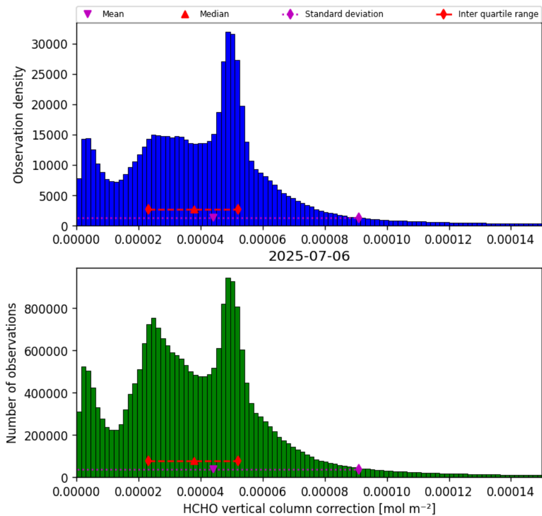
Figure 37: Histogram of “HCHO vertical column correction” for 2025-07-05 to 2025-07-07
