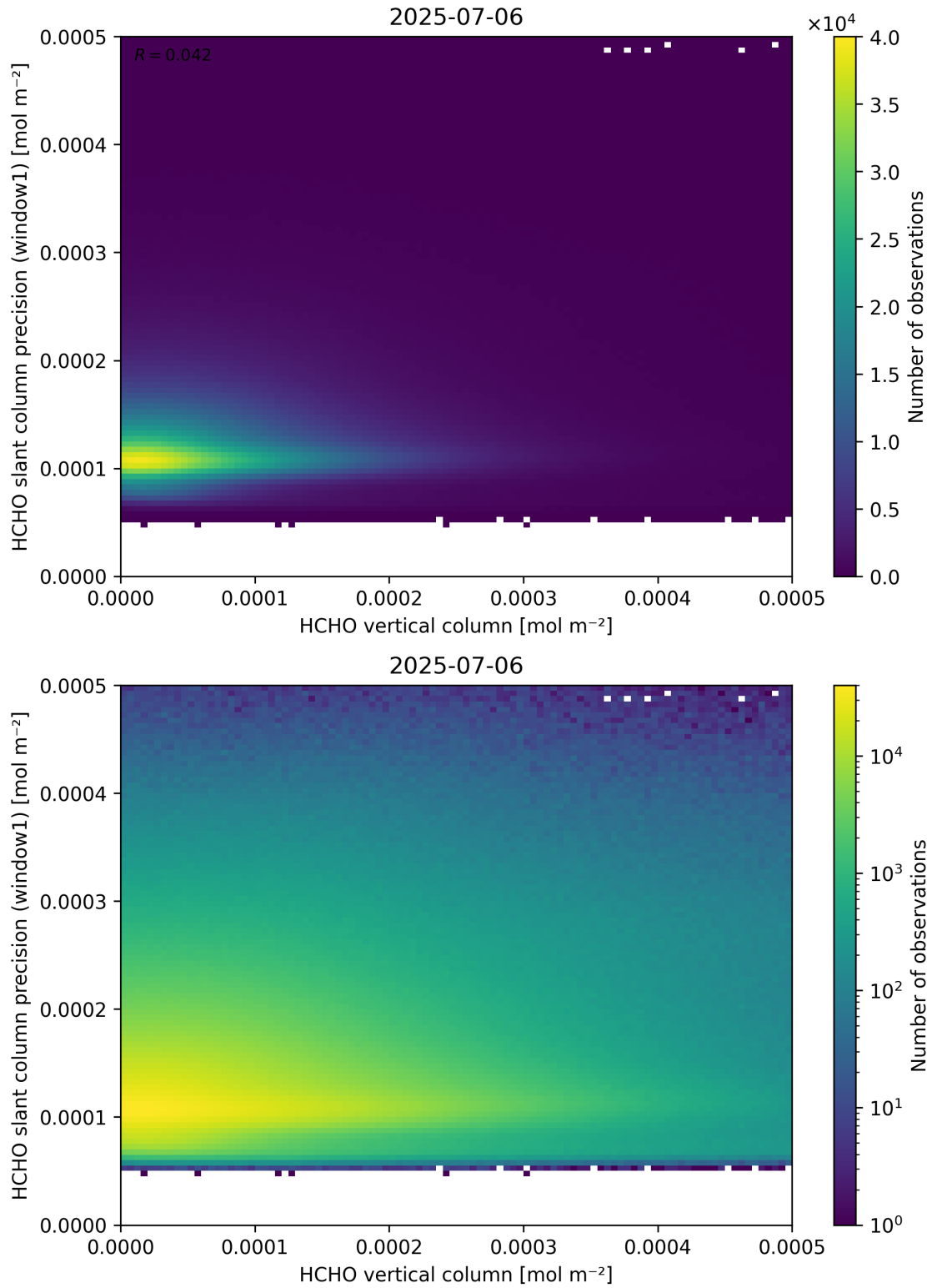
Figure 130: Scatter density plot of “HCHO vertical column” against “HCHO slant column precision (window1)” for 2025-07-05 to 2025-07-07.
