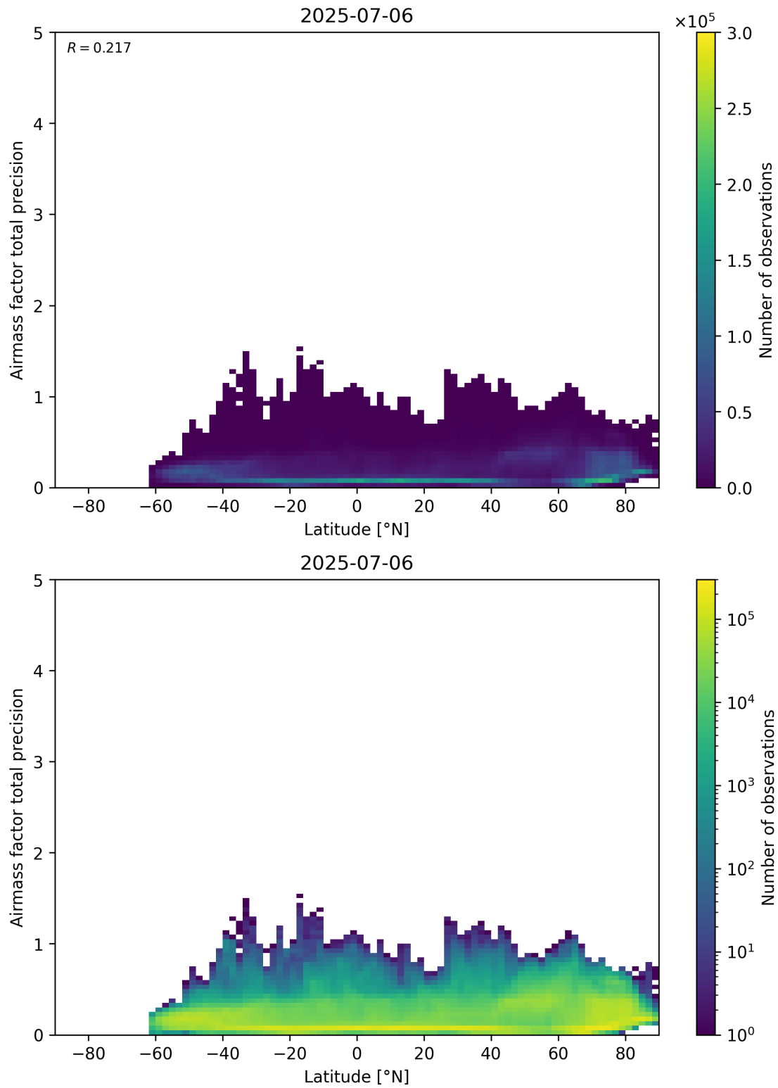
Figure 162: Scatter density plot of “Latitude” against “Airmass factor total precision” for 2025-07-05 to 2025-07-07.
