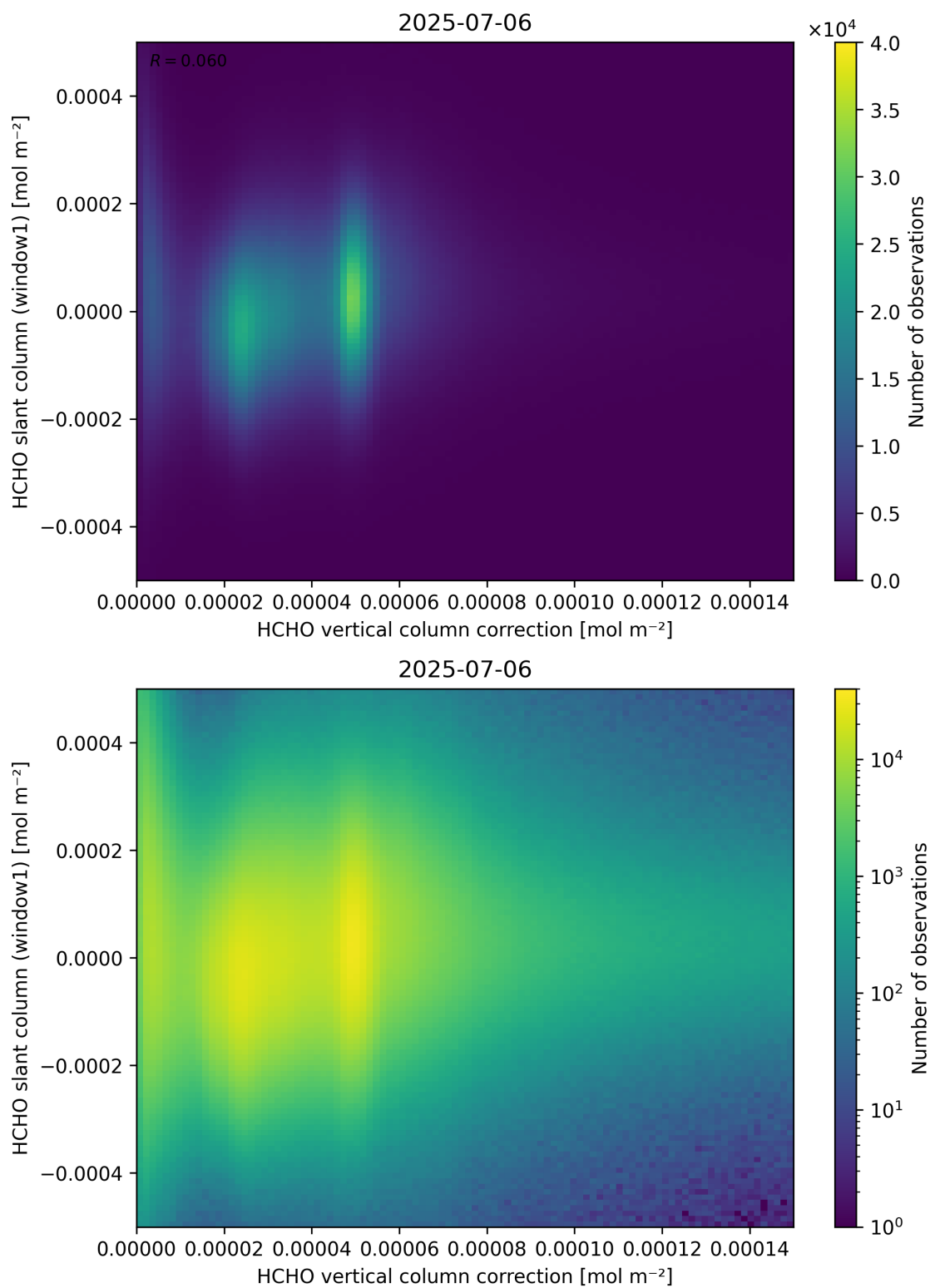
Figure 118: Scatter density plot of “HCHO vertical column correction” against “HCHO slant column (window1)” for 2025-07-05 to 2025-07-07.
