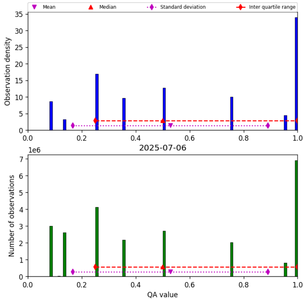
Figure 34: Histogram of “QA value” for 2025-07-05 to 2025-07-07
