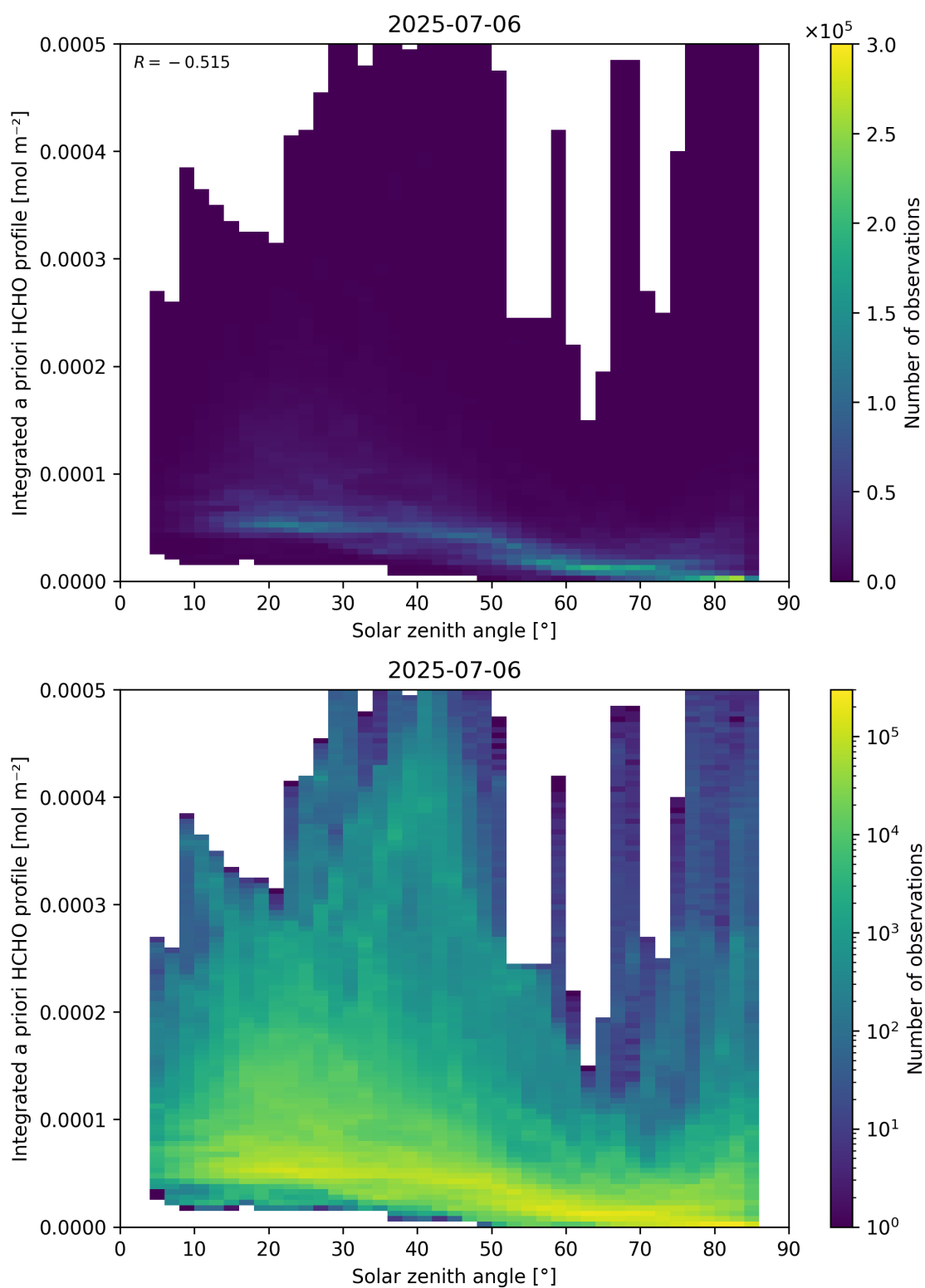
Figure 180: Scatter density plot of “Solar zenith angle” against “Integrated a priori HCHO profile” for 2025-07-05 to 2025-07-07.
