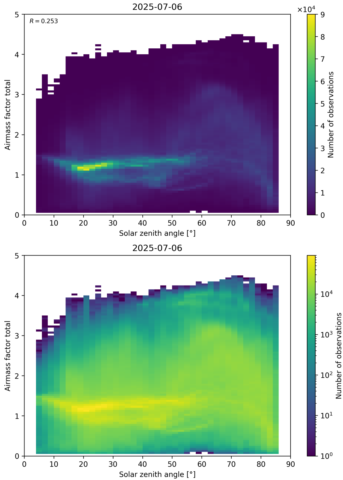
Figure 175: Scatter density plot of “Solar zenith angle” against “Airmass factor total” for 2025-07-05 to 2025-07-07.
