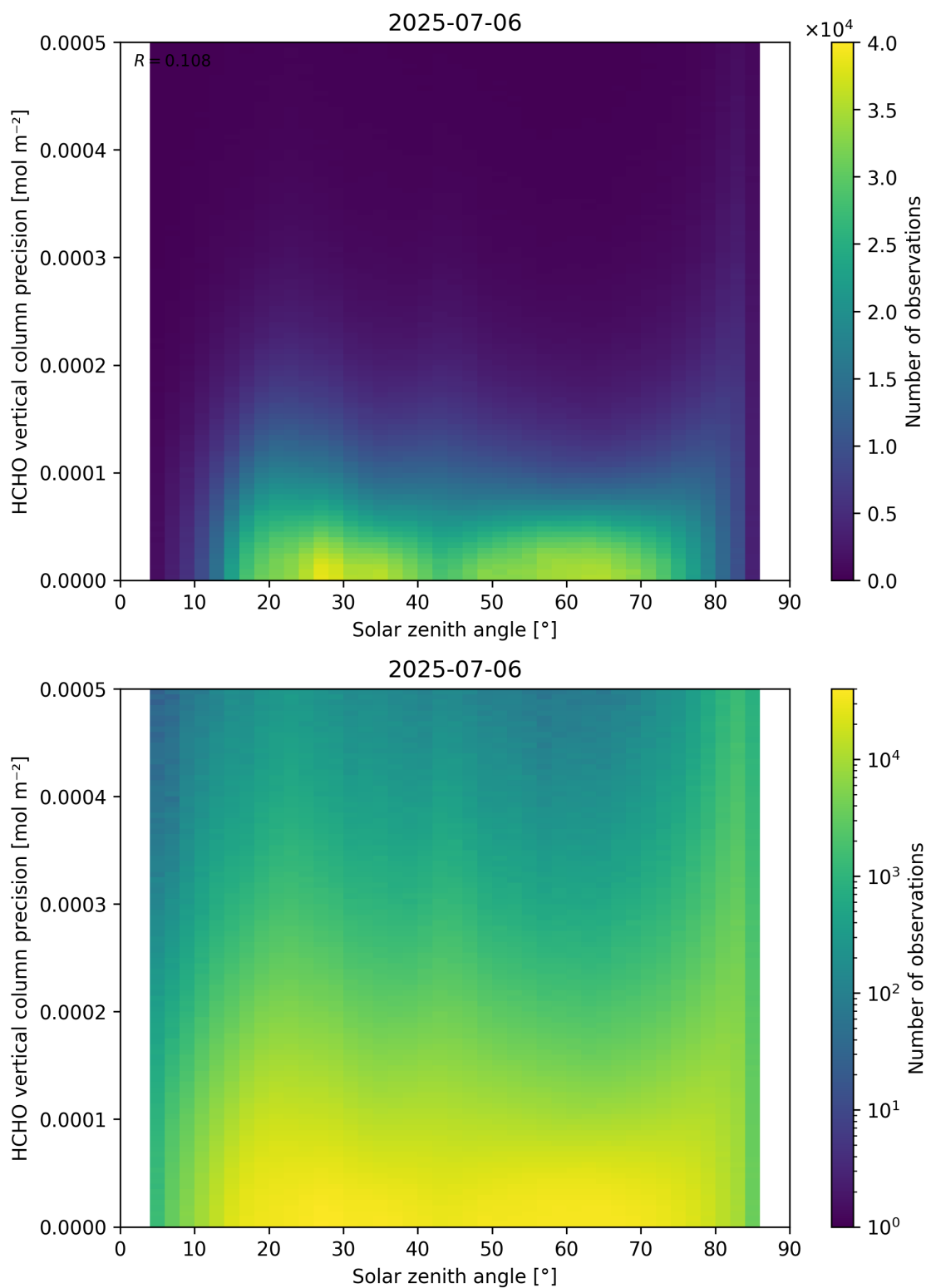
Figure 179: Scatter density plot of “Solar zenith angle” against “HCHO vertical column precision” for 2025-07-05 to 2025-07-07.
