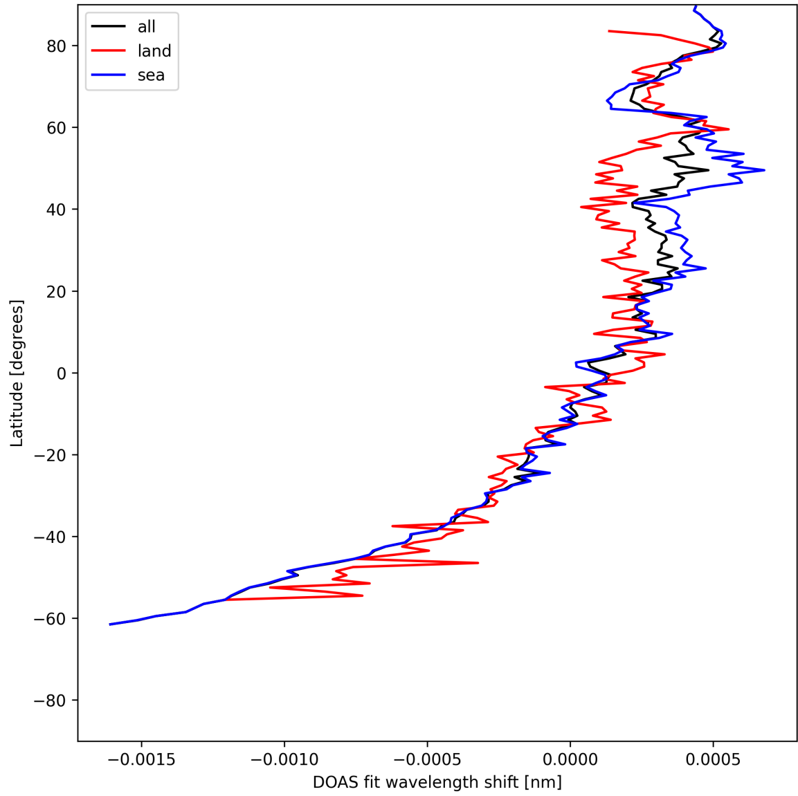
Figure 30: Zonal average of “DOAS fit wavelength shift” for 2025-07-05 to 2025-07-07.
