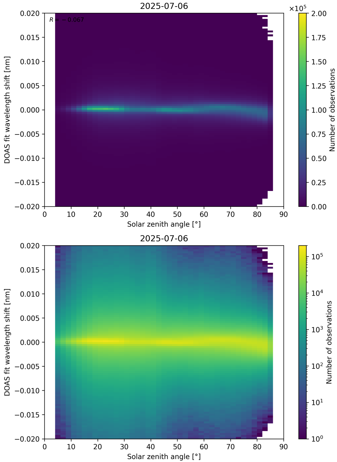
Figure 168: Scatter density plot of “Solar zenith angle” against “DOAS fit wavelength shift” for 2025-07-05 to 2025-07-07.
