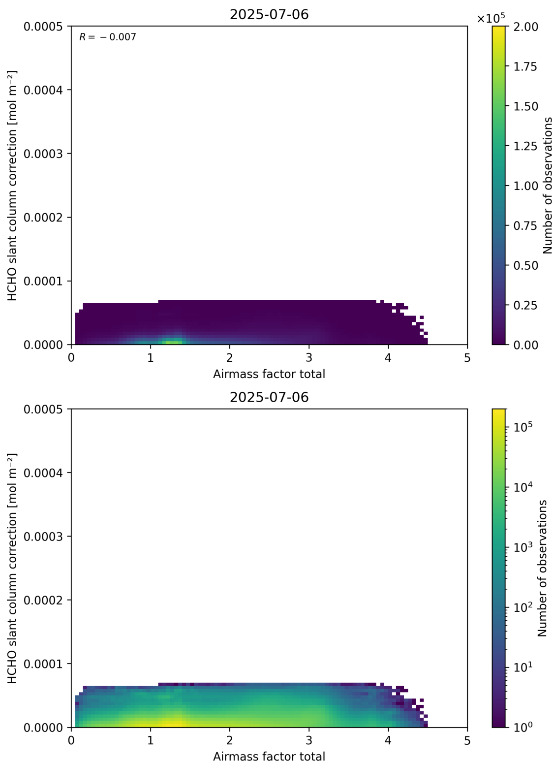
Figure 102: Scatter density plot of “Airmass factor total” against “HCHO slant column correction” for 2025-07-05 to 2025-07-07.
