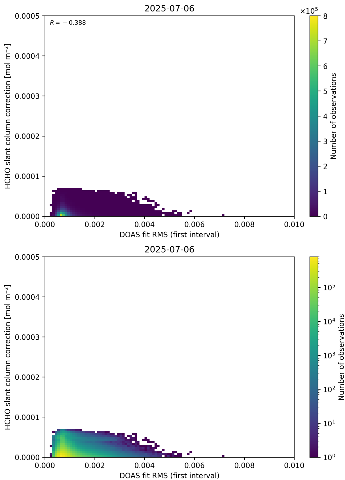
Figure 63: Scatter density plot of “DOAS fit RMS (first interval)” against “HCHO slant column correction” for 2025-07-05 to 2025-07-07.
