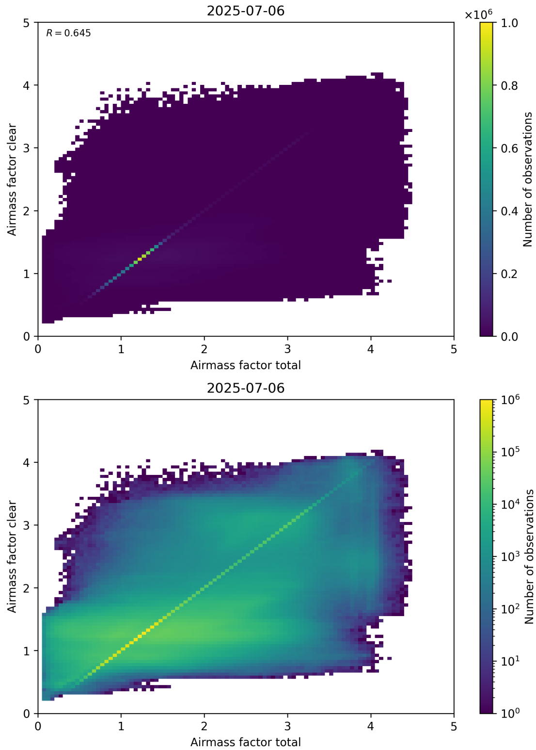
Figure 100: Scatter density plot of “Airmass factor total” against “Airmass factor clear” for 2025-07-05 to 2025-07-07.
