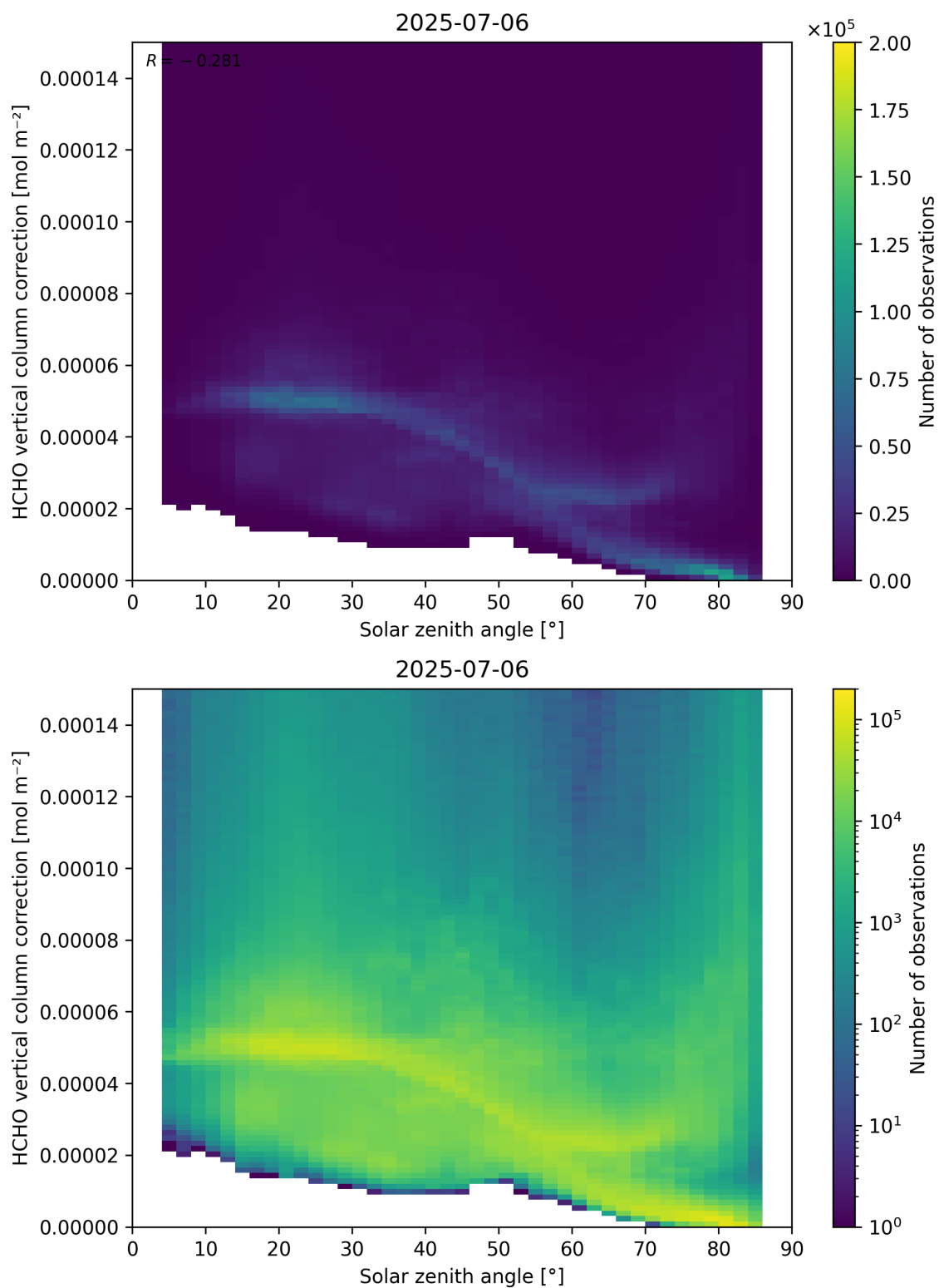
Figure 178: Scatter density plot of “Solar zenith angle” against “HCHO vertical column correction” for 2025-07-05 to 2025-07-07.
