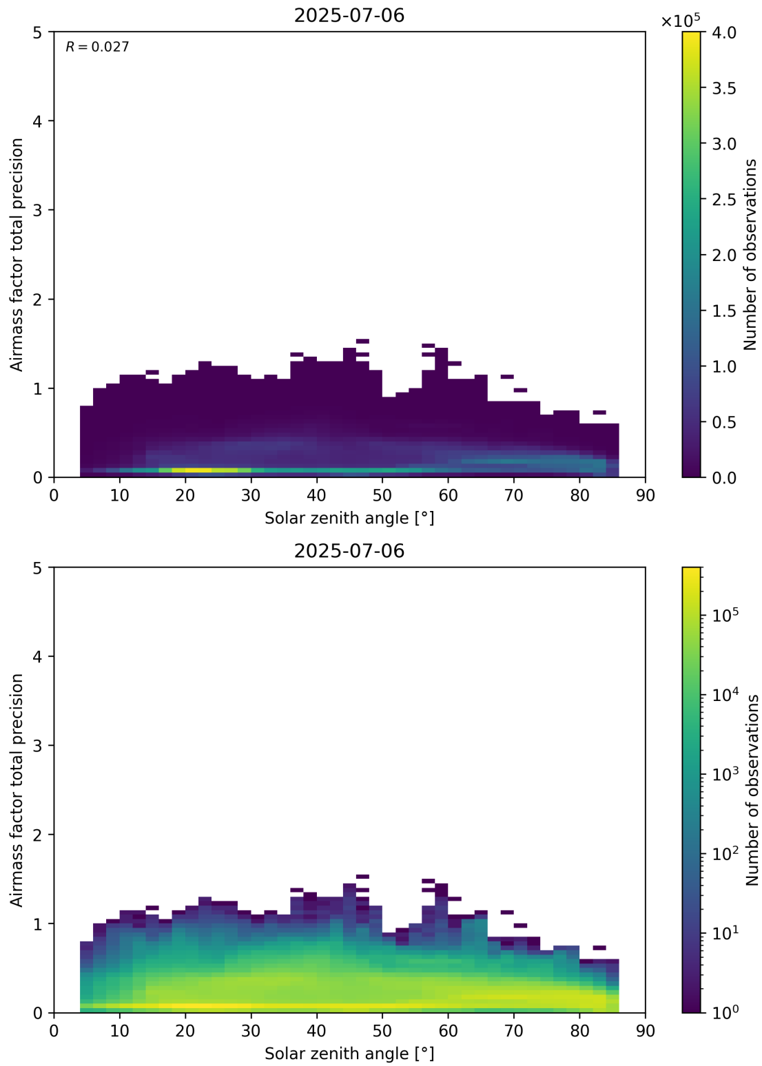
Figure 176: Scatter density plot of “Solar zenith angle” against “Airmass factor total precision” for 2025-07-05 to 2025-07-07.
