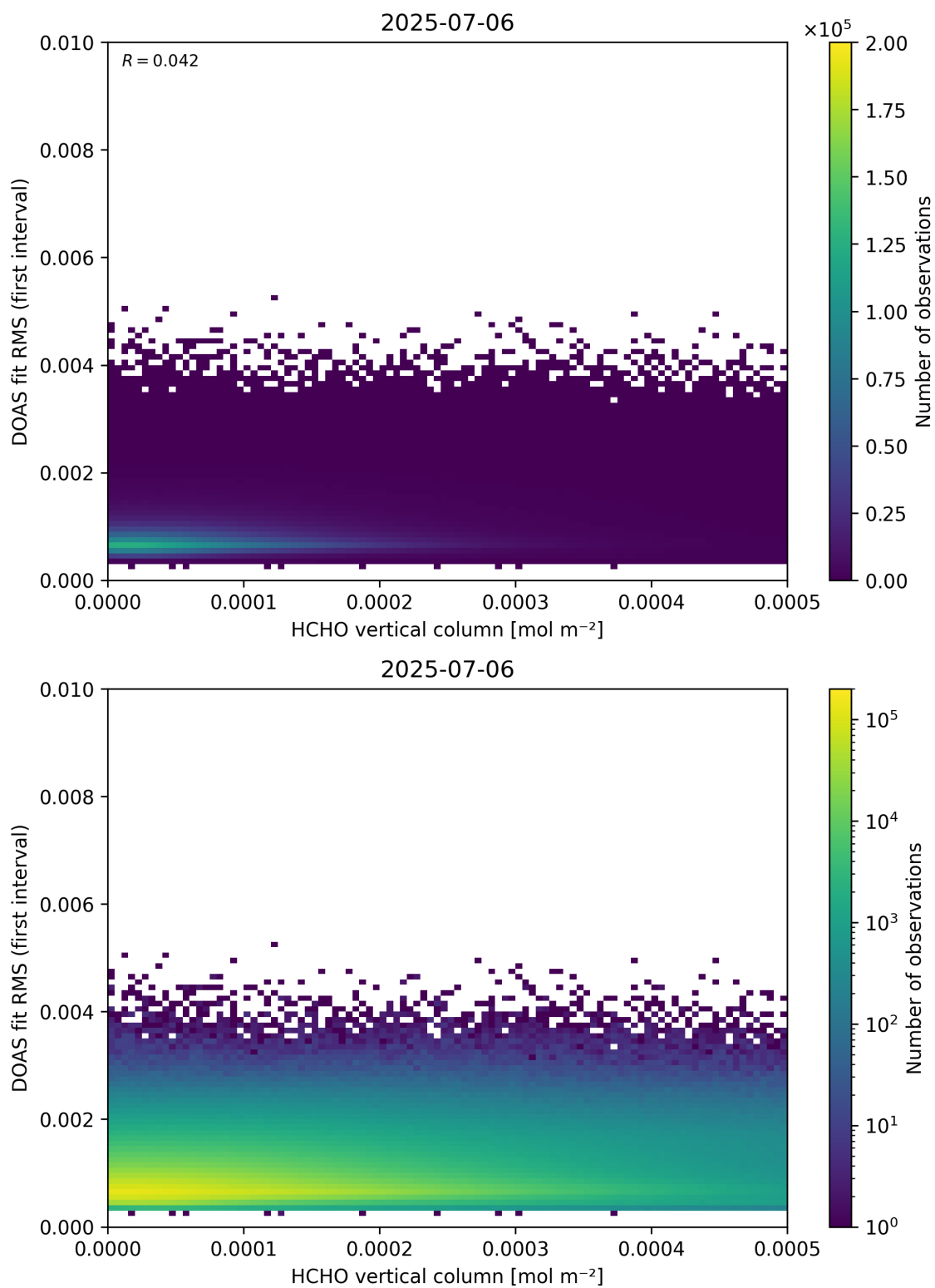
Figure 123: Scatter density plot of “HCHO vertical column” against “DOAS fit RMS (first interval)” for 2025-07-05 to 2025-07-07.
