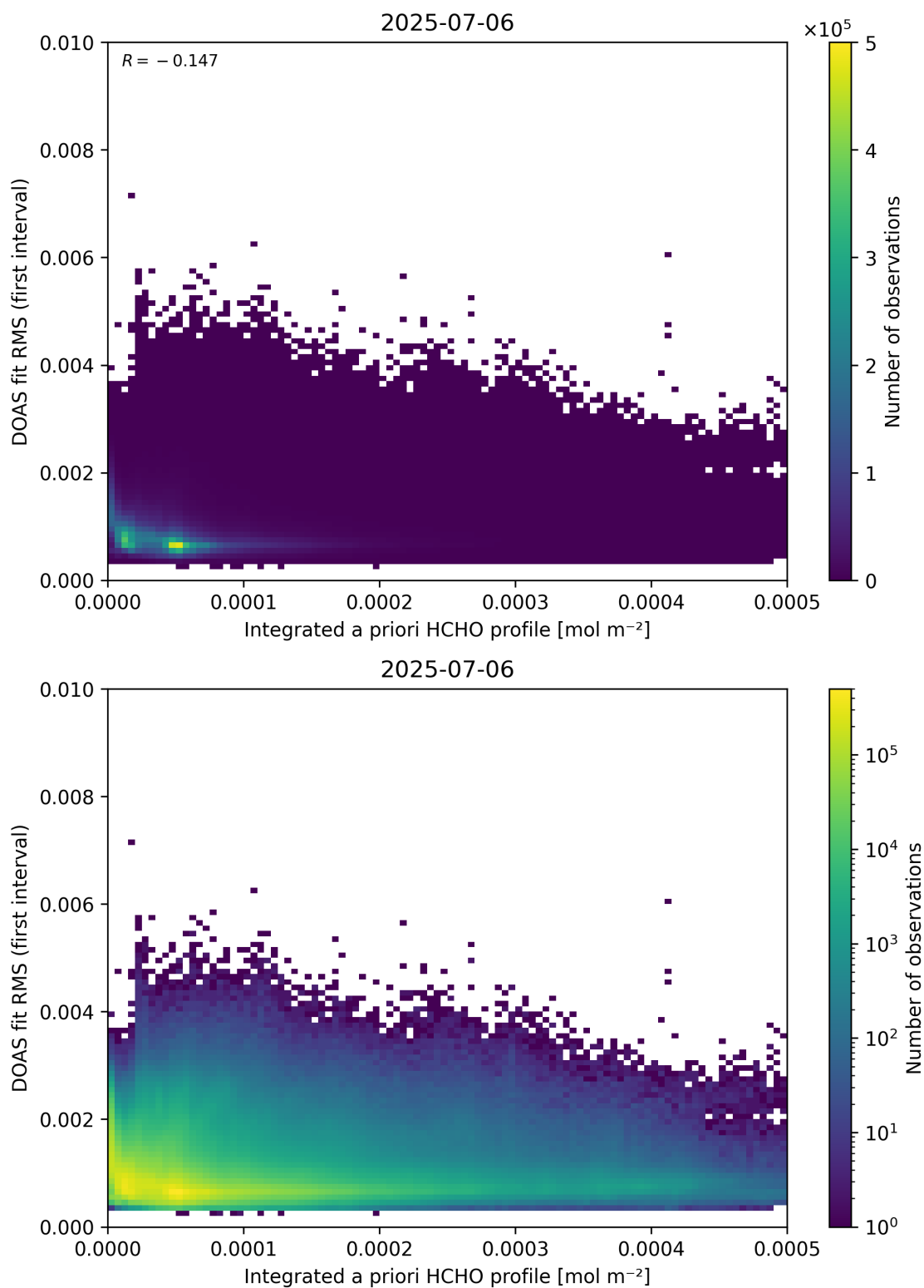
Figure 148: Scatter density plot of “Integrated a priori HCHO profile” against “DOAS fit RMS (first interval)” for 2025-07-05 to 2025-07-07.
