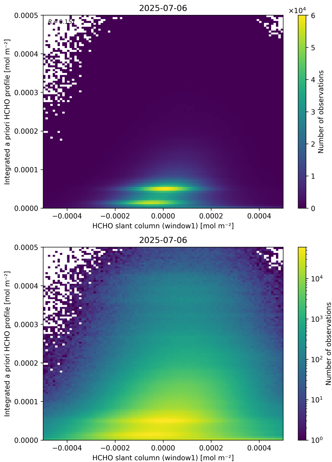
Figure 87: Scatter density plot of “HCHO slant column (window1)” against “Integrated a priori HCHO profile” for 2025-07-05 to 2025-07-07.
