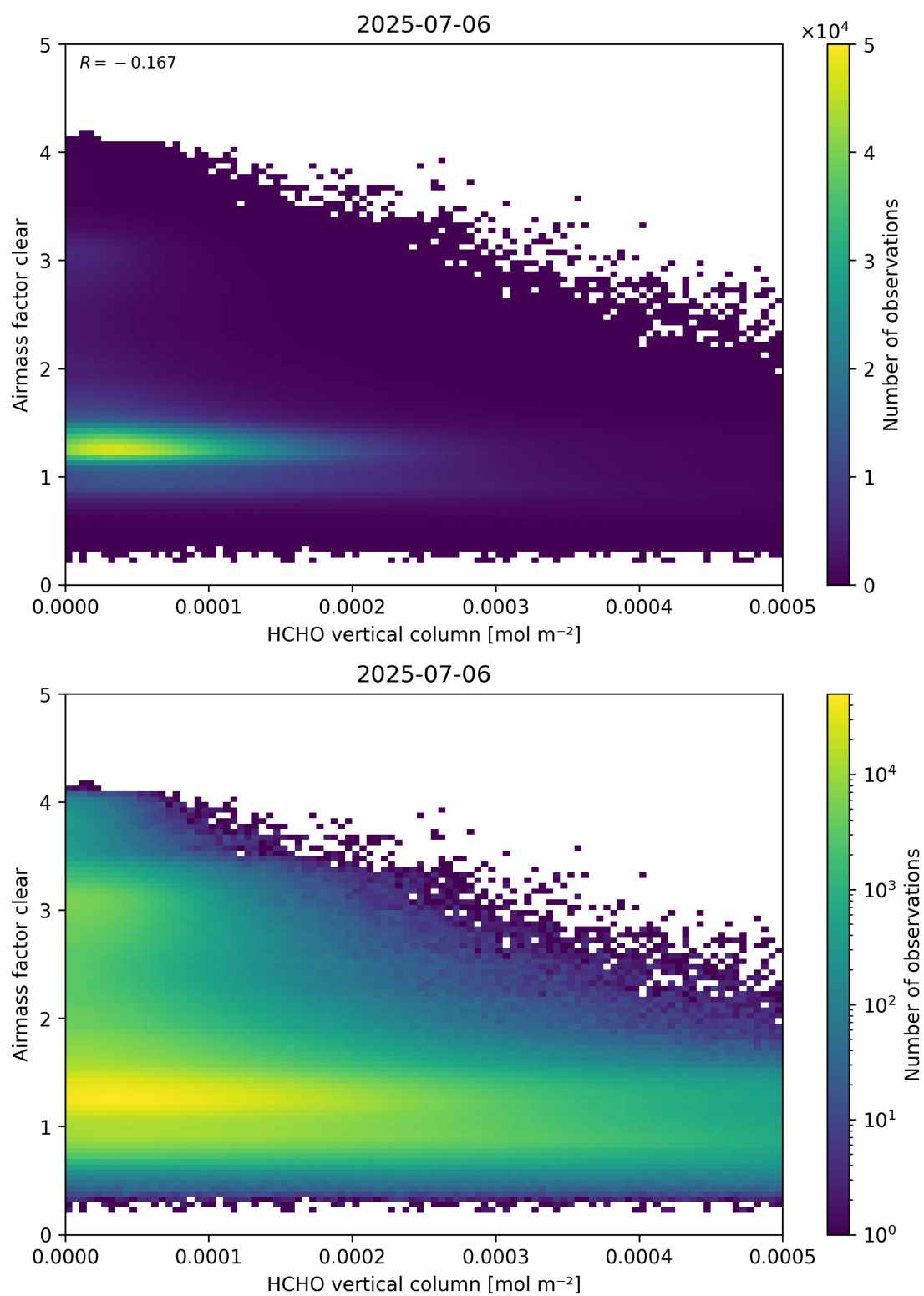
Figure 126: Scatter density plot of “HCHO vertical column” against “Airmass factor clear” for 2025-07-05 to 2025-07-07.
