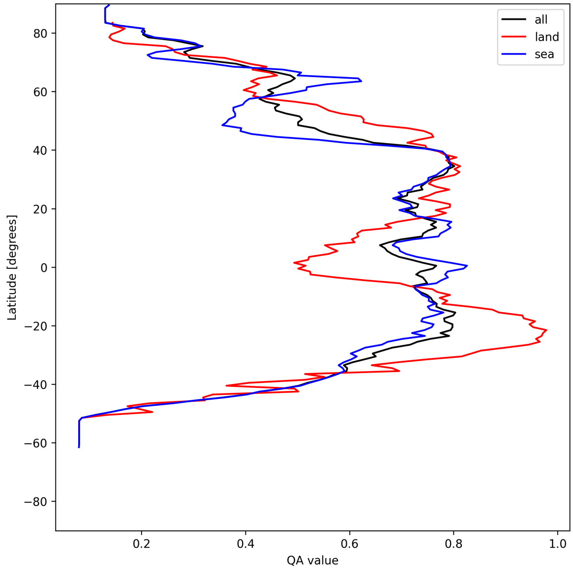
Figure 20: Zonal average of “QA value” for 2025-07-05 to 2025-07-07.
