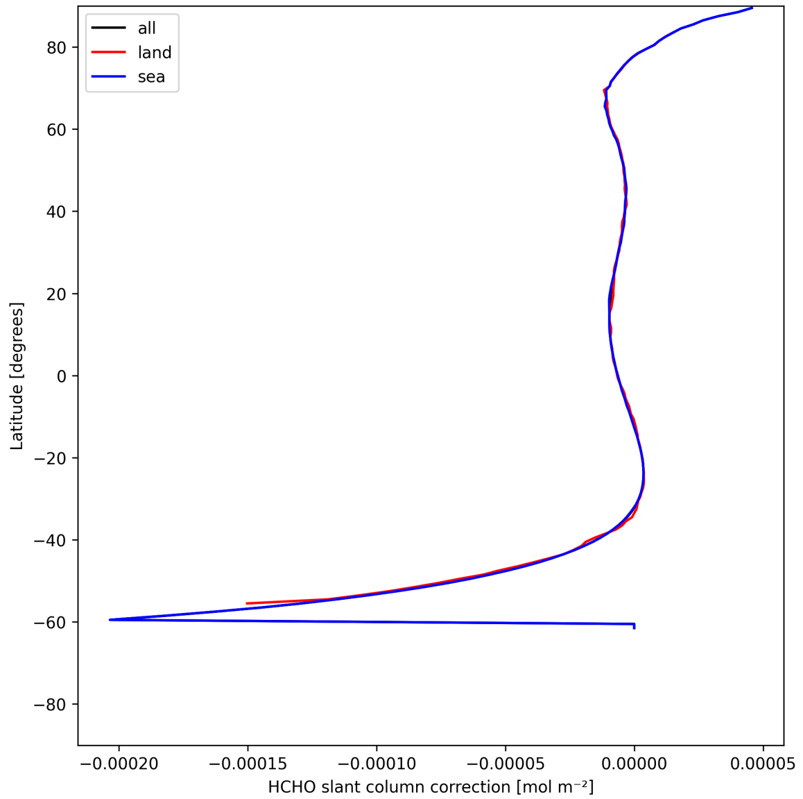
Figure 33: Zonal average of “HCHO slant column correction” for 2025-07-05 to 2025-07-07.
