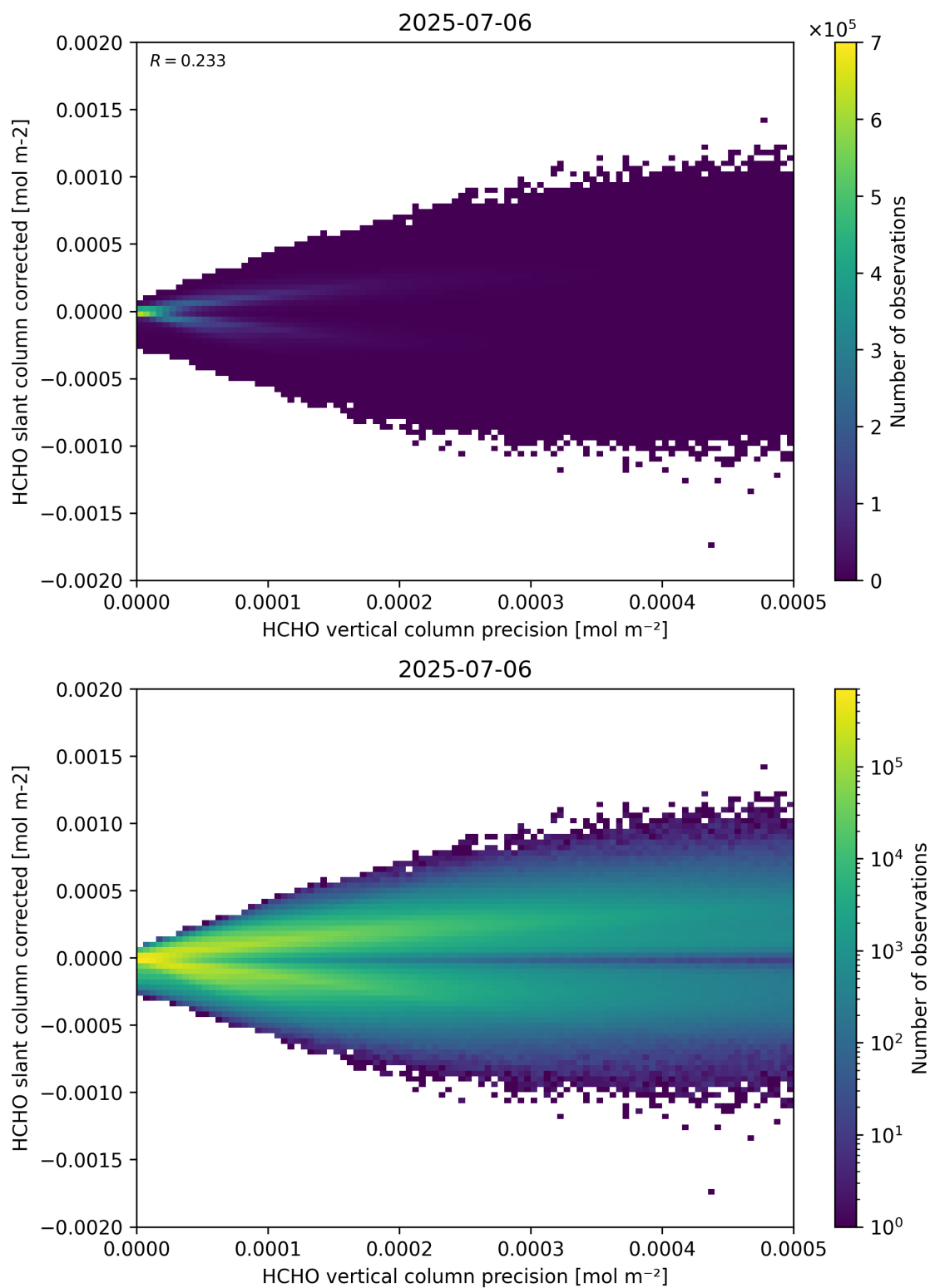
Figure 140: Scatter density plot of “HCHO vertical column precision” against “HCHO slant column corrected” for 2025-07-05 to 2025-07-07.
