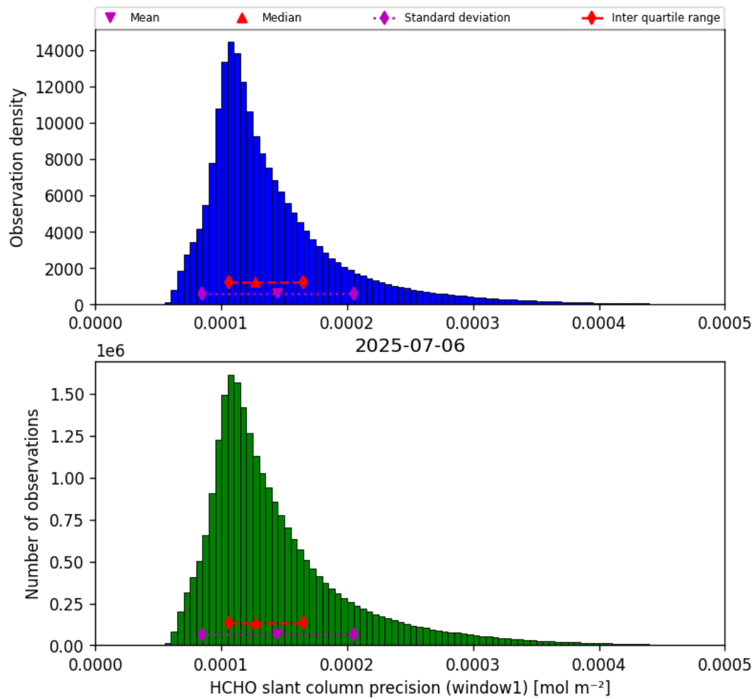
Figure 39: Histogram of “HCHO slant column precision (window1)” for 2025-07-05 to 2025-07-07
