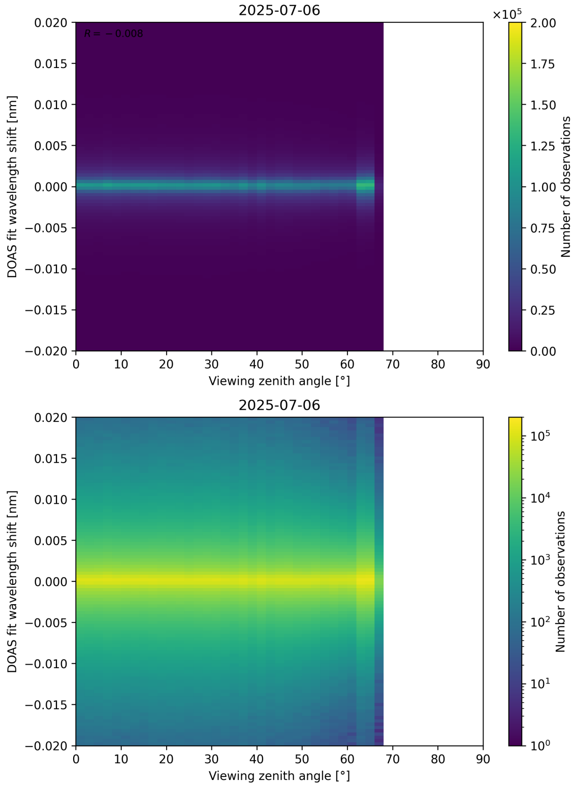
Figure 183: Scatter density plot of “Viewing zenith angle” against “DOAS fit wavelength shift” for 2025-07-05 to 2025-07-07.
