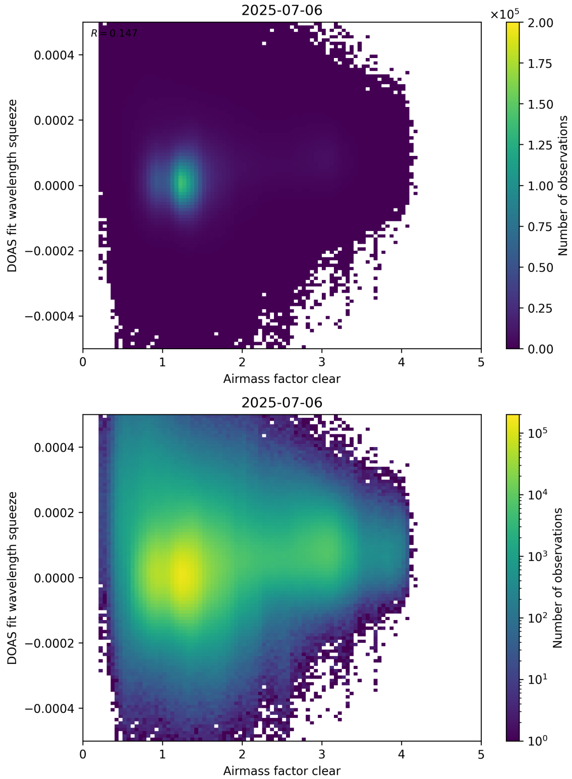
Figure 73: Scatter density plot of “Airmass factor clear” against “DOAS fit wavelength squeeze” for 2025-07-05 to 2025-07-07.
