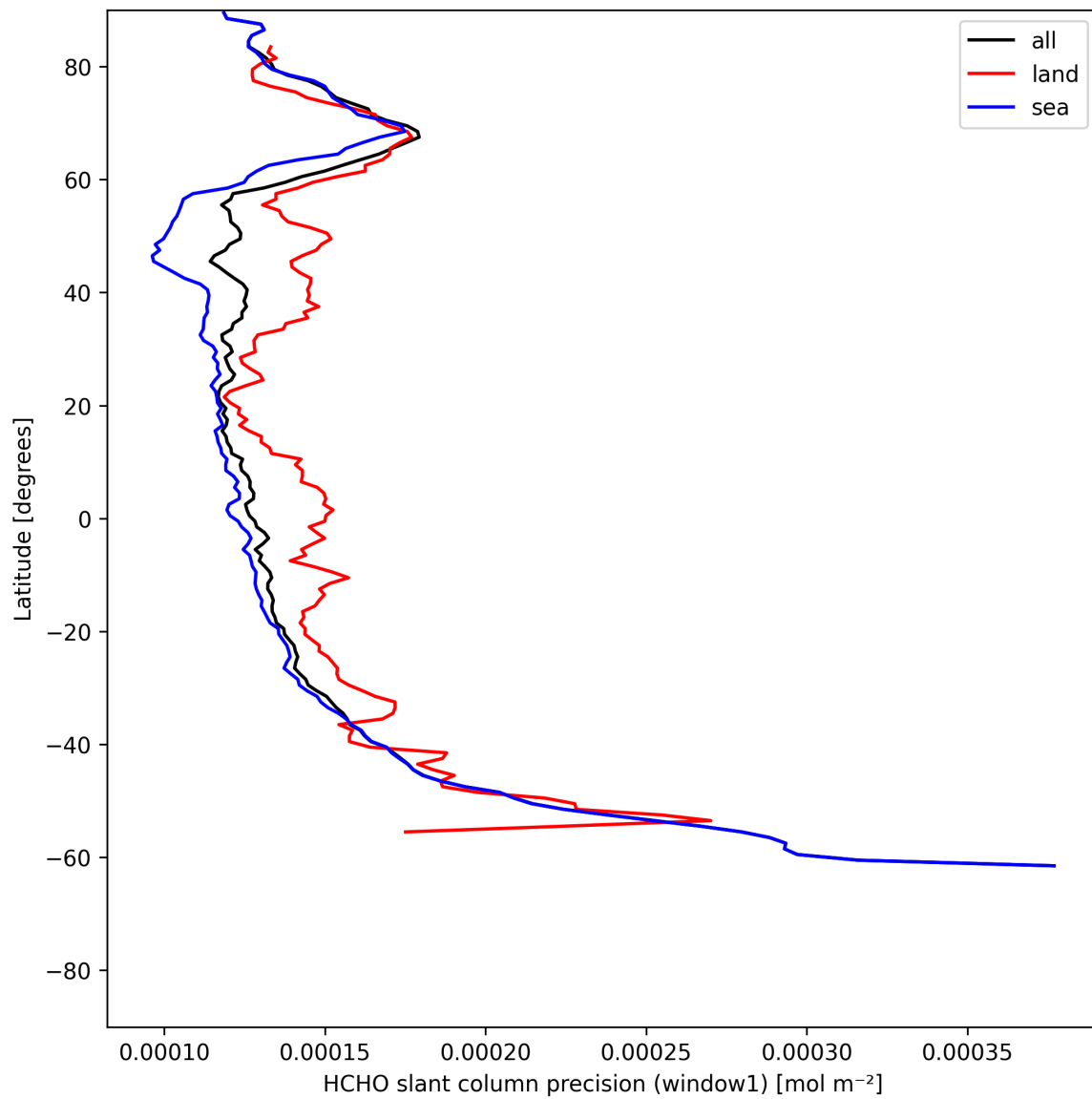
Figure 25: Zonal average of “HCHO slant column precision (window1)” for 2025-07-05 to 2025-07-07.
