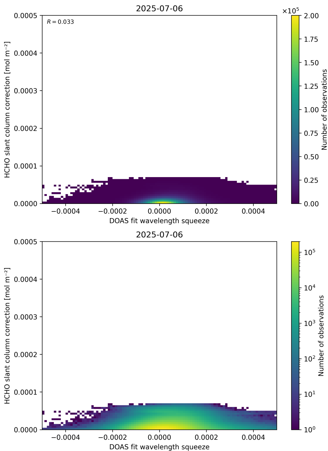
Figure 70: Scatter density plot of “DOAS fit wavelength squeeze” against “HCHO slant column correction” for 2025-07-05 to 2025-07-07.
