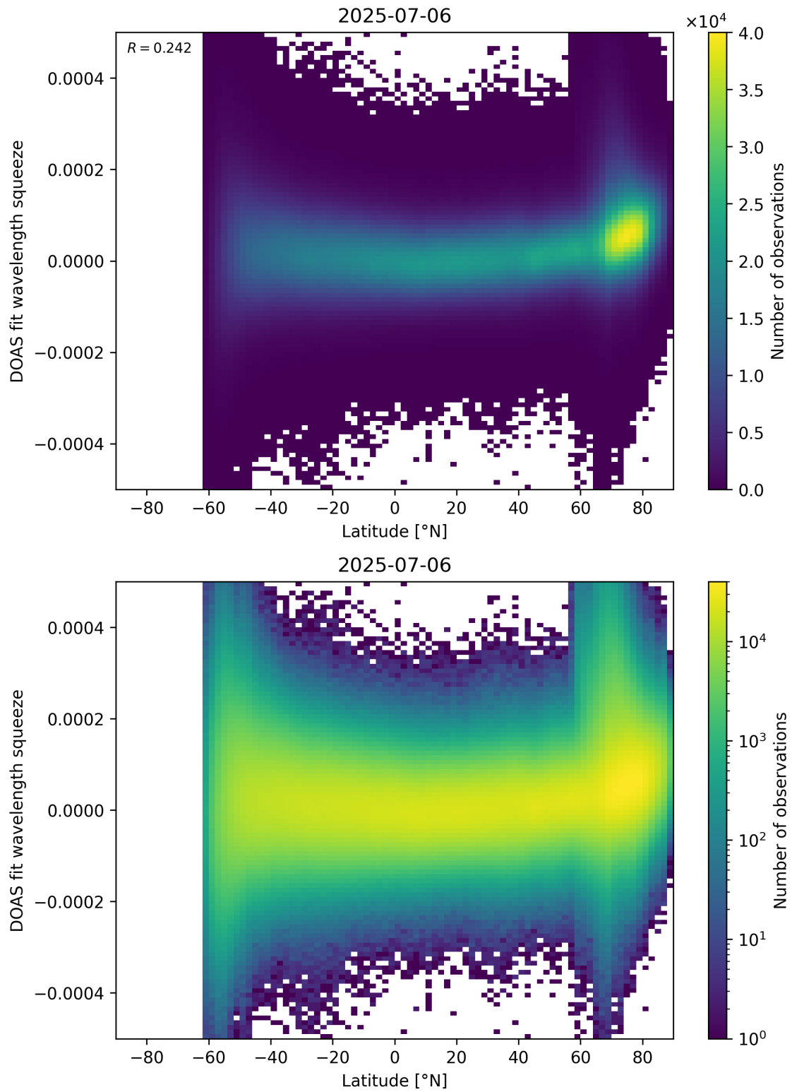
Figure 155: Scatter density plot of “Latitude” against “DOAS fit wavelength squeeze” for 2025-07-05 to 2025-07-07.
