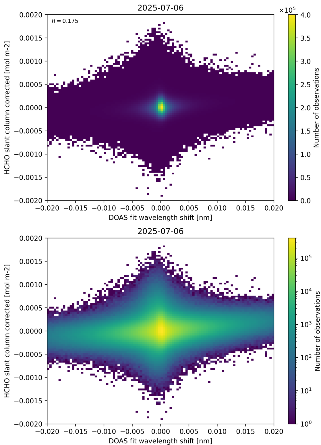
Figure 66: Scatter density plot of “DOAS fit wavelength shift” against “HCHO slant column corrected” for 2025-07-05 to 2025-07-07.
