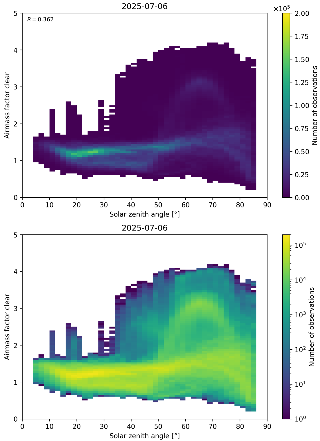
Figure 170: Scatter density plot of “Solar zenith angle” against “Airmass factor clear” for 2025-07-05 to 2025-07-07.
