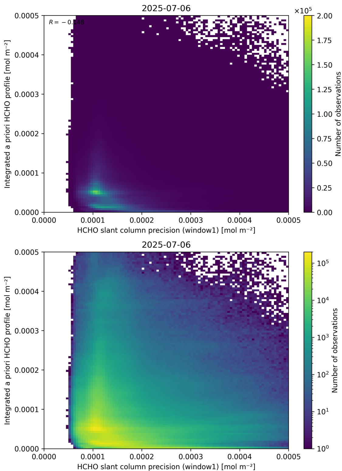
Figure 96: Scatter density plot of “HCHO slant column precision (window1)” against “Integrated a priori HCHO profile” for 2025-07-05 to 2025-07-07.
