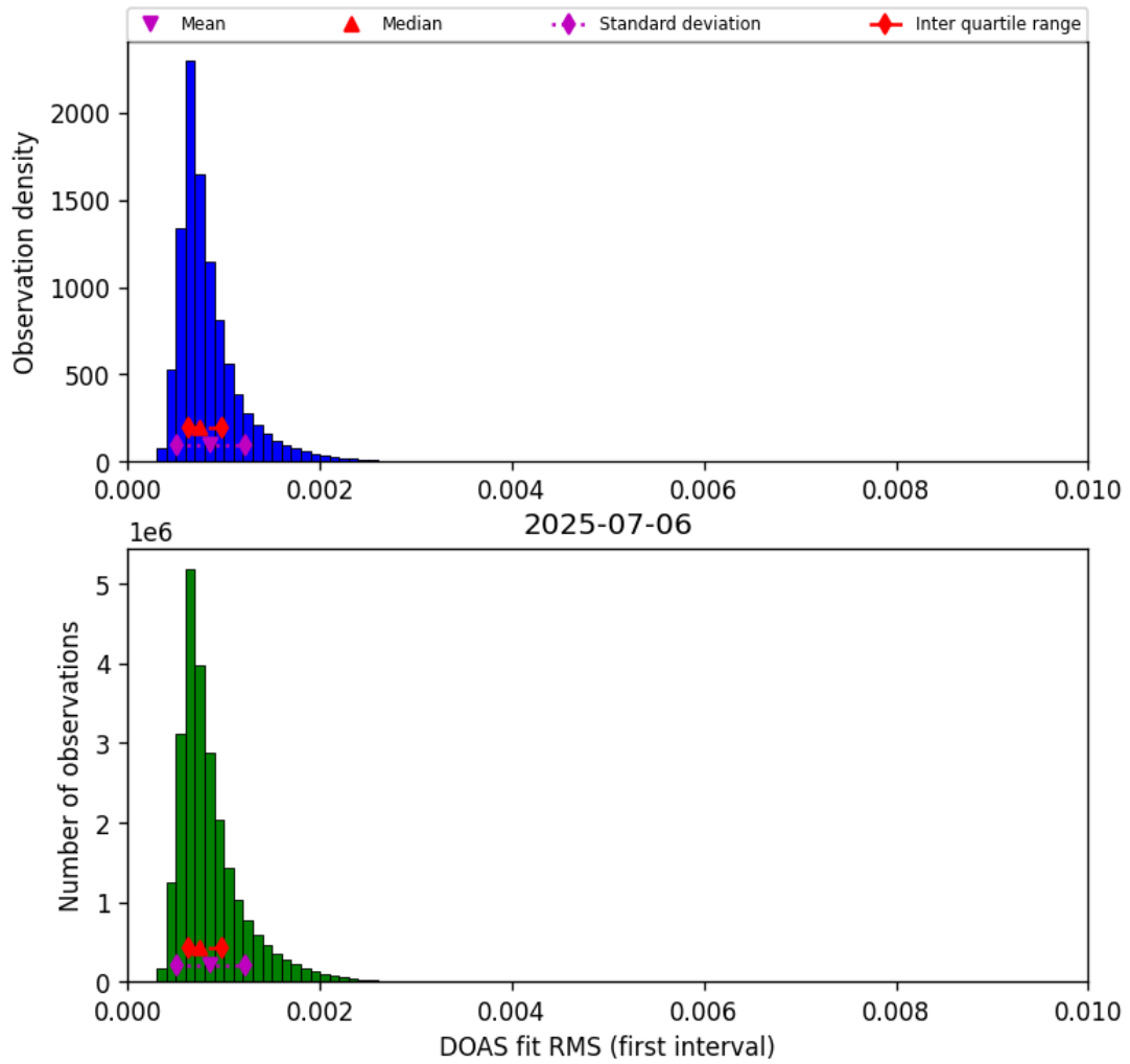
Figure 46: Histogram of “DOAS fit RMS (first interval)” for 2025-07-05 to 2025-07-07
