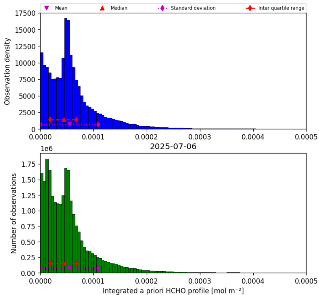
Figure 43: Histogram of “Integrated a priori HCHO profile” for 2025-07-05 to 2025-07-07
