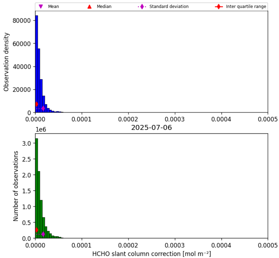
Figure 47: Histogram of “HCHO slant column correction” for 2025-07-05 to 2025-07-07
