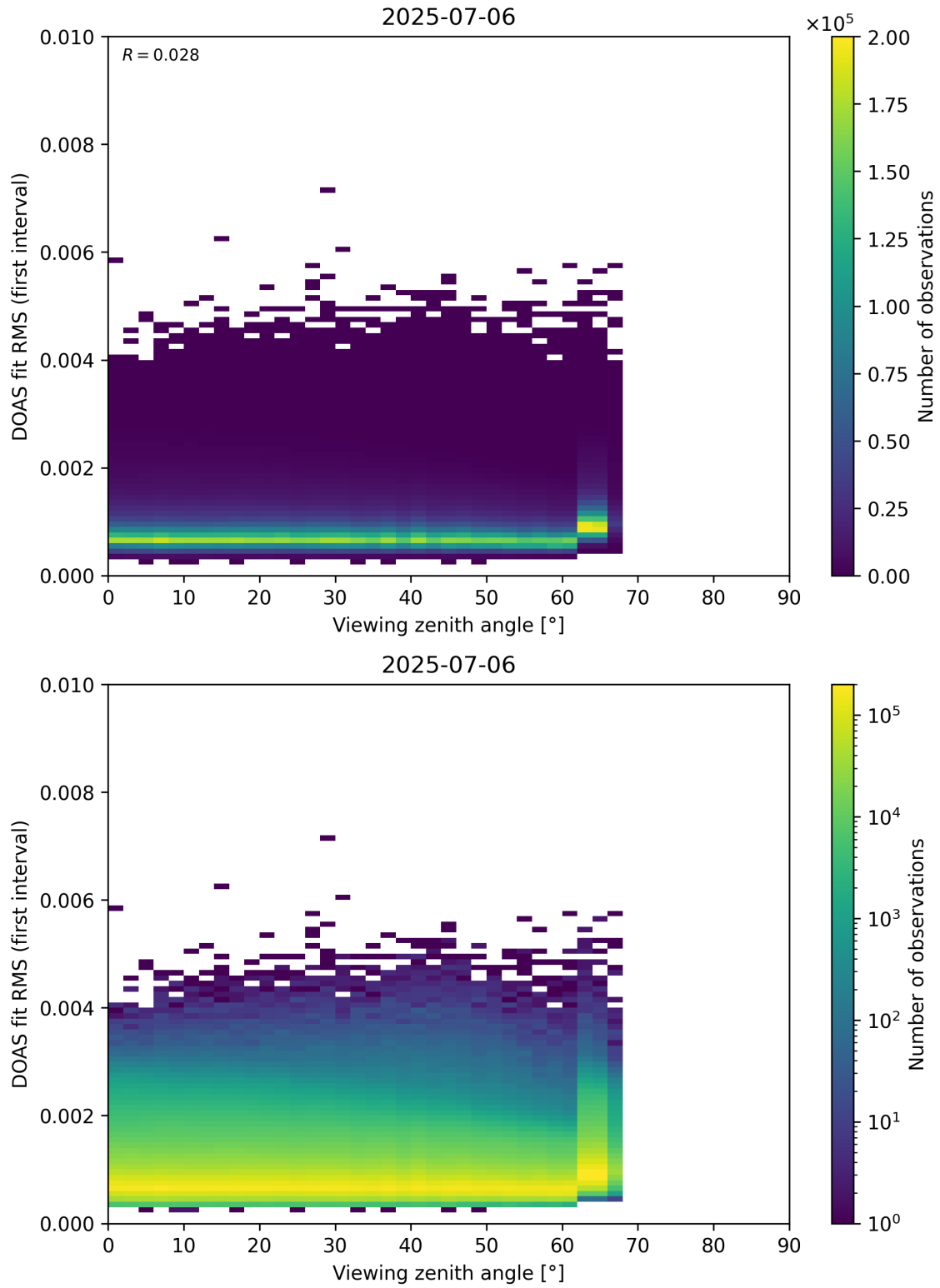
Figure 182: Scatter density plot of “Viewing zenith angle” against “DOAS fit RMS (first interval)” for 2025-07-05 to 2025-07-07.
