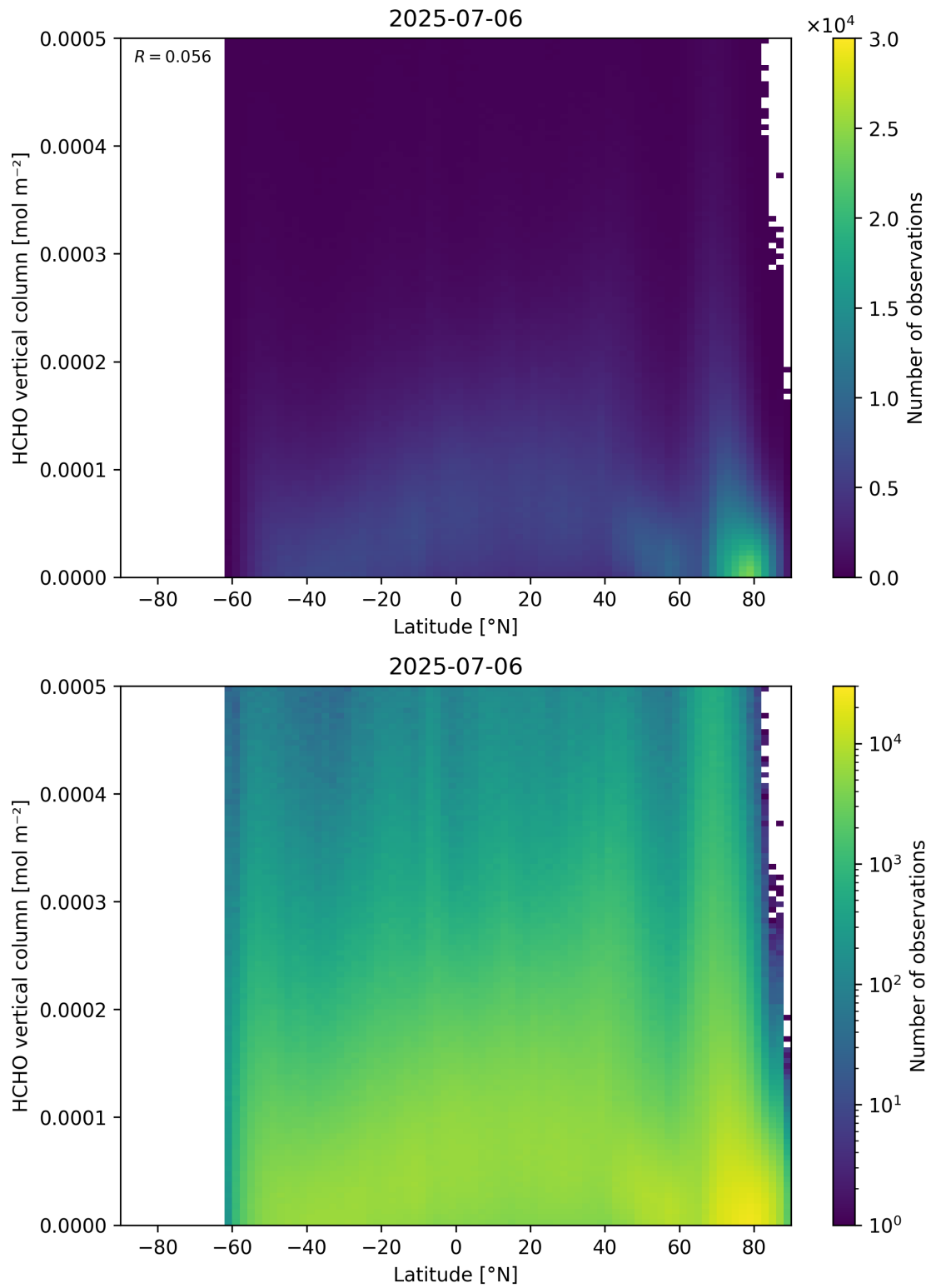
Figure 163: Scatter density plot of “Latitude” against “HCHO vertical column” for 2025-07-05 to 2025-07-07.
