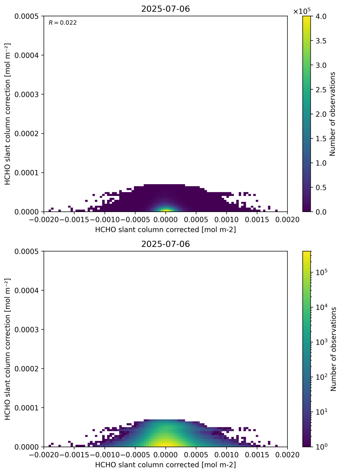
Figure 77: Scatter density plot of “HCHO slant column corrected” against “HCHO slant column correction” for 2025-07-05 to 2025-07-07.
