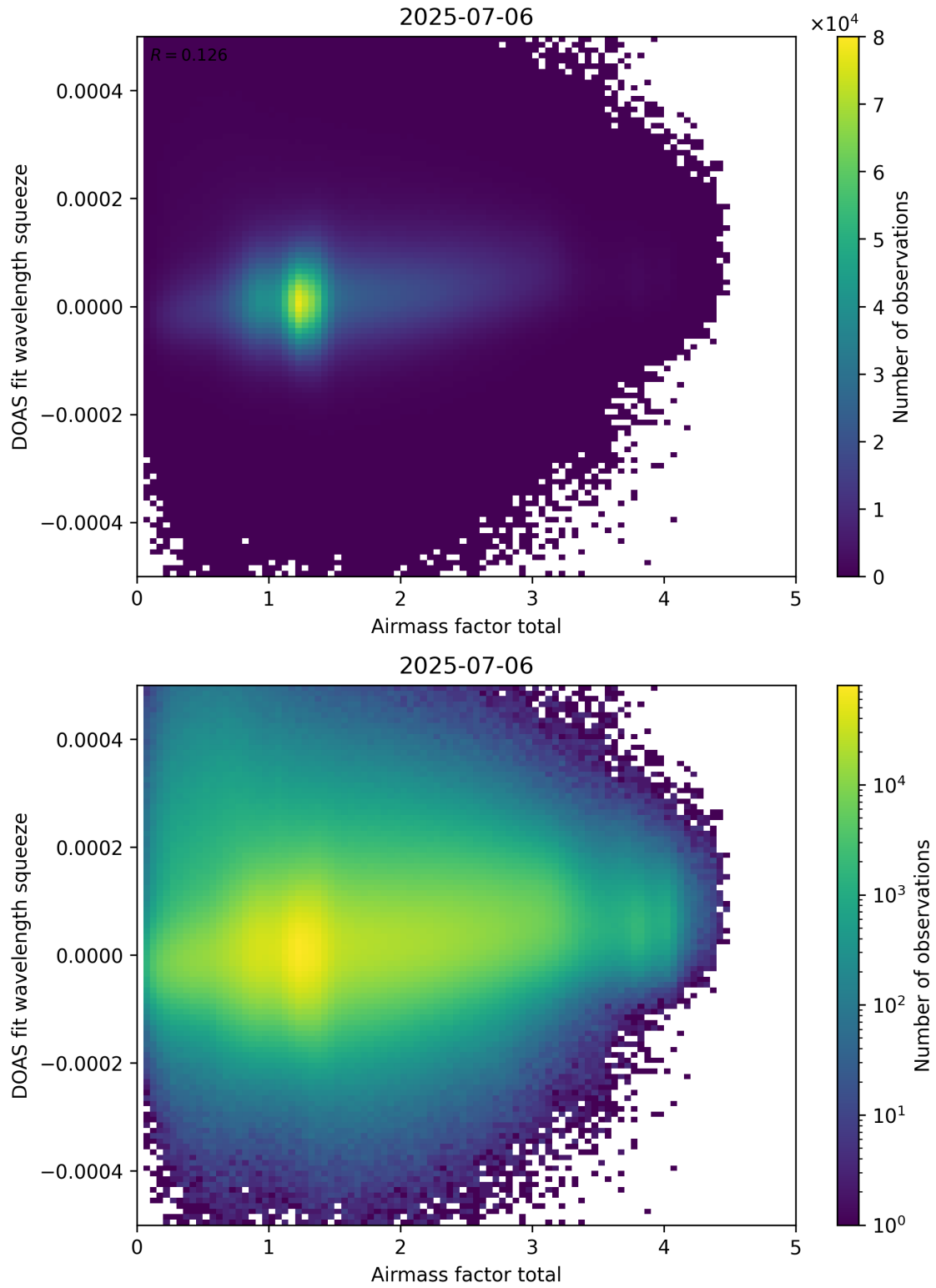
Figure 99: Scatter density plot of “Airmass factor total” against “DOAS fit wavelength squeeze” for 2025-07-05 to 2025-07-07.
