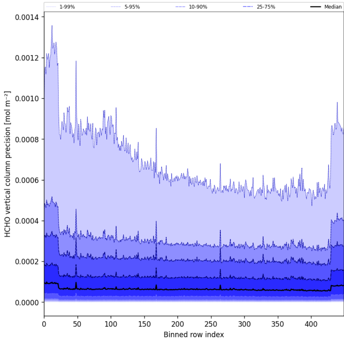
Figure 50: Along track statistics of “HCHO vertical column precision” for 2025-07-05 to 2025-07-07
