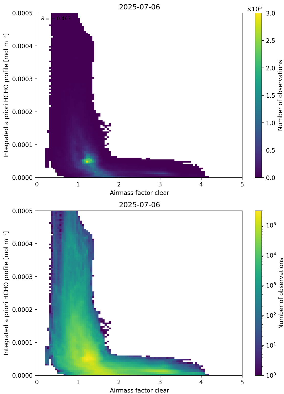
Figure 76: Scatter density plot of “Airmass factor clear” against “Integrated a priori HCHO profile” for 2025-07-05 to 2025-07-07.
