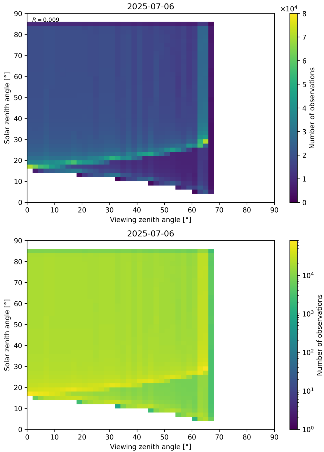
Figure 197: Scatter density plot of “Viewing zenith angle” against “Solar zenith angle” for 2025-07-05 to 2025-07-07.
