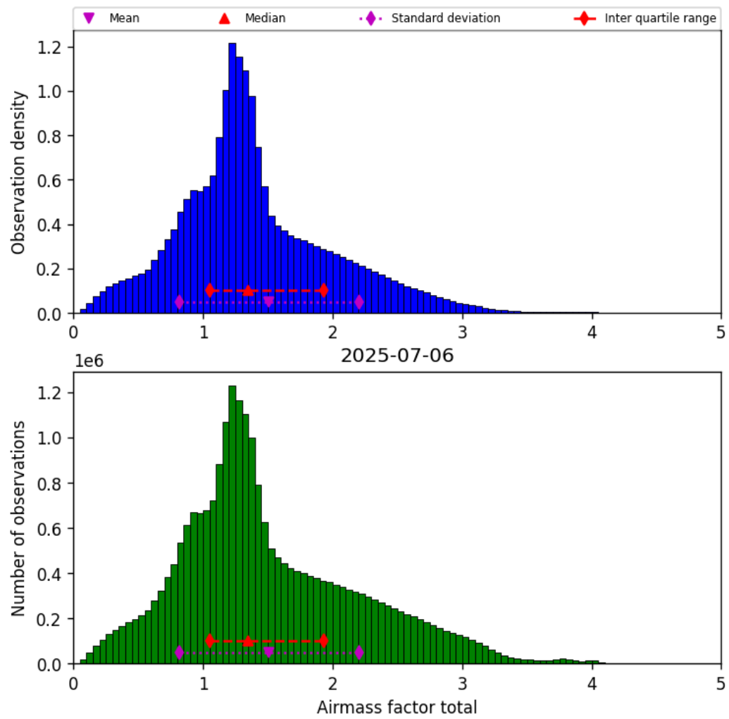
Figure 40: Histogram of “Airmass factor total” for 2025-07-05 to 2025-07-07
