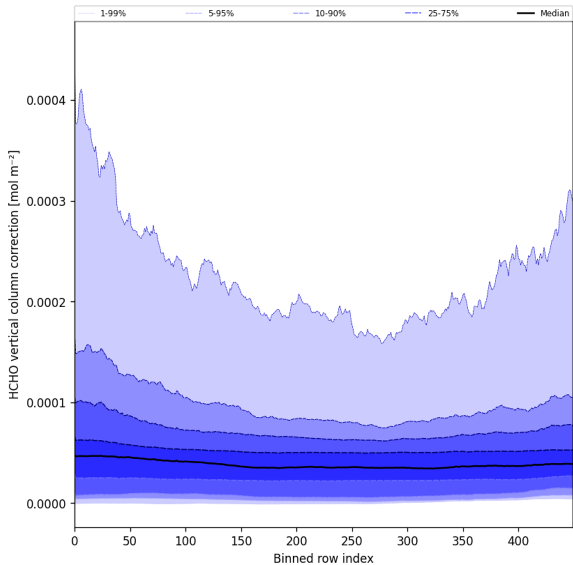
Figure 51: Along track statistics of “HCHO vertical column correction” for 2025-07-05 to 2025-07-07
