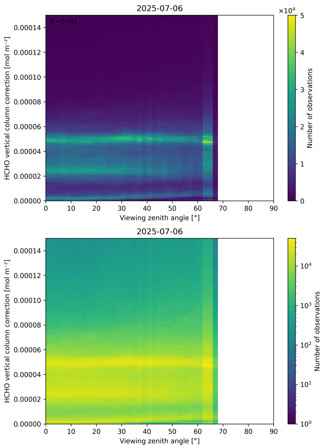
Figure 193: Scatter density plot of “Viewing zenith angle” against “HCHO vertical column correction” for 2025-07-05 to 2025-07-07.
