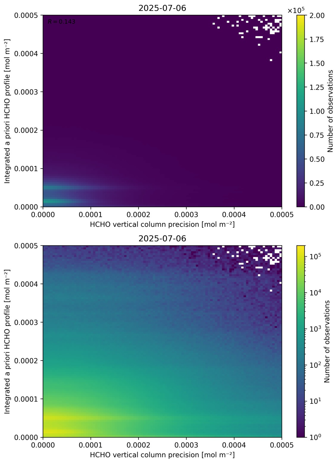
Figure 147: Scatter density plot of “HCHO vertical column precision” against “Integrated a priori HCHO profile” for 2025-07-05 to 2025-07-07.
