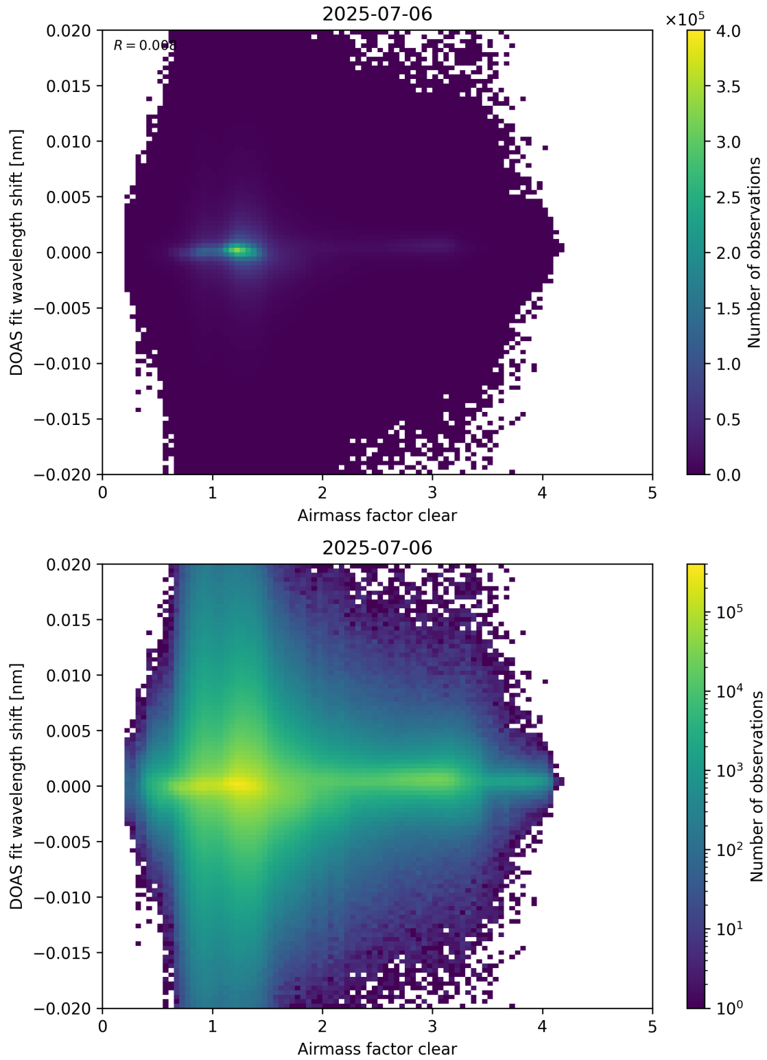
Figure 72: Scatter density plot of “Airmass factor clear” against “DOAS fit wavelength shift” for 2025-07-05 to 2025-07-07.
