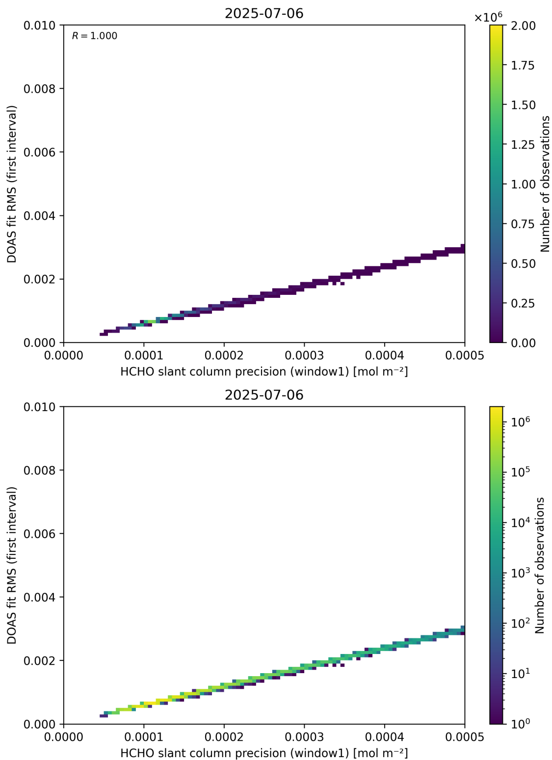
Figure 88: Scatter density plot of “HCHO slant column precision (window1)” against “DOAS fit RMS (first interval)” for 2025-07-05 to 2025-07-07.
