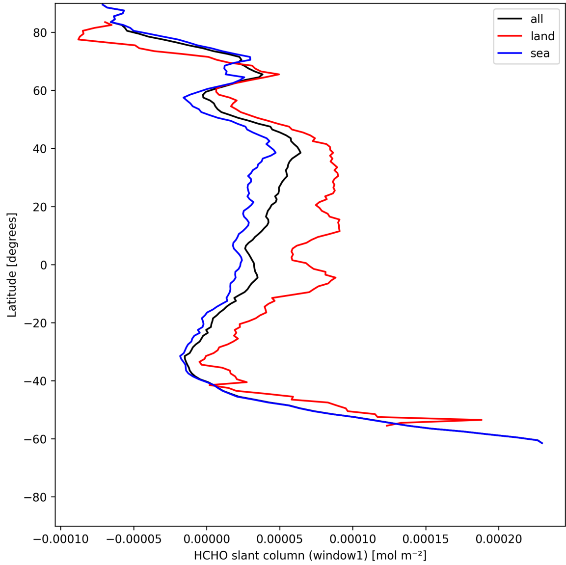
Figure 24: Zonal average of “HCHO slant column (window1)” for 2025-07-05 to 2025-07-07.
