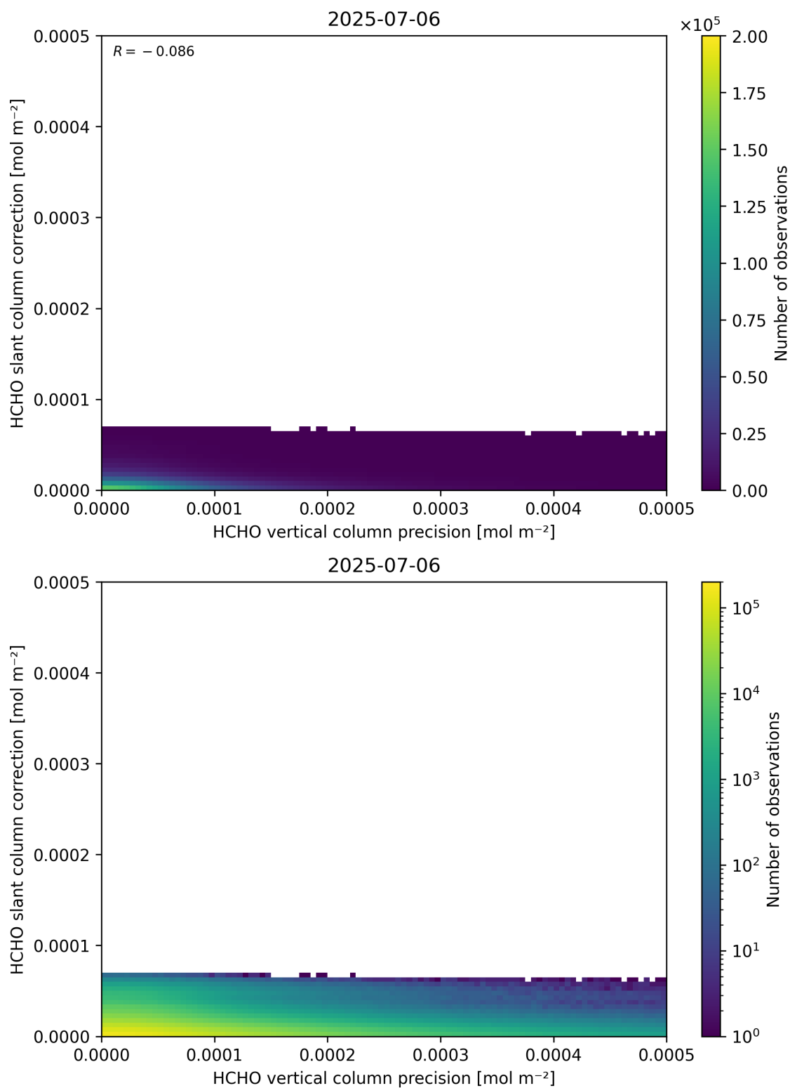
Figure 141: Scatter density plot of “HCHO vertical column precision” against “HCHO slant column correction” for 2025-07-05 to 2025-07-07.
