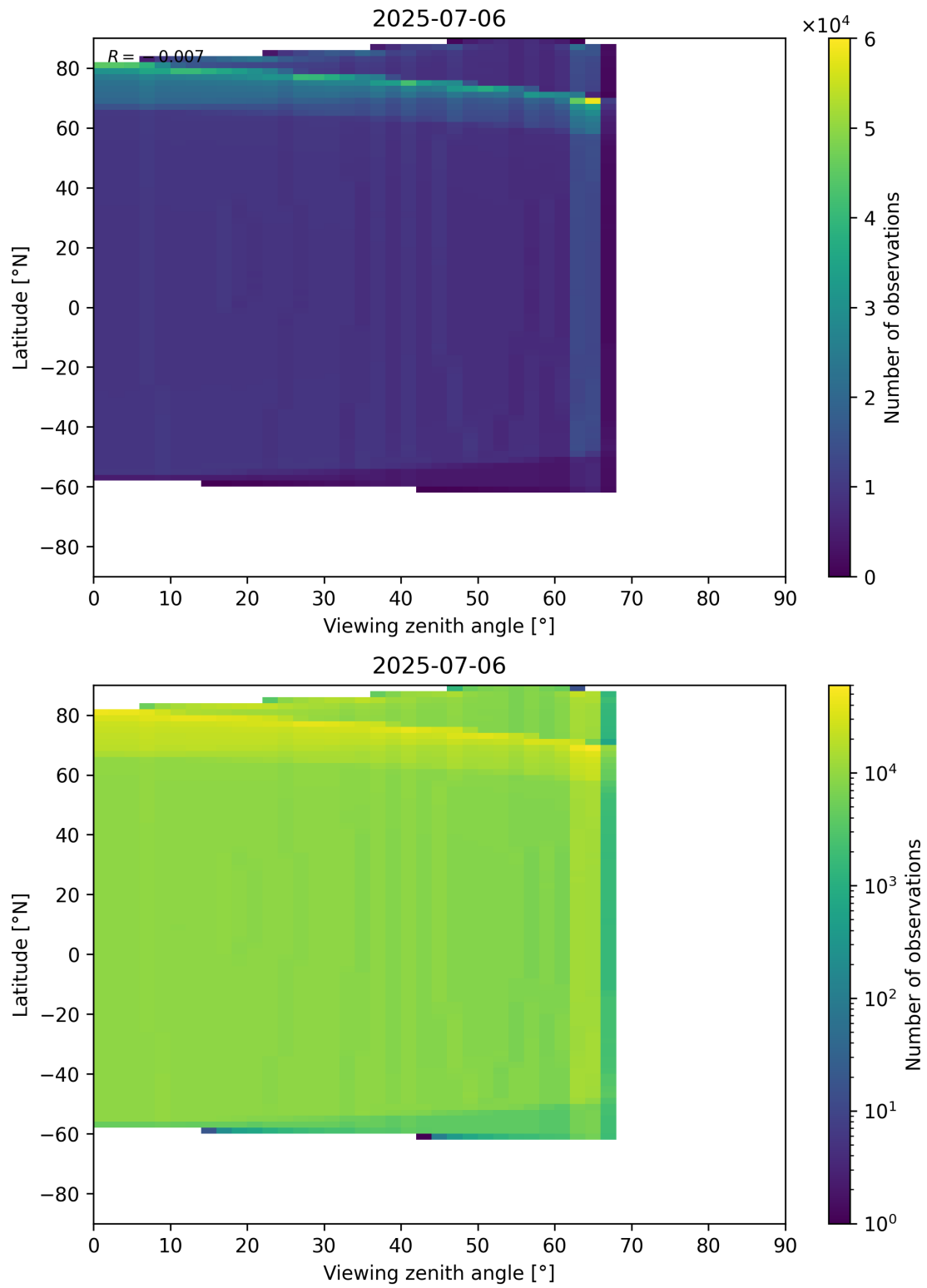
Figure 196: Scatter density plot of “Viewing zenith angle” against “Latitude” for 2025-07-05 to 2025-07-07.
