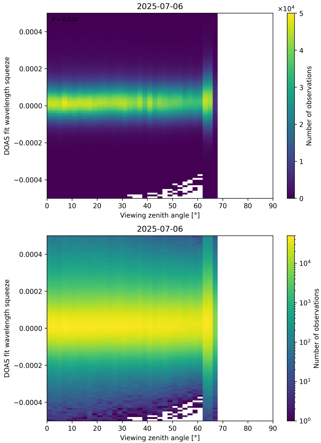
Figure 184: Scatter density plot of “Viewing zenith angle” against “DOAS fit wavelength squeeze” for 2025-07-05 to 2025-07-07.
