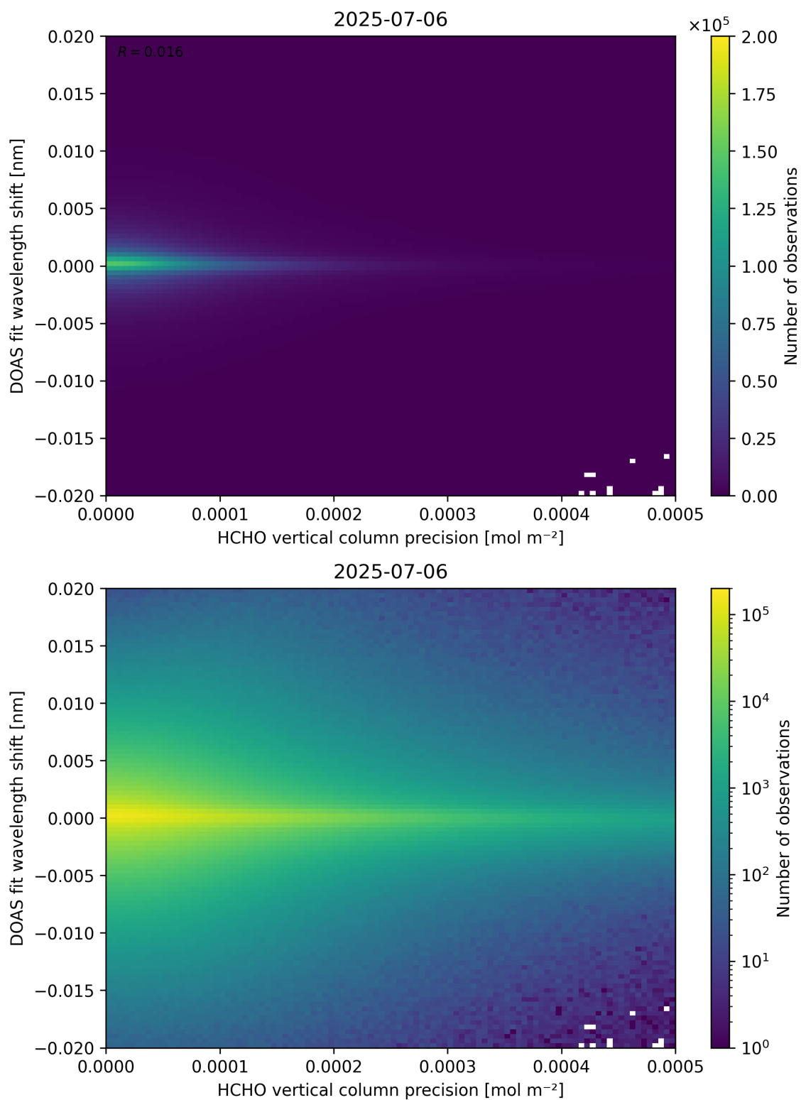
Figure 137: Scatter density plot of “HCHO vertical column precision” against “DOAS fit wavelength shift” for 2025-07-05 to 2025-07-07.
