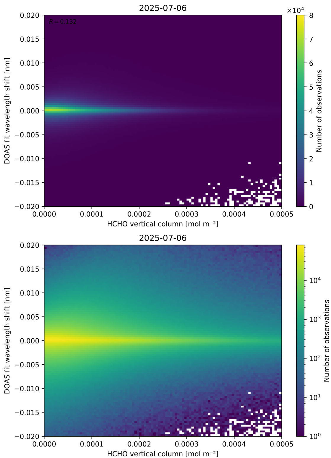
Figure 124: Scatter density plot of “HCHO vertical column” against “DOAS fit wavelength shift” for 2025-07-05 to 2025-07-07.
