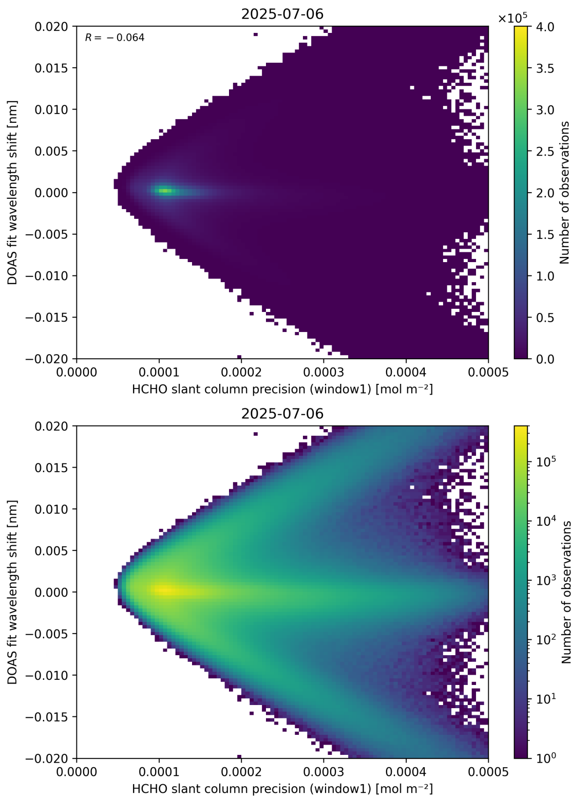
Figure 89: Scatter density plot of “HCHO slant column precision (window1)” against “DOAS fit wavelength shift” for 2025-07-05 to 2025-07-07.
