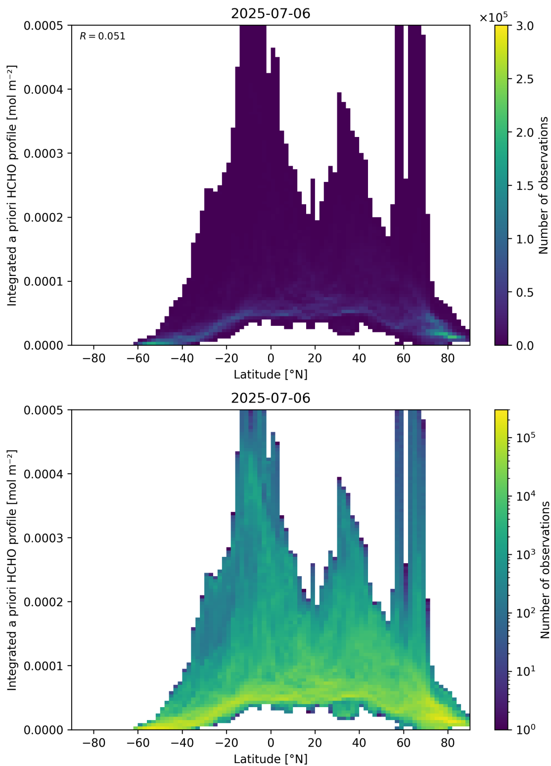
Figure 166: Scatter density plot of “Latitude” against “Integrated a priori HCHO profile” for 2025-07-05 to 2025-07-07.
