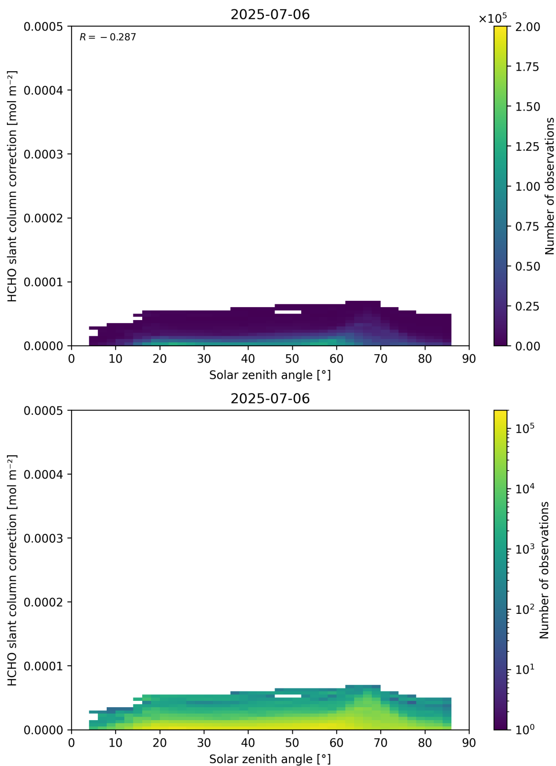
Figure 172: Scatter density plot of “Solar zenith angle” against “HCHO slant column correction” for 2025-07-05 to 2025-07-07.
