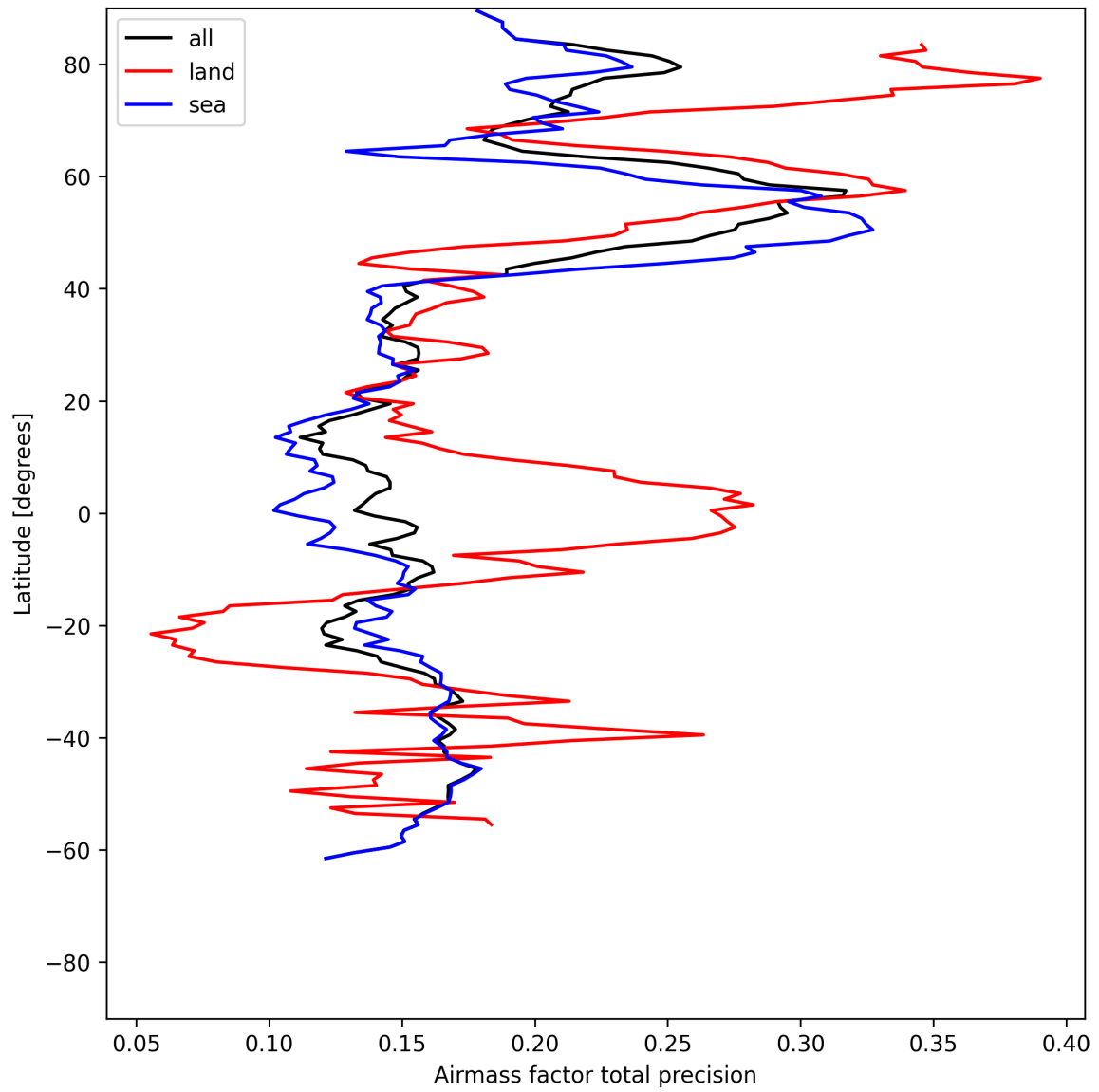
Figure 27: Zonal average of “Airmass factor total precision” for 2025-07-05 to 2025-07-07.
