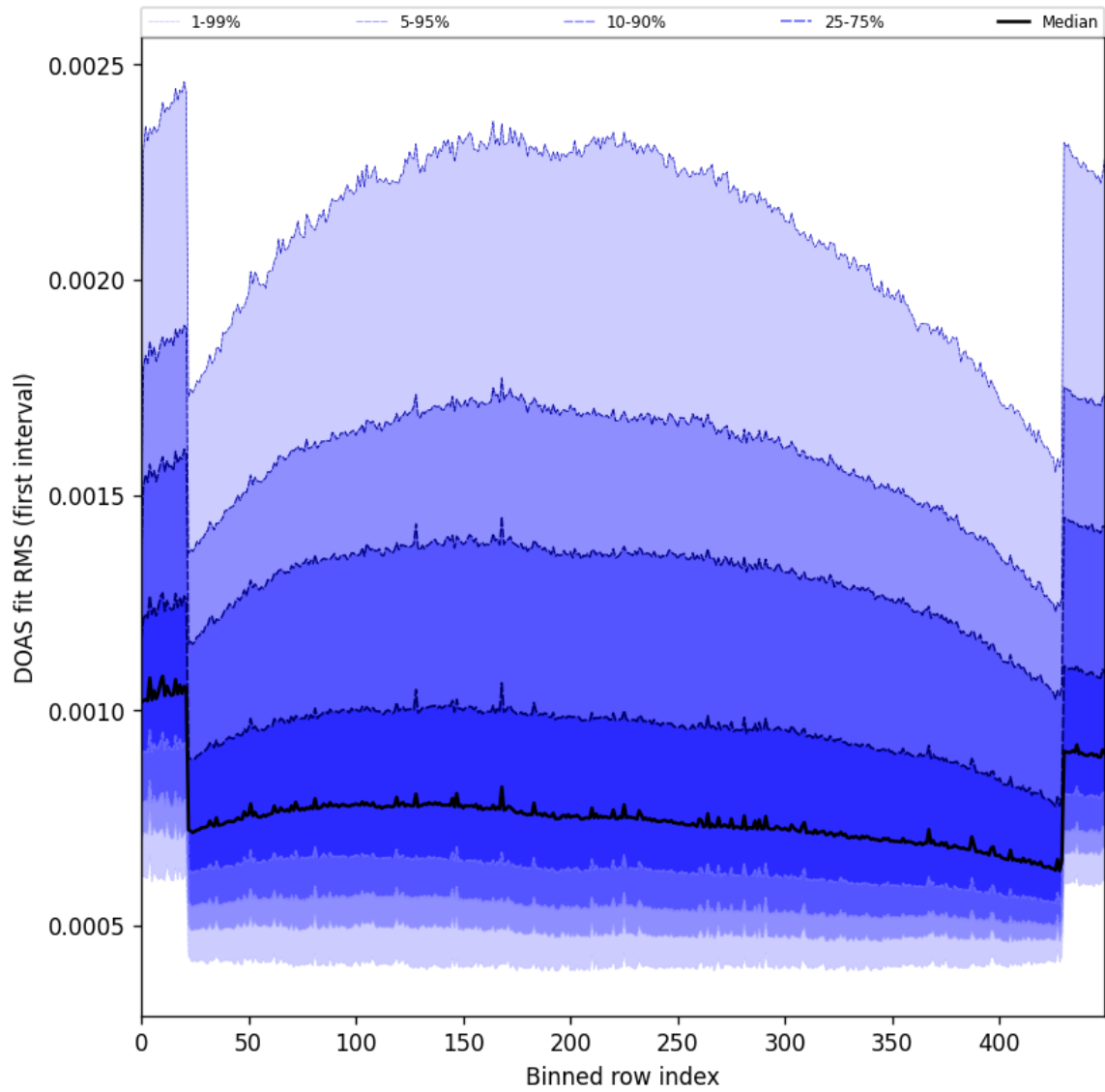
Figure 60: Along track statistics of “DOAS fit RMS (first interval)” for 2025-07-05 to 2025-07-07
