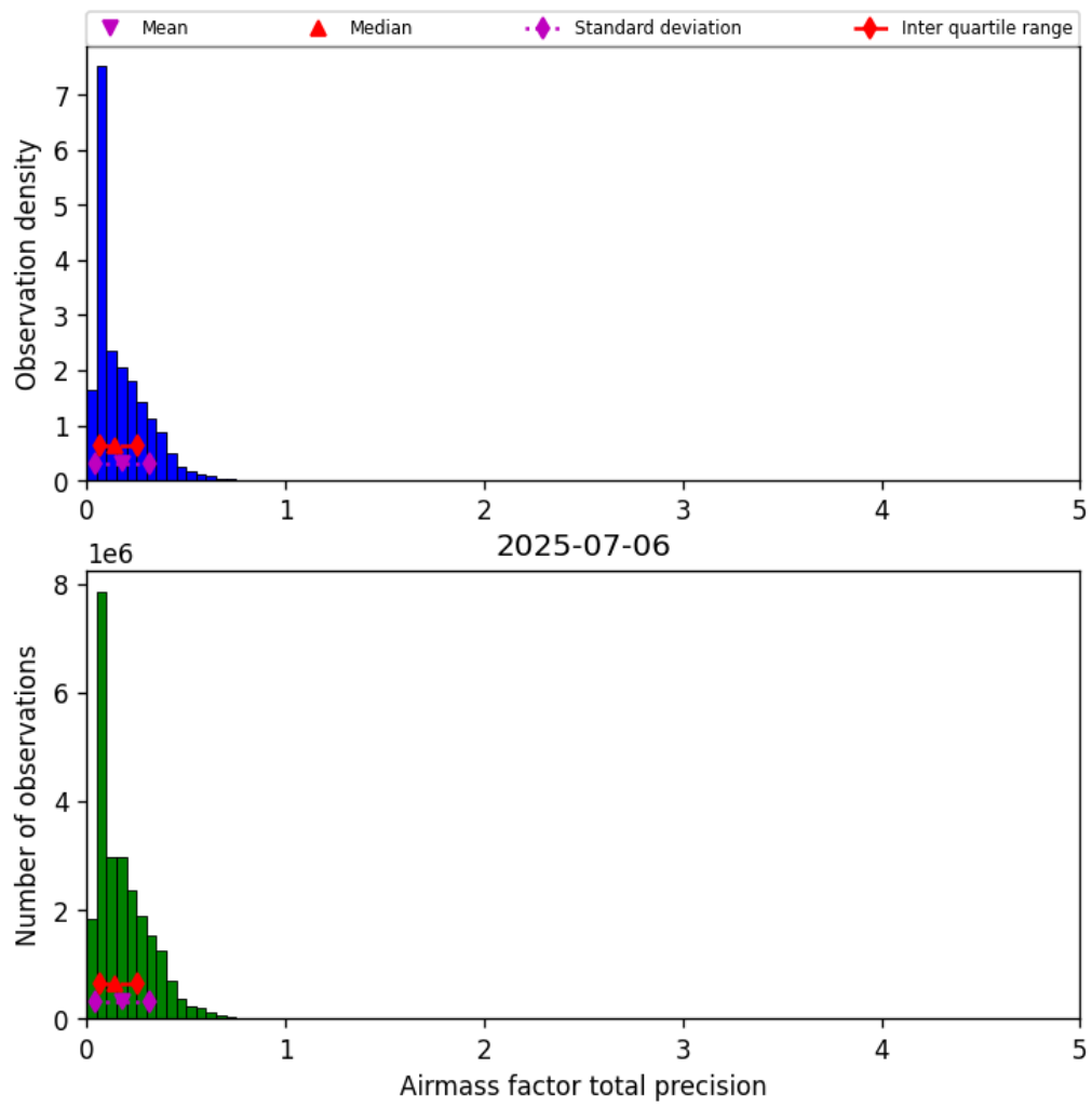
Figure 41: Histogram of “Airmass factor total precision” for 2025-07-05 to 2025-07-07
