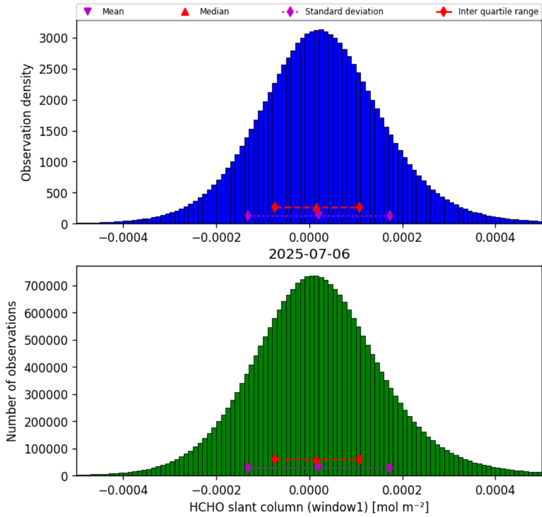
Figure 38: Histogram of “HCHO slant column (window1)” for 2025-07-05 to 2025-07-07
