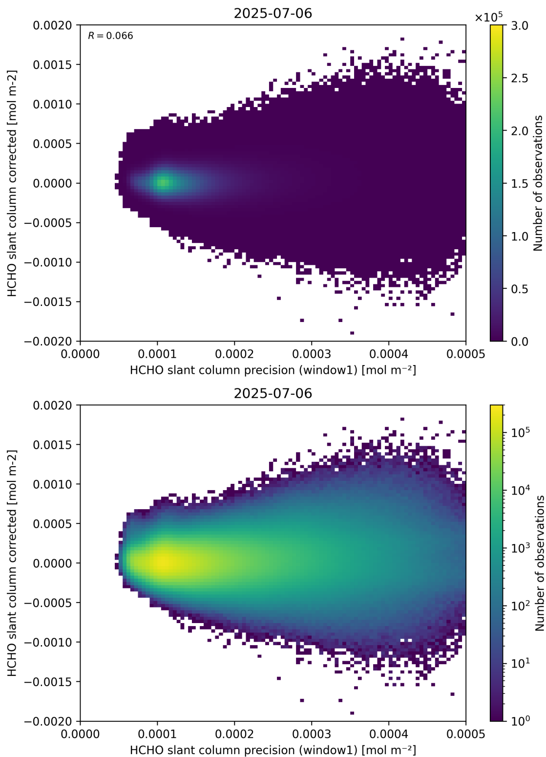
Figure 92: Scatter density plot of “HCHO slant column precision (window1)” against “HCHO slant column corrected” for 2025-07-05 to 2025-07-07.
