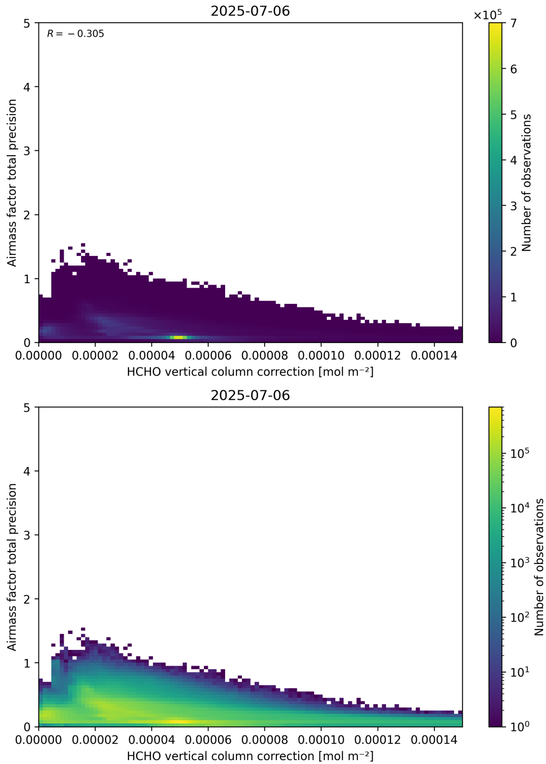
Figure 121: Scatter density plot of “HCHO vertical column correction” against “Airmass factor total precision” for 2025-07-05 to 2025-07-07.
