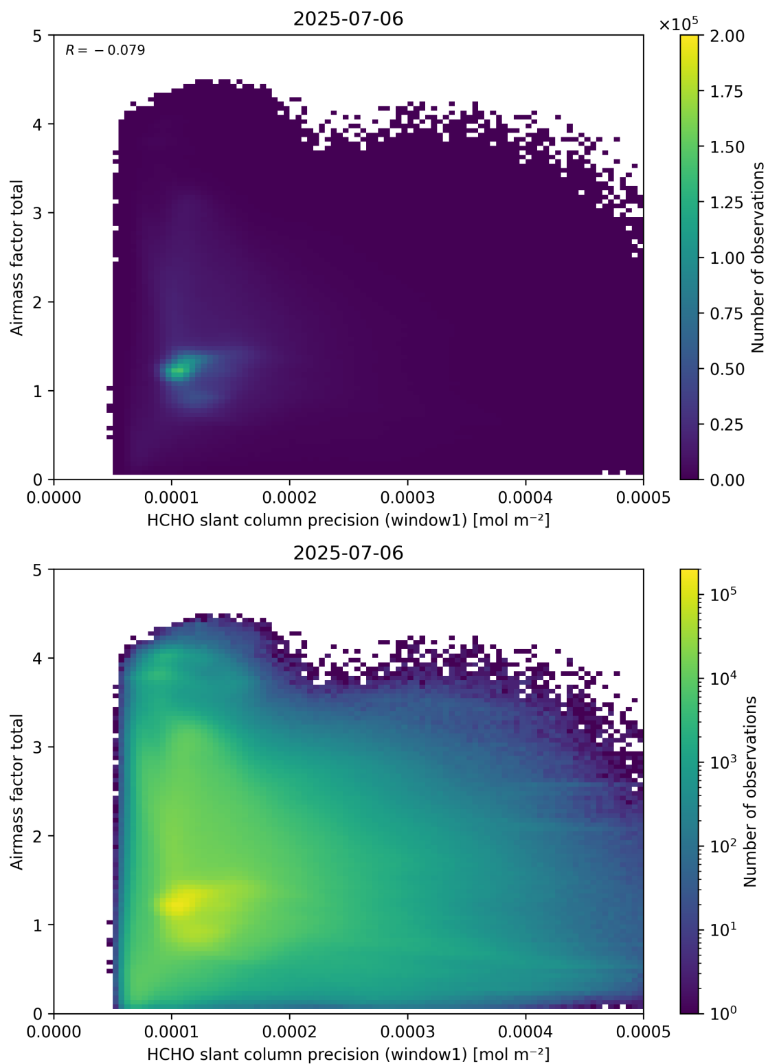
Figure 94: Scatter density plot of “HCHO slant column precision (window1)” against “Airmass factor total” for 2025-07-05 to 2025-07-07.
