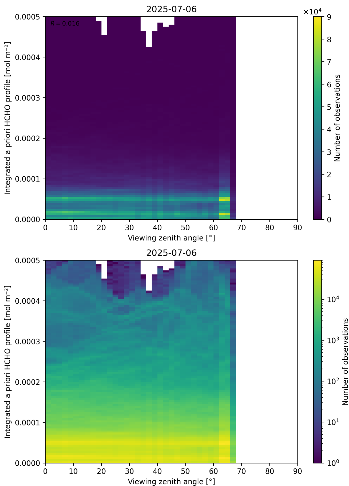
Figure 195: Scatter density plot of “Viewing zenith angle” against “Integrated a priori HCHO profile” for 2025-07-05 to 2025-07-07.
