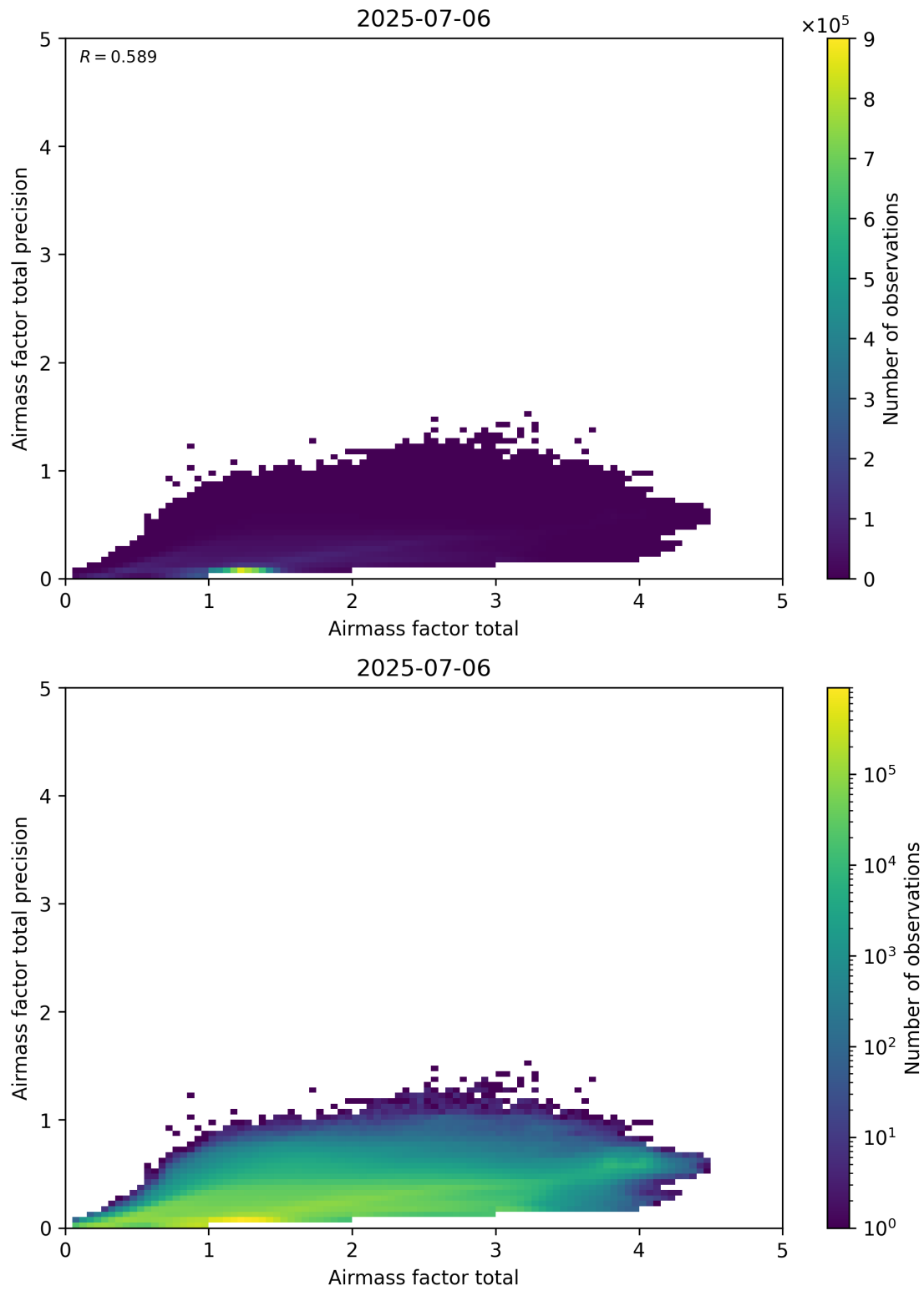
Figure 103: Scatter density plot of “Airmass factor total” against “Airmass factor total precision” for 2025-07-05 to 2025-07-07.
