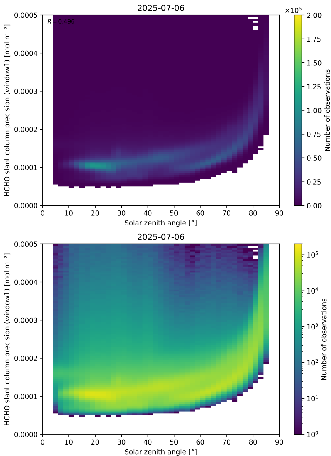
Figure 174: Scatter density plot of “Solar zenith angle” against “HCHO slant column precision (window1)” for 2025-07-05 to 2025-07-07.
