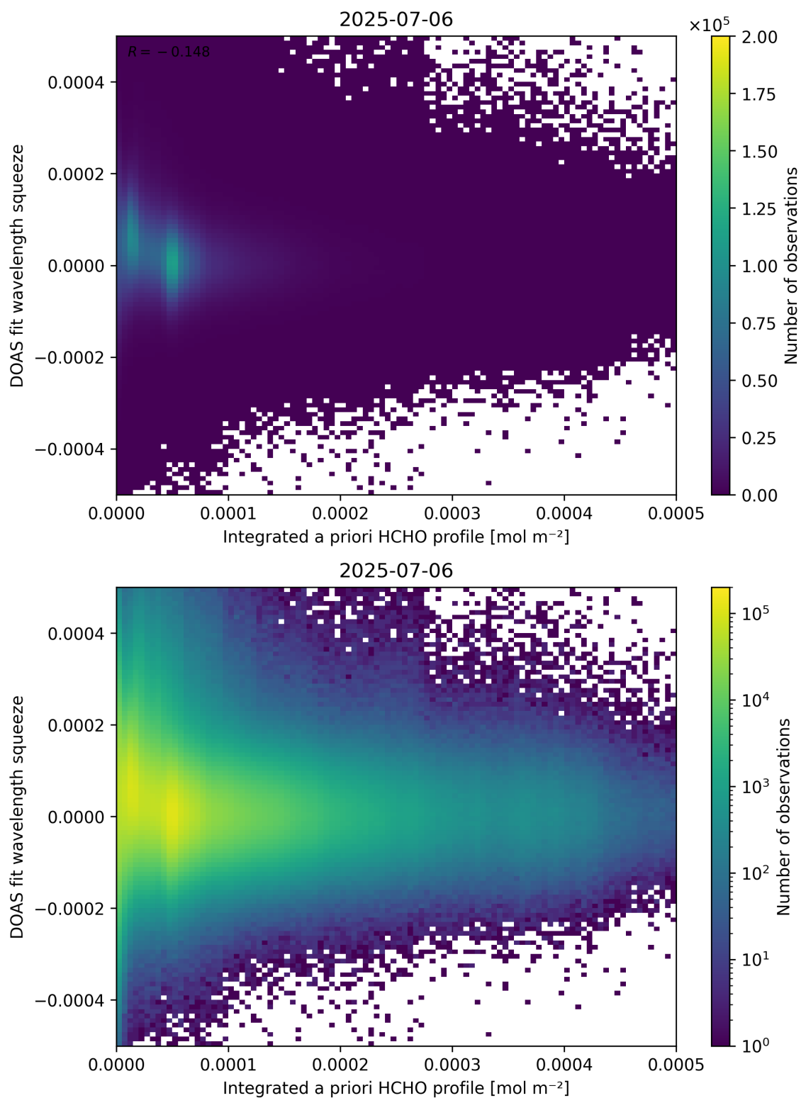
Figure 150: Scatter density plot of “Integrated a priori HCHO profile” against “DOAS fit wavelength squeeze” for 2025-07-05 to 2025-07-07.
