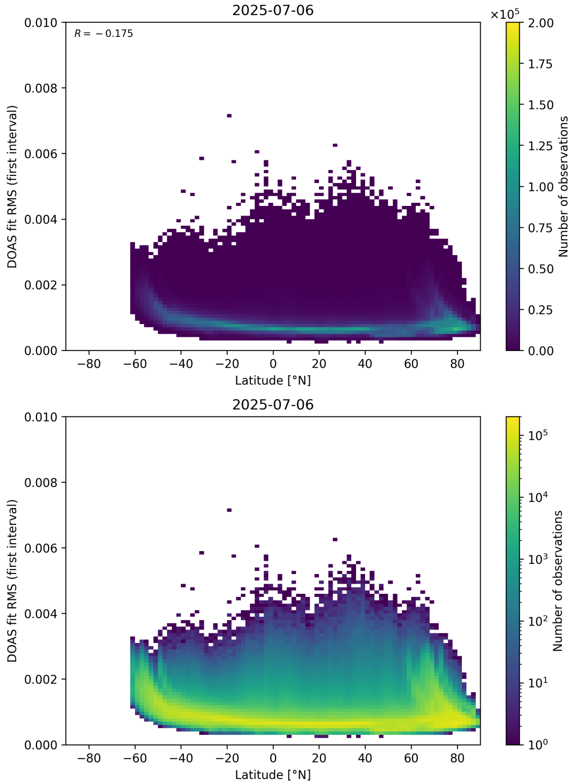
Figure 153: Scatter density plot of “Latitude” against “DOAS fit RMS (first interval)” for 2025-07-05 to 2025-07-07.
