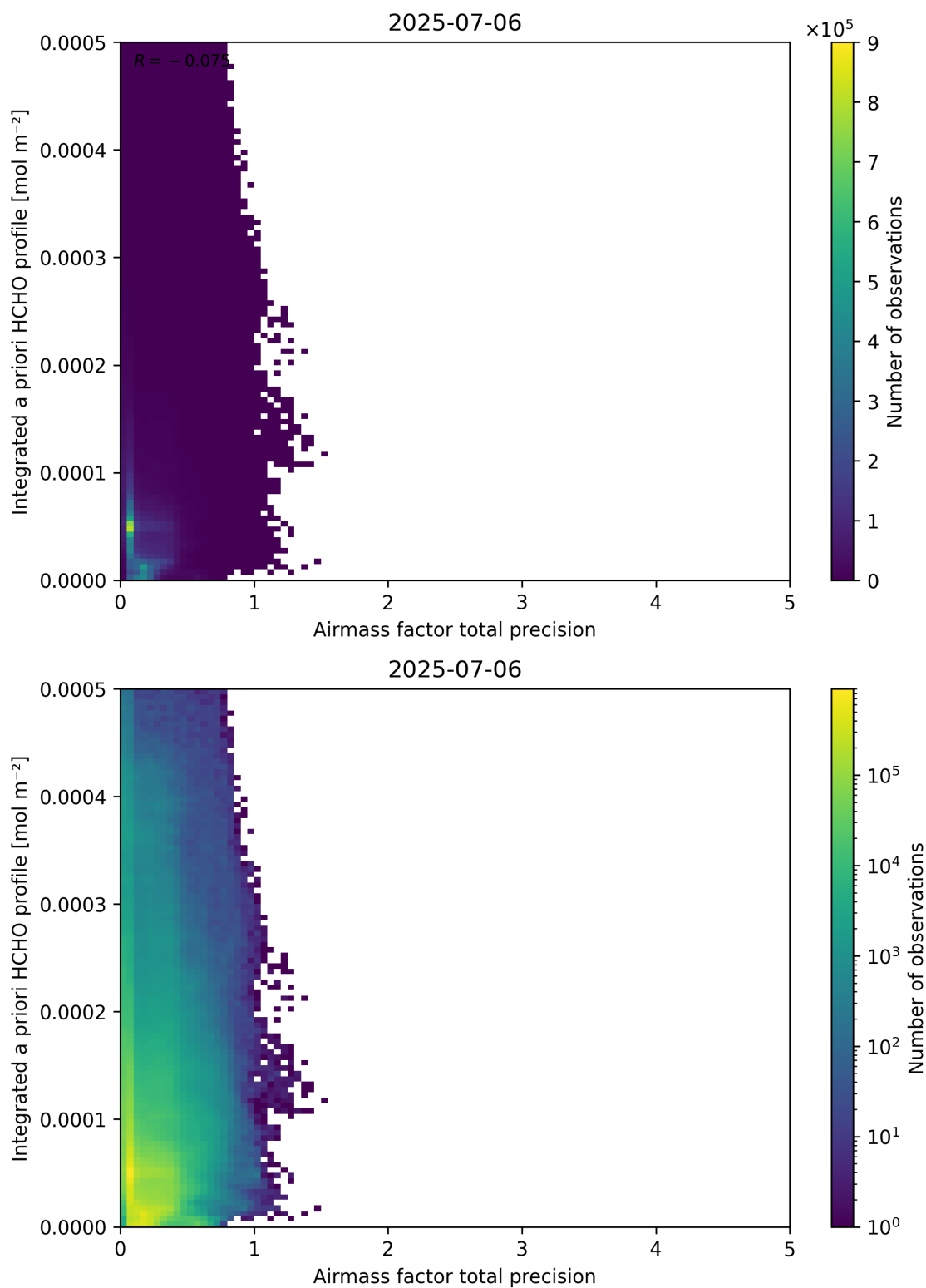
Figure 111: Scatter density plot of “Airmass factor total precision” against “Integrated a priori HCHO profile” for 2025-07-05 to 2025-07-07.
