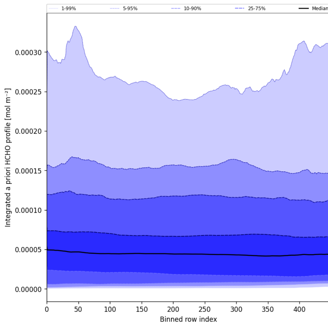
Figure 57: Along track statistics of "Integrated a priori HCHO profile" for 2025-07-05 to 2025-07-07
