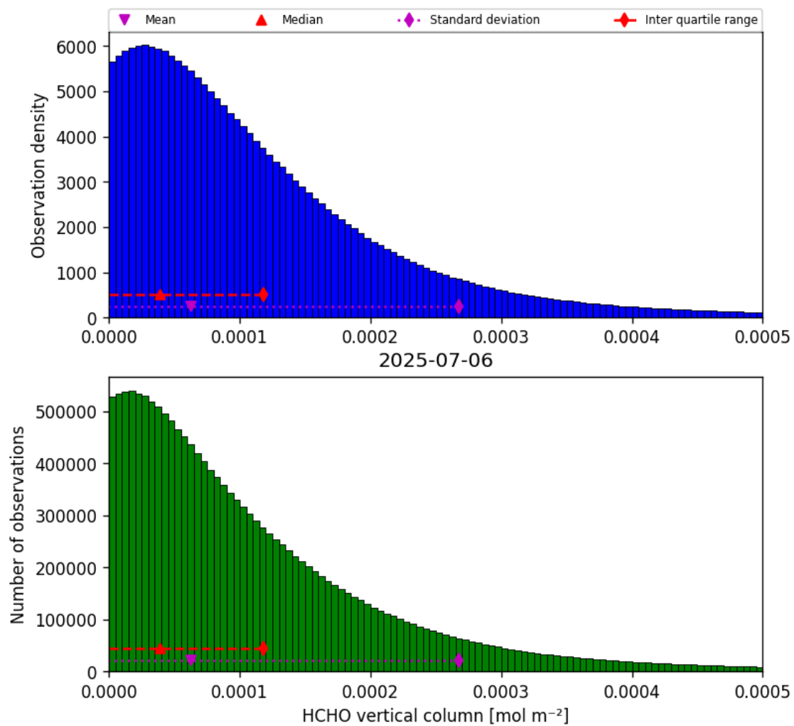
Figure 35: Histogram of “HCHO vertical column” for 2025-07-05 to 2025-07-07
