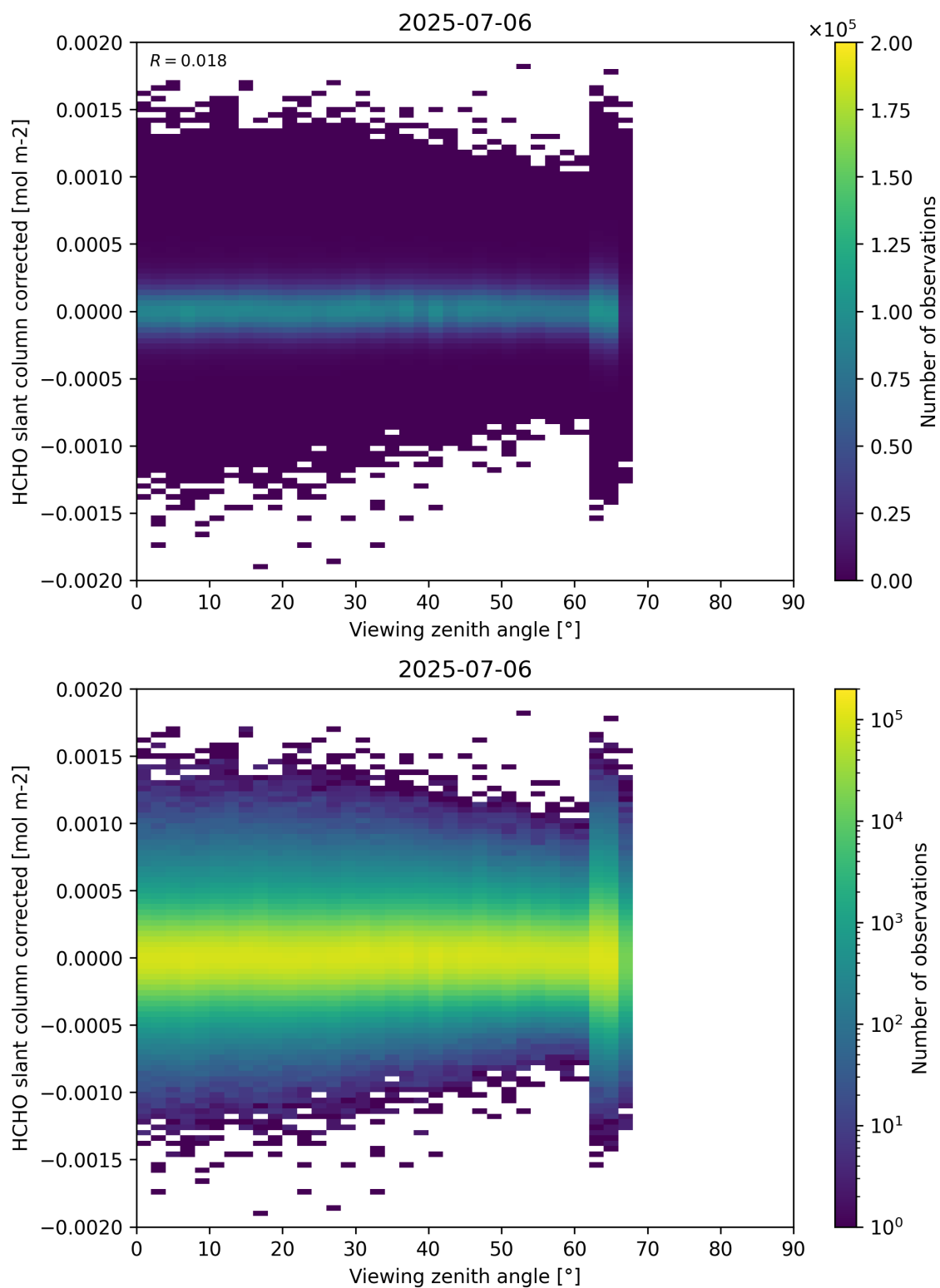
Figure 186: Scatter density plot of “Viewing zenith angle” against “HCHO slant column corrected” for 2025-07-05 to 2025-07-07.
