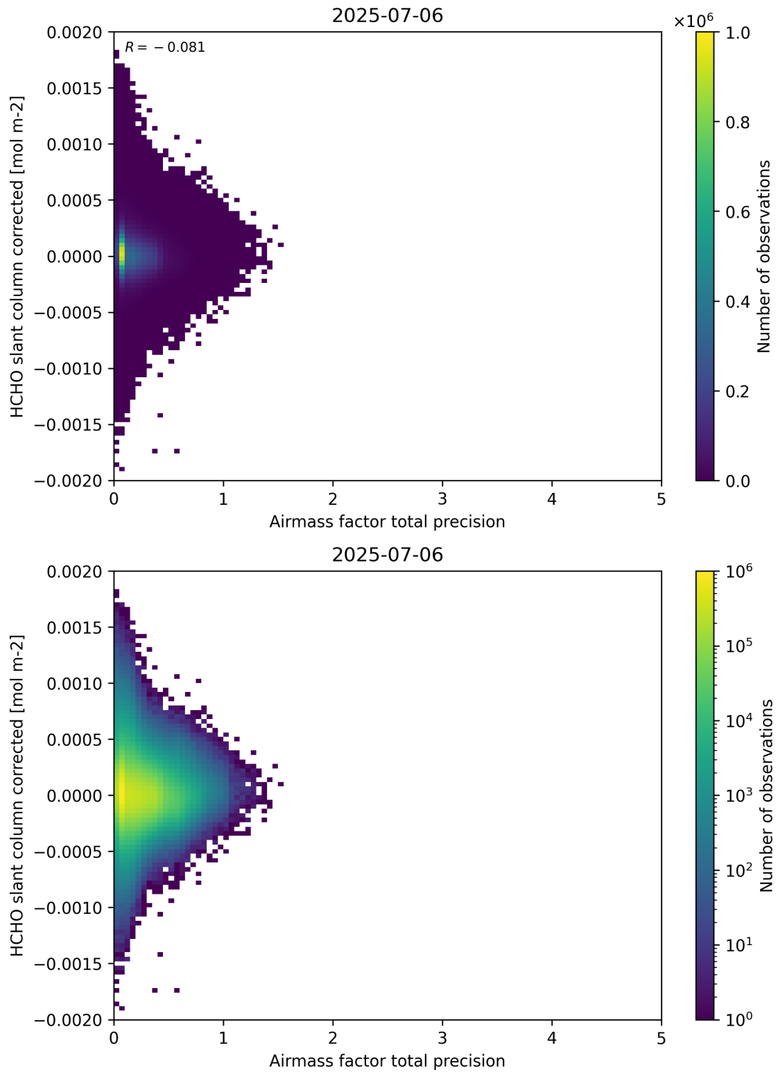
Figure 109: Scatter density plot of “Airmass factor total precision” against “HCHO slant column corrected” for 2025-07-05 to 2025-07-07.
