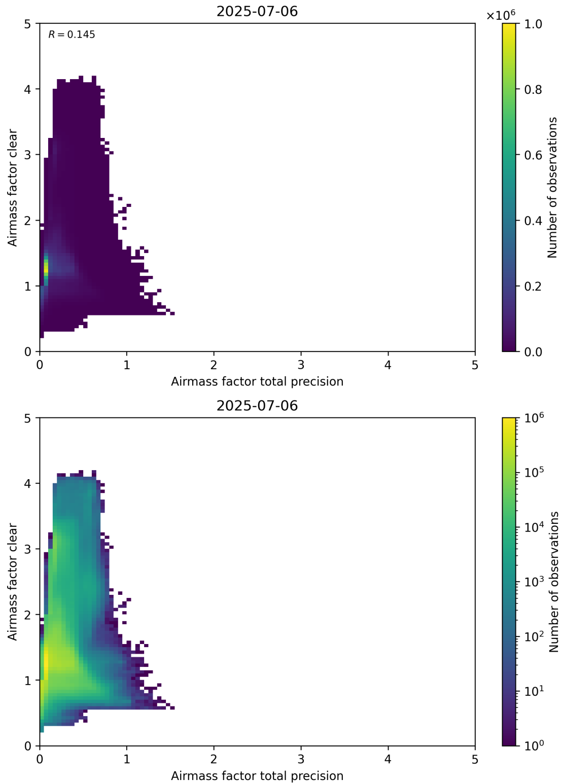
Figure 108: Scatter density plot of “Airmass factor total precision” against “Airmass factor clear” for 2025-07-05 to 2025-07-07.
