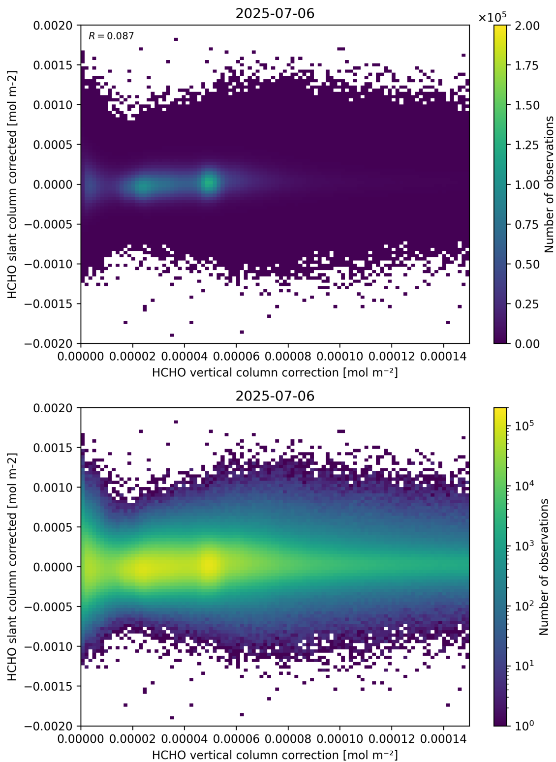
Figure 116: Scatter density plot of “HCHO vertical column correction” against “HCHO slant column corrected” for 2025-07-05 to 2025-07-07.
