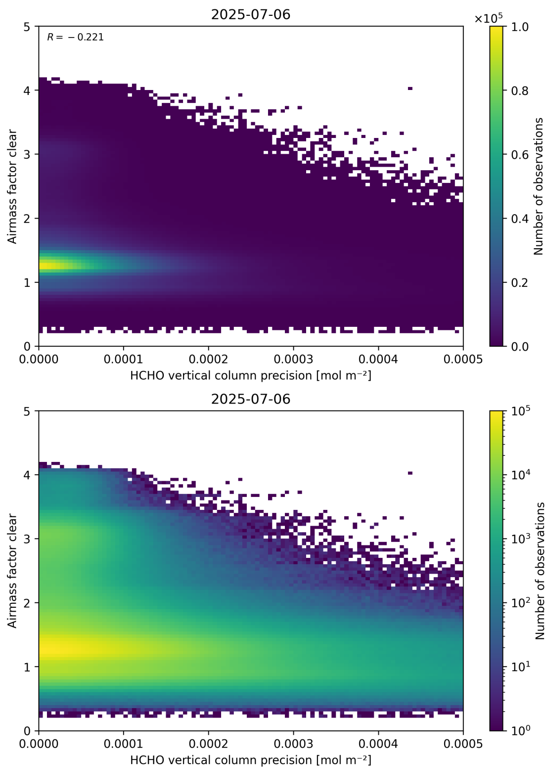
Figure 139: Scatter density plot of “HCHO vertical column precision” against “Airmass factor clear” for 2025-07-05 to 2025-07-07.
