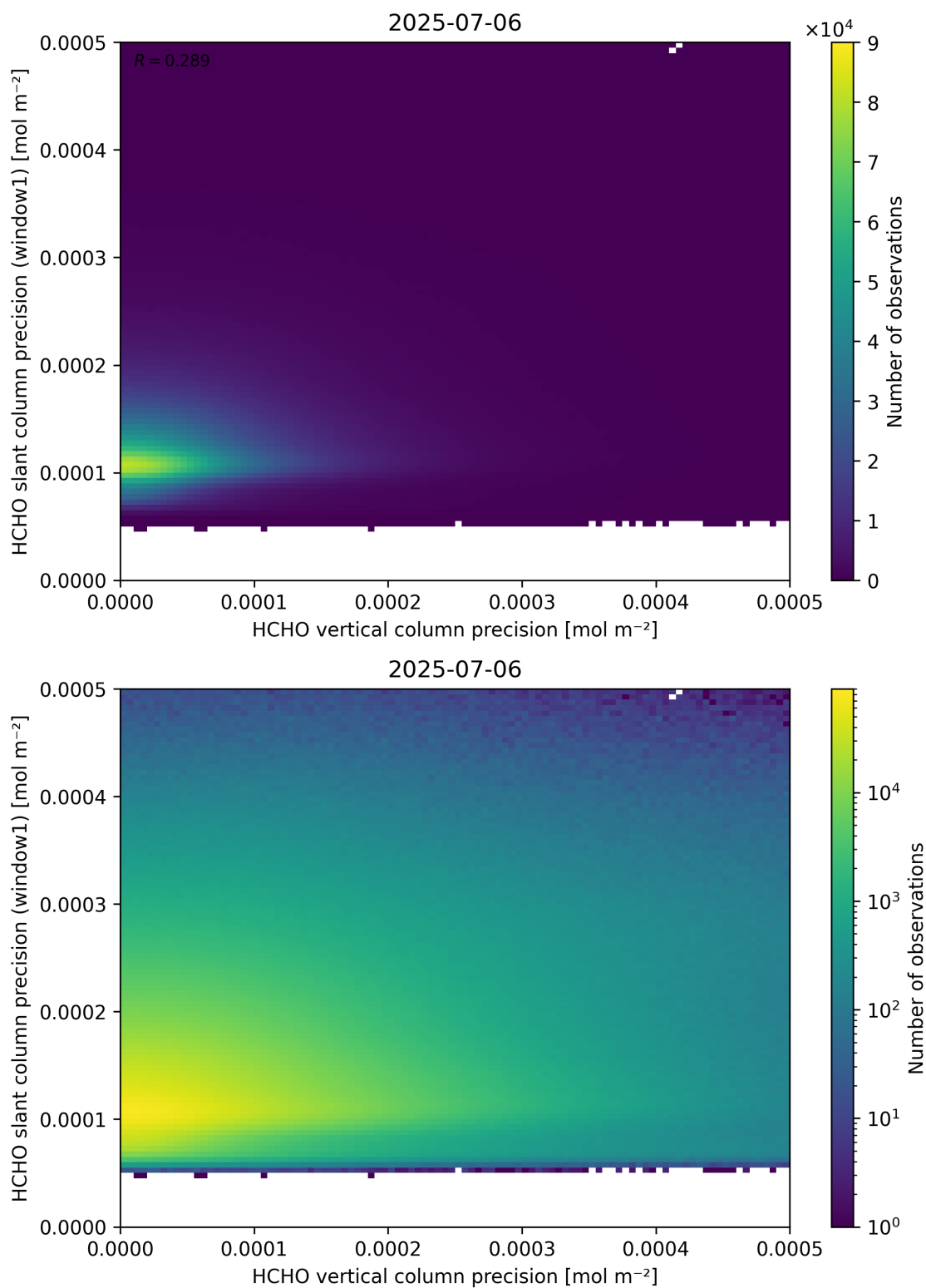
Figure 143: Scatter density plot of “HCHO vertical column precision” against “HCHO slant column precision (window1)” for 2025-07-05 to 2025-07-07.
