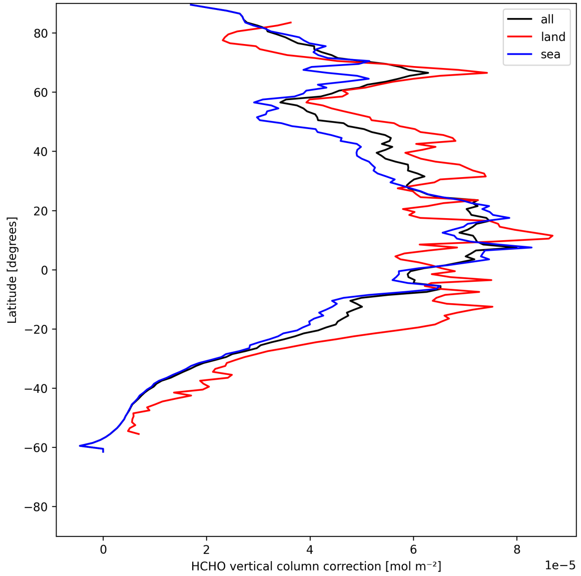
Figure 23: Zonal average of “HCHO vertical column correction” for 2025-07-05 to 2025-07-07.
