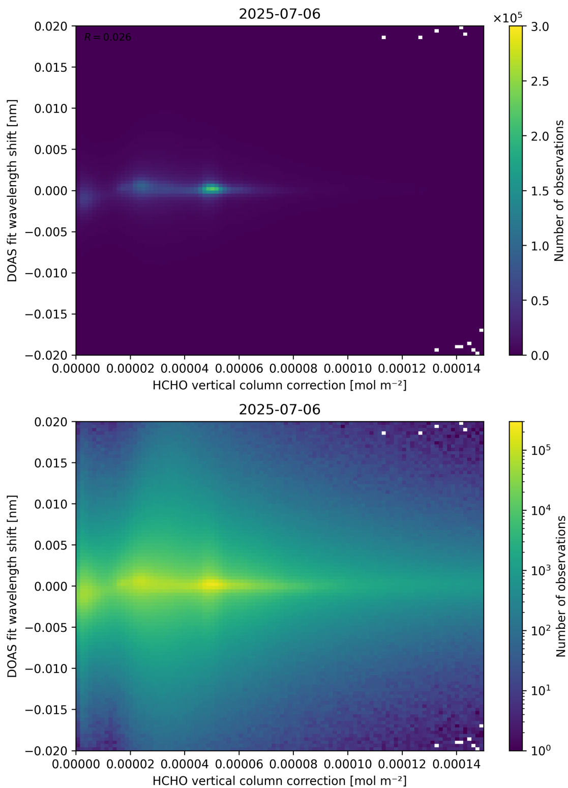
Figure 113: Scatter density plot of “HCHO vertical column correction” against “DOAS fit wavelength shift” for 2025-07-05 to 2025-07-07.
