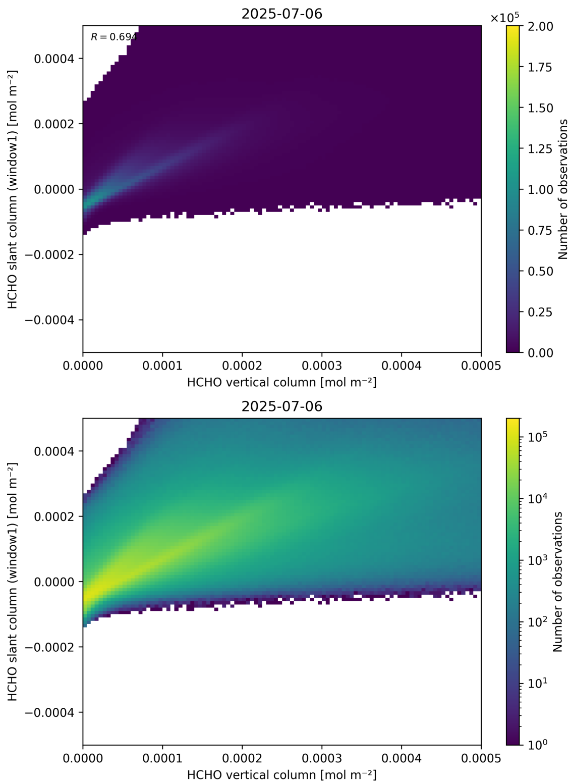
Figure 129: Scatter density plot of “HCHO vertical column” against “HCHO slant column (window1)” for 2025-07-05 to 2025-07-07.
