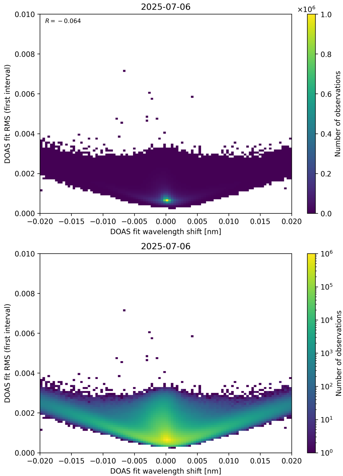
Figure 64: Scatter density plot of “DOAS fit wavelength shift” against “DOAS fit RMS (first interval)” for 2025-07-05 to 2025-07-07.
