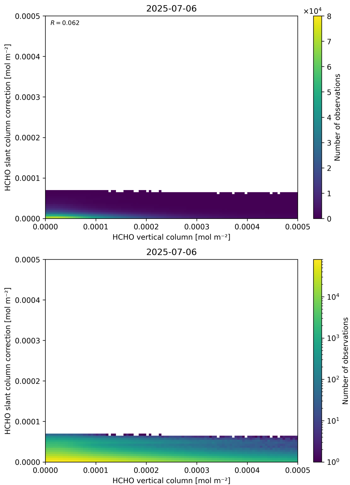
Figure 128: Scatter density plot of “HCHO vertical column” against “HCHO slant column correction” for 2025-07-05 to 2025-07-07.
