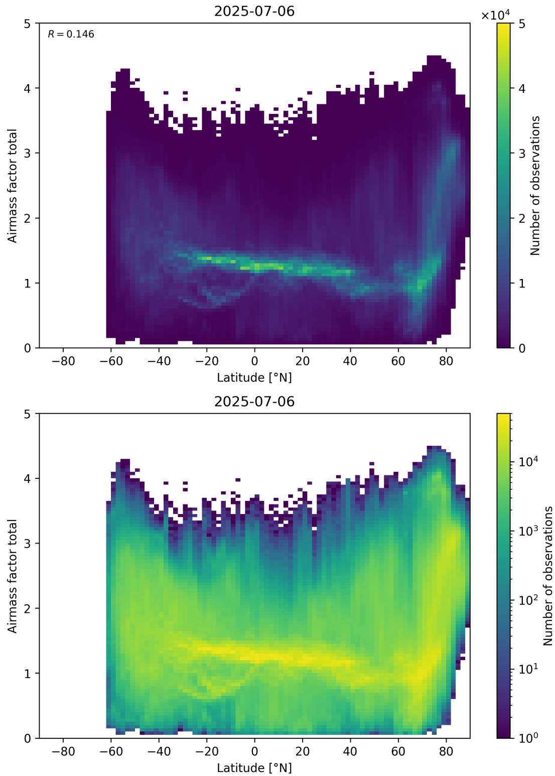
Figure 161: Scatter density plot of “Latitude” against “Airmass factor total” for 2025-07-05 to 2025-07-07.
