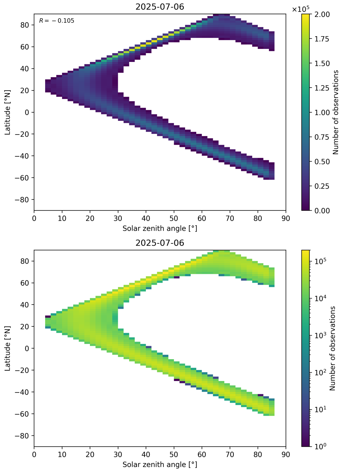
Figure 181: Scatter density plot of “Solar zenith angle” against “Latitude” for 2025-07-05 to 2025-07-07.
