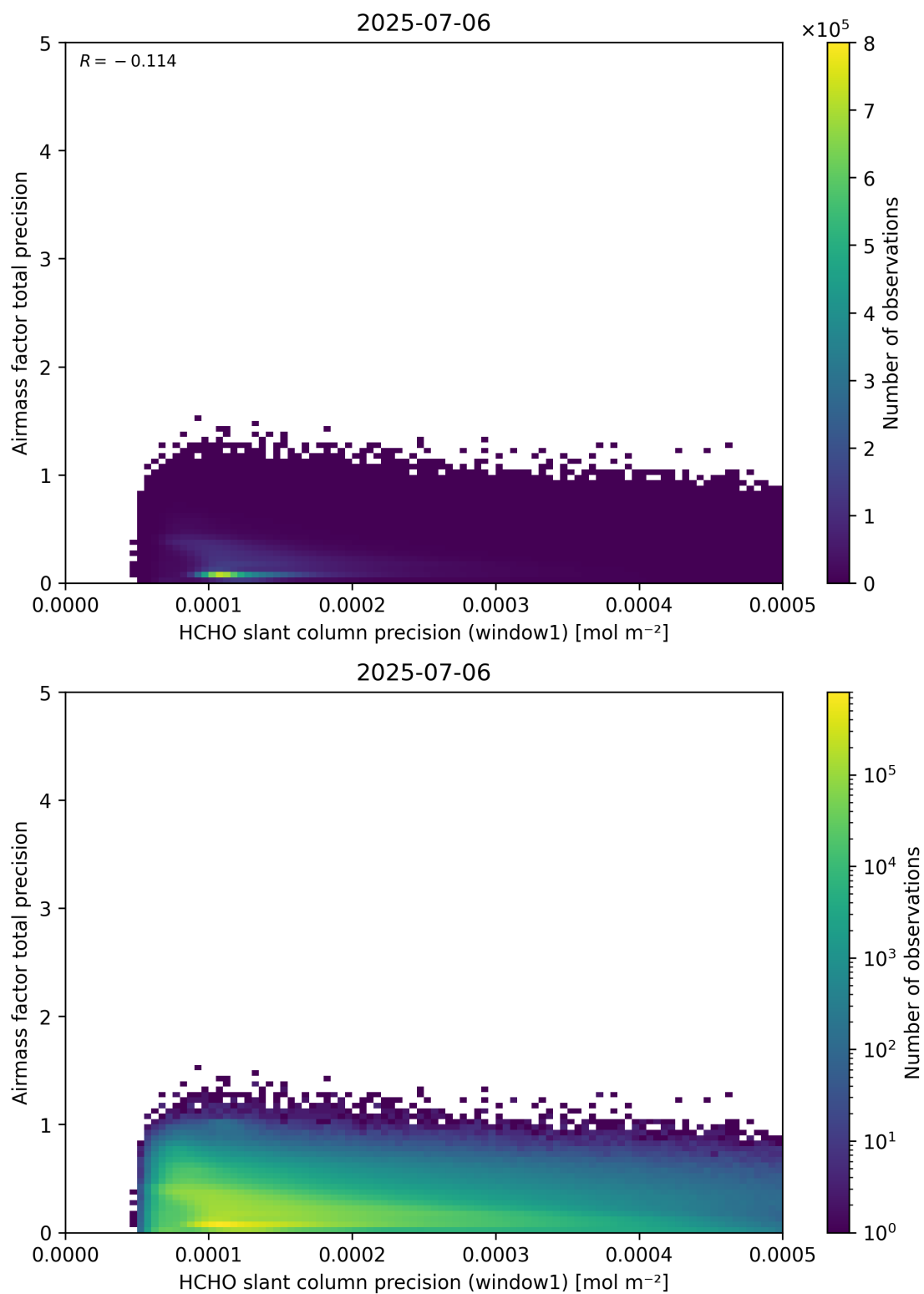
Figure 95: Scatter density plot of “HCHO slant column precision (window1)” against “Airmass factor total precision” for 2025-07-05 to 2025-07-07.
