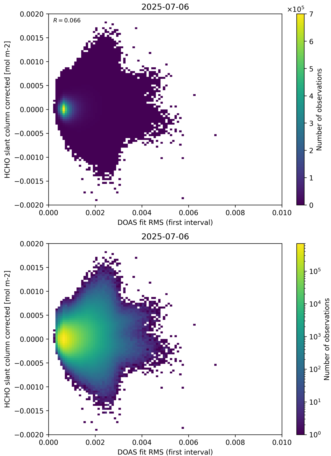
Figure 62: Scatter density plot of “DOAS fit RMS (first interval)” against “HCHO slant column corrected” for 2025-07-05 to 2025-07-07.
