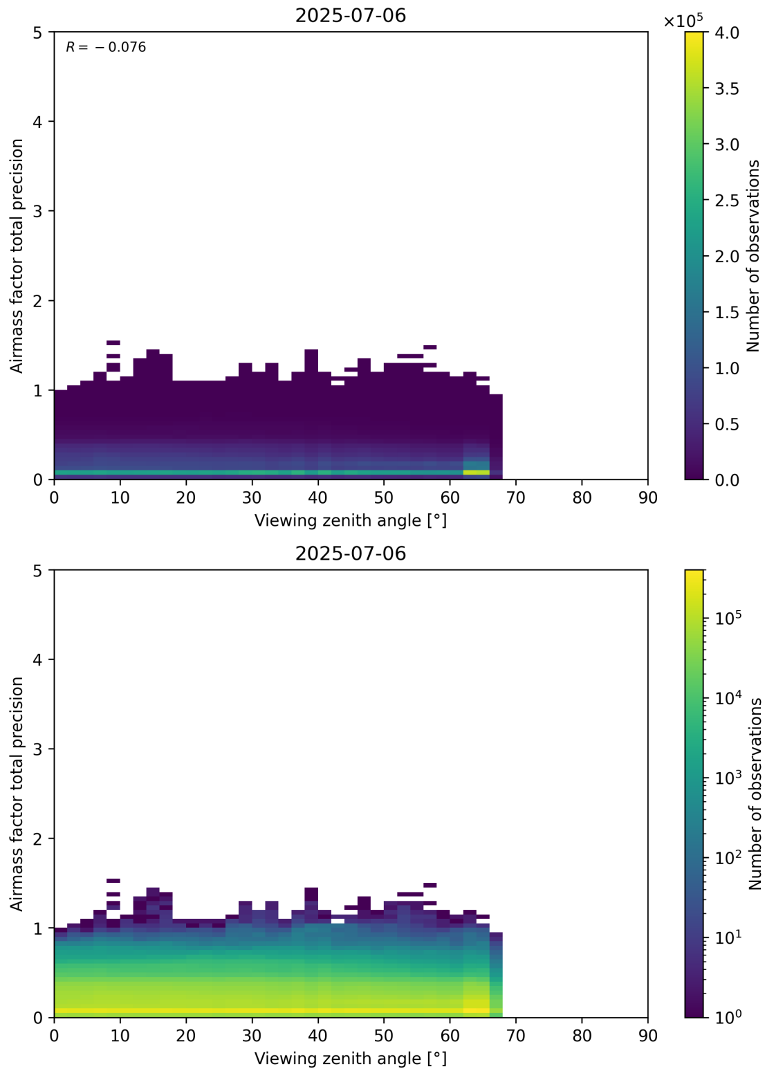
Figure 191: Scatter density plot of “Viewing zenith angle” against “Airmass factor total precision” for 2025-07-05 to 2025-07-07.
