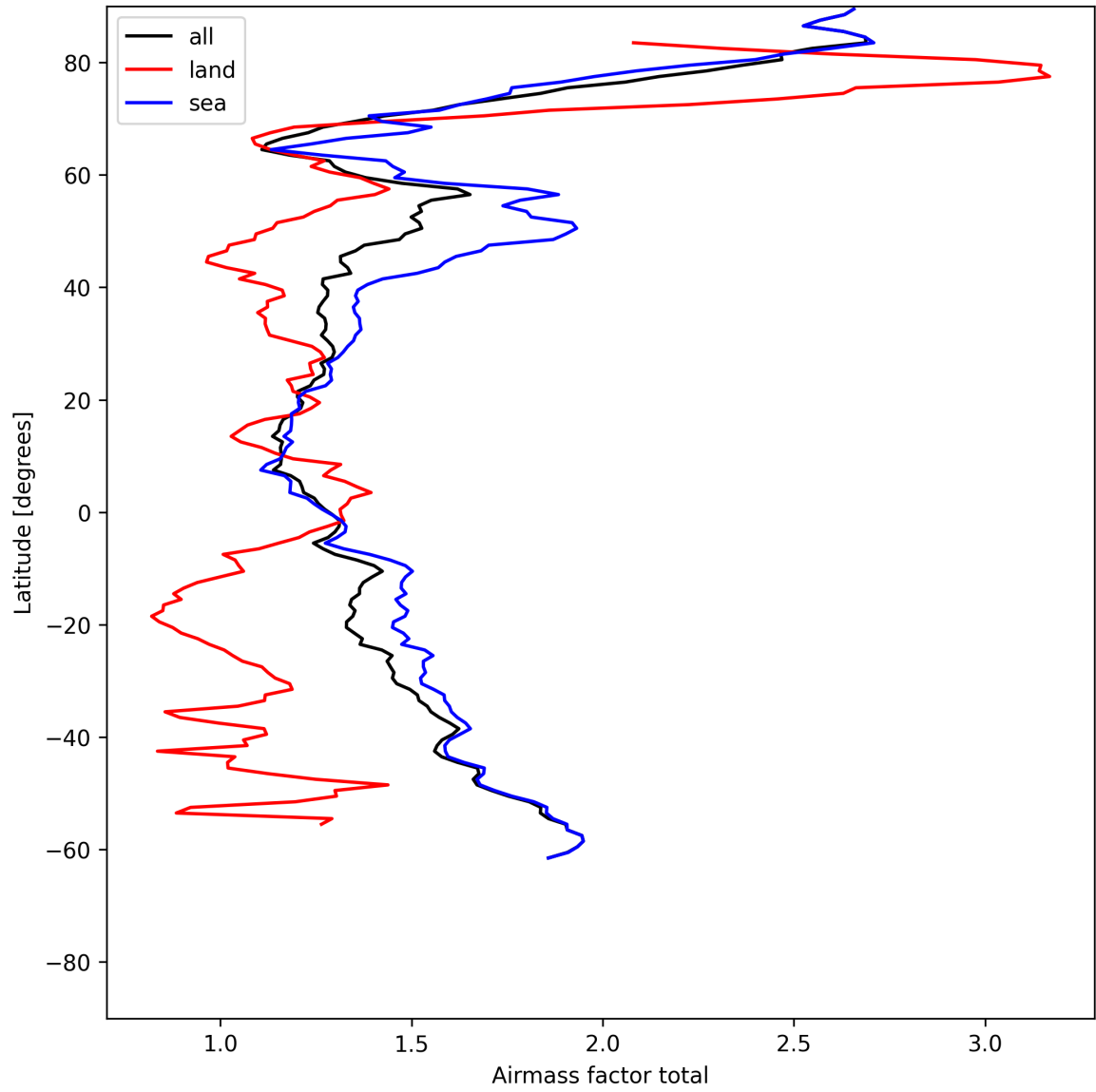
Figure 26: Zonal average of “Airmass factor total” for 2025-07-05 to 2025-07-07.
