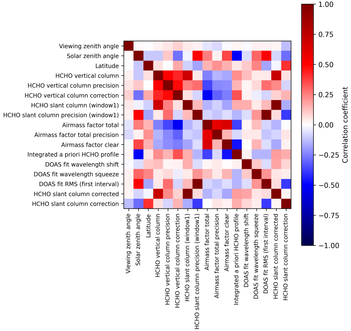
Figure 2: Map of correlation matrix for 2025-07-05 to 2025-07-07.
