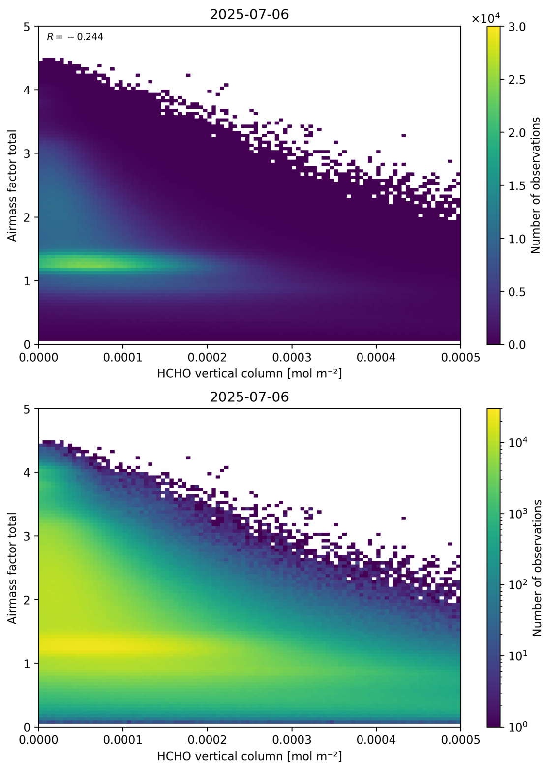
Figure 131: Scatter density plot of “HCHO vertical column” against “Airmass factor total” for 2025-07-05 to 2025-07-07.
