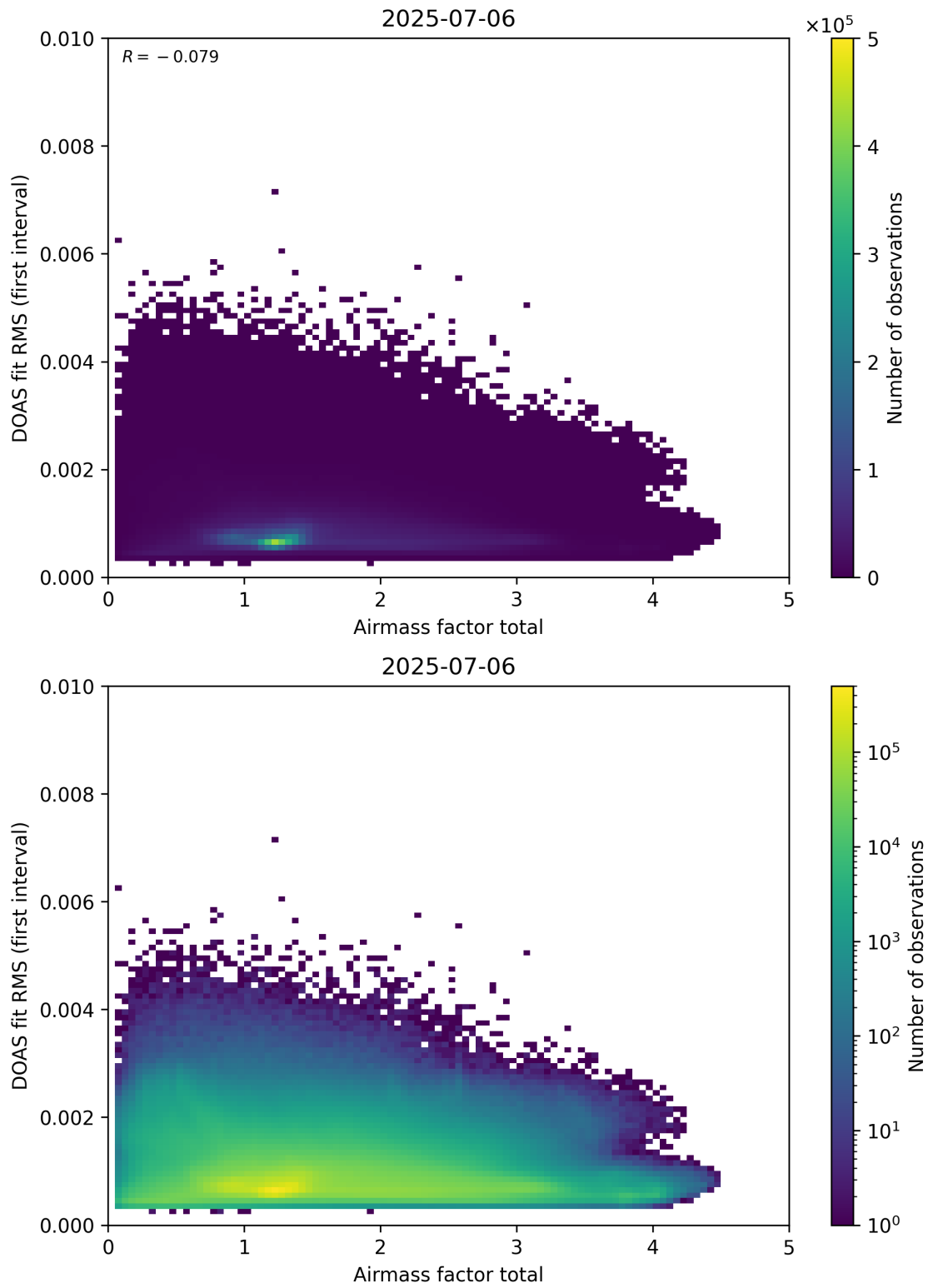
Figure 97: Scatter density plot of “Airmass factor total” against “DOAS fit RMS (first interval)” for 2025-07-05 to 2025-07-07.
