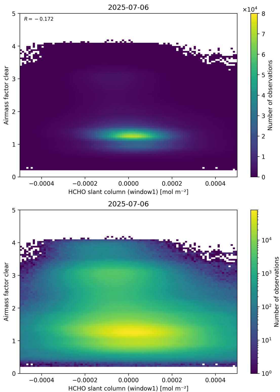
Figure 81: Scatter density plot of “HCHO slant column (window1)” against “Airmass factor clear” for 2025-07-05 to 2025-07-07.
