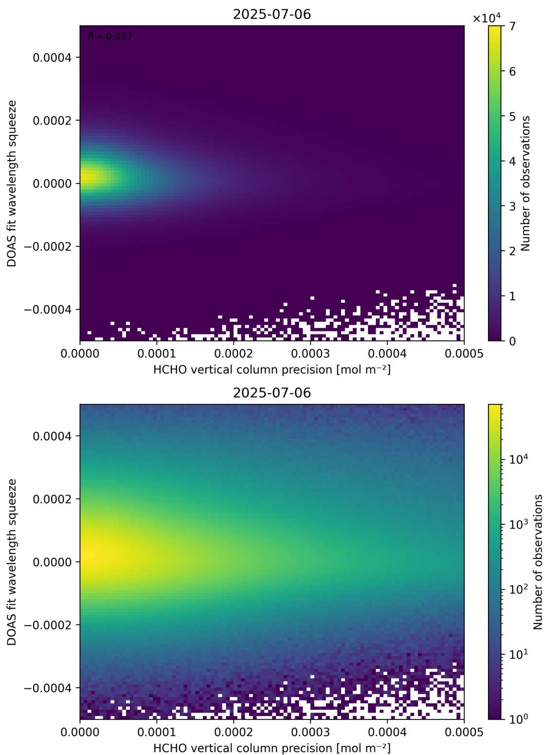
Figure 138: Scatter density plot of “HCHO vertical column precision” against “DOAS fit wavelength squeeze” for 2025-07-05 to 2025-07-07.
