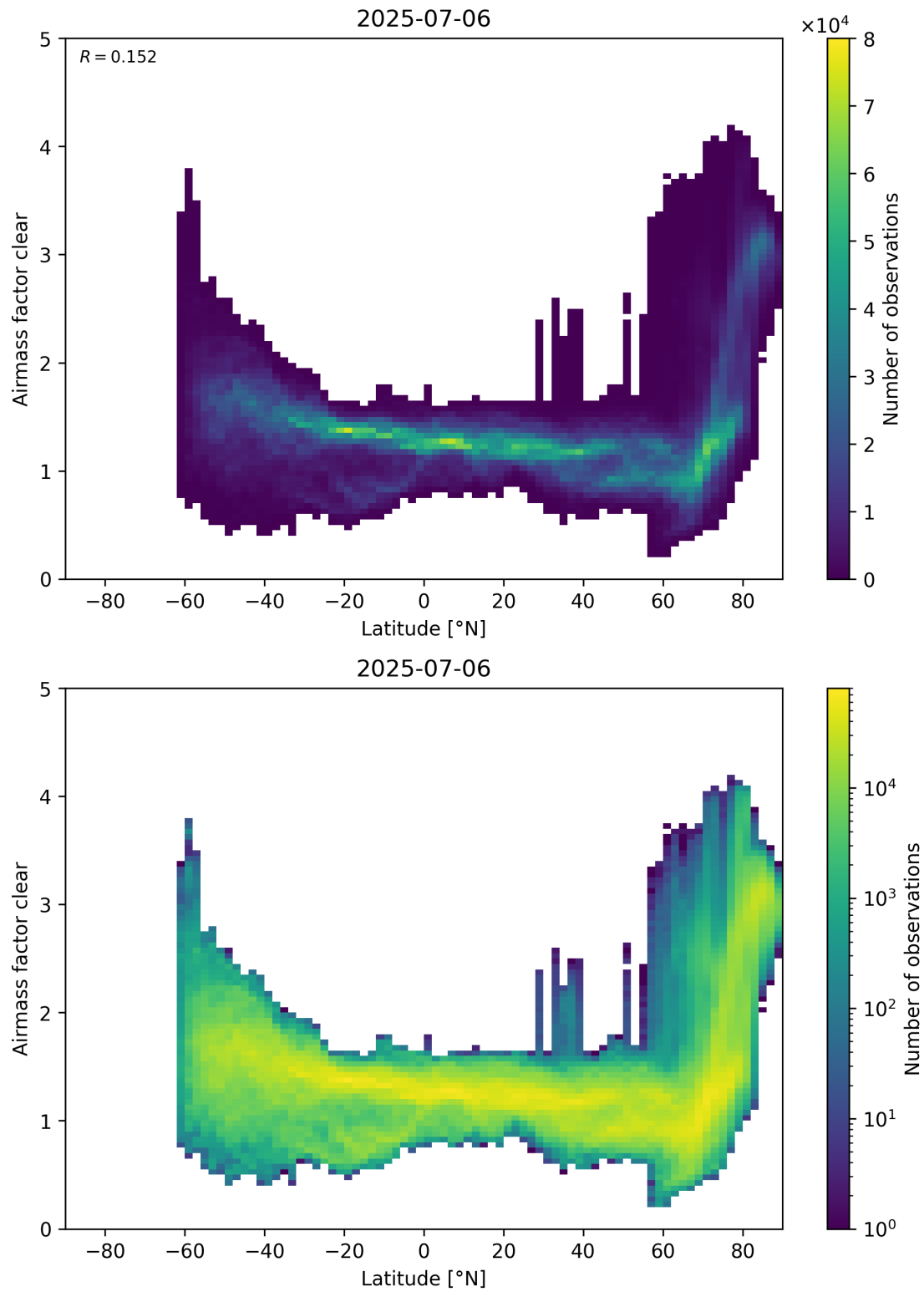
Figure 156: Scatter density plot of “Latitude” against “Airmass factor clear” for 2025-07-05 to 2025-07-07.
