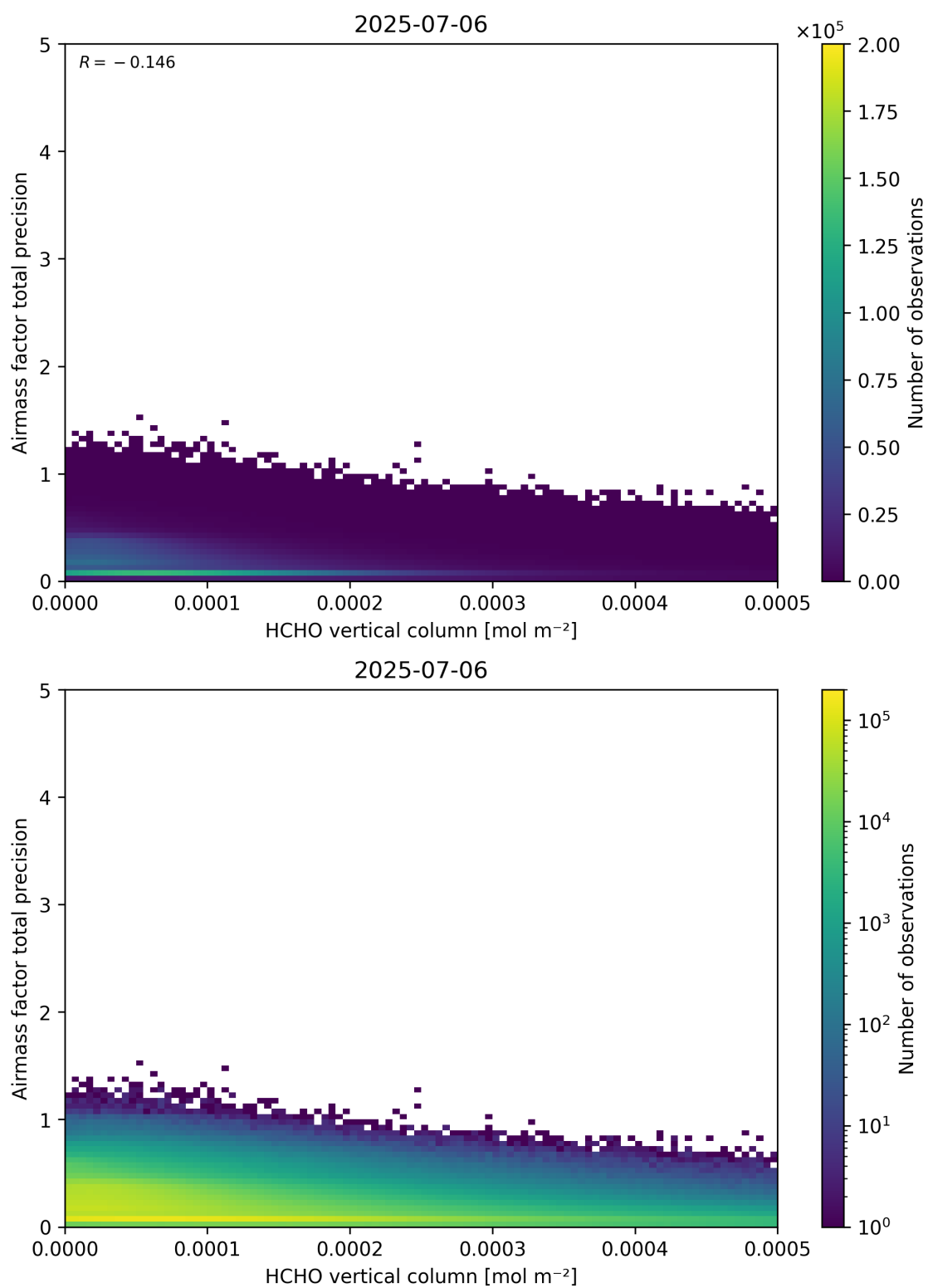
Figure 132: Scatter density plot of “HCHO vertical column” against “Airmass factor total precision” for 2025-07-05 to 2025-07-07.
