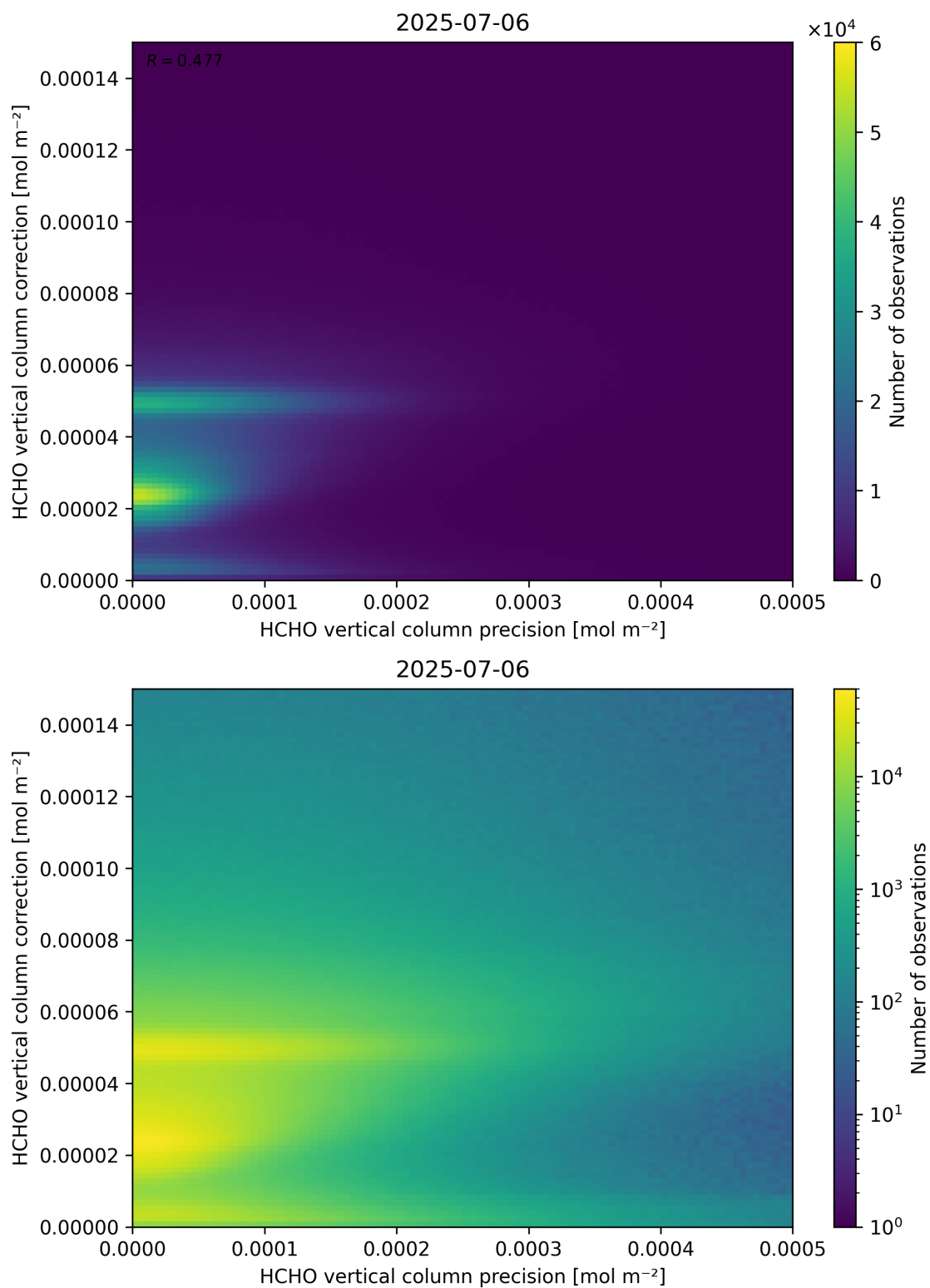
Figure 146: Scatter density plot of “HCHO vertical column precision” against “HCHO vertical column correction” for 2025-07-05 to 2025-07-07.
