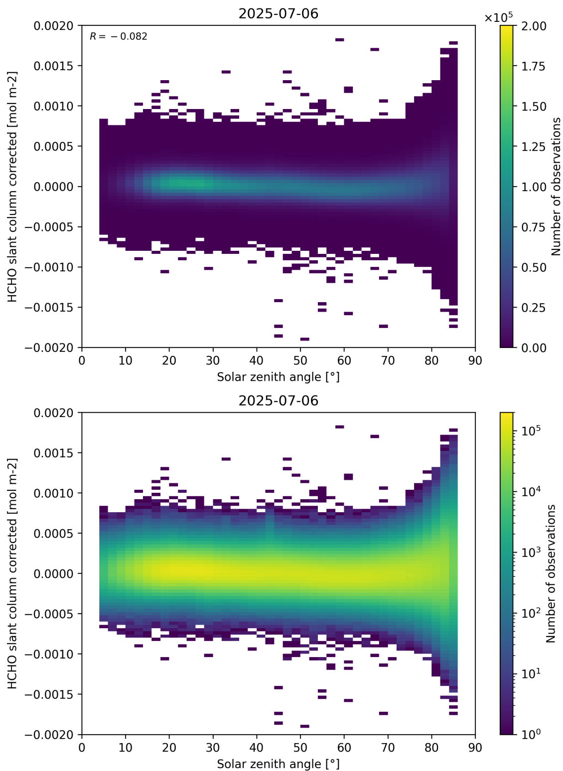
Figure 171: Scatter density plot of “Solar zenith angle” against “HCHO slant column corrected” for 2025-07-05 to 2025-07-07.
