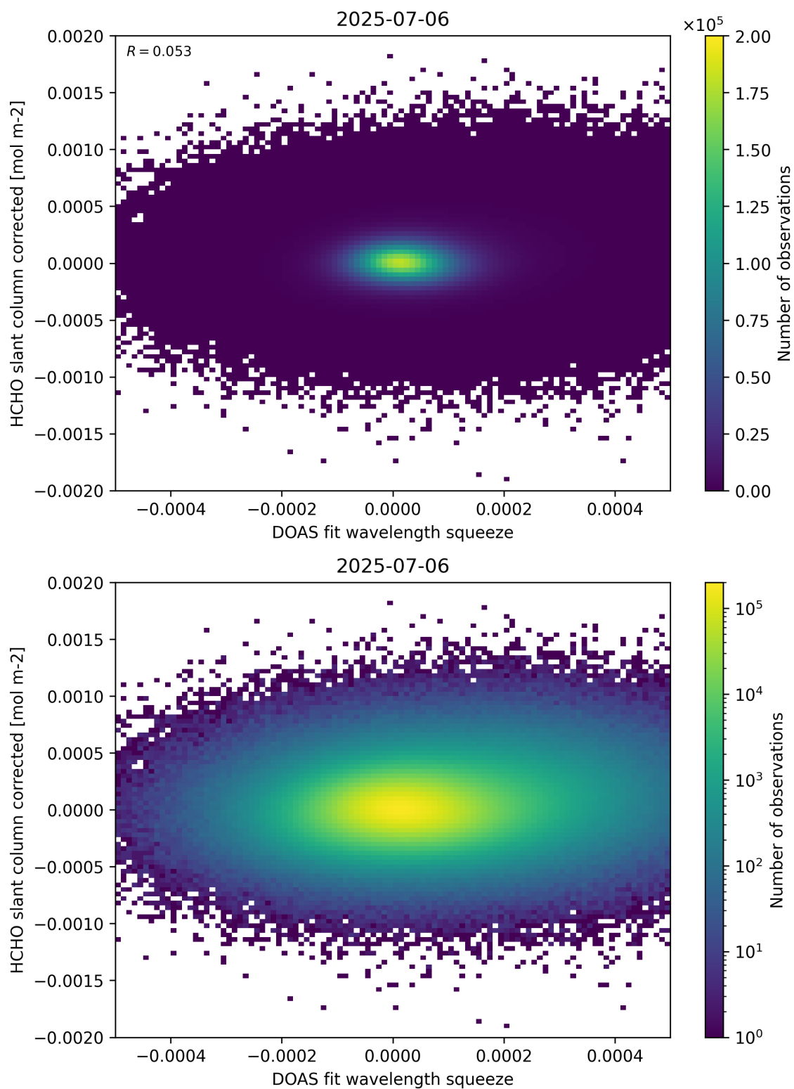
Figure 69: Scatter density plot of “DOAS fit wavelength squeeze” against “HCHO slant column corrected” for 2025-07-05 to 2025-07-07.
