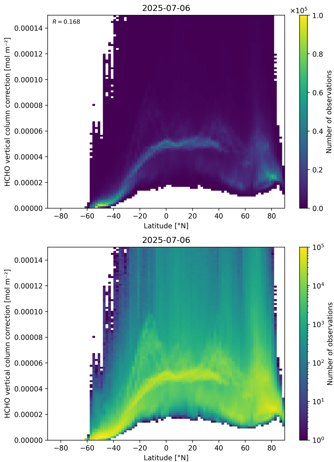
Figure 164: Scatter density plot of “Latitude” against “HCHO vertical column correction” for 2025-07-05 to 2025-07-07.
