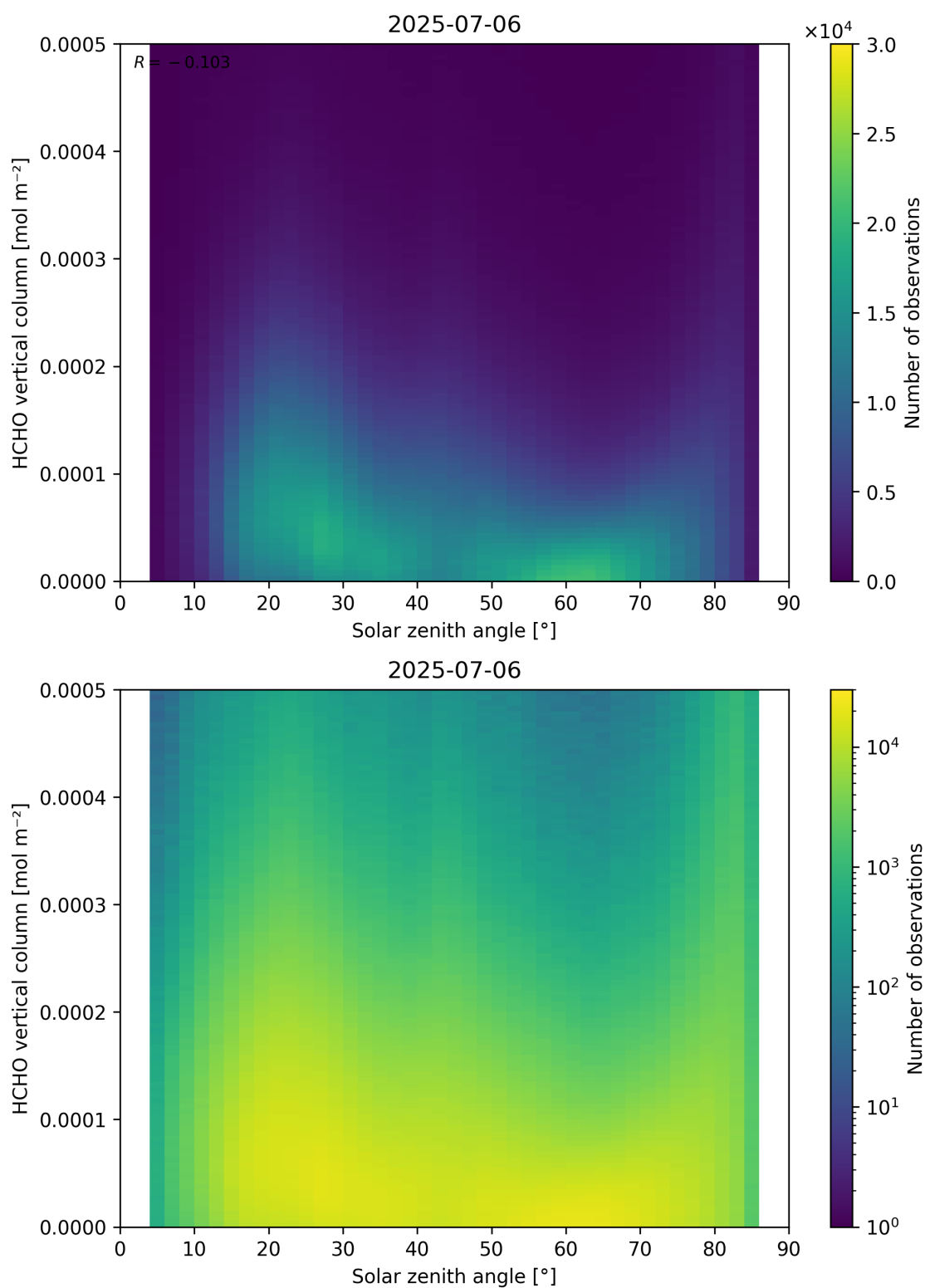
Figure 177: Scatter density plot of “Solar zenith angle” against “HCHO vertical column” for 2025-07-05 to 2025-07-07.
