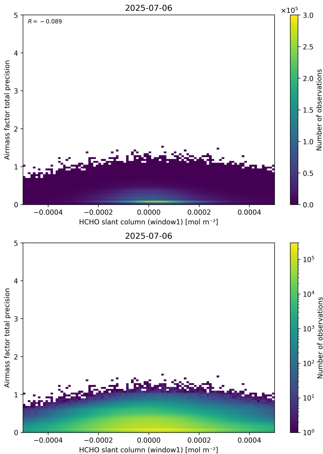
Figure 86: Scatter density plot of “HCHO slant column (window1)” against “Airmass factor total precision” for 2025-07-05 to 2025-07-07.
