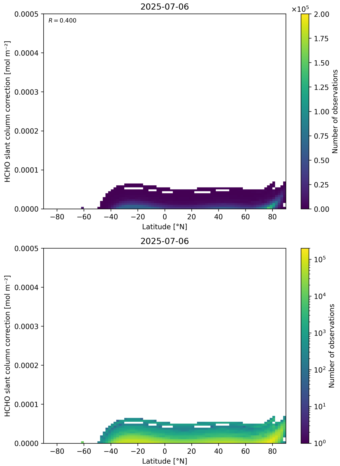
Figure 158: Scatter density plot of “Latitude” against “HCHO slant column correction” for 2025-07-05 to 2025-07-07.
