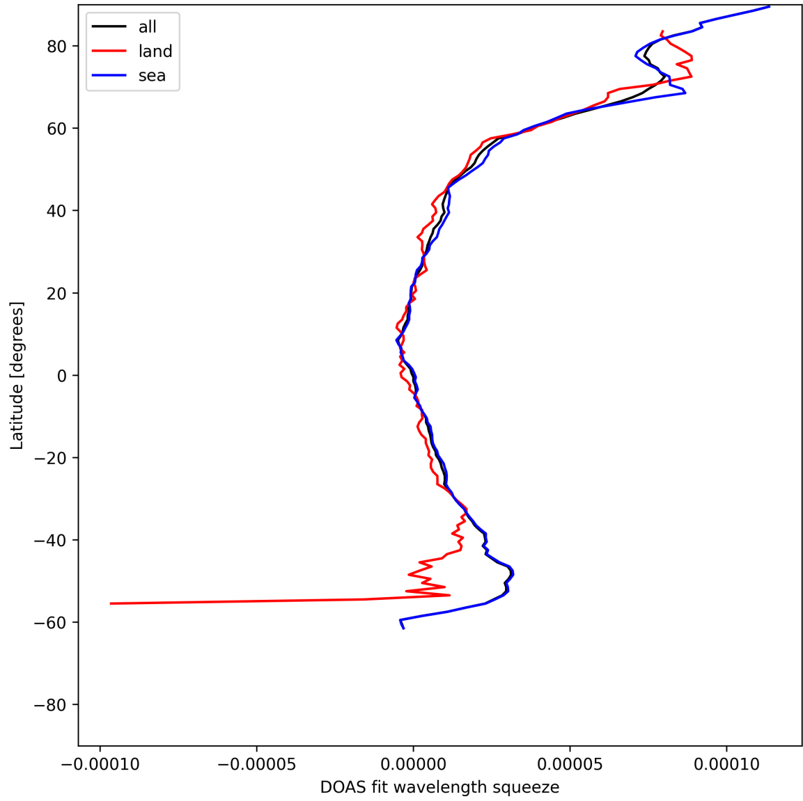
Figure 31: Zonal average of “DOAS fit wavelength squeeze” for 2025-07-05 to 2025-07-07.
