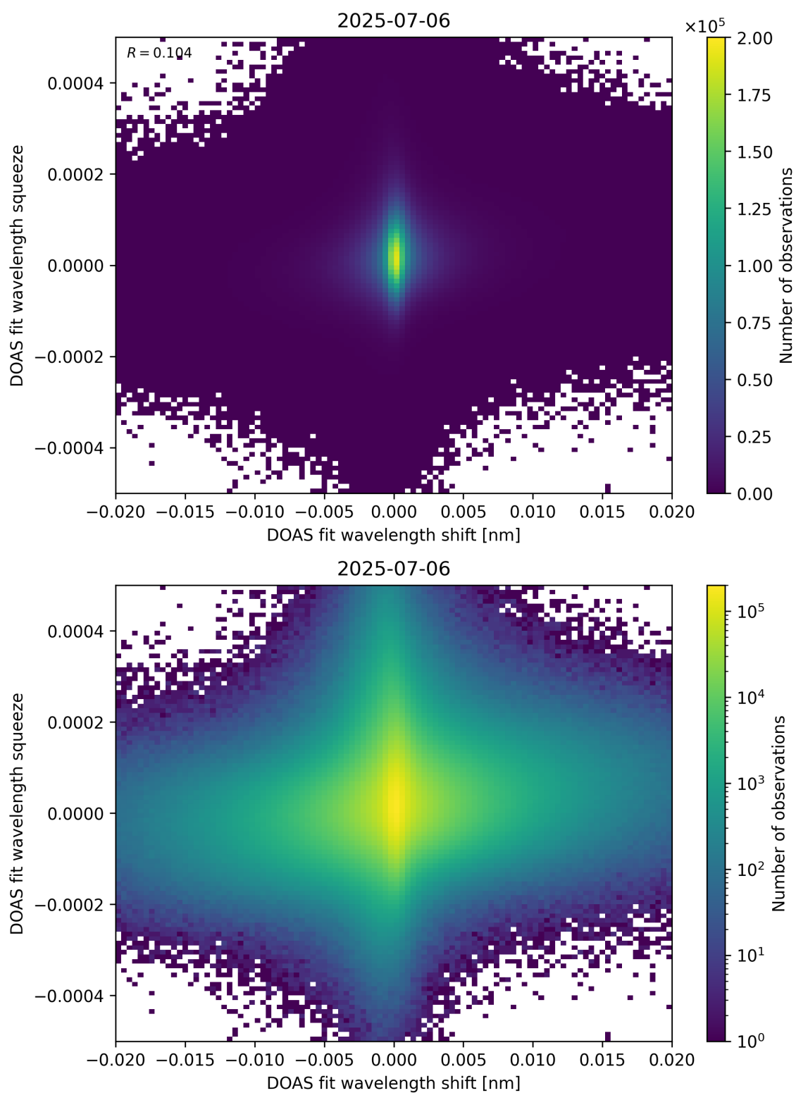
Figure 65: Scatter density plot of “DOAS fit wavelength shift” against “DOAS fit wavelength squeeze” for 2025-07-05 to 2025-07-07.
