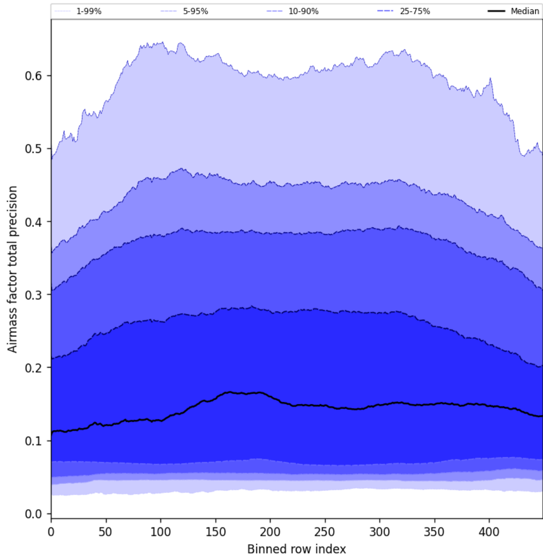
Figure 55: Along track statistics of “Airmass factor total precision” for 2025-07-05 to 2025-07-07
