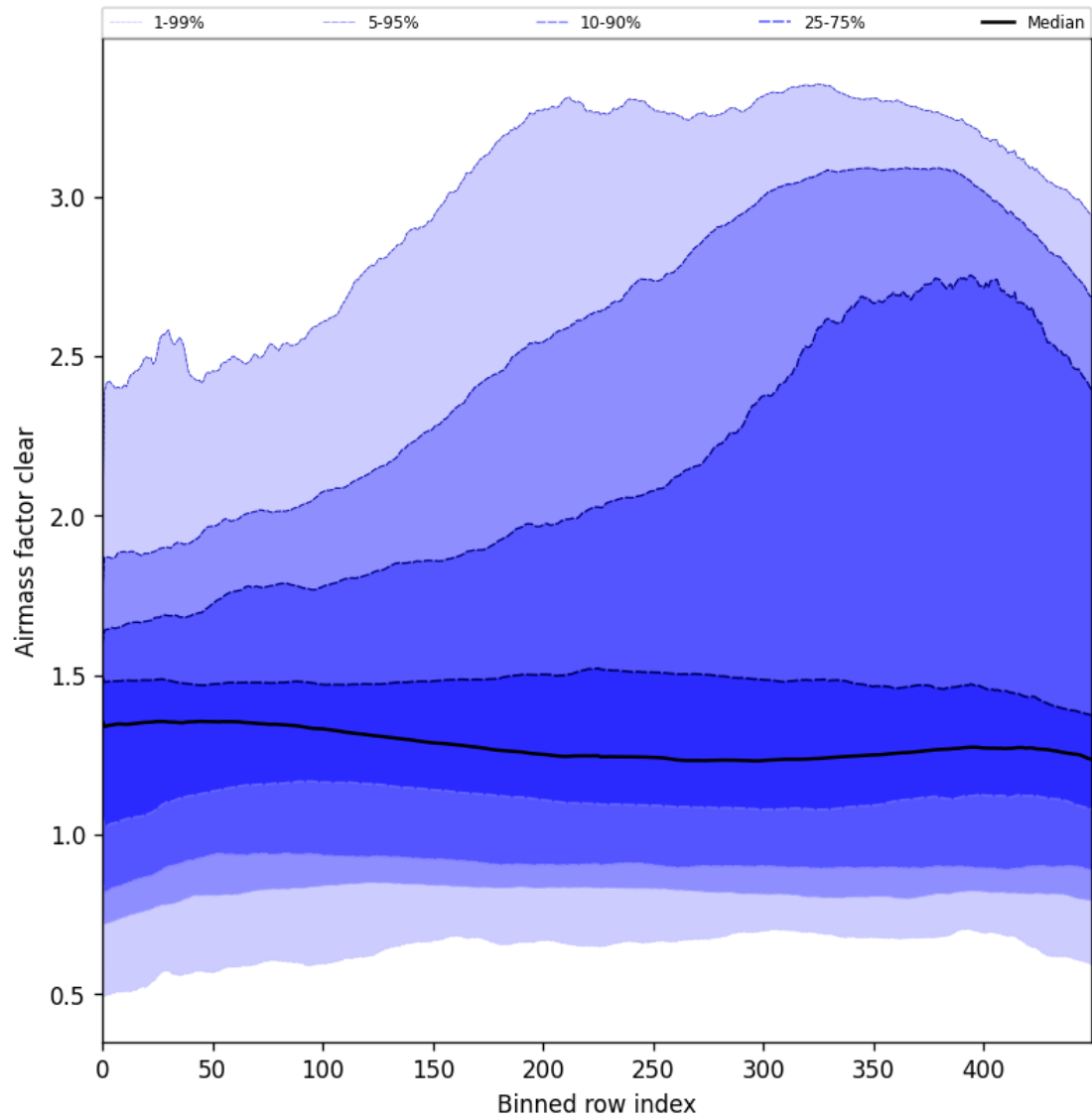
Figure 56: Along track statistics of “Airmass factor clear” for 2025-07-05 to 2025-07-07
