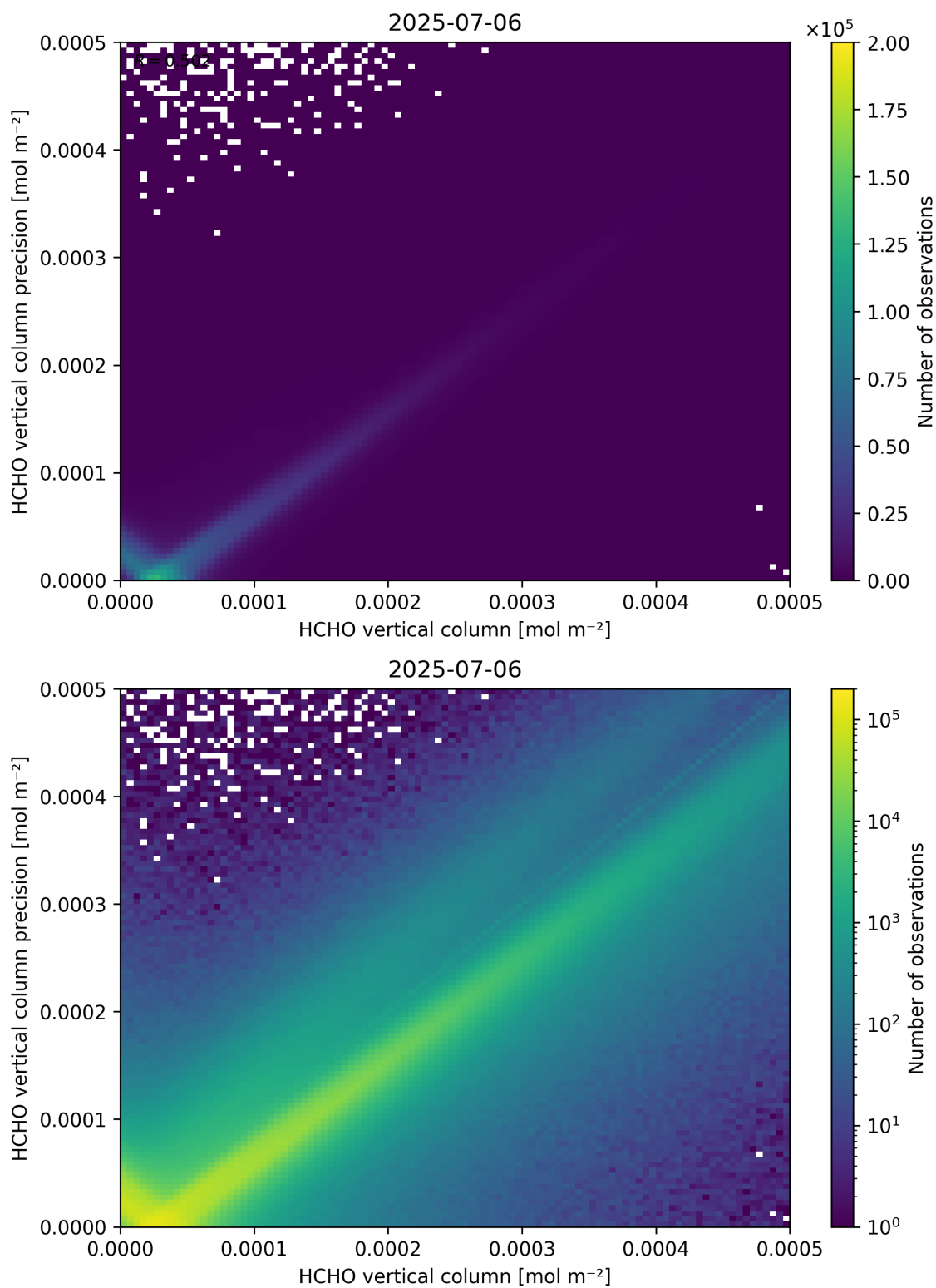
Figure 134: Scatter density plot of “HCHO vertical column” against “HCHO vertical column precision” for 2025-07-05 to 2025-07-07.
