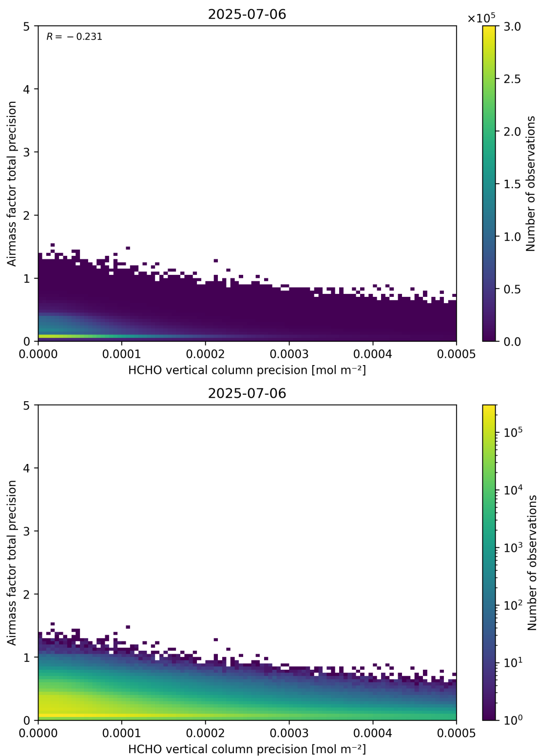
Figure 145: Scatter density plot of “HCHO vertical column precision” against “Airmass factor total precision” for 2025-07-05 to 2025-07-07.
