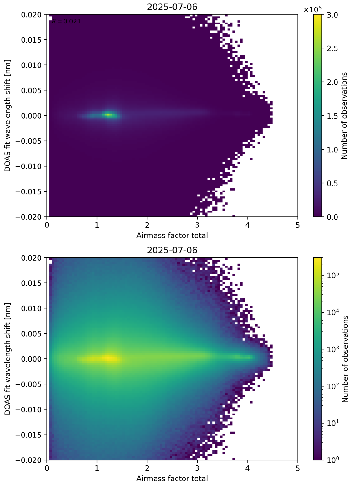
Figure 98: Scatter density plot of “Airmass factor total” against “DOAS fit wavelength shift” for 2025-07-05 to 2025-07-07.
