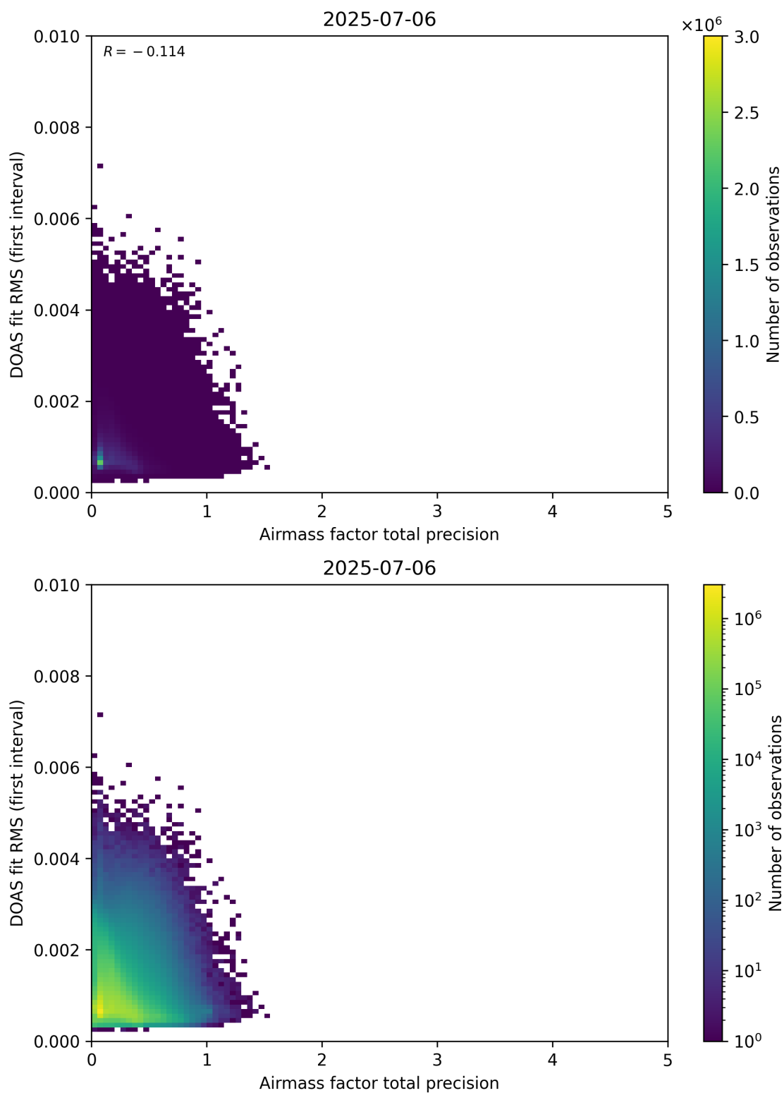
Figure 105: Scatter density plot of “Airmass factor total precision” against “DOAS fit RMS (first interval)” for 2025-07-05 to 2025-07-07.
