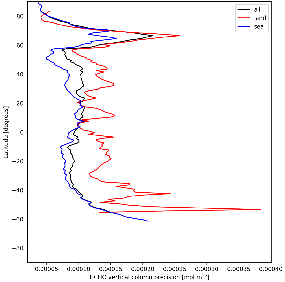
Figure 22: Zonal average of “HCHO vertical column precision” for 2025-07-05 to 2025-07-07.
