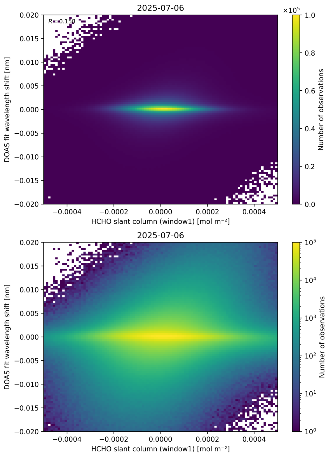
Figure 79: Scatter density plot of “HCHO slant column (window1)” against “DOAS fit wavelength shift” for 2025-07-05 to 2025-07-07.
