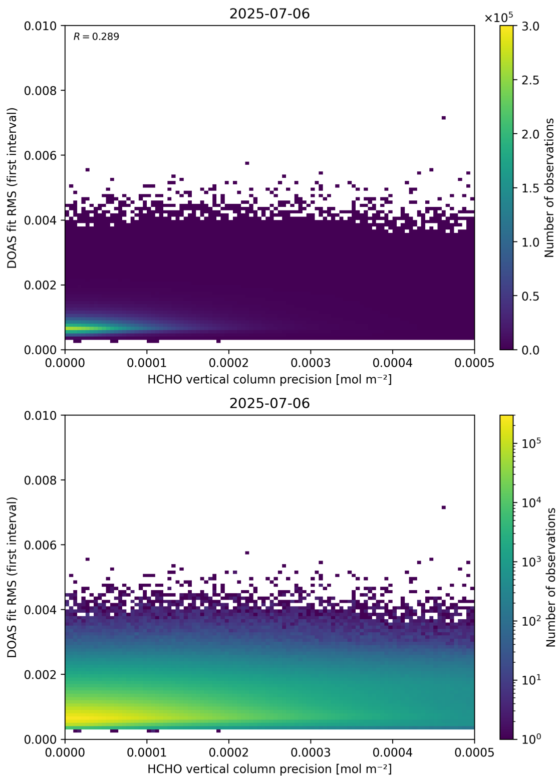
Figure 136: Scatter density plot of “HCHO vertical column precision” against “DOAS fit RMS (first interval)” for 2025-07-05 to 2025-07-07.
