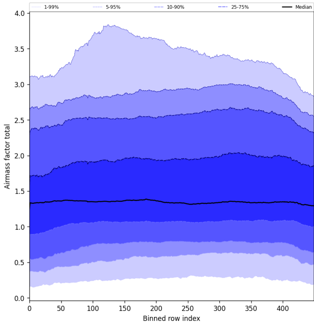
Figure 54: Along track statistics of “Airmass factor total” for 2025-07-05 to 2025-07-07
