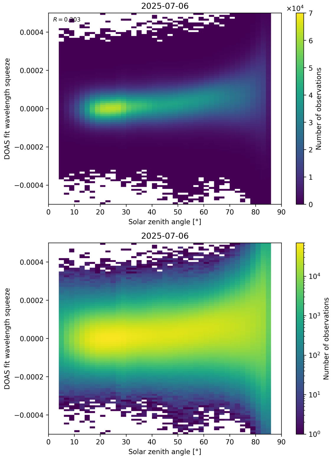
Figure 169: Scatter density plot of “Solar zenith angle” against “DOAS fit wavelength squeeze” for 2025-07-05 to 2025-07-07.
