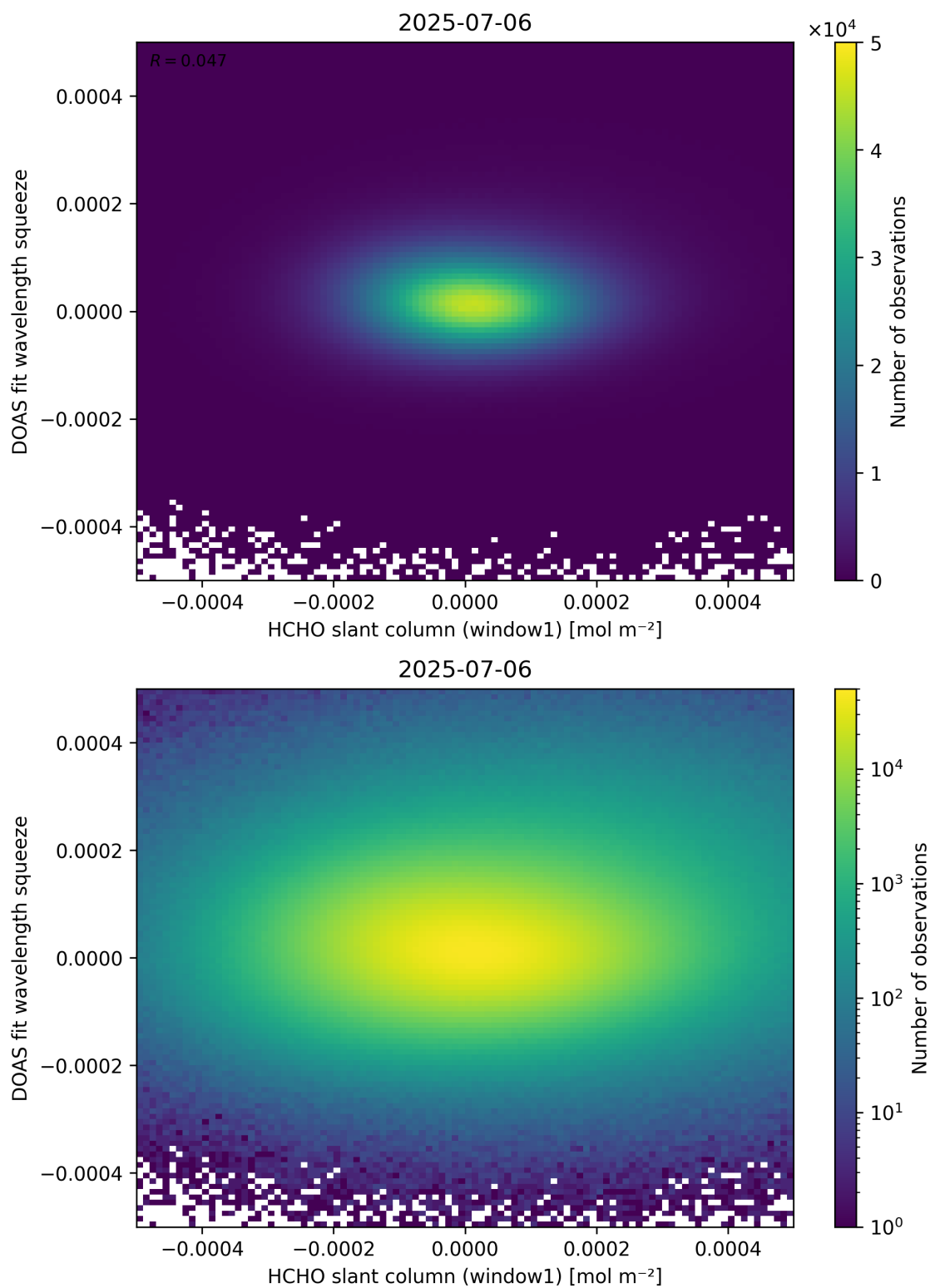
Figure 80: Scatter density plot of “HCHO slant column (window1)” against “DOAS fit wavelength squeeze” for 2025-07-05 to 2025-07-07.
