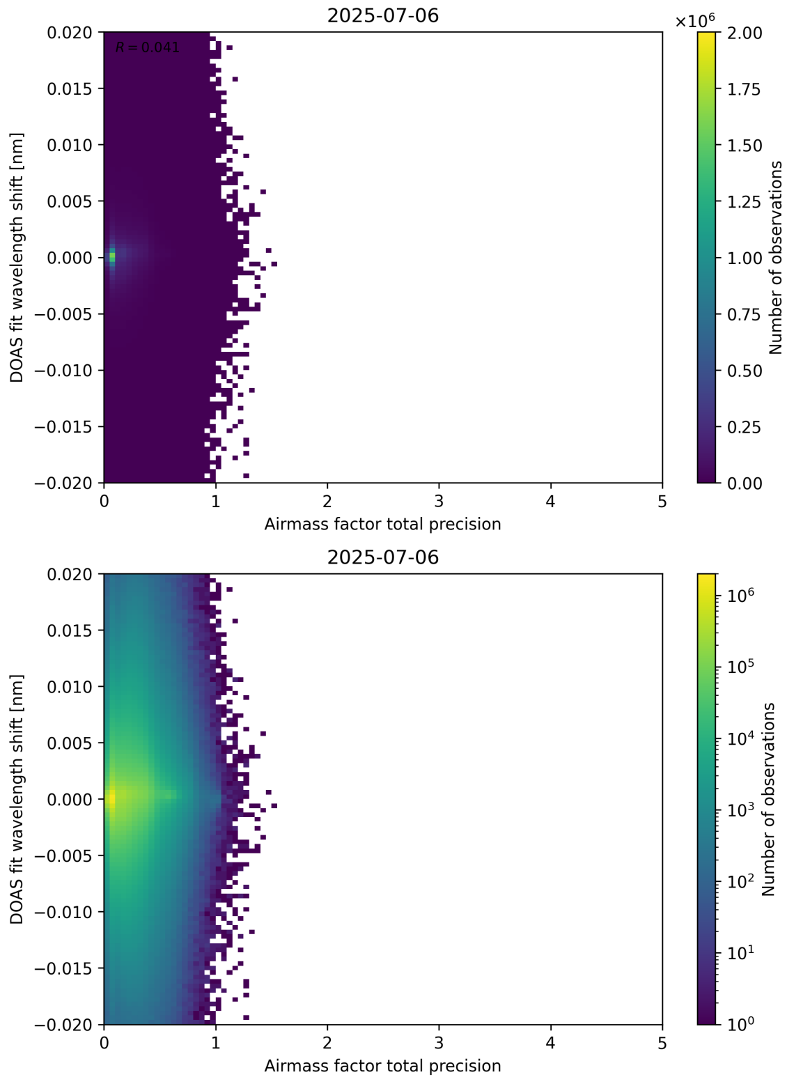
Figure 106: Scatter density plot of “Airmass factor total precision” against “DOAS fit wavelength shift” for 2025-07-05 to 2025-07-07.
