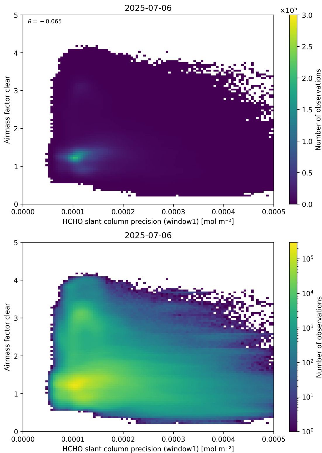
Figure 91: Scatter density plot of “HCHO slant column precision (window1)” against “Airmass factor clear” for 2025-07-05 to 2025-07-07.
