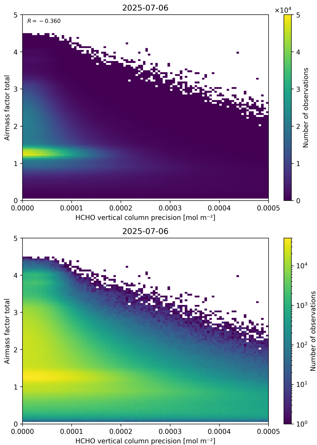
Figure 144: Scatter density plot of “HCHO vertical column precision” against “Airmass factor total” for 2025-07-05 to 2025-07-07.
