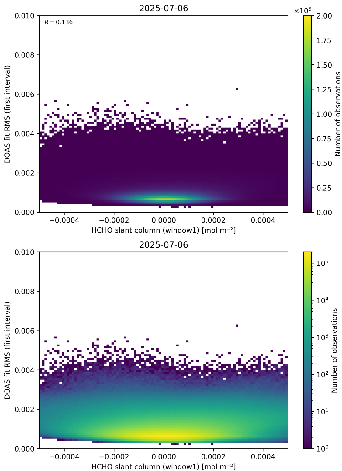
Figure 78: Scatter density plot of “HCHO slant column (window1)” against “DOAS fit RMS (first interval)” for 2025-07-05 to 2025-07-07.
