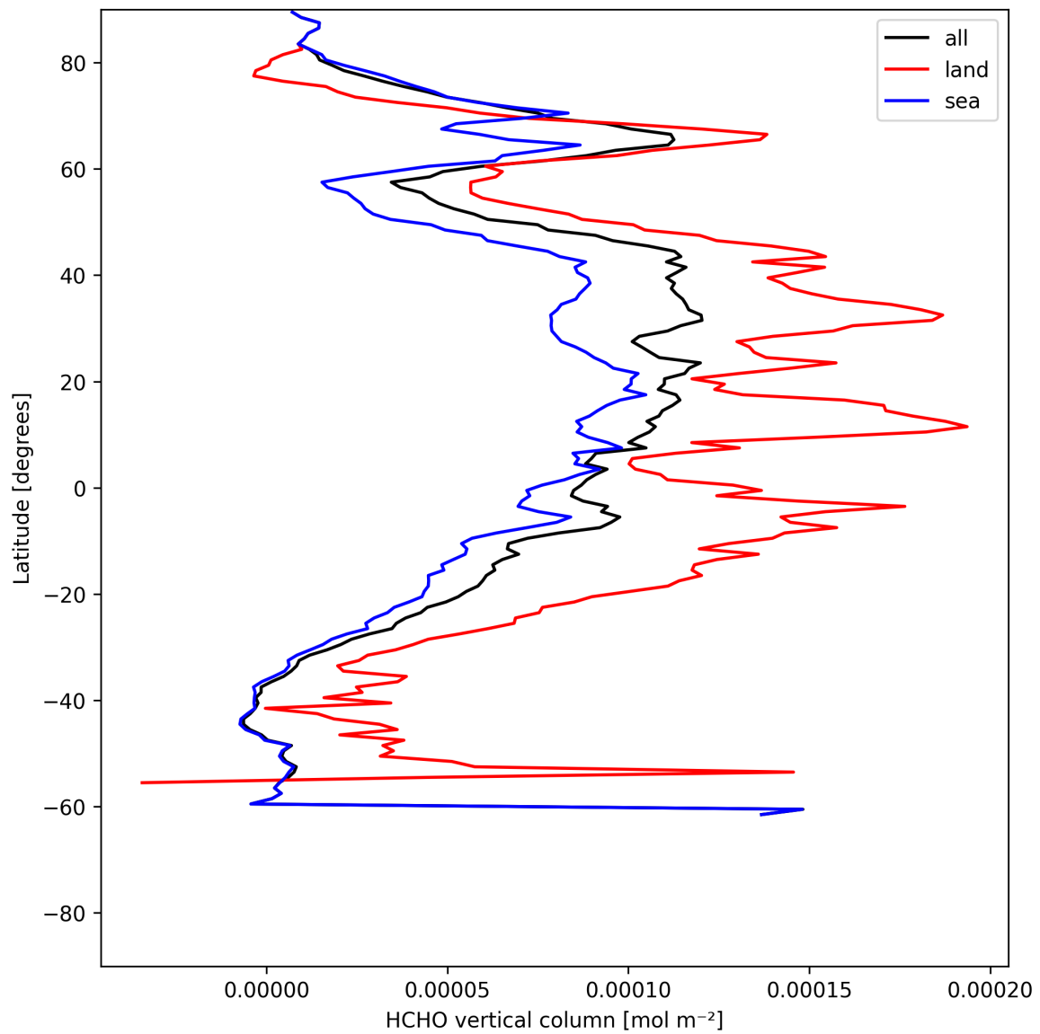
Figure 21: Zonal average of “HCHO vertical column” for 2025-07-05 to 2025-07-07.
