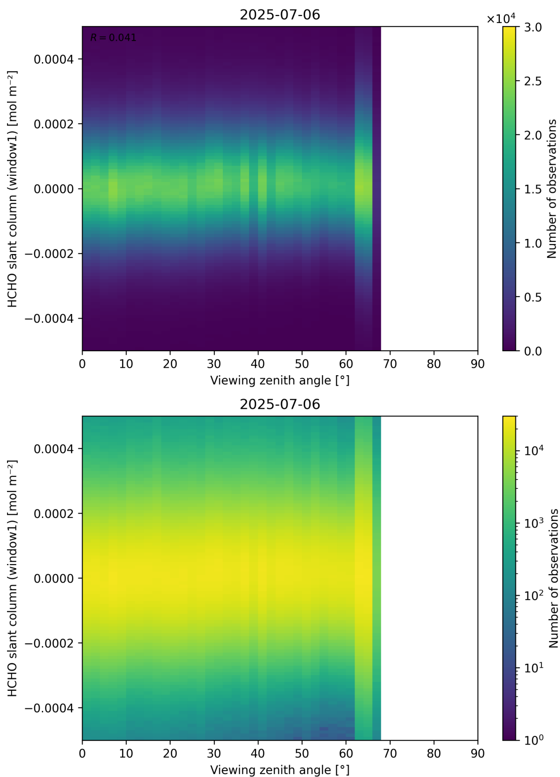
Figure 188: Scatter density plot of “Viewing zenith angle” against “HCHO slant column (window1)” for 2025-07-05 to 2025-07-07.
