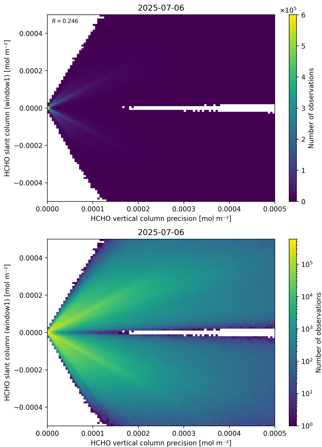
Figure 142: Scatter density plot of “HCHO vertical column precision” against “HCHO slant column (window1)” for 2025-07-05 to 2025-07-07.
