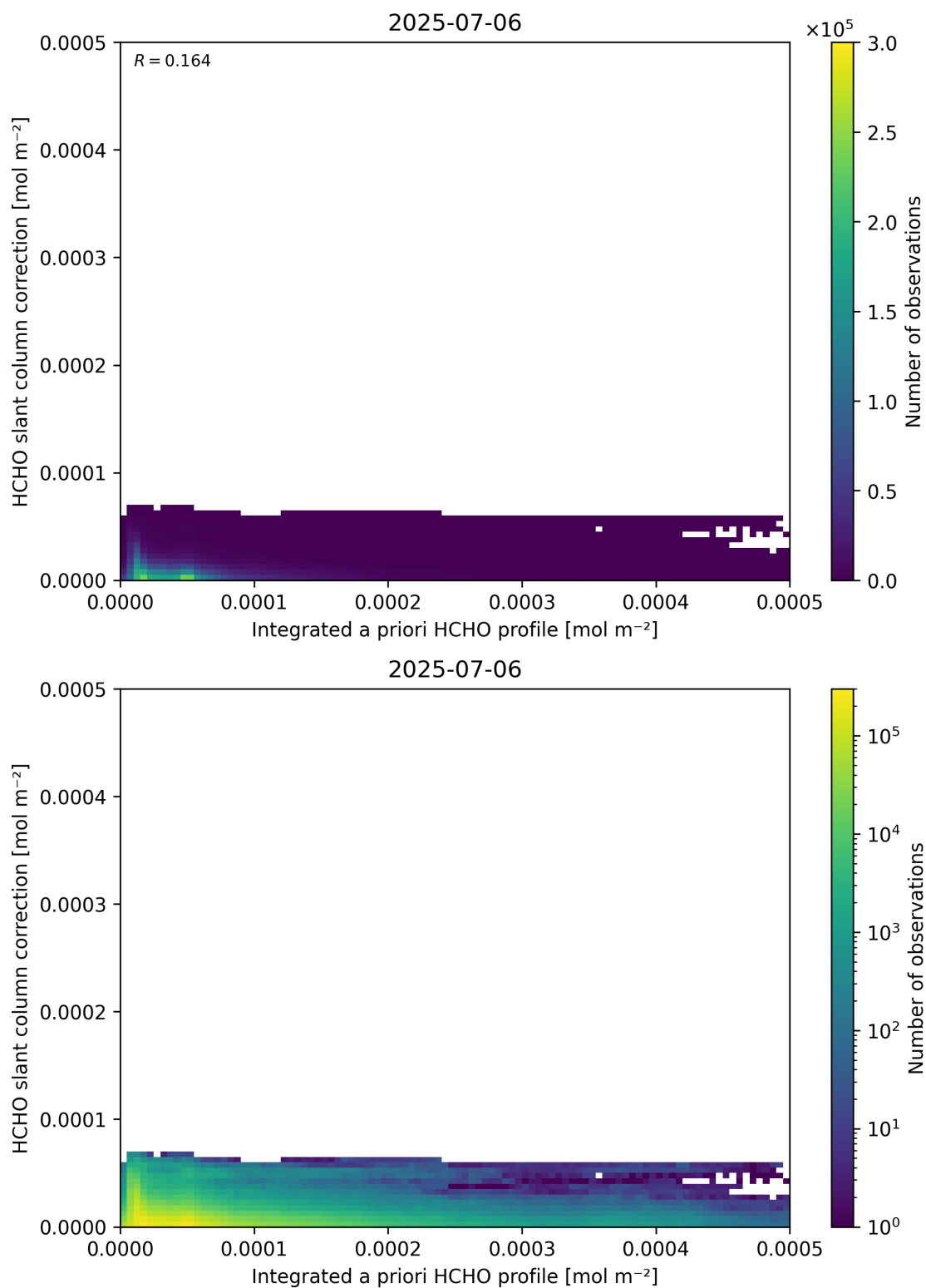
Figure 152: Scatter density plot of “Integrated a priori HCHO profile” against “HCHO slant column correction” for 2025-07-05 to 2025-07-07.
