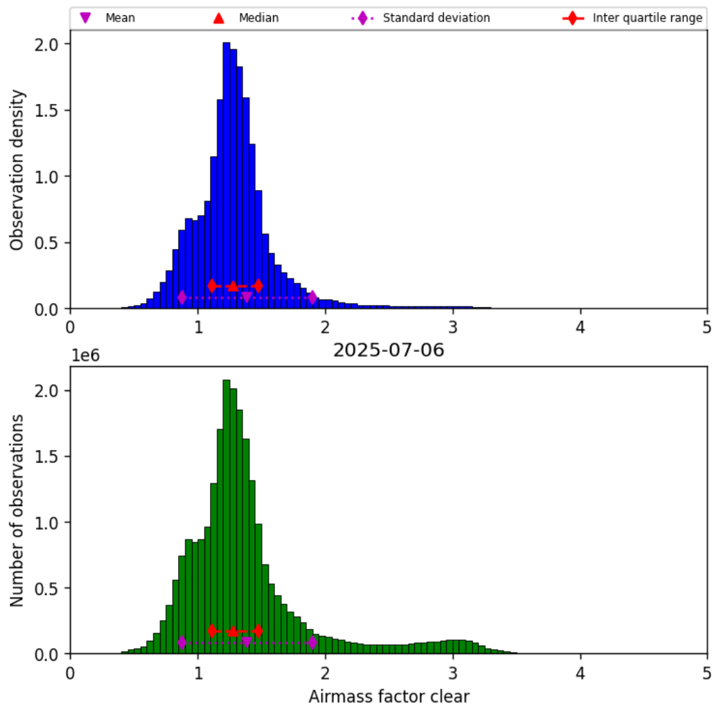
Figure 42: Histogram of “Airmass factor clear” for 2025-07-05 to 2025-07-07
