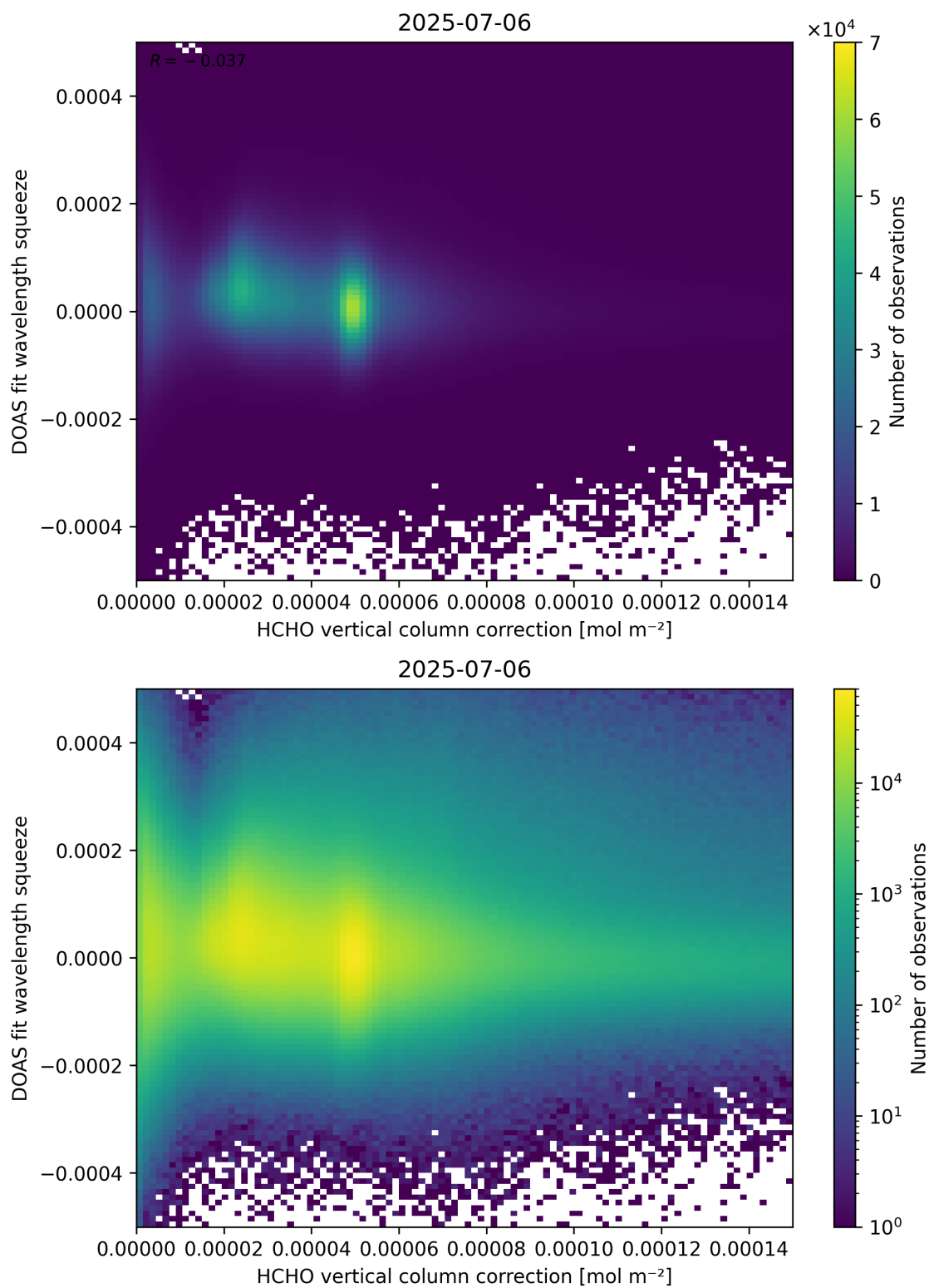
Figure 114: Scatter density plot of “HCHO vertical column correction” against “DOAS fit wavelength squeeze” for 2025-07-05 to 2025-07-07.
