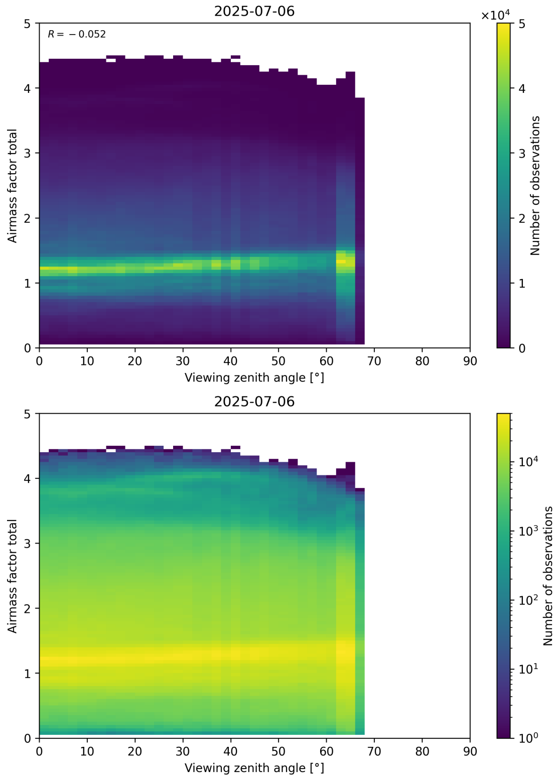
Figure 190: Scatter density plot of “Viewing zenith angle” against “Airmass factor total” for 2025-07-05 to 2025-07-07.
