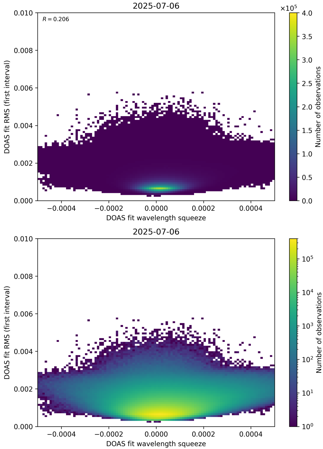
Figure 68: Scatter density plot of “DOAS fit wavelength squeeze” against “DOAS fit RMS (first interval)” for 2025-07-05 to 2025-07-07.
