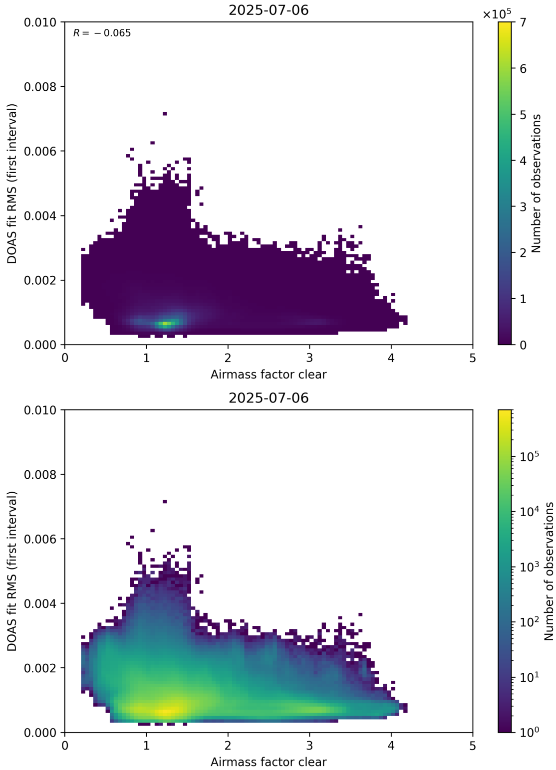
Figure 71: Scatter density plot of “Airmass factor clear” against “DOAS fit RMS (first interval)” for 2025-07-05 to 2025-07-07.
