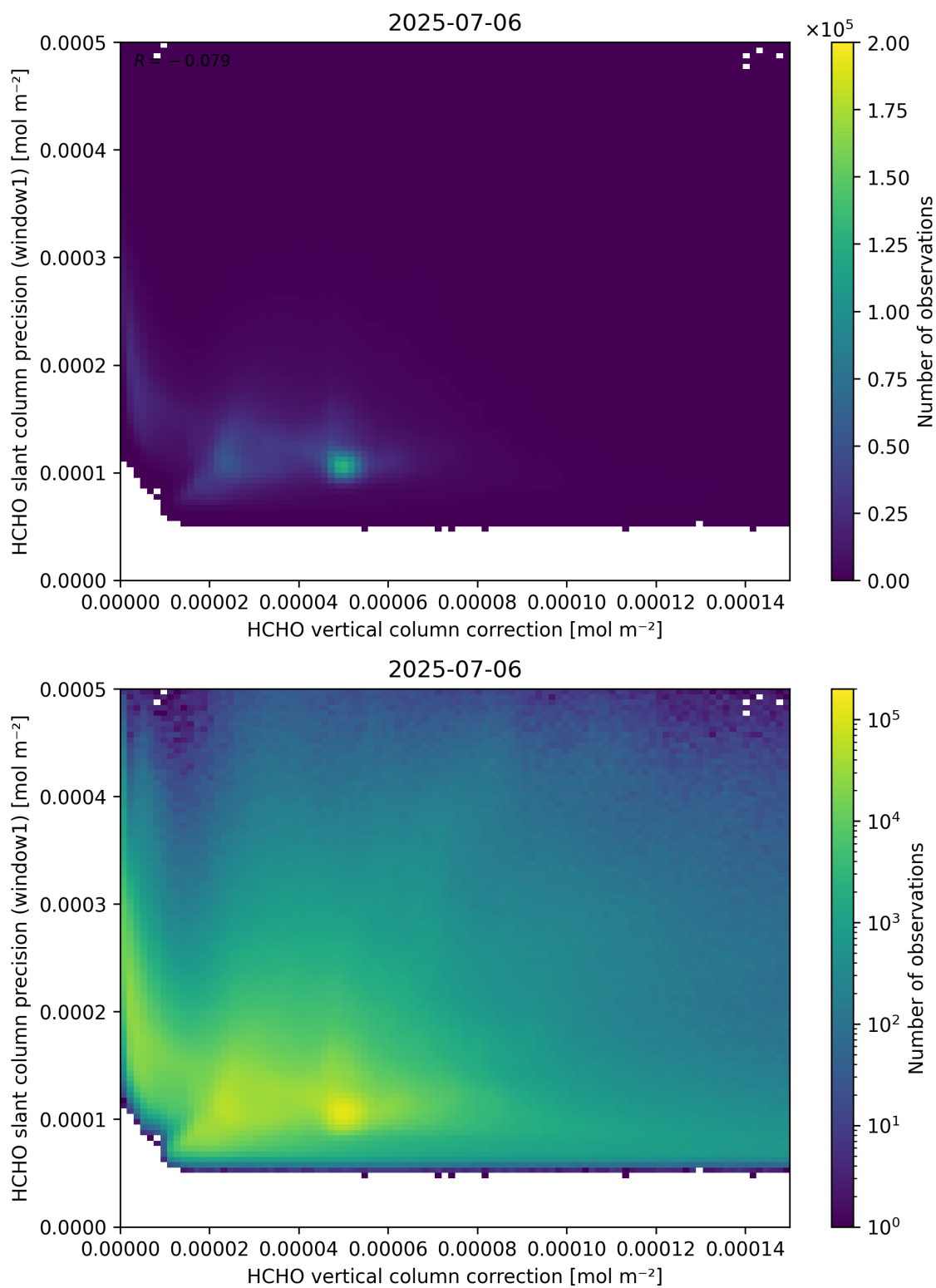
Figure 119: Scatter density plot of “HCHO vertical column correction” against “HCHO slant column precision (window1)” for 2025-07-05 to 2025-07-07.
