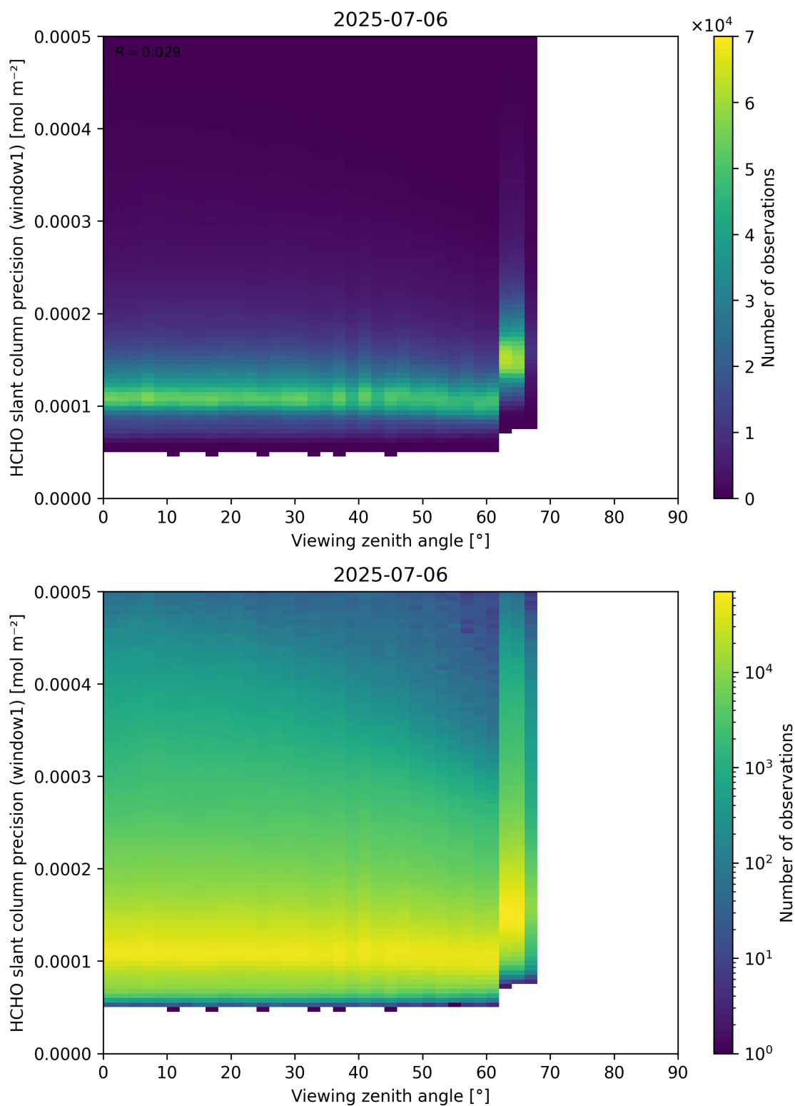
Figure 189: Scatter density plot of “Viewing zenith angle” against “HCHO slant column precision (window1)” for 2025-07-05 to 2025-07-07.
