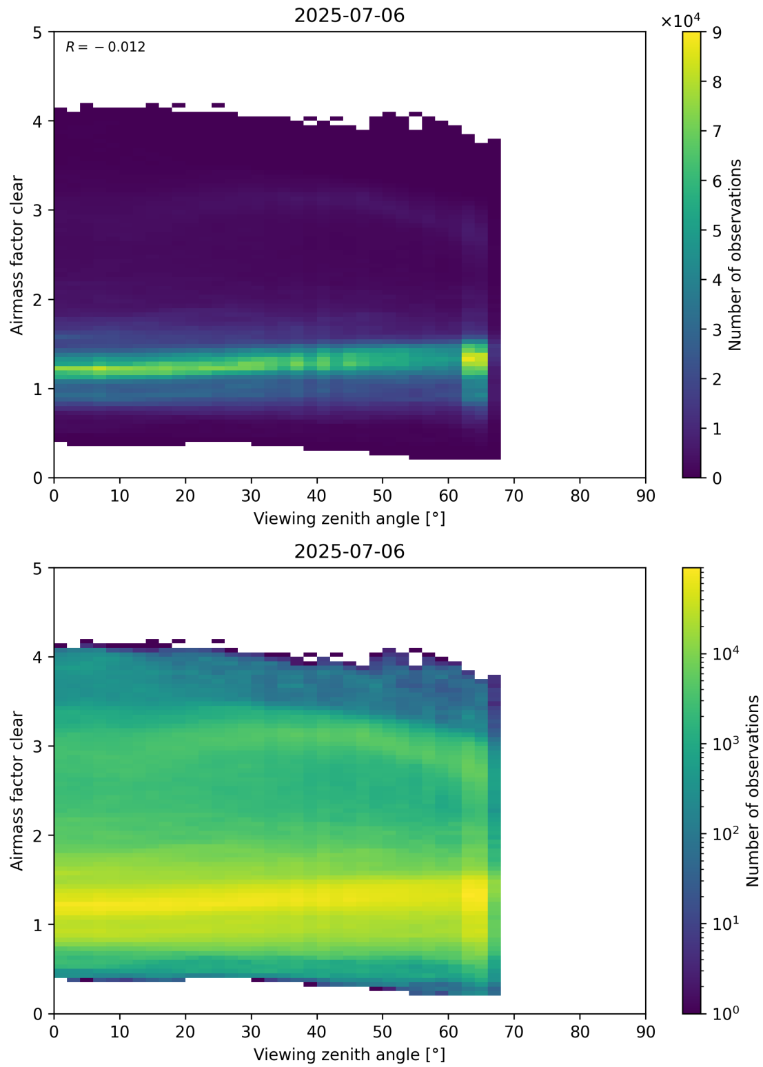
Figure 185: Scatter density plot of “Viewing zenith angle” against “Airmass factor clear” for 2025-07-05 to 2025-07-07.
