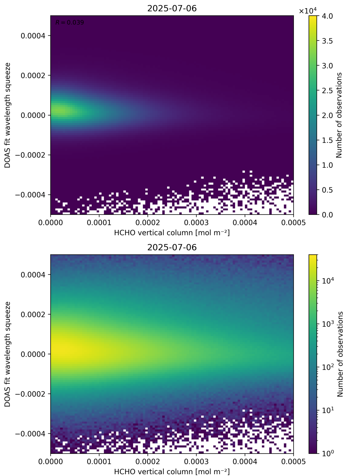
Figure 125: Scatter density plot of “HCHO vertical column” against “DOAS fit wavelength squeeze” for 2025-07-05 to 2025-07-07.
