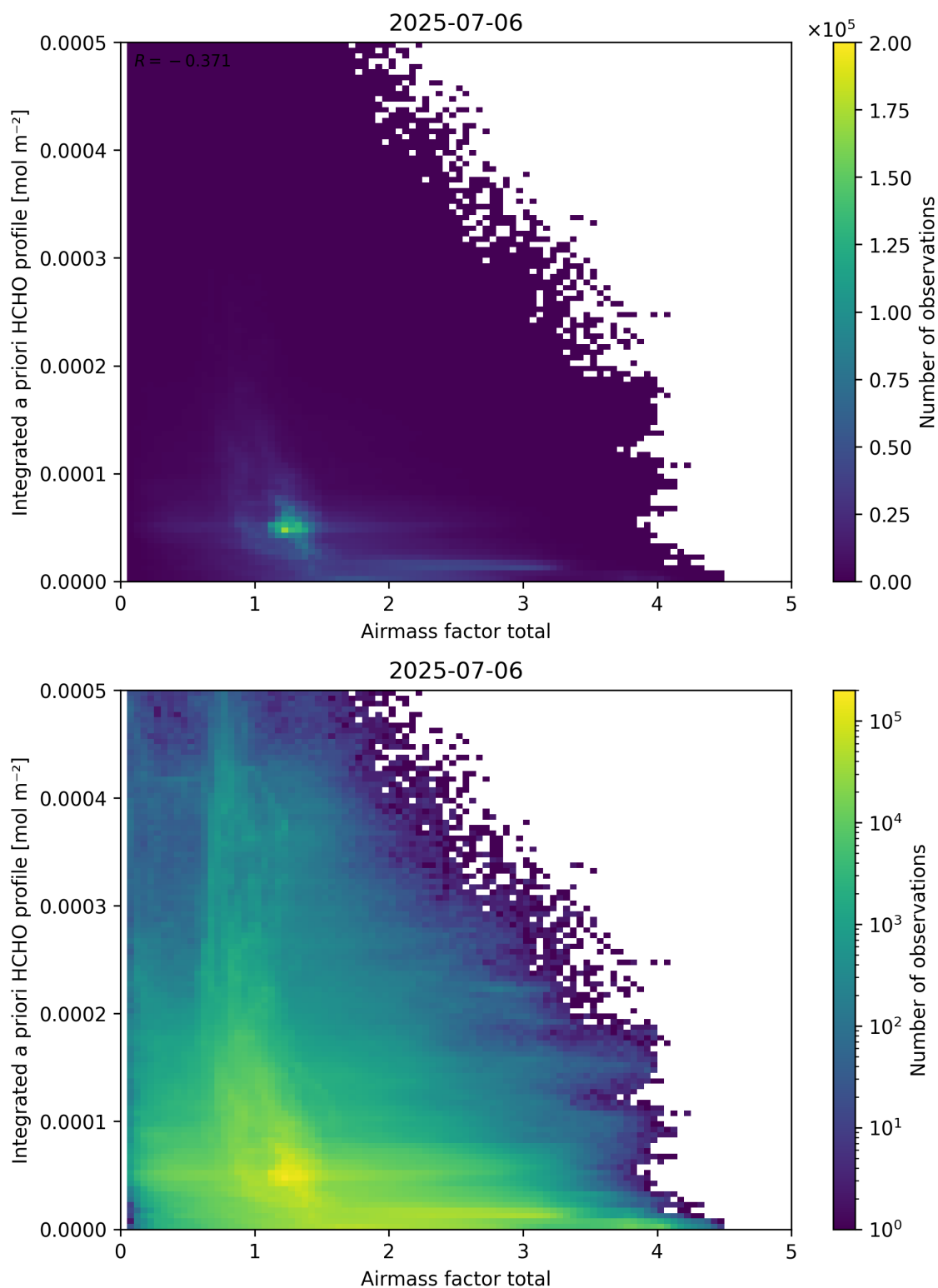
Figure 104: Scatter density plot of “Airmass factor total” against “Integrated a priori HCHO profile” for 2025-07-05 to 2025-07-07.
