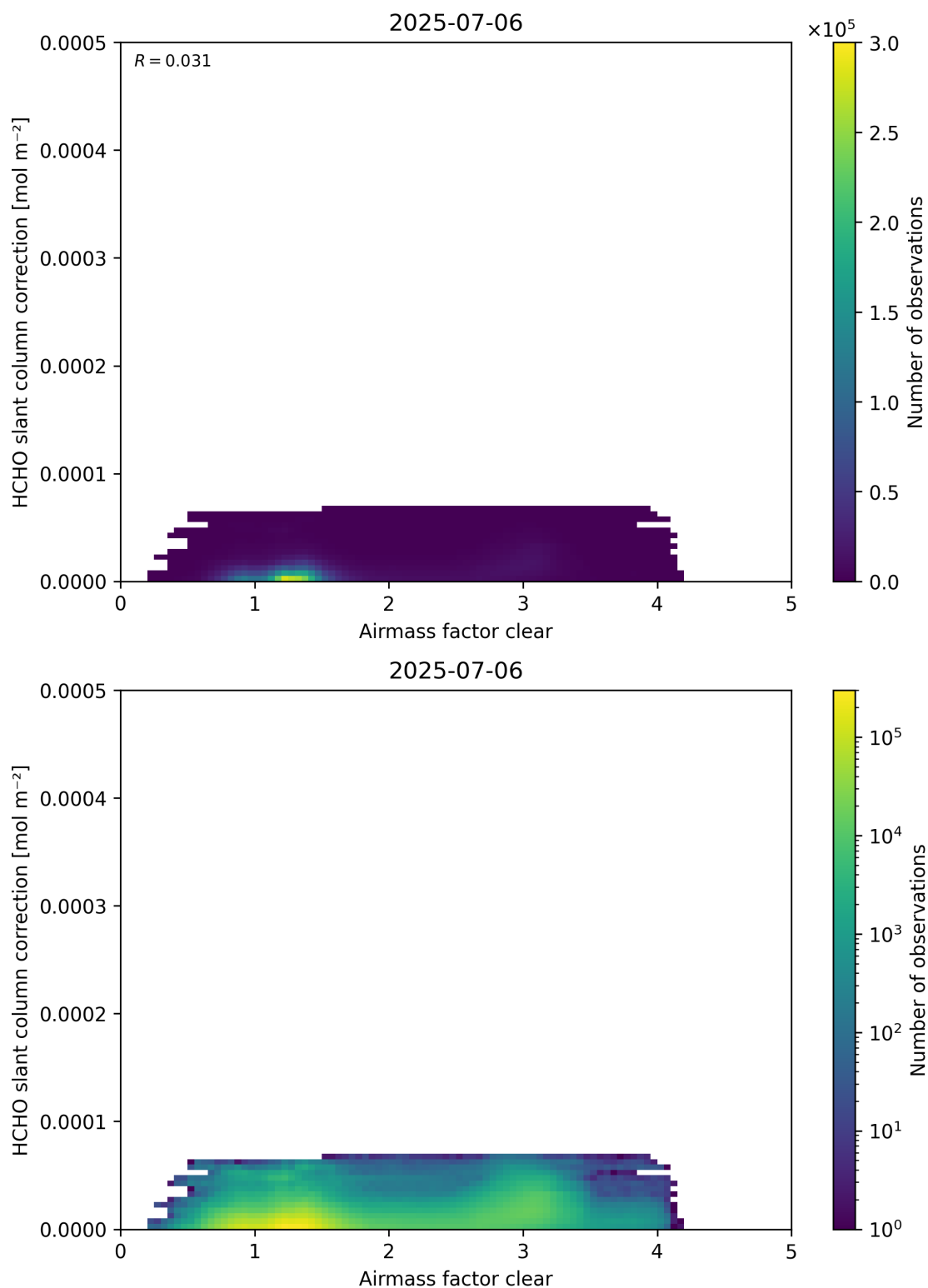
Figure 75: Scatter density plot of “Airmass factor clear” against “HCHO slant column correction” for 2025-07-05 to 2025-07-07.
