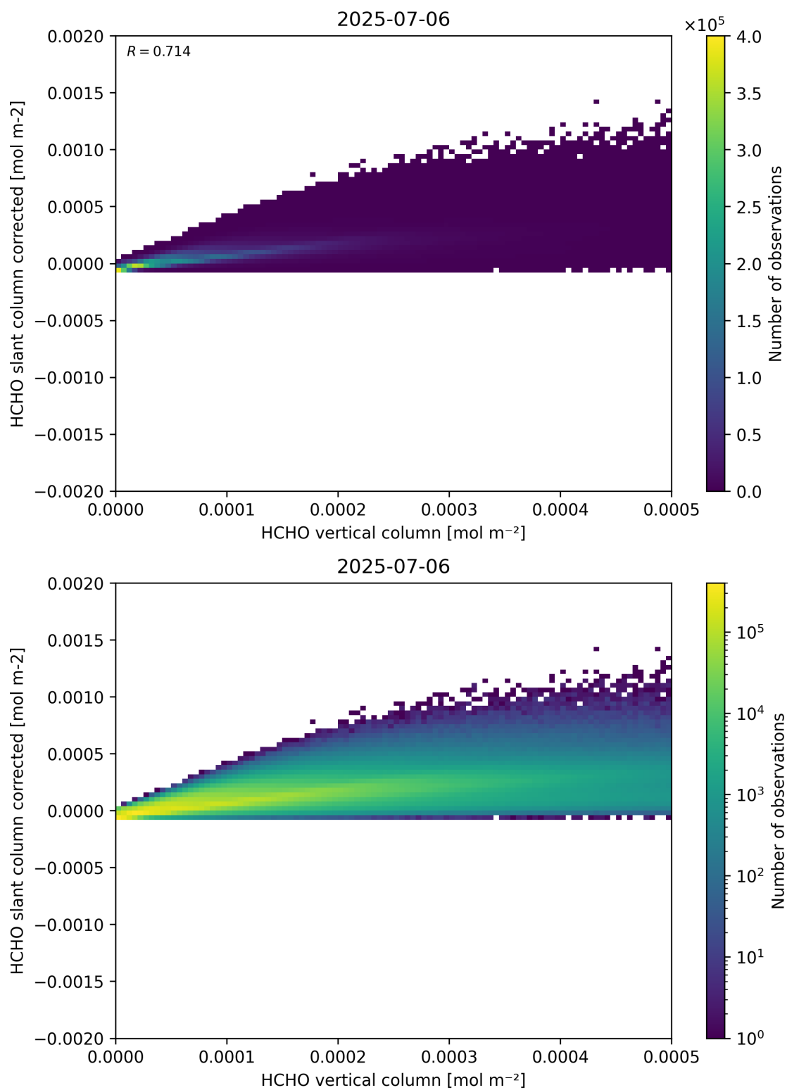
Figure 127: Scatter density plot of “HCHO vertical column” against “HCHO slant column corrected” for 2025-07-05 to 2025-07-07.
