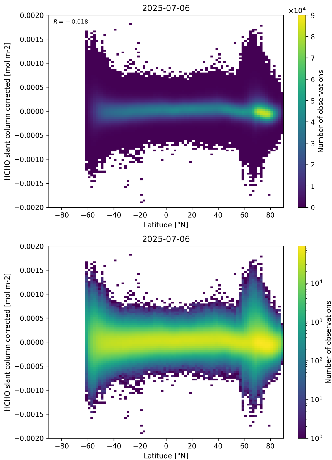
Figure 157: Scatter density plot of “Latitude” against “HCHO slant column corrected” for 2025-07-05 to 2025-07-07.
