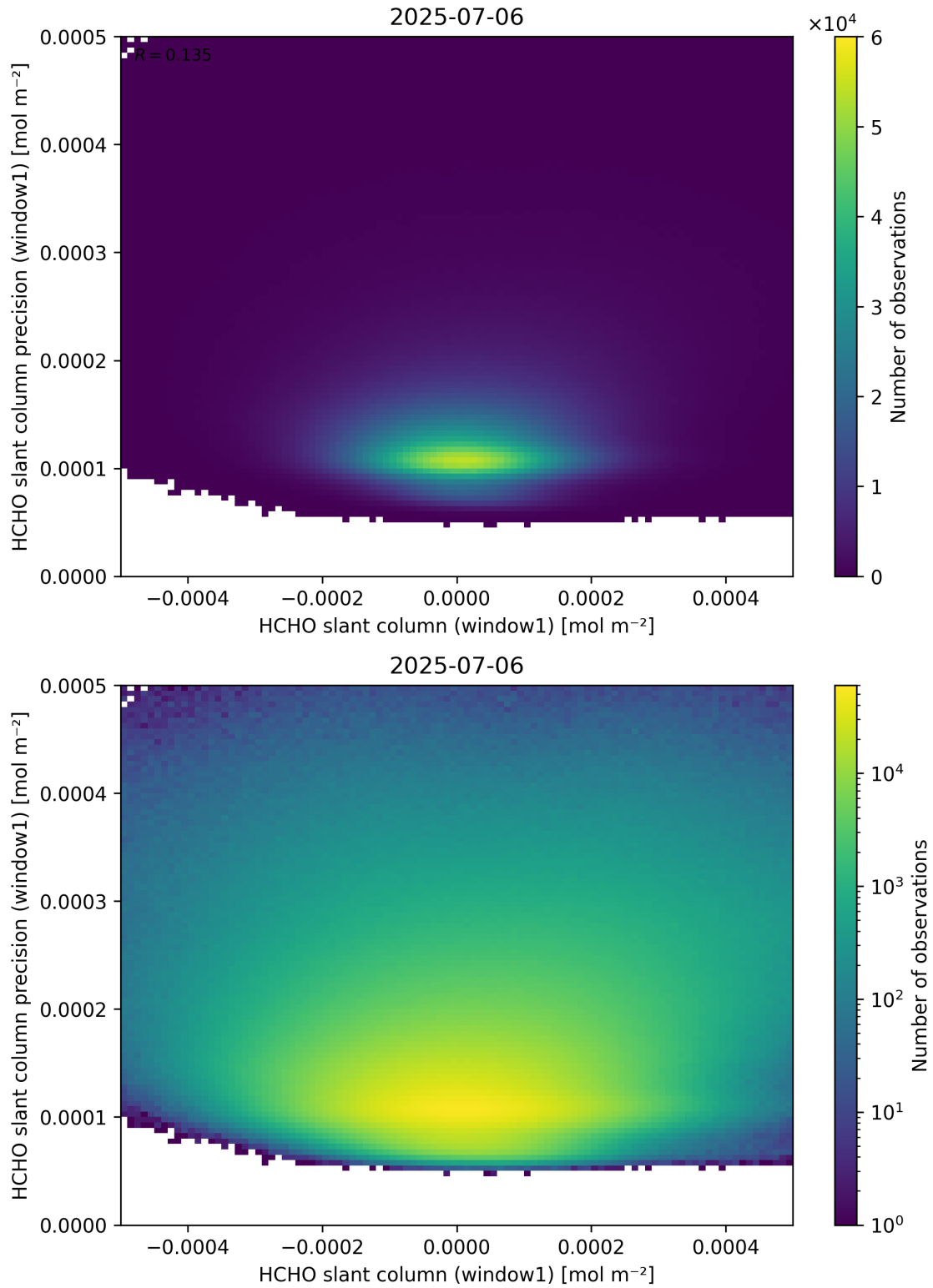
Figure 84: Scatter density plot of “HCHO slant column (window1)” against “HCHO slant column precision (window1)” for 2025-07-05 to 2025-07-07.
