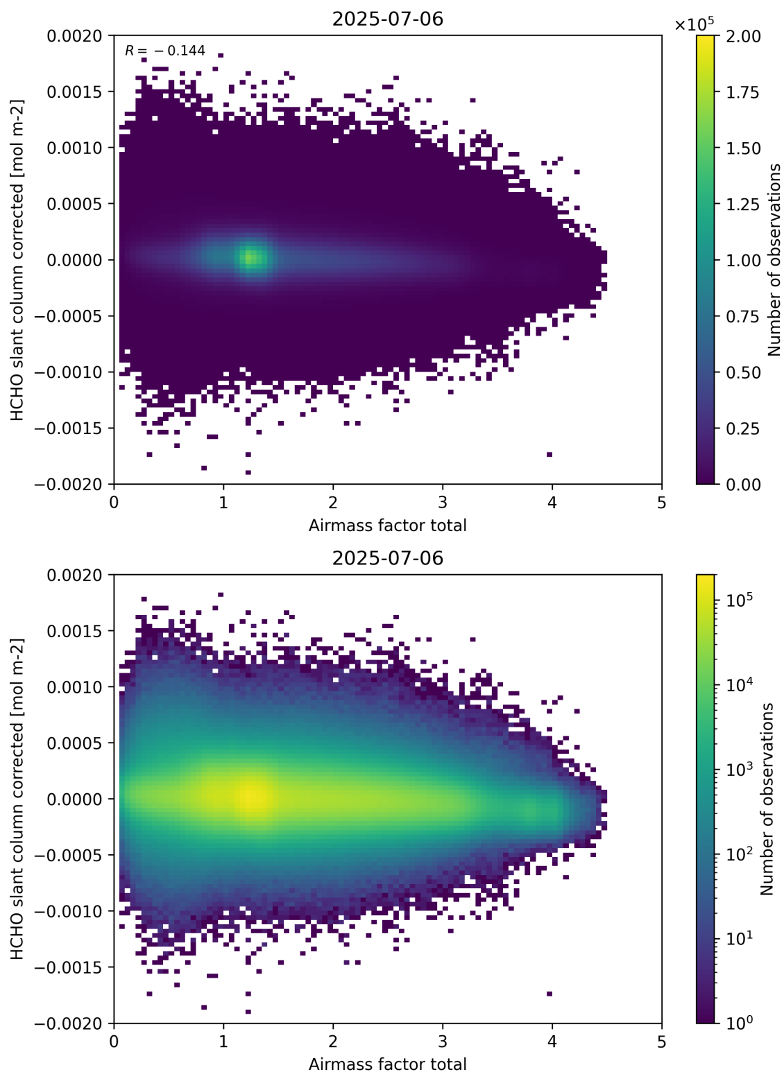
Figure 101: Scatter density plot of “Airmass factor total” against “HCHO slant column corrected” for 2025-07-05 to 2025-07-07.
