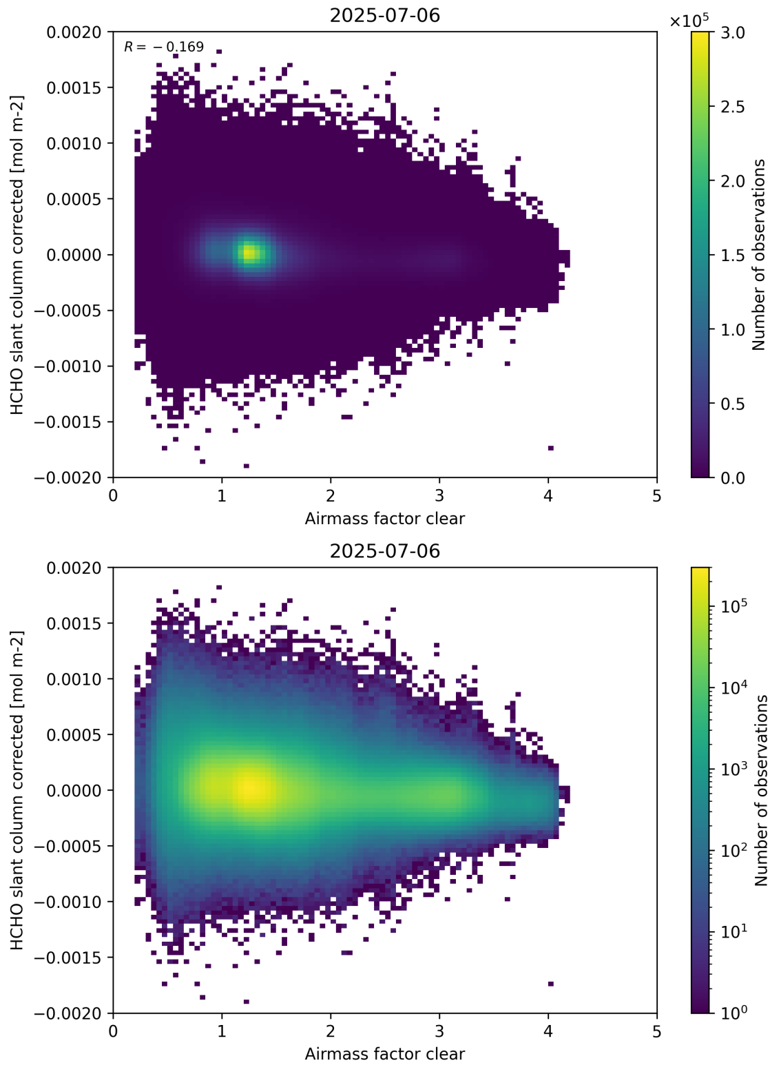
Figure 74: Scatter density plot of “Airmass factor clear” against “HCHO slant column corrected” for 2025-07-05 to 2025-07-07.
