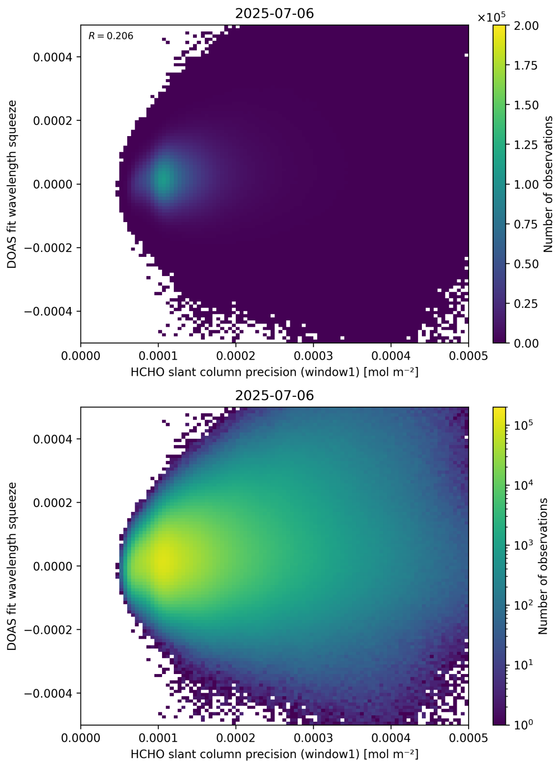
Figure 90: Scatter density plot of “HCHO slant column precision (window1)” against “DOAS fit wavelength squeeze” for 2025-07-05 to 2025-07-07.
