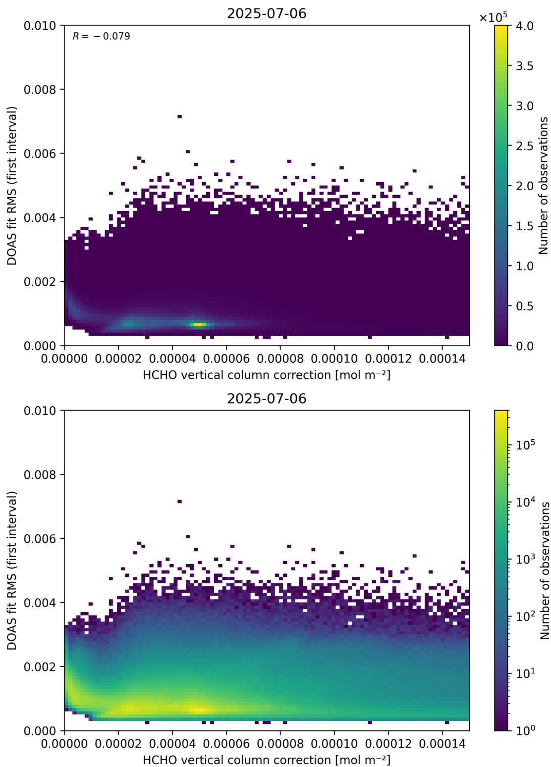
Figure 112: Scatter density plot of “HCHO vertical column correction” against “DOAS fit RMS (first interval)” for 2025-07-05 to 2025-07-07.
