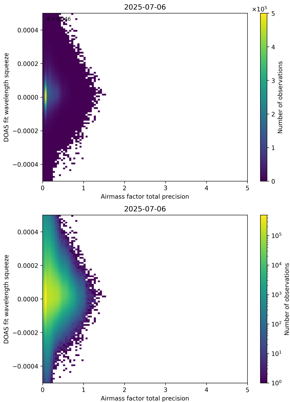
Figure 107: Scatter density plot of “Airmass factor total precision” against “DOAS fit wavelength squeeze” for 2025-07-05 to 2025-07-07.
