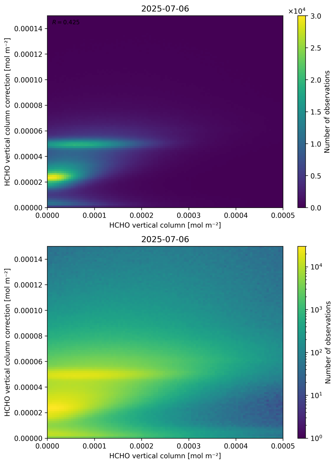
Figure 133: Scatter density plot of “HCHO vertical column” against “HCHO vertical column correction” for 2025-07-05 to 2025-07-07.
