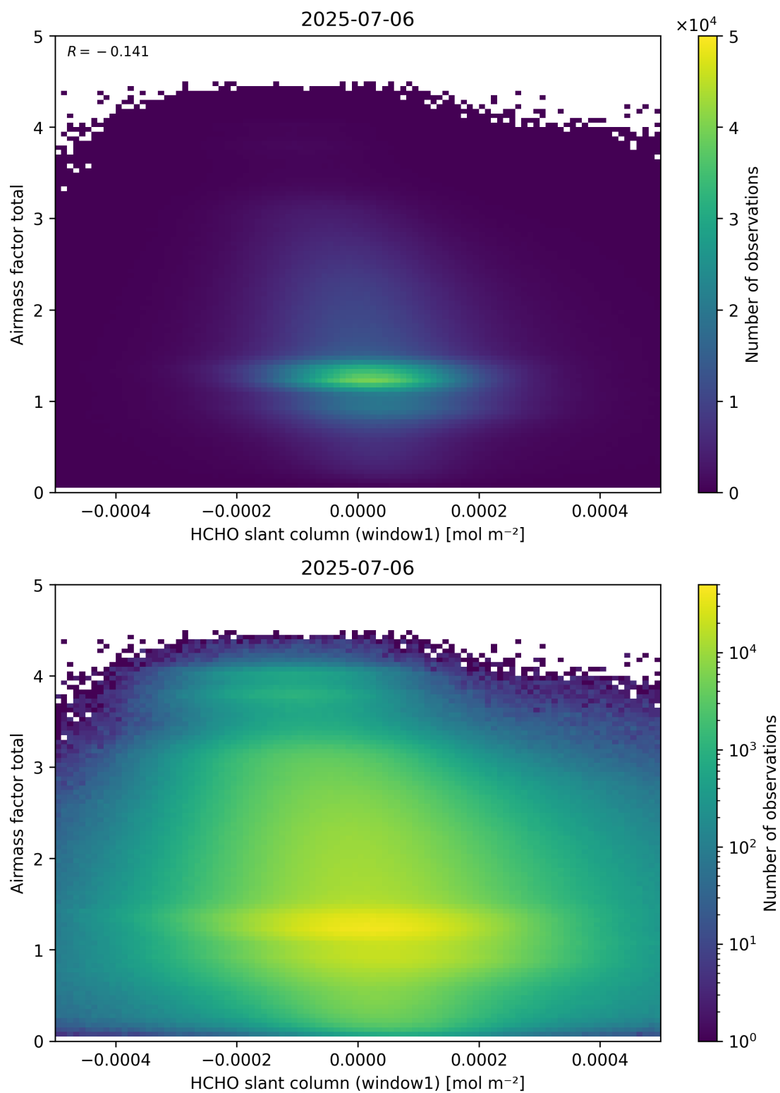
Figure 85: Scatter density plot of “HCHO slant column (window1)” against “Airmass factor total” for 2025-07-05 to 2025-07-07.
