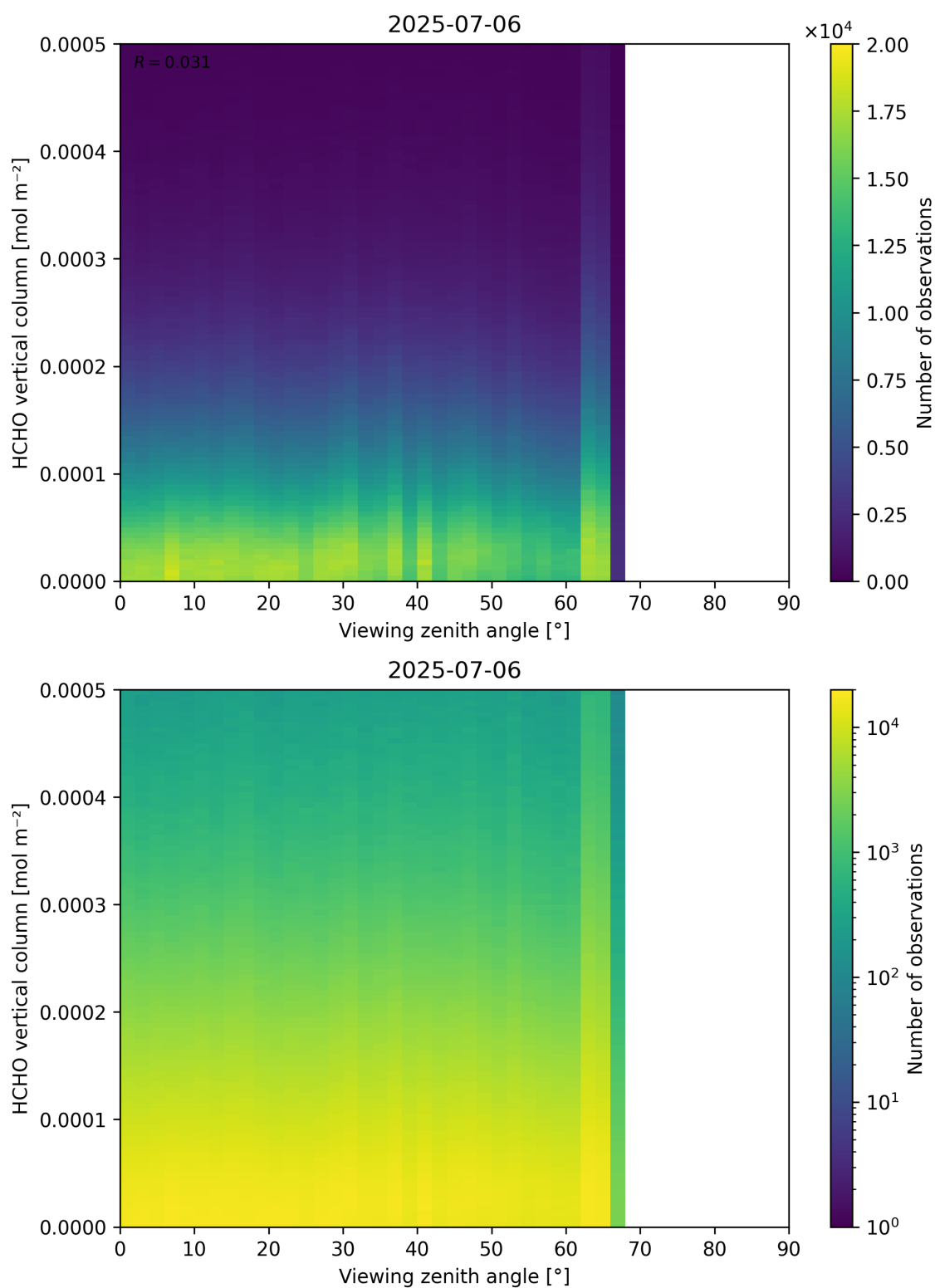
Figure 192: Scatter density plot of “Viewing zenith angle” against “HCHO vertical column” for 2025-07-05 to 2025-07-07.
