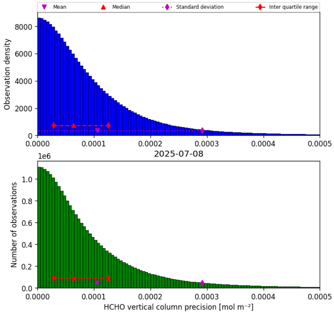
Figure 36: Histogram of “HCHO vertical column precision” for 2025-07-08 to 2025-07-09
