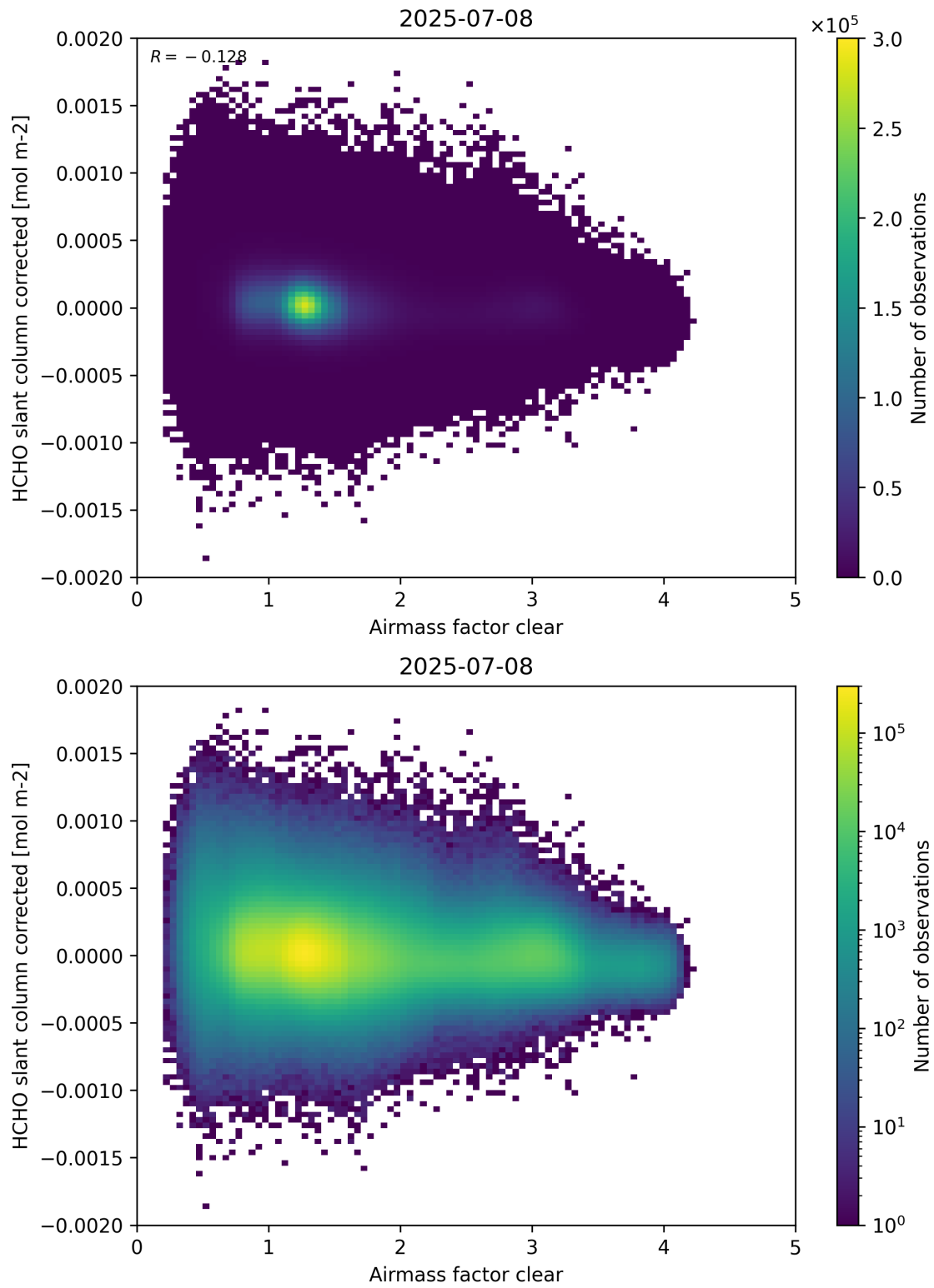
Figure 74: Scatter density plot of “Airmass factor clear” against “HCHO slant column corrected” for 2025-07-08 to 2025-07-09.
