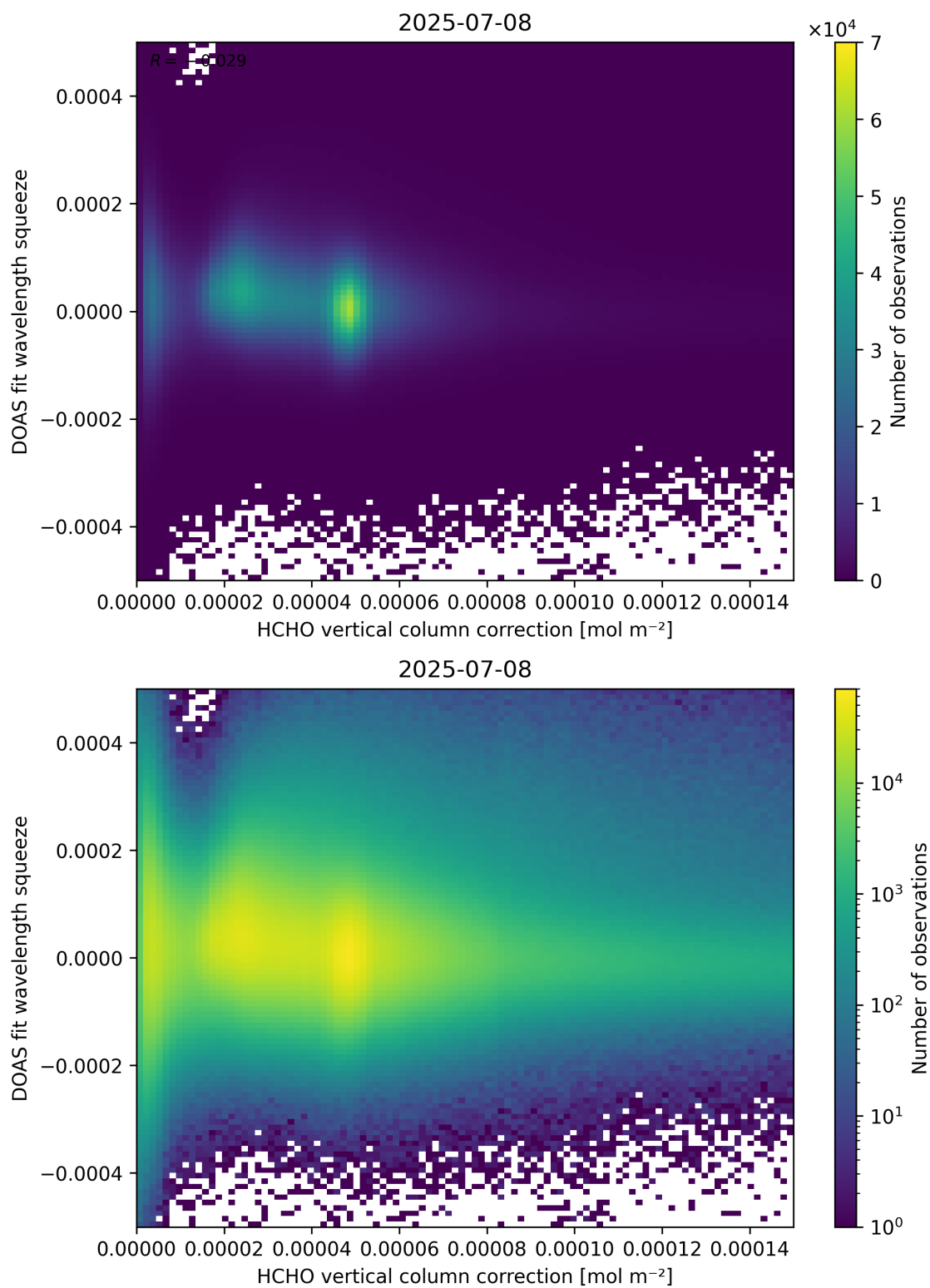
Figure 114: Scatter density plot of “HCHO vertical column correction” against “DOAS fit wavelength squeeze” for 2025-07-08 to 2025-07-09.
