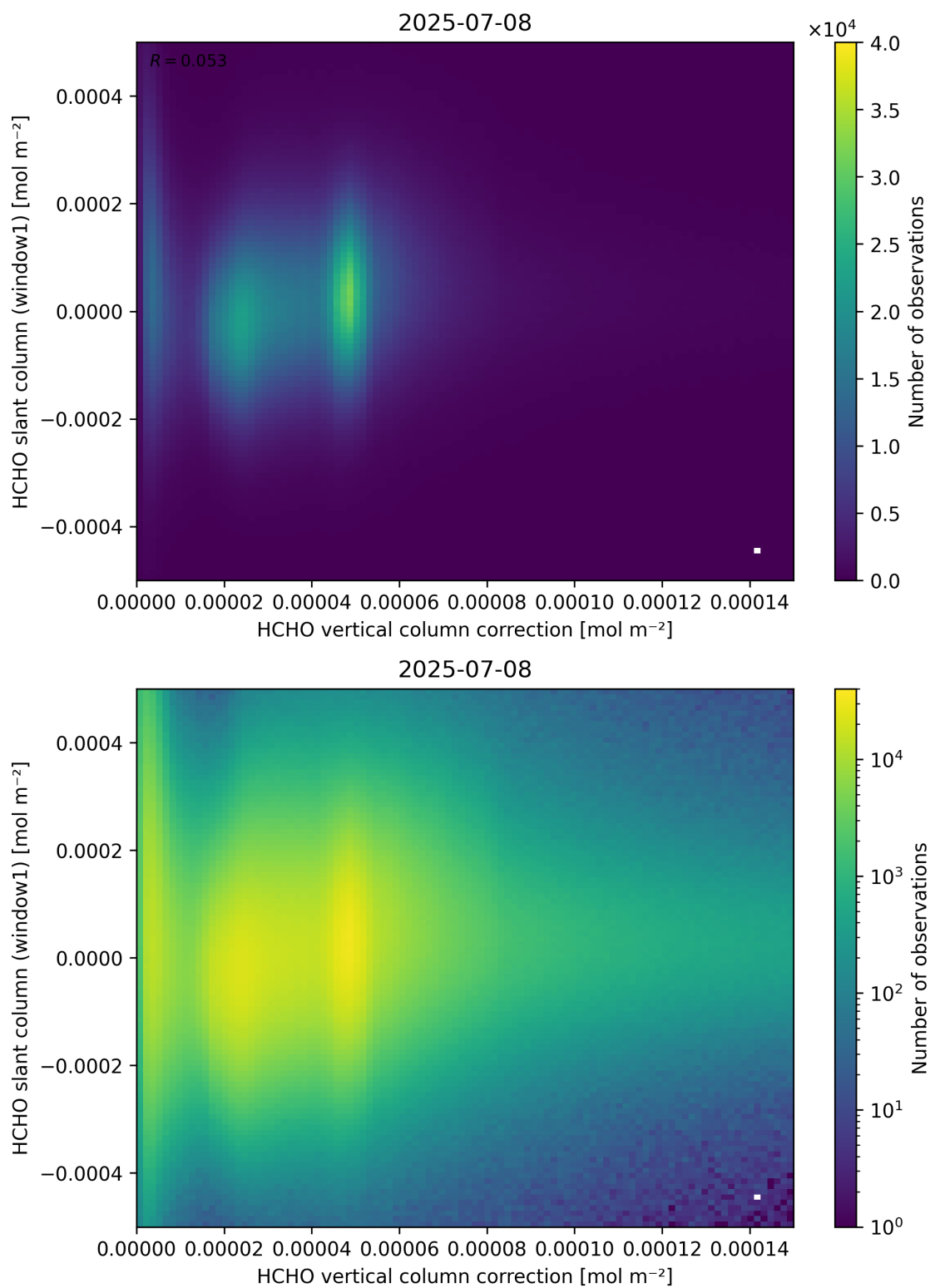
Figure 118: Scatter density plot of “HCHO vertical column correction” against “HCHO slant column (window1)” for 2025-07-08 to 2025-07-09.
