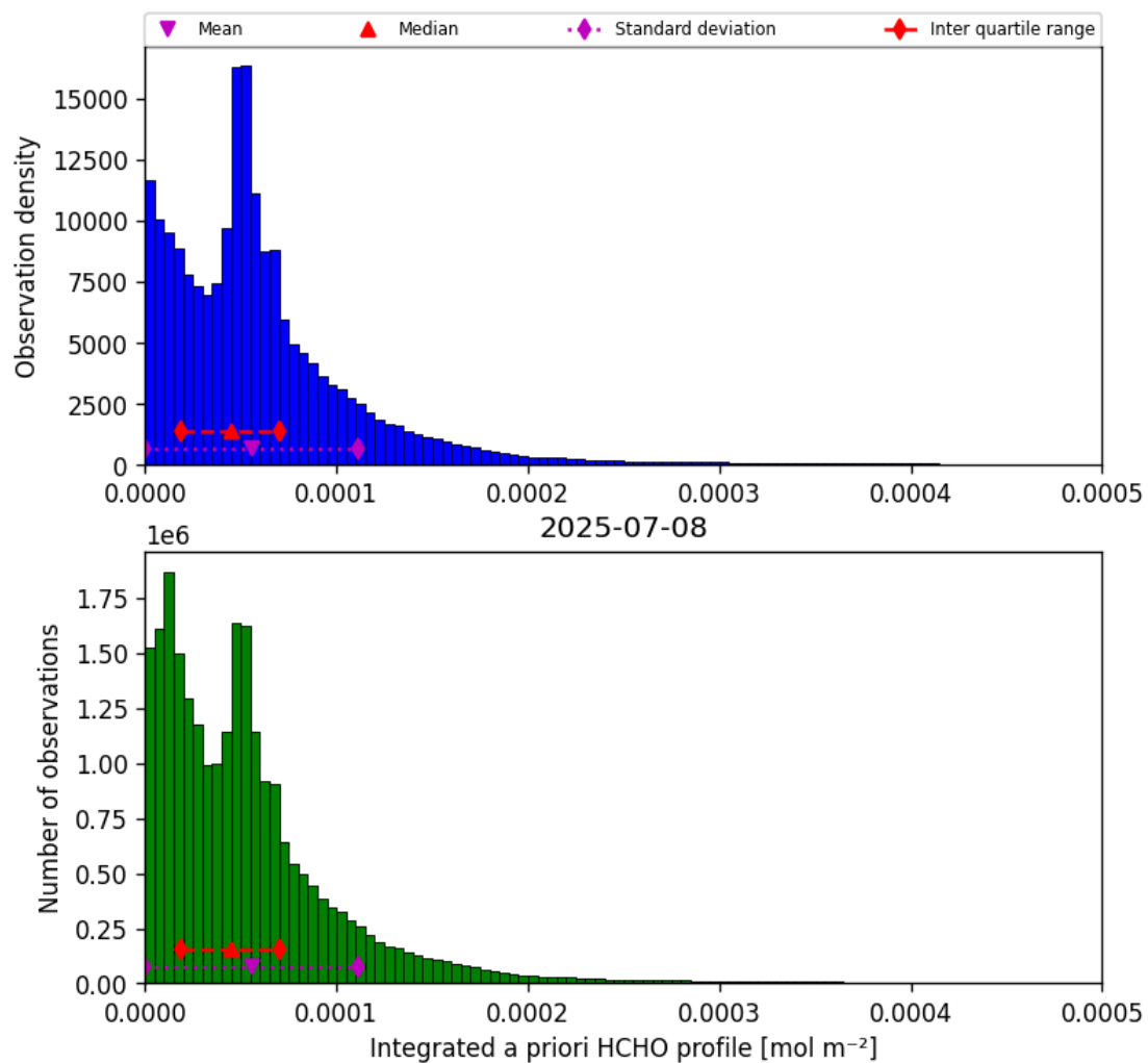
Figure 43: Histogram of “Integrated a priori HCHO profile” for 2025-07-08 to 2025-07-09
