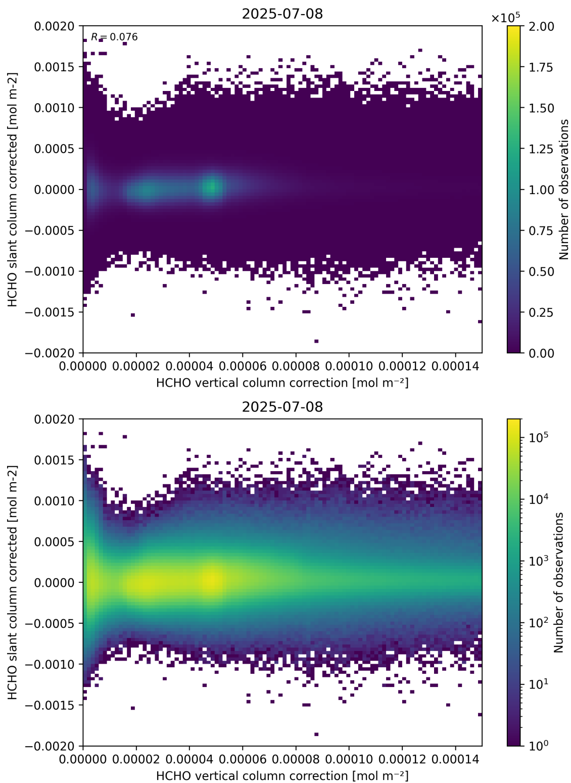
Figure 116: Scatter density plot of “HCHO vertical column correction” against “HCHO slant column corrected” for 2025-07-08 to 2025-07-09.
