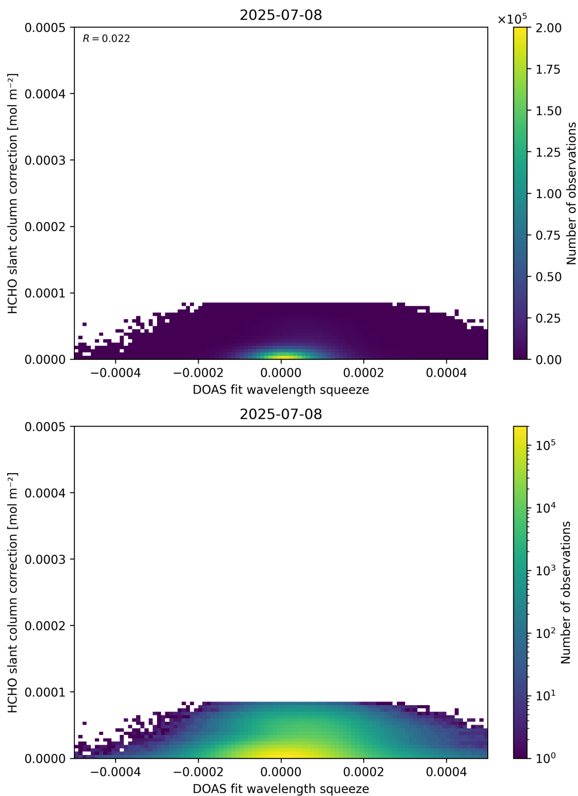
Figure 70: Scatter density plot of “DOAS fit wavelength squeeze” against “HCHO slant column correction” for 2025-07-08 to 2025-07-09.
