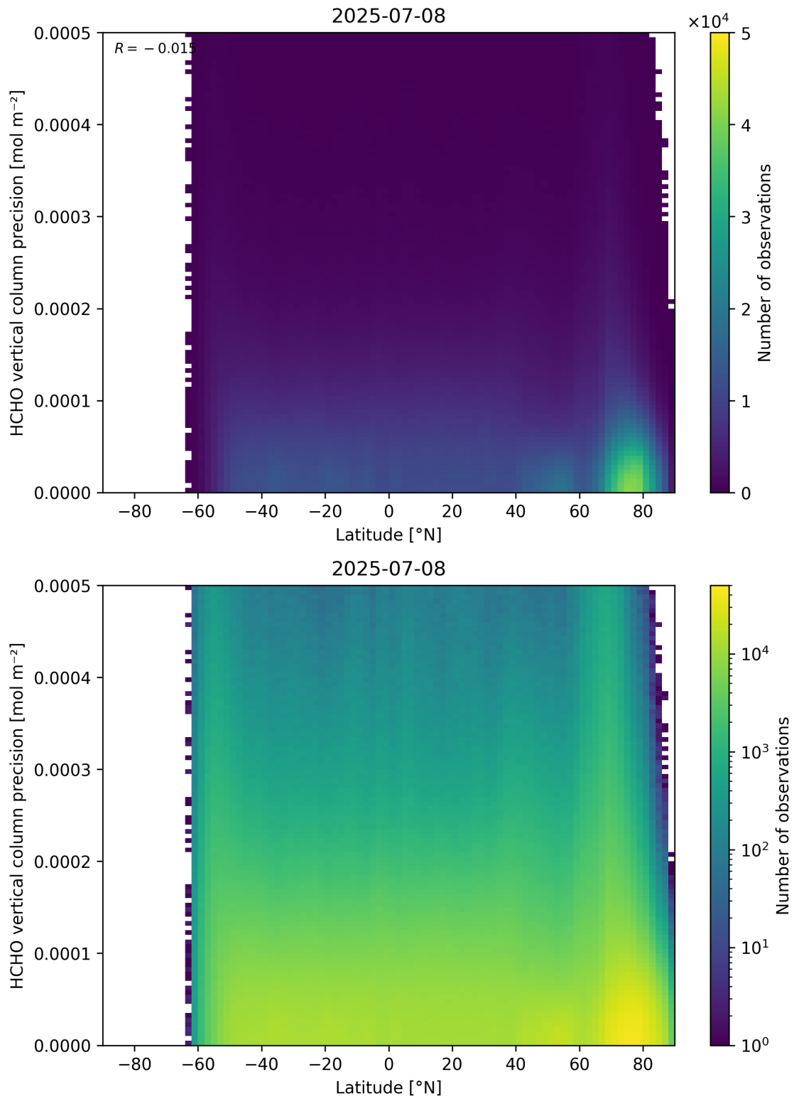
Figure 165: Scatter density plot of “Latitude” against “HCHO vertical column precision” for 2025-07-08 to 2025-07-09.
