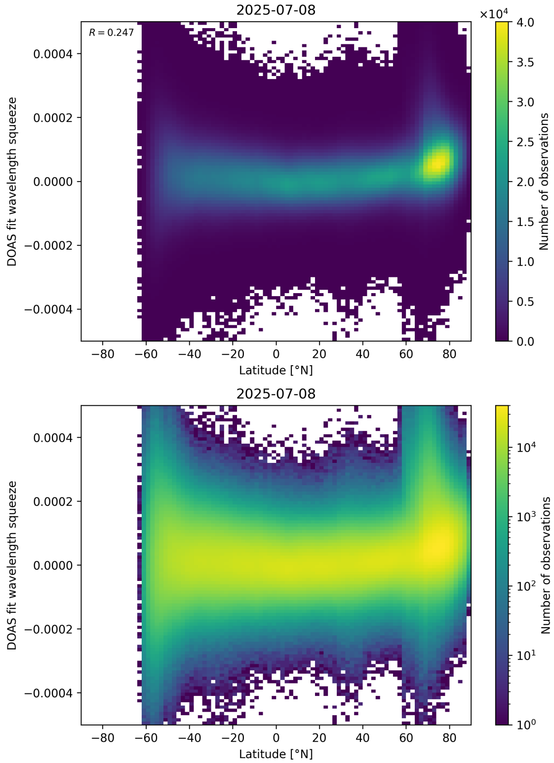
Figure 155: Scatter density plot of “Latitude” against “DOAS fit wavelength squeeze” for 2025-07-08 to 2025-07-09.
