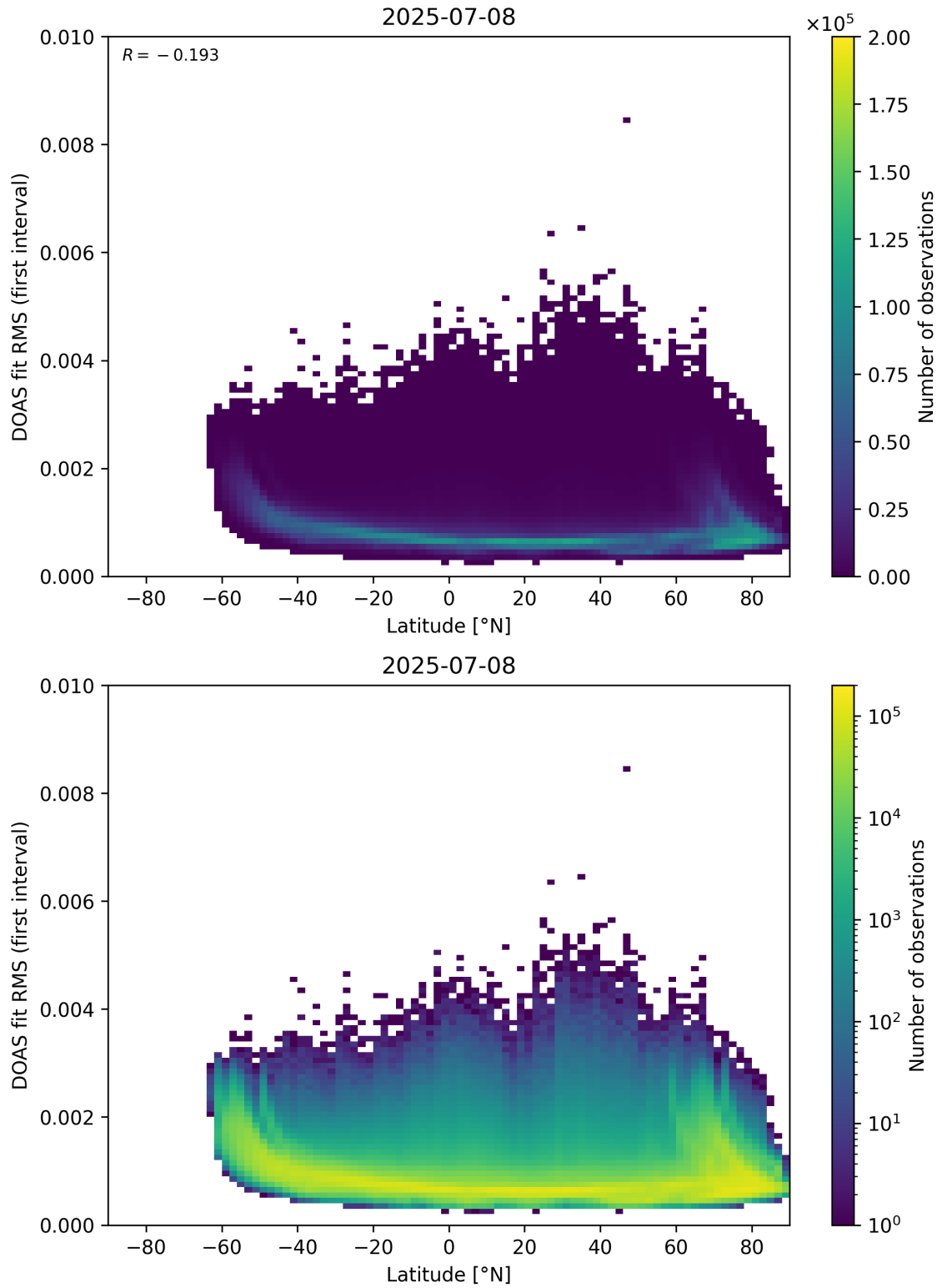
Figure 153: Scatter density plot of “Latitude” against “DOAS fit RMS (first interval)” for 2025-07-08 to 2025-07-09.
