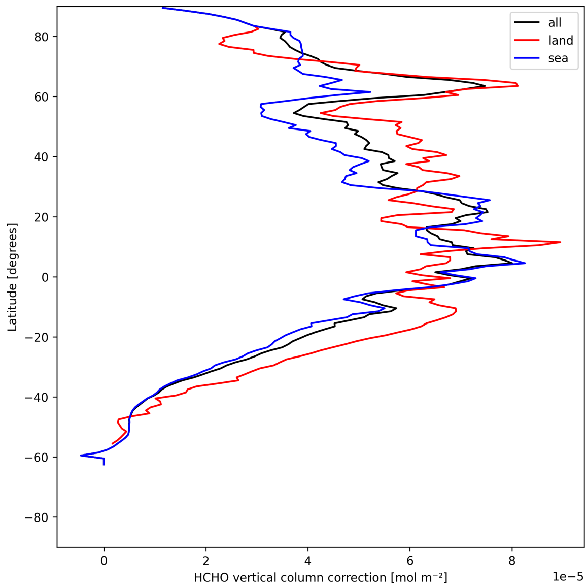
Figure 23: Zonal average of “HCHO vertical column correction” for 2025-07-08 to 2025-07-09.
