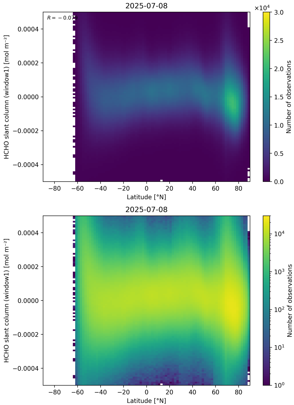
Figure 159: Scatter density plot of “Latitude” against “HCHO slant column (window1)” for 2025-07-08 to 2025-07-09.
