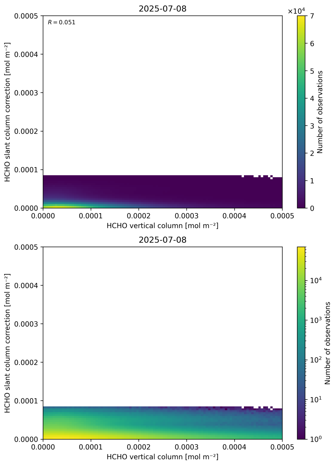
Figure 128: Scatter density plot of “HCHO vertical column” against “HCHO slant column correction” for 2025-07-08 to 2025-07-09.
