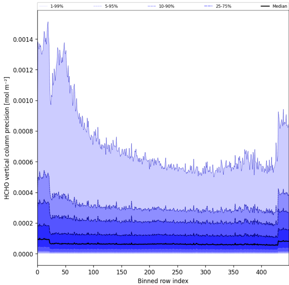
Figure 50: Along track statistics of “HCHO vertical column precision” for 2025-07-08 to 2025-07-09
