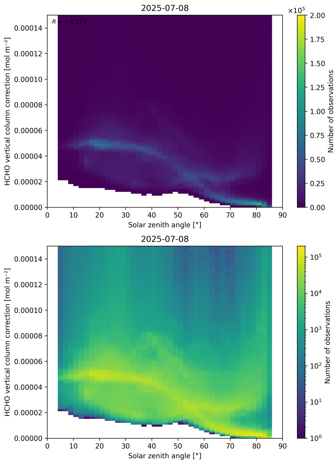
Figure 178: Scatter density plot of “Solar zenith angle” against “HCHO vertical column correction” for 2025-07-08 to 2025-07-09.
