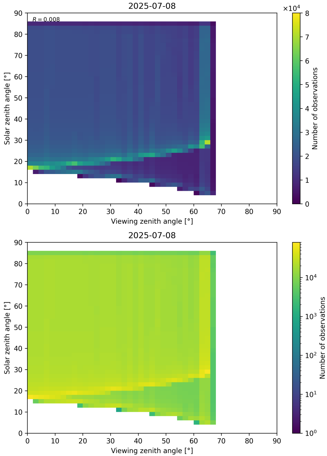
Figure 197: Scatter density plot of “Viewing zenith angle” against “Solar zenith angle” for 2025-07-08 to 2025-07-09.
