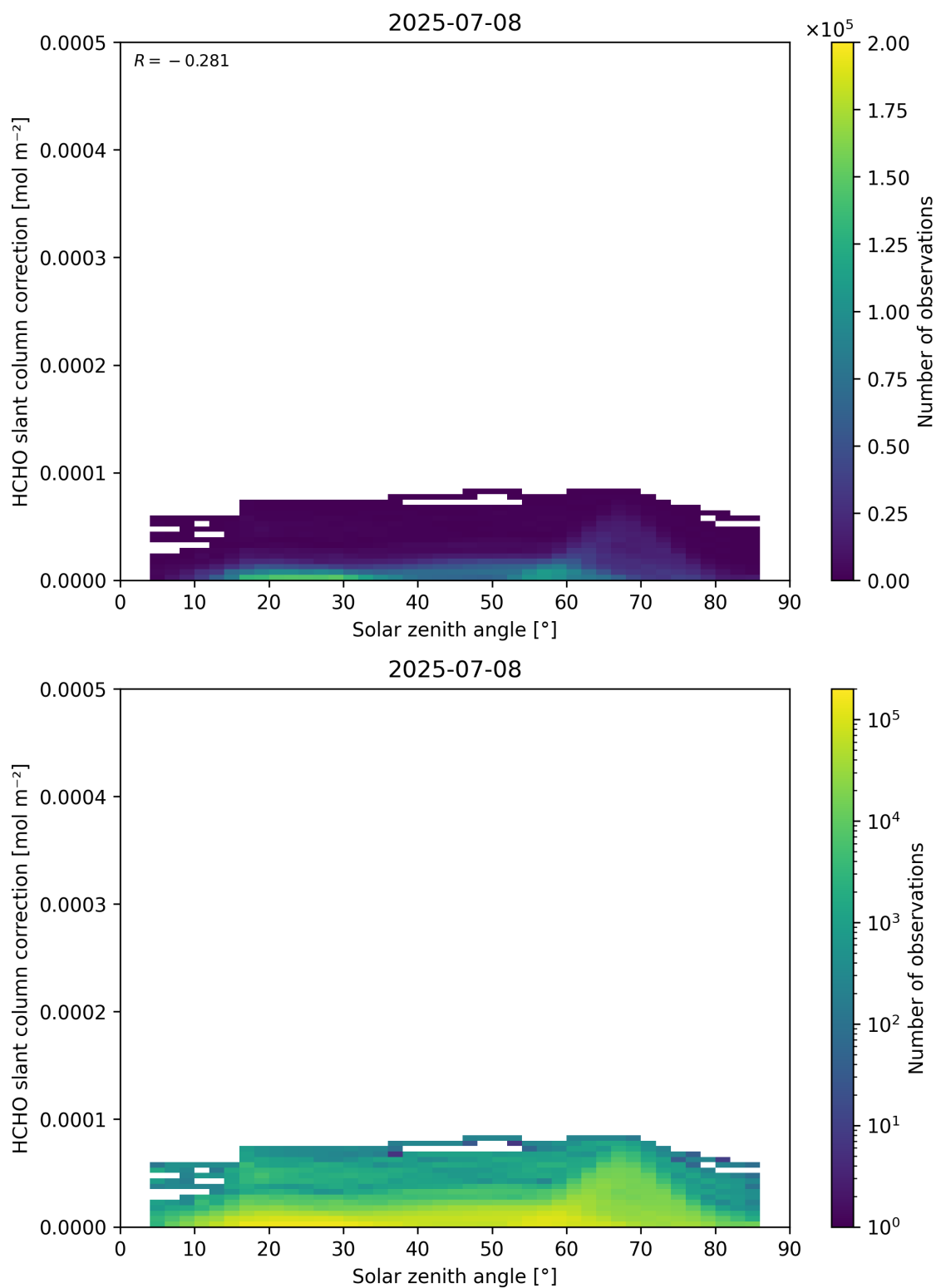
Figure 172: Scatter density plot of “Solar zenith angle” against “HCHO slant column correction” for 2025-07-08 to 2025-07-09.
