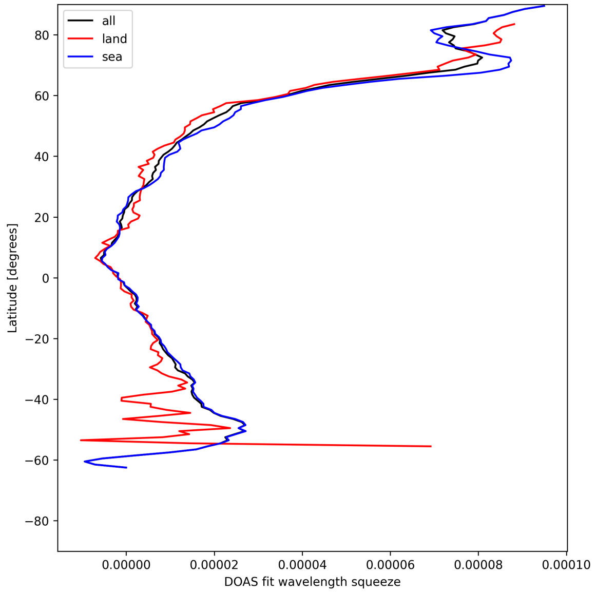
Figure 31: Zonal average of “DOAS fit wavelength squeeze” for 2025-07-08 to 2025-07-09.
