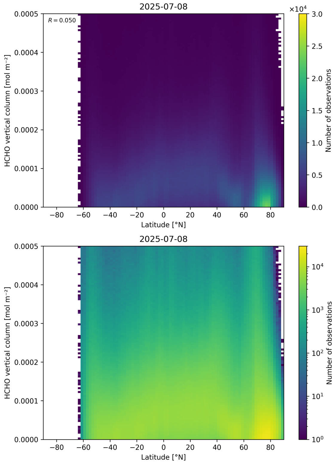
Figure 163: Scatter density plot of “Latitude” against “HCHO vertical column” for 2025-07-08 to 2025-07-09.
