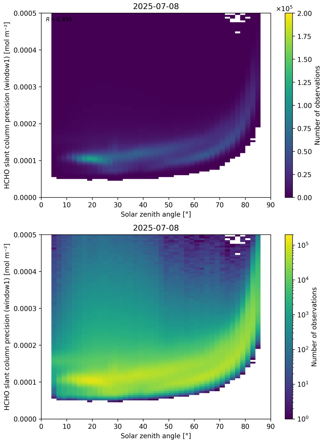
Figure 174: Scatter density plot of “Solar zenith angle” against “HCHO slant column precision (window1)” for 2025-07-08 to 2025-07-09.
