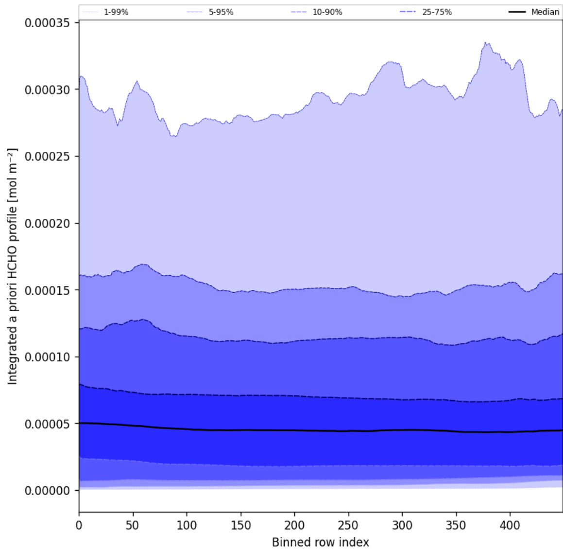
Figure 57: Along track statistics of “Integrated a priori HCHO profile” for 2025-07-08 to 2025-07-09
