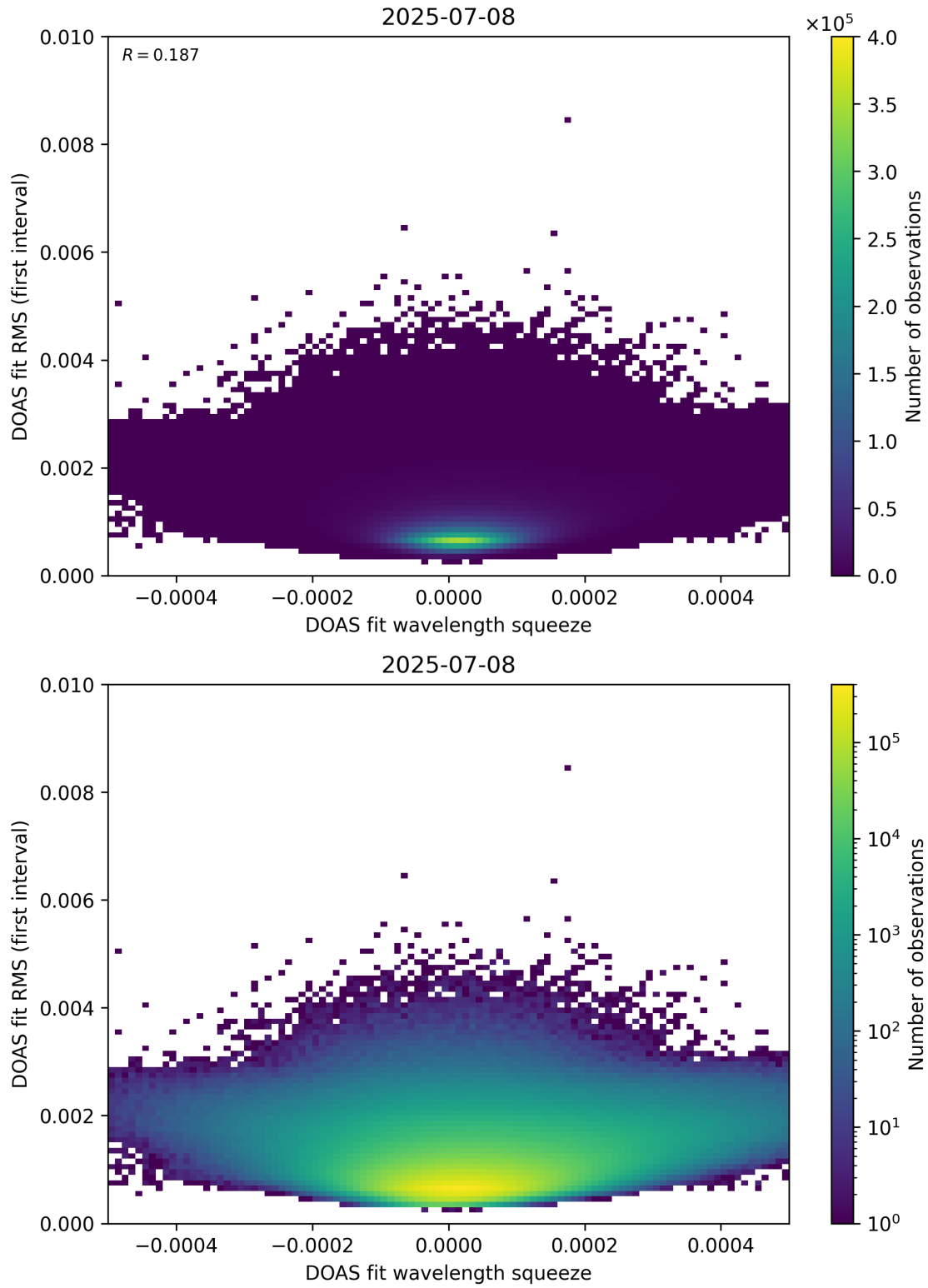
Figure 68: Scatter density plot of “DOAS fit wavelength squeeze” against “DOAS fit RMS (first interval)” for 2025-07-08 to 2025-07-09.
