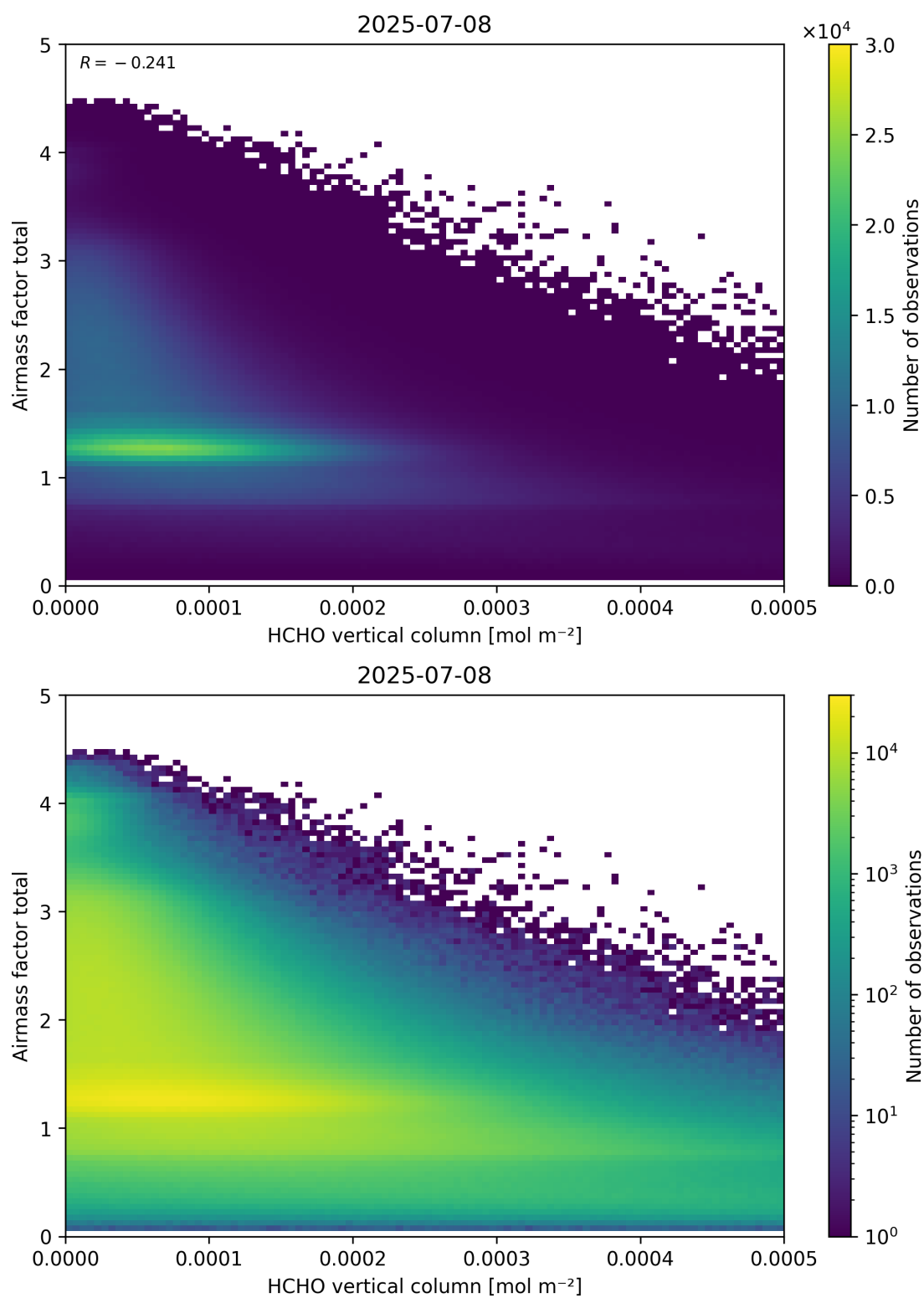
Figure 131: Scatter density plot of “HCHO vertical column” against “Airmass factor total” for 2025-07-08 to 2025-07-09.
