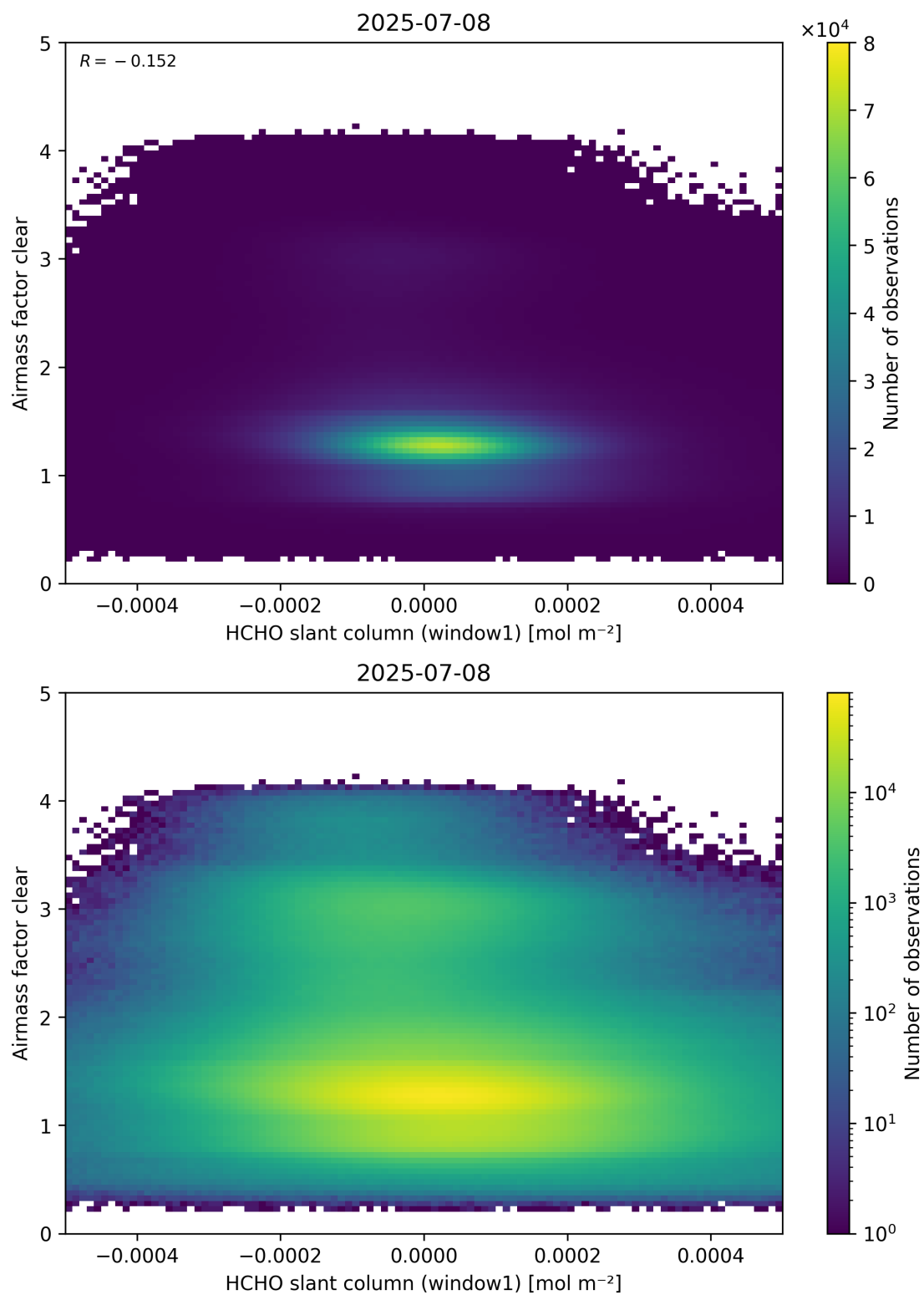
Figure 81: Scatter density plot of “HCHO slant column (window1)” against “Airmass factor clear” for 2025-07-08 to 2025-07-09.
