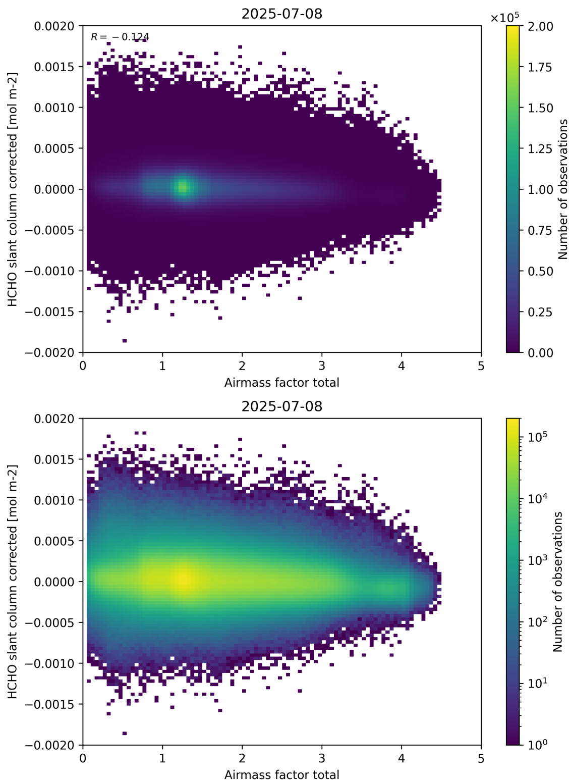
Figure 101: Scatter density plot of “Airmass factor total” against “HCHO slant column corrected” for 2025-07-08 to 2025-07-09.
