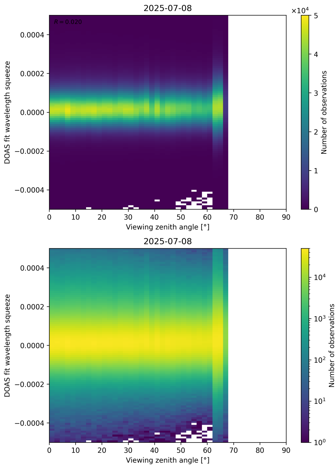
Figure 184: Scatter density plot of “Viewing zenith angle” against “DOAS fit wavelength squeeze” for 2025-07-08 to 2025-07-09.
