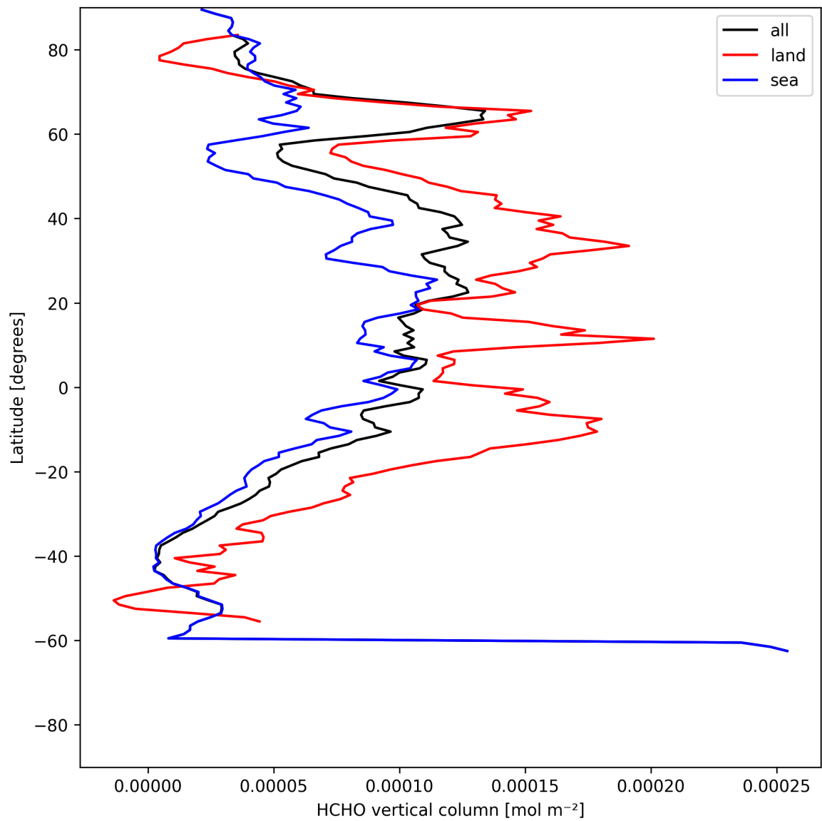
Figure 21: Zonal average of “HCHO vertical column” for 2025-07-08 to 2025-07-09.
