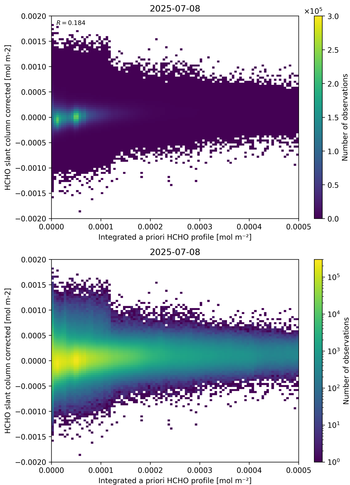
Figure 151: Scatter density plot of “Integrated a priori HCHO profile” against “HCHO slant column corrected” for 2025-07-08 to 2025-07-09.
