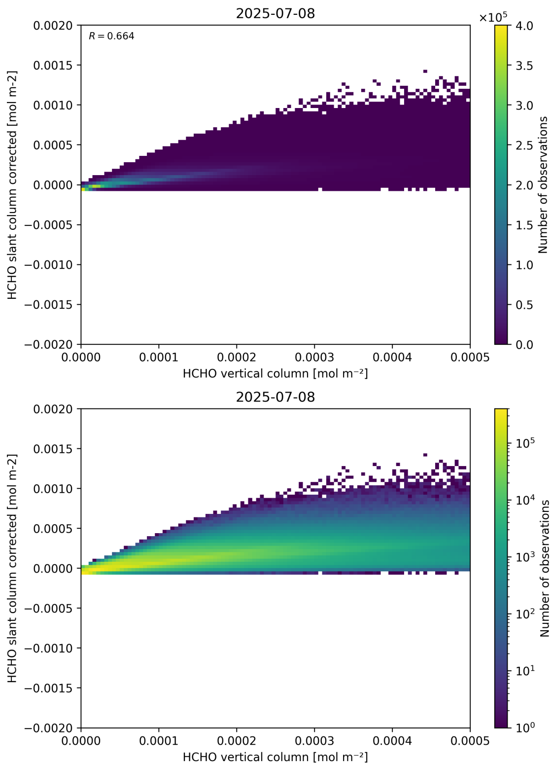
Figure 127: Scatter density plot of “HCHO vertical column” against “HCHO slant column corrected” for 2025-07-08 to 2025-07-09.
