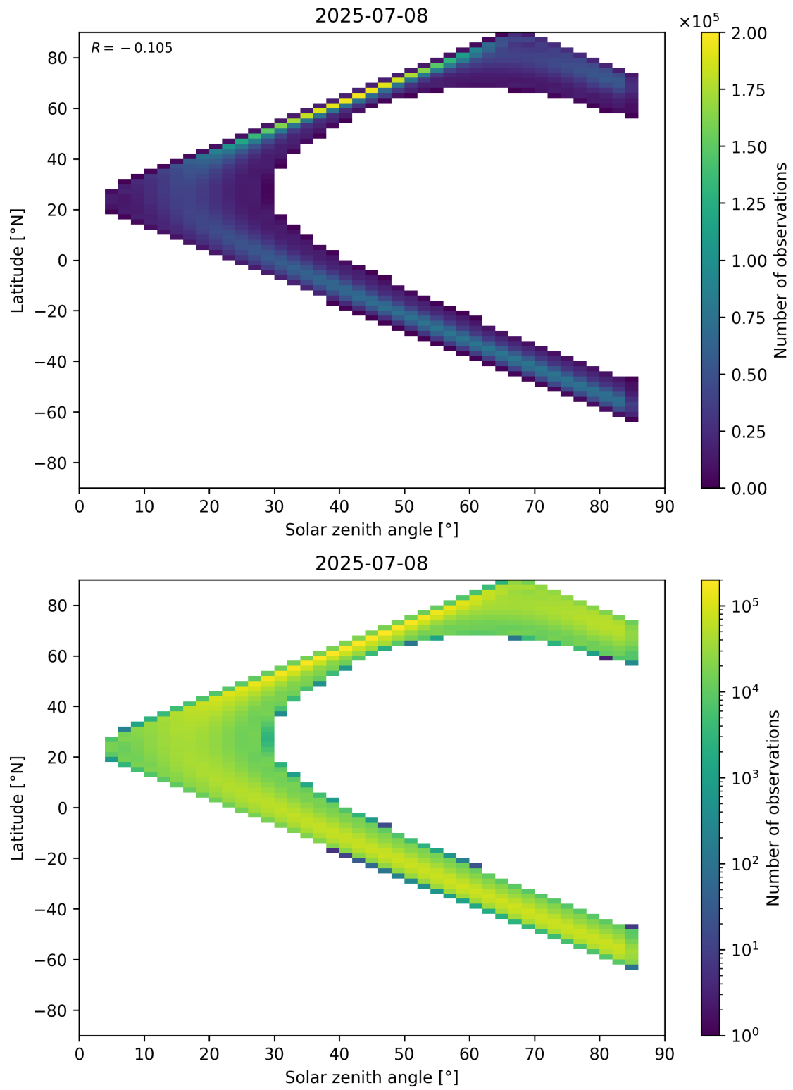
Figure 181: Scatter density plot of “Solar zenith angle” against “Latitude” for 2025-07-08 to 2025-07-09.
