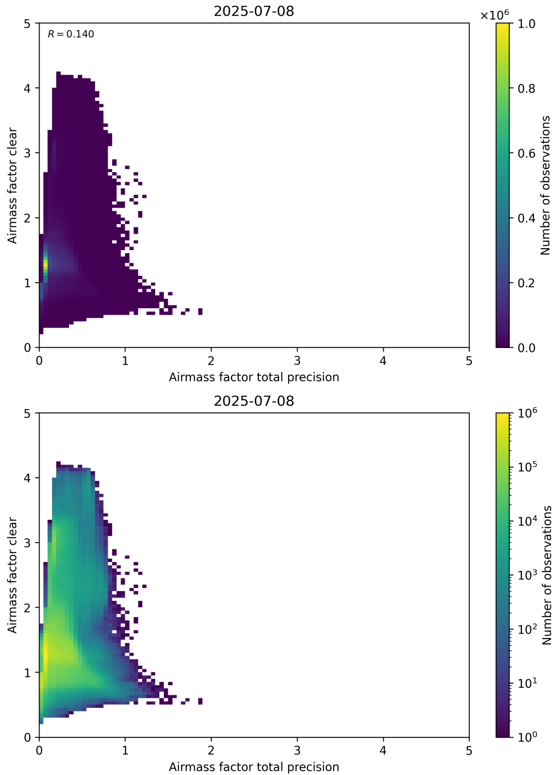
Figure 108: Scatter density plot of “Airmass factor total precision” against “Airmass factor clear” for 2025-07-08 to 2025-07-09.
