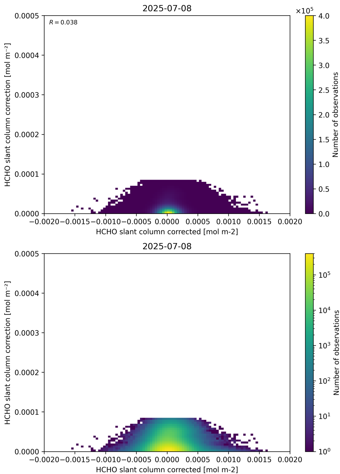
Figure 77: Scatter density plot of “HCHO slant column corrected” against “HCHO slant column correction” for 2025-07-08 to 2025-07-09.
