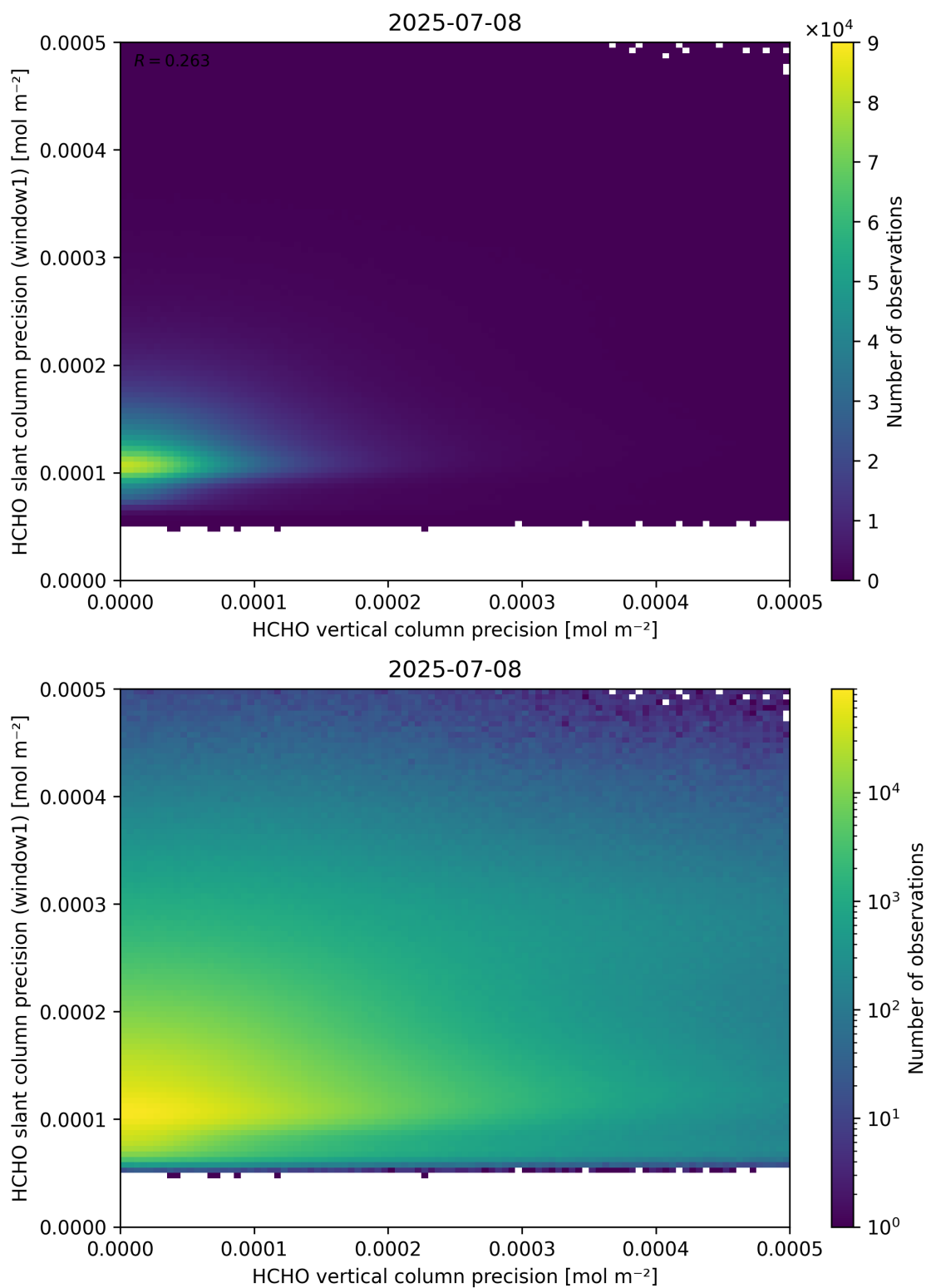
Figure 143: Scatter density plot of “HCHO vertical column precision” against “HCHO slant column precision (window1)” for 2025-07-08 to 2025-07-09.
