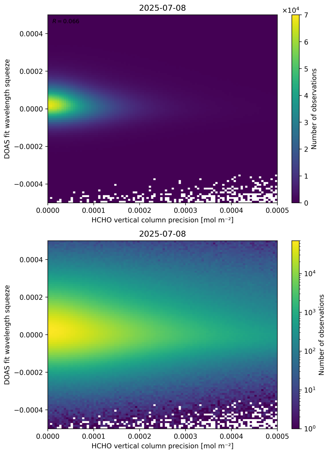
Figure 138: Scatter density plot of “HCHO vertical column precision” against “DOAS fit wavelength squeeze” for 2025-07-08 to 2025-07-09.
