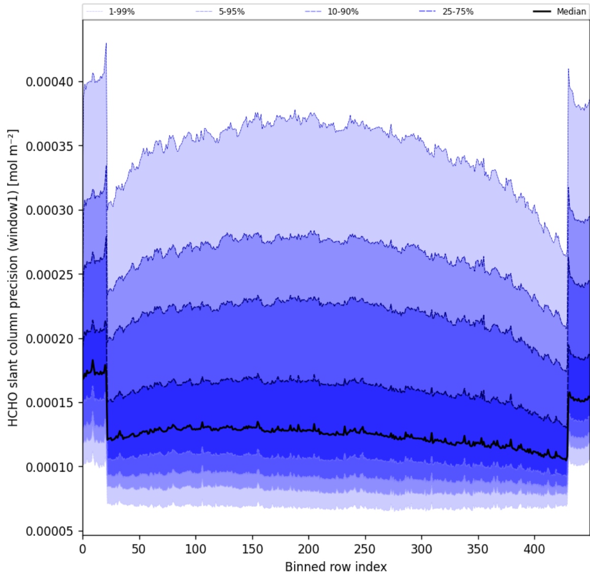
Figure 53: Along track statistics of “HCHO slant column precision (window1)” for 2025-07-08 to 2025-07-09
