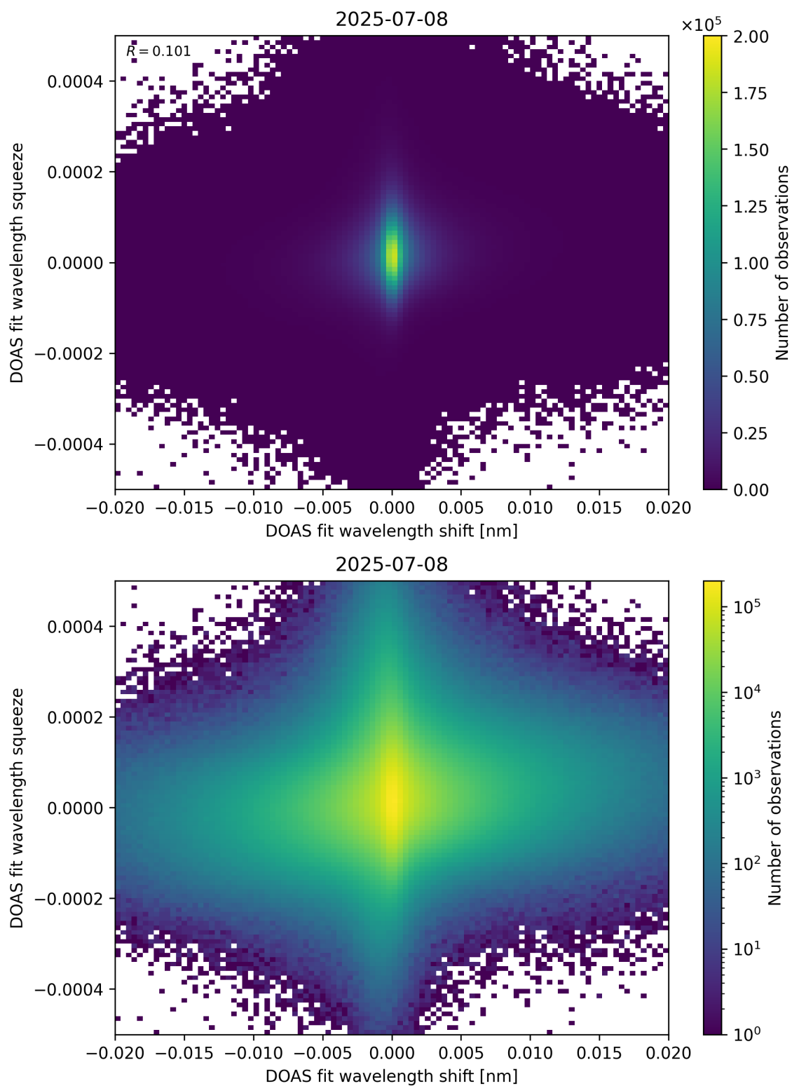
Figure 65: Scatter density plot of “DOAS fit wavelength shift” against “DOAS fit wavelength squeeze” for 2025-07-08 to 2025-07-09.
