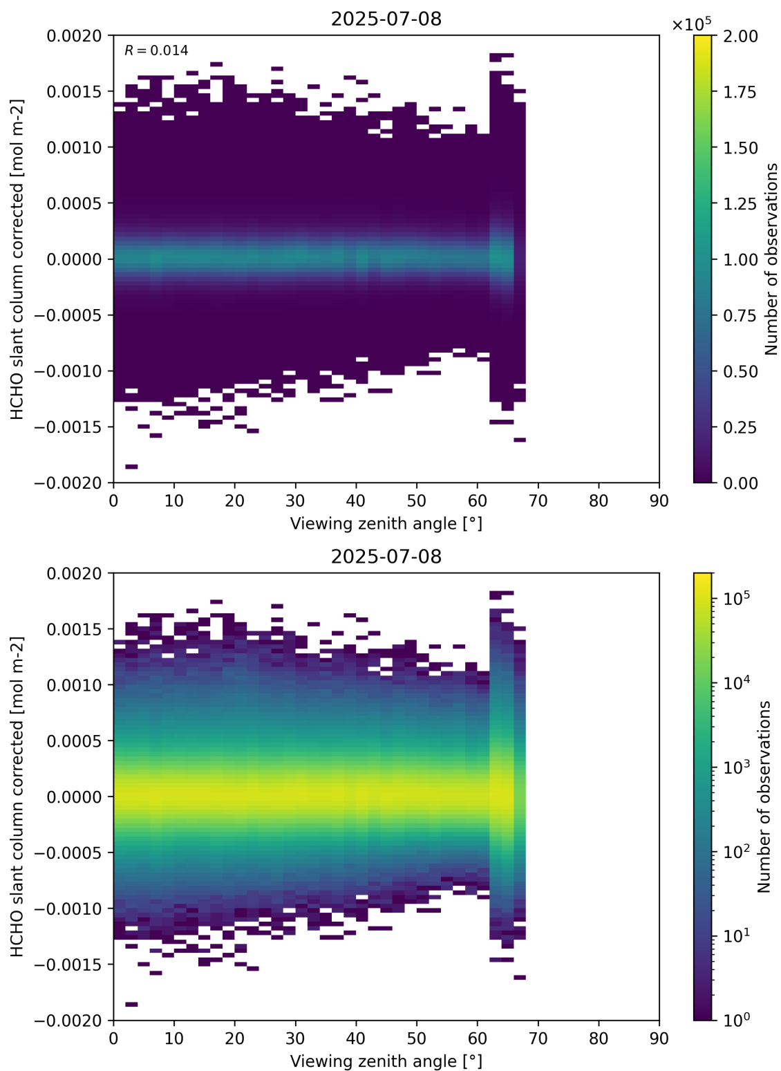
Figure 186: Scatter density plot of “Viewing zenith angle” against “HCHO slant column corrected” for 2025-07-08 to 2025-07-09.
