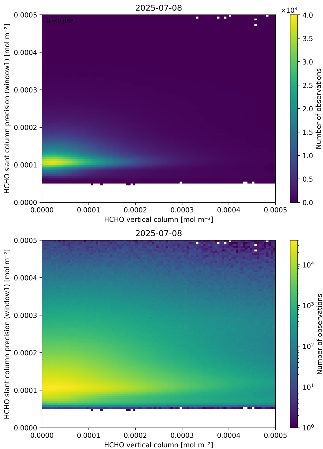
Figure 130: Scatter density plot of “HCHO vertical column” against “HCHO slant column precision (window1)” for 2025-07-08 to 2025-07-09.
