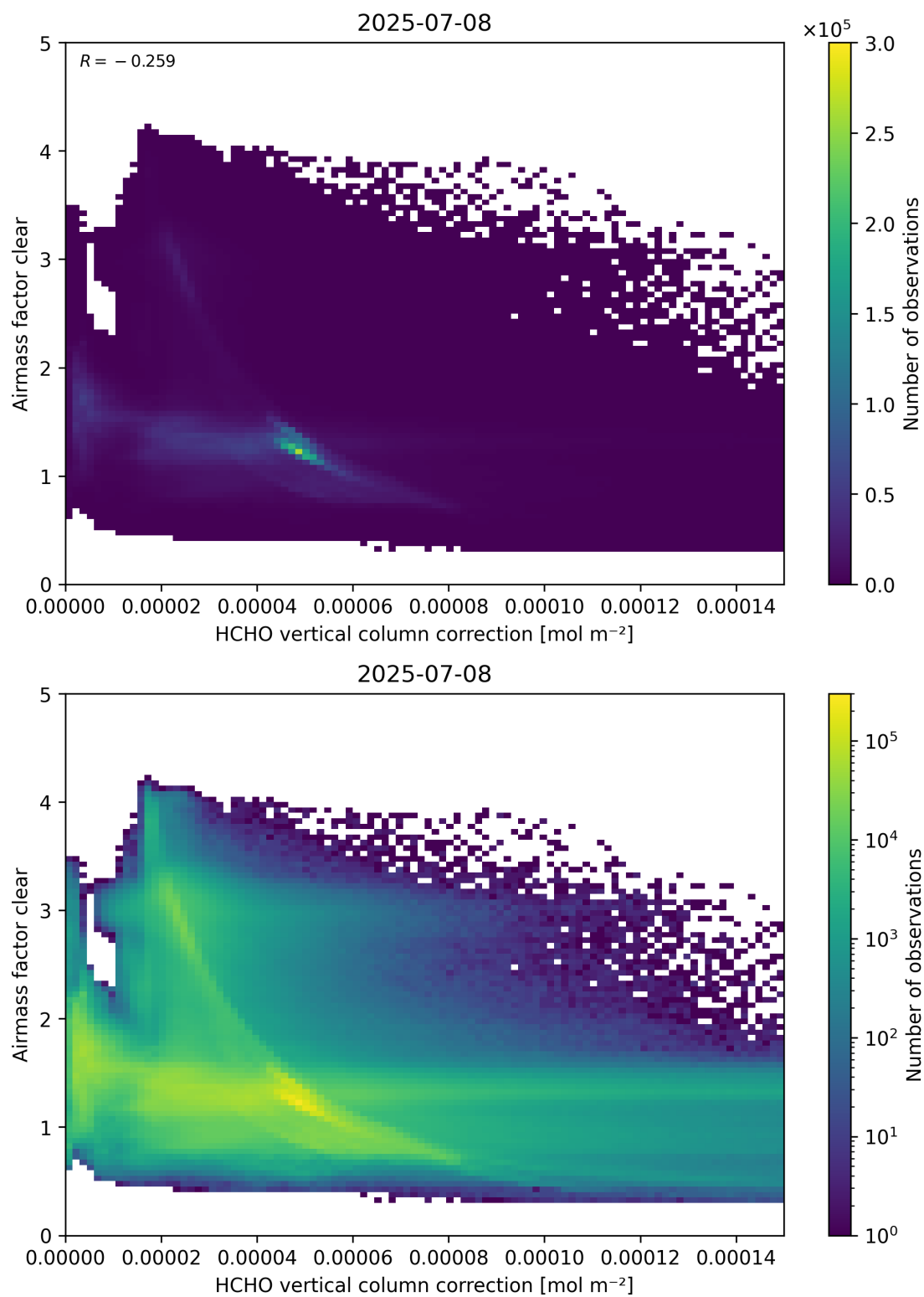
Figure 115: Scatter density plot of “HCHO vertical column correction” against “Airmass factor clear” for 2025-07-08 to 2025-07-09.
