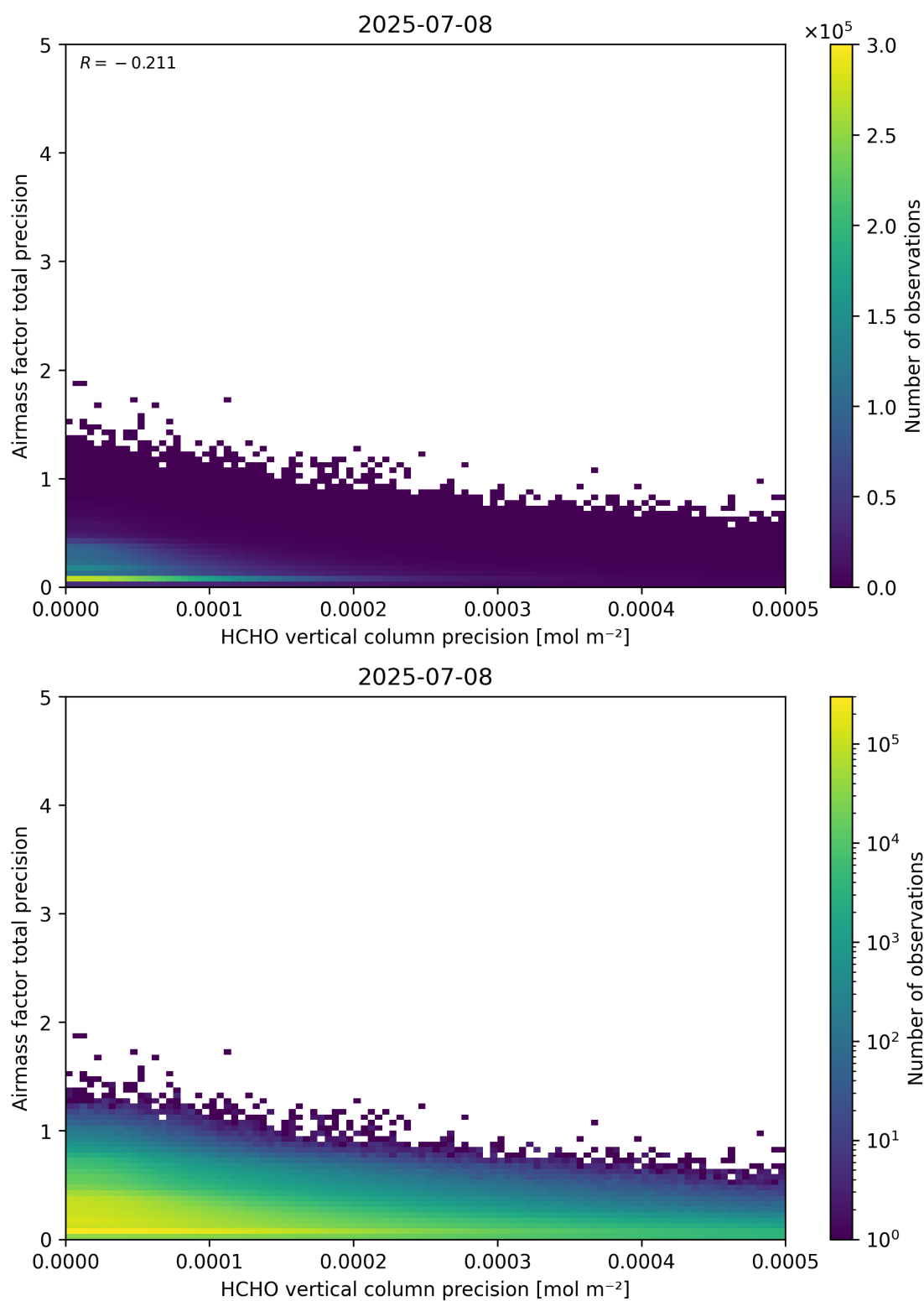
Figure 145: Scatter density plot of “HCHO vertical column precision” against “Airmass factor total precision” for 2025-07-08 to 2025-07-09.
