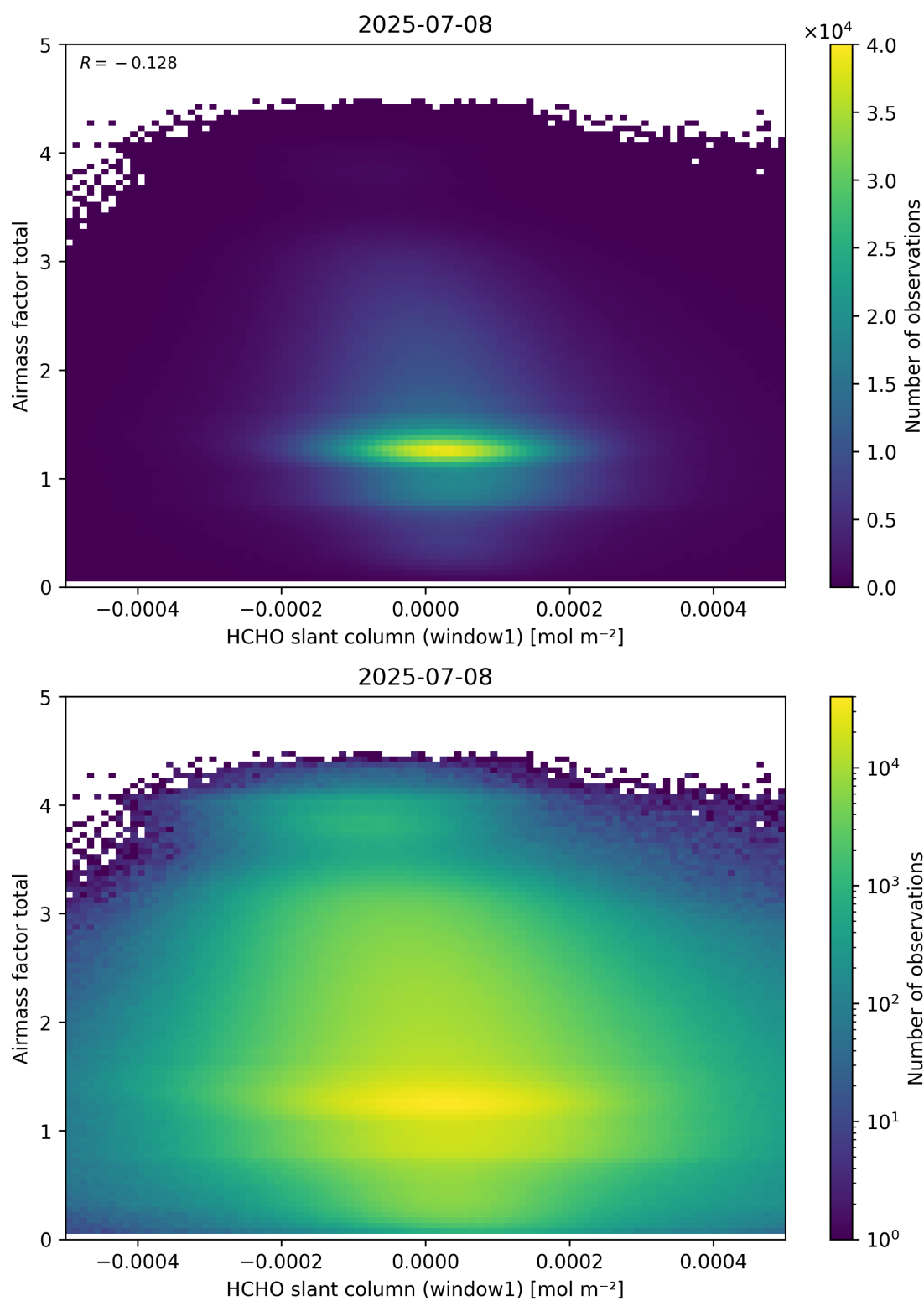
Figure 85: Scatter density plot of “HCHO slant column (window1)” against “Airmass factor total” for 2025-07-08 to 2025-07-09.
