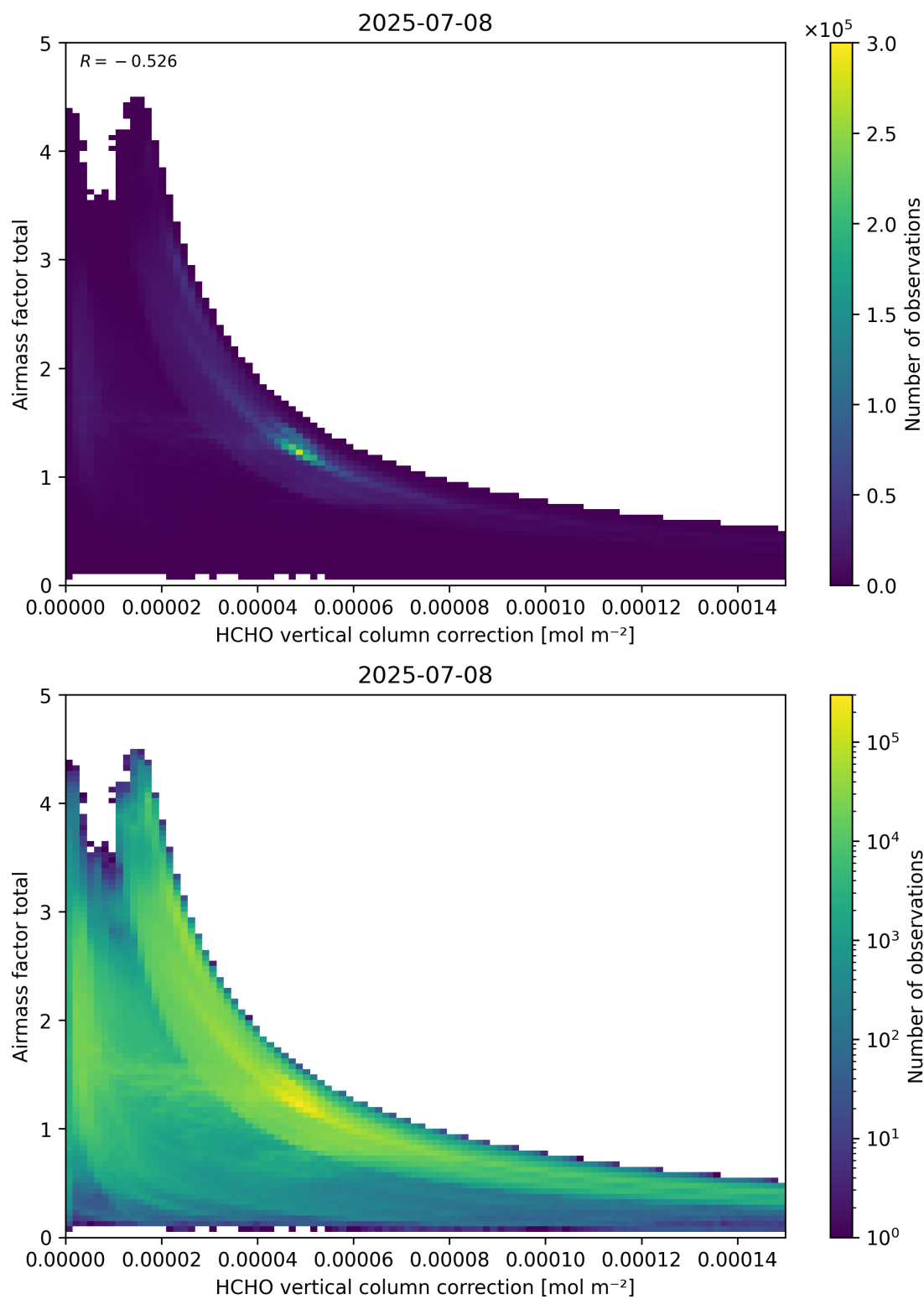
Figure 120: Scatter density plot of “HCHO vertical column correction” against “Airmass factor total” for 2025-07-08 to 2025-07-09.
