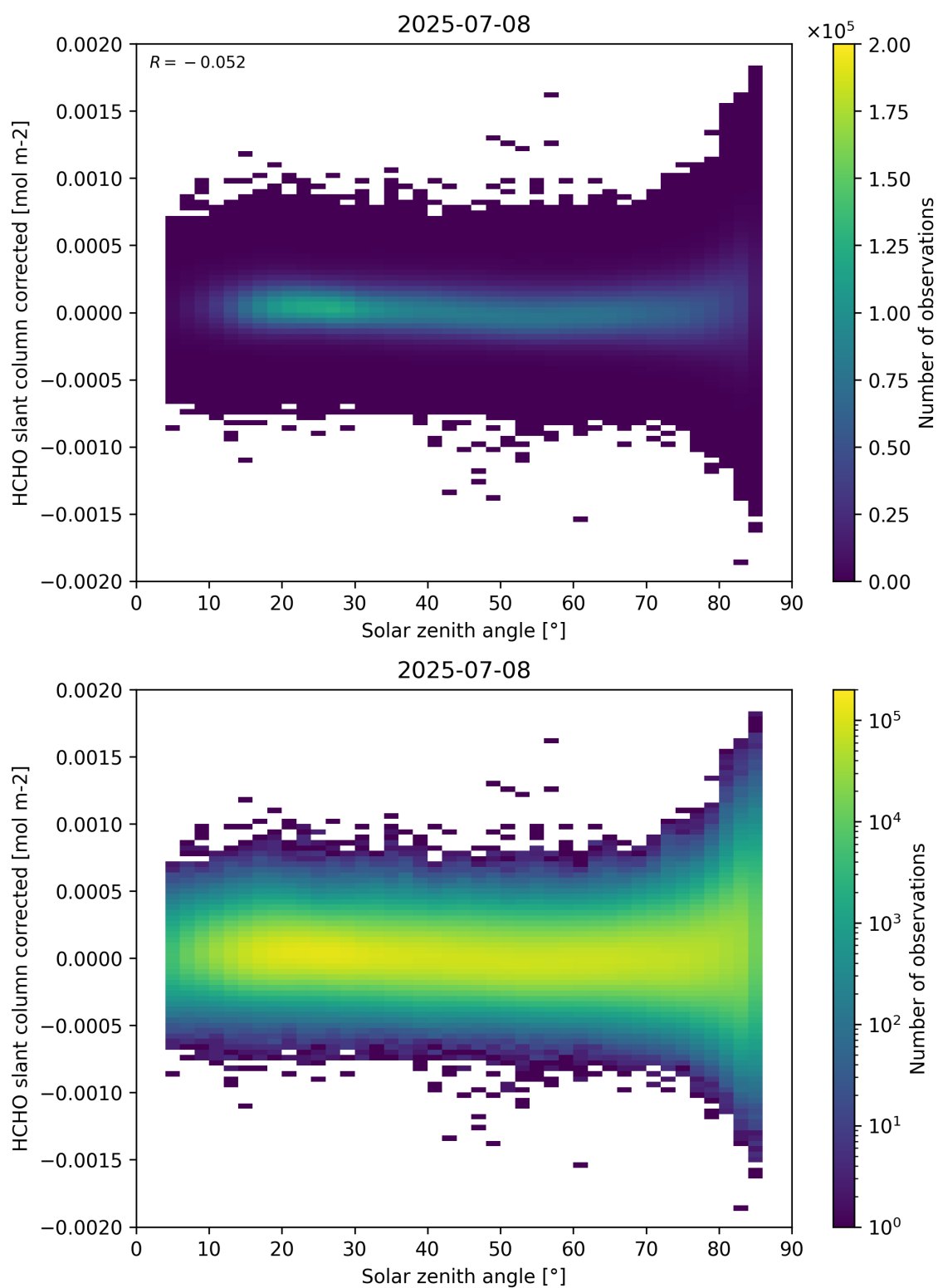
Figure 171: Scatter density plot of “Solar zenith angle” against “HCHO slant column corrected” for 2025-07-08 to 2025-07-09.
