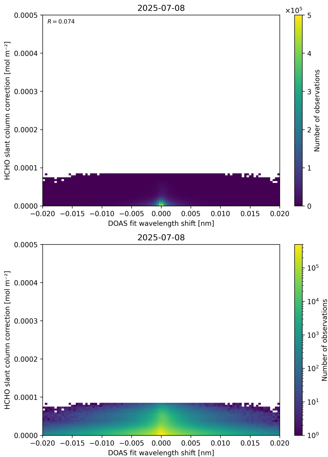
Figure 67: Scatter density plot of “DOAS fit wavelength shift” against “HCHO slant column correction” for 2025-07-08 to 2025-07-09.
