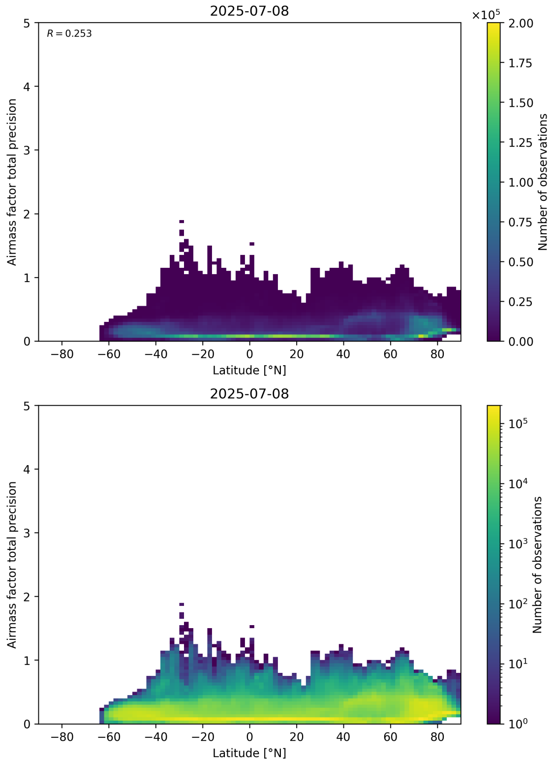
Figure 162: Scatter density plot of “Latitude” against “Airmass factor total precision” for 2025-07-08 to 2025-07-09.
