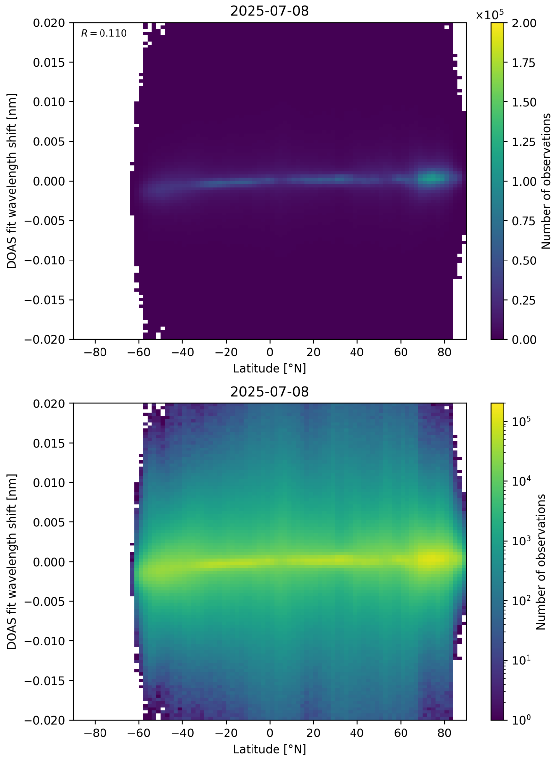
Figure 154: Scatter density plot of “Latitude” against “DOAS fit wavelength shift” for 2025-07-08 to 2025-07-09.
