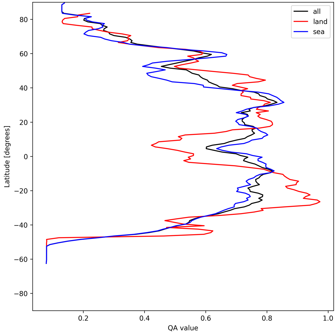
Figure 20: Zonal average of “QA value” for 2025-07-08 to 2025-07-09.
