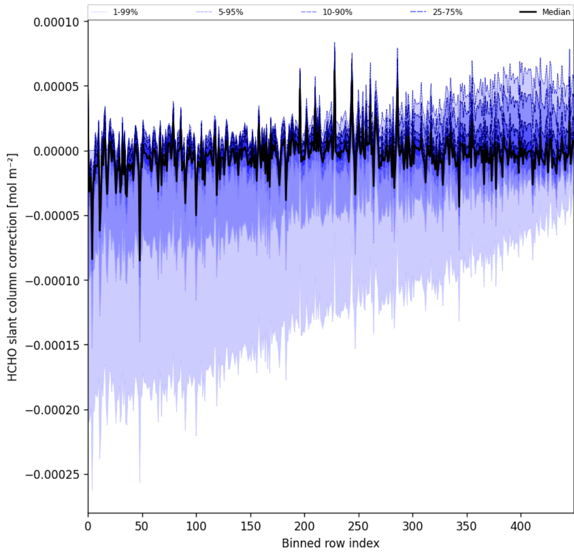
Figure 61: Along track statistics of “HCHO slant column correction” for 2025-07-08 to 2025-07-09
