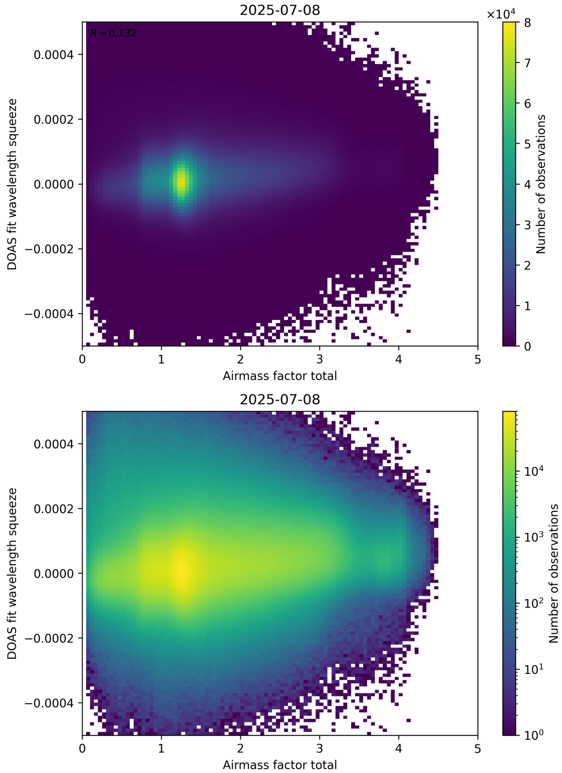
Figure 99: Scatter density plot of “Airmass factor total” against “DOAS fit wavelength squeeze” for 2025-07-08 to 2025-07-09.
