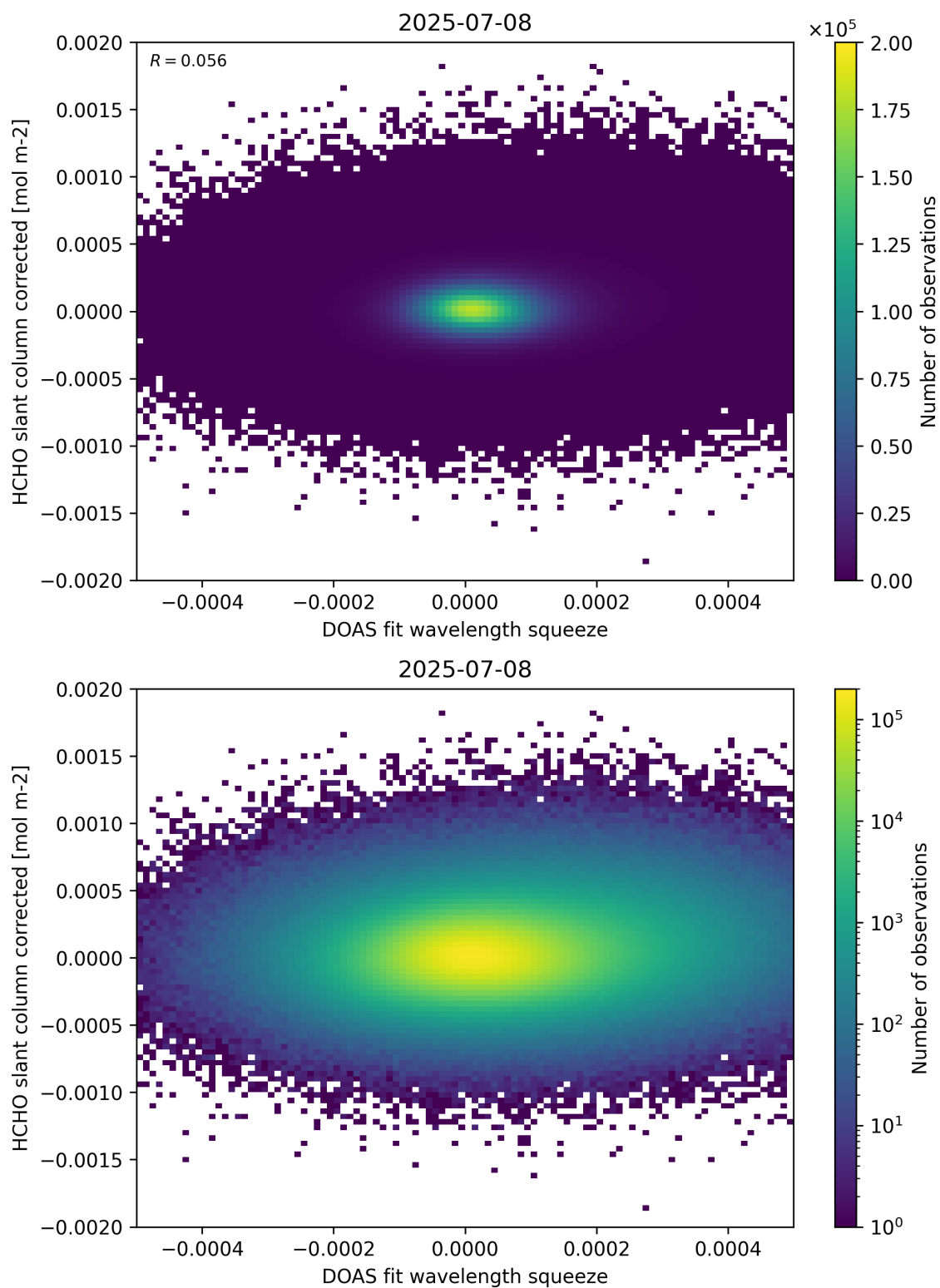
Figure 69: Scatter density plot of “DOAS fit wavelength squeeze” against “HCHO slant column corrected” for 2025-07-08 to 2025-07-09.
