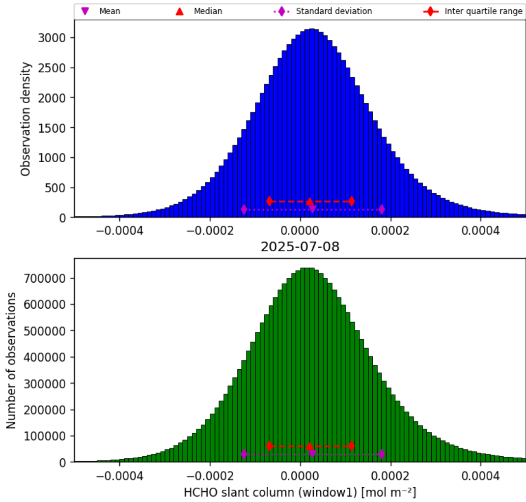
Figure 38: Histogram of “HCHO slant column (window1)” for 2025-07-08 to 2025-07-09
