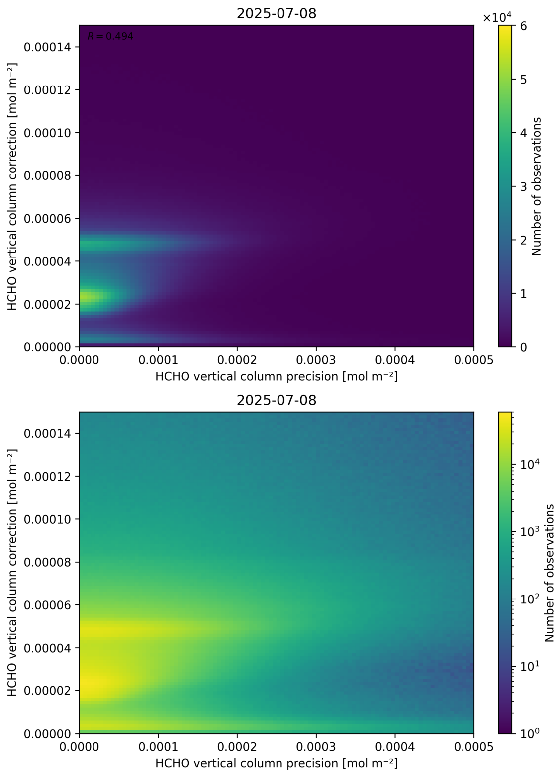
Figure 146: Scatter density plot of “HCHO vertical column precision” against “HCHO vertical column correction” for 2025-07-08 to 2025-07-09.
