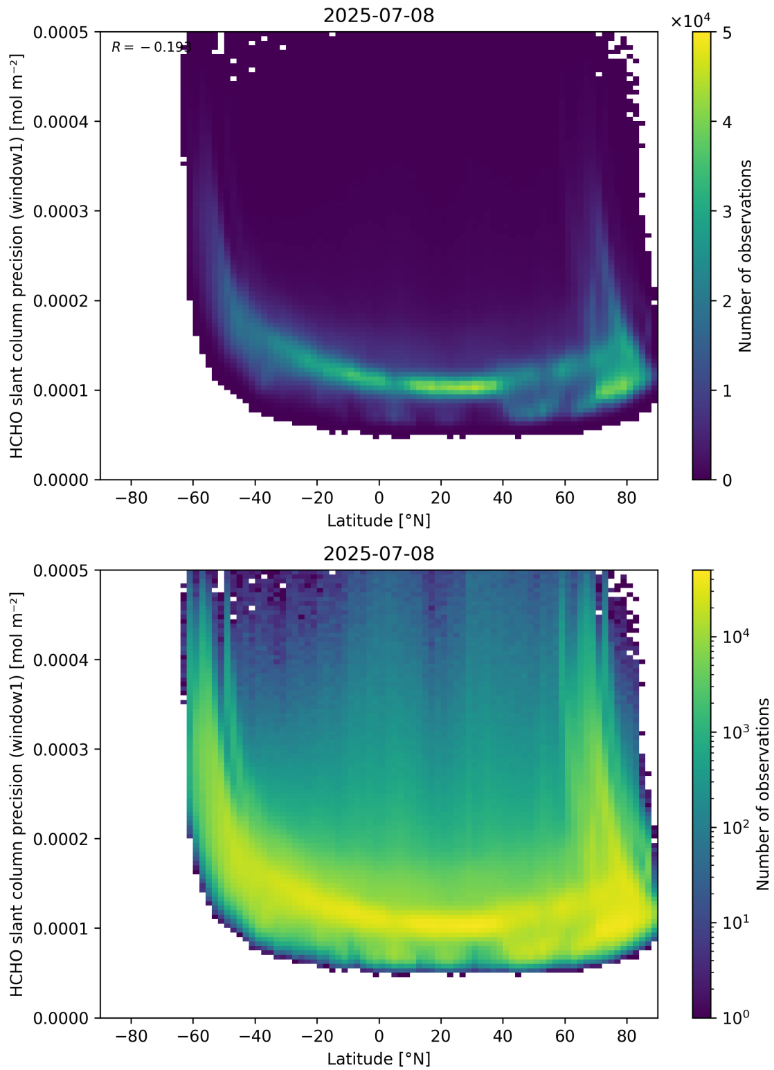
Figure 160: Scatter density plot of “Latitude” against “HCHO slant column precision (window1)” for 2025-07-08 to 2025-07-09.
