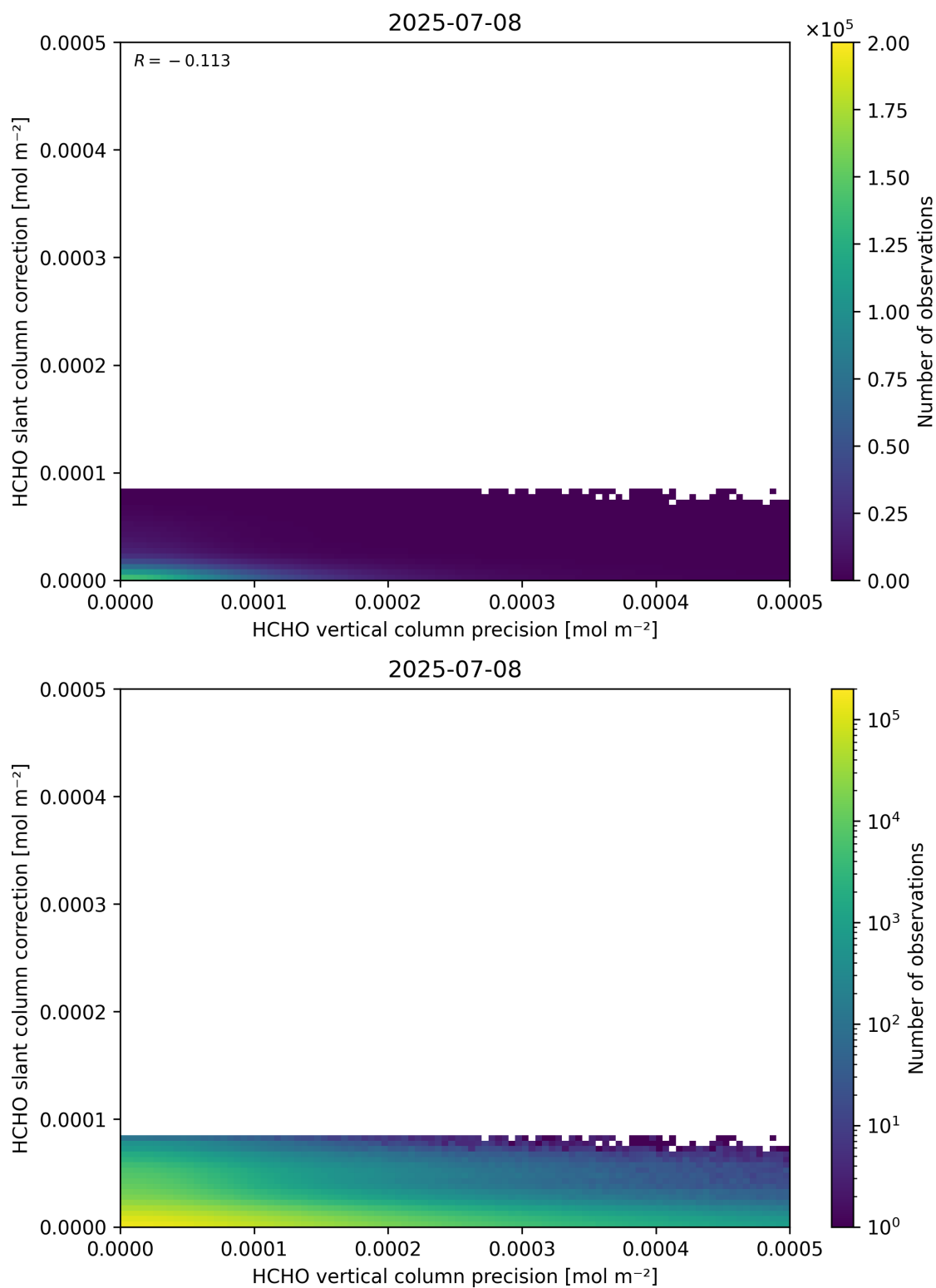
Figure 141: Scatter density plot of “HCHO vertical column precision” against “HCHO slant column correction” for 2025-07-08 to 2025-07-09.
