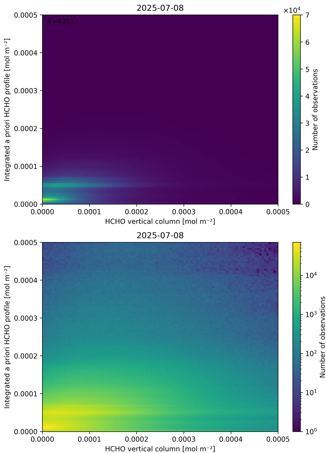
Figure 135: Scatter density plot of “HCHO vertical column” against “Integrated a priori HCHO profile” for 2025-07-08 to 2025-07-09.
