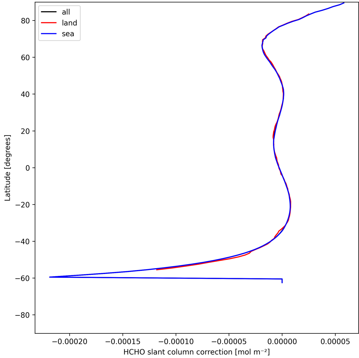
Figure 33: Zonal average of “HCHO slant column correction” for 2025-07-08 to 2025-07-09.
