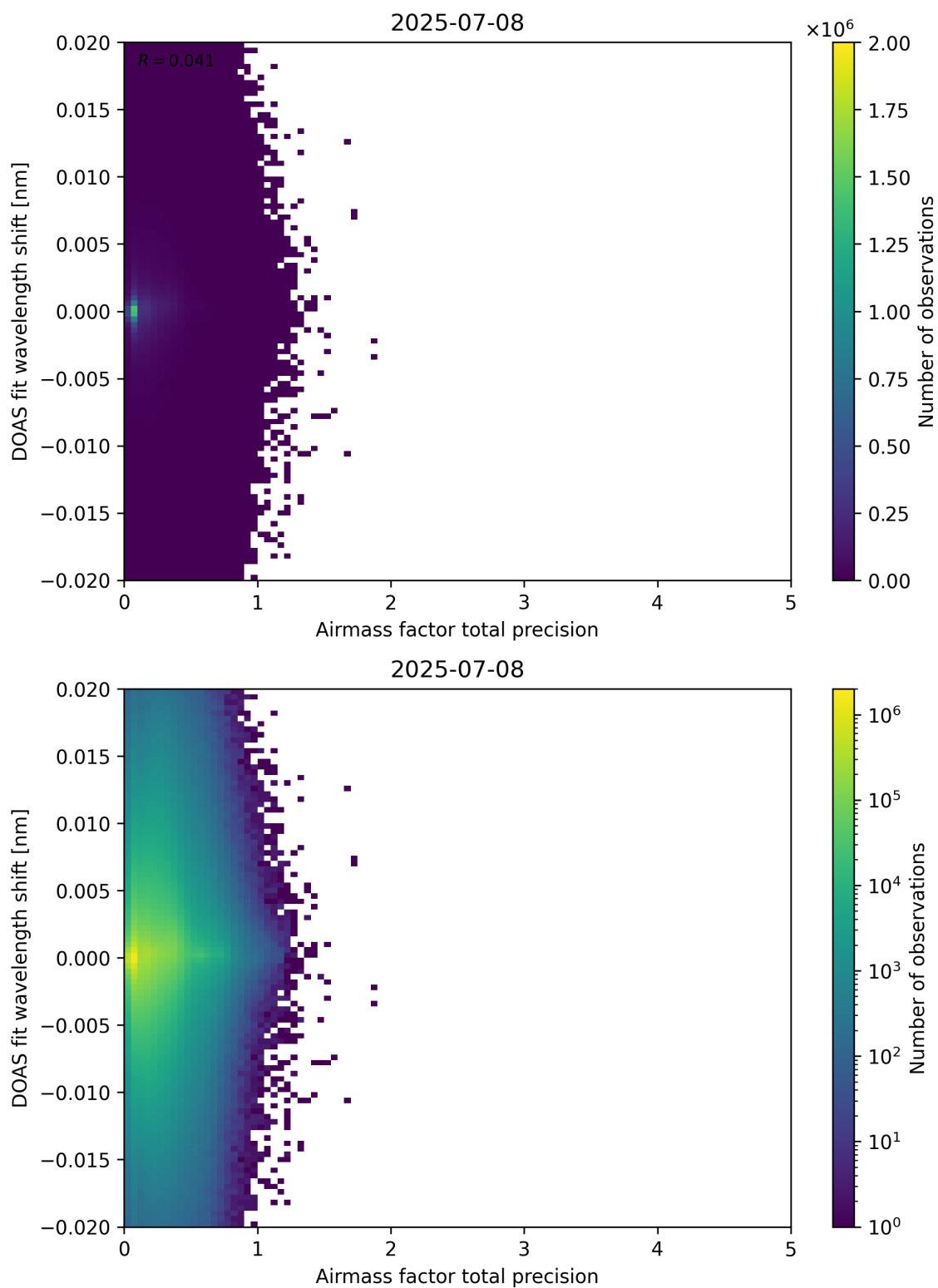
Figure 106: Scatter density plot of “Airmass factor total precision” against “DOAS fit wavelength shift” for 2025-07-08 to 2025-07-09.
