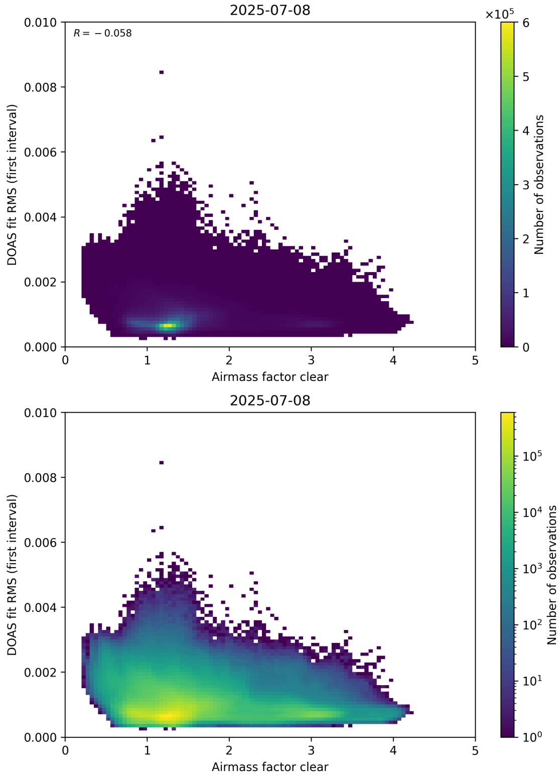
Figure 71: Scatter density plot of “Airmass factor clear” against “DOAS fit RMS (first interval)” for 2025-07-08 to 2025-07-09.
