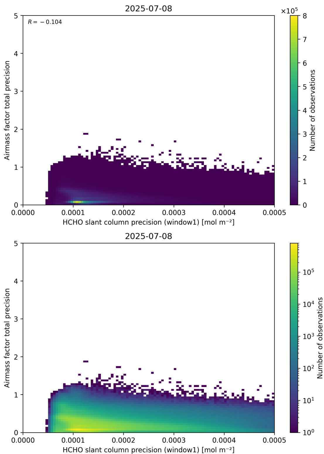
Figure 95: Scatter density plot of “HCHO slant column precision (window1)” against “Airmass factor total precision” for 2025-07-08 to 2025-07-09.
