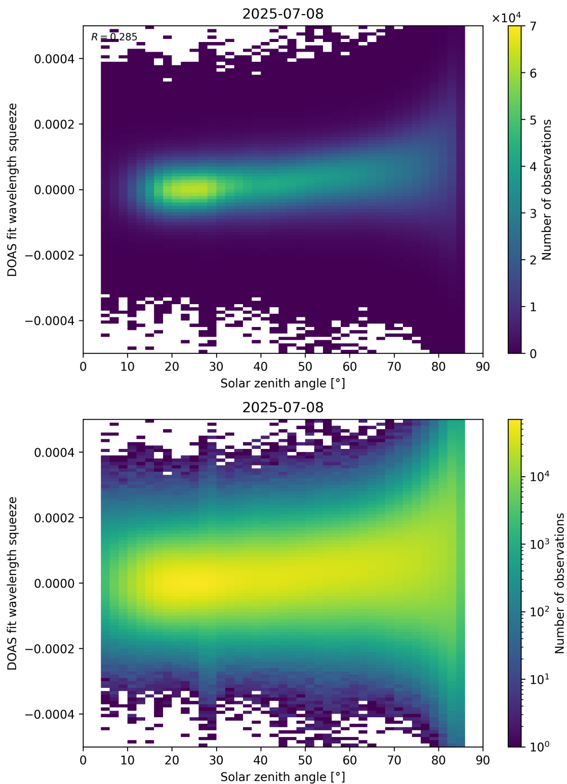
Figure 169: Scatter density plot of “Solar zenith angle” against “DOAS fit wavelength squeeze” for 2025-07-08 to 2025-07-09.
