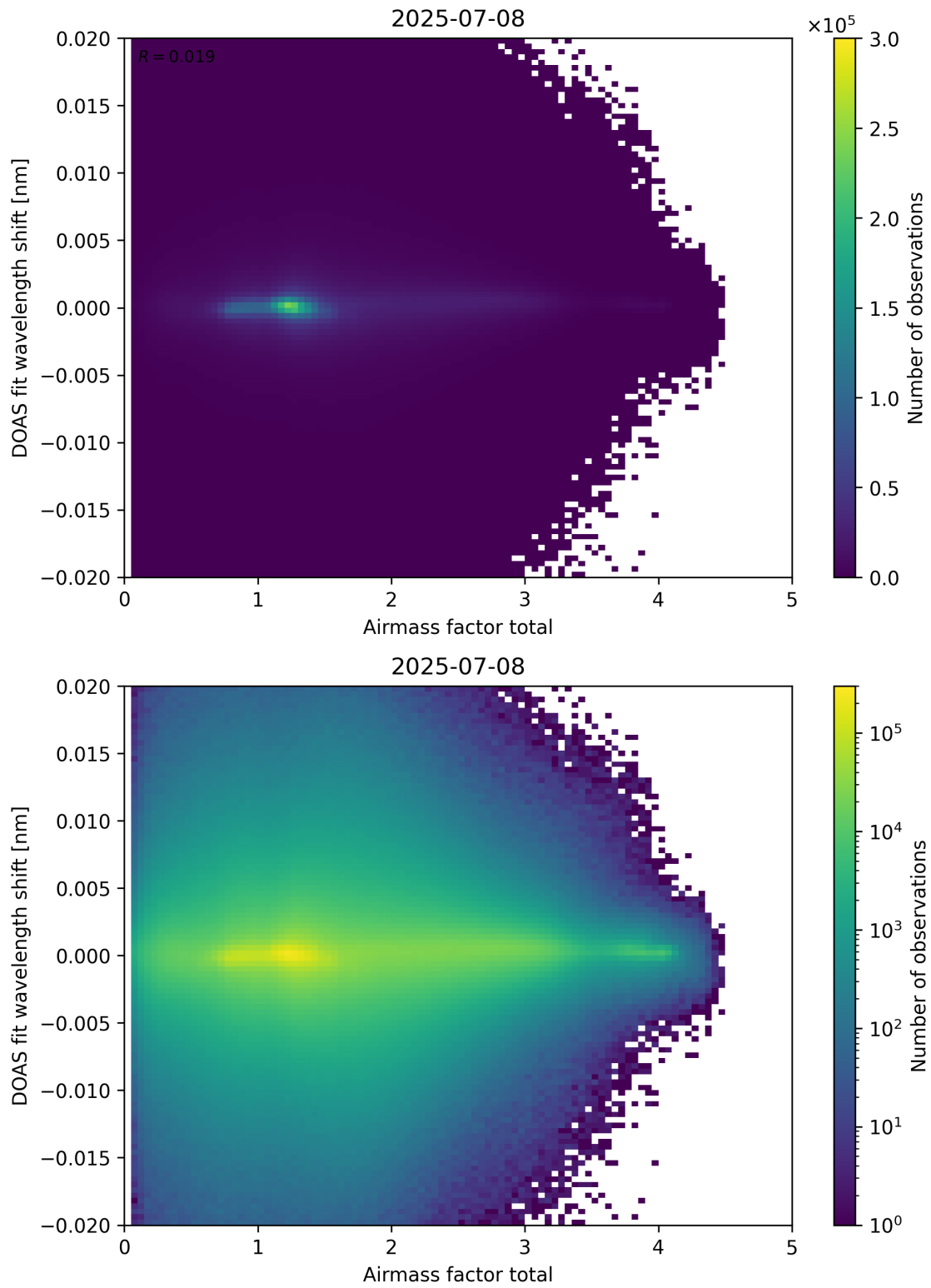
Figure 98: Scatter density plot of “Airmass factor total” against “DOAS fit wavelength shift” for 2025-07-08 to 2025-07-09.
