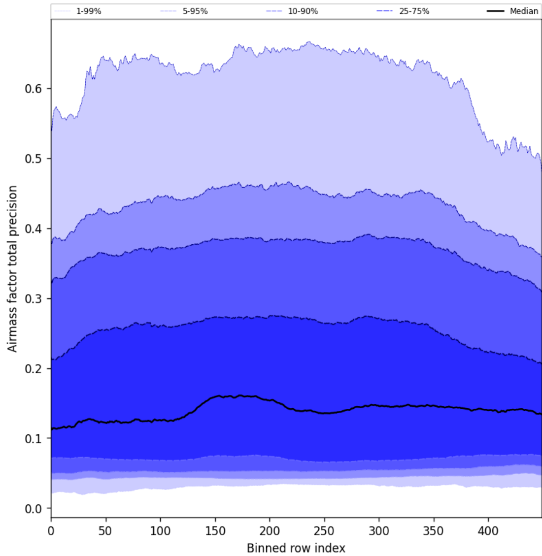
Figure 55: Along track statistics of “Airmass factor total precision” for 2025-07-08 to 2025-07-09
