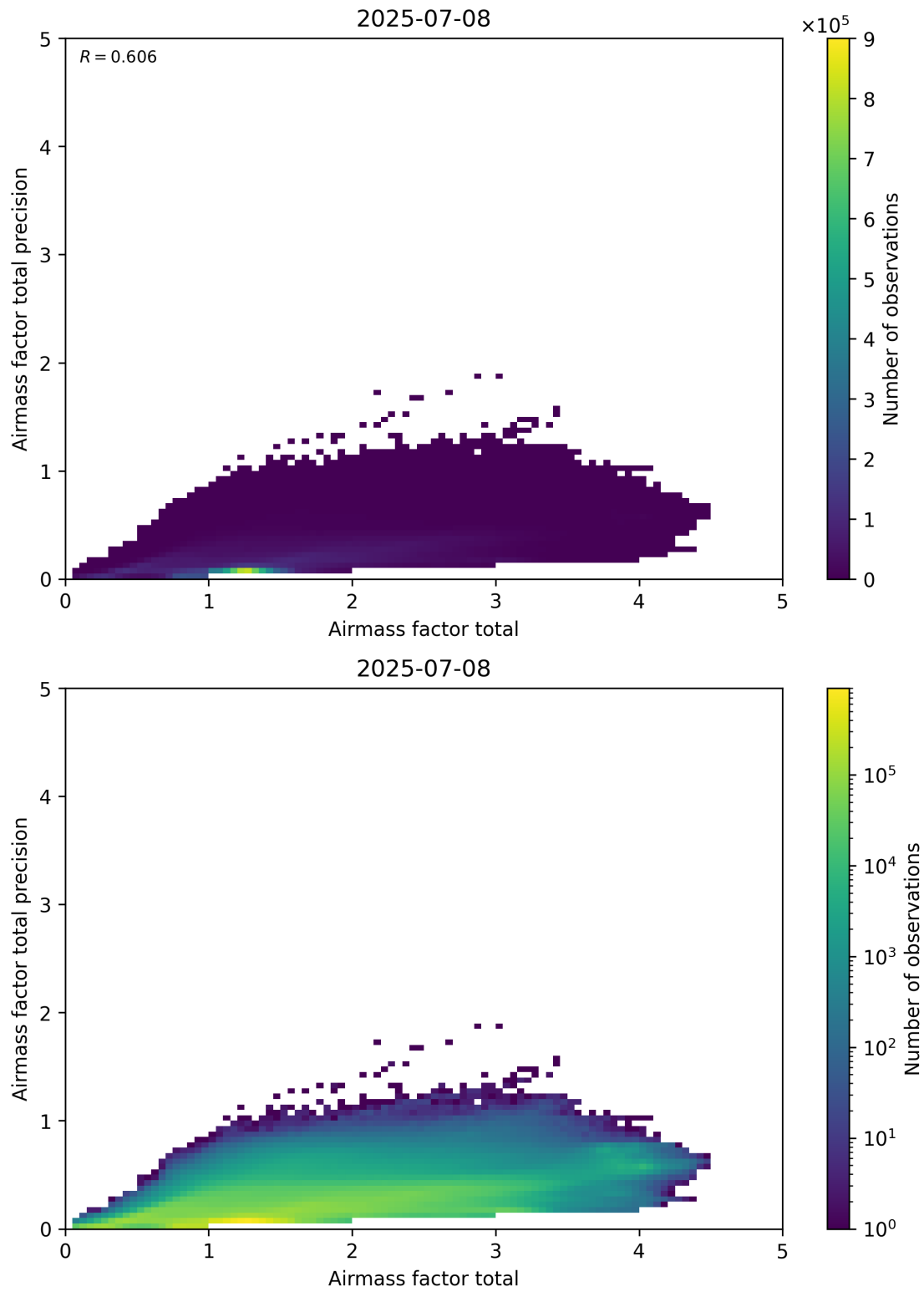
Figure 103: Scatter density plot of “Airmass factor total” against “Airmass factor total precision” for 2025-07-08 to 2025-07-09.
