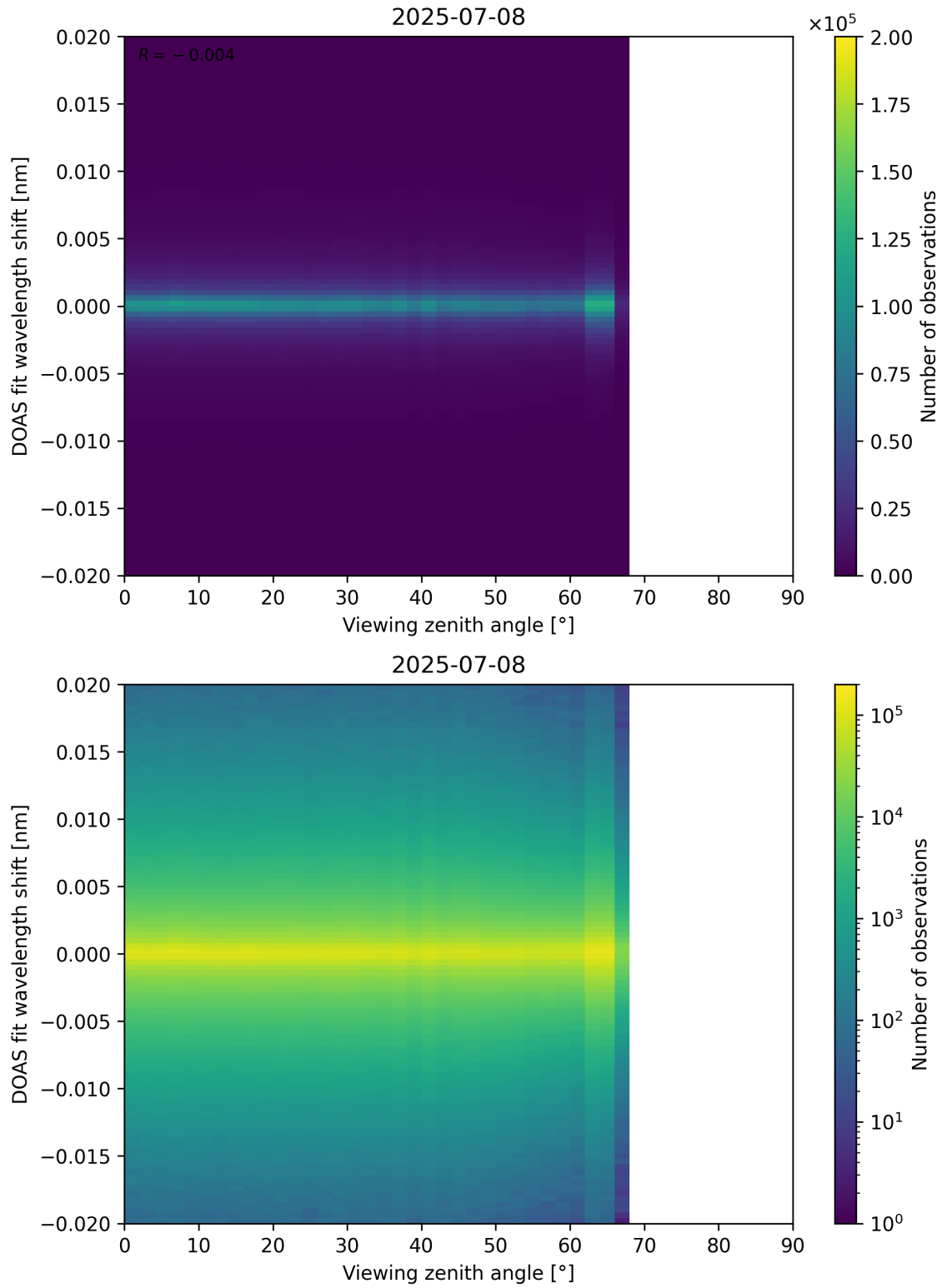
Figure 183: Scatter density plot of “Viewing zenith angle” against “DOAS fit wavelength shift” for 2025-07-08 to 2025-07-09.
