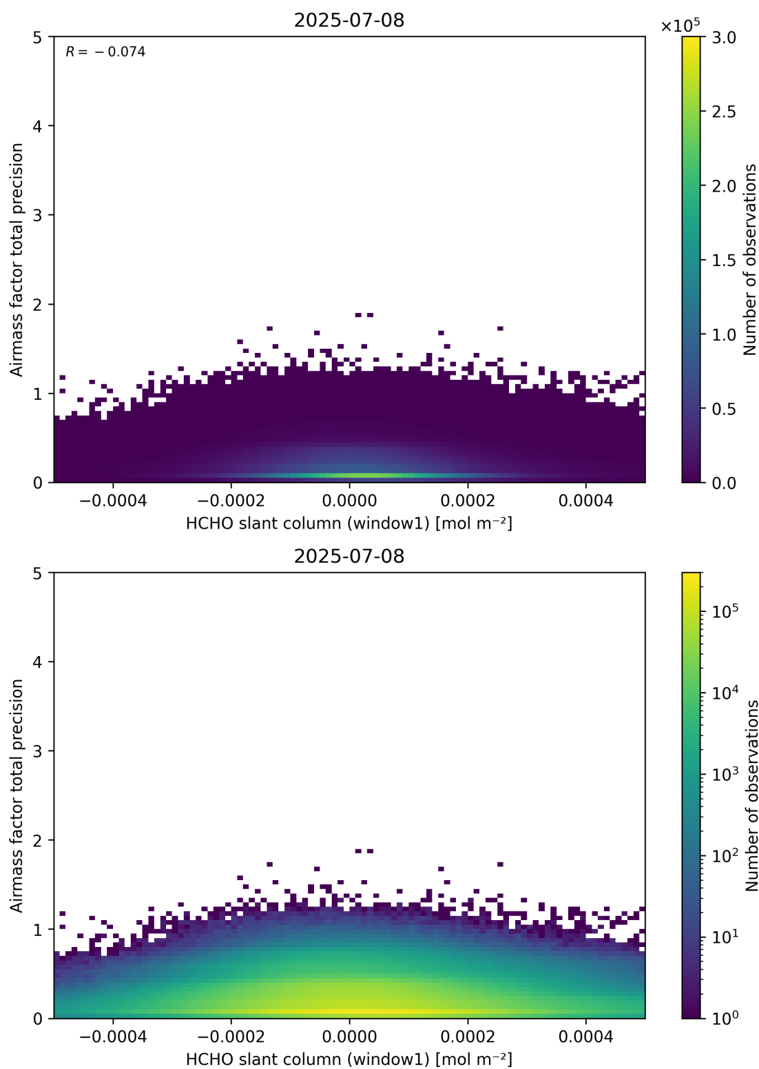
Figure 86: Scatter density plot of “HCHO slant column (window1)” against “Airmass factor total precision” for 2025-07-08 to 2025-07-09.
