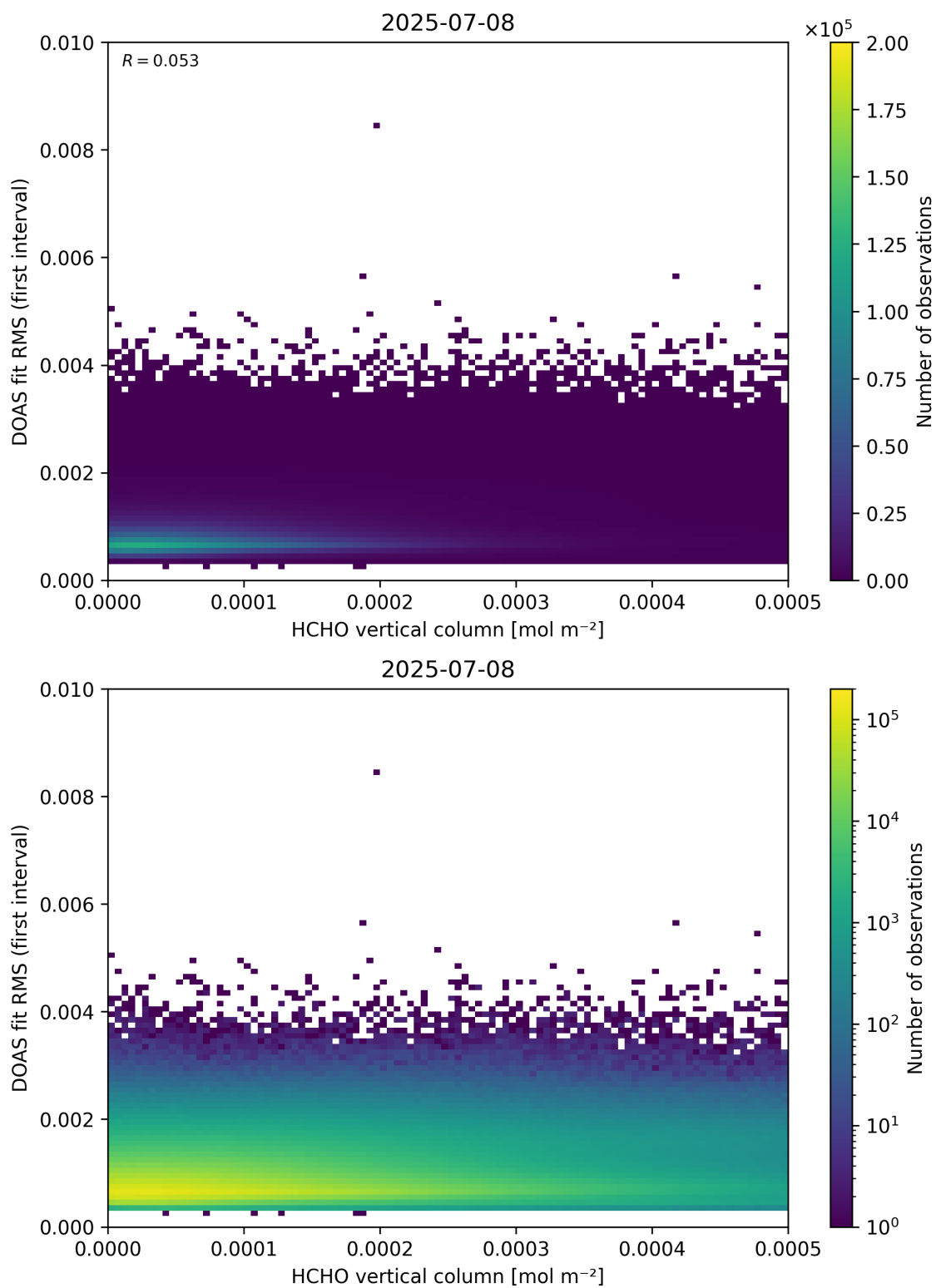
Figure 123: Scatter density plot of “HCHO vertical column” against “DOAS fit RMS (first interval)” for 2025-07-08 to 2025-07-09.
