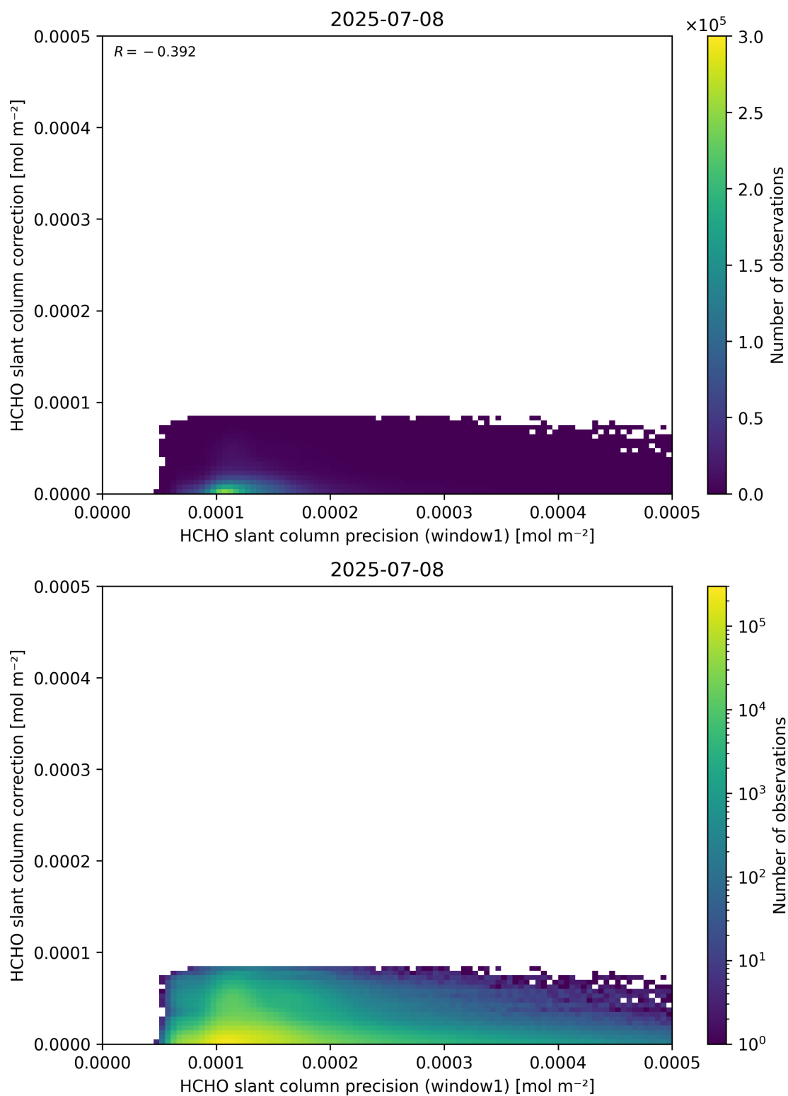
Figure 93: Scatter density plot of “HCHO slant column precision (window1)” against “HCHO slant column correction” for 2025-07-08 to 2025-07-09.
