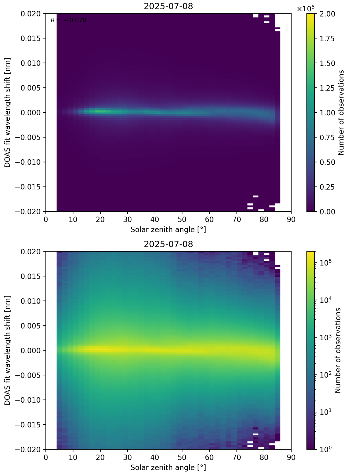
Figure 168: Scatter density plot of “Solar zenith angle” against “DOAS fit wavelength shift” for 2025-07-08 to 2025-07-09.
