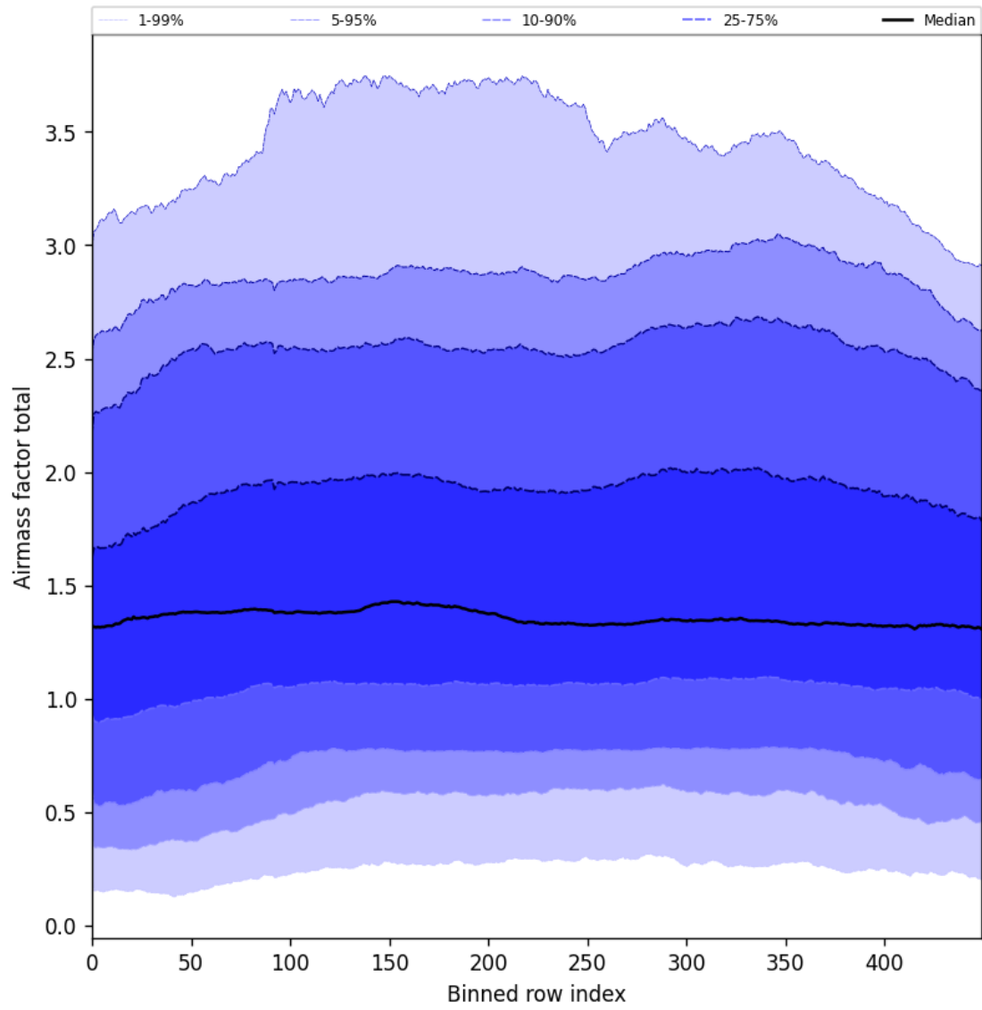
Figure 54: Along track statistics of “Airmass factor total” for 2025-07-08 to 2025-07-09
