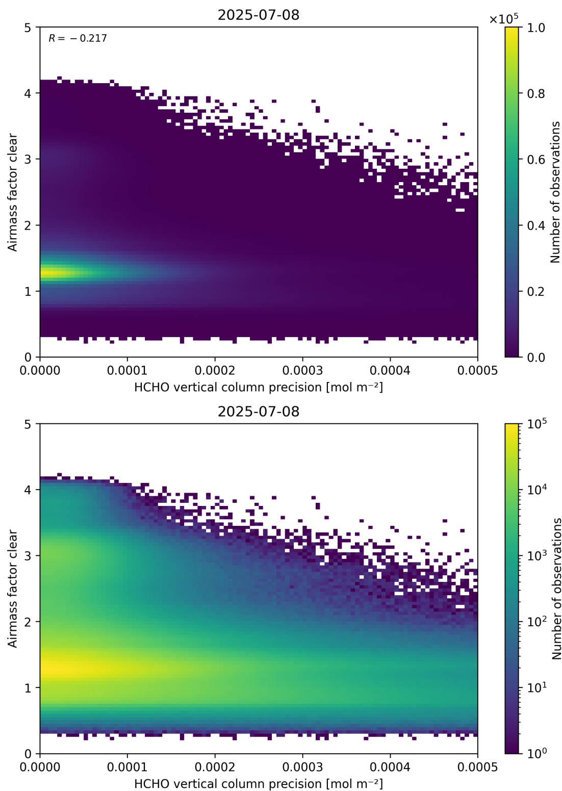
Figure 139: Scatter density plot of “HCHO vertical column precision” against “Airmass factor clear” for 2025-07-08 to 2025-07-09.
