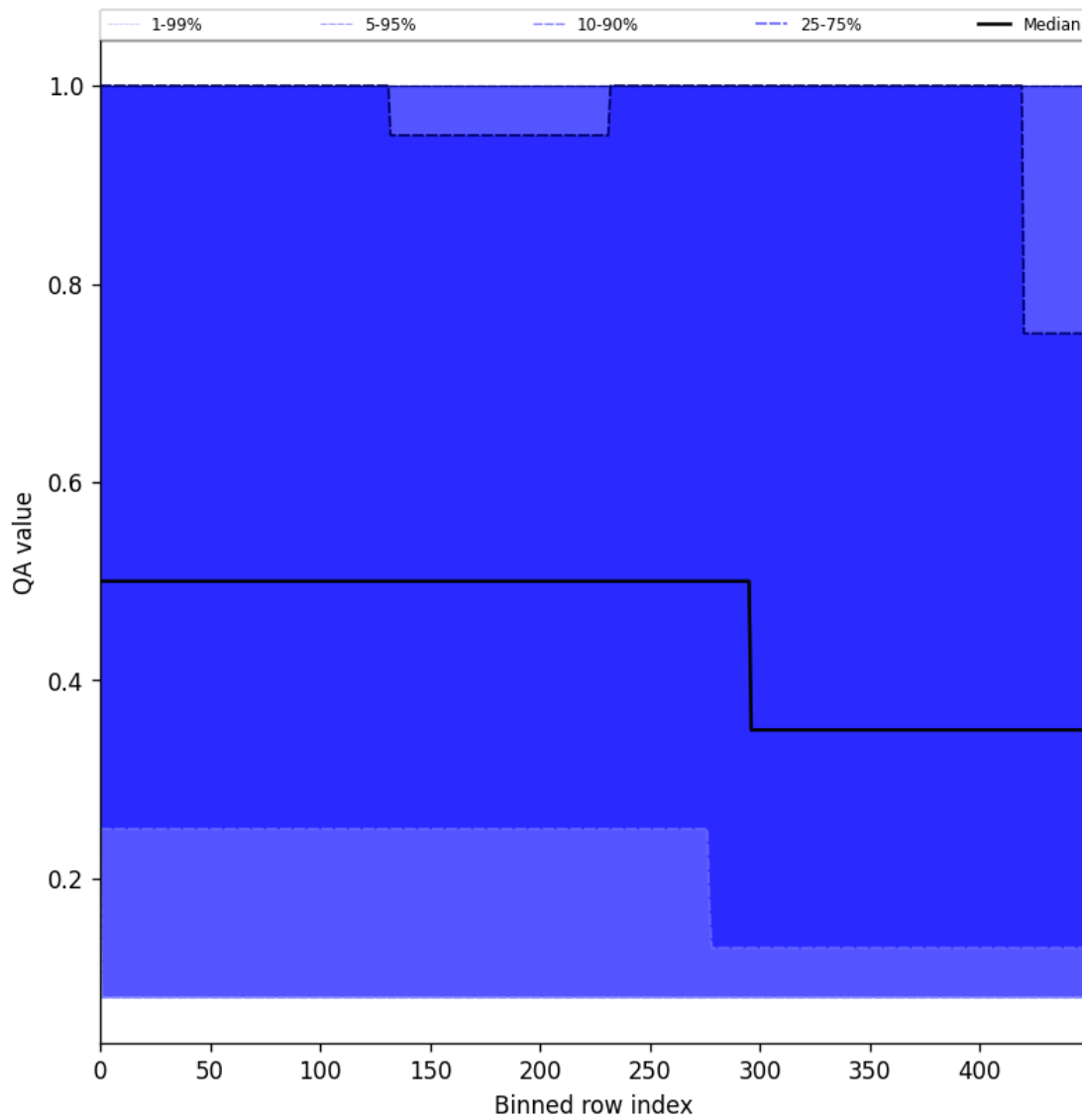
Figure 48: Along track statistics of “QA value” for 2025-07-08 to 2025-07-09
