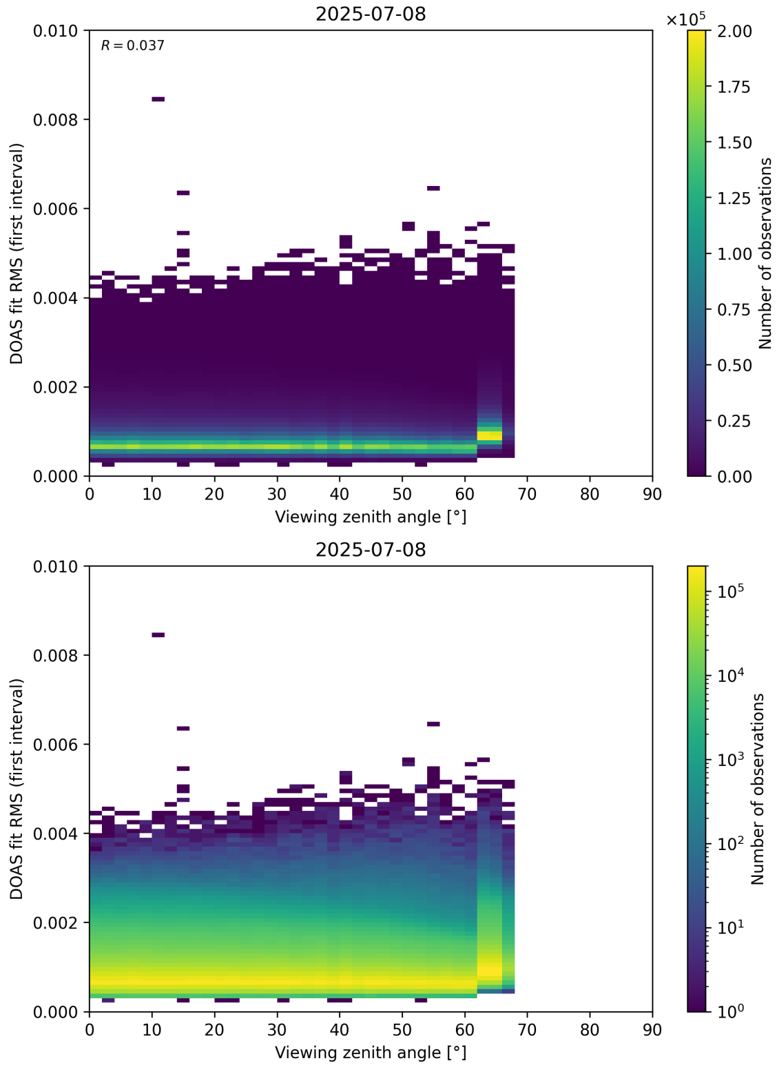
Figure 182: Scatter density plot of “Viewing zenith angle” against “DOAS fit RMS (first interval)” for 2025-07-08 to 2025-07-09.
