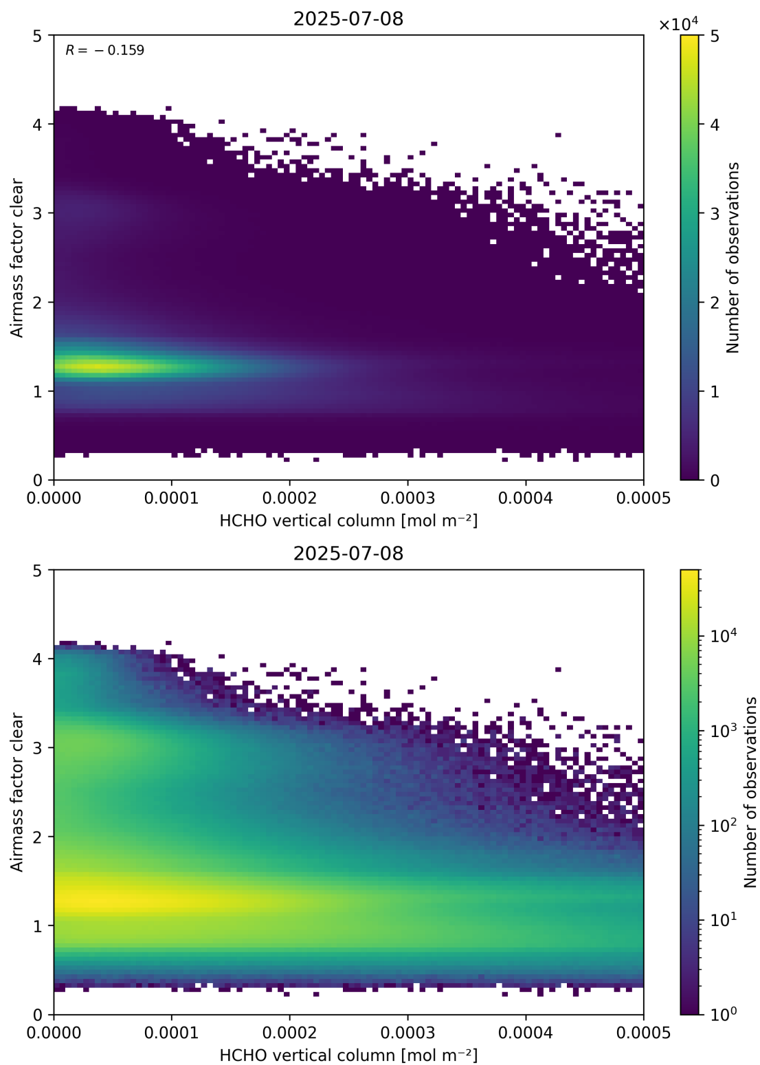
Figure 126: Scatter density plot of “HCHO vertical column” against “Airmass factor clear” for 2025-07-08 to 2025-07-09.
