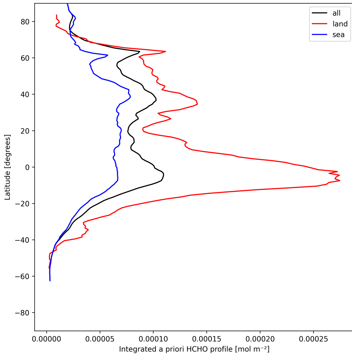
Figure 29: Zonal average of “Integrated a priori HCHO profile” for 2025-07-08 to 2025-07-09.
