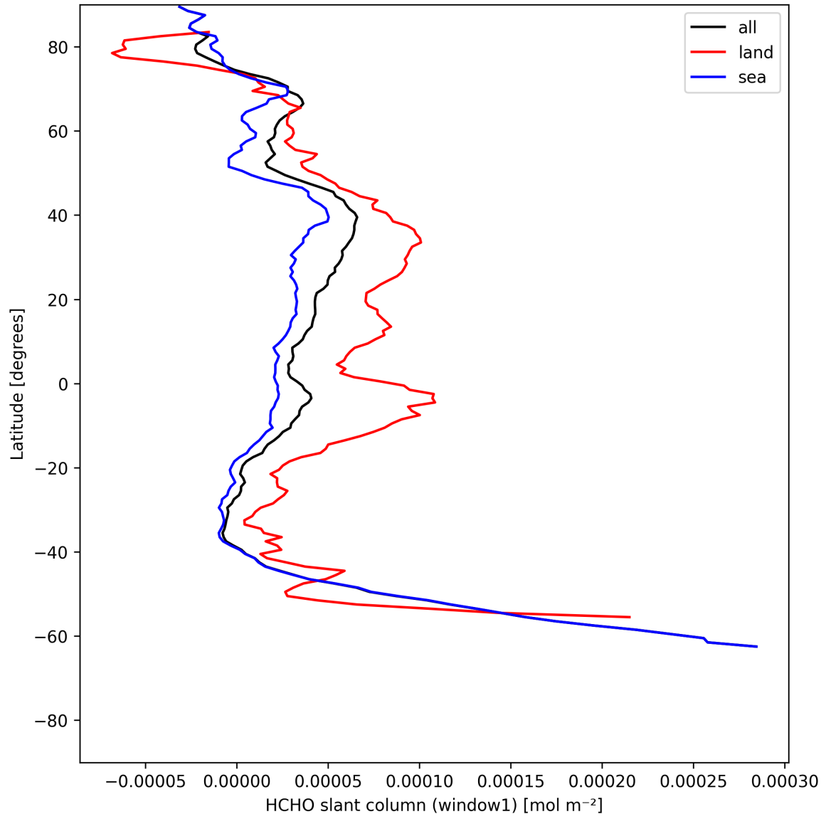
Figure 24: Zonal average of “HCHO slant column (window1)” for 2025-07-08 to 2025-07-09.
