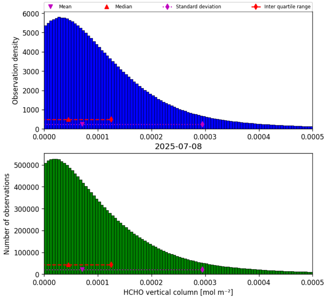
Figure 35: Histogram of “HCHO vertical column” for 2025-07-08 to 2025-07-09
