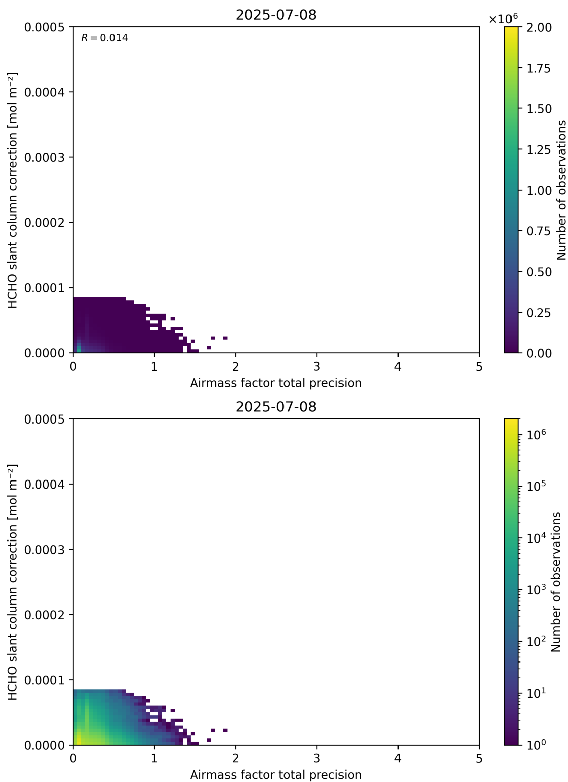
Figure 110: Scatter density plot of “Airmass factor total precision” against “HCHO slant column correction” for 2025-07-08 to 2025-07-09.
