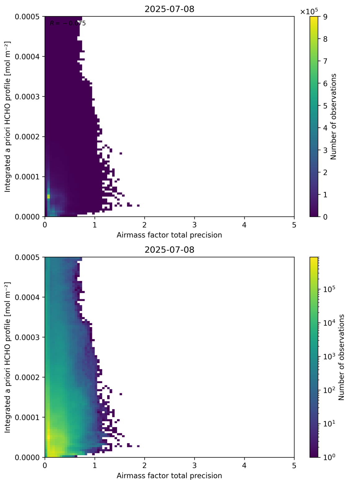
Figure 111: Scatter density plot of “Airmass factor total precision” against “Integrated a priori HCHO profile” for 2025-07-08 to 2025-07-09.
