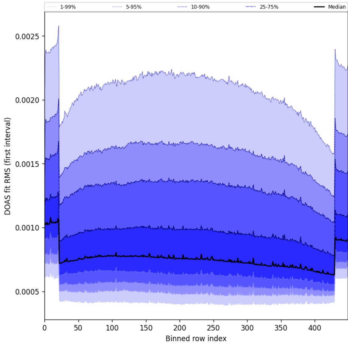
Figure 60: Along track statistics of “DOAS fit RMS (first interval)” for 2025-07-08 to 2025-07-09
