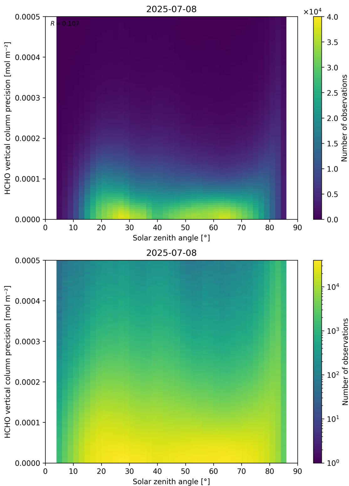
Figure 179: Scatter density plot of “Solar zenith angle” against “HCHO vertical column precision” for 2025-07-08 to 2025-07-09.
