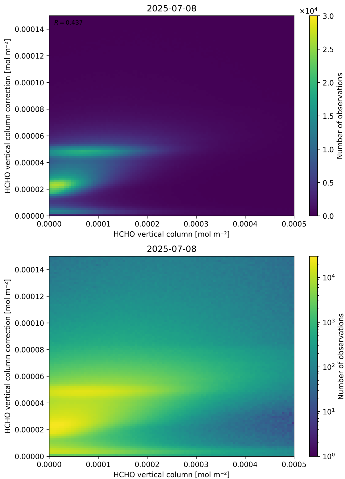
Figure 133: Scatter density plot of “HCHO vertical column” against “HCHO vertical column correction” for 2025-07-08 to 2025-07-09.
