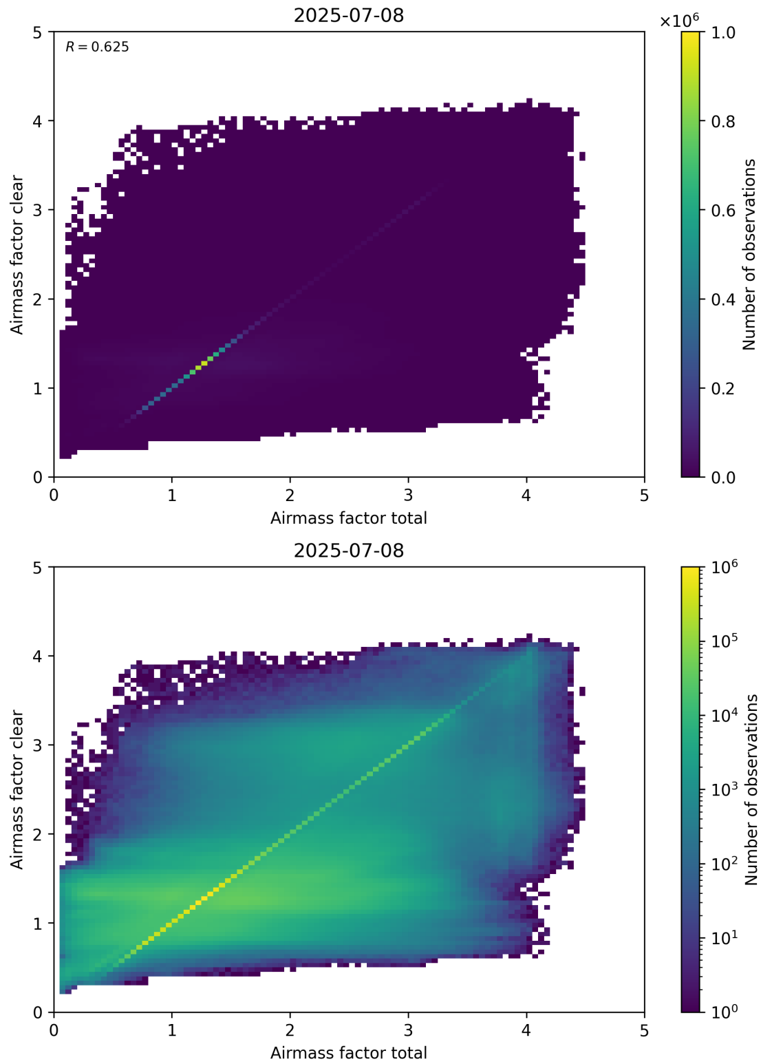
Figure 100: Scatter density plot of “Airmass factor total” against “Airmass factor clear” for 2025-07-08 to 2025-07-09.
