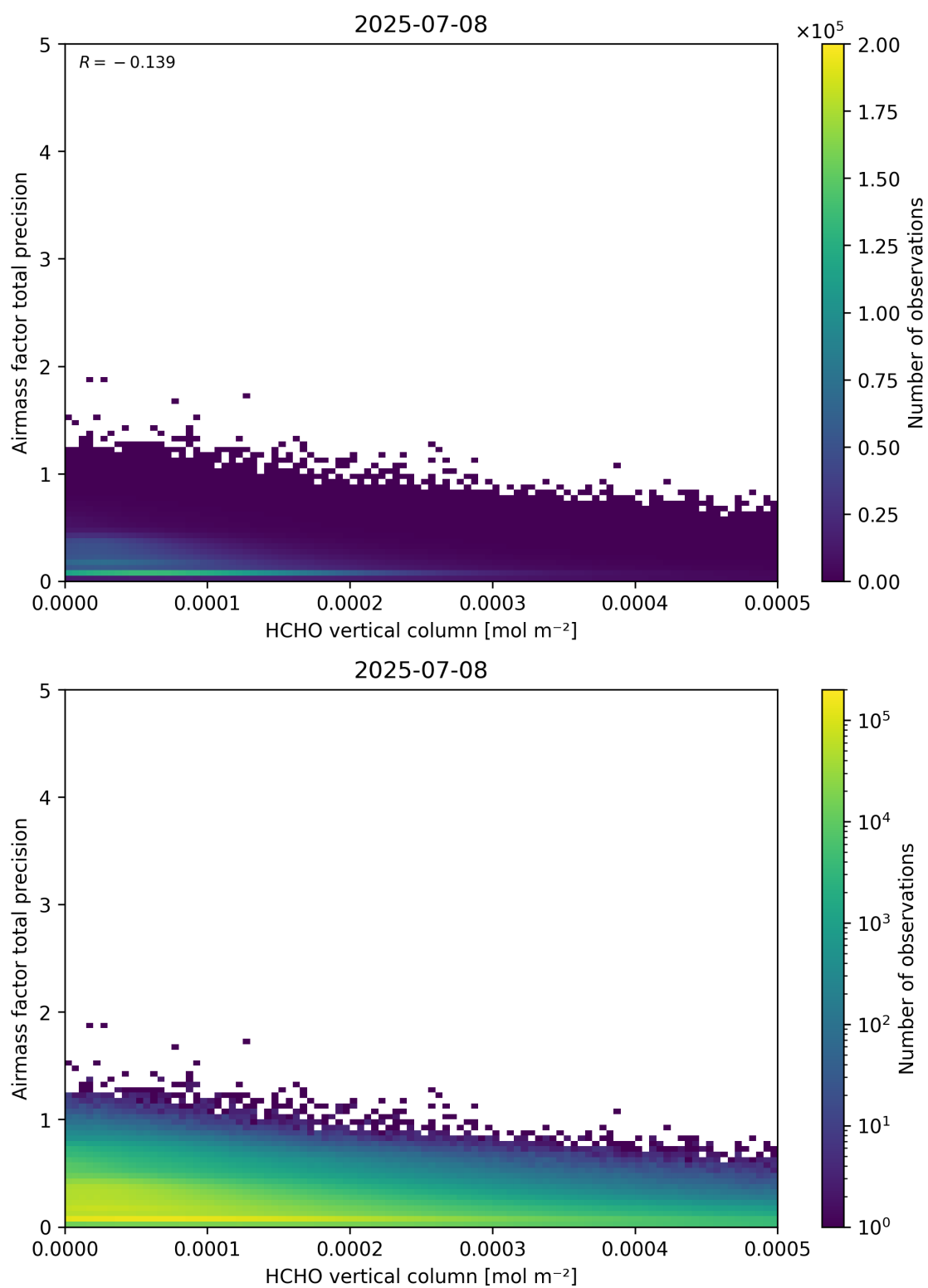
Figure 132: Scatter density plot of “HCHO vertical column” against “Airmass factor total precision” for 2025-07-08 to 2025-07-09.
