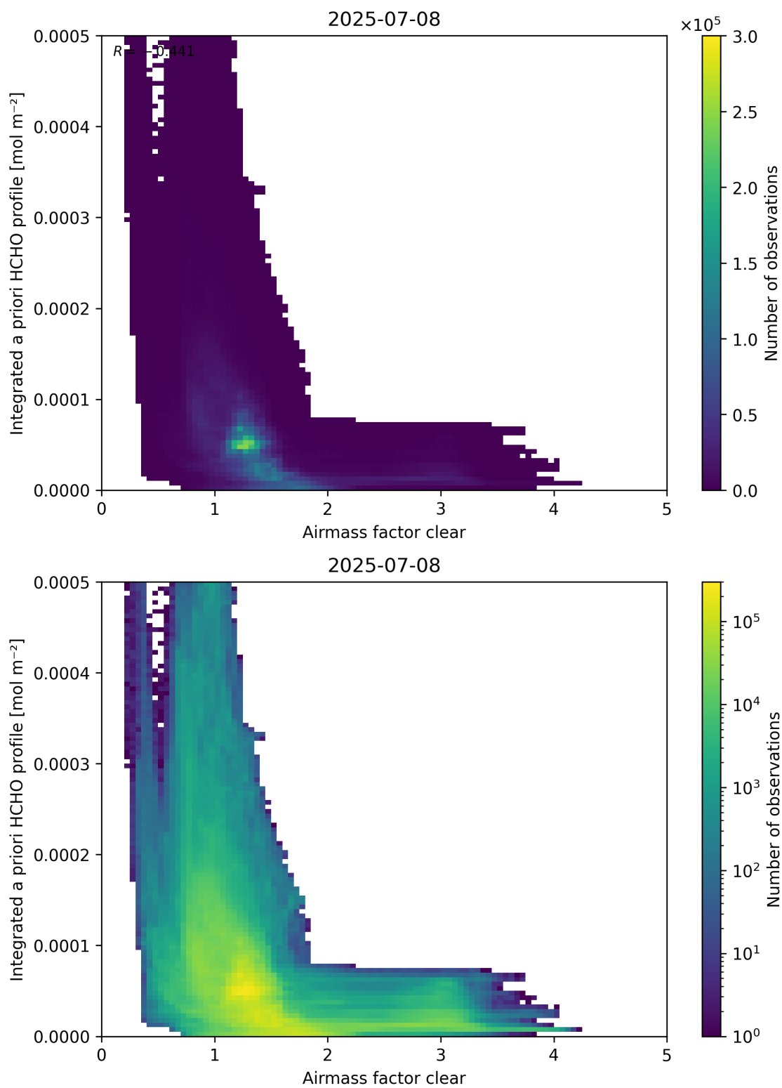
Figure 76: Scatter density plot of “Airmass factor clear” against “Integrated a priori HCHO profile” for 2025-07-08 to 2025-07-09.
