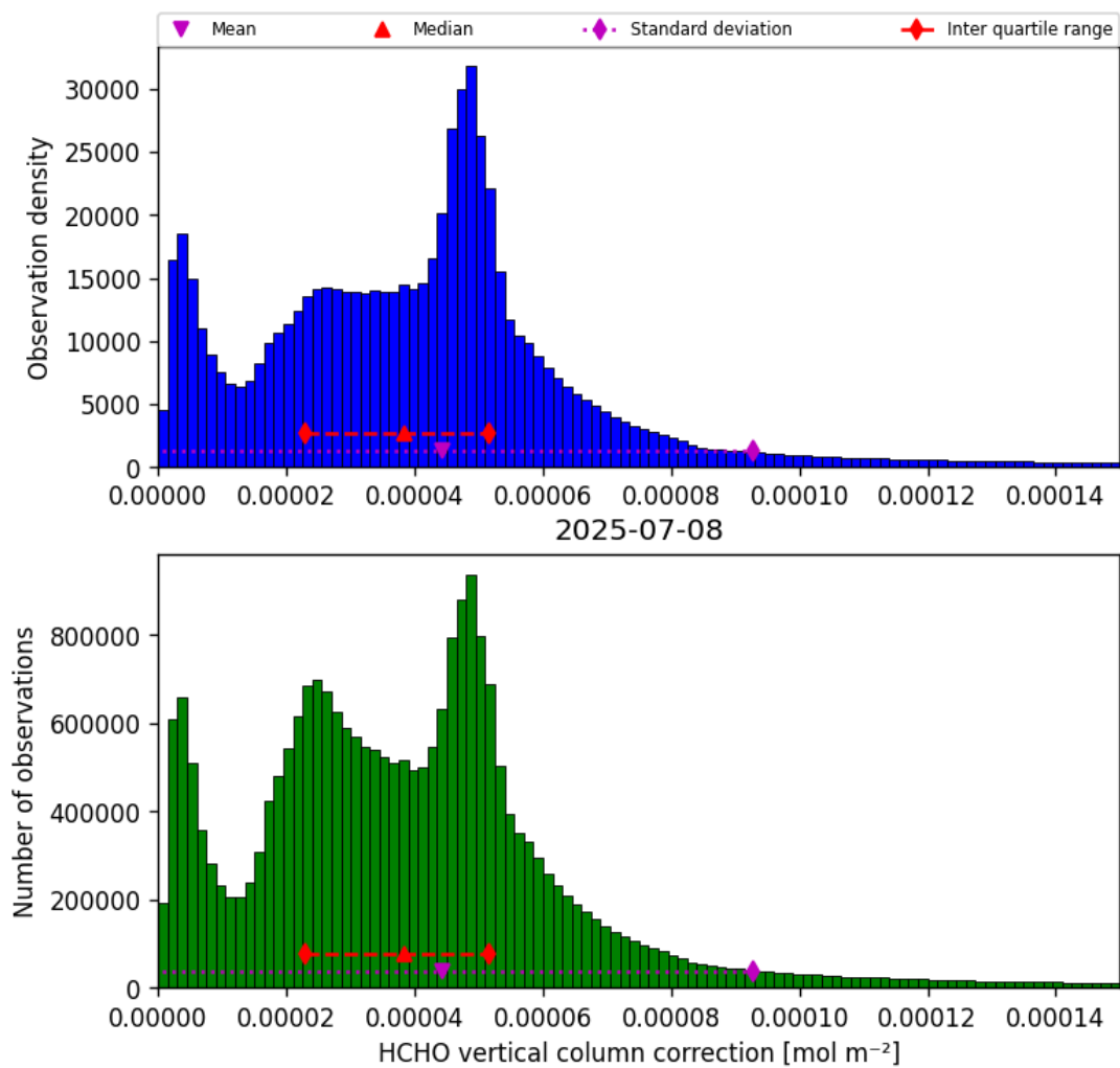
Figure 37: Histogram of “HCHO vertical column correction” for 2025-07-08 to 2025-07-09
