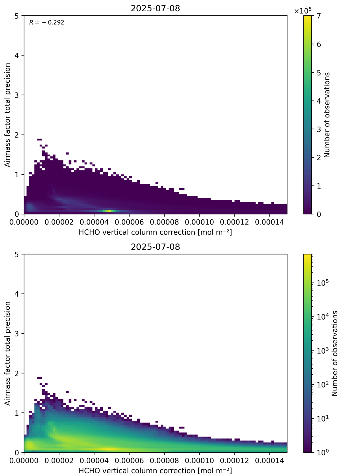
Figure 121: Scatter density plot of “HCHO vertical column correction” against “Airmass factor total precision” for 2025-07-08 to 2025-07-09.
