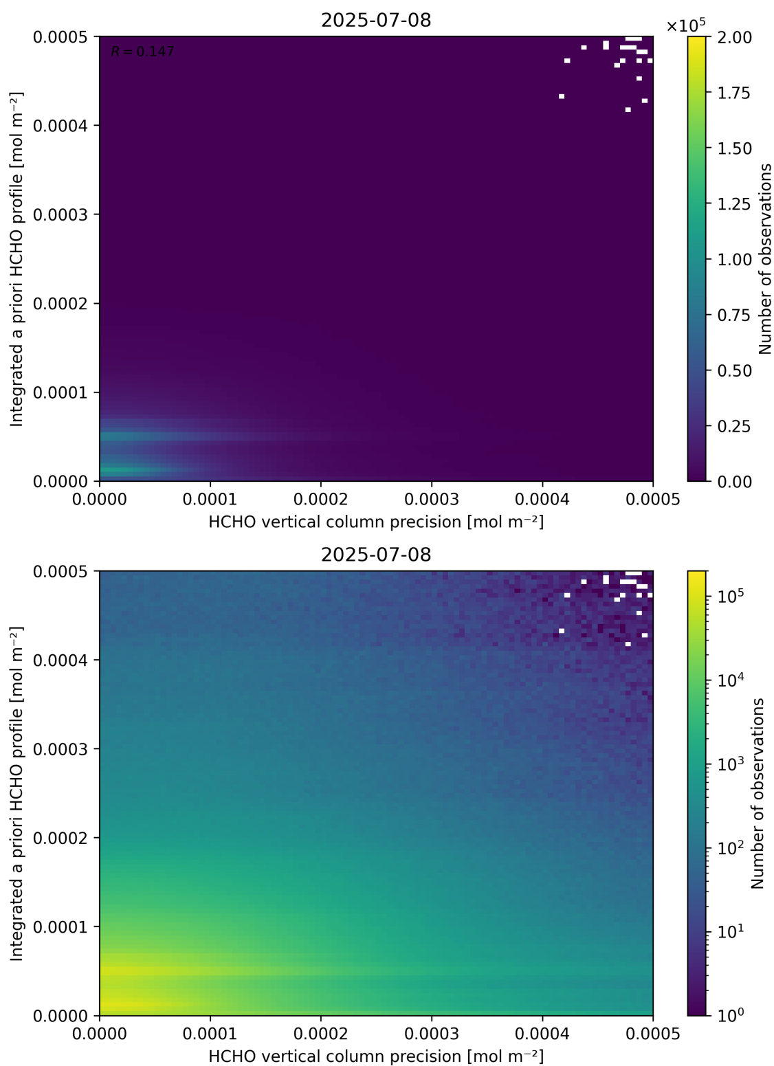
Figure 147: Scatter density plot of “HCHO vertical column precision” against “Integrated a priori HCHO profile” for 2025-07-08 to 2025-07-09.
