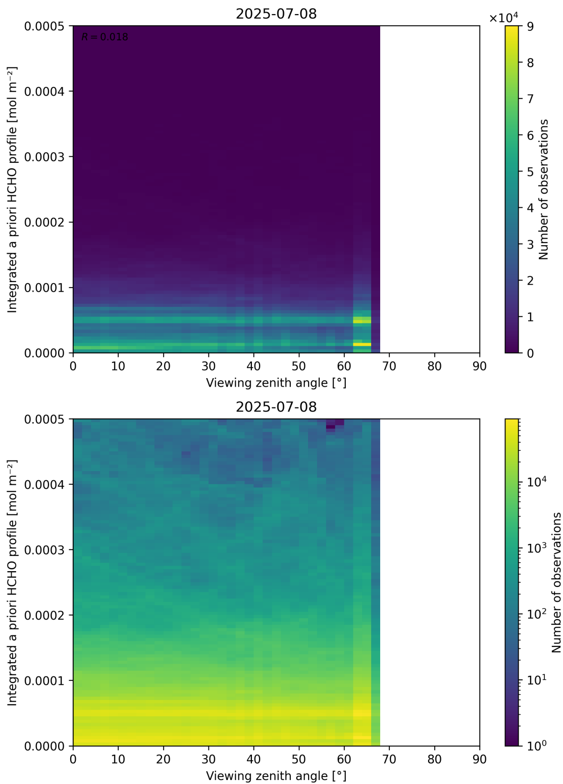
Figure 195: Scatter density plot of “Viewing zenith angle” against “Integrated a priori HCHO profile” for 2025-07-08 to 2025-07-09.
