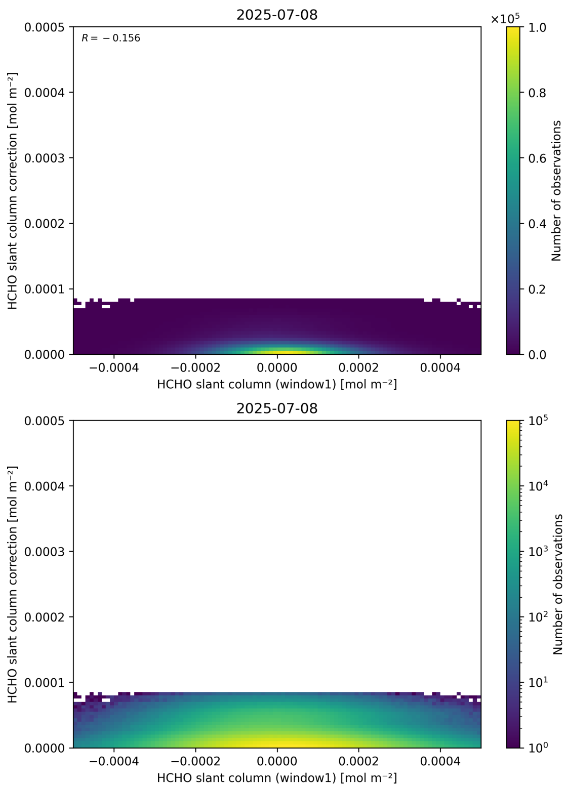
Figure 83: Scatter density plot of “HCHO slant column (window1)” against “HCHO slant column correction” for 2025-07-08 to 2025-07-09.
