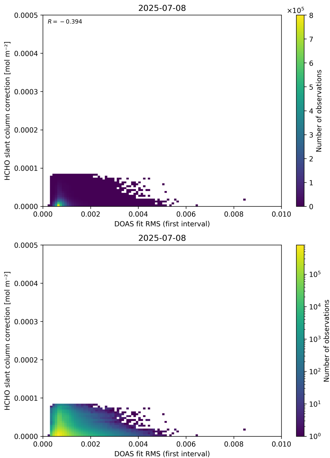
Figure 63: Scatter density plot of “DOAS fit RMS (first interval)” against “HCHO slant column correction” for 2025-07-08 to 2025-07-09.
