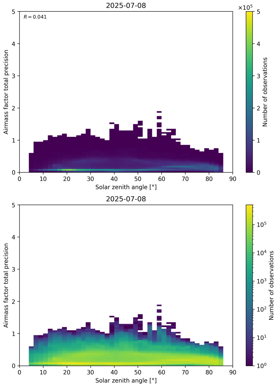
Figure 176: Scatter density plot of “Solar zenith angle” against “Airmass factor total precision” for 2025-07-08 to 2025-07-09.
