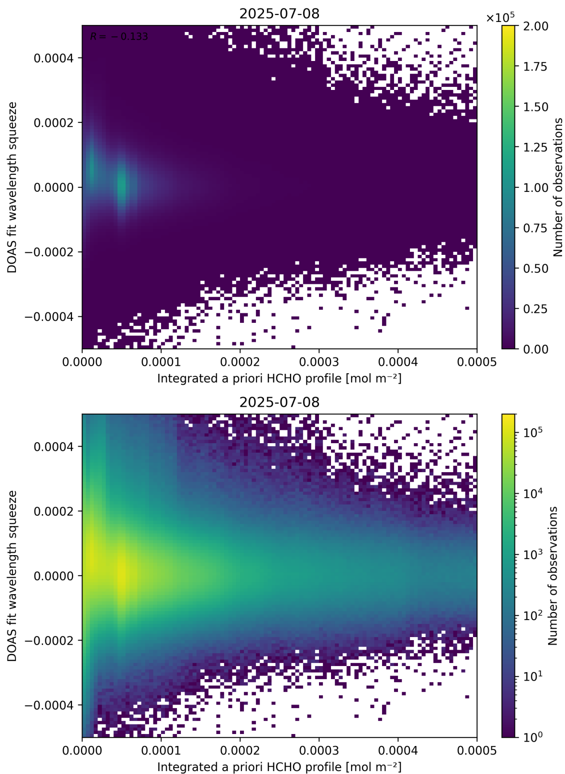
Figure 150: Scatter density plot of “Integrated a priori HCHO profile” against “DOAS fit wavelength squeeze” for 2025-07-08 to 2025-07-09.
