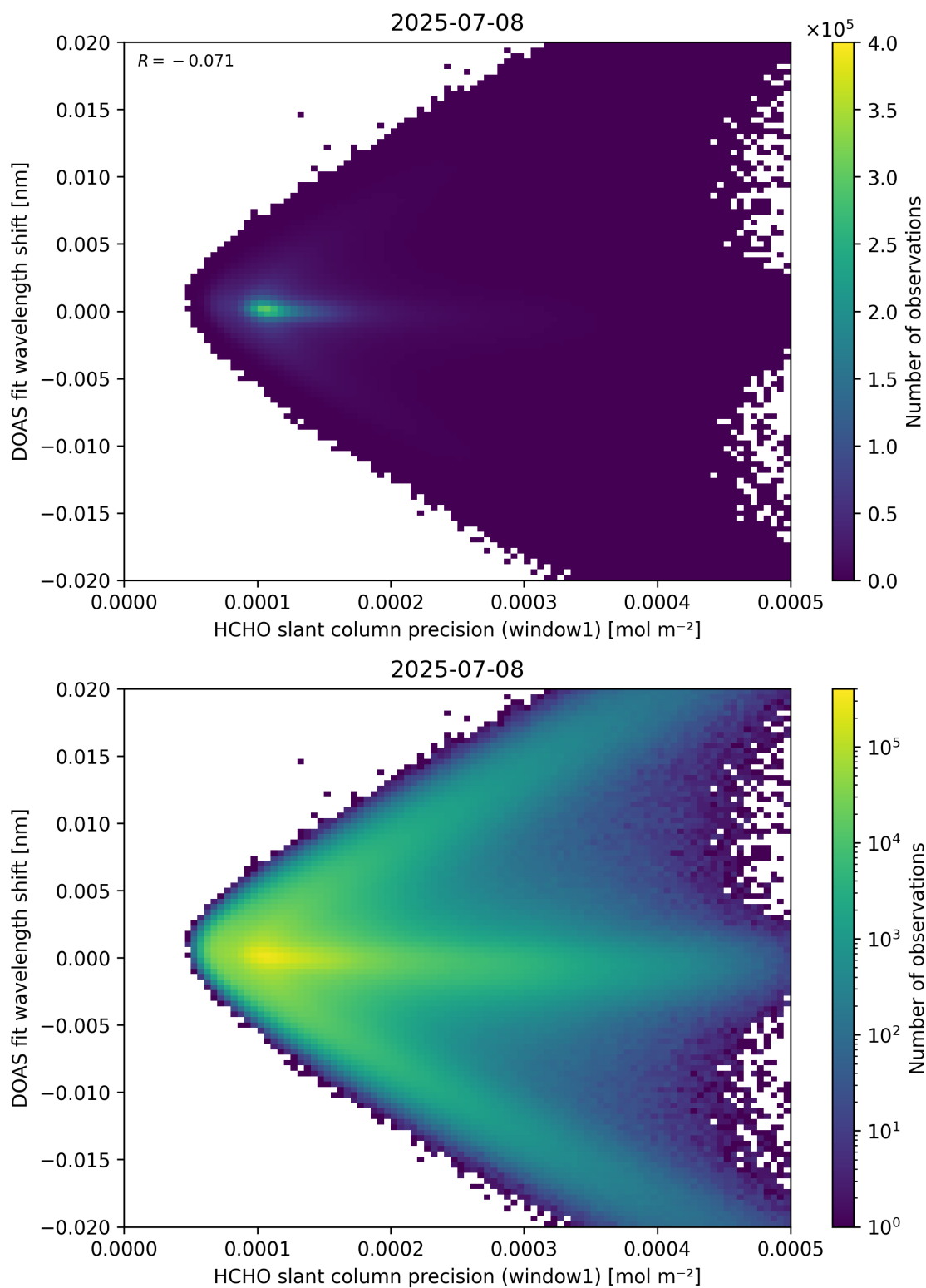
Figure 89: Scatter density plot of “HCHO slant column precision (window1)” against “DOAS fit wavelength shift” for 2025-07-08 to 2025-07-09.
