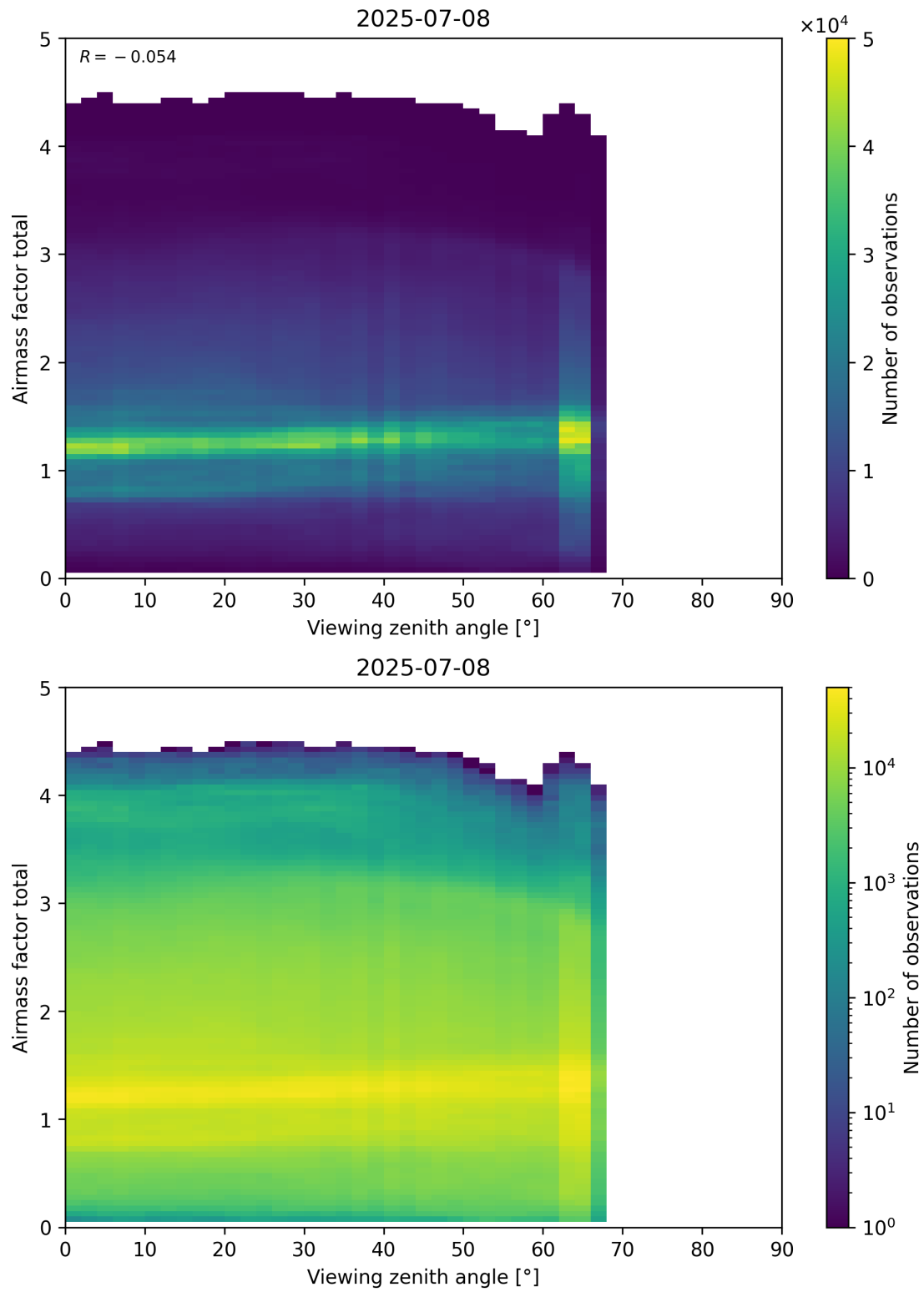
Figure 190: Scatter density plot of “Viewing zenith angle” against “Airmass factor total” for 2025-07-08 to 2025-07-09.
