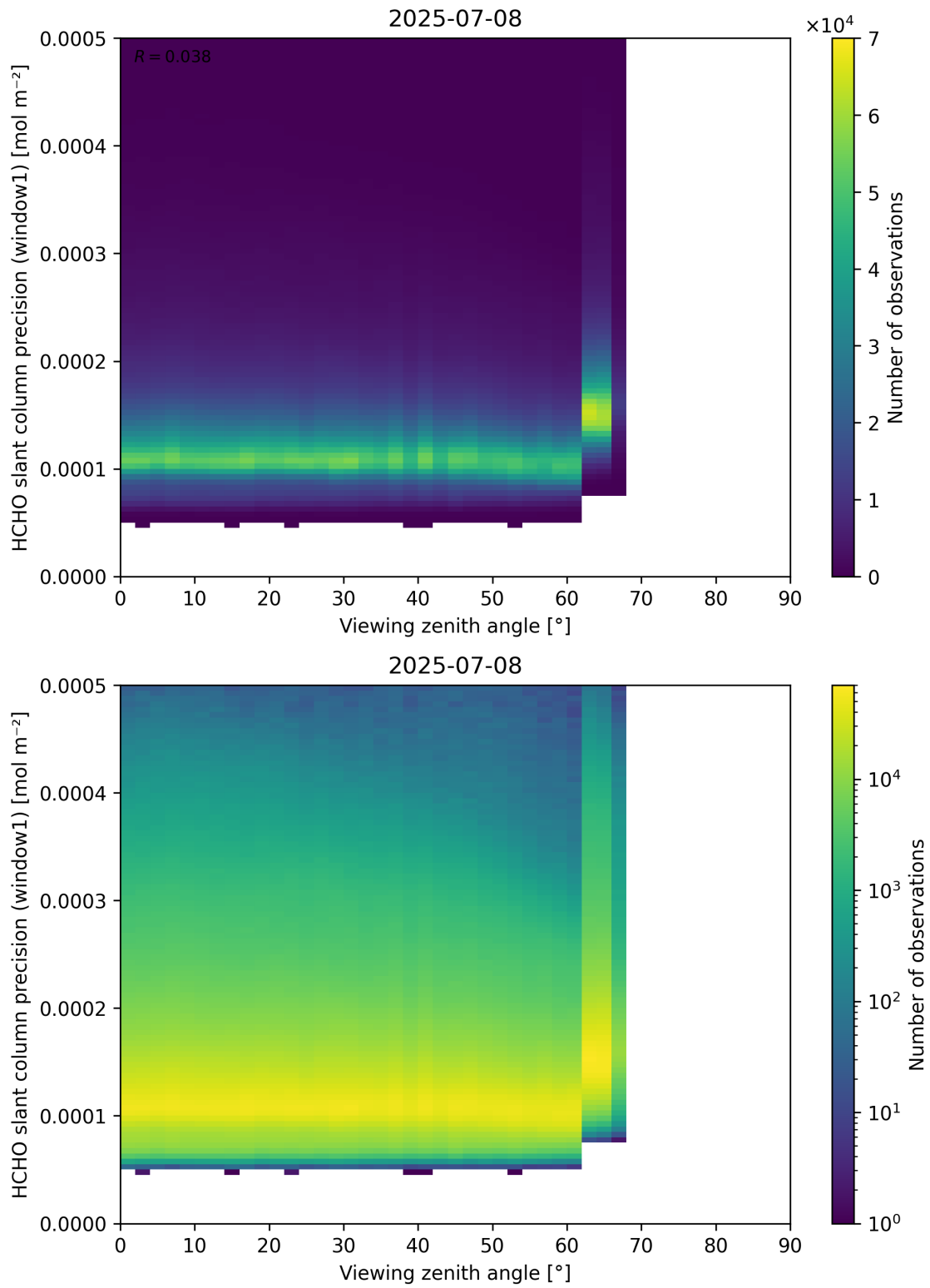
Figure 189: Scatter density plot of “Viewing zenith angle” against “HCHO slant column precision (window1)” for 2025-07-08 to 2025-07-09.
