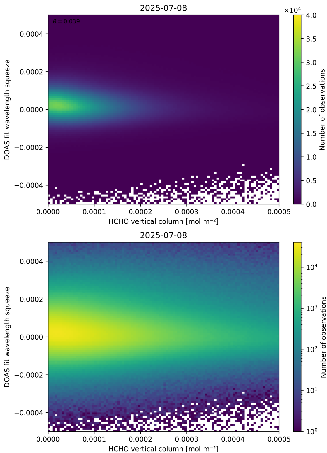
Figure 125: Scatter density plot of “HCHO vertical column” against “DOAS fit wavelength squeeze” for 2025-07-08 to 2025-07-09.
