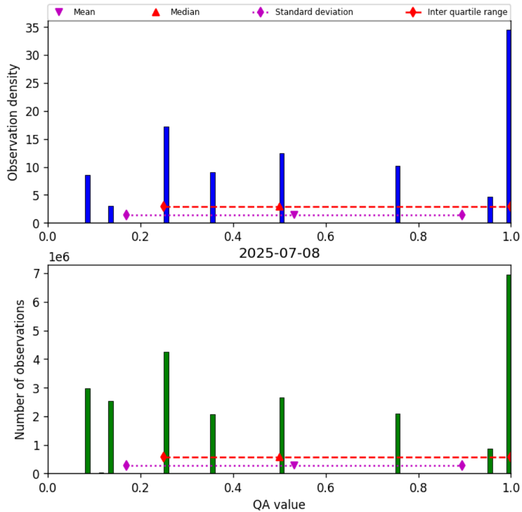
Figure 34: Histogram of “QA value” for 2025-07-08 to 2025-07-09
