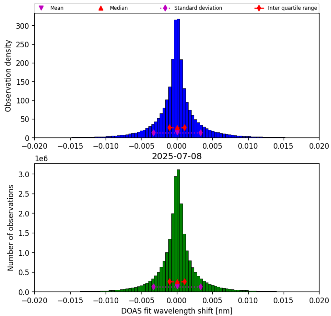
Figure 44: Histogram of “DOAS fit wavelength shift” for 2025-07-08 to 2025-07-09
