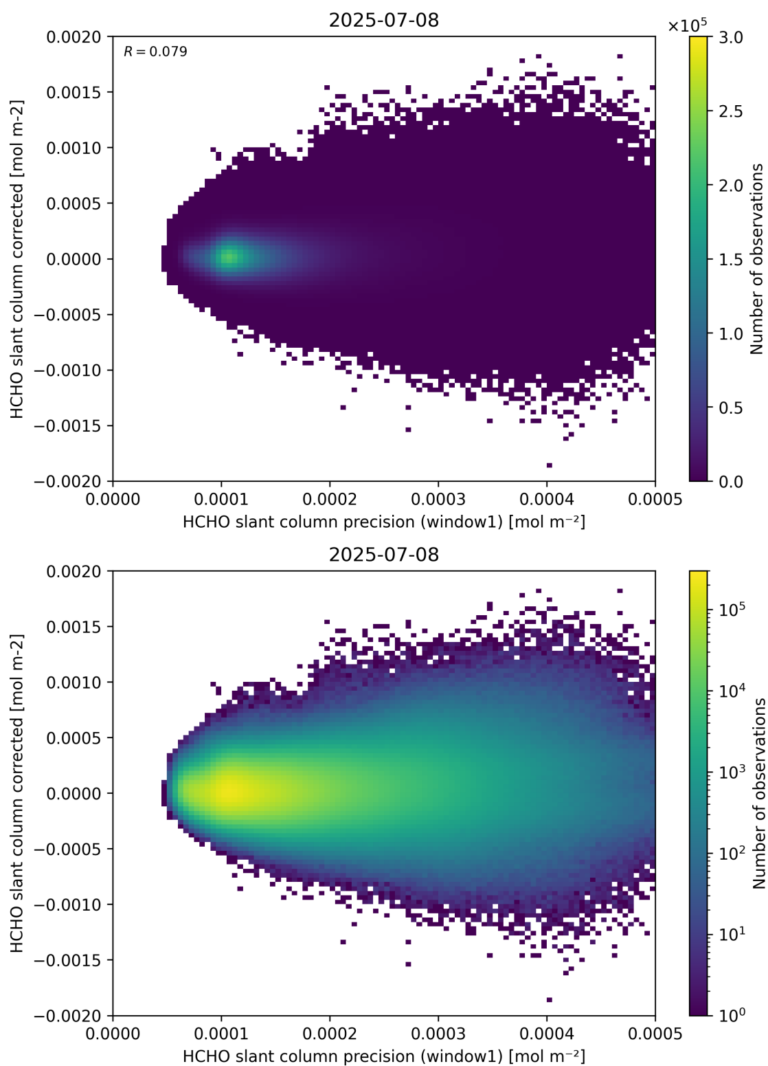
Figure 92: Scatter density plot of “HCHO slant column precision (window1)” against “HCHO slant column corrected” for 2025-07-08 to 2025-07-09.
