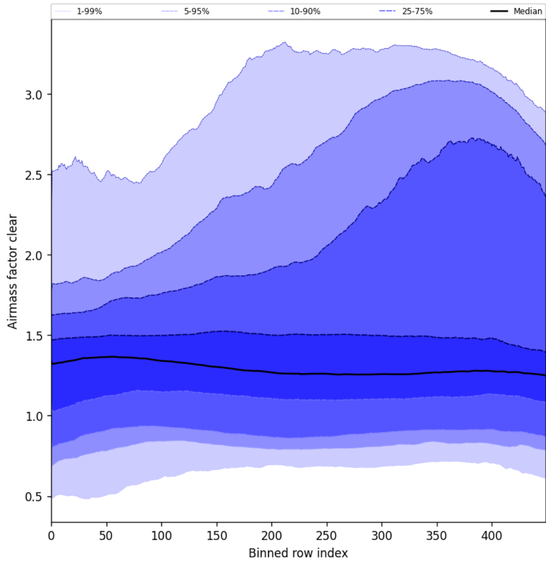
Figure 56: Along track statistics of “Airmass factor clear” for 2025-07-08 to 2025-07-09
