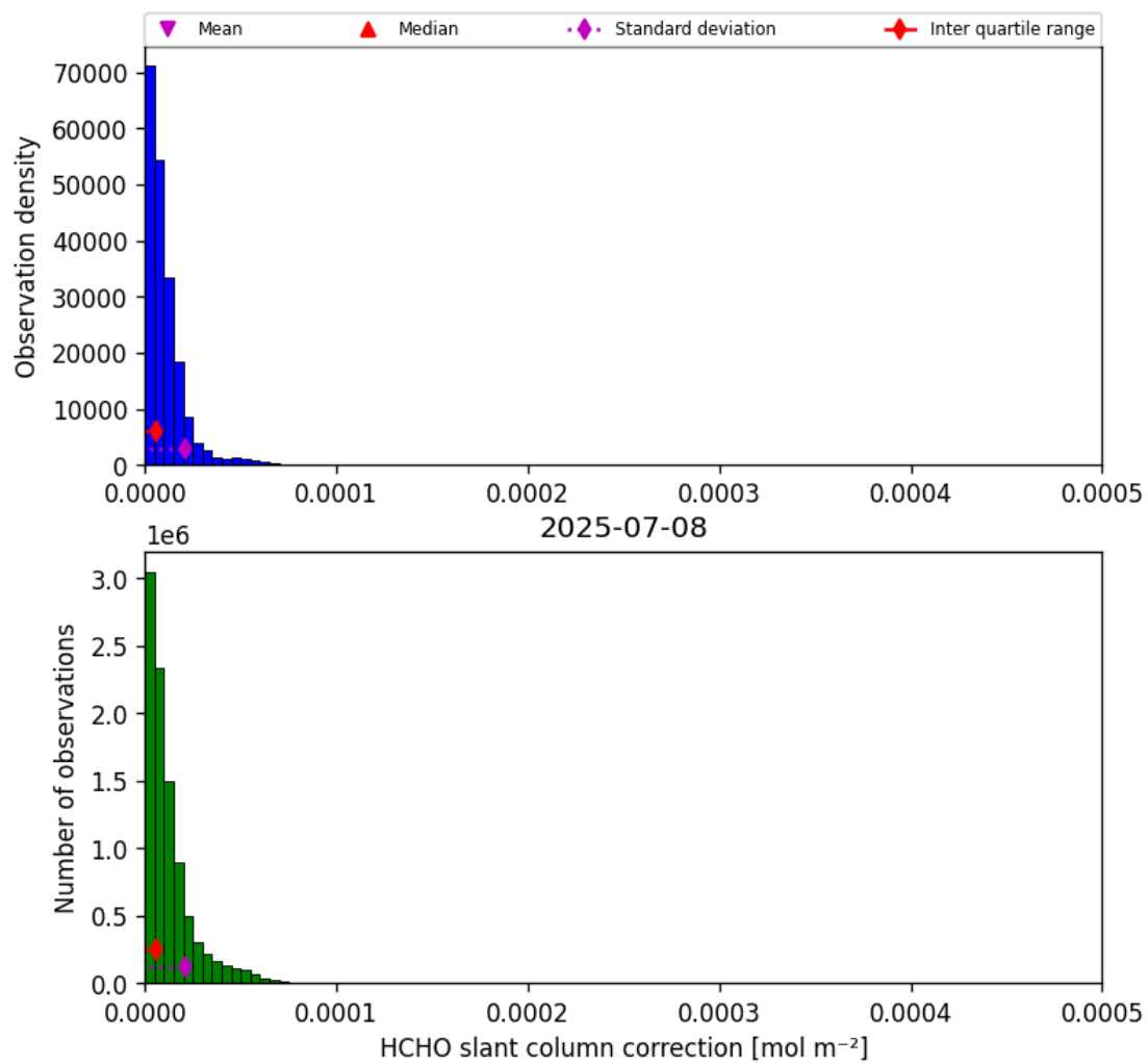
Figure 47: Histogram of “HCHO slant column correction” for 2025-07-08 to 2025-07-09
