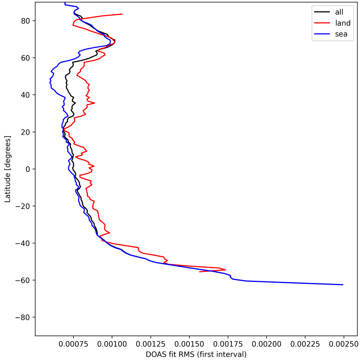
Figure 32: Zonal average of “DOAS fit RMS (first interval)” for 2025-07-08 to 2025-07-09.
