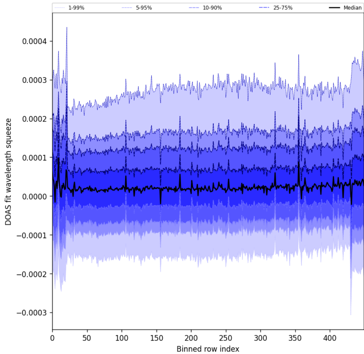
Figure 59: Along track statistics of “DOAS fit wavelength squeeze” for 2025-07-08 to 2025-07-09
