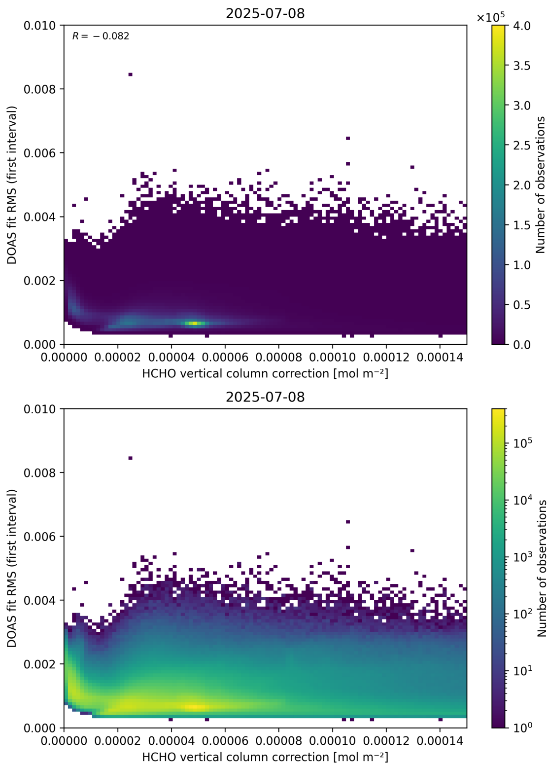
Figure 112: Scatter density plot of “HCHO vertical column correction” against “DOAS fit RMS (first interval)” for 2025-07-08 to 2025-07-09.
