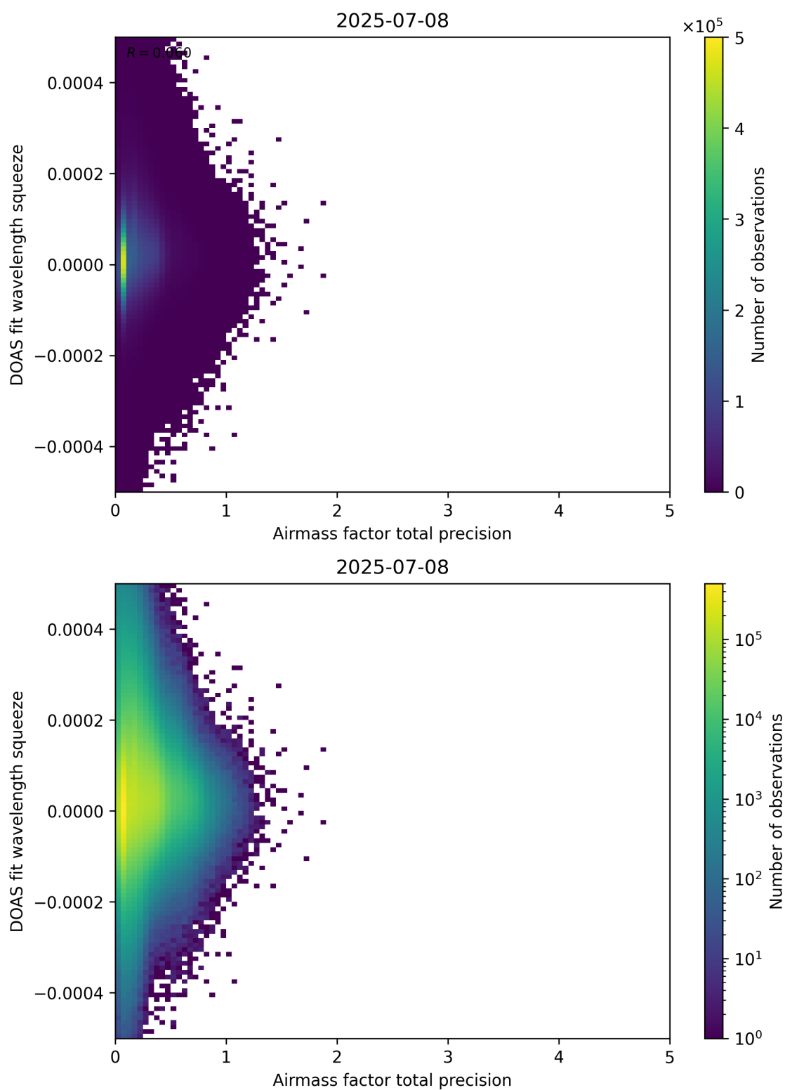
Figure 107: Scatter density plot of “Airmass factor total precision” against “DOAS fit wavelength squeeze” for 2025-07-08 to 2025-07-09.
