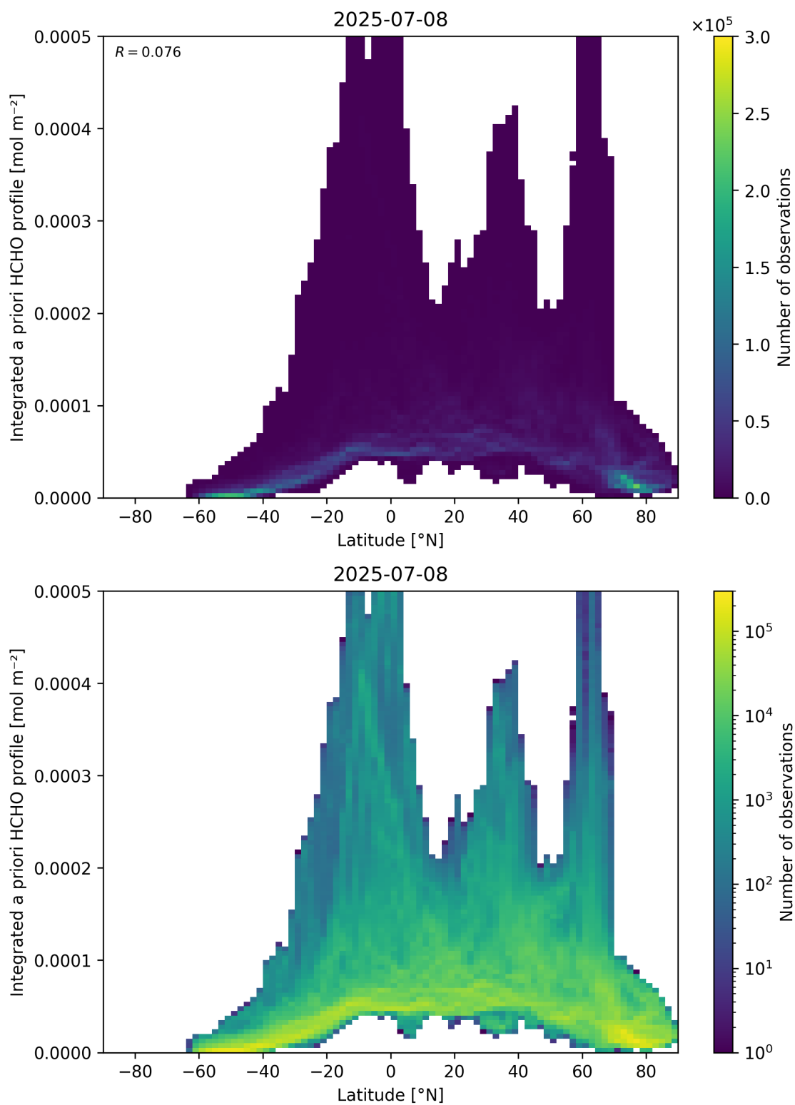
Figure 166: Scatter density plot of “Latitude” against “Integrated a priori HCHO profile” for 2025-07-08 to 2025-07-09.
