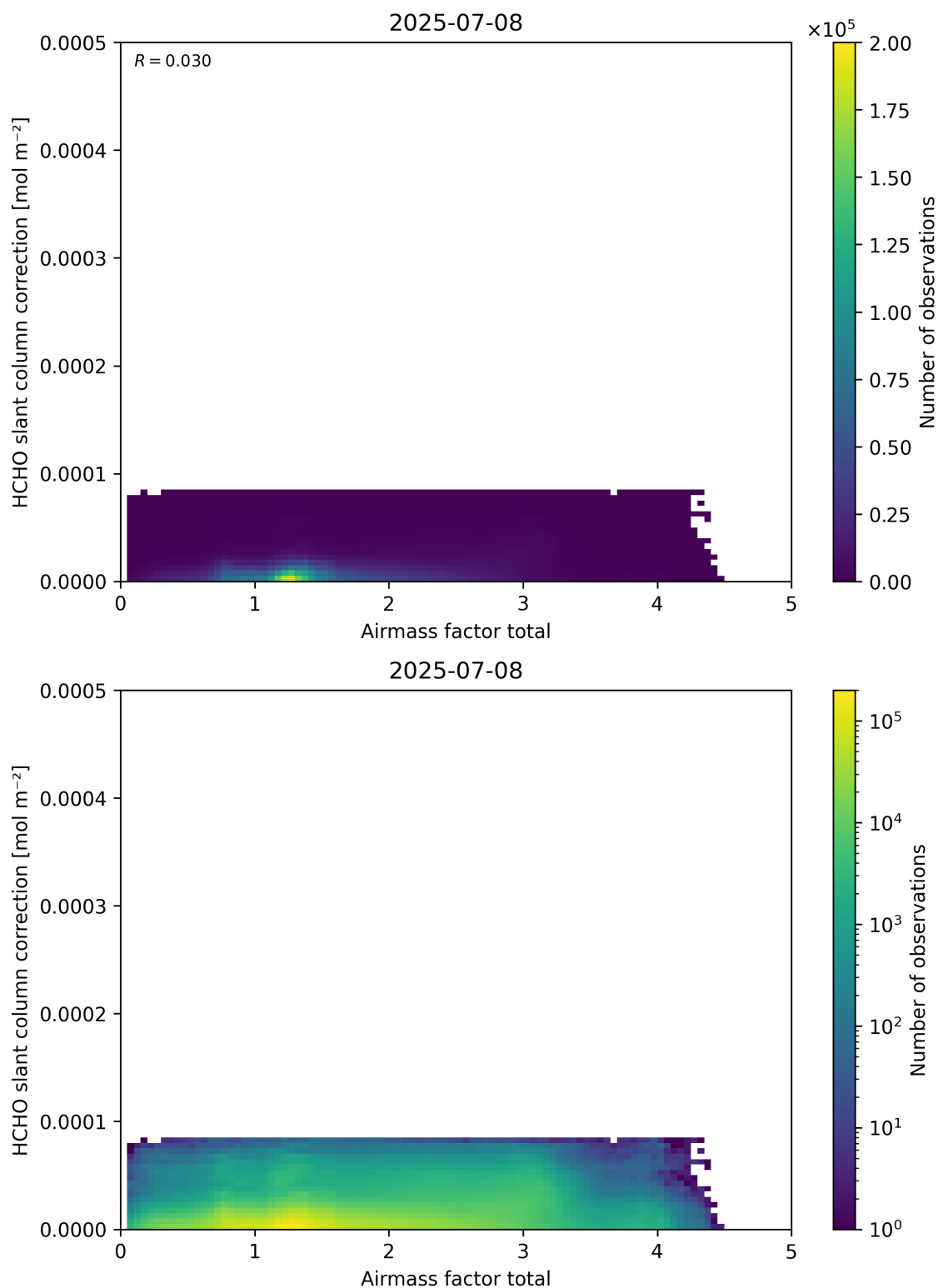
Figure 102: Scatter density plot of “Airmass factor total” against “HCHO slant column correction” for 2025-07-08 to 2025-07-09.
