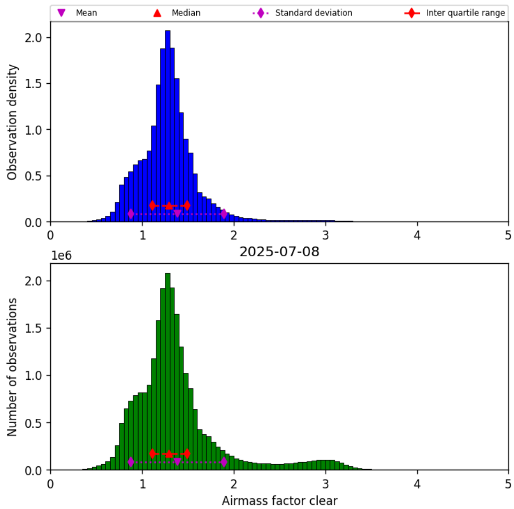
Figure 42: Histogram of “Airmass factor clear” for 2025-07-08 to 2025-07-09
