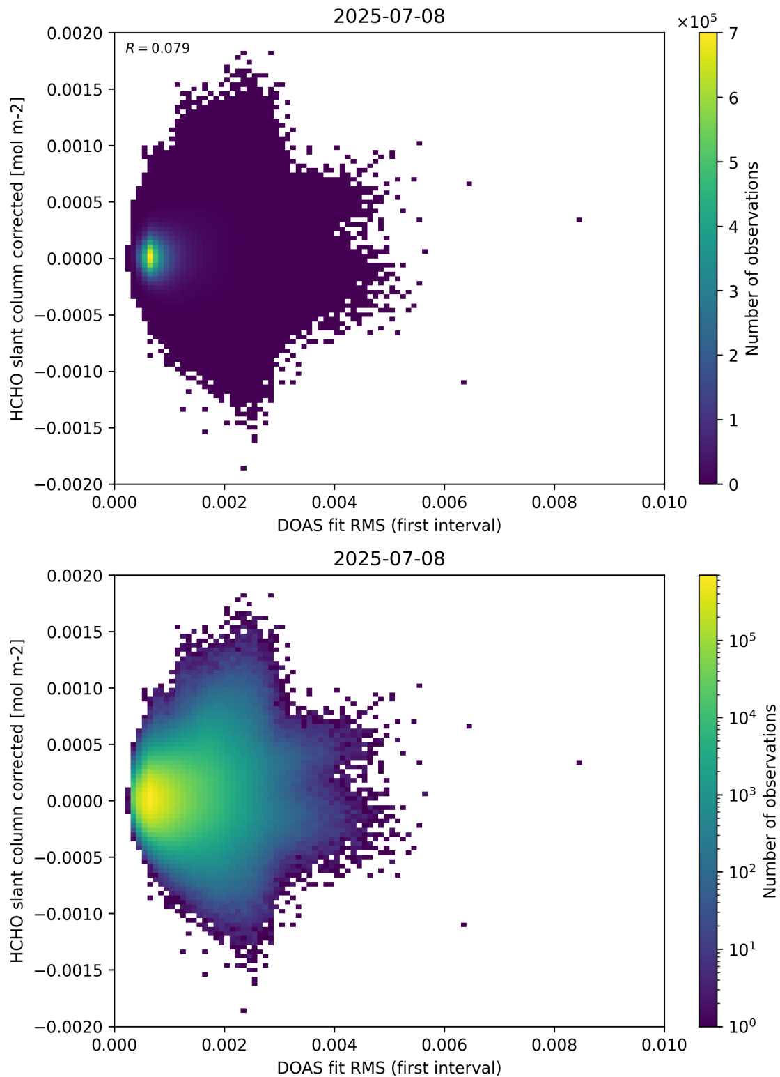
Figure 62: Scatter density plot of “DOAS fit RMS (first interval)” against “HCHO slant column corrected” for 2025-07-08 to 2025-07-09.
