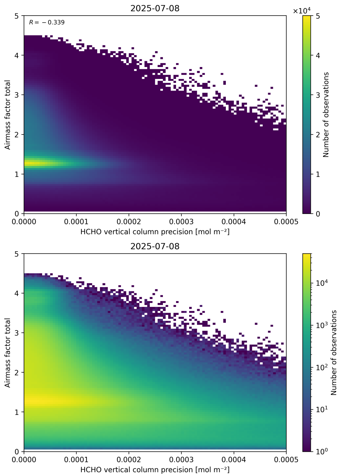
Figure 144: Scatter density plot of “HCHO vertical column precision” against “Airmass factor total” for 2025-07-08 to 2025-07-09.
