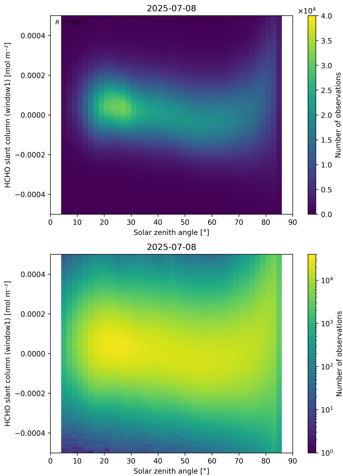
Figure 173: Scatter density plot of “Solar zenith angle” against “HCHO slant column (window1)” for 2025-07-08 to 2025-07-09.
