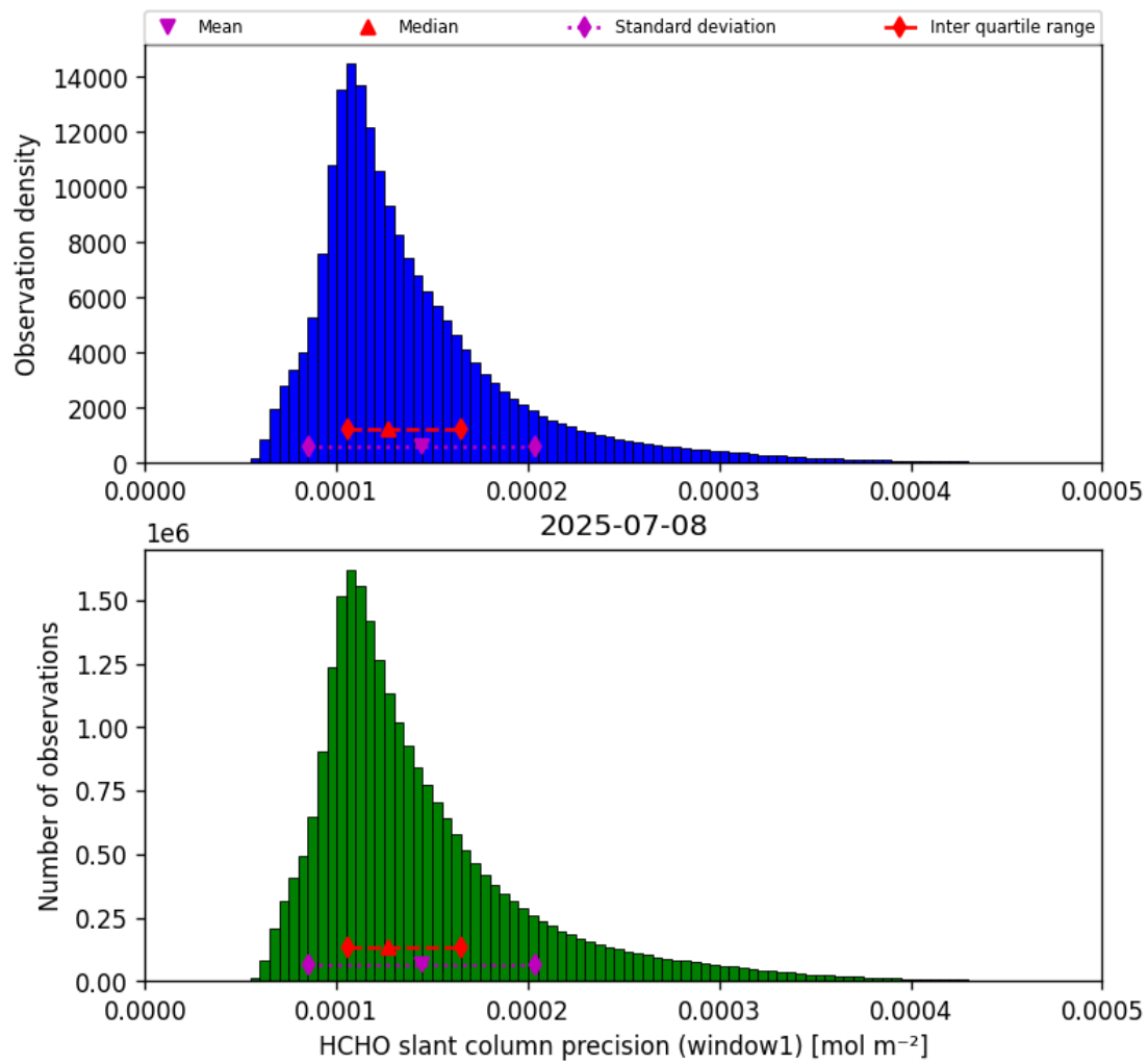
Figure 39: Histogram of “HCHO slant column precision (window1)” for 2025-07-08 to 2025-07-09
