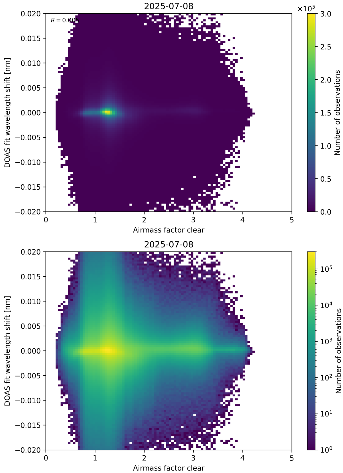
Figure 72: Scatter density plot of “Airmass factor clear” against “DOAS fit wavelength shift” for 2025-07-08 to 2025-07-09.
