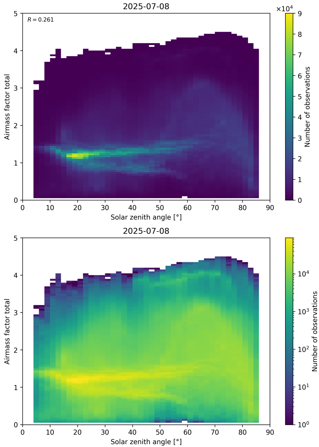
Figure 175: Scatter density plot of “Solar zenith angle” against “Airmass factor total” for 2025-07-08 to 2025-07-09.
