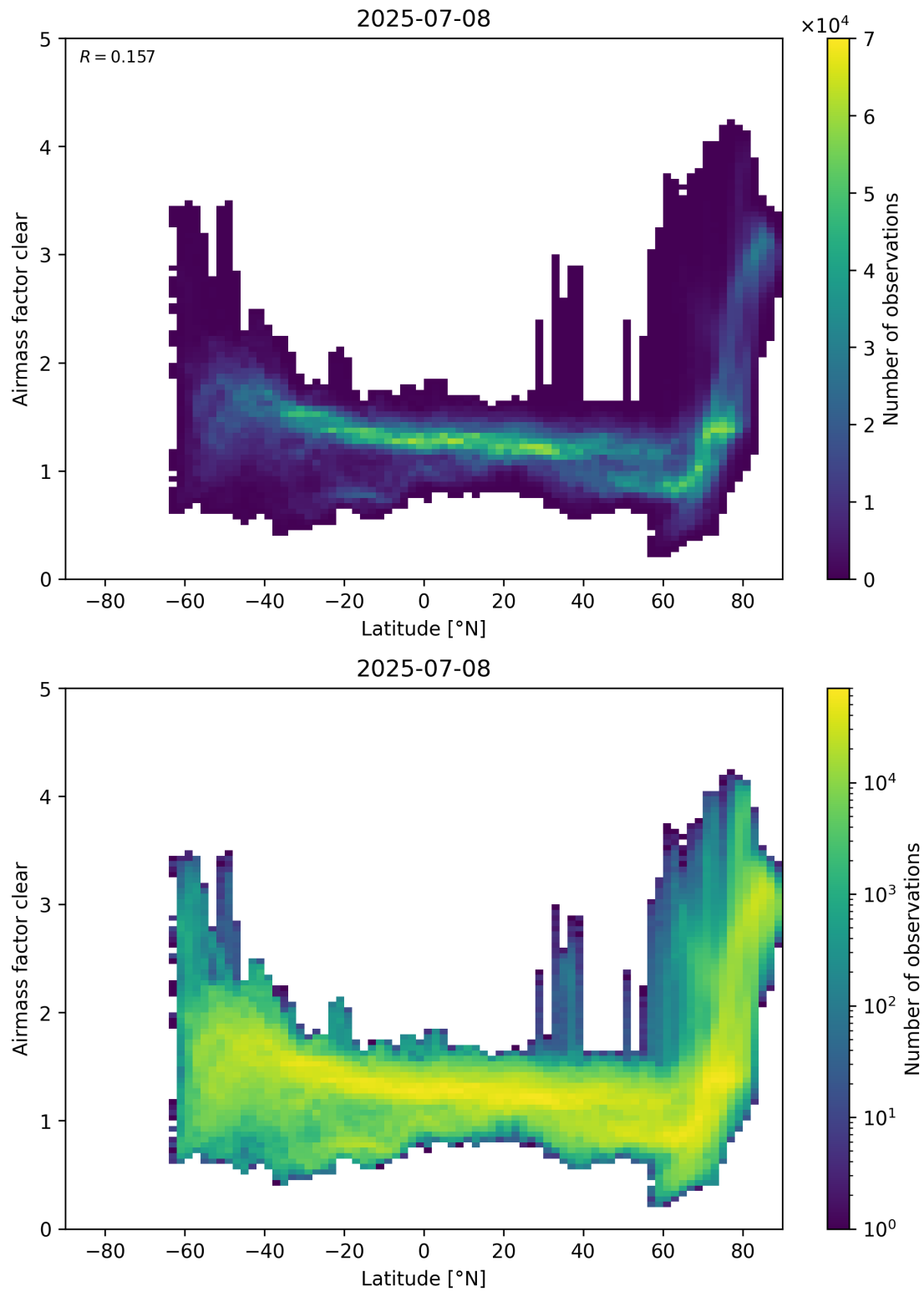
Figure 156: Scatter density plot of “Latitude” against “Airmass factor clear” for 2025-07-08 to 2025-07-09.
