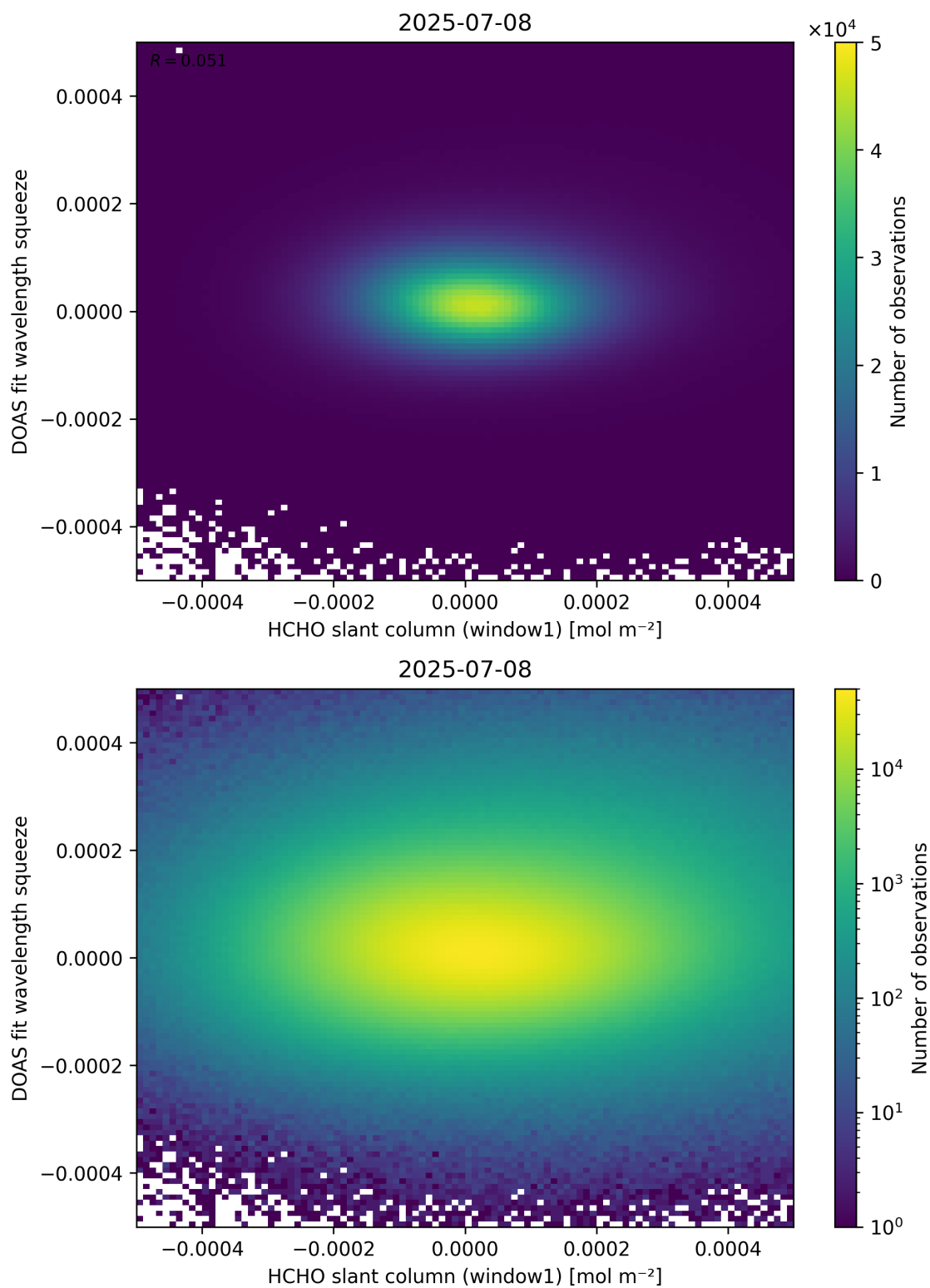
Figure 80: Scatter density plot of “HCHO slant column (window1)” against “DOAS fit wavelength squeeze” for 2025-07-08 to 2025-07-09.
