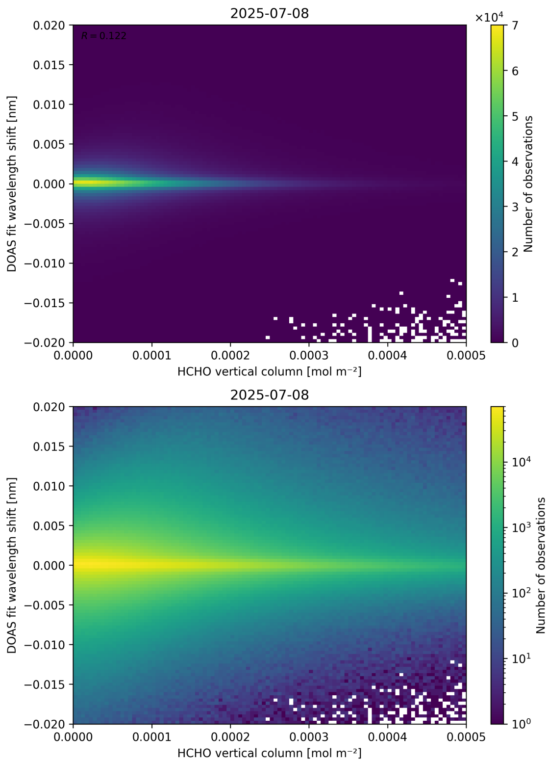
Figure 124: Scatter density plot of “HCHO vertical column” against “DOAS fit wavelength shift” for 2025-07-08 to 2025-07-09.
