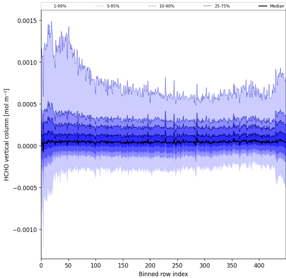
Figure 49: Along track statistics of “HCHO vertical column” for 2025-07-08 to 2025-07-09
