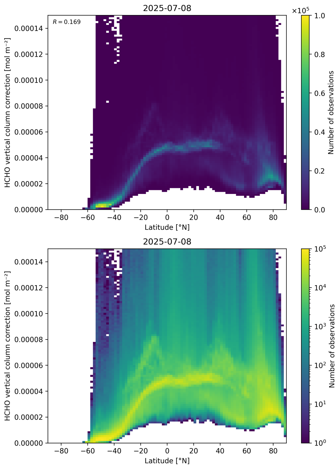
Figure 164: Scatter density plot of “Latitude” against “HCHO vertical column correction” for 2025-07-08 to 2025-07-09.
