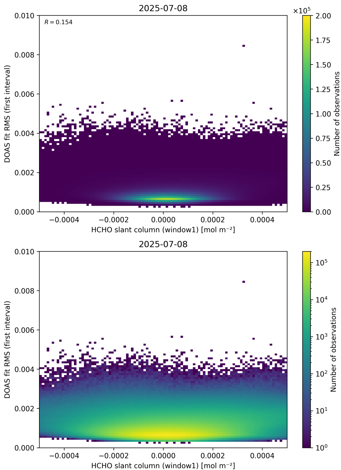
Figure 78: Scatter density plot of “HCHO slant column (window1)” against “DOAS fit RMS (first interval)” for 2025-07-08 to 2025-07-09.
