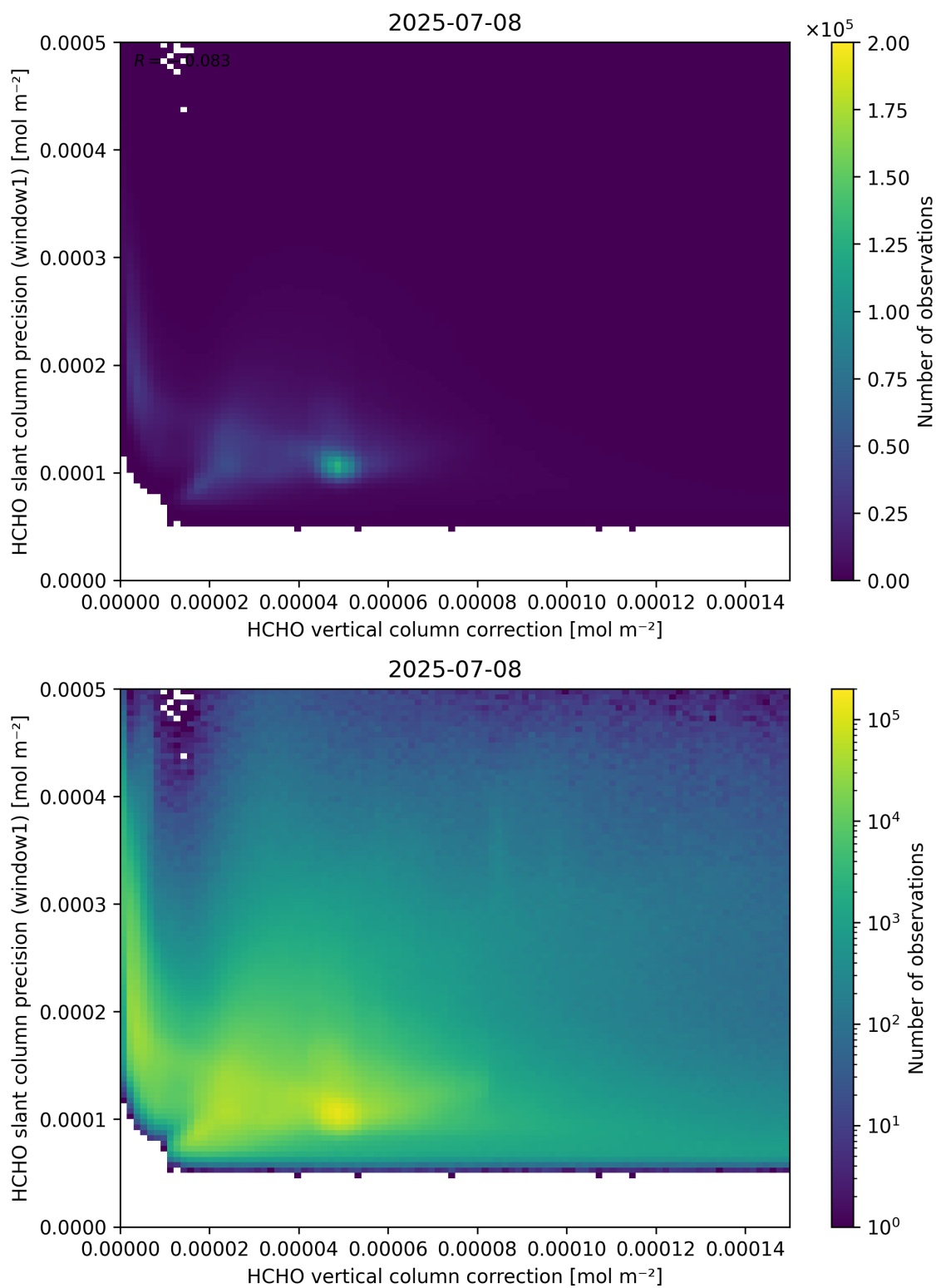
Figure 119: Scatter density plot of “HCHO vertical column correction” against “HCHO slant column precision (window1)” for 2025-07-08 to 2025-07-09.
