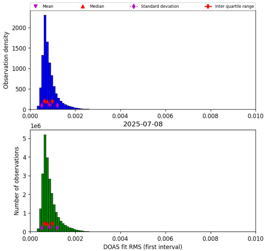
Figure 46: Histogram of "DOAS fit RMS (first interval)" for 2025-07-08 to 2025-07-09
