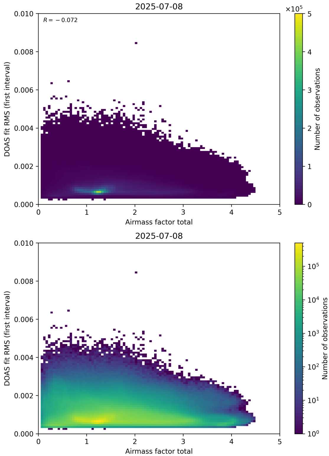
Figure 97: Scatter density plot of “Airmass factor total” against “DOAS fit RMS (first interval)” for 2025-07-08 to 2025-07-09.
