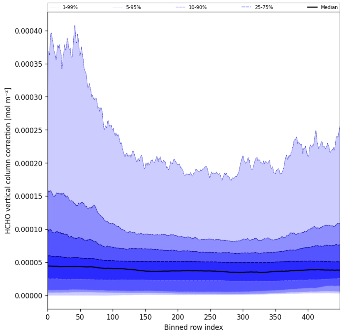
Figure 51: Along track statistics of “HCHO vertical column correction” for 2025-07-08 to 2025-07-09
