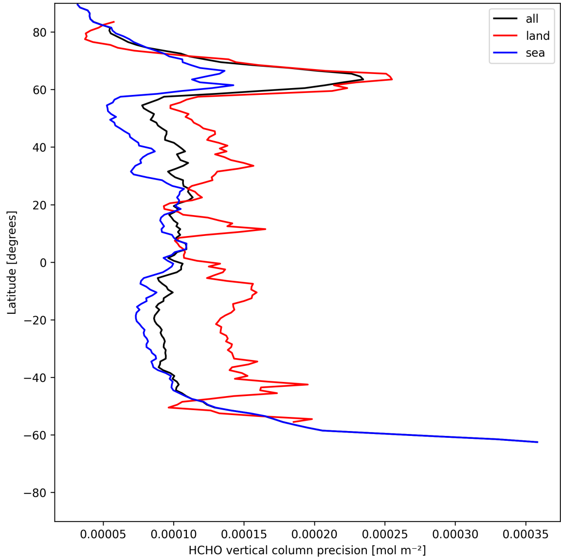
Figure 22: Zonal average of “HCHO vertical column precision” for 2025-07-08 to 2025-07-09.
