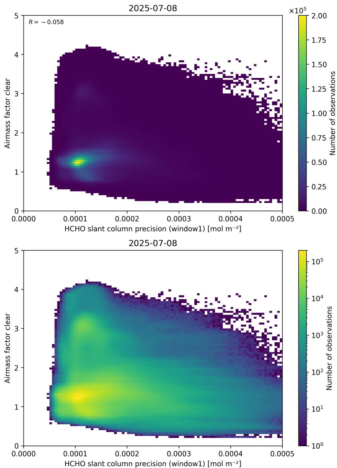
Figure 91: Scatter density plot of “HCHO slant column precision (window1)” against “Airmass factor clear” for 2025-07-08 to 2025-07-09.
