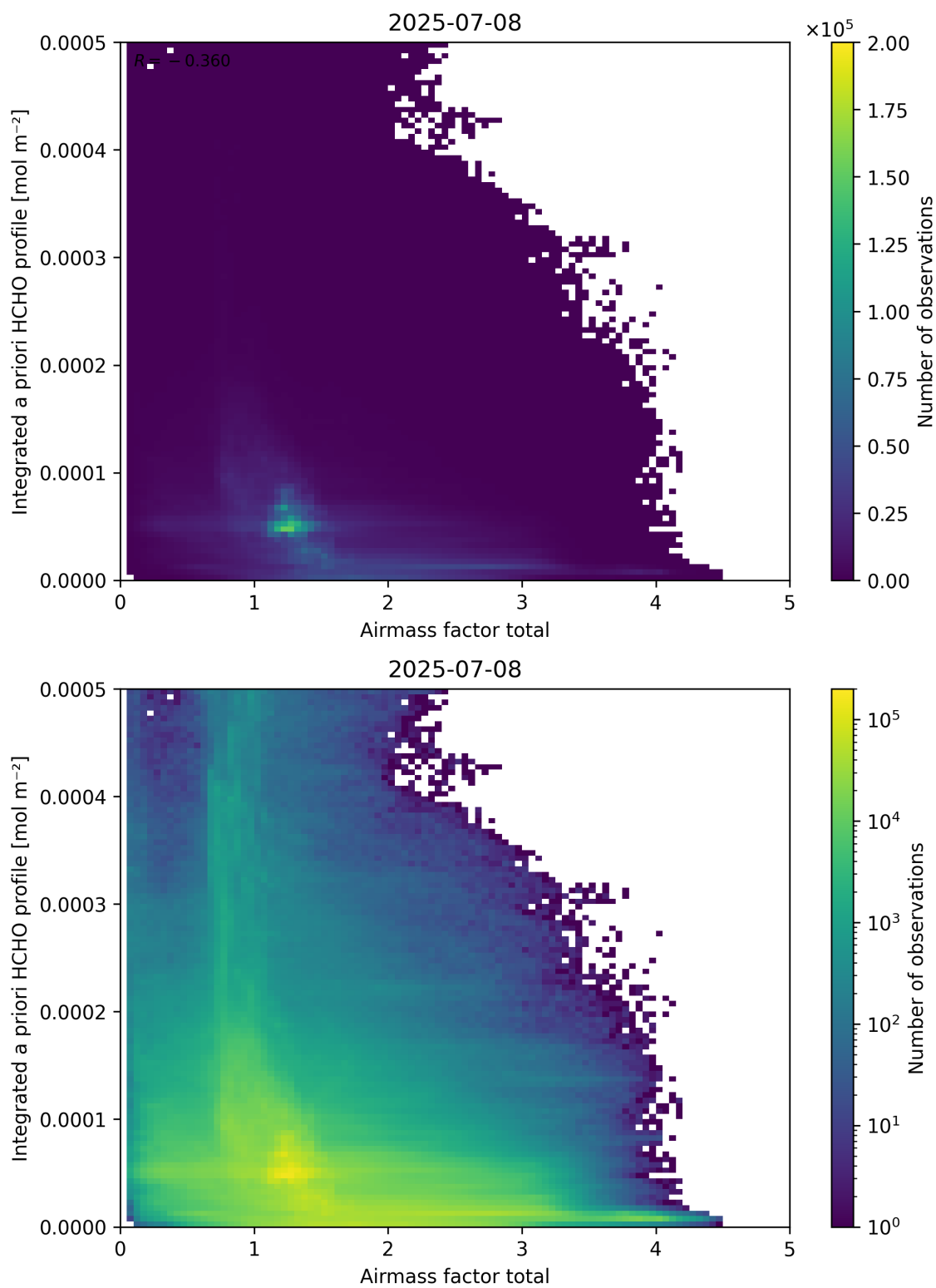
Figure 104: Scatter density plot of “Airmass factor total” against “Integrated a priori HCHO profile” for 2025-07-08 to 2025-07-09.
