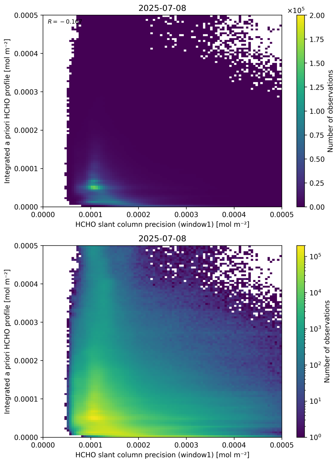
Figure 96: Scatter density plot of “HCHO slant column precision (window1)” against “Integrated a priori HCHO profile” for 2025-07-08 to 2025-07-09.
