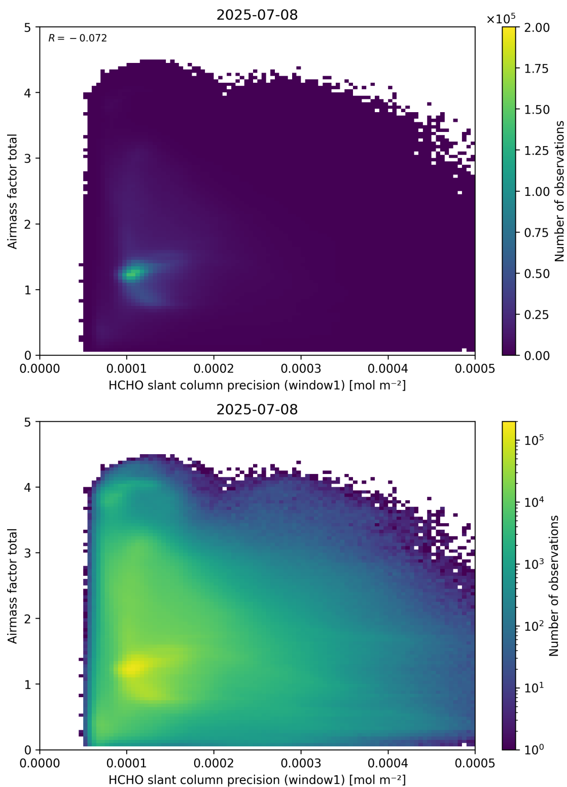
Figure 94: Scatter density plot of “HCHO slant column precision (window1)” against “Airmass factor total” for 2025-07-08 to 2025-07-09.
