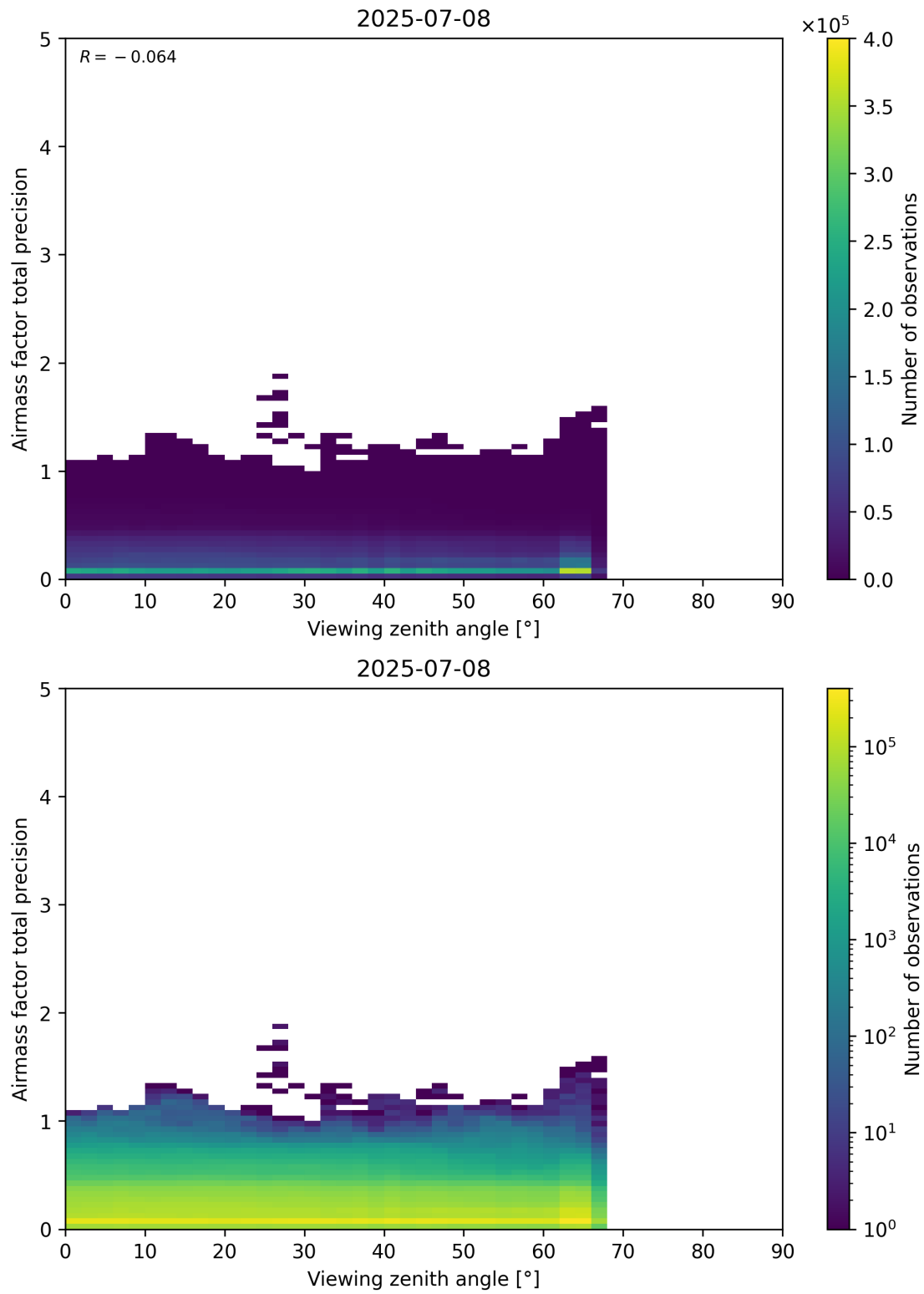
Figure 191: Scatter density plot of “Viewing zenith angle” against “Airmass factor total precision” for 2025-07-08 to 2025-07-09.
