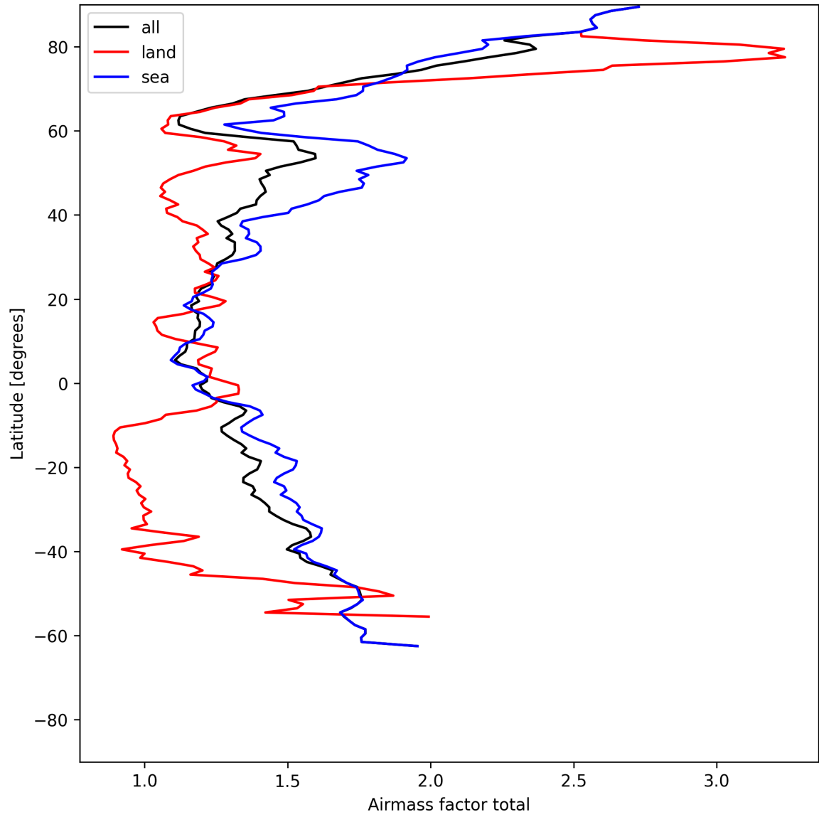
Figure 26: Zonal average of “Airmass factor total” for 2025-07-08 to 2025-07-09.
