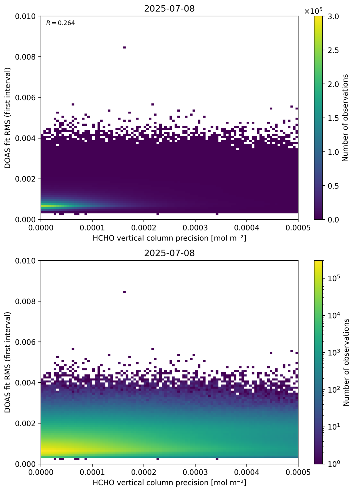
Figure 136: Scatter density plot of “HCHO vertical column precision” against “DOAS fit RMS (first interval)” for 2025-07-08 to 2025-07-09.
