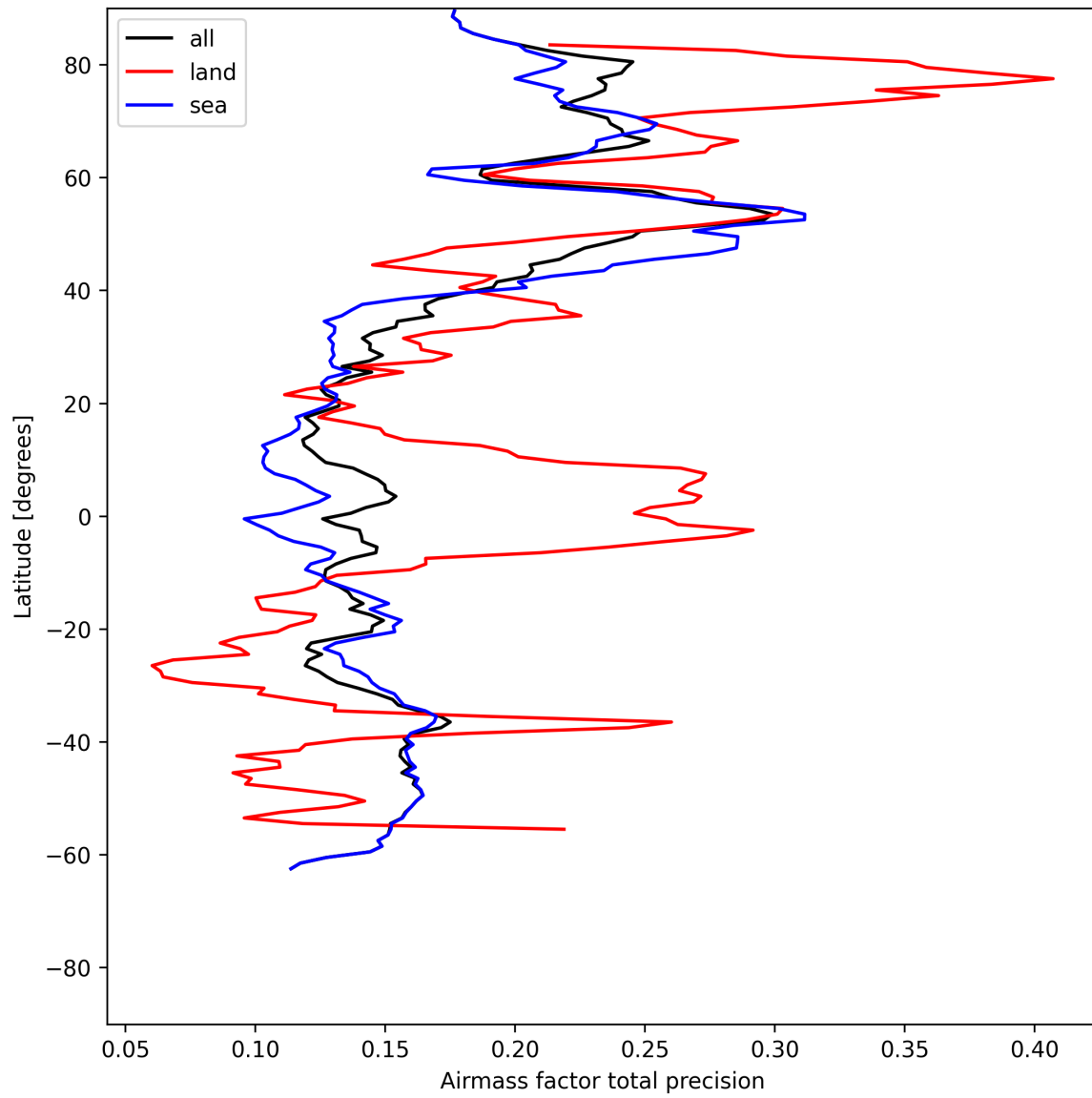
Figure 27: Zonal average of “Airmass factor total precision” for 2025-07-08 to 2025-07-09.
