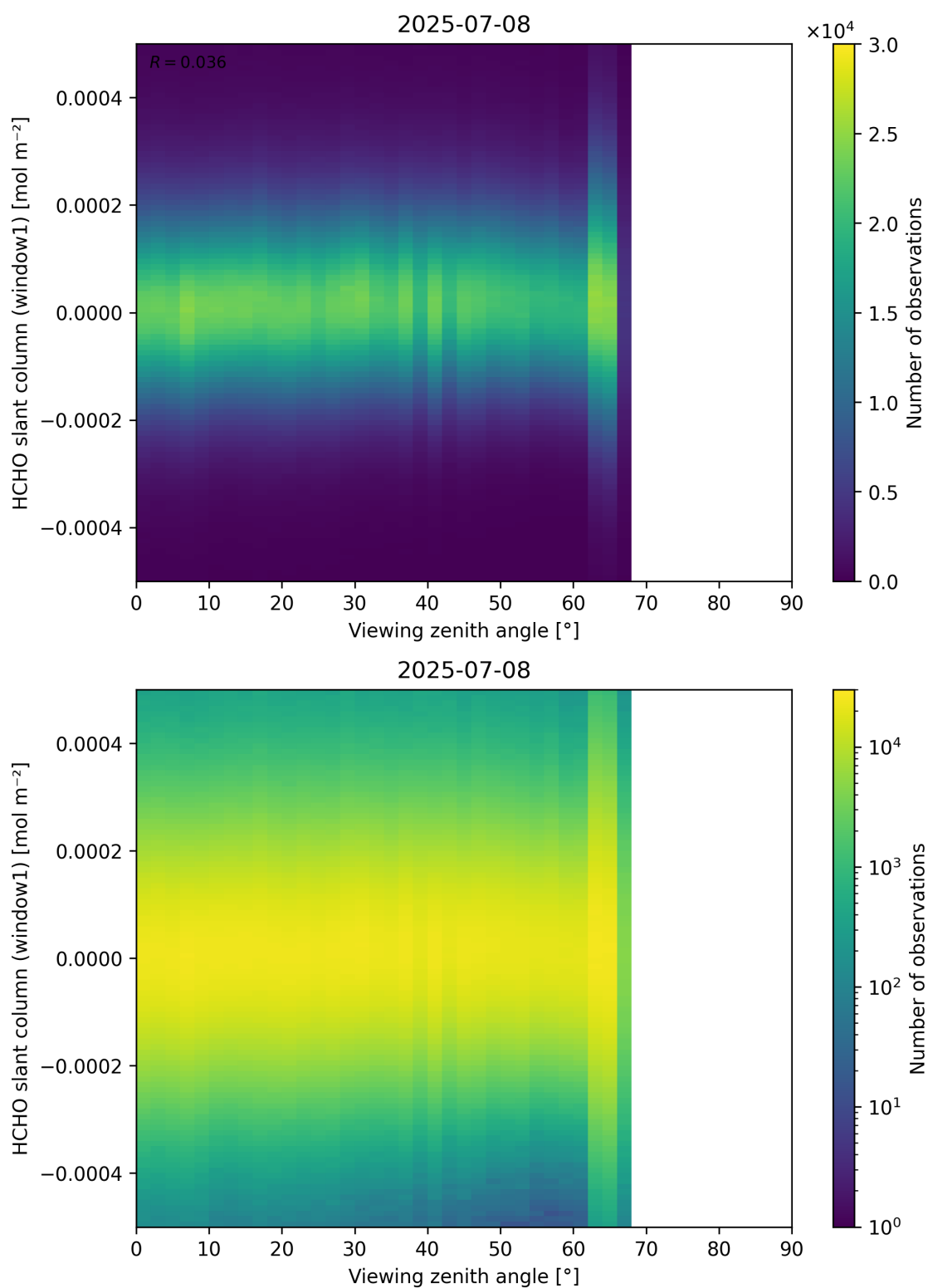
Figure 188: Scatter density plot of “Viewing zenith angle” against “HCHO slant column (window1)” for 2025-07-08 to 2025-07-09.
