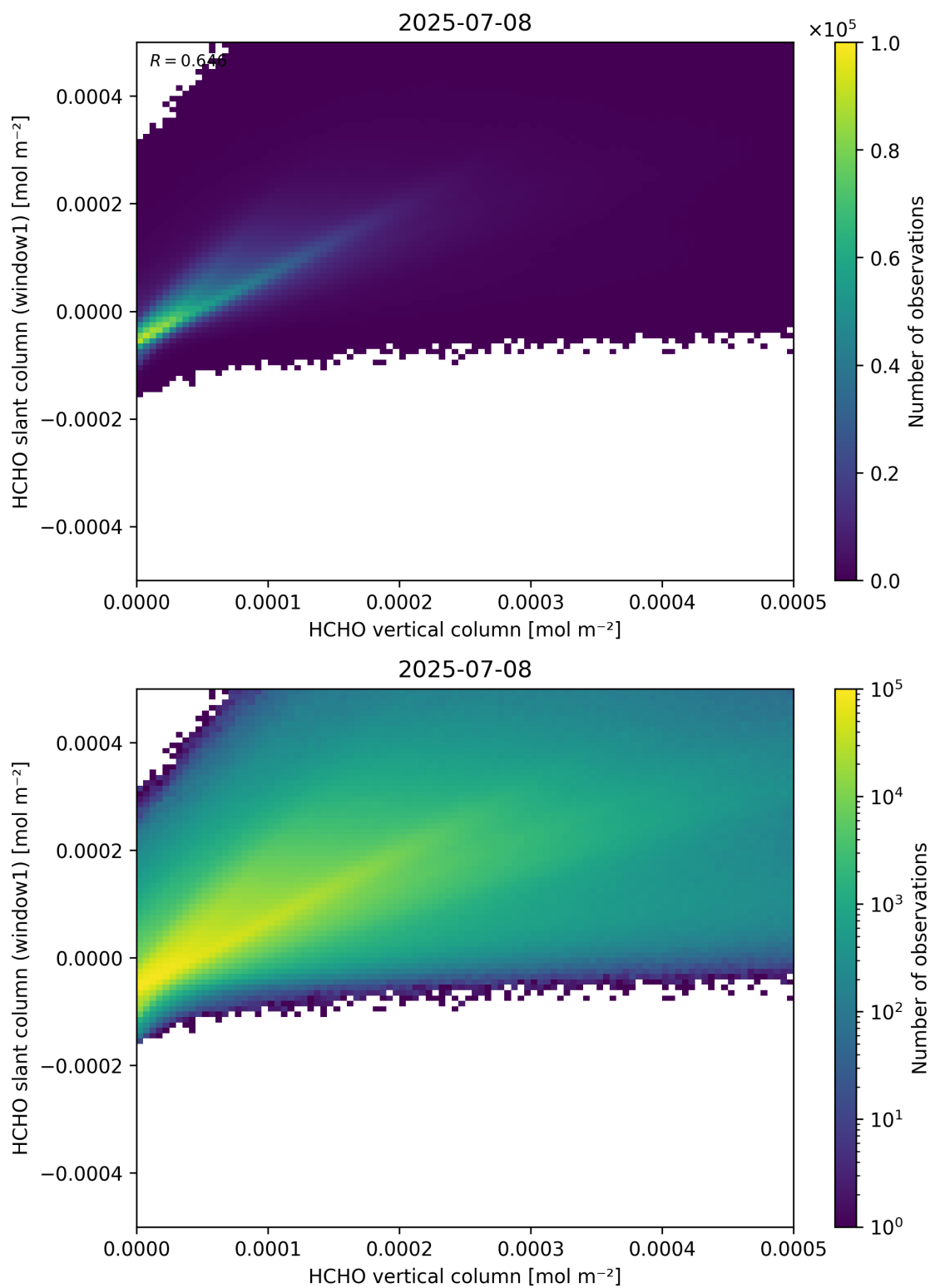
Figure 129: Scatter density plot of “HCHO vertical column” against “HCHO slant column (window1)” for 2025-07-08 to 2025-07-09.
