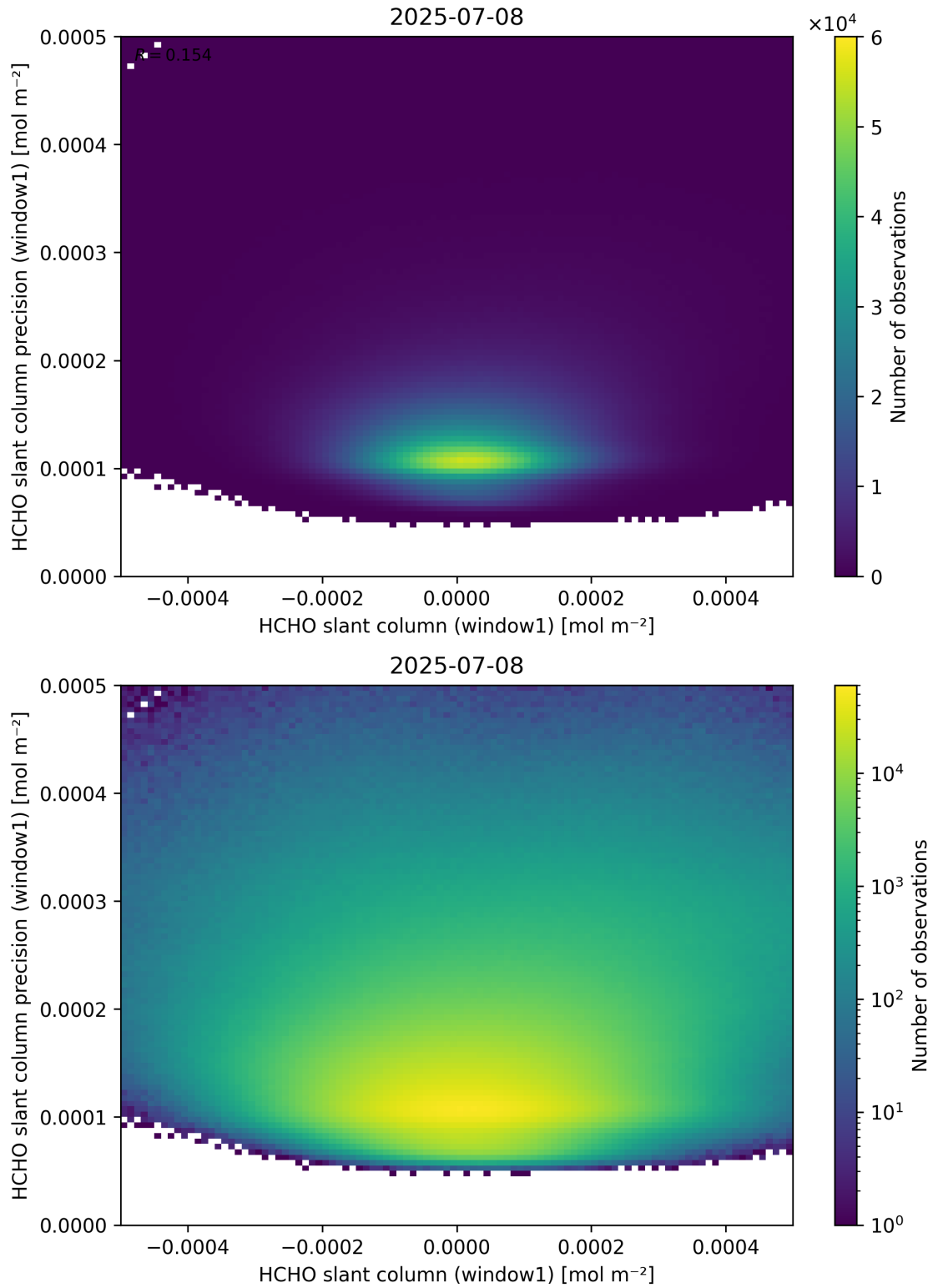
Figure 84: Scatter density plot of “HCHO slant column (window1)” against “HCHO slant column precision (window1)” for 2025-07-08 to 2025-07-09.
