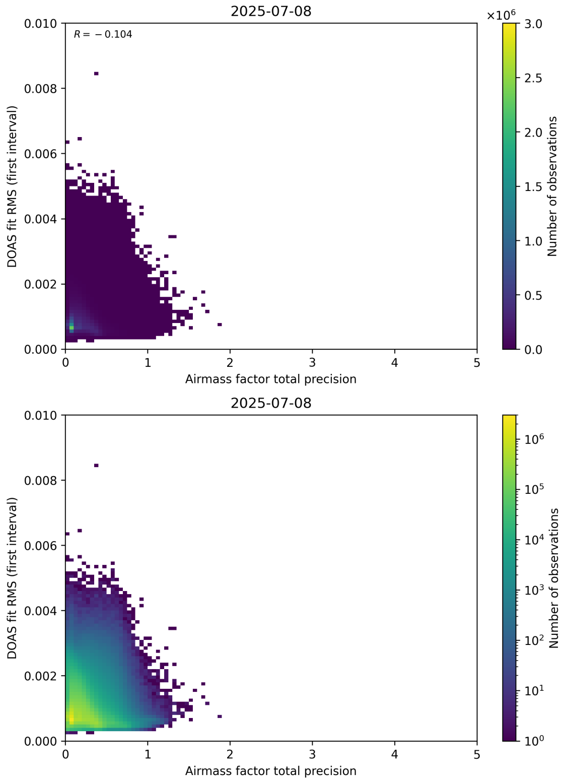
Figure 105: Scatter density plot of “Airmass factor total precision” against “DOAS fit RMS (first interval)” for 2025-07-08 to 2025-07-09.
