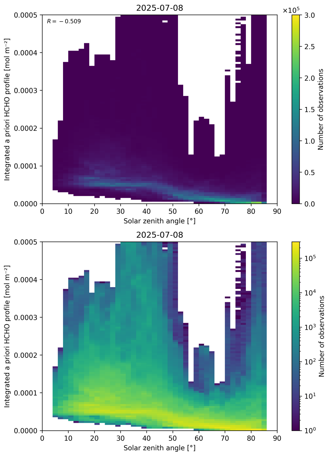
Figure 180: Scatter density plot of “Solar zenith angle” against “Integrated a priori HCHO profile” for 2025-07-08 to 2025-07-09.
