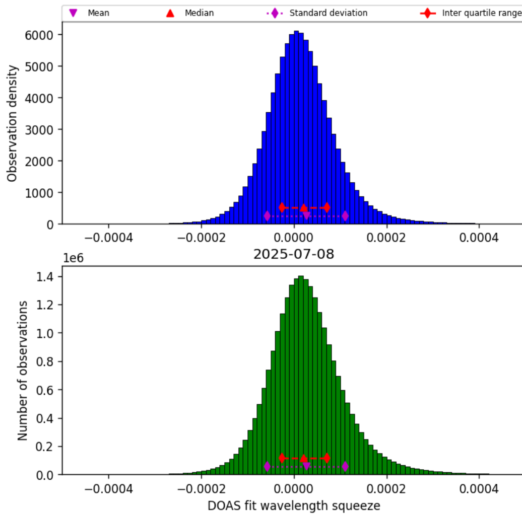
Figure 45: Histogram of “DOAS fit wavelength squeeze” for 2025-07-08 to 2025-07-09
