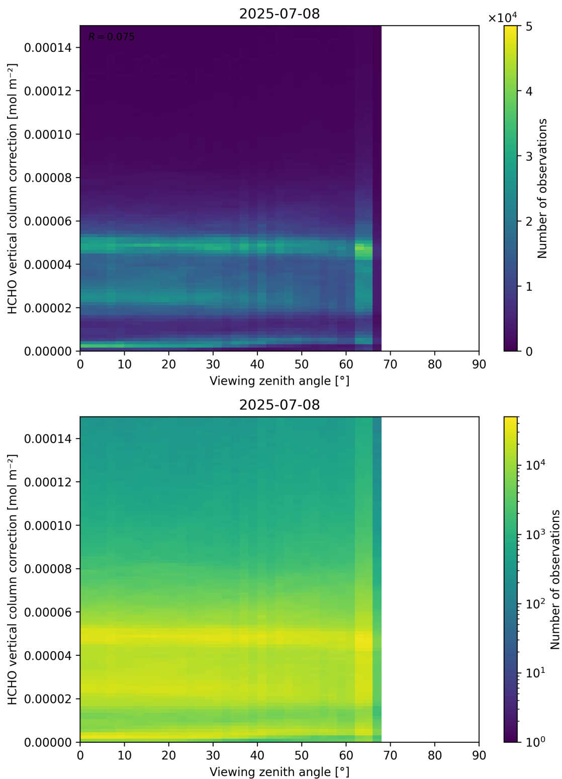
Figure 193: Scatter density plot of “Viewing zenith angle” against “HCHO vertical column correction” for 2025-07-08 to 2025-07-09.
