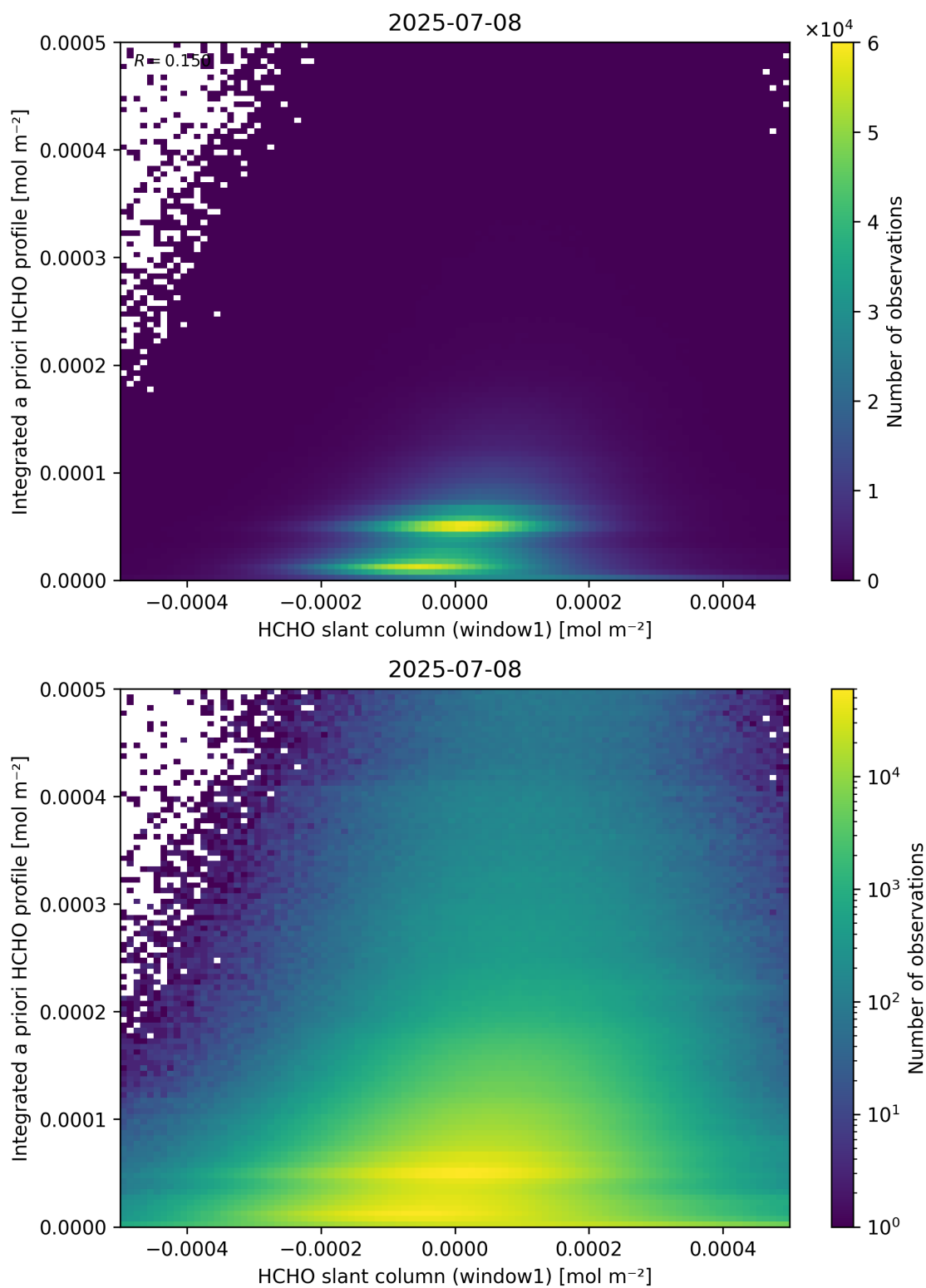
Figure 87: Scatter density plot of “HCHO slant column (window1)” against “Integrated a priori HCHO profile” for 2025-07-08 to 2025-07-09.
