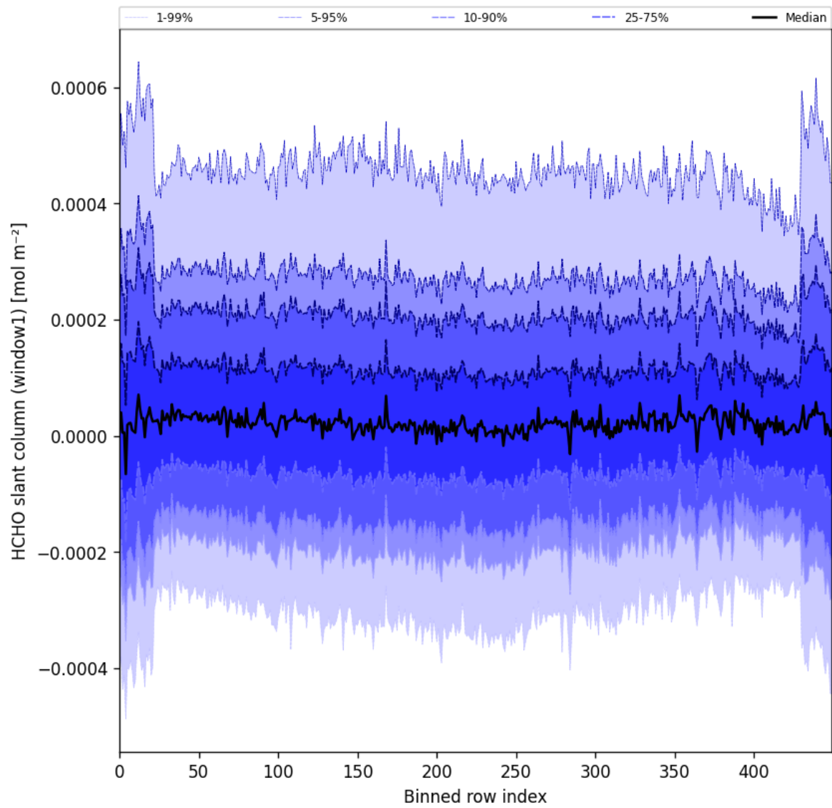
Figure 52: Along track statistics of “HCHO slant column (window1)” for 2025-07-08 to 2025-07-09
