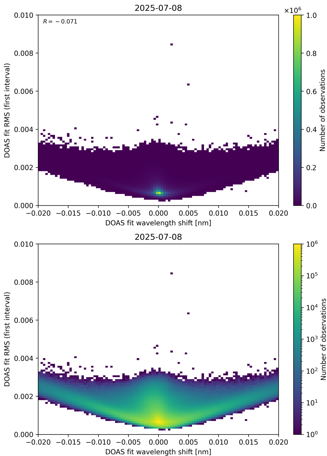
Figure 64: Scatter density plot of “DOAS fit wavelength shift” against “DOAS fit RMS (first interval)” for 2025-07-08 to 2025-07-09.
