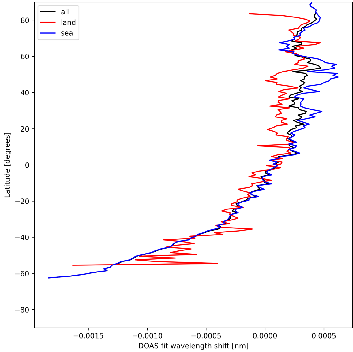
Figure 30: Zonal average of "DOAS fit wavelength shift" for 2025-07-08 to 2025-07-09.
