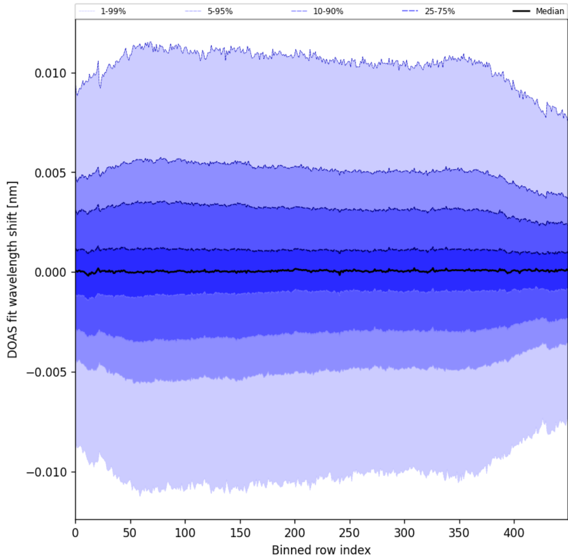
Figure 58: Along track statistics of “DOAS fit wavelength shift” for 2025-07-08 to 2025-07-09
