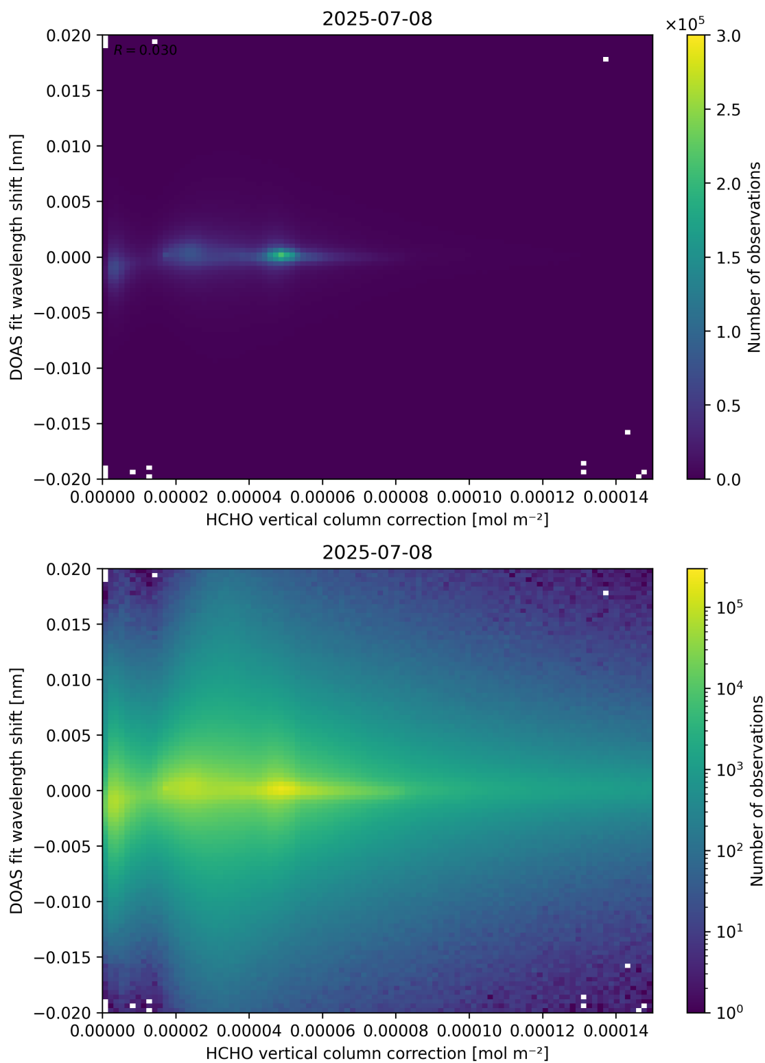
Figure 113: Scatter density plot of “HCHO vertical column correction” against “DOAS fit wavelength shift” for 2025-07-08 to 2025-07-09.
