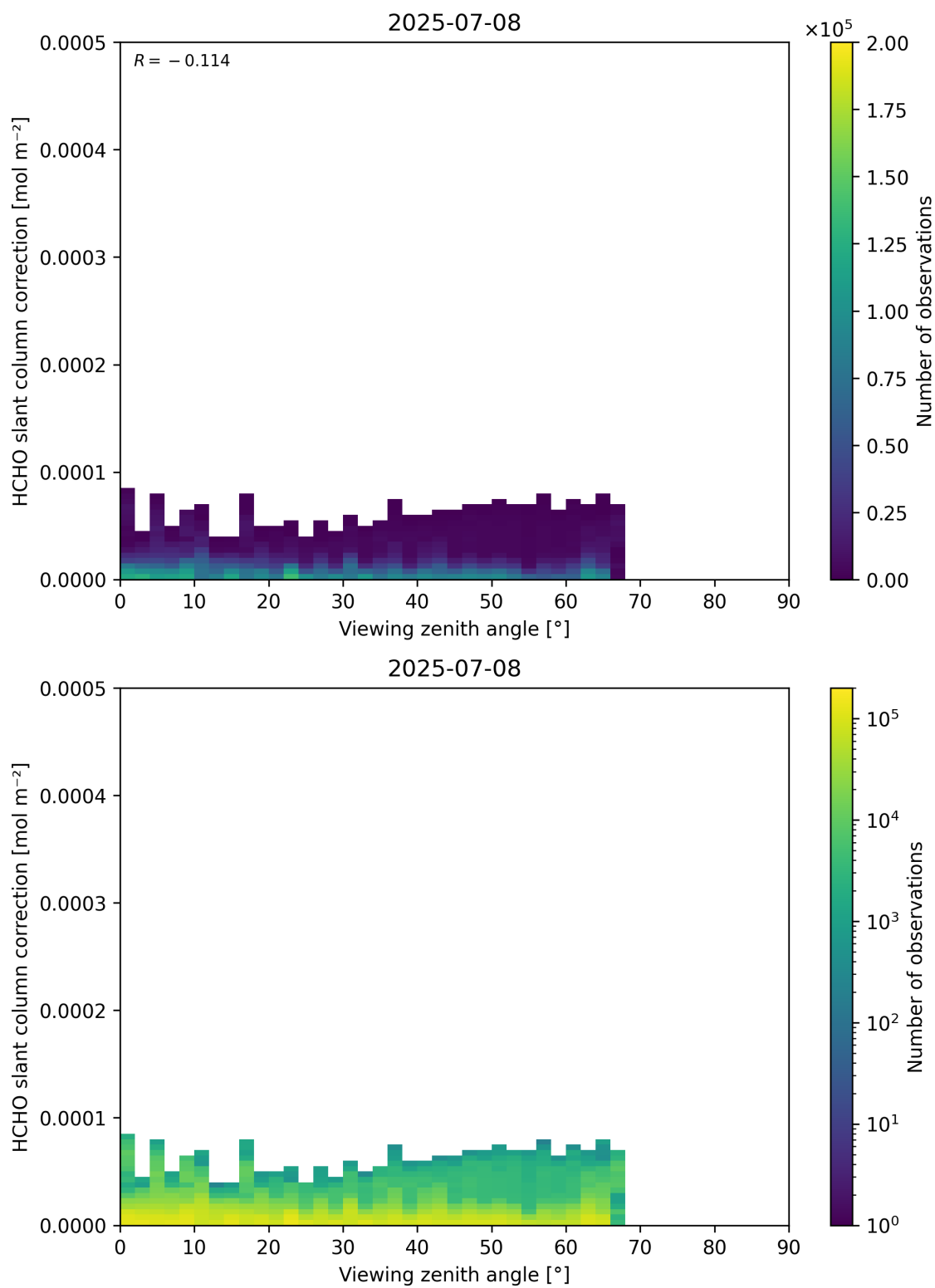
Figure 187: Scatter density plot of “Viewing zenith angle” against “HCHO slant column correction” for 2025-07-08 to 2025-07-09.
