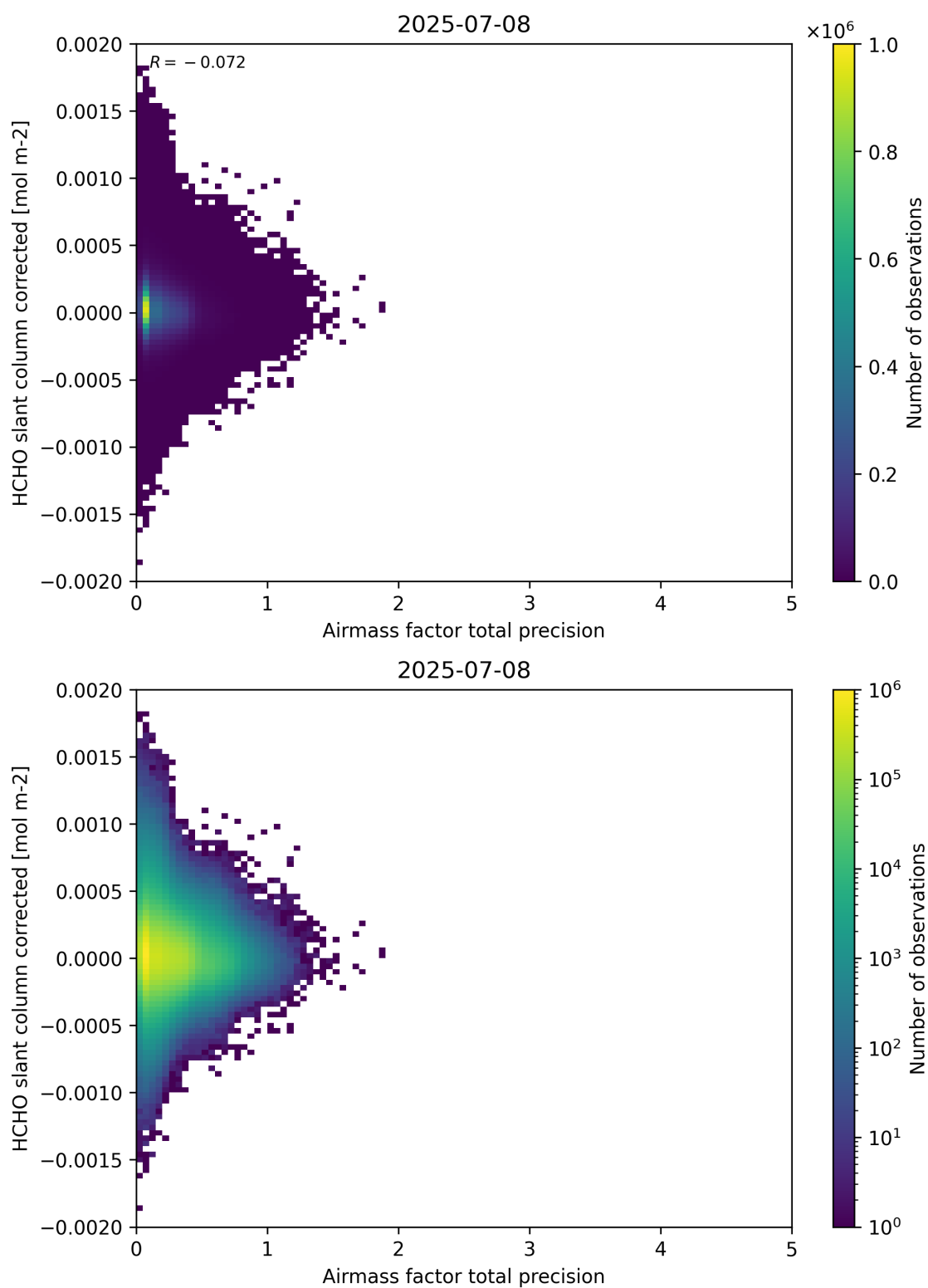
Figure 109: Scatter density plot of “Airmass factor total precision” against “HCHO slant column corrected” for 2025-07-08 to 2025-07-09.
