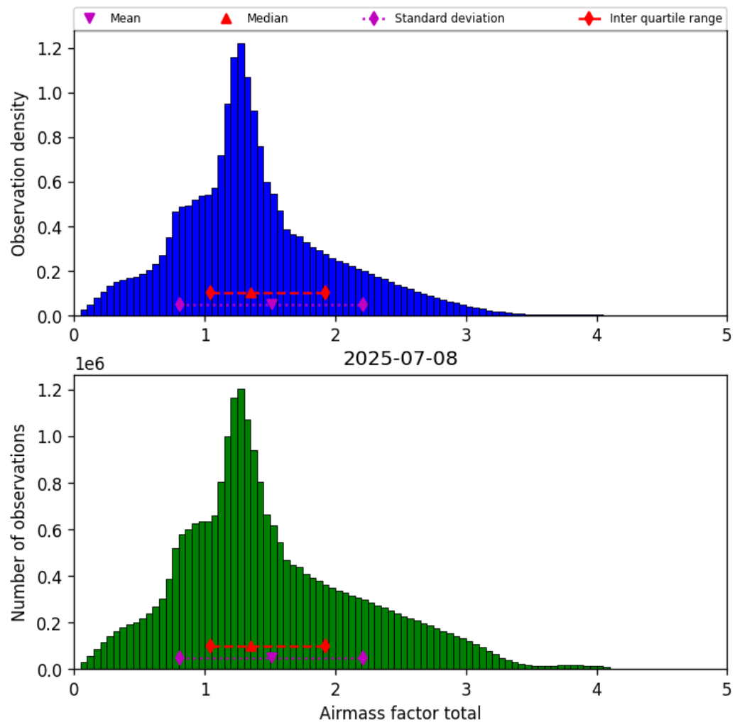
Figure 40: Histogram of “Airmass factor total” for 2025-07-08 to 2025-07-09
