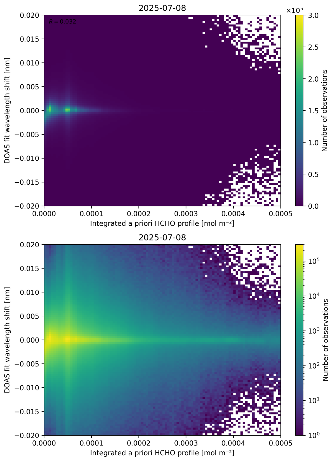
Figure 149: Scatter density plot of “Integrated a priori HCHO profile” against “DOAS fit wavelength shift” for 2025-07-08 to 2025-07-09.
