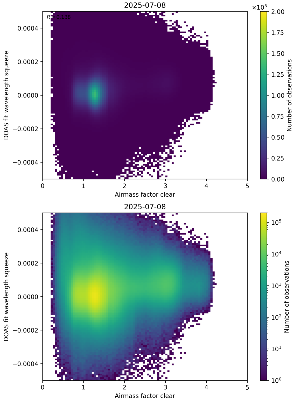
Figure 73: Scatter density plot of “Airmass factor clear” against “DOAS fit wavelength squeeze” for 2025-07-08 to 2025-07-09.
