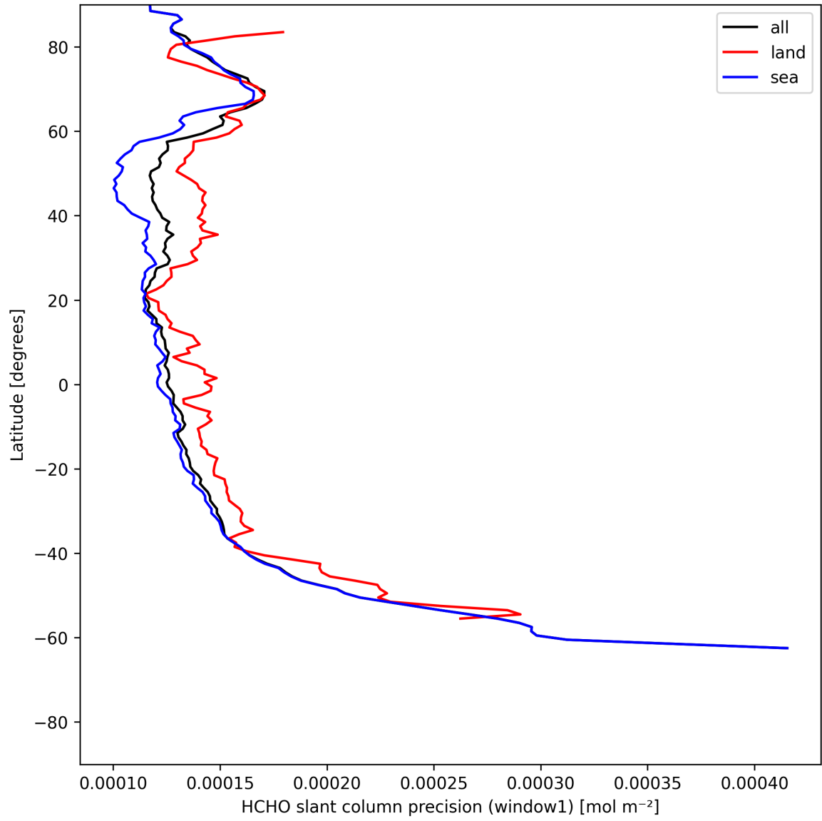
Figure 25: Zonal average of “HCHO slant column precision (window1)” for 2025-07-08 to 2025-07-09.
