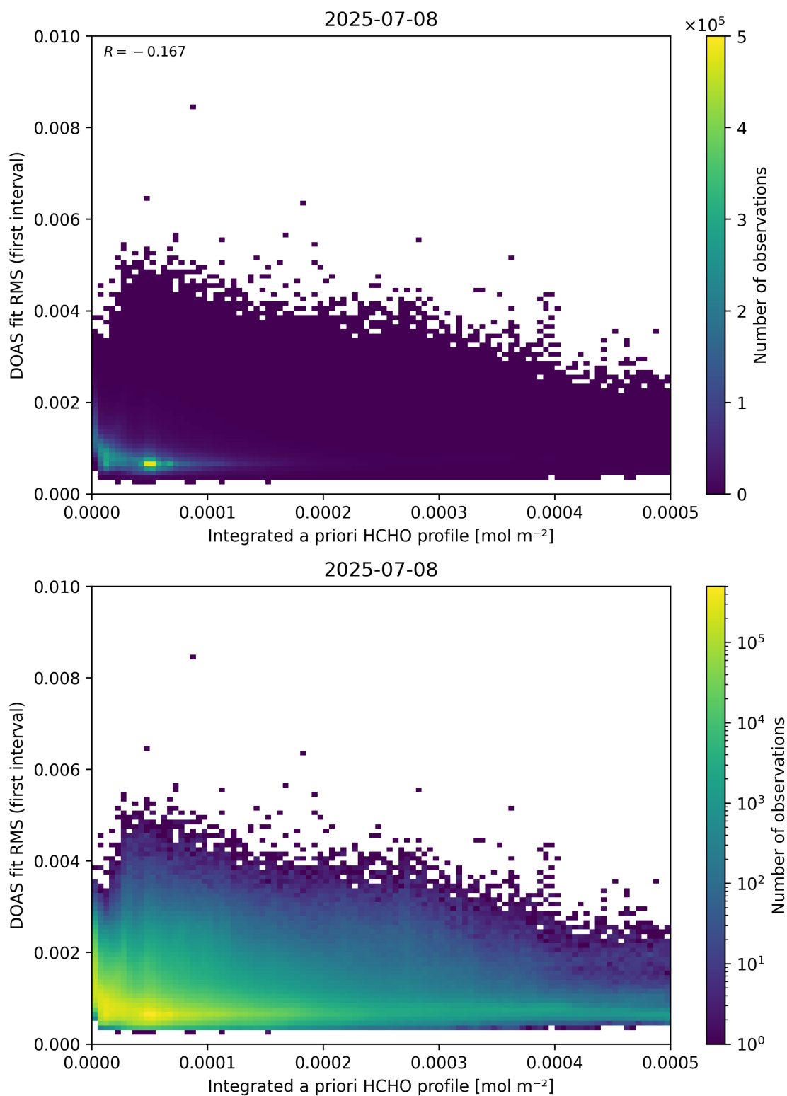
Figure 148: Scatter density plot of “Integrated a priori HCHO profile” against “DOAS fit RMS (first interval)” for 2025-07-08 to 2025-07-09.
