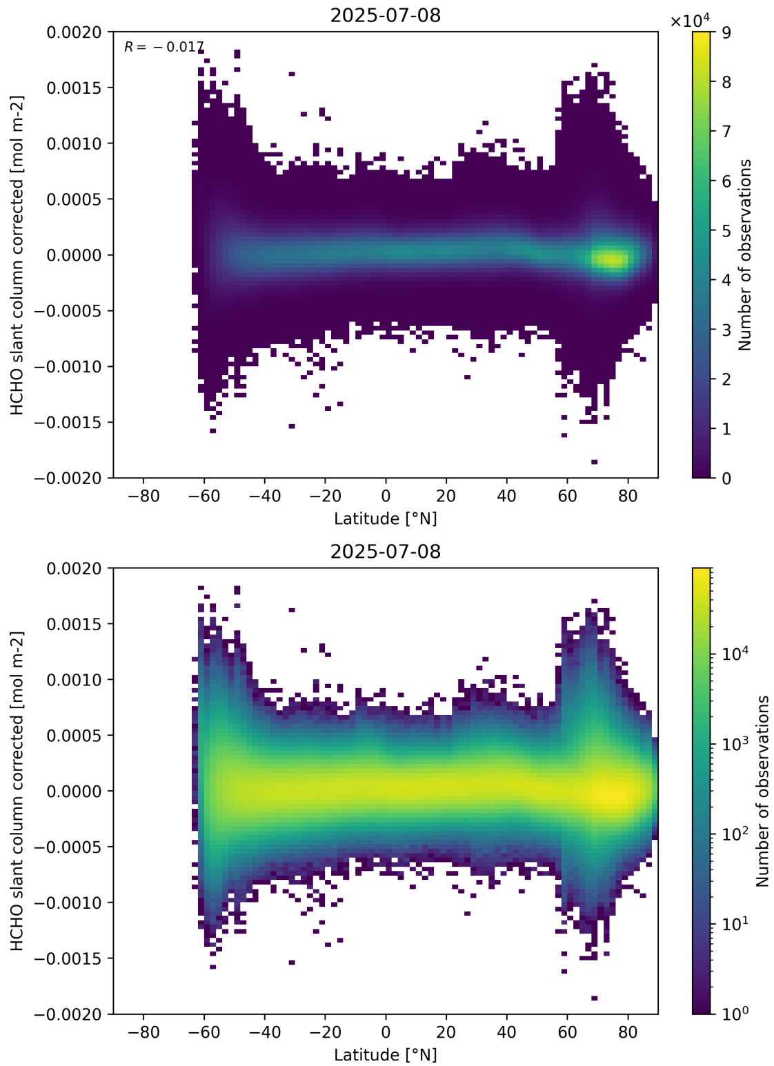
Figure 157: Scatter density plot of “Latitude” against “HCHO slant column corrected” for 2025-07-08 to 2025-07-09.
