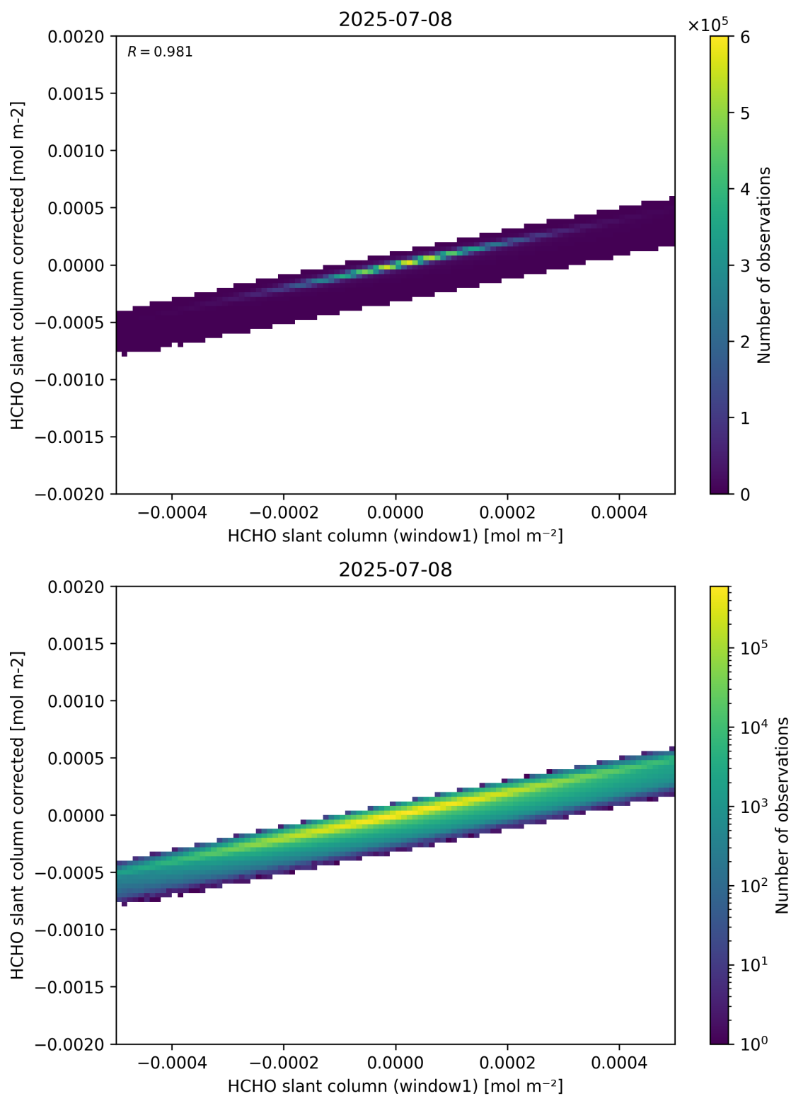
Figure 82: Scatter density plot of “HCHO slant column (window1)” against “HCHO slant column corrected” for 2025-07-08 to 2025-07-09.
