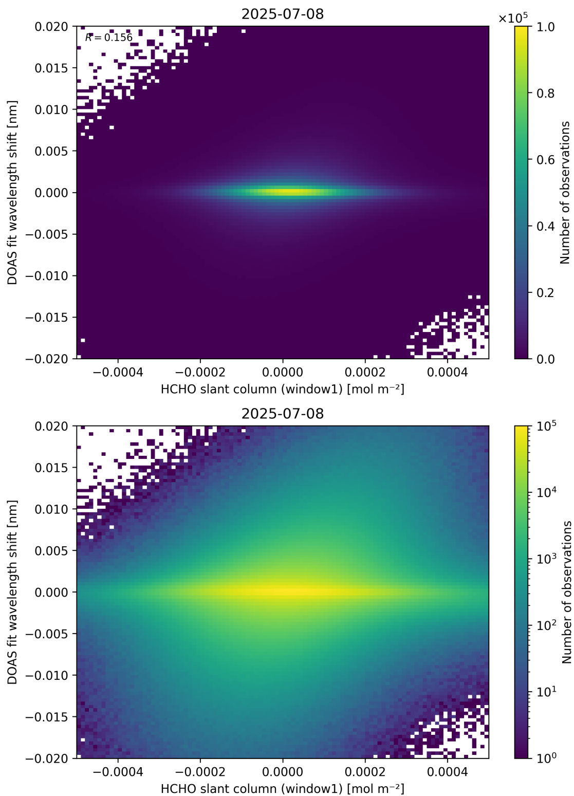
Figure 79: Scatter density plot of “HCHO slant column (window1)” against “DOAS fit wavelength shift” for 2025-07-08 to 2025-07-09.
