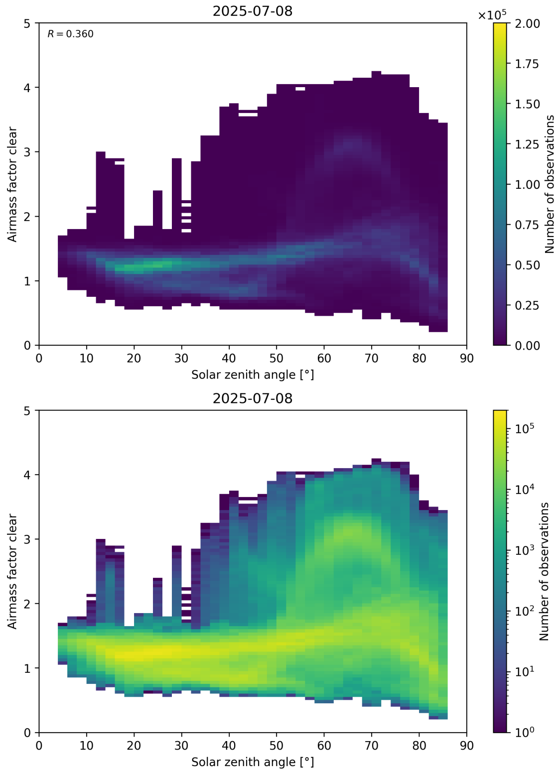
Figure 170: Scatter density plot of “Solar zenith angle” against “Airmass factor clear” for 2025-07-08 to 2025-07-09.
