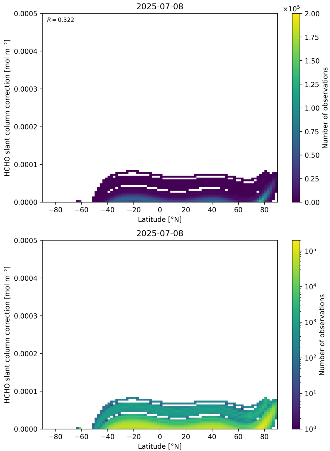
Figure 158: Scatter density plot of “Latitude” against “HCHO slant column correction” for 2025-07-08 to 2025-07-09.
