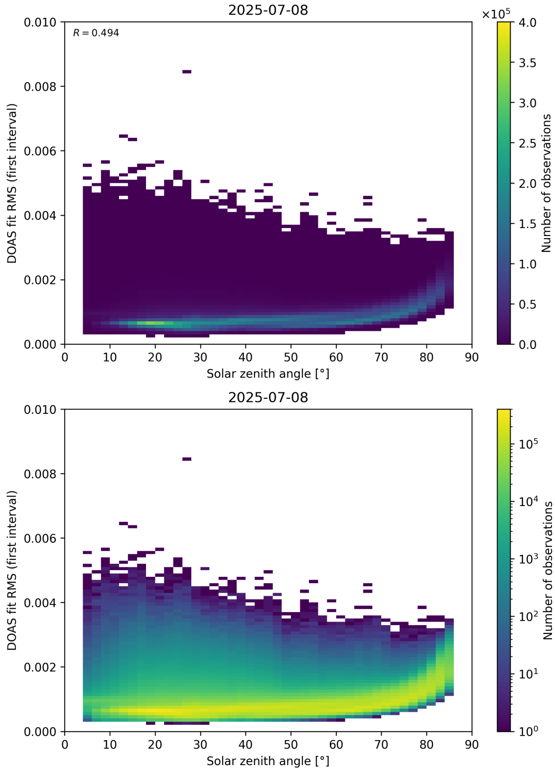
Figure 167: Scatter density plot of “Solar zenith angle” against “DOAS fit RMS (first interval)” for 2025-07-08 to 2025-07-09.
