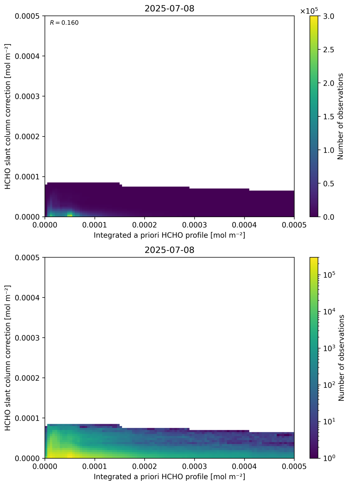
Figure 152: Scatter density plot of “Integrated a priori HCHO profile” against “HCHO slant column correction” for 2025-07-08 to 2025-07-09.
