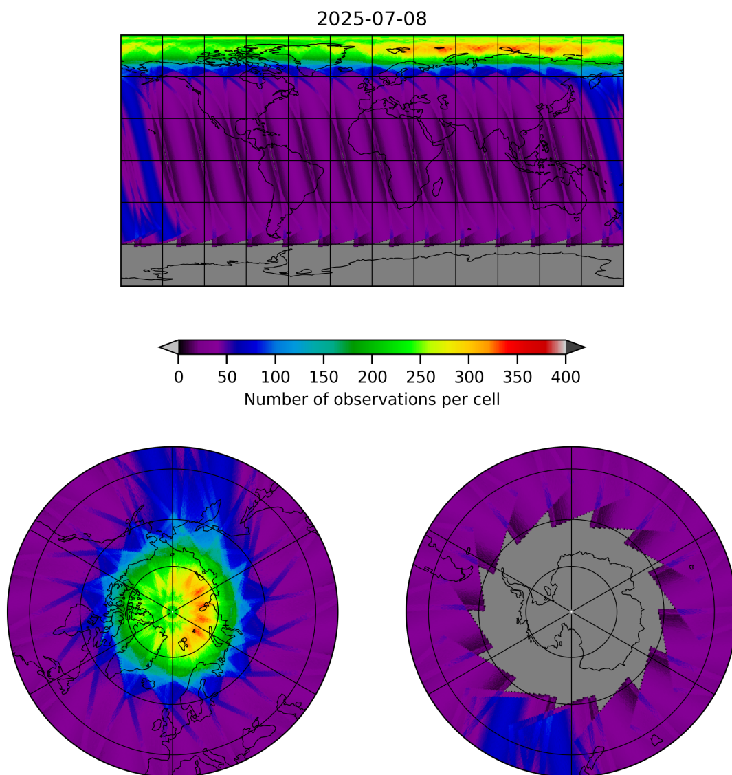
Figure 19: Map of the number of observations for 2025-07-08 to 2025-07-09
