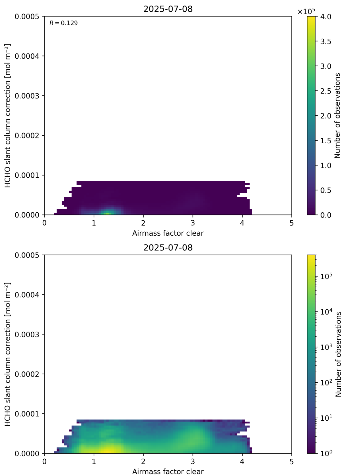
Figure 75: Scatter density plot of “Airmass factor clear” against “HCHO slant column correction” for 2025-07-08 to 2025-07-09.
