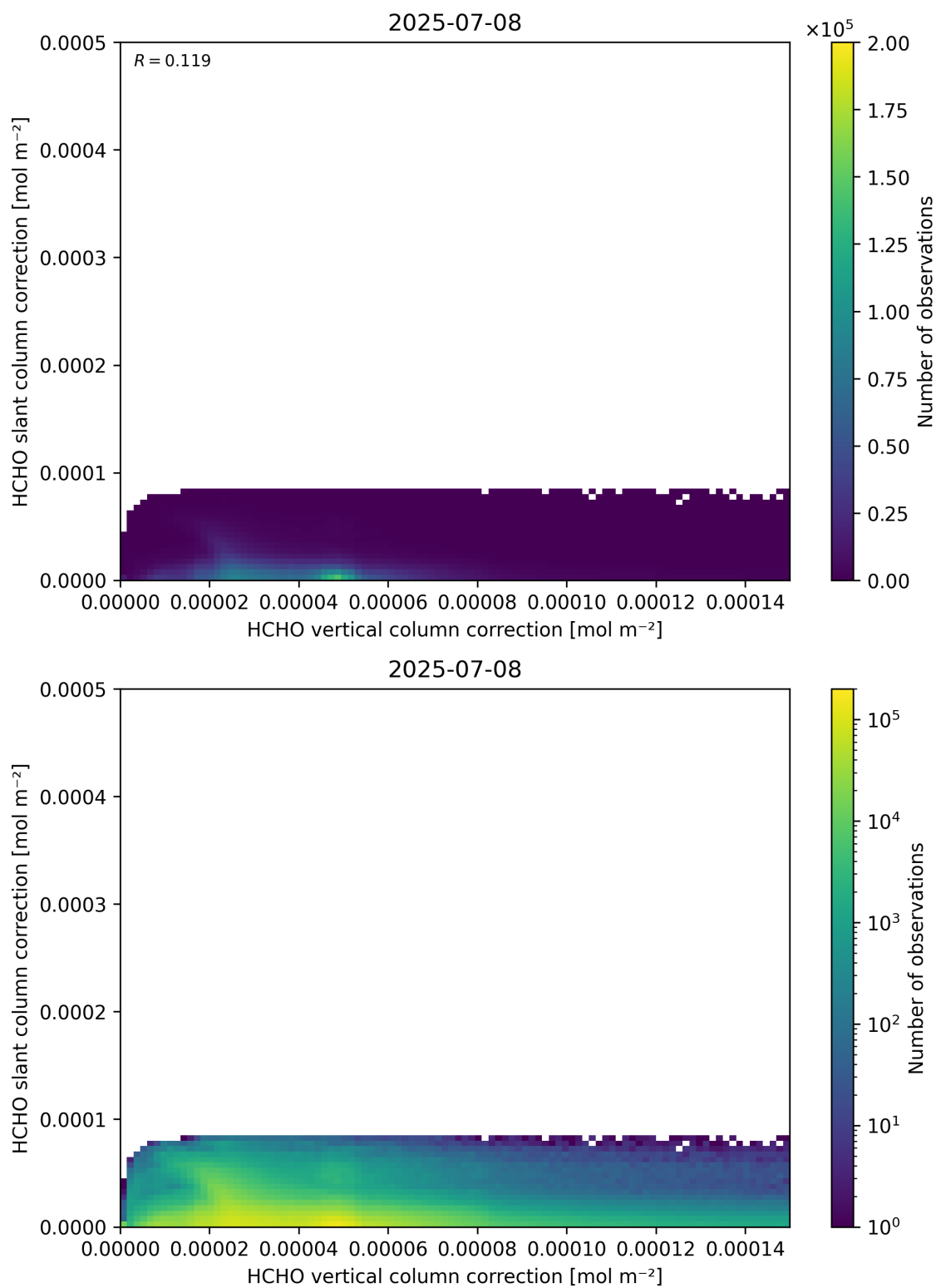
Figure 117: Scatter density plot of “HCHO vertical column correction” against “HCHO slant column correction” for 2025-07-08 to 2025-07-09.
