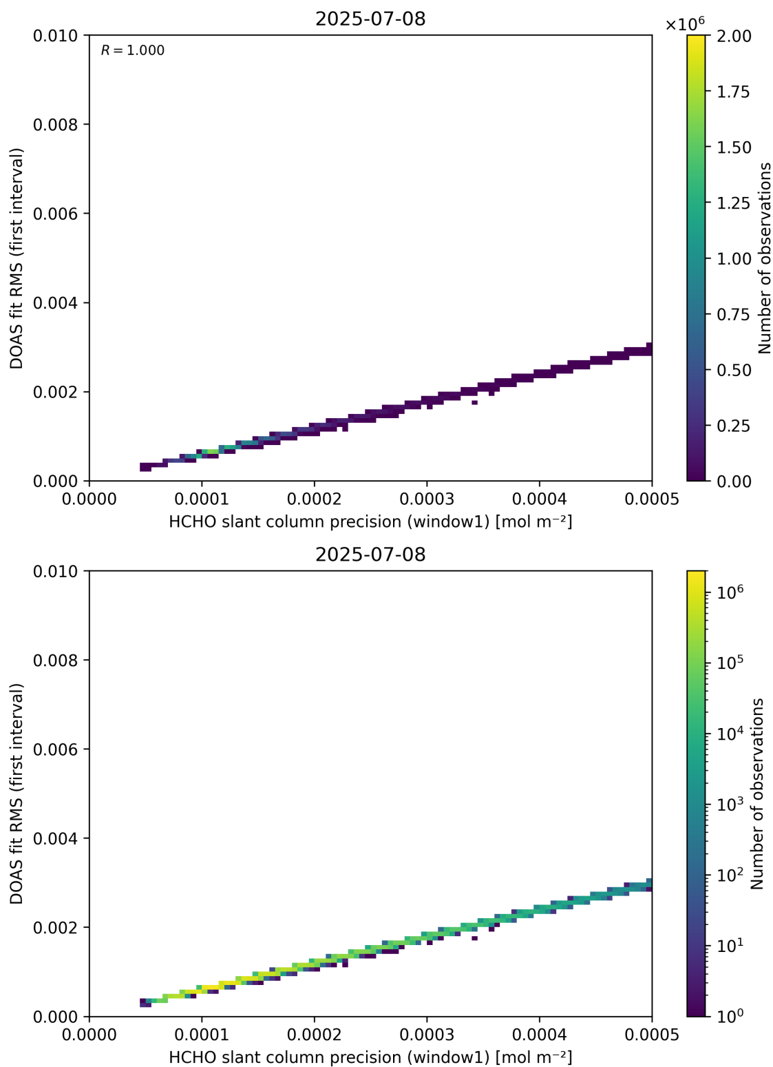
Figure 88: Scatter density plot of “HCHO slant column precision (window1)” against “DOAS fit RMS (first interval)” for 2025-07-08 to 2025-07-09.
