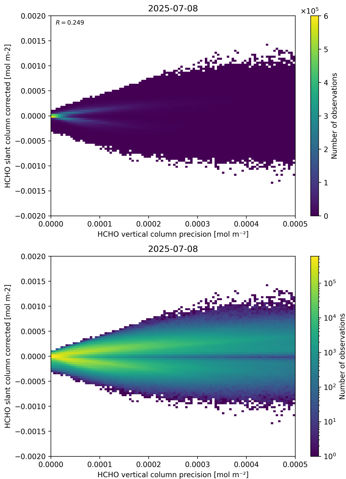
Figure 140: Scatter density plot of “HCHO vertical column precision” against “HCHO slant column corrected” for 2025-07-08 to 2025-07-09.
