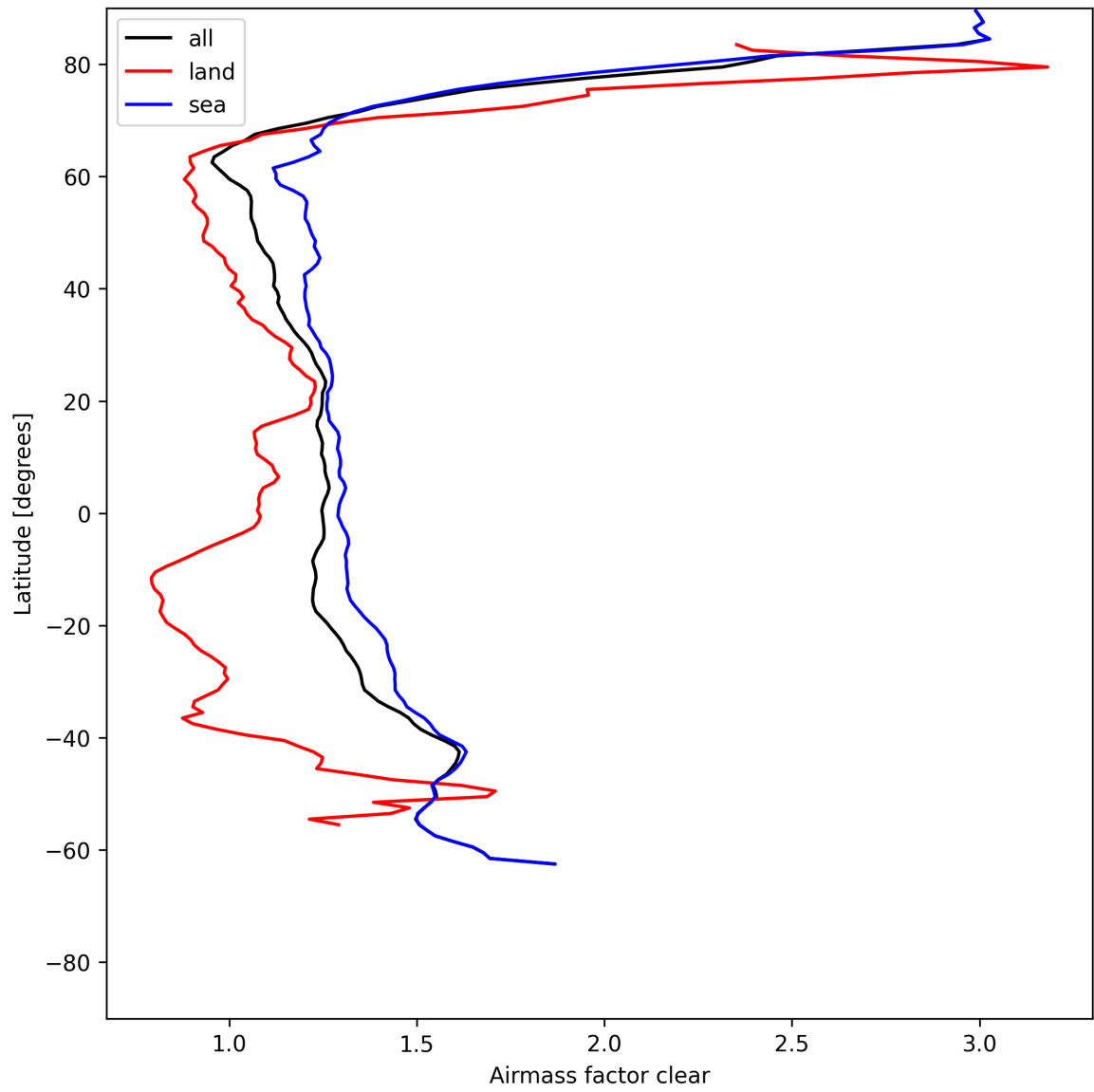
Figure 28: Zonal average of “Airmass factor clear” for 2025-07-08 to 2025-07-09.
