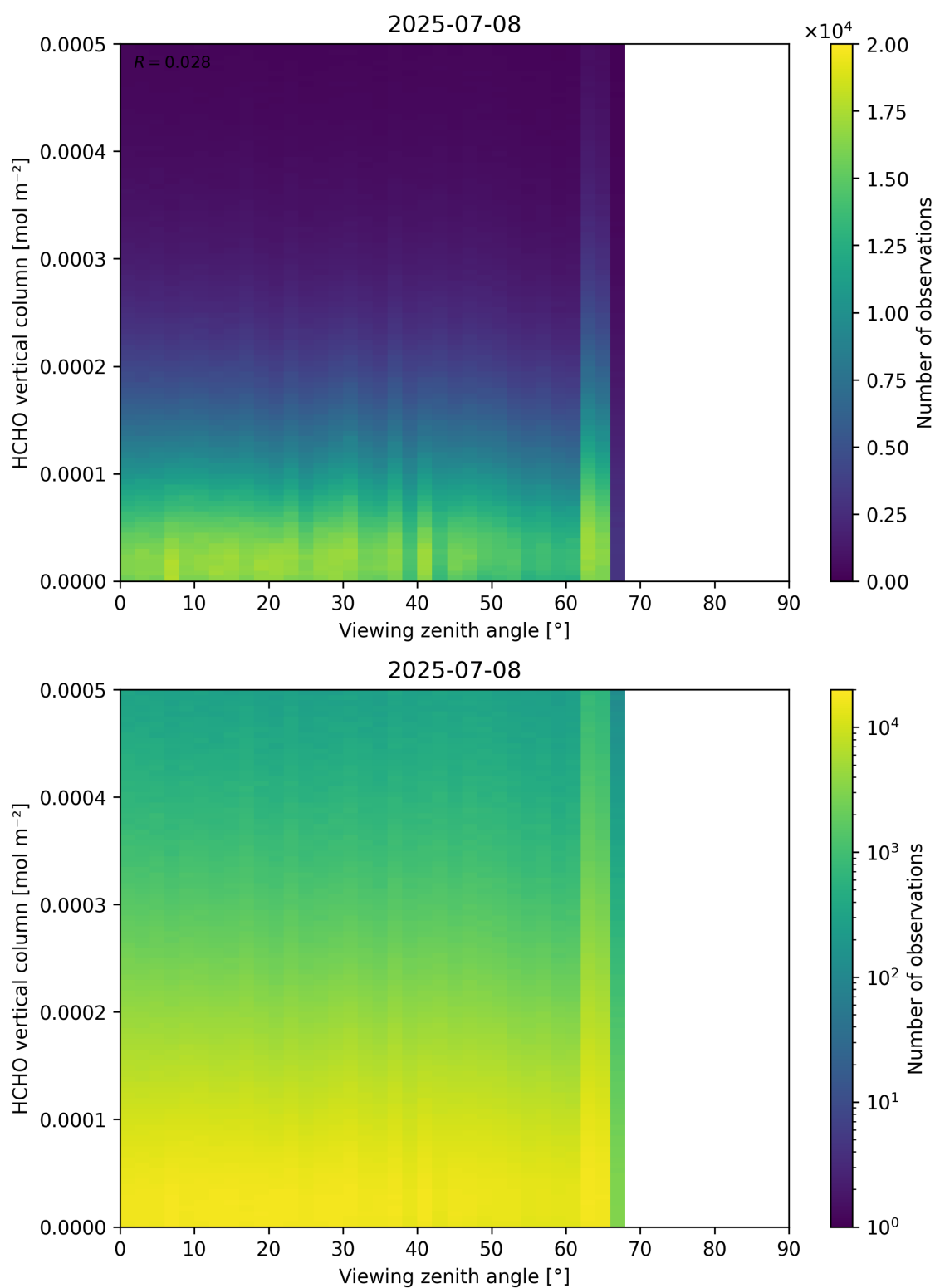
Figure 192: Scatter density plot of “Viewing zenith angle” against “HCHO vertical column” for 2025-07-08 to 2025-07-09.
