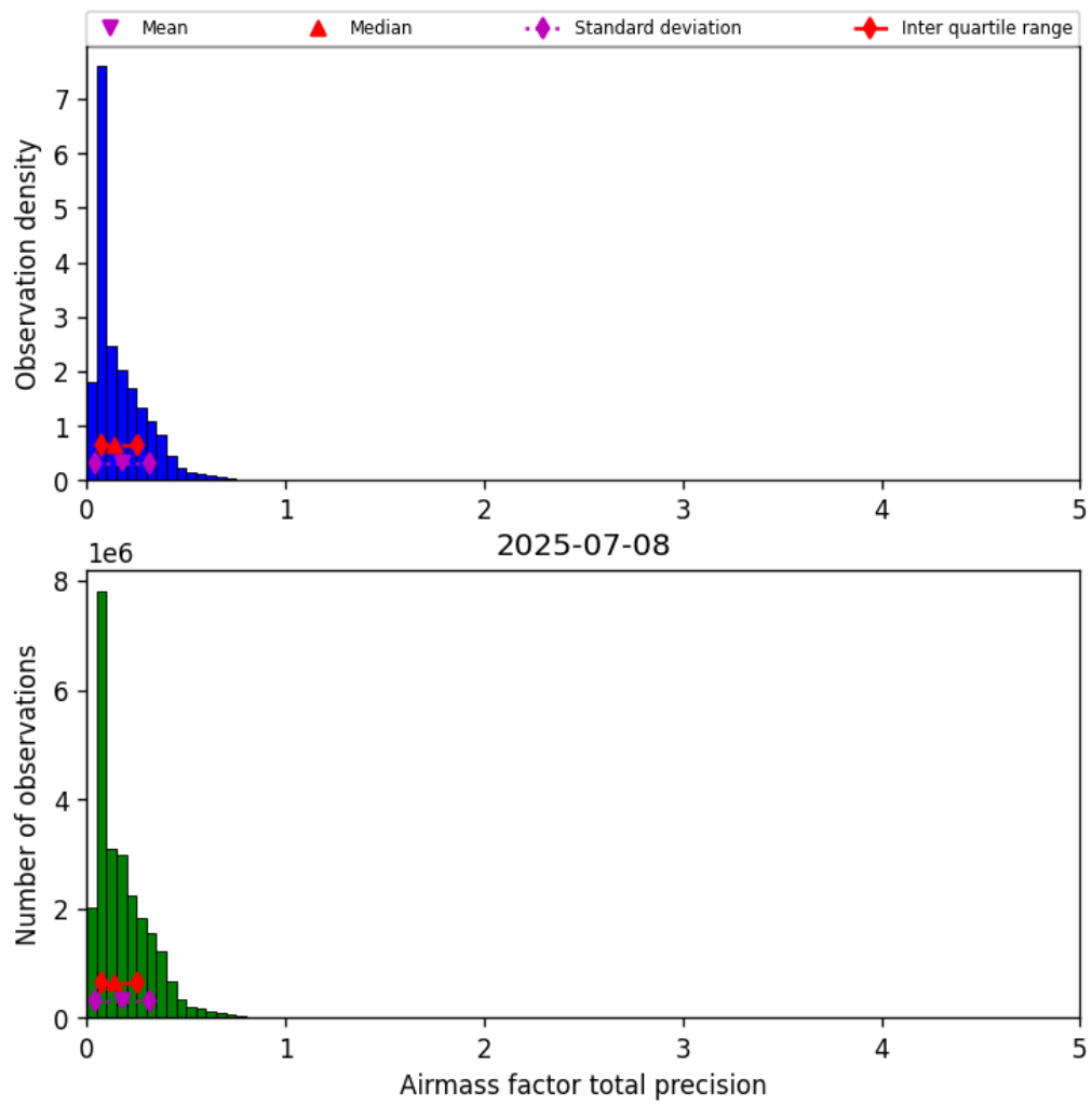
Figure 41: Histogram of “Airmass factor total precision” for 2025-07-08 to 2025-07-09
