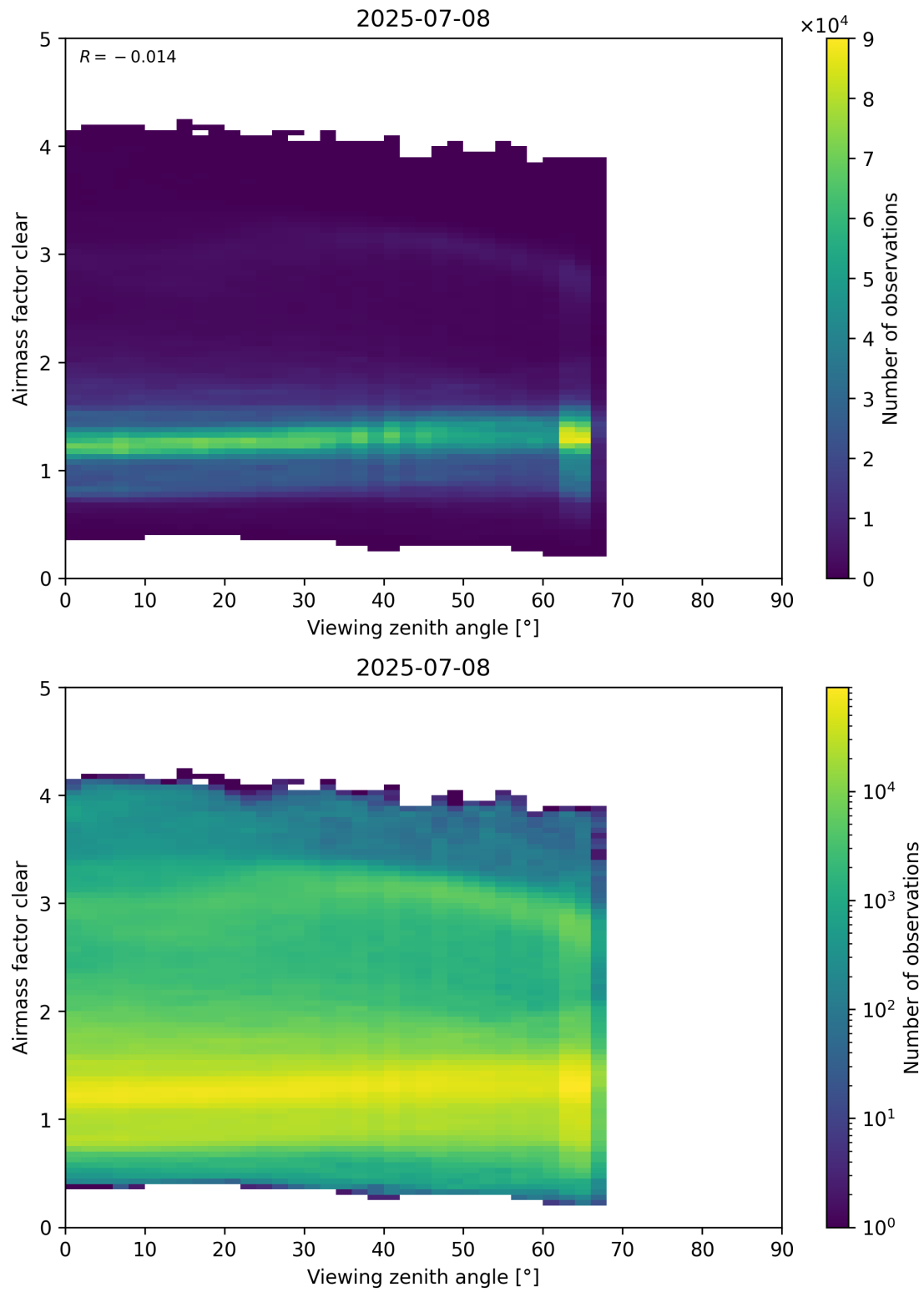
Figure 185: Scatter density plot of “Viewing zenith angle” against “Airmass factor clear” for 2025-07-08 to 2025-07-09.
