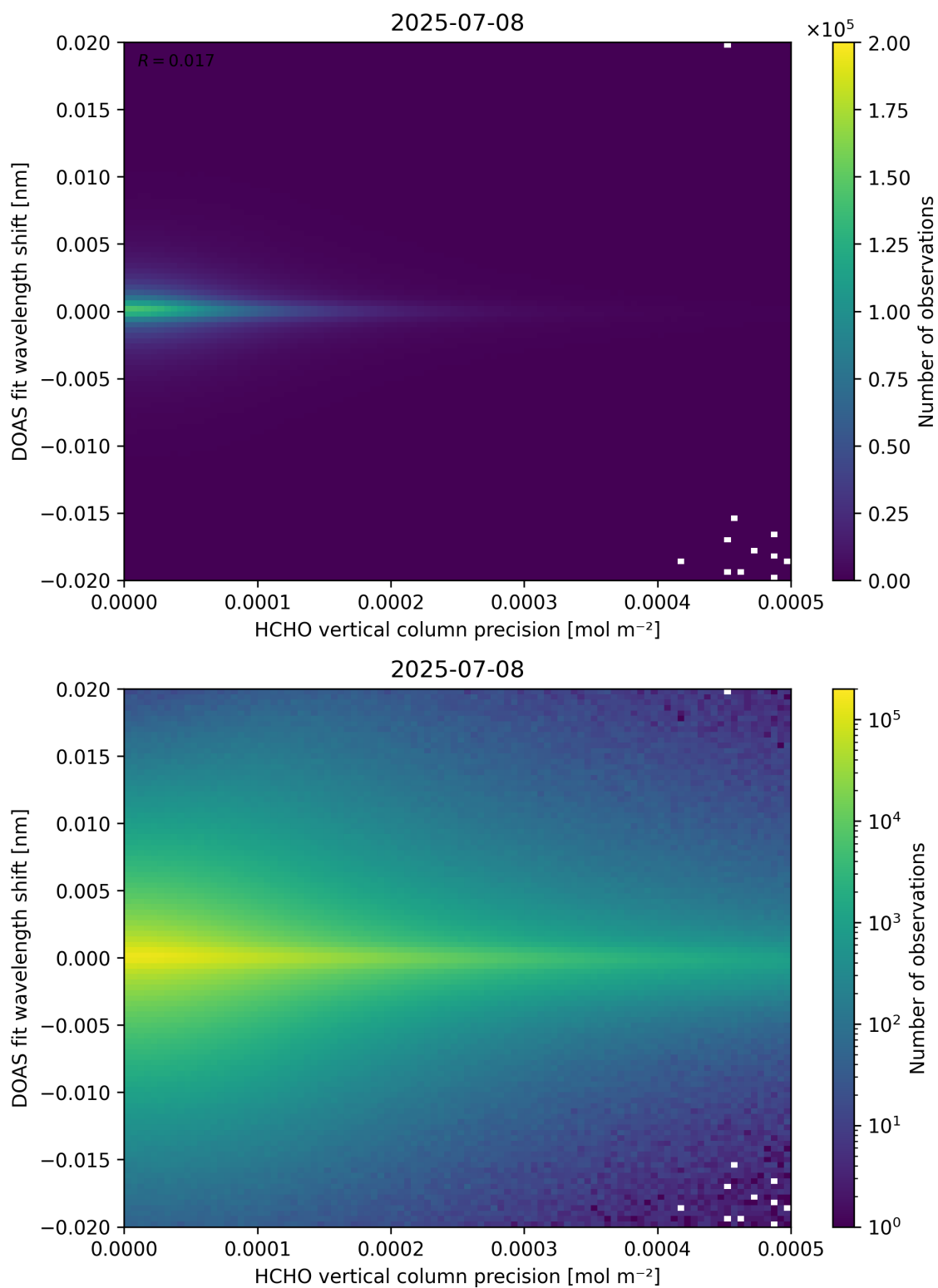
Figure 137: Scatter density plot of “HCHO vertical column precision” against “DOAS fit wavelength shift” for 2025-07-08 to 2025-07-09.
