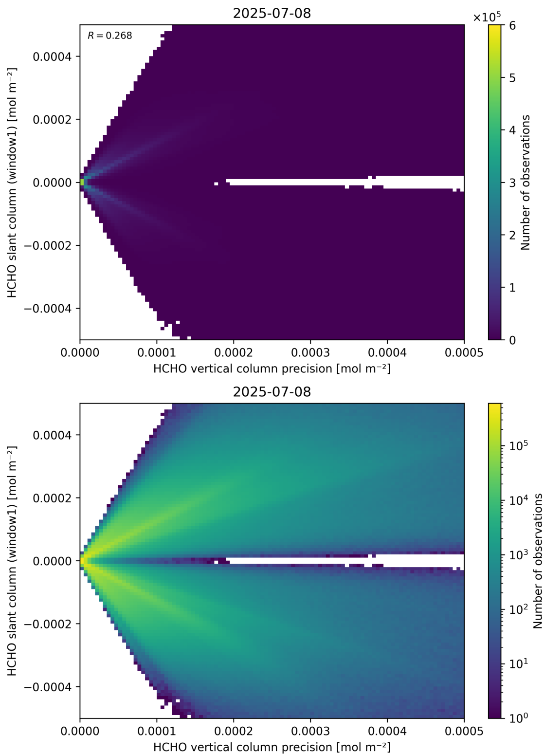
Figure 142: Scatter density plot of “HCHO vertical column precision” against “HCHO slant column (window1)” for 2025-07-08 to 2025-07-09.
