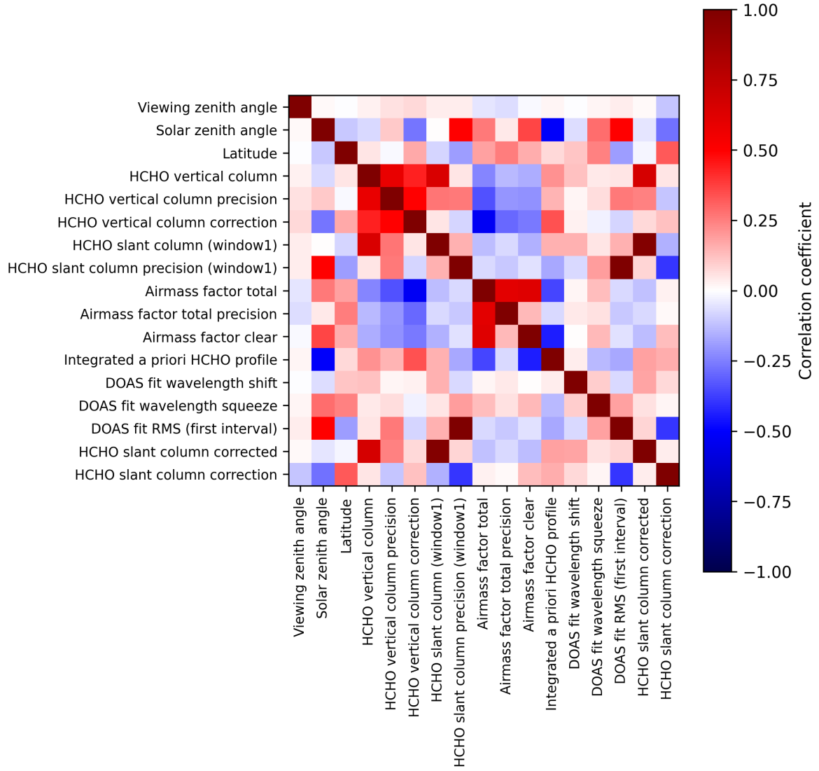
Figure 2: Map of correlation matrix for 2025-07-08 to 2025-07-09.
