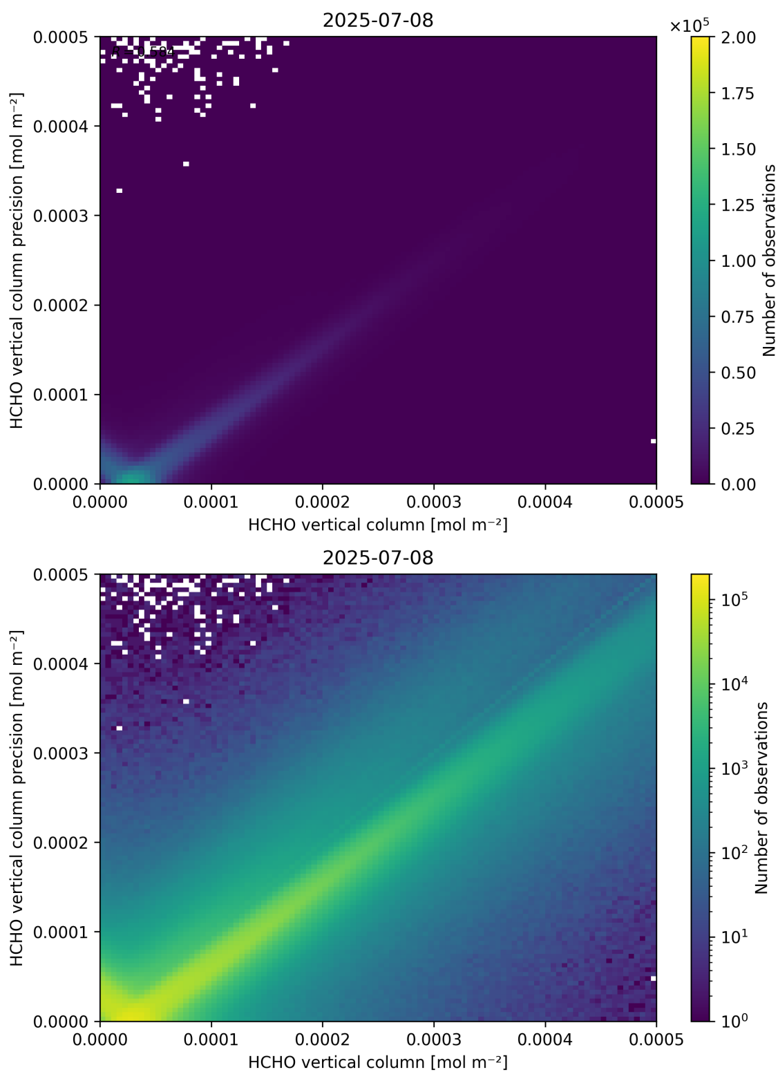
Figure 134: Scatter density plot of “HCHO vertical column” against “HCHO vertical column precision” for 2025-07-08 to 2025-07-09.
