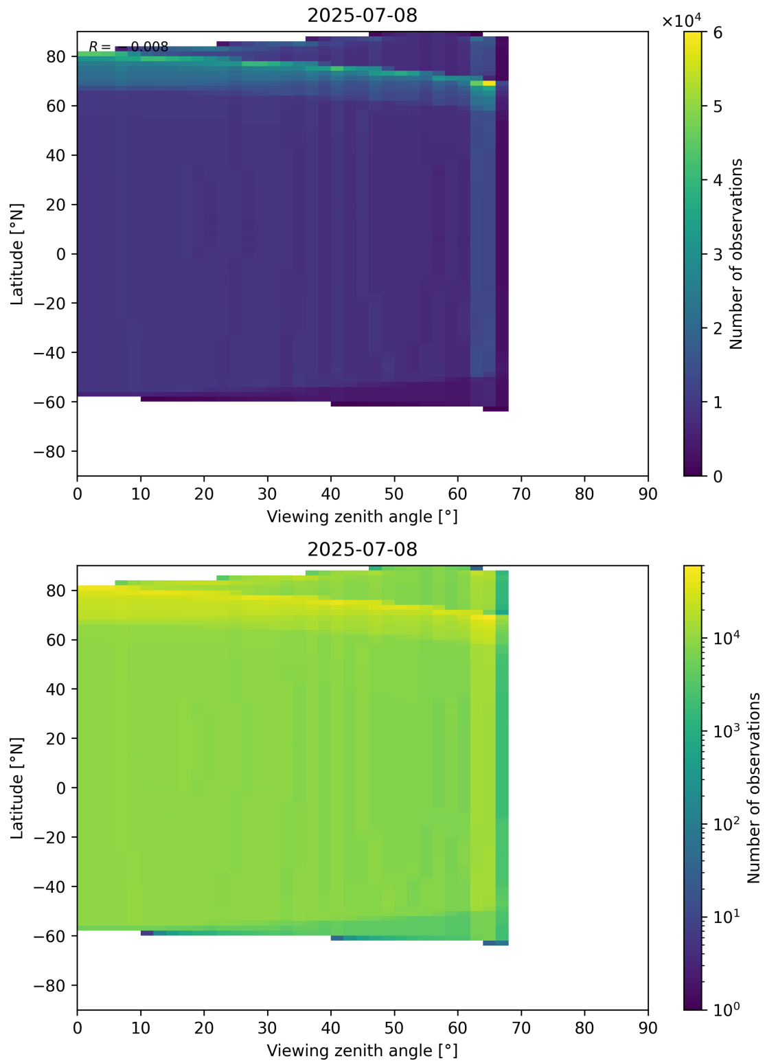
Figure 196: Scatter density plot of “Viewing zenith angle” against “Latitude” for 2025-07-08 to 2025-07-09.
