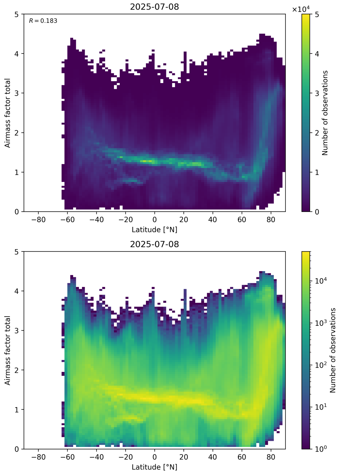
Figure 161: Scatter density plot of “Latitude” against “Airmass factor total” for 2025-07-08 to 2025-07-09.
