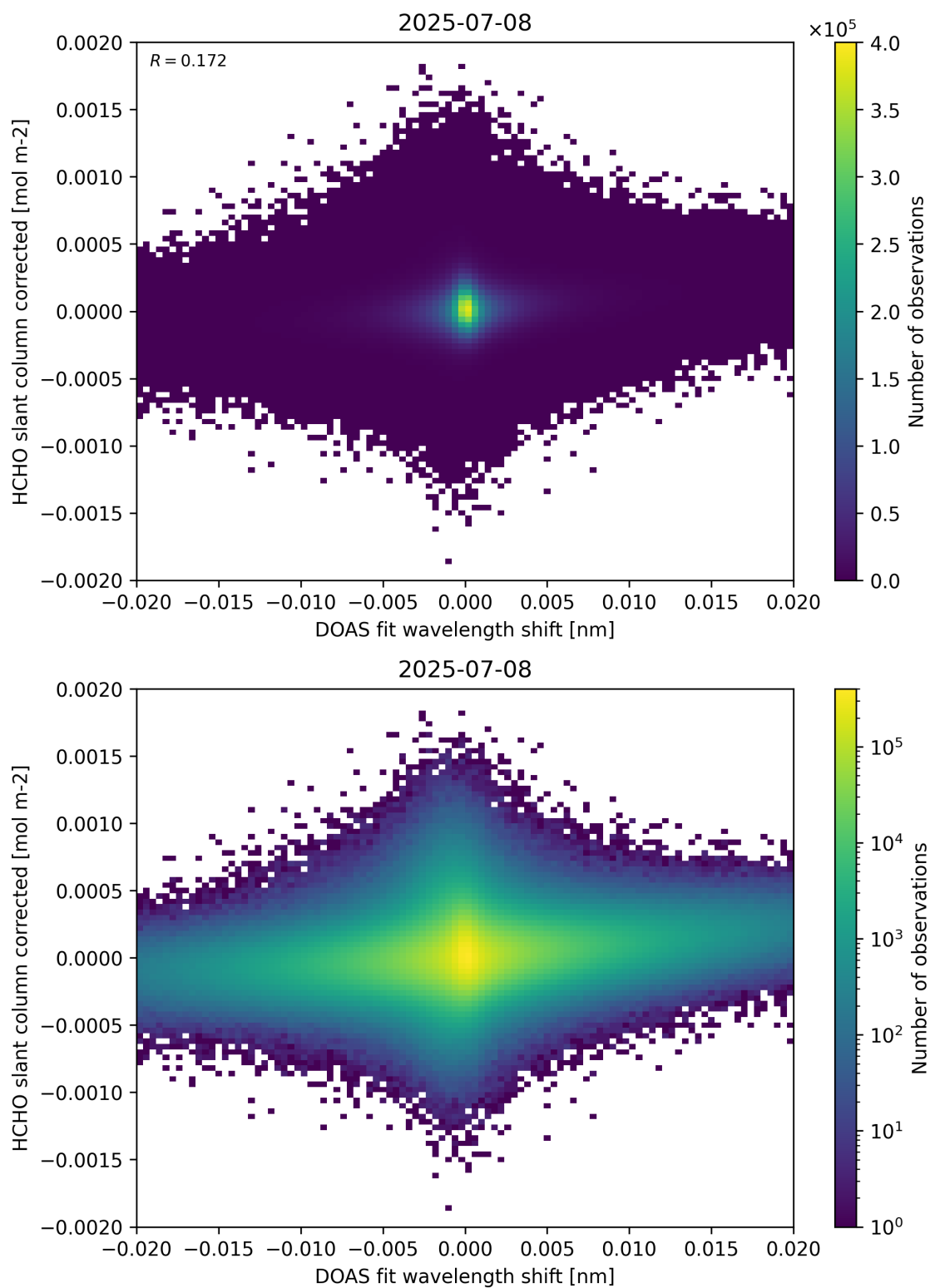
Figure 66: Scatter density plot of “DOAS fit wavelength shift” against “HCHO slant column corrected” for 2025-07-08 to 2025-07-09.
