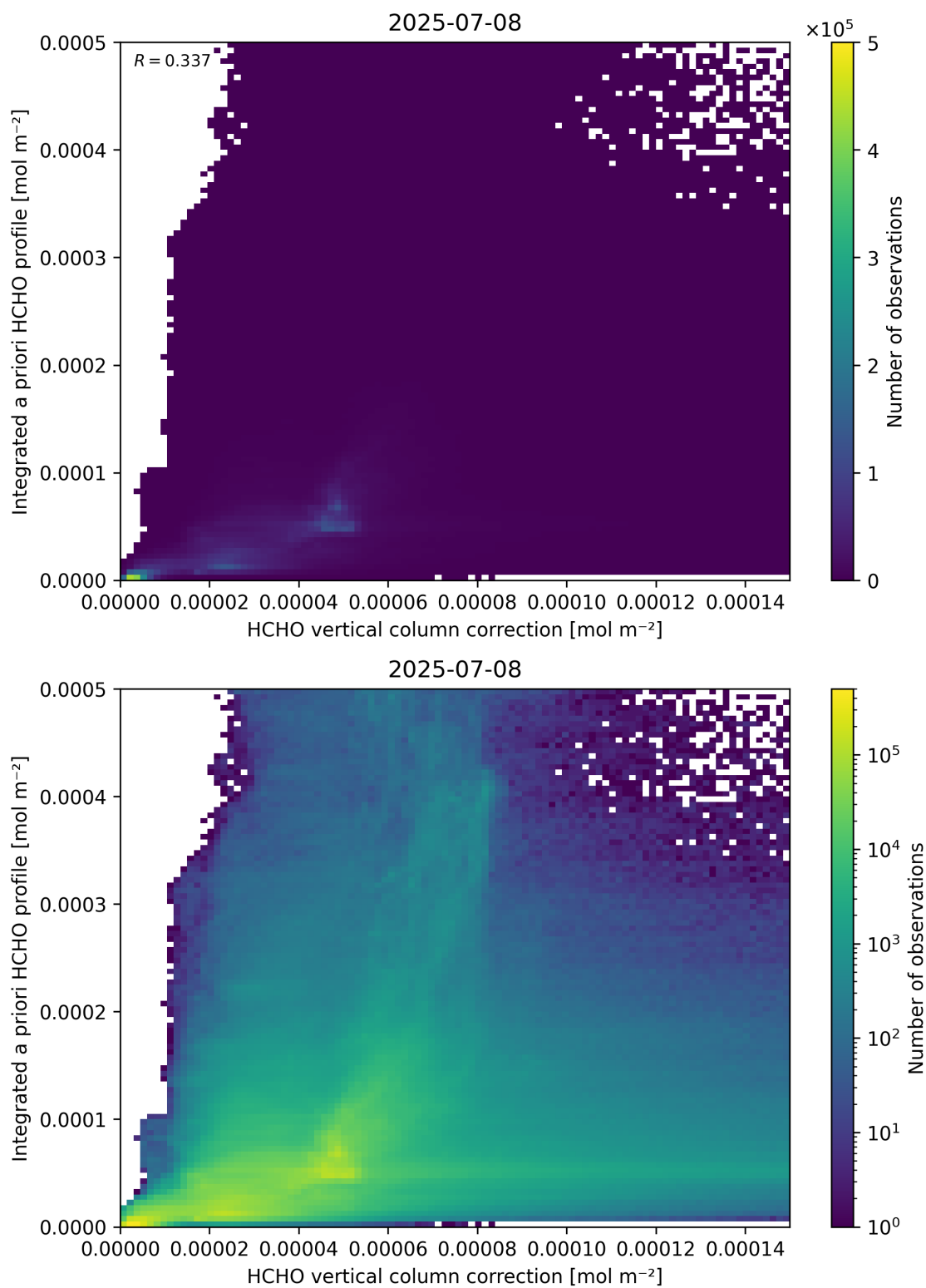
Figure 122: Scatter density plot of “HCHO vertical column correction” against “Integrated a priori HCHO profile” for 2025-07-08 to 2025-07-09.
