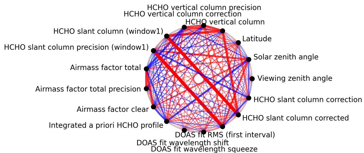
Figure 1: Map of correlation graph for 2025-07-08 to 2025-07-09.
