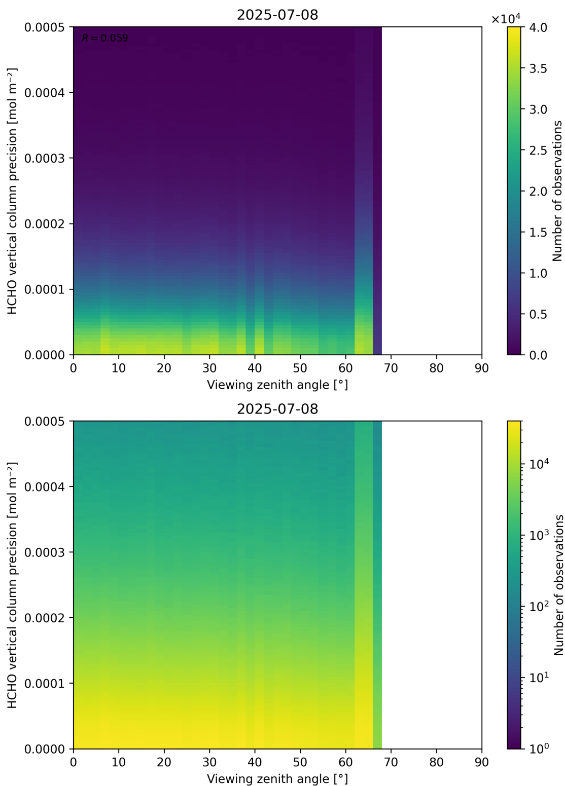
Figure 194: Scatter density plot of “Viewing zenith angle” against “HCHO vertical column precision” for 2025-07-08 to 2025-07-09.
