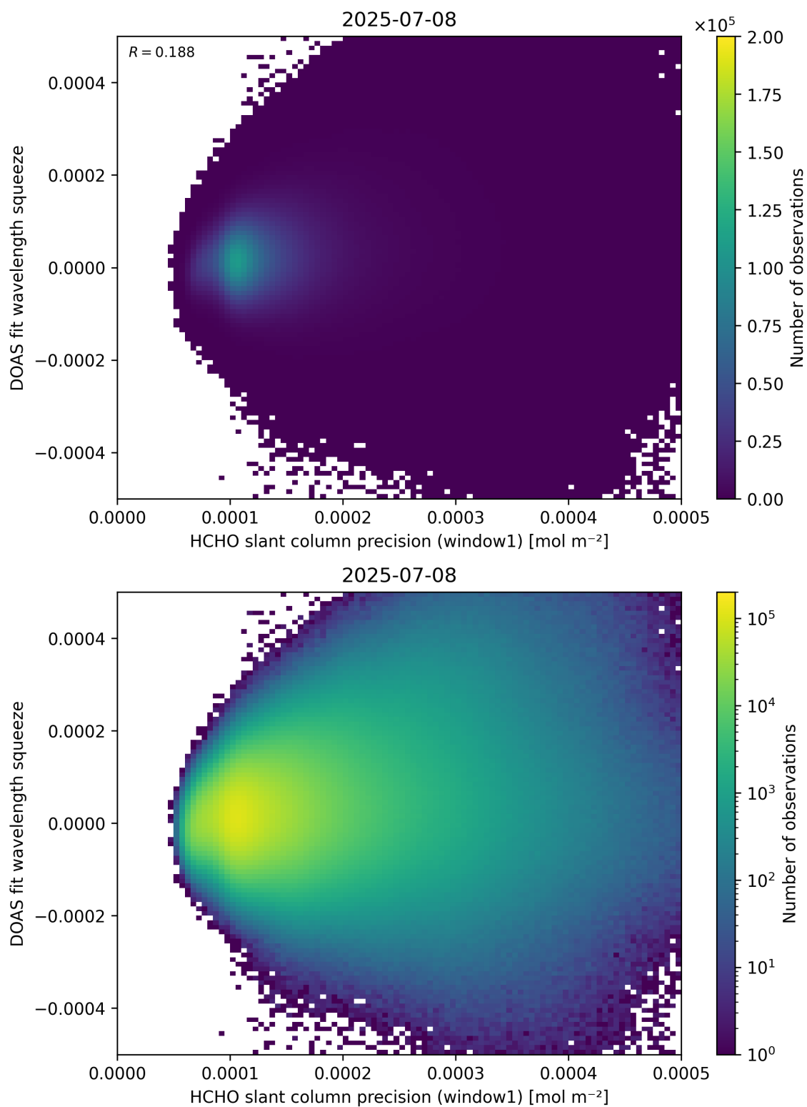
Figure 90: Scatter density plot of “HCHO slant column precision (window1)” against “DOAS fit wavelength squeeze” for 2025-07-08 to 2025-07-09.
