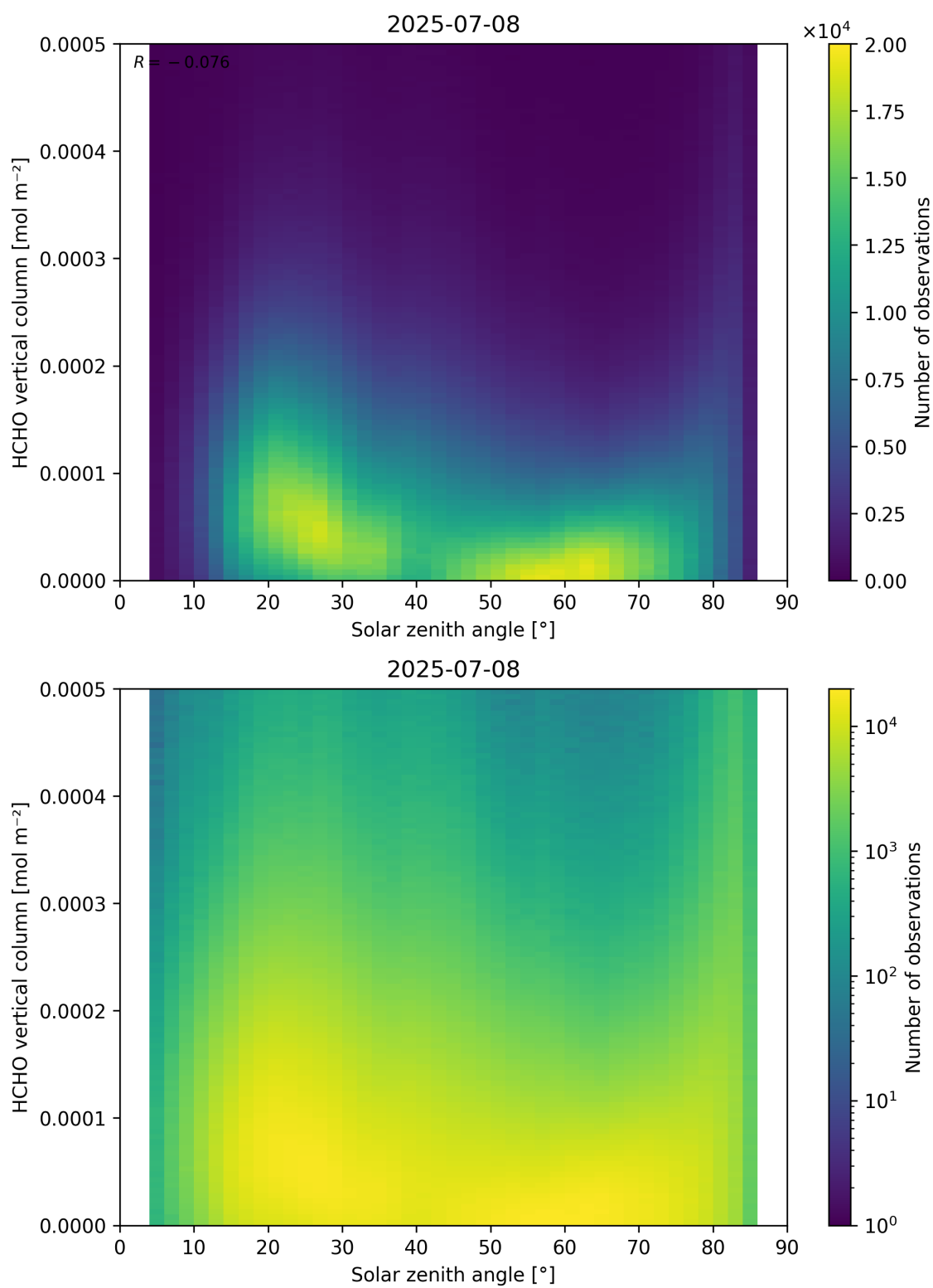
Figure 177: Scatter density plot of “Solar zenith angle” against “HCHO vertical column” for 2025-07-08 to 2025-07-09.
