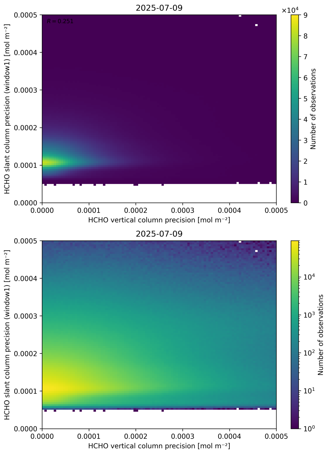
Figure 143: Scatter density plot of “HCHO vertical column precision” against “HCHO slant column precision (window1)” for 2025-07-08 to 2025-07-10.
