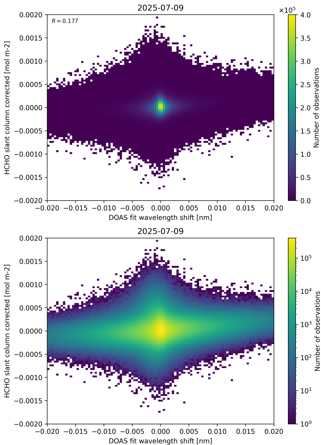
Figure 66: Scatter density plot of “DOAS fit wavelength shift” against “HCHO slant column corrected” for 2025-07-08 to 2025-07-10.
