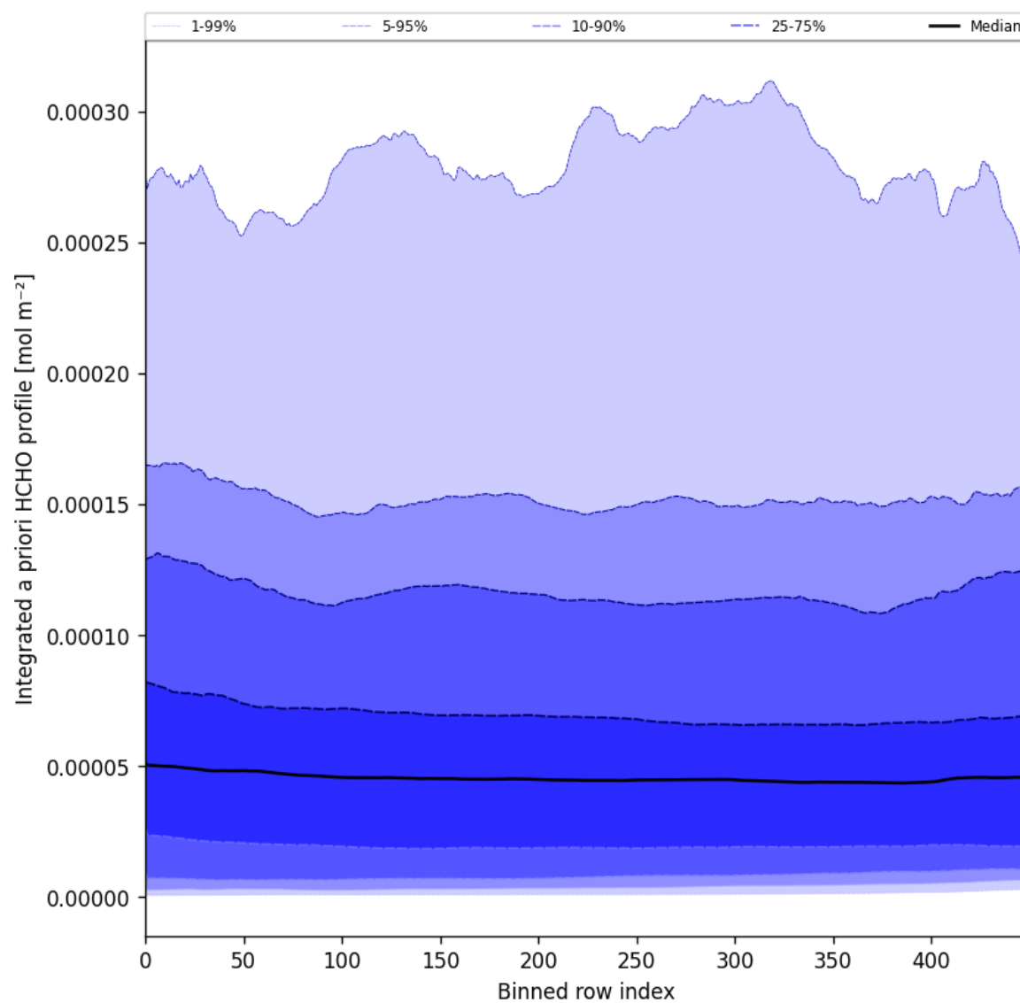
Figure 57: Along track statistics of "Integrated a priori HCHO profile" for 2025-07-08 to 2025-07-10
