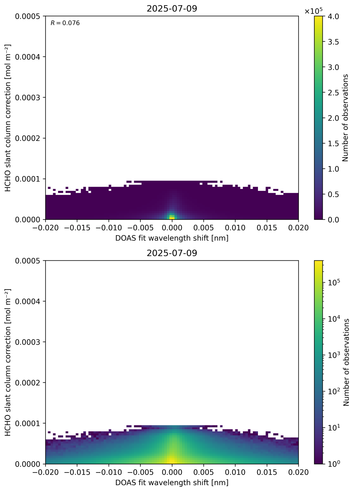
Figure 67: Scatter density plot of “DOAS fit wavelength shift” against “HCHO slant column correction” for 2025-07-08 to 2025-07-10.
