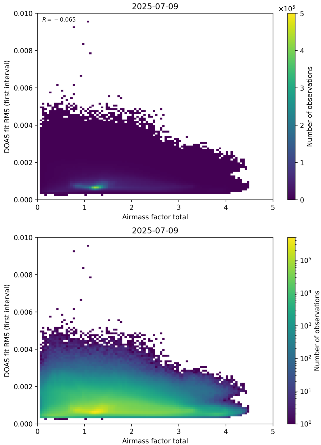
Figure 97: Scatter density plot of “Airmass factor total” against “DOAS fit RMS (first interval)” for 2025-07-08 to 2025-07-10.
