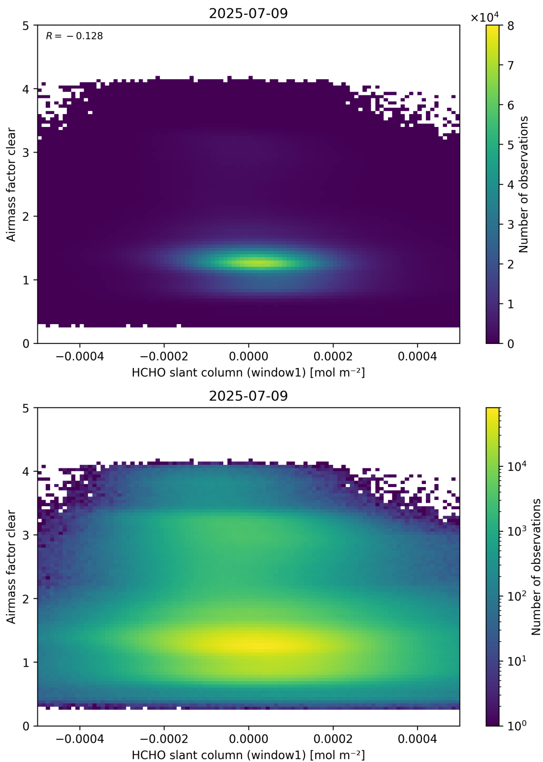
Figure 81: Scatter density plot of “HCHO slant column (window1)” against “Airmass factor clear” for 2025-07-08 to 2025-07-10.
