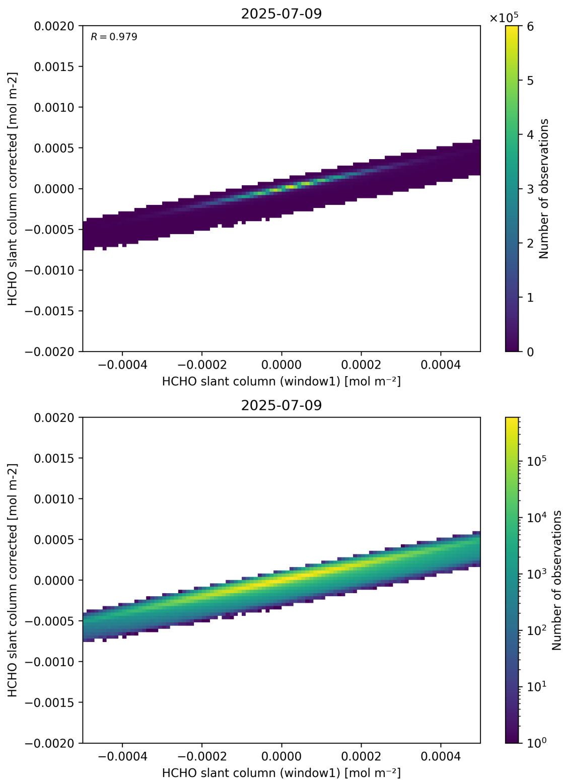
Figure 82: Scatter density plot of “HCHO slant column (window1)” against “HCHO slant column corrected” for 2025-07-08 to 2025-07-10.
