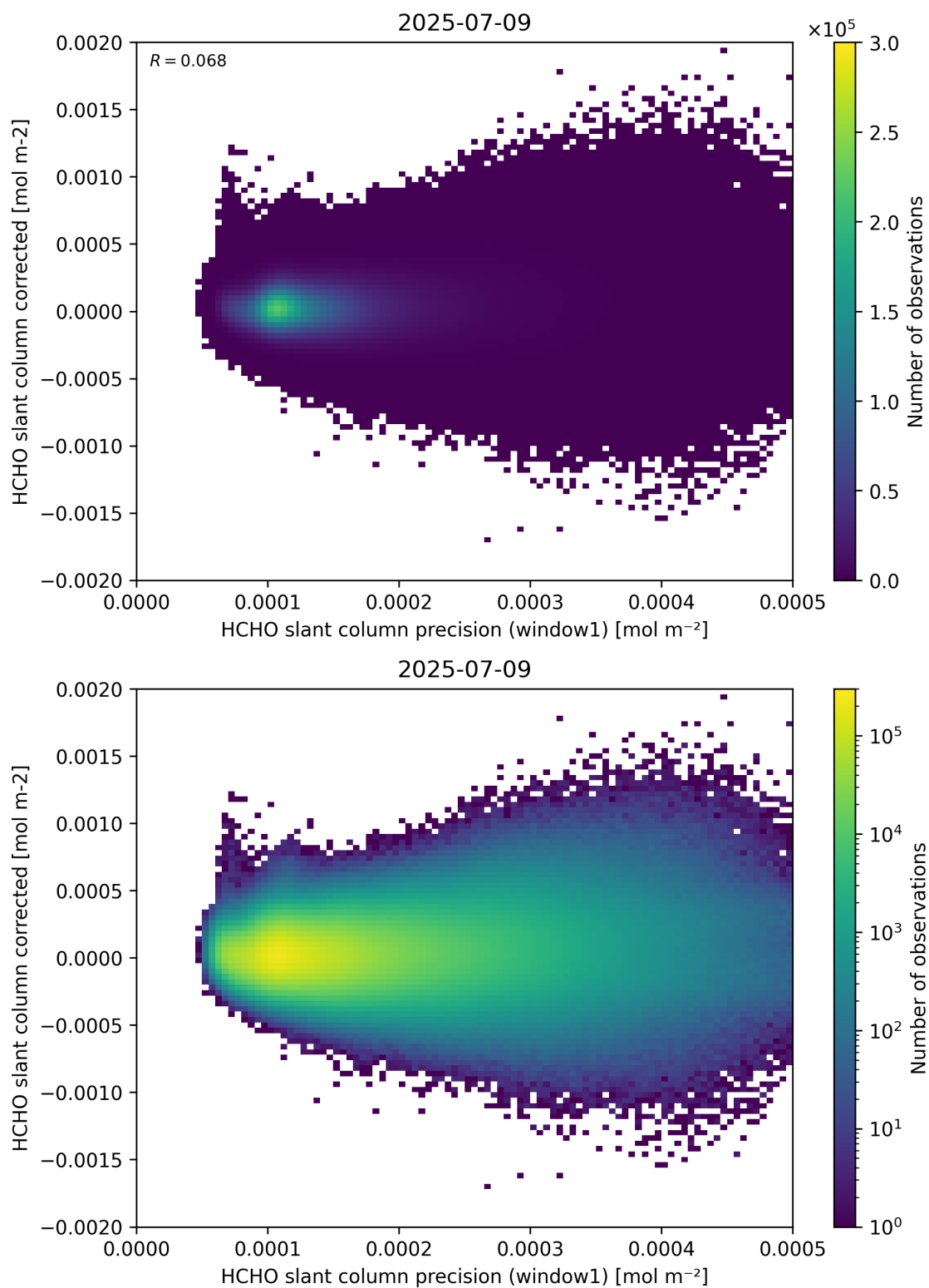
Figure 92: Scatter density plot of “HCHO slant column precision (window1)” against “HCHO slant column corrected” for 2025-07-08 to 2025-07-10.
