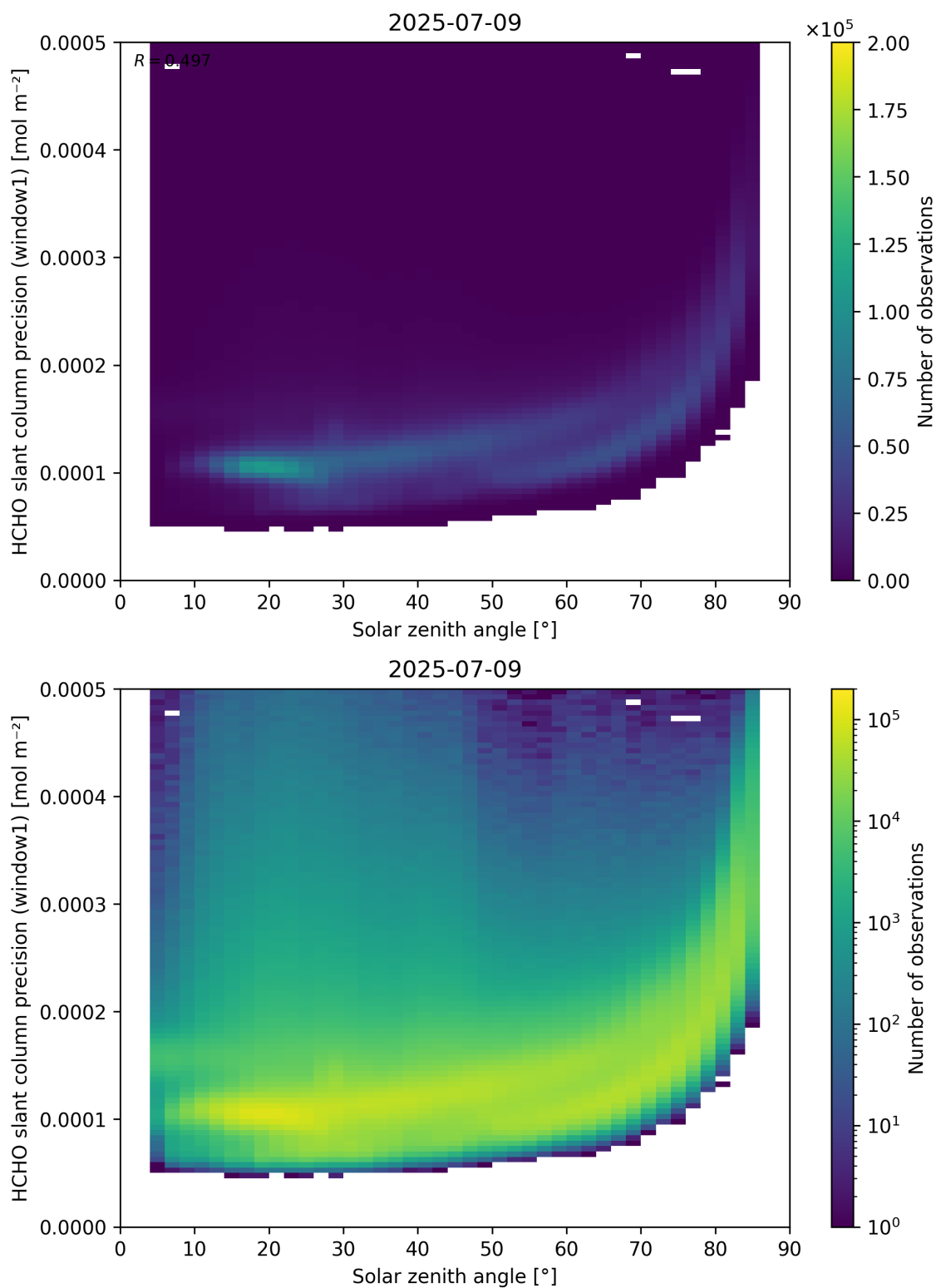
Figure 174: Scatter density plot of “Solar zenith angle” against “HCHO slant column precision (window1)” for 2025-07-08 to 2025-07-10.
