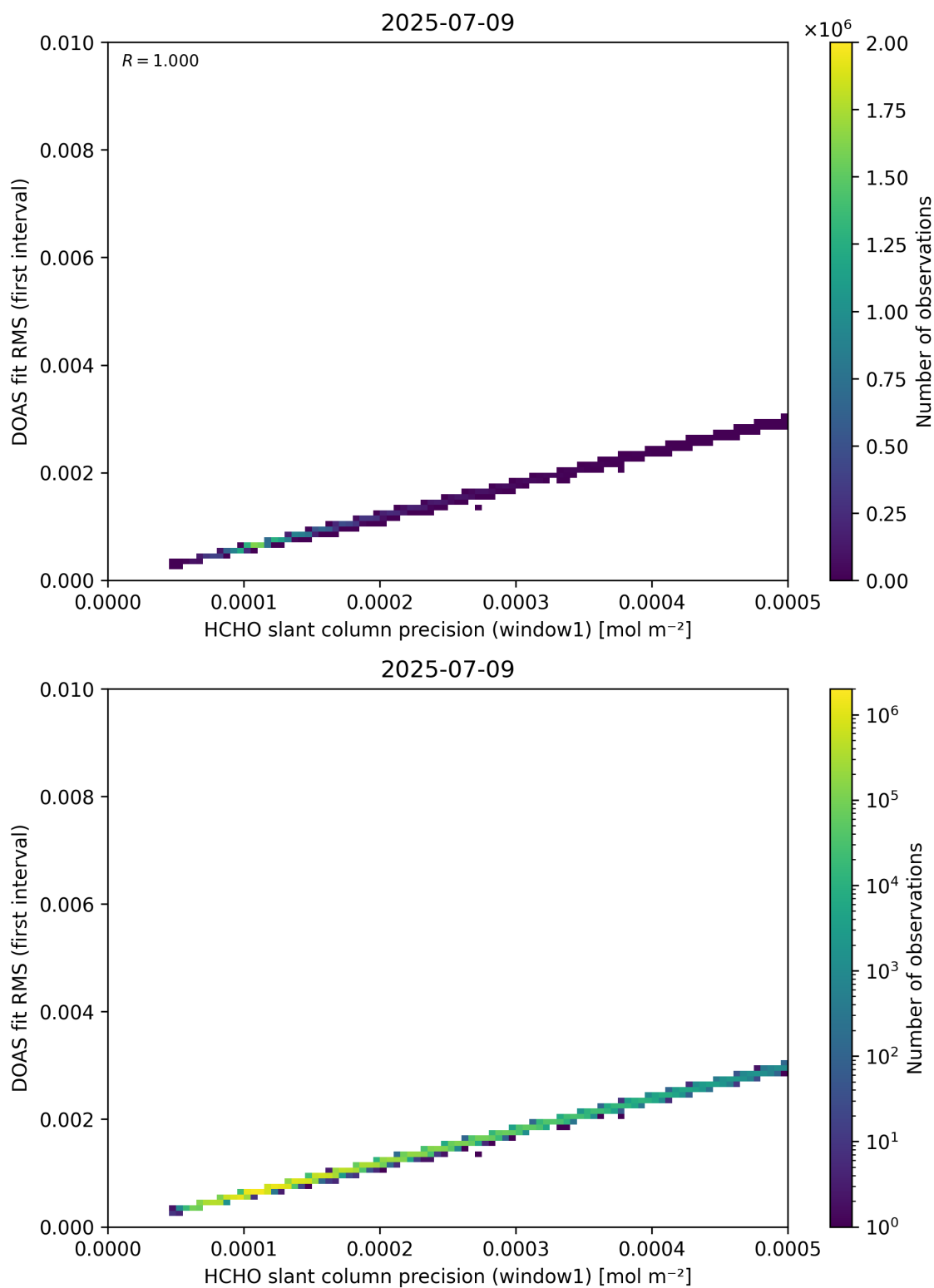
Figure 88: Scatter density plot of “HCHO slant column precision (window1)” against “DOAS fit RMS (first interval)” for 2025-07-08 to 2025-07-10.
