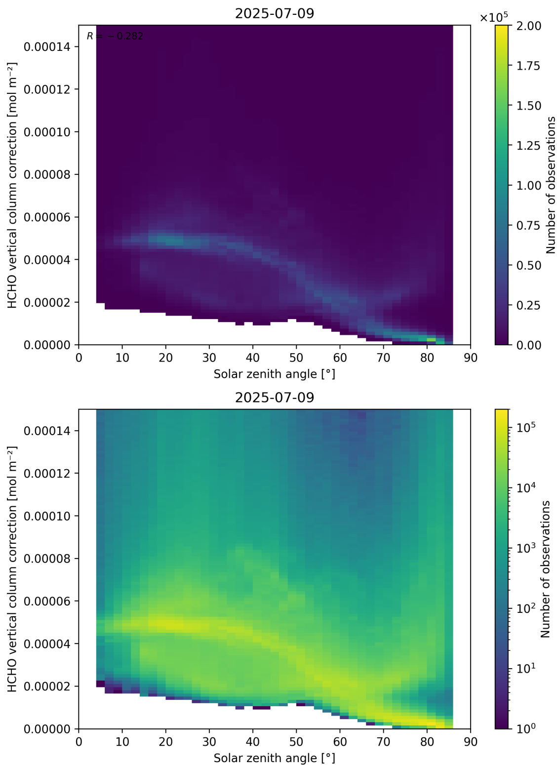
Figure 178: Scatter density plot of “Solar zenith angle” against “HCHO vertical column correction” for 2025-07-08 to 2025-07-10.
