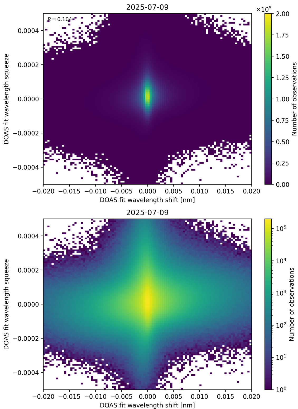
Figure 65: Scatter density plot of “DOAS fit wavelength shift” against “DOAS fit wavelength squeeze” for 2025-07-08 to 2025-07-10.
