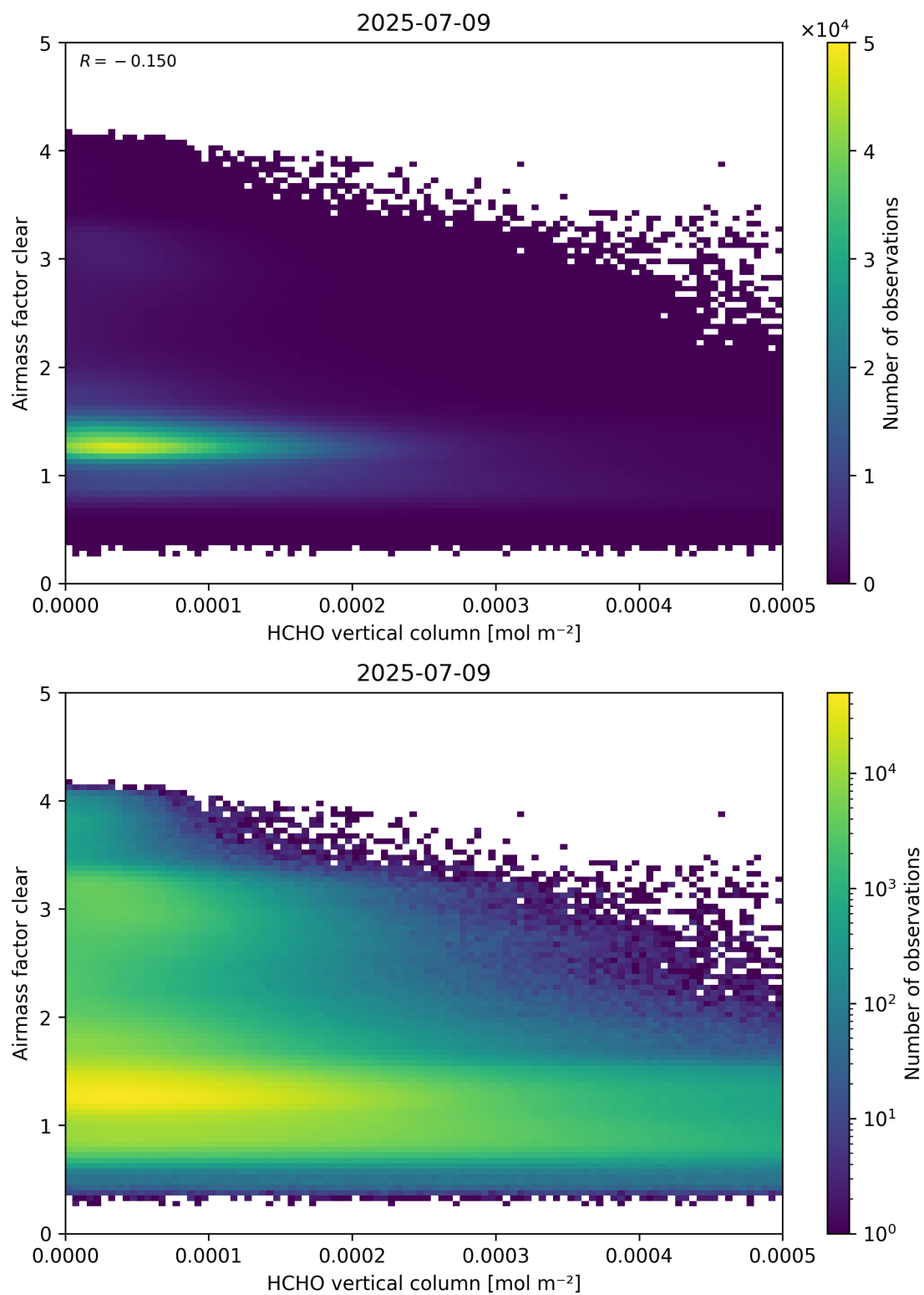
Figure 126: Scatter density plot of “HCHO vertical column” against “Airmass factor clear” for 2025-07-08 to 2025-07-10.
