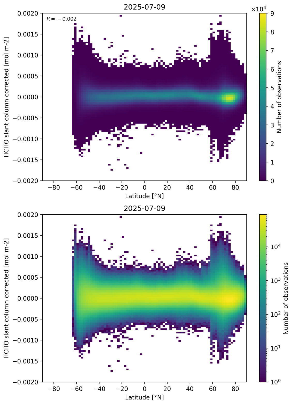
Figure 157: Scatter density plot of “Latitude” against “HCHO slant column corrected” for 2025-07-08 to 2025-07-10.
