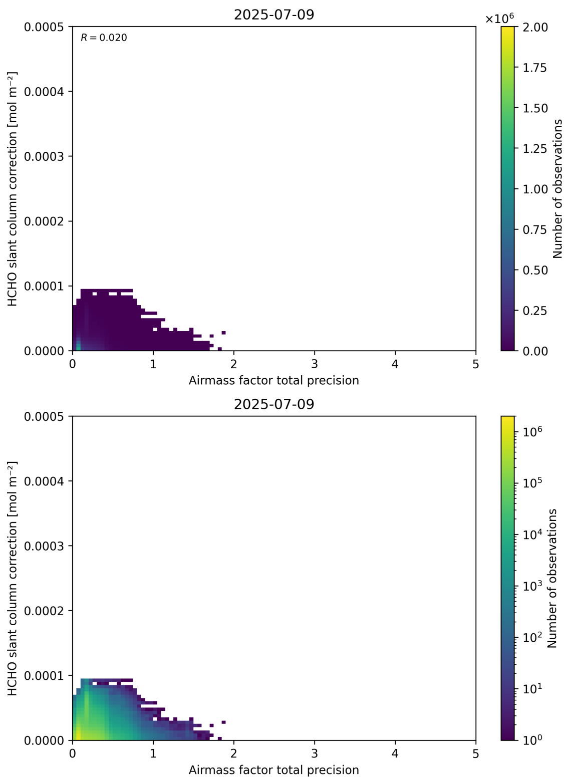
Figure 110: Scatter density plot of “Airmass factor total precision” against “HCHO slant column correction” for 2025-07-08 to 2025-07-10.
