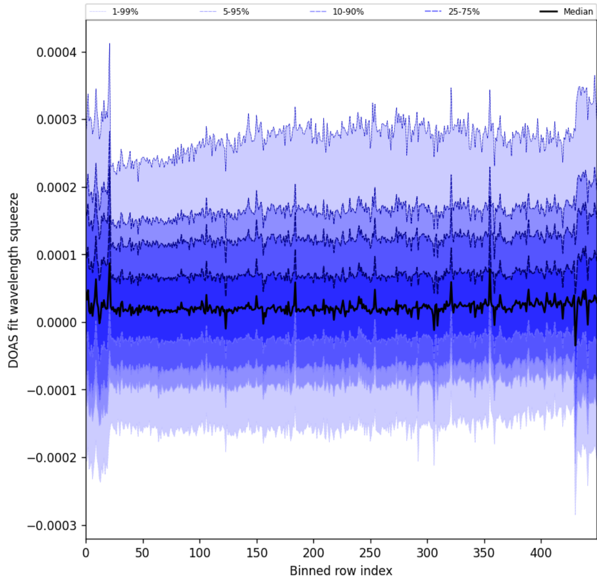
Figure 59: Along track statistics of “DOAS fit wavelength squeeze” for 2025-07-08 to 2025-07-10
