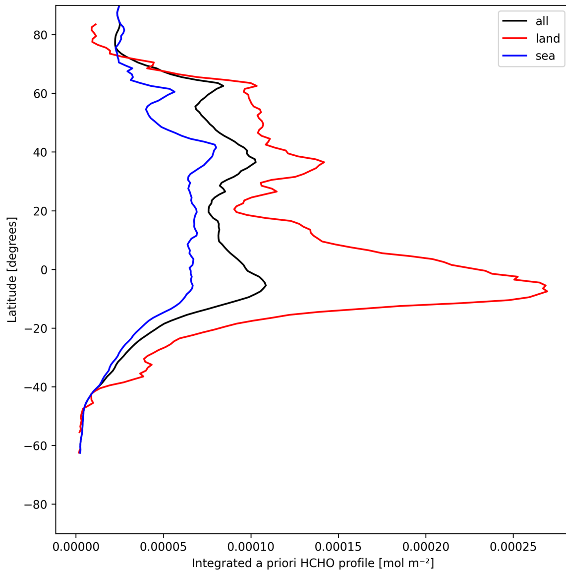
Figure 29: Zonal average of “Integrated a priori HCHO profile” for 2025-07-08 to 2025-07-10.
