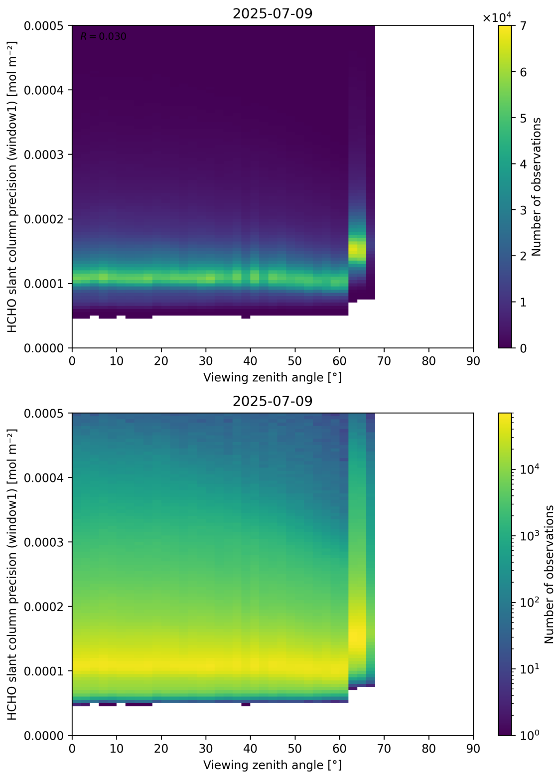
Figure 189: Scatter density plot of “Viewing zenith angle” against “HCHO slant column precision (window1)” for 2025-07-08 to 2025-07-10.
