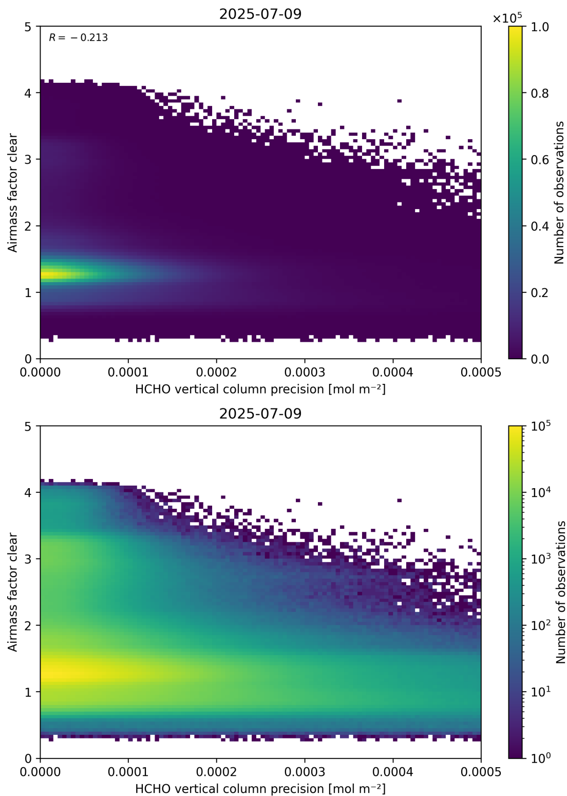
Figure 139: Scatter density plot of “HCHO vertical column precision” against “Airmass factor clear” for 2025-07-08 to 2025-07-10.
