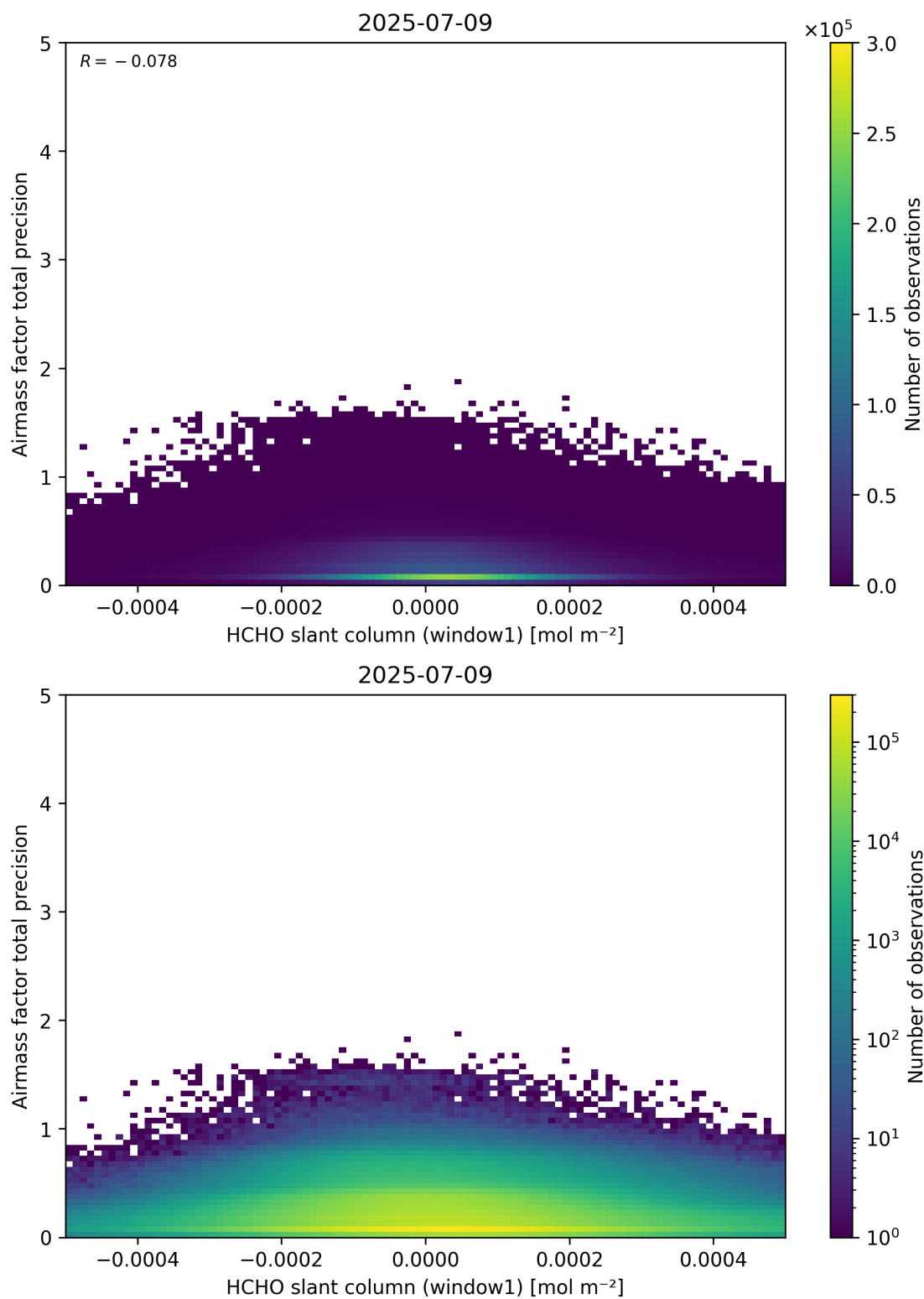
Figure 86: Scatter density plot of “HCHO slant column (window1)” against “Airmass factor total precision” for 2025-07-08 to 2025-07-10.
