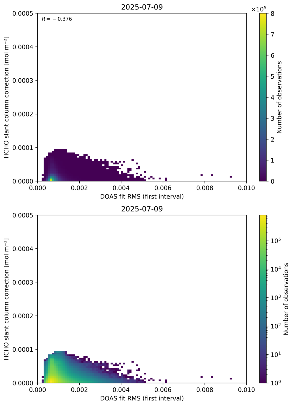
Figure 63: Scatter density plot of “DOAS fit RMS (first interval)” against “HCHO slant column correction” for 2025-07-08 to 2025-07-10.
