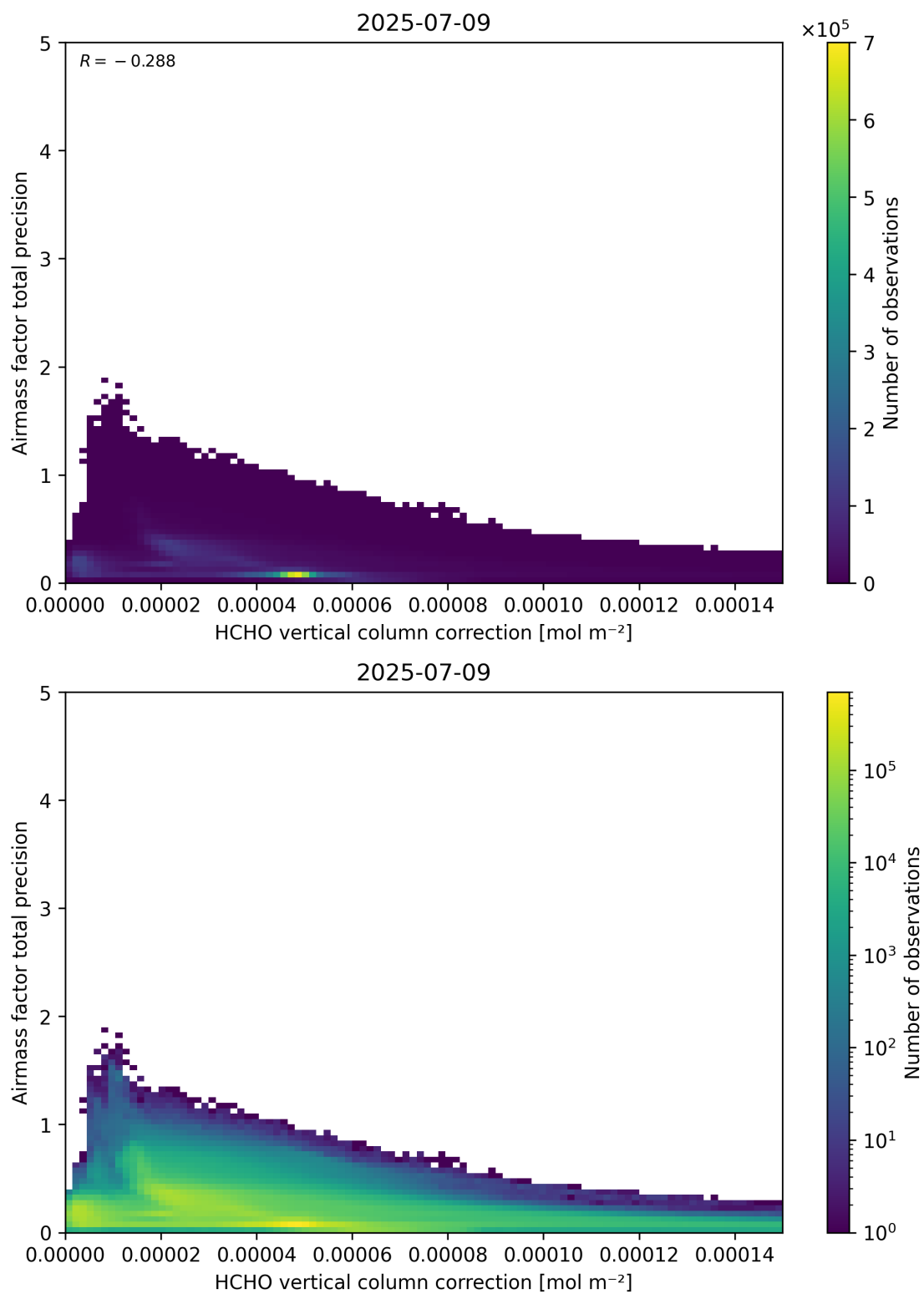
Figure 121: Scatter density plot of “HCHO vertical column correction” against “Airmass factor total precision” for 2025-07-08 to 2025-07-10.
