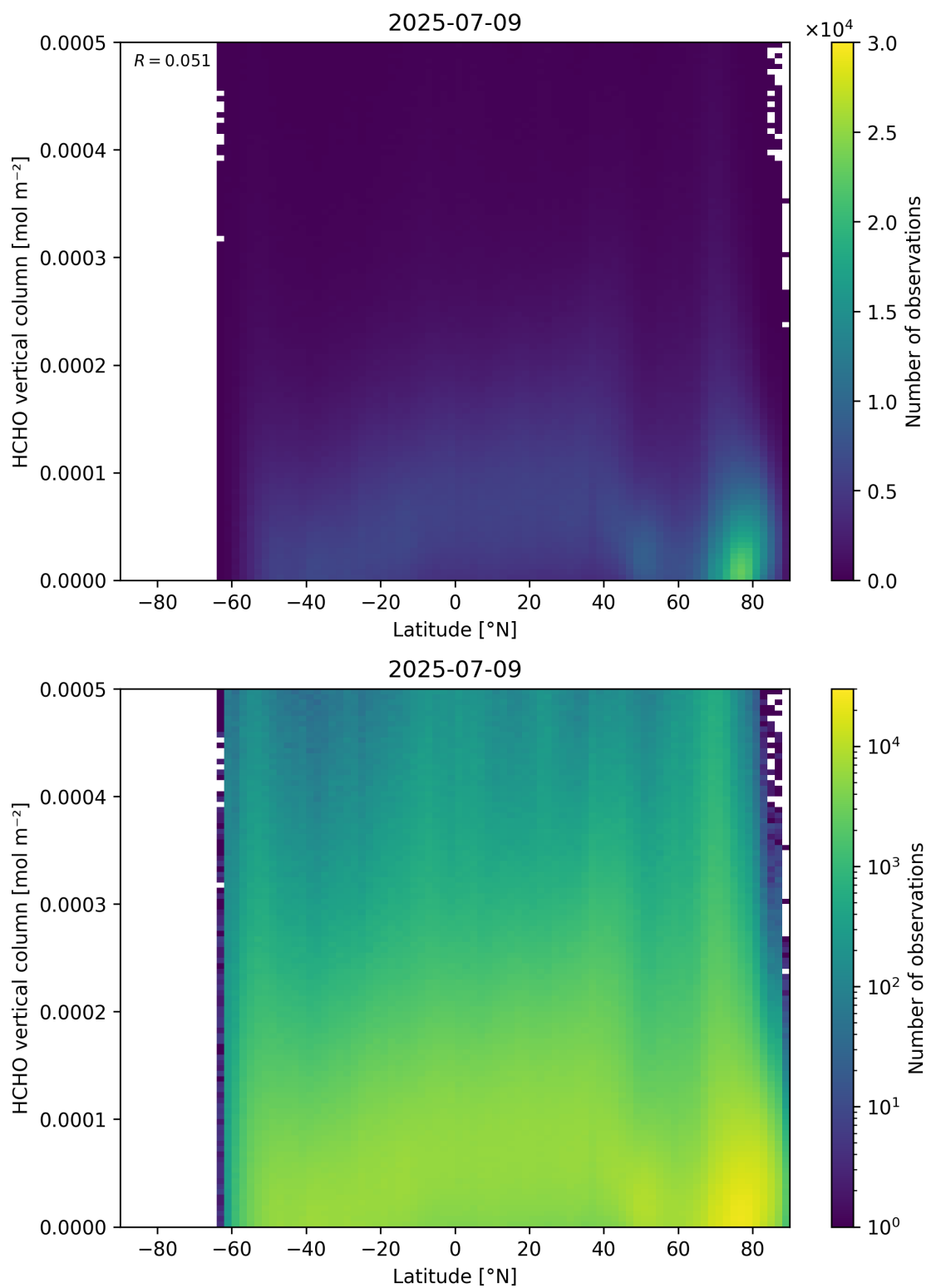
Figure 163: Scatter density plot of “Latitude” against “HCHO vertical column” for 2025-07-08 to 2025-07-10.
