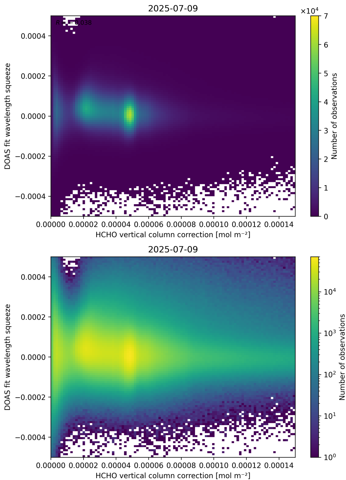
Figure 114: Scatter density plot of “HCHO vertical column correction” against “DOAS fit wavelength squeeze” for 2025-07-08 to 2025-07-10.
