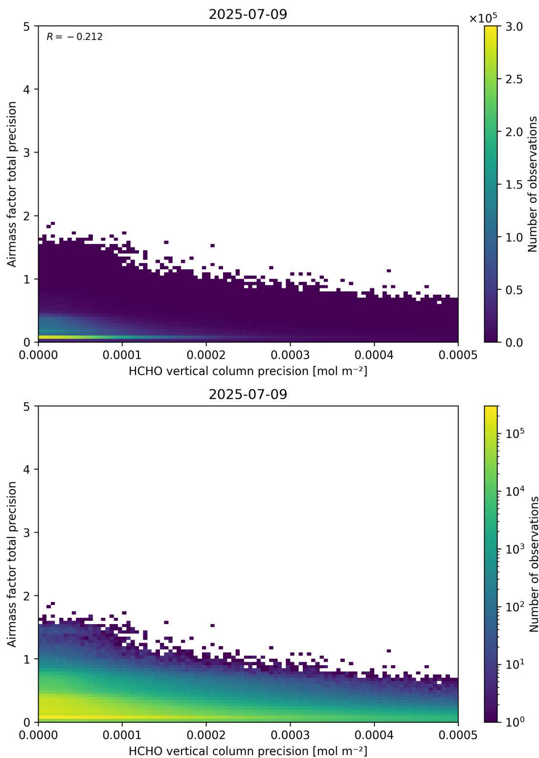
Figure 145: Scatter density plot of “HCHO vertical column precision” against “Airmass factor total precision” for 2025-07-08 to 2025-07-10.
