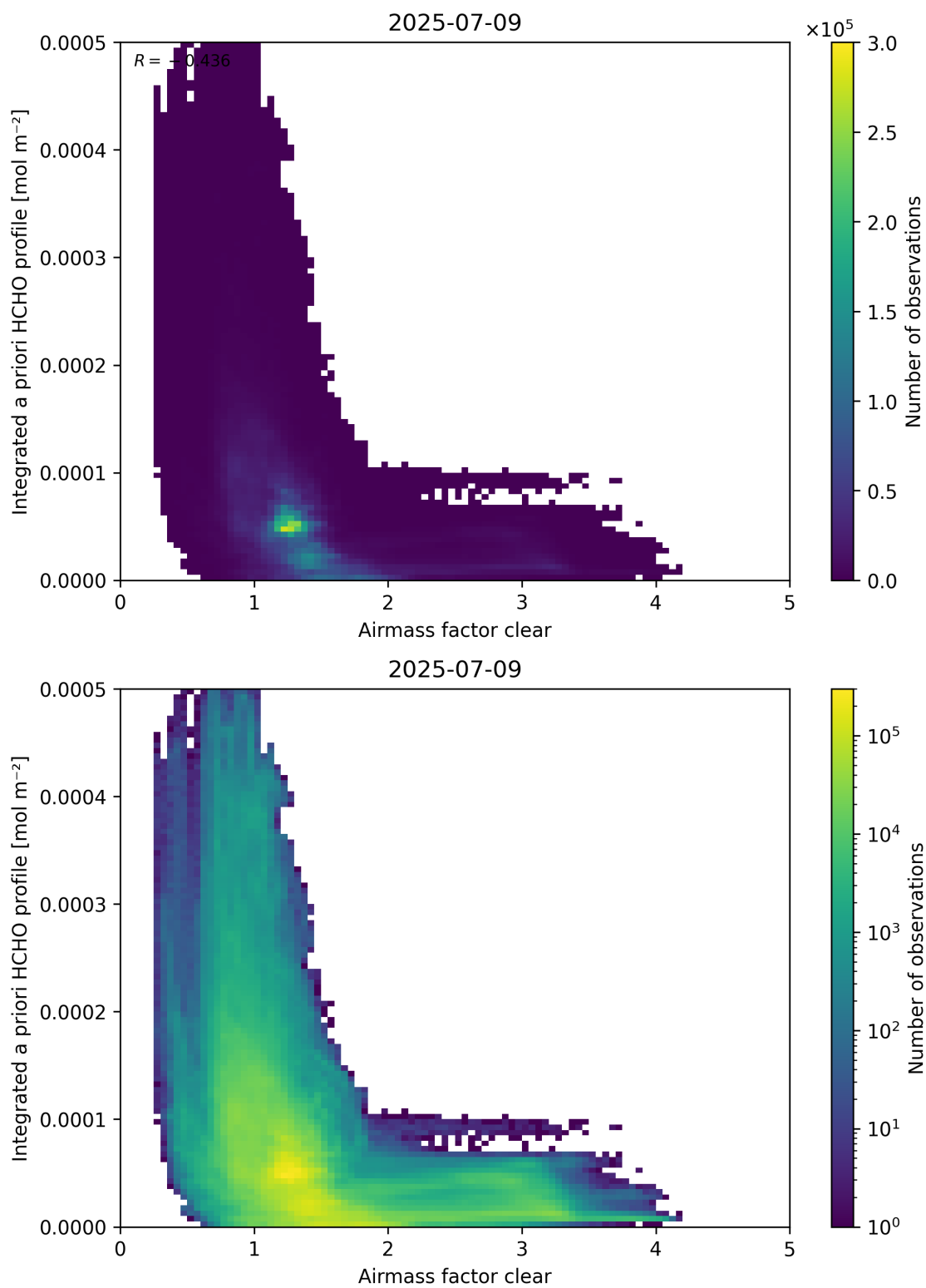
Figure 76: Scatter density plot of “Airmass factor clear” against “Integrated a priori HCHO profile” for 2025-07-08 to 2025-07-10.
