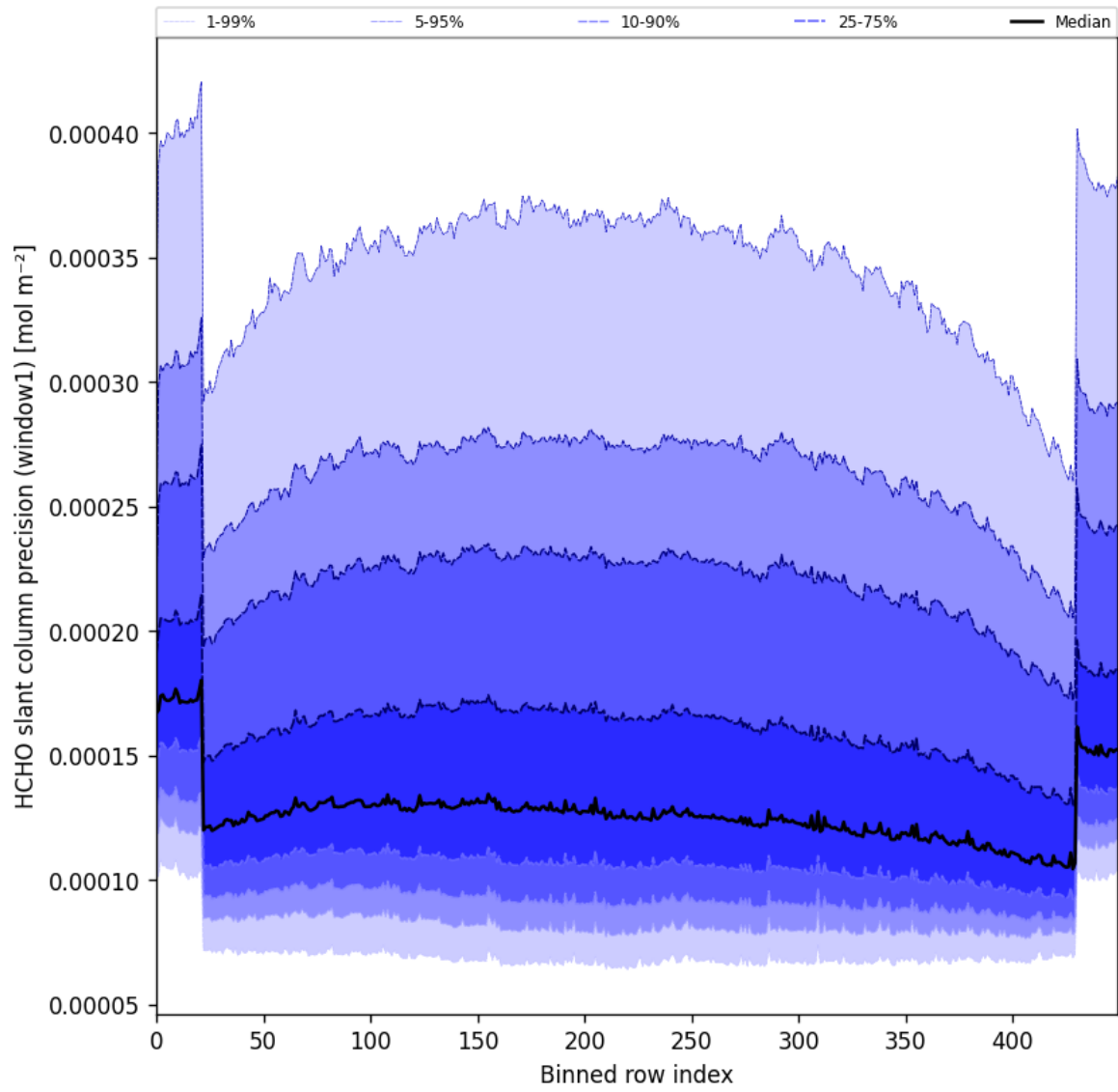
Figure 53: Along track statistics of “HCHO slant column precision (window1)” for 2025-07-08 to 2025-07-10
