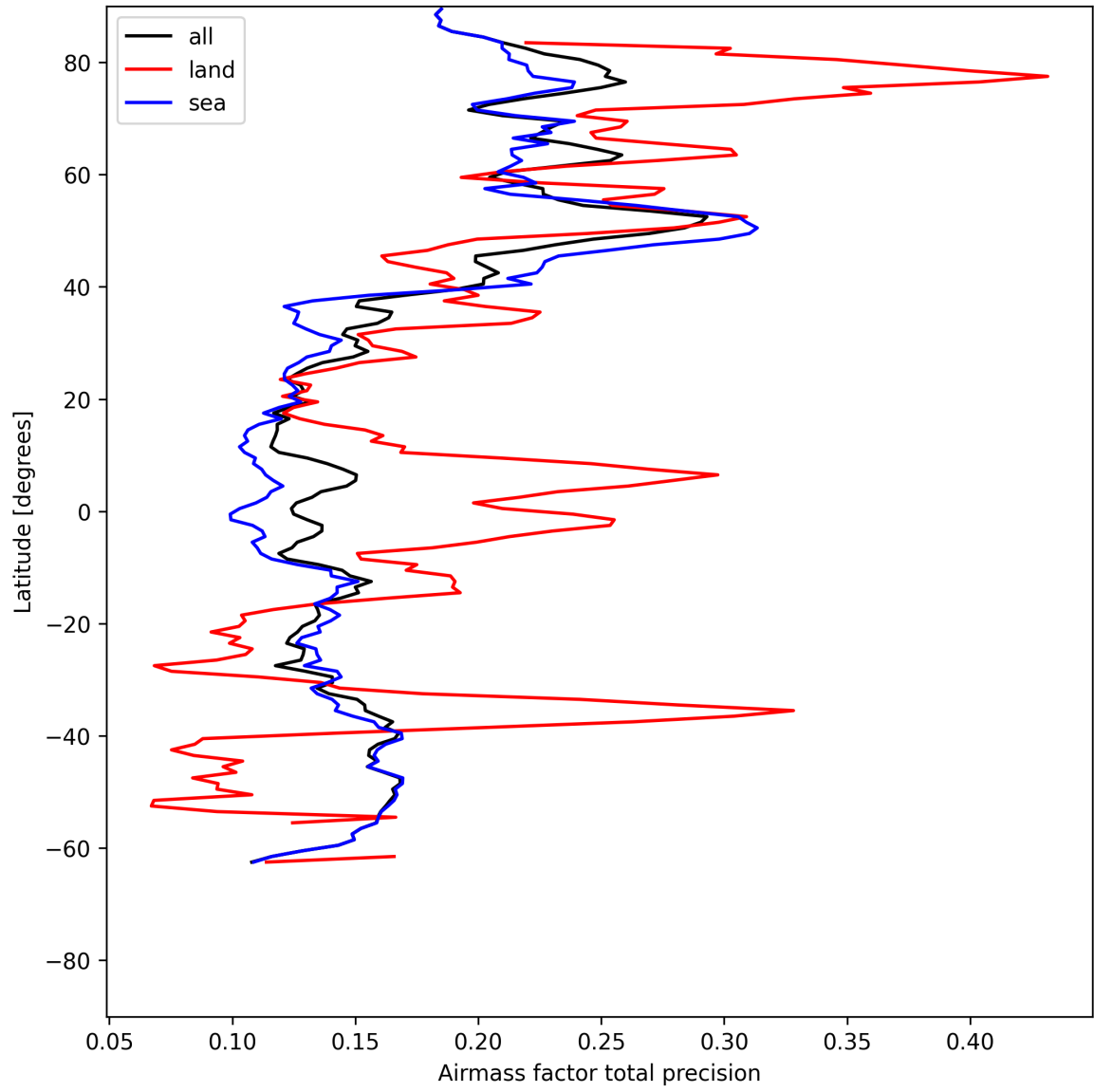
Figure 27: Zonal average of “Airmass factor total precision” for 2025-07-08 to 2025-07-10.
