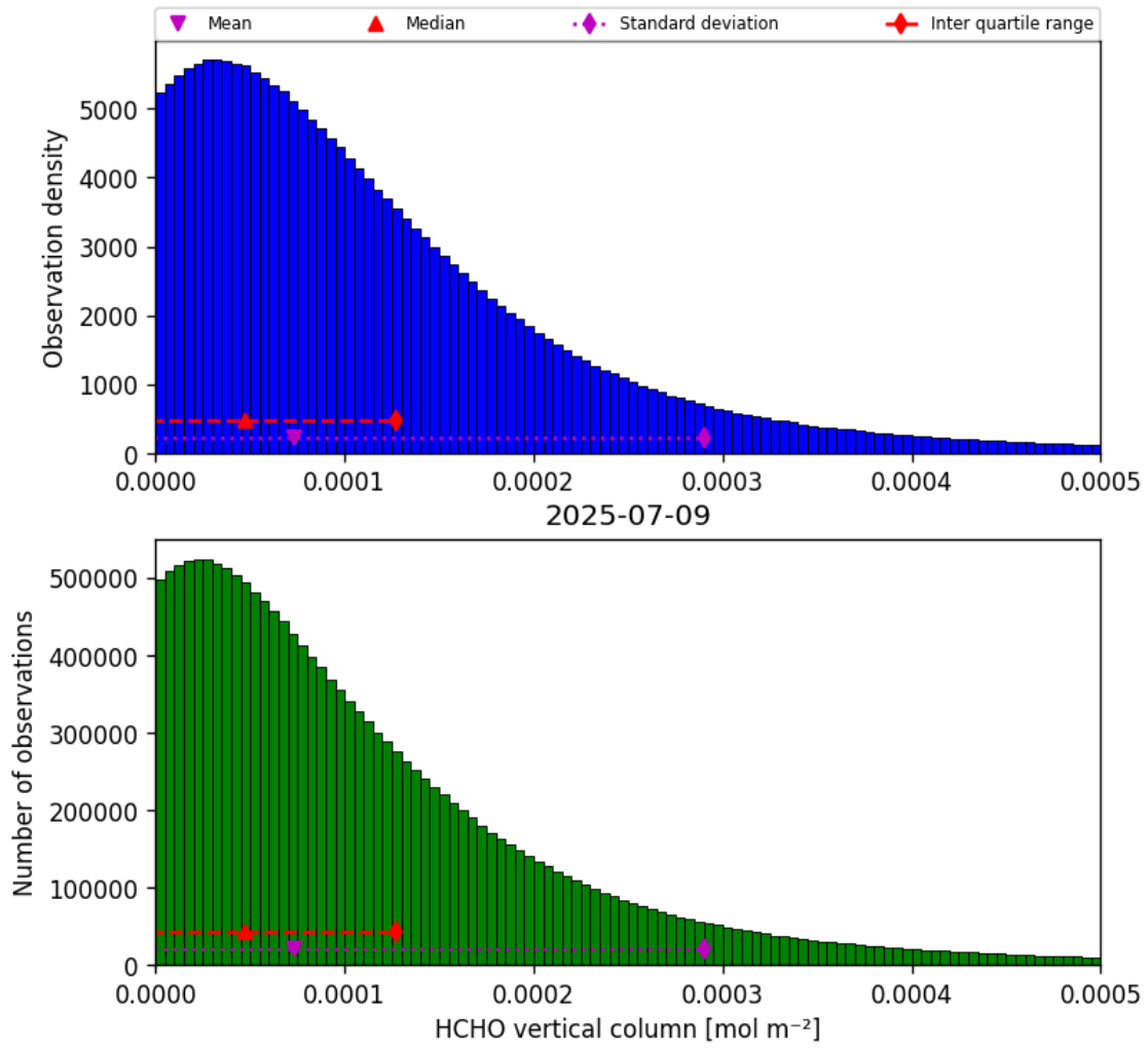
Figure 35: Histogram of “HCHO vertical column” for 2025-07-08 to 2025-07-10
