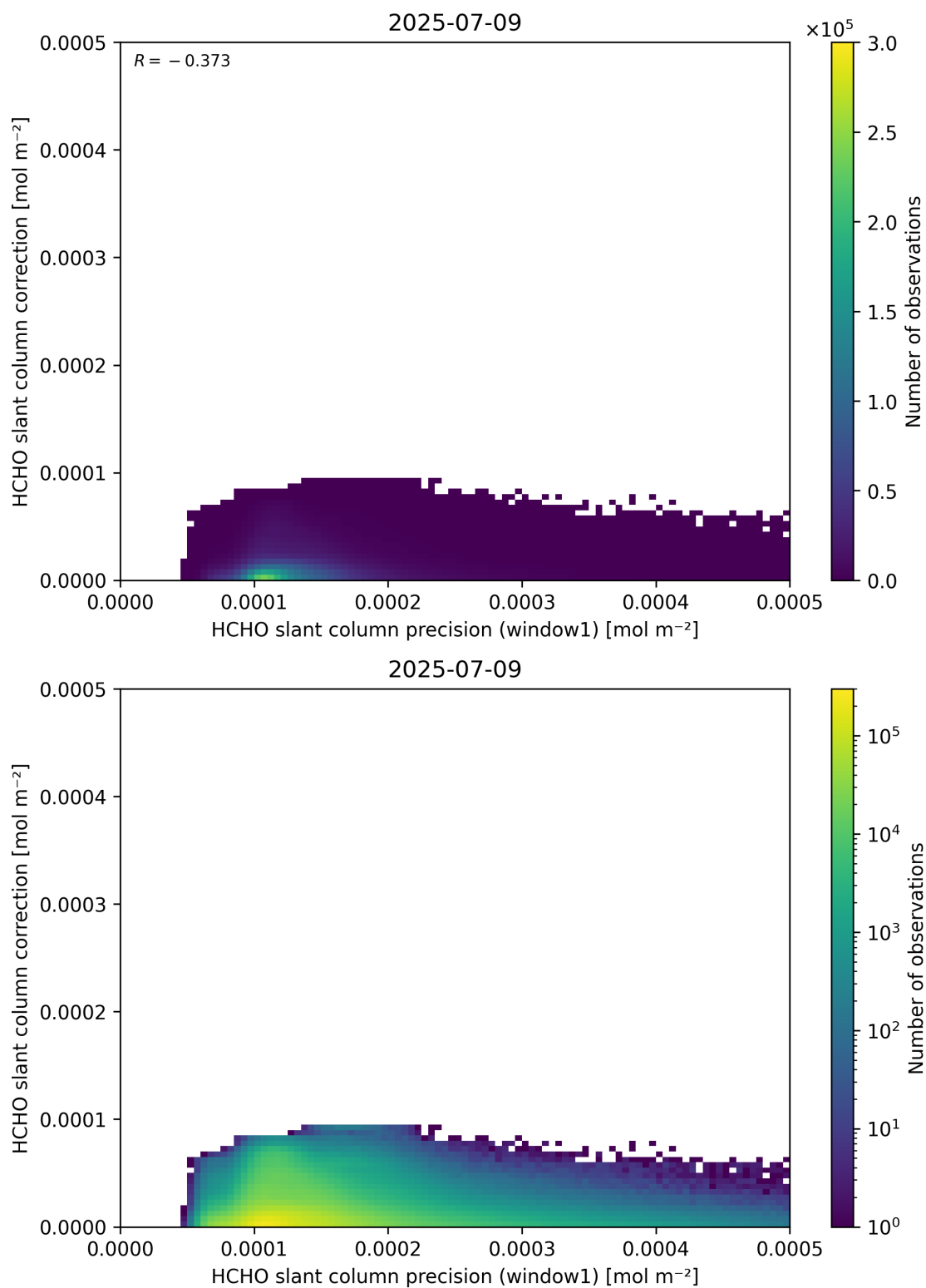
Figure 93: Scatter density plot of “HCHO slant column precision (window1)” against “HCHO slant column correction” for 2025-07-08 to 2025-07-10.
