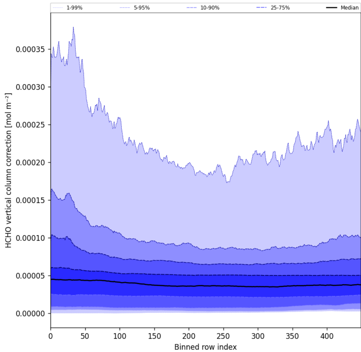
Figure 51: Along track statistics of “HCHO vertical column correction” for 2025-07-08 to 2025-07-10
