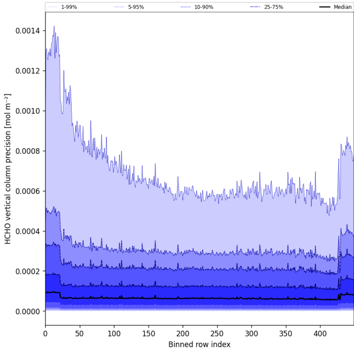
Figure 50: Along track statistics of “HCHO vertical column precision” for 2025-07-08 to 2025-07-10
