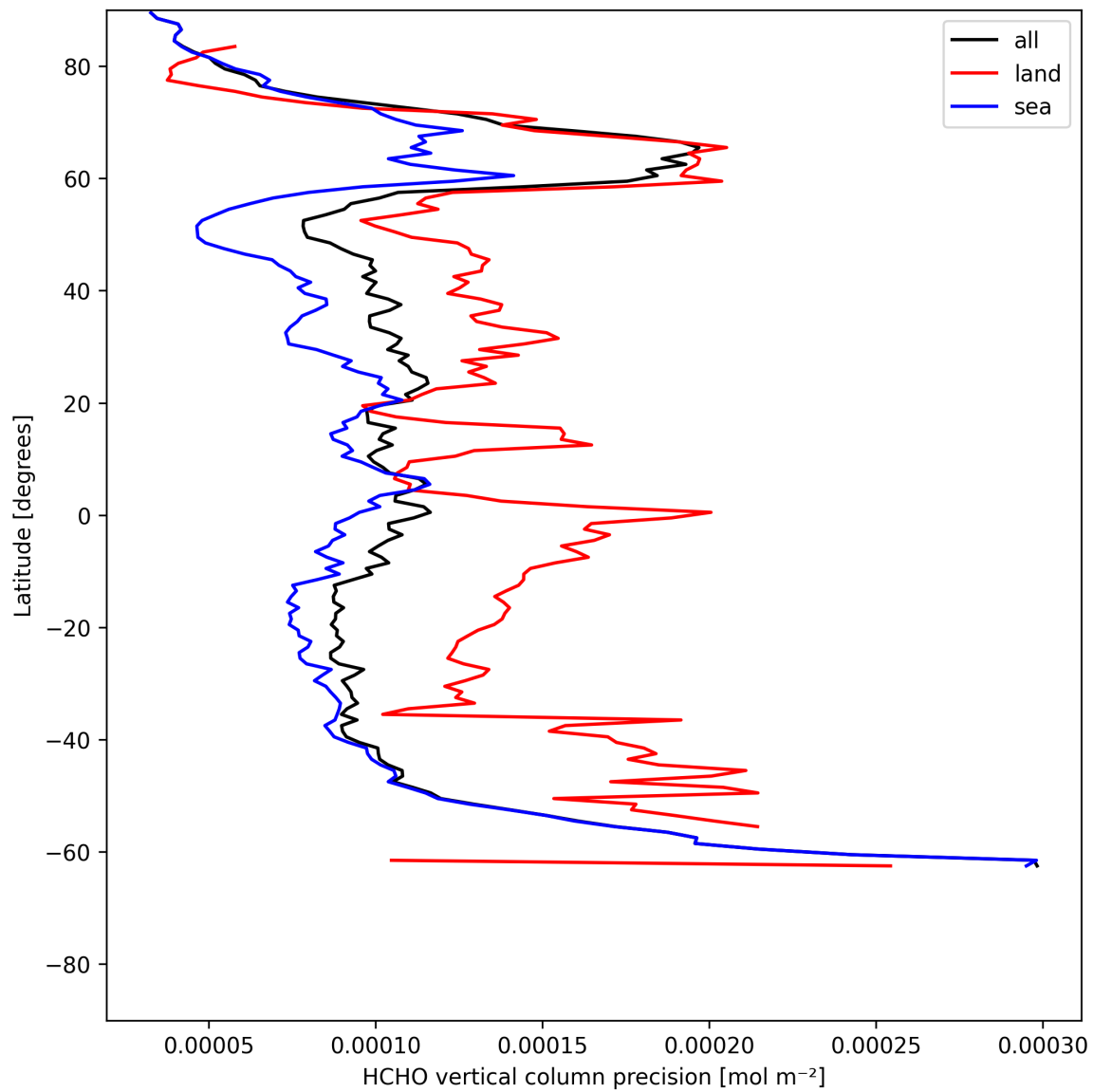
Figure 22: Zonal average of “HCHO vertical column precision” for 2025-07-08 to 2025-07-10.
