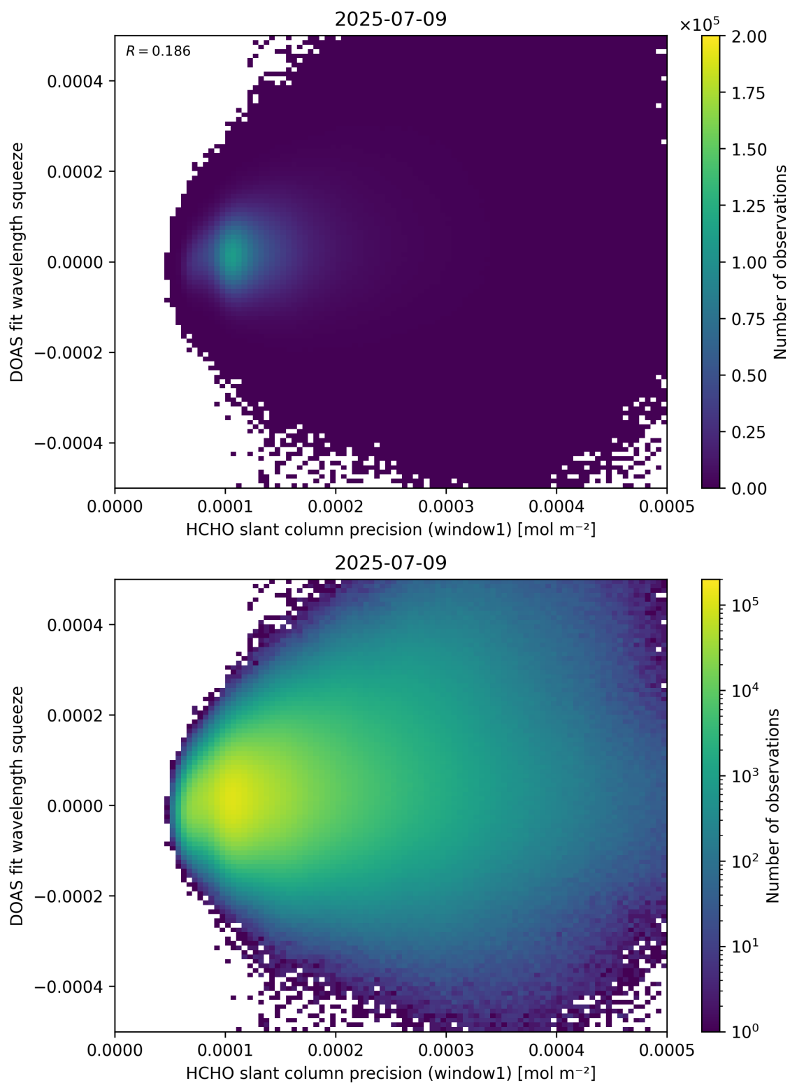
Figure 90: Scatter density plot of “HCHO slant column precision (window1)” against “DOAS fit wavelength squeeze” for 2025-07-08 to 2025-07-10.
