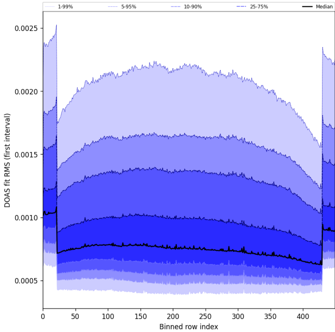
Figure 60: Along track statistics of “DOAS fit RMS (first interval)” for 2025-07-08 to 2025-07-10
