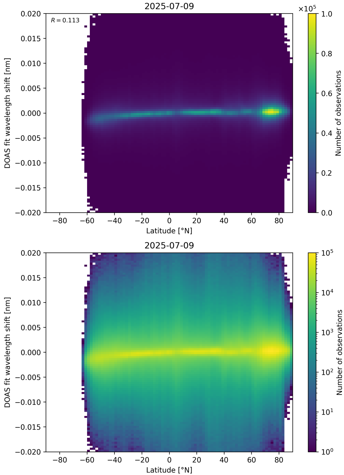
Figure 154: Scatter density plot of “Latitude” against “DOAS fit wavelength shift” for 2025-07-08 to 2025-07-10.
