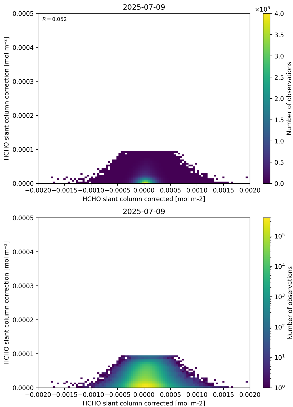
Figure 77: Scatter density plot of “HCHO slant column corrected” against “HCHO slant column correction” for 2025-07-08 to 2025-07-10.
