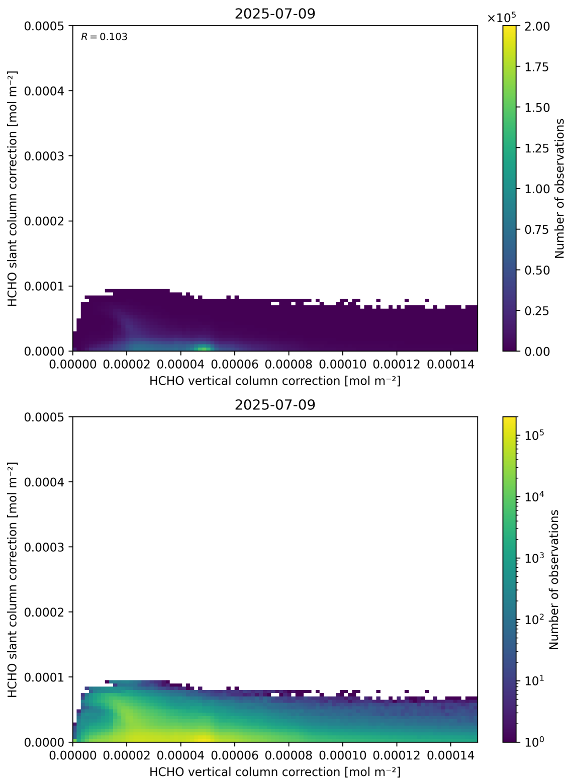
Figure 117: Scatter density plot of “HCHO vertical column correction” against “HCHO slant column correction” for 2025-07-08 to 2025-07-10.
