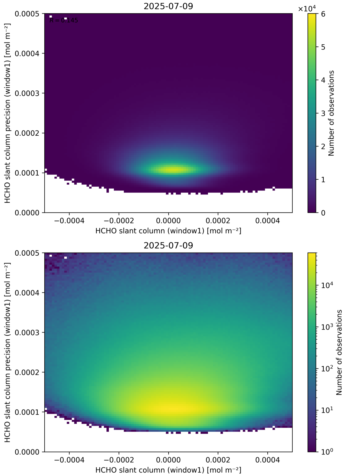
Figure 84: Scatter density plot of “HCHO slant column (window1)” against “HCHO slant column precision (window1)” for 2025-07-08 to 2025-07-10.
