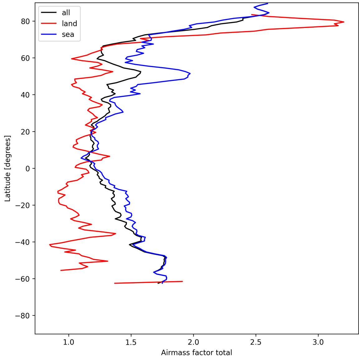
Figure 26: Zonal average of “Airmass factor total” for 2025-07-08 to 2025-07-10.
