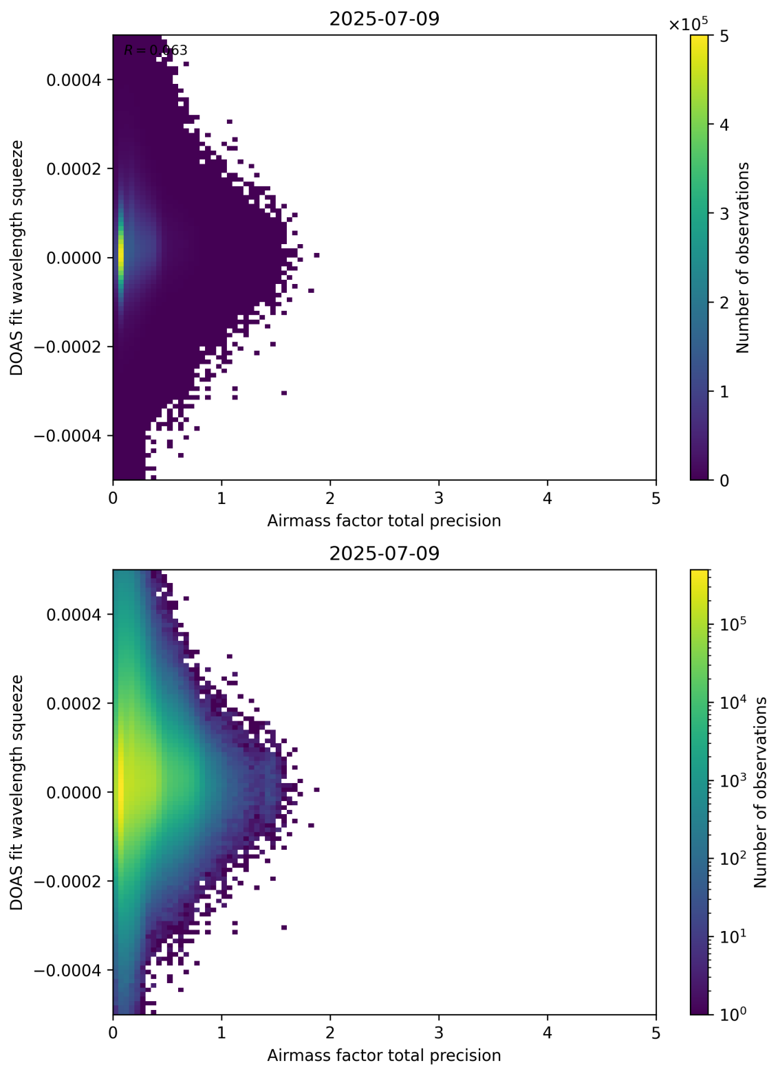
Figure 107: Scatter density plot of “Airmass factor total precision” against “DOAS fit wavelength squeeze” for 2025-07-08 to 2025-07-10.
