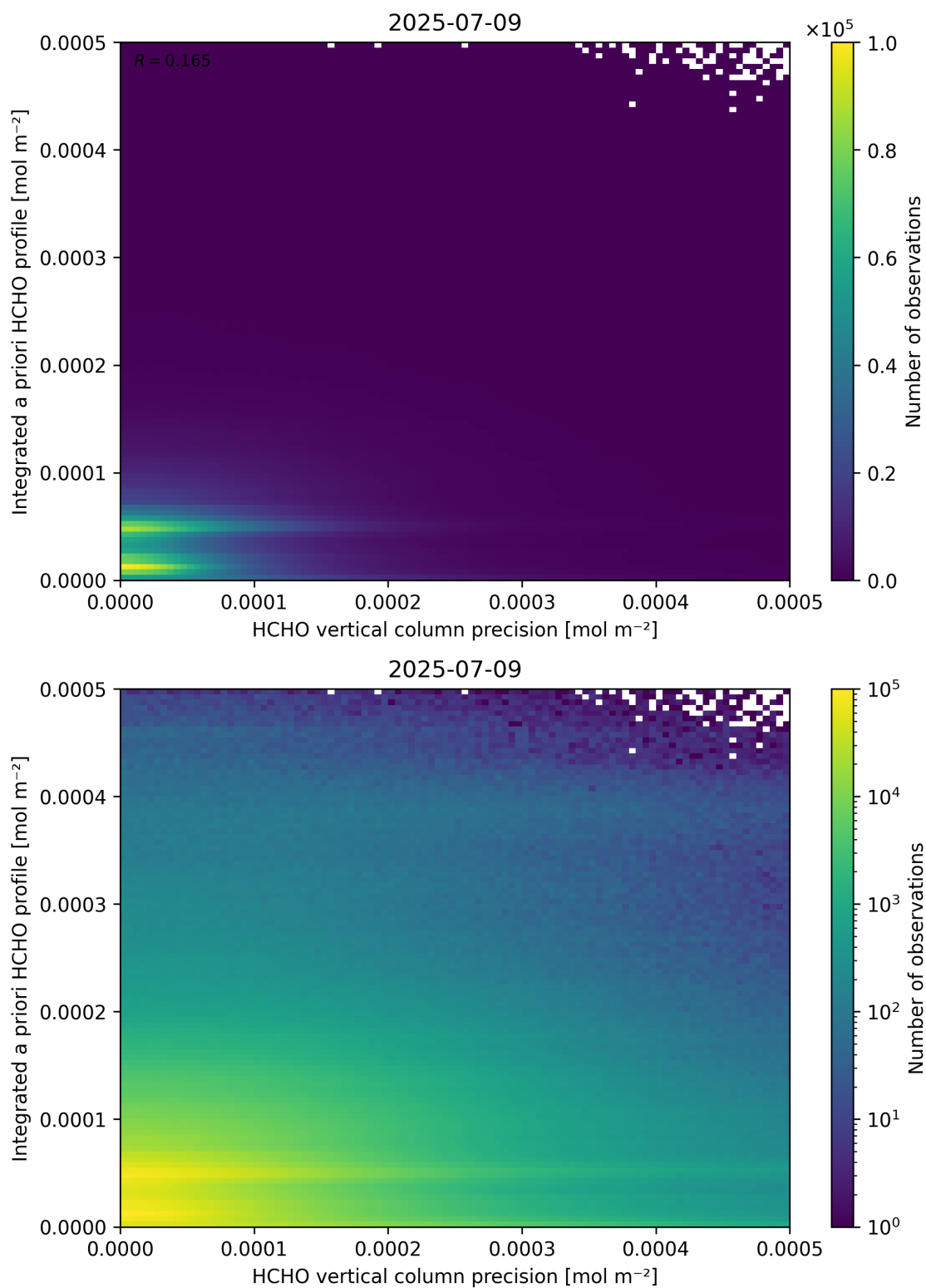
Figure 147: Scatter density plot of “HCHO vertical column precision” against “Integrated a priori HCHO profile” for 2025-07-08 to 2025-07-10.
