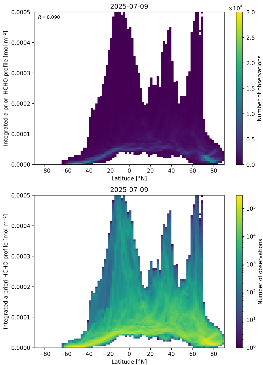
Figure 166: Scatter density plot of “Latitude” against “Integrated a priori HCHO profile” for 2025-07-08 to 2025-07-10.
