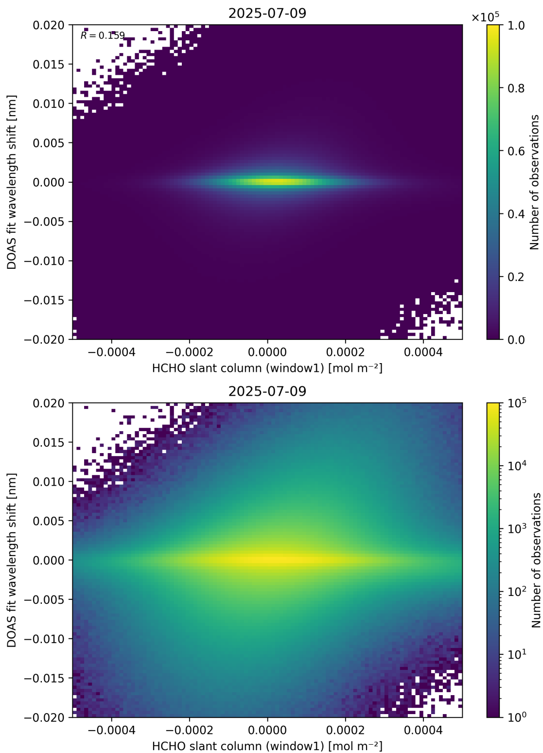
Figure 79: Scatter density plot of “HCHO slant column (window1)” against “DOAS fit wavelength shift” for 2025-07-08 to 2025-07-10.
