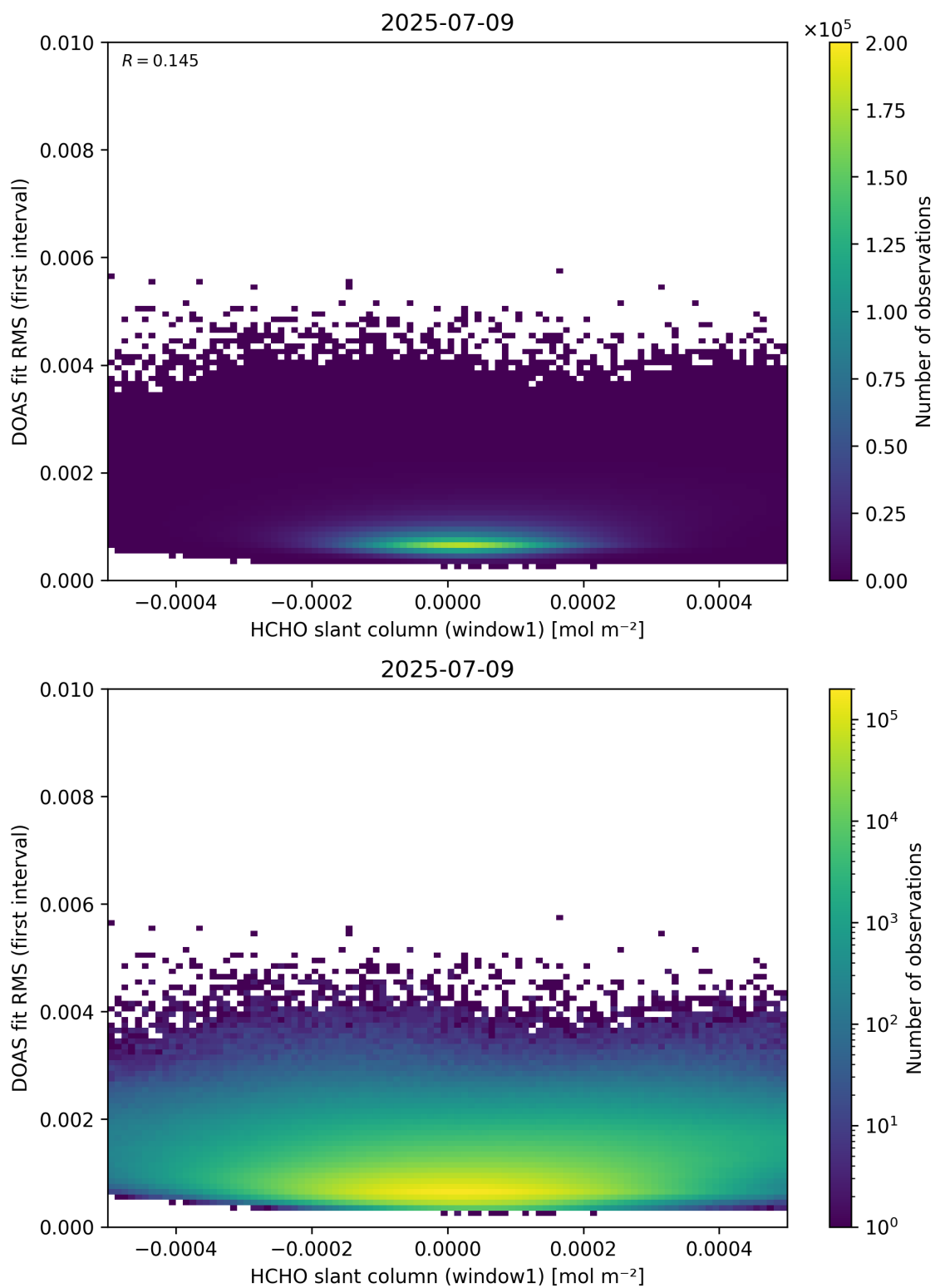
Figure 78: Scatter density plot of “HCHO slant column (window1)” against “DOAS fit RMS (first interval)” for 2025-07-08 to 2025-07-10.
