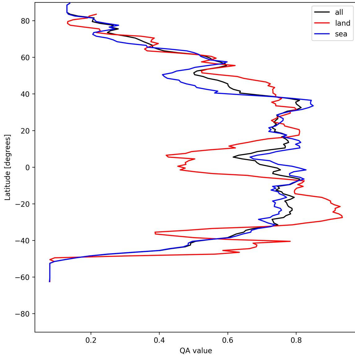
Figure 20: Zonal average of “QA value” for 2025-07-08 to 2025-07-10.
