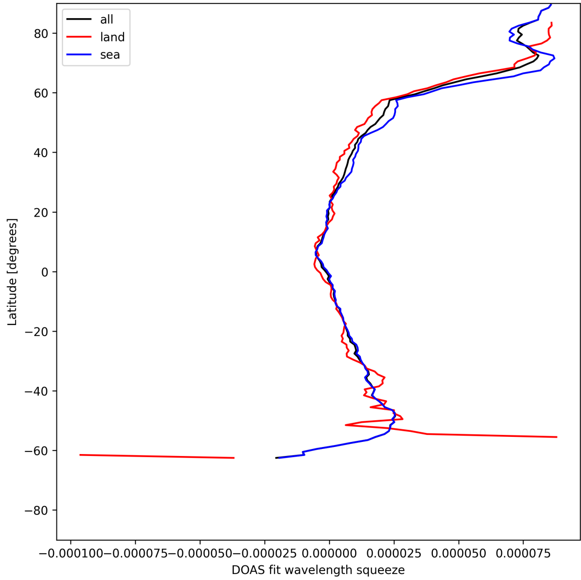
Figure 31: Zonal average of “DOAS fit wavelength squeeze” for 2025-07-08 to 2025-07-10.
