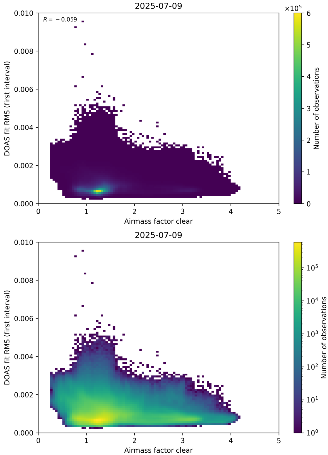
Figure 71: Scatter density plot of “Airmass factor clear” against “DOAS fit RMS (first interval)” for 2025-07-08 to 2025-07-10.
