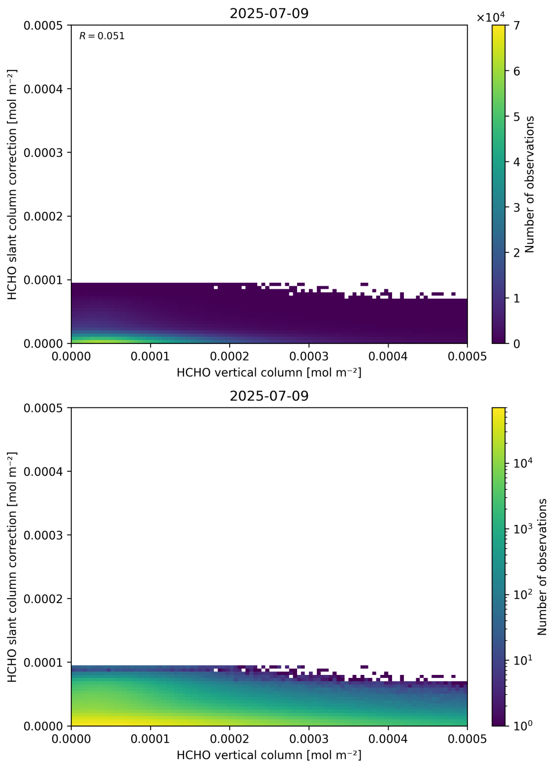
Figure 128: Scatter density plot of “HCHO vertical column” against “HCHO slant column correction” for 2025-07-08 to 2025-07-10.
