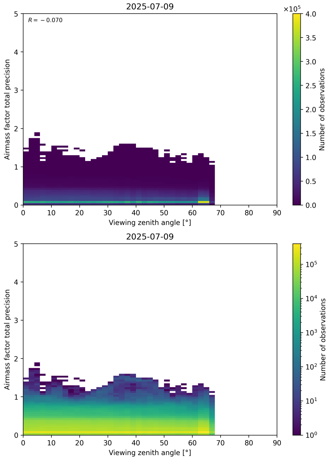
Figure 191: Scatter density plot of “Viewing zenith angle” against “Airmass factor total precision” for 2025-07-08 to 2025-07-10.
