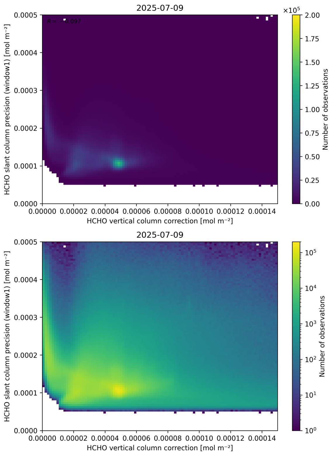
Figure 119: Scatter density plot of “HCHO vertical column correction” against “HCHO slant column precision (window1)” for 2025-07-08 to 2025-07-10.
