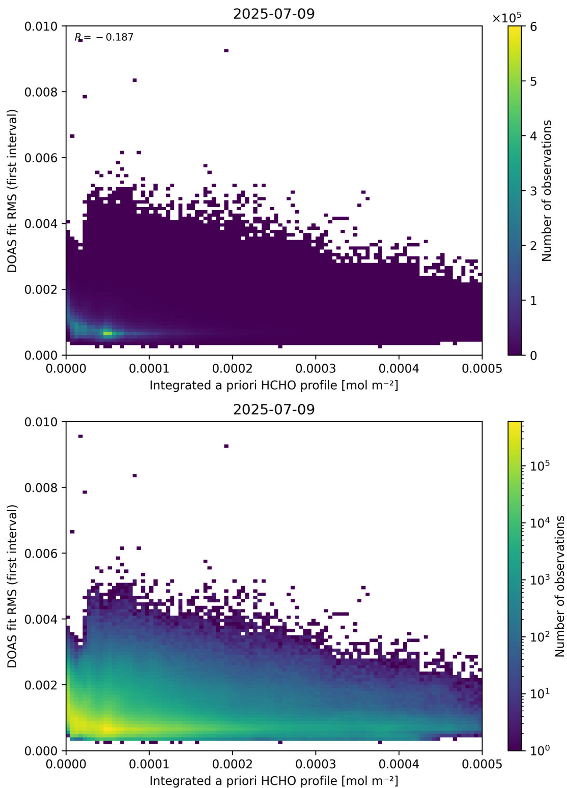
Figure 148: Scatter density plot of “Integrated a priori HCHO profile” against “DOAS fit RMS (first interval)” for 2025-07-08 to 2025-07-10.
