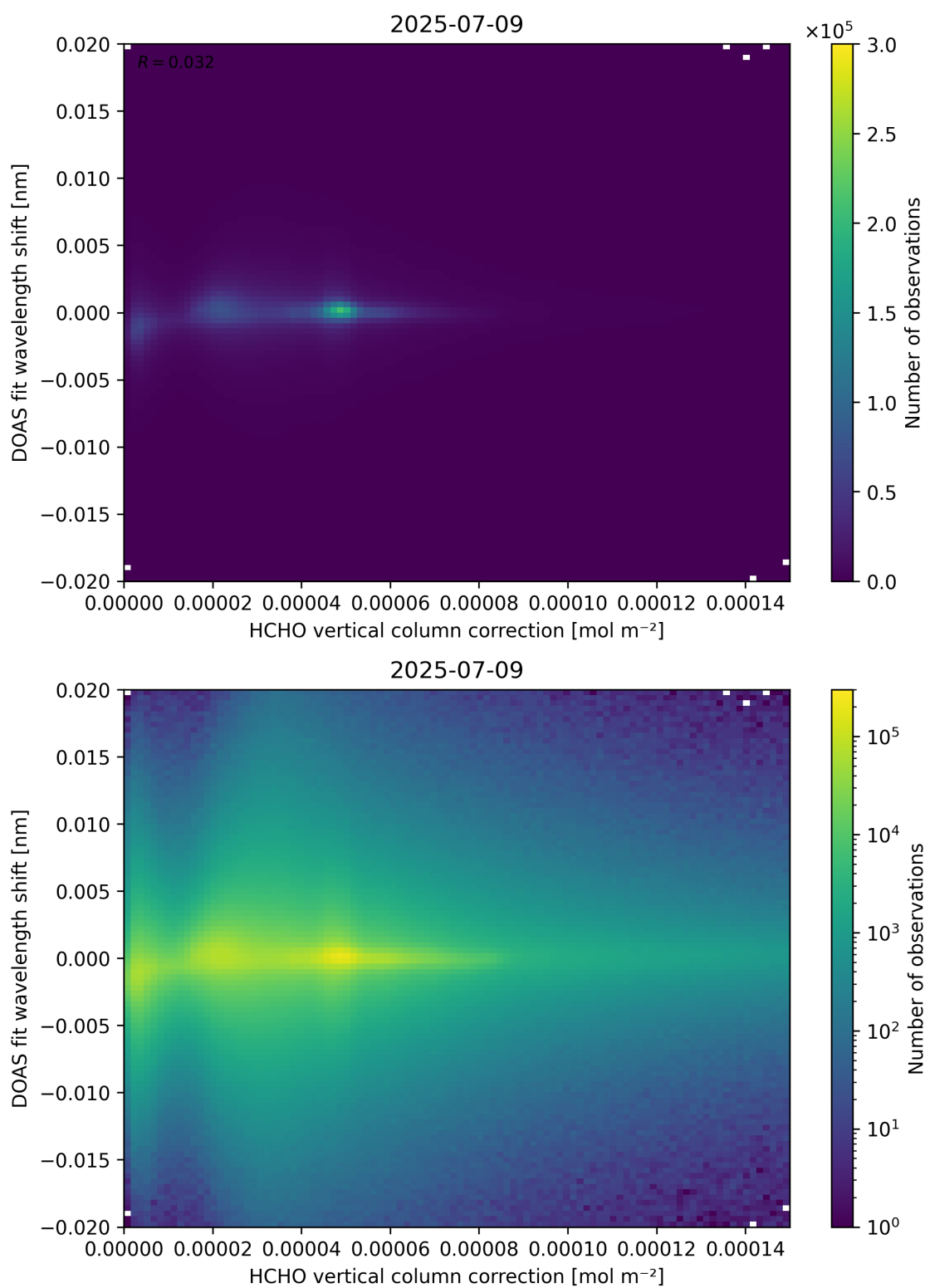
Figure 113: Scatter density plot of “HCHO vertical column correction” against “DOAS fit wavelength shift” for 2025-07-08 to 2025-07-10.
