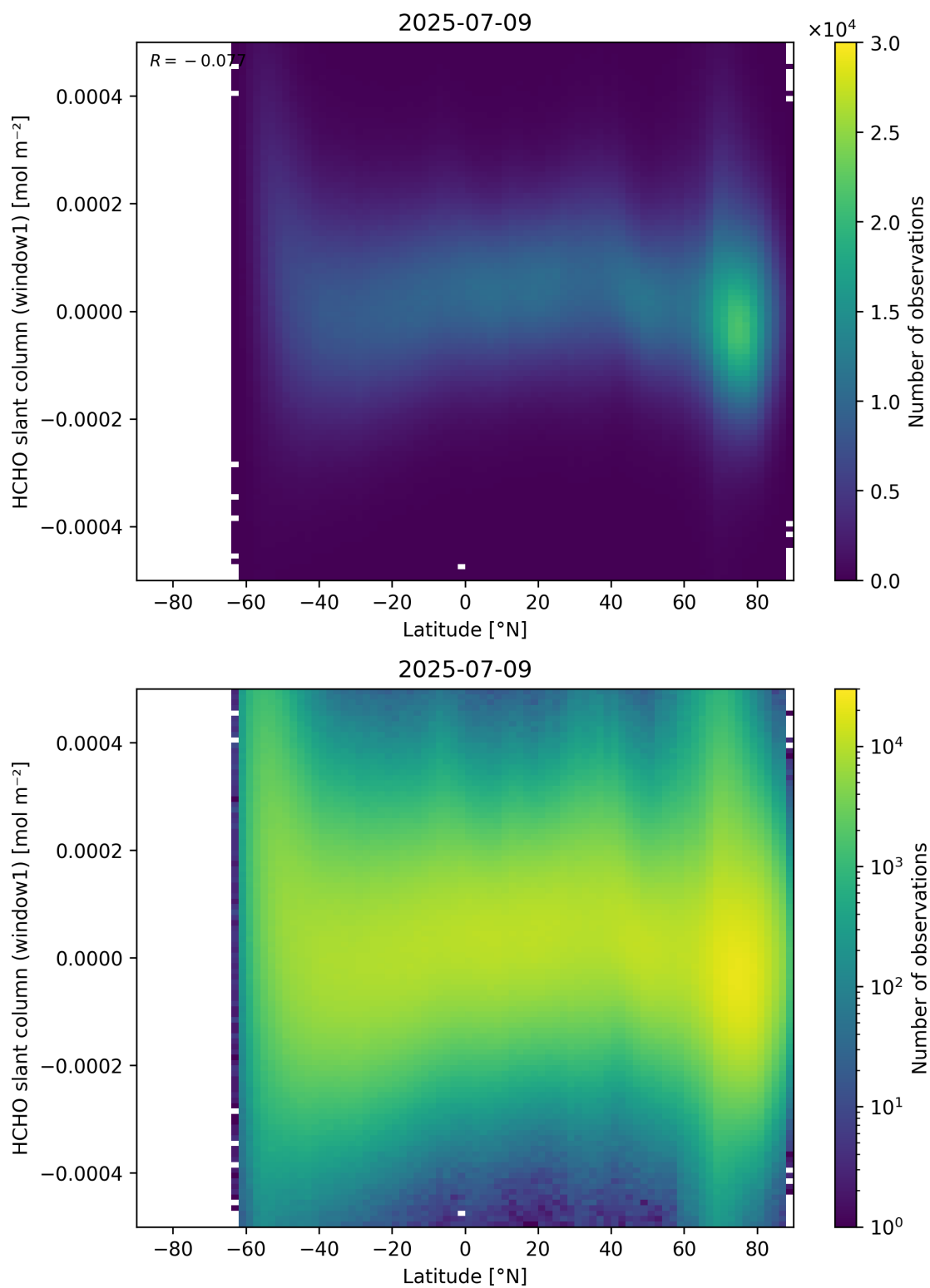
Figure 159: Scatter density plot of “Latitude” against “HCHO slant column (window1)” for 2025-07-08 to 2025-07-10.
