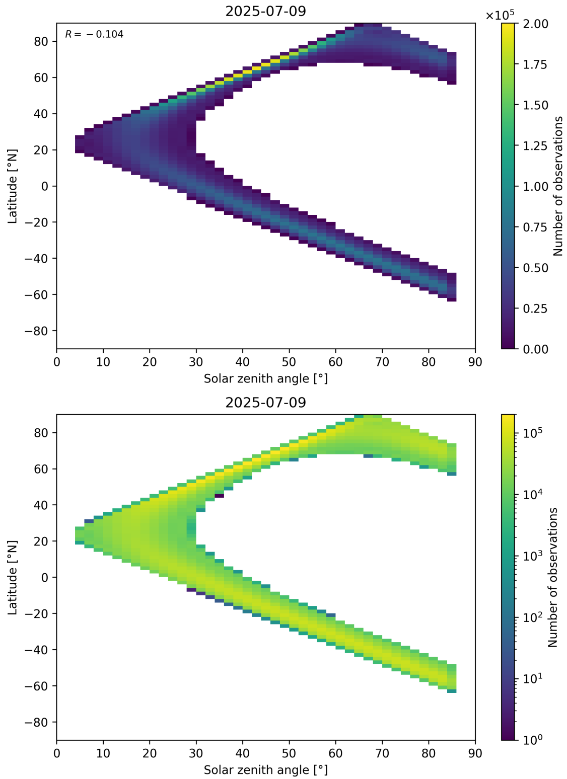
Figure 181: Scatter density plot of “Solar zenith angle” against “Latitude” for 2025-07-08 to 2025-07-10.
