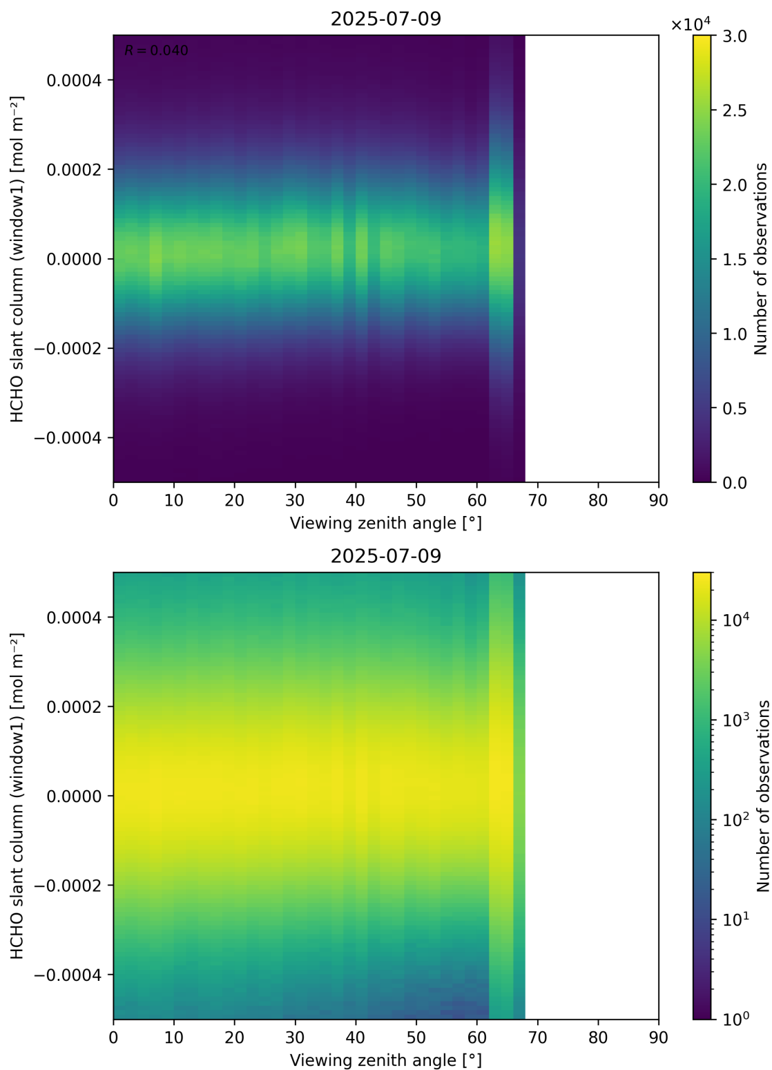
Figure 188: Scatter density plot of “Viewing zenith angle” against “HCHO slant column (window1)” for 2025-07-08 to 2025-07-10.
