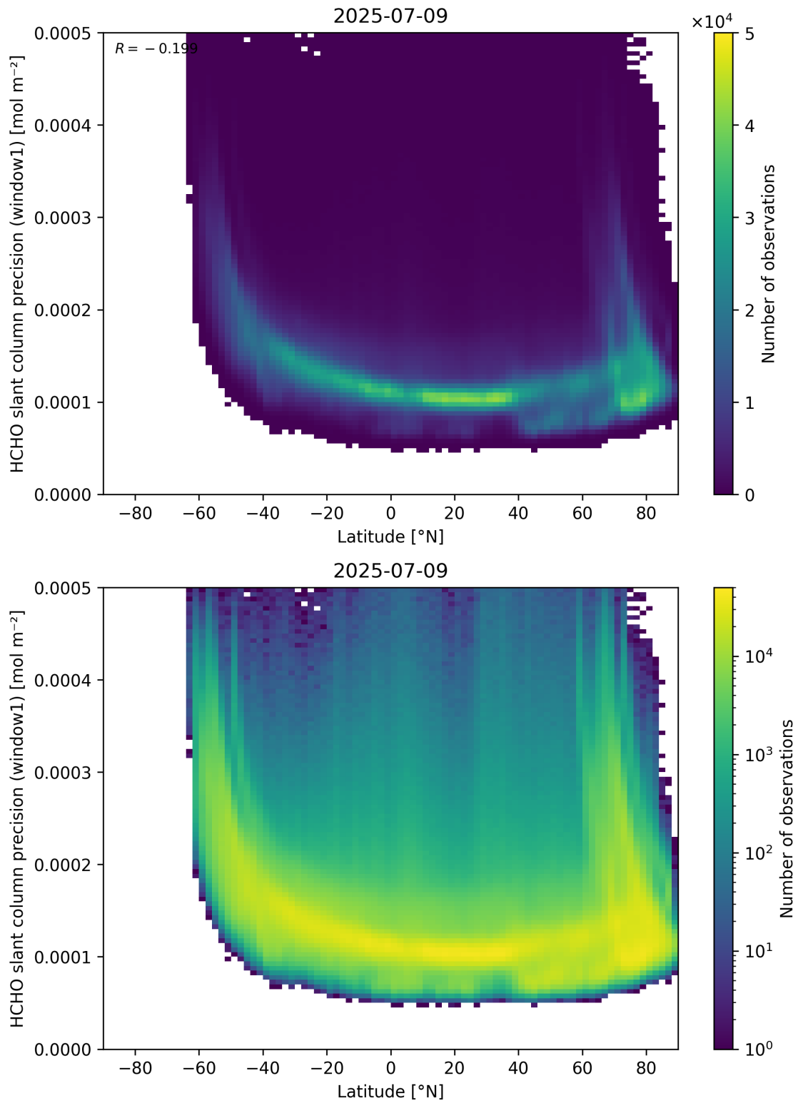
Figure 160: Scatter density plot of “Latitude” against “HCHO slant column precision (window1)” for 2025-07-08 to 2025-07-10.
