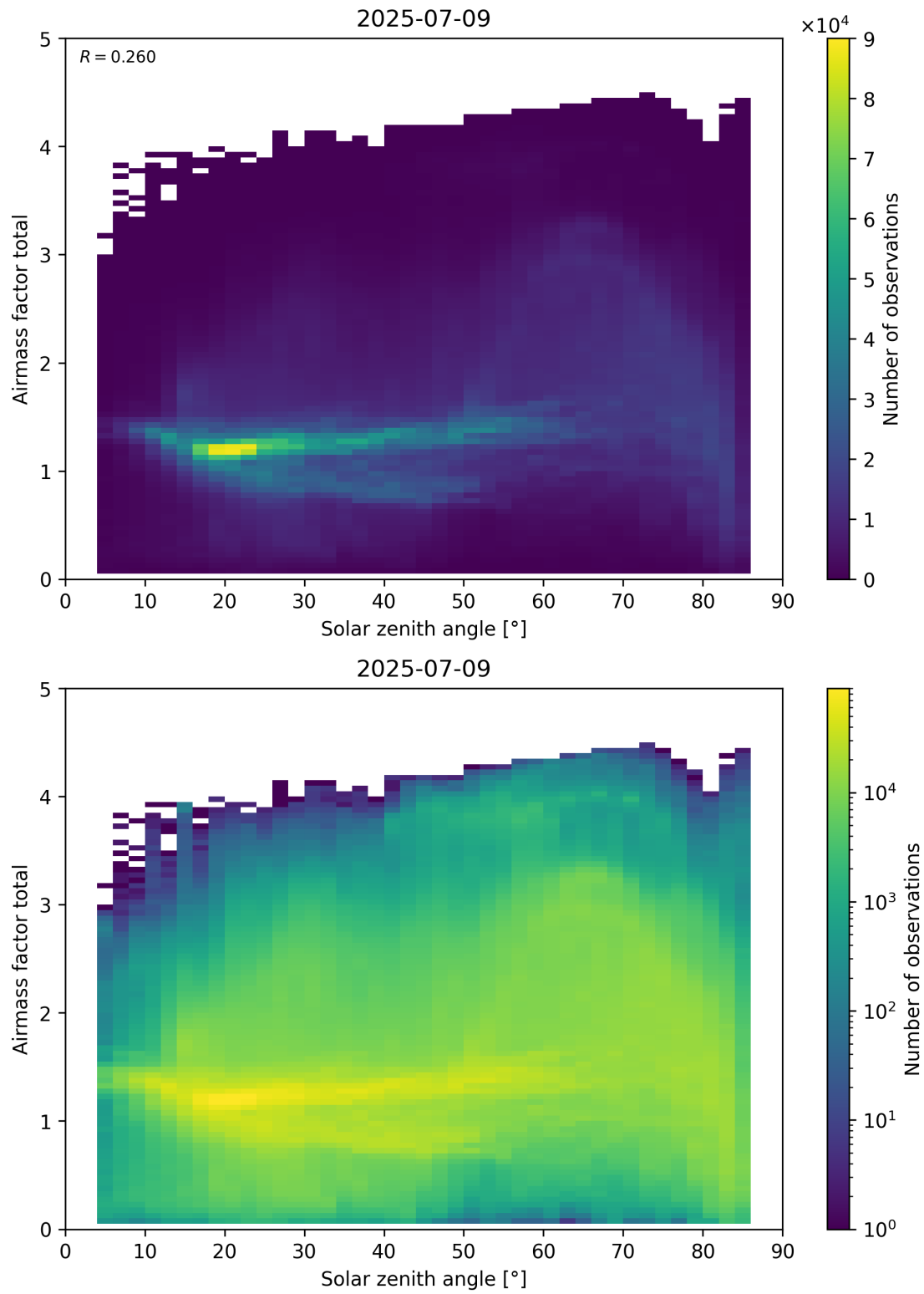
Figure 175: Scatter density plot of “Solar zenith angle” against “Airmass factor total” for 2025-07-08 to 2025-07-10.
