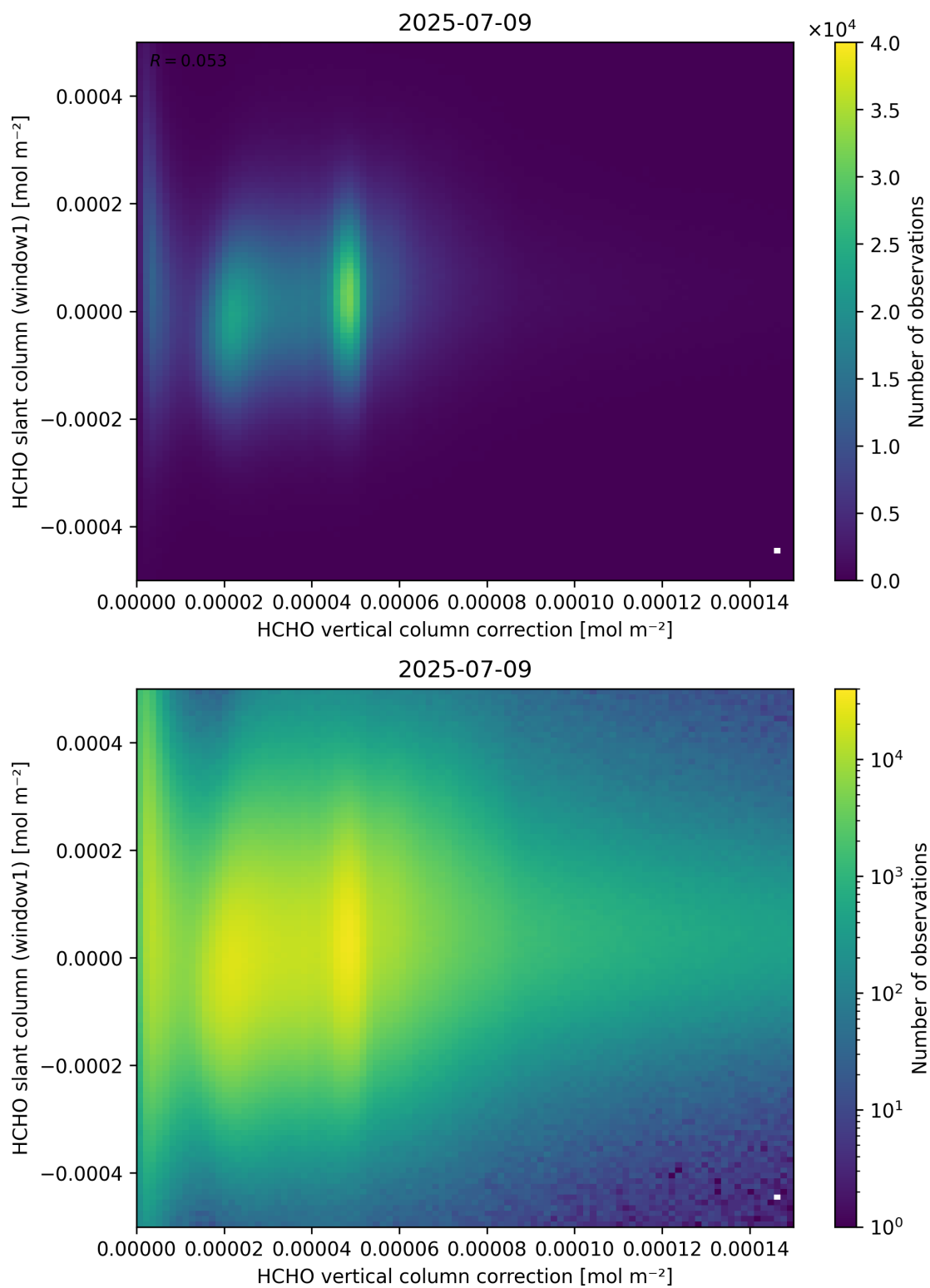
Figure 118: Scatter density plot of “HCHO vertical column correction” against “HCHO slant column (window1)” for 2025-07-08 to 2025-07-10.
