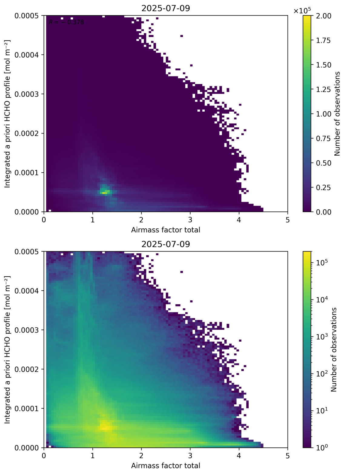
Figure 104: Scatter density plot of “Airmass factor total” against “Integrated a priori HCHO profile” for 2025-07-08 to 2025-07-10.
