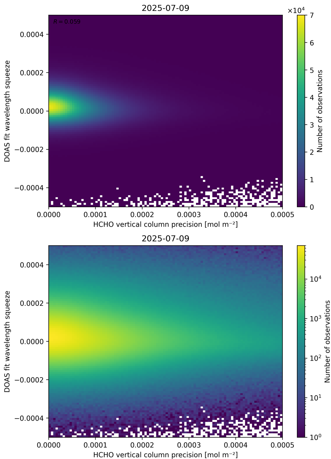
Figure 138: Scatter density plot of “HCHO vertical column precision” against “DOAS fit wavelength squeeze” for 2025-07-08 to 2025-07-10.
