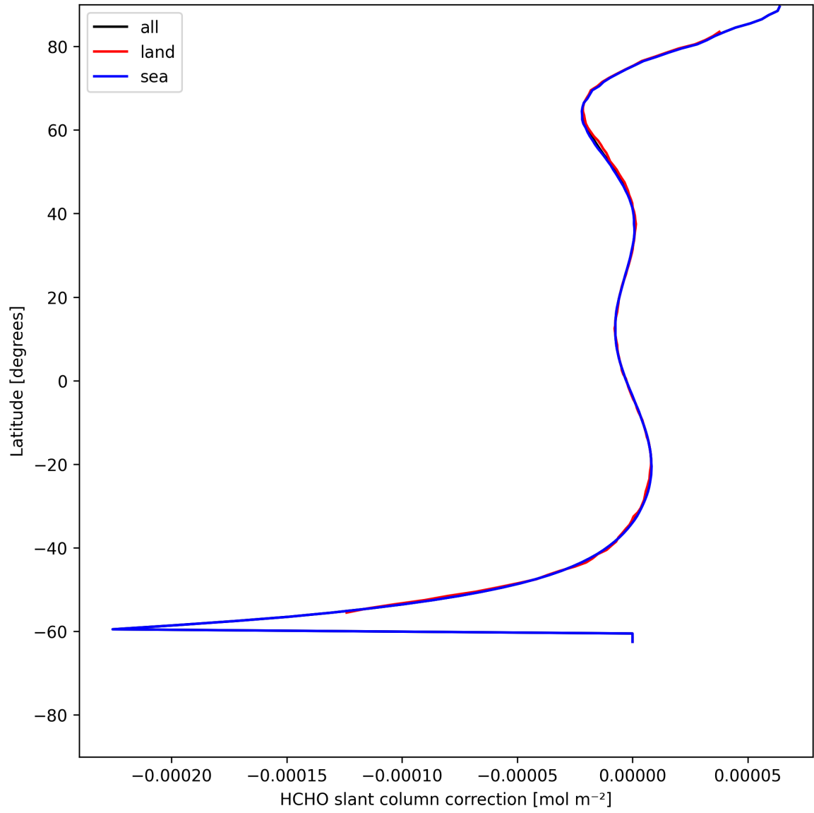
Figure 33: Zonal average of “HCHO slant column correction” for 2025-07-08 to 2025-07-10.
