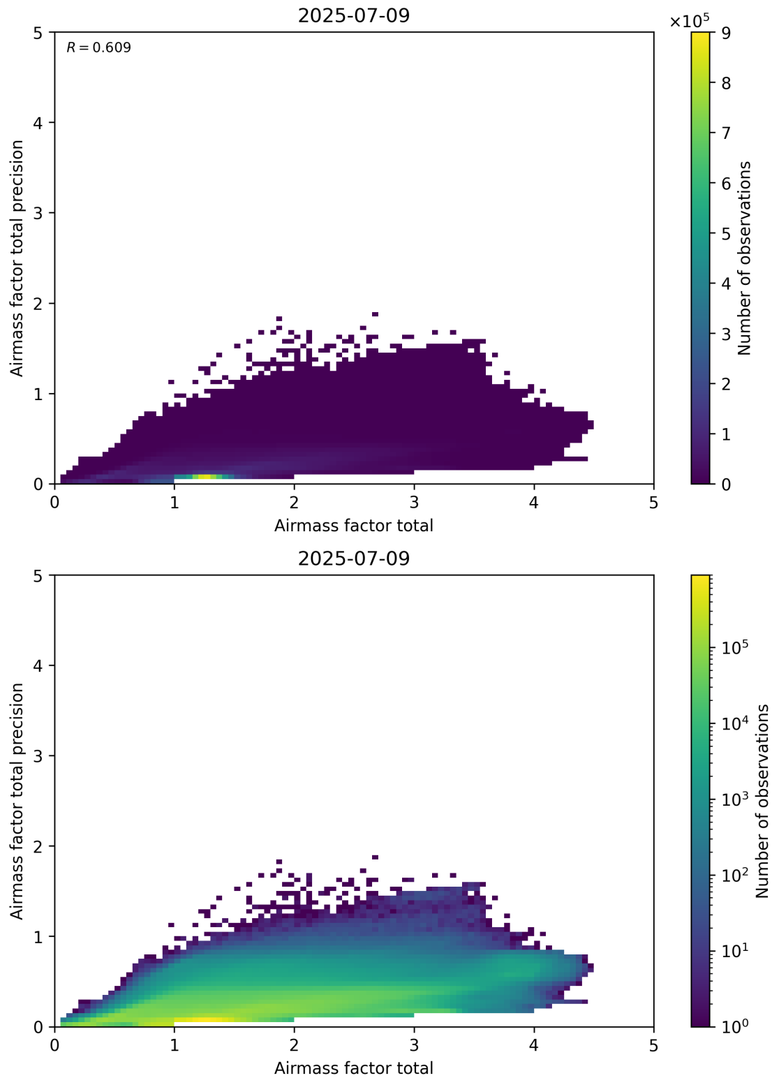
Figure 103: Scatter density plot of “Airmass factor total” against “Airmass factor total precision” for 2025-07-08 to 2025-07-10.
