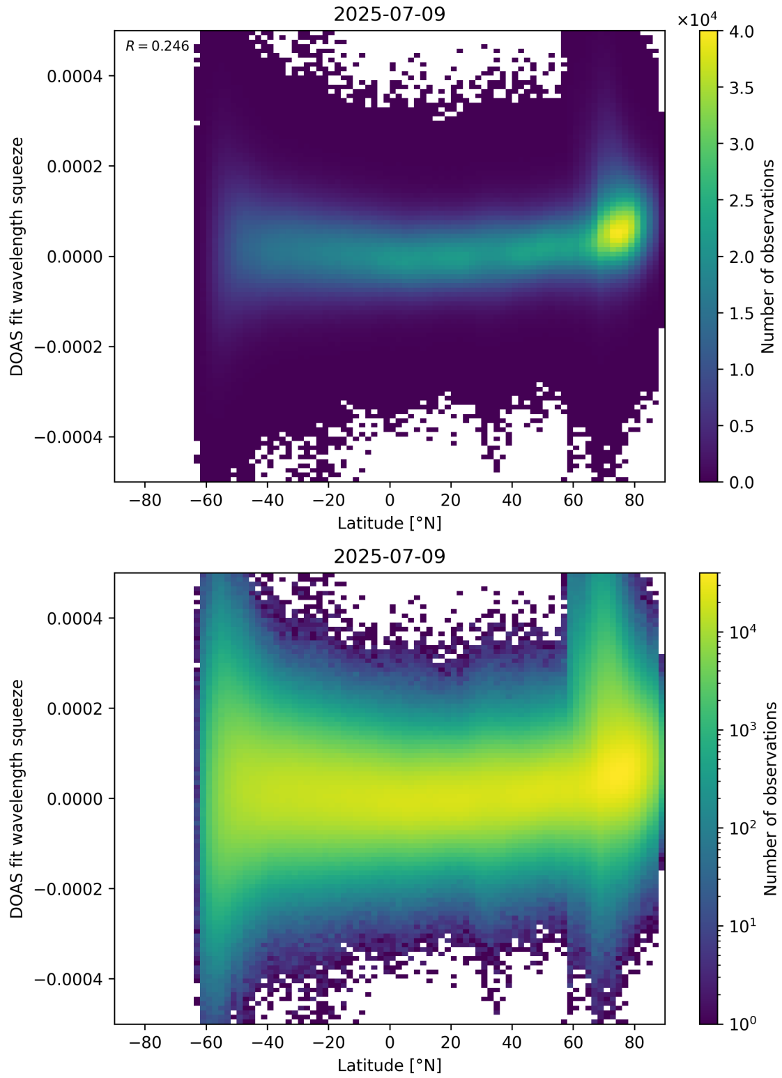
Figure 155: Scatter density plot of “Latitude” against “DOAS fit wavelength squeeze” for 2025-07-08 to 2025-07-10.
