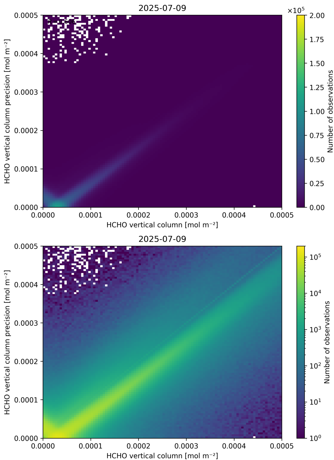
Figure 134: Scatter density plot of “HCHO vertical column” against “HCHO vertical column precision” for 2025-07-08 to 2025-07-10.
