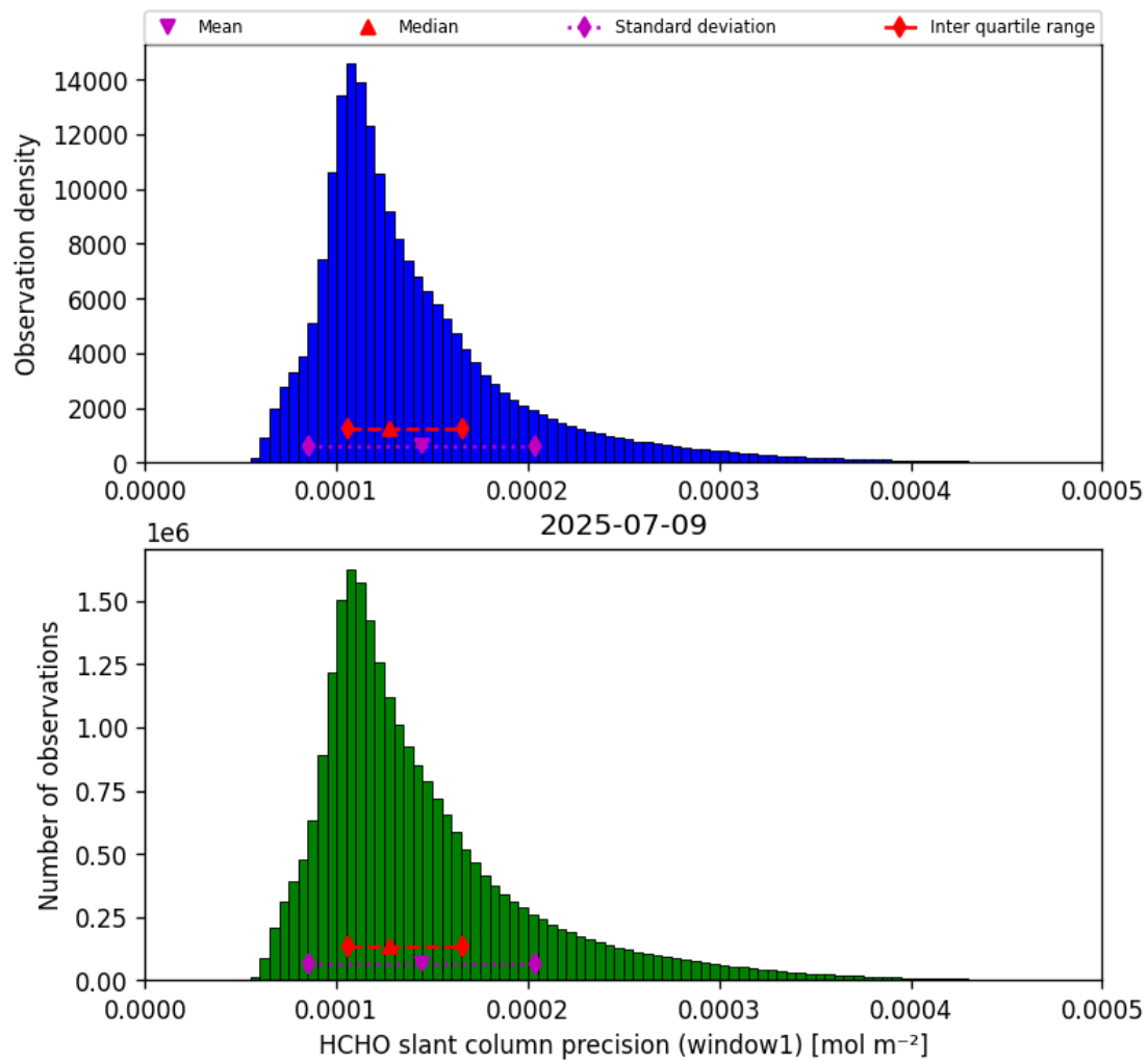
Figure 39: Histogram of “HCHO slant column precision (window1)” for 2025-07-08 to 2025-07-10
