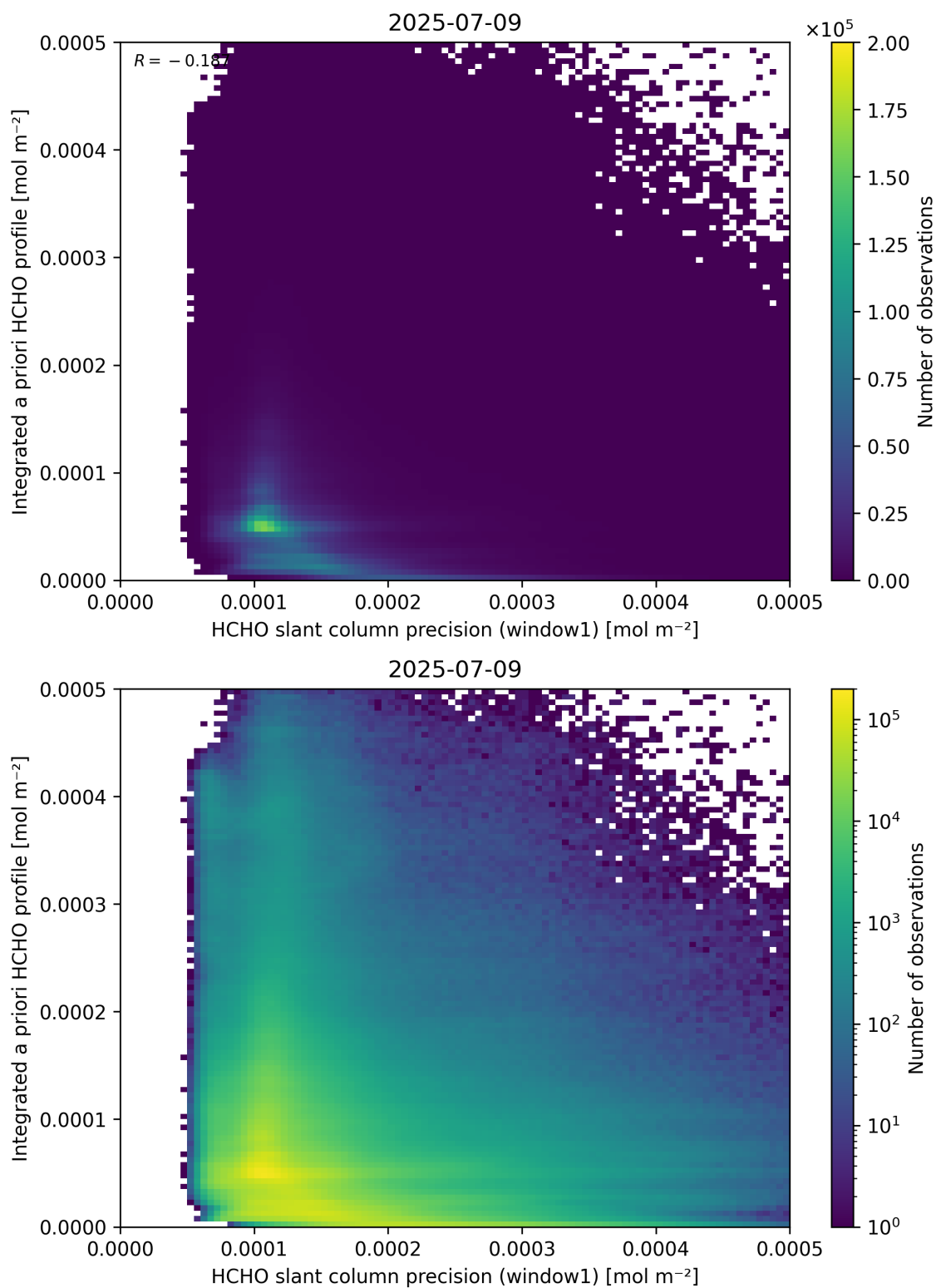
Figure 96: Scatter density plot of “HCHO slant column precision (window1)” against “Integrated a priori HCHO profile” for 2025-07-08 to 2025-07-10.
