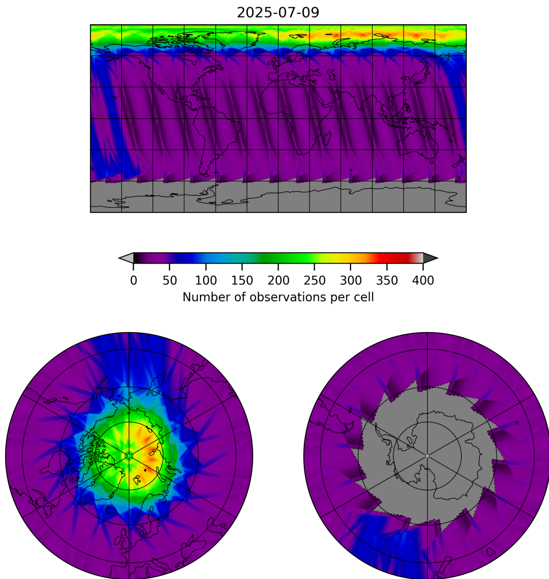
Figure 19: Map of the number of observations for 2025-07-08 to 2025-07-10
