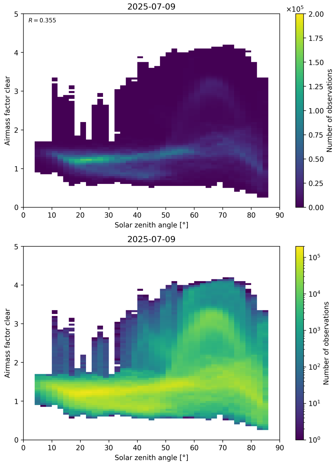
Figure 170: Scatter density plot of “Solar zenith angle” against “Airmass factor clear” for 2025-07-08 to 2025-07-10.
