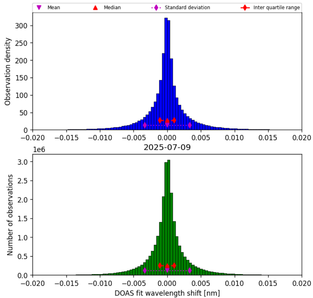
Figure 44: Histogram of “DOAS fit wavelength shift” for 2025-07-08 to 2025-07-10
