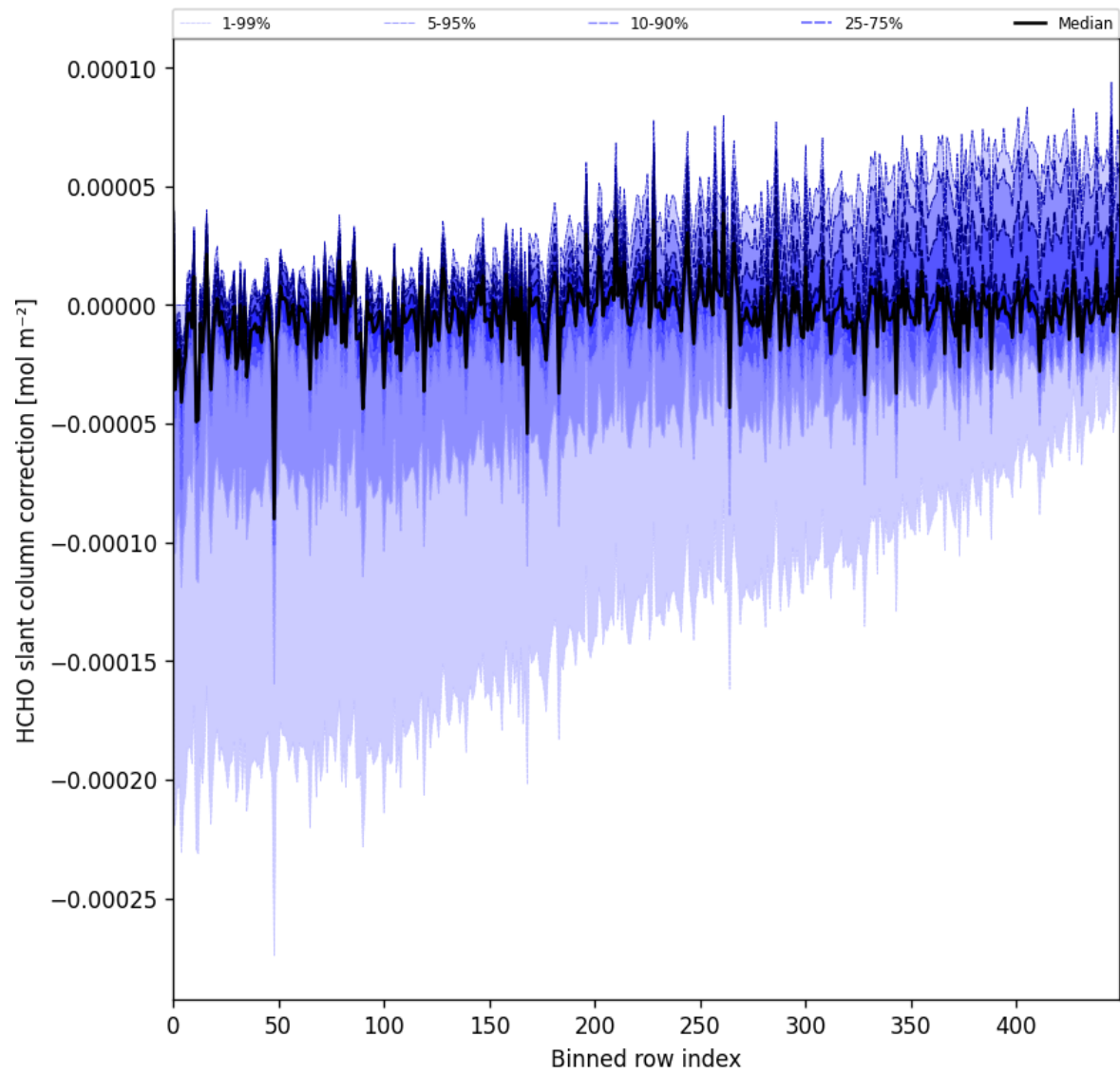
Figure 61: Along track statistics of “HCHO slant column correction” for 2025-07-08 to 2025-07-10
