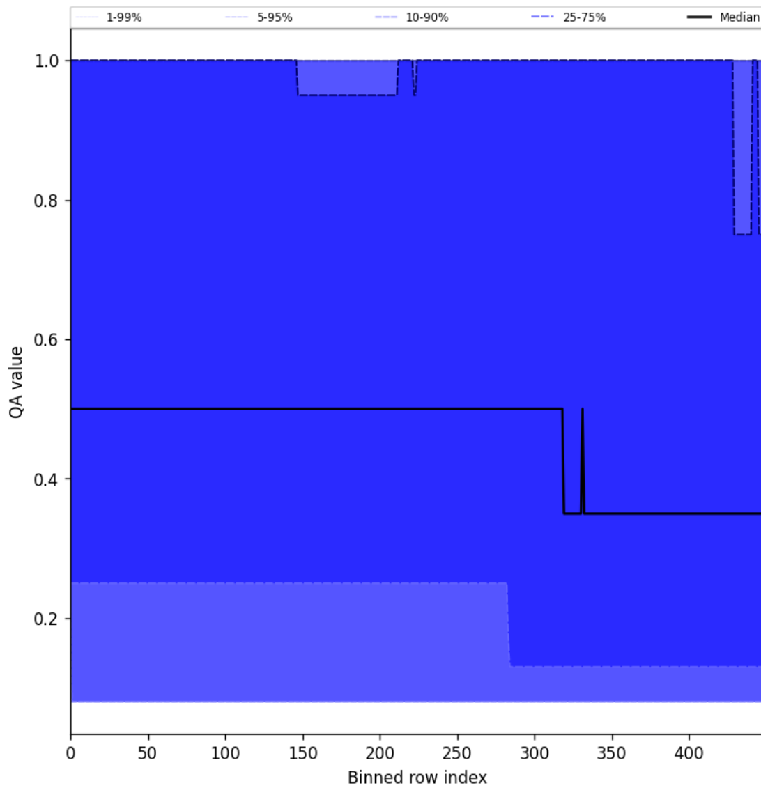
Figure 48: Along track statistics of “QA value” for 2025-07-08 to 2025-07-10
