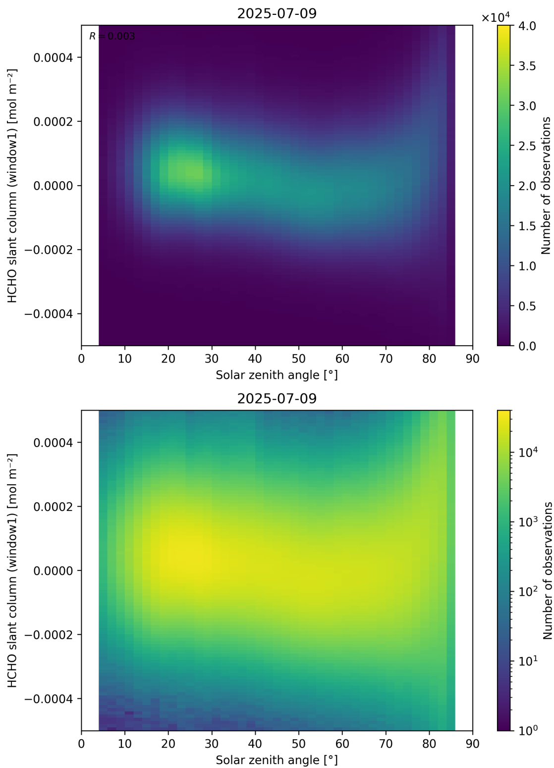
Figure 173: Scatter density plot of “Solar zenith angle” against “HCHO slant column (window1)” for 2025-07-08 to 2025-07-10.
