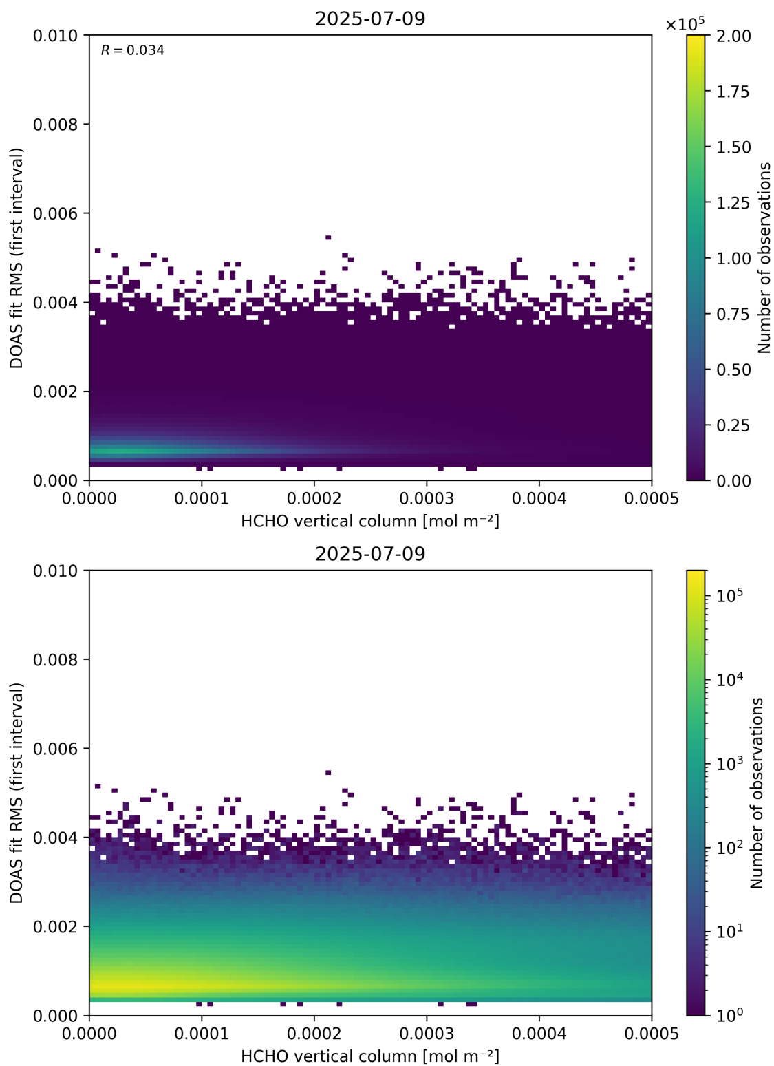
Figure 123: Scatter density plot of “HCHO vertical column” against “DOAS fit RMS (first interval)” for 2025-07-08 to 2025-07-10.
