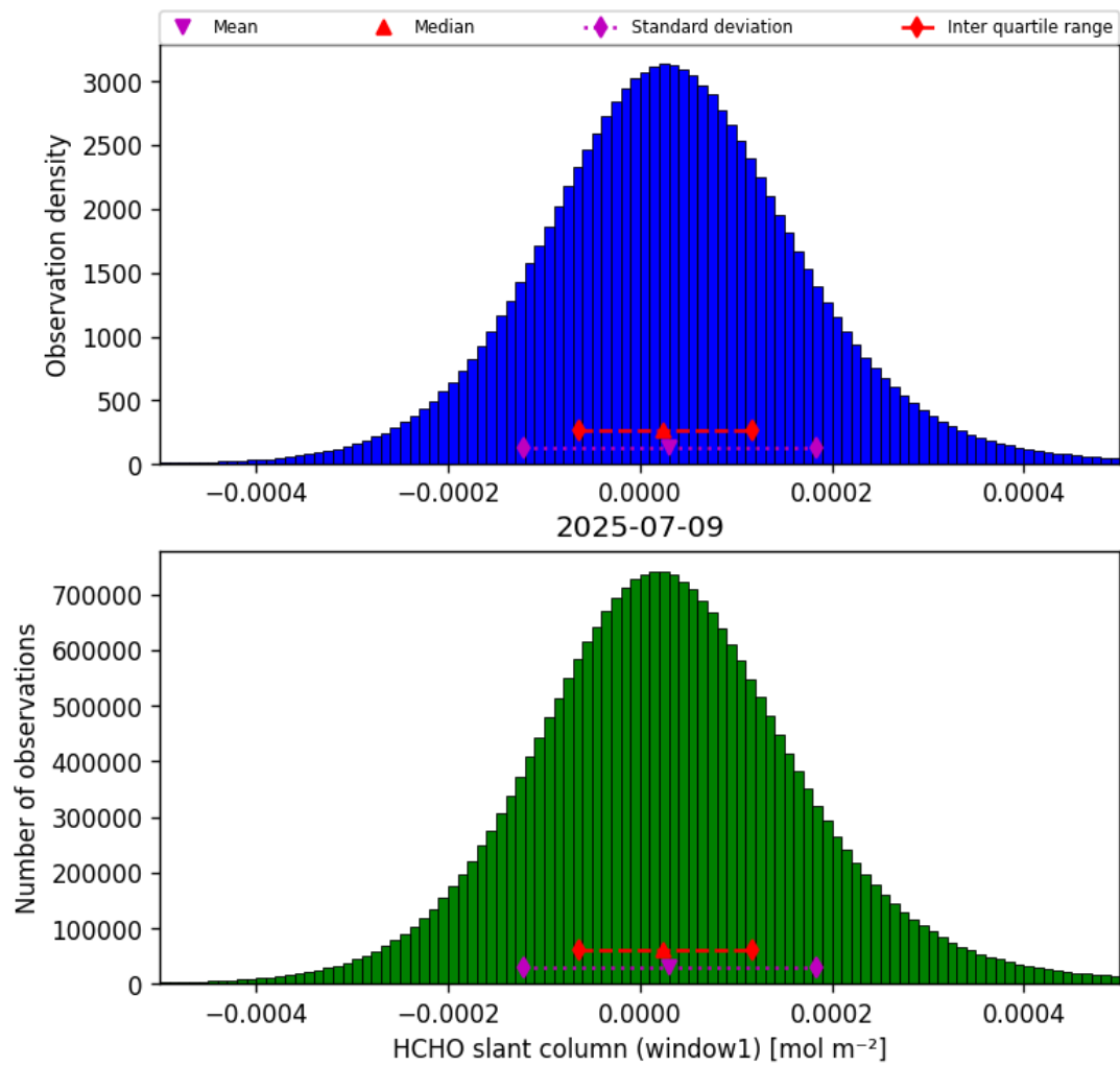
Figure 38: Histogram of “HCHO slant column (window1)” for 2025-07-08 to 2025-07-10
