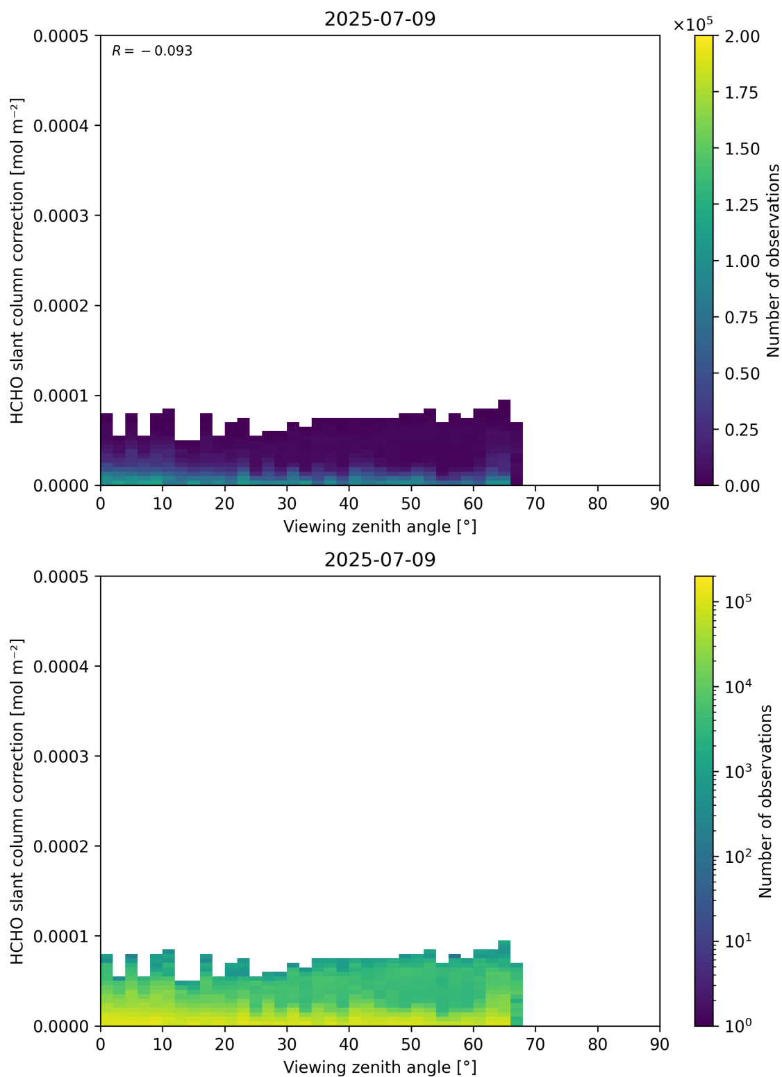
Figure 187: Scatter density plot of “Viewing zenith angle” against “HCHO slant column correction” for 2025-07-08 to 2025-07-10.
