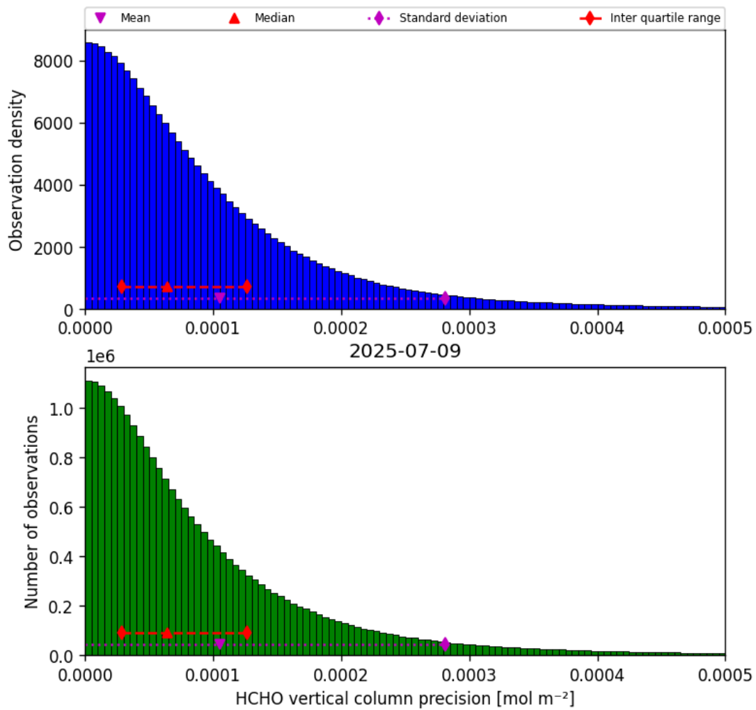
Figure 36: Histogram of “HCHO vertical column precision” for 2025-07-08 to 2025-07-10
