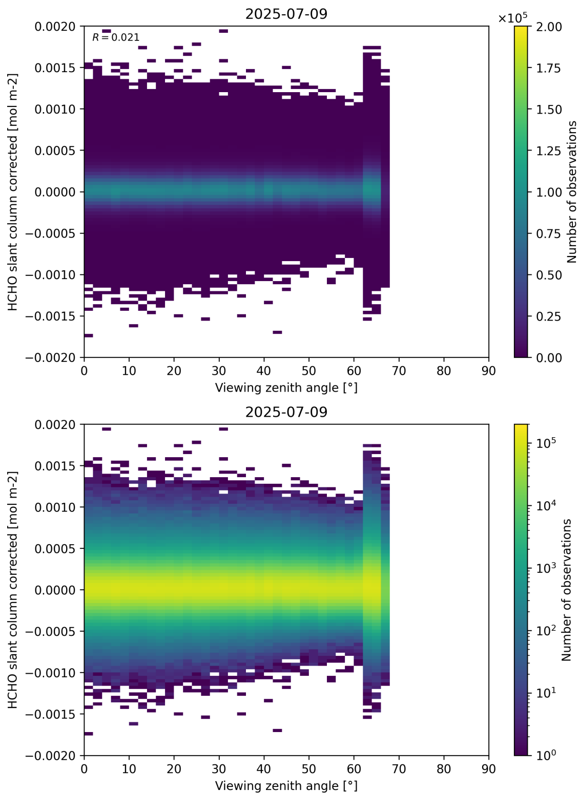
Figure 186: Scatter density plot of “Viewing zenith angle” against “HCHO slant column corrected” for 2025-07-08 to 2025-07-10.
