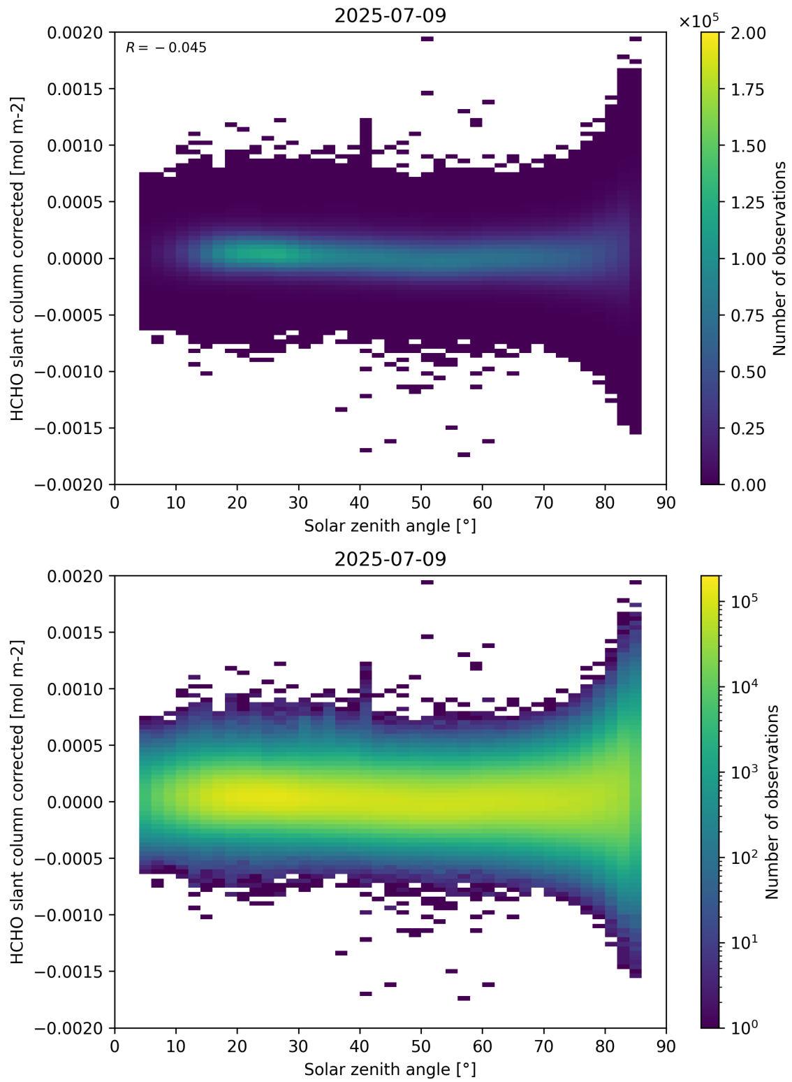
Figure 171: Scatter density plot of “Solar zenith angle” against “HCHO slant column corrected” for 2025-07-08 to 2025-07-10.
