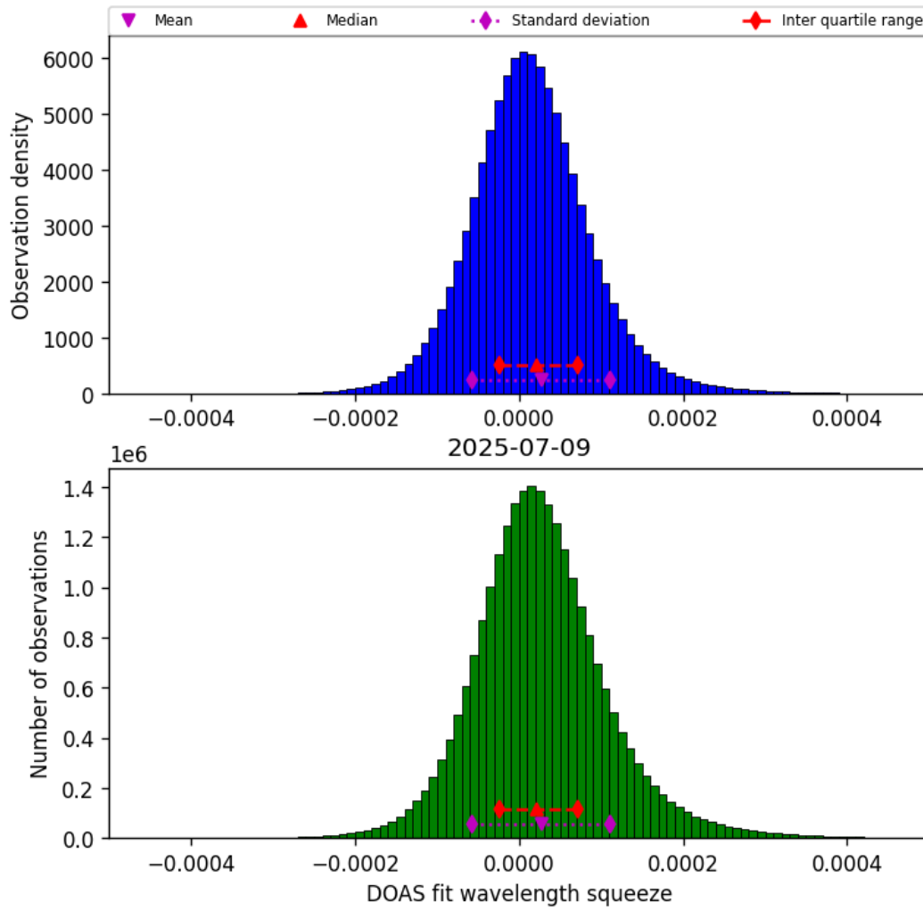
Figure 45: Histogram of “DOAS fit wavelength squeeze” for 2025-07-08 to 2025-07-10
