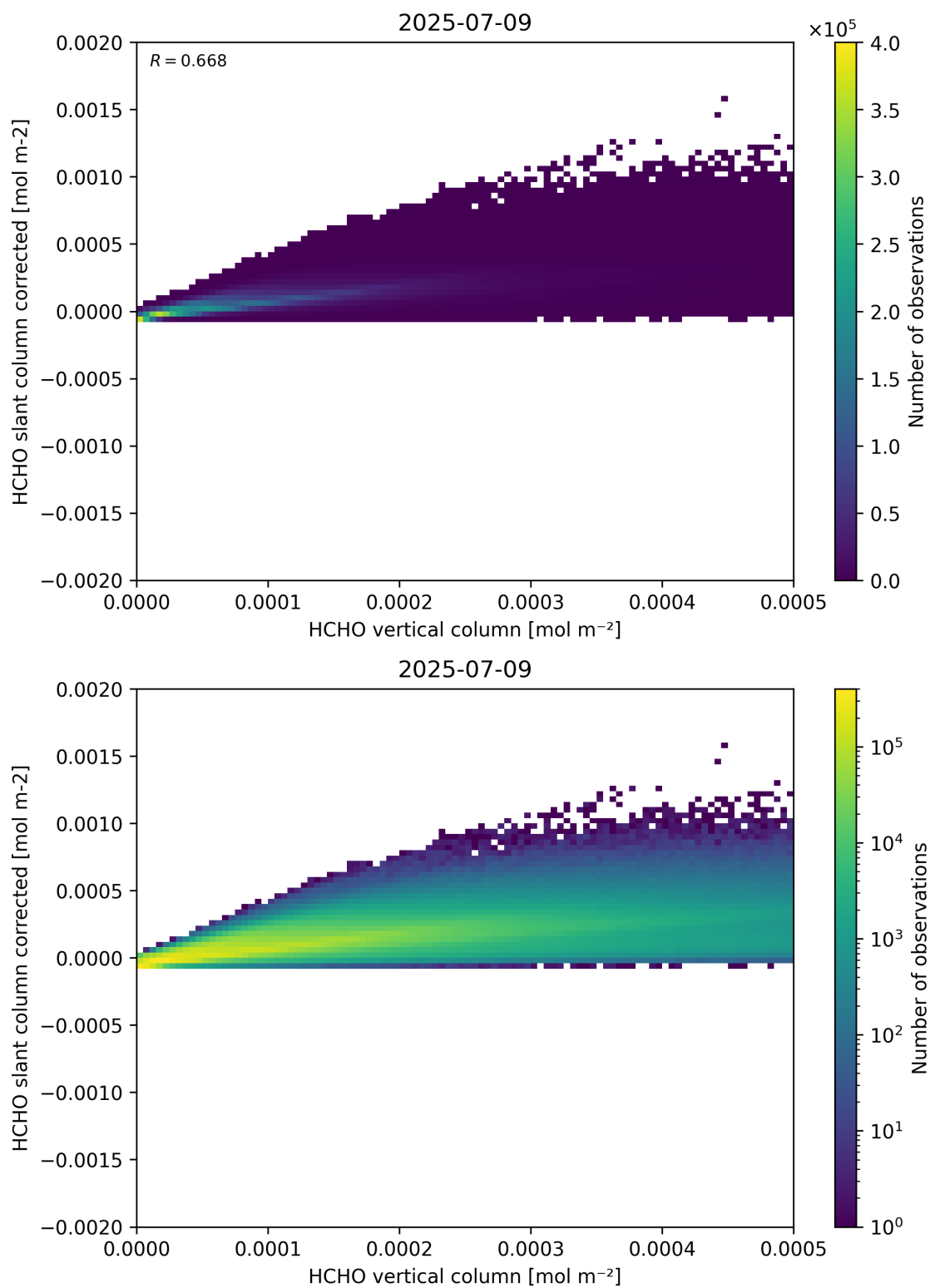
Figure 127: Scatter density plot of “HCHO vertical column” against “HCHO slant column corrected” for 2025-07-08 to 2025-07-10.
