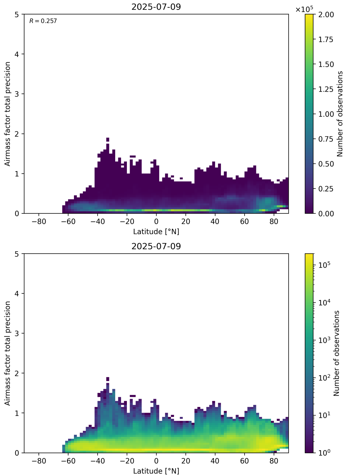
Figure 162: Scatter density plot of “Latitude” against “Airmass factor total precision” for 2025-07-08 to 2025-07-10.
