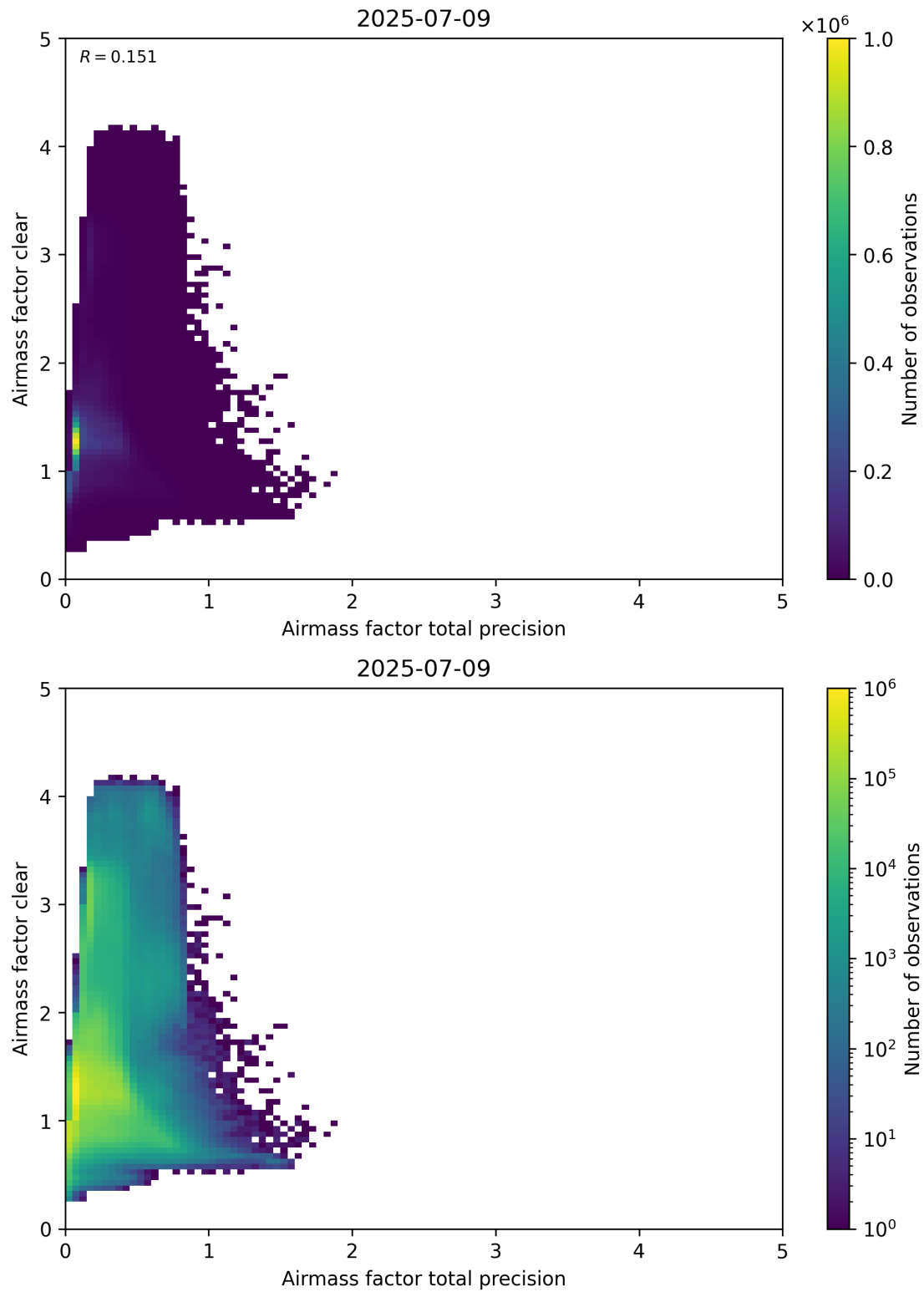
Figure 108: Scatter density plot of “Airmass factor total precision” against “Airmass factor clear” for 2025-07-08 to 2025-07-10.
