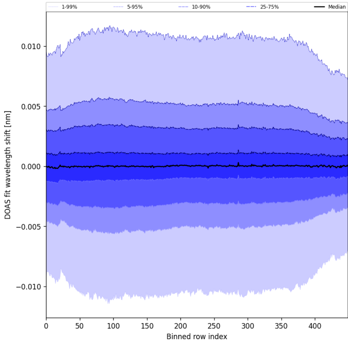
Figure 58: Along track statistics of “DOAS fit wavelength shift” for 2025-07-08 to 2025-07-10
