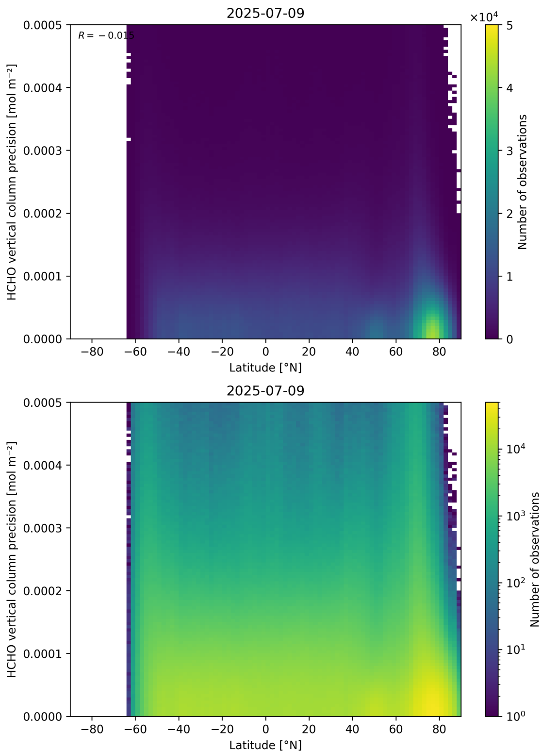
Figure 165: Scatter density plot of “Latitude” against “HCHO vertical column precision” for 2025-07-08 to 2025-07-10.
