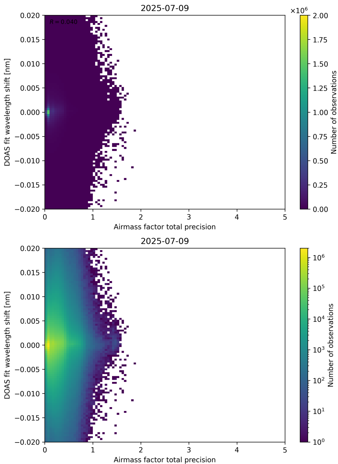
Figure 106: Scatter density plot of “Airmass factor total precision” against “DOAS fit wavelength shift” for 2025-07-08 to 2025-07-10.
