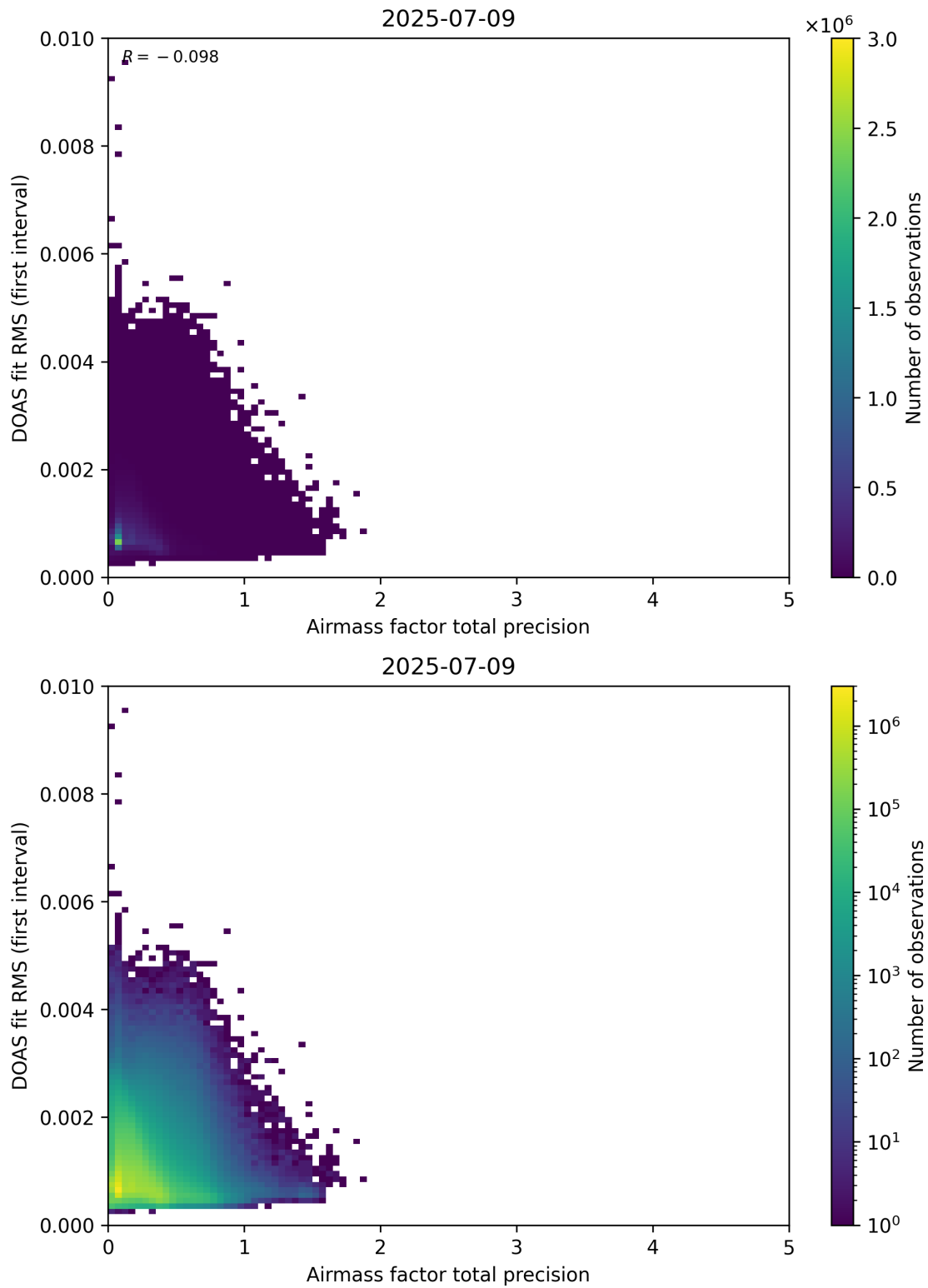
Figure 105: Scatter density plot of “Airmass factor total precision” against “DOAS fit RMS (first interval)” for 2025-07-08 to 2025-07-10.
