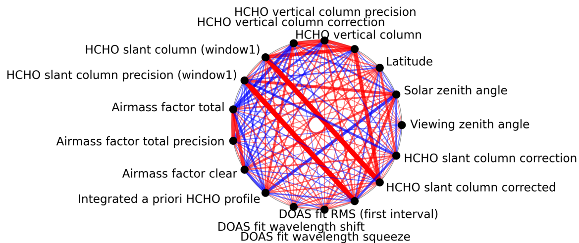
Figure 1: Map of correlation graph for 2025-07-08 to 2025-07-10.
