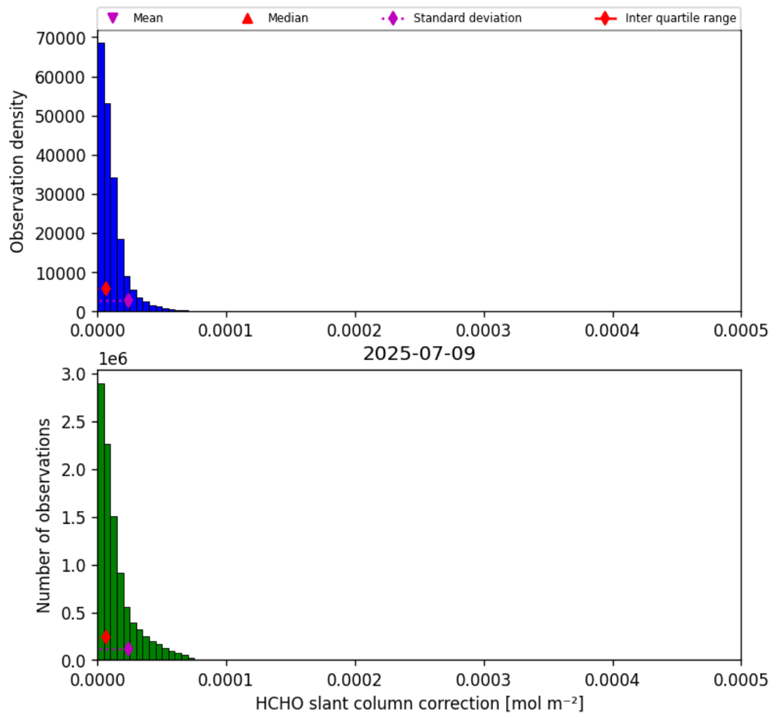
Figure 47: Histogram of “HCHO slant column correction” for 2025-07-08 to 2025-07-10
