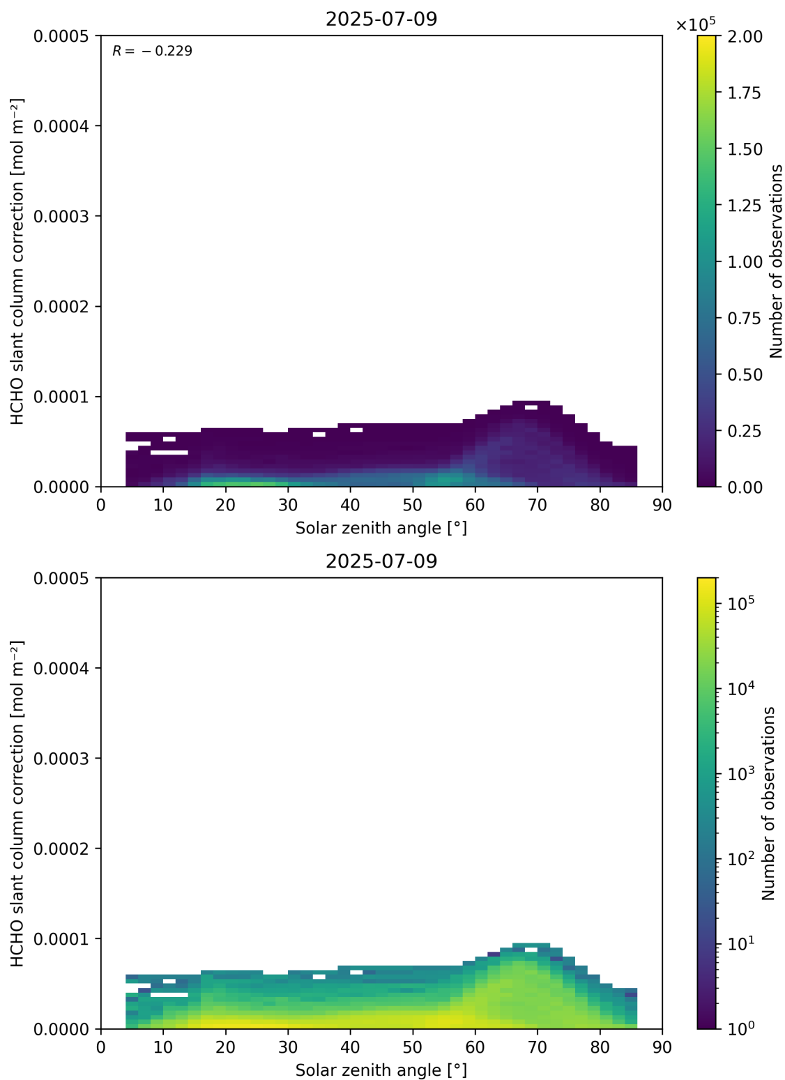
Figure 172: Scatter density plot of “Solar zenith angle” against “HCHO slant column correction” for 2025-07-08 to 2025-07-10.
