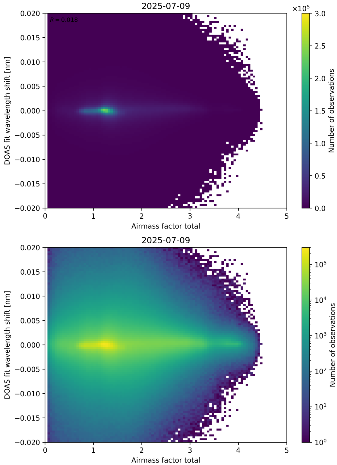
Figure 98: Scatter density plot of “Airmass factor total” against “DOAS fit wavelength shift” for 2025-07-08 to 2025-07-10.
