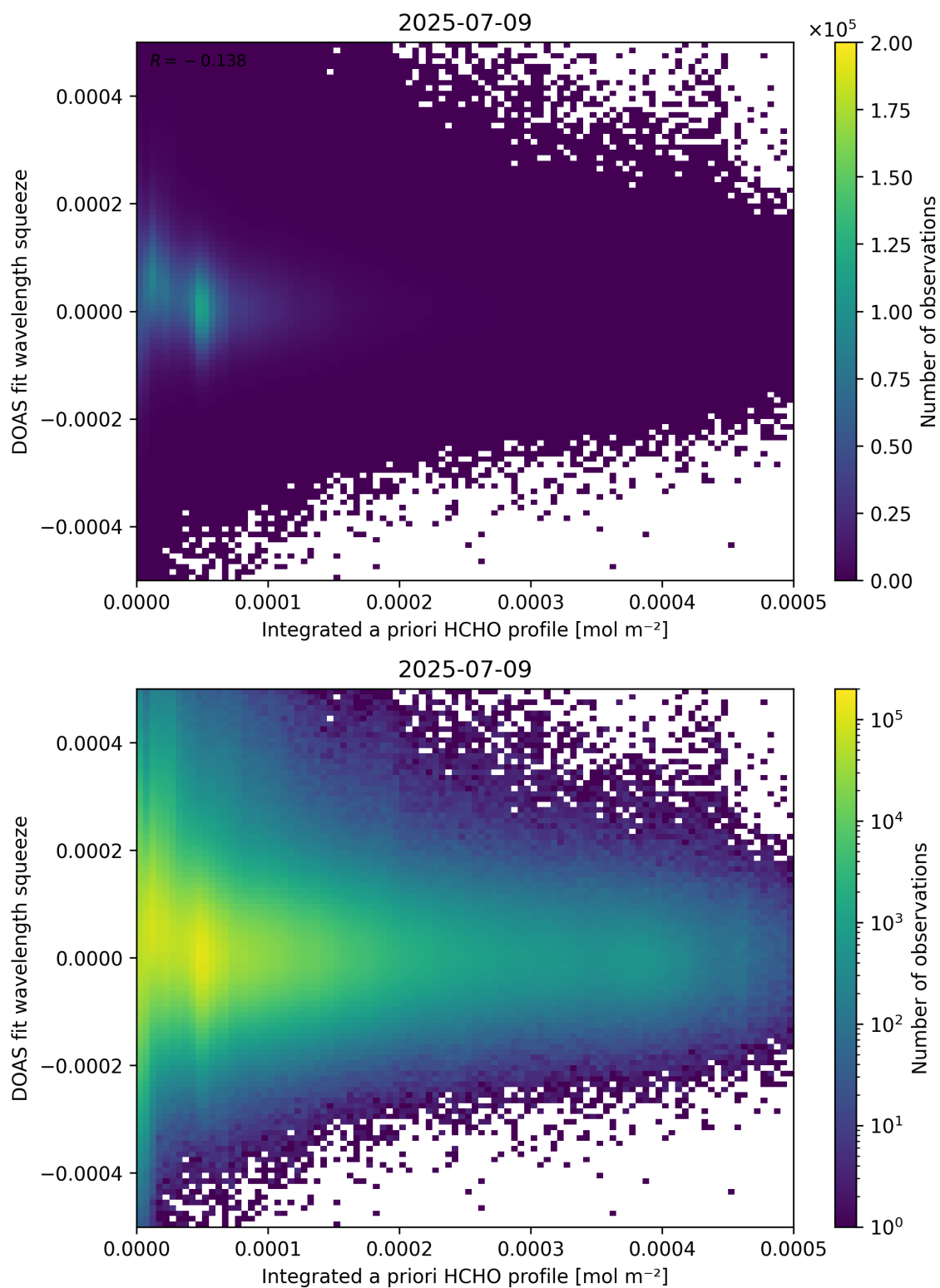
Figure 150: Scatter density plot of “Integrated a priori HCHO profile” against “DOAS fit wavelength squeeze” for 2025-07-08 to 2025-07-10.
