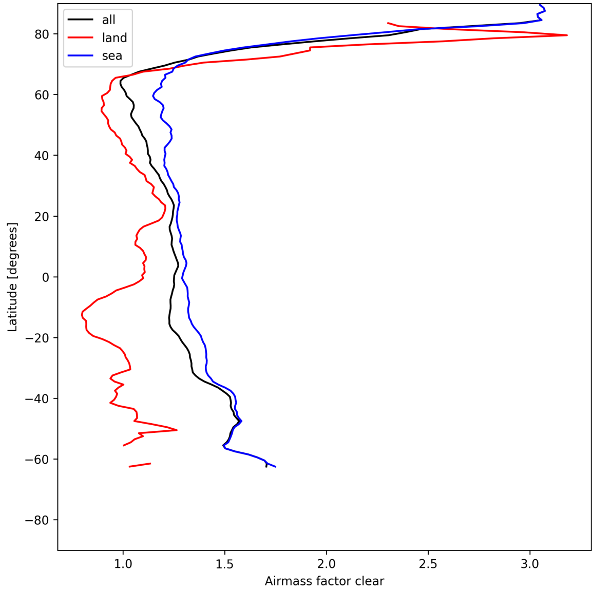
Figure 28: Zonal average of “Airmass factor clear” for 2025-07-08 to 2025-07-10.
