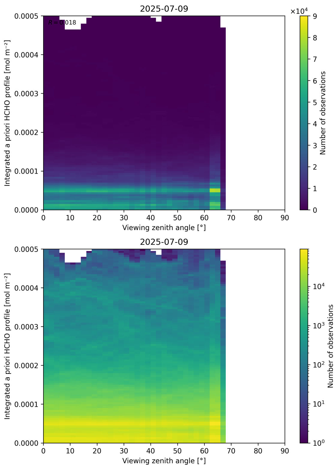
Figure 195: Scatter density plot of “Viewing zenith angle” against “Integrated a priori HCHO profile” for 2025-07-08 to 2025-07-10.
