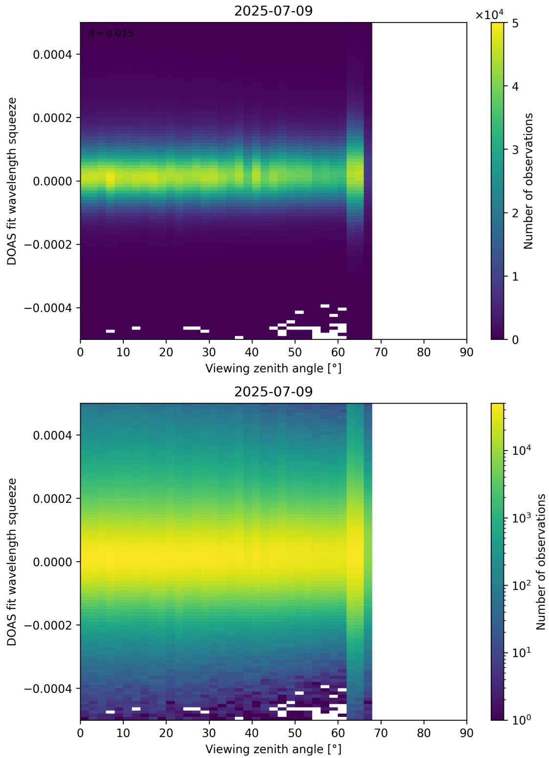
Figure 184: Scatter density plot of “Viewing zenith angle” against “DOAS fit wavelength squeeze” for 2025-07-08 to 2025-07-10.
