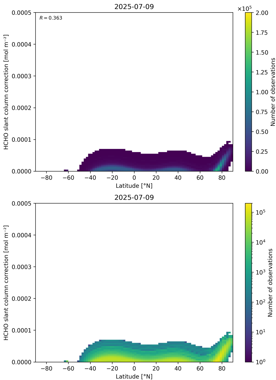
Figure 158: Scatter density plot of “Latitude” against “HCHO slant column correction” for 2025-07-08 to 2025-07-10.
