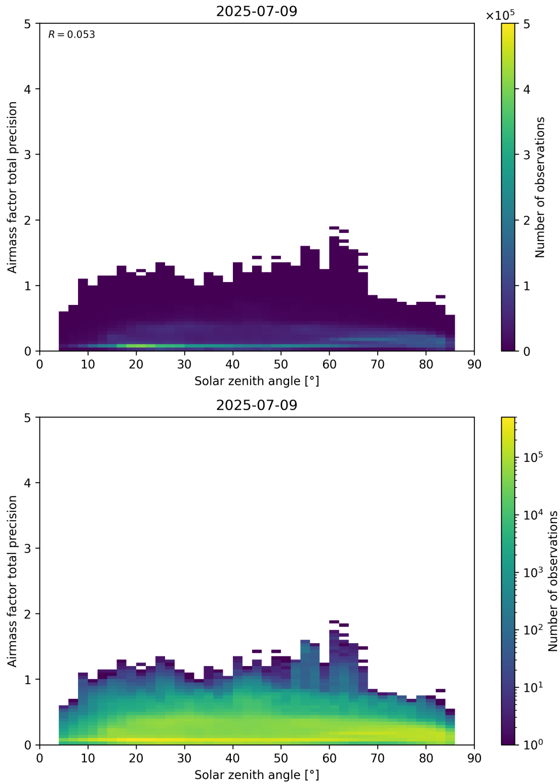
Figure 176: Scatter density plot of “Solar zenith angle” against “Airmass factor total precision” for 2025-07-08 to 2025-07-10.
