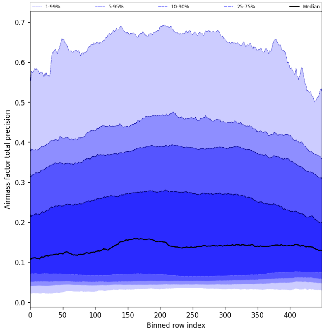
Figure 55: Along track statistics of “Airmass factor total precision” for 2025-07-08 to 2025-07-10
