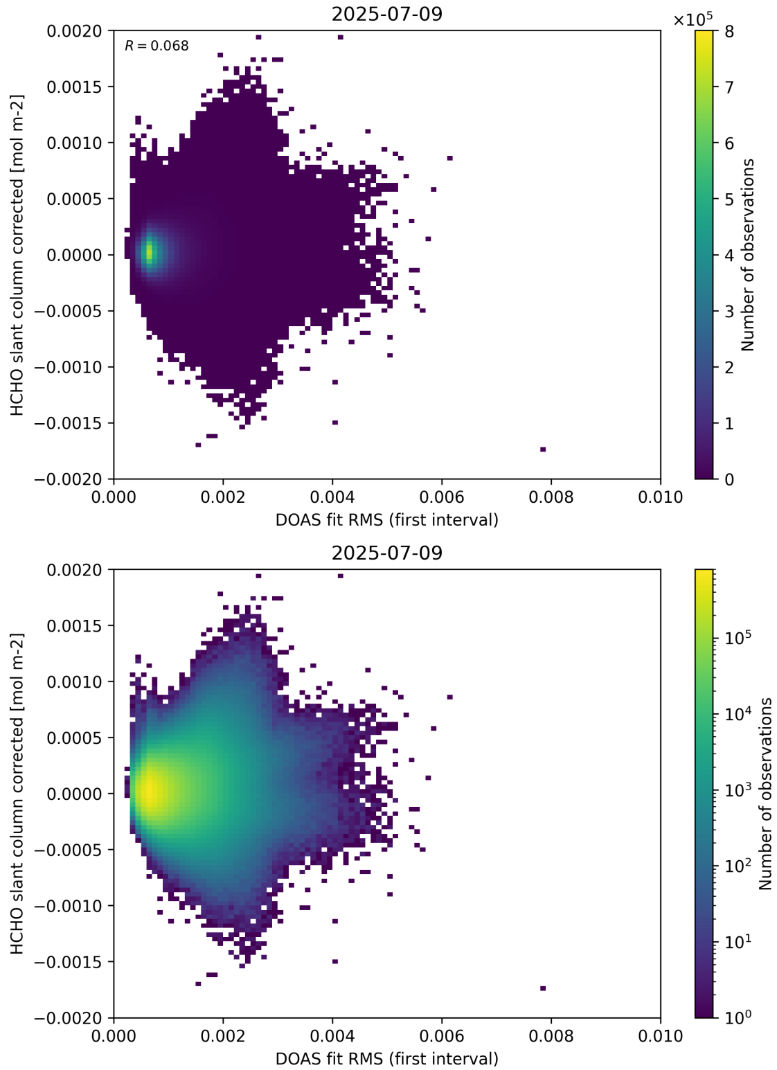
Figure 62: Scatter density plot of “DOAS fit RMS (first interval)” against “HCHO slant column corrected” for 2025-07-08 to 2025-07-10.
