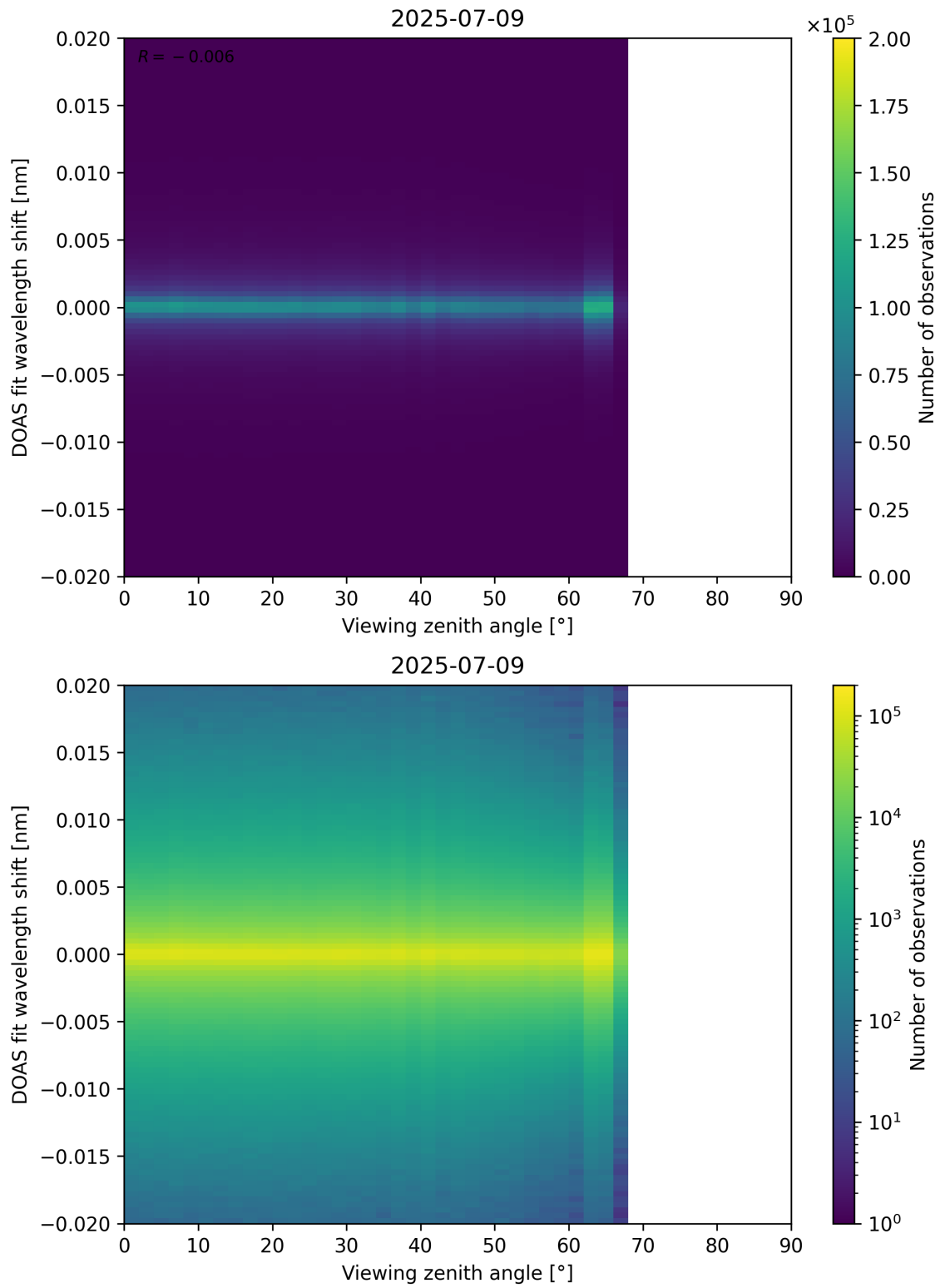
Figure 183: Scatter density plot of “Viewing zenith angle” against “DOAS fit wavelength shift” for 2025-07-08 to 2025-07-10.
