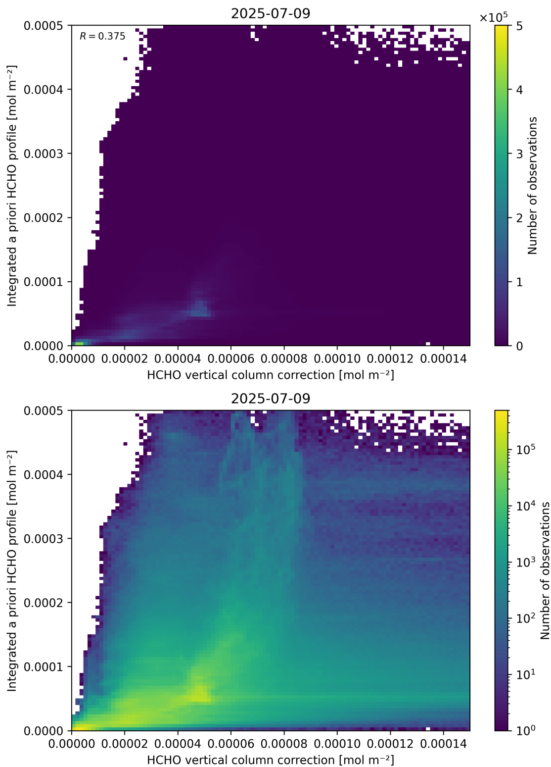
Figure 122: Scatter density plot of “HCHO vertical column correction” against “Integrated a priori HCHO profile” for 2025-07-08 to 2025-07-10.
