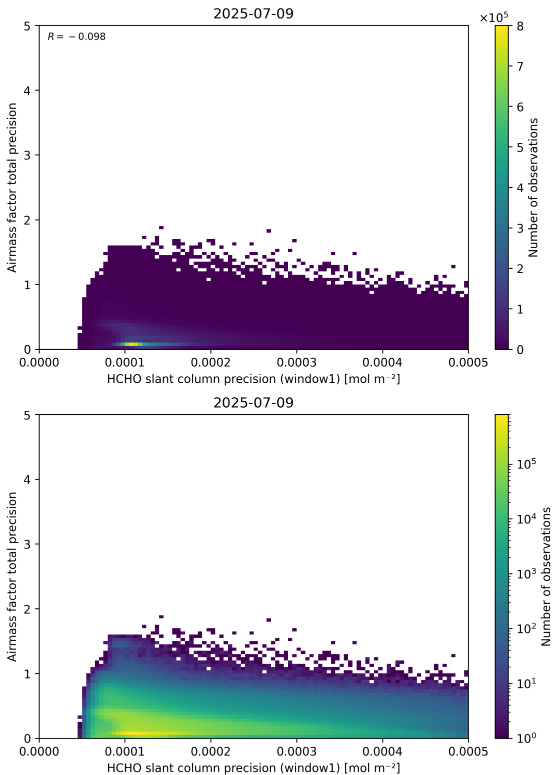
Figure 95: Scatter density plot of “HCHO slant column precision (window1)” against “Airmass factor total precision” for 2025-07-08 to 2025-07-10.
