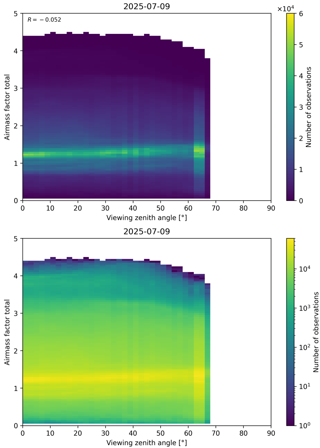
Figure 190: Scatter density plot of “Viewing zenith angle” against “Airmass factor total” for 2025-07-08 to 2025-07-10.
