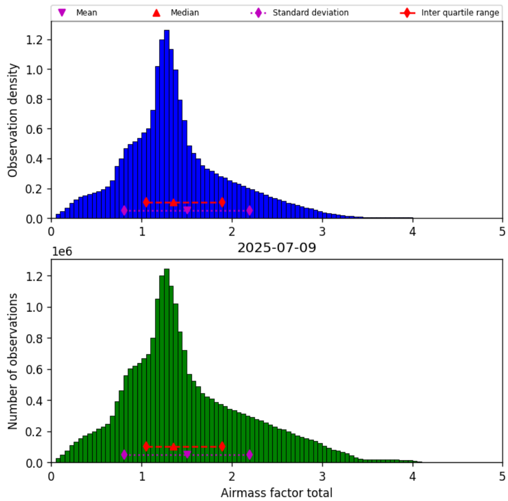
Figure 40: Histogram of “Airmass factor total” for 2025-07-08 to 2025-07-10
