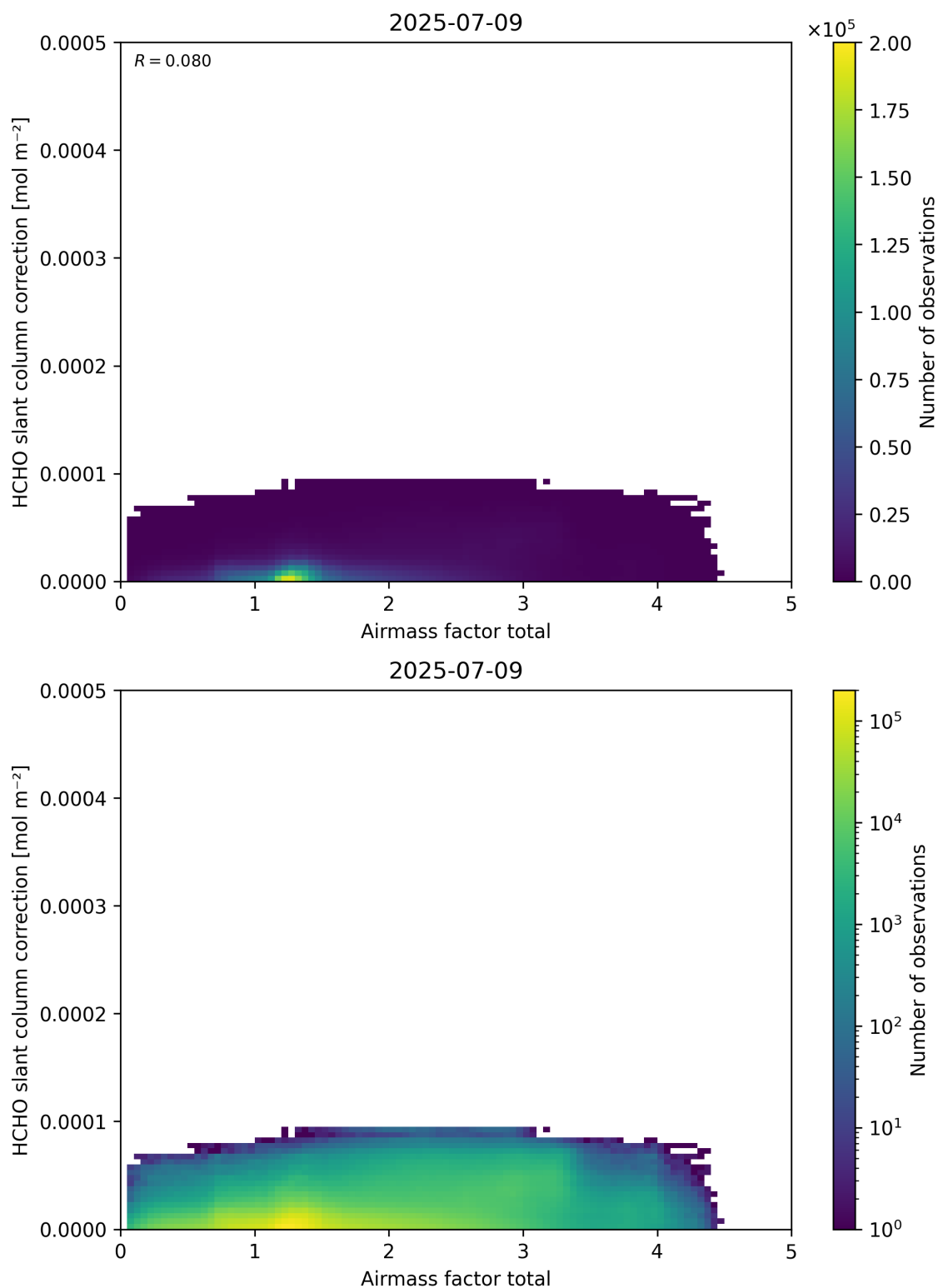
Figure 102: Scatter density plot of “Airmass factor total” against “HCHO slant column correction” for 2025-07-08 to 2025-07-10.
