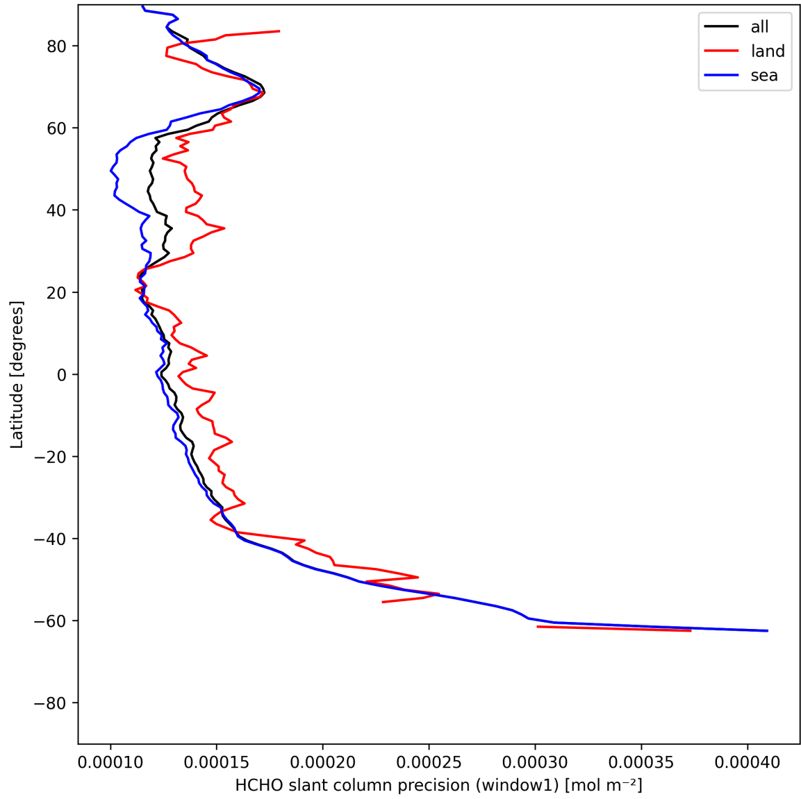
Figure 25: Zonal average of “HCHO slant column precision (window1)” for 2025-07-08 to 2025-07-10.
