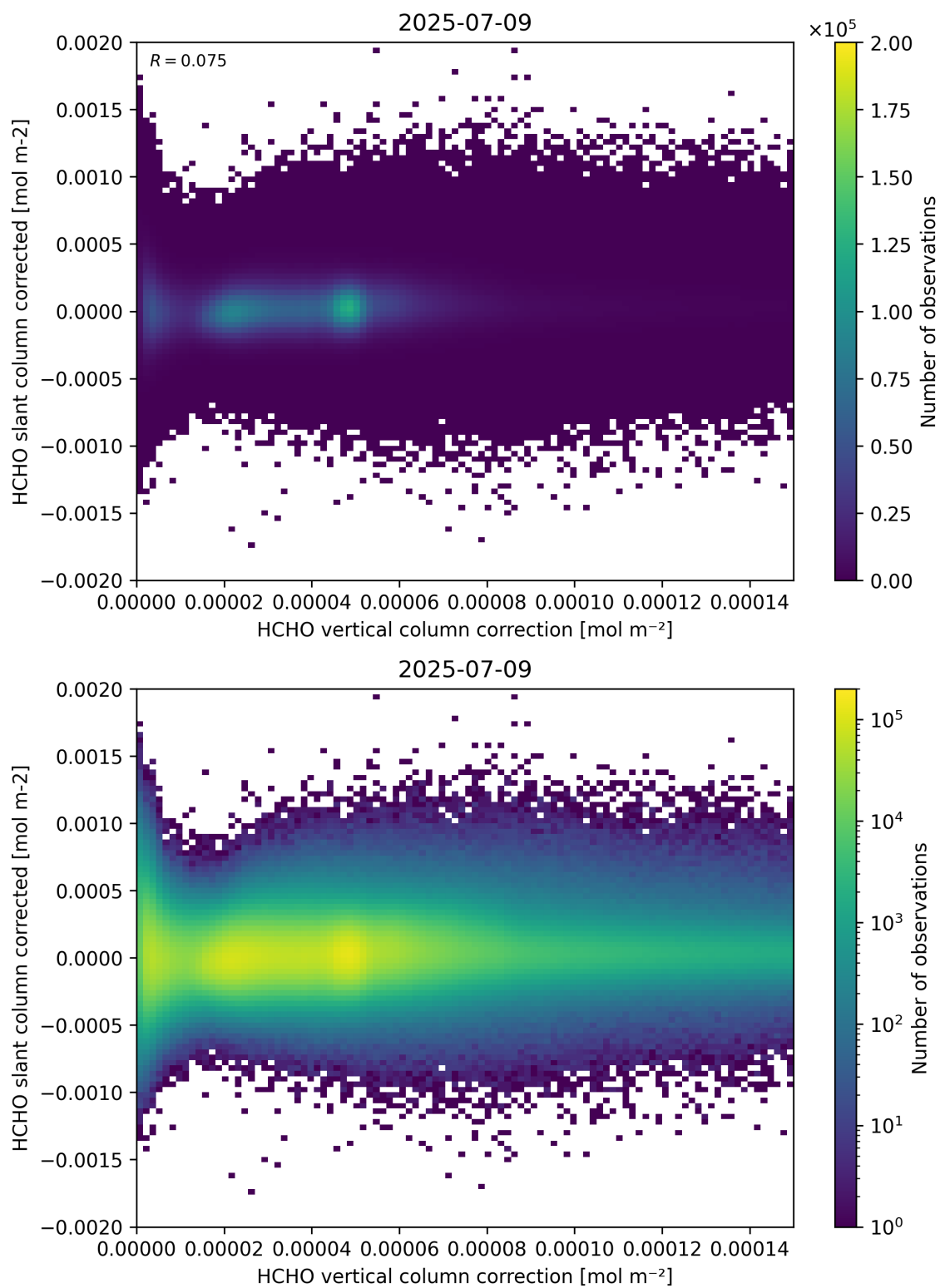
Figure 116: Scatter density plot of “HCHO vertical column correction” against “HCHO slant column corrected” for 2025-07-08 to 2025-07-10.
