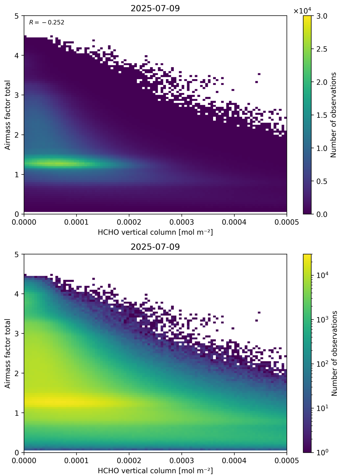
Figure 131: Scatter density plot of “HCHO vertical column” against “Airmass factor total” for 2025-07-08 to 2025-07-10.
