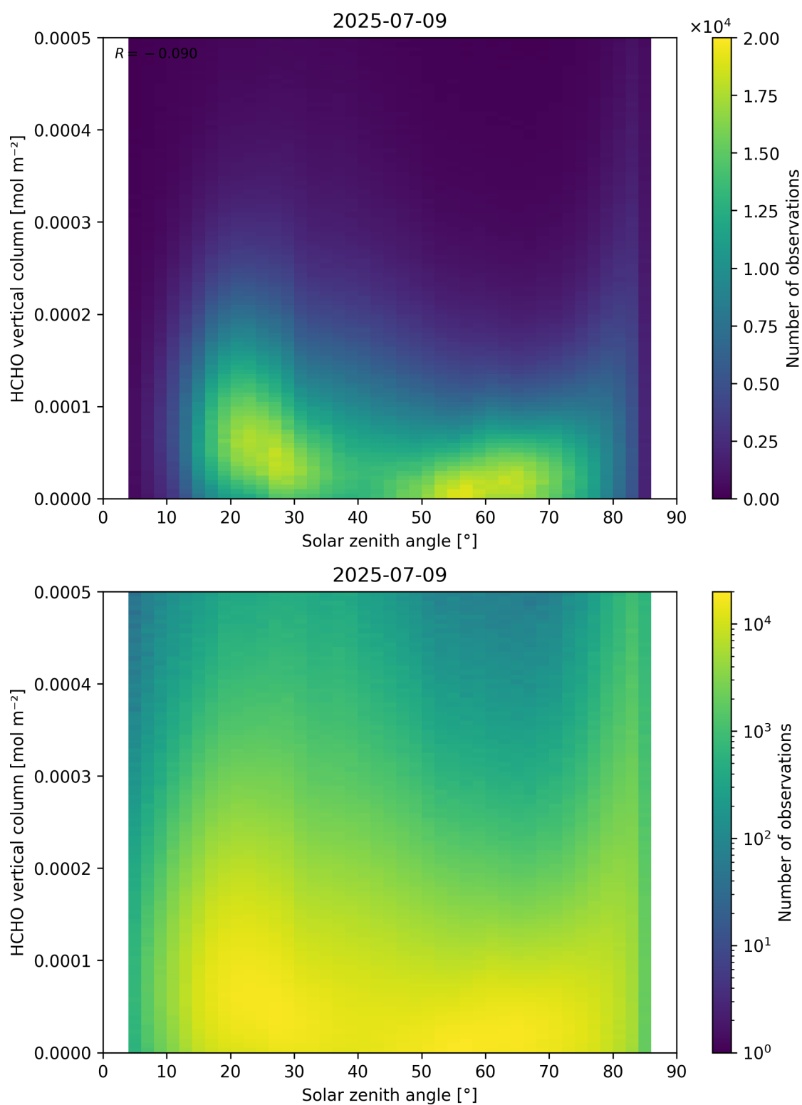
Figure 177: Scatter density plot of “Solar zenith angle” against “HCHO vertical column” for 2025-07-08 to 2025-07-10.
