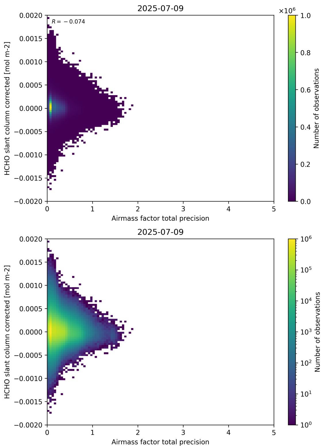
Figure 109: Scatter density plot of “Airmass factor total precision” against “HCHO slant column corrected” for 2025-07-08 to 2025-07-10.
