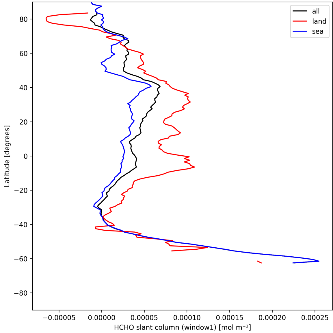
Figure 24: Zonal average of “HCHO slant column (window1)” for 2025-07-08 to 2025-07-10.
