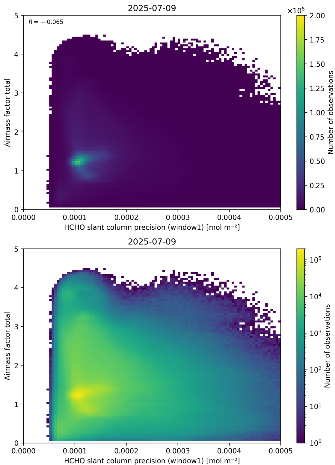
Figure 94: Scatter density plot of “HCHO slant column precision (window1)” against “Airmass factor total” for 2025-07-08 to 2025-07-10.
