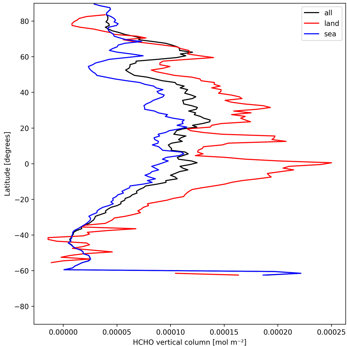
Figure 21: Zonal average of “HCHO vertical column” for 2025-07-08 to 2025-07-10.
