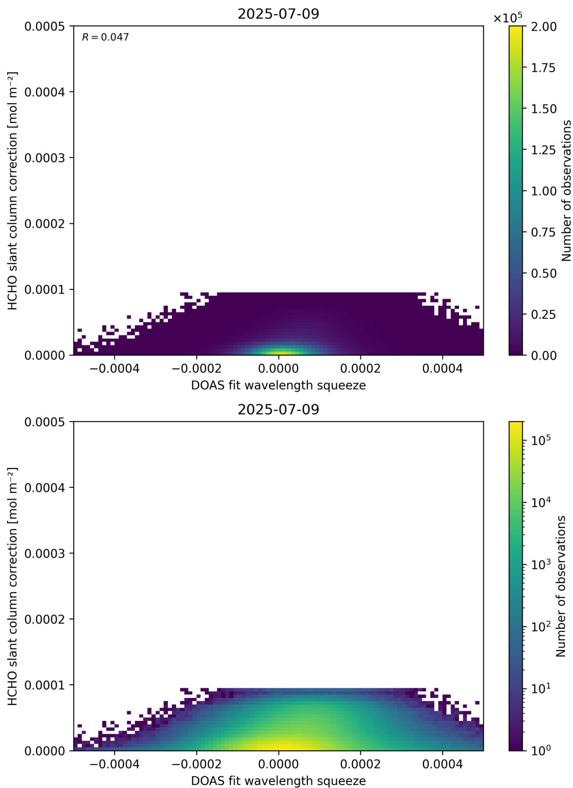
Figure 70: Scatter density plot of “DOAS fit wavelength squeeze” against “HCHO slant column correction” for 2025-07-08 to 2025-07-10.
