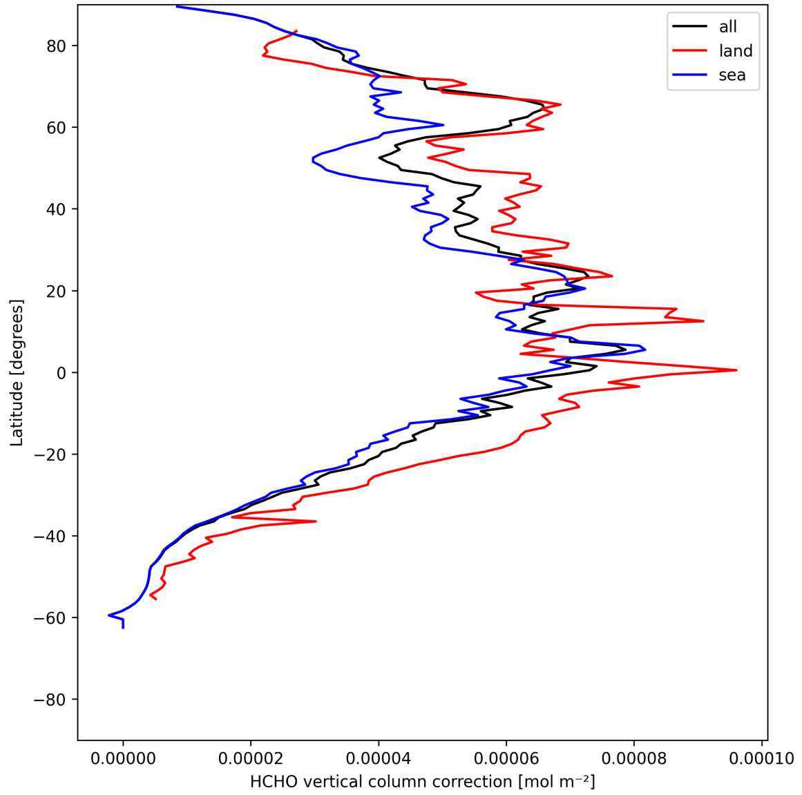
Figure 23: Zonal average of “HCHO vertical column correction” for 2025-07-08 to 2025-07-10.
