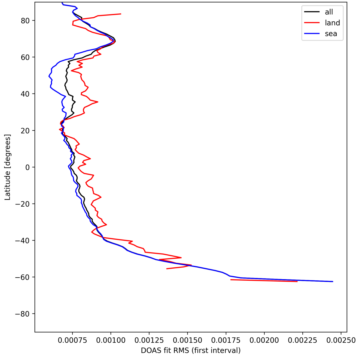
Figure 32: Zonal average of “DOAS fit RMS (first interval)” for 2025-07-08 to 2025-07-10.
