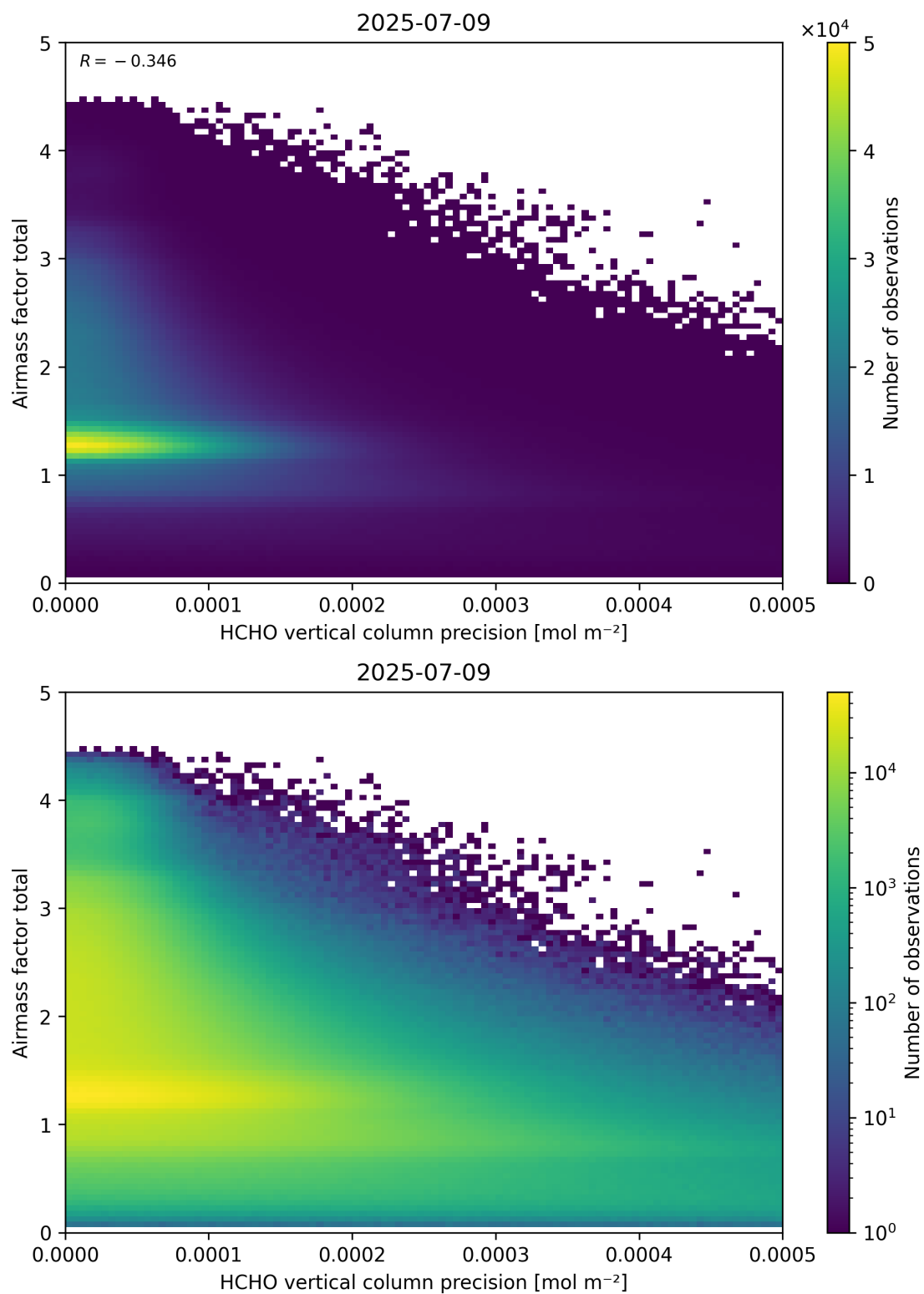
Figure 144: Scatter density plot of “HCHO vertical column precision” against “Airmass factor total” for 2025-07-08 to 2025-07-10.
