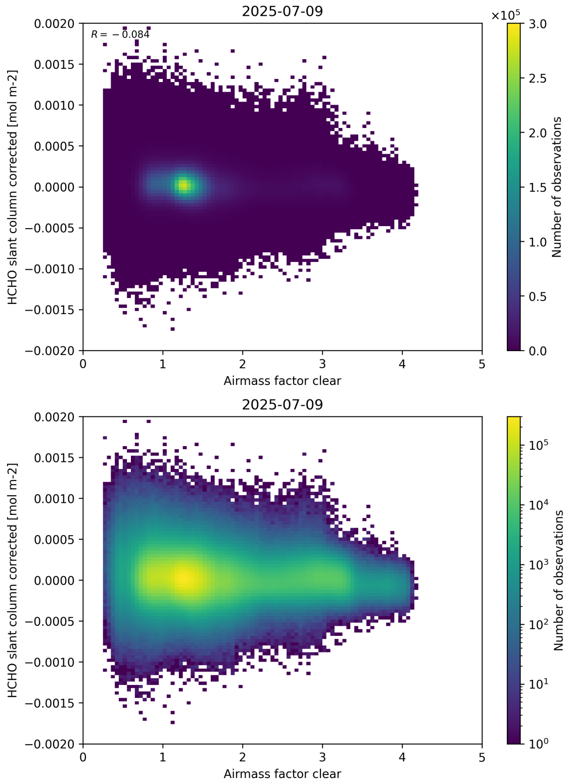
Figure 74: Scatter density plot of “Airmass factor clear” against “HCHO slant column corrected” for 2025-07-08 to 2025-07-10.
