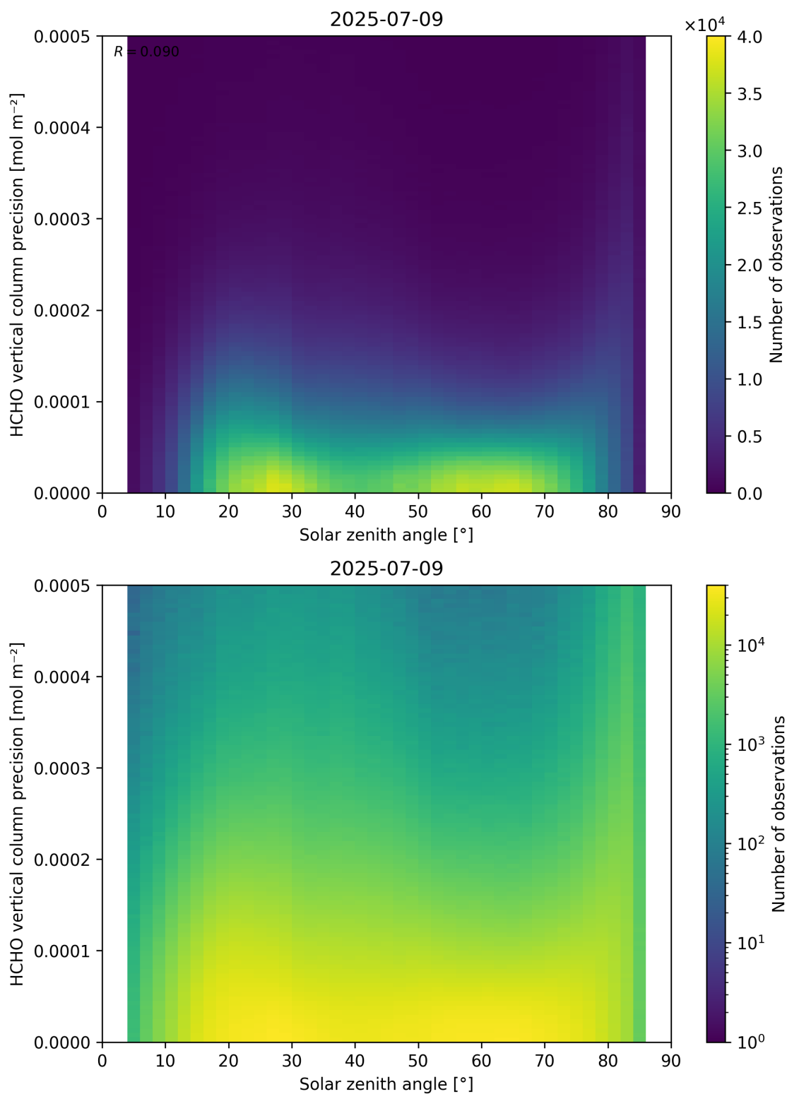
Figure 179: Scatter density plot of “Solar zenith angle” against “HCHO vertical column precision” for 2025-07-08 to 2025-07-10.
