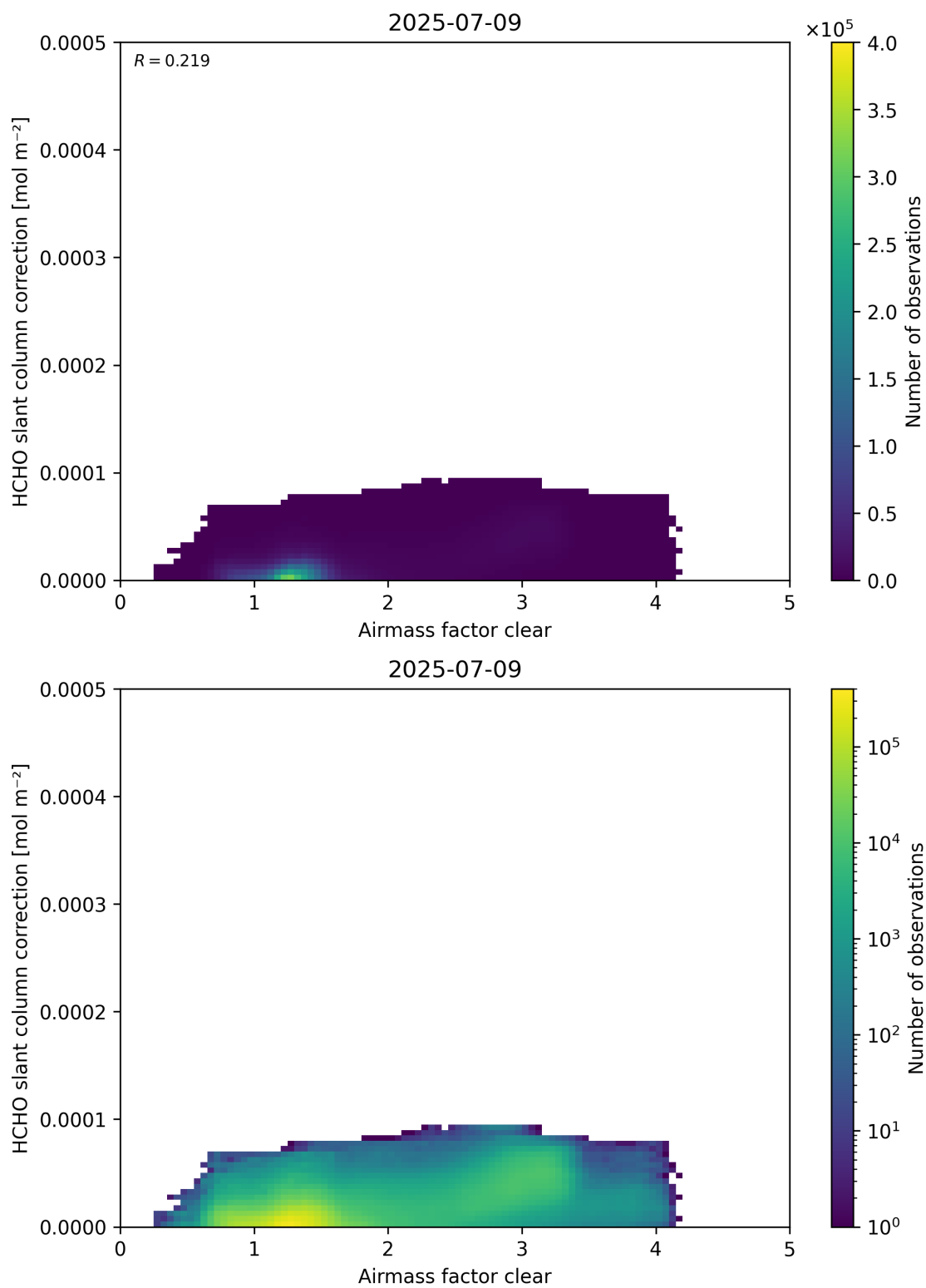
Figure 75: Scatter density plot of “Air mass factor clear” against “HCHO slant column correction” for 2025-07-08 to 2025-07-10.
