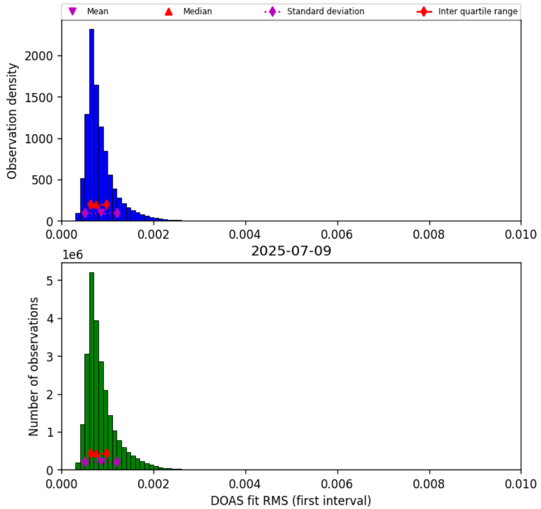
Figure 46: Histogram of “DOAS fit RMS (first interval)” for 2025-07-08 to 2025-07-10
