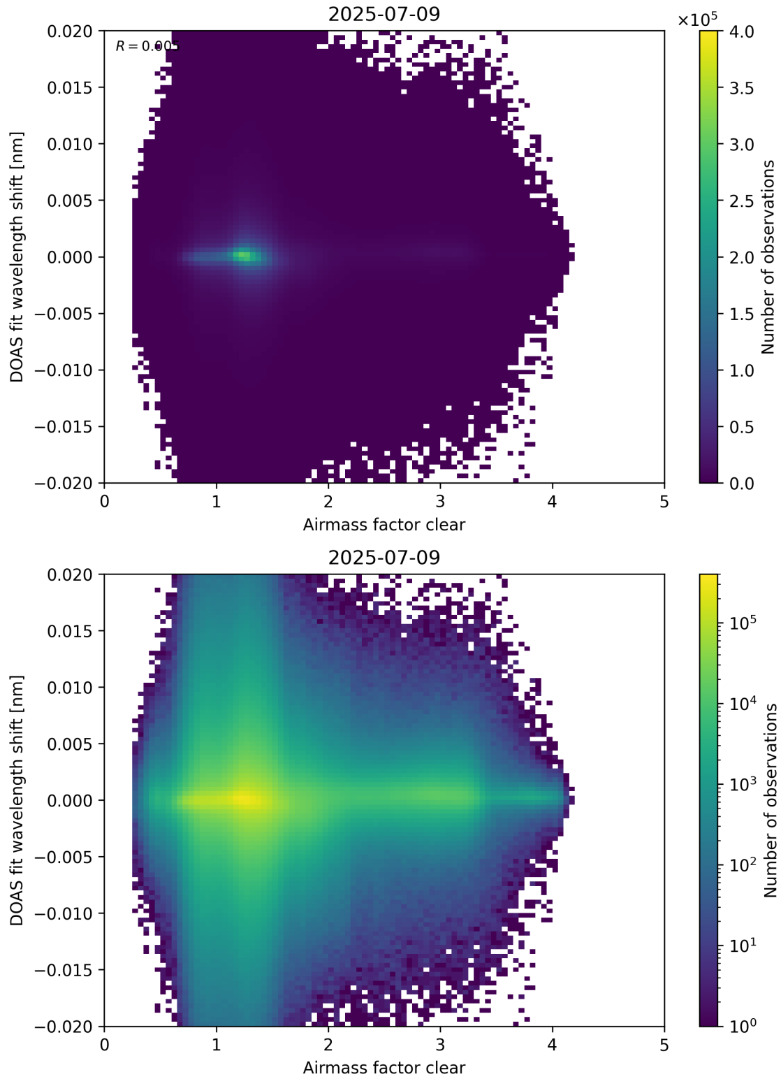
Figure 72: Scatter density plot of “Airmass factor clear” against “DOAS fit wavelength shift” for 2025-07-08 to 2025-07-10.
