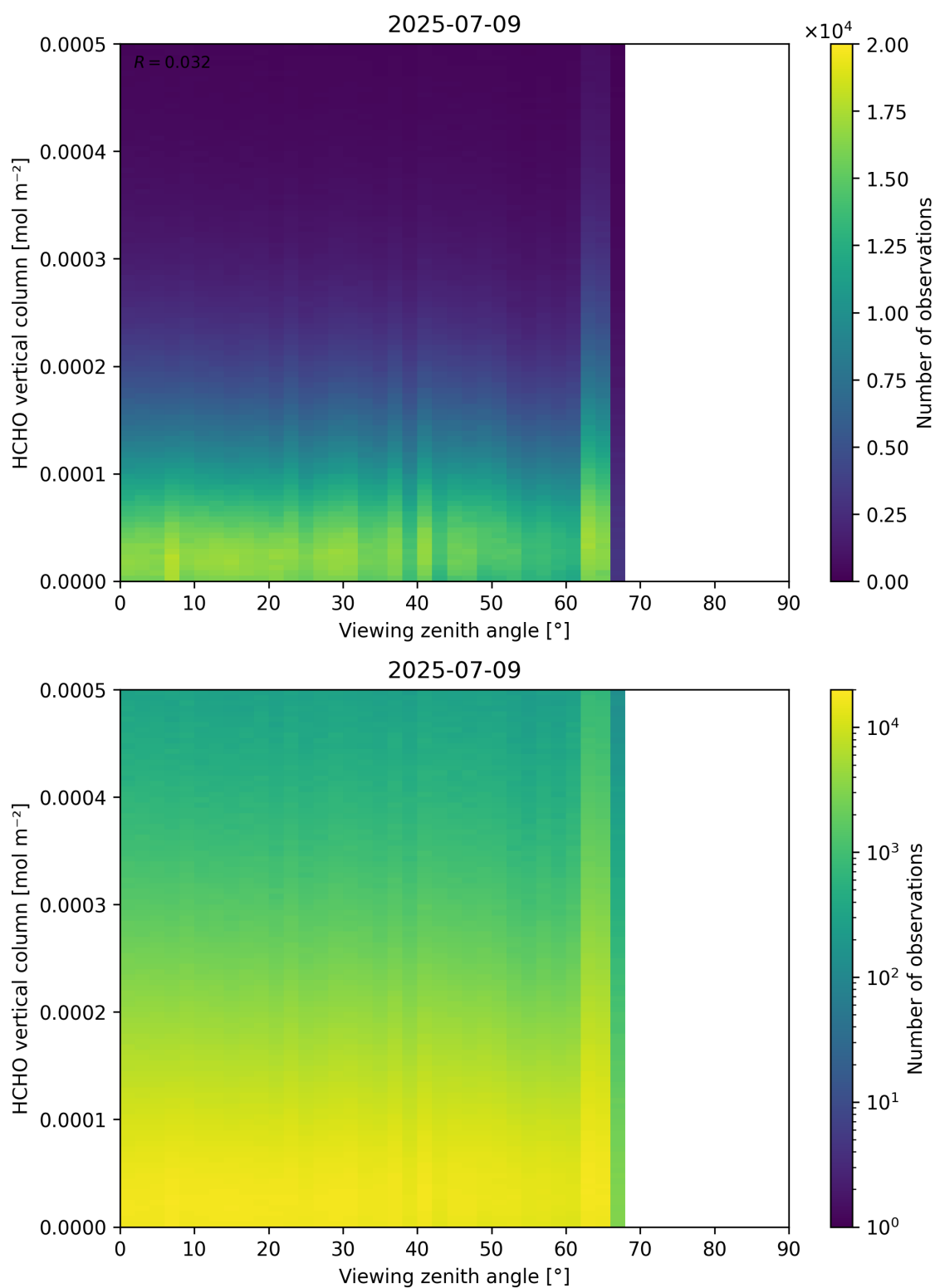
Figure 192: Scatter density plot of “Viewing zenith angle” against “HCHO vertical column” for 2025-07-08 to 2025-07-10.
