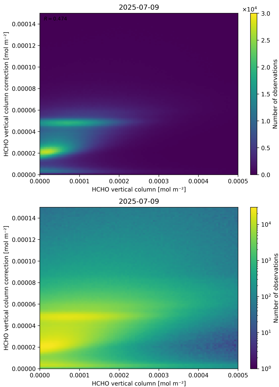
Figure 133: Scatter density plot of “HCHO vertical column” against “HCHO vertical column correction” for 2025-07-08 to 2025-07-10.
