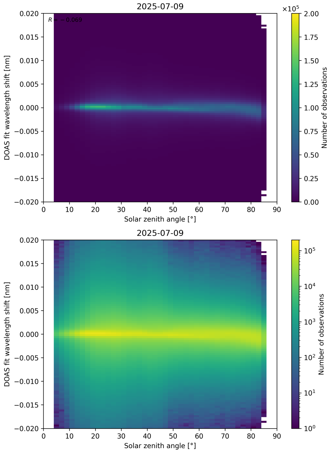
Figure 168: Scatter density plot of “Solar zenith angle” against “DOAS fit wavelength shift” for 2025-07-08 to 2025-07-10.
