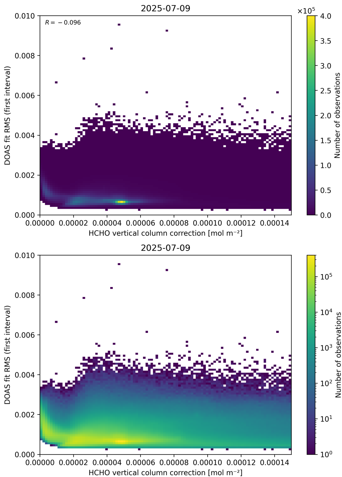
Figure 112: Scatter density plot of “HCHO vertical column correction” against “DOAS fit RMS (first interval)” for 2025-07-08 to 2025-07-10.
