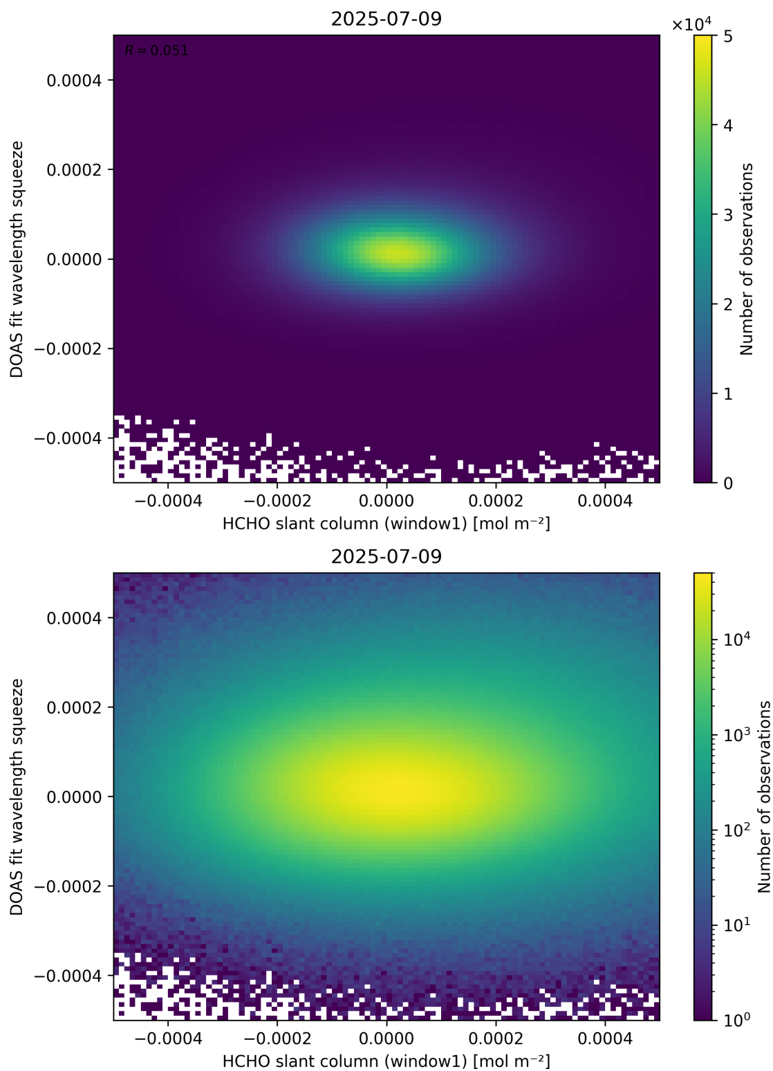
Figure 80: Scatter density plot of “HCHO slant column (window1)” against “DOAS fit wavelength squeeze” for 2025-07-08 to 2025-07-10.
