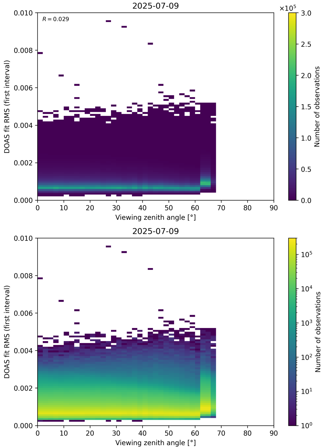
Figure 182: Scatter density plot of “Viewing zenith angle” against “DOAS fit RMS (first interval)” for 2025-07-08 to 2025-07-10.
