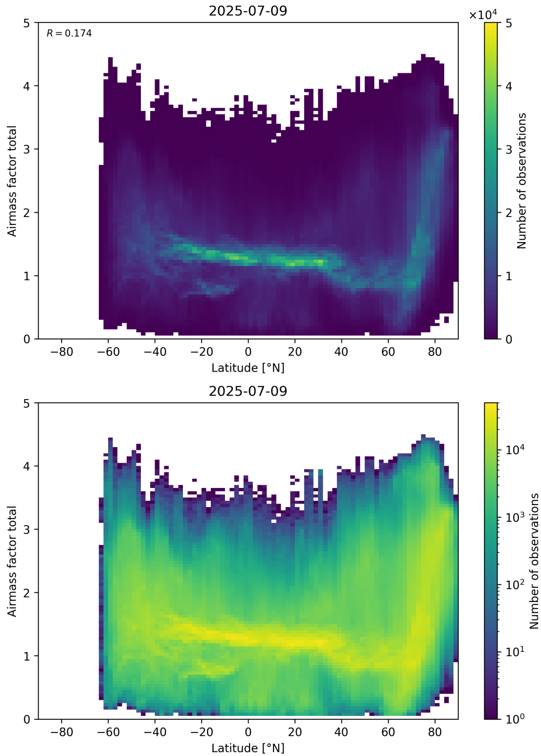
Figure 161: Scatter density plot of “Latitude” against “Airmass factor total” for 2025-07-08 to 2025-07-10.
