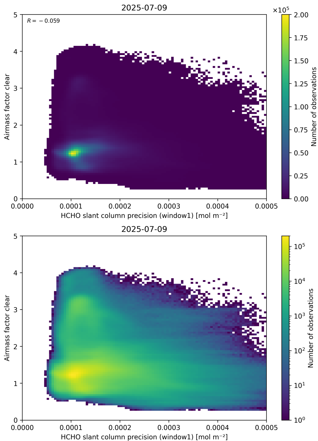
Figure 91: Scatter density plot of “HCHO slant column precision (window1)” against “Airmass factor clear” for 2025-07-08 to 2025-07-10.
