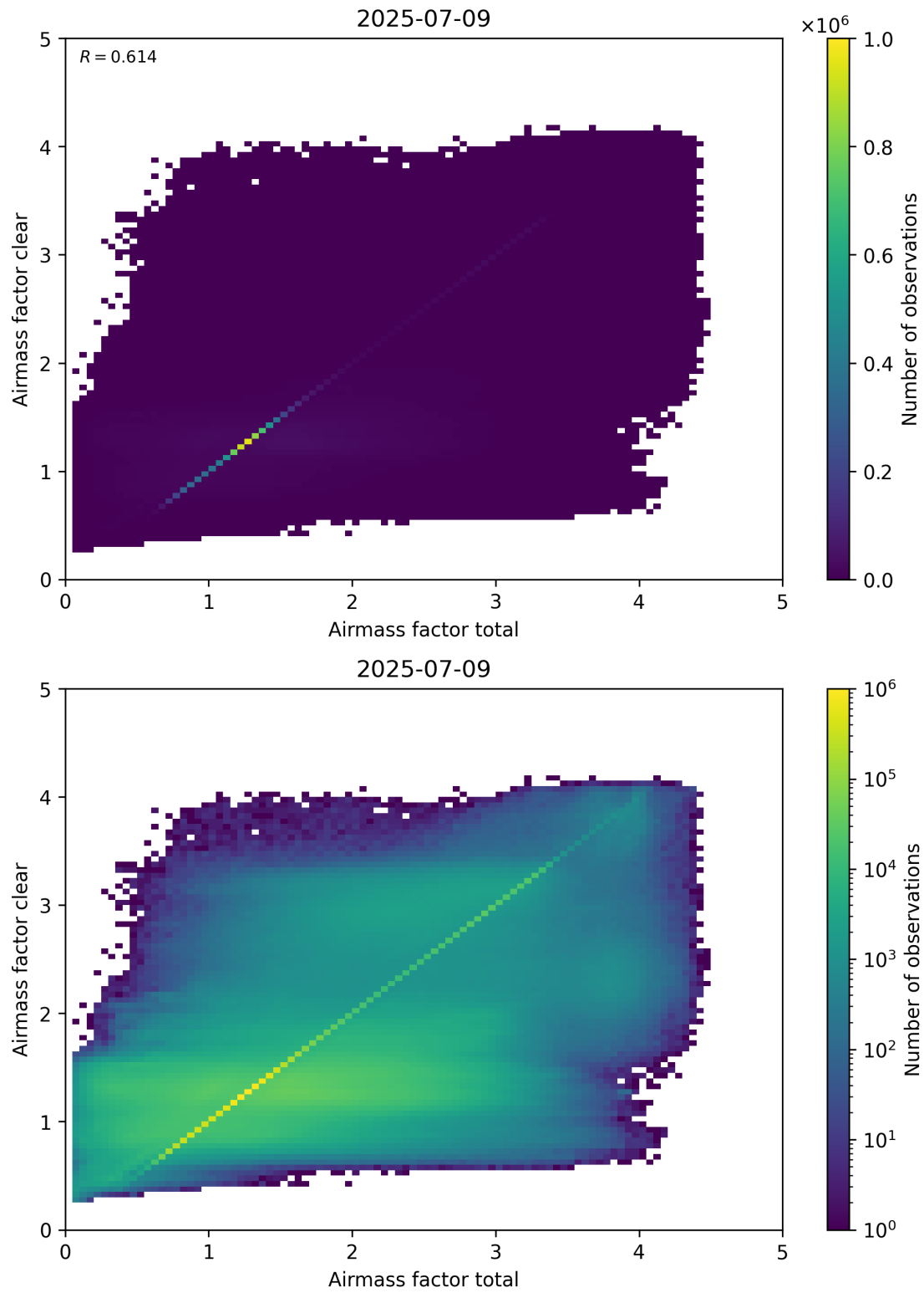
Figure 100: Scatter density plot of “Airmass factor total” against “Airmass factor clear” for 2025-07-08 to 2025-07-10.
