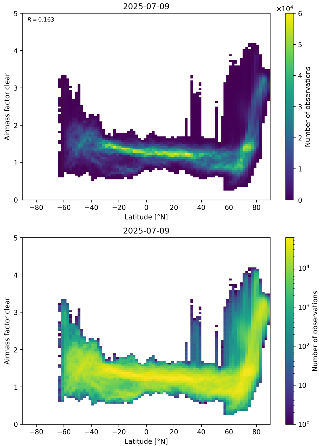
Figure 156: Scatter density plot of “Latitude” against “Airmass factor clear” for 2025-07-08 to 2025-07-10.
