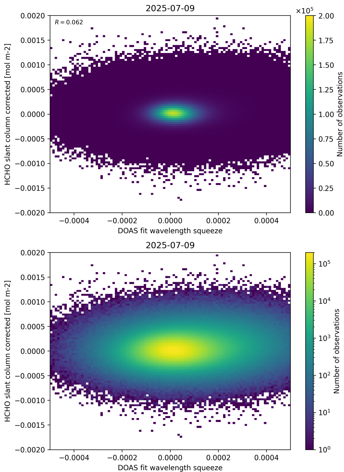
Figure 69: Scatter density plot of “DOAS fit wavelength squeeze” against “HCHO slant column corrected” for 2025-07-08 to 2025-07-10.
