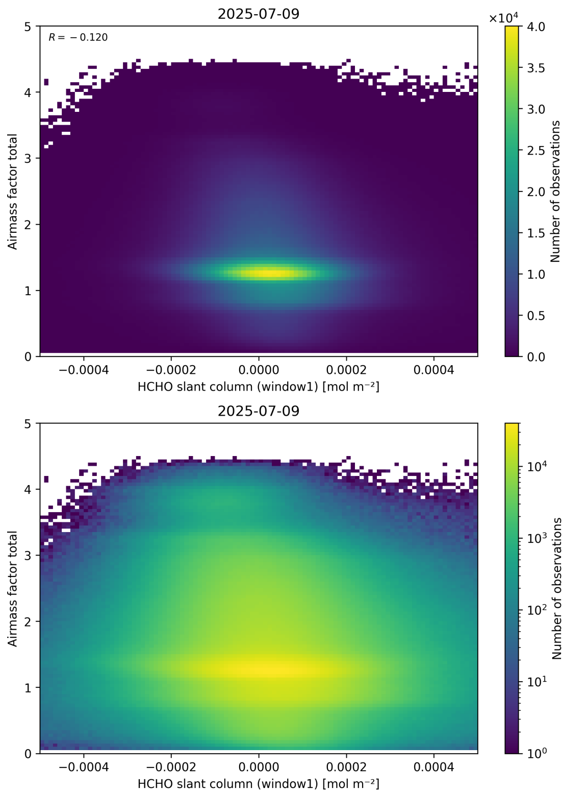
Figure 85: Scatter density plot of “HCHO slant column (window1)” against “Airmass factor total” for 2025-07-08 to 2025-07-10.
