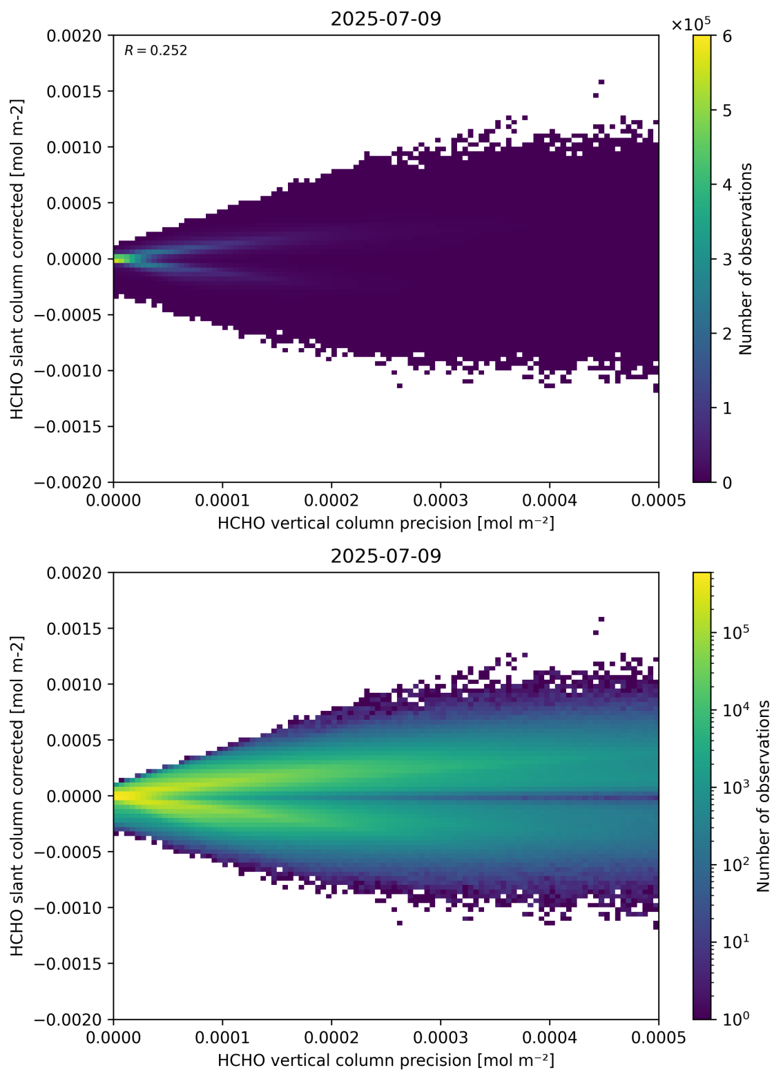
Figure 140: Scatter density plot of “HCHO vertical column precision” against “HCHO slant column corrected” for 2025-07-08 to 2025-07-10.
