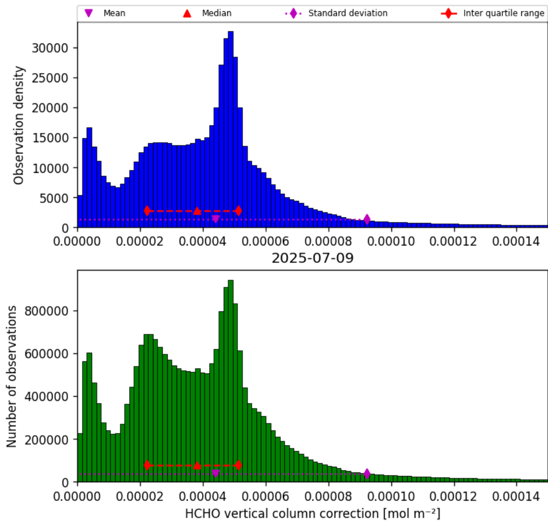
Figure 37: Histogram of “HCHO vertical column correction” for 2025-07-08 to 2025-07-10
