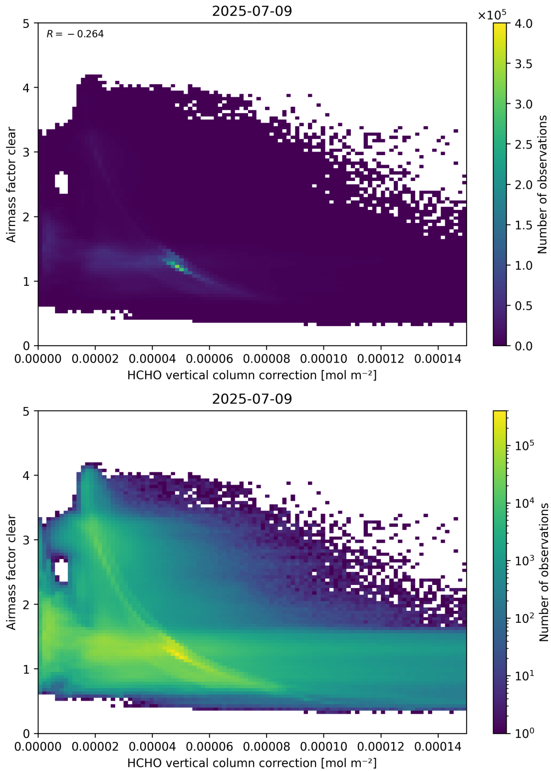
Figure 115: Scatter density plot of “HCHO vertical column correction” against “Airmass factor clear” for 2025-07-08 to 2025-07-10.
