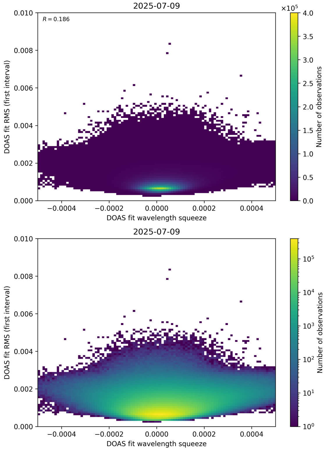
Figure 68: Scatter density plot of “DOAS fit wavelength squeeze” against “DOAS fit RMS (first interval)” for 2025-07-08 to 2025-07-10.
