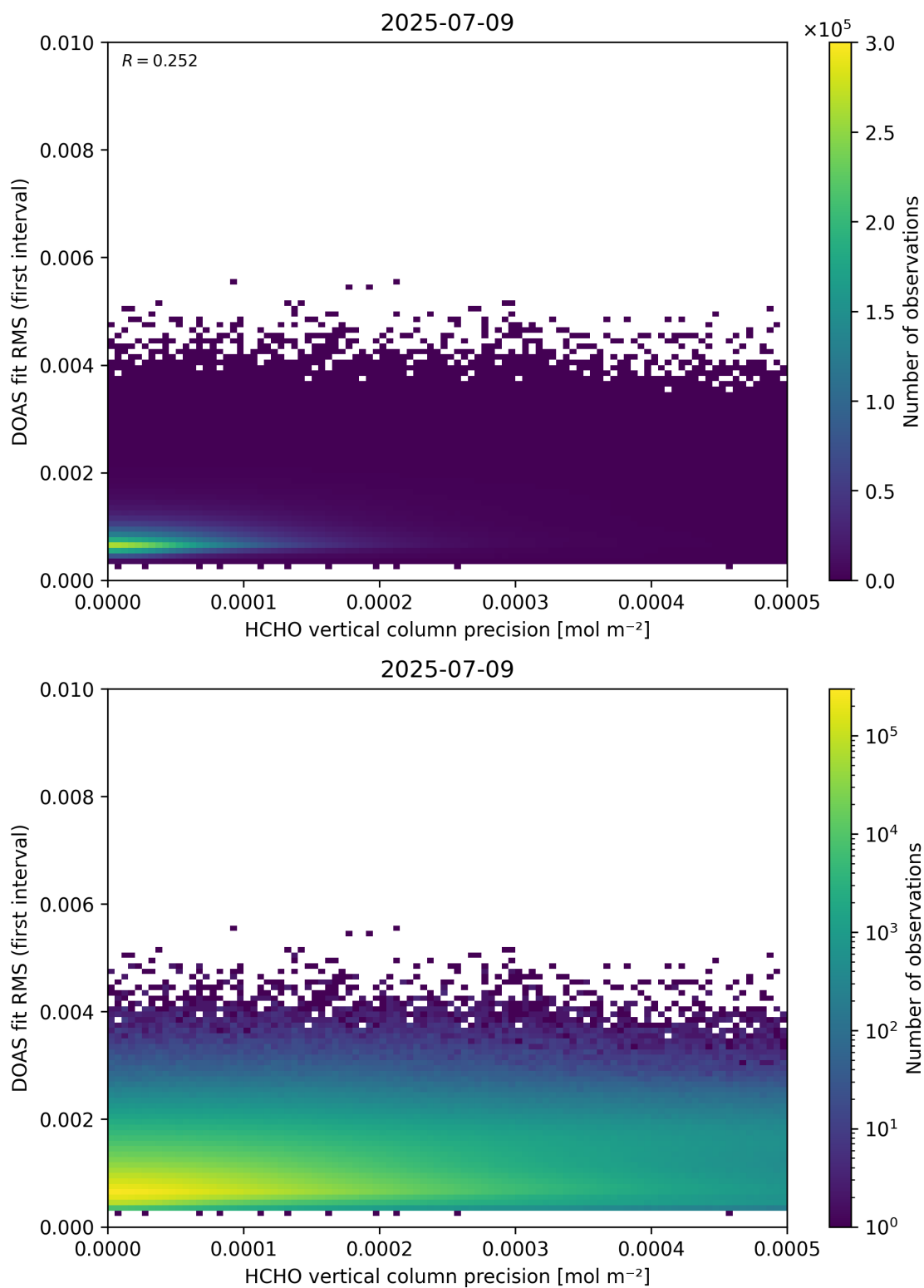
Figure 136: Scatter density plot of “HCHO vertical column precision” against “DOAS fit RMS (first interval)” for 2025-07-08 to 2025-07-10.
