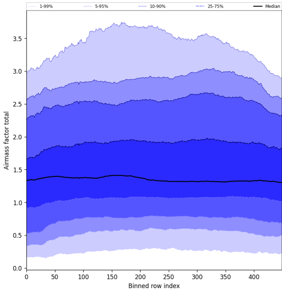
Figure 54: Along track statistics of “Airmass factor total” for 2025-07-08 to 2025-07-10
