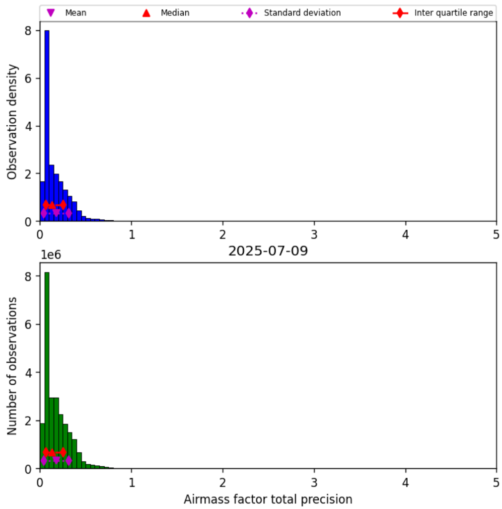
Figure 41: Histogram of “Airmass factor total precision” for 2025-07-08 to 2025-07-10
