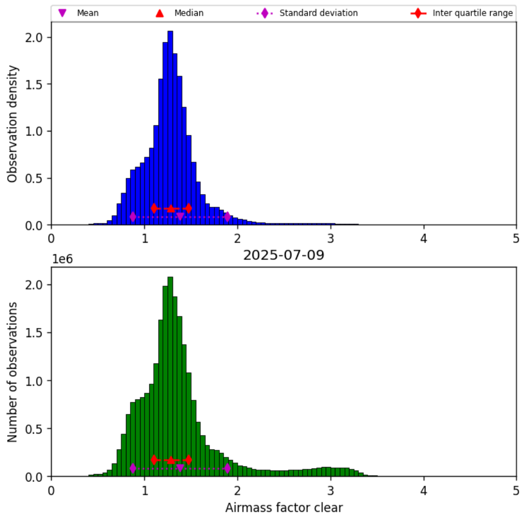
Figure 42: Histogram of “Airmass factor clear” for 2025-07-08 to 2025-07-10
