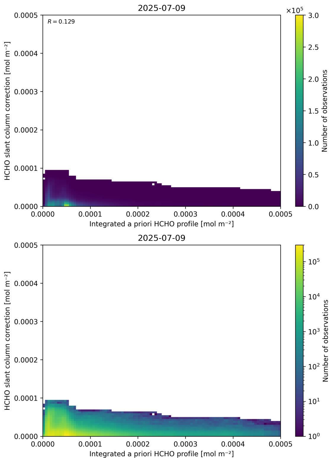
Figure 152: Scatter density plot of “Integrated a priori HCHO profile” against “HCHO slant column correction” for 2025-07-08 to 2025-07-10.
