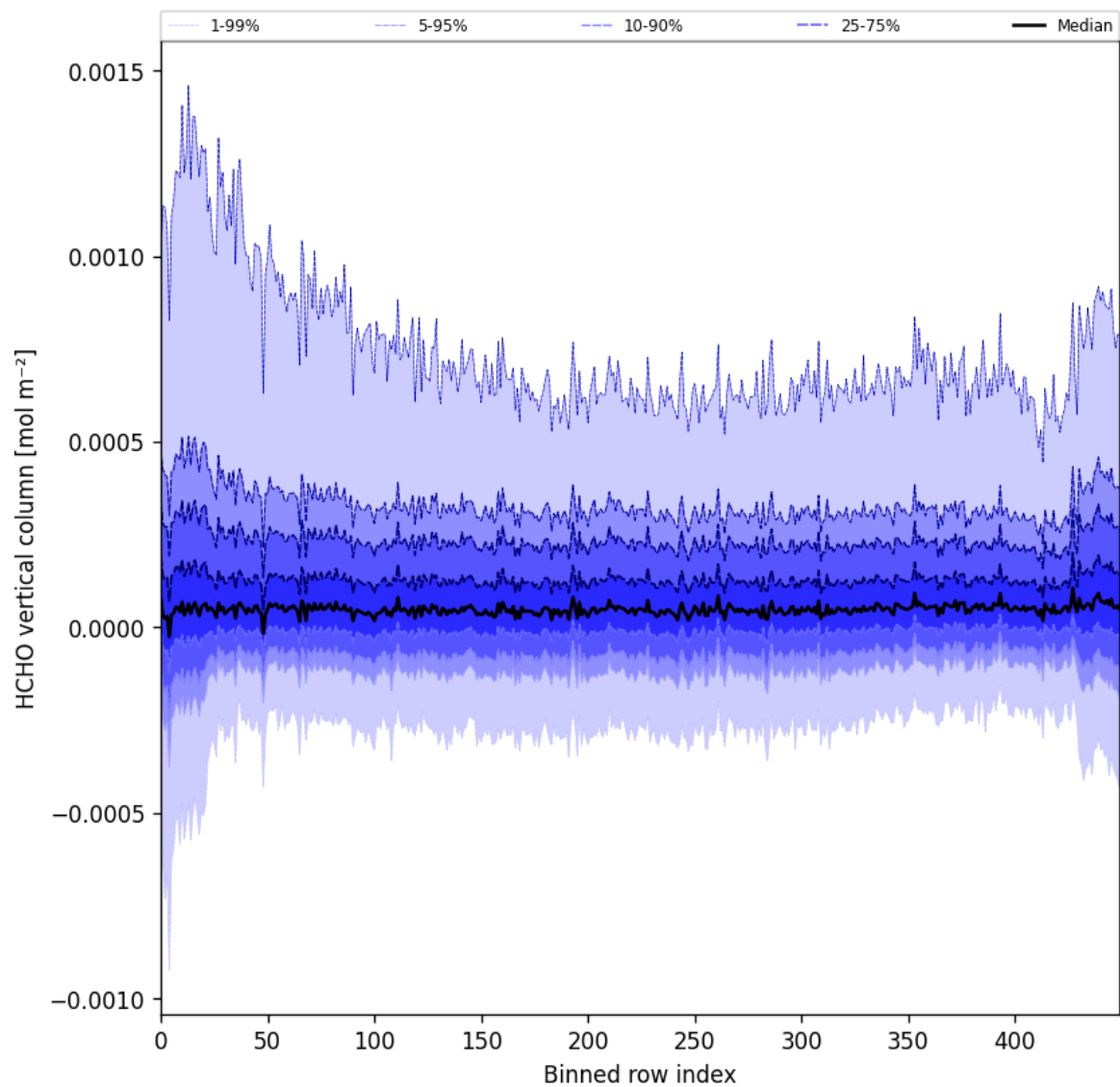
Figure 49: Along track statistics of “HCHO vertical column” for 2025-07-08 to 2025-07-10
