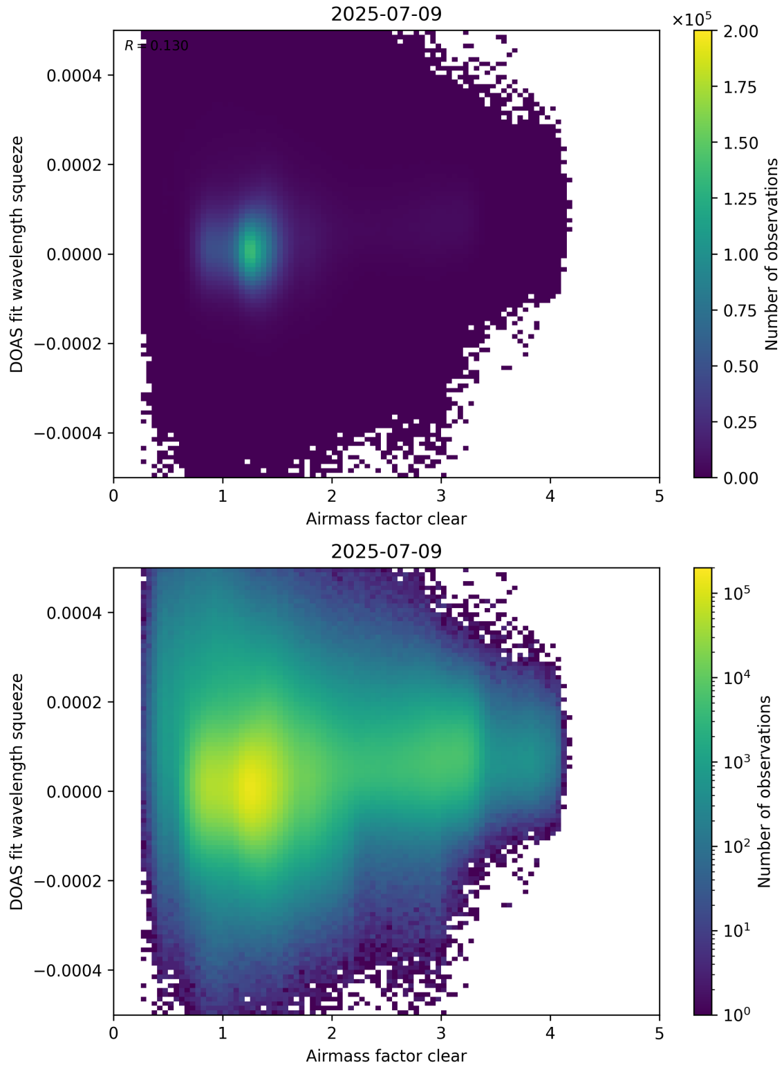
Figure 73: Scatter density plot of “Airmass factor clear” against “DOAS fit wavelength squeeze” for 2025-07-08 to 2025-07-10.
