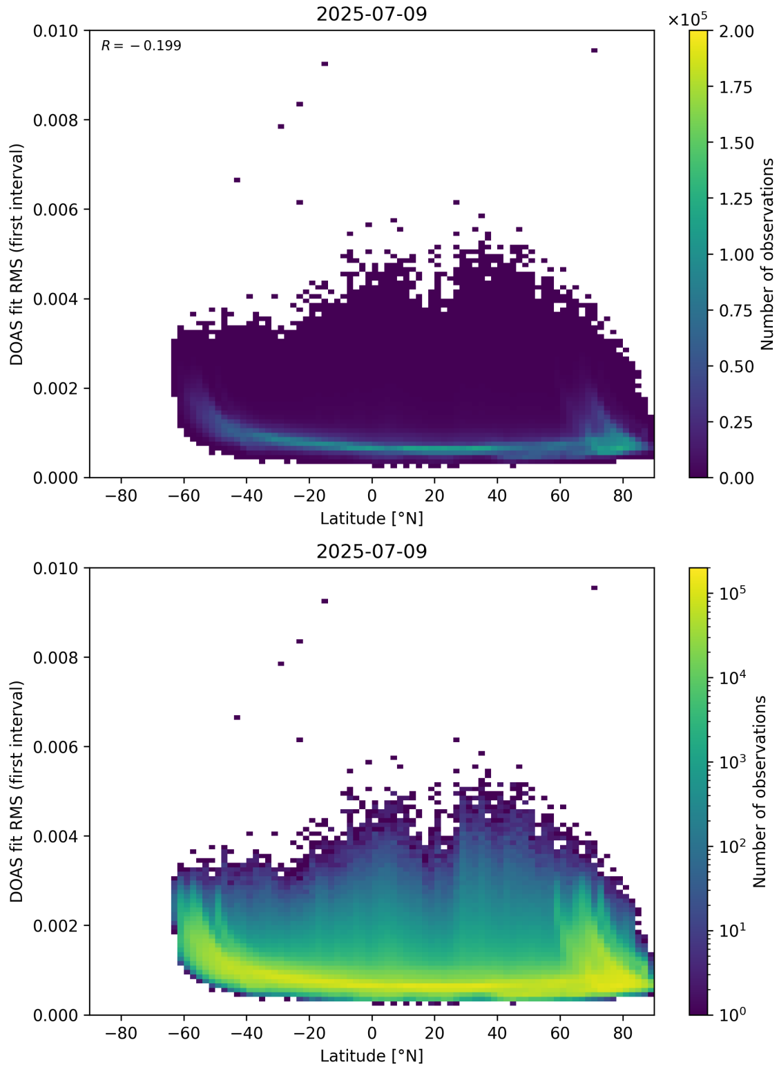
Figure 153: Scatter density plot of “Latitude” against “DOAS fit RMS (first interval)” for 2025-07-08 to 2025-07-10.
