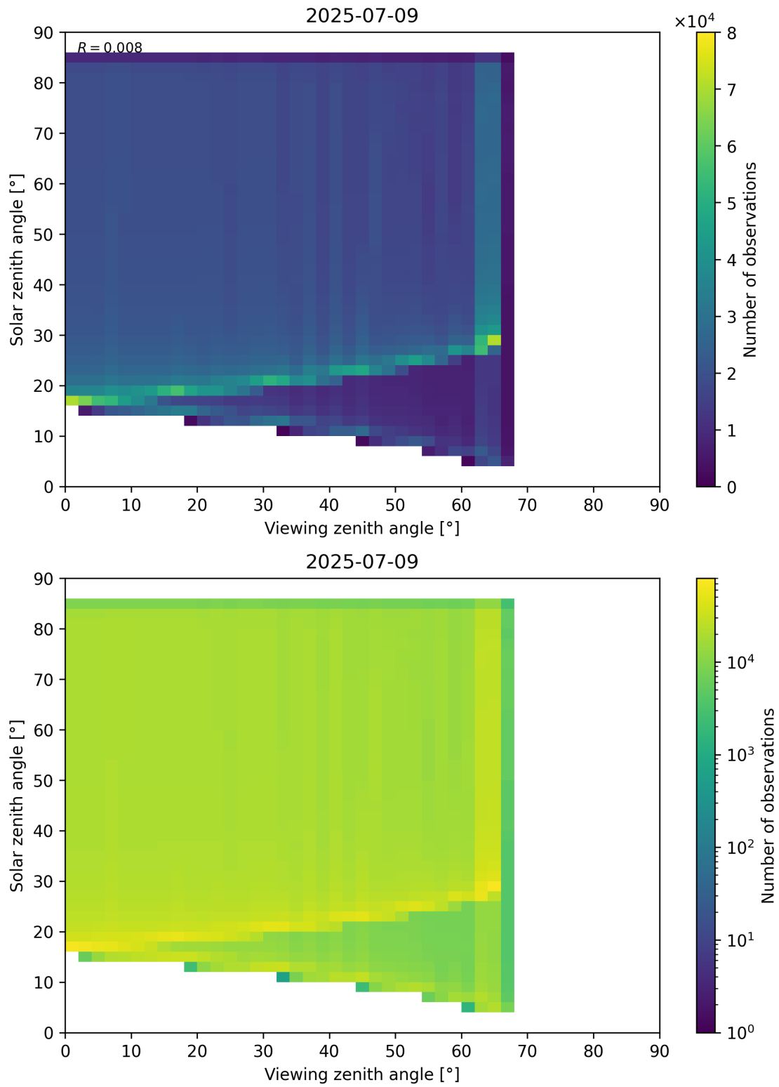
Figure 197: Scatter density plot of “Viewing zenith angle” against “Solar zenith angle” for 2025-07-08 to 2025-07-10.
