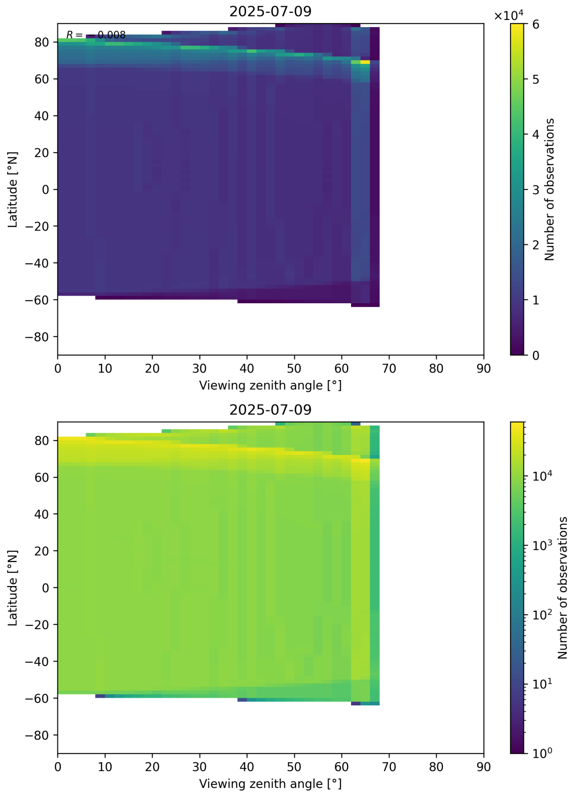
Figure 196: Scatter density plot of “Viewing zenith angle” against “Latitude” for 2025-07-08 to 2025-07-10.
