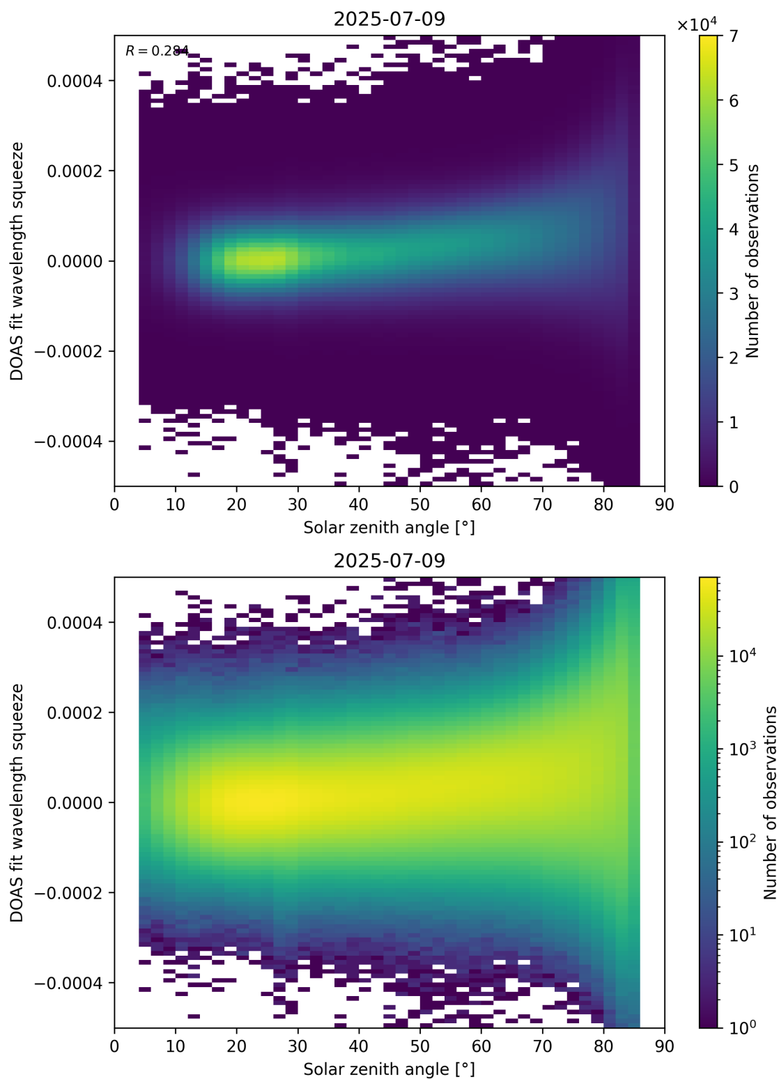
Figure 169: Scatter density plot of “Solar zenith angle” against “DOAS fit wavelength squeeze” for 2025-07-08 to 2025-07-10.
