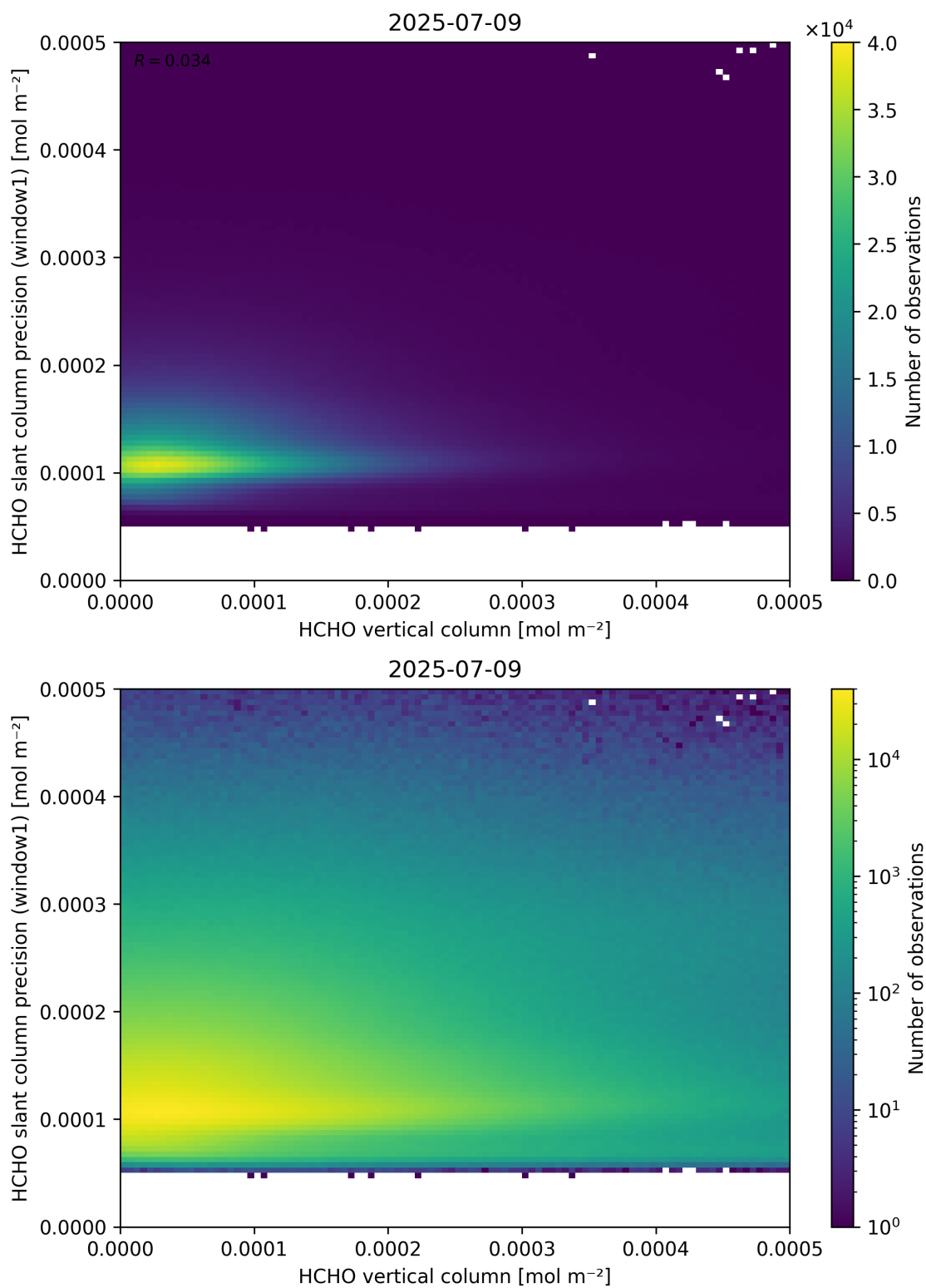
Figure 130: Scatter density plot of “HCHO vertical column” against “HCHO slant column precision (window1)” for 2025-07-08 to 2025-07-10.
