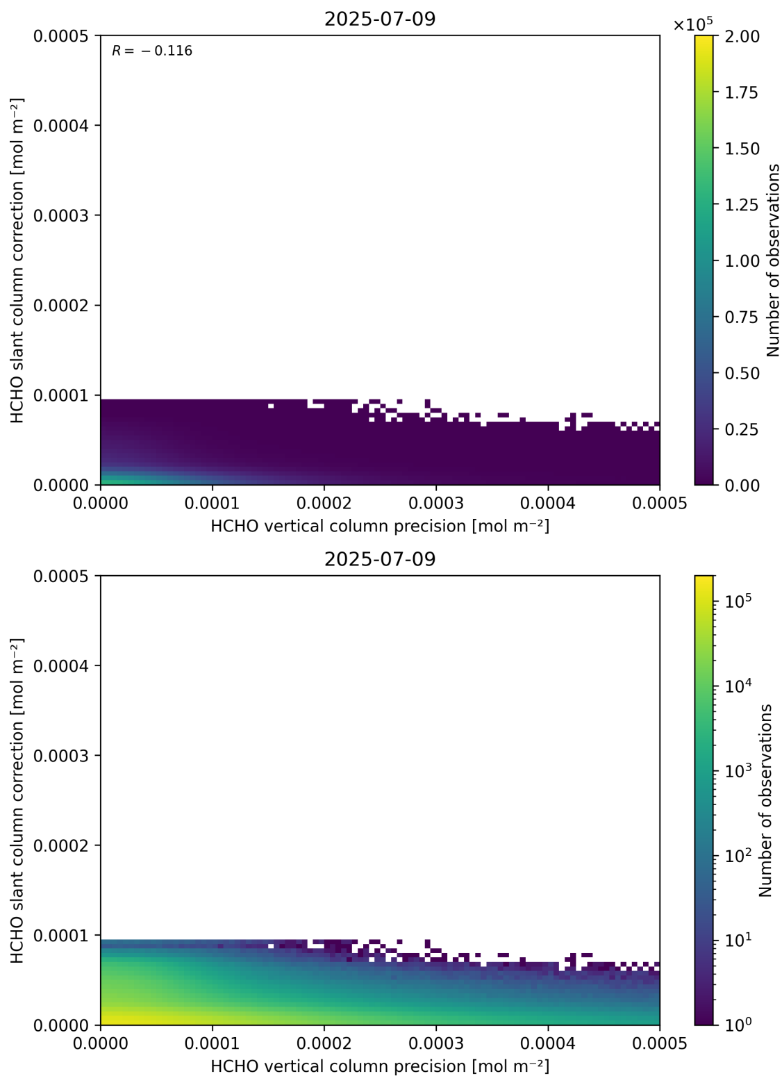
Figure 141: Scatter density plot of “HCHO vertical column precision” against “HCHO slant column correction” for 2025-07-08 to 2025-07-10.
