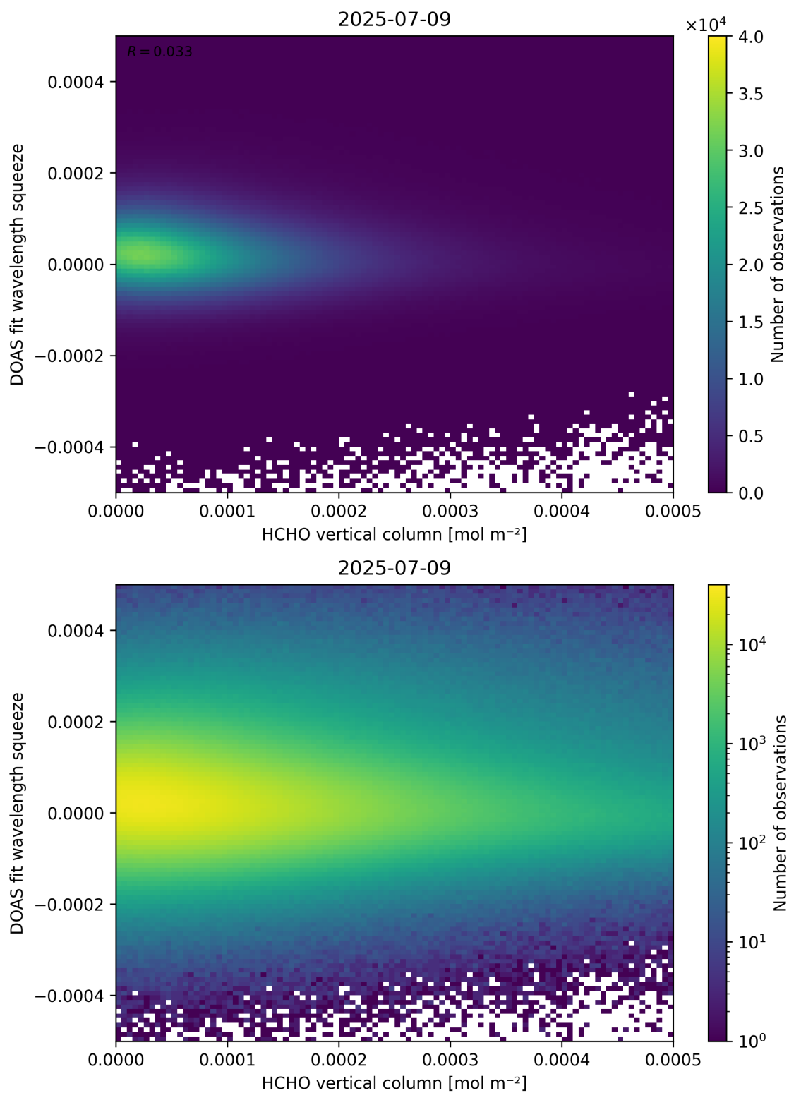
Figure 125: Scatter density plot of “HCHO vertical column” against “DOAS fit wavelength squeeze” for 2025-07-08 to 2025-07-10.
