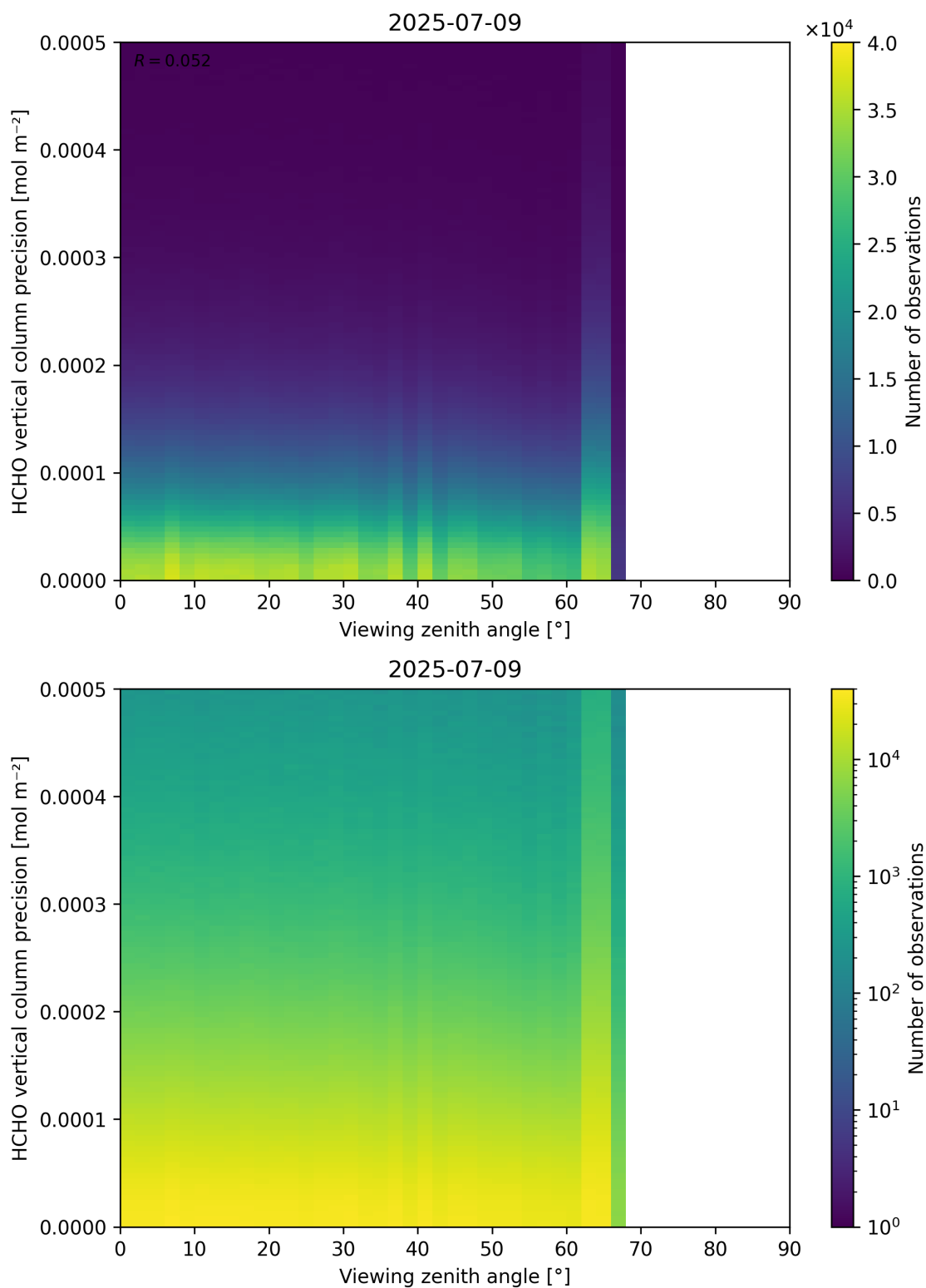
Figure 194: Scatter density plot of “Viewing zenith angle” against “HCHO vertical column precision” for 2025-07-08 to 2025-07-10.
