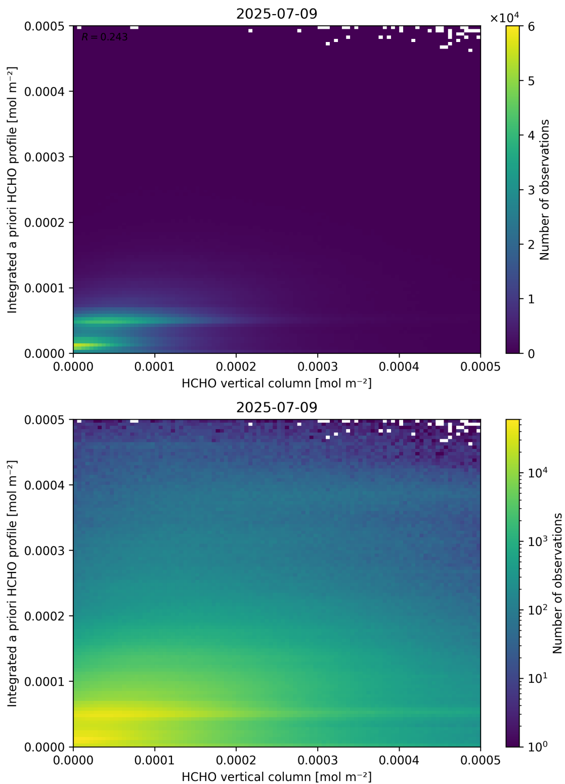
Figure 135: Scatter density plot of “HCHO vertical column” against “Integrated a priori HCHO profile” for 2025-07-08 to 2025-07-10.
