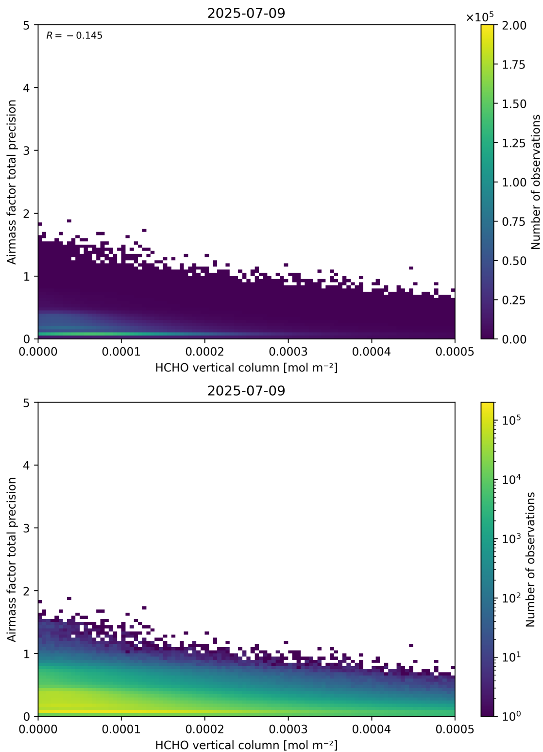
Figure 132: Scatter density plot of “HCHO vertical column” against “Airmass factor total precision” for 2025-07-08 to 2025-07-10.
