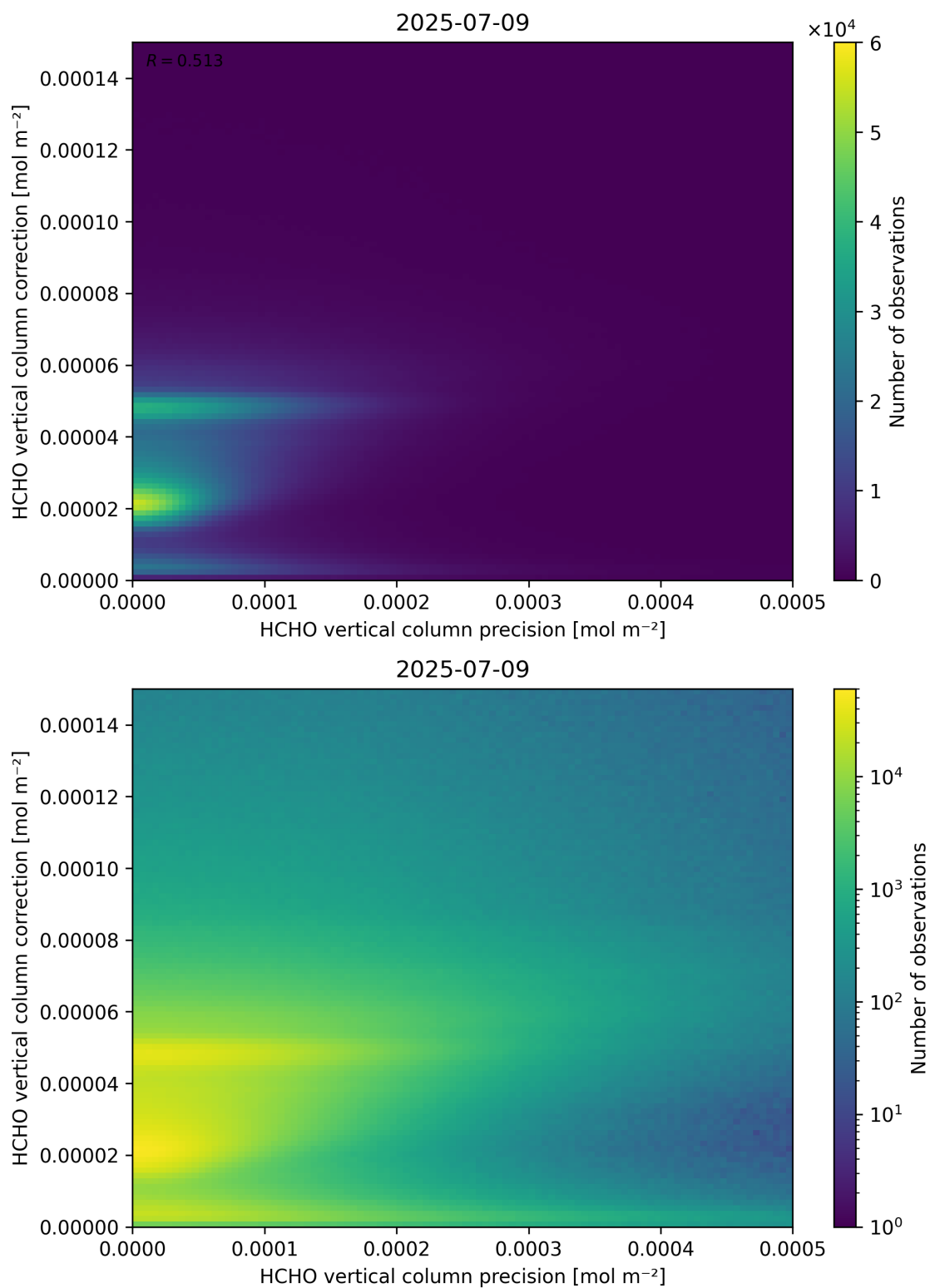
Figure 146: Scatter density plot of “HCHO vertical column precision” against “HCHO vertical column correction” for 2025-07-08 to 2025-07-10.
