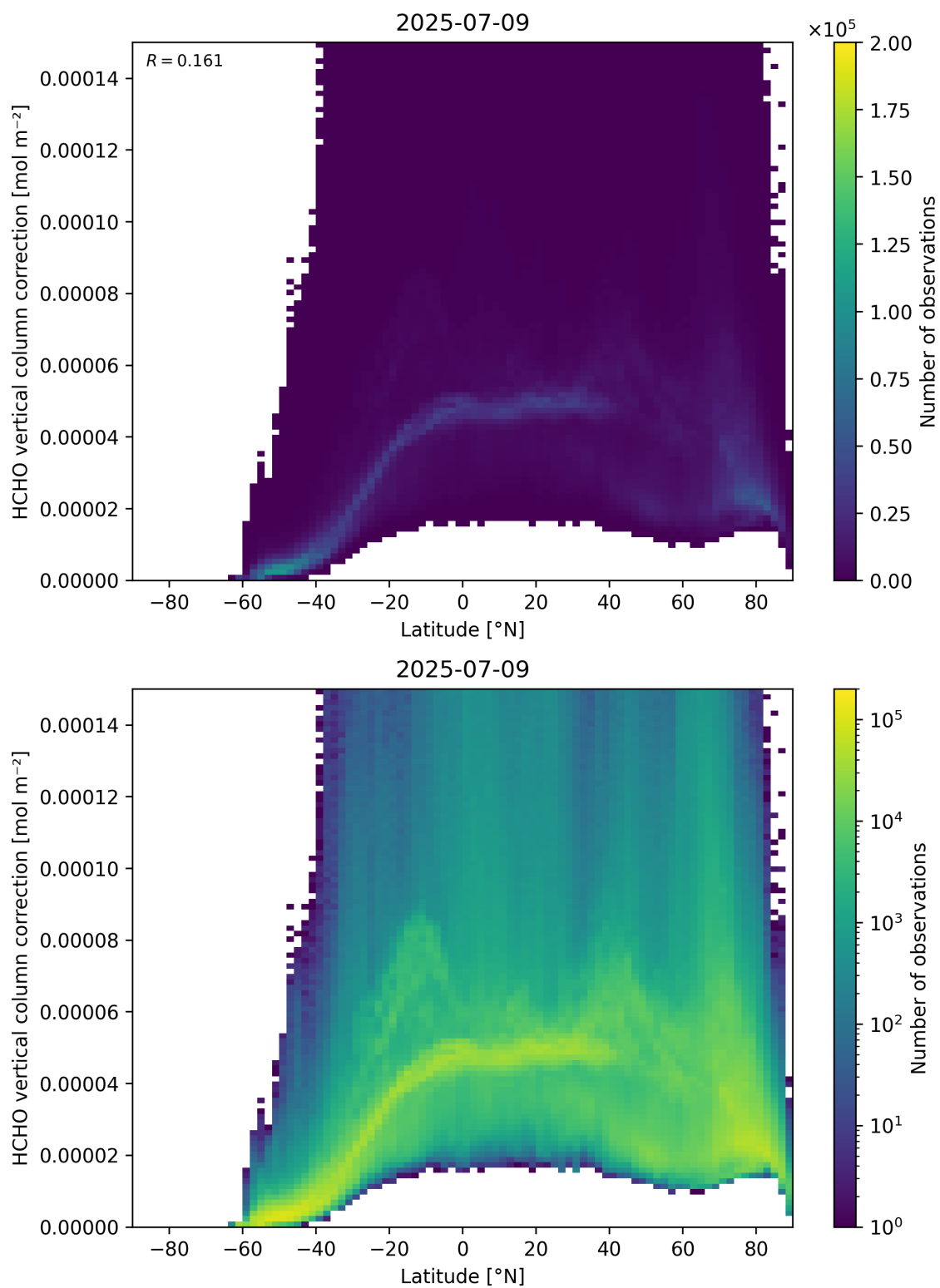
Figure 164: Scatter density plot of “Latitude” against “HCHO vertical column correction” for 2025-07-08 to 2025-07-10.
