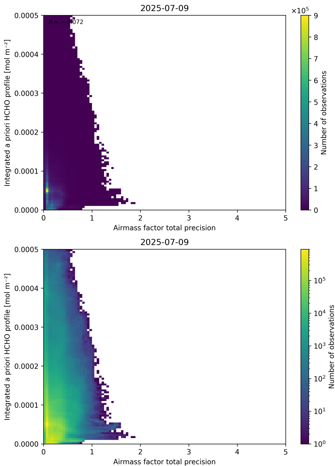
Figure 111: Scatter density plot of “Airmass factor total precision” against “Integrated a priori HCHO profile” for 2025-07-08 to 2025-07-10.
