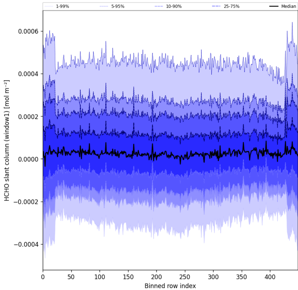
Figure 52: Along track statistics of "HCHO slant column (window1)" for 2025-07-08 to 2025-07-10
