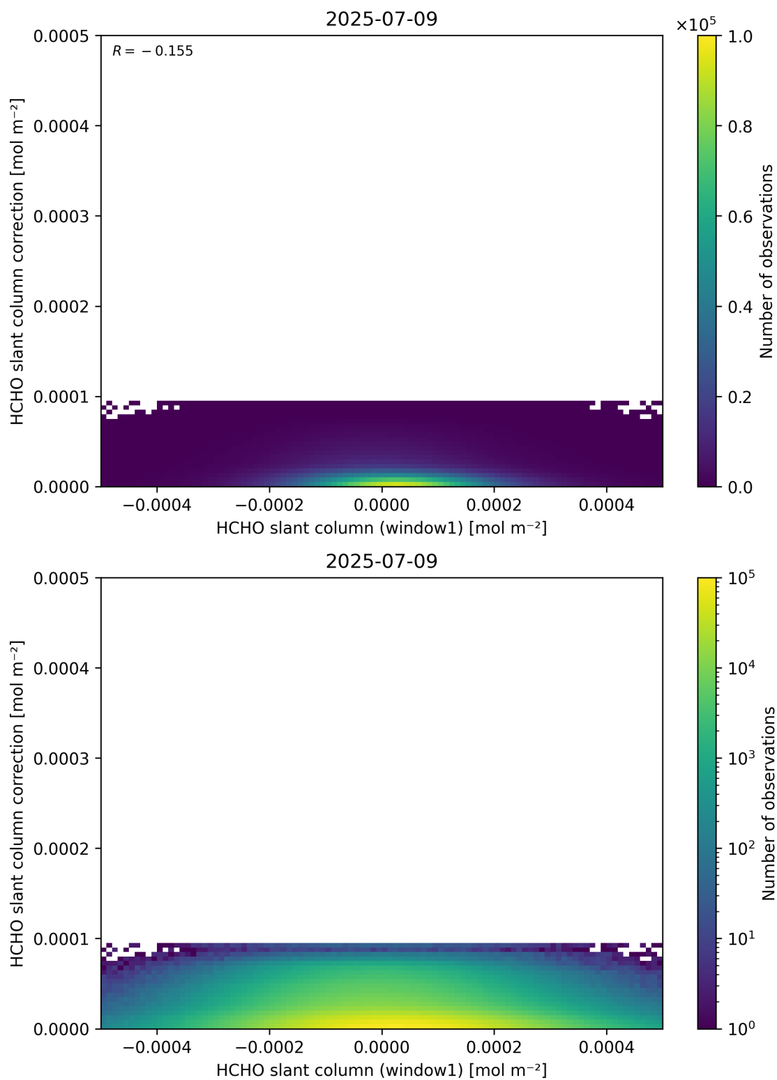
Figure 83: Scatter density plot of “HCHO slant column (window1)” against “HCHO slant column correction” for 2025-07-08 to 2025-07-10.
