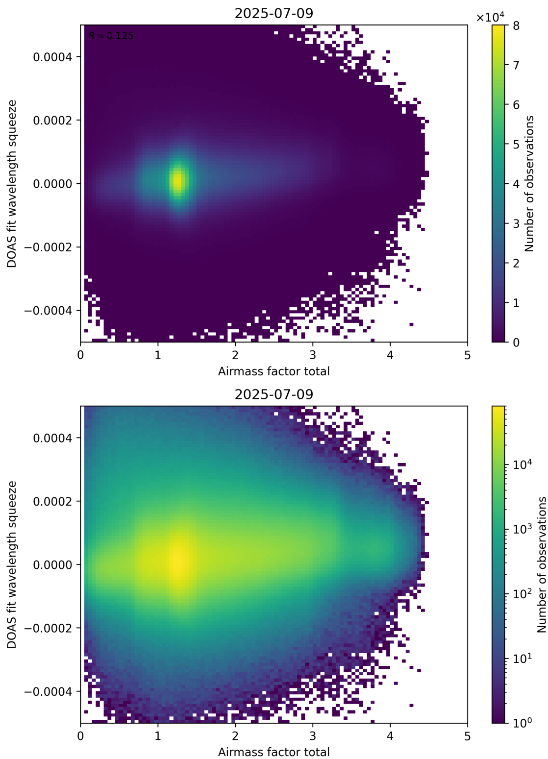
Figure 99: Scatter density plot of “Airmass factor total” against “DOAS fit wavelength squeeze” for 2025-07-08 to 2025-07-10.
