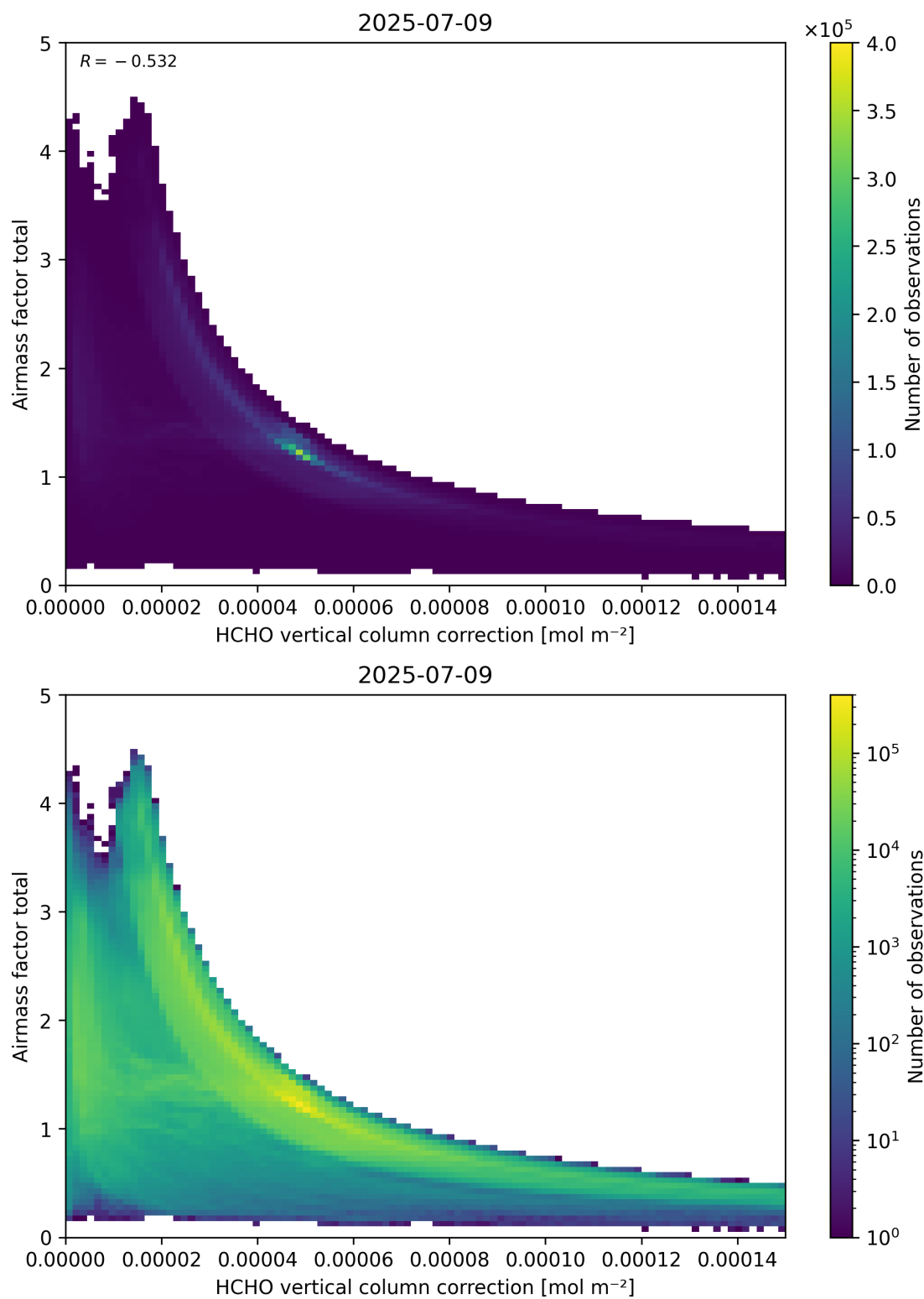
Figure 120: Scatter density plot of “HCHO vertical column correction” against “Airmass factor total” for 2025-07-08 to 2025-07-10.
