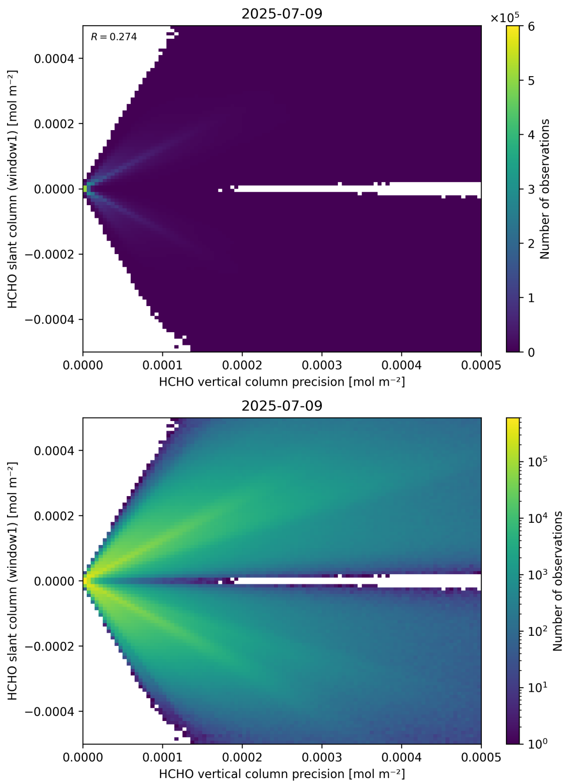
Figure 142: Scatter density plot of “HCHO vertical column precision” against “HCHO slant column (window1)” for 2025-07-08 to 2025-07-10.
