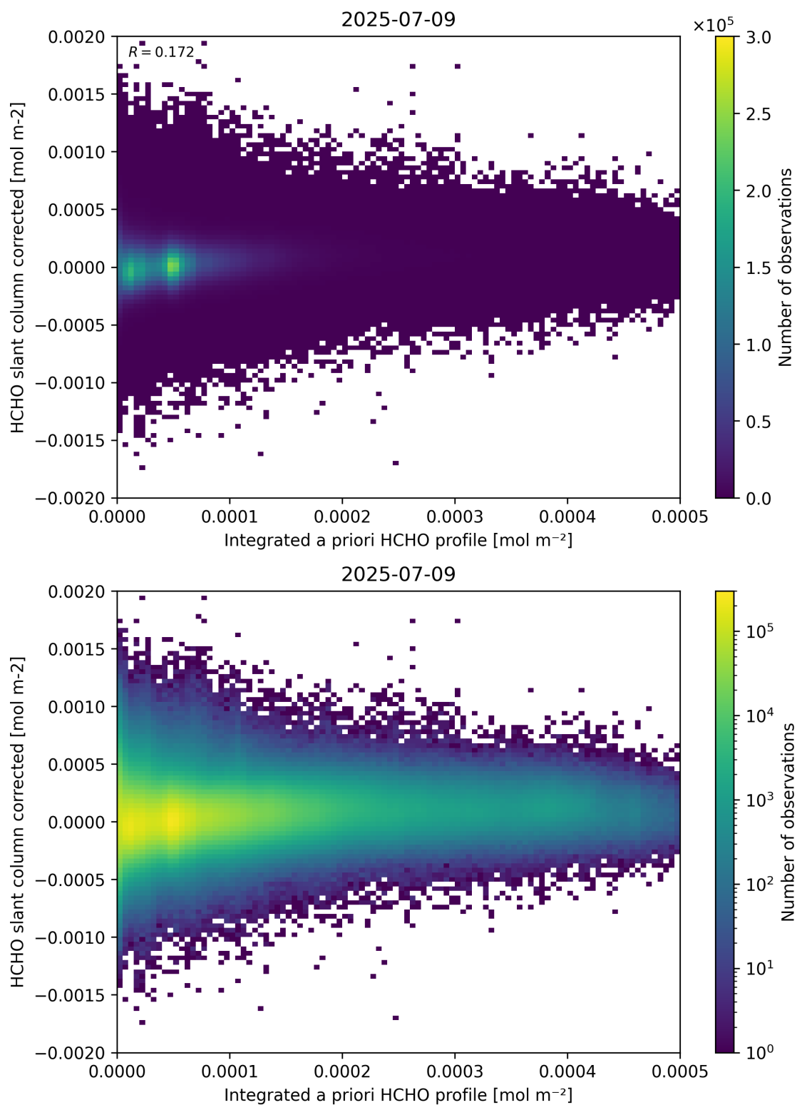
Figure 151: Scatter density plot of “Integrated a priori HCHO profile” against “HCHO slant column corrected” for 2025-07-08 to 2025-07-10.
