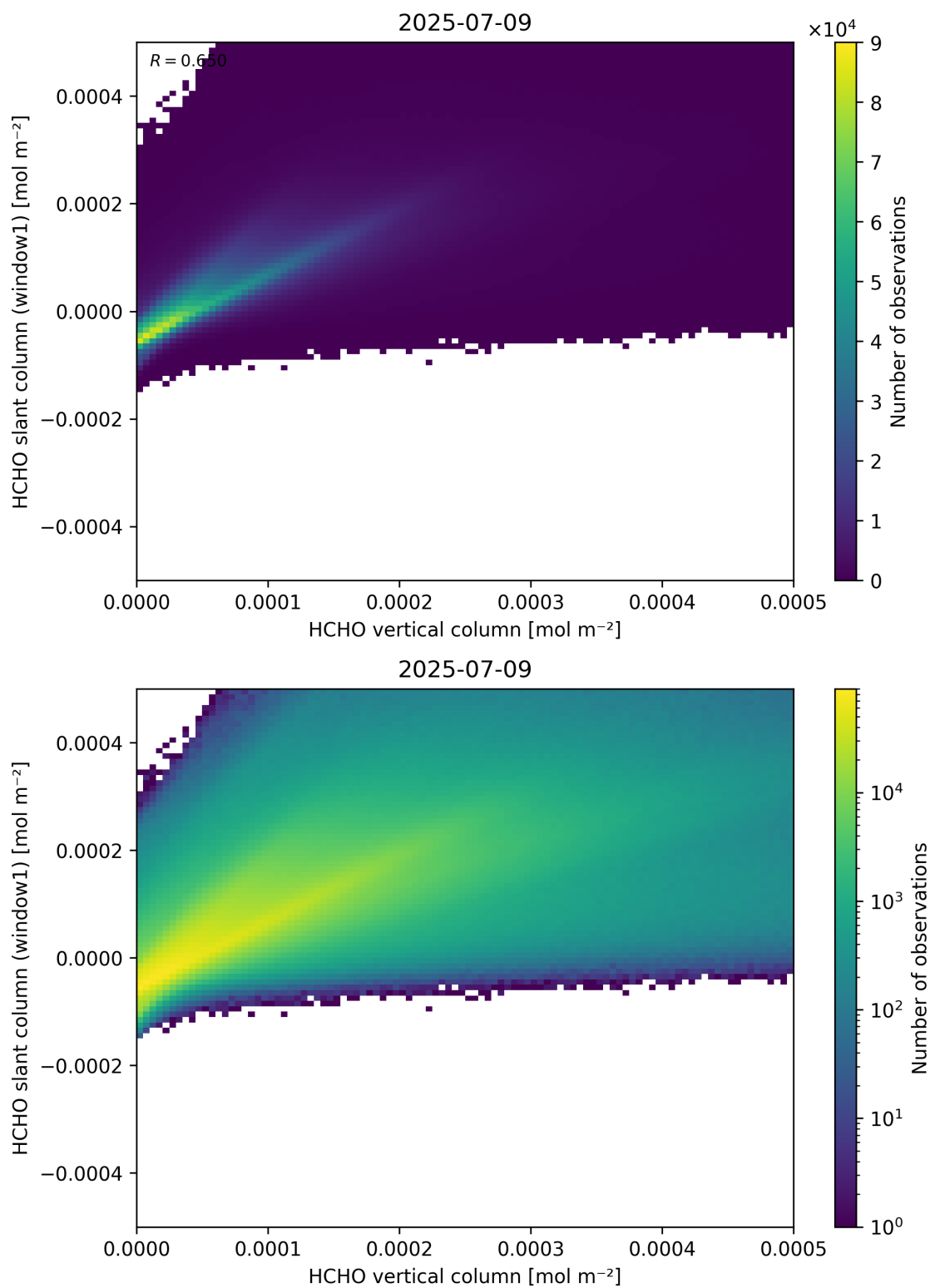
Figure 129: Scatter density plot of “HCHO vertical column” against “HCHO slant column (window1)” for 2025-07-08 to 2025-07-10.
