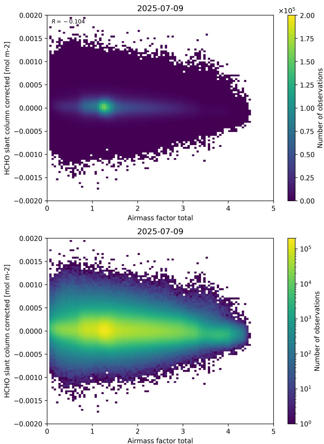
Figure 101: Scatter density plot of “Airmass factor total” against “HCHO slant column corrected” for 2025-07-08 to 2025-07-10.
