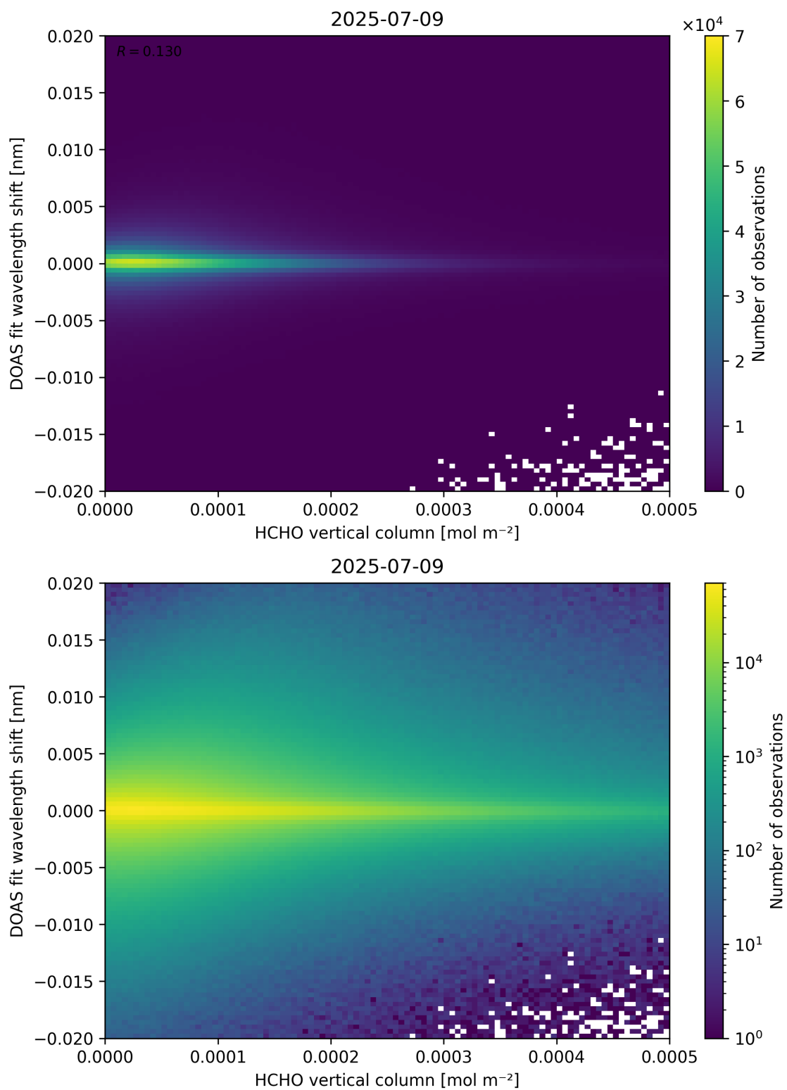
Figure 124: Scatter density plot of “HCHO vertical column” against “DOAS fit wavelength shift” for 2025-07-08 to 2025-07-10.
