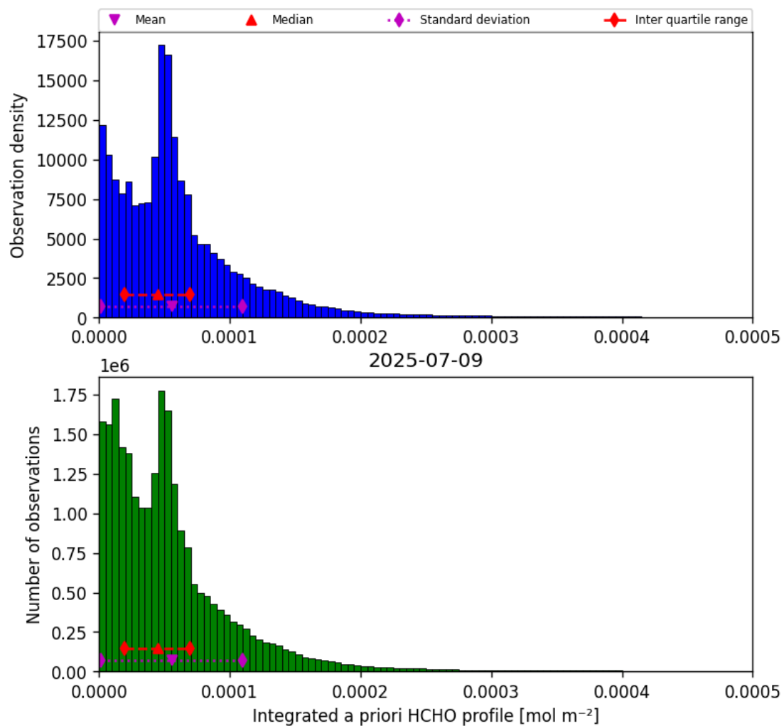
Figure 43: Histogram of “Integrated a priori HCHO profile” for 2025-07-08 to 2025-07-10
