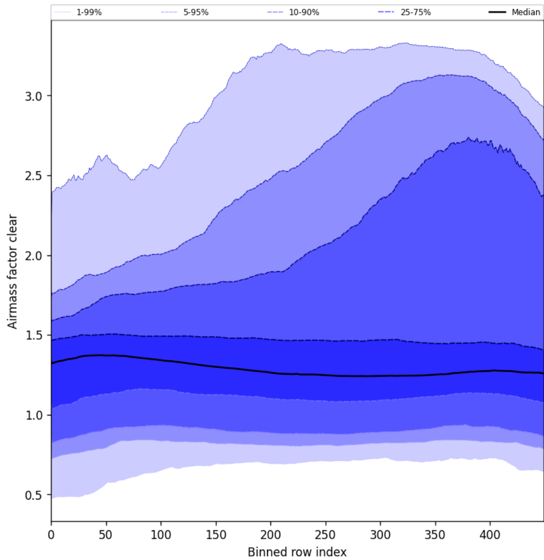
Figure 56: Along track statistics of “Airmass factor clear” for 2025-07-08 to 2025-07-10
