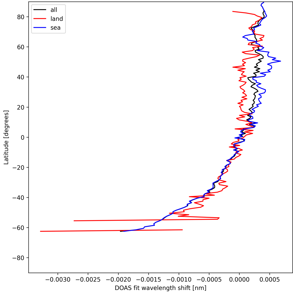
Figure 30: Zonal average of “DOAS fit wavelength shift” for 2025-07-08 to 2025-07-10.
