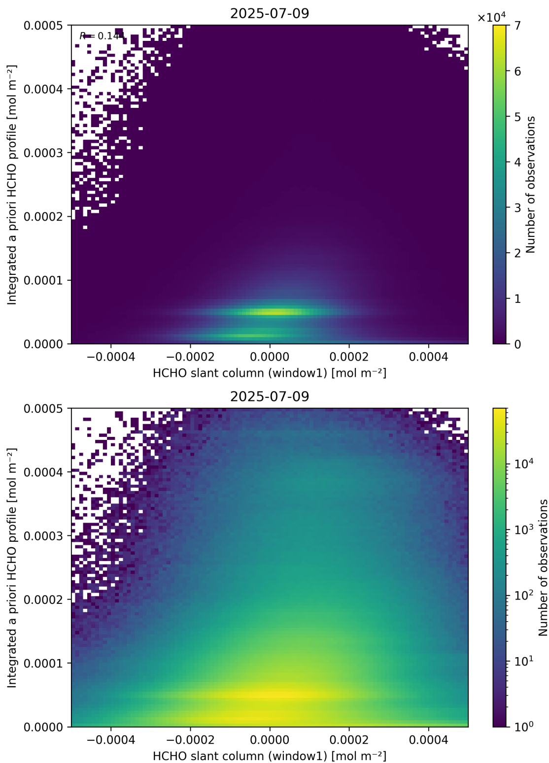
Figure 87: Scatter density plot of “HCHO slant column (window1)” against “Integrated a priori HCHO profile” for 2025-07-08 to 2025-07-10.
