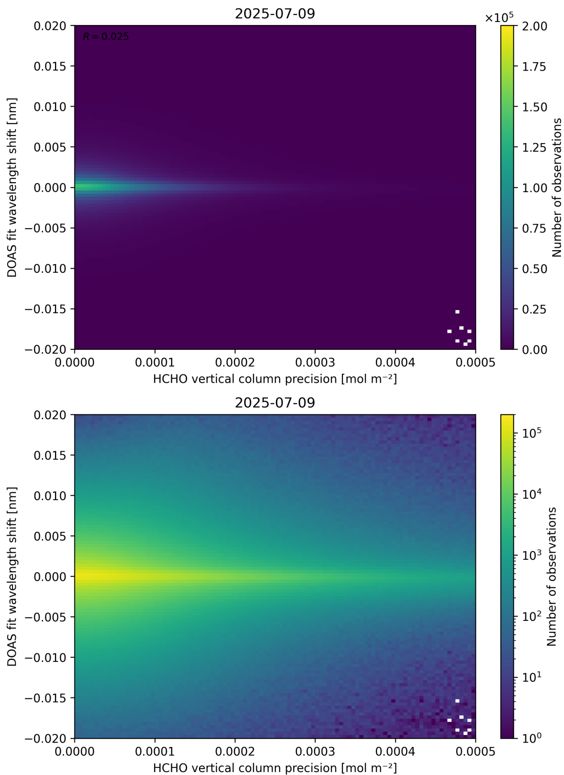
Figure 137: Scatter density plot of “HCHO vertical column precision” against “DOAS fit wavelength shift” for 2025-07-08 to 2025-07-10.
