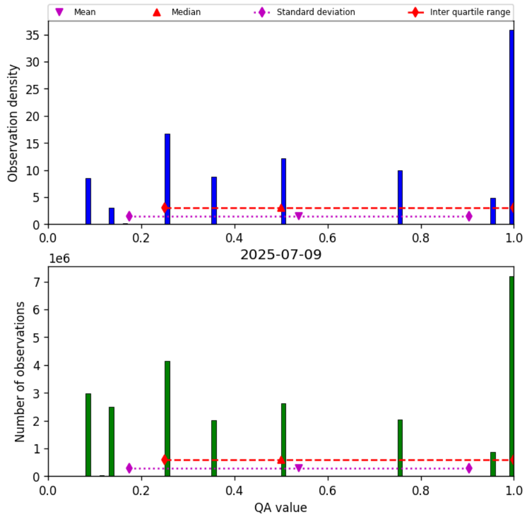
Figure 34: Histogram of “QA value” for 2025-07-08 to 2025-07-10
