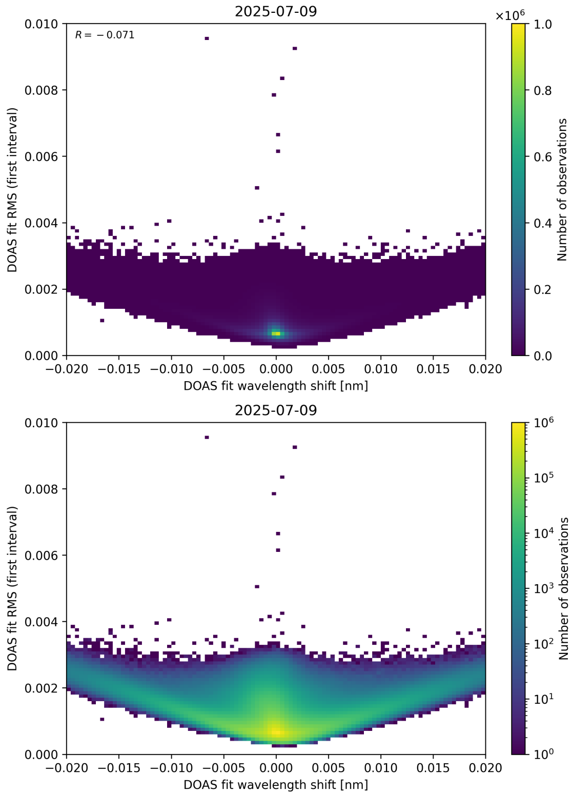
Figure 64: Scatter density plot of “DOAS fit wavelength shift” against “DOAS fit RMS (first interval)” for 2025-07-08 to 2025-07-10.
