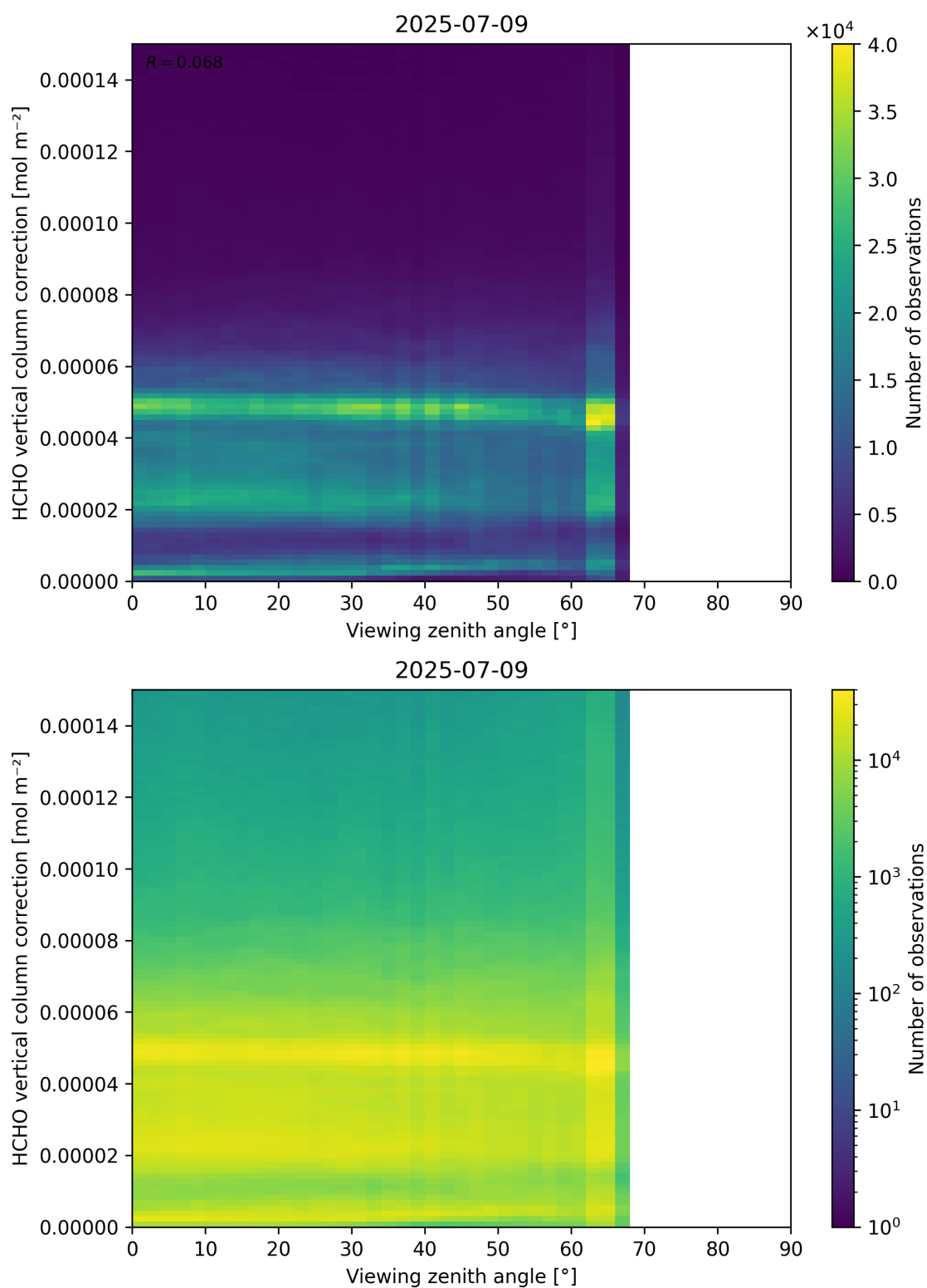
Figure 193: Scatter density plot of “Viewing zenith angle” against “HCHO vertical column correction” for 2025-07-08 to 2025-07-10.
