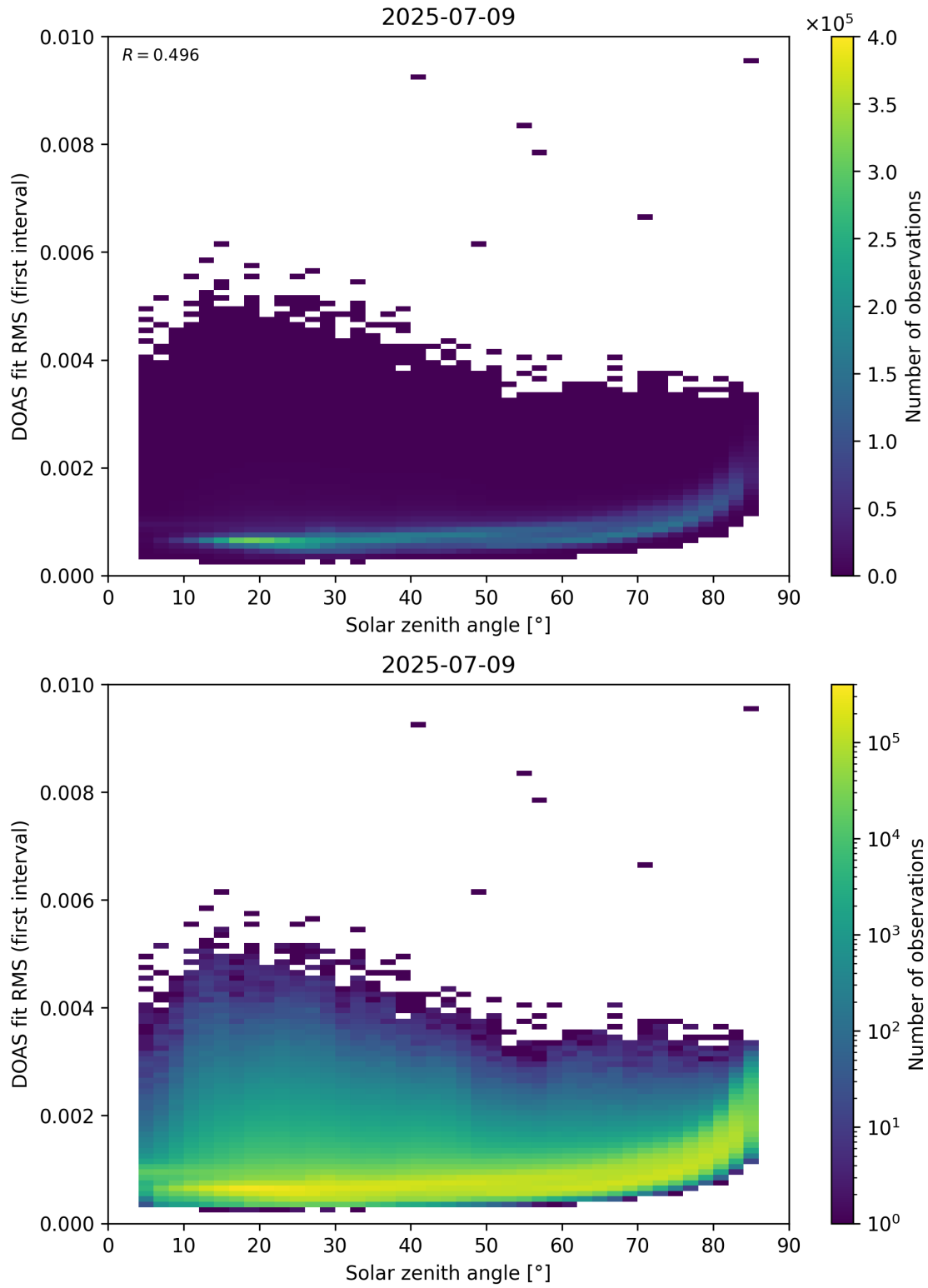
Figure 167: Scatter density plot of “Solar zenith angle” against “DOAS fit RMS (first interval)” for 2025-07-08 to 2025-07-10.
