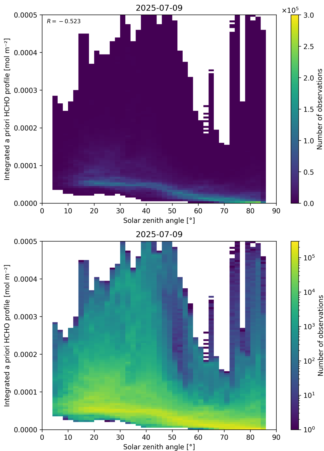
Figure 180: Scatter density plot of “Solar zenith angle” against “Integrated a priori HCHO profile” for 2025-07-08 to 2025-07-10.
