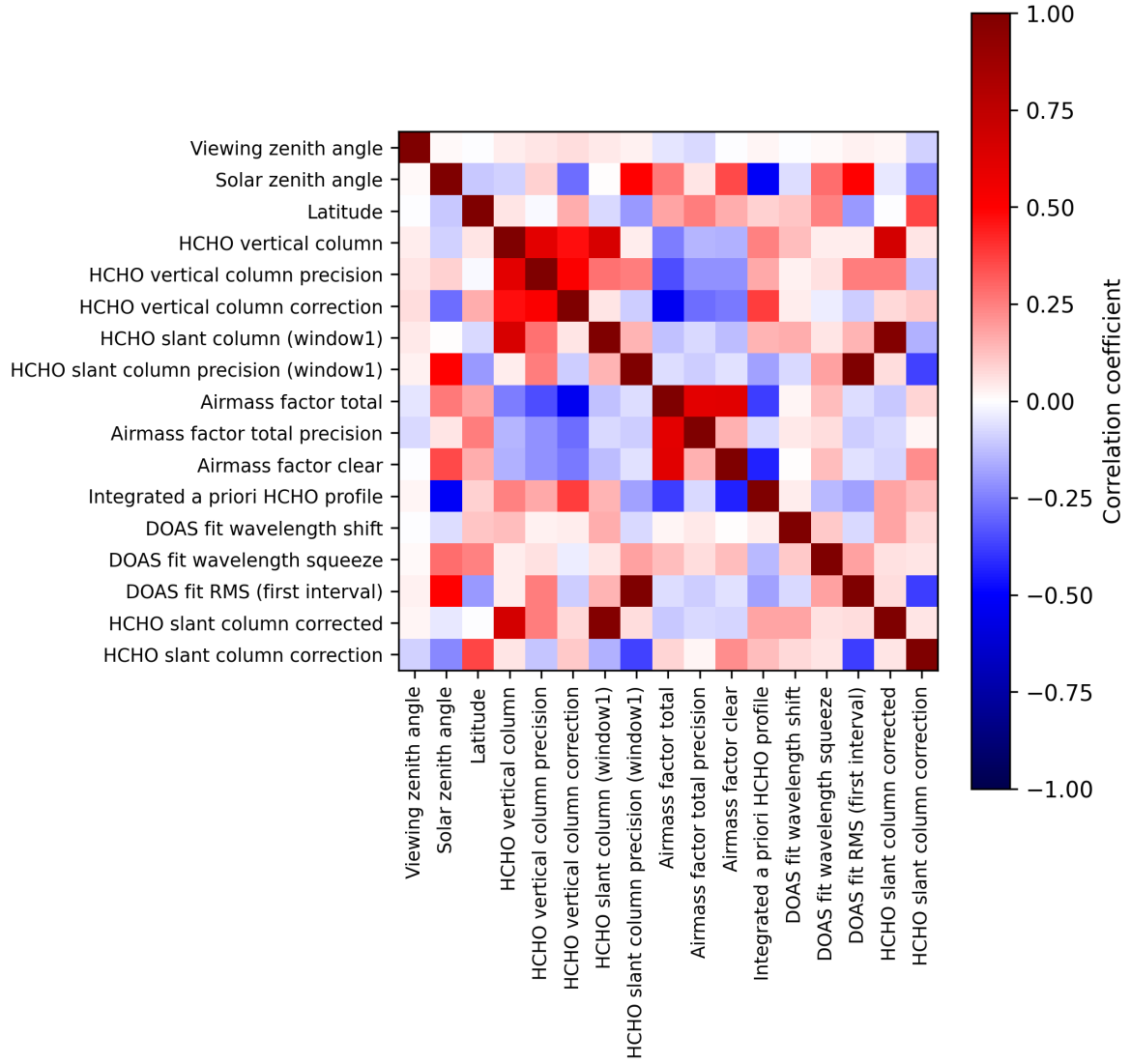
Figure 2: Map of correlation matrix for 2025-07-08 to 2025-07-10.
