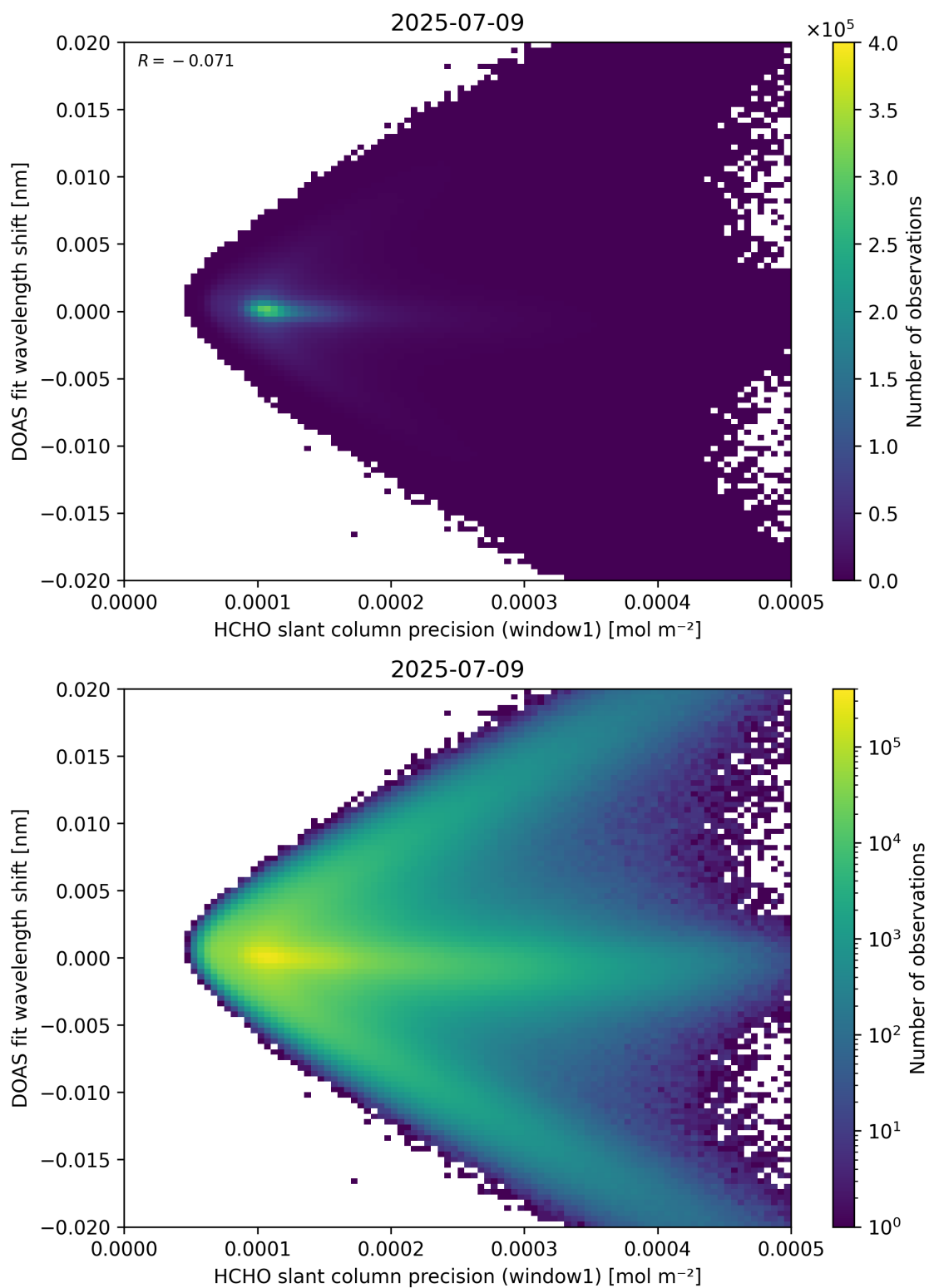
Figure 89: Scatter density plot of “HCHO slant column precision (window1)” against “DOAS fit wavelength shift” for 2025-07-08 to 2025-07-10.
