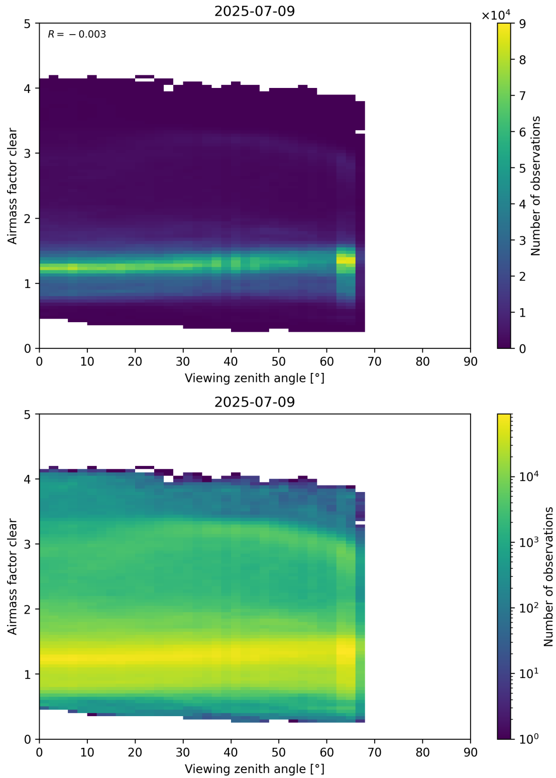
Figure 185: Scatter density plot of “Viewing zenith angle” against “Airmass factor clear” for 2025-07-08 to 2025-07-10.
