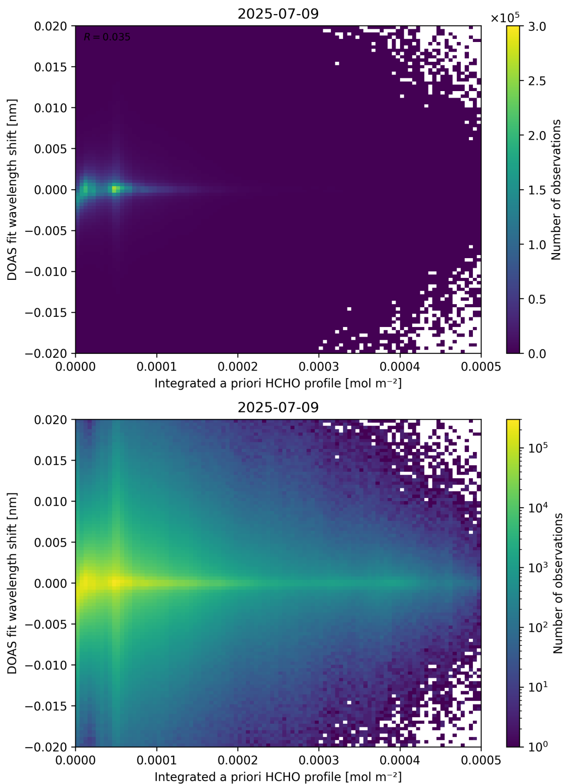
Figure 149: Scatter density plot of “Integrated a priori HCHO profile” against “DOAS fit wavelength shift” for 2025-07-08 to 2025-07-10.
