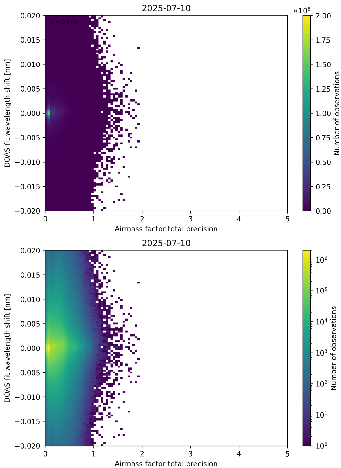
Figure 106: Scatter density plot of “Airmass factor total precision” against “DOAS fit wavelength shift” for 2025-07-09 to 2025-07-11.
