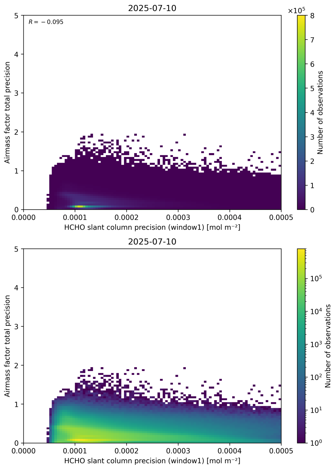
Figure 95: Scatter density plot of “HCHO slant column precision (window1)” against “Airmass factor total precision” for 2025-07-09 to 2025-07-11.
