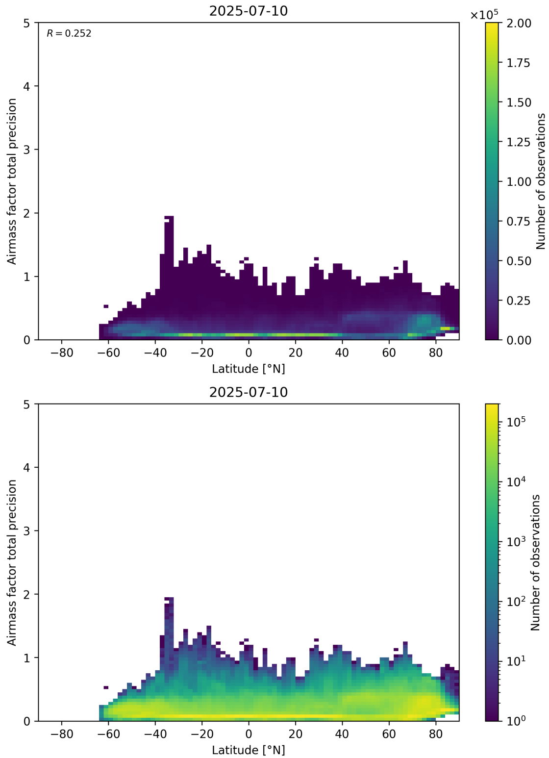
Figure 162: Scatter density plot of “Latitude” against “Airmass factor total precision” for 2025-07-09 to 2025-07-11.
