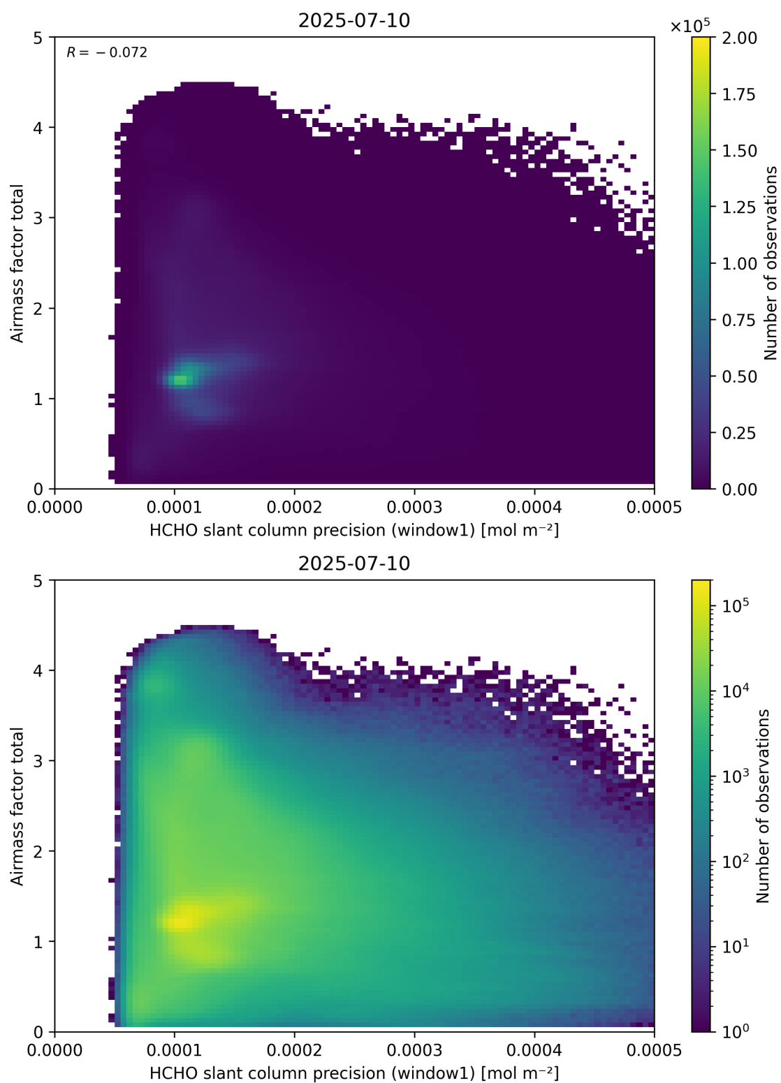
Figure 94: Scatter density plot of “HCHO slant column precision (window1)” against “Airmass factor total” for 2025-07-09 to 2025-07-11.
