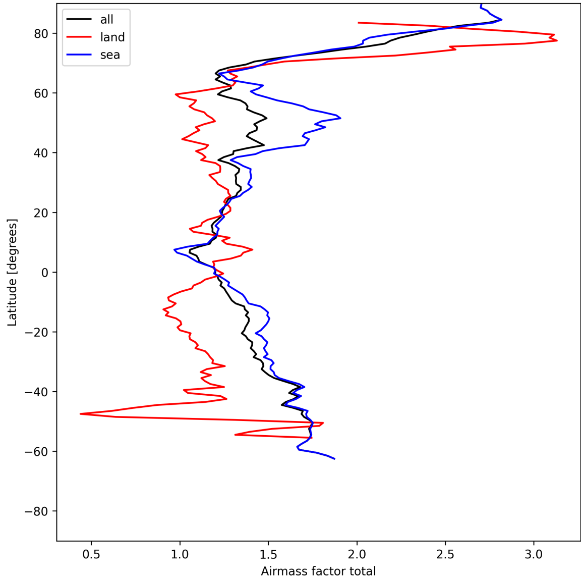
Figure 26: Zonal average of “Airmass factor total” for 2025-07-09 to 2025-07-11.
