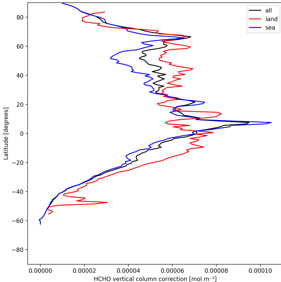
Figure 23: Zonal average of “HCHO vertical column correction” for 2025-07-09 to 2025-07-11.
