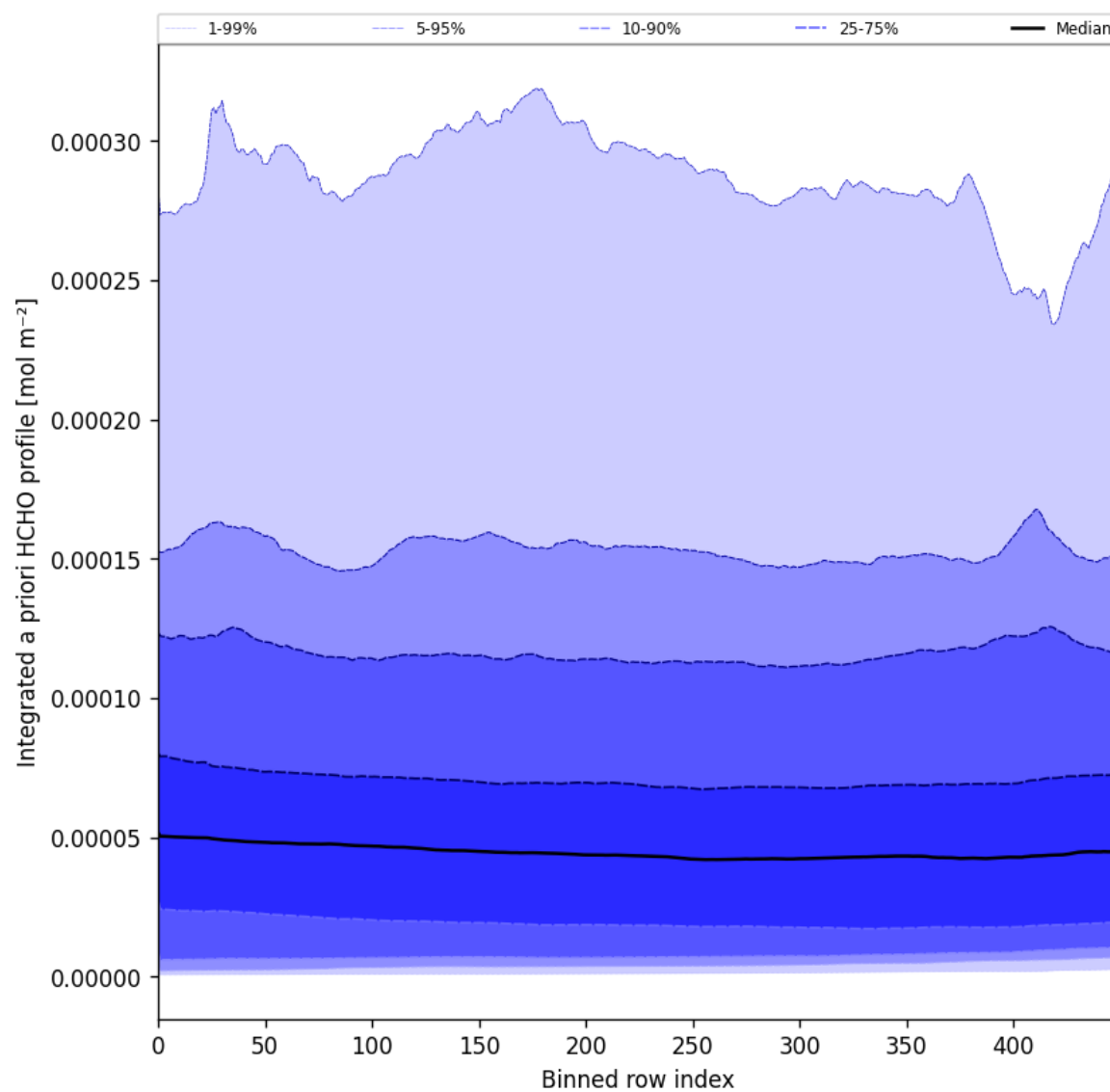
Figure 57: Along track statistics of “Integrated a priori HCHO profile” for 2025-07-09 to 2025-07-11
