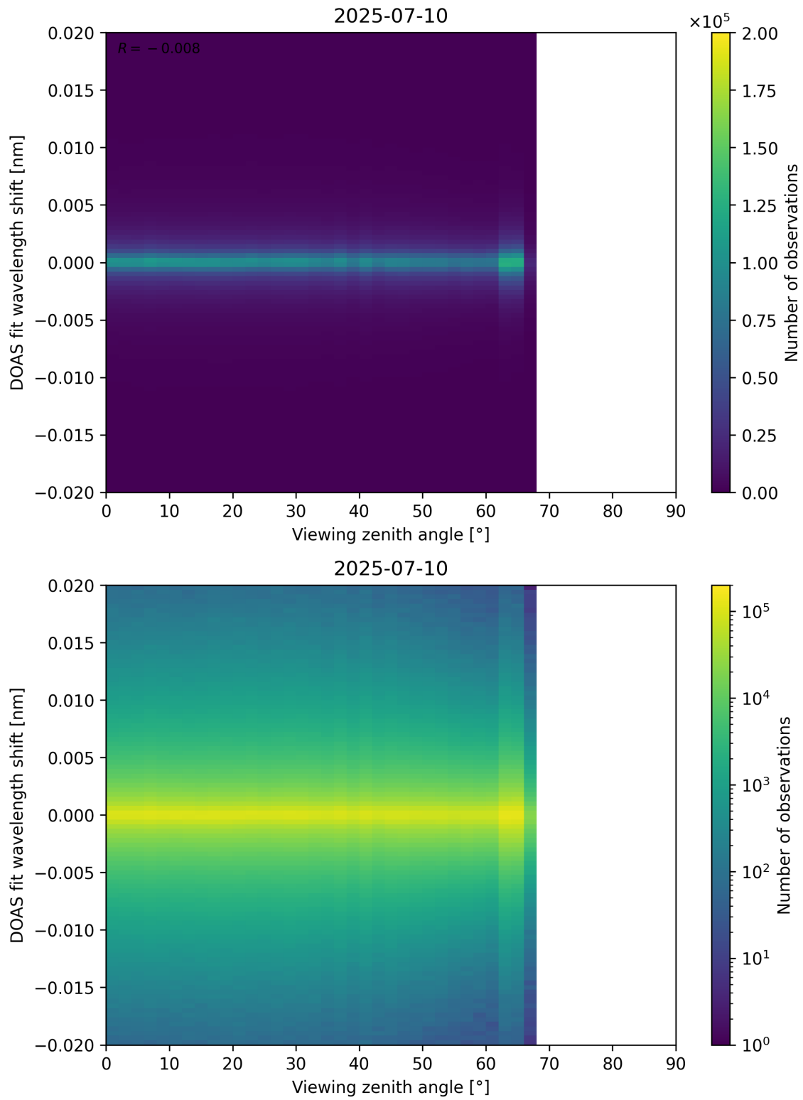
Figure 183: Scatter density plot of “Viewing zenith angle” against “DOAS fit wavelength shift” for 2025-07-09 to 2025-07-11.
