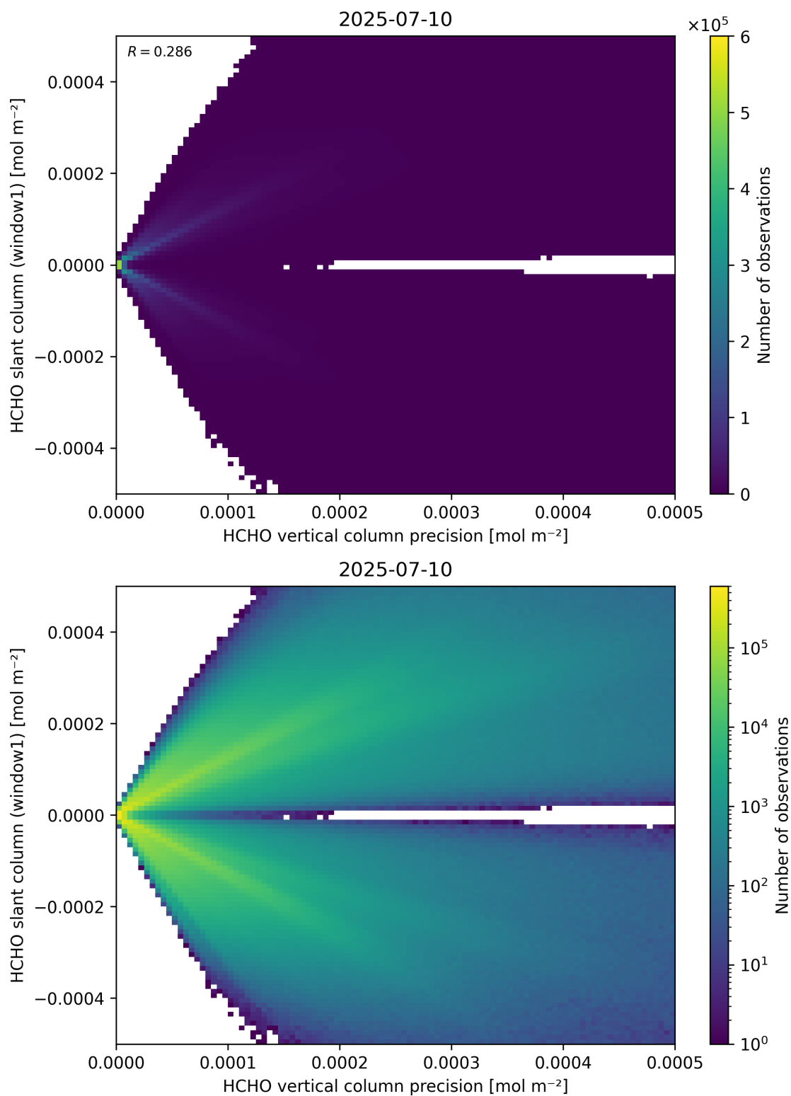
Figure 142: Scatter density plot of “HCHO vertical column precision” against “HCHO slant column (window1)” for 2025-07-09 to 2025-07-11.
