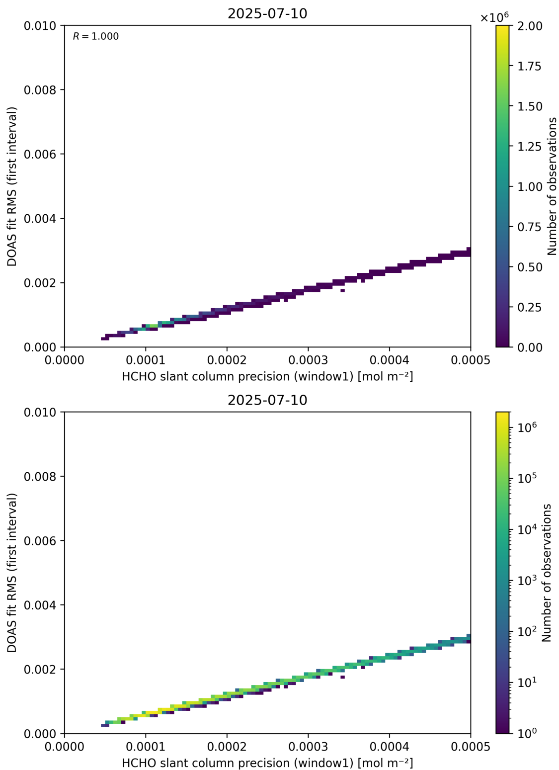
Figure 88: Scatter density plot of “HCHO slant column precision (window1)” against “DOAS fit RMS (first interval)” for 2025-07-09 to 2025-07-11.
