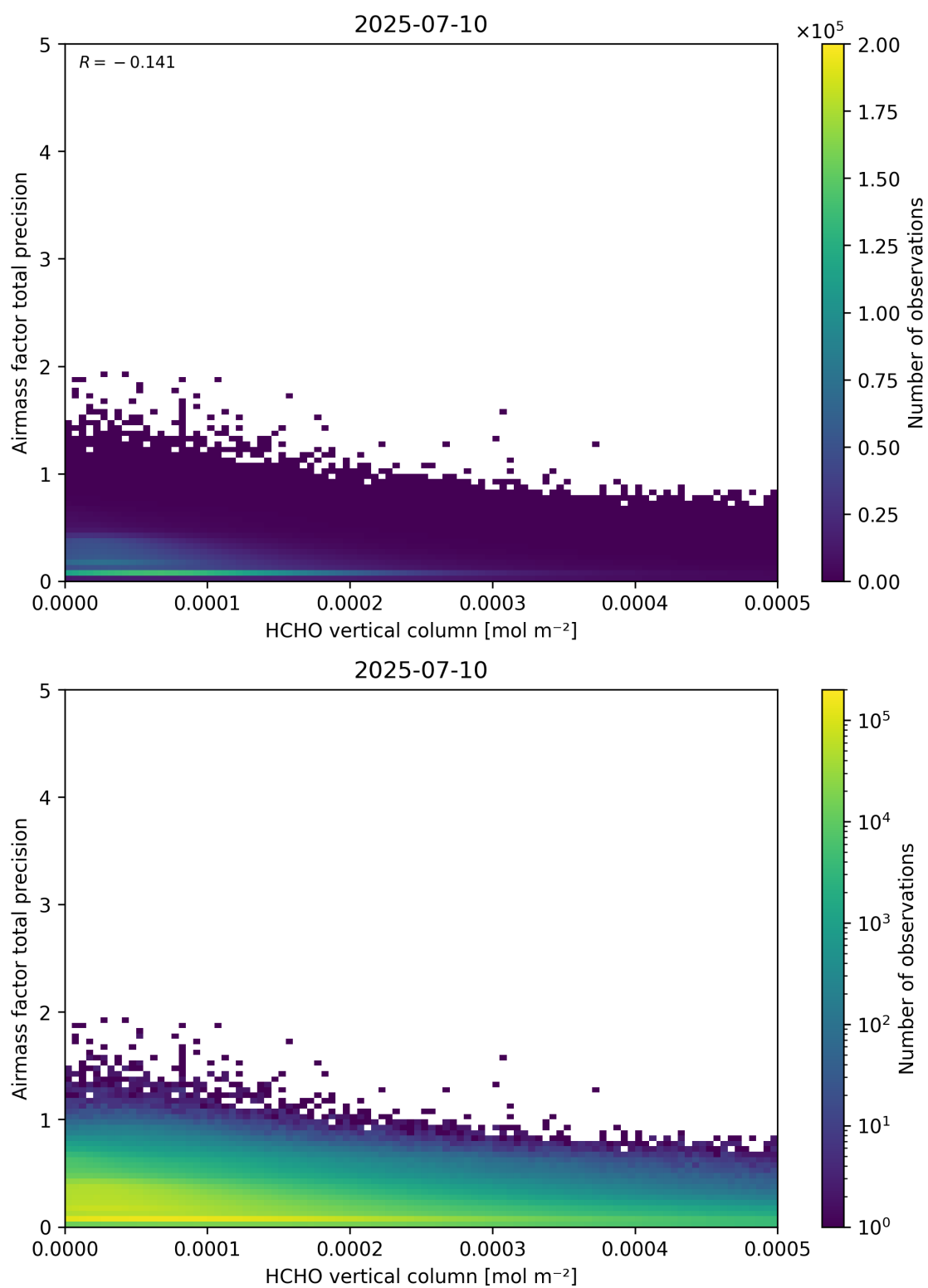
Figure 132: Scatter density plot of “HCHO vertical column” against “Airmass factor total precision” for 2025-07-09 to 2025-07-11.
