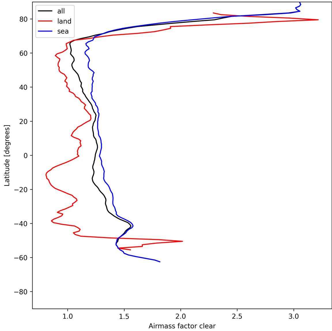
Figure 28: Zonal average of “Airmass factor clear” for 2025-07-09 to 2025-07-11.
