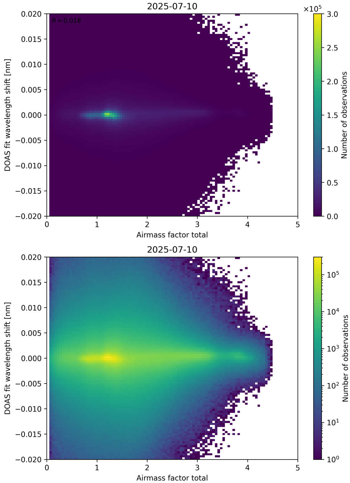
Figure 98: Scatter density plot of “Airmass factor total” against “DOAS fit wavelength shift” for 2025-07-09 to 2025-07-11.
