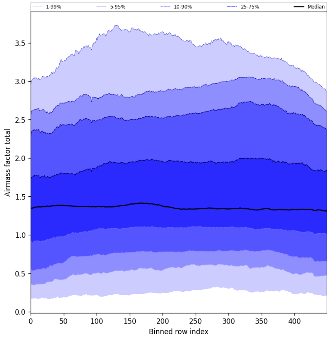
Figure 54: Along track statistics of “Airmass factor total” for 2025-07-09 to 2025-07-11
