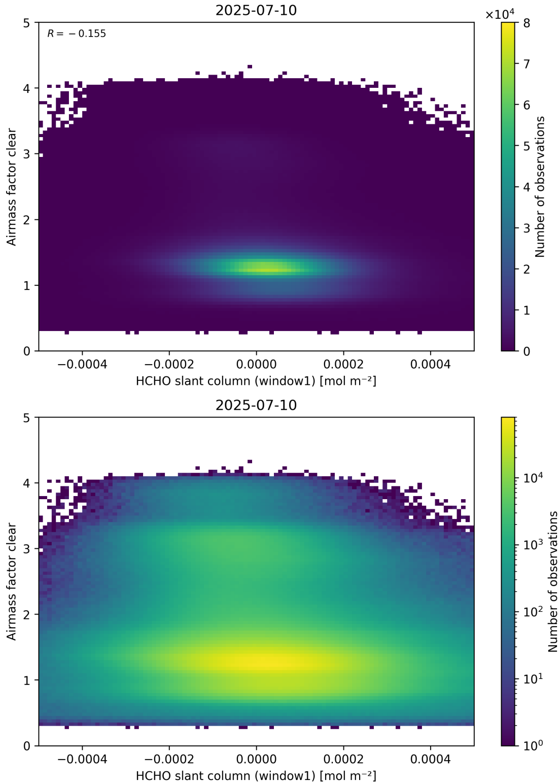
Figure 81: Scatter density plot of “HCHO slant column (window1)” against “Airmass factor clear” for 2025-07-09 to 2025-07-11.
