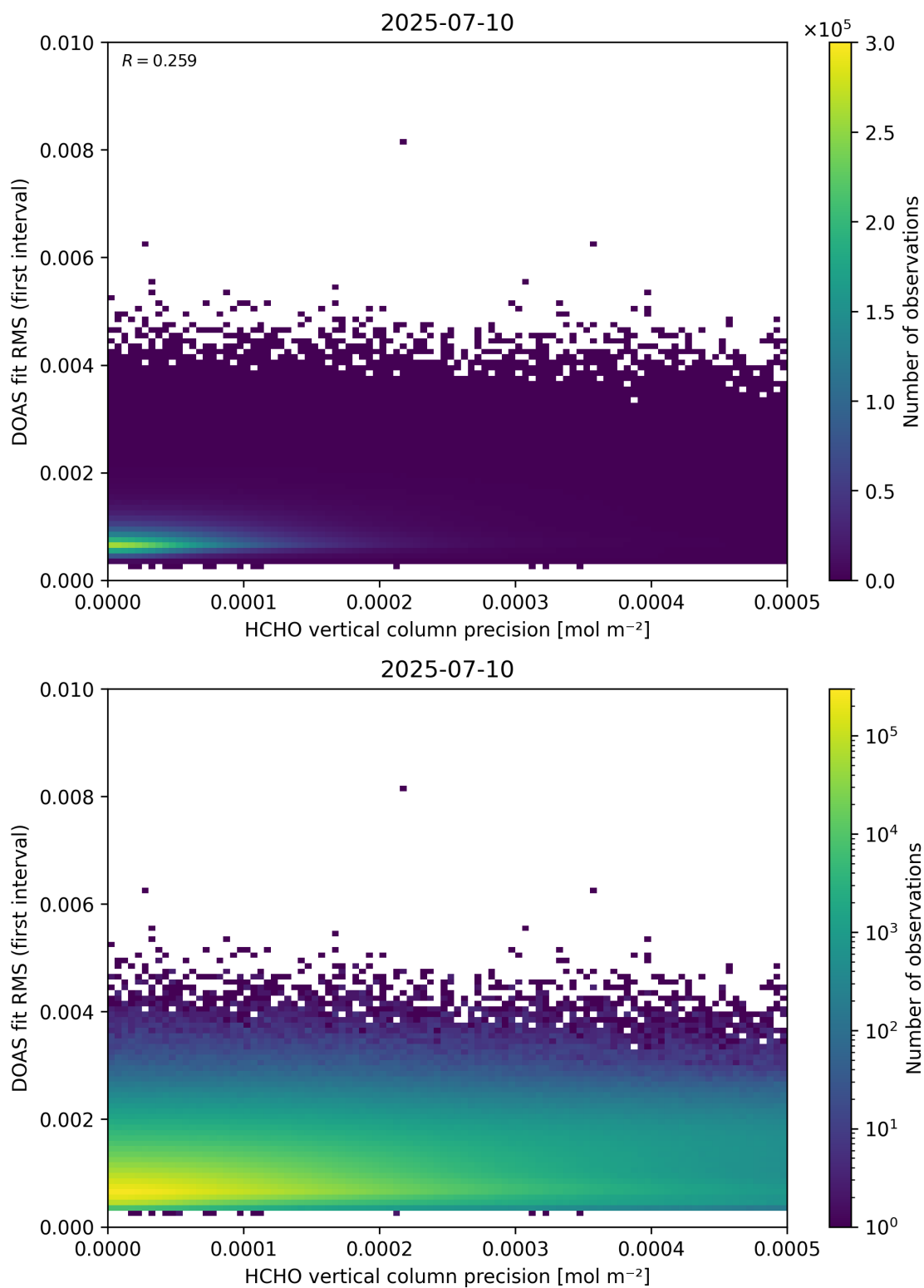
Figure 136: Scatter density plot of “HCHO vertical column precision” against “DOAS fit RMS (first interval)” for 2025-07-09 to 2025-07-11.
