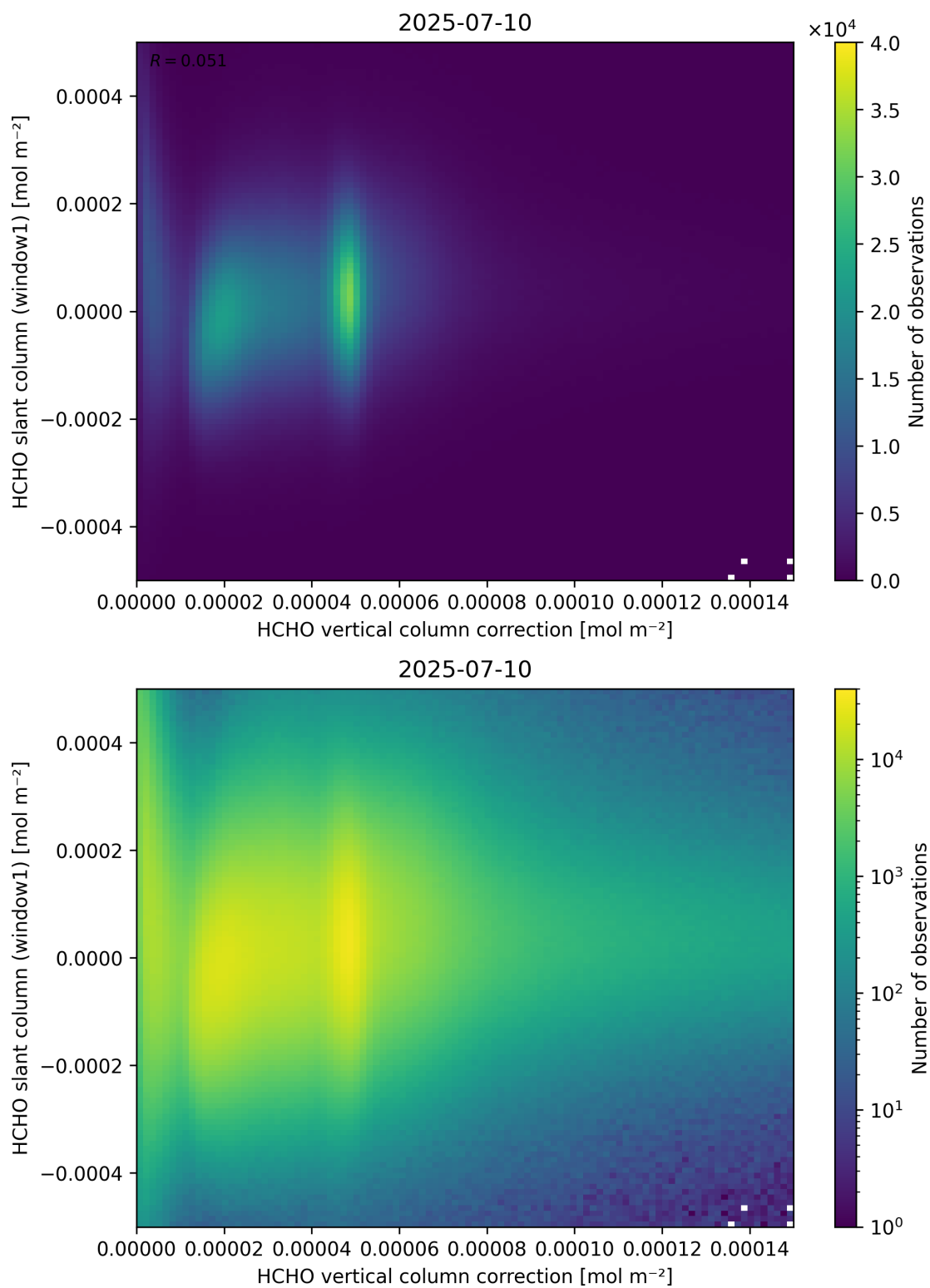
Figure 118: Scatter density plot of “HCHO vertical column correction” against “HCHO slant column (window1)” for 2025-07-09 to 2025-07-11.
