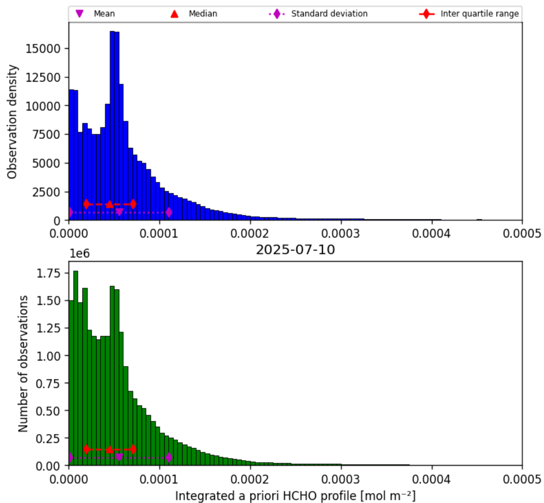
Figure 43: Histogram of “Integrated a priori HCHO profile” for 2025-07-09 to 2025-07-11
