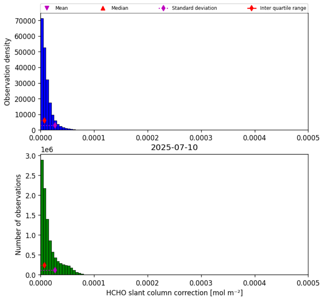
Figure 47: Histogram of “HCHO slant column correction” for 2025-07-09 to 2025-07-11
