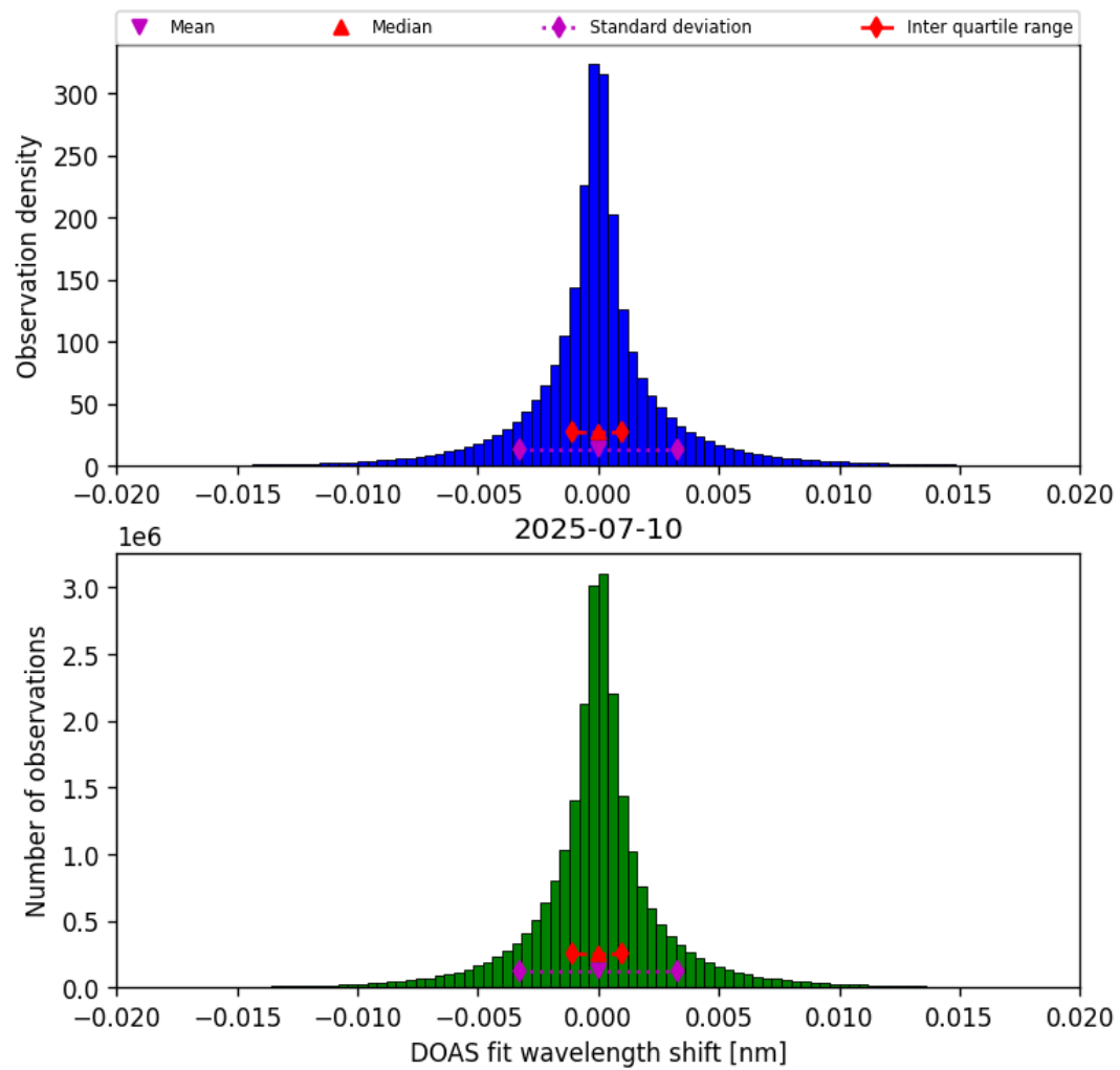
Figure 44: Histogram of “DOAS fit wavelength shift” for 2025-07-09 to 2025-07-11
