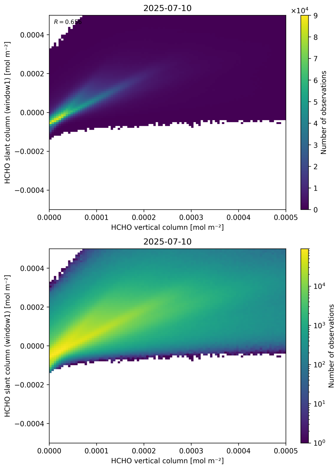
Figure 129: Scatter density plot of “HCHO vertical column” against “HCHO slant column (window1)” for 2025-07-09 to 2025-07-11.
