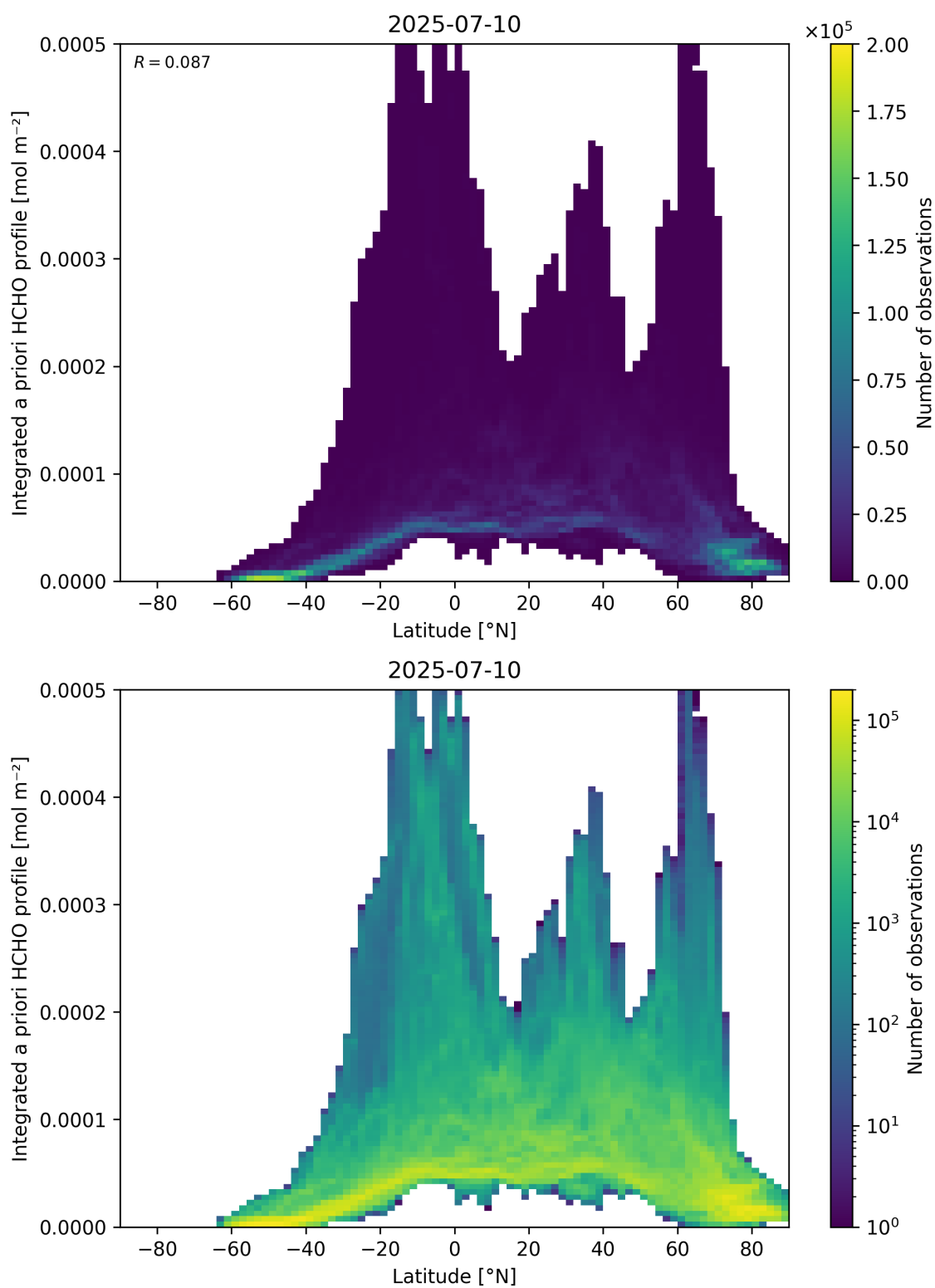
Figure 166: Scatter density plot of “Latitude” against “Integrated a priori HCHO profile” for 2025-07-09 to 2025-07-11.
