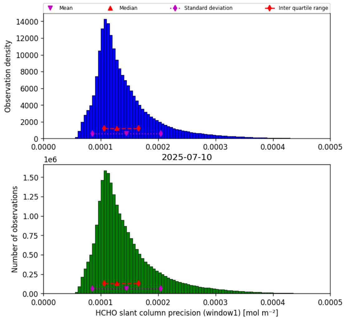
Figure 39: Histogram of “HCHO slant column precision (window1)” for 2025-07-09 to 2025-07-11
