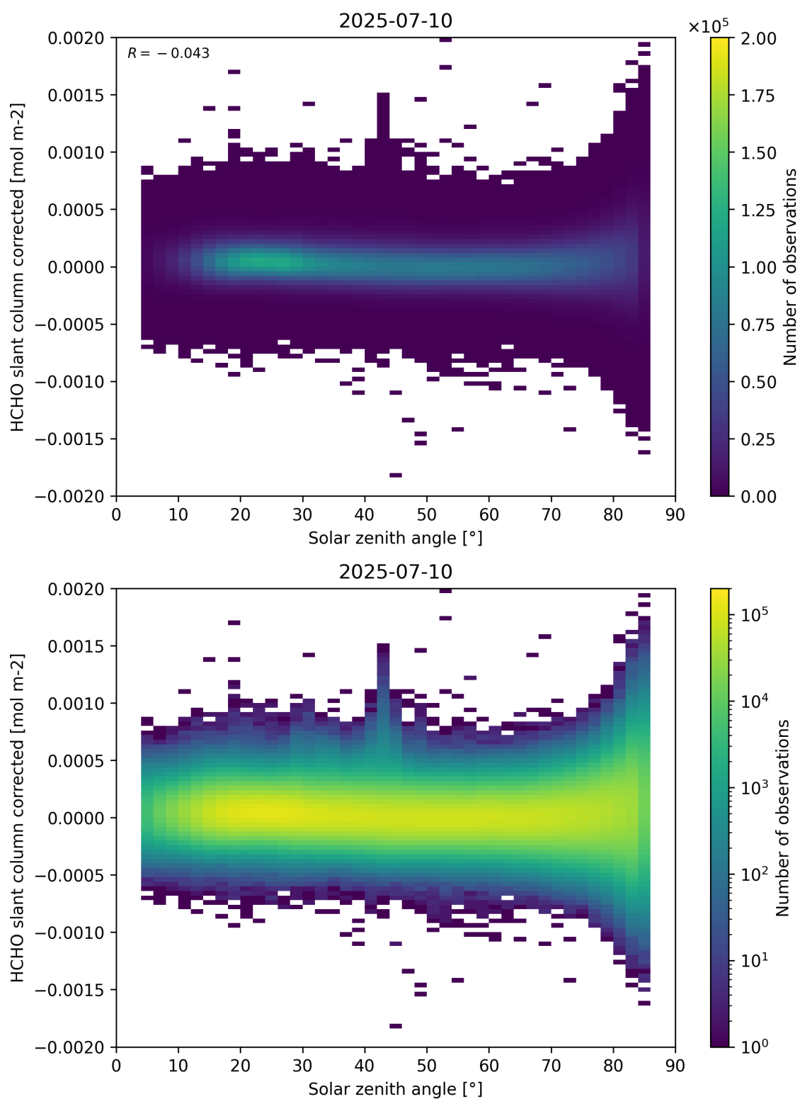
Figure 171: Scatter density plot of “Solar zenith angle” against “HCHO slant column corrected” for 2025-07-09 to 2025-07-11.
