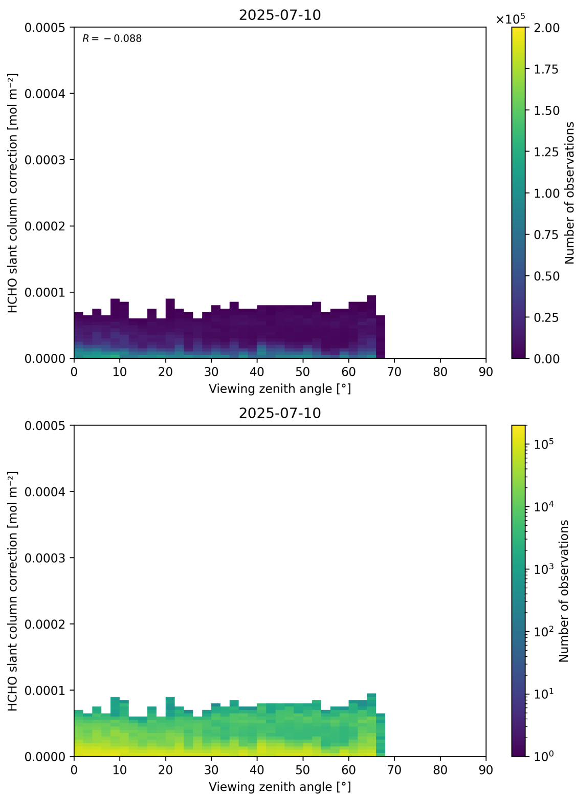
Figure 187: Scatter density plot of “Viewing zenith angle” against “HCHO slant column correction” for 2025-07-09 to 2025-07-11.
