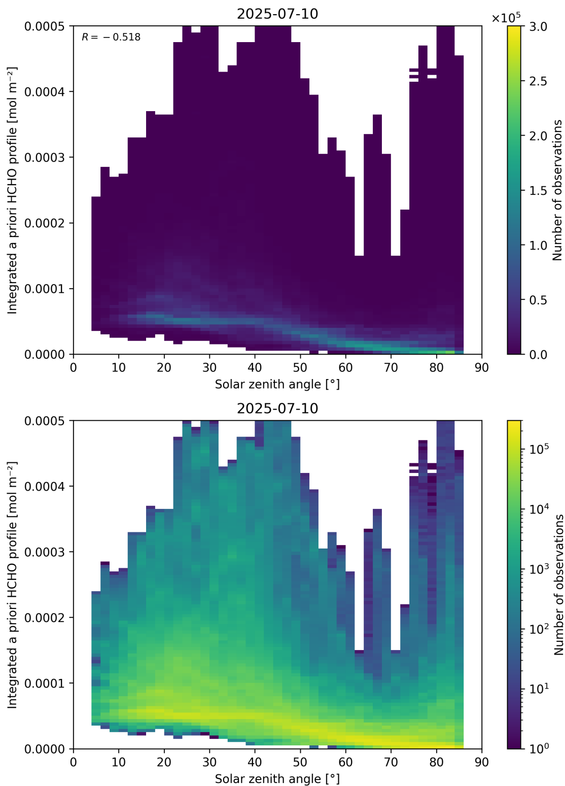
Figure 180: Scatter density plot of “Solar zenith angle” against “Integrated a priori HCHO profile” for 2025-07-09 to 2025-07-11.
