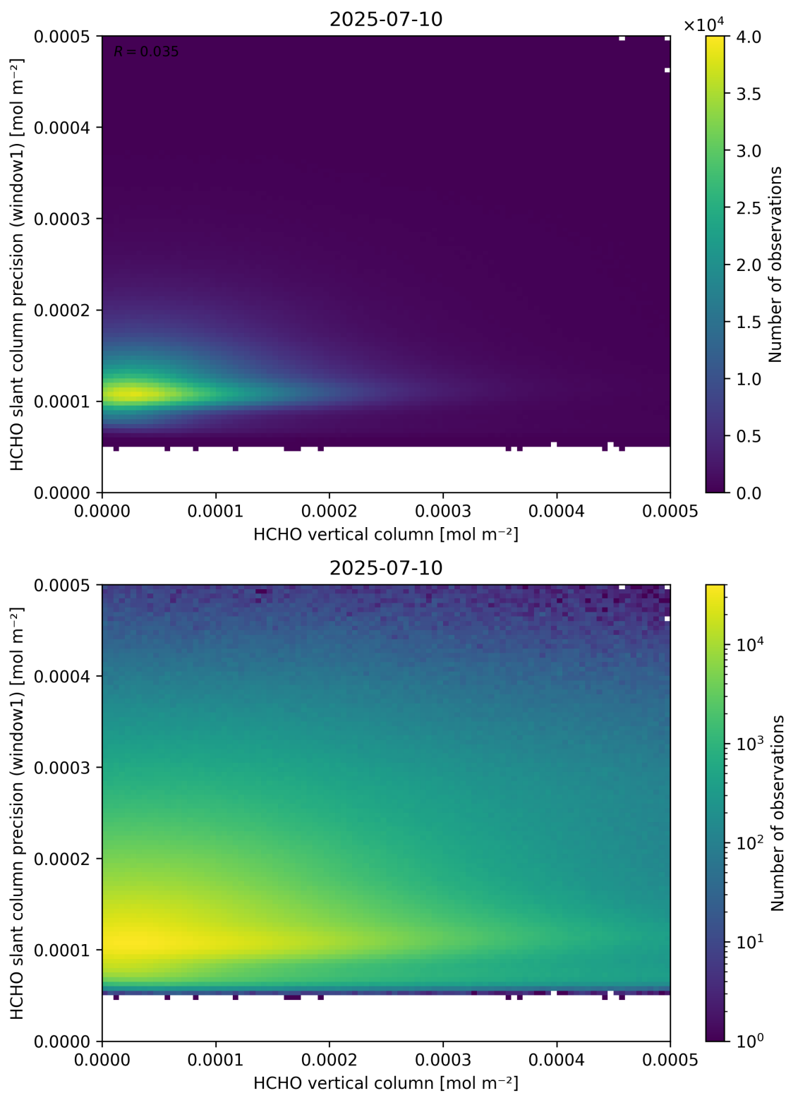
Figure 130: Scatter density plot of “HCHO vertical column” against “HCHO slant column precision (window1)” for 2025-07-09 to 2025-07-11.
