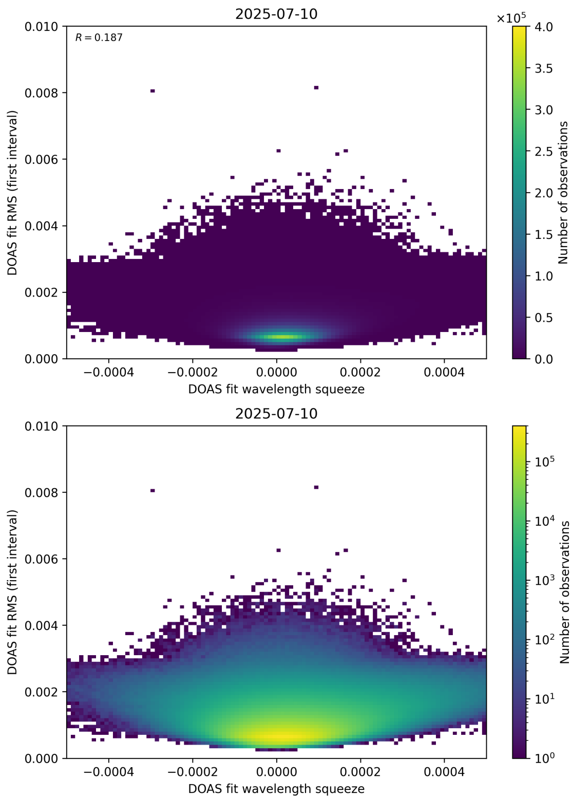
Figure 68: Scatter density plot of “DOAS fit wavelength squeeze” against “DOAS fit RMS (first interval)” for 2025-07-09 to 2025-07-11.
