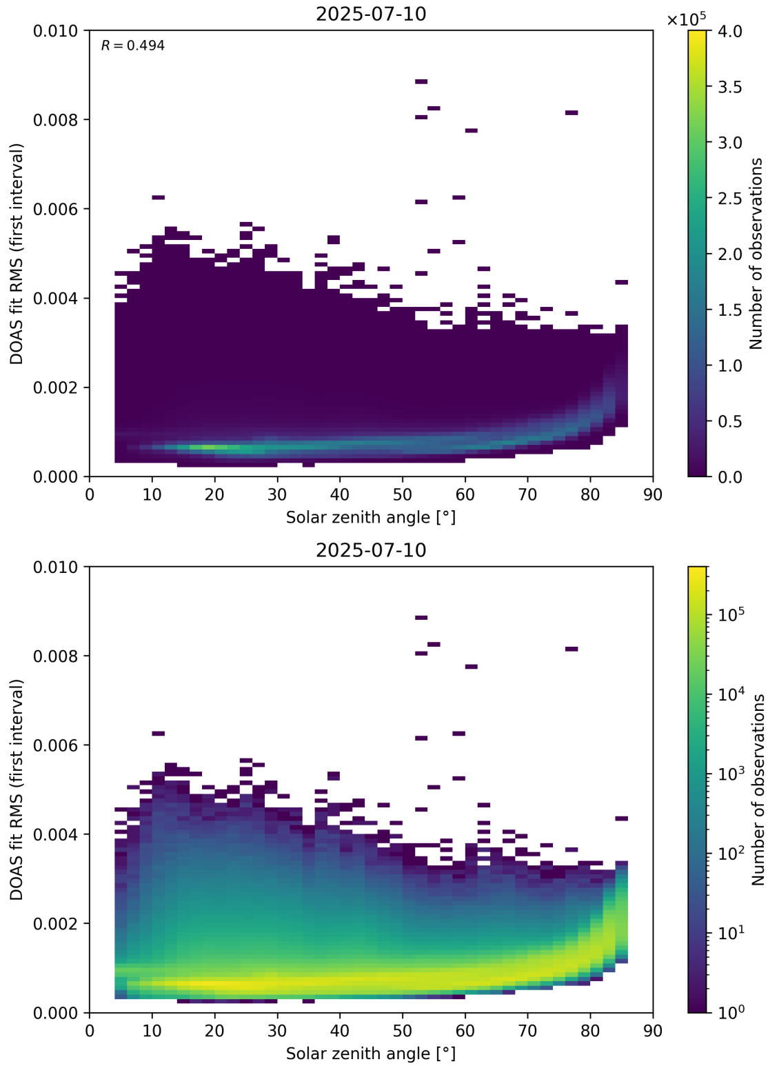
Figure 167: Scatter density plot of “Solar zenith angle” against “DOAS fit RMS (first interval)” for 2025-07-09 to 2025-07-11.
