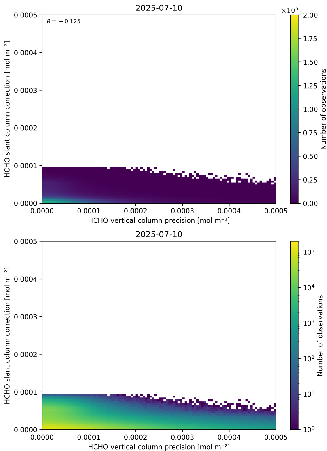
Figure 141: Scatter density plot of “HCHO vertical column precision” against “HCHO slant column correction” for 2025-07-09 to 2025-07-11.
