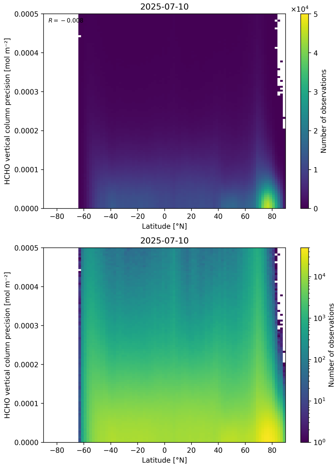
Figure 165: Scatter density plot of “Latitude” against “HCHO vertical column precision” for 2025-07-09 to 2025-07-11.
