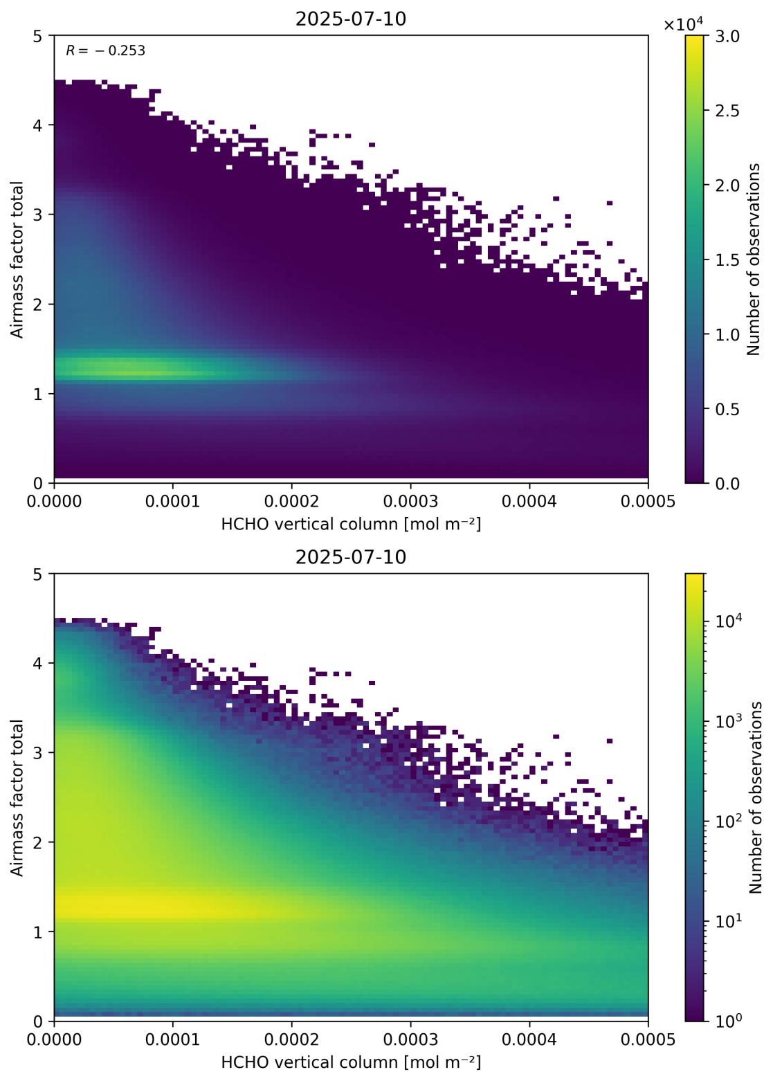
Figure 131: Scatter density plot of “HCHO vertical column” against “Airmass factor total” for 2025-07-09 to 2025-07-11.
