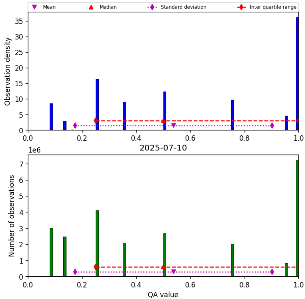
Figure 34: Histogram of “QA value” for 2025-07-09 to 2025-07-11
