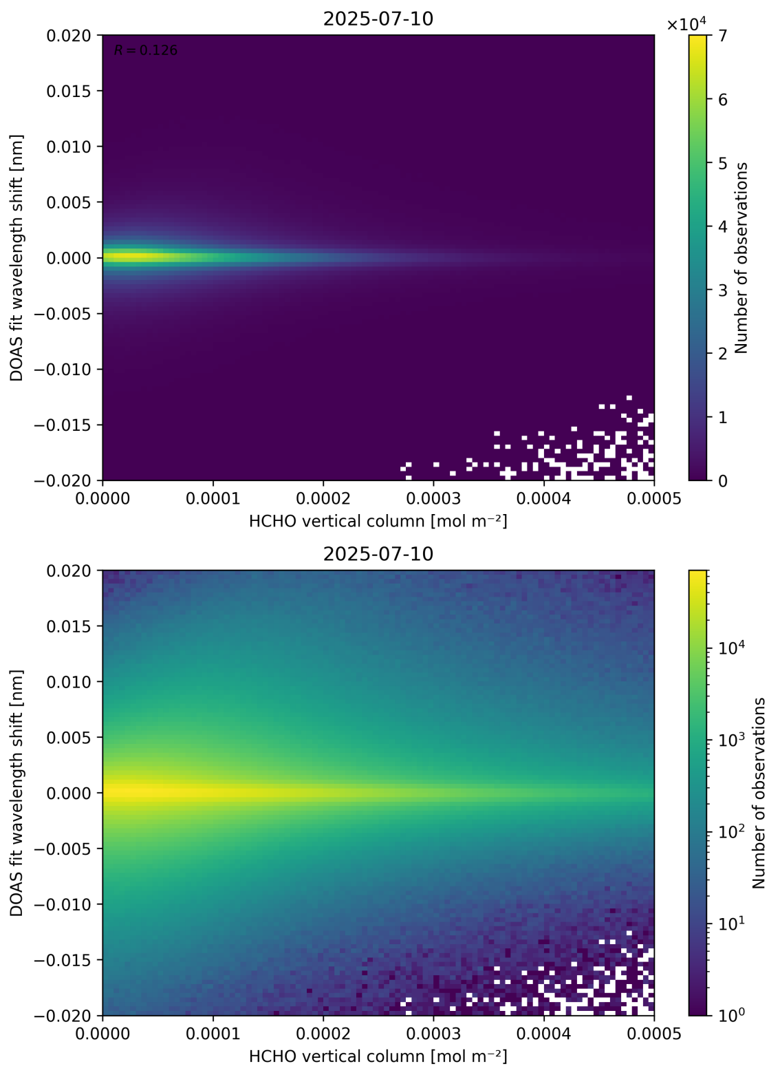
Figure 124: Scatter density plot of “HCHO vertical column” against “DOAS fit wavelength shift” for 2025-07-09 to 2025-07-11.
