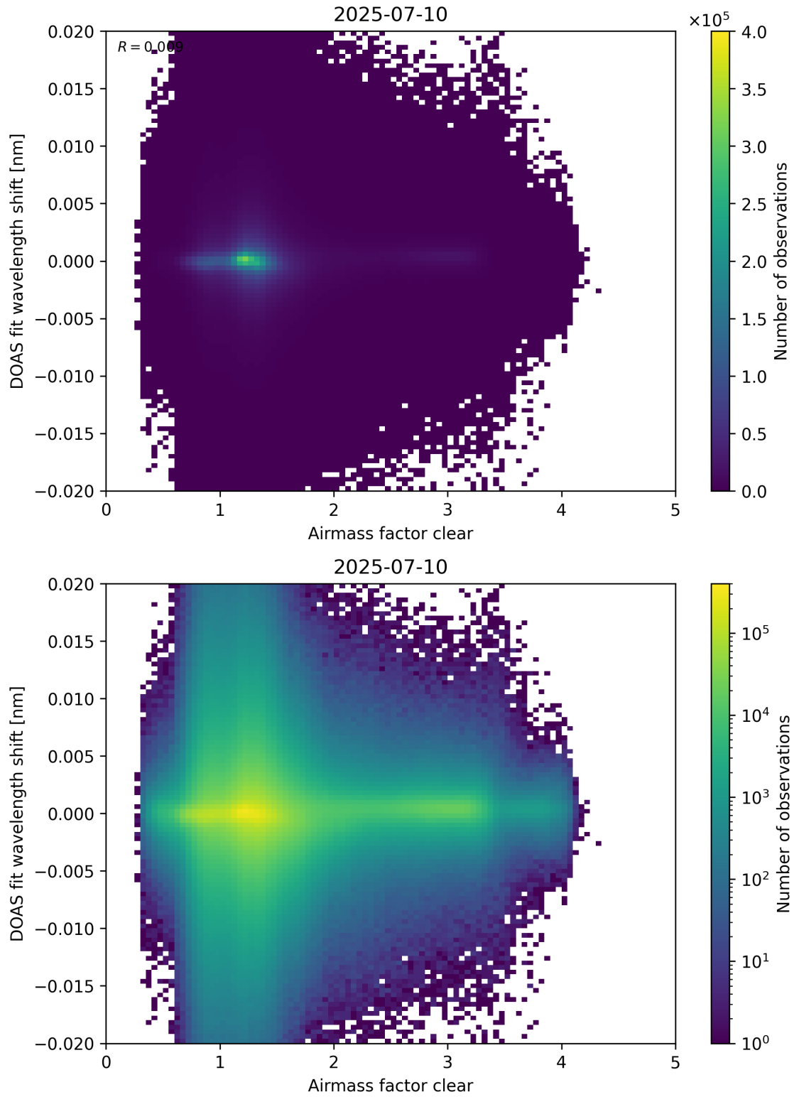
Figure 72: Scatter density plot of “Airmass factor clear” against “DOAS fit wavelength shift” for 2025-07-09 to 2025-07-11.
