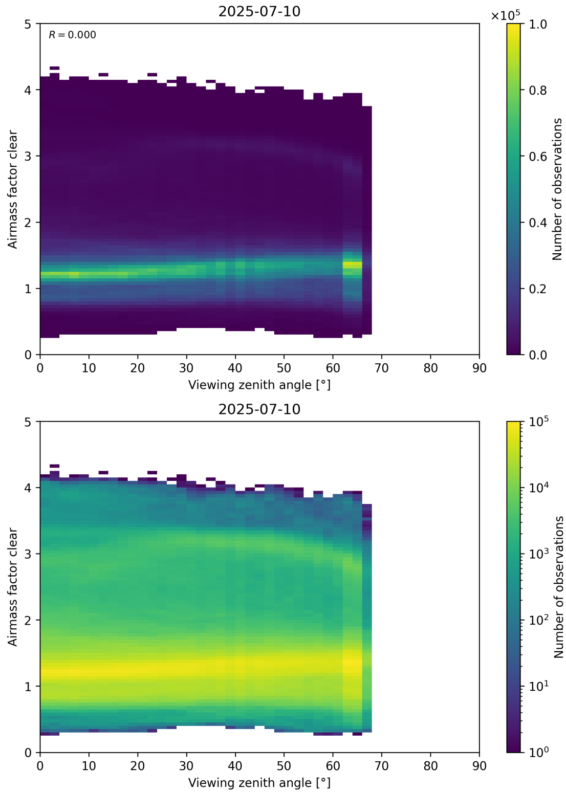
Figure 185: Scatter density plot of “Viewing zenith angle” against “Airmass factor clear” for 2025-07-09 to 2025-07-11.
