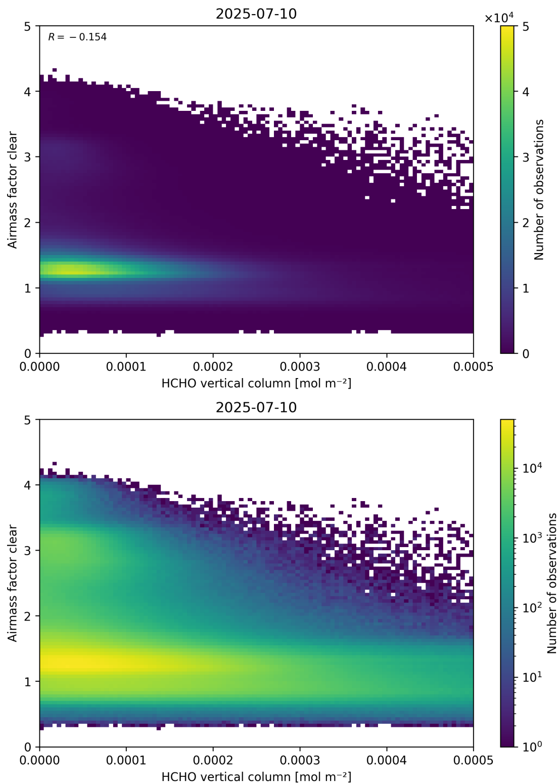
Figure 126: Scatter density plot of “HCHO vertical column” against “Airmass factor clear” for 2025-07-09 to 2025-07-11.
