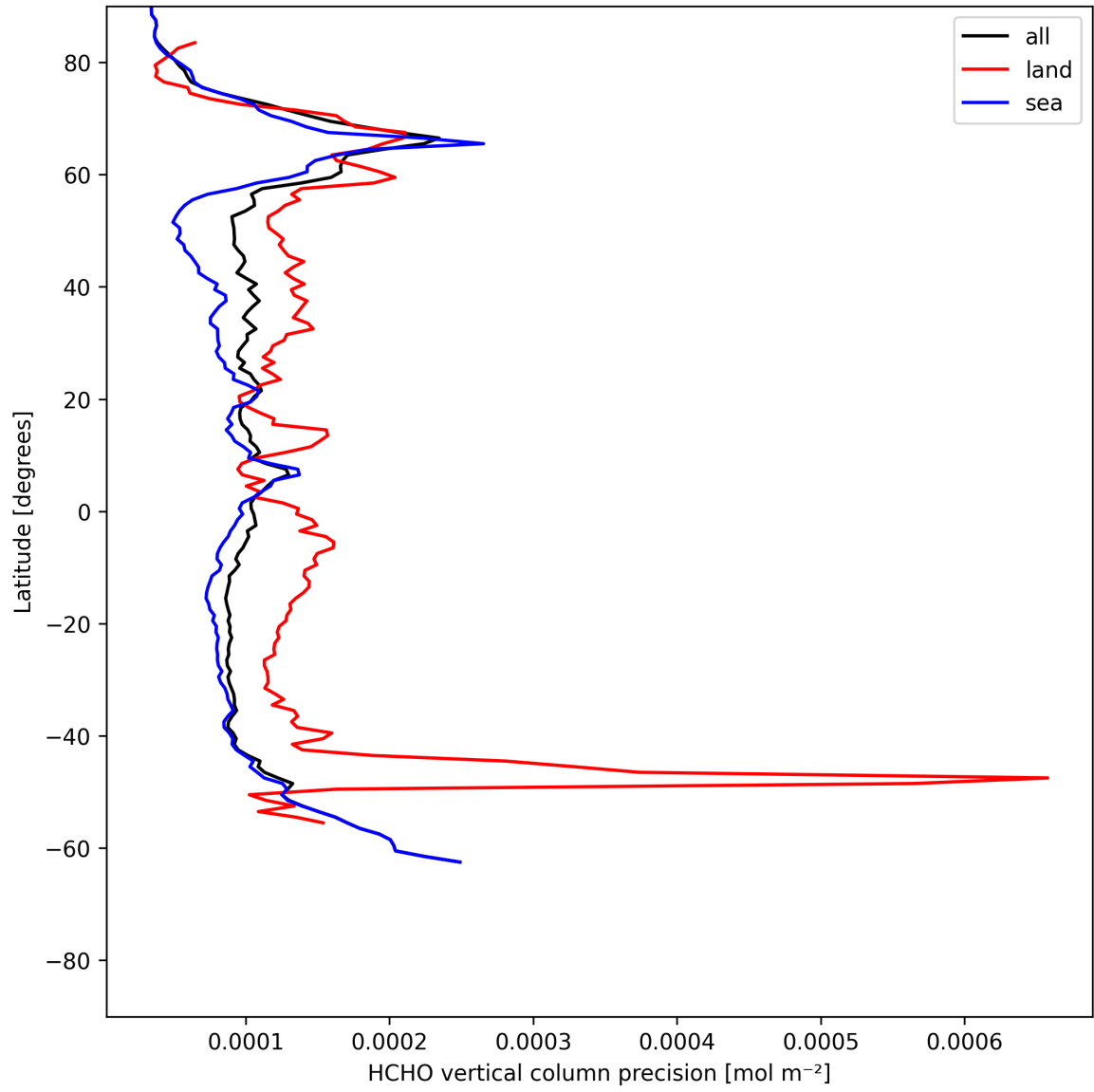
Figure 22: Zonal average of “HCHO vertical column precision” for 2025-07-09 to 2025-07-11.
