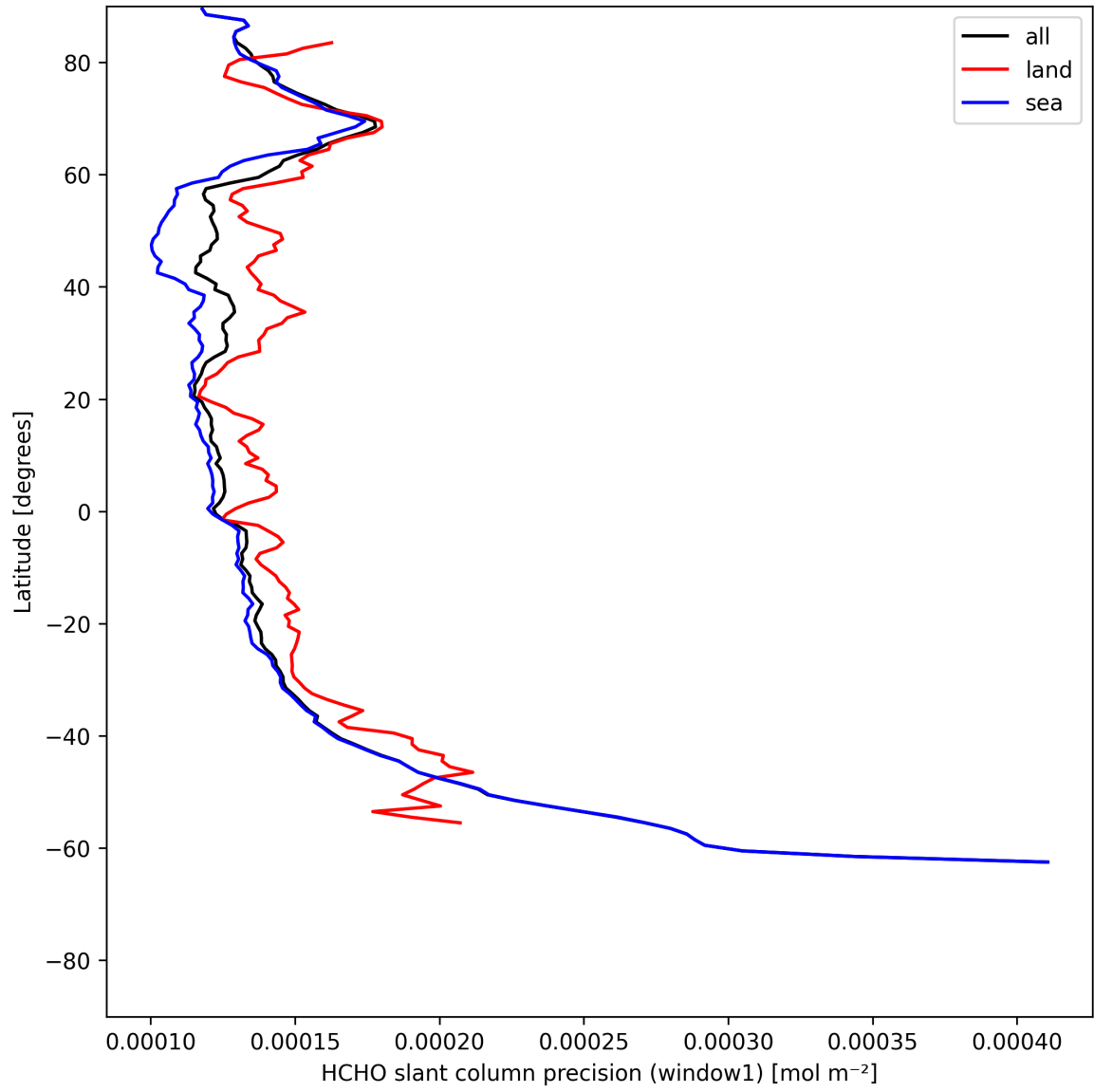
Figure 25: Zonal average of “HCHO slant column precision (window1)” for 2025-07-09 to 2025-07-11.
