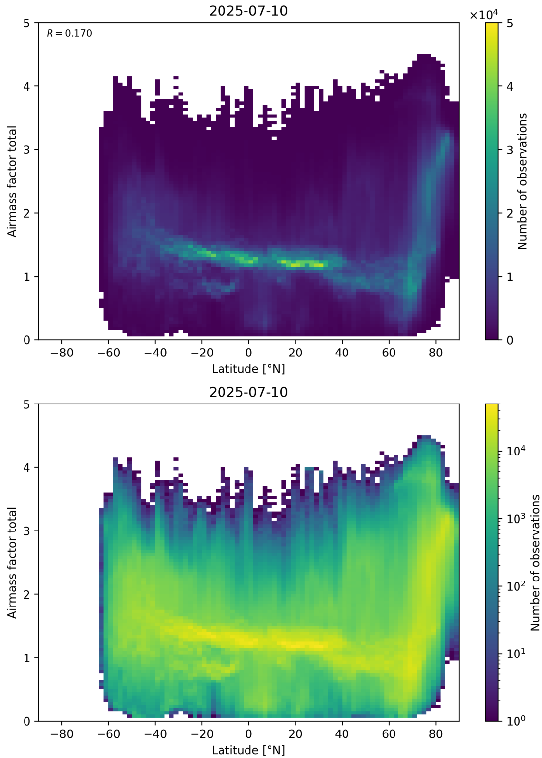
Figure 161: Scatter density plot of “Latitude” against “Airmass factor total” for 2025-07-09 to 2025-07-11.
