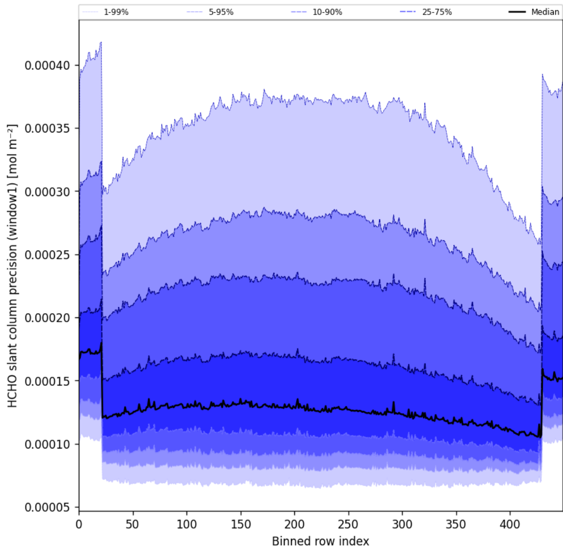
Figure 53: Along track statistics of “HCHO slant column precision (window1)” for 2025-07-09 to 2025-07-11
