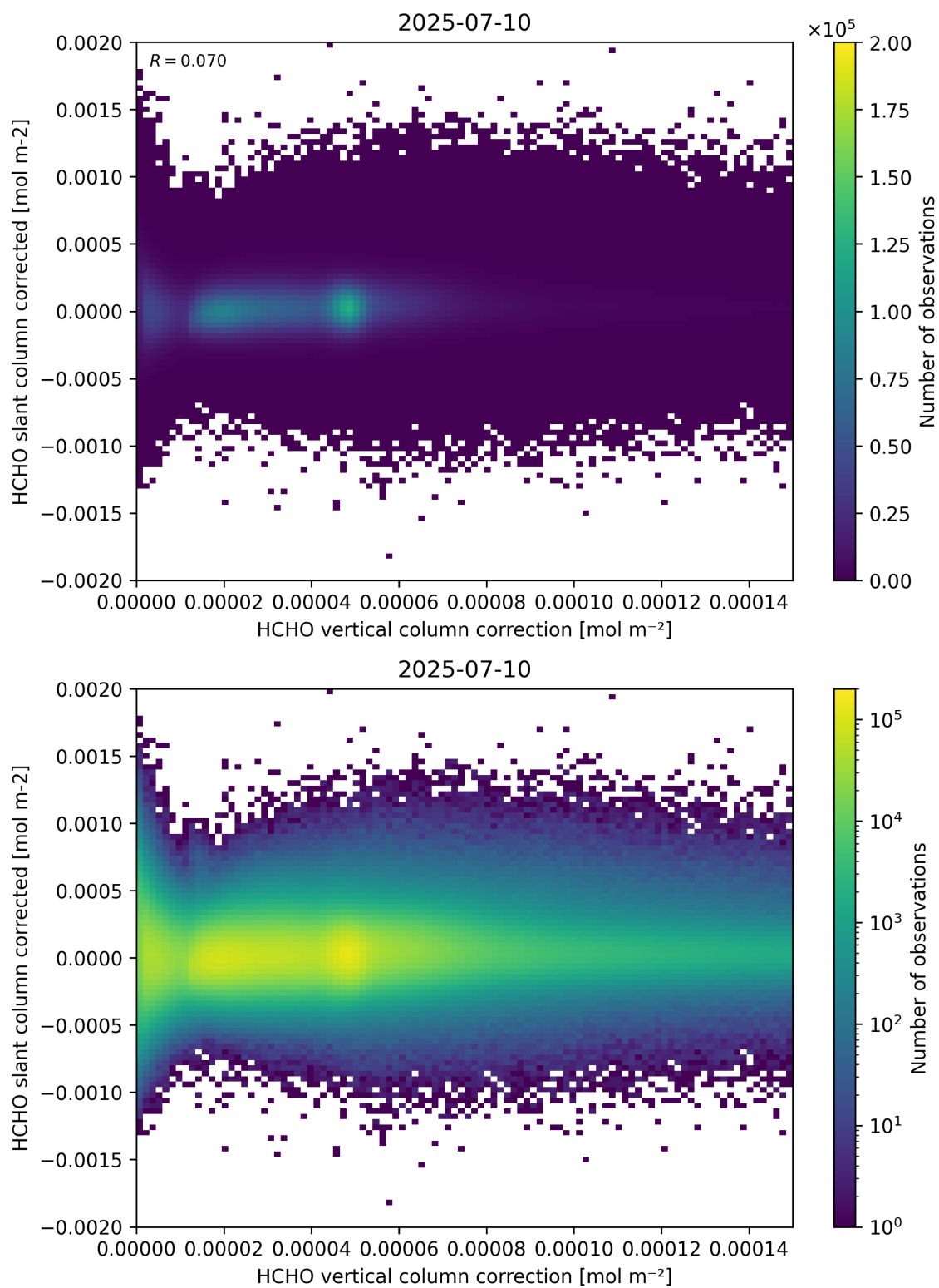
Figure 116: Scatter density plot of “HCHO vertical column correction” against “HCHO slant column corrected” for 2025-07-09 to 2025-07-11.
