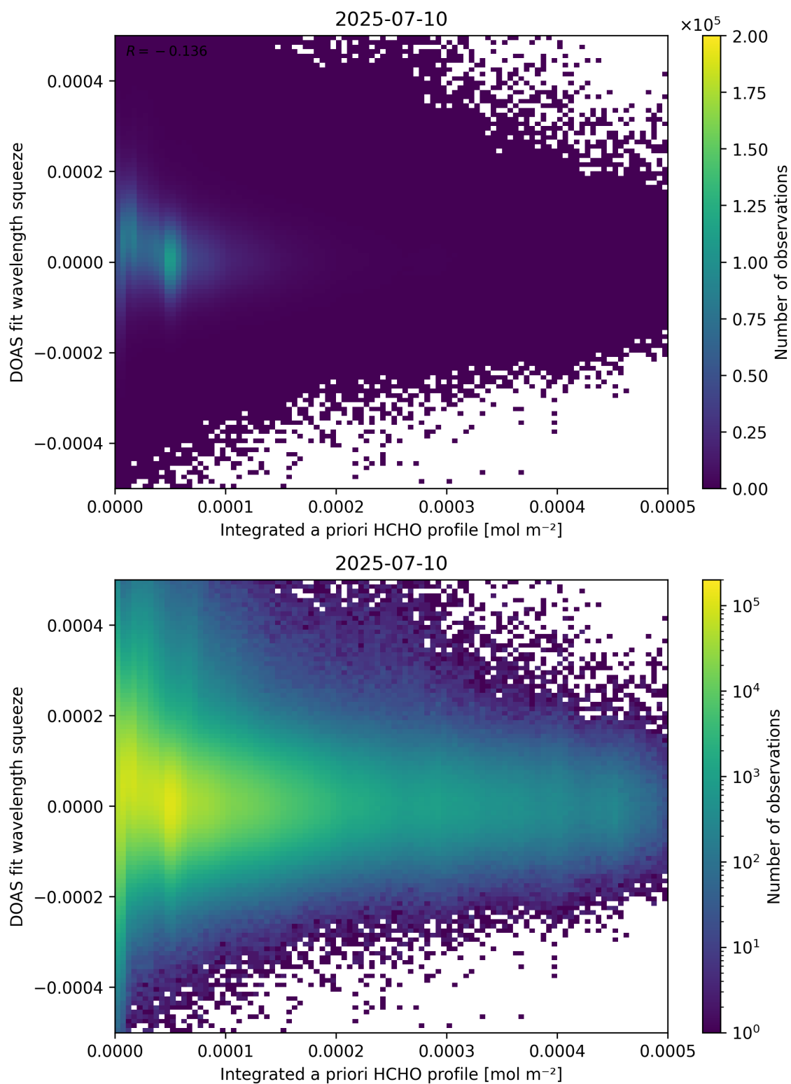
Figure 150: Scatter density plot of “Integrated a priori HCHO profile” against “DOAS fit wavelength squeeze” for 2025-07-09 to 2025-07-11.
