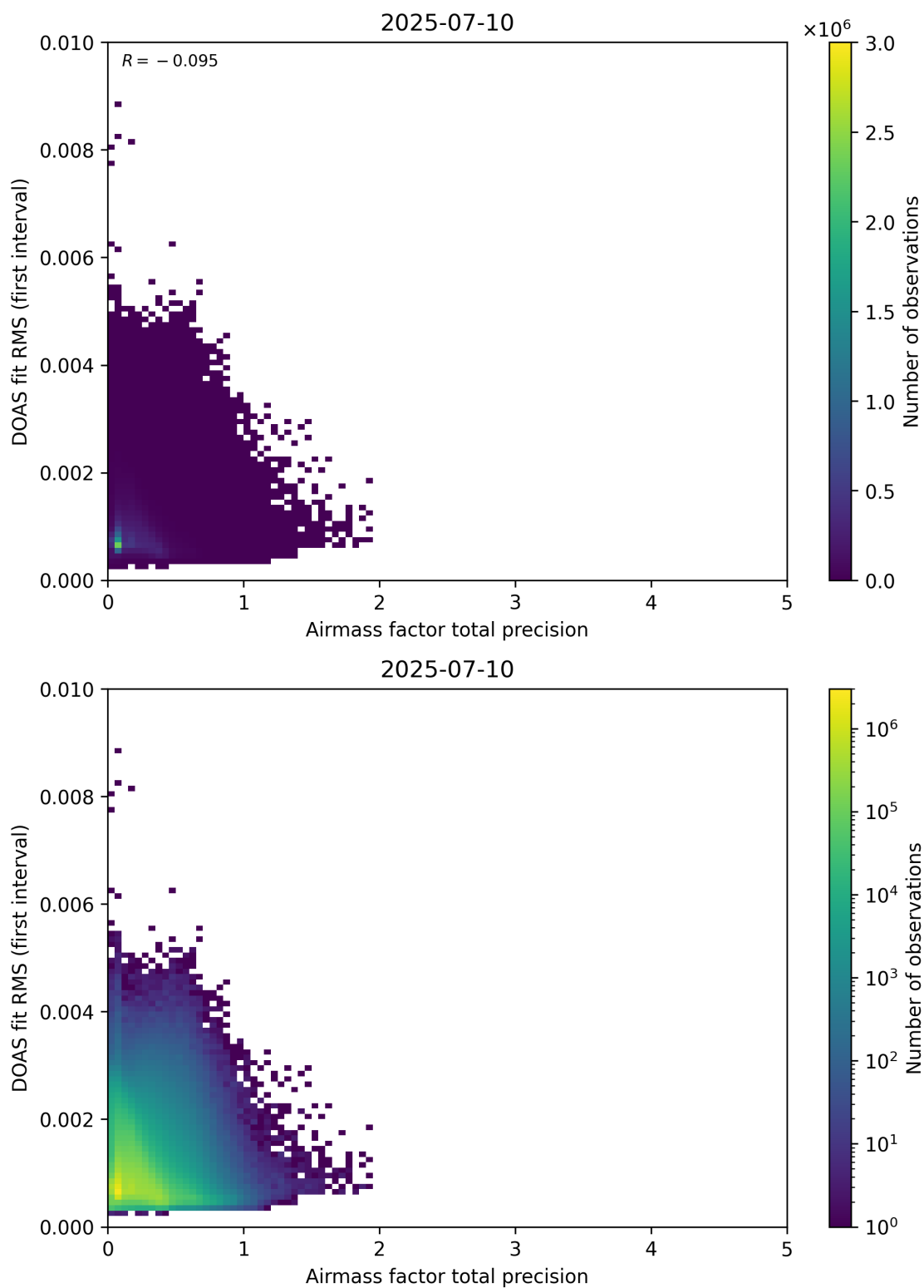
Figure 105: Scatter density plot of “Airmass factor total precision” against “DOAS fit RMS (first interval)” for 2025-07-09 to 2025-07-11.
