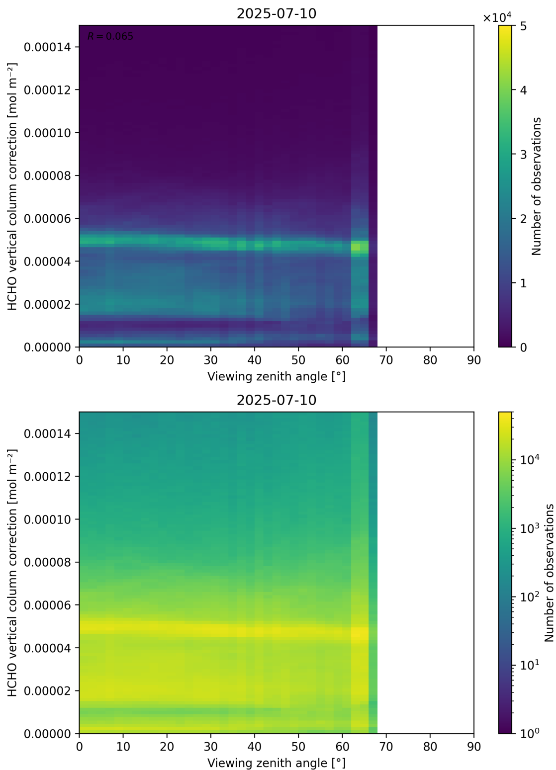
Figure 193: Scatter density plot of “Viewing zenith angle” against “HCHO vertical column correction” for 2025-07-09 to 2025-07-11.
