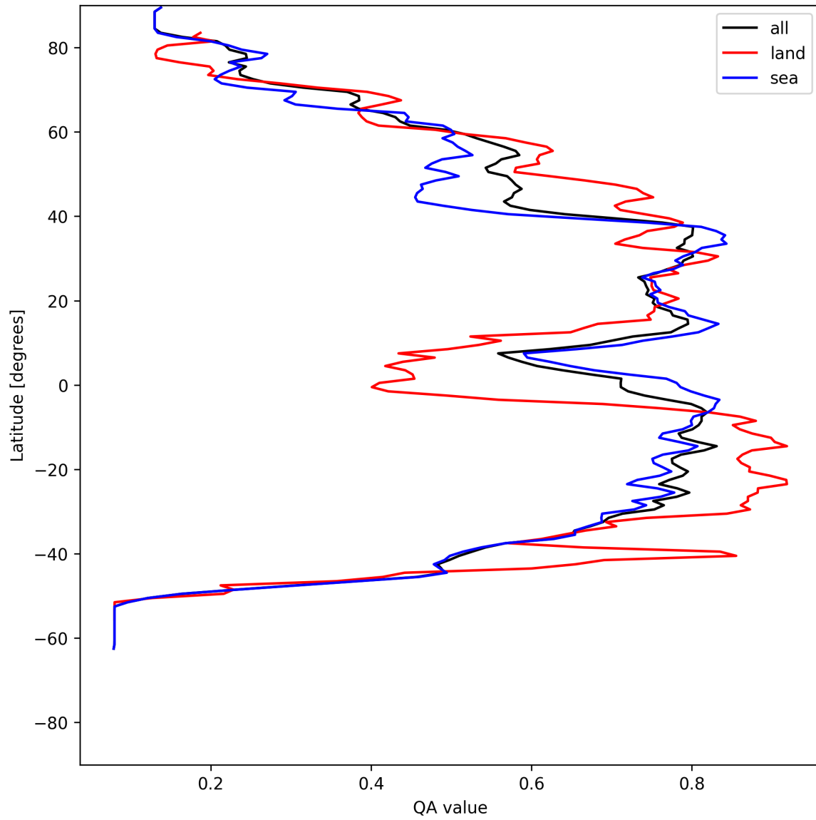
Figure 20: Zonal average of “QA value” for 2025-07-09 to 2025-07-11.
