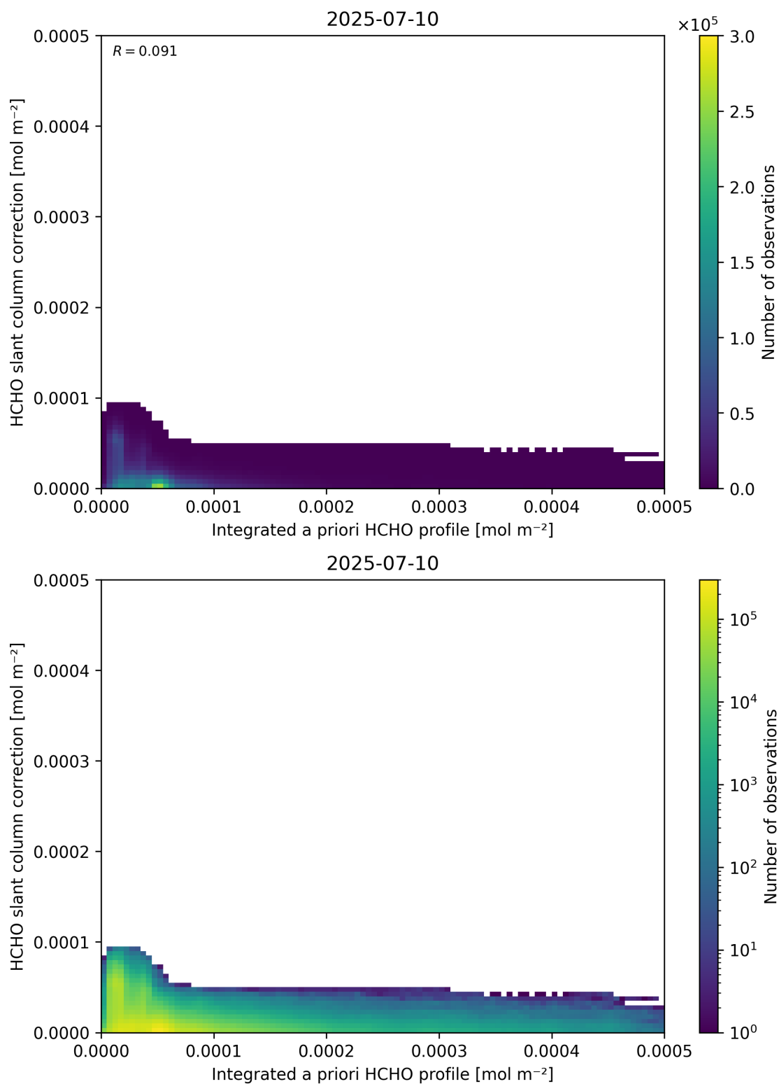
Figure 152: Scatter density plot of “Integrated a priori HCHO profile” against “HCHO slant column correction” for 2025-07-09 to 2025-07-11.
