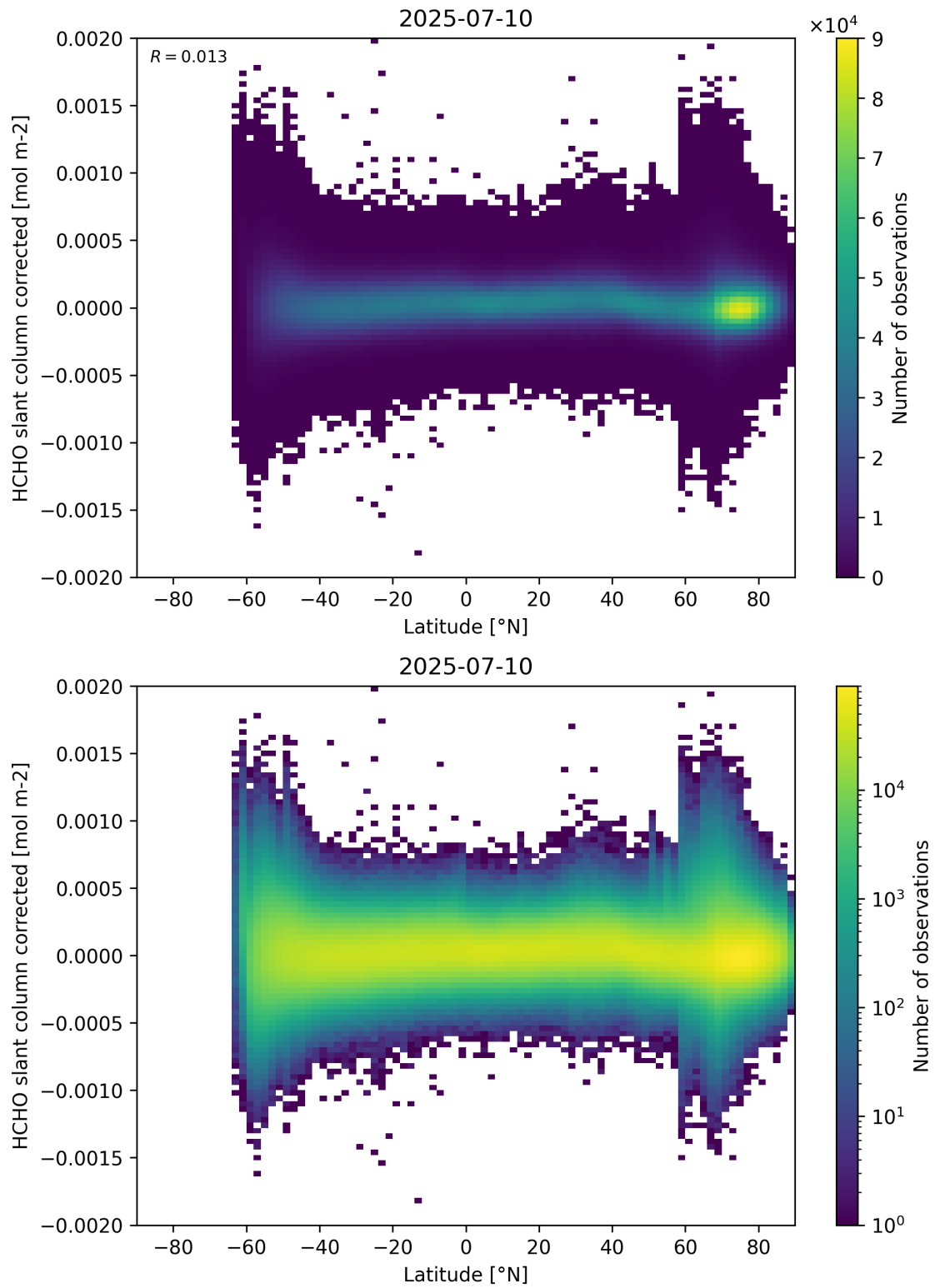
Figure 157: Scatter density plot of “Latitude” against “HCHO slant column corrected” for 2025-07-09 to 2025-07-11.
