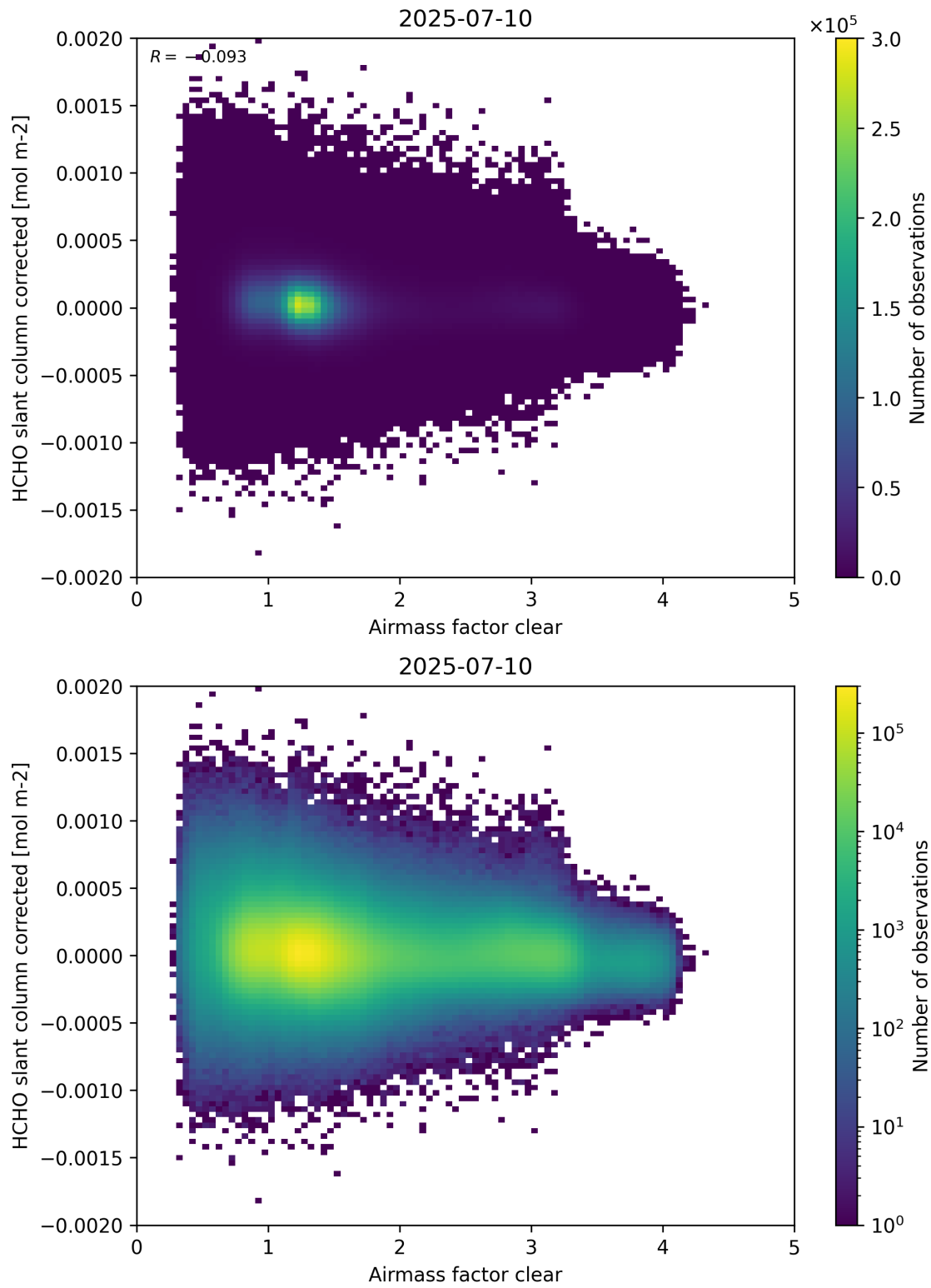
Figure 74: Scatter density plot of “Airmass factor clear” against “HCHO slant column corrected” for 2025-07-09 to 2025-07-11.
