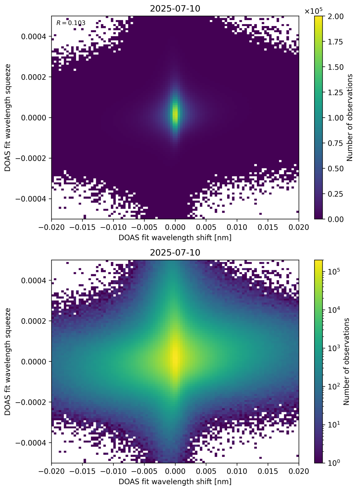
Figure 65: Scatter density plot of “DOAS fit wavelength shift” against “DOAS fit wavelength squeeze” for 2025-07-09 to 2025-07-11.
