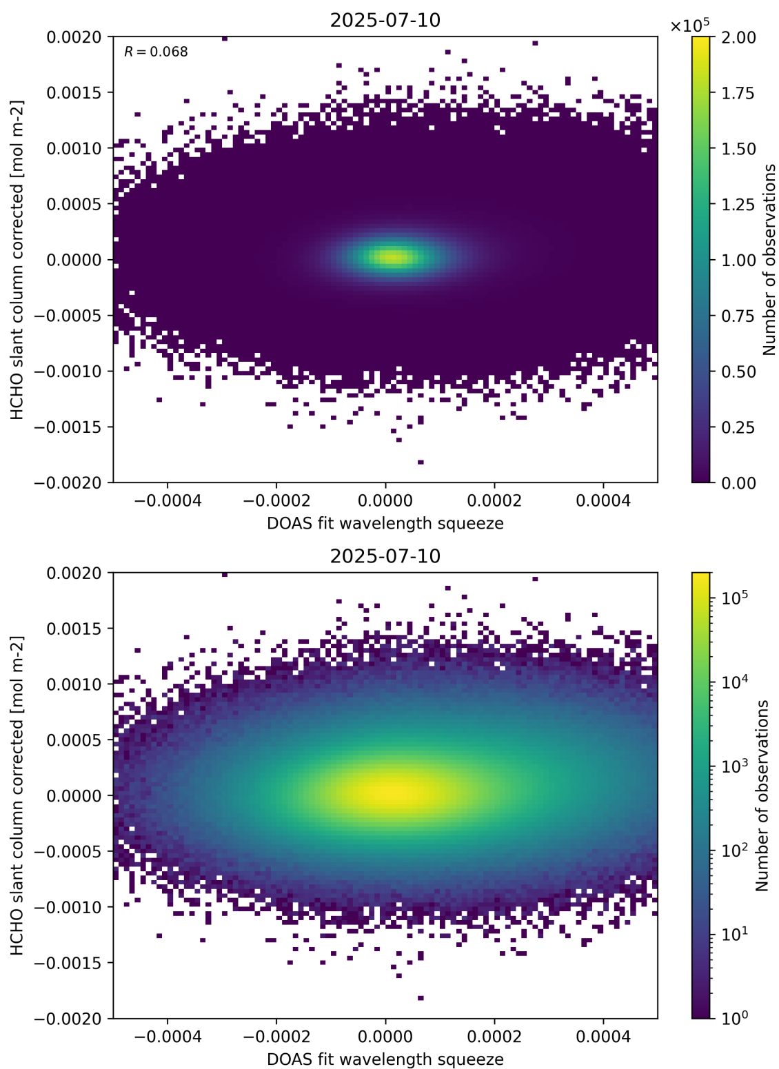
Figure 69: Scatter density plot of “DOAS fit wavelength squeeze” against “HCHO slant column corrected” for 2025-07-09 to 2025-07-11.
