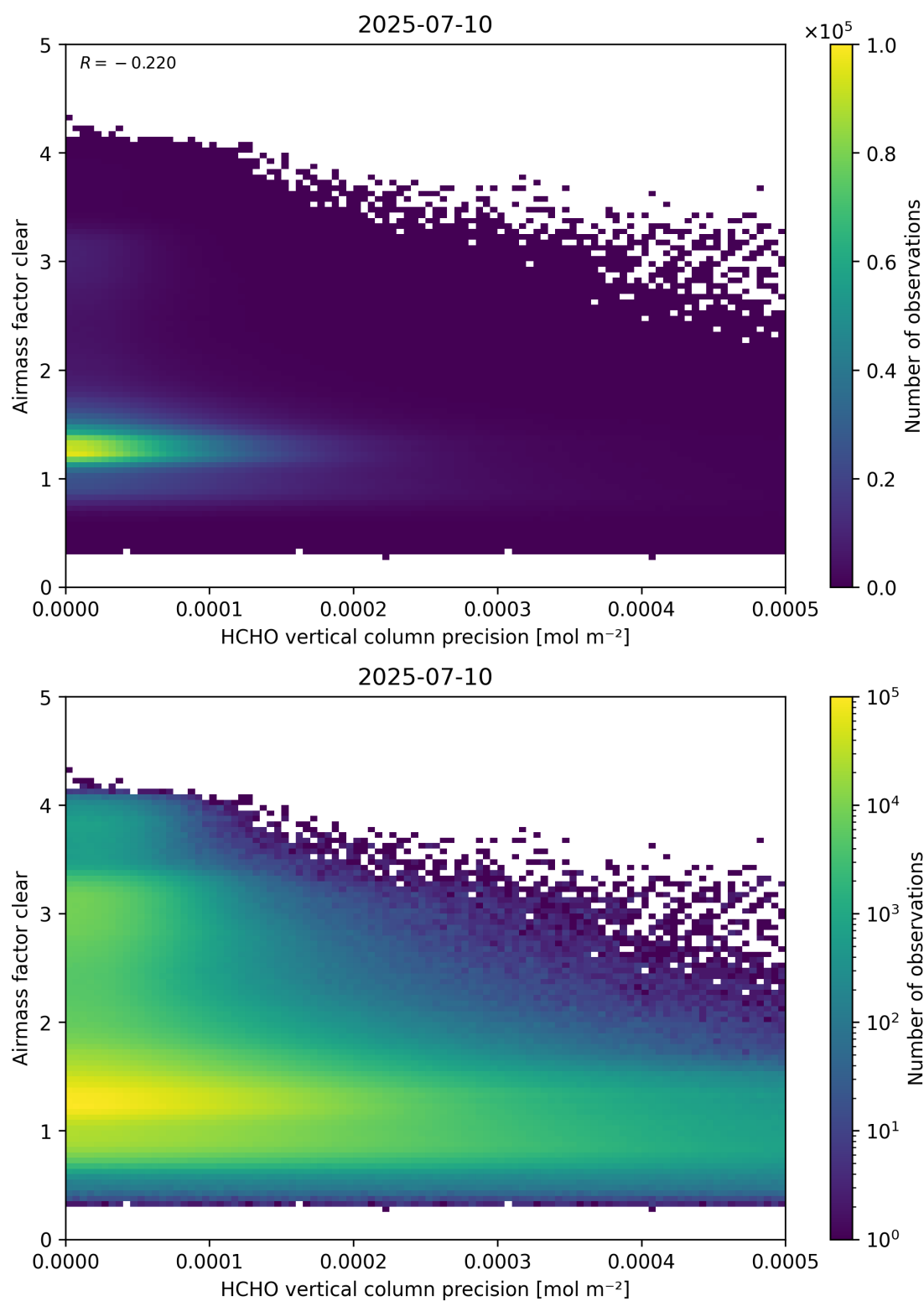
Figure 139: Scatter density plot of “HCHO vertical column precision” against “Airmass factor clear” for 2025-07-09 to 2025-07-11.
