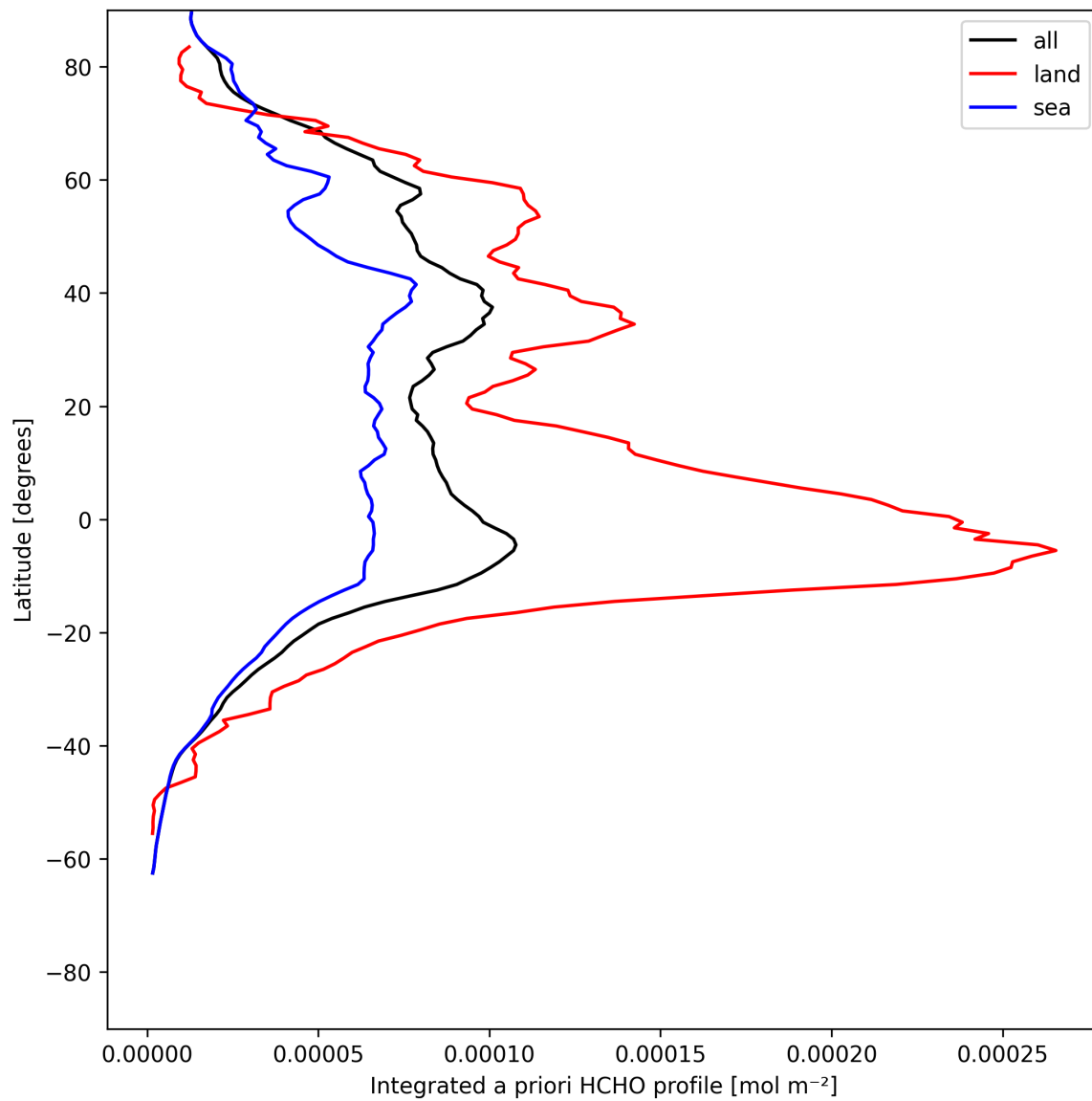
Figure 29: Zonal average of “Integrated a priori HCHO profile” for 2025-07-09 to 2025-07-11.
