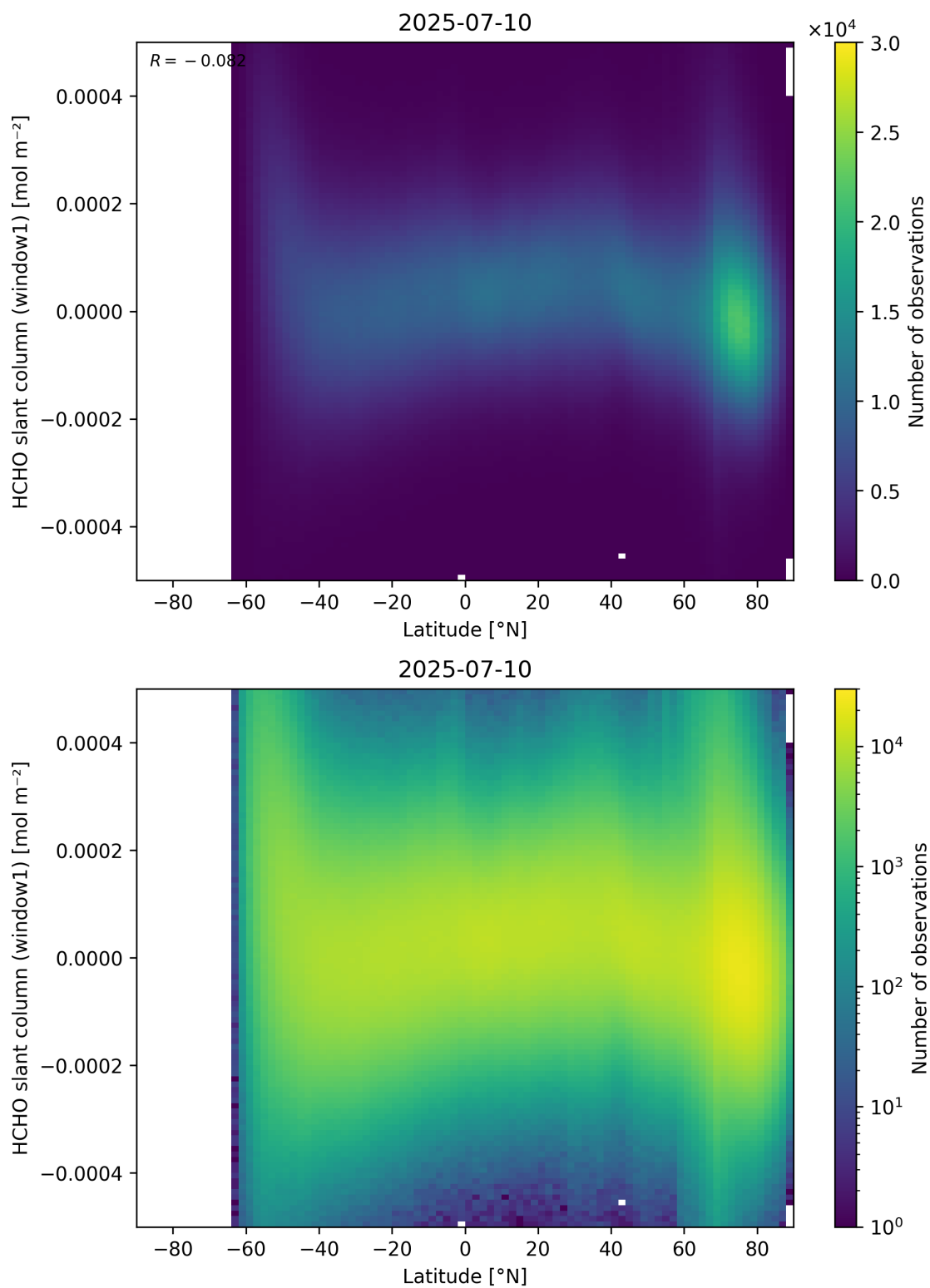
Figure 159: Scatter density plot of “Latitude” against “HCHO slant column (window1)” for 2025-07-09 to 2025-07-11.
