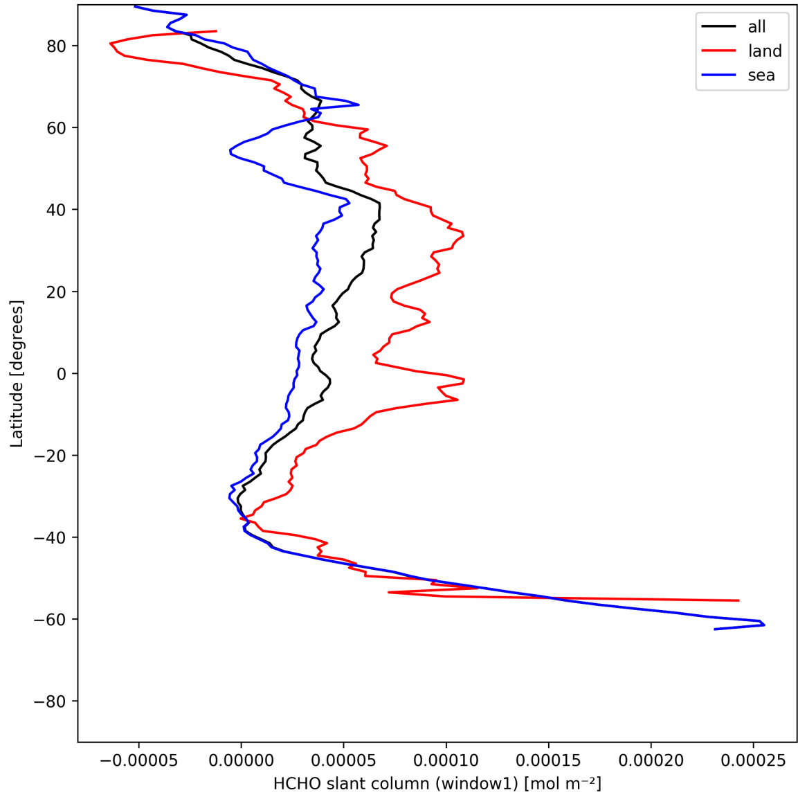
Figure 24: Zonal average of “HCHO slant column (window1)” for 2025-07-09 to 2025-07-11.
