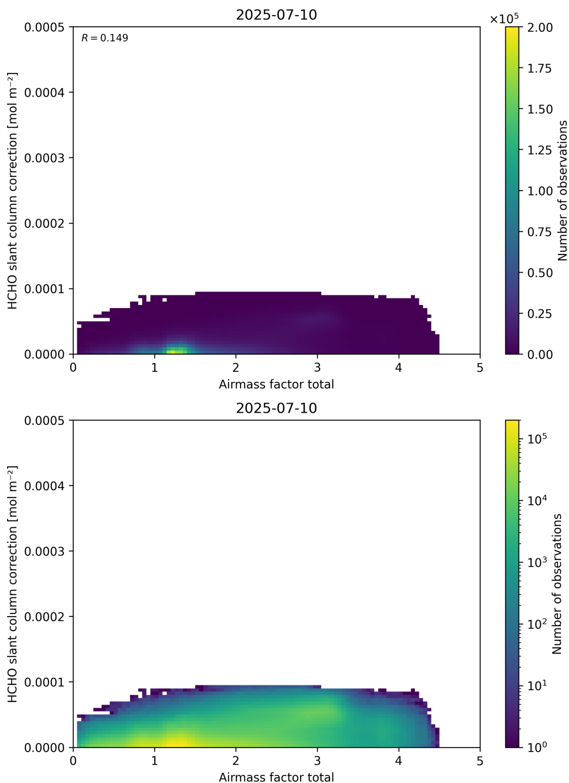
Figure 102: Scatter density plot of “Airmass factor total” against “HCHO slant column correction” for 2025-07-09 to 2025-07-11.
