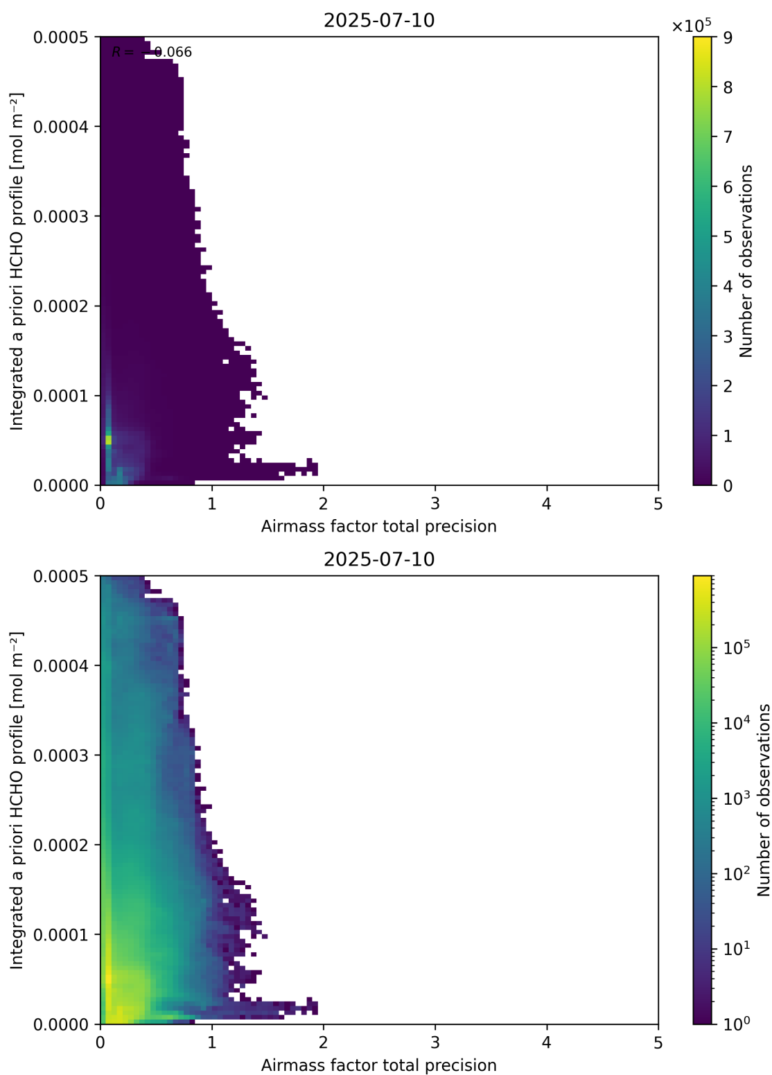
Figure 111: Scatter density plot of “Airmass factor total precision” against “Integrated a priori HCHO profile” for 2025-07-09 to 2025-07-11.
