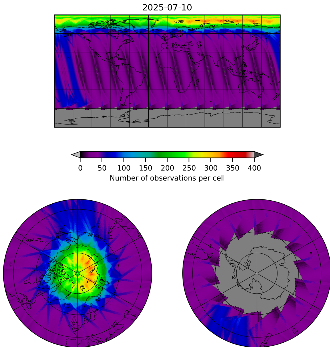
Figure 19: Map of the number of observations for 2025-07-09 to 2025-07-11
