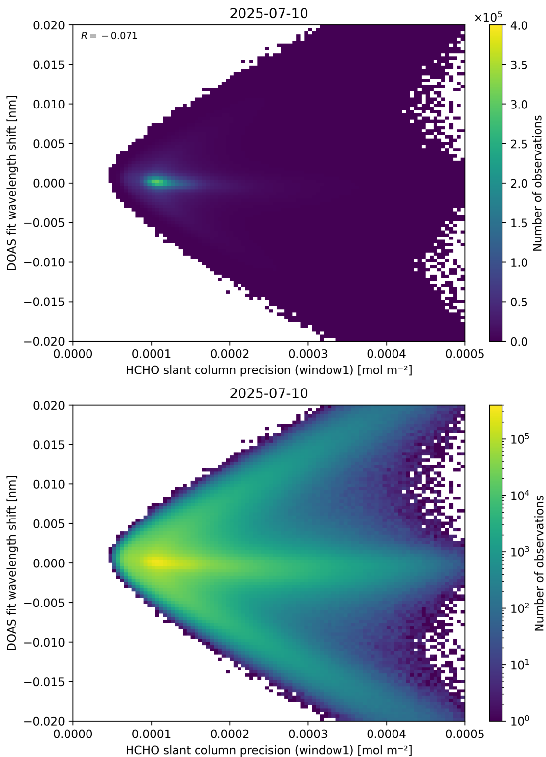
Figure 89: Scatter density plot of “HCHO slant column precision (window1)” against “DOAS fit wavelength shift” for 2025-07-09 to 2025-07-11.
