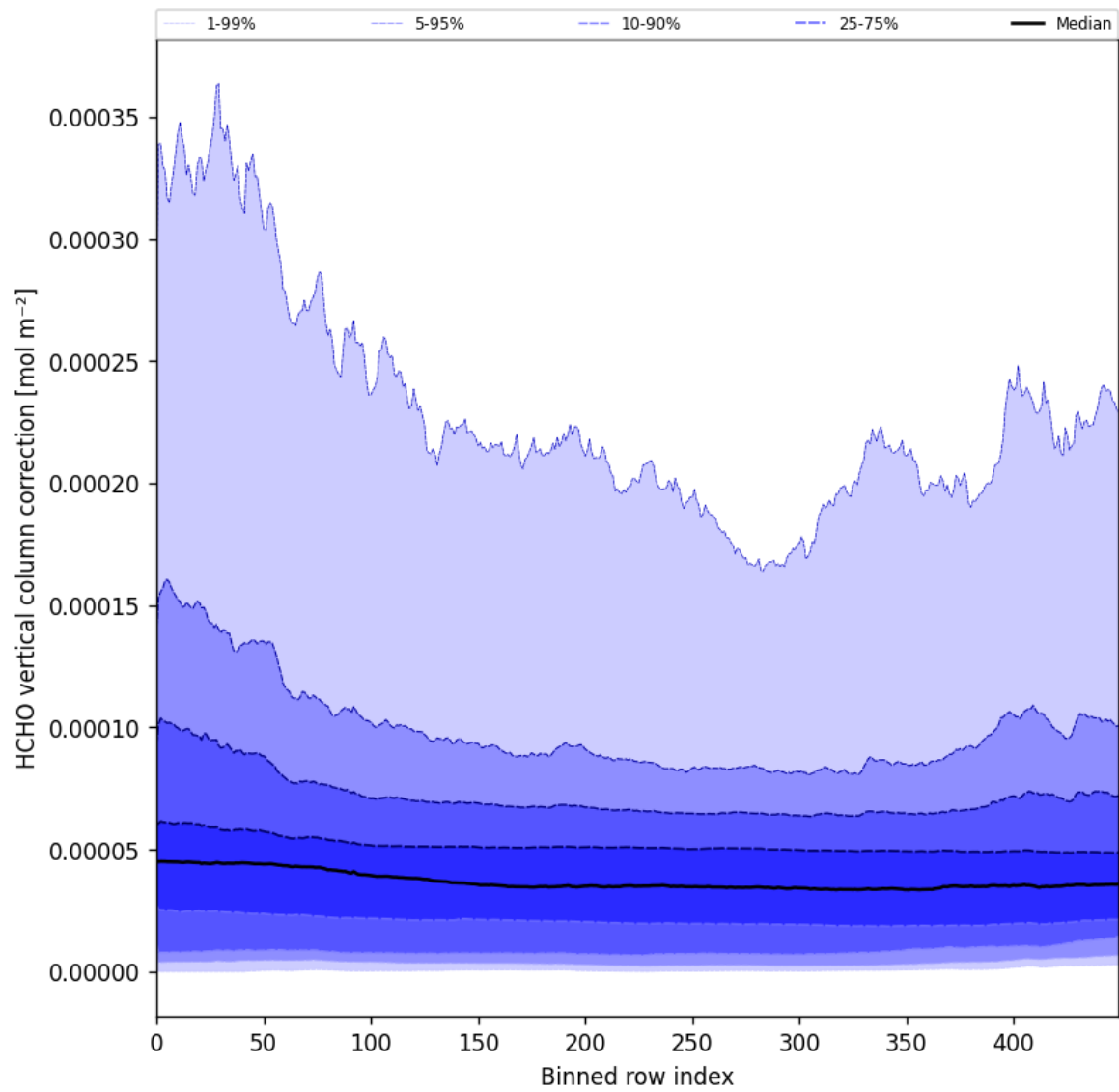
Figure 51: Along track statistics of "HCHO vertical column correction" for 2025-07-09 to 2025-07-11
