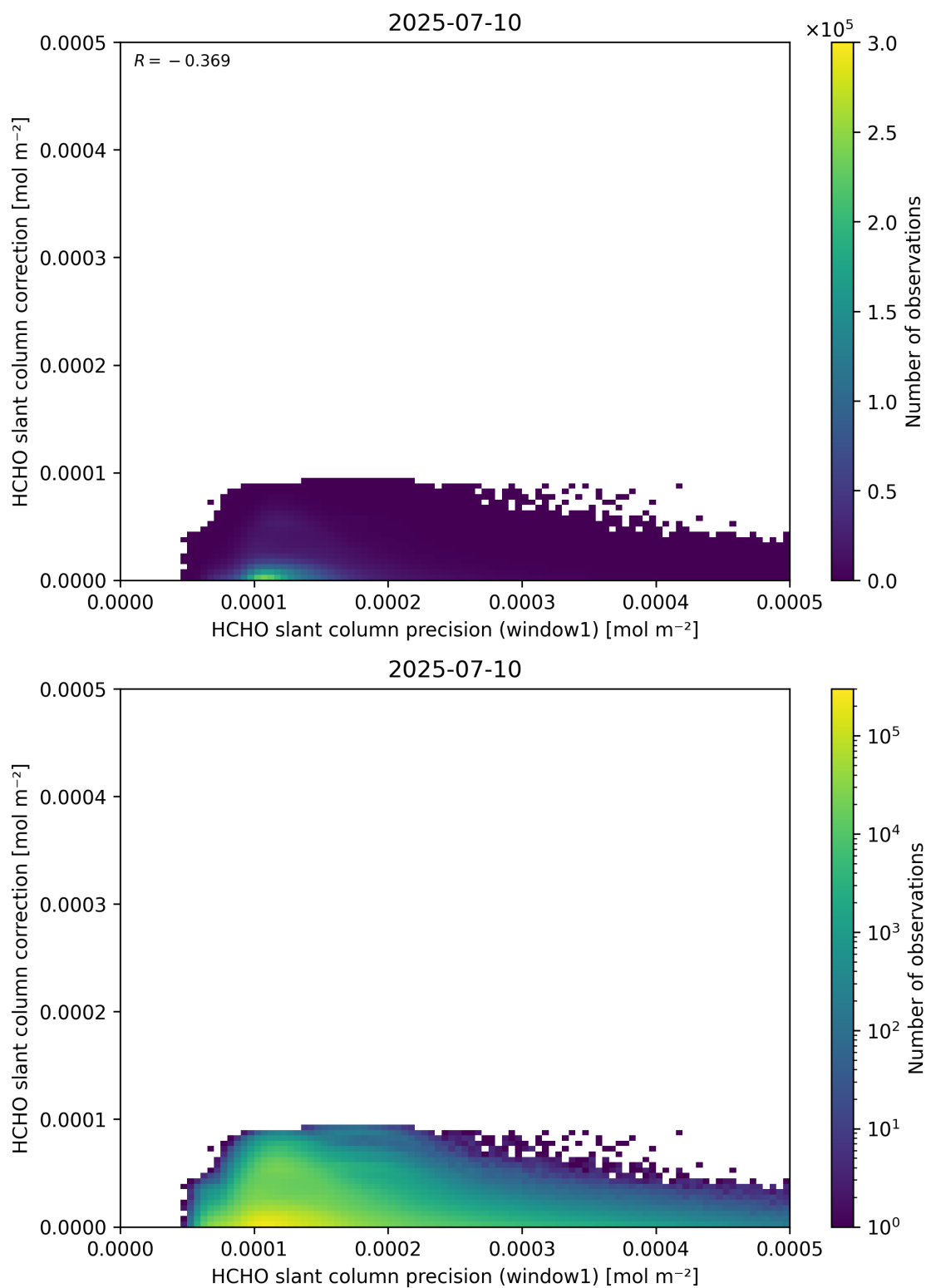
Figure 93: Scatter density plot of “HCHO slant column precision (window1)” against “HCHO slant column correction” for 2025-07-09 to 2025-07-11.
