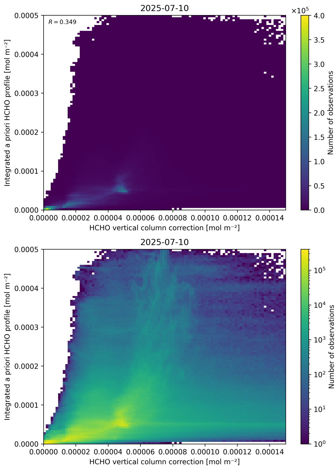
Figure 122: Scatter density plot of “HCHO vertical column correction” against “Integrated a priori HCHO profile” for 2025-07-09 to 2025-07-11.
