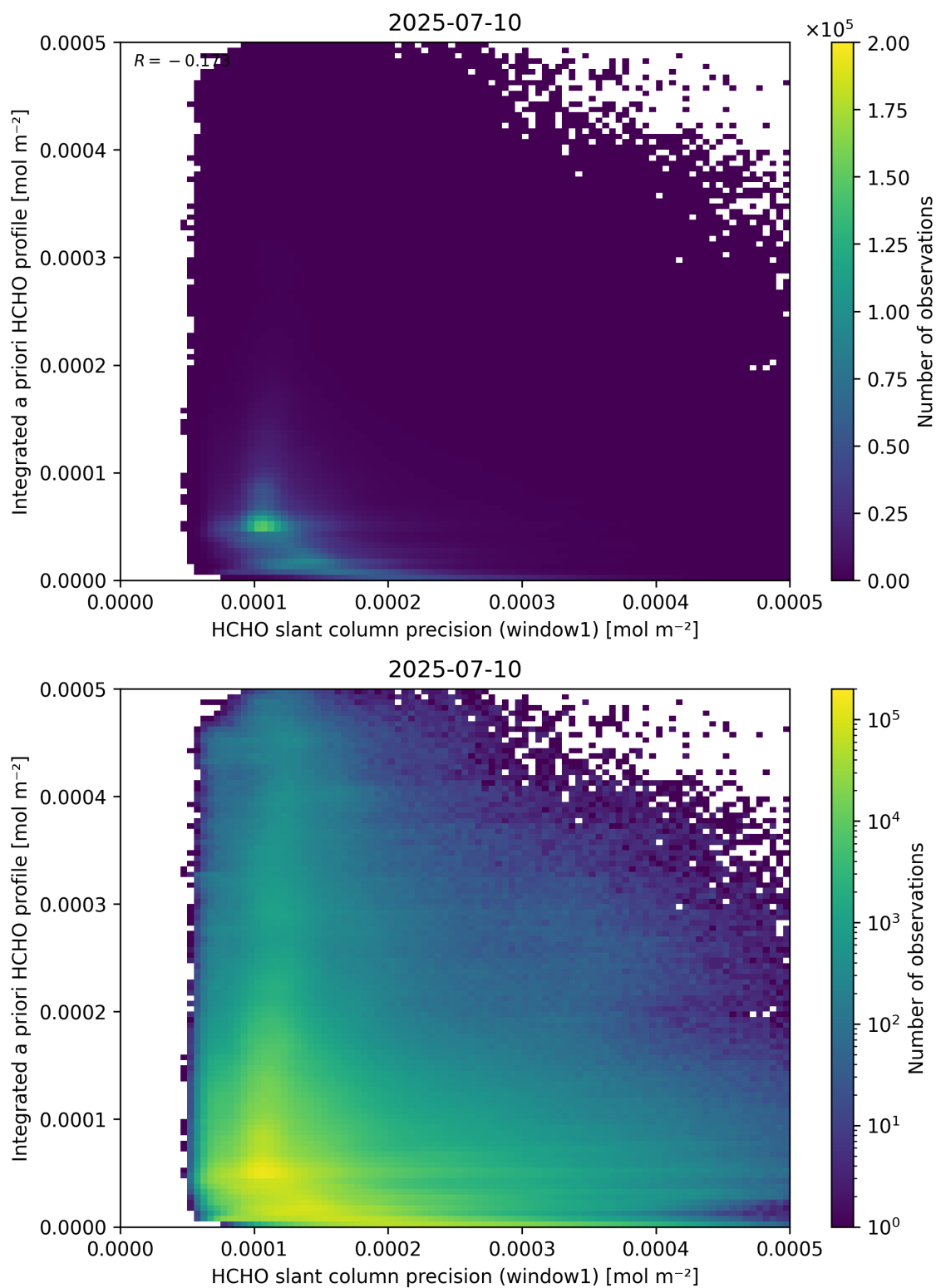
Figure 96: Scatter density plot of “HCHO slant column precision (window1)” against “Integrated a priori HCHO profile” for 2025-07-09 to 2025-07-11.
