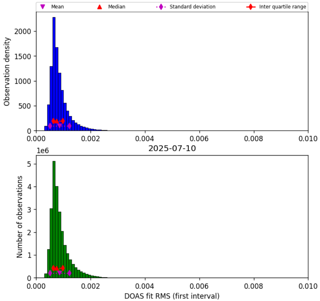
Figure 46: Histogram of “DOAS fit RMS (first interval)” for 2025-07-09 to 2025-07-11
