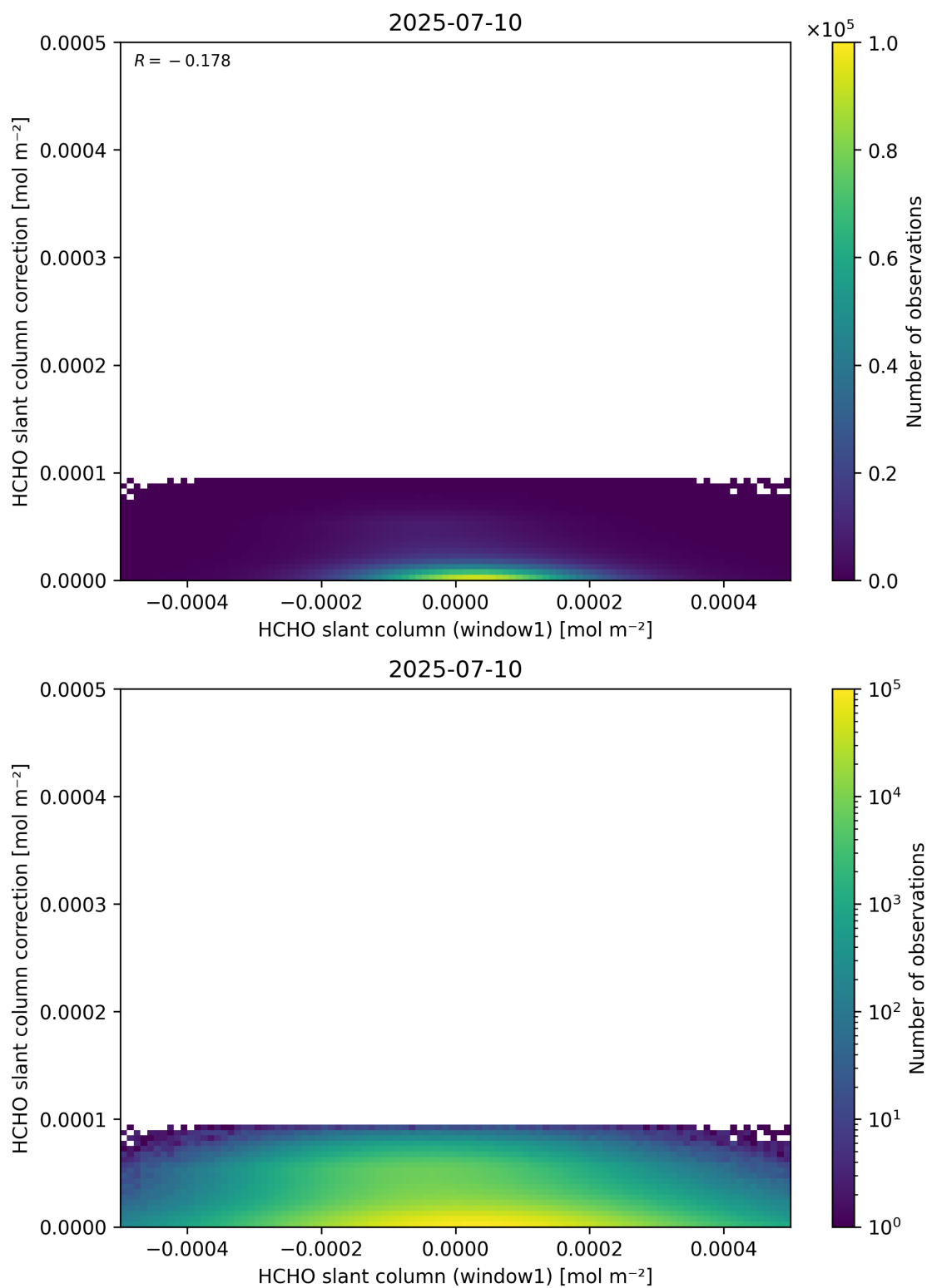
Figure 83: Scatter density plot of “HCHO slant column (window1)” against “HCHO slant column correction” for 2025-07-09 to 2025-07-11.
