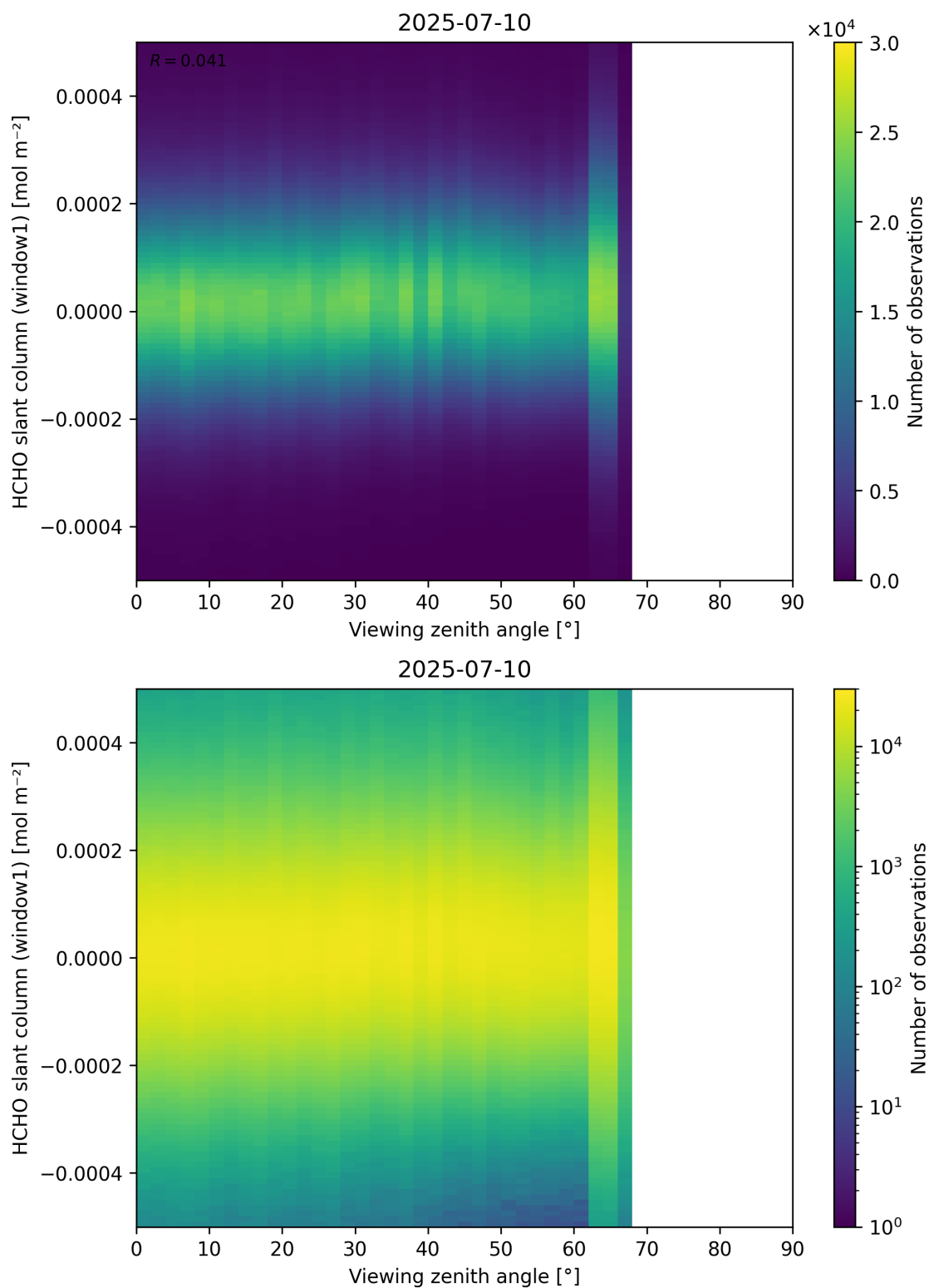
Figure 188: Scatter density plot of “Viewing zenith angle” against “HCHO slant column (window1)” for 2025-07-09 to 2025-07-11.
