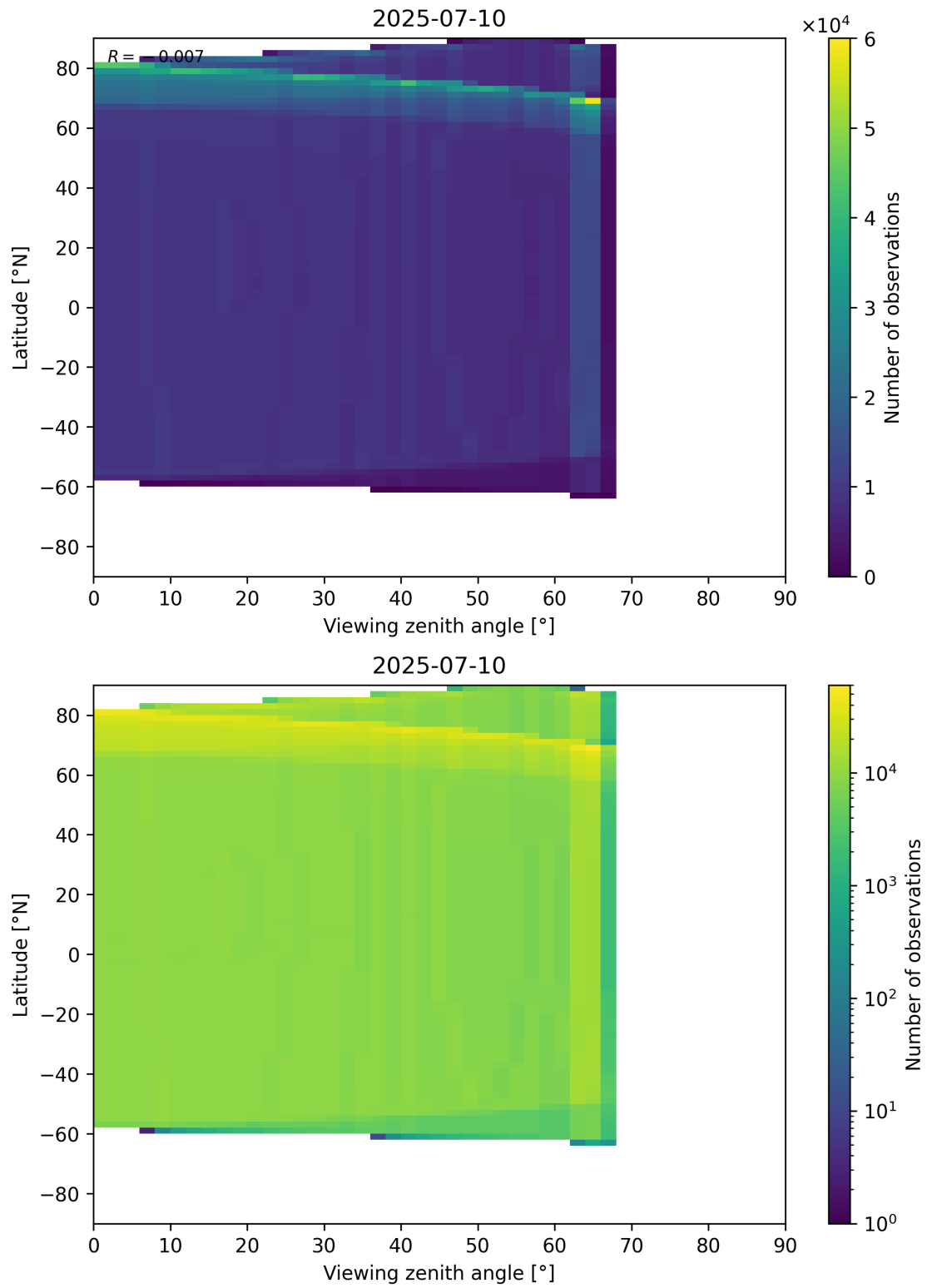
Figure 196: Scatter density plot of “Viewing zenith angle” against “Latitude” for 2025-07-09 to 2025-07-11.
