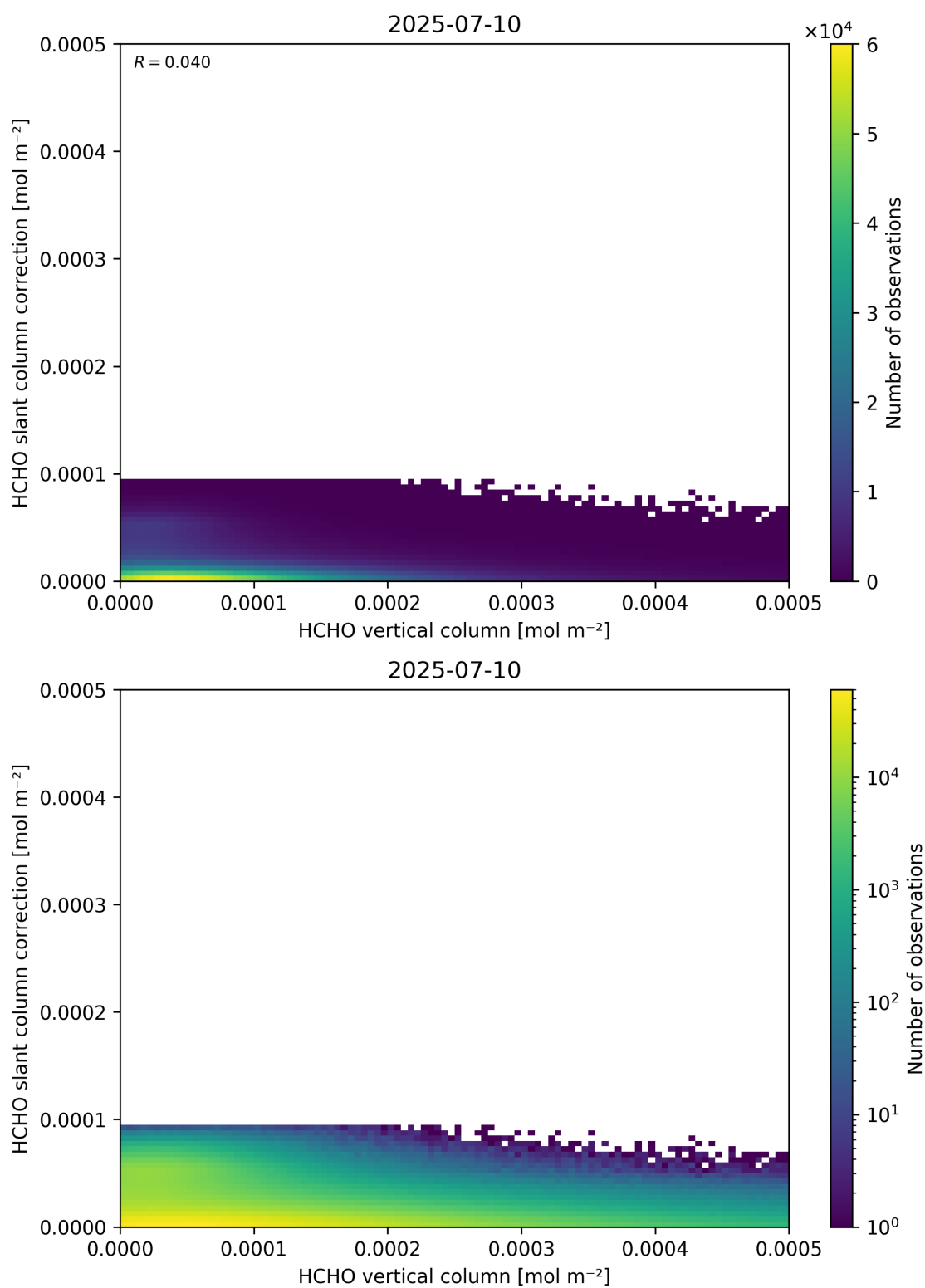
Figure 128: Scatter density plot of “HCHO vertical column” against “HCHO slant column correction” for 2025-07-09 to 2025-07-11.
