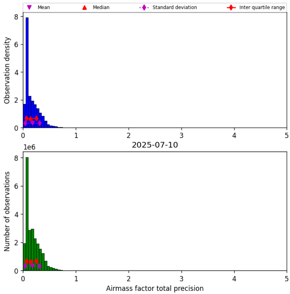
Figure 41: Histogram of “Airmass factor total precision” for 2025-07-09 to 2025-07-11
