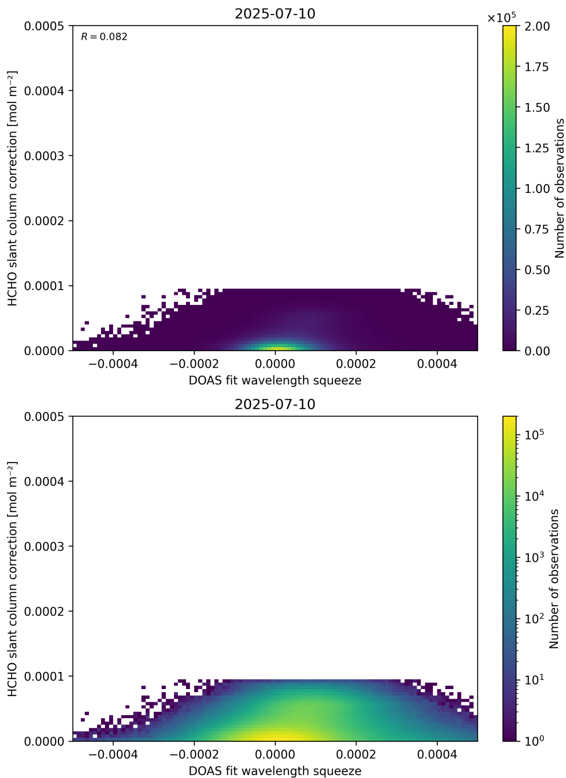
Figure 70: Scatter density plot of “DOAS fit wavelength squeeze” against “HCHO slant column correction” for 2025-07-09 to 2025-07-11.
