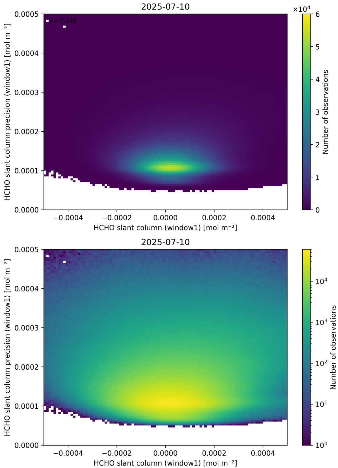
Figure 84: Scatter density plot of “HCHO slant column (window1)” against “HCHO slant column precision (window1)” for 2025-07-09 to 2025-07-11.
