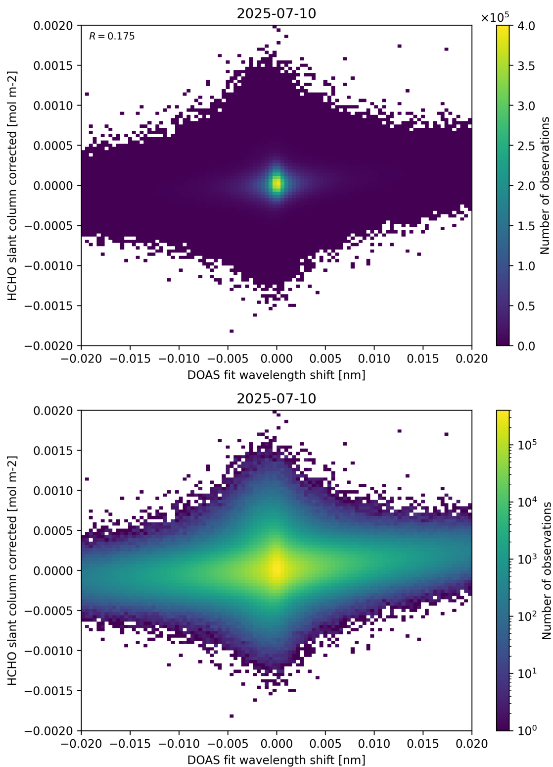
Figure 66: Scatter density plot of “DOAS fit wavelength shift” against “HCHO slant column corrected” for 2025-07-09 to 2025-07-11.
