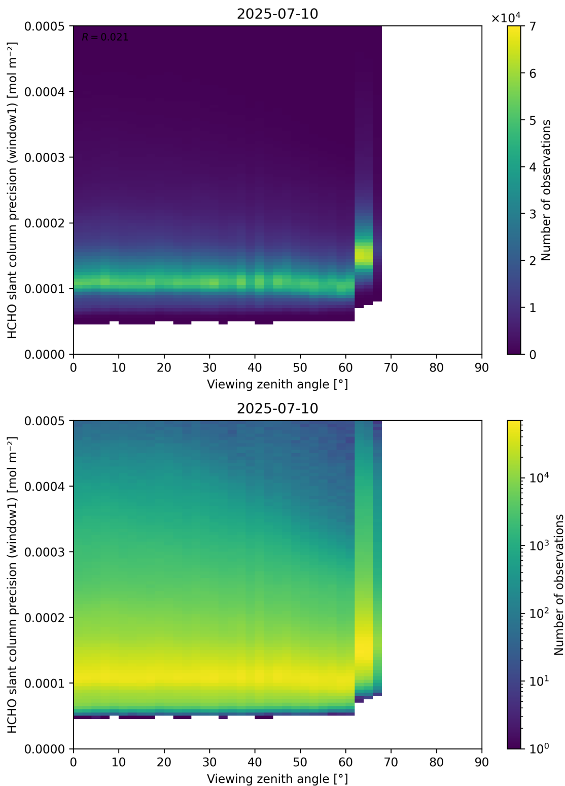
Figure 189: Scatter density plot of “Viewing zenith angle” against “HCHO slant column precision (window1)” for 2025-07-09 to 2025-07-11.
