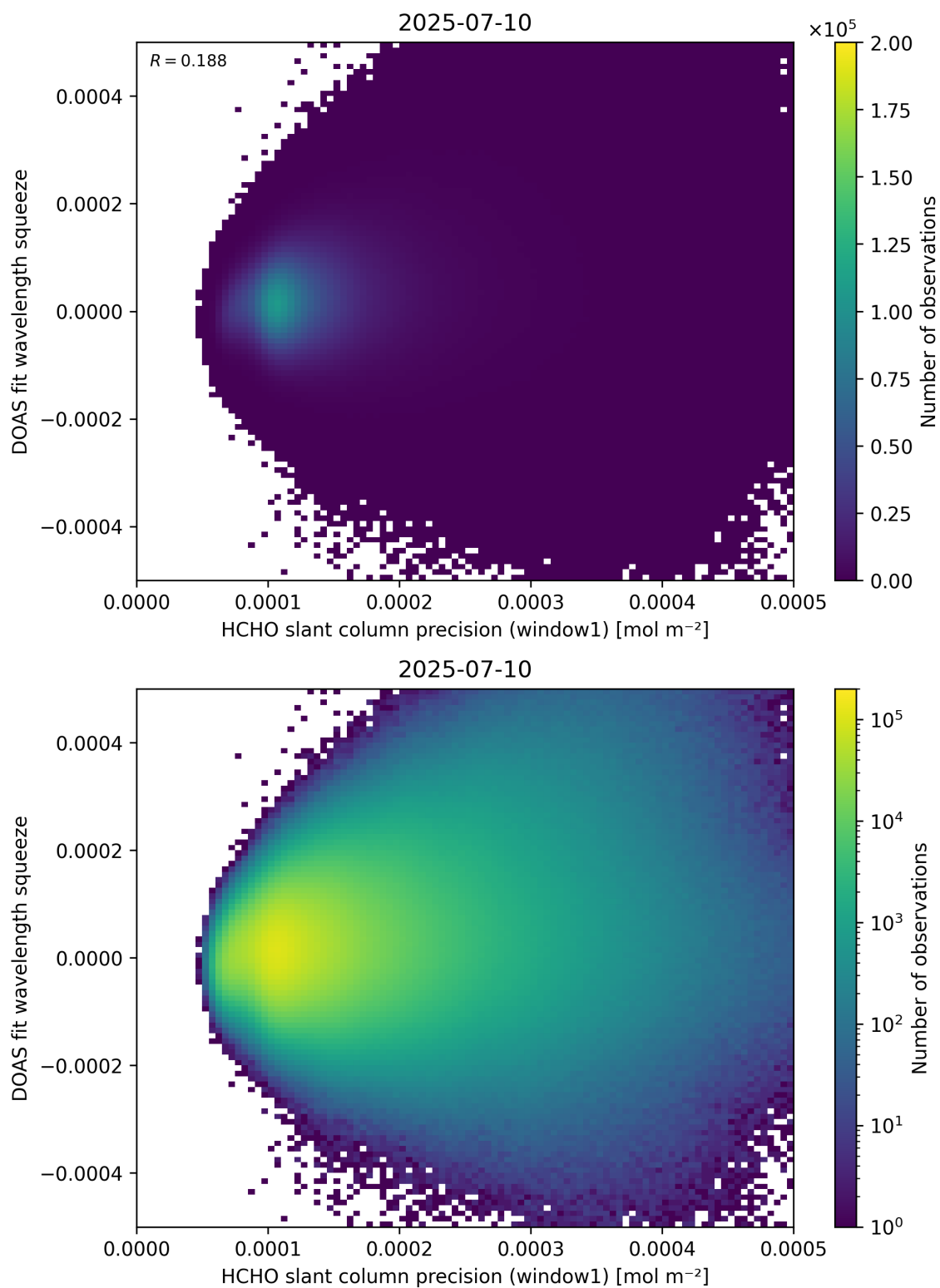
Figure 90: Scatter density plot of “HCHO slant column precision (window1)” against “DOAS fit wavelength squeeze” for 2025-07-09 to 2025-07-11.
