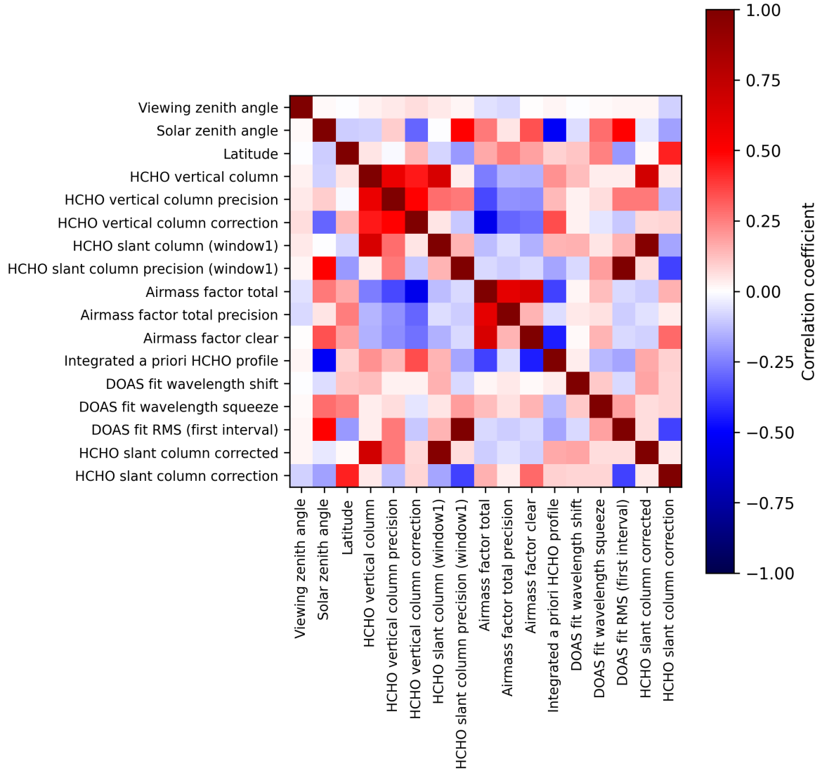
Figure 2: Map of correlation matrix for 2025-07-09 to 2025-07-11.
