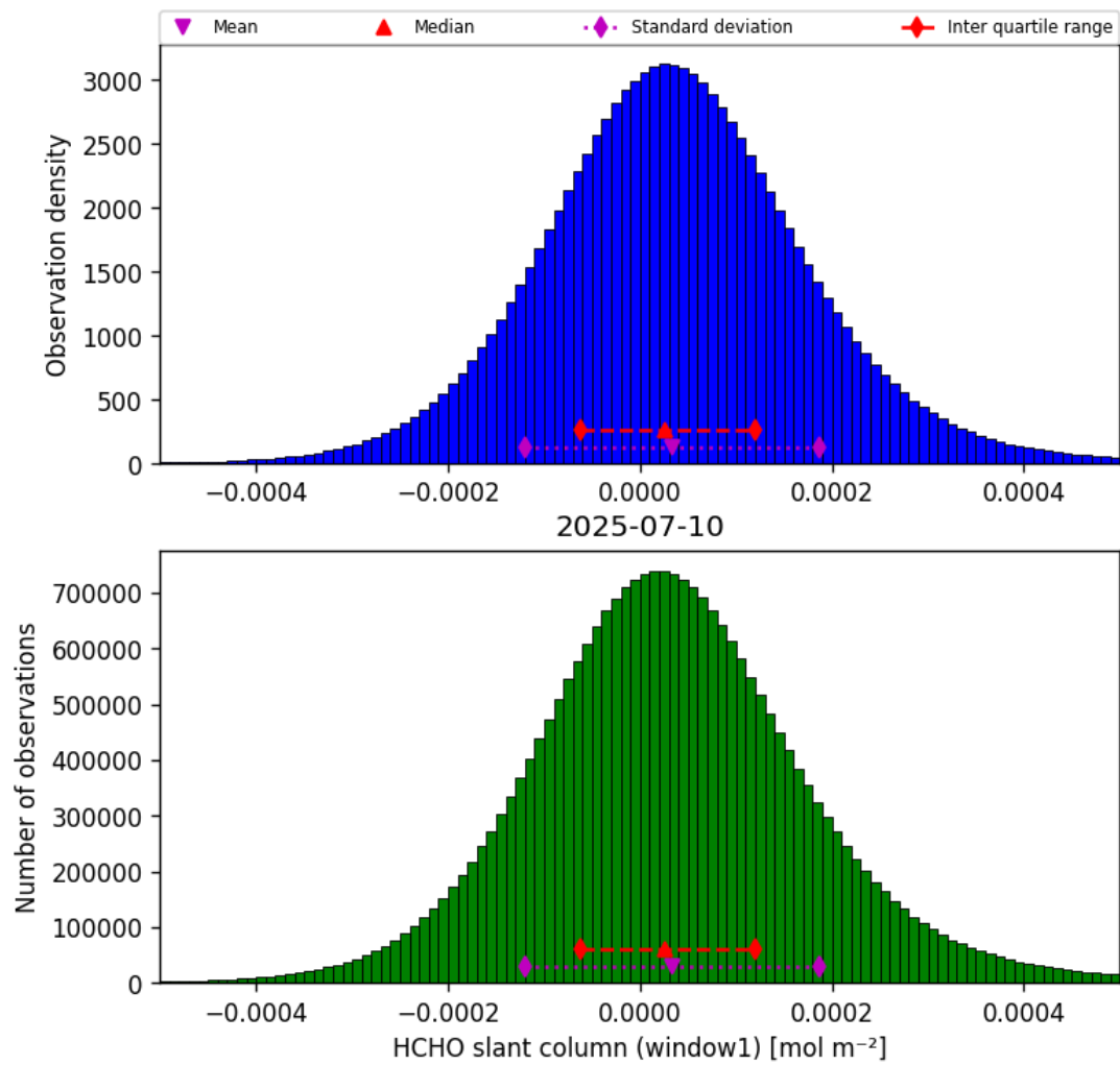
Figure 38: Histogram of “HCHO slant column (window1)” for 2025-07-09 to 2025-07-11
