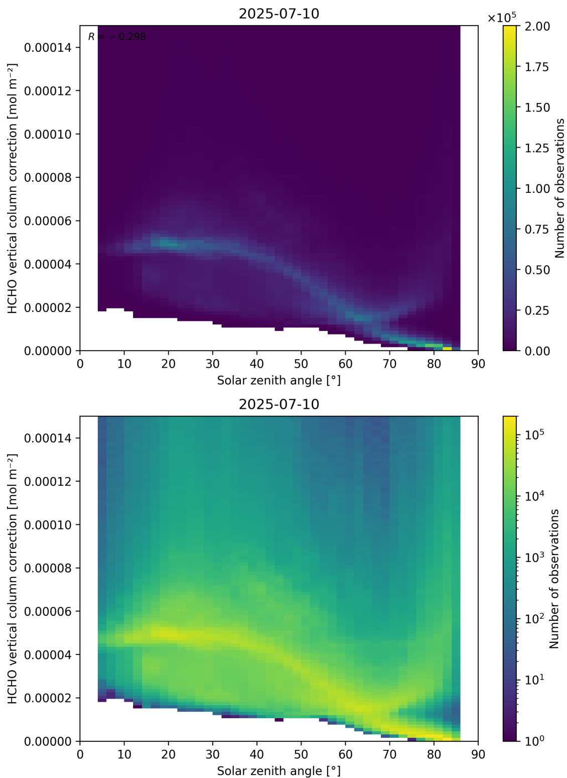
Figure 178: Scatter density plot of “Solar zenith angle” against “HCHO vertical column correction” for 2025-07-09 to 2025-07-11.
