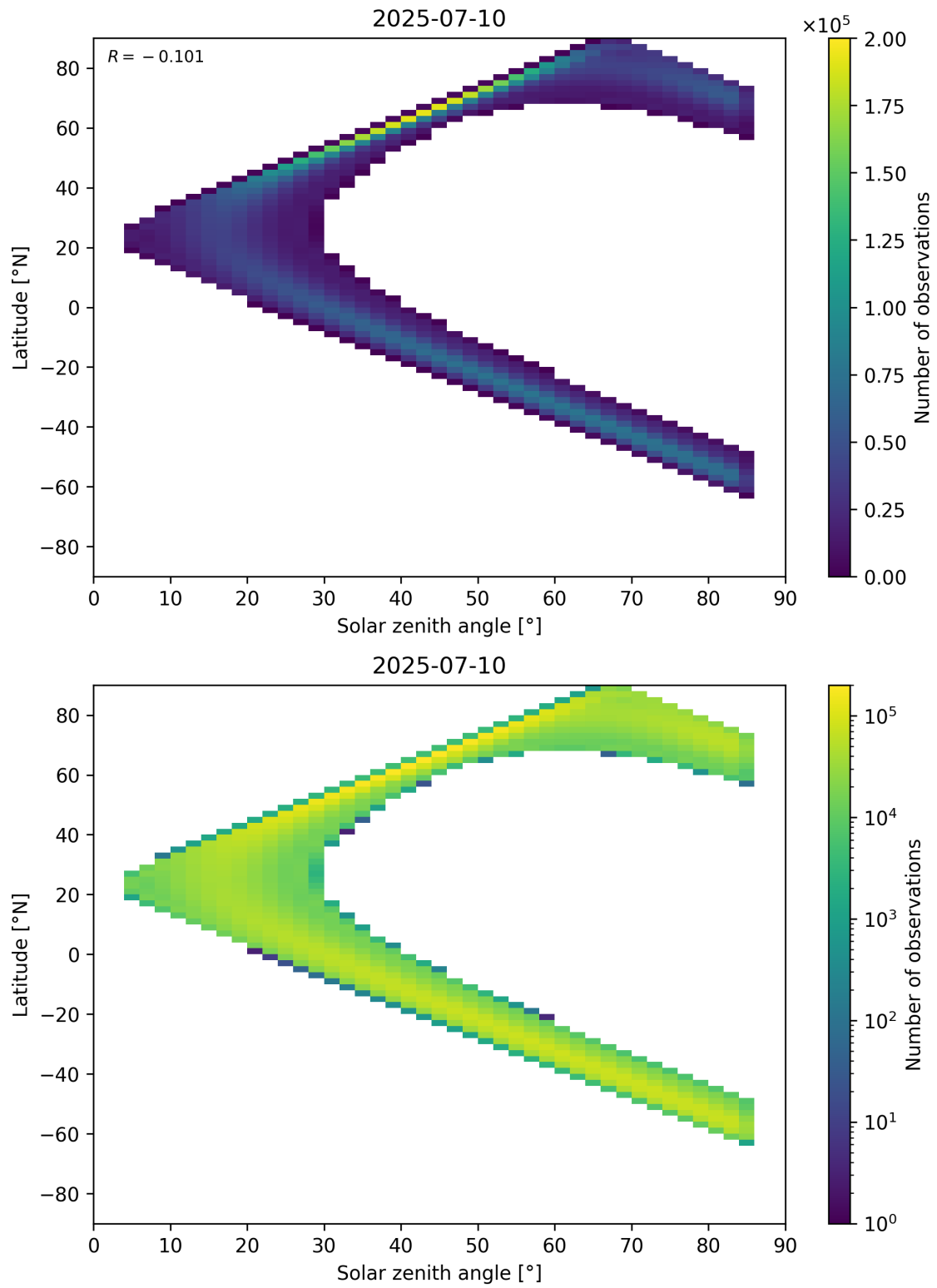
Figure 181: Scatter density plot of “Solar zenith angle” against “Latitude” for 2025-07-09 to 2025-07-11.
