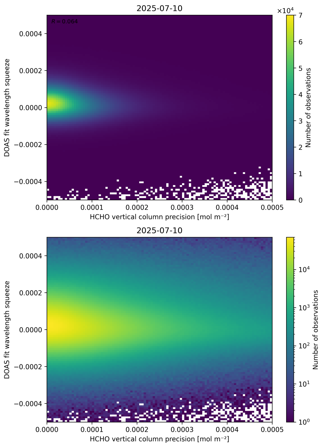
Figure 138: Scatter density plot of “HCHO vertical column precision” against “DOAS fit wavelength squeeze” for 2025-07-09 to 2025-07-11.
