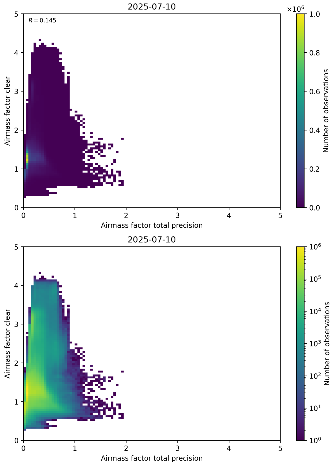
Figure 108: Scatter density plot of “Airmass factor total precision” against “Airmass factor clear” for 2025-07-09 to 2025-07-11.
