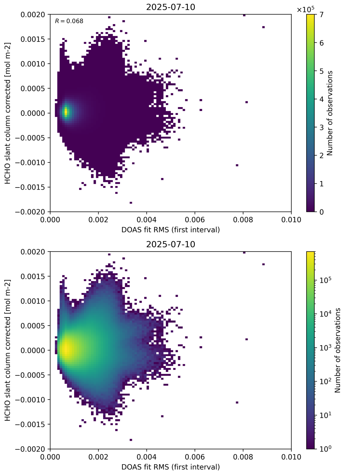
Figure 62: Scatter density plot of “DOAS fit RMS (first interval)” against “HCHO slant column corrected” for 2025-07-09 to 2025-07-11.
