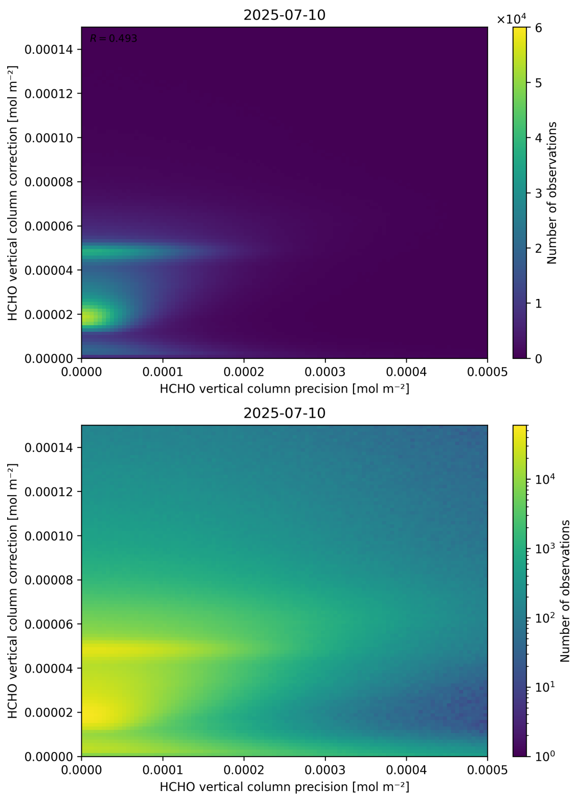
Figure 146: Scatter density plot of “HCHO vertical column precision” against “HCHO vertical column correction” for 2025-07-09 to 2025-07-11.
