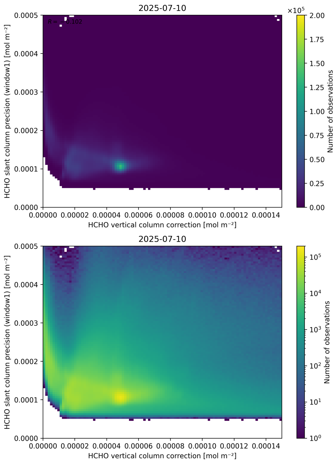
Figure 119: Scatter density plot of “HCHO vertical column correction” against “HCHO slant column precision (window1)” for 2025-07-09 to 2025-07-11.
