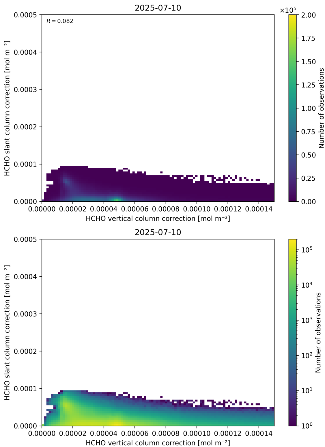
Figure 117: Scatter density plot of “HCHO vertical column correction” against “HCHO slant column correction” for 2025-07-09 to 2025-07-11.
