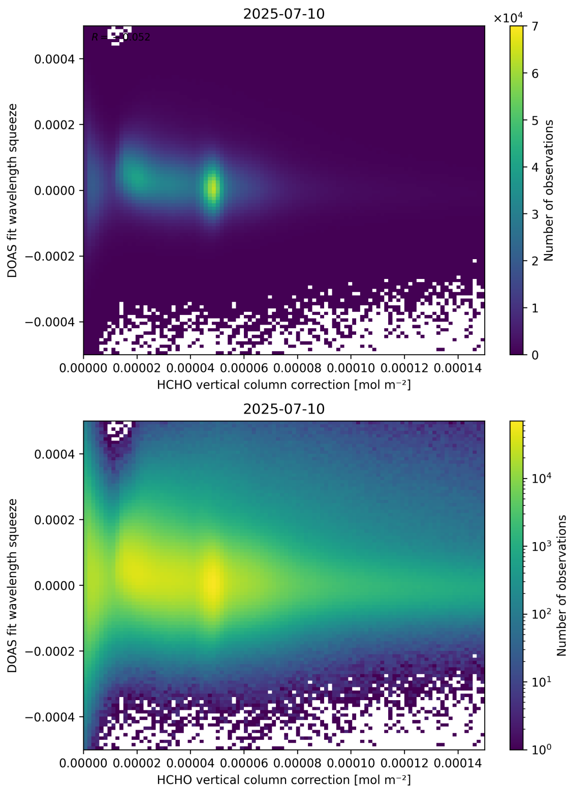
Figure 114: Scatter density plot of “HCHO vertical column correction” against “DOAS fit wavelength squeeze” for 2025-07-09 to 2025-07-11.
