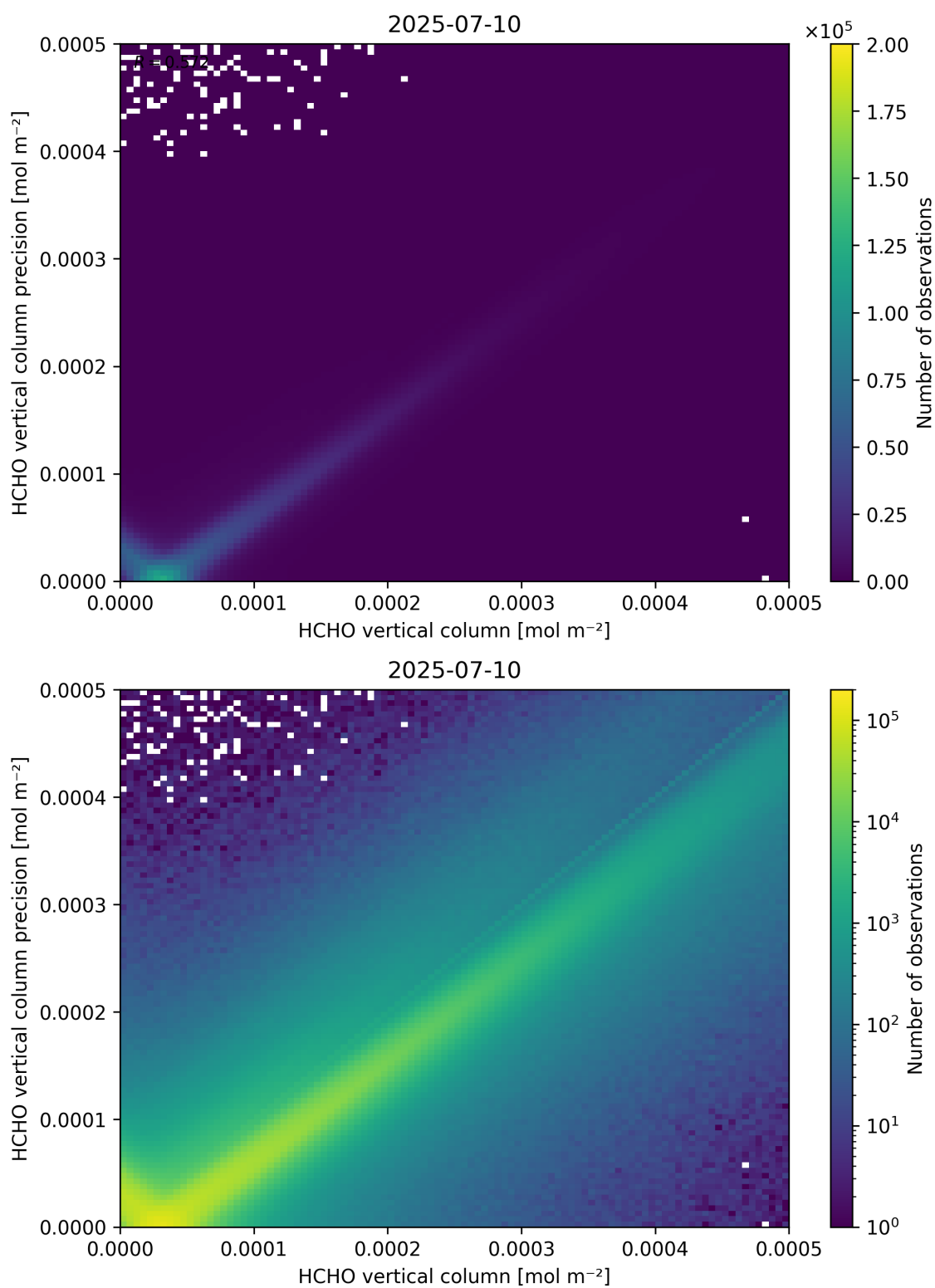
Figure 134: Scatter density plot of “HCHO vertical column” against “HCHO vertical column precision” for 2025-07-09 to 2025-07-11.
