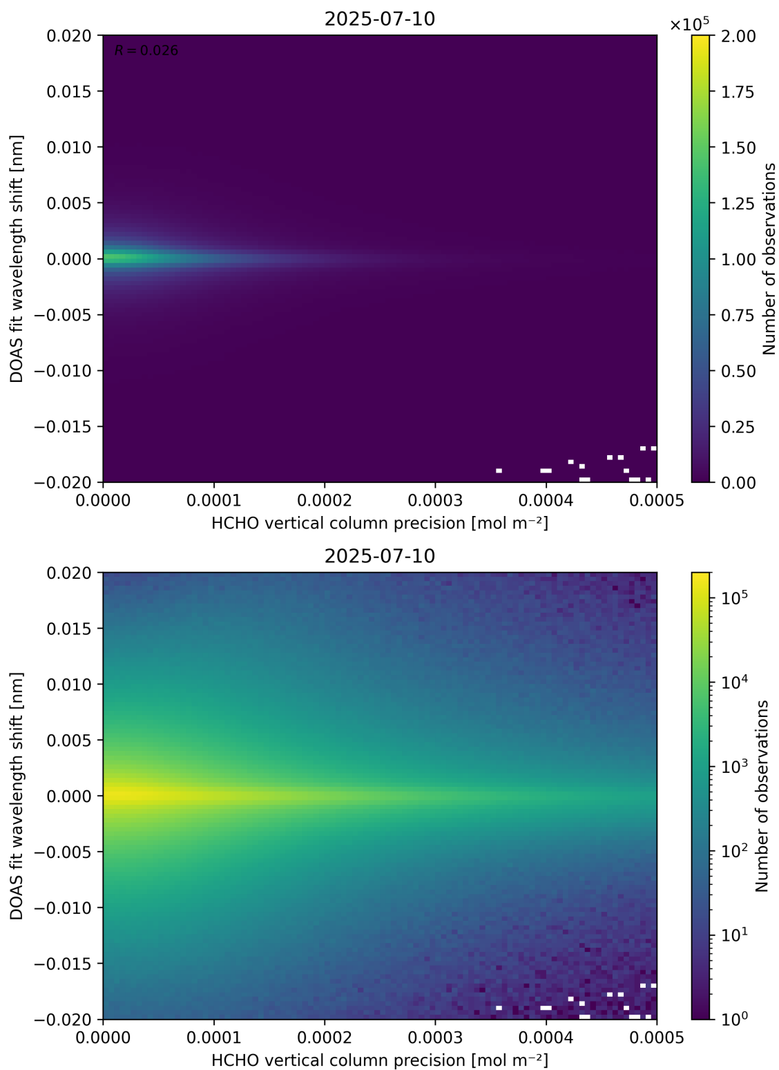
Figure 137: Scatter density plot of “HCHO vertical column precision” against “DOAS fit wavelength shift” for 2025-07-09 to 2025-07-11.
