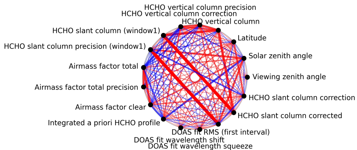
Figure 1: Map of correlation graph for 2025-07-09 to 2025-07-11.
