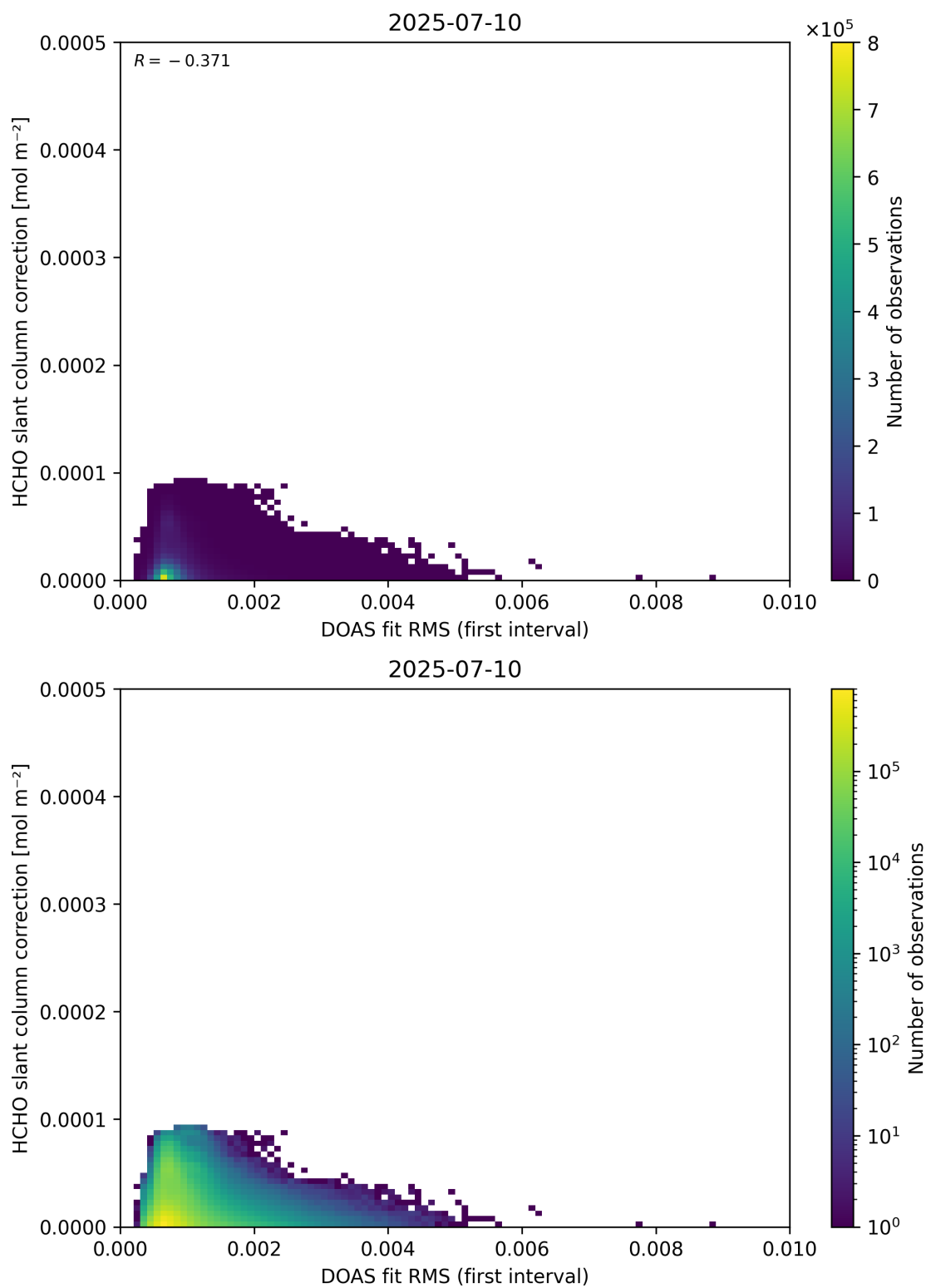
Figure 63: Scatter density plot of “DOAS fit RMS (first interval)” against “HCHO slant column correction” for 2025-07-09 to 2025-07-11.
