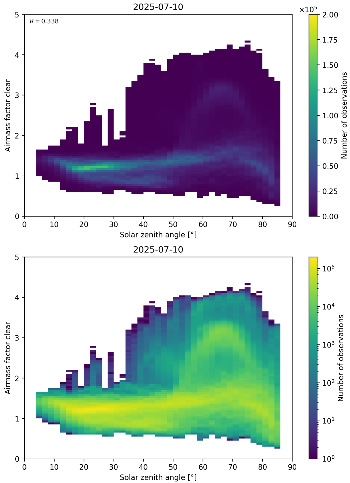
Figure 170: Scatter density plot of “Solar zenith angle” against “Airmass factor clear” for 2025-07-09 to 2025-07-11.
