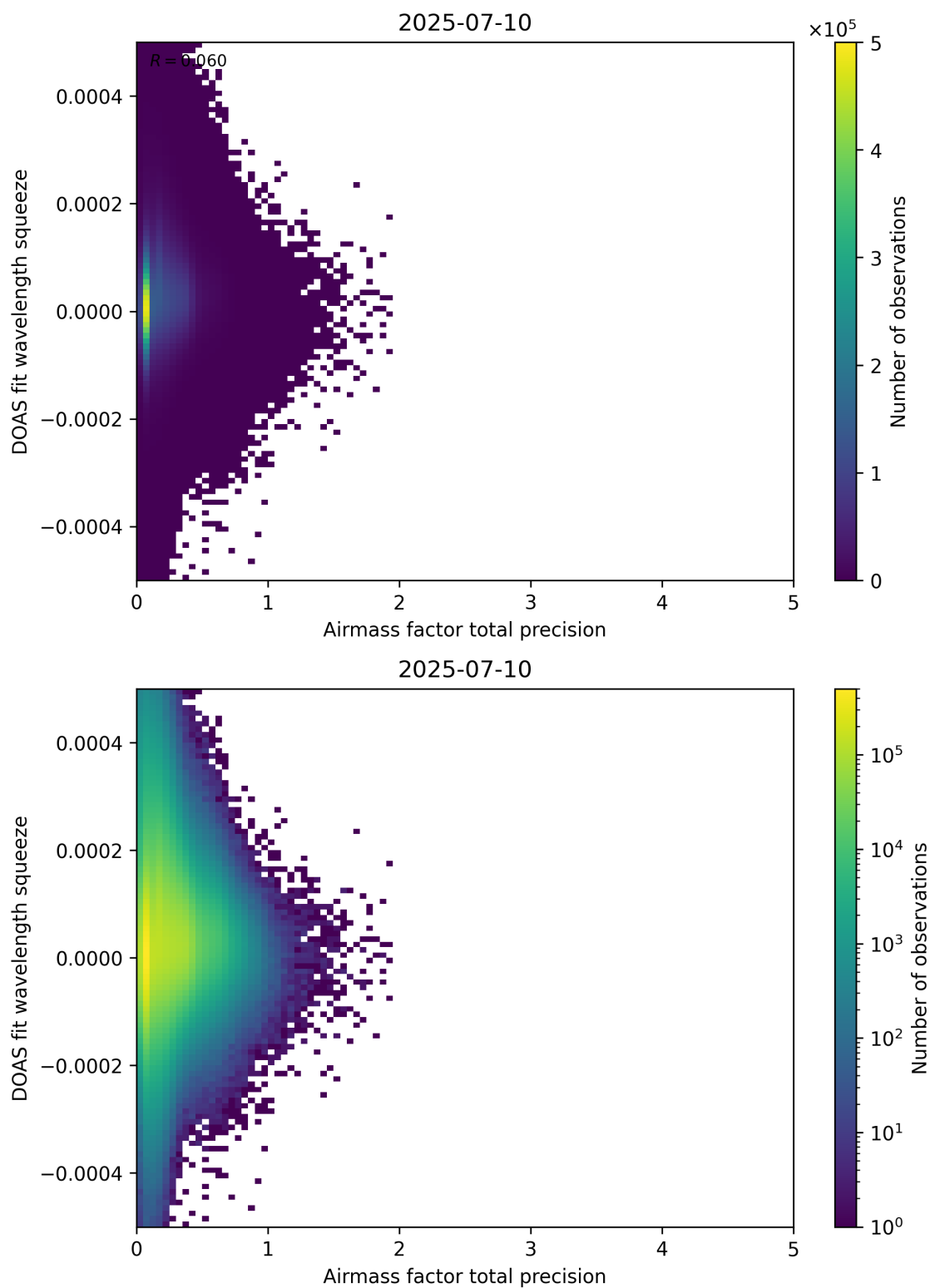
Figure 107: Scatter density plot of “Airmass factor total precision” against “DOAS fit wavelength squeeze” for 2025-07-09 to 2025-07-11.
