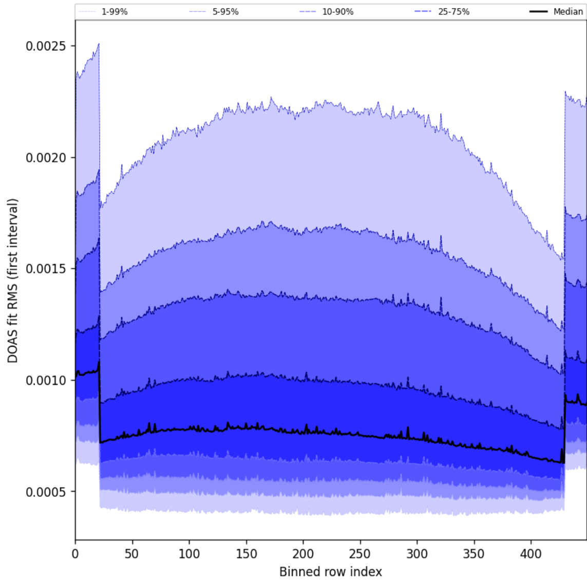
Figure 60: Along track statistics of “DOAS fit RMS (first interval)” for 2025-07-09 to 2025-07-11
