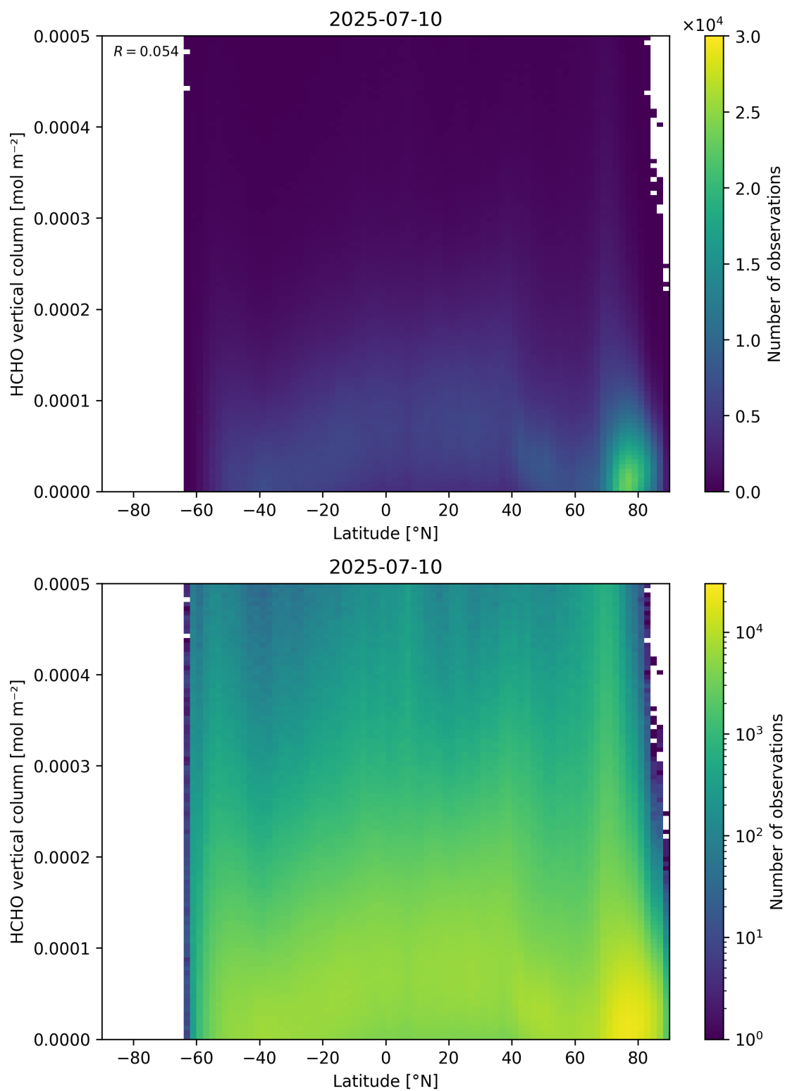
Figure 163: Scatter density plot of “Latitude” against “HCHO vertical column” for 2025-07-09 to 2025-07-11.
