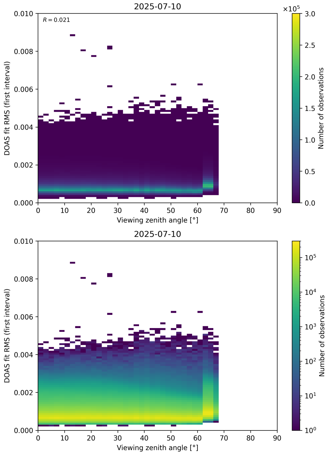
Figure 182: Scatter density plot of “Viewing zenith angle” against “DOAS fit RMS (first interval)” for 2025-07-09 to 2025-07-11.
