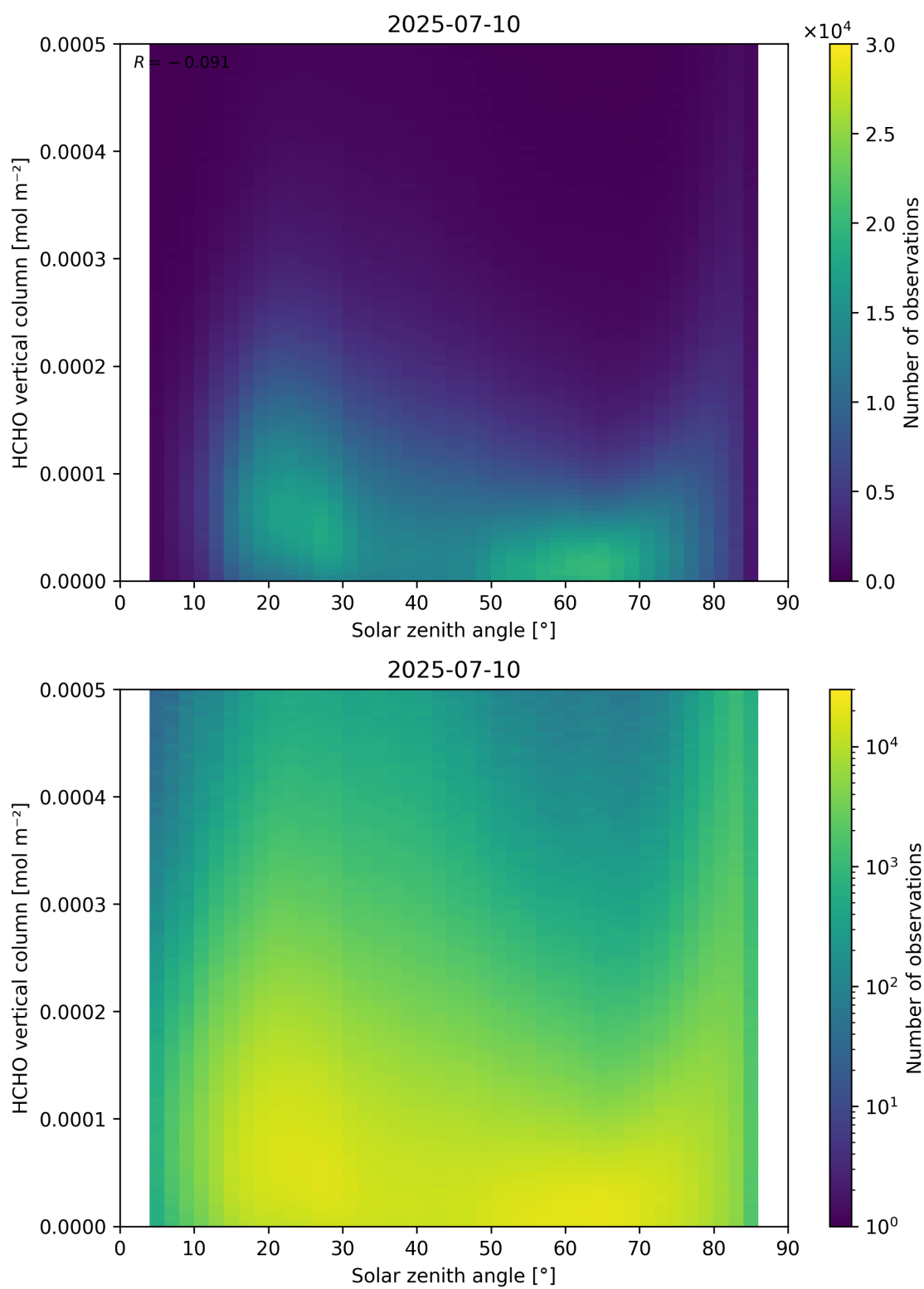
Figure 177: Scatter density plot of “Solar zenith angle” against “HCHO vertical column” for 2025-07-09 to 2025-07-11.
