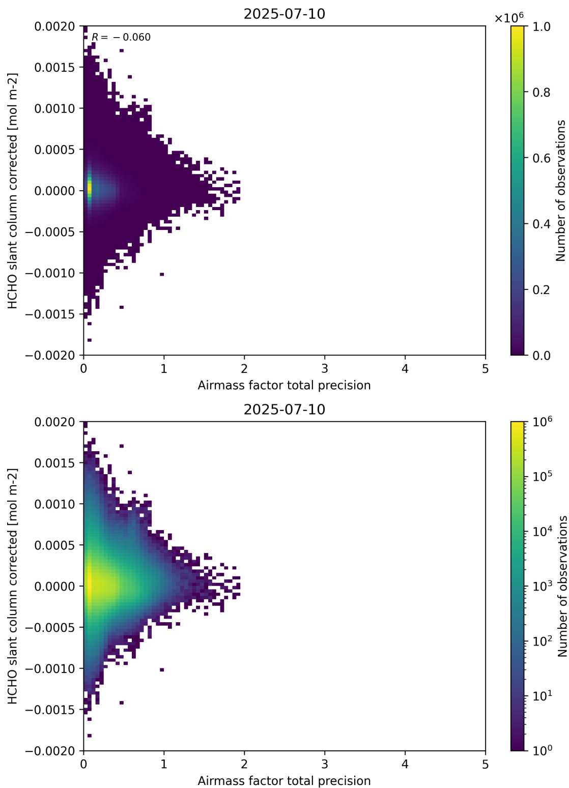
Figure 109: Scatter density plot of “Airmass factor total precision” against “HCHO slant column corrected” for 2025-07-09 to 2025-07-11.
