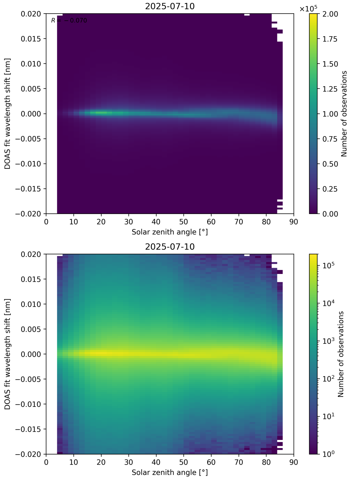
Figure 168: Scatter density plot of “Solar zenith angle” against “DOAS fit wavelength shift” for 2025-07-09 to 2025-07-11.
