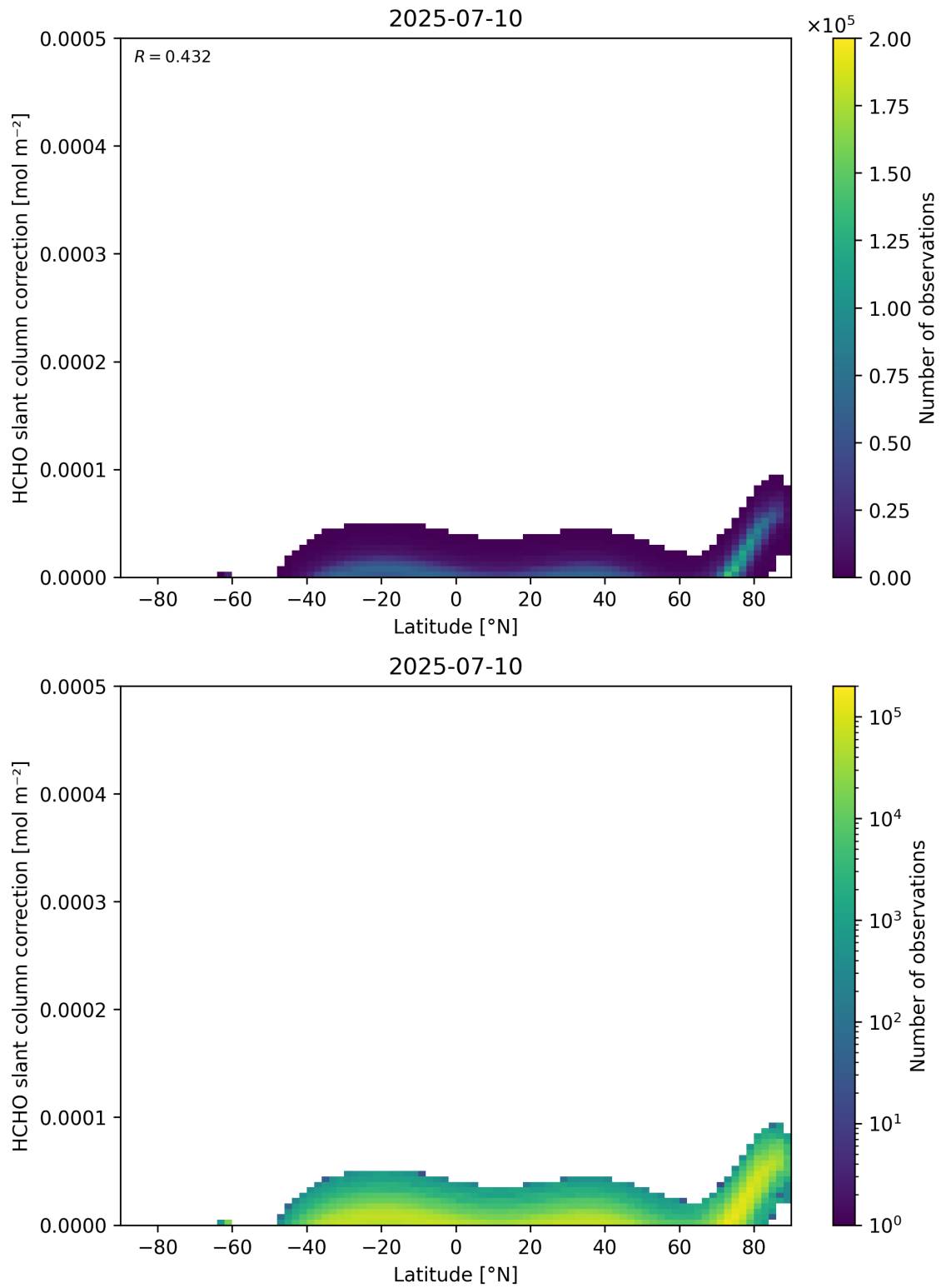
Figure 158: Scatter density plot of “Latitude” against “HCHO slant column correction” for 2025-07-09 to 2025-07-11.
