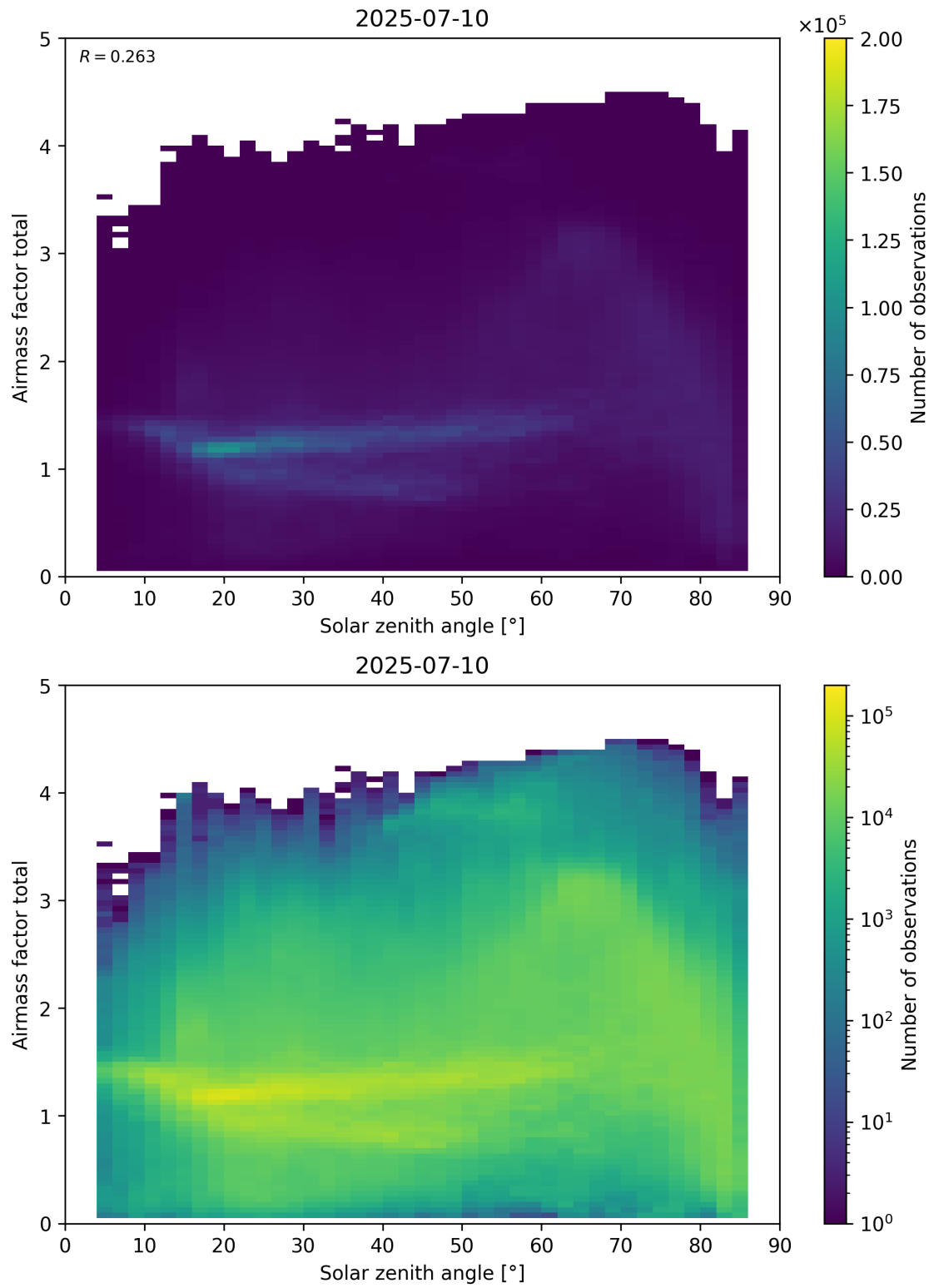
Figure 175: Scatter density plot of “Solar zenith angle” against “Airmass factor total” for 2025-07-09 to 2025-07-11.
