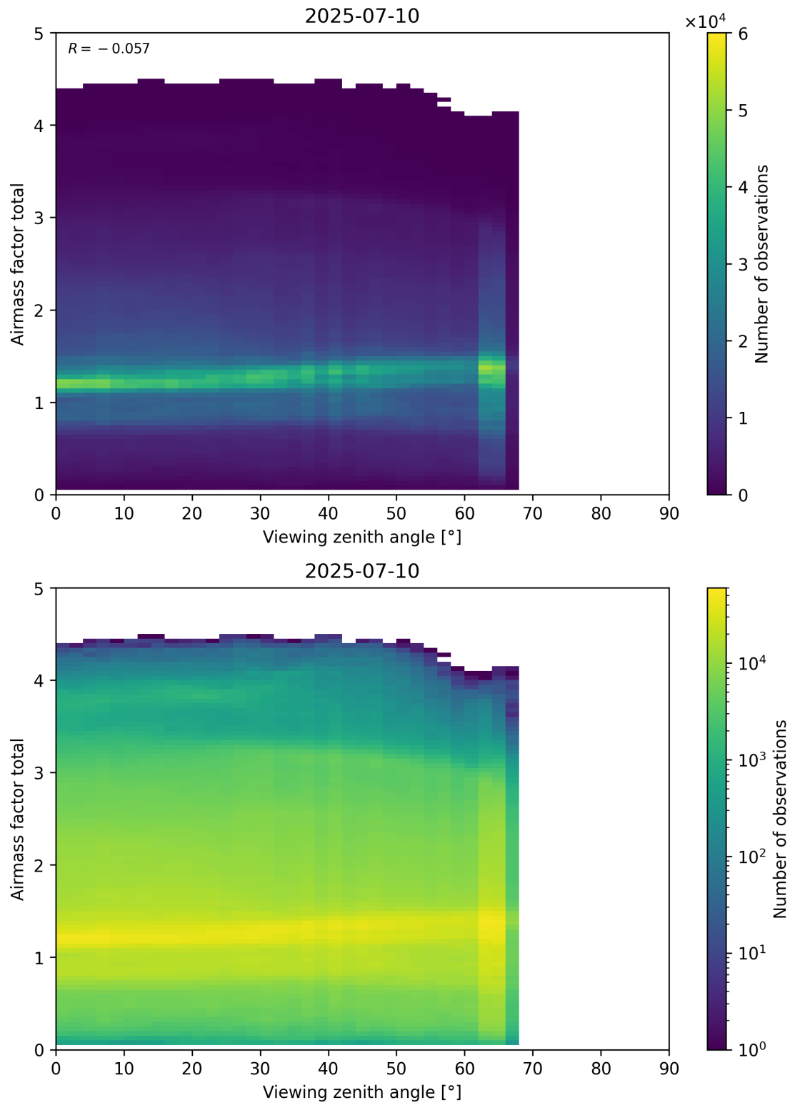
Figure 190: Scatter density plot of “Viewing zenith angle” against “Airmass factor total” for 2025-07-09 to 2025-07-11.
