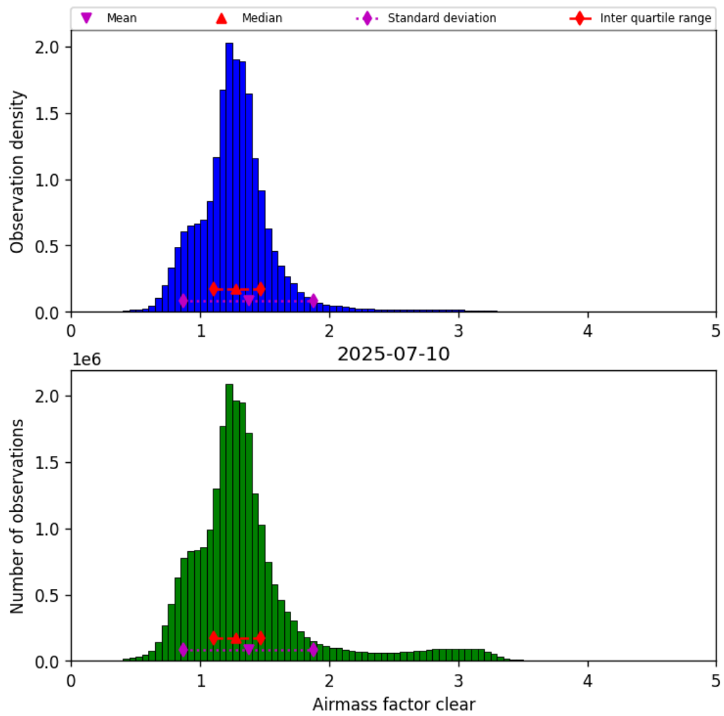
Figure 42: Histogram of “Airmass factor clear” for 2025-07-09 to 2025-07-11
