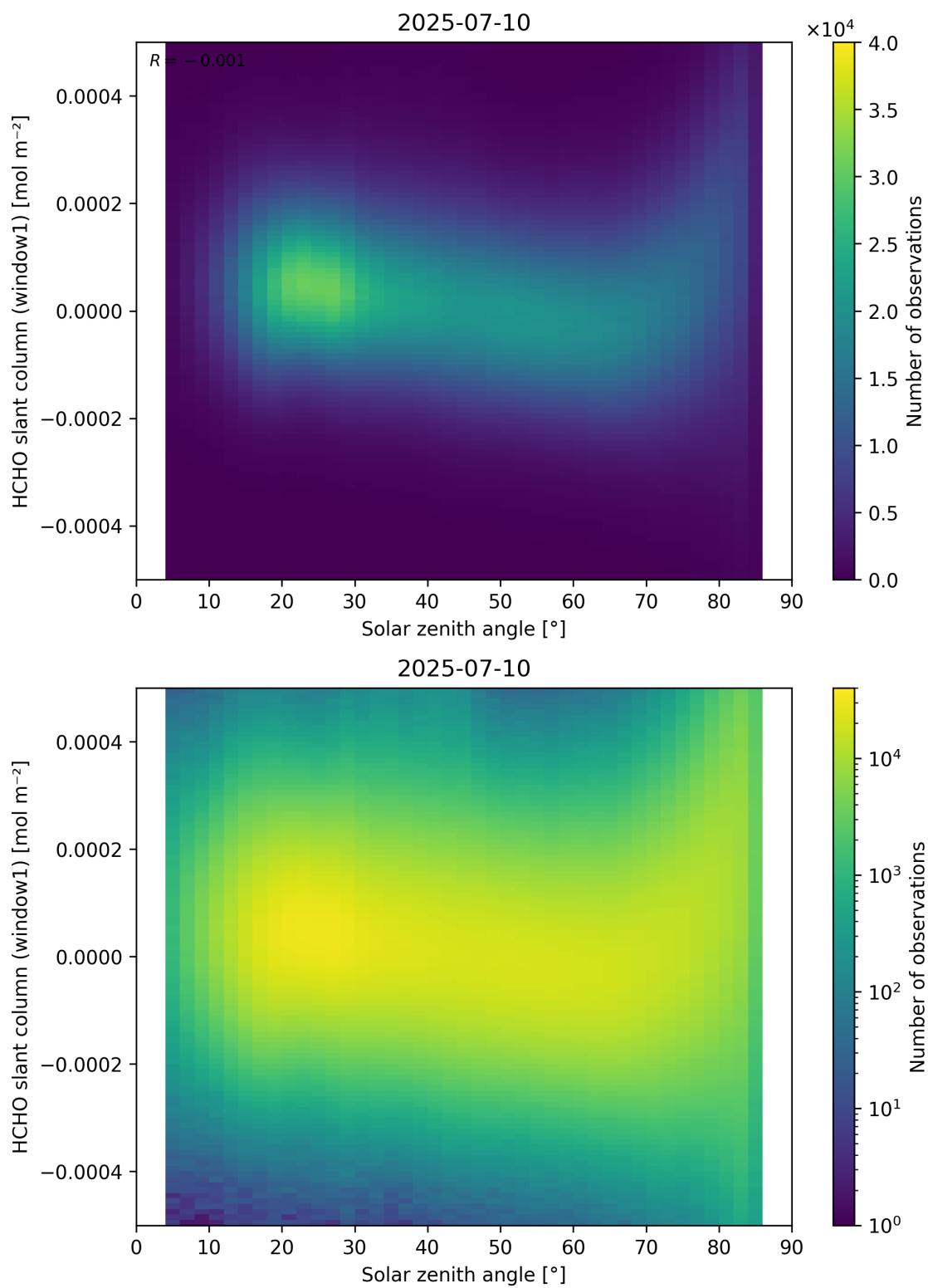
Figure 173: Scatter density plot of “Solar zenith angle” against “HCHO slant column (window1)” for 2025-07-09 to 2025-07-11.
