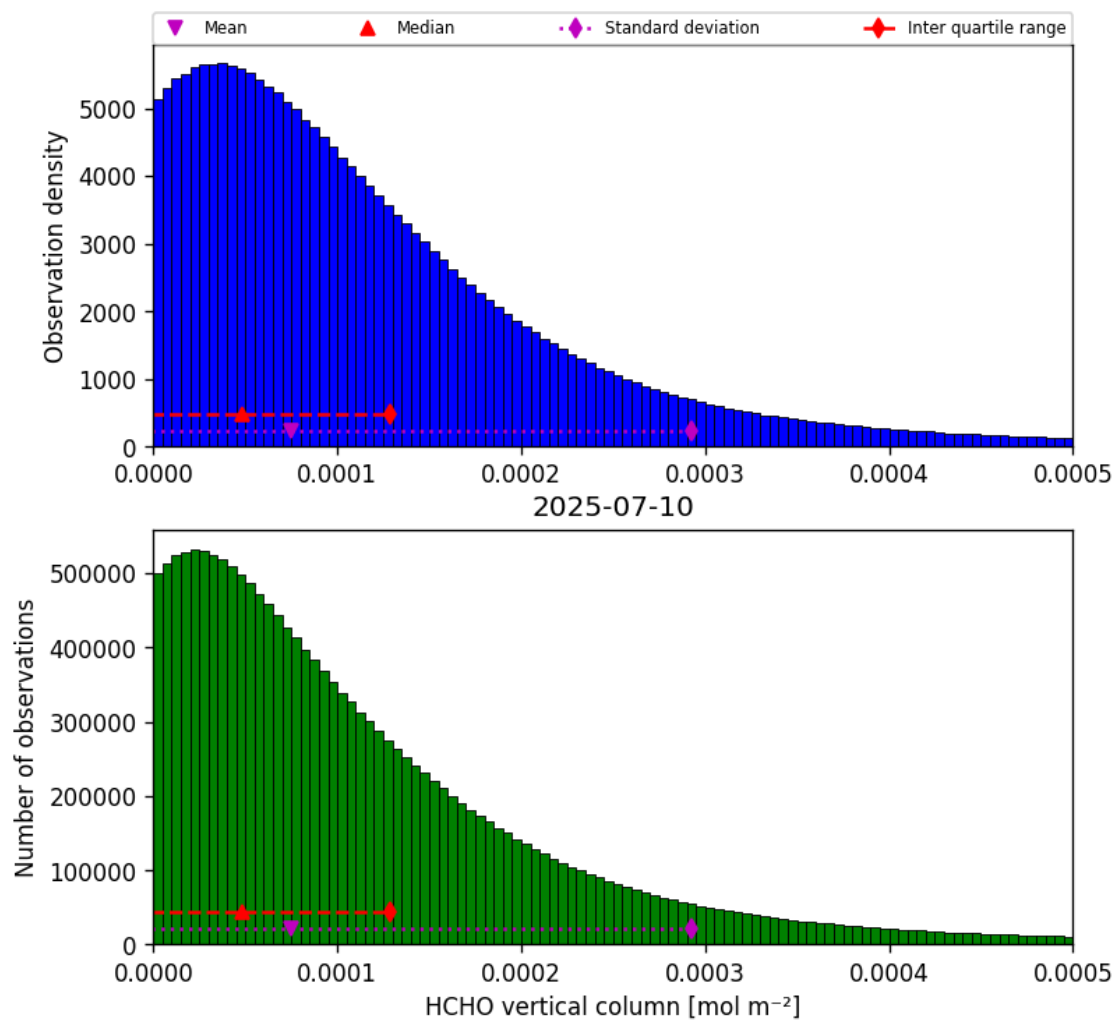
Figure 35: Histogram of “HCHO vertical column” for 2025-07-09 to 2025-07-11
