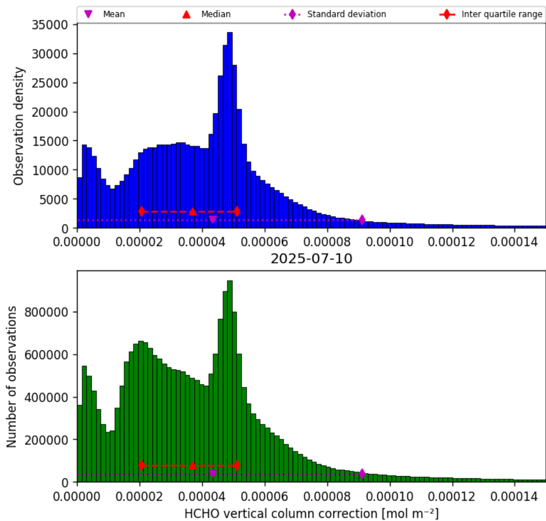
Figure 37: Histogram of “HCHO vertical column correction” for 2025-07-09 to 2025-07-11
