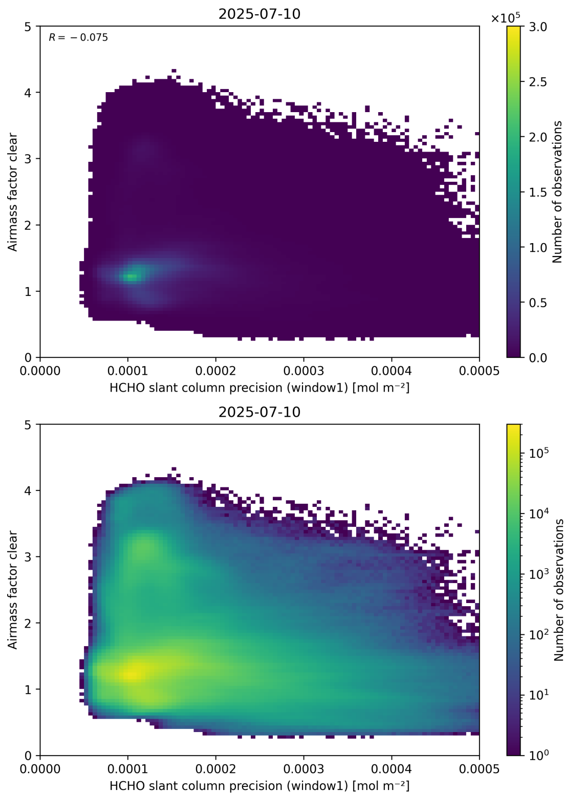
Figure 91: Scatter density plot of “HCHO slant column precision (window1)” against “Airmass factor clear” for 2025-07-09 to 2025-07-11.
