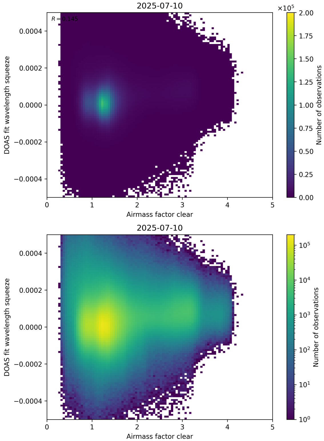
Figure 73: Scatter density plot of “Airmass factor clear” against “DOAS fit wavelength squeeze” for 2025-07-09 to 2025-07-11.
