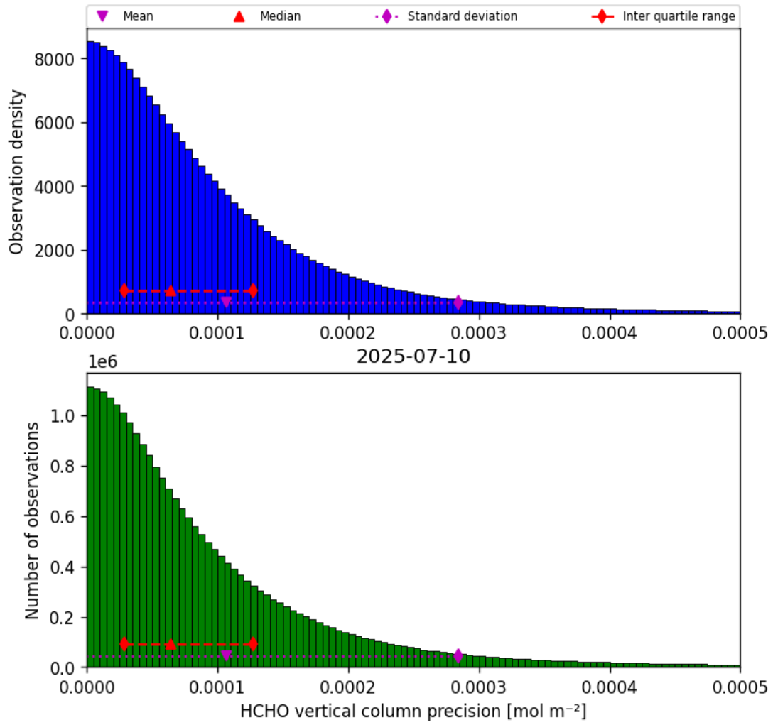
Figure 36: Histogram of “HCHO vertical column precision” for 2025-07-09 to 2025-07-11
