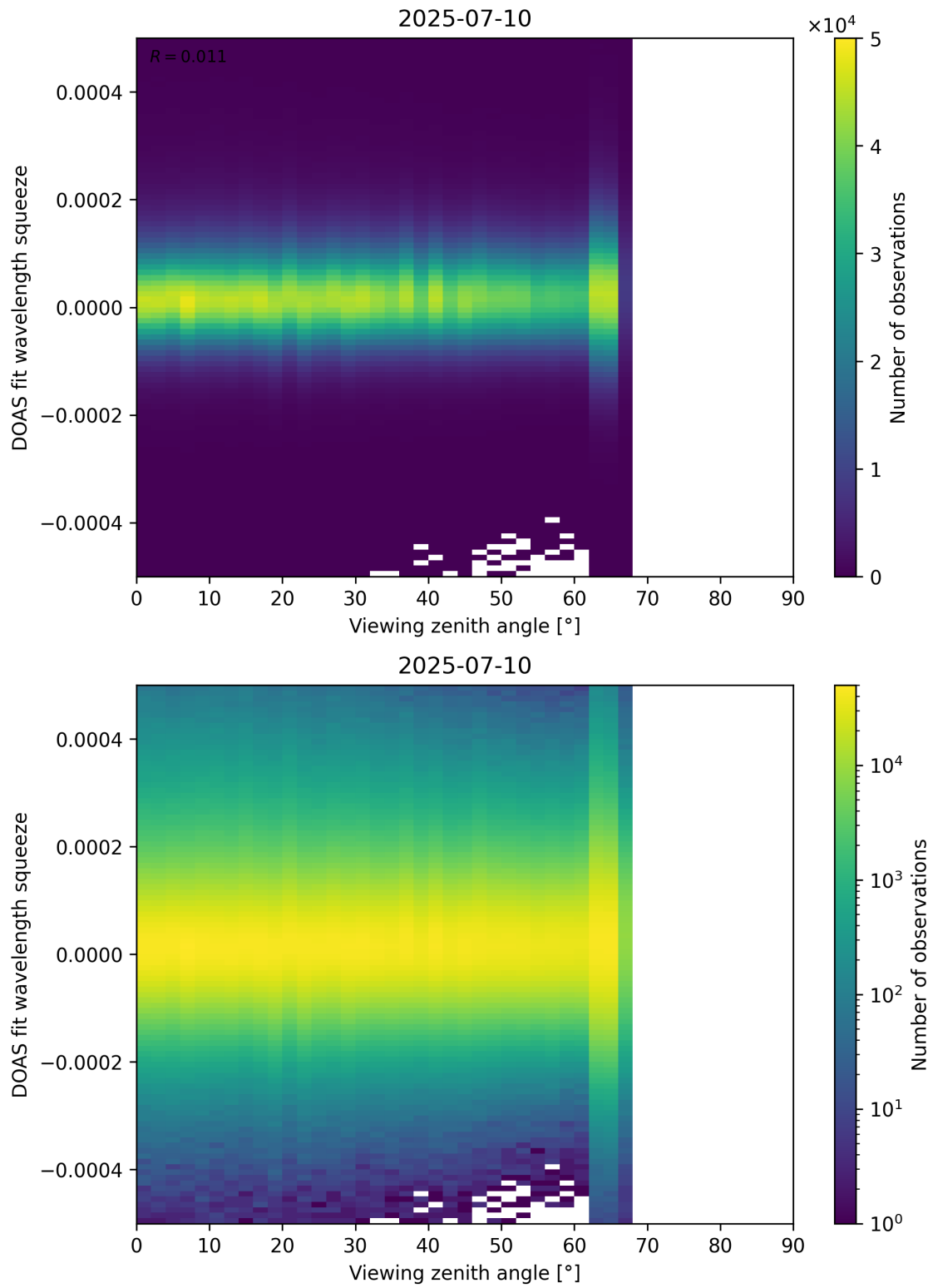
Figure 184: Scatter density plot of “Viewing zenith angle” against “DOAS fit wavelength squeeze” for 2025-07-09 to 2025-07-11.
