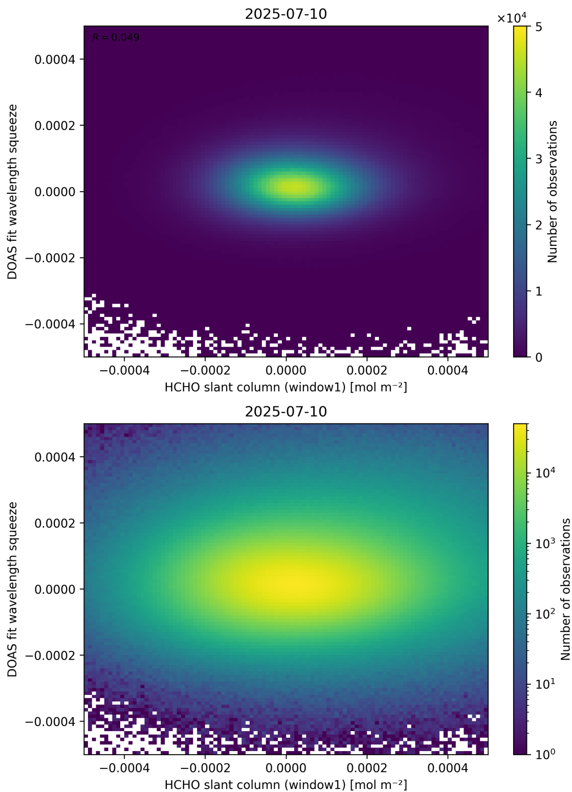
Figure 80: Scatter density plot of “HCHO slant column (window1)” against “DOAS fit wavelength squeeze” for 2025-07-09 to 2025-07-11.
