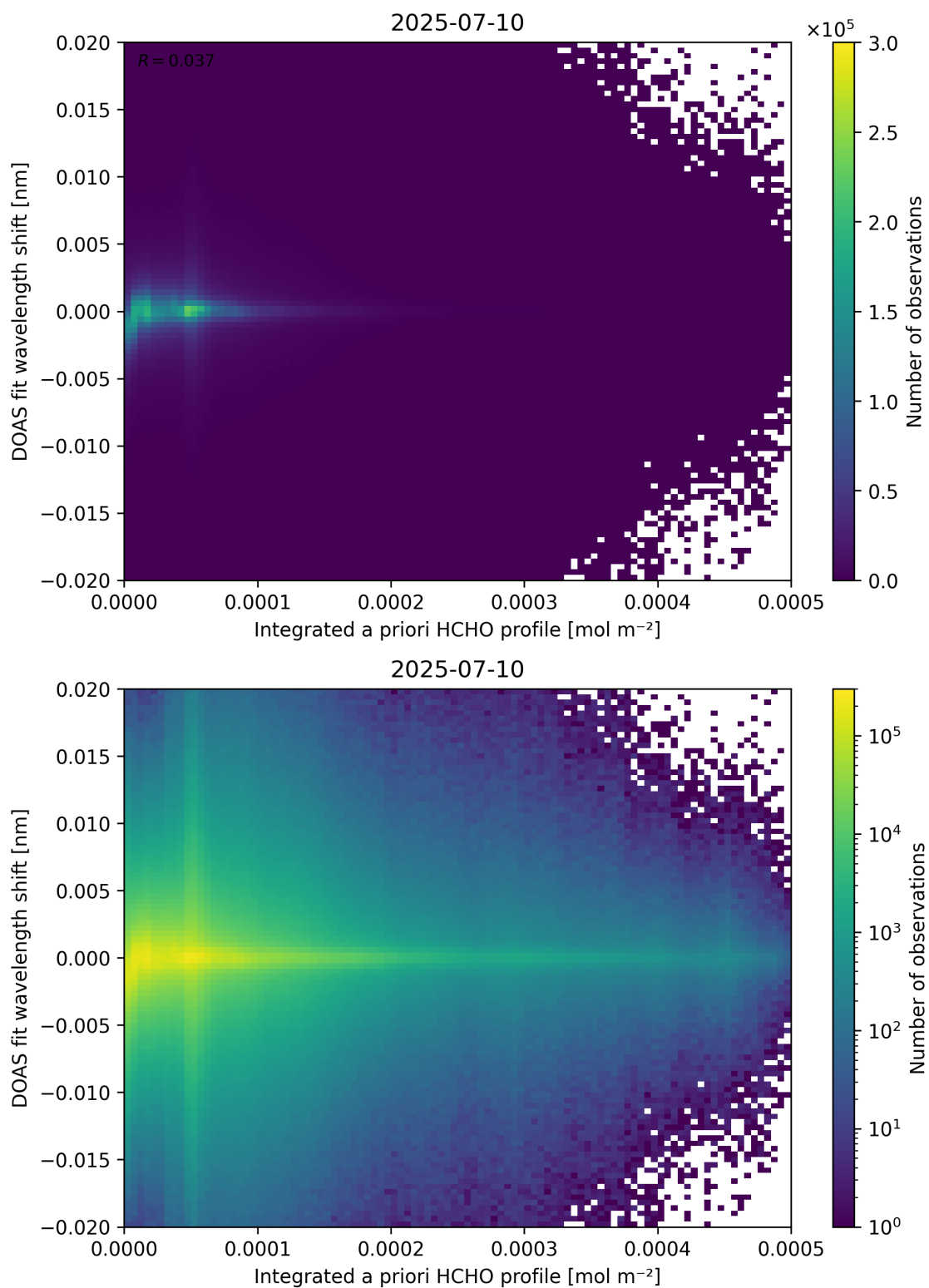
Figure 149: Scatter density plot of “Integrated a priori HCHO profile” against “DOAS fit wavelength shift” for 2025-07-09 to 2025-07-11.
