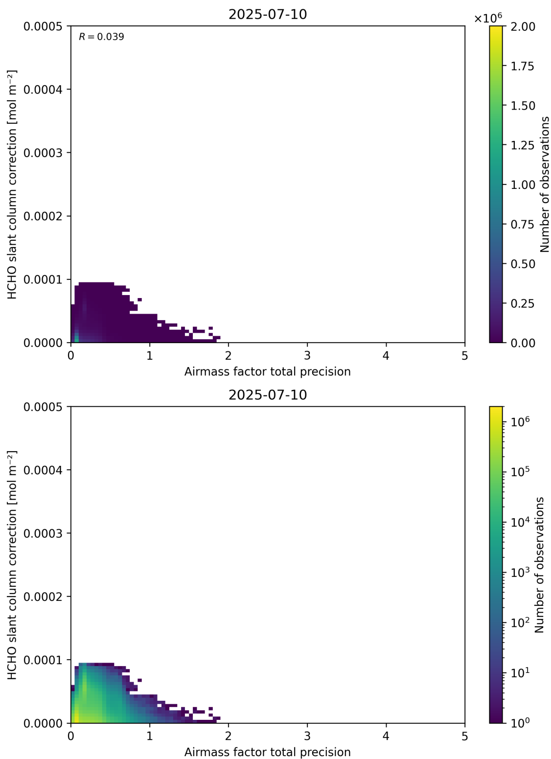
Figure 110: Scatter density plot of “Airmass factor total precision” against “HCHO slant column correction” for 2025-07-09 to 2025-07-11.
