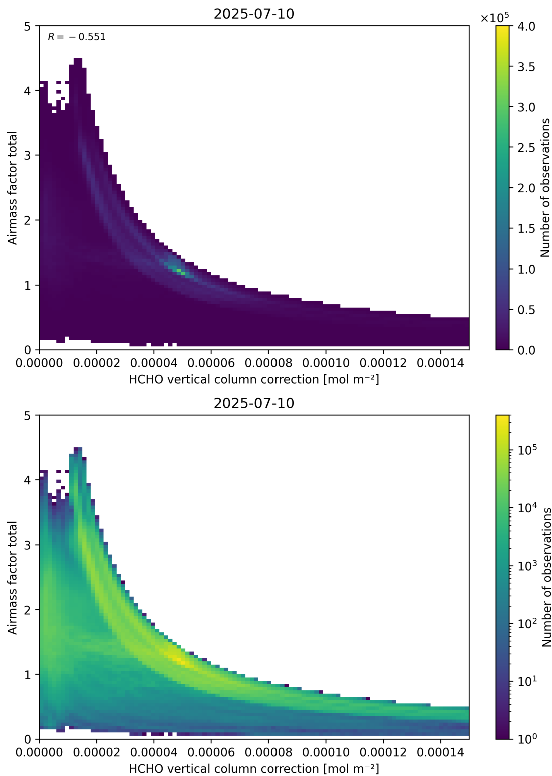
Figure 120: Scatter density plot of “HCHO vertical column correction” against “Airmass factor total” for 2025-07-09 to 2025-07-11.
