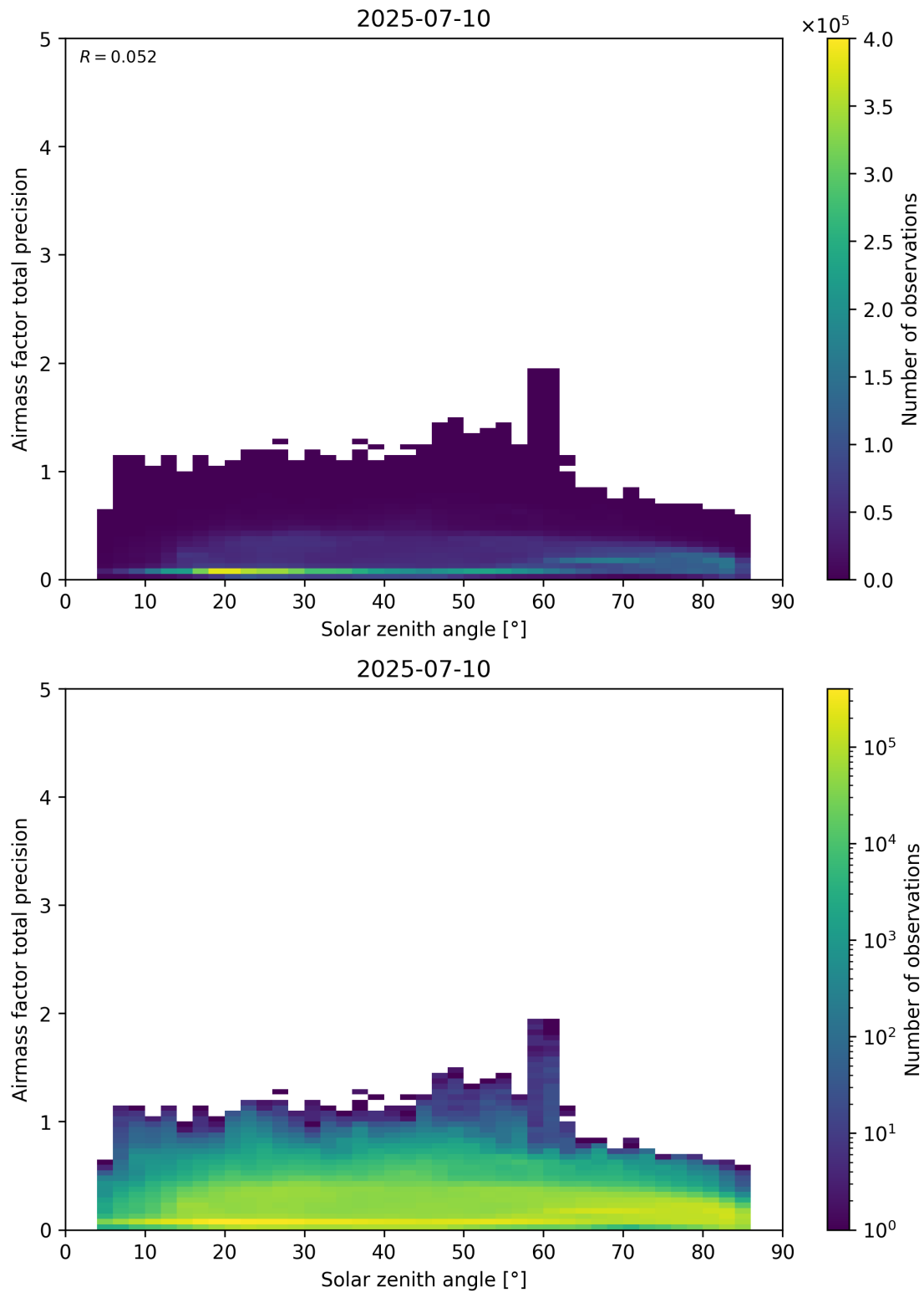
Figure 176: Scatter density plot of “Solar zenith angle” against “Airmass factor total precision” for 2025-07-09 to 2025-07-11.
