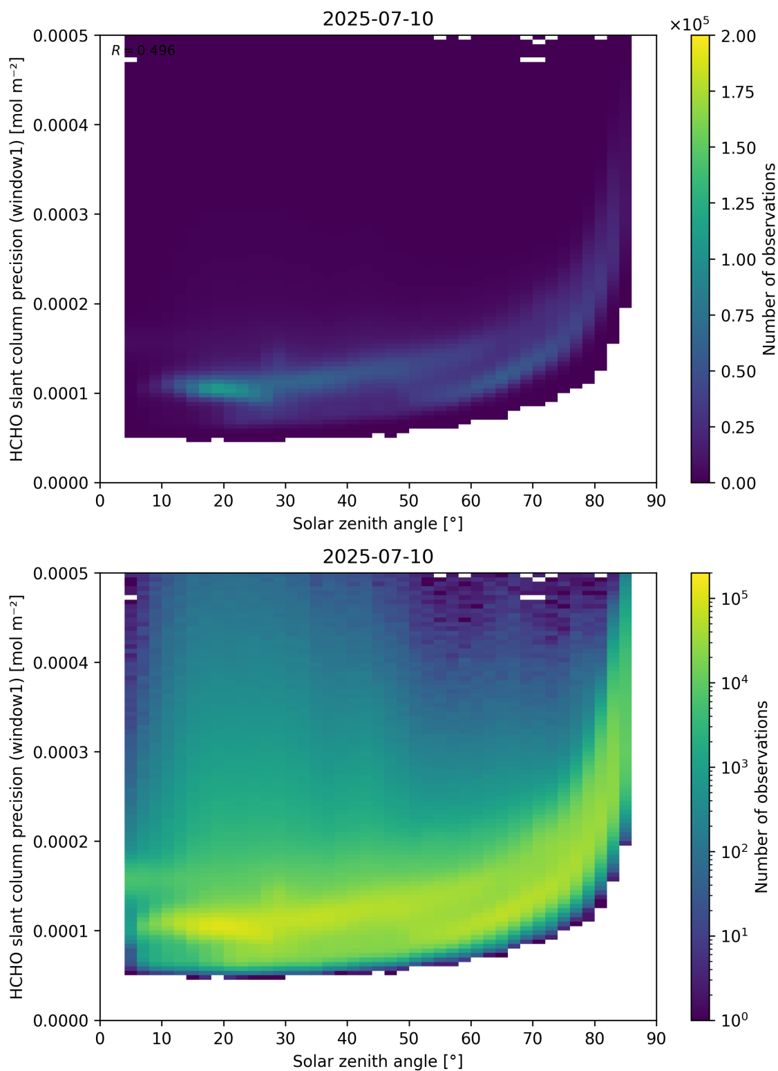
Figure 174: Scatter density plot of “Solar zenith angle” against “HCHO slant column precision (window1)” for 2025-07-09 to 2025-07-11.
