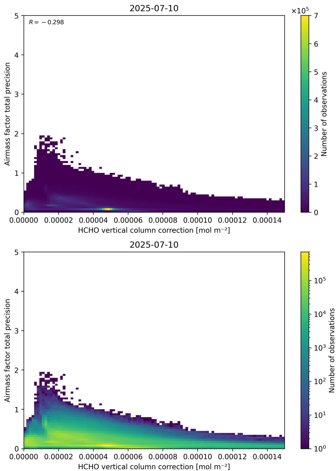
Figure 121: Scatter density plot of “HCHO vertical column correction” against “Airmass factor total precision” for 2025-07-09 to 2025-07-11.
