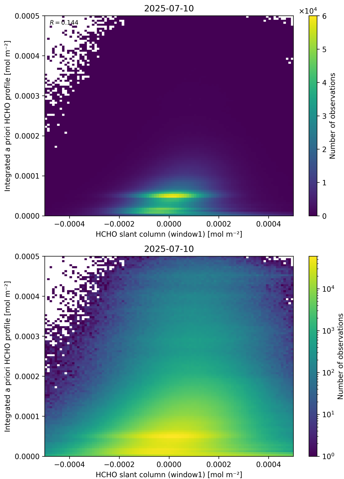
Figure 87: Scatter density plot of “HCHO slant column (window1)” against “Integrated a priori HCHO profile” for 2025-07-09 to 2025-07-11.
