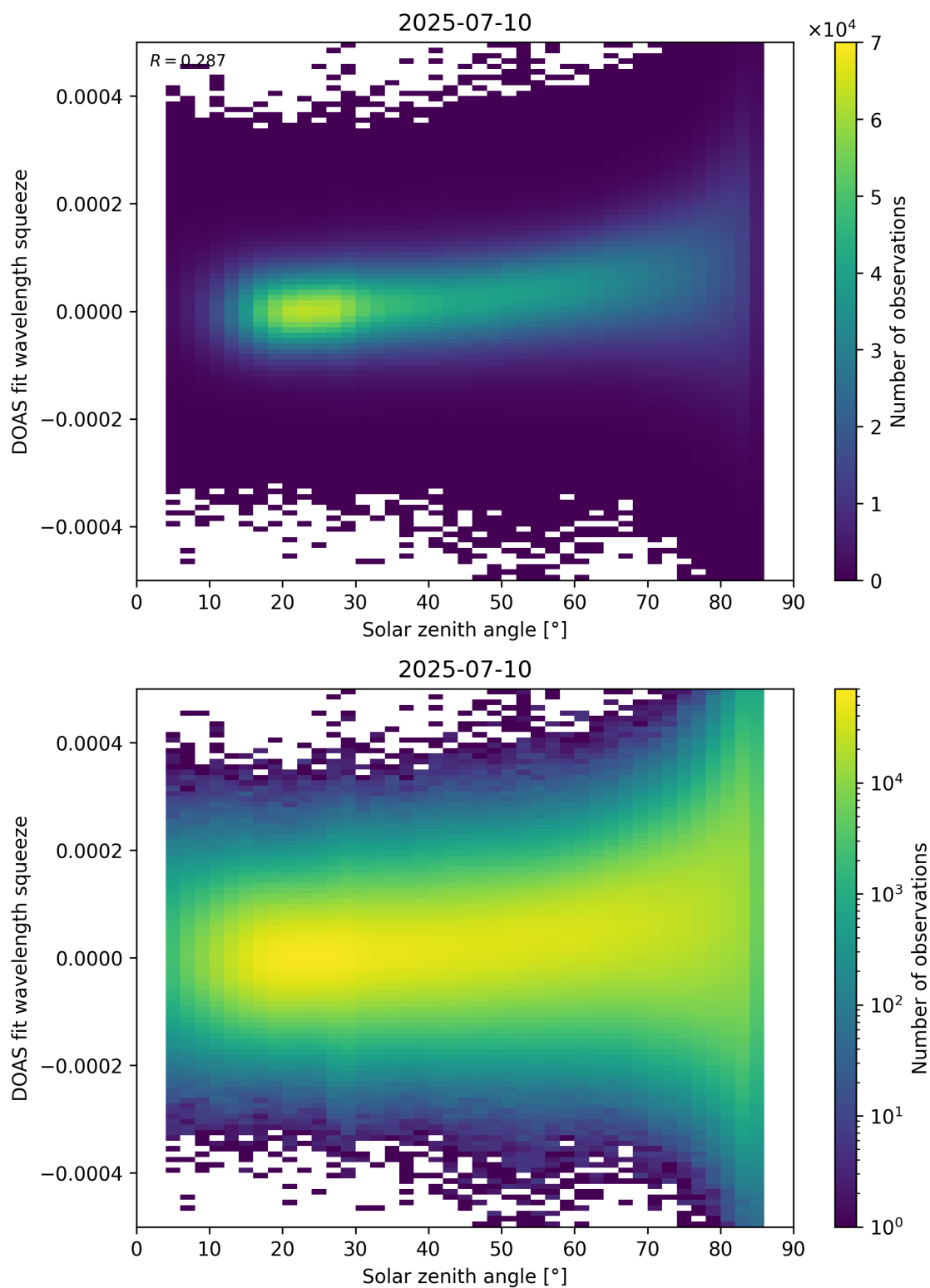
Figure 169: Scatter density plot of “Solar zenith angle” against “DOAS fit wavelength squeeze” for 2025-07-09 to 2025-07-11.
