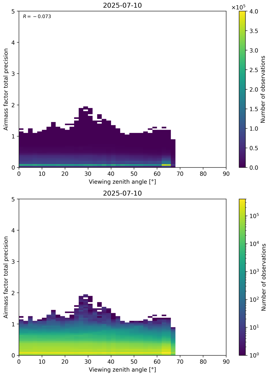
Figure 191: Scatter density plot of “Viewing zenith angle” against “Airmass factor total precision” for 2025-07-09 to 2025-07-11.
