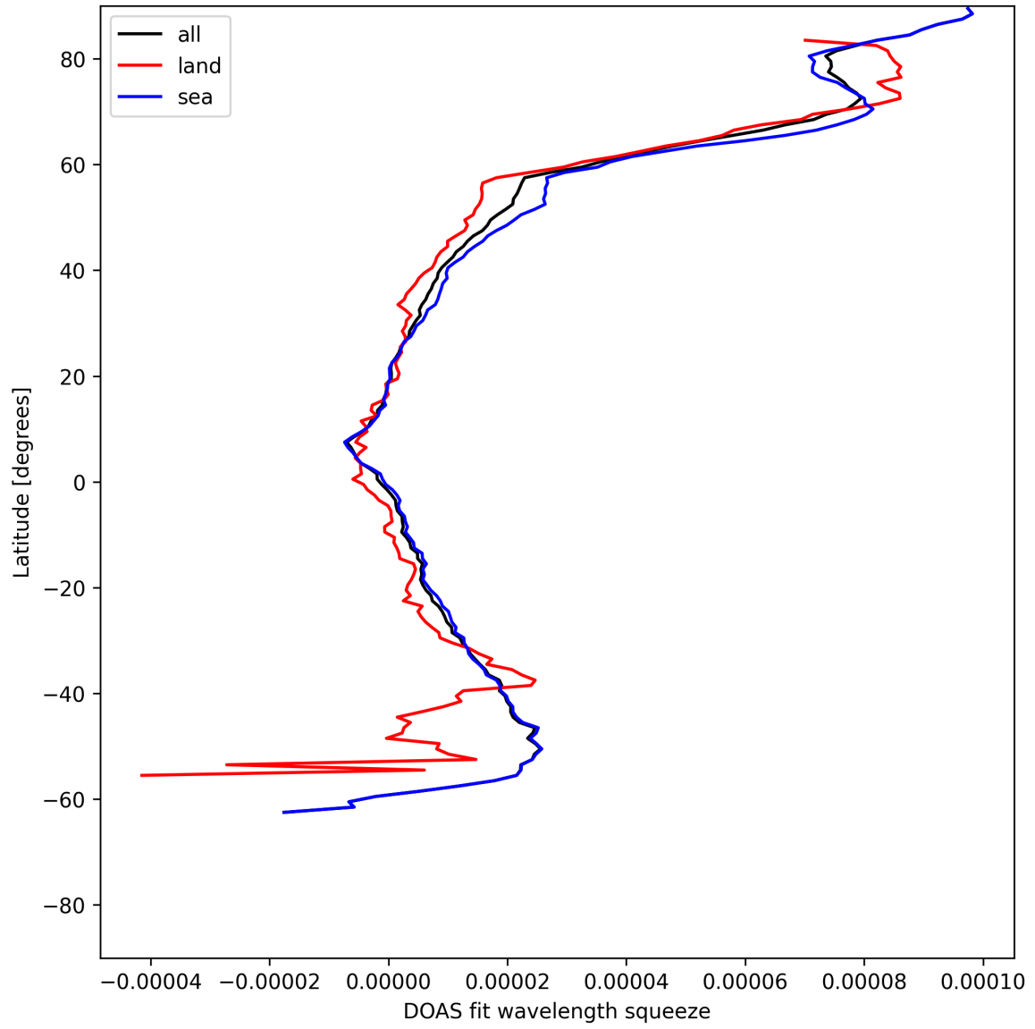
Figure 31: Zonal average of “DOAS fit wavelength squeeze” for 2025-07-09 to 2025-07-11.
