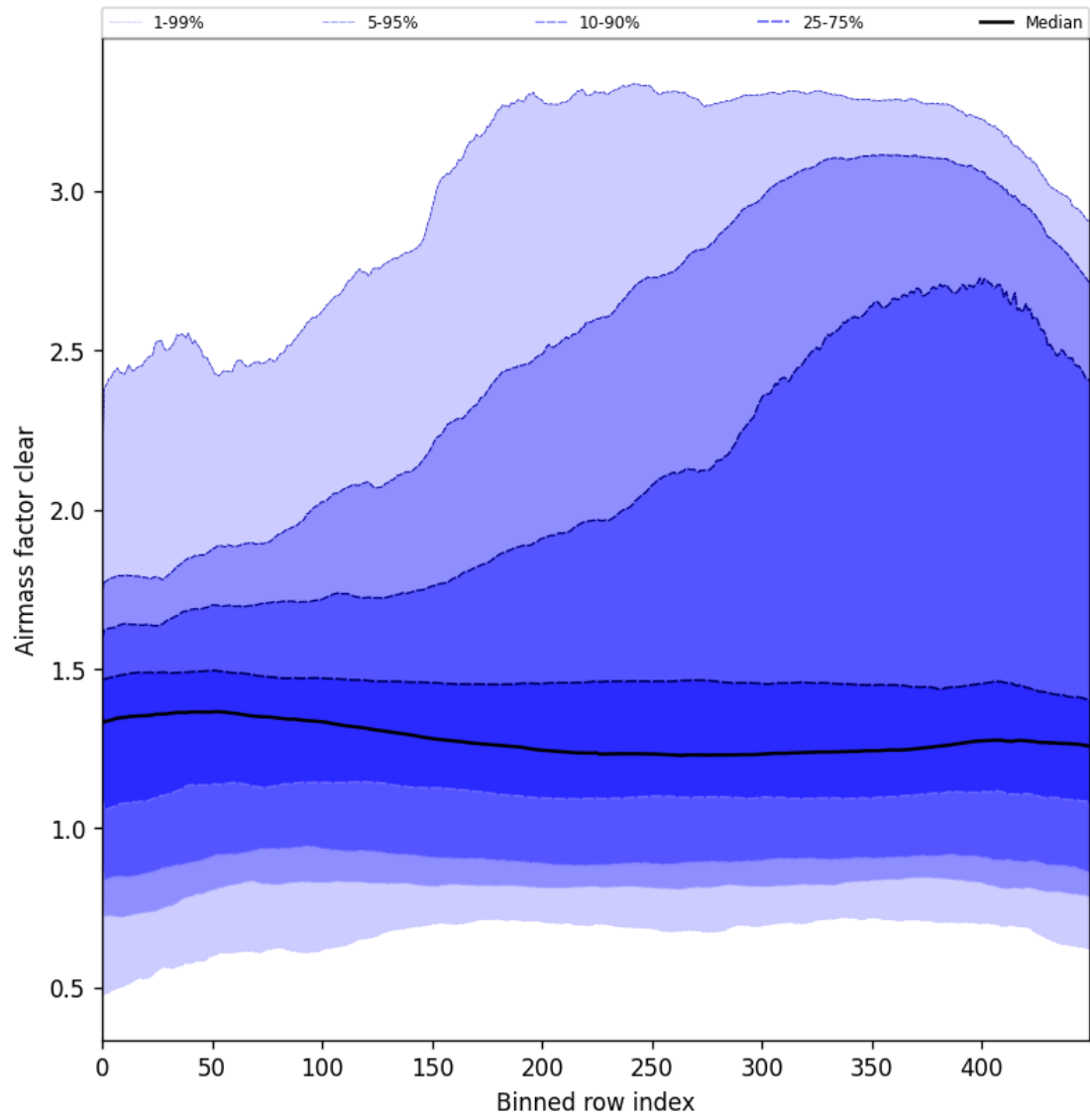
Figure 56: Along track statistics of “Airmass factor clear” for 2025-07-09 to 2025-07-11
