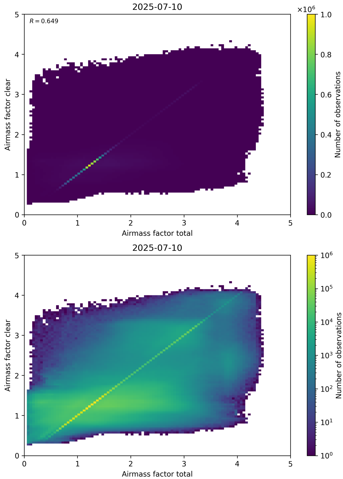
Figure 100: Scatter density plot of “Airmass factor total” against “Airmass factor clear” for 2025-07-09 to 2025-07-11.
