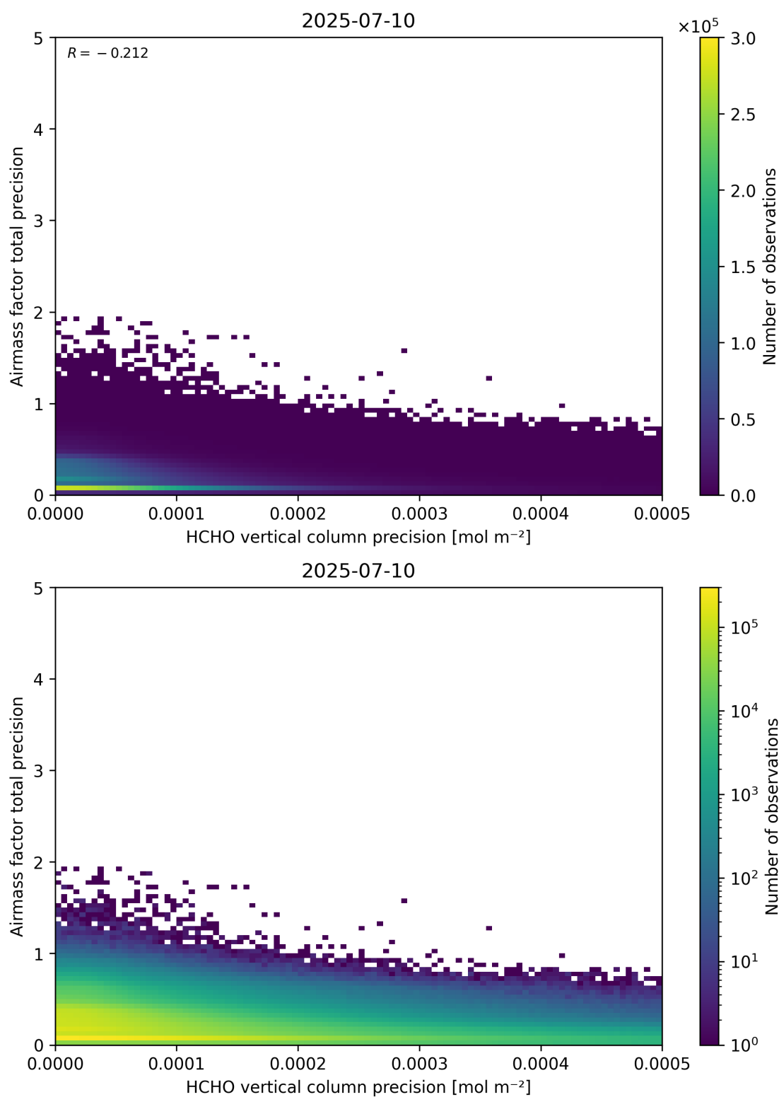
Figure 145: Scatter density plot of “HCHO vertical column precision” against “Airmass factor total precision” for 2025-07-09 to 2025-07-11.
