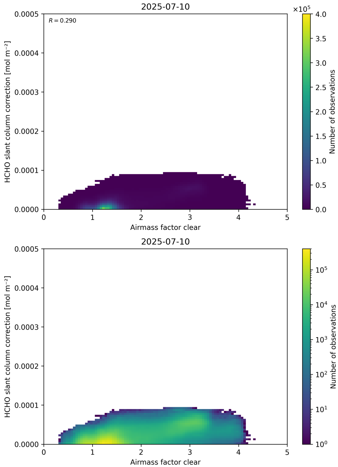
Figure 75: Scatter density plot of “Airmass factor clear” against “HCHO slant column correction” for 2025-07-09 to 2025-07-11.
