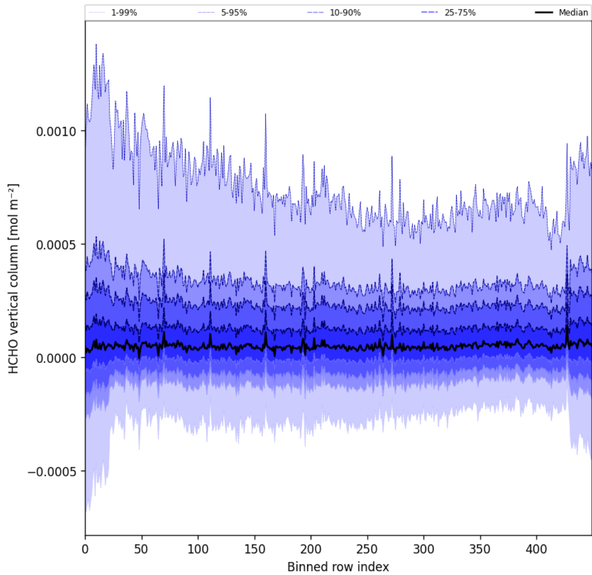
Figure 49: Along track statistics of "HCHO vertical column" for 2025-07-09 to 2025-07-11
