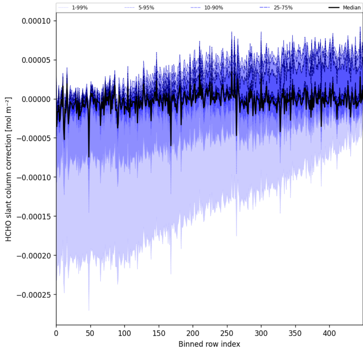
Figure 61: Along track statistics of “HCHO slant column correction” for 2025-07-09 to 2025-07-11
