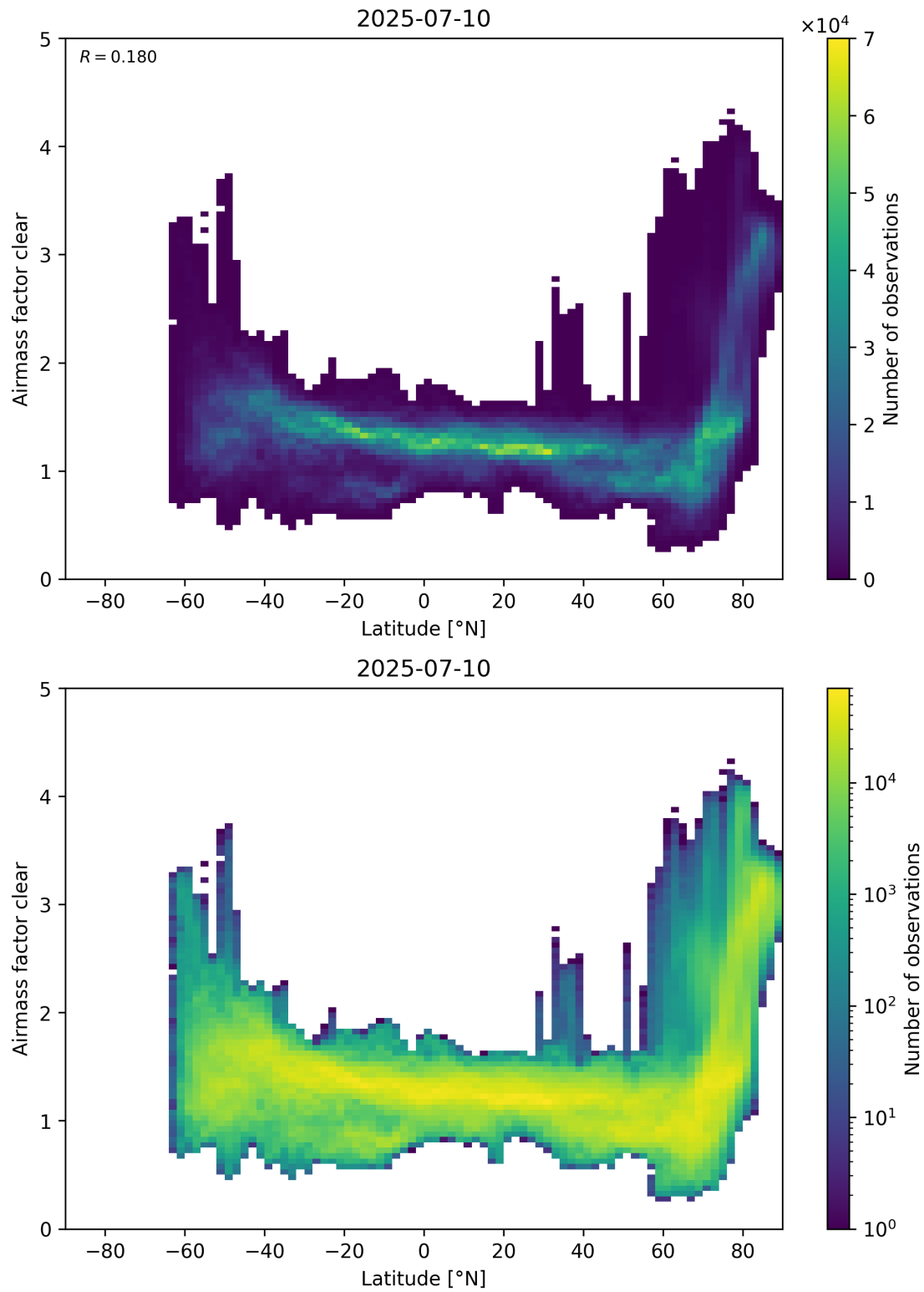
Figure 156: Scatter density plot of “Latitude” against “Airmass factor clear” for 2025-07-09 to 2025-07-11.
