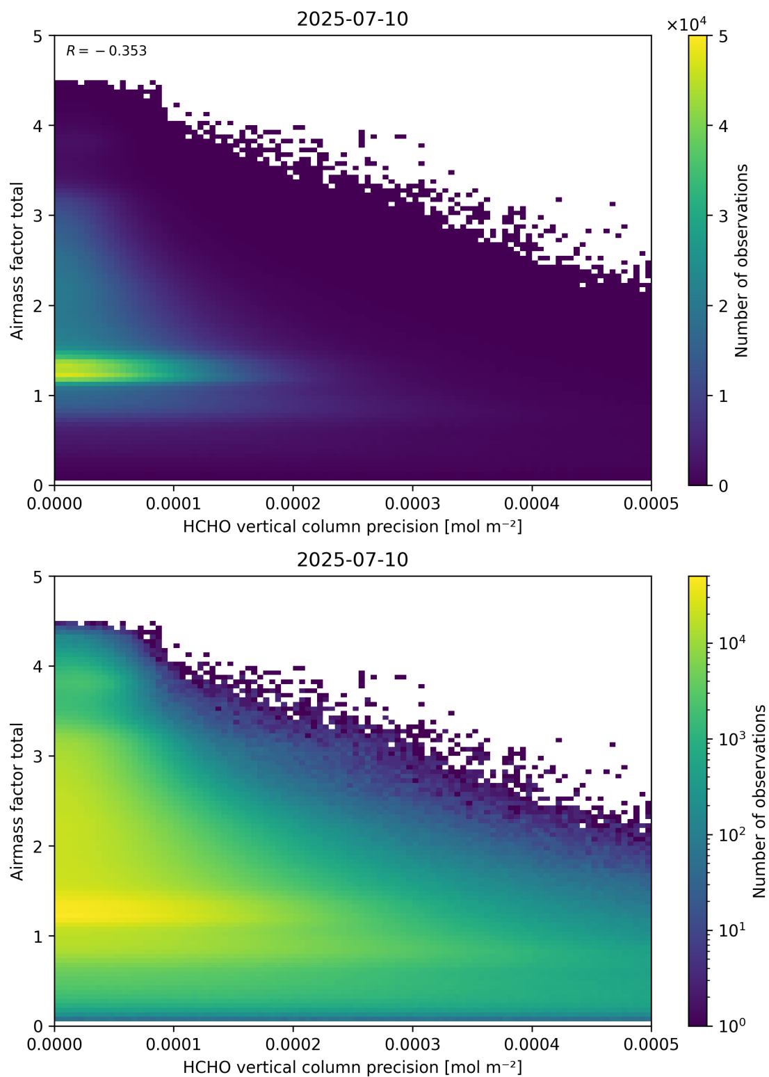
Figure 144: Scatter density plot of “HCHO vertical column precision” against “Airmass factor total” for 2025-07-09 to 2025-07-11.
