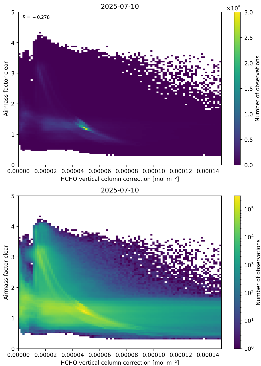
Figure 115: Scatter density plot of “HCHO vertical column correction” against “Airmass factor clear” for 2025-07-09 to 2025-07-11.
