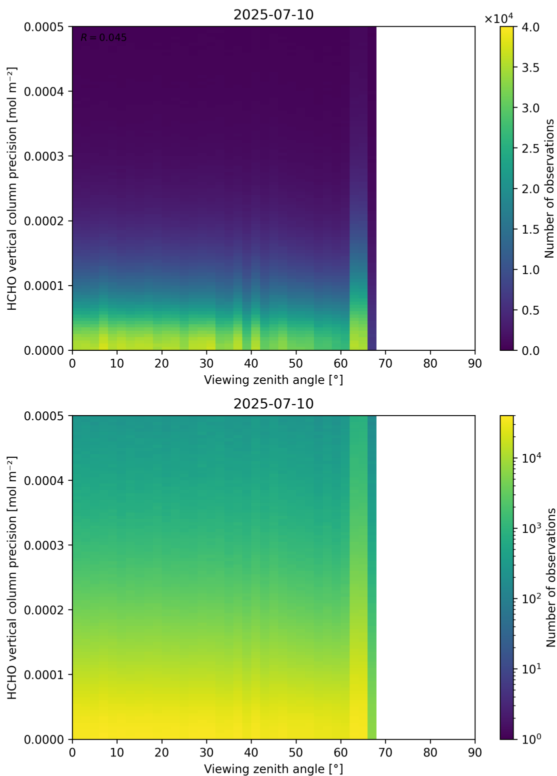
Figure 194: Scatter density plot of “Viewing zenith angle” against “HCHO vertical column precision” for 2025-07-09 to 2025-07-11.
