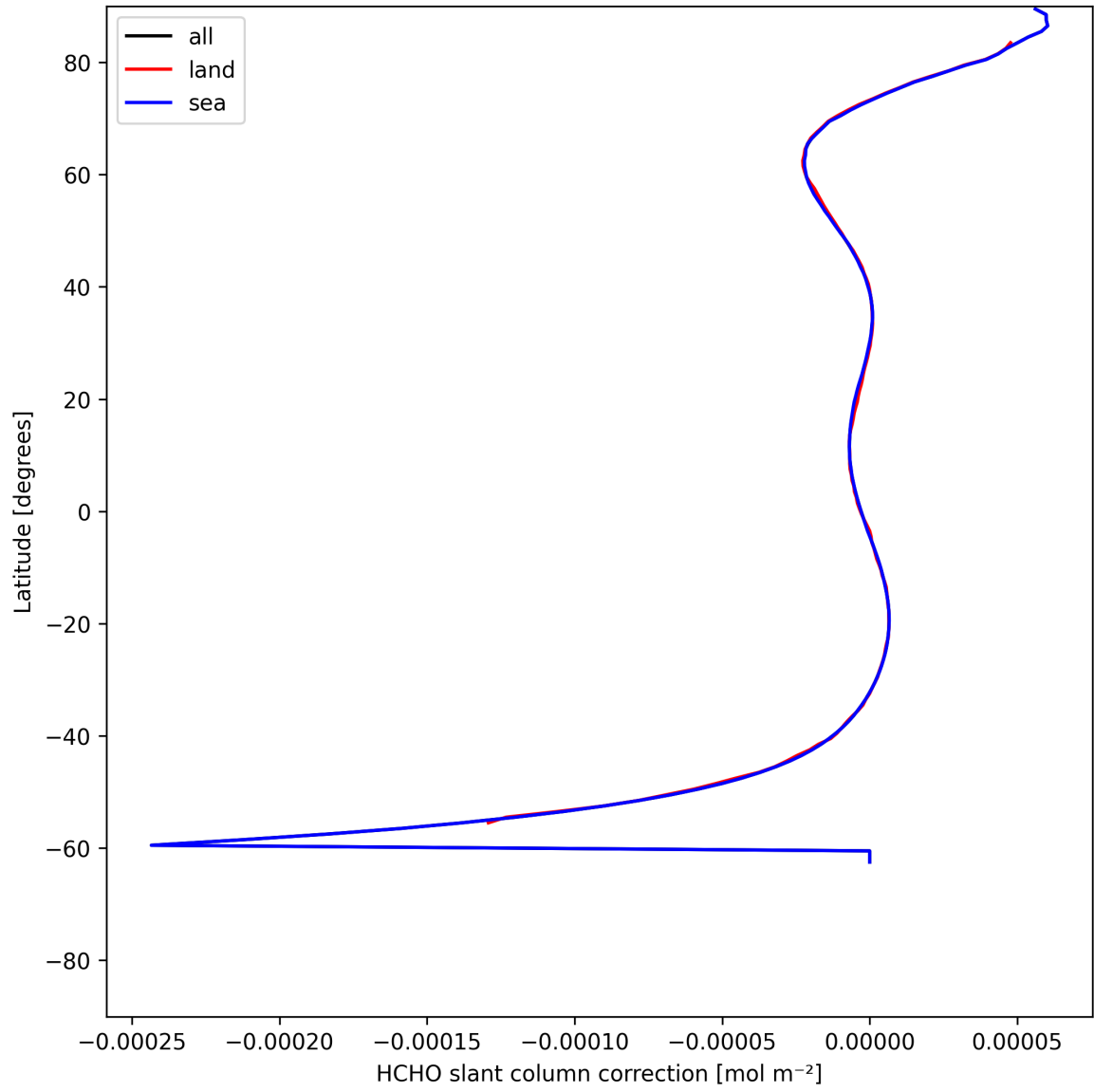
Figure 33: Zonal average of “HCHO slant column correction” for 2025-07-09 to 2025-07-11.
