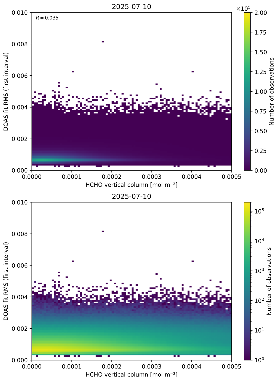
Figure 123: Scatter density plot of “HCHO vertical column” against “DOAS fit RMS (first interval)” for 2025-07-09 to 2025-07-11.
