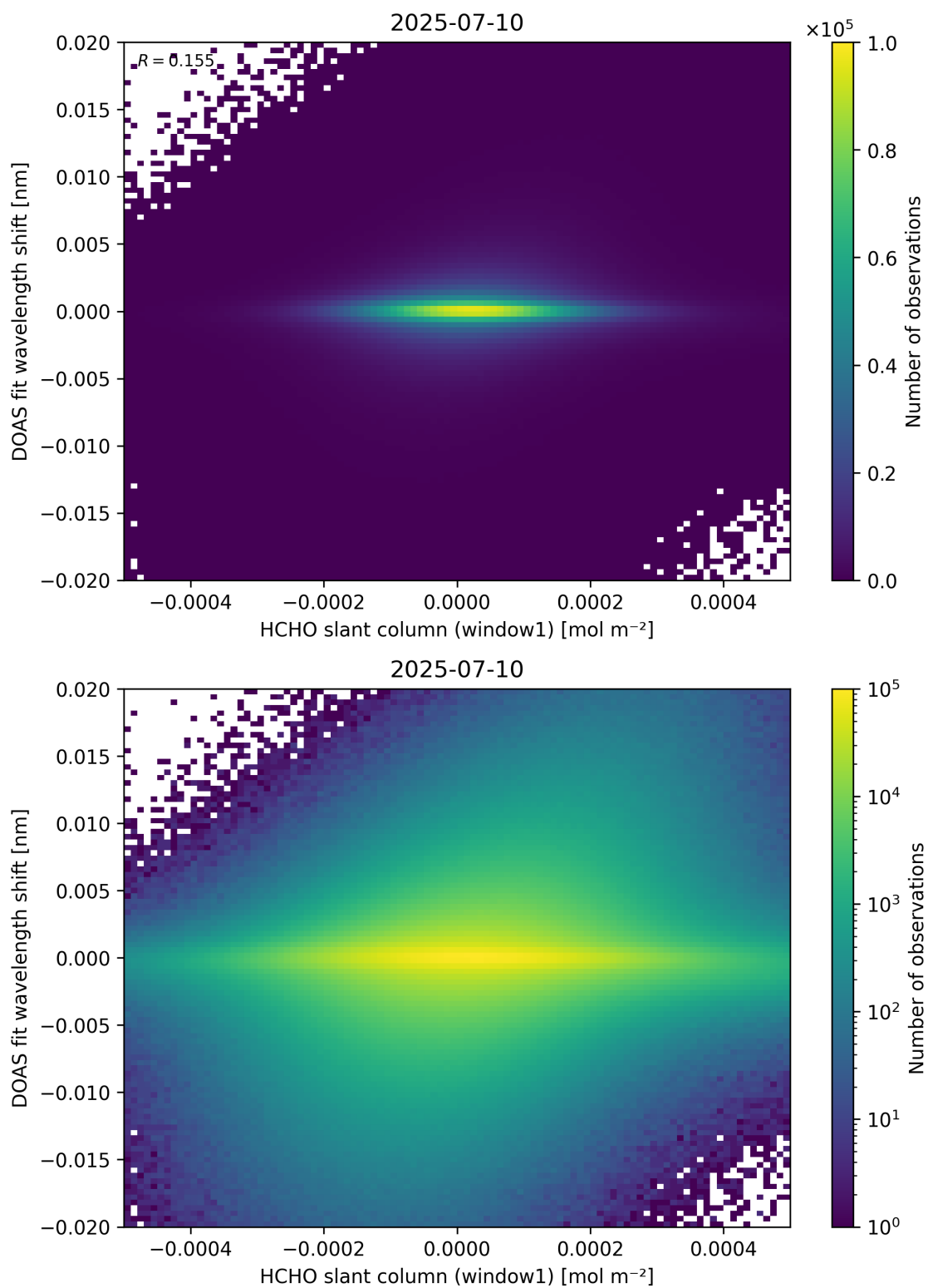
Figure 79: Scatter density plot of “HCHO slant column (window1)” against “DOAS fit wavelength shift” for 2025-07-09 to 2025-07-11.
