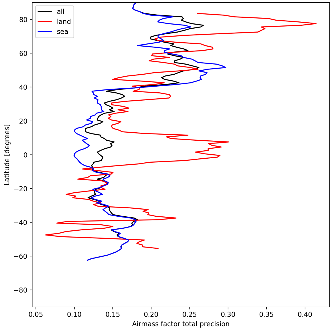
Figure 27: Zonal average of “Airmass factor total precision” for 2025-07-09 to 2025-07-11.
