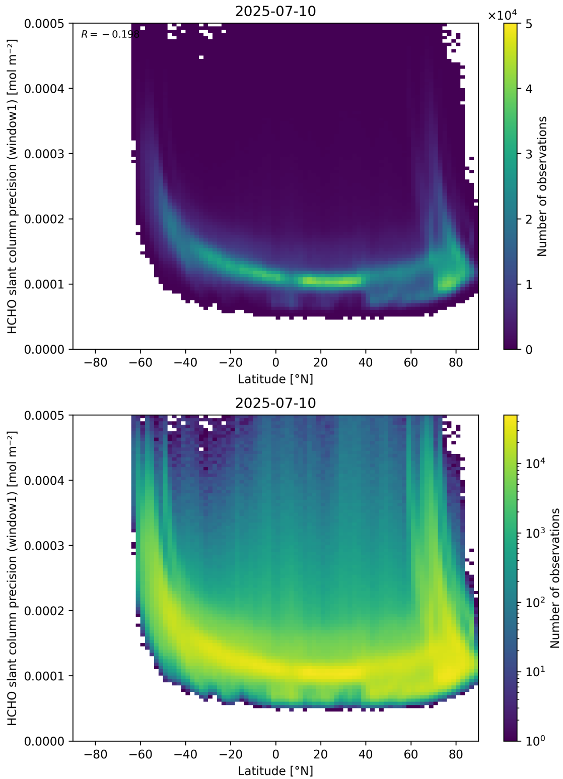
Figure 160: Scatter density plot of “Latitude” against “HCHO slant column precision (window1)” for 2025-07-09 to 2025-07-11.
