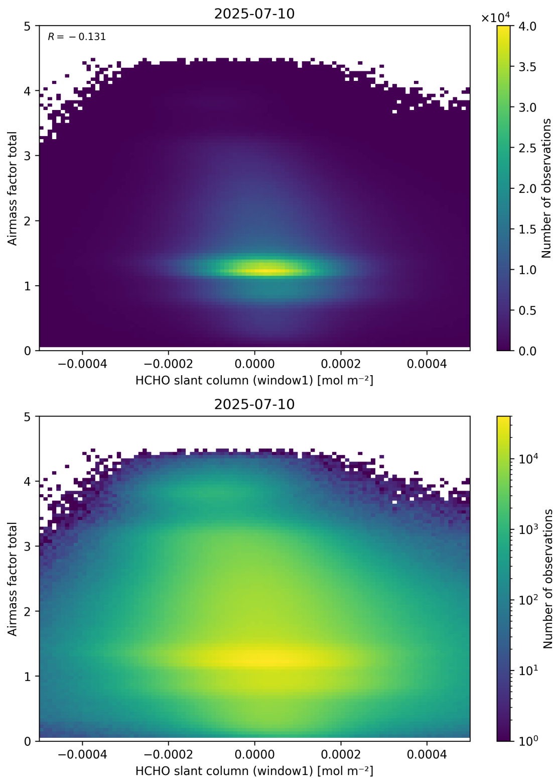
Figure 85: Scatter density plot of “HCHO slant column (window1)” against “Airmass factor total” for 2025-07-09 to 2025-07-11.
