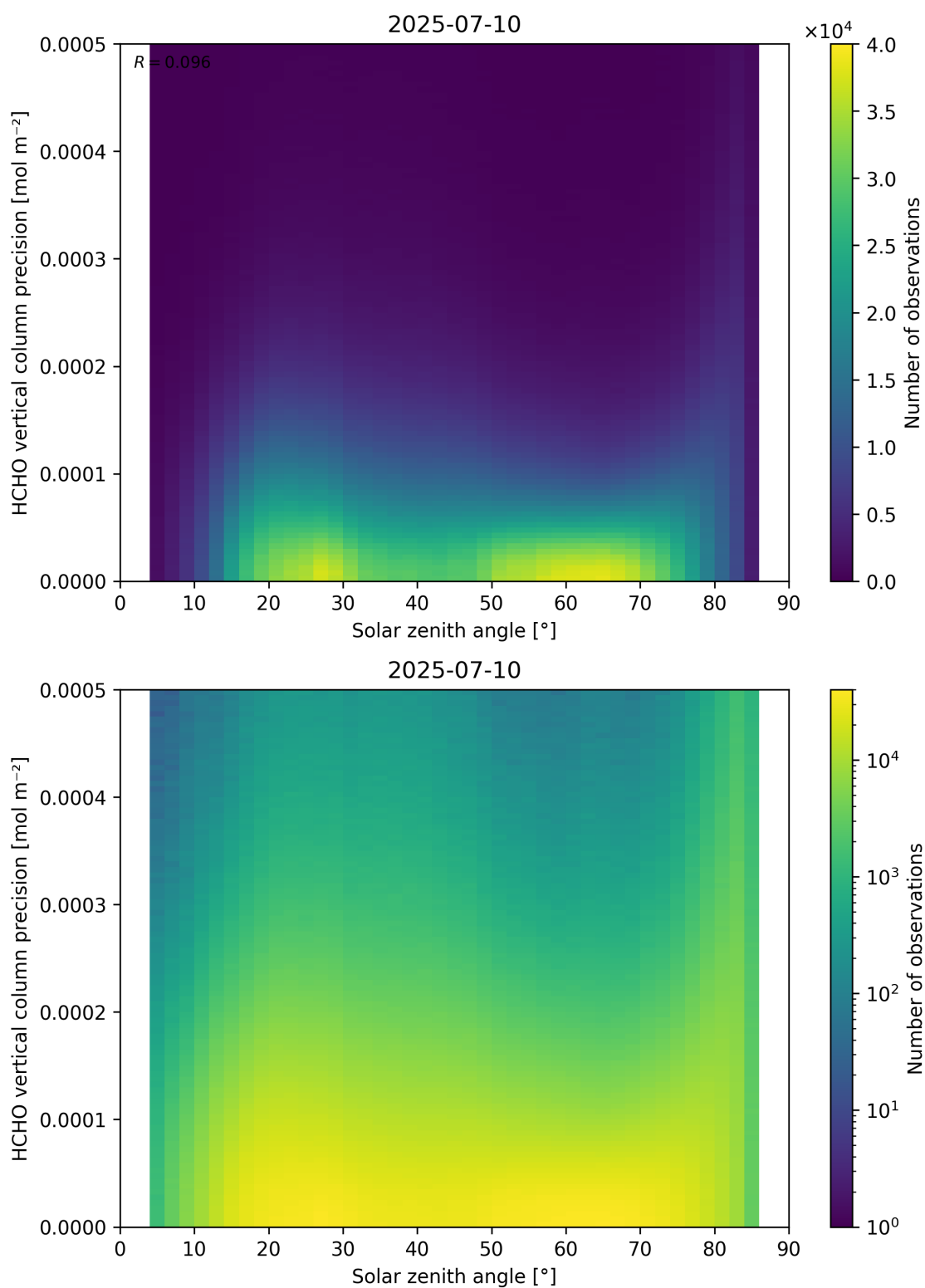
Figure 179: Scatter density plot of “Solar zenith angle” against “HCHO vertical column precision” for 2025-07-09 to 2025-07-11.
