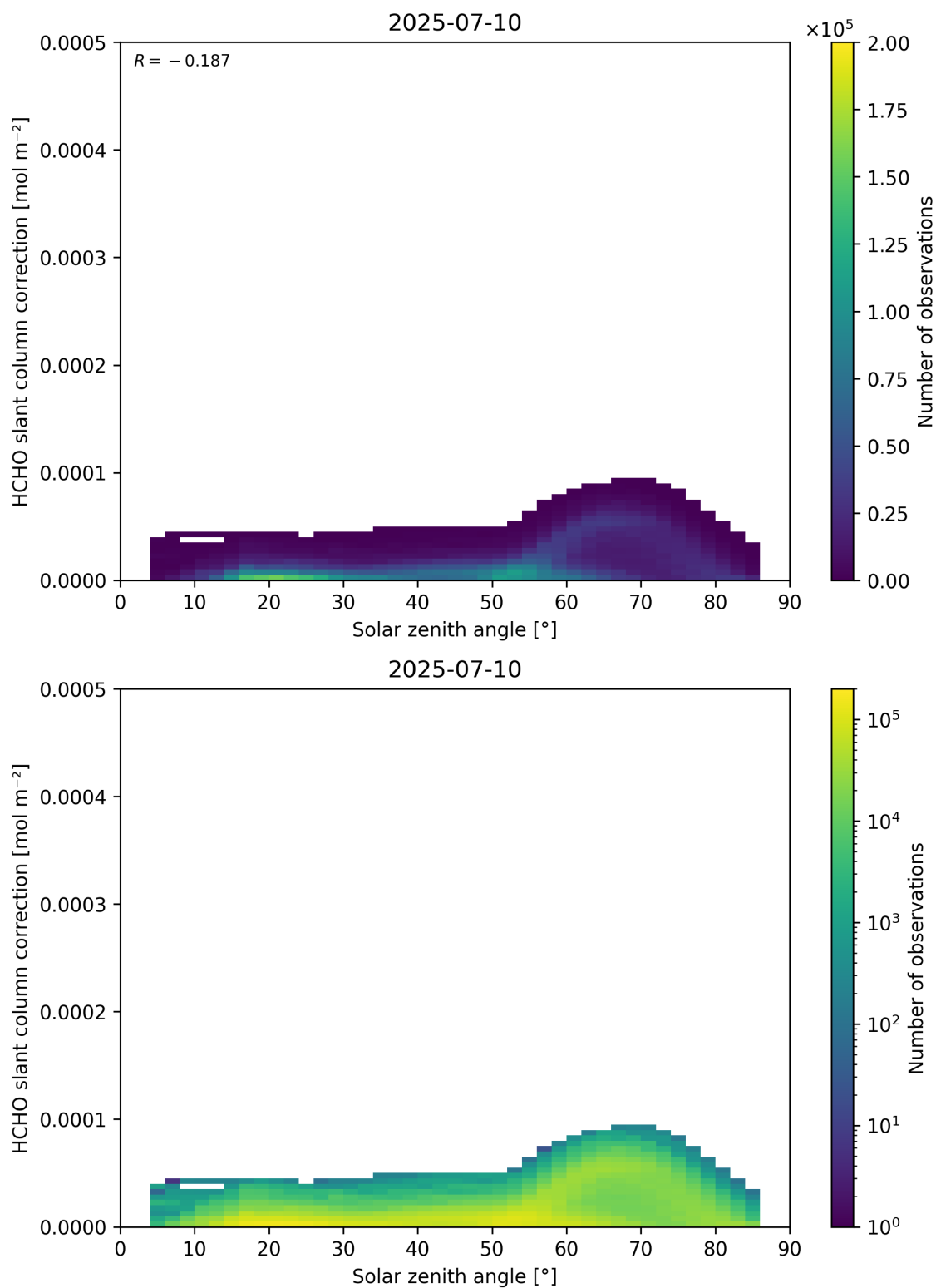
Figure 172: Scatter density plot of “Solar zenith angle” against “HCHO slant column correction” for 2025-07-09 to 2025-07-11.
