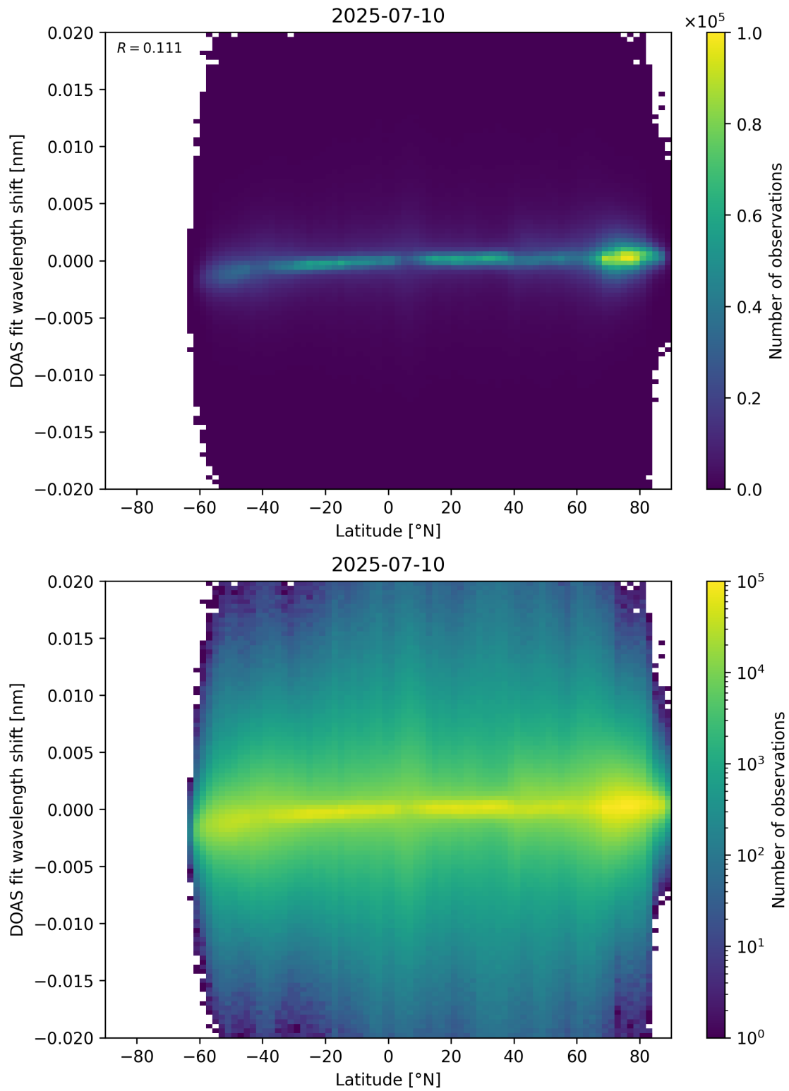
Figure 154: Scatter density plot of “Latitude” against “DOAS fit wavelength shift” for 2025-07-09 to 2025-07-11.
