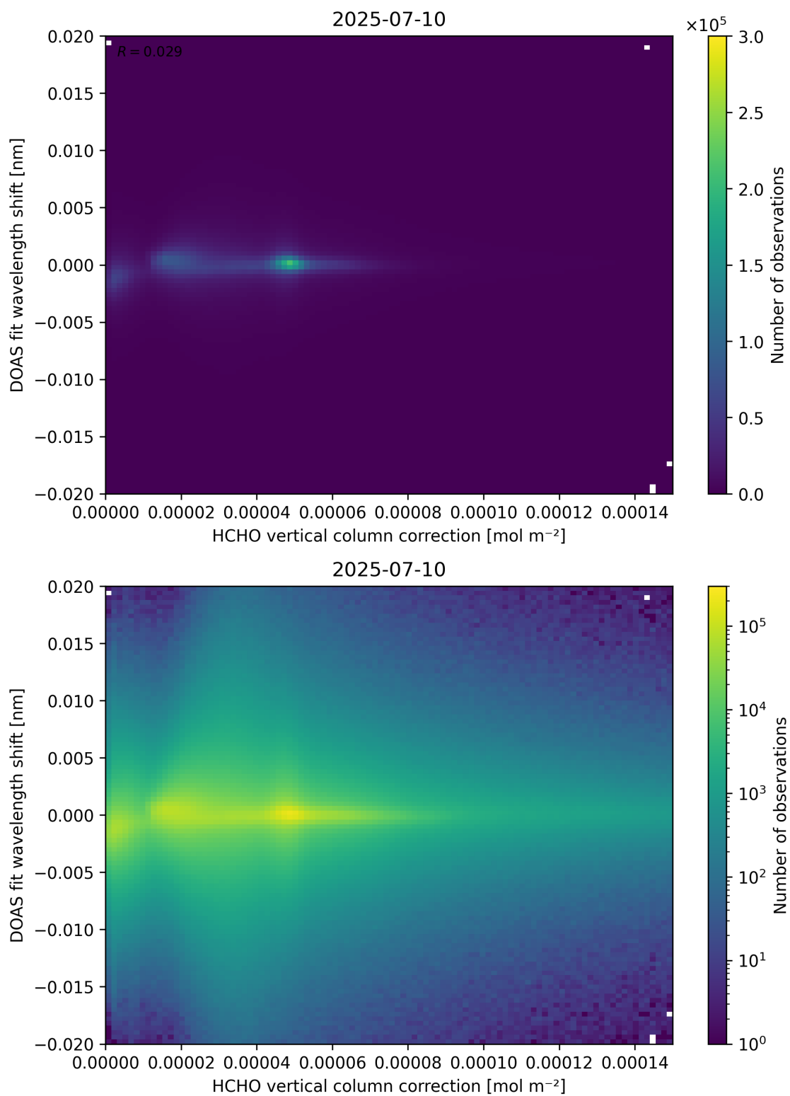
Figure 113: Scatter density plot of “HCHO vertical column correction” against “DOAS fit wavelength shift” for 2025-07-09 to 2025-07-11.
