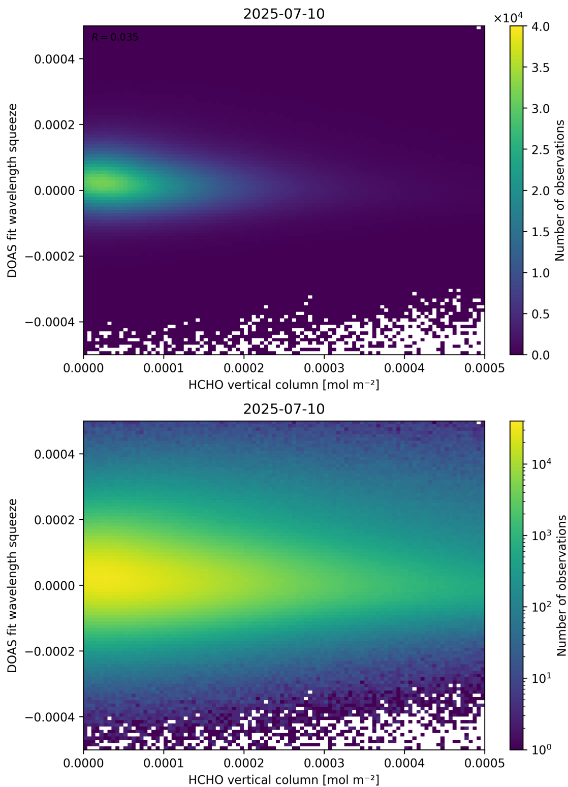
Figure 125: Scatter density plot of “HCHO vertical column” against “DOAS fit wavelength squeeze” for 2025-07-09 to 2025-07-11.
