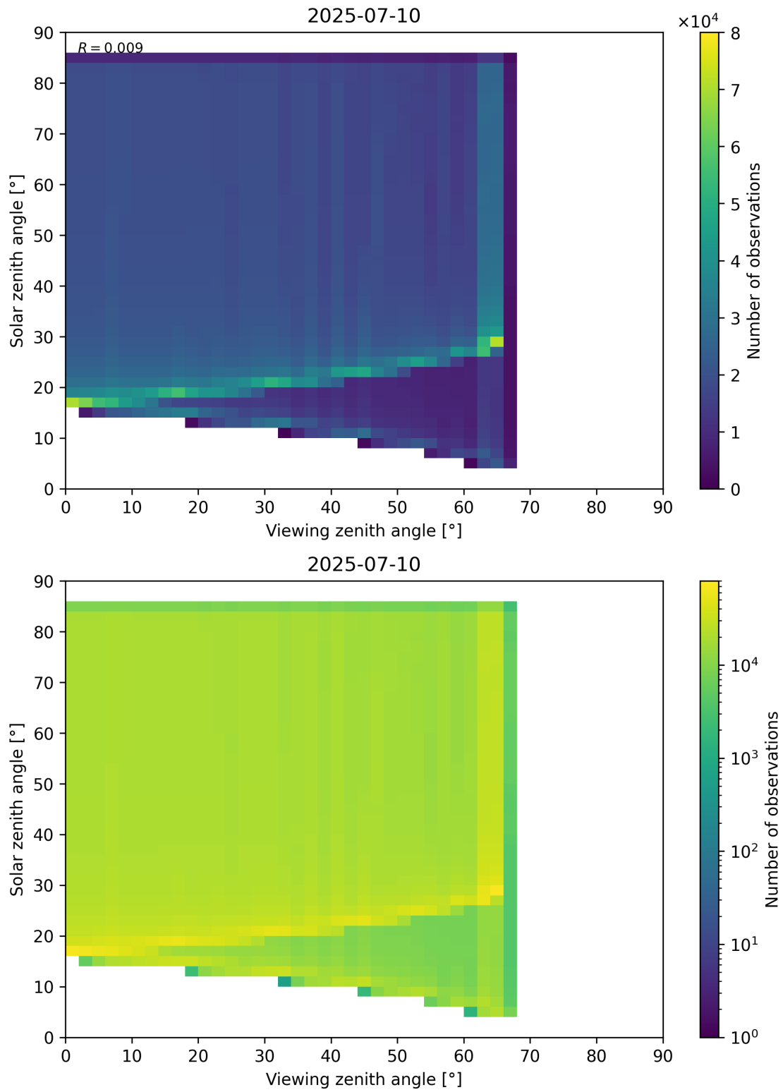
Figure 197: Scatter density plot of “Viewing zenith angle” against “Solar zenith angle” for 2025-07-09 to 2025-07-11.
