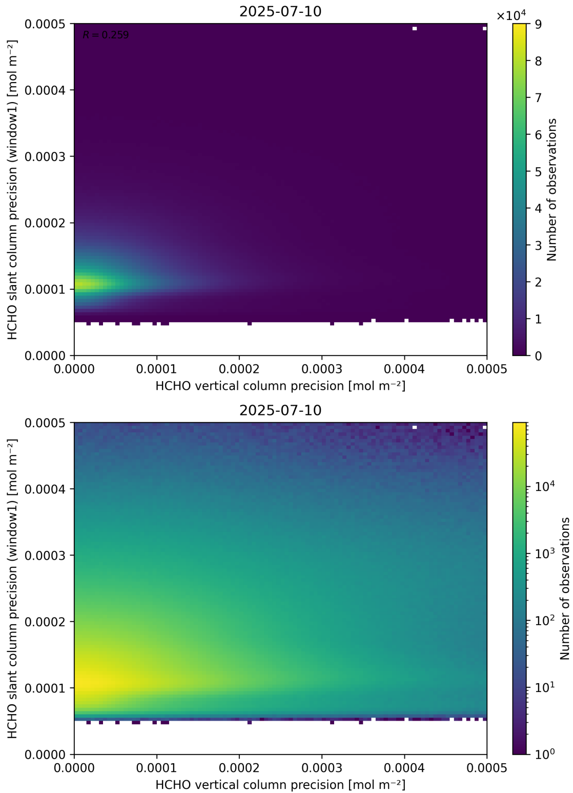
Figure 143: Scatter density plot of “HCHO vertical column precision” against “HCHO slant column precision (window1)” for 2025-07-09 to 2025-07-11.
