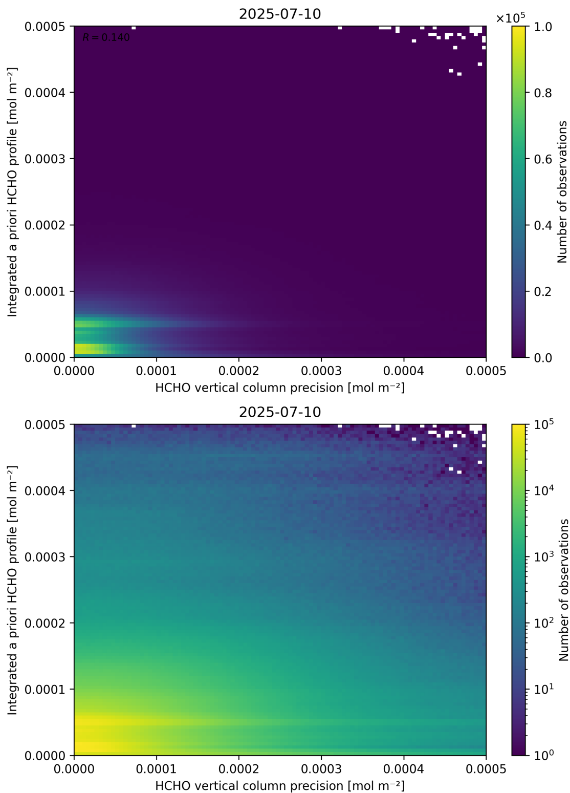
Figure 147: Scatter density plot of “HCHO vertical column precision” against “Integrated a priori HCHO profile” for 2025-07-09 to 2025-07-11.
