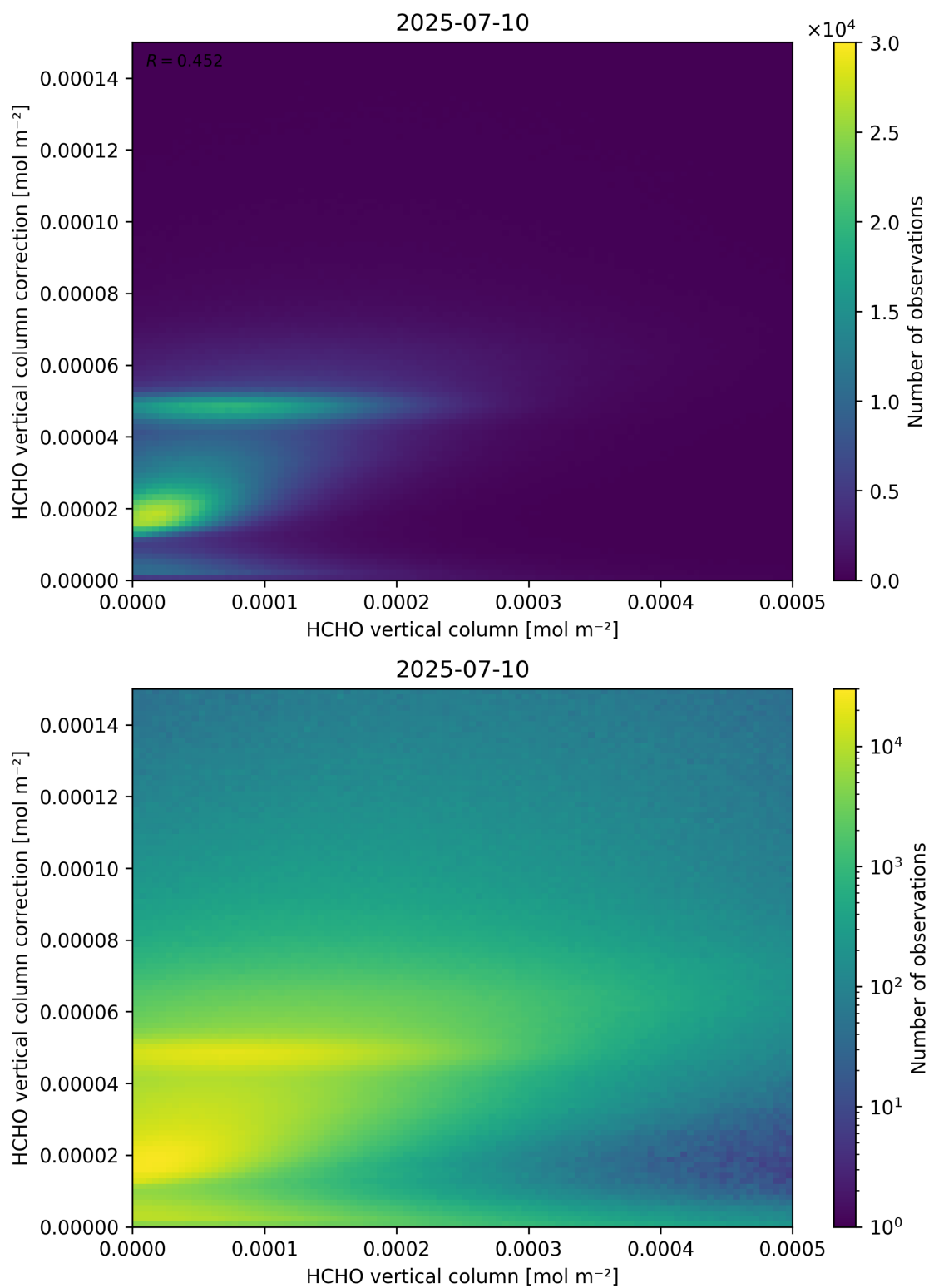
Figure 133: Scatter density plot of “HCHO vertical column” against “HCHO vertical column correction” for 2025-07-09 to 2025-07-11.
