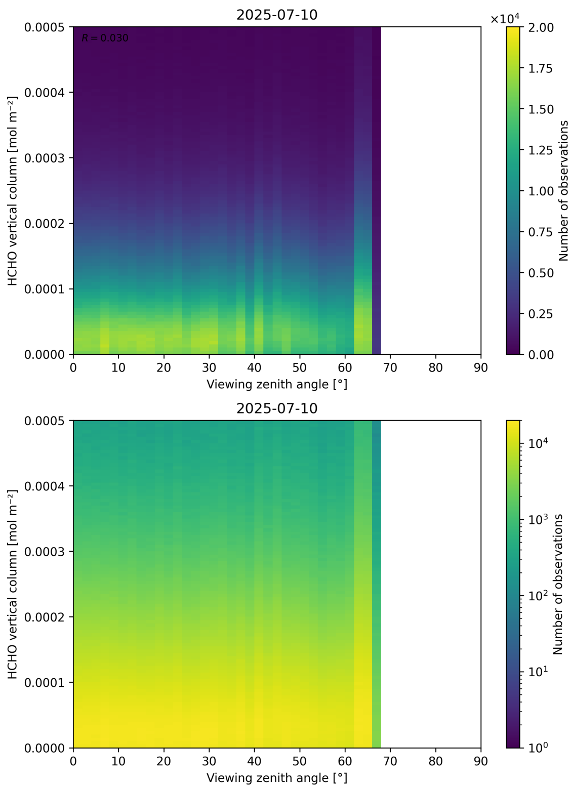
Figure 192: Scatter density plot of “Viewing zenith angle” against “HCHO vertical column” for 2025-07-09 to 2025-07-11.
