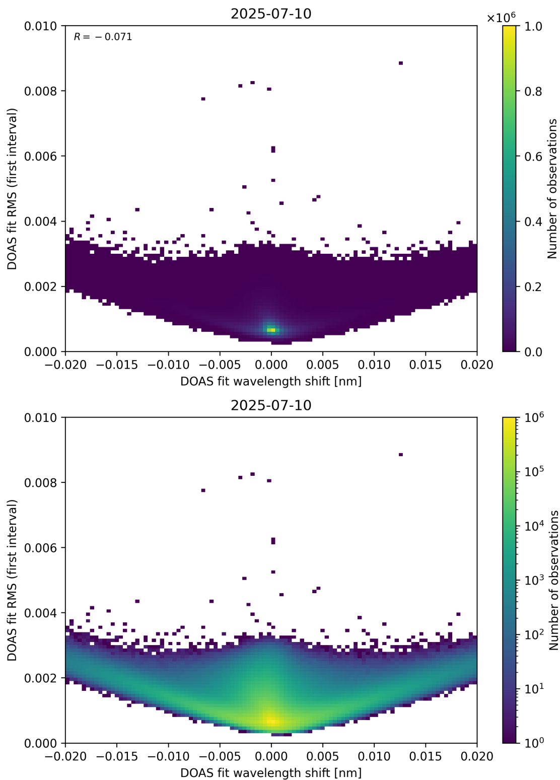
Figure 64: Scatter density plot of “DOAS fit wavelength shift” against “DOAS fit RMS (first interval)” for 2025-07-09 to 2025-07-11.
