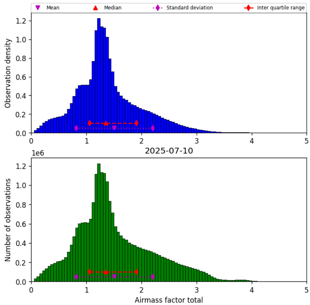
Figure 40: Histogram of “Airmass factor total” for 2025-07-09 to 2025-07-11
