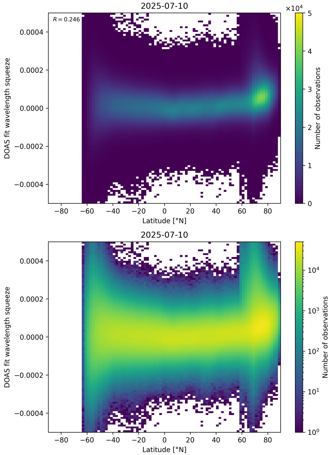
Figure 155: Scatter density plot of “Latitude” against “DOAS fit wavelength squeeze” for 2025-07-09 to 2025-07-11.
