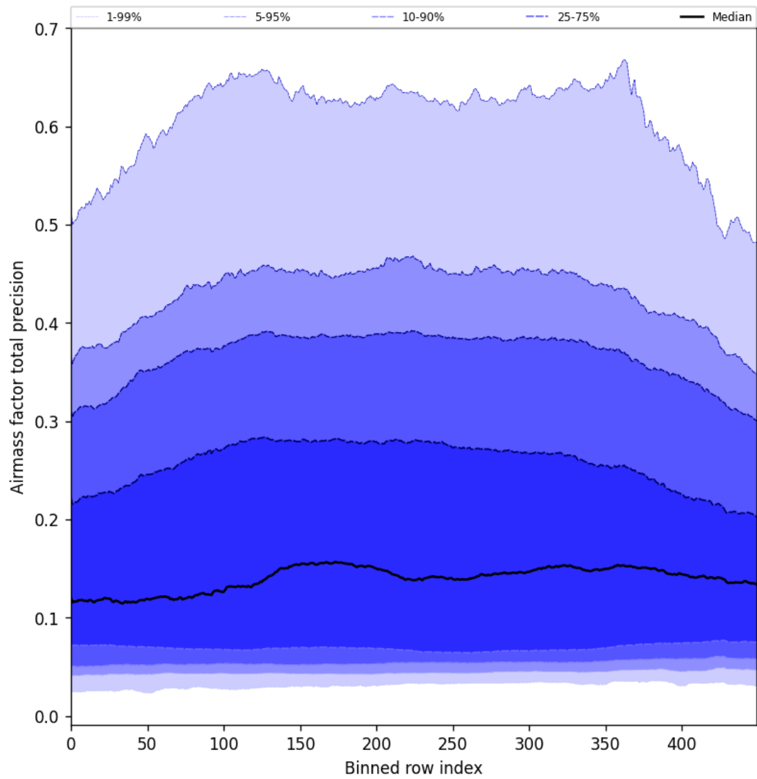
Figure 55: Along track statistics of “Airmass factor total precision” for 2025-07-09 to 2025-07-11
