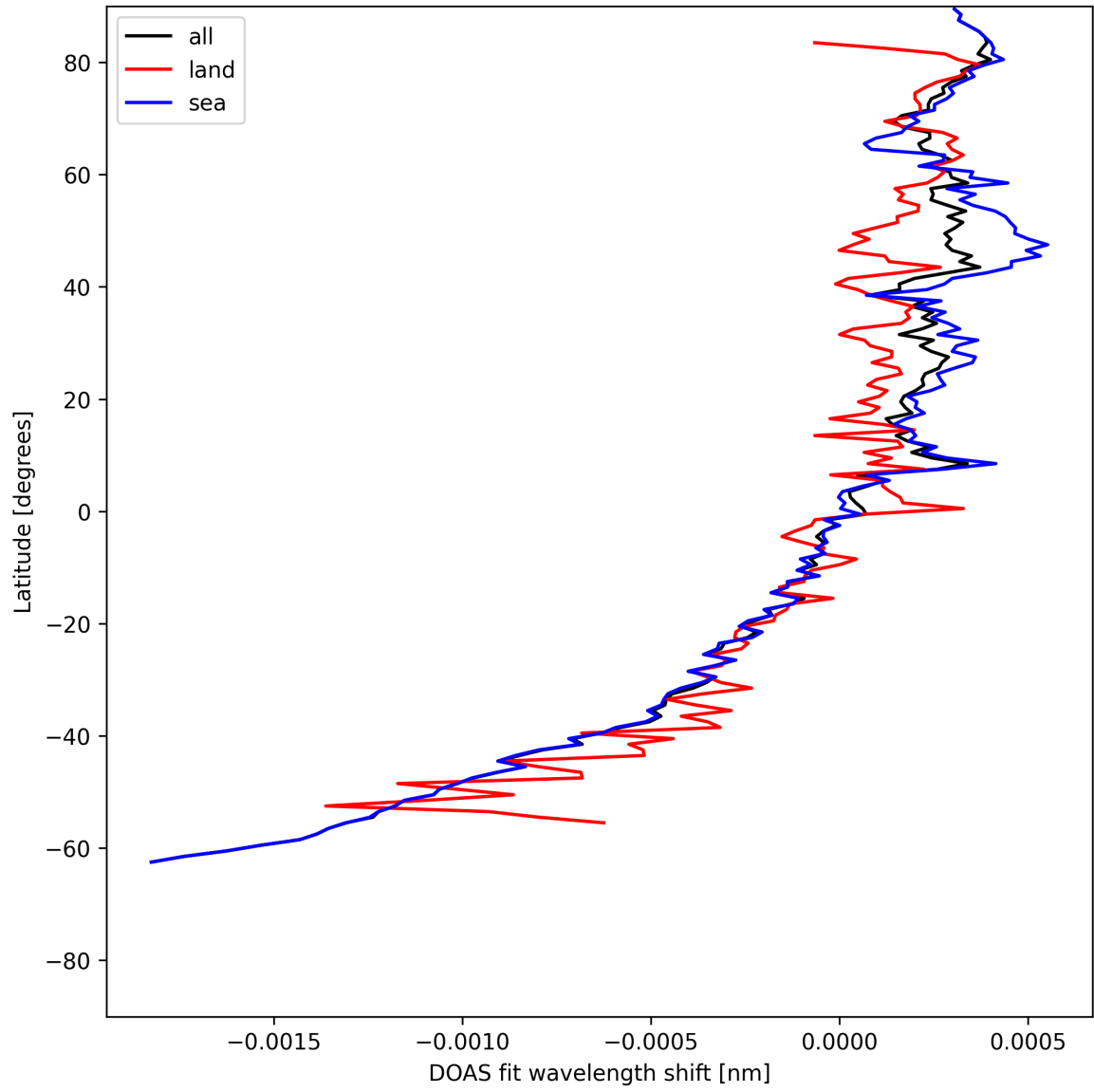
Figure 30: Zonal average of “DOAS fit wavelength shift” for 2025-07-09 to 2025-07-11.
