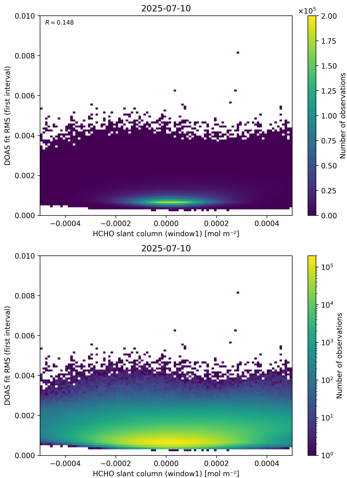
Figure 78: Scatter density plot of “HCHO slant column (window1)” against “DOAS fit RMS (first interval)” for 2025-07-09 to 2025-07-11.
