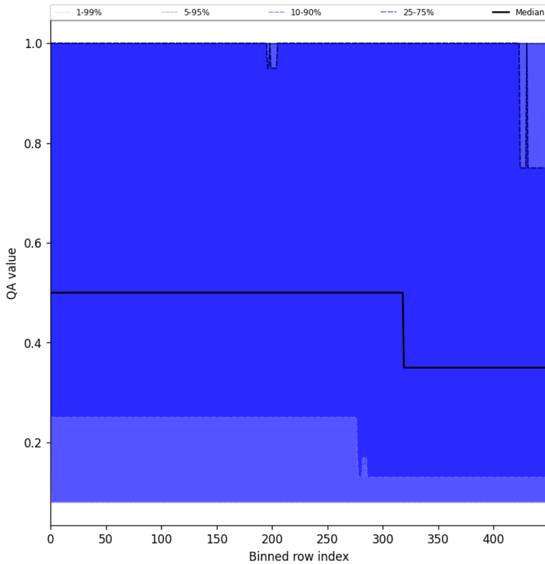
Figure 48: Along track statistics of “QA value” for 2025-07-09 to 2025-07-11
