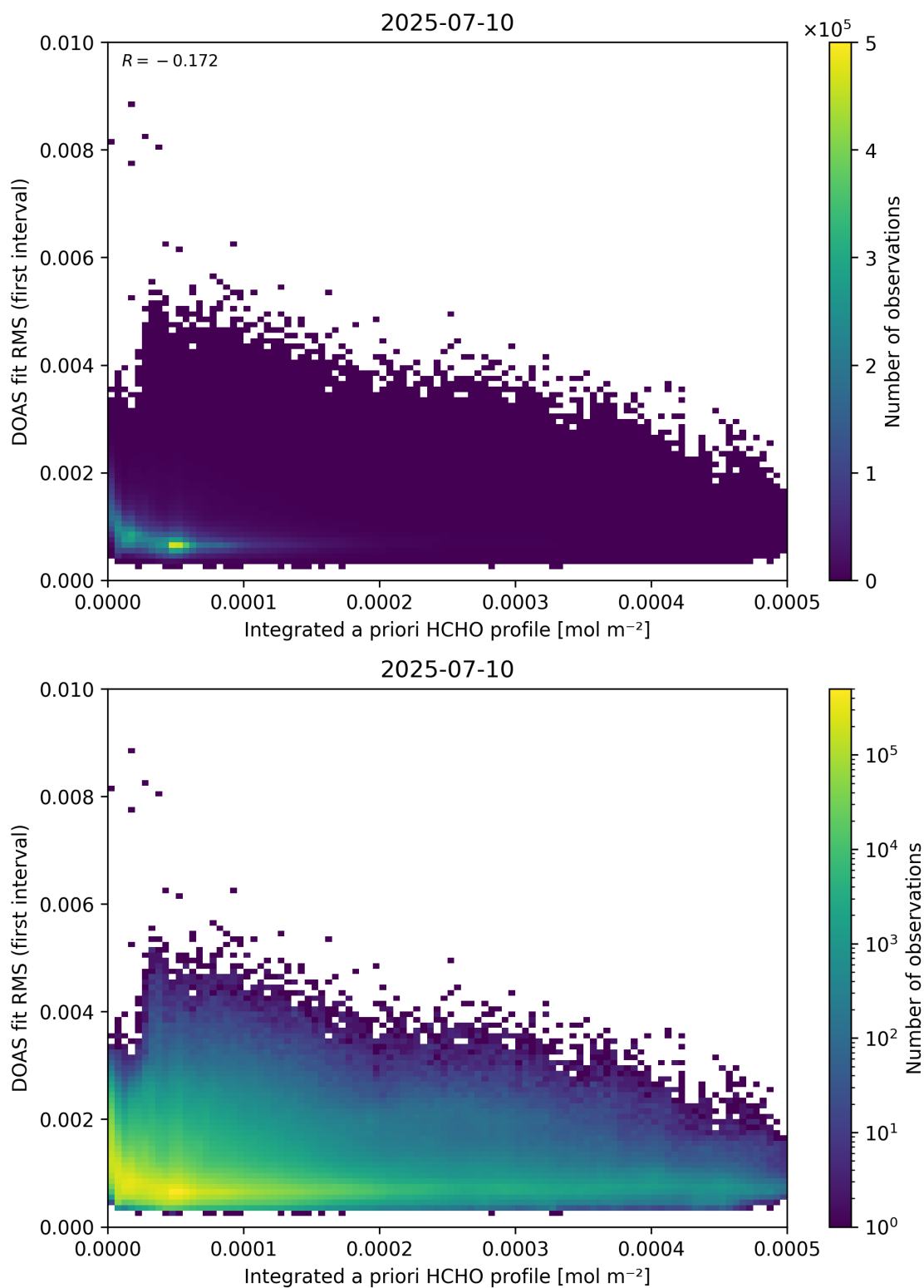
Figure 148: Scatter density plot of “Integrated a priori HCHO profile” against “DOAS fit RMS (first interval)” for 2025-07-09 to 2025-07-11.
