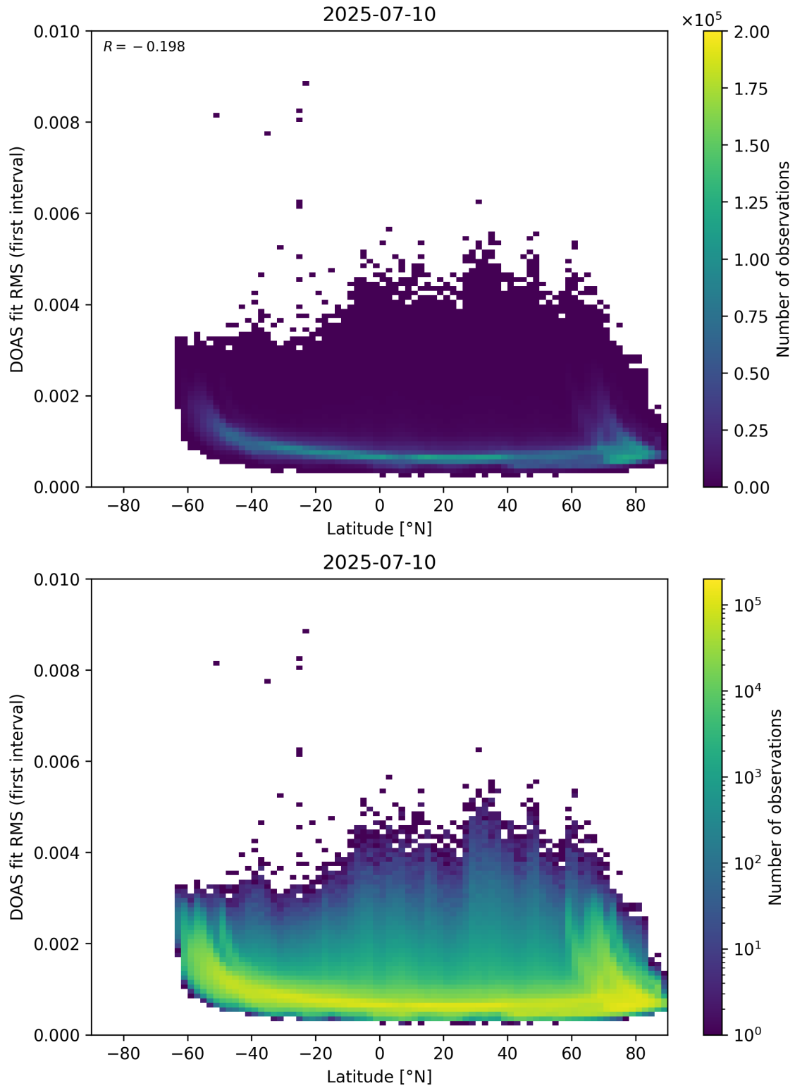
Figure 153: Scatter density plot of “Latitude” against “DOAS fit RMS (first interval)” for 2025-07-09 to 2025-07-11.
