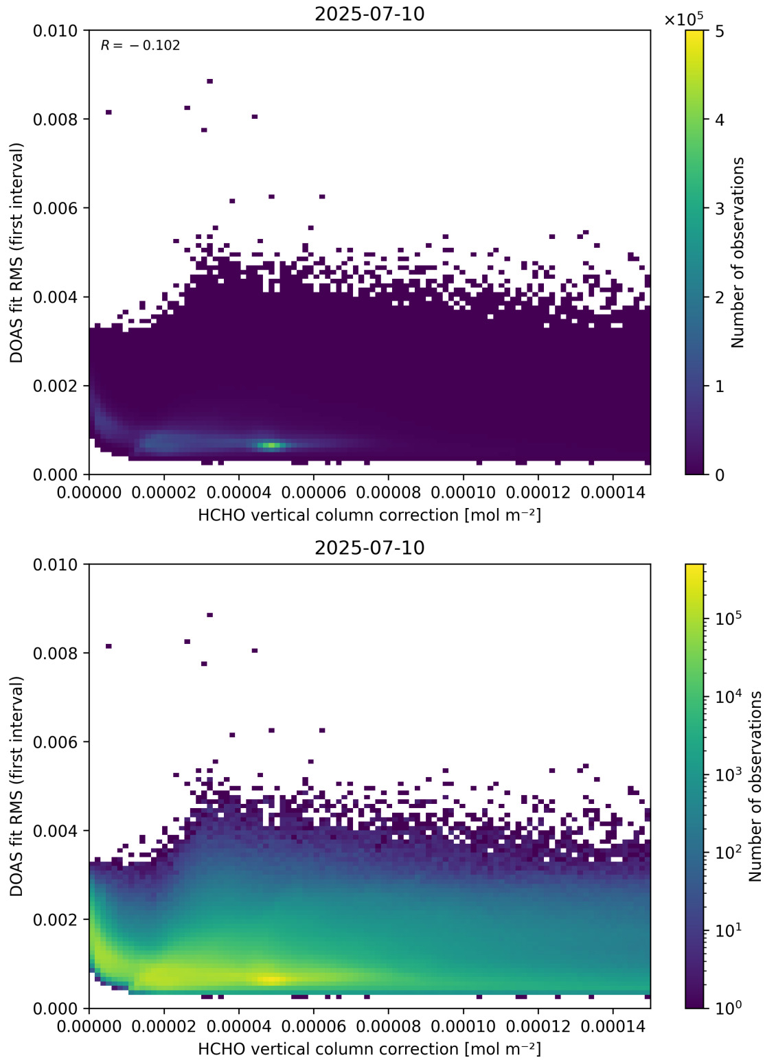
Figure 112: Scatter density plot of “HCHO vertical column correction” against “DOAS fit RMS (first interval)” for 2025-07-09 to 2025-07-11.
