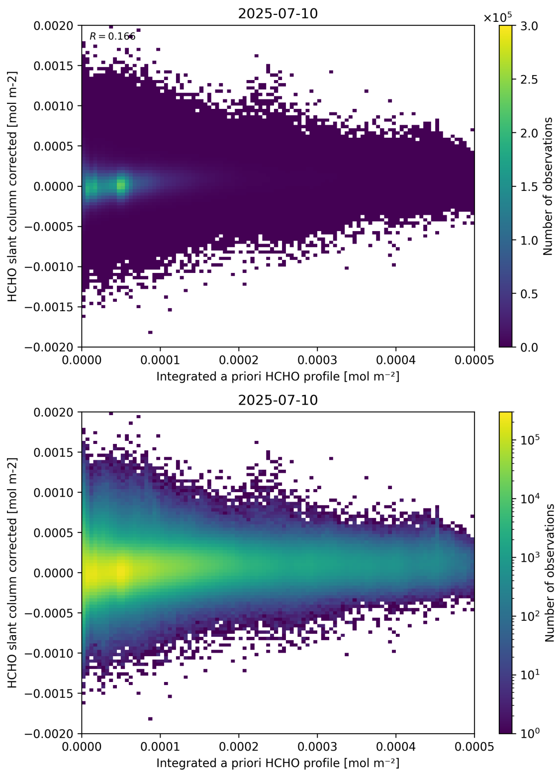
Figure 151: Scatter density plot of “Integrated a priori HCHO profile” against “HCHO slant column corrected” for 2025-07-09 to 2025-07-11.
