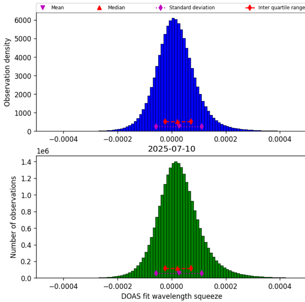
Figure 45: Histogram of “DOAS fit wavelength squeeze” for 2025-07-09 to 2025-07-11
