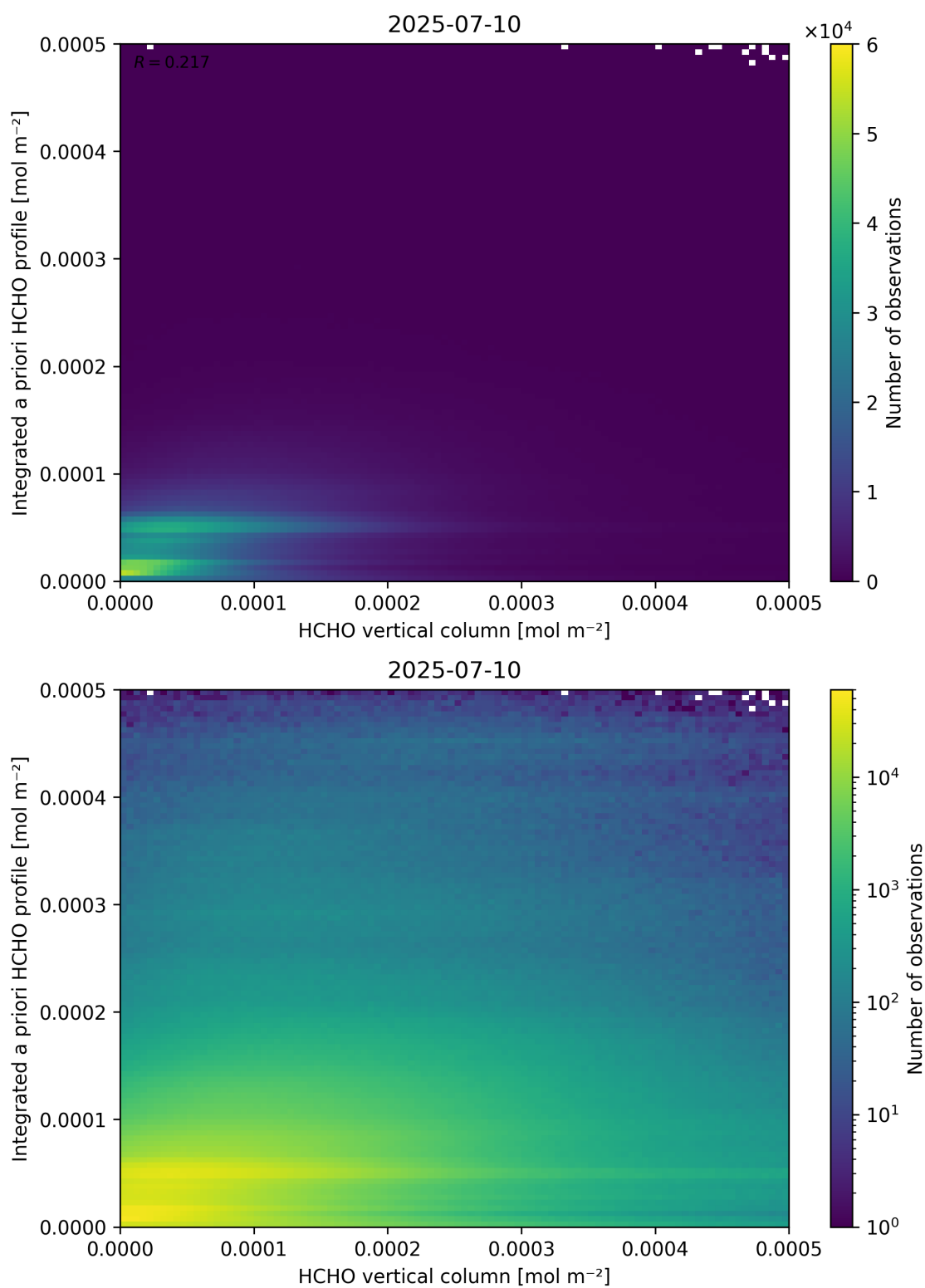
Figure 135: Scatter density plot of “HCHO vertical column” against “Integrated a priori HCHO profile” for 2025-07-09 to 2025-07-11.
