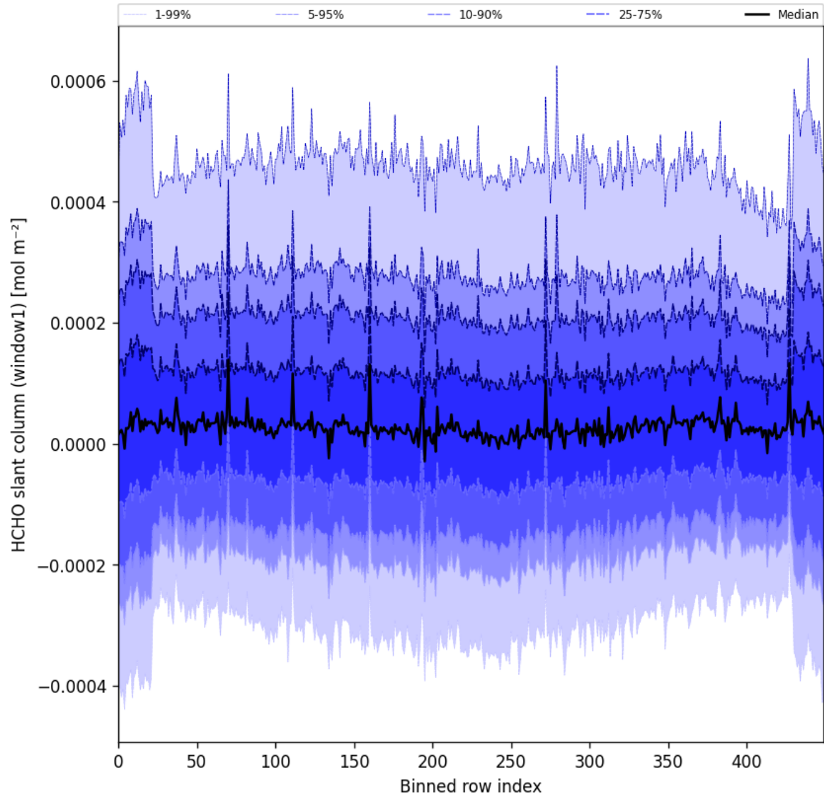
Figure 52: Along track statistics of “HCHO slant column (window1)” for 2025-07-09 to 2025-07-11
