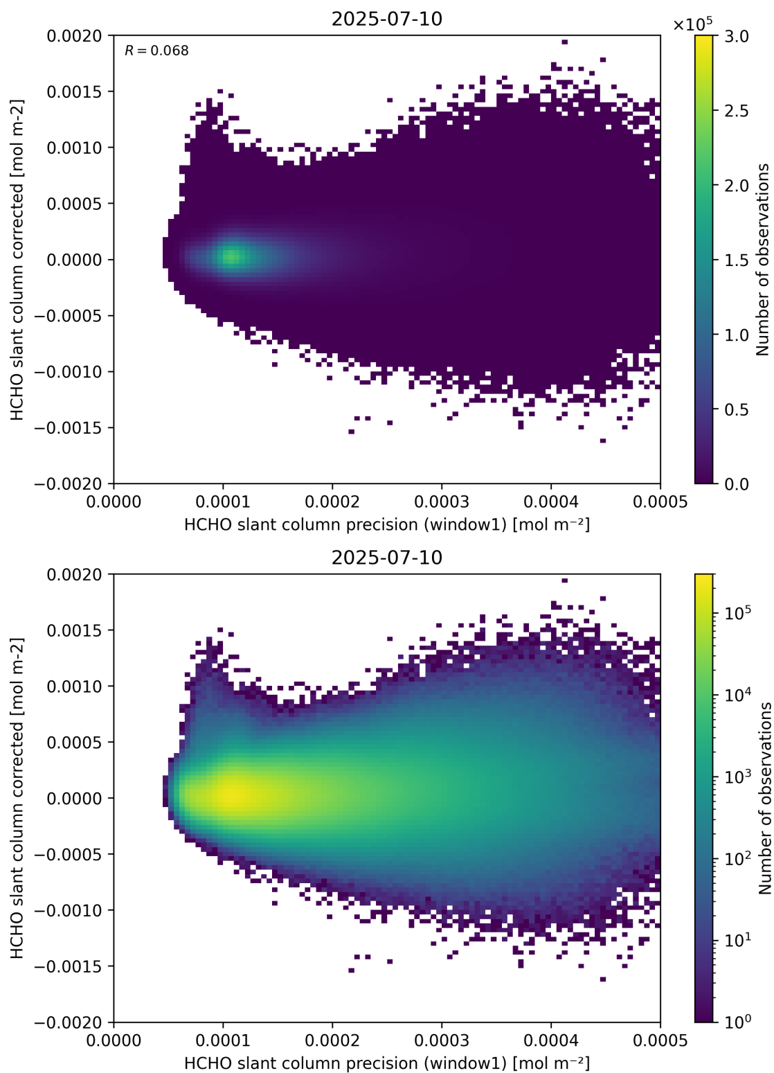
Figure 92: Scatter density plot of “HCHO slant column precision (window1)” against “HCHO slant column corrected” for 2025-07-09 to 2025-07-11.
