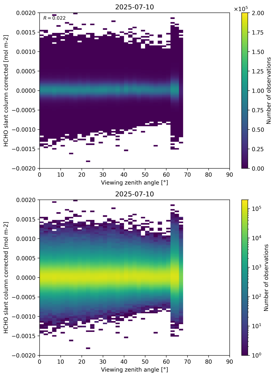
Figure 186: Scatter density plot of “Viewing zenith angle” against “HCHO slant column corrected” for 2025-07-09 to 2025-07-11.
