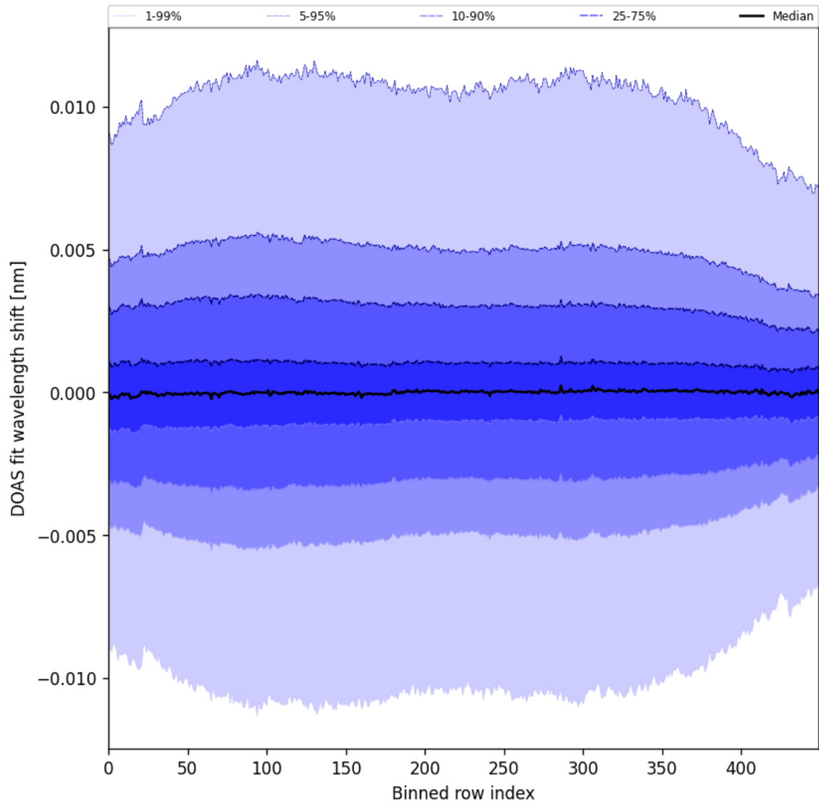
Figure 58: Along track statistics of “DOAS fit wavelength shift” for 2025-07-09 to 2025-07-11
