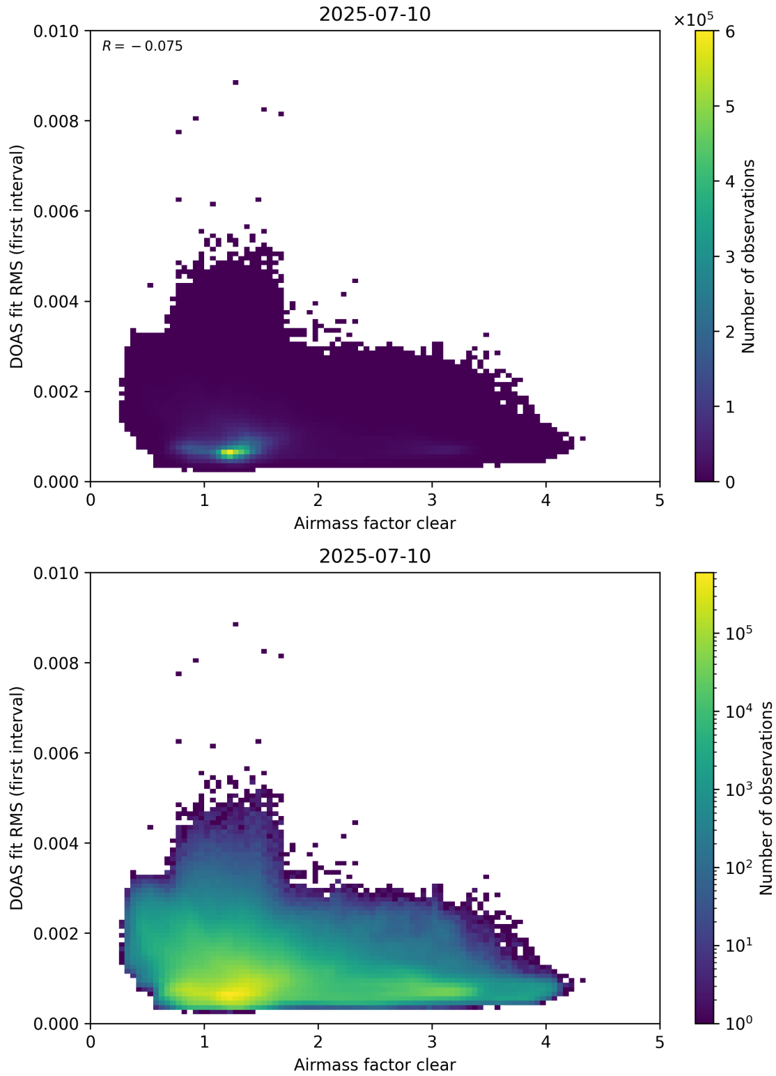
Figure 71: Scatter density plot of “Airmass factor clear” against “DOAS fit RMS (first interval)” for 2025-07-09 to 2025-07-11.
