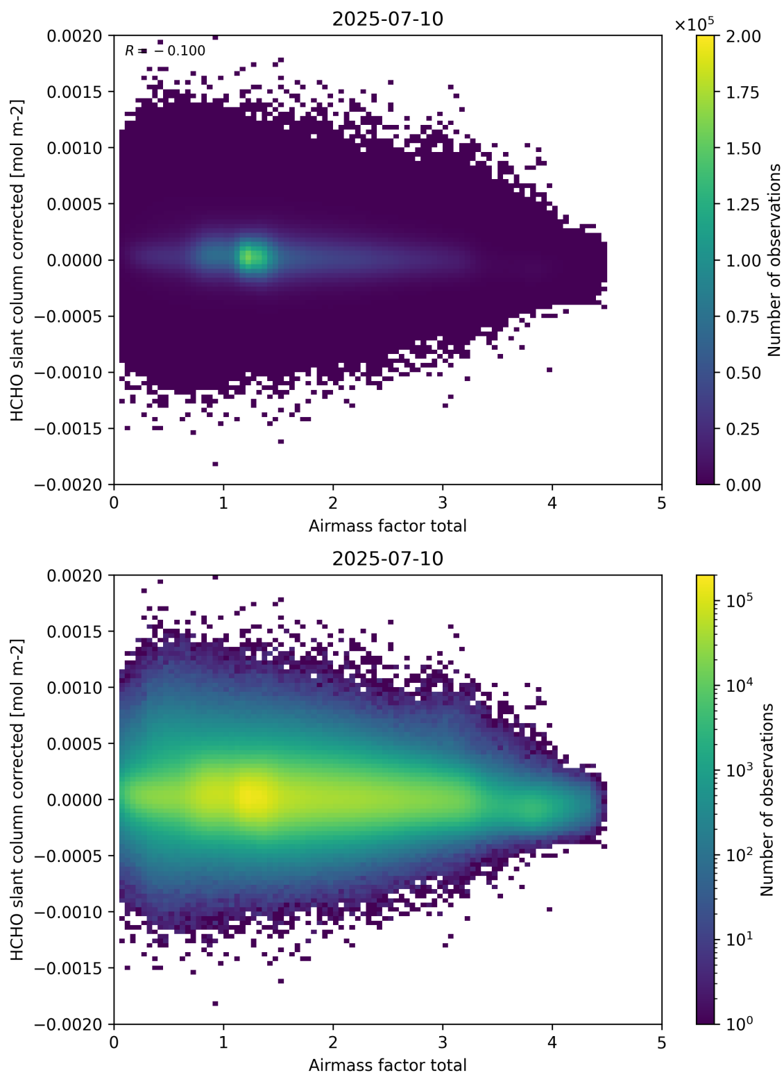
Figure 101: Scatter density plot of “Airmass factor total” against “HCHO slant column corrected” for 2025-07-09 to 2025-07-11.
