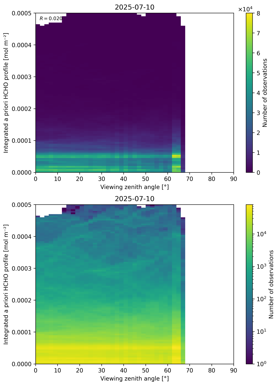
Figure 195: Scatter density plot of “Viewing zenith angle” against “Integrated a priori HCHO profile” for 2025-07-09 to 2025-07-11.
