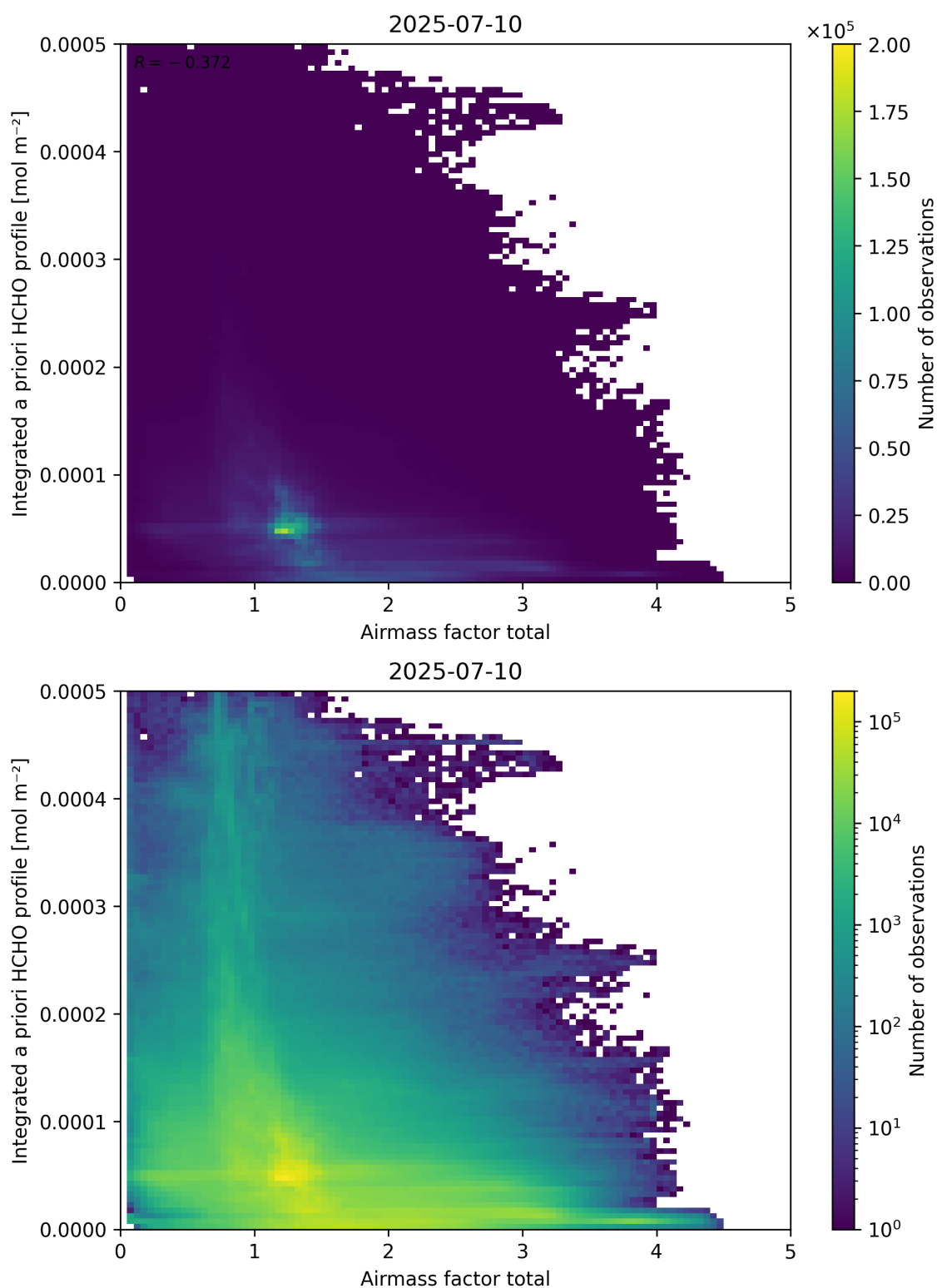
Figure 104: Scatter density plot of “Airmass factor total” against “Integrated a priori HCHO profile” for 2025-07-09 to 2025-07-11.
