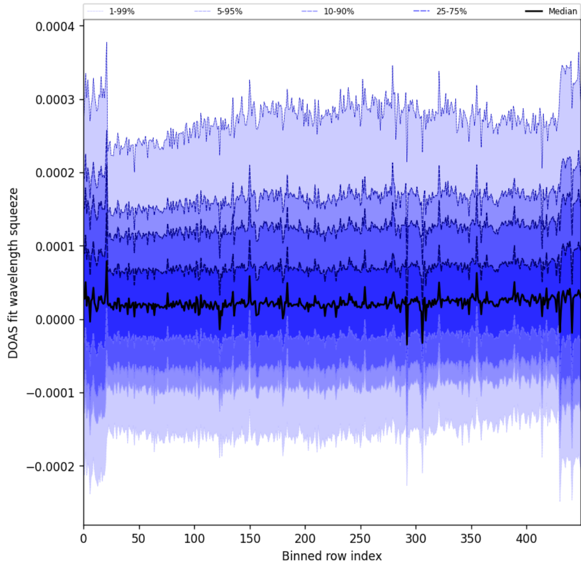
Figure 59: Along track statistics of “DOAS fit wavelength squeeze” for 2025-07-09 to 2025-07-11
