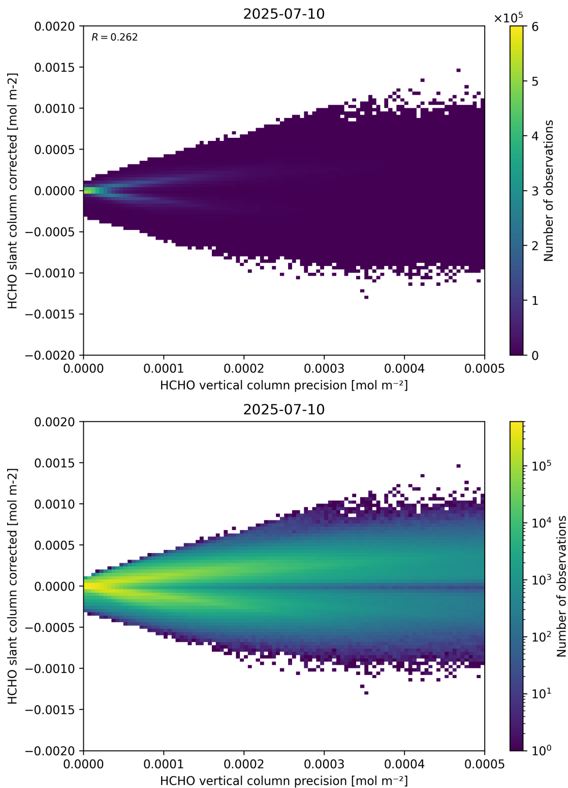
Figure 140: Scatter density plot of “HCHO vertical column precision” against “HCHO slant column corrected” for 2025-07-09 to 2025-07-11.
