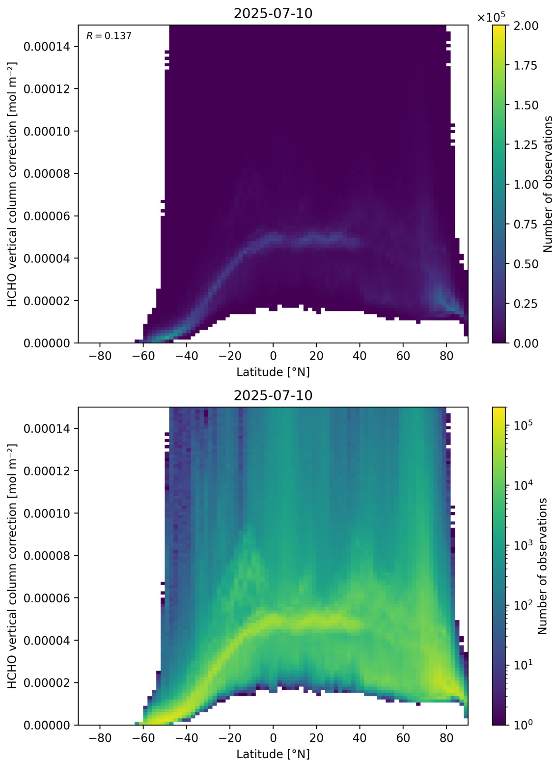
Figure 164: Scatter density plot of “Latitude” against “HCHO vertical column correction” for 2025-07-09 to 2025-07-11.
