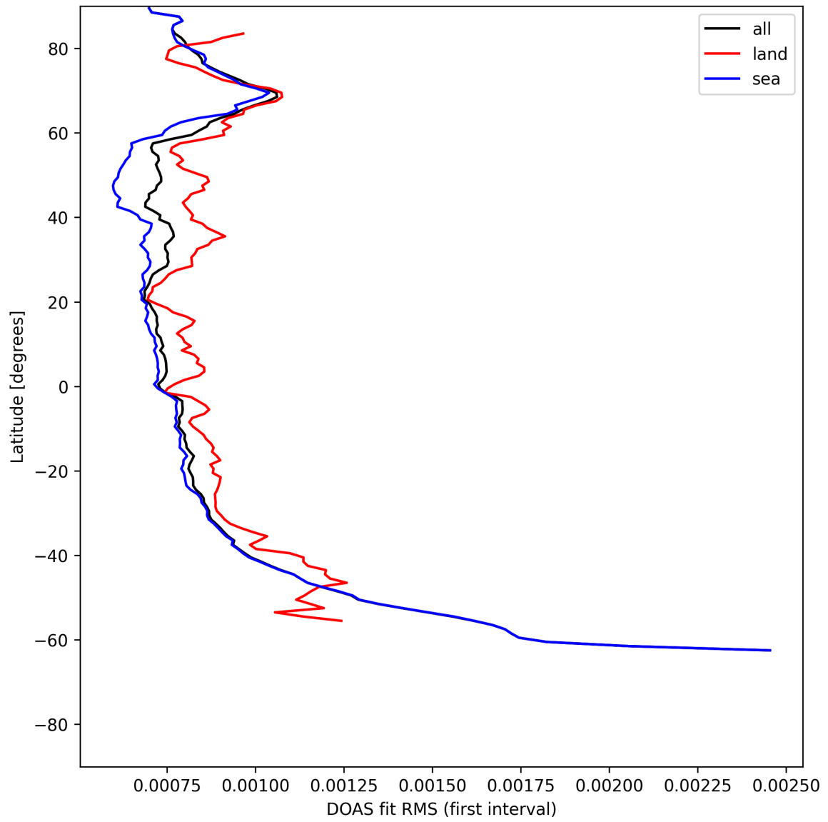
Figure 32: Zonal average of "DOAS fit RMS (first interval)" for 2025-07-09 to 2025-07-11.
