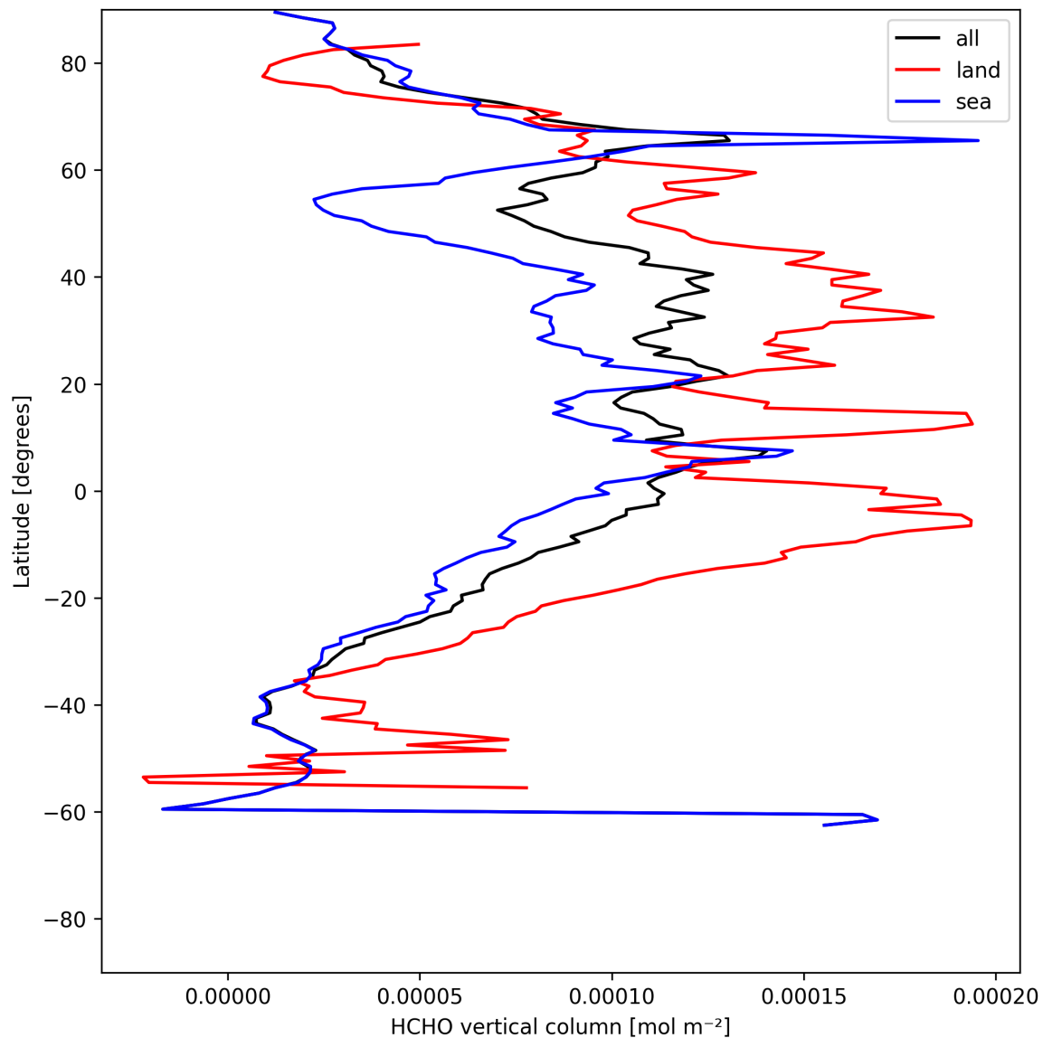
Figure 21: Zonal average of “HCHO vertical column” for 2025-07-09 to 2025-07-11.
