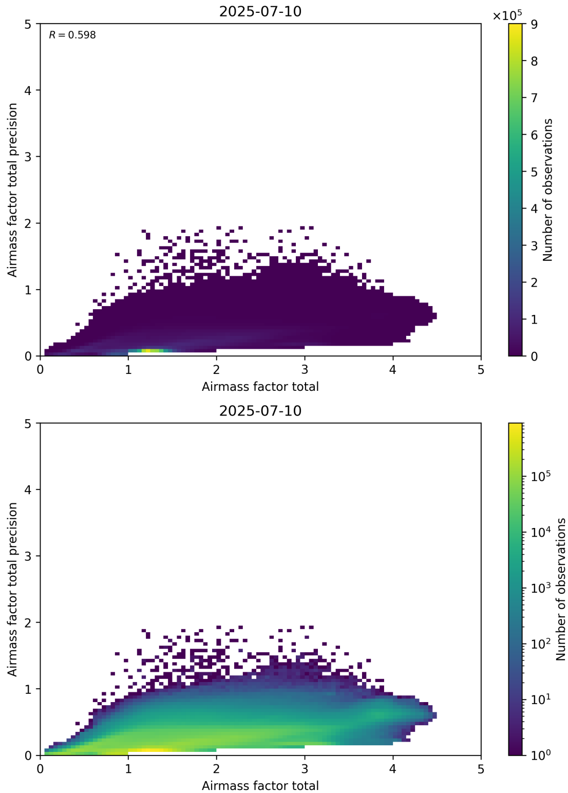
Figure 103: Scatter density plot of “Airmass factor total” against “Airmass factor total precision” for 2025-07-09 to 2025-07-11.
