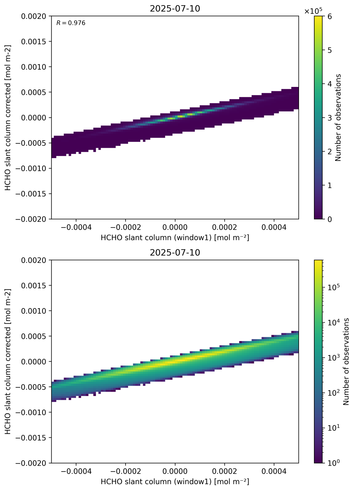
Figure 82: Scatter density plot of “HCHO slant column (window1)” against “HCHO slant column corrected” for 2025-07-09 to 2025-07-11.
