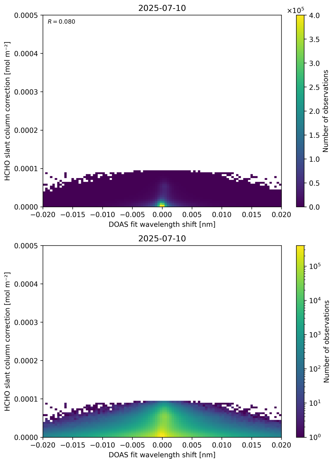
Figure 67: Scatter density plot of “DOAS fit wavelength shift” against “HCHO slant column correction” for 2025-07-09 to 2025-07-11.
