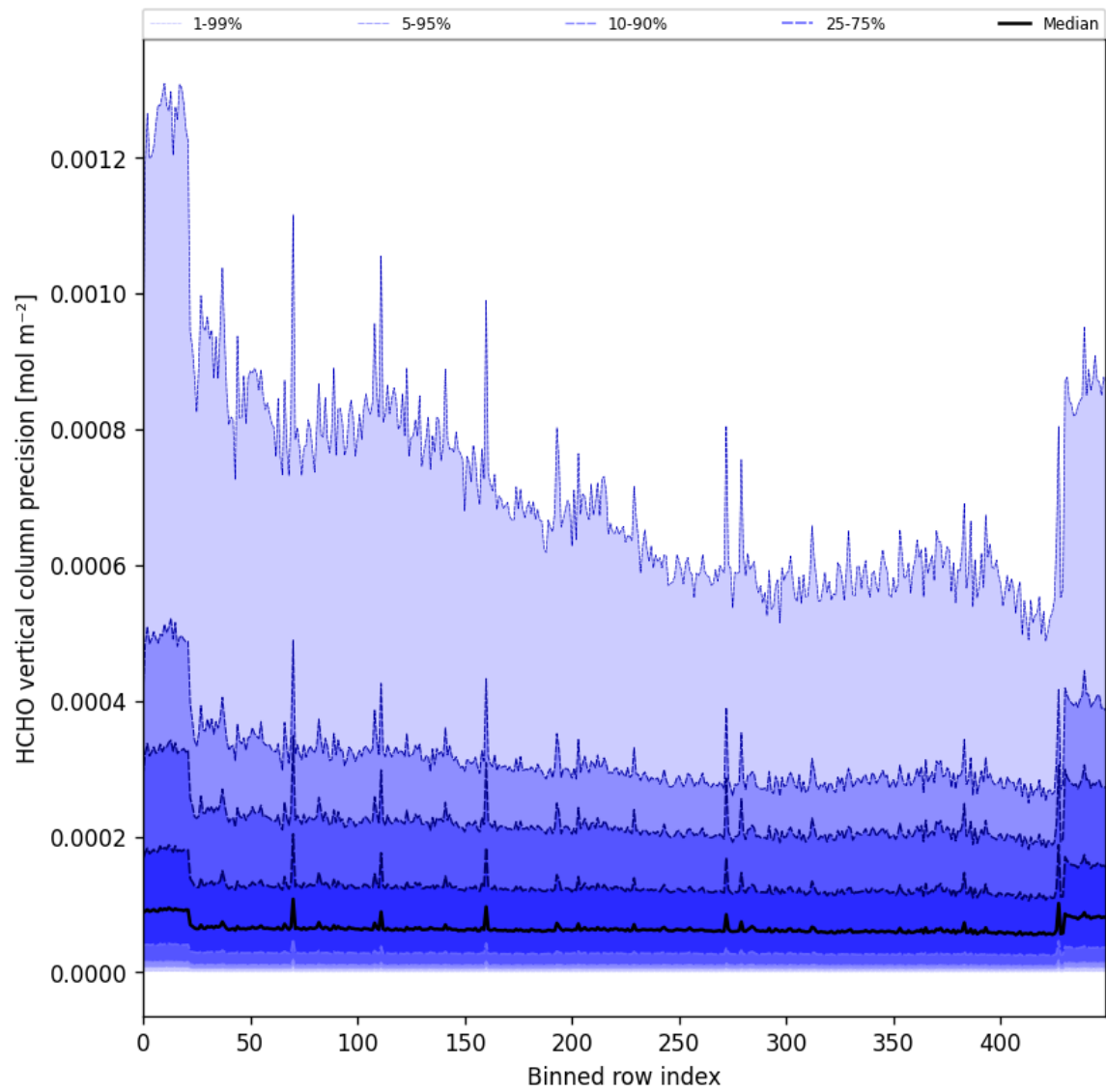
Figure 50: Along track statistics of “HCHO vertical column precision” for 2025-07-09 to 2025-07-11
