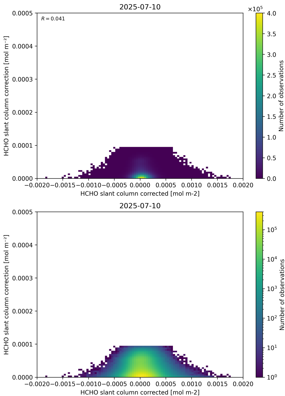
Figure 77: Scatter density plot of “HCHO slant column corrected” against “HCHO slant column correction” for 2025-07-09 to 2025-07-11.
