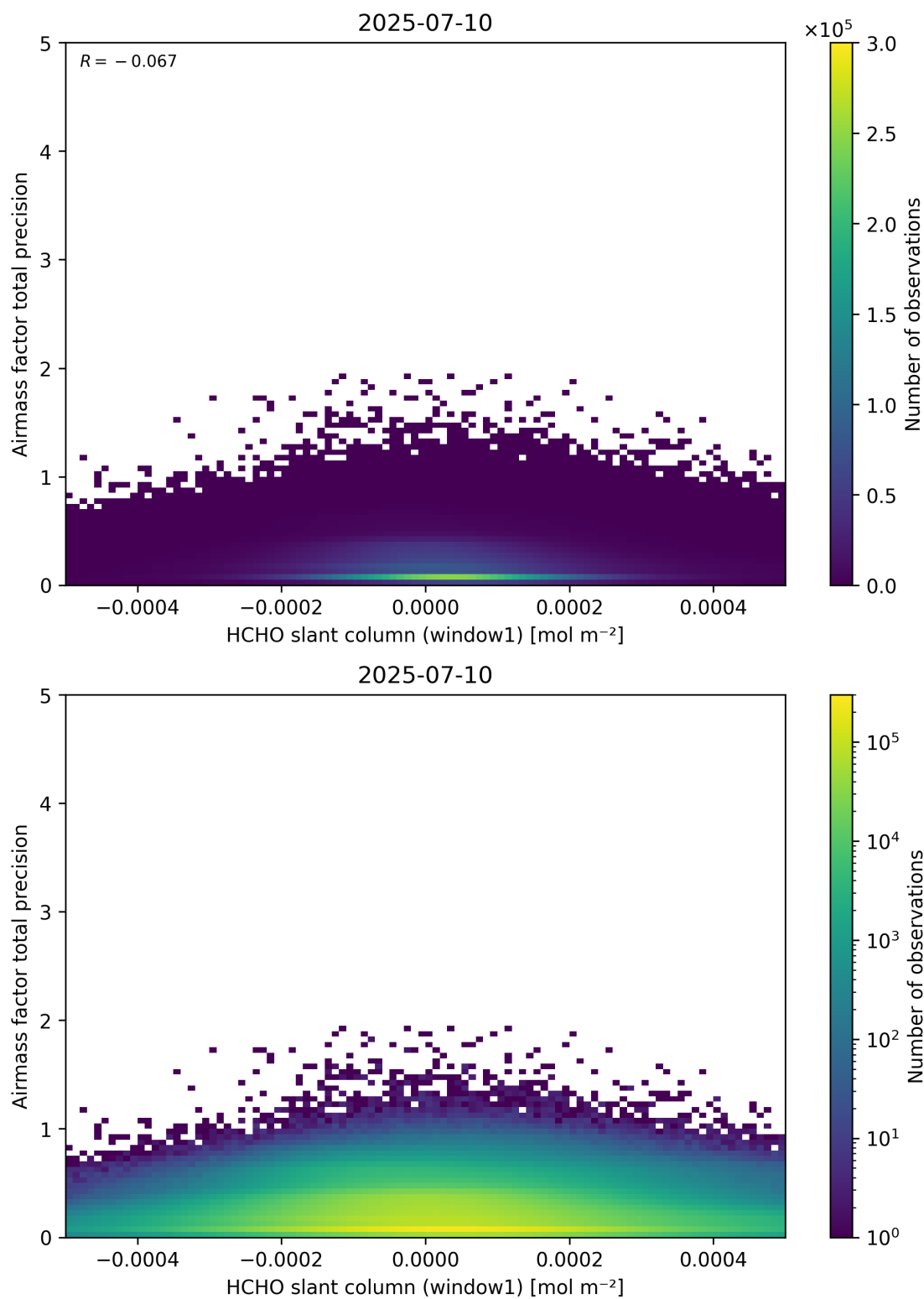
Figure 86: Scatter density plot of “HCHO slant column (window1)” against “Airmass factor total precision” for 2025-07-09 to 2025-07-11.
