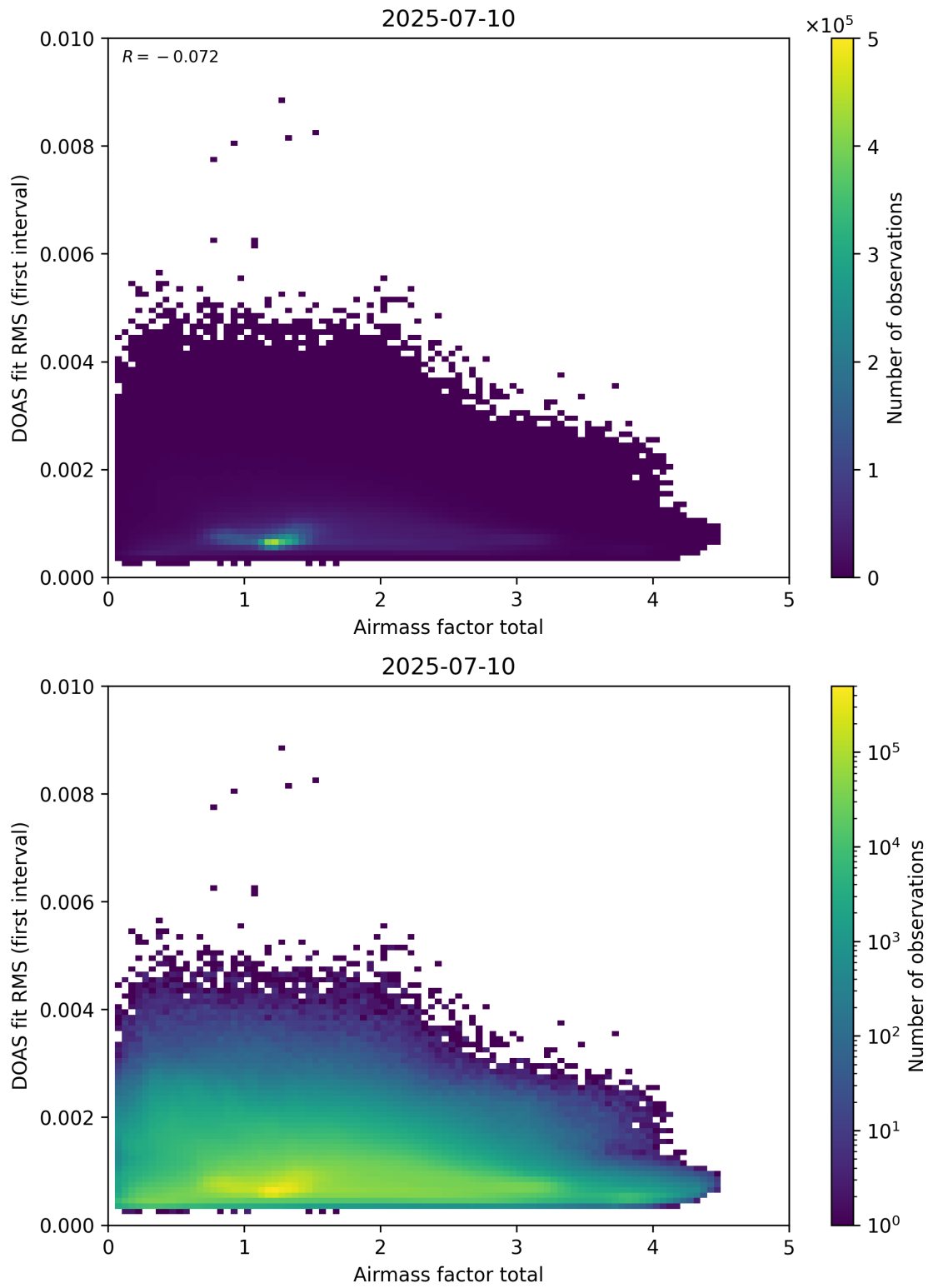
Figure 97: Scatter density plot of “Airmass factor total” against “DOAS fit RMS (first interval)” for 2025-07-09 to 2025-07-11.
