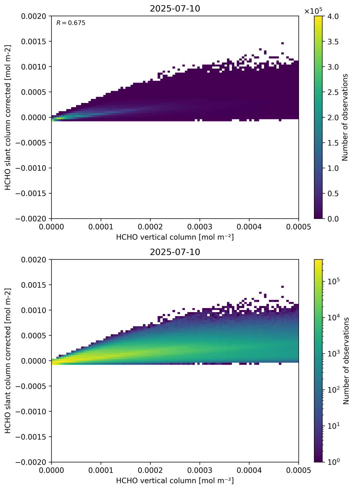
Figure 127: Scatter density plot of “HCHO vertical column” against “HCHO slant column corrected” for 2025-07-09 to 2025-07-11.
