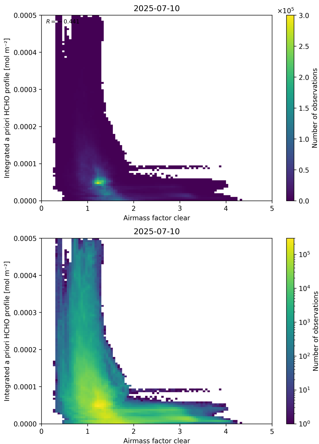
Figure 76: Scatter density plot of “Airmass factor clear” against “Integrated a priori HCHO profile” for 2025-07-09 to 2025-07-11.
