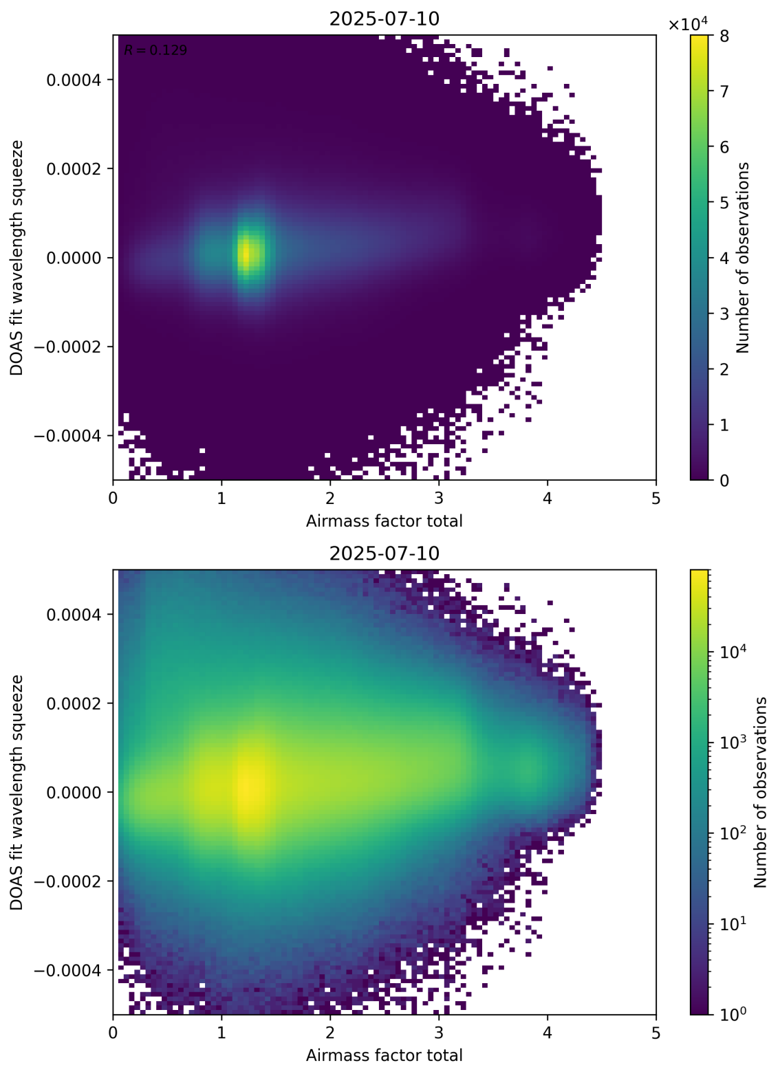
Figure 99: Scatter density plot of “Airmass factor total” against “DOAS fit wavelength squeeze” for 2025-07-09 to 2025-07-11.
