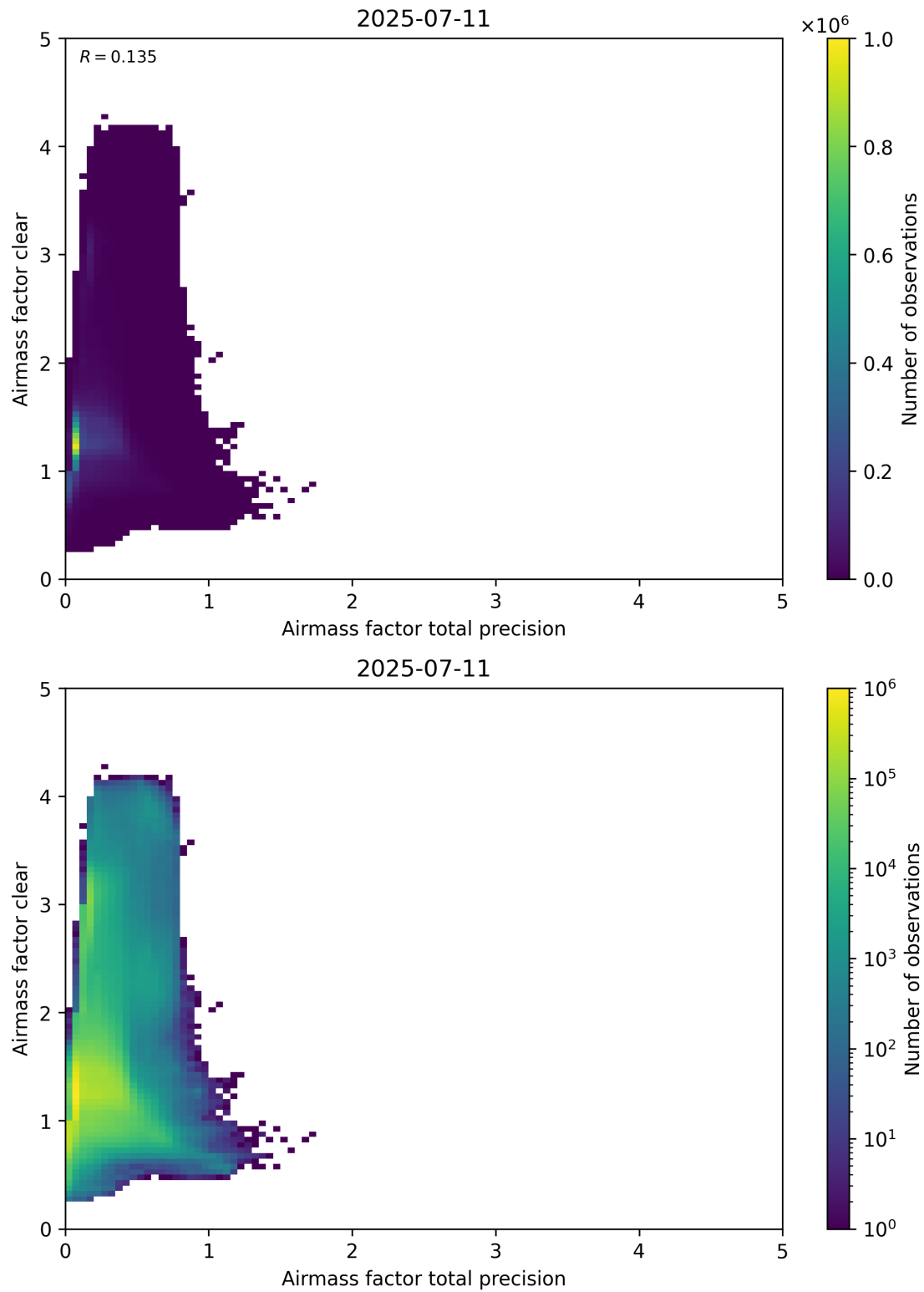
Figure 108: Scatter density plot of “Airmass factor total precision” against “Airmass factor clear” for 2025-07-10 to 2025-07-12.
