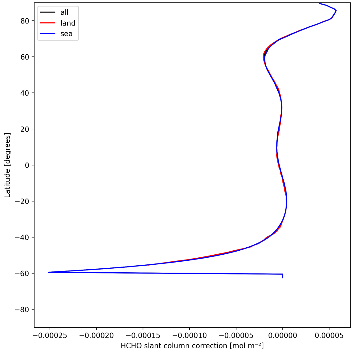
Figure 33: Zonal average of “HCHO slant column correction” for 2025-07-10 to 2025-07-12.
