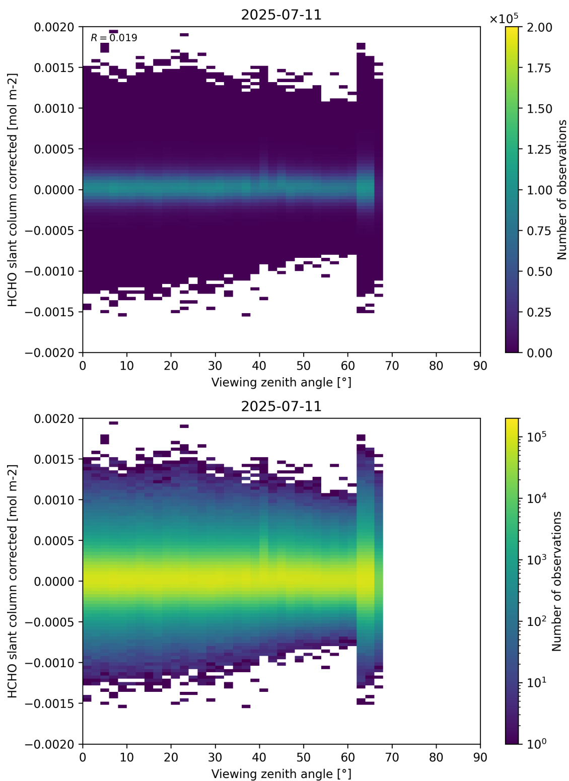
Figure 186: Scatter density plot of “Viewing zenith angle” against “HCHO slant column corrected” for 2025-07-10 to 2025-07-12.
