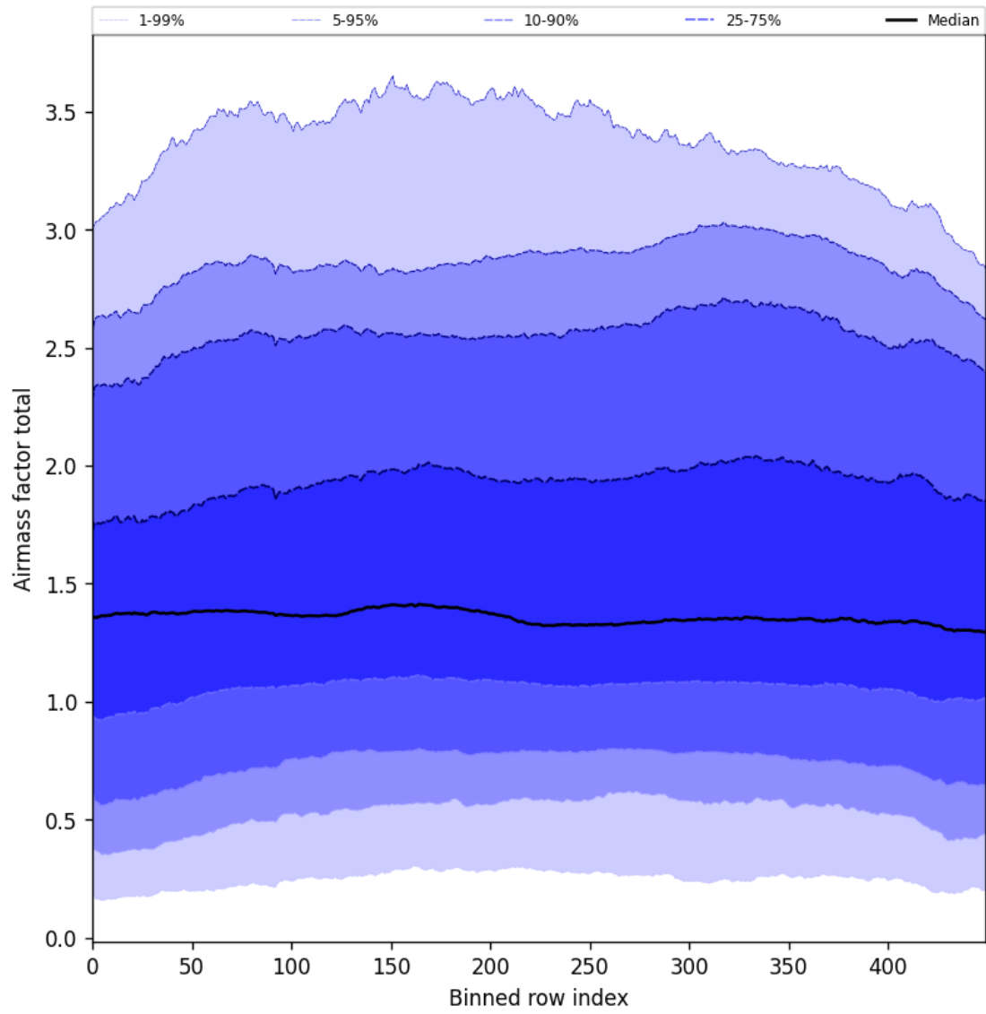
Figure 54: Along track statistics of “Airmass factor total” for 2025-07-10 to 2025-07-12
