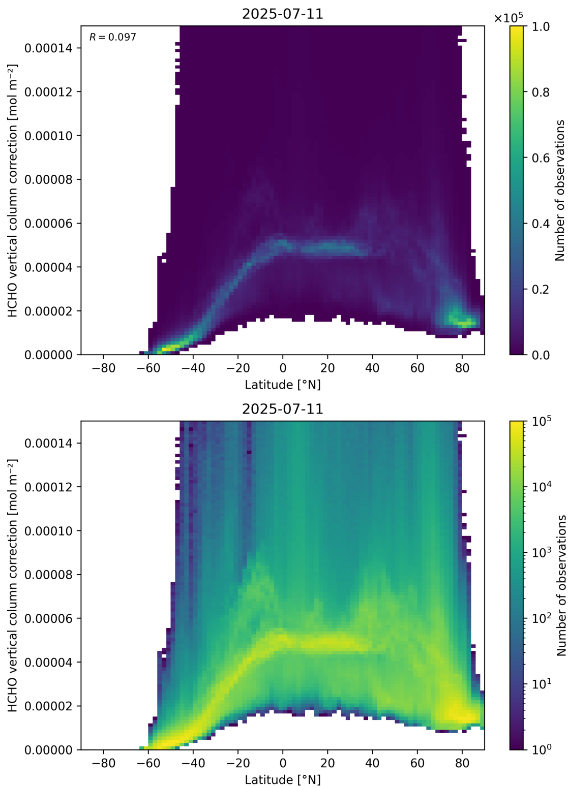
Figure 164: Scatter density plot of “Latitude” against “HCHO vertical column correction” for 2025-07-10 to 2025-07-12.
