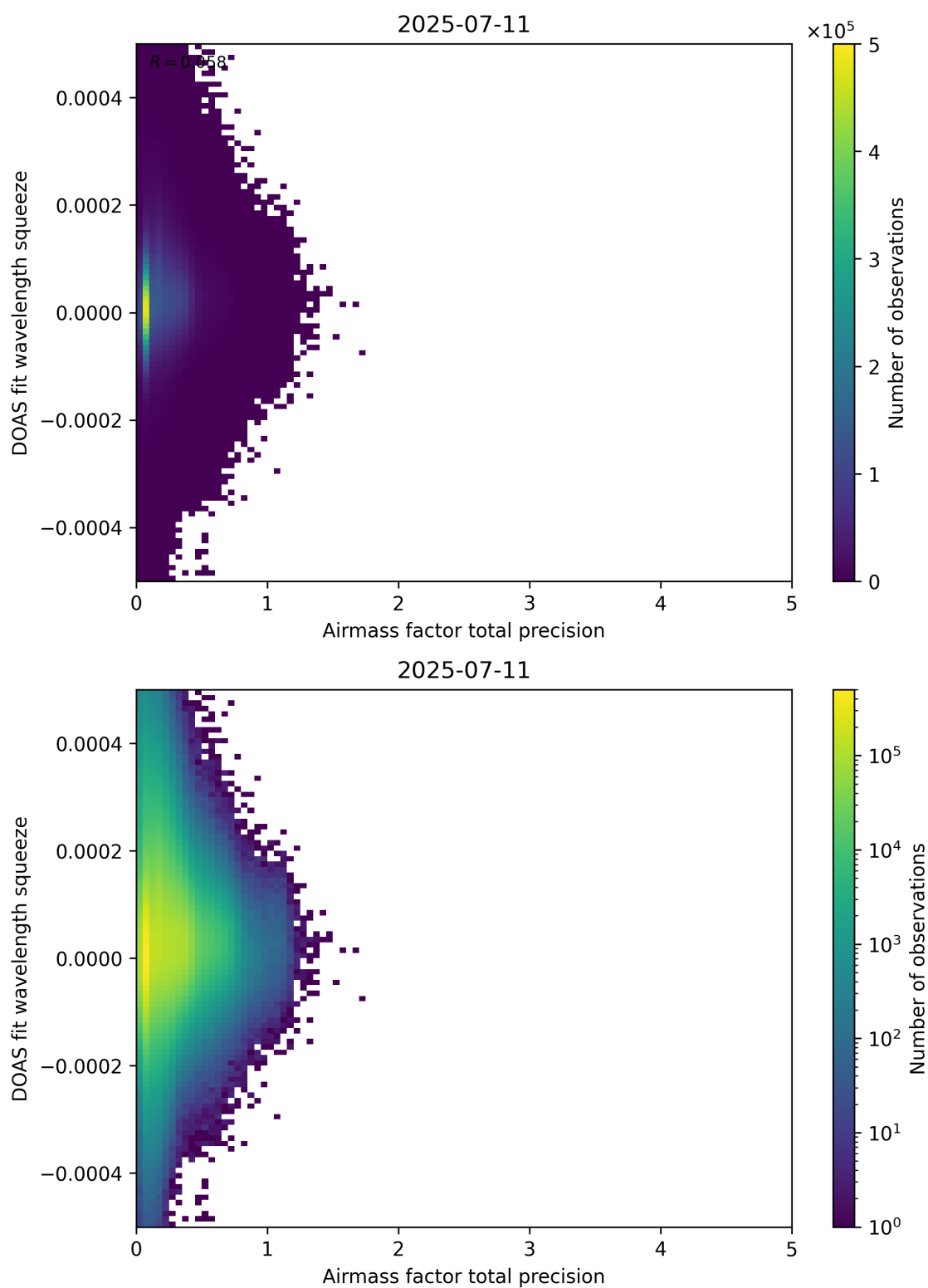
Figure 107: Scatter density plot of “Airmass factor total precision” against “DOAS fit wavelength squeeze” for 2025-07-10 to 2025-07-12.
