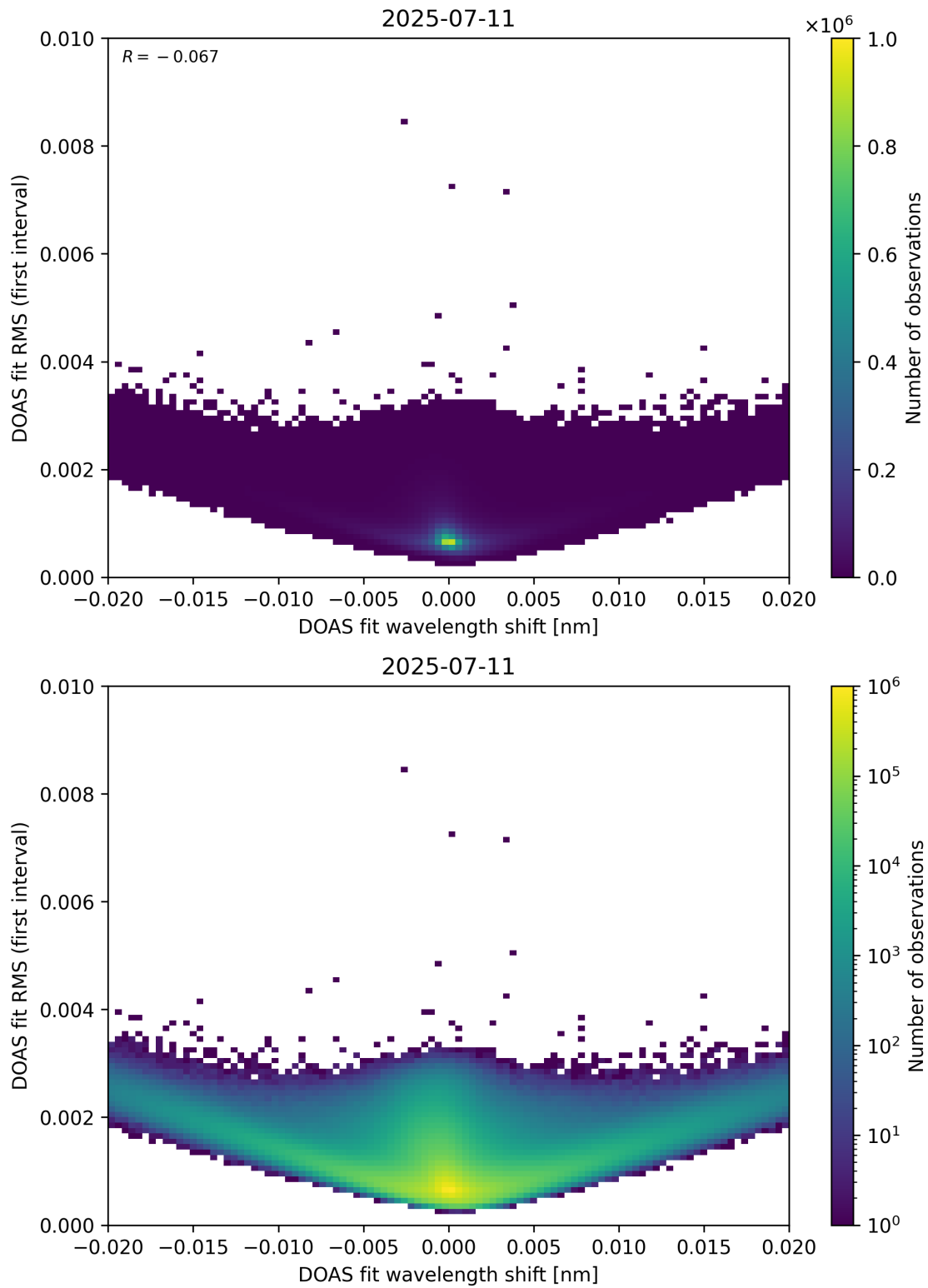
Figure 64: Scatter density plot of “DOAS fit wavelength shift” against “DOAS fit RMS (first interval)” for 2025-07-10 to 2025-07-12.
