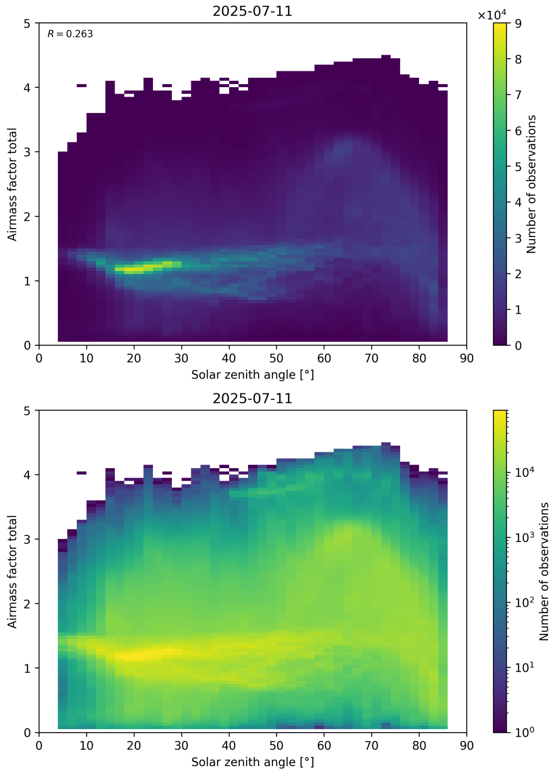
Figure 175: Scatter density plot of “Solar zenith angle” against “Airmass factor total” for 2025-07-10 to 2025-07-12.
