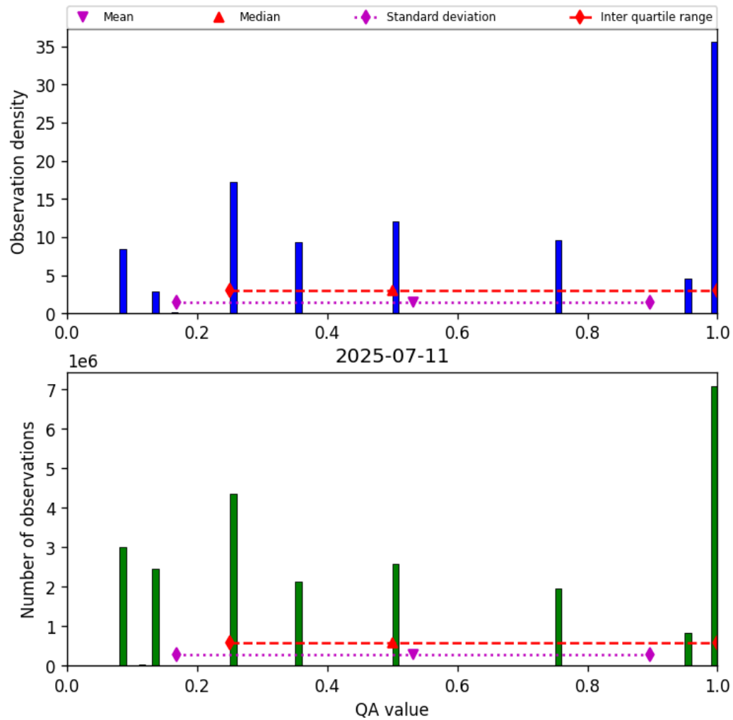
Figure 34: Histogram of “QA value” for 2025-07-10 to 2025-07-12
