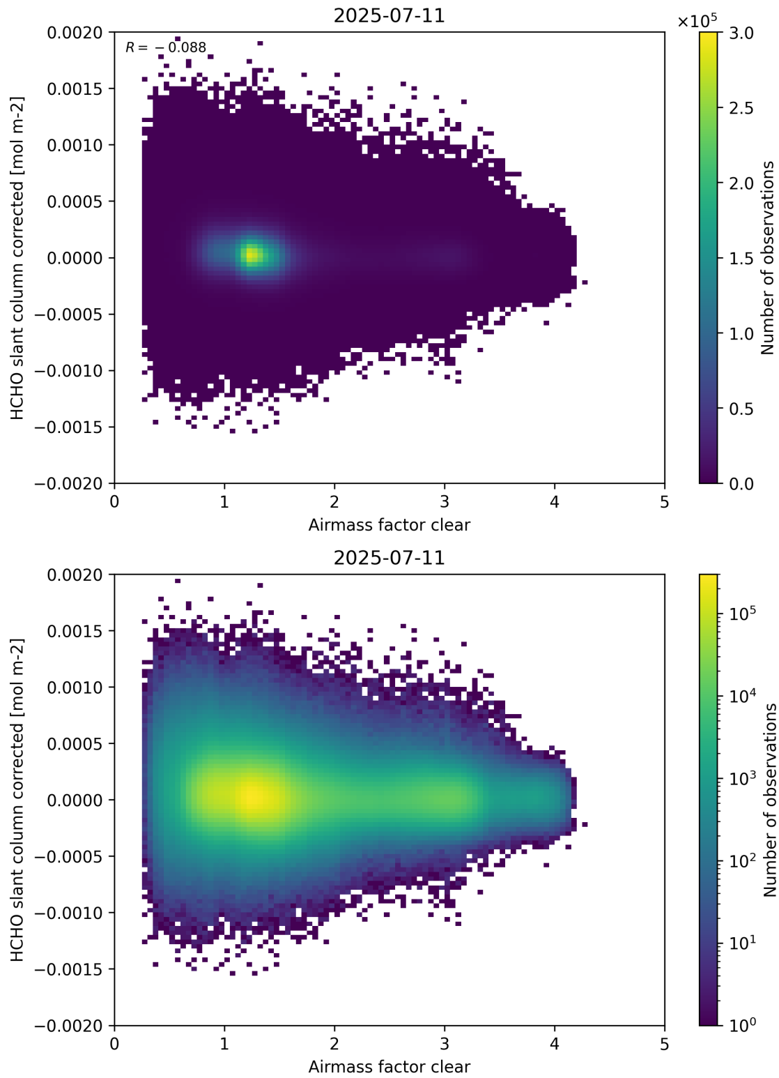
Figure 74: Scatter density plot of “Airmass factor clear” against “HCHO slant column corrected” for 2025-07-10 to 2025-07-12.
