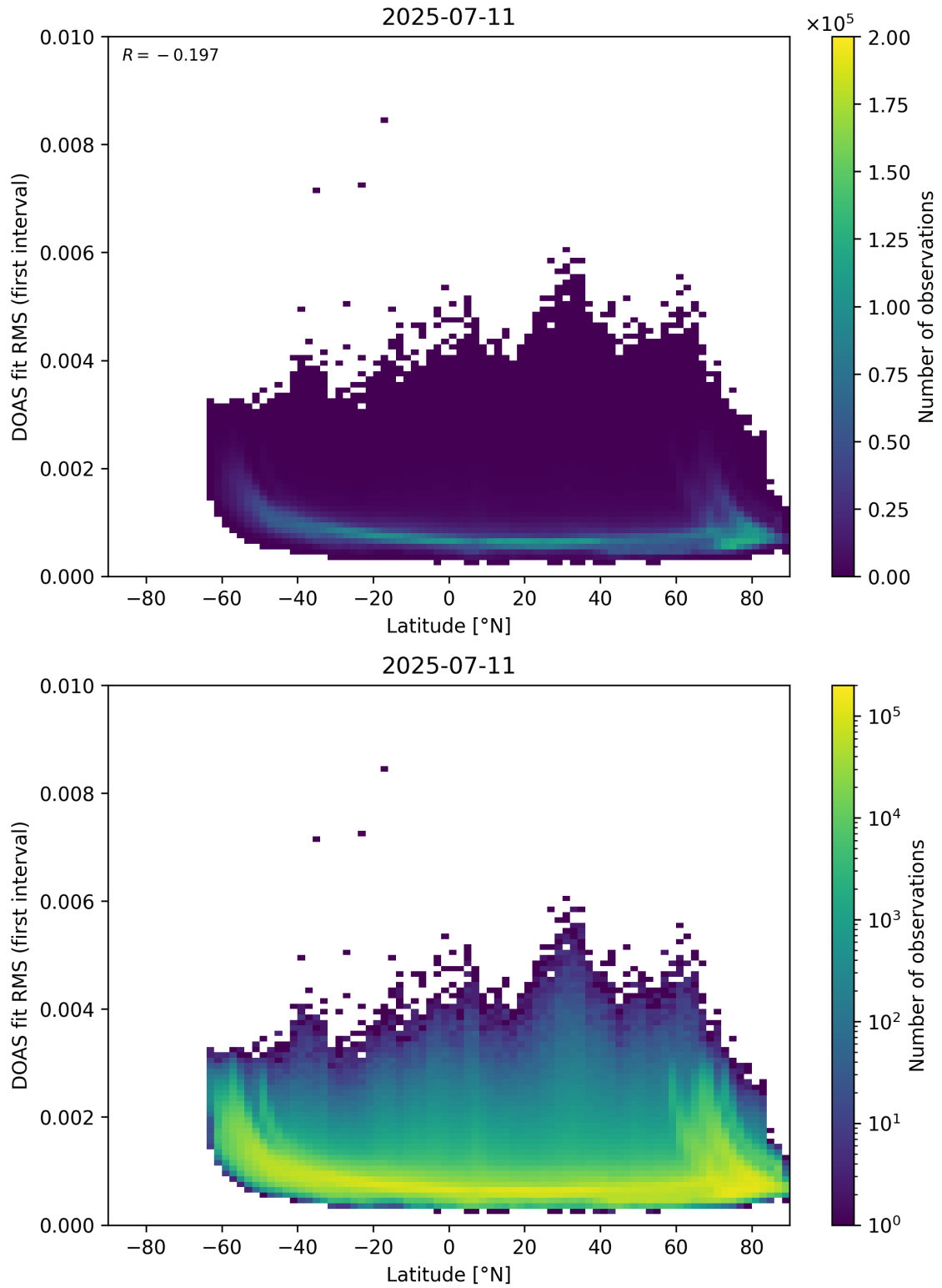
Figure 153: Scatter density plot of “Latitude” against “DOAS fit RMS (first interval)” for 2025-07-10 to 2025-07-12.
