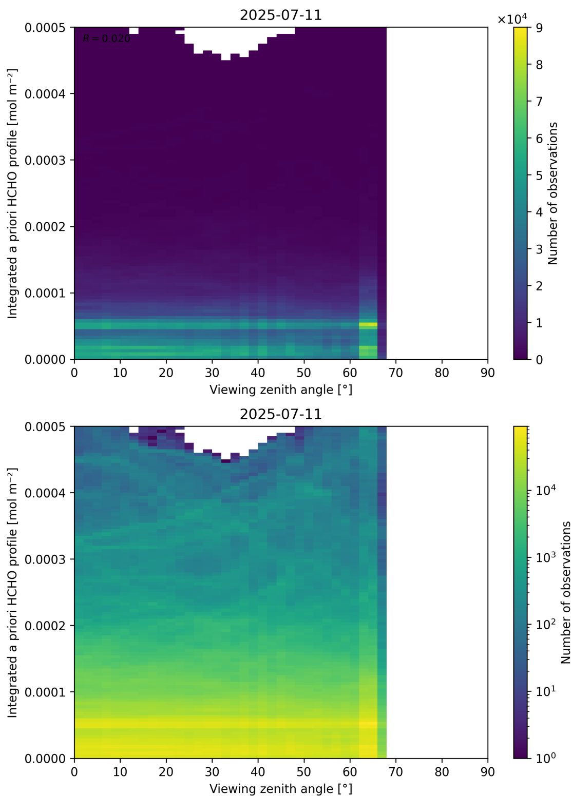
Figure 195: Scatter density plot of “Viewing zenith angle” against “Integrated a priori HCHO profile” for 2025-07-10 to 2025-07-12.
