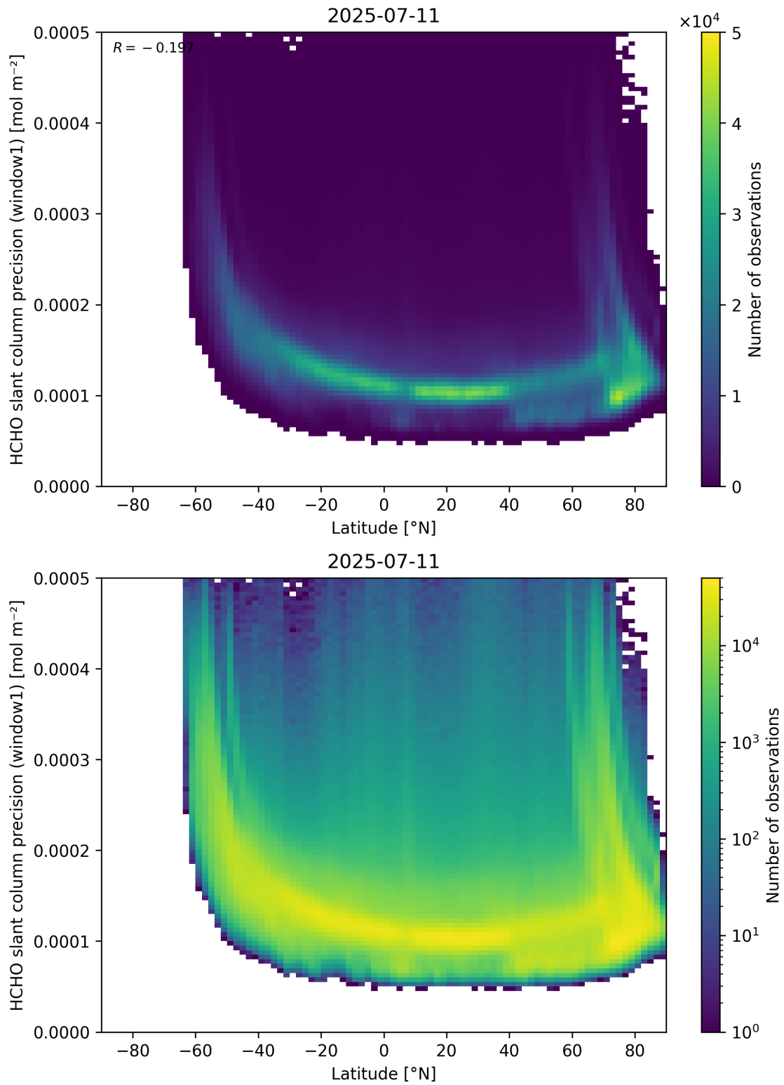
Figure 160: Scatter density plot of “Latitude” against “HCHO slant column precision (window1)” for 2025-07-10 to 2025-07-12.
