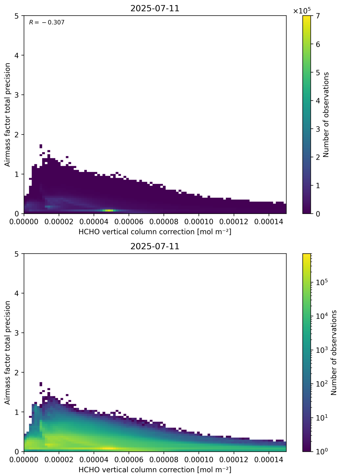
Figure 121: Scatter density plot of “HCHO vertical column correction” against “Airmass factor total precision” for 2025-07-10 to 2025-07-12.
