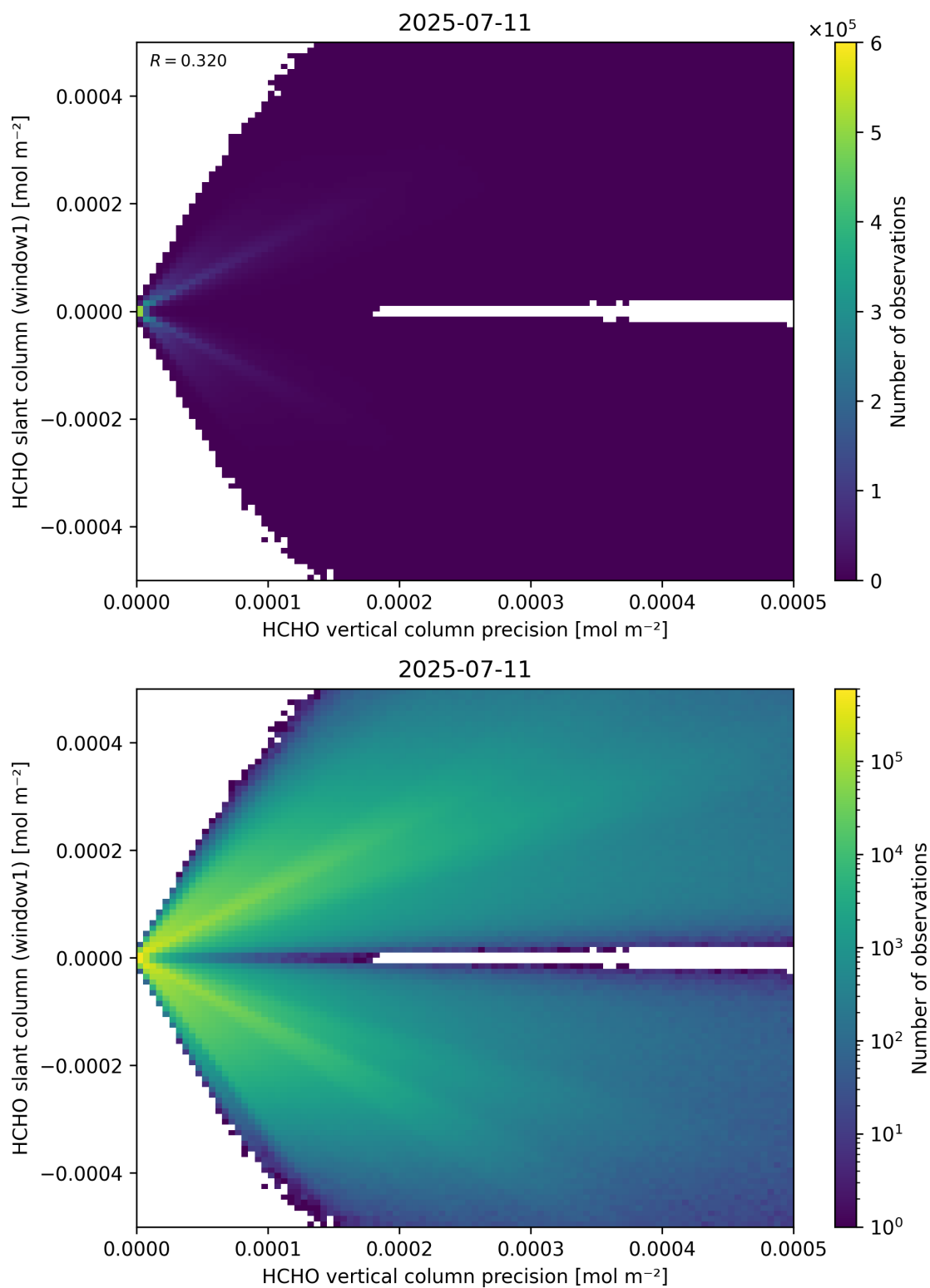
Figure 142: Scatter density plot of “HCHO vertical column precision” against “HCHO slant column (window1)” for 2025-07-10 to 2025-07-12.
