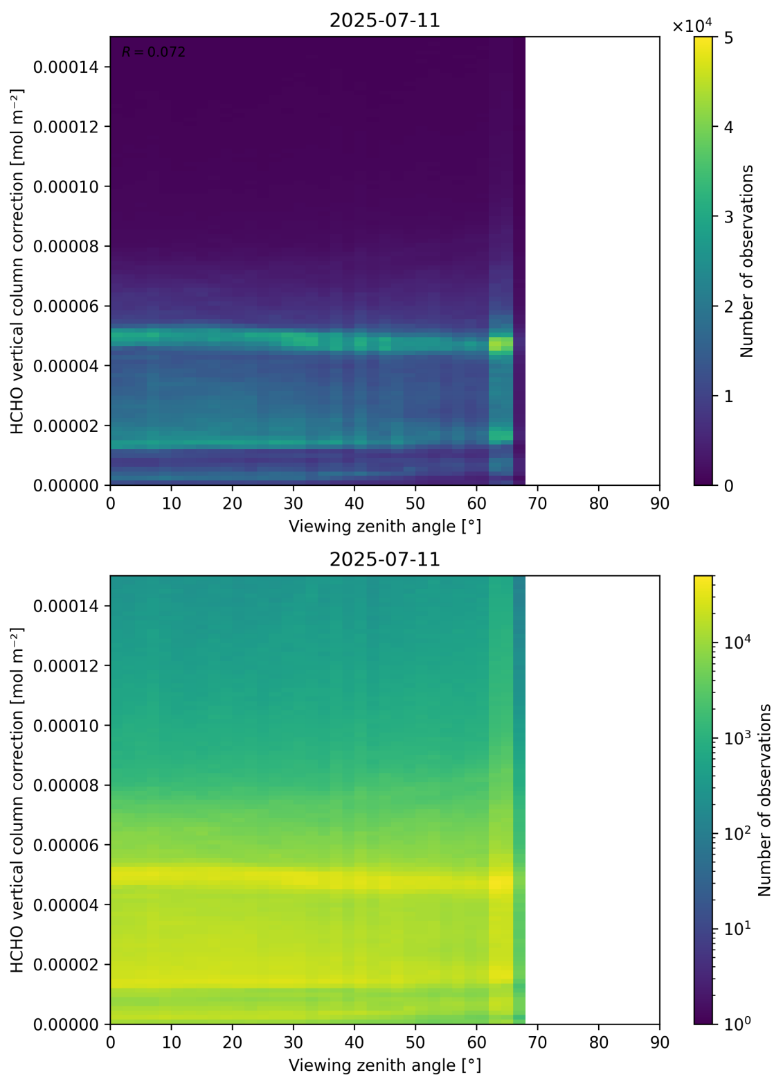
Figure 193: Scatter density plot of “Viewing zenith angle” against “HCHO vertical column correction” for 2025-07-10 to 2025-07-12.
