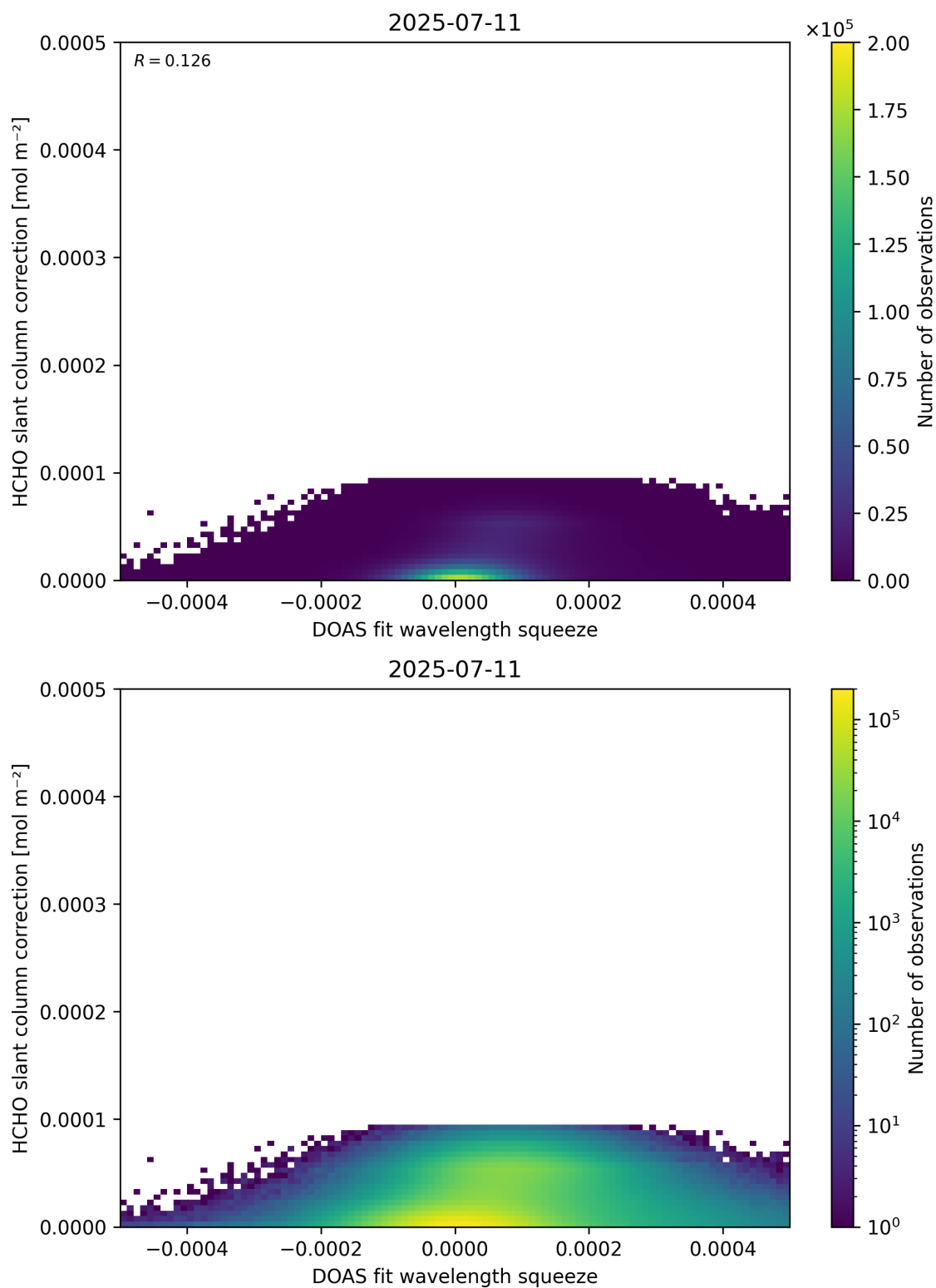
Figure 70: Scatter density plot of “DOAS fit wavelength squeeze” against “HCHO slant column correction” for 2025-07-10 to 2025-07-12.
