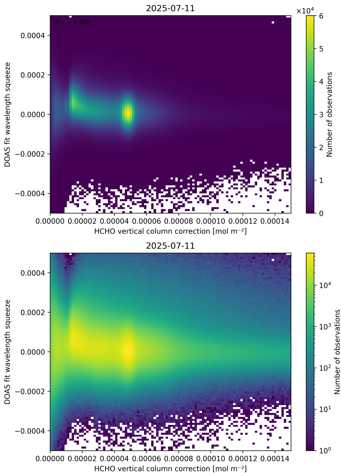
Figure 114: Scatter density plot of “HCHO vertical column correction” against “DOAS fit wavelength squeeze” for 2025-07-10 to 2025-07-12.
