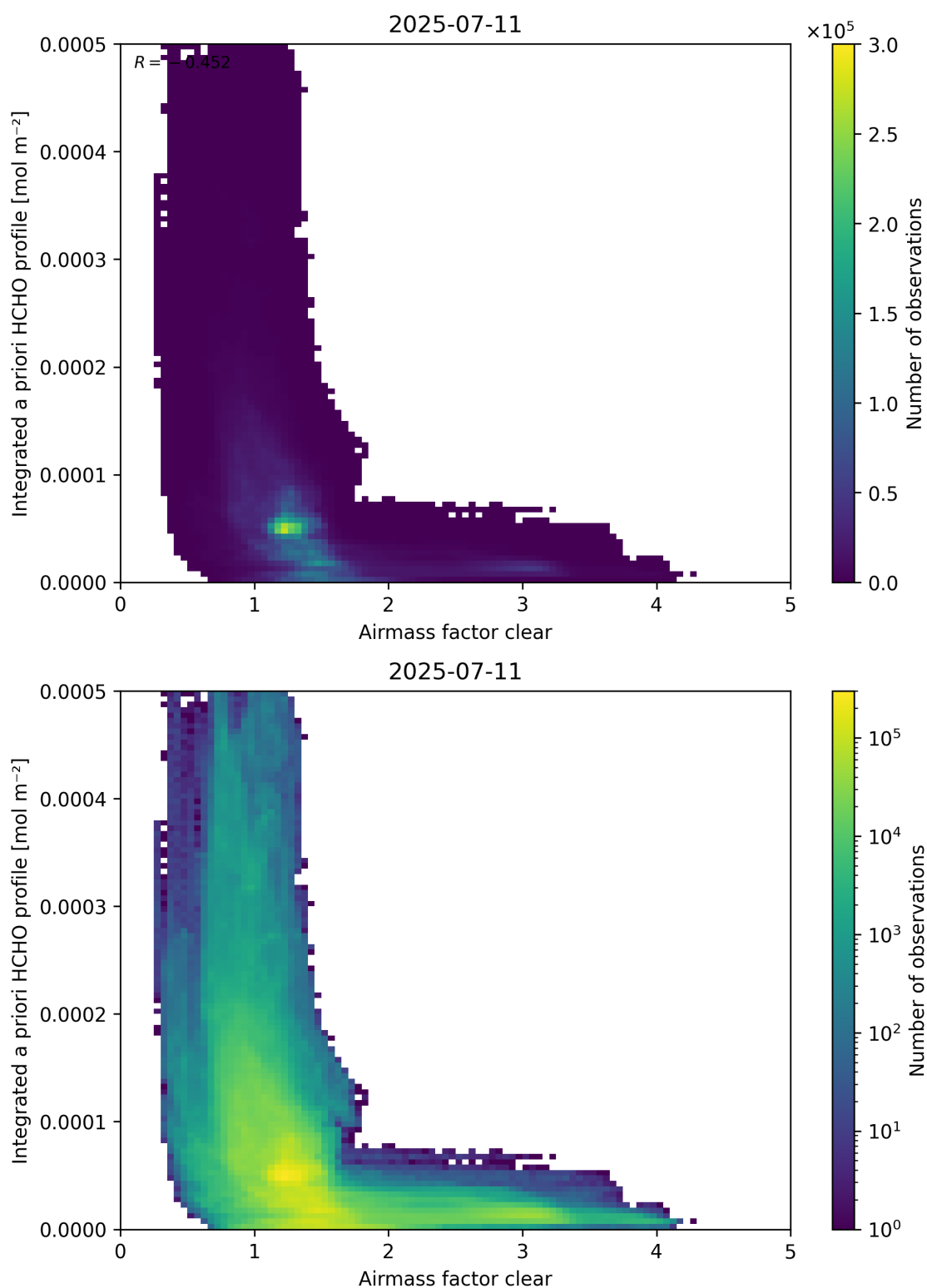
Figure 76: Scatter density plot of “Airmass factor clear” against “Integrated a priori HCHO profile” for 2025-07-10 to 2025-07-12.
