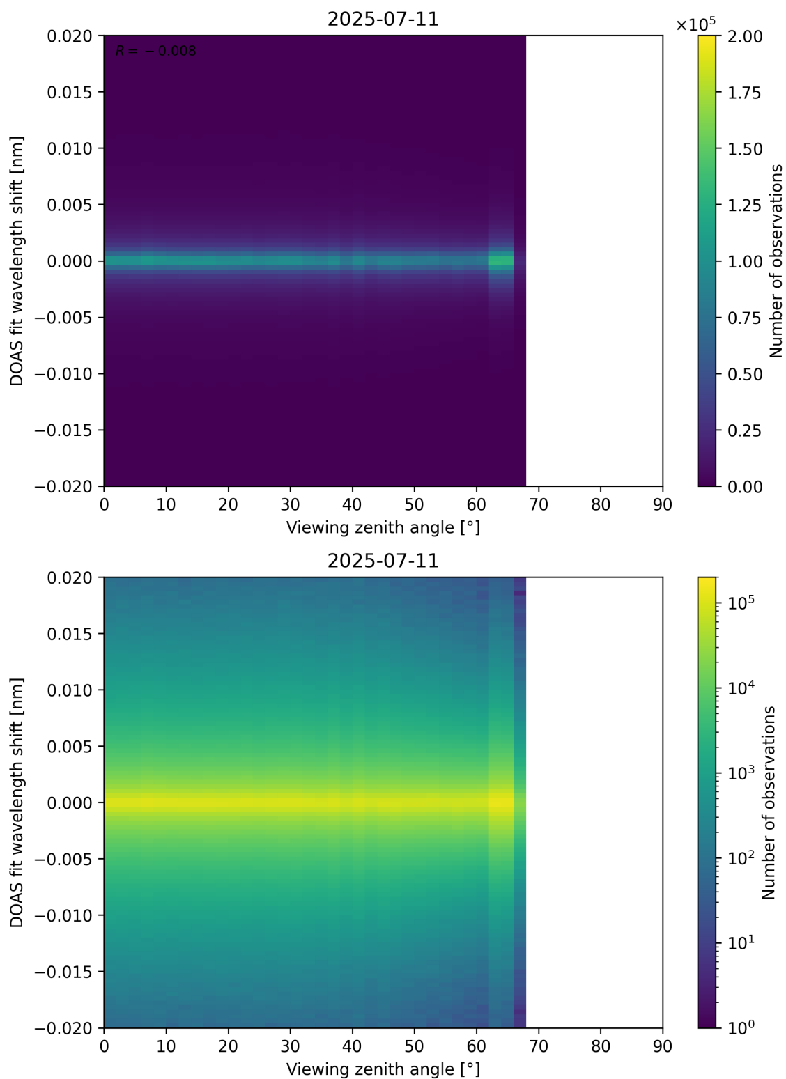
Figure 183: Scatter density plot of “Viewing zenith angle” against “DOAS fit wavelength shift” for 2025-07-10 to 2025-07-12.
