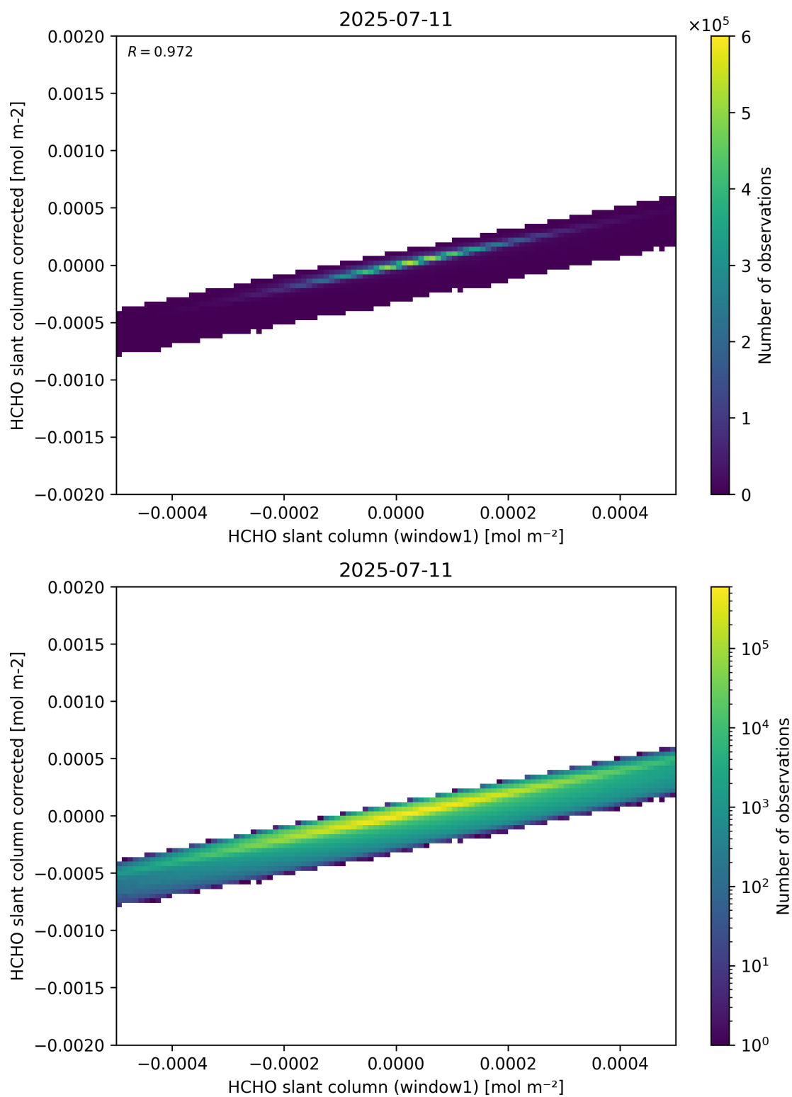
Figure 82: Scatter density plot of “HCHO slant column (window1)” against “HCHO slant column corrected” for 2025-07-10 to 2025-07-12.
