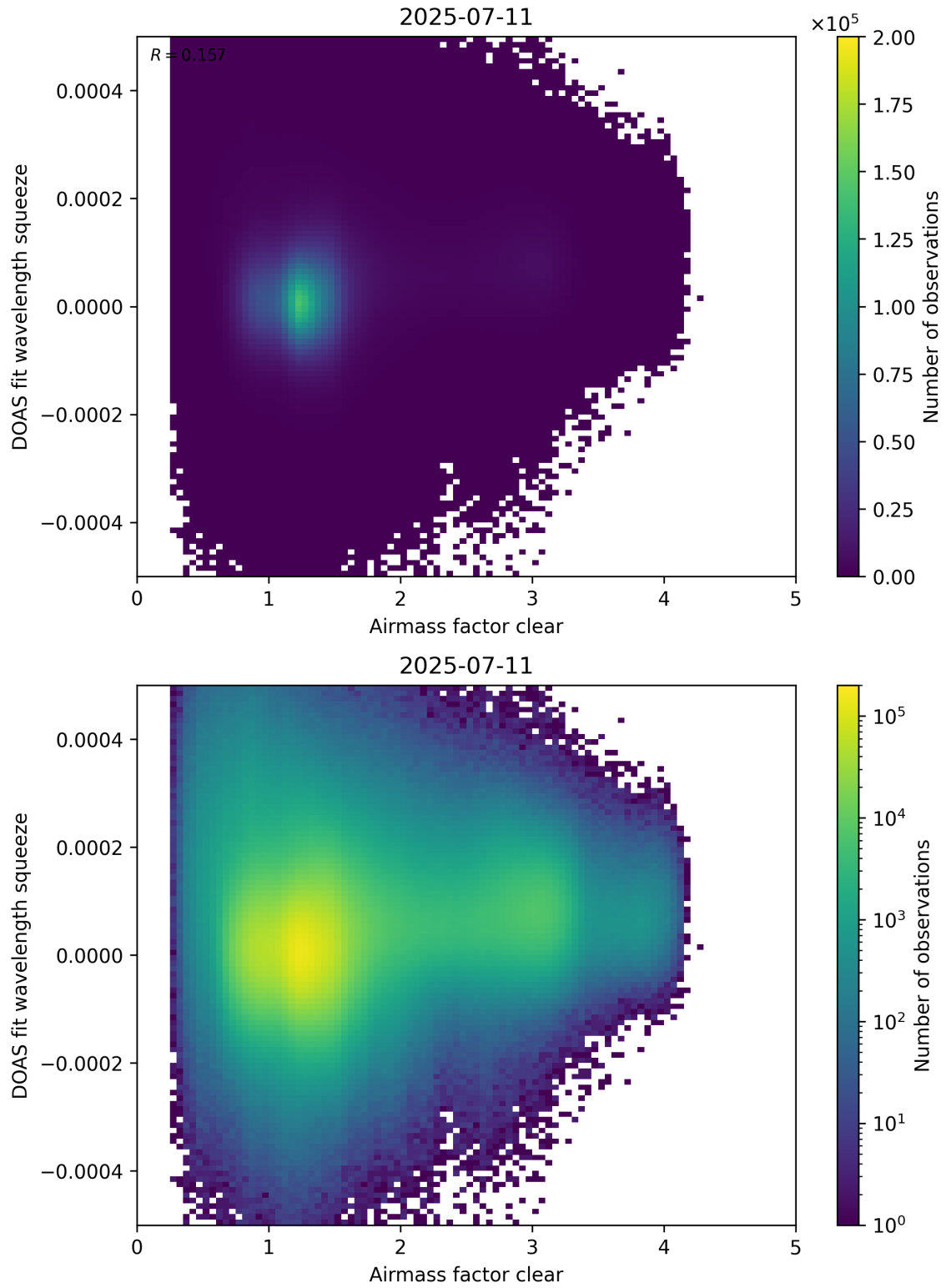
Figure 73: Scatter density plot of “Airmass factor clear” against “DOAS fit wavelength squeeze” for 2025-07-10 to 2025-07-12.
