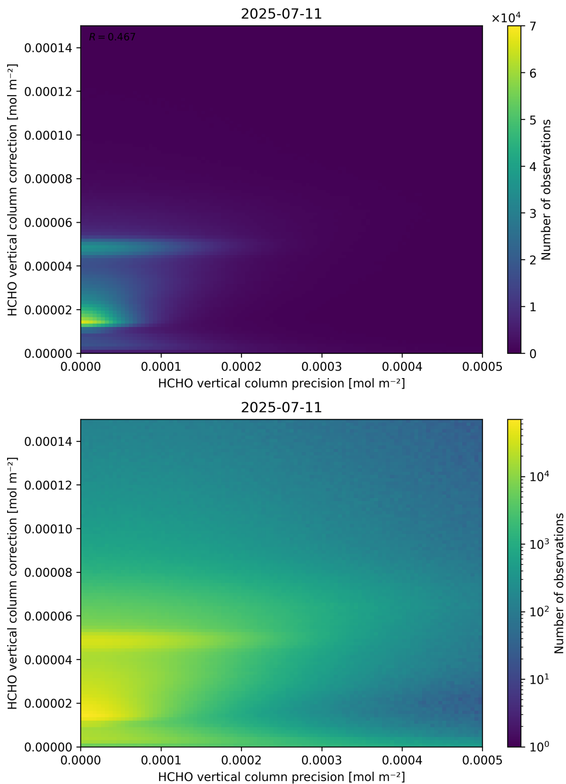
Figure 146: Scatter density plot of “HCHO vertical column precision” against “HCHO vertical column correction” for 2025-07-10 to 2025-07-12.
