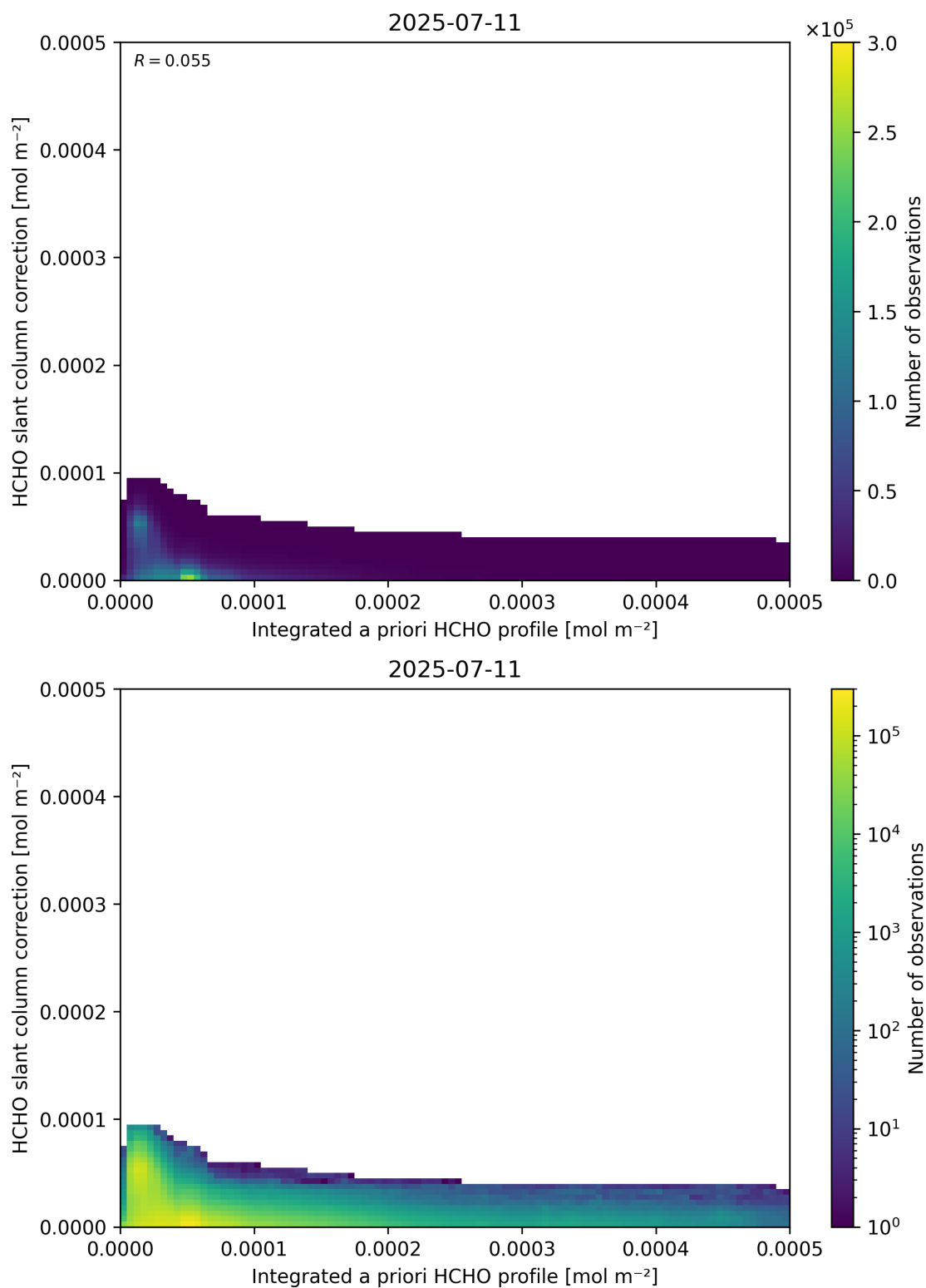
Figure 152: Scatter density plot of “Integrated a priori HCHO profile” against “HCHO slant column correction” for 2025-07-10 to 2025-07-12.
