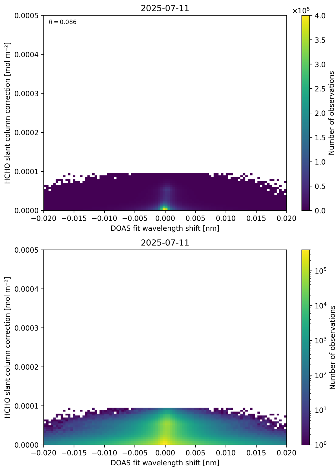
Figure 67: Scatter density plot of “DOAS fit wavelength shift” against “HCHO slant column correction” for 2025-07-10 to 2025-07-12.
