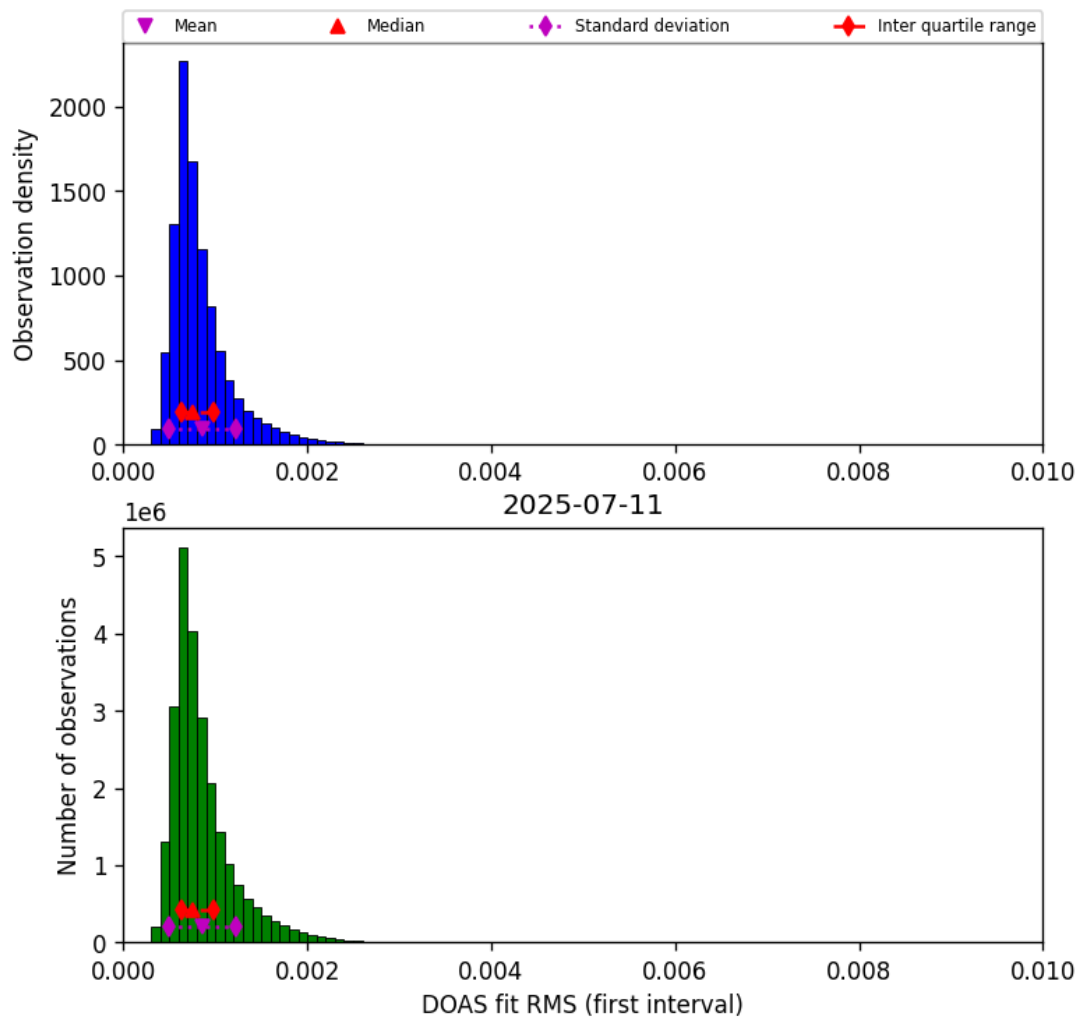
Figure 46: Histogram of “DOAS fit RMS (first interval)” for 2025-07-10 to 2025-07-12
