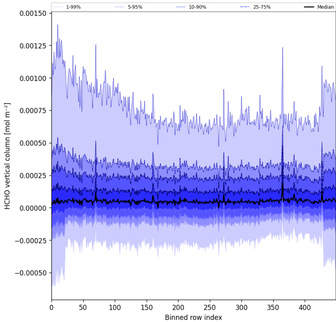
Figure 49: Along track statistics of “HCHO vertical column” for 2025-07-10 to 2025-07-12
