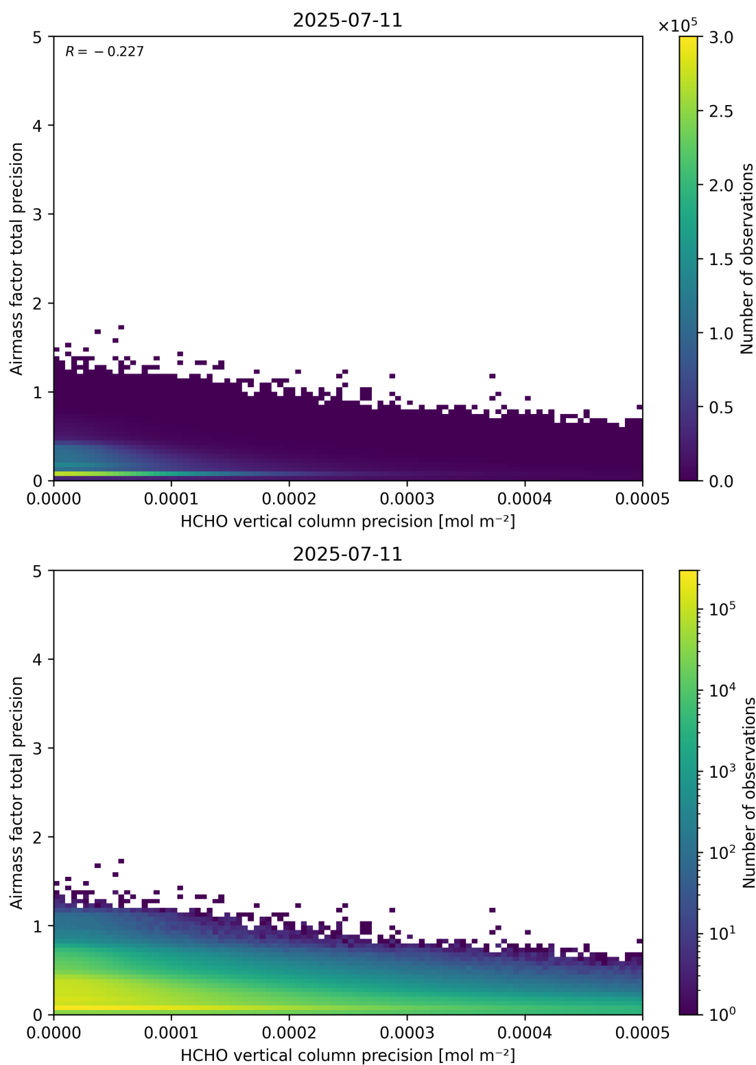
Figure 145: Scatter density plot of “HCHO vertical column precision” against “Airmass factor total precision” for 2025-07-10 to 2025-07-12.
