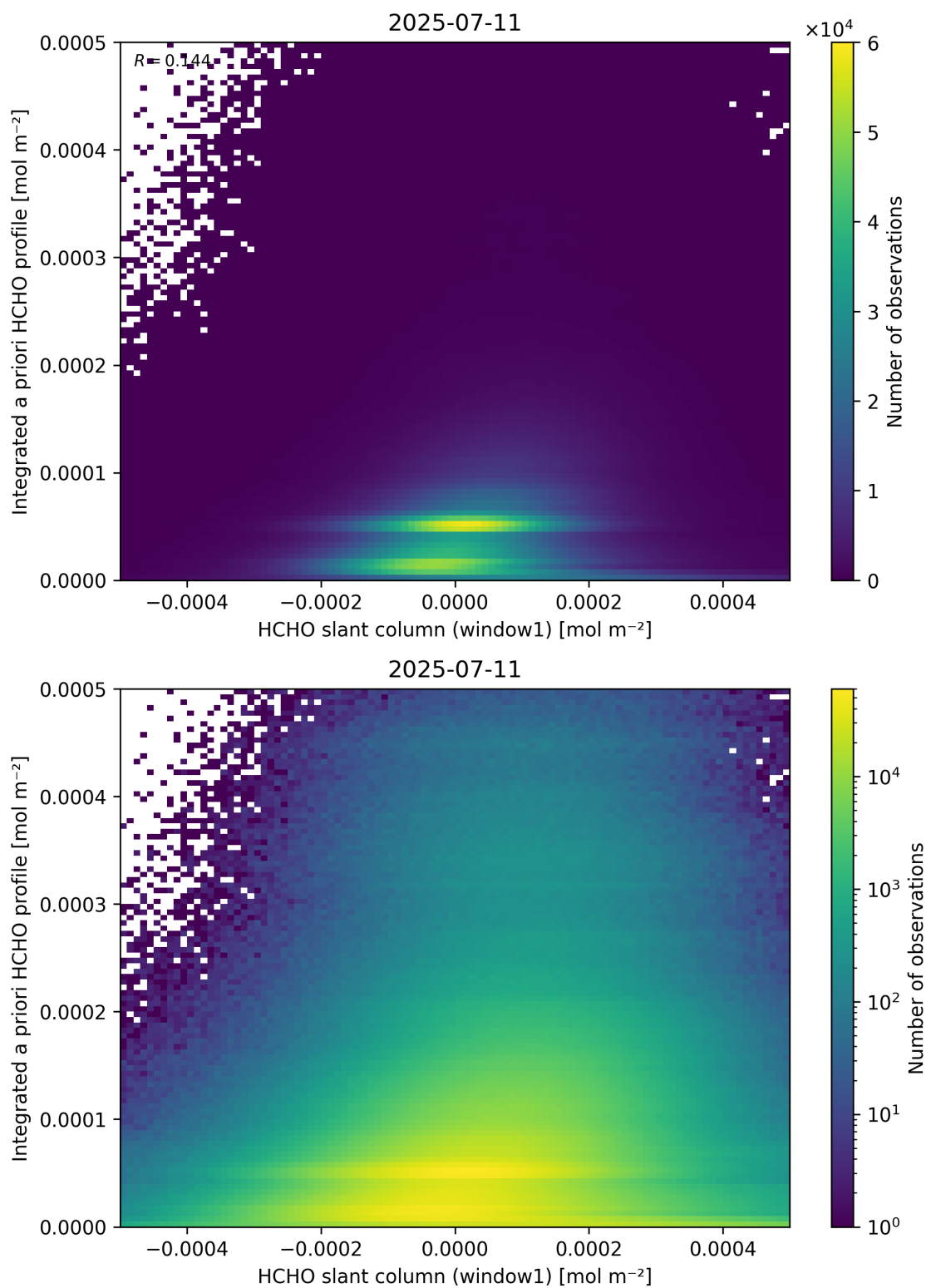
Figure 87: Scatter density plot of “HCHO slant column (window1)” against “Integrated a priori HCHO profile” for 2025-07-10 to 2025-07-12.
