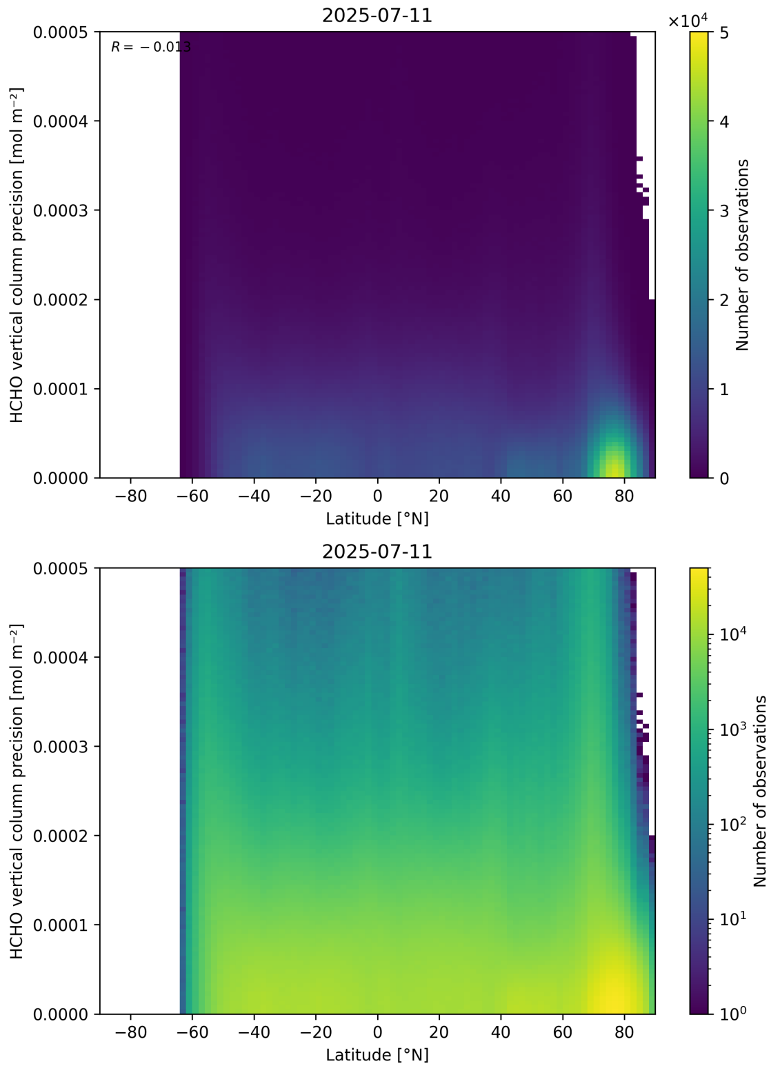
Figure 165: Scatter density plot of “Latitude” against “HCHO vertical column precision” for 2025-07-10 to 2025-07-12.
