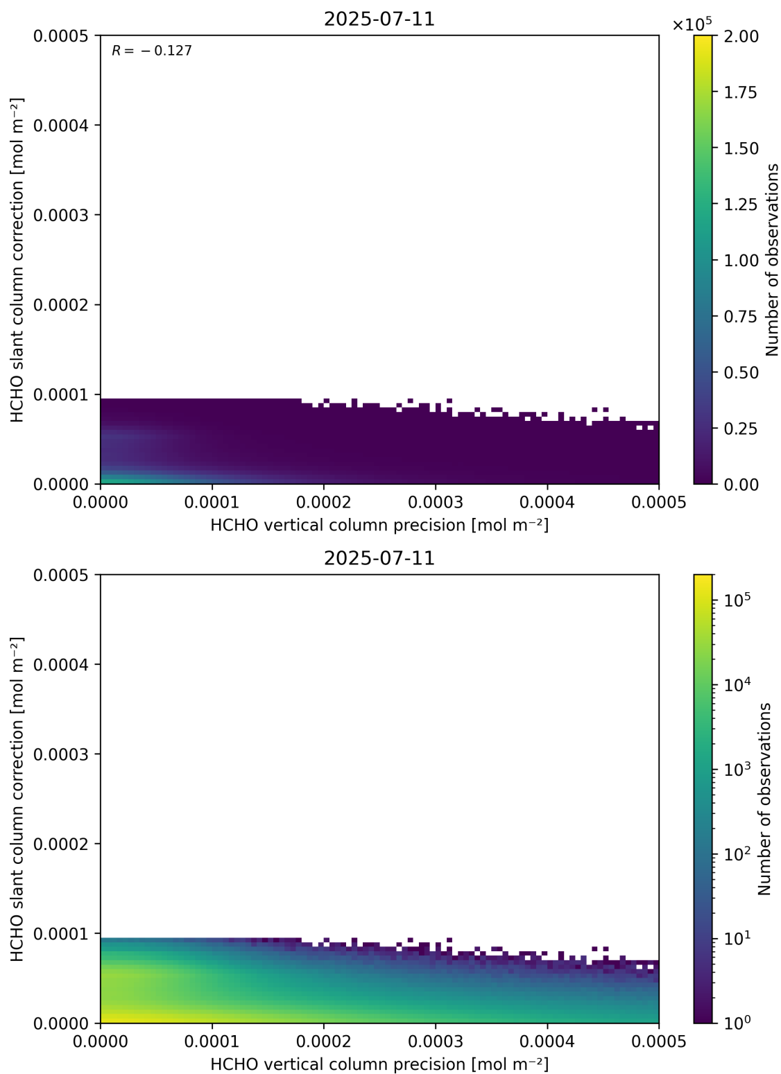
Figure 141: Scatter density plot of “HCHO vertical column precision” against “HCHO slant column correction” for 2025-07-10 to 2025-07-12.
