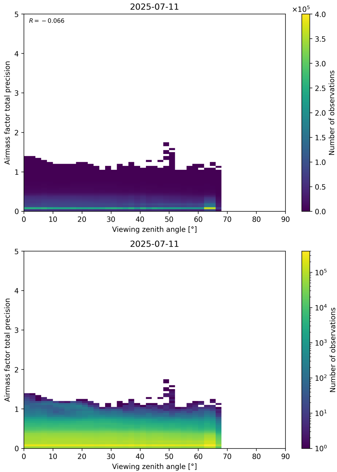
Figure 191: Scatter density plot of “Viewing zenith angle” against “Airmass factor total precision” for 2025-07-10 to 2025-07-12.
