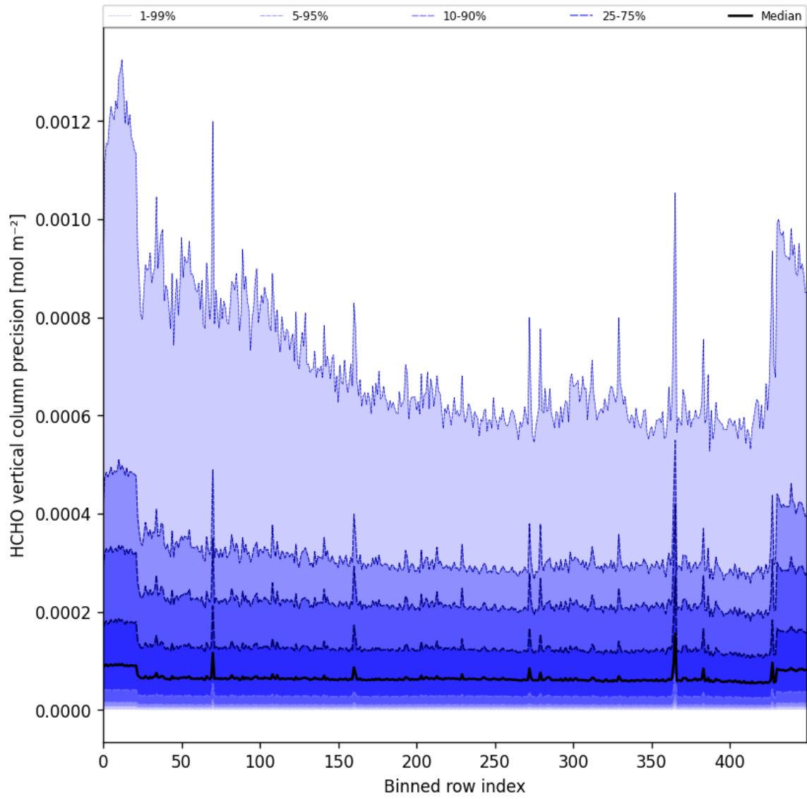
Figure 50: Along track statistics of “HCHO vertical column precision” for 2025-07-10 to 2025-07-12
