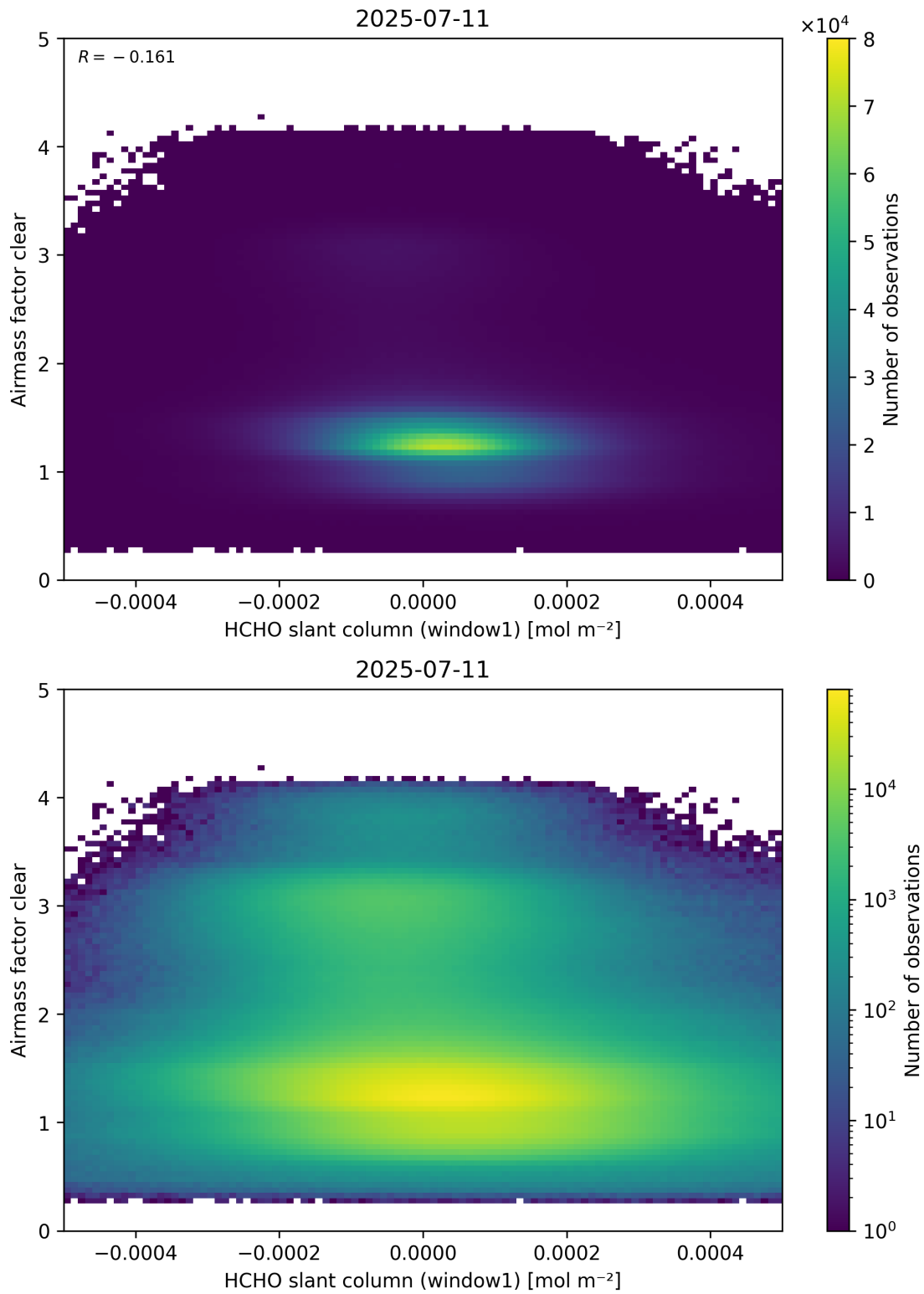
Figure 81: Scatter density plot of “HCHO slant column (window1)” against “Airmass factor clear” for 2025-07-10 to 2025-07-12.
