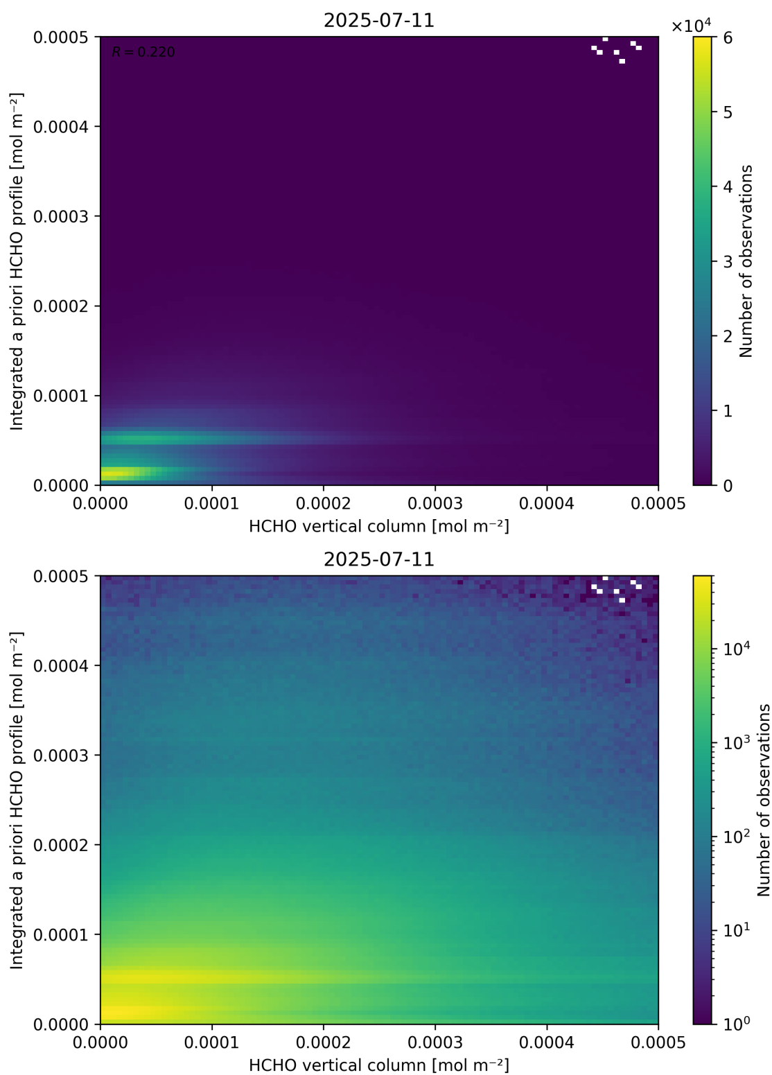
Figure 135: Scatter density plot of “HCHO vertical column” against “Integrated a priori HCHO profile” for 2025-07-10 to 2025-07-12.
