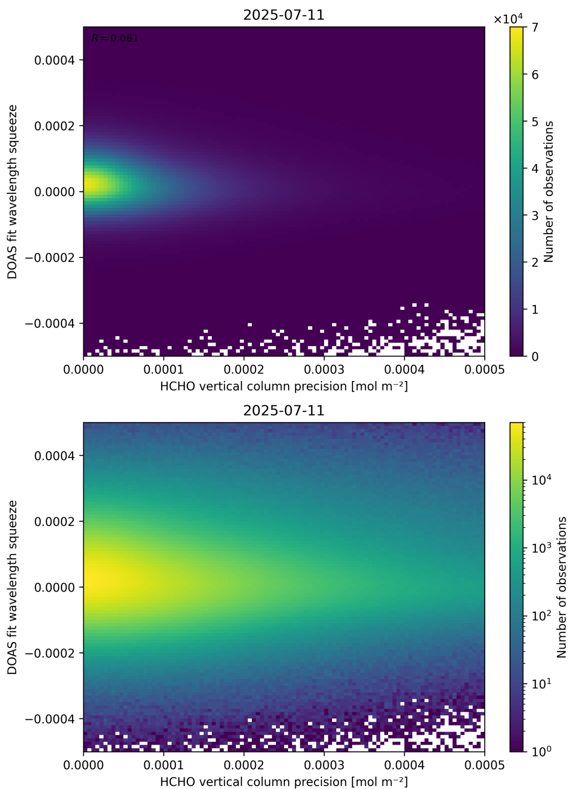
Figure 138: Scatter density plot of “HCHO vertical column precision” against “DOAS fit wavelength squeeze” for 2025-07-10 to 2025-07-12.
