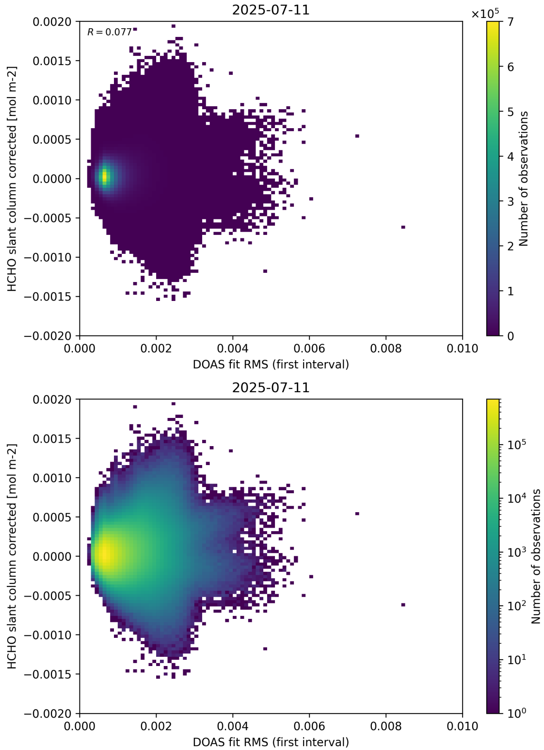
Figure 62: Scatter density plot of “DOAS fit RMS (first interval)” against “HCHO slant column corrected” for 2025-07-10 to 2025-07-12.
