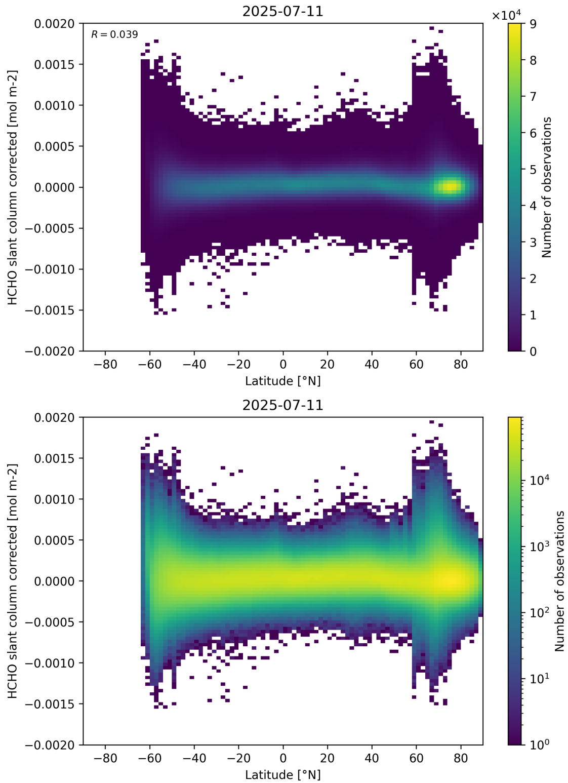
Figure 157: Scatter density plot of “Latitude” against “HCHO slant column corrected” for 2025-07-10 to 2025-07-12.
