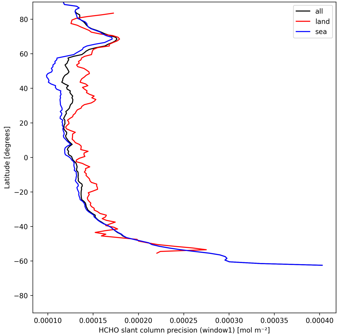
Figure 25: Zonal average of “HCHO slant column precision (window1)” for 2025-07-10 to 2025-07-12.
