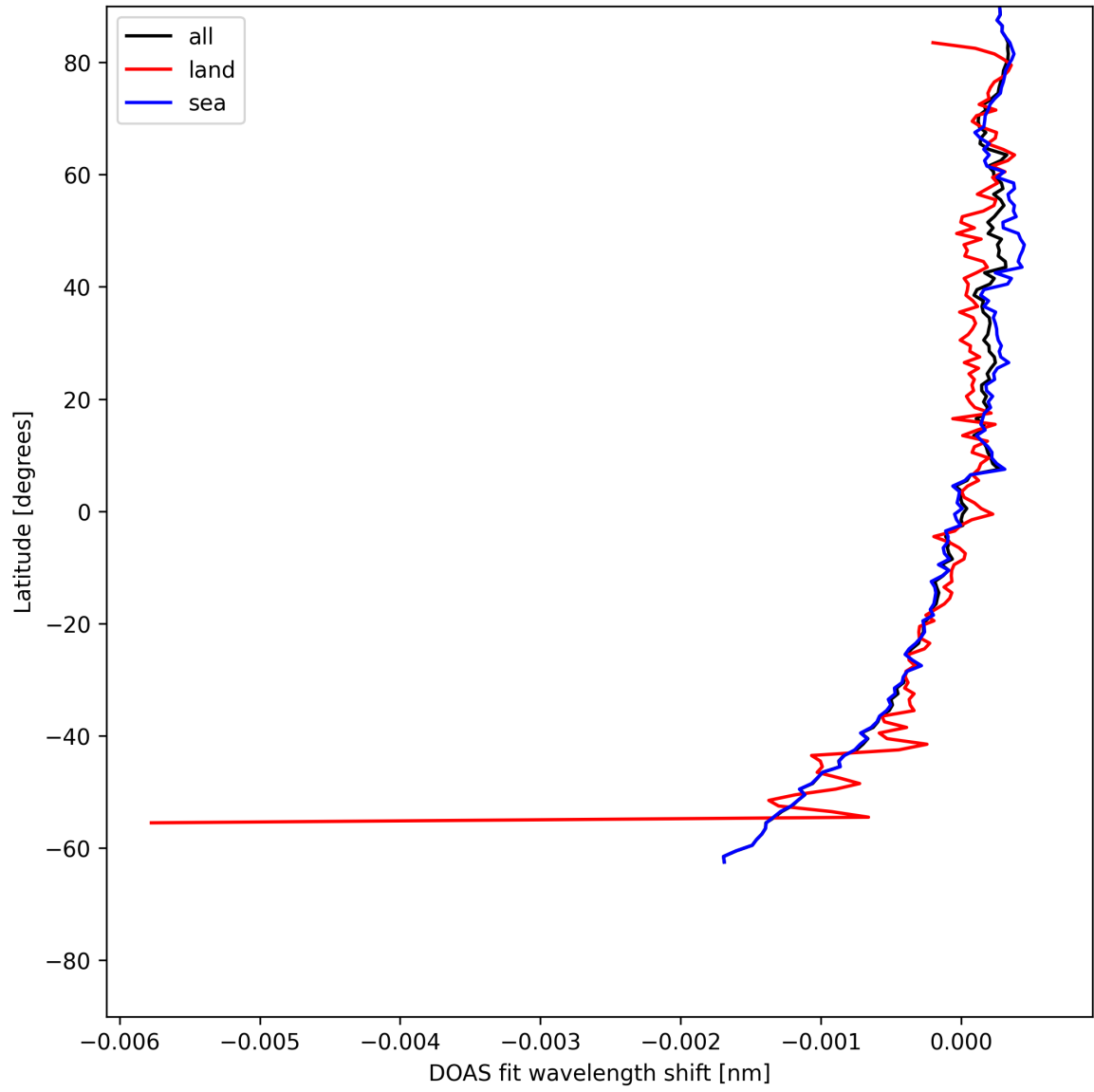
Figure 30: Zonal average of “DOAS fit wavelength shift” for 2025-07-10 to 2025-07-12.
