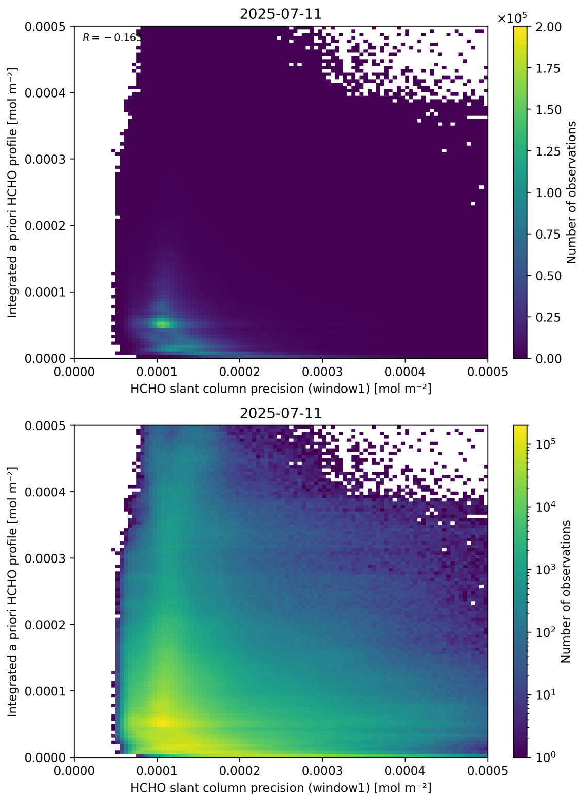
Figure 96: Scatter density plot of “HCHO slant column precision (window1)” against “Integrated a priori HCHO profile” for 2025-07-10 to 2025-07-12.
