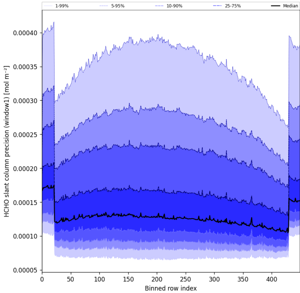
Figure 53: Along track statistics of "HCHO slant column precision (window1)" for 2025-07-10 to 2025-07-12
