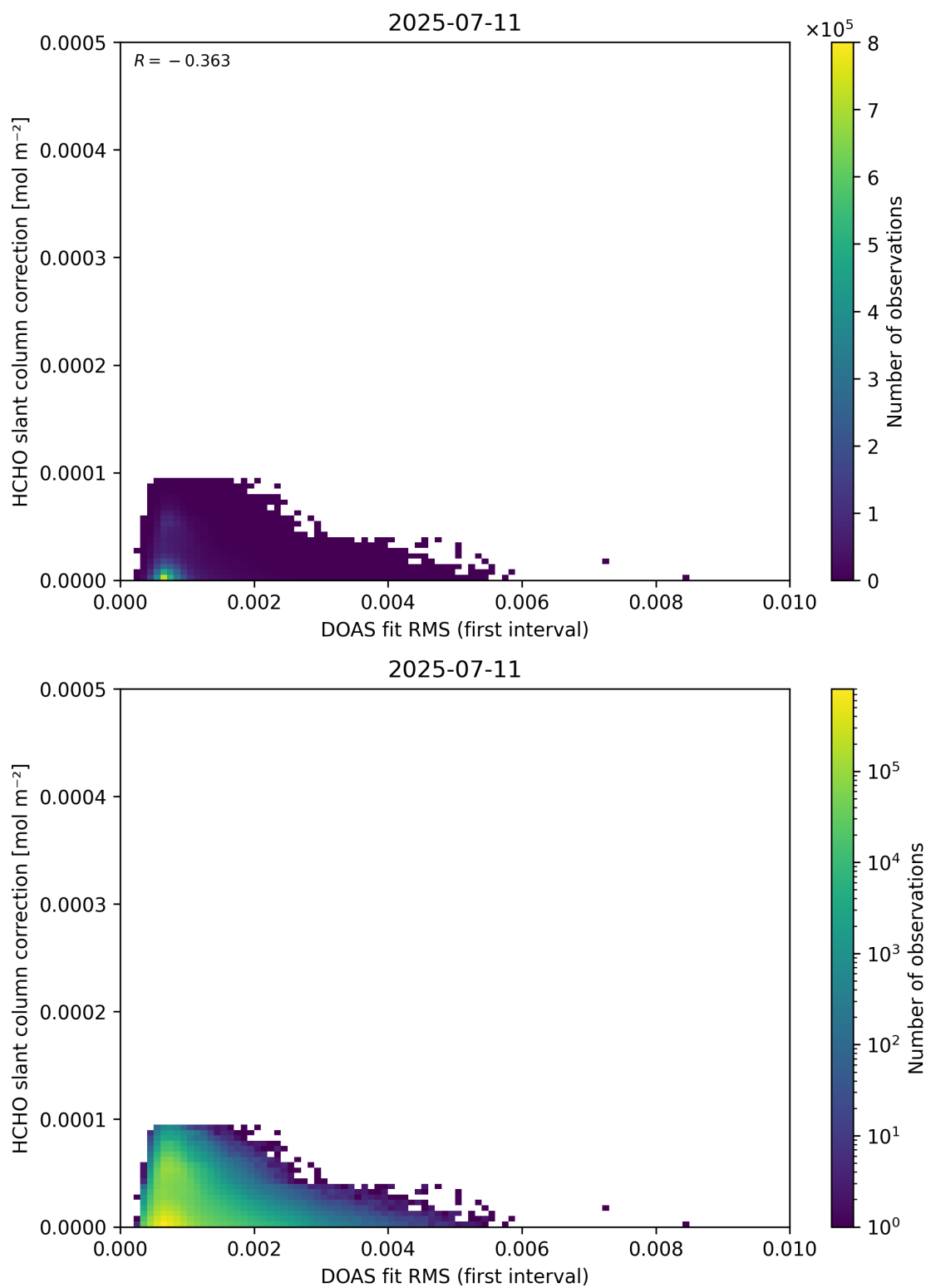
Figure 63: Scatter density plot of “DOAS fit RMS (first interval)” against “HCHO slant column correction” for 2025-07-10 to 2025-07-12.
