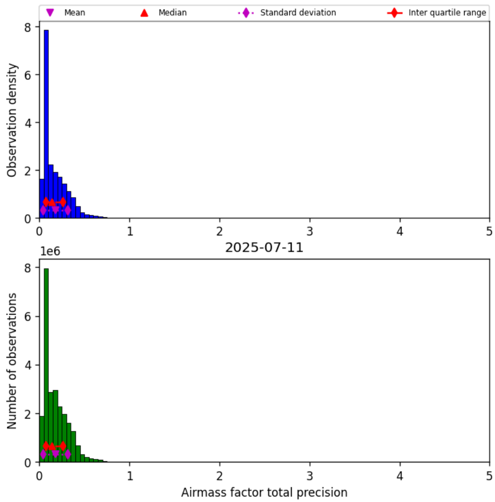
Figure 41: Histogram of “Airmass factor total precision” for 2025-07-10 to 2025-07-12
