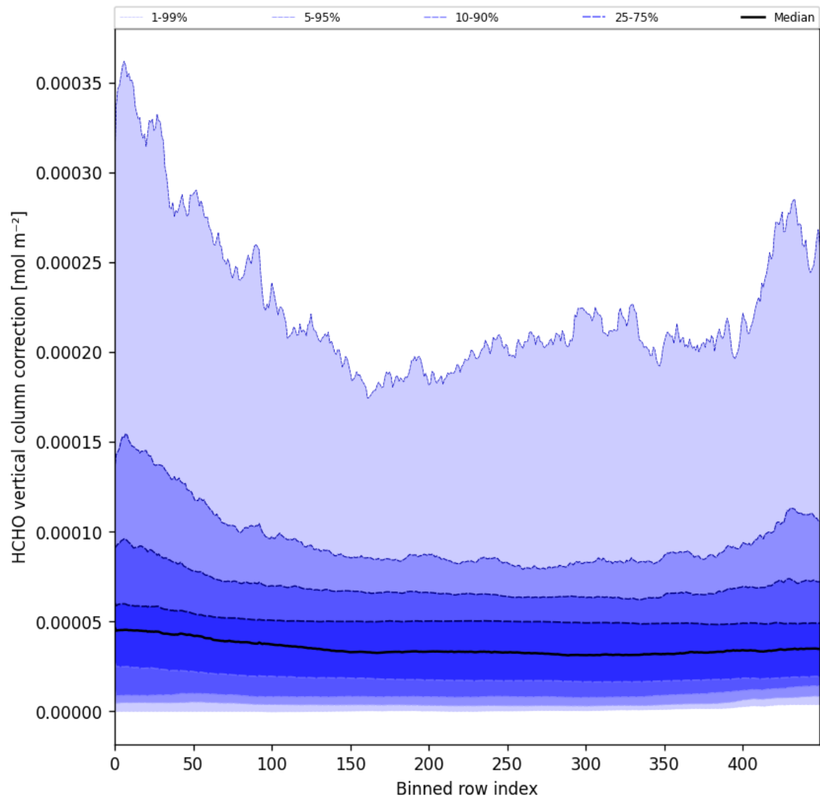
Figure 51: Along track statistics of “HCHO vertical column correction” for 2025-07-10 to 2025-07-12
