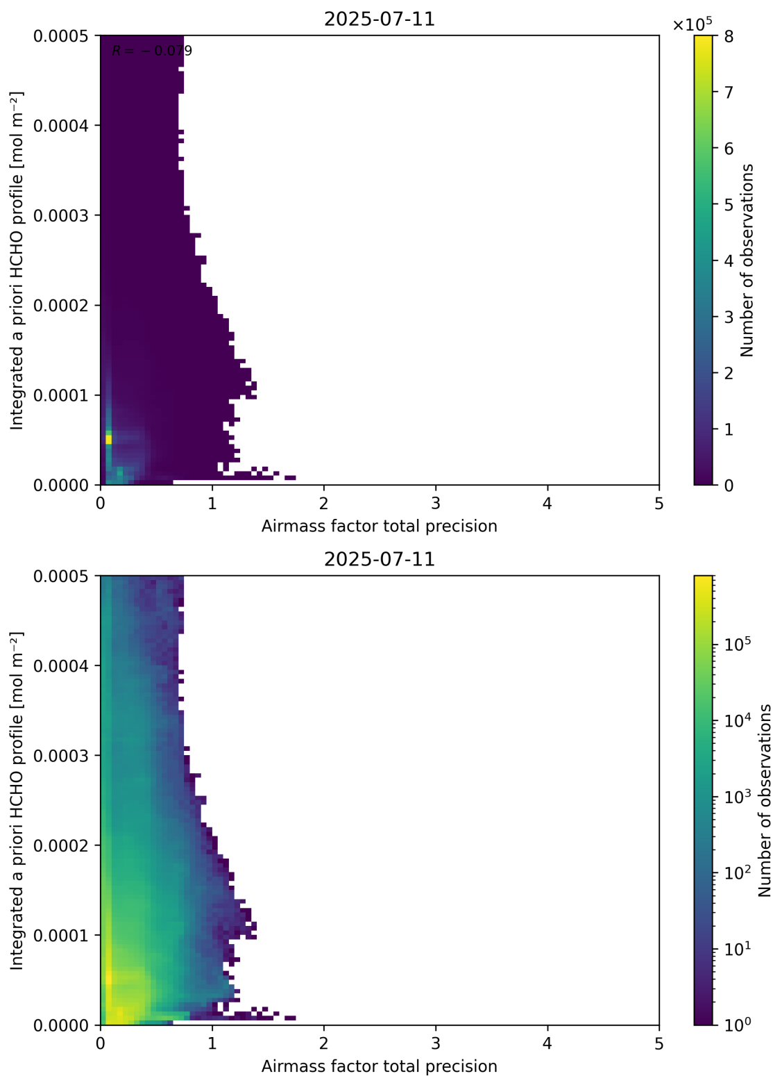
Figure 111: Scatter density plot of “Airmass factor total precision” against “Integrated a priori HCHO profile” for 2025-07-10 to 2025-07-12.
