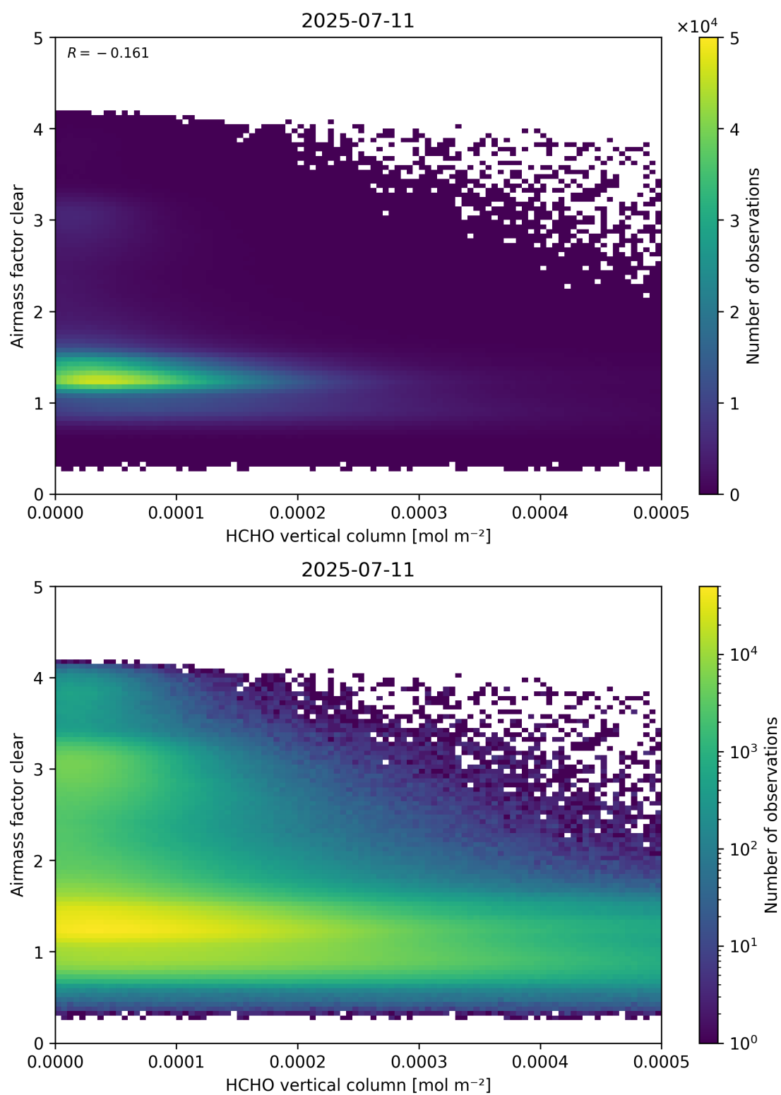
Figure 126: Scatter density plot of “HCHO vertical column” against “Airmass factor clear” for 2025-07-10 to 2025-07-12.
