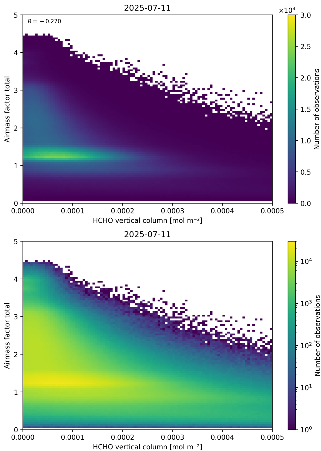
Figure 131: Scatter density plot of “HCHO vertical column” against “Airmass factor total” for 2025-07-10 to 2025-07-12.
