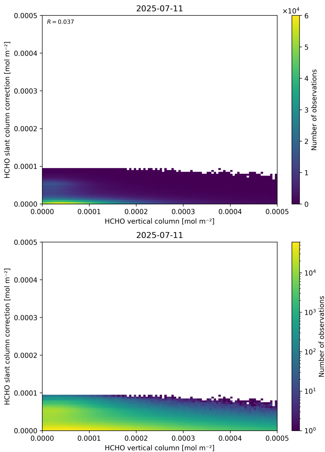
Figure 128: Scatter density plot of “HCHO vertical column” against “HCHO slant column correction” for 2025-07-10 to 2025-07-12.
