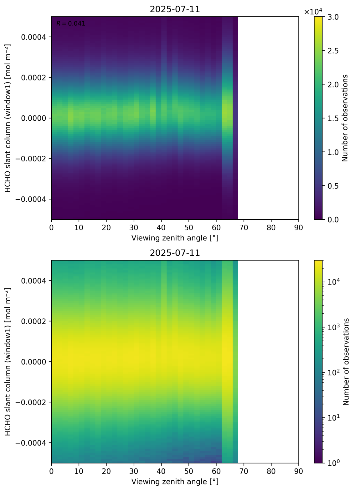
Figure 188: Scatter density plot of “Viewing zenith angle” against “HCHO slant column (window1)” for 2025-07-10 to 2025-07-12.
