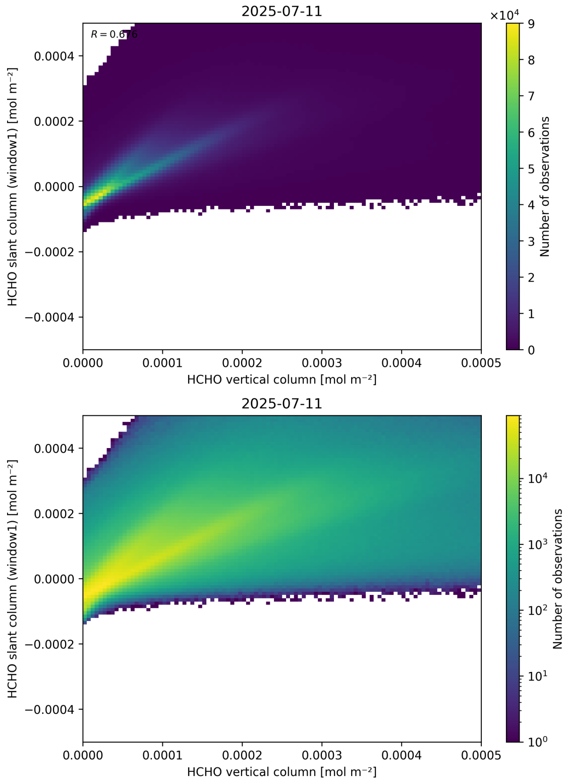
Figure 129: Scatter density plot of “HCHO vertical column” against “HCHO slant column (window1)” for 2025-07-10 to 2025-07-12.
