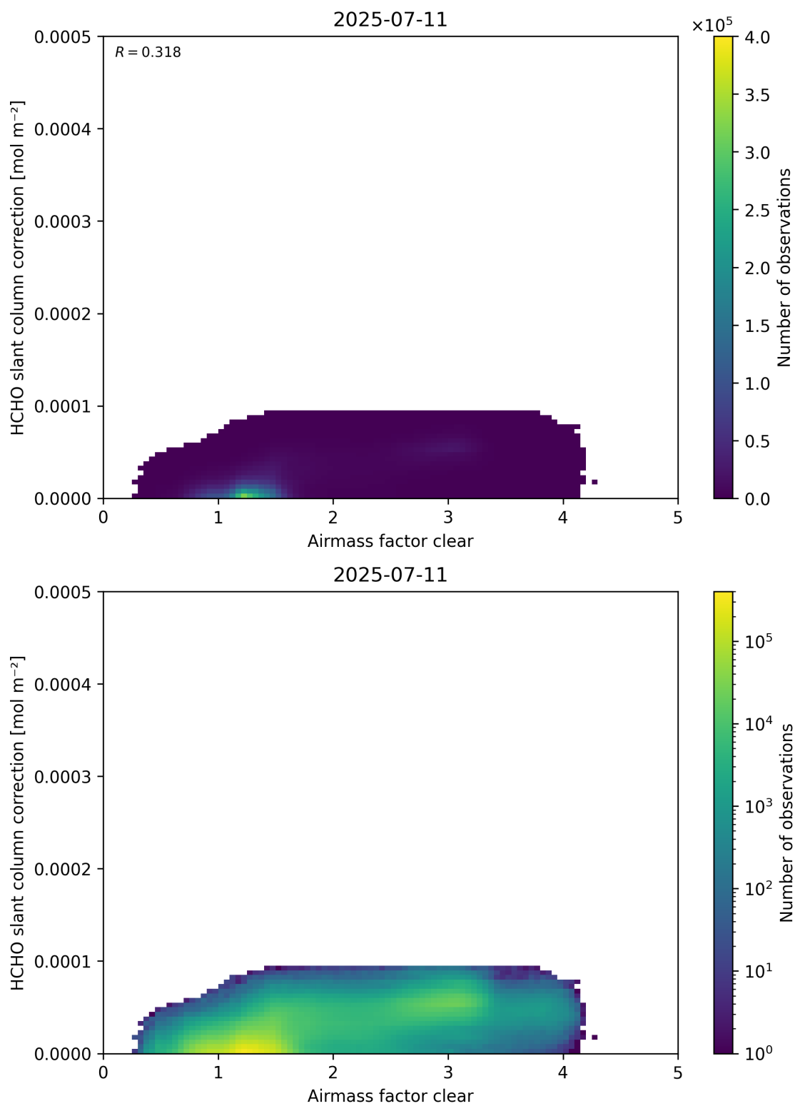
Figure 75: Scatter density plot of “Airmass factor clear” against “HCHO slant column correction” for 2025-07-10 to 2025-07-12.
