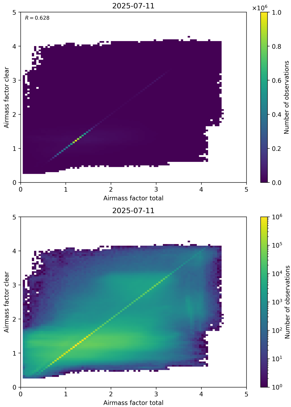
Figure 100: Scatter density plot of “Airmass factor total” against “Airmass factor clear” for 2025-07-10 to 2025-07-12.
