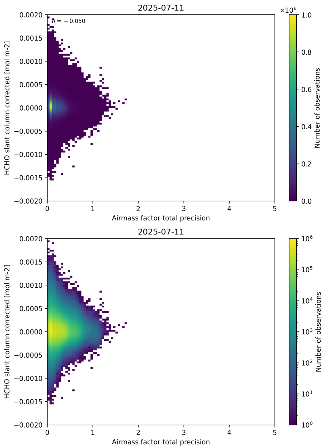
Figure 109: Scatter density plot of “Airmass factor total precision” against “HCHO slant column corrected” for 2025-07-10 to 2025-07-12.
