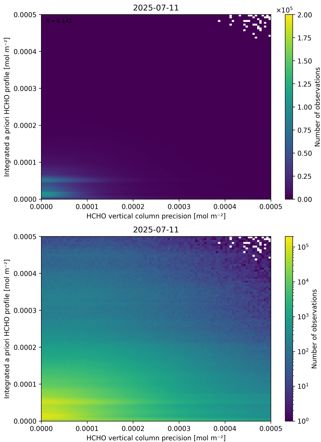
Figure 147: Scatter density plot of “HCHO vertical column precision” against “Integrated a priori HCHO profile” for 2025-07-10 to 2025-07-12.
