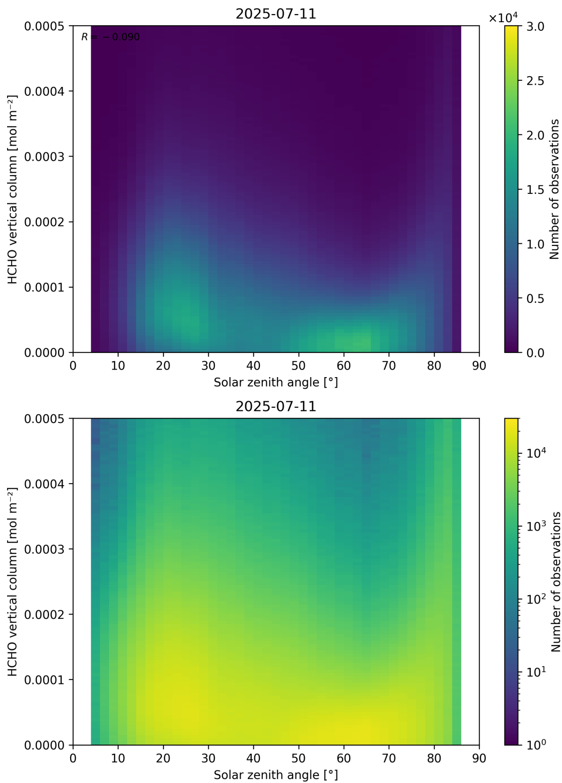
Figure 177: Scatter density plot of “Solar zenith angle” against “HCHO vertical column” for 2025-07-10 to 2025-07-12.
