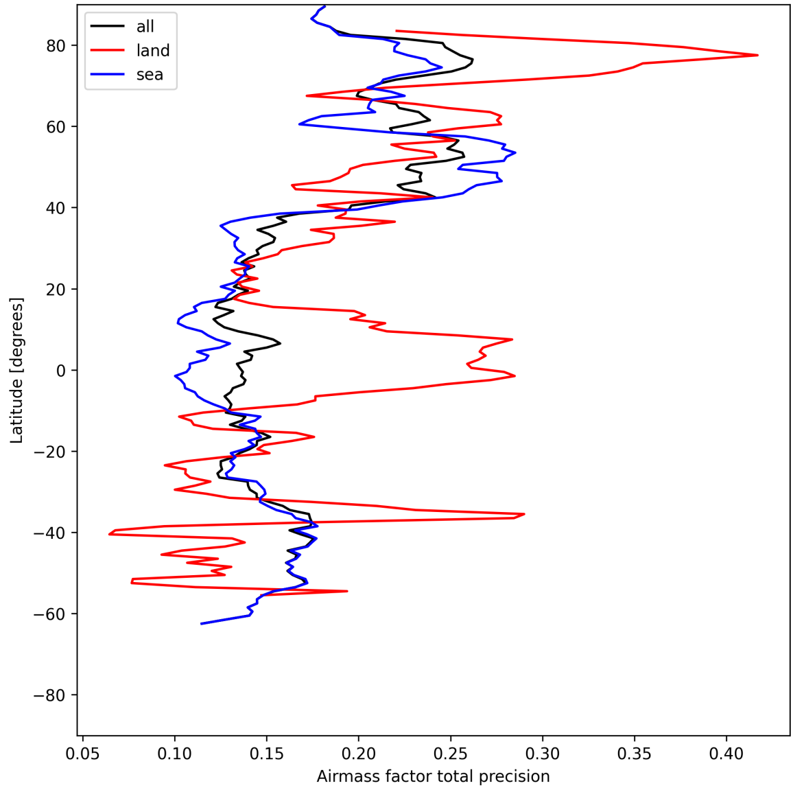
Figure 27: Zonal average of “Airmass factor total precision” for 2025-07-10 to 2025-07-12.
