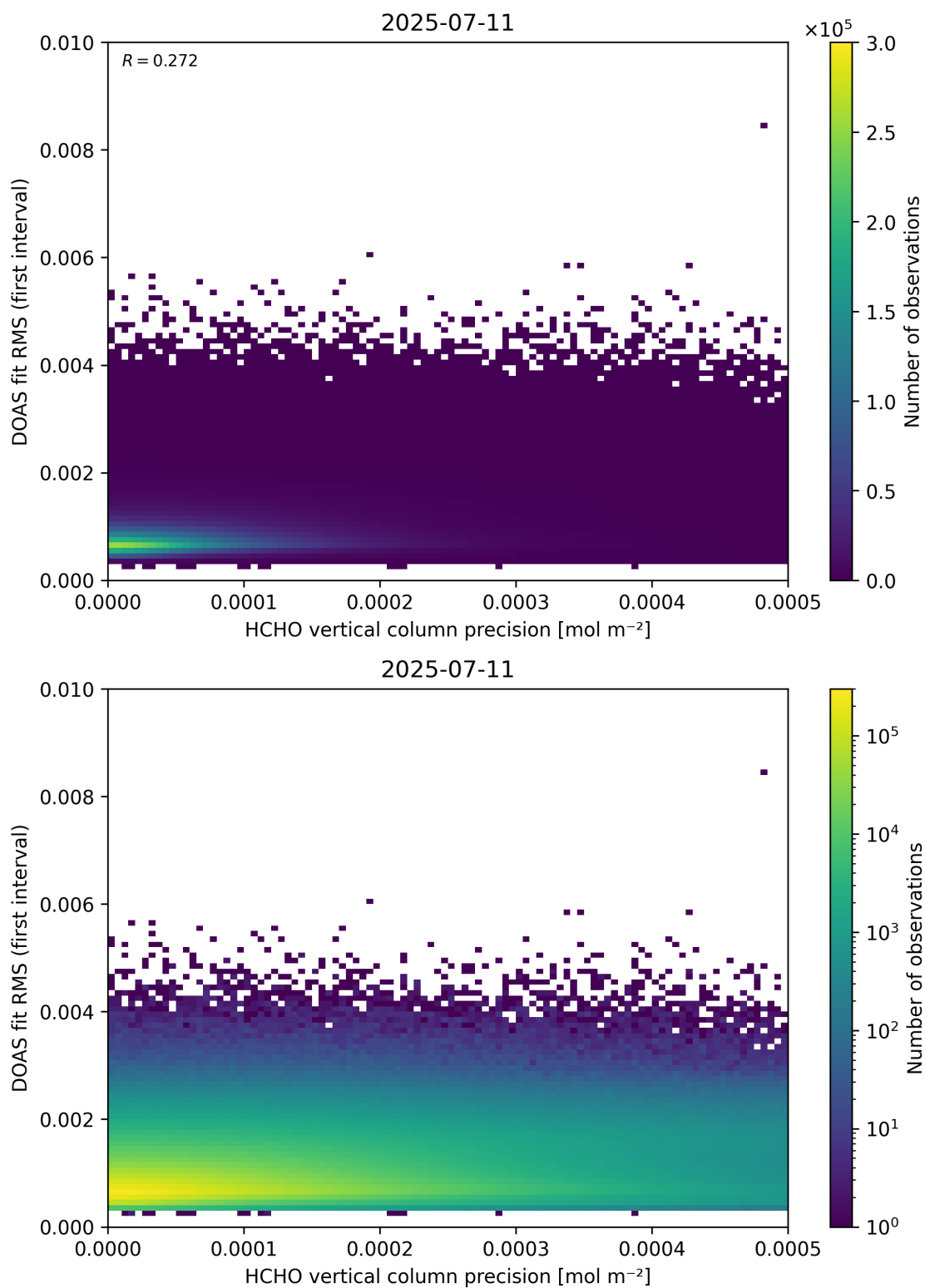
Figure 136: Scatter density plot of “HCHO vertical column precision” against “DOAS fit RMS (first interval)” for 2025-07-10 to 2025-07-12.
