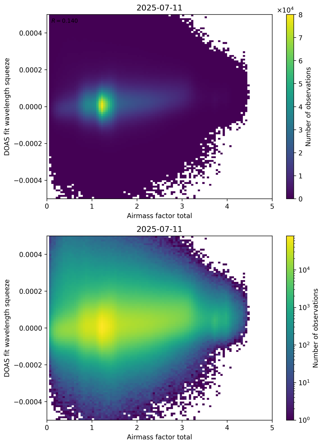
Figure 99: Scatter density plot of “Airmass factor total” against “DOAS fit wavelength squeeze” for 2025-07-10 to 2025-07-12.
