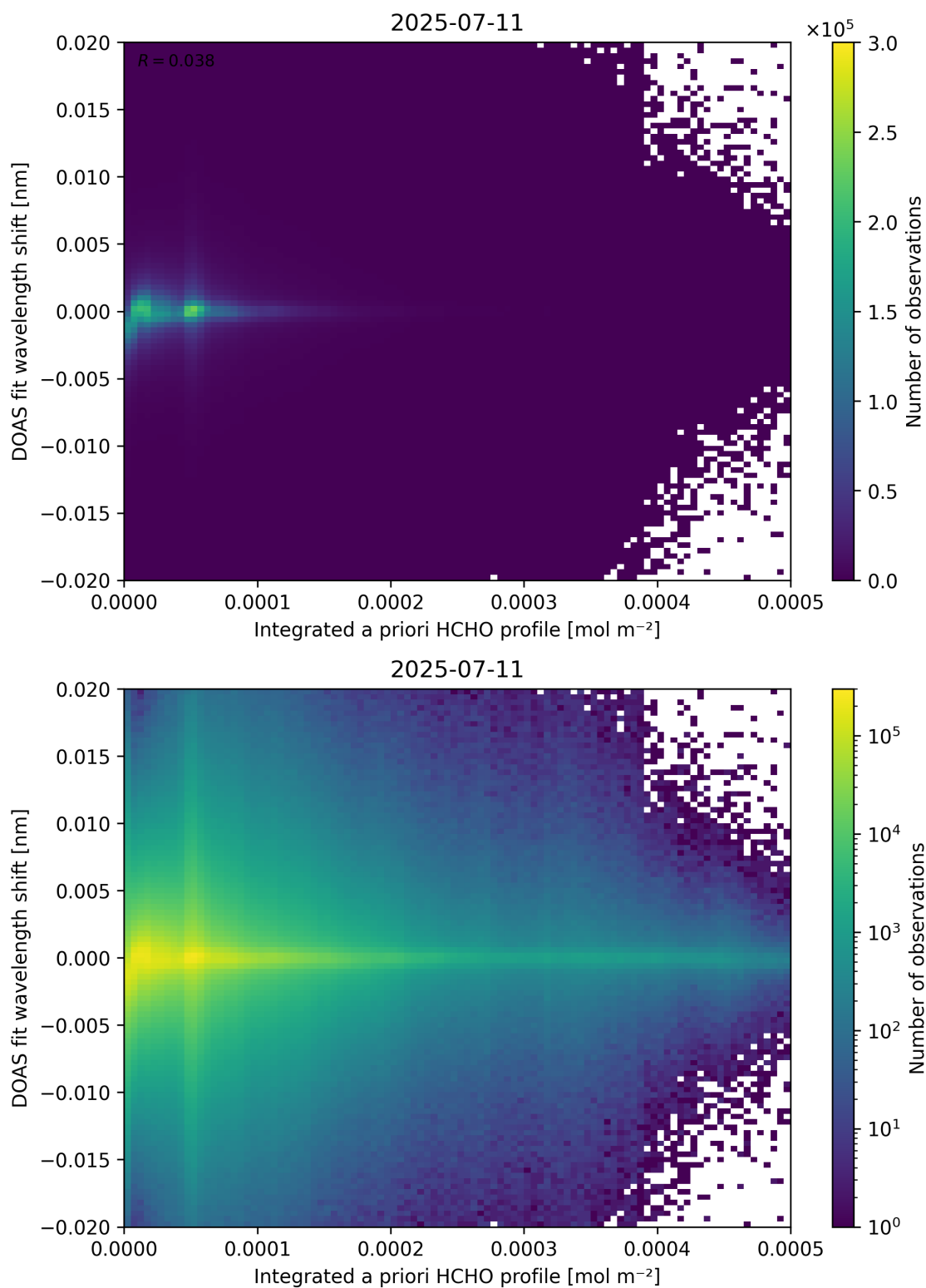
Figure 149: Scatter density plot of “Integrated a priori HCHO profile” against “DOAS fit wavelength shift” for 2025-07-10 to 2025-07-12.
