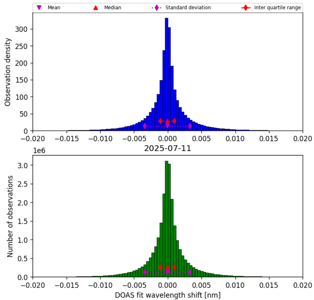
Figure 44: Histogram of “DOAS fit wavelength shift” for 2025-07-10 to 2025-07-12
