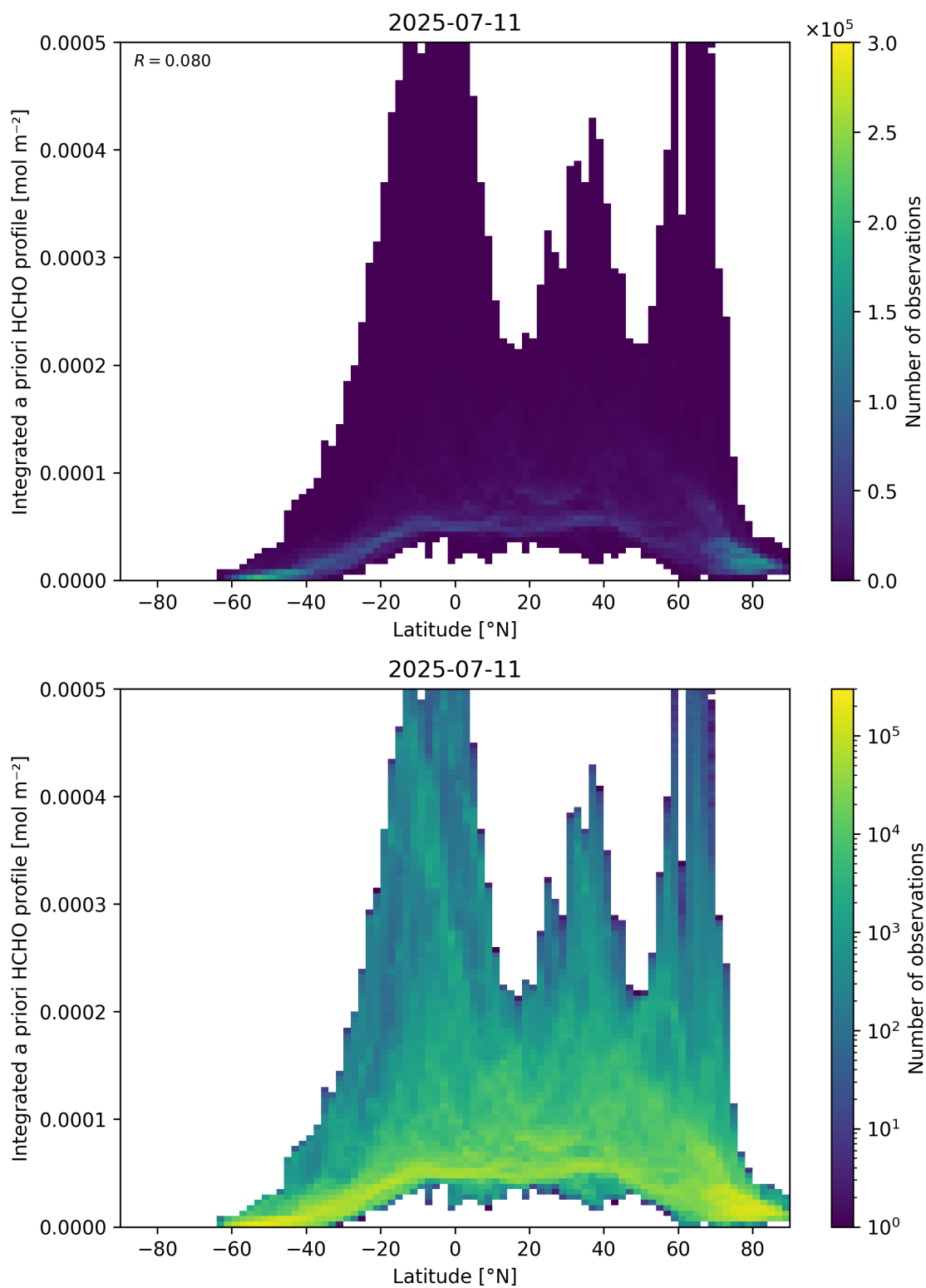
Figure 166: Scatter density plot of “Latitude” against “Integrated a priori HCHO profile” for 2025-07-10 to 2025-07-12.
