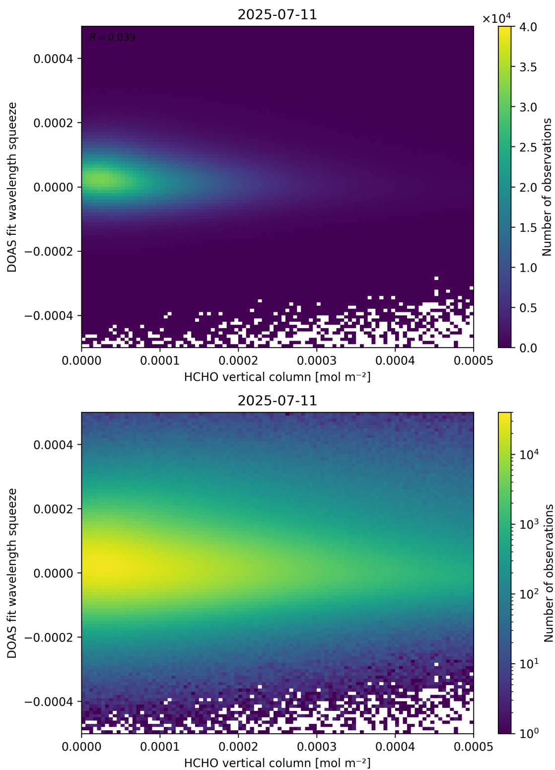
Figure 125: Scatter density plot of “HCHO vertical column” against “DOAS fit wavelength squeeze” for 2025-07-10 to 2025-07-12.
