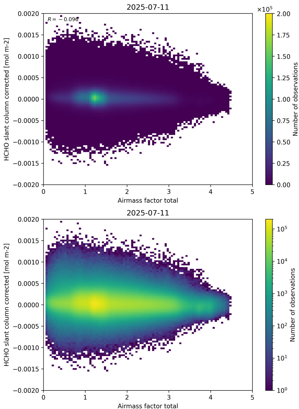
Figure 101: Scatter density plot of “Airmass factor total” against “HCHO slant column corrected” for 2025-07-10 to 2025-07-12.
