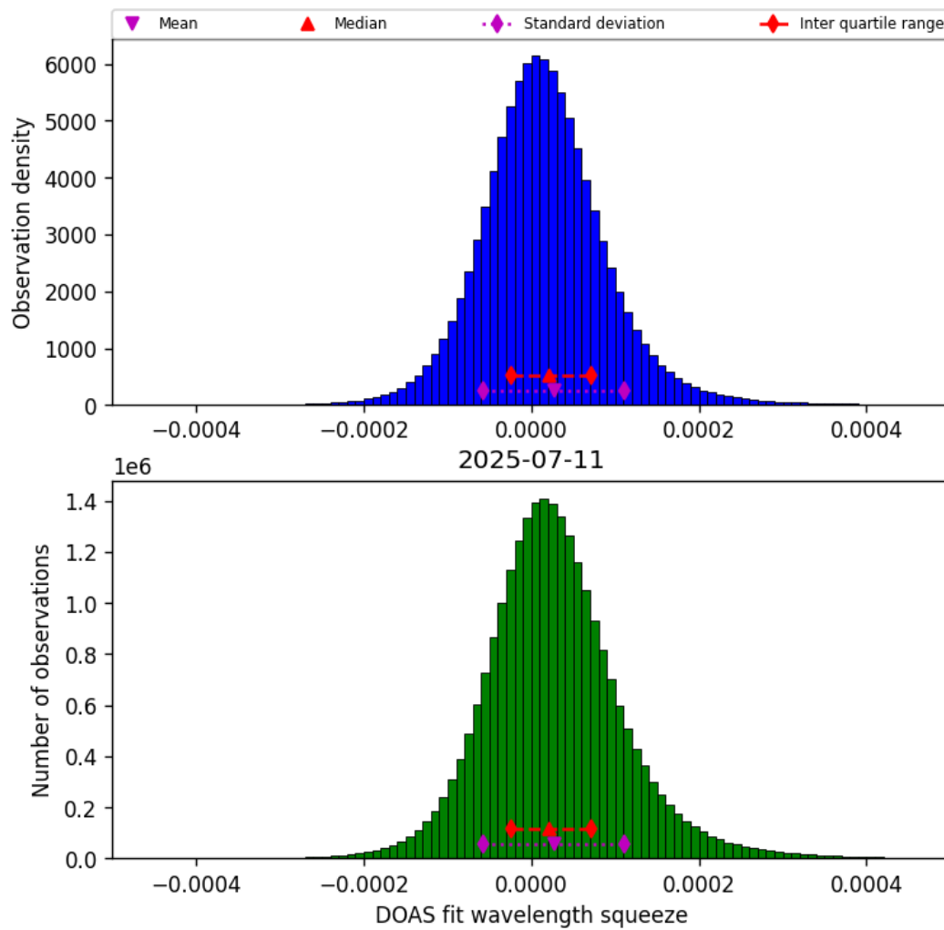
Figure 45: Histogram of “DOAS fit wavelength squeeze” for 2025-07-10 to 2025-07-12
