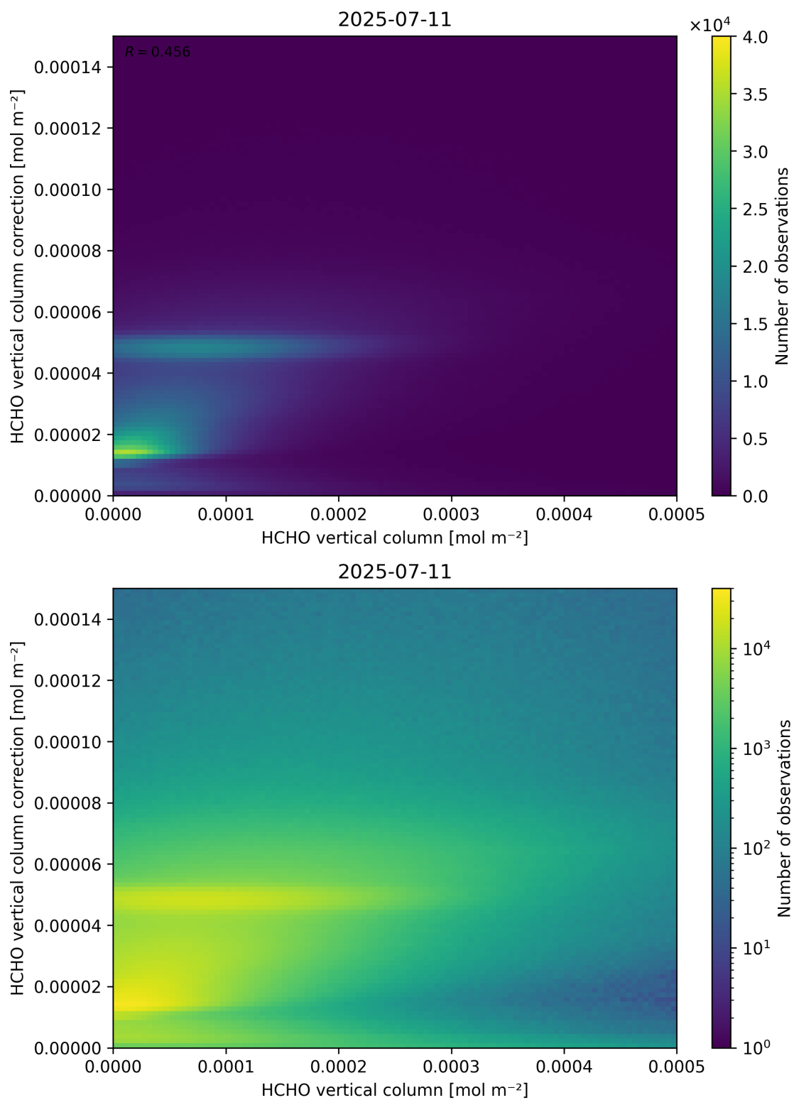
Figure 133: Scatter density plot of “HCHO vertical column” against “HCHO vertical column correction” for 2025-07-10 to 2025-07-12.
