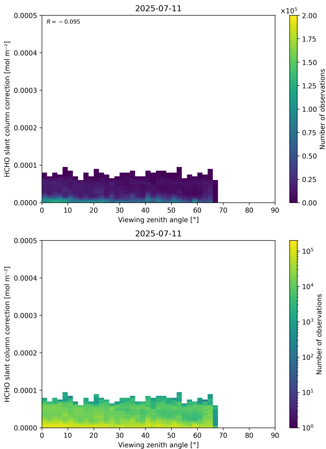
Figure 187: Scatter density plot of “Viewing zenith angle” against “HCHO slant column correction” for 2025-07-10 to 2025-07-12.
