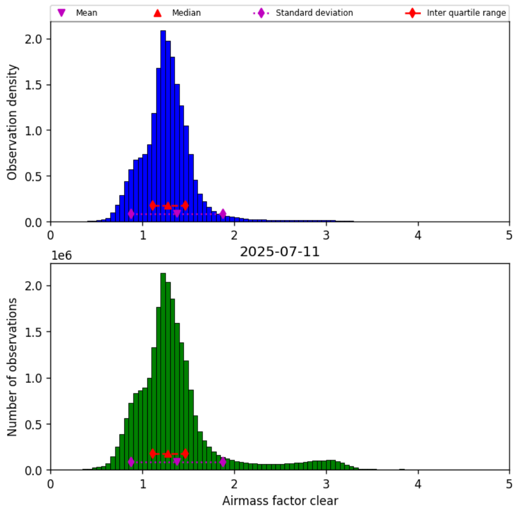
Figure 42: Histogram of “Airmass factor clear” for 2025-07-10 to 2025-07-12
