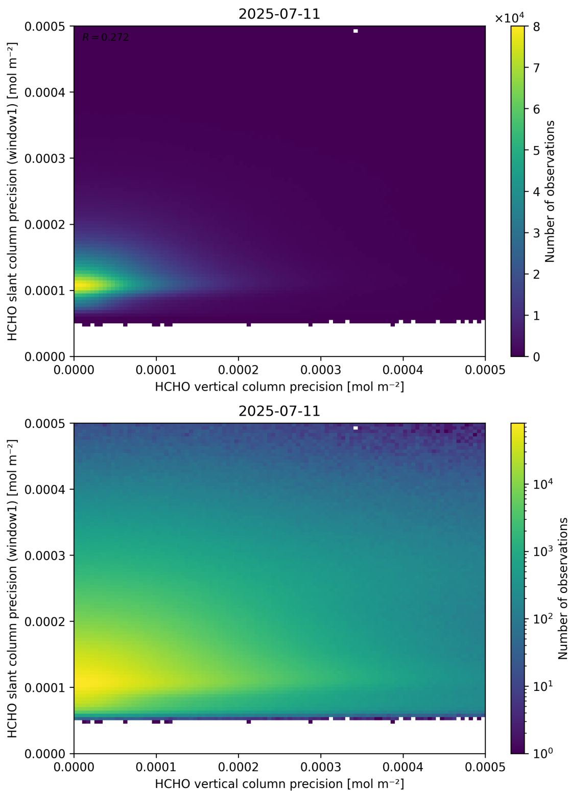
Figure 143: Scatter density plot of “HCHO vertical column precision” against “HCHO slant column precision (window1)” for 2025-07-10 to 2025-07-12.
