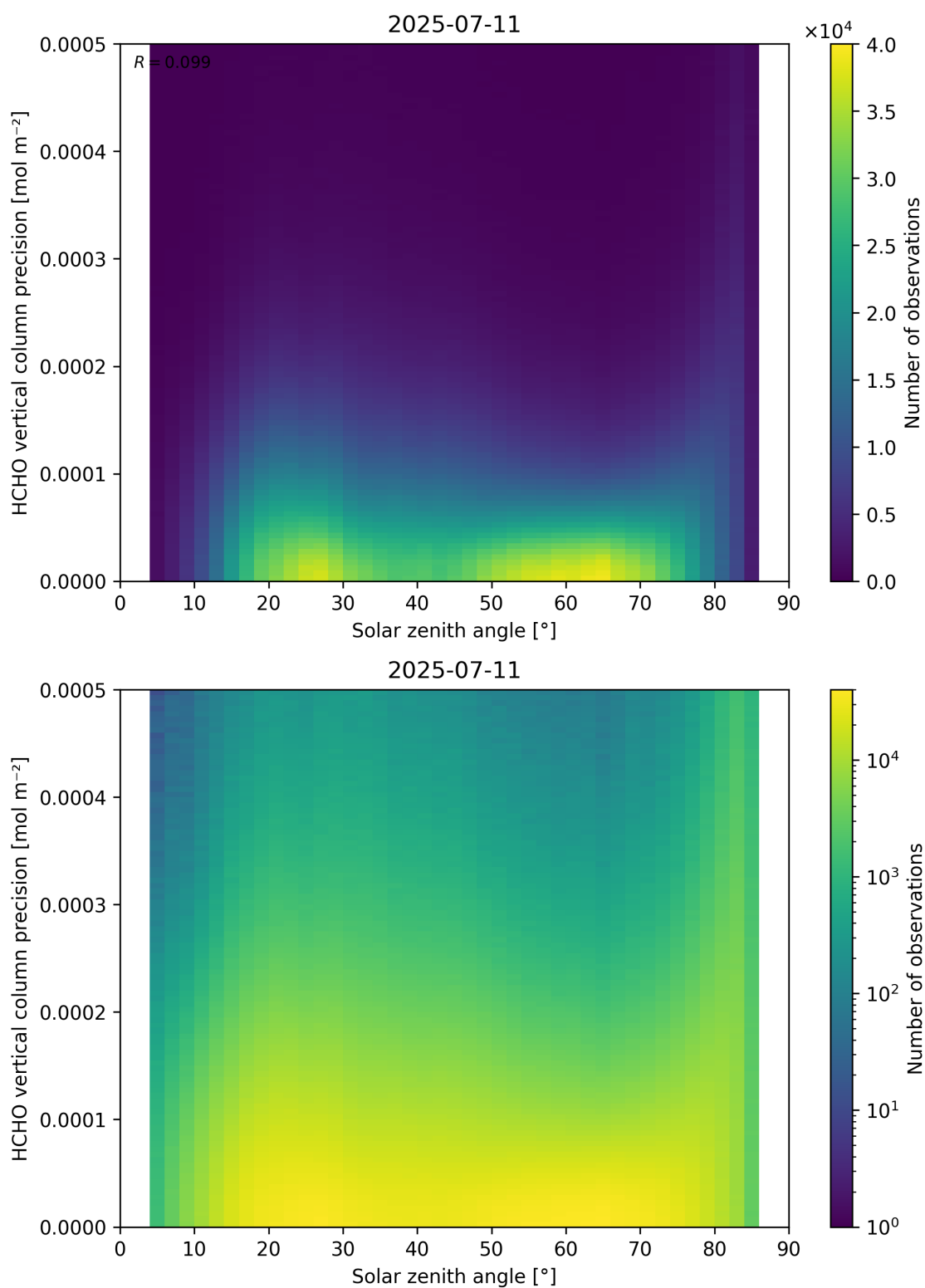
Figure 179: Scatter density plot of “Solar zenith angle” against “HCHO vertical column precision” for 2025-07-10 to 2025-07-12.
