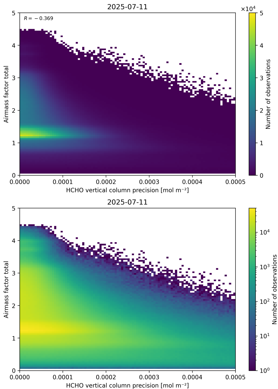
Figure 144: Scatter density plot of “HCHO vertical column precision” against “Airmass factor total” for 2025-07-10 to 2025-07-12.
