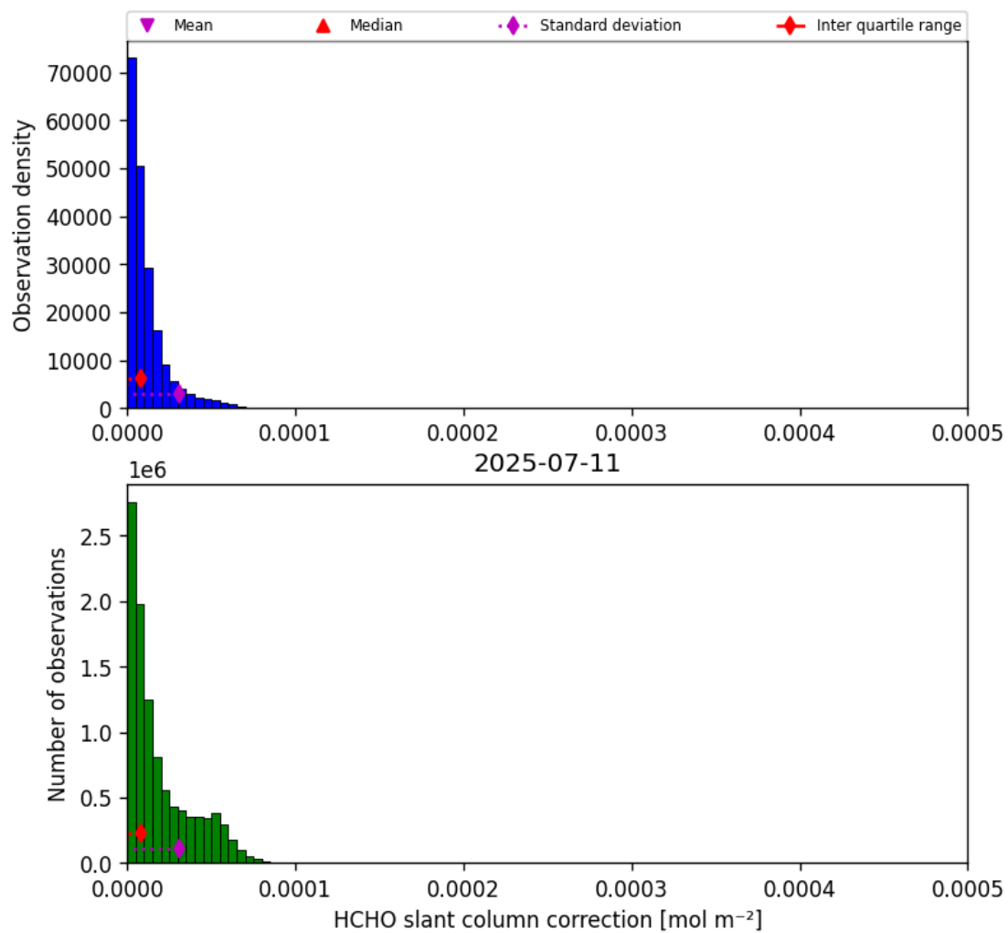
Figure 47: Histogram of “HCHO slant column correction” for 2025-07-10 to 2025-07-12
