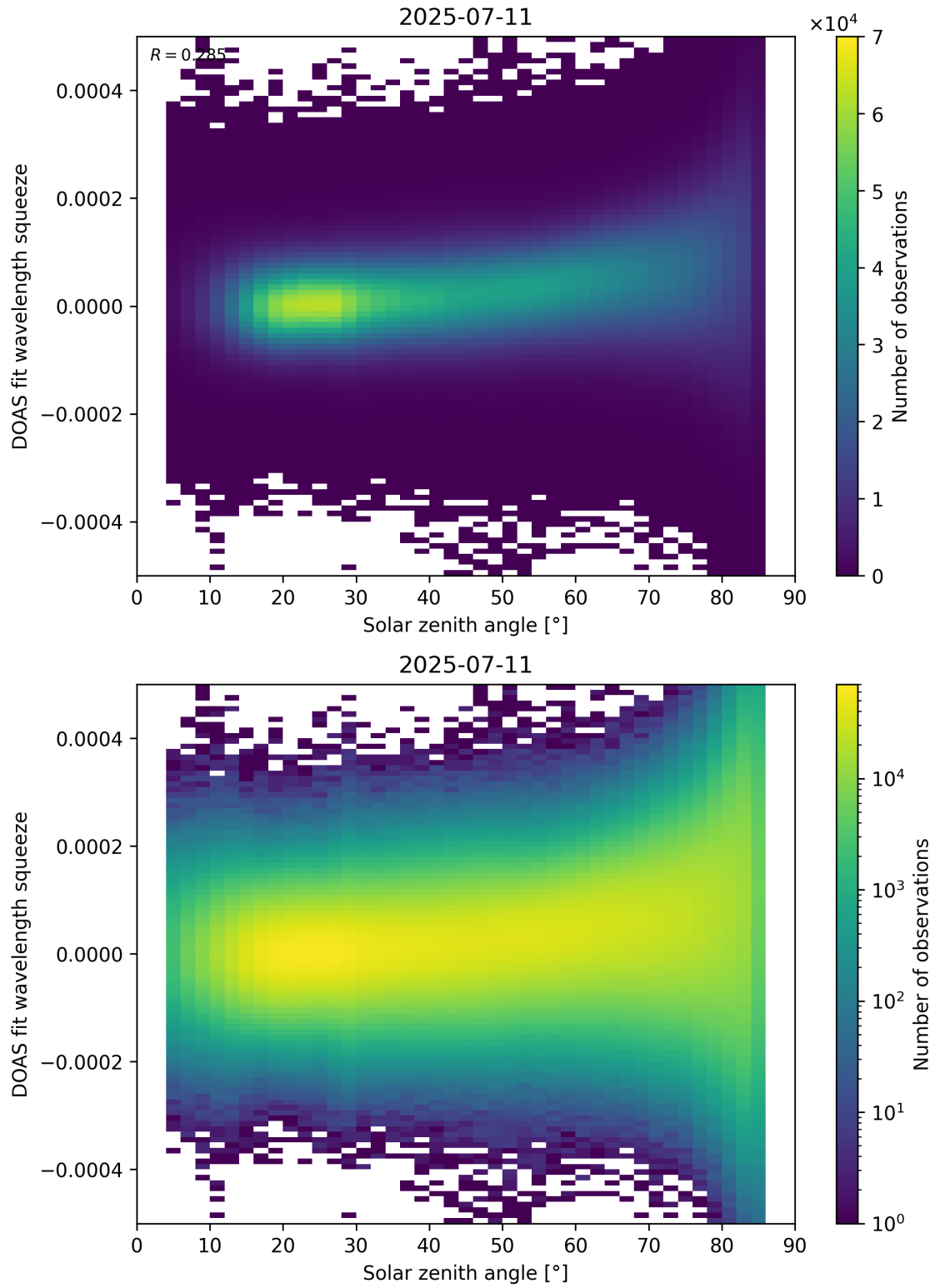
Figure 169: Scatter density plot of “Solar zenith angle” against “DOAS fit wavelength squeeze” for 2025-07-10 to 2025-07-12.
