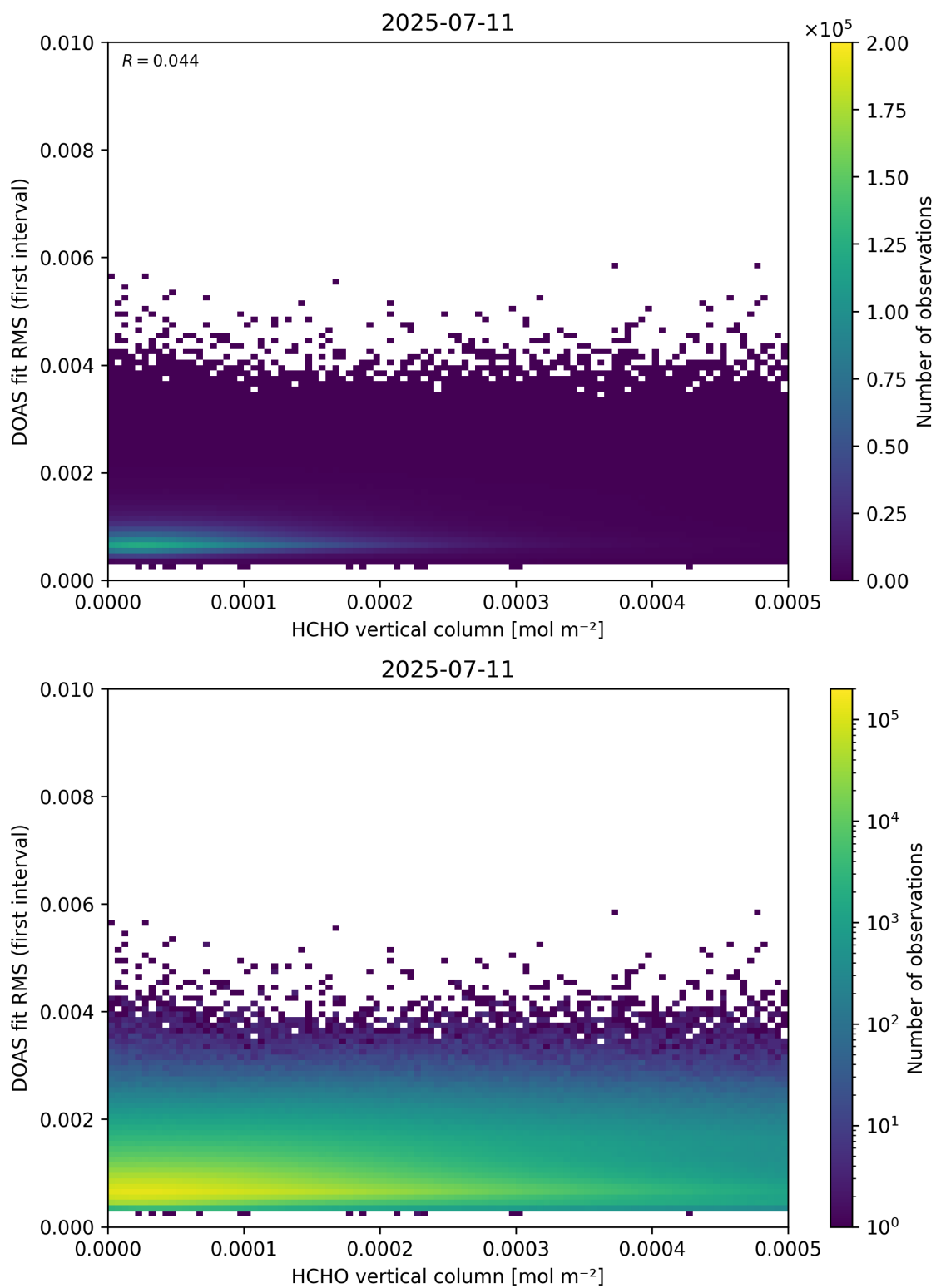
Figure 123: Scatter density plot of “HCHO vertical column” against “DOAS fit RMS (first interval)” for 2025-07-10 to 2025-07-12.
