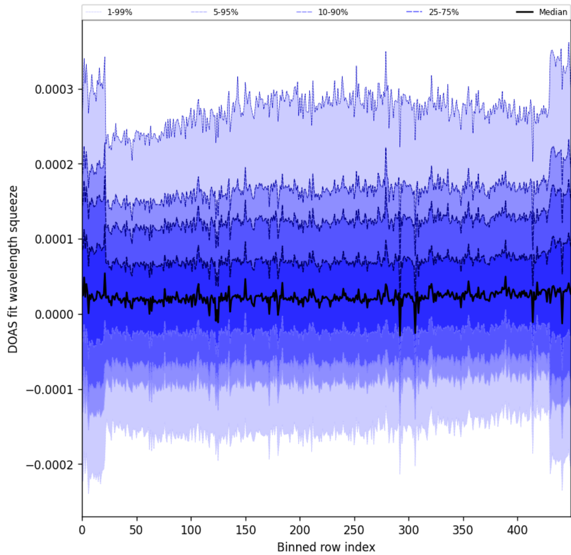
Figure 59: Along track statistics of “DOAS fit wavelength squeeze” for 2025-07-10 to 2025-07-12
