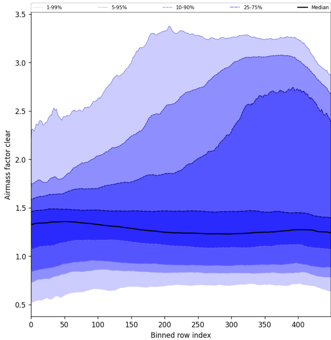
Figure 56: Along track statistics of “Airmass factor clear” for 2025-07-10 to 2025-07-12
