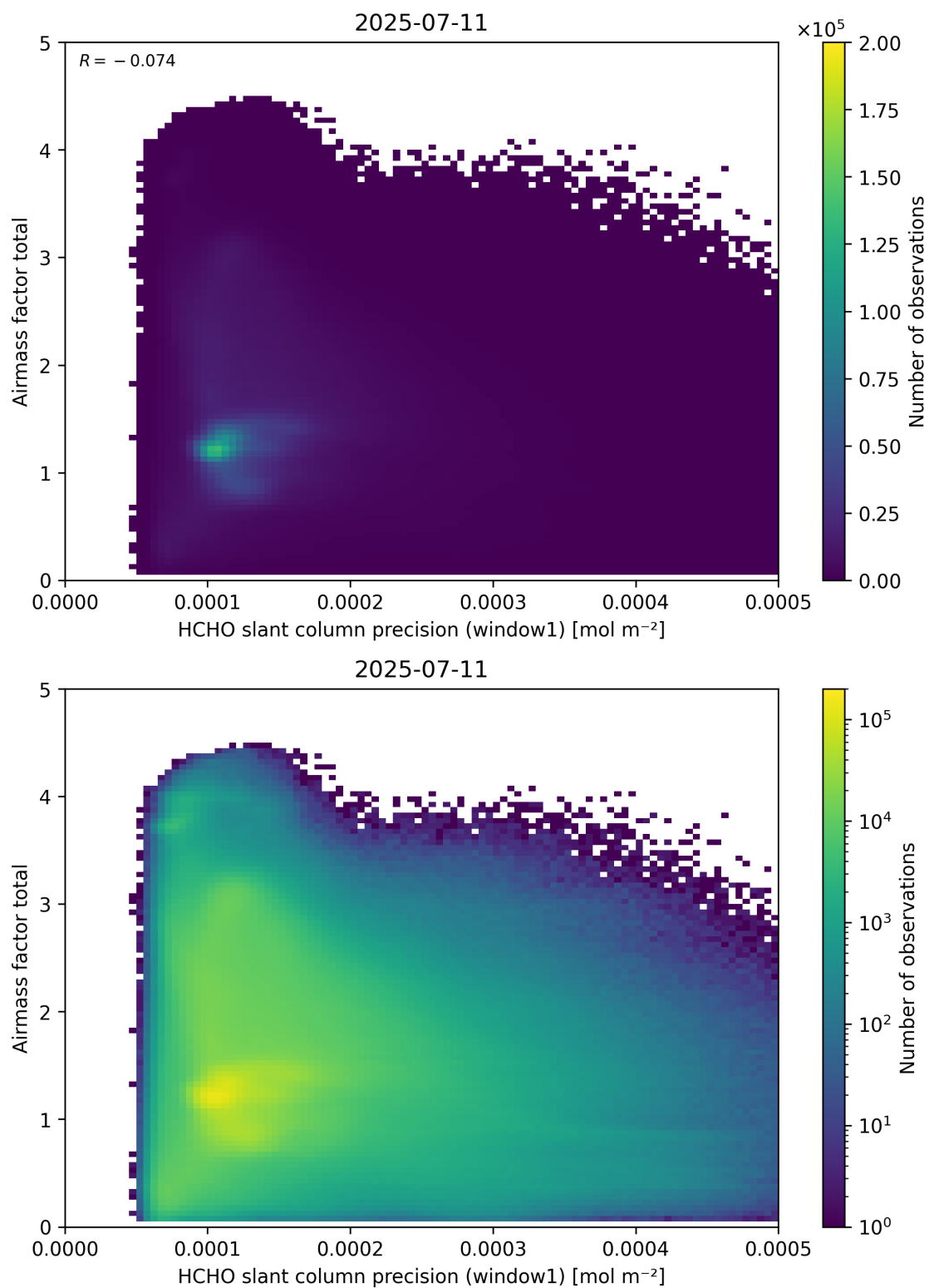
Figure 94: Scatter density plot of “HCHO slant column precision (window1)” against “Airmass factor total” for 2025-07-10 to 2025-07-12.
