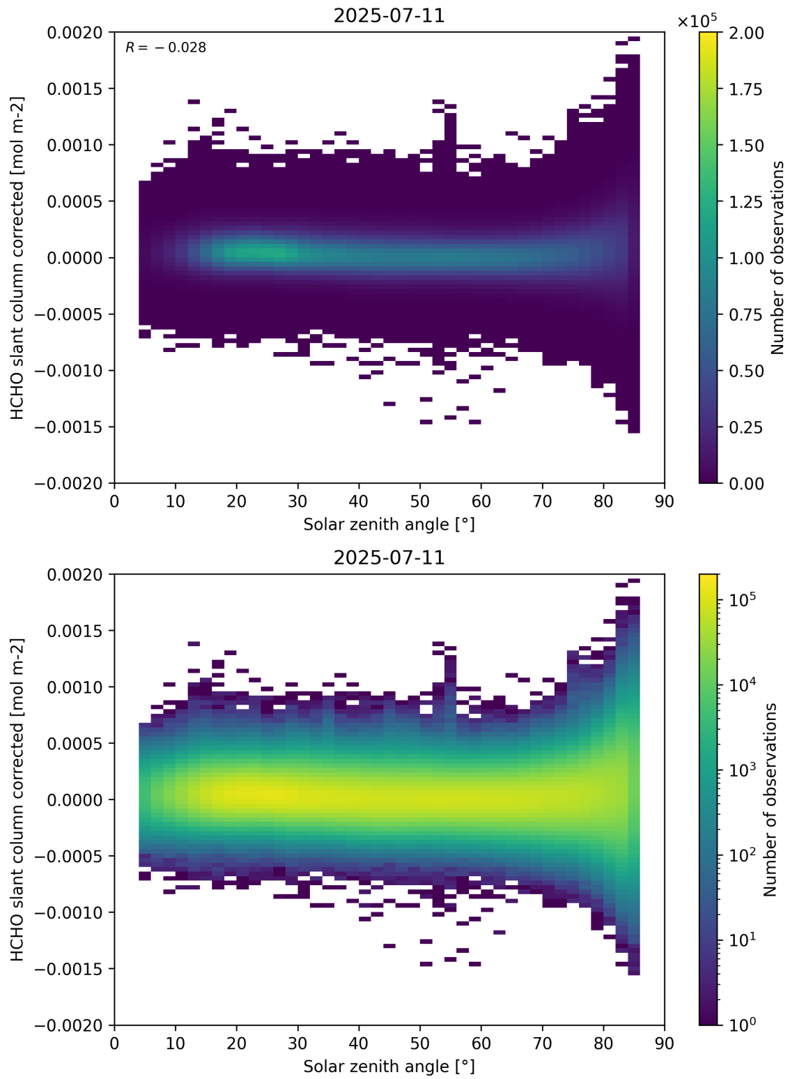
Figure 171: Scatter density plot of “Solar zenith angle” against “HCHO slant column corrected” for 2025-07-10 to 2025-07-12.
