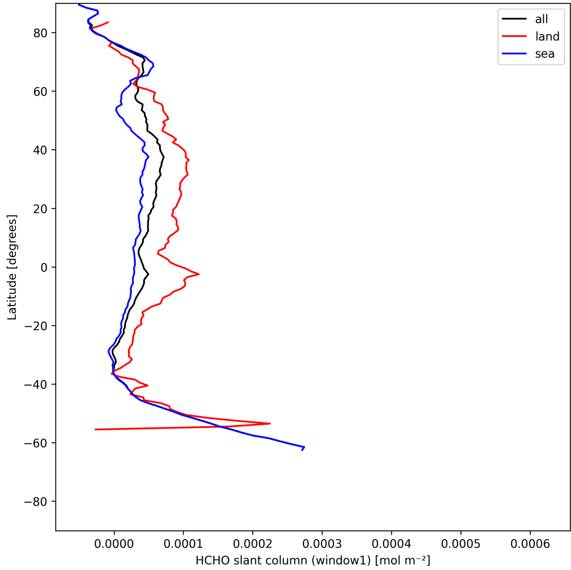
Figure 24: Zonal average of “HCHO slant column (window1)” for 2025-07-10 to 2025-07-12.
