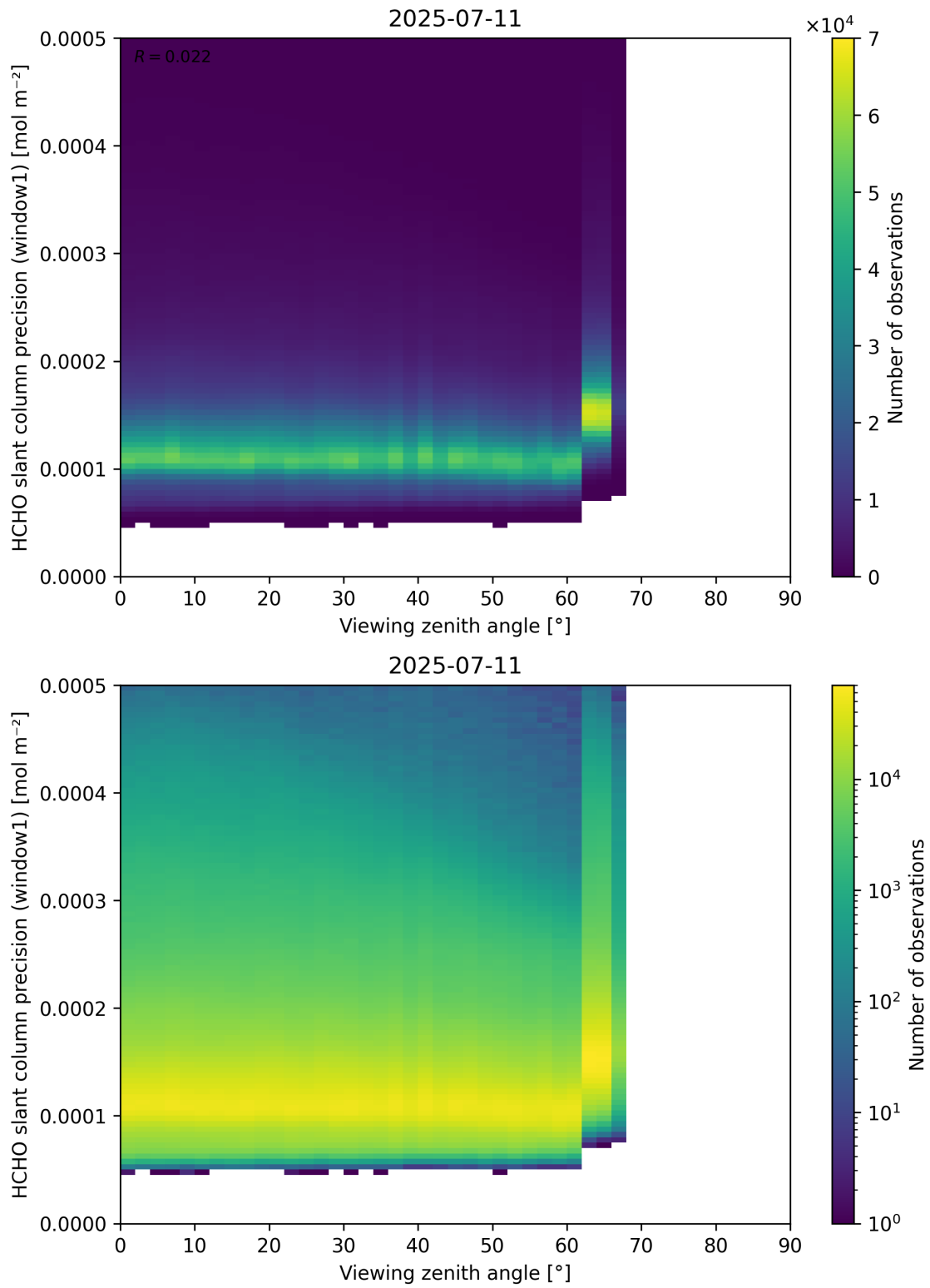
Figure 189: Scatter density plot of “Viewing zenith angle” against “HCHO slant column precision (window1)” for 2025-07-10 to 2025-07-12.
