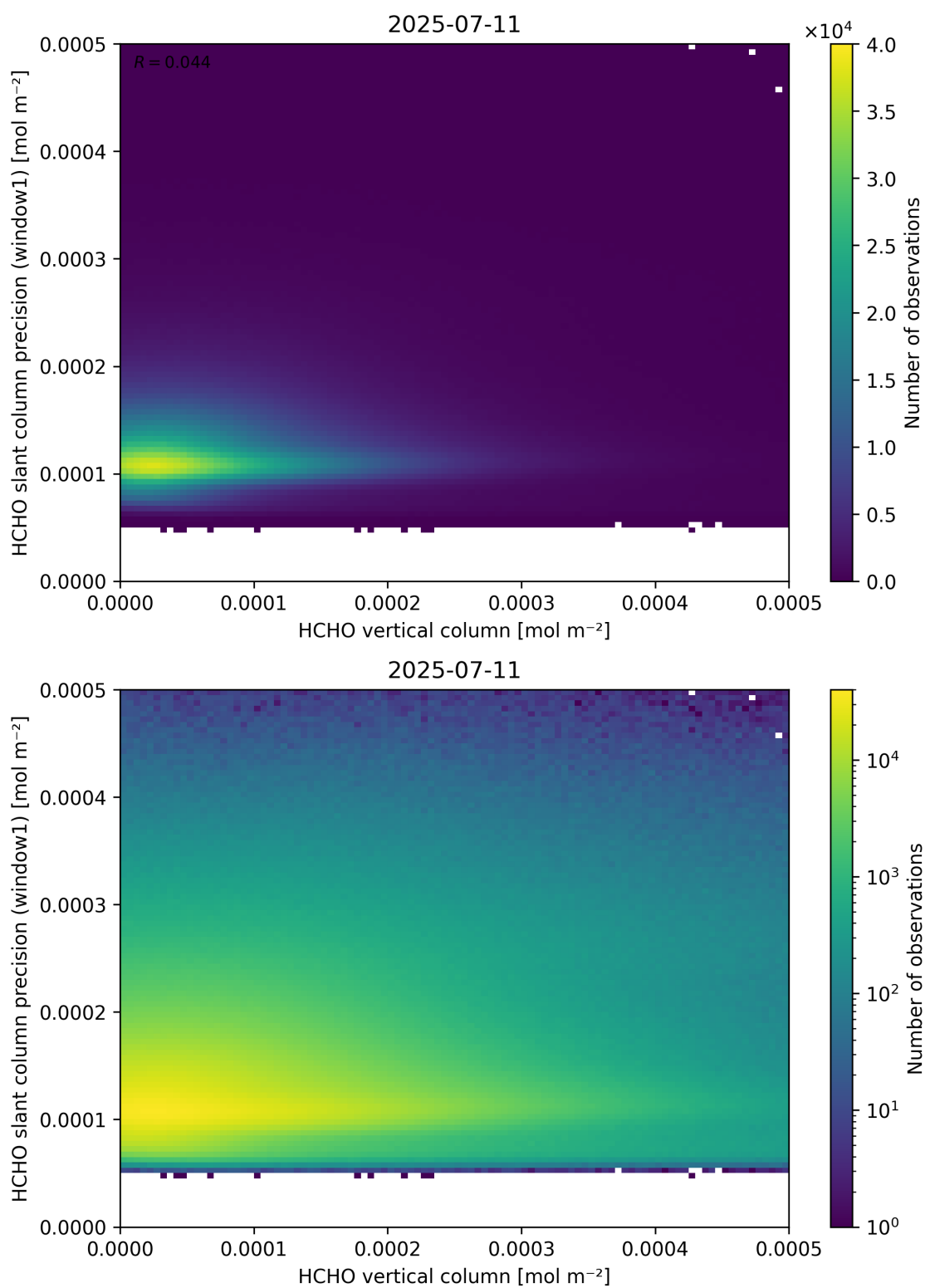
Figure 130: Scatter density plot of “HCHO vertical column” against “HCHO slant column precision (window1)” for 2025-07-10 to 2025-07-12.
