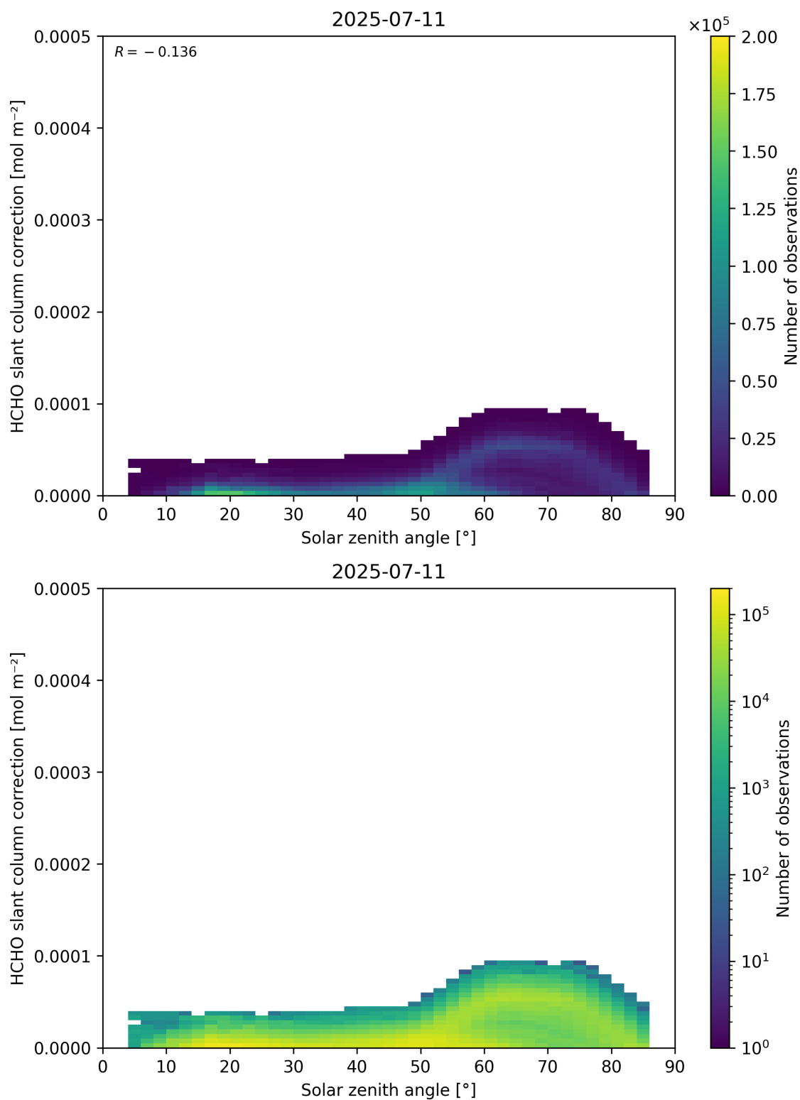
Figure 172: Scatter density plot of “Solar zenith angle” against “HCHO slant column correction” for 2025-07-10 to 2025-07-12.
