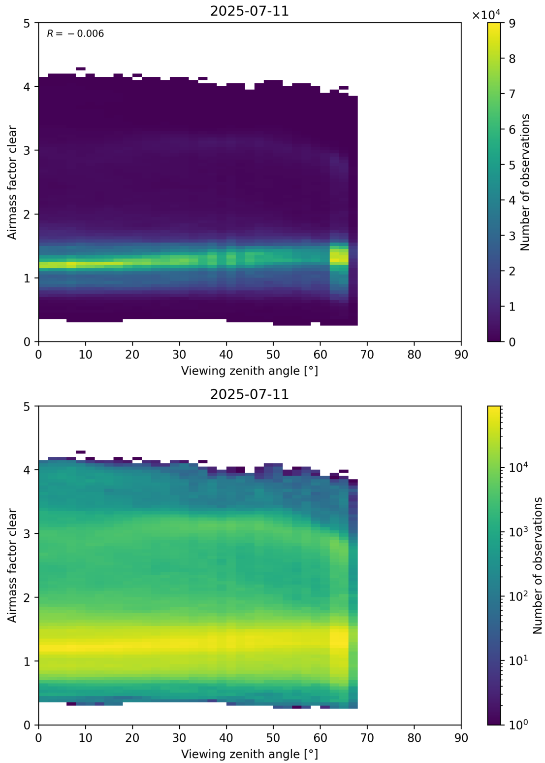
Figure 185: Scatter density plot of “Viewing zenith angle” against “Airmass factor clear” for 2025-07-10 to 2025-07-12.
