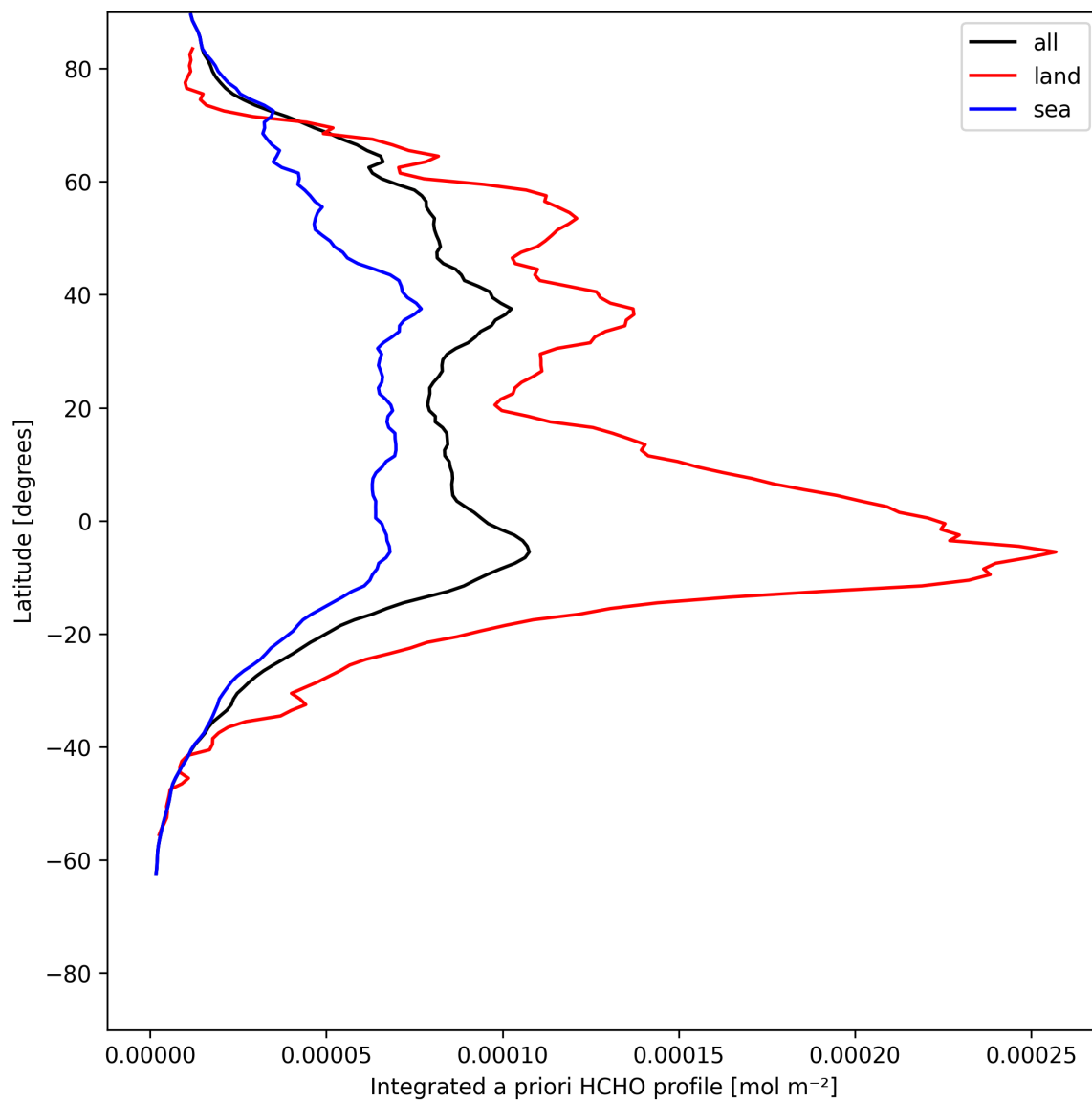
Figure 29: Zonal average of “Integrated a priori HCHO profile” for 2025-07-10 to 2025-07-12.
