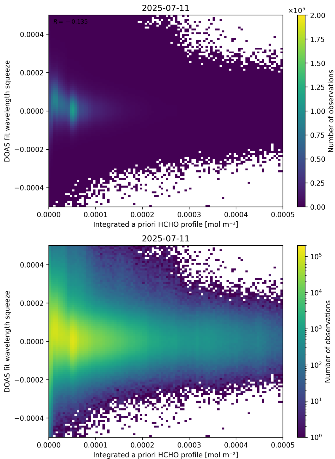
Figure 150: Scatter density plot of “Integrated a priori HCHO profile” against “DOAS fit wavelength squeeze” for 2025-07-10 to 2025-07-12.
