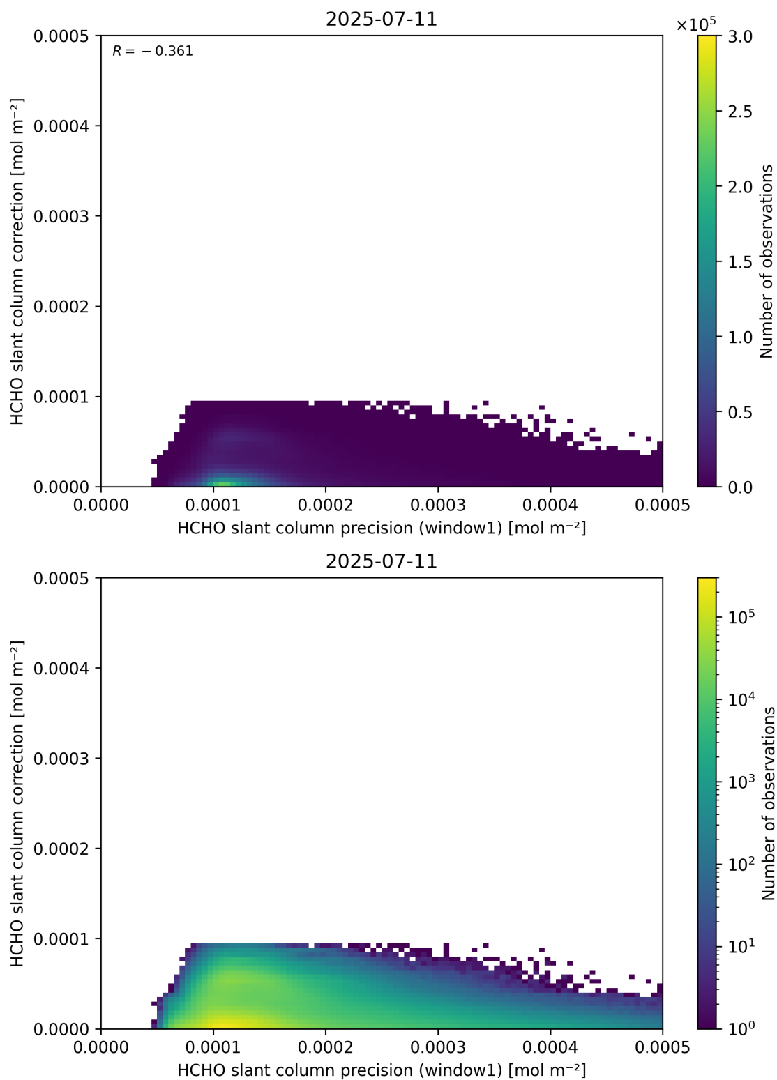
Figure 93: Scatter density plot of “HCHO slant column precision (window1)” against “HCHO slant column correction” for 2025-07-10 to 2025-07-12.
