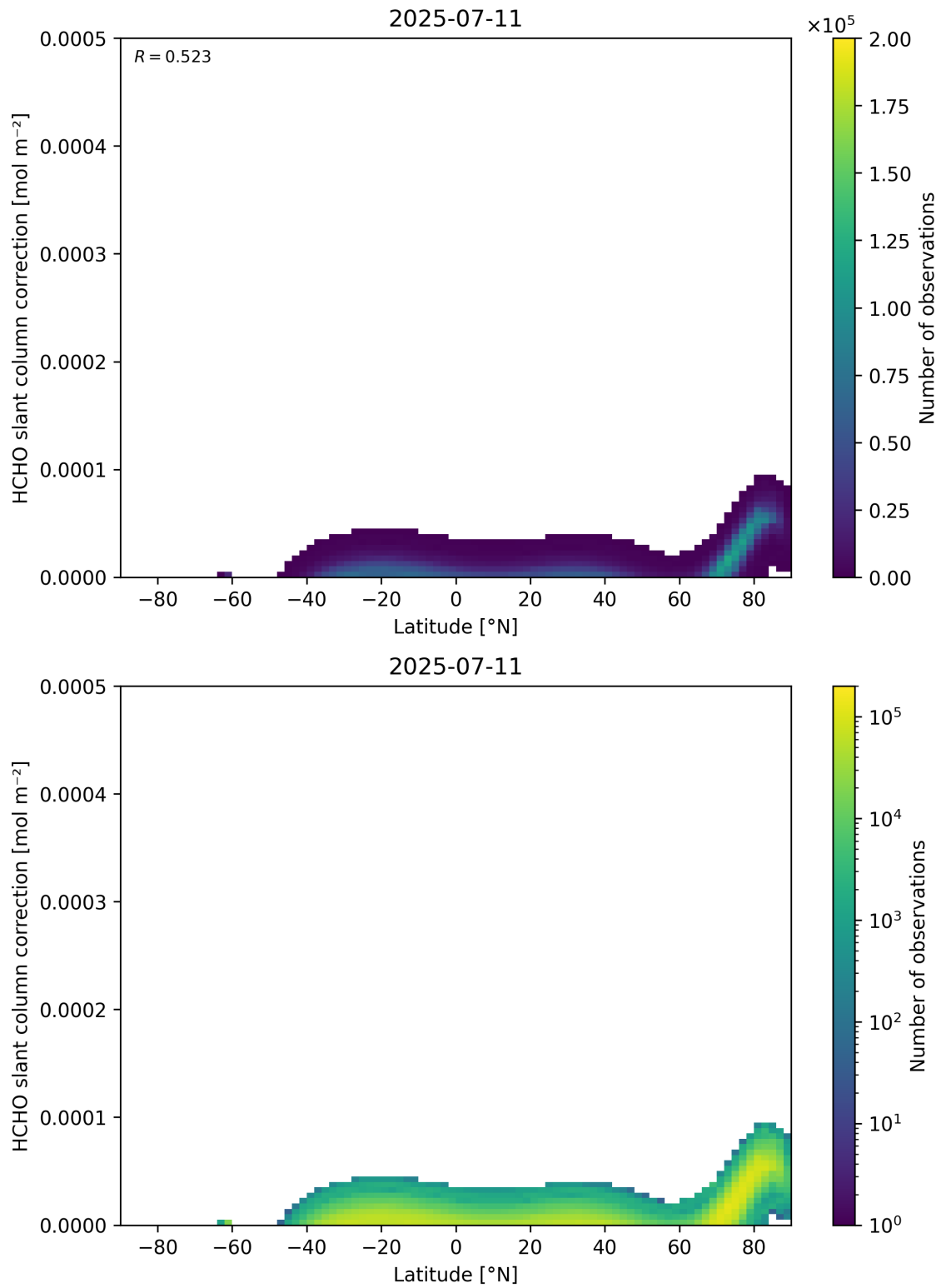
Figure 158: Scatter density plot of “Latitude” against “HCHO slant column correction” for 2025-07-10 to 2025-07-12.
