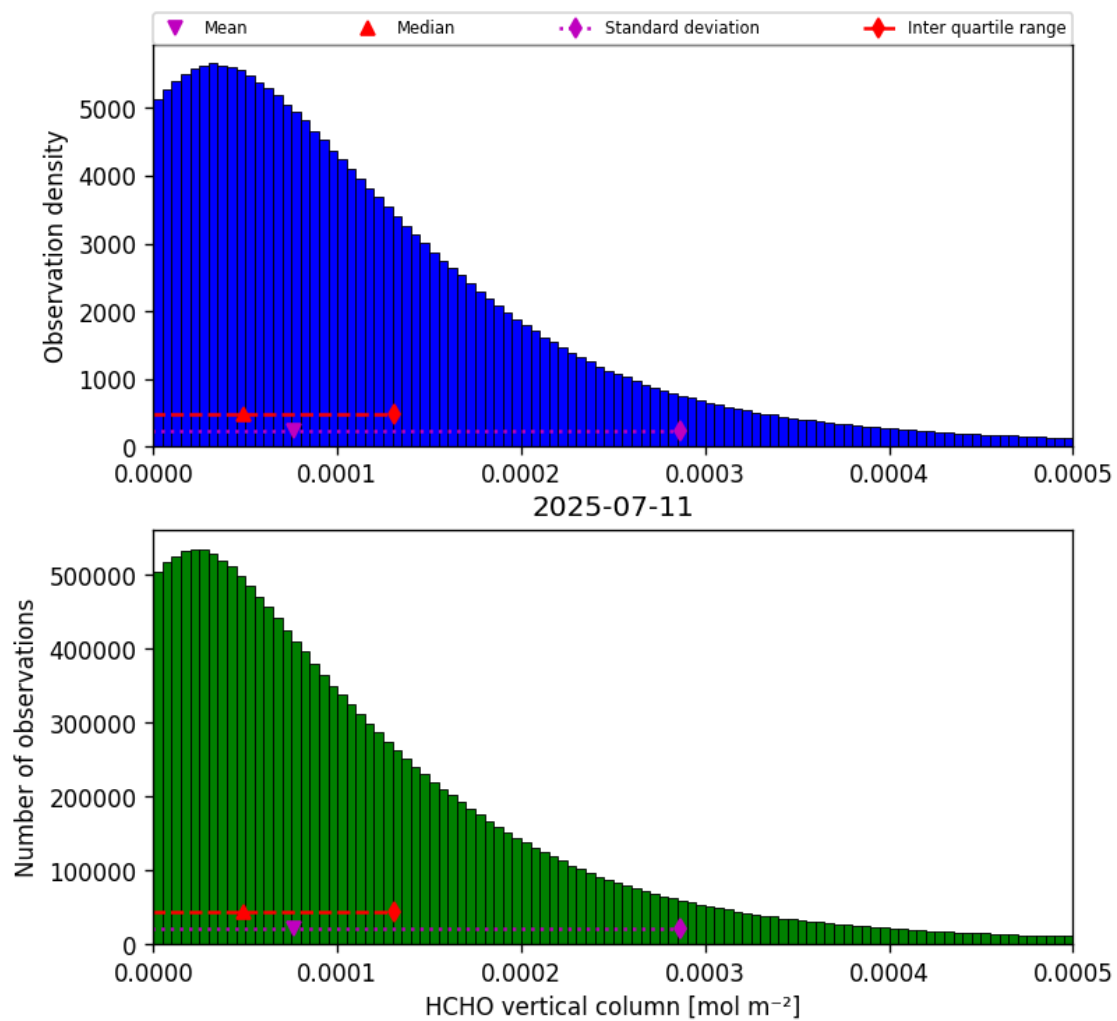
Figure 35: Histogram of “HCHO vertical column” for 2025-07-10 to 2025-07-12
