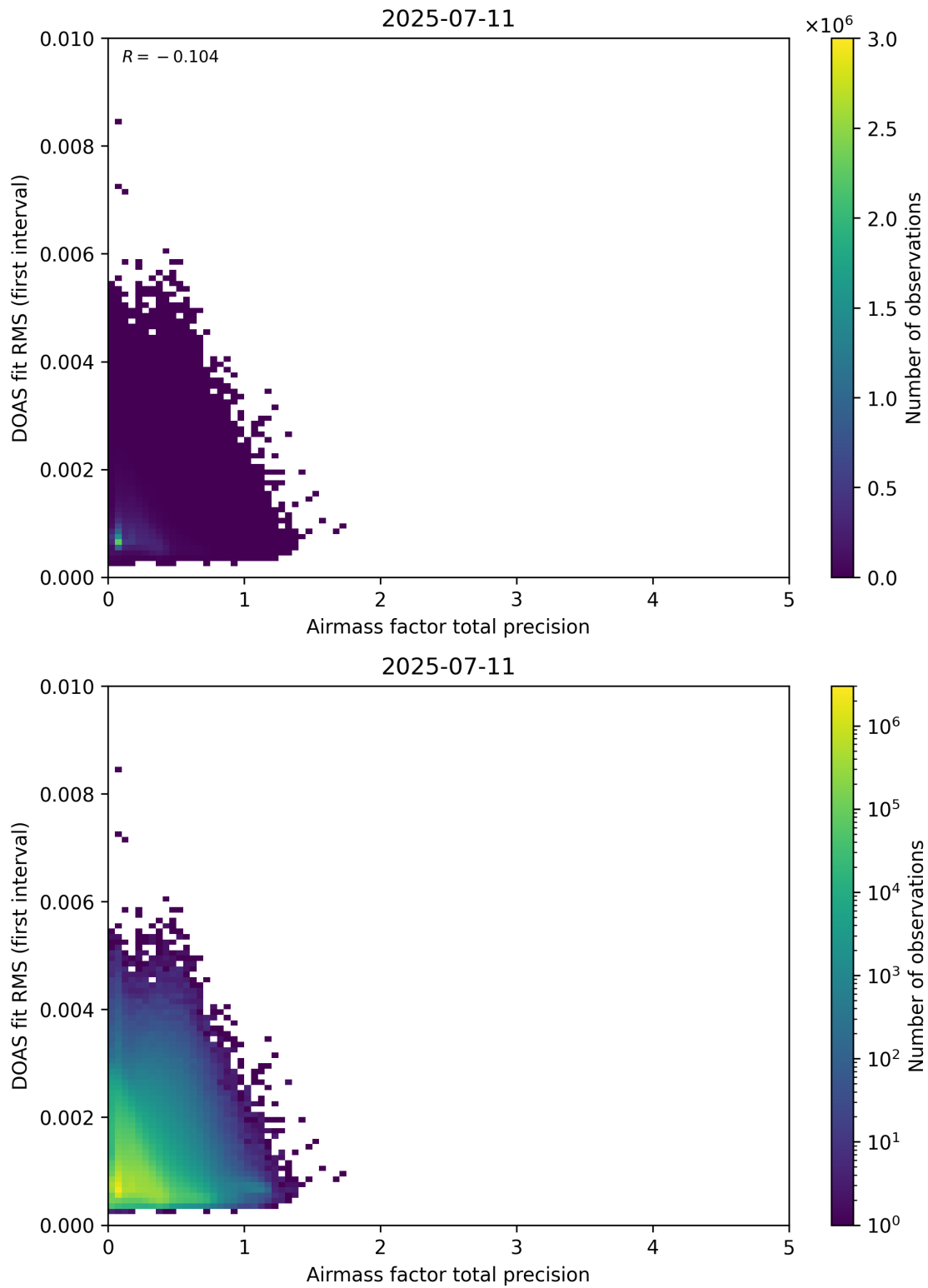
Figure 105: Scatter density plot of “Airmass factor total precision” against “DOAS fit RMS (first interval)” for 2025-07-10 to 2025-07-12.
