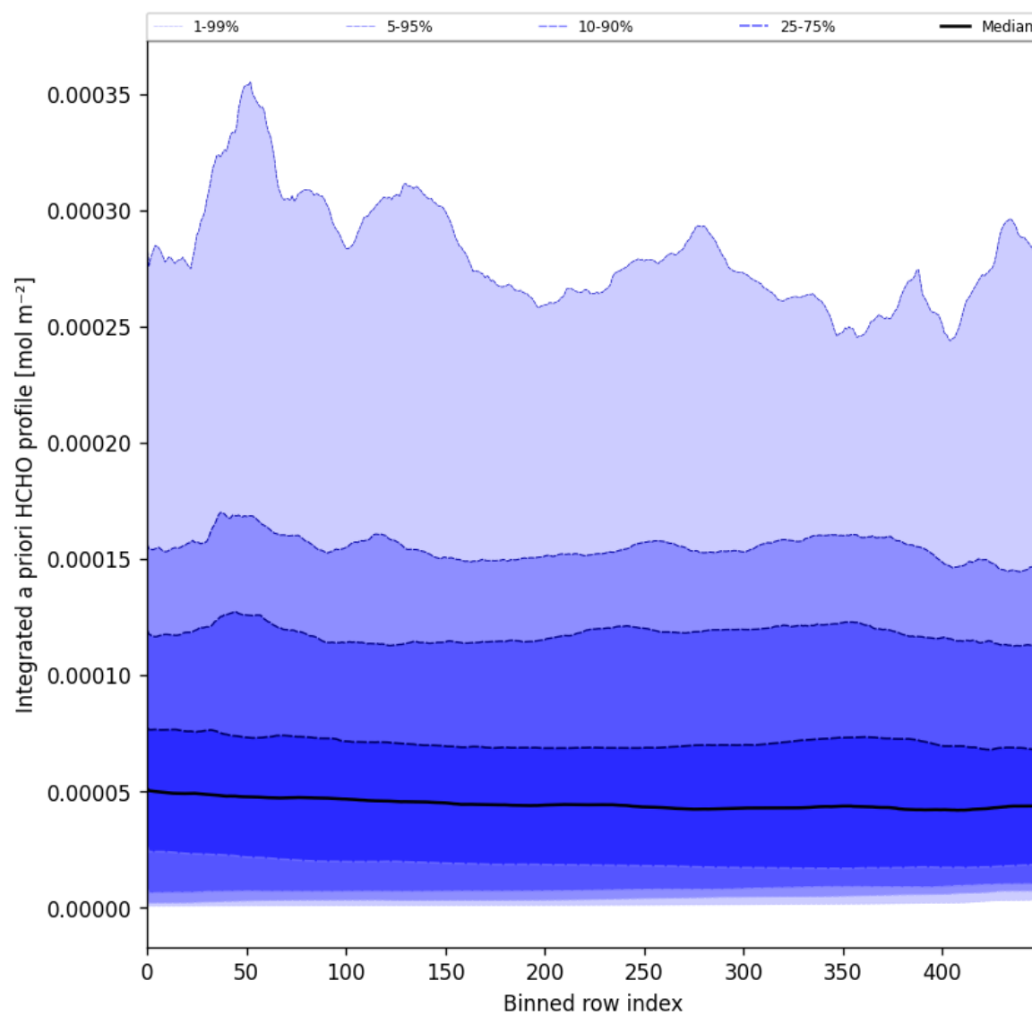
Figure 57: Along track statistics of "Integrated a priori HCHO profile" for 2025-07-10 to 2025-07-12
