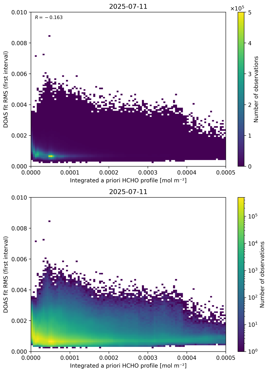
Figure 148: Scatter density plot of “Integrated a priori HCHO profile” against “DOAS fit RMS (first interval)” for 2025-07-10 to 2025-07-12.
