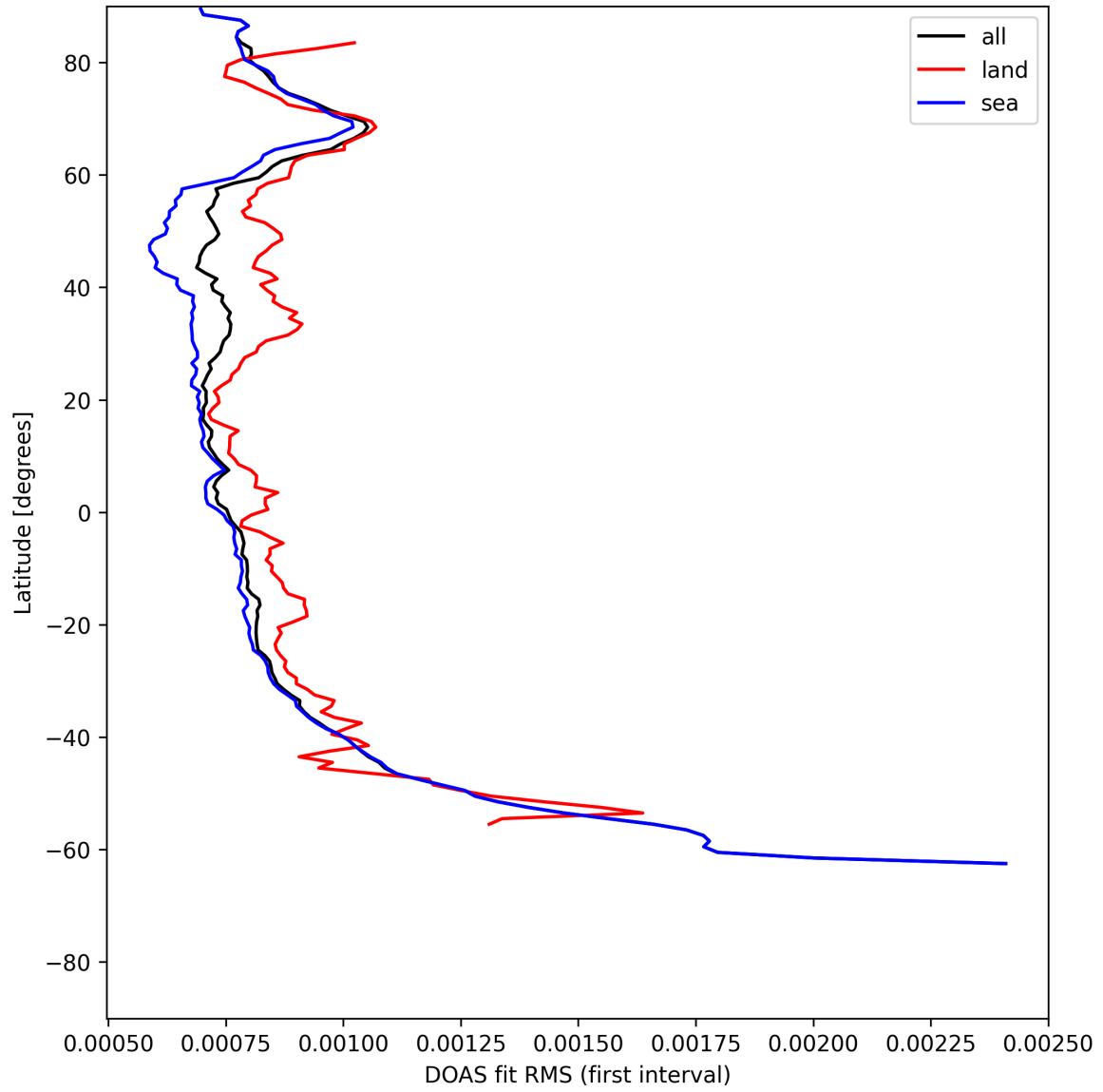
Figure 32: Zonal average of "DOAS fit RMS (first interval)" for 2025-07-10 to 2025-07-12.
