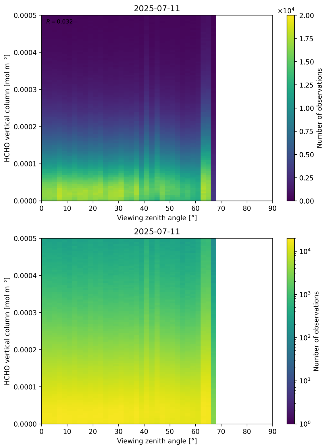
Figure 192: Scatter density plot of “Viewing zenith angle” against “HCHO vertical column” for 2025-07-10 to 2025-07-12.
