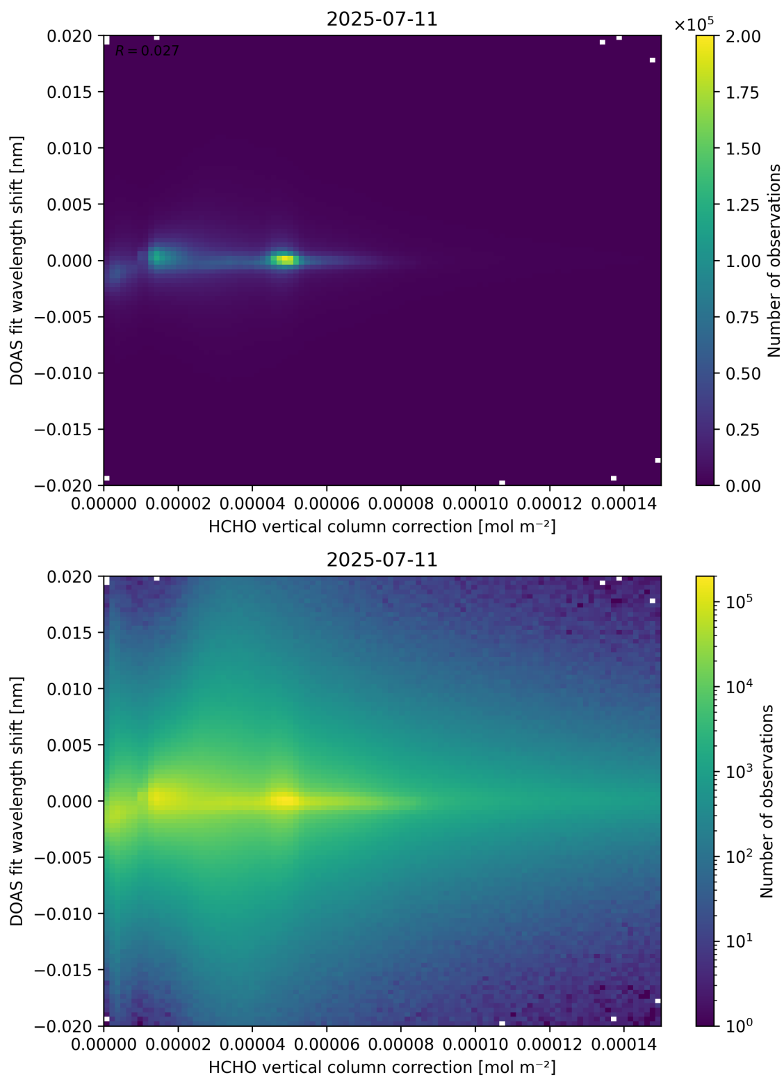
Figure 113: Scatter density plot of “HCHO vertical column correction” against “DOAS fit wavelength shift” for 2025-07-10 to 2025-07-12.
