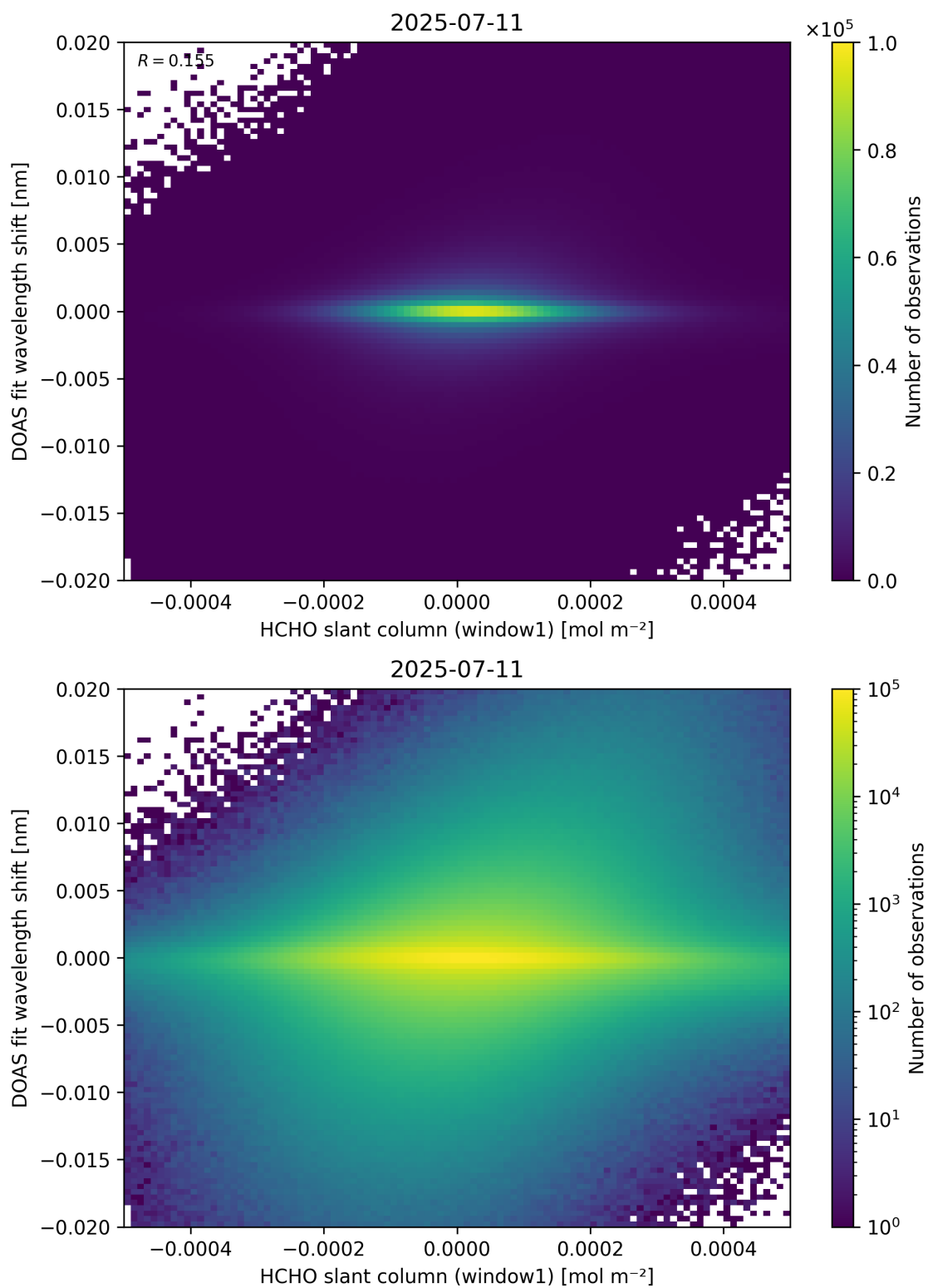
Figure 79: Scatter density plot of “HCHO slant column (window1)” against “DOAS fit wavelength shift” for 2025-07-10 to 2025-07-12.
