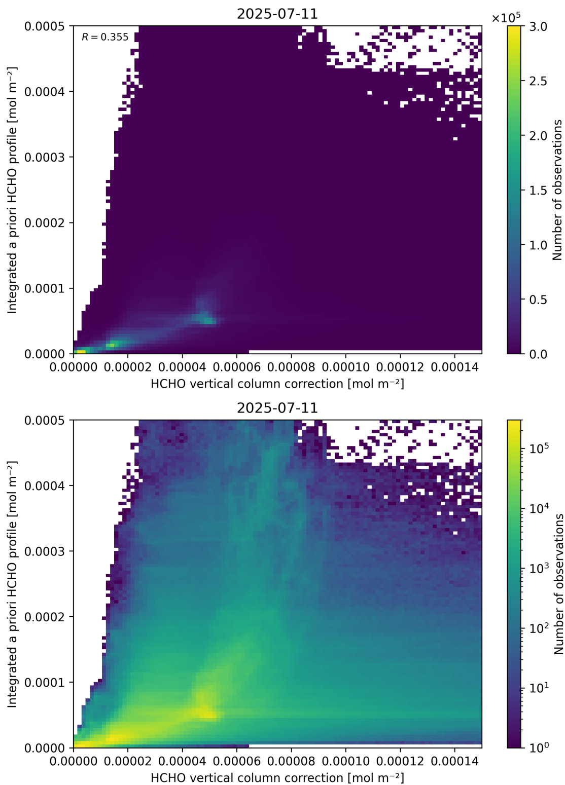
Figure 122: Scatter density plot of “HCHO vertical column correction” against “Integrated a priori HCHO profile” for 2025-07-10 to 2025-07-12.
