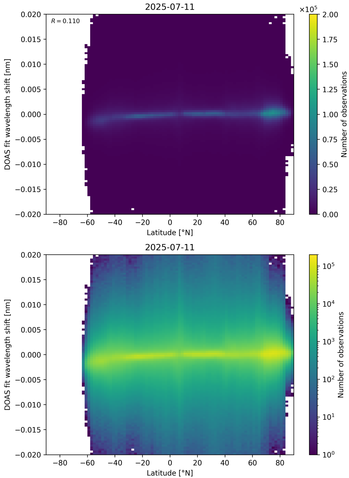
Figure 154: Scatter density plot of “Latitude” against “DOAS fit wavelength shift” for 2025-07-10 to 2025-07-12.
