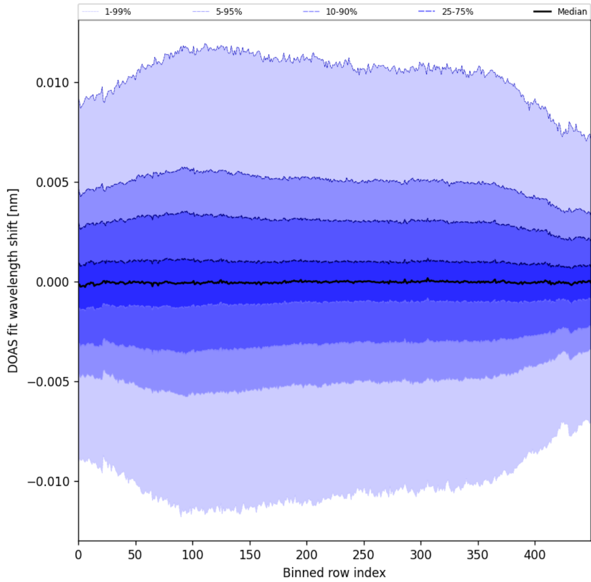
Figure 58: Along track statistics of “DOAS fit wavelength shift” for 2025-07-10 to 2025-07-12
