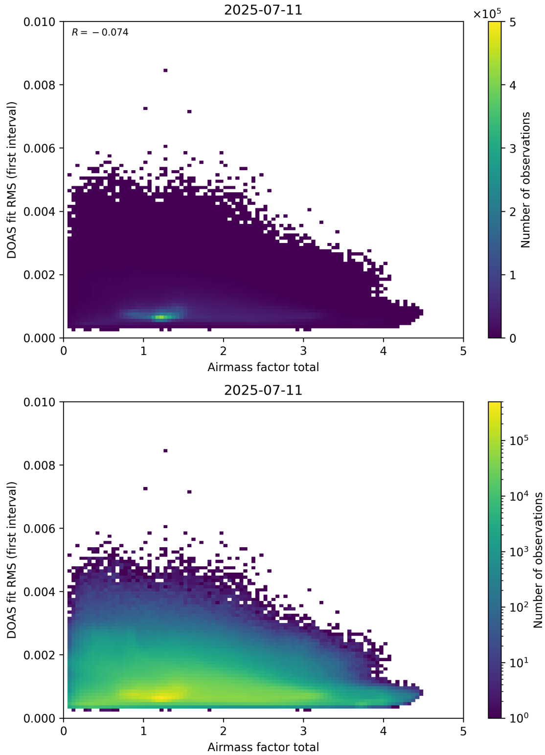
Figure 97: Scatter density plot of “Airmass factor total” against “DOAS fit RMS (first interval)” for 2025-07-10 to 2025-07-12.
