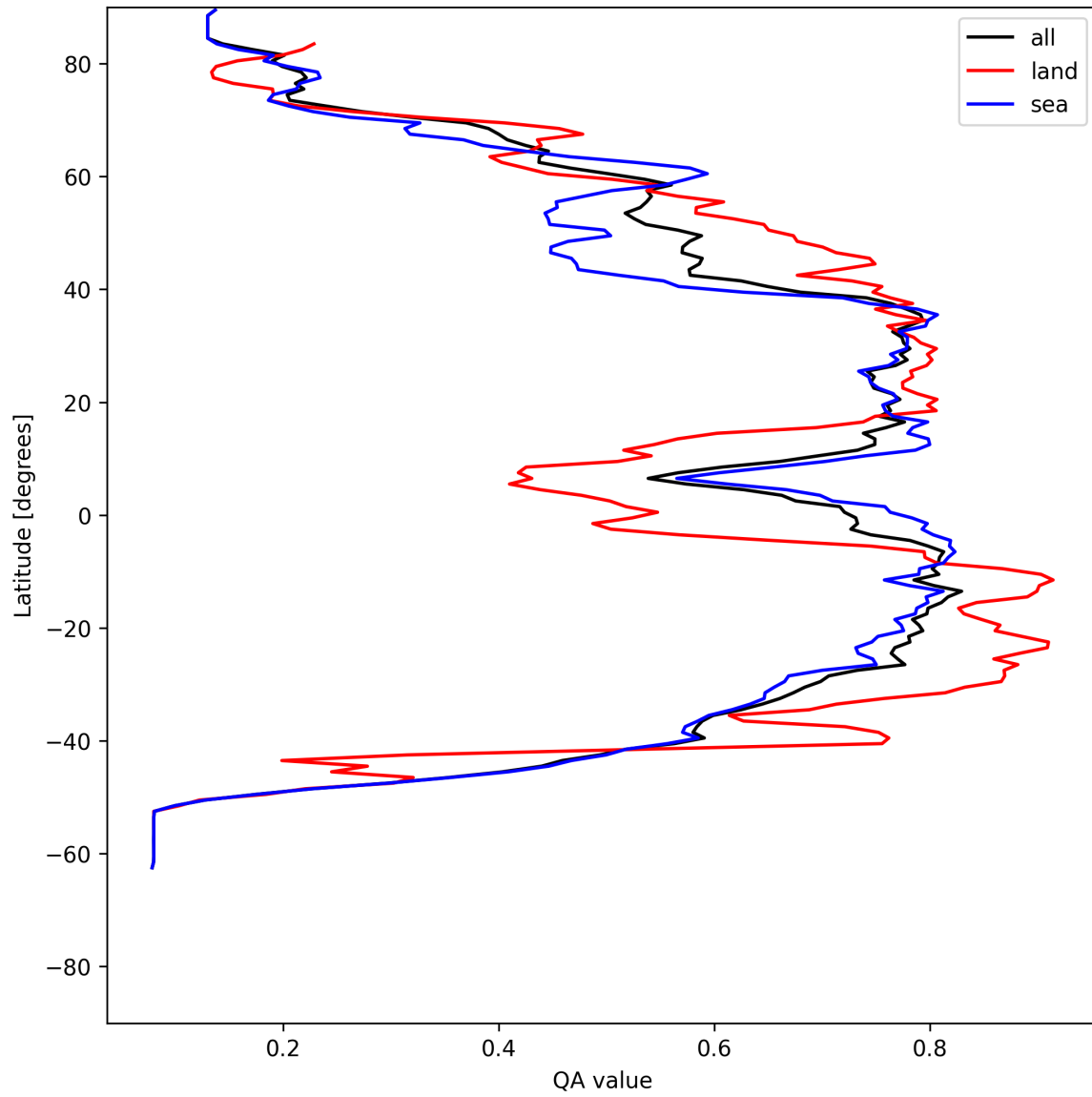
Figure 20: Zonal average of “QA value” for 2025-07-10 to 2025-07-12.
