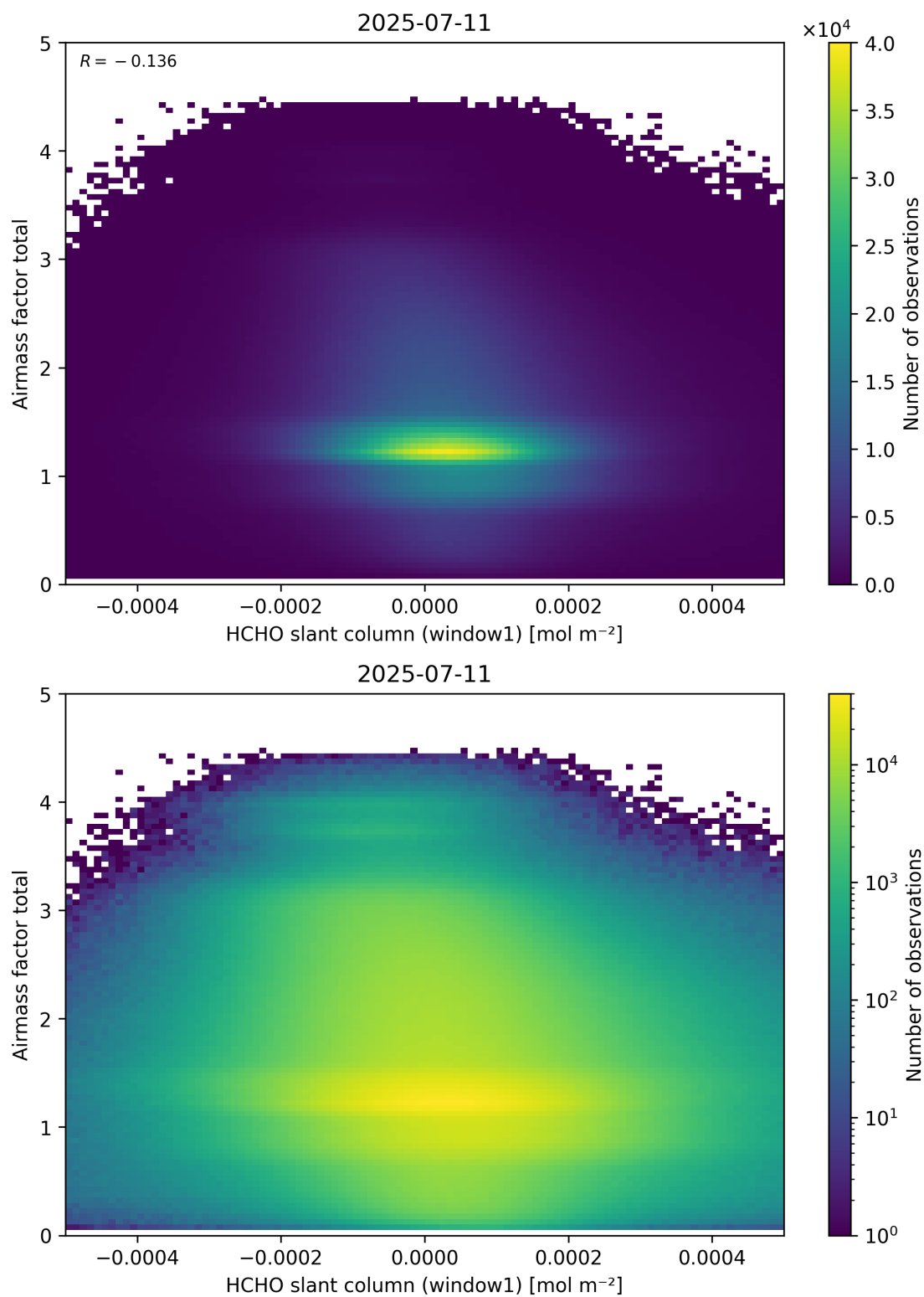
Figure 85: Scatter density plot of “HCHO slant column (window1)” against “Airmass factor total” for 2025-07-10 to 2025-07-12.
