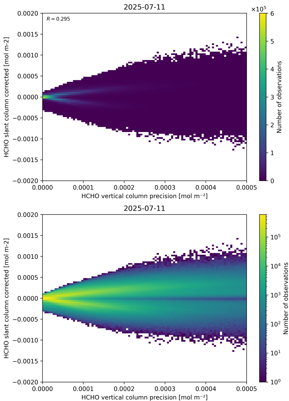
Figure 140: Scatter density plot of “HCHO vertical column precision” against “HCHO slant column corrected” for 2025-07-10 to 2025-07-12.
