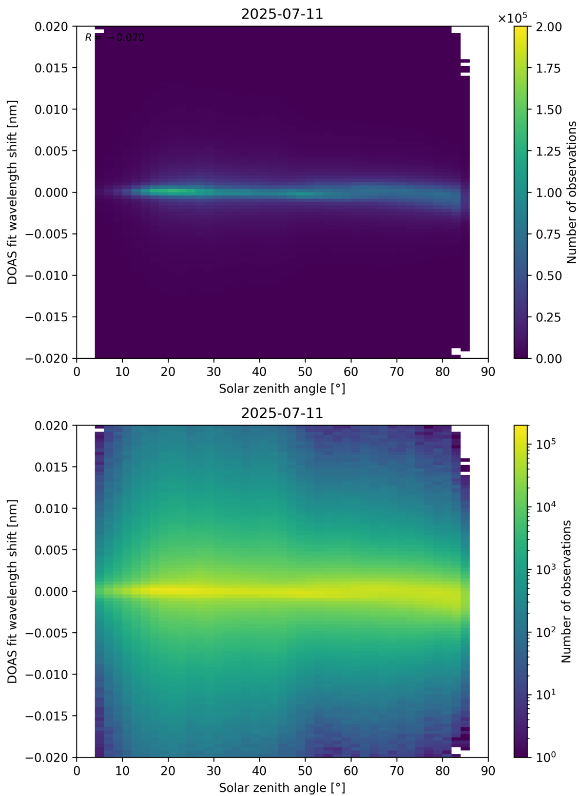
Figure 168: Scatter density plot of “Solar zenith angle” against “DOAS fit wavelength shift” for 2025-07-10 to 2025-07-12.
