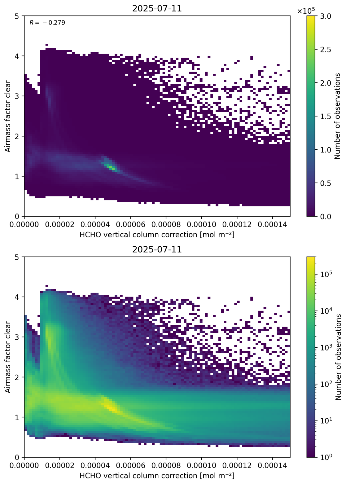
Figure 115: Scatter density plot of “HCHO vertical column correction” against “Airmass factor clear” for 2025-07-10 to 2025-07-12.
