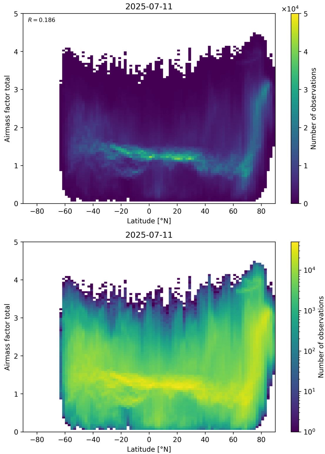
Figure 161: Scatter density plot of “Latitude” against “Airmass factor total” for 2025-07-10 to 2025-07-12.
