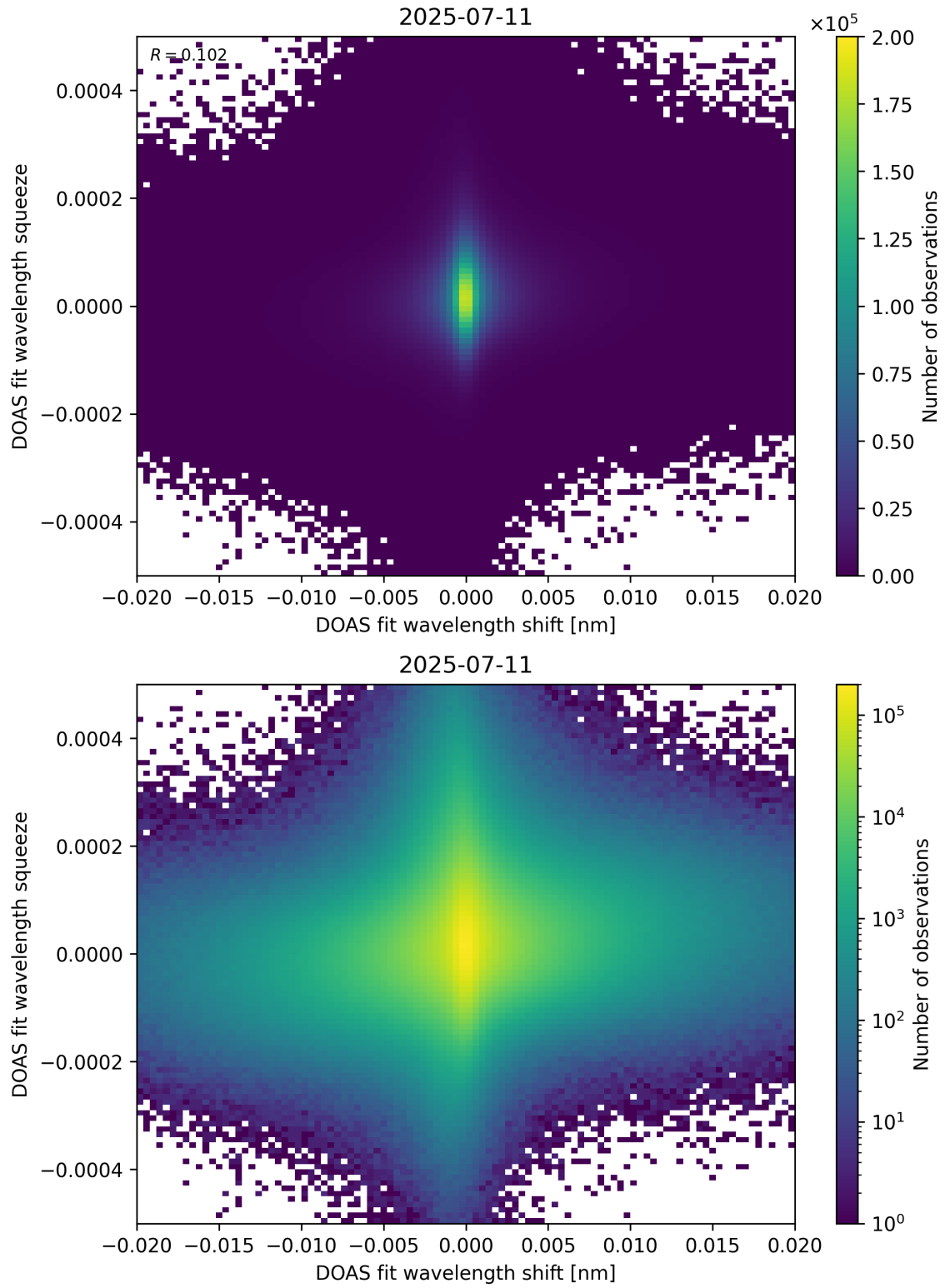
Figure 65: Scatter density plot of “DOAS fit wavelength shift” against “DOAS fit wavelength squeeze” for 2025-07-10 to 2025-07-12.
