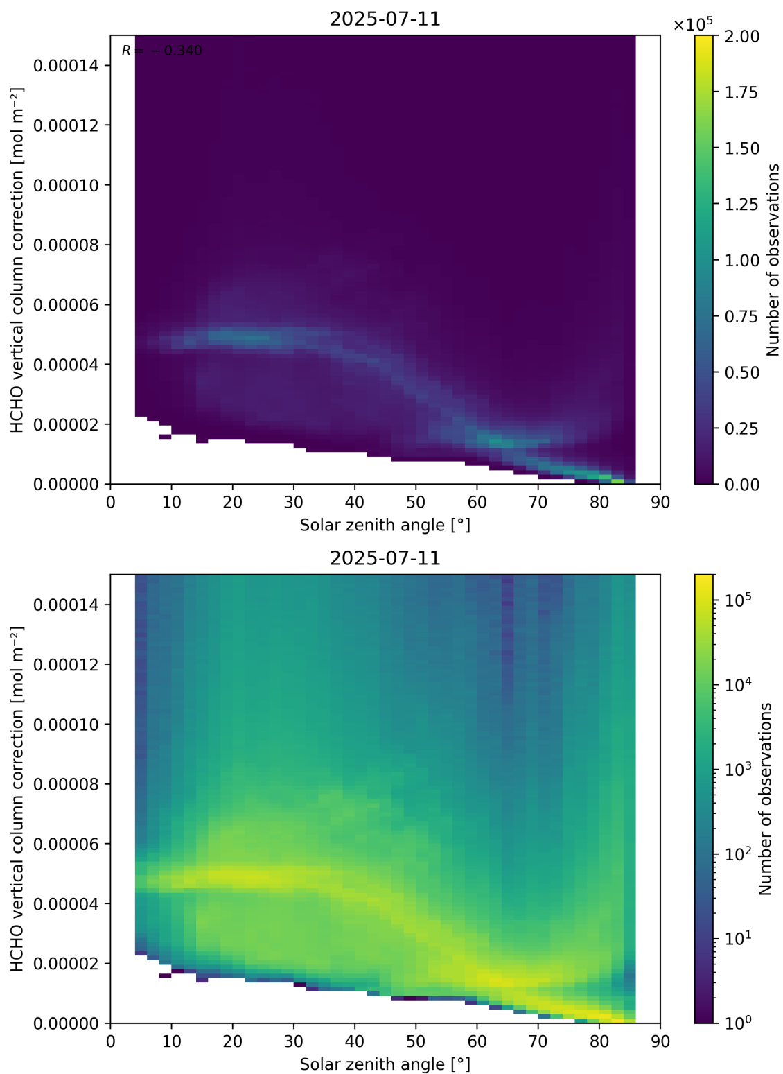
Figure 178: Scatter density plot of “Solar zenith angle” against “HCHO vertical column correction” for 2025-07-10 to 2025-07-12.
