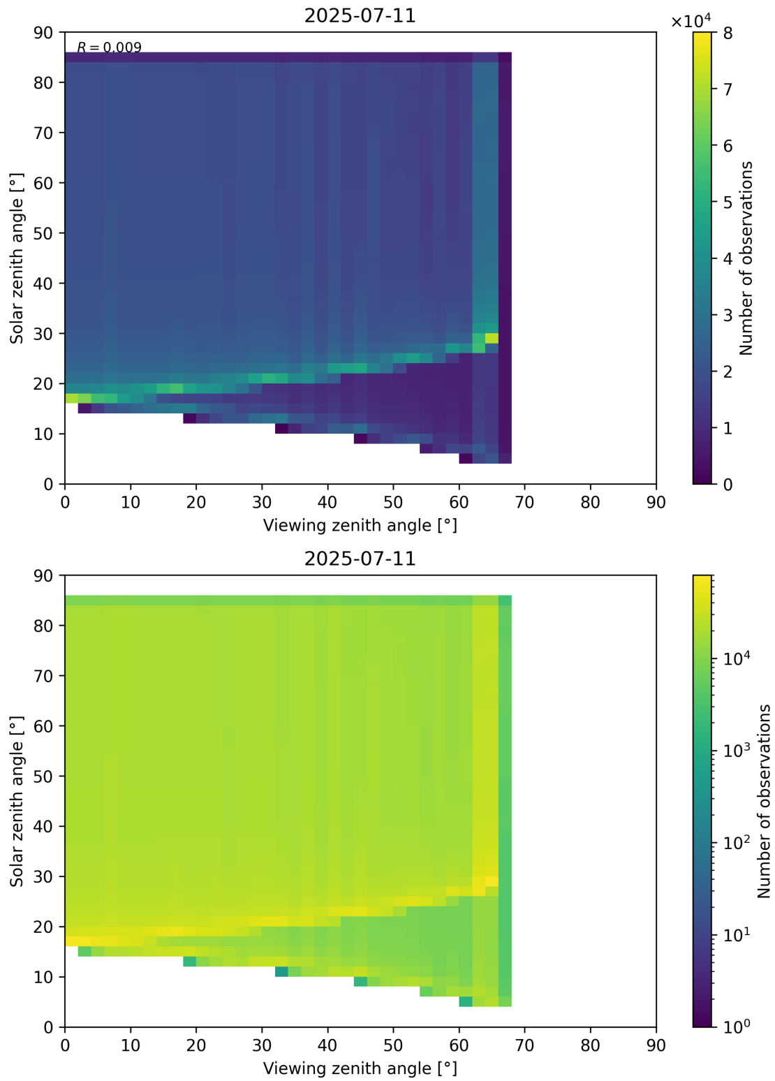
Figure 197: Scatter density plot of “Viewing zenith angle” against “Solar zenith angle” for 2025-07-10 to 2025-07-12.
