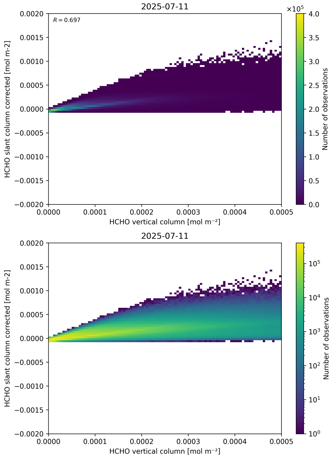
Figure 127: Scatter density plot of “HCHO vertical column” against “HCHO slant column corrected” for 2025-07-10 to 2025-07-12.
