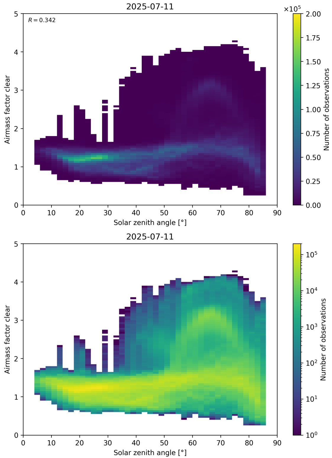
Figure 170: Scatter density plot of “Solar zenith angle” against “Airmass factor clear” for 2025-07-10 to 2025-07-12.
