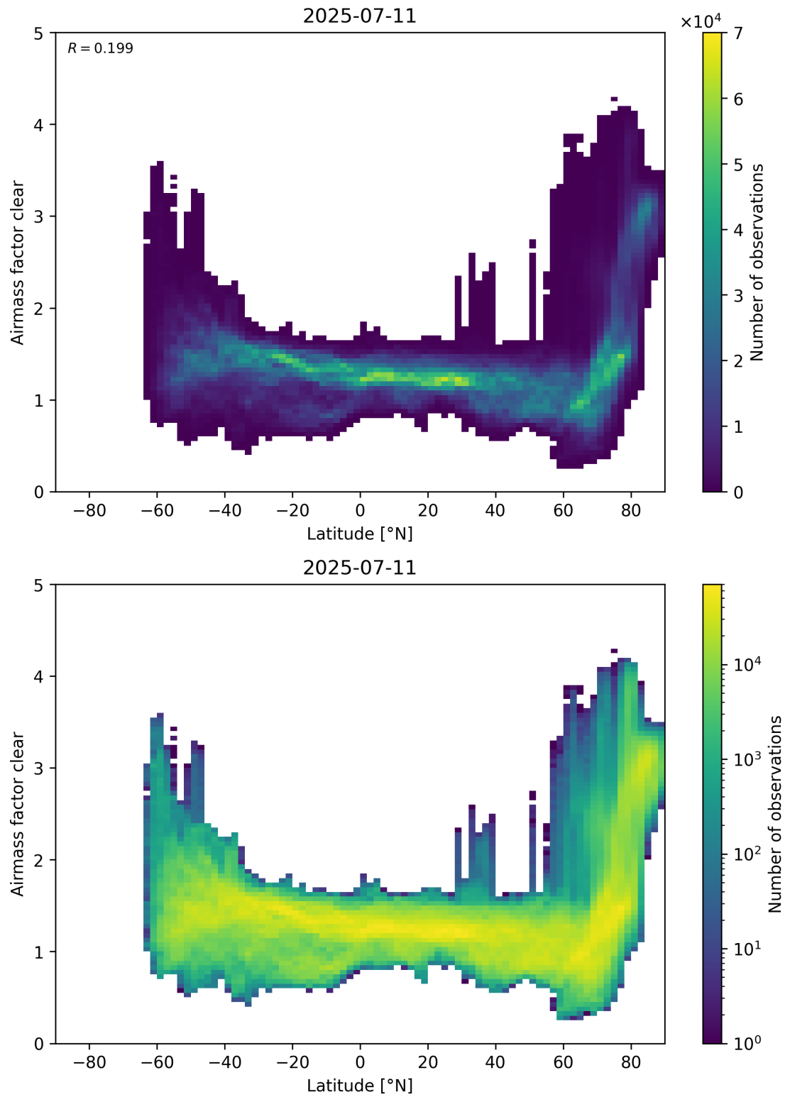
Figure 156: Scatter density plot of “Latitude” against “Airmass factor clear” for 2025-07-10 to 2025-07-12.
