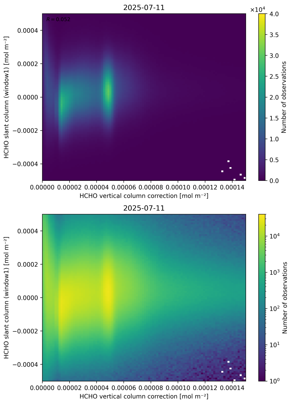
Figure 118: Scatter density plot of “HCHO vertical column correction” against “HCHO slant column (window1)” for 2025-07-10 to 2025-07-12.
