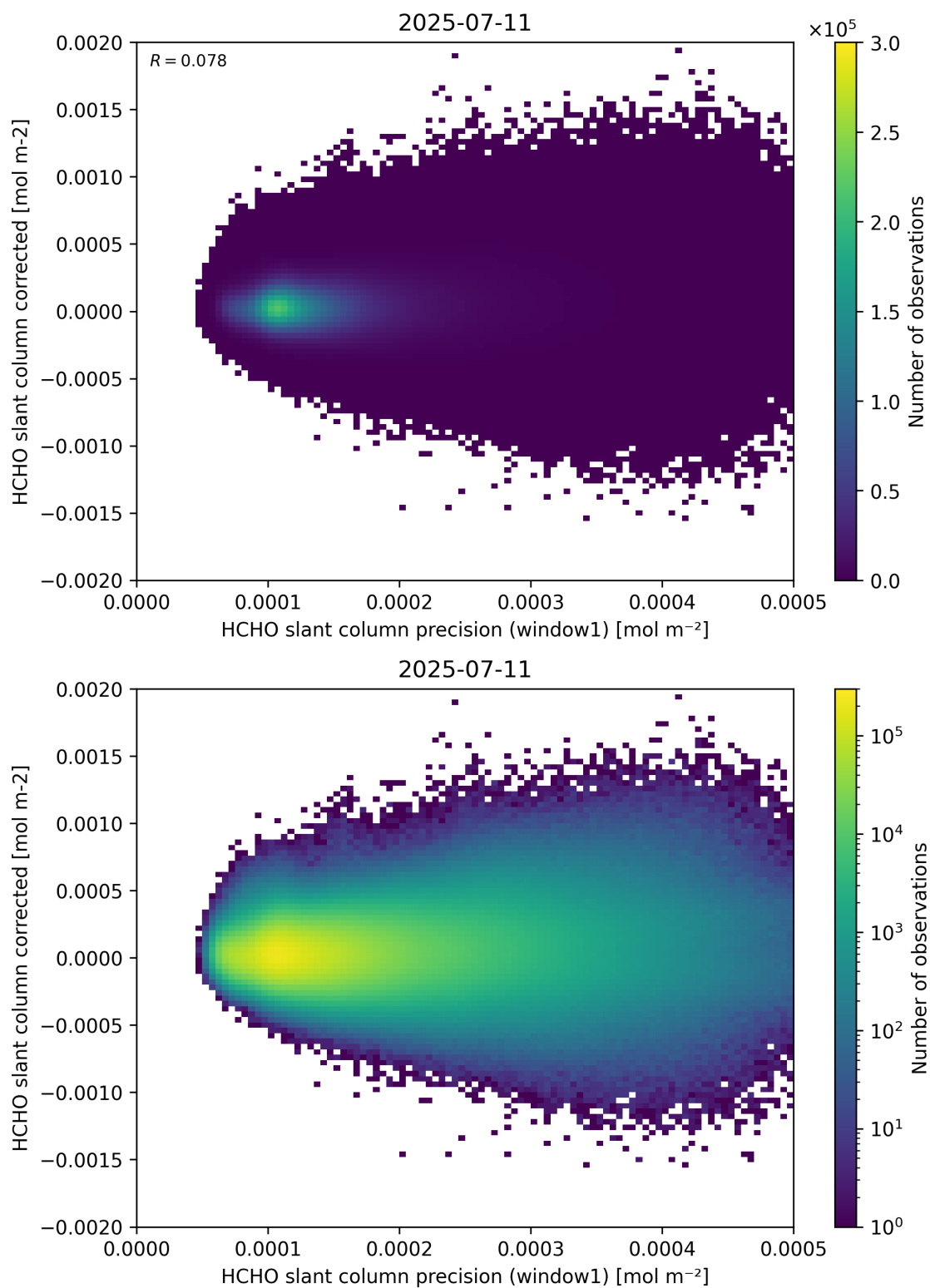
Figure 92: Scatter density plot of “HCHO slant column precision (window1)” against “HCHO slant column corrected” for 2025-07-10 to 2025-07-12.
