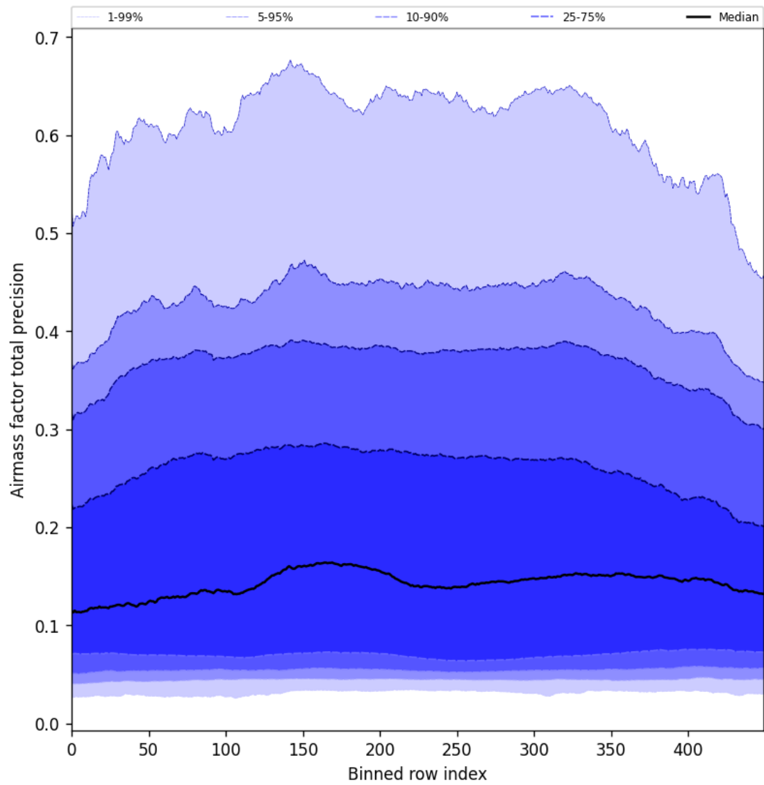
Figure 55: Along track statistics of “Airmass factor total precision” for 2025-07-10 to 2025-07-12
