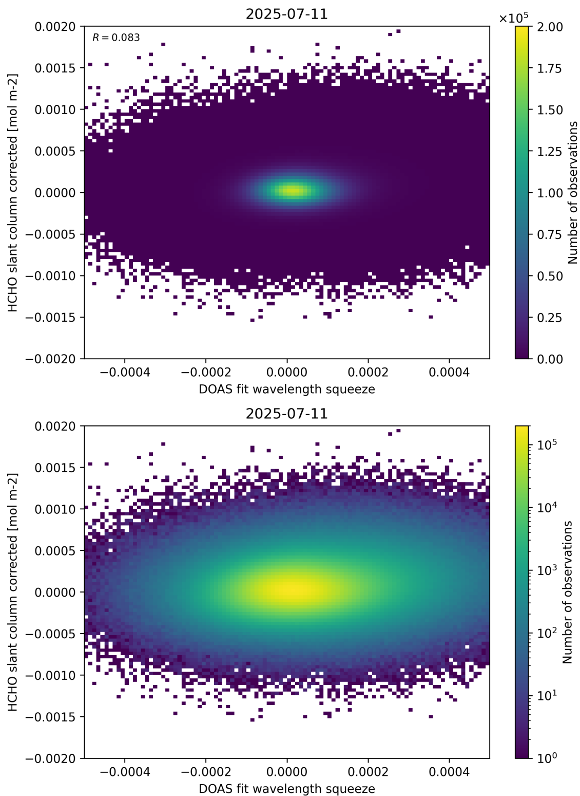
Figure 69: Scatter density plot of “DOAS fit wavelength squeeze” against “HCHO slant column corrected” for 2025-07-10 to 2025-07-12.
