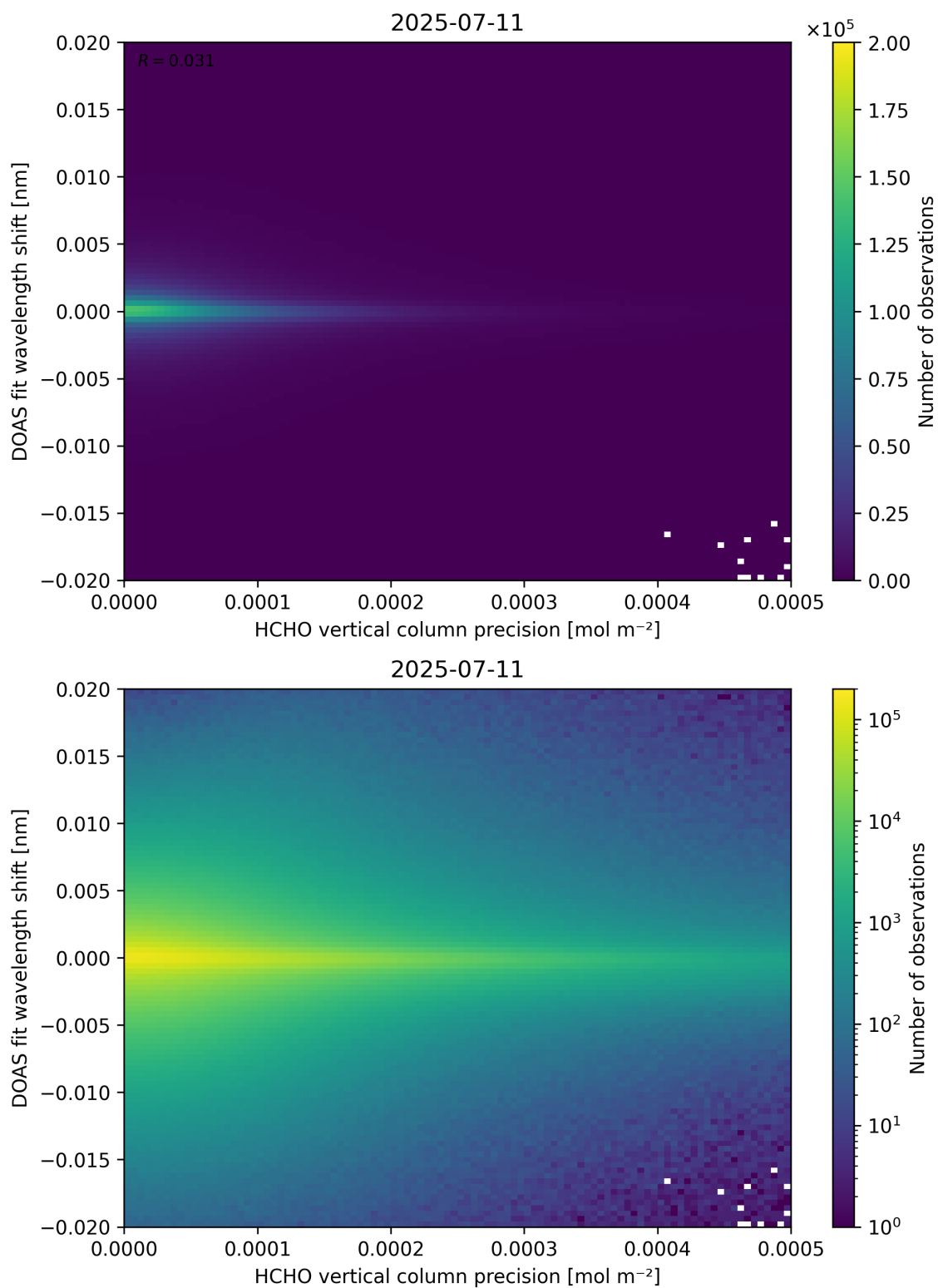
Figure 137: Scatter density plot of “HCHO vertical column precision” against “DOAS fit wavelength shift” for 2025-07-10 to 2025-07-12.
