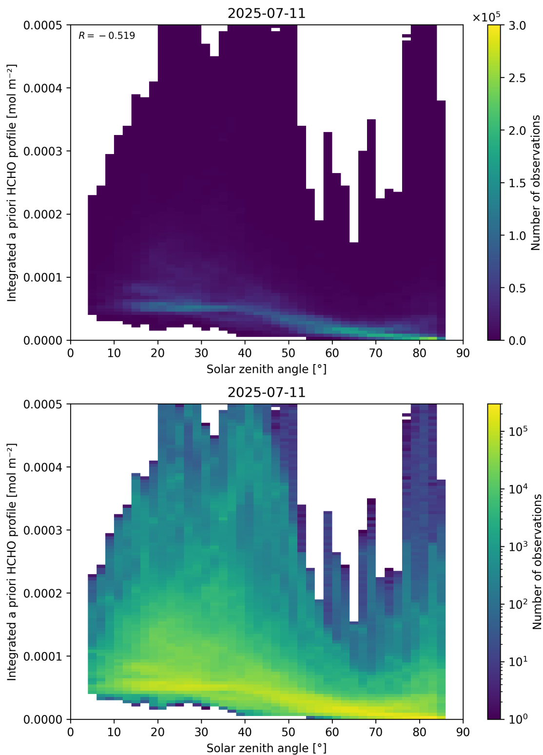
Figure 180: Scatter density plot of “Solar zenith angle” against “Integrated a priori HCHO profile” for 2025-07-10 to 2025-07-12.
