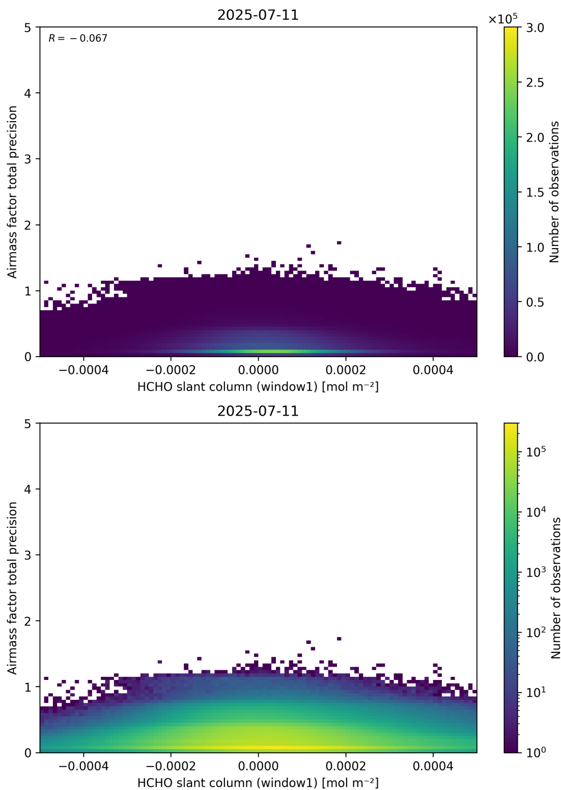
Figure 86: Scatter density plot of “HCHO slant column (window1)” against “Airmass factor total precision” for 2025-07-10 to 2025-07-12.
