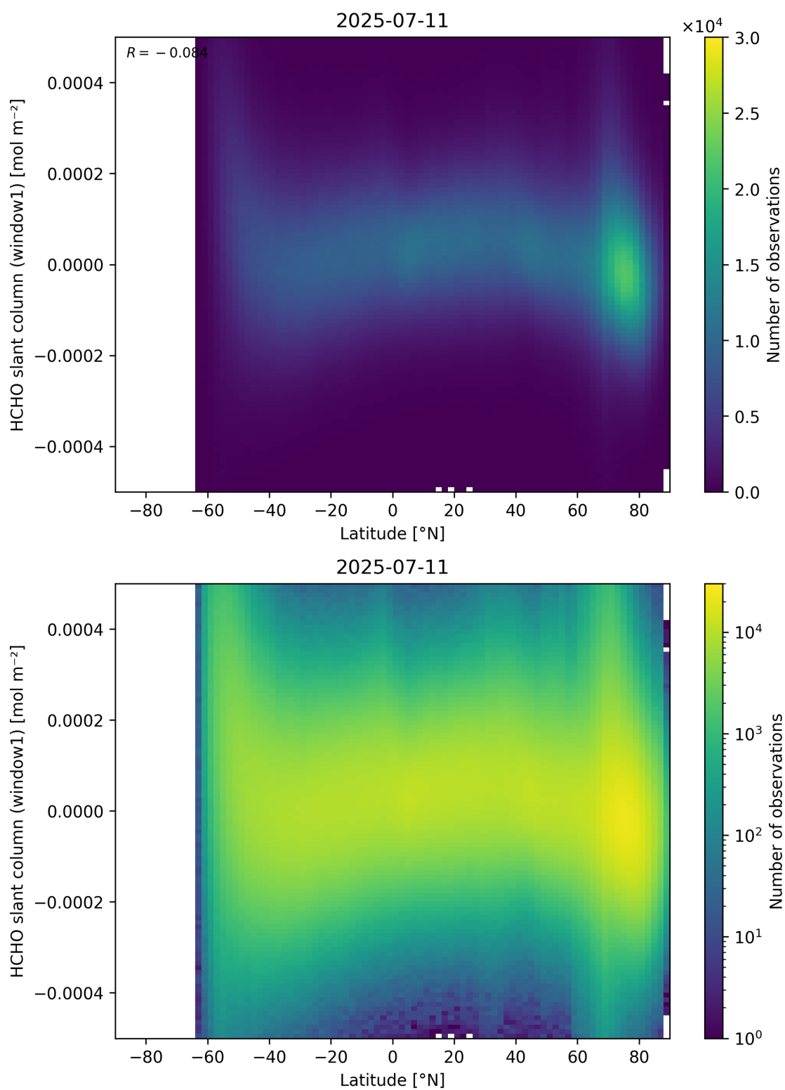
Figure 159: Scatter density plot of “Latitude” against “HCHO slant column (window1)” for 2025-07-10 to 2025-07-12.
