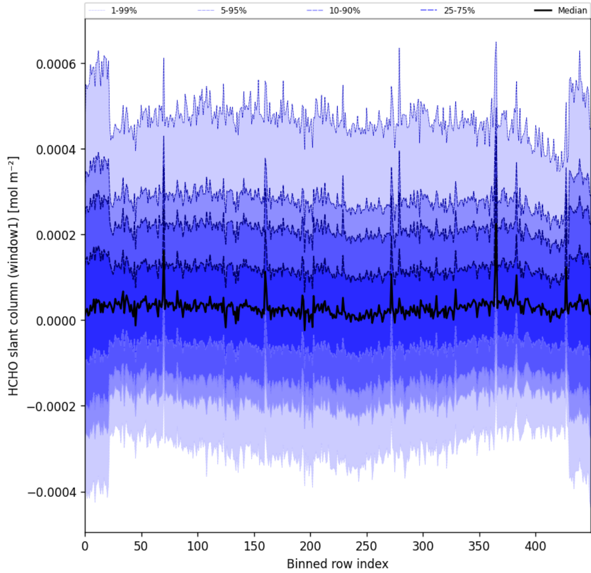
Figure 52: Along track statistics of “HCHO slant column (window1)” for 2025-07-10 to 2025-07-12
