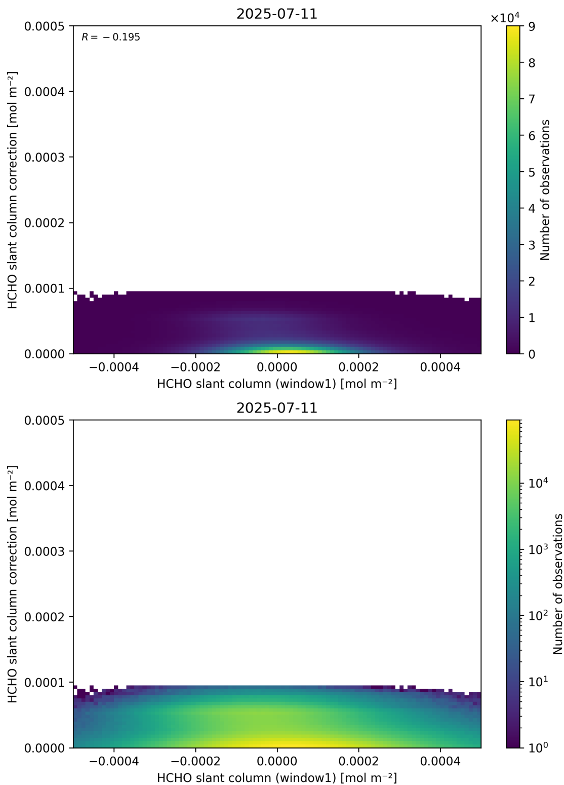
Figure 83: Scatter density plot of “HCHO slant column (window1)” against “HCHO slant column correction” for 2025-07-10 to 2025-07-12.
