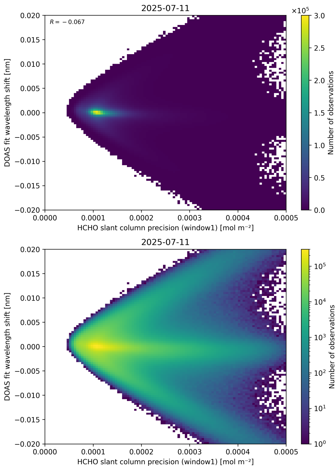
Figure 89: Scatter density plot of “HCHO slant column precision (window1)” against “DOAS fit wavelength shift” for 2025-07-10 to 2025-07-12.
