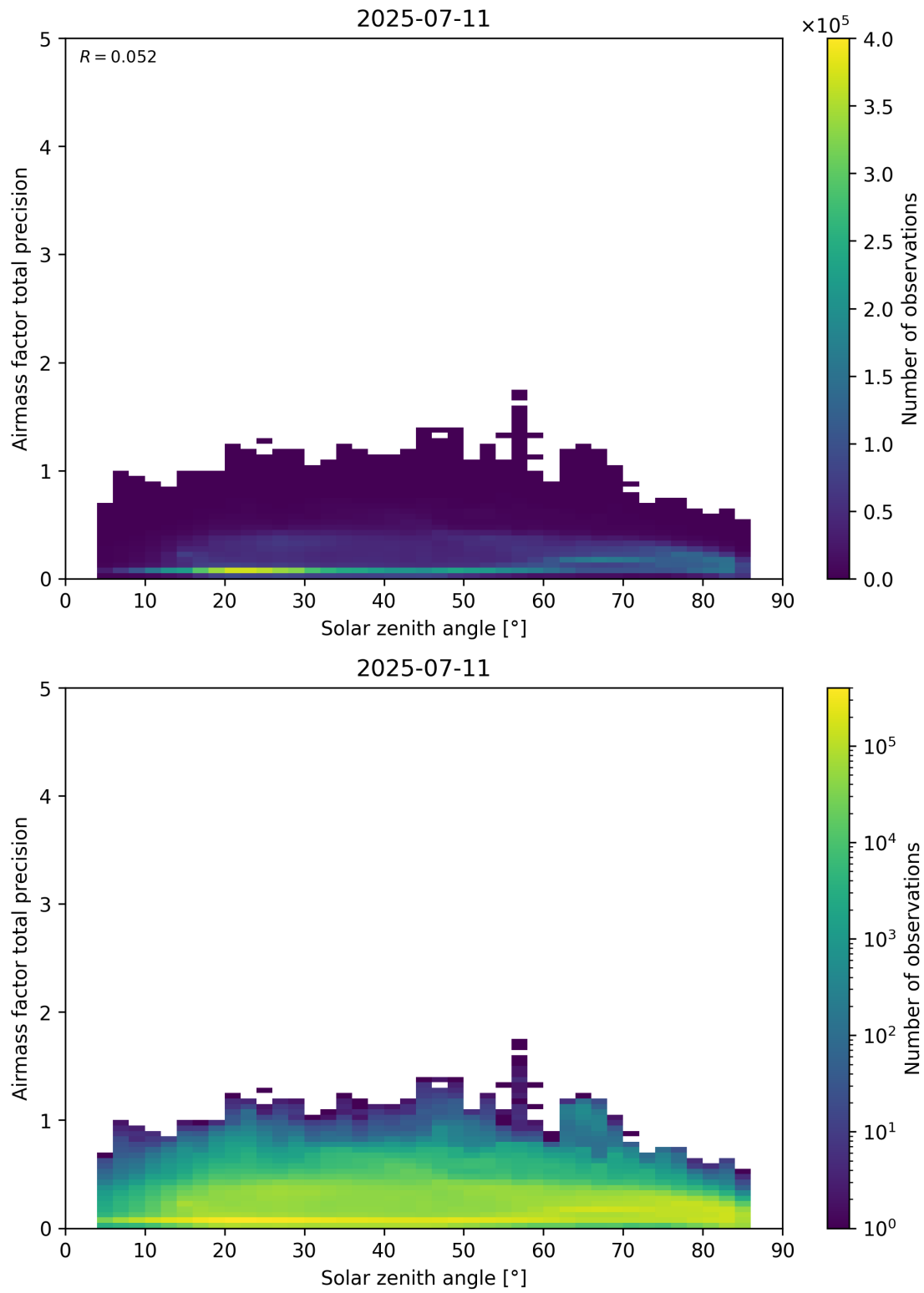
Figure 176: Scatter density plot of “Solar zenith angle” against “Airmass factor total precision” for 2025-07-10 to 2025-07-12.
