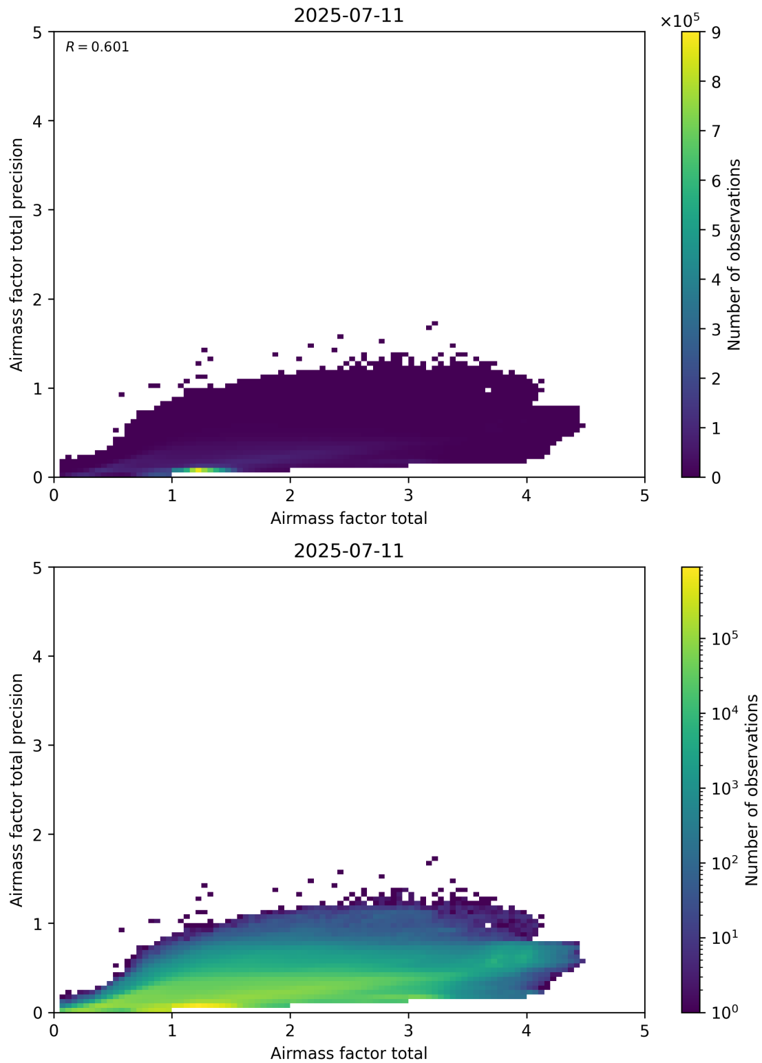
Figure 103: Scatter density plot of “Airmass factor total” against “Airmass factor total precision” for 2025-07-10 to 2025-07-12.
