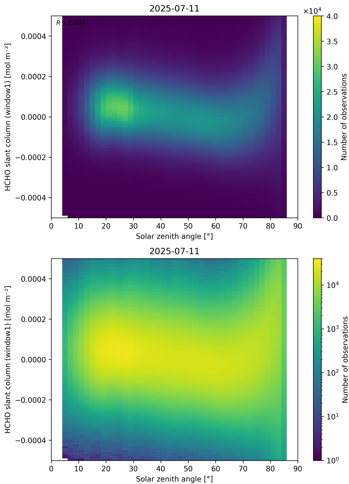
Figure 173: Scatter density plot of “Solar zenith angle” against “HCHO slant column (window1)” for 2025-07-10 to 2025-07-12.
