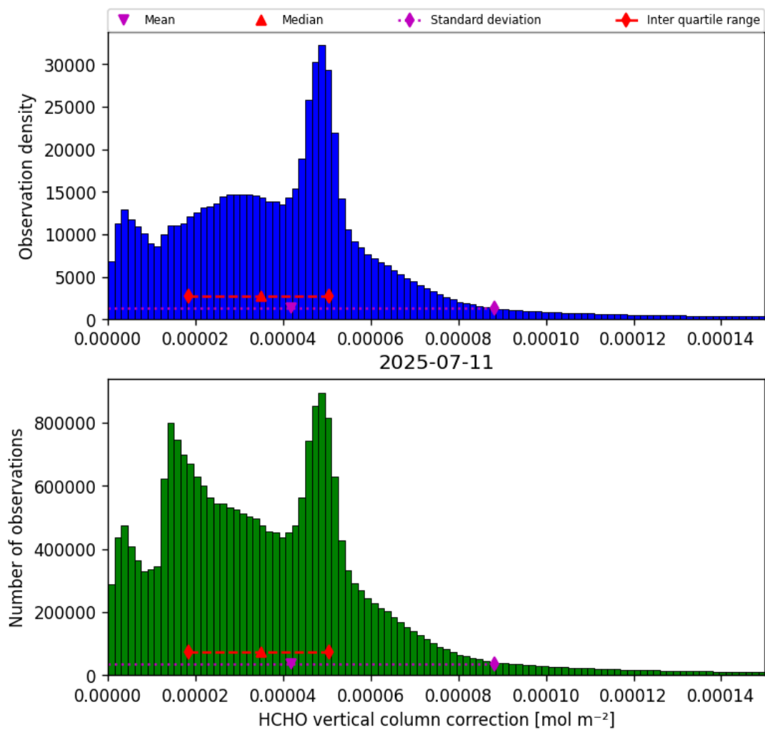
Figure 37: Histogram of “HCHO vertical column correction” for 2025-07-10 to 2025-07-12
