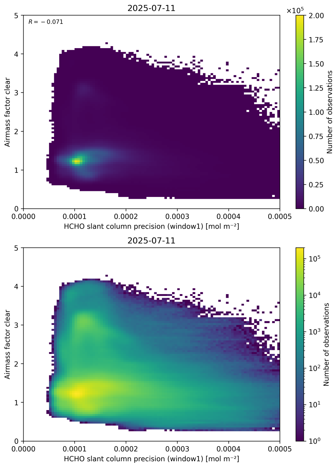
Figure 91: Scatter density plot of “HCHO slant column precision (window1)” against “Airmass factor clear” for 2025-07-10 to 2025-07-12.
