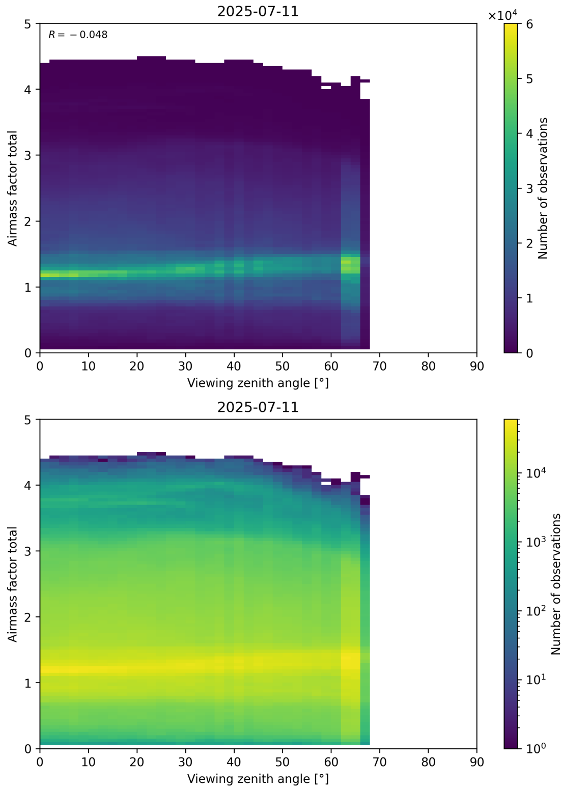
Figure 190: Scatter density plot of “Viewing zenith angle” against “Airmass factor total” for 2025-07-10 to 2025-07-12.
