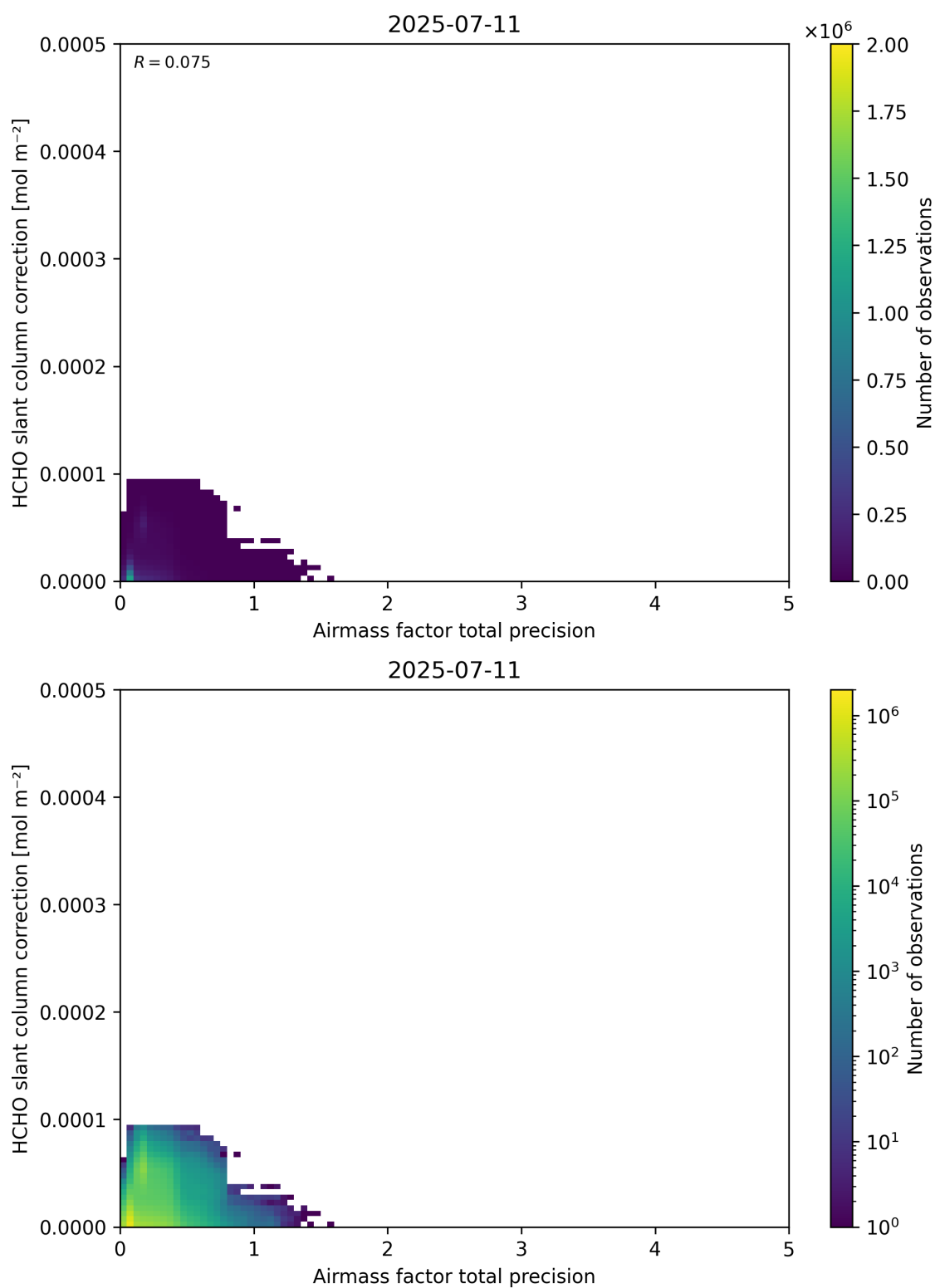
Figure 110: Scatter density plot of “Airmass factor total precision” against “HCHO slant column correction” for 2025-07-10 to 2025-07-12.
