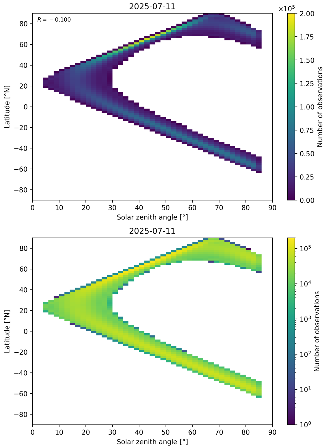
Figure 181: Scatter density plot of “Solar zenith angle” against “Latitude” for 2025-07-10 to 2025-07-12.
