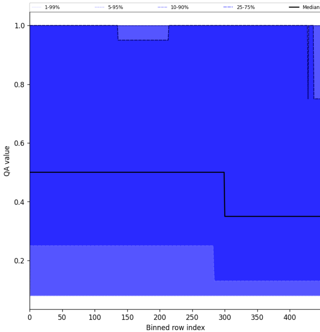
Figure 48: Along track statistics of “QA value” for 2025-07-10 to 2025-07-12
