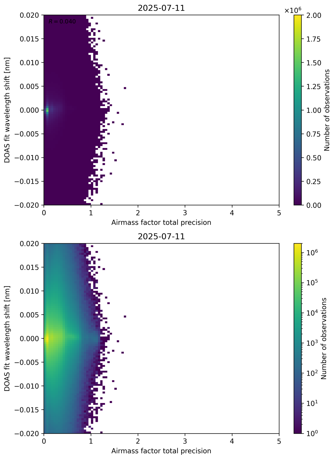
Figure 106: Scatter density plot of “Airmass factor total precision” against “DOAS fit wavelength shift” for 2025-07-10 to 2025-07-12.
