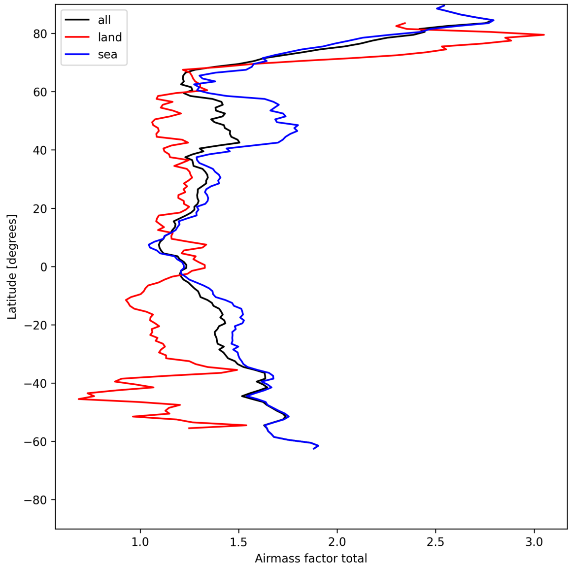
Figure 26: Zonal average of “Airmass factor total” for 2025-07-10 to 2025-07-12.
