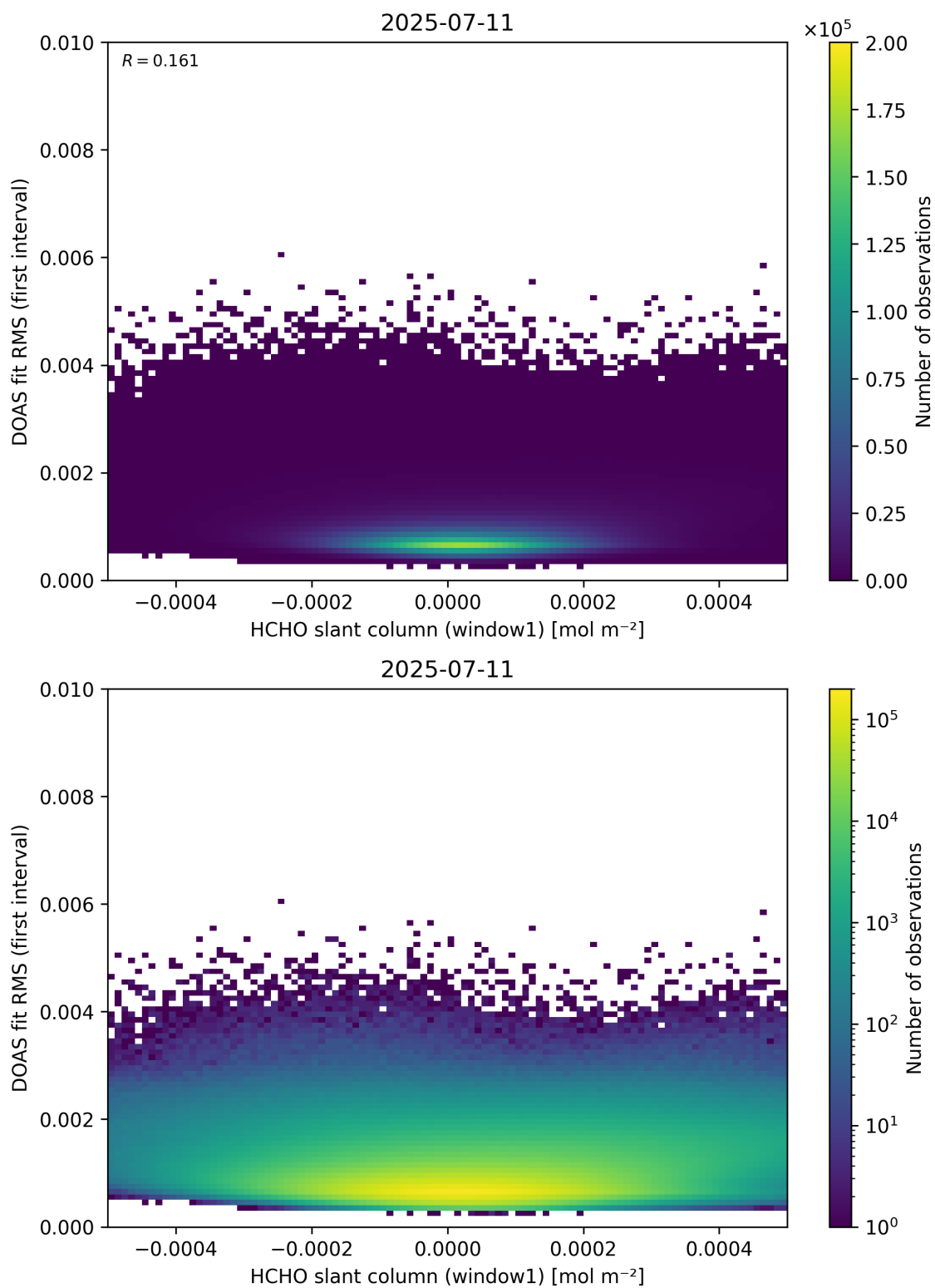
Figure 78: Scatter density plot of “HCHO slant column (window1)” against “DOAS fit RMS (first interval)” for 2025-07-10 to 2025-07-12.
