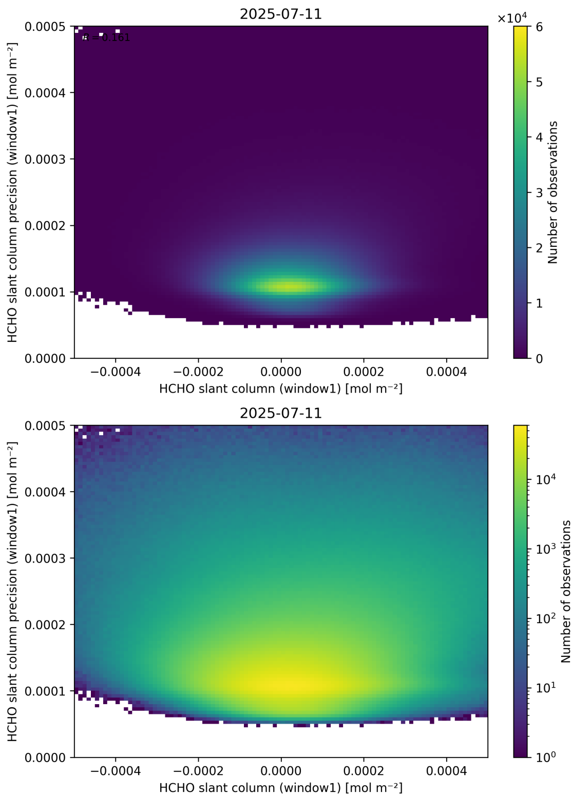
Figure 84: Scatter density plot of “HCHO slant column (window1)” against “HCHO slant column precision (window1)” for 2025-07-10 to 2025-07-12.
