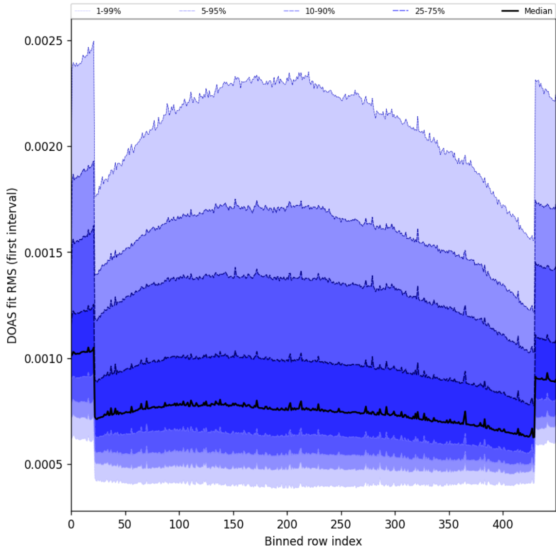
Figure 60: Along track statistics of “DOAS fit RMS (first interval)” for 2025-07-10 to 2025-07-12
