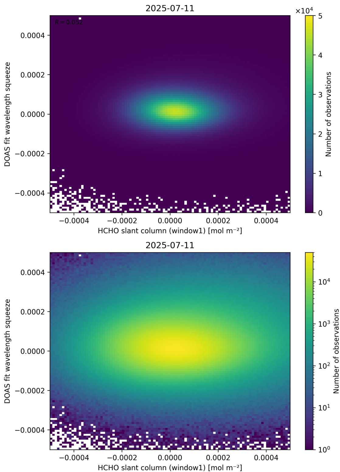
Figure 80: Scatter density plot of “HCHO slant column (window1)” against “DOAS fit wavelength squeeze” for 2025-07-10 to 2025-07-12.
