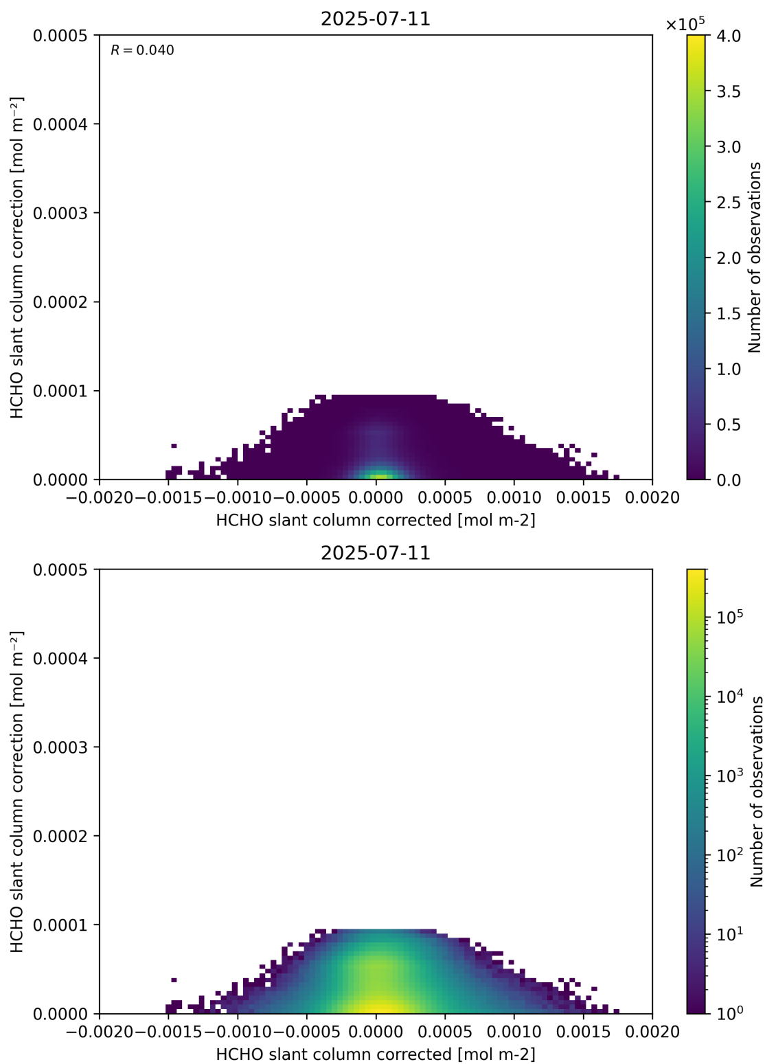
Figure 77: Scatter density plot of “HCHO slant column corrected” against “HCHO slant column correction” for 2025-07-10 to 2025-07-12.
