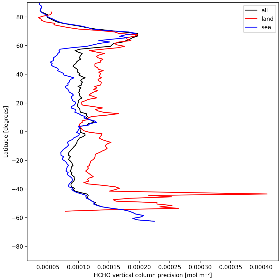
Figure 22: Zonal average of “HCHO vertical column precision” for 2025-07-10 to 2025-07-12.
