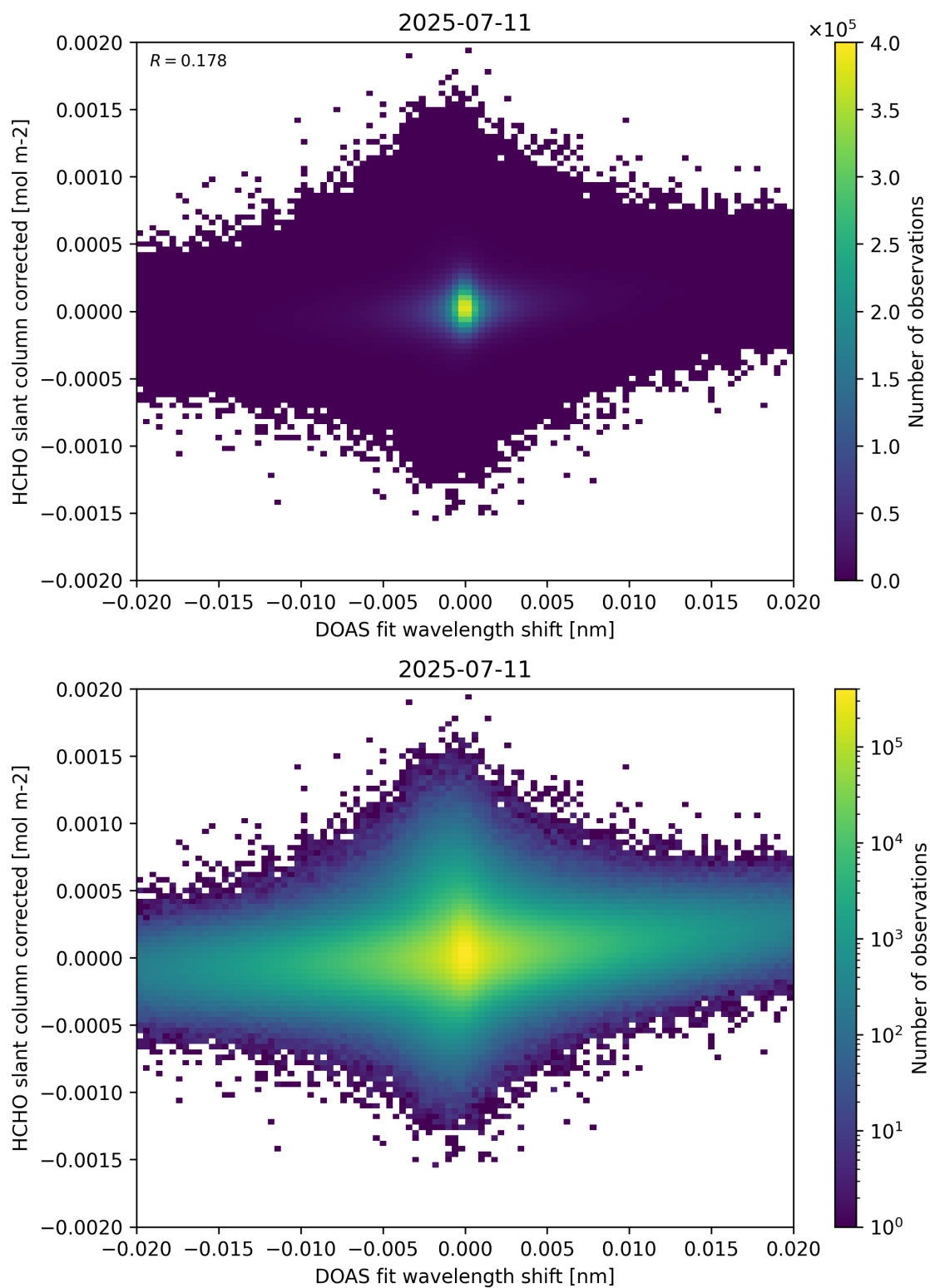
Figure 66: Scatter density plot of “DOAS fit wavelength shift” against “HCHO slant column corrected” for 2025-07-10 to 2025-07-12.
