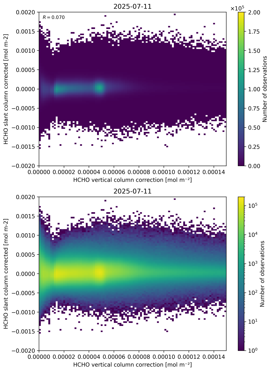
Figure 116: Scatter density plot of “HCHO vertical column correction” against “HCHO slant column corrected” for 2025-07-10 to 2025-07-12.
