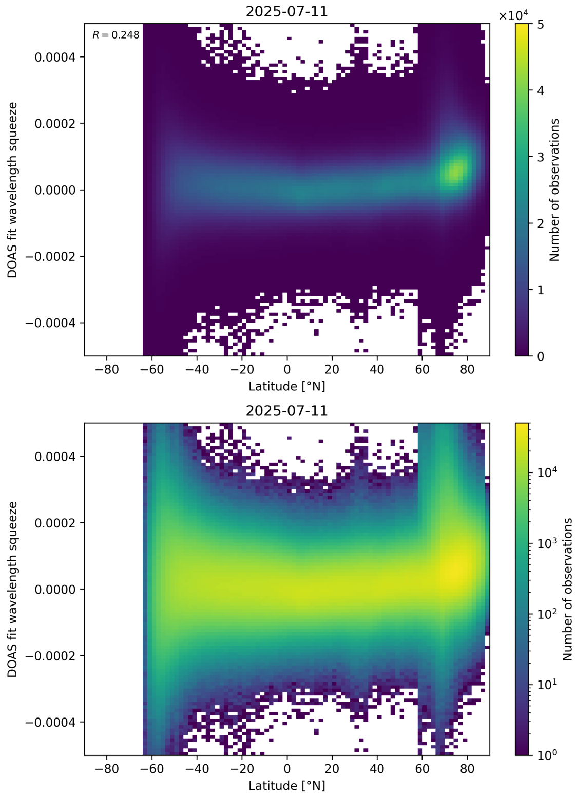
Figure 155: Scatter density plot of “Latitude” against “DOAS fit wavelength squeeze” for 2025-07-10 to 2025-07-12.
