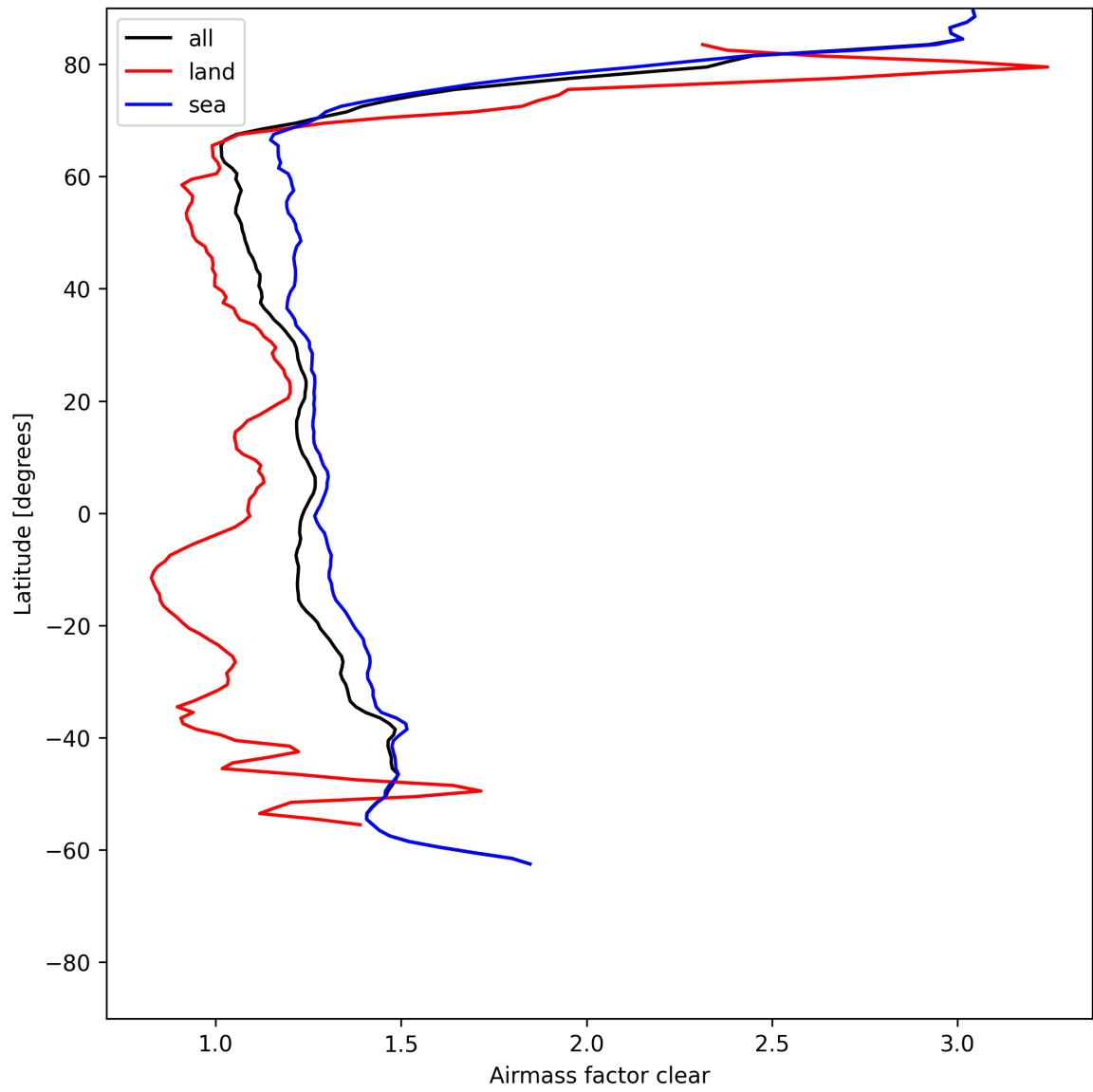
Figure 28: Zonal average of “Airmass factor clear” for 2025-07-10 to 2025-07-12.
