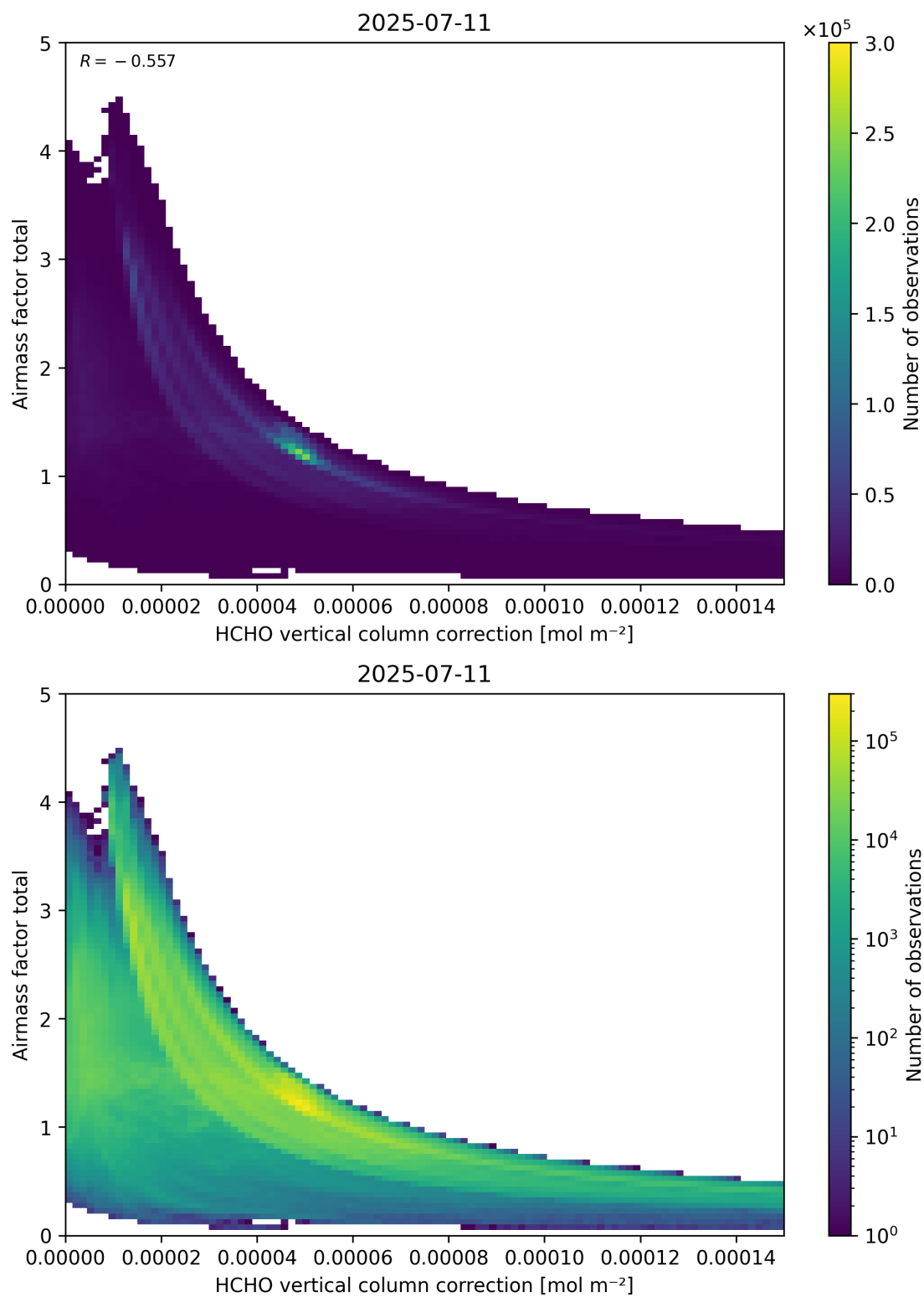
Figure 120: Scatter density plot of “HCHO vertical column correction” against “Airmass factor total” for 2025-07-10 to 2025-07-12.
