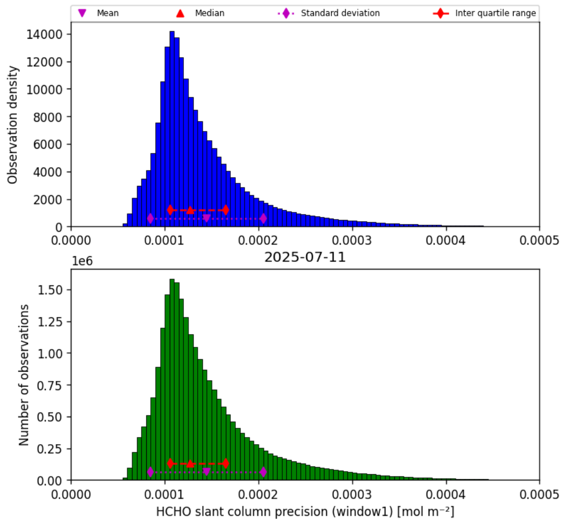
Figure 39: Histogram of “HCHO slant column precision (window1)” for 2025-07-10 to 2025-07-12
