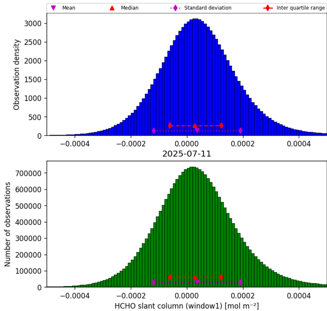
Figure 38: Histogram of “HCHO slant column (window1)” for 2025-07-10 to 2025-07-12
