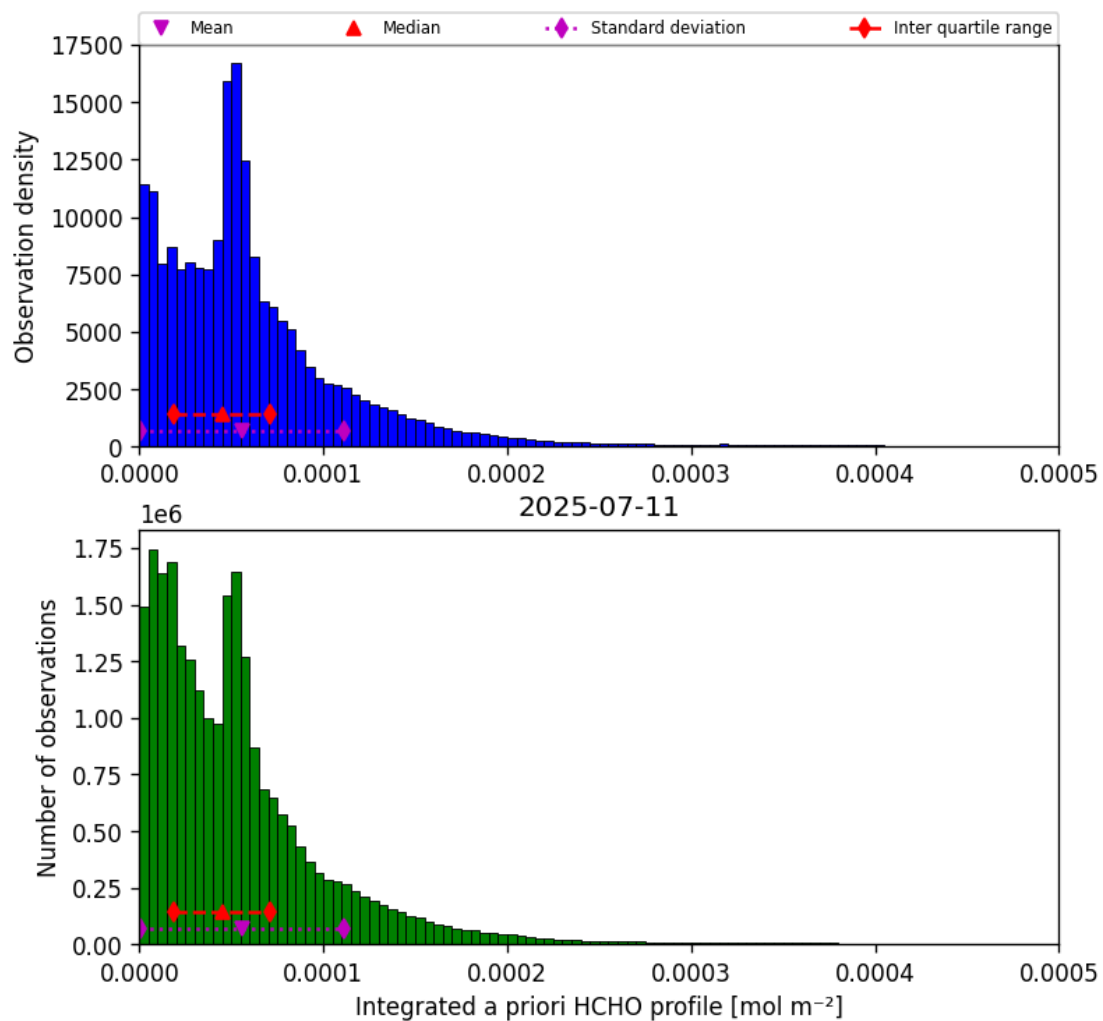
Figure 43: Histogram of “Integrated a priori HCHO profile” for 2025-07-10 to 2025-07-12
