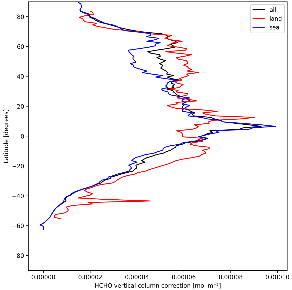
Figure 23: Zonal average of “HCHO vertical column correction” for 2025-07-10 to 2025-07-12.
