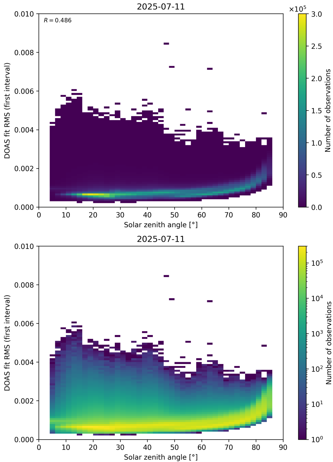
Figure 167: Scatter density plot of “Solar zenith angle” against “DOAS fit RMS (first interval)” for 2025-07-10 to 2025-07-12.
