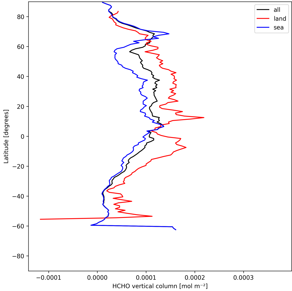
Figure 21: Zonal average of “HCHO vertical column” for 2025-07-10 to 2025-07-12.
