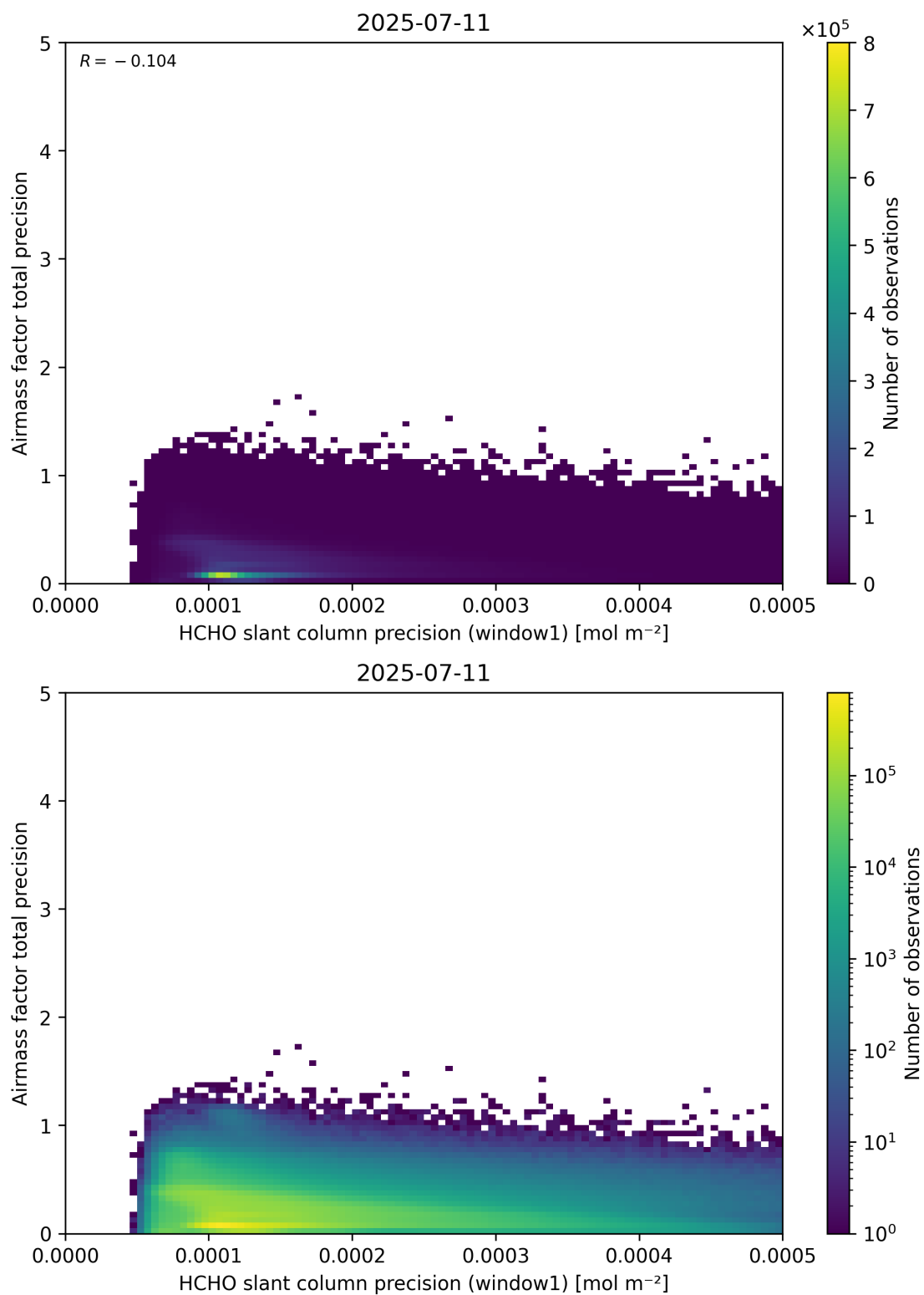
Figure 95: Scatter density plot of “HCHO slant column precision (window1)” against “Airmass factor total precision” for 2025-07-10 to 2025-07-12.
