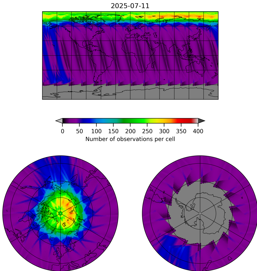
Figure 19: Map of the number of observations for 2025-07-10 to 2025-07-12
