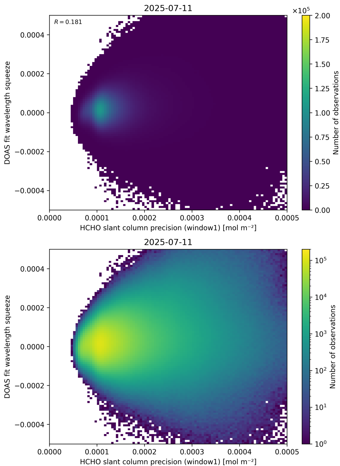
Figure 90: Scatter density plot of “HCHO slant column precision (window1)” against “DOAS fit wavelength squeeze” for 2025-07-10 to 2025-07-12.
