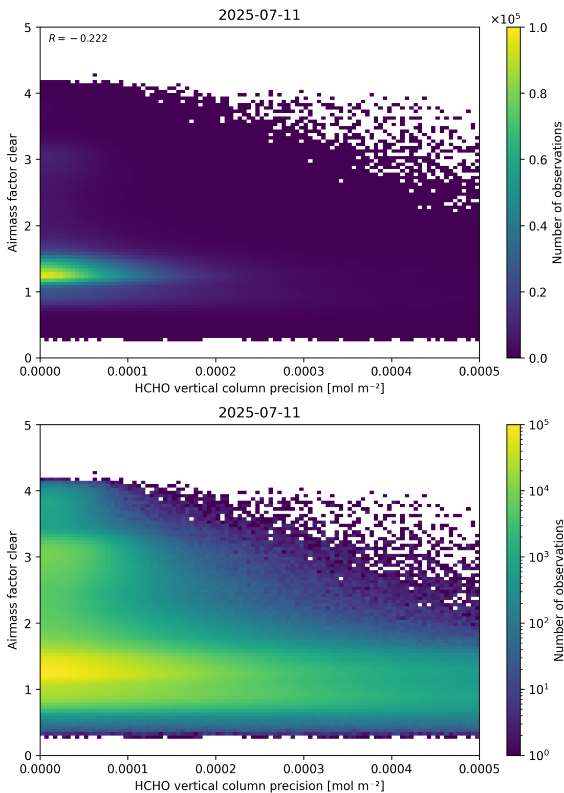
Figure 139: Scatter density plot of “HCHO vertical column precision” against “Airmass factor clear” for 2025-07-10 to 2025-07-12.
