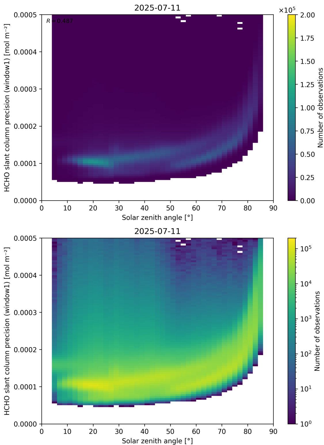
Figure 174: Scatter density plot of “Solar zenith angle” against “HCHO slant column precision (window1)” for 2025-07-10 to 2025-07-12.
