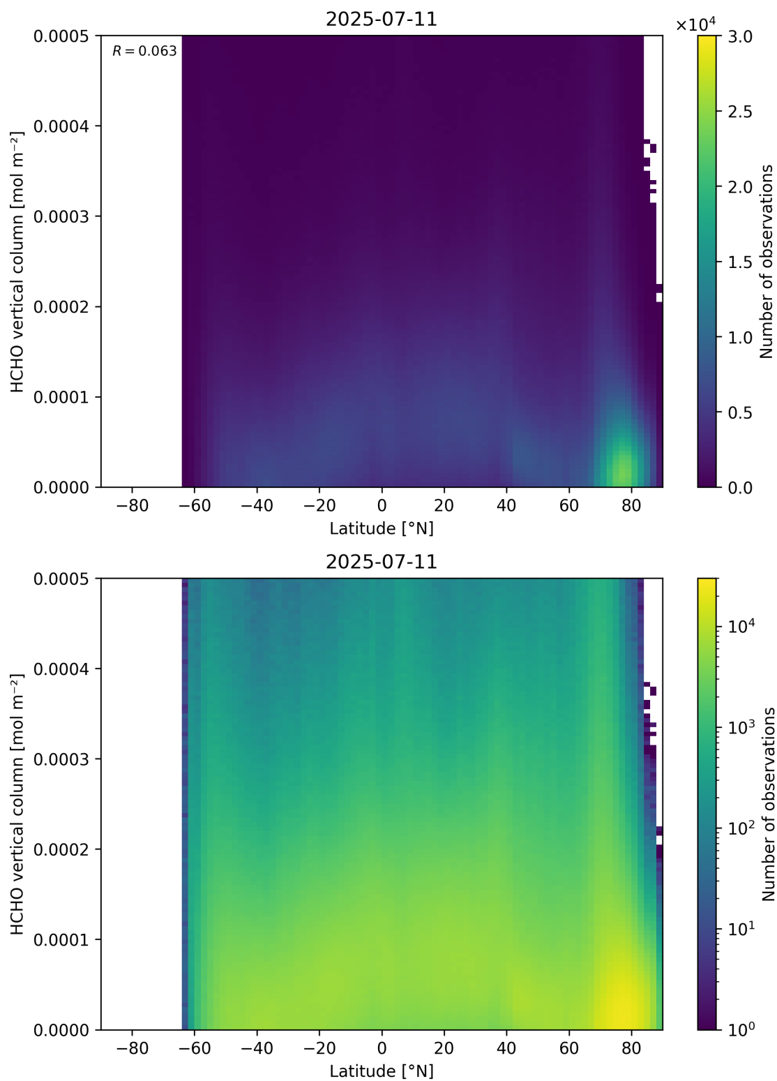
Figure 163: Scatter density plot of “Latitude” against “HCHO vertical column” for 2025-07-10 to 2025-07-12.
