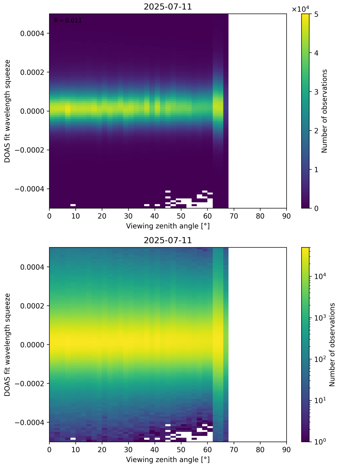
Figure 184: Scatter density plot of “Viewing zenith angle” against “DOAS fit wavelength squeeze” for 2025-07-10 to 2025-07-12.
