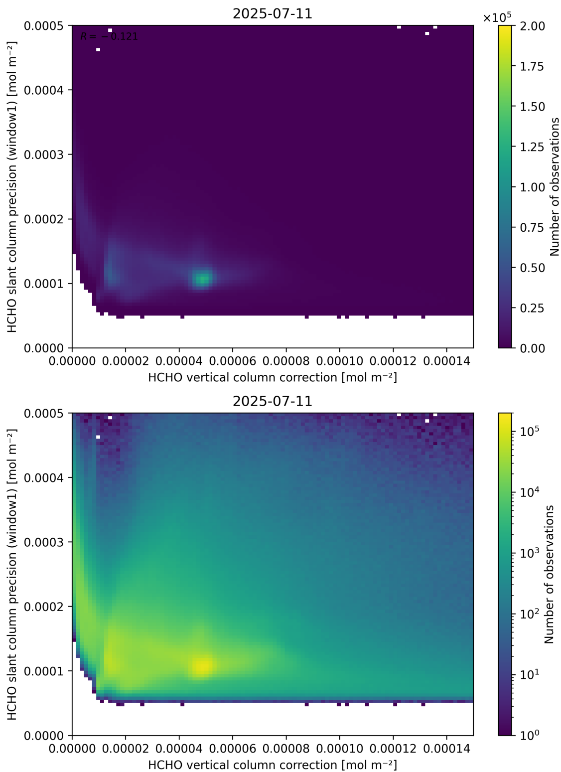
Figure 119: Scatter density plot of “HCHO vertical column correction” against “HCHO slant column precision (window1)” for 2025-07-10 to 2025-07-12.
