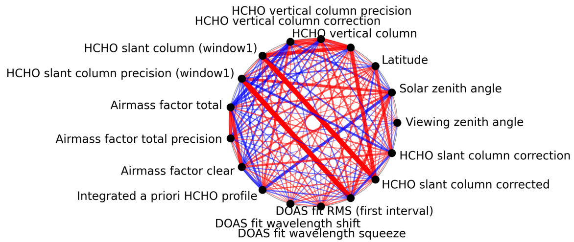
Figure 1: Map of correlation graph for 2025-07-10 to 2025-07-12.
