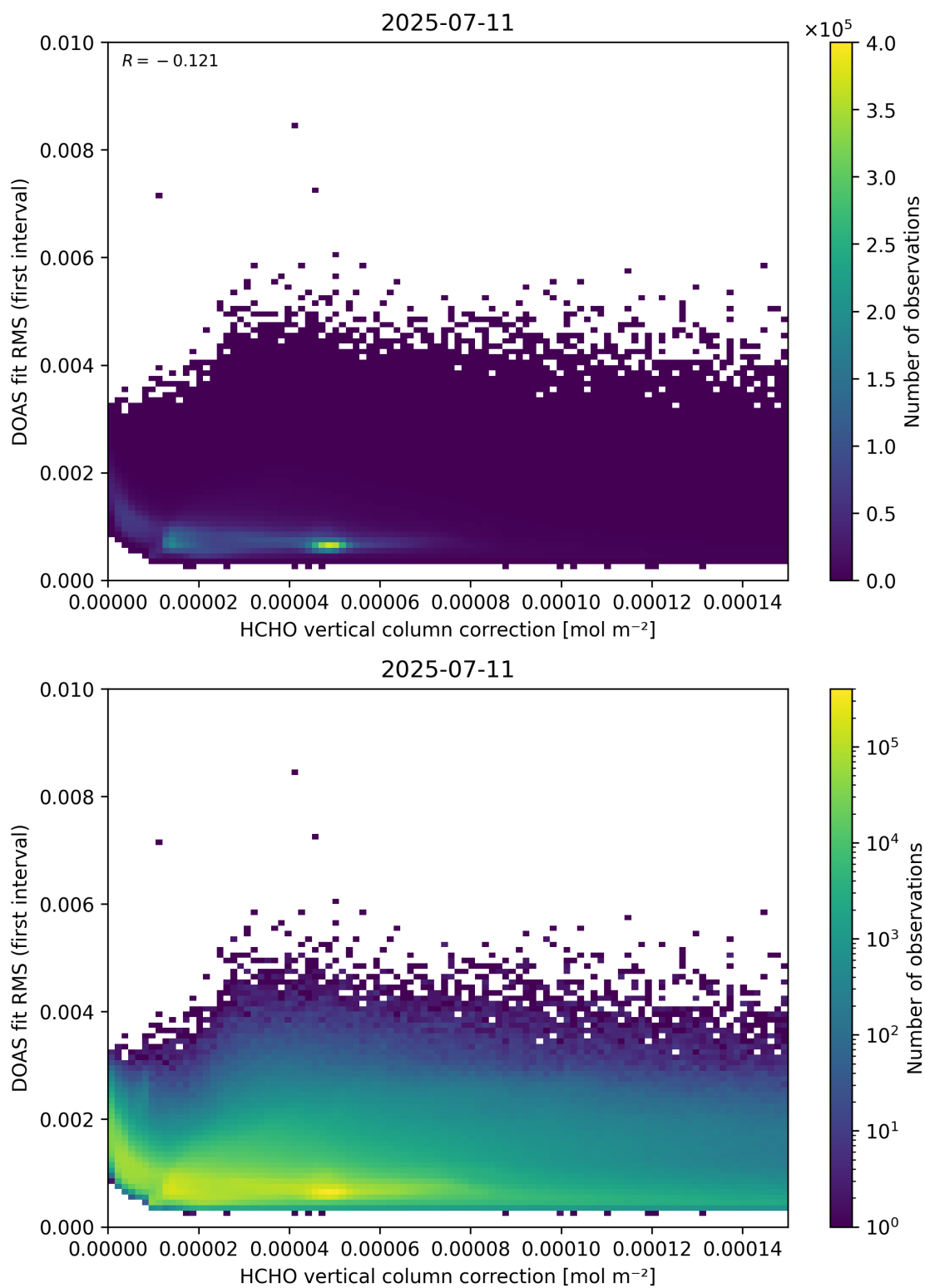
Figure 112: Scatter density plot of “HCHO vertical column correction” against “DOAS fit RMS (first interval)” for 2025-07-10 to 2025-07-12.
