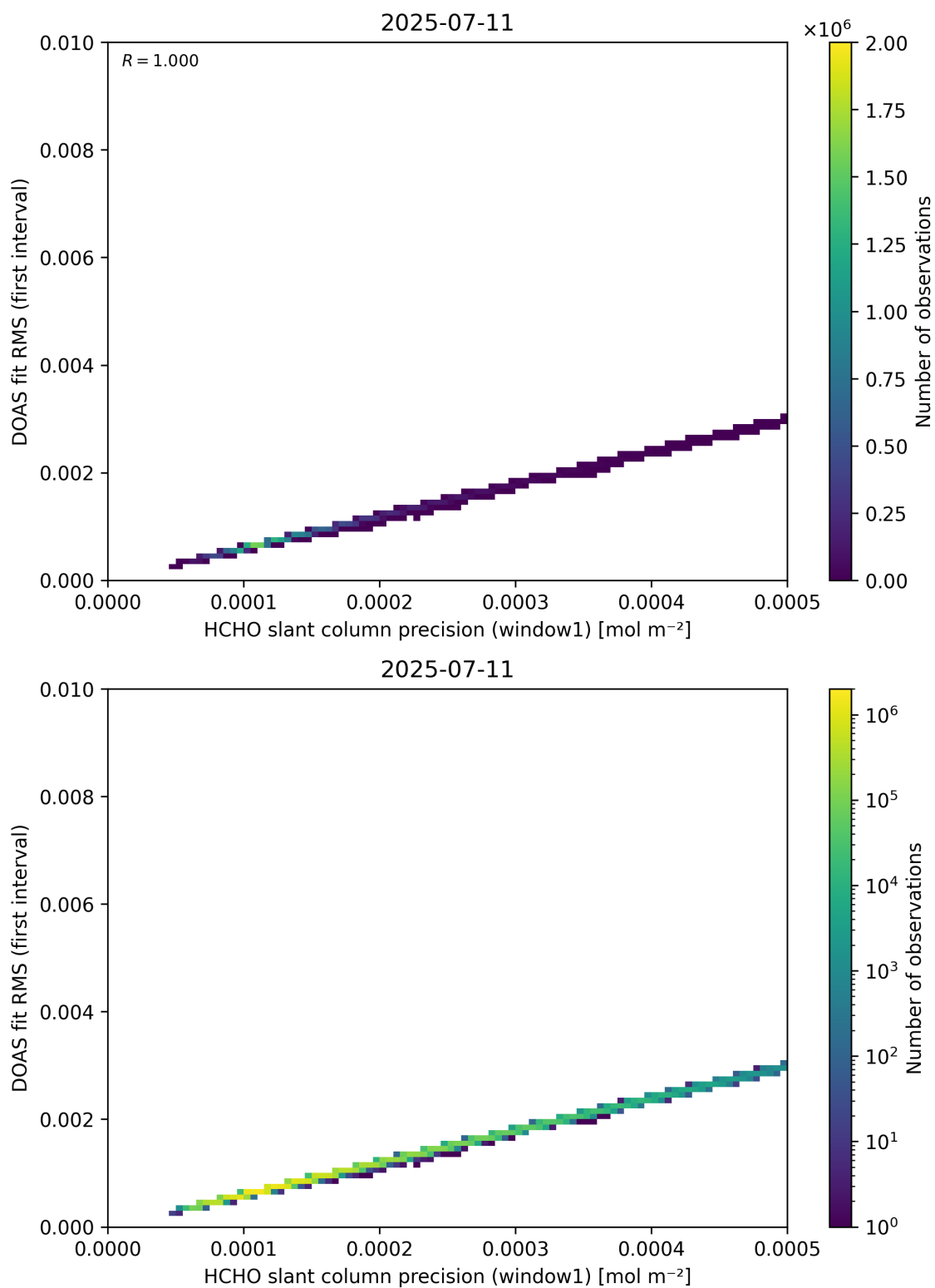
Figure 88: Scatter density plot of “HCHO slant column precision (window1)” against “DOAS fit RMS (first interval)” for 2025-07-10 to 2025-07-12.
