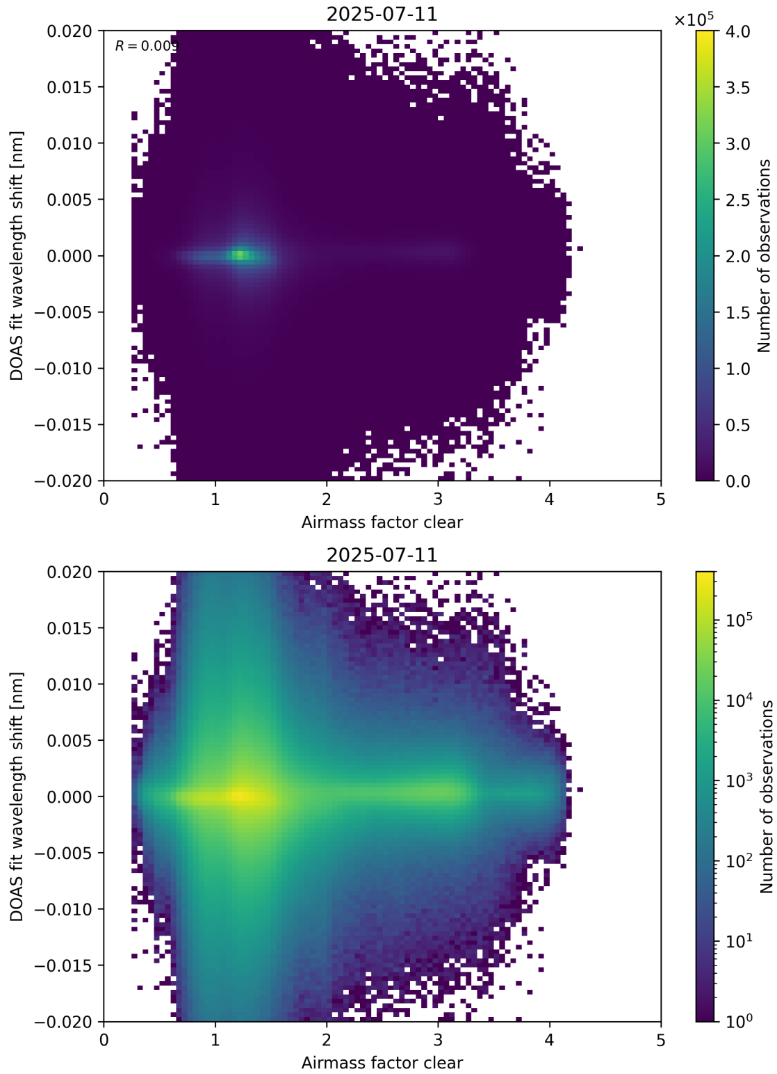
Figure 72: Scatter density plot of “Airmass factor clear” against “DOAS fit wavelength shift” for 2025-07-10 to 2025-07-12.
