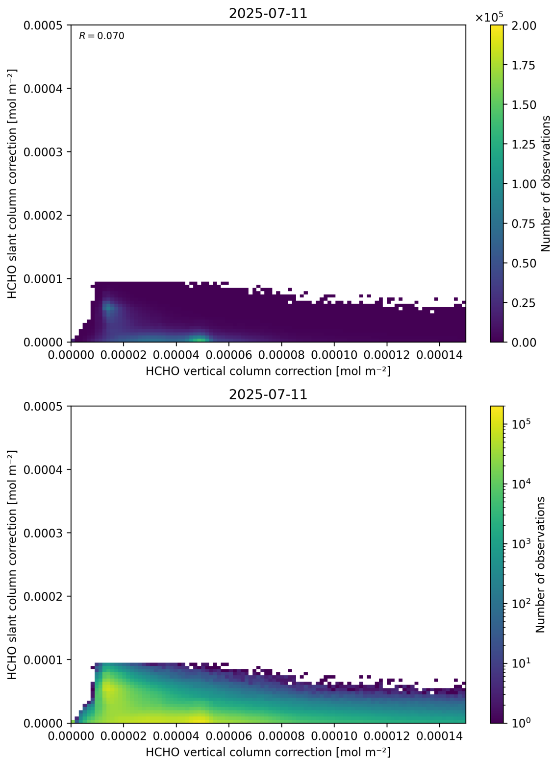
Figure 117: Scatter density plot of “HCHO vertical column correction” against “HCHO slant column correction” for 2025-07-10 to 2025-07-12.
