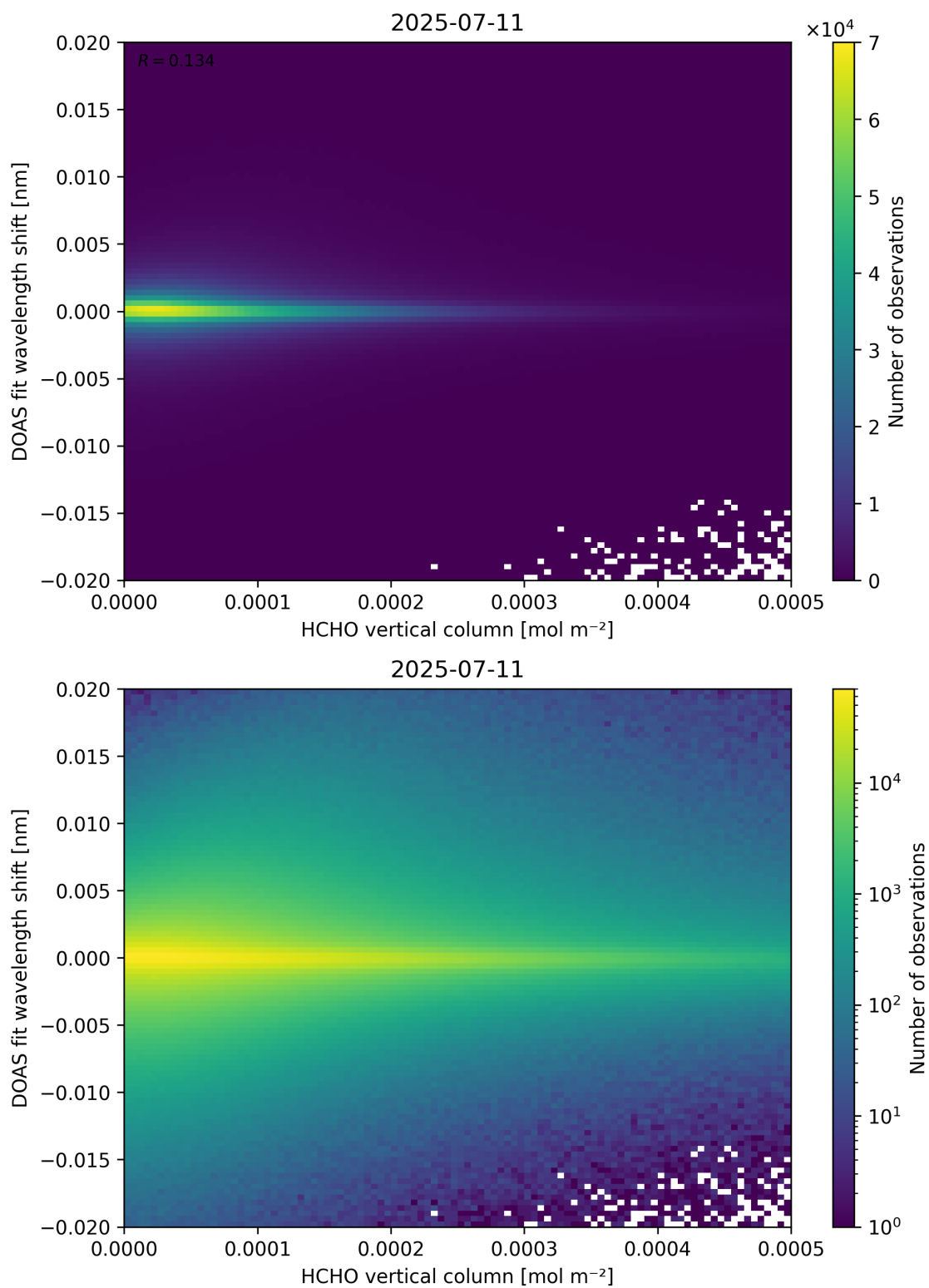
Figure 124: Scatter density plot of “HCHO vertical column” against “DOAS fit wavelength shift” for 2025-07-10 to 2025-07-12.
