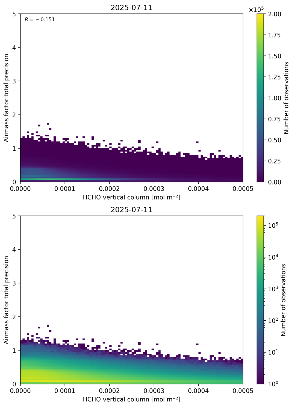
Figure 132: Scatter density plot of “HCHO vertical column” against “Airmass factor total precision” for 2025-07-10 to 2025-07-12.
