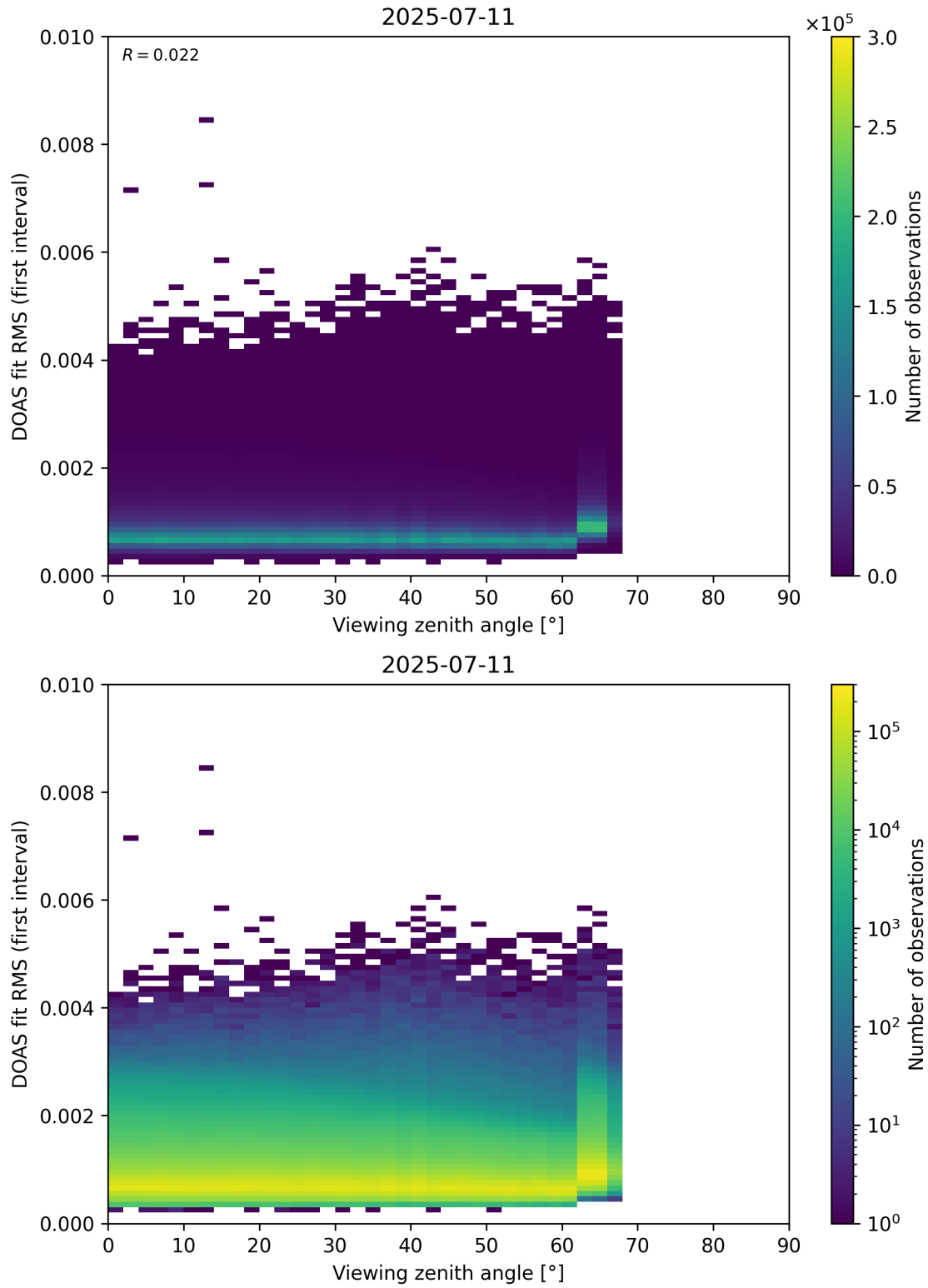
Figure 182: Scatter density plot of “Viewing zenith angle” against “DOAS fit RMS (first interval)” for 2025-07-10 to 2025-07-12.
