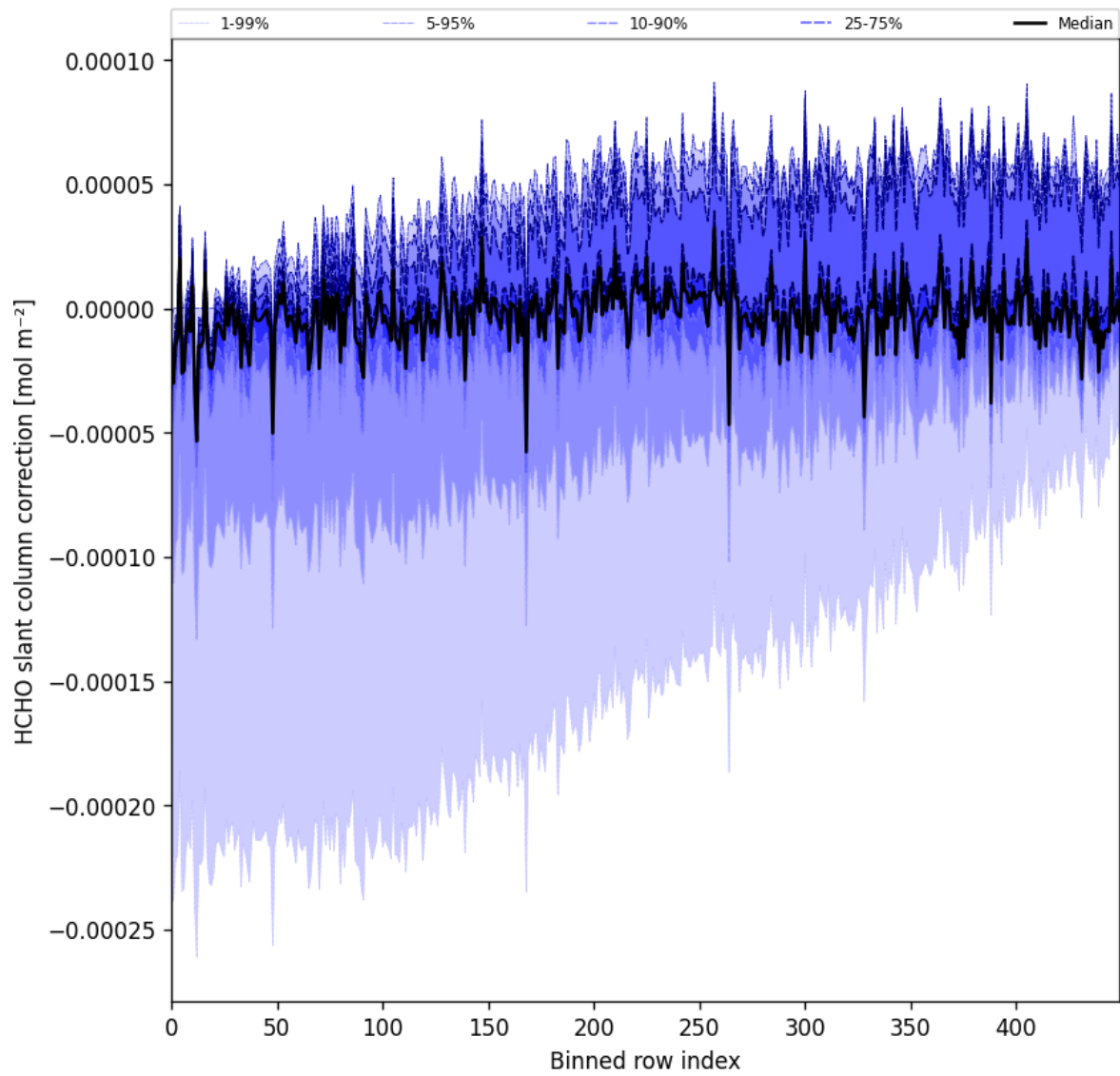
Figure 61: Along track statistics of “HCHO slant column correction” for 2025-07-10 to 2025-07-12
