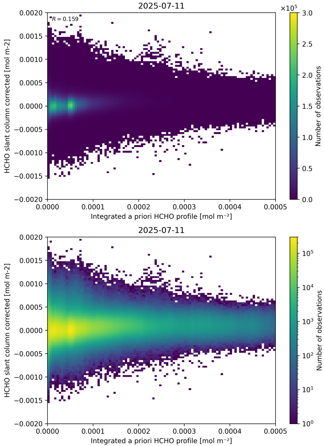
Figure 151: Scatter density plot of “Integrated a priori HCHO profile” against “HCHO slant column corrected” for 2025-07-10 to 2025-07-12.
