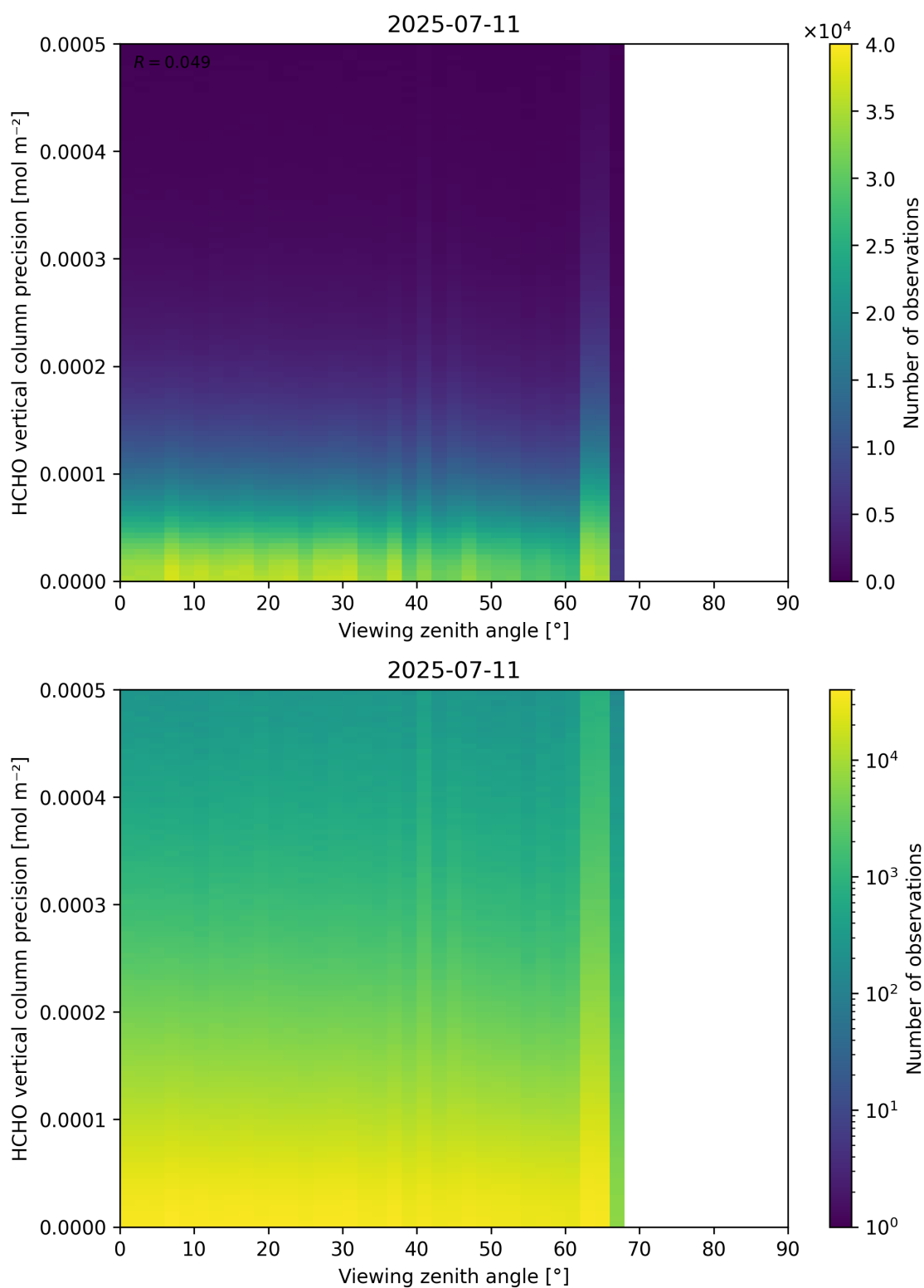
Figure 194: Scatter density plot of “Viewing zenith angle” against “HCHO vertical column precision” for 2025-07-10 to 2025-07-12.
