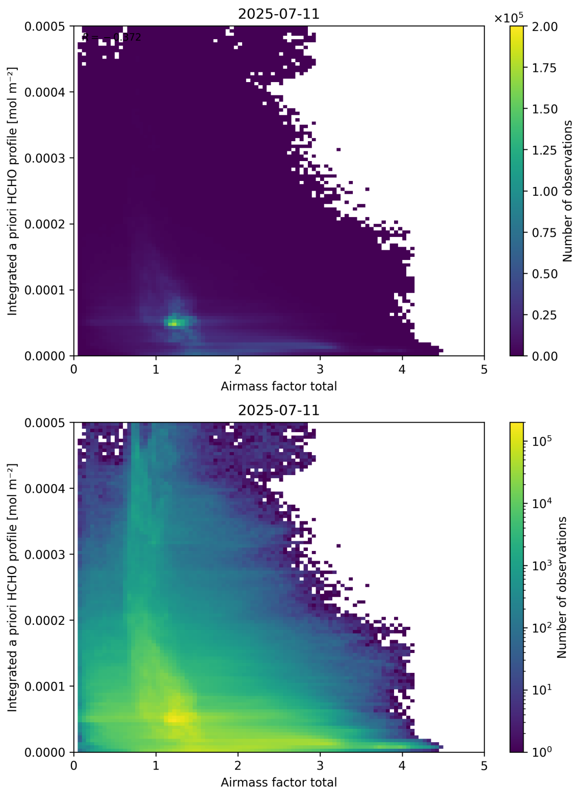
Figure 104: Scatter density plot of “Airmass factor total” against “Integrated a priori HCHO profile” for 2025-07-10 to 2025-07-12.
