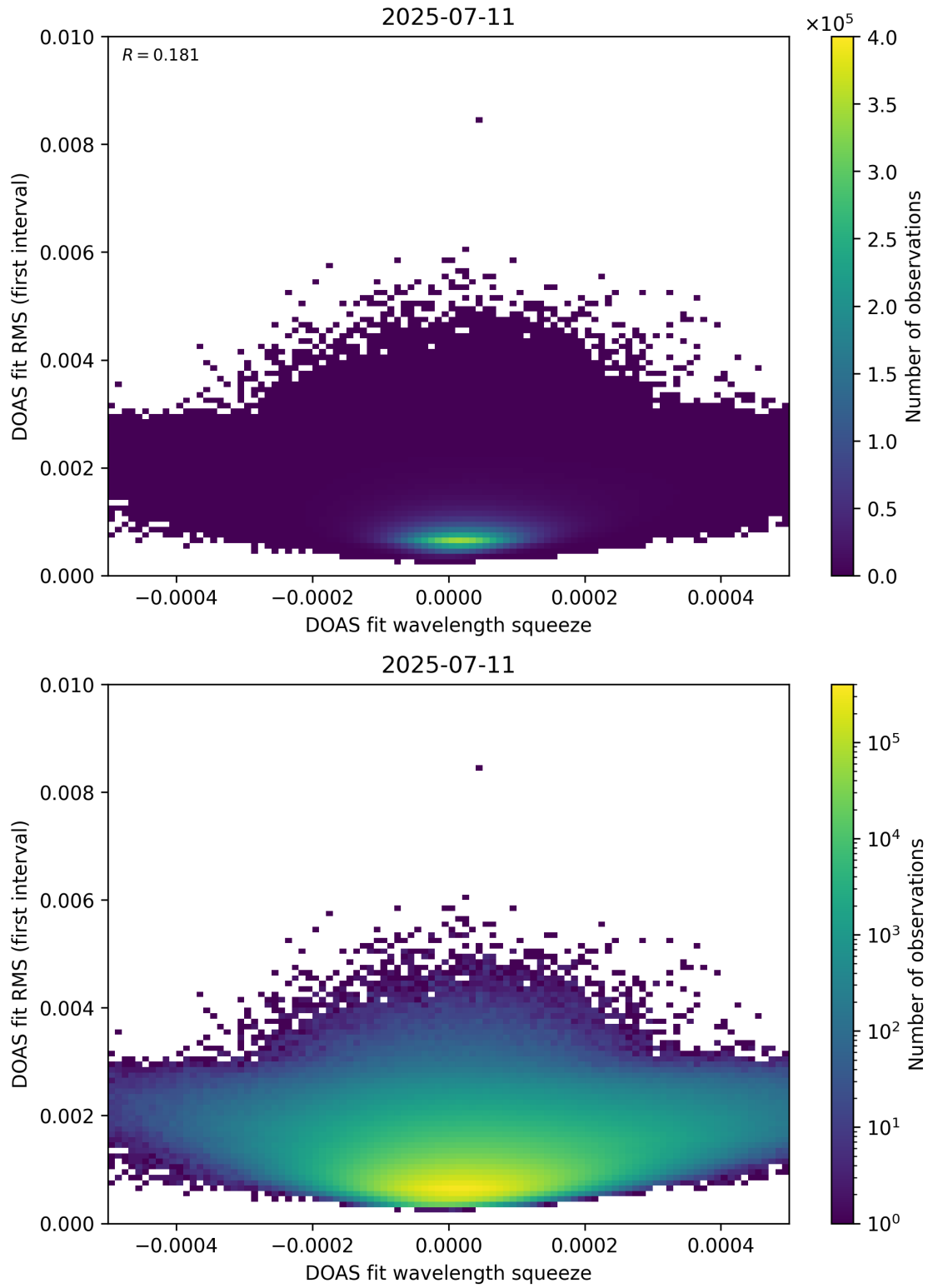
Figure 68: Scatter density plot of “DOAS fit wavelength squeeze” against “DOAS fit RMS (first interval)” for 2025-07-10 to 2025-07-12.
