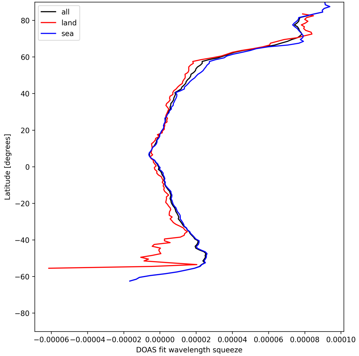
Figure 31: Zonal average of “DOAS fit wavelength squeeze” for 2025-07-10 to 2025-07-12.
