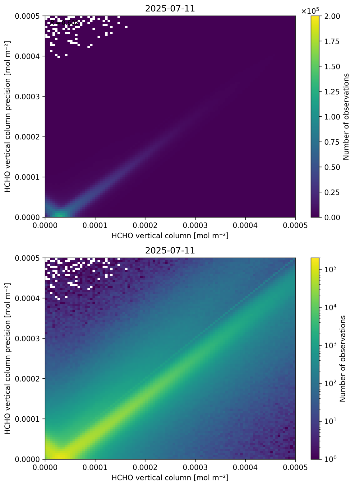
Figure 134: Scatter density plot of “HCHO vertical column” against “HCHO vertical column precision” for 2025-07-10 to 2025-07-12.
