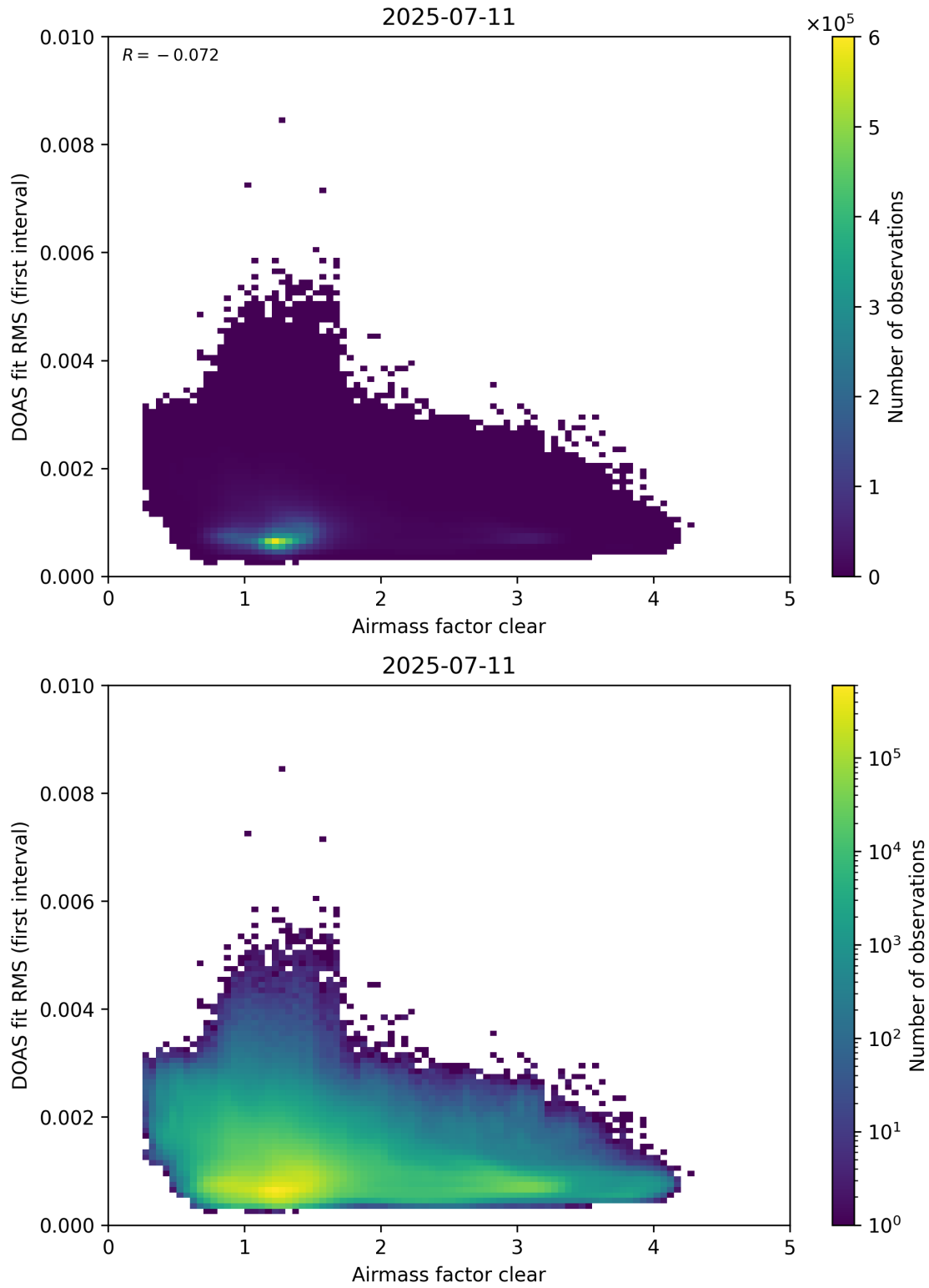
Figure 71: Scatter density plot of “Airmass factor clear” against “DOAS fit RMS (first interval)” for 2025-07-10 to 2025-07-12.
