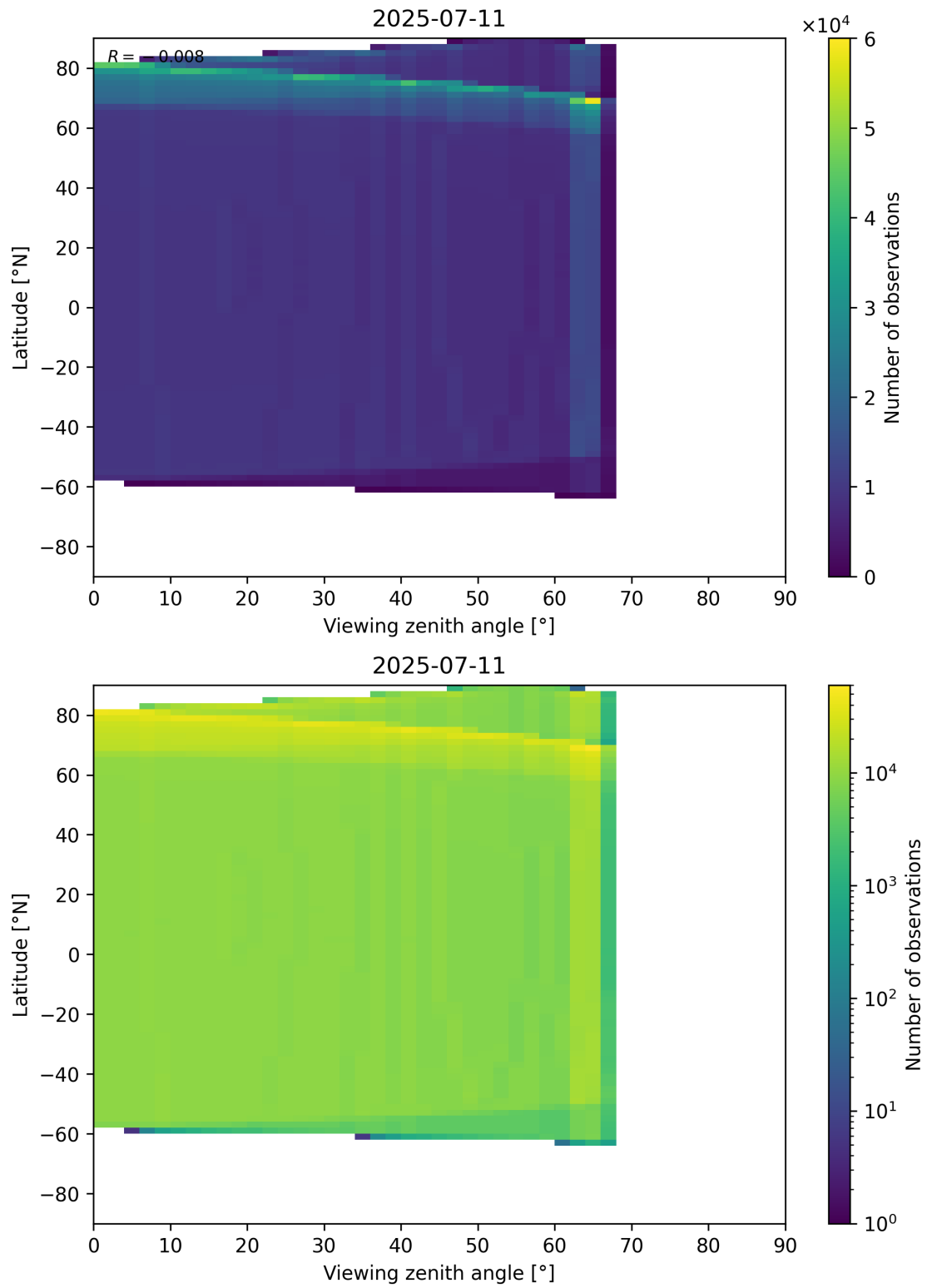
Figure 196: Scatter density plot of “Viewing zenith angle” against “Latitude” for 2025-07-10 to 2025-07-12.
