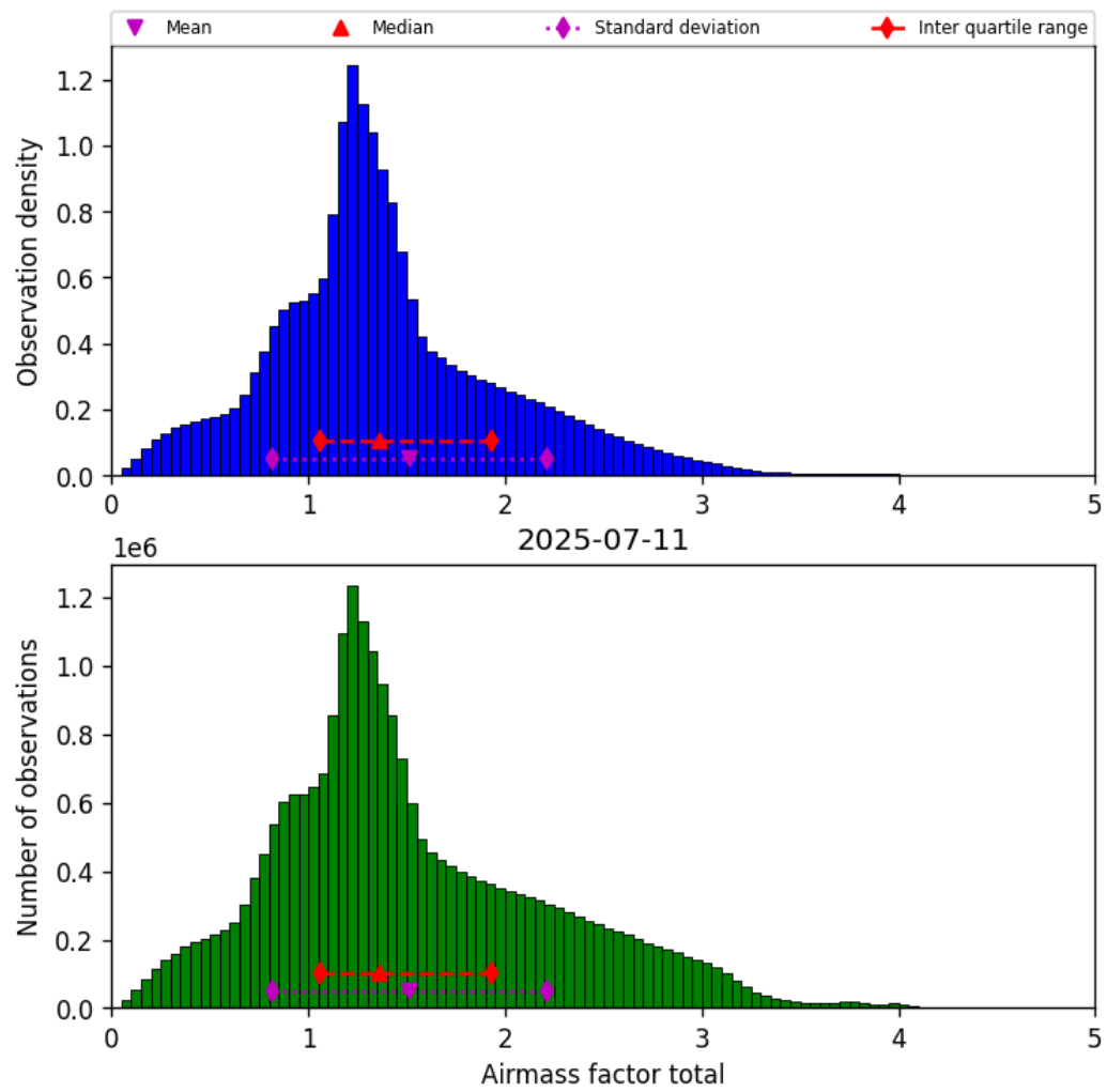
Figure 40: Histogram of “Airmass factor total” for 2025-07-10 to 2025-07-12
