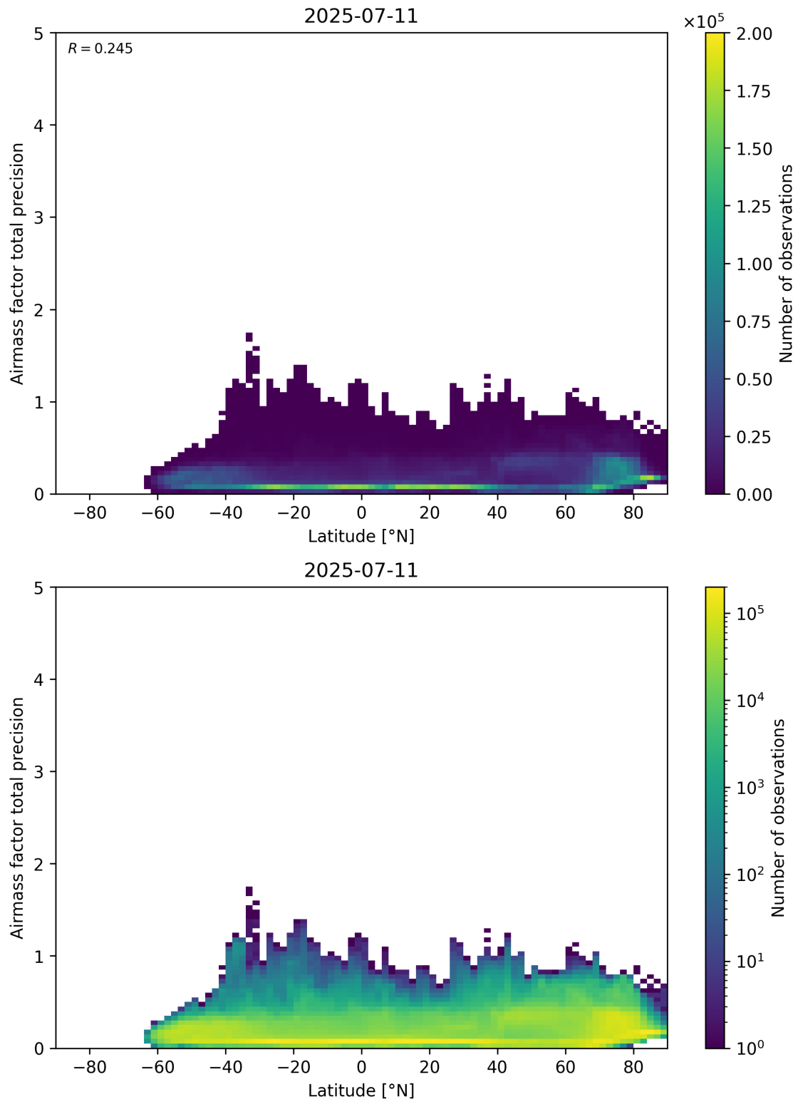
Figure 162: Scatter density plot of “Latitude” against “Airmass factor total precision” for 2025-07-10 to 2025-07-12.
