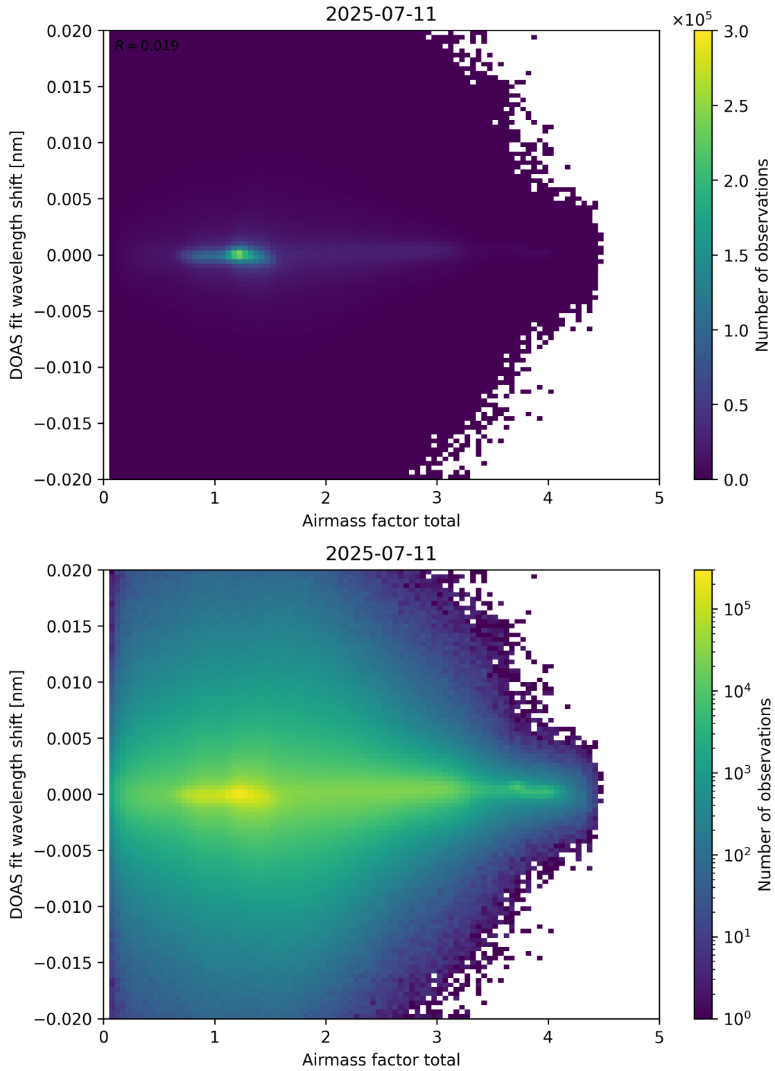
Figure 98: Scatter density plot of “Airmass factor total” against “DOAS fit wavelength shift” for 2025-07-10 to 2025-07-12.
