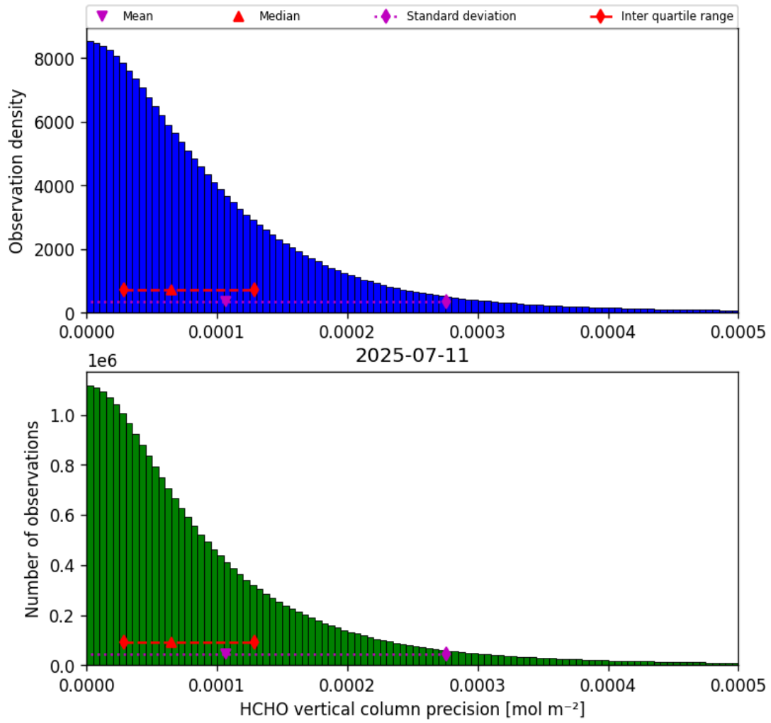
Figure 36: Histogram of “HCHO vertical column precision” for 2025-07-10 to 2025-07-12
