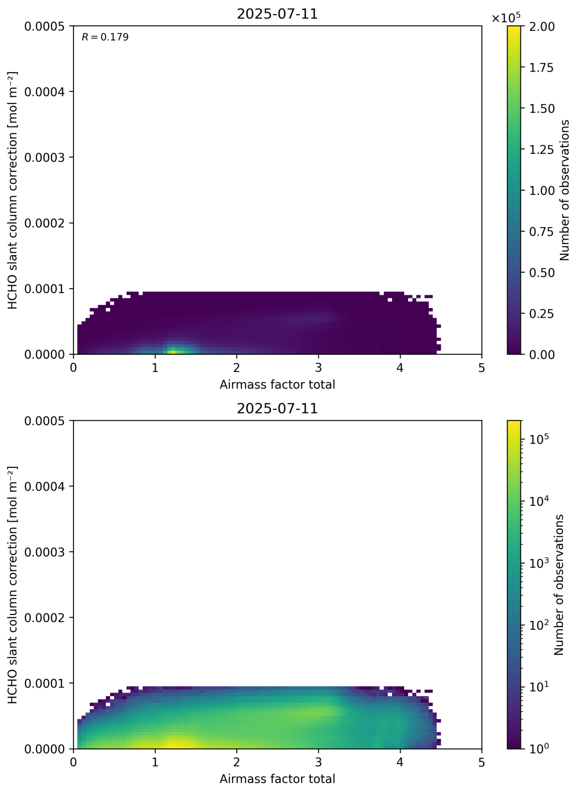
Figure 102: Scatter density plot of “Airmass factor total” against “HCHO slant column correction” for 2025-07-10 to 2025-07-12.
