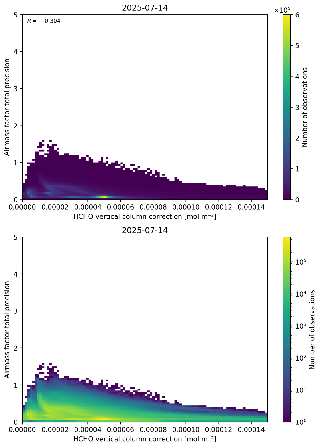
Figure 121: Scatter density plot of “HCHO vertical column correction” against “Airmass factor total precision” for 2025-07-13 to 2025-07-15.
