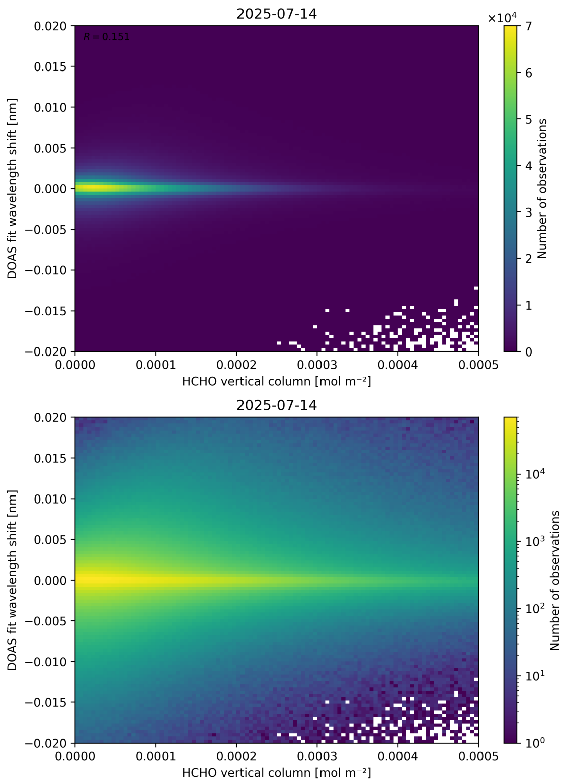
Figure 124: Scatter density plot of “HCHO vertical column” against “DOAS fit wavelength shift” for 2025-07-13 to 2025-07-15.
