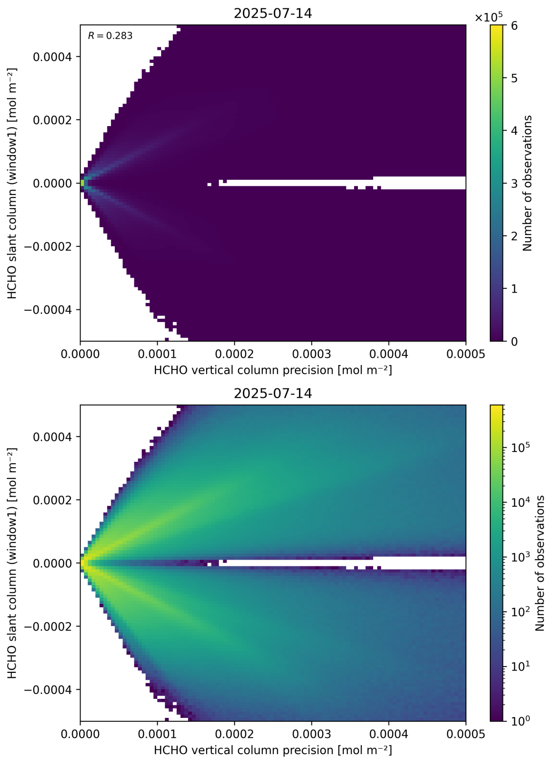
Figure 142: Scatter density plot of “HCHO vertical column precision” against “HCHO slant column (window1)” for 2025-07-13 to 2025-07-15.
