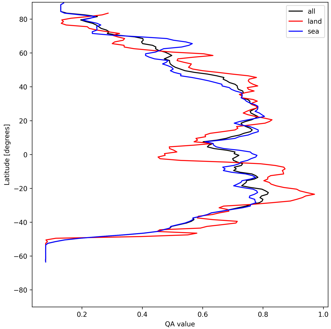
Figure 20: Zonal average of “QA value” for 2025-07-13 to 2025-07-15.
