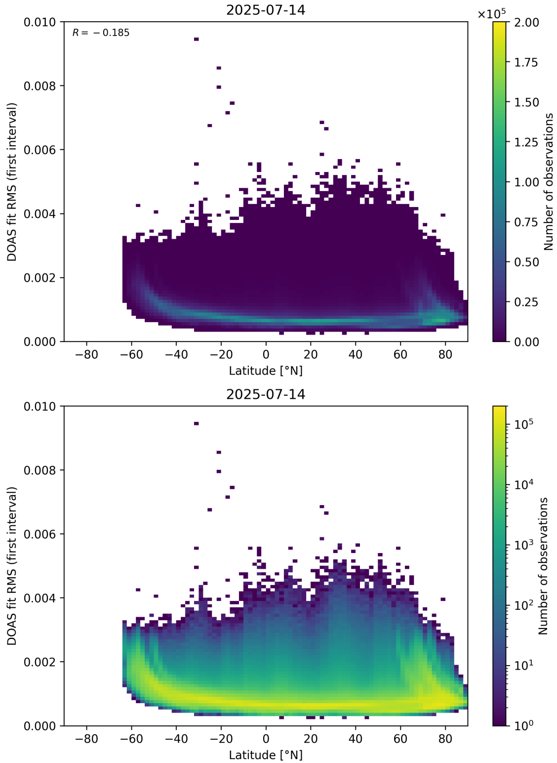
Figure 153: Scatter density plot of “Latitude” against “DOAS fit RMS (first interval)” for 2025-07-13 to 2025-07-15.
