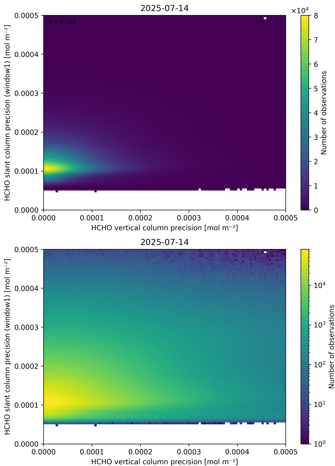
Figure 143: Scatter density plot of “HCHO vertical column precision” against “HCHO slant column precision (window1)” for 2025-07-13 to 2025-07-15.
