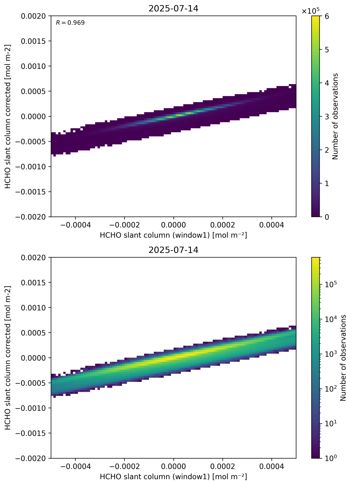
Figure 82: Scatter density plot of “HCHO slant column (window1)” against “HCHO slant column corrected” for 2025-07-13 to 2025-07-15.
