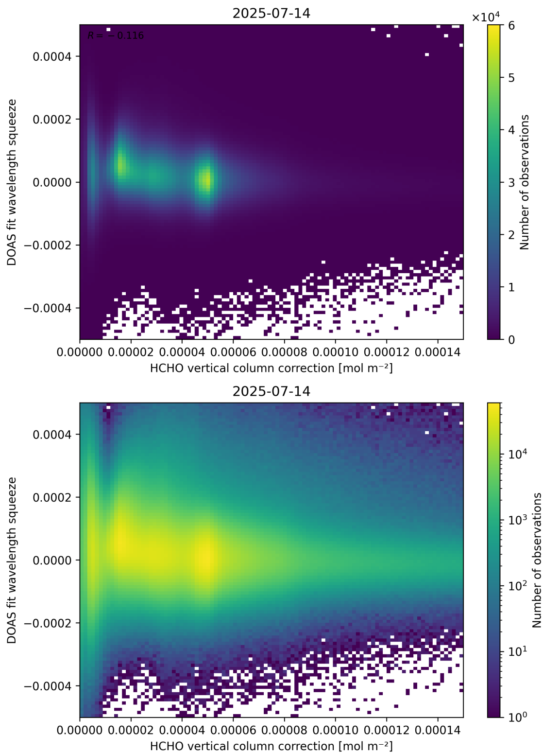
Figure 114: Scatter density plot of “HCHO vertical column correction” against “DOAS fit wavelength squeeze” for 2025-07-13 to 2025-07-15.
