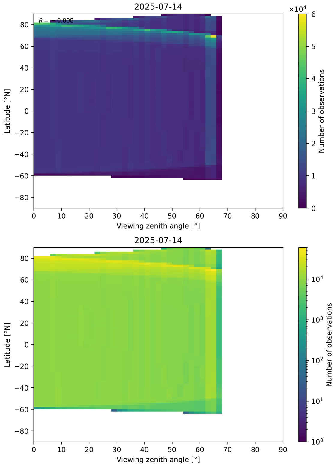
Figure 196: Scatter density plot of “Viewing zenith angle” against “Latitude” for 2025-07-13 to 2025-07-15.
