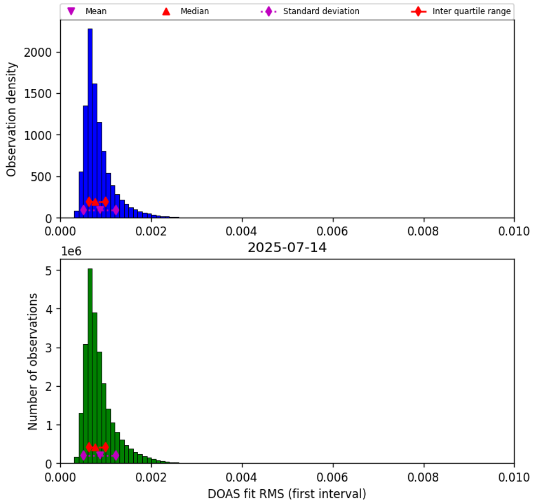
Figure 46: Histogram of “DOAS fit RMS (first interval)” for 2025-07-13 to 2025-07-15
