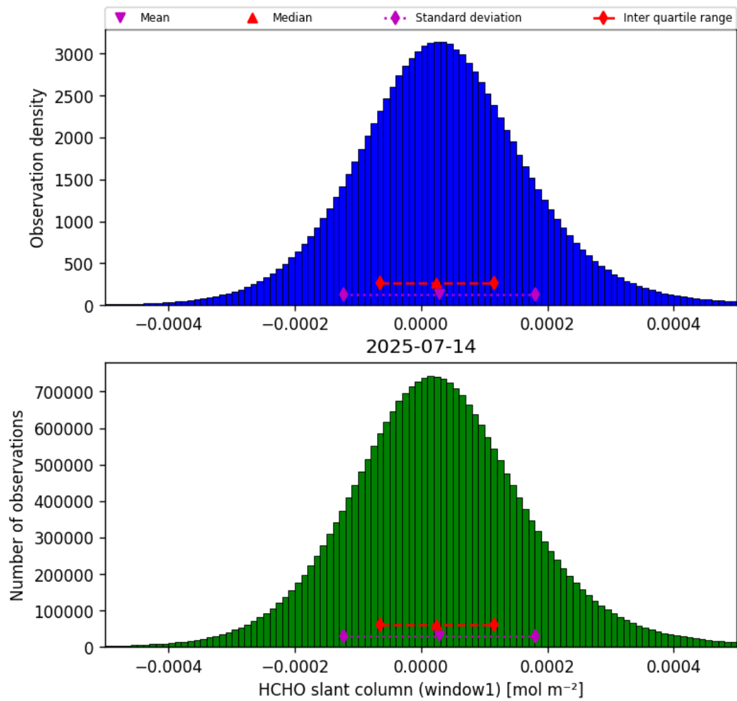
Figure 38: Histogram of “HCHO slant column (window1)” for 2025-07-13 to 2025-07-15
