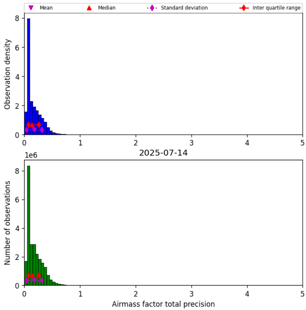
Figure 41: Histogram of “Airmass factor total precision” for 2025-07-13 to 2025-07-15
