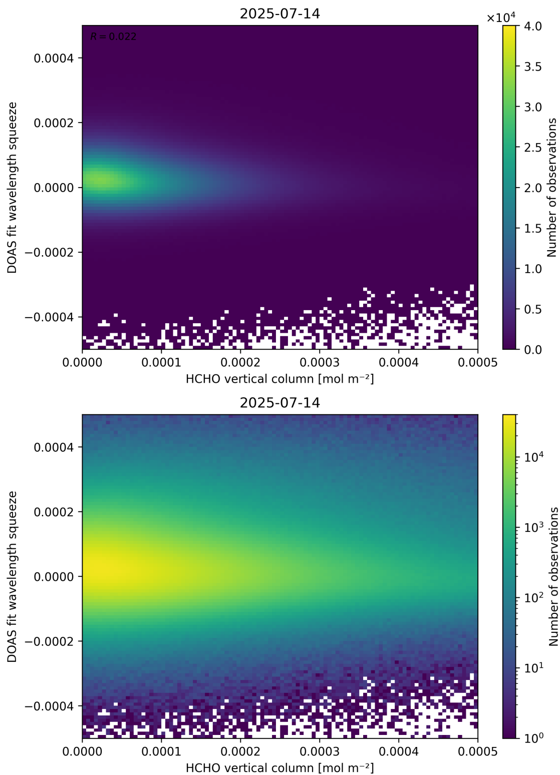
Figure 125: Scatter density plot of “HCHO vertical column” against “DOAS fit wavelength squeeze” for 2025-07-13 to 2025-07-15.
