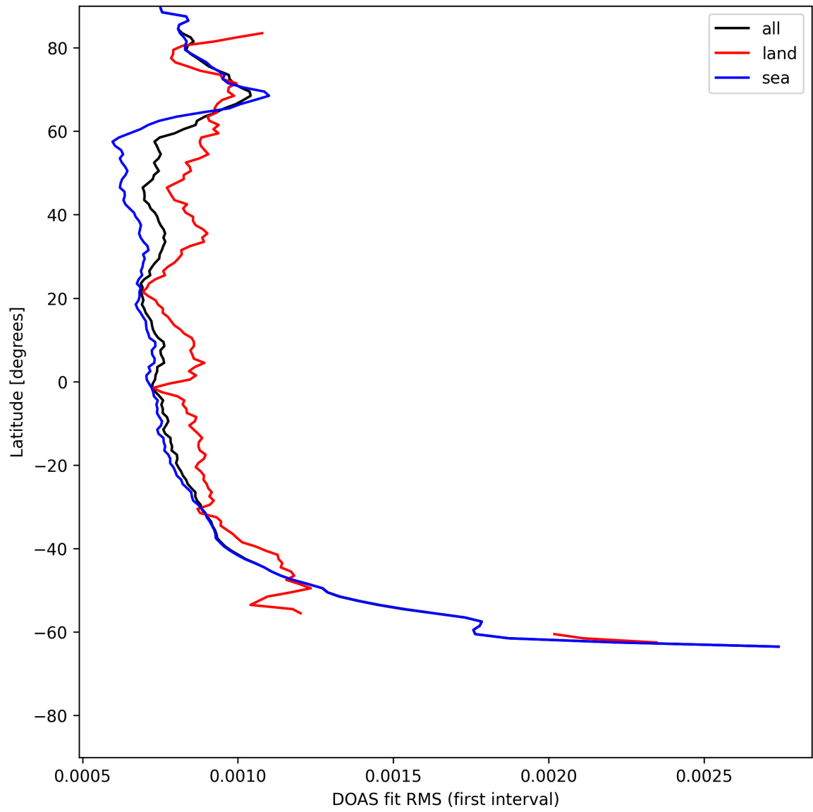
Figure 32: Zonal average of "DOAS fit RMS (first interval)" for 2025-07-13 to 2025-07-15.
