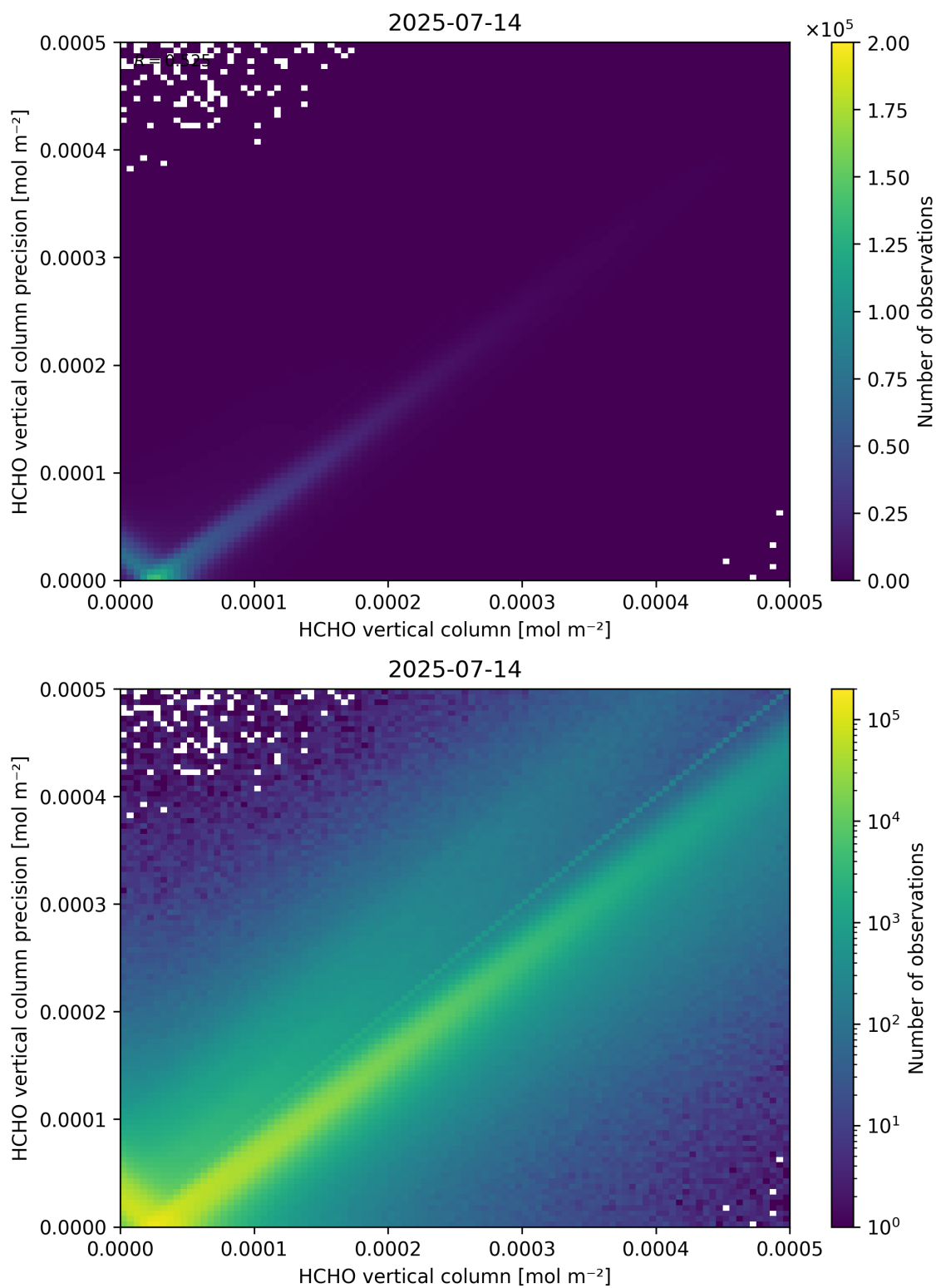
Figure 134: Scatter density plot of “HCHO vertical column” against “HCHO vertical column precision” for 2025-07-13 to 2025-07-15.
