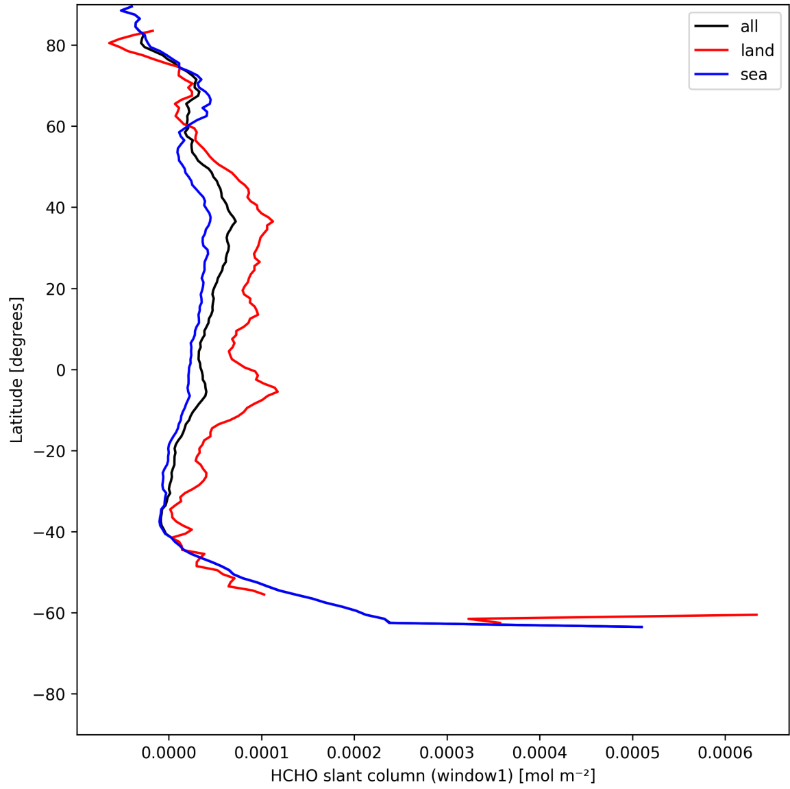
Figure 24: Zonal average of “HCHO slant column (window1)” for 2025-07-13 to 2025-07-15.
