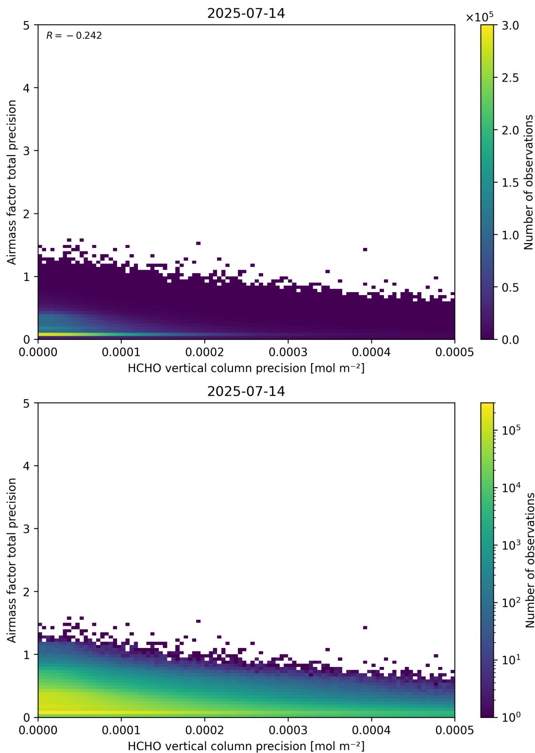
Figure 145: Scatter density plot of “HCHO vertical column precision” against “Airmass factor total precision” for 2025-07-13 to 2025-07-15.
