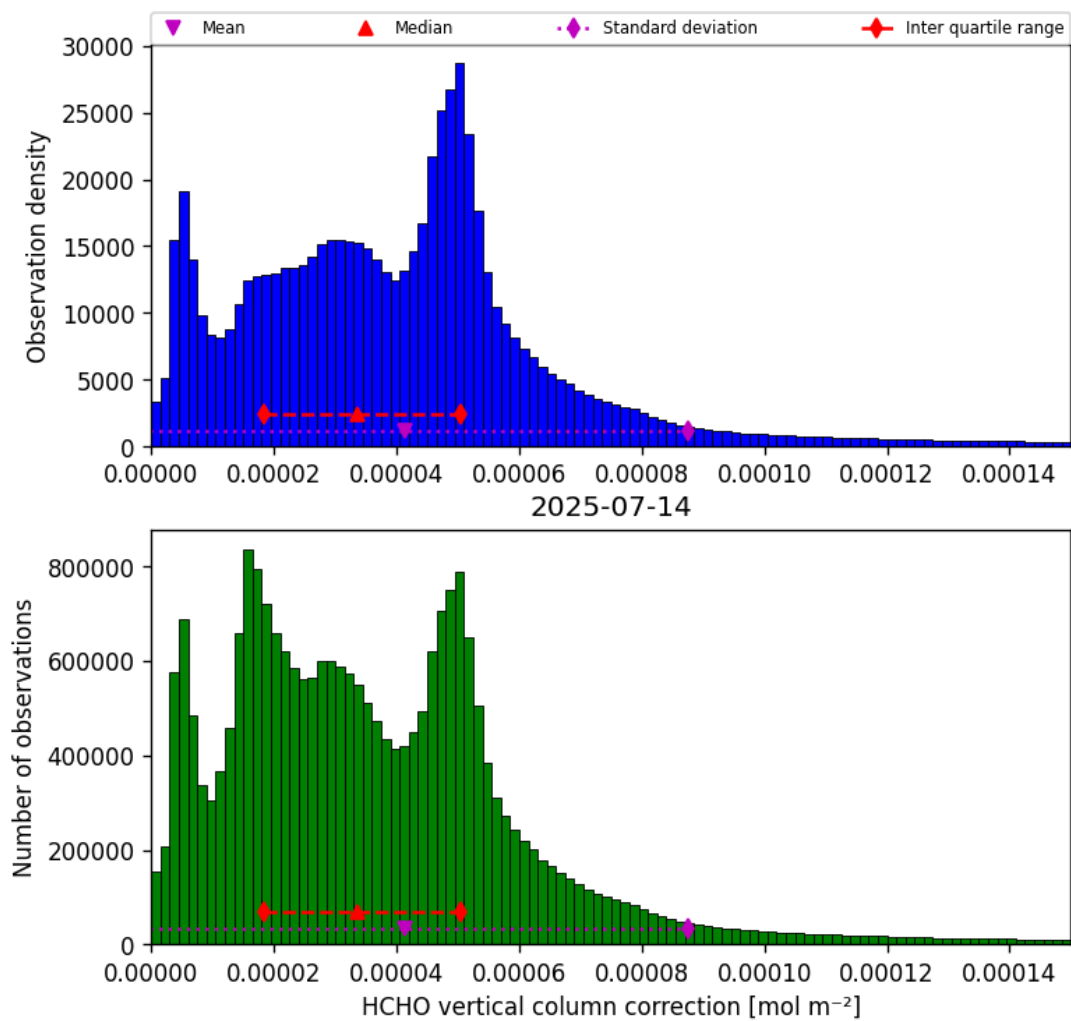
Figure 37: Histogram of “HCHO vertical column correction” for 2025-07-13 to 2025-07-15
