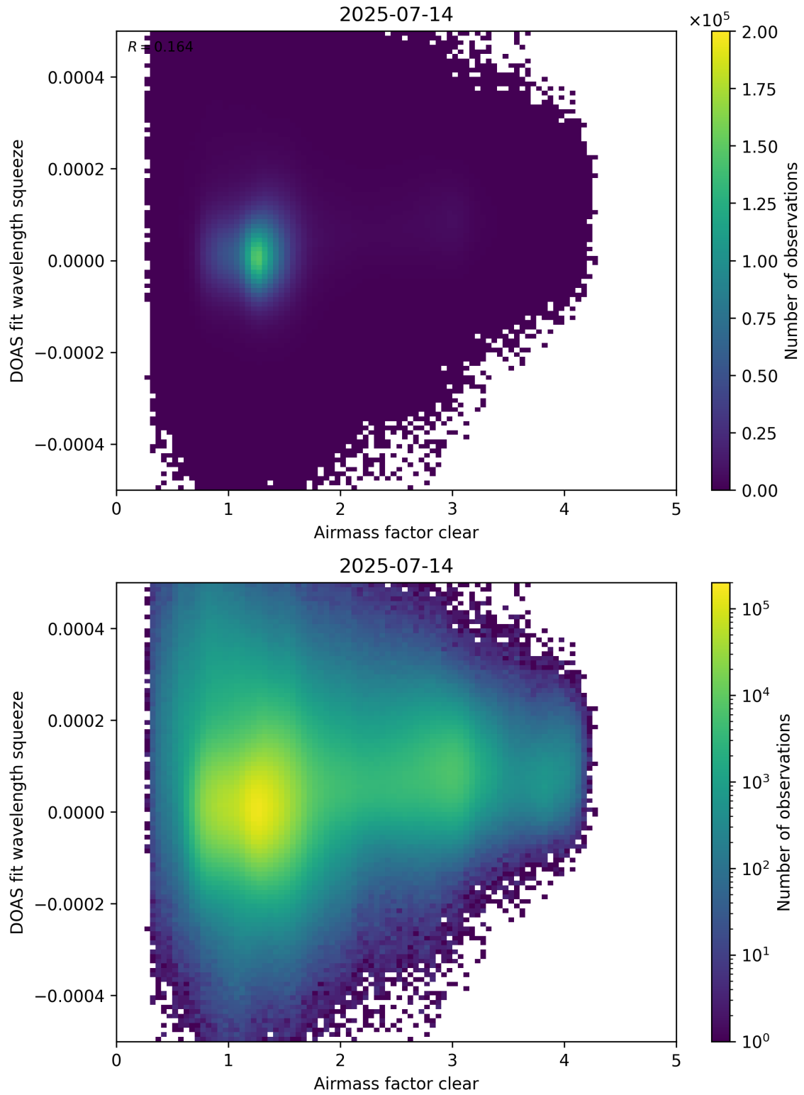
Figure 73: Scatter density plot of “Airmass factor clear” against “DOAS fit wavelength squeeze” for 2025-07-13 to 2025-07-15.
