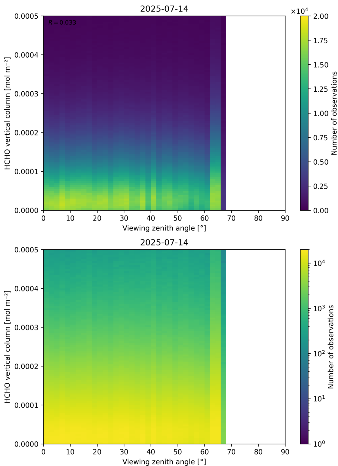
Figure 192: Scatter density plot of “Viewing zenith angle” against “HCHO vertical column” for 2025-07-13 to 2025-07-15.
