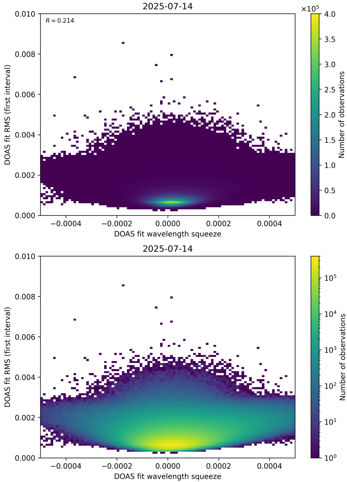
Figure 68: Scatter density plot of “DOAS fit wavelength squeeze” against “DOAS fit RMS (first interval)” for 2025-07-13 to 2025-07-15.
