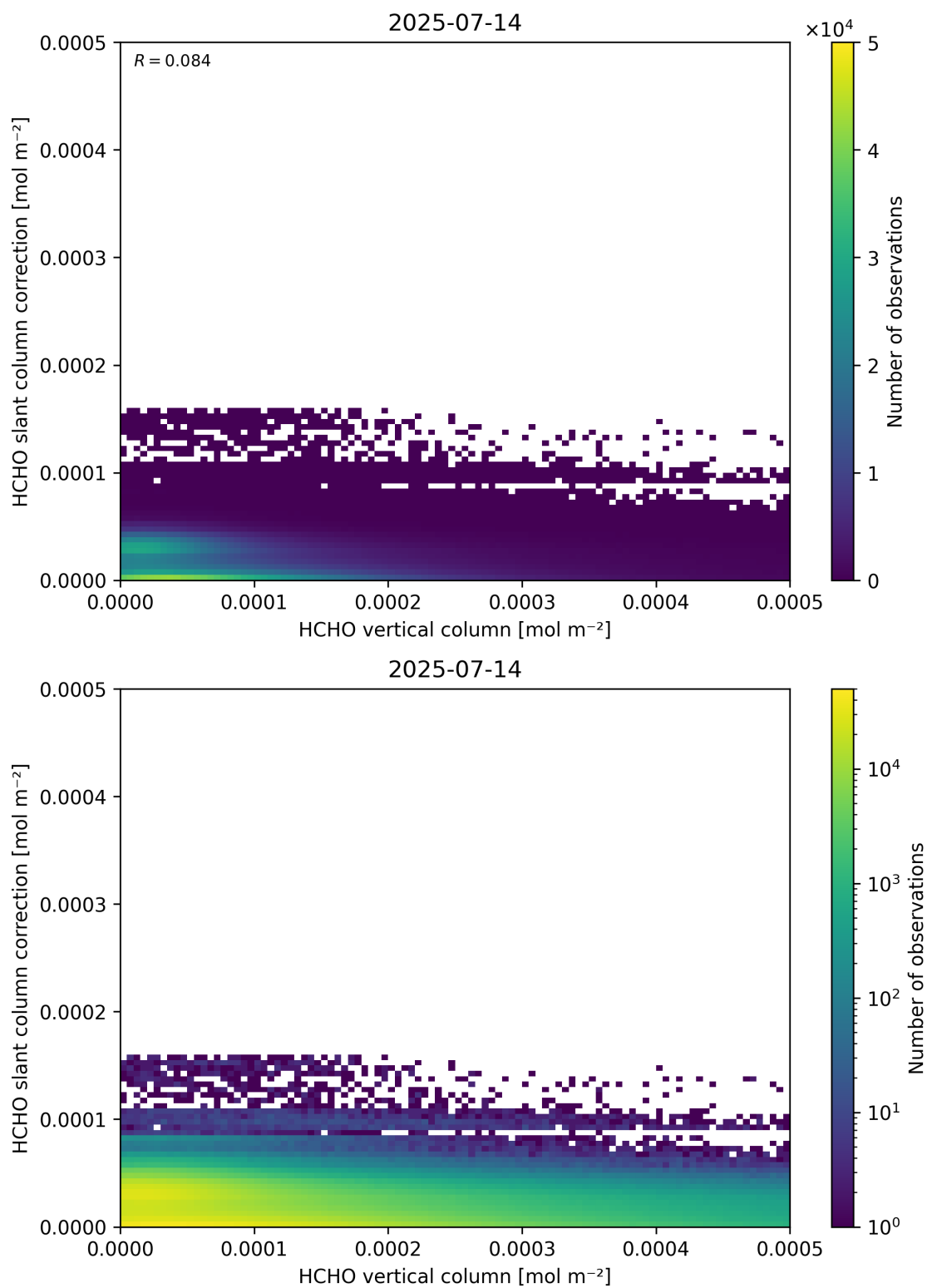
Figure 128: Scatter density plot of “HCHO vertical column” against “HCHO slant column correction” for 2025-07-13 to 2025-07-15.
