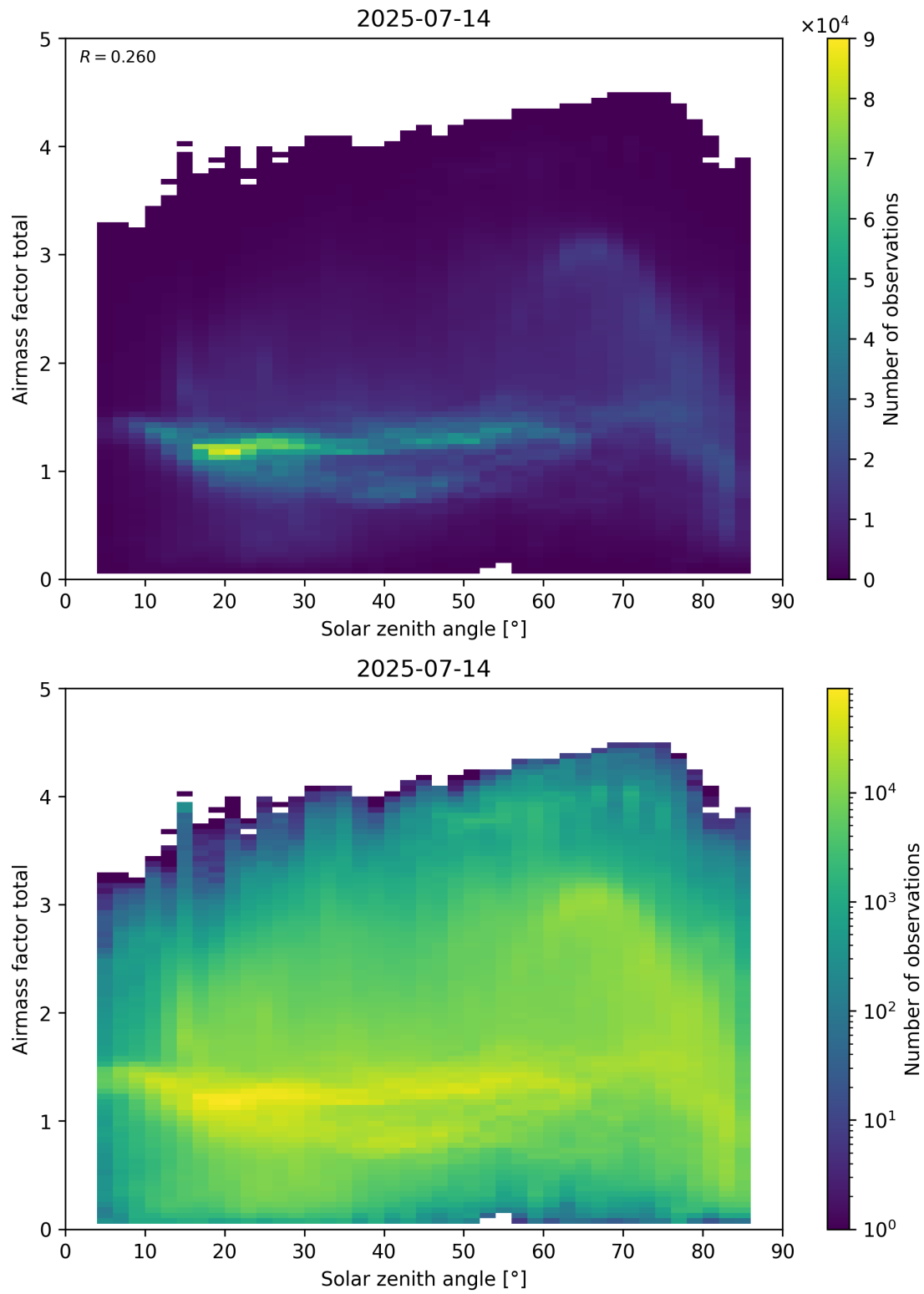
Figure 175: Scatter density plot of “Solar zenith angle” against “Airmass factor total” for 2025-07-13 to 2025-07-15.
