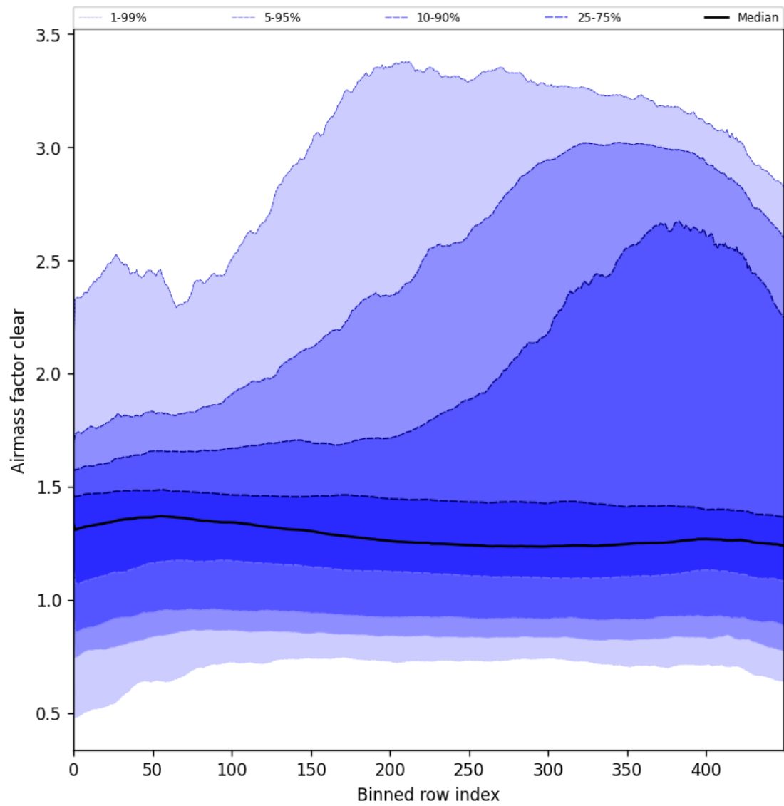
Figure 56: Along track statistics of “Air mass factor clear” for 2025-07-13 to 2025-07-15
