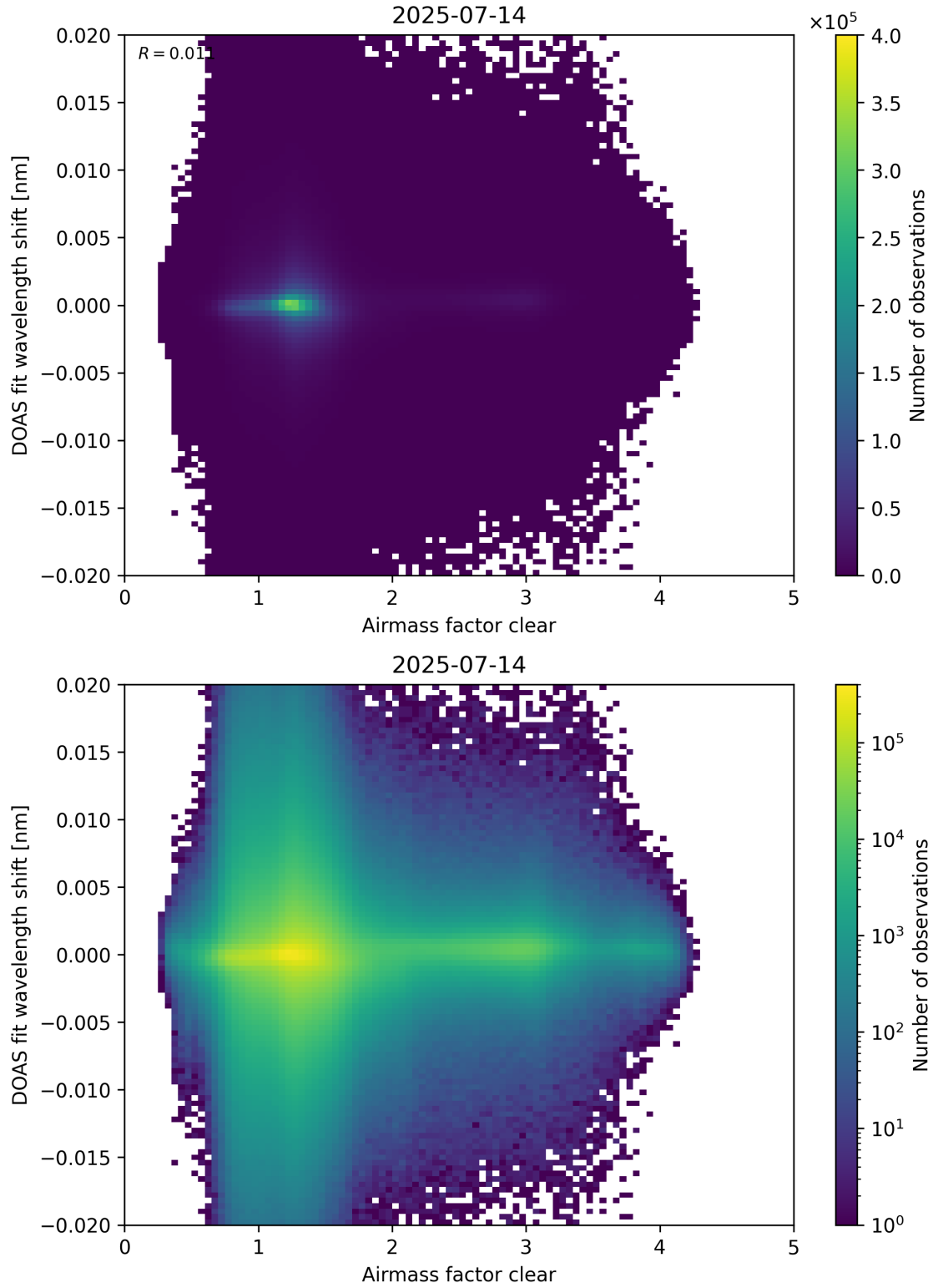
Figure 72: Scatter density plot of “Airmass factor clear” against “DOAS fit wavelength shift” for 2025-07-13 to 2025-07-15.
