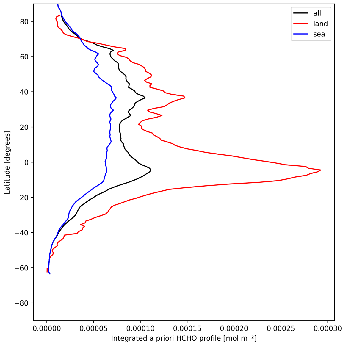
Figure 29: Zonal average of “Integrated a priori HCHO profile” for 2025-07-13 to 2025-07-15.
