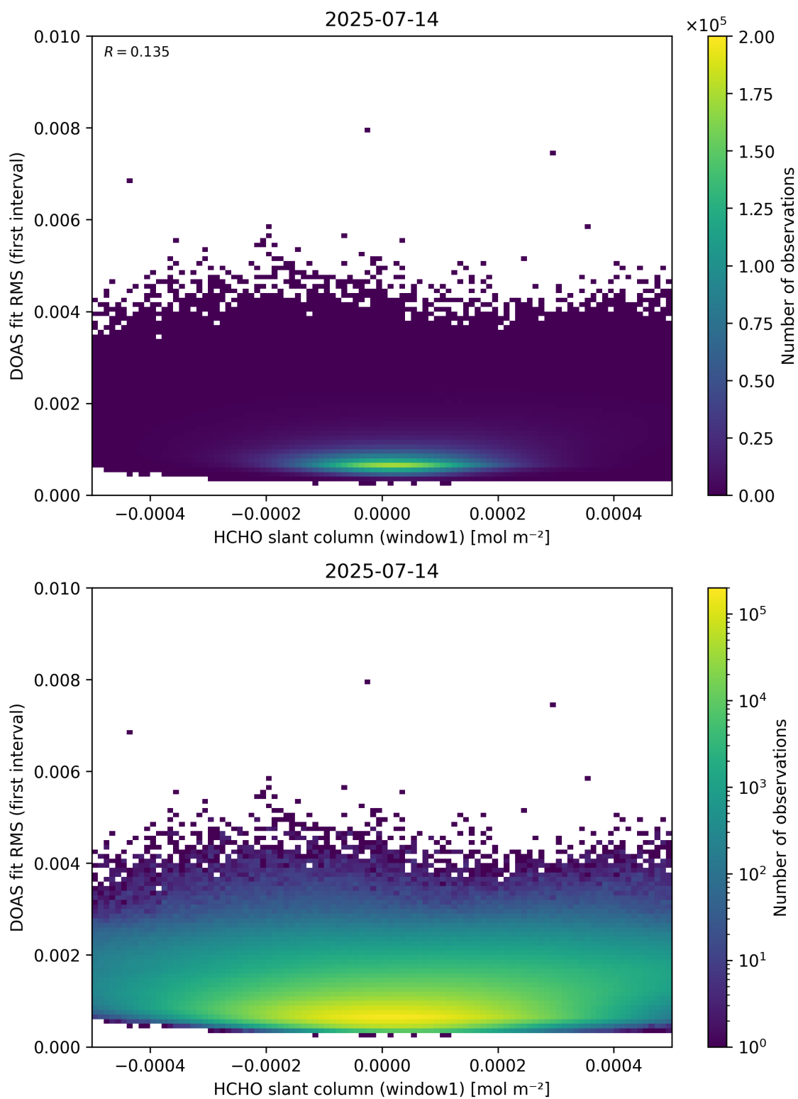
Figure 78: Scatter density plot of “HCHO slant column (window1)” against “DOAS fit RMS (first interval)” for 2025-07-13 to 2025-07-15.
