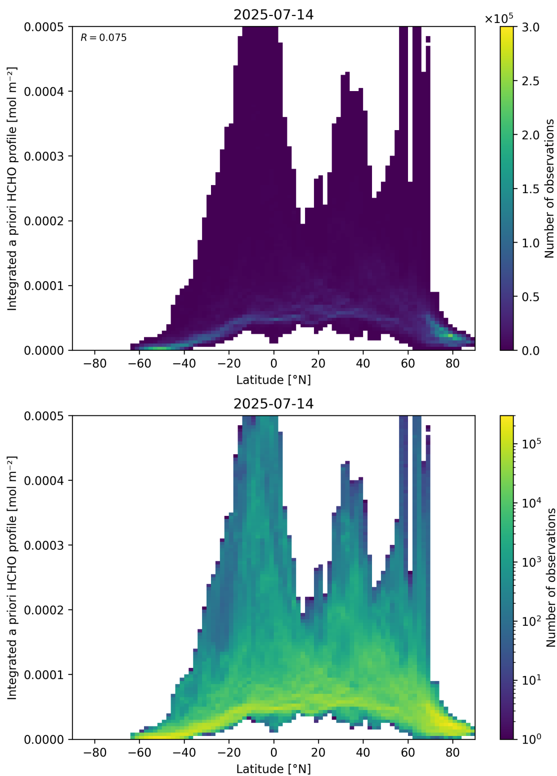
Figure 166: Scatter density plot of “Latitude” against “Integrated a priori HCHO profile” for 2025-07-13 to 2025-07-15.
