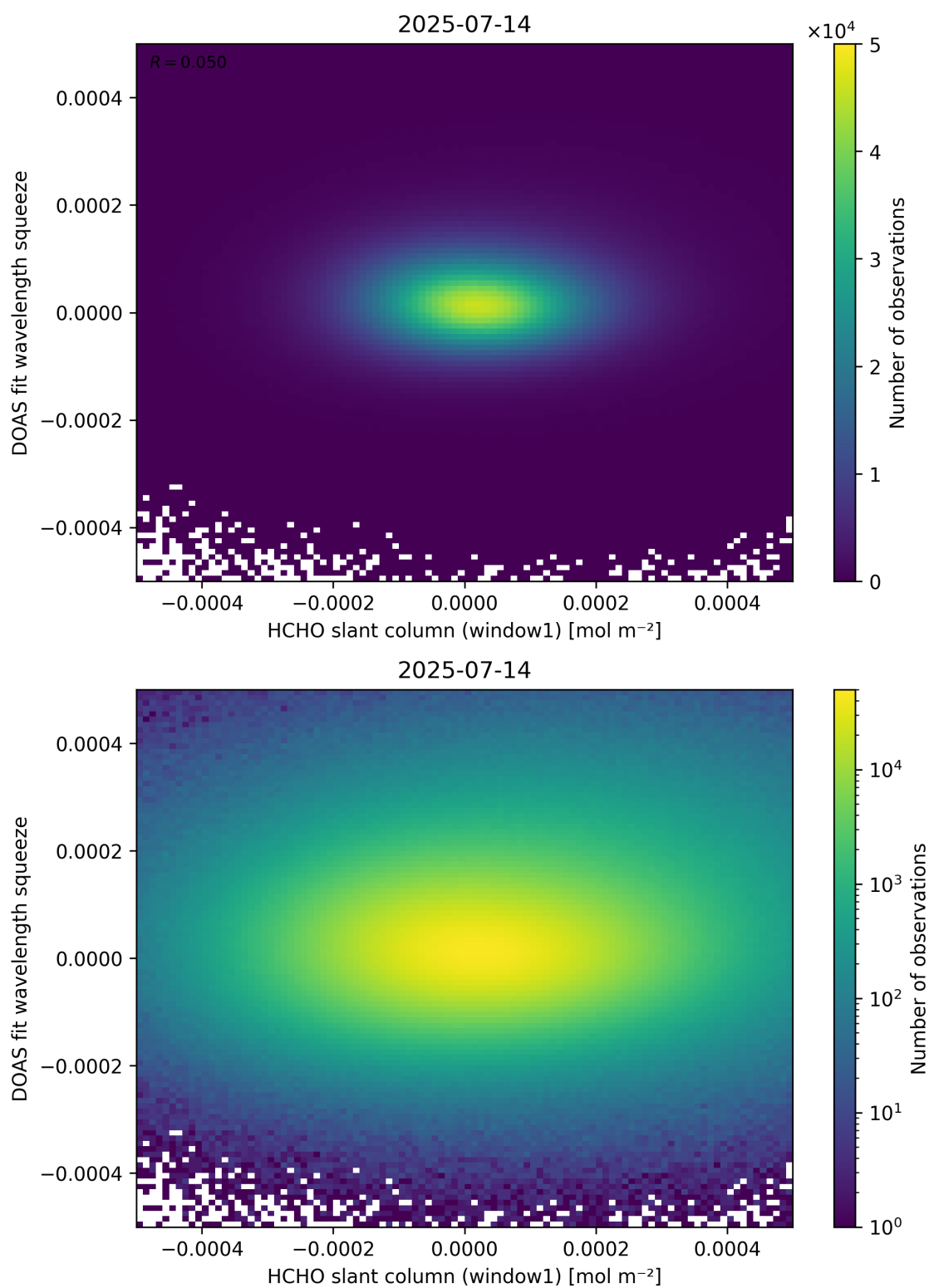
Figure 80: Scatter density plot of “HCHO slant column (window1)” against “DOAS fit wavelength squeeze” for 2025-07-13 to 2025-07-15.
