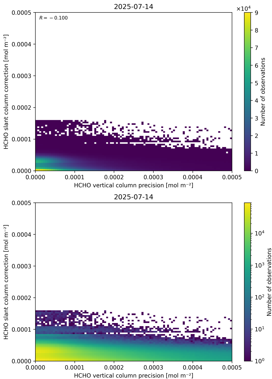
Figure 141: Scatter density plot of “HCHO vertical column precision” against “HCHO slant column correction” for 2025-07-13 to 2025-07-15.
