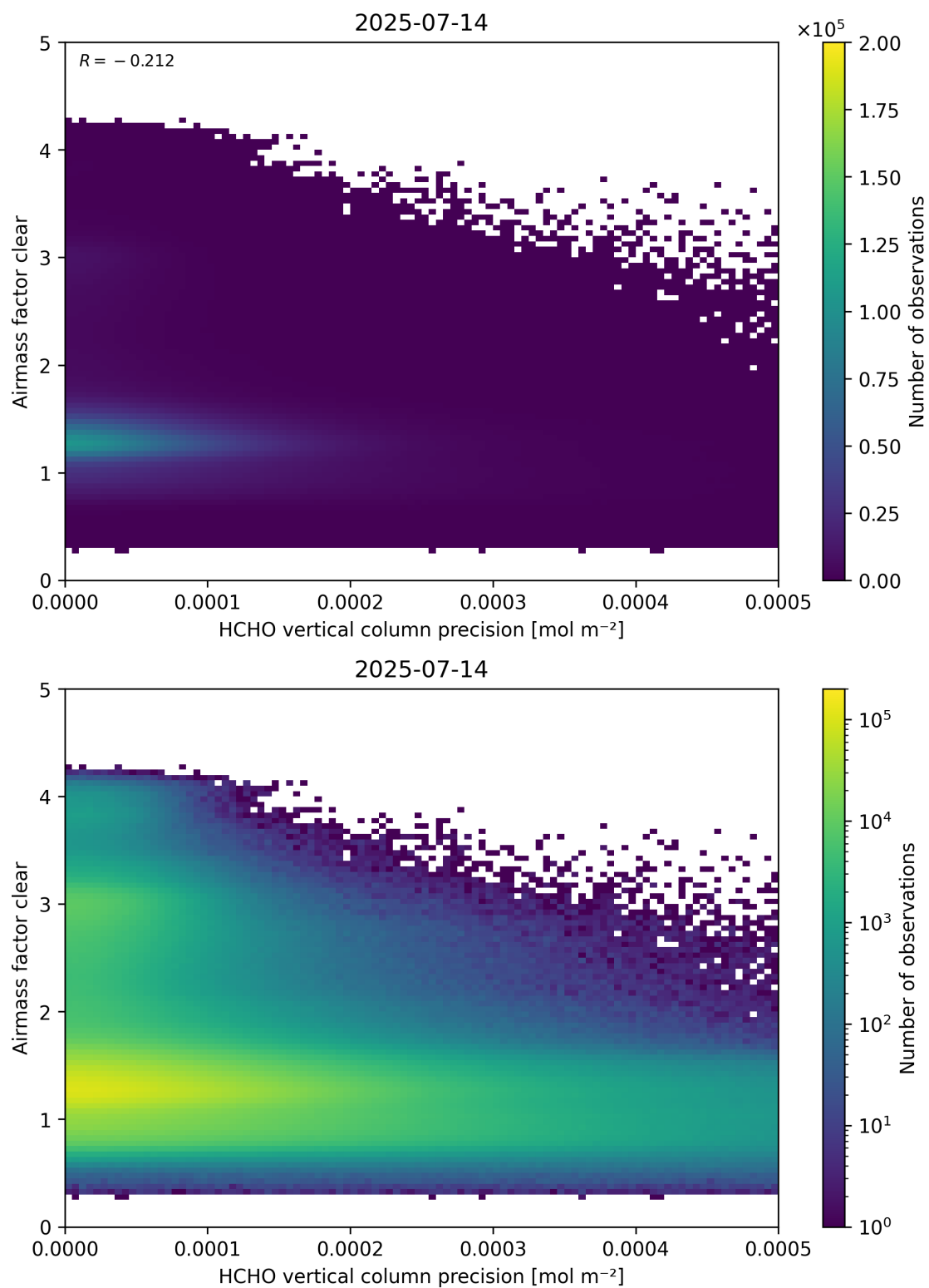
Figure 139: Scatter density plot of “HCHO vertical column precision” against “Airmass factor clear” for 2025-07-13 to 2025-07-15.
