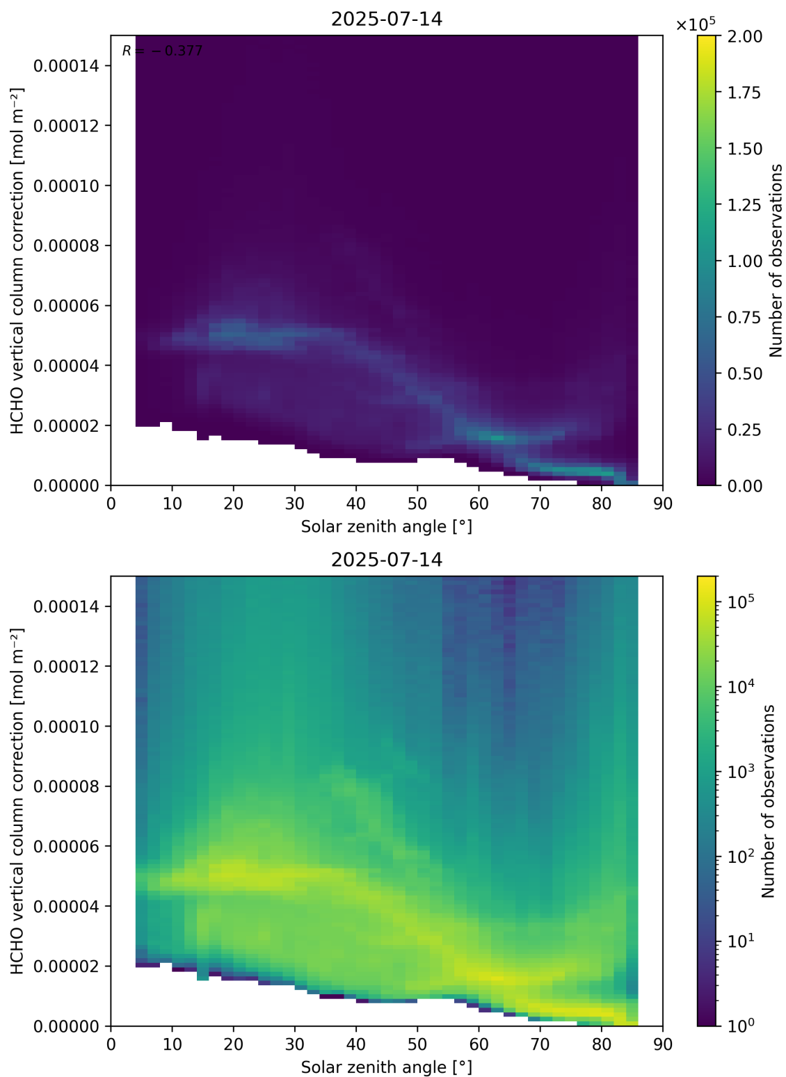
Figure 178: Scatter density plot of “Solar zenith angle” against “HCHO vertical column correction” for 2025-07-13 to 2025-07-15.
