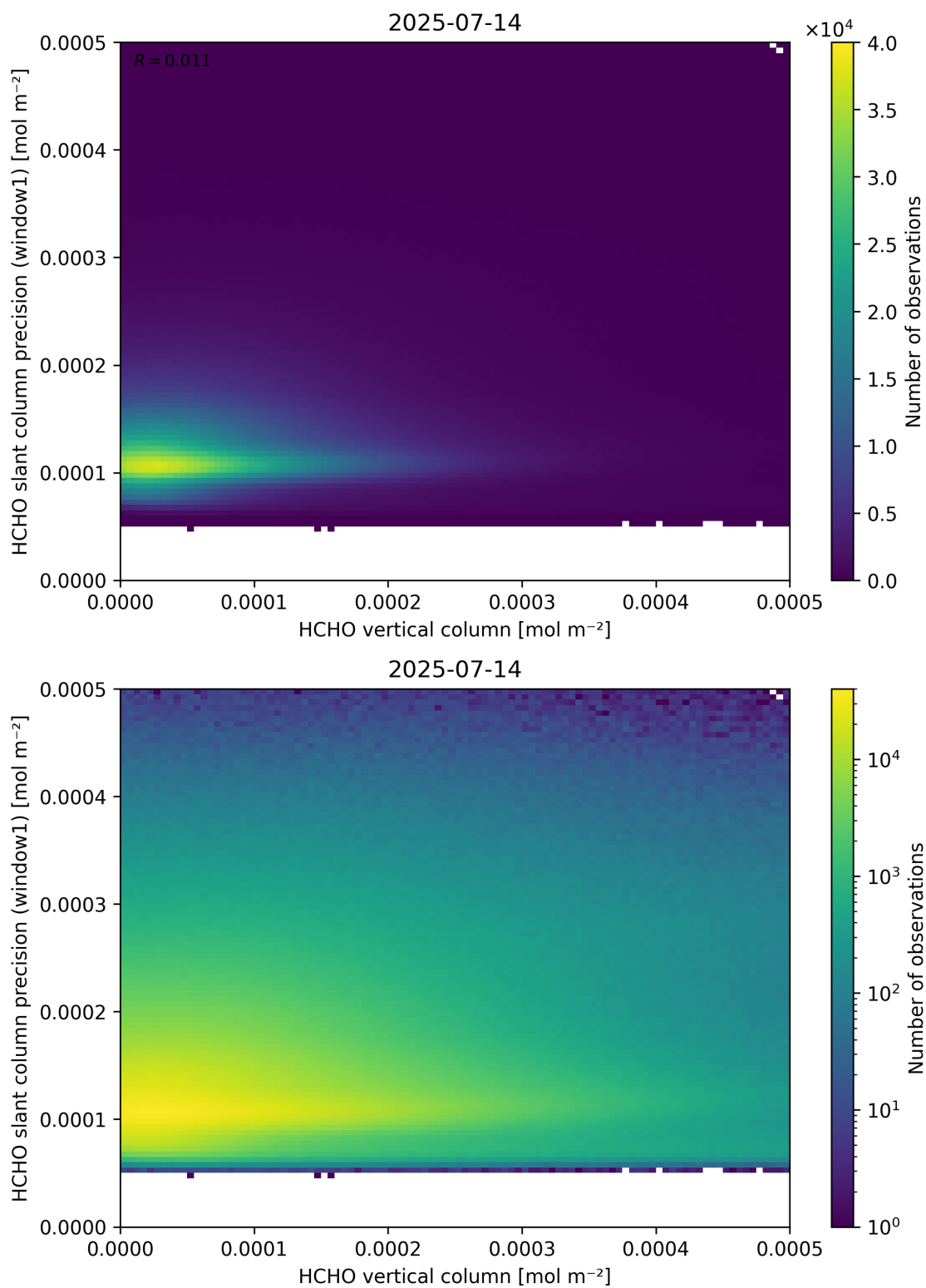
Figure 130: Scatter density plot of “HCHO vertical column” against “HCHO slant column precision (window1)” for 2025-07-13 to 2025-07-15.
