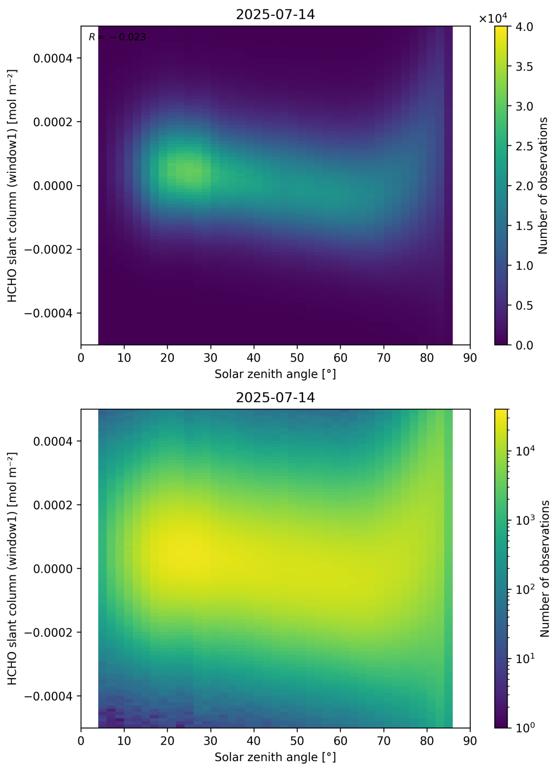
Figure 173: Scatter density plot of “Solar zenith angle” against “HCHO slant column (window1)” for 2025-07-13 to 2025-07-15.
