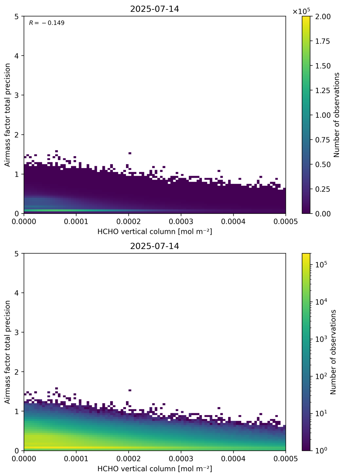
Figure 132: Scatter density plot of “HCHO vertical column” against “Airmass factor total precision” for 2025-07-13 to 2025-07-15.
