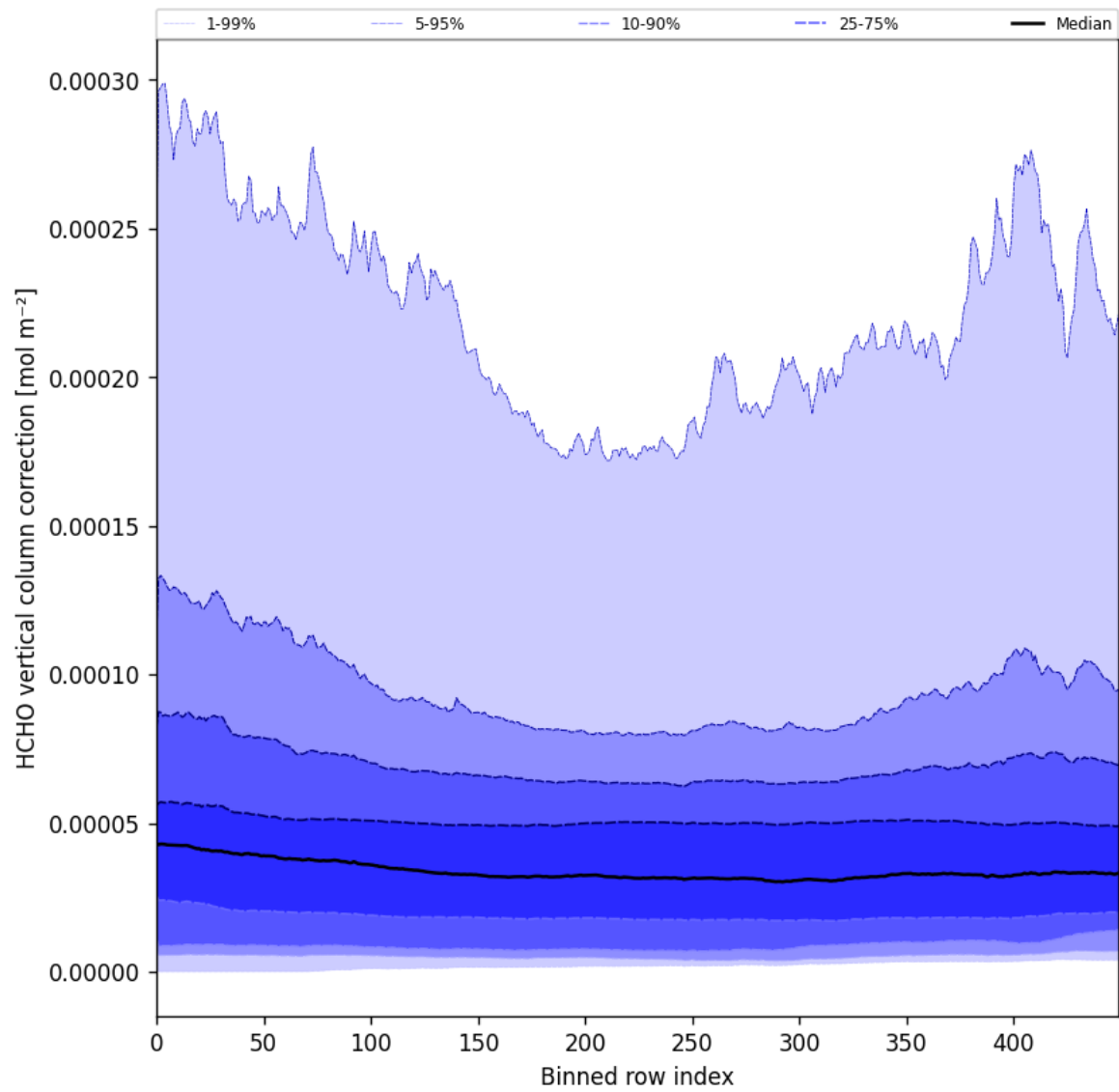
Figure 51: Along track statistics of “HCHO vertical column correction” for 2025-07-13 to 2025-07-15
