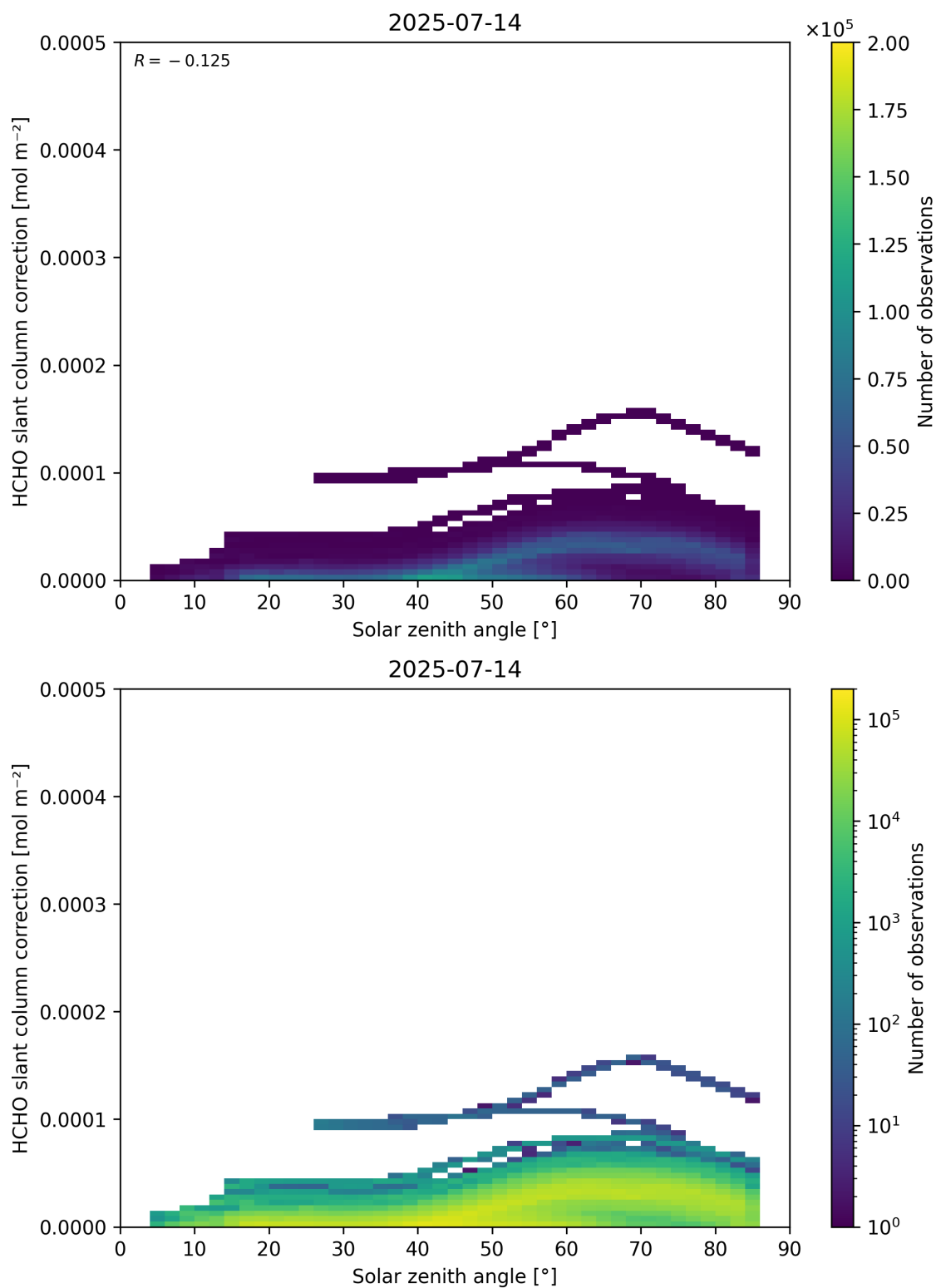
Figure 172: Scatter density plot of “Solar zenith angle” against “HCHO slant column correction” for 2025-07-13 to 2025-07-15.
