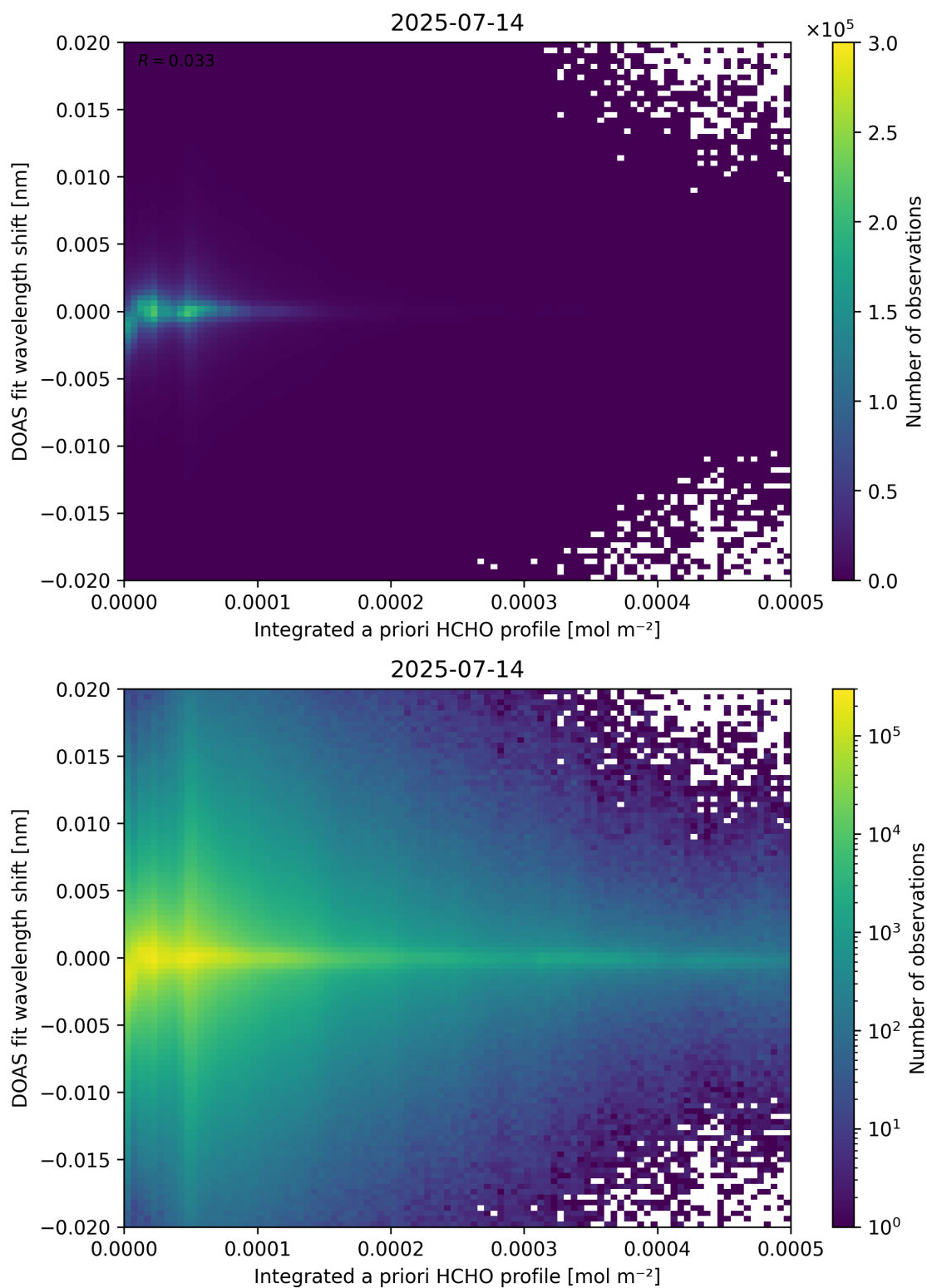
Figure 149: Scatter density plot of “Integrated a priori HCHO profile” against “DOAS fit wavelength shift” for 2025-07-13 to 2025-07-15.
