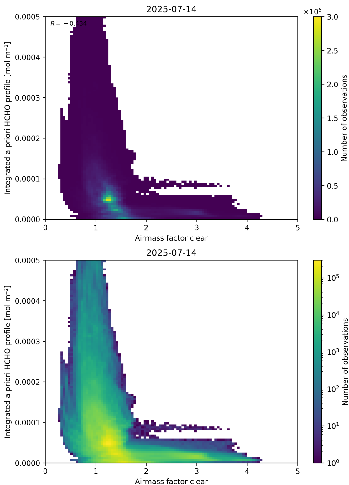
Figure 76: Scatter density plot of “Airmass factor clear” against “Integrated a priori HCHO profile” for 2025-07-13 to 2025-07-15.
