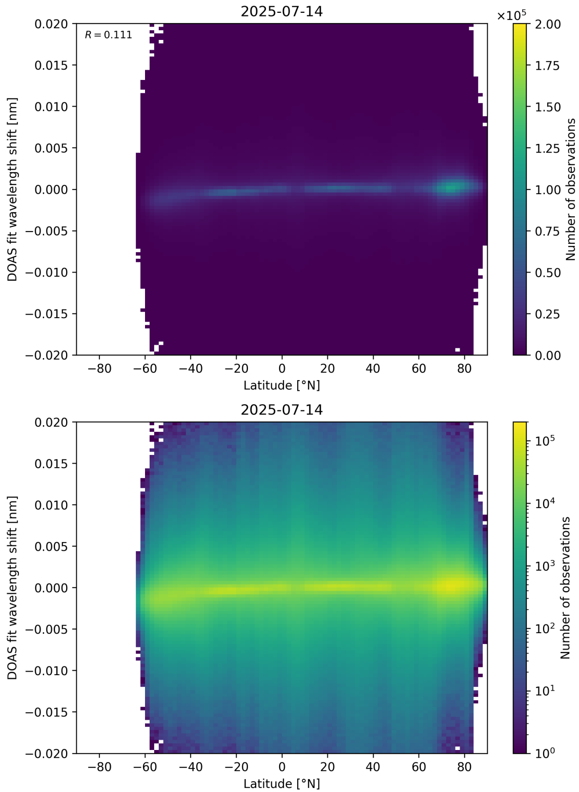
Figure 154: Scatter density plot of “Latitude” against “DOAS fit wavelength shift” for 2025-07-13 to 2025-07-15.
