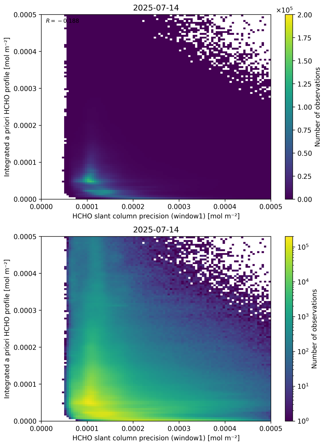
Figure 96: Scatter density plot of “HCHO slant column precision (window1)” against “Integrated a priori HCHO profile” for 2025-07-13 to 2025-07-15.
