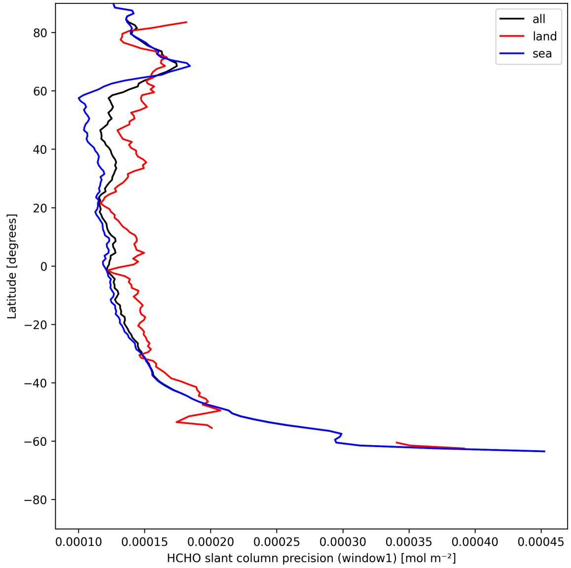
Figure 25: Zonal average of “HCHO slant column precision (window1)” for 2025-07-13 to 2025-07-15.
