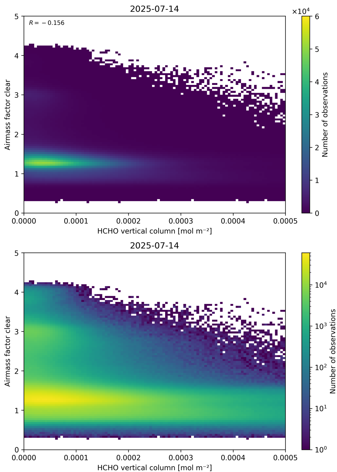
Figure 126: Scatter density plot of “HCHO vertical column” against “Airmass factor clear” for 2025-07-13 to 2025-07-15.
