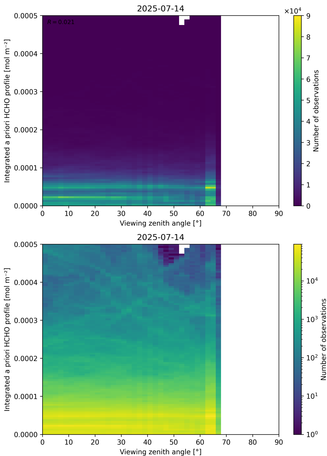
Figure 195: Scatter density plot of “Viewing zenith angle” against “Integrated a priori HCHO profile” for 2025-07-13 to 2025-07-15.
