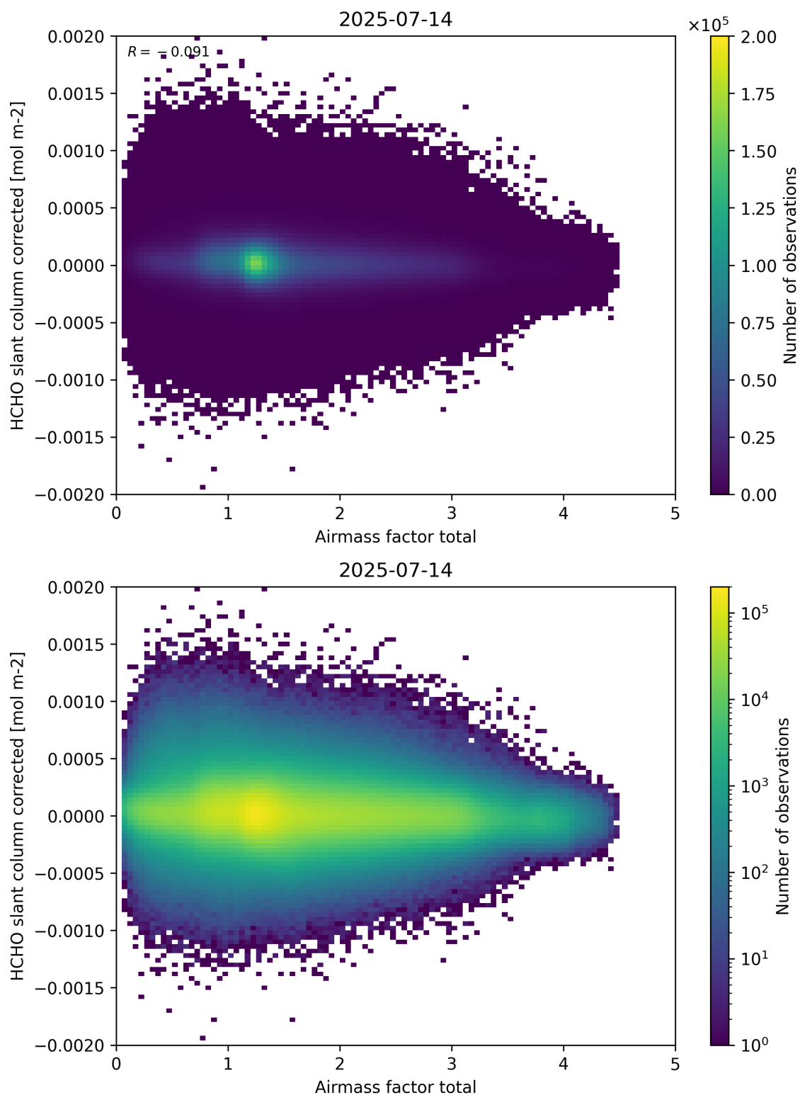
Figure 101: Scatter density plot of “Airmass factor total” against “HCHO slant column corrected” for 2025-07-13 to 2025-07-15.
