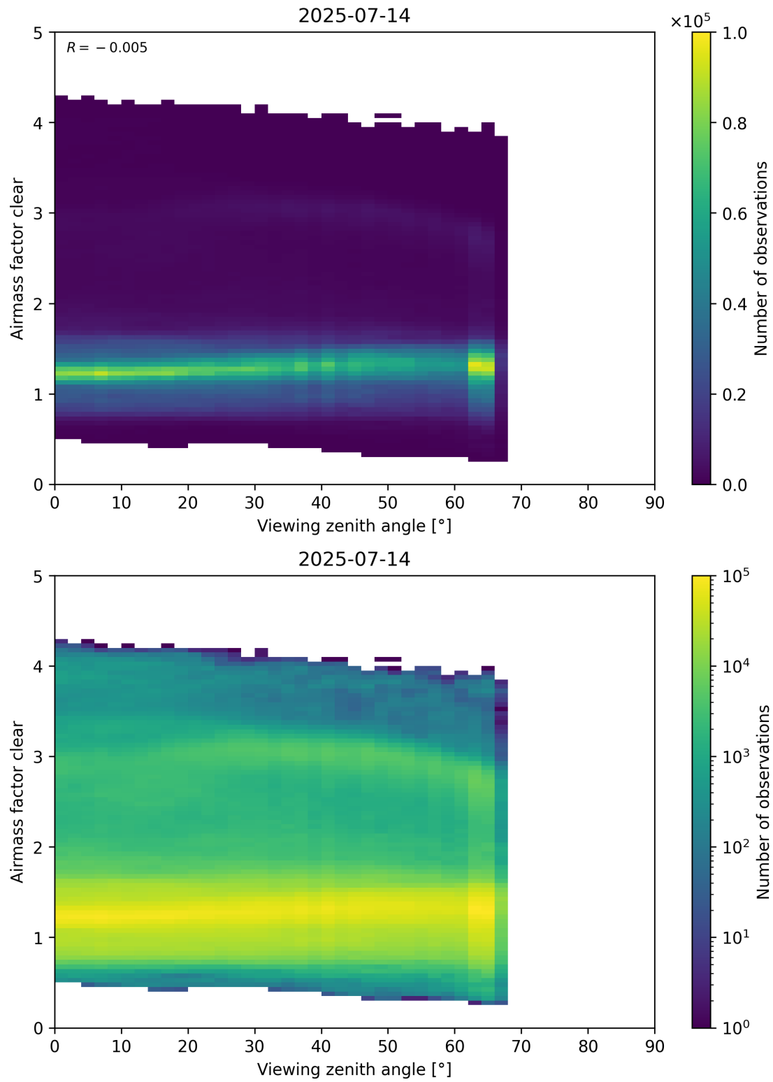
Figure 185: Scatter density plot of “Viewing zenith angle” against “Airmass factor clear” for 2025-07-13 to 2025-07-15.
