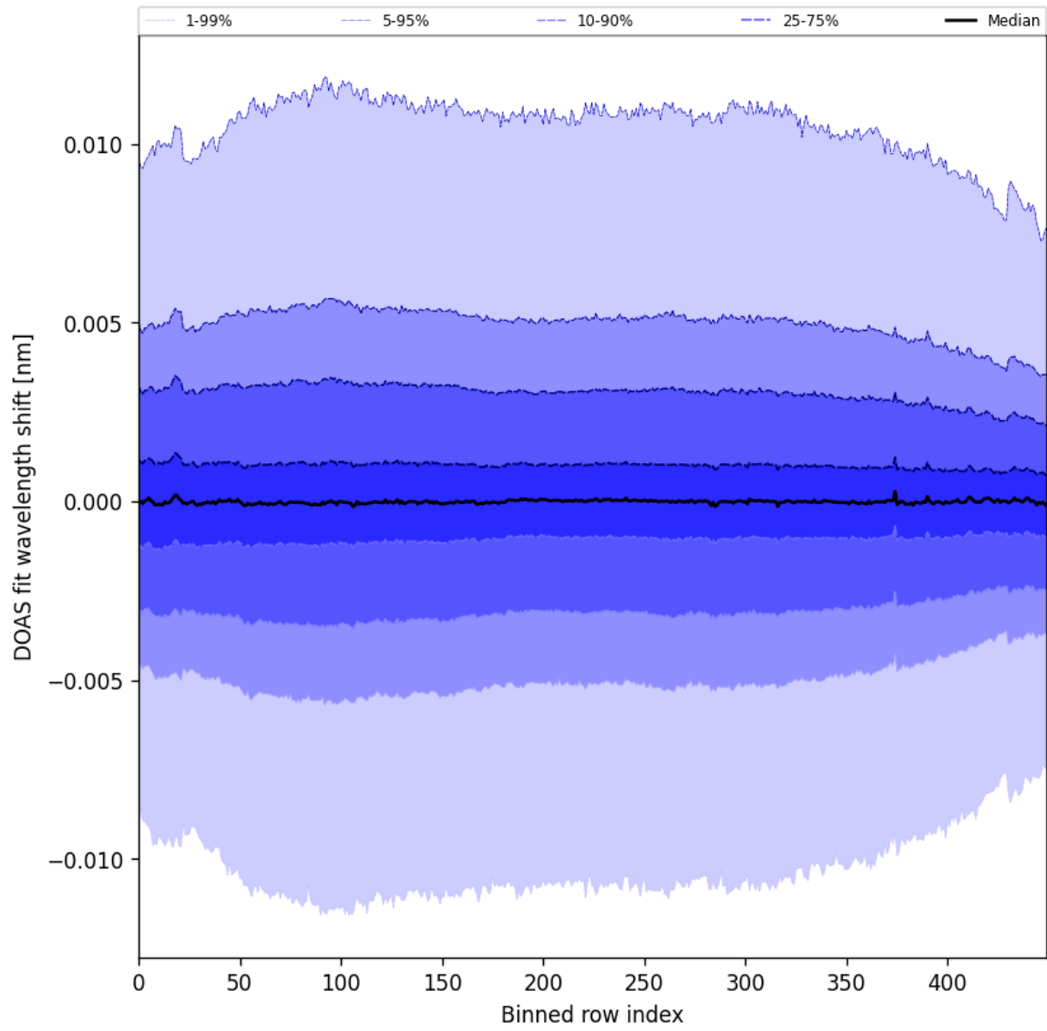
Figure 58: Along track statistics of “DOAS fit wavelength shift” for 2025-07-13 to 2025-07-15
