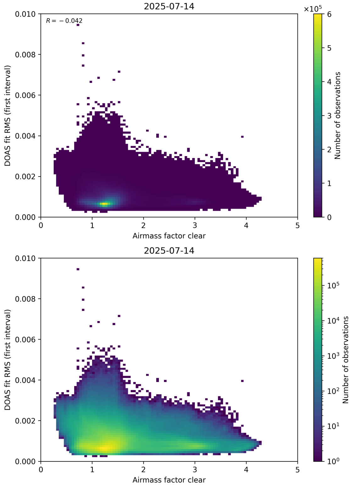
Figure 71: Scatter density plot of “Airmass factor clear” against “DOAS fit RMS (first interval)” for 2025-07-13 to 2025-07-15.
