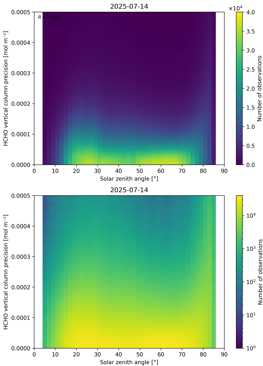
Figure 179: Scatter density plot of “Solar zenith angle” against “HCHO vertical column precision” for 2025-07-13 to 2025-07-15.
