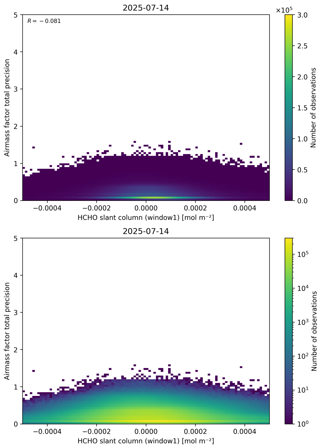
Figure 86: Scatter density plot of “HCHO slant column (window1)” against “Airmass factor total precision” for 2025-07-13 to 2025-07-15.
