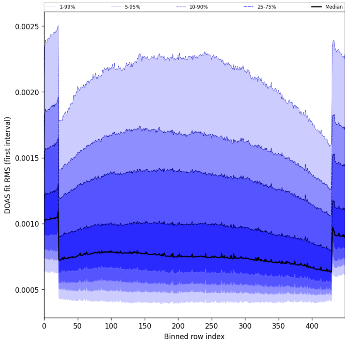
Figure 60: Along track statistics of “DOAS fit RMS (first interval)” for 2025-07-13 to 2025-07-15
