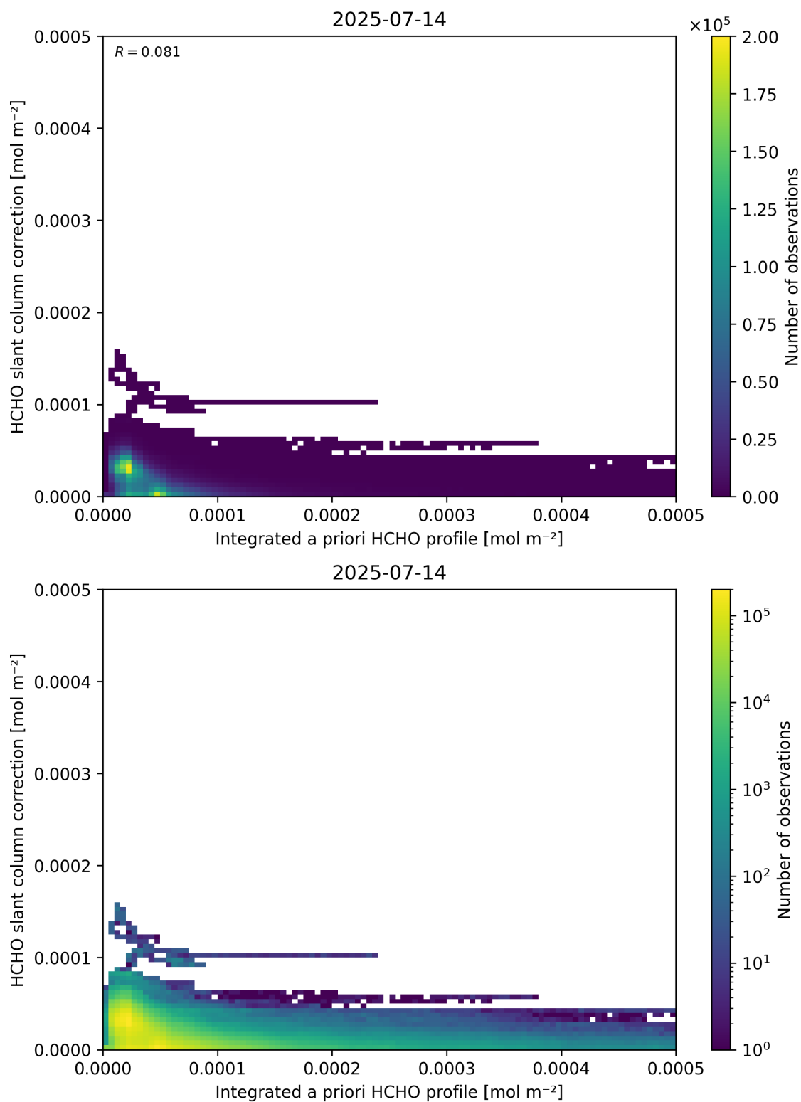
Figure 152: Scatter density plot of “Integrated a priori HCHO profile” against “HCHO slant column correction” for 2025-07-13 to 2025-07-15.
