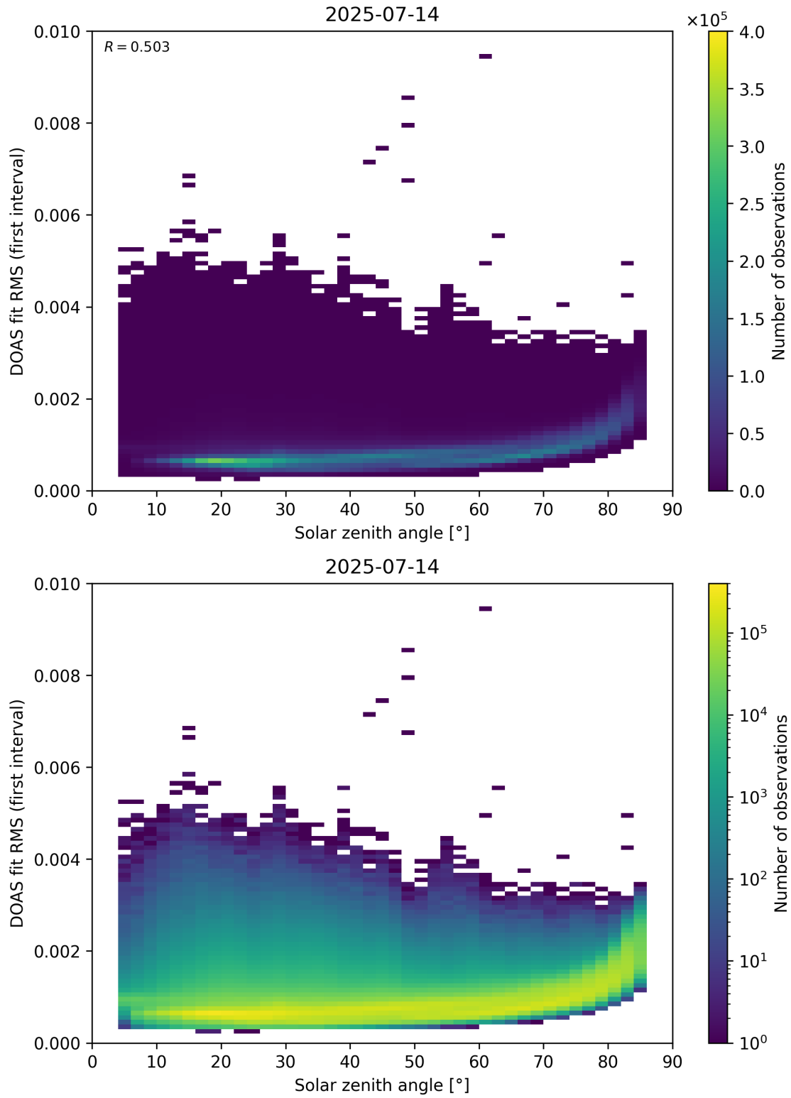
Figure 167: Scatter density plot of “Solar zenith angle” against “DOAS fit RMS (first interval)” for 2025-07-13 to 2025-07-15.
