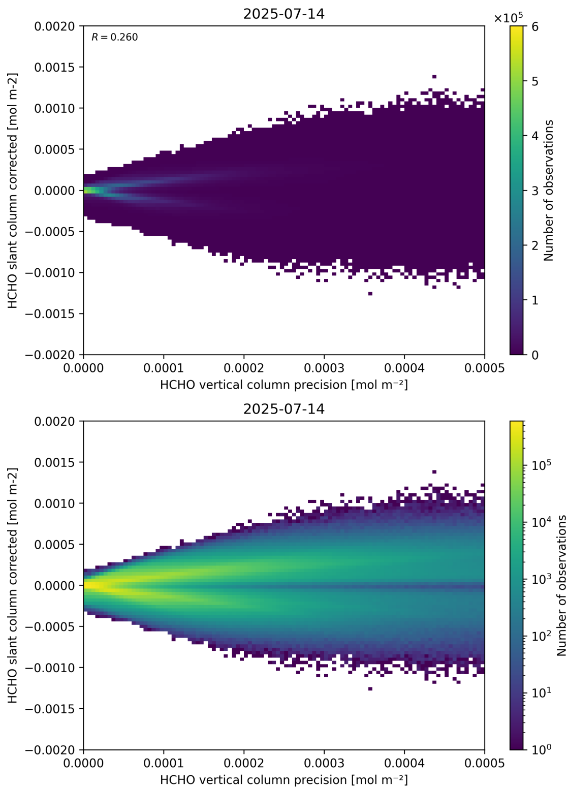
Figure 140: Scatter density plot of “HCHO vertical column precision” against “HCHO slant column corrected” for 2025-07-13 to 2025-07-15.
