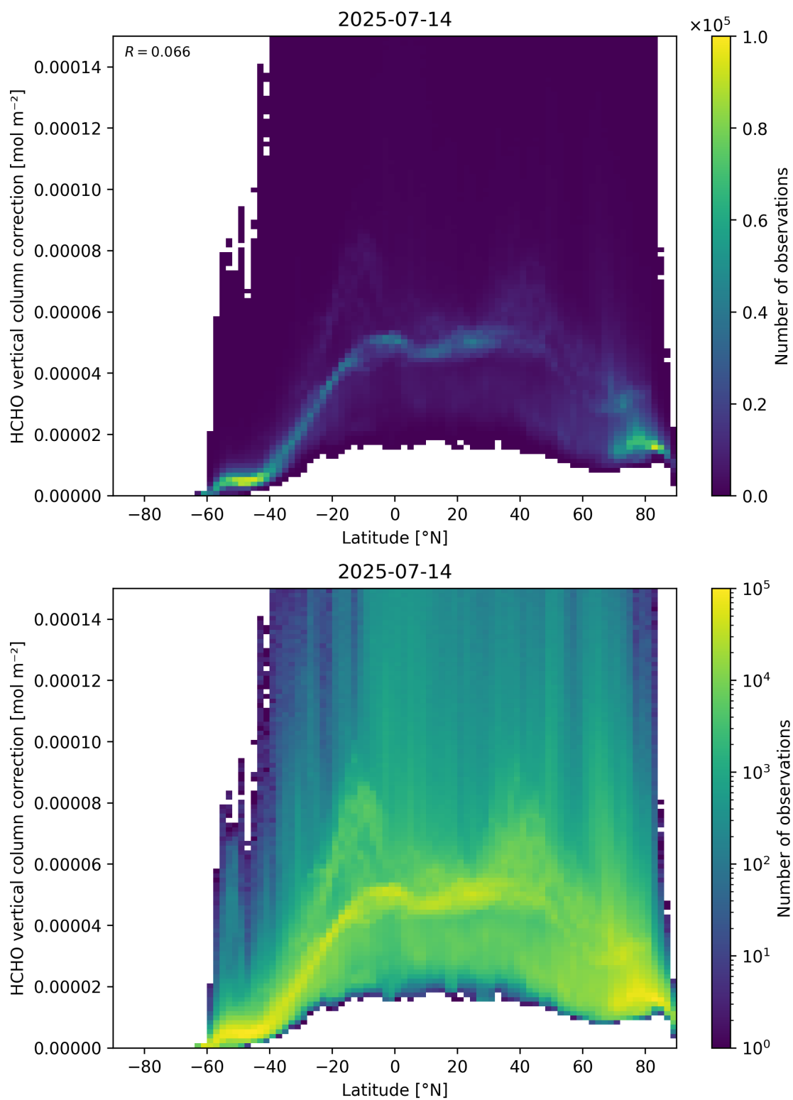
Figure 164: Scatter density plot of “Latitude” against “HCHO vertical column correction” for 2025-07-13 to 2025-07-15.
