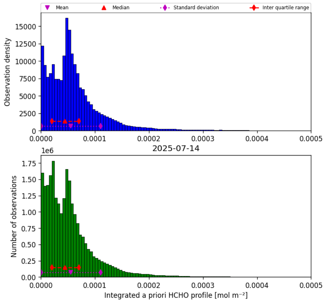
Figure 43: Histogram of “Integrated a priori HCHO profile” for 2025-07-13 to 2025-07-15
