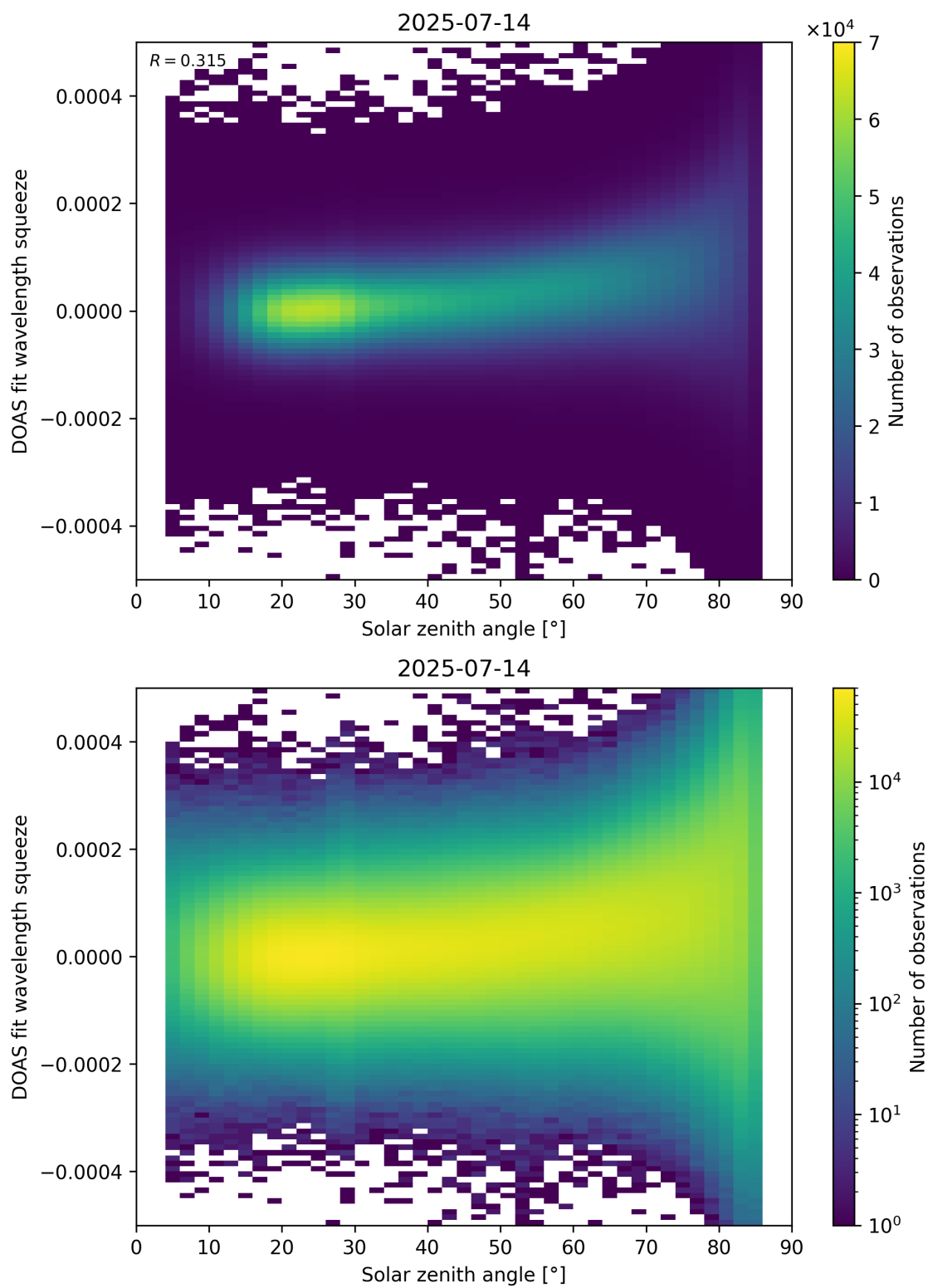
Figure 169: Scatter density plot of “Solar zenith angle” against “DOAS fit wavelength squeeze” for 2025-07-13 to 2025-07-15.
