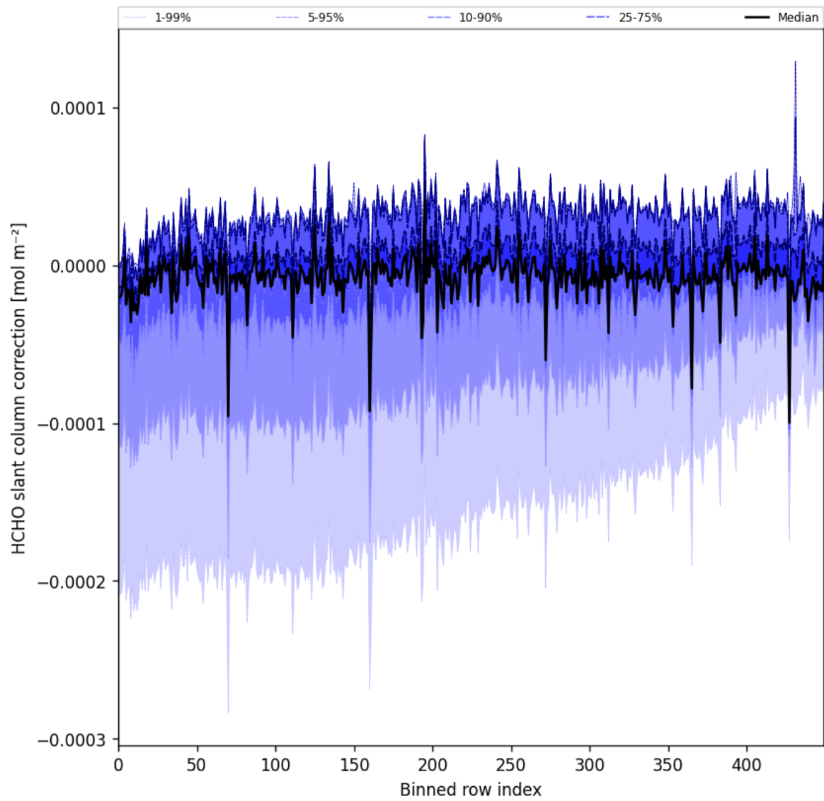
Figure 61: Along track statistics of "HCHO slant column correction" for 2025-07-13 to 2025-07-15
