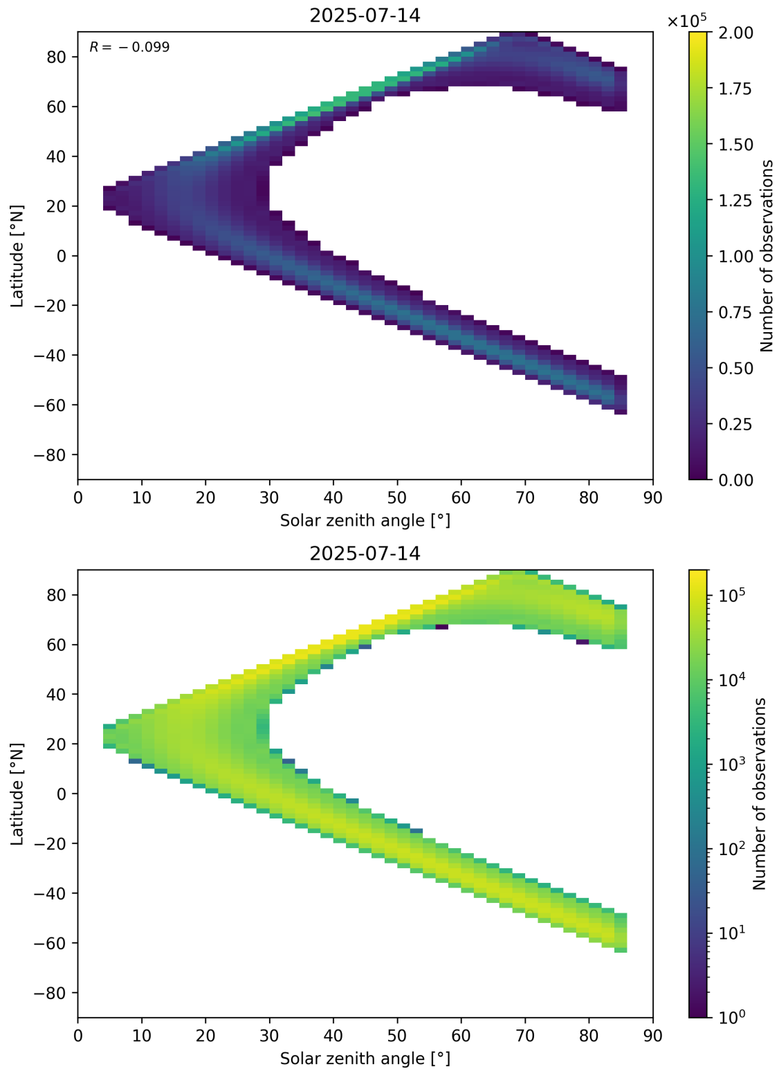
Figure 181: Scatter density plot of “Solar zenith angle” against “Latitude” for 2025-07-13 to 2025-07-15.
