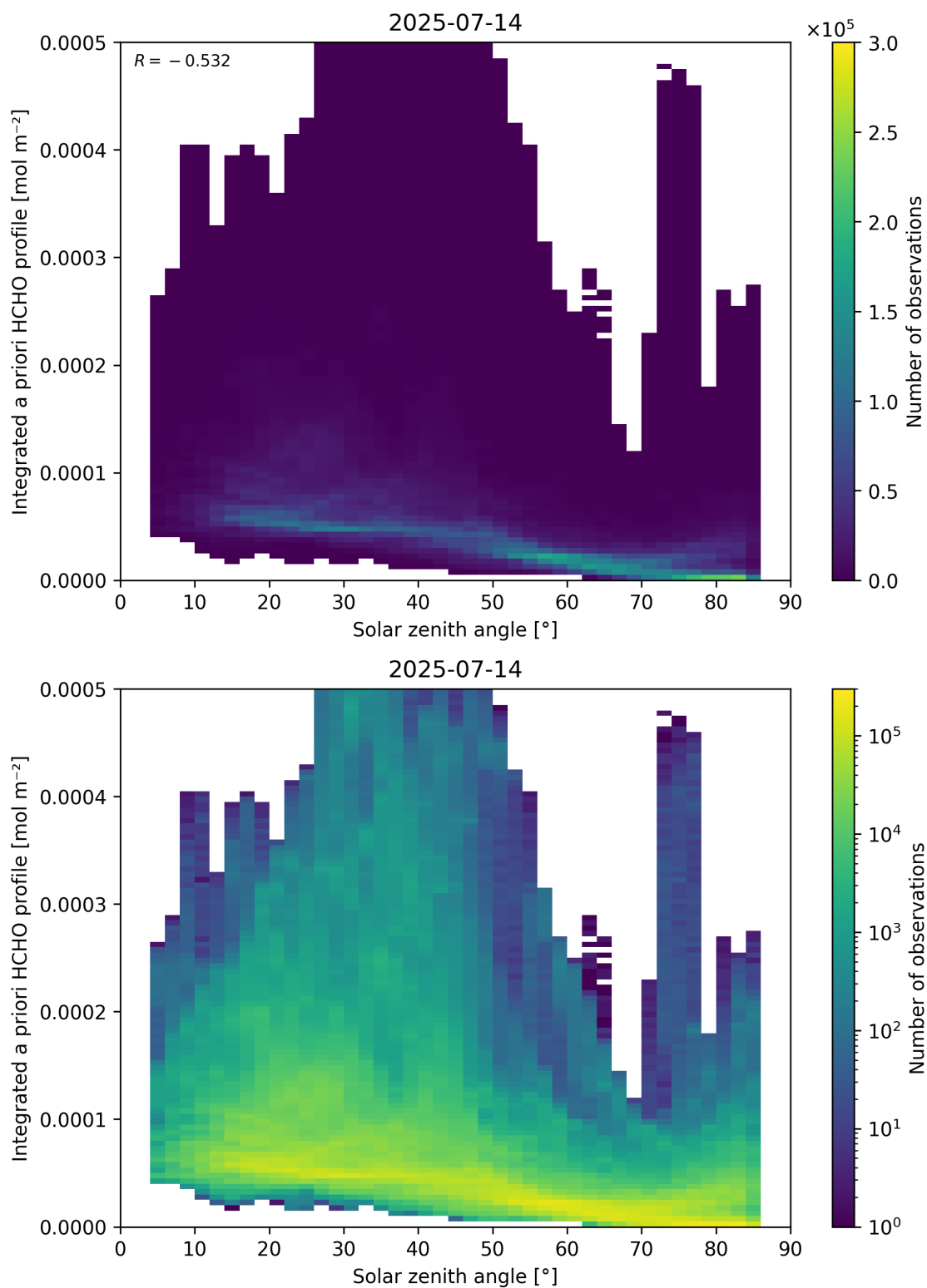
Figure 180: Scatter density plot of “Solar zenith angle” against “Integrated a priori HCHO profile” for 2025-07-13 to 2025-07-15.
