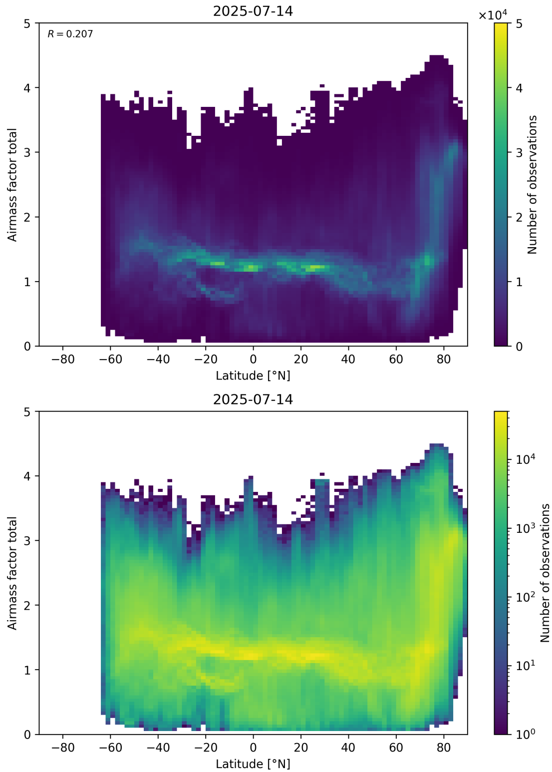
Figure 161: Scatter density plot of “Latitude” against “Airmass factor total” for 2025-07-13 to 2025-07-15.
