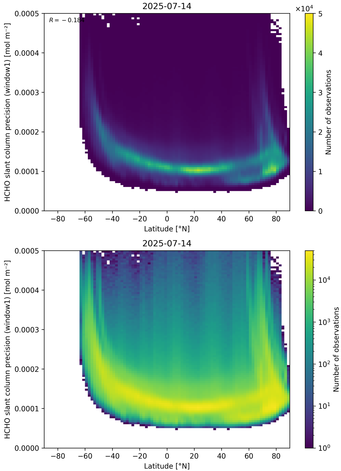
Figure 160: Scatter density plot of “Latitude” against “HCHO slant column precision (window1)” for 2025-07-13 to 2025-07-15.
