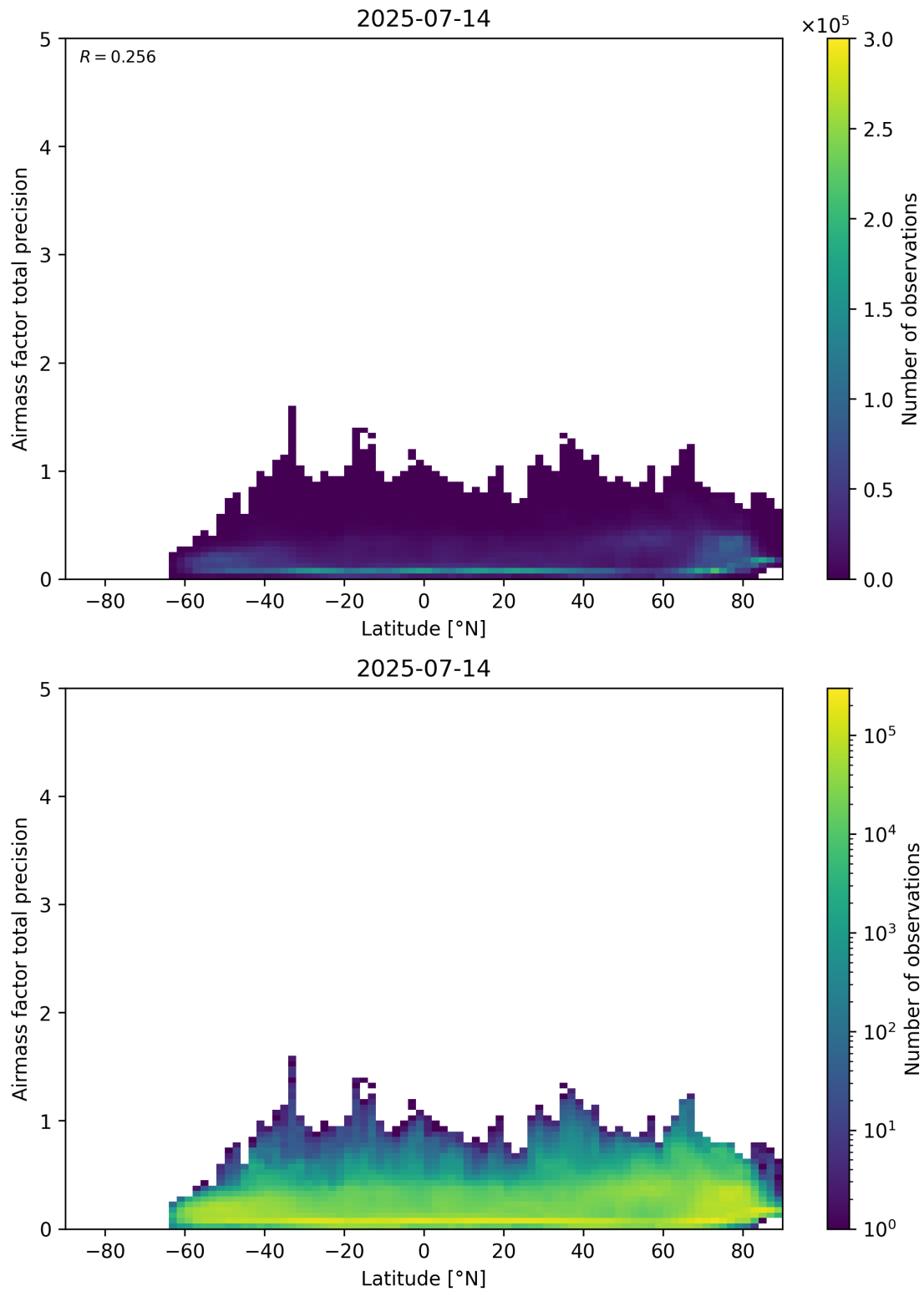
Figure 162: Scatter density plot of “Latitude” against “Airmass factor total precision” for 2025-07-13 to 2025-07-15.
