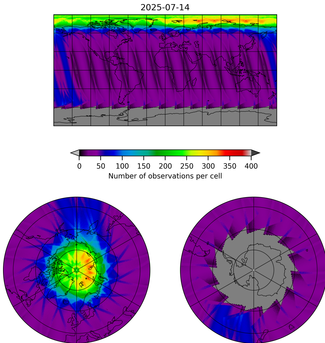
Figure 19: Map of the number of observations for 2025-07-13 to 2025-07-15
