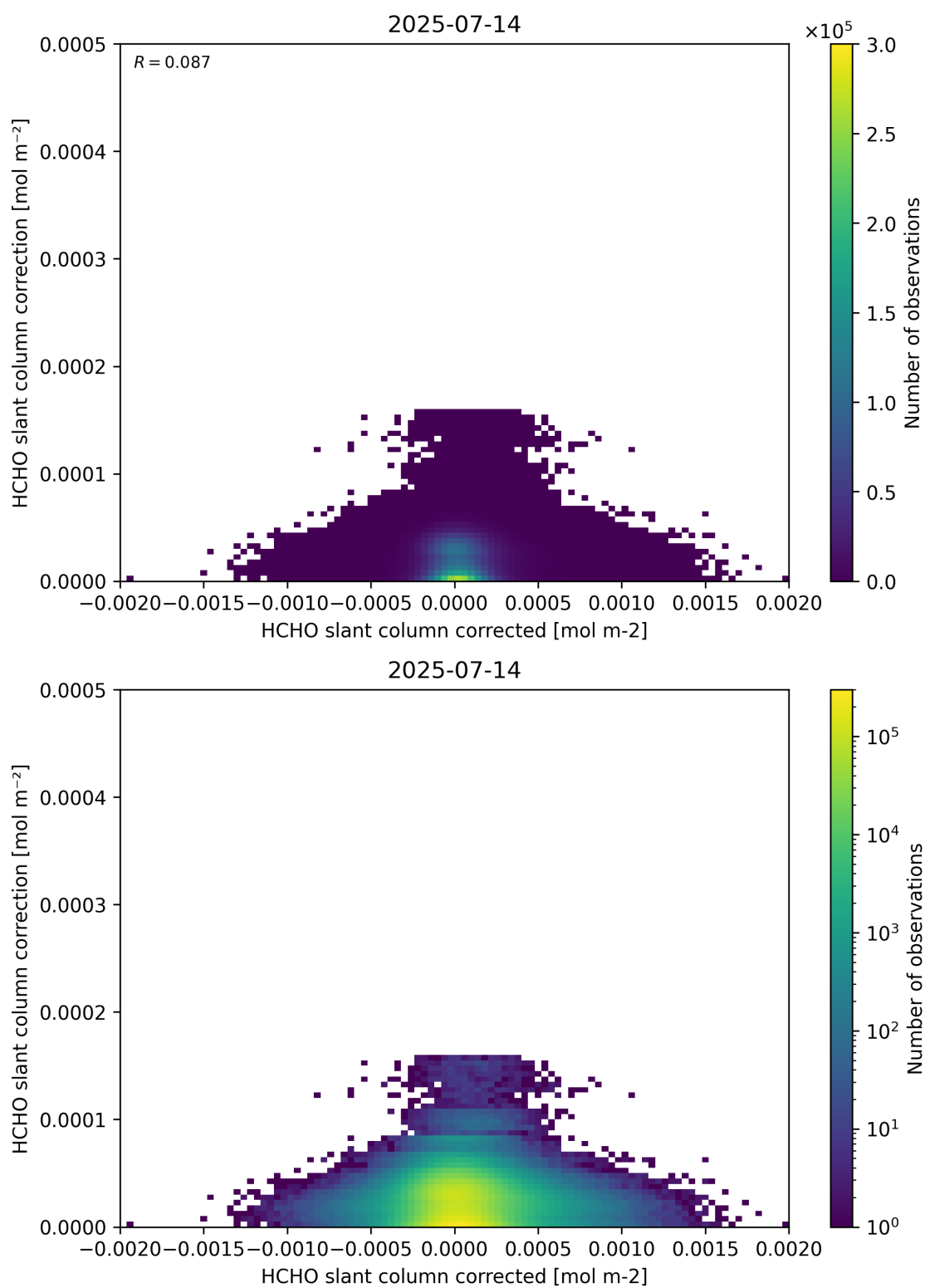
Figure 77: Scatter density plot of “HCHO slant column corrected” against “HCHO slant column correction” for 2025-07-13 to 2025-07-15.
