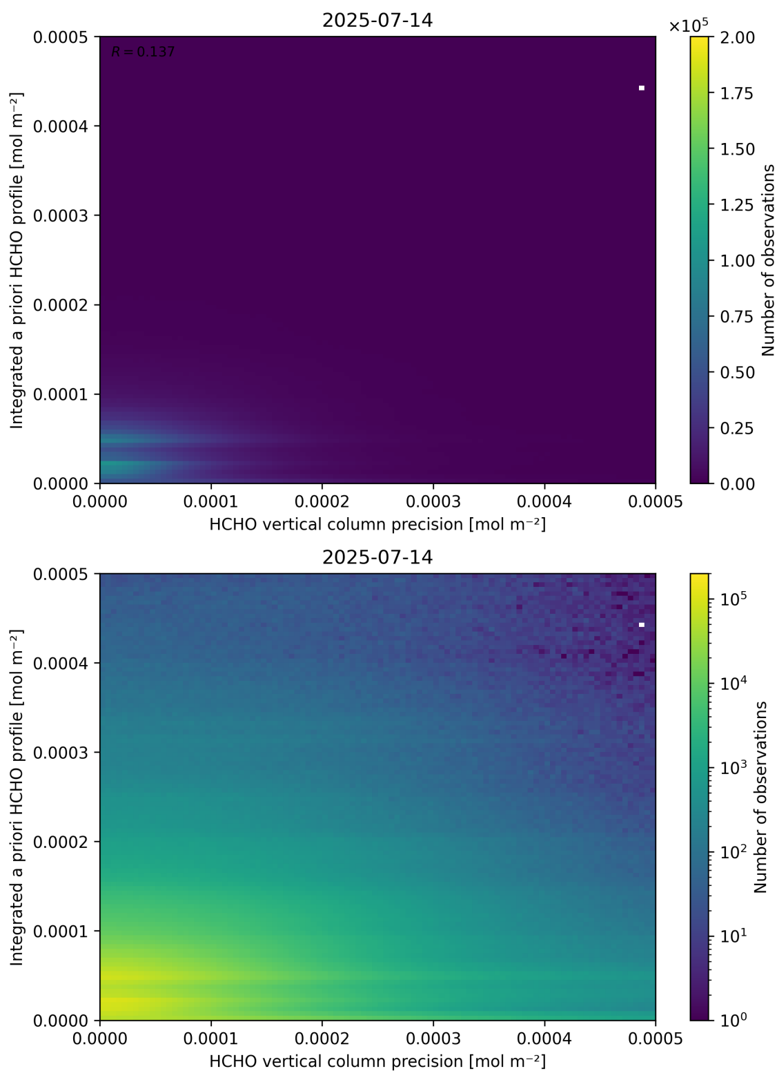
Figure 147: Scatter density plot of “HCHO vertical column precision” against “Integrated a priori HCHO profile” for 2025-07-13 to 2025-07-15.
