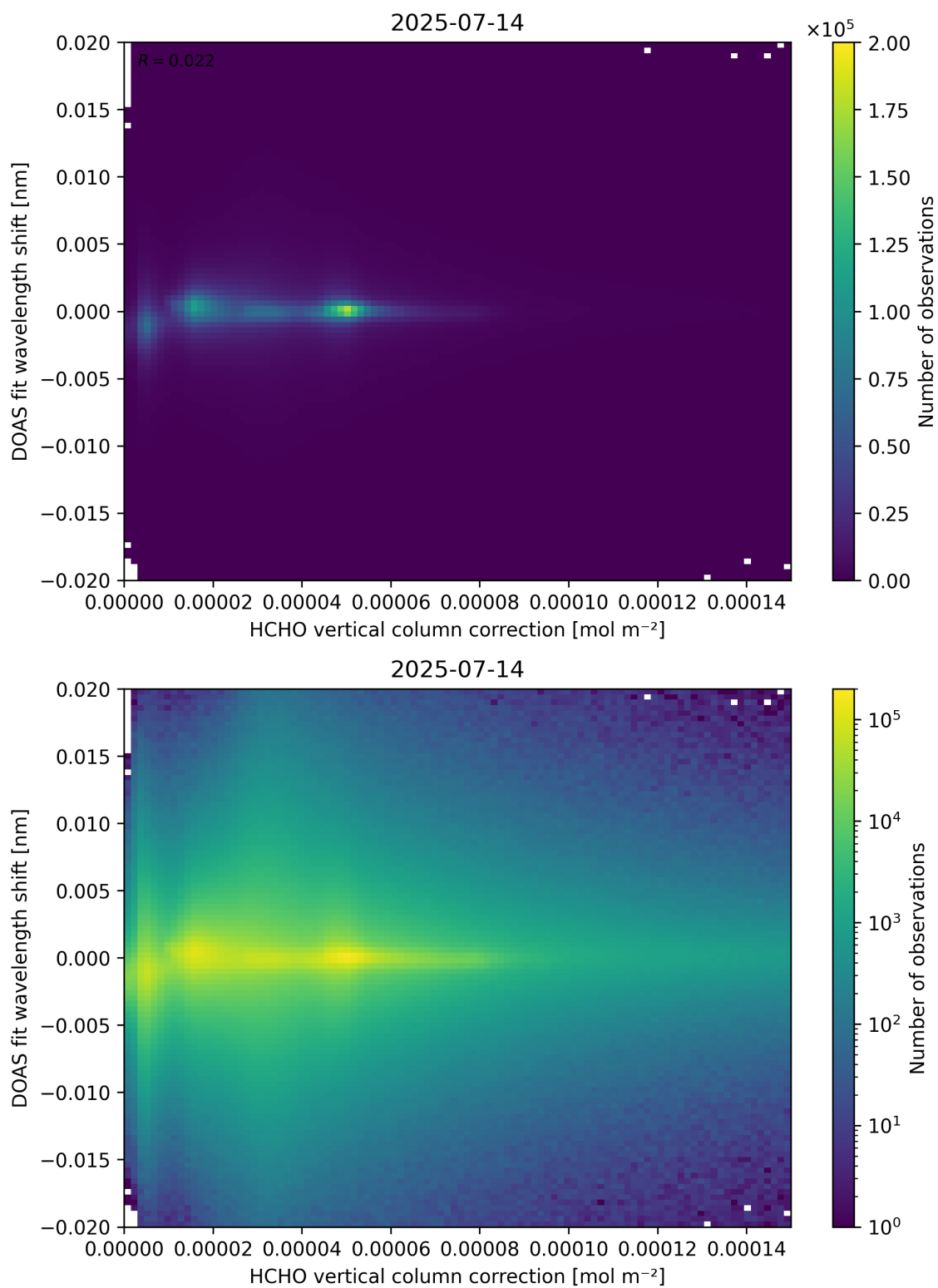
Figure 113: Scatter density plot of “HCHO vertical column correction” against “DOAS fit wavelength shift” for 2025-07-13 to 2025-07-15.
