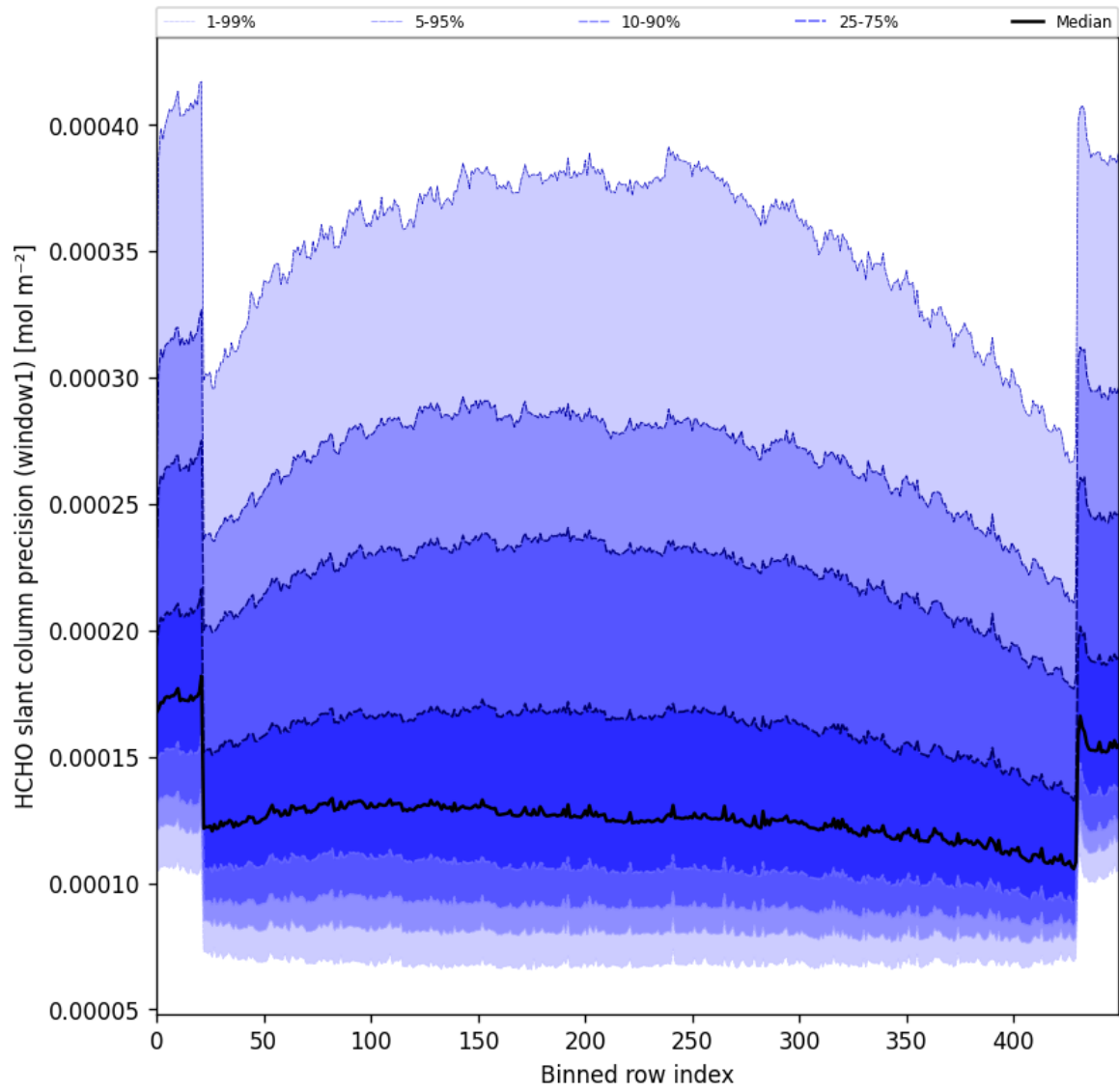
Figure 53: Along track statistics of “HCHO slant column precision (window1)” for 2025-07-13 to 2025-07-15
