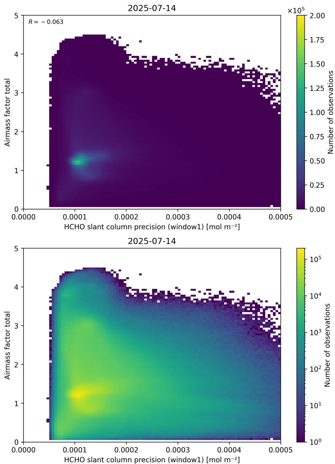
Figure 94: Scatter density plot of “HCHO slant column precision (window1)” against “Airmass factor total” for 2025-07-13 to 2025-07-15.
