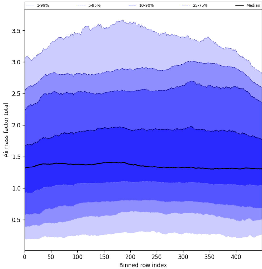
Figure 54: Along track statistics of “Airmass factor total” for 2025-07-13 to 2025-07-15
