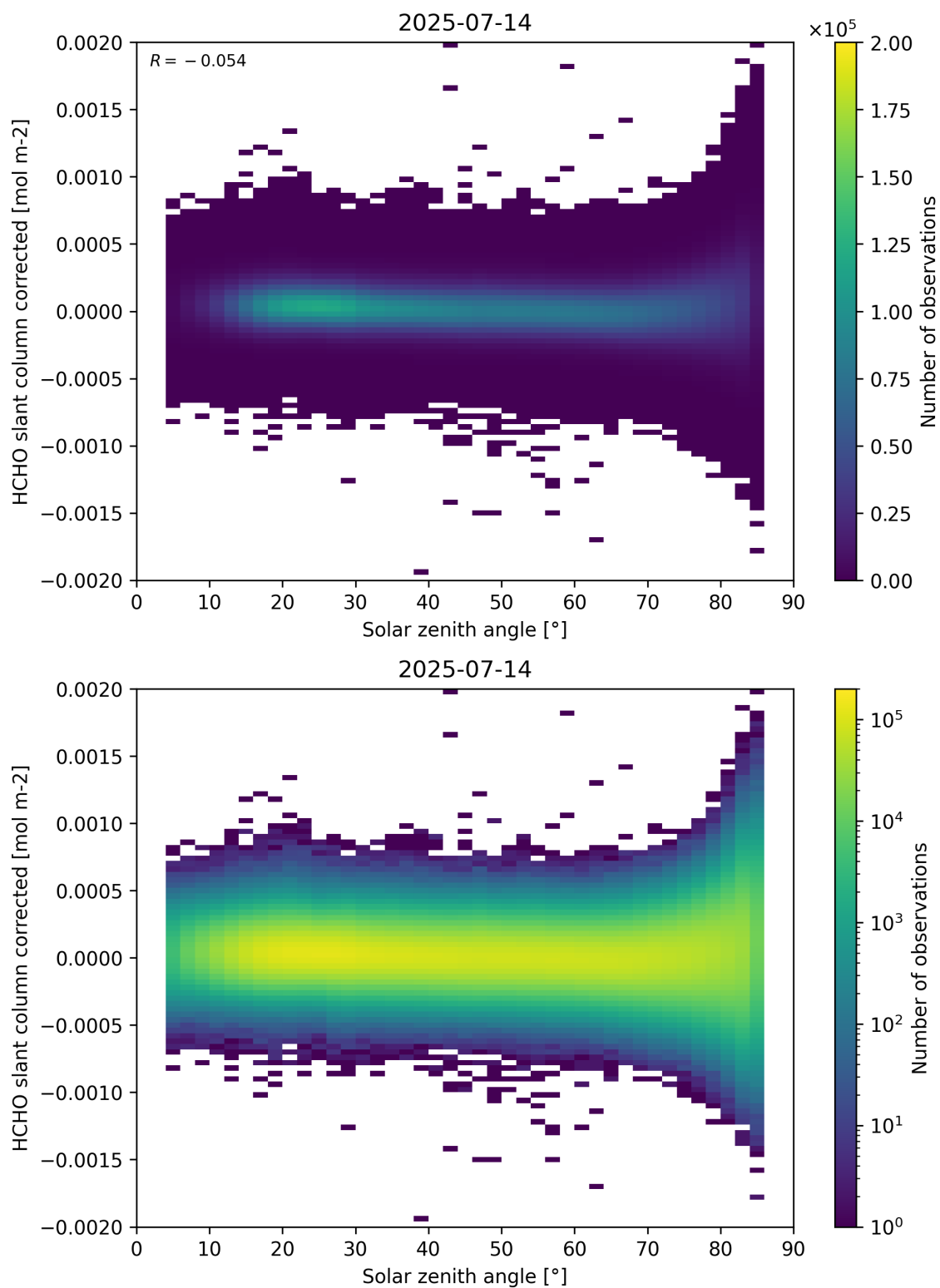
Figure 171: Scatter density plot of “Solar zenith angle” against “HCHO slant column corrected” for 2025-07-13 to 2025-07-15.
