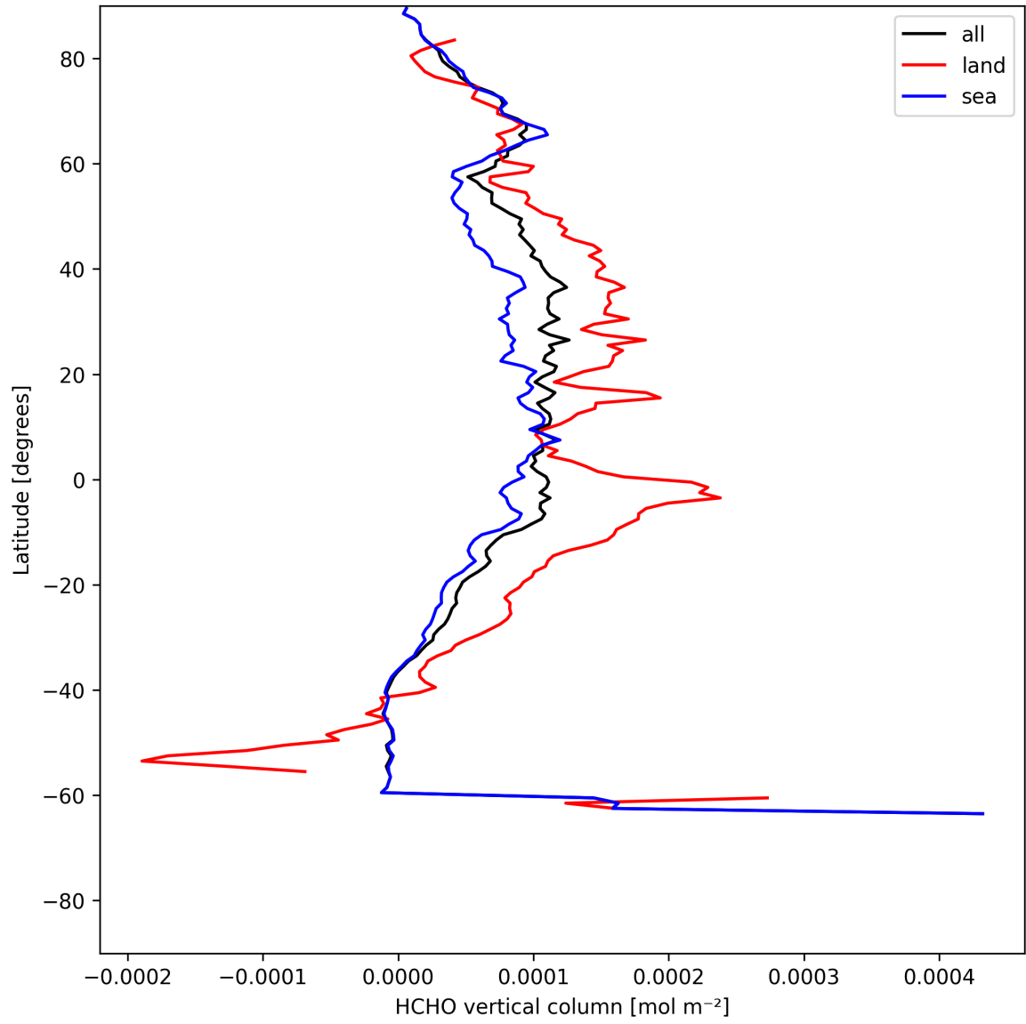
Figure 21: Zonal average of “HCHO vertical column” for 2025-07-13 to 2025-07-15.
