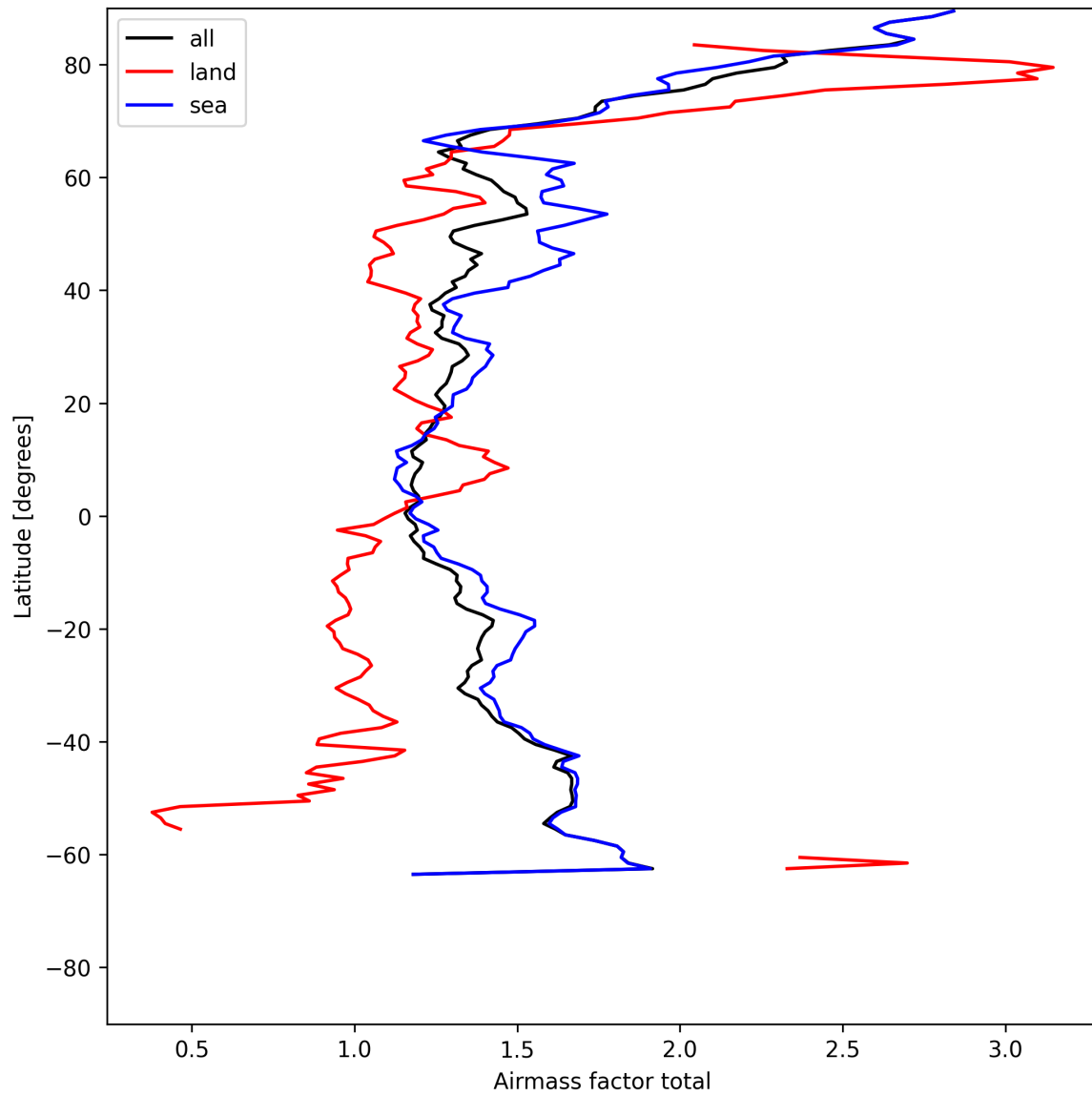
Figure 26: Zonal average of “Airmass factor total” for 2025-07-13 to 2025-07-15.
