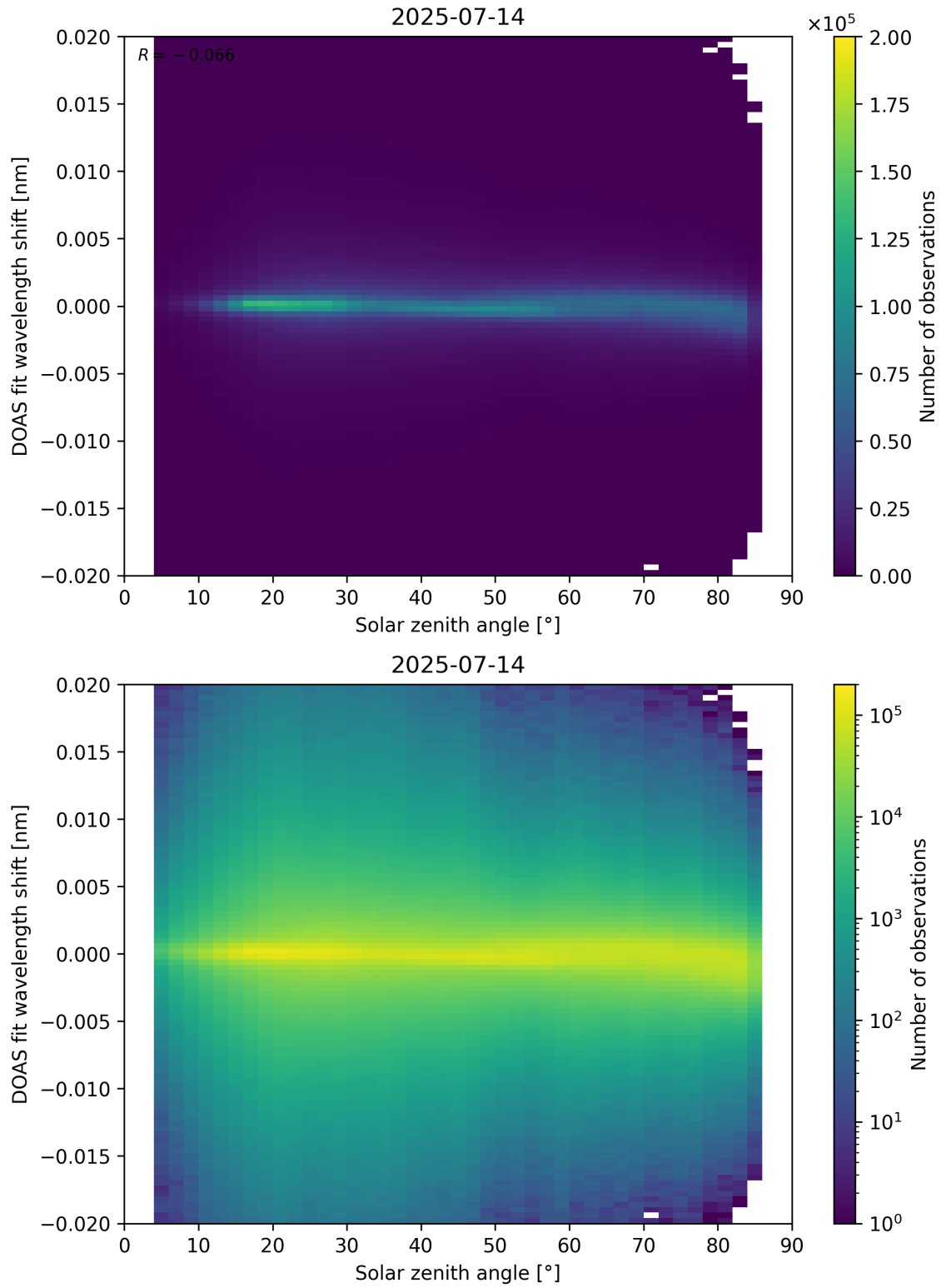
Figure 168: Scatter density plot of “Solar zenith angle” against “DOAS fit wavelength shift” for 2025-07-13 to 2025-07-15.
