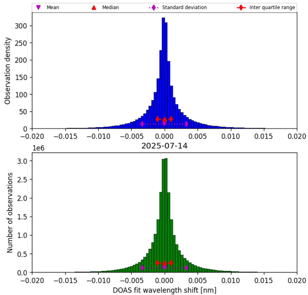
Figure 44: Histogram of “DOAS fit wavelength shift” for 2025-07-13 to 2025-07-15
