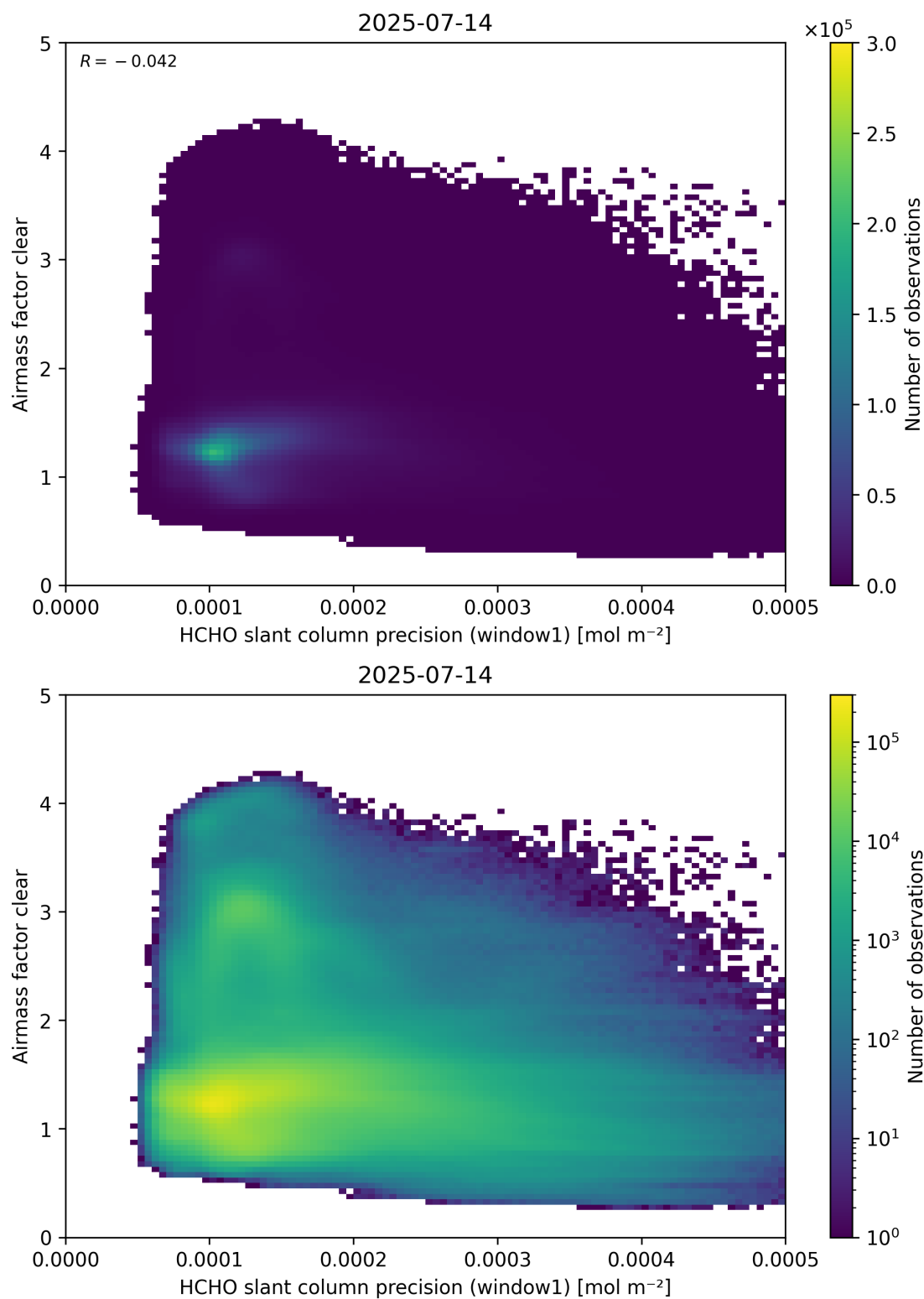
Figure 91: Scatter density plot of “HCHO slant column precision (window1)” against “Airmass factor clear” for 2025-07-13 to 2025-07-15.
