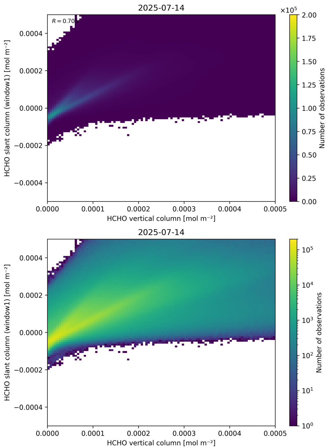
Figure 129: Scatter density plot of “HCHO vertical column” against “HCHO slant column (window1)” for 2025-07-13 to 2025-07-15.
