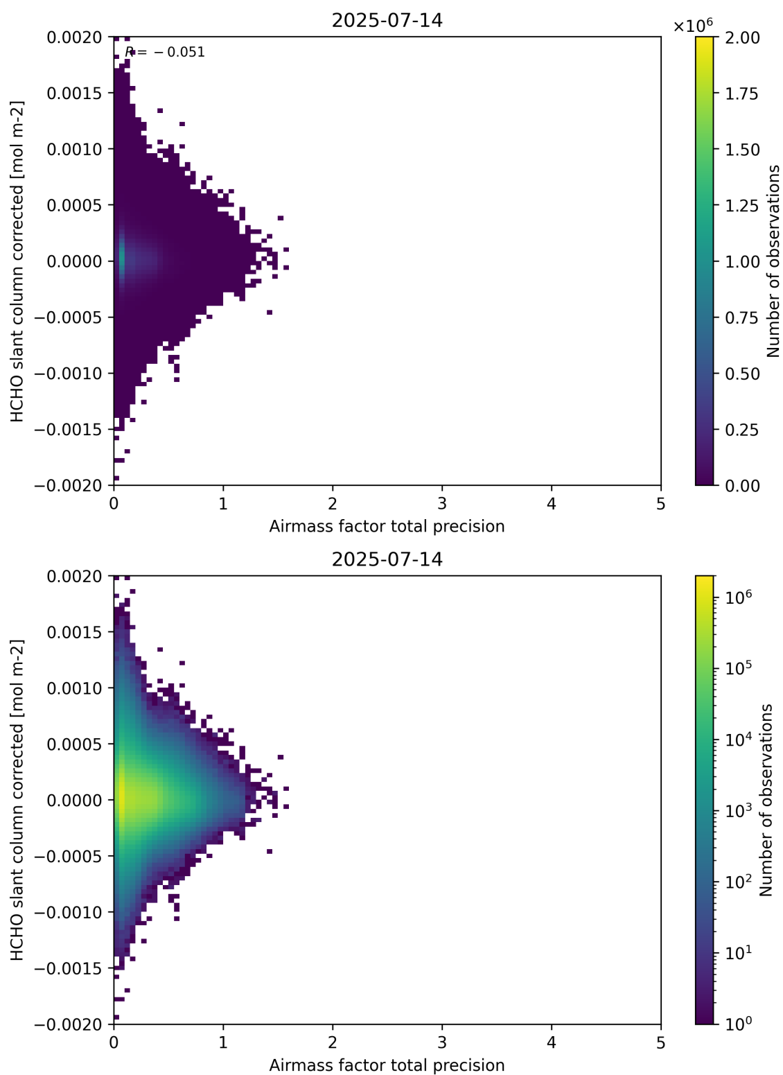
Figure 109: Scatter density plot of “Airmass factor total precision” against “HCHO slant column corrected” for 2025-07-13 to 2025-07-15.
