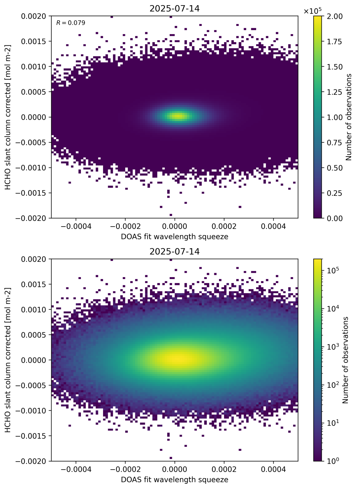
Figure 69: Scatter density plot of “DOAS fit wavelength squeeze” against “HCHO slant column corrected” for 2025-07-13 to 2025-07-15.
