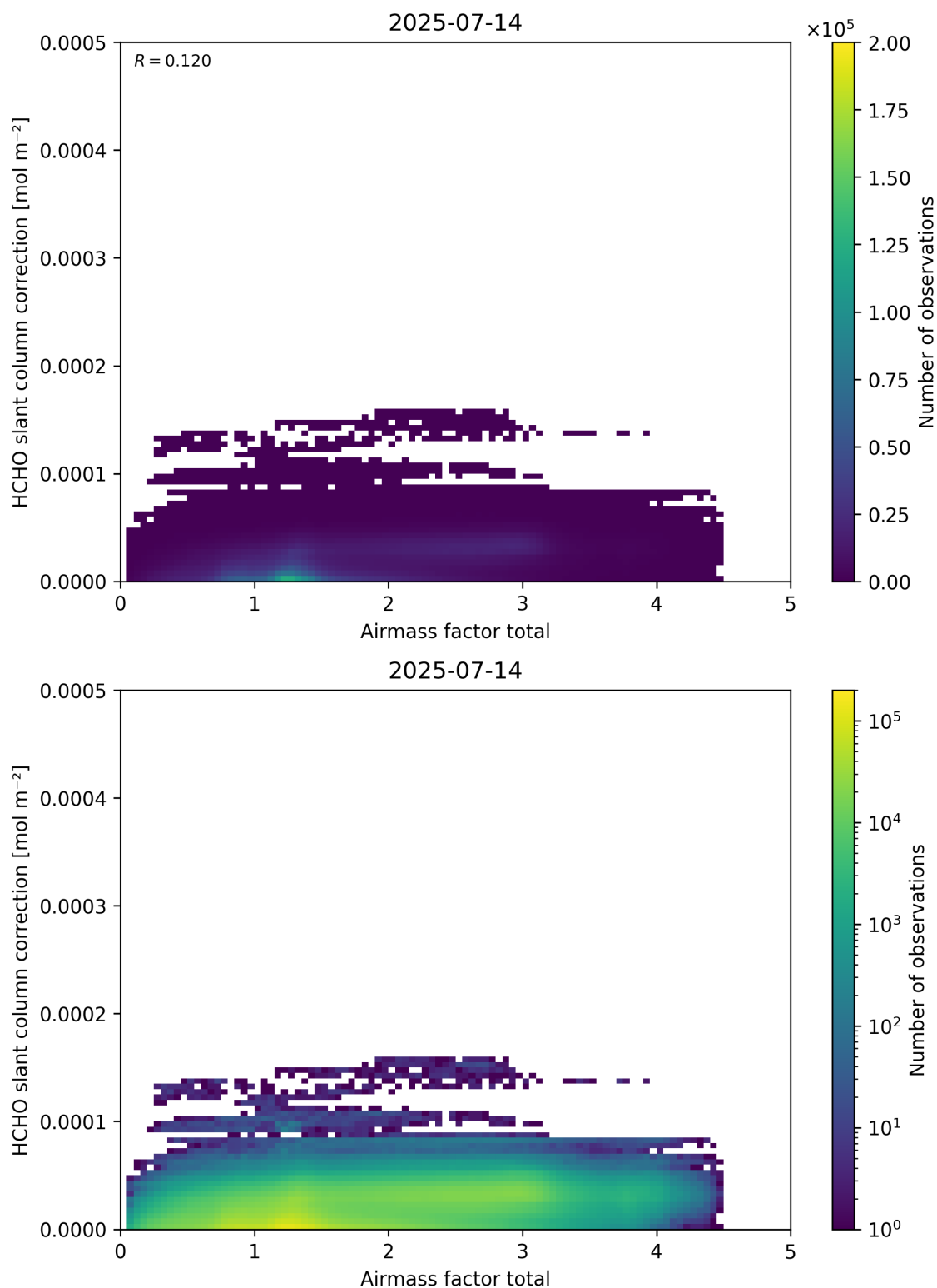
Figure 102: Scatter density plot of “Airmass factor total” against “HCHO slant column correction” for 2025-07-13 to 2025-07-15.
