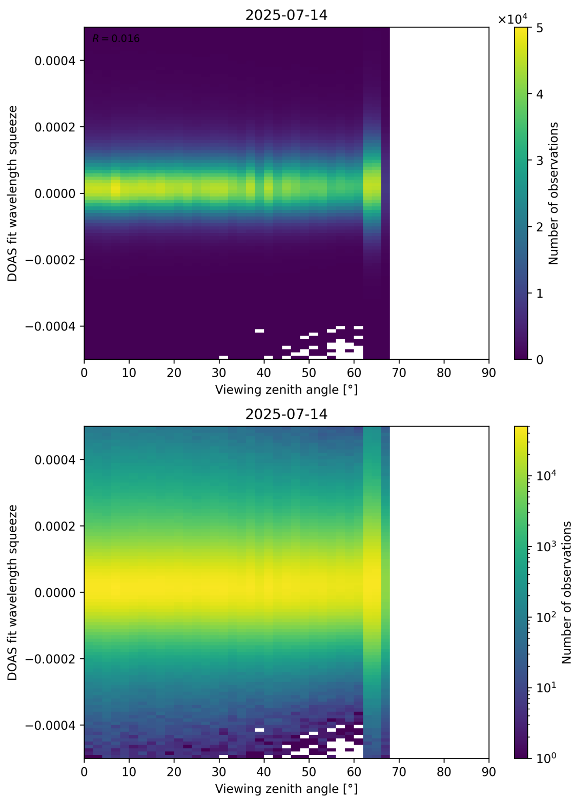
Figure 184: Scatter density plot of “Viewing zenith angle” against “DOAS fit wavelength squeeze” for 2025-07-13 to 2025-07-15.
