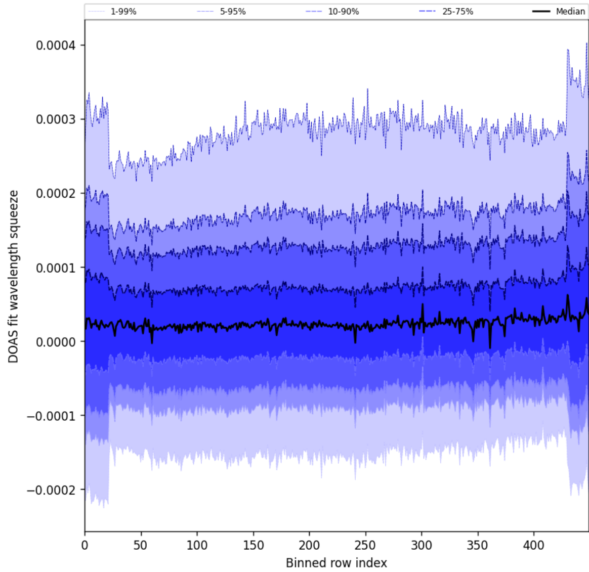
Figure 59: Along track statistics of “DOAS fit wavelength squeeze” for 2025-07-13 to 2025-07-15
