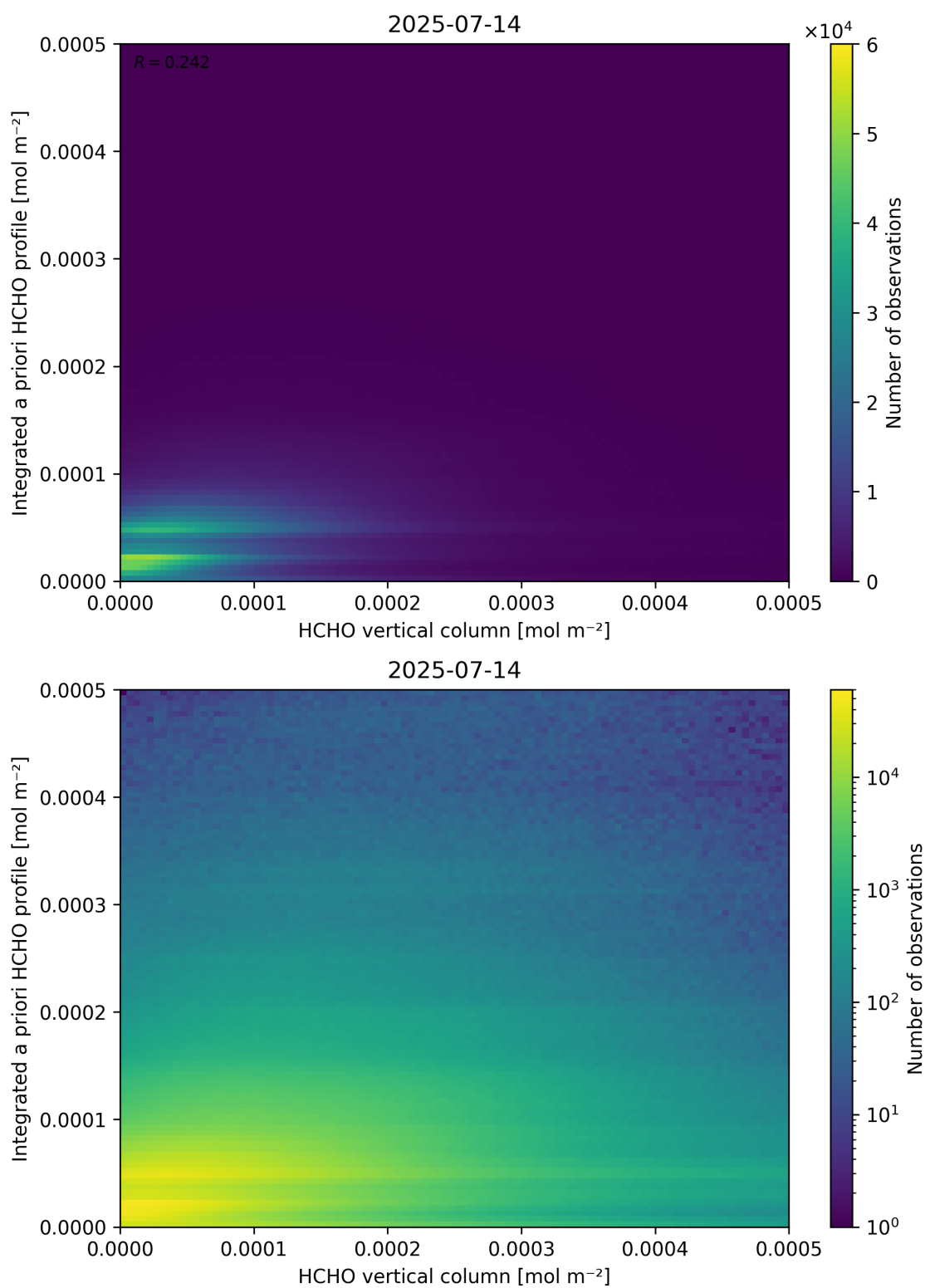
Figure 135: Scatter density plot of “HCHO vertical column” against “Integrated a priori HCHO profile” for 2025-07-13 to 2025-07-15.
