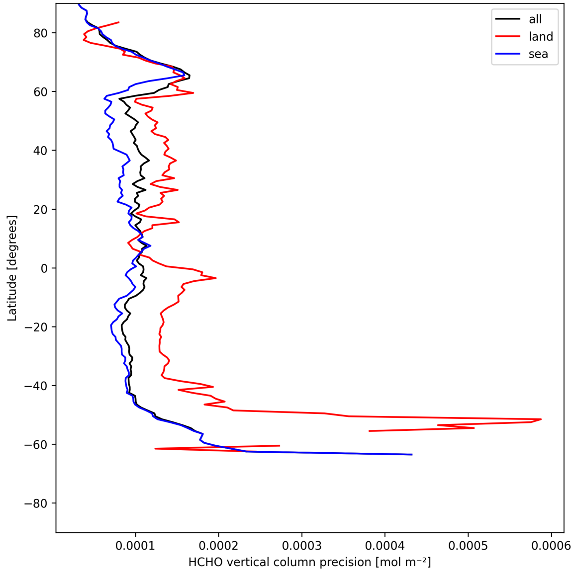
Figure 22: Zonal average of “HCHO vertical column precision” for 2025-07-13 to 2025-07-15.
