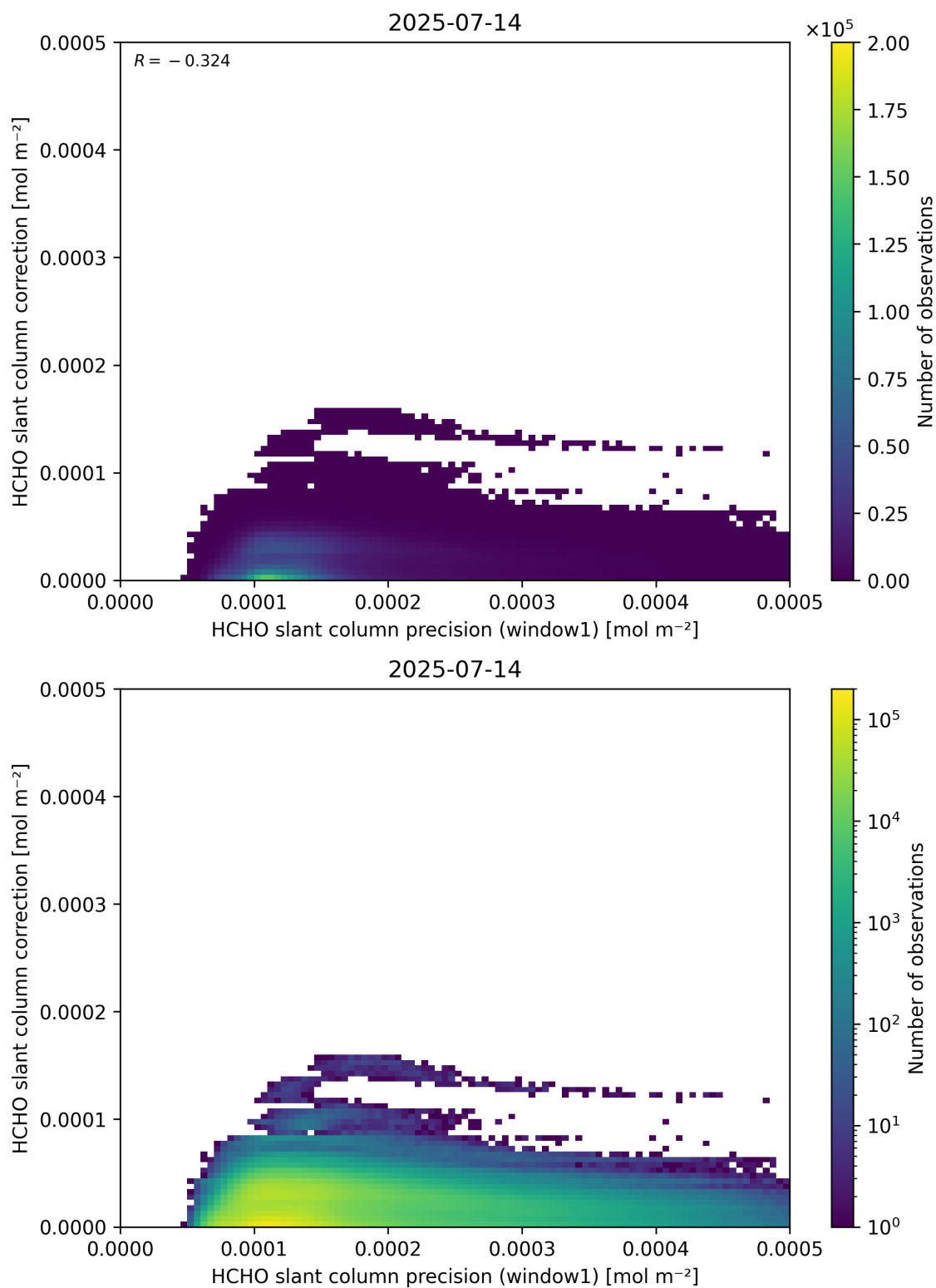
Figure 93: Scatter density plot of “HCHO slant column precision (window1)” against “HCHO slant column correction” for 2025-07-13 to 2025-07-15.
