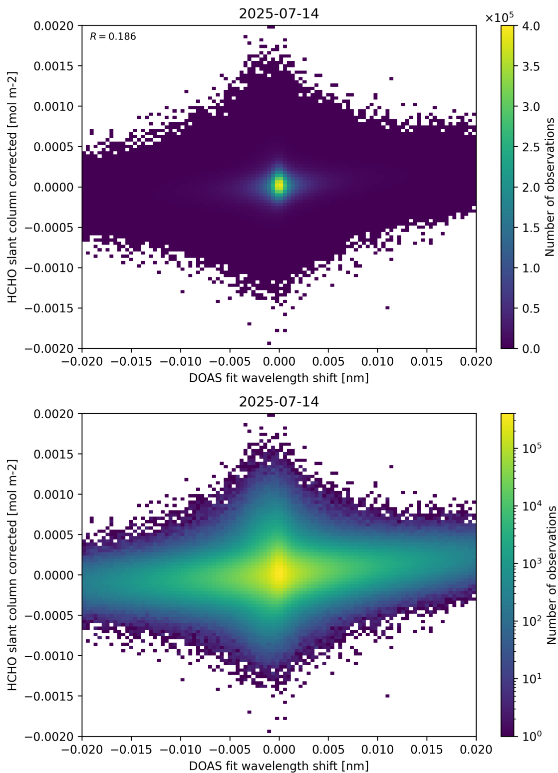
Figure 66: Scatter density plot of “DOAS fit wavelength shift” against “HCHO slant column corrected” for 2025-07-13 to 2025-07-15.
