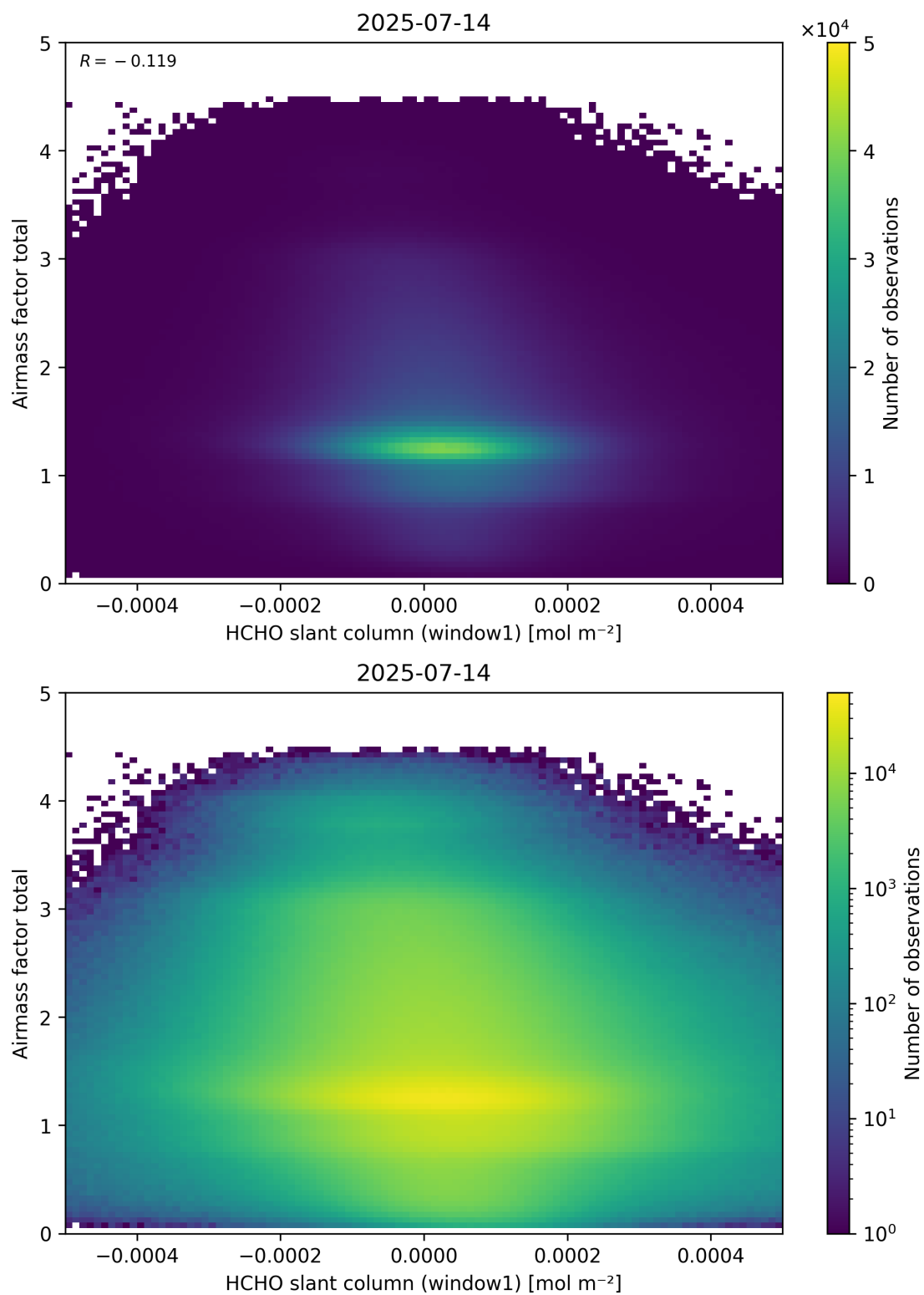
Figure 85: Scatter density plot of “HCHO slant column (window1)” against “Airmass factor total” for 2025-07-13 to 2025-07-15.
