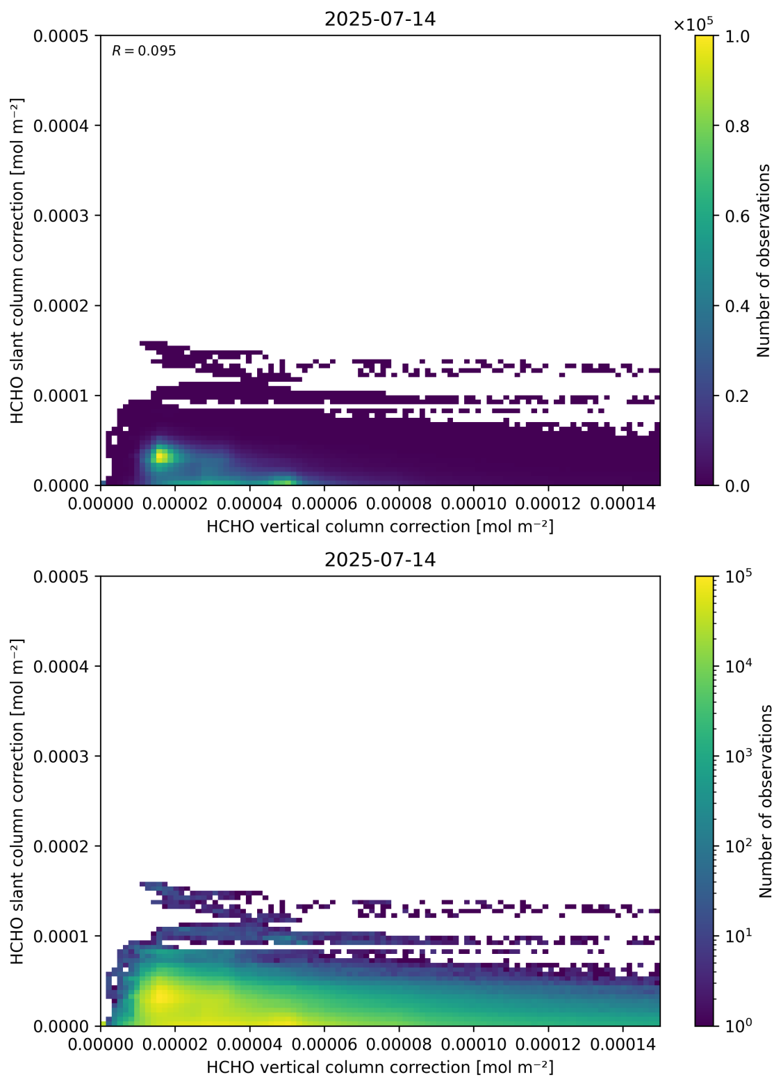
Figure 117: Scatter density plot of “HCHO vertical column correction” against “HCHO slant column correction” for 2025-07-13 to 2025-07-15.
