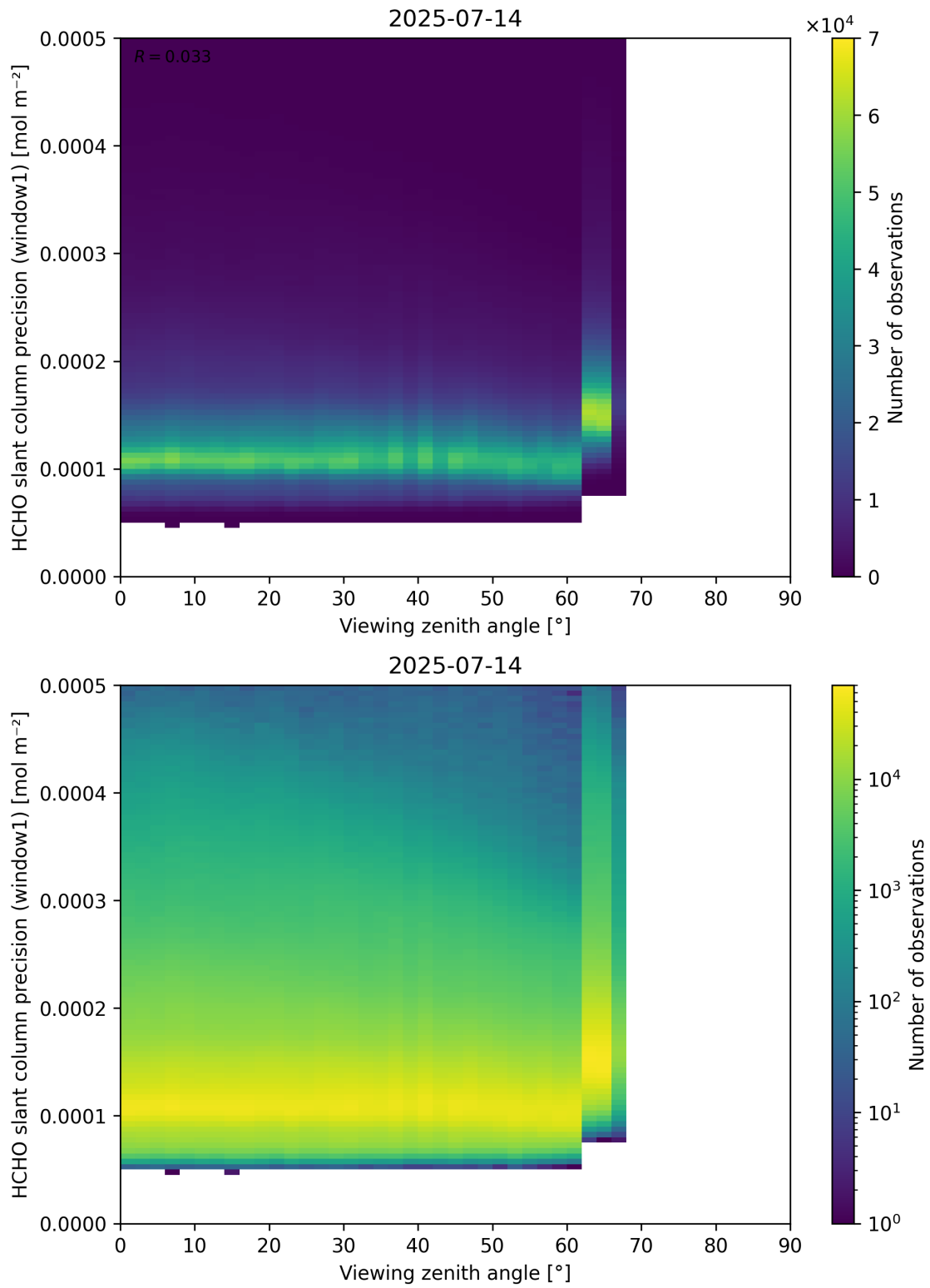
Figure 189: Scatter density plot of “Viewing zenith angle” against “HCHO slant column precision (window1)” for 2025-07-13 to 2025-07-15.
