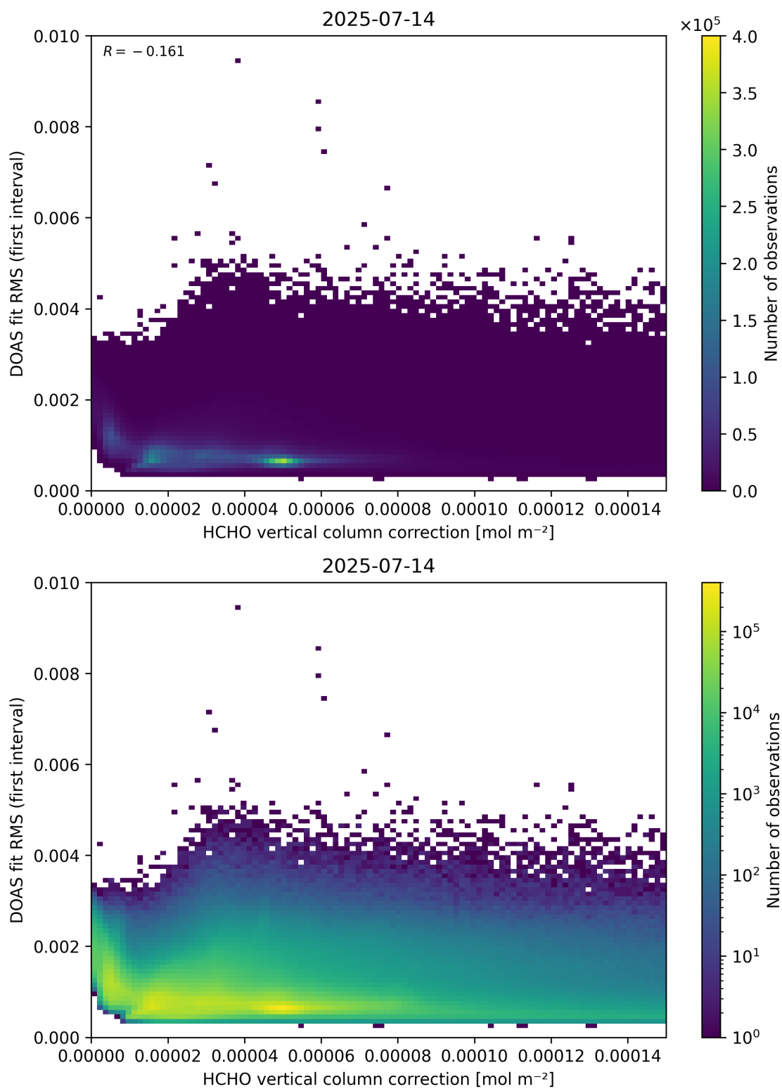
Figure 112: Scatter density plot of “HCHO vertical column correction” against “DOAS fit RMS (first interval)” for 2025-07-13 to 2025-07-15.
