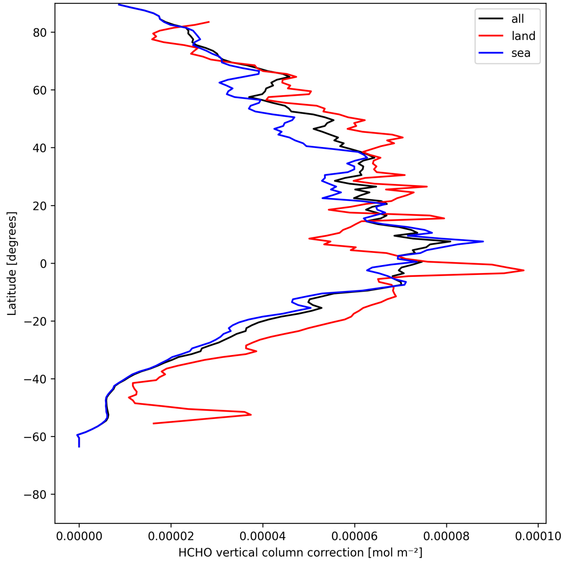
Figure 23: Zonal average of “HCHO vertical column correction” for 2025-07-13 to 2025-07-15.
