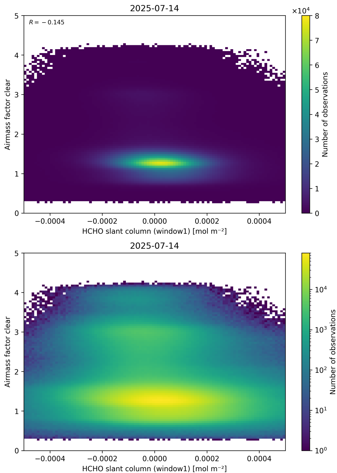
Figure 81: Scatter density plot of “HCHO slant column (window1)” against “Airmass factor clear” for 2025-07-13 to 2025-07-15.
