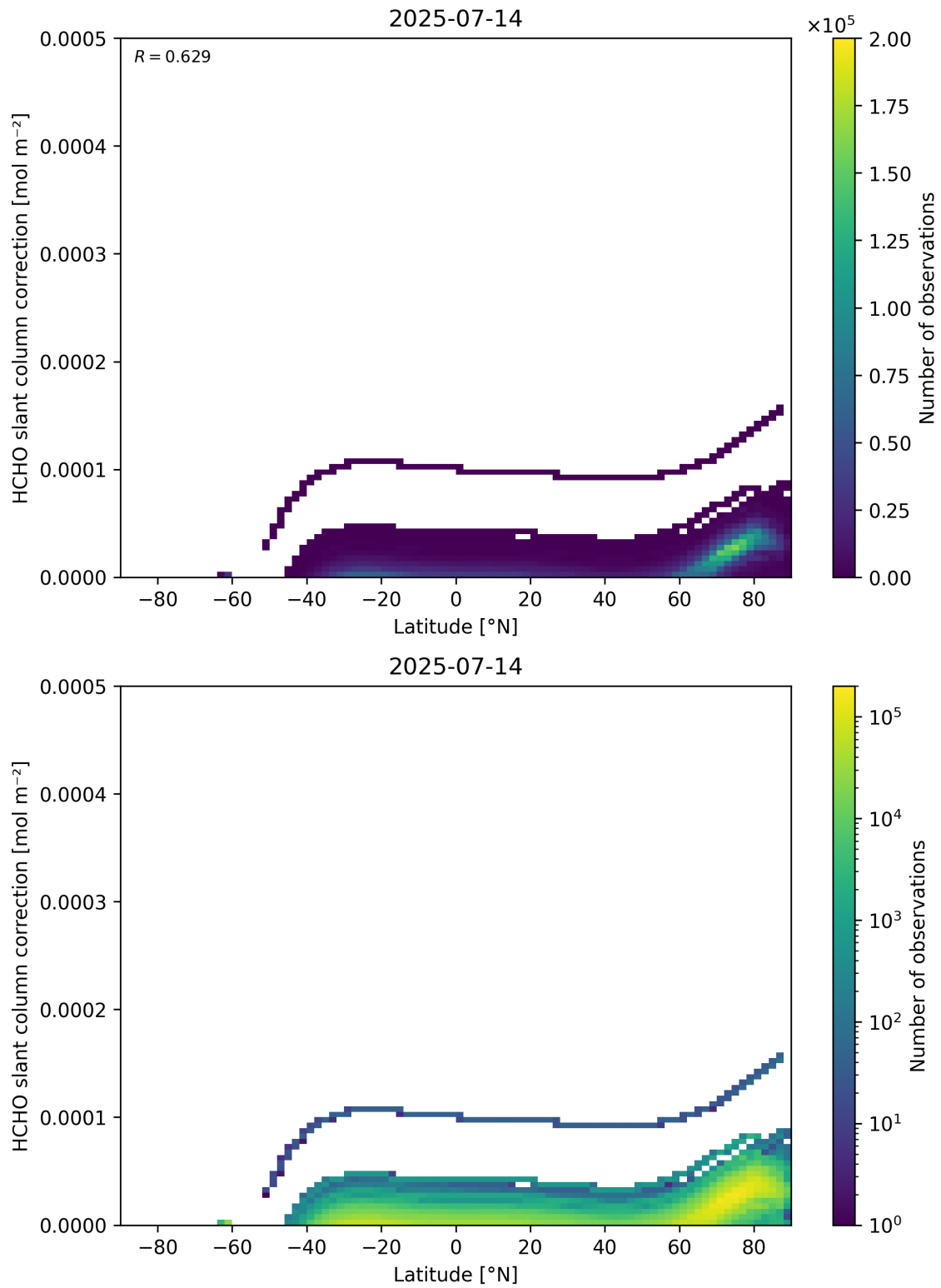
Figure 158: Scatter density plot of “Latitude” against “HCHO slant column correction” for 2025-07-13 to 2025-07-15.
