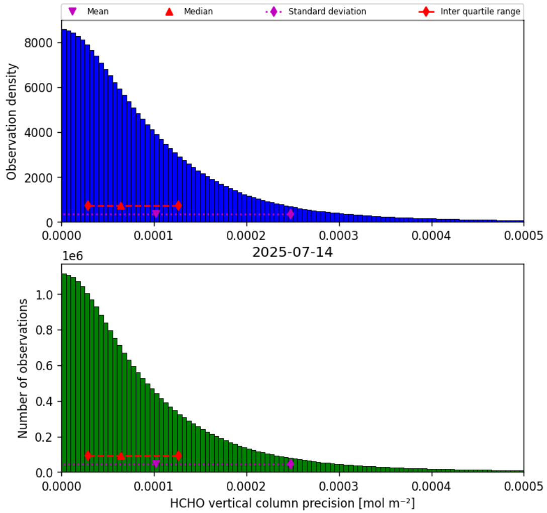
Figure 36: Histogram of “HCHO vertical column precision” for 2025-07-13 to 2025-07-15
