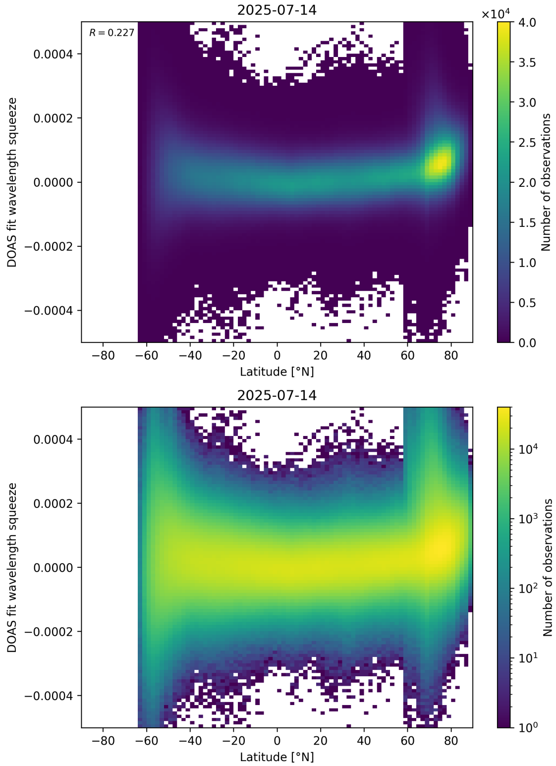
Figure 155: Scatter density plot of “Latitude” against “DOAS fit wavelength squeeze” for 2025-07-13 to 2025-07-15.
