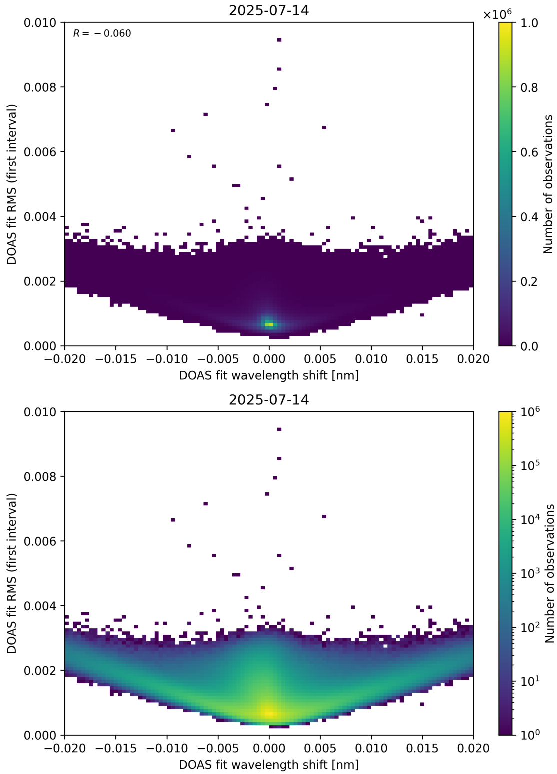
Figure 64: Scatter density plot of “DOAS fit wavelength shift” against “DOAS fit RMS (first interval)” for 2025-07-13 to 2025-07-15.
