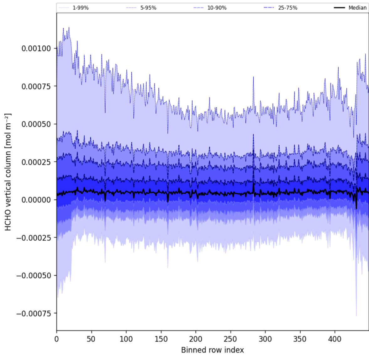
Figure 49: Along track statistics of “HCHO vertical column” for 2025-07-13 to 2025-07-15
