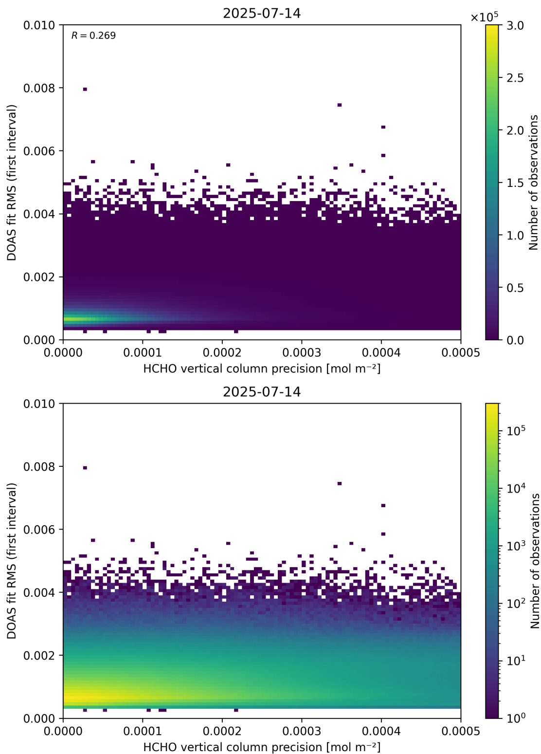
Figure 136: Scatter density plot of “HCHO vertical column precision” against “DOAS fit RMS (first interval)” for 2025-07-13 to 2025-07-15.
