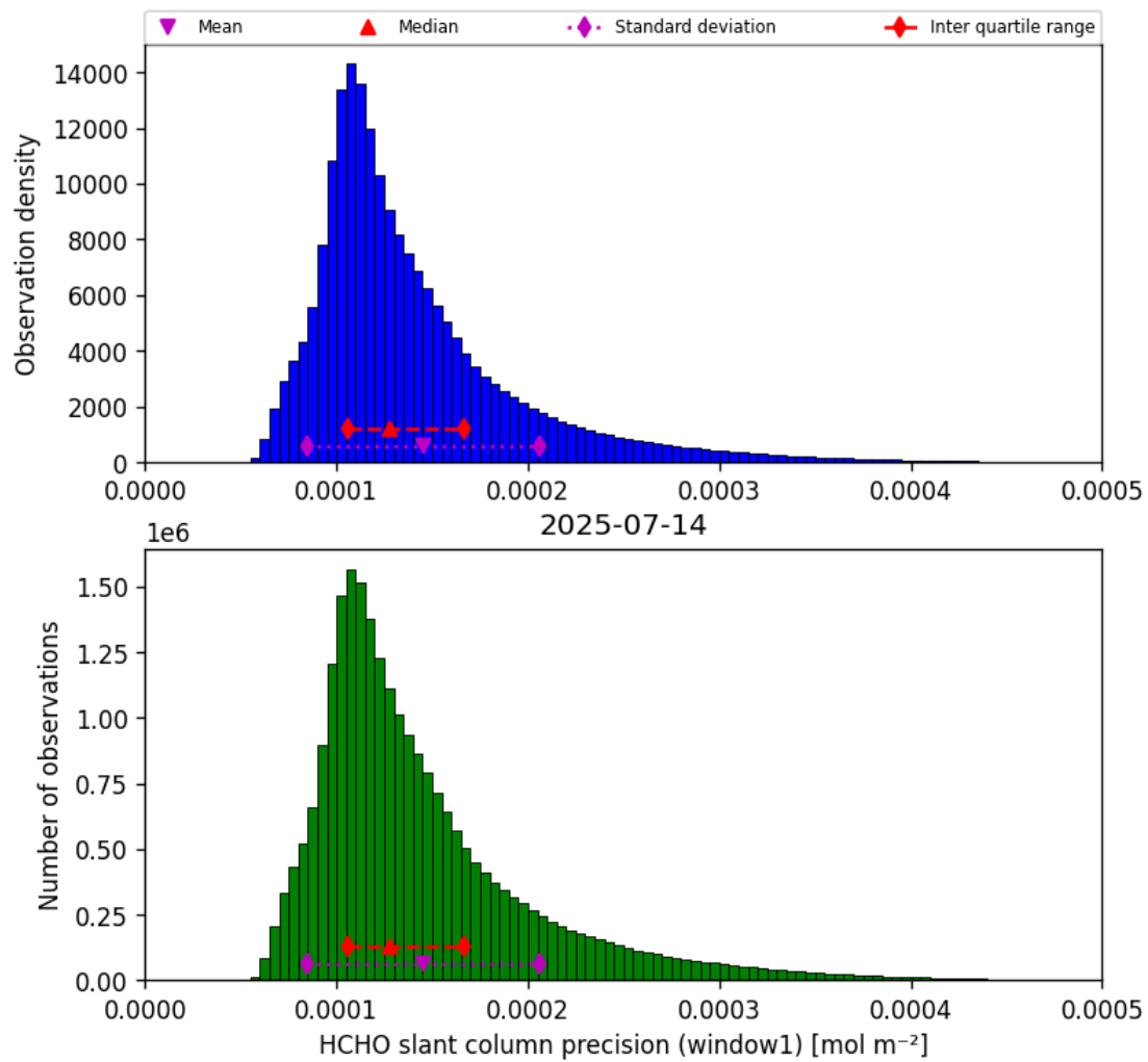
Figure 39: Histogram of “HCHO slant column precision (window1)” for 2025-07-13 to 2025-07-15
