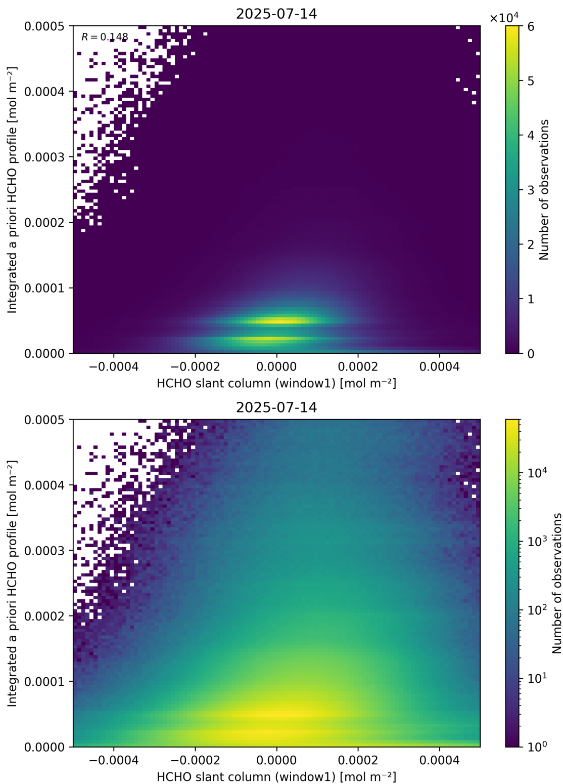
Figure 87: Scatter density plot of “HCHO slant column (window1)” against “Integrated a priori HCHO profile” for 2025-07-13 to 2025-07-15.
