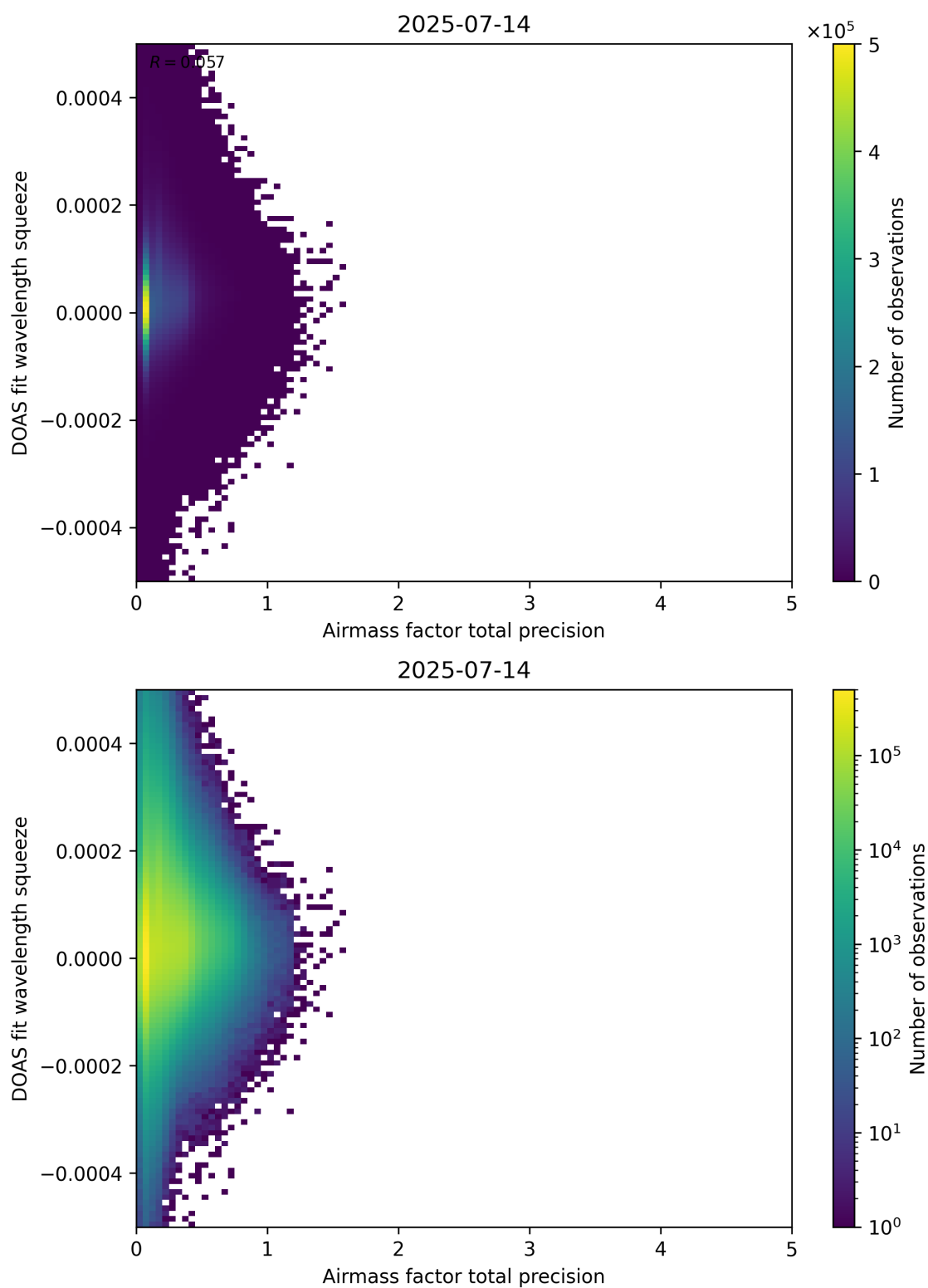
Figure 107: Scatter density plot of “Airmass factor total precision” against “DOAS fit wavelength squeeze” for 2025-07-13 to 2025-07-15.
