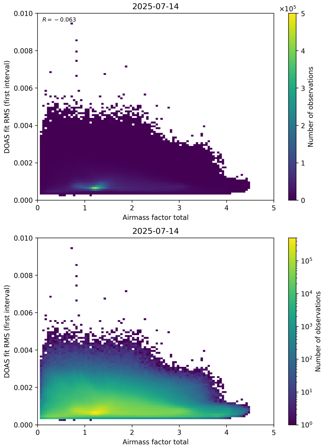
Figure 97: Scatter density plot of “Airmass factor total” against “DOAS fit RMS (first interval)” for 2025-07-13 to 2025-07-15.
