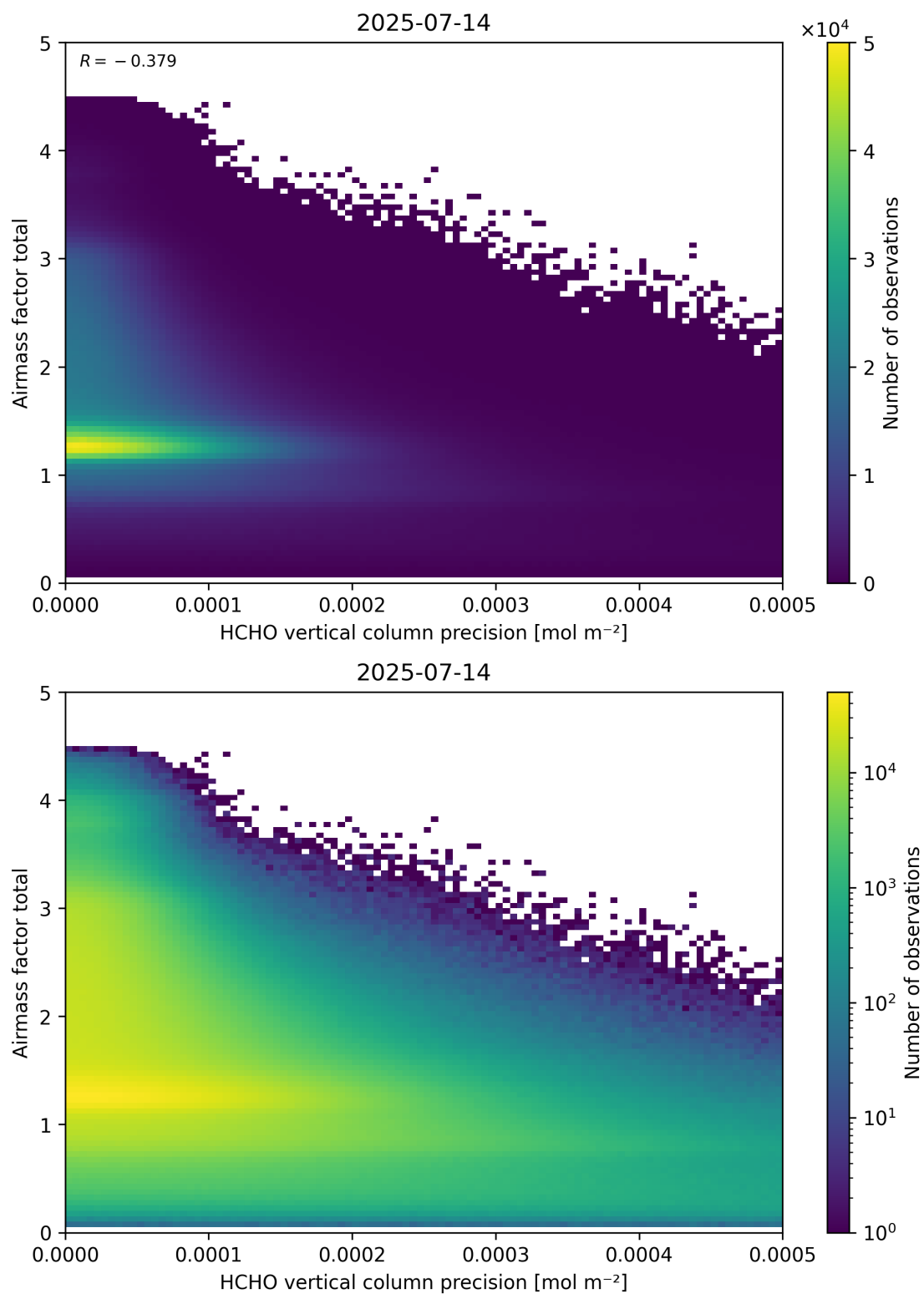
Figure 144: Scatter density plot of “HCHO vertical column precision” against “Airmass factor total” for 2025-07-13 to 2025-07-15.
