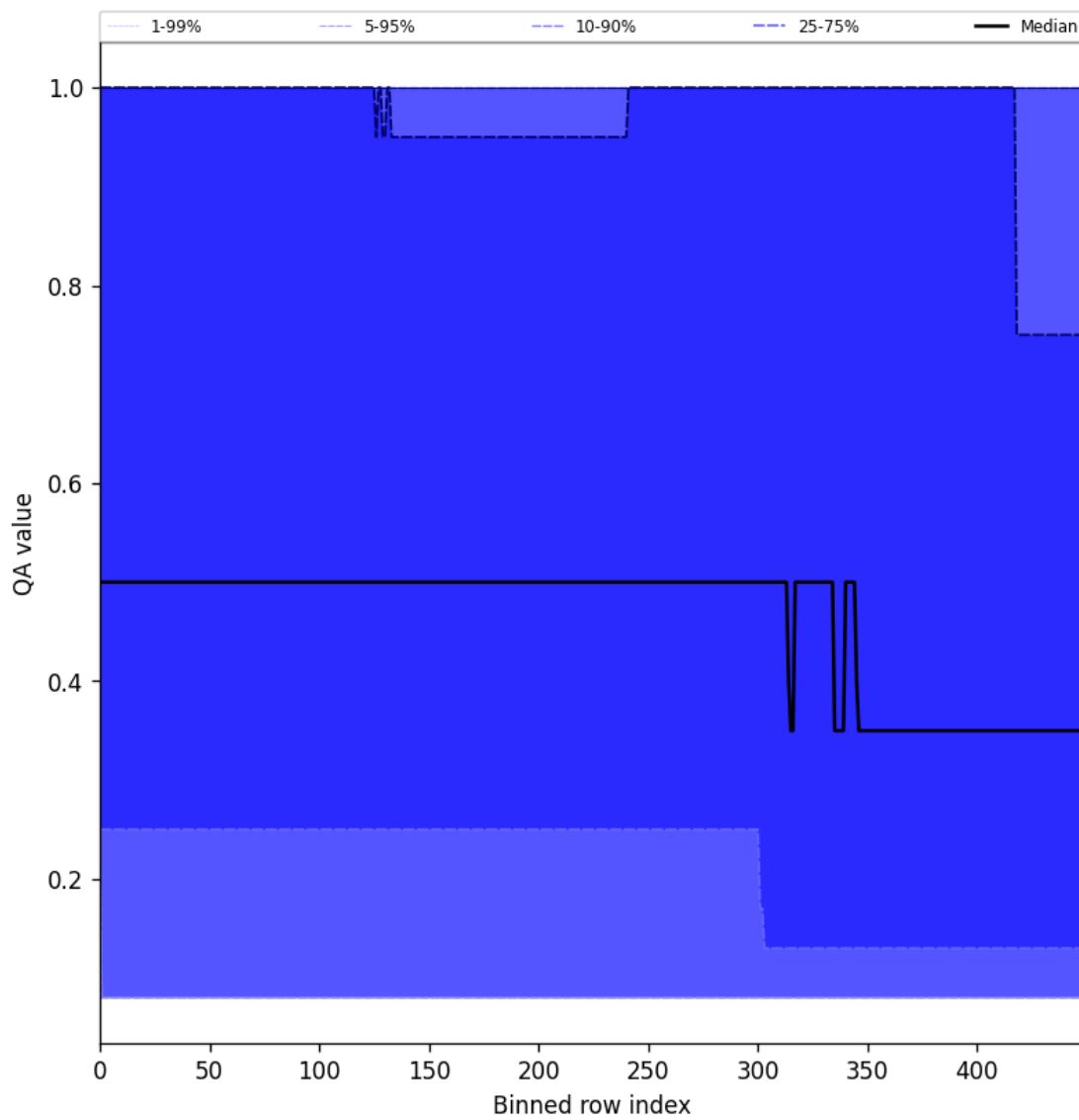
Figure 48: Along track statistics of “QA value” for 2025-07-13 to 2025-07-15
