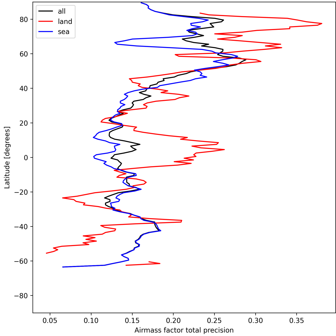
Figure 27: Zonal average of “Airmass factor total precision” for 2025-07-13 to 2025-07-15.
