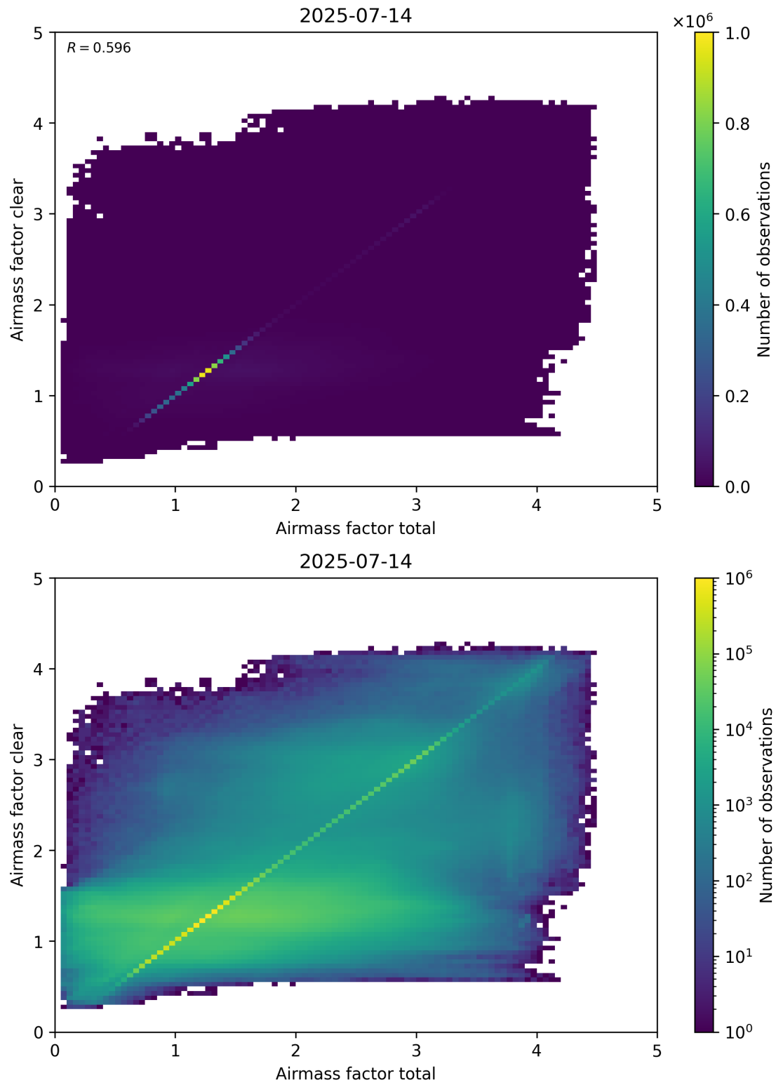
Figure 100: Scatter density plot of “Airmass factor total” against “Airmass factor clear” for 2025-07-13 to 2025-07-15.
