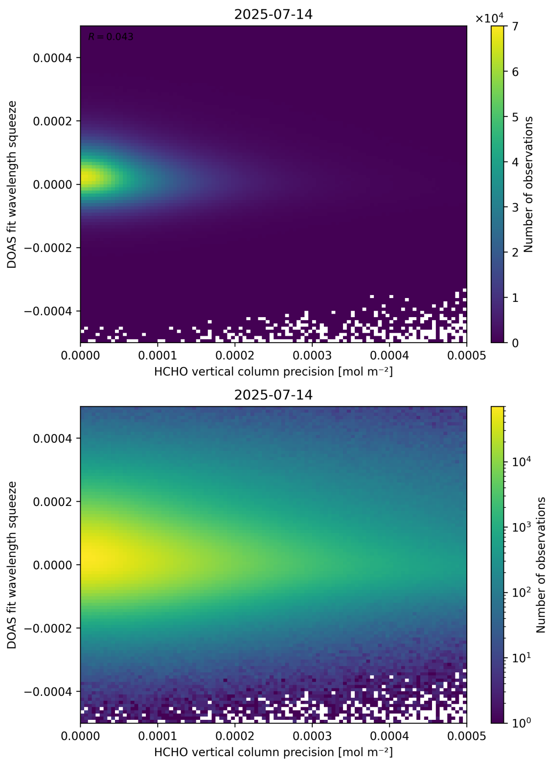
Figure 138: Scatter density plot of “HCHO vertical column precision” against “DOAS fit wavelength squeeze” for 2025-07-13 to 2025-07-15.
