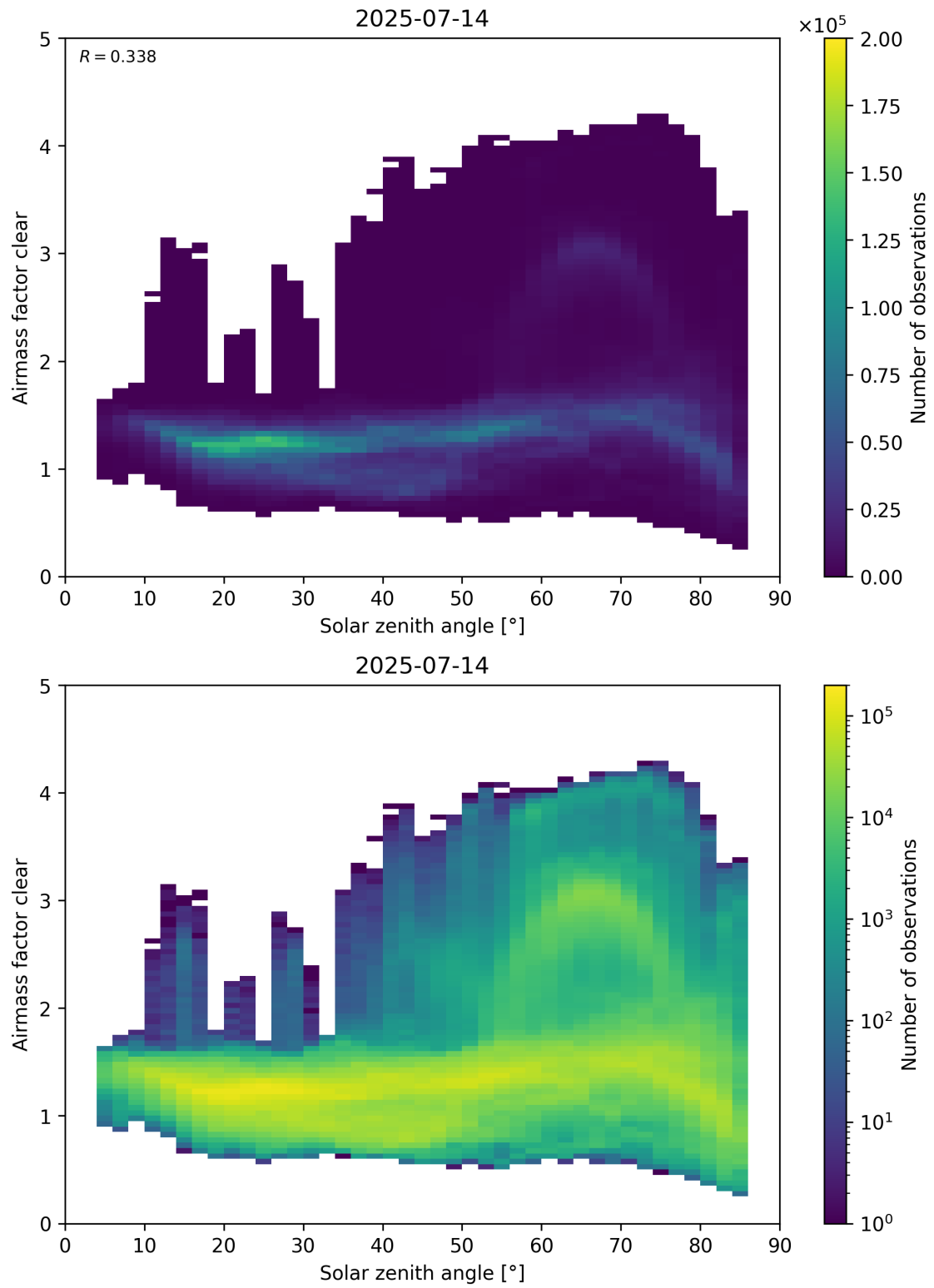
Figure 170: Scatter density plot of “Solar zenith angle” against “Airmass factor clear” for 2025-07-13 to 2025-07-15.
