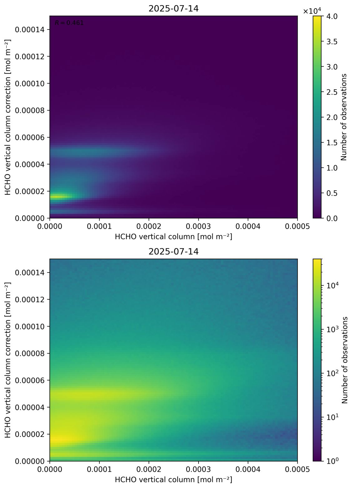
Figure 133: Scatter density plot of “HCHO vertical column” against “HCHO vertical column correction” for 2025-07-13 to 2025-07-15.
