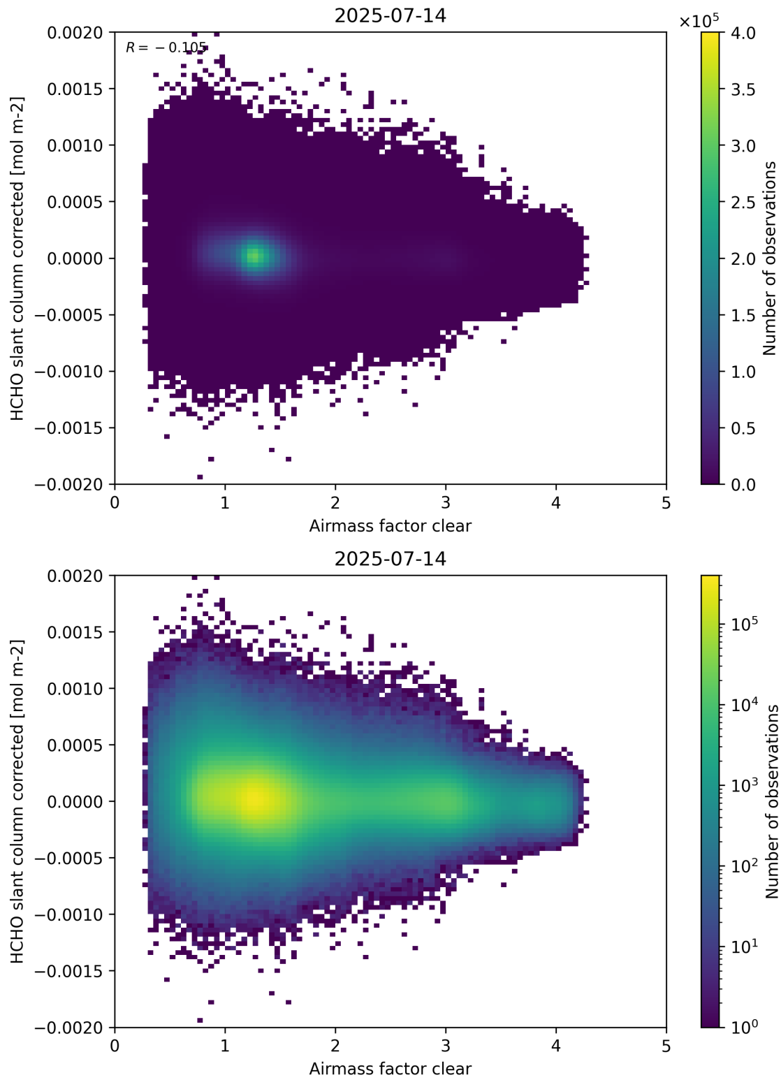
Figure 74: Scatter density plot of “Airmass factor clear” against “HCHO slant column corrected” for 2025-07-13 to 2025-07-15.
