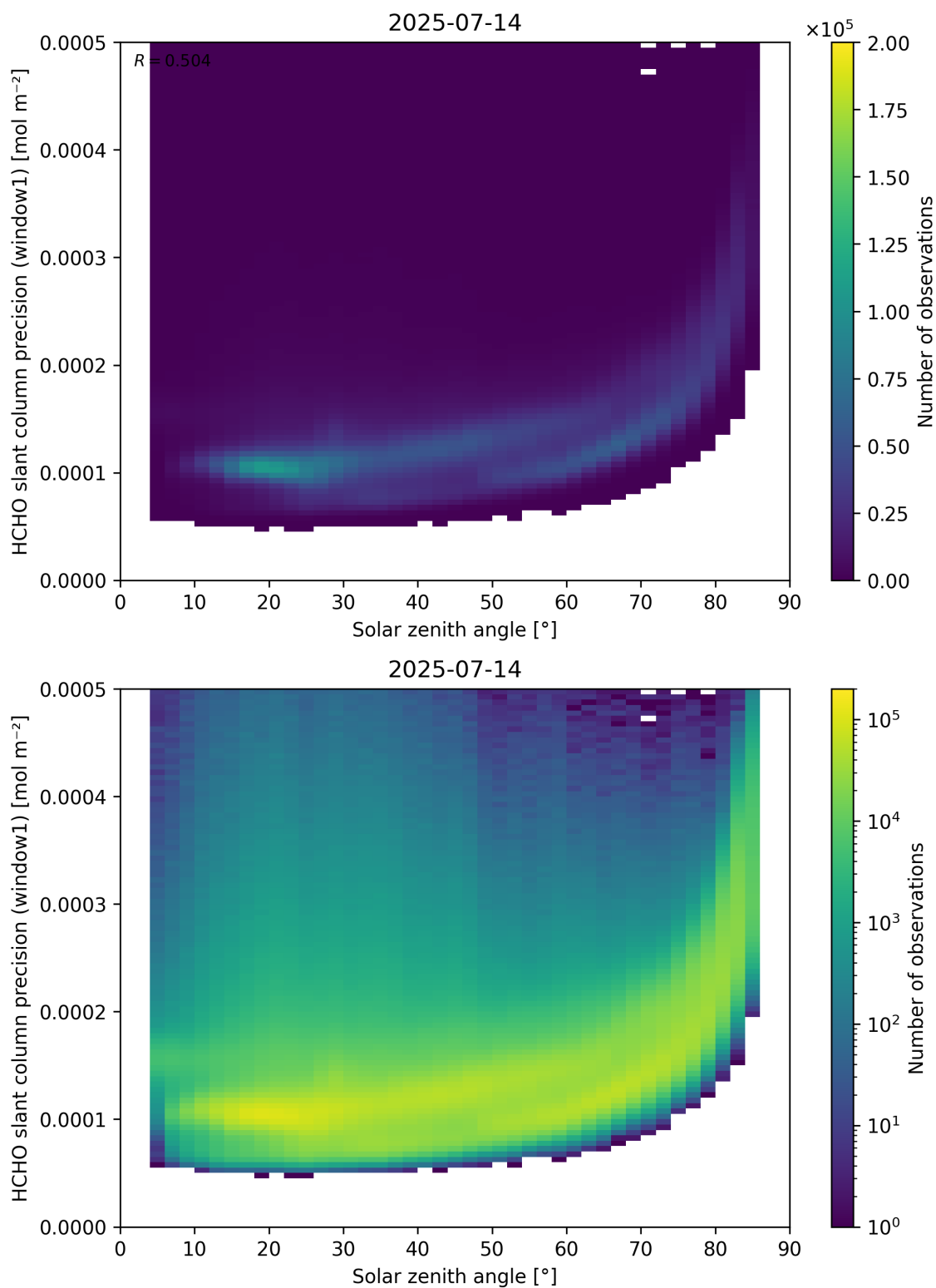
Figure 174: Scatter density plot of “Solar zenith angle” against “HCHO slant column precision (window1)” for 2025-07-13 to 2025-07-15.
