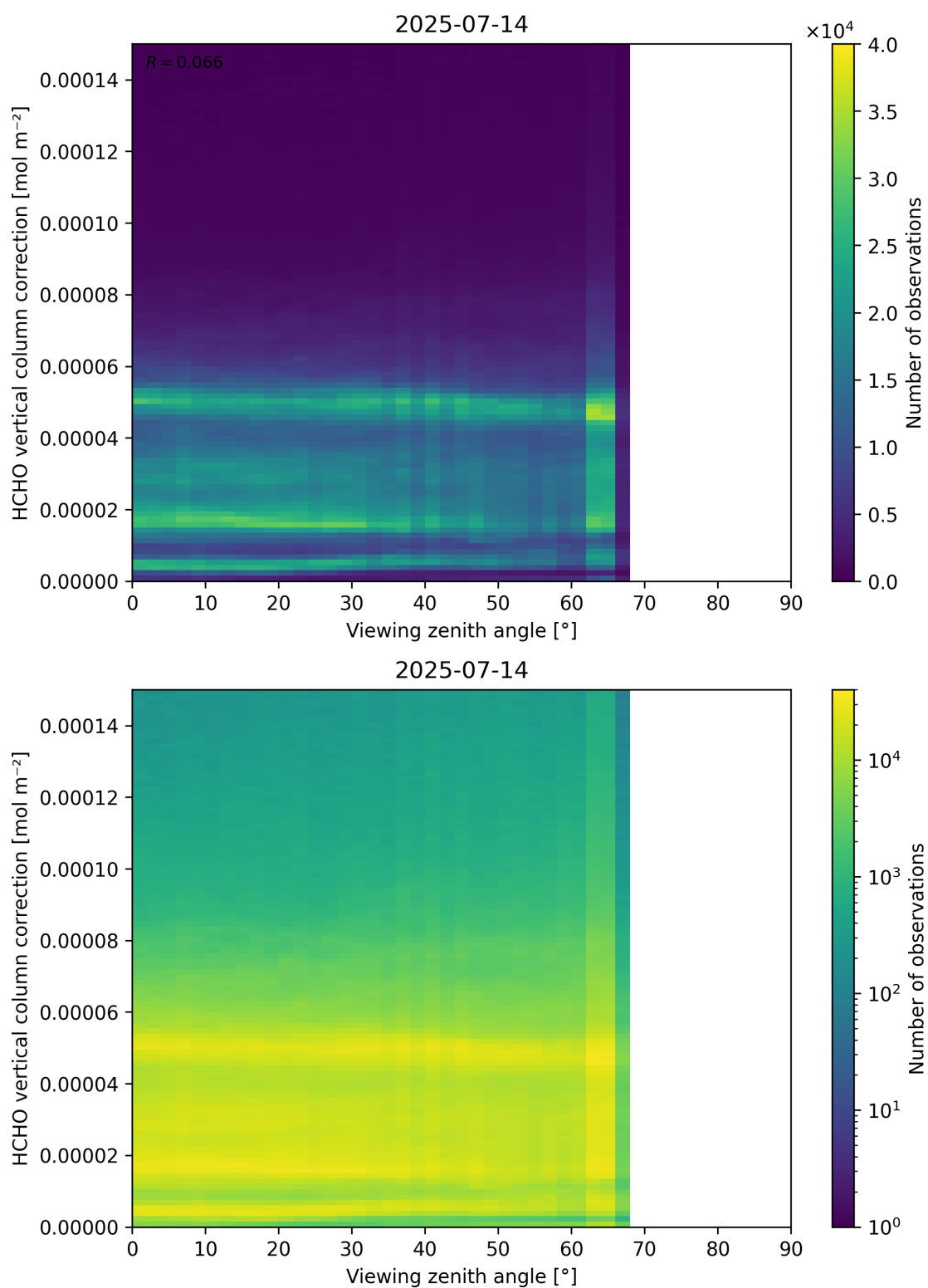
Figure 193: Scatter density plot of “Viewing zenith angle” against “HCHO vertical column correction” for 2025-07-13 to 2025-07-15.
