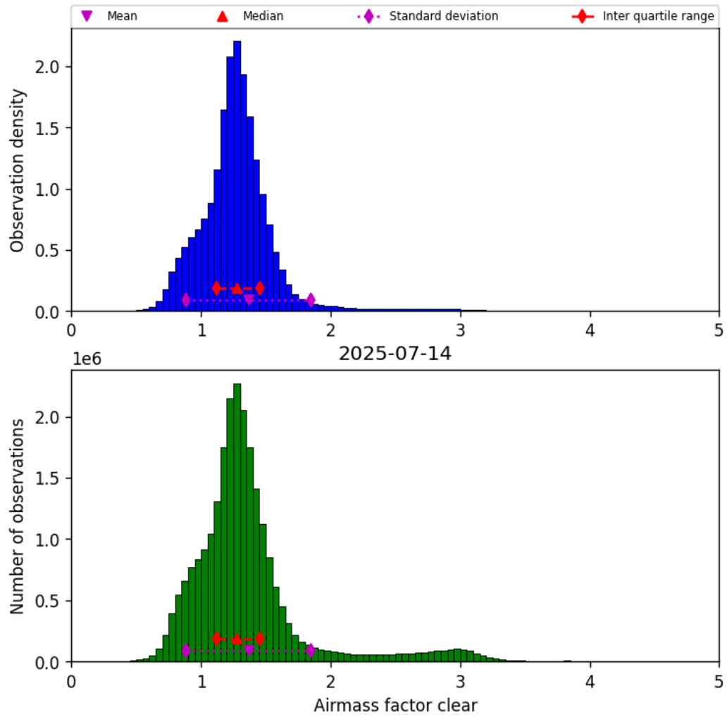
Figure 42: Histogram of “Airmass factor clear” for 2025-07-13 to 2025-07-15
