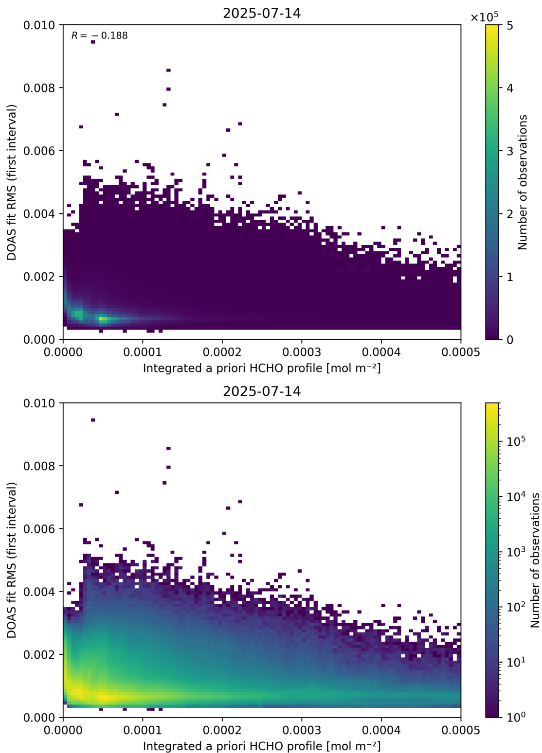
Figure 148: Scatter density plot of “Integrated a priori HCHO profile” against “DOAS fit RMS (first interval)” for 2025-07-13 to 2025-07-15.
