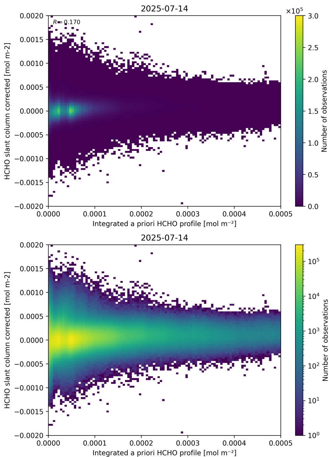
Figure 151: Scatter density plot of “Integrated a priori HCHO profile” against “HCHO slant column corrected” for 2025-07-13 to 2025-07-15.
