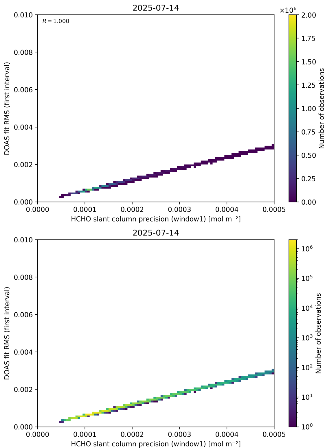
Figure 88: Scatter density plot of “HCHO slant column precision (window1)” against “DOAS fit RMS (first interval)” for 2025-07-13 to 2025-07-15.
