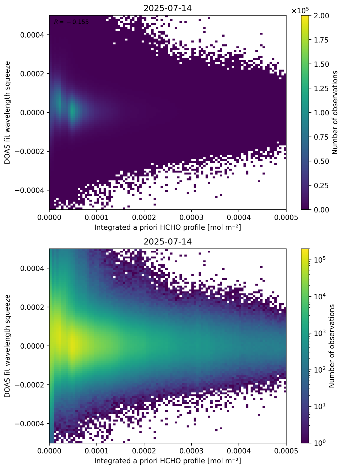
Figure 150: Scatter density plot of “Integrated a priori HCHO profile” against “DOAS fit wavelength squeeze” for 2025-07-13 to 2025-07-15.
