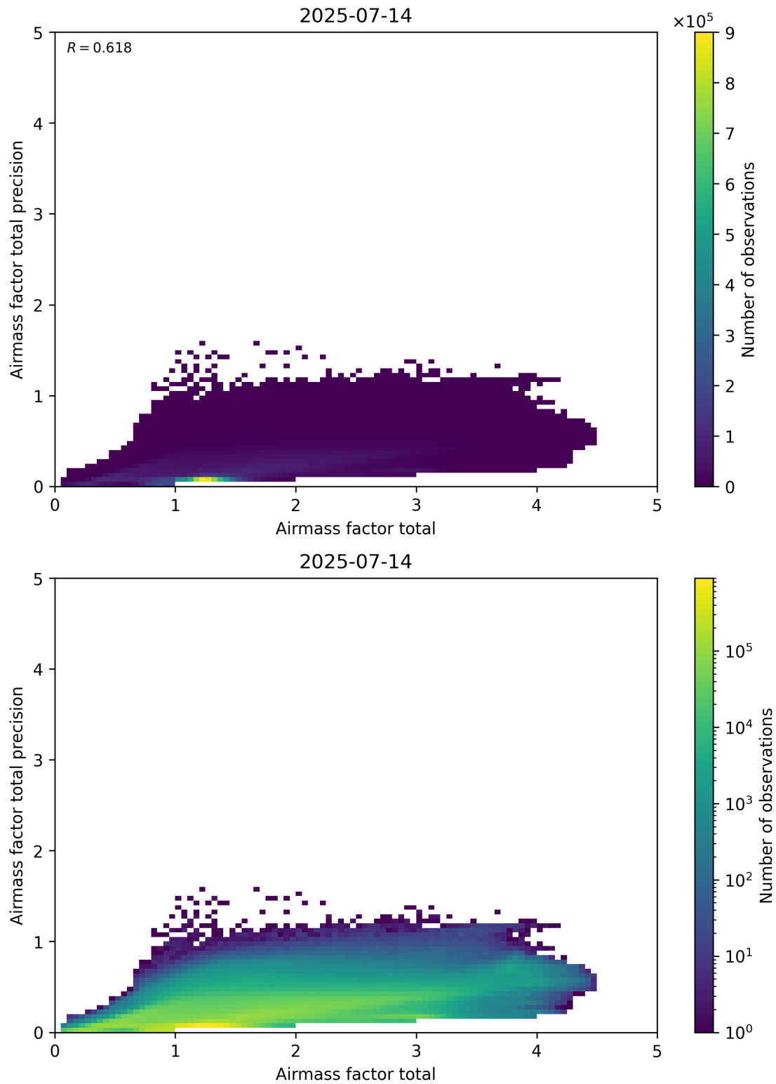
Figure 103: Scatter density plot of “Airmass factor total” against “Airmass factor total precision” for 2025-07-13 to 2025-07-15.
