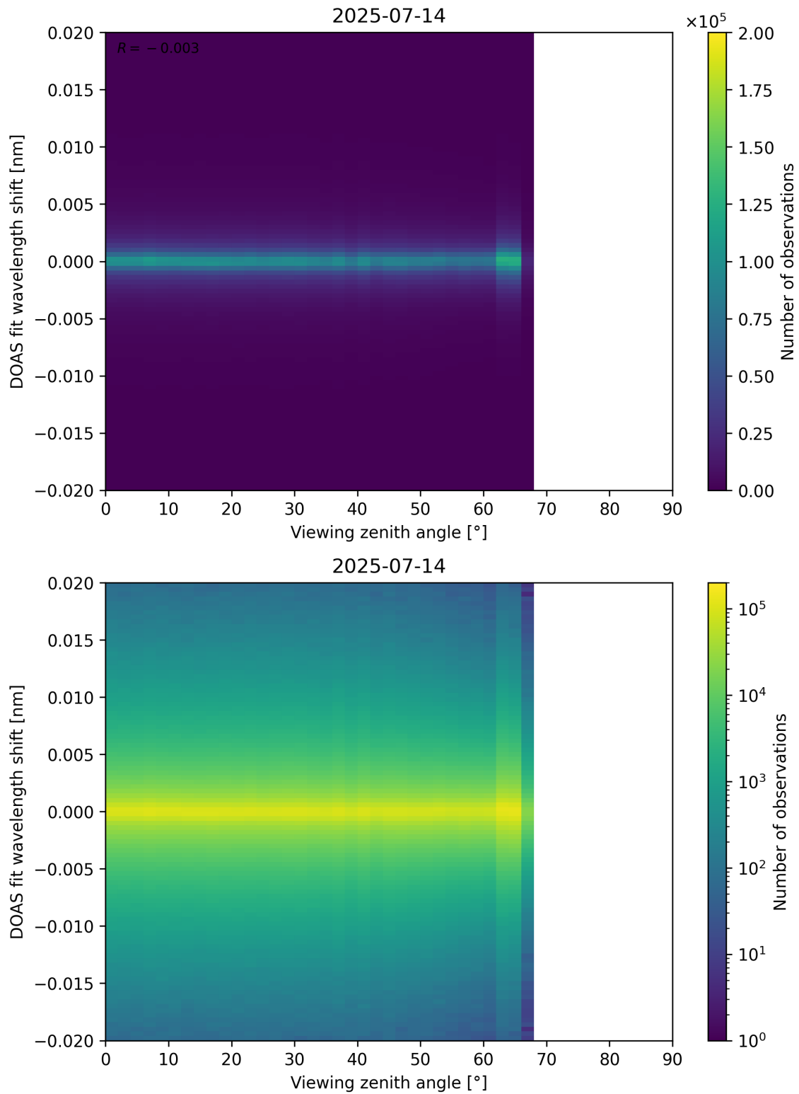
Figure 183: Scatter density plot of “Viewing zenith angle” against “DOAS fit wavelength shift” for 2025-07-13 to 2025-07-15.
