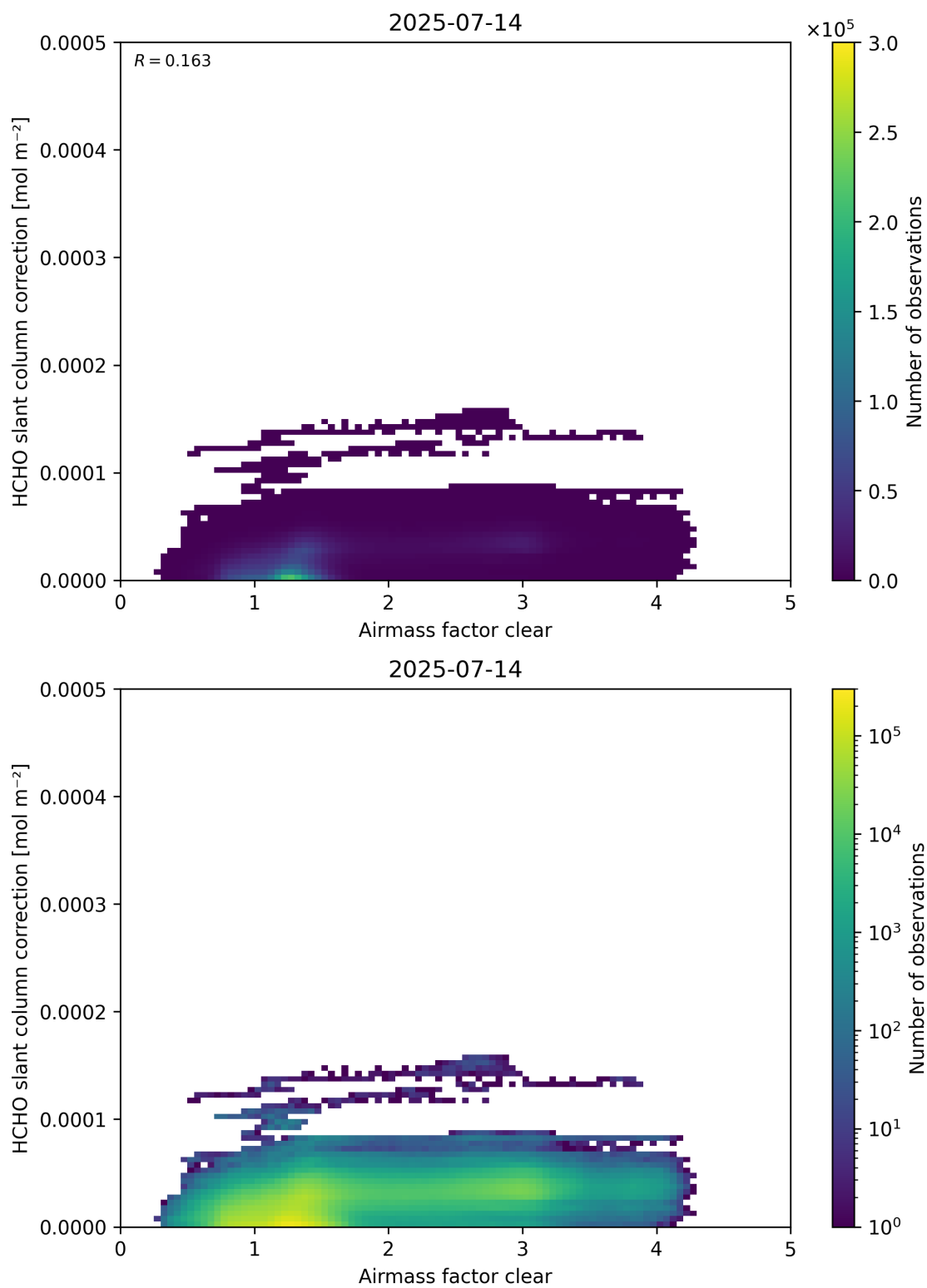
Figure 75: Scatter density plot of “Airmass factor clear” against “HCHO slant column correction” for 2025-07-13 to 2025-07-15.
