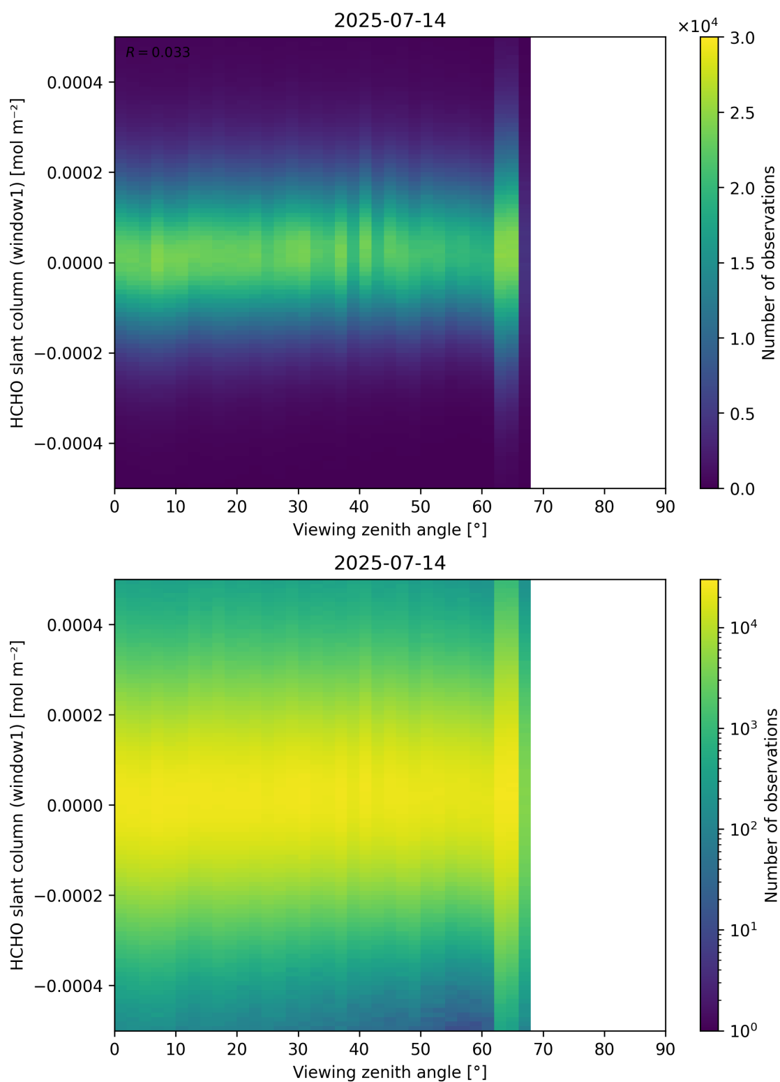
Figure 188: Scatter density plot of “Viewing zenith angle” against “HCHO slant column (window1)” for 2025-07-13 to 2025-07-15.
