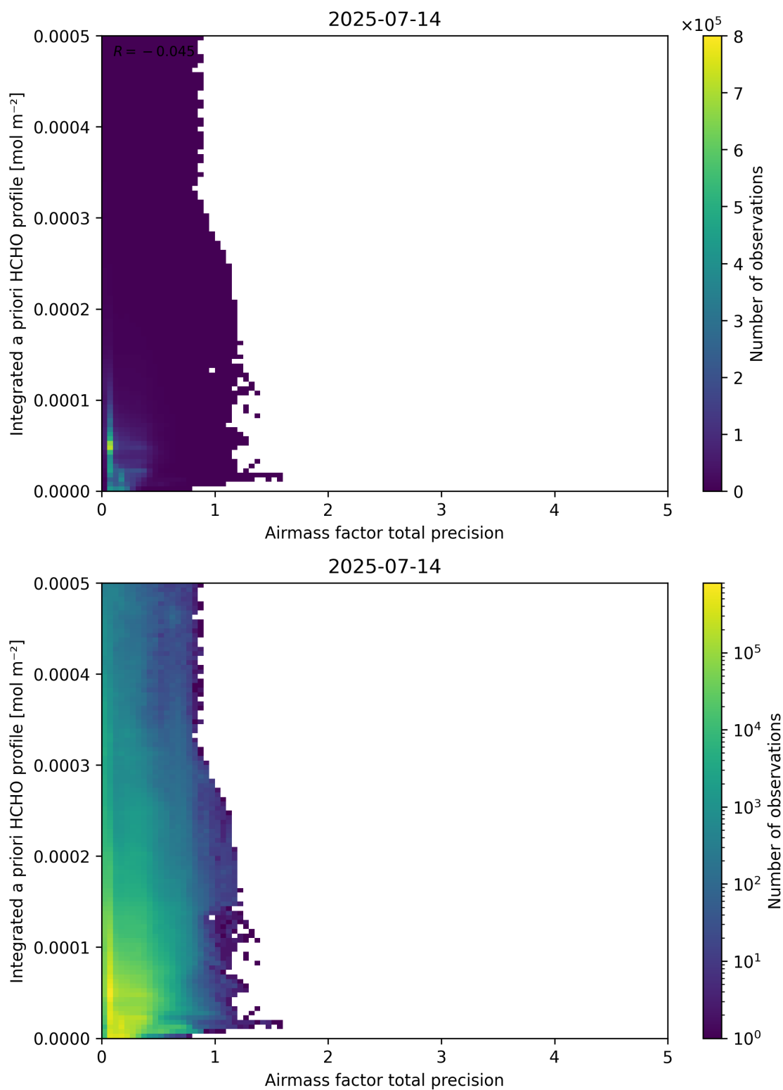
Figure 111: Scatter density plot of “Airmass factor total precision” against “Integrated a priori HCHO profile” for 2025-07-13 to 2025-07-15.
