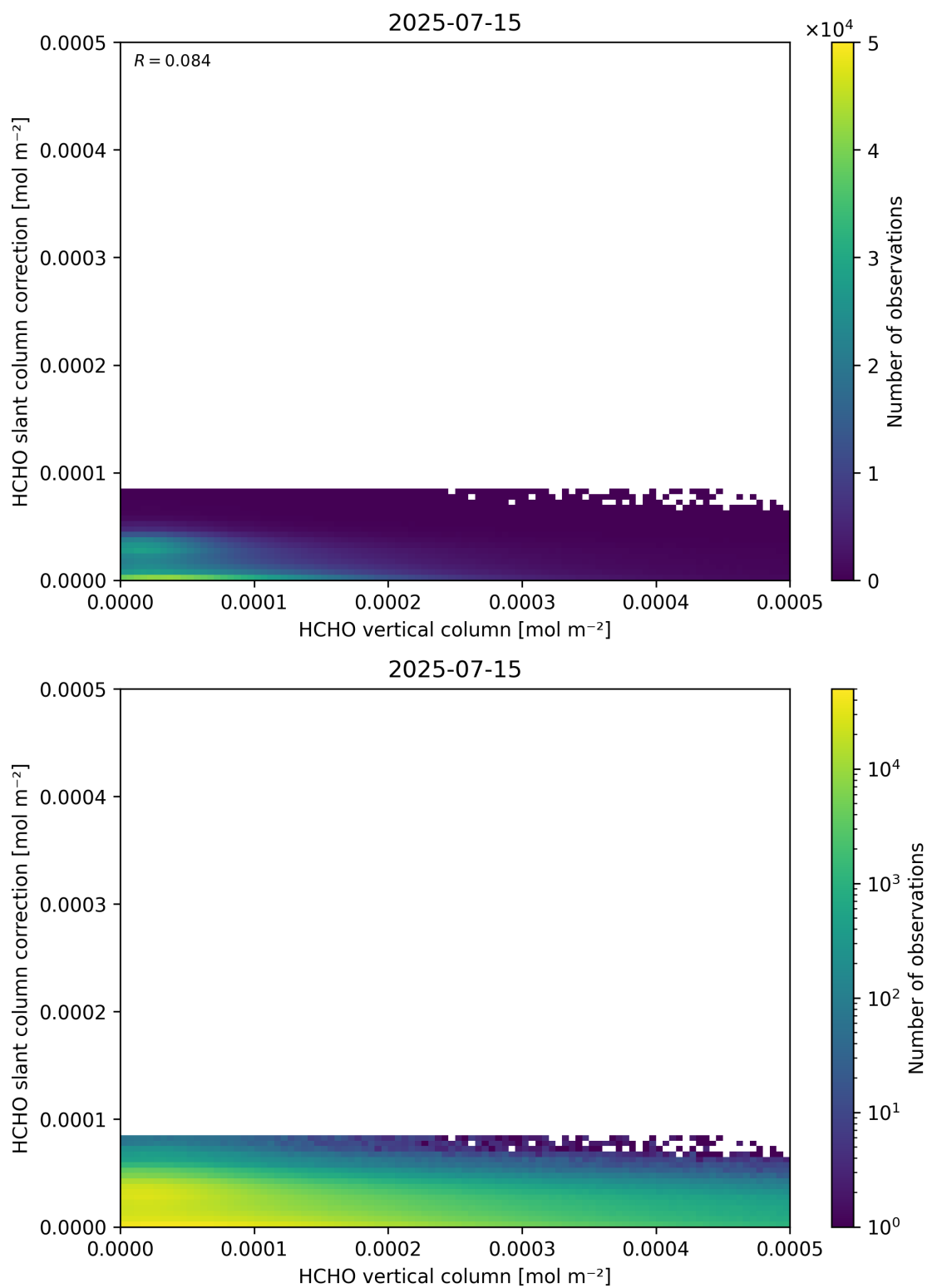
Figure 128: Scatter density plot of “HCHO vertical column” against “HCHO slant column correction” for 2025-07-14 to 2025-07-16.
