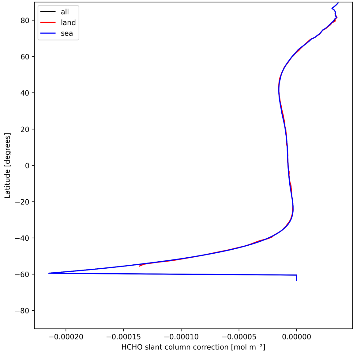
Figure 33: Zonal average of “HCHO slant column correction” for 2025-07-14 to 2025-07-16.
