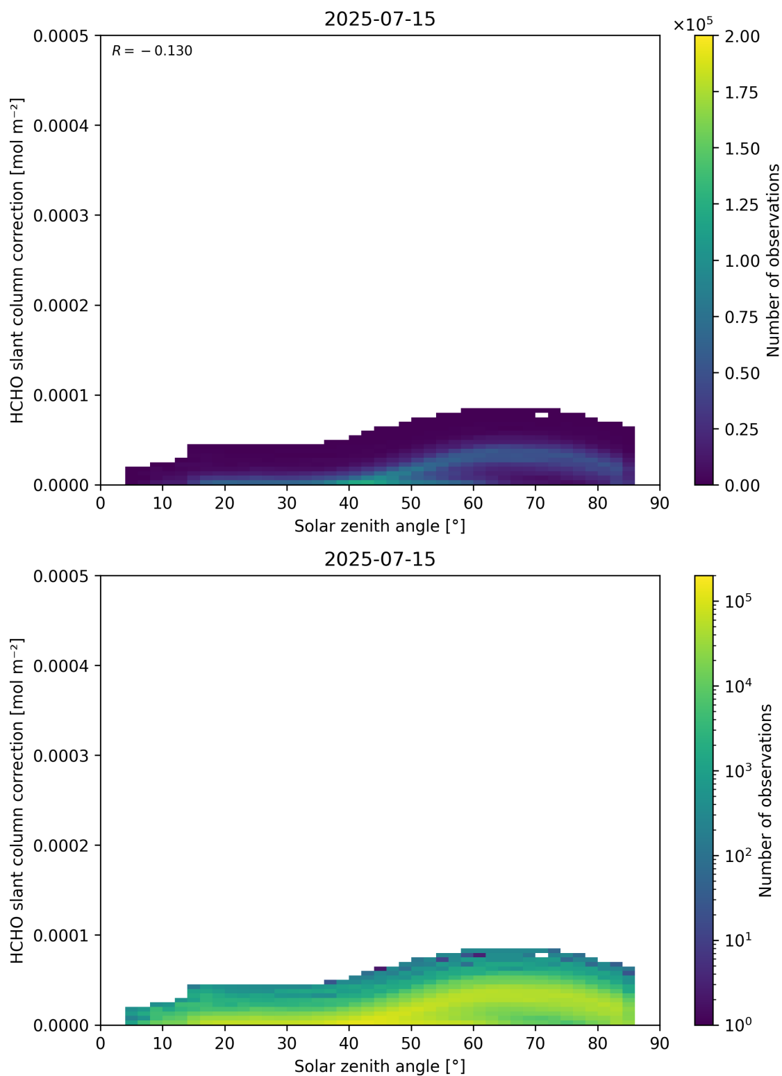
Figure 172: Scatter density plot of “Solar zenith angle” against “HCHO slant column correction” for 2025-07-14 to 2025-07-16.
