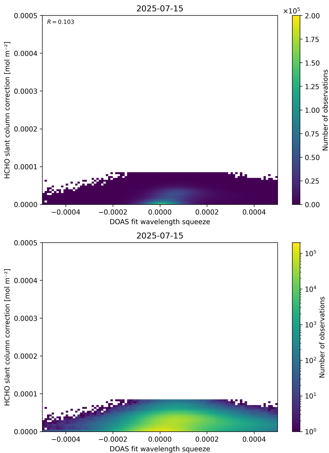
Figure 70: Scatter density plot of “DOAS fit wavelength squeeze” against “HCHO slant column correction” for 2025-07-14 to 2025-07-16.
