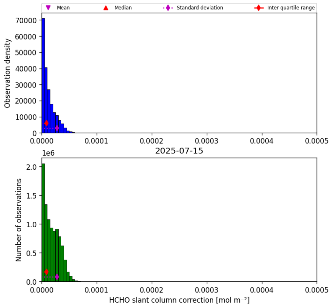
Figure 47: Histogram of “HCHO slant column correction” for 2025-07-14 to 2025-07-16
