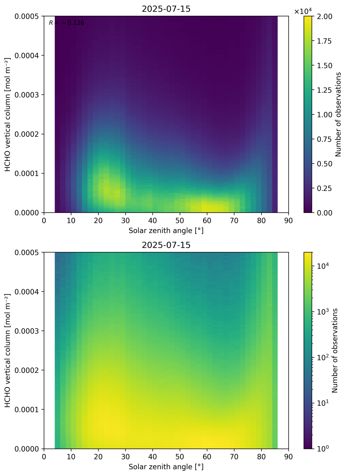
Figure 177: Scatter density plot of “Solar zenith angle” against “HCHO vertical column” for 2025-07-14 to 2025-07-16.
