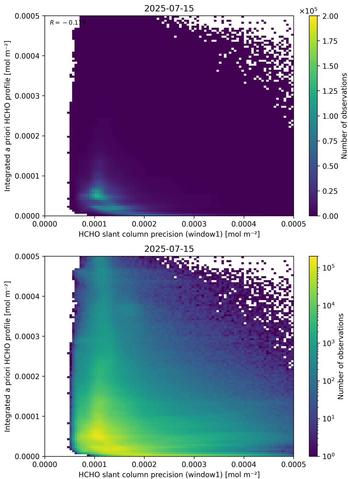
Figure 96: Scatter density plot of “HCHO slant column precision (window1)” against “Integrated a priori HCHO profile” for 2025-07-14 to 2025-07-16.
