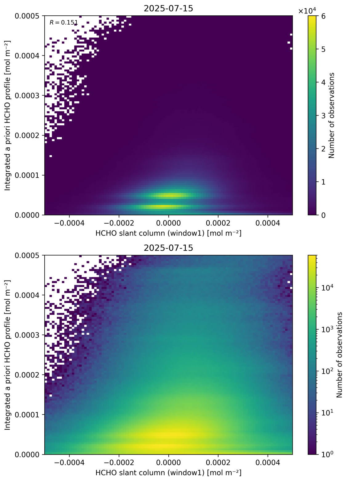
Figure 87: Scatter density plot of “HCHO slant column (window1)” against “Integrated a priori HCHO profile” for 2025-07-14 to 2025-07-16.
