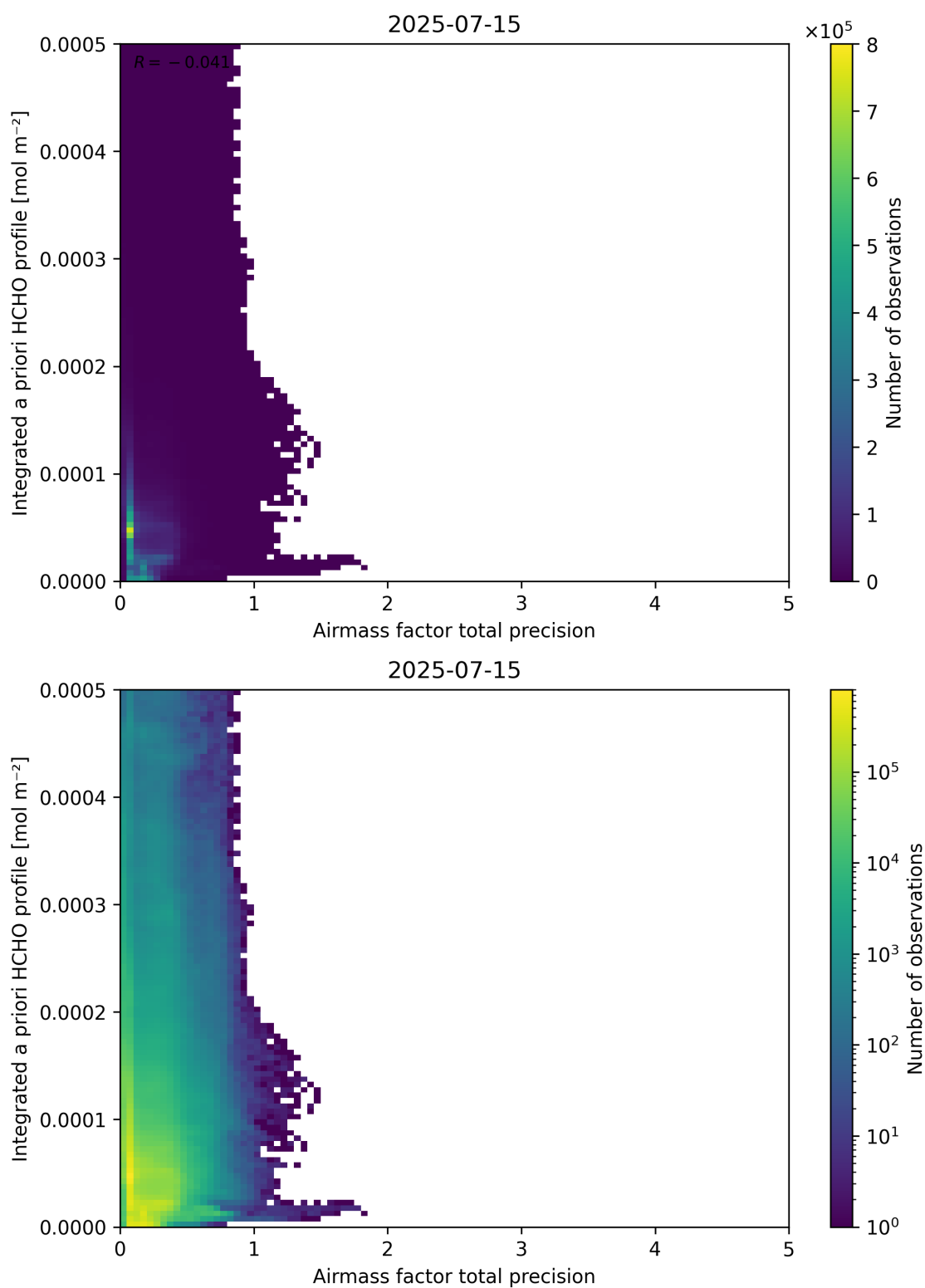
Figure 111: Scatter density plot of “Airmass factor total precision” against “Integrated a priori HCHO profile” for 2025-07-14 to 2025-07-16.
