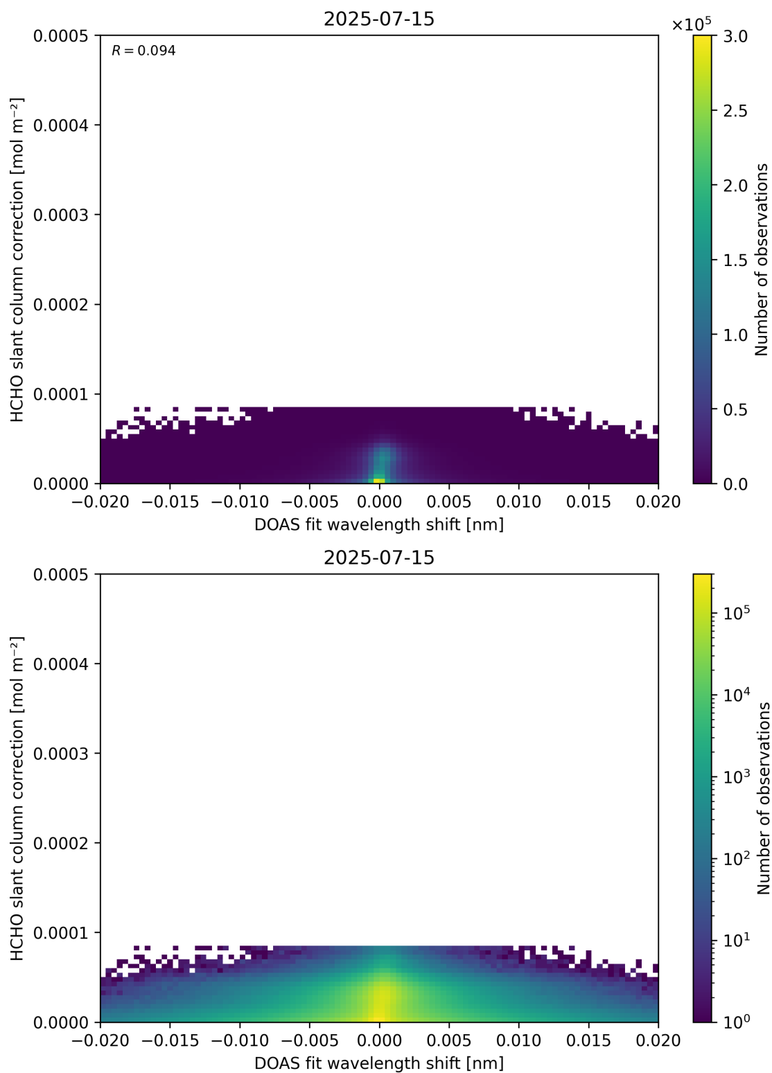
Figure 67: Scatter density plot of “DOAS fit wavelength shift” against “HCHO slant column correction” for 2025-07-14 to 2025-07-16.
