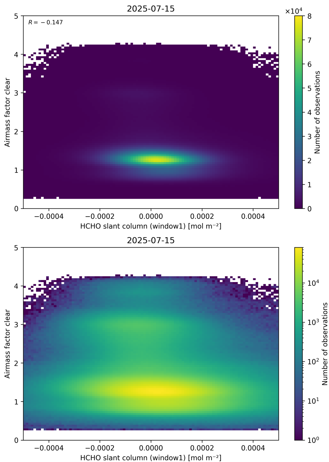
Figure 81: Scatter density plot of “HCHO slant column (window1)” against “Airmass factor clear” for 2025-07-14 to 2025-07-16.
