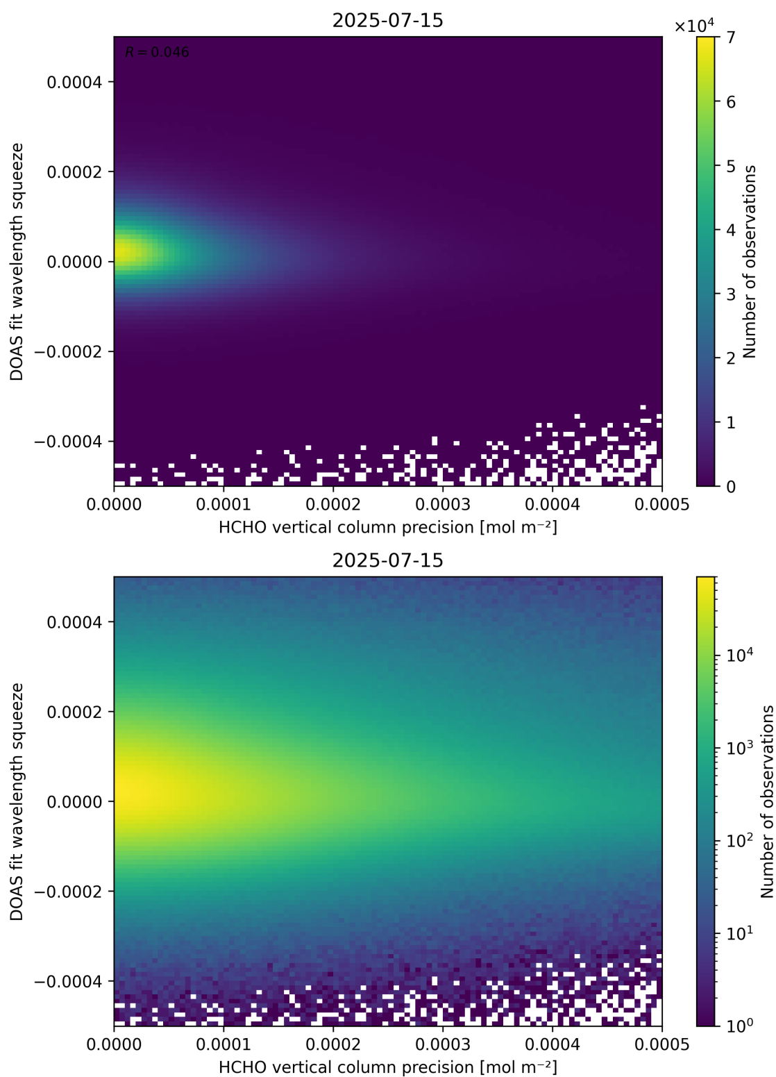
Figure 138: Scatter density plot of “HCHO vertical column precision” against “DOAS fit wavelength squeeze” for 2025-07-14 to 2025-07-16.
