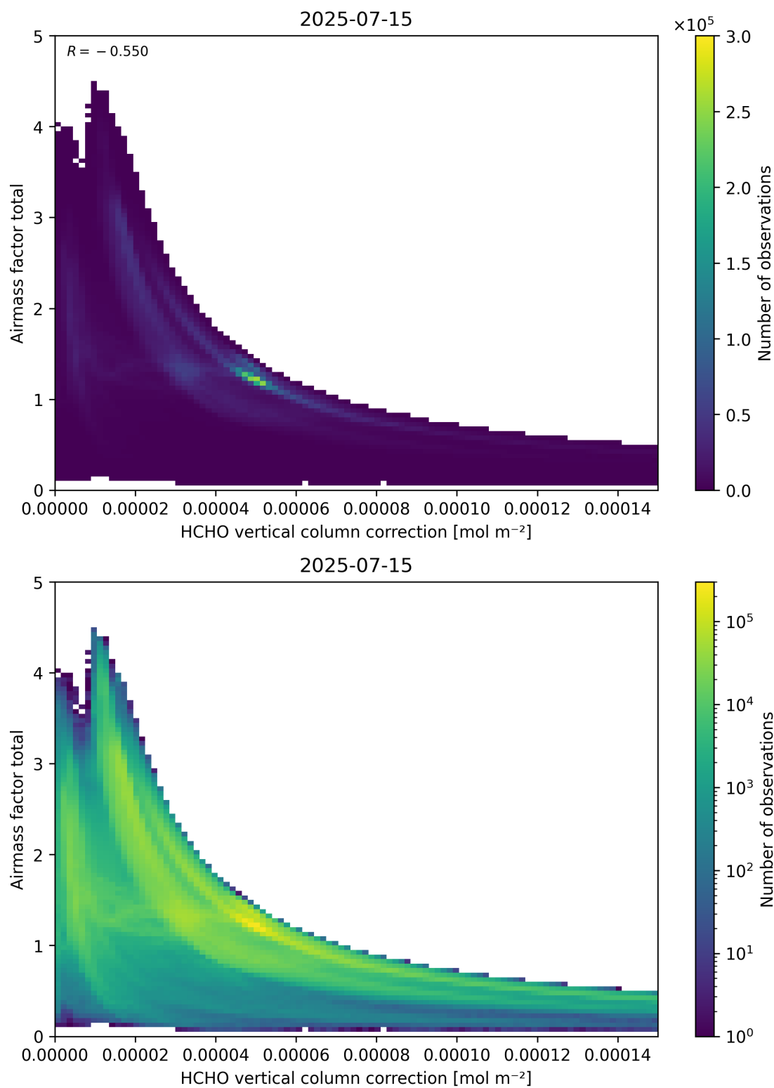
Figure 120: Scatter density plot of “HCHO vertical column correction” against “Airmass factor total” for 2025-07-14 to 2025-07-16.
