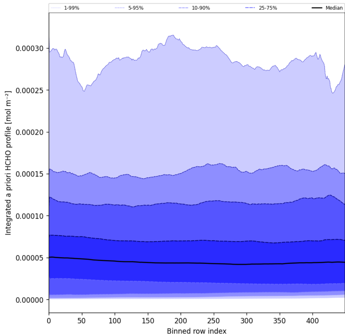
Figure 57: Along track statistics of “Integrated a priori HCHO profile” for 2025-07-14 to 2025-07-16
