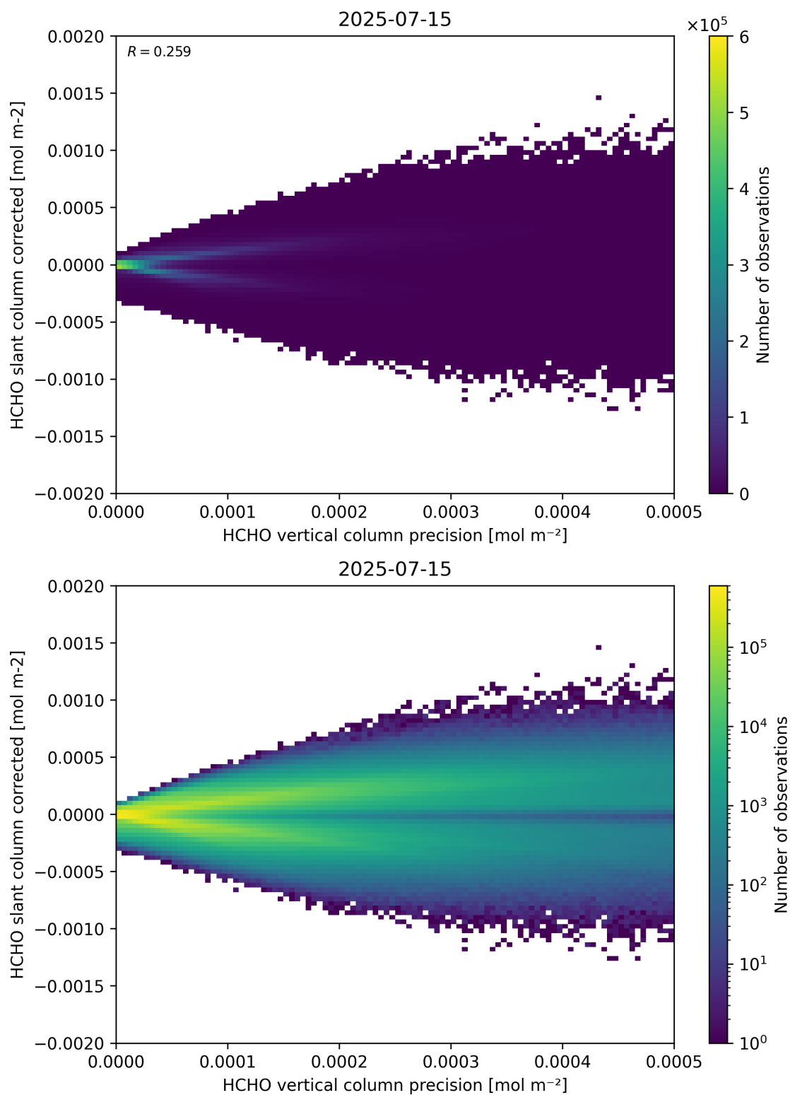
Figure 140: Scatter density plot of “HCHO vertical column precision” against “HCHO slant column corrected” for 2025-07-14 to 2025-07-16.
