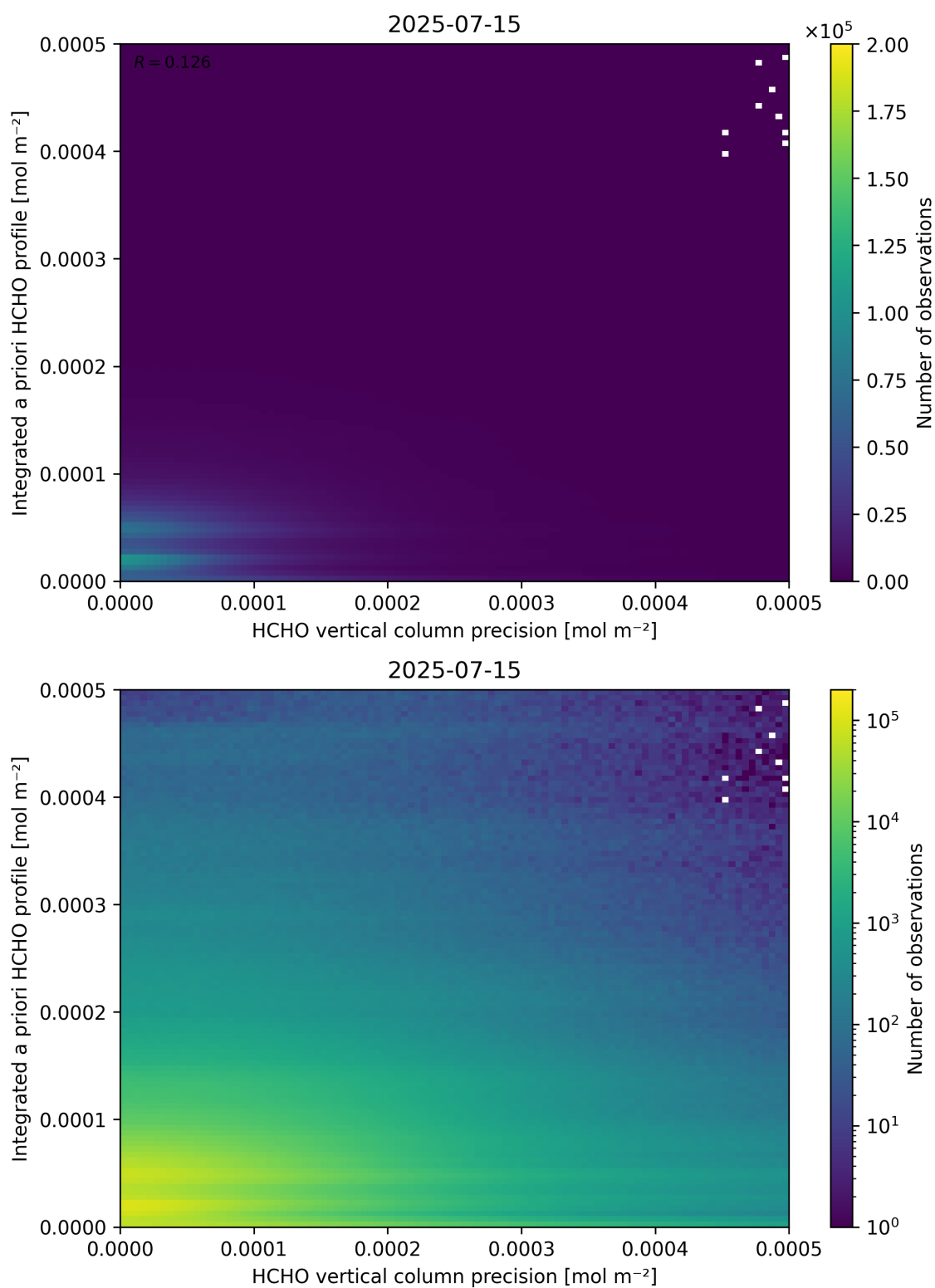
Figure 147: Scatter density plot of “HCHO vertical column precision” against “Integrated a priori HCHO profile” for 2025-07-14 to 2025-07-16.
