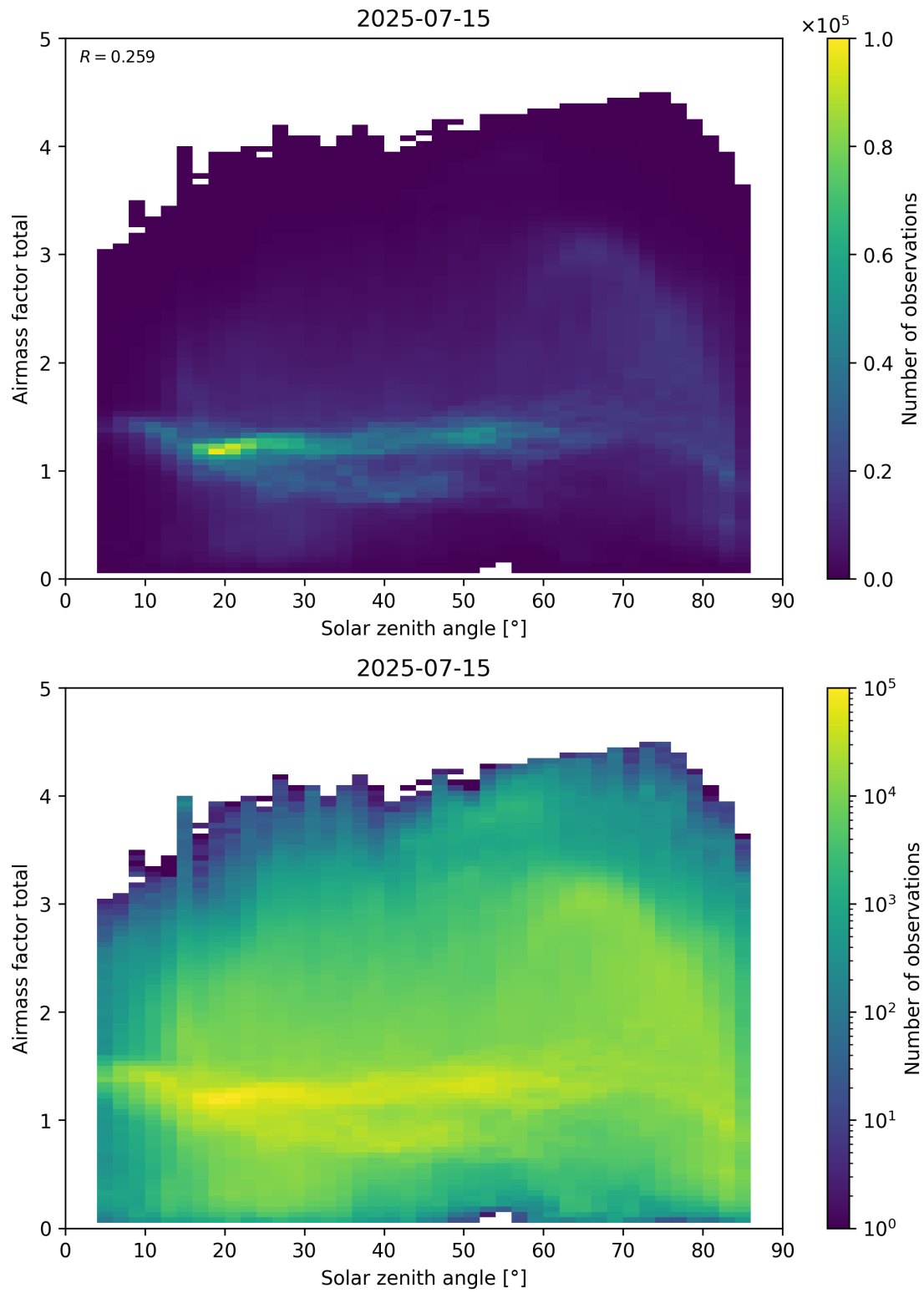
Figure 175: Scatter density plot of “Solar zenith angle” against “Airmass factor total” for 2025-07-14 to 2025-07-16.
