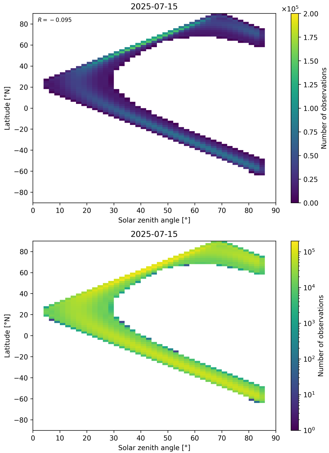
Figure 181: Scatter density plot of “Solar zenith angle” against “Latitude” for 2025-07-14 to 2025-07-16.
