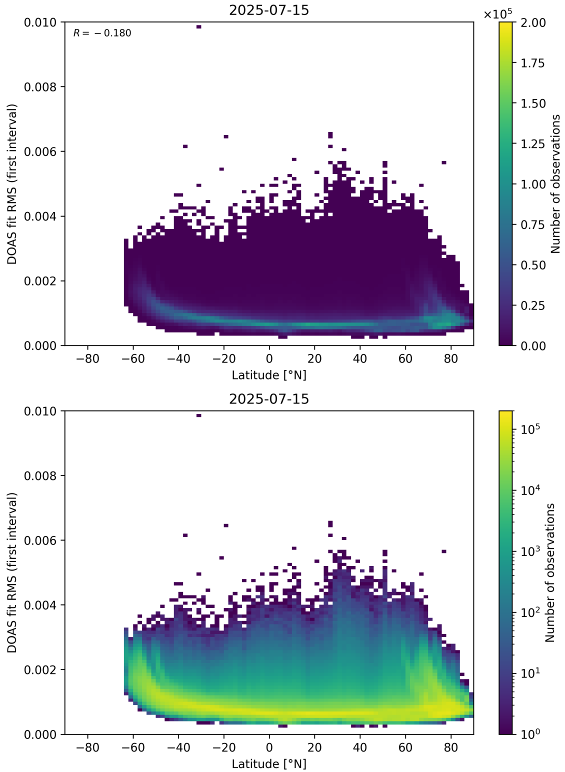
Figure 153: Scatter density plot of “Latitude” against “DOAS fit RMS (first interval)” for 2025-07-14 to 2025-07-16.
