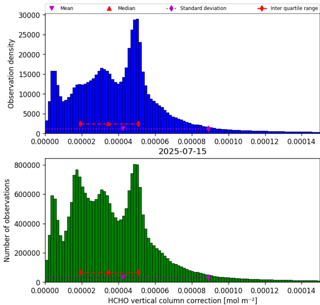
Figure 37: Histogram of “HCHO vertical column correction” for 2025-07-14 to 2025-07-16
