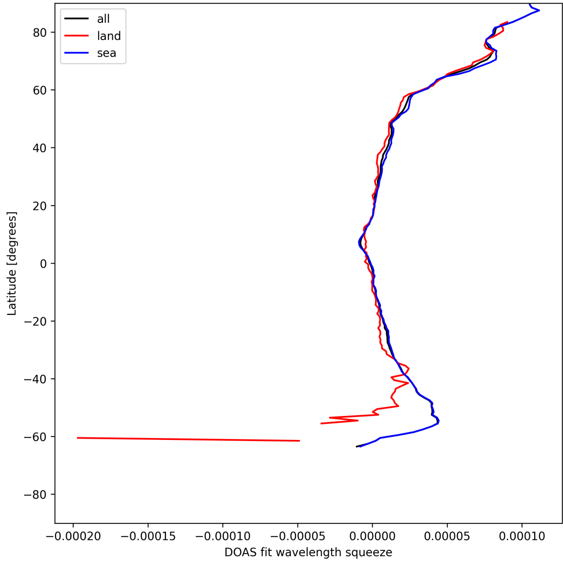
Figure 31: Zonal average of “DOAS fit wavelength squeeze” for 2025-07-14 to 2025-07-16.
