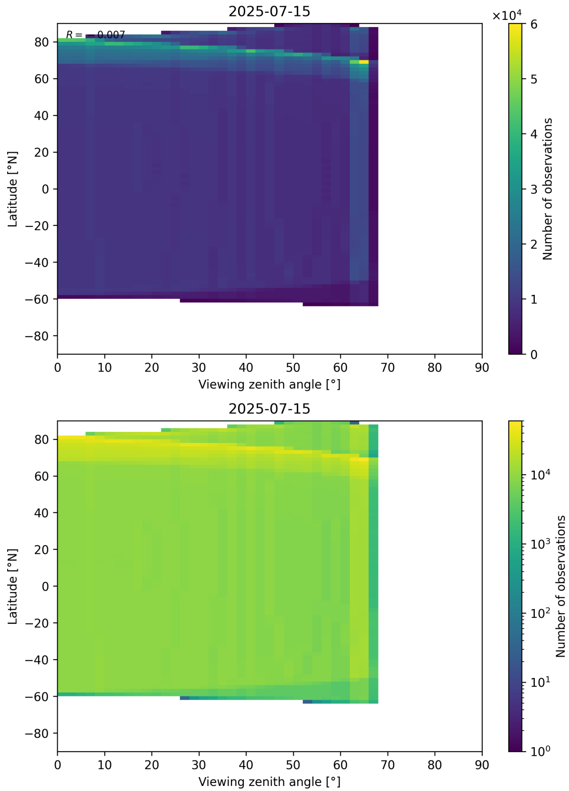
Figure 196: Scatter density plot of “Viewing zenith angle” against “Latitude” for 2025-07-14 to 2025-07-16.
