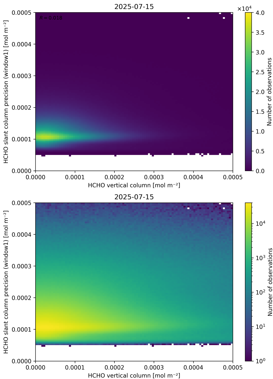
Figure 130: Scatter density plot of “HCHO vertical column” against “HCHO slant column precision (window1)” for 2025-07-14 to 2025-07-16.
