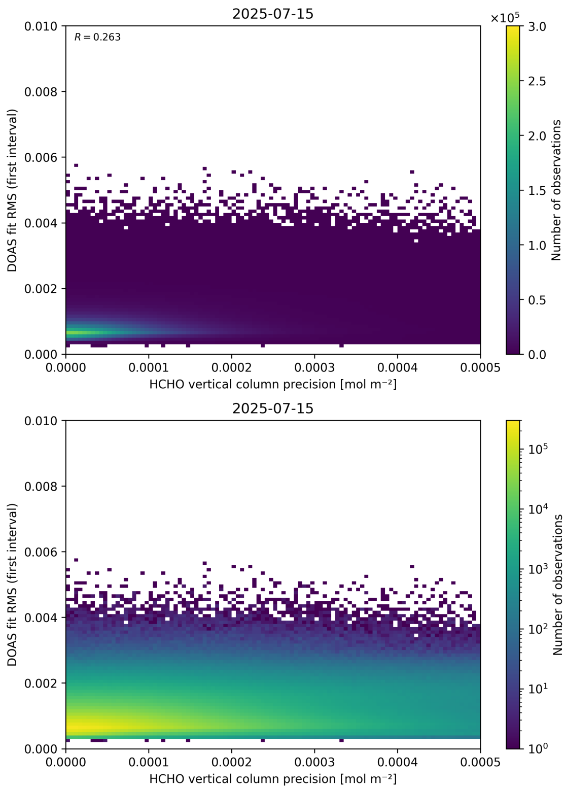
Figure 136: Scatter density plot of “HCHO vertical column precision” against “DOAS fit RMS (first interval)” for 2025-07-14 to 2025-07-16.
