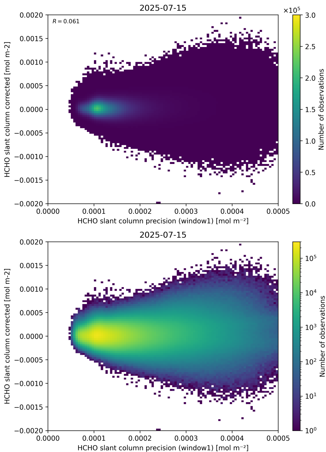
Figure 92: Scatter density plot of “HCHO slant column precision (window1)” against “HCHO slant column corrected” for 2025-07-14 to 2025-07-16.
