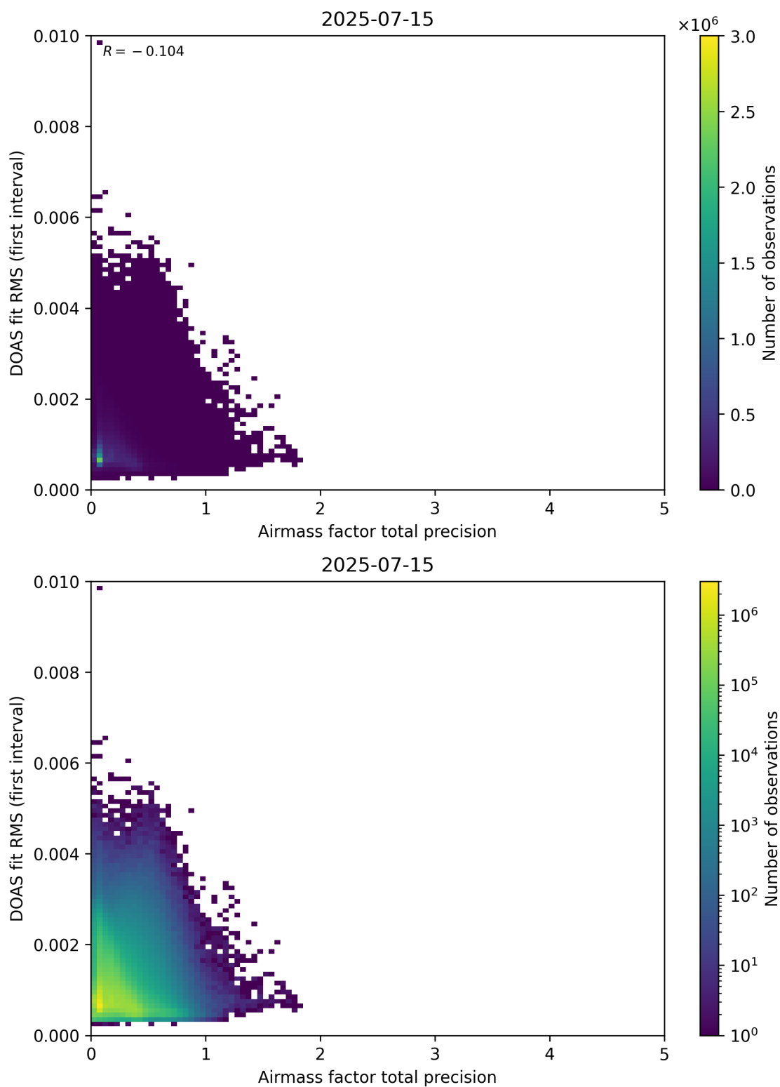
Figure 105: Scatter density plot of “Airmass factor total precision” against “DOAS fit RMS (first interval)” for 2025-07-14 to 2025-07-16.
