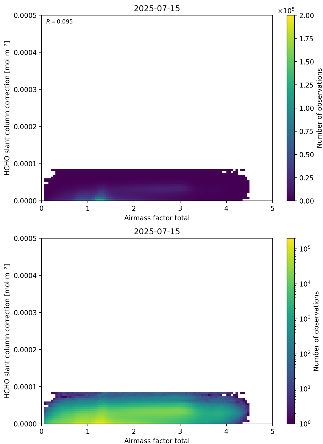
Figure 102: Scatter density plot of “Airmass factor total” against “HCHO slant column correction” for 2025-07-14 to 2025-07-16.
