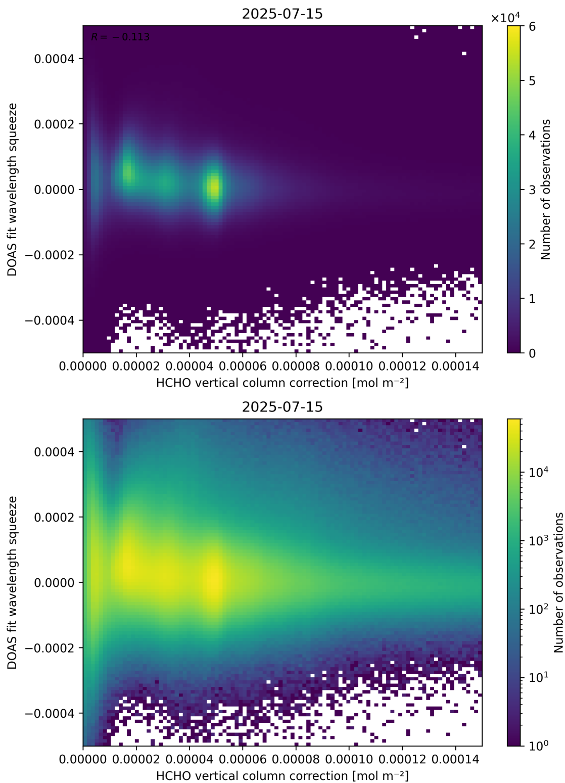
Figure 114: Scatter density plot of “HCHO vertical column correction” against “DOAS fit wavelength squeeze” for 2025-07-14 to 2025-07-16.
