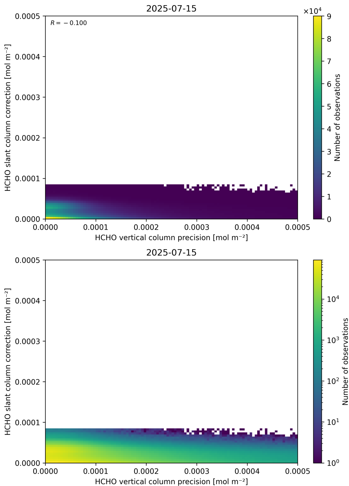
Figure 141: Scatter density plot of “HCHO vertical column precision” against “HCHO slant column correction” for 2025-07-14 to 2025-07-16.
