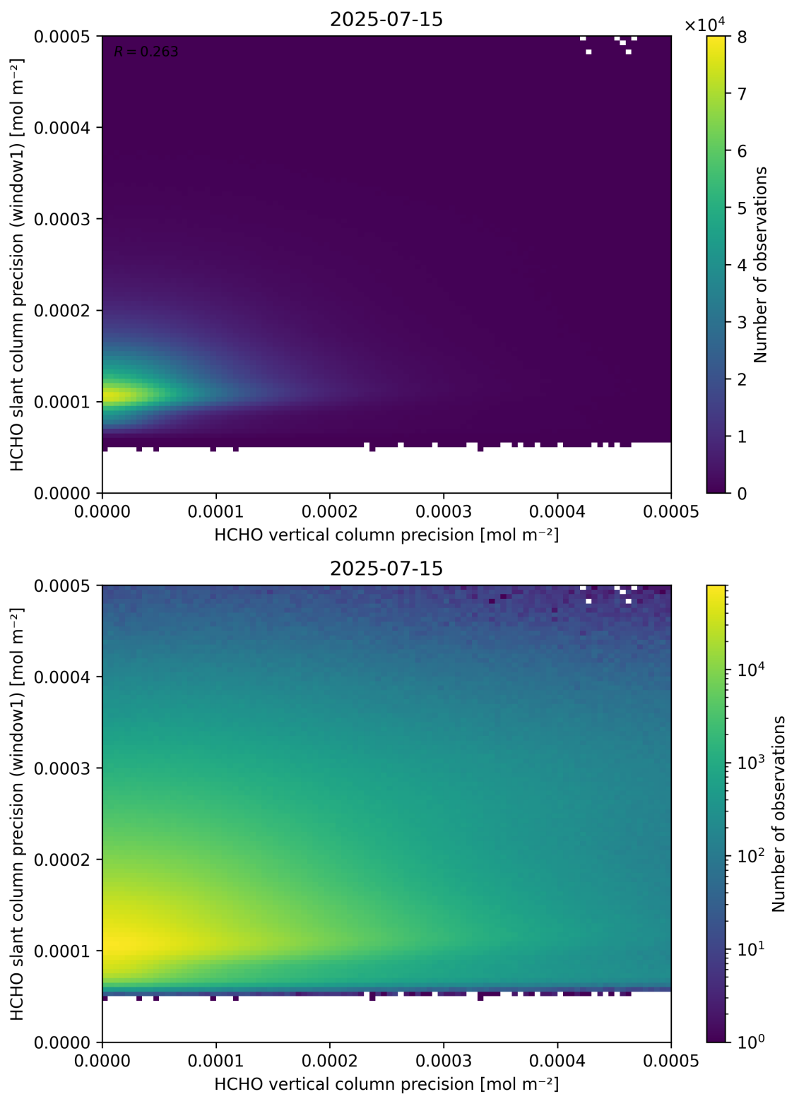
Figure 143: Scatter density plot of “HCHO vertical column precision” against “HCHO slant column precision (window1)” for 2025-07-14 to 2025-07-16.
