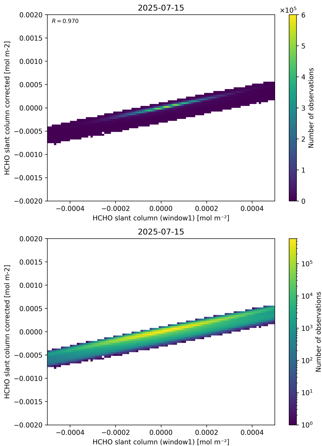
Figure 82: Scatter density plot of “HCHO slant column (window1)” against “HCHO slant column corrected” for 2025-07-14 to 2025-07-16.
