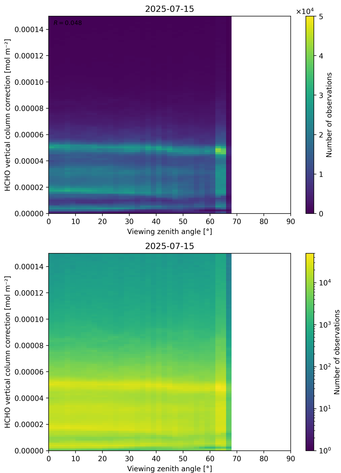
Figure 193: Scatter density plot of “Viewing zenith angle” against “HCHO vertical column correction” for 2025-07-14 to 2025-07-16.
