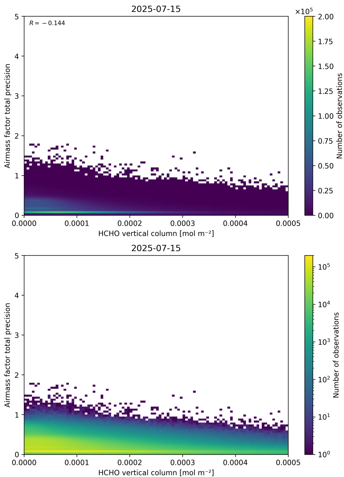
Figure 132: Scatter density plot of “HCHO vertical column” against “Airmass factor total precision” for 2025-07-14 to 2025-07-16.
