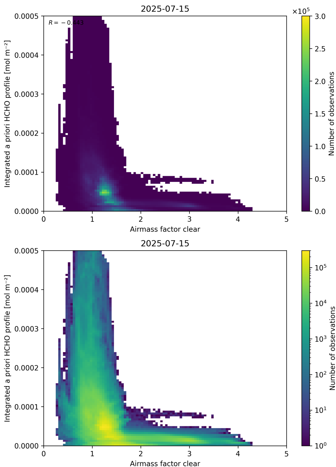
Figure 76: Scatter density plot of “Airmass factor clear” against “Integrated a priori HCHO profile” for 2025-07-14 to 2025-07-16.
