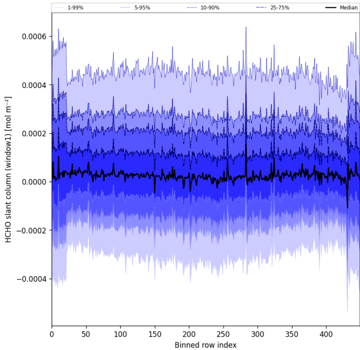
Figure 52: Along track statistics of “HCHO slant column (window1)” for 2025-07-14 to 2025-07-16
