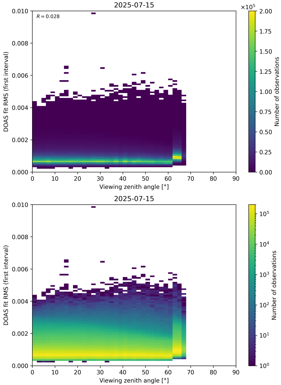
Figure 182: Scatter density plot of “Viewing zenith angle” against “DOAS fit RMS (first interval)” for 2025-07-14 to 2025-07-16.
