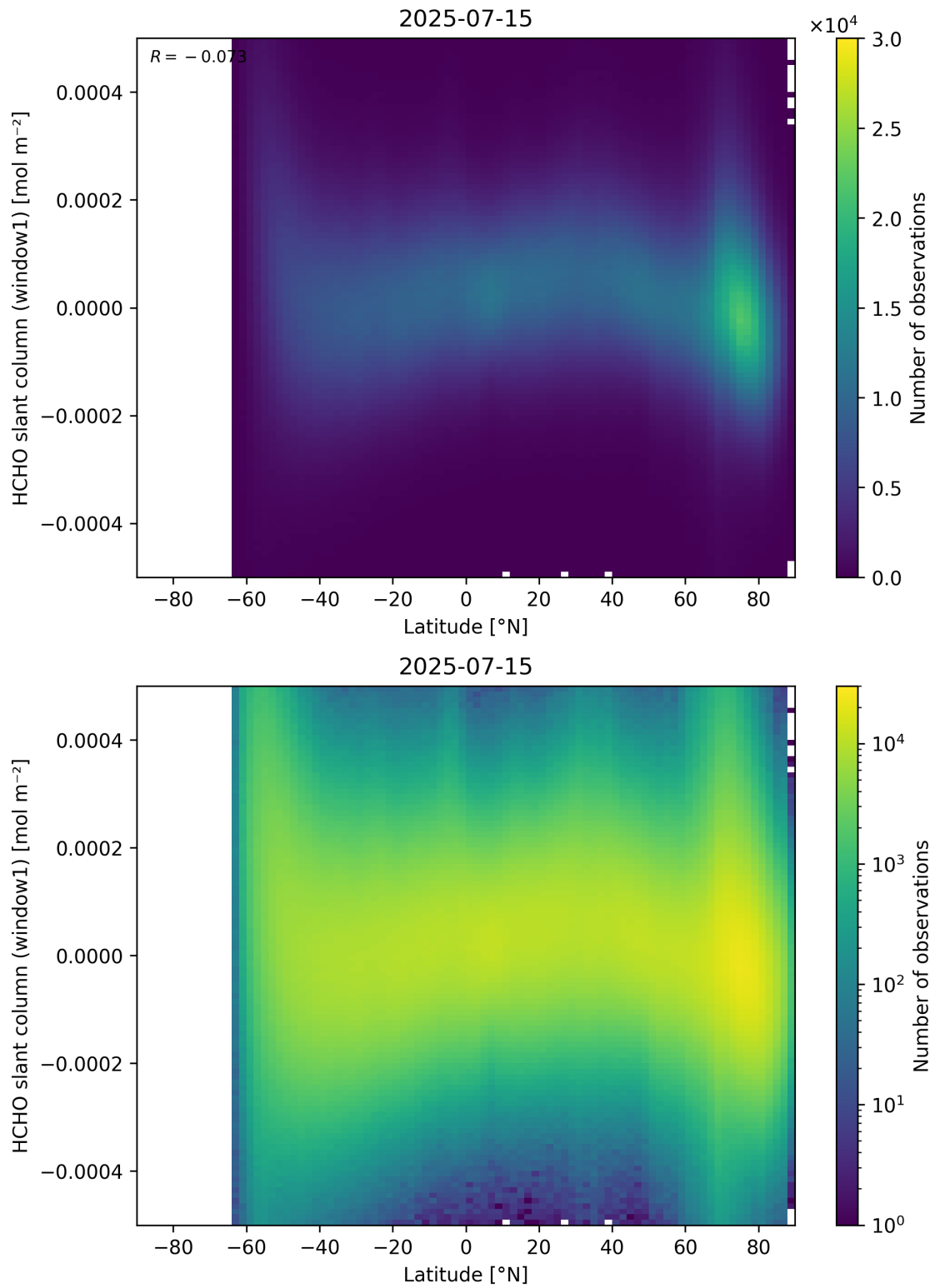
Figure 159: Scatter density plot of “Latitude” against “HCHO slant column (window1)” for 2025-07-14 to 2025-07-16.
