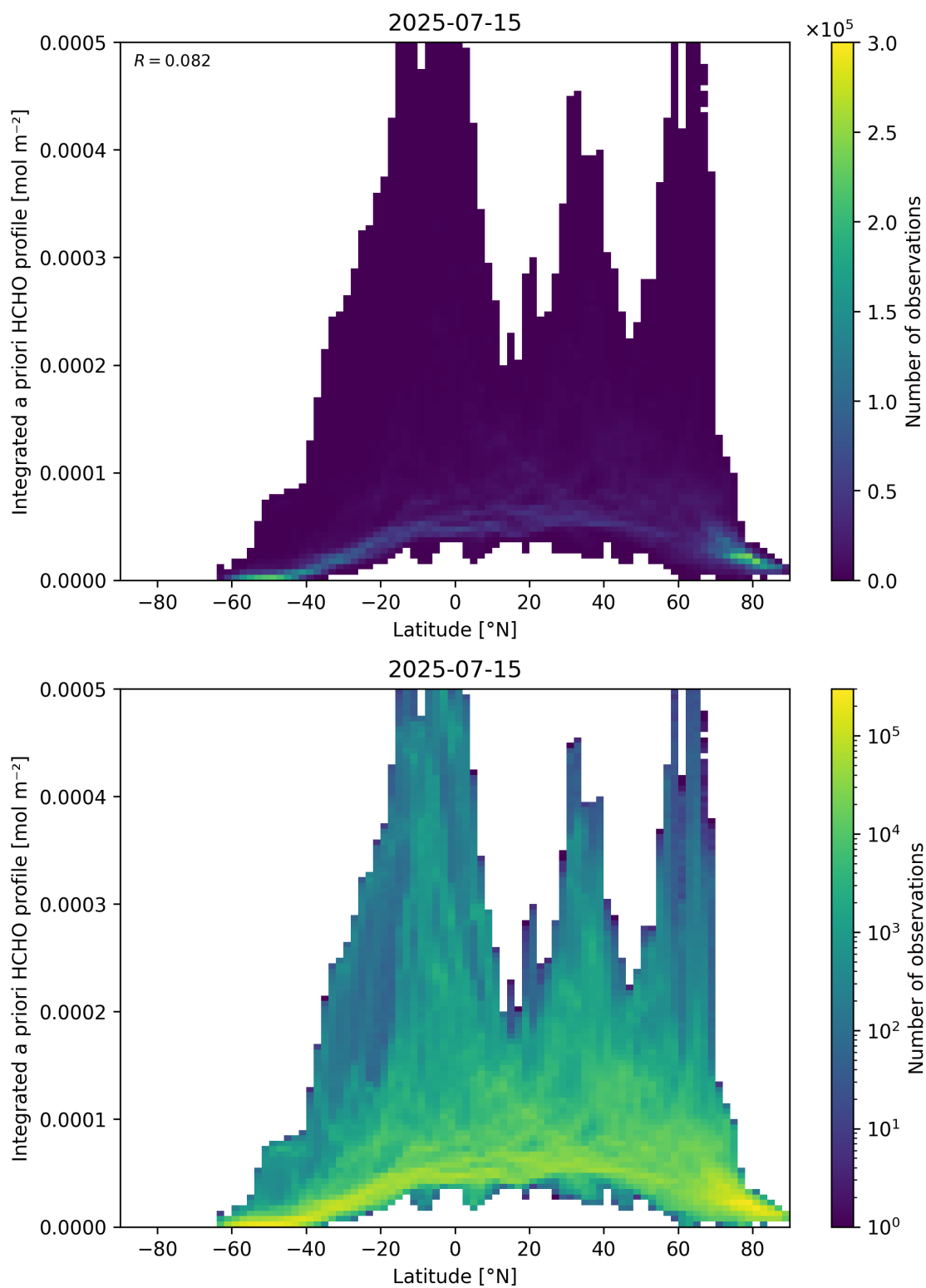
Figure 166: Scatter density plot of “Latitude” against “Integrated a priori HCHO profile” for 2025-07-14 to 2025-07-16.
