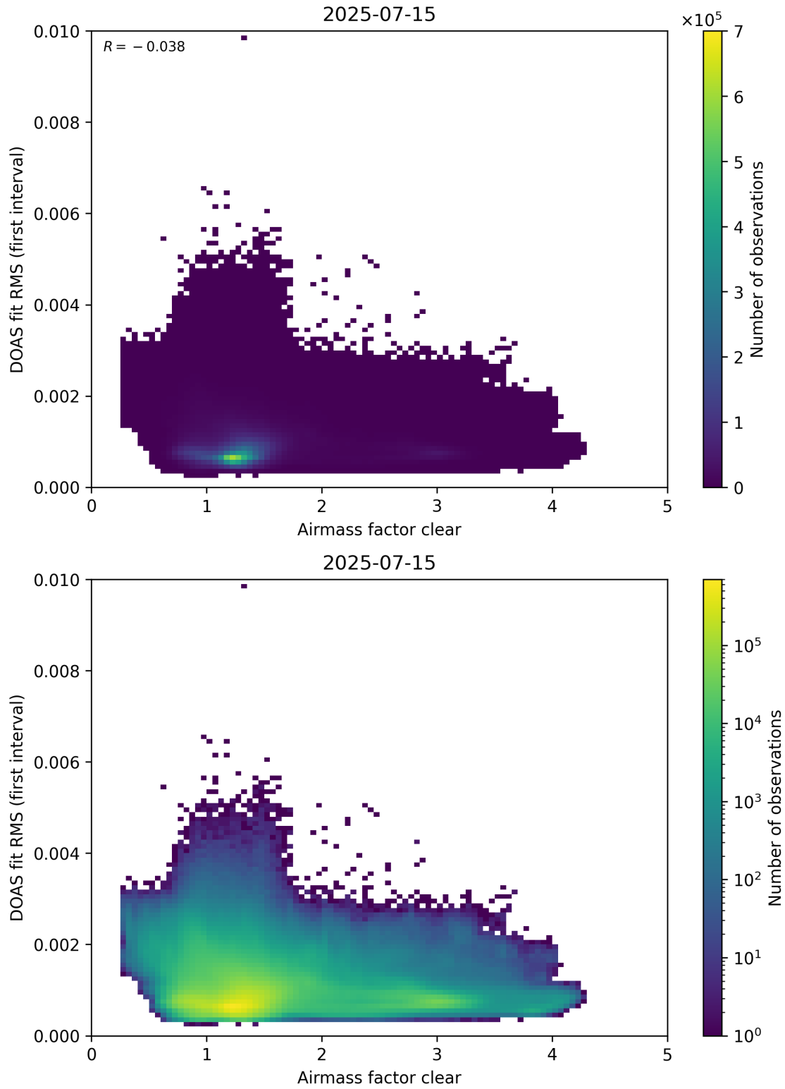
Figure 71: Scatter density plot of “Airmass factor clear” against “DOAS fit RMS (first interval)” for 2025-07-14 to 2025-07-16.
