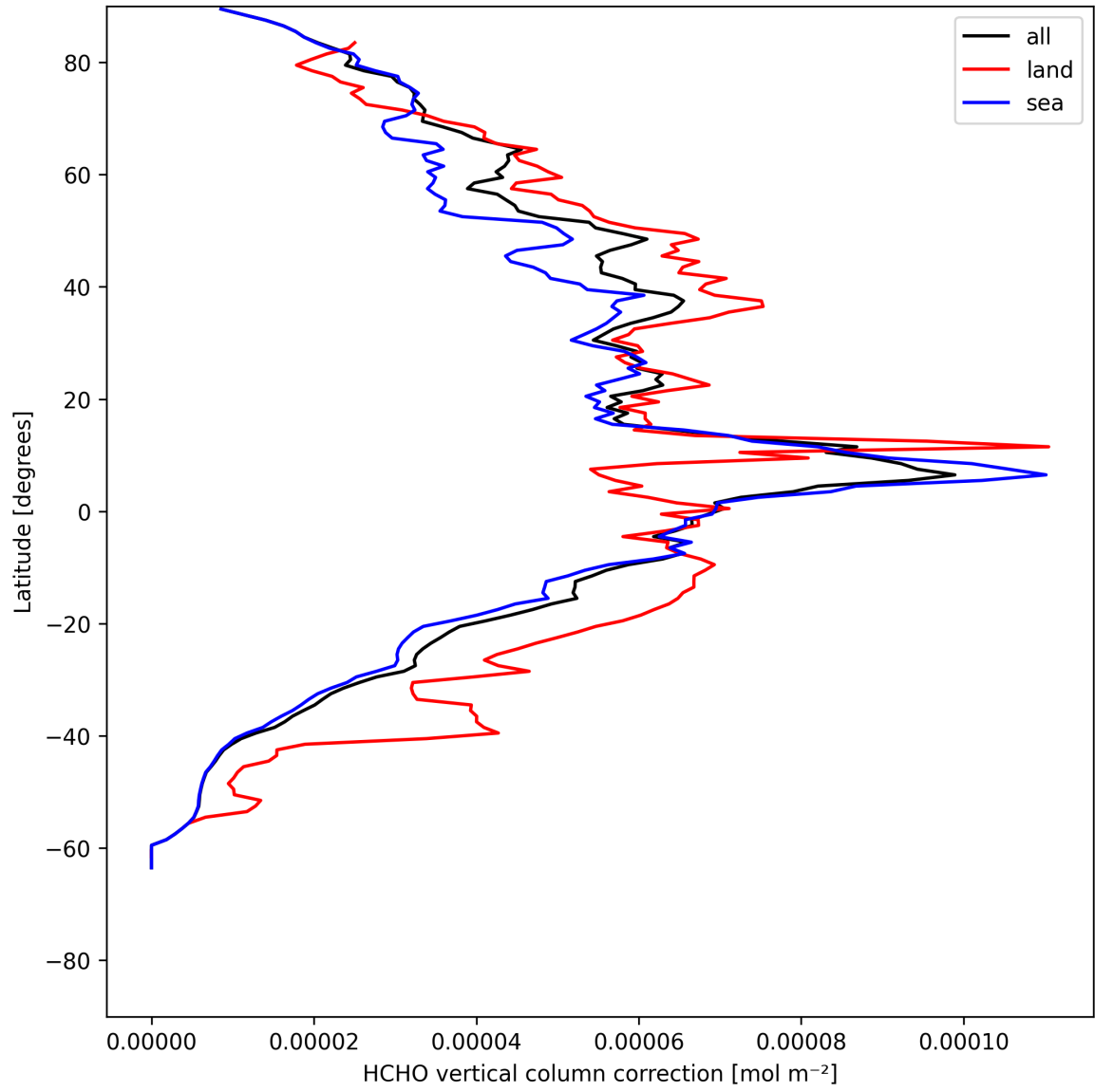
Figure 23: Zonal average of “HCHO vertical column correction” for 2025-07-14 to 2025-07-16.
