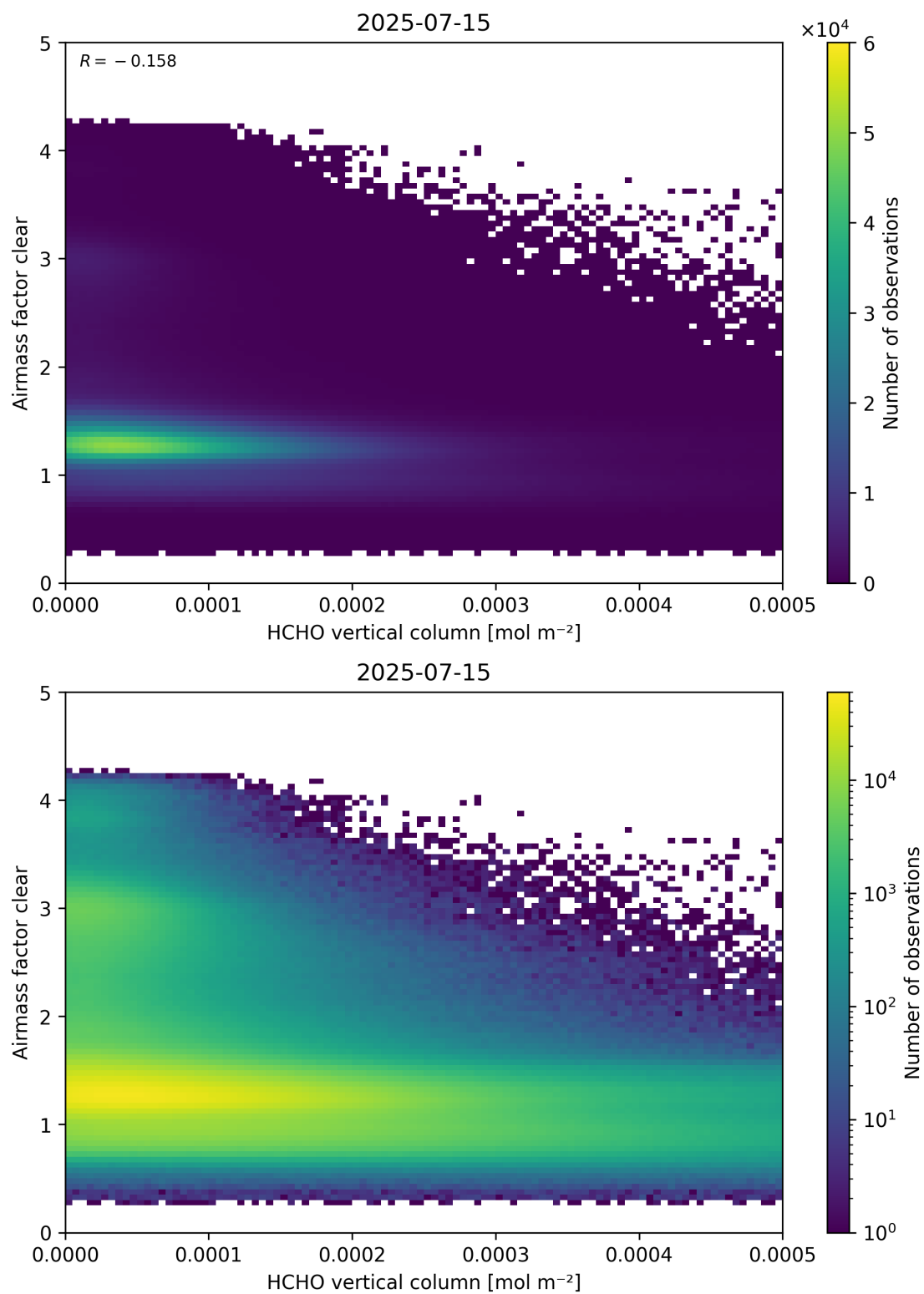
Figure 126: Scatter density plot of “HCHO vertical column” against “Airmass factor clear” for 2025-07-14 to 2025-07-16.
