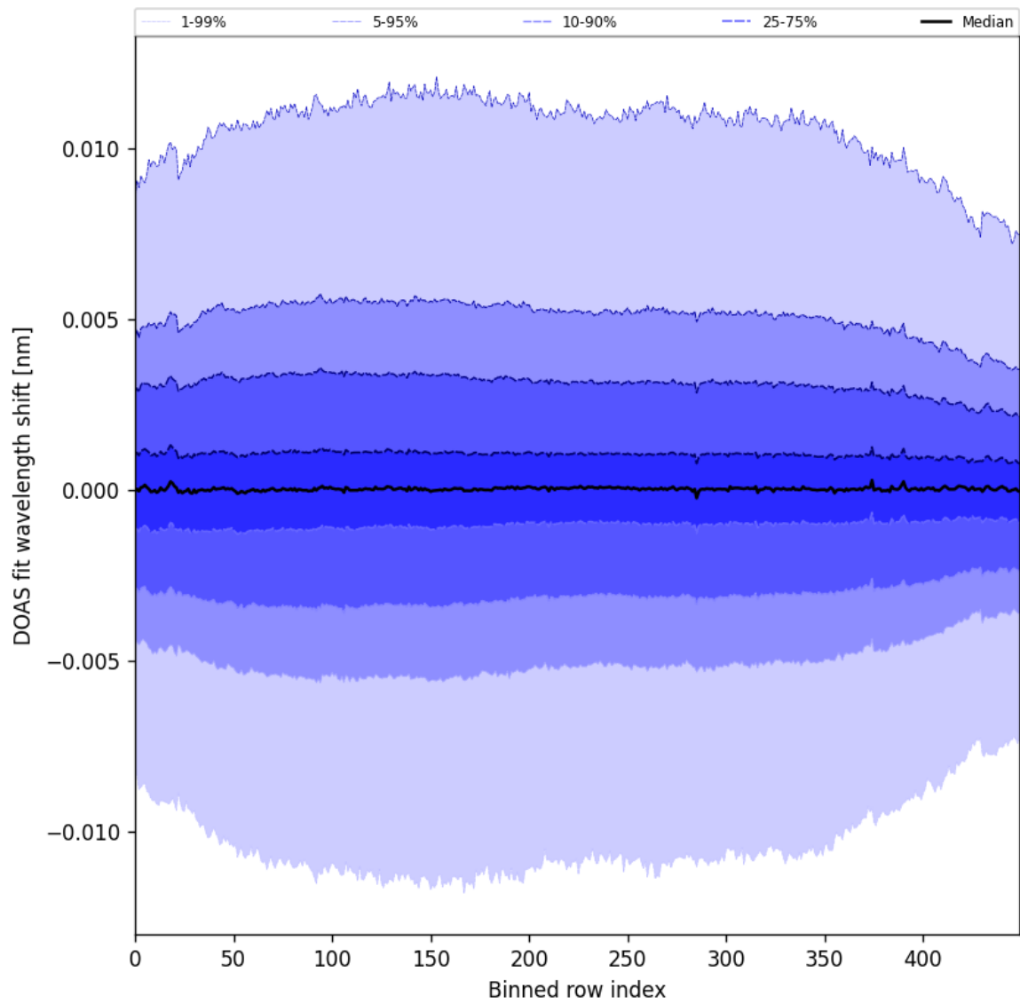
Figure 58: Along track statistics of “DOAS fit wavelength shift” for 2025-07-14 to 2025-07-16
