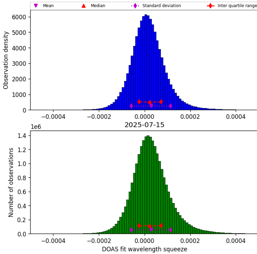
Figure 45: Histogram of “DOAS fit wavelength squeeze” for 2025-07-14 to 2025-07-16
