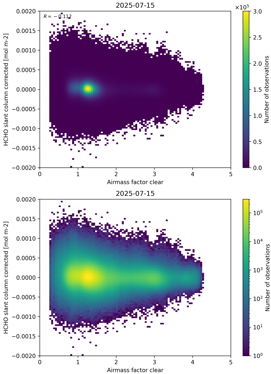
Figure 74: Scatter density plot of “Airmass factor clear” against “HCHO slant column corrected” for 2025-07-14 to 2025-07-16.
