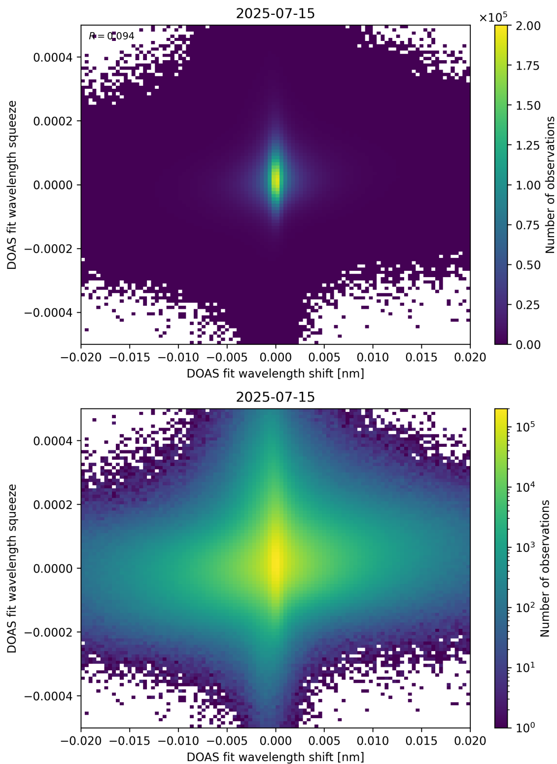
Figure 65: Scatter density plot of “DOAS fit wavelength shift” against “DOAS fit wavelength squeeze” for 2025-07-14 to 2025-07-16.
