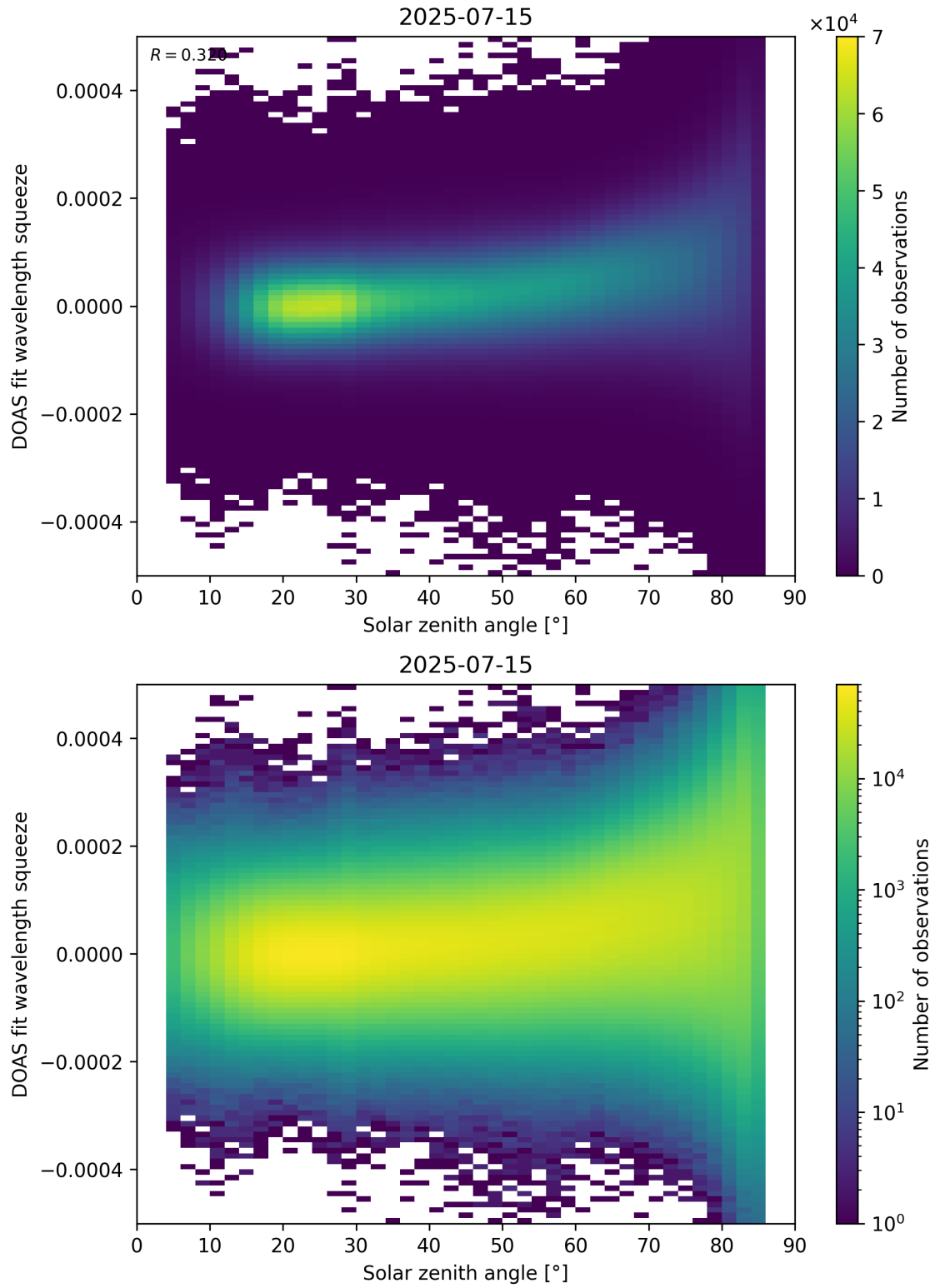
Figure 169: Scatter density plot of “Solar zenith angle” against “DOAS fit wavelength squeeze” for 2025-07-14 to 2025-07-16.
