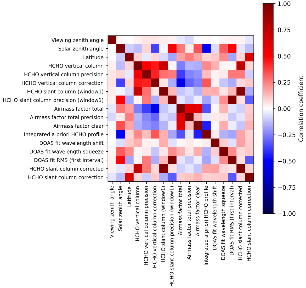
Figure 2: Map of correlation matrix for 2025-07-14 to 2025-07-16.
