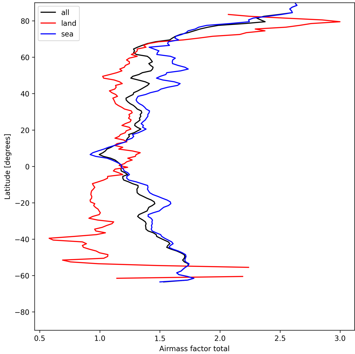
Figure 26: Zonal average of “Airmass factor total” for 2025-07-14 to 2025-07-16.
