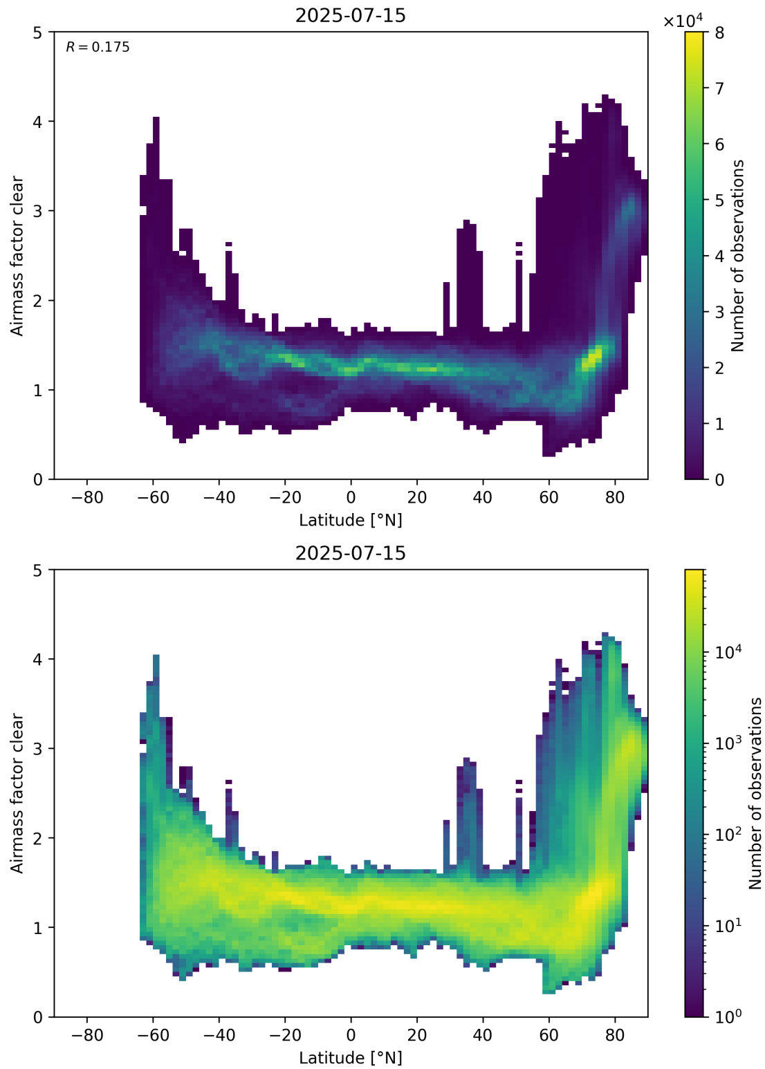
Figure 156: Scatter density plot of “Latitude” against “Airmass factor clear” for 2025-07-14 to 2025-07-16.
