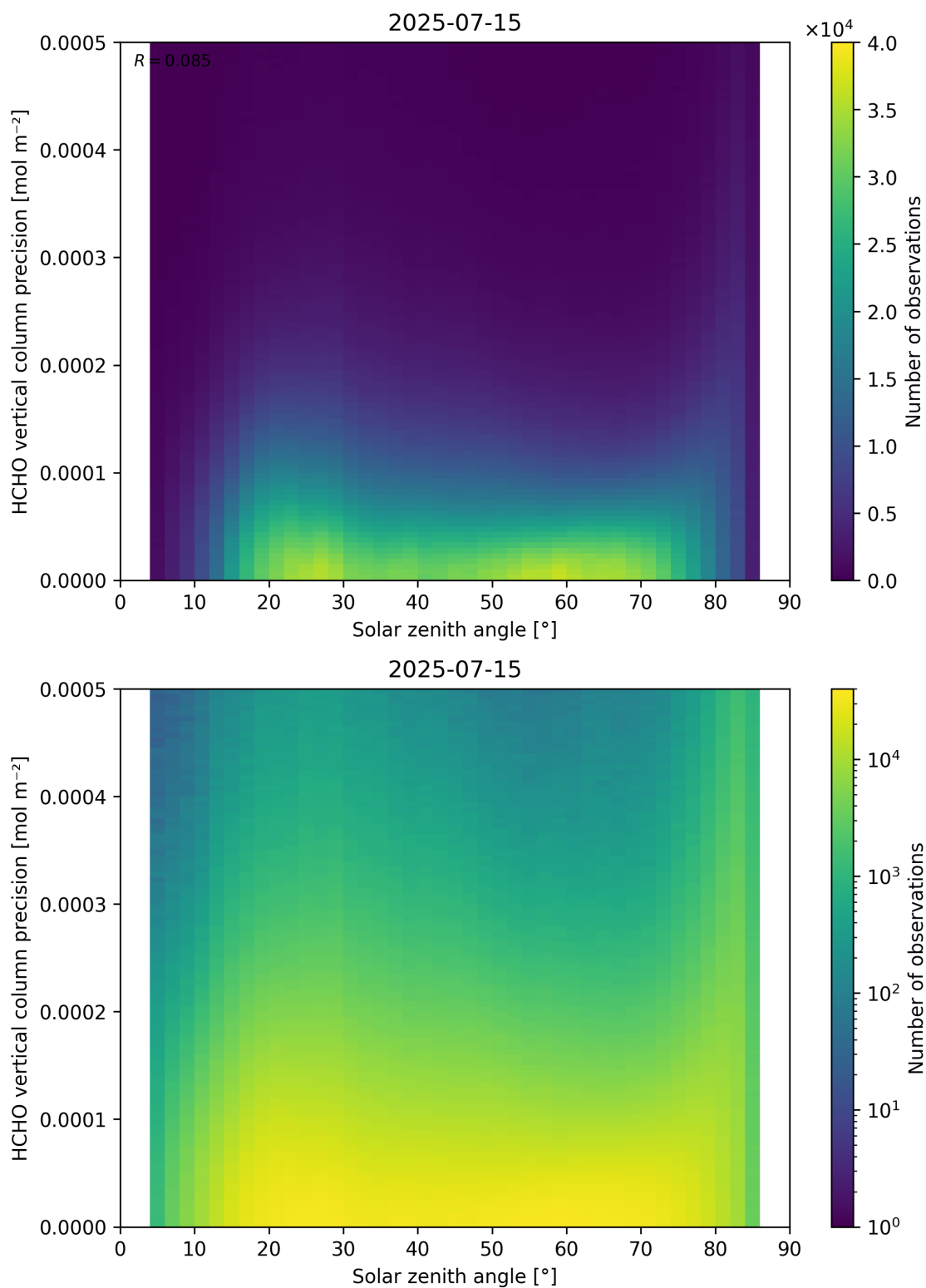
Figure 179: Scatter density plot of “Solar zenith angle” against “HCHO vertical column precision” for 2025-07-14 to 2025-07-16.
