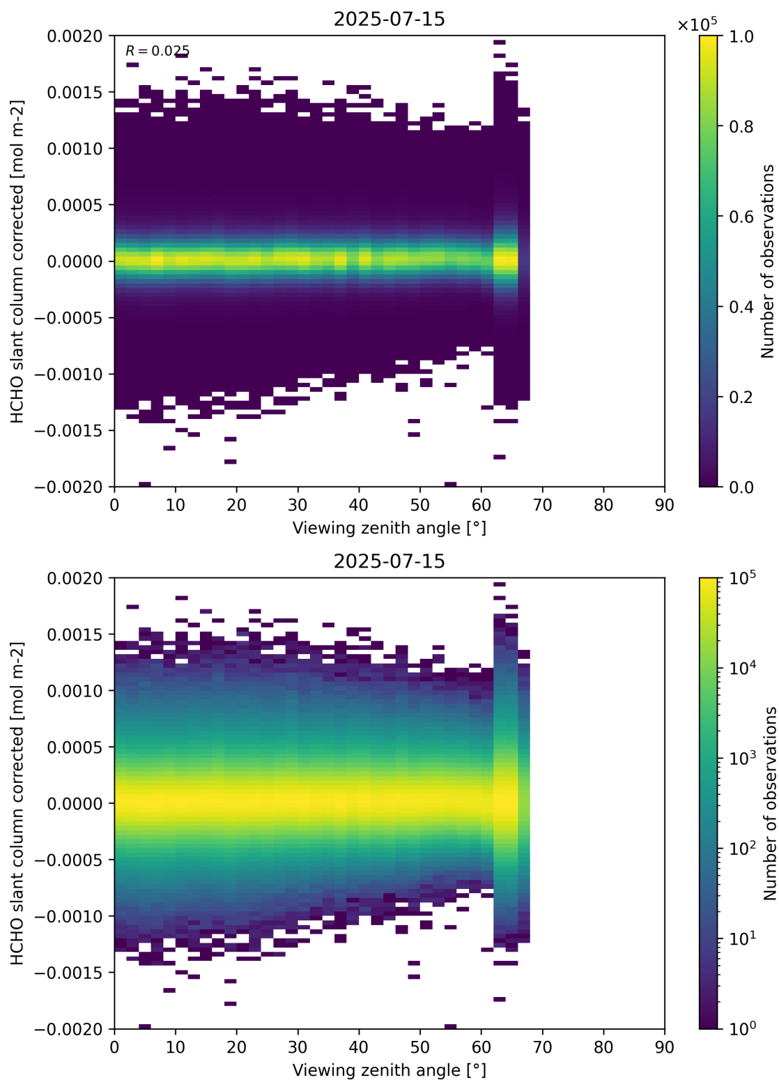
Figure 186: Scatter density plot of “Viewing zenith angle” against “HCHO slant column corrected” for 2025-07-14 to 2025-07-16.
