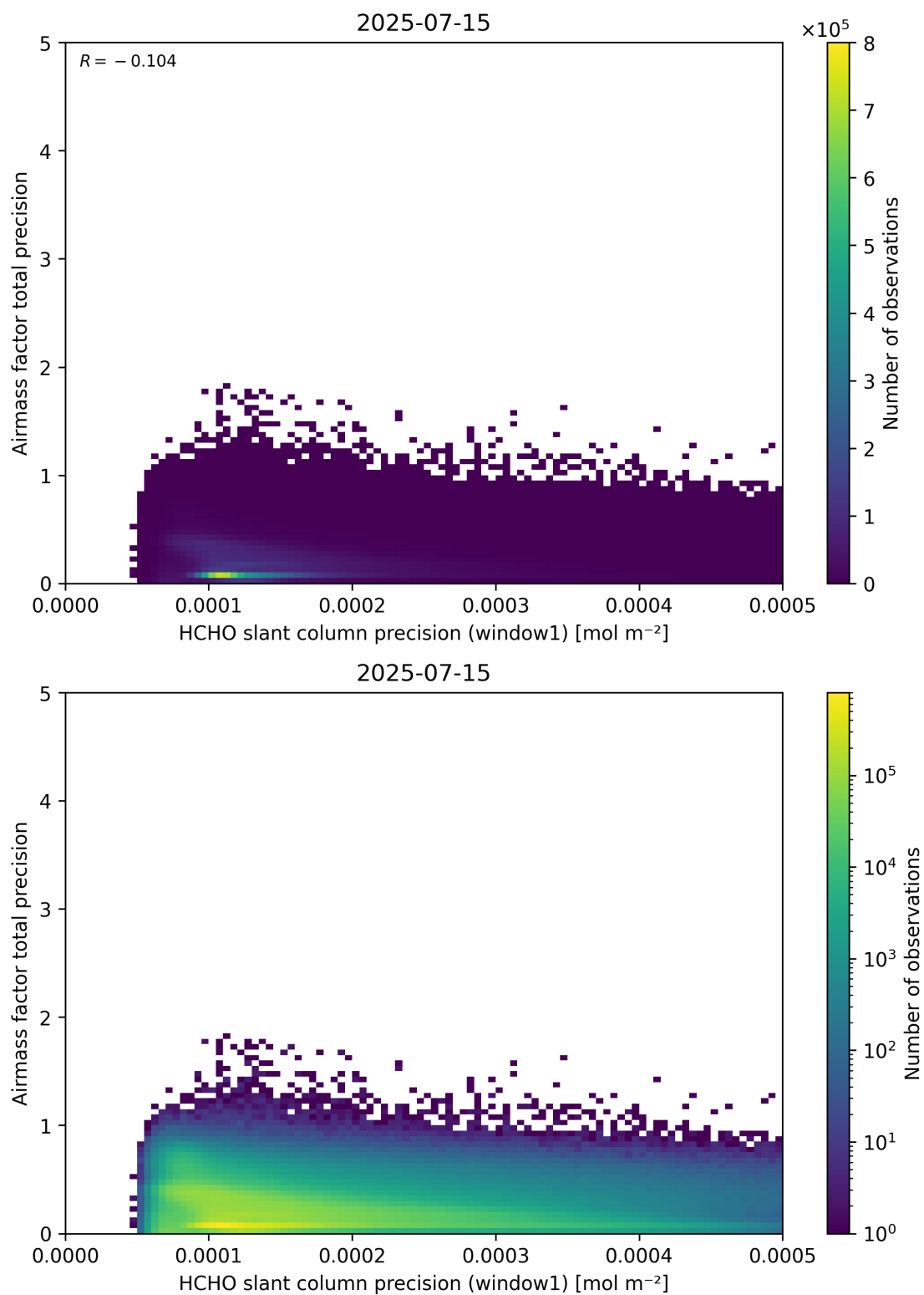
Figure 95: Scatter density plot of “HCHO slant column precision (window1)” against “Airmass factor total precision” for 2025-07-14 to 2025-07-16.
