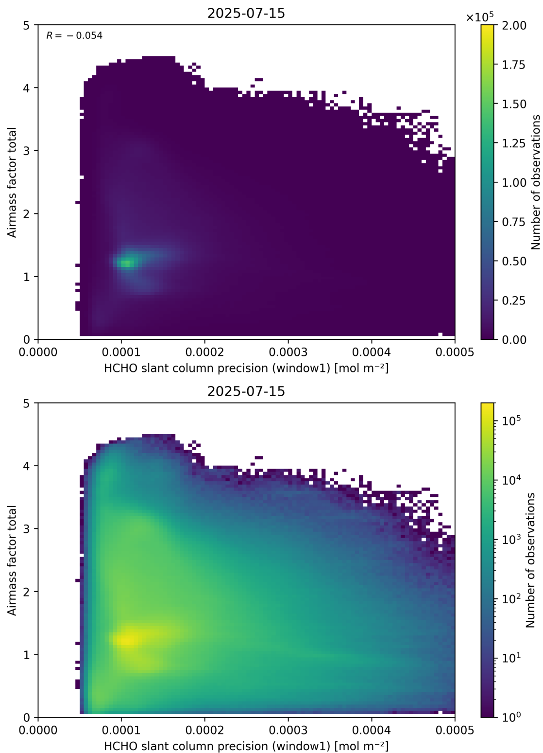
Figure 94: Scatter density plot of “HCHO slant column precision (window1)” against “Airmass factor total” for 2025-07-14 to 2025-07-16.
