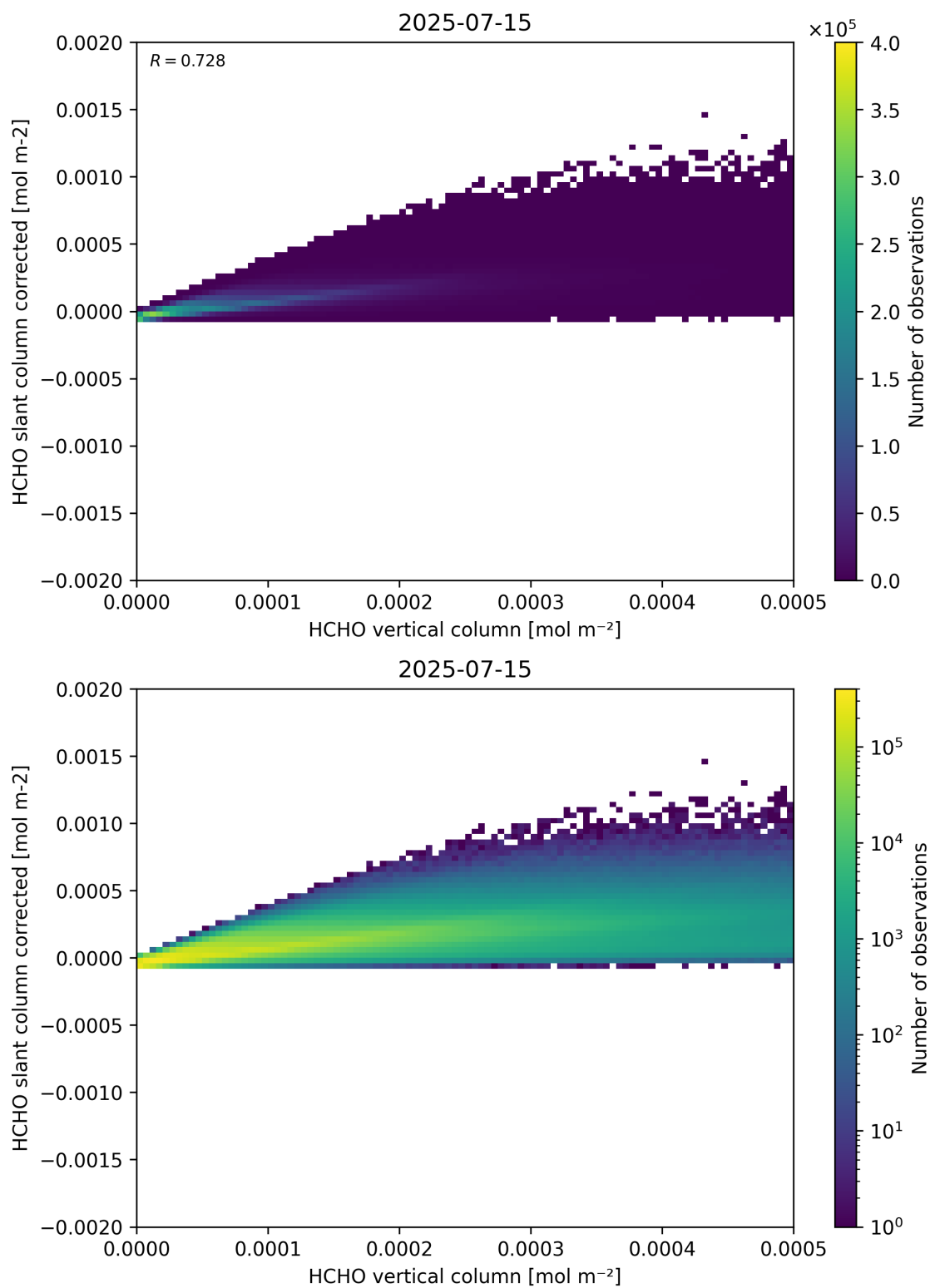
Figure 127: Scatter density plot of “HCHO vertical column” against “HCHO slant column corrected” for 2025-07-14 to 2025-07-16.
