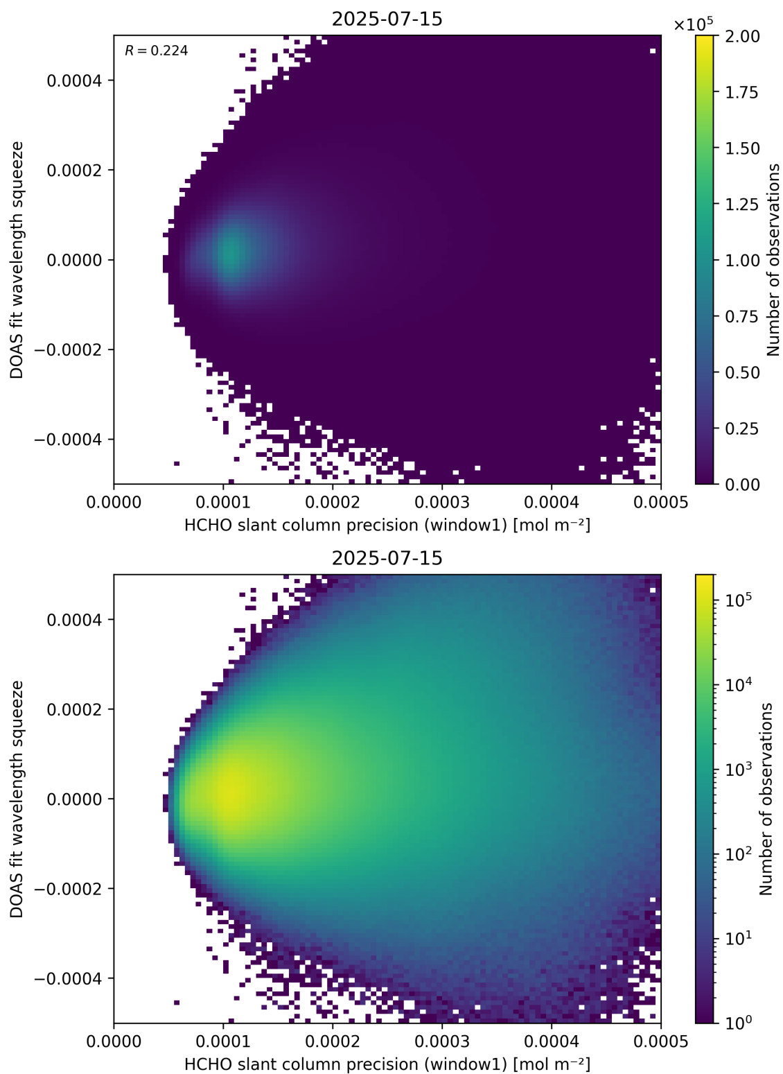
Figure 90: Scatter density plot of “HCHO slant column precision (window1)” against “DOAS fit wavelength squeeze” for 2025-07-14 to 2025-07-16.
