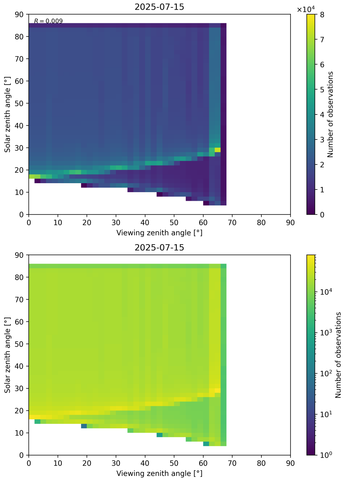
Figure 197: Scatter density plot of “Viewing zenith angle” against “Solar zenith angle” for 2025-07-14 to 2025-07-16.
