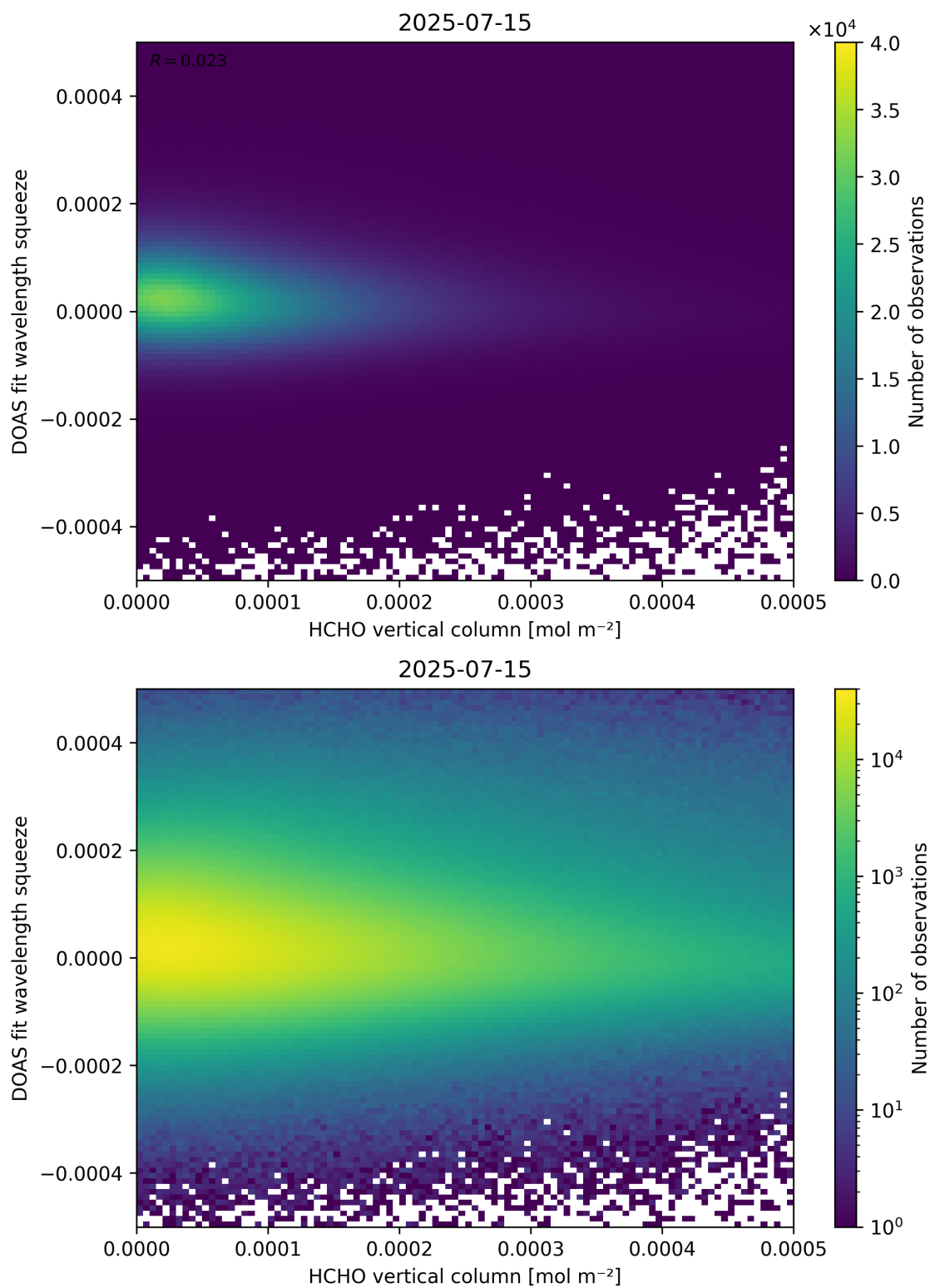
Figure 125: Scatter density plot of “HCHO vertical column” against “DOAS fit wavelength squeeze” for 2025-07-14 to 2025-07-16.
