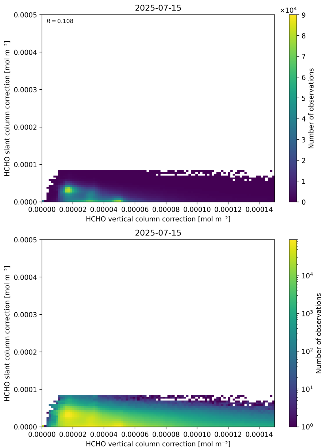
Figure 117: Scatter density plot of “HCHO vertical column correction” against “HCHO slant column correction” for 2025-07-14 to 2025-07-16.
