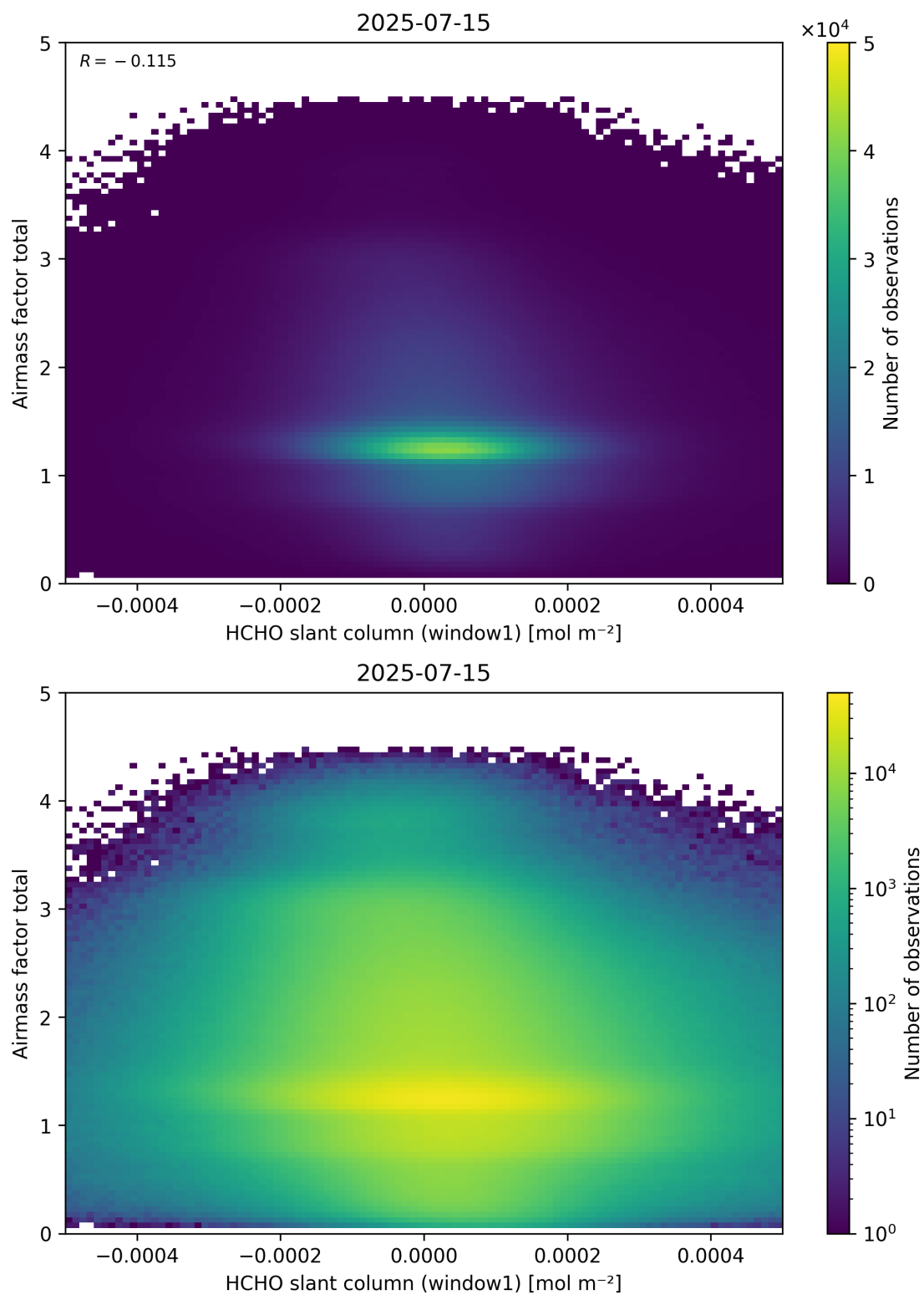
Figure 85: Scatter density plot of “HCHO slant column (window1)” against “Airmass factor total” for 2025-07-14 to 2025-07-16.
