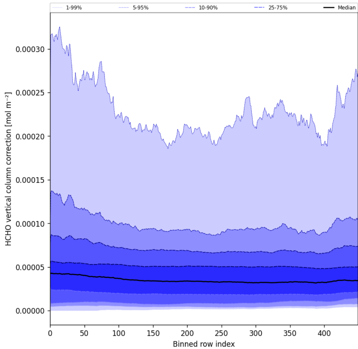
Figure 51: Along track statistics of “HCHO vertical column correction” for 2025-07-14 to 2025-07-16
