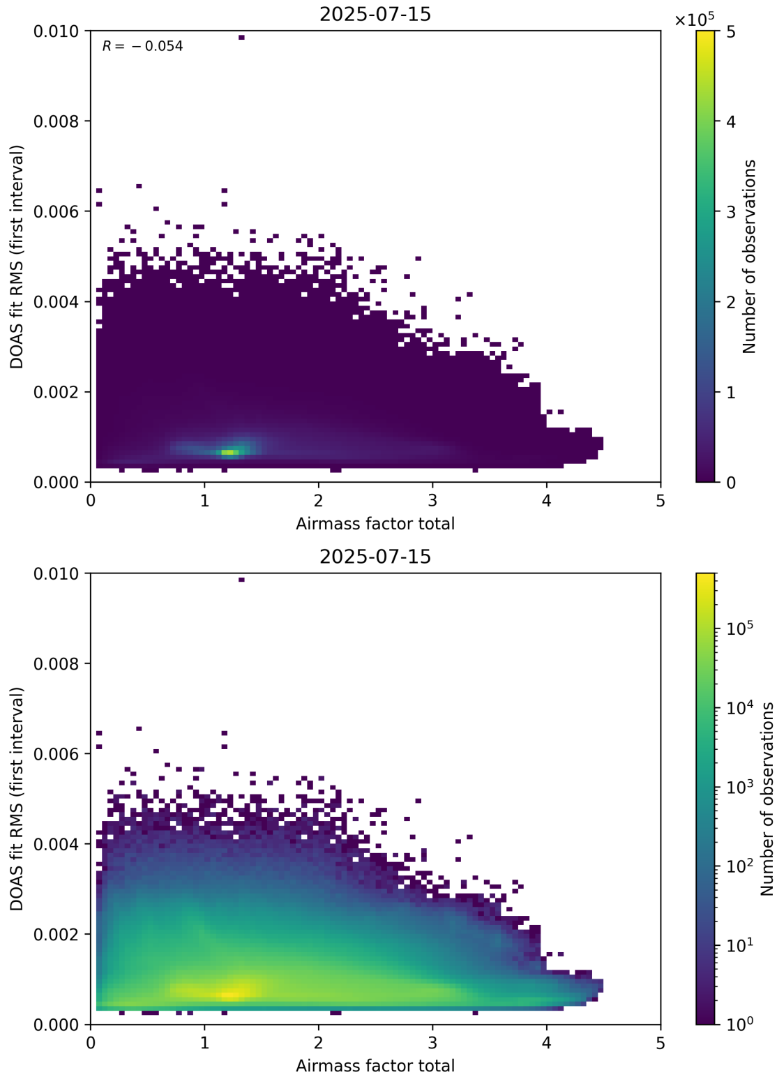
Figure 97: Scatter density plot of “Airmass factor total” against “DOAS fit RMS (first interval)” for 2025-07-14 to 2025-07-16.
