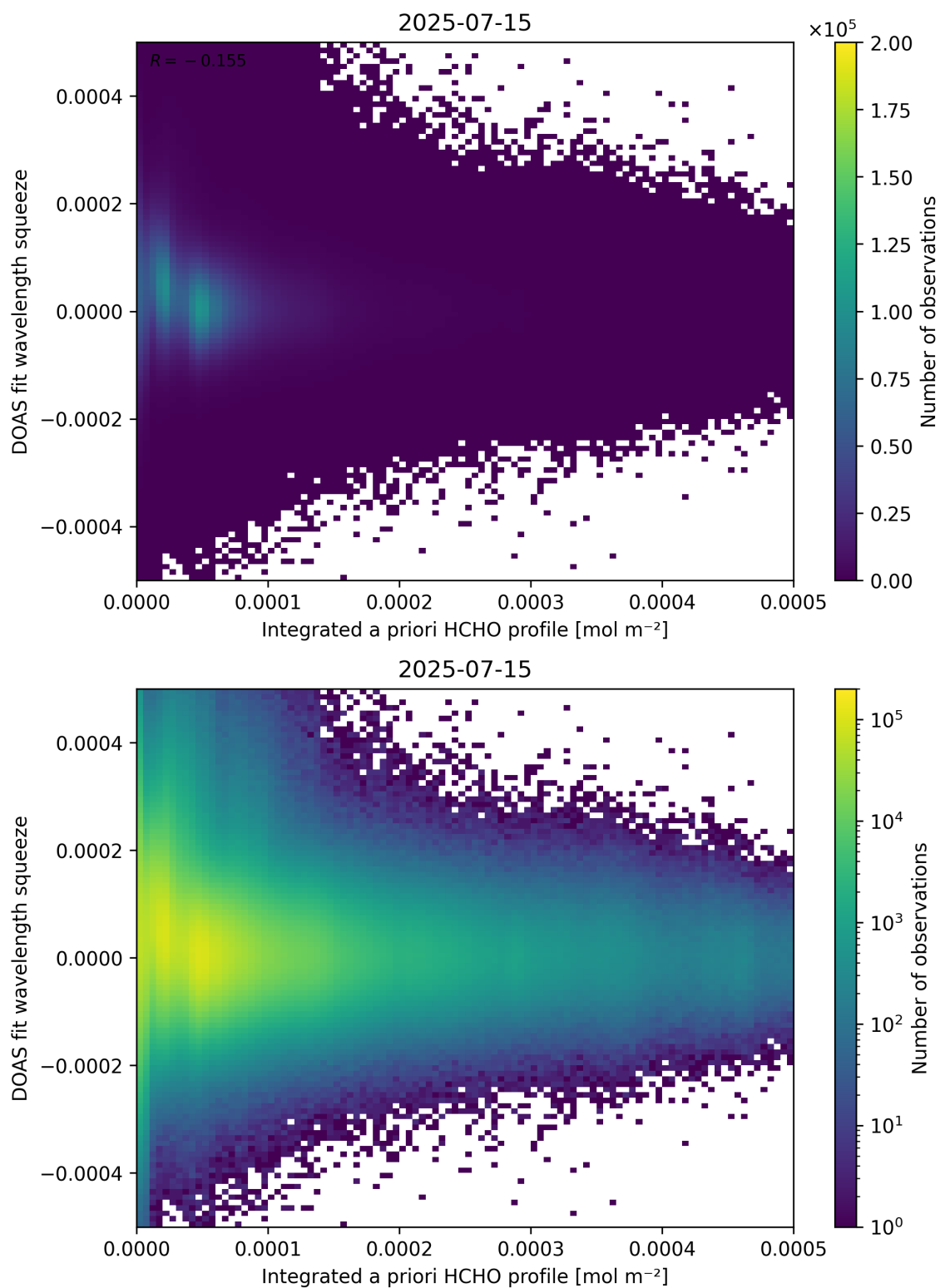
Figure 150: Scatter density plot of “Integrated a priori HCHO profile” against “DOAS fit wavelength squeeze” for 2025-07-14 to 2025-07-16.
