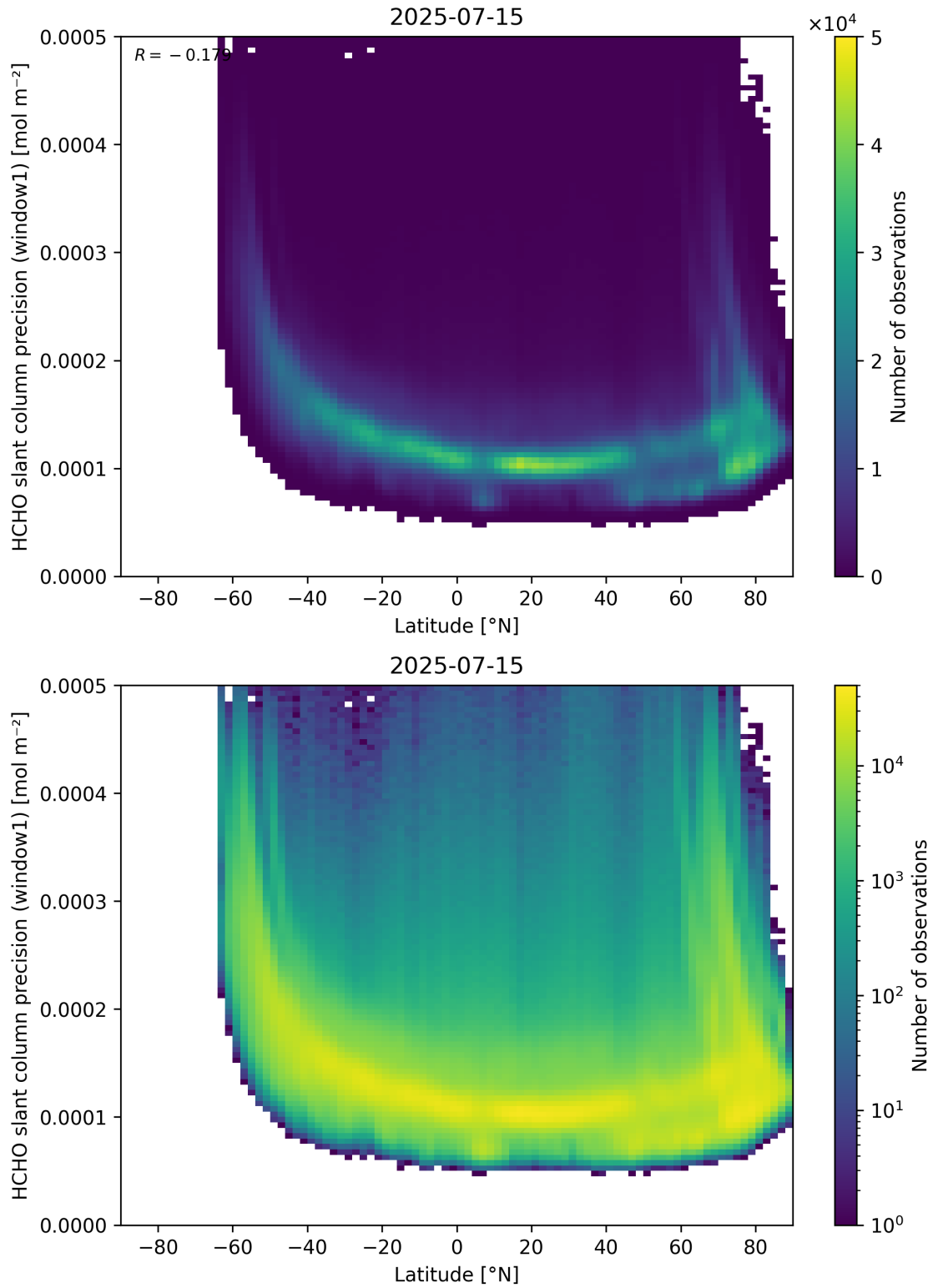
Figure 160: Scatter density plot of “Latitude” against “HCHO slant column precision (window1)” for 2025-07-14 to 2025-07-16.
