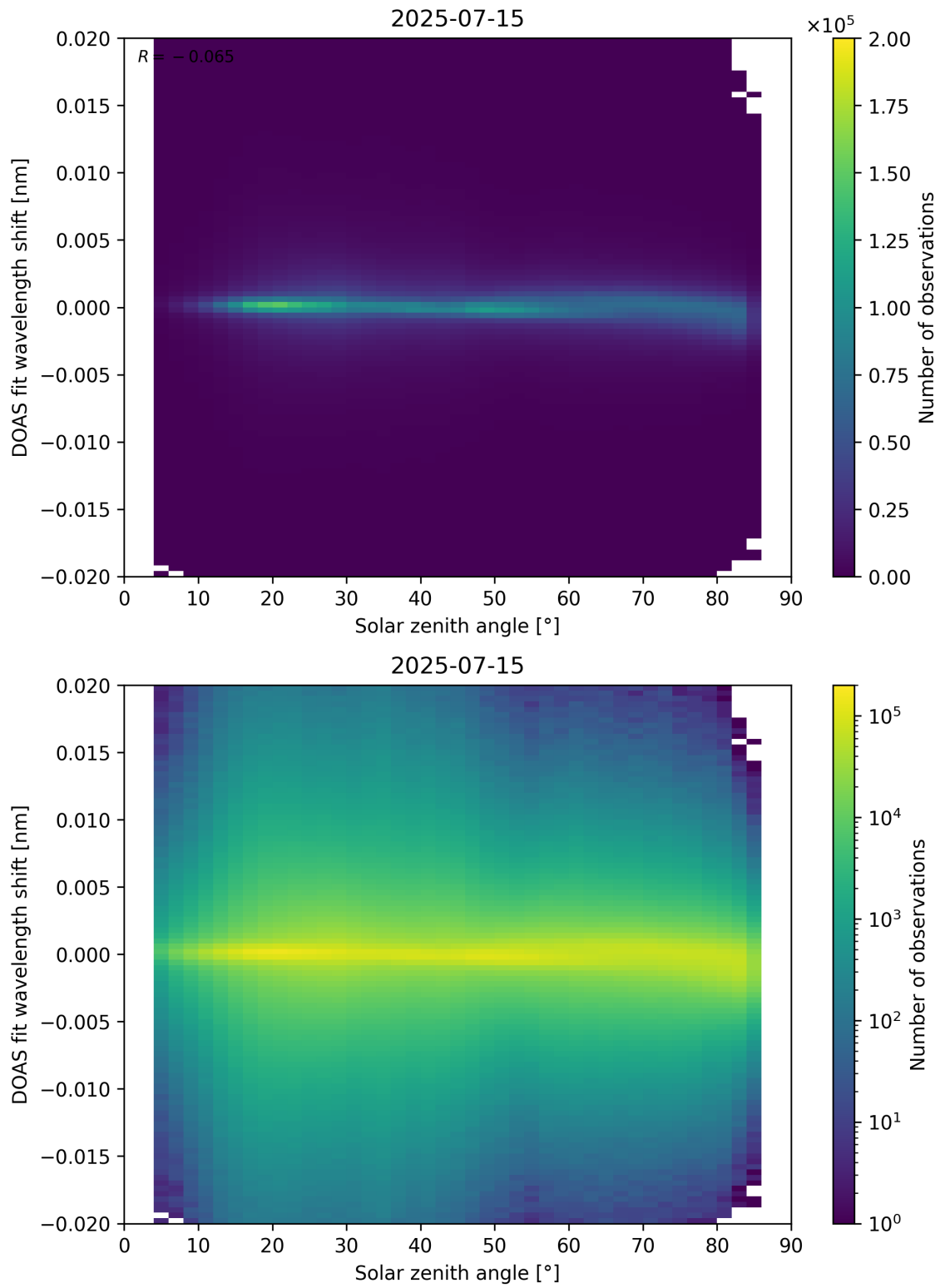
Figure 168: Scatter density plot of “Solar zenith angle” against “DOAS fit wavelength shift” for 2025-07-14 to 2025-07-16.
