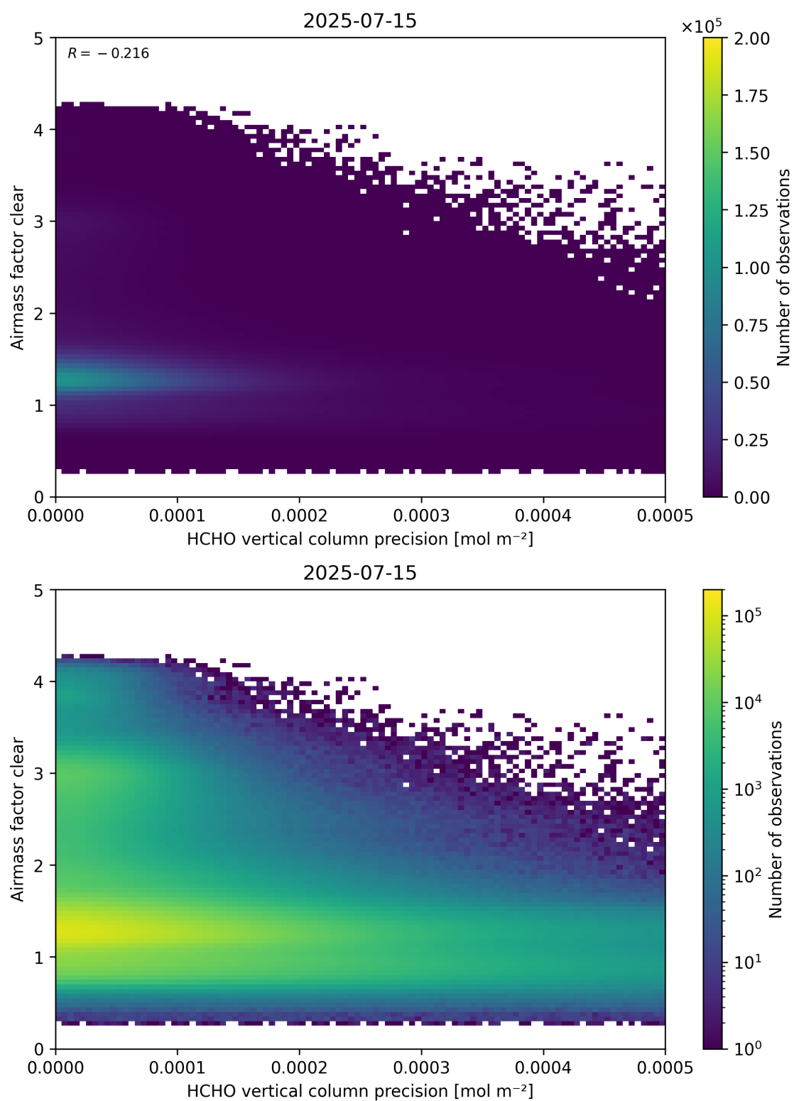
Figure 139: Scatter density plot of “HCHO vertical column precision” against “Airmass factor clear” for 2025-07-14 to 2025-07-16.
