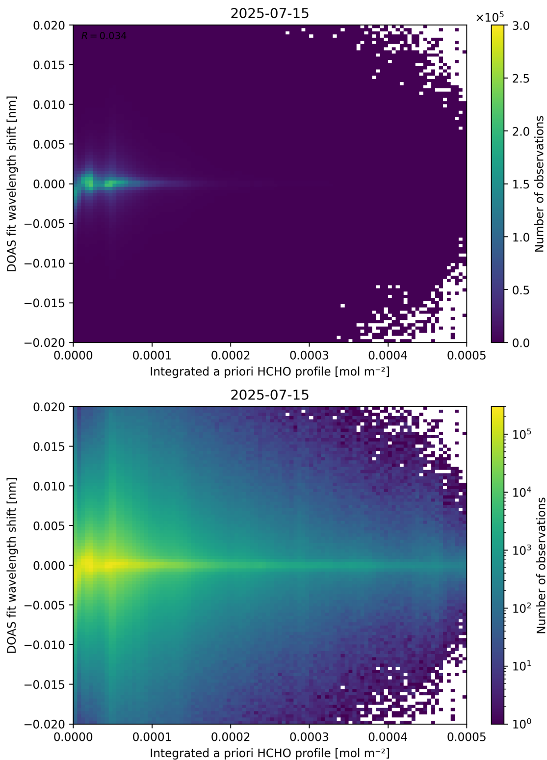
Figure 149: Scatter density plot of “Integrated a priori HCHO profile” against “DOAS fit wavelength shift” for 2025-07-14 to 2025-07-16.
