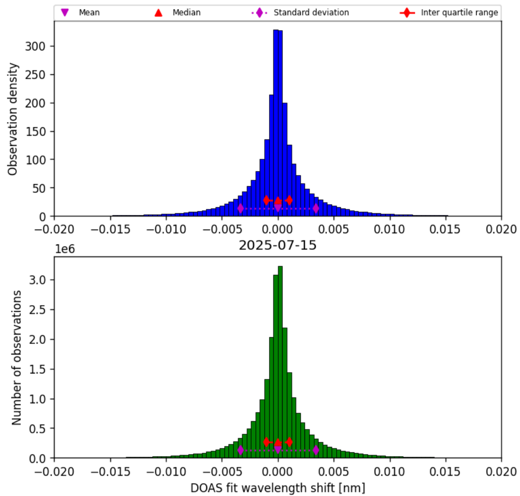
Figure 44: Histogram of “DOAS fit wavelength shift” for 2025-07-14 to 2025-07-16
