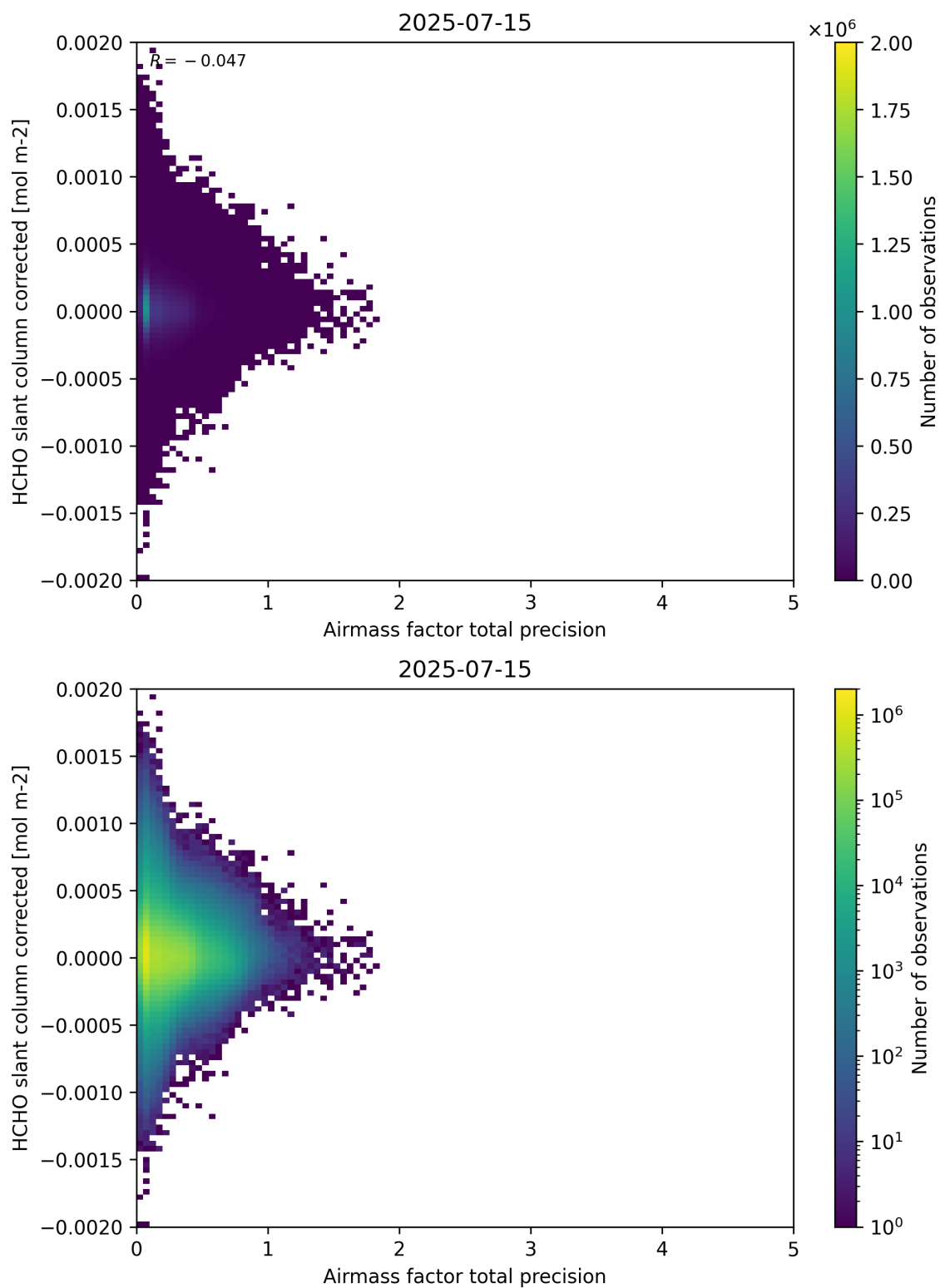
Figure 109: Scatter density plot of “Airmass factor total precision” against “HCHO slant column corrected” for 2025-07-14 to 2025-07-16.
