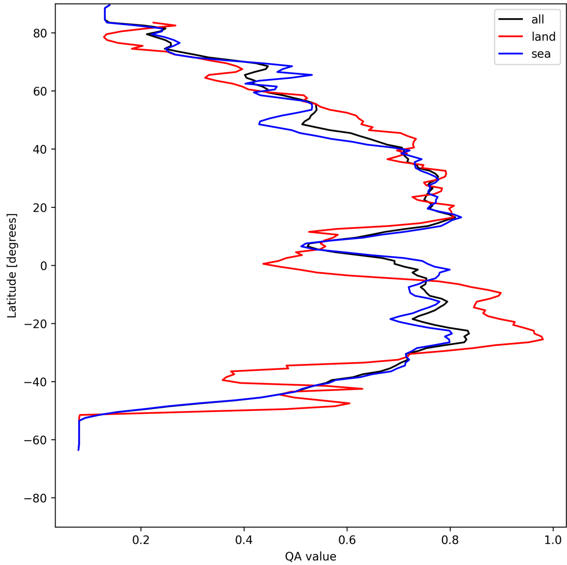
Figure 20: Zonal average of “QA value” for 2025-07-14 to 2025-07-16.
