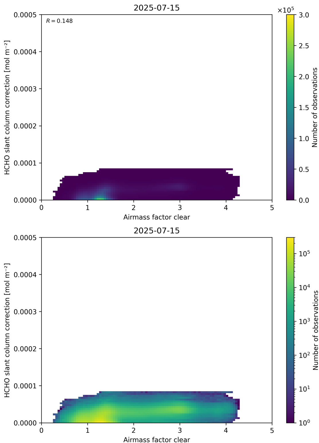
Figure 75: Scatter density plot of “Airmass factor clear” against “HCHO slant column correction” for 2025-07-14 to 2025-07-16.
