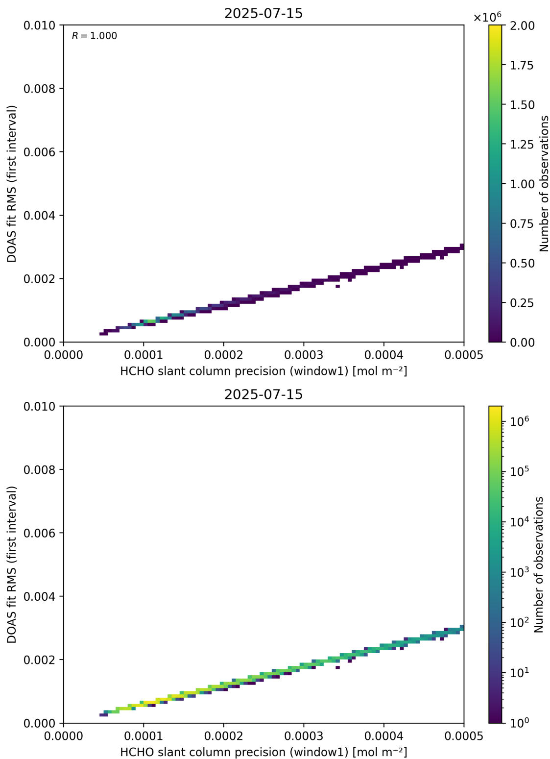
Figure 88: Scatter density plot of “HCHO slant column precision (window1)” against “DOAS fit RMS (first interval)” for 2025-07-14 to 2025-07-16.
