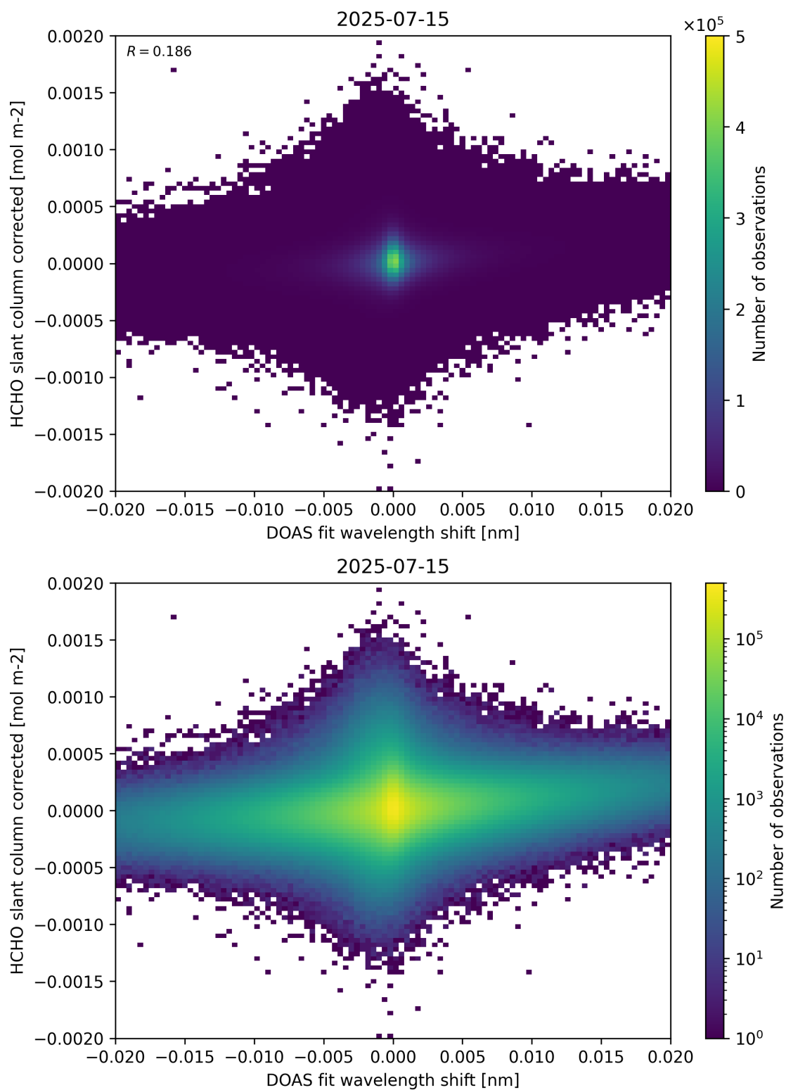
Figure 66: Scatter density plot of “DOAS fit wavelength shift” against “HCHO slant column corrected” for 2025-07-14 to 2025-07-16.
