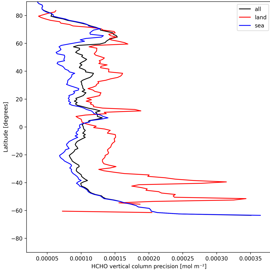
Figure 22: Zonal average of “HCHO vertical column precision” for 2025-07-14 to 2025-07-16.
