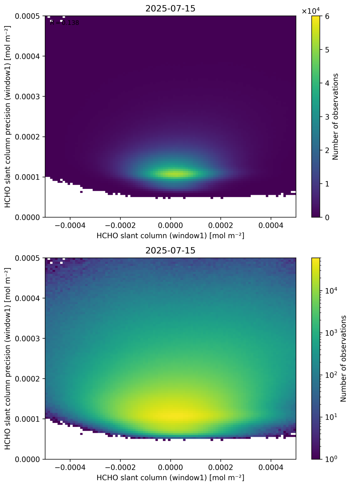
Figure 84: Scatter density plot of “HCHO slant column (window1)” against “HCHO slant column precision (window1)” for 2025-07-14 to 2025-07-16.
