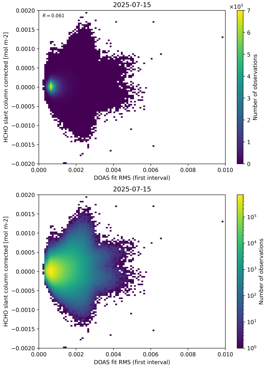
Figure 62: Scatter density plot of “DOAS fit RMS (first interval)” against “HCHO slant column corrected” for 2025-07-14 to 2025-07-16.
