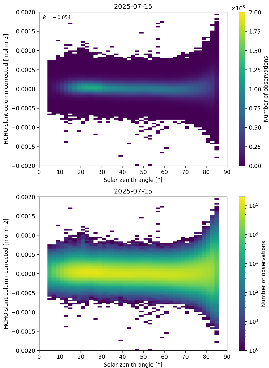
Figure 171: Scatter density plot of “Solar zenith angle” against “HCHO slant column corrected” for 2025-07-14 to 2025-07-16.
