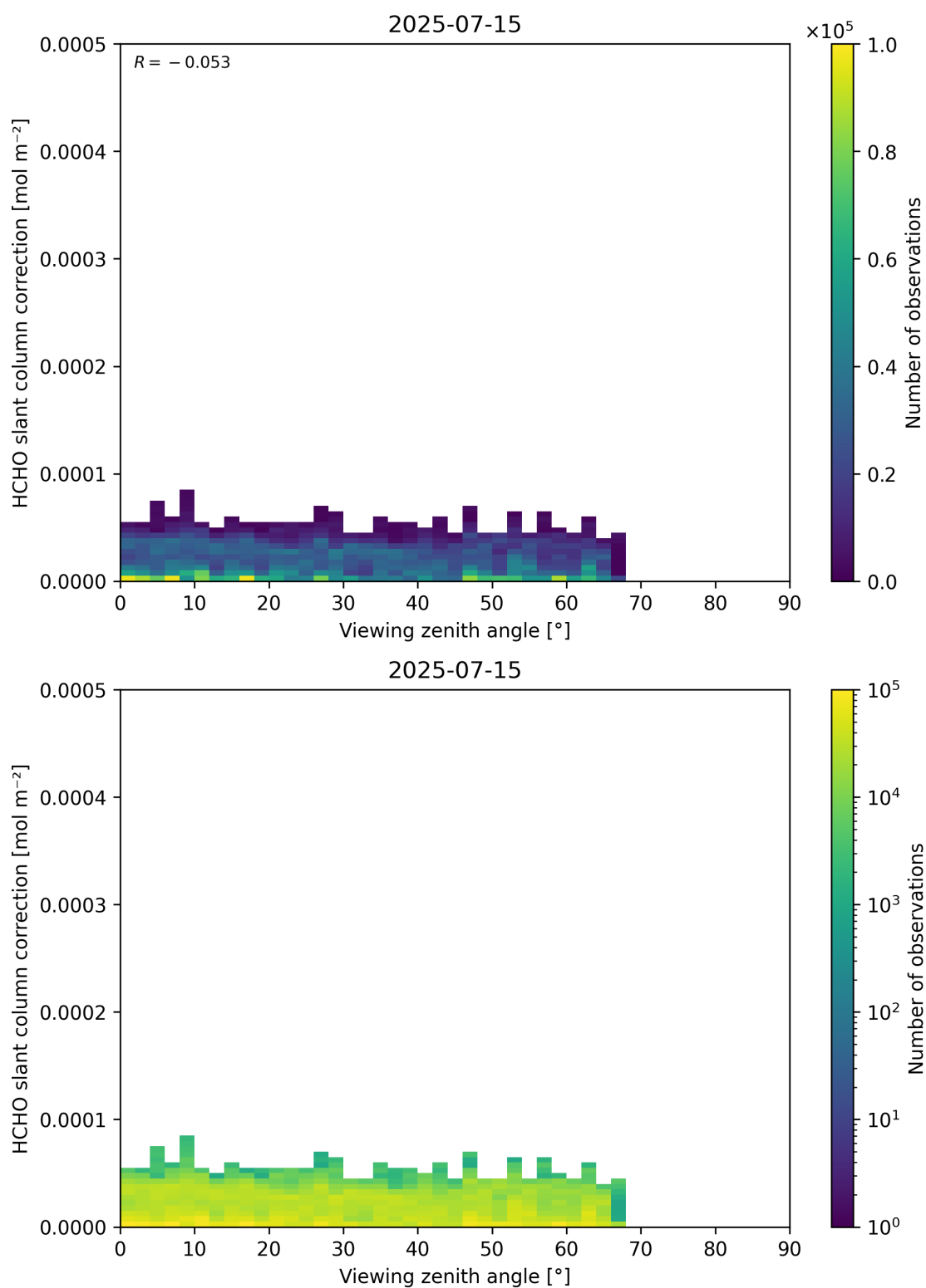
Figure 187: Scatter density plot of “Viewing zenith angle” against “HCHO slant column correction” for 2025-07-14 to 2025-07-16.
