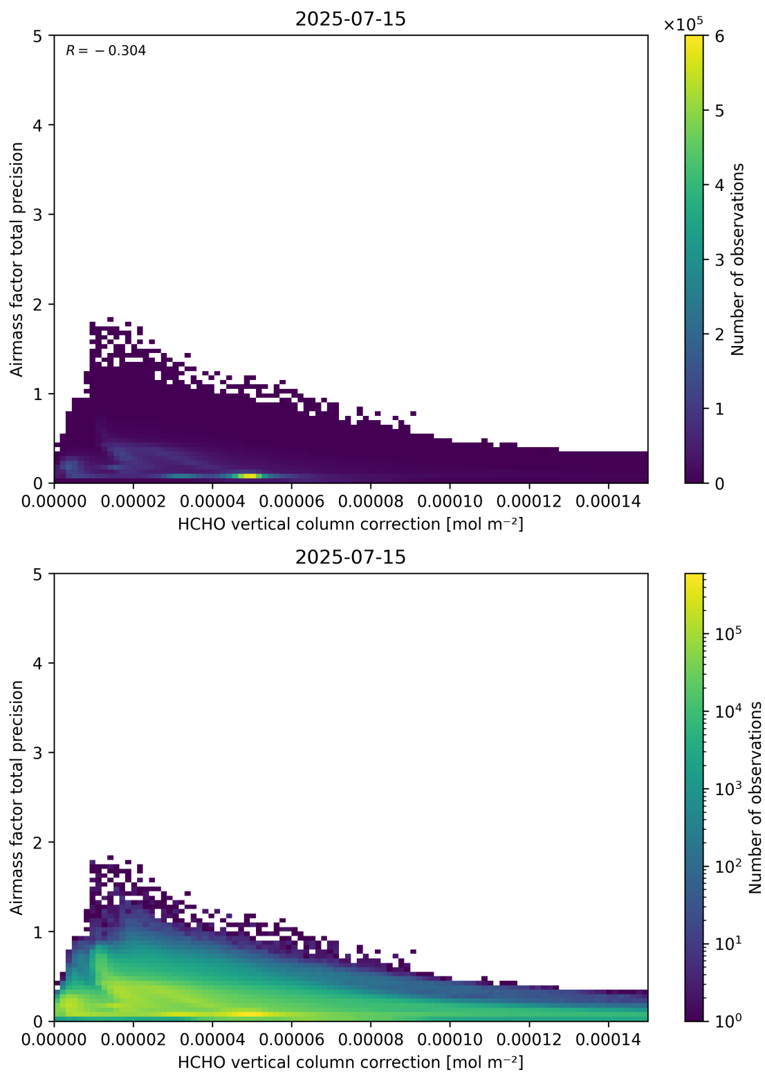
Figure 121: Scatter density plot of “HCHO vertical column correction” against “Airmass factor total precision” for 2025-07-14 to 2025-07-16.
