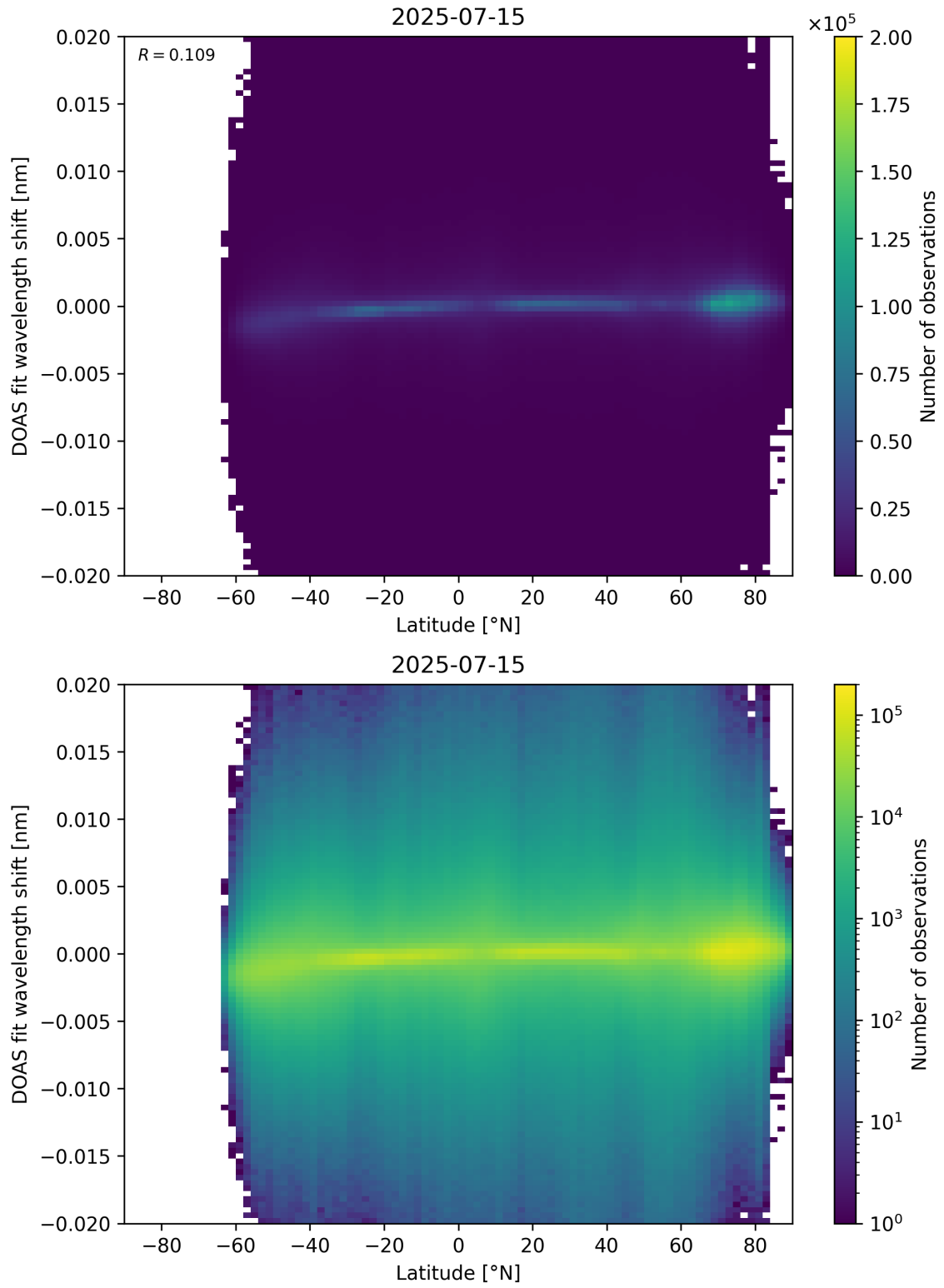
Figure 154: Scatter density plot of “Latitude” against “DOAS fit wavelength shift” for 2025-07-14 to 2025-07-16.
