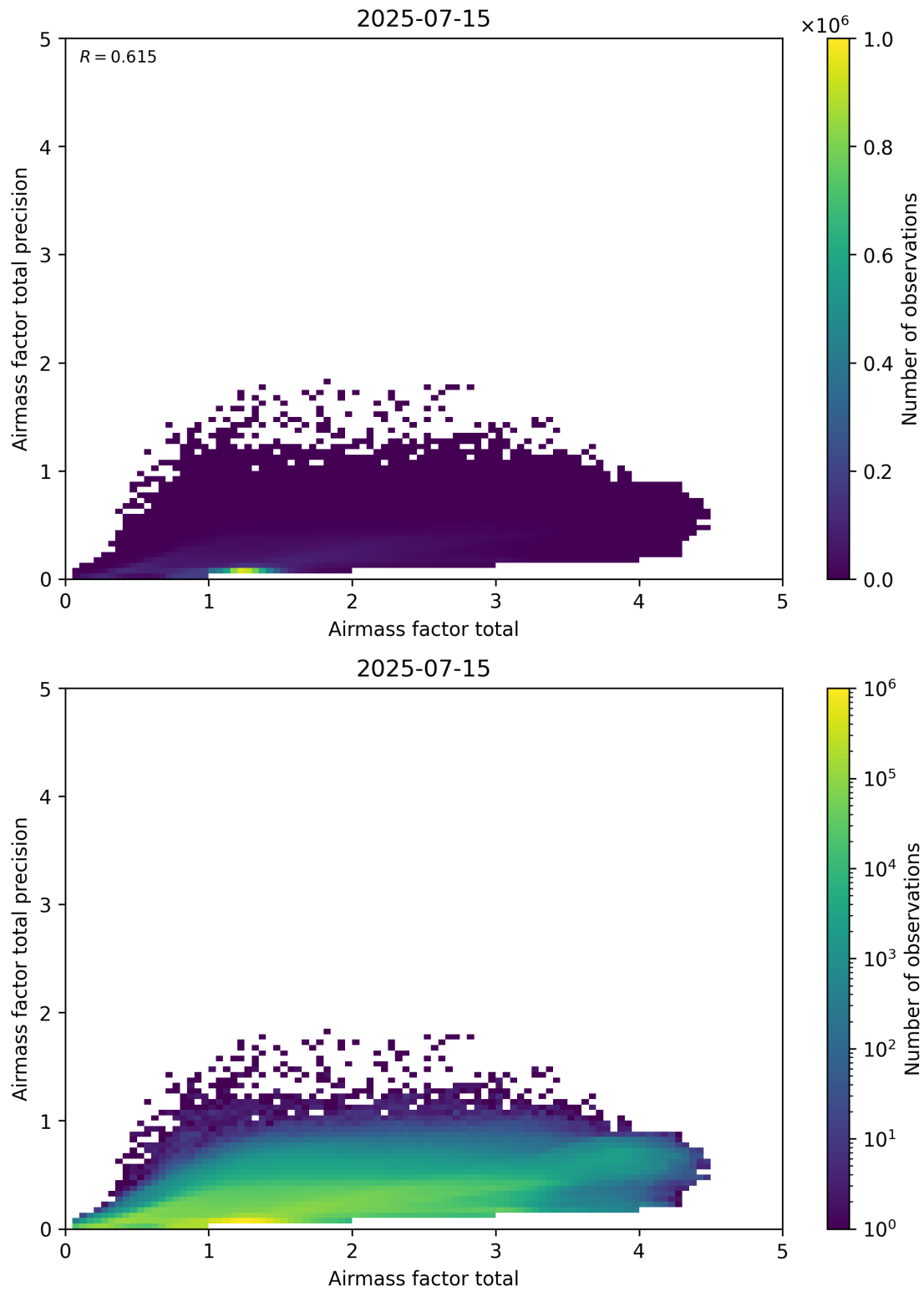
Figure 103: Scatter density plot of “Airmass factor total” against “Airmass factor total precision” for 2025-07-14 to 2025-07-16.
