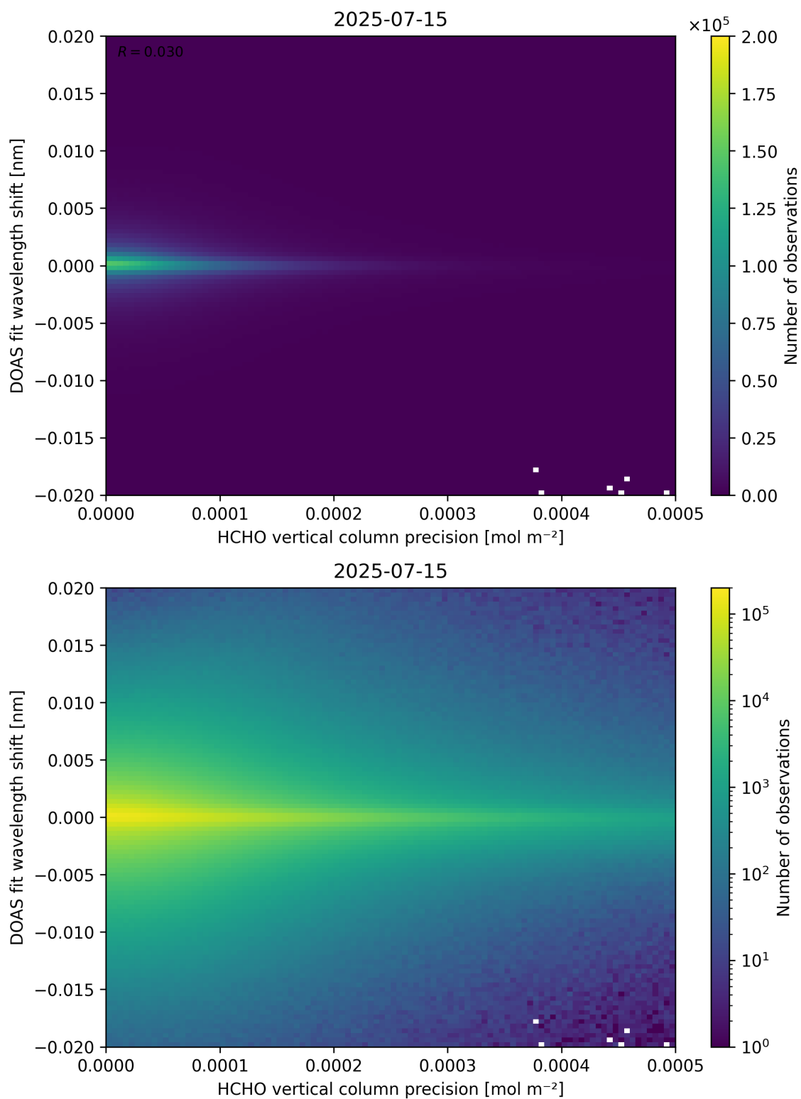
Figure 137: Scatter density plot of “HCHO vertical column precision” against “DOAS fit wavelength shift” for 2025-07-14 to 2025-07-16.
