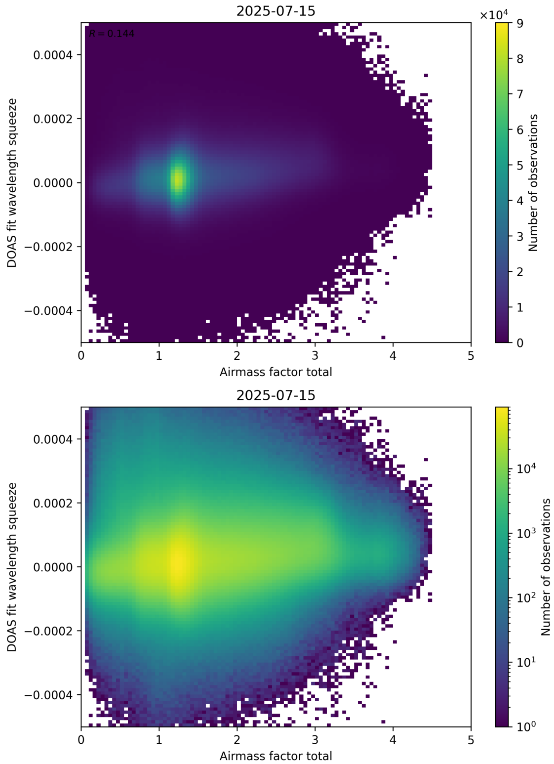
Figure 99: Scatter density plot of “Airmass factor total” against “DOAS fit wavelength squeeze” for 2025-07-14 to 2025-07-16.
