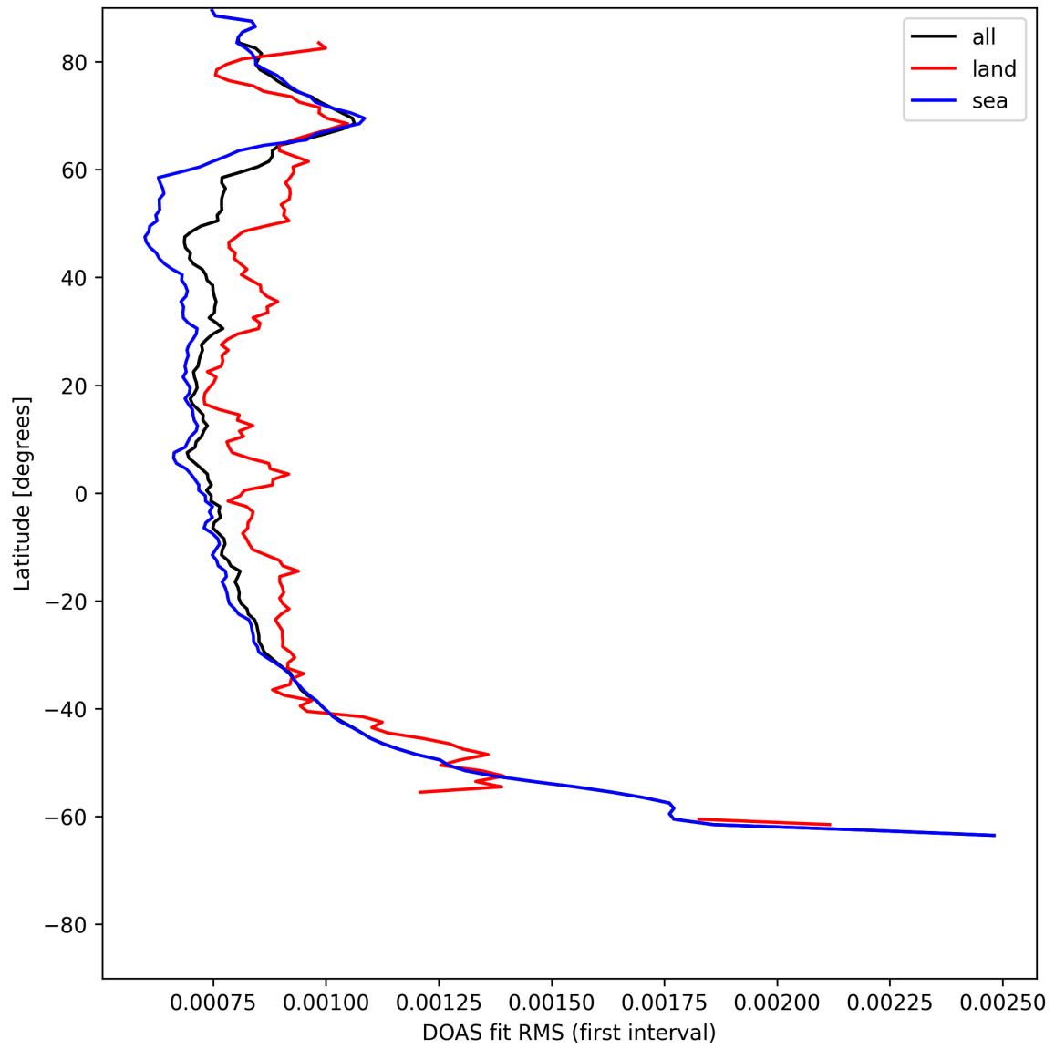
Figure 32: Zonal average of “DOAS fit RMS (first interval)” for 2025-07-14 to 2025-07-16.
