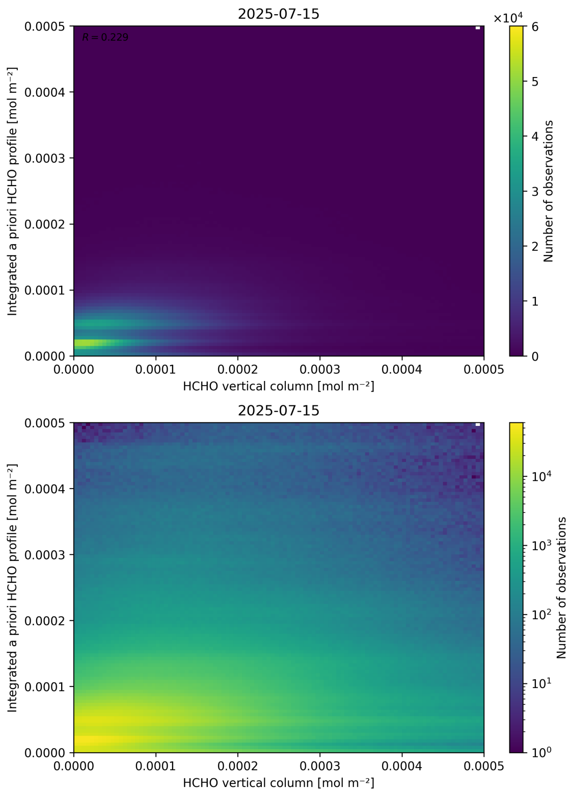
Figure 135: Scatter density plot of “HCHO vertical column” against “Integrated a priori HCHO profile” for 2025-07-14 to 2025-07-16.
