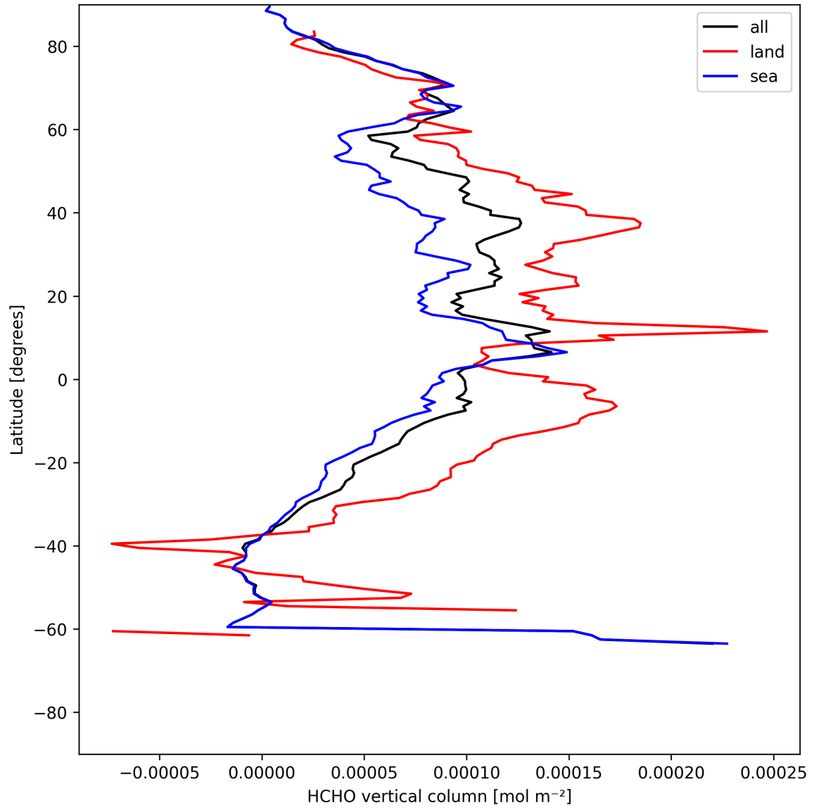
Figure 21: Zonal average of “HCHO vertical column” for 2025-07-14 to 2025-07-16.
