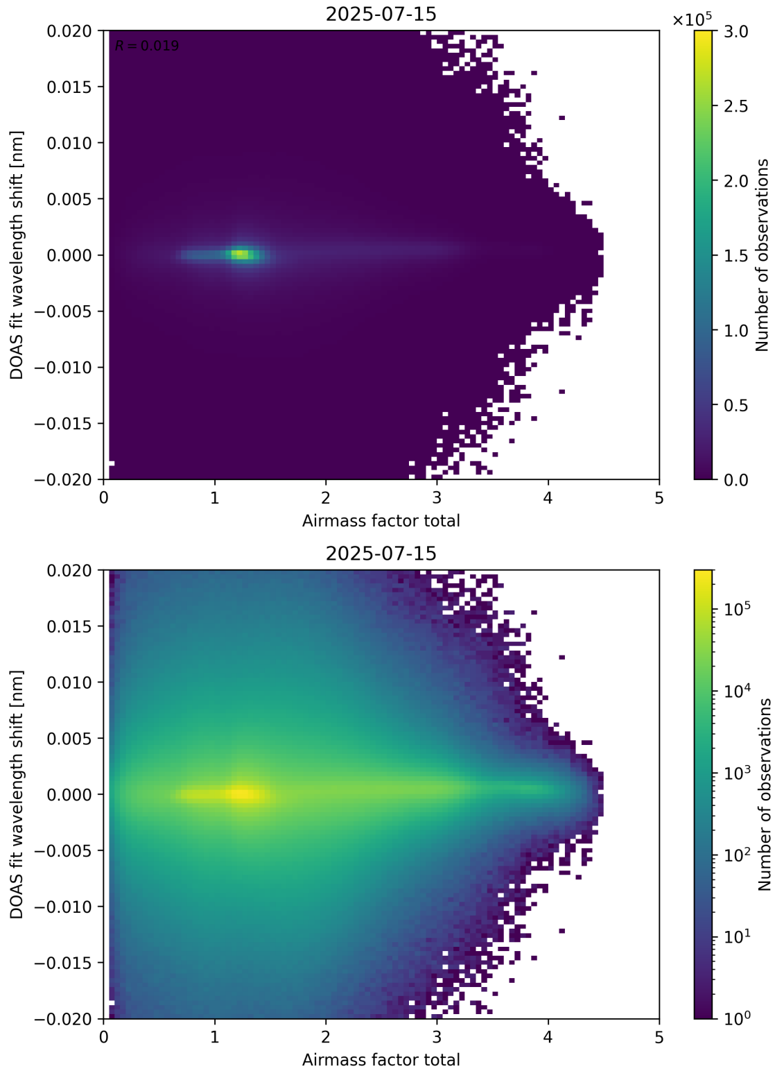
Figure 98: Scatter density plot of “Airmass factor total” against “DOAS fit wavelength shift” for 2025-07-14 to 2025-07-16.
