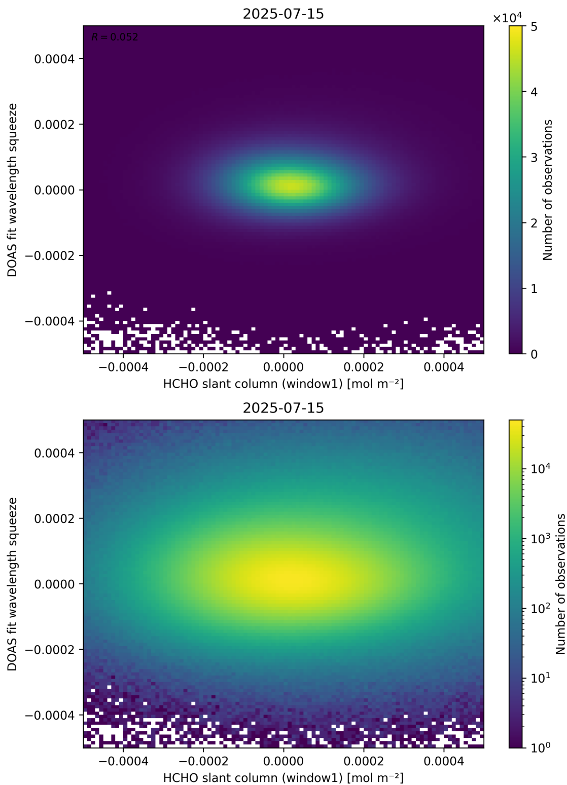
Figure 80: Scatter density plot of “HCHO slant column (window1)” against “DOAS fit wavelength squeeze” for 2025-07-14 to 2025-07-16.
