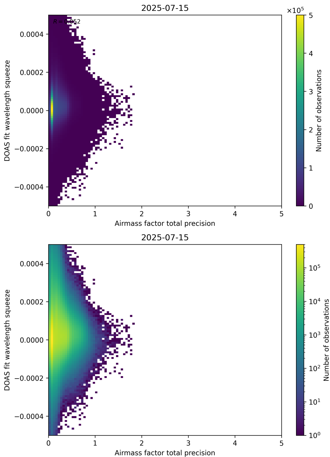
Figure 107: Scatter density plot of “Airmass factor total precision” against “DOAS fit wavelength squeeze” for 2025-07-14 to 2025-07-16.
