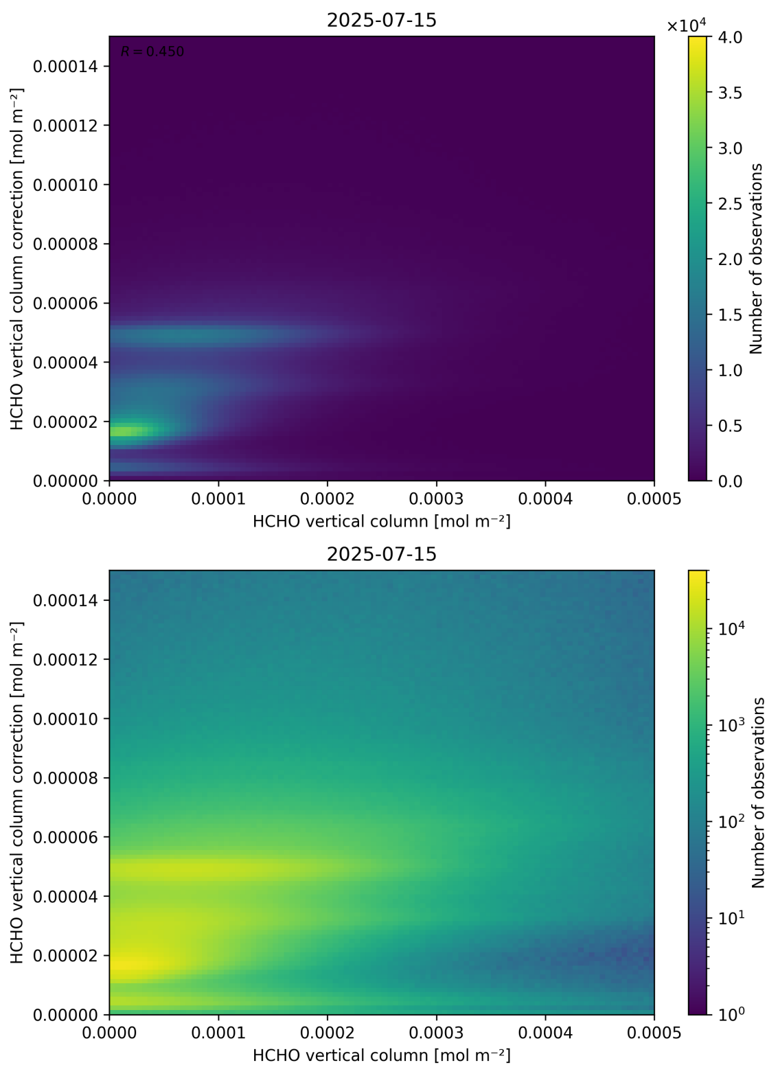
Figure 133: Scatter density plot of “HCHO vertical column” against “HCHO vertical column correction” for 2025-07-14 to 2025-07-16.
