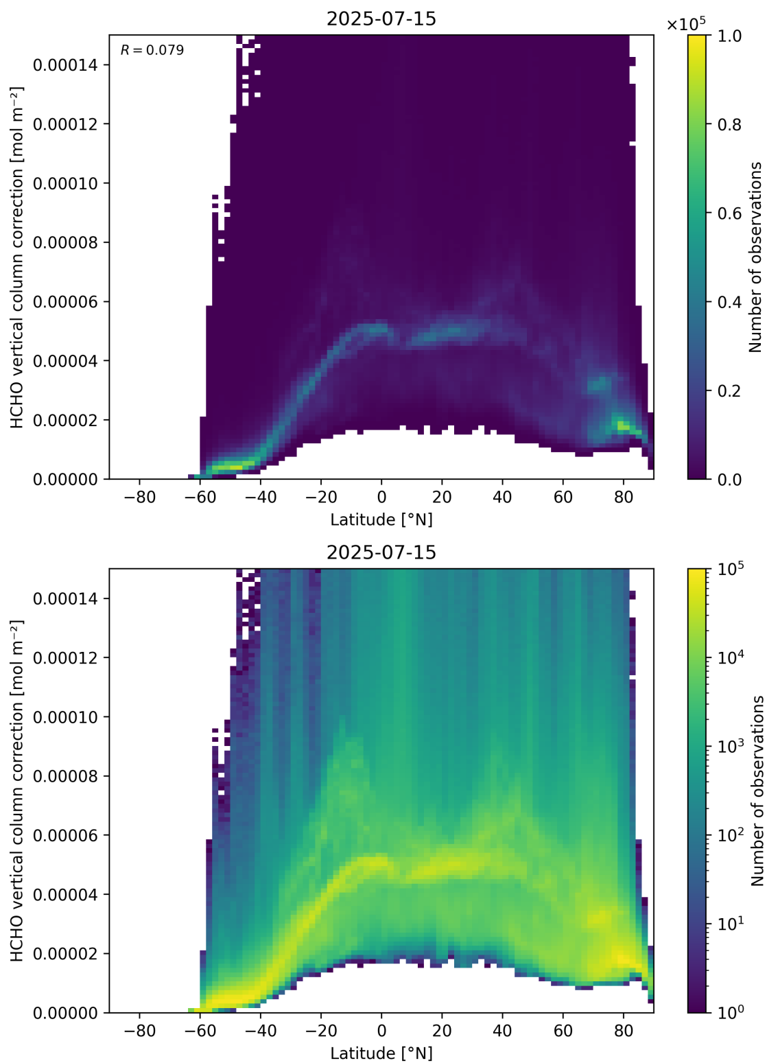
Figure 164: Scatter density plot of “Latitude” against “HCHO vertical column correction” for 2025-07-14 to 2025-07-16.
