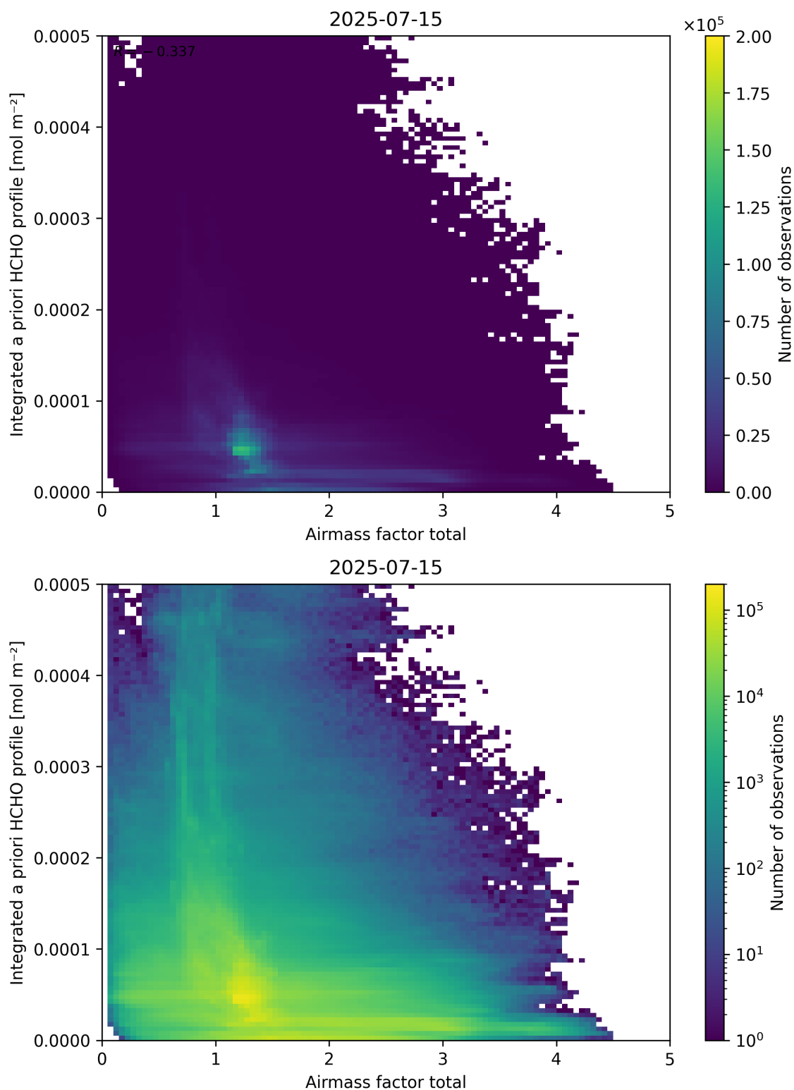
Figure 104: Scatter density plot of “Airmass factor total” against “Integrated a priori HCHO profile” for 2025-07-14 to 2025-07-16.
