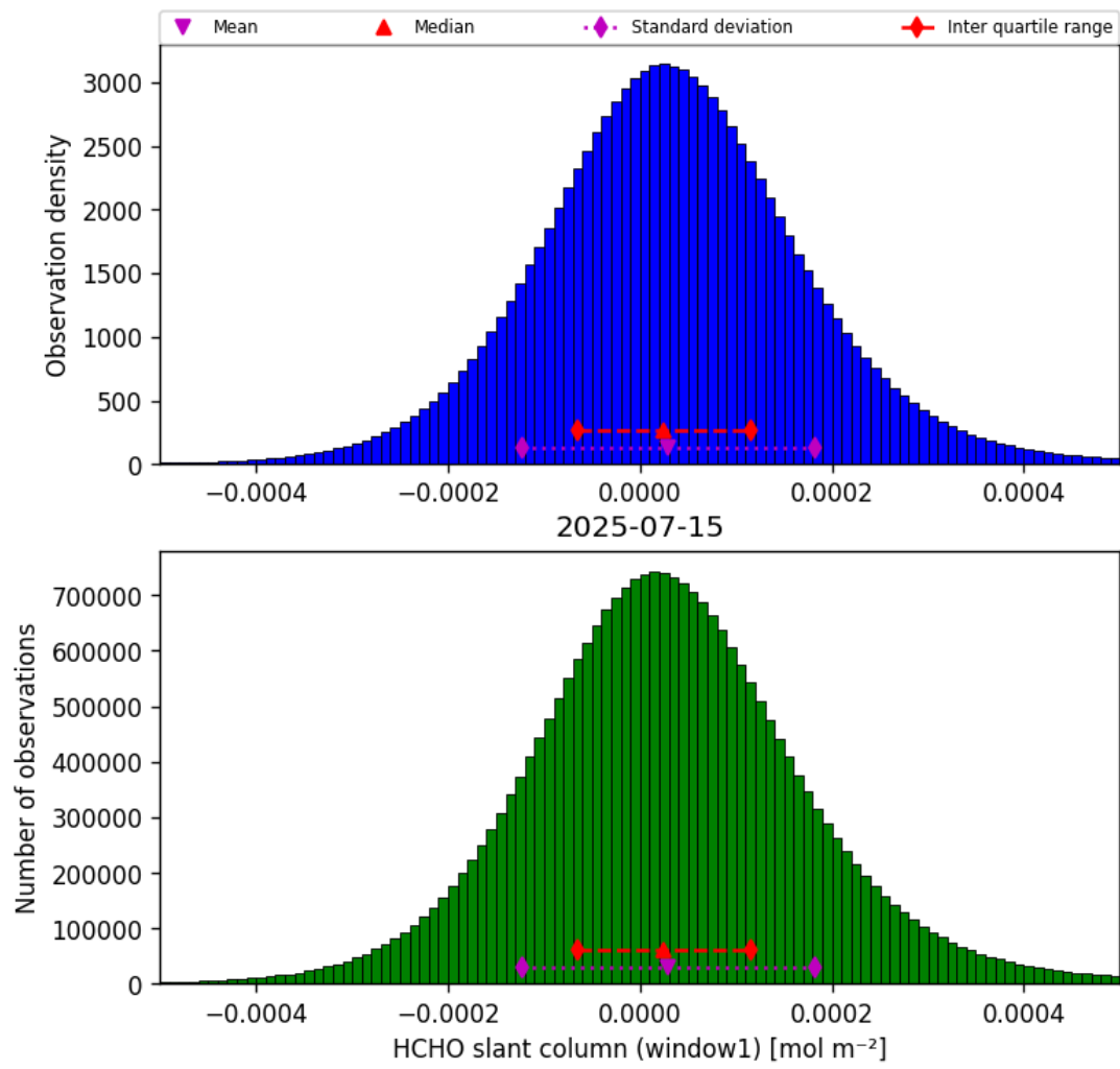
Figure 38: Histogram of “HCHO slant column (window1)” for 2025-07-14 to 2025-07-16
