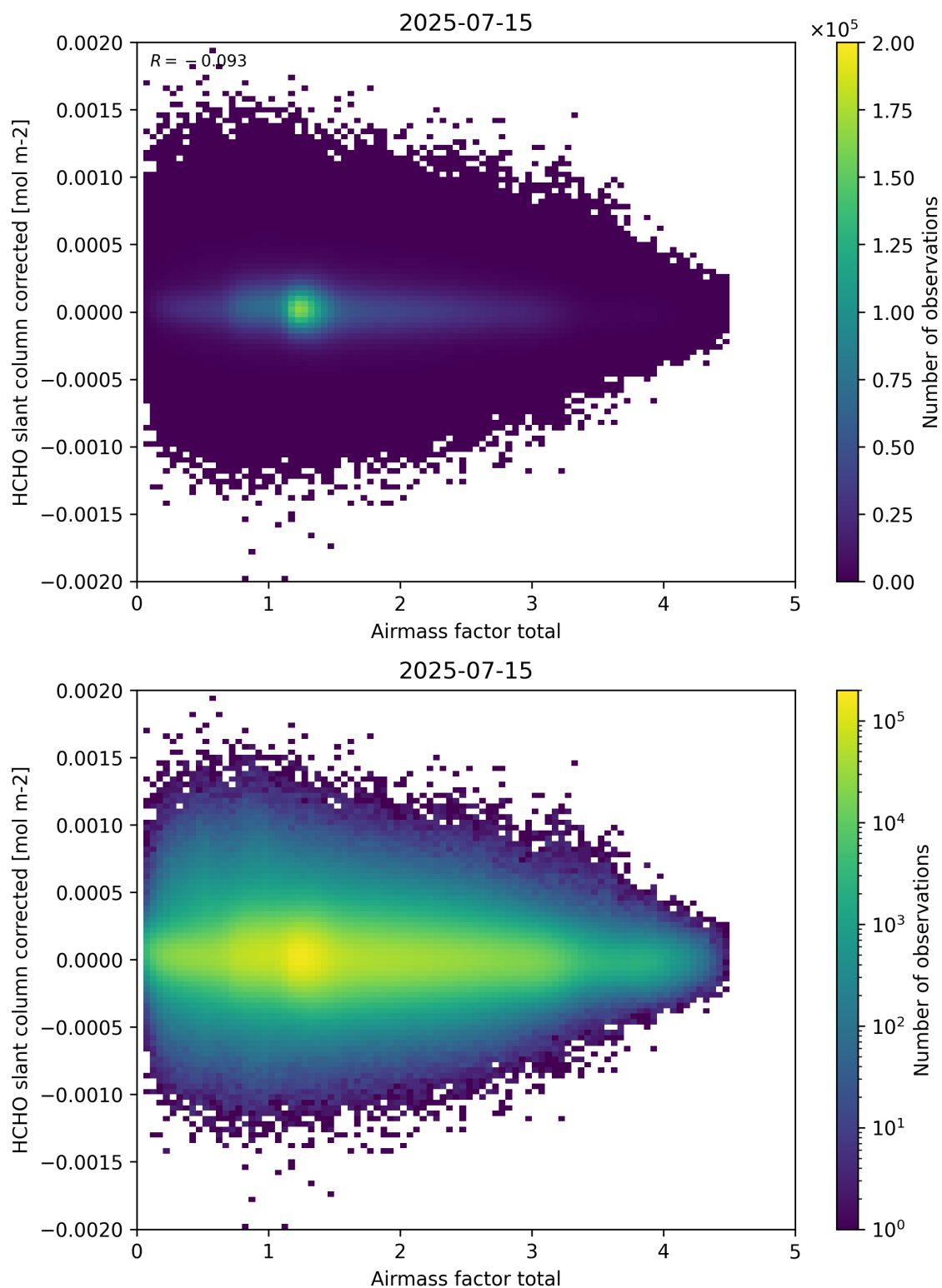
Figure 101: Scatter density plot of “Airmass factor total” against “HCHO slant column corrected” for 2025-07-14 to 2025-07-16.
