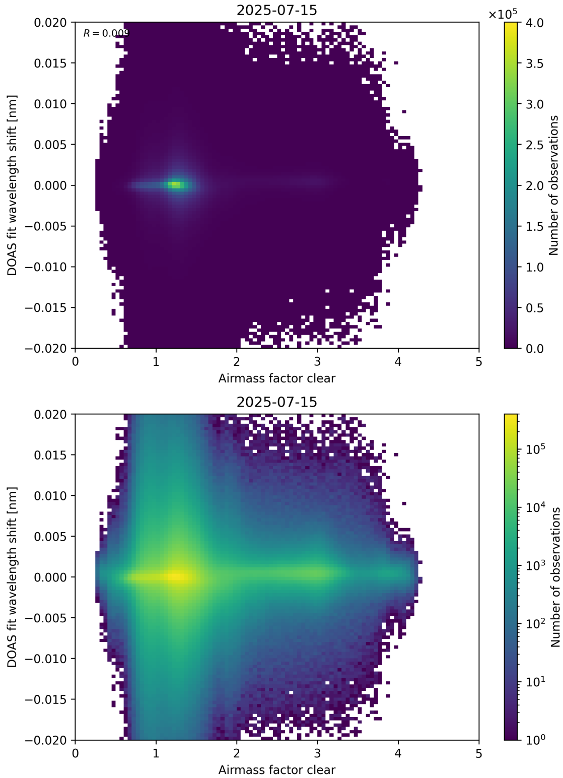
Figure 72: Scatter density plot of “Airmass factor clear” against “DOAS fit wavelength shift” for 2025-07-14 to 2025-07-16.
