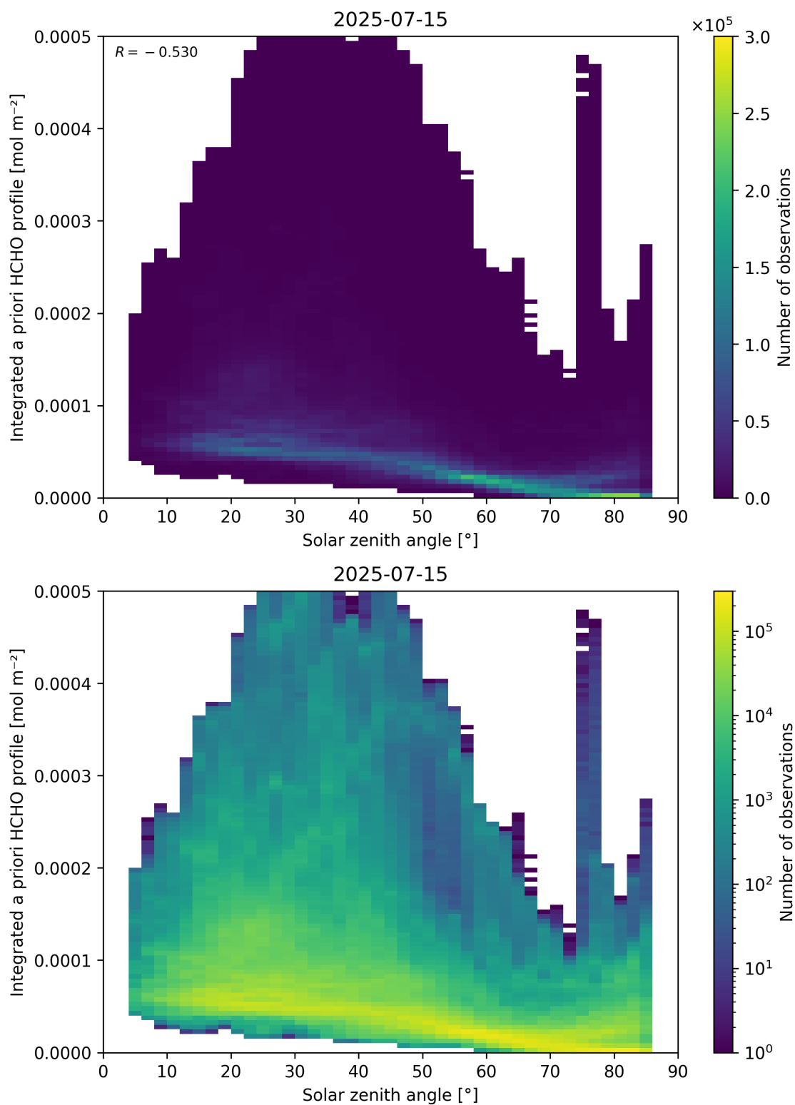
Figure 180: Scatter density plot of “Solar zenith angle” against “Integrated a priori HCHO profile” for 2025-07-14 to 2025-07-16.
