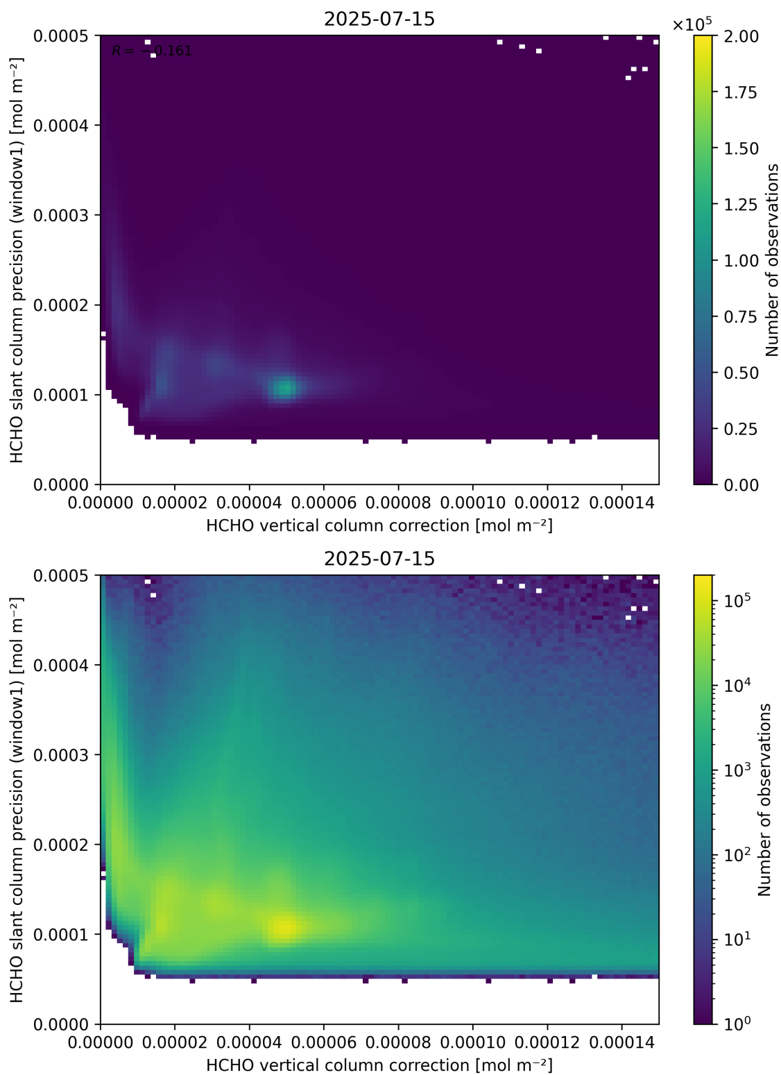
Figure 119: Scatter density plot of “HCHO vertical column correction” against “HCHO slant column precision (window1)” for 2025-07-14 to 2025-07-16.
