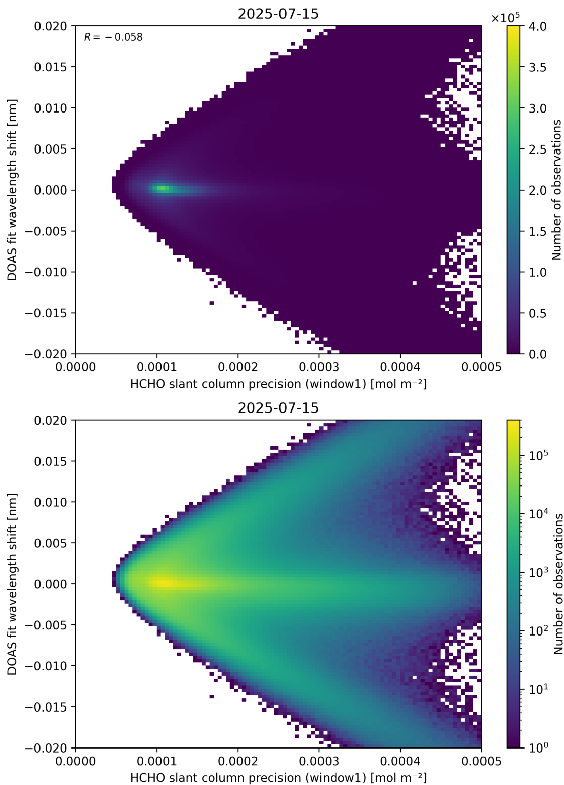
Figure 89: Scatter density plot of “HCHO slant column precision (window1)” against “DOAS fit wavelength shift” for 2025-07-14 to 2025-07-16.
