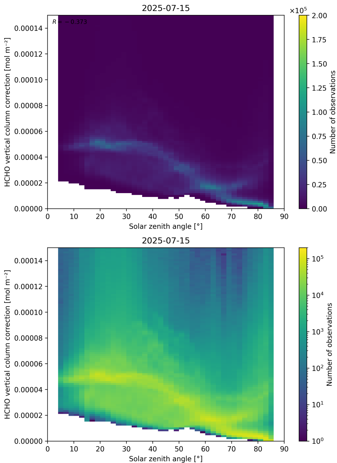
Figure 178: Scatter density plot of “Solar zenith angle” against “HCHO vertical column correction” for 2025-07-14 to 2025-07-16.
