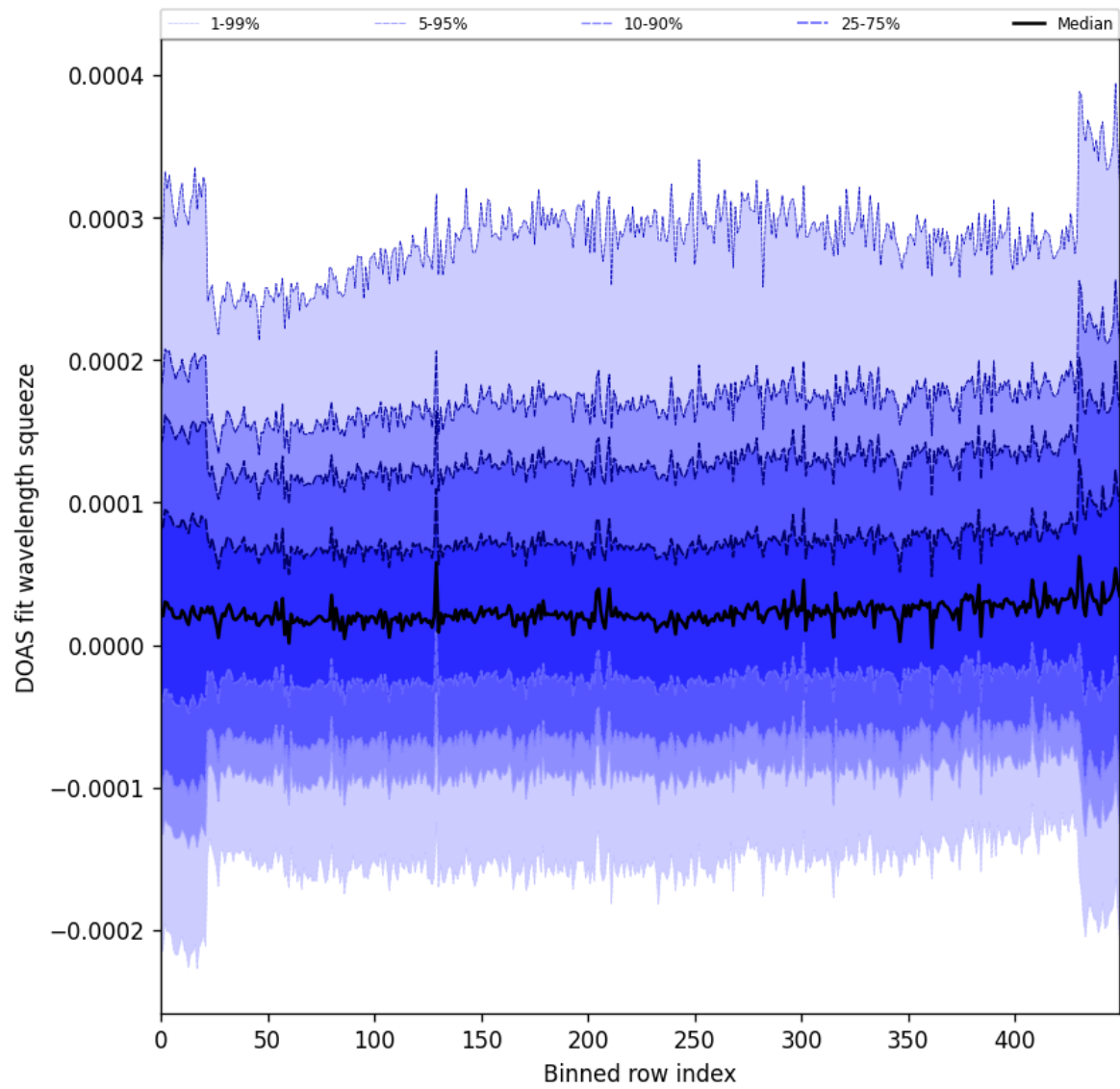
Figure 59: Along track statistics of “DOAS fit wavelength squeeze” for 2025-07-14 to 2025-07-16
