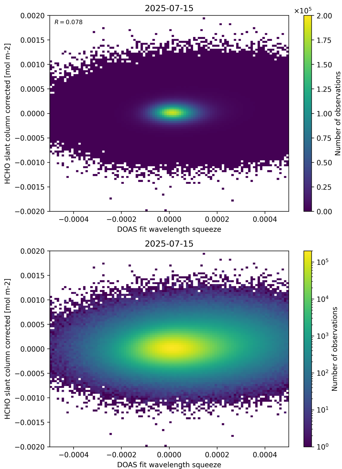
Figure 69: Scatter density plot of “DOAS fit wavelength squeeze” against “HCHO slant column corrected” for 2025-07-14 to 2025-07-16.
