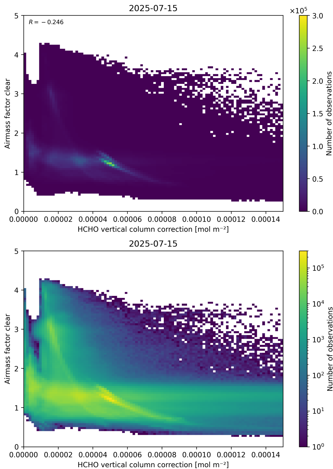
Figure 115: Scatter density plot of “HCHO vertical column correction” against “Airmass factor clear” for 2025-07-14 to 2025-07-16.
