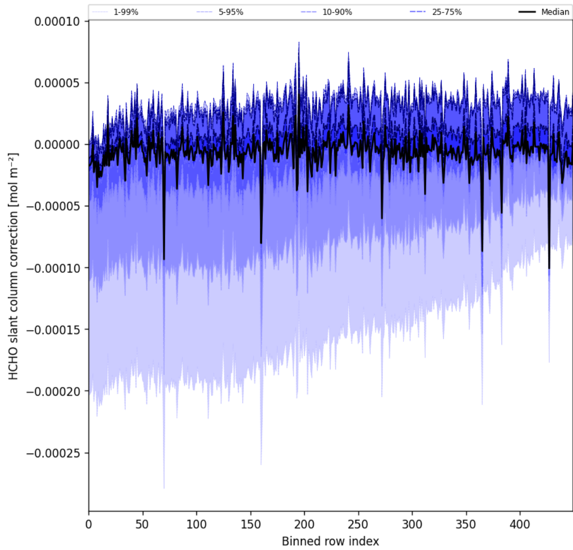
Figure 61: Along track statistics of “HCHO slant column correction” for 2025-07-14 to 2025-07-16
