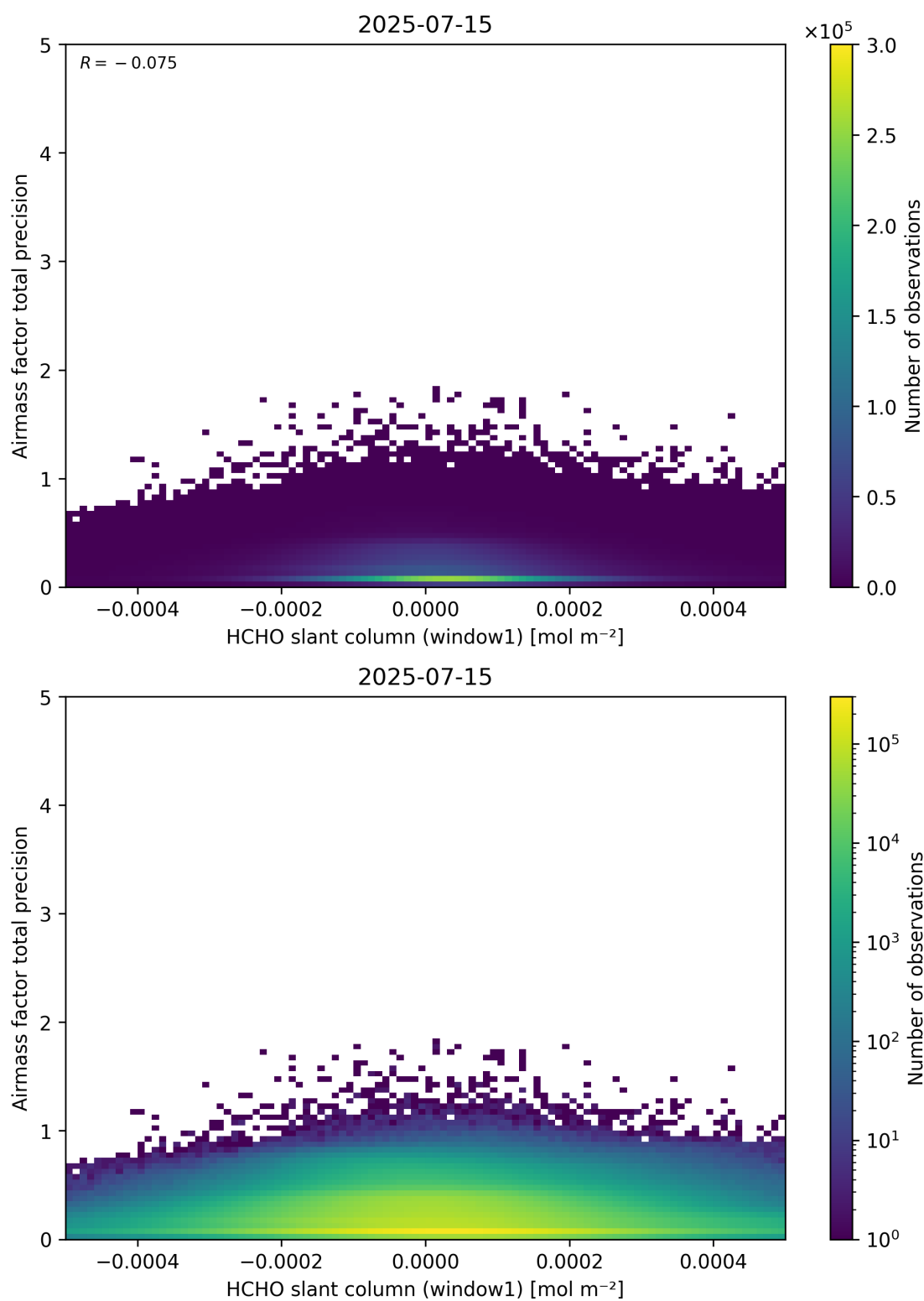
Figure 86: Scatter density plot of “HCHO slant column (window1)” against “Airmass factor total precision” for 2025-07-14 to 2025-07-16.
