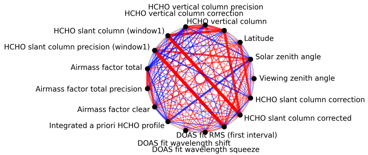
Figure 1: Map of correlation graph for 2025-07-14 to 2025-07-16.
