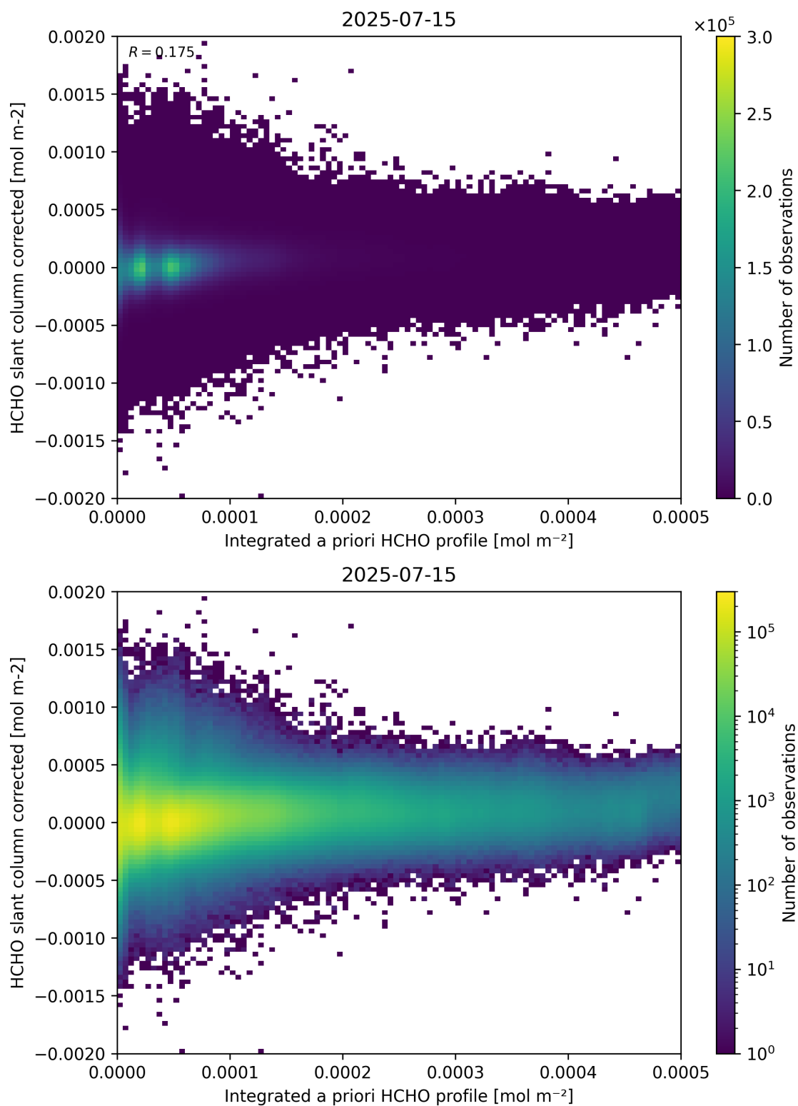
Figure 151: Scatter density plot of “Integrated a priori HCHO profile” against “HCHO slant column corrected” for 2025-07-14 to 2025-07-16.
