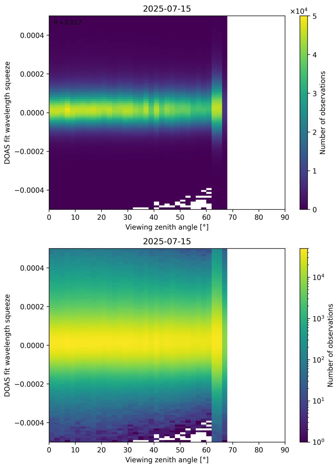
Figure 184: Scatter density plot of “Viewing zenith angle” against “DOAS fit wavelength squeeze” for 2025-07-14 to 2025-07-16.
