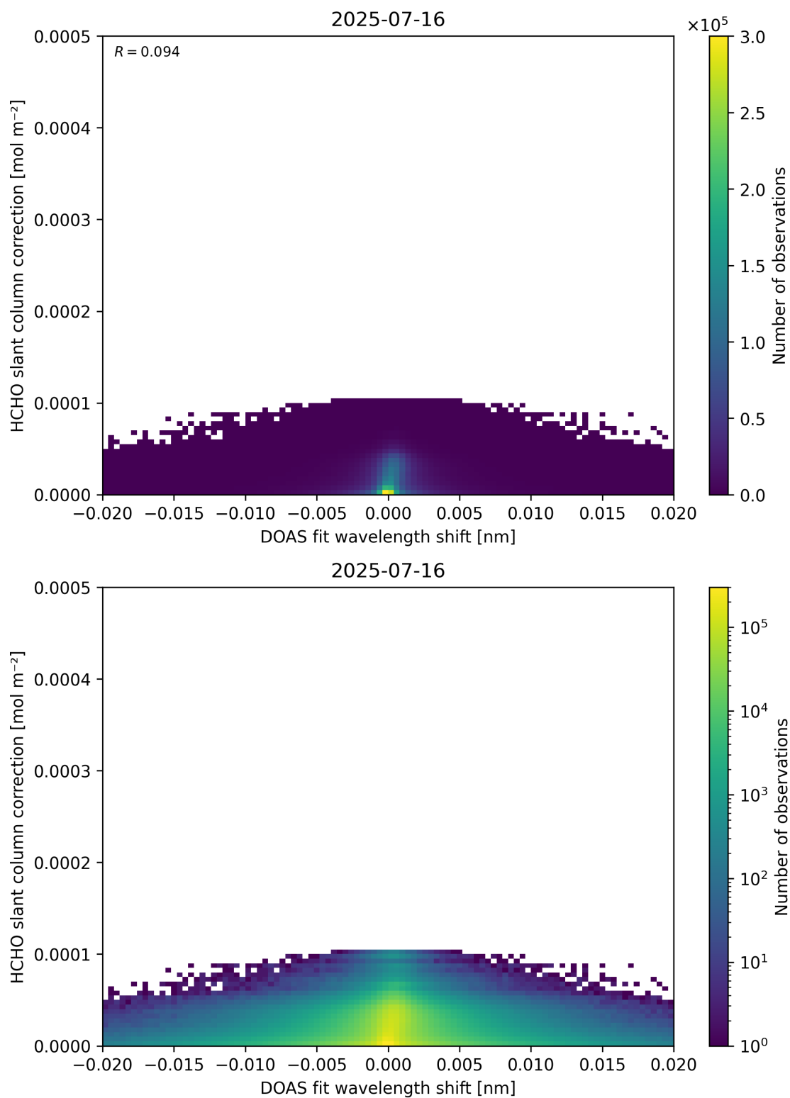
Figure 67: Scatter density plot of “DOAS fit wavelength shift” against “HCHO slant column correction” for 2025-07-15 to 2025-07-17.
