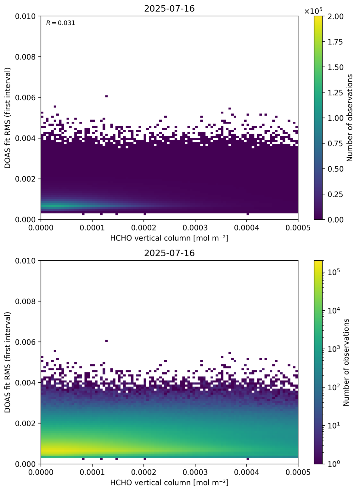
Figure 123: Scatter density plot of “HCHO vertical column” against “DOAS fit RMS (first interval)” for 2025-07-15 to 2025-07-17.
