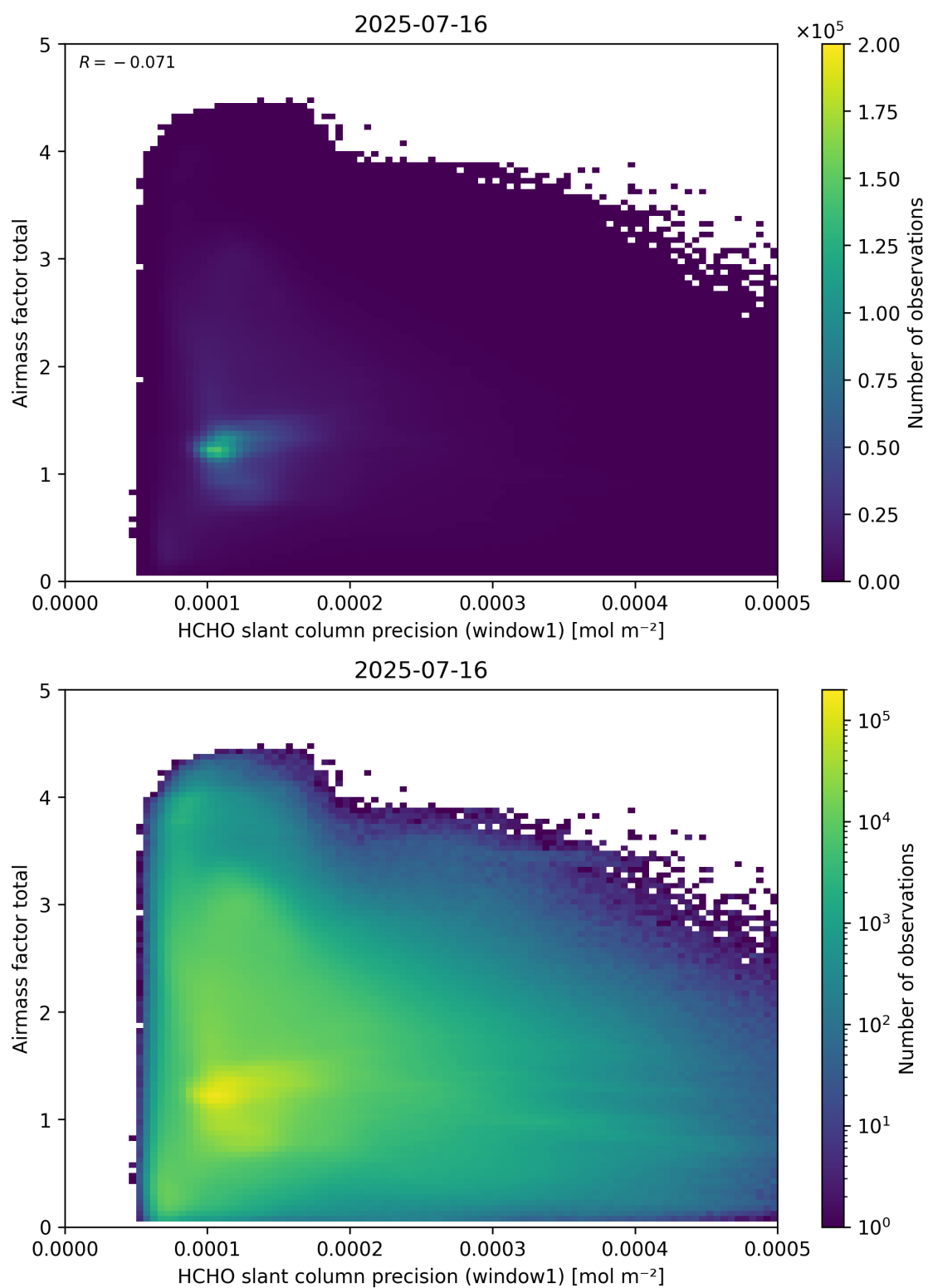
Figure 94: Scatter density plot of “HCHO slant column precision (window1)” against “Airmass factor total” for 2025-07-15 to 2025-07-17.
