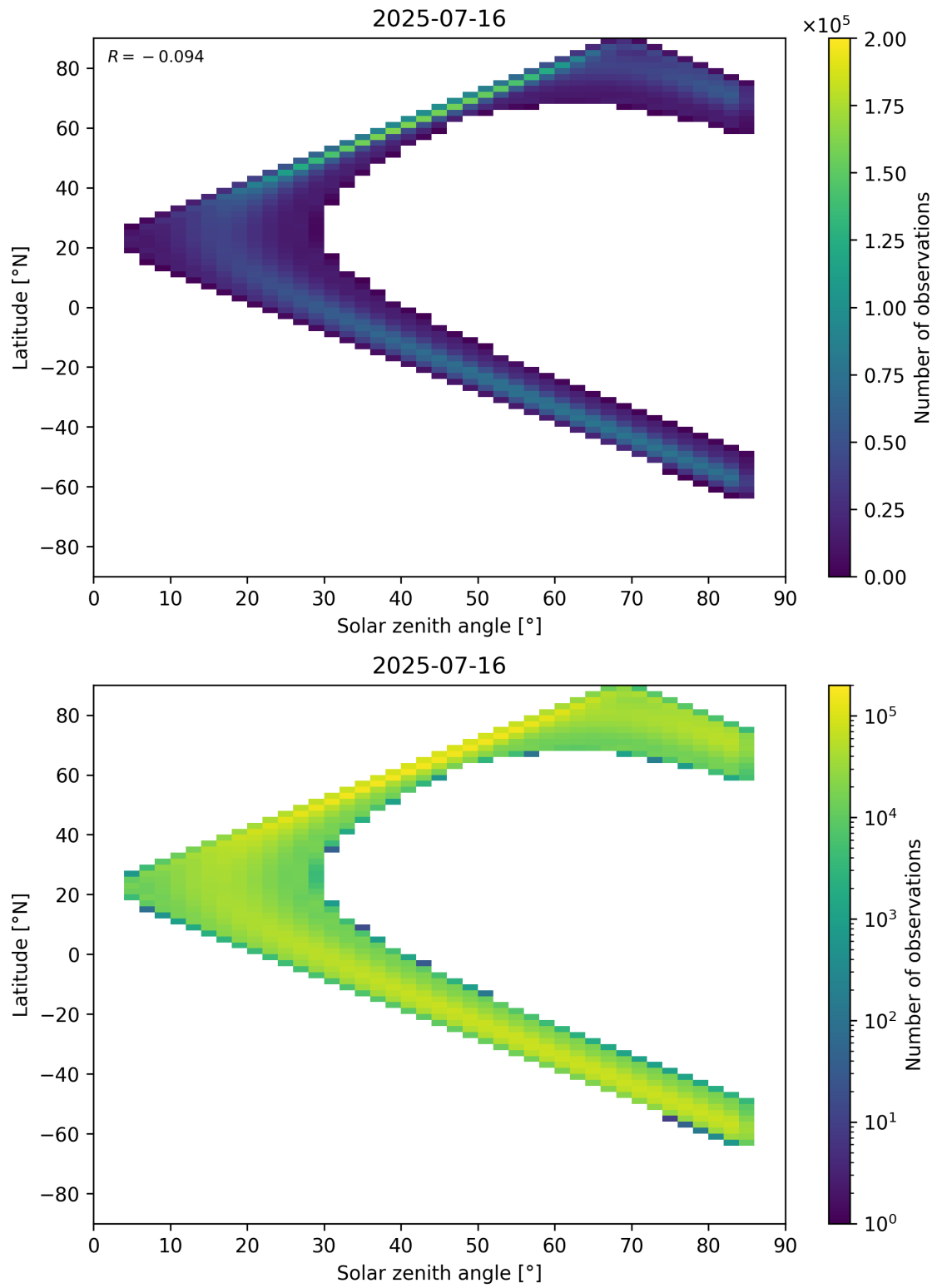
Figure 181: Scatter density plot of “Solar zenith angle” against “Latitude” for 2025-07-15 to 2025-07-17.
