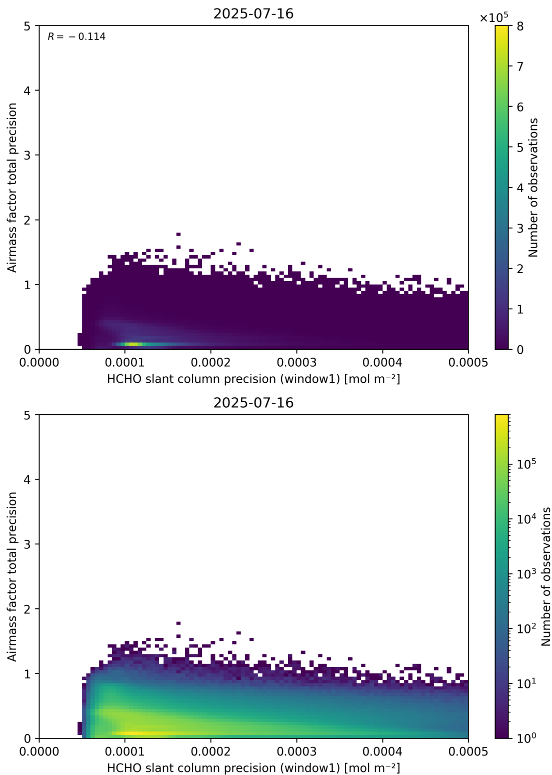
Figure 95: Scatter density plot of “HCHO slant column precision (window1)” against “Airmass factor total precision” for 2025-07-15 to 2025-07-17.
