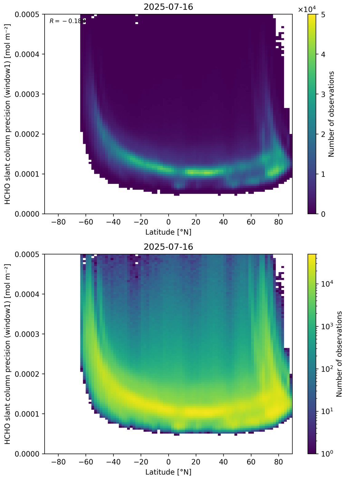
Figure 160: Scatter density plot of “Latitude” against “HCHO slant column precision (window1)” for 2025-07-15 to 2025-07-17.
