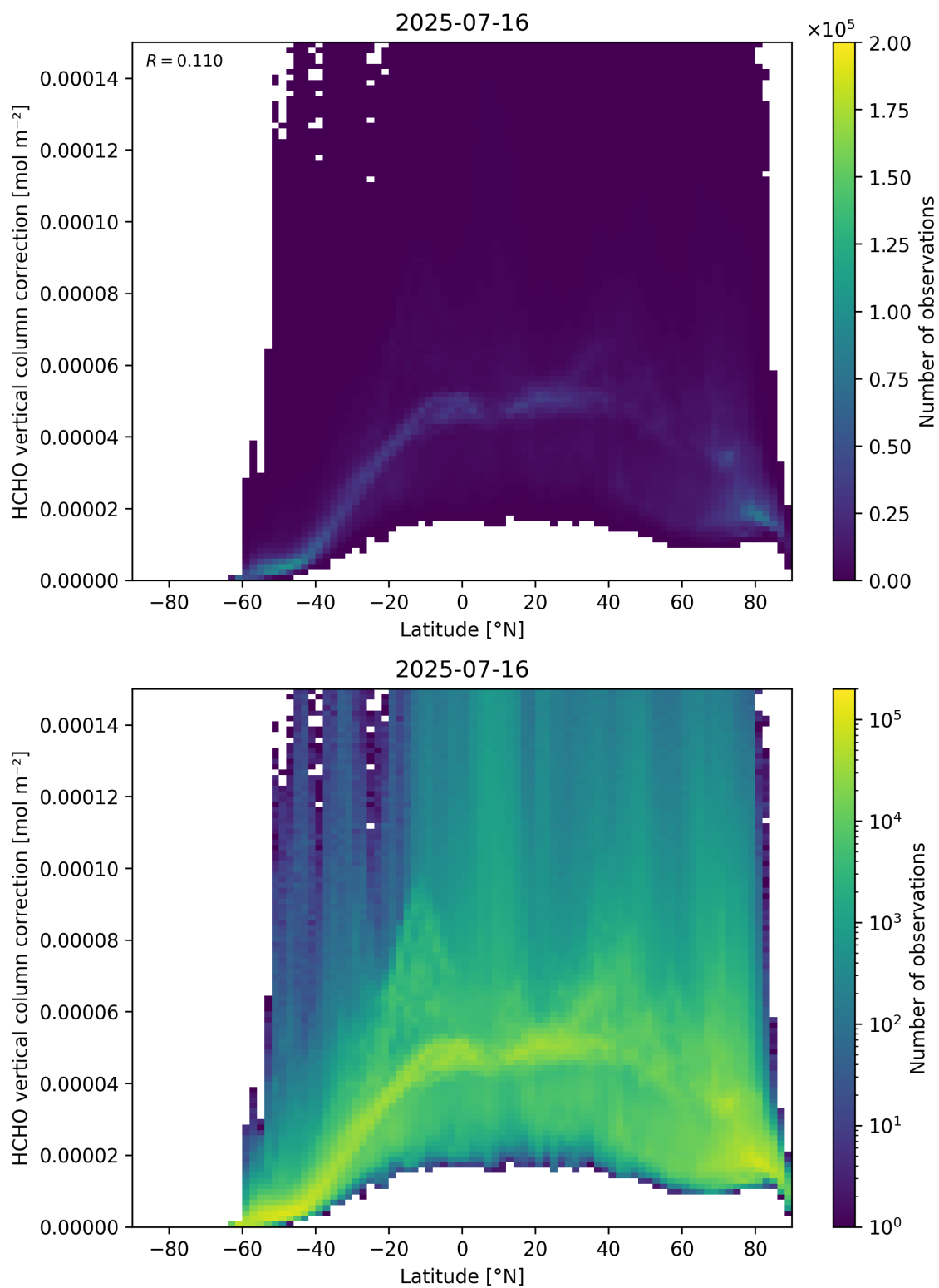
Figure 164: Scatter density plot of “Latitude” against “HCHO vertical column correction” for 2025-07-15 to 2025-07-17.
