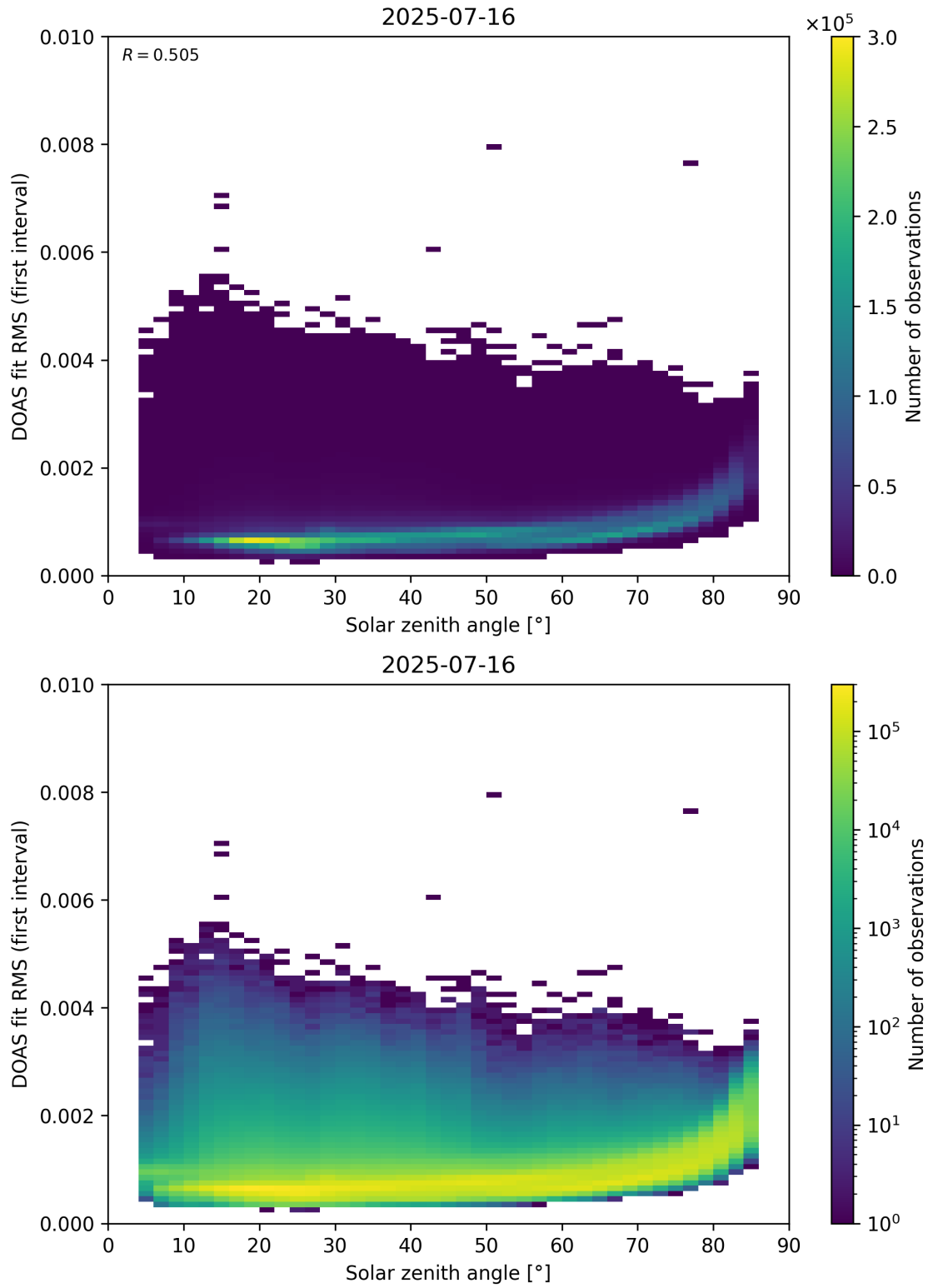
Figure 167: Scatter density plot of “Solar zenith angle” against “DOAS fit RMS (first interval)” for 2025-07-15 to 2025-07-17.
