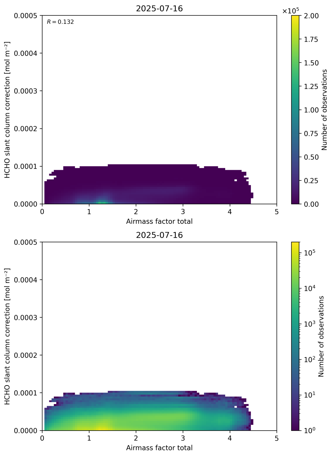
Figure 102: Scatter density plot of “Airmass factor total” against “HCHO slant column correction” for 2025-07-15 to 2025-07-17.
