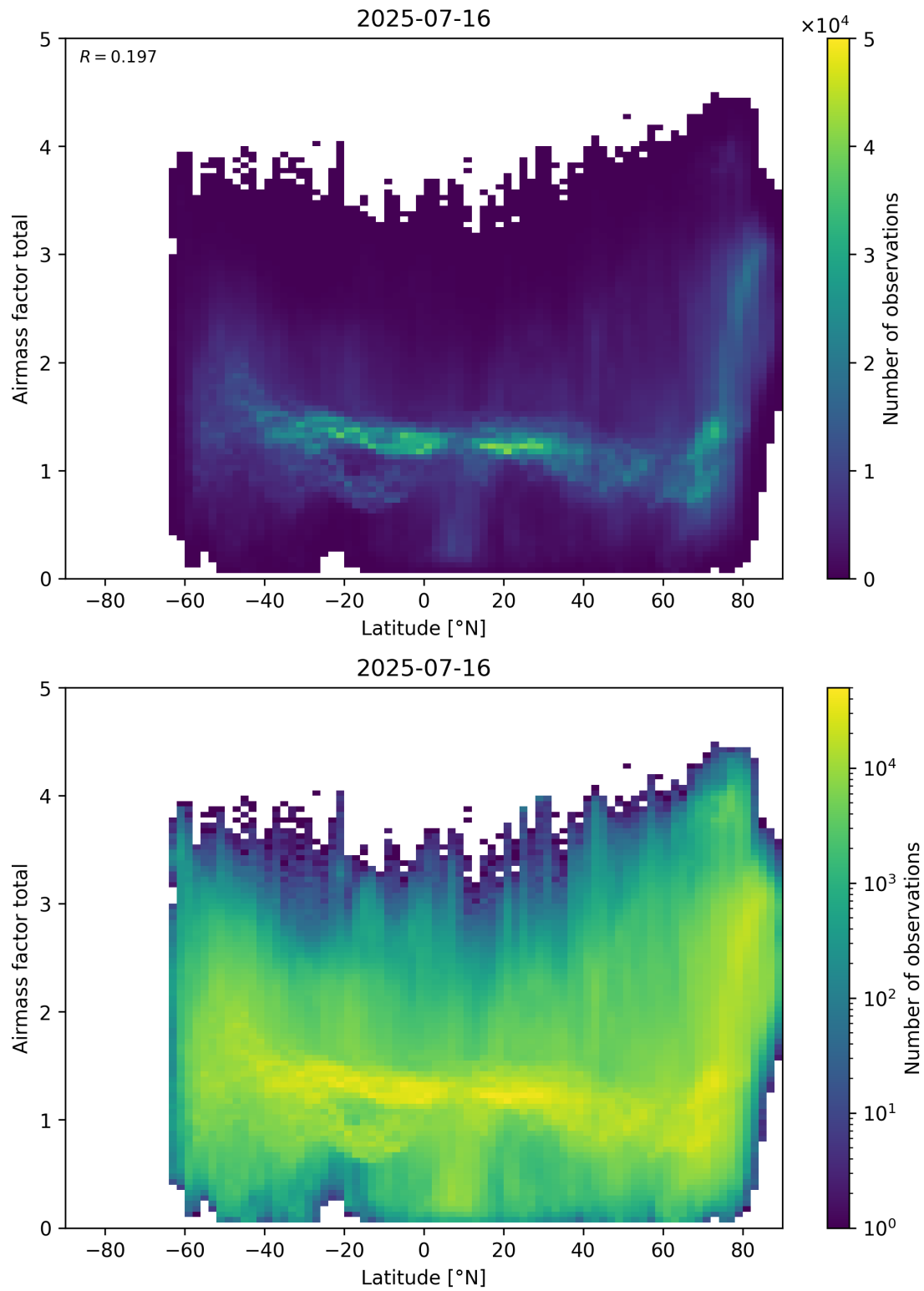
Figure 161: Scatter density plot of “Latitude” against “Airmass factor total” for 2025-07-15 to 2025-07-17.
