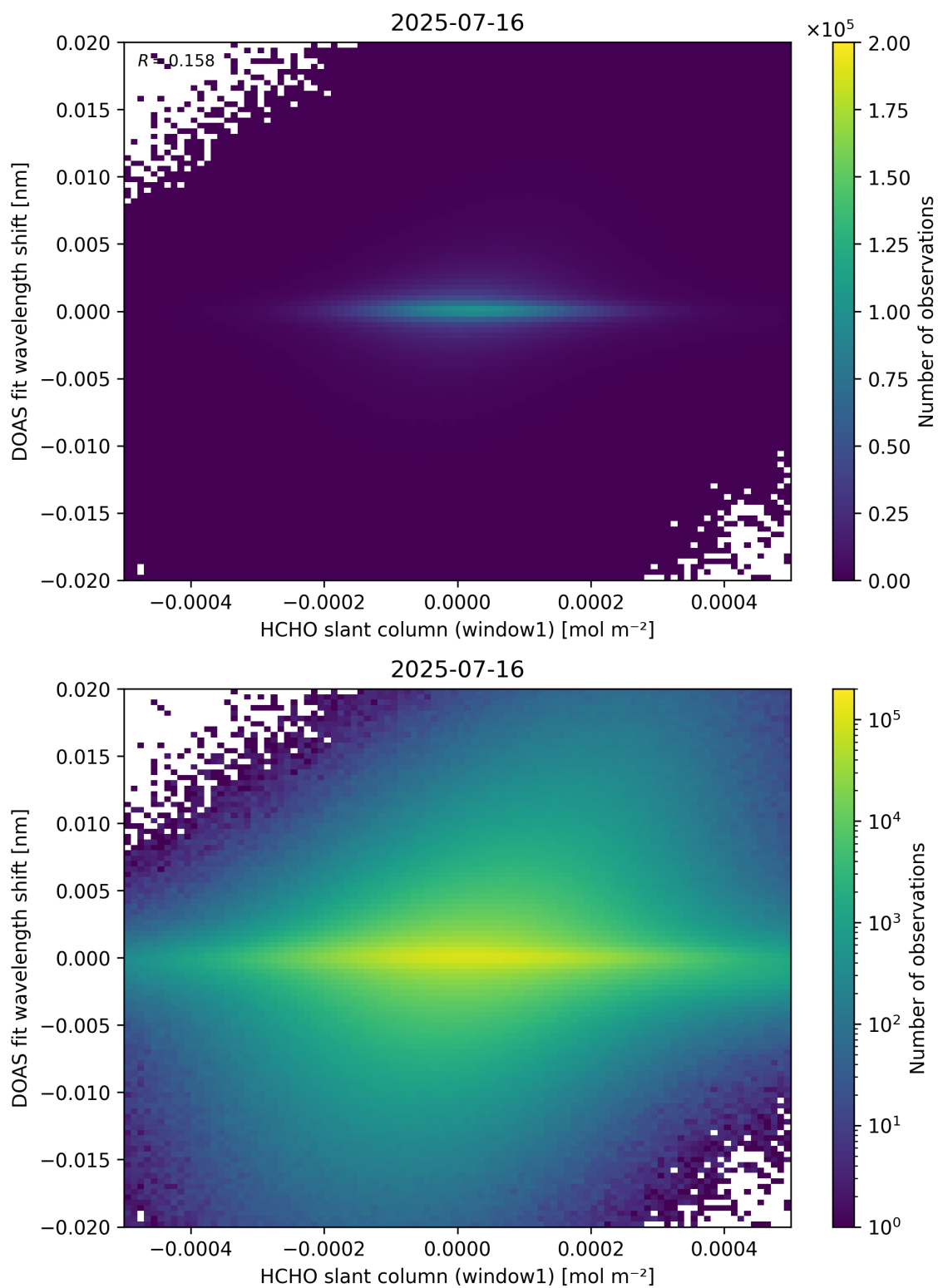
Figure 79: Scatter density plot of “HCHO slant column (window1)” against “DOAS fit wavelength shift” for 2025-07-15 to 2025-07-17.
