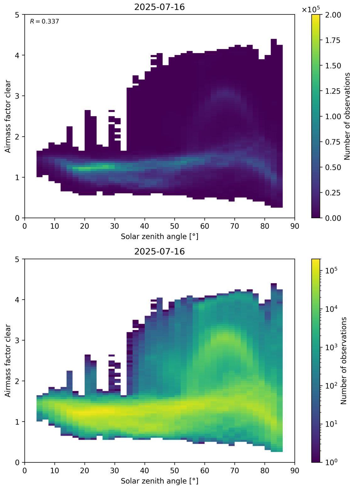
Figure 170: Scatter density plot of “Solar zenith angle” against “Airmass factor clear” for 2025-07-15 to 2025-07-17.
