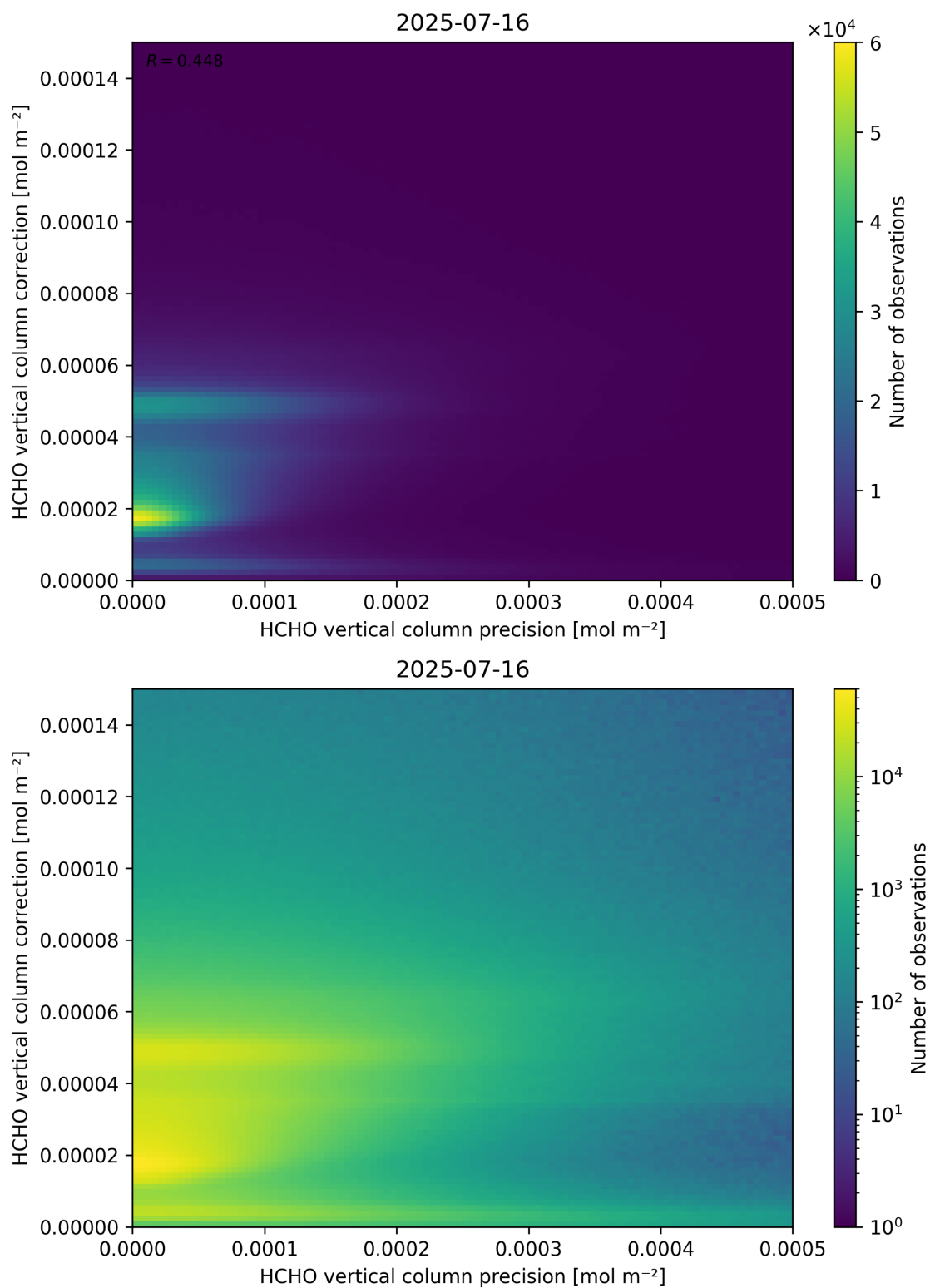
Figure 146: Scatter density plot of “HCHO vertical column precision” against “HCHO vertical column correction” for 2025-07-15 to 2025-07-17.
