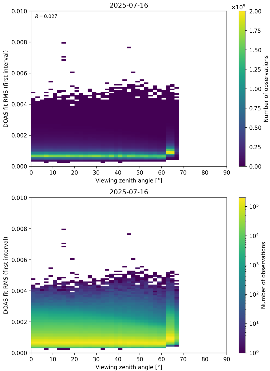
Figure 182: Scatter density plot of “Viewing zenith angle” against “DOAS fit RMS (first interval)” for 2025-07-15 to 2025-07-17.
