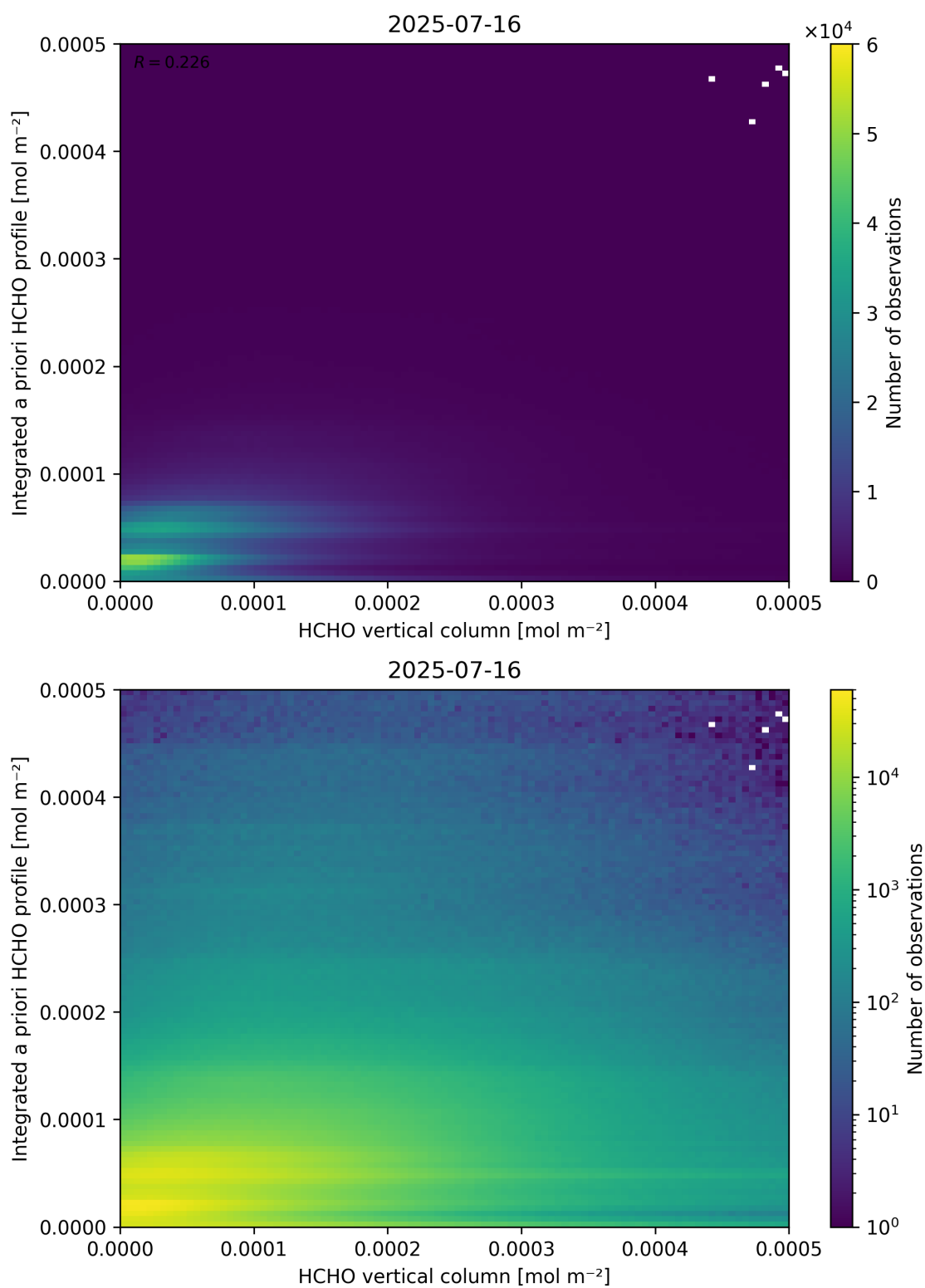
Figure 135: Scatter density plot of “HCHO vertical column” against “Integrated a priori HCHO profile” for 2025-07-15 to 2025-07-17.
