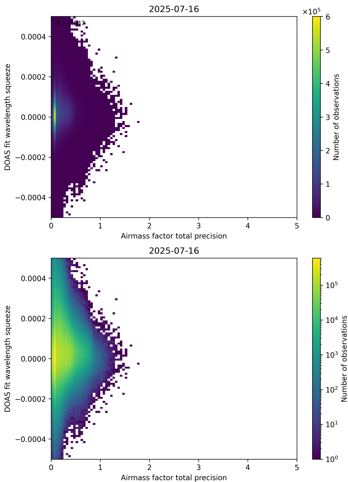
Figure 107: Scatter density plot of “Airmass factor total precision” against “DOAS fit wavelength squeeze” for 2025-07-15 to 2025-07-17.
