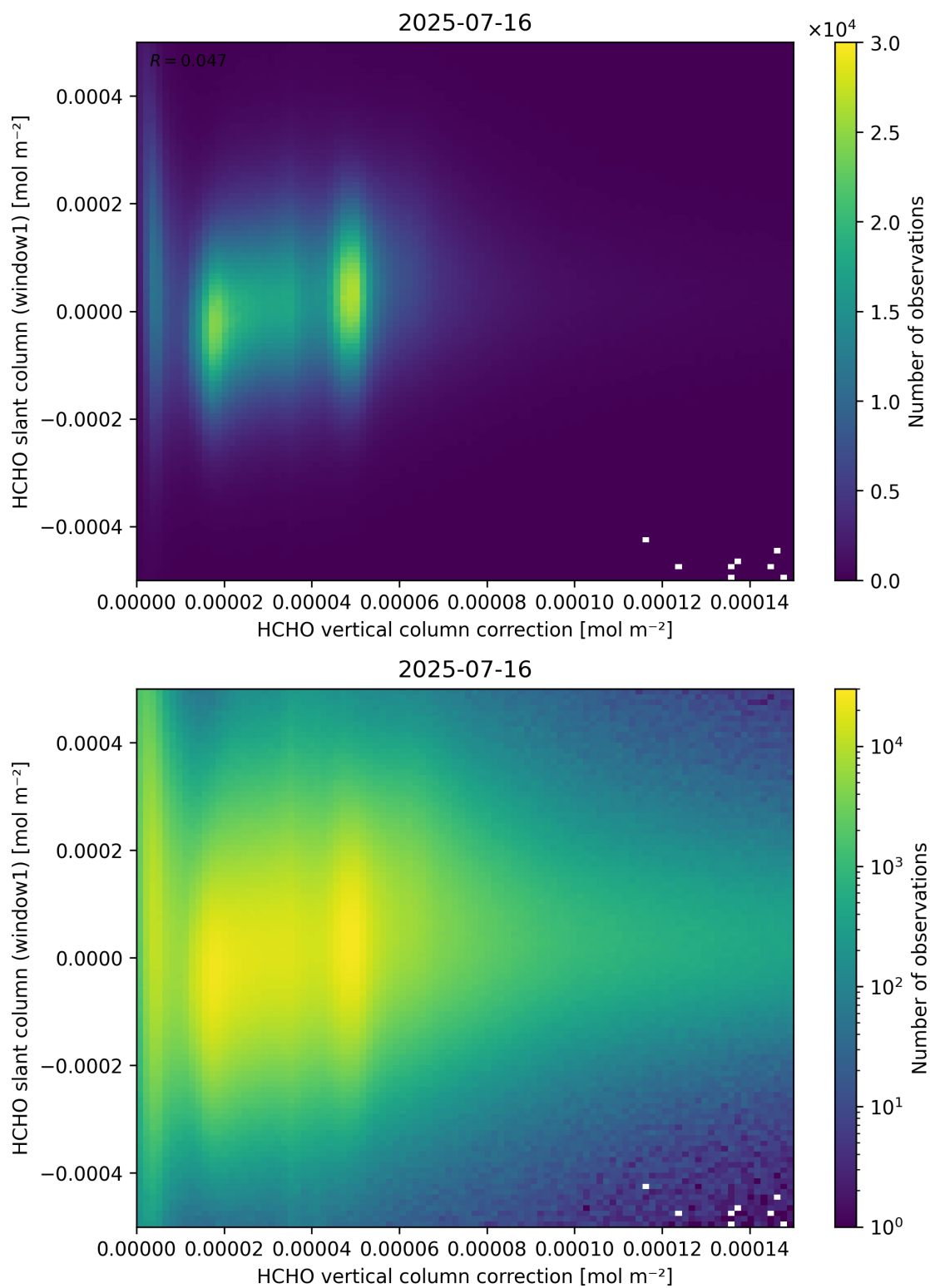
Figure 118: Scatter density plot of “HCHO vertical column correction” against “HCHO slant column (window1)” for 2025-07-15 to 2025-07-17.
