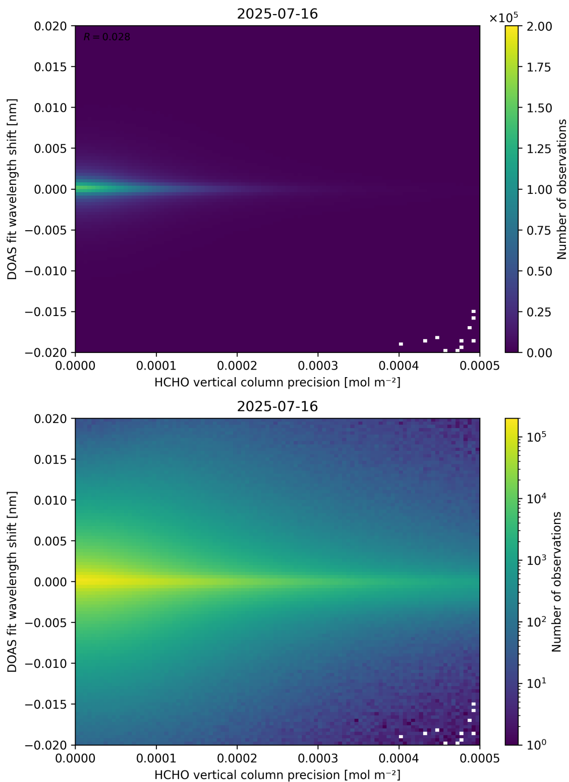
Figure 137: Scatter density plot of “HCHO vertical column precision” against “DOAS fit wavelength shift” for 2025-07-15 to 2025-07-17.
