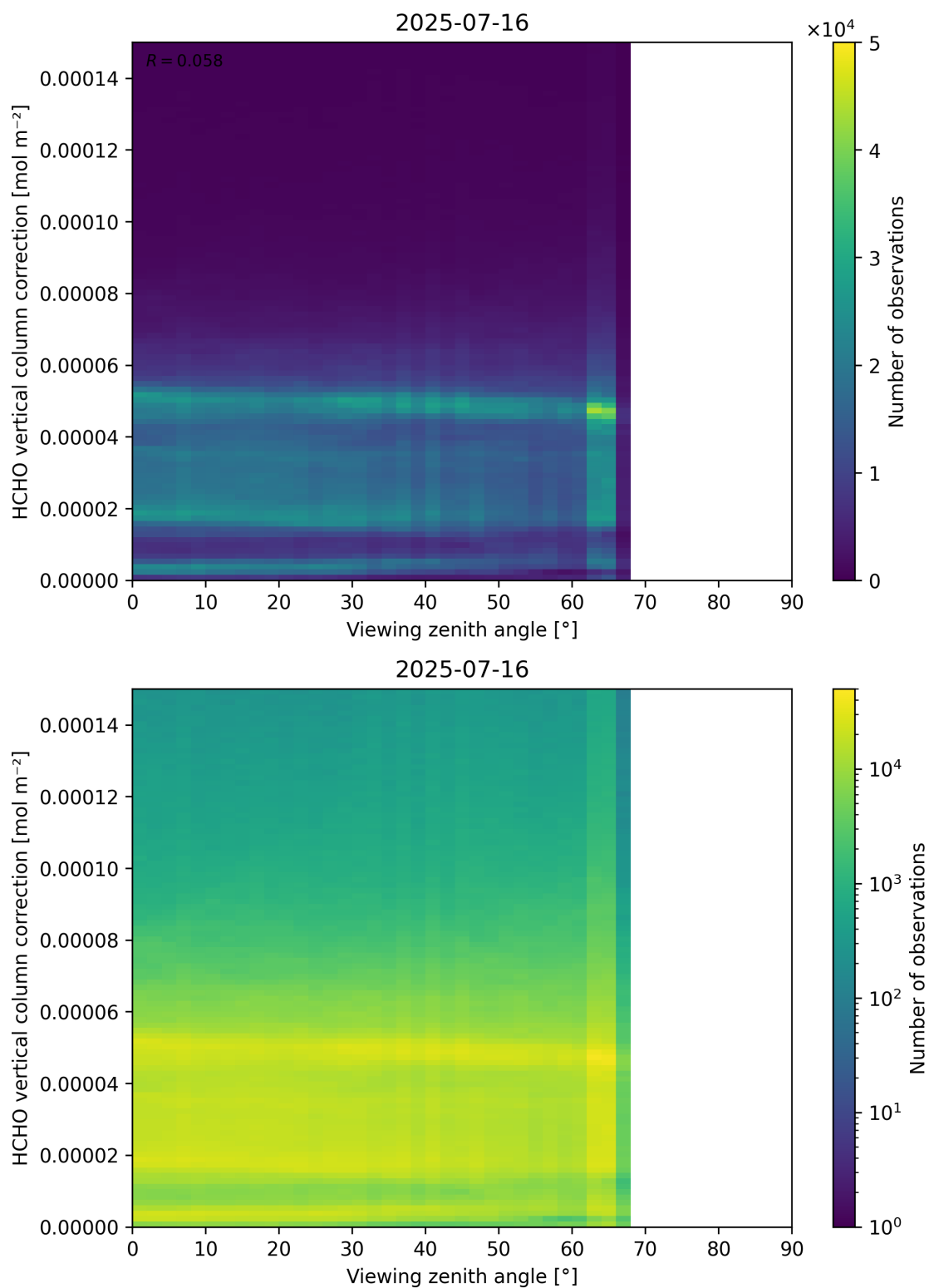
Figure 193: Scatter density plot of “Viewing zenith angle” against “HCHO vertical column correction” for 2025-07-15 to 2025-07-17.
