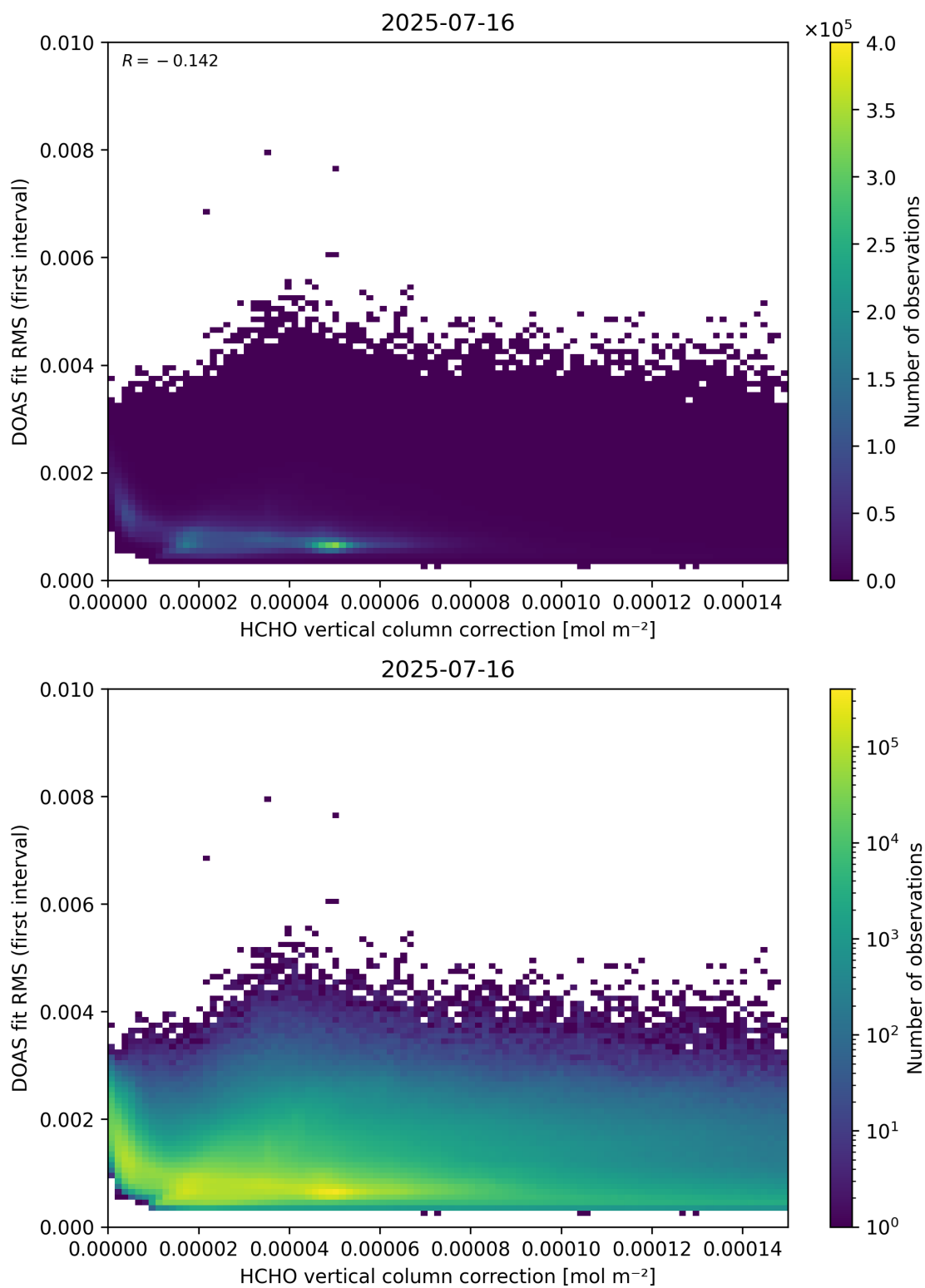
Figure 112: Scatter density plot of “HCHO vertical column correction” against “DOAS fit RMS (first interval)” for 2025-07-15 to 2025-07-17.
