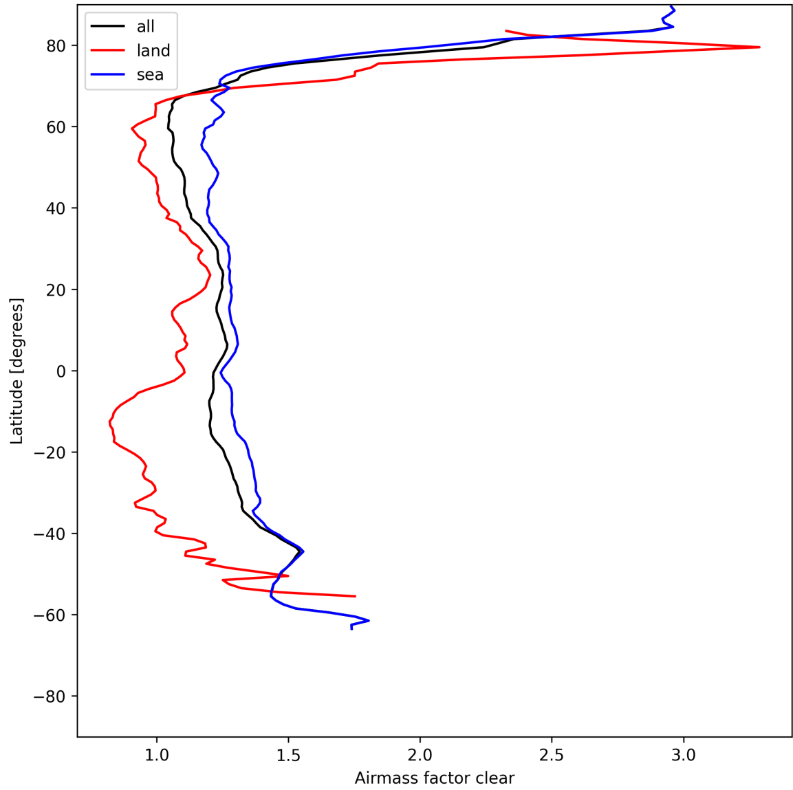
Figure 28: Zonal average of “Airmass factor clear” for 2025-07-15 to 2025-07-17.
