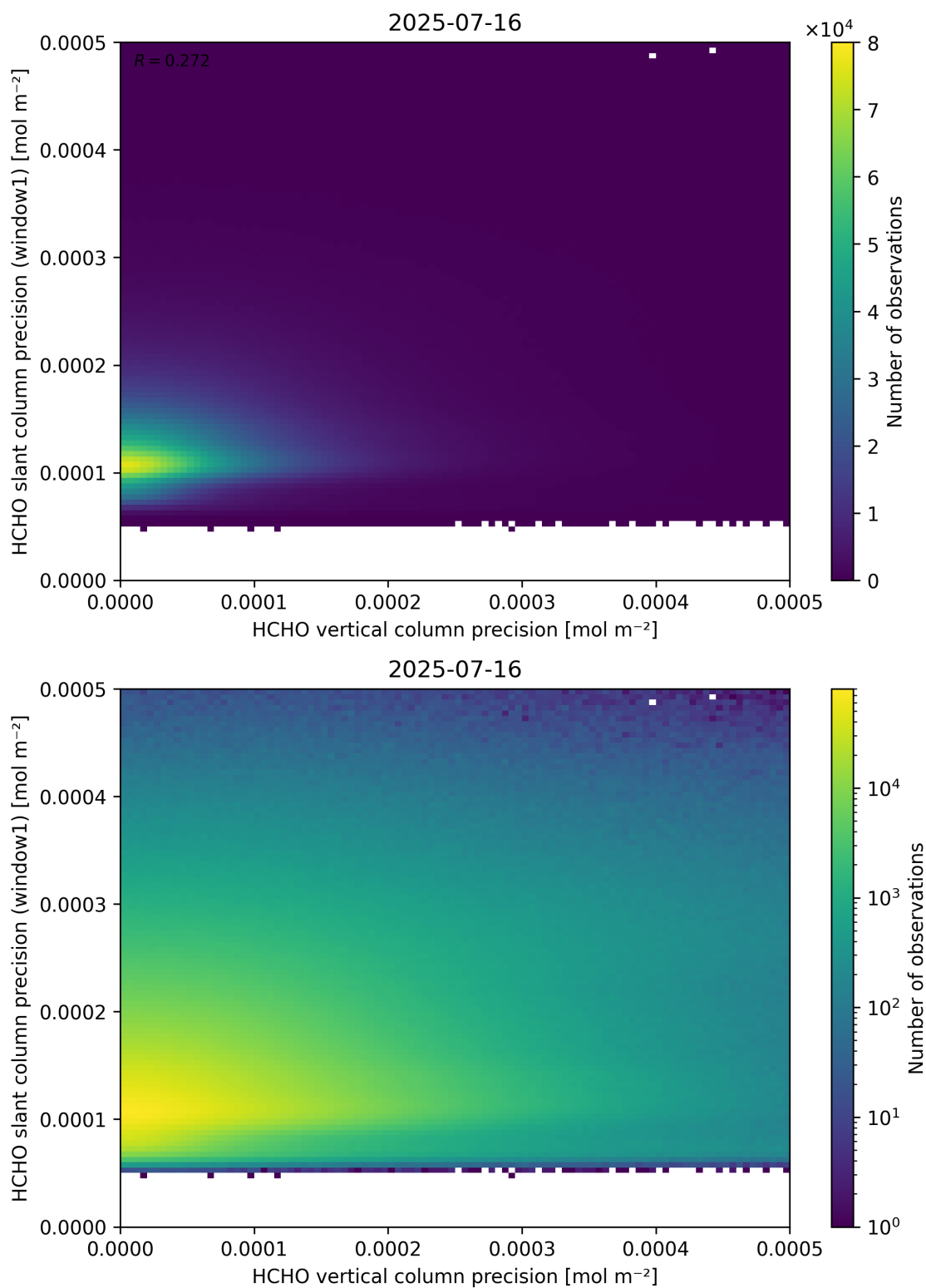
Figure 143: Scatter density plot of “HCHO vertical column precision” against “HCHO slant column precision (window1)” for 2025-07-15 to 2025-07-17.
