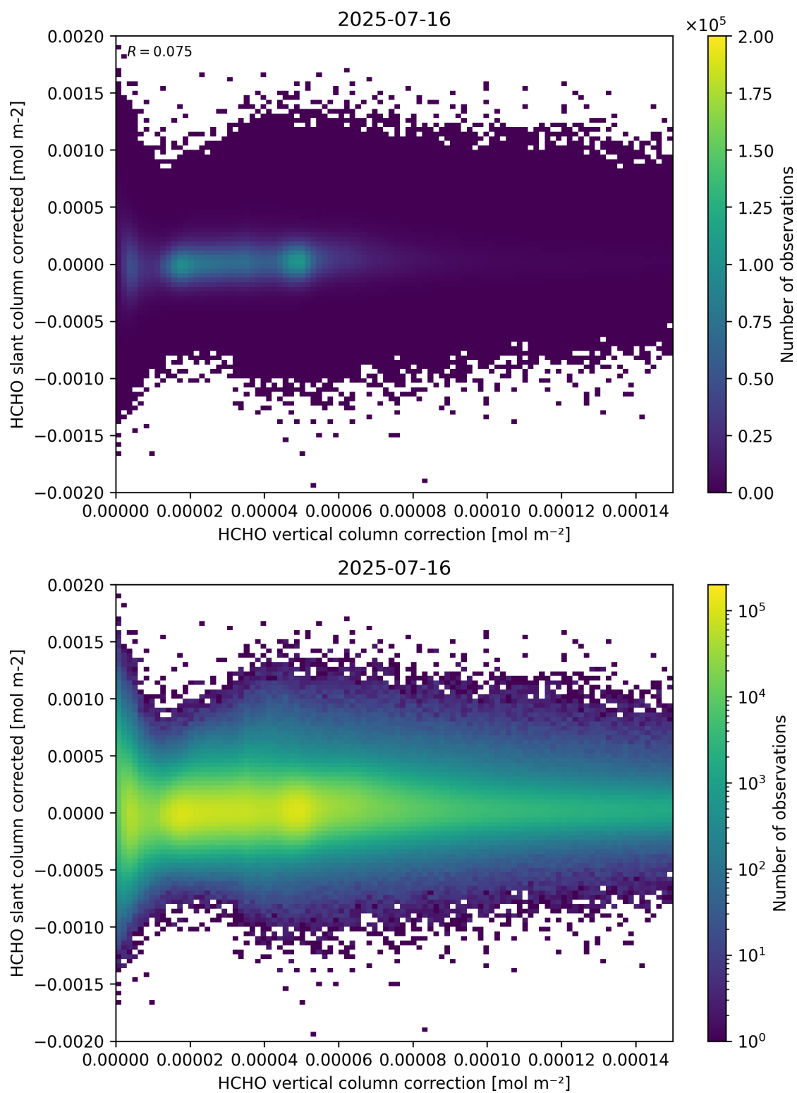
Figure 116: Scatter density plot of “HCHO vertical column correction” against “HCHO slant column corrected” for 2025-07-15 to 2025-07-17.
