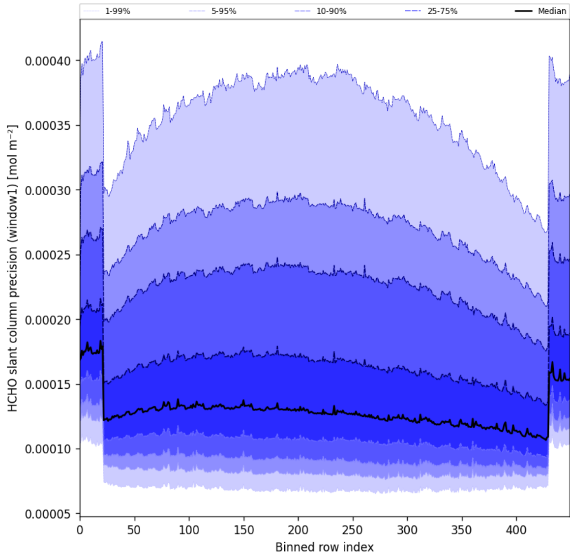
Figure 53: Along track statistics of “HCHO slant column precision (window1)” for 2025-07-15 to 2025-07-17
