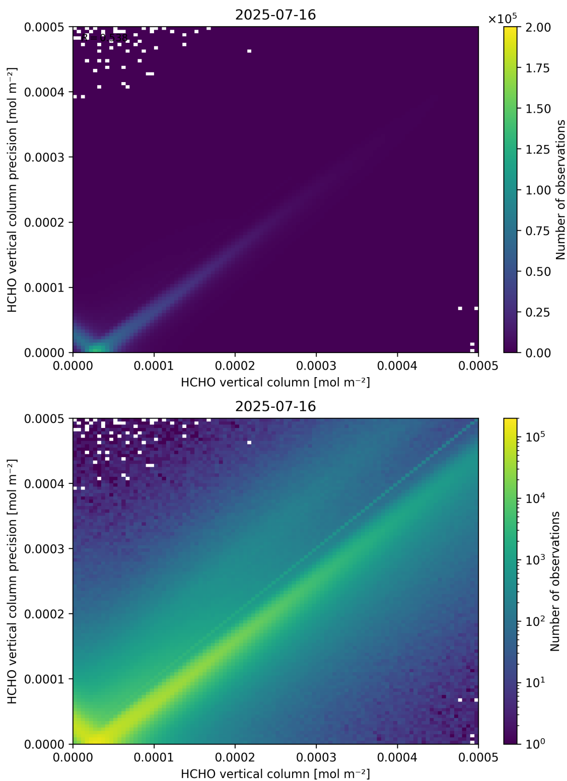
Figure 134: Scatter density plot of “HCHO vertical column” against “HCHO vertical column precision” for 2025-07-15 to 2025-07-17.
