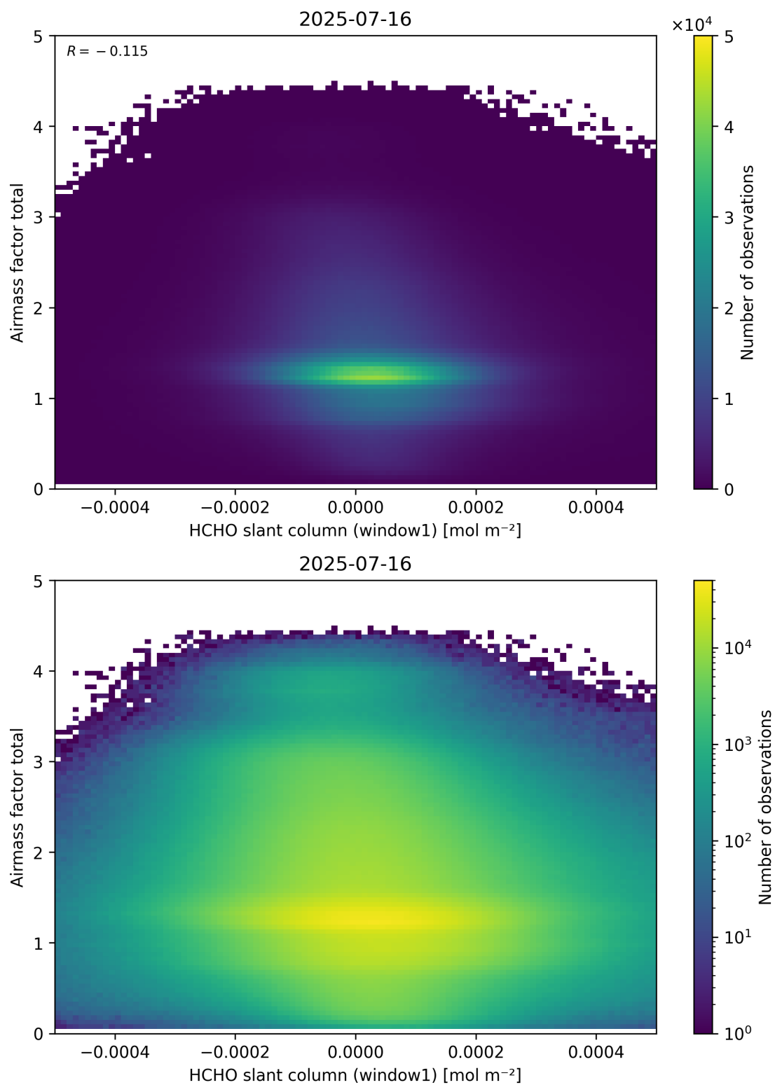
Figure 85: Scatter density plot of “HCHO slant column (window1)” against “Airmass factor total” for 2025-07-15 to 2025-07-17.
