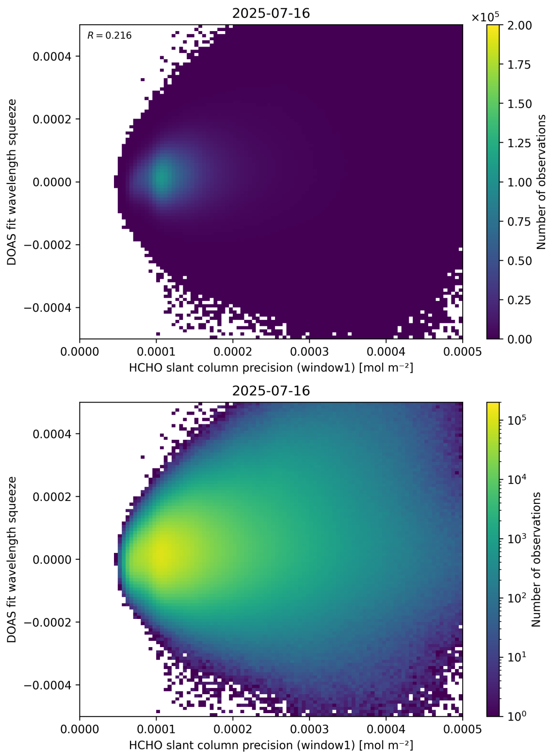
Figure 90: Scatter density plot of “HCHO slant column precision (window1)” against “DOAS fit wavelength squeeze” for 2025-07-15 to 2025-07-17.
