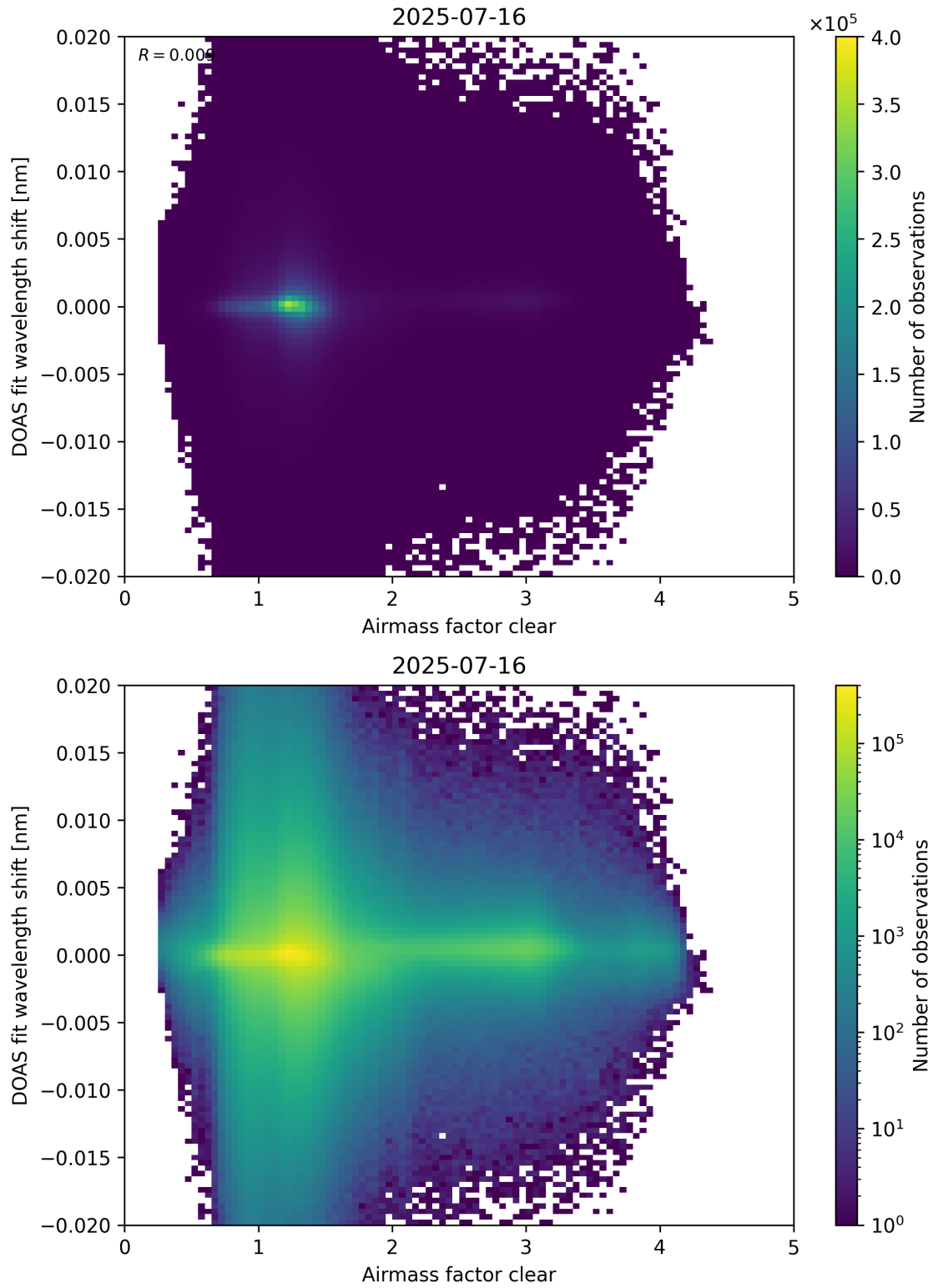
Figure 72: Scatter density plot of “Airmass factor clear” against “DOAS fit wavelength shift” for 2025-07-15 to 2025-07-17.
