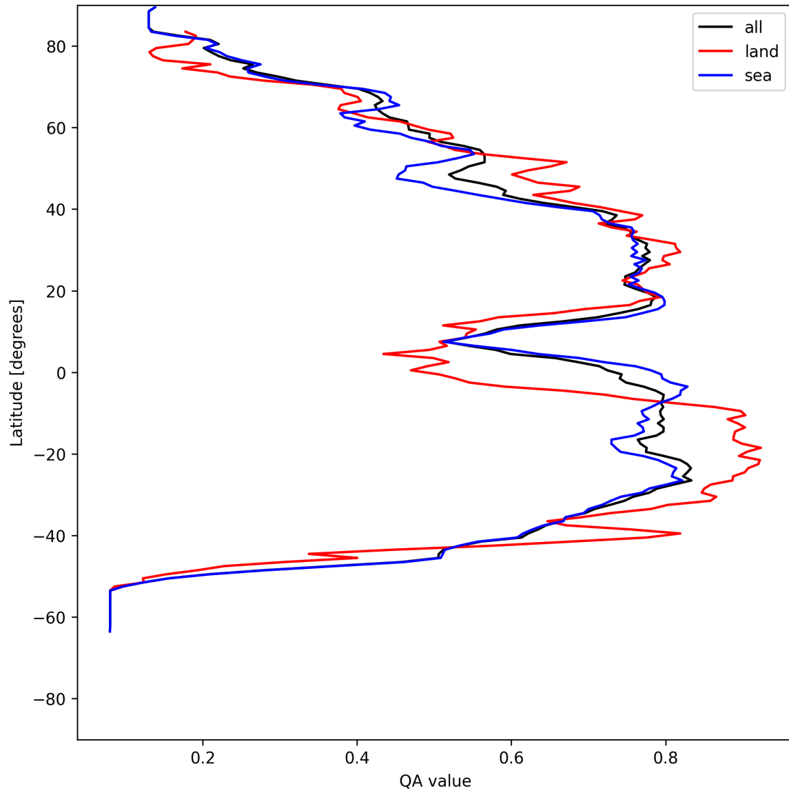
Figure 20: Zonal average of “QA value” for 2025-07-15 to 2025-07-17.
