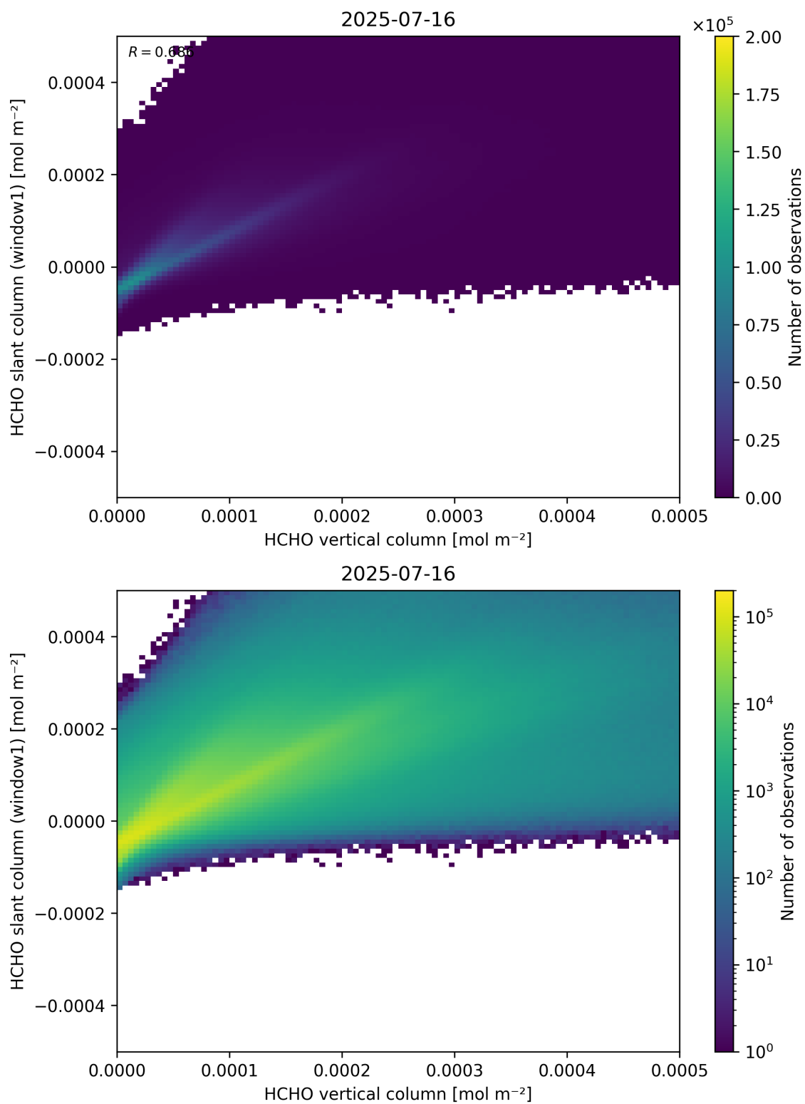
Figure 129: Scatter density plot of “HCHO vertical column” against “HCHO slant column (window1)” for 2025-07-15 to 2025-07-17.
