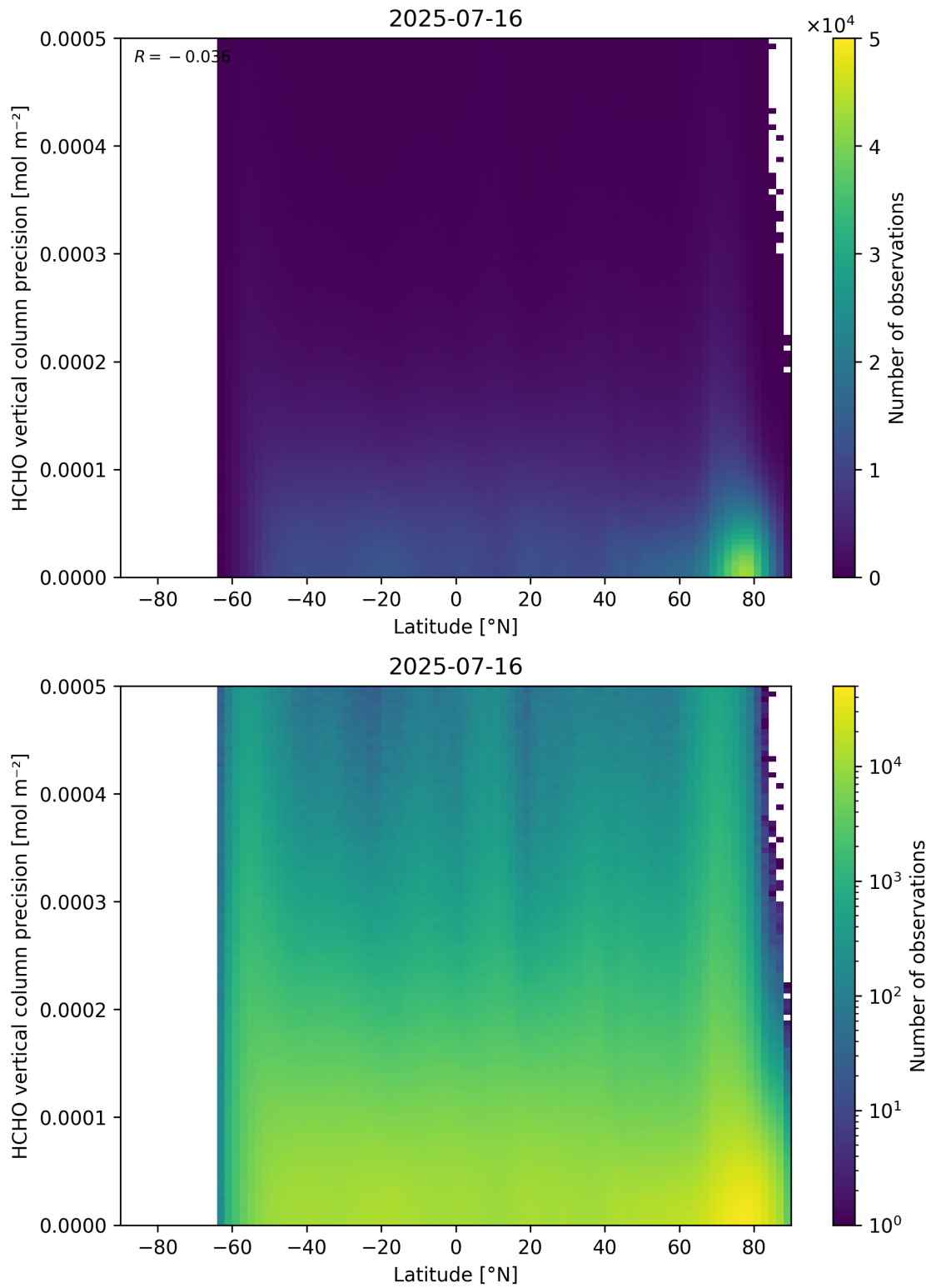
Figure 165: Scatter density plot of “Latitude” against “HCHO vertical column precision” for 2025-07-15 to 2025-07-17.
