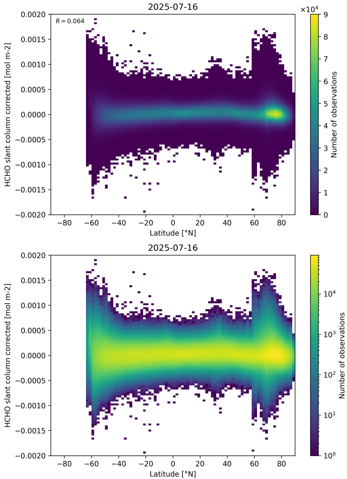
Figure 157: Scatter density plot of “Latitude” against “HCHO slant column corrected” for 2025-07-15 to 2025-07-17.
