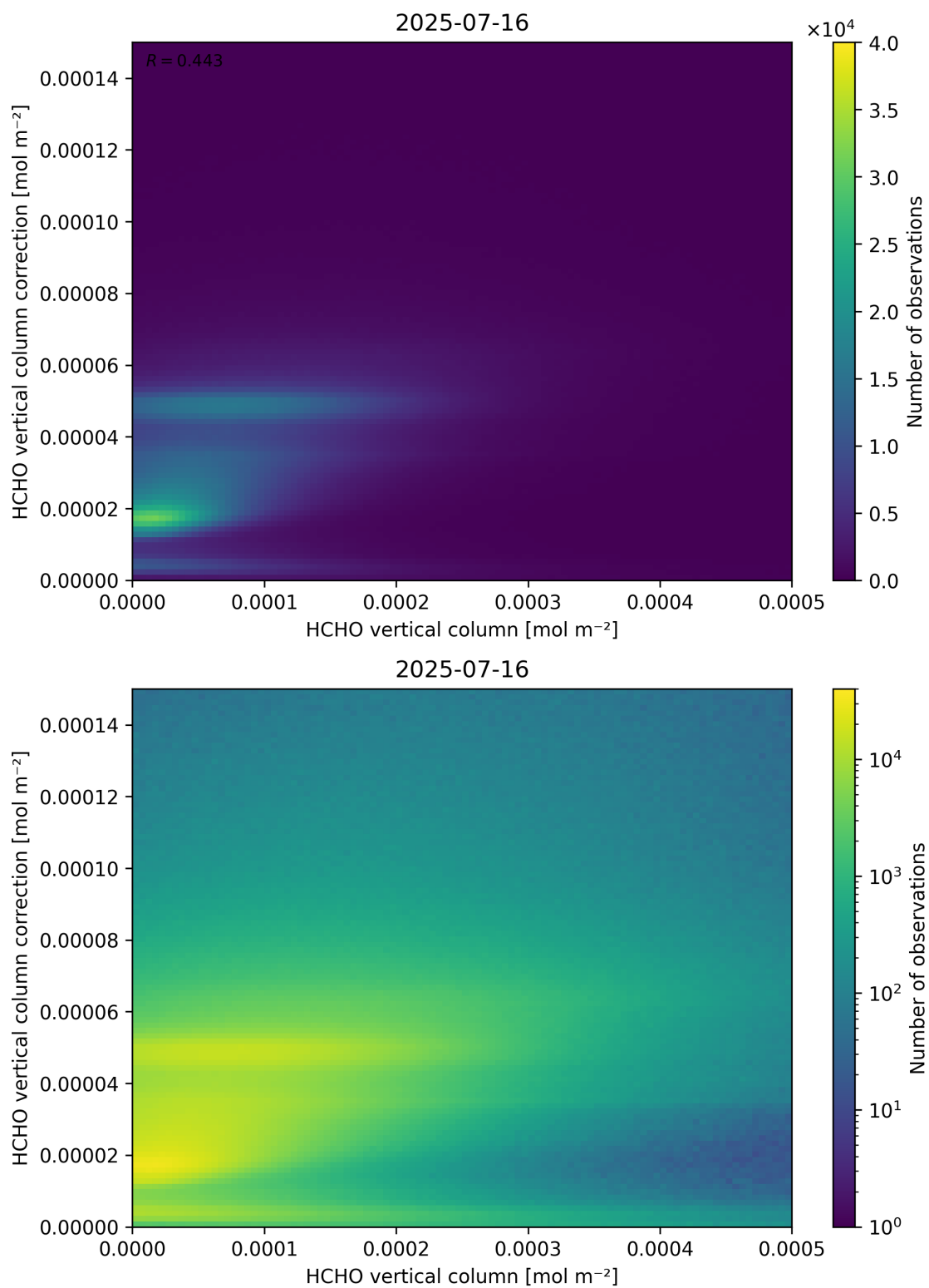
Figure 133: Scatter density plot of “HCHO vertical column” against “HCHO vertical column correction” for 2025-07-15 to 2025-07-17.
