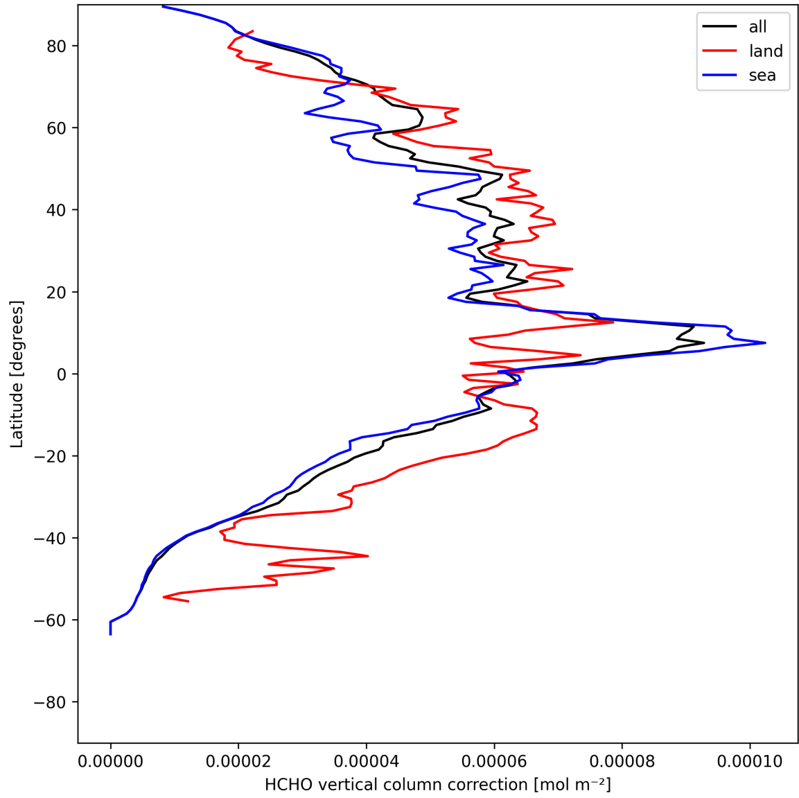
Figure 23: Zonal average of “HCHO vertical column correction” for 2025-07-15 to 2025-07-17.
