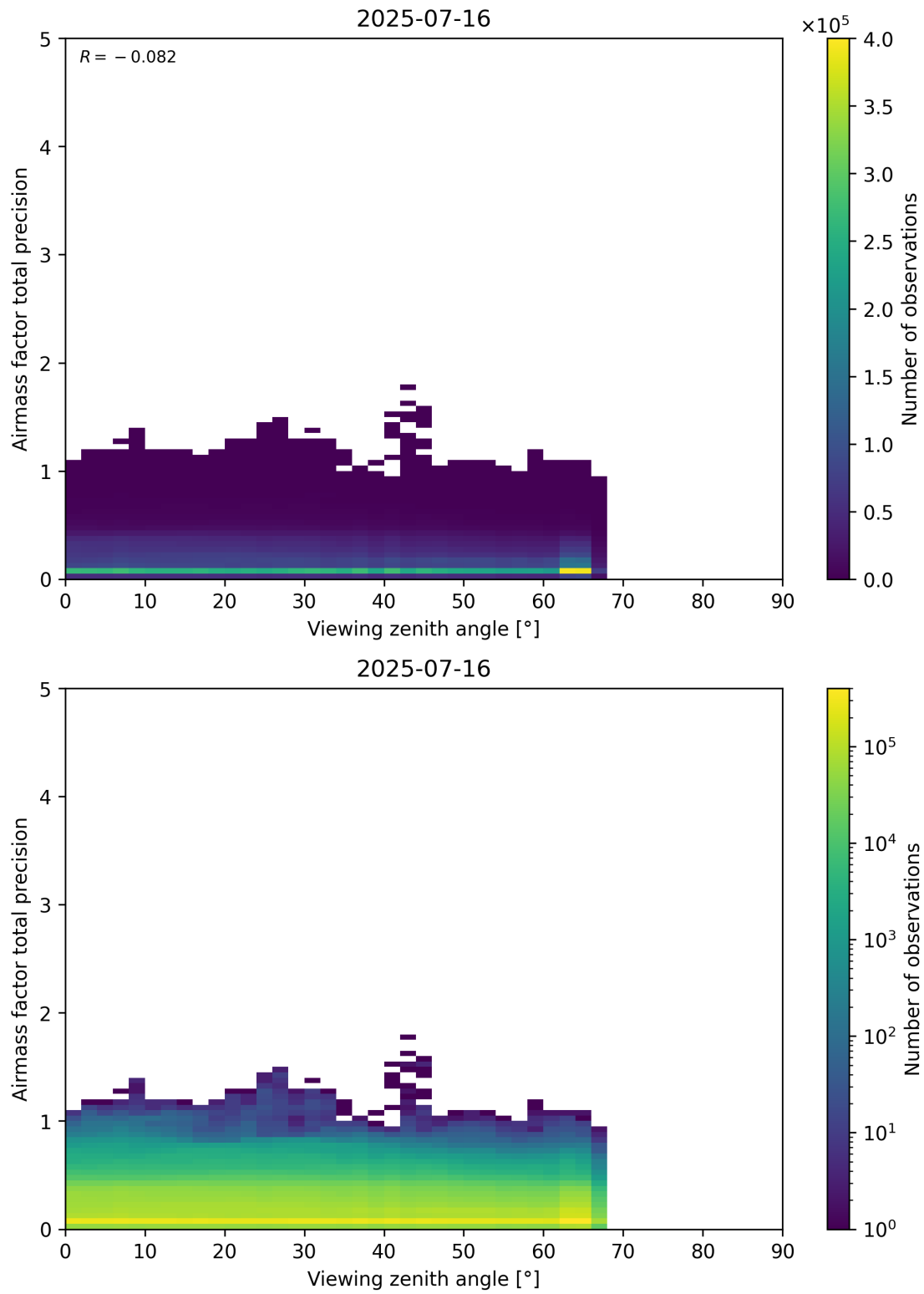
Figure 191: Scatter density plot of “Viewing zenith angle” against “Airmass factor total precision” for 2025-07-15 to 2025-07-17.
