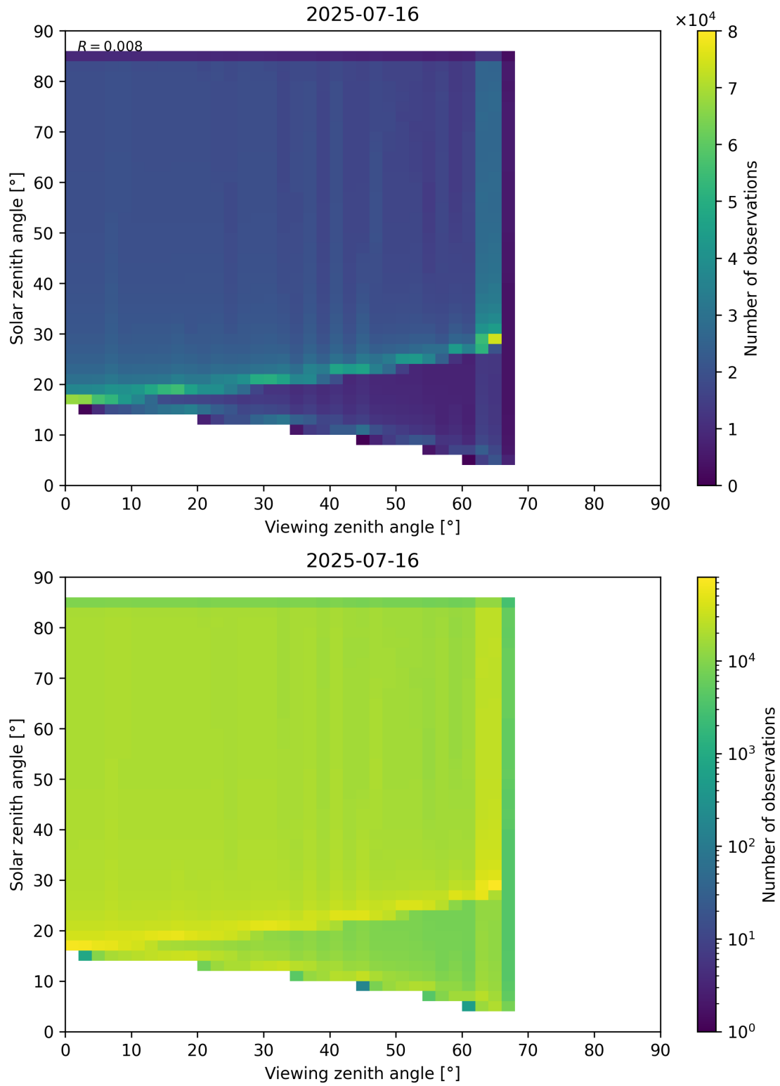
Figure 197: Scatter density plot of “Viewing zenith angle” against “Solar zenith angle” for 2025-07-15 to 2025-07-17.
