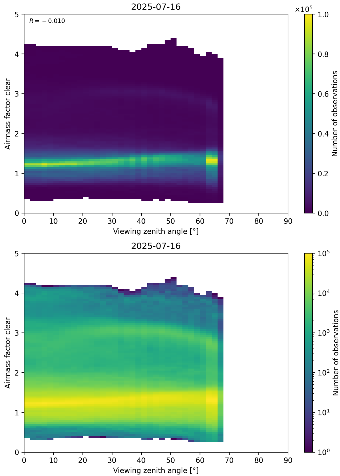
Figure 185: Scatter density plot of “Viewing zenith angle” against “Airmass factor clear” for 2025-07-15 to 2025-07-17.
