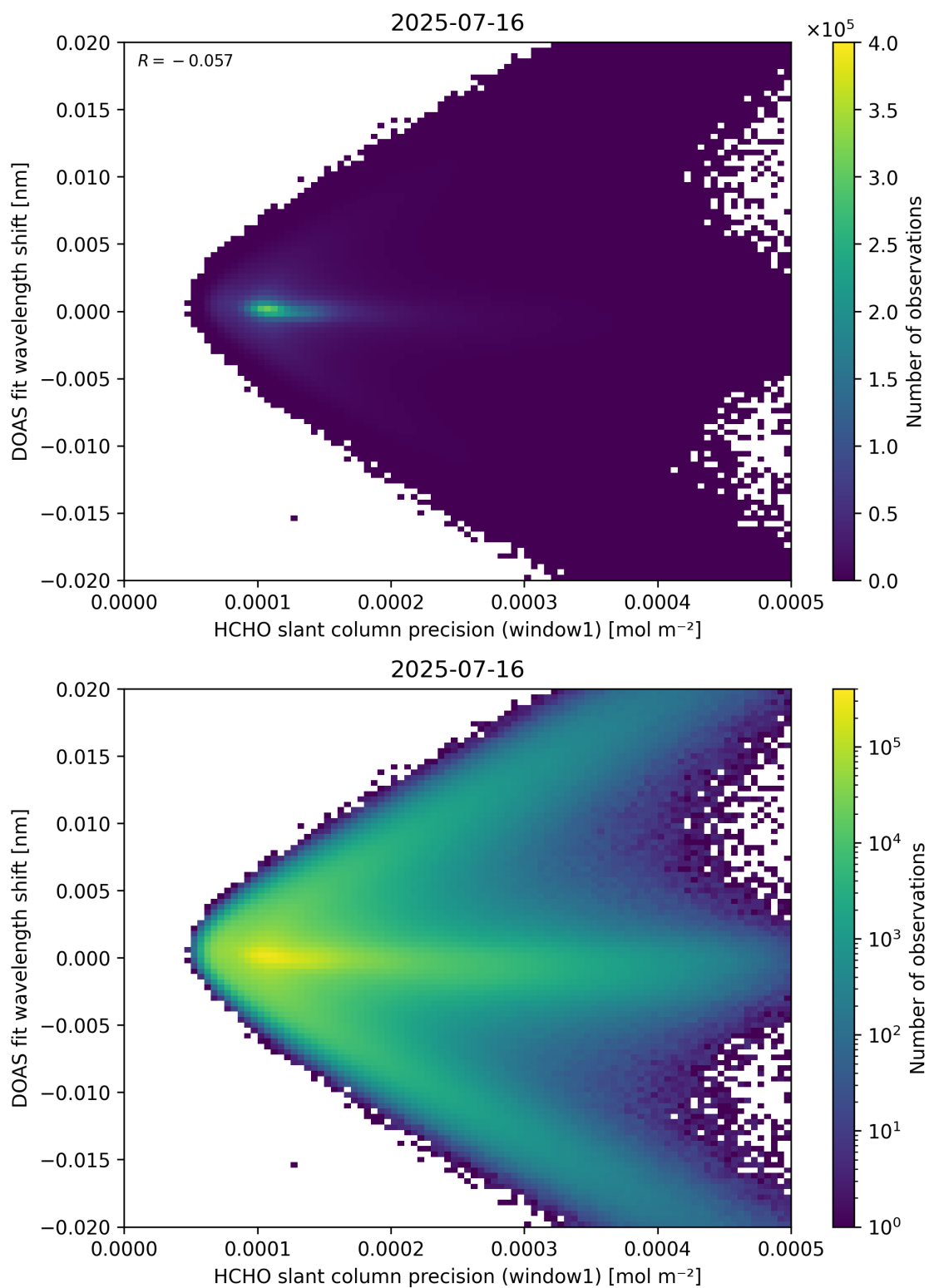
Figure 89: Scatter density plot of “HCHO slant column precision (window1)” against “DOAS fit wavelength shift” for 2025-07-15 to 2025-07-17.
