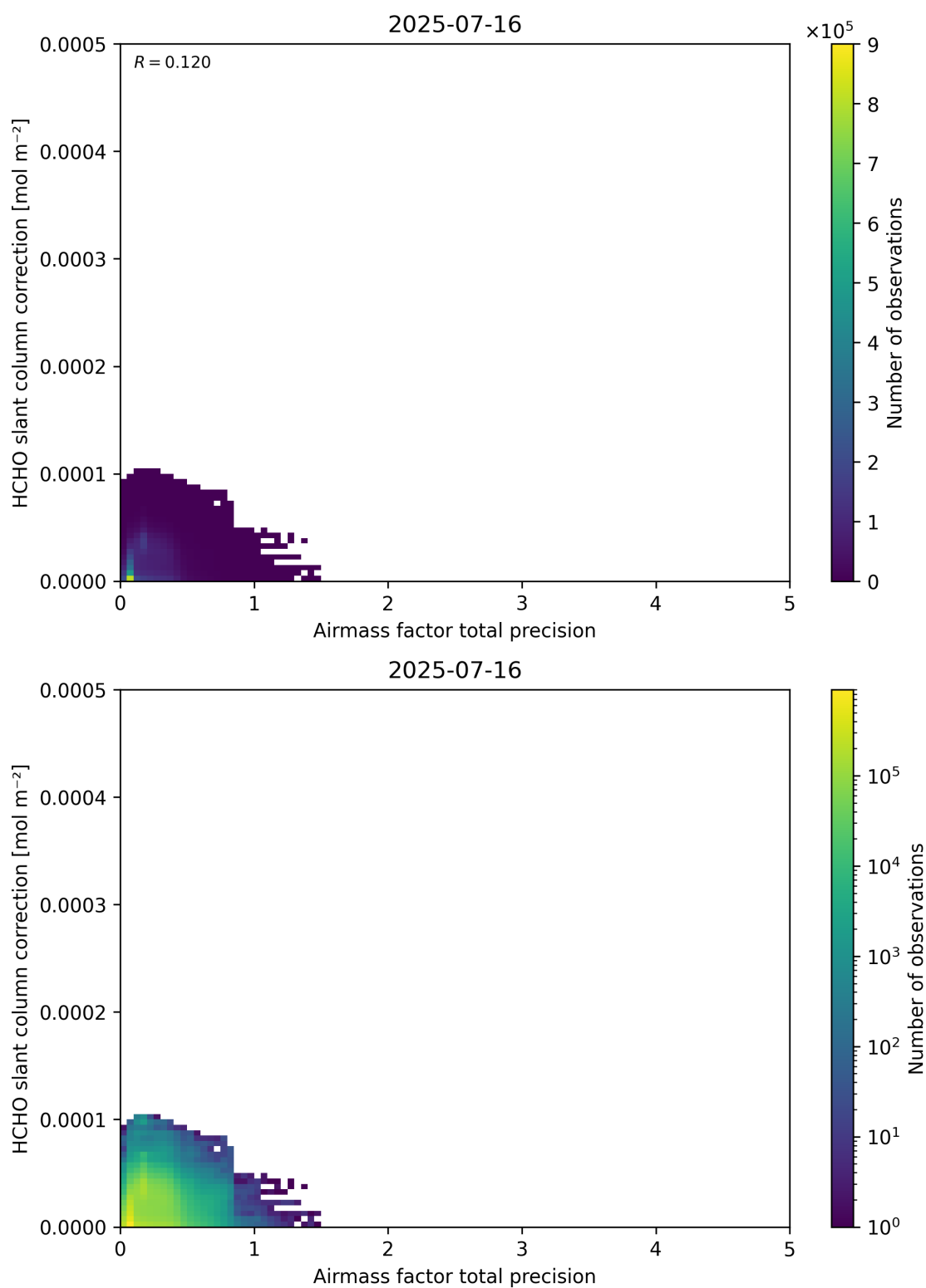
Figure 110: Scatter density plot of “Airmass factor total precision” against “HCHO slant column correction” for 2025-07-15 to 2025-07-17.
