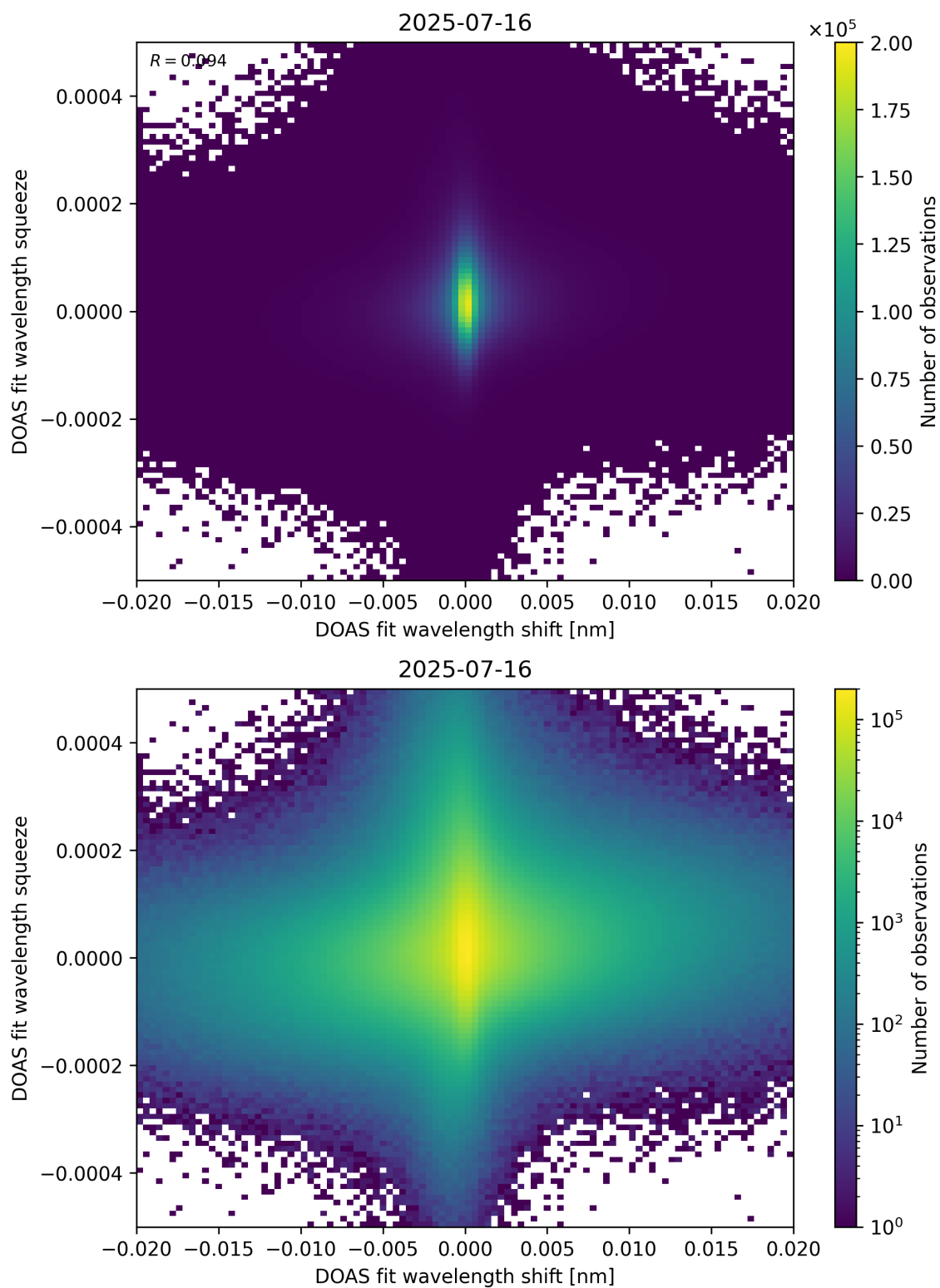
Figure 65: Scatter density plot of “DOAS fit wavelength shift” against “DOAS fit wavelength squeeze” for 2025-07-15 to 2025-07-17.
