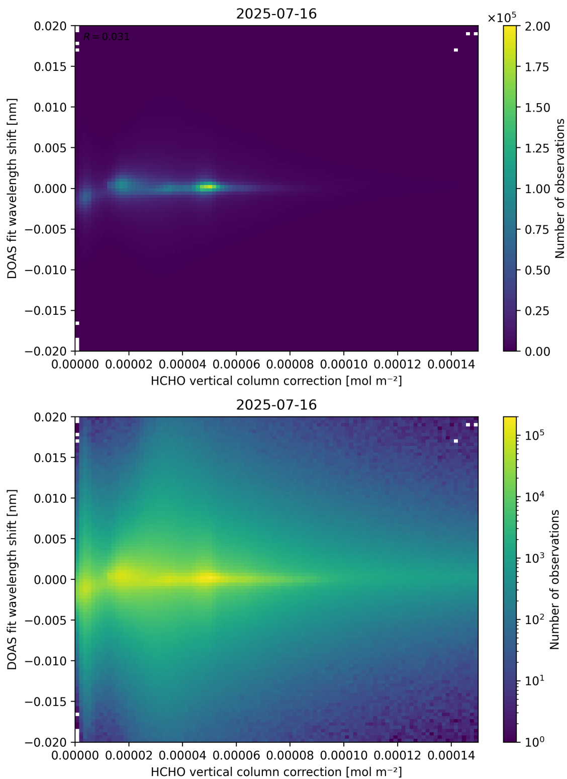
Figure 113: Scatter density plot of “HCHO vertical column correction” against “DOAS fit wavelength shift” for 2025-07-15 to 2025-07-17.
