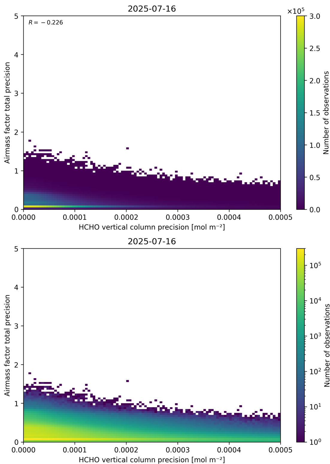
Figure 145: Scatter density plot of “HCHO vertical column precision” against “Airmass factor total precision” for 2025-07-15 to 2025-07-17.
