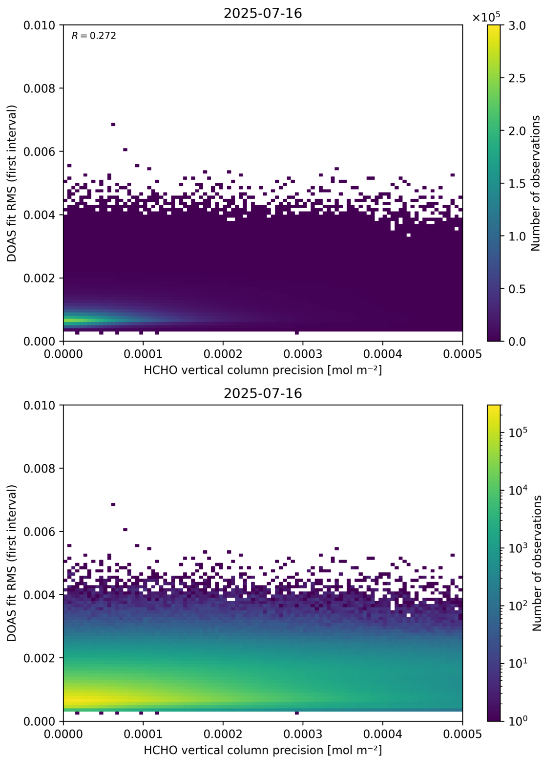
Figure 136: Scatter density plot of “HCHO vertical column precision” against “DOAS fit RMS (first interval)” for 2025-07-15 to 2025-07-17.
