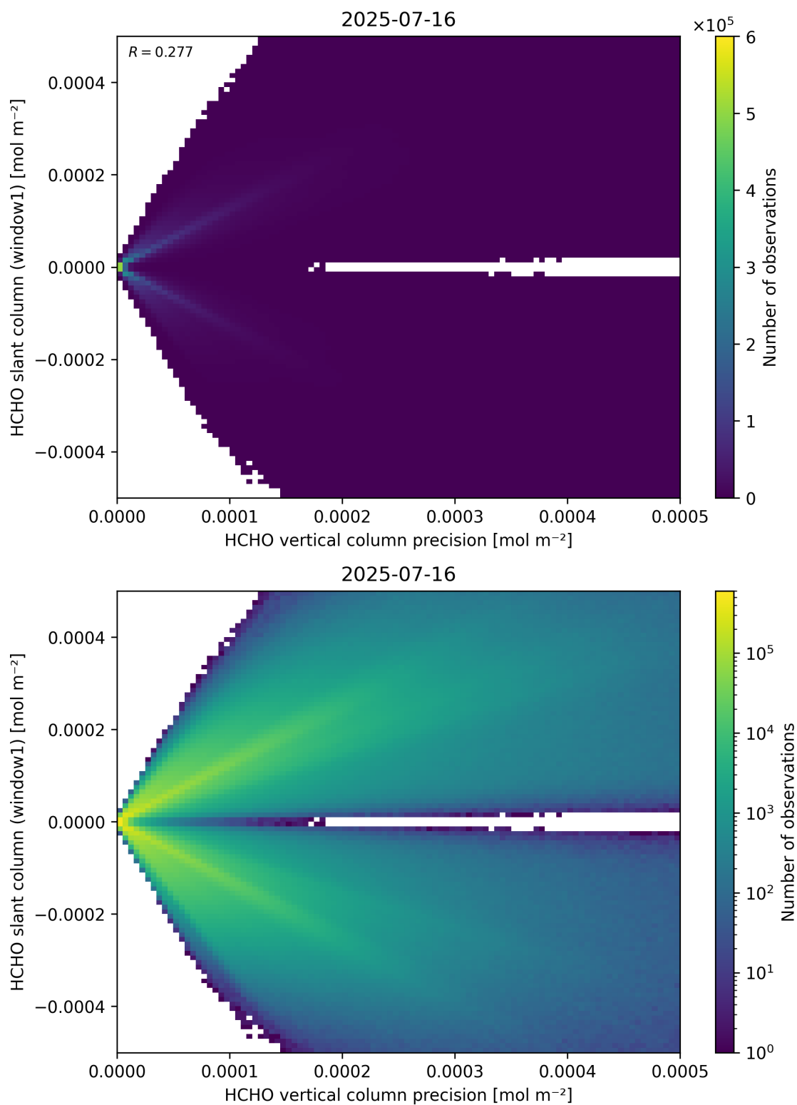
Figure 142: Scatter density plot of “HCHO vertical column precision” against “HCHO slant column (window1)” for 2025-07-15 to 2025-07-17.
