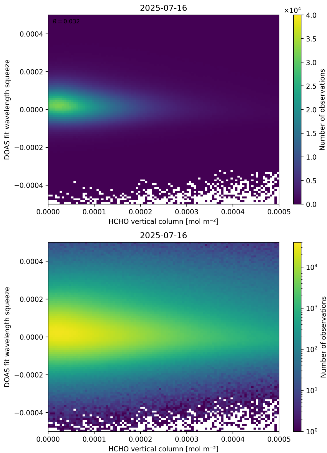
Figure 125: Scatter density plot of “HCHO vertical column” against “DOAS fit wavelength squeeze” for 2025-07-15 to 2025-07-17.
