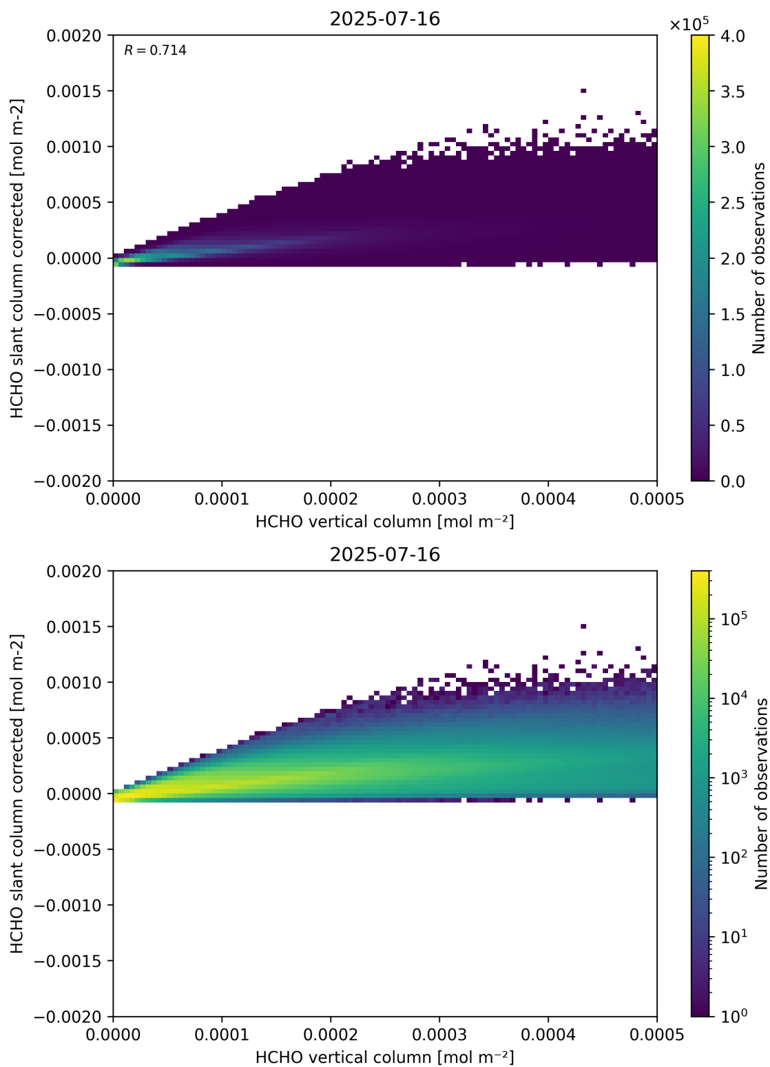
Figure 127: Scatter density plot of “HCHO vertical column” against “HCHO slant column corrected” for 2025-07-15 to 2025-07-17.
