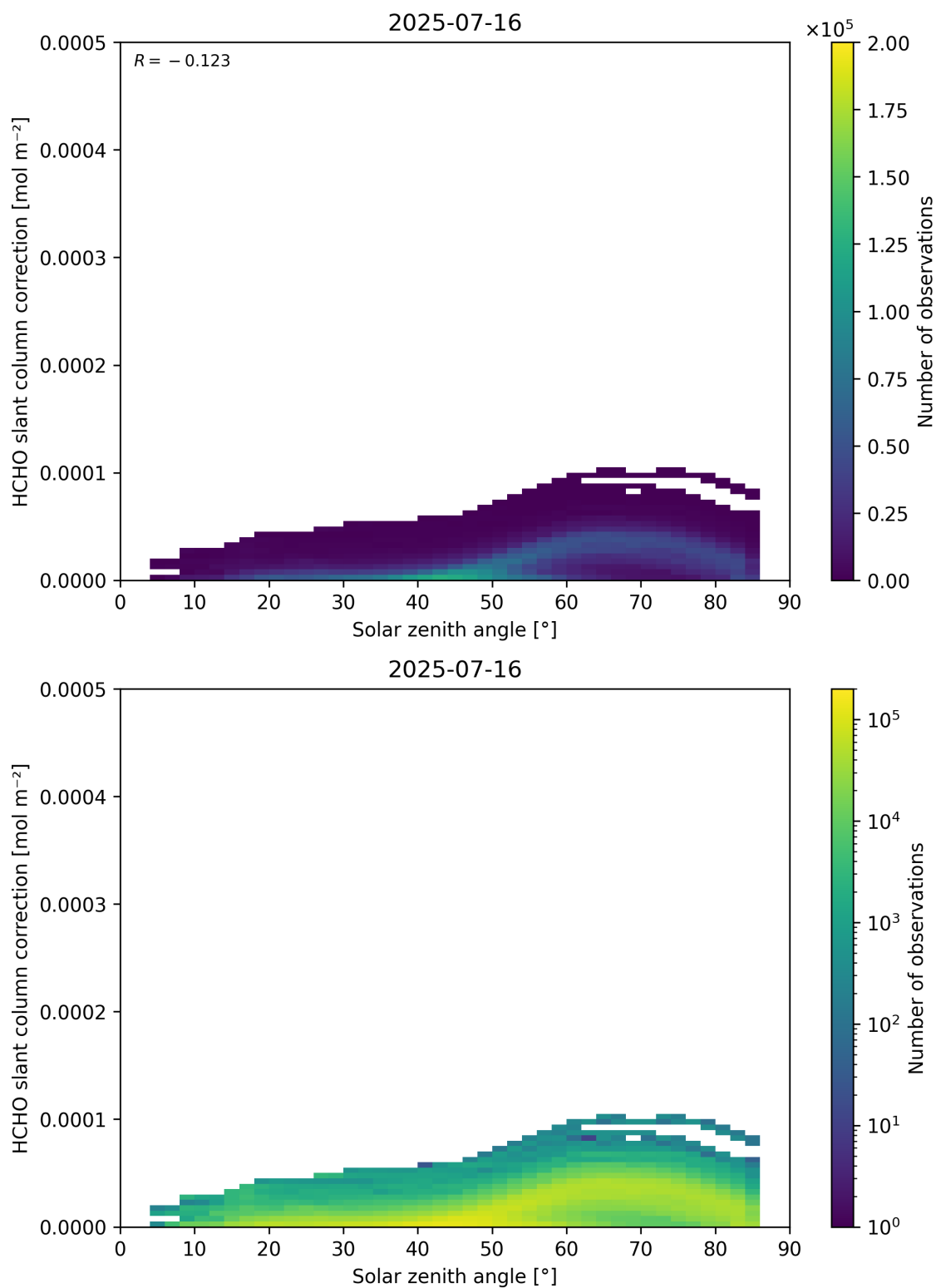
Figure 172: Scatter density plot of “Solar zenith angle” against “HCHO slant column correction” for 2025-07-15 to 2025-07-17.
