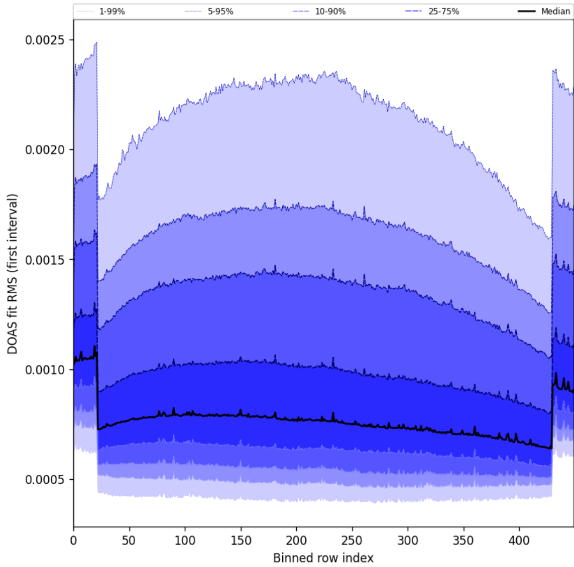
Figure 60: Along track statistics of “DOAS fit RMS (first interval)” for 2025-07-15 to 2025-07-17
