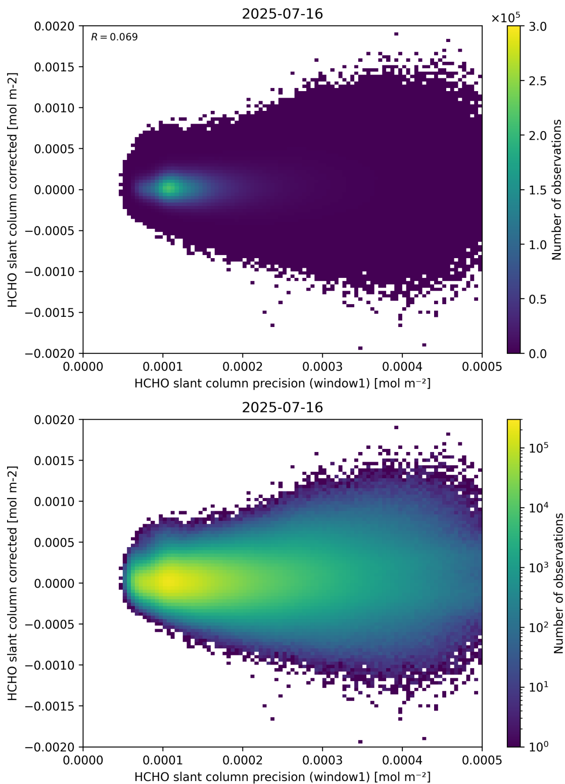
Figure 92: Scatter density plot of “HCHO slant column precision (window1)” against “HCHO slant column corrected” for 2025-07-15 to 2025-07-17.
