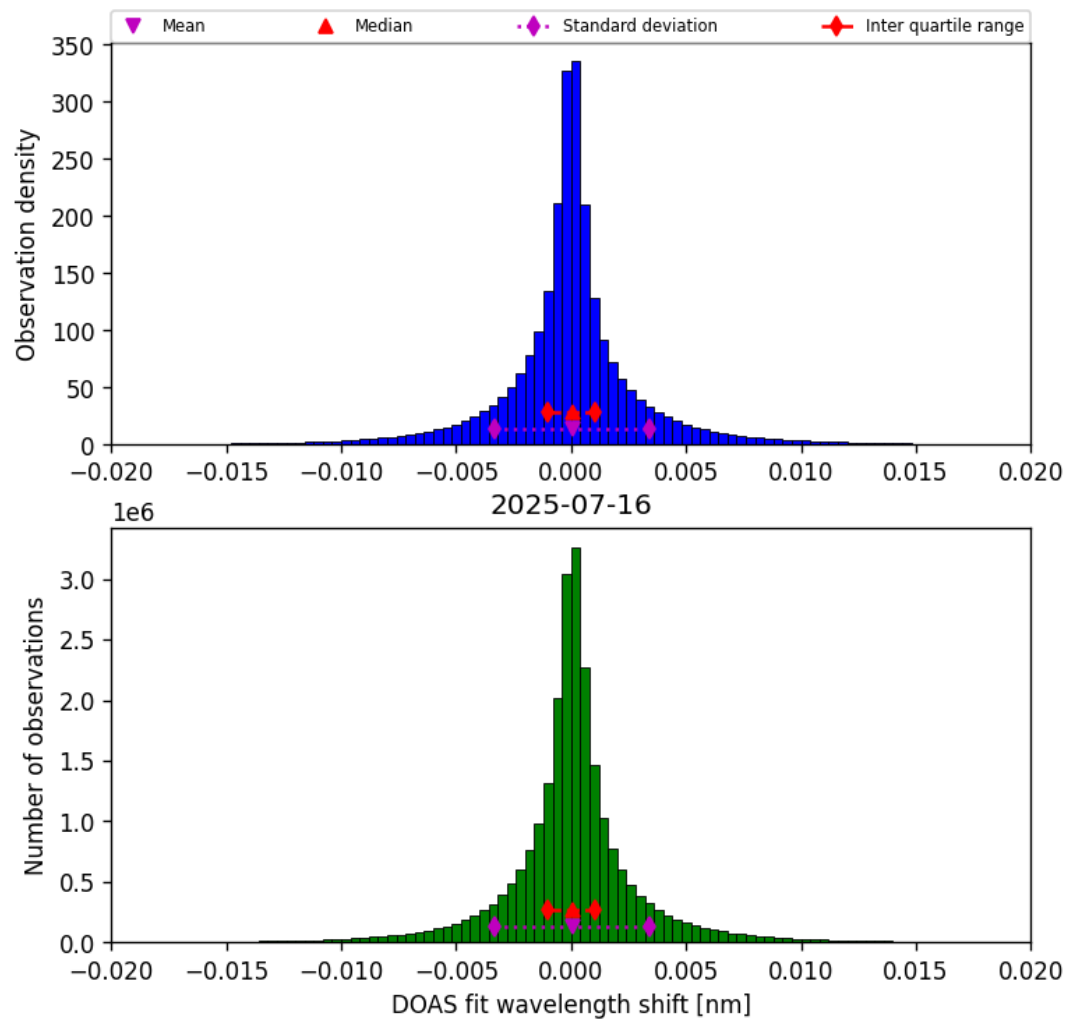
Figure 44: Histogram of “DOAS fit wavelength shift” for 2025-07-15 to 2025-07-17
