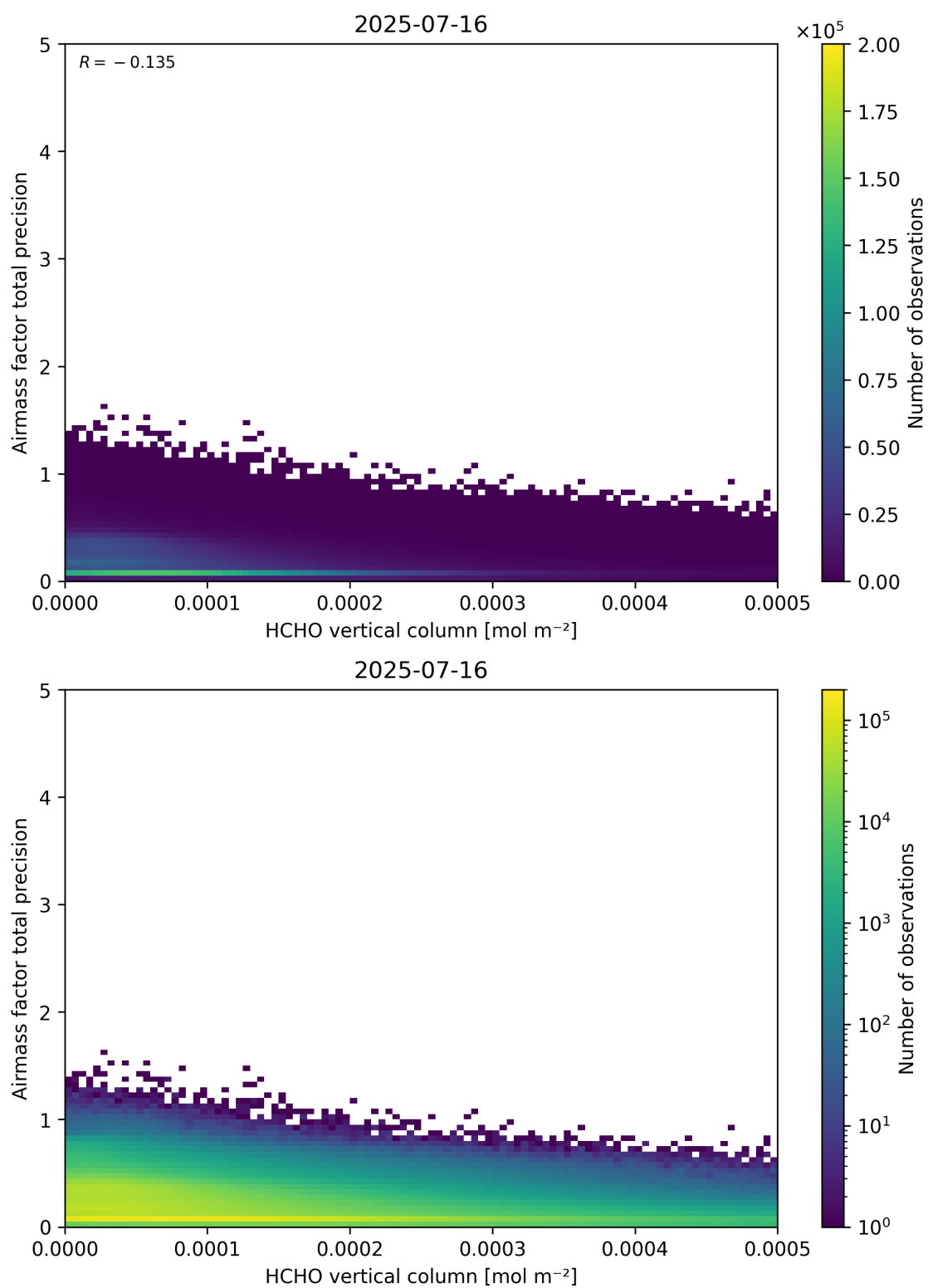
Figure 132: Scatter density plot of “HCHO vertical column” against “Airmass factor total precision” for 2025-07-15 to 2025-07-17.
