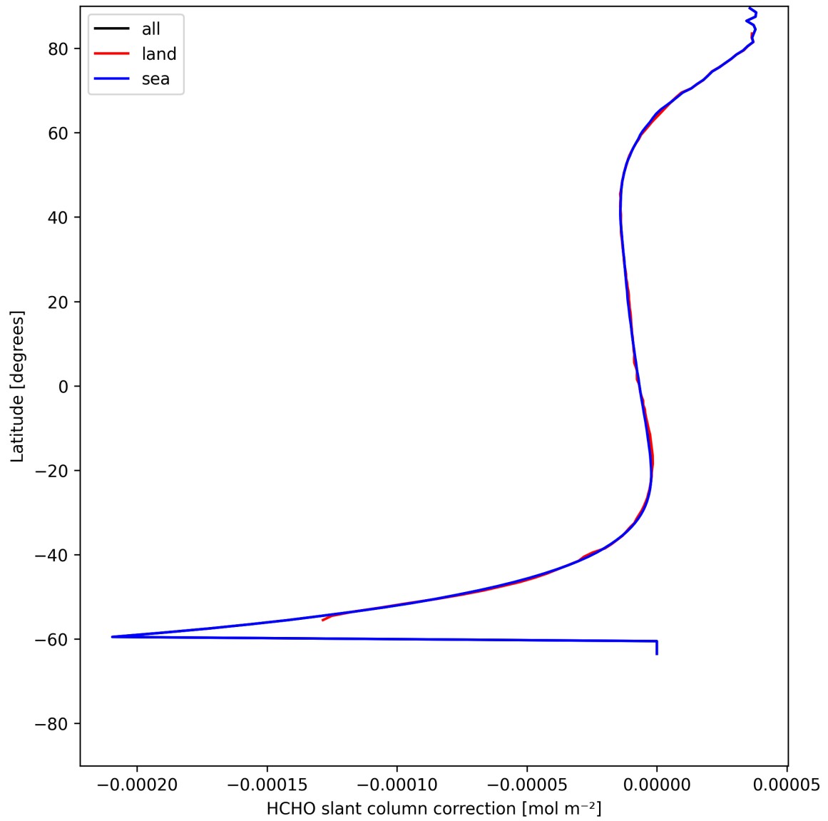
Figure 33: Zonal average of “HCHO slant column correction” for 2025-07-15 to 2025-07-17.
