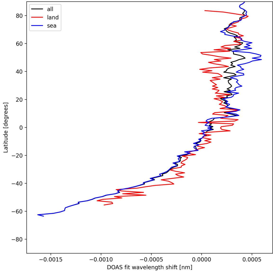
Figure 30: Zonal average of “DOAS fit wavelength shift” for 2025-07-15 to 2025-07-17.
