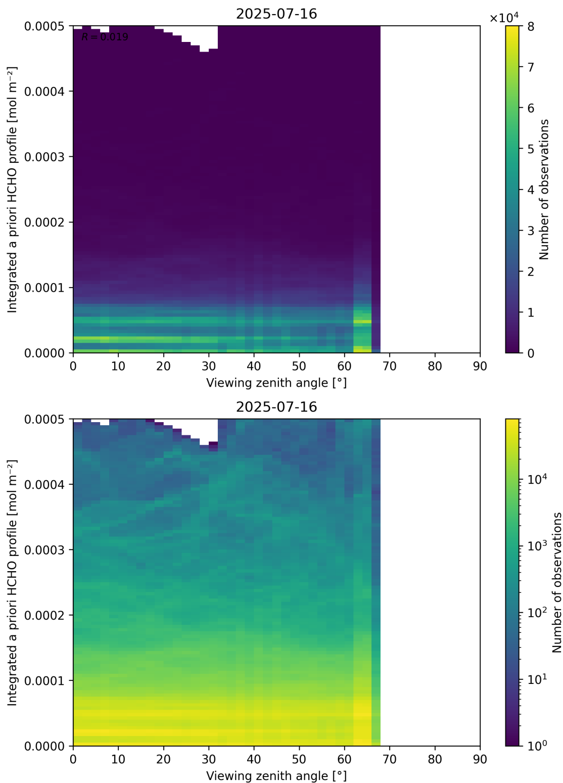
Figure 195: Scatter density plot of “Viewing zenith angle” against “Integrated a priori HCHO profile” for 2025-07-15 to 2025-07-17.
