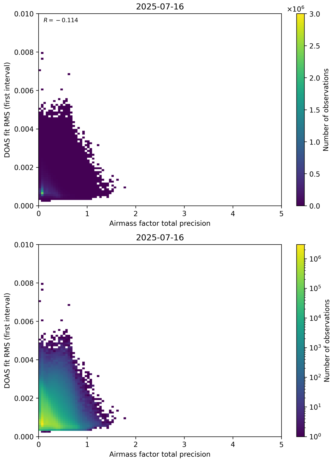
Figure 105: Scatter density plot of “Airmass factor total precision” against “DOAS fit RMS (first interval)” for 2025-07-15 to 2025-07-17.
