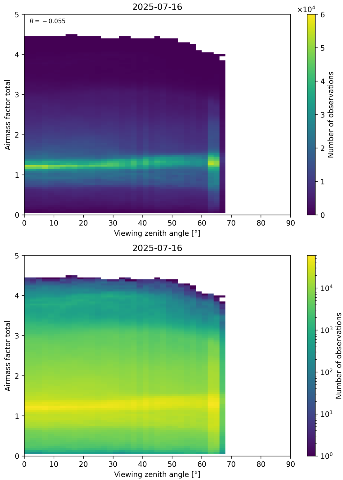
Figure 190: Scatter density plot of “Viewing zenith angle” against “Airmass factor total” for 2025-07-15 to 2025-07-17.
