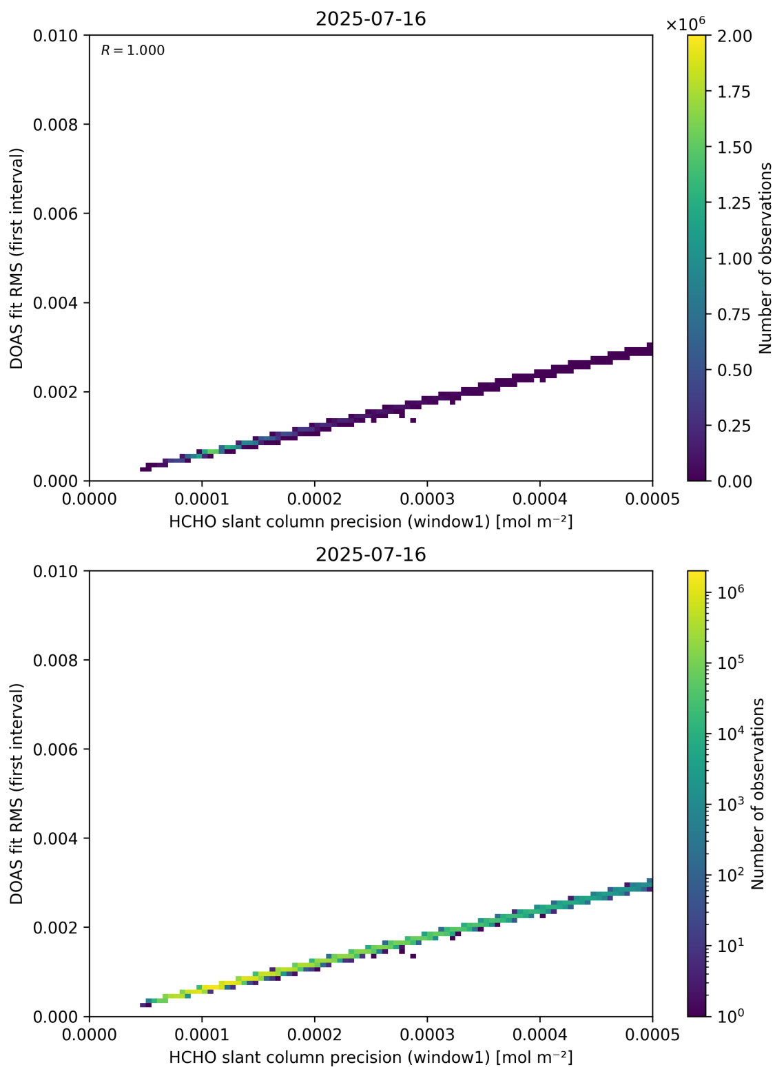
Figure 88: Scatter density plot of “HCHO slant column precision (window1)” against “DOAS fit RMS (first interval)” for 2025-07-15 to 2025-07-17.
