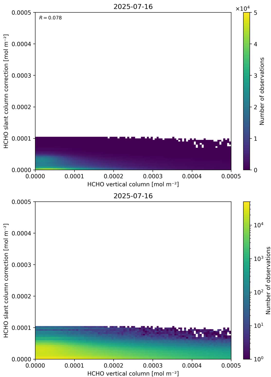
Figure 128: Scatter density plot of “HCHO vertical column” against “HCHO slant column correction” for 2025-07-15 to 2025-07-17.
