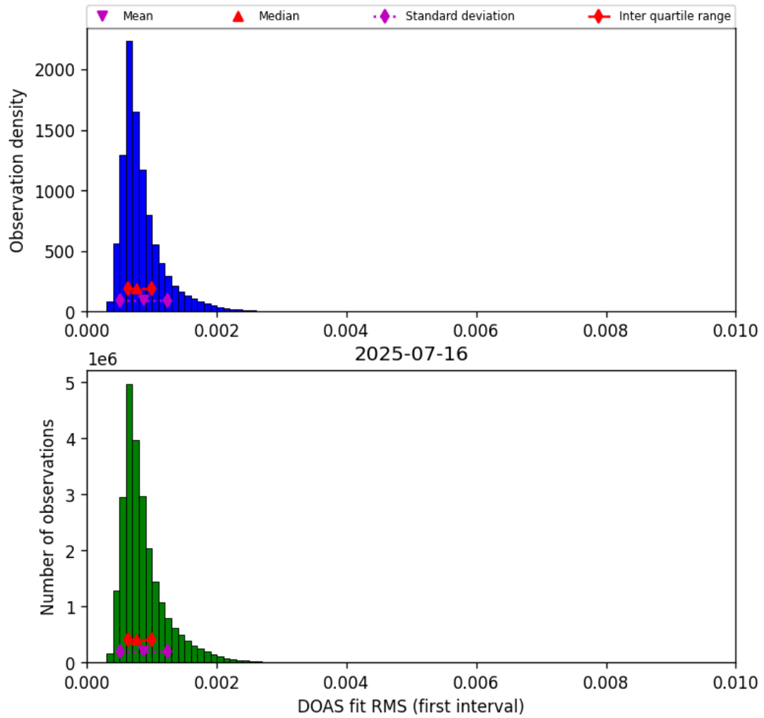
Figure 46: Histogram of “DOAS fit RMS (first interval)” for 2025-07-15 to 2025-07-17
