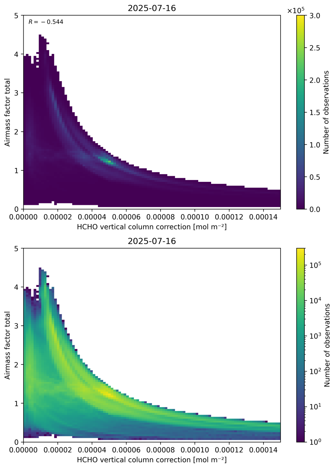
Figure 120: Scatter density plot of “HCHO vertical column correction” against “Airmass factor total” for 2025-07-15 to 2025-07-17.
