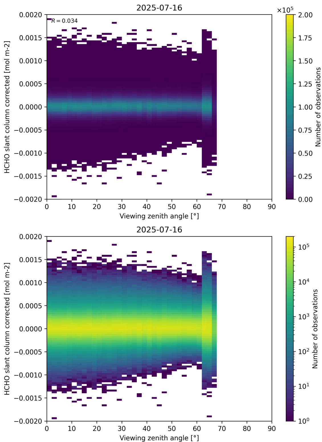
Figure 186: Scatter density plot of “Viewing zenith angle” against “HCHO slant column corrected” for 2025-07-15 to 2025-07-17.
