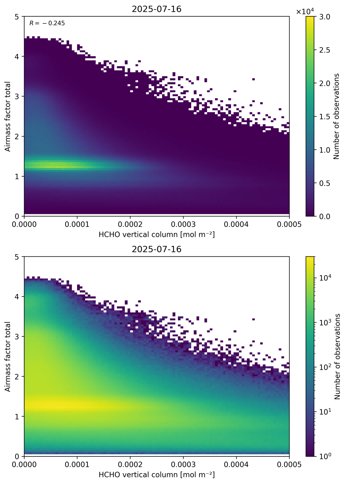
Figure 131: Scatter density plot of “HCHO vertical column” against “Airmass factor total” for 2025-07-15 to 2025-07-17.
