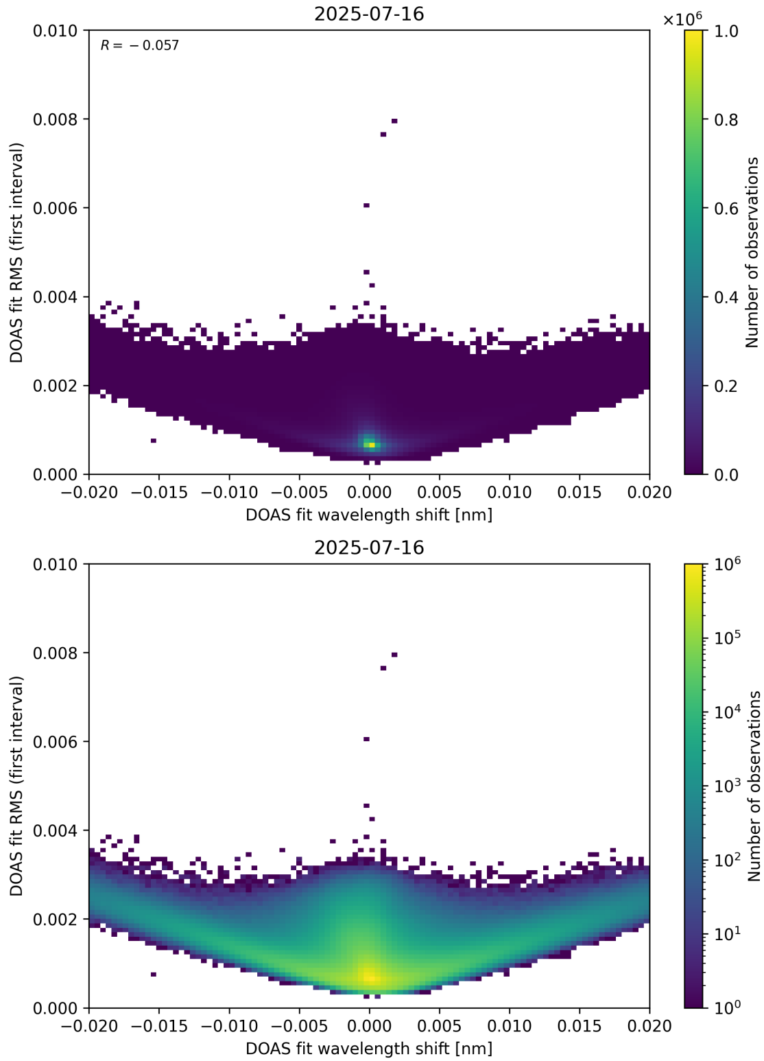
Figure 64: Scatter density plot of “DOAS fit wavelength shift” against “DOAS fit RMS (first interval)” for 2025-07-15 to 2025-07-17.
