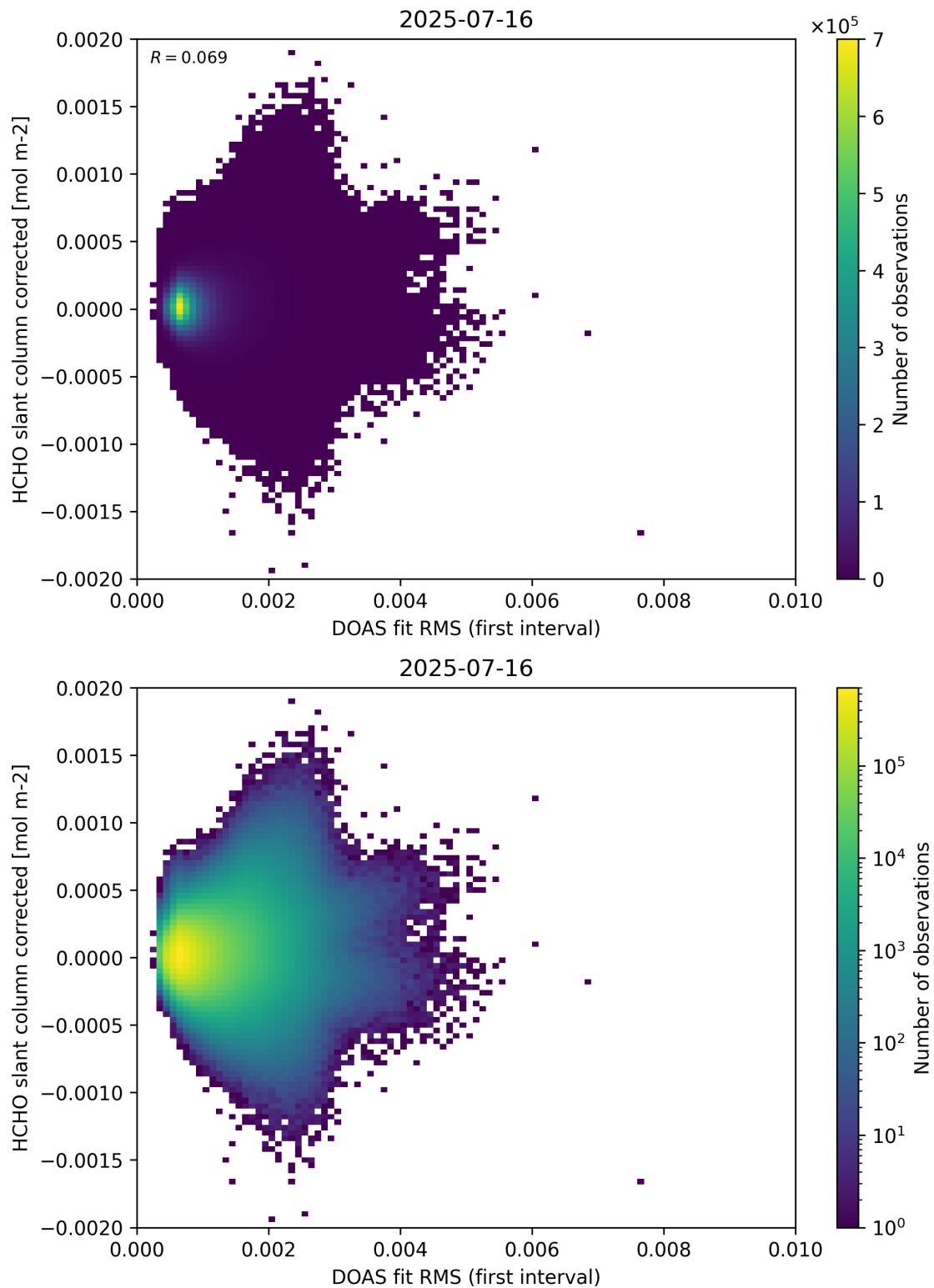
Figure 62: Scatter density plot of “DOAS fit RMS (first interval)” against “HCHO slant column corrected” for 2025-07-15 to 2025-07-17.
