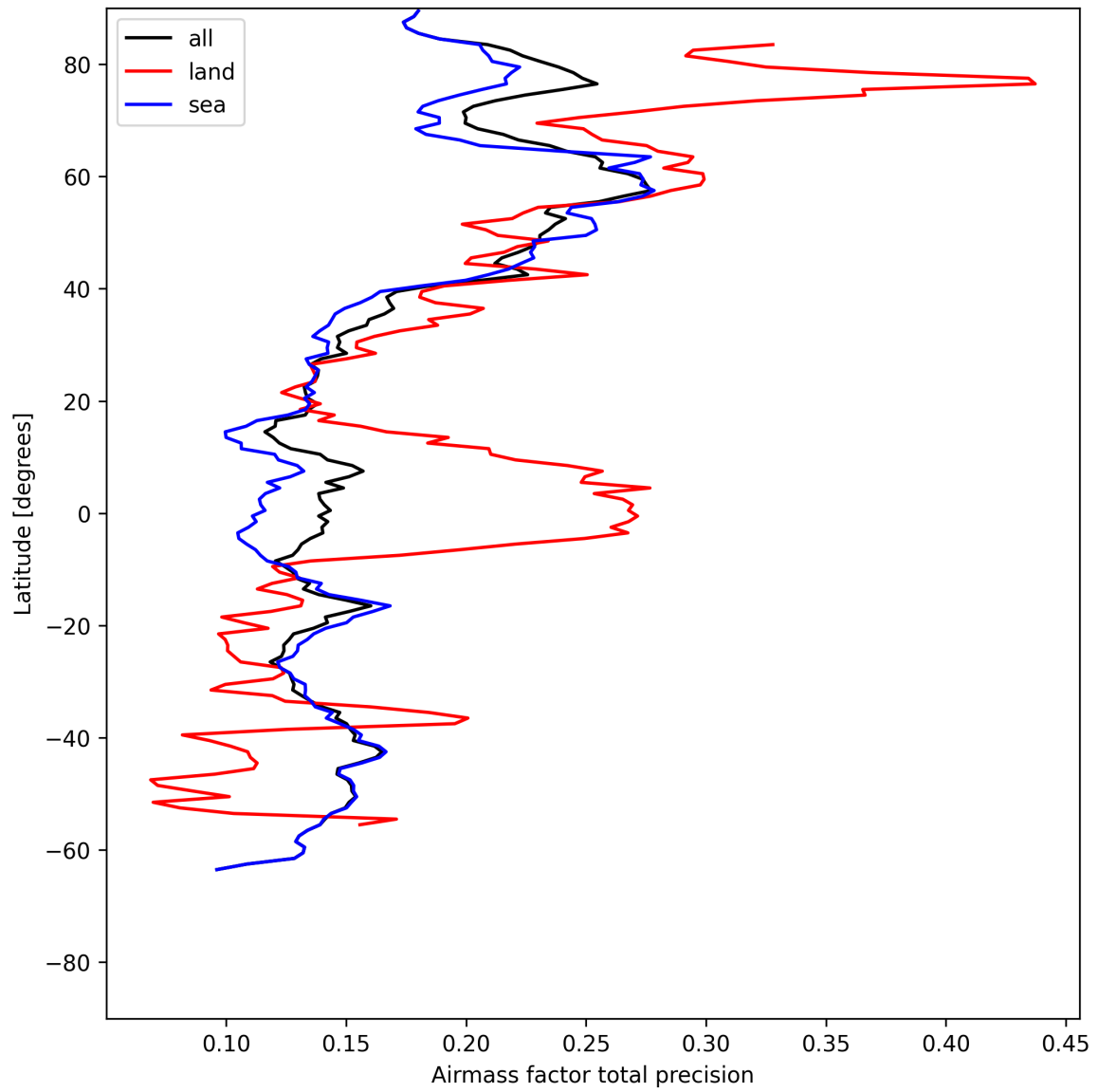
Figure 27: Zonal average of “Airmass factor total precision” for 2025-07-15 to 2025-07-17.
