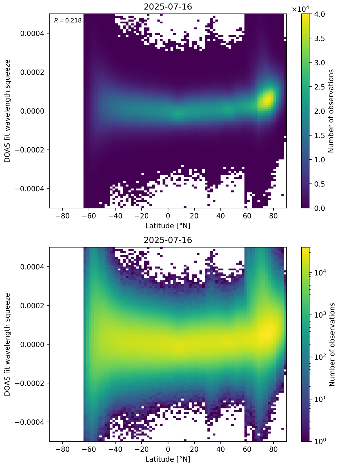
Figure 155: Scatter density plot of “Latitude” against “DOAS fit wavelength squeeze” for 2025-07-15 to 2025-07-17.
