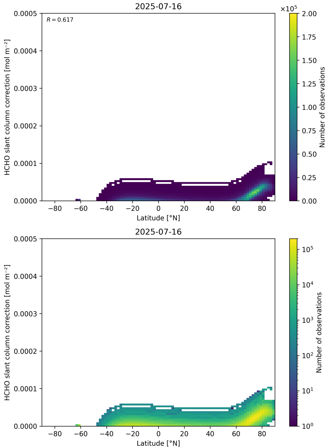
Figure 158: Scatter density plot of “Latitude” against “HCHO slant column correction” for 2025-07-15 to 2025-07-17.
