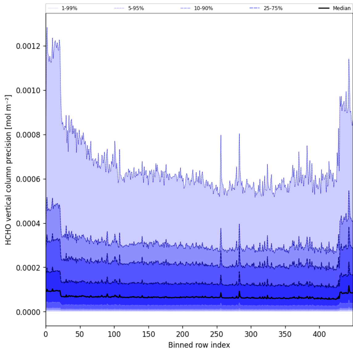
Figure 50: Along track statistics of “HCHO vertical column precision” for 2025-07-15 to 2025-07-17
