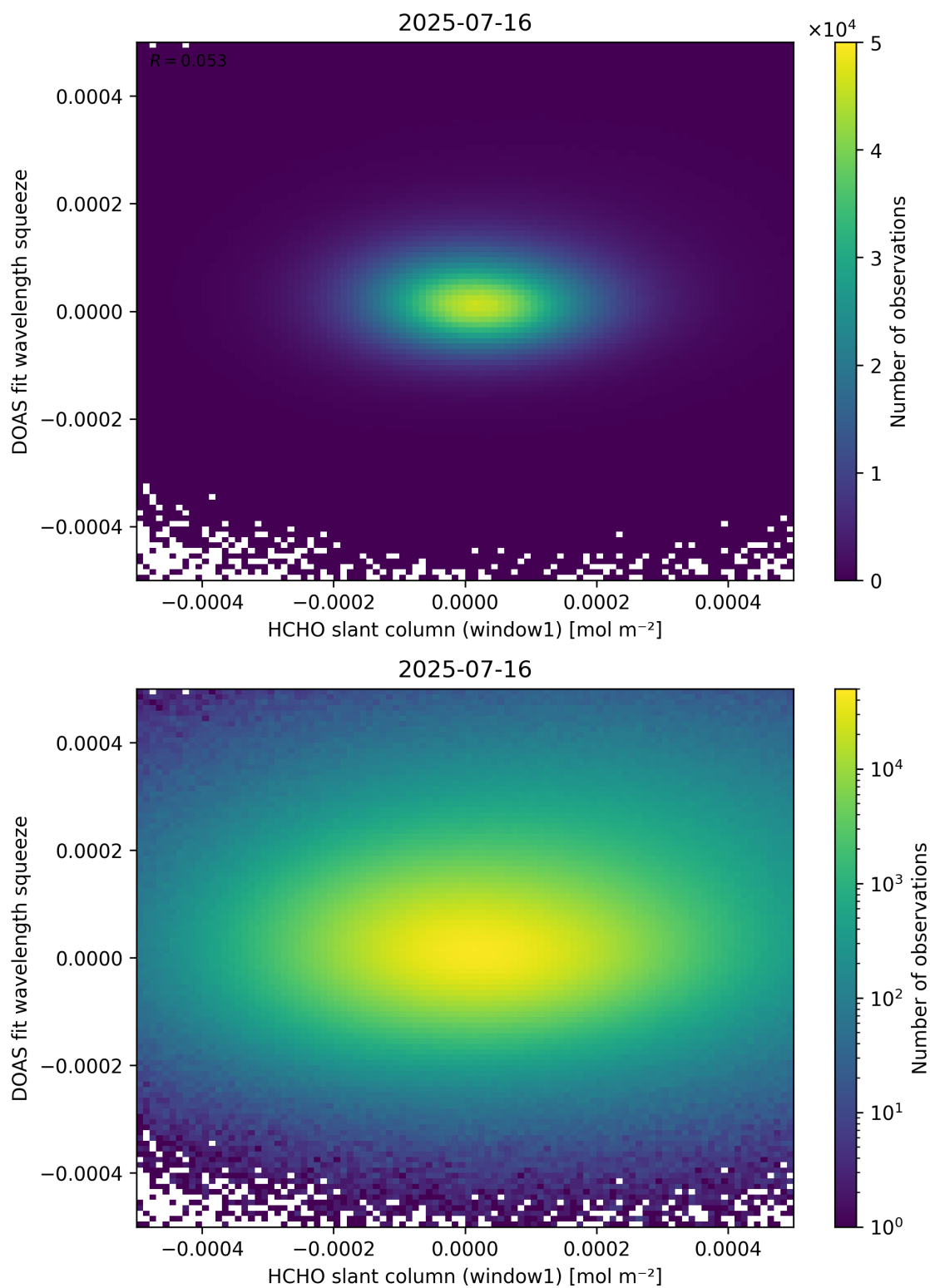
Figure 80: Scatter density plot of “HCHO slant column (window1)” against “DOAS fit wavelength squeeze” for 2025-07-15 to 2025-07-17.
