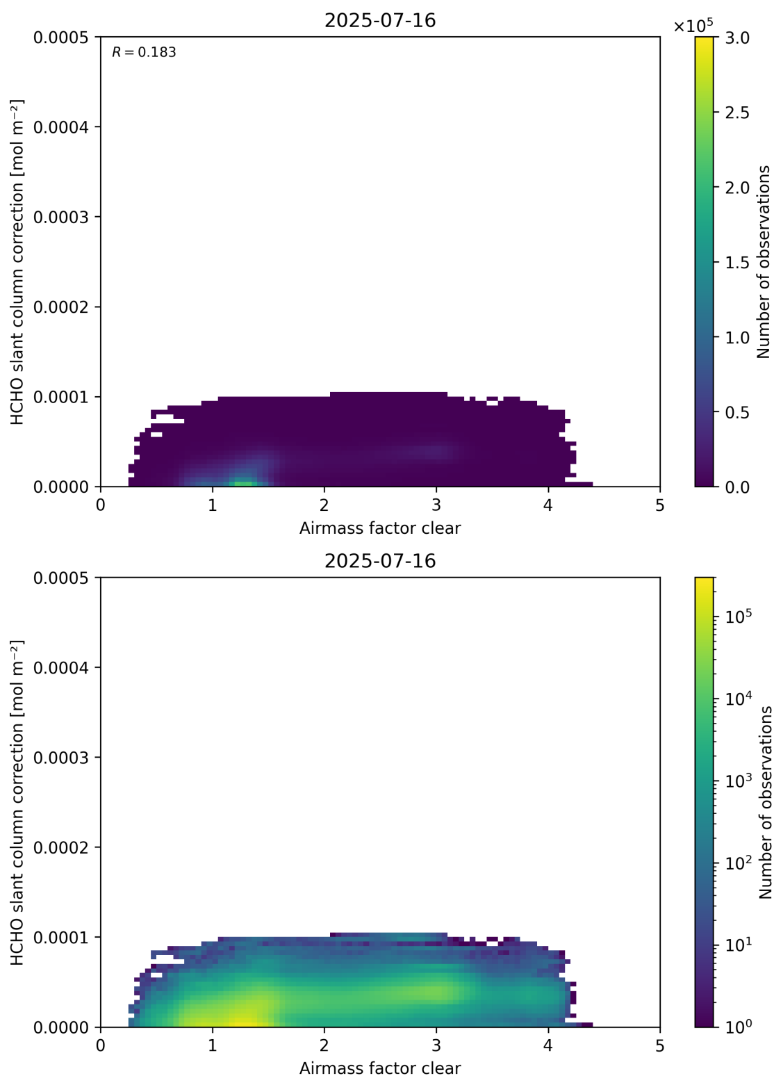
Figure 75: Scatter density plot of “Airmass factor clear” against “HCHO slant column correction” for 2025-07-15 to 2025-07-17.
