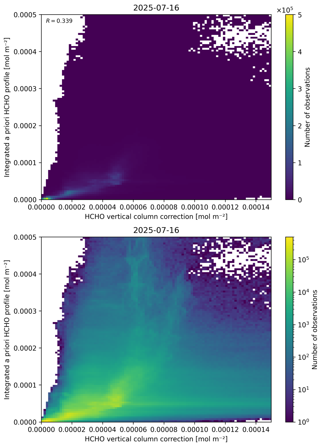
Figure 122: Scatter density plot of “HCHO vertical column correction” against “Integrated a priori HCHO profile” for 2025-07-15 to 2025-07-17.
