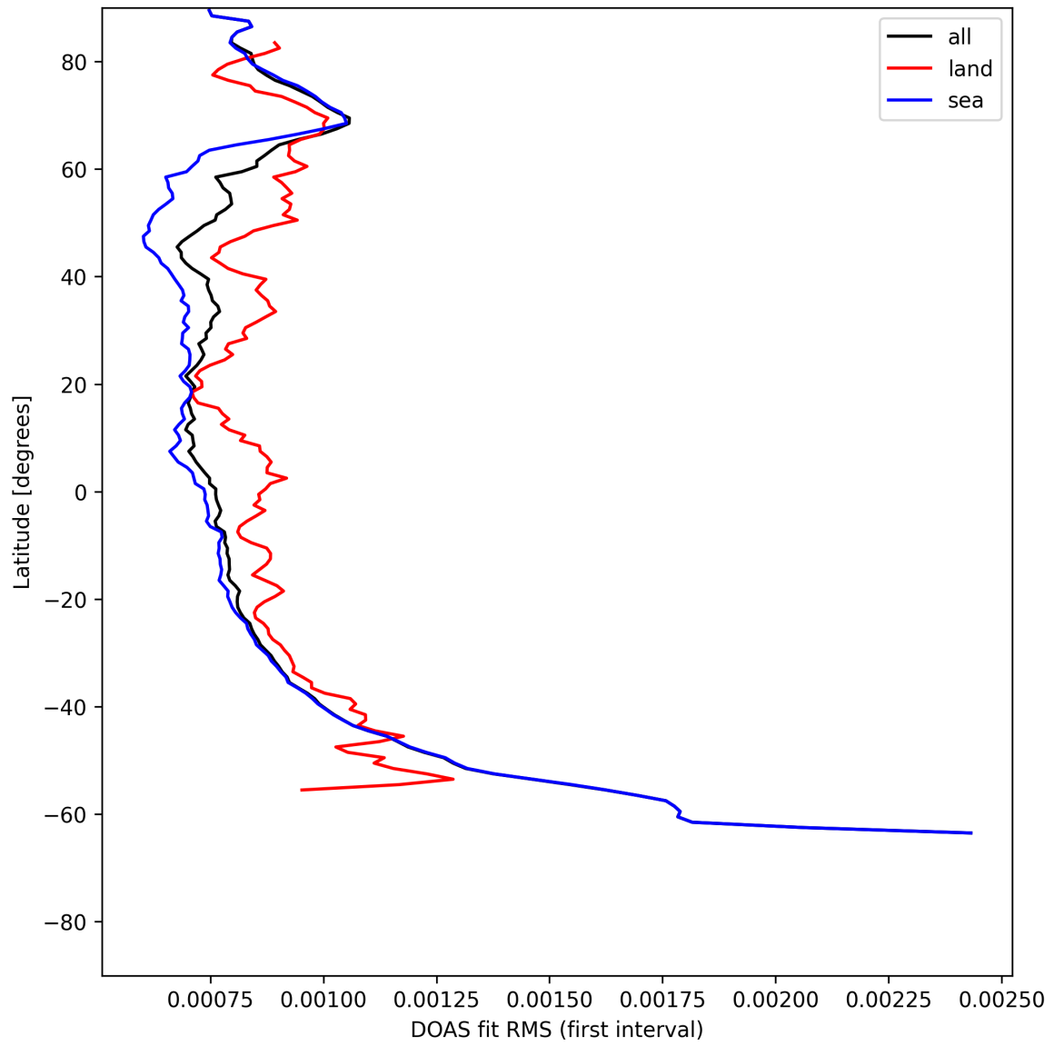
Figure 32: Zonal average of "DOAS fit RMS (first interval)" for 2025-07-15 to 2025-07-17.
