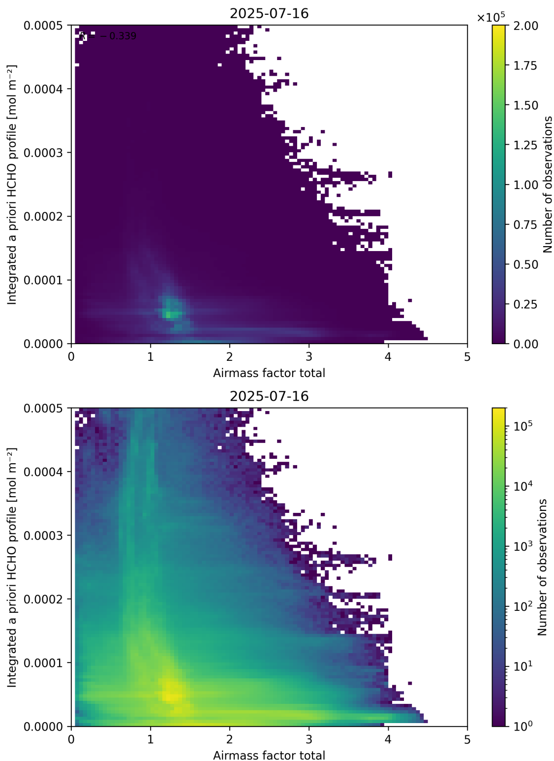
Figure 104: Scatter density plot of “Airmass factor total” against “Integrated a priori HCHO profile” for 2025-07-15 to 2025-07-17.
