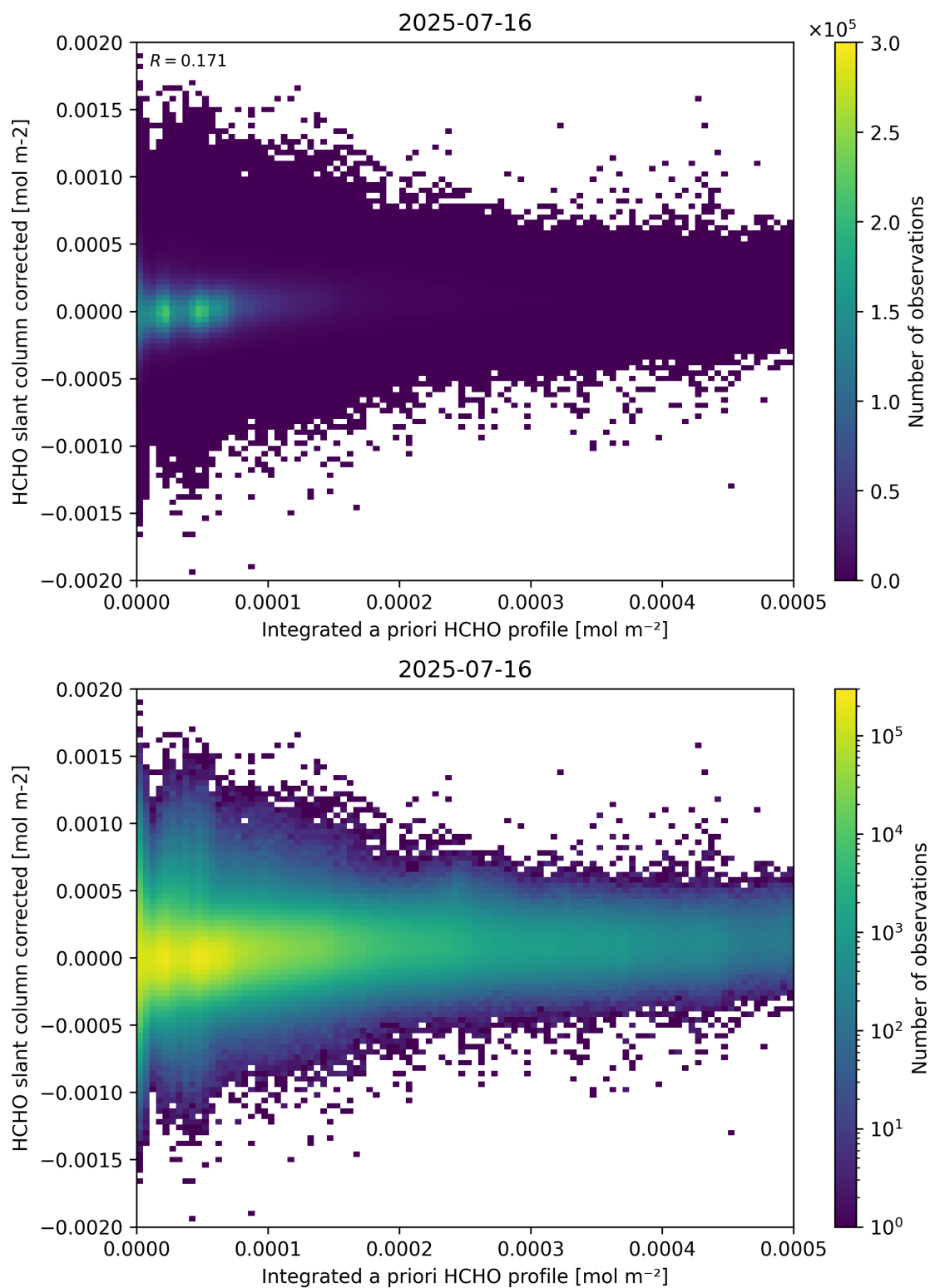
Figure 151: Scatter density plot of “Integrated a priori HCHO profile” against “HCHO slant column corrected” for 2025-07-15 to 2025-07-17.
