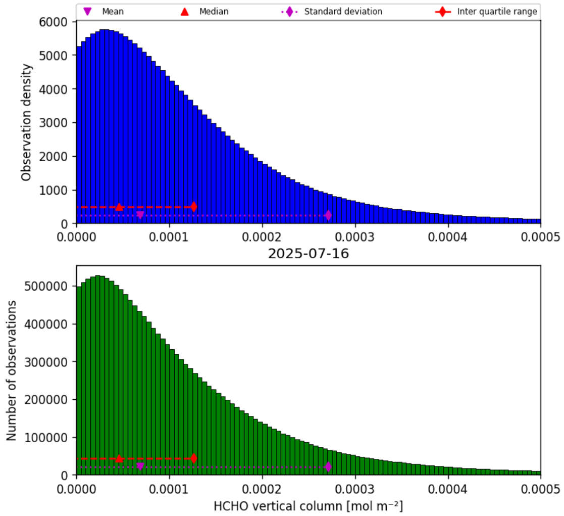
Figure 35: Histogram of “HCHO vertical column” for 2025-07-15 to 2025-07-17
