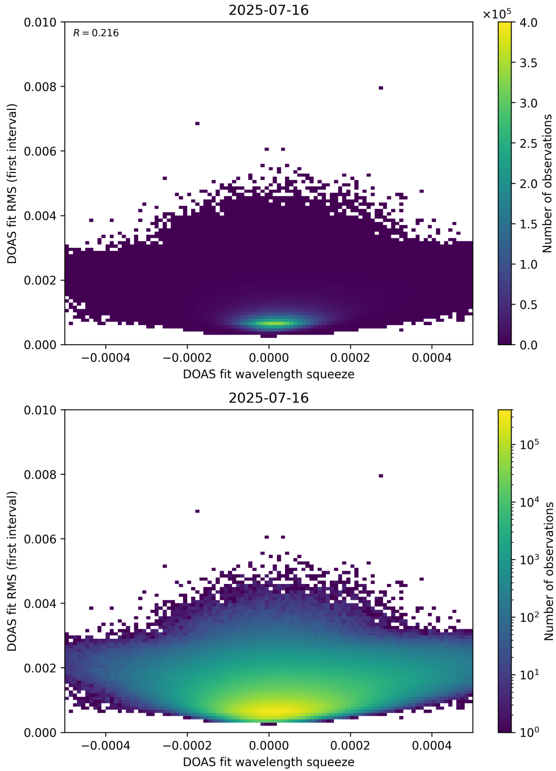
Figure 68: Scatter density plot of “DOAS fit wavelength squeeze” against “DOAS fit RMS (first interval)” for 2025-07-15 to 2025-07-17.
