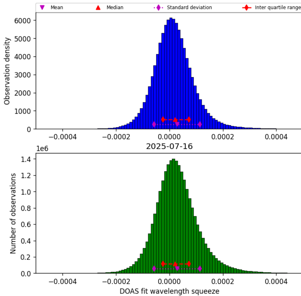
Figure 45: Histogram of “DOAS fit wavelength squeeze” for 2025-07-15 to 2025-07-17
