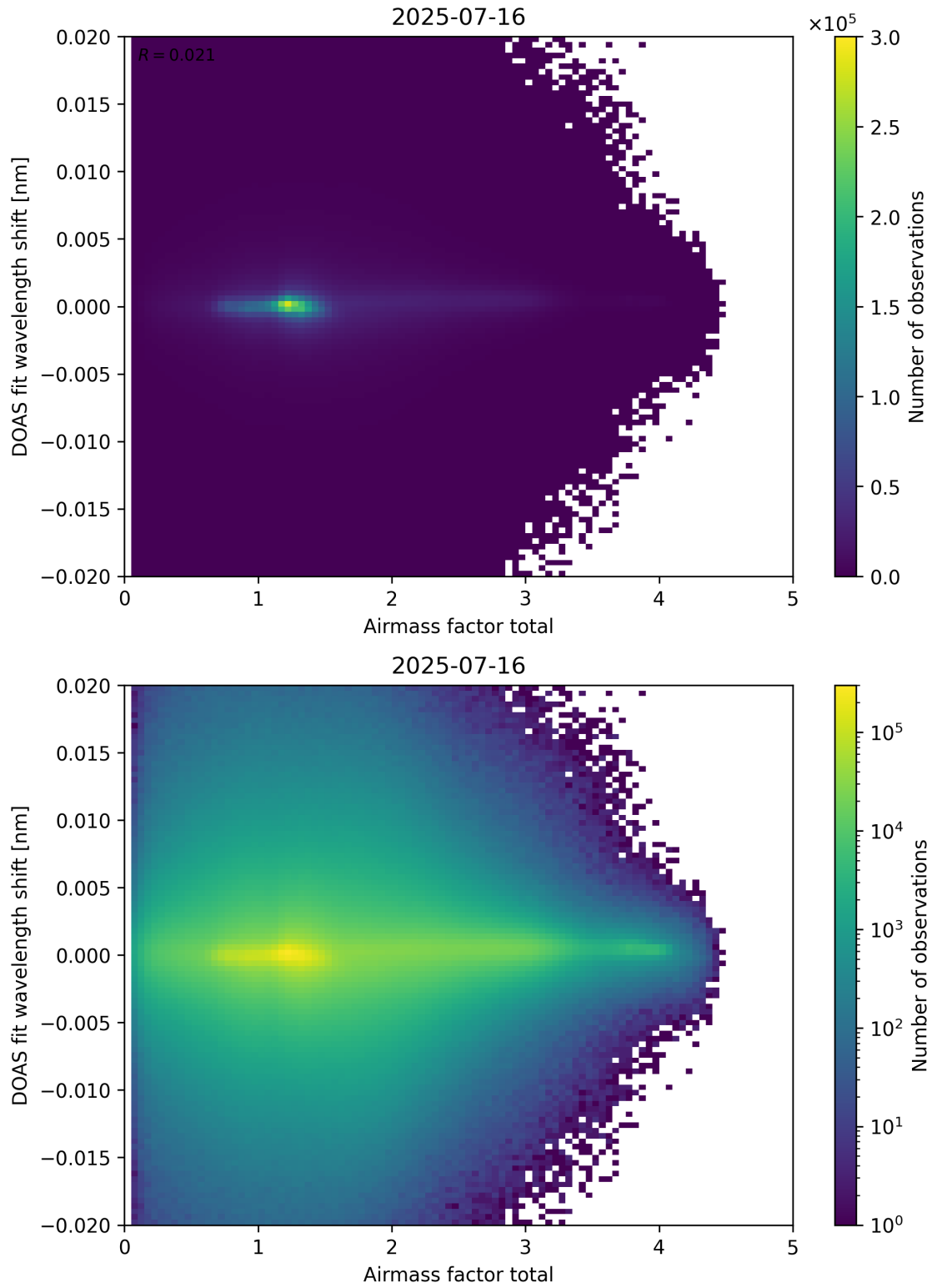
Figure 98: Scatter density plot of “Airmass factor total” against “DOAS fit wavelength shift” for 2025-07-15 to 2025-07-17.
