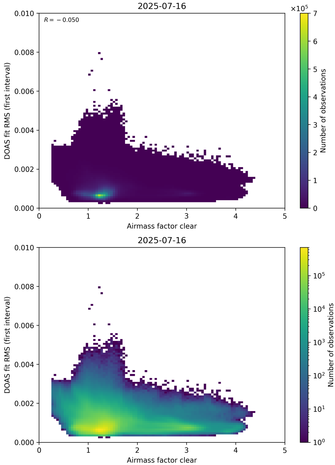
Figure 71: Scatter density plot of “Airmass factor clear” against “DOAS fit RMS (first interval)” for 2025-07-15 to 2025-07-17.
