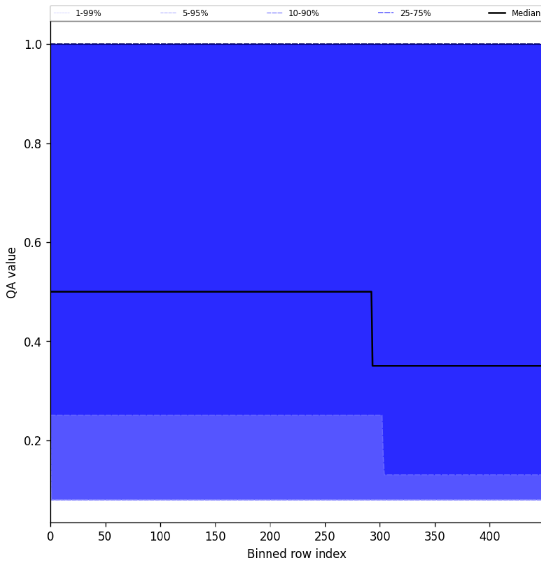
Figure 48: Along track statistics of “QA value” for 2025-07-15 to 2025-07-17
