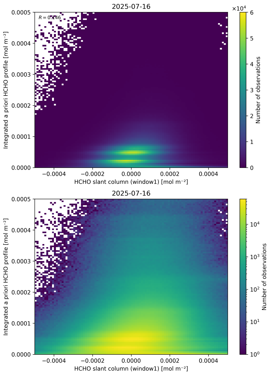
Figure 87: Scatter density plot of “HCHO slant column (window1)” against “Integrated a priori HCHO profile” for 2025-07-15 to 2025-07-17.
