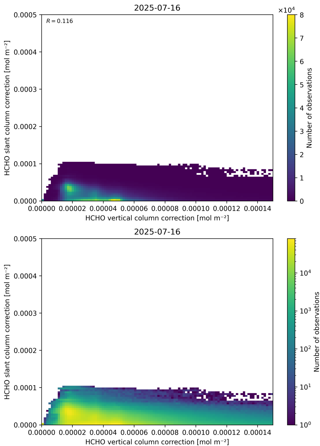
Figure 117: Scatter density plot of “HCHO vertical column correction” against “HCHO slant column correction” for 2025-07-15 to 2025-07-17.
