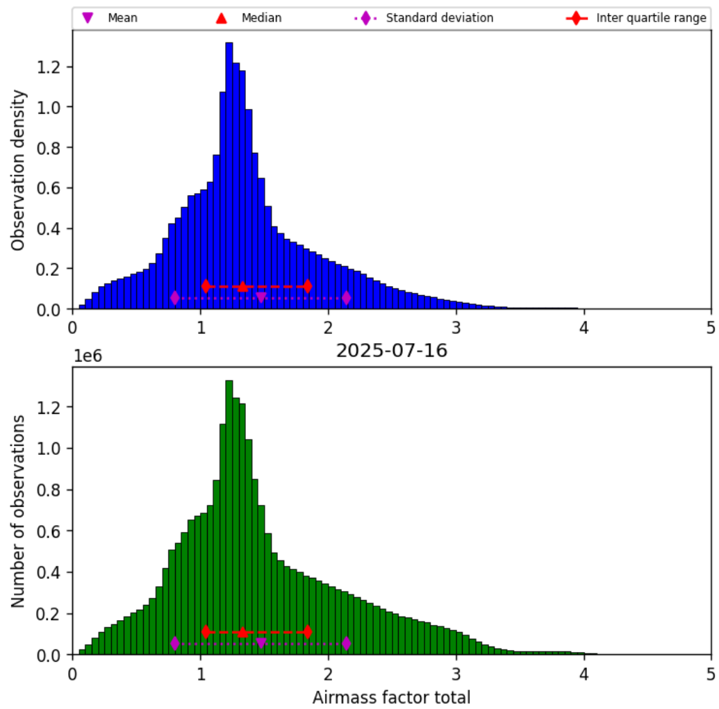
Figure 40: Histogram of “Airmass factor total” for 2025-07-15 to 2025-07-17
