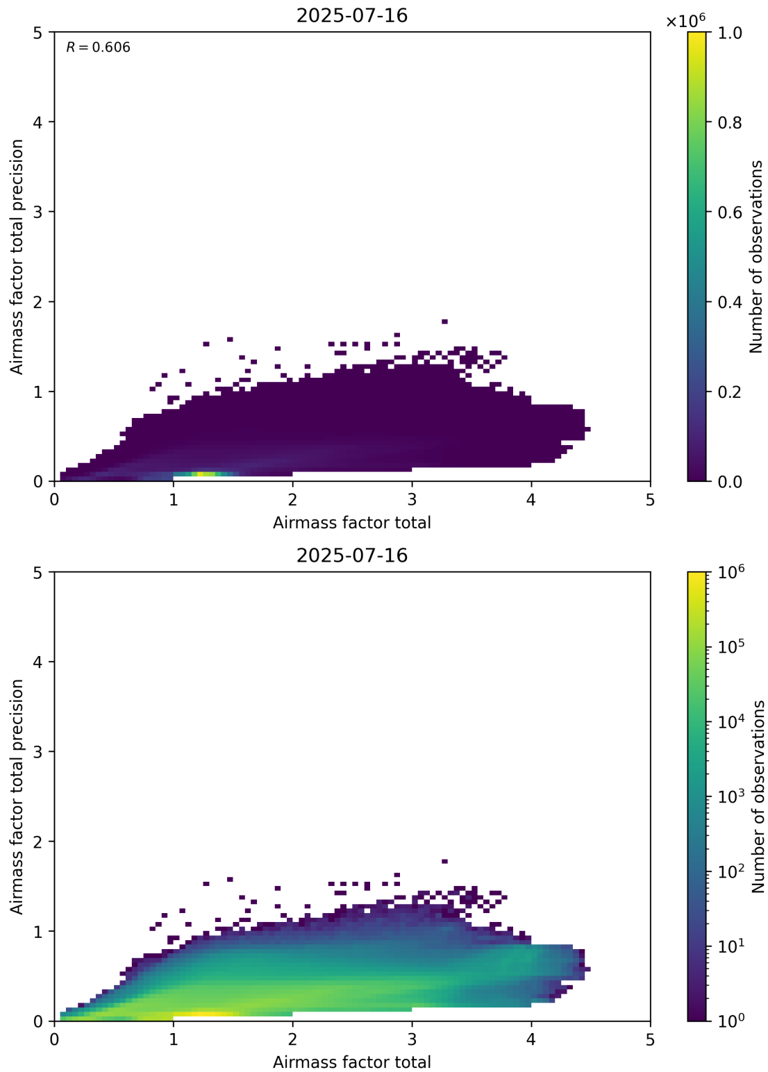
Figure 103: Scatter density plot of “Airmass factor total” against “Airmass factor total precision” for 2025-07-15 to 2025-07-17.
