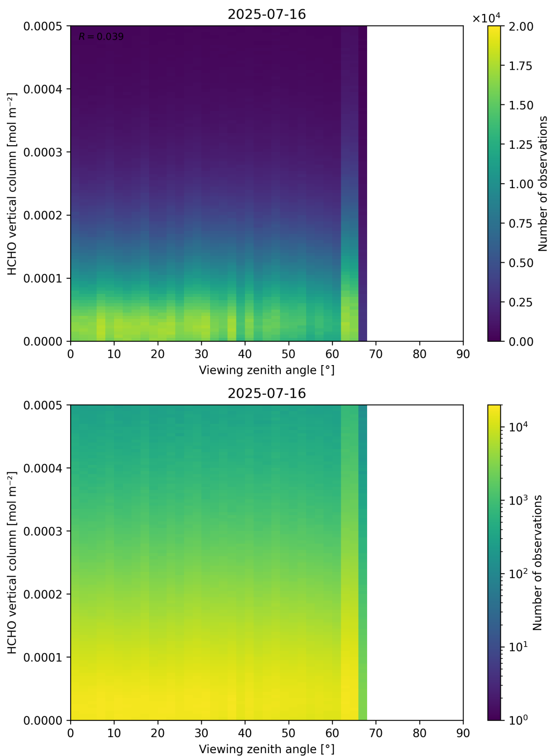
Figure 192: Scatter density plot of “Viewing zenith angle” against “HCHO vertical column” for 2025-07-15 to 2025-07-17.
