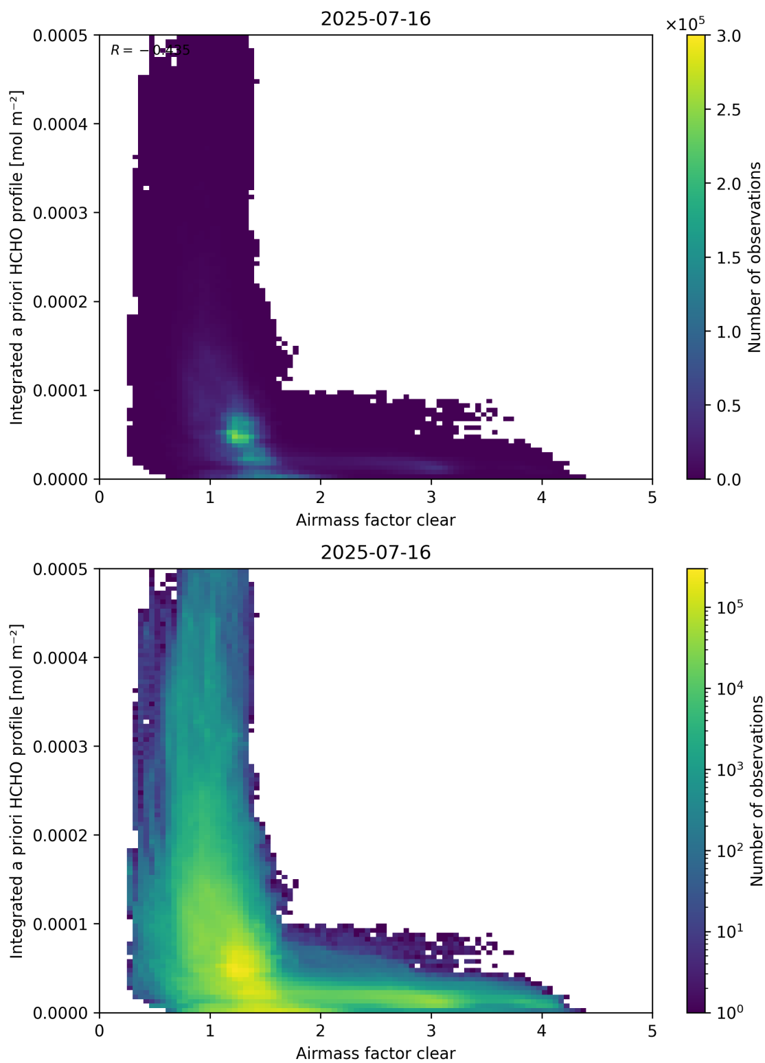
Figure 76: Scatter density plot of “Airmass factor clear” against “Integrated a priori HCHO profile” for 2025-07-15 to 2025-07-17.
