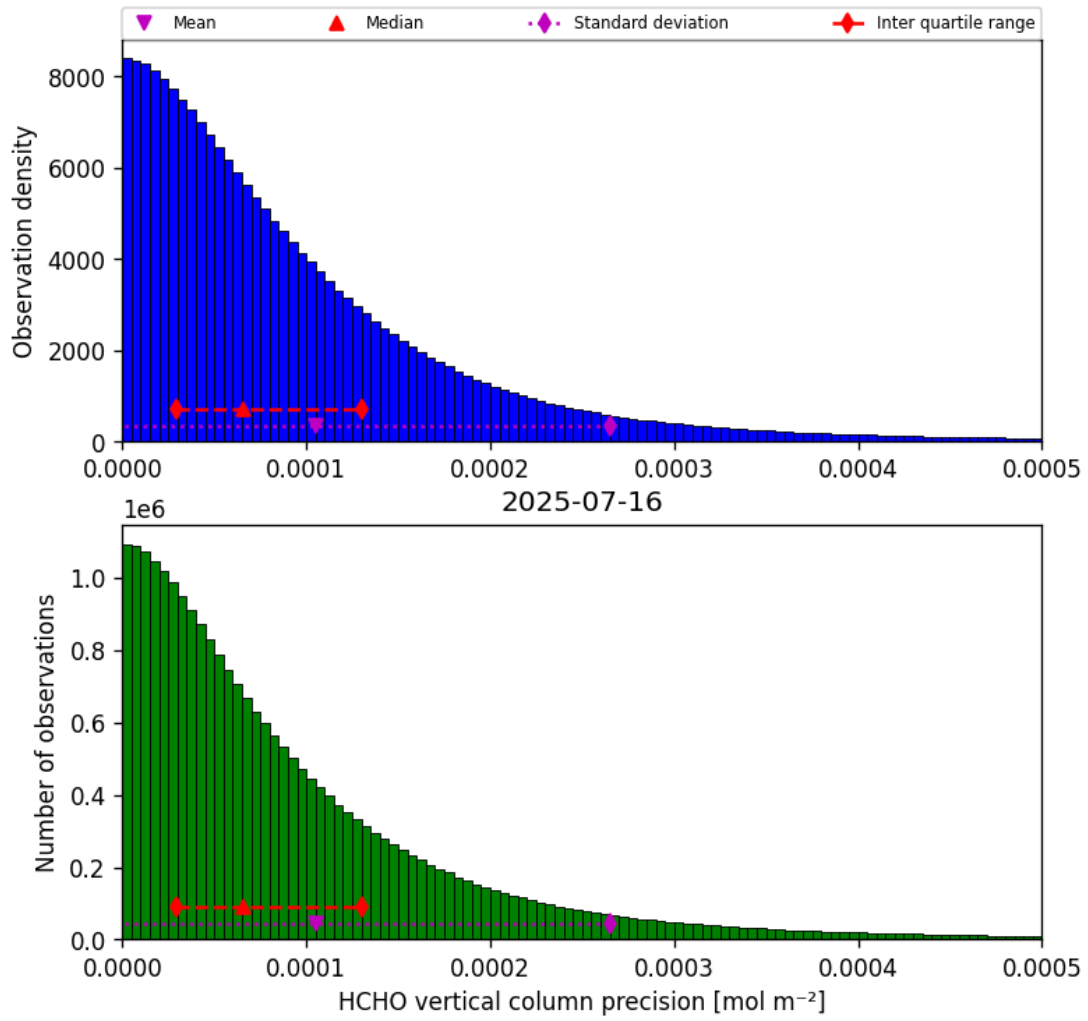
Figure 36: Histogram of “HCHO vertical column precision” for 2025-07-15 to 2025-07-17
