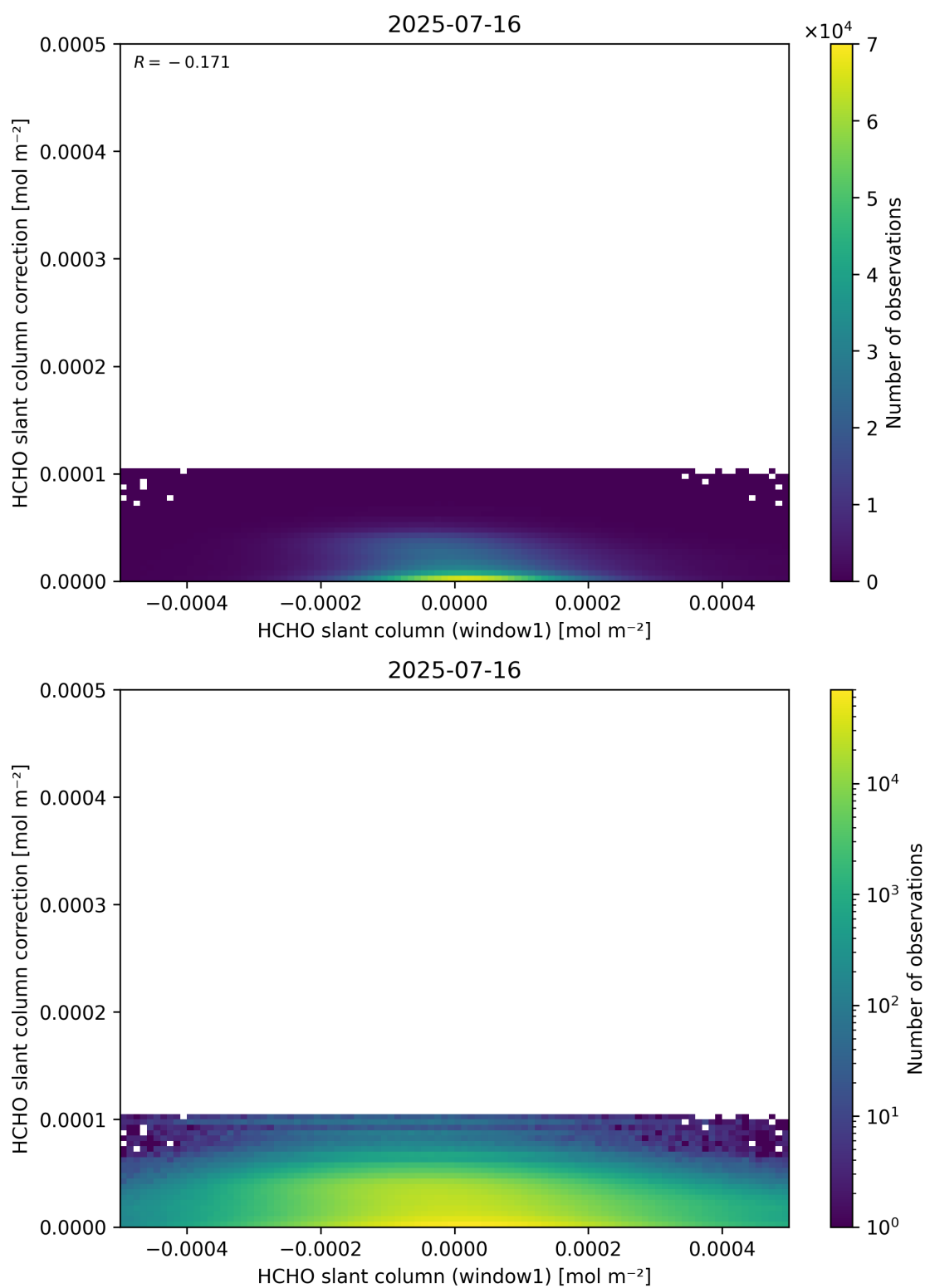
Figure 83: Scatter density plot of “HCHO slant column (window1)” against “HCHO slant column correction” for 2025-07-15 to 2025-07-17.
