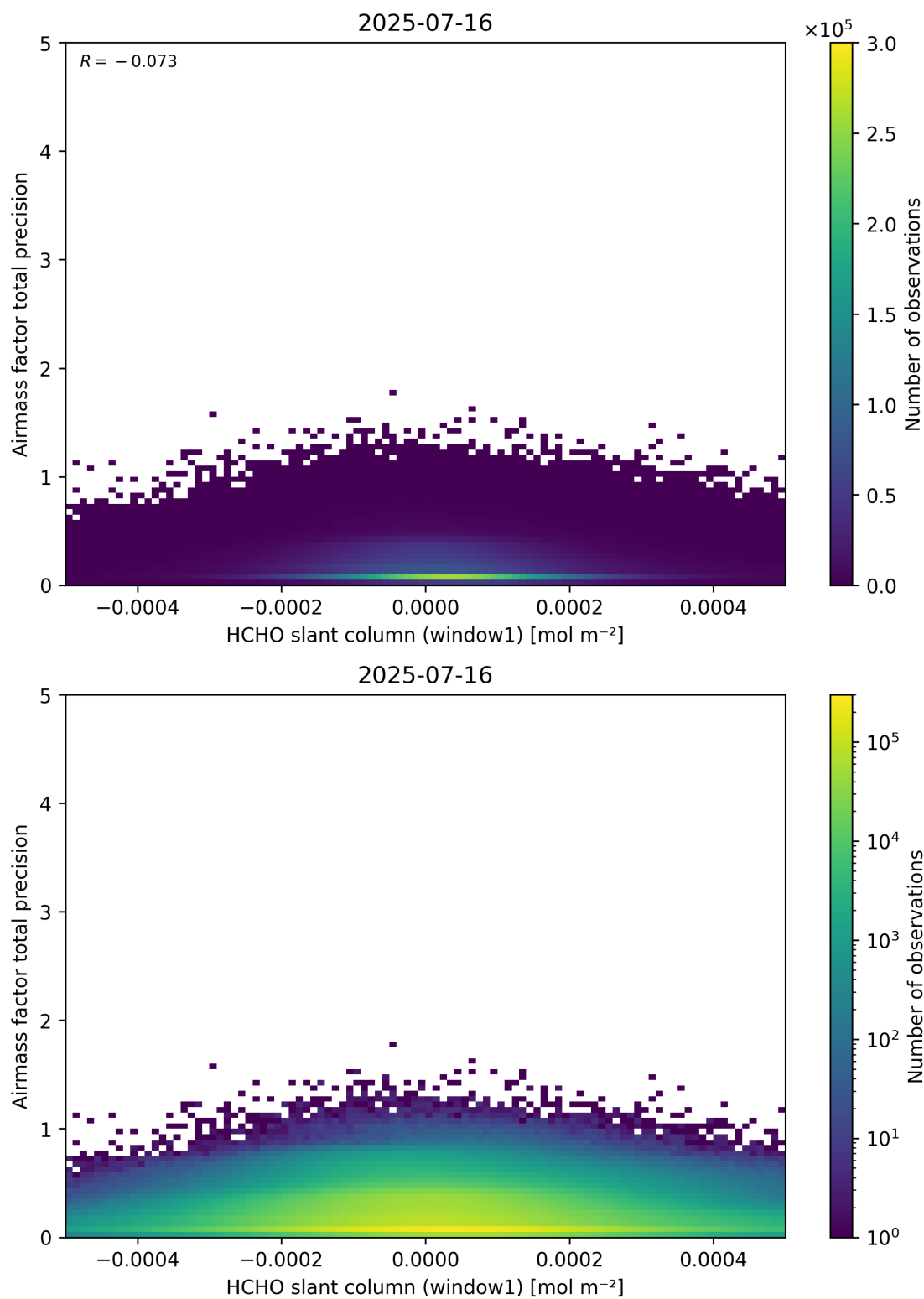
Figure 86: Scatter density plot of “HCHO slant column (window1)” against “Airmass factor total precision” for 2025-07-15 to 2025-07-17.
