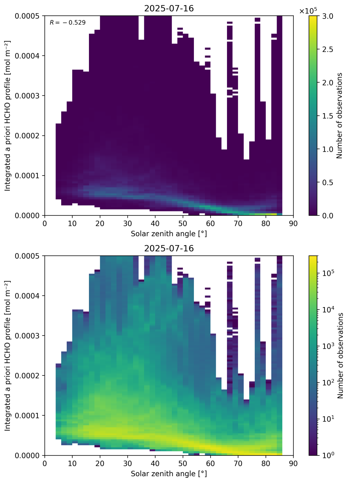
Figure 180: Scatter density plot of “Solar zenith angle” against “Integrated a priori HCHO profile” for 2025-07-15 to 2025-07-17.
