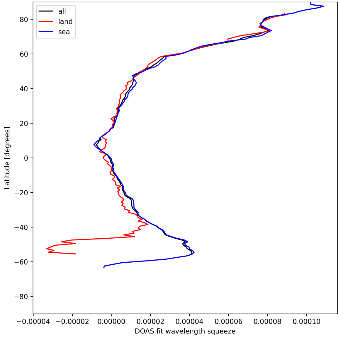
Figure 31: Zonal average of “DOAS fit wavelength squeeze” for 2025-07-15 to 2025-07-17.
