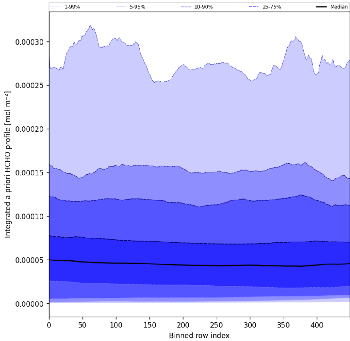
Figure 57: Along track statistics of “Integrated a priori HCHO profile” for 2025-07-15 to 2025-07-17
