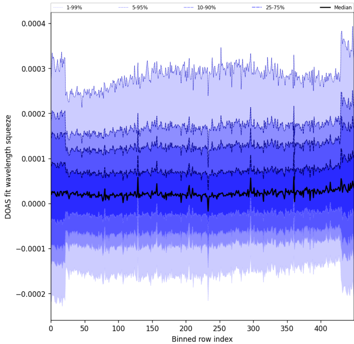
Figure 59: Along track statistics of “DOAS fit wavelength squeeze” for 2025-07-15 to 2025-07-17
