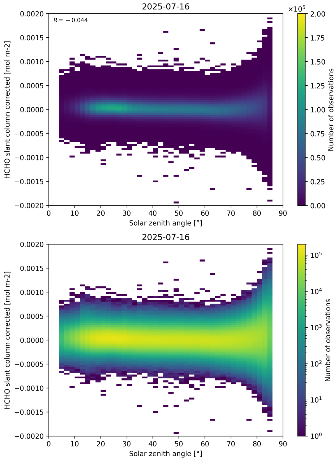
Figure 171: Scatter density plot of “Solar zenith angle” against “HCHO slant column corrected” for 2025-07-15 to 2025-07-17.
