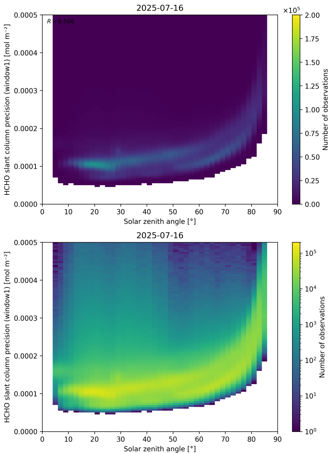
Figure 174: Scatter density plot of “Solar zenith angle” against “HCHO slant column precision (window1)” for 2025-07-15 to 2025-07-17.
