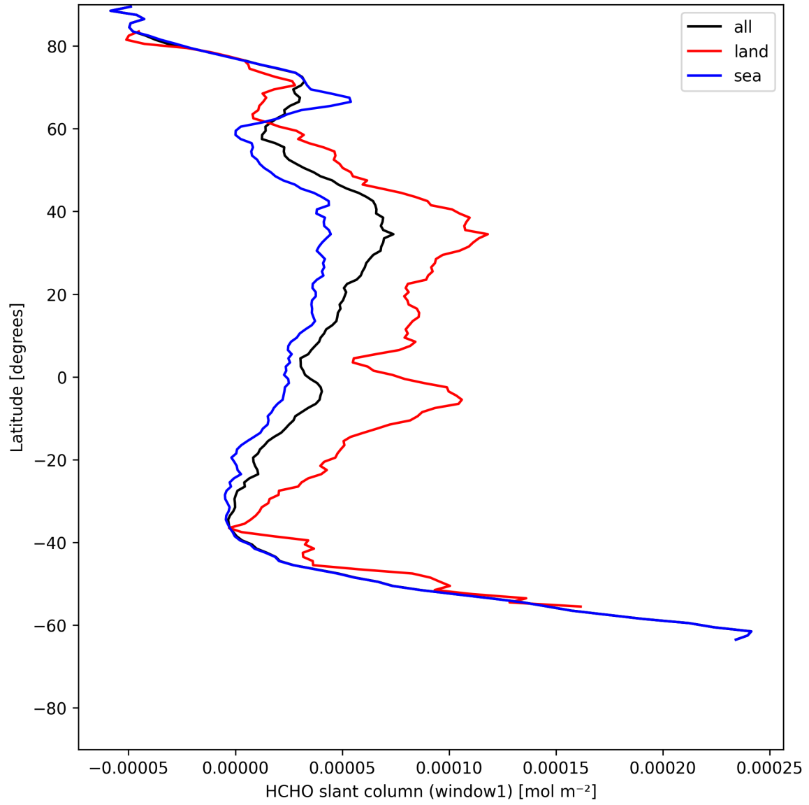
Figure 24: Zonal average of “HCHO slant column (window1)” for 2025-07-15 to 2025-07-17.
