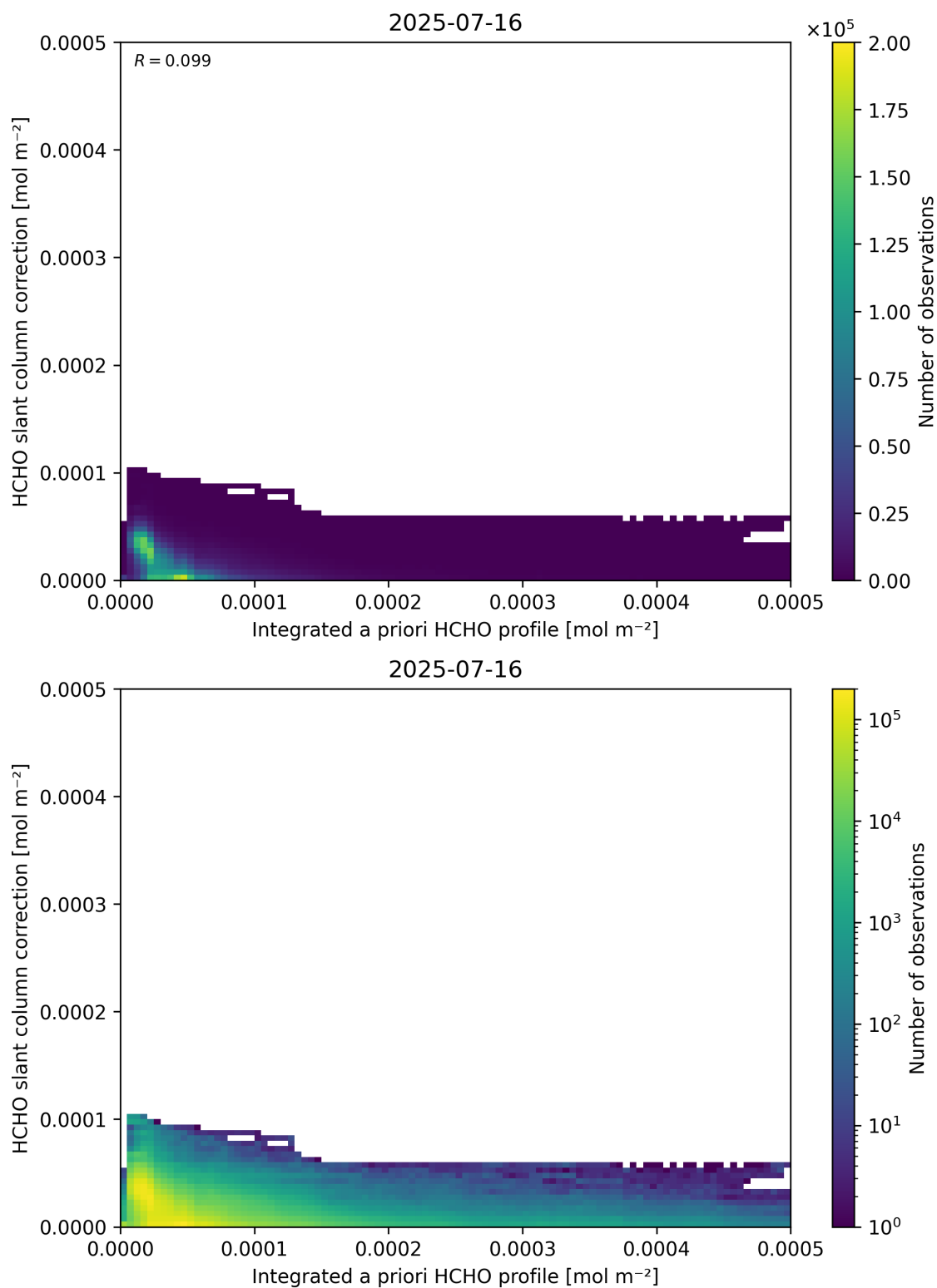
Figure 152: Scatter density plot of “Integrated a priori HCHO profile” against “HCHO slant column correction” for 2025-07-15 to 2025-07-17.
