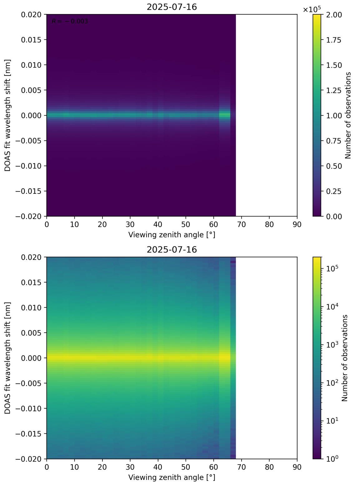
Figure 183: Scatter density plot of “Viewing zenith angle” against “DOAS fit wavelength shift” for 2025-07-15 to 2025-07-17.
