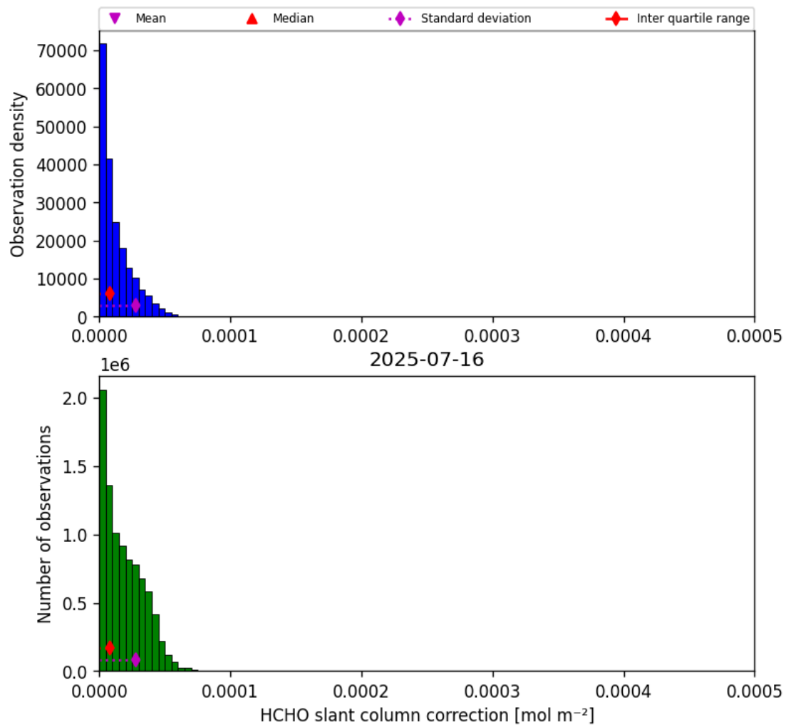
Figure 47: Histogram of “HCHO slant column correction” for 2025-07-15 to 2025-07-17
