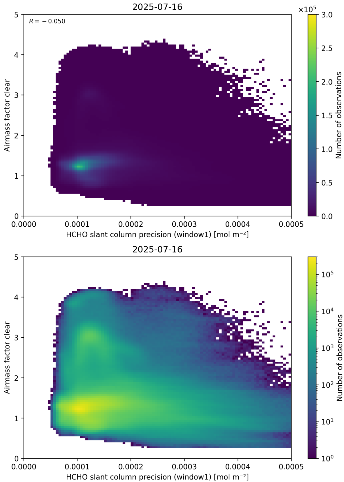
Figure 91: Scatter density plot of “HCHO slant column precision (window1)” against “Airmass factor clear” for 2025-07-15 to 2025-07-17.
