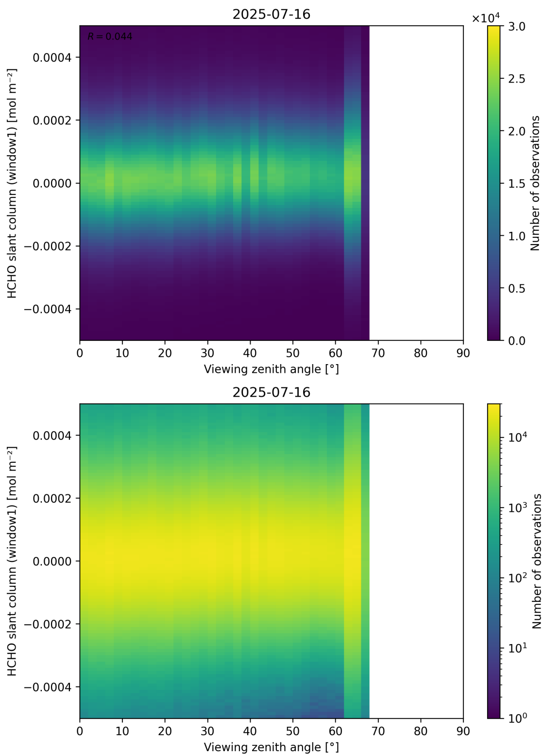
Figure 188: Scatter density plot of “Viewing zenith angle” against “HCHO slant column (window1)” for 2025-07-15 to 2025-07-17.
