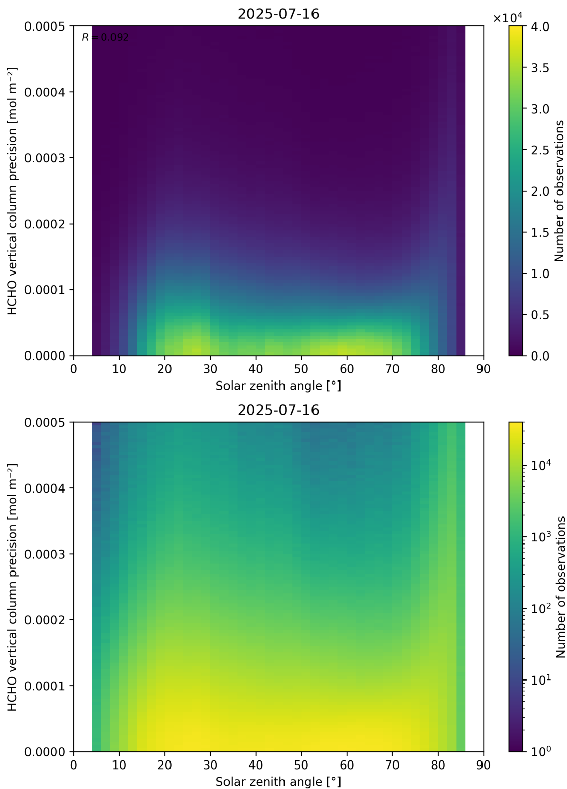
Figure 179: Scatter density plot of “Solar zenith angle” against “HCHO vertical column precision” for 2025-07-15 to 2025-07-17.
