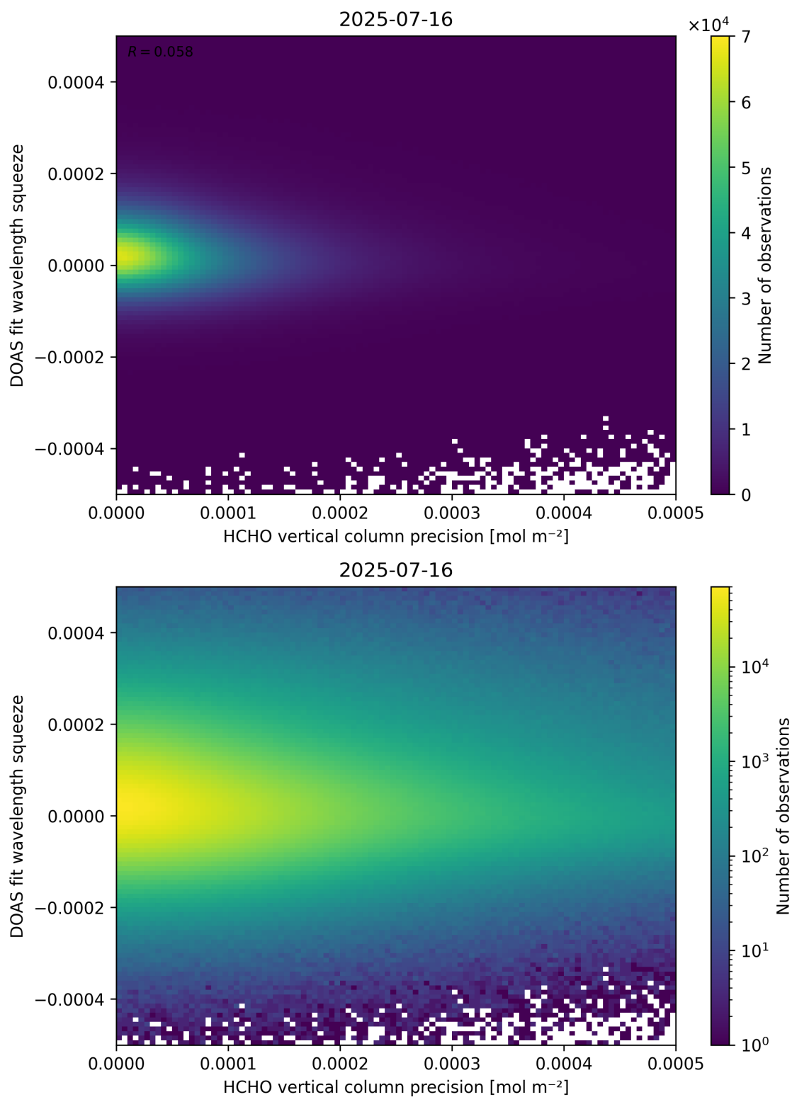
Figure 138: Scatter density plot of “HCHO vertical column precision” against “DOAS fit wavelength squeeze” for 2025-07-15 to 2025-07-17.
