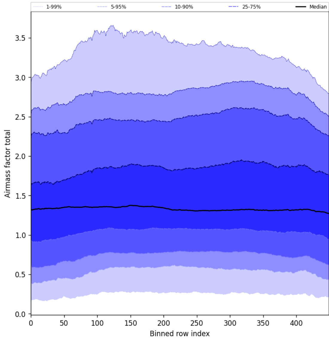
Figure 54: Along track statistics of “Airmass factor total” for 2025-07-15 to 2025-07-17
