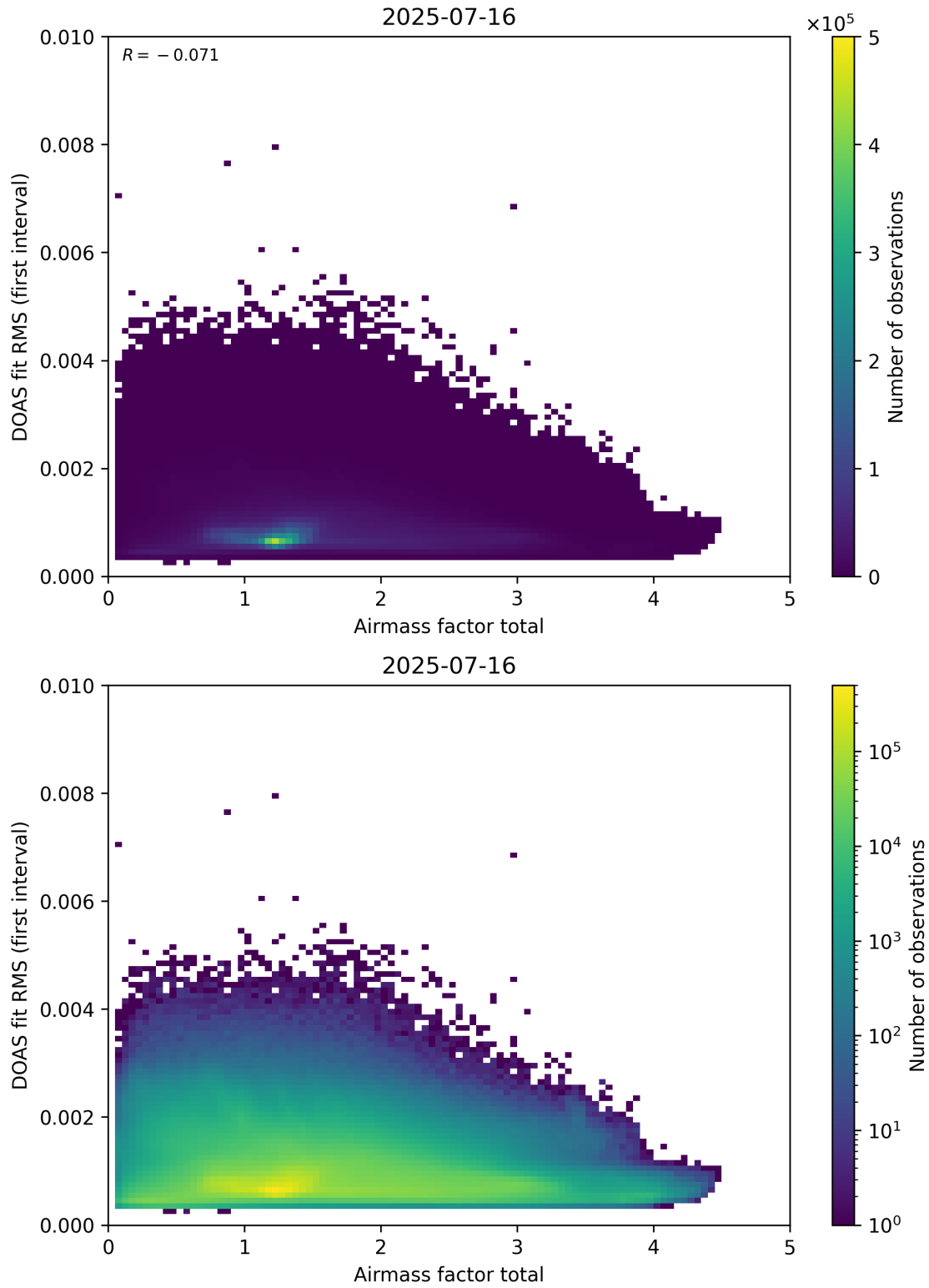
Figure 97: Scatter density plot of “Airmass factor total” against “DOAS fit RMS (first interval)” for 2025-07-15 to 2025-07-17.
