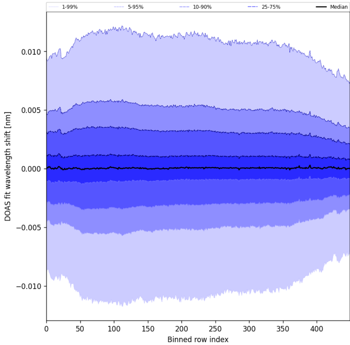
Figure 58: Along track statistics of “DOAS fit wavelength shift” for 2025-07-15 to 2025-07-17
