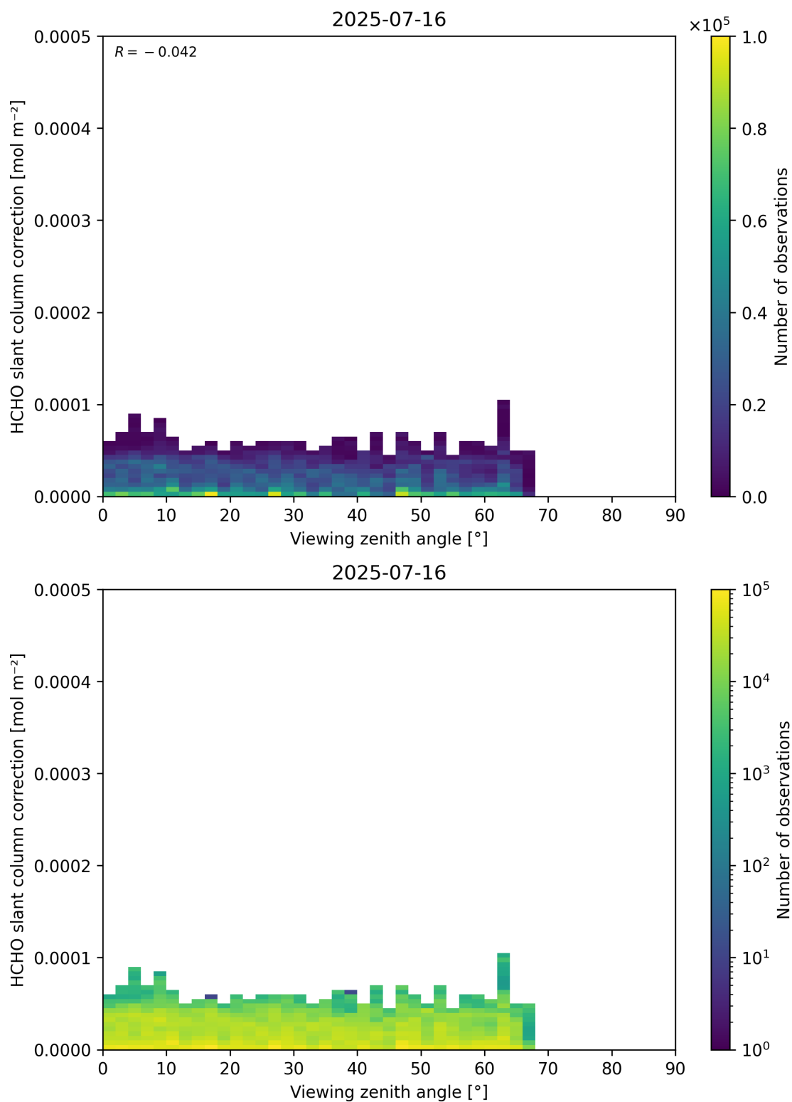
Figure 187: Scatter density plot of “Viewing zenith angle” against “HCHO slant column correction” for 2025-07-15 to 2025-07-17.
