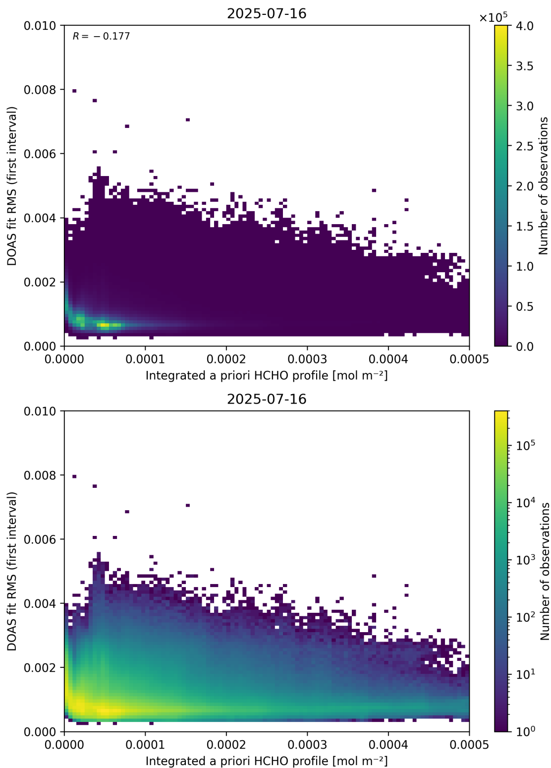
Figure 148: Scatter density plot of “Integrated a priori HCHO profile” against “DOAS fit RMS (first interval)” for 2025-07-15 to 2025-07-17.
