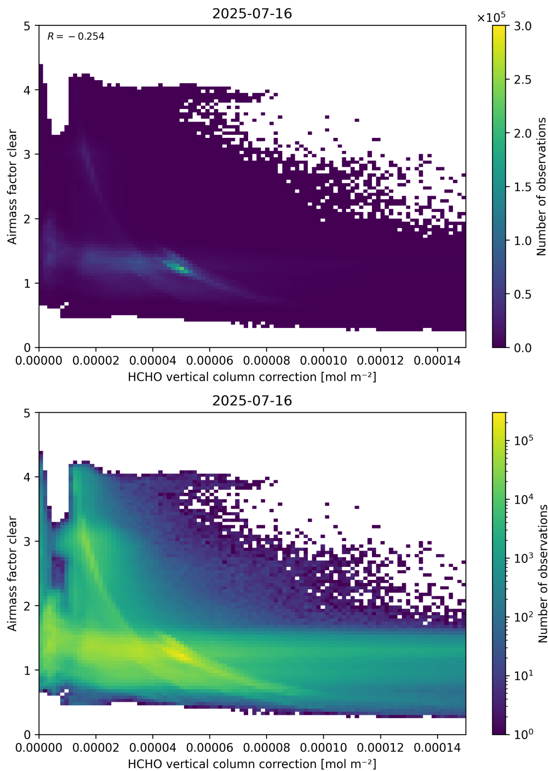
Figure 115: Scatter density plot of “HCHO vertical column correction” against “Airmass factor clear” for 2025-07-15 to 2025-07-17.
