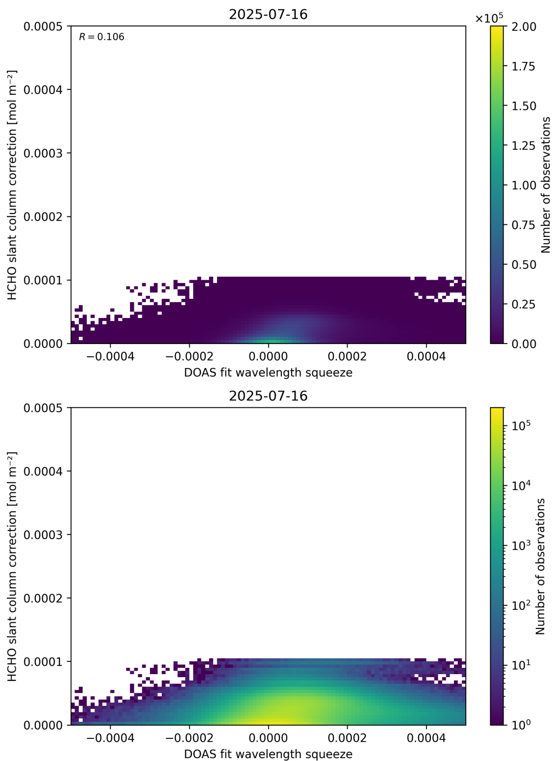
Figure 70: Scatter density plot of “DOAS fit wavelength squeeze” against “HCHO slant column correction” for 2025-07-15 to 2025-07-17.
