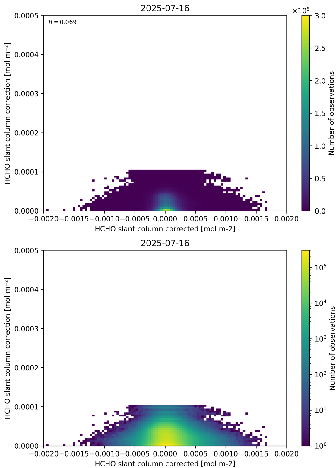
Figure 77: Scatter density plot of “HCHO slant column corrected” against “HCHO slant column correction” for 2025-07-15 to 2025-07-17.
