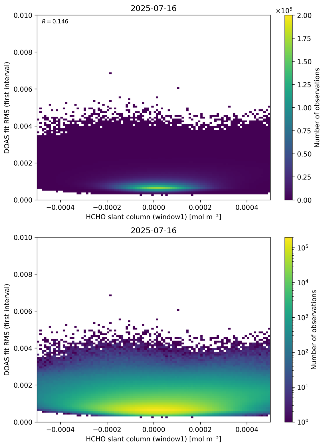
Figure 78: Scatter density plot of “HCHO slant column (window1)” against “DOAS fit RMS (first interval)” for 2025-07-15 to 2025-07-17.
