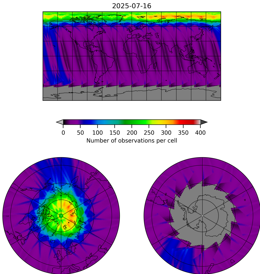
Figure 19: Map of the number of observations for 2025-07-15 to 2025-07-17
