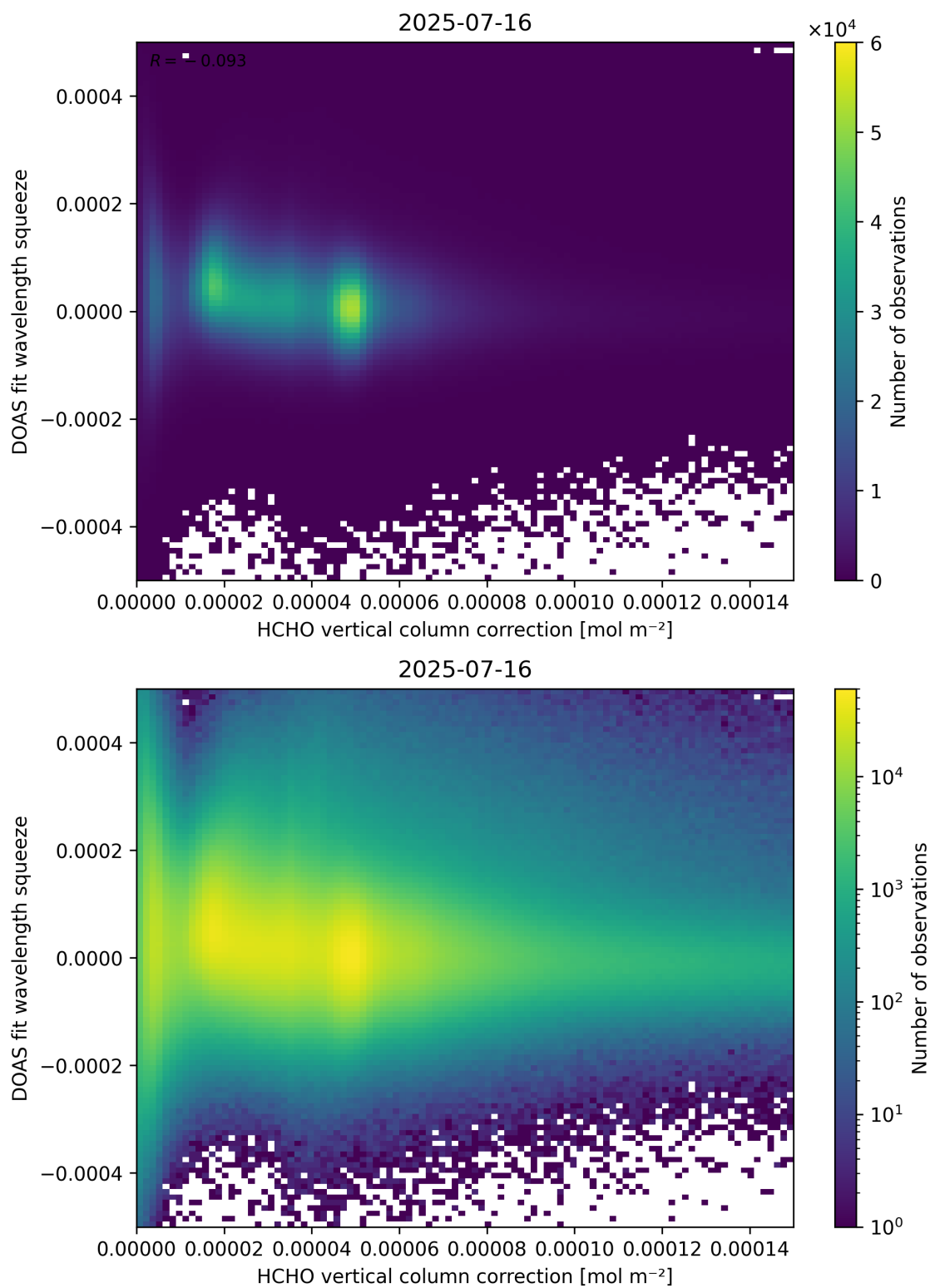
Figure 114: Scatter density plot of “HCHO vertical column correction” against “DOAS fit wavelength squeeze” for 2025-07-15 to 2025-07-17.
