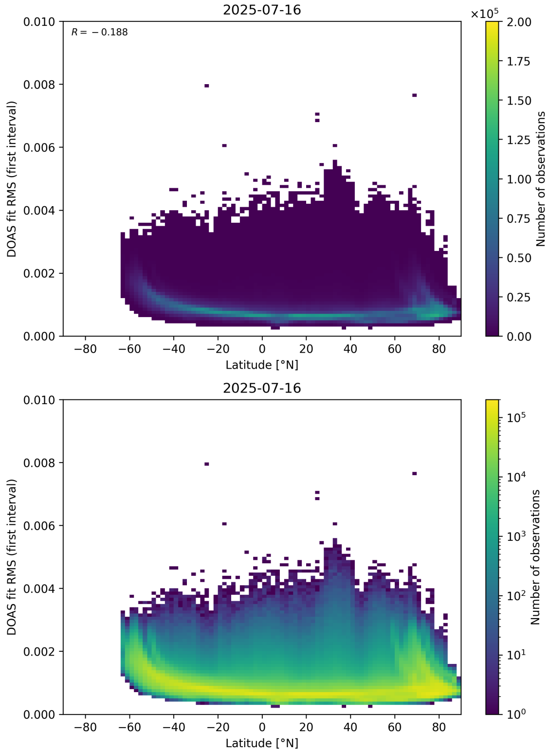
Figure 153: Scatter density plot of “Latitude” against “DOAS fit RMS (first interval)” for 2025-07-15 to 2025-07-17.
