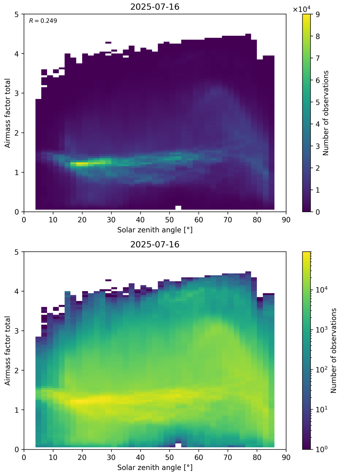
Figure 175: Scatter density plot of “Solar zenith angle” against “Airmass factor total” for 2025-07-15 to 2025-07-17.
