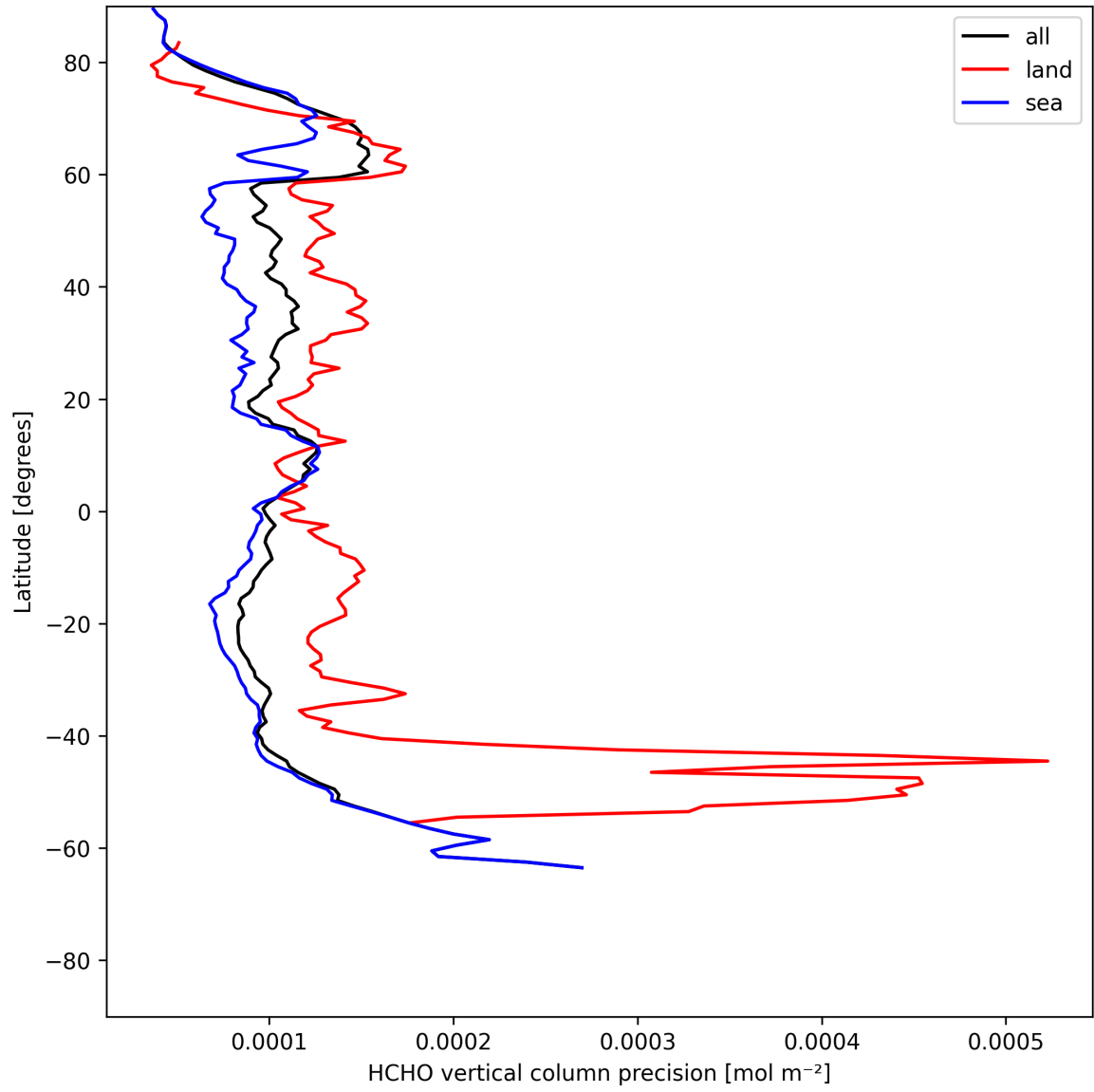
Figure 22: Zonal average of “HCHO vertical column precision” for 2025-07-15 to 2025-07-17.
