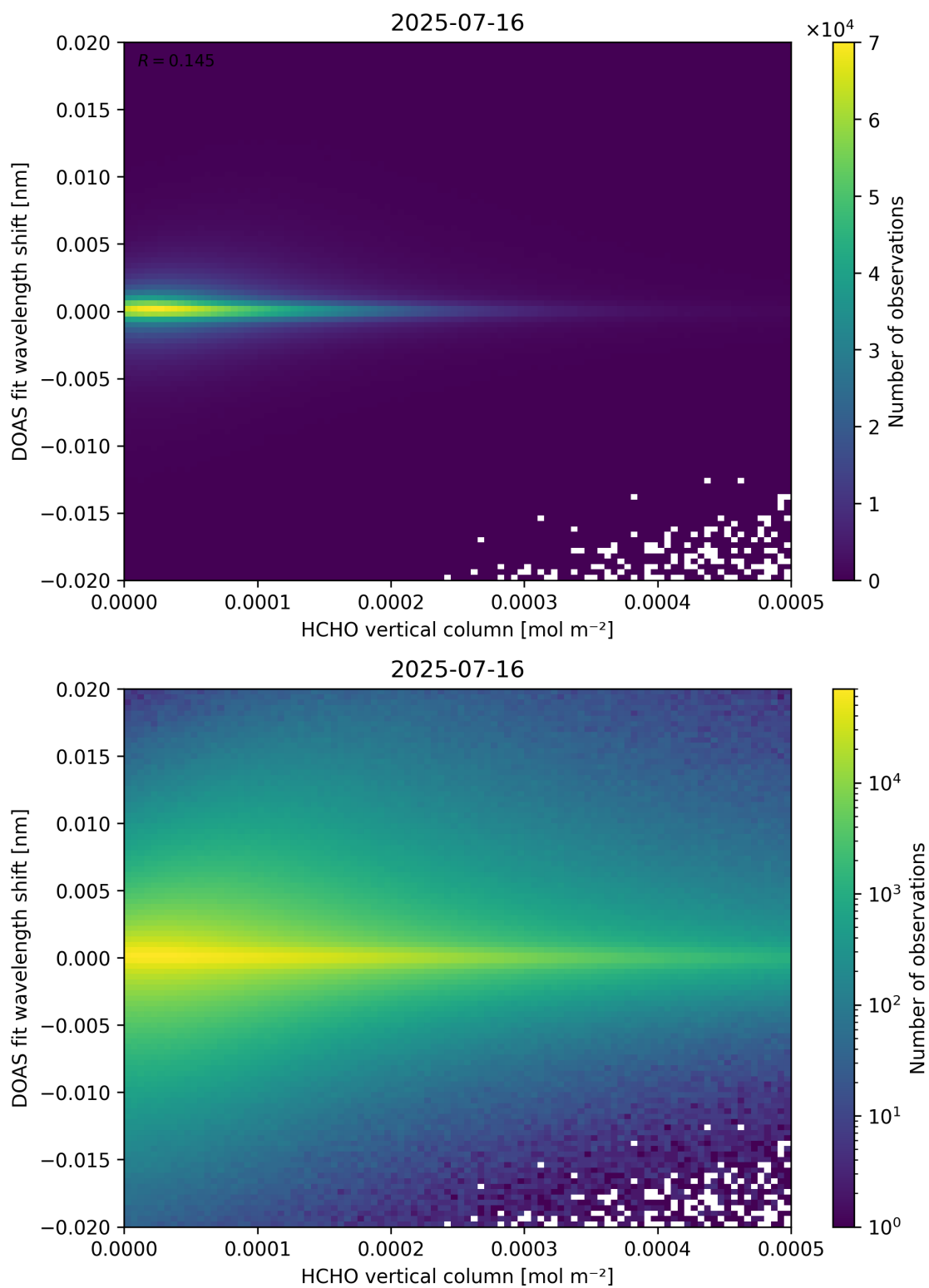
Figure 124: Scatter density plot of “HCHO vertical column” against “DOAS fit wavelength shift” for 2025-07-15 to 2025-07-17.
