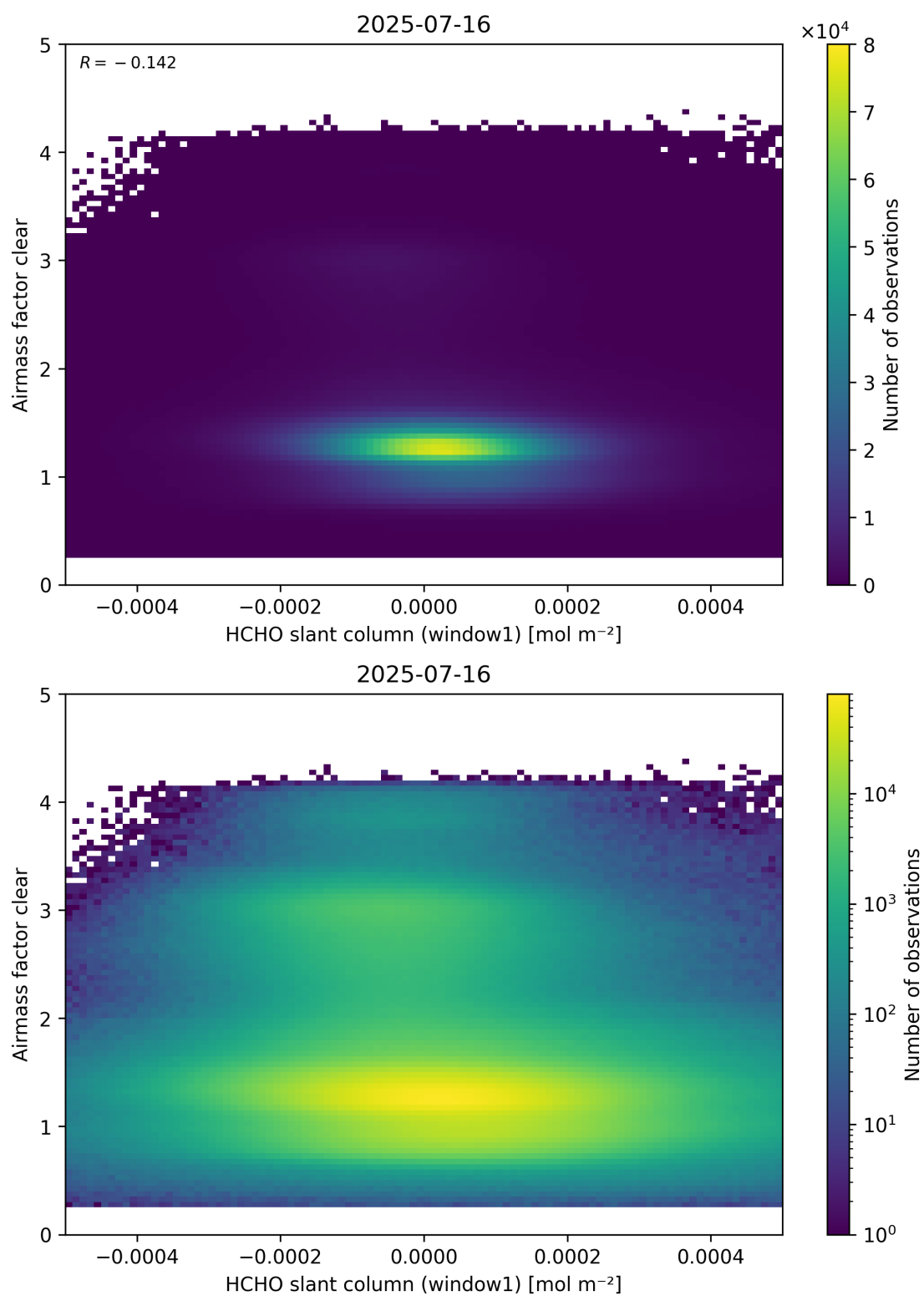
Figure 81: Scatter density plot of “HCHO slant column (window1)” against “Airmass factor clear” for 2025-07-15 to 2025-07-17.
