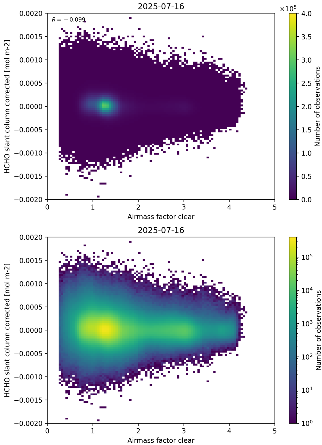
Figure 74: Scatter density plot of “Airmass factor clear” against “HCHO slant column corrected” for 2025-07-15 to 2025-07-17.
