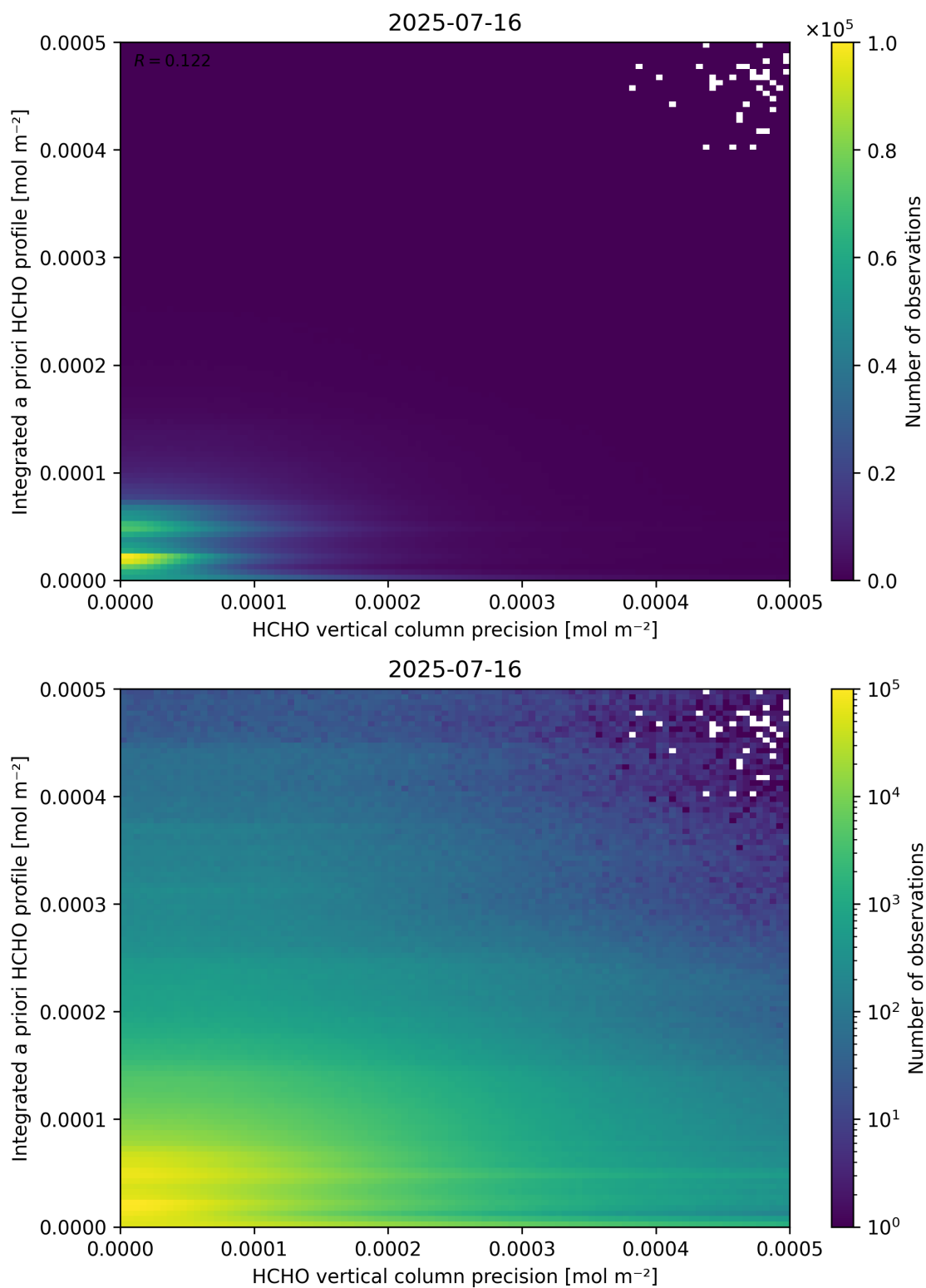
Figure 147: Scatter density plot of “HCHO vertical column precision” against “Integrated a priori HCHO profile” for 2025-07-15 to 2025-07-17.
