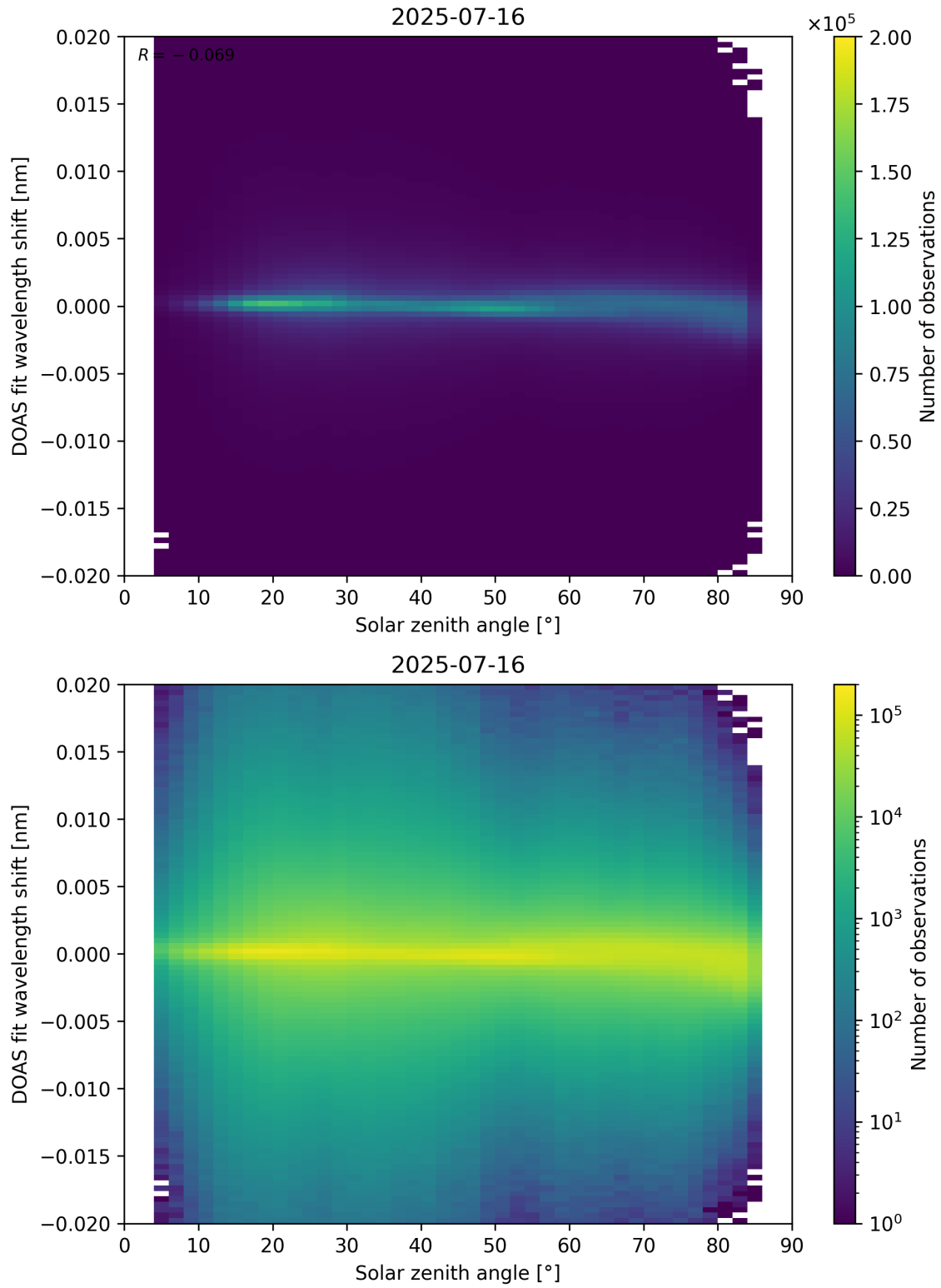
Figure 168: Scatter density plot of “Solar zenith angle” against “DOAS fit wavelength shift” for 2025-07-15 to 2025-07-17.
