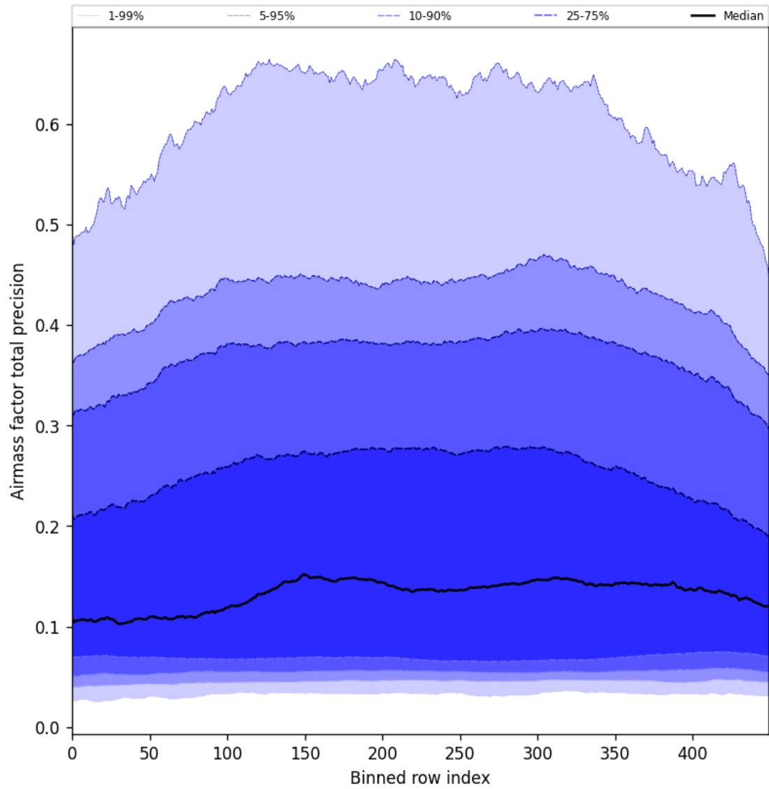
Figure 55: Along track statistics of “Airmass factor total precision” for 2025-07-15 to 2025-07-17
