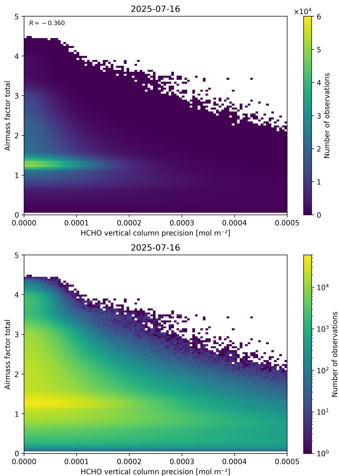
Figure 144: Scatter density plot of “HCHO vertical column precision” against “Airmass factor total” for 2025-07-15 to 2025-07-17.
