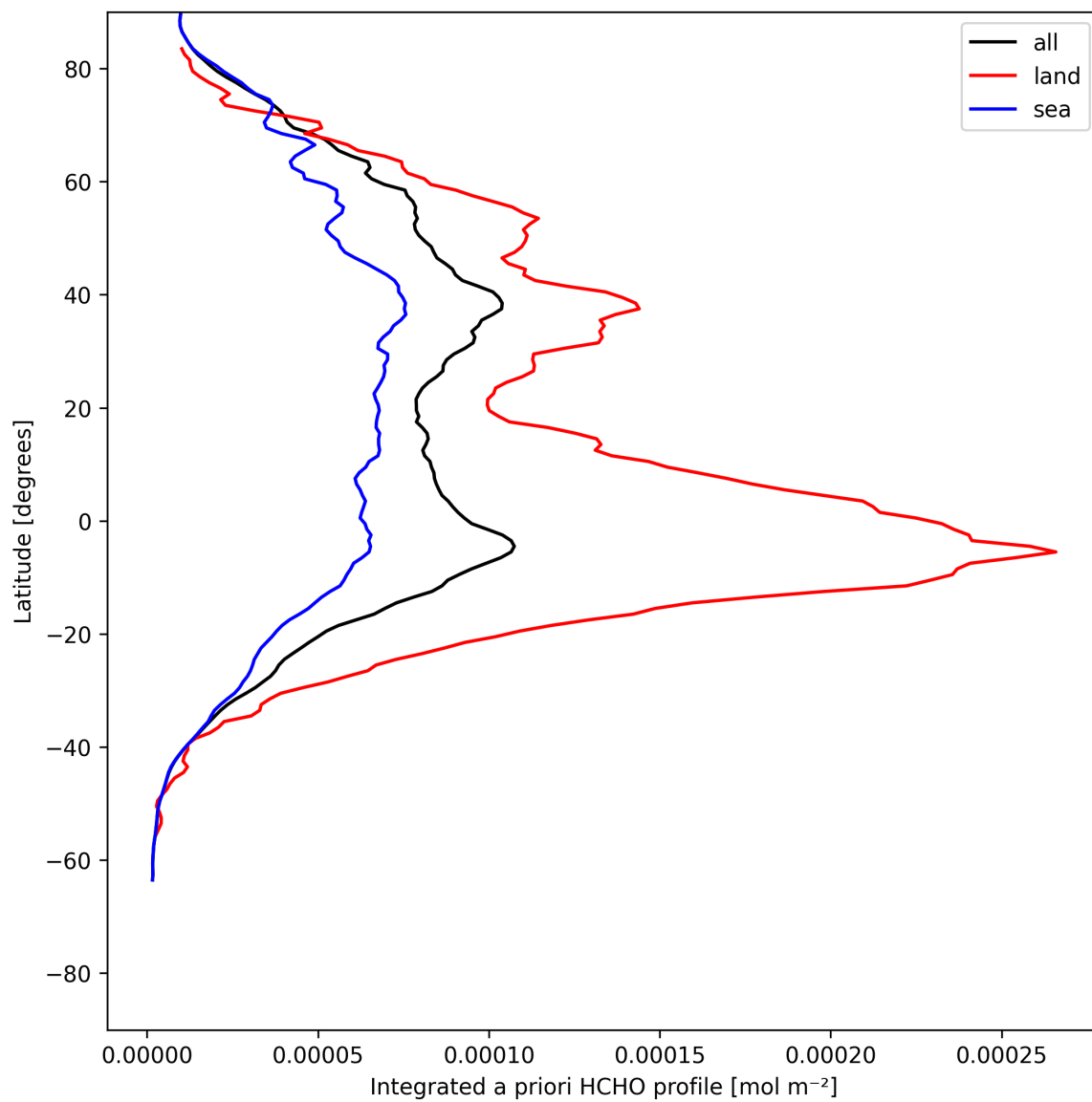
Figure 29: Zonal average of “Integrated a priori HCHO profile” for 2025-07-15 to 2025-07-17.
