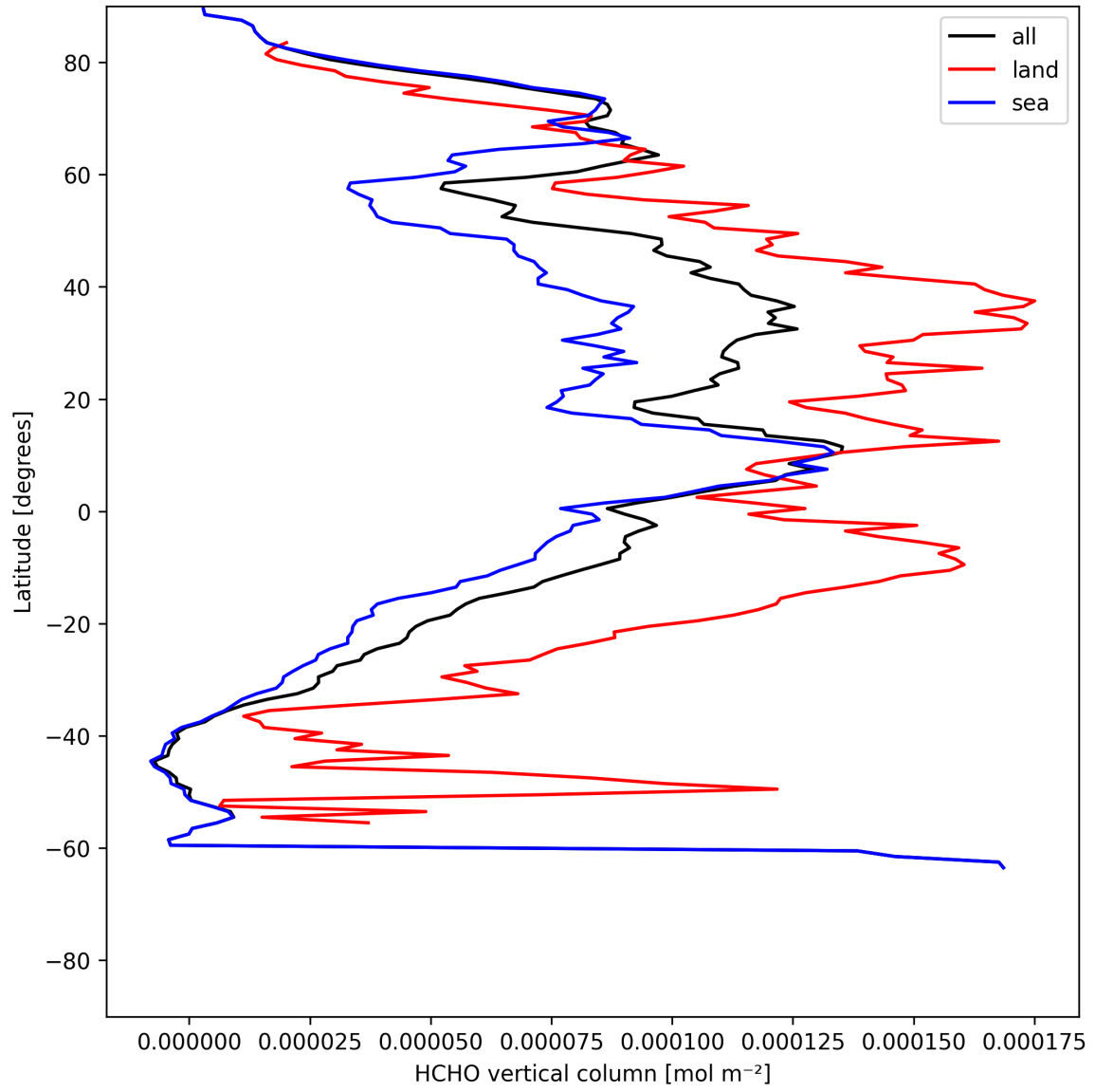
Figure 21: Zonal average of “HCHO vertical column” for 2025-07-15 to 2025-07-17.
