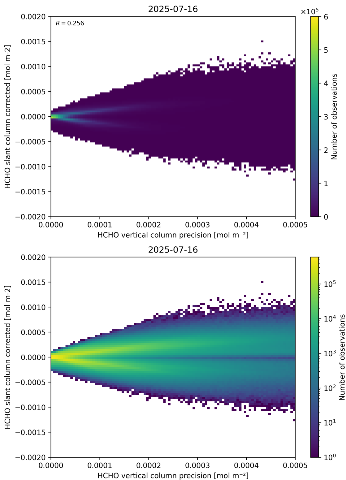
Figure 140: Scatter density plot of “HCHO vertical column precision” against “HCHO slant column corrected” for 2025-07-15 to 2025-07-17.
