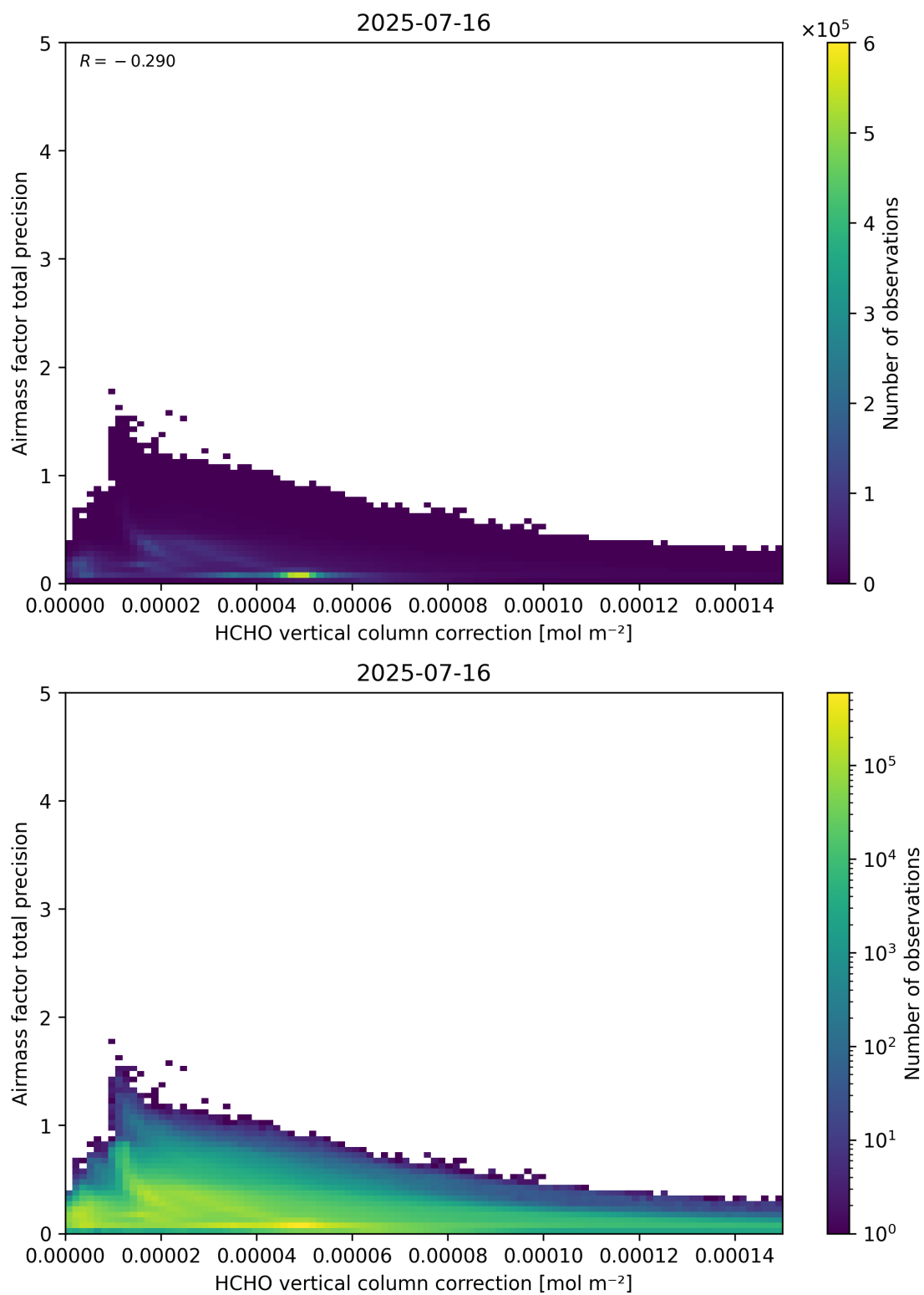
Figure 121: Scatter density plot of “HCHO vertical column correction” against “Airmass factor total precision” for 2025-07-15 to 2025-07-17.
