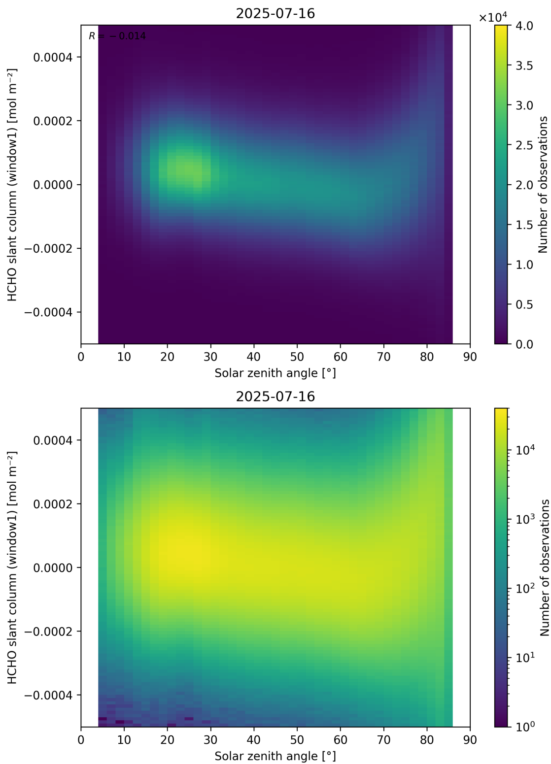
Figure 173: Scatter density plot of “Solar zenith angle” against “HCHO slant column (window1)” for 2025-07-15 to 2025-07-17.
