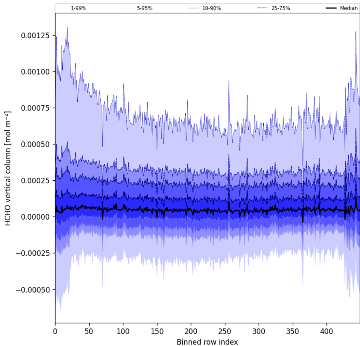
Figure 49: Along track statistics of “HCHO vertical column” for 2025-07-15 to 2025-07-17
