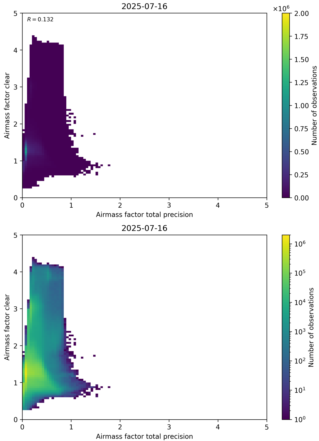
Figure 108: Scatter density plot of “Airmass factor total precision” against “Airmass factor clear” for 2025-07-15 to 2025-07-17.
