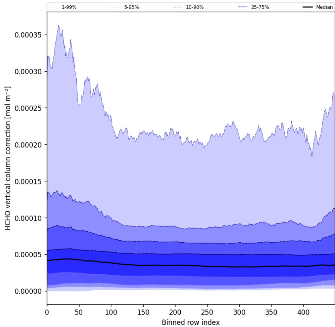
Figure 51: Along track statistics of “HCHO vertical column correction” for 2025-07-15 to 2025-07-17
