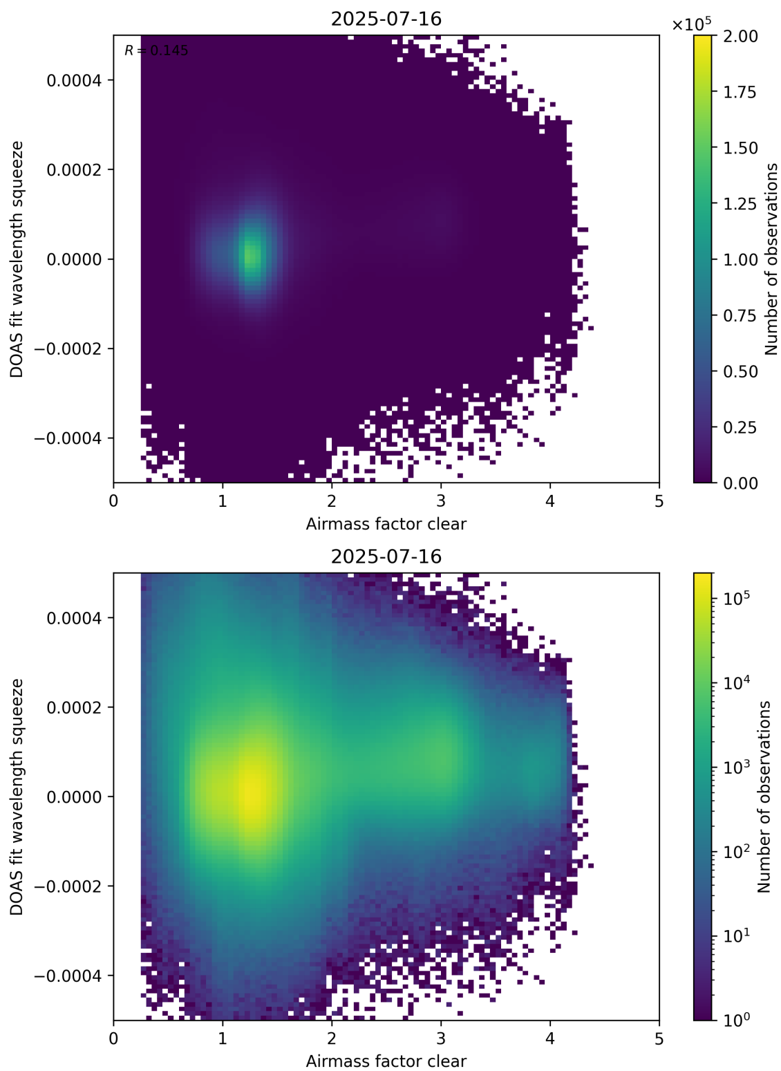
Figure 73: Scatter density plot of “Airmass factor clear” against “DOAS fit wavelength squeeze” for 2025-07-15 to 2025-07-17.
