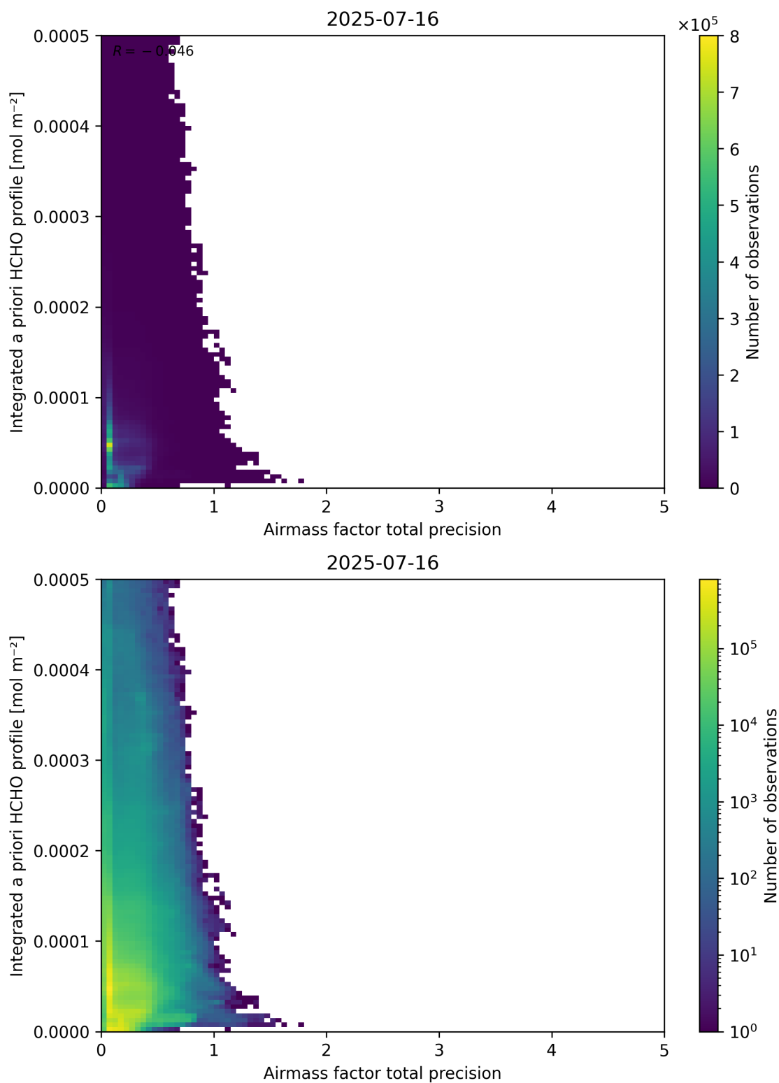
Figure 111: Scatter density plot of “Airmass factor total precision” against “Integrated a priori HCHO profile” for 2025-07-15 to 2025-07-17.
