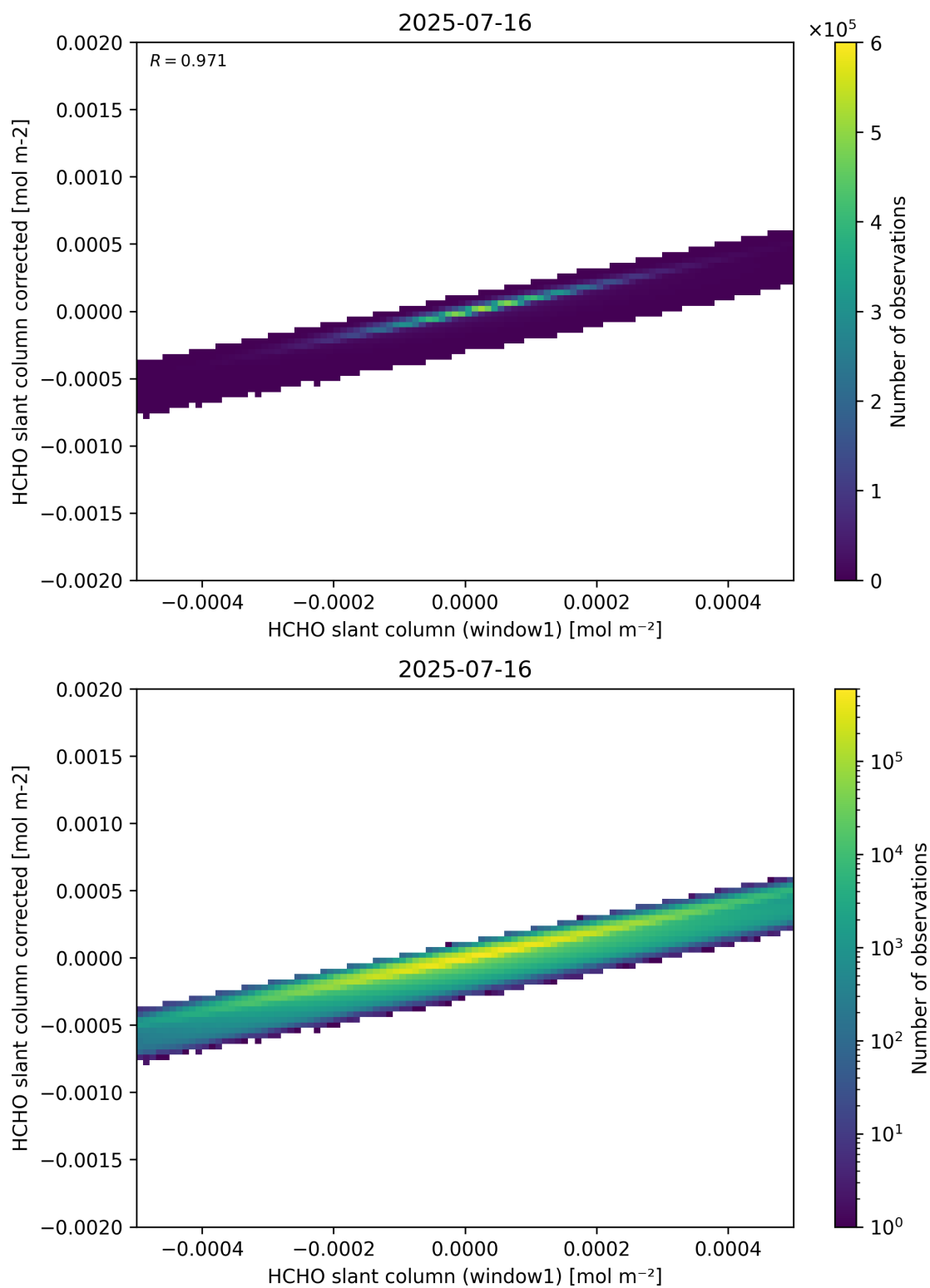
Figure 82: Scatter density plot of “HCHO slant column (window1)” against “HCHO slant column corrected” for 2025-07-15 to 2025-07-17.
