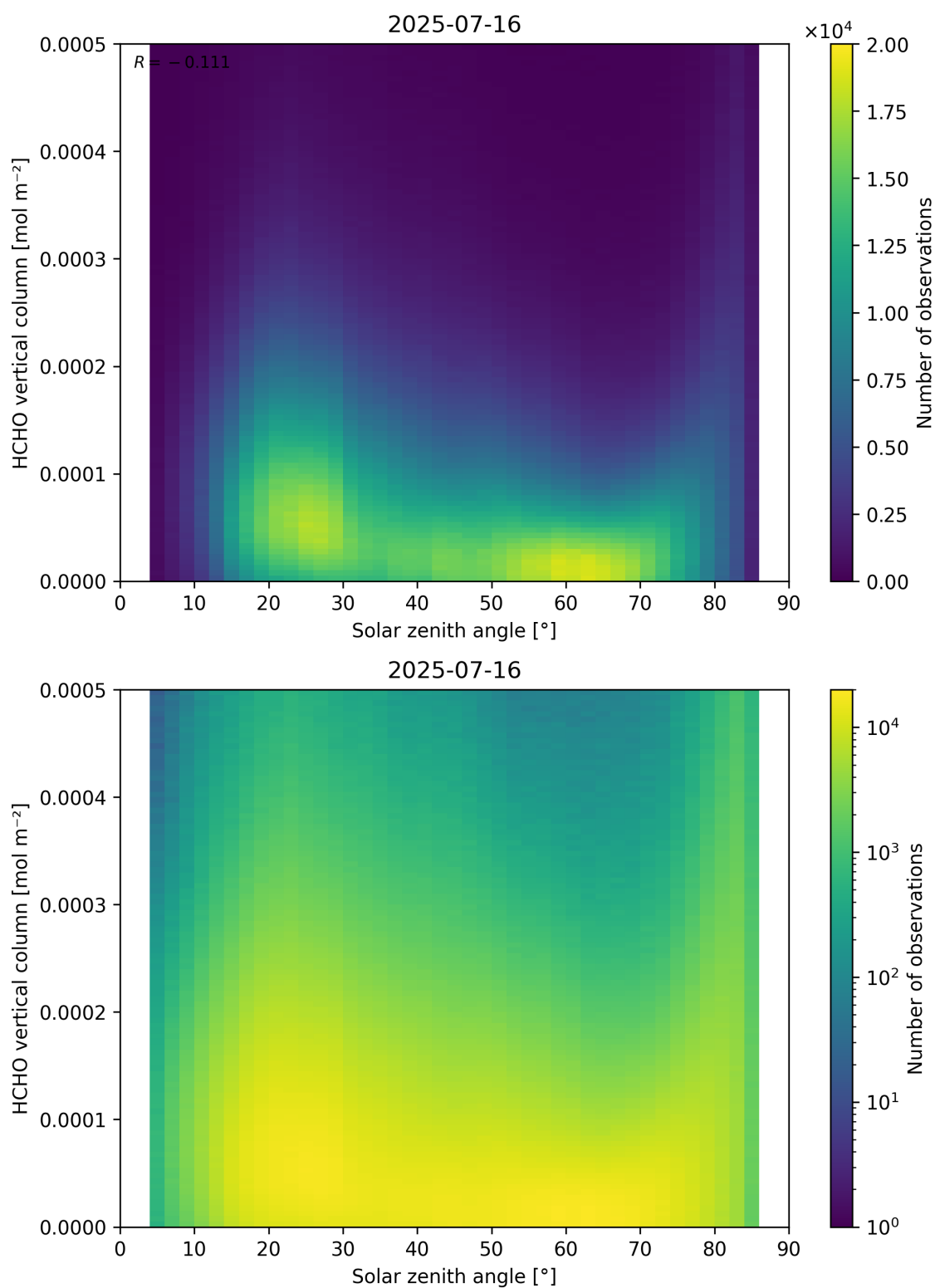
Figure 177: Scatter density plot of “Solar zenith angle” against “HCHO vertical column” for 2025-07-15 to 2025-07-17.
