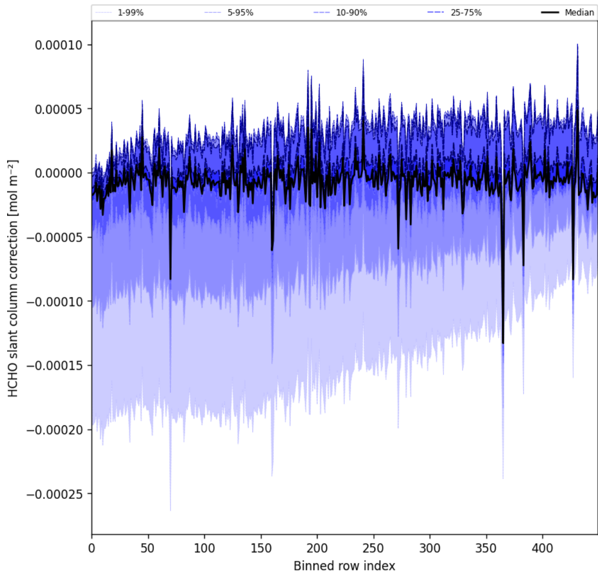
Figure 61: Along track statistics of “HCHO slant column correction” for 2025-07-15 to 2025-07-17
