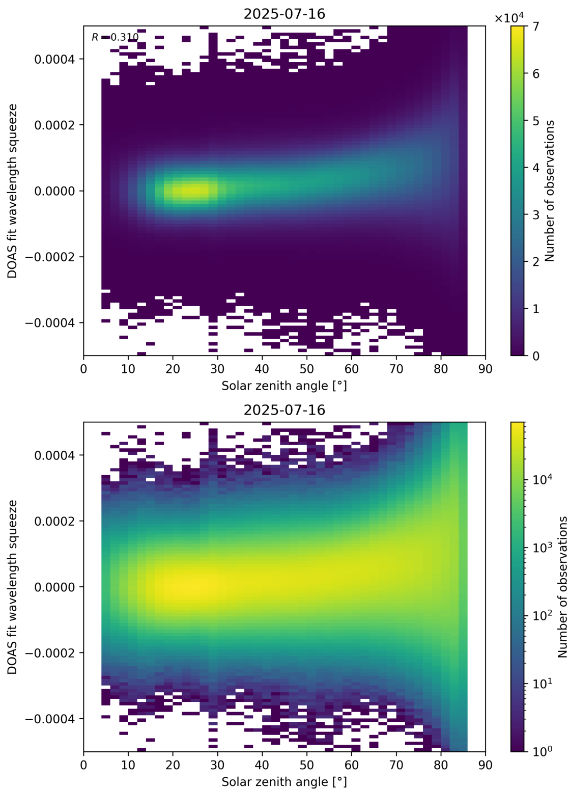
Figure 169: Scatter density plot of “Solar zenith angle” against “DOAS fit wavelength squeeze” for 2025-07-15 to 2025-07-17.
