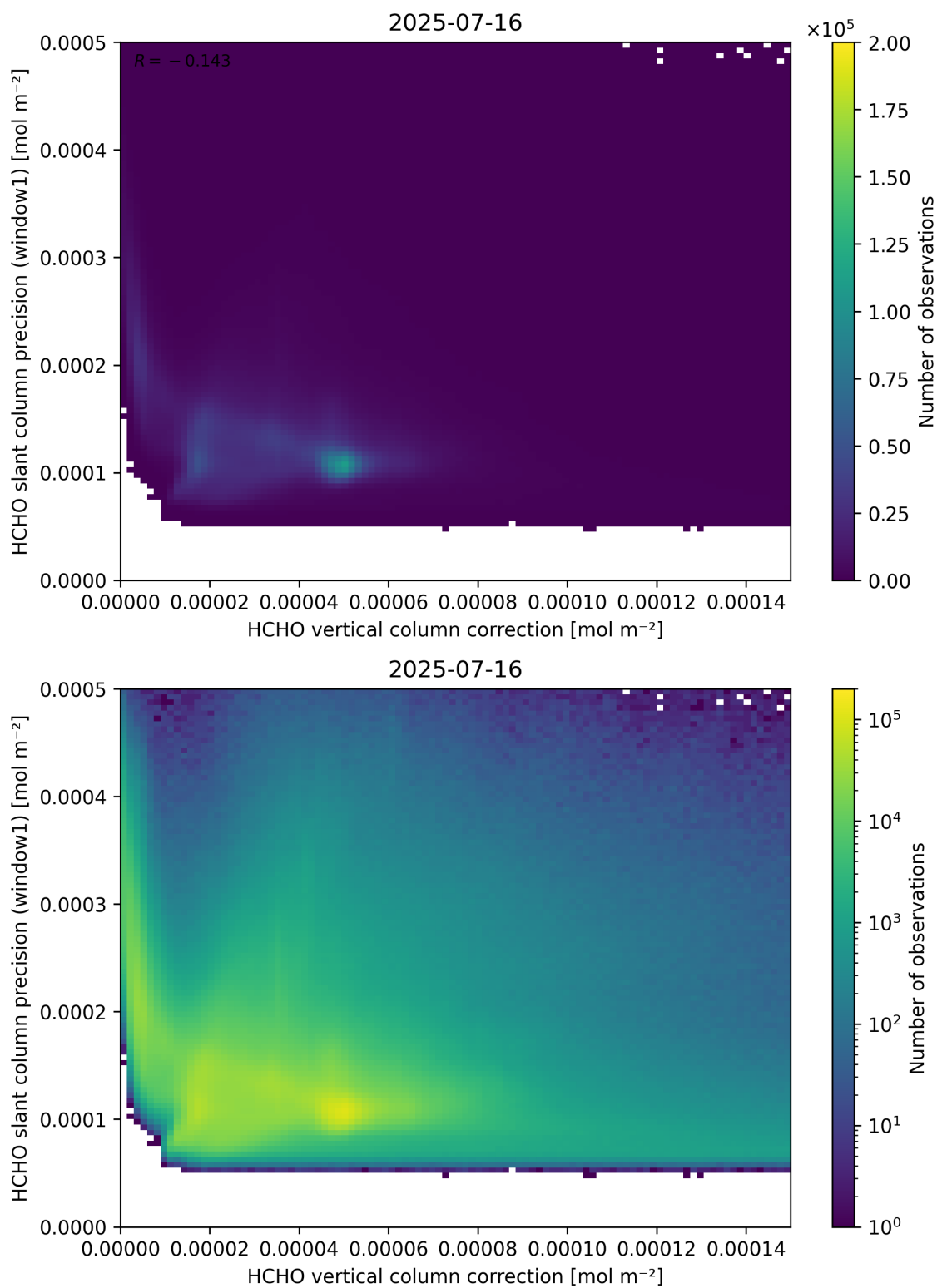
Figure 119: Scatter density plot of “HCHO vertical column correction” against “HCHO slant column precision (window1)” for 2025-07-15 to 2025-07-17.
