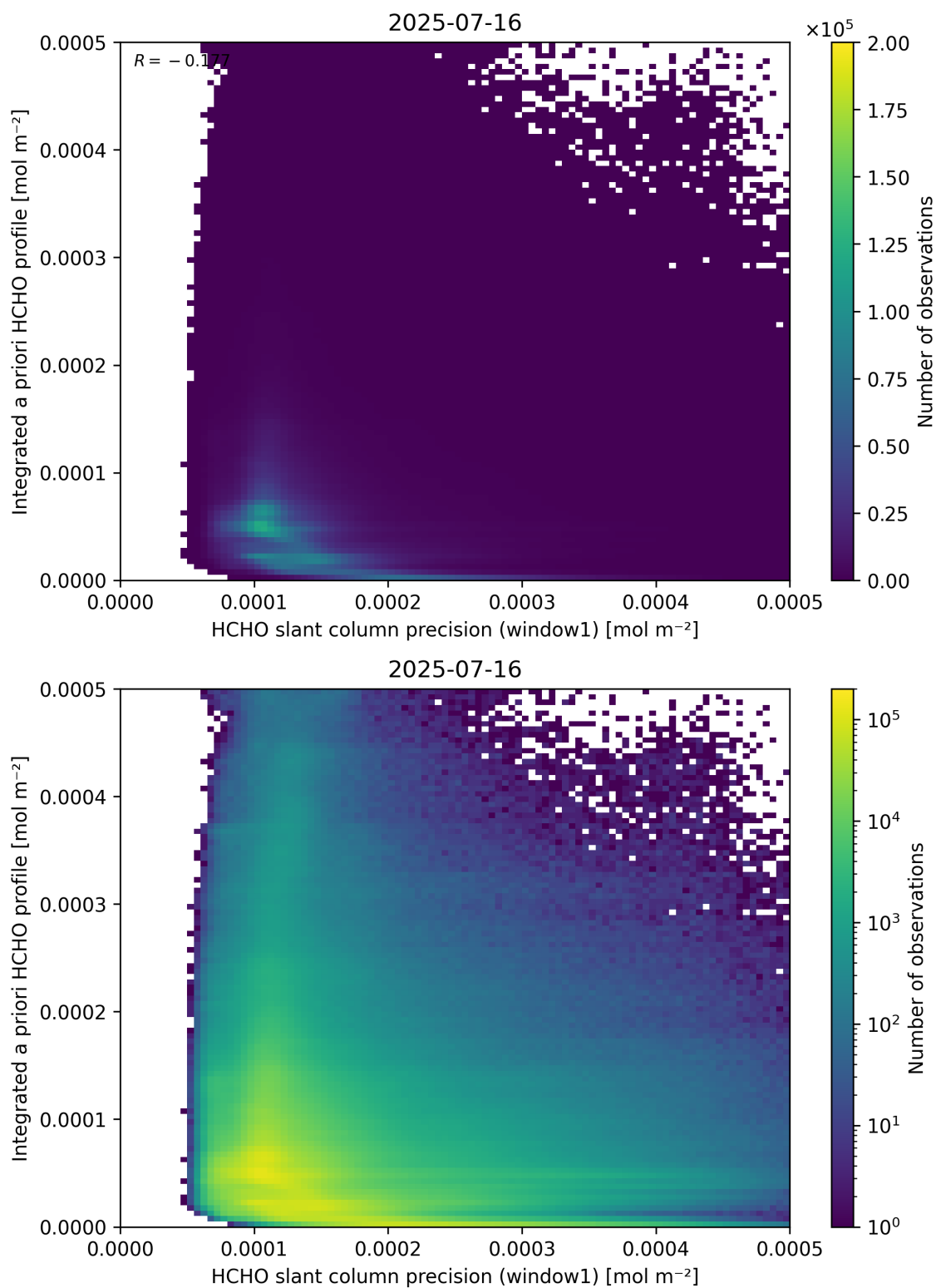
Figure 96: Scatter density plot of “HCHO slant column precision (window1)” against “Integrated a priori HCHO profile” for 2025-07-15 to 2025-07-17.
