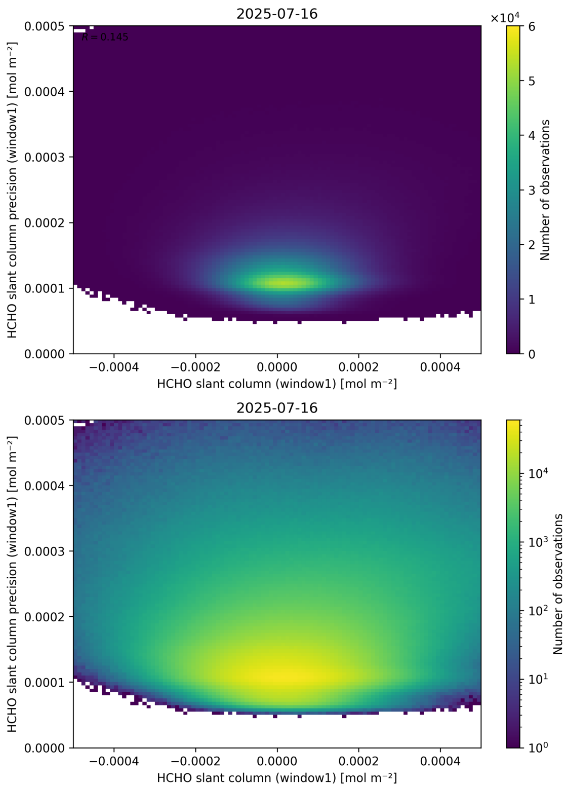
Figure 84: Scatter density plot of “HCHO slant column (window1)” against “HCHO slant column precision (window1)” for 2025-07-15 to 2025-07-17.
