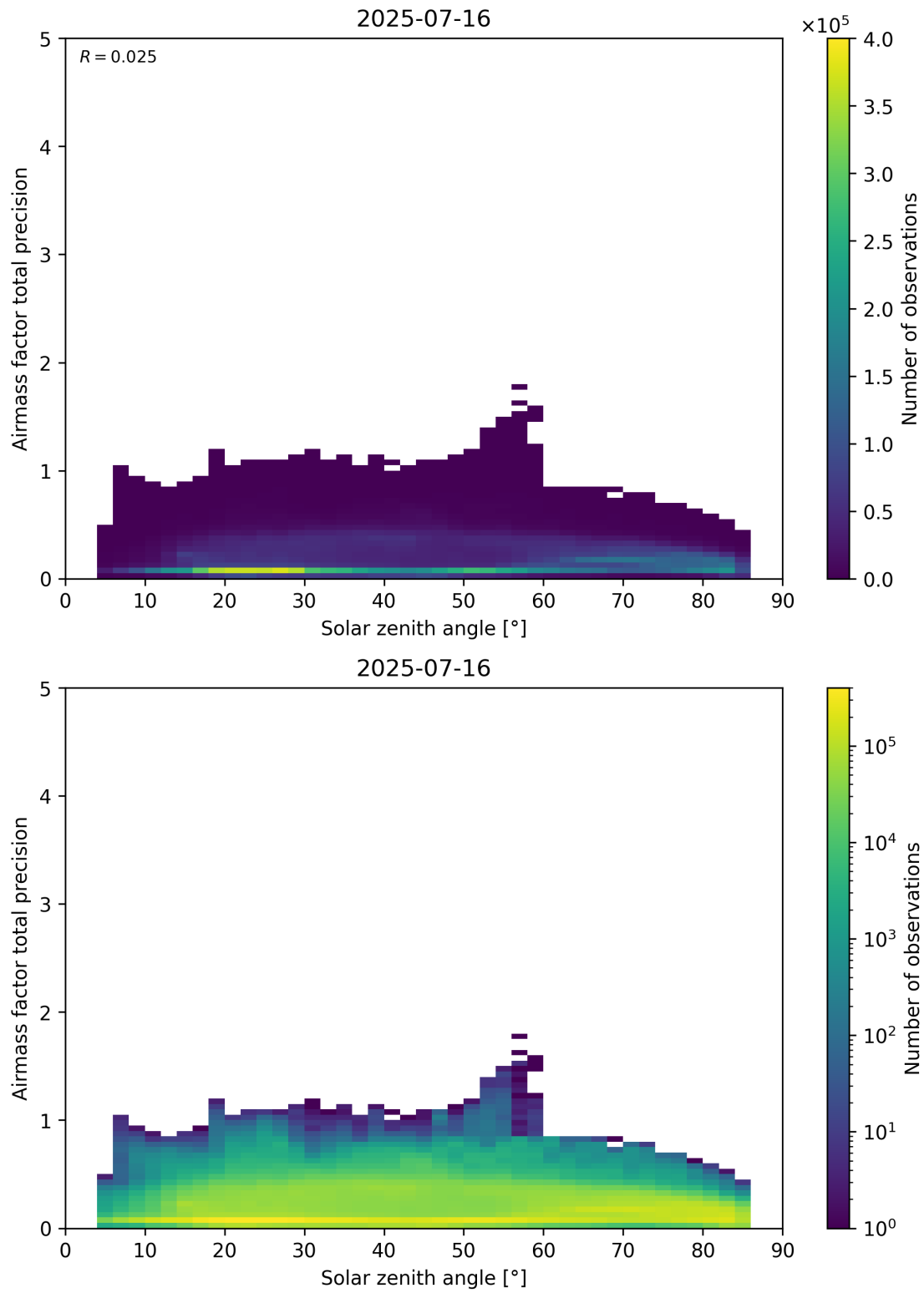
Figure 176: Scatter density plot of “Solar zenith angle” against “Airmass factor total precision” for 2025-07-15 to 2025-07-17.
