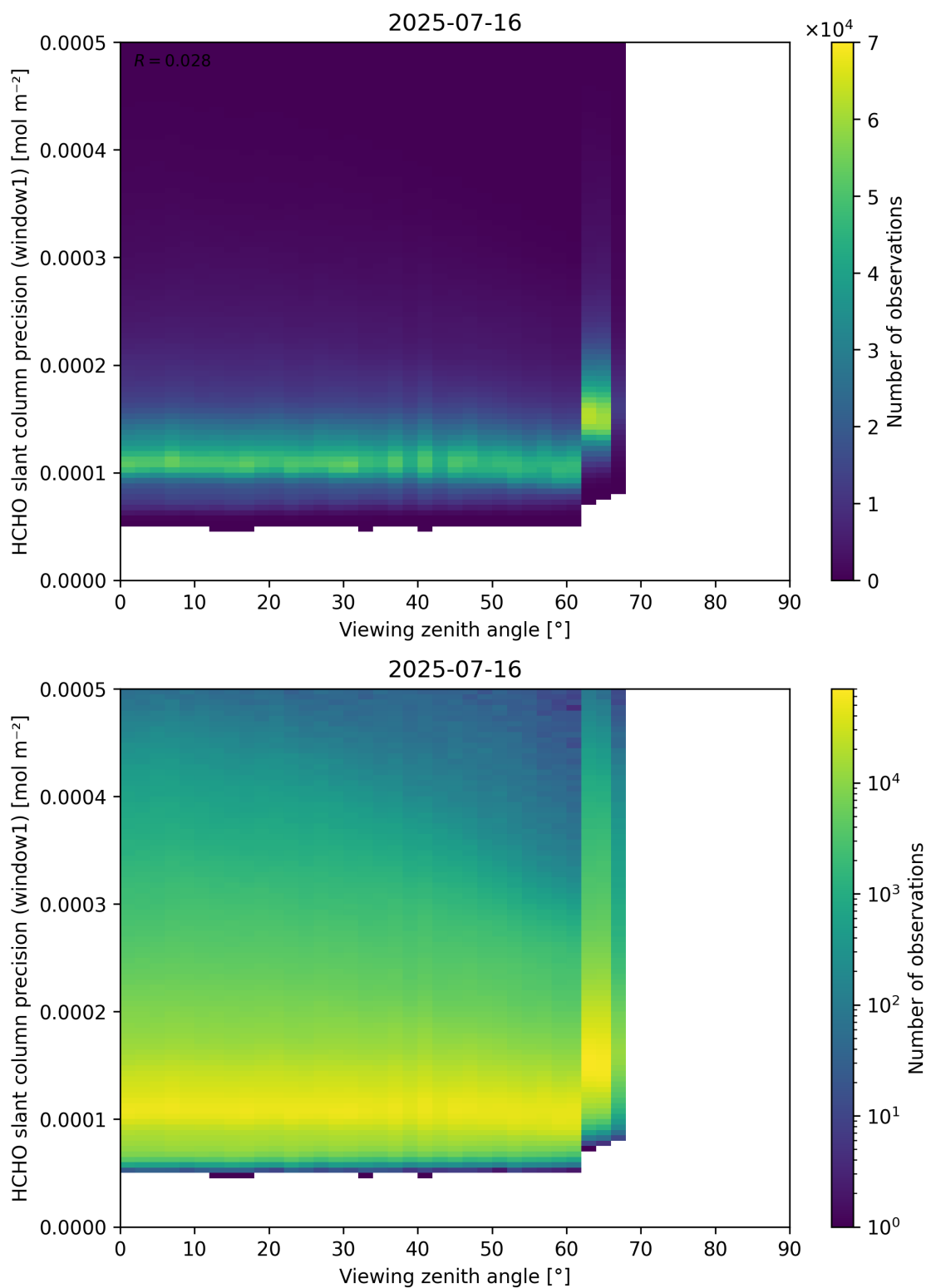
Figure 189: Scatter density plot of “Viewing zenith angle” against “HCHO slant column precision (window1)” for 2025-07-15 to 2025-07-17.
