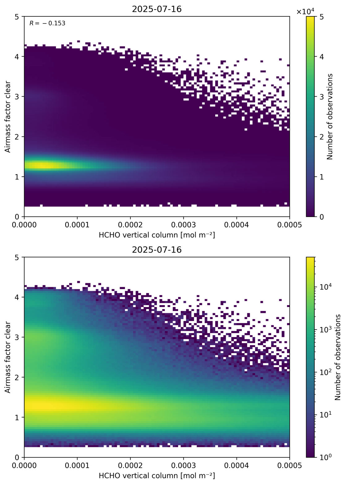
Figure 126: Scatter density plot of “HCHO vertical column” against “Airmass factor clear” for 2025-07-15 to 2025-07-17.
