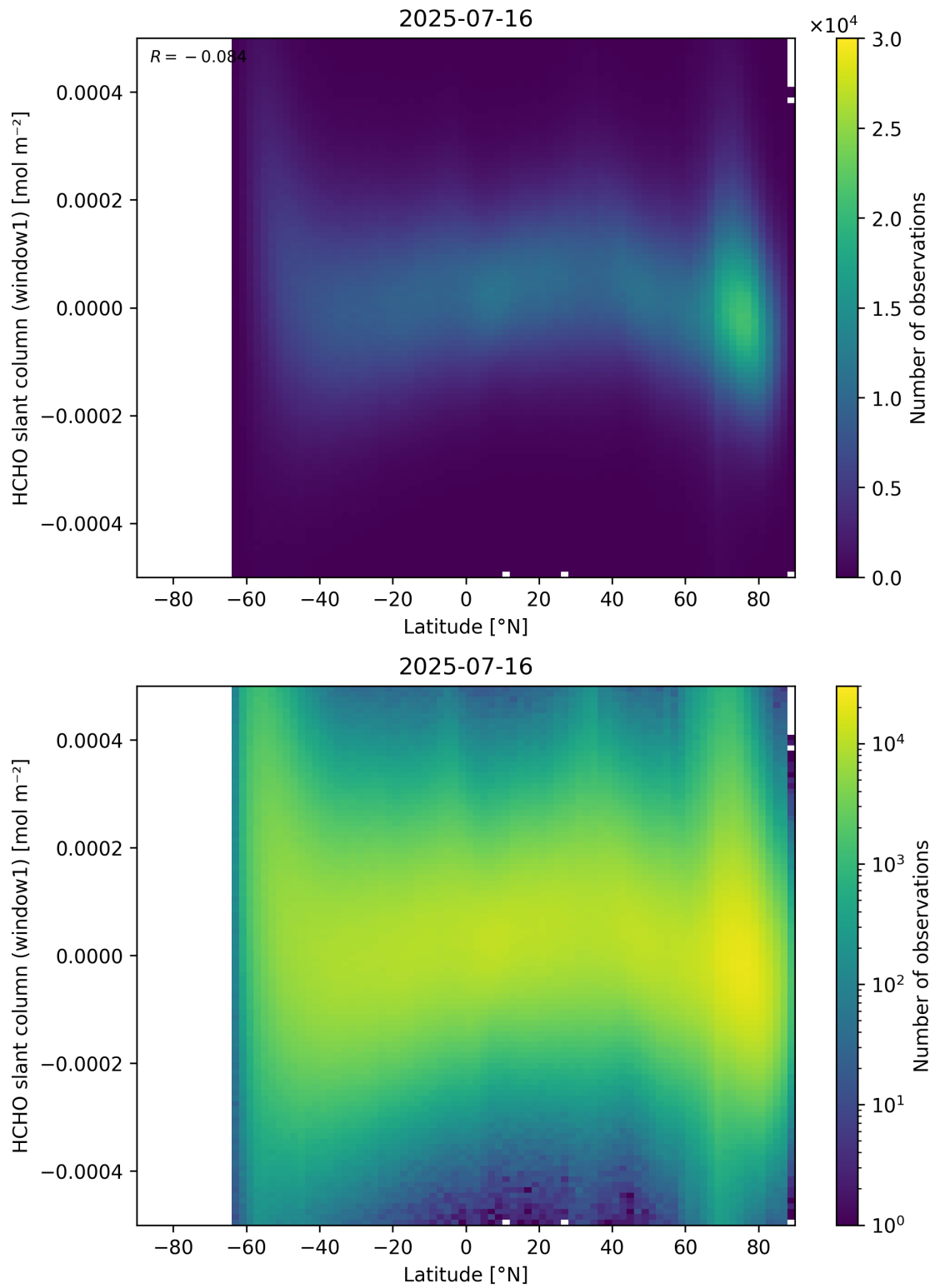
Figure 159: Scatter density plot of “Latitude” against “HCHO slant column (window1)” for 2025-07-15 to 2025-07-17.
