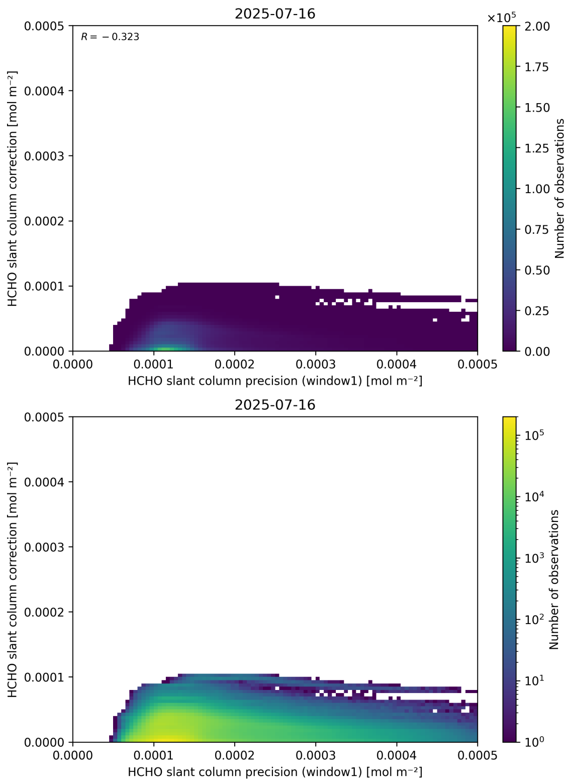
Figure 93: Scatter density plot of “HCHO slant column precision (window1)” against “HCHO slant column correction” for 2025-07-15 to 2025-07-17.
