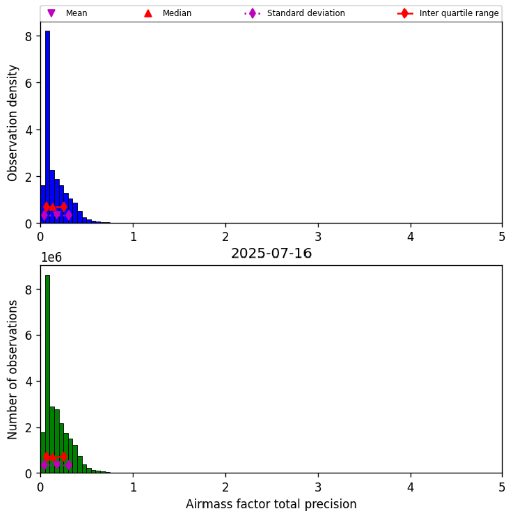
Figure 41: Histogram of “Airmass factor total precision” for 2025-07-15 to 2025-07-17
