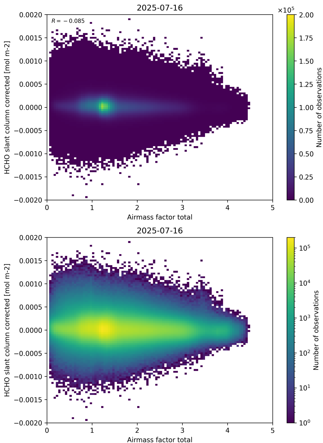
Figure 101: Scatter density plot of “Airmass factor total” against “HCHO slant column corrected” for 2025-07-15 to 2025-07-17.
