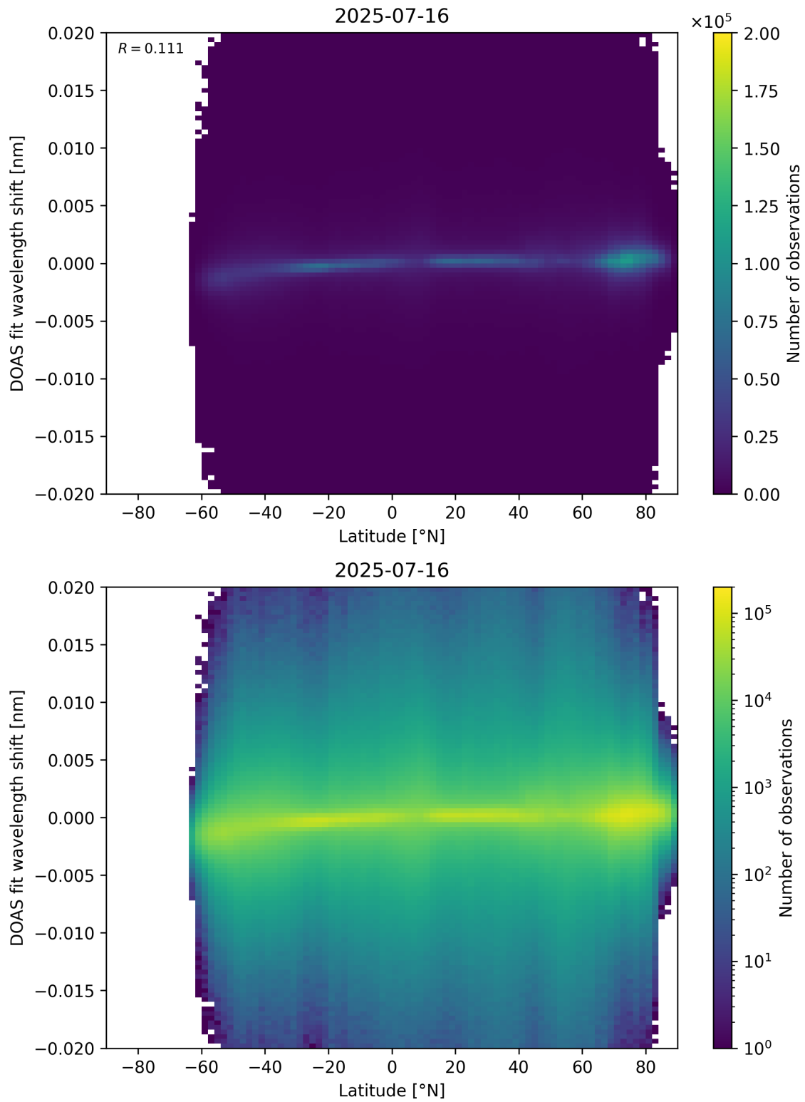
Figure 154: Scatter density plot of “Latitude” against “DOAS fit wavelength shift” for 2025-07-15 to 2025-07-17.
