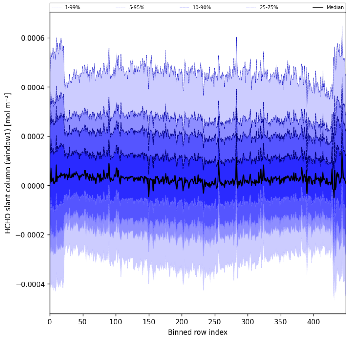
Figure 52: Along track statistics of “HCHO slant column (window1)” for 2025-07-15 to 2025-07-17
