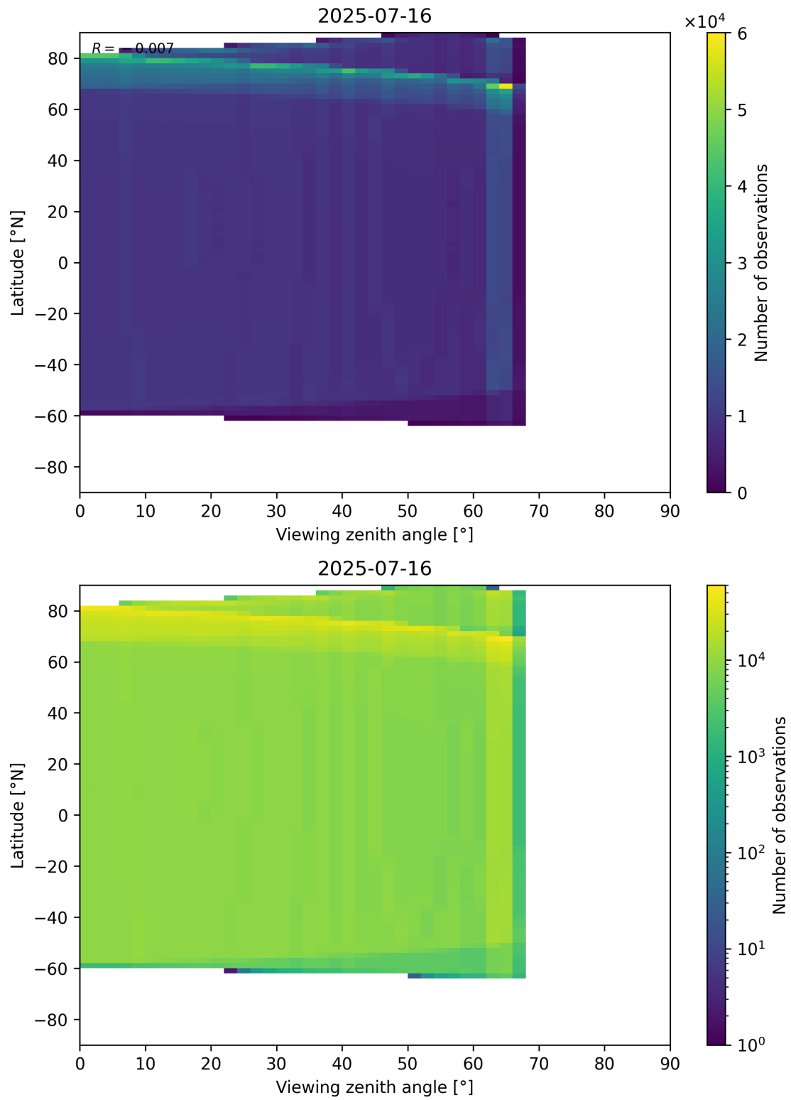
Figure 196: Scatter density plot of “Viewing zenith angle” against “Latitude” for 2025-07-15 to 2025-07-17.
