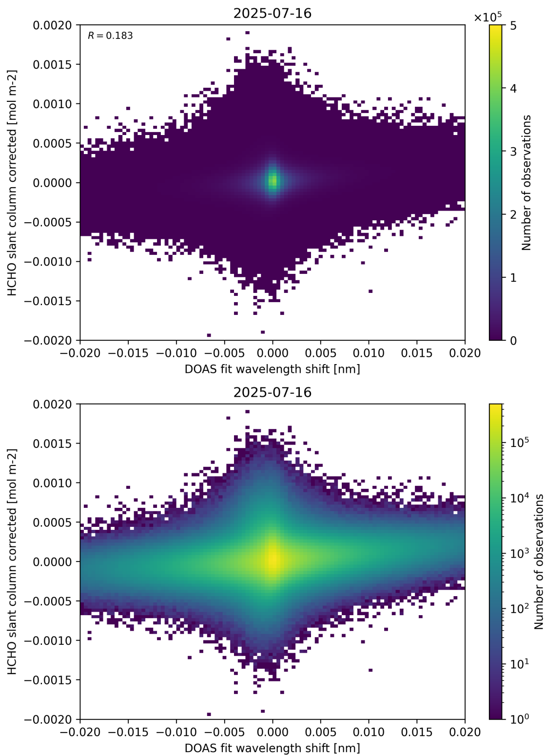
Figure 66: Scatter density plot of “DOAS fit wavelength shift” against “HCHO slant column corrected” for 2025-07-15 to 2025-07-17.
