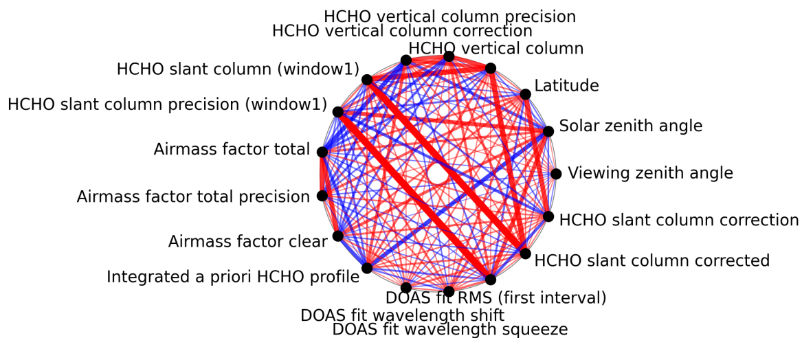
Figure 1: Map of correlation graph for 2025-07-15 to 2025-07-17.
