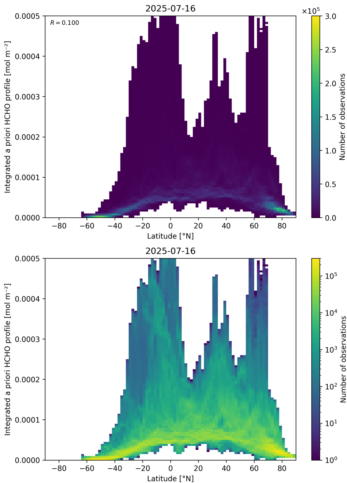
Figure 166: Scatter density plot of “Latitude” against “Integrated a priori HCHO profile” for 2025-07-15 to 2025-07-17.
