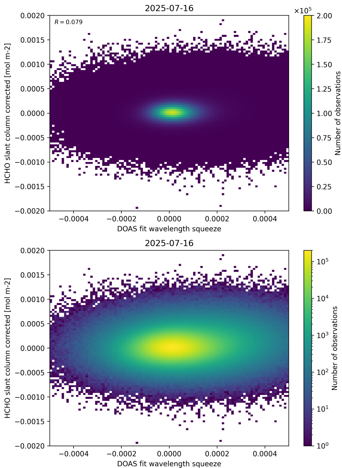
Figure 69: Scatter density plot of “DOAS fit wavelength squeeze” against “HCHO slant column corrected” for 2025-07-15 to 2025-07-17.
