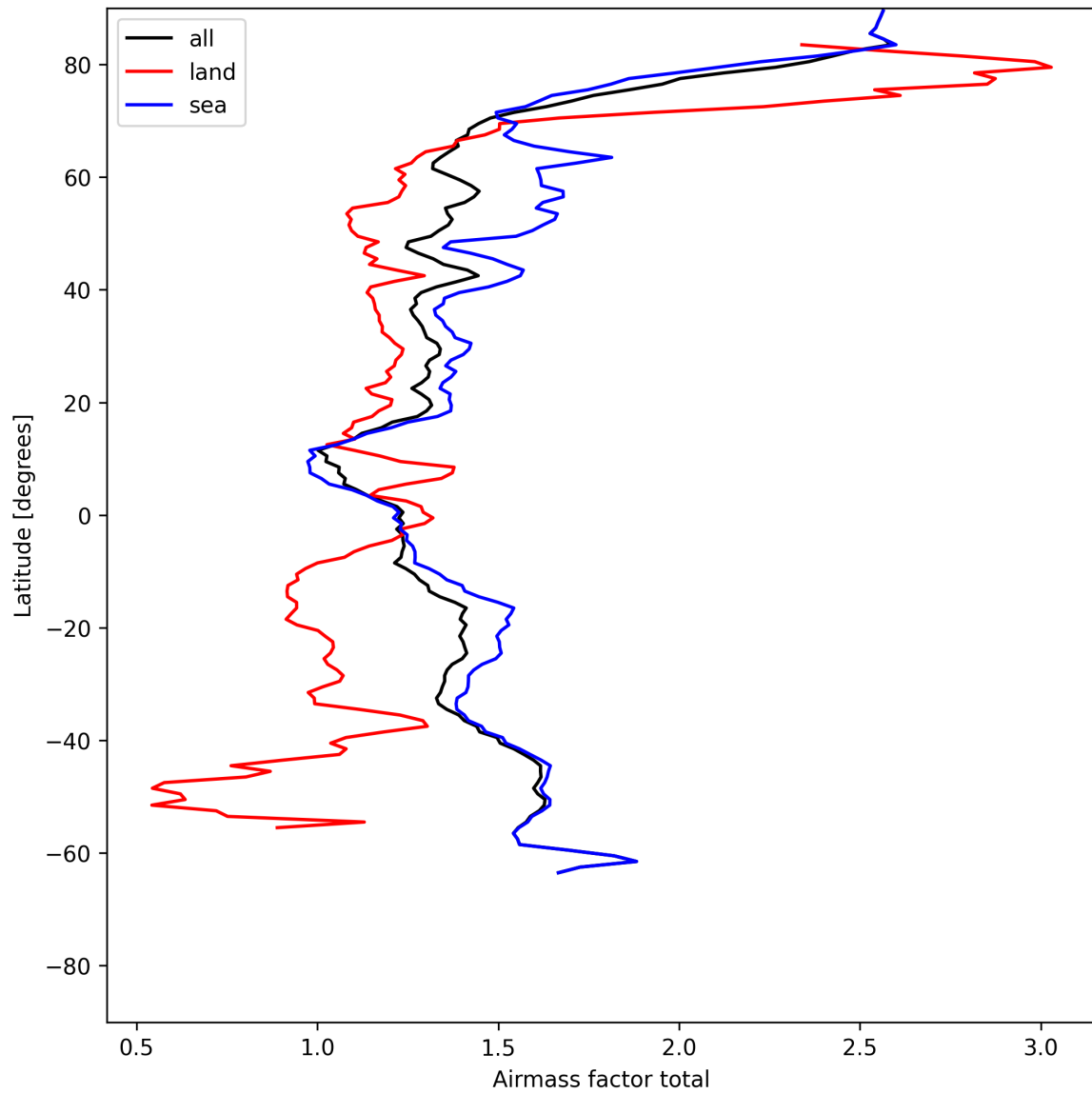
Figure 26: Zonal average of “Airmass factor total” for 2025-07-15 to 2025-07-17.
