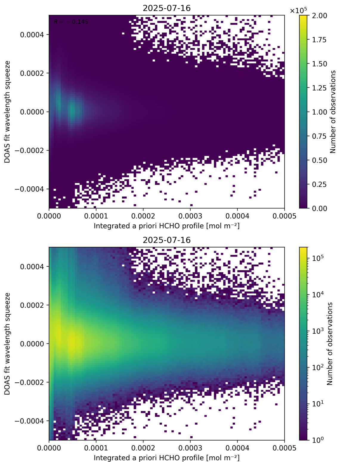
Figure 150: Scatter density plot of “Integrated a priori HCHO profile” against “DOAS fit wavelength squeeze” for 2025-07-15 to 2025-07-17.
