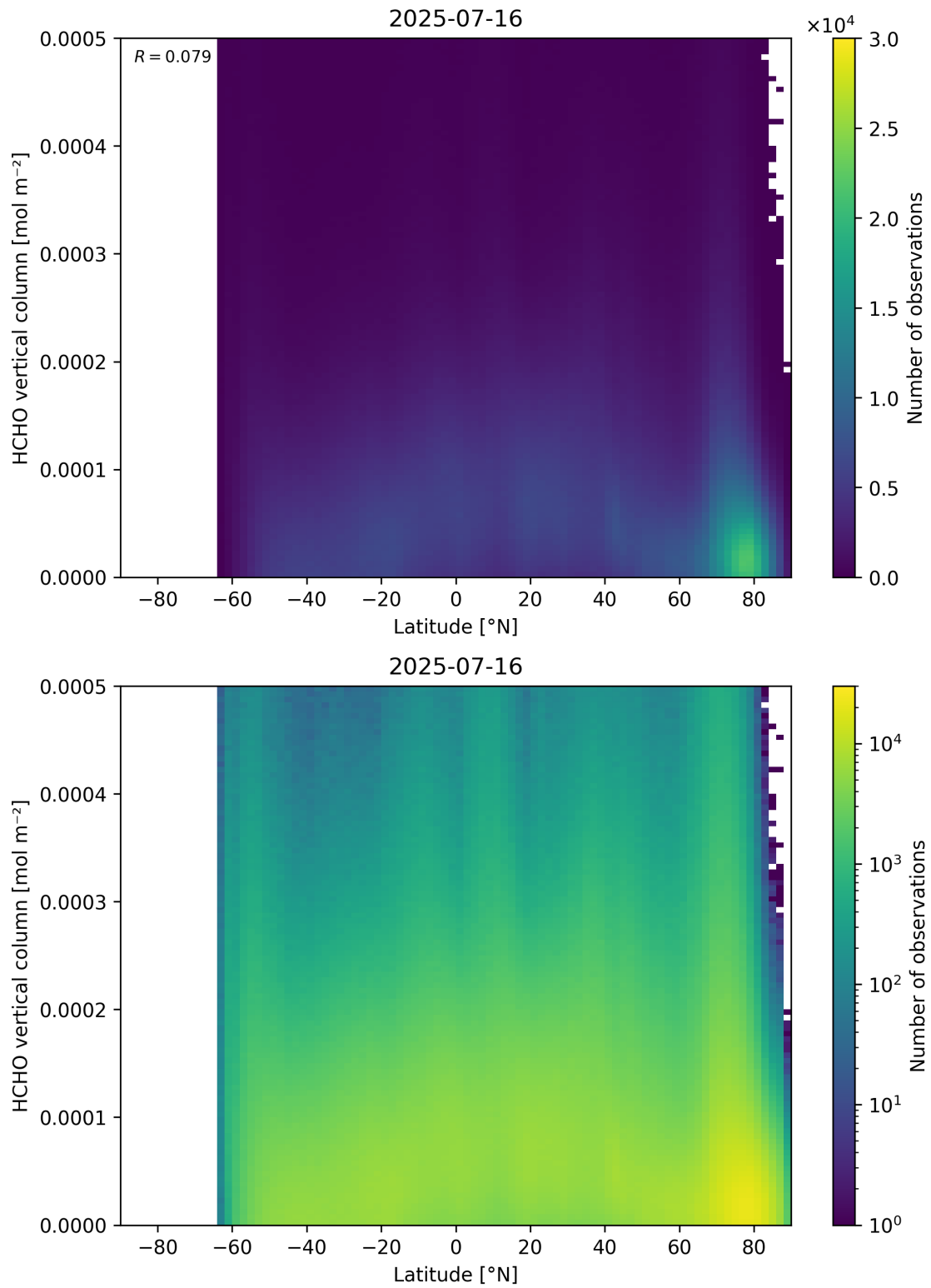
Figure 163: Scatter density plot of “Latitude” against “HCHO vertical column” for 2025-07-15 to 2025-07-17.
