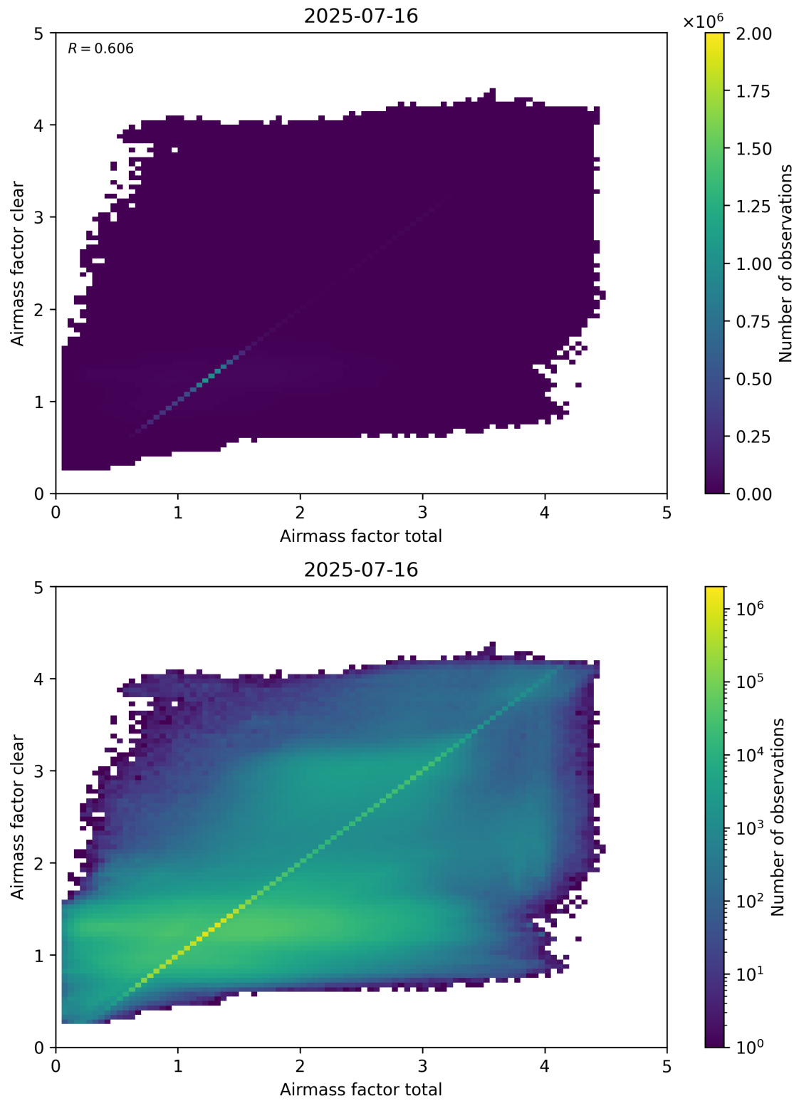
Figure 100: Scatter density plot of “Airmass factor total” against “Airmass factor clear” for 2025-07-15 to 2025-07-17.
