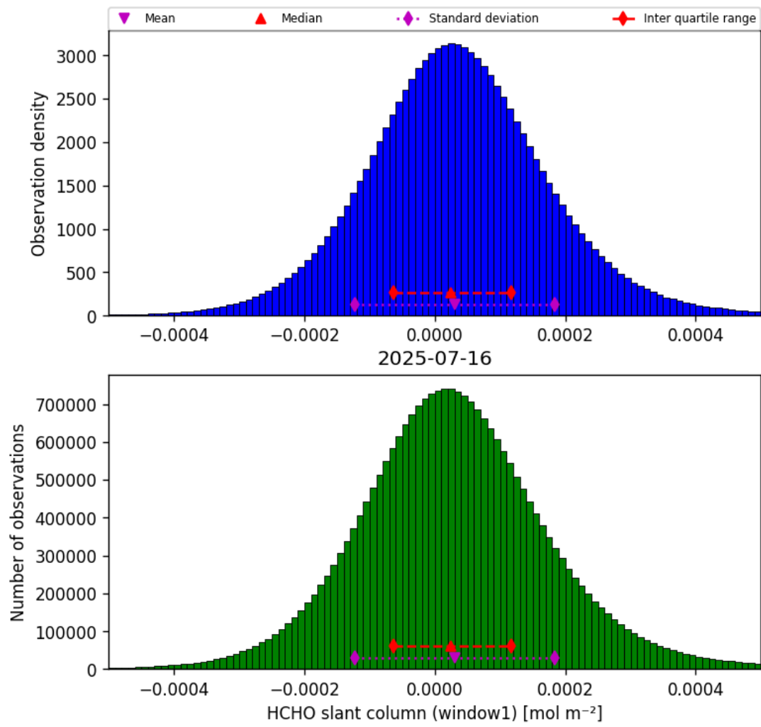
Figure 38: Histogram of “HCHO slant column (window1)” for 2025-07-15 to 2025-07-17
