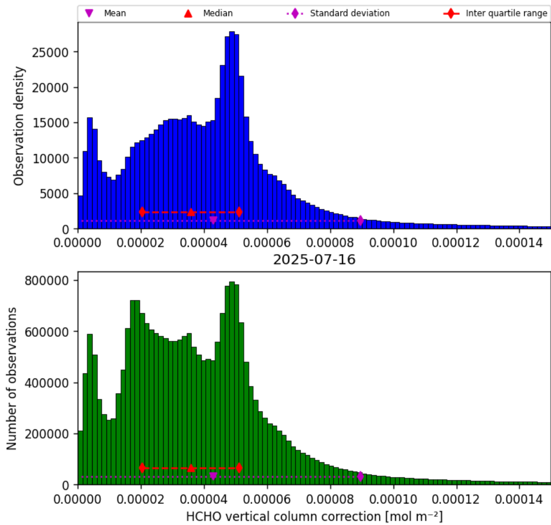
Figure 37: Histogram of “HCHO vertical column correction” for 2025-07-15 to 2025-07-17
