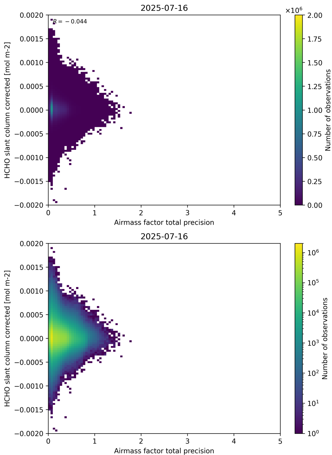
Figure 109: Scatter density plot of “Airmass factor total precision” against “HCHO slant column corrected” for 2025-07-15 to 2025-07-17.
