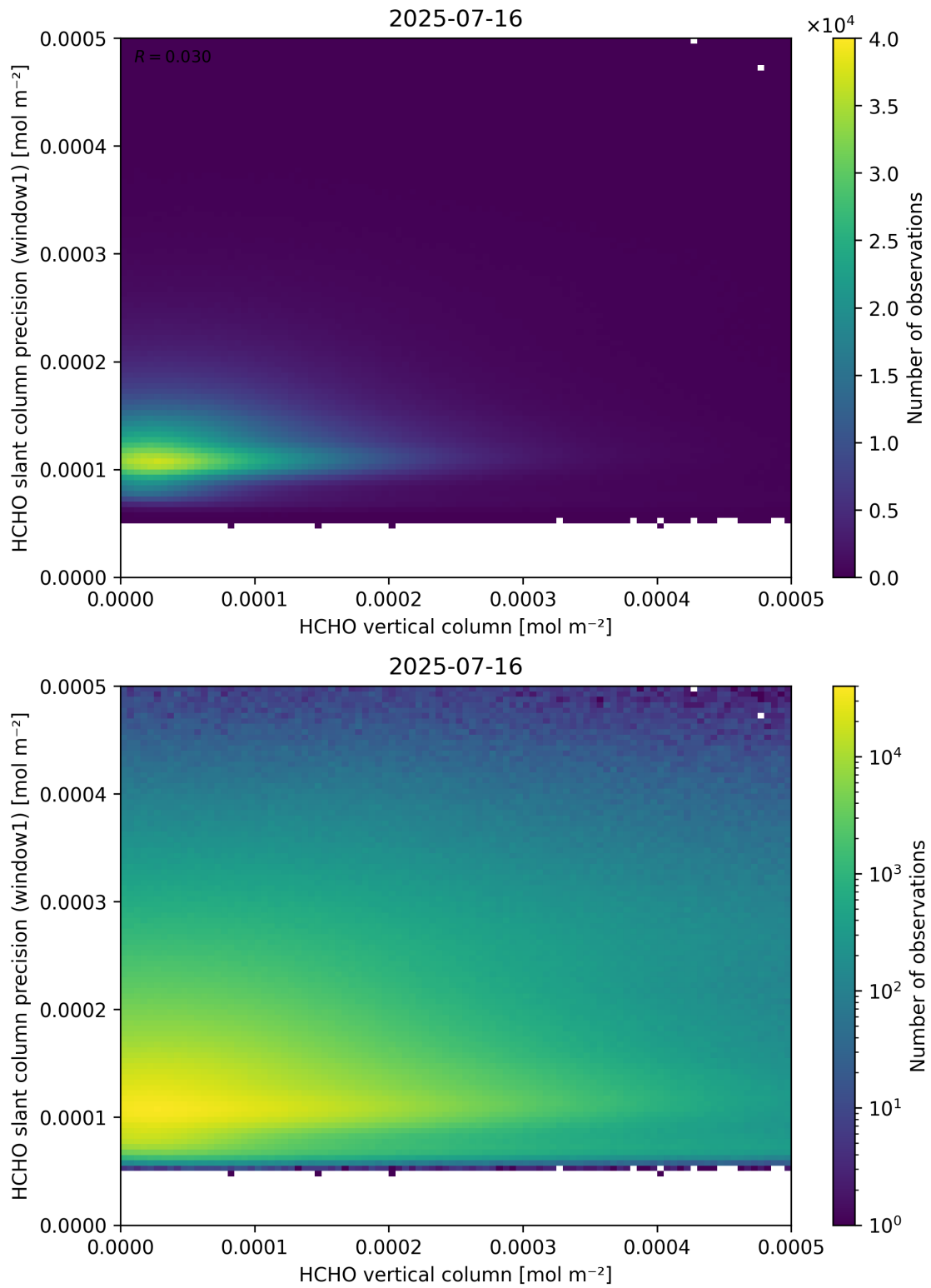
Figure 130: Scatter density plot of “HCHO vertical column” against “HCHO slant column precision (window1)” for 2025-07-15 to 2025-07-17.
