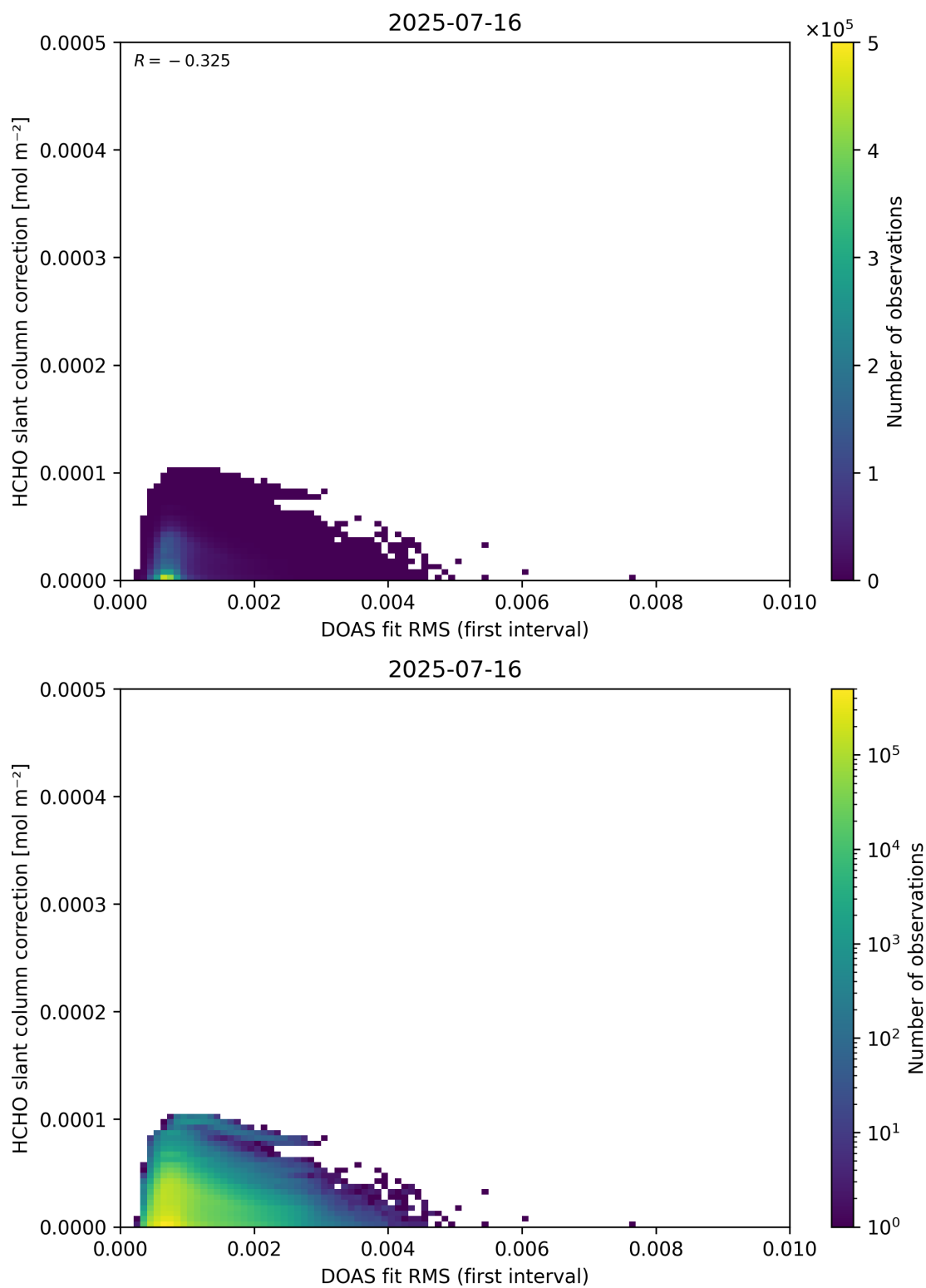
Figure 63: Scatter density plot of “DOAS fit RMS (first interval)” against “HCHO slant column correction” for 2025-07-15 to 2025-07-17.
