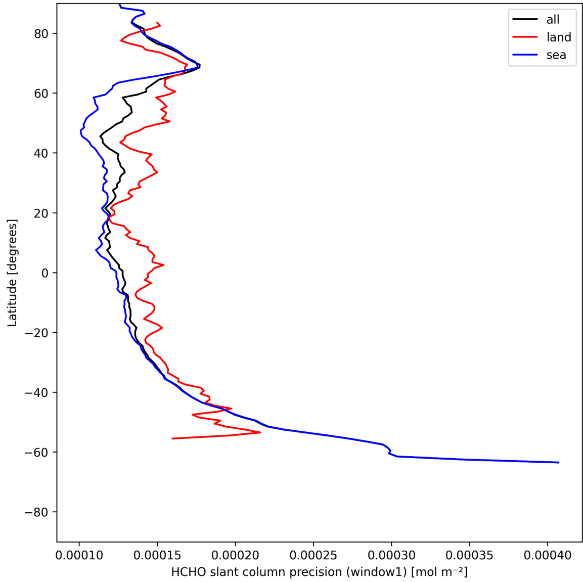
Figure 25: Zonal average of "HCHO slant column precision (window1)" for 2025-07-15 to 2025-07-17.
