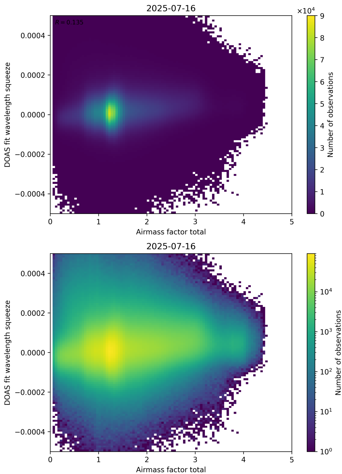
Figure 99: Scatter density plot of “Airmass factor total” against “DOAS fit wavelength squeeze” for 2025-07-15 to 2025-07-17.
