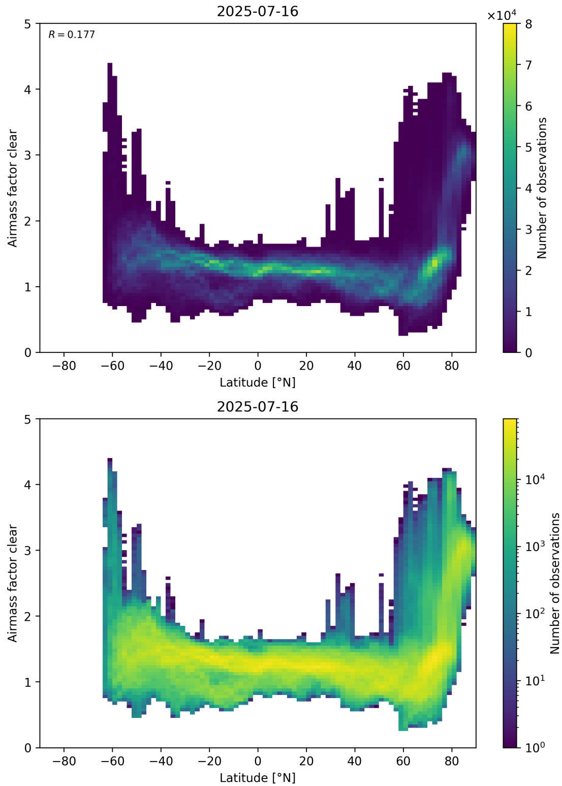
Figure 156: Scatter density plot of “Latitude” against “Airmass factor clear” for 2025-07-15 to 2025-07-17.
