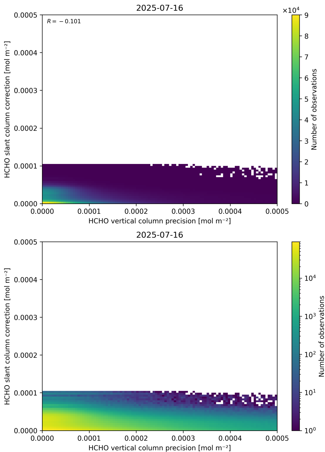
Figure 141: Scatter density plot of “HCHO vertical column precision” against “HCHO slant column correction” for 2025-07-15 to 2025-07-17.
