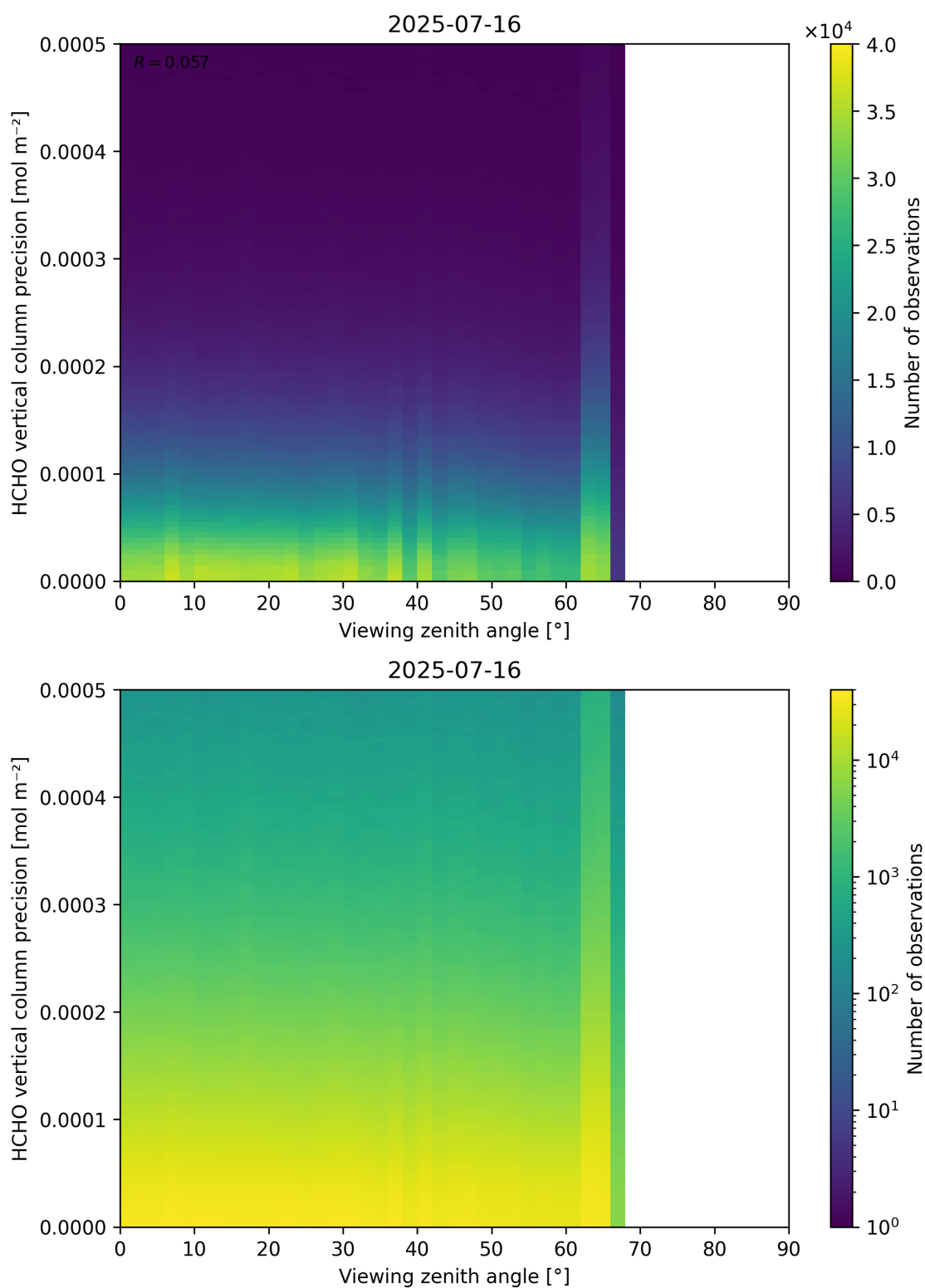
Figure 194: Scatter density plot of “Viewing zenith angle” against “HCHO vertical column precision” for 2025-07-15 to 2025-07-17.
