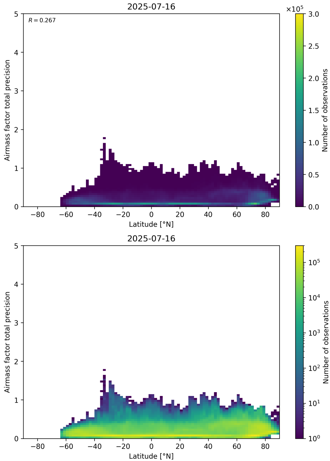
Figure 162: Scatter density plot of “Latitude” against “Airmass factor total precision” for 2025-07-15 to 2025-07-17.
