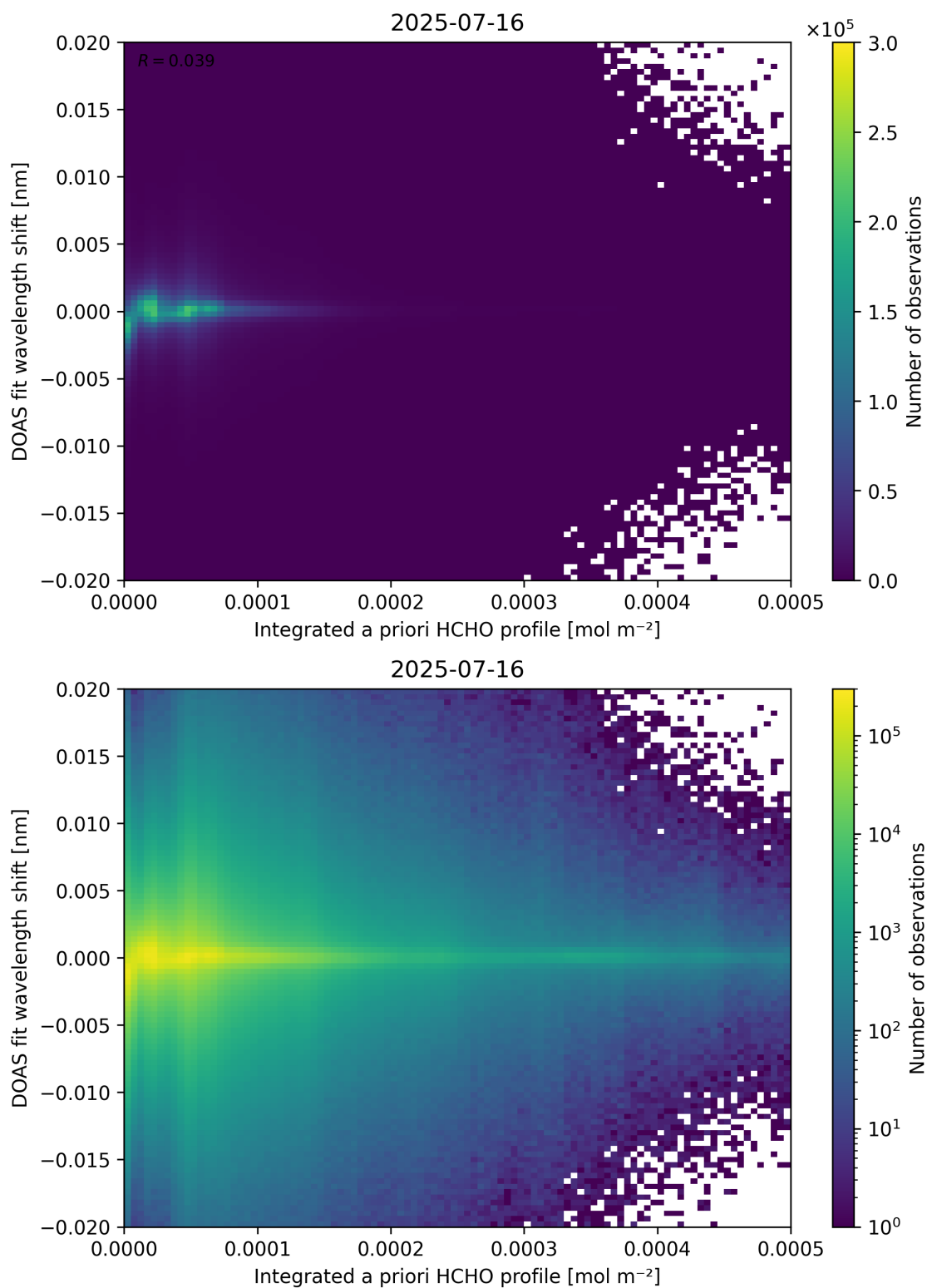
Figure 149: Scatter density plot of “Integrated a priori HCHO profile” against “DOAS fit wavelength shift” for 2025-07-15 to 2025-07-17.
