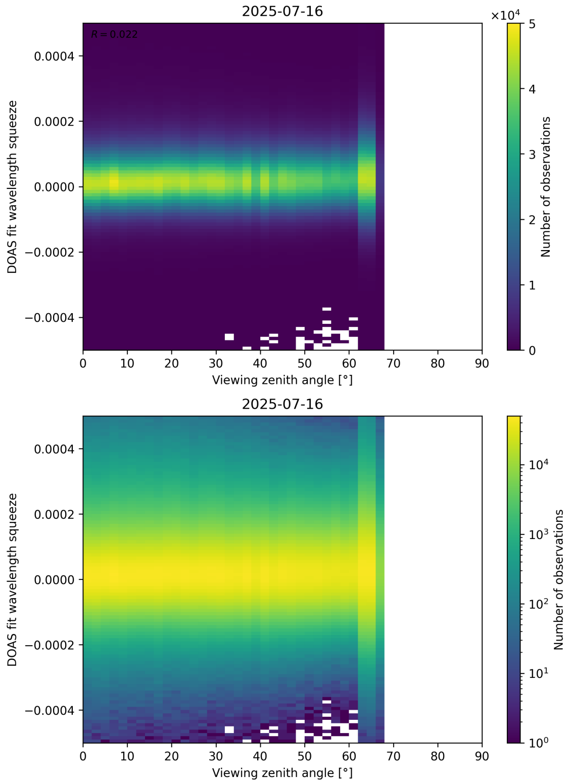
Figure 184: Scatter density plot of “Viewing zenith angle” against “DOAS fit wavelength squeeze” for 2025-07-15 to 2025-07-17.
