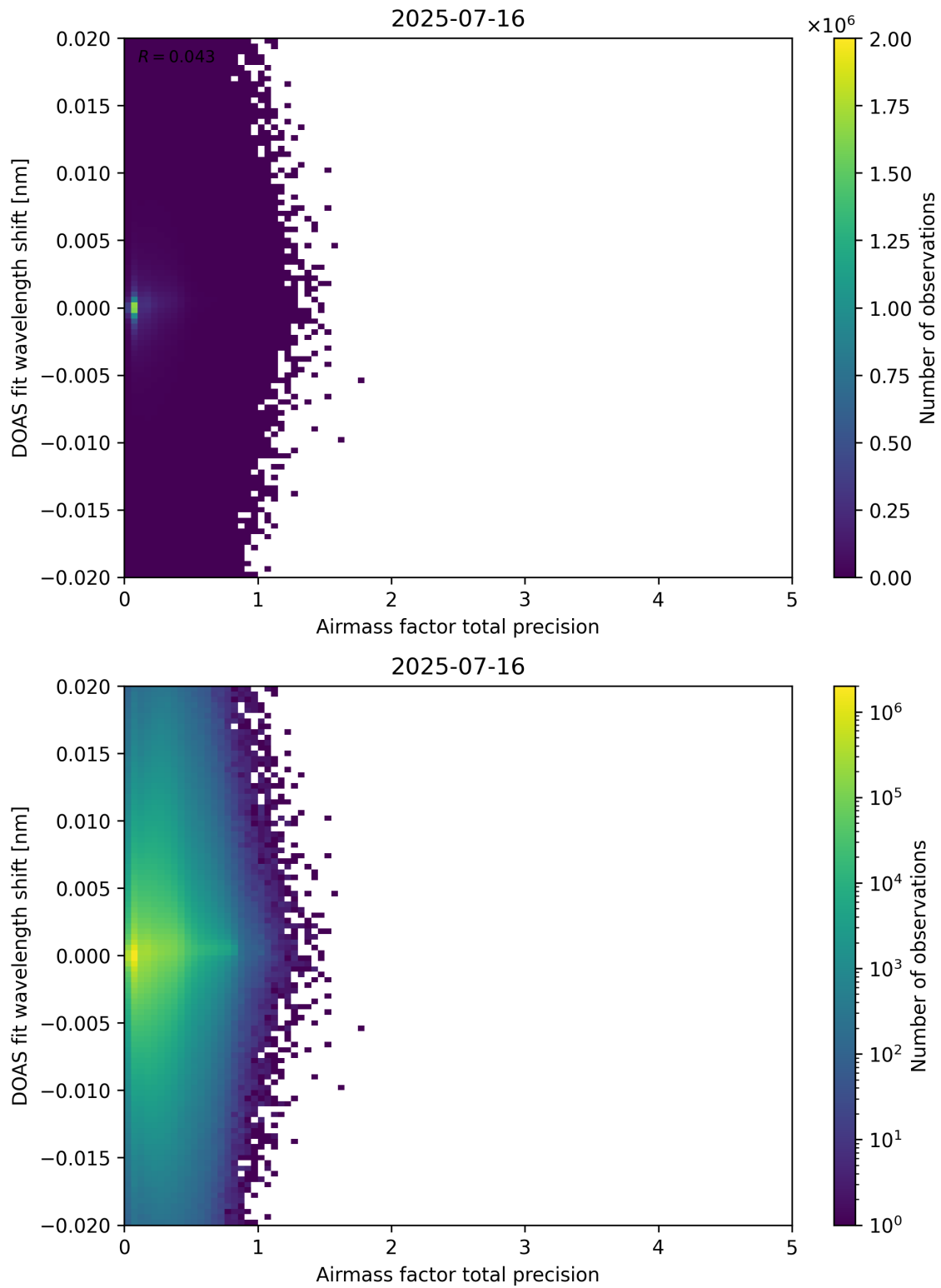
Figure 106: Scatter density plot of “Airmass factor total precision” against “DOAS fit wavelength shift” for 2025-07-15 to 2025-07-17.
