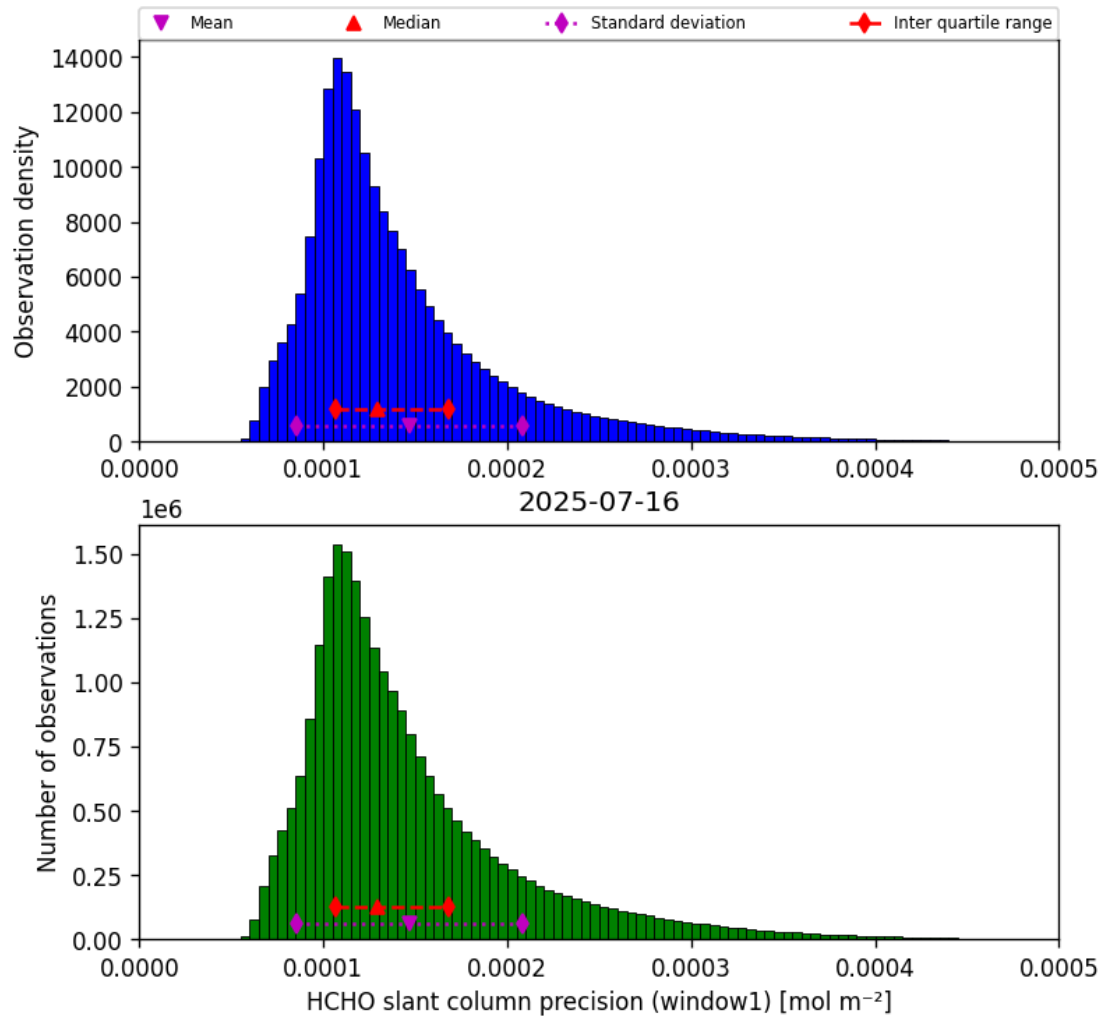
Figure 39: Histogram of “HCHO slant column precision (window1)” for 2025-07-15 to 2025-07-17
