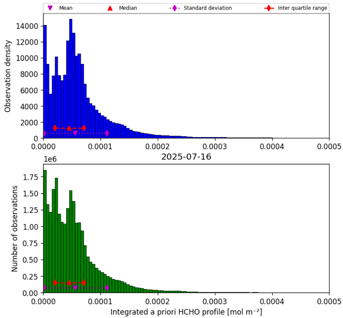
Figure 43: Histogram of “Integrated a priori HCHO profile” for 2025-07-15 to 2025-07-17
