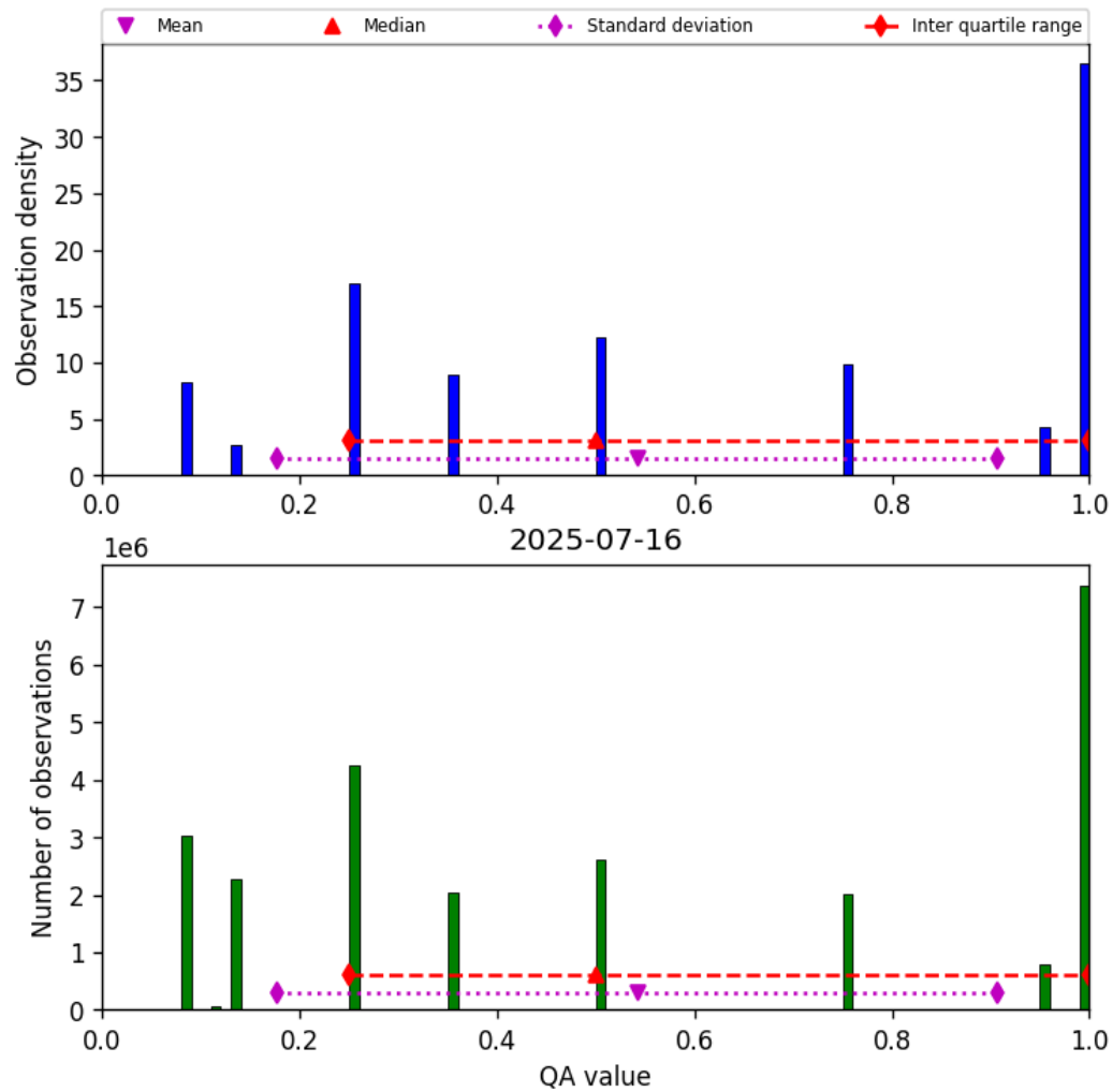
Figure 34: Histogram of “QA value” for 2025-07-15 to 2025-07-17
