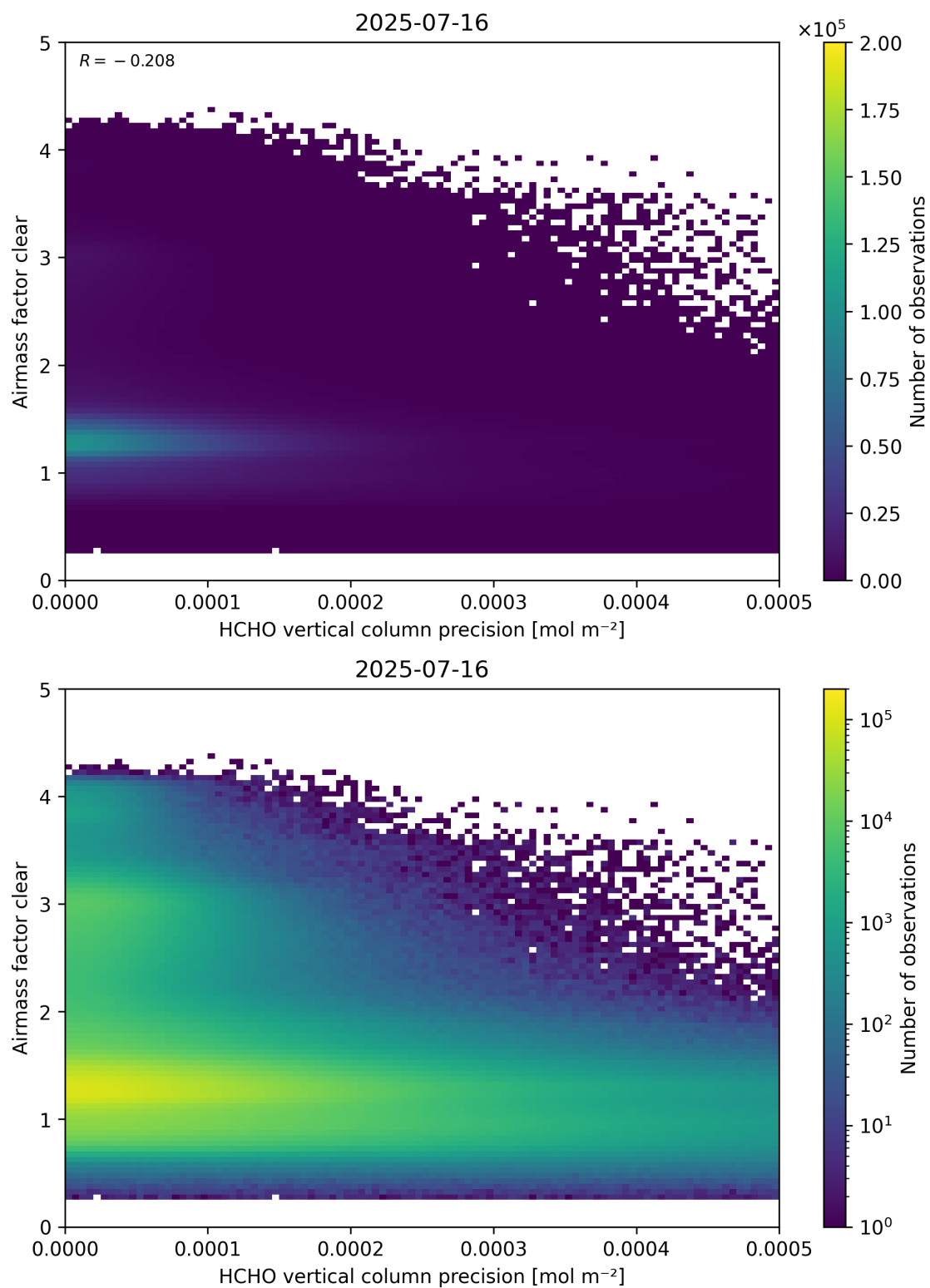
Figure 139: Scatter density plot of “HCHO vertical column precision” against “Airmass factor clear” for 2025-07-15 to 2025-07-17.
