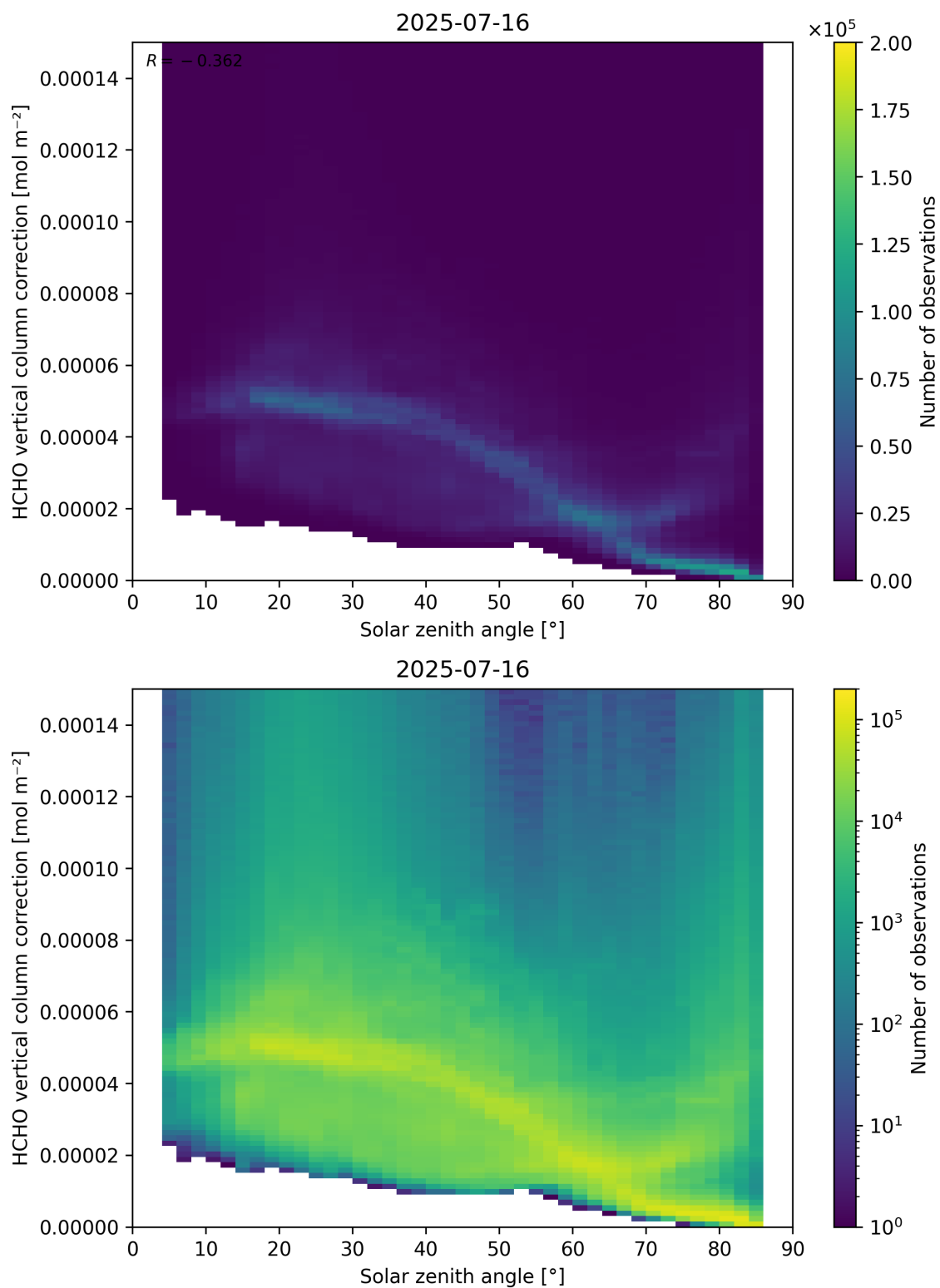
Figure 178: Scatter density plot of “Solar zenith angle” against “HCHO vertical column correction” for 2025-07-15 to 2025-07-17.
