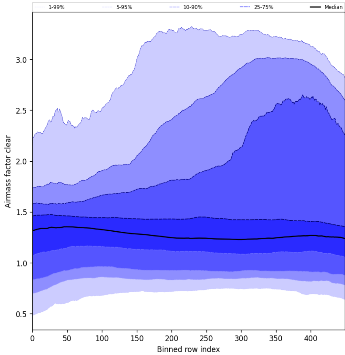
Figure 56: Along track statistics of “Air mass factor clear” for 2025-07-15 to 2025-07-17
