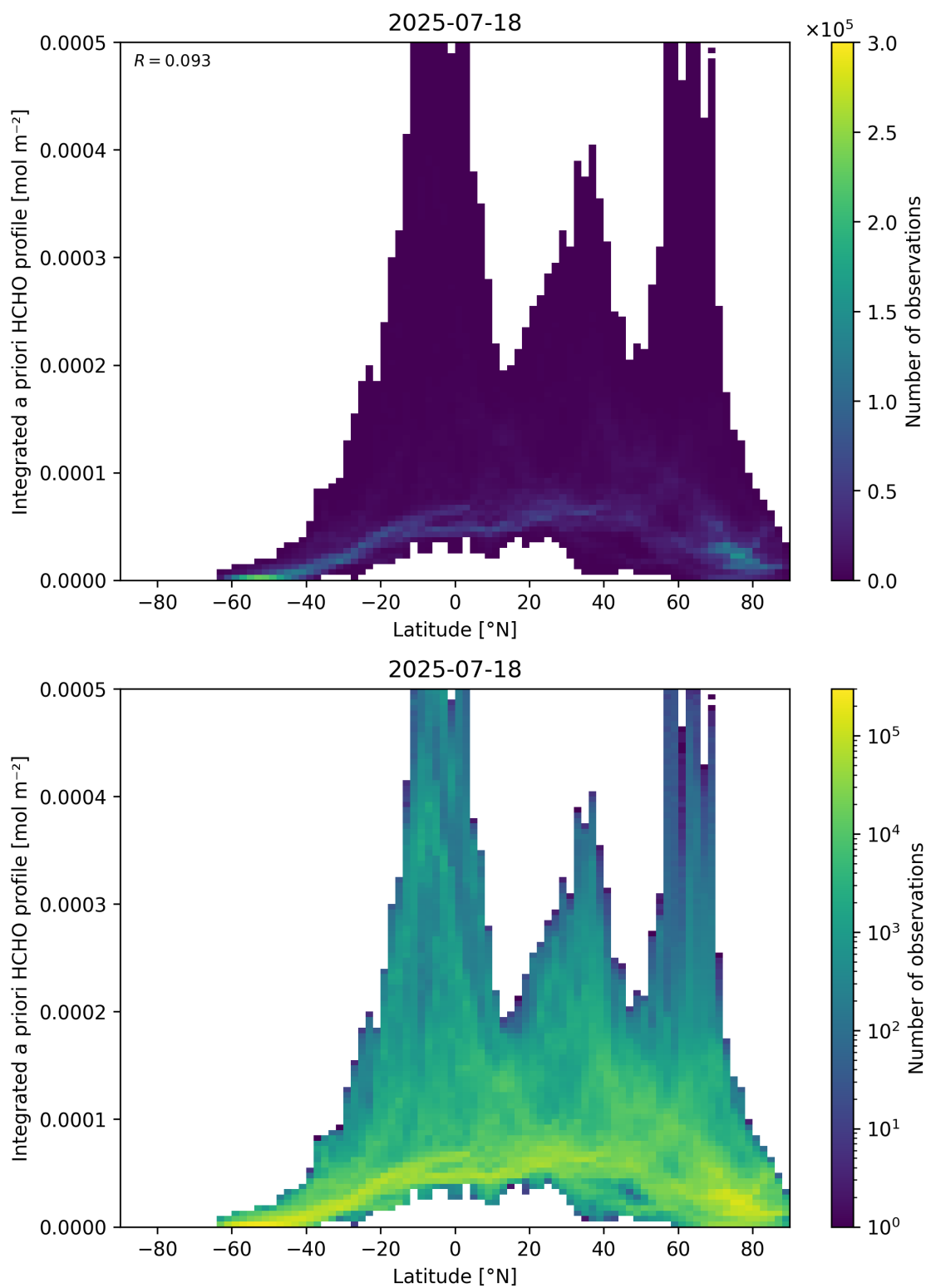
Figure 166: Scatter density plot of “Latitude” against “Integrated a priori HCHO profile” for 2025-07-18 to 2025-07-19.
