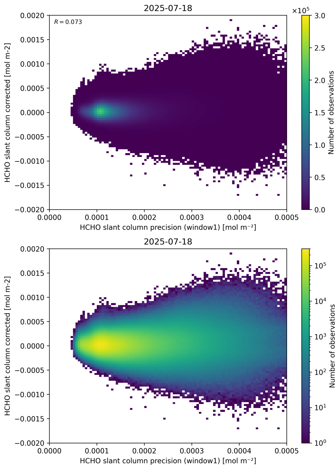
Figure 92: Scatter density plot of “HCHO slant column precision (window1)” against “HCHO slant column corrected” for 2025-07-18 to 2025-07-19.
