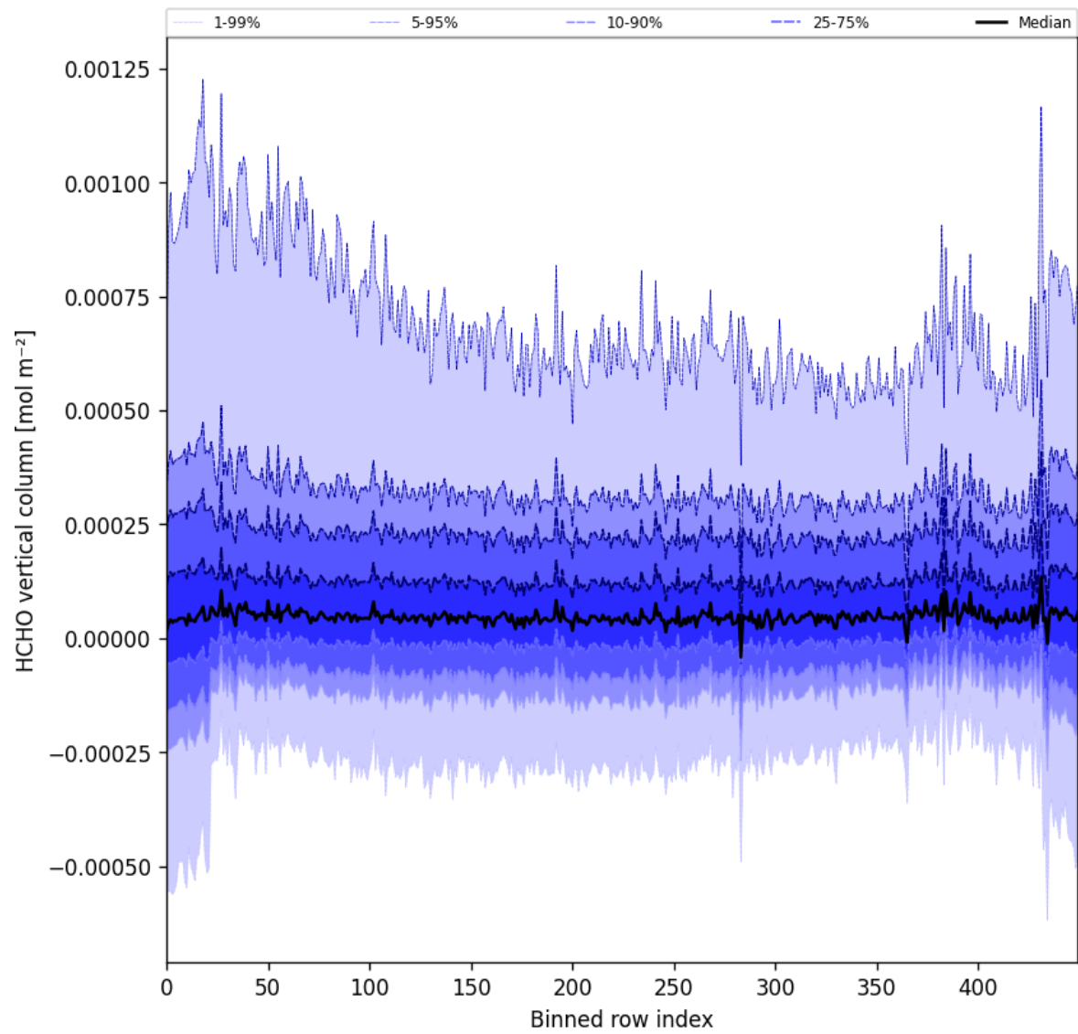
Figure 49: Along track statistics of “HCHO vertical column” for 2025-07-18 to 2025-07-19
