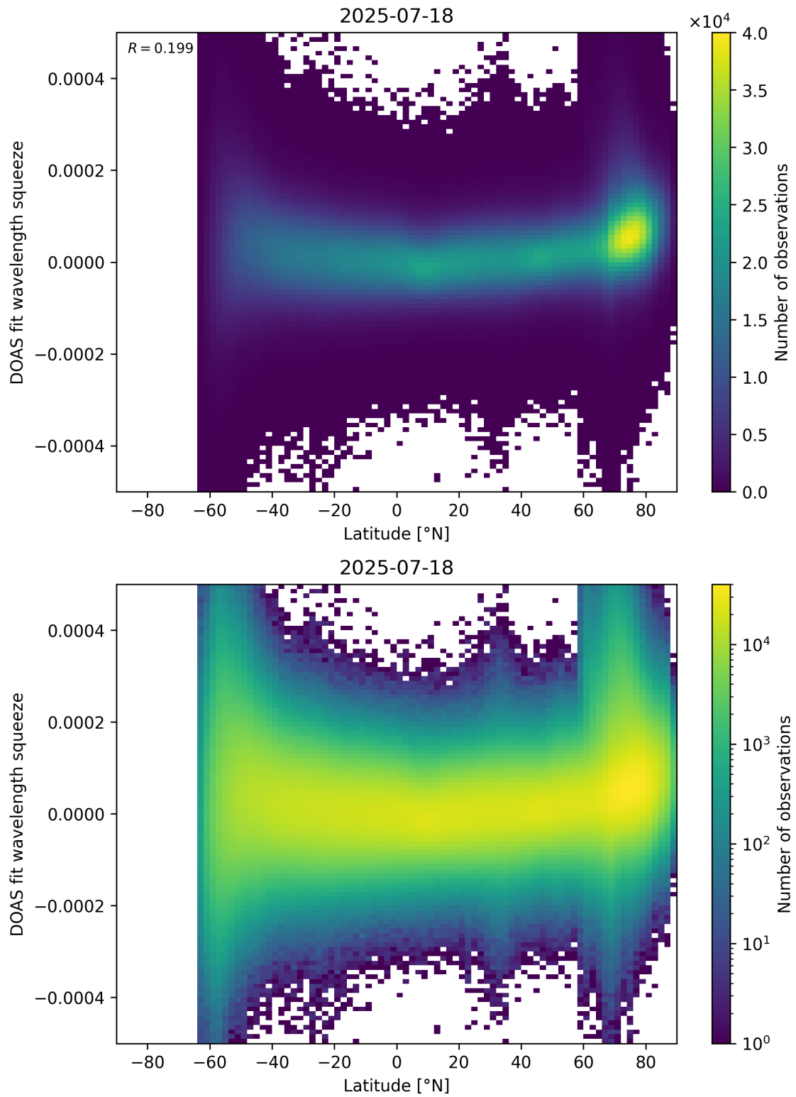
Figure 155: Scatter density plot of “Latitude” against “DOAS fit wavelength squeeze” for 2025-07-18 to 2025-07-19.
