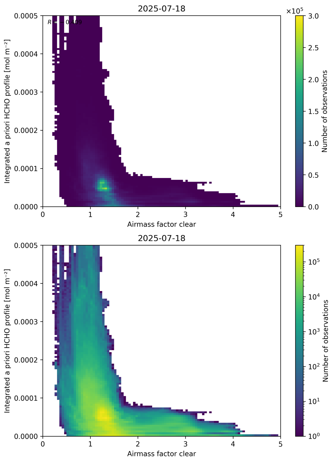
Figure 76: Scatter density plot of “Airmass factor clear” against “Integrated a priori HCHO profile” for 2025-07-18 to 2025-07-19.
