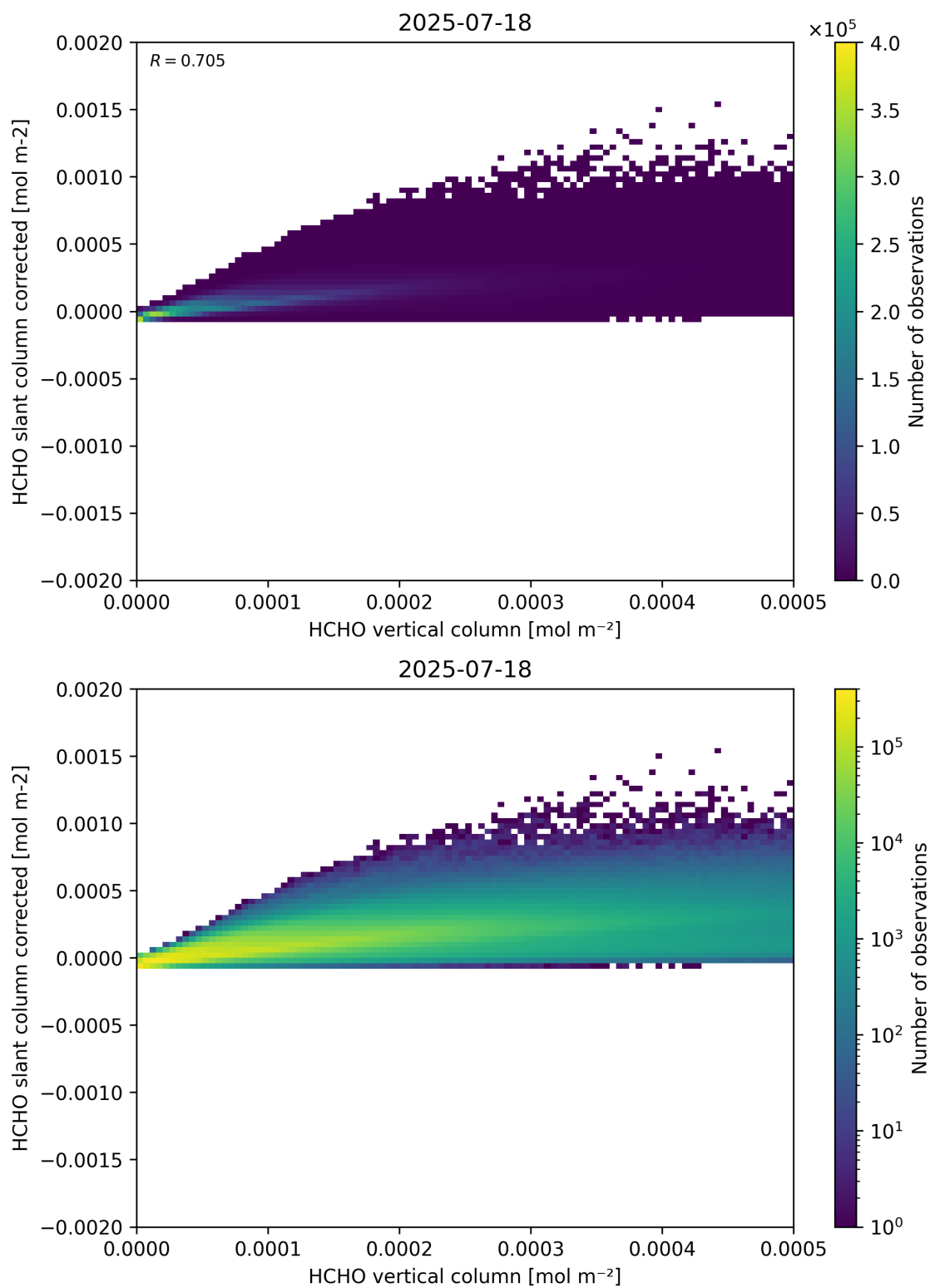
Figure 127: Scatter density plot of “HCHO vertical column” against “HCHO slant column corrected” for 2025-07-18 to 2025-07-19.
