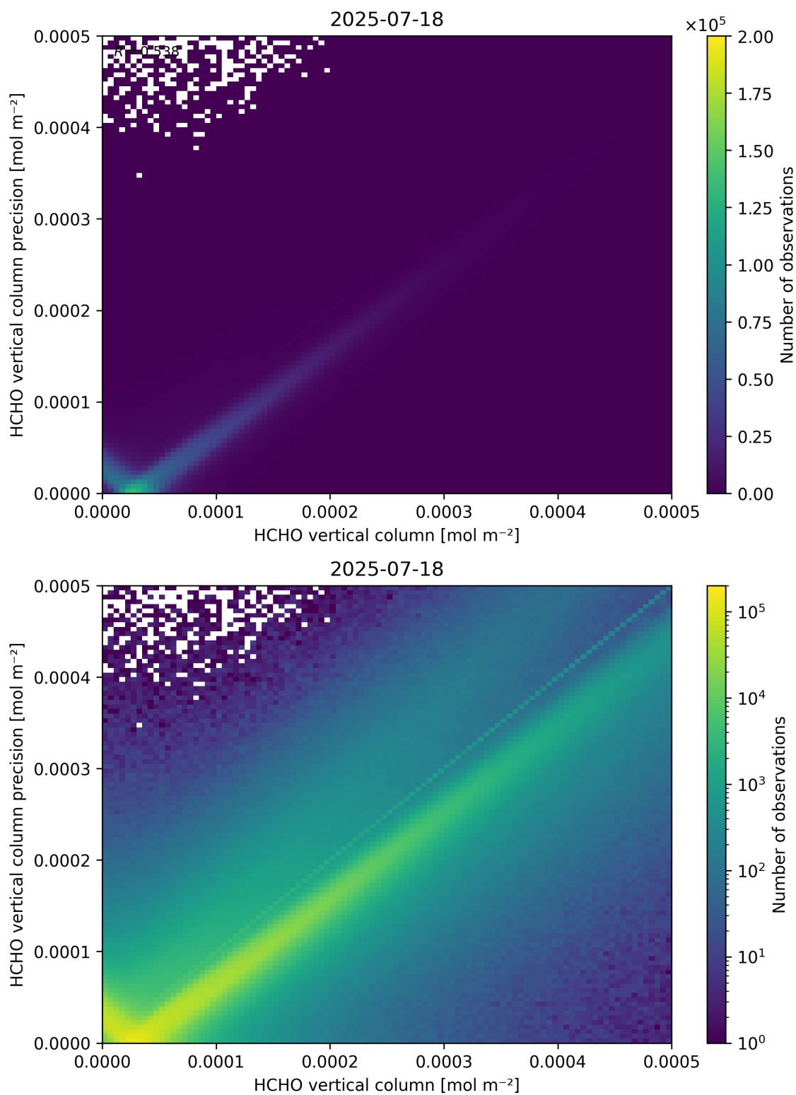
Figure 134: Scatter density plot of “HCHO vertical column” against “HCHO vertical column precision” for 2025-07-18 to 2025-07-19.
