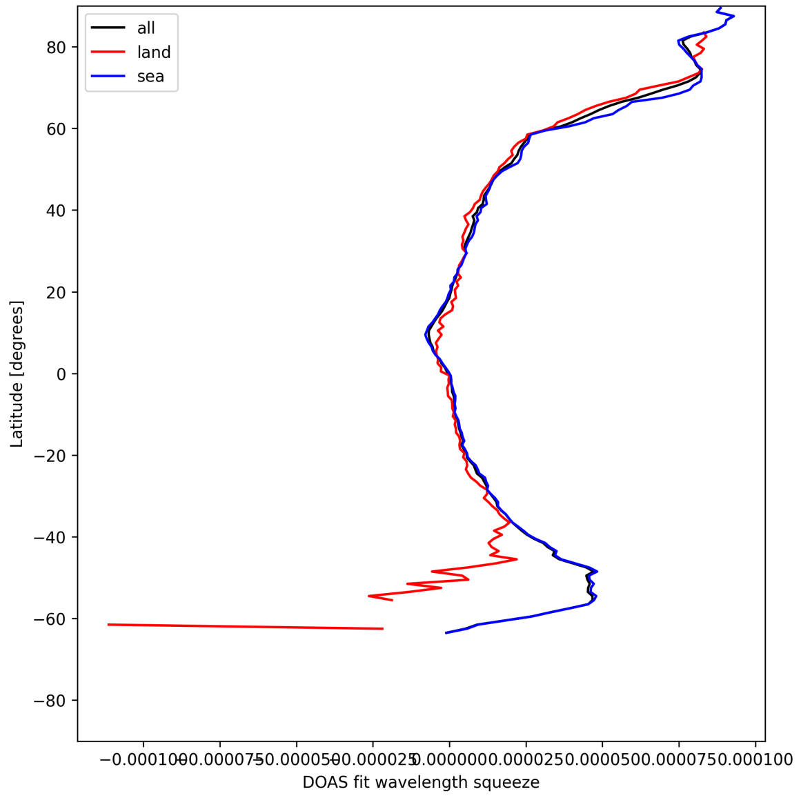
Figure 31: Zonal average of "DOAS fit wavelength squeeze" for 2025-07-18 to 2025-07-19.
