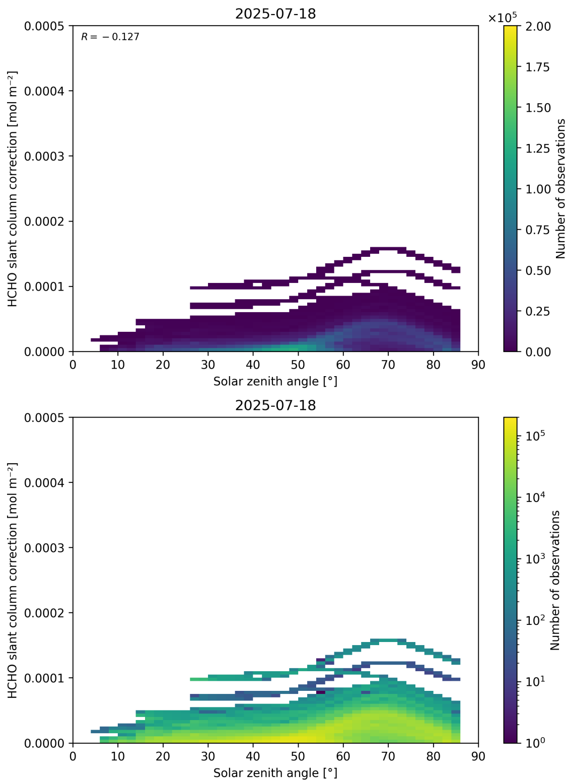
Figure 172: Scatter density plot of “Solar zenith angle” against “HCHO slant column correction” for 2025-07-18 to 2025-07-19.
