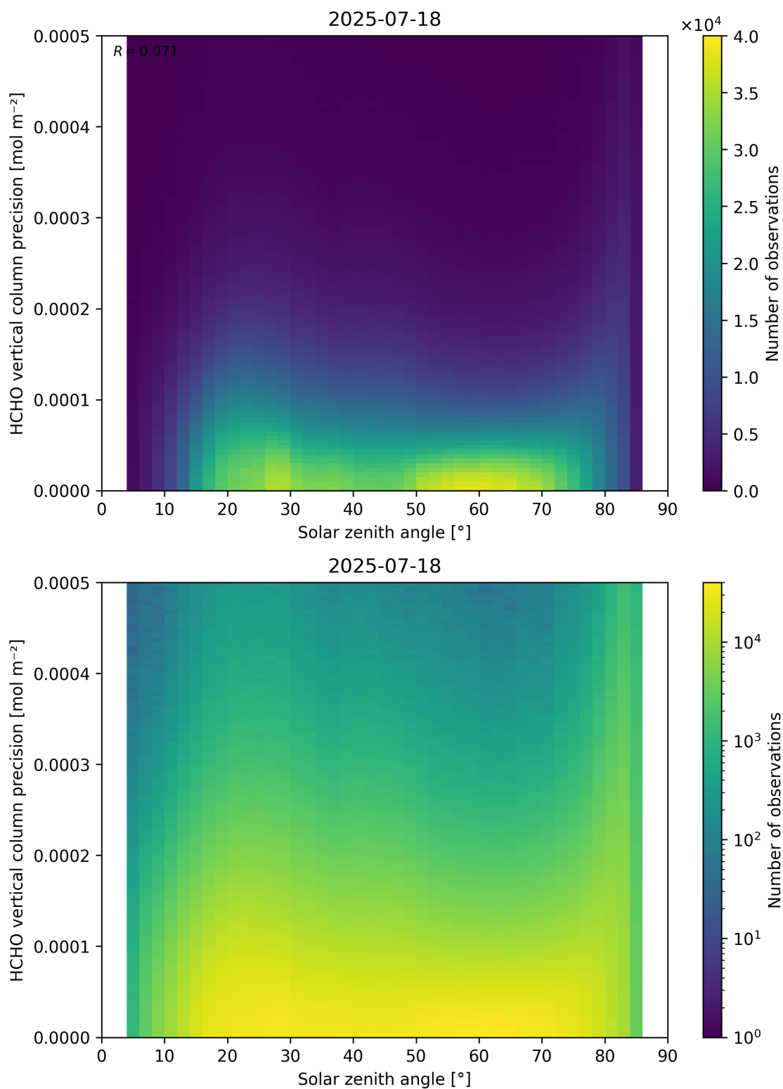
Figure 179: Scatter density plot of “Solar zenith angle” against “HCHO vertical column precision” for 2025-07-18 to 2025-07-19.
