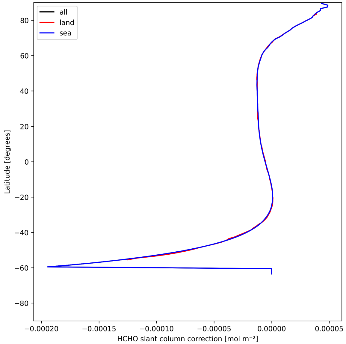
Figure 33: Zonal average of “HCHO slant column correction” for 2025-07-18 to 2025-07-19.
