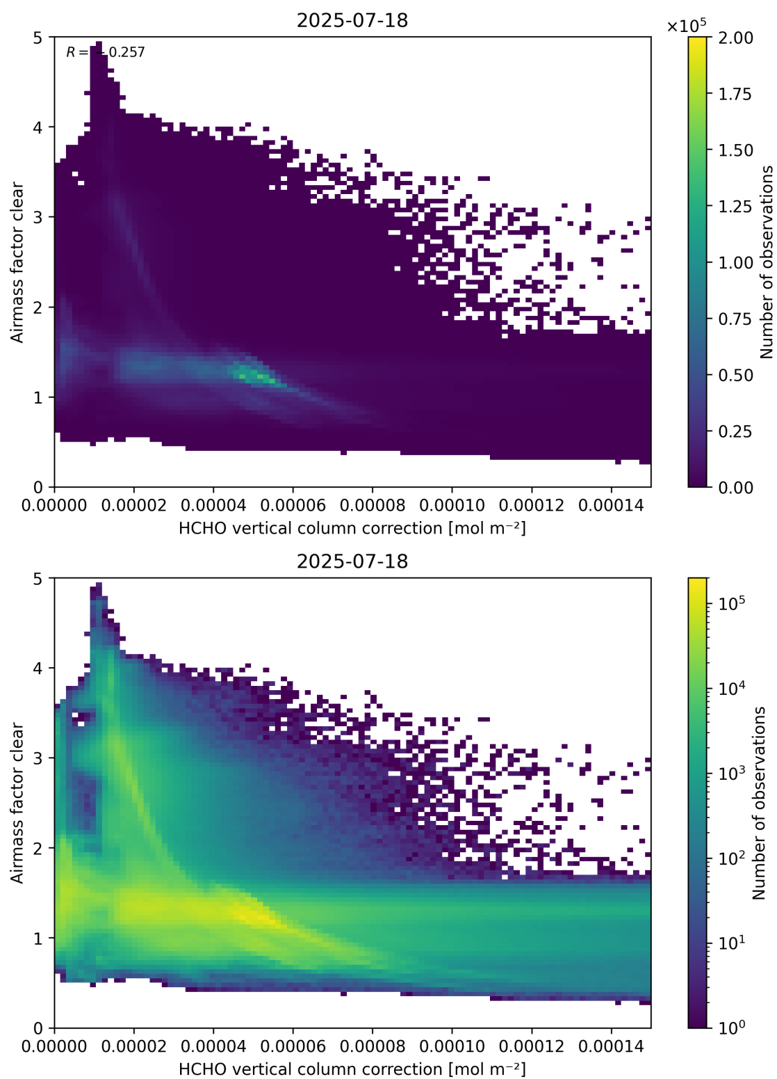
Figure 115: Scatter density plot of “HCHO vertical column correction” against “Air mass factor clear” for 2025-07-18 to 2025-07-19.
