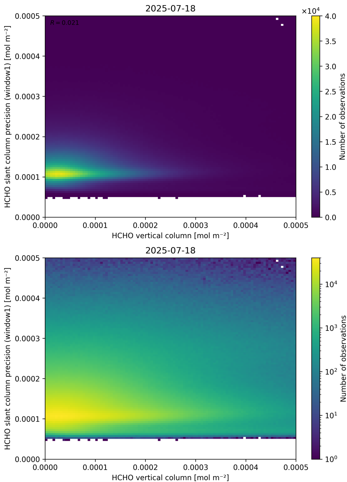
Figure 130: Scatter density plot of “HCHO vertical column” against “HCHO slant column precision (window1)” for 2025-07-18 to 2025-07-19.
