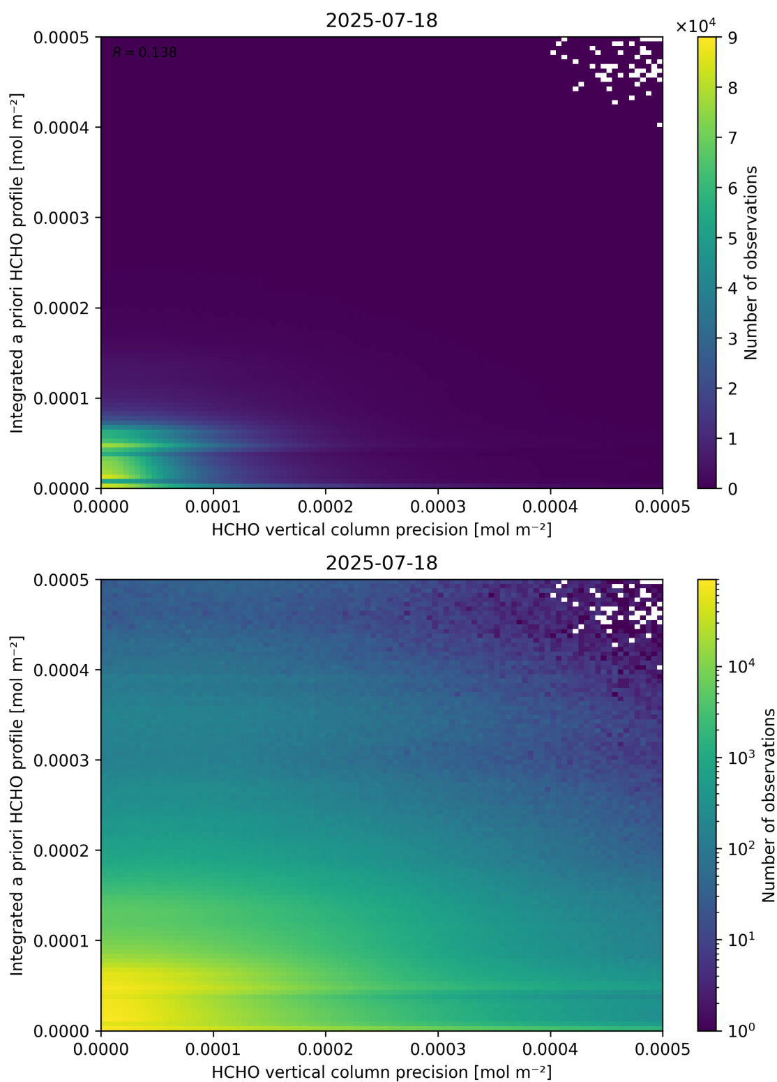
Figure 147: Scatter density plot of “HCHO vertical column precision” against “Integrated a priori HCHO profile” for 2025-07-18 to 2025-07-19.
