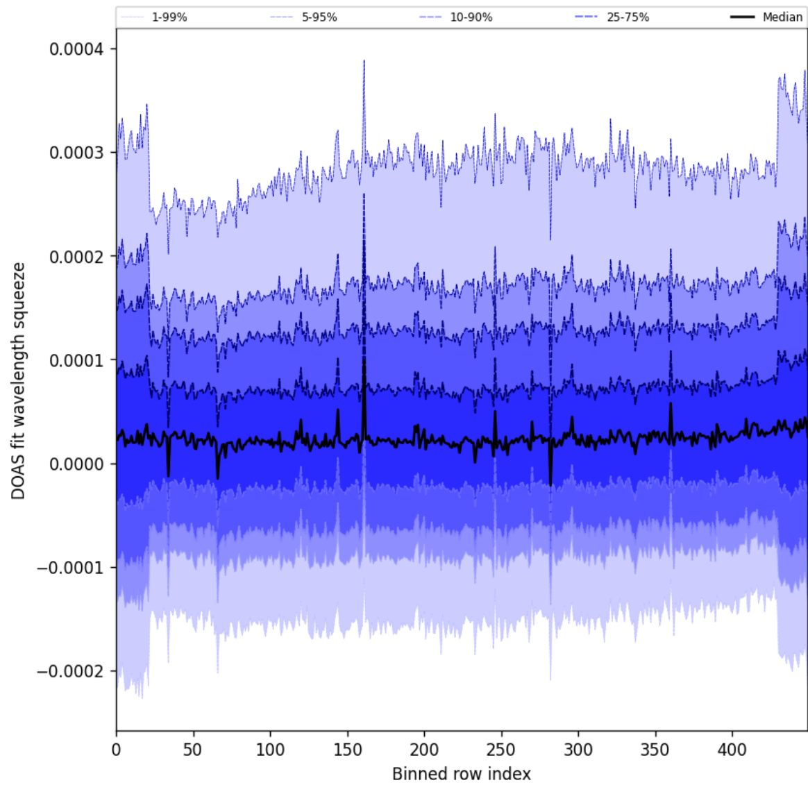
Figure 59: Along track statistics of “DOAS fit wavelength squeeze” for 2025-07-18 to 2025-07-19
