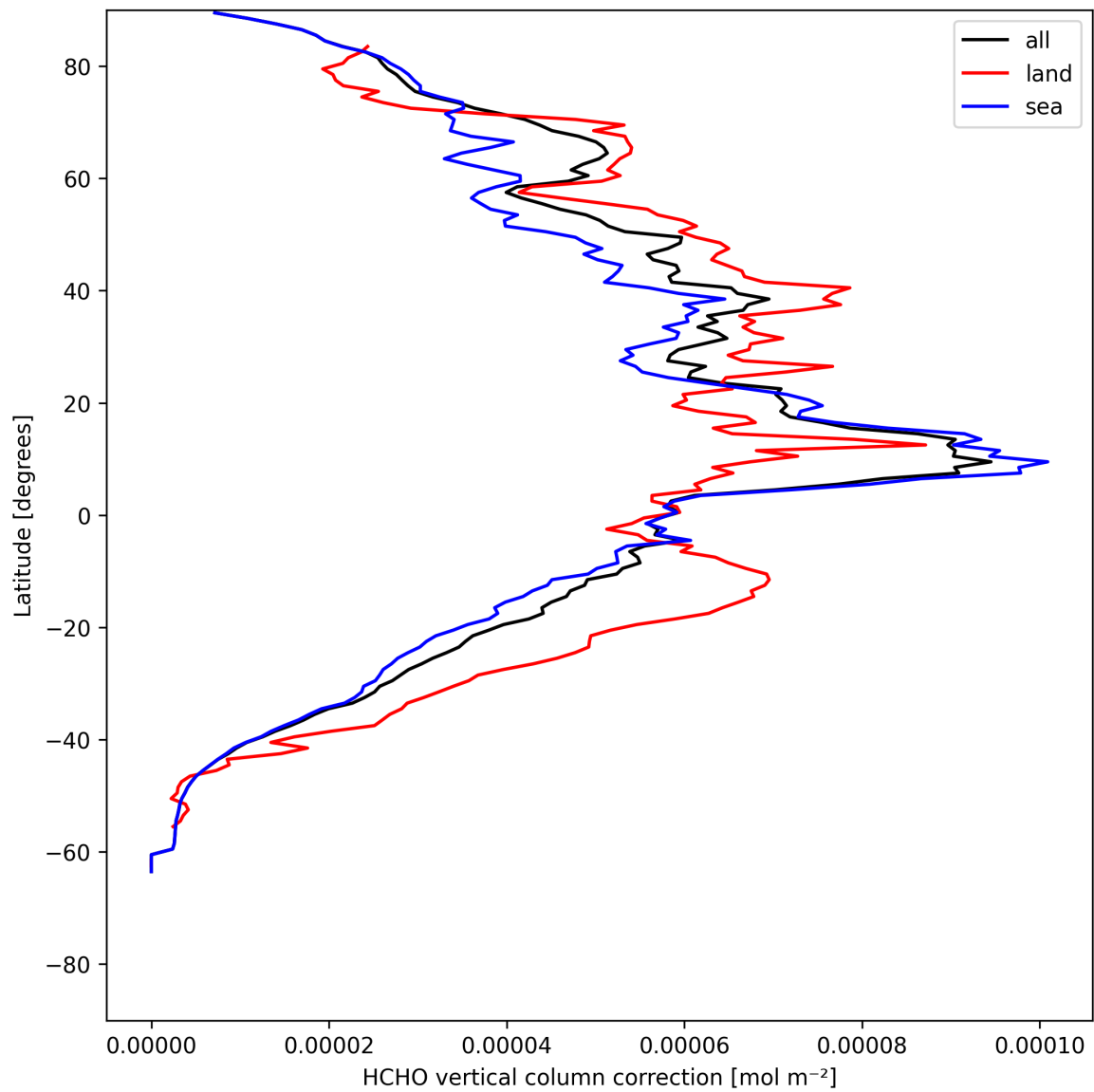
Figure 23: Zonal average of “HCHO vertical column correction” for 2025-07-18 to 2025-07-19.
