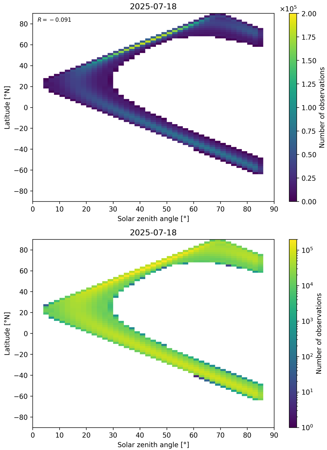
Figure 181: Scatter density plot of “Solar zenith angle” against “Latitude” for 2025-07-18 to 2025-07-19.
