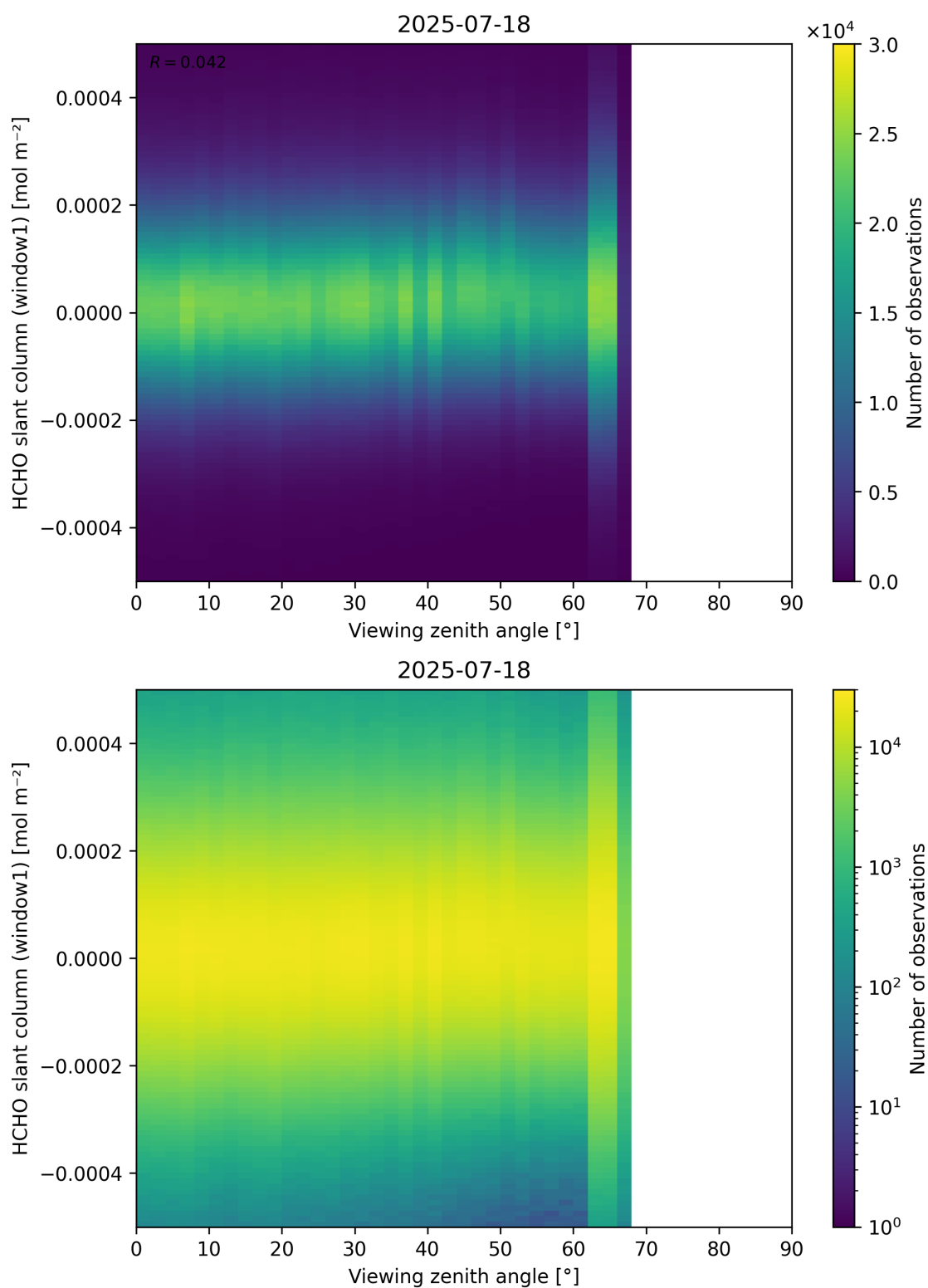
Figure 188: Scatter density plot of “Viewing zenith angle” against “HCHO slant column (window1)” for 2025-07-18 to 2025-07-19.
