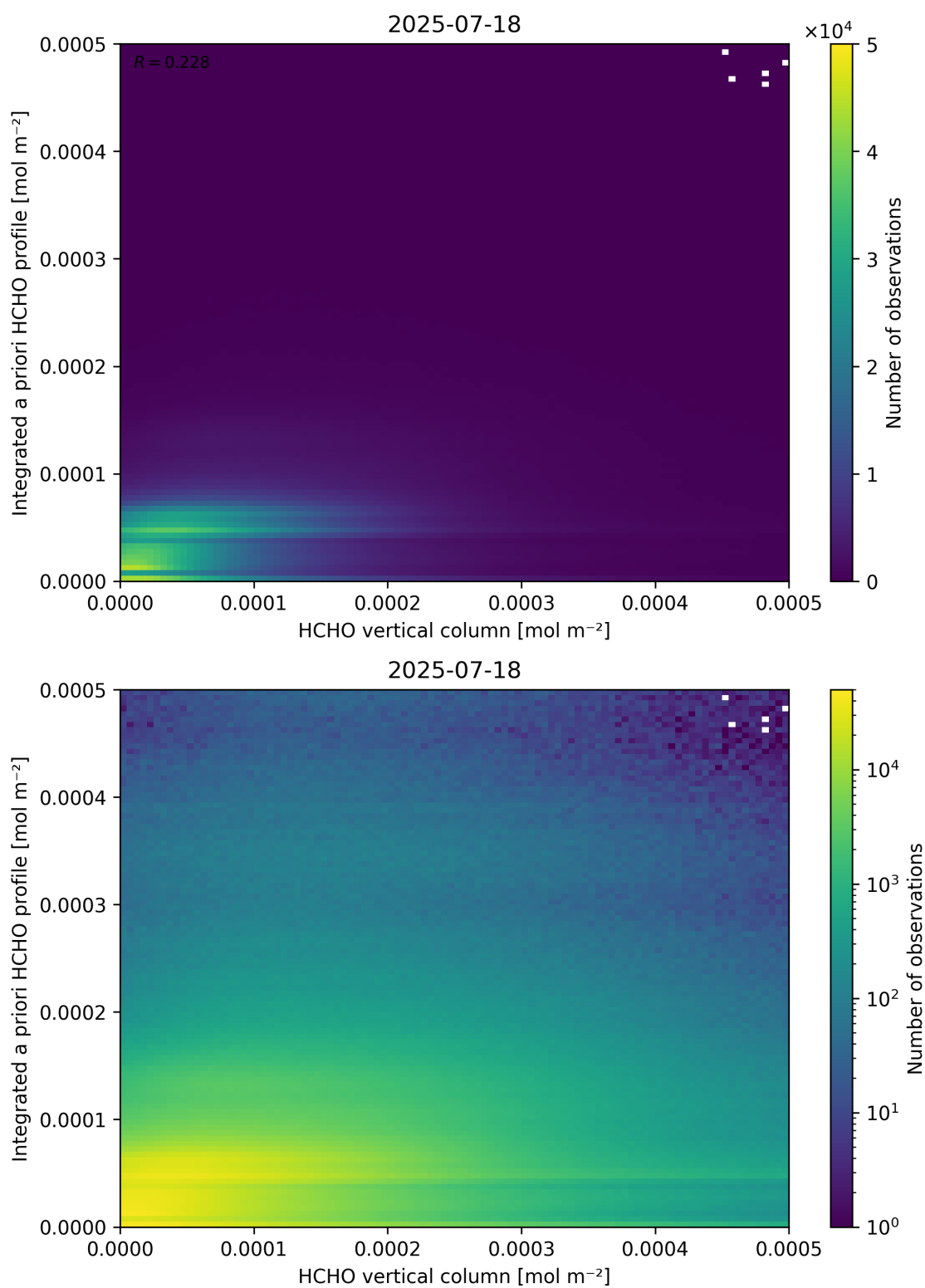
Figure 135: Scatter density plot of “HCHO vertical column” against “Integrated a priori HCHO profile” for 2025-07-18 to 2025-07-19.
