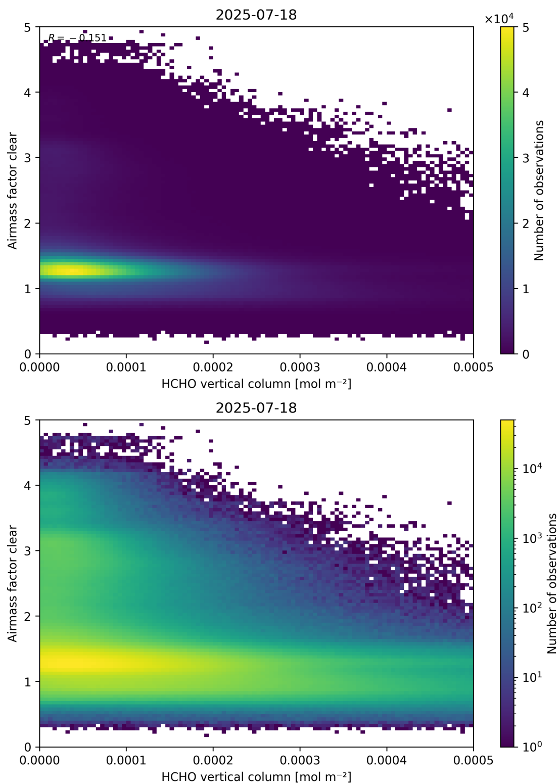
Figure 126: Scatter density plot of “HCHO vertical column” against “Airmass factor clear” for 2025-07-18 to 2025-07-19.
