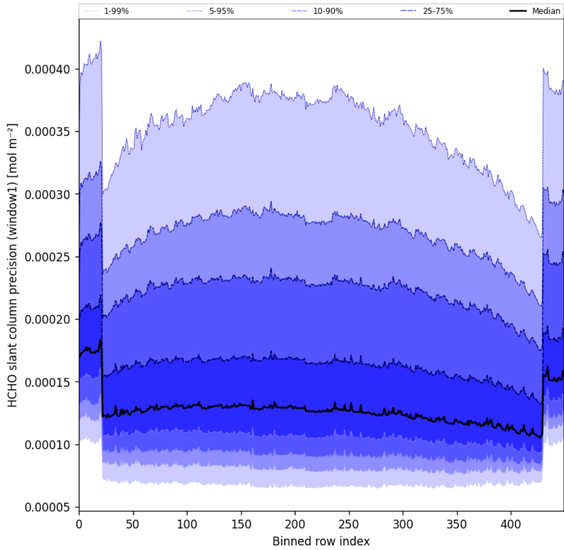
Figure 53: Along track statistics of “HCHO slant column precision (window1)” for 2025-07-18 to 2025-07-19
