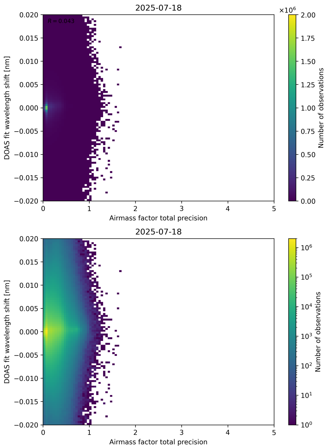
Figure 106: Scatter density plot of “Airmass factor total precision” against “DOAS fit wavelength shift” for 2025-07-18 to 2025-07-19.
