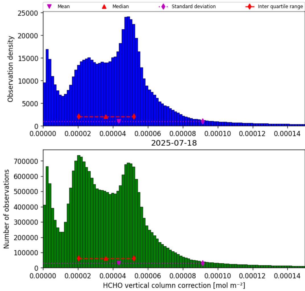
Figure 37: Histogram of “HCHO vertical column correction” for 2025-07-18 to 2025-07-19
