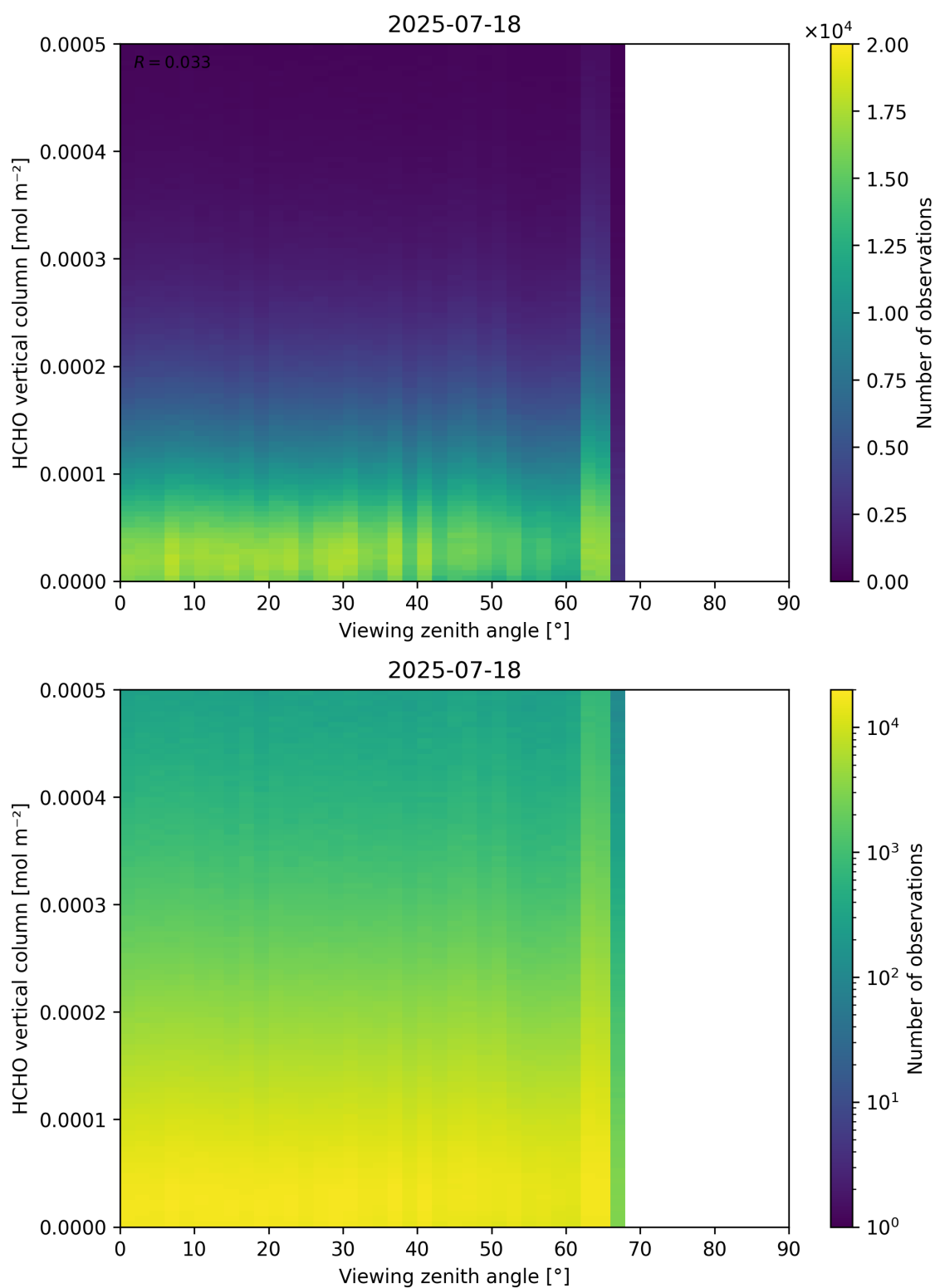
Figure 192: Scatter density plot of “Viewing zenith angle” against “HCHO vertical column” for 2025-07-18 to 2025-07-19.
