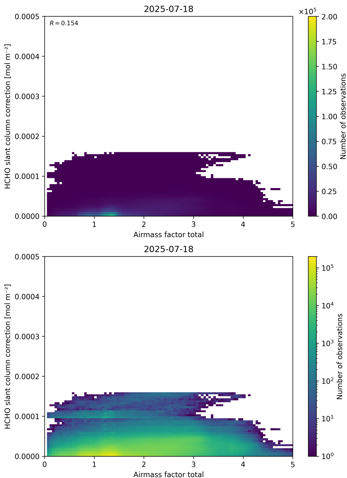
Figure 102: Scatter density plot of “Airmass factor total” against “HCHO slant column correction” for 2025-07-18 to 2025-07-19.
