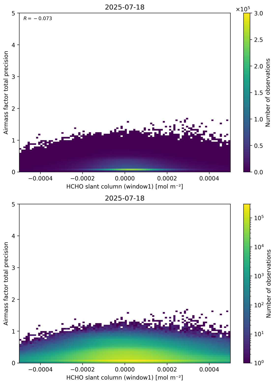
Figure 86: Scatter density plot of “HCHO slant column (window1)” against “Airmass factor total precision” for 2025-07-18 to 2025-07-19.
