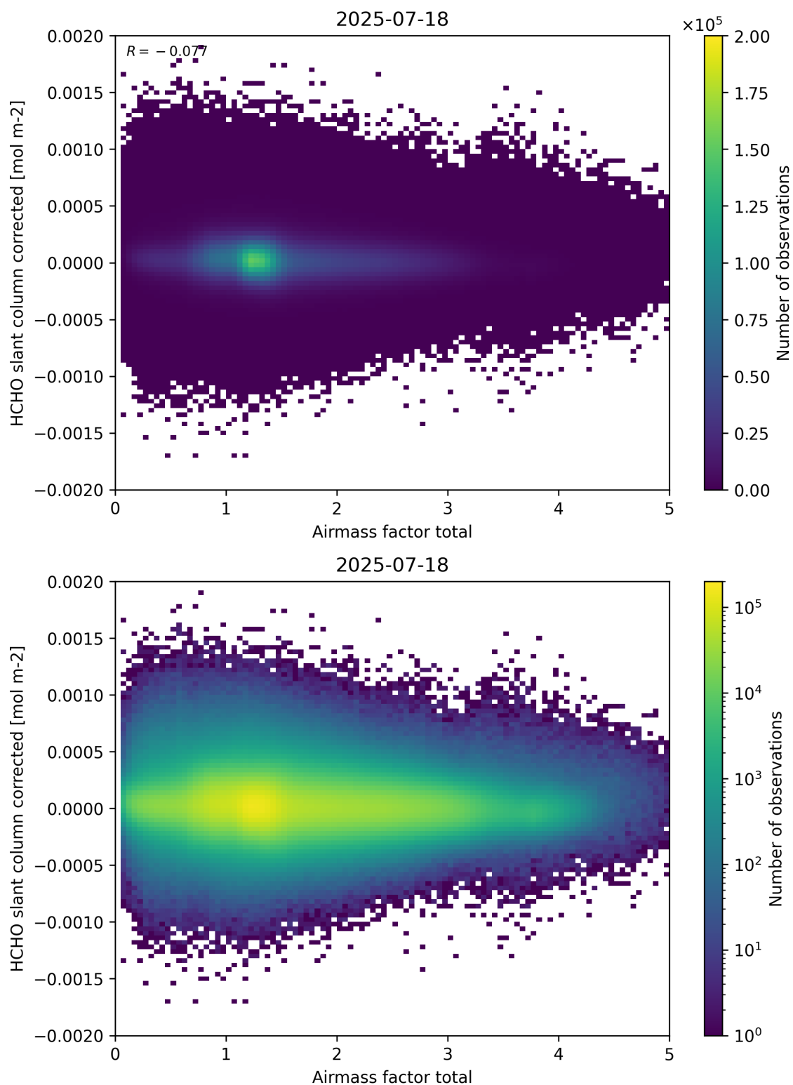
Figure 101: Scatter density plot of “Airmass factor total” against “HCHO slant column corrected” for 2025-07-18 to 2025-07-19.
