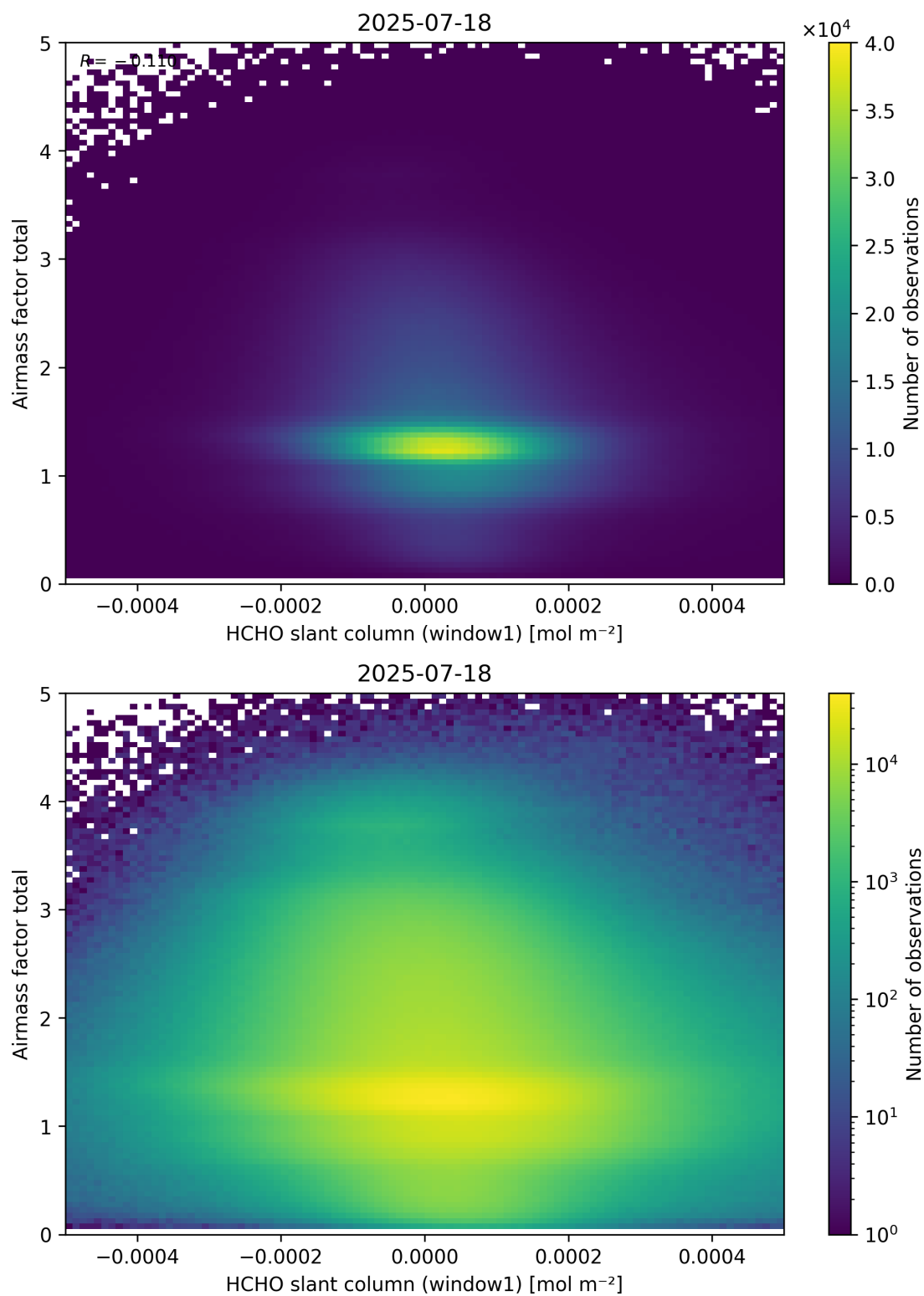
Figure 85: Scatter density plot of “HCHO slant column (window1)” against “Airmass factor total” for 2025-07-18 to 2025-07-19.
