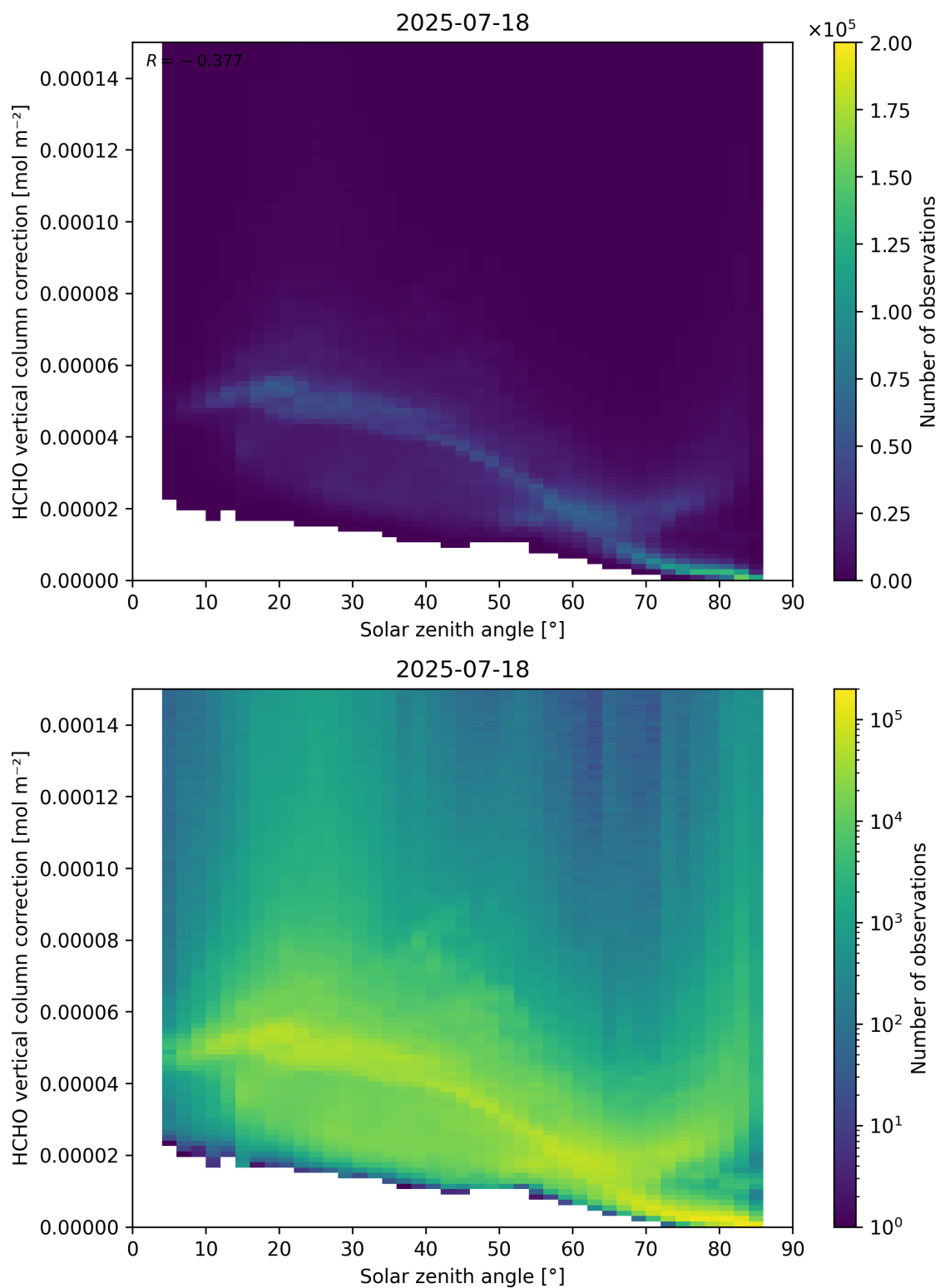
Figure 178: Scatter density plot of “Solar zenith angle” against “HCHO vertical column correction” for 2025-07-18 to 2025-07-19.
