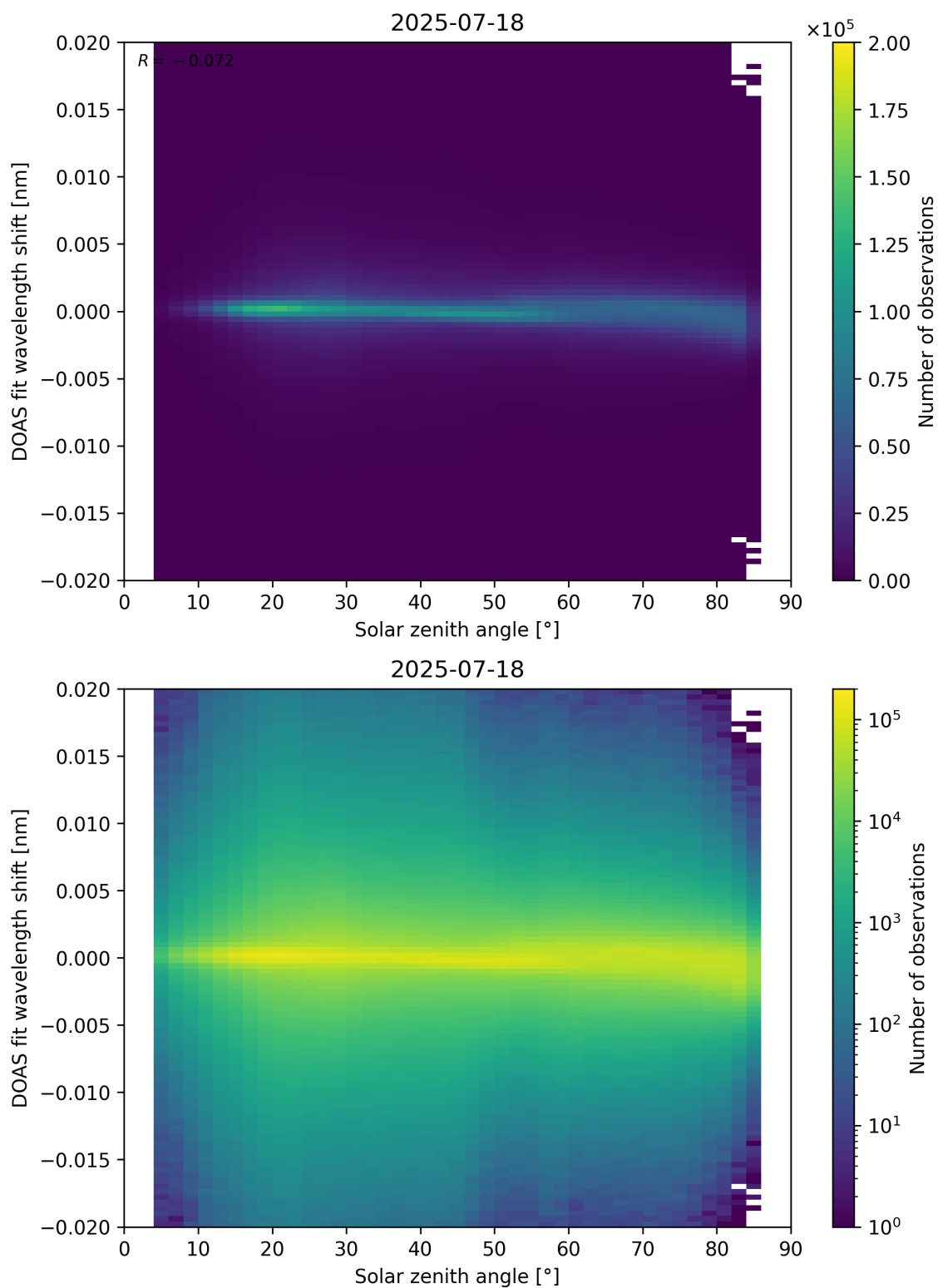
Figure 168: Scatter density plot of “Solar zenith angle” against “DOAS fit wavelength shift” for 2025-07-18 to 2025-07-19.
