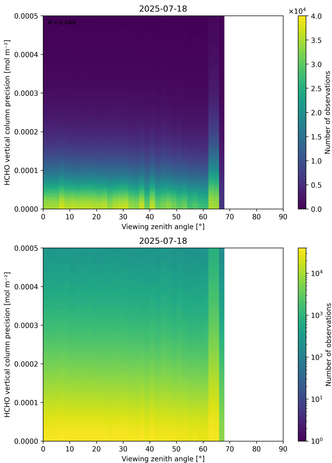
Figure 194: Scatter density plot of “Viewing zenith angle” against “HCHO vertical column precision” for 2025-07-18 to 2025-07-19.
