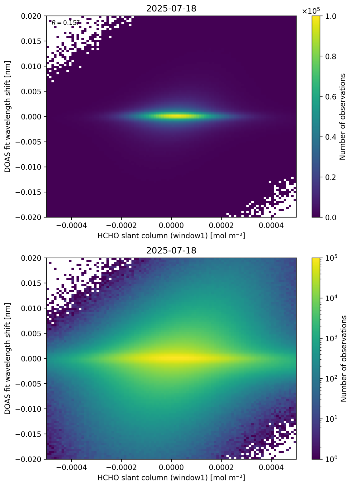
Figure 79: Scatter density plot of “HCHO slant column (window1)” against “DOAS fit wavelength shift” for 2025-07-18 to 2025-07-19.
