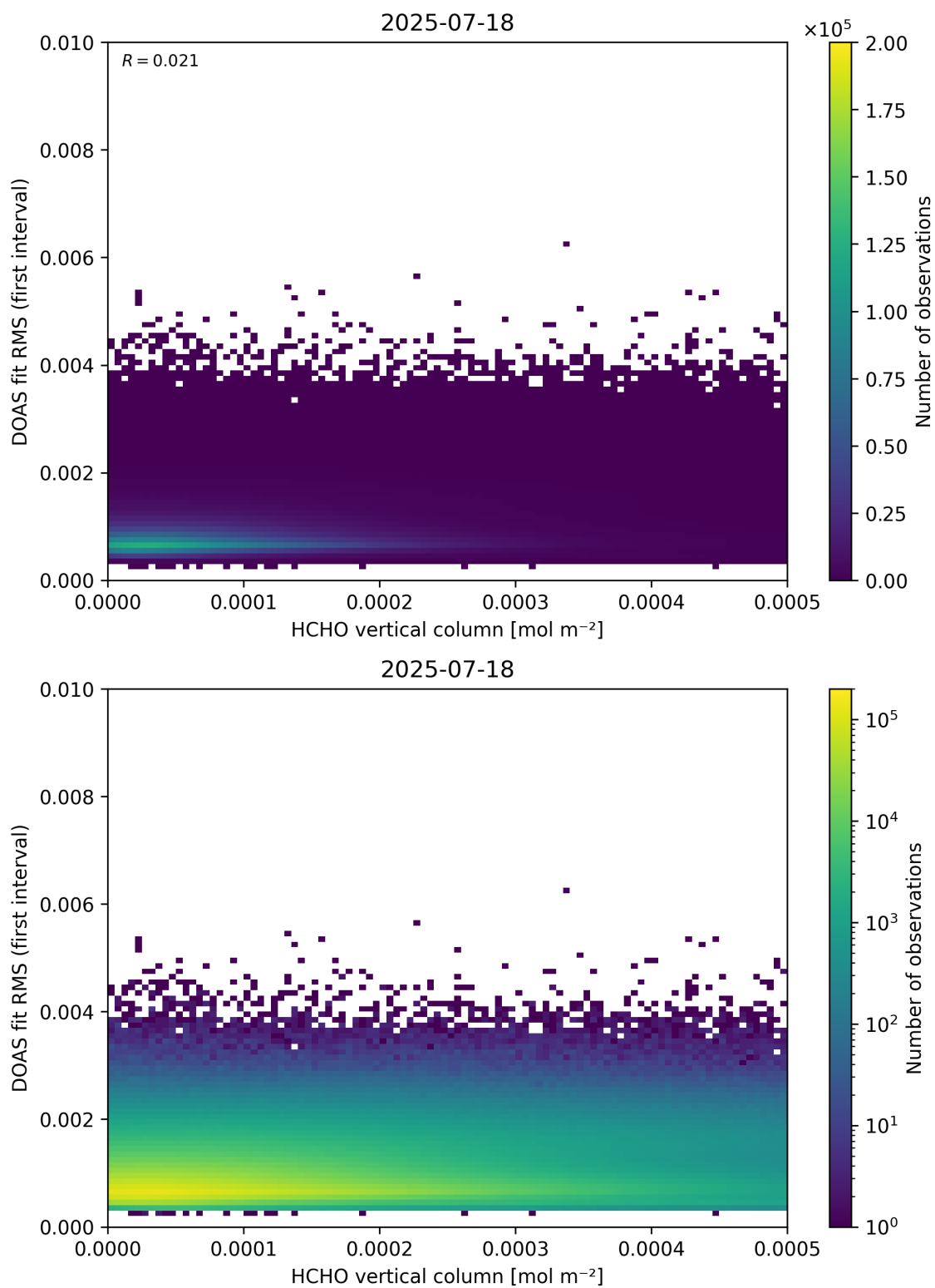
Figure 123: Scatter density plot of “HCHO vertical column” against “DOAS fit RMS (first interval)” for 2025-07-18 to 2025-07-19.
