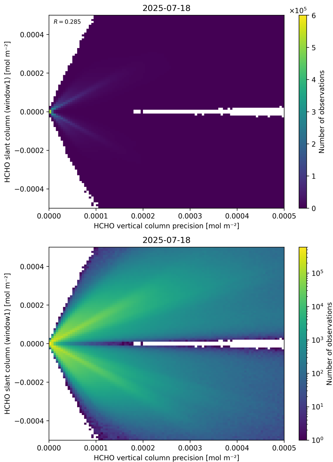
Figure 142: Scatter density plot of “HCHO vertical column precision” against “HCHO slant column (window1)” for 2025-07-18 to 2025-07-19.
