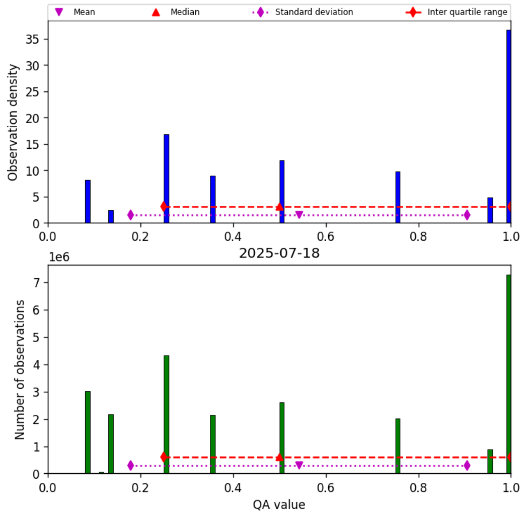
Figure 34: Histogram of “QA value” for 2025-07-18 to 2025-07-19
