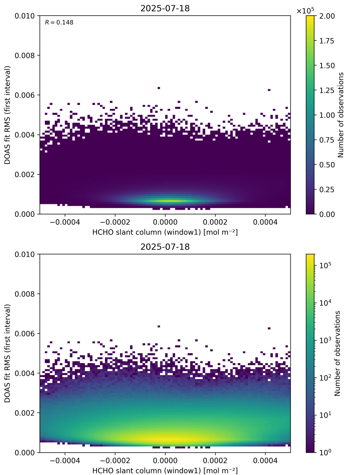
Figure 78: Scatter density plot of “HCHO slant column (window1)” against “DOAS fit RMS (first interval)” for 2025-07-18 to 2025-07-19.
