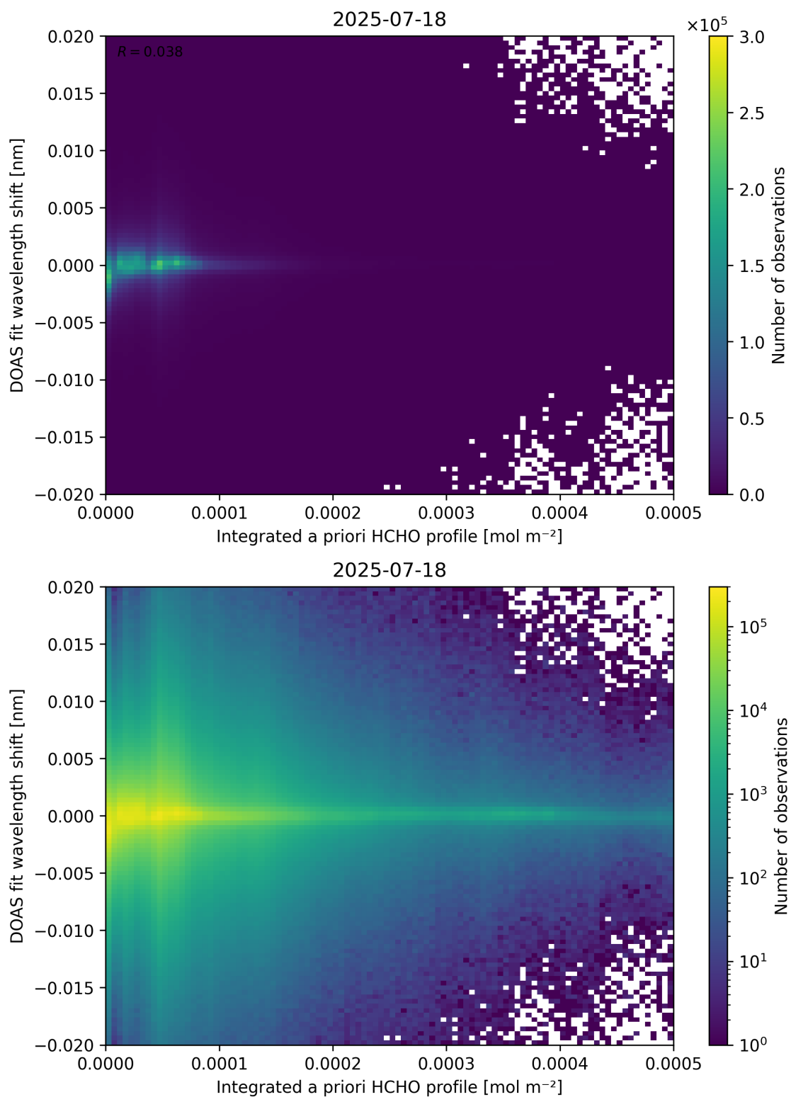
Figure 149: Scatter density plot of “Integrated a priori HCHO profile” against “DOAS fit wavelength shift” for 2025-07-18 to 2025-07-19.
