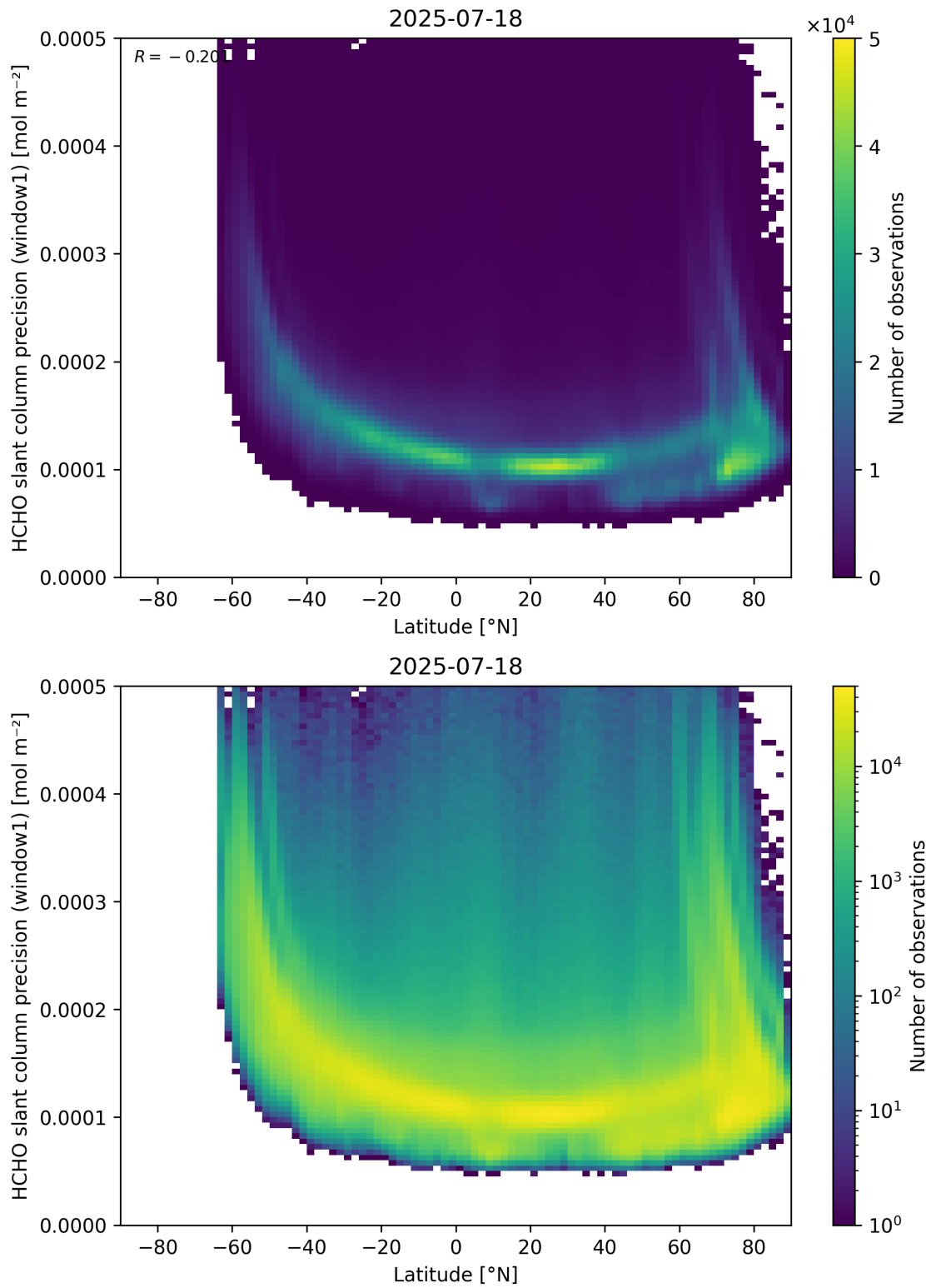
Figure 160: Scatter density plot of “Latitude” against “HCHO slant column precision (window1)” for 2025-07-18 to 2025-07-19.
