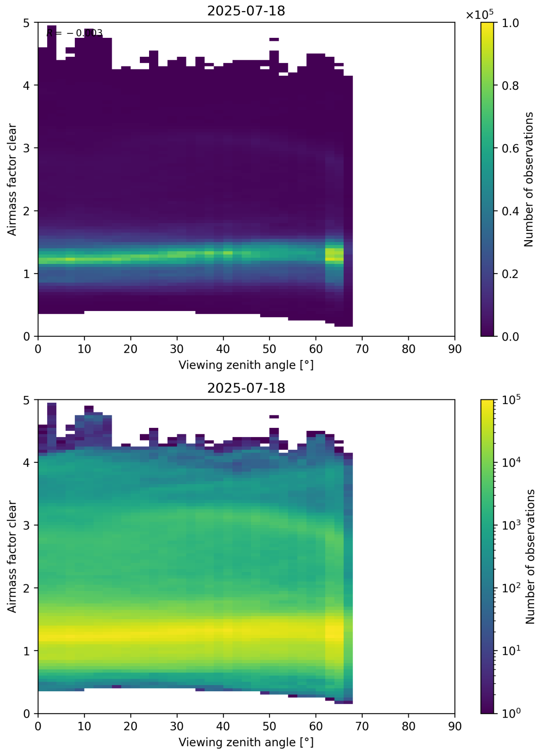
Figure 185: Scatter density plot of “Viewing zenith angle” against “Airmass factor clear” for 2025-07-18 to 2025-07-19.
