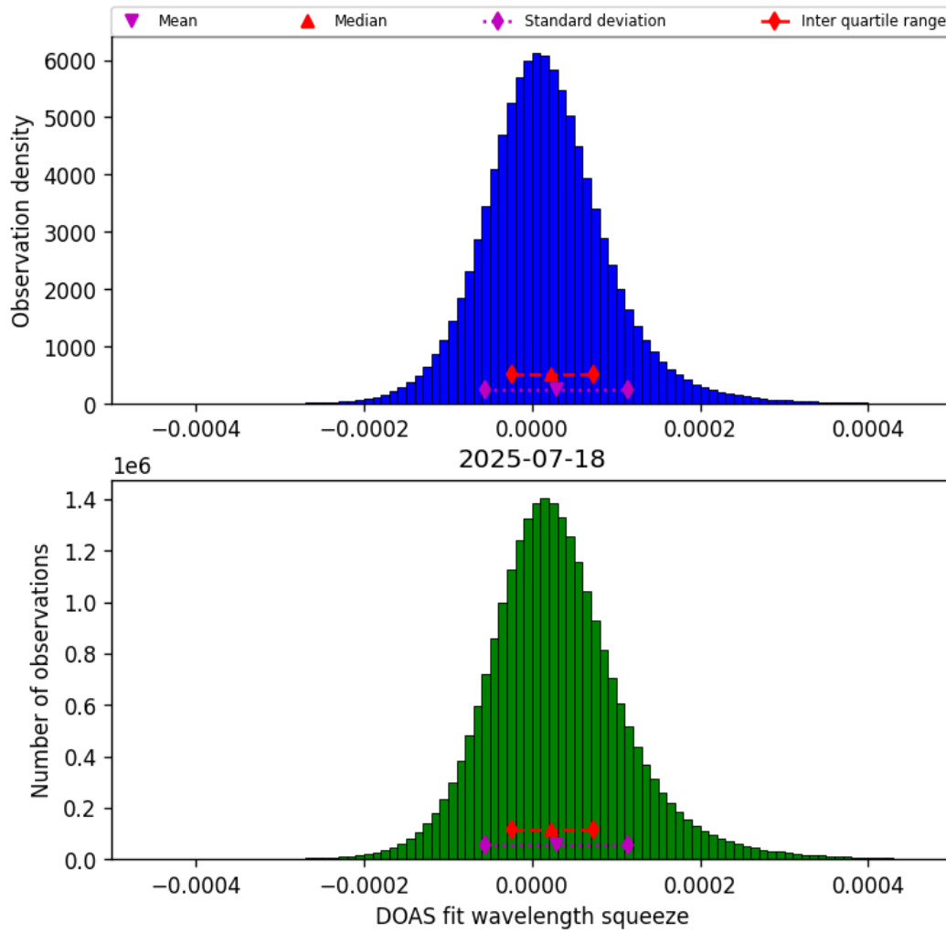
Figure 45: Histogram of “DOAS fit wavelength squeeze” for 2025-07-18 to 2025-07-19
