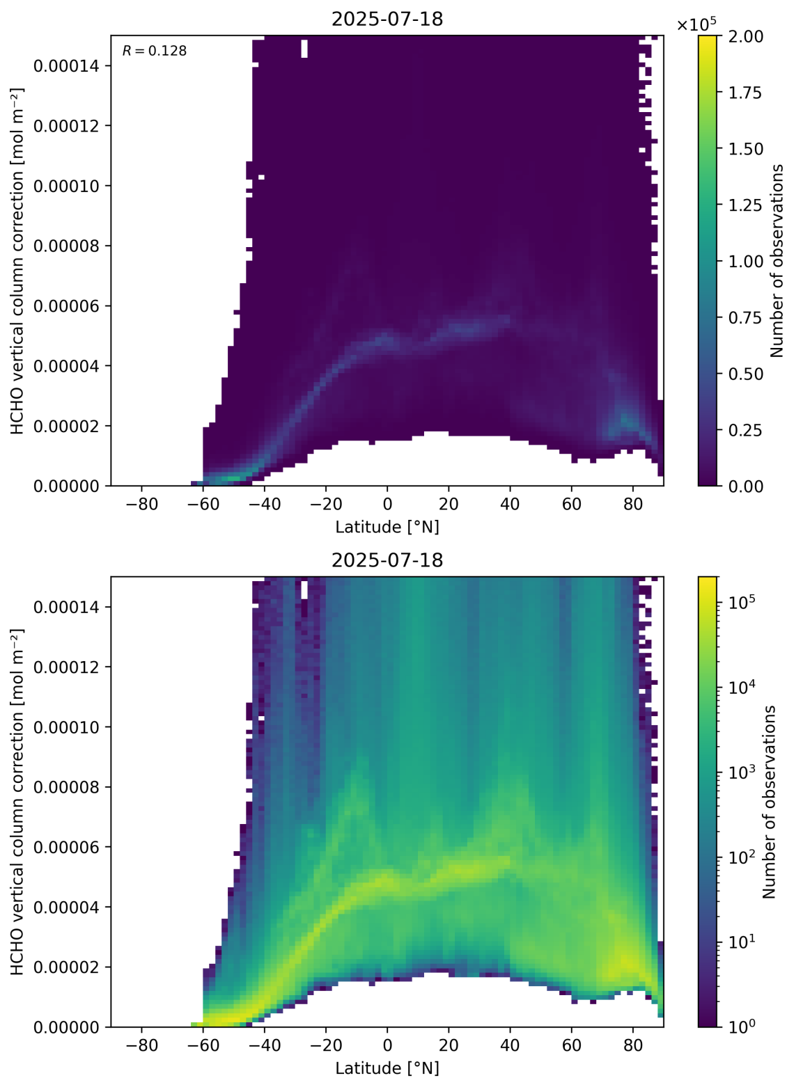
Figure 164: Scatter density plot of “Latitude” against “HCHO vertical column correction” for 2025-07-18 to 2025-07-19.
