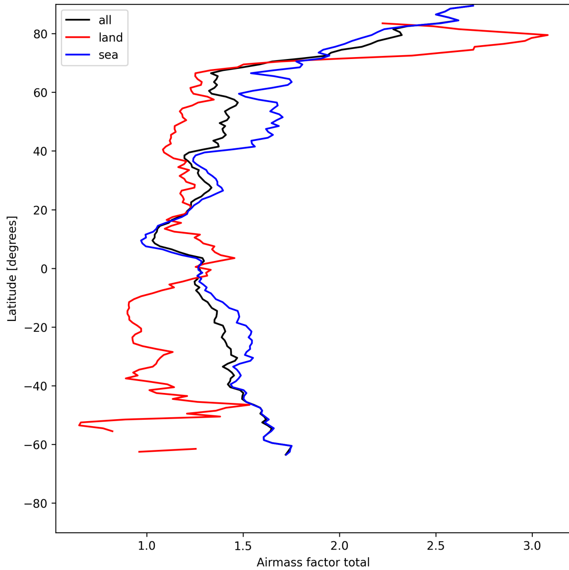
Figure 26: Zonal average of “Airmass factor total” for 2025-07-18 to 2025-07-19.
