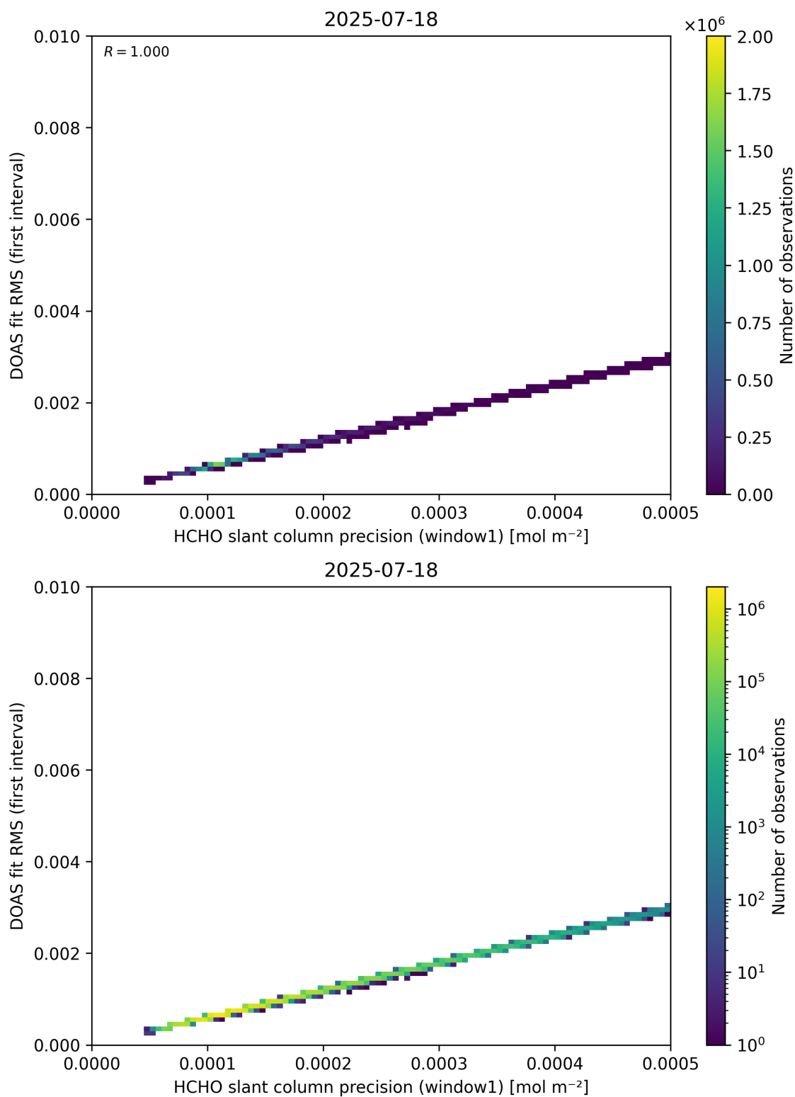
Figure 88: Scatter density plot of “HCHO slant column precision (window1)” against “DOAS fit RMS (first interval)” for 2025-07-18 to 2025-07-19.
