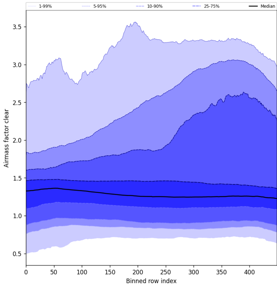
Figure 56: Along track statistics of “Air mass factor clear” for 2025-07-18 to 2025-07-19
