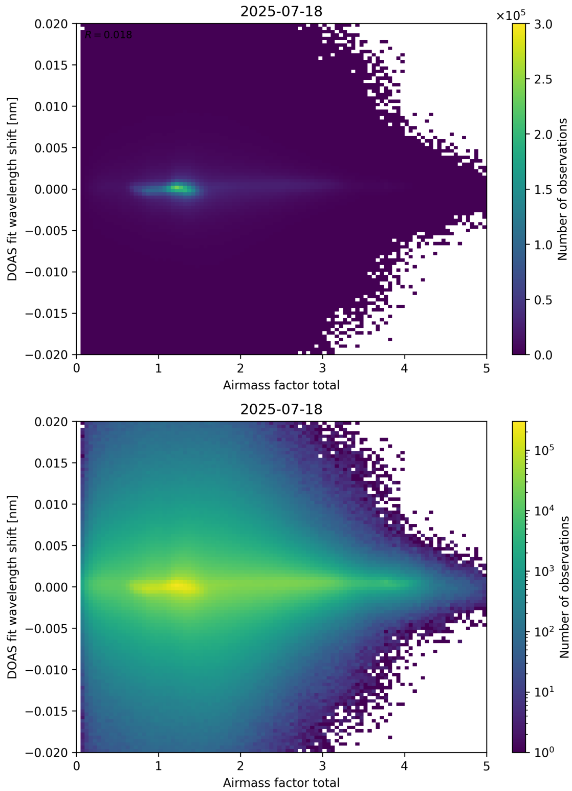
Figure 98: Scatter density plot of “Airmass factor total” against “DOAS fit wavelength shift” for 2025-07-18 to 2025-07-19.
