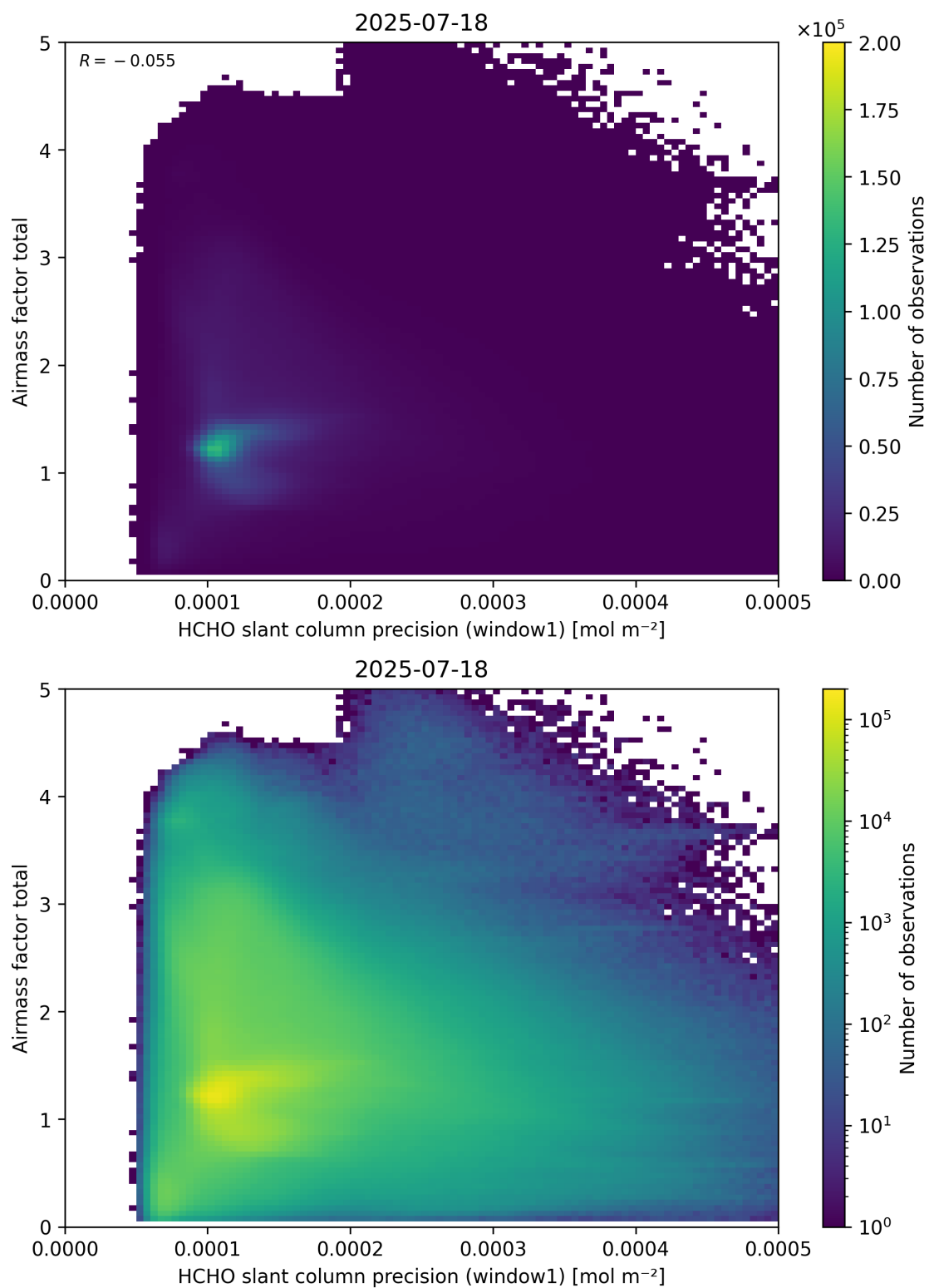
Figure 94: Scatter density plot of “HCHO slant column precision (window1)” against “Airmass factor total” for 2025-07-18 to 2025-07-19.
