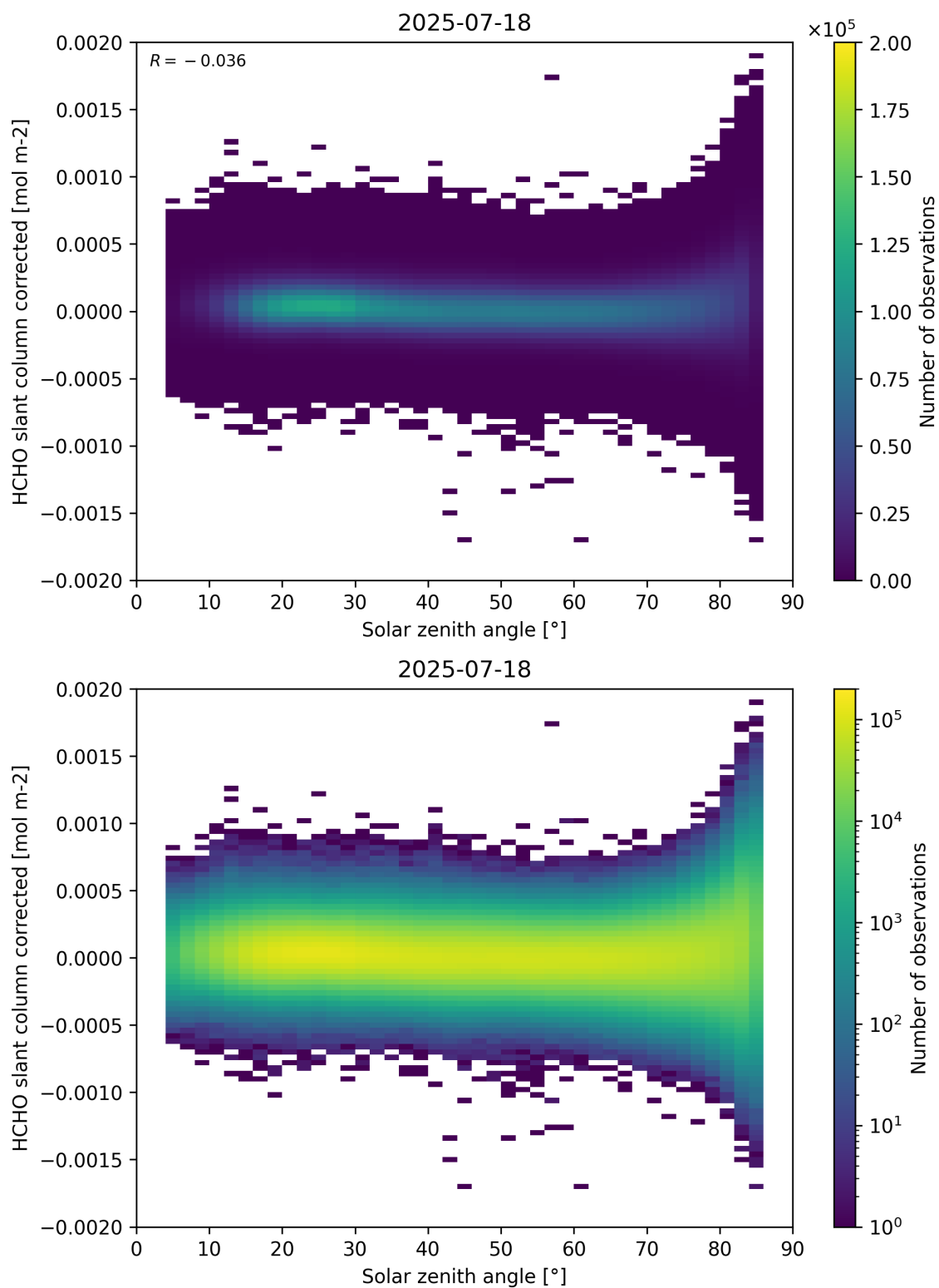
Figure 171: Scatter density plot of “Solar zenith angle” against “HCHO slant column corrected” for 2025-07-18 to 2025-07-19.
