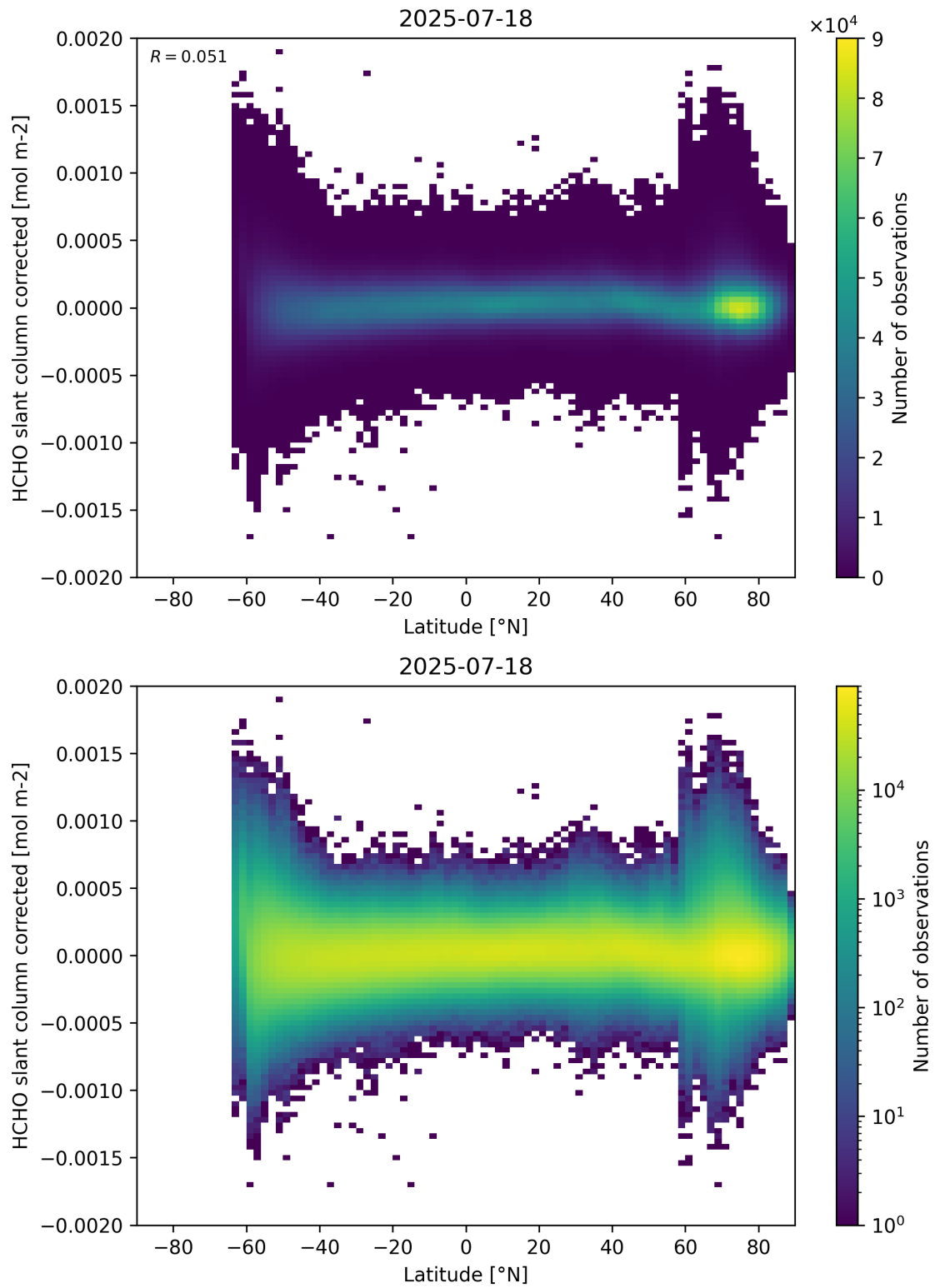
Figure 157: Scatter density plot of “Latitude” against “HCHO slant column corrected” for 2025-07-18 to 2025-07-19.
