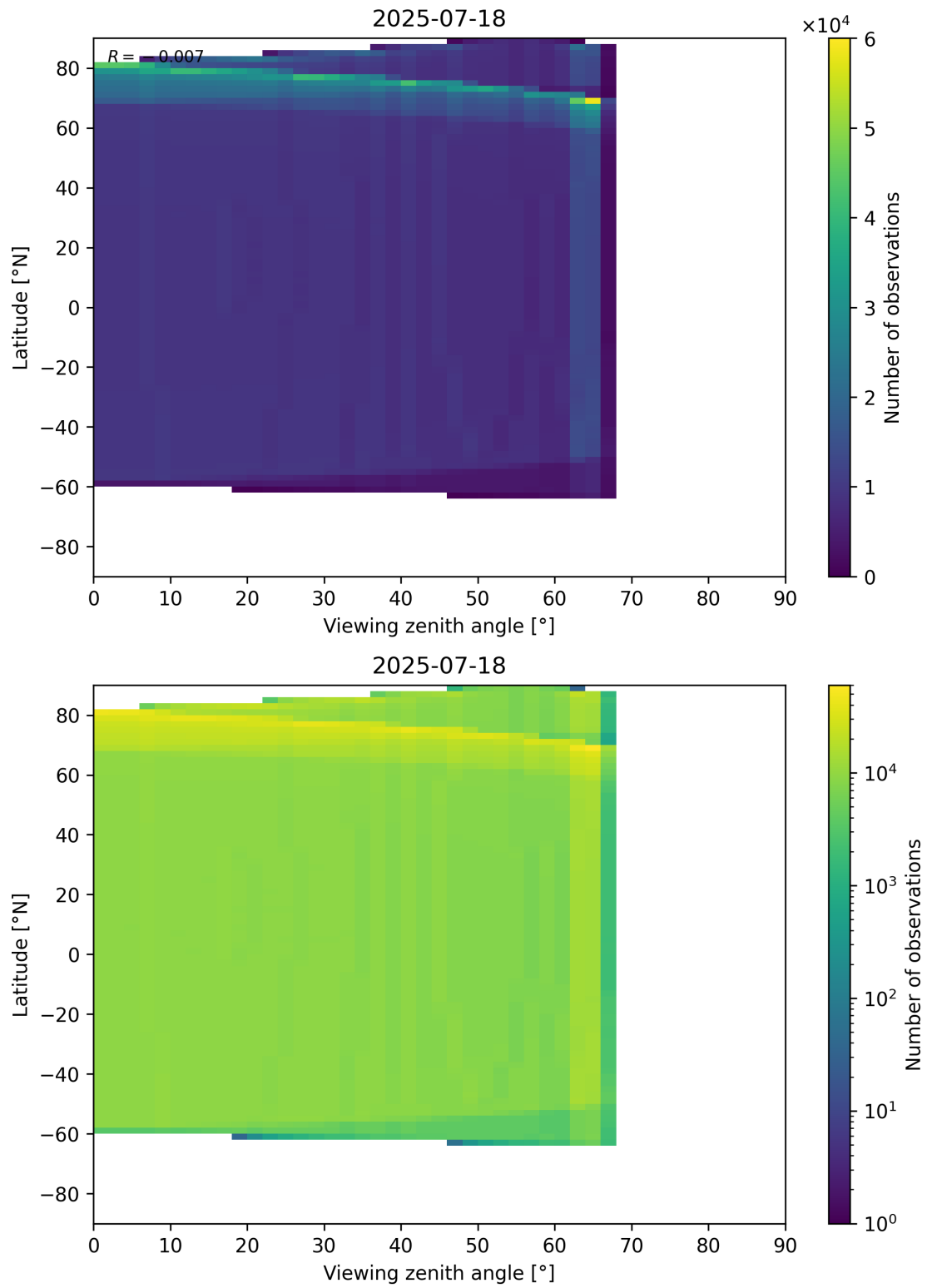
Figure 196: Scatter density plot of “Viewing zenith angle” against “Latitude” for 2025-07-18 to 2025-07-19.
