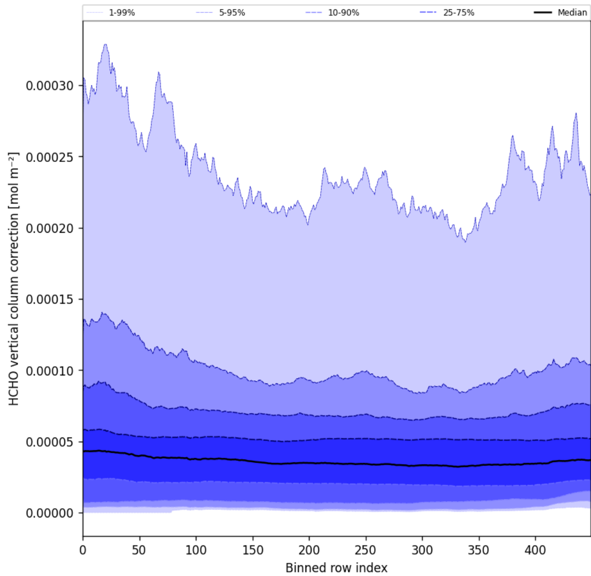
Figure 51: Along track statistics of “HCHO vertical column correction” for 2025-07-18 to 2025-07-19
