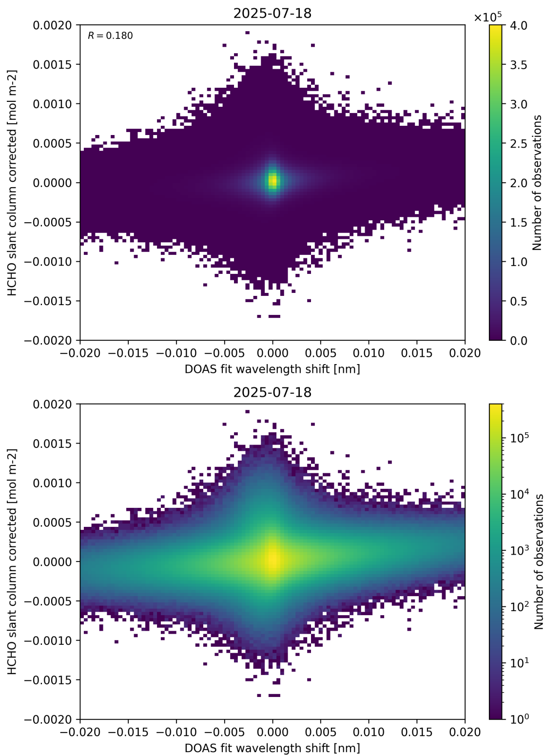
Figure 66: Scatter density plot of “DOAS fit wavelength shift” against “HCHO slant column corrected” for 2025-07-18 to 2025-07-19.
