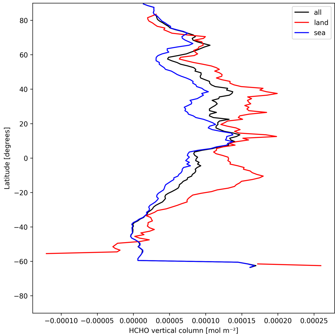
Figure 21: Zonal average of “HCHO vertical column” for 2025-07-18 to 2025-07-19.
