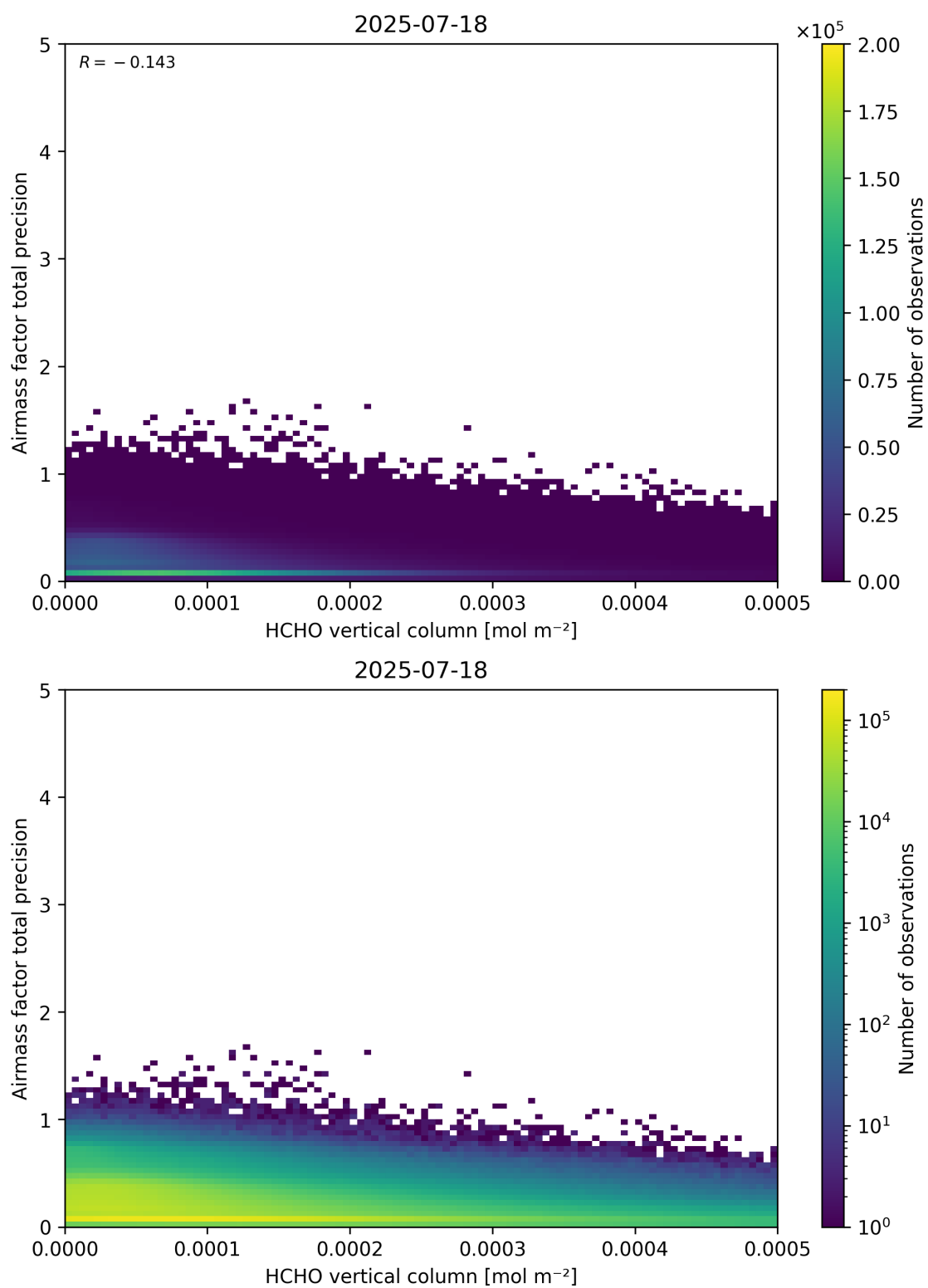
Figure 132: Scatter density plot of “HCHO vertical column” against “Airmass factor total precision” for 2025-07-18 to 2025-07-19.
