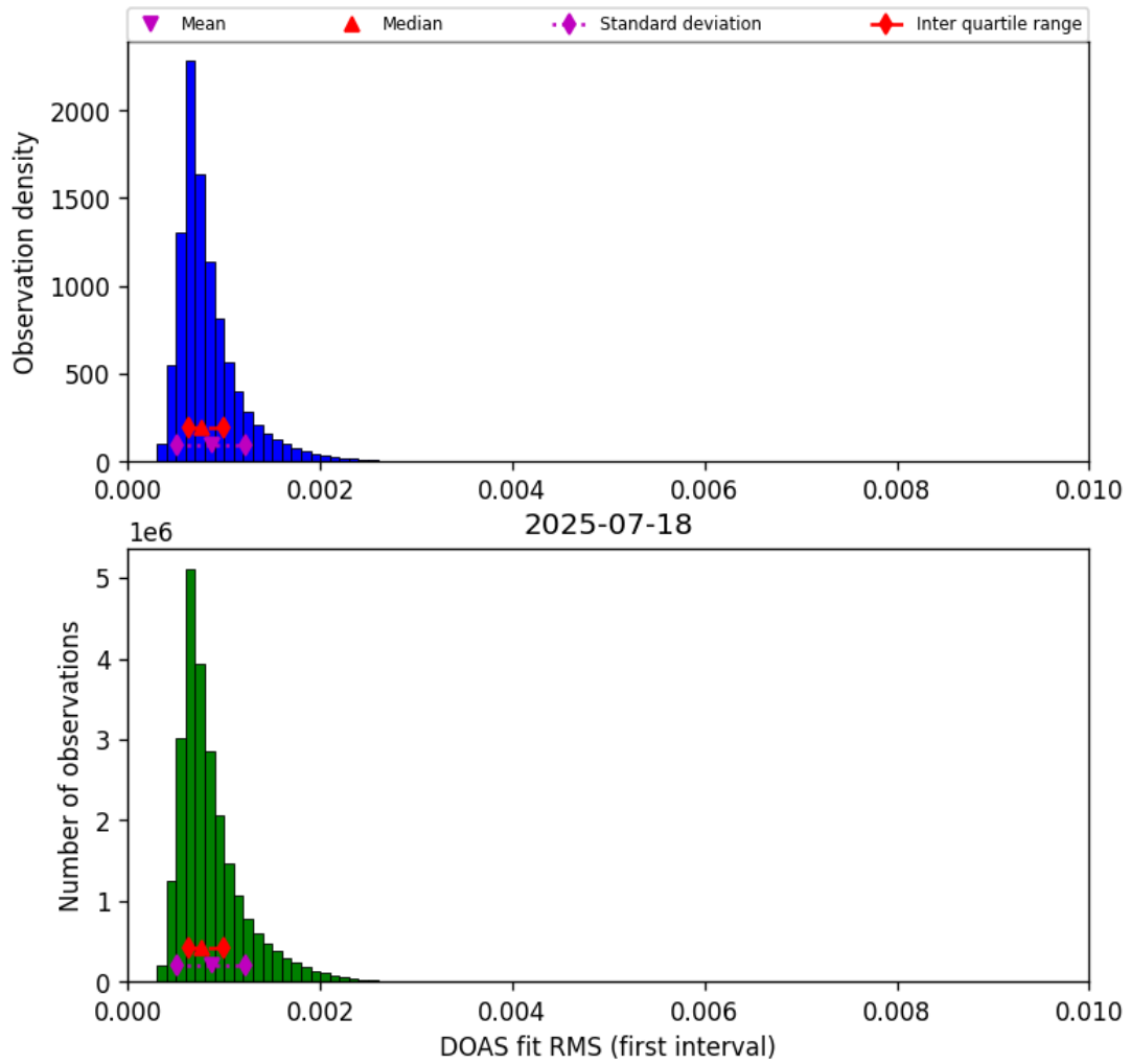
Figure 46: Histogram of "DOAS fit RMS (first interval)" for 2025-07-18 to 2025-07-19
