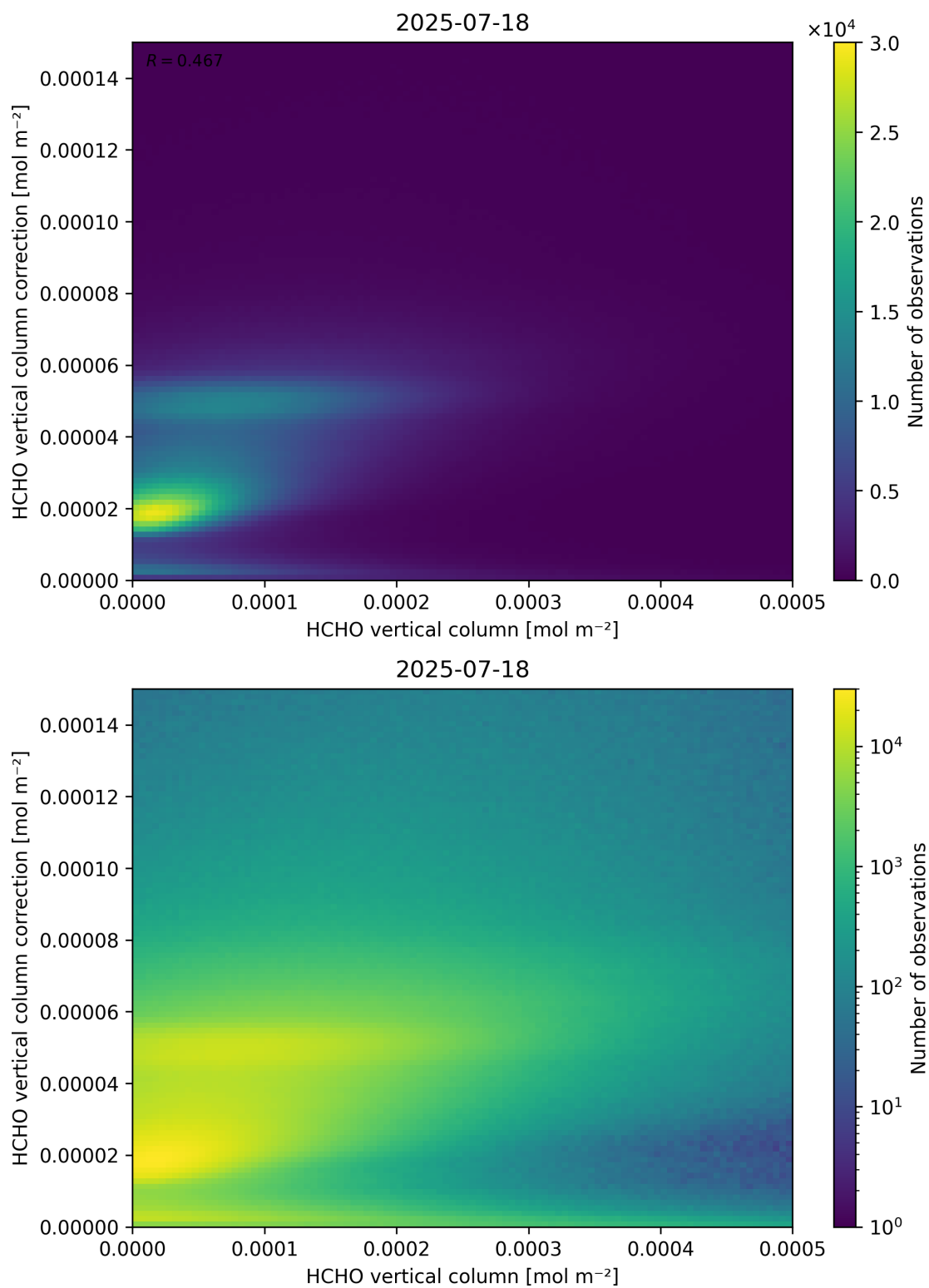
Figure 133: Scatter density plot of “HCHO vertical column” against “HCHO vertical column correction” for 2025-07-18 to 2025-07-19.
