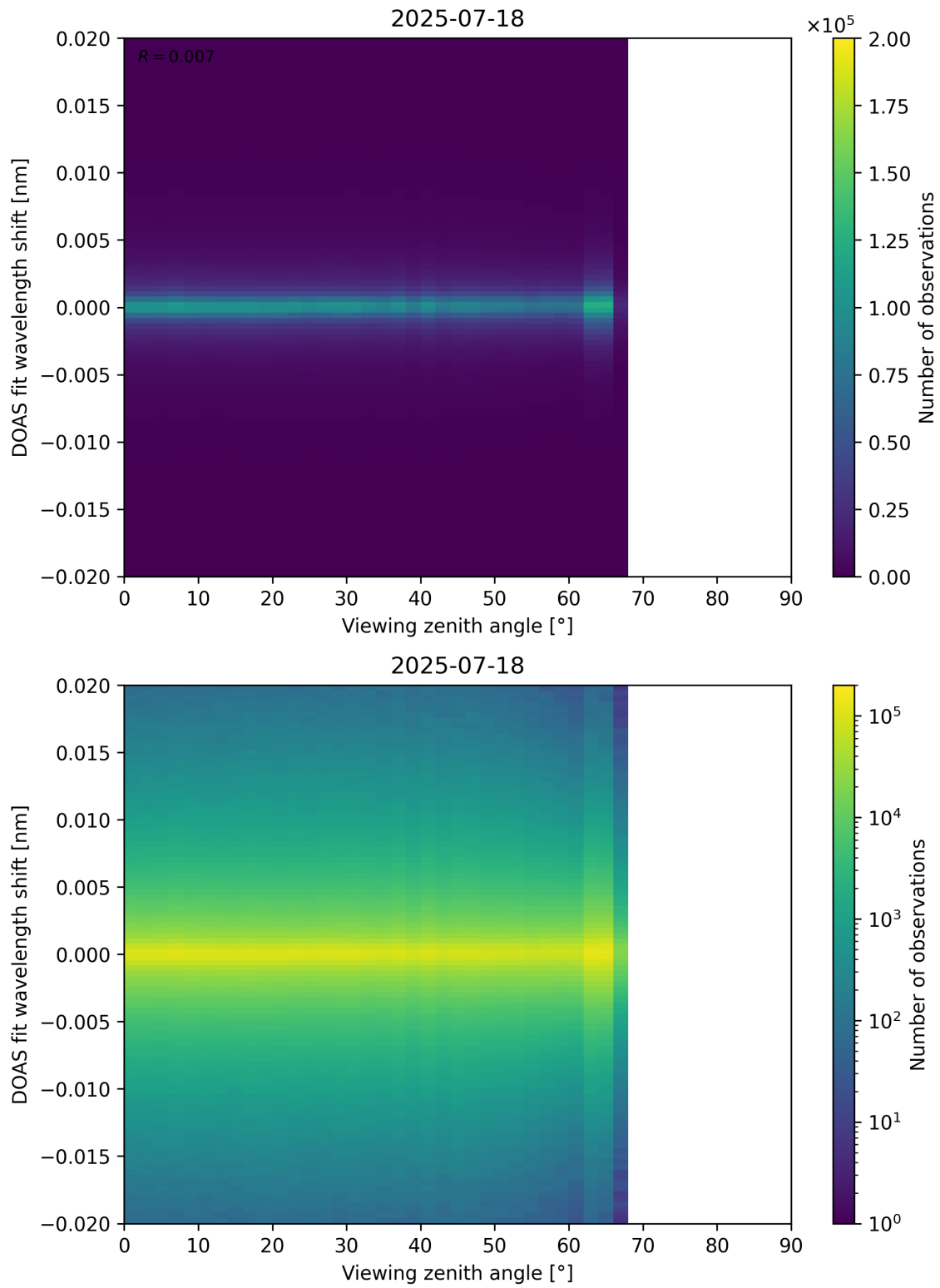
Figure 183: Scatter density plot of “Viewing zenith angle” against “DOAS fit wavelength shift” for 2025-07-18 to 2025-07-19.
