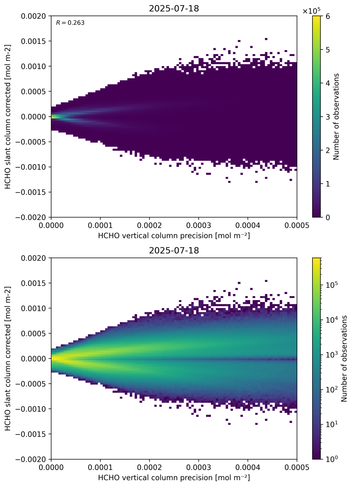
Figure 140: Scatter density plot of “HCHO vertical column precision” against “HCHO slant column corrected” for 2025-07-18 to 2025-07-19.
