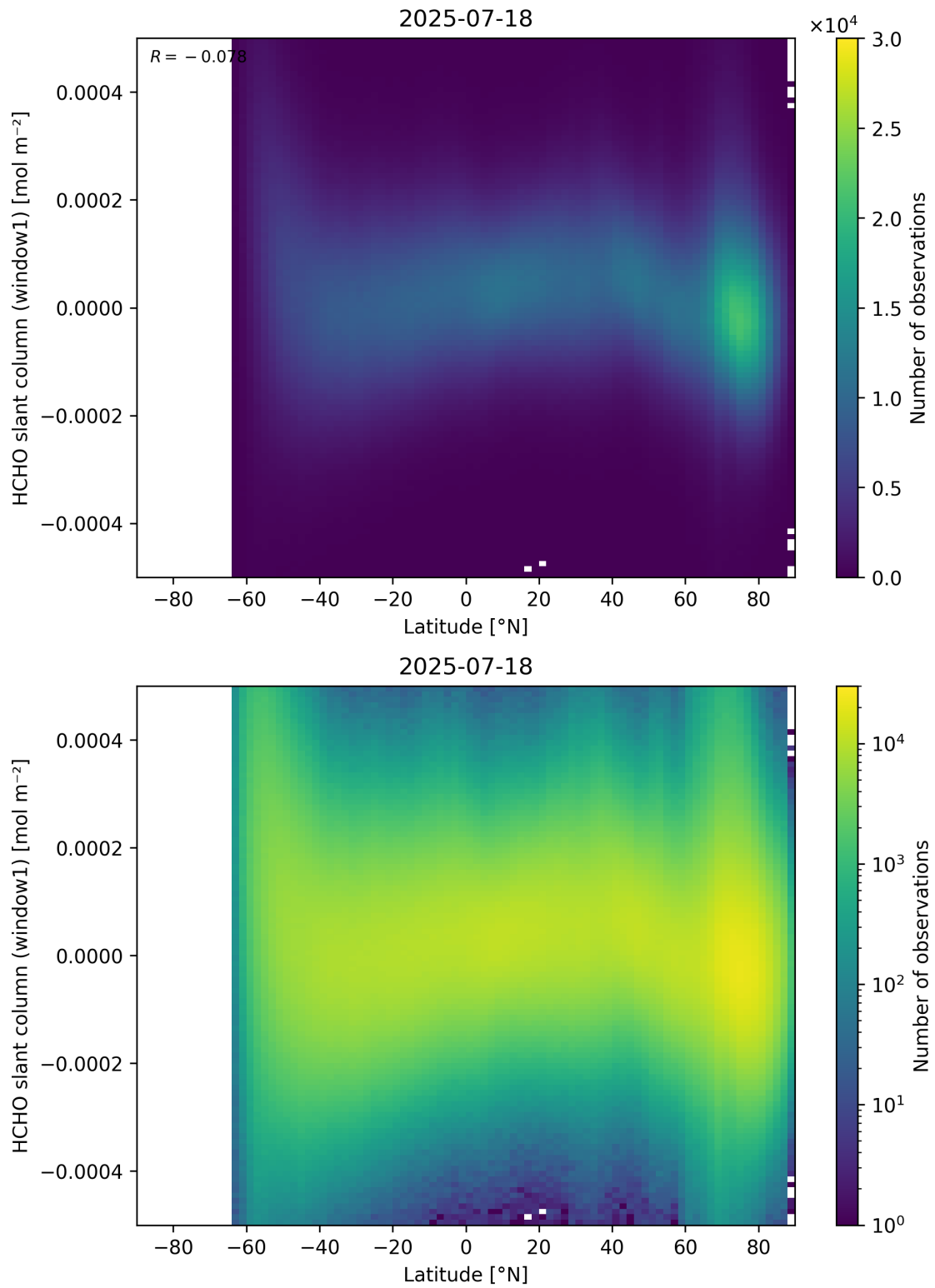
Figure 159: Scatter density plot of “Latitude” against “HCHO slant column (window1)” for 2025-07-18 to 2025-07-19.
