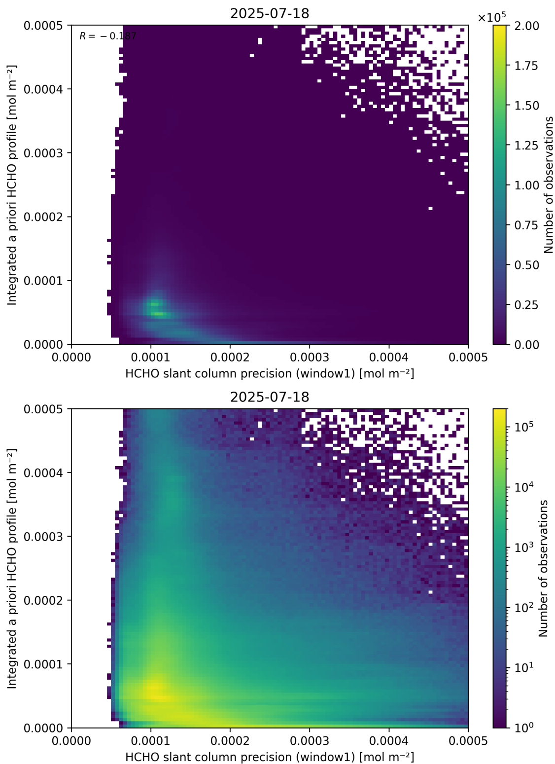
Figure 96: Scatter density plot of “HCHO slant column precision (window1)” against “Integrated a priori HCHO profile” for 2025-07-18 to 2025-07-19.
