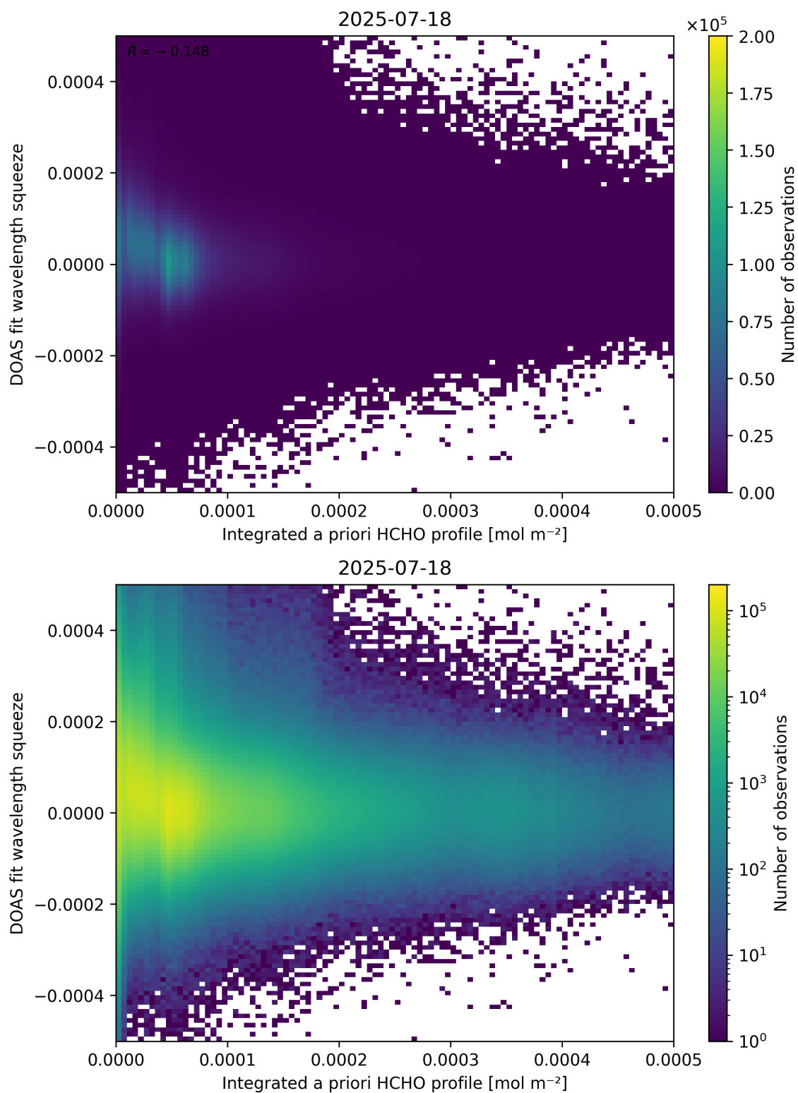
Figure 150: Scatter density plot of “Integrated a priori HCHO profile” against “DOAS fit wavelength squeeze” for 2025-07-18 to 2025-07-19.
