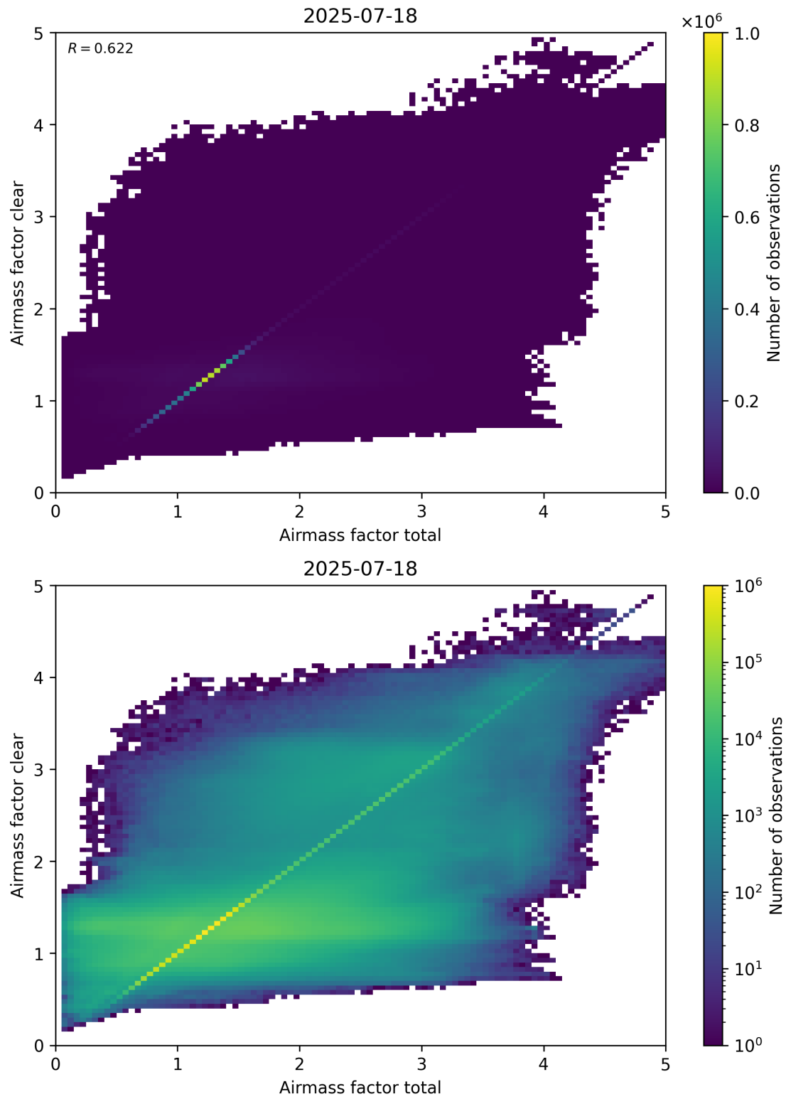
Figure 100: Scatter density plot of “Airmass factor total” against “Airmass factor clear” for 2025-07-18 to 2025-07-19.
