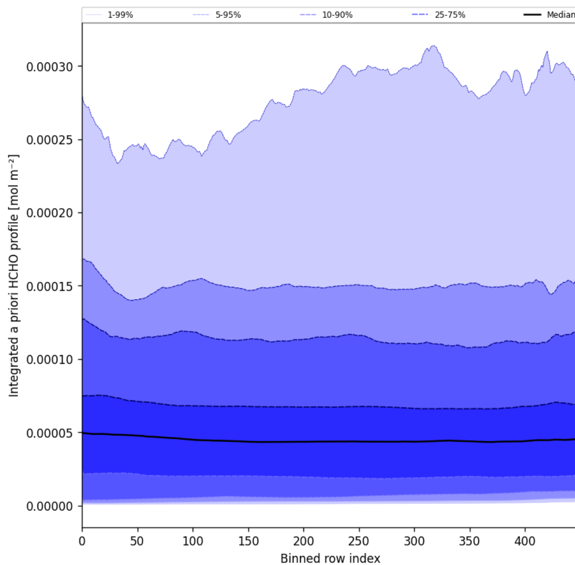
Figure 57: Along track statistics of “Integrated a priori HCHO profile” for 2025-07-18 to 2025-07-19
