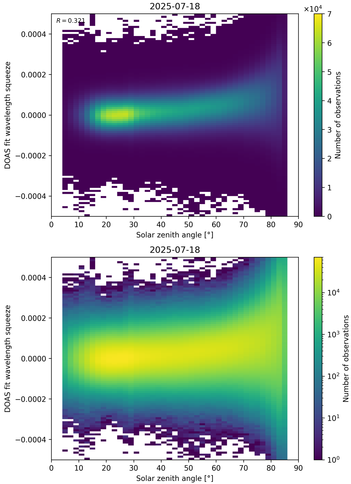
Figure 169: Scatter density plot of “Solar zenith angle” against “DOAS fit wavelength squeeze” for 2025-07-18 to 2025-07-19.
