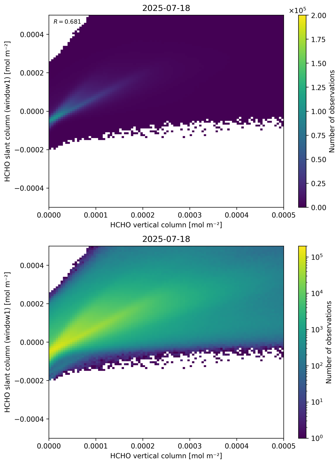
Figure 129: Scatter density plot of “HCHO vertical column” against “HCHO slant column (window1)” for 2025-07-18 to 2025-07-19.
