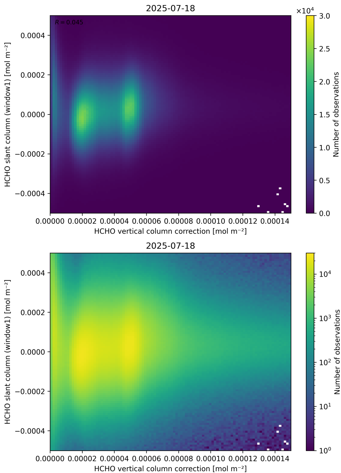
Figure 118: Scatter density plot of “HCHO vertical column correction” against “HCHO slant column (window1)” for 2025-07-18 to 2025-07-19.
