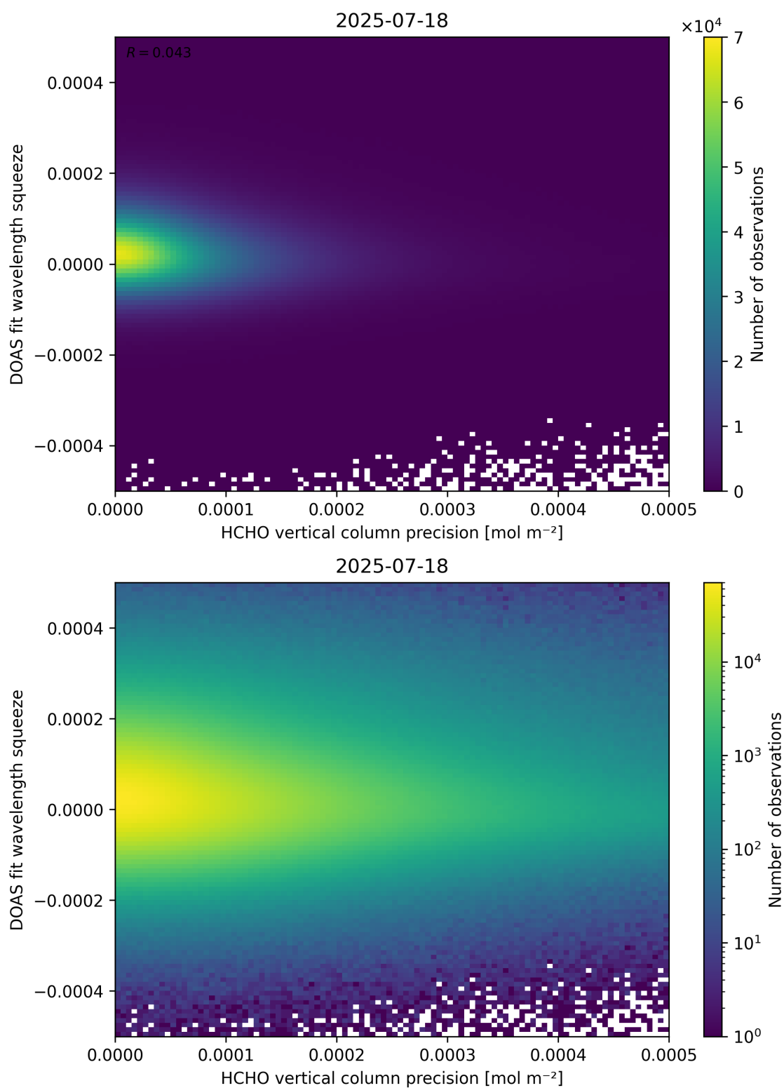
Figure 138: Scatter density plot of “HCHO vertical column precision” against “DOAS fit wavelength squeeze” for 2025-07-18 to 2025-07-19.
