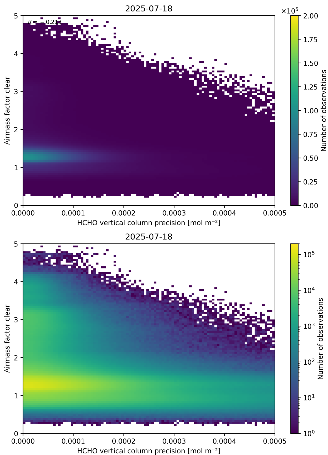
Figure 139: Scatter density plot of “HCHO vertical column precision” against “Airmass factor clear” for 2025-07-18 to 2025-07-19.
