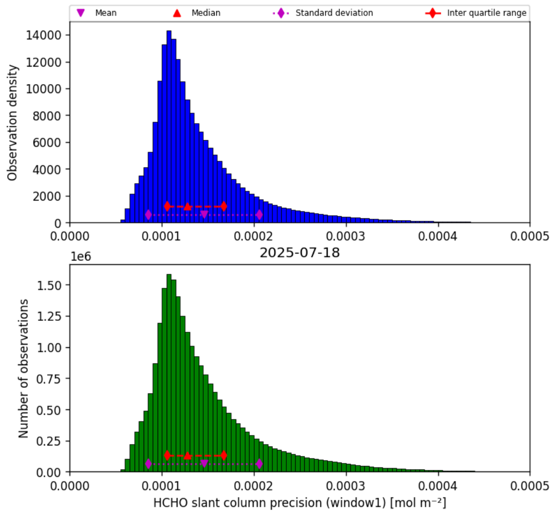
Figure 39: Histogram of “HCHO slant column precision (window1)” for 2025-07-18 to 2025-07-19
