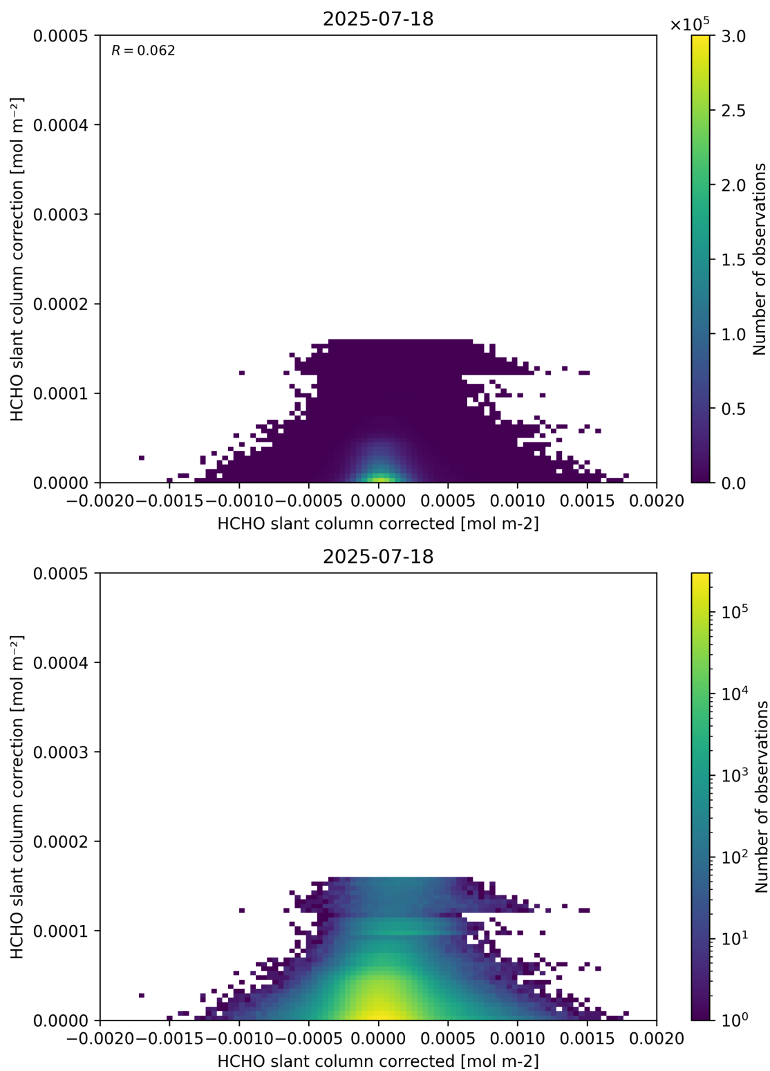
Figure 77: Scatter density plot of “HCHO slant column corrected” against “HCHO slant column correction” for 2025-07-18 to 2025-07-19.
