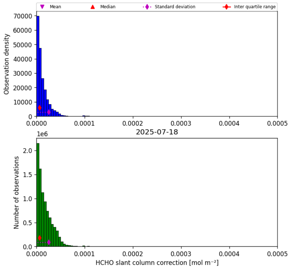
Figure 47: Histogram of “HCHO slant column correction” for 2025-07-18 to 2025-07-19
