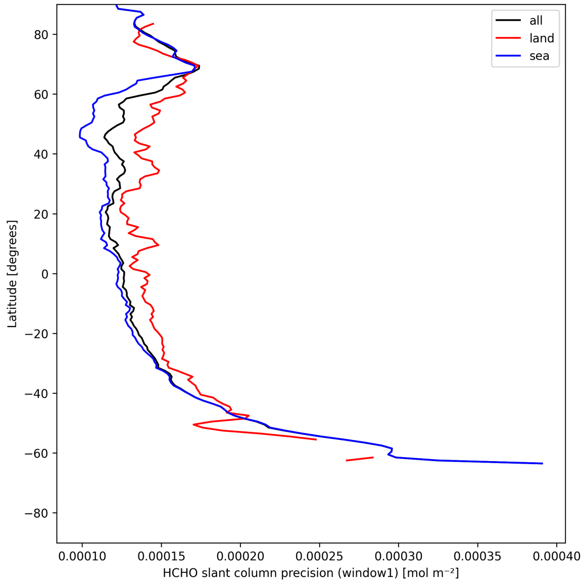
Figure 25: Zonal average of “HCHO slant column precision (window1)” for 2025-07-18 to 2025-07-19.
