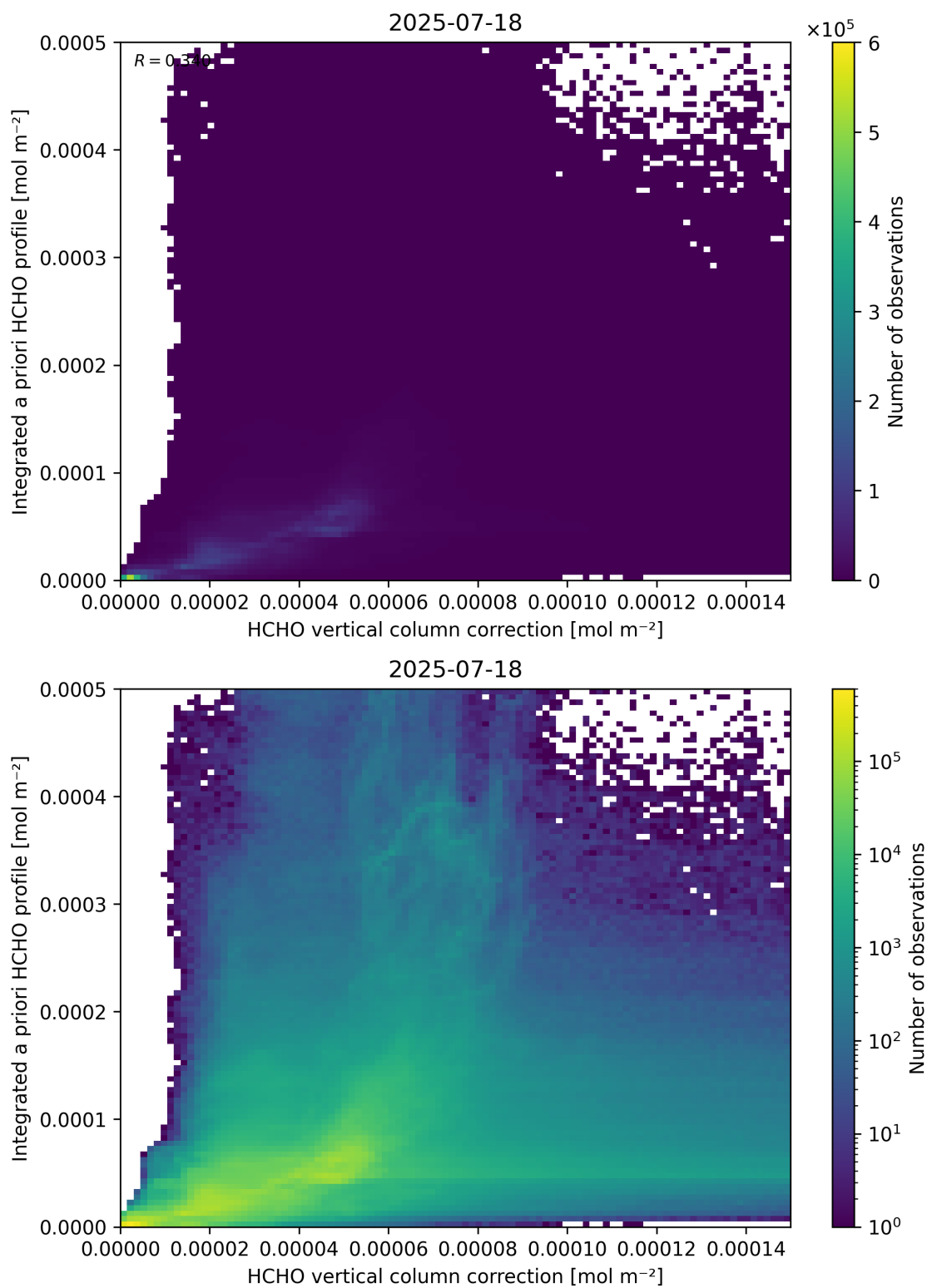
Figure 122: Scatter density plot of “HCHO vertical column correction” against “Integrated a priori HCHO profile” for 2025-07-18 to 2025-07-19.
