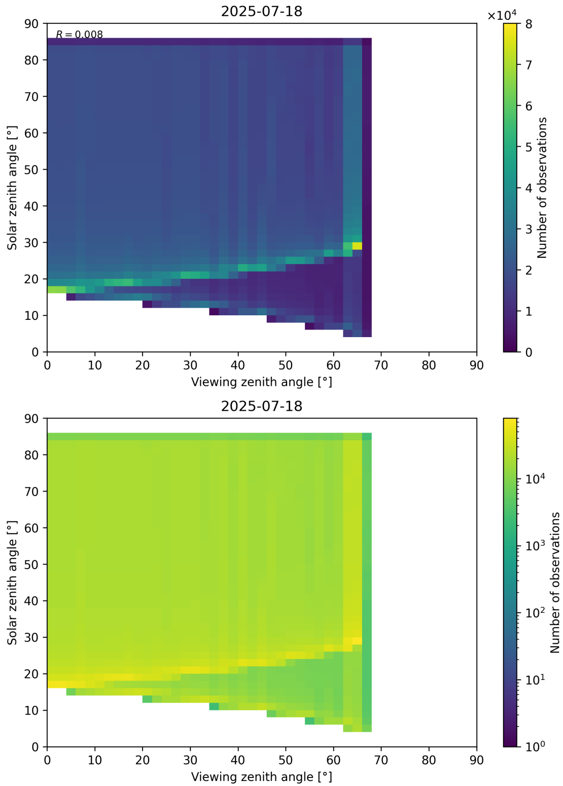
Figure 197: Scatter density plot of “Viewing zenith angle” against “Solar zenith angle” for 2025-07-18 to 2025-07-19.
