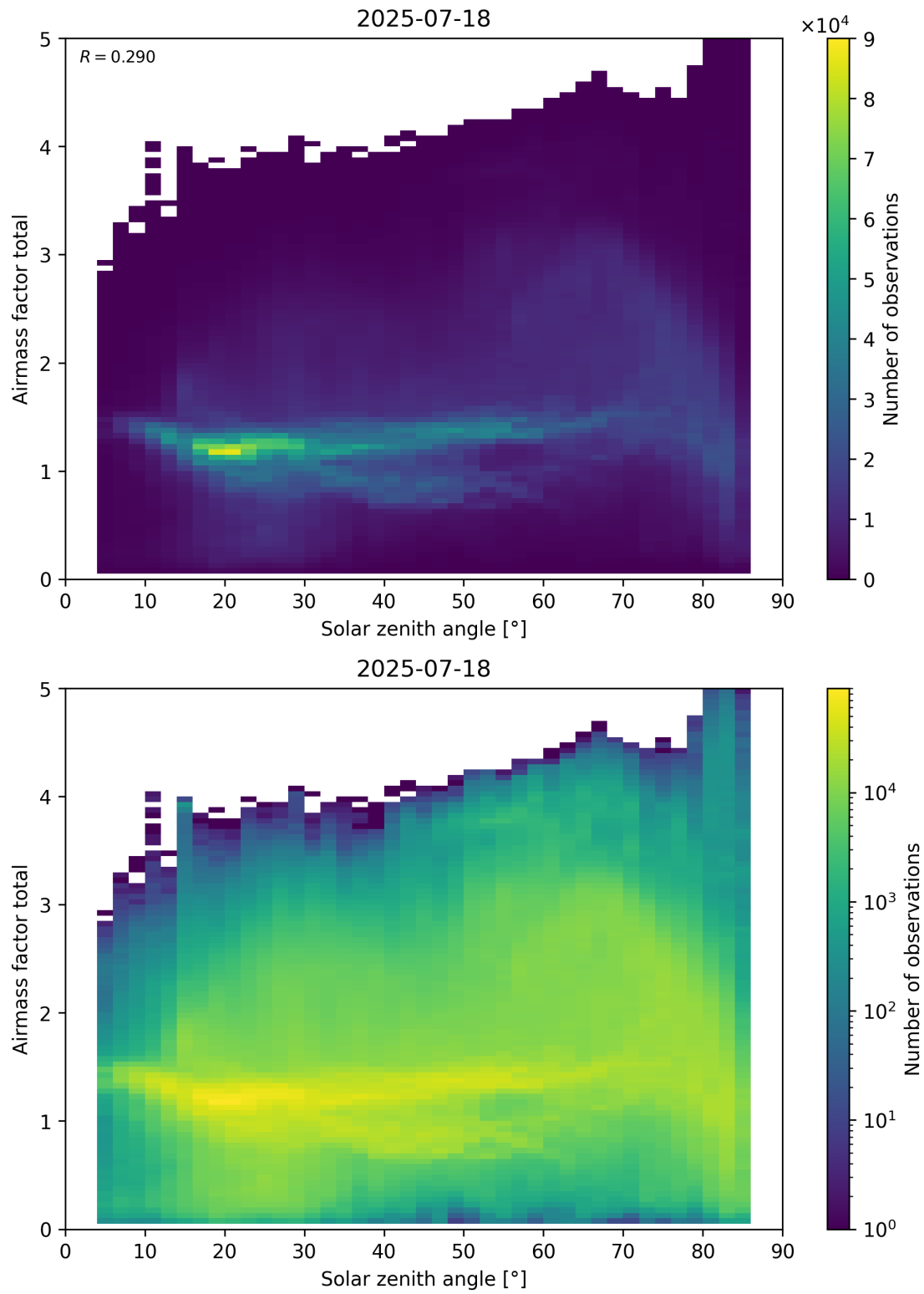
Figure 175: Scatter density plot of “Solar zenith angle” against “Airmass factor total” for 2025-07-18 to 2025-07-19.
