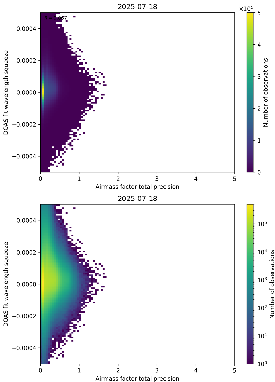
Figure 107: Scatter density plot of “Airmass factor total precision” against “DOAS fit wavelength squeeze” for 2025-07-18 to 2025-07-19.
