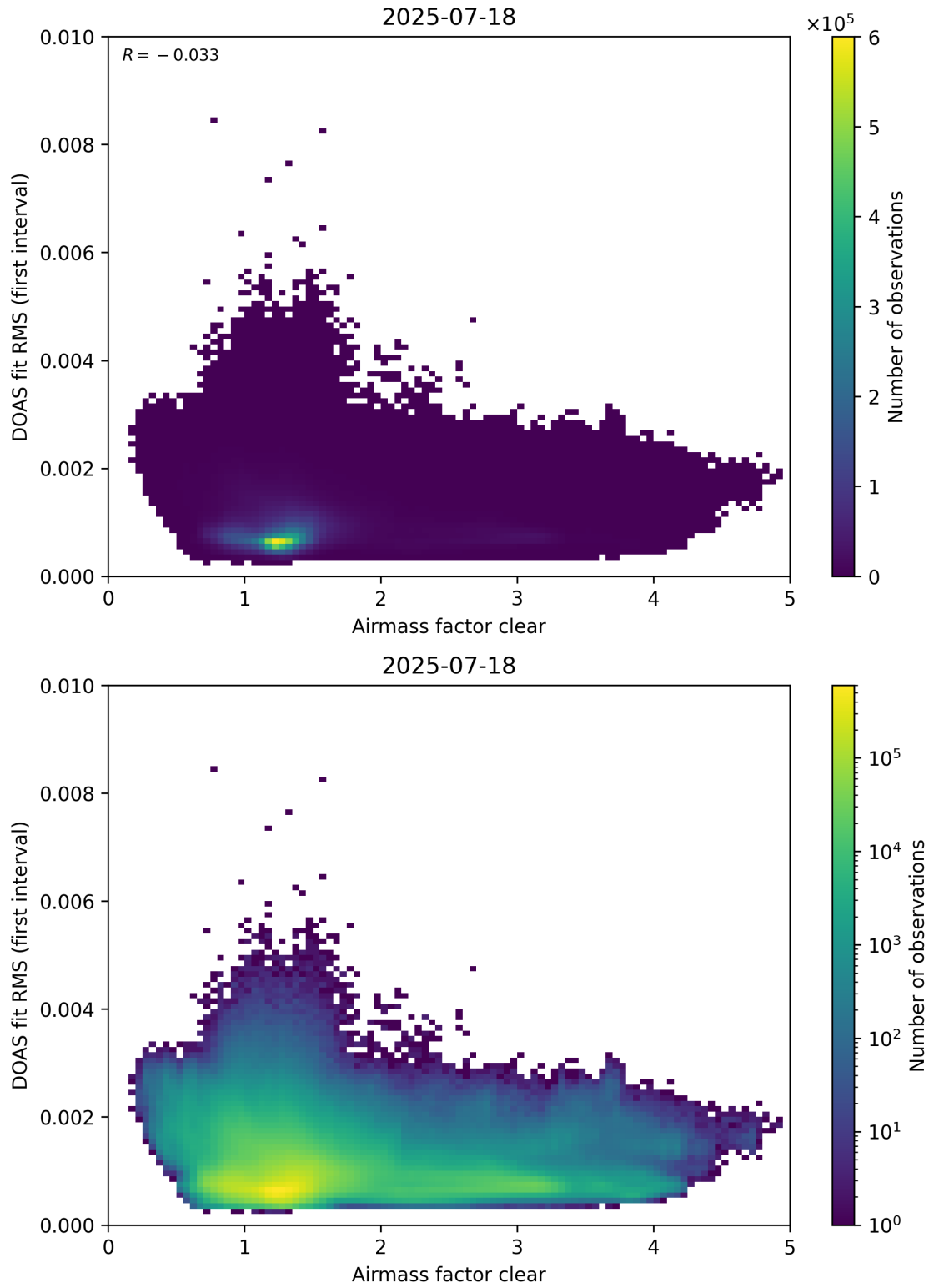
Figure 71: Scatter density plot of “Airmass factor clear” against “DOAS fit RMS (first interval)” for 2025-07-18 to 2025-07-19.
