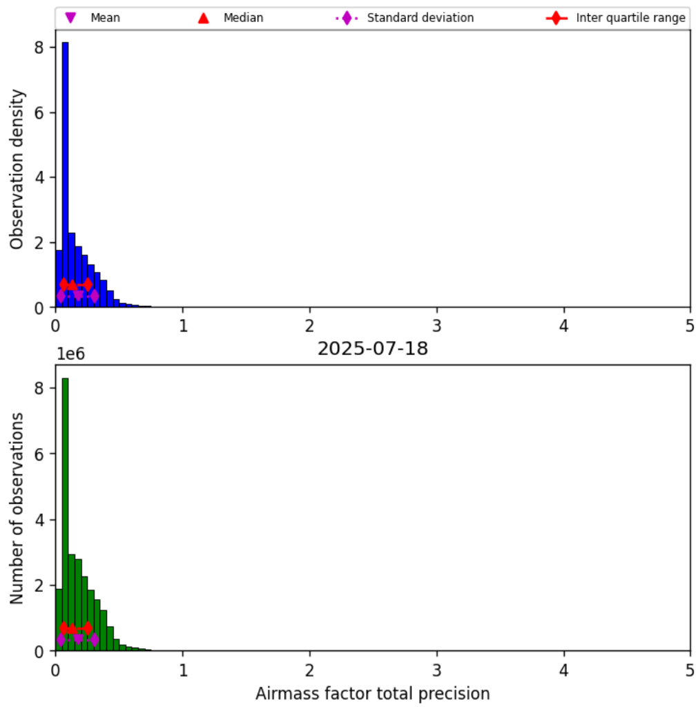
Figure 41: Histogram of “Airmass factor total precision” for 2025-07-18 to 2025-07-19
