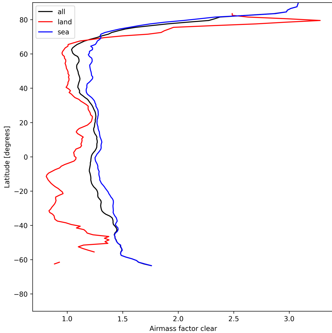
Figure 28: Zonal average of “Airmass factor clear” for 2025-07-18 to 2025-07-19.
