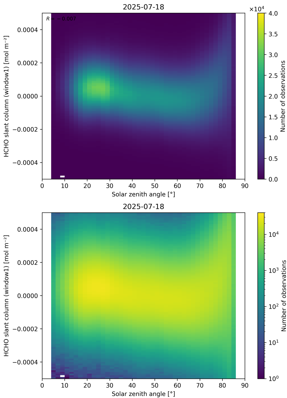
Figure 173: Scatter density plot of “Solar zenith angle” against “HCHO slant column (window1)” for 2025-07-18 to 2025-07-19.
