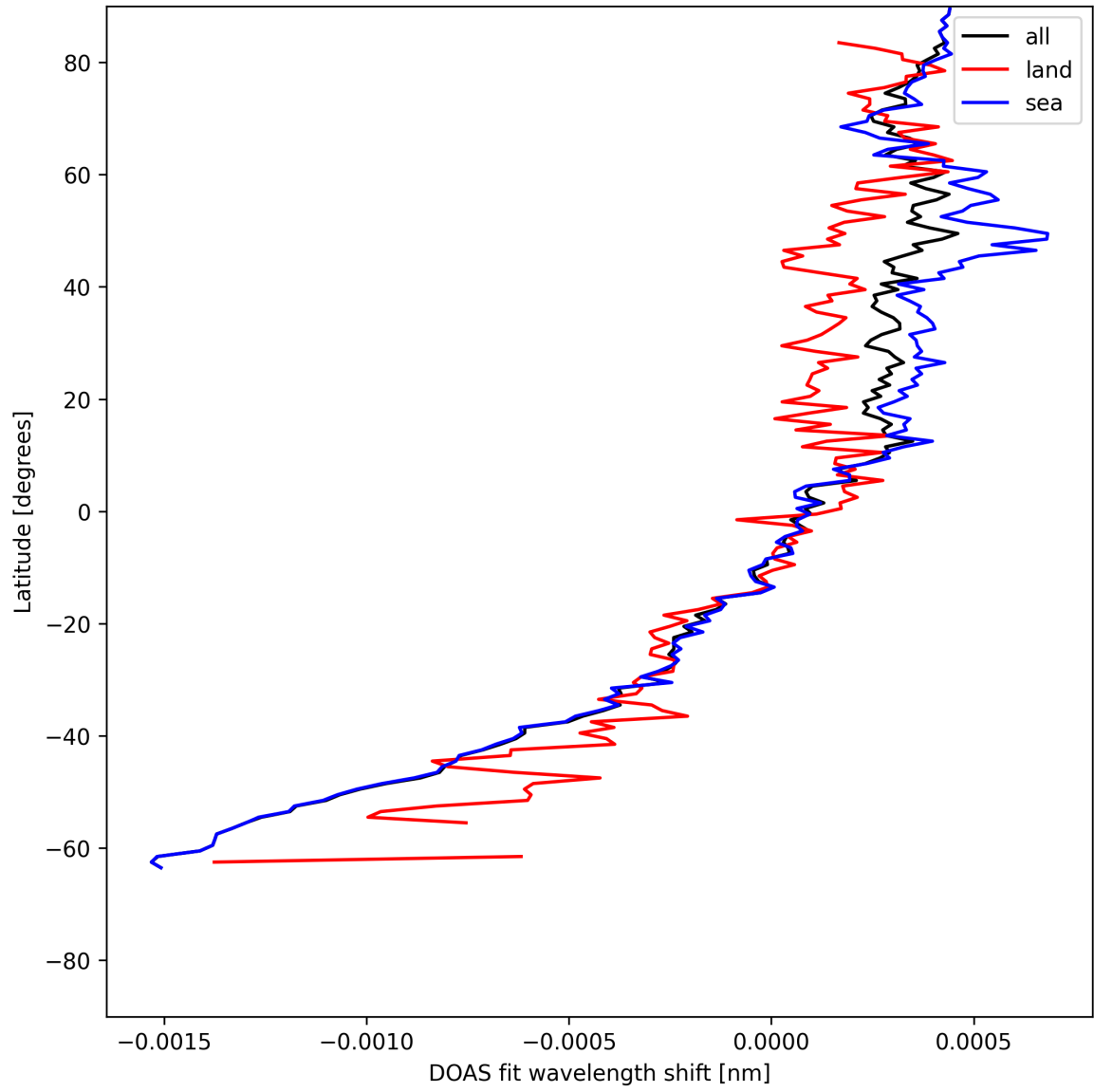
Figure 30: Zonal average of "DOAS fit wavelength shift" for 2025-07-18 to 2025-07-19.
