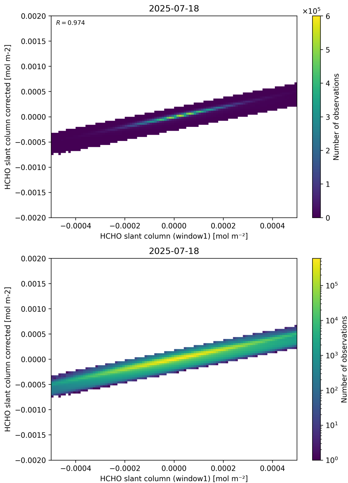
Figure 82: Scatter density plot of “HCHO slant column (window1)” against “HCHO slant column corrected” for 2025-07-18 to 2025-07-19.
