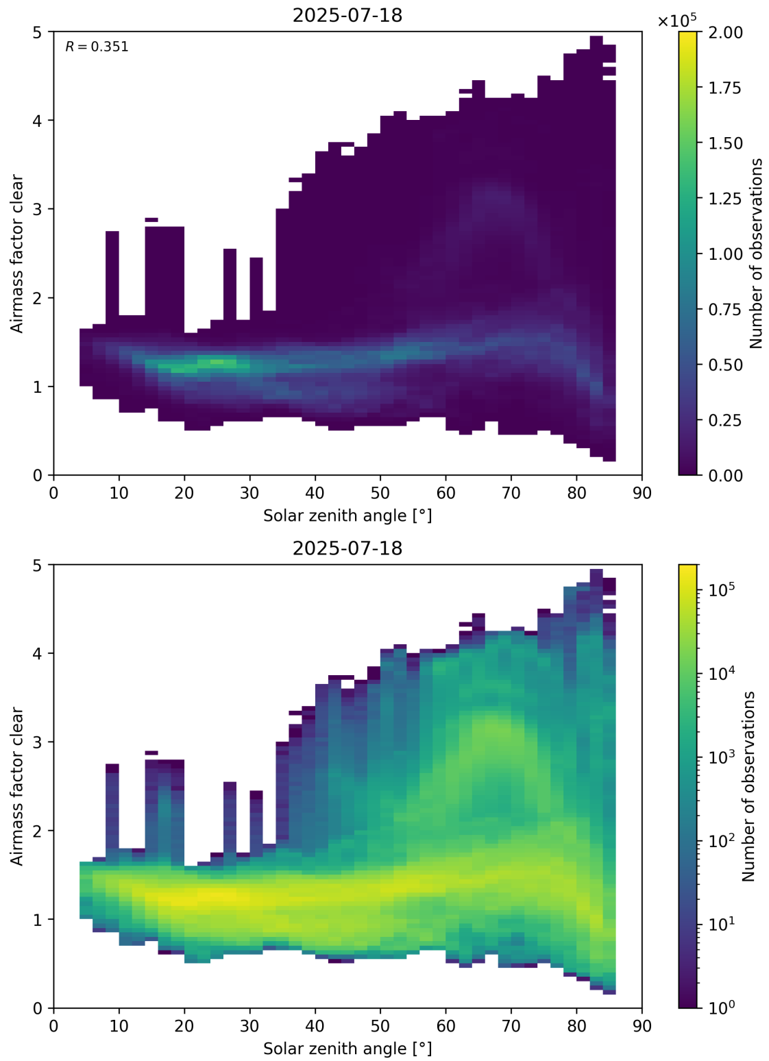
Figure 170: Scatter density plot of “Solar zenith angle” against “Airmass factor clear” for 2025-07-18 to 2025-07-19.
