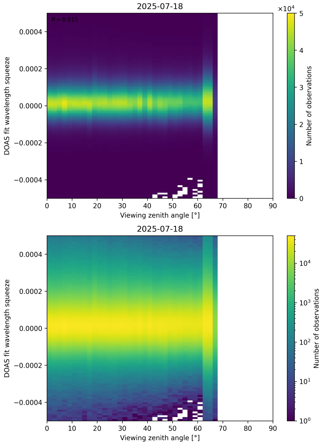
Figure 184: Scatter density plot of “Viewing zenith angle” against “DOAS fit wavelength squeeze” for 2025-07-18 to 2025-07-19.
