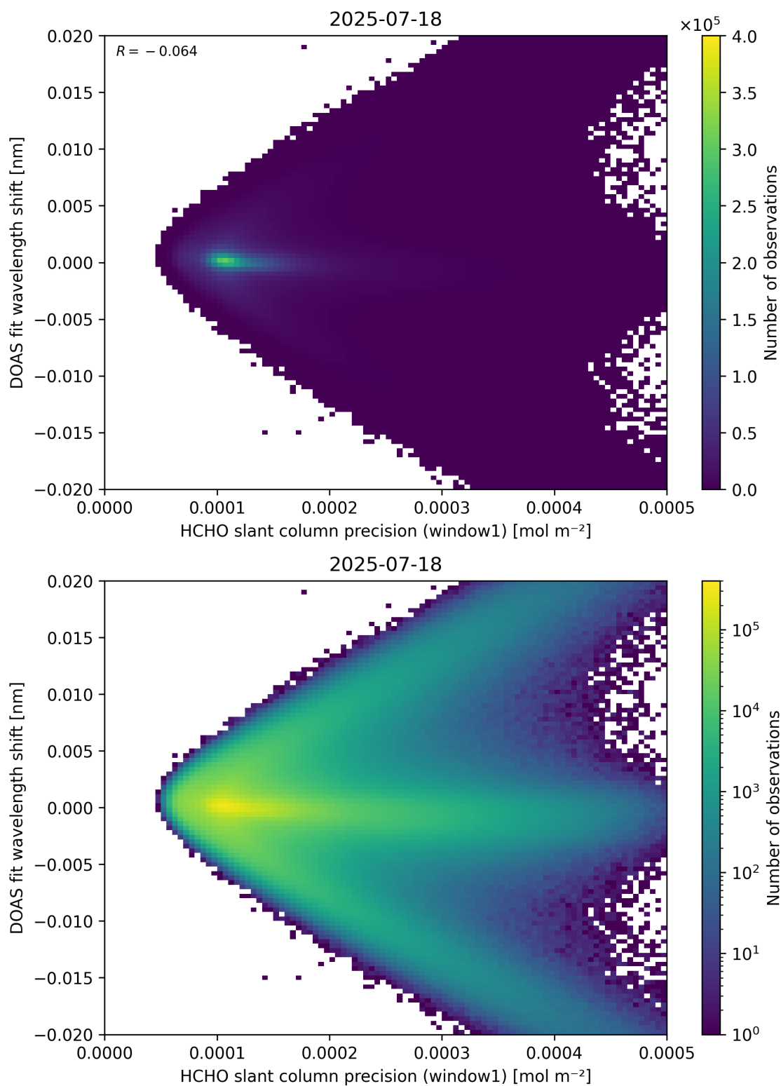
Figure 89: Scatter density plot of “HCHO slant column precision (window1)” against “DOAS fit wavelength shift” for 2025-07-18 to 2025-07-19.
