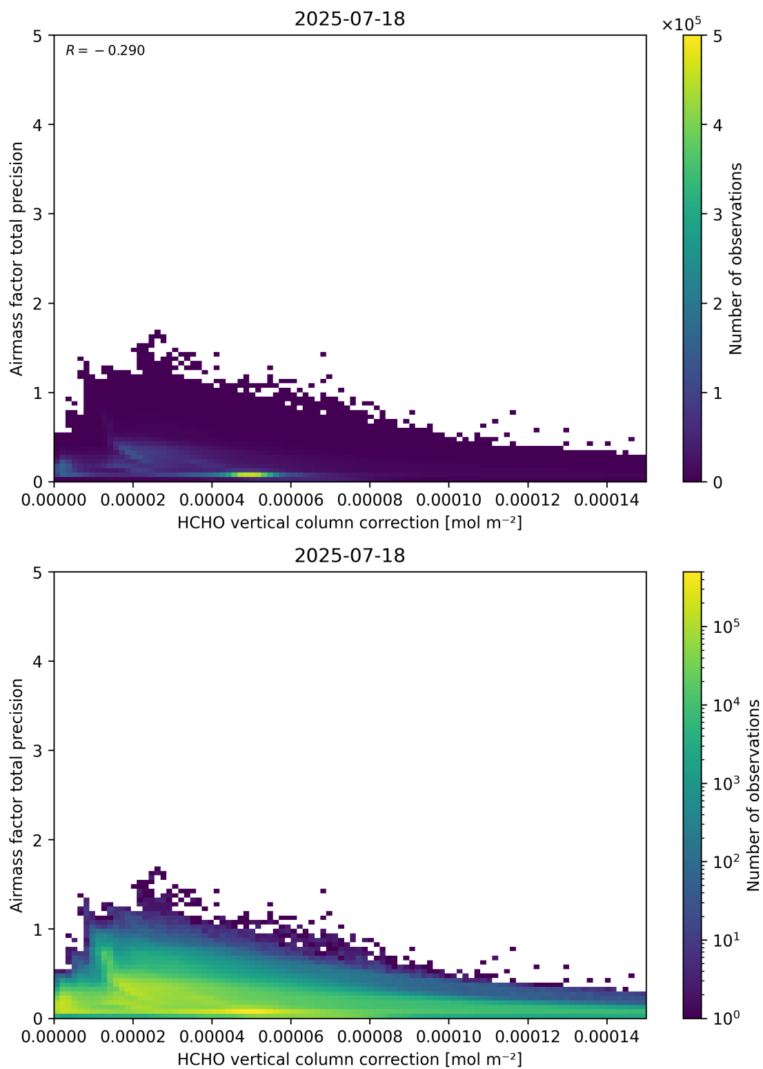
Figure 121: Scatter density plot of “HCHO vertical column correction” against “Airmass factor total precision” for 2025-07-18 to 2025-07-19.
