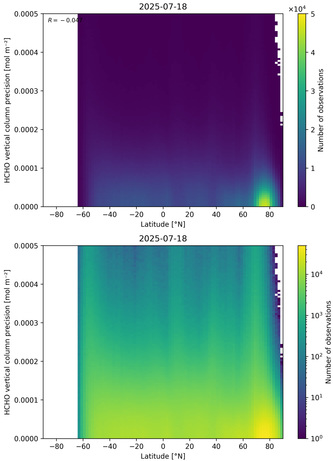
Figure 165: Scatter density plot of “Latitude” against “HCHO vertical column precision” for 2025-07-18 to 2025-07-19.
