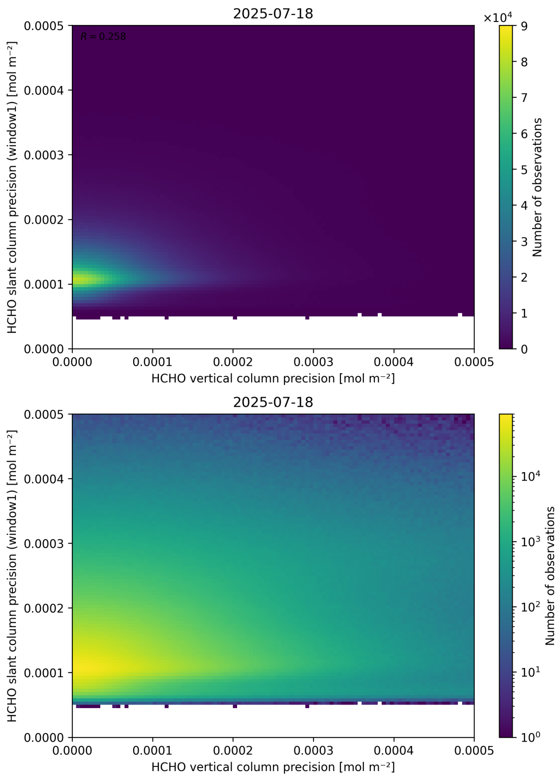
Figure 143: Scatter density plot of “HCHO vertical column precision” against “HCHO slant column precision (window1)” for 2025-07-18 to 2025-07-19.
