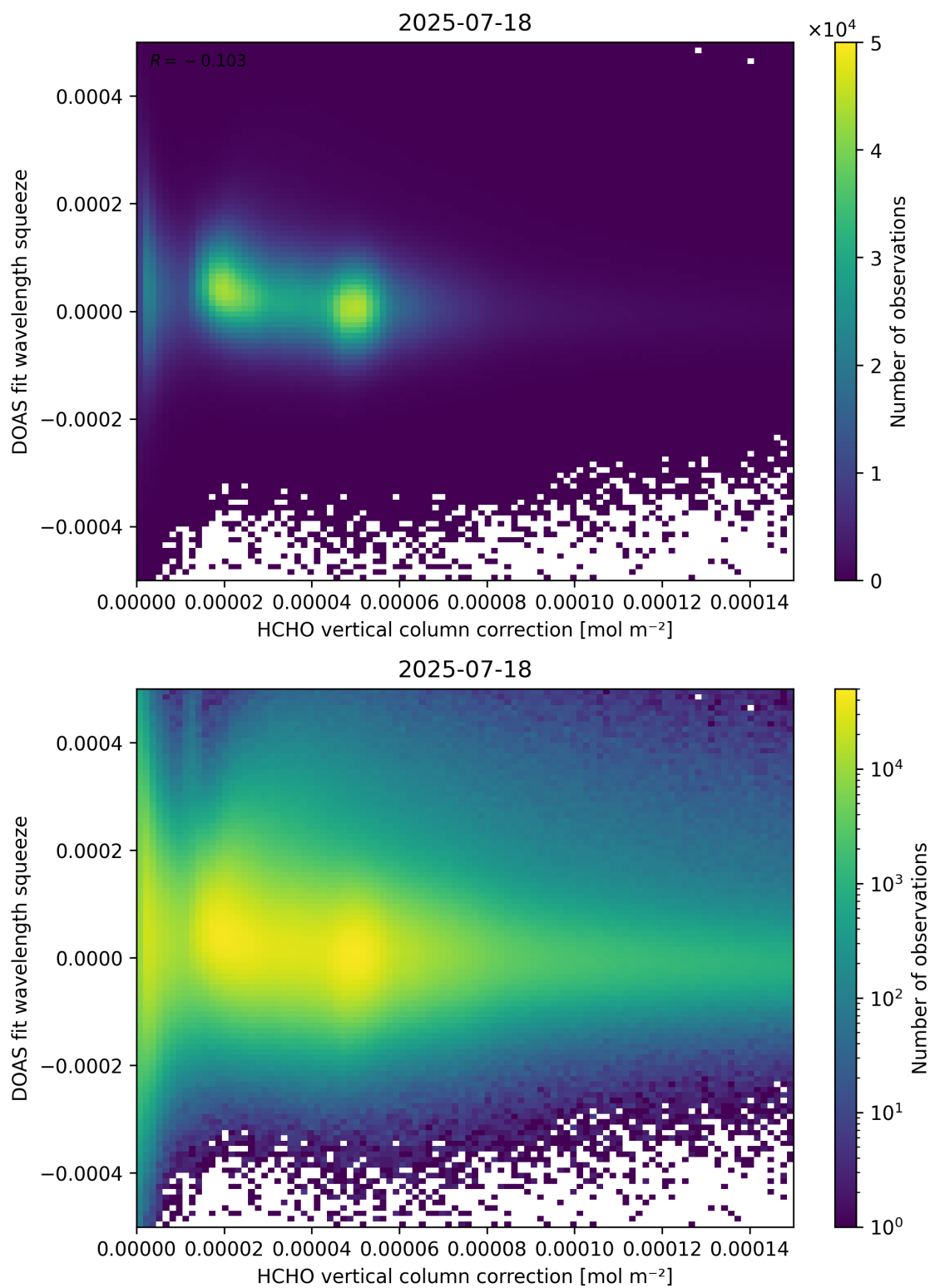
Figure 114: Scatter density plot of “HCHO vertical column correction” against “DOAS fit wavelength squeeze” for 2025-07-18 to 2025-07-19.
