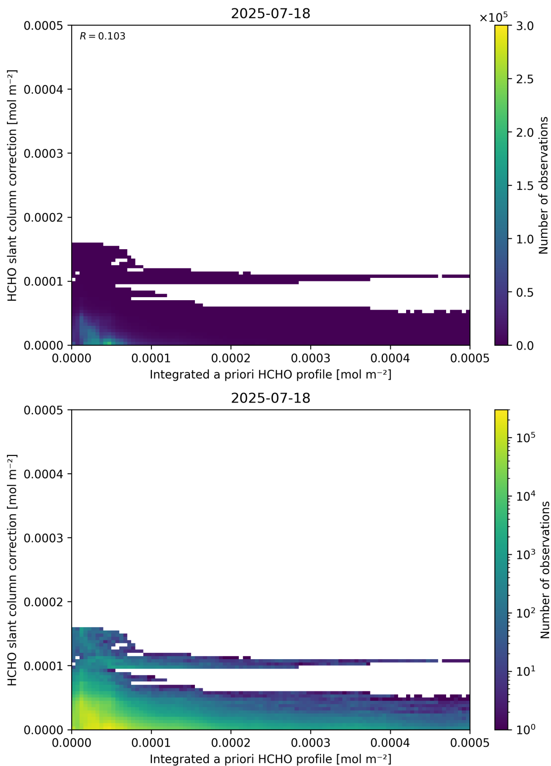
Figure 152: Scatter density plot of “Integrated a priori HCHO profile” against “HCHO slant column correction” for 2025-07-18 to 2025-07-19.
