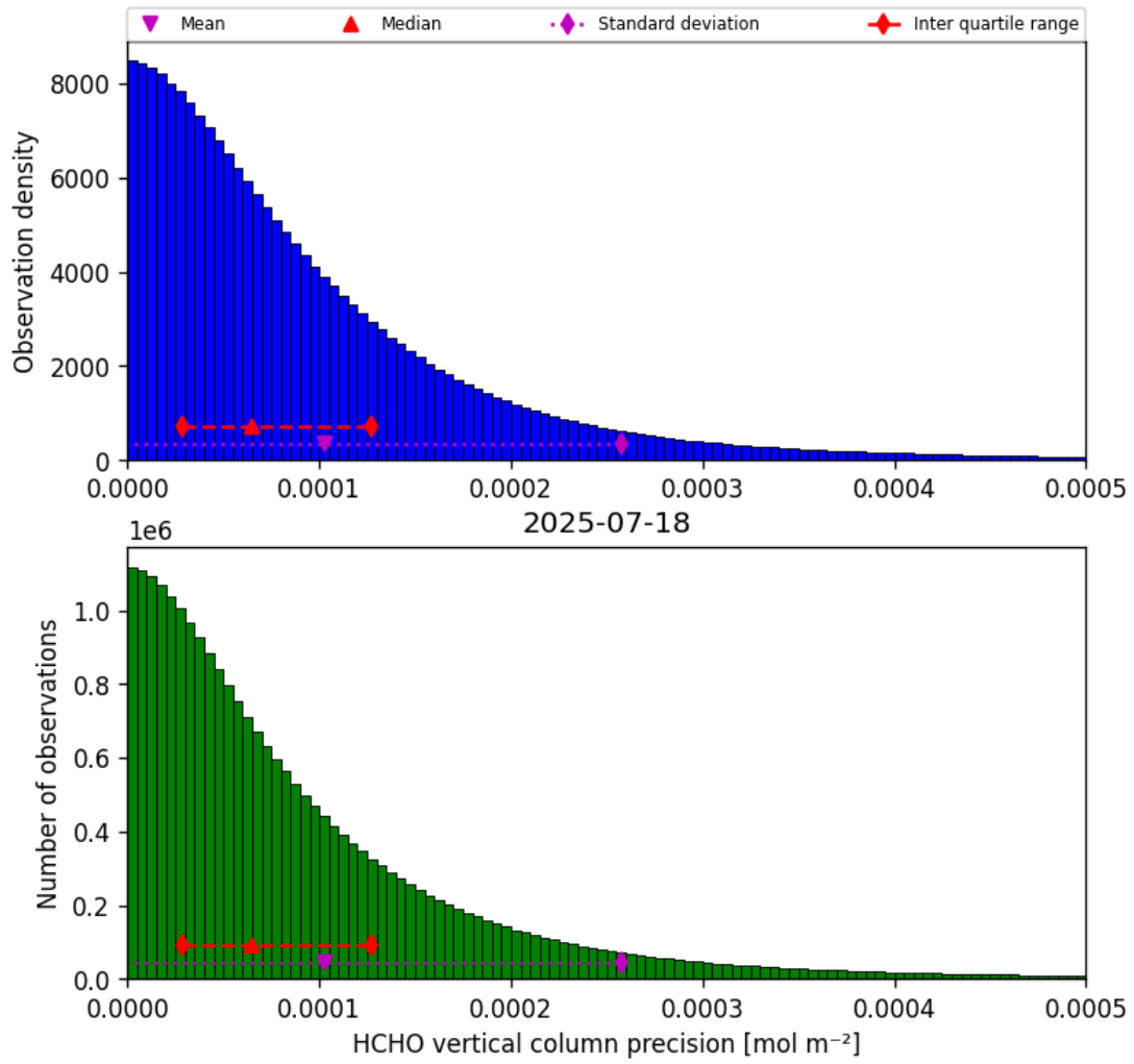
Figure 36: Histogram of “HCHO vertical column precision” for 2025-07-18 to 2025-07-19
