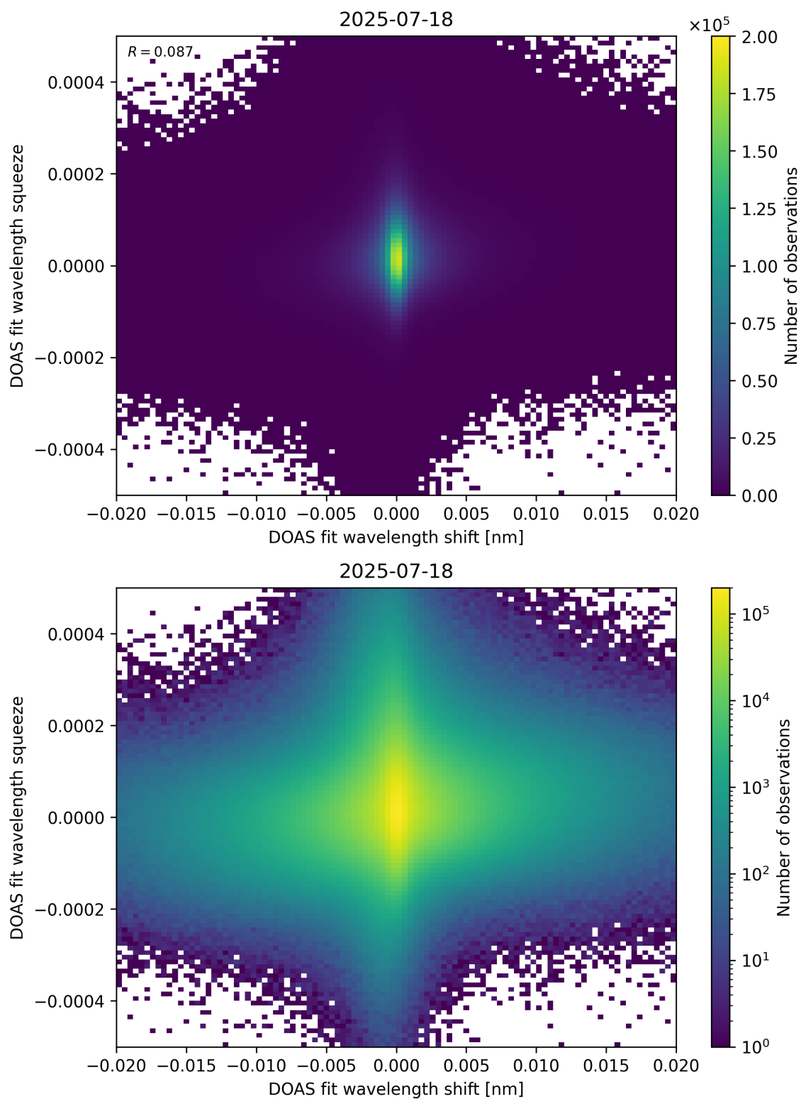
Figure 65: Scatter density plot of “DOAS fit wavelength shift” against “DOAS fit wavelength squeeze” for 2025-07-18 to 2025-07-19.
