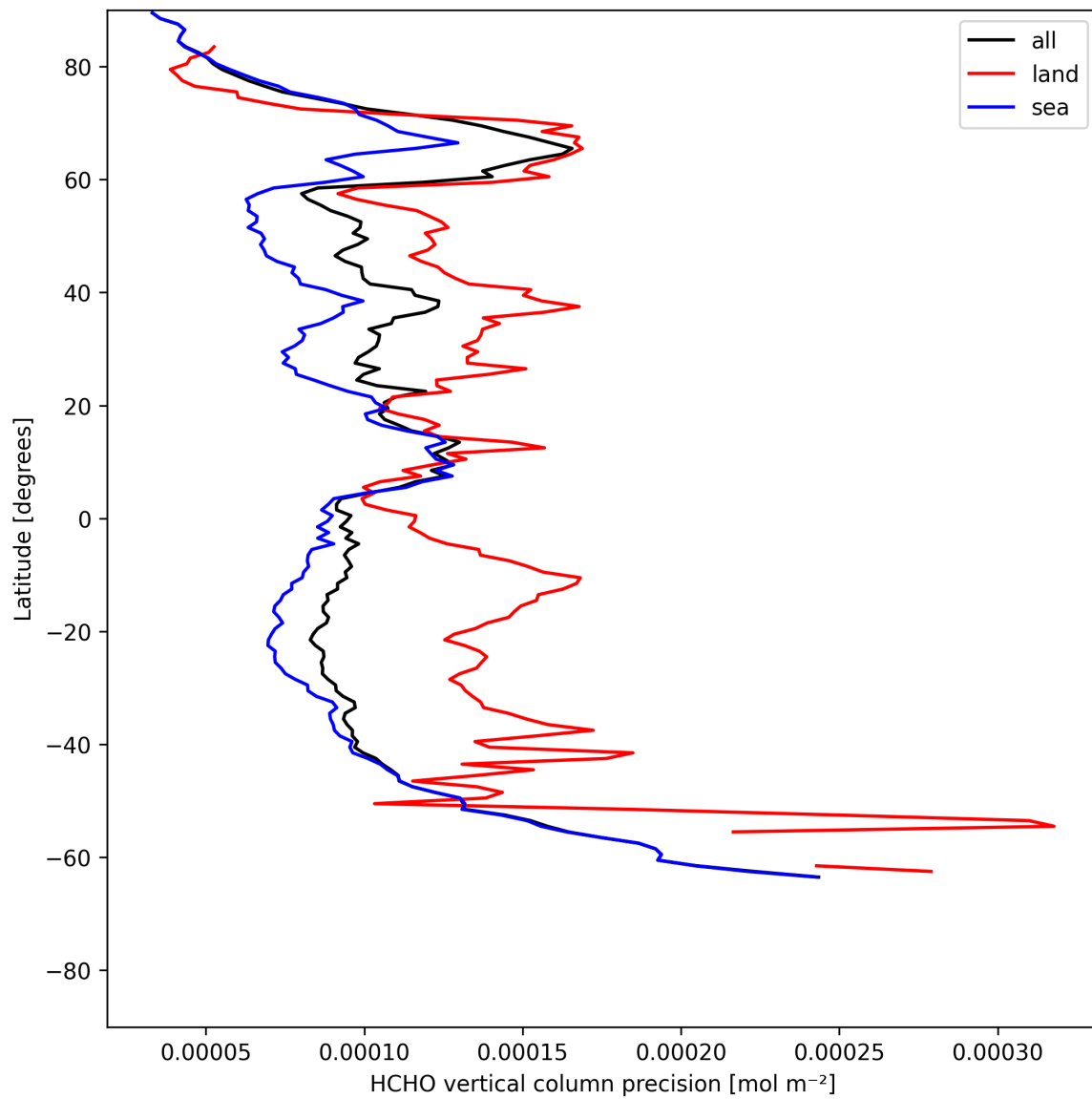
Figure 22: Zonal average of “HCHO vertical column precision” for 2025-07-18 to 2025-07-19.
