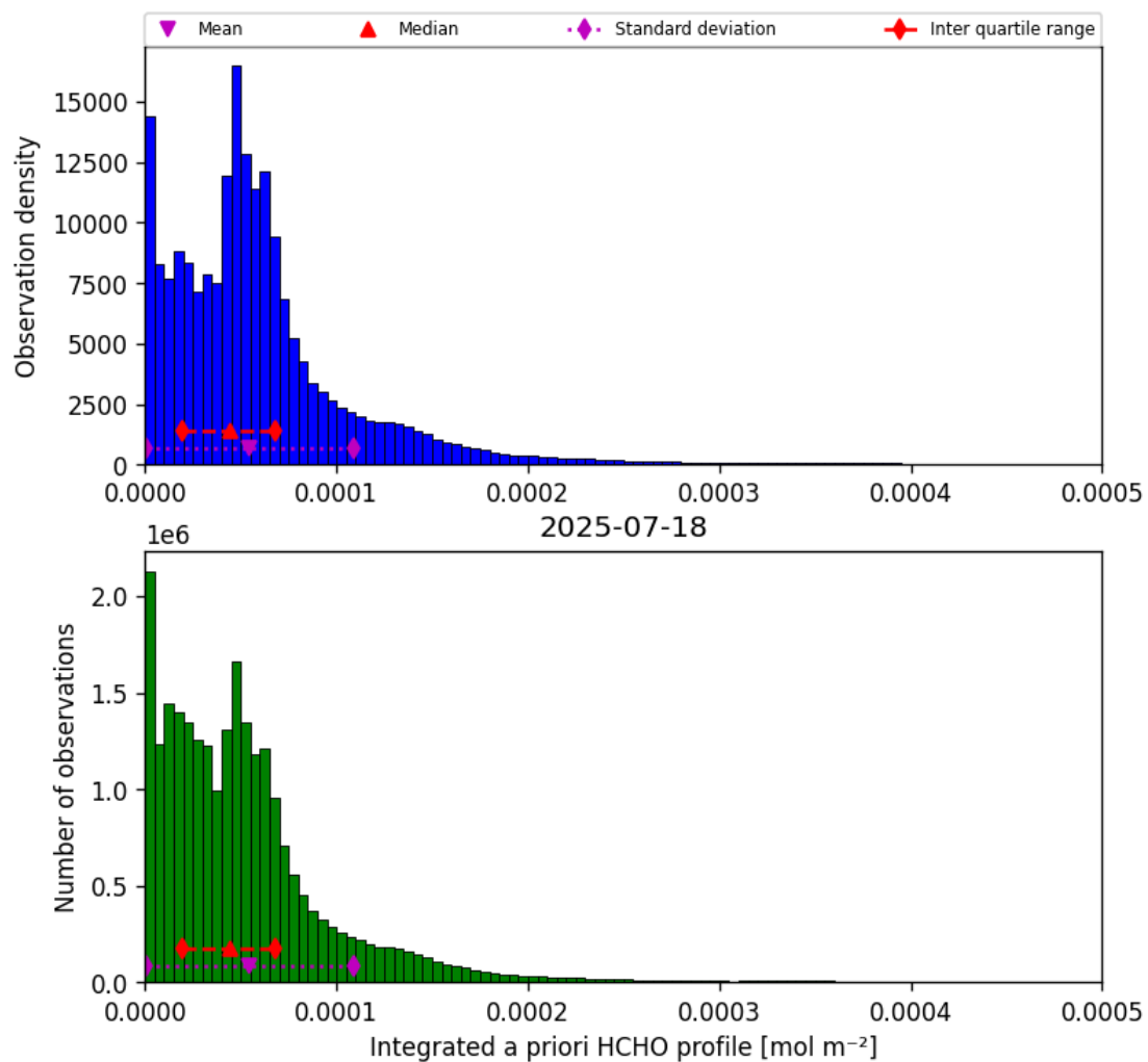
Figure 43: Histogram of “Integrated a priori HCHO profile” for 2025-07-18 to 2025-07-19
