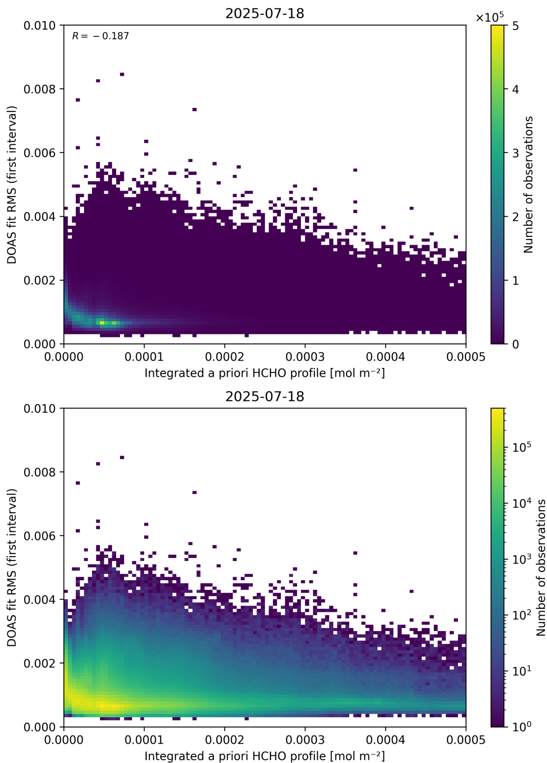
Figure 148: Scatter density plot of “Integrated a priori HCHO profile” against “DOAS fit RMS (first interval)” for 2025-07-18 to 2025-07-19.
