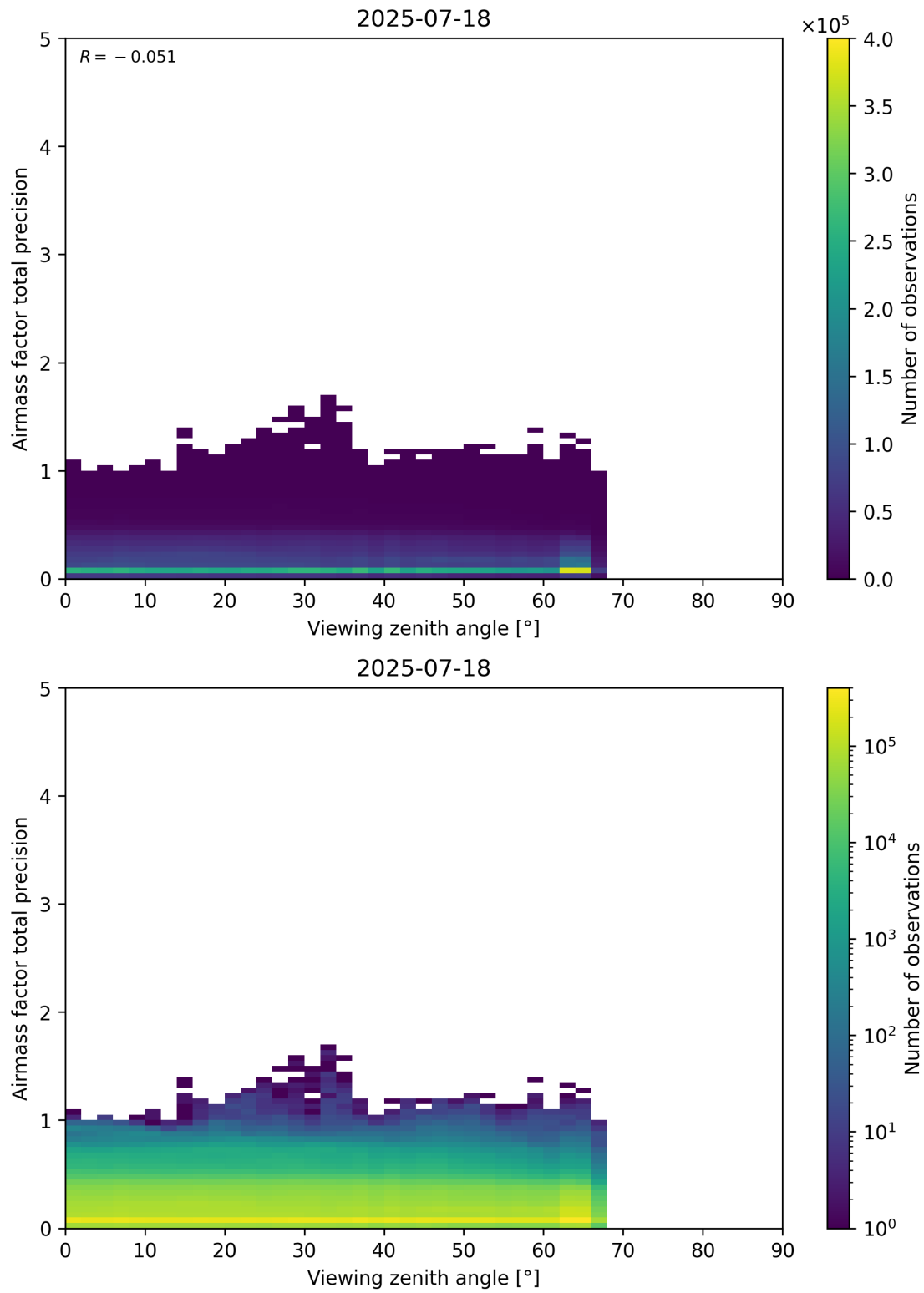
Figure 191: Scatter density plot of “Viewing zenith angle” against “Airmass factor total precision” for 2025-07-18 to 2025-07-19.
