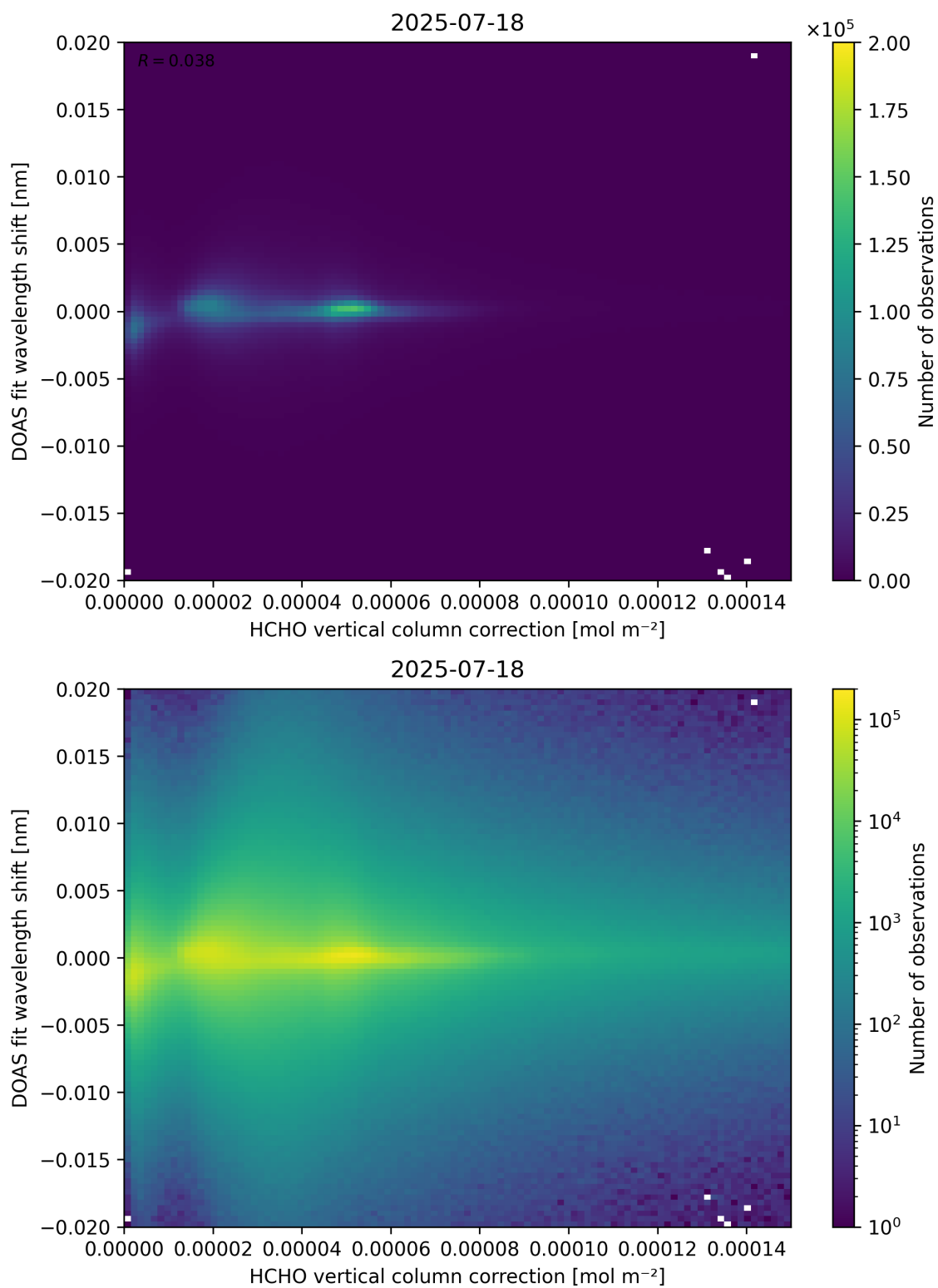
Figure 113: Scatter density plot of “HCHO vertical column correction” against “DOAS fit wavelength shift” for 2025-07-18 to 2025-07-19.
