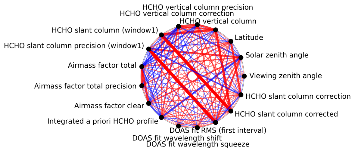
Figure 1: Map of correlation graph for 2025-07-18 to 2025-07-19.
