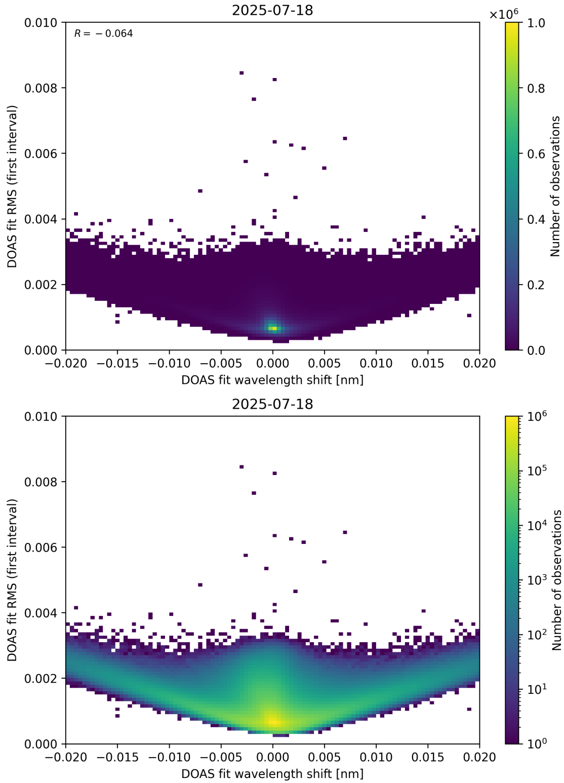
Figure 64: Scatter density plot of “DOAS fit wavelength shift” against “DOAS fit RMS (first interval)” for 2025-07-18 to 2025-07-19.
