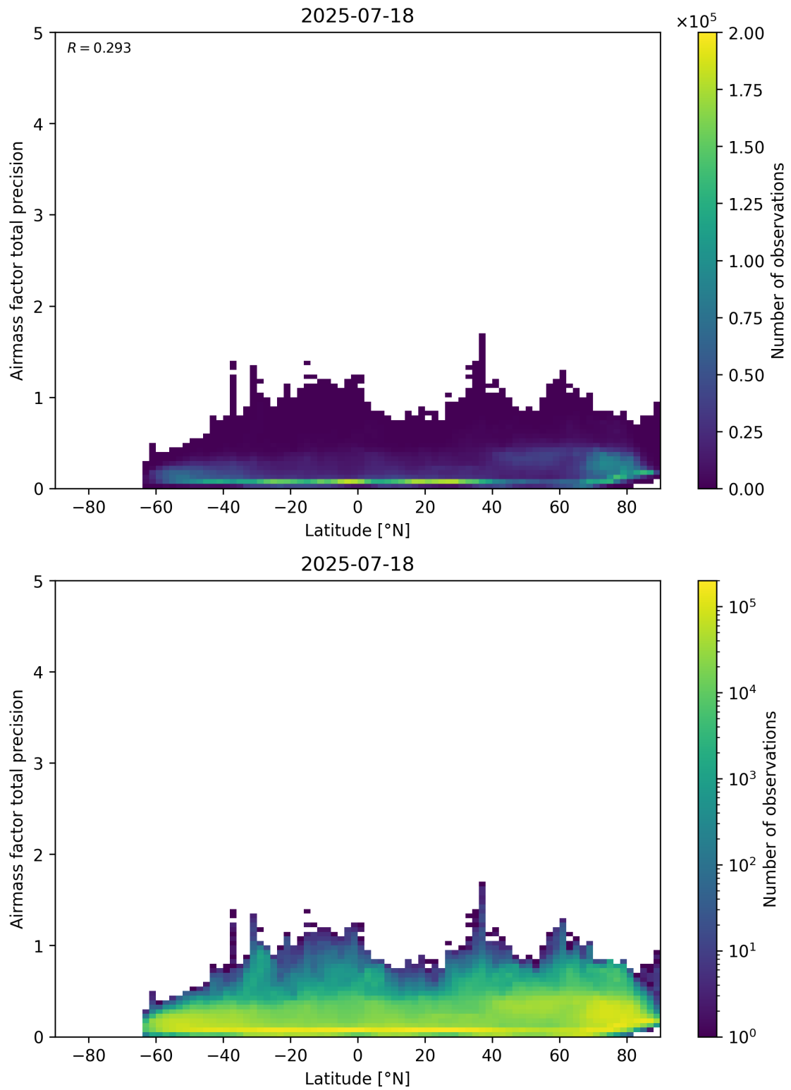
Figure 162: Scatter density plot of “Latitude” against “Airmass factor total precision” for 2025-07-18 to 2025-07-19.
