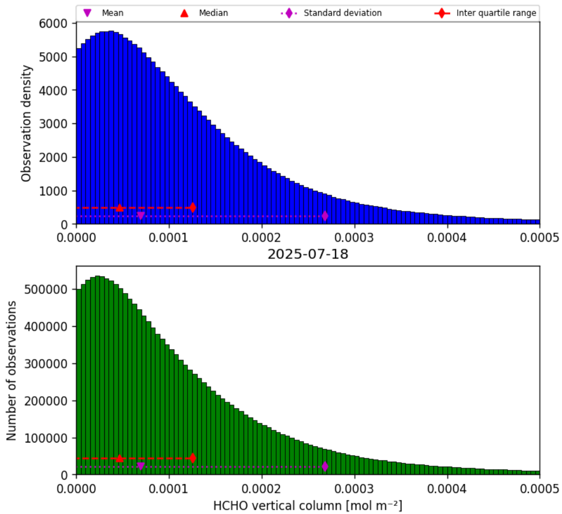
Figure 35: Histogram of “HCHO vertical column” for 2025-07-18 to 2025-07-19
