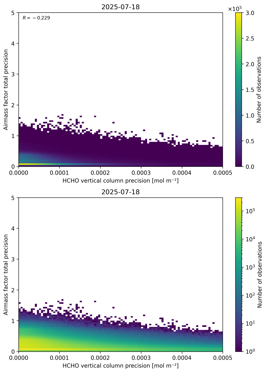
Figure 145: Scatter density plot of “HCHO vertical column precision” against “Airmass factor total precision” for 2025-07-18 to 2025-07-19.
