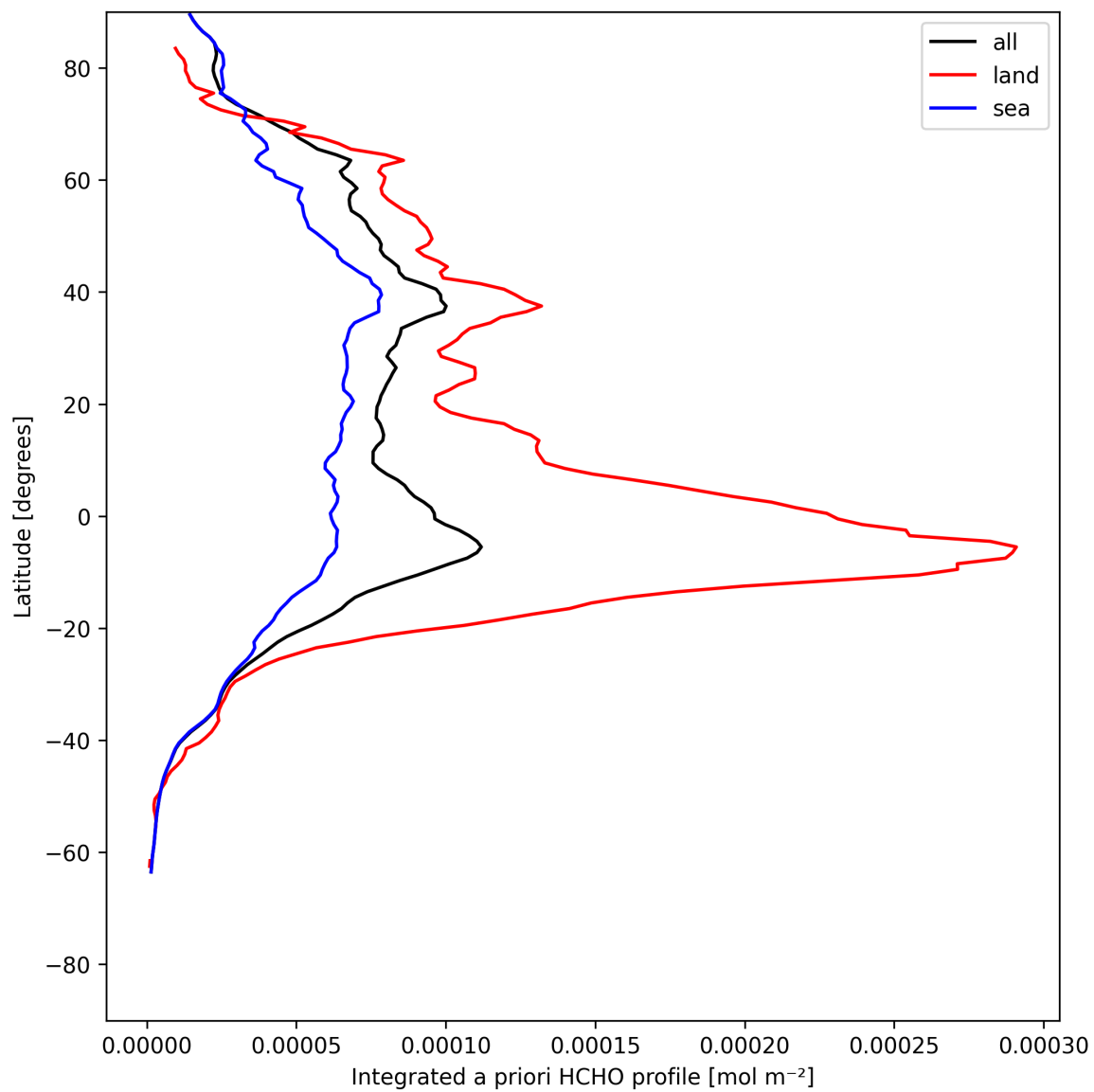
Figure 29: Zonal average of “Integrated a priori HCHO profile” for 2025-07-18 to 2025-07-19.
