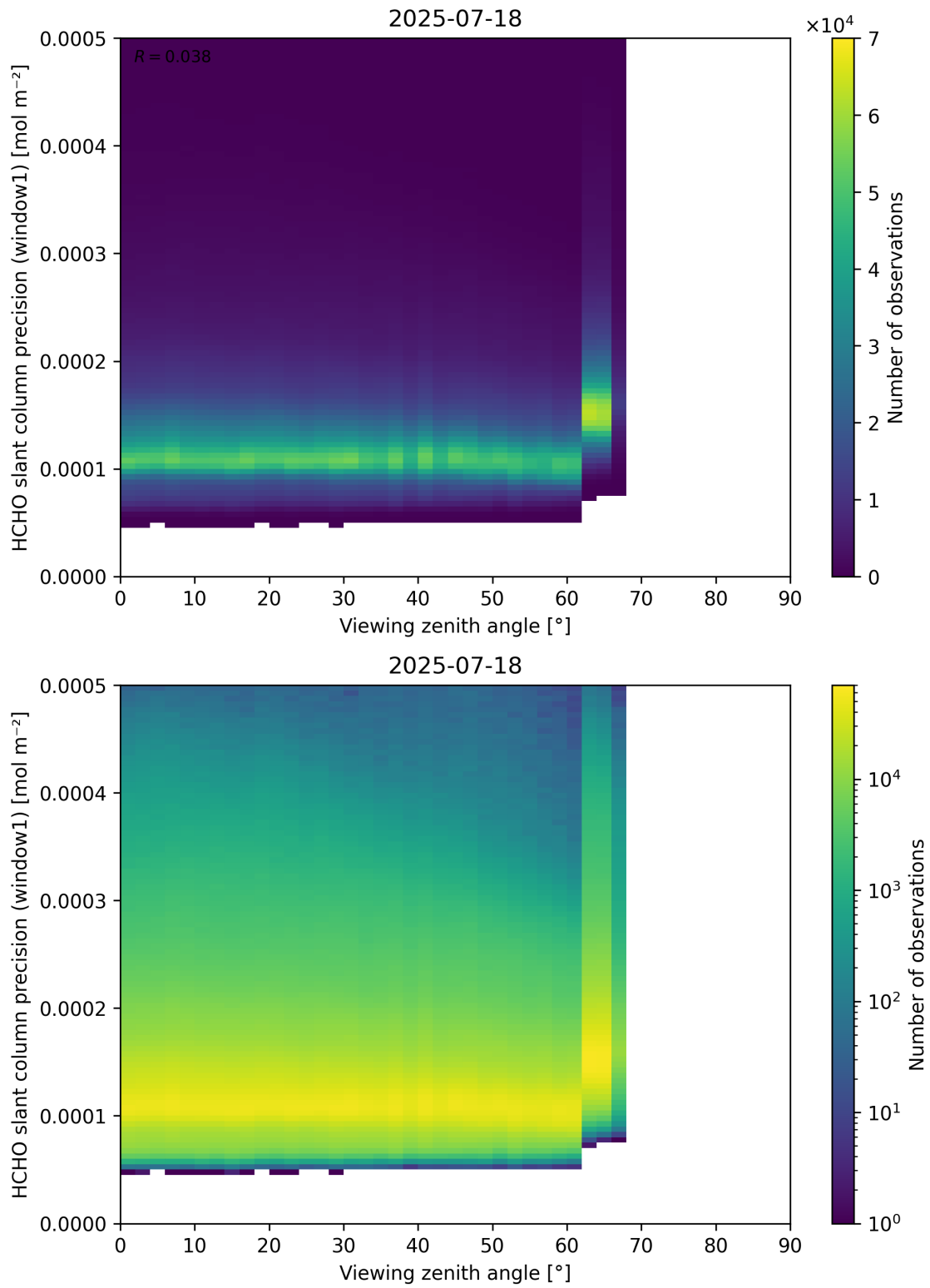
Figure 189: Scatter density plot of “Viewing zenith angle” against “HCHO slant column precision (window1)” for 2025-07-18 to 2025-07-19.
