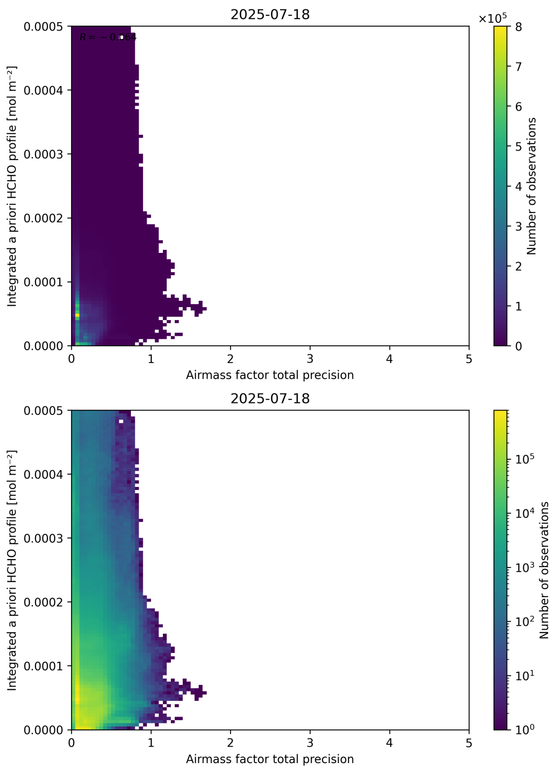
Figure 111: Scatter density plot of “Airmass factor total precision” against “Integrated a priori HCHO profile” for 2025-07-18 to 2025-07-19.
