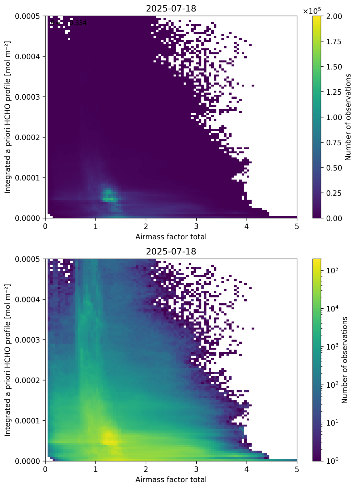
Figure 104: Scatter density plot of “Airmass factor total” against “Integrated a priori HCHO profile” for 2025-07-18 to 2025-07-19.
