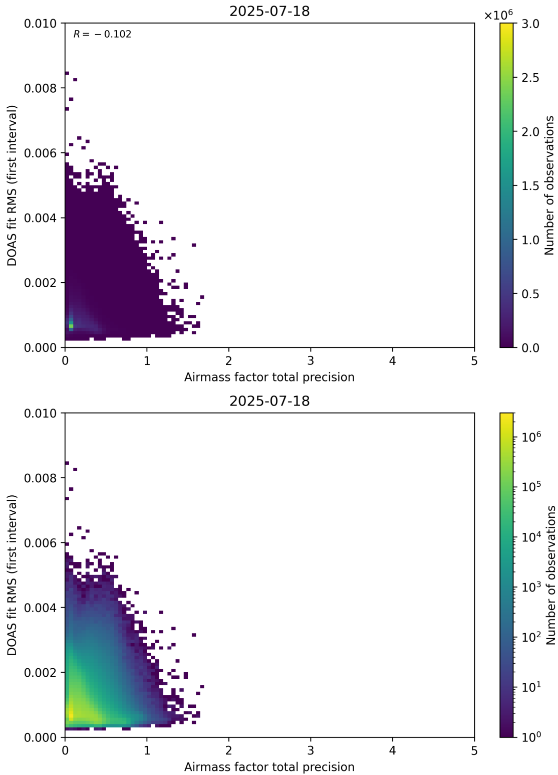
Figure 105: Scatter density plot of “Airmass factor total precision” against “DOAS fit RMS (first interval)” for 2025-07-18 to 2025-07-19.
