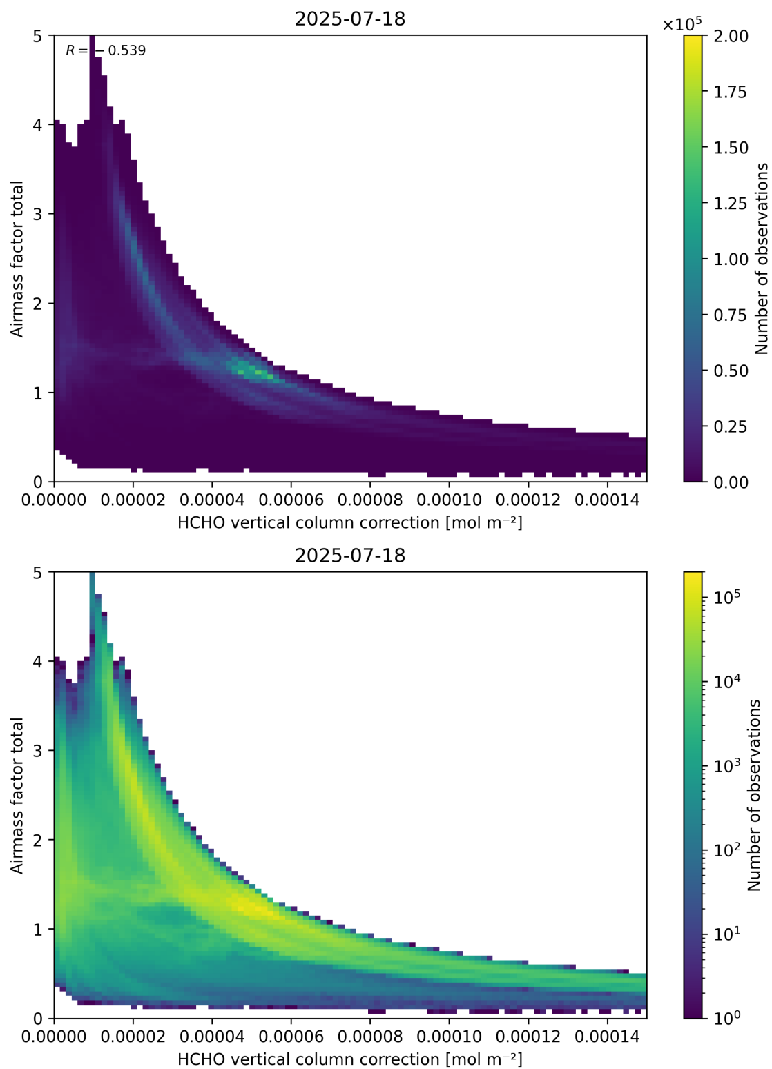
Figure 120: Scatter density plot of “HCHO vertical column correction” against “Airmass factor total” for 2025-07-18 to 2025-07-19.
