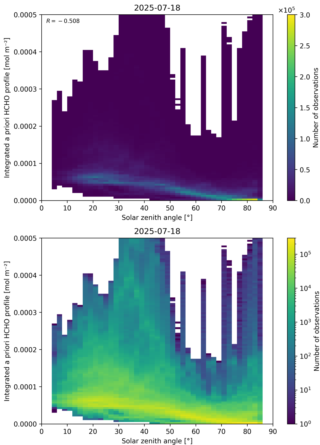
Figure 180: Scatter density plot of “Solar zenith angle” against “Integrated a priori HCHO profile” for 2025-07-18 to 2025-07-19.
