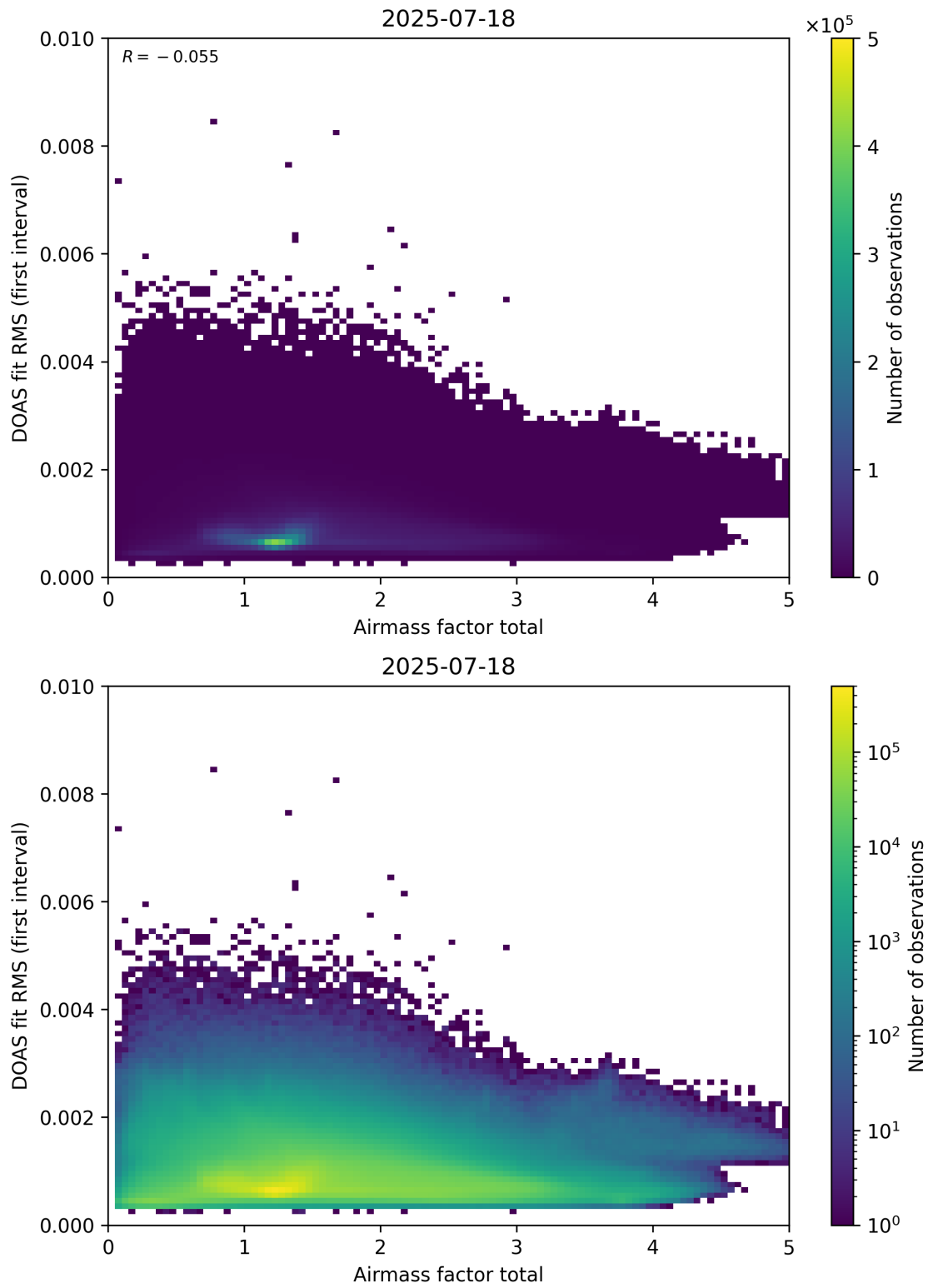
Figure 97: Scatter density plot of “Airmass factor total” against “DOAS fit RMS (first interval)” for 2025-07-18 to 2025-07-19.
