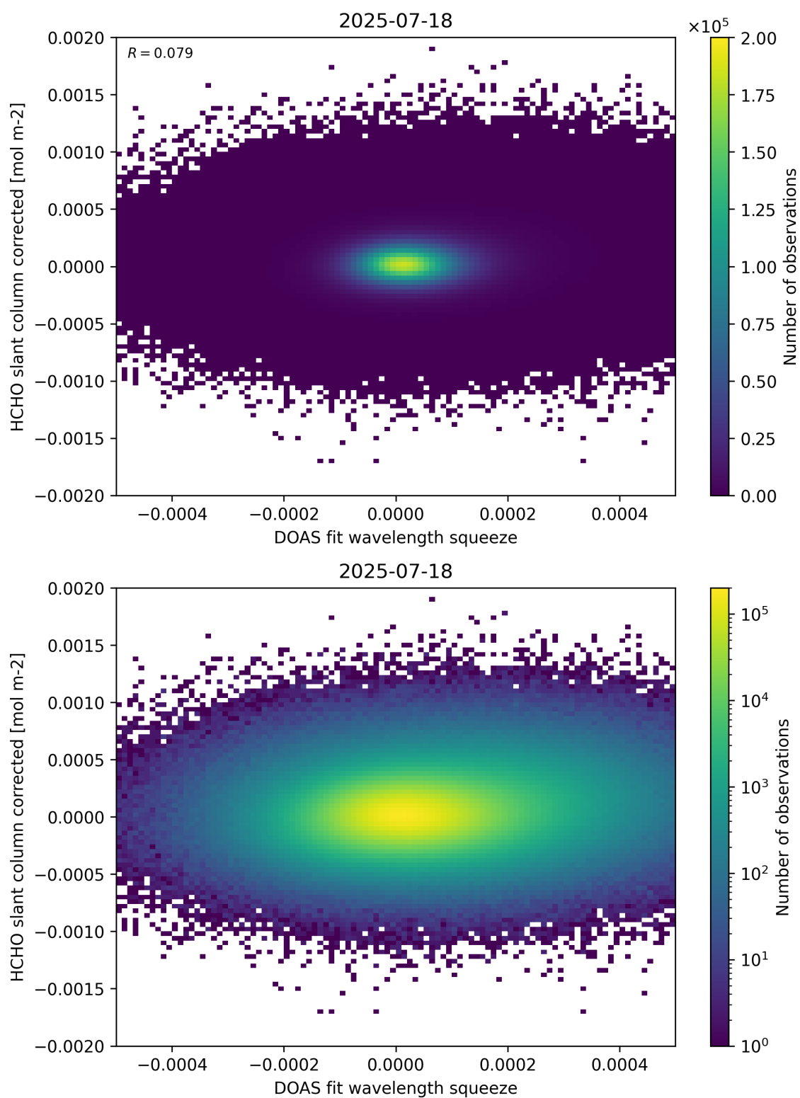
Figure 69: Scatter density plot of “DOAS fit wavelength squeeze” against “HCHO slant column corrected” for 2025-07-18 to 2025-07-19.
