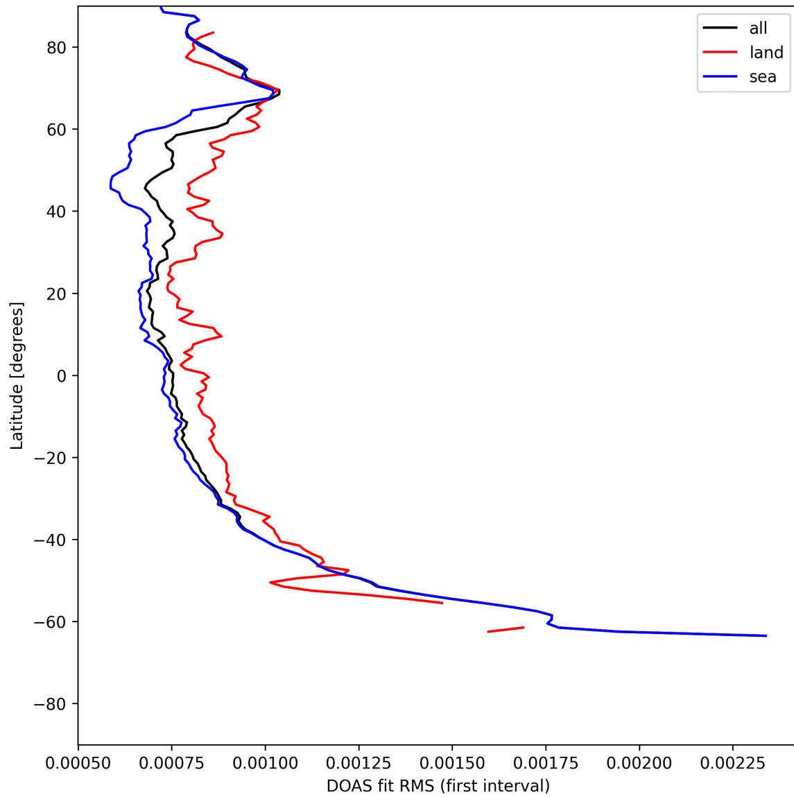
Figure 32: Zonal average of “DOAS fit RMS (first interval)” for 2025-07-18 to 2025-07-19.
