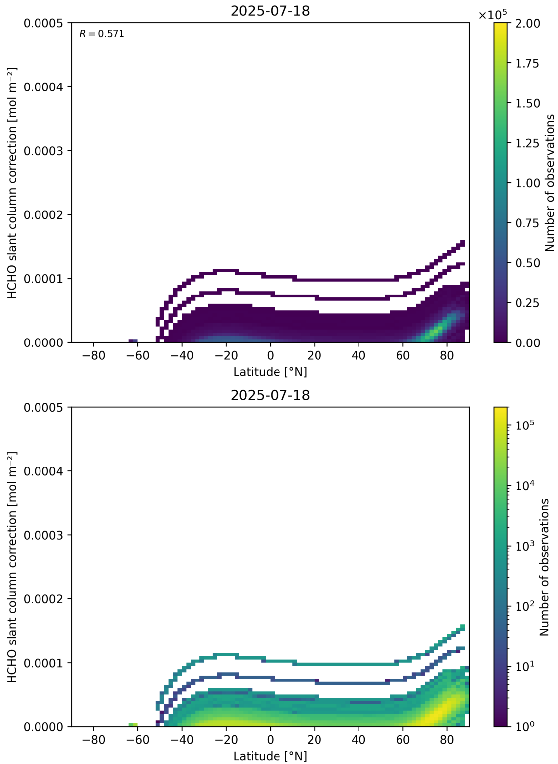
Figure 158: Scatter density plot of “Latitude” against “HCHO slant column correction” for 2025-07-18 to 2025-07-19.
