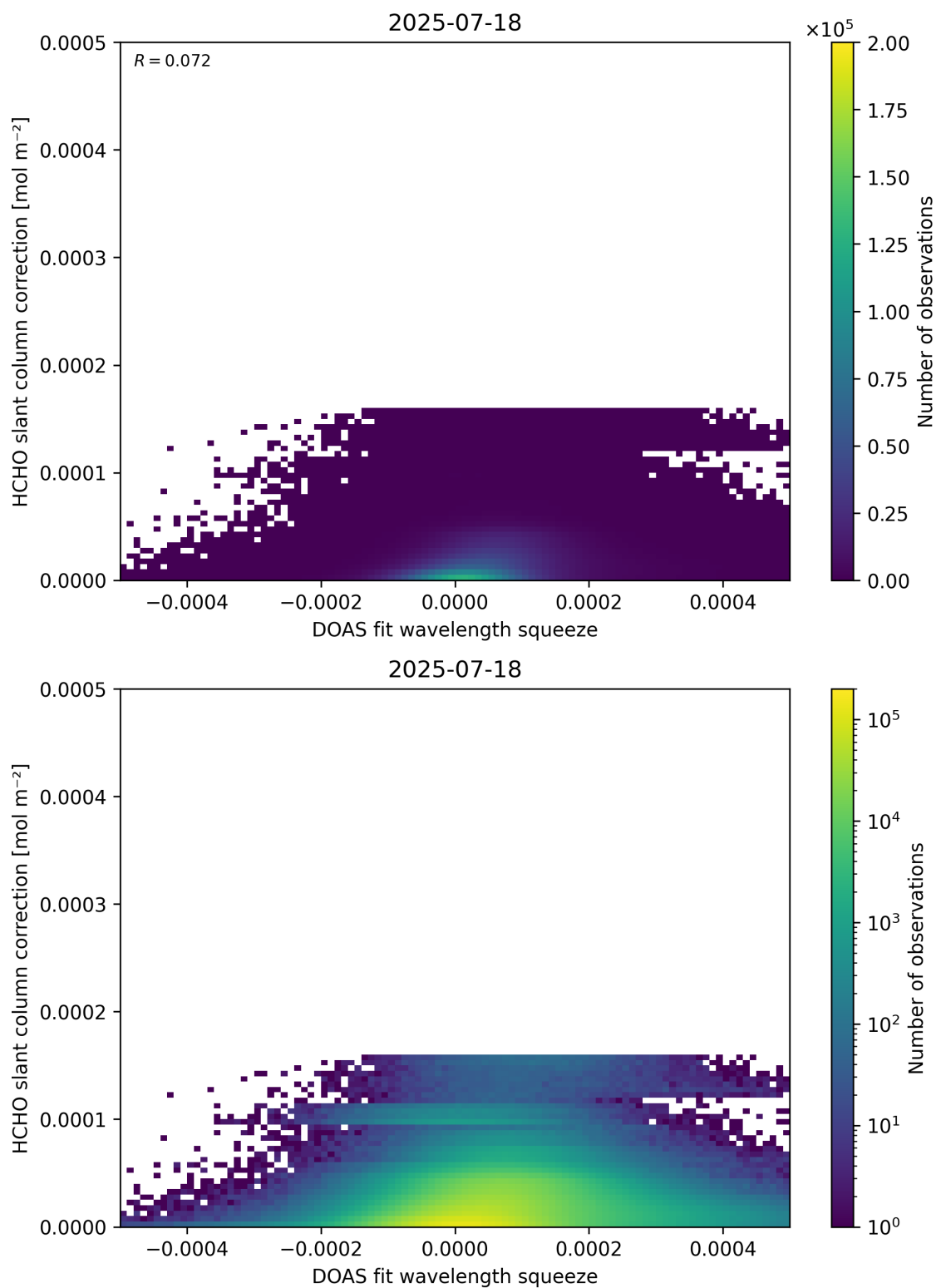
Figure 70: Scatter density plot of “DOAS fit wavelength squeeze” against “HCHO slant column correction” for 2025-07-18 to 2025-07-19.
