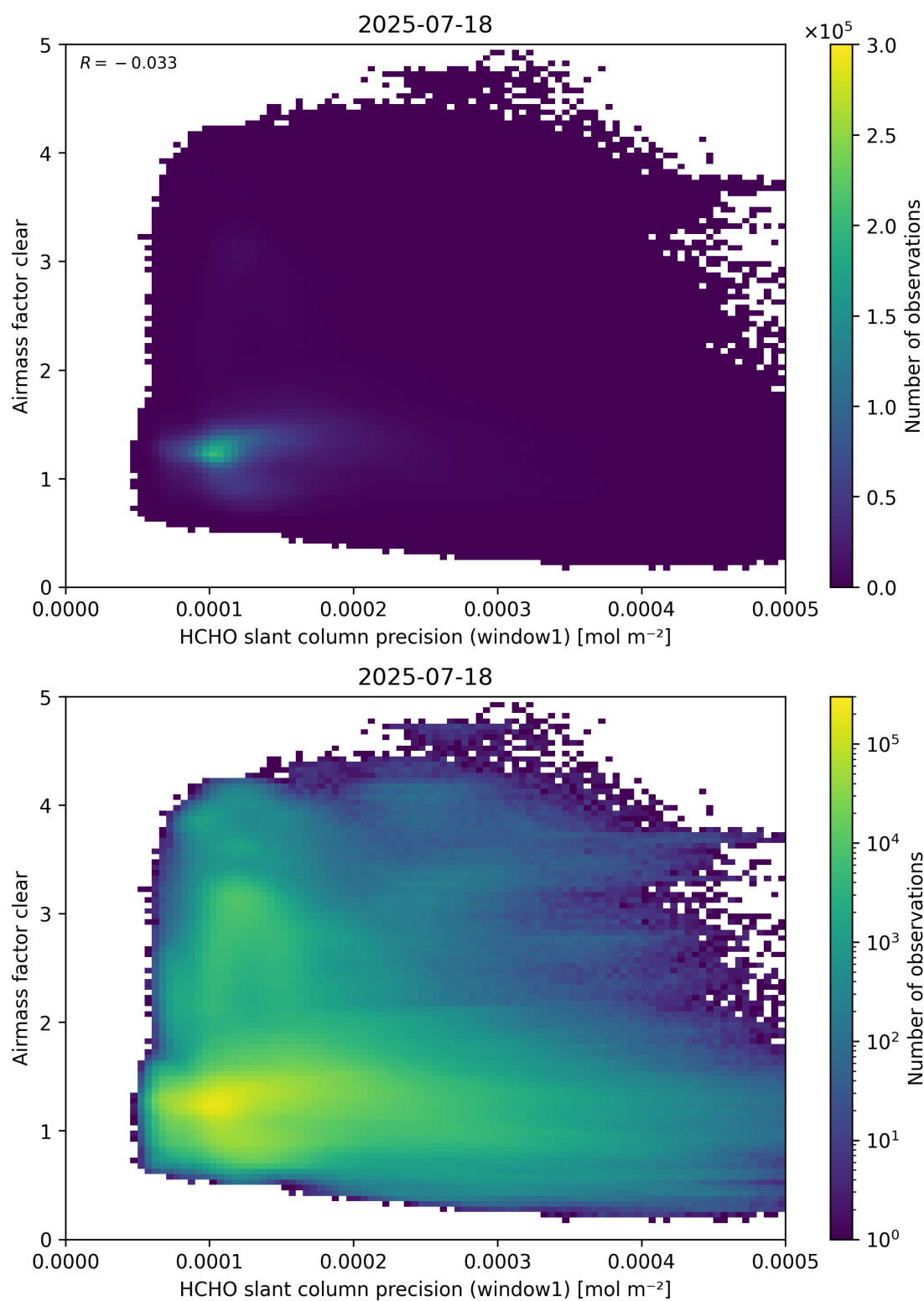
Figure 91: Scatter density plot of “HCHO slant column precision (window1)” against “Airmass factor clear” for 2025-07-18 to 2025-07-19.
