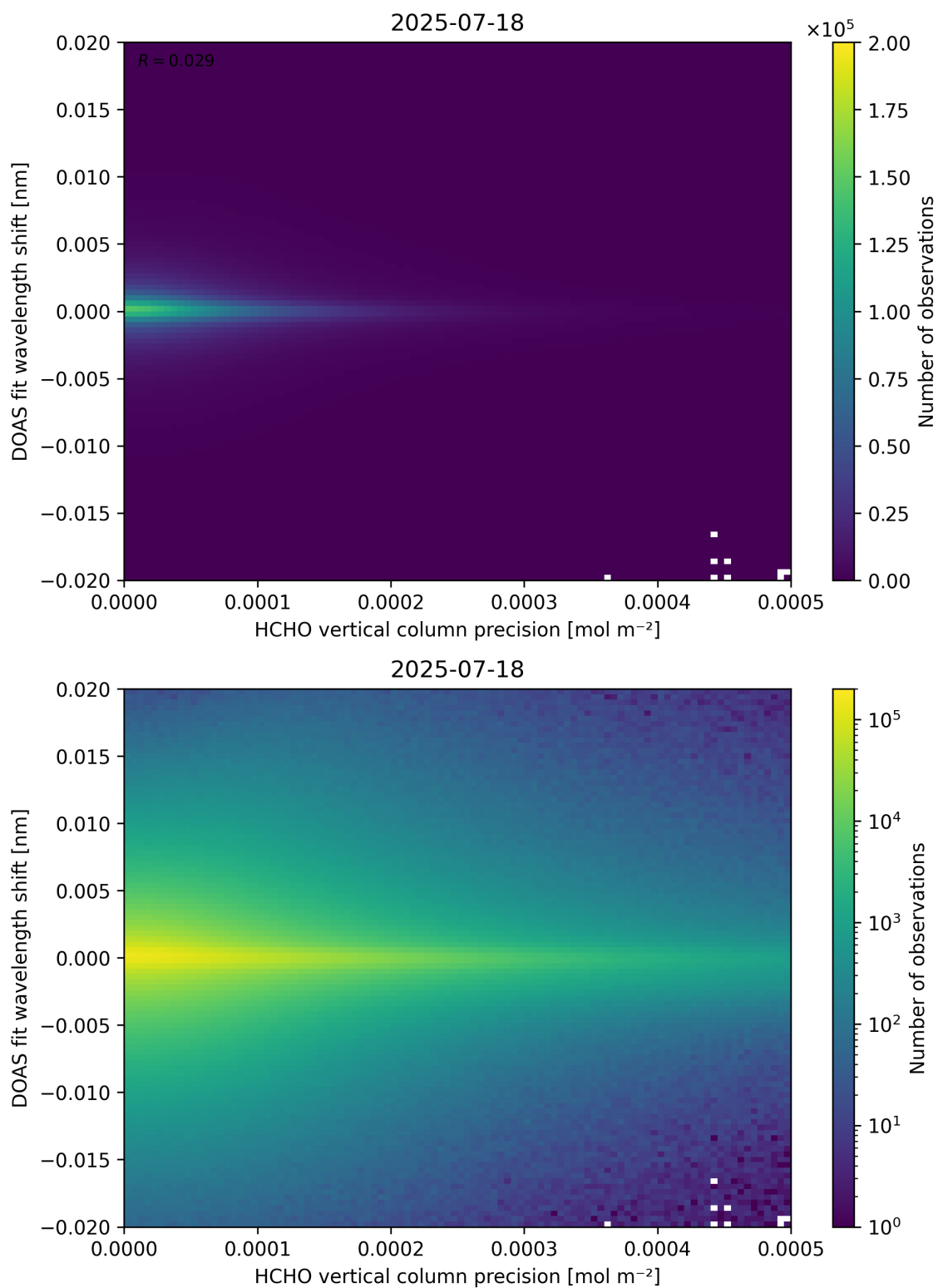
Figure 137: Scatter density plot of “HCHO vertical column precision” against “DOAS fit wavelength shift” for 2025-07-18 to 2025-07-19.
