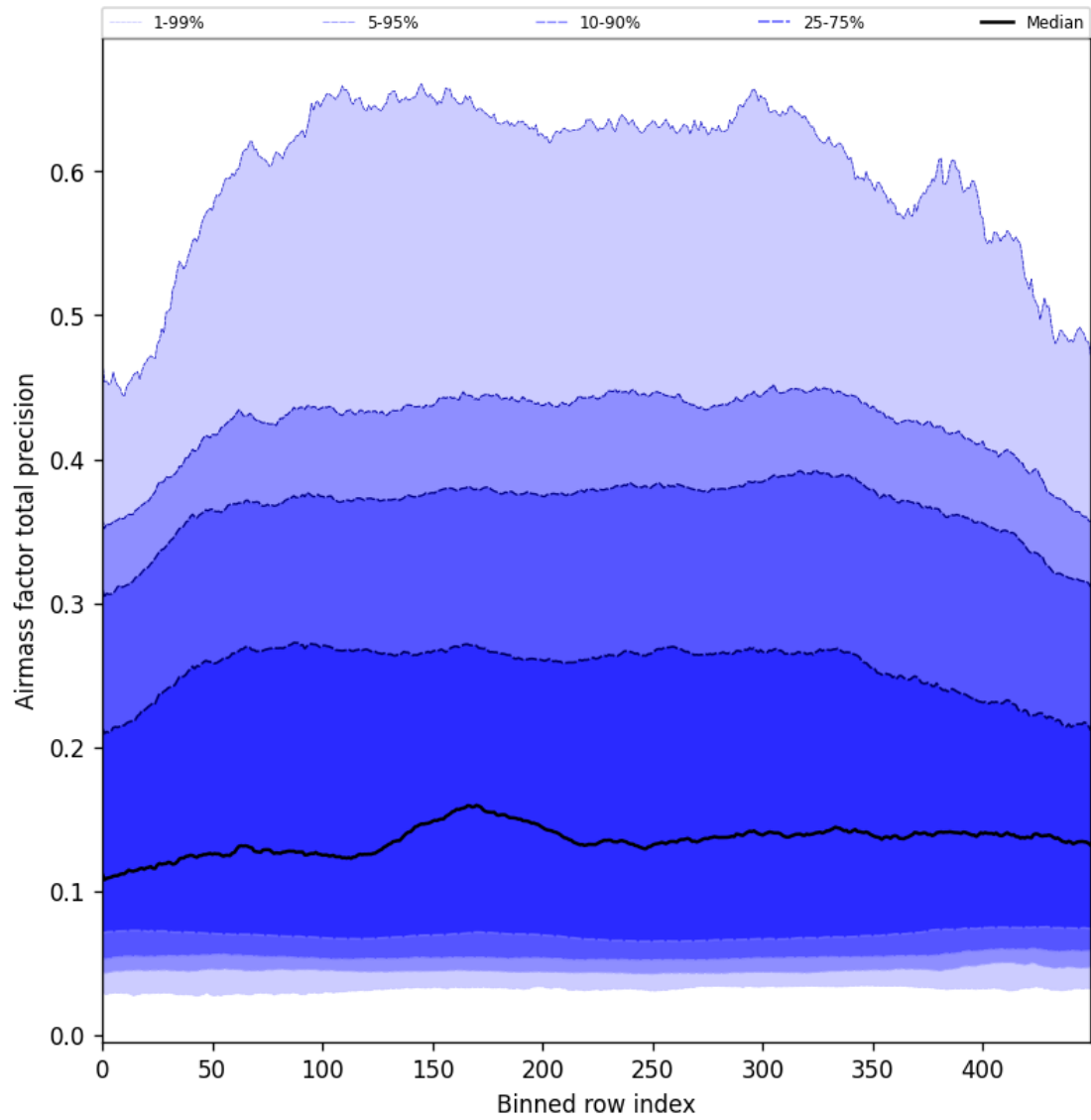
Figure 55: Along track statistics of “Airmass factor total precision” for 2025-07-18 to 2025-07-19
