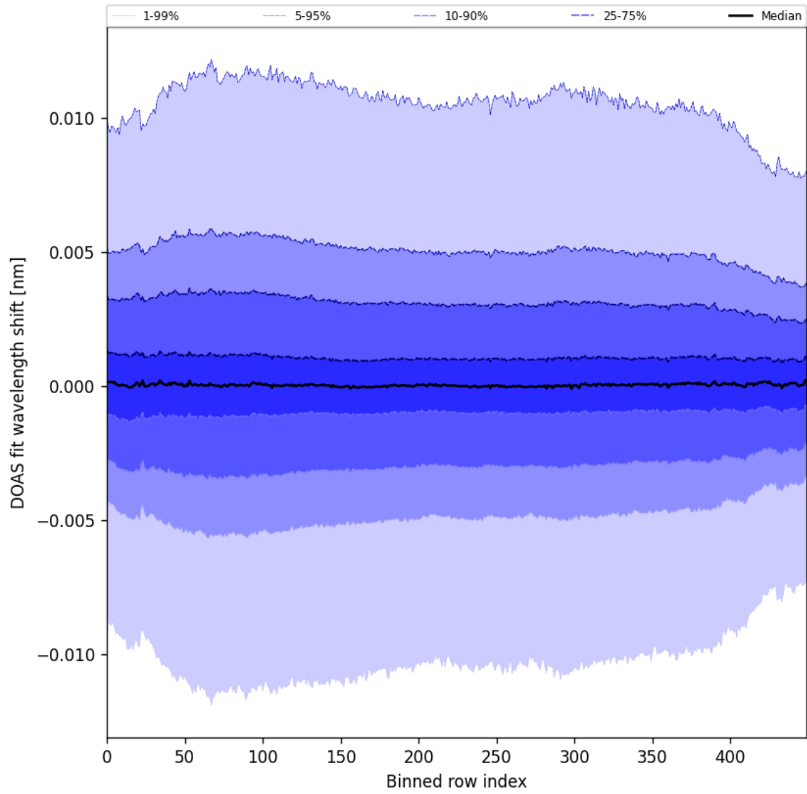
Figure 58: Along track statistics of “DOAS fit wavelength shift” for 2025-07-18 to 2025-07-19
