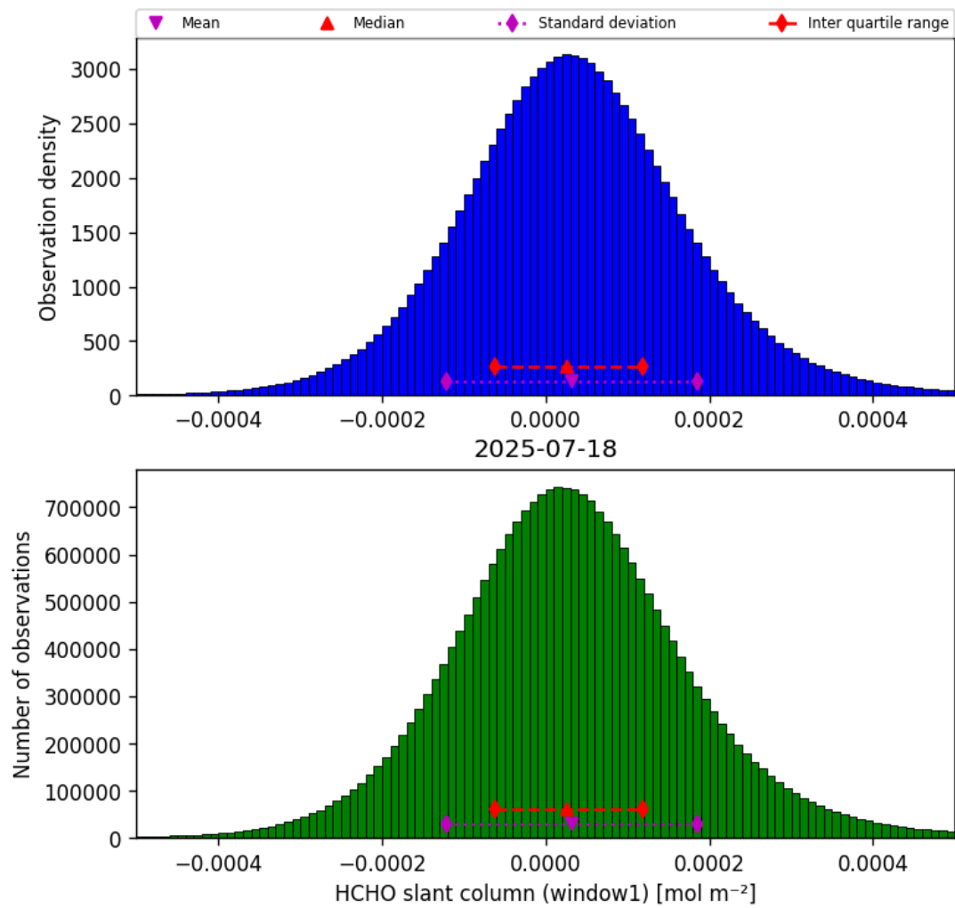
Figure 38: Histogram of “HCHO slant column (window1)” for 2025-07-18 to 2025-07-19
