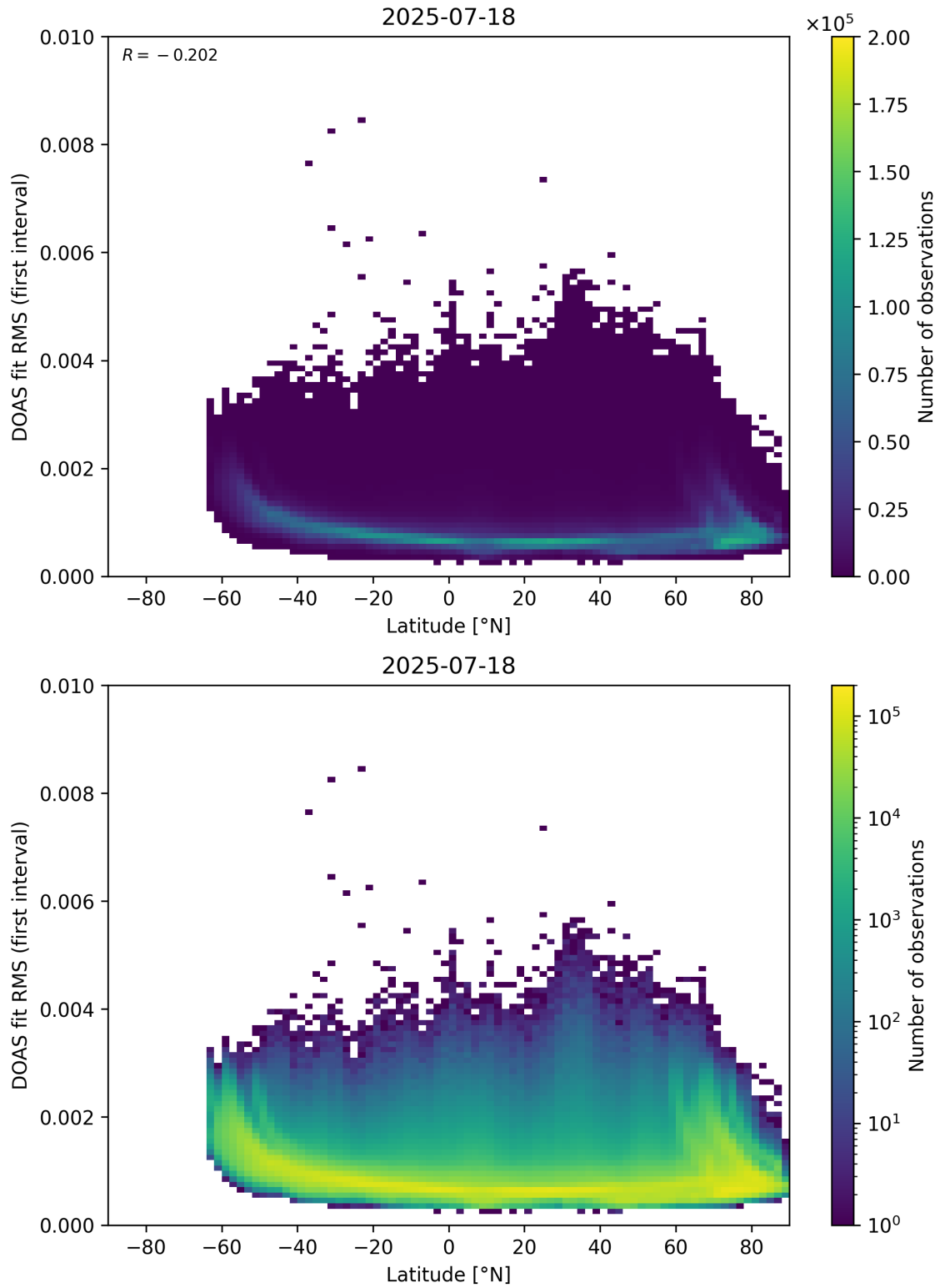
Figure 153: Scatter density plot of “Latitude” against “DOAS fit RMS (first interval)” for 2025-07-18 to 2025-07-19.
