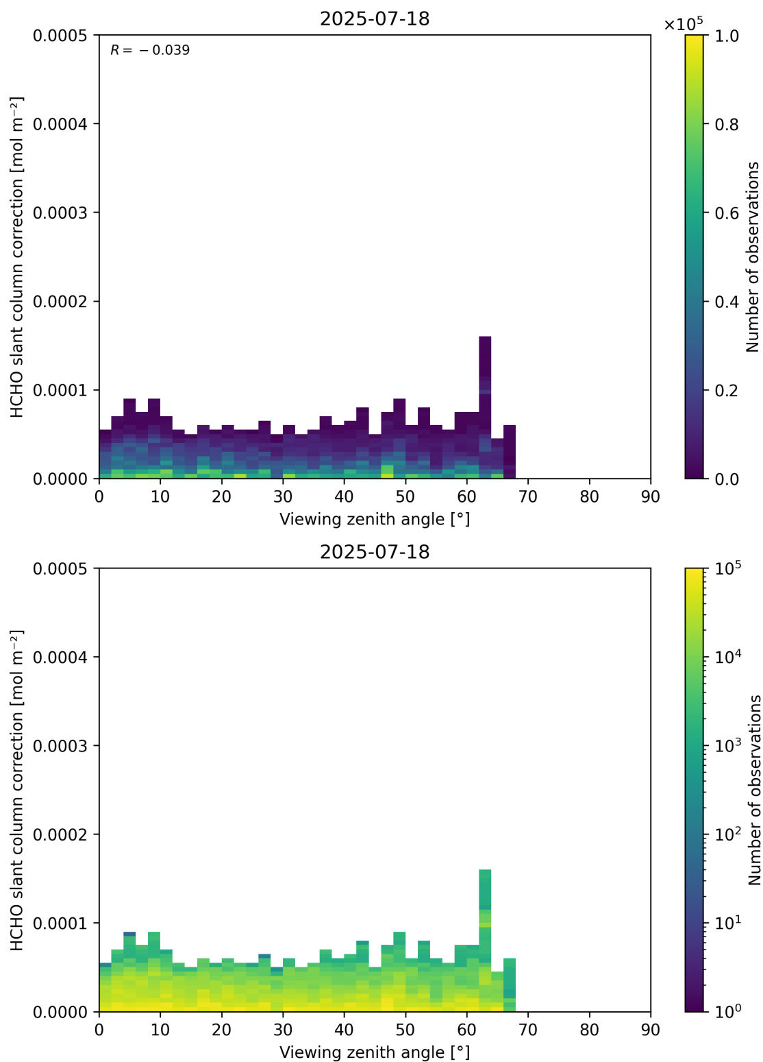
Figure 187: Scatter density plot of “Viewing zenith angle” against “HCHO slant column correction” for 2025-07-18 to 2025-07-19.
