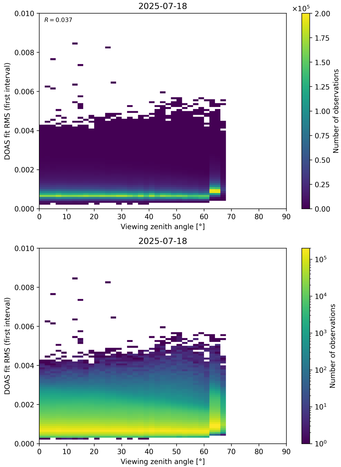
Figure 182: Scatter density plot of “Viewing zenith angle” against “DOAS fit RMS (first interval)” for 2025-07-18 to 2025-07-19.
