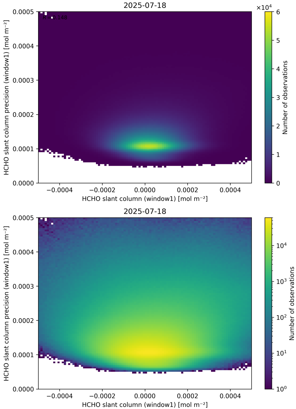
Figure 84: Scatter density plot of “HCHO slant column (window1)” against “HCHO slant column precision (window1)” for 2025-07-18 to 2025-07-19.
