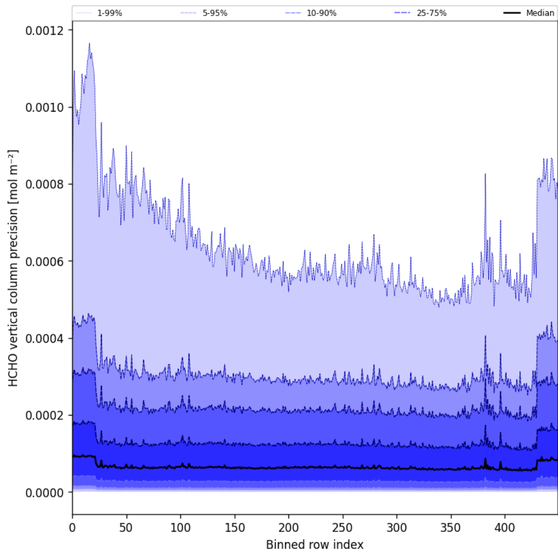
Figure 50: Along track statistics of “HCHO vertical column precision” for 2025-07-18 to 2025-07-19
