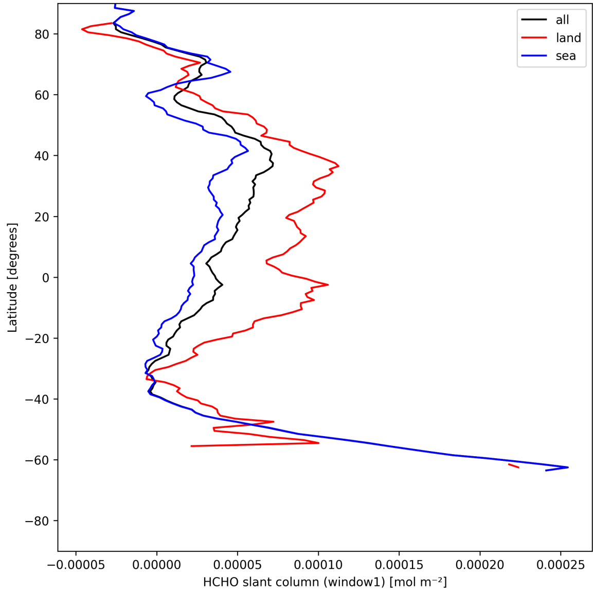
Figure 24: Zonal average of “HCHO slant column (window1)” for 2025-07-18 to 2025-07-19.
