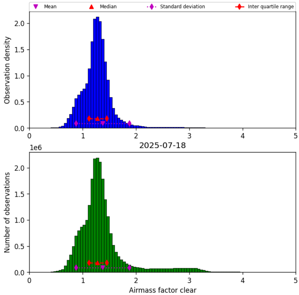
Figure 42: Histogram of “Airmass factor clear” for 2025-07-18 to 2025-07-19
