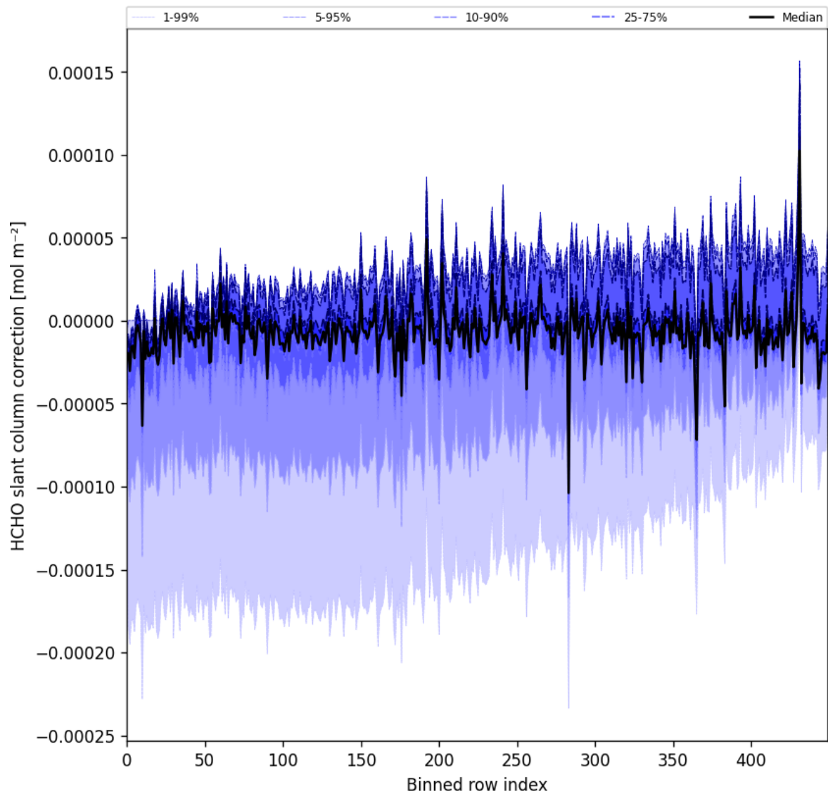
Figure 61: Along track statistics of “HCHO slant column correction” for 2025-07-18 to 2025-07-19
