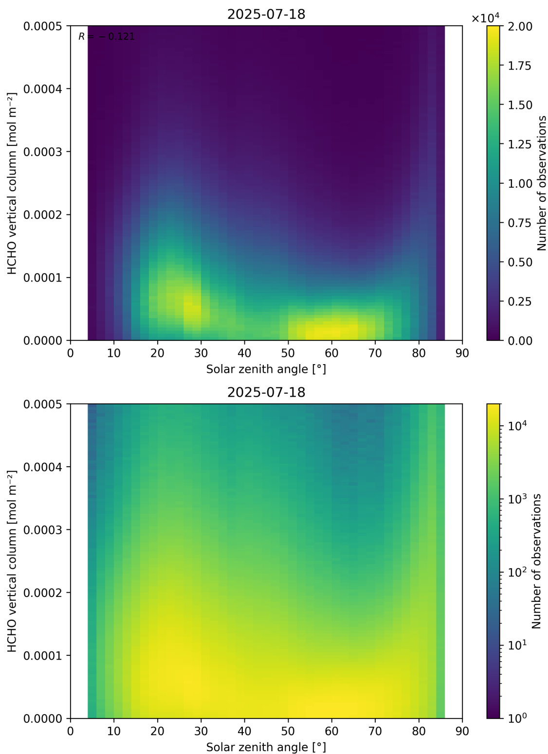
Figure 177: Scatter density plot of “Solar zenith angle” against “HCHO vertical column” for 2025-07-18 to 2025-07-19.
