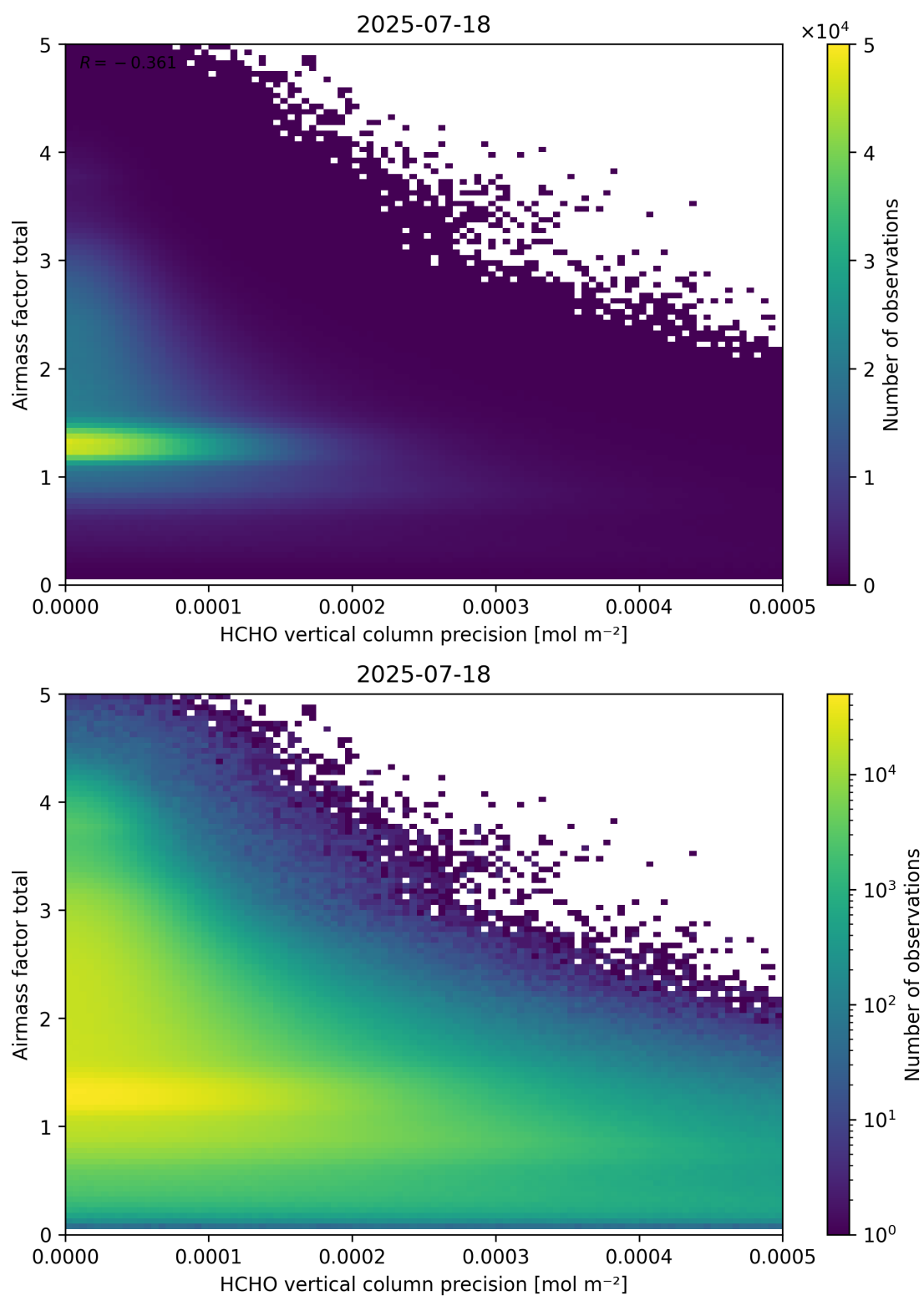
Figure 144: Scatter density plot of “HCHO vertical column precision” against “Airmass factor total” for 2025-07-18 to 2025-07-19.
