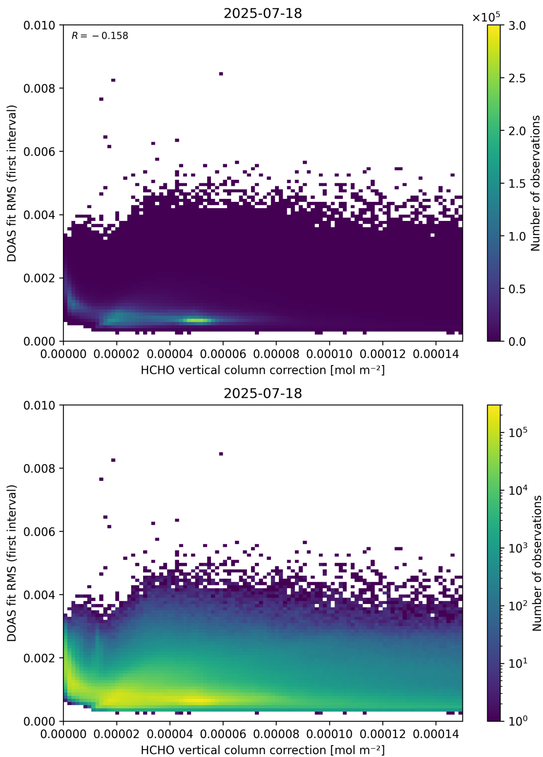
Figure 112: Scatter density plot of “HCHO vertical column correction” against “DOAS fit RMS (first interval)” for 2025-07-18 to 2025-07-19.
