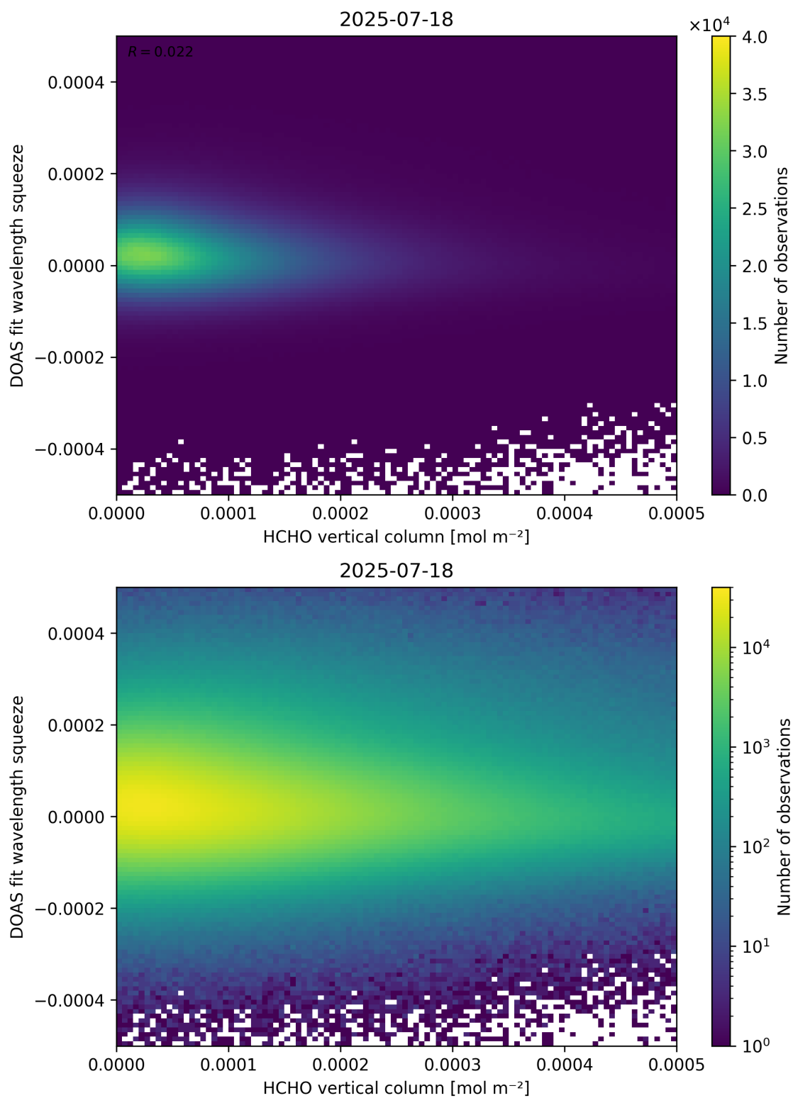
Figure 125: Scatter density plot of “HCHO vertical column” against “DOAS fit wavelength squeeze” for 2025-07-18 to 2025-07-19.
