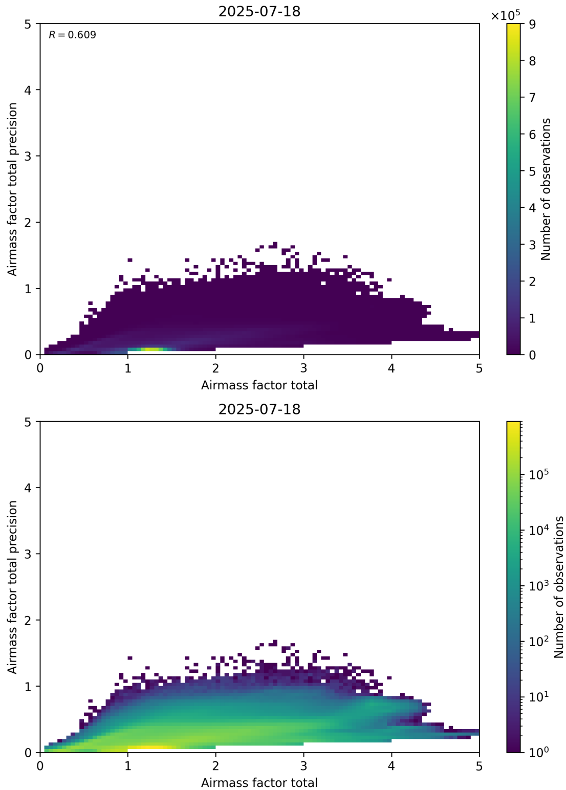
Figure 103: Scatter density plot of “Airmass factor total” against “Airmass factor total precision” for 2025-07-18 to 2025-07-19.
