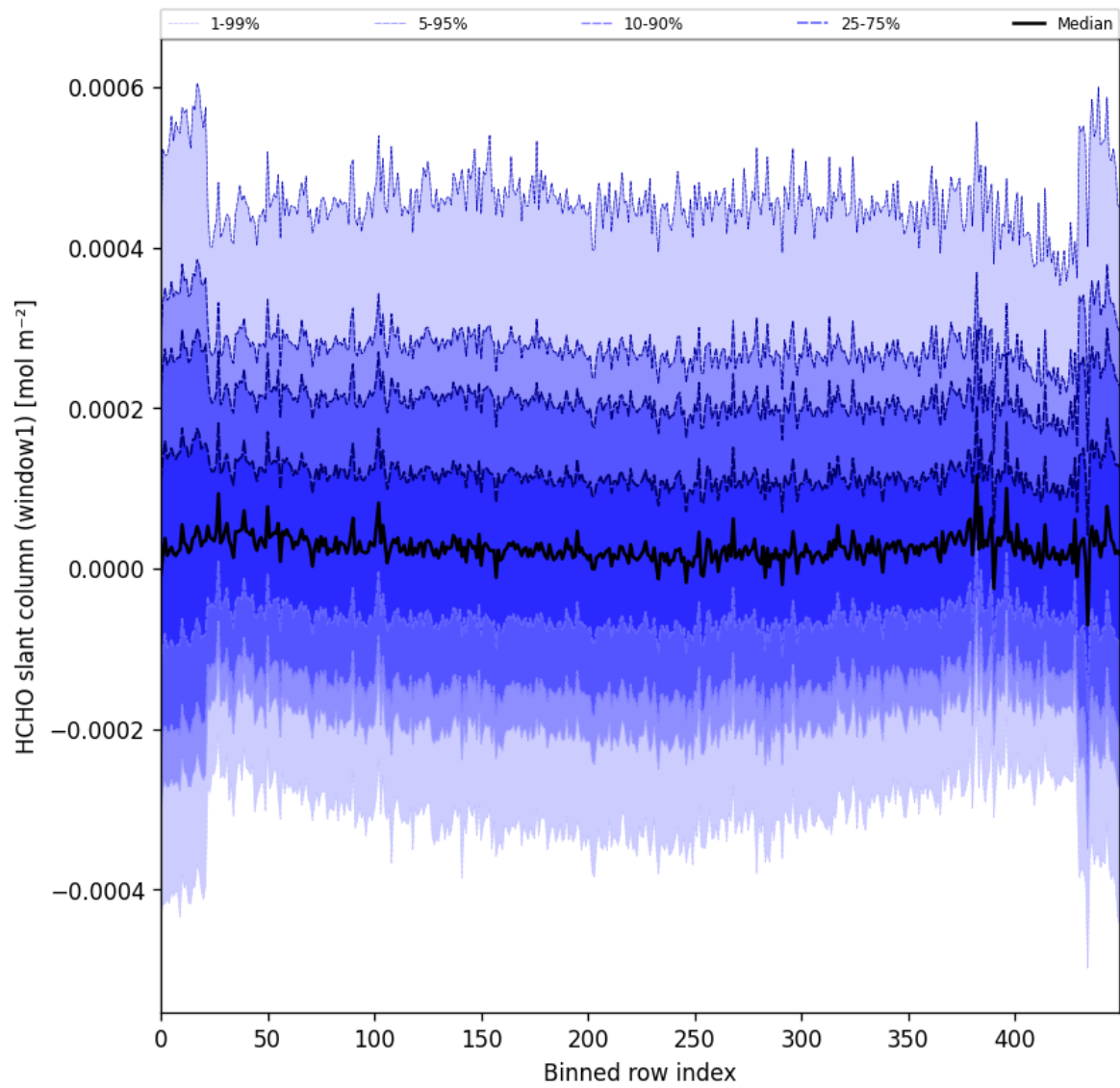
Figure 52: Along track statistics of "HCHO slant column (window1)" for 2025-07-18 to 2025-07-19
