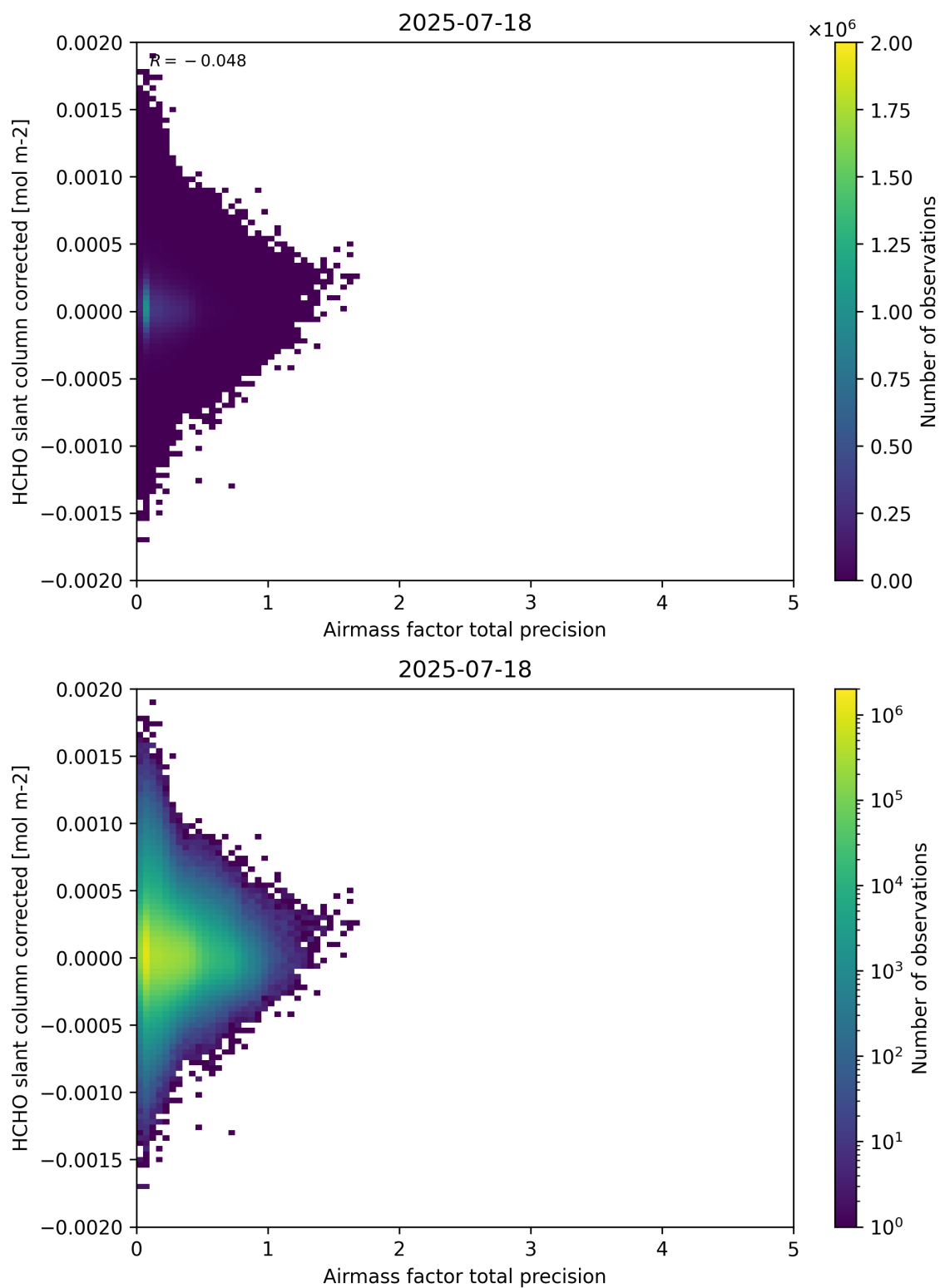
Figure 109: Scatter density plot of “Airmass factor total precision” against “HCHO slant column corrected” for 2025-07-18 to 2025-07-19.
