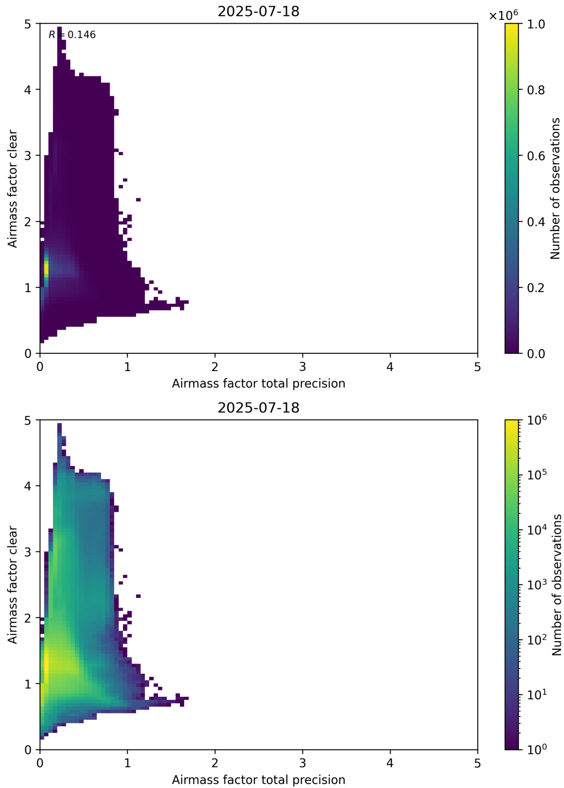
Figure 108: Scatter density plot of “Airmass factor total precision” against “Airmass factor clear” for 2025-07-18 to 2025-07-19.
