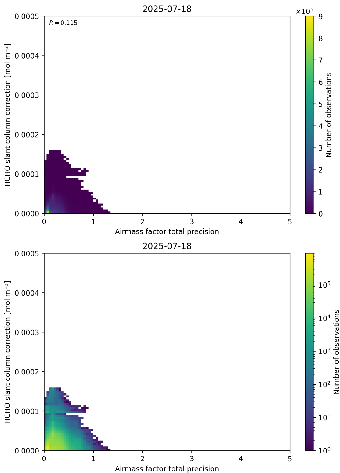
Figure 110: Scatter density plot of “Airmass factor total precision” against “HCHO slant column correction” for 2025-07-18 to 2025-07-19.
