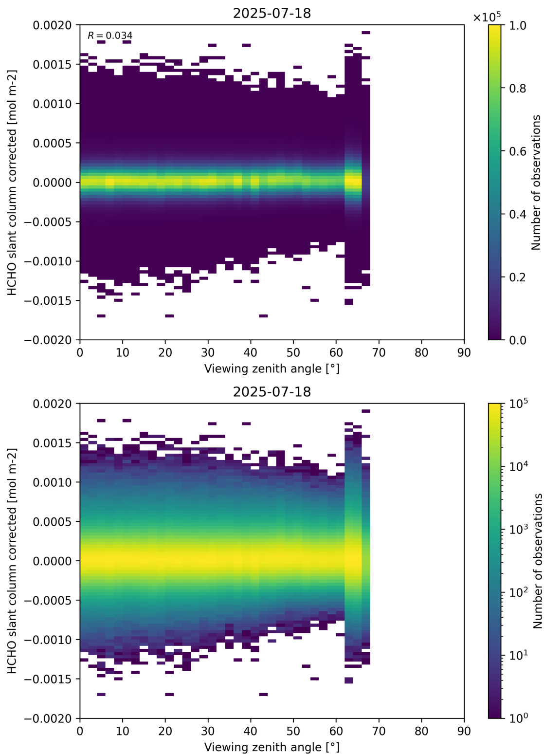
Figure 186: Scatter density plot of “Viewing zenith angle” against “HCHO slant column corrected” for 2025-07-18 to 2025-07-19.
