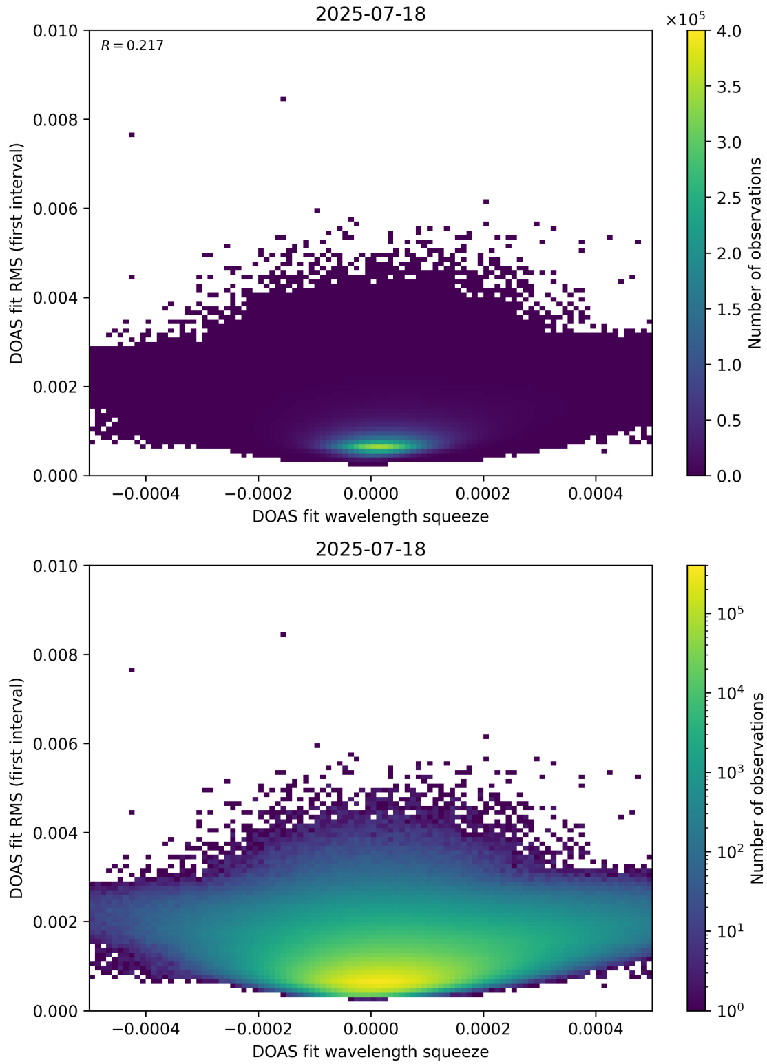
Figure 68: Scatter density plot of “DOAS fit wavelength squeeze” against “DOAS fit RMS (first interval)” for 2025-07-18 to 2025-07-19.
