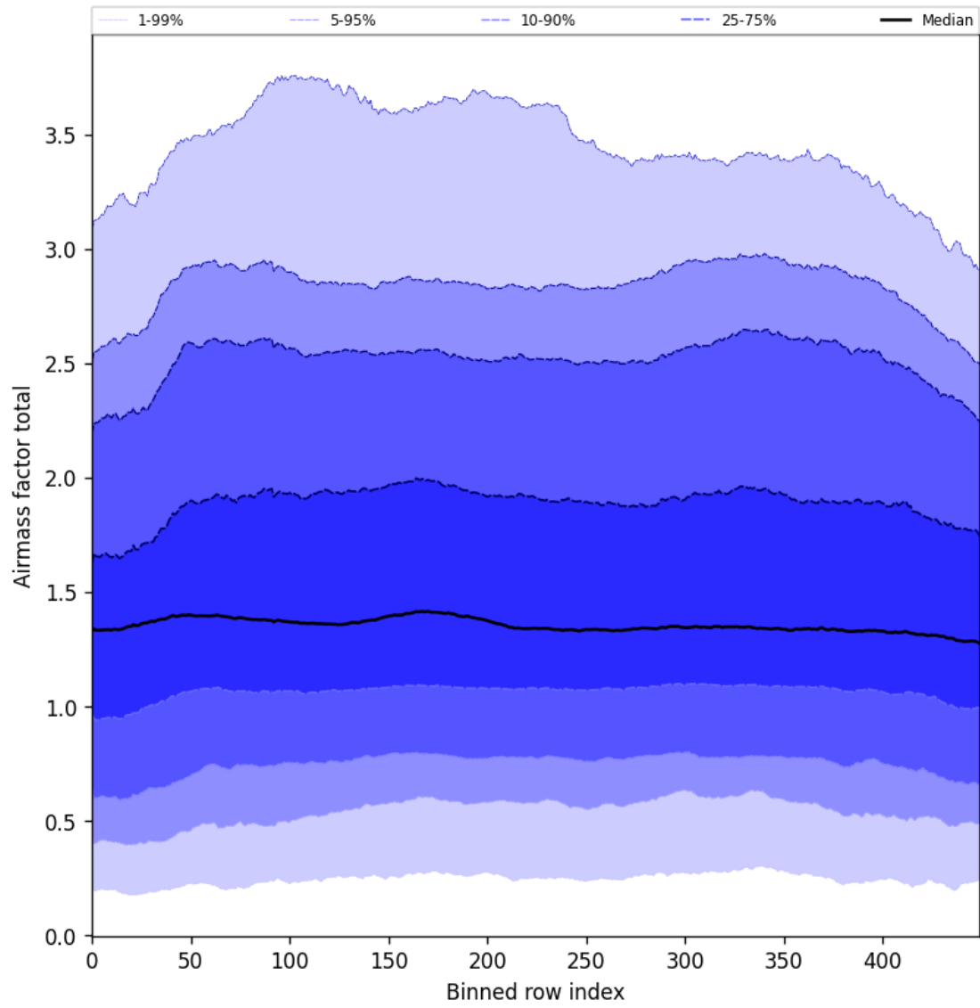
Figure 54: Along track statistics of “Airmass factor total” for 2025-07-18 to 2025-07-19
