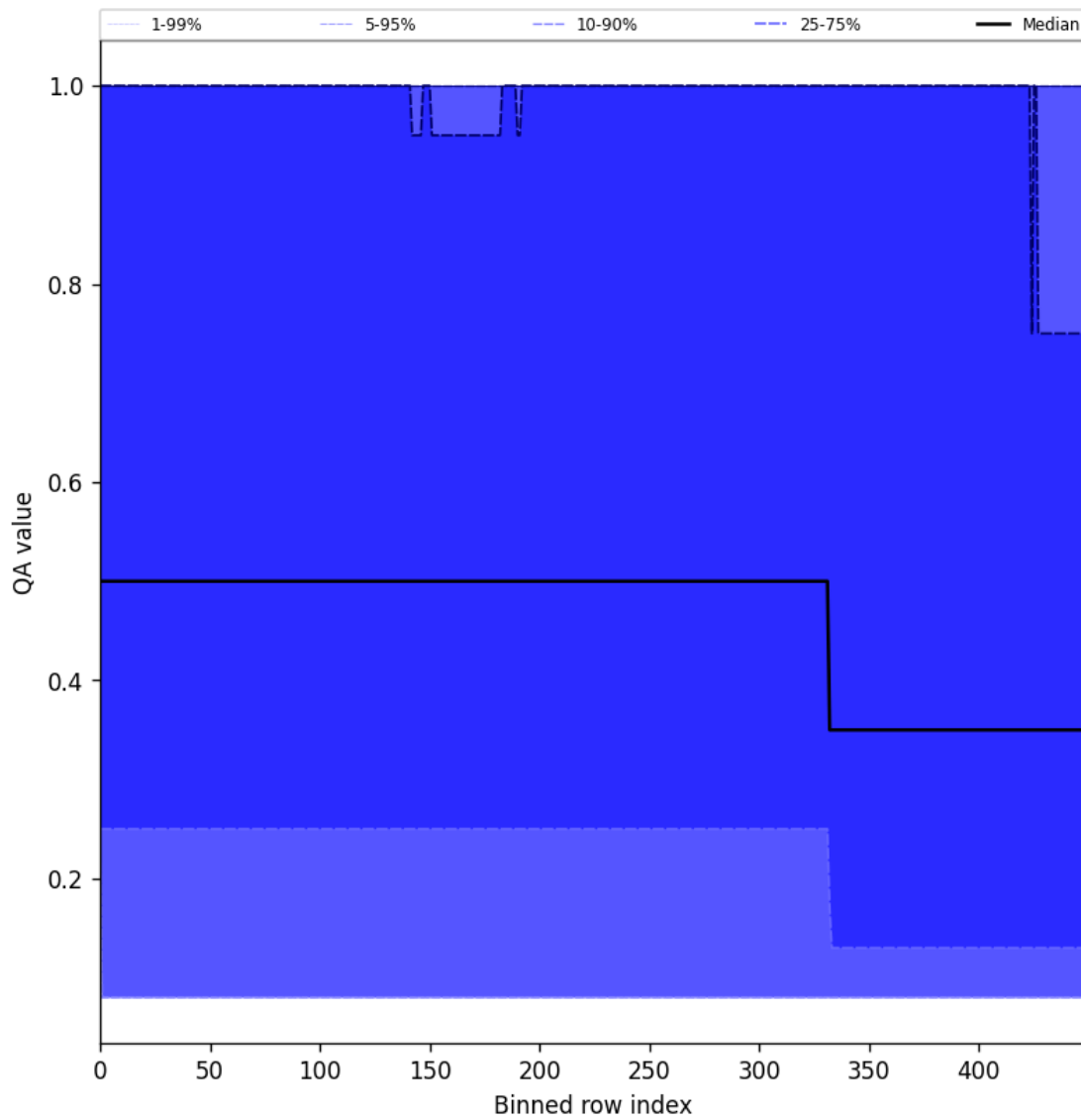
Figure 48: Along track statistics of “QA value” for 2025-07-18 to 2025-07-19
