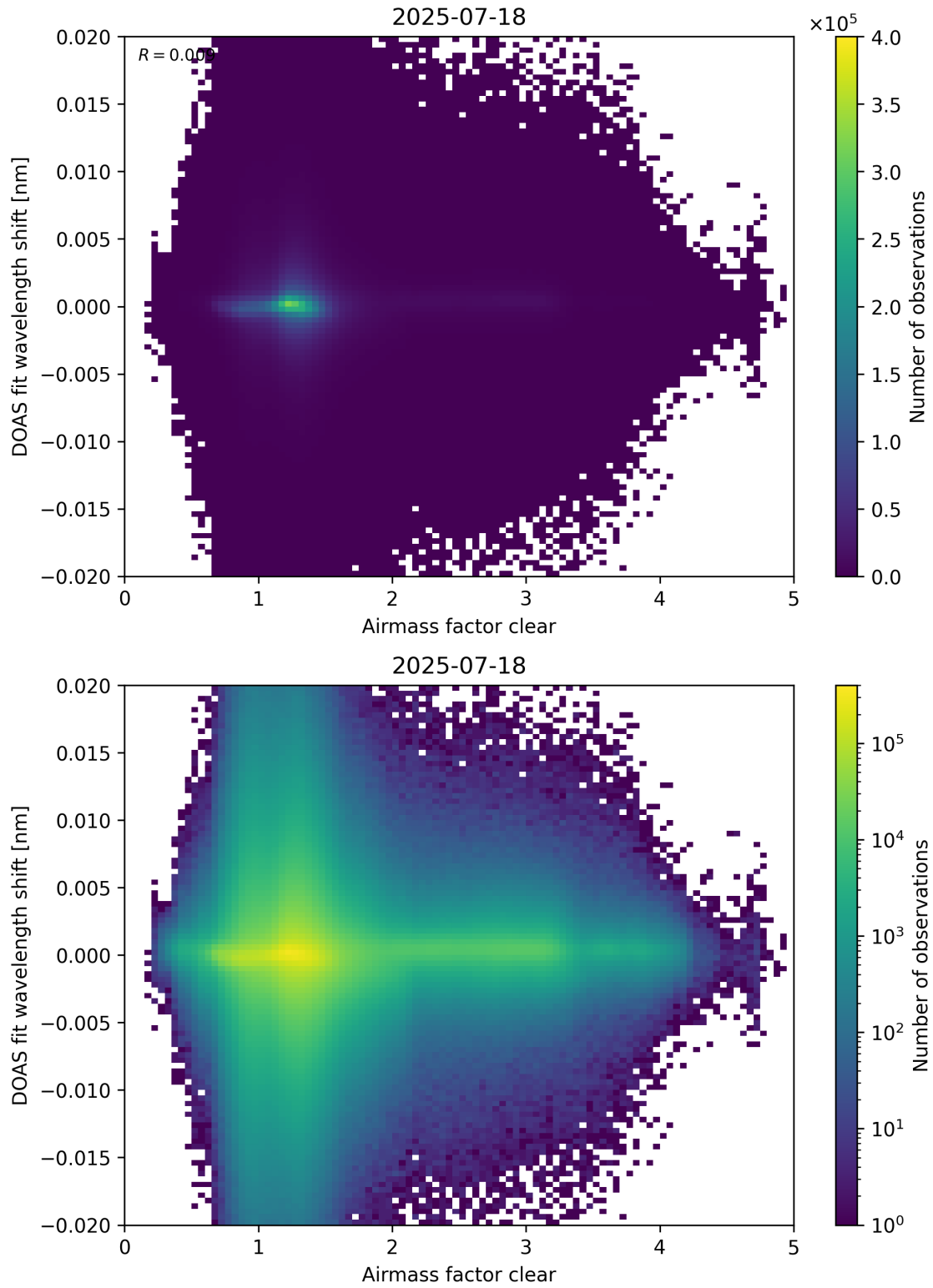
Figure 72: Scatter density plot of “Airmass factor clear” against “DOAS fit wavelength shift” for 2025-07-18 to 2025-07-19.
