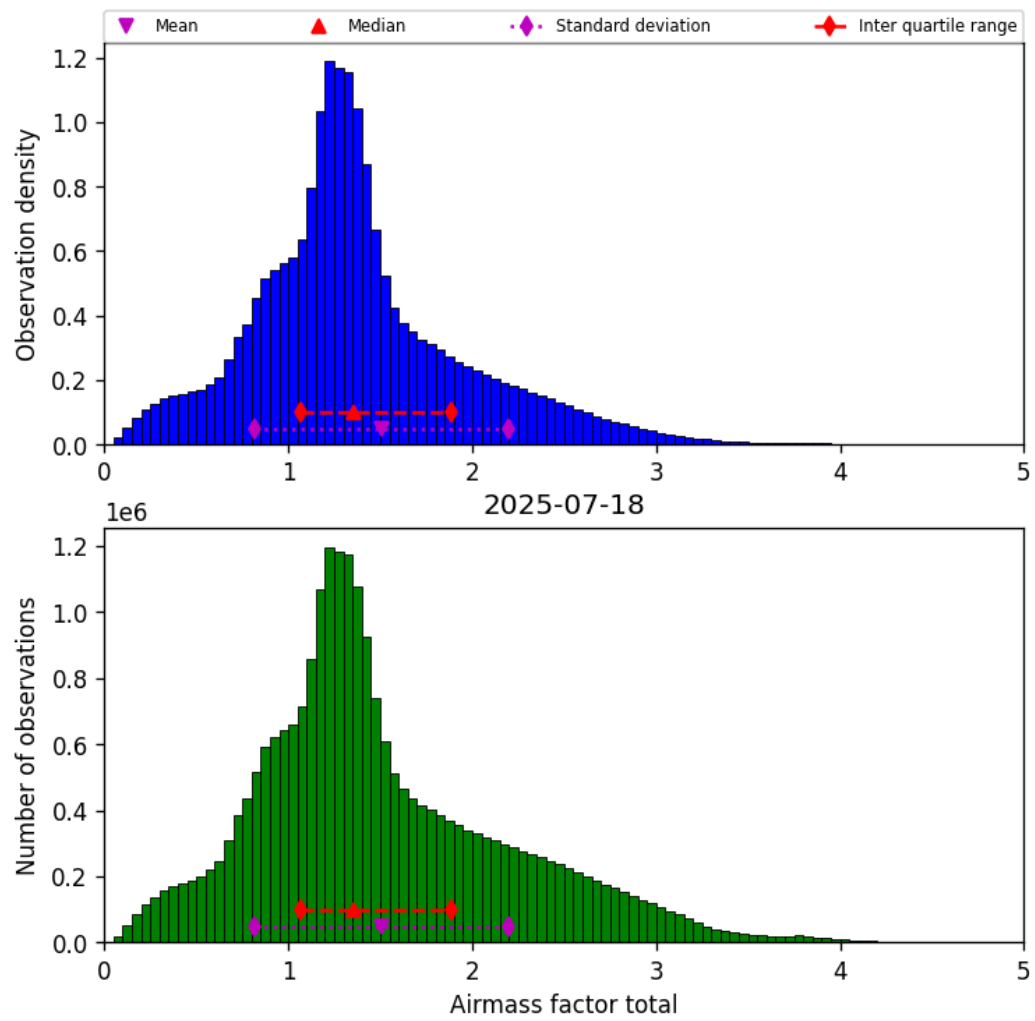
Figure 40: Histogram of “Airmass factor total” for 2025-07-18 to 2025-07-19
