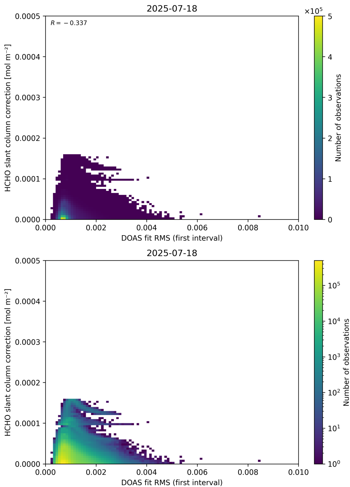
Figure 63: Scatter density plot of “DOAS fit RMS (first interval)” against “HCHO slant column correction” for 2025-07-18 to 2025-07-19.
