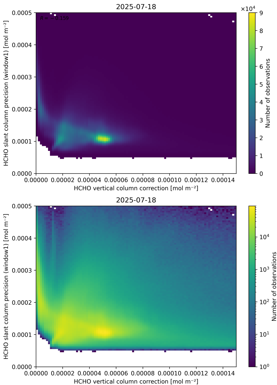
Figure 119: Scatter density plot of “HCHO vertical column correction” against “HCHO slant column precision (window1)” for 2025-07-18 to 2025-07-19.
