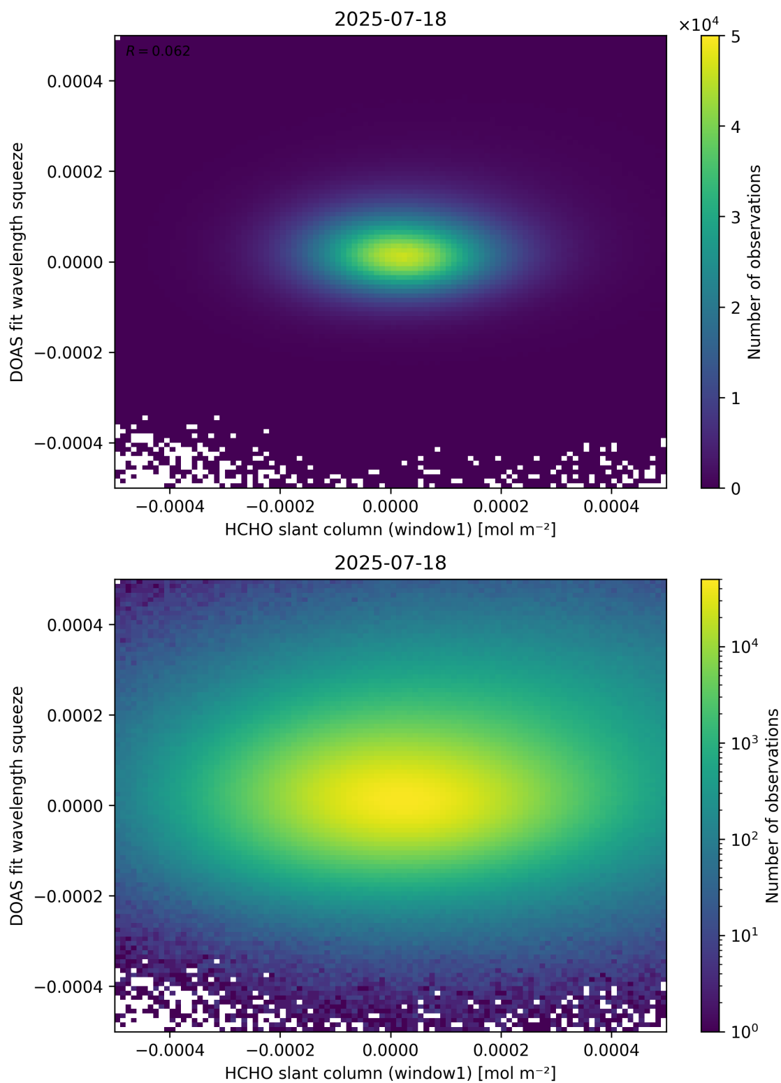
Figure 80: Scatter density plot of “HCHO slant column (window1)” against “DOAS fit wavelength squeeze” for 2025-07-18 to 2025-07-19.
