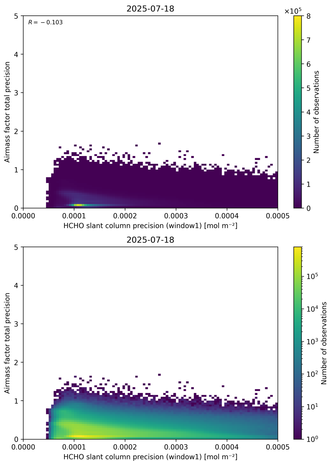
Figure 95: Scatter density plot of “HCHO slant column precision (window1)” against “Airmass factor total precision” for 2025-07-18 to 2025-07-19.
