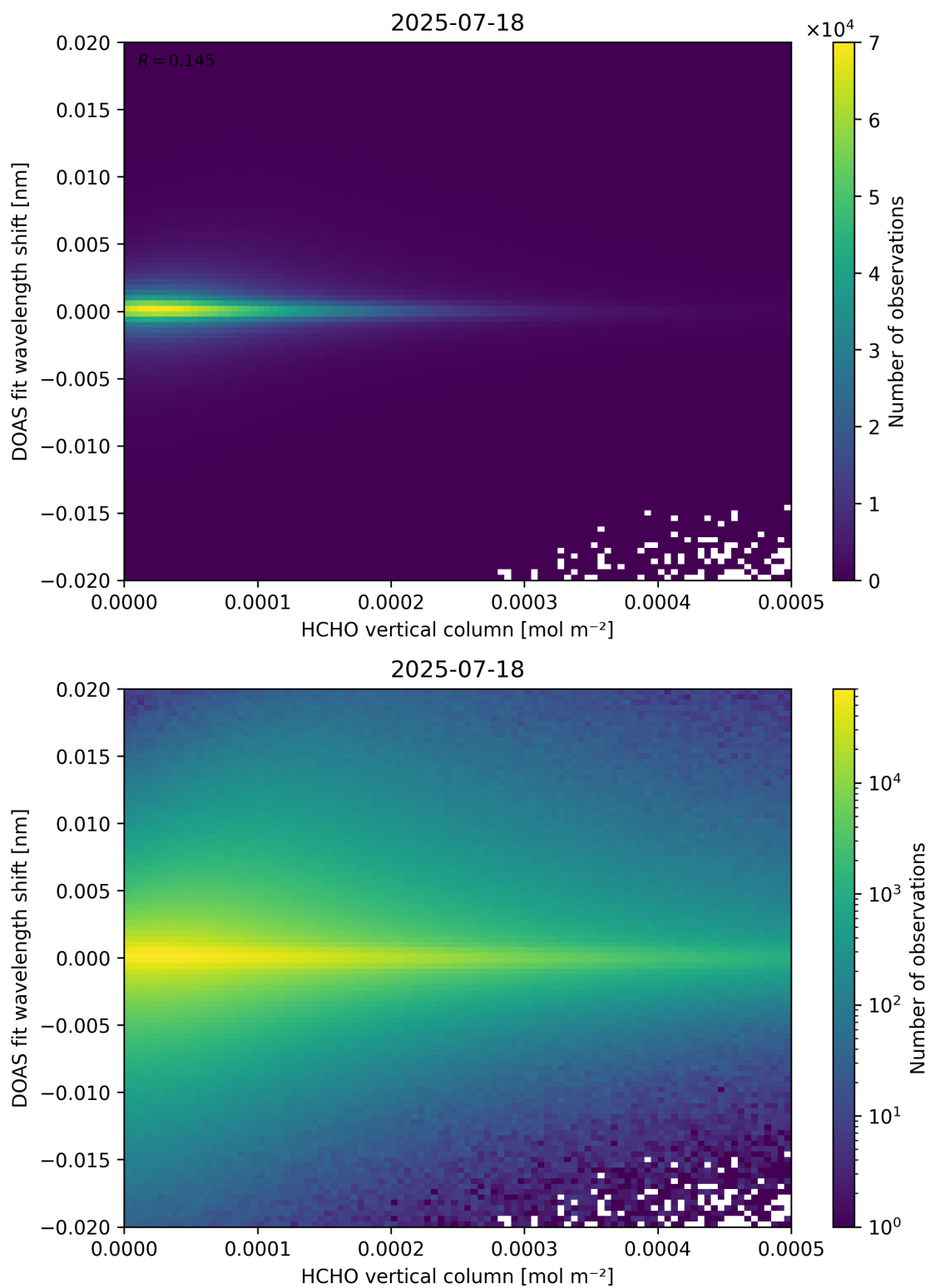
Figure 124: Scatter density plot of “HCHO vertical column” against “DOAS fit wavelength shift” for 2025-07-18 to 2025-07-19.
