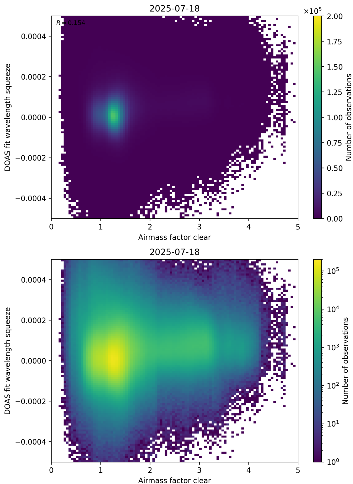
Figure 73: Scatter density plot of “Airmass factor clear” against “DOAS fit wavelength squeeze” for 2025-07-18 to 2025-07-19.
