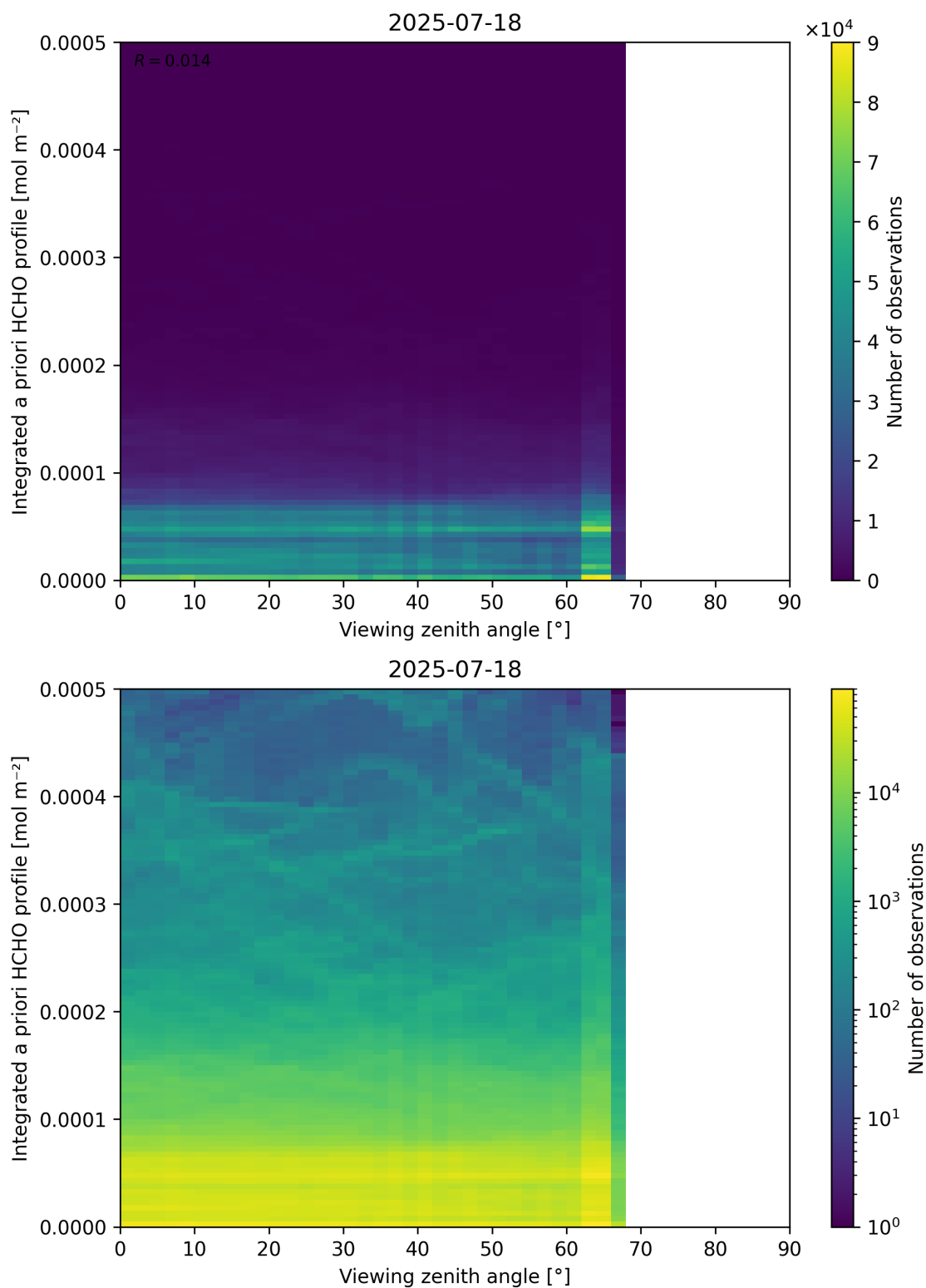
Figure 195: Scatter density plot of “Viewing zenith angle” against “Integrated a priori HCHO profile” for 2025-07-18 to 2025-07-19.
