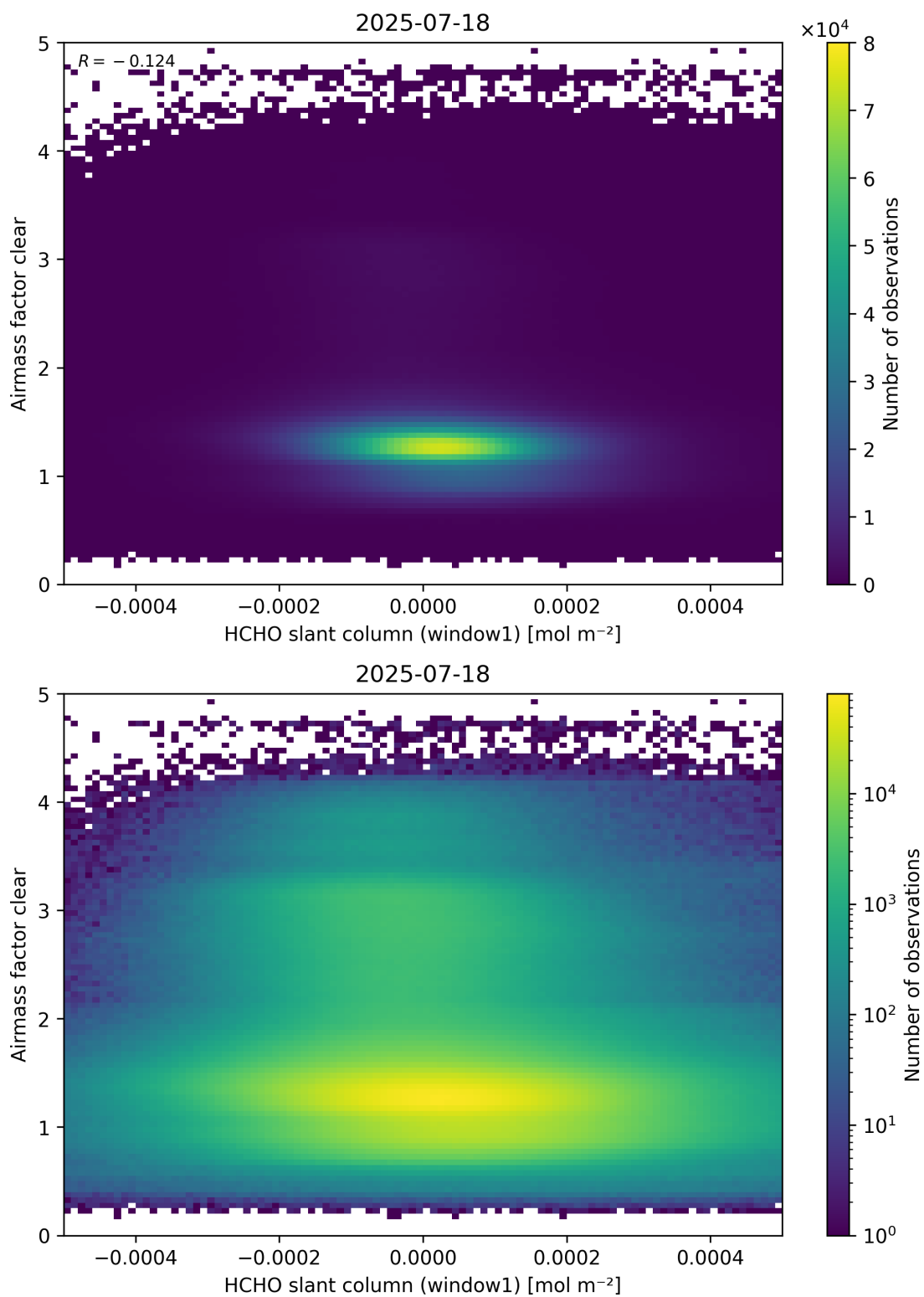
Figure 81: Scatter density plot of “HCHO slant column (window1)” against “Airmass factor clear” for 2025-07-18 to 2025-07-19.
