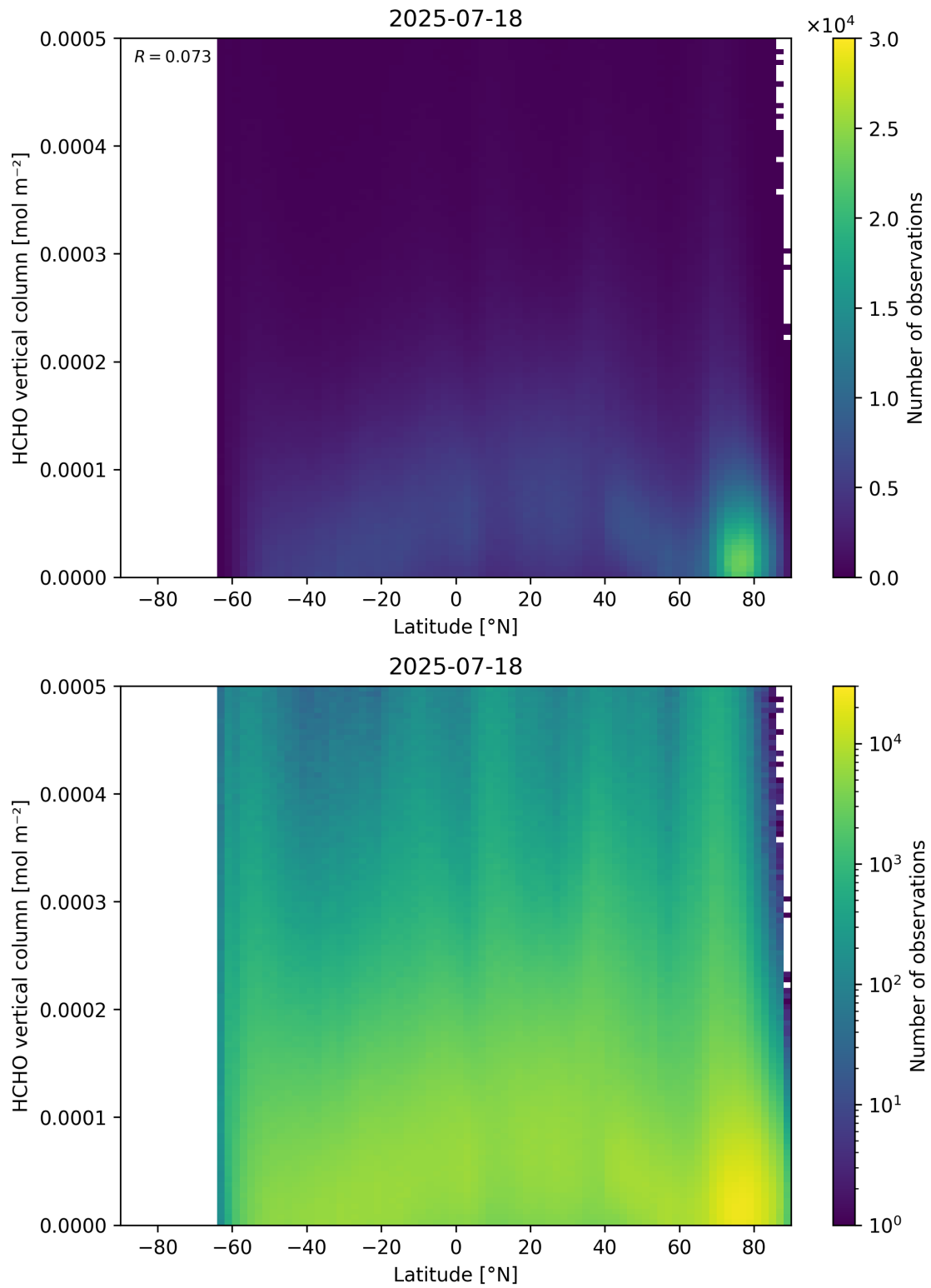
Figure 163: Scatter density plot of “Latitude” against “HCHO vertical column” for 2025-07-18 to 2025-07-19.
