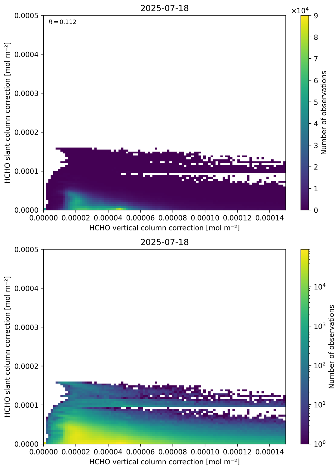
Figure 117: Scatter density plot of “HCHO vertical column correction” against “HCHO slant column correction” for 2025-07-18 to 2025-07-19.
