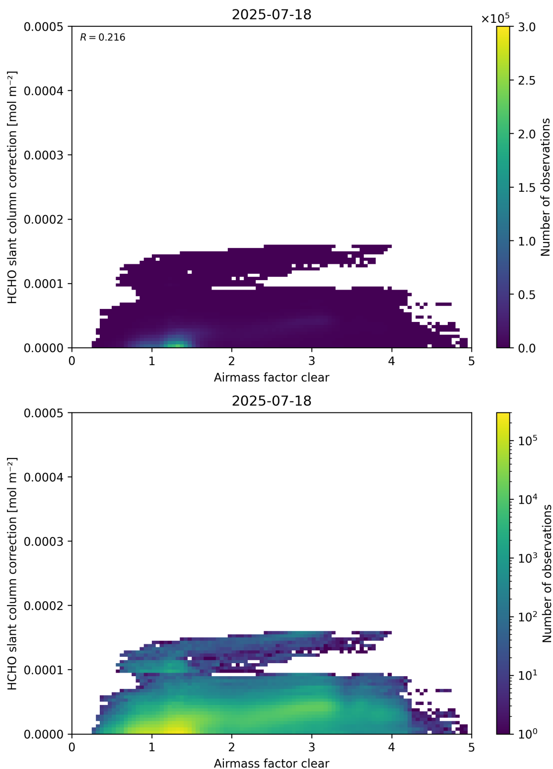
Figure 75: Scatter density plot of “Airmass factor clear” against “HCHO slant column correction” for 2025-07-18 to 2025-07-19.
