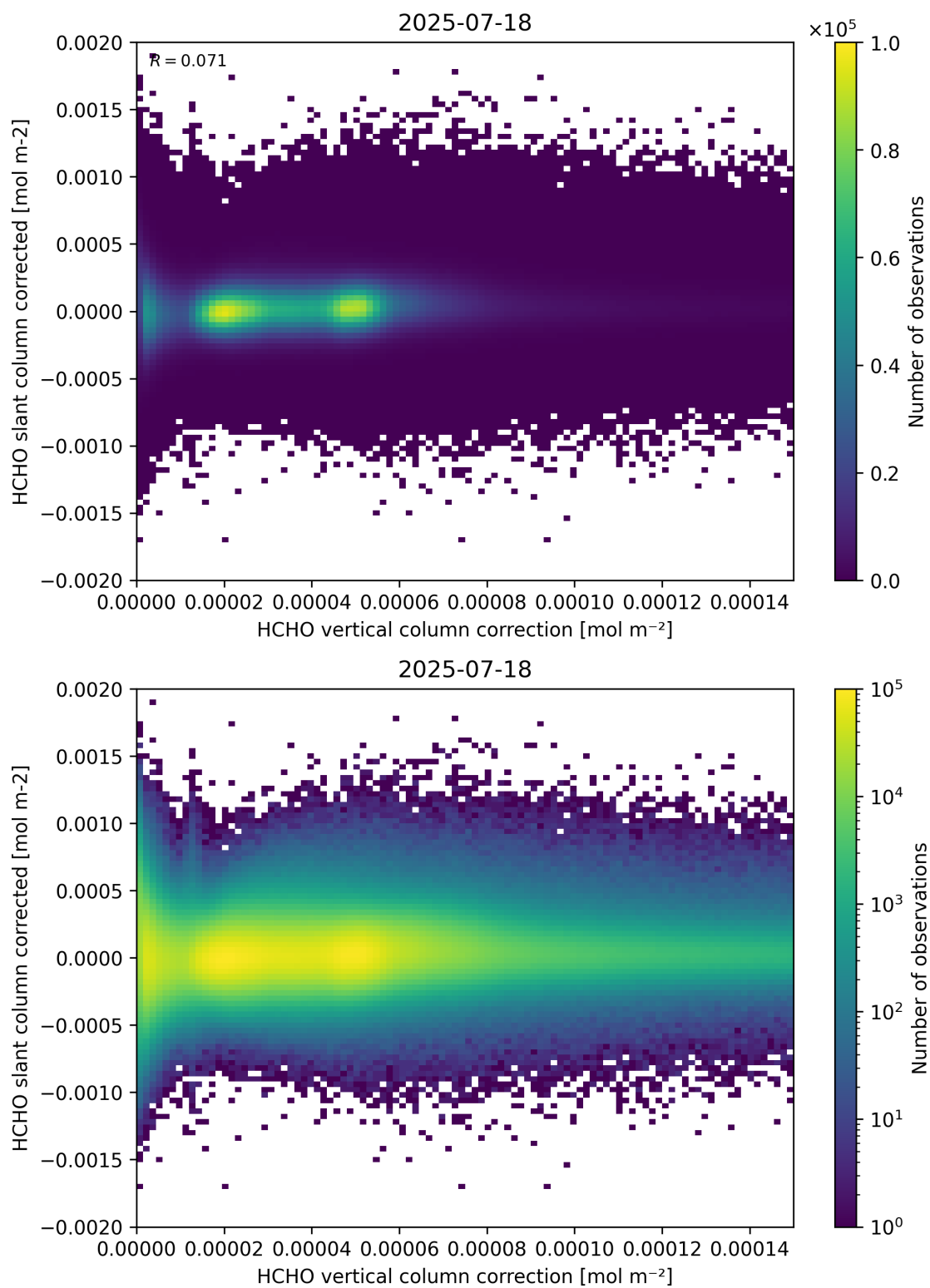
Figure 116: Scatter density plot of “HCHO vertical column correction” against “HCHO slant column corrected” for 2025-07-18 to 2025-07-19.
