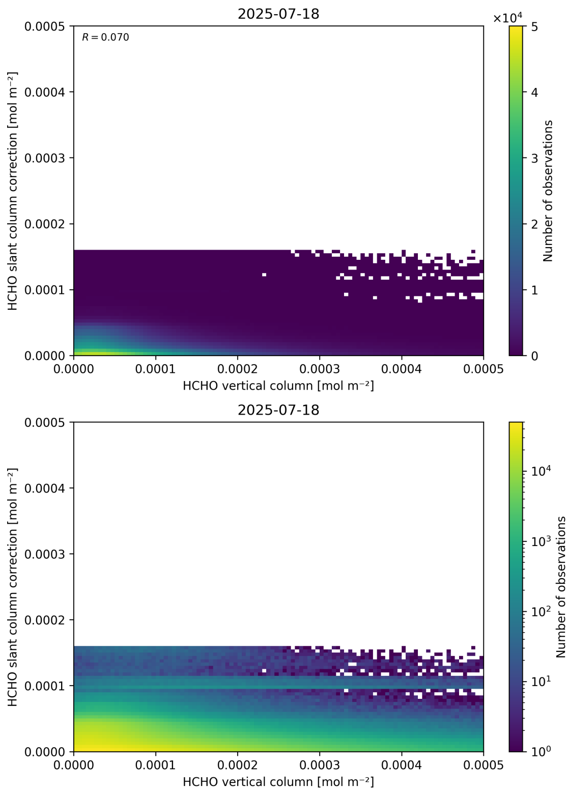
Figure 128: Scatter density plot of “HCHO vertical column” against “HCHO slant column correction” for 2025-07-18 to 2025-07-19.
