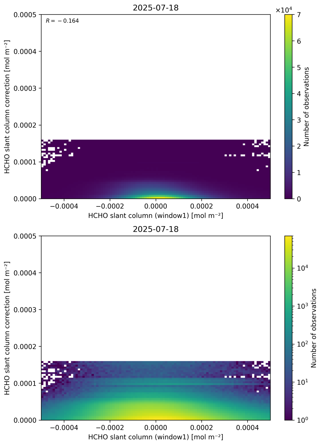
Figure 83: Scatter density plot of “HCHO slant column (window1)” against “HCHO slant column correction” for 2025-07-18 to 2025-07-19.
