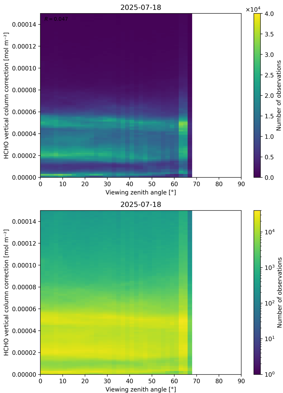
Figure 193: Scatter density plot of “Viewing zenith angle” against “HCHO vertical column correction” for 2025-07-18 to 2025-07-19.
