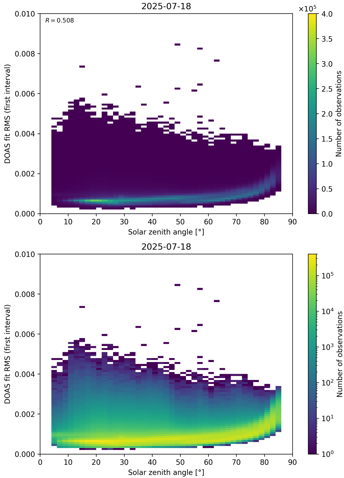
Figure 167: Scatter density plot of “Solar zenith angle” against “DOAS fit RMS (first interval)” for 2025-07-18 to 2025-07-19.
