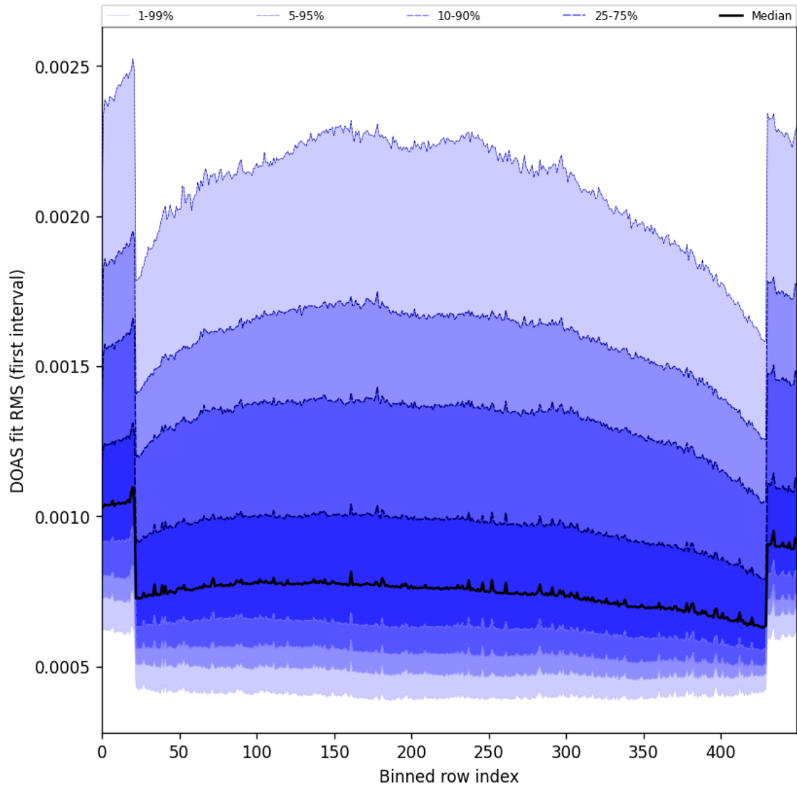
Figure 60: Along track statistics of “DOAS fit RMS (first interval)” for 2025-07-18 to 2025-07-19
