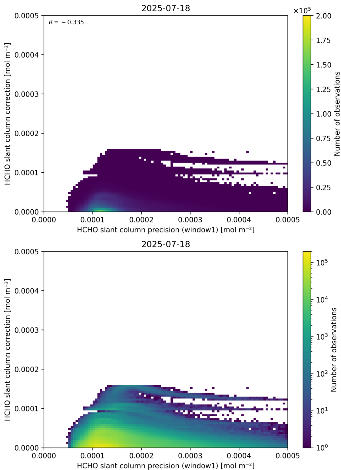
Figure 93: Scatter density plot of “HCHO slant column precision (window1)” against “HCHO slant column correction” for 2025-07-18 to 2025-07-19.
