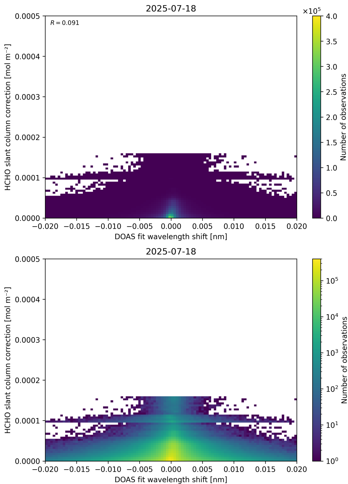
Figure 67: Scatter density plot of “DOAS fit wavelength shift” against “HCHO slant column correction” for 2025-07-18 to 2025-07-19.
