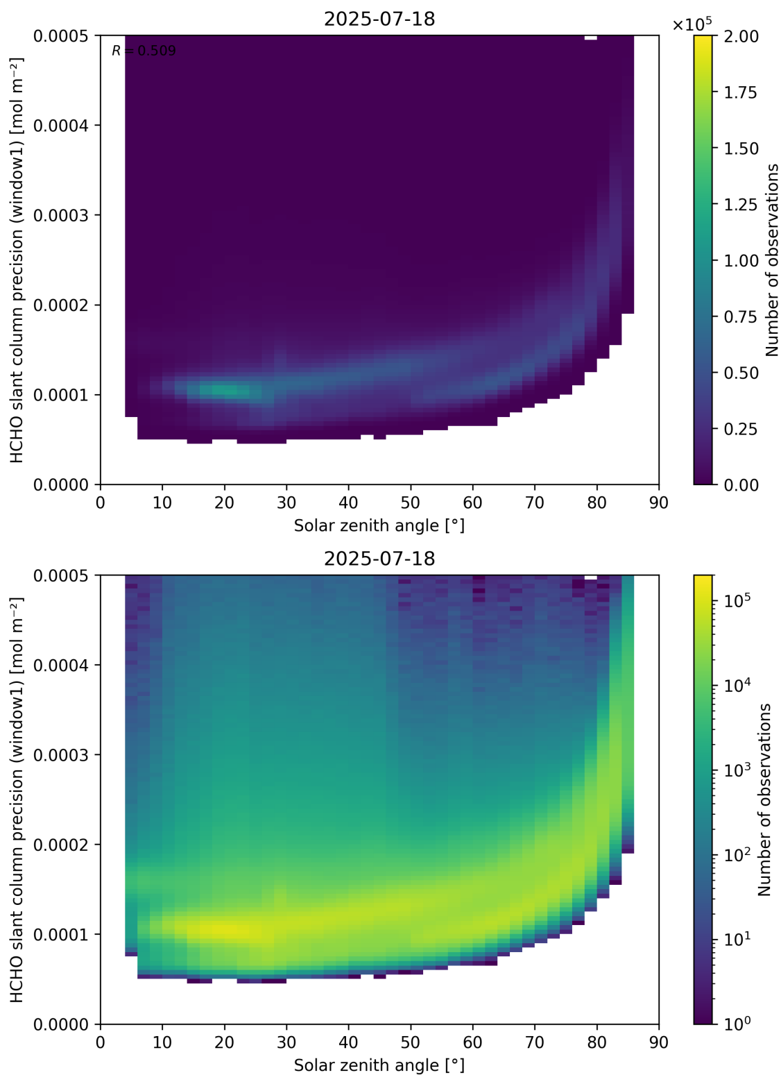
Figure 174: Scatter density plot of “Solar zenith angle” against “HCHO slant column precision (window1)” for 2025-07-18 to 2025-07-19.
