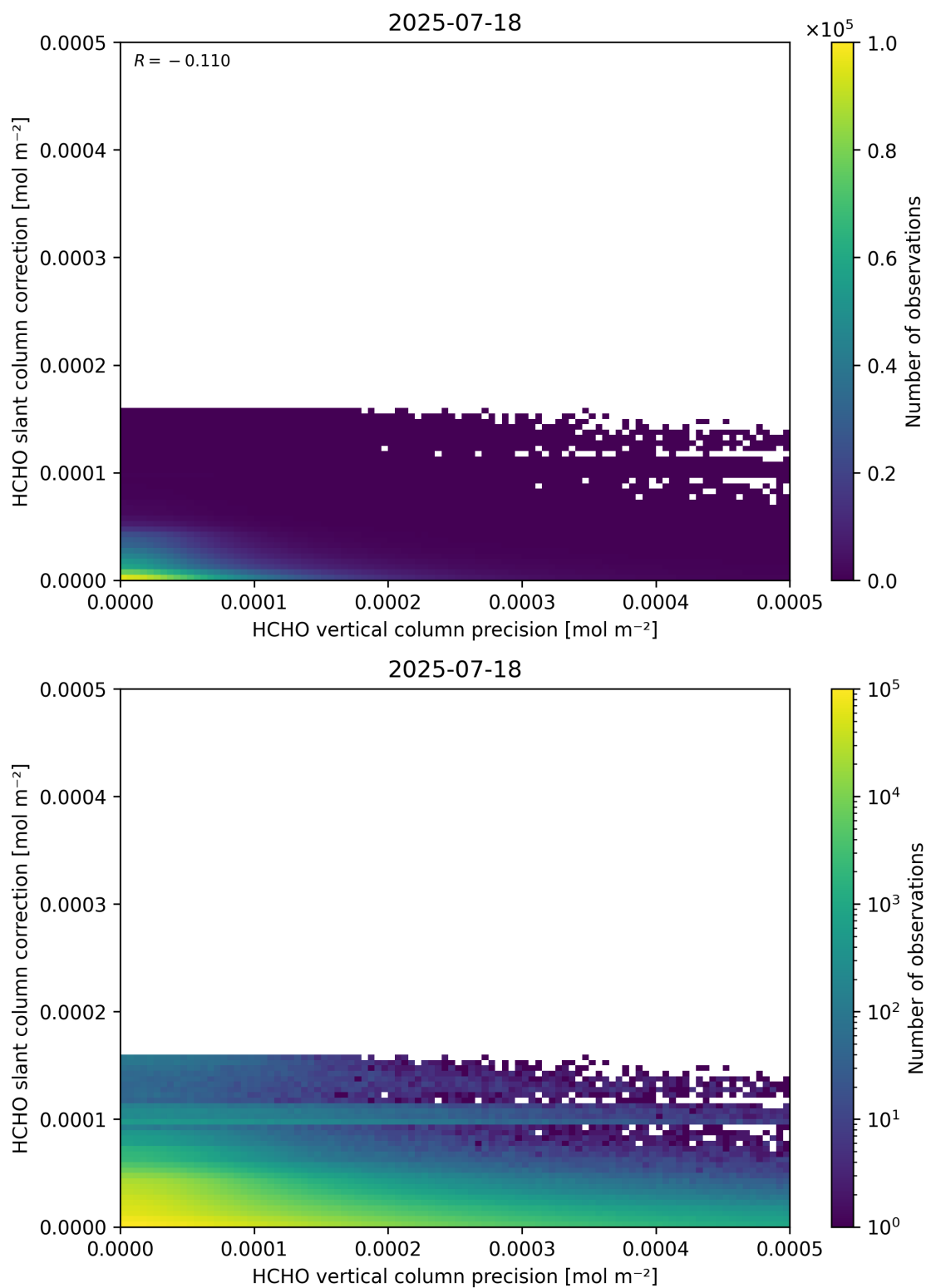
Figure 141: Scatter density plot of “HCHO vertical column precision” against “HCHO slant column correction” for 2025-07-18 to 2025-07-19.
