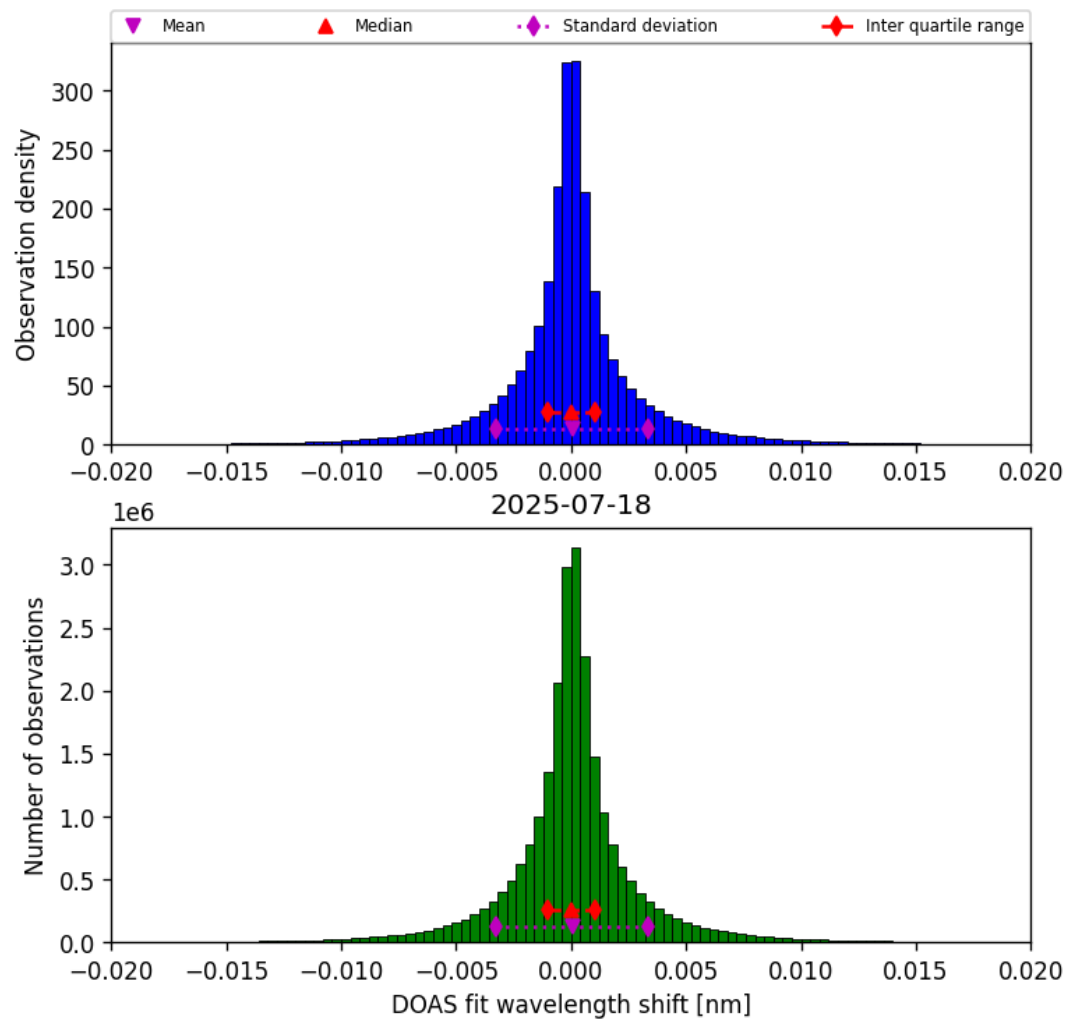
Figure 44: Histogram of “DOAS fit wavelength shift” for 2025-07-18 to 2025-07-19
