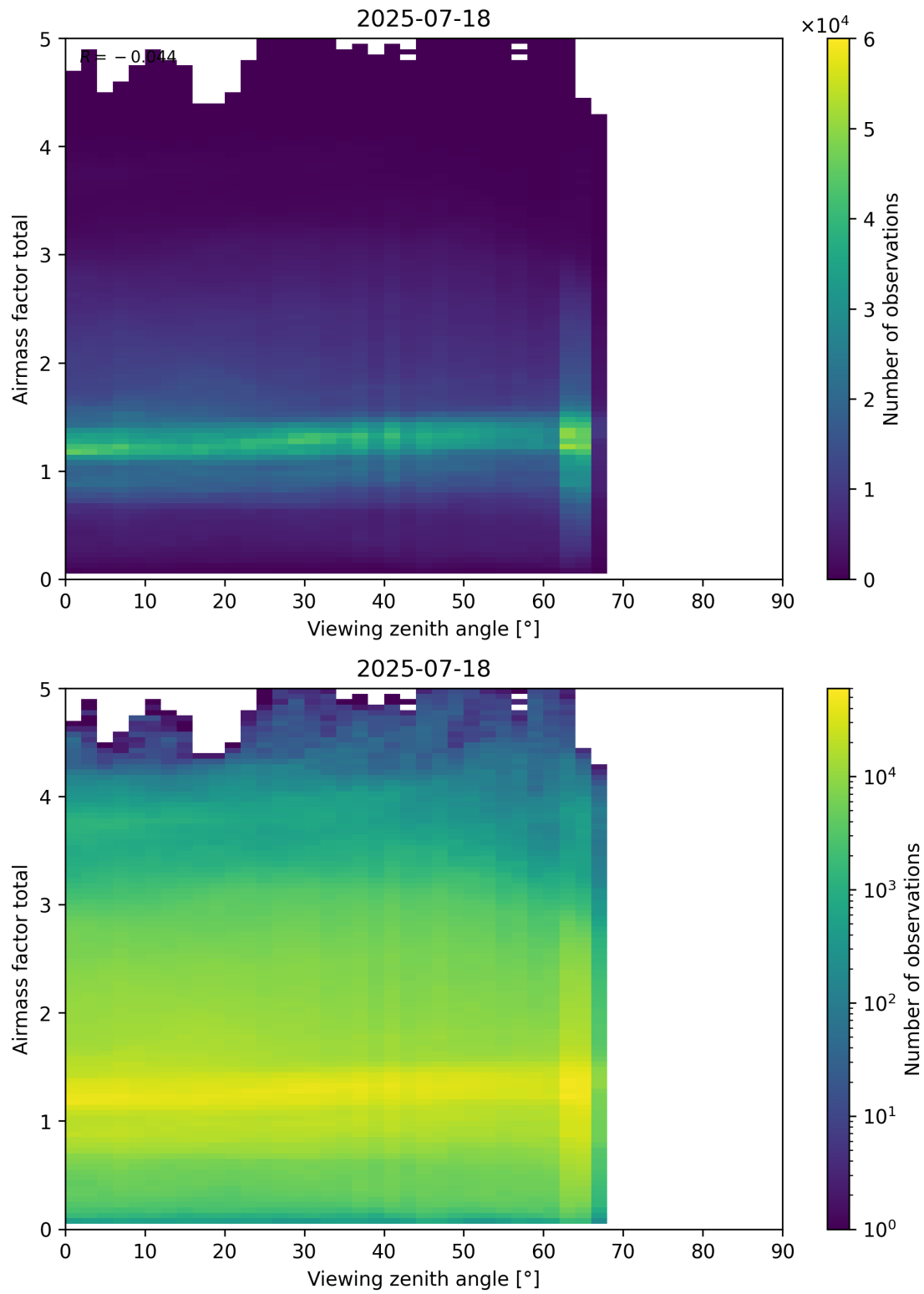
Figure 190: Scatter density plot of “Viewing zenith angle” against “Airmass factor total” for 2025-07-18 to 2025-07-19.
