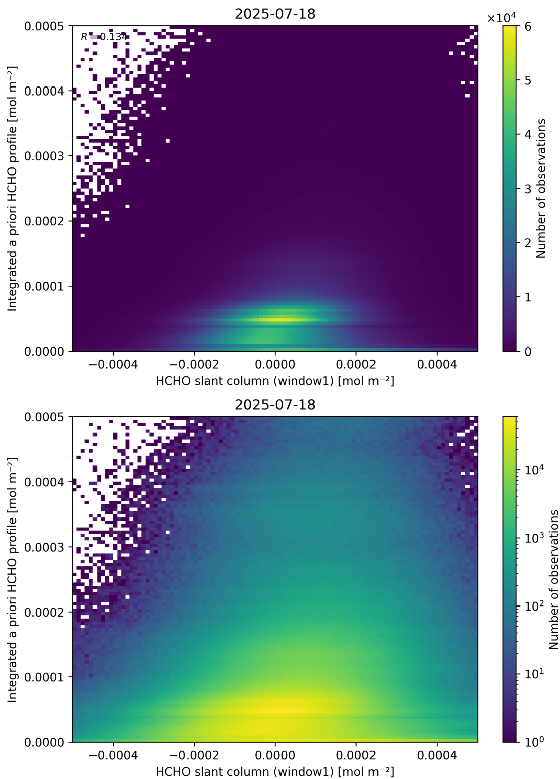
Figure 87: Scatter density plot of “HCHO slant column (window1)” against “Integrated a priori HCHO profile” for 2025-07-18 to 2025-07-19.
