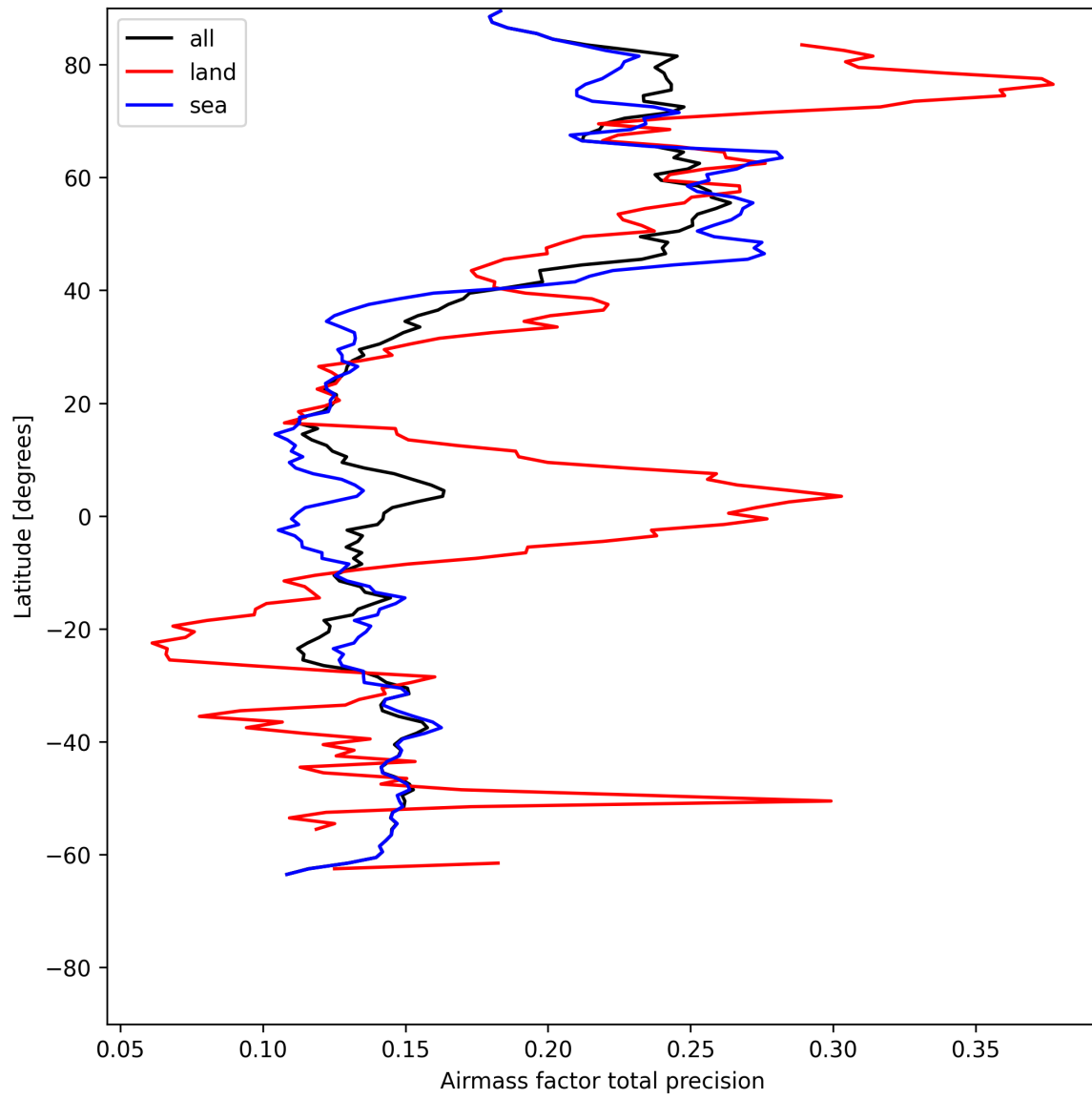
Figure 27: Zonal average of “Airmass factor total precision” for 2025-07-18 to 2025-07-19.
