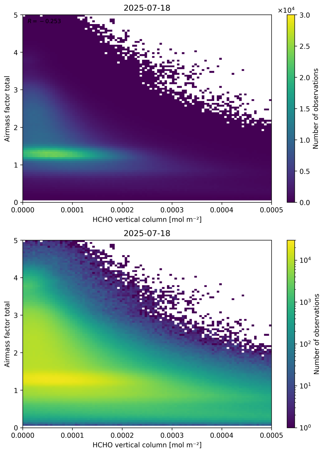
Figure 131: Scatter density plot of “HCHO vertical column” against “Airmass factor total” for 2025-07-18 to 2025-07-19.
