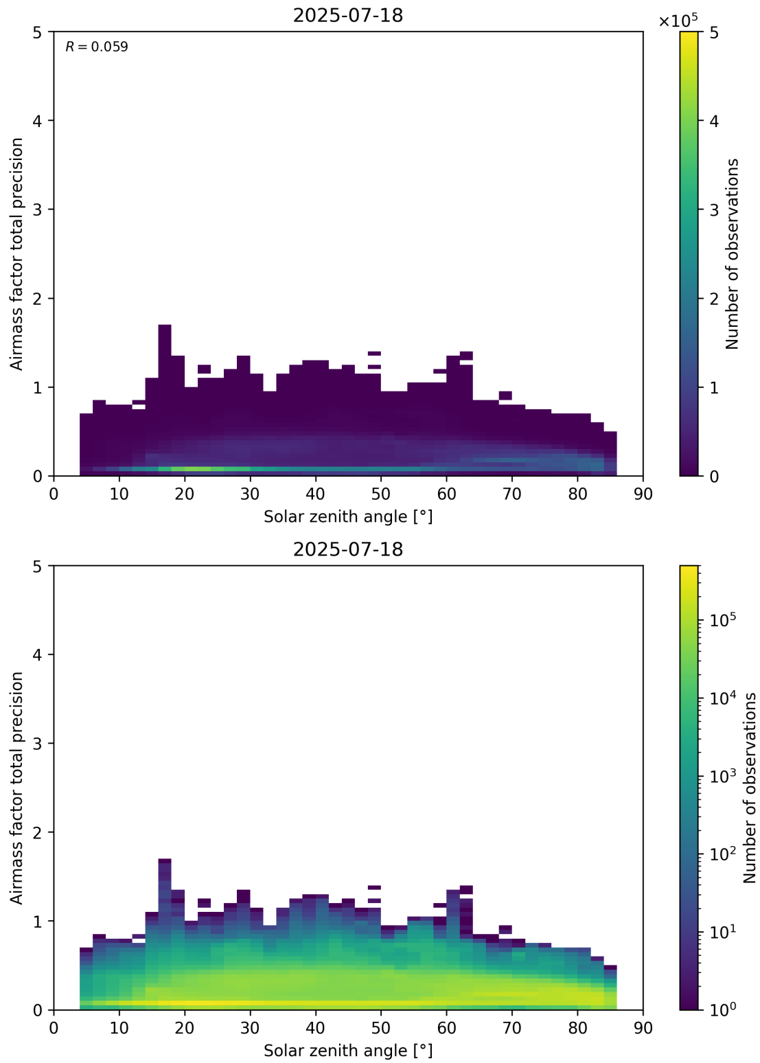
Figure 176: Scatter density plot of “Solar zenith angle” against “Airmass factor total precision” for 2025-07-18 to 2025-07-19.
