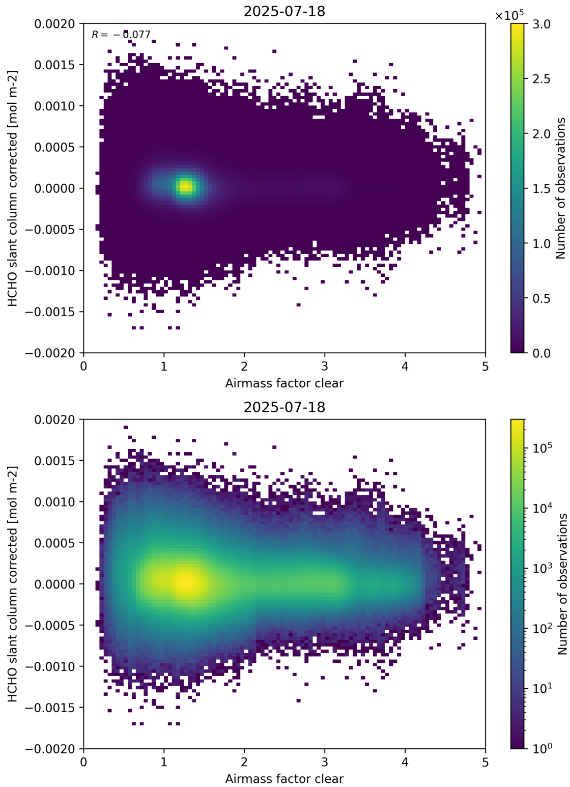
Figure 74: Scatter density plot of “Airmass factor clear” against “HCHO slant column corrected” for 2025-07-18 to 2025-07-19.
