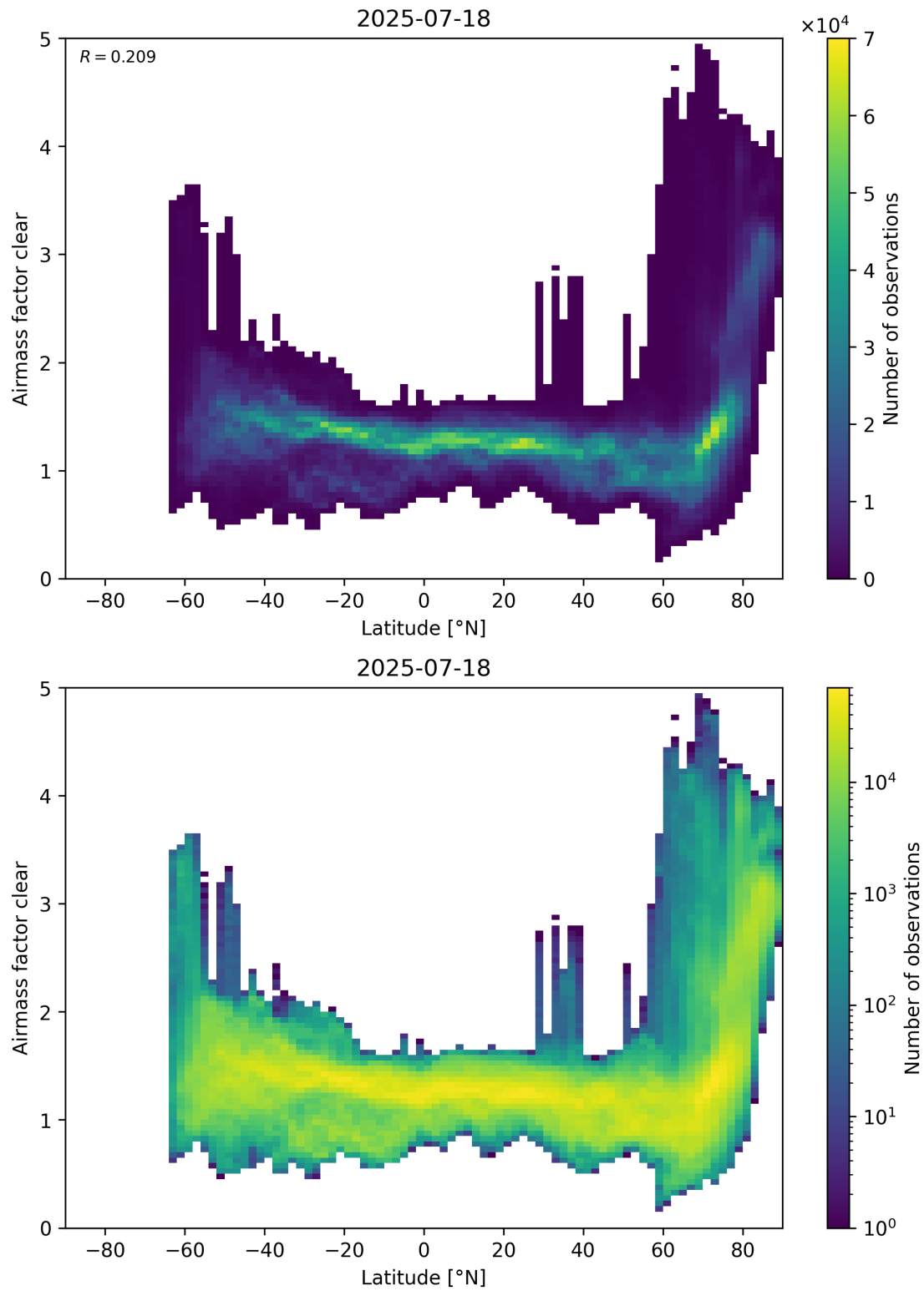
Figure 156: Scatter density plot of “Latitude” against “Airmass factor clear” for 2025-07-18 to 2025-07-19.
