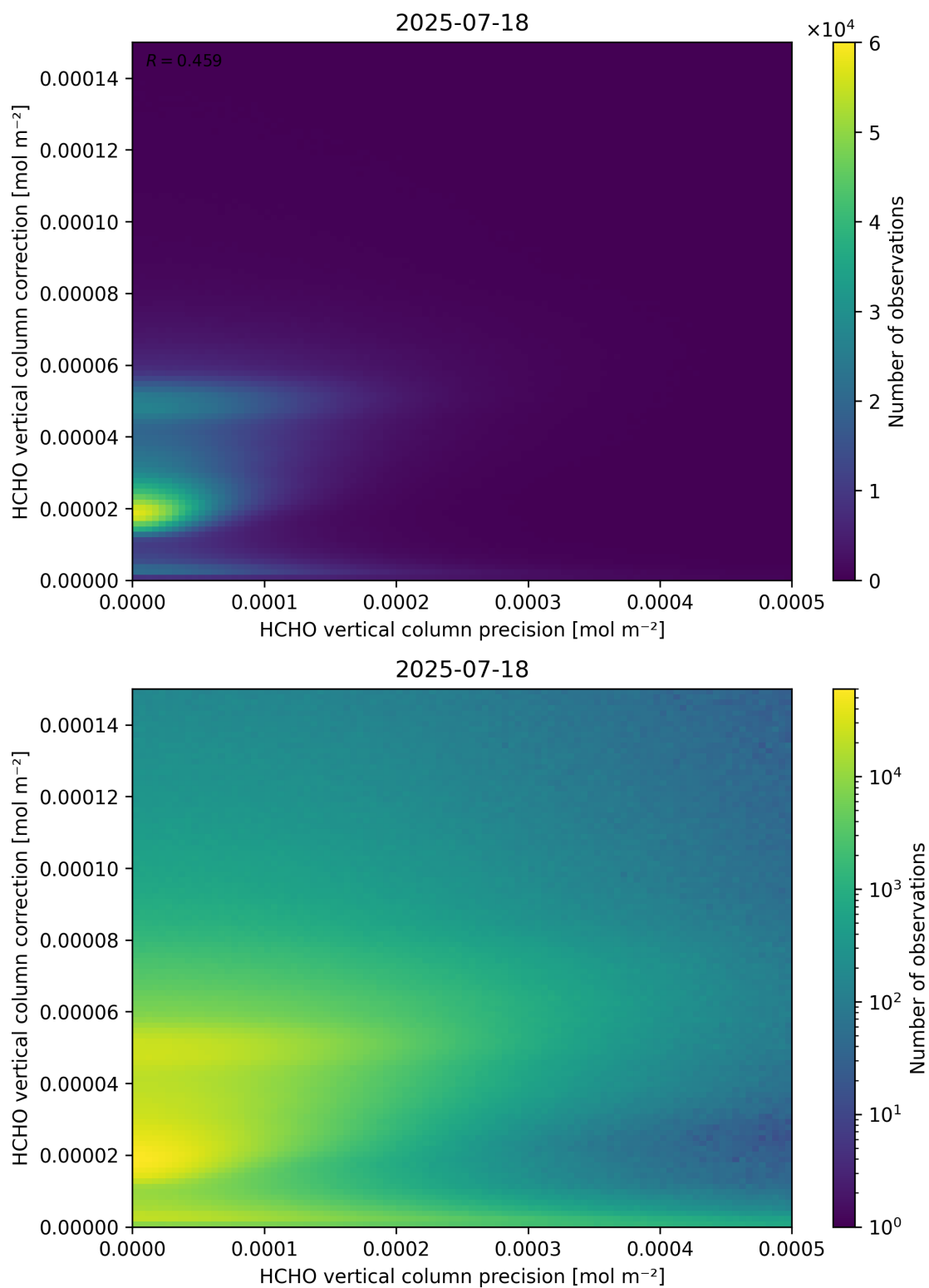
Figure 146: Scatter density plot of “HCHO vertical column precision” against “HCHO vertical column correction” for 2025-07-18 to 2025-07-19.
