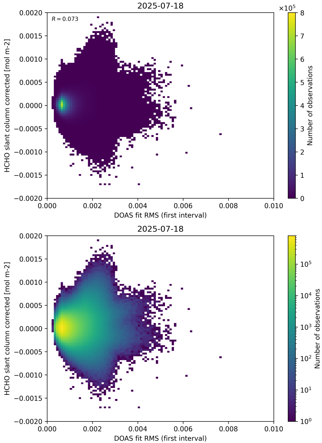
Figure 62: Scatter density plot of “DOAS fit RMS (first interval)” against “HCHO slant column corrected” for 2025-07-18 to 2025-07-19.
