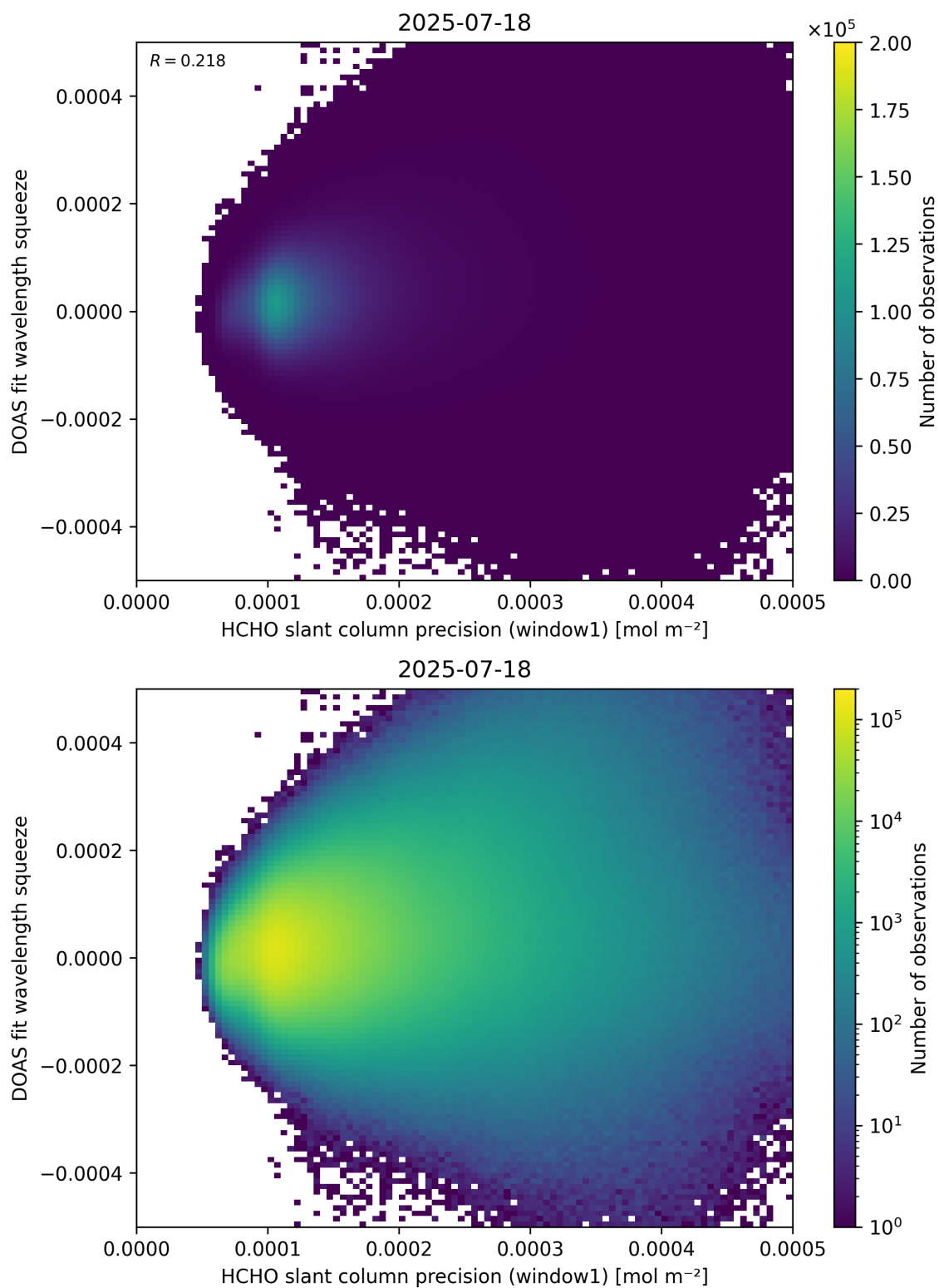
Figure 90: Scatter density plot of “HCHO slant column precision (window1)” against “DOAS fit wavelength squeeze” for 2025-07-18 to 2025-07-19.
