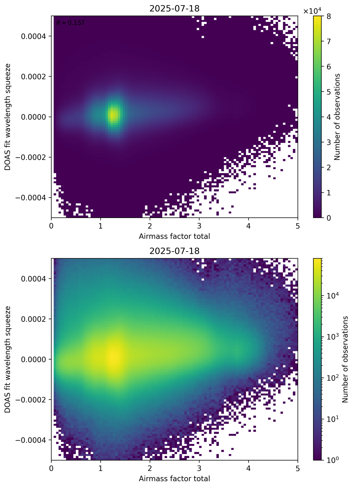
Figure 99: Scatter density plot of “Airmass factor total” against “DOAS fit wavelength squeeze” for 2025-07-18 to 2025-07-19.
