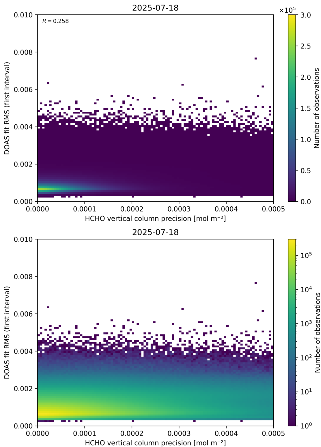
Figure 136: Scatter density plot of “HCHO vertical column precision” against “DOAS fit RMS (first interval)” for 2025-07-18 to 2025-07-19.
