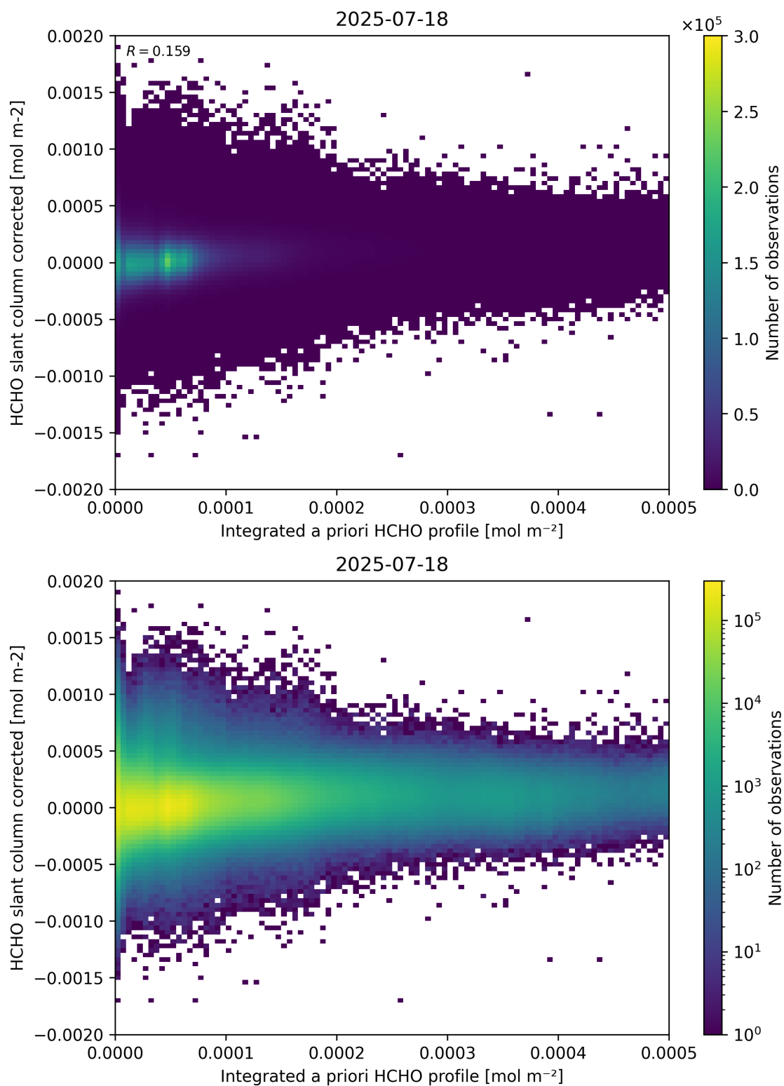
Figure 151: Scatter density plot of “Integrated a priori HCHO profile” against “HCHO slant column corrected” for 2025-07-18 to 2025-07-19.
