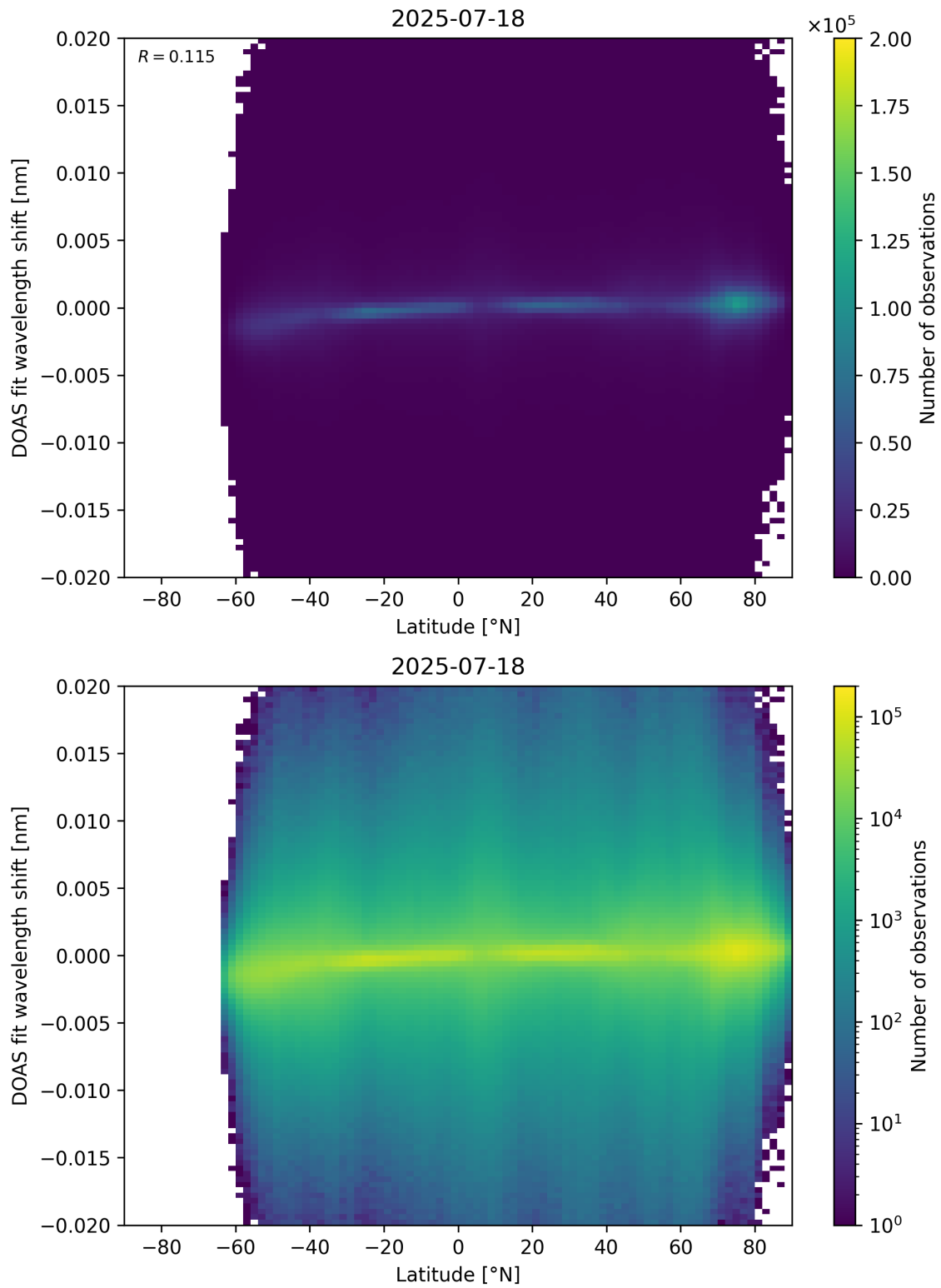
Figure 154: Scatter density plot of “Latitude” against “DOAS fit wavelength shift” for 2025-07-18 to 2025-07-19.
