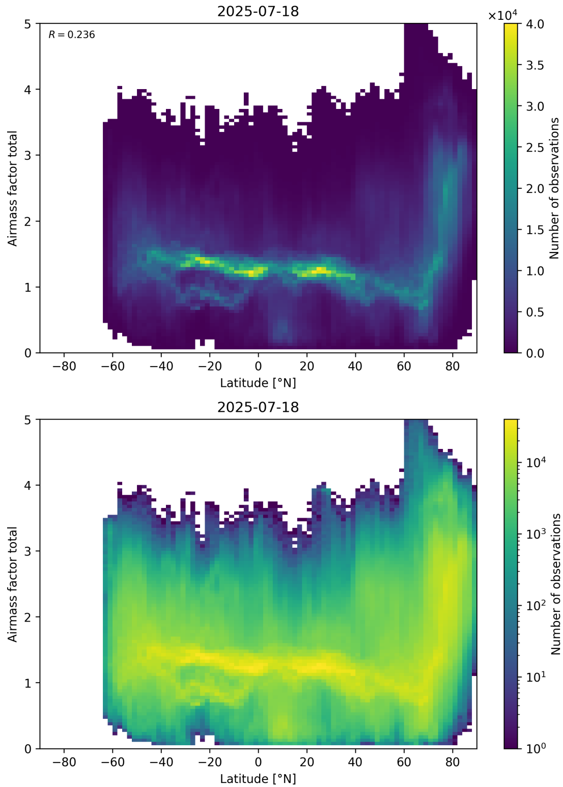
Figure 161: Scatter density plot of “Latitude” against “Airmass factor total” for 2025-07-18 to 2025-07-19.
