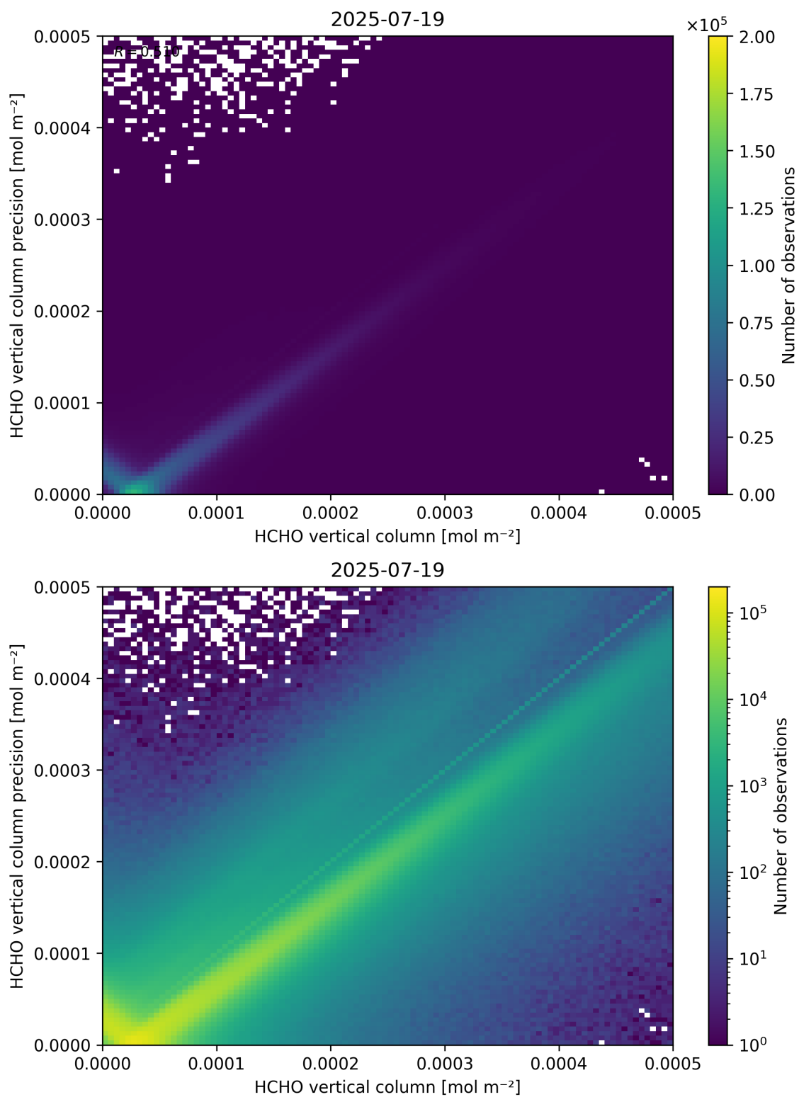
Figure 134: Scatter density plot of “HCHO vertical column” against “HCHO vertical column precision” for 2025-07-19 to 2025-07-20.
