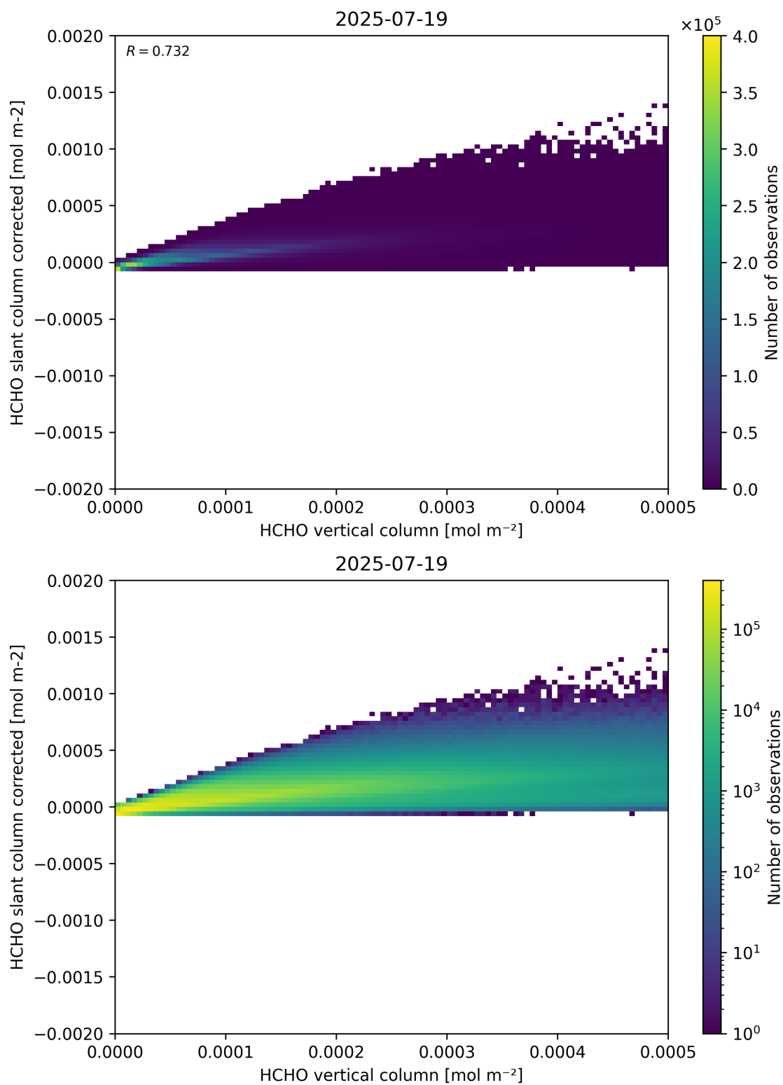
Figure 127: Scatter density plot of “HCHO vertical column” against “HCHO slant column corrected” for 2025-07-19 to 2025-07-20.
