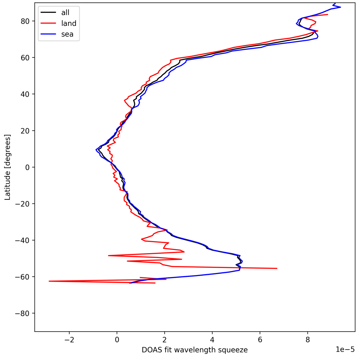
Figure 31: Zonal average of “DOAS fit wavelength squeeze” for 2025-07-19 to 2025-07-20.
