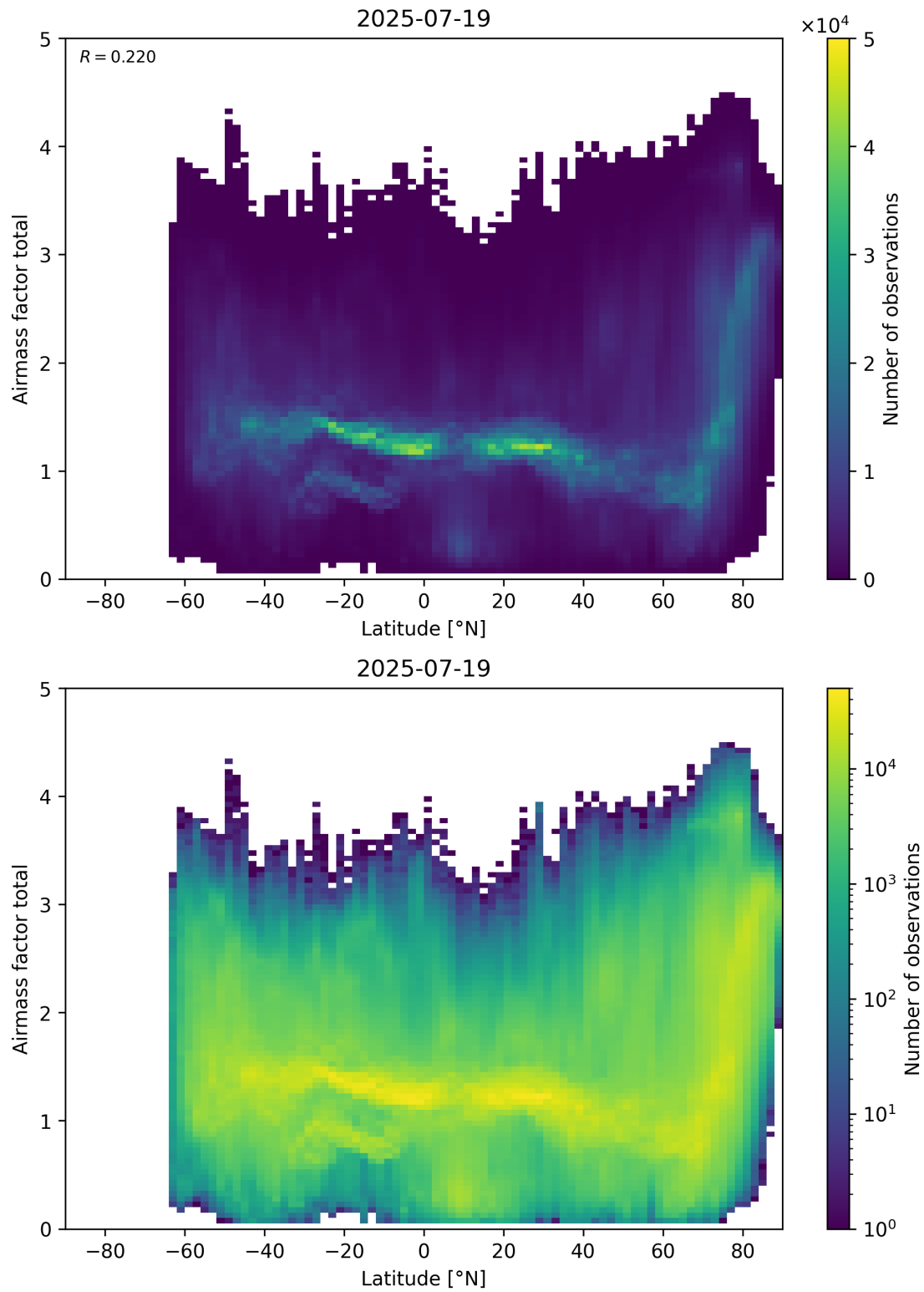
Figure 161: Scatter density plot of “Latitude” against “Airmass factor total” for 2025-07-19 to 2025-07-20.
