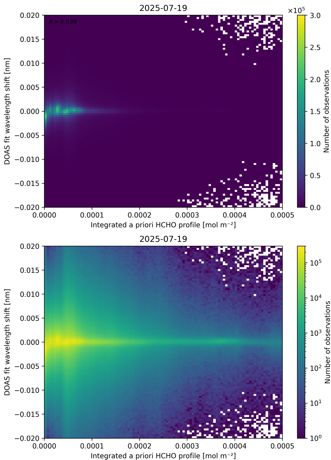
Figure 149: Scatter density plot of “Integrated a priori HCHO profile” against “DOAS fit wavelength shift” for 2025-07-19 to 2025-07-20.
