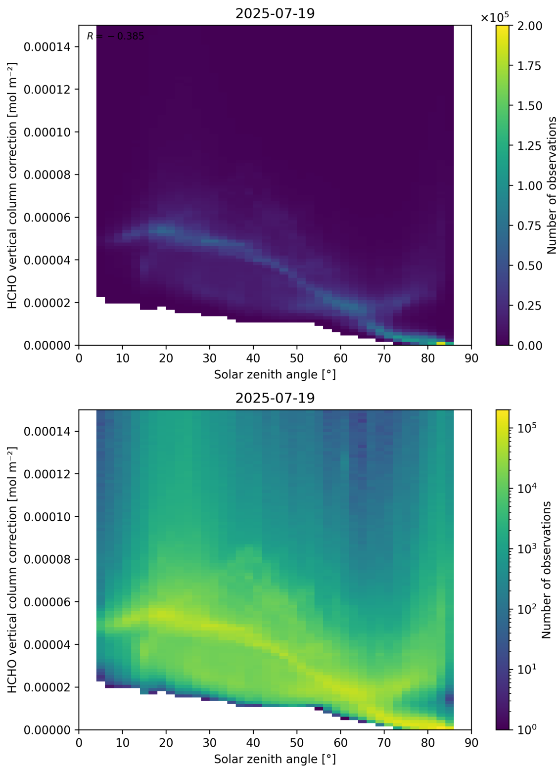
Figure 178: Scatter density plot of “Solar zenith angle” against “HCHO vertical column correction” for 2025-07-19 to 2025-07-20.
