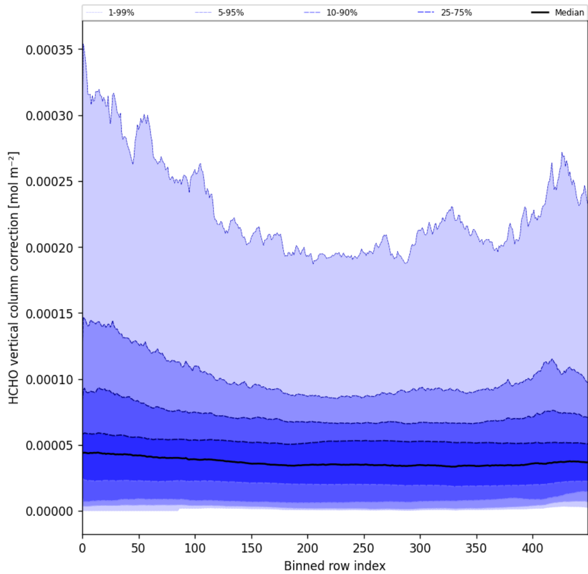
Figure 51: Along track statistics of “HCHO vertical column correction” for 2025-07-19 to 2025-07-20
