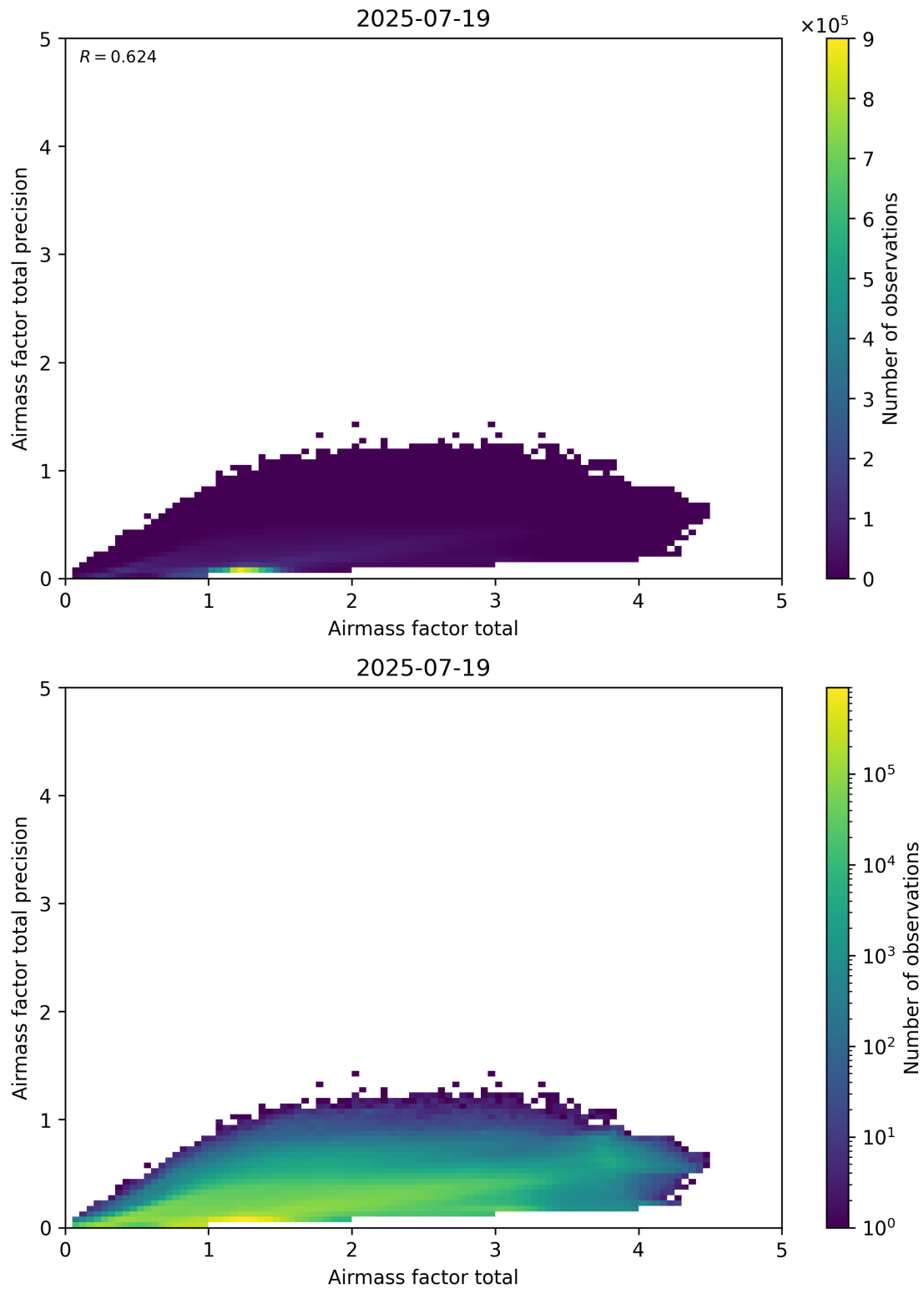
Figure 103: Scatter density plot of “Airmass factor total” against “Airmass factor total precision” for 2025-07-19 to 2025-07-20.
