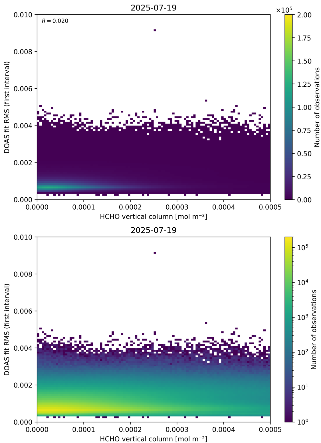
Figure 123: Scatter density plot of “HCHO vertical column” against “DOAS fit RMS (first interval)” for 2025-07-19 to 2025-07-20.
