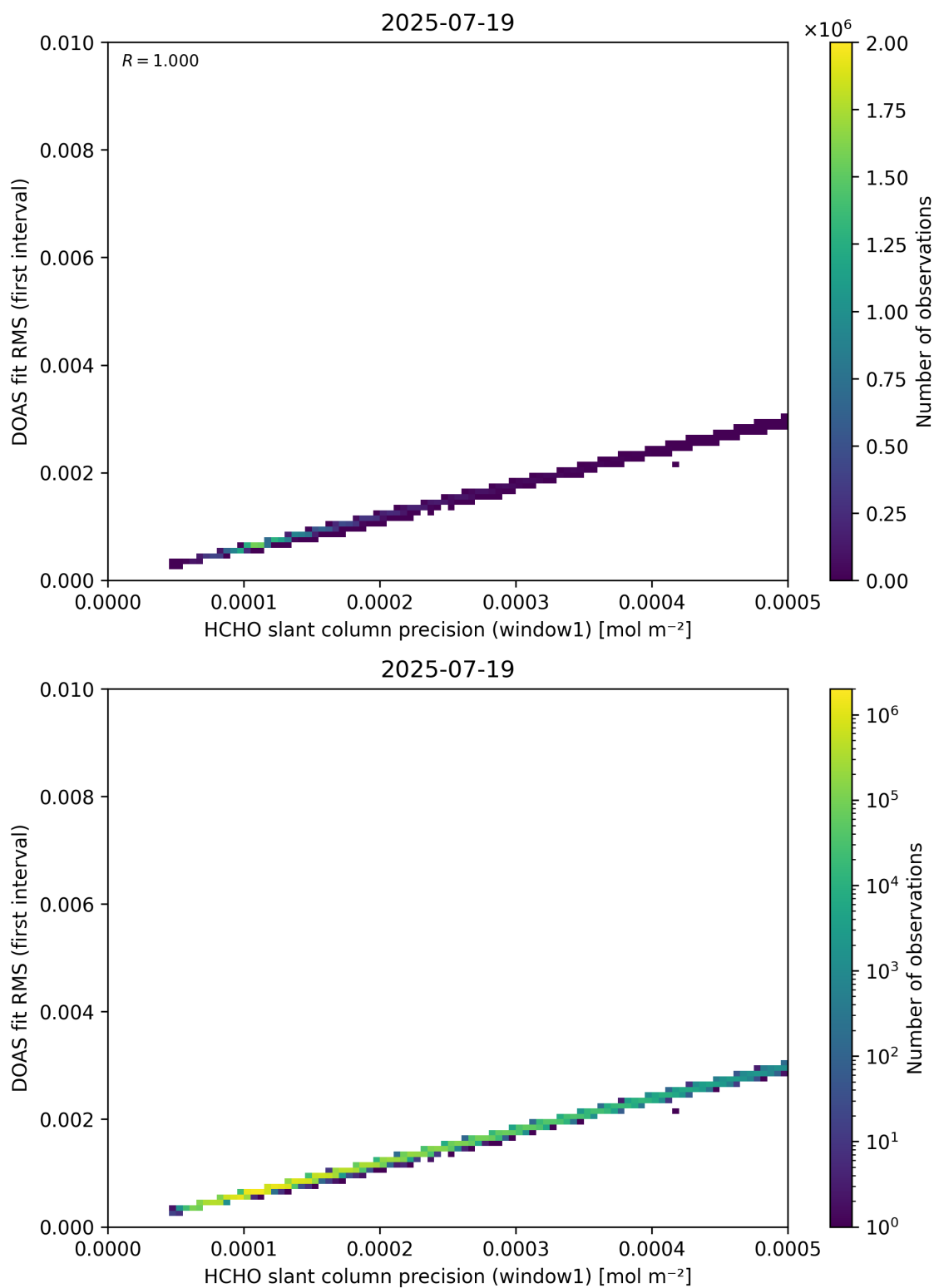
Figure 88: Scatter density plot of “HCHO slant column precision (window1)” against “DOAS fit RMS (first interval)” for 2025-07-19 to 2025-07-20.
