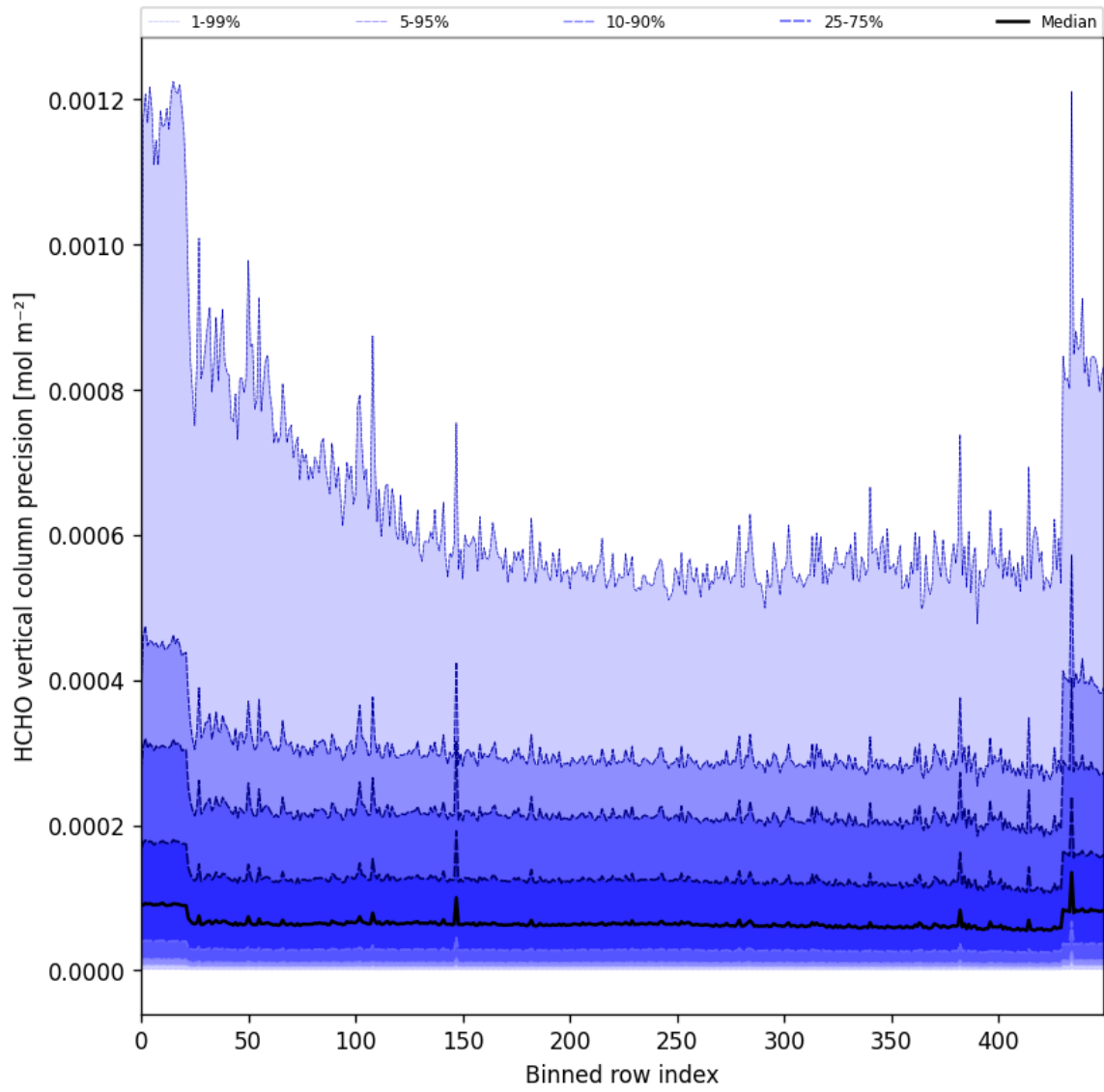
Figure 50: Along track statistics of “HCHO vertical column precision” for 2025-07-19 to 2025-07-20
