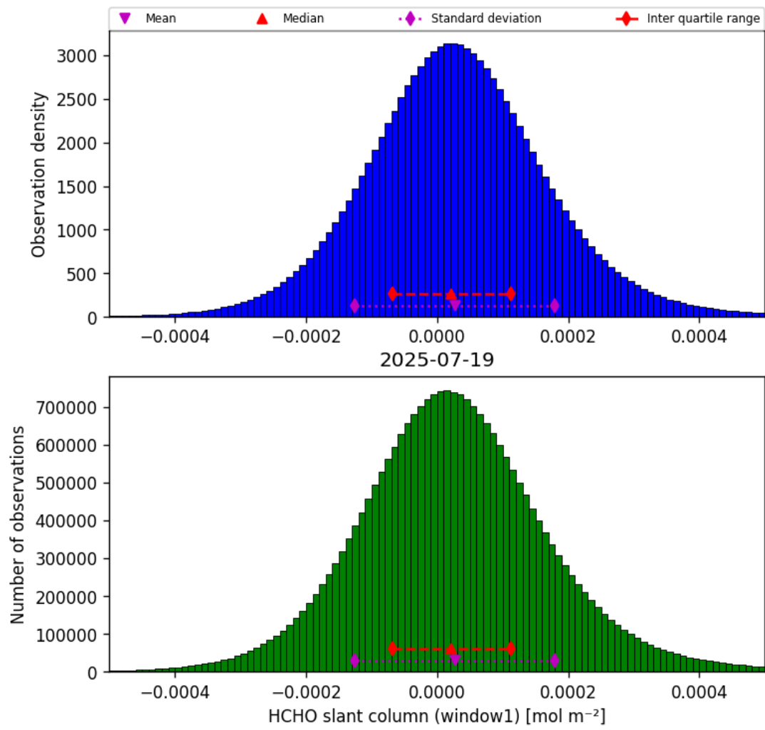
Figure 38: Histogram of “HCHO slant column (window1)” for 2025-07-19 to 2025-07-20
