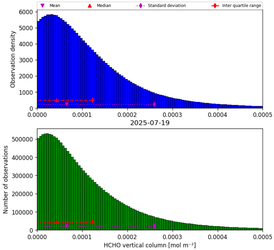
Figure 35: Histogram of “HCHO vertical column” for 2025-07-19 to 2025-07-20
