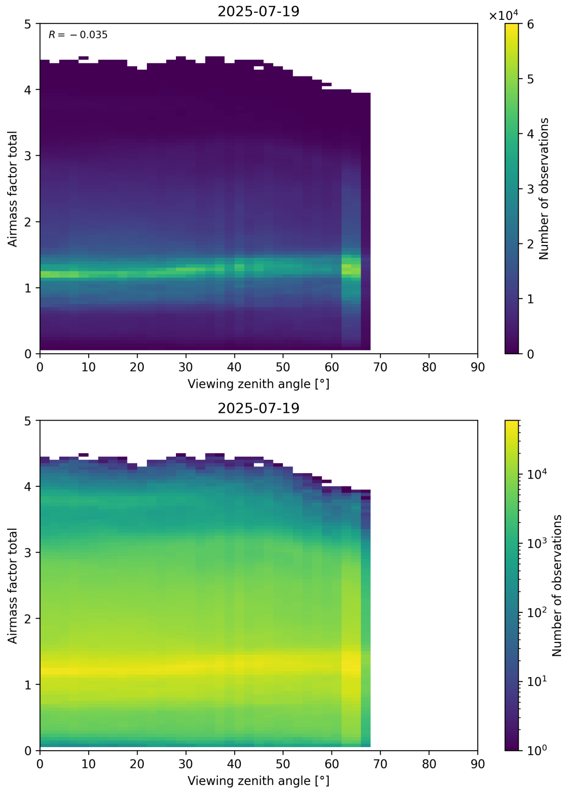
Figure 190: Scatter density plot of “Viewing zenith angle” against “Airmass factor total” for 2025-07-19 to 2025-07-20.
