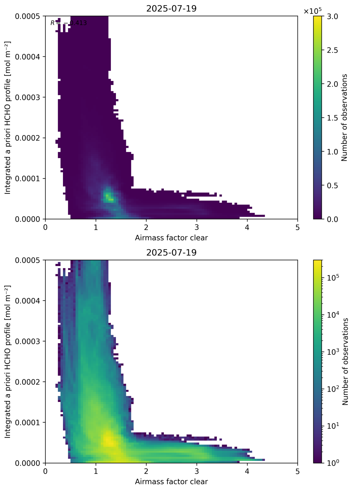
Figure 76: Scatter density plot of “Airmass factor clear” against “Integrated a priori HCHO profile” for 2025-07-19 to 2025-07-20.
