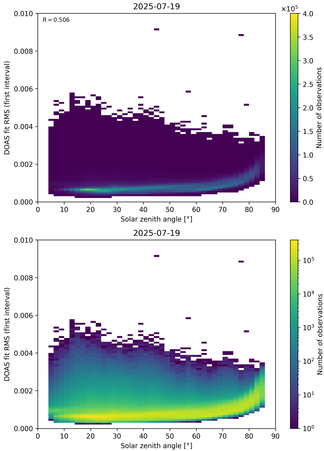
Figure 167: Scatter density plot of “Solar zenith angle” against “DOAS fit RMS (first interval)” for 2025-07-19 to 2025-07-20.
