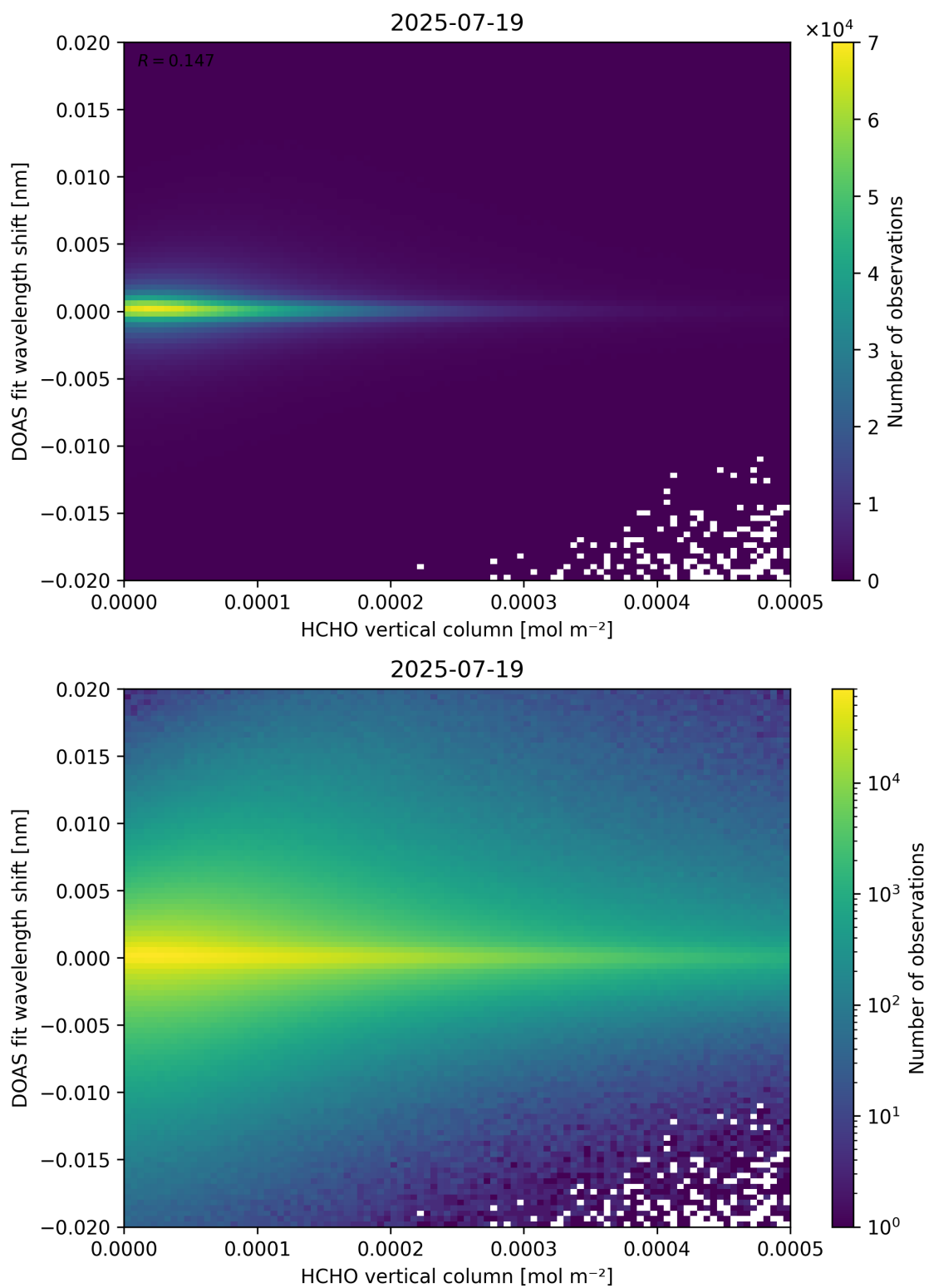
Figure 124: Scatter density plot of “HCHO vertical column” against “DOAS fit wavelength shift” for 2025-07-19 to 2025-07-20.
