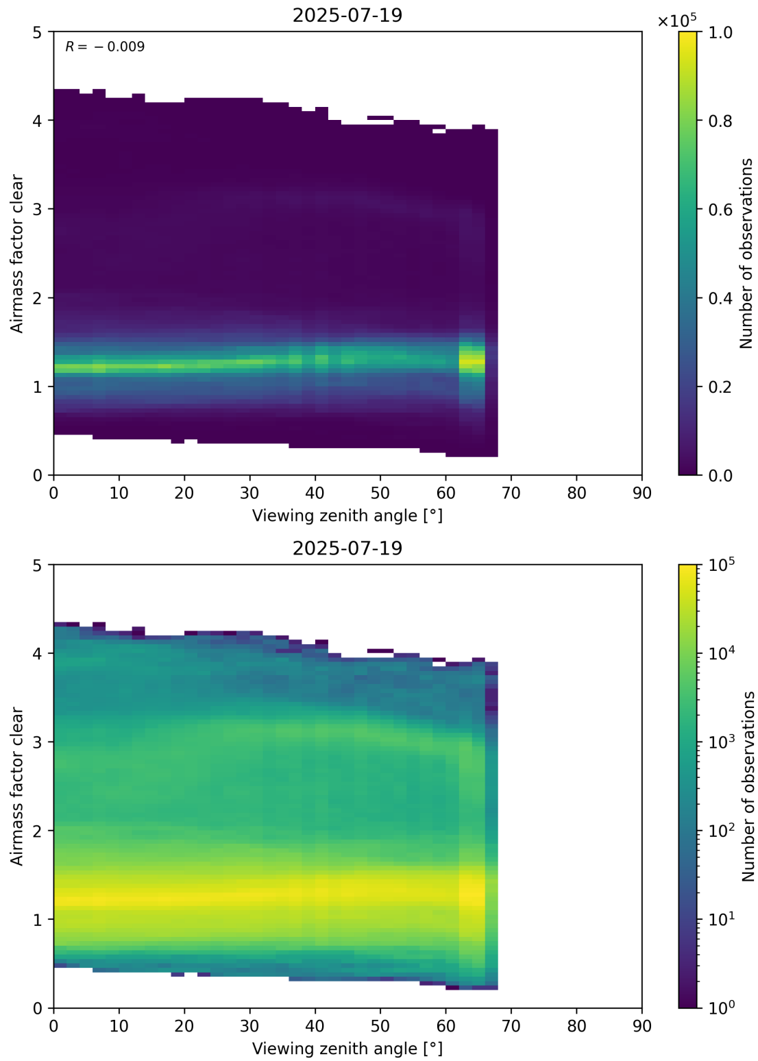
Figure 185: Scatter density plot of “Viewing zenith angle” against “Airmass factor clear” for 2025-07-19 to 2025-07-20.
