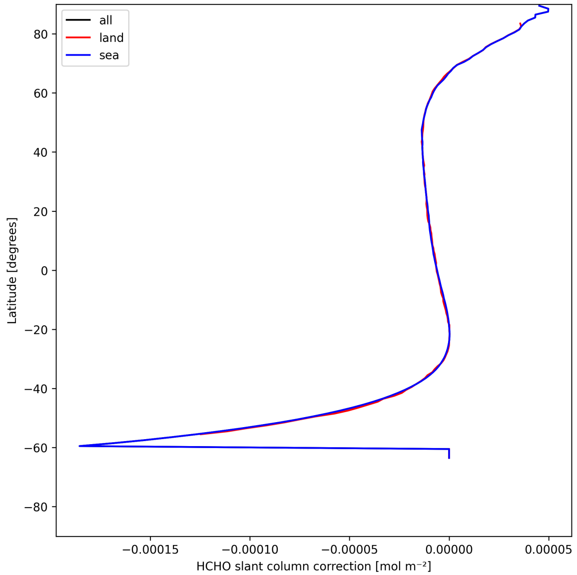
Figure 33: Zonal average of “HCHO slant column correction” for 2025-07-19 to 2025-07-20.
