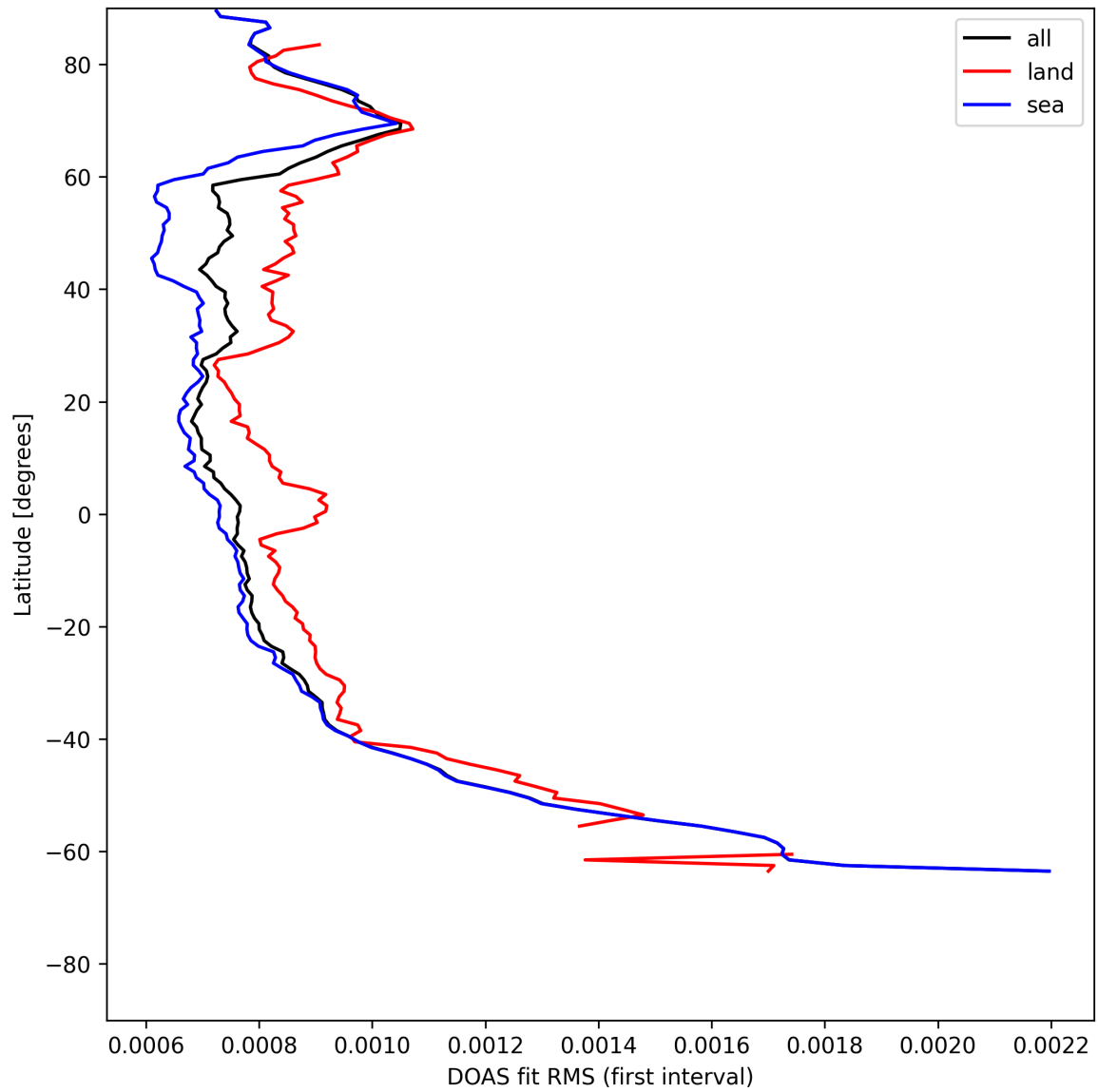
Figure 32: Zonal average of “DOAS fit RMS (first interval)” for 2025-07-19 to 2025-07-20.
