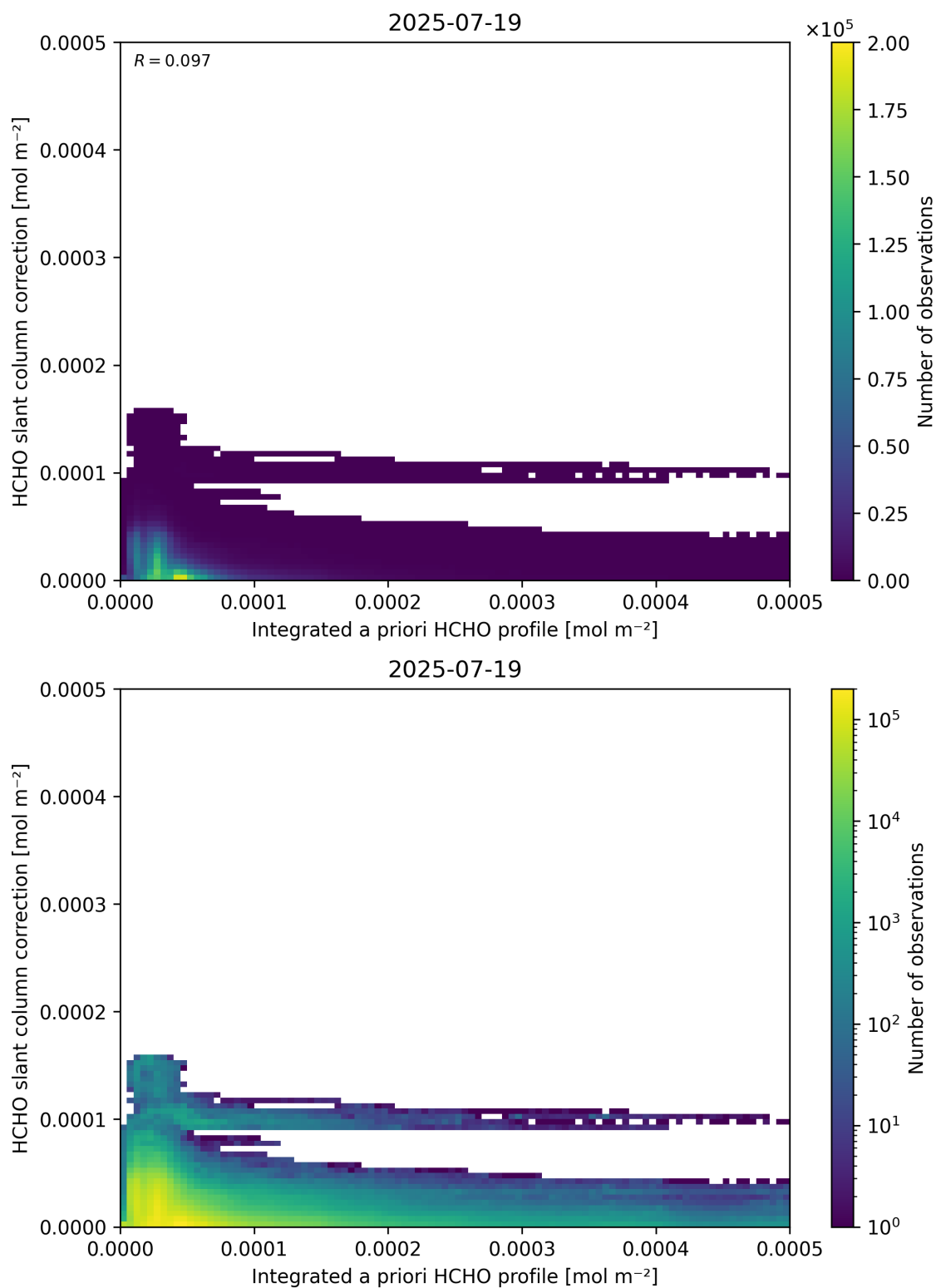
Figure 152: Scatter density plot of “Integrated a priori HCHO profile” against “HCHO slant column correction” for 2025-07-19 to 2025-07-20.
