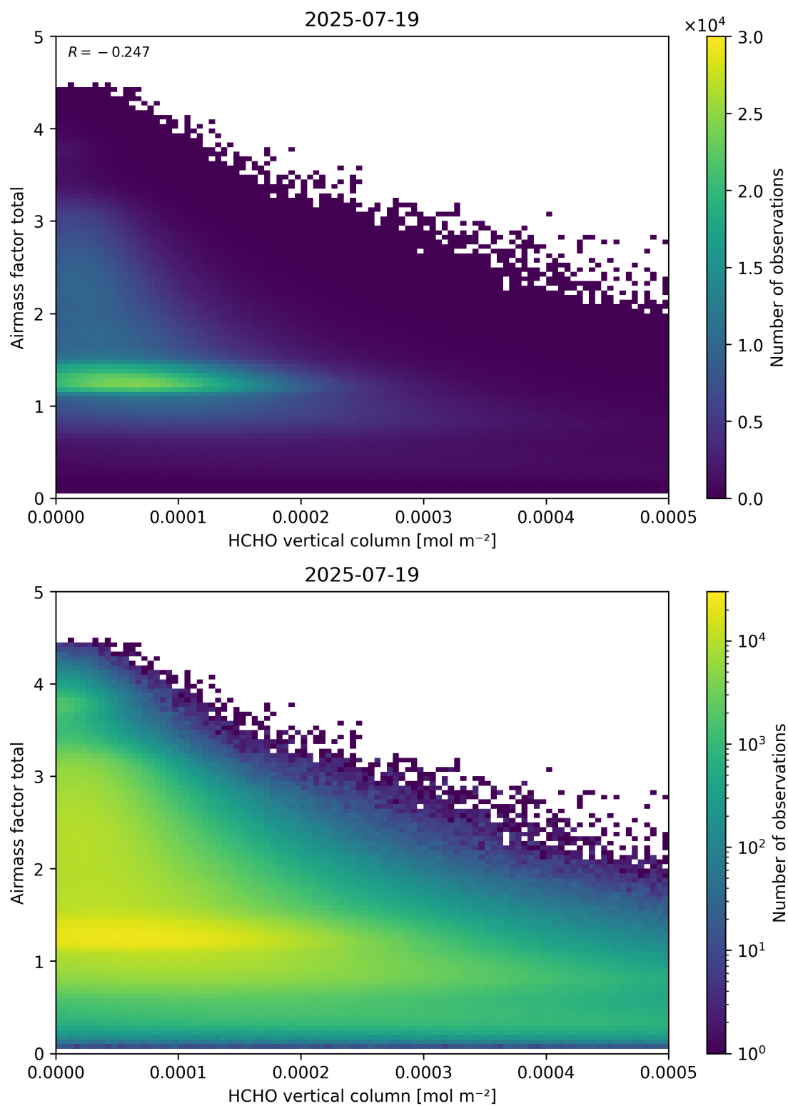
Figure 131: Scatter density plot of “HCHO vertical column” against “Airmass factor total” for 2025-07-19 to 2025-07-20.
