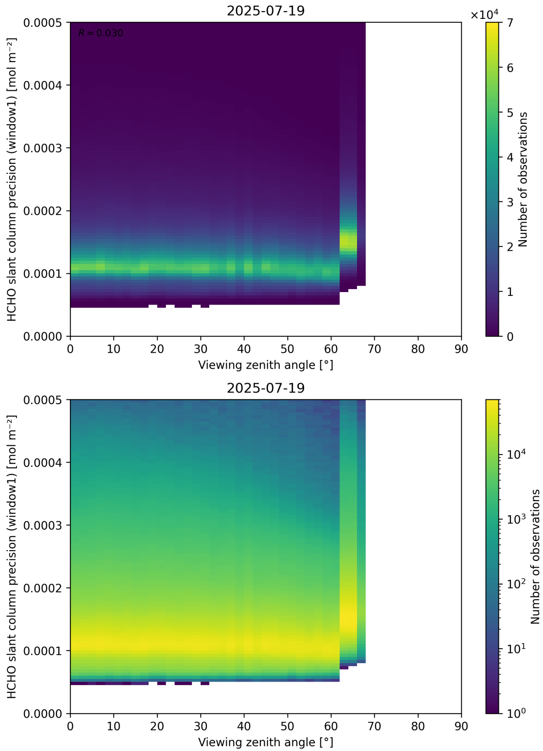
Figure 189: Scatter density plot of “Viewing zenith angle” against “HCHO slant column precision (window1)” for 2025-07-19 to 2025-07-20.
