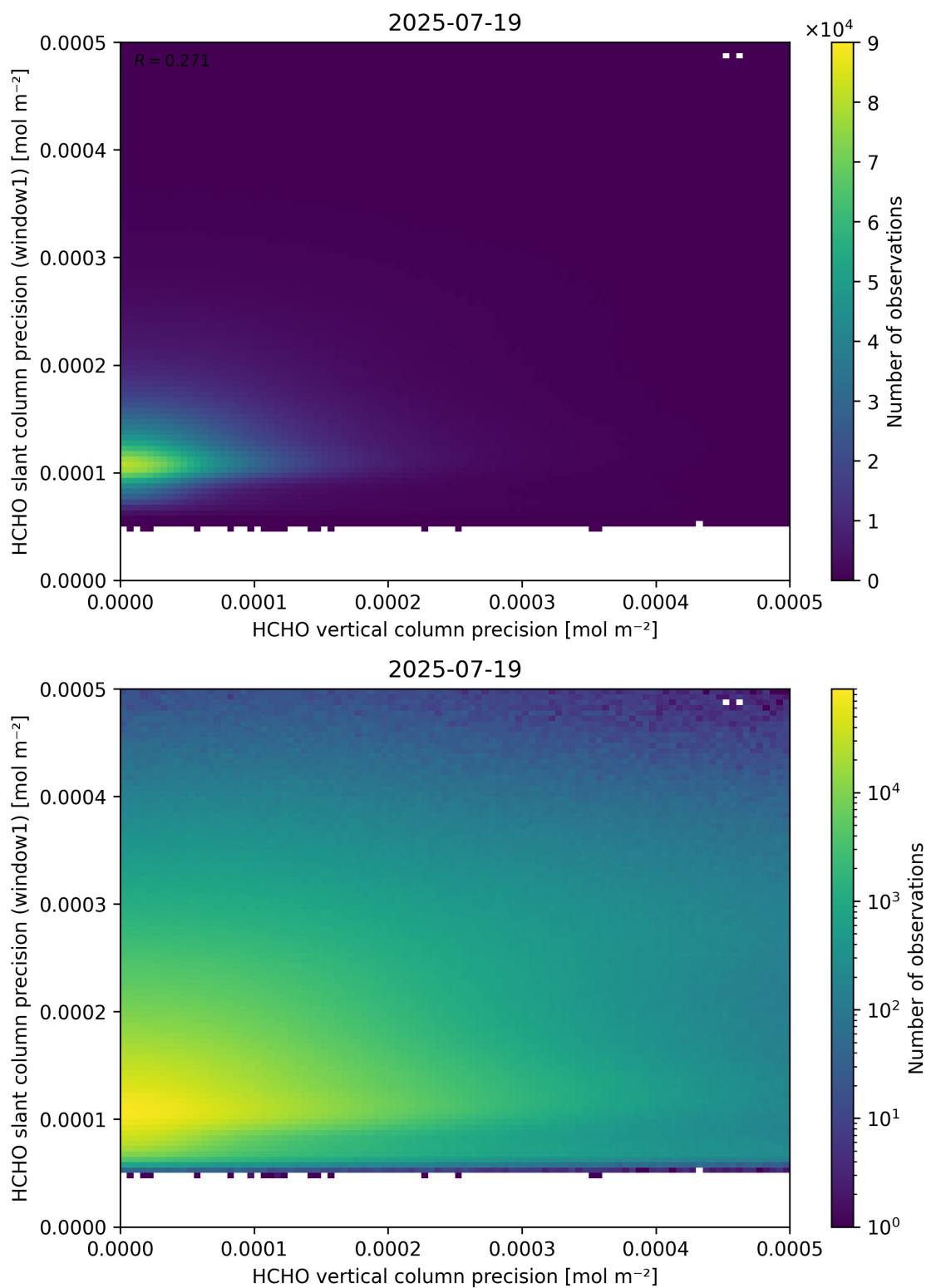
Figure 143: Scatter density plot of “HCHO vertical column precision” against “HCHO slant column precision (window1)” for 2025-07-19 to 2025-07-20.
