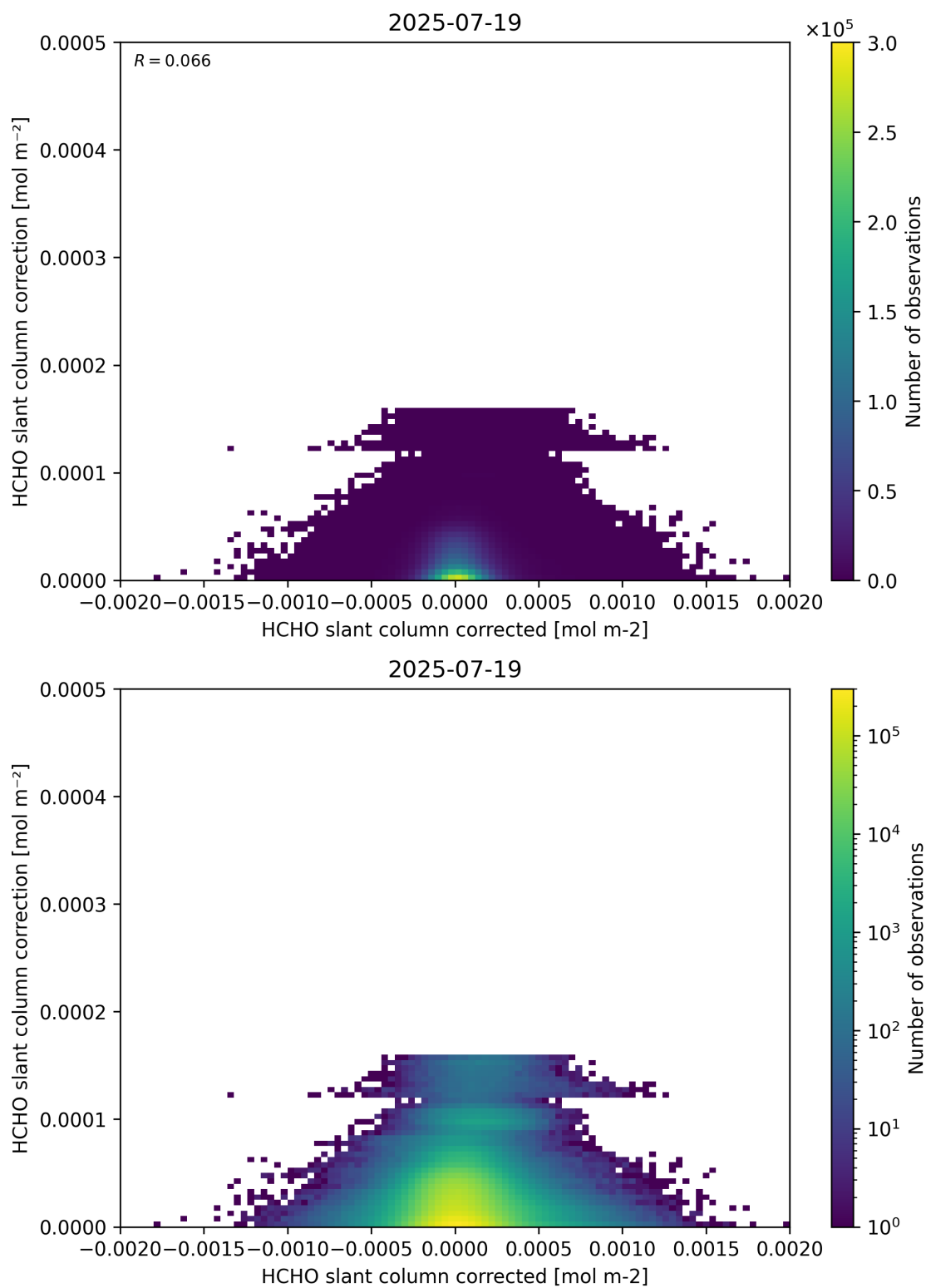
Figure 77: Scatter density plot of “HCHO slant column corrected” against “HCHO slant column correction” for 2025-07-19 to 2025-07-20.
