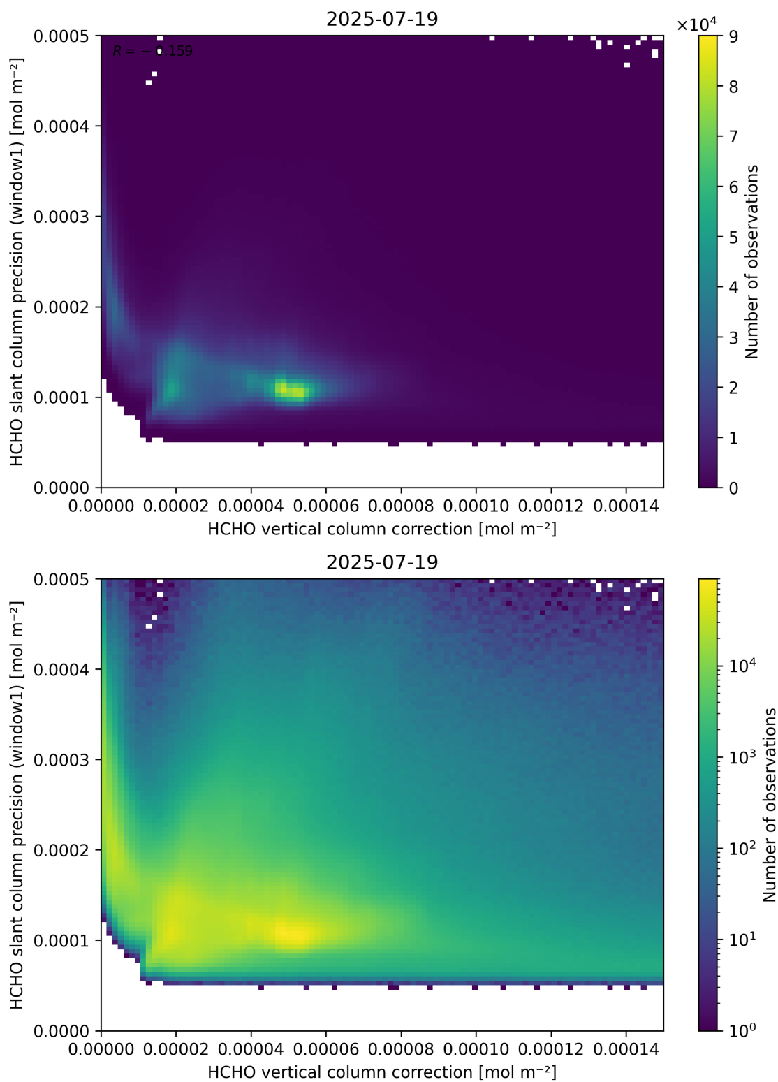
Figure 119: Scatter density plot of “HCHO vertical column correction” against “HCHO slant column precision (window1)” for 2025-07-19 to 2025-07-20.
