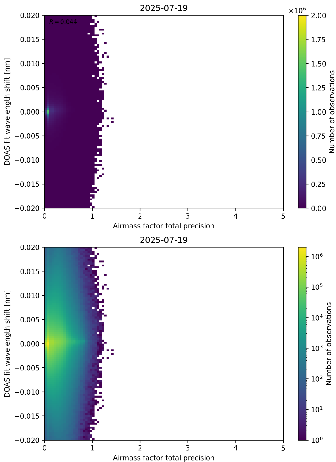
Figure 106: Scatter density plot of “Airmass factor total precision” against “DOAS fit wavelength shift” for 2025-07-19 to 2025-07-20.
