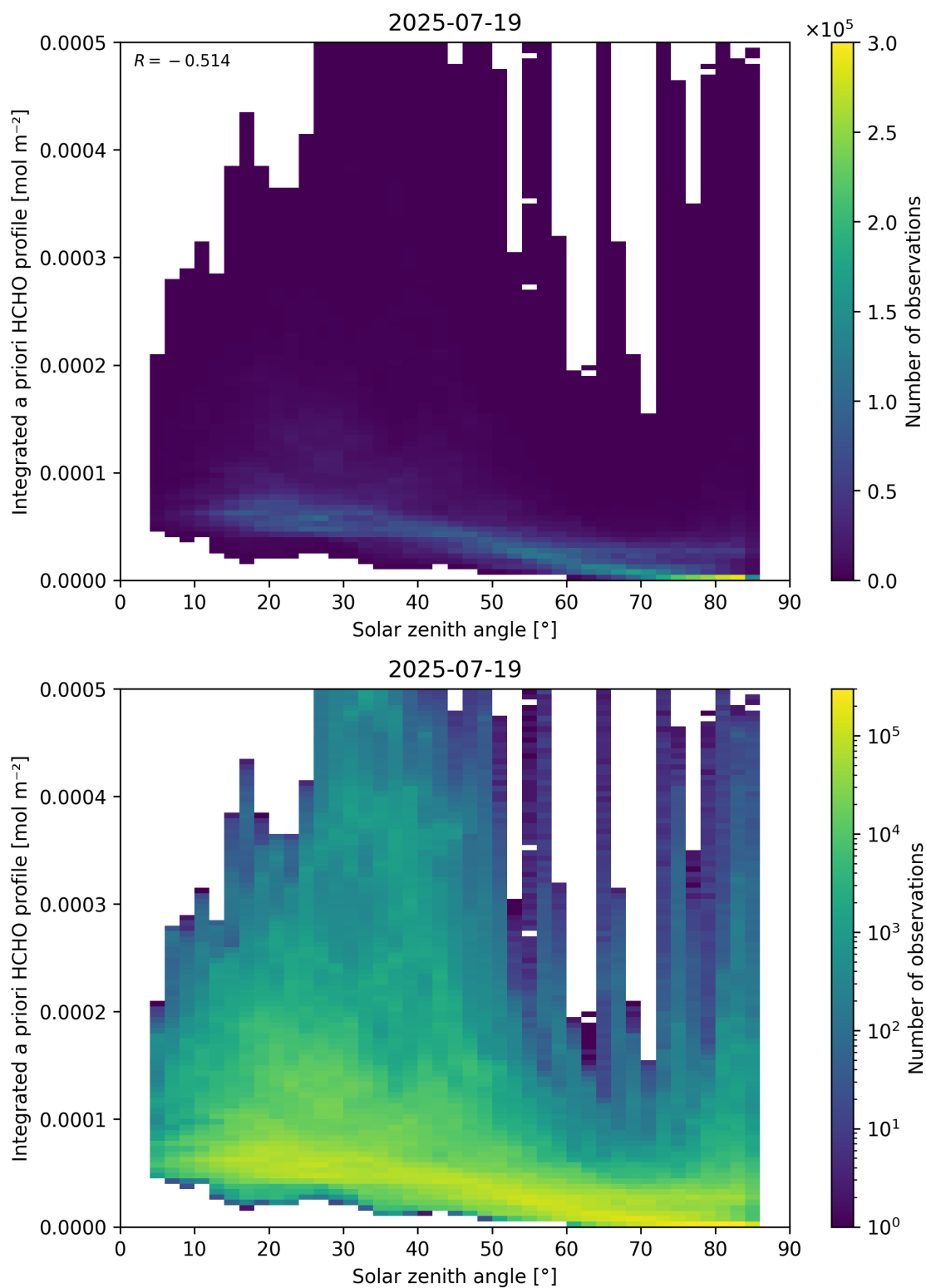
Figure 180: Scatter density plot of “Solar zenith angle” against “Integrated a priori HCHO profile” for 2025-07-19 to 2025-07-20.
