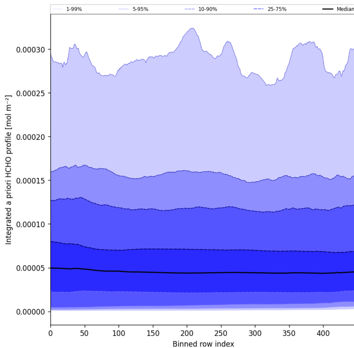
Figure 57: Along track statistics of "Integrated a priori HCHO profile" for 2025-07-19 to 2025-07-20
