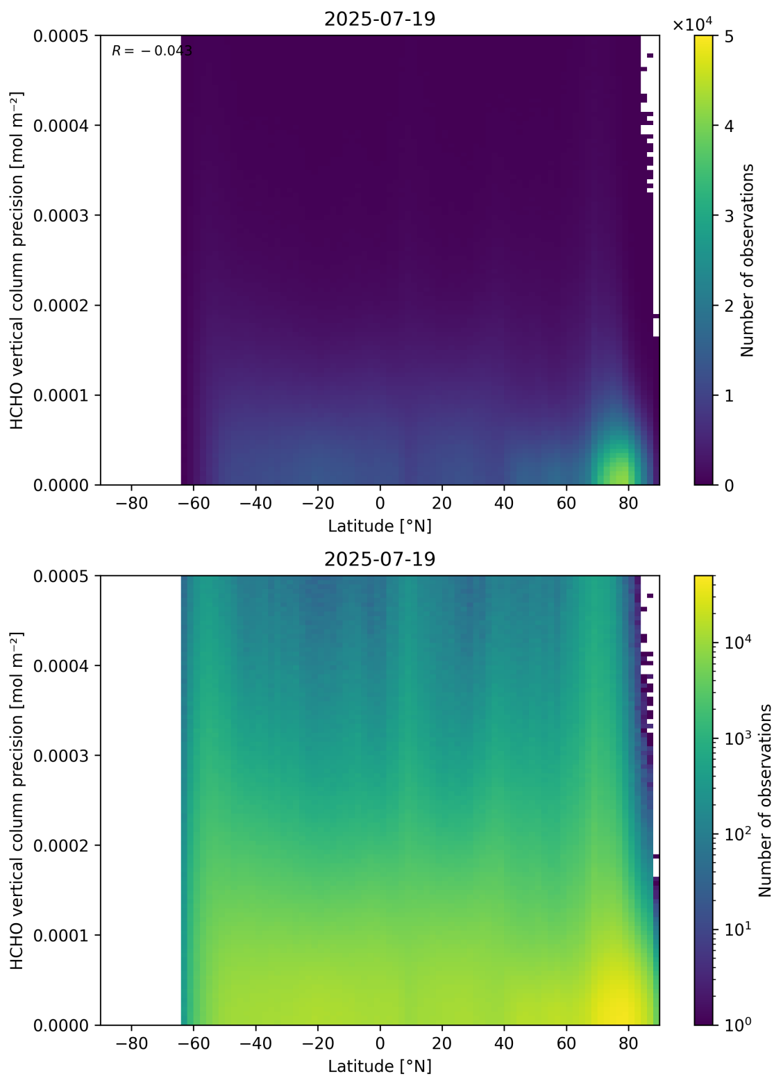
Figure 165: Scatter density plot of “Latitude” against “HCHO vertical column precision” for 2025-07-19 to 2025-07-20.
