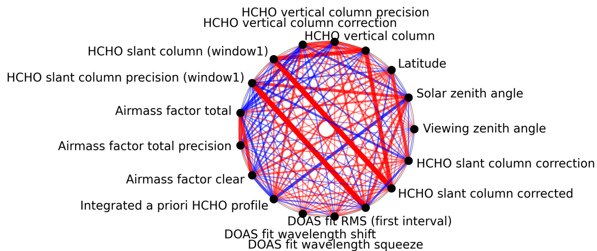
Figure 1: Map of correlation graph for 2025-07-19 to 2025-07-20.
