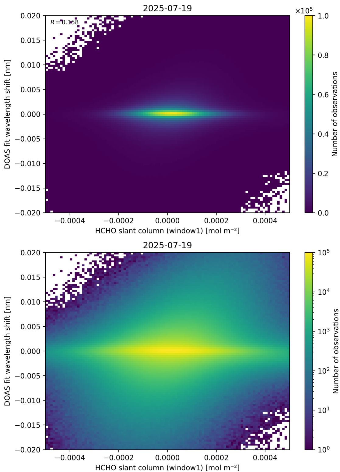
Figure 79: Scatter density plot of “HCHO slant column (window1)” against “DOAS fit wavelength shift” for 2025-07-19 to 2025-07-20.
