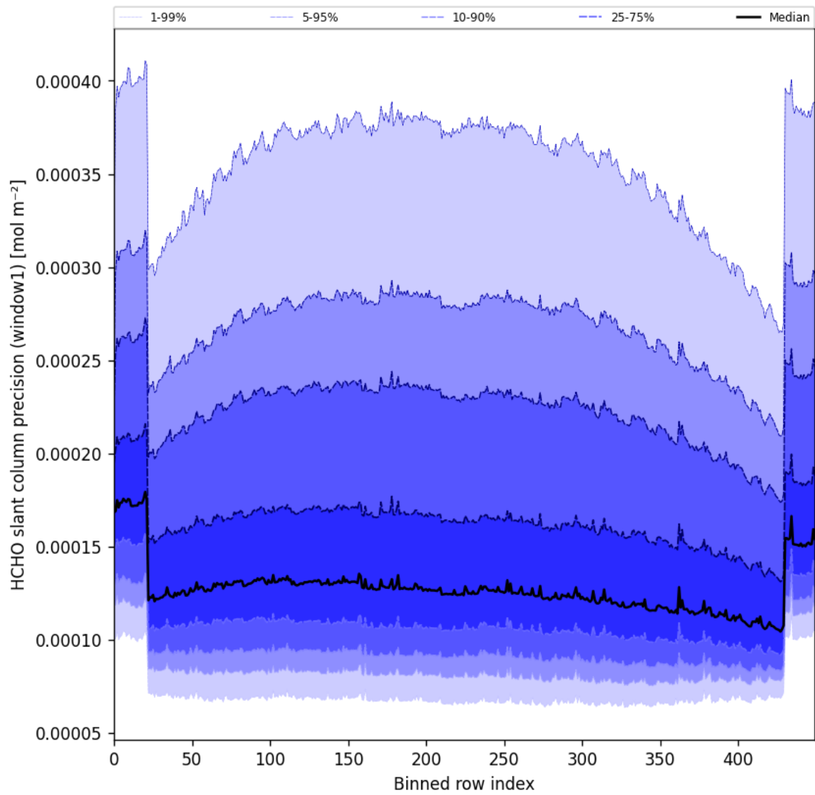
Figure 53: Along track statistics of “HCHO slant column precision (window1)” for 2025-07-19 to 2025-07-20
