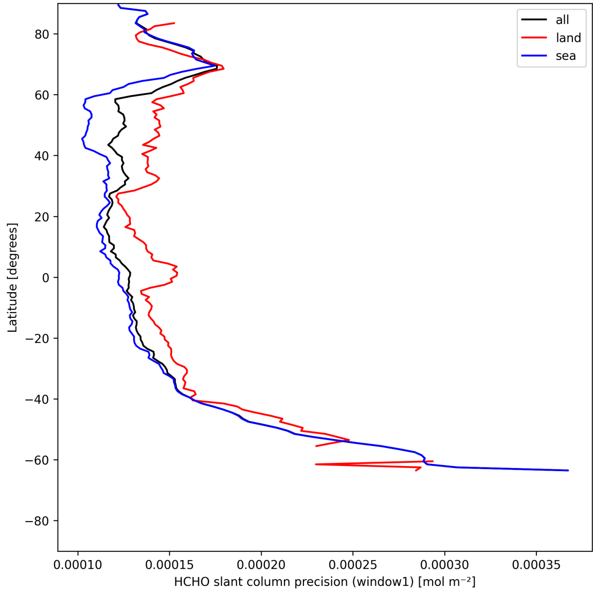
Figure 25: Zonal average of “HCHO slant column precision (window1)” for 2025-07-19 to 2025-07-20.
