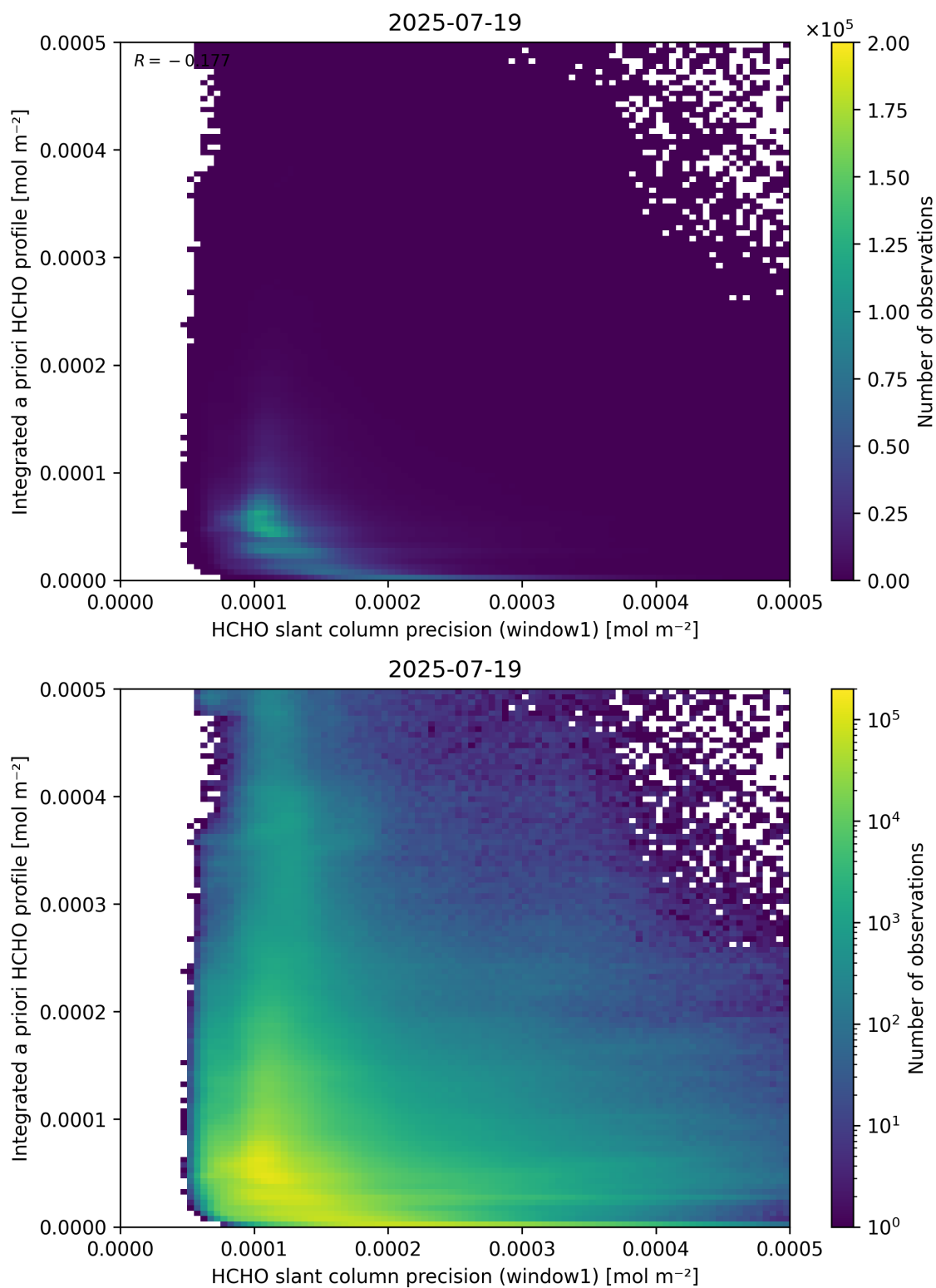
Figure 96: Scatter density plot of “HCHO slant column precision (window1)” against “Integrated a priori HCHO profile” for 2025-07-19 to 2025-07-20.
