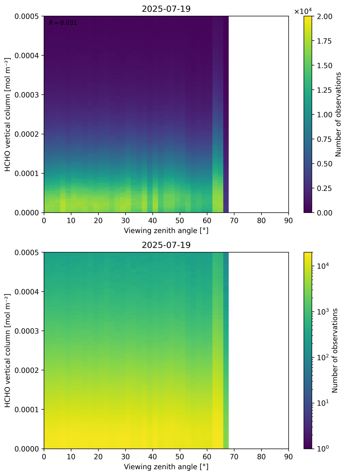
Figure 192: Scatter density plot of “Viewing zenith angle” against “HCHO vertical column” for 2025-07-19 to 2025-07-20.
