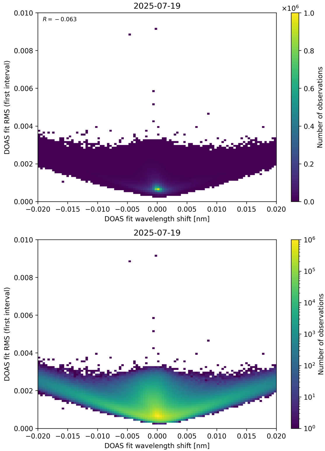
Figure 64: Scatter density plot of “DOAS fit wavelength shift” against “DOAS fit RMS (first interval)” for 2025-07-19 to 2025-07-20.
