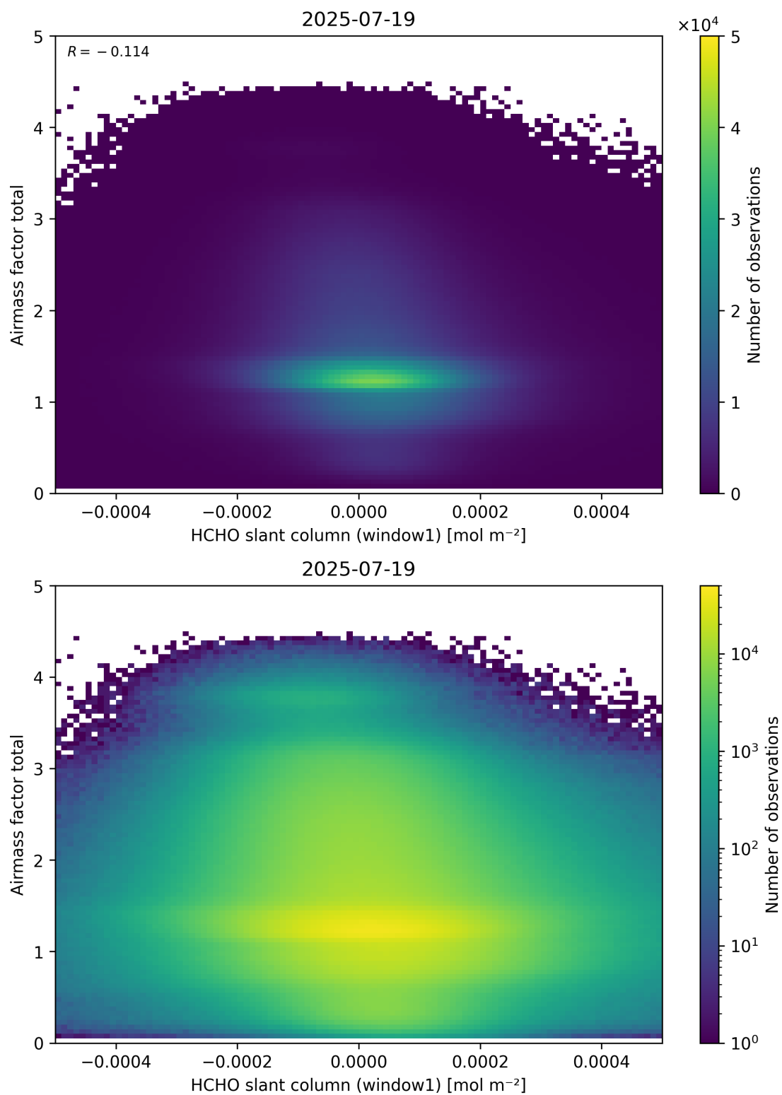
Figure 85: Scatter density plot of “HCHO slant column (window1)” against “Airmass factor total” for 2025-07-19 to 2025-07-20.
