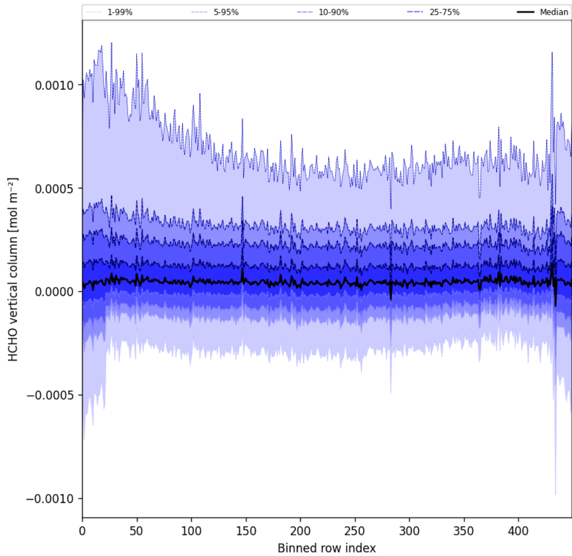
Figure 49: Along track statistics of “HCHO vertical column” for 2025-07-19 to 2025-07-20
