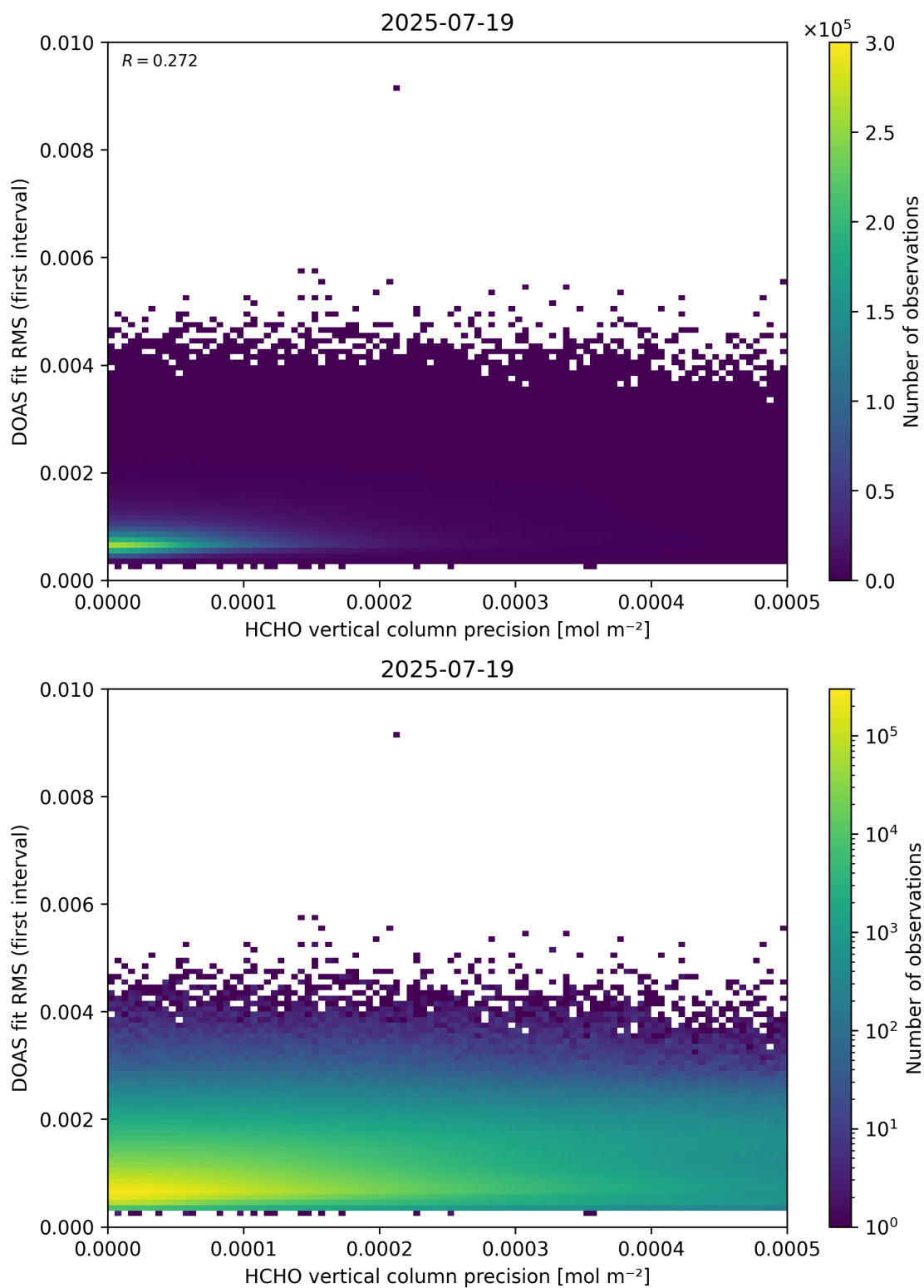
Figure 136: Scatter density plot of “HCHO vertical column precision” against “DOAS fit RMS (first interval)” for 2025-07-19 to 2025-07-20.
