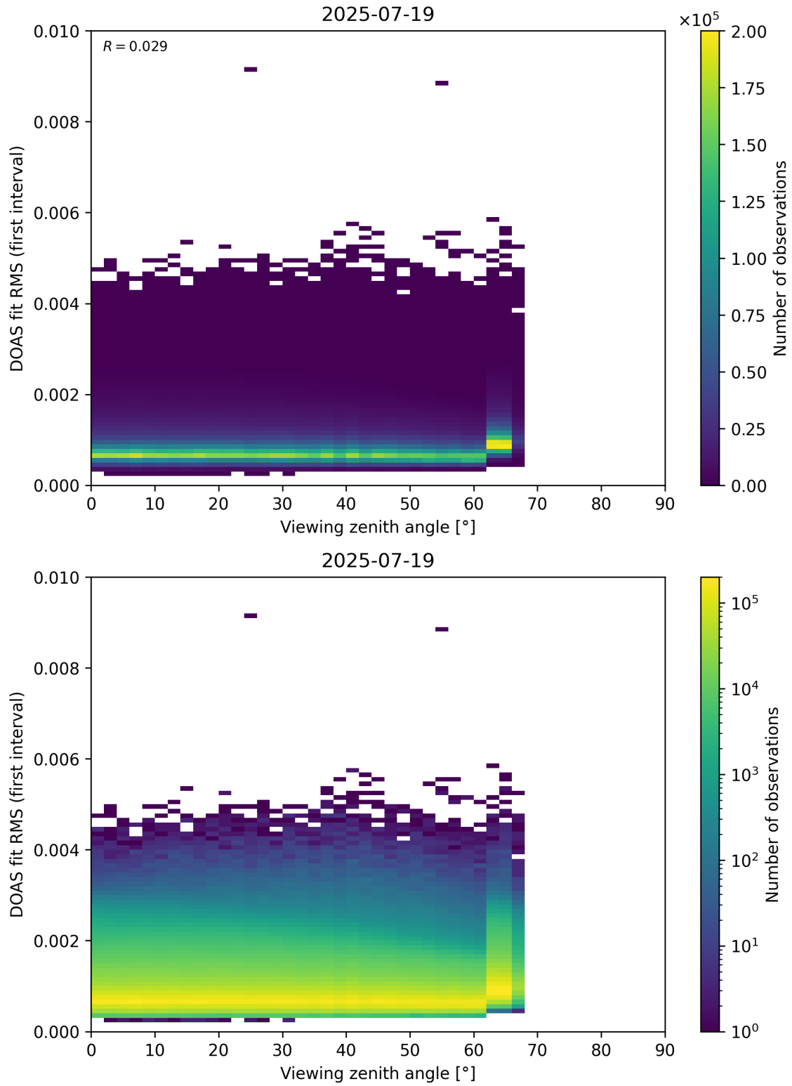
Figure 182: Scatter density plot of “Viewing zenith angle” against “DOAS fit RMS (first interval)” for 2025-07-19 to 2025-07-20.
