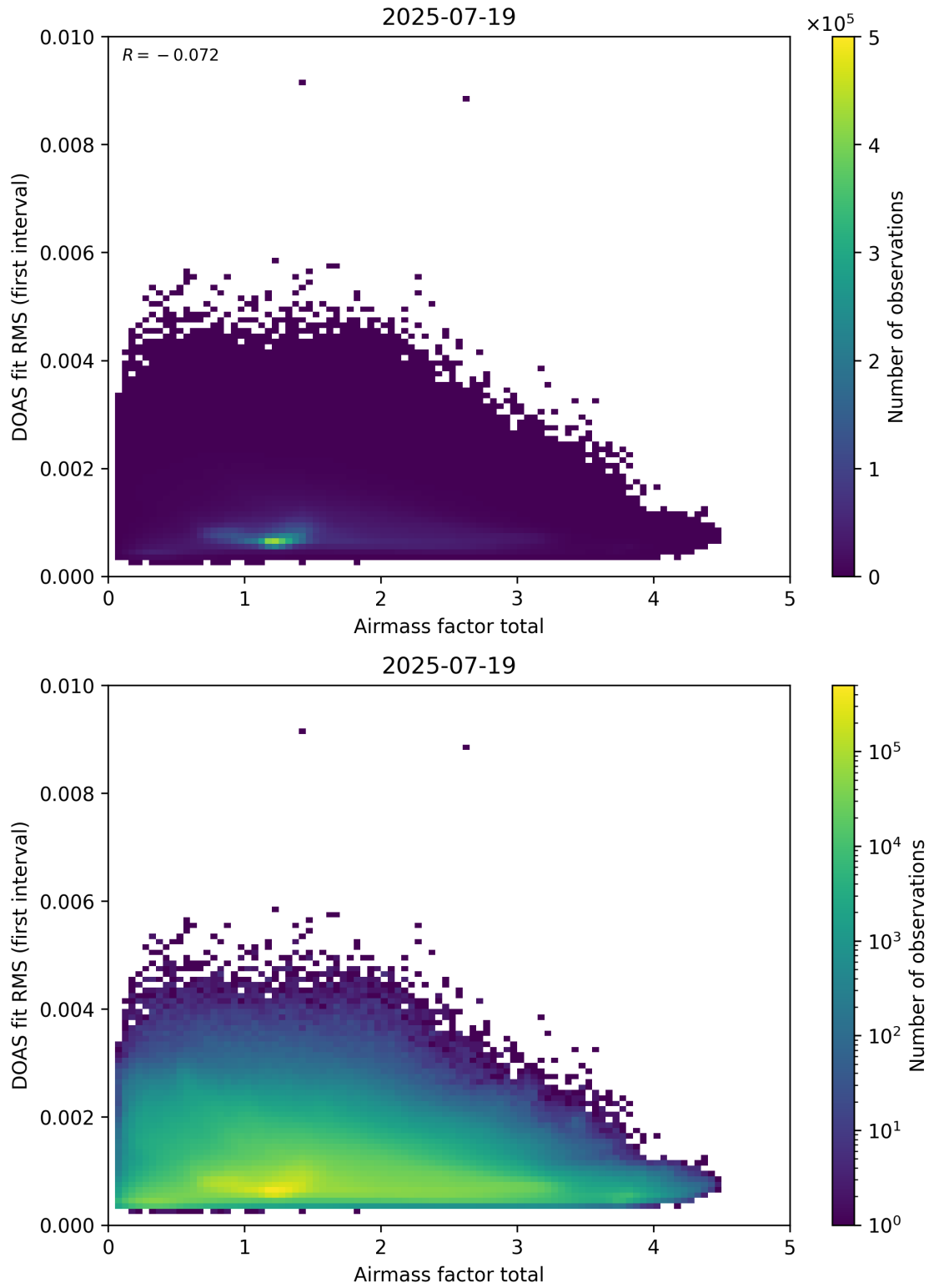
Figure 97: Scatter density plot of “Airmass factor total” against “DOAS fit RMS (first interval)” for 2025-07-19 to 2025-07-20.
