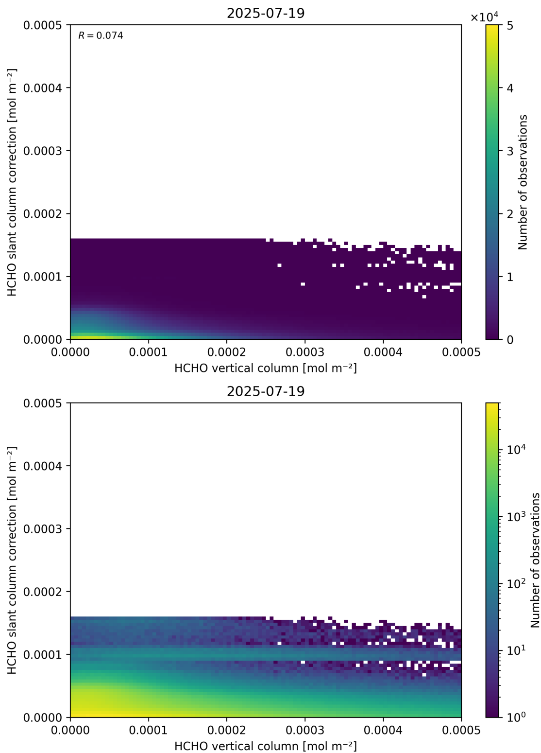
Figure 128: Scatter density plot of “HCHO vertical column” against “HCHO slant column correction” for 2025-07-19 to 2025-07-20.
