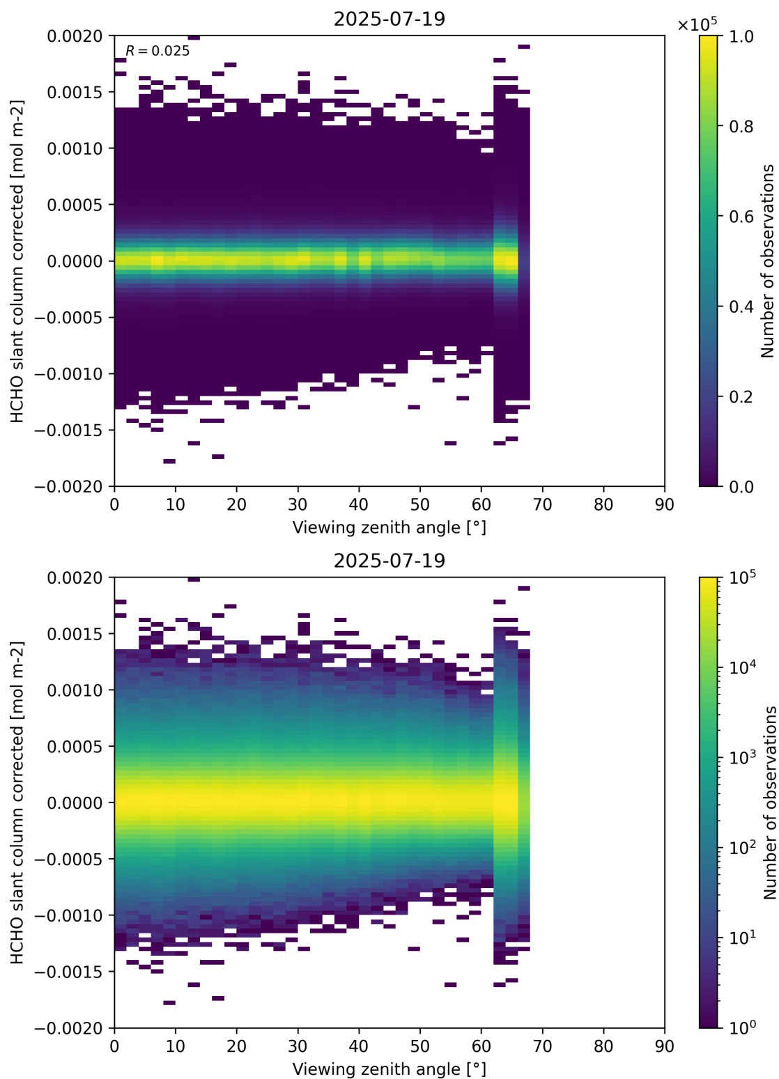
Figure 186: Scatter density plot of “Viewing zenith angle” against “HCHO slant column corrected” for 2025-07-19 to 2025-07-20.
