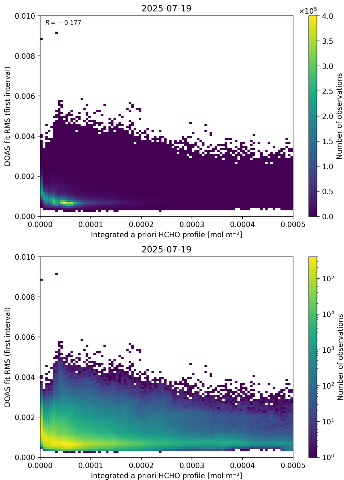
Figure 148: Scatter density plot of “Integrated a priori HCHO profile” against “DOAS fit RMS (first interval)” for 2025-07-19 to 2025-07-20.
