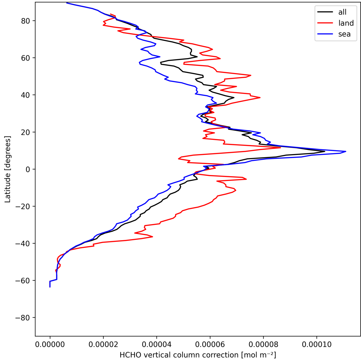
Figure 23: Zonal average of “HCHO vertical column correction” for 2025-07-19 to 2025-07-20.
