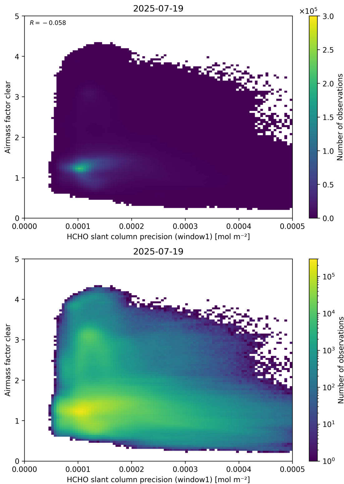
Figure 91: Scatter density plot of “HCHO slant column precision (window1)” against “Airmass factor clear” for 2025-07-19 to 2025-07-20.
