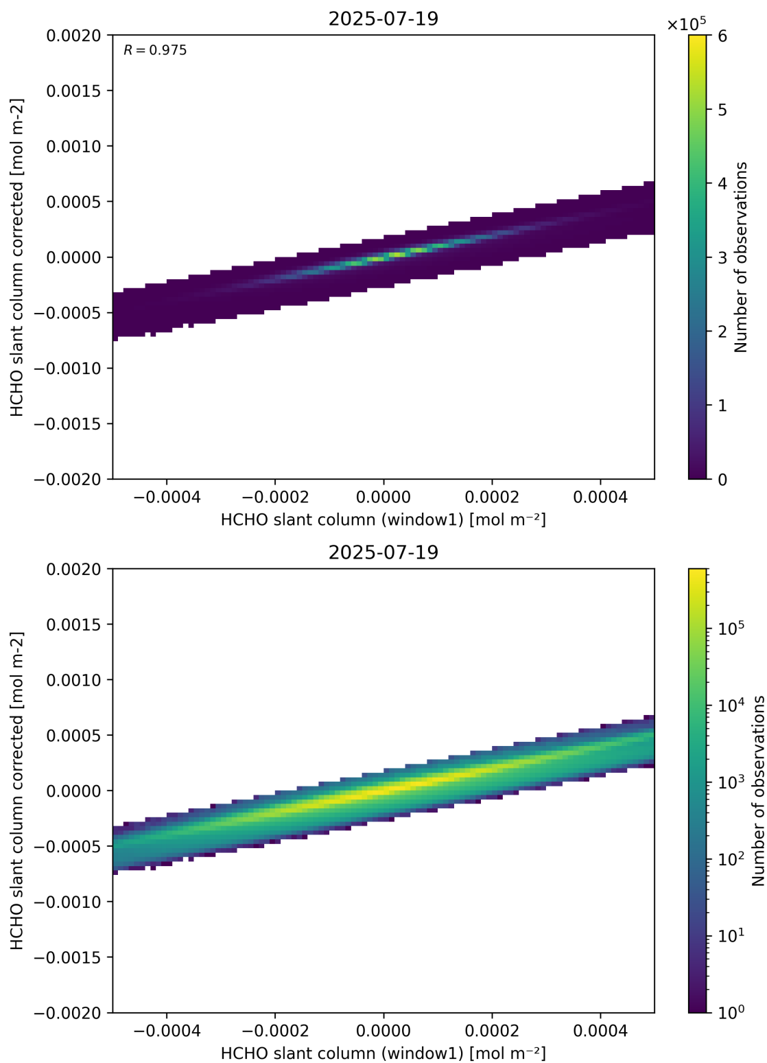
Figure 82: Scatter density plot of “HCHO slant column (window1)” against “HCHO slant column corrected” for 2025-07-19 to 2025-07-20.
