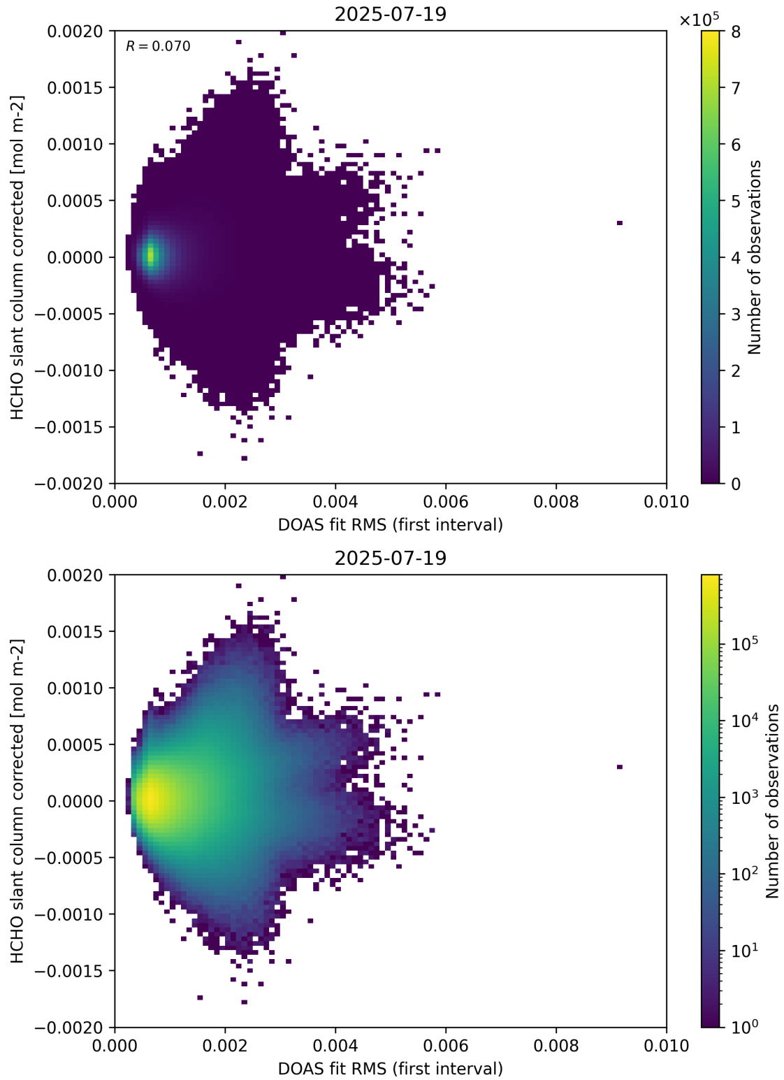
Figure 62: Scatter density plot of “DOAS fit RMS (first interval)” against “HCHO slant column corrected” for 2025-07-19 to 2025-07-20.
