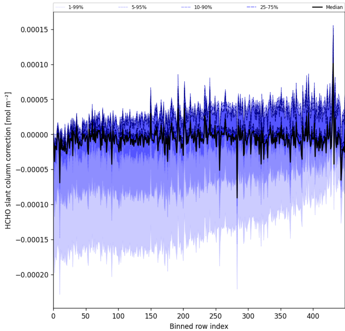
Figure 61: Along track statistics of “HCHO slant column correction” for 2025-07-19 to 2025-07-20
