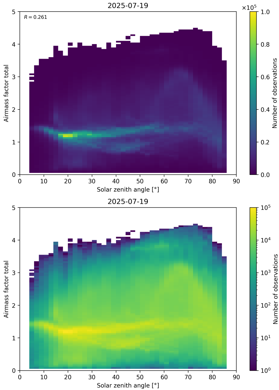
Figure 175: Scatter density plot of “Solar zenith angle” against “Airmass factor total” for 2025-07-19 to 2025-07-20.
