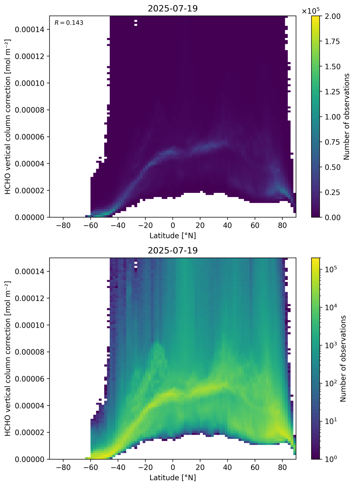
Figure 164: Scatter density plot of “Latitude” against “HCHO vertical column correction” for 2025-07-19 to 2025-07-20.
