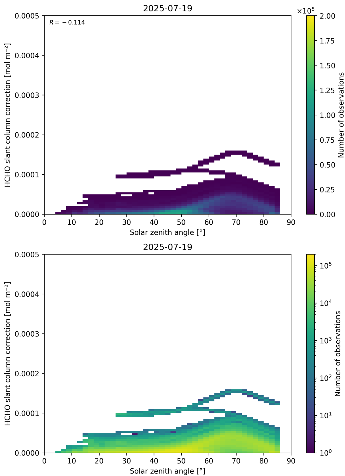
Figure 172: Scatter density plot of “Solar zenith angle” against “HCHO slant column correction” for 2025-07-19 to 2025-07-20.
