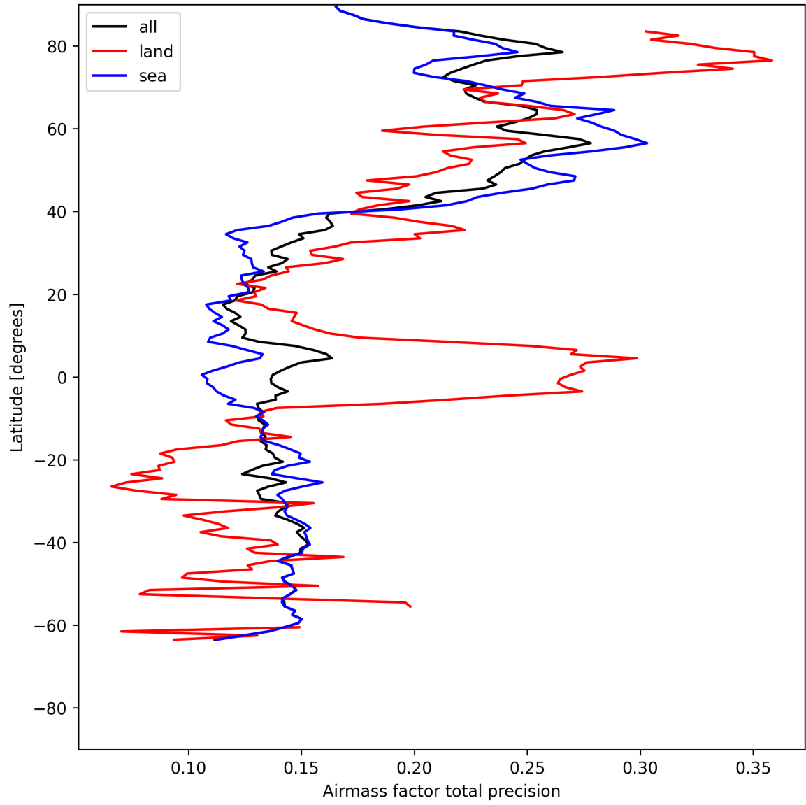
Figure 27: Zonal average of “Airmass factor total precision” for 2025-07-19 to 2025-07-20.
