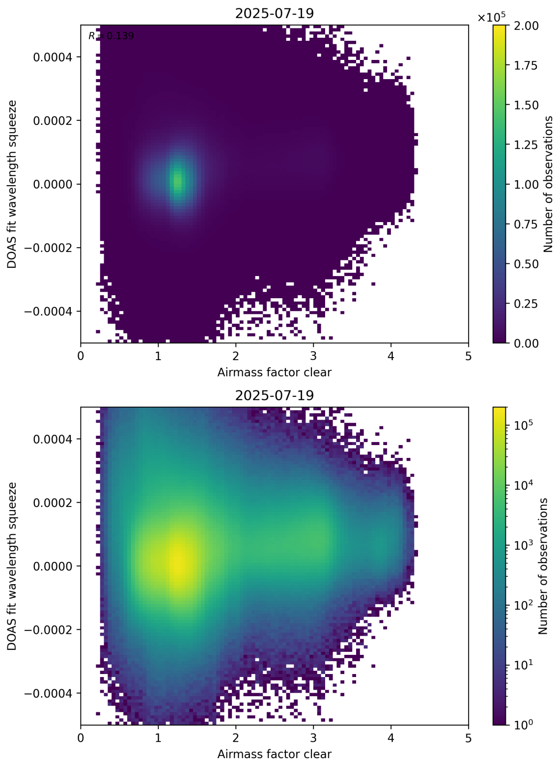
Figure 73: Scatter density plot of “Airmass factor clear” against “DOAS fit wavelength squeeze” for 2025-07-19 to 2025-07-20.
