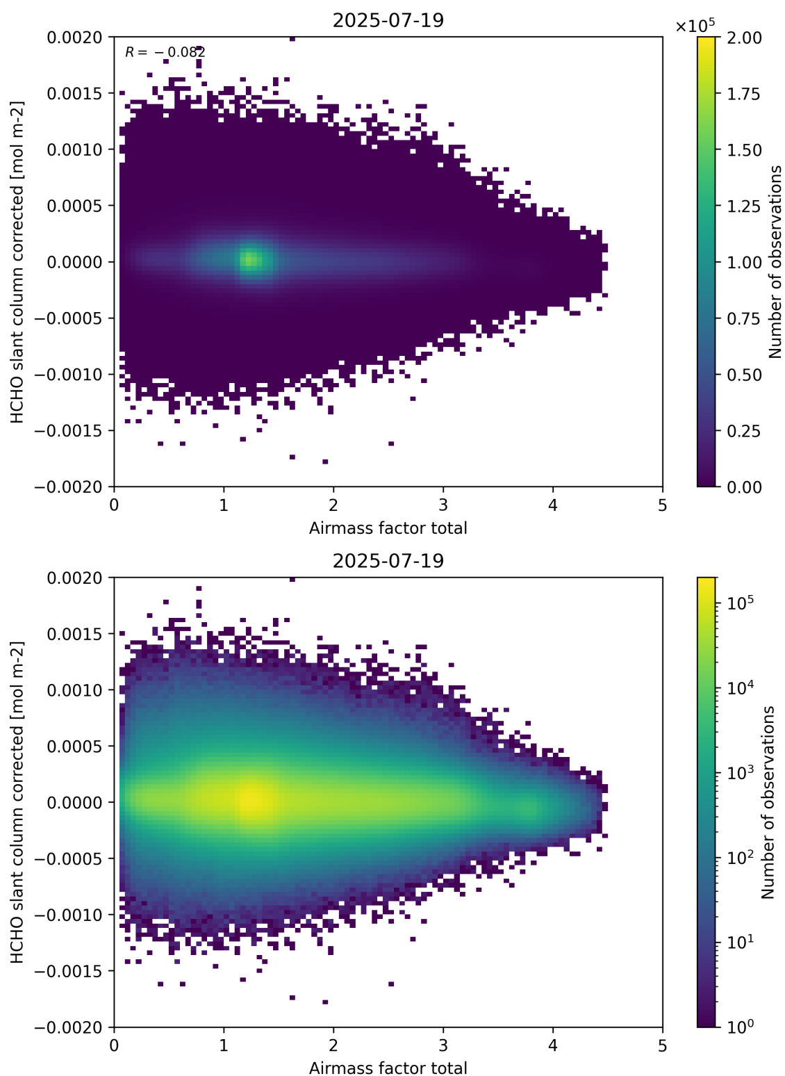
Figure 101: Scatter density plot of “Airmass factor total” against “HCHO slant column corrected” for 2025-07-19 to 2025-07-20.
