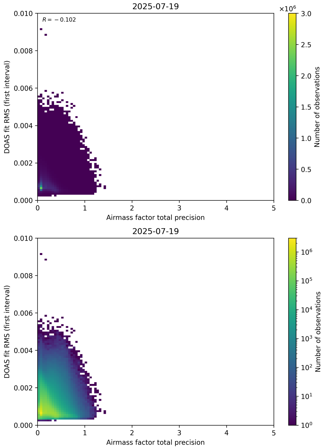
Figure 105: Scatter density plot of “Airmass factor total precision” against “DOAS fit RMS (first interval)” for 2025-07-19 to 2025-07-20.
