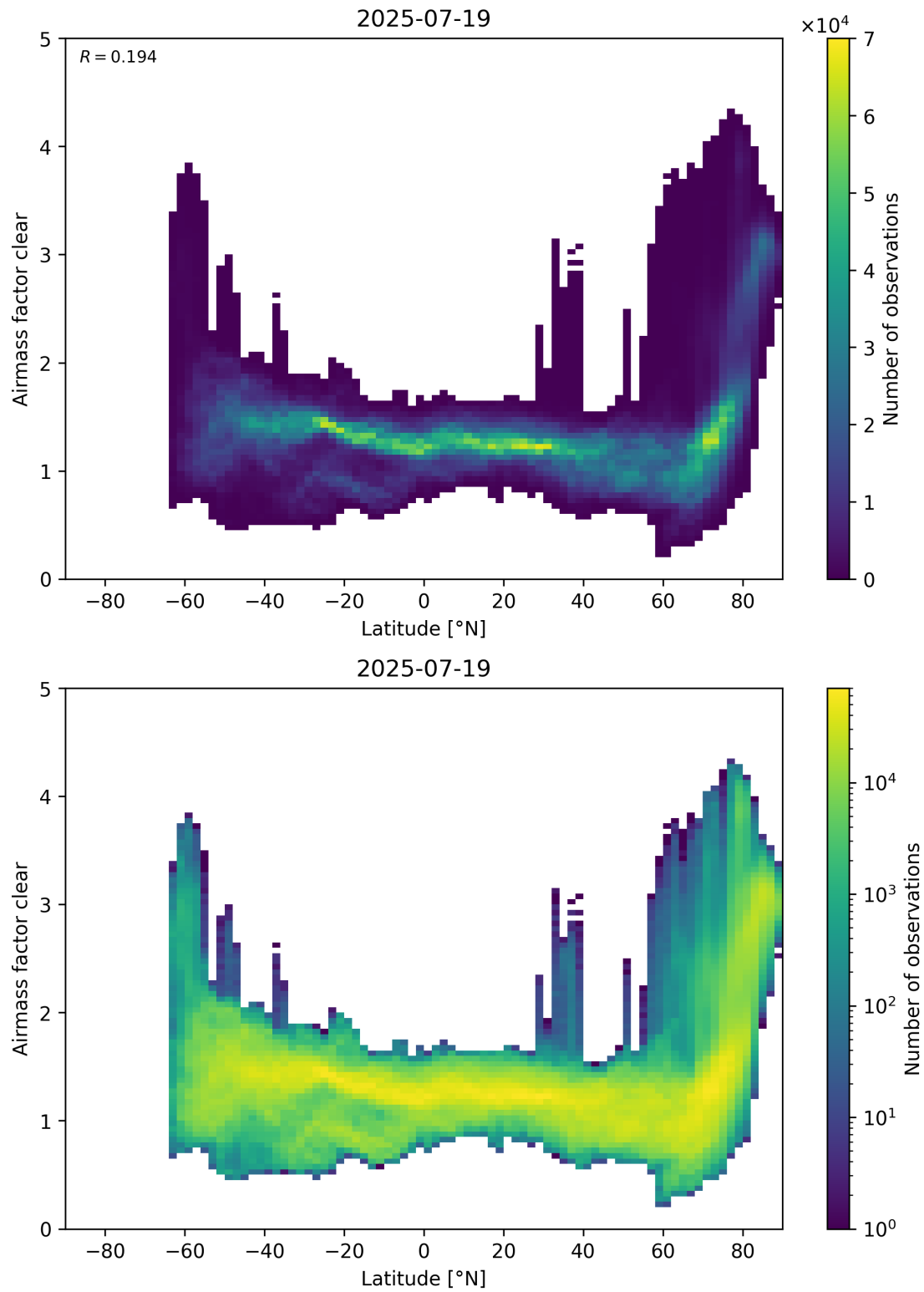
Figure 156: Scatter density plot of “Latitude” against “Airmass factor clear” for 2025-07-19 to 2025-07-20.
