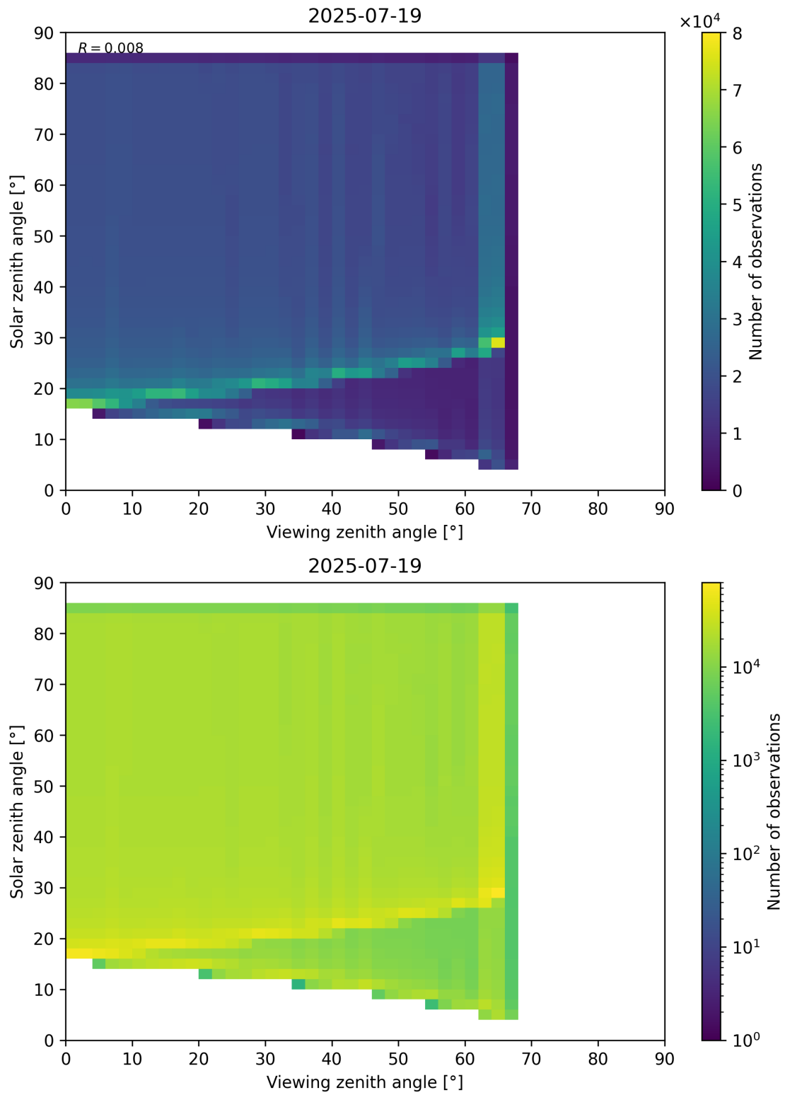
Figure 197: Scatter density plot of “Viewing zenith angle” against “Solar zenith angle” for 2025-07-19 to 2025-07-20.
