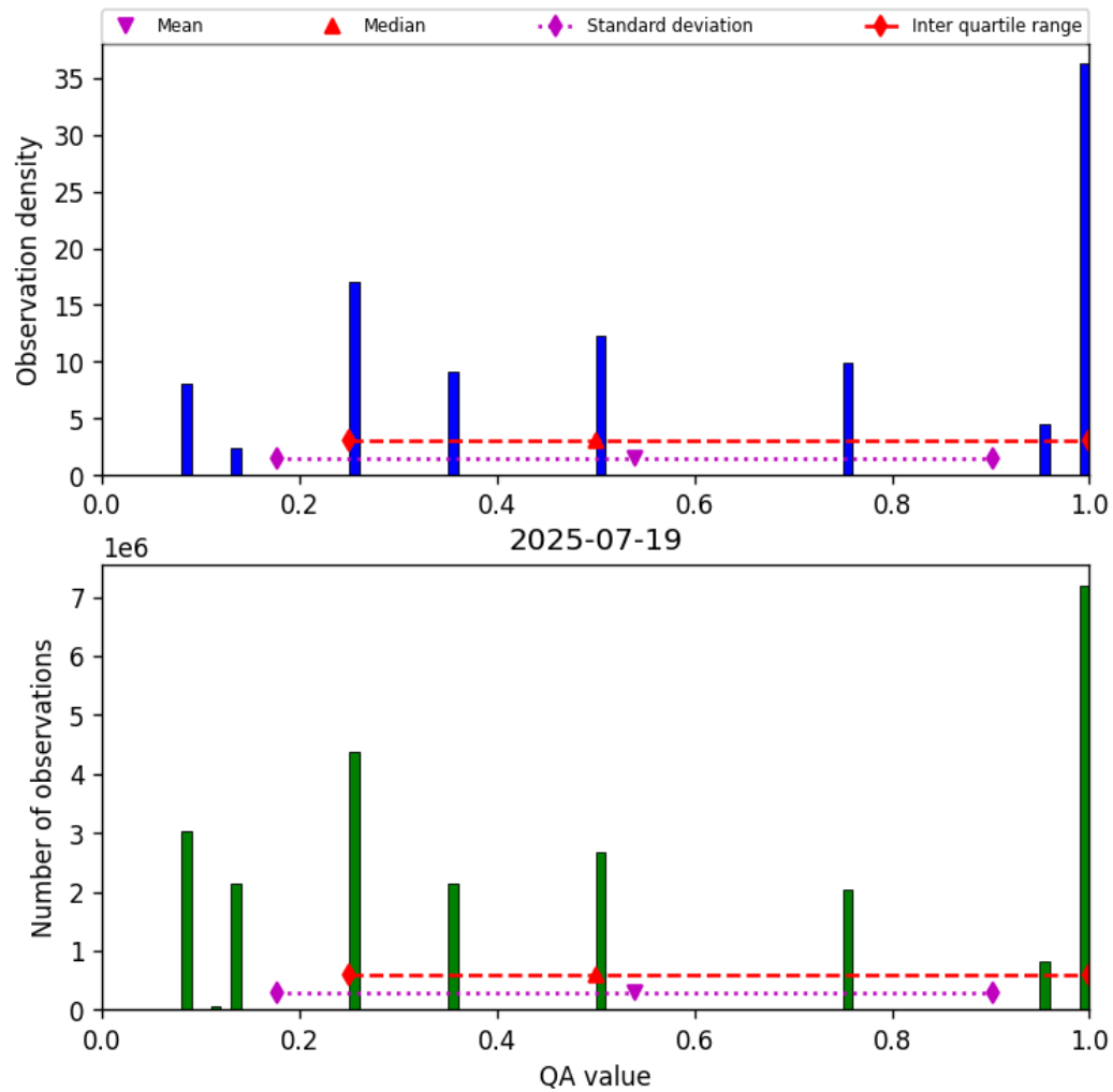
Figure 34: Histogram of “QA value” for 2025-07-19 to 2025-07-20
