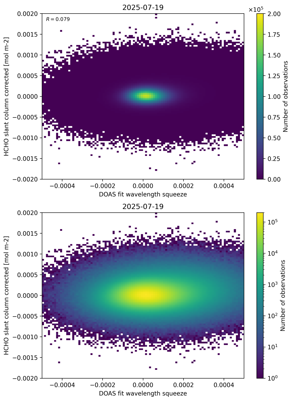
Figure 69: Scatter density plot of “DOAS fit wavelength squeeze” against “HCHO slant column corrected” for 2025-07-19 to 2025-07-20.
