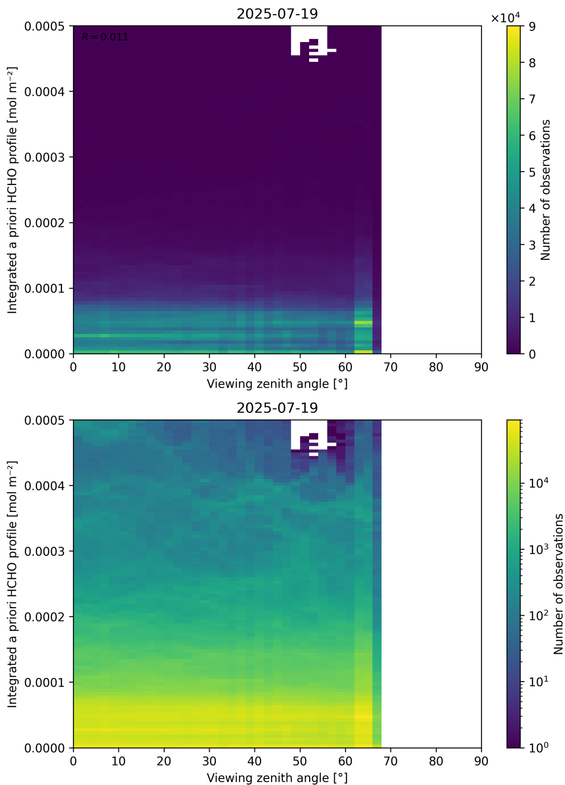
Figure 195: Scatter density plot of “Viewing zenith angle” against “Integrated a priori HCHO profile” for 2025-07-19 to 2025-07-20.
