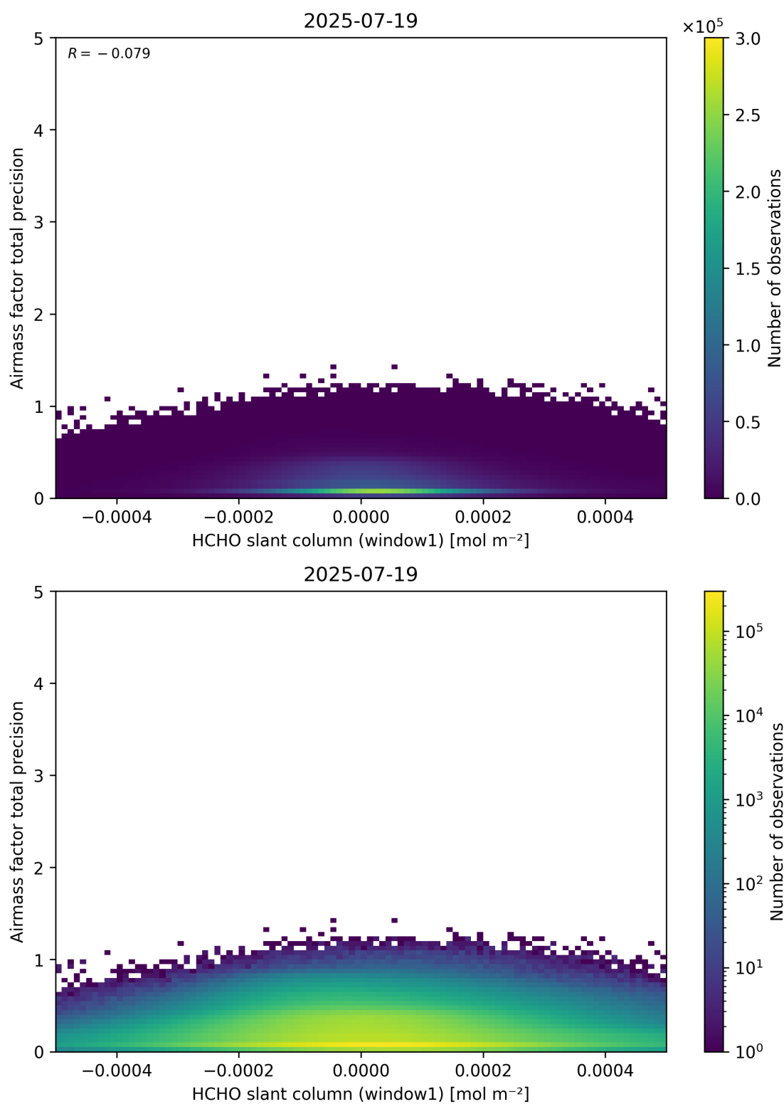
Figure 86: Scatter density plot of “HCHO slant column (window1)” against “Airmass factor total precision” for 2025-07-19 to 2025-07-20.
