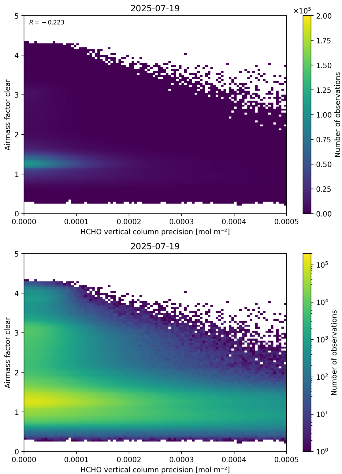
Figure 139: Scatter density plot of “HCHO vertical column precision” against “Airmass factor clear” for 2025-07-19 to 2025-07-20.
