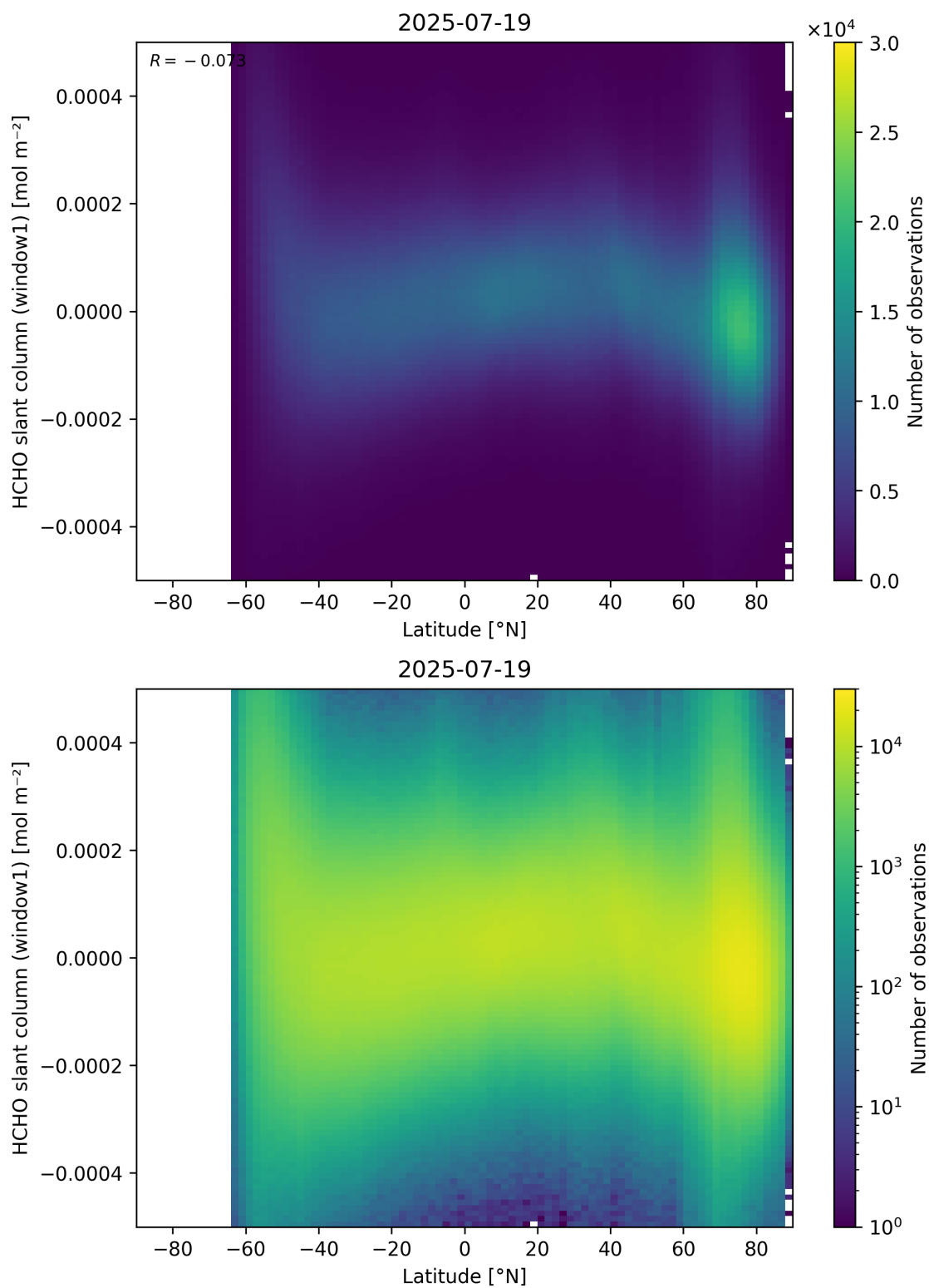
Figure 159: Scatter density plot of “Latitude” against “HCHO slant column (window1)” for 2025-07-19 to 2025-07-20.
