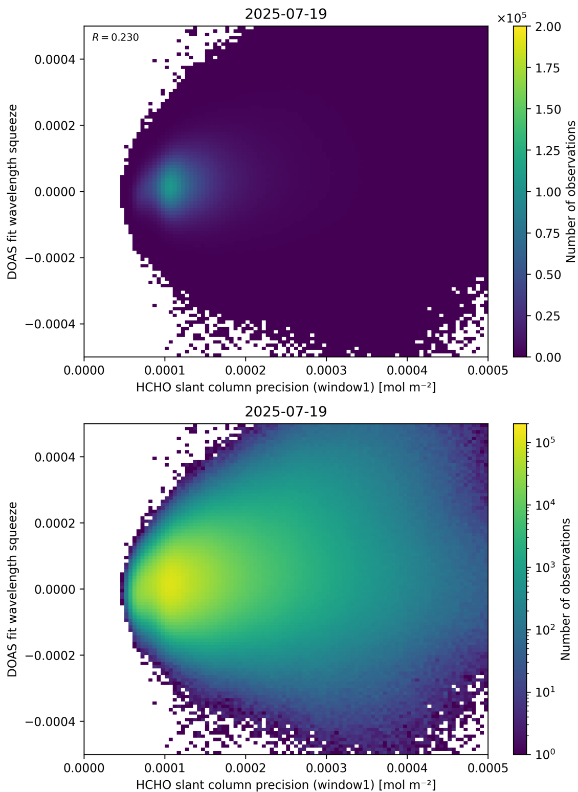
Figure 90: Scatter density plot of “HCHO slant column precision (window1)” against “DOAS fit wavelength squeeze” for 2025-07-19 to 2025-07-20.
