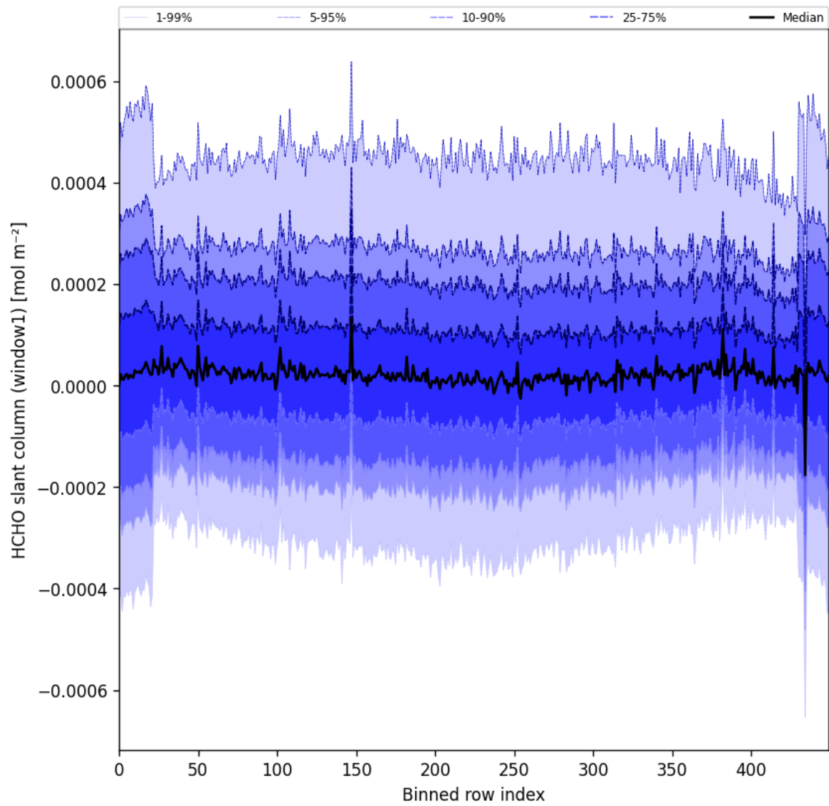
Figure 52: Along track statistics of “HCHO slant column (window1)” for 2025-07-19 to 2025-07-20
