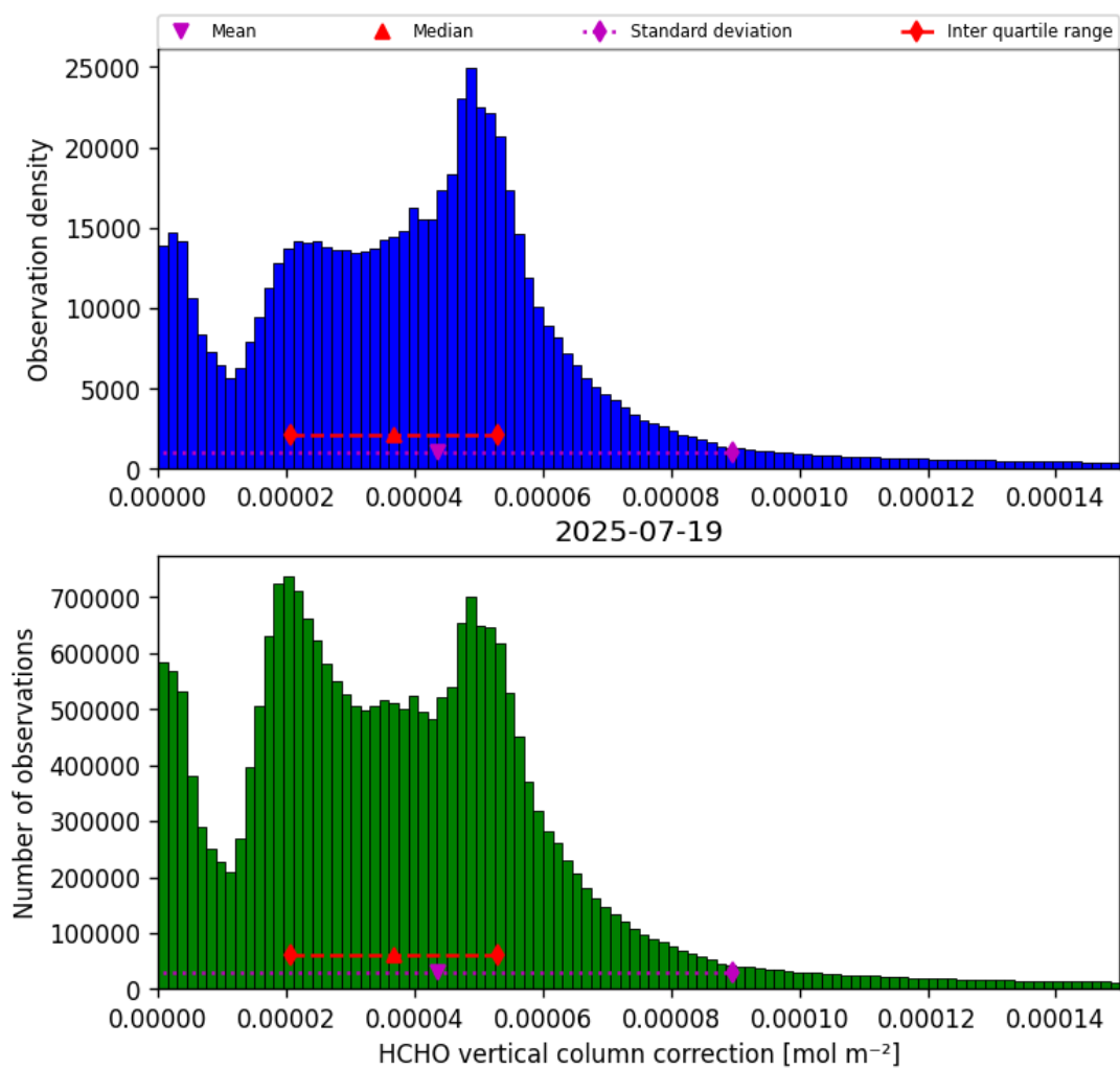
Figure 37: Histogram of “HCHO vertical column correction” for 2025-07-19 to 2025-07-20
