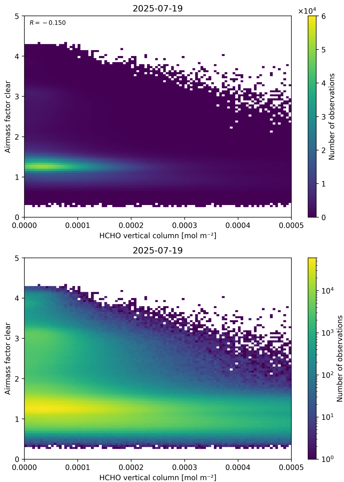
Figure 126: Scatter density plot of “HCHO vertical column” against “Airmass factor clear” for 2025-07-19 to 2025-07-20.
