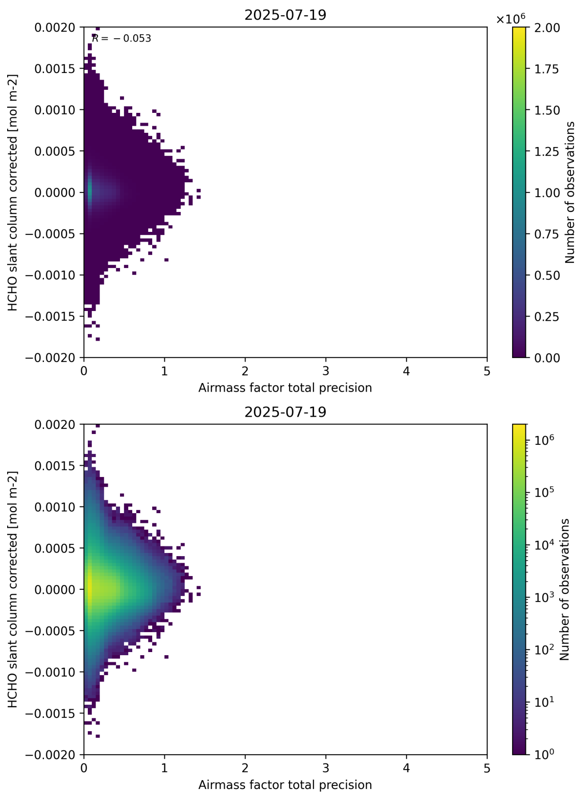
Figure 109: Scatter density plot of “Airmass factor total precision” against “HCHO slant column corrected” for 2025-07-19 to 2025-07-20.
