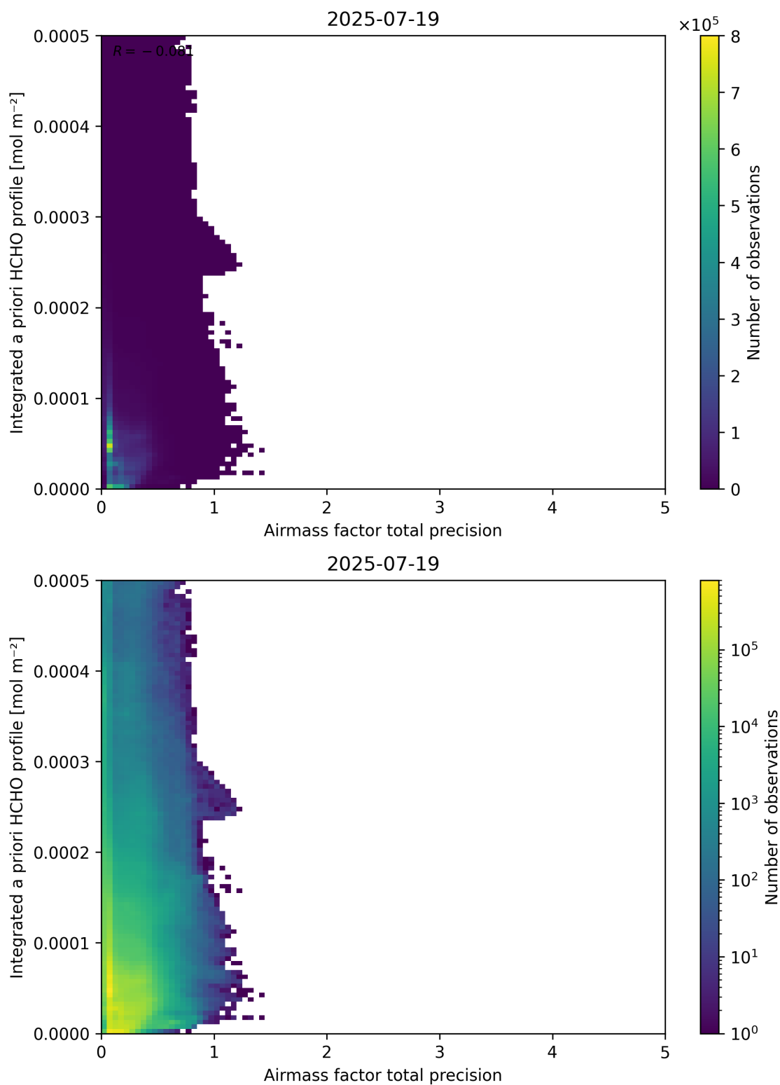
Figure 111: Scatter density plot of “Airmass factor total precision” against “Integrated a priori HCHO profile” for 2025-07-19 to 2025-07-20.
