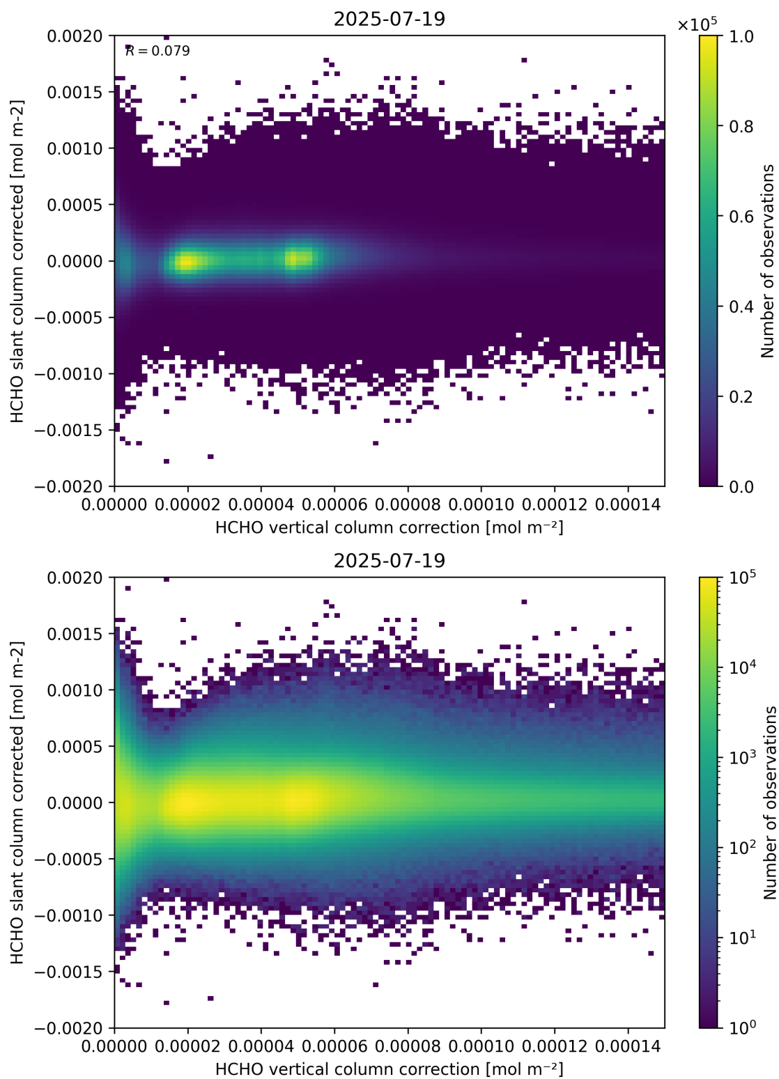
Figure 116: Scatter density plot of “HCHO vertical column correction” against “HCHO slant column corrected” for 2025-07-19 to 2025-07-20.
