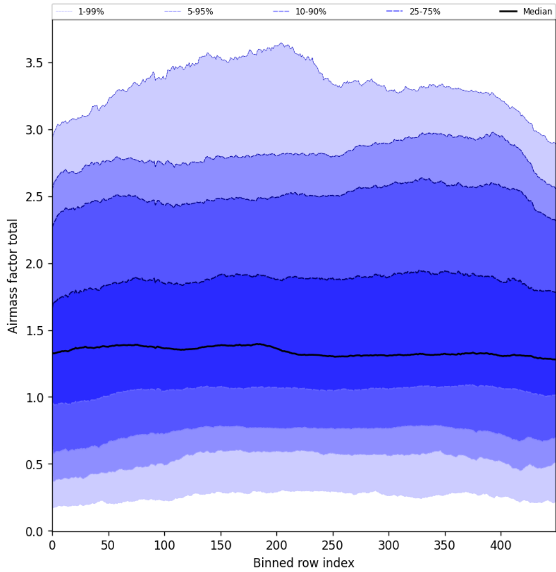
Figure 54: Along track statistics of “Airmass factor total” for 2025-07-19 to 2025-07-20
