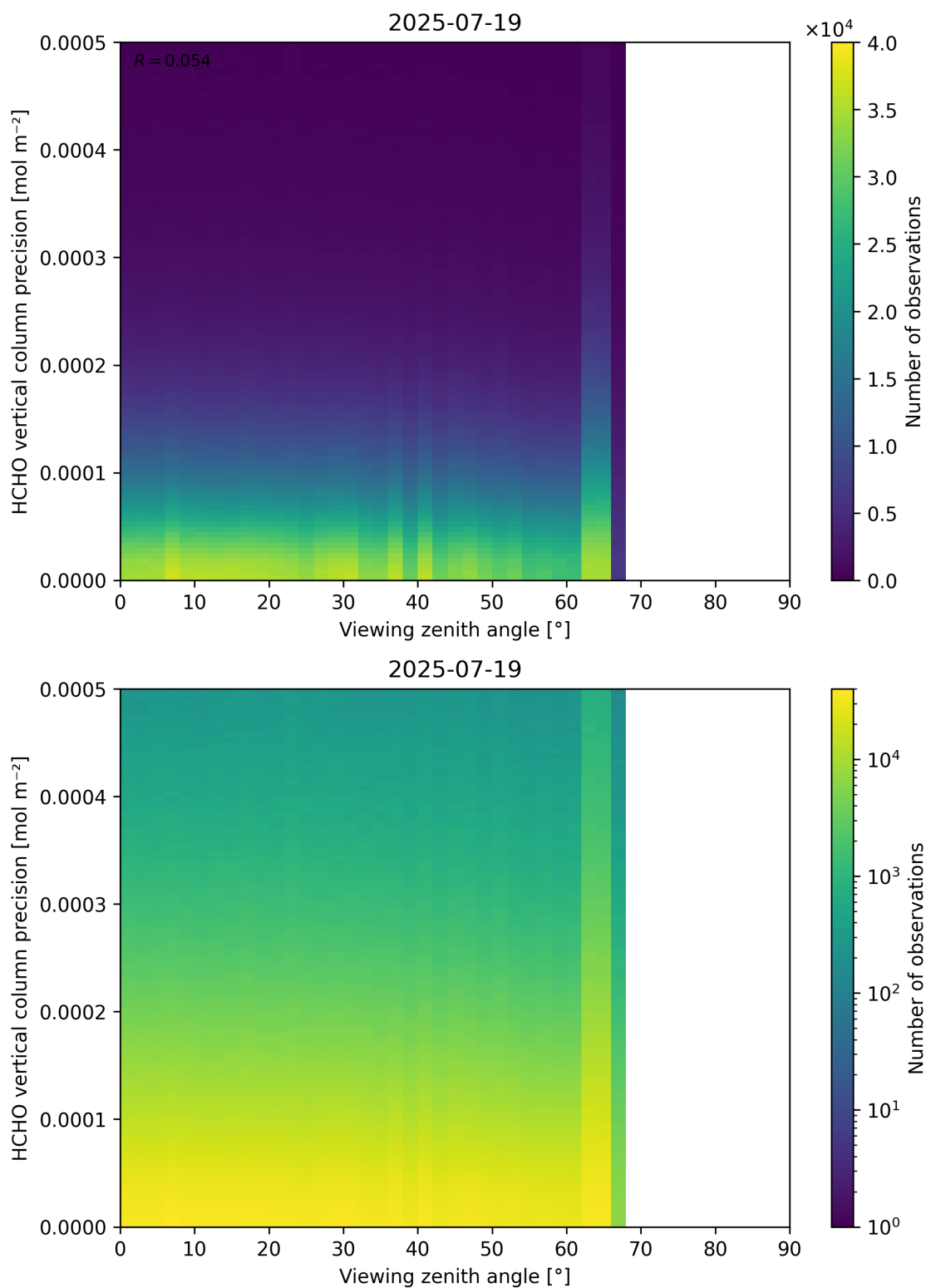
Figure 194: Scatter density plot of “Viewing zenith angle” against “HCHO vertical column precision” for 2025-07-19 to 2025-07-20.
