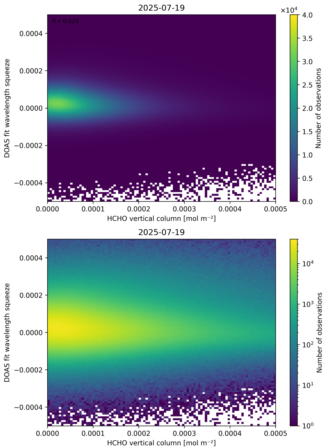
Figure 125: Scatter density plot of “HCHO vertical column” against “DOAS fit wavelength squeeze” for 2025-07-19 to 2025-07-20.
