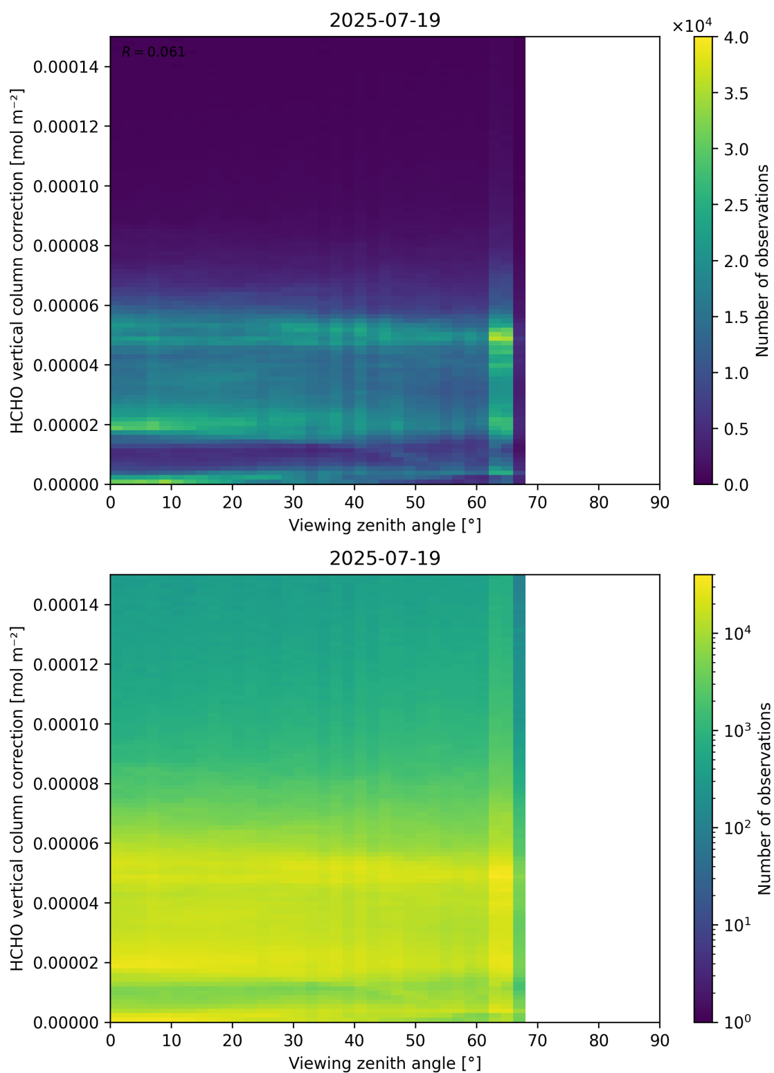
Figure 193: Scatter density plot of “Viewing zenith angle” against “HCHO vertical column correction” for 2025-07-19 to 2025-07-20.
