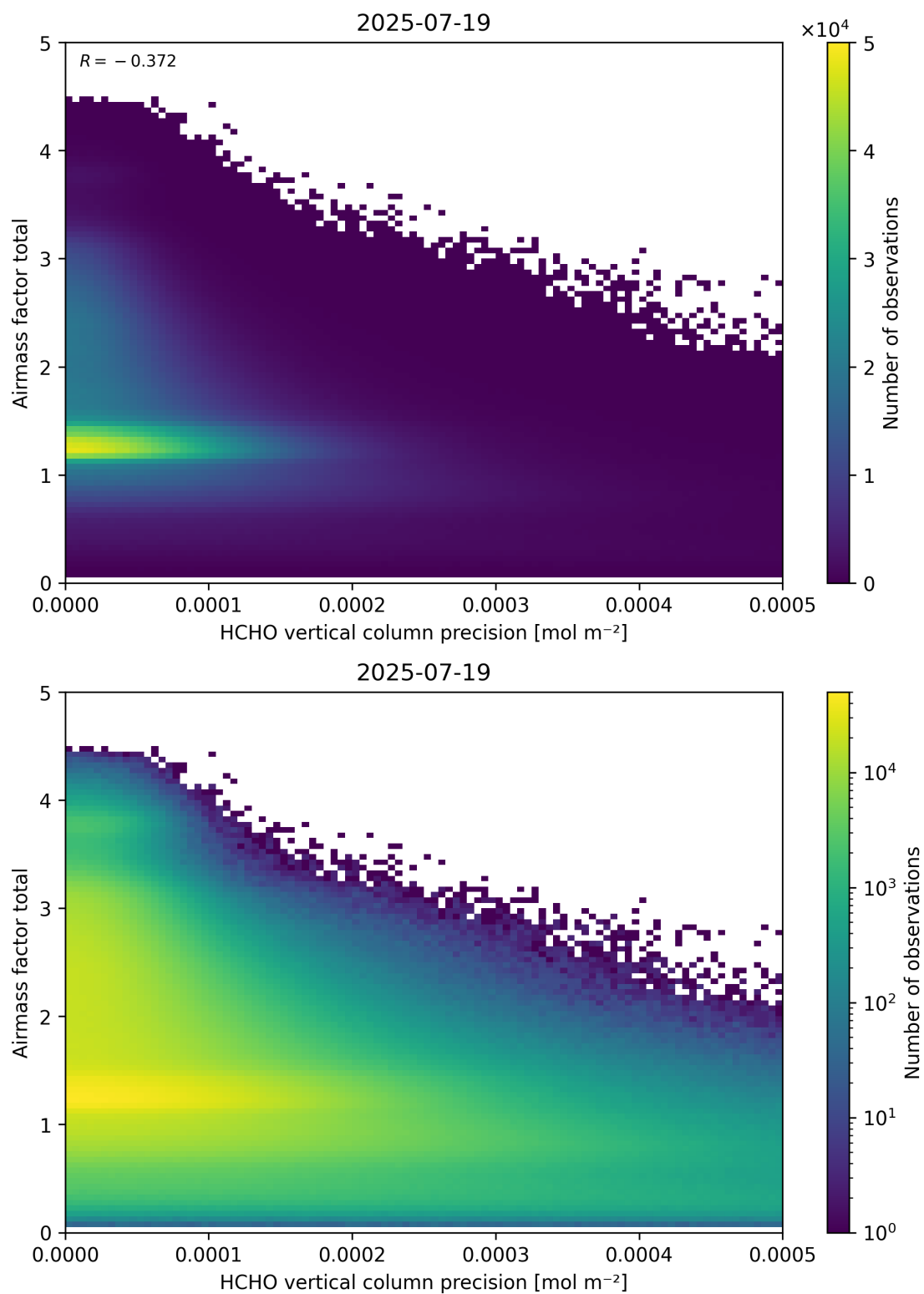
Figure 144: Scatter density plot of “HCHO vertical column precision” against “Airmass factor total” for 2025-07-19 to 2025-07-20.
