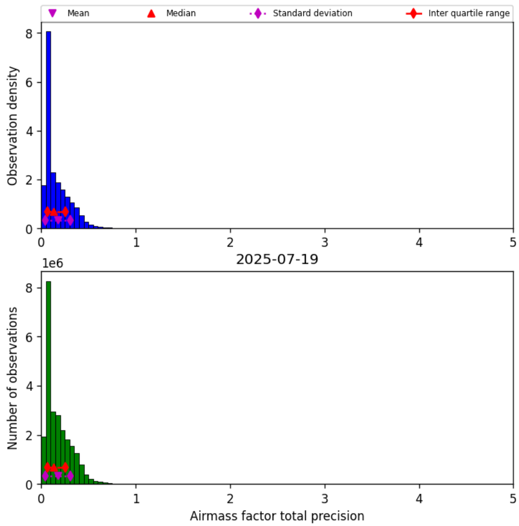
Figure 41: Histogram of “Airmass factor total precision” for 2025-07-19 to 2025-07-20
