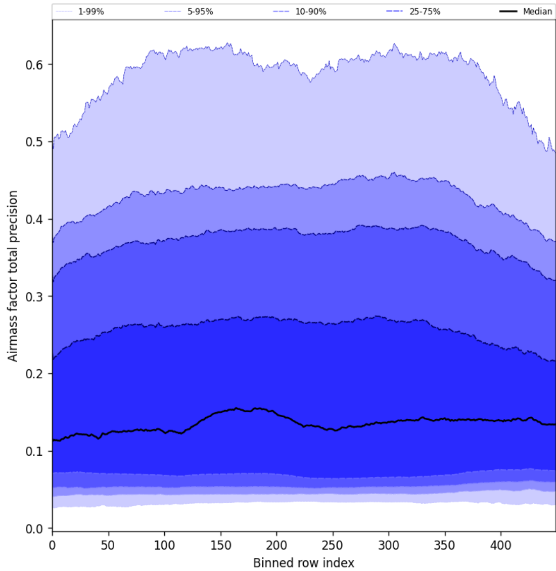
Figure 55: Along track statistics of “Airmass factor total precision” for 2025-07-19 to 2025-07-20
