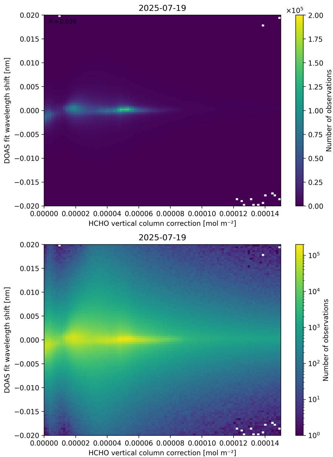
Figure 113: Scatter density plot of “HCHO vertical column correction” against “DOAS fit wavelength shift” for 2025-07-19 to 2025-07-20.
