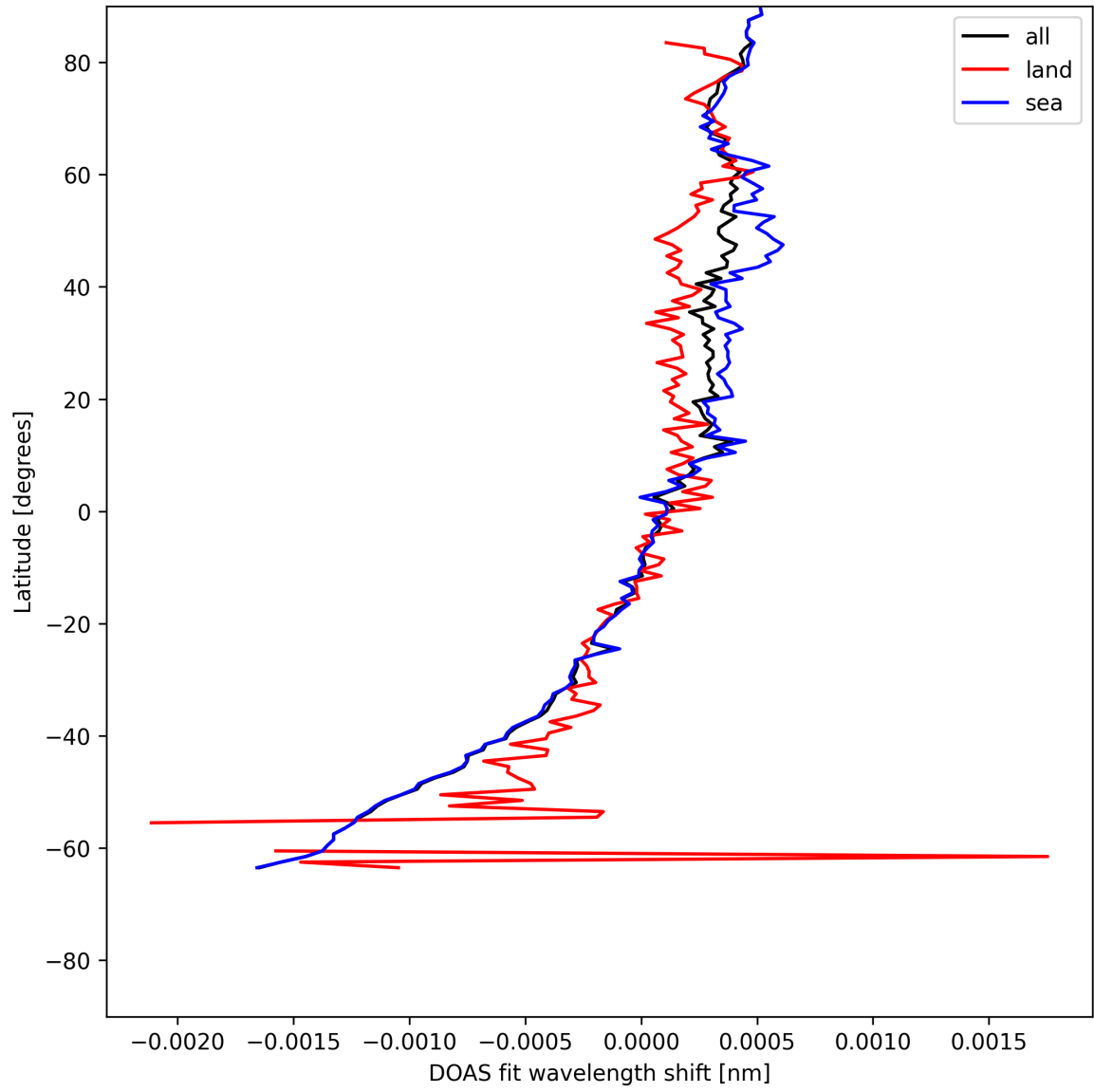
Figure 30: Zonal average of "DOAS fit wavelength shift" for 2025-07-19 to 2025-07-20.
