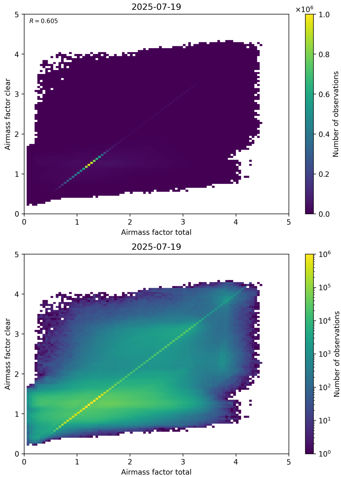
Figure 100: Scatter density plot of “Airmass factor total” against “Airmass factor clear” for 2025-07-19 to 2025-07-20.
