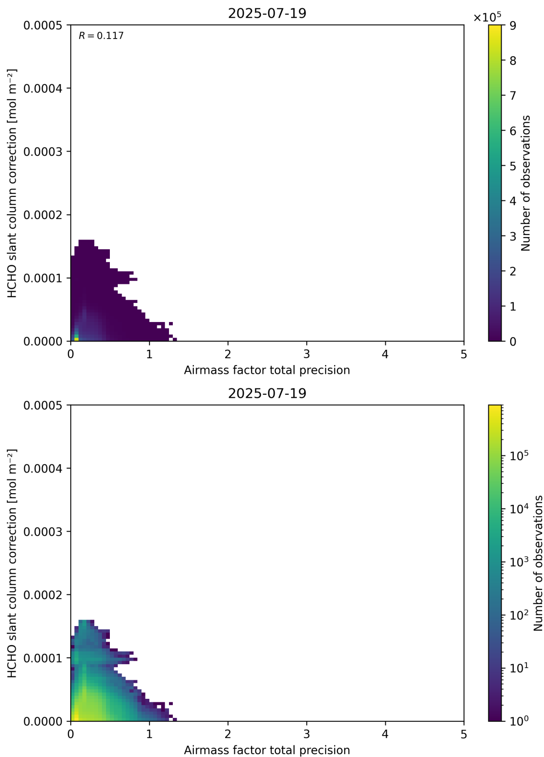
Figure 110: Scatter density plot of “Airmass factor total precision” against “HCHO slant column correction” for 2025-07-19 to 2025-07-20.
