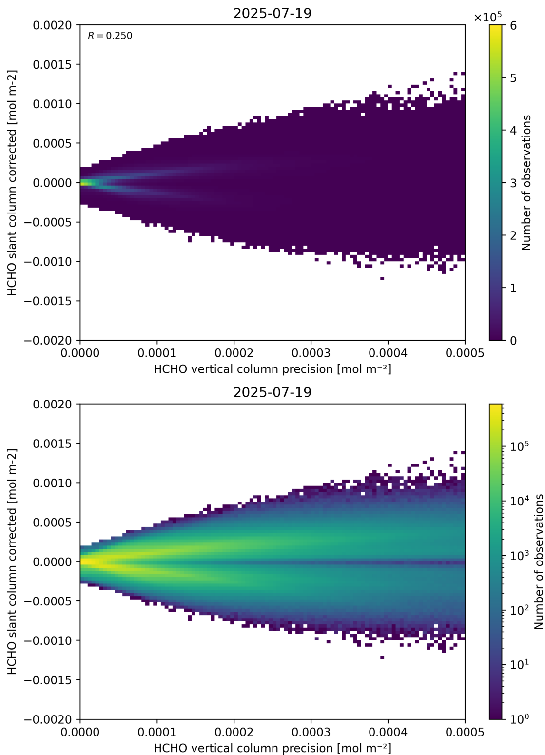
Figure 140: Scatter density plot of “HCHO vertical column precision” against “HCHO slant column corrected” for 2025-07-19 to 2025-07-20.
