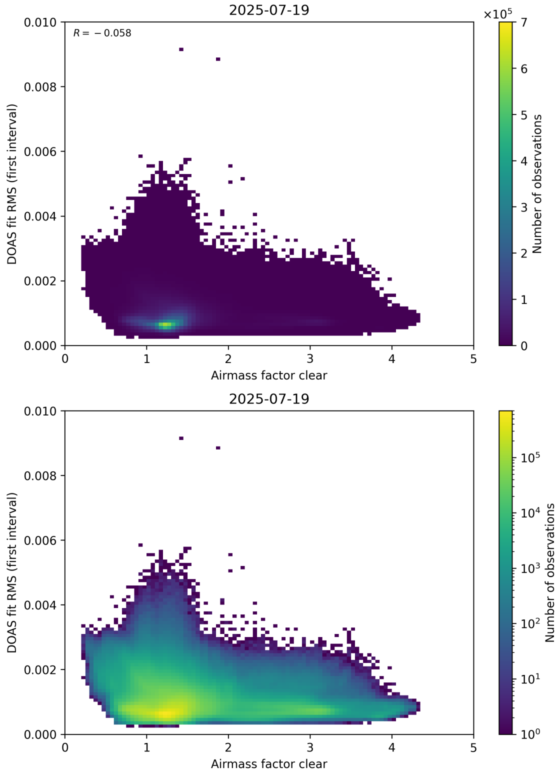
Figure 71: Scatter density plot of “Airmass factor clear” against “DOAS fit RMS (first interval)” for 2025-07-19 to 2025-07-20.
