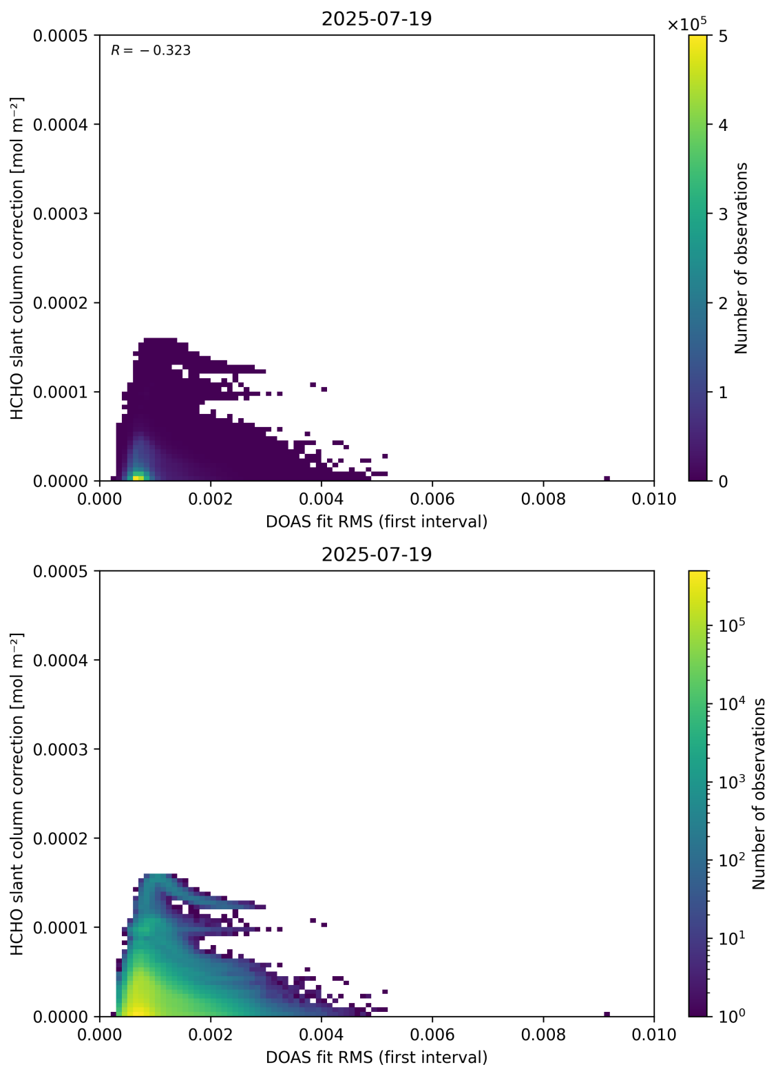
Figure 63: Scatter density plot of “DOAS fit RMS (first interval)” against “HCHO slant column correction” for 2025-07-19 to 2025-07-20.
