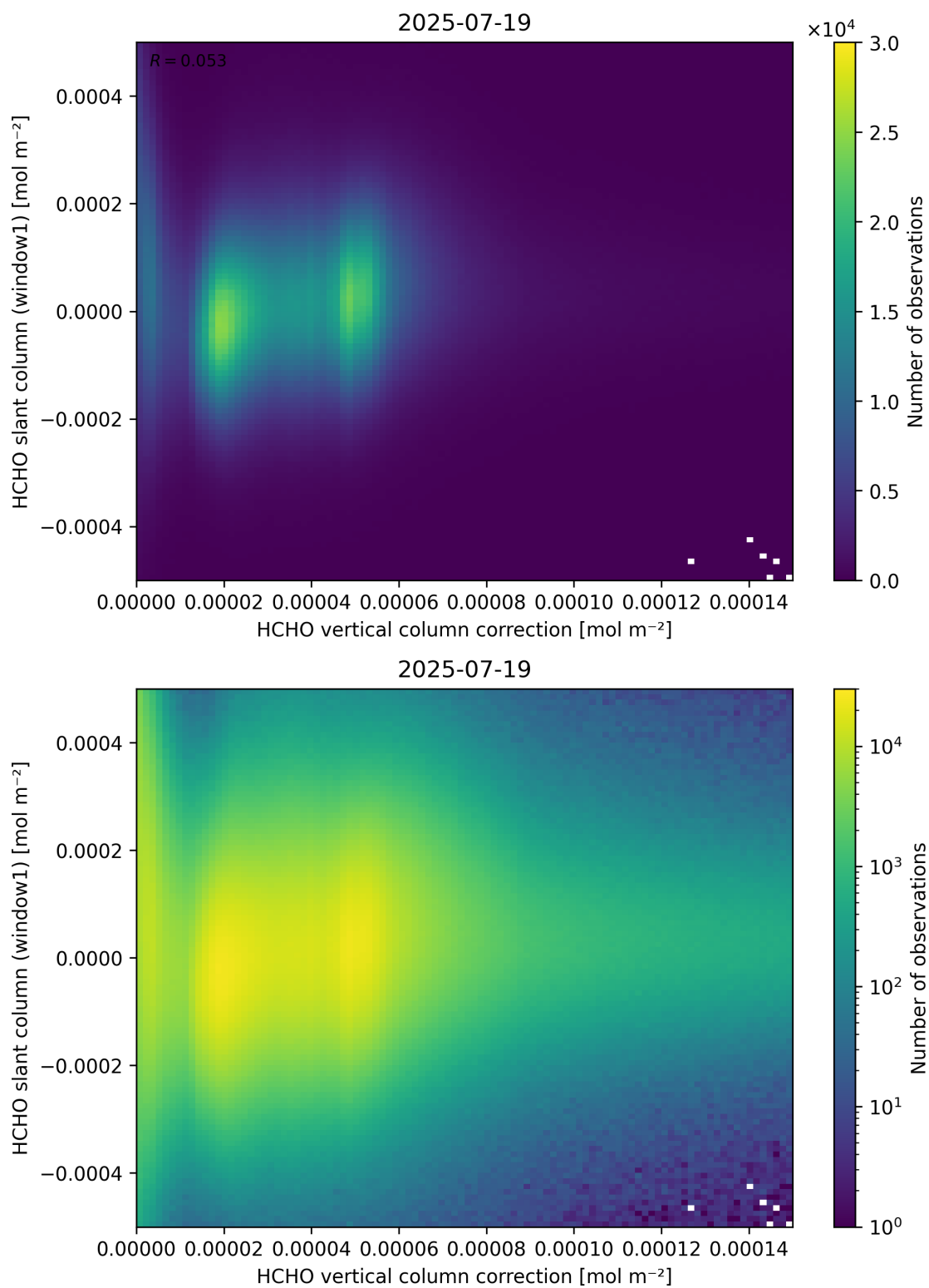
Figure 118: Scatter density plot of “HCHO vertical column correction” against “HCHO slant column (window1)” for 2025-07-19 to 2025-07-20.
