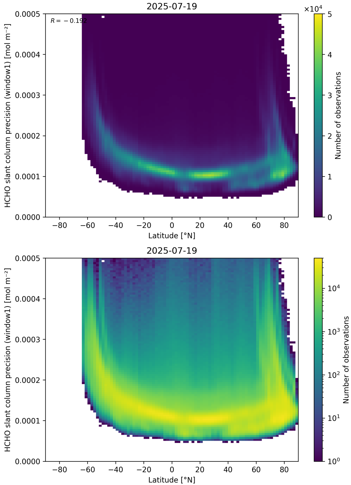
Figure 160: Scatter density plot of “Latitude” against “HCHO slant column precision (window1)” for 2025-07-19 to 2025-07-20.
