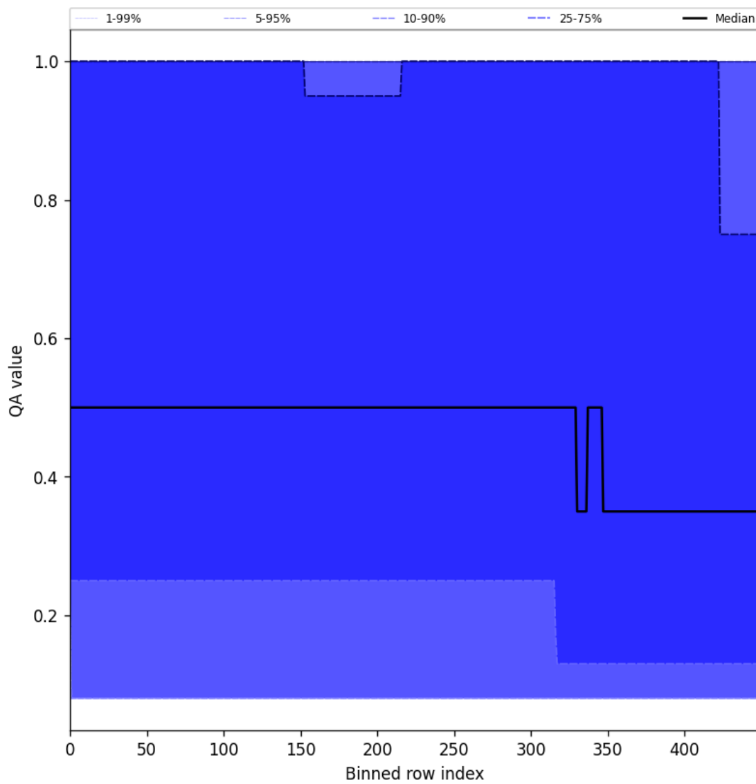
Figure 48: Along track statistics of “QA value” for 2025-07-19 to 2025-07-20
