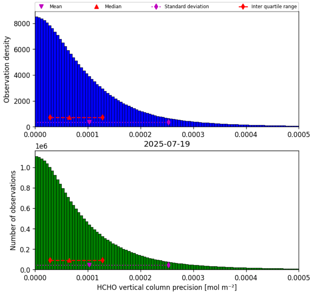
Figure 36: Histogram of “HCHO vertical column precision” for 2025-07-19 to 2025-07-20
