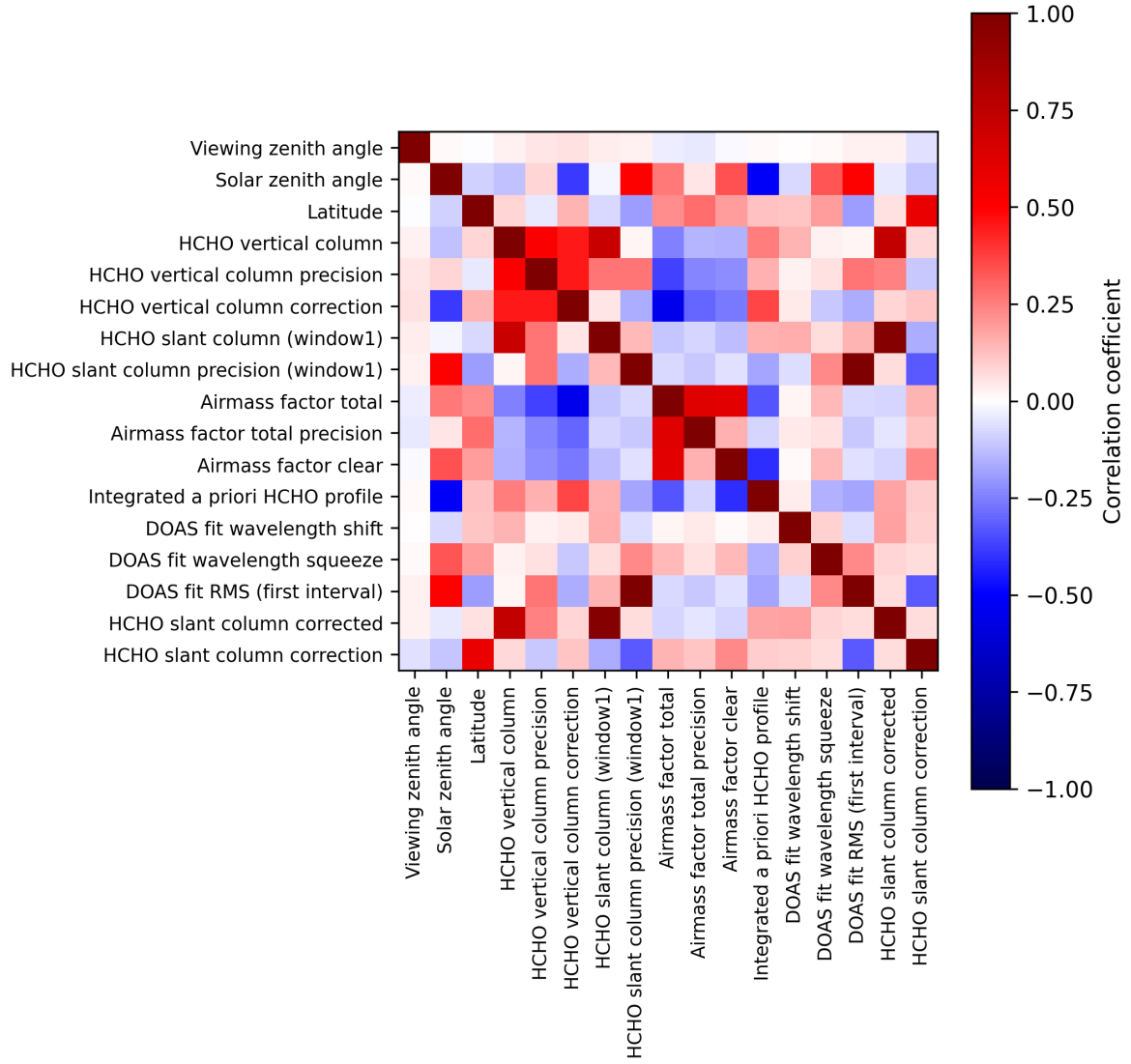
Figure 2: Map of correlation matrix for 2025-07-19 to 2025-07-20.
