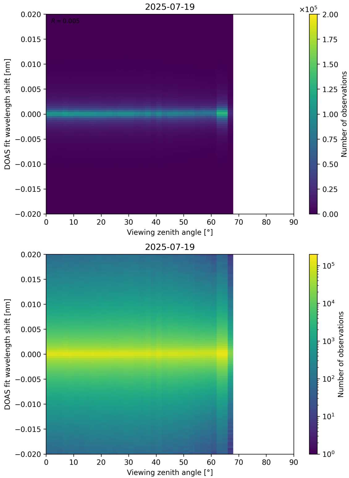
Figure 183: Scatter density plot of “Viewing zenith angle” against “DOAS fit wavelength shift” for 2025-07-19 to 2025-07-20.
