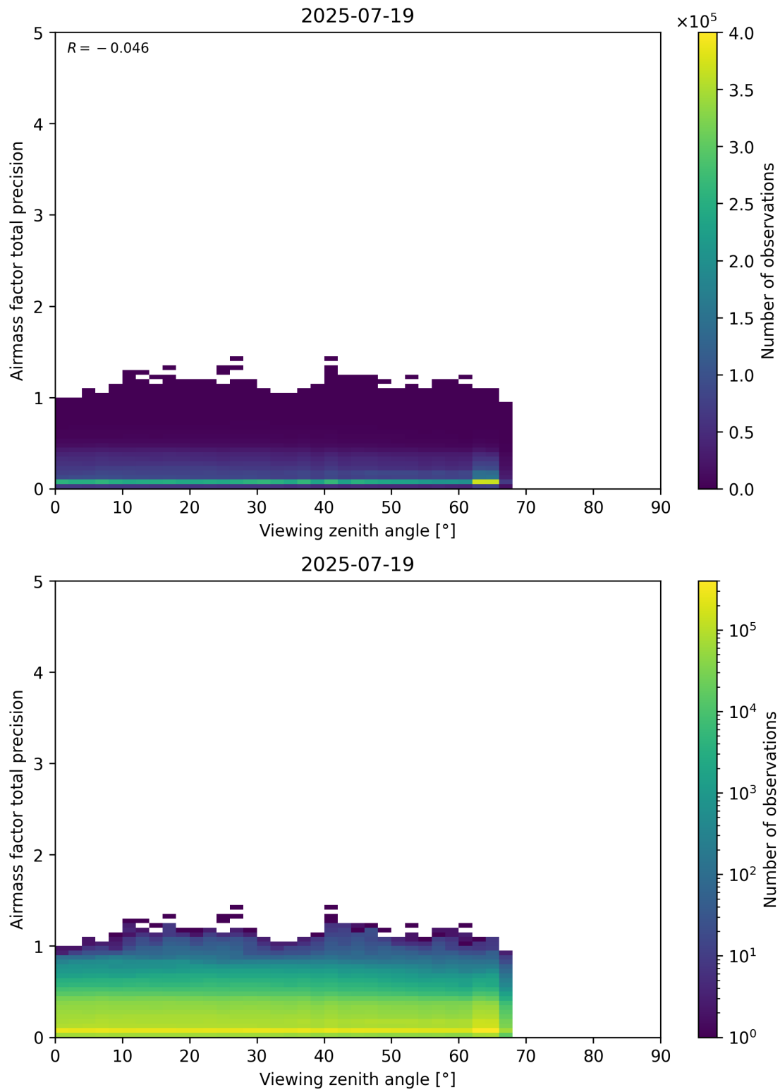
Figure 191: Scatter density plot of “Viewing zenith angle” against “Airmass factor total precision” for 2025-07-19 to 2025-07-20.
