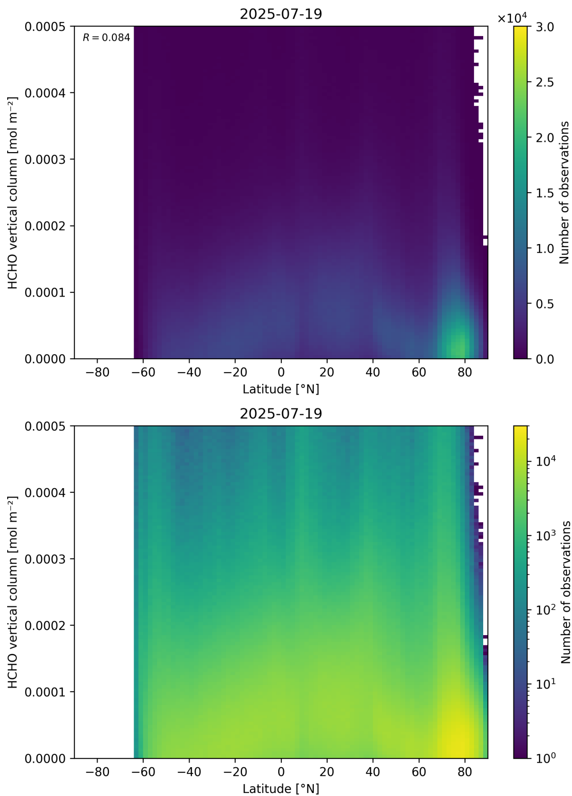
Figure 163: Scatter density plot of “Latitude” against “HCHO vertical column” for 2025-07-19 to 2025-07-20.
