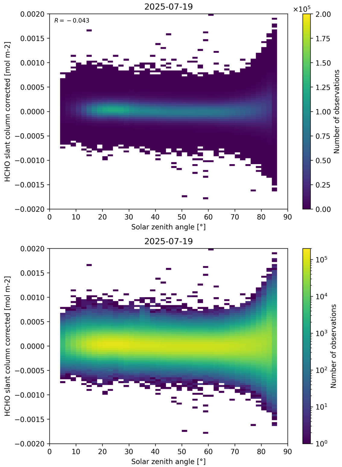
Figure 171: Scatter density plot of “Solar zenith angle” against “HCHO slant column corrected” for 2025-07-19 to 2025-07-20.
