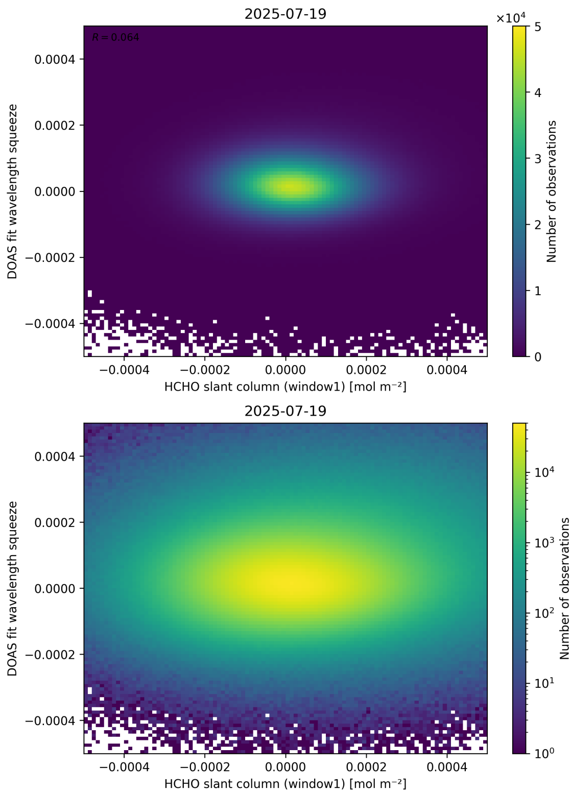
Figure 80: Scatter density plot of “HCHO slant column (window1)” against “DOAS fit wavelength squeeze” for 2025-07-19 to 2025-07-20.
