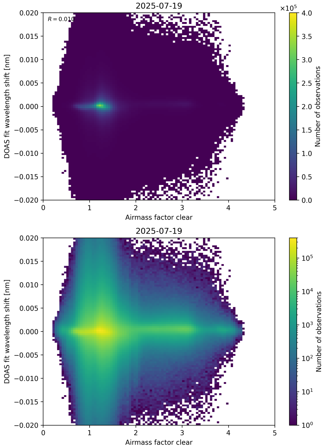
Figure 72: Scatter density plot of “Airmass factor clear” against “DOAS fit wavelength shift” for 2025-07-19 to 2025-07-20.
