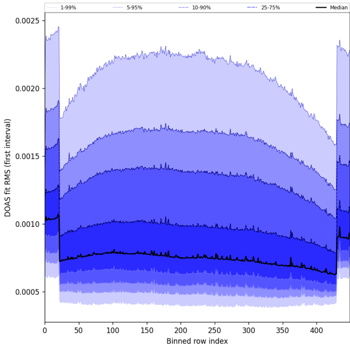
Figure 60: Along track statistics of “DOAS fit RMS (first interval)” for 2025-07-19 to 2025-07-20
