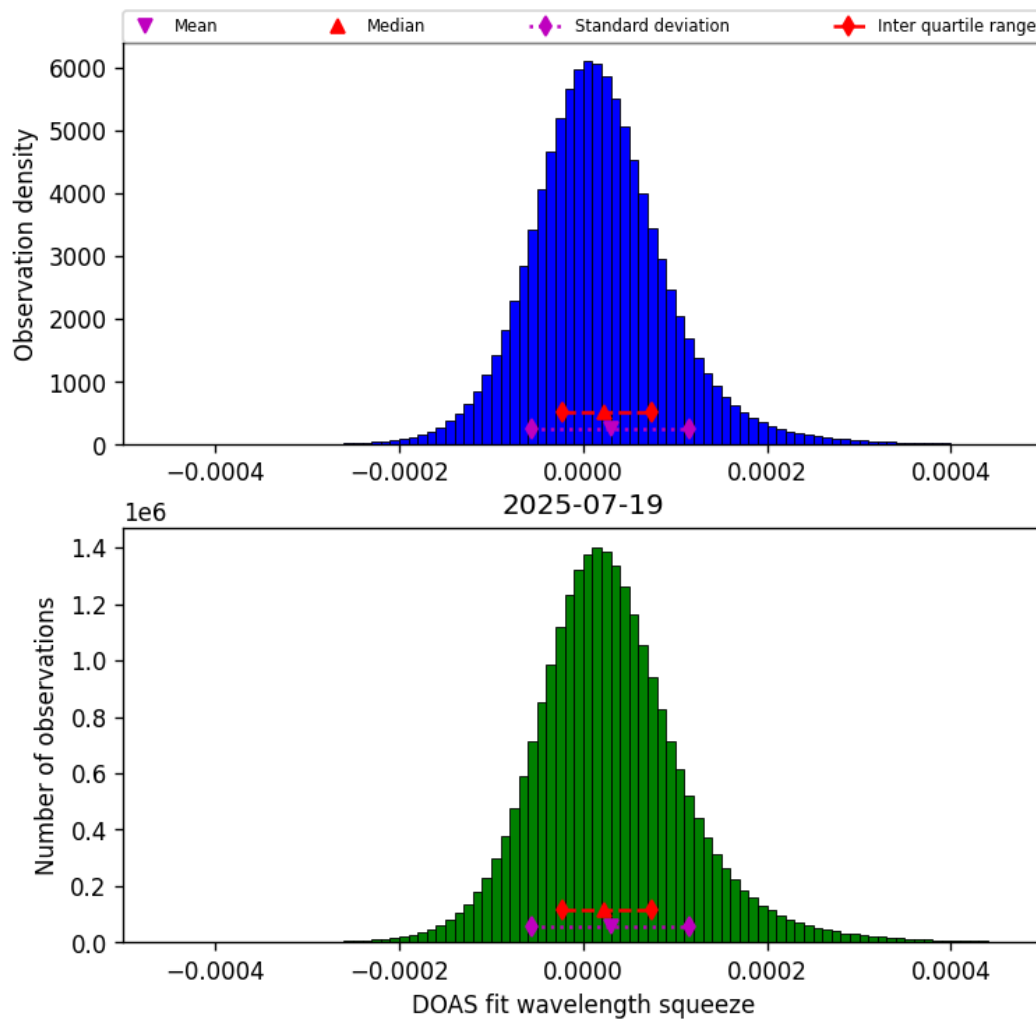
Figure 45: Histogram of “DOAS fit wavelength squeeze” for 2025-07-19 to 2025-07-20
