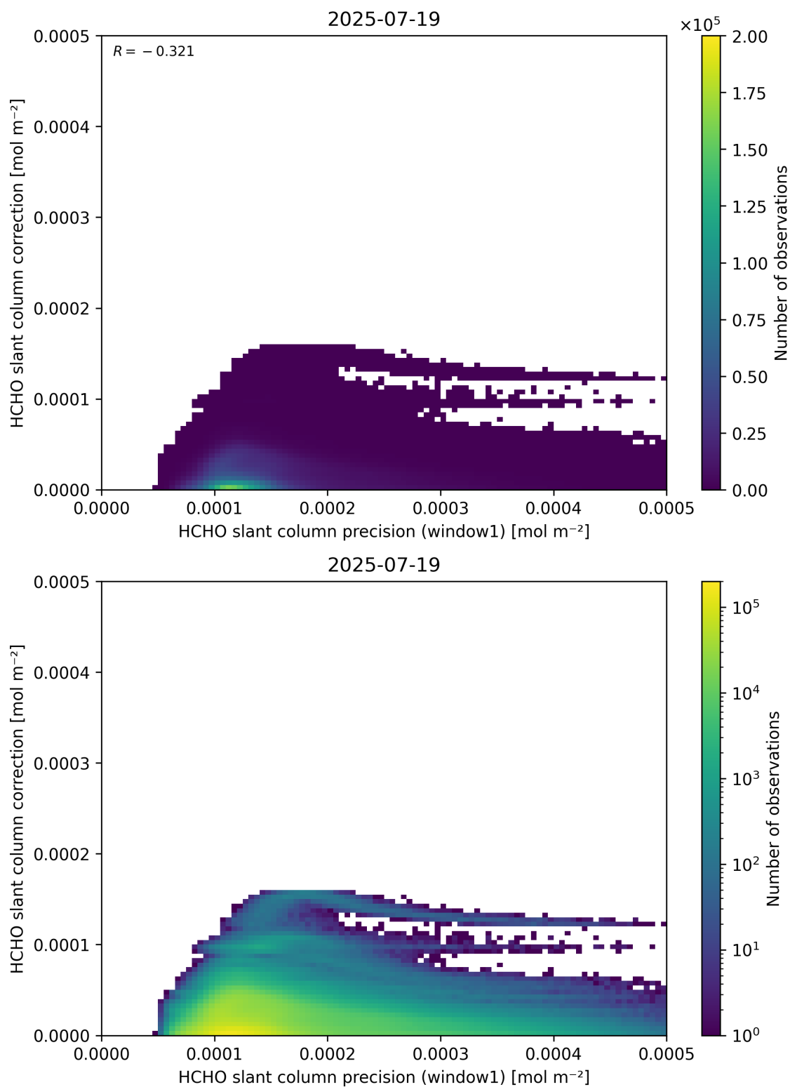
Figure 93: Scatter density plot of “HCHO slant column precision (window1)” against “HCHO slant column correction” for 2025-07-19 to 2025-07-20.
