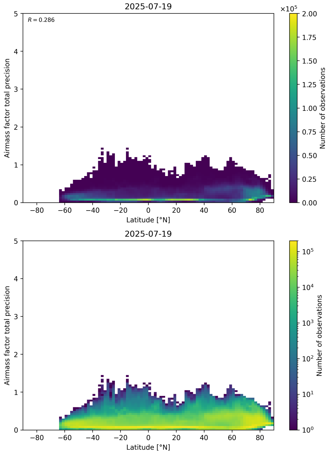
Figure 162: Scatter density plot of “Latitude” against “Airmass factor total precision” for 2025-07-19 to 2025-07-20.
