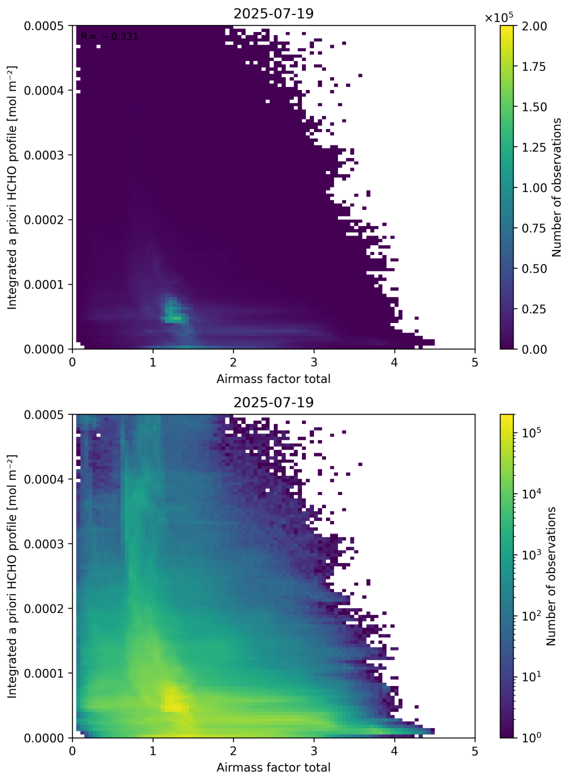
Figure 104: Scatter density plot of “Airmass factor total” against “Integrated a priori HCHO profile” for 2025-07-19 to 2025-07-20.
