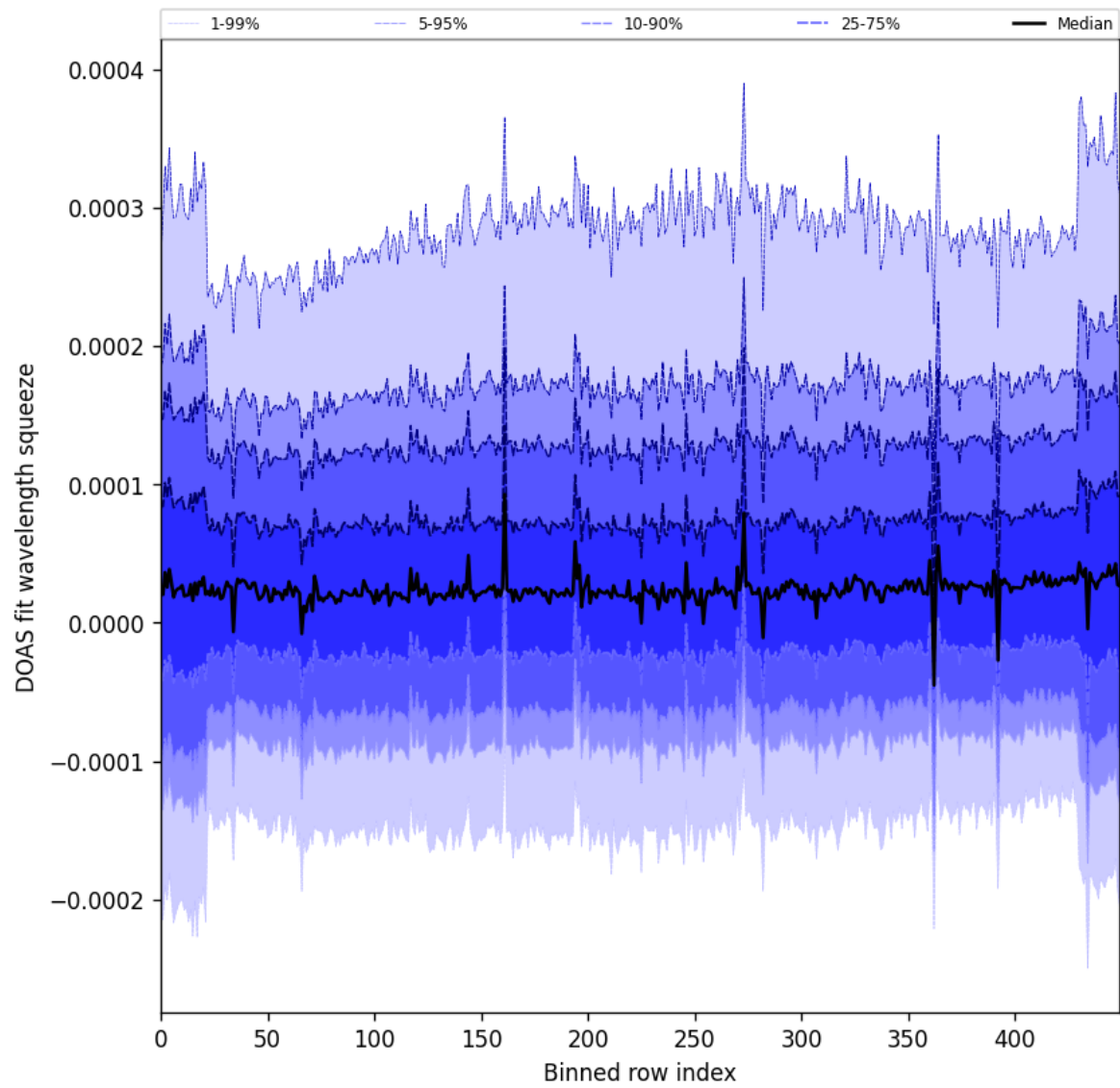
Figure 59: Along track statistics of “DOAS fit wavelength squeeze” for 2025-07-19 to 2025-07-20
