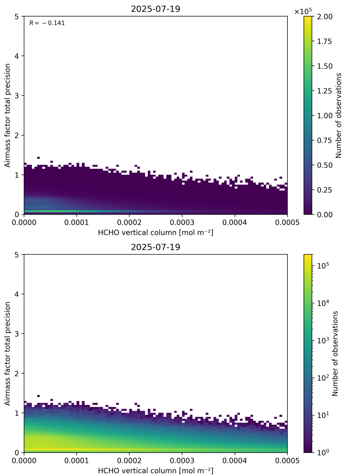
Figure 132: Scatter density plot of “HCHO vertical column” against “Airmass factor total precision” for 2025-07-19 to 2025-07-20.
