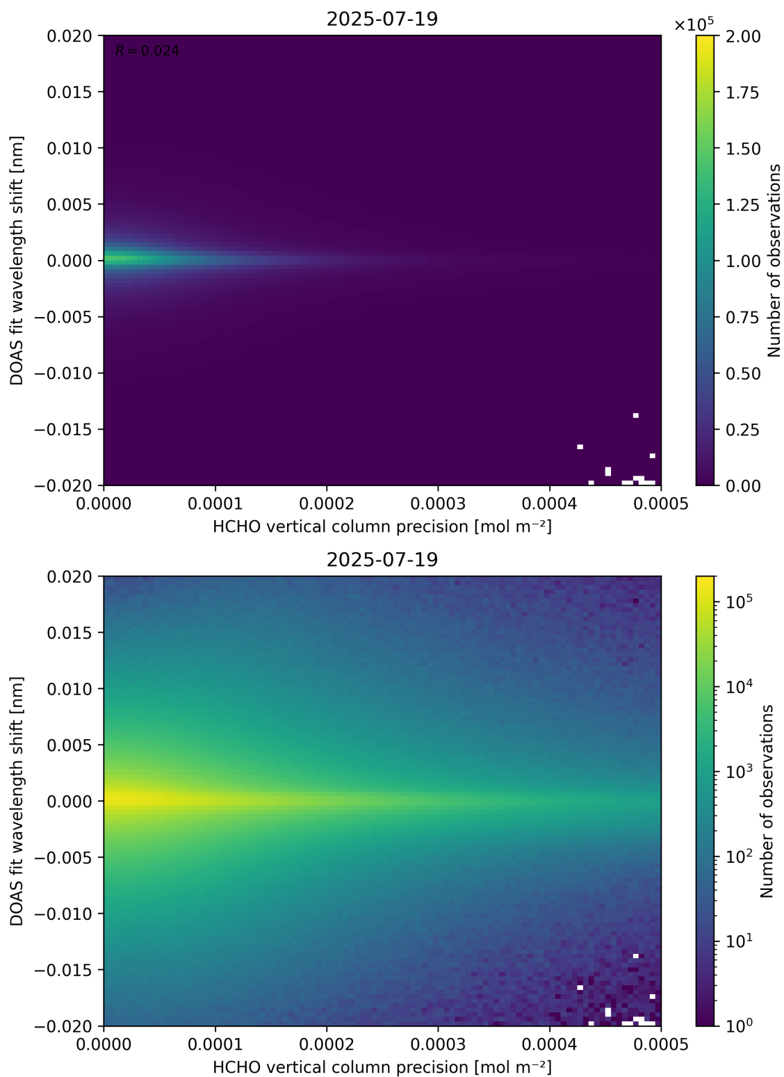
Figure 137: Scatter density plot of “HCHO vertical column precision” against “DOAS fit wavelength shift” for 2025-07-19 to 2025-07-20.
