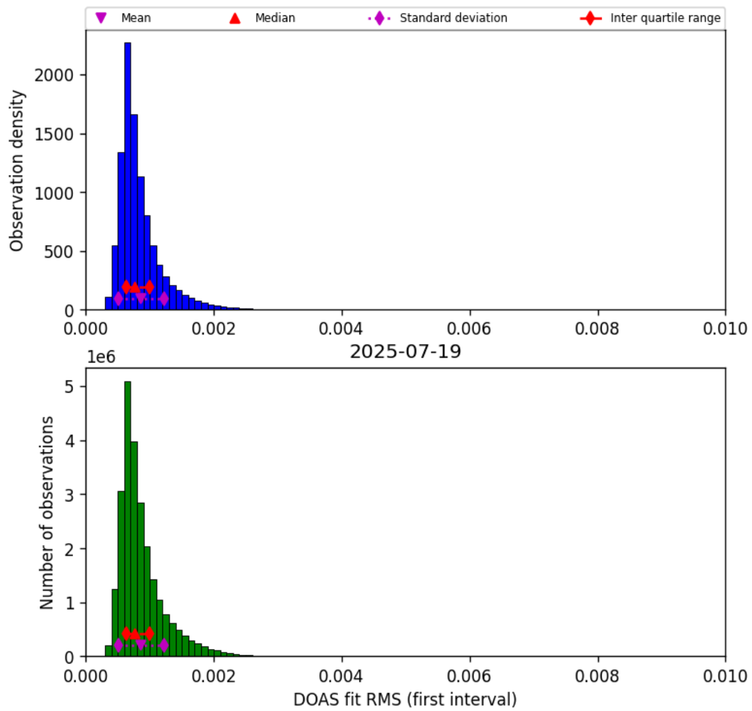
Figure 46: Histogram of “DOAS fit RMS (first interval)” for 2025-07-19 to 2025-07-20
