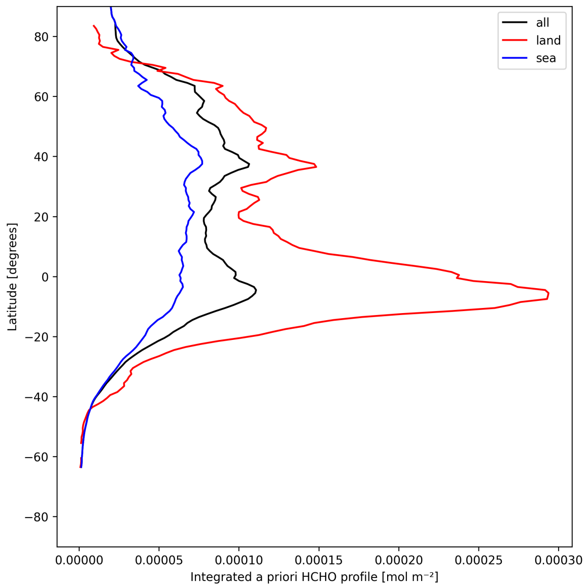
Figure 29: Zonal average of “Integrated a priori HCHO profile” for 2025-07-19 to 2025-07-20.
