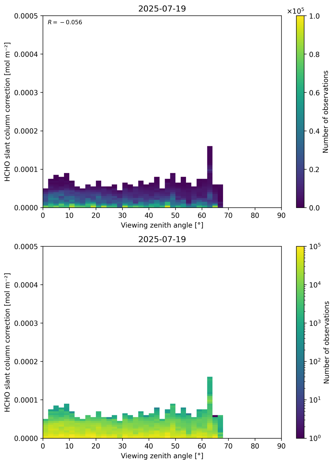
Figure 187: Scatter density plot of “Viewing zenith angle” against “HCHO slant column correction” for 2025-07-19 to 2025-07-20.
