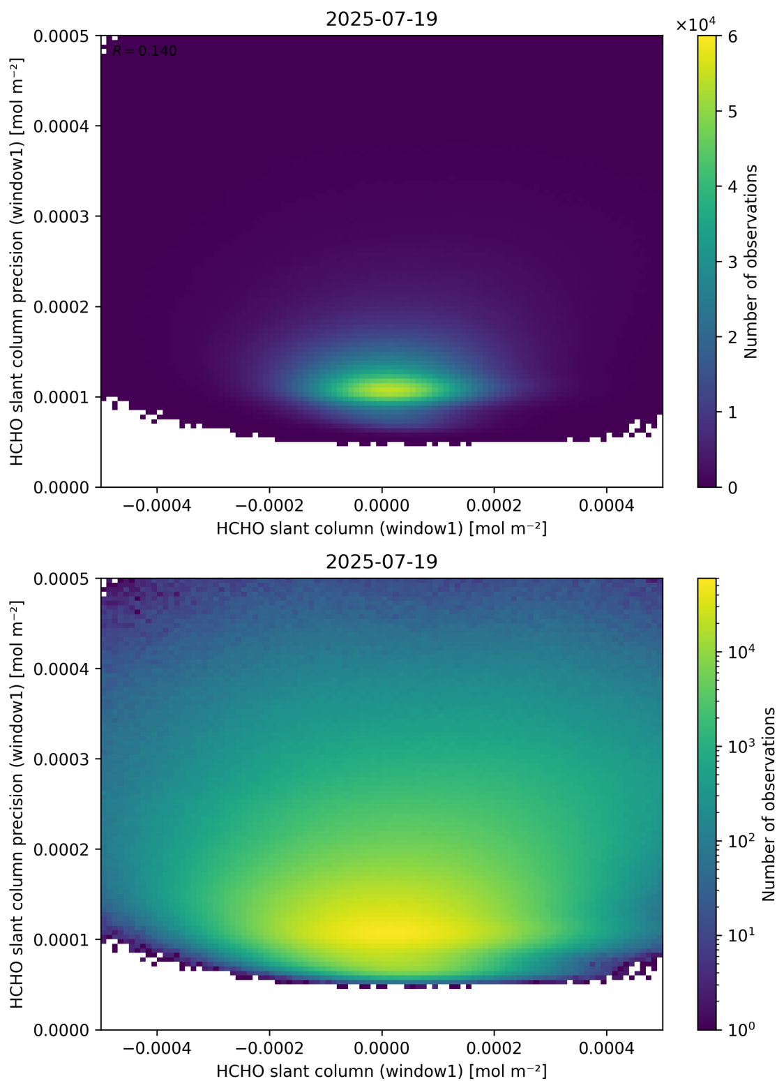
Figure 84: Scatter density plot of “HCHO slant column (window1)” against “HCHO slant column precision (window1)” for 2025-07-19 to 2025-07-20.
