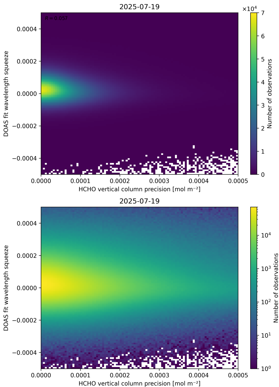
Figure 138: Scatter density plot of “HCHO vertical column precision” against “DOAS fit wavelength squeeze” for 2025-07-19 to 2025-07-20.
