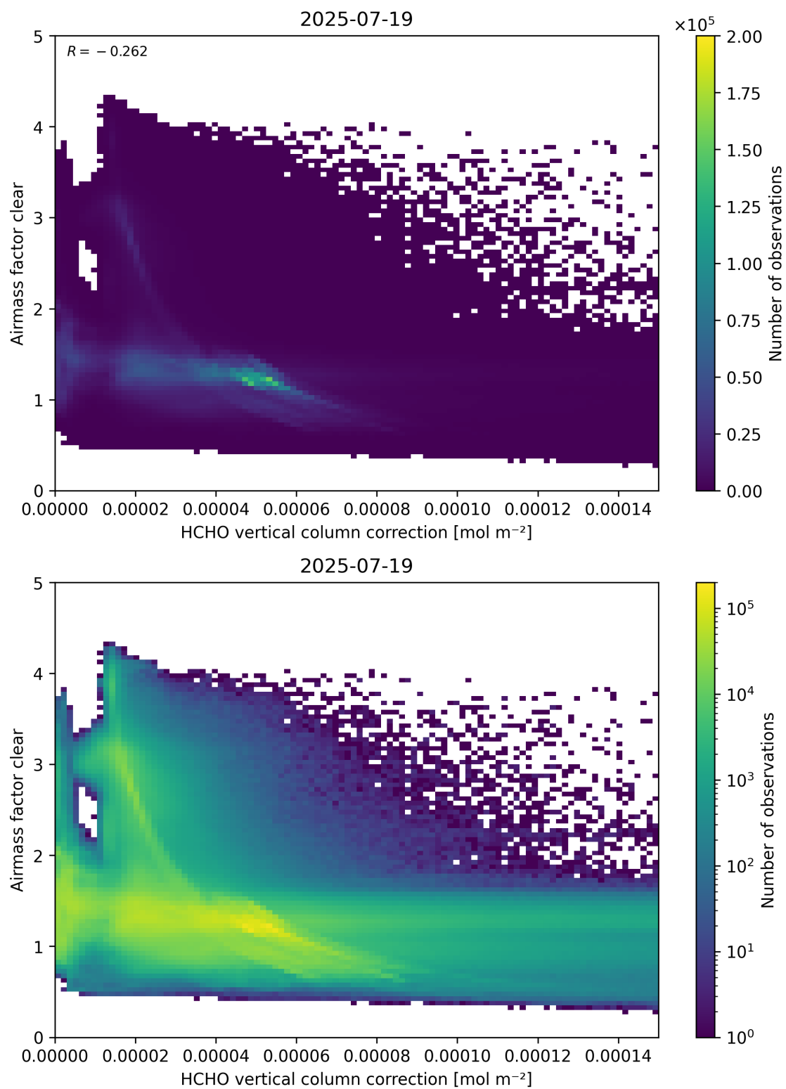
Figure 115: Scatter density plot of “HCHO vertical column correction” against “Airmass factor clear” for 2025-07-19 to 2025-07-20.
