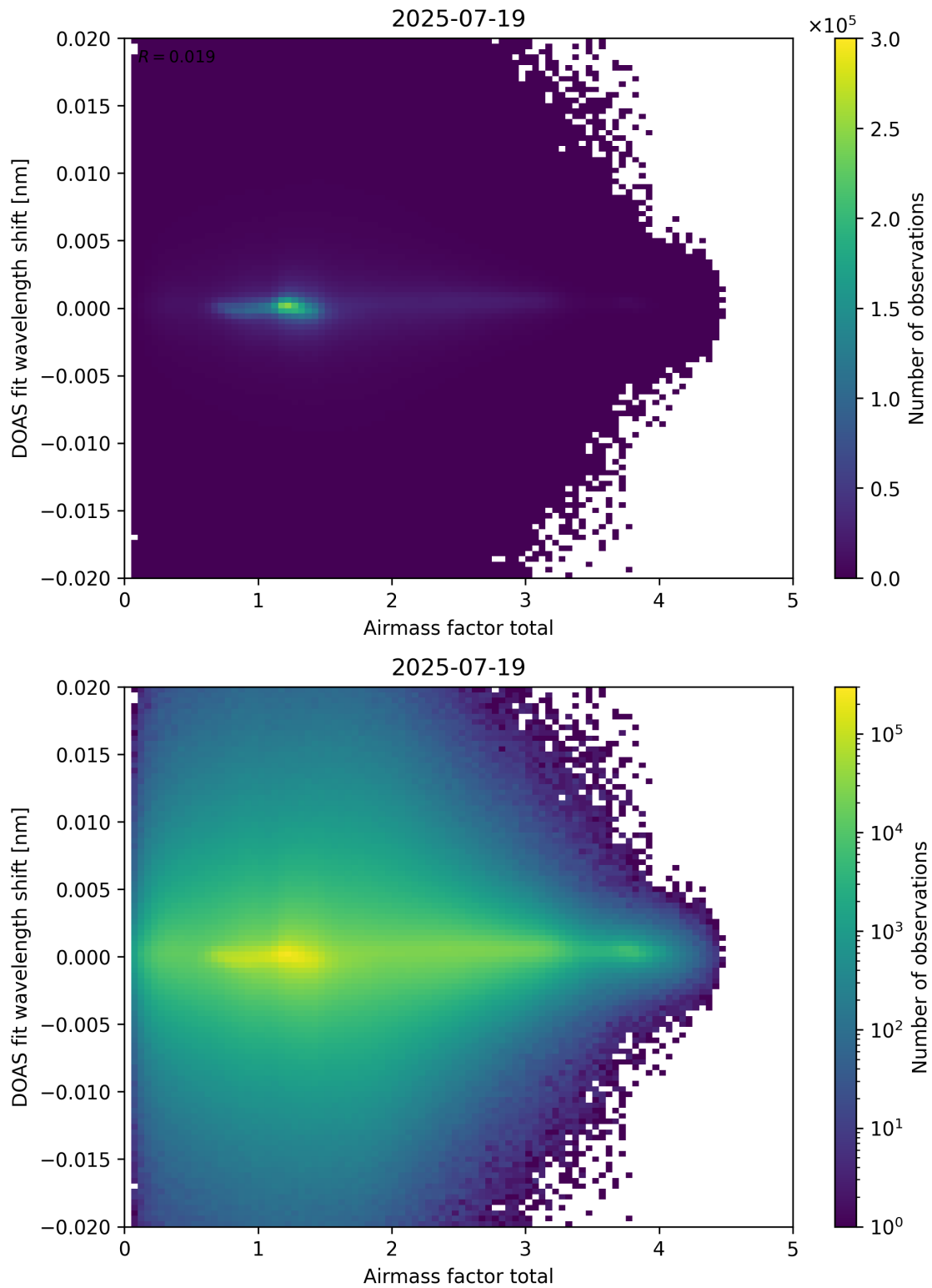
Figure 98: Scatter density plot of “Airmass factor total” against “DOAS fit wavelength shift” for 2025-07-19 to 2025-07-20.
