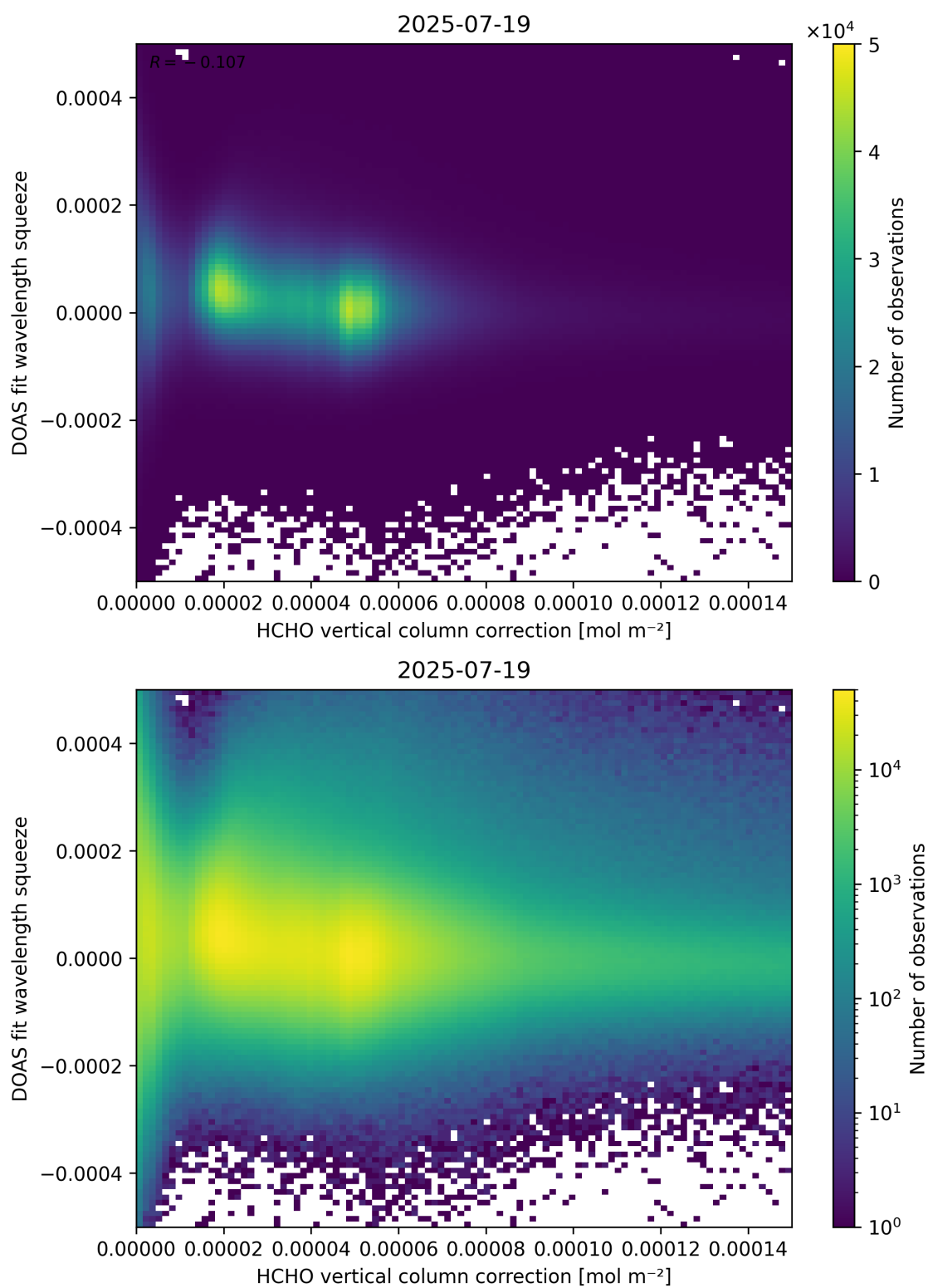
Figure 114: Scatter density plot of “HCHO vertical column correction” against “DOAS fit wavelength squeeze” for 2025-07-19 to 2025-07-20.
