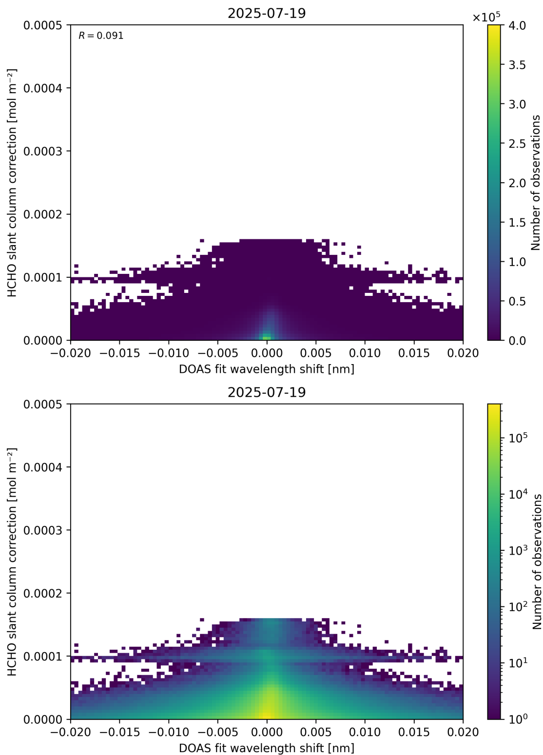
Figure 67: Scatter density plot of “DOAS fit wavelength shift” against “HCHO slant column correction” for 2025-07-19 to 2025-07-20.
