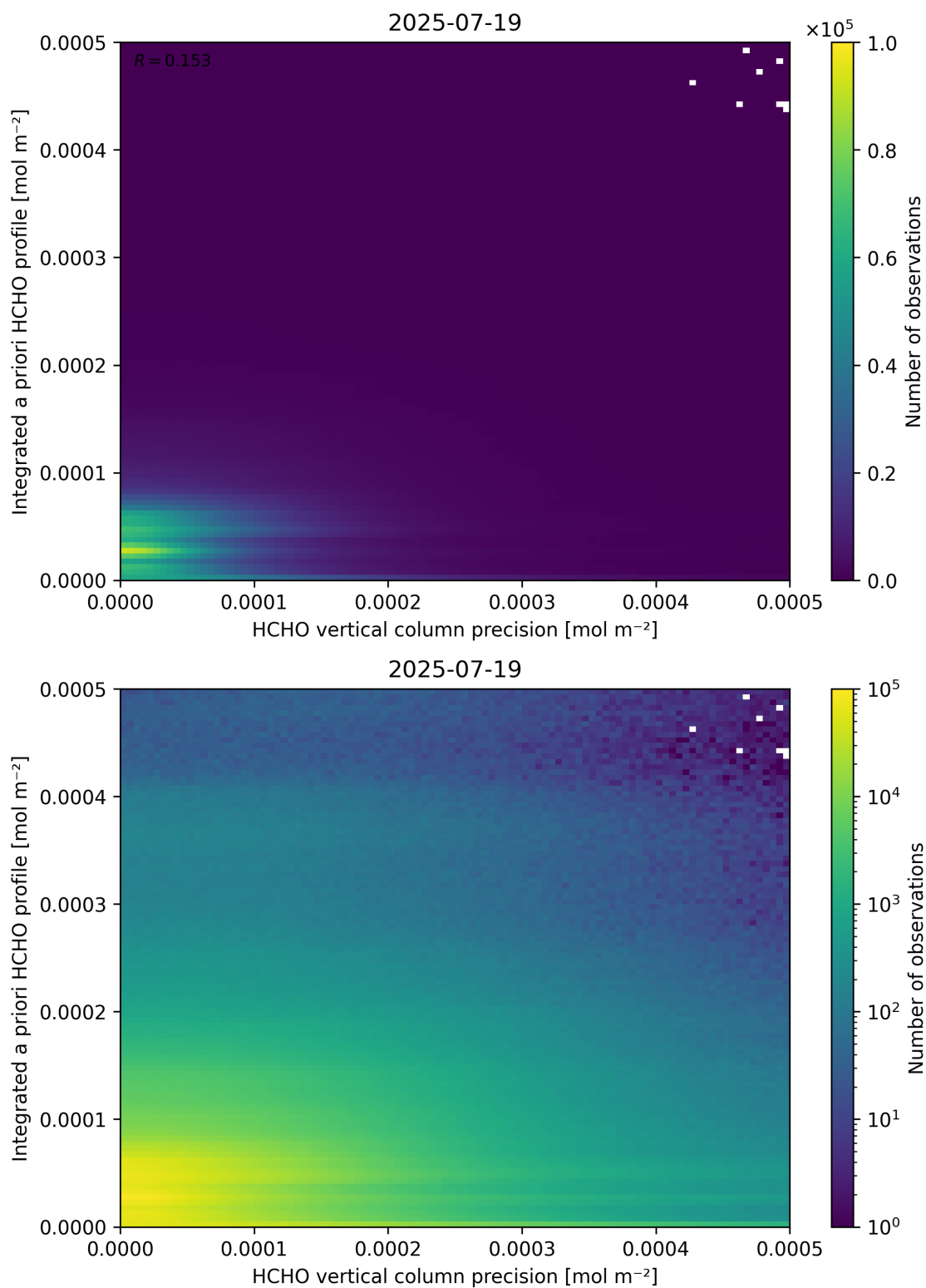
Figure 147: Scatter density plot of “HCHO vertical column precision” against “Integrated a priori HCHO profile” for 2025-07-19 to 2025-07-20.
