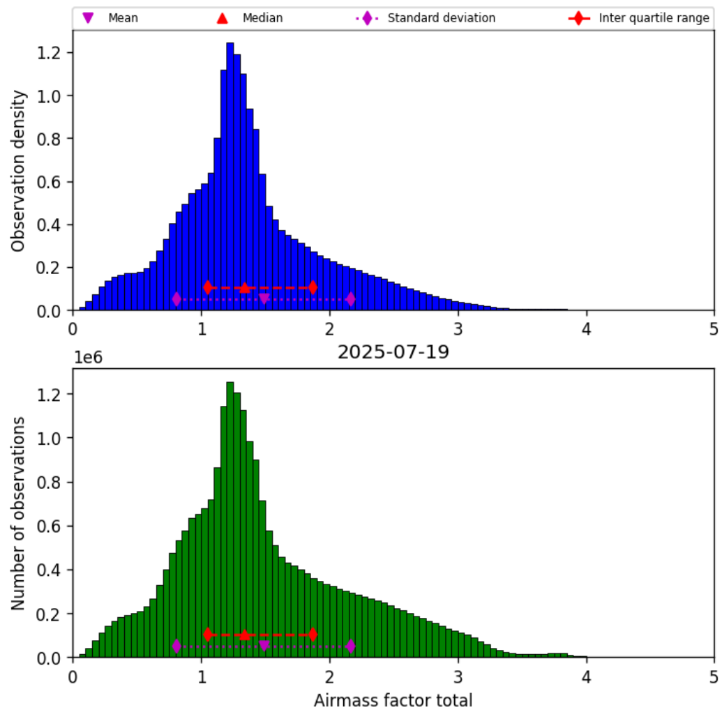
Figure 40: Histogram of “Airmass factor total” for 2025-07-19 to 2025-07-20
