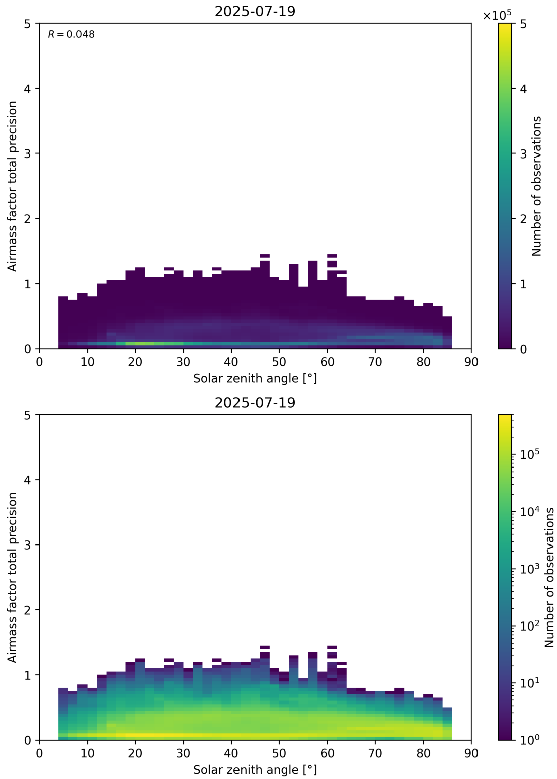
Figure 176: Scatter density plot of “Solar zenith angle” against “Airmass factor total precision” for 2025-07-19 to 2025-07-20.
