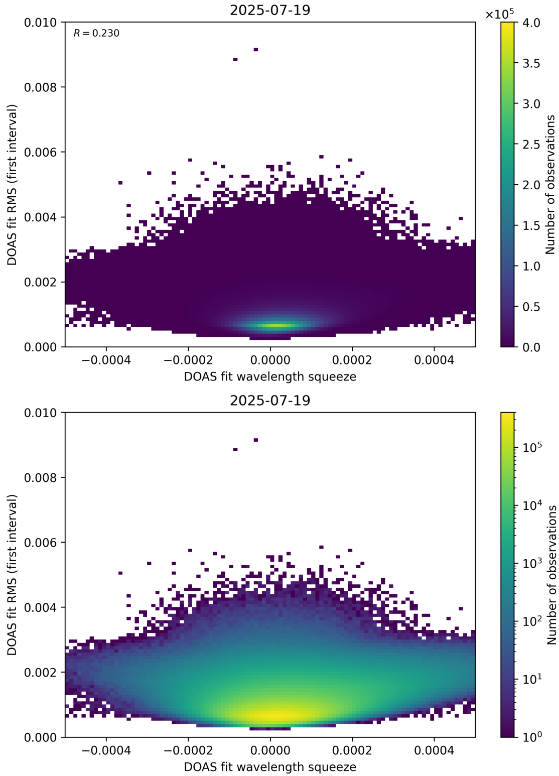
Figure 68: Scatter density plot of “DOAS fit wavelength squeeze” against “DOAS fit RMS (first interval)” for 2025-07-19 to 2025-07-20.
