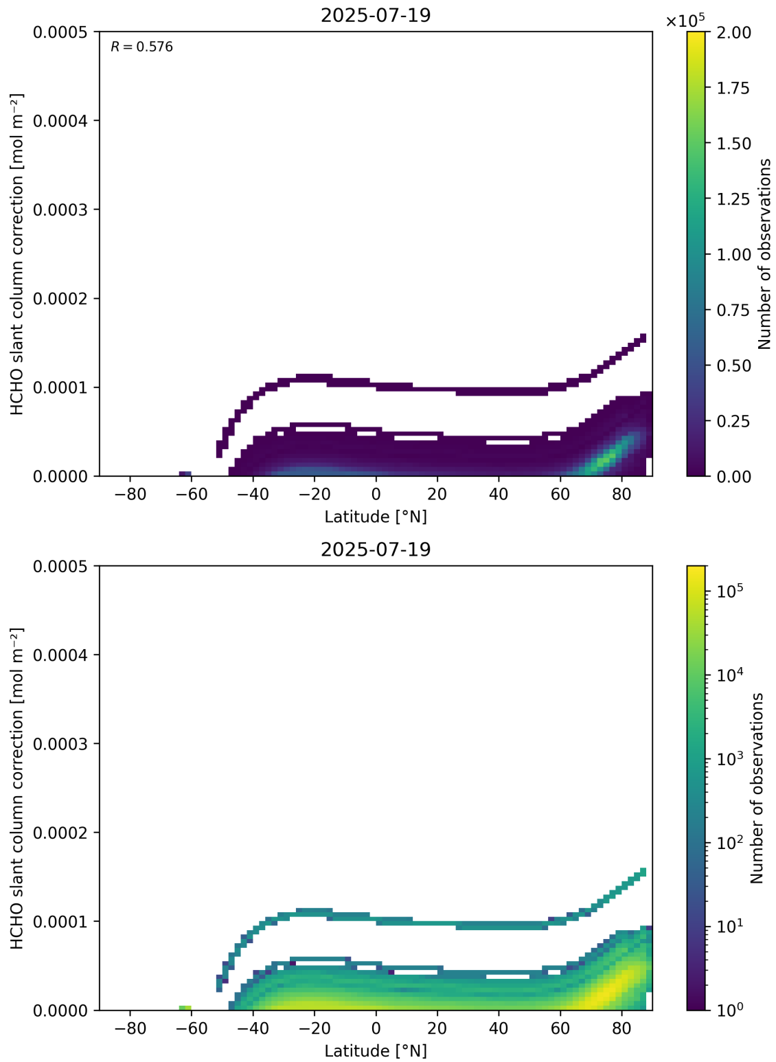
Figure 158: Scatter density plot of “Latitude” against “HCHO slant column correction” for 2025-07-19 to 2025-07-20.
