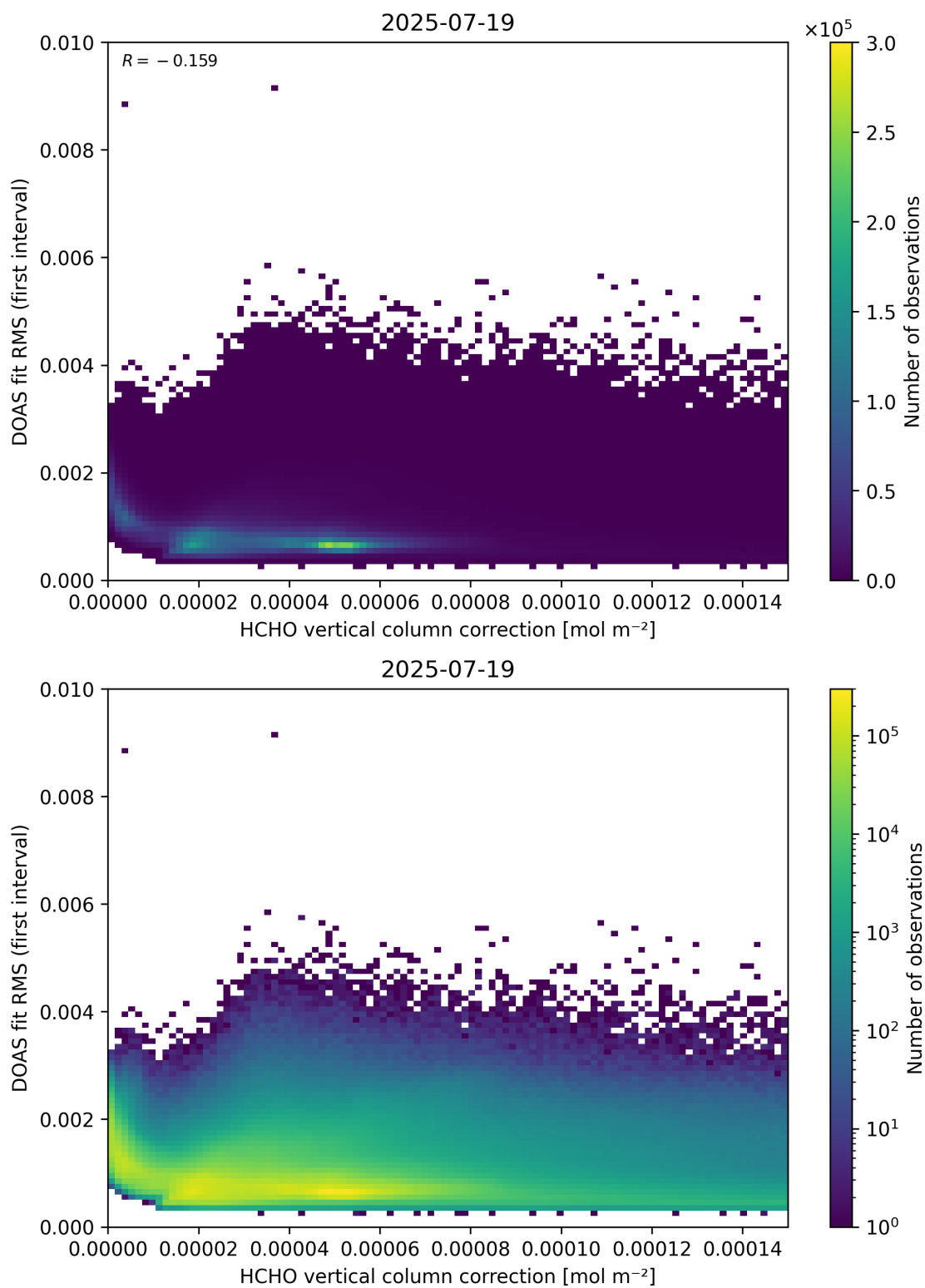
Figure 112: Scatter density plot of “HCHO vertical column correction” against “DOAS fit RMS (first interval)” for 2025-07-19 to 2025-07-20.
