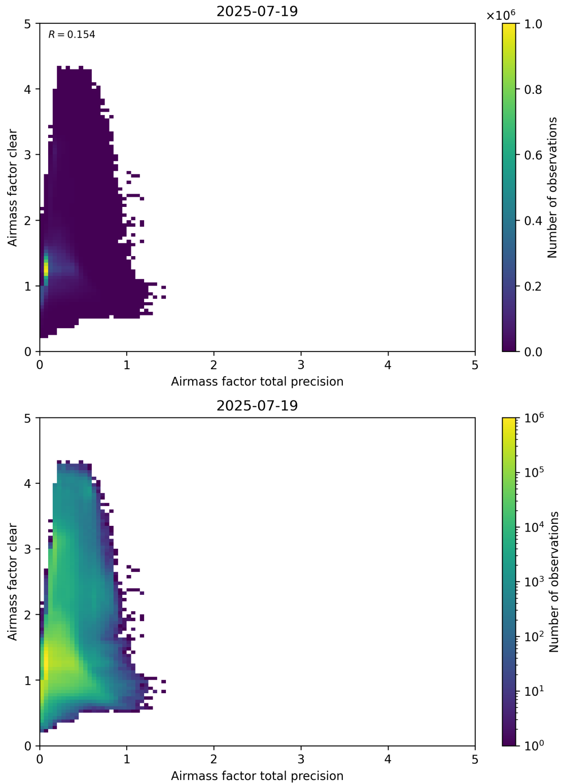
Figure 108: Scatter density plot of “Airmass factor total precision” against “Airmass factor clear” for 2025-07-19 to 2025-07-20.
