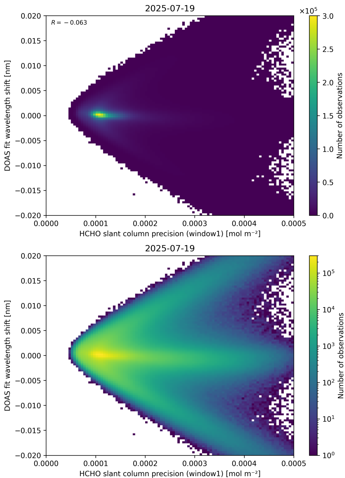
Figure 89: Scatter density plot of “HCHO slant column precision (window1)” against “DOAS fit wavelength shift” for 2025-07-19 to 2025-07-20.
