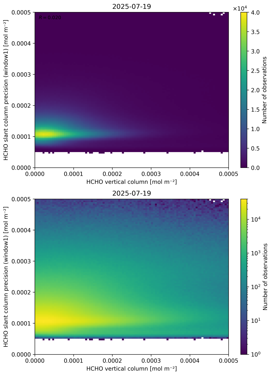
Figure 130: Scatter density plot of “HCHO vertical column” against “HCHO slant column precision (window1)” for 2025-07-19 to 2025-07-20.
