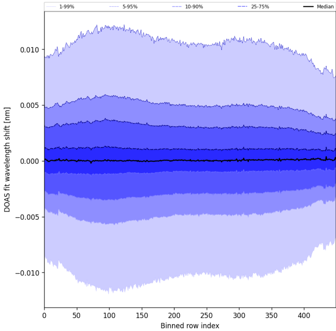
Figure 58: Along track statistics of “DOAS fit wavelength shift” for 2025-07-19 to 2025-07-20
