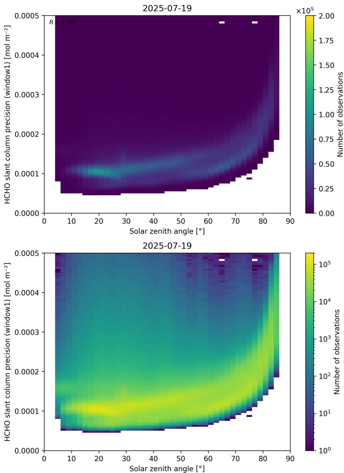
Figure 174: Scatter density plot of “Solar zenith angle” against “HCHO slant column precision (window1)” for 2025-07-19 to 2025-07-20.
