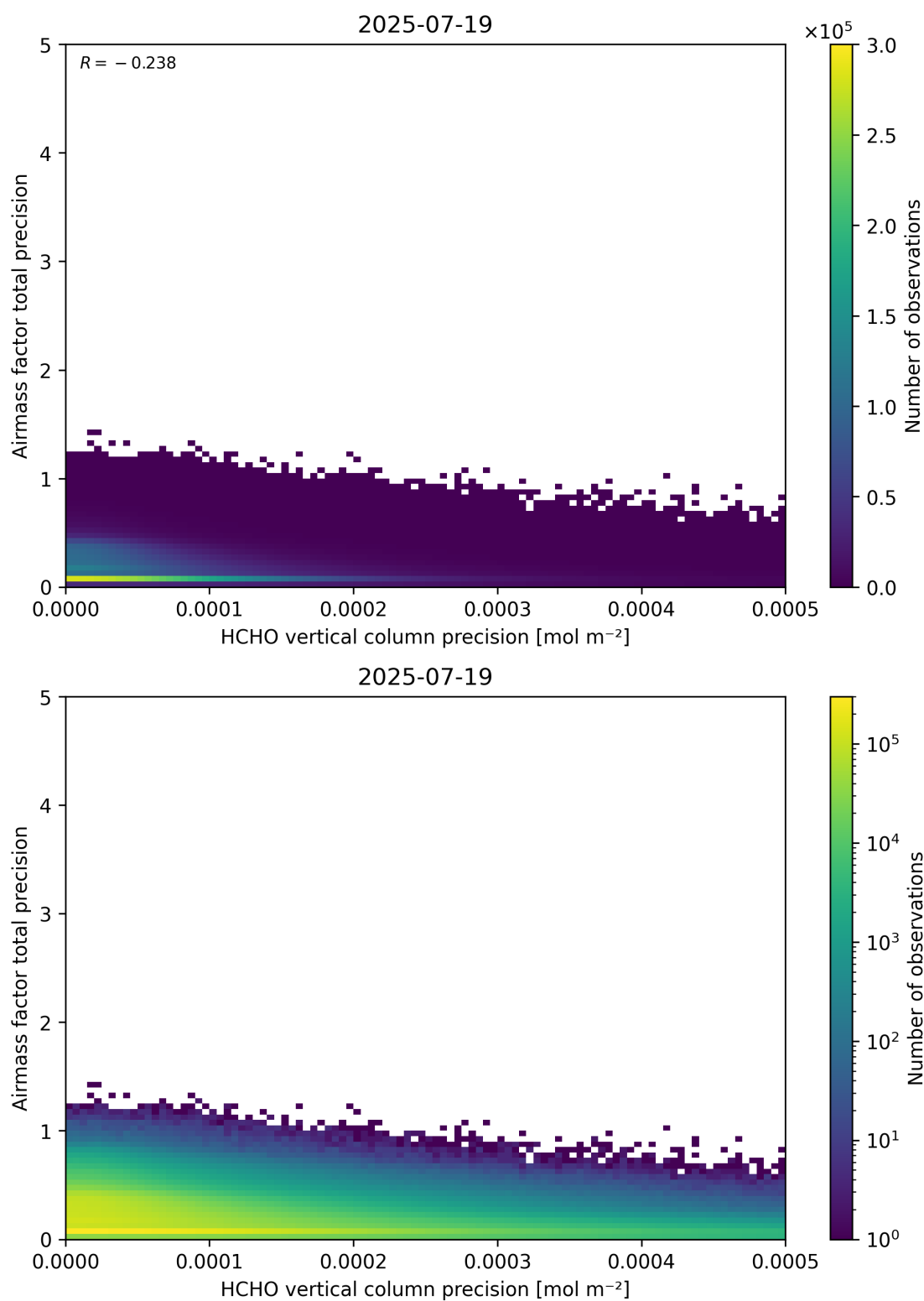
Figure 145: Scatter density plot of “HCHO vertical column precision” against “Airmass factor total precision” for 2025-07-19 to 2025-07-20.
