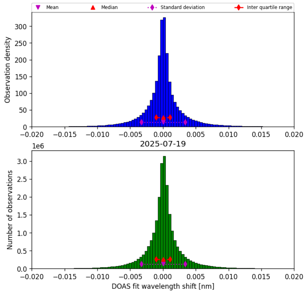
Figure 44: Histogram of “DOAS fit wavelength shift” for 2025-07-19 to 2025-07-20
