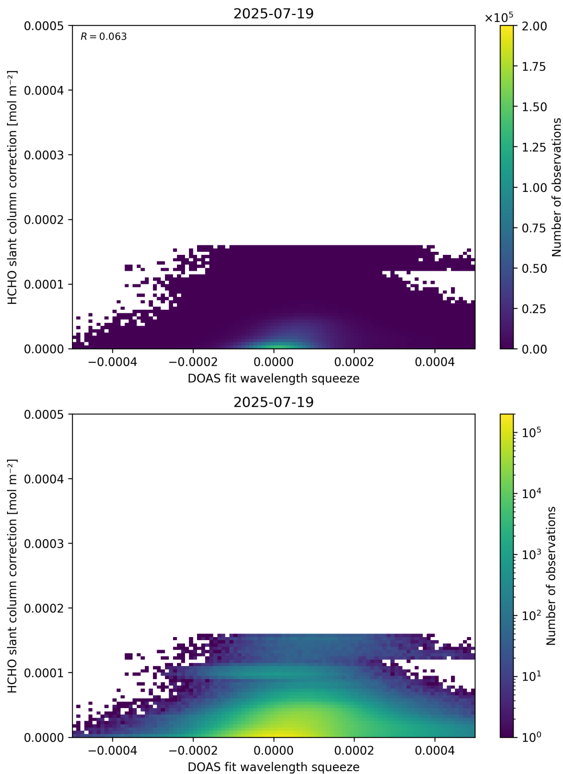
Figure 70: Scatter density plot of “DOAS fit wavelength squeeze” against “HCHO slant column correction” for 2025-07-19 to 2025-07-20.
