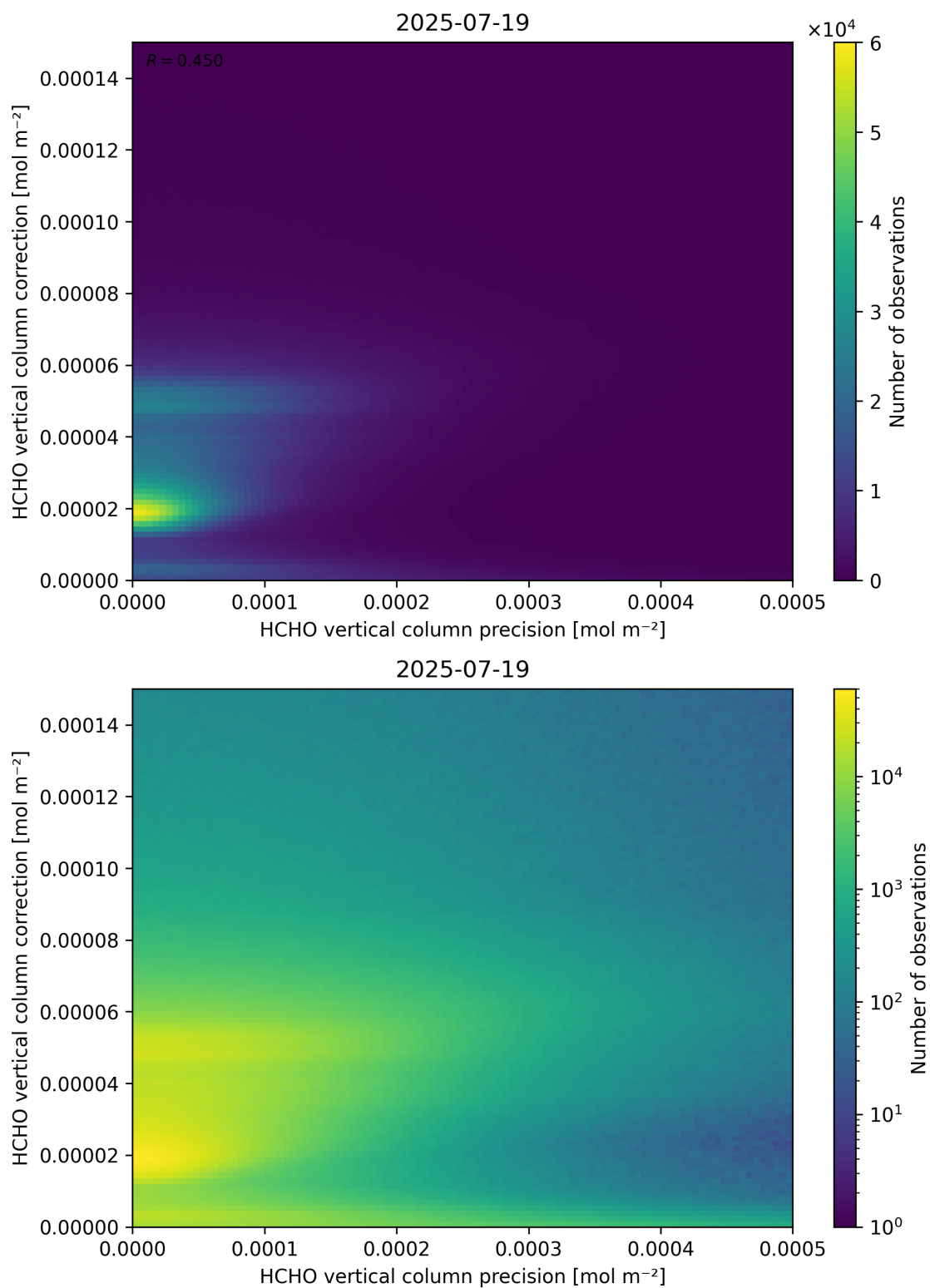
Figure 146: Scatter density plot of “HCHO vertical column precision” against “HCHO vertical column correction” for 2025-07-19 to 2025-07-20.
