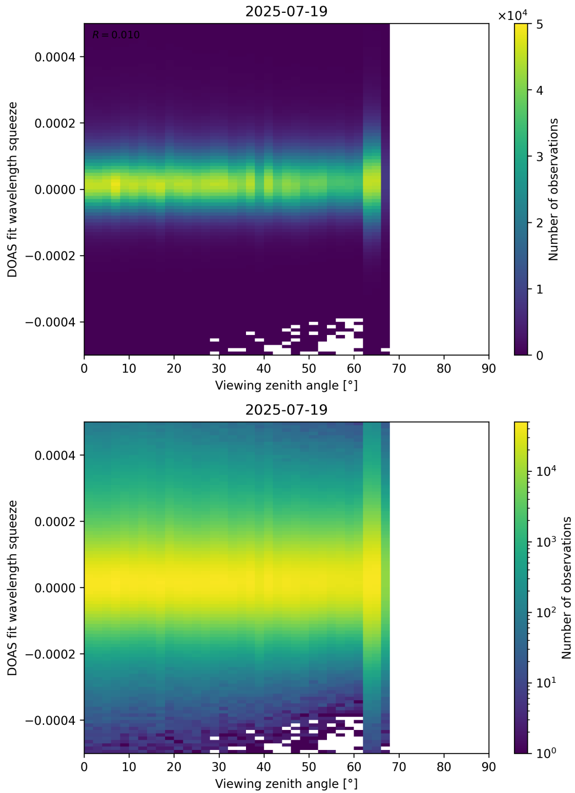
Figure 184: Scatter density plot of “Viewing zenith angle” against “DOAS fit wavelength squeeze” for 2025-07-19 to 2025-07-20.
