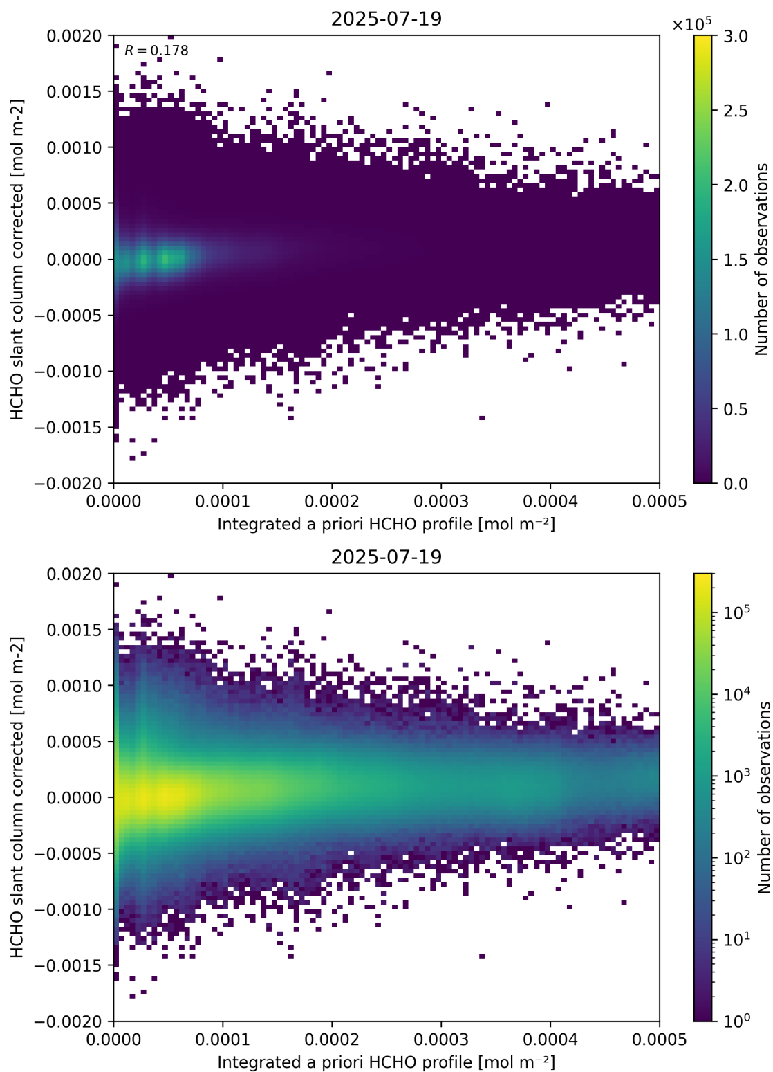
Figure 151: Scatter density plot of “Integrated a priori HCHO profile” against “HCHO slant column corrected” for 2025-07-19 to 2025-07-20.
