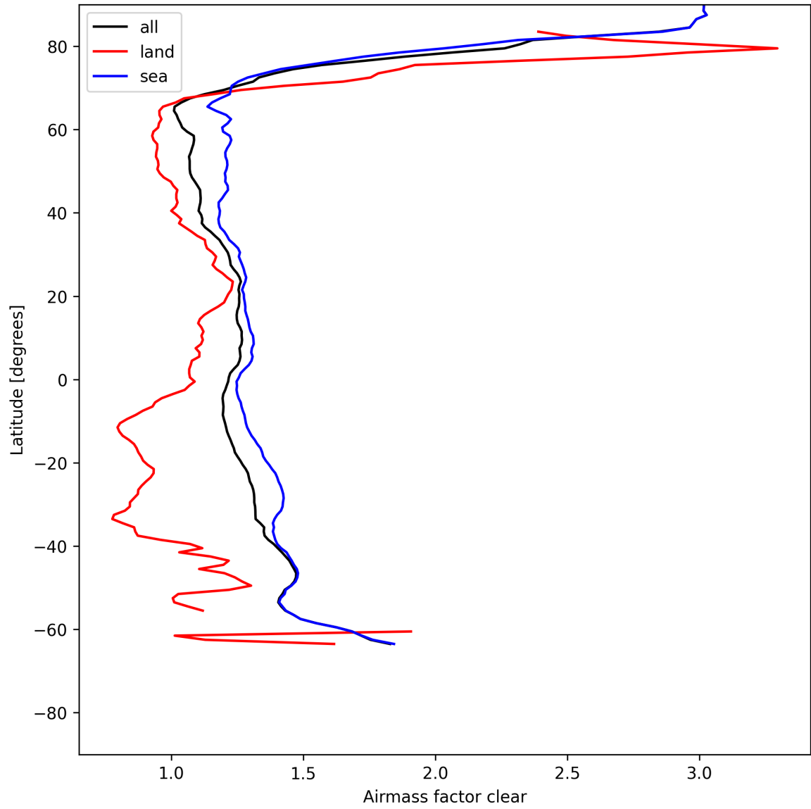
Figure 28: Zonal average of “Airmass factor clear” for 2025-07-19 to 2025-07-20.
