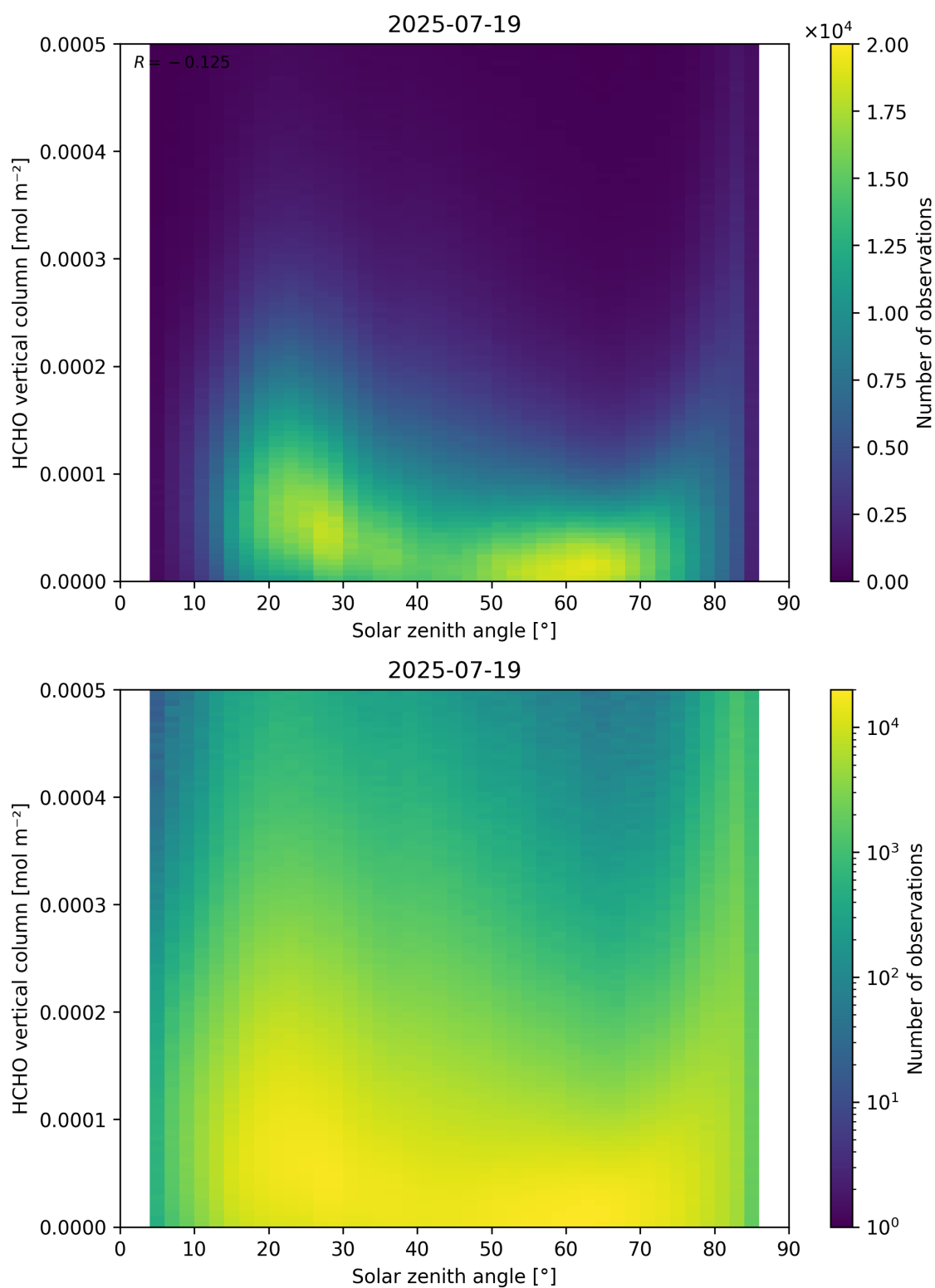
Figure 177: Scatter density plot of “Solar zenith angle” against “HCHO vertical column” for 2025-07-19 to 2025-07-20.
