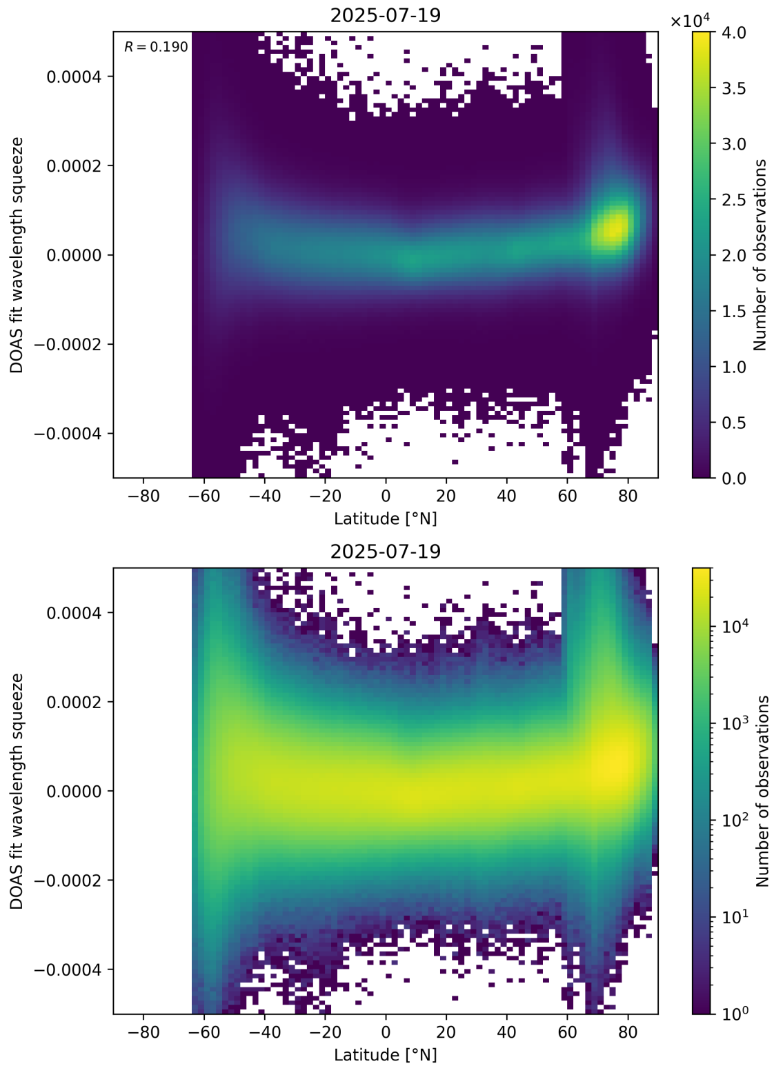
Figure 155: Scatter density plot of “Latitude” against “DOAS fit wavelength squeeze” for 2025-07-19 to 2025-07-20.
