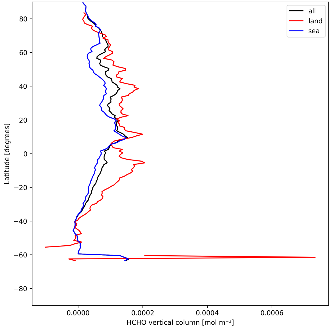
Figure 21: Zonal average of “HCHO vertical column” for 2025-07-19 to 2025-07-20.
