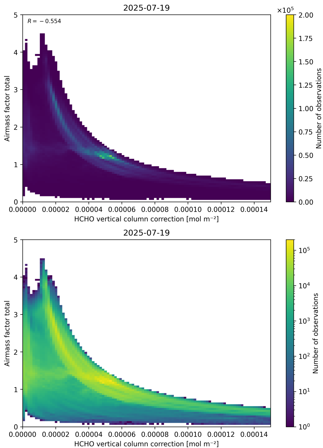
Figure 120: Scatter density plot of “HCHO vertical column correction” against “Airmass factor total” for 2025-07-19 to 2025-07-20.
