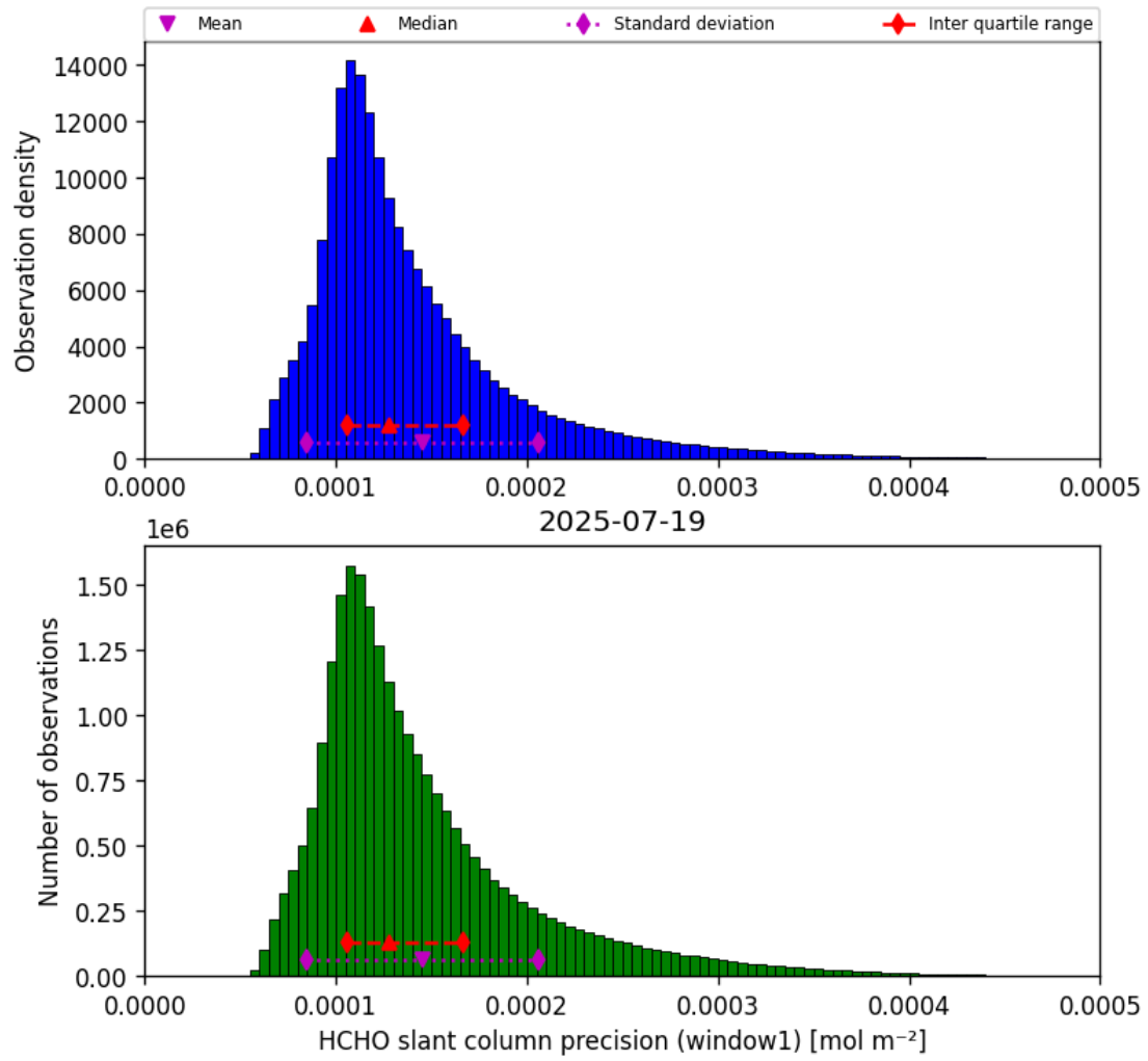
Figure 39: Histogram of “HCHO slant column precision (window1)” for 2025-07-19 to 2025-07-20
