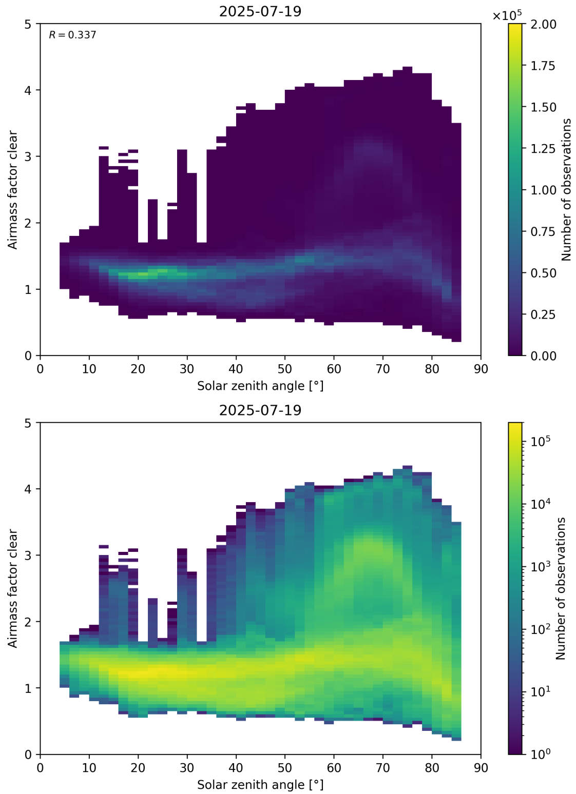
Figure 170: Scatter density plot of “Solar zenith angle” against “Airmass factor clear” for 2025-07-19 to 2025-07-20.
