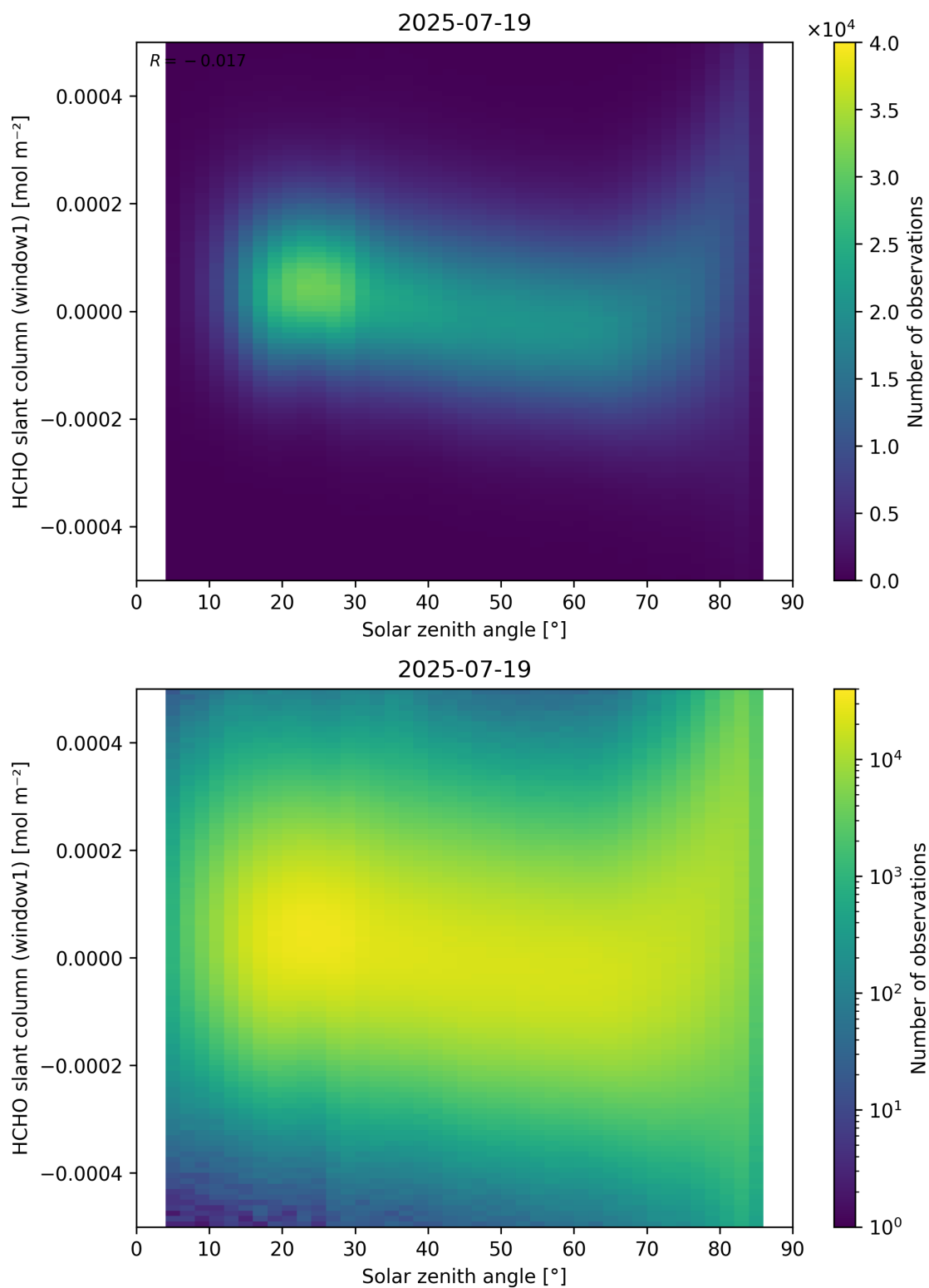
Figure 173: Scatter density plot of “Solar zenith angle” against “HCHO slant column (window1)” for 2025-07-19 to 2025-07-20.
