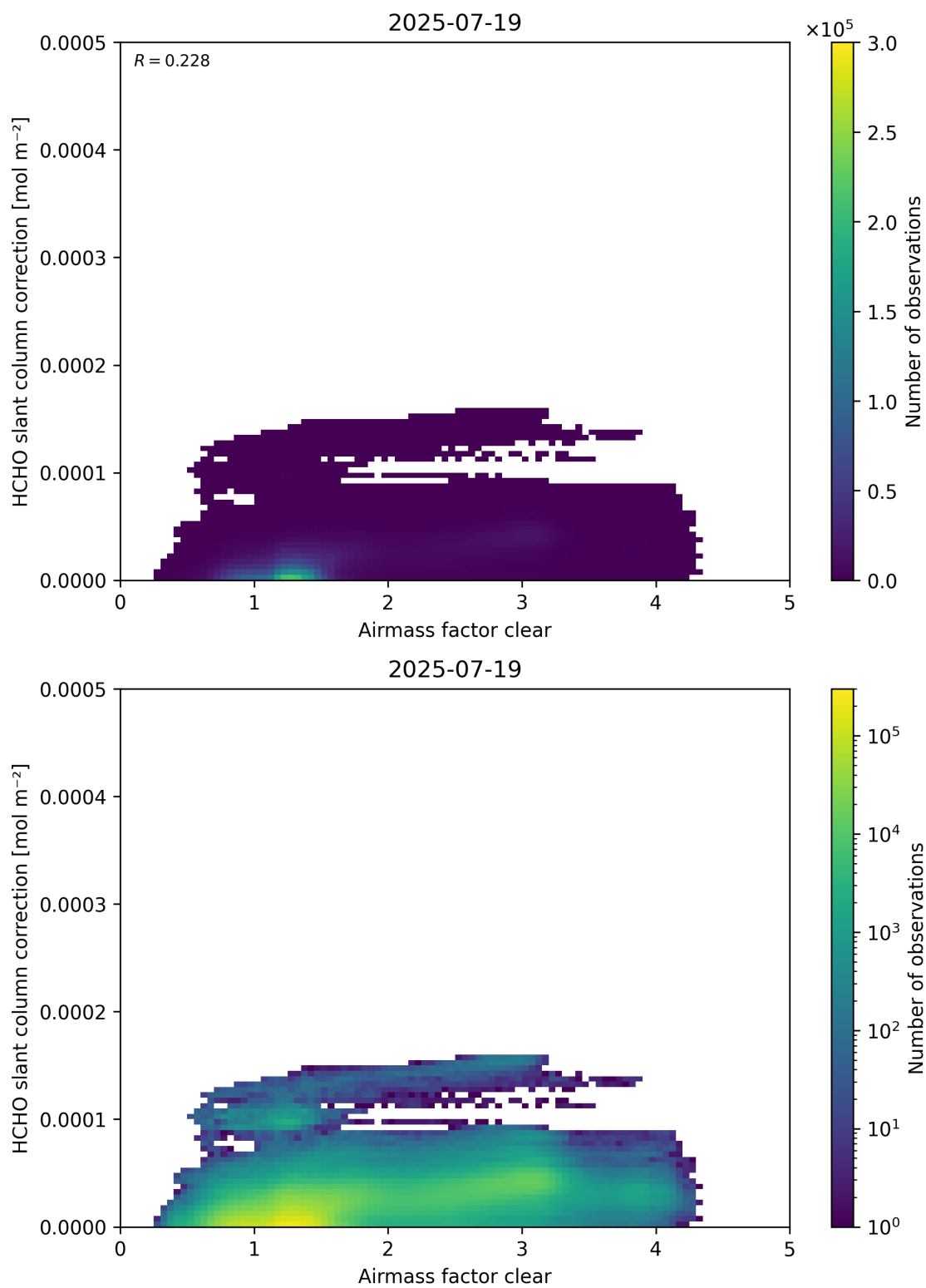
Figure 75: Scatter density plot of “Airmass factor clear” against “HCHO slant column correction” for 2025-07-19 to 2025-07-20.
