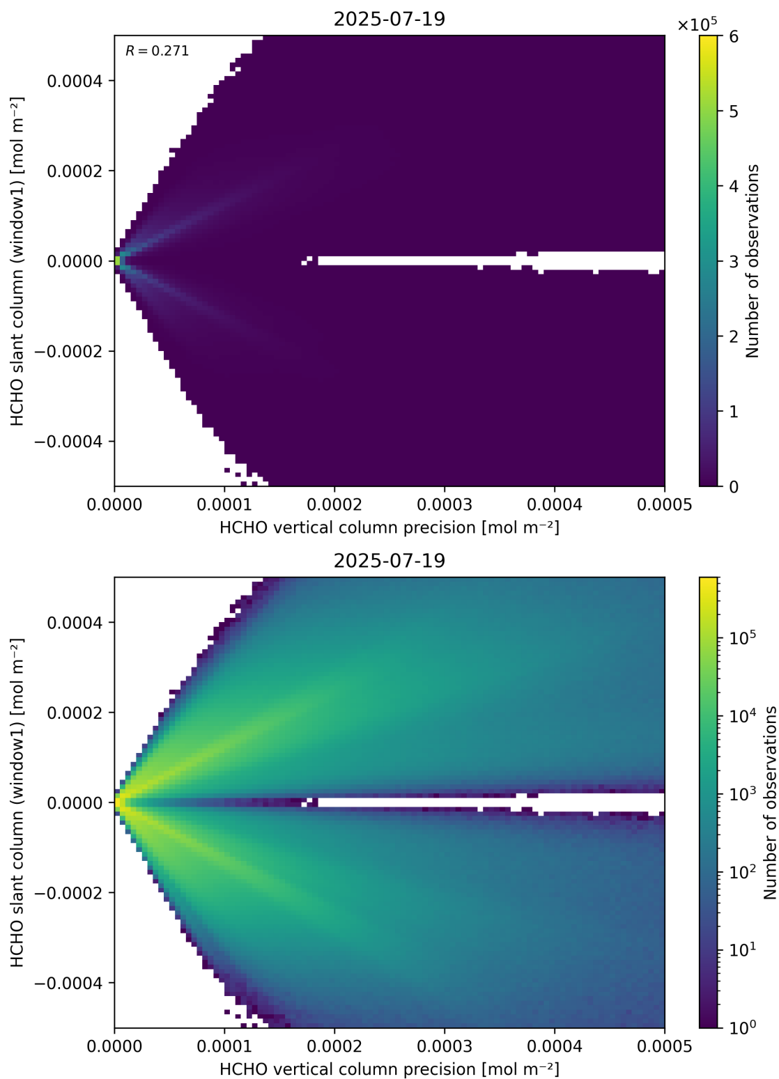
Figure 142: Scatter density plot of “HCHO vertical column precision” against “HCHO slant column (window1)” for 2025-07-19 to 2025-07-20.
