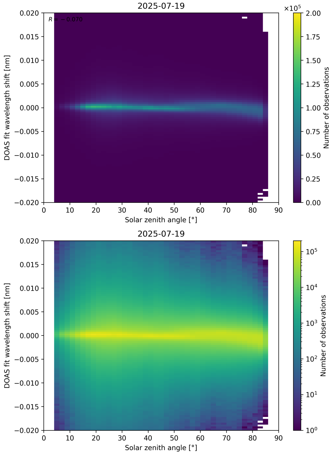
Figure 168: Scatter density plot of “Solar zenith angle” against “DOAS fit wavelength shift” for 2025-07-19 to 2025-07-20.
