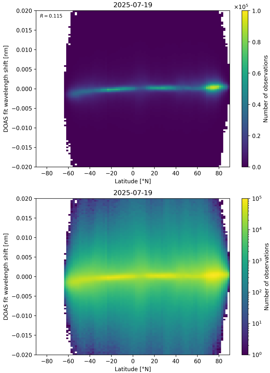
Figure 154: Scatter density plot of “Latitude” against “DOAS fit wavelength shift” for 2025-07-19 to 2025-07-20.
