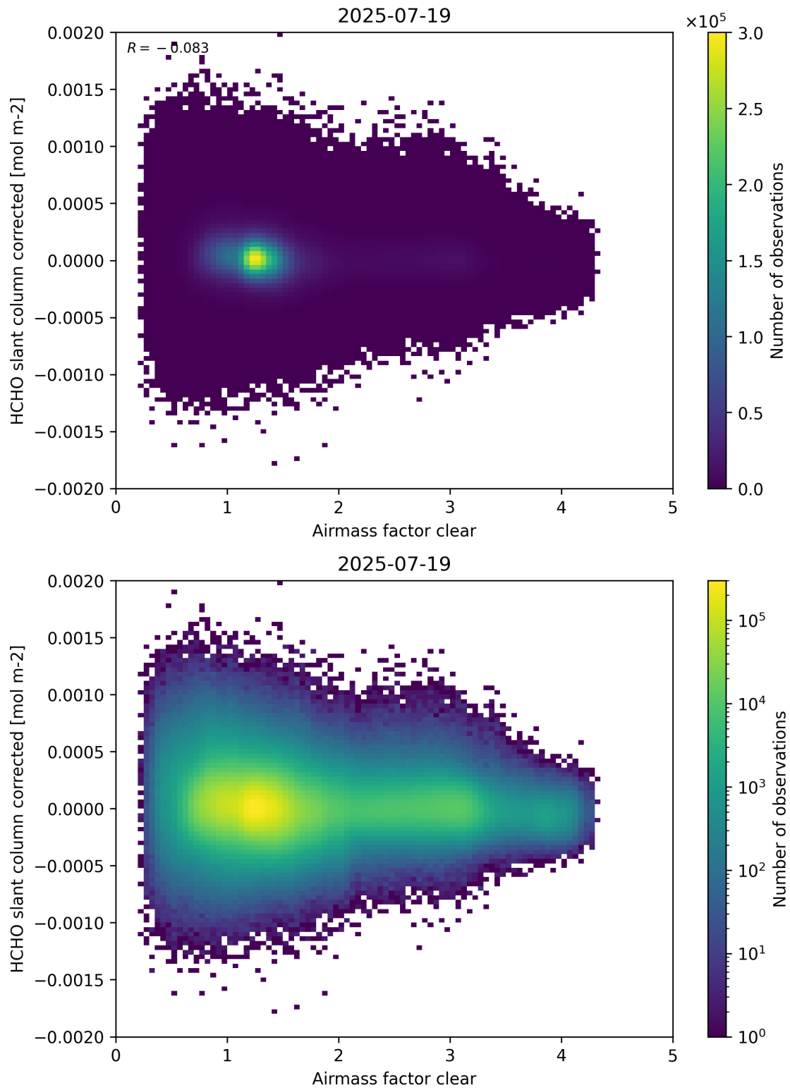
Figure 74: Scatter density plot of “Airmass factor clear” against “HCHO slant column corrected” for 2025-07-19 to 2025-07-20.
