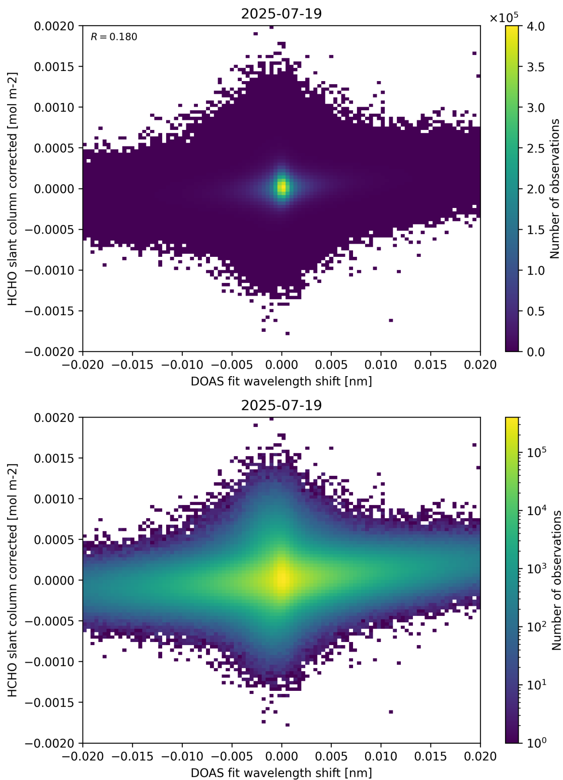
Figure 66: Scatter density plot of “DOAS fit wavelength shift” against “HCHO slant column corrected” for 2025-07-19 to 2025-07-20.
