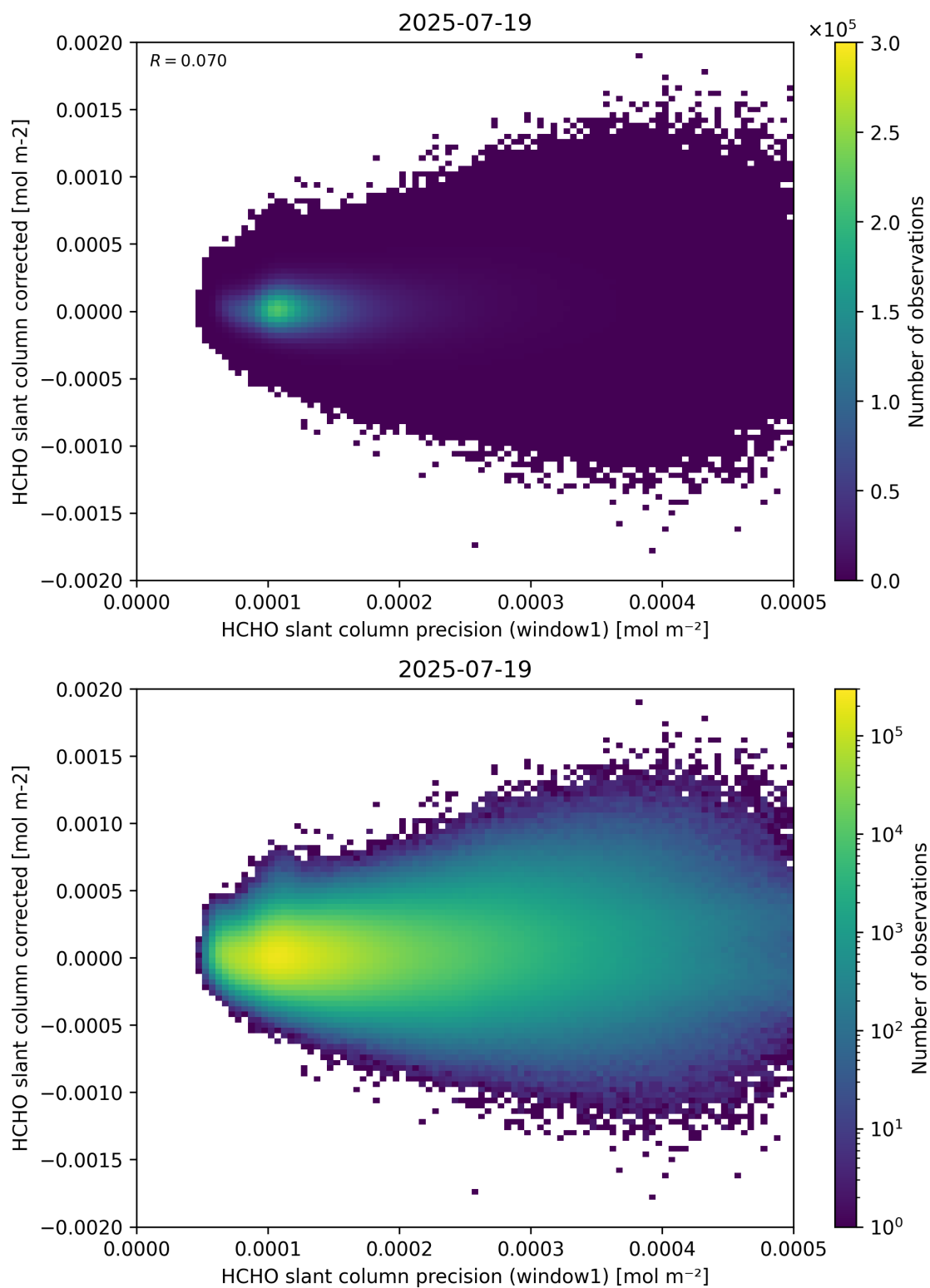
Figure 92: Scatter density plot of “HCHO slant column precision (window1)” against “HCHO slant column corrected” for 2025-07-19 to 2025-07-20.
