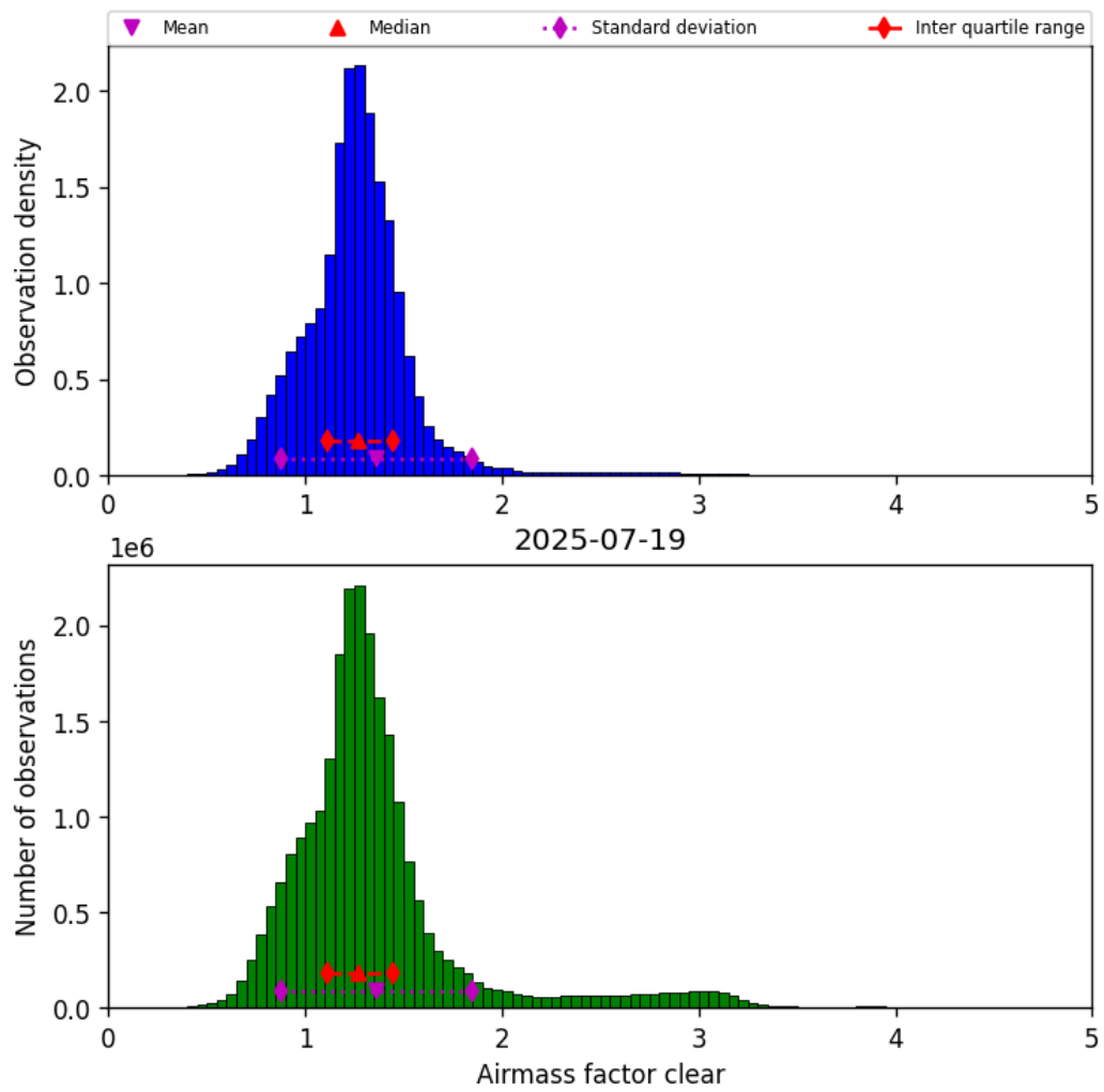
Figure 42: Histogram of “Airmass factor clear” for 2025-07-19 to 2025-07-20
