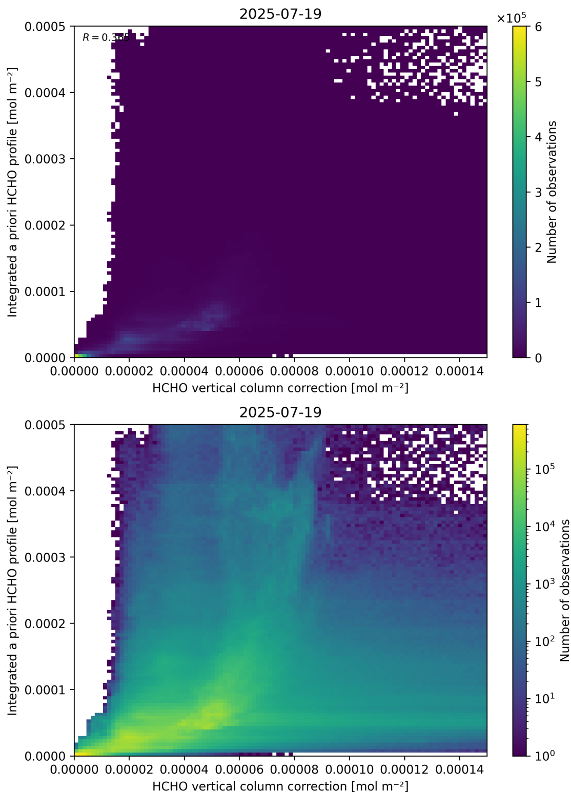
Figure 122: Scatter density plot of “HCHO vertical column correction” against “Integrated a priori HCHO profile” for 2025-07-19 to 2025-07-20.
