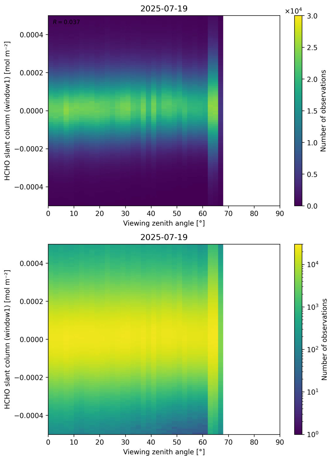
Figure 188: Scatter density plot of “Viewing zenith angle” against “HCHO slant column (window1)” for 2025-07-19 to 2025-07-20.
