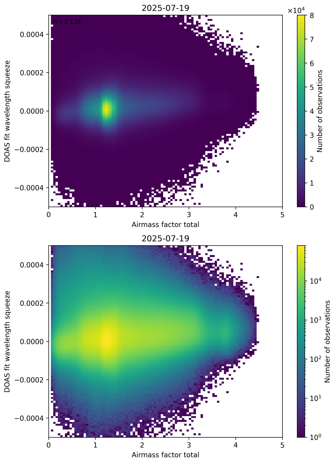
Figure 99: Scatter density plot of “Airmass factor total” against “DOAS fit wavelength squeeze” for 2025-07-19 to 2025-07-20.
