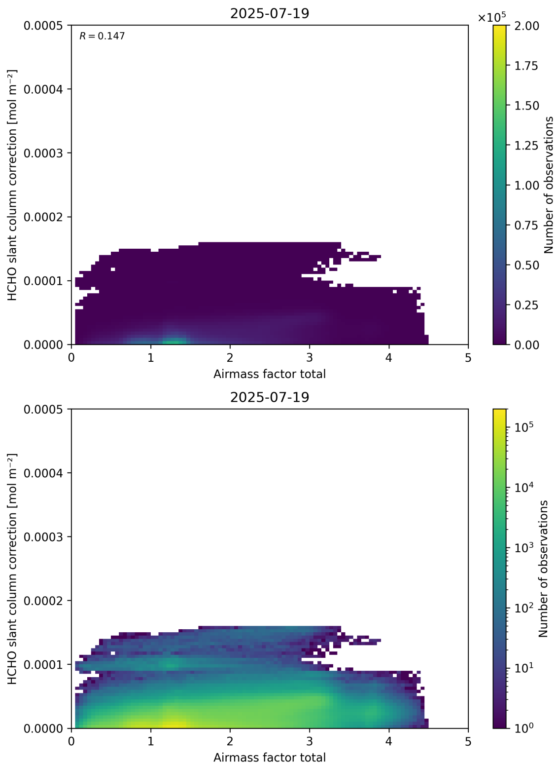
Figure 102: Scatter density plot of “Airmass factor total” against “HCHO slant column correction” for 2025-07-19 to 2025-07-20.
