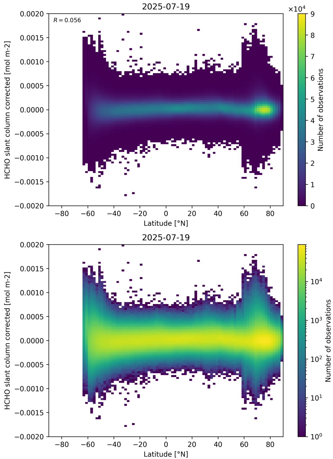
Figure 157: Scatter density plot of “Latitude” against “HCHO slant column corrected” for 2025-07-19 to 2025-07-20.
