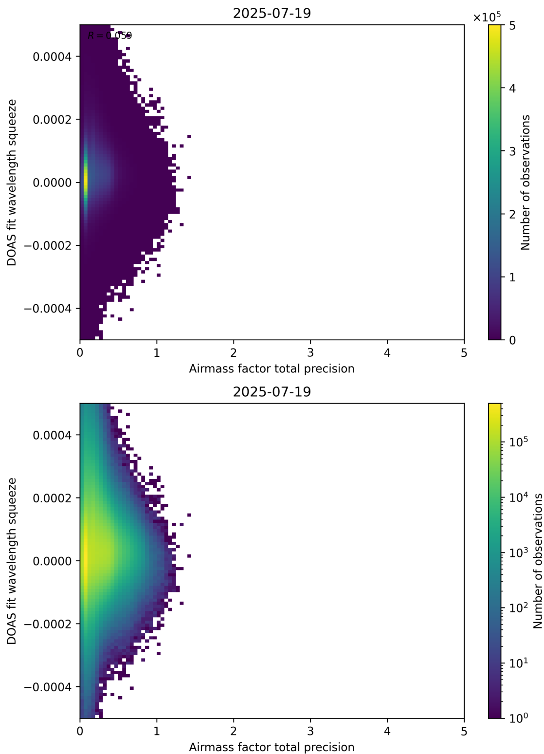
Figure 107: Scatter density plot of “Airmass factor total precision” against “DOAS fit wavelength squeeze” for 2025-07-19 to 2025-07-20.
