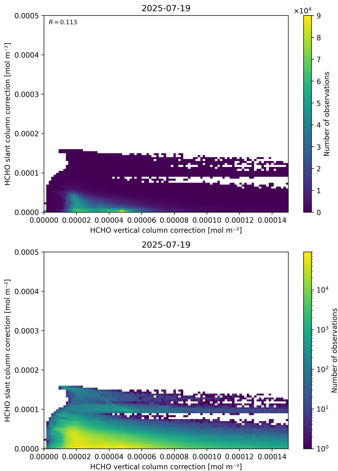
Figure 117: Scatter density plot of “HCHO vertical column correction” against “HCHO slant column correction” for 2025-07-19 to 2025-07-20.
