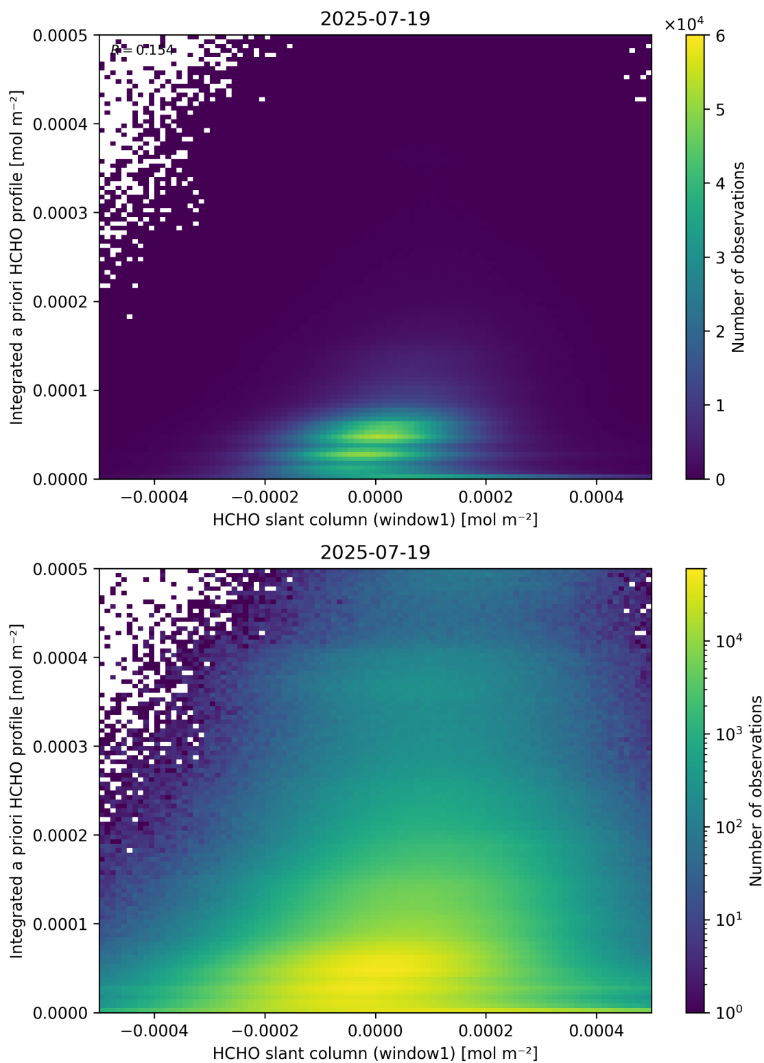
Figure 87: Scatter density plot of “HCHO slant column (window1)” against “Integrated a priori HCHO profile” for 2025-07-19 to 2025-07-20.
