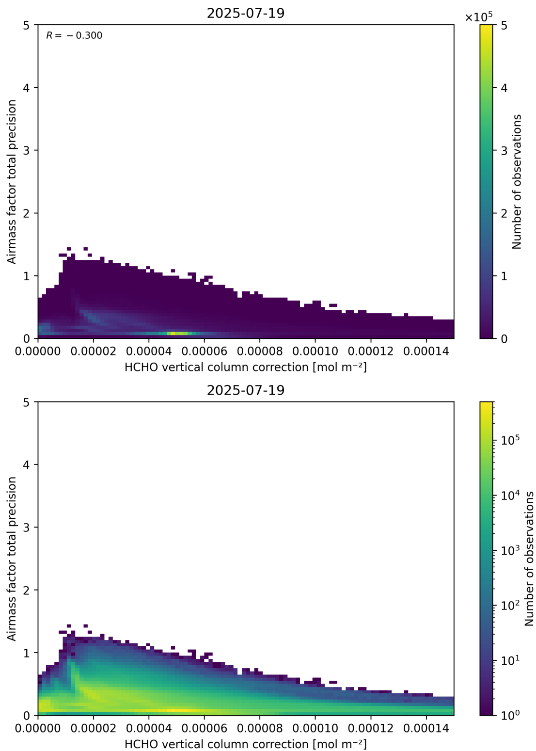
Figure 121: Scatter density plot of “HCHO vertical column correction” against “Airmass factor total precision” for 2025-07-19 to 2025-07-20.
