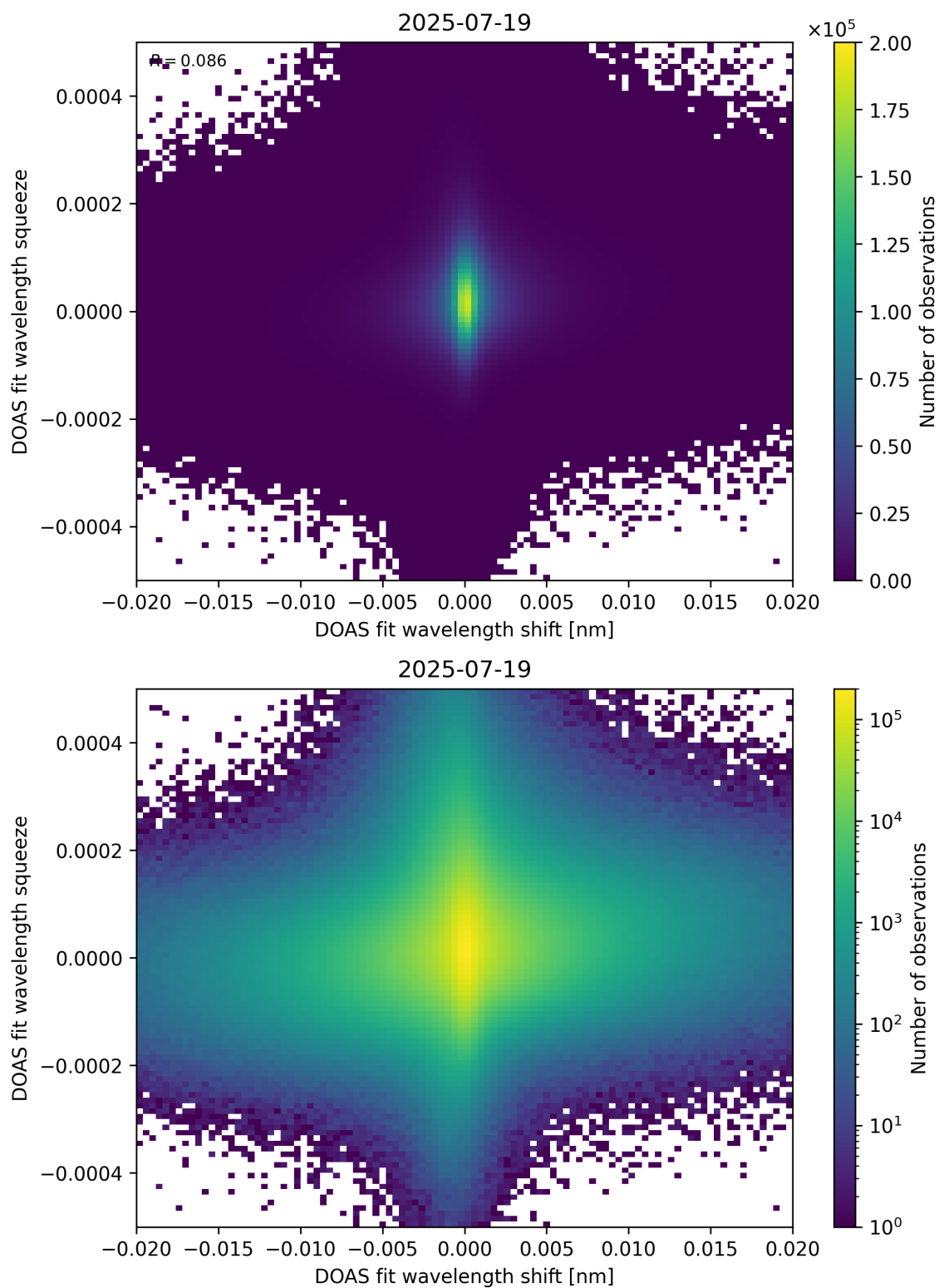
Figure 65: Scatter density plot of “DOAS fit wavelength shift” against “DOAS fit wavelength squeeze” for 2025-07-19 to 2025-07-20.
