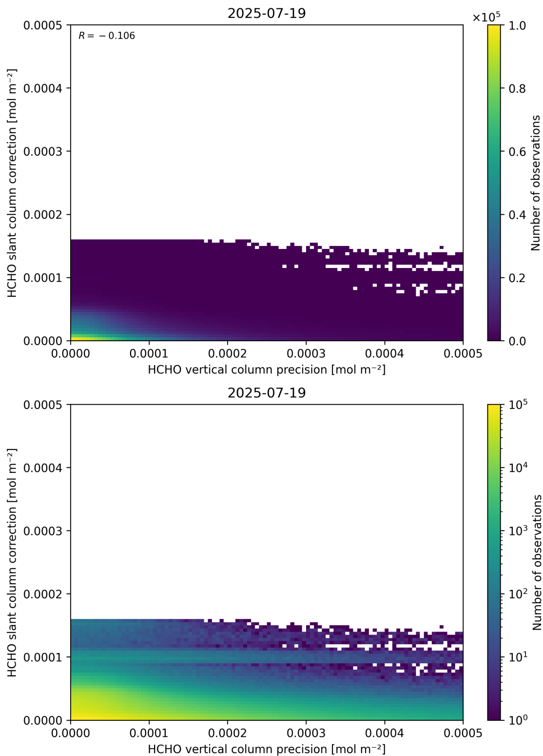
Figure 141: Scatter density plot of “HCHO vertical column precision” against “HCHO slant column correction” for 2025-07-19 to 2025-07-20.
