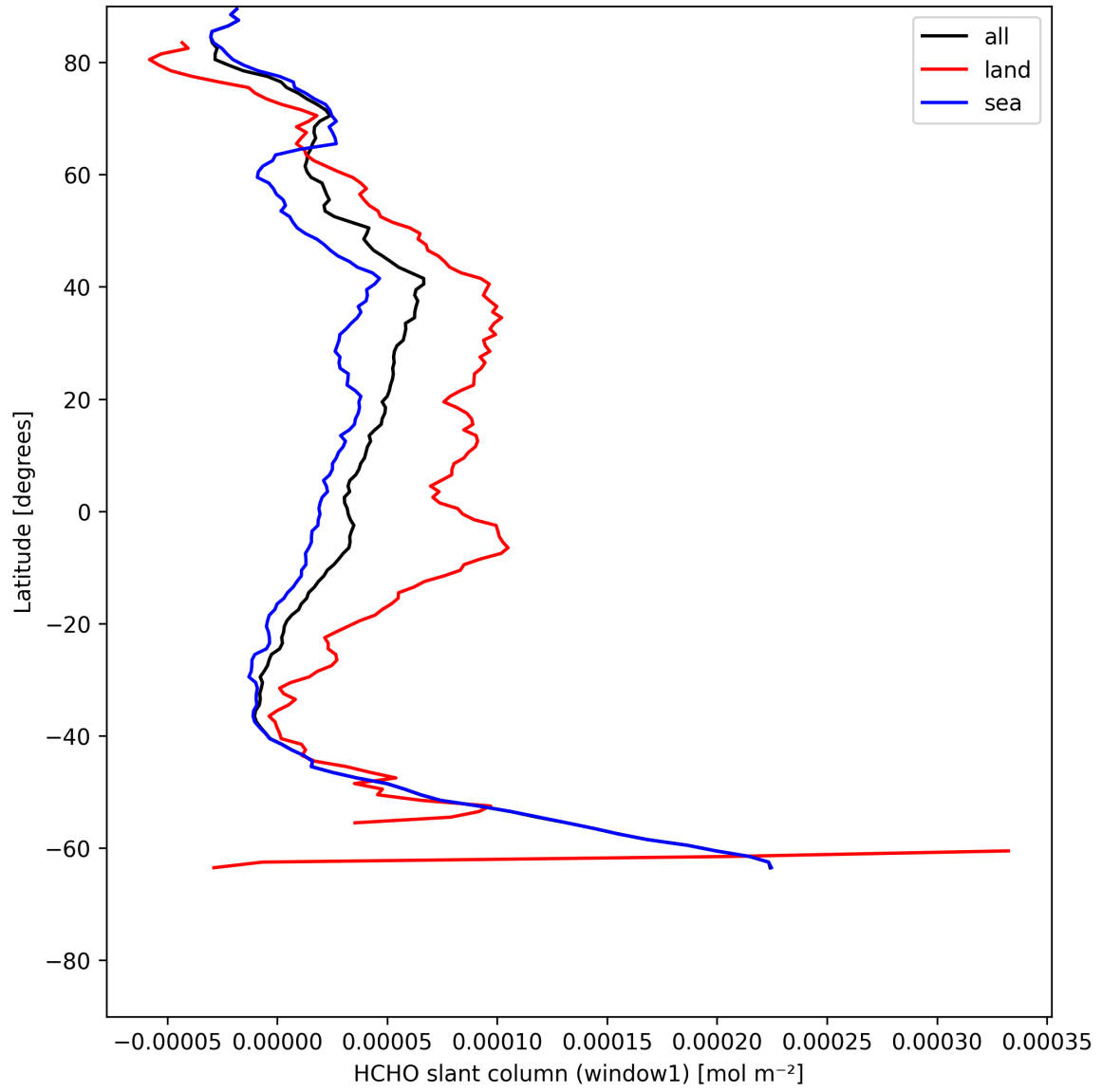
Figure 24: Zonal average of “HCHO slant column (window1)” for 2025-07-19 to 2025-07-20.
