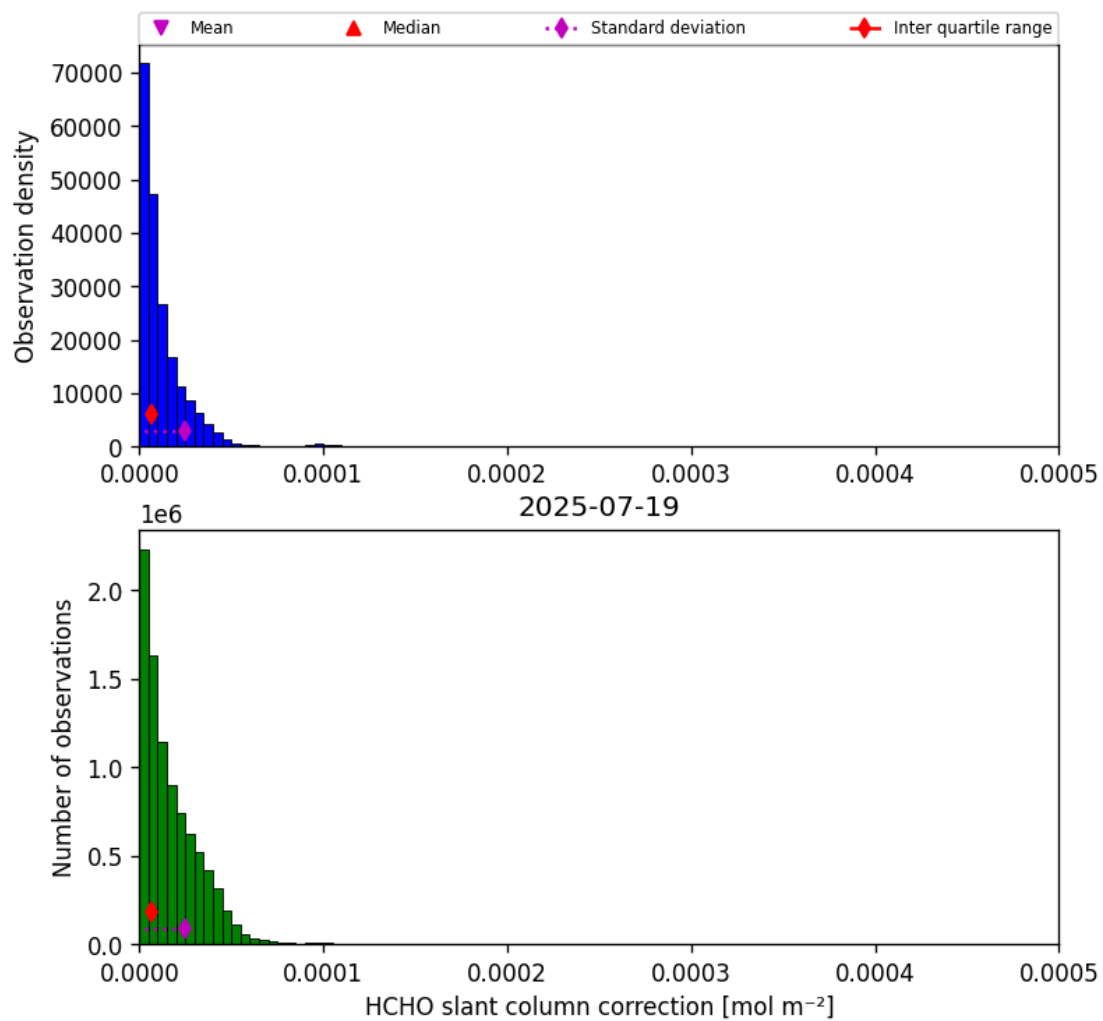
Figure 47: Histogram of “HCHO slant column correction” for 2025-07-19 to 2025-07-20
