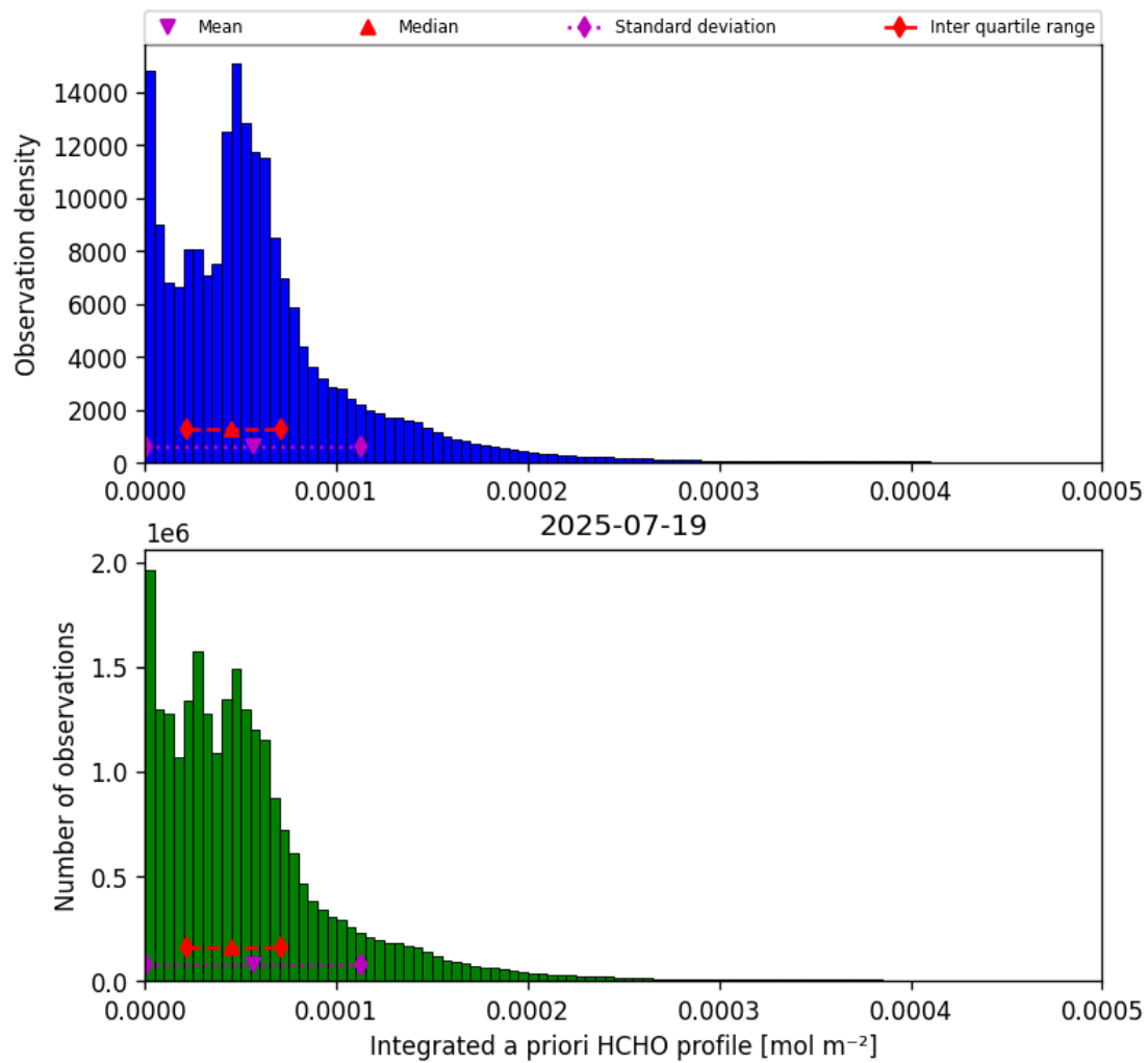
Figure 43: Histogram of “Integrated a priori HCHO profile” for 2025-07-19 to 2025-07-20
