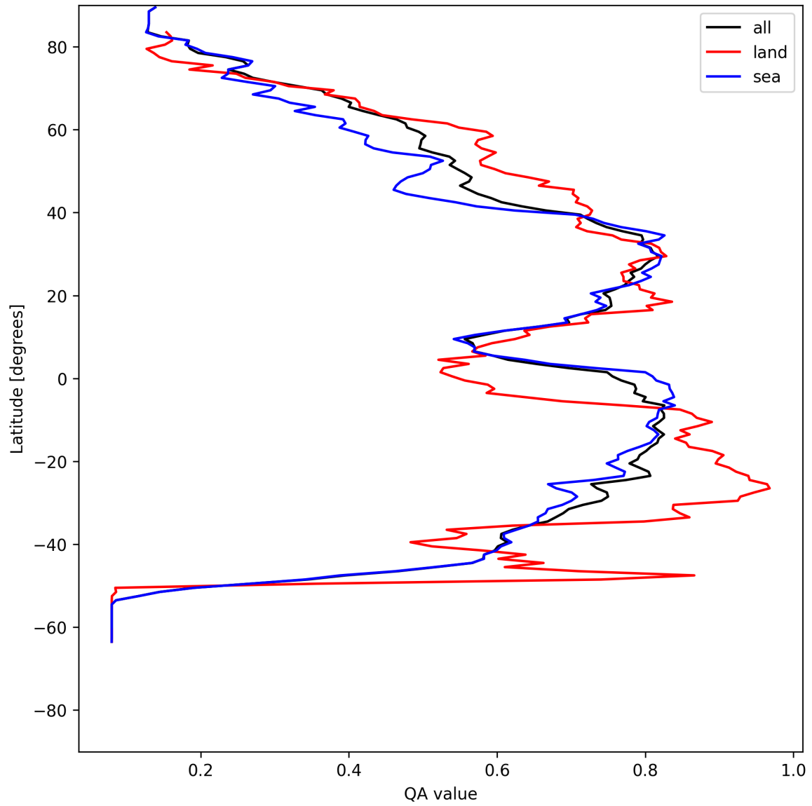
Figure 20: Zonal average of “QA value” for 2025-07-19 to 2025-07-20.
