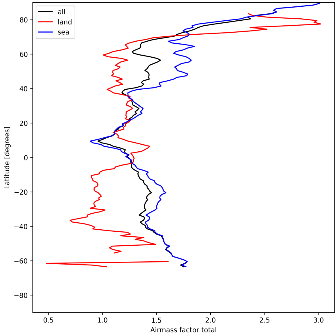
Figure 26: Zonal average of “Airmass factor total” for 2025-07-19 to 2025-07-20.
