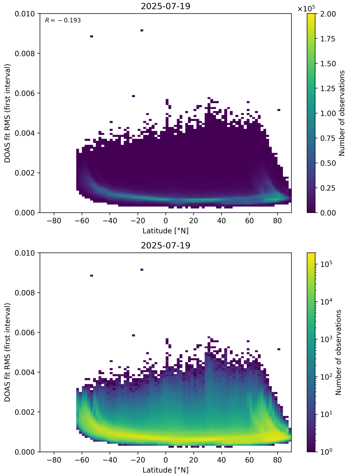
Figure 153: Scatter density plot of “Latitude” against “DOAS fit RMS (first interval)” for 2025-07-19 to 2025-07-20.
