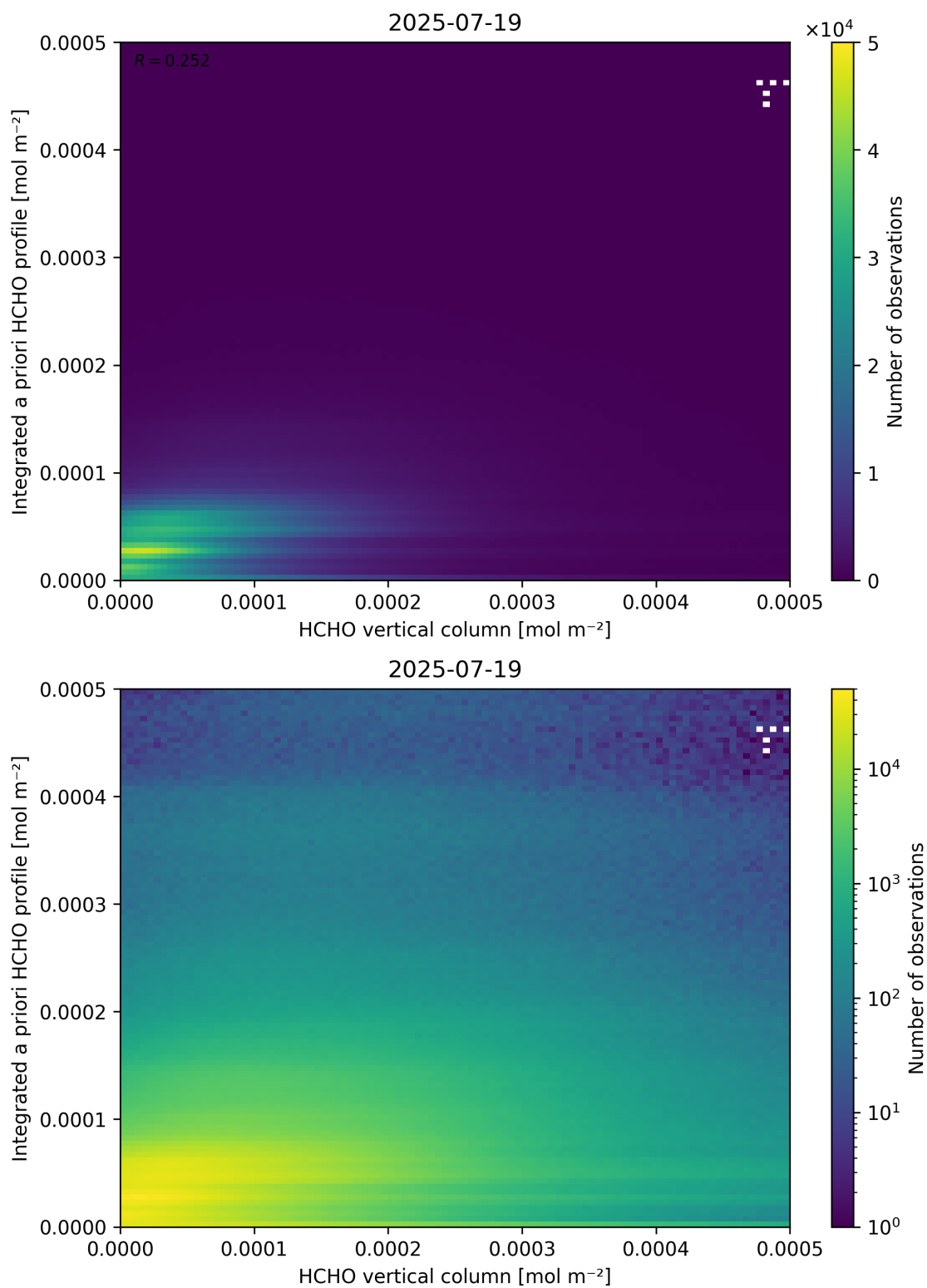
Figure 135: Scatter density plot of “HCHO vertical column” against “Integrated a priori HCHO profile” for 2025-07-19 to 2025-07-20.
