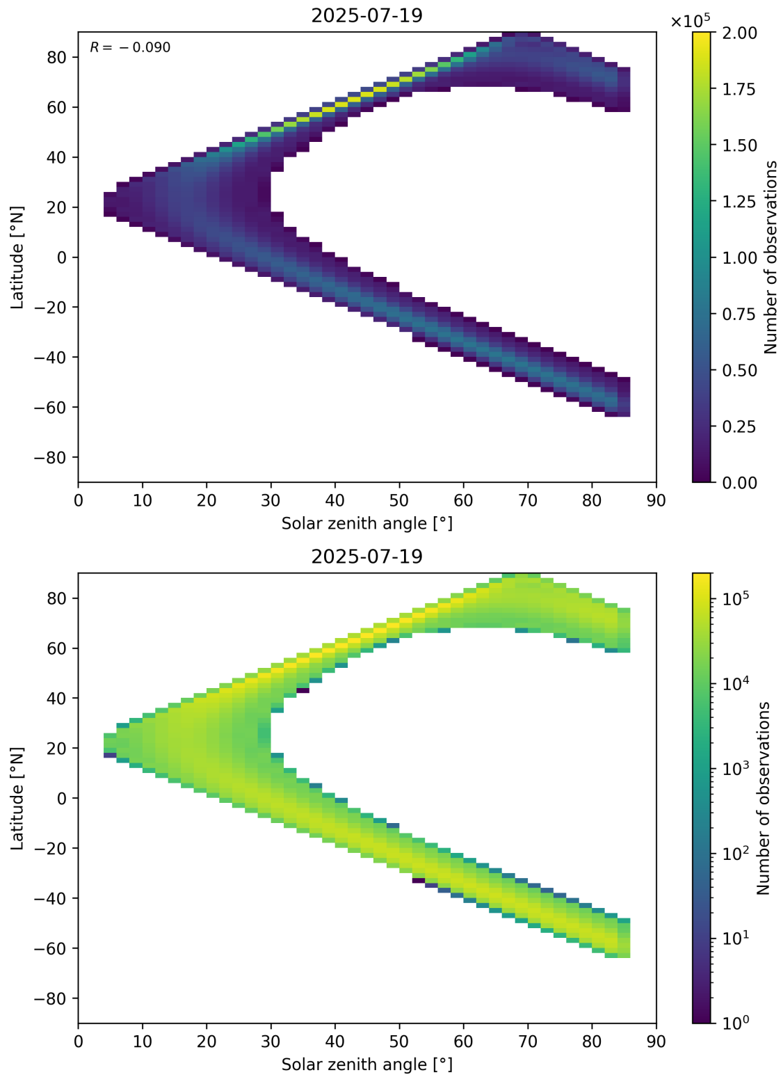
Figure 181: Scatter density plot of “Solar zenith angle” against “Latitude” for 2025-07-19 to 2025-07-20.
