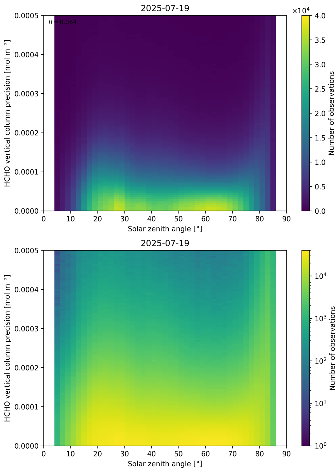
Figure 179: Scatter density plot of “Solar zenith angle” against “HCHO vertical column precision” for 2025-07-19 to 2025-07-20.
