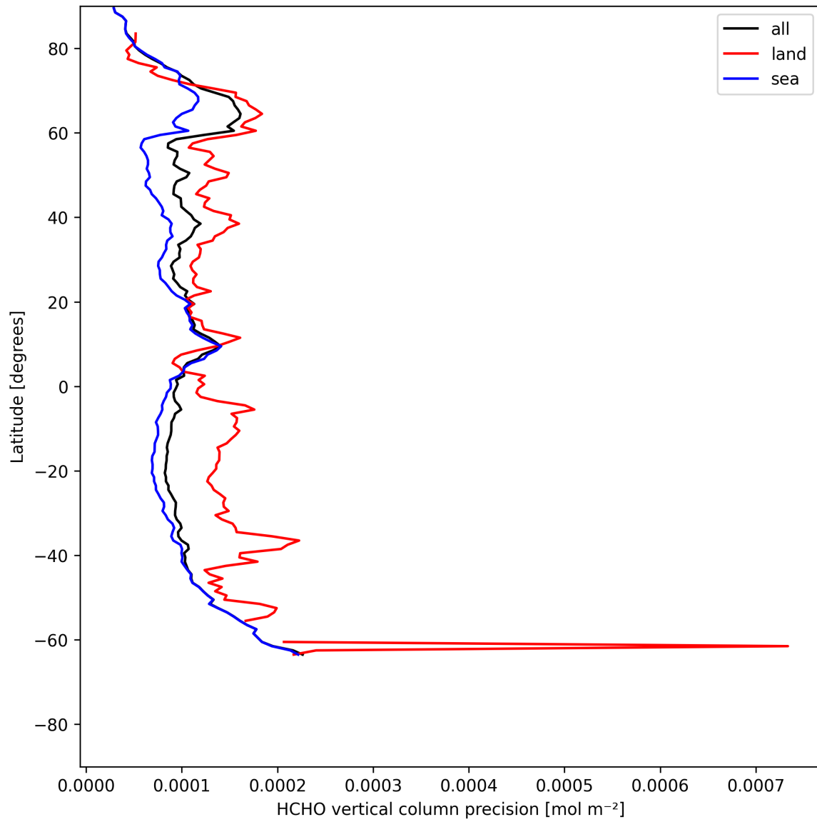
Figure 22: Zonal average of “HCHO vertical column precision” for 2025-07-19 to 2025-07-20.
