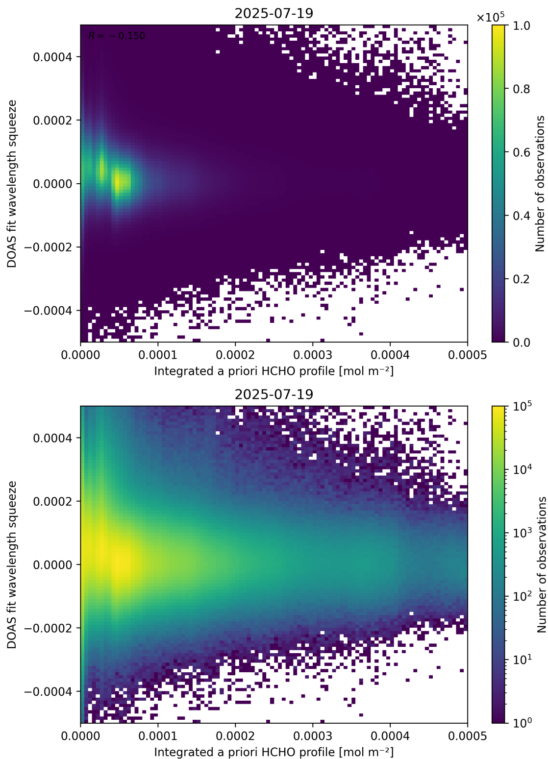
Figure 150: Scatter density plot of “Integrated a priori HCHO profile” against “DOAS fit wavelength squeeze” for 2025-07-19 to 2025-07-20.
