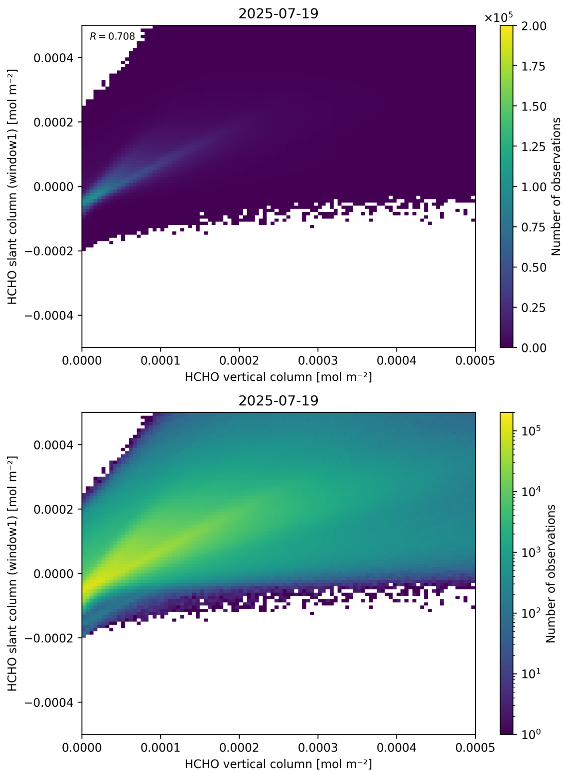
Figure 129: Scatter density plot of “HCHO vertical column” against “HCHO slant column (window1)” for 2025-07-19 to 2025-07-20.
