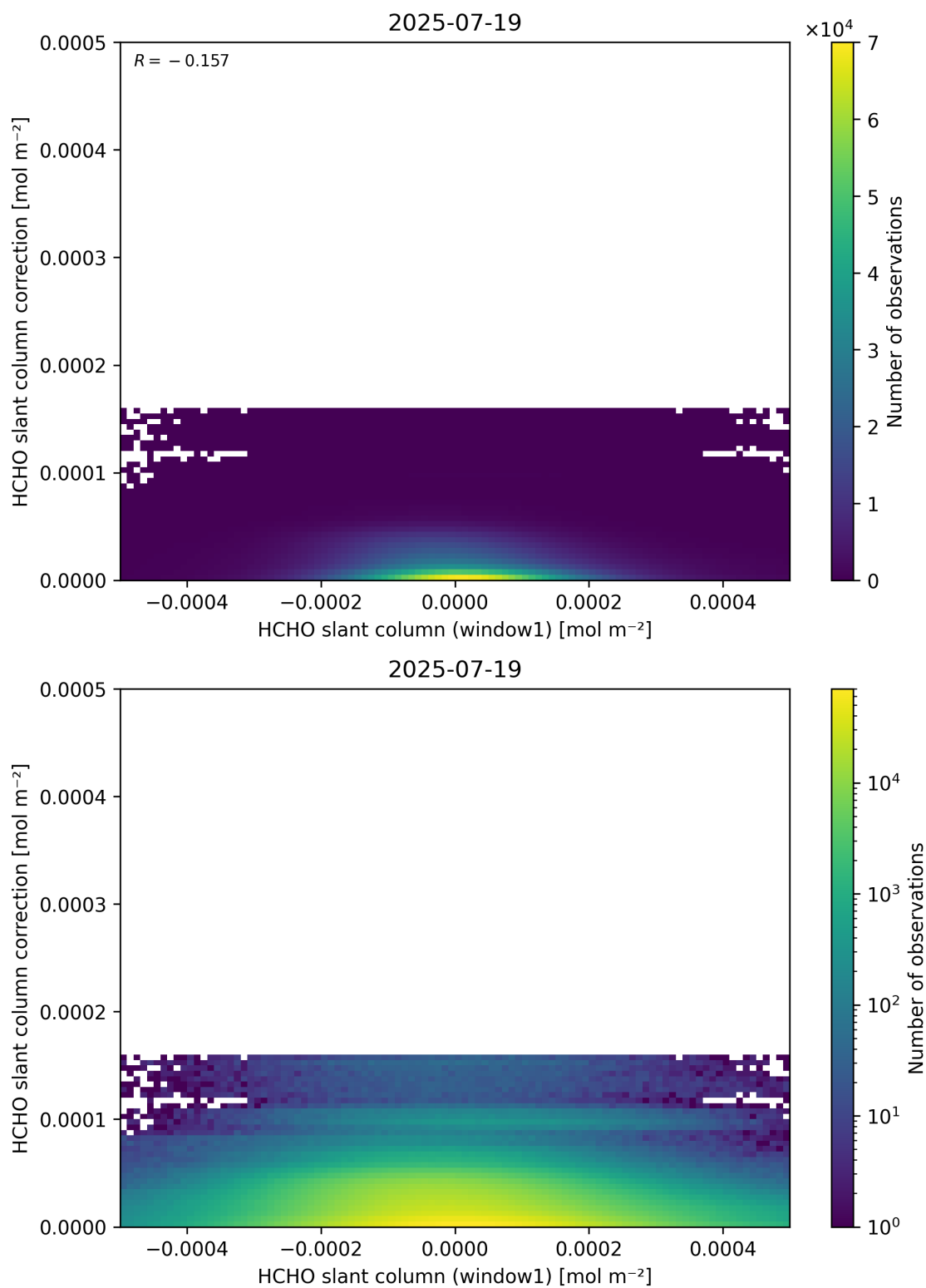
Figure 83: Scatter density plot of “HCHO slant column (window1)” against “HCHO slant column correction” for 2025-07-19 to 2025-07-20.
