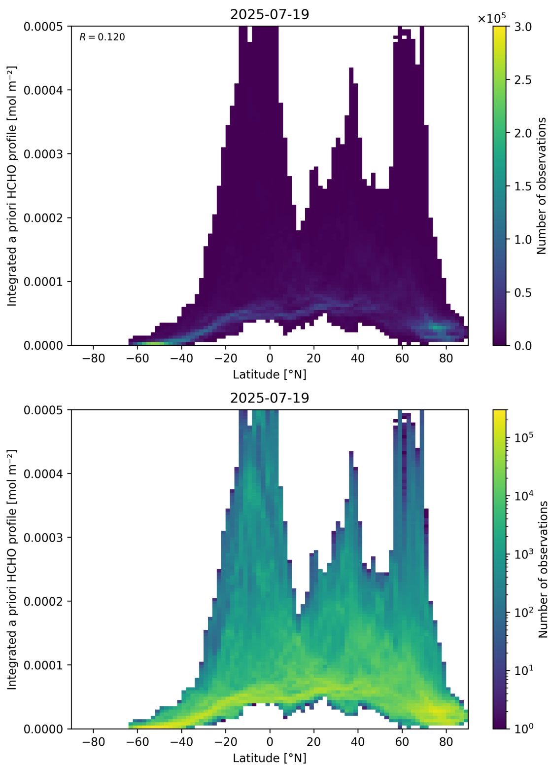
Figure 166: Scatter density plot of “Latitude” against “Integrated a priori HCHO profile” for 2025-07-19 to 2025-07-20.
