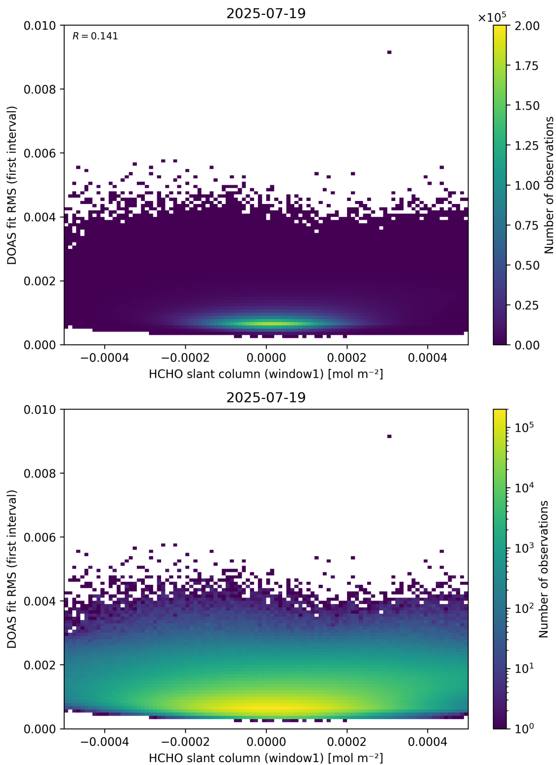
Figure 78: Scatter density plot of “HCHO slant column (window1)” against “DOAS fit RMS (first interval)” for 2025-07-19 to 2025-07-20.
