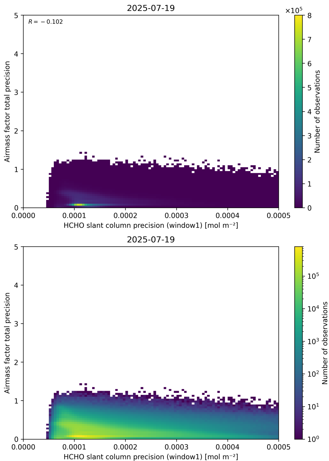
Figure 95: Scatter density plot of “HCHO slant column precision (window1)” against “Airmass factor total precision” for 2025-07-19 to 2025-07-20.
