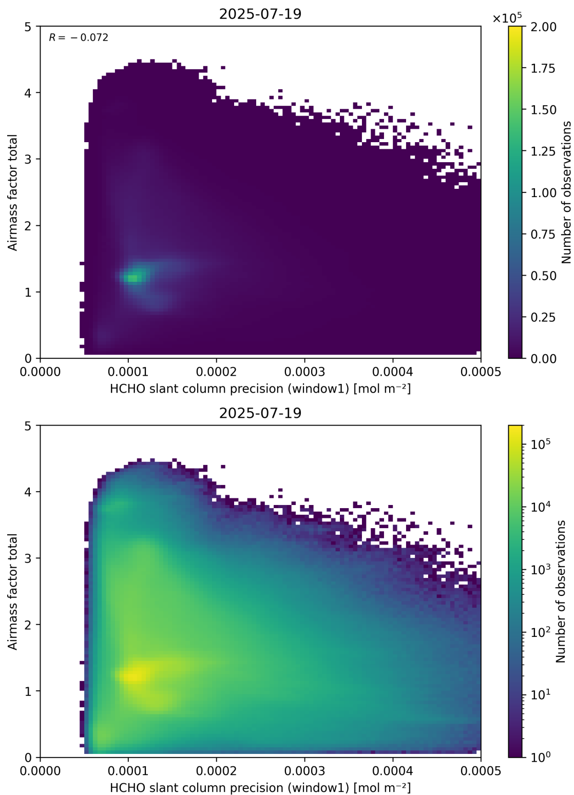
Figure 94: Scatter density plot of “HCHO slant column precision (window1)” against “Airmass factor total” for 2025-07-19 to 2025-07-20.
