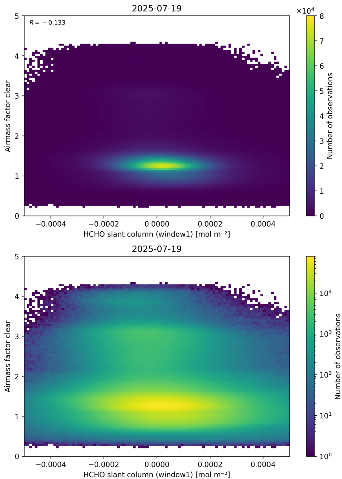
Figure 81: Scatter density plot of “HCHO slant column (window1)” against “Airmass factor clear” for 2025-07-19 to 2025-07-20.
