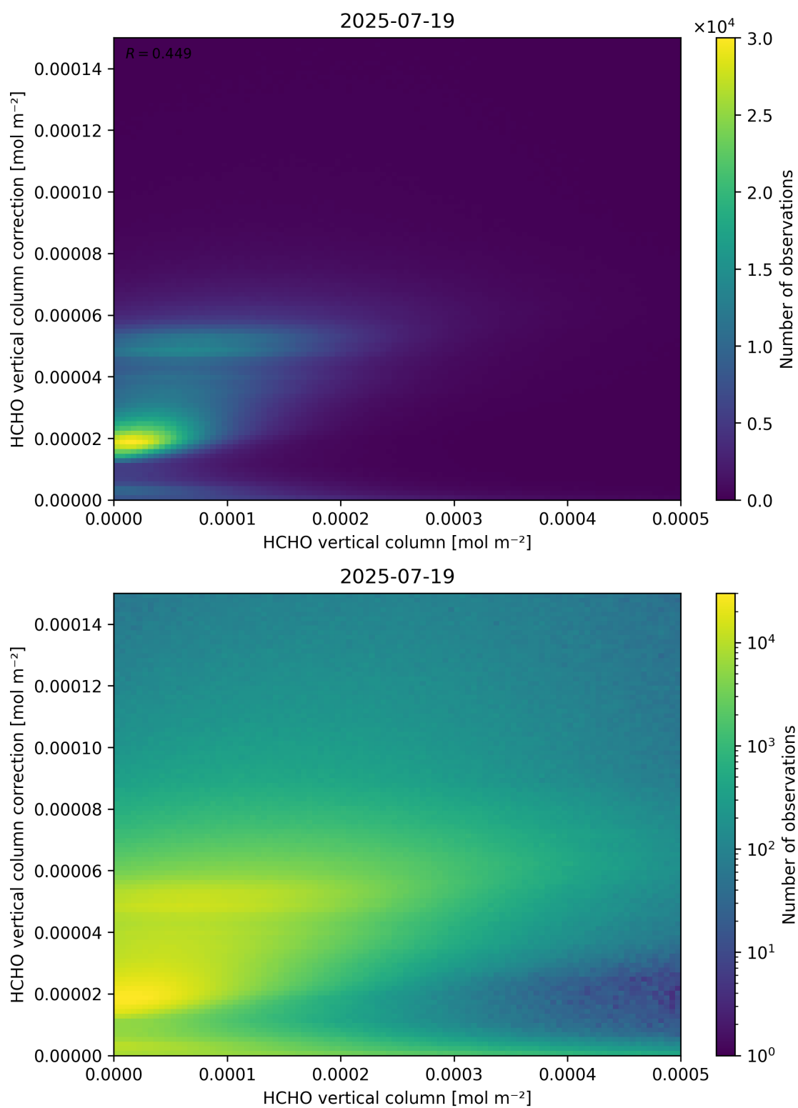
Figure 133: Scatter density plot of “HCHO vertical column” against “HCHO vertical column correction” for 2025-07-19 to 2025-07-20.
