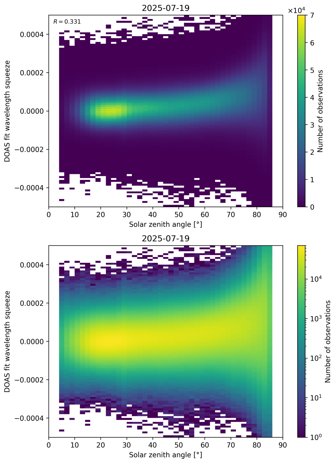
Figure 169: Scatter density plot of “Solar zenith angle” against “DOAS fit wavelength squeeze” for 2025-07-19 to 2025-07-20.
