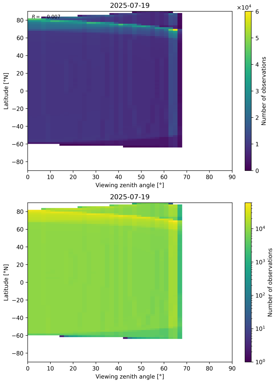
Figure 196: Scatter density plot of “Viewing zenith angle” against “Latitude” for 2025-07-19 to 2025-07-20.
