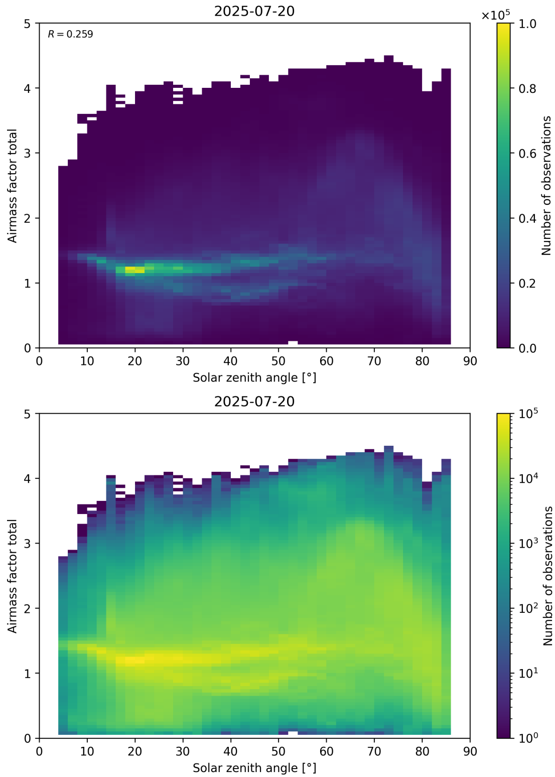
Figure 175: Scatter density plot of “Solar zenith angle” against “Airmass factor total” for 2025-07-19 to 2025-07-21.
