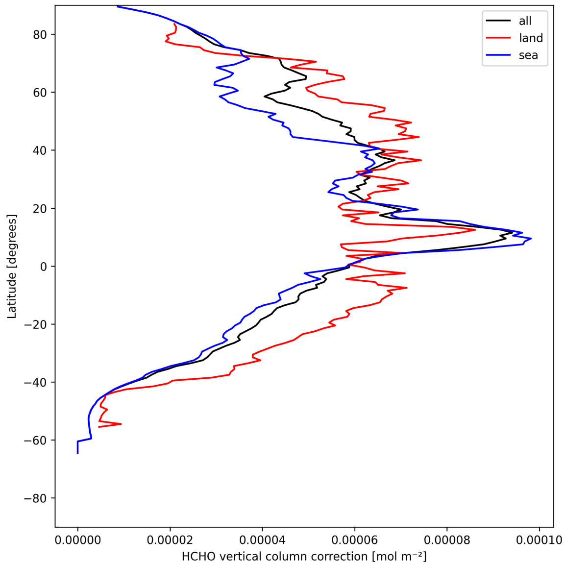
Figure 23: Zonal average of “HCHO vertical column correction” for 2025-07-19 to 2025-07-21.
