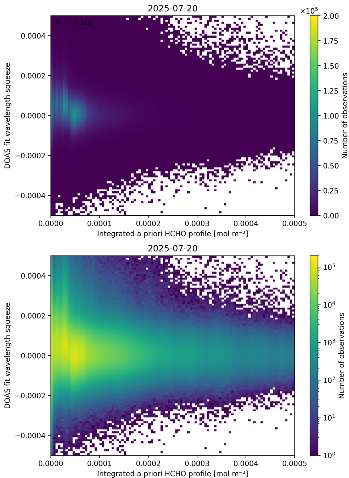
Figure 150: Scatter density plot of “Integrated a priori HCHO profile” against “DOAS fit wavelength squeeze” for 2025-07-19 to 2025-07-21.
