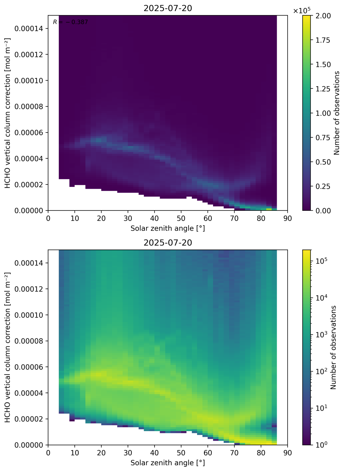
Figure 178: Scatter density plot of “Solar zenith angle” against “HCHO vertical column correction” for 2025-07-19 to 2025-07-21.
