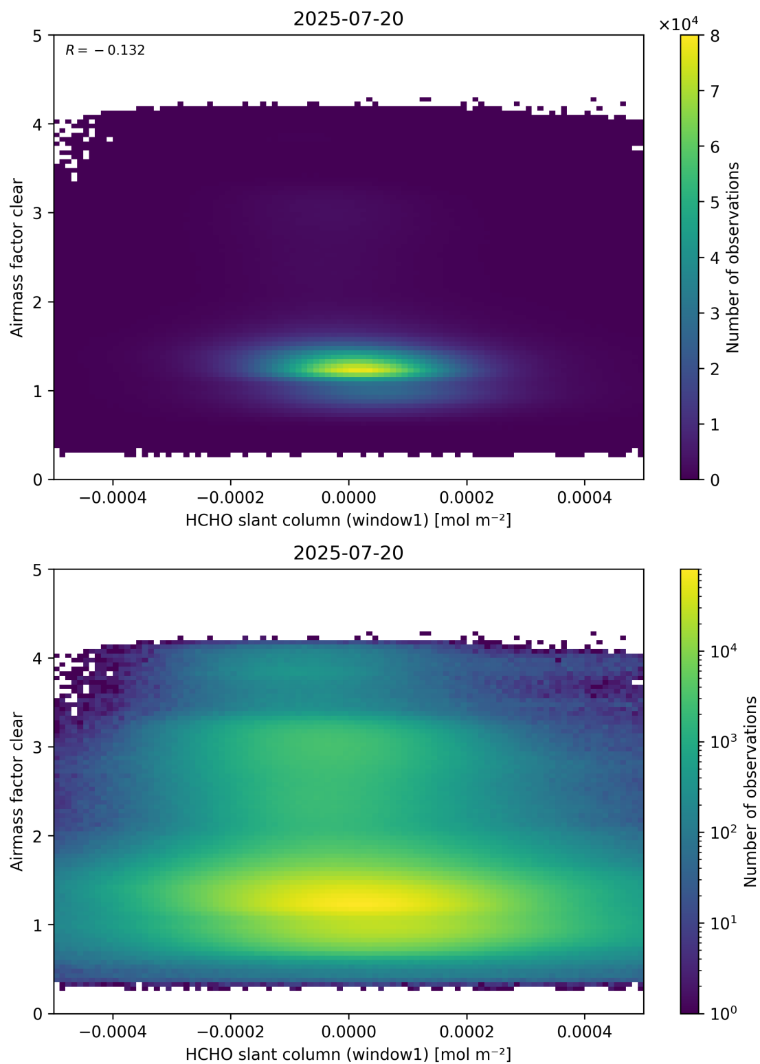
Figure 81: Scatter density plot of “HCHO slant column (window1)” against “Airmass factor clear” for 2025-07-19 to 2025-07-21.
