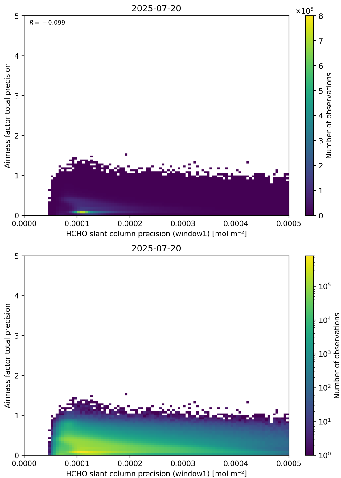
Figure 95: Scatter density plot of “HCHO slant column precision (window1)” against “Airmass factor total precision” for 2025-07-19 to 2025-07-21.
