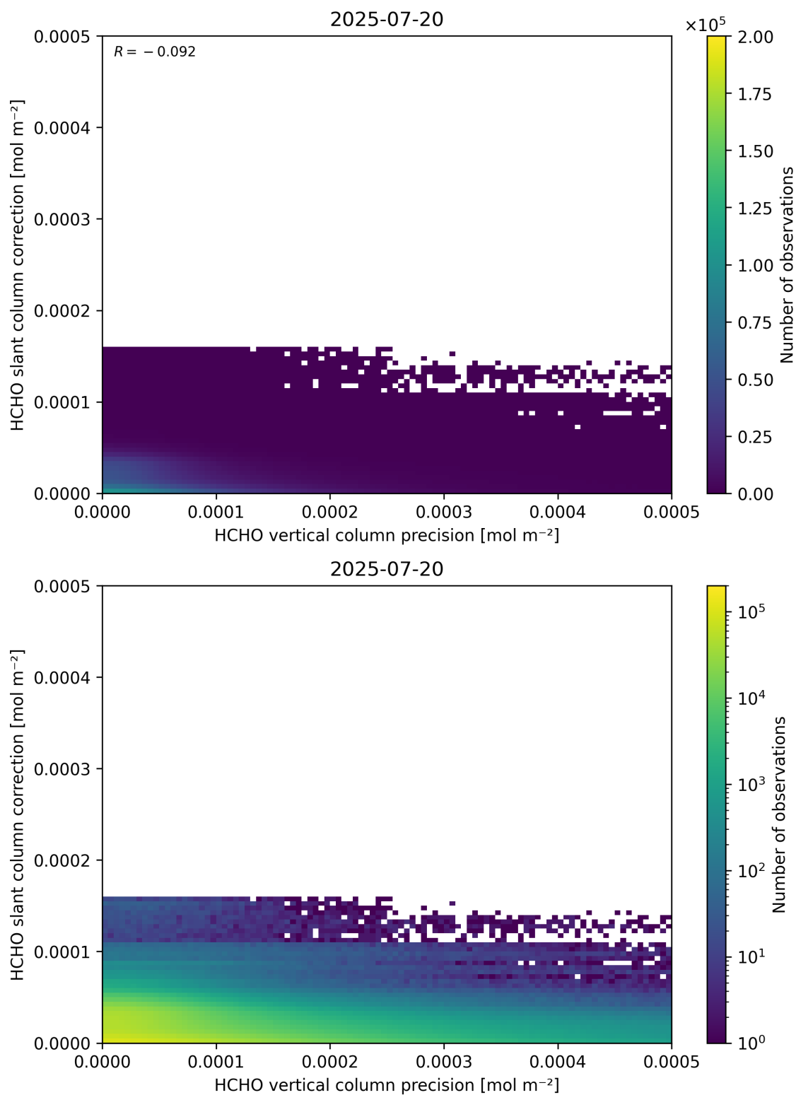
Figure 141: Scatter density plot of “HCHO vertical column precision” against “HCHO slant column correction” for 2025-07-19 to 2025-07-21.
