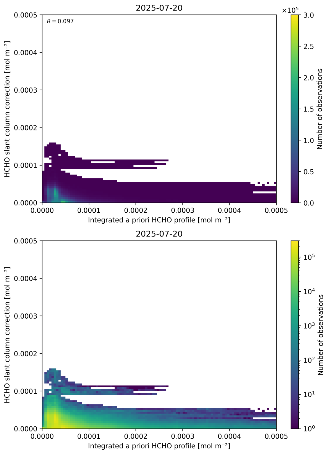
Figure 152: Scatter density plot of “Integrated a priori HCHO profile” against “HCHO slant column correction” for 2025-07-19 to 2025-07-21.
