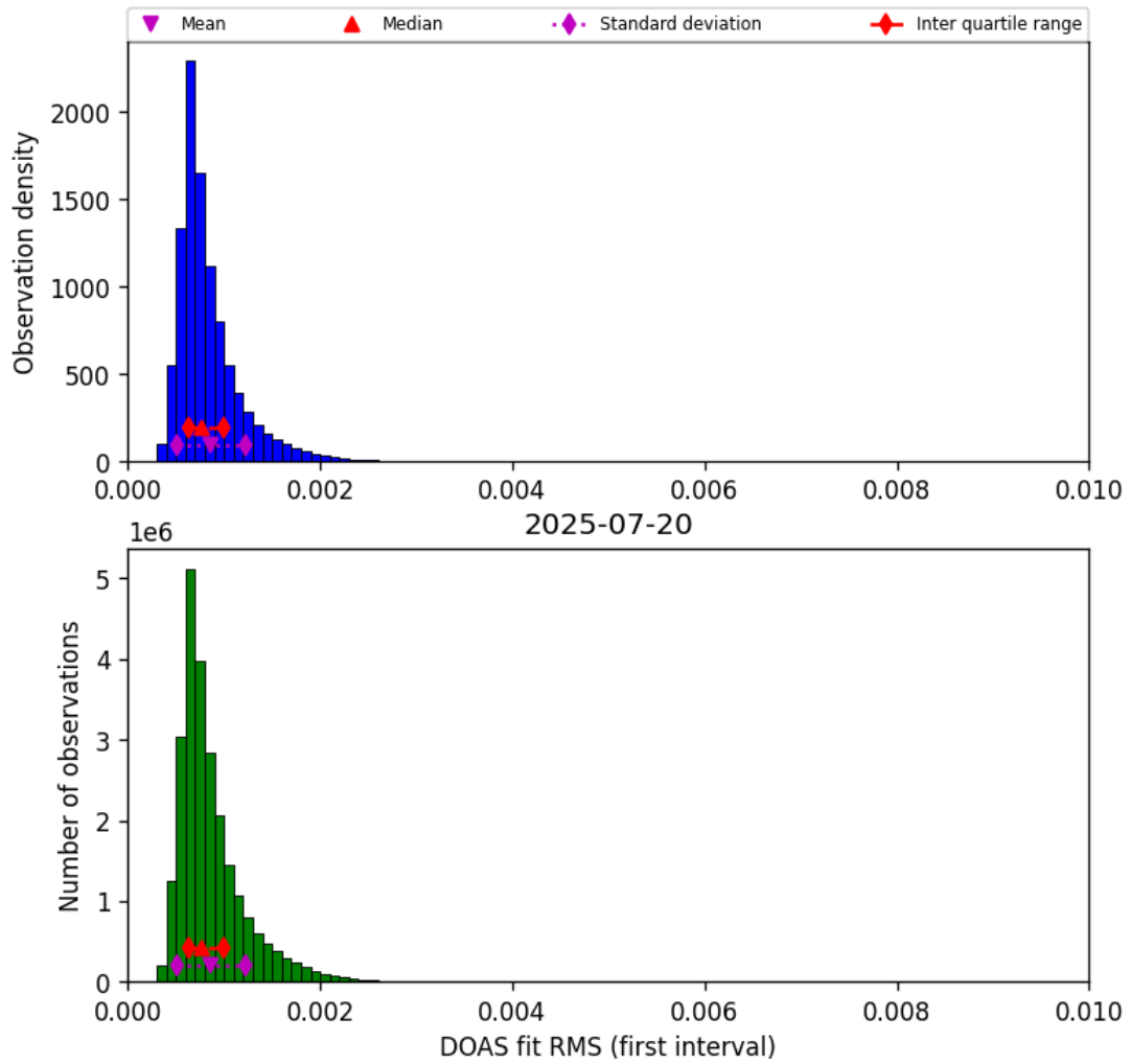
Figure 46: Histogram of “DOAS fit RMS (first interval)” for 2025-07-19 to 2025-07-21
