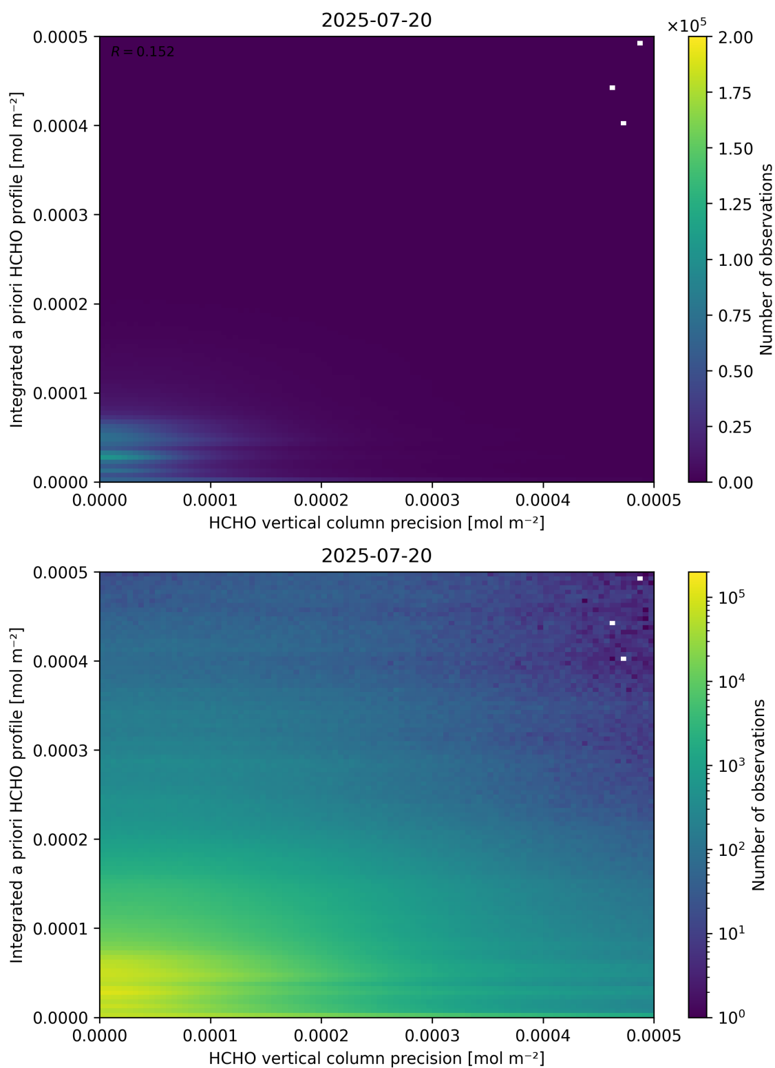
Figure 147: Scatter density plot of “HCHO vertical column precision” against “Integrated a priori HCHO profile” for 2025-07-19 to 2025-07-21.
