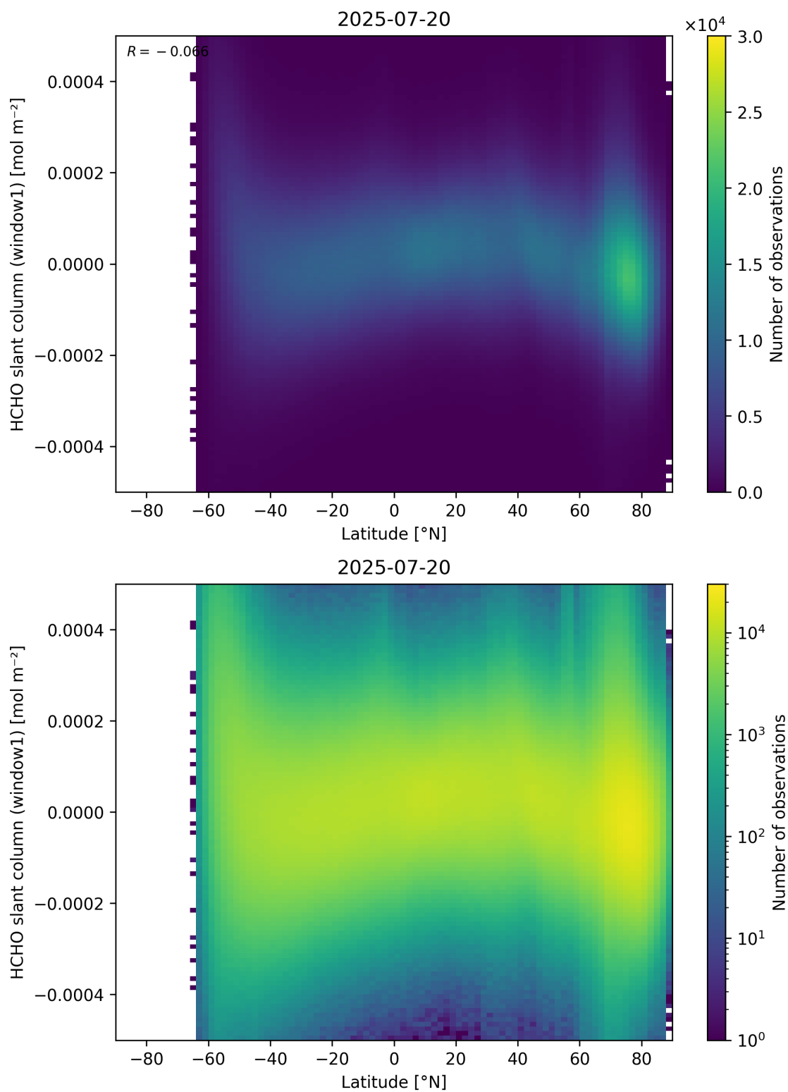
Figure 159: Scatter density plot of “Latitude” against “HCHO slant column (window1)” for 2025-07-19 to 2025-07-21.
