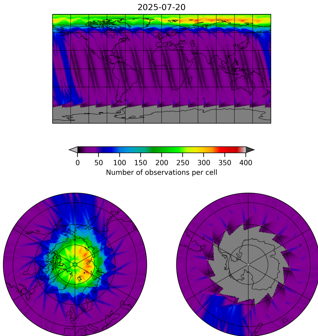
Figure 19: Map of the number of observations for 2025-07-19 to 2025-07-21
