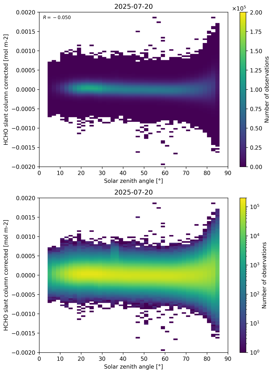
Figure 171: Scatter density plot of “Solar zenith angle” against “HCHO slant column corrected” for 2025-07-19 to 2025-07-21.
