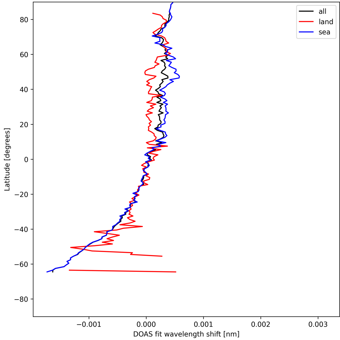
Figure 30: Zonal average of “DOAS fit wavelength shift” for 2025-07-19 to 2025-07-21.
