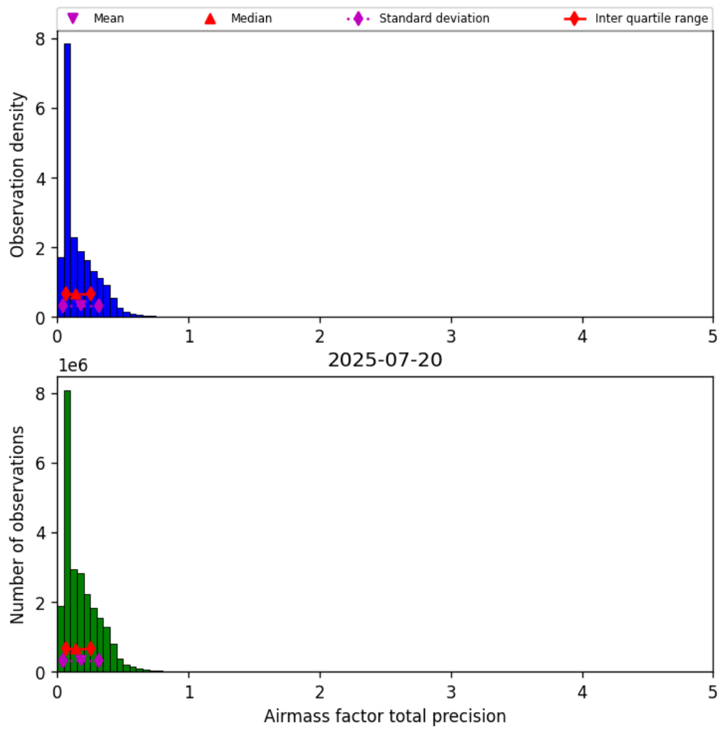
Figure 41: Histogram of “Airmass factor total precision” for 2025-07-19 to 2025-07-21
