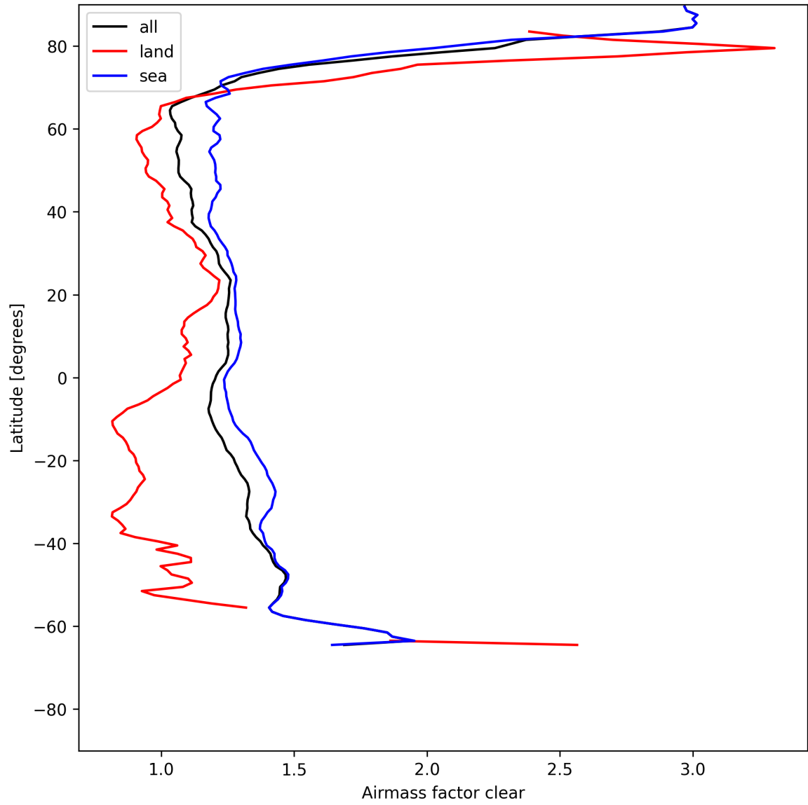
Figure 28: Zonal average of “Airmass factor clear” for 2025-07-19 to 2025-07-21.
