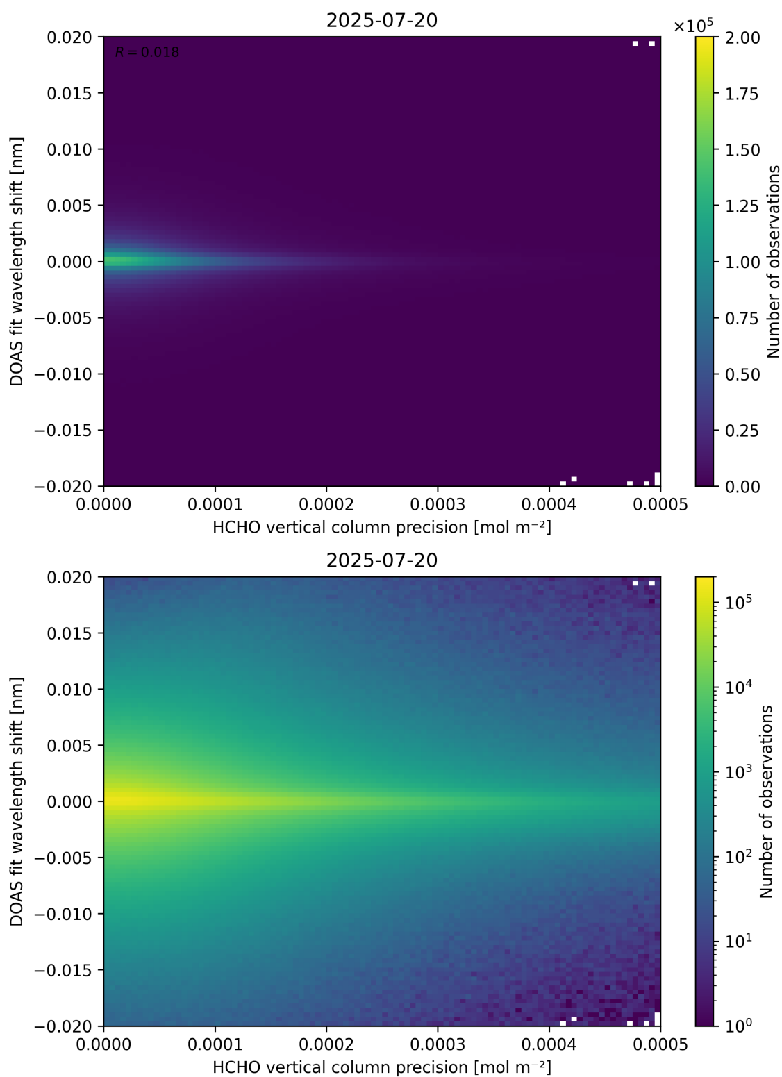
Figure 137: Scatter density plot of “HCHO vertical column precision” against “DOAS fit wavelength shift” for 2025-07-19 to 2025-07-21.
