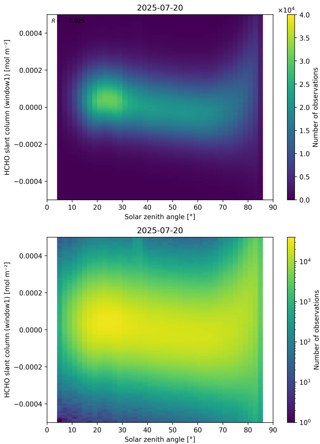
Figure 173: Scatter density plot of “Solar zenith angle” against “HCHO slant column (window1)” for 2025-07-19 to 2025-07-21.
