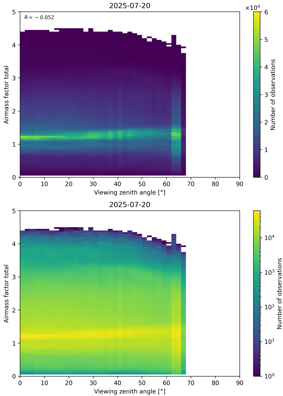
Figure 190: Scatter density plot of “Viewing zenith angle” against “Airmass factor total” for 2025-07-19 to 2025-07-21.
