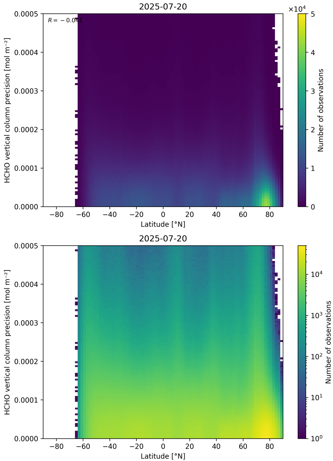
Figure 165: Scatter density plot of “Latitude” against “HCHO vertical column precision” for 2025-07-19 to 2025-07-21.
