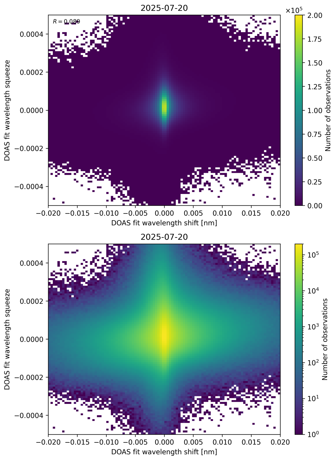
Figure 65: Scatter density plot of “DOAS fit wavelength shift” against “DOAS fit wavelength squeeze” for 2025-07-19 to 2025-07-21.
