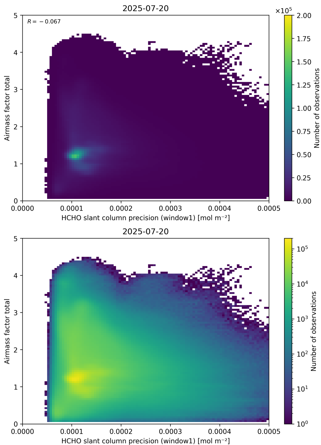
Figure 94: Scatter density plot of “HCHO slant column precision (window1)” against “Airmass factor total” for 2025-07-19 to 2025-07-21.
