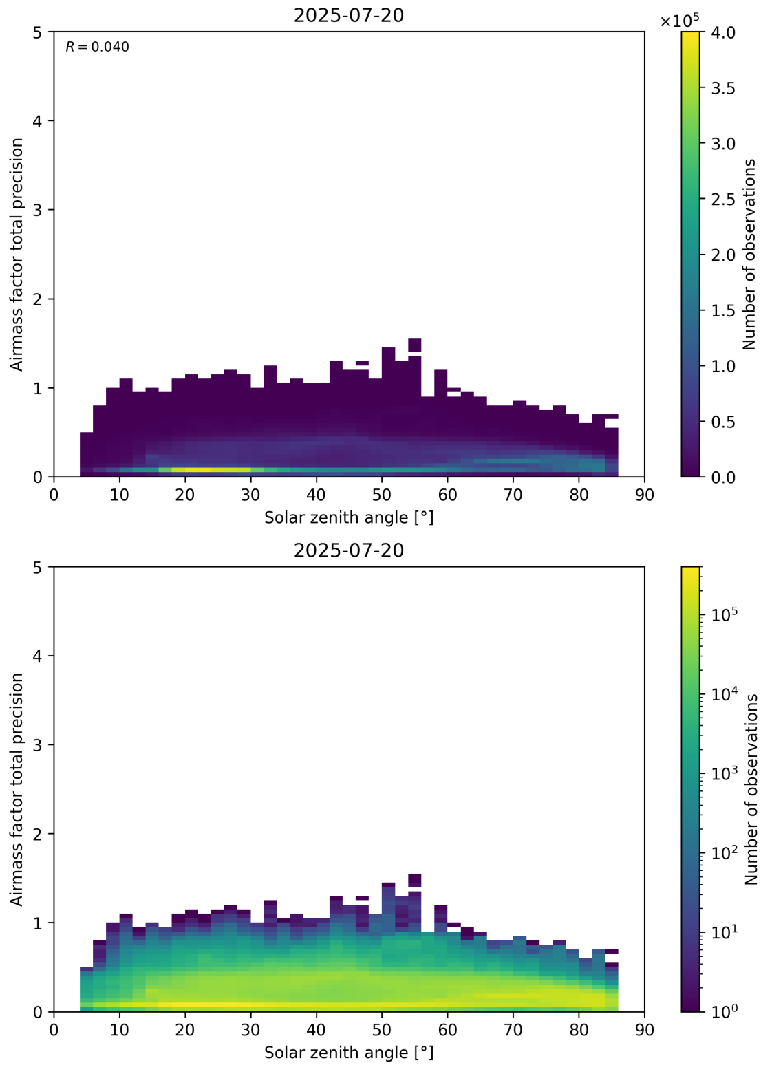
Figure 176: Scatter density plot of “Solar zenith angle” against “Airmass factor total precision” for 2025-07-19 to 2025-07-21.
