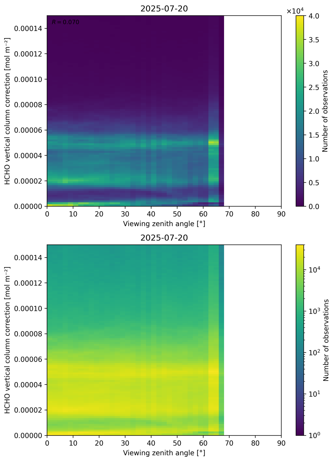
Figure 193: Scatter density plot of “Viewing zenith angle” against “HCHO vertical column correction” for 2025-07-19 to 2025-07-21.
