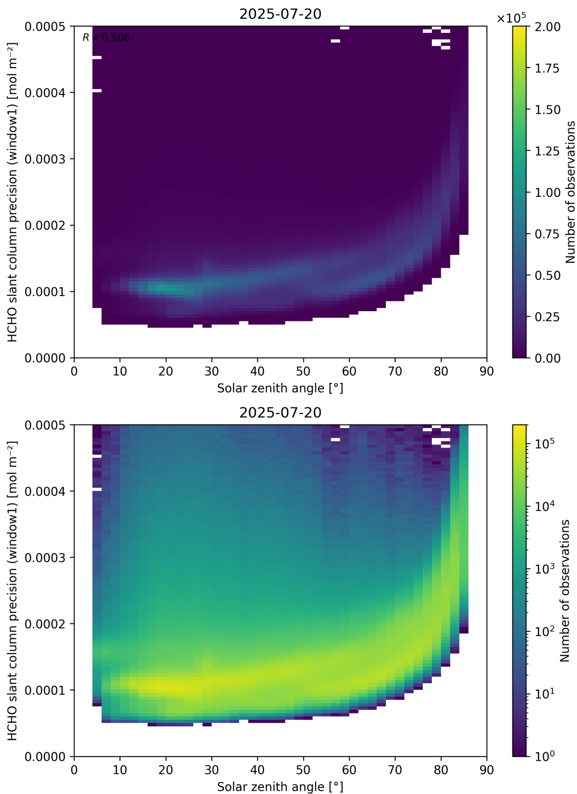
Figure 174: Scatter density plot of “Solar zenith angle” against “HCHO slant column precision (window1)” for 2025-07-19 to 2025-07-21.
