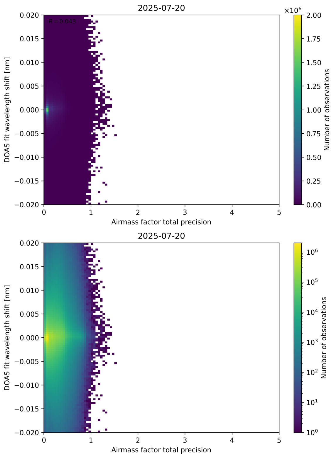
Figure 106: Scatter density plot of “Airmass factor total precision” against “DOAS fit wavelength shift” for 2025-07-19 to 2025-07-21.
