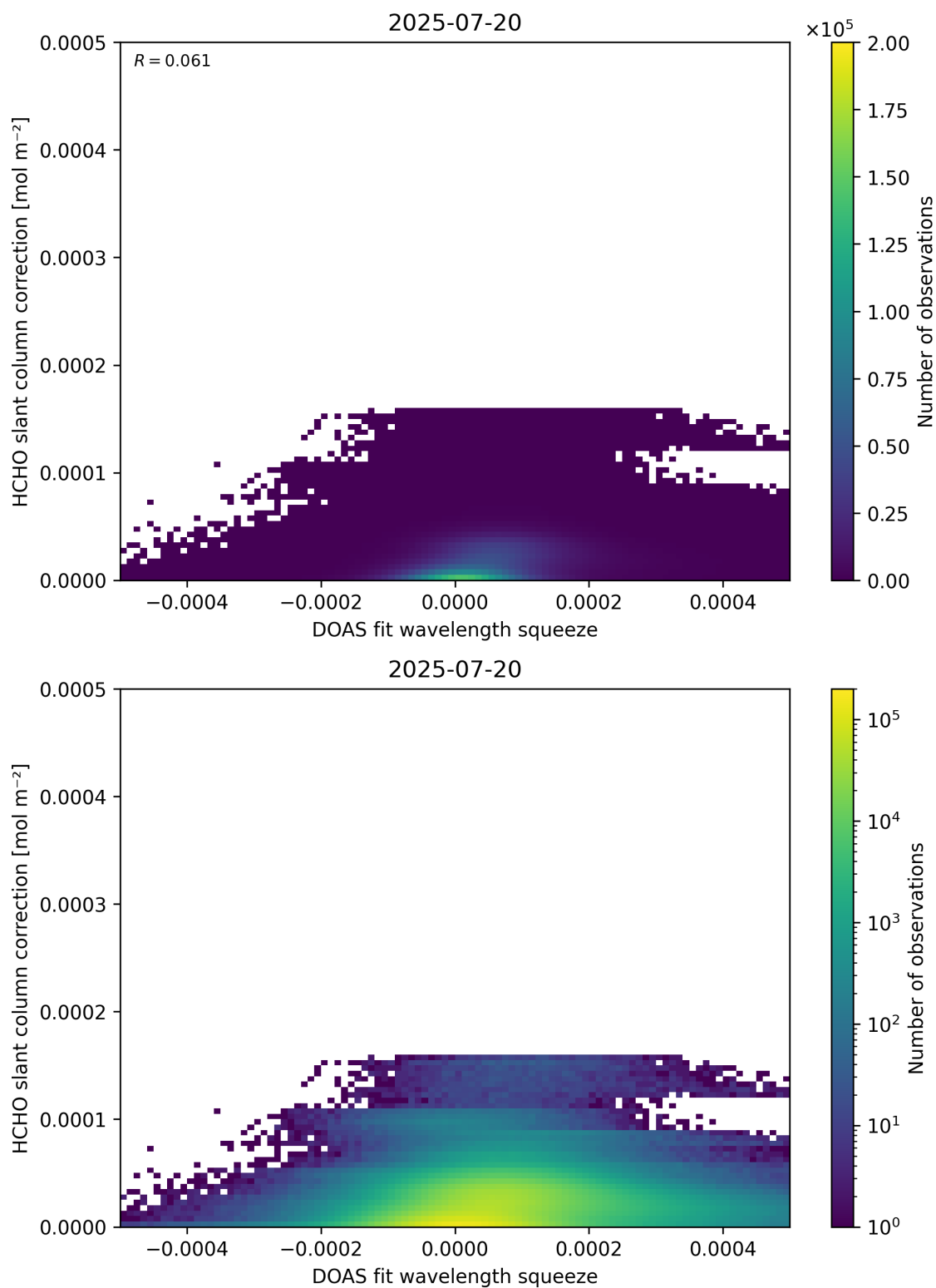
Figure 70: Scatter density plot of “DOAS fit wavelength squeeze” against “HCHO slant column correction” for 2025-07-19 to 2025-07-21.
