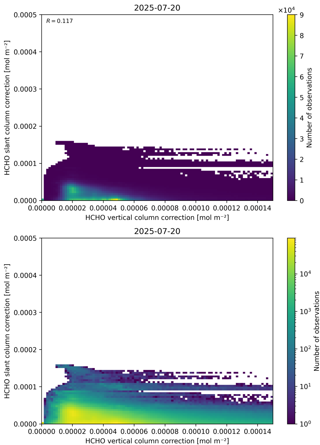
Figure 117: Scatter density plot of “HCHO vertical column correction” against “HCHO slant column correction” for 2025-07-19 to 2025-07-21.
