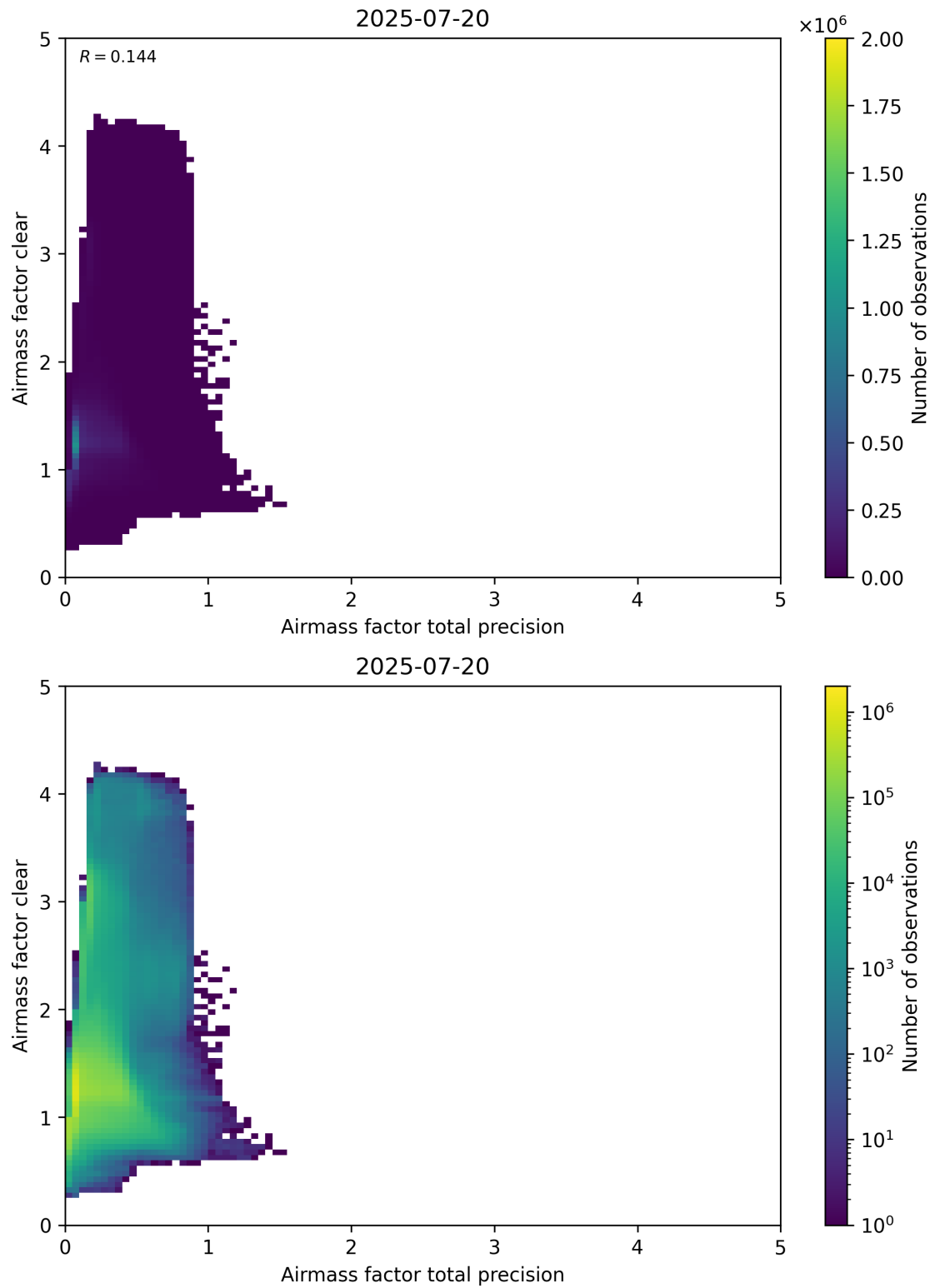
Figure 108: Scatter density plot of “Airmass factor total precision” against “Airmass factor clear” for 2025-07-19 to 2025-07-21.
