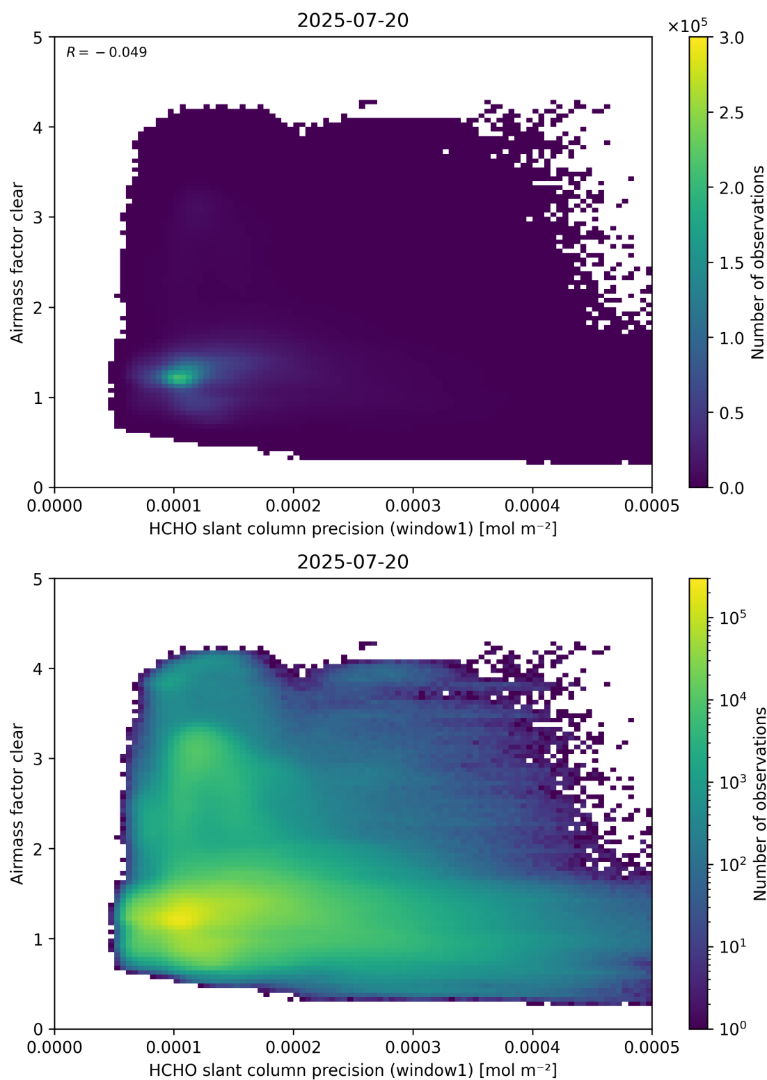
Figure 91: Scatter density plot of “HCHO slant column precision (window1)” against “Airmass factor clear” for 2025-07-19 to 2025-07-21.
