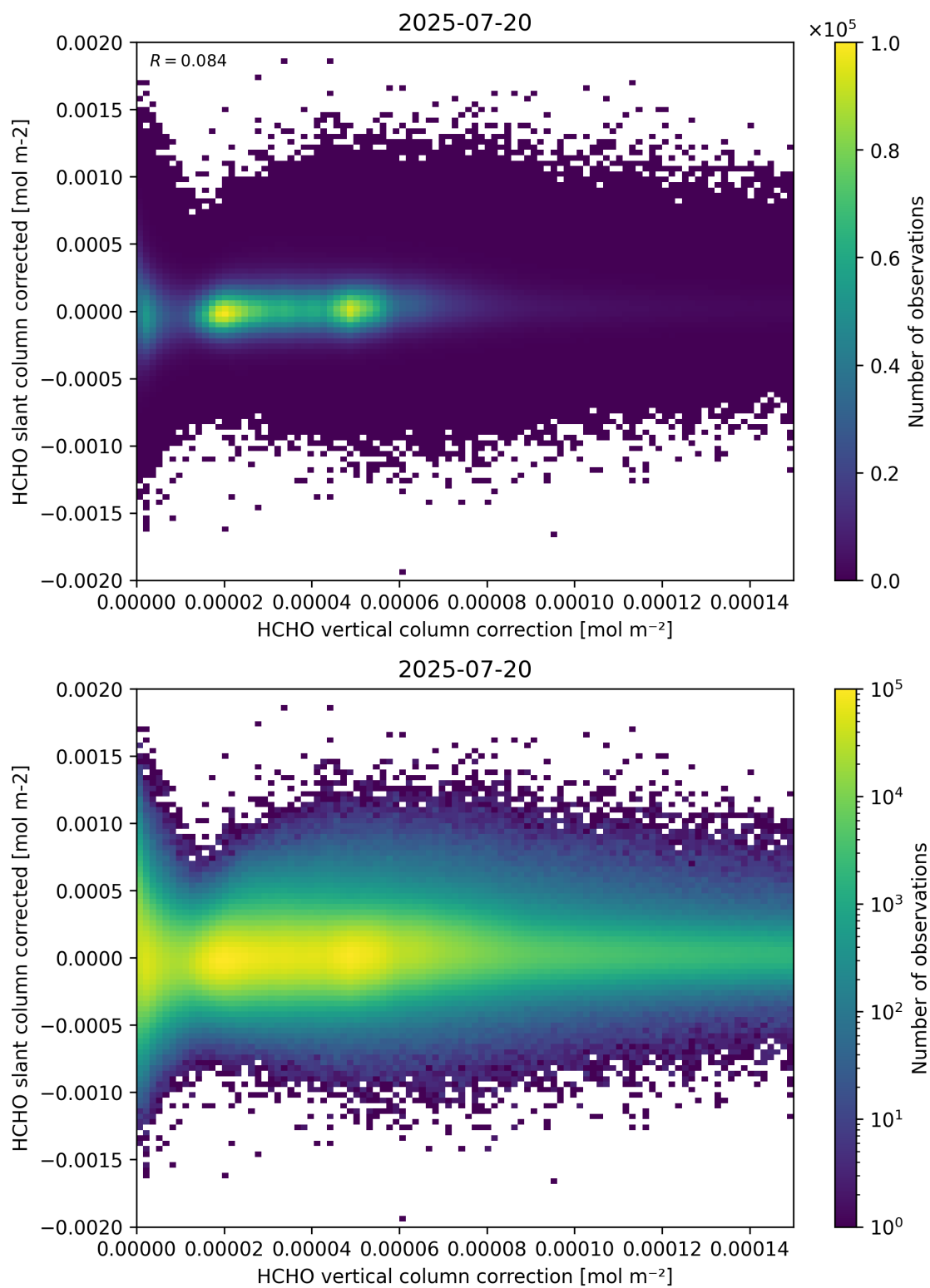
Figure 116: Scatter density plot of “HCHO vertical column correction” against “HCHO slant column corrected” for 2025-07-19 to 2025-07-21.
