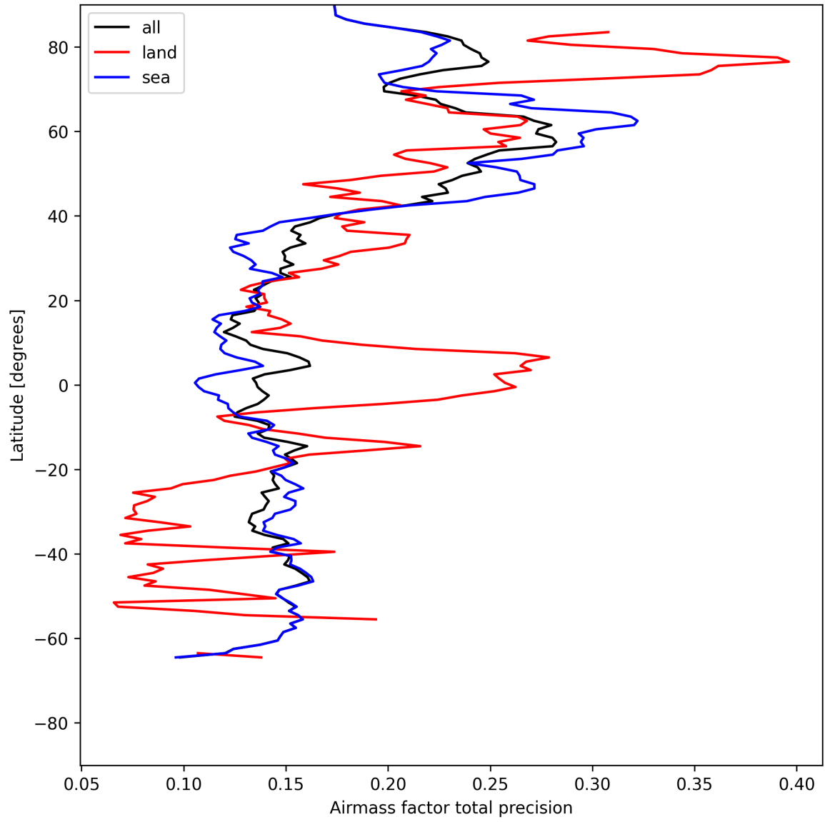
Figure 27: Zonal average of “Airmass factor total precision” for 2025-07-19 to 2025-07-21.
