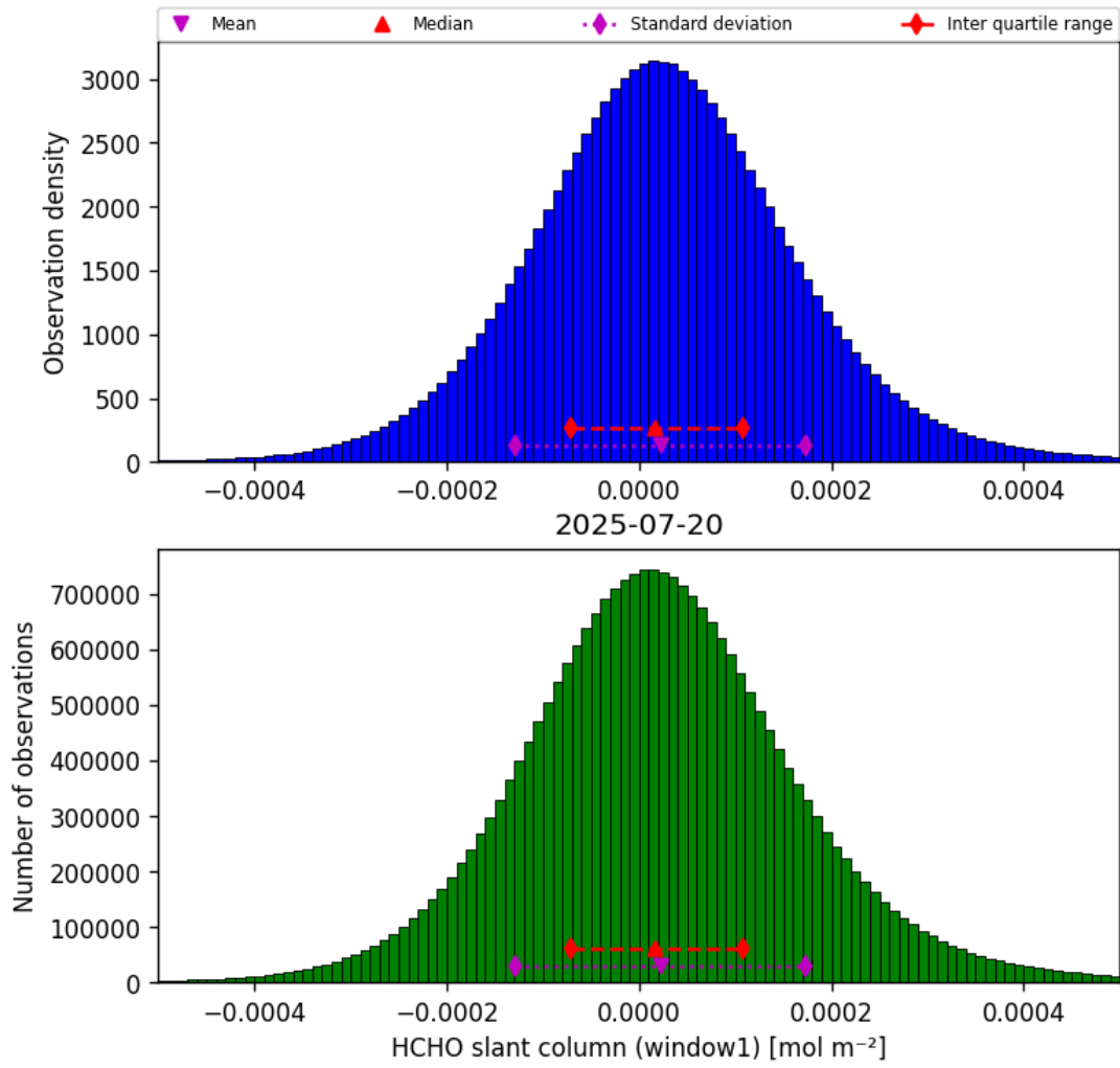
Figure 38: Histogram of “HCHO slant column (window1)” for 2025-07-19 to 2025-07-21
