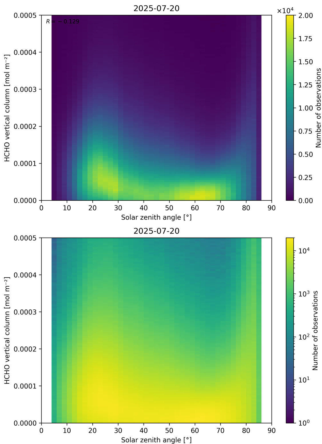
Figure 177: Scatter density plot of “Solar zenith angle” against “HCHO vertical column” for 2025-07-19 to 2025-07-21.
