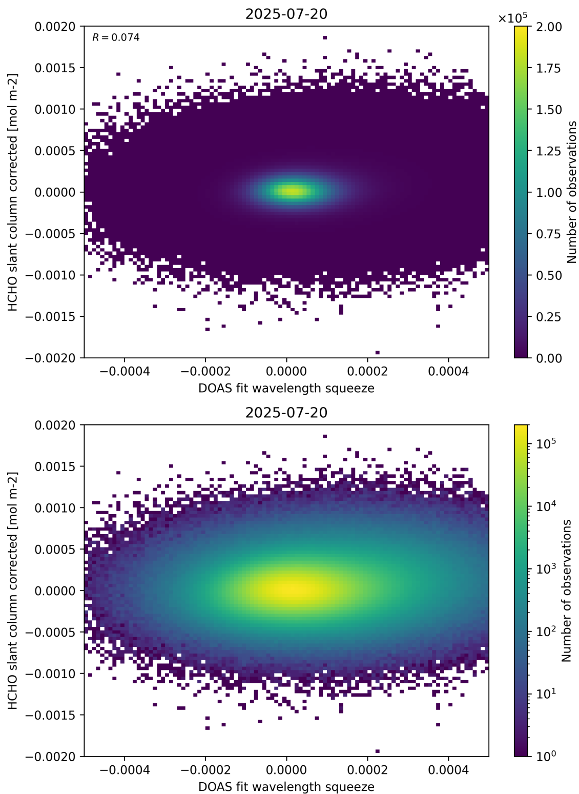
Figure 69: Scatter density plot of “DOAS fit wavelength squeeze” against “HCHO slant column corrected” for 2025-07-19 to 2025-07-21.
