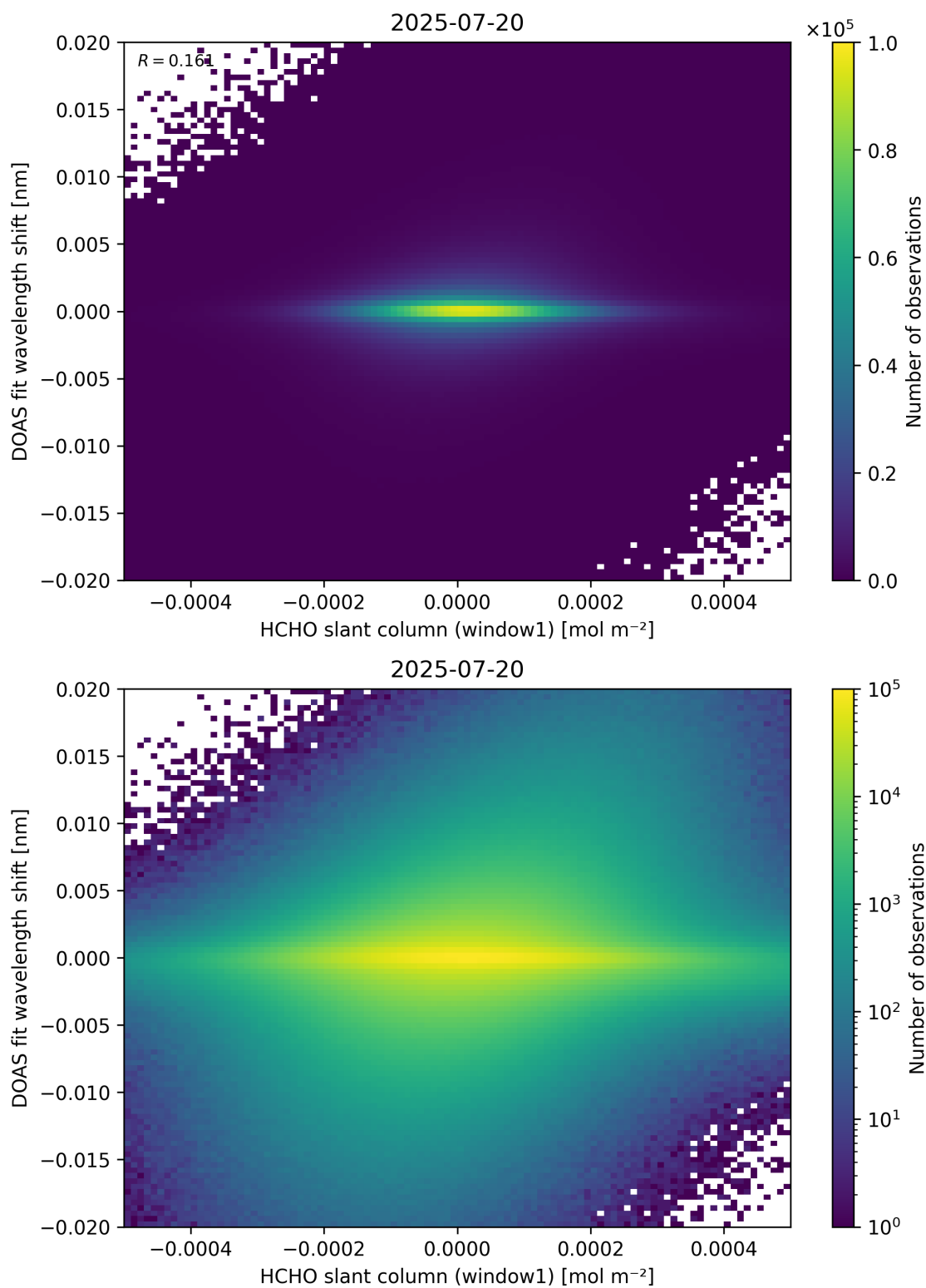
Figure 79: Scatter density plot of “HCHO slant column (window1)” against “DOAS fit wavelength shift” for 2025-07-19 to 2025-07-21.
