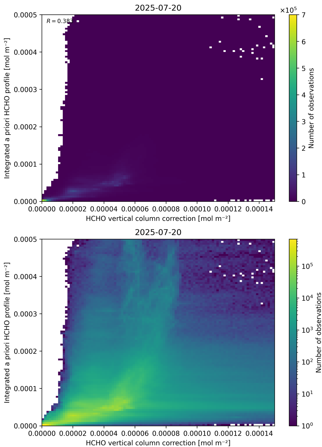
Figure 122: Scatter density plot of “HCHO vertical column correction” against “Integrated a priori HCHO profile” for 2025-07-19 to 2025-07-21.
