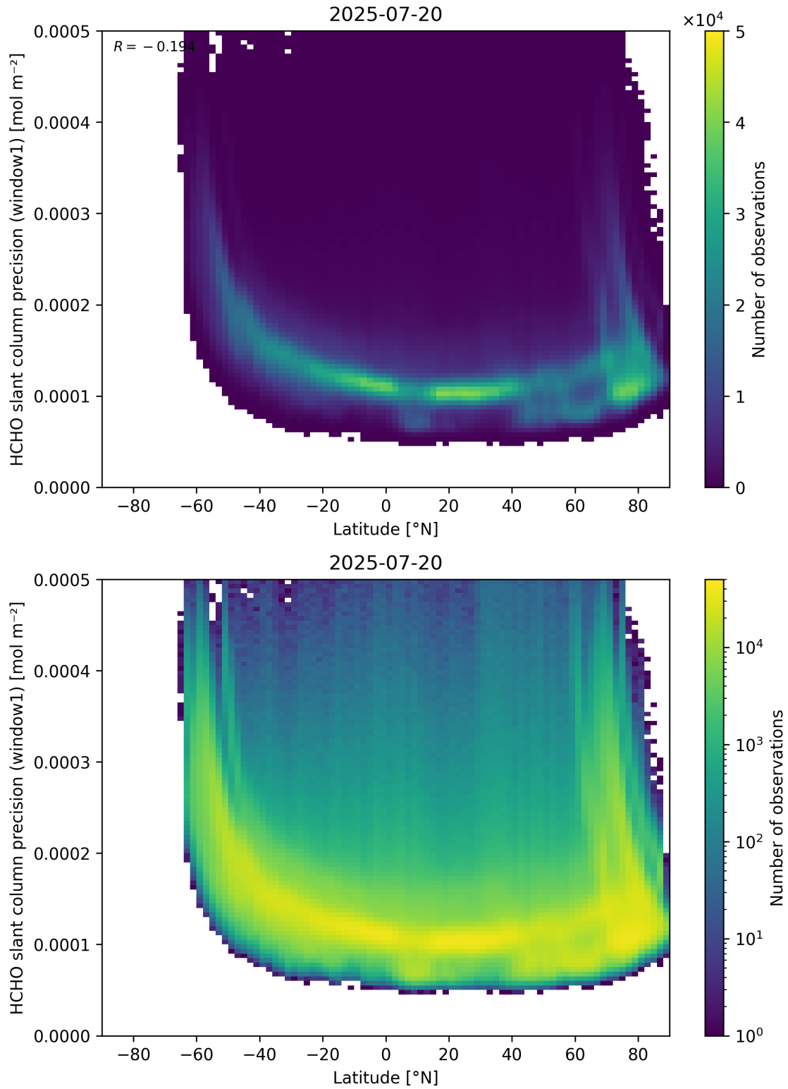
Figure 160: Scatter density plot of “Latitude” against “HCHO slant column precision (window1)” for 2025-07-19 to 2025-07-21.
