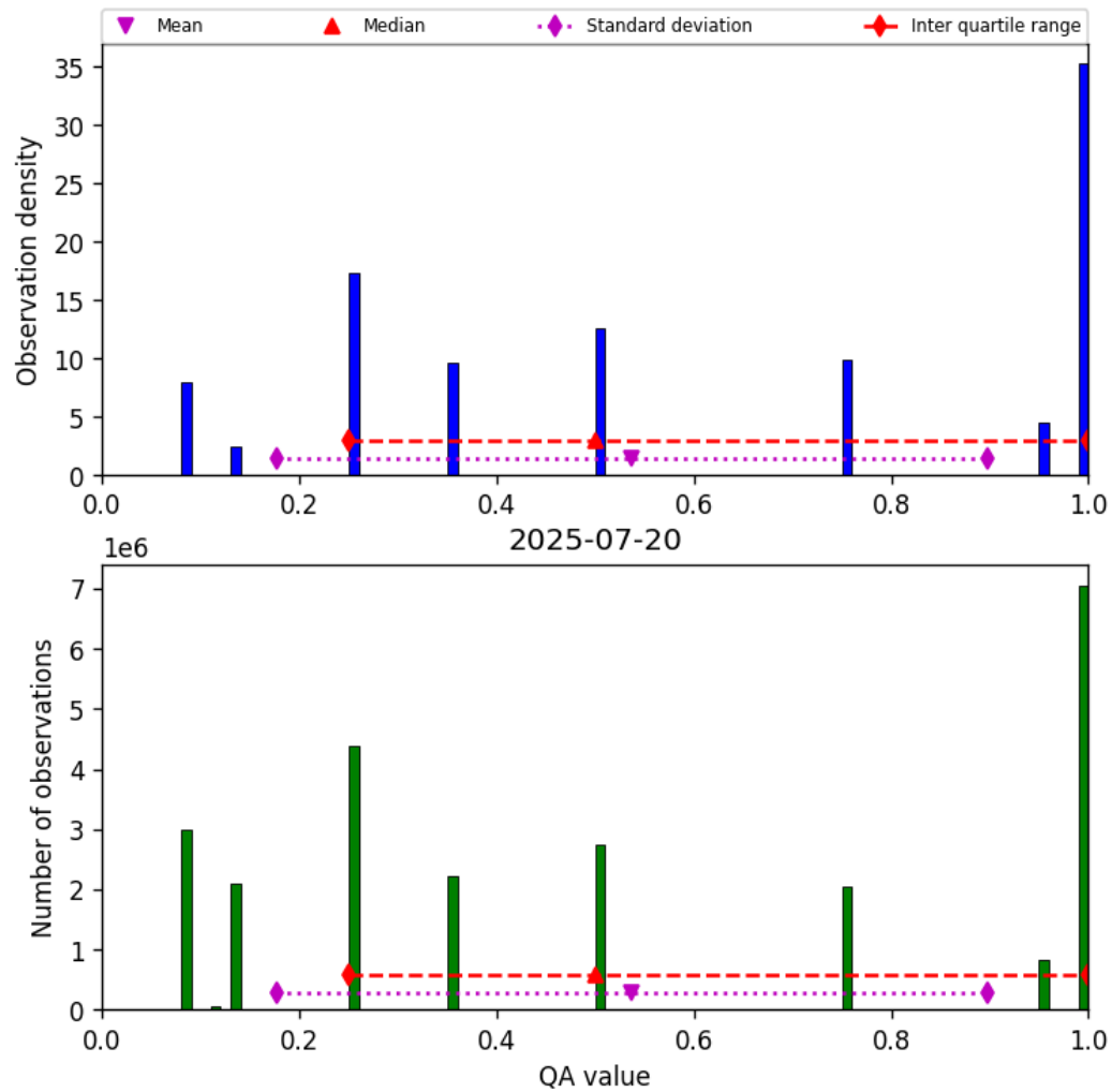
Figure 34: Histogram of “QA value” for 2025-07-19 to 2025-07-21
