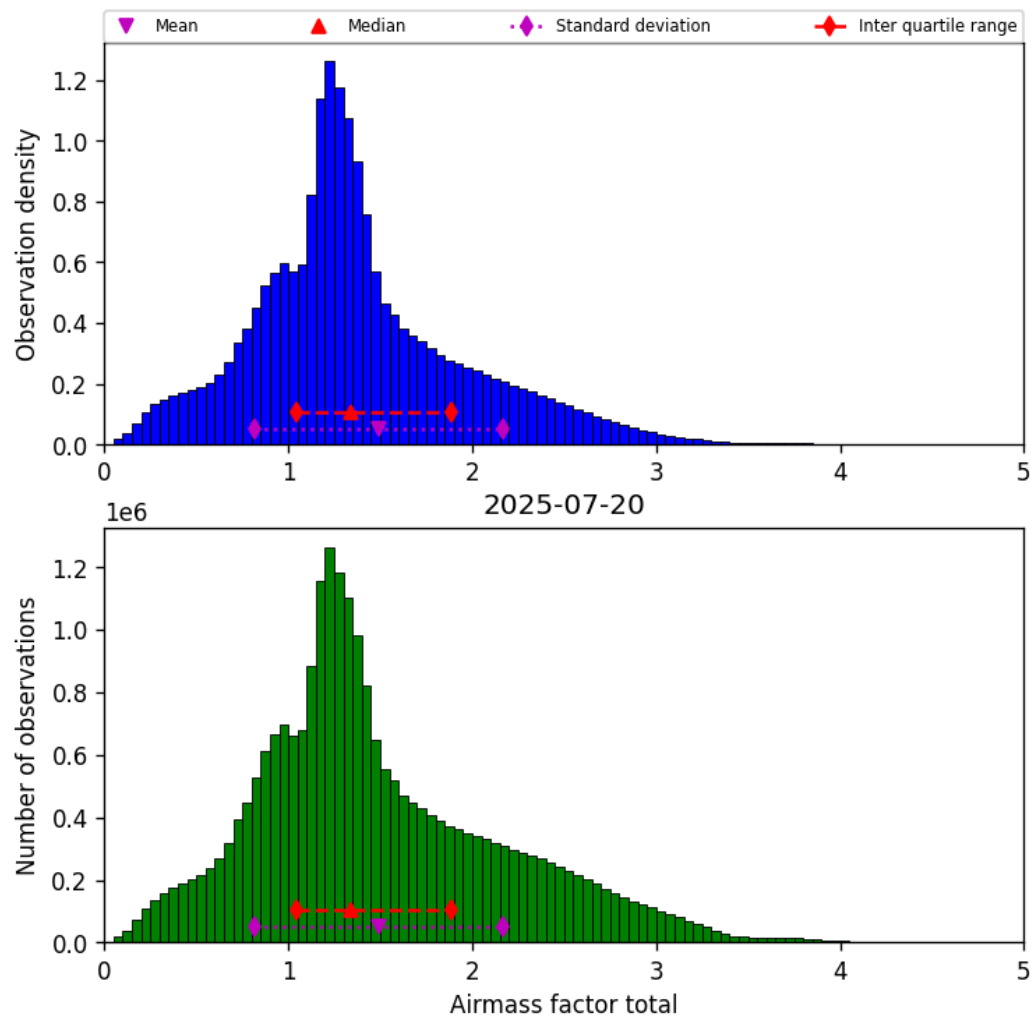
Figure 40: Histogram of “Airmass factor total” for 2025-07-19 to 2025-07-21
