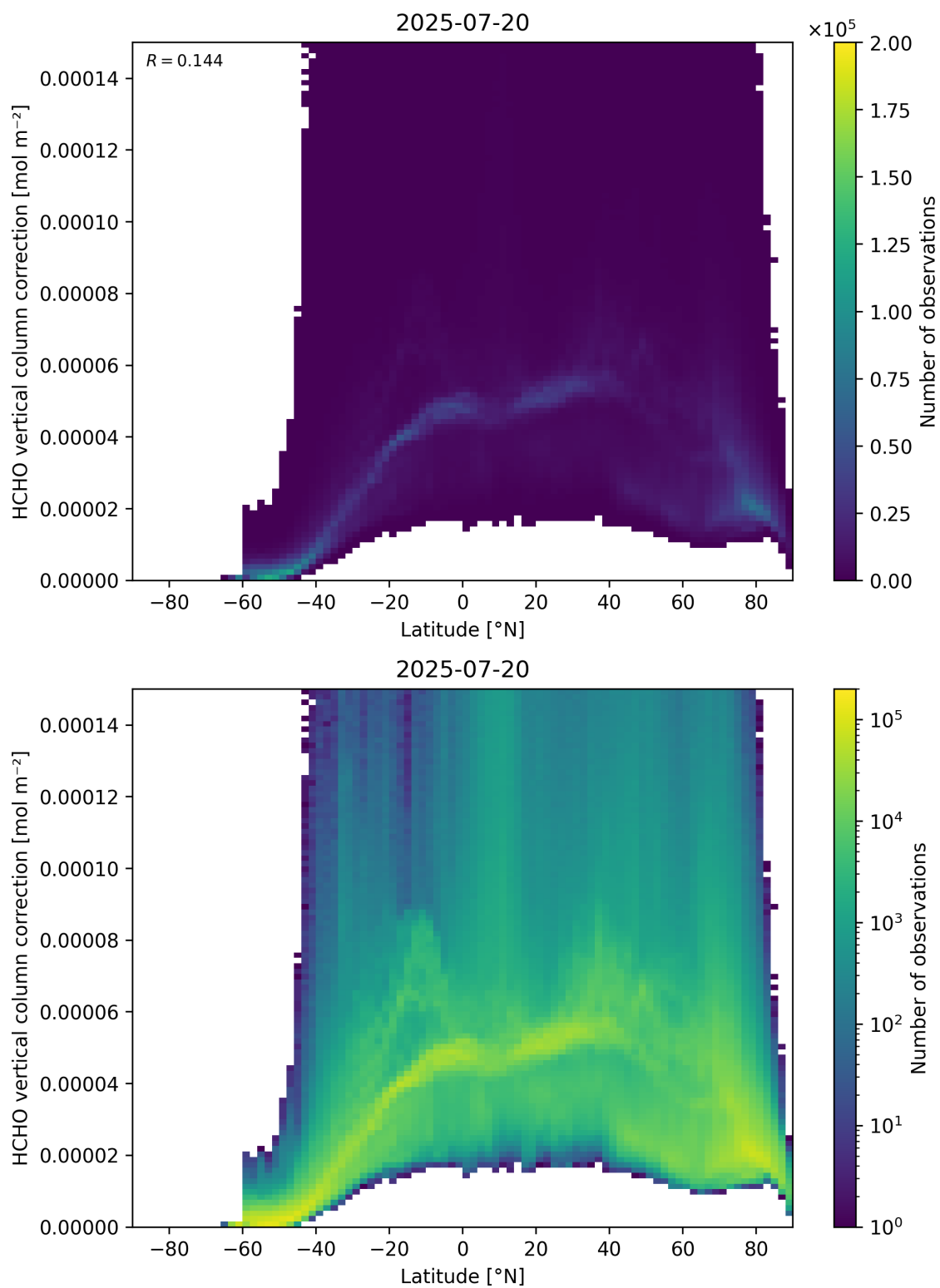
Figure 164: Scatter density plot of “Latitude” against “HCHO vertical column correction” for 2025-07-19 to 2025-07-21.
