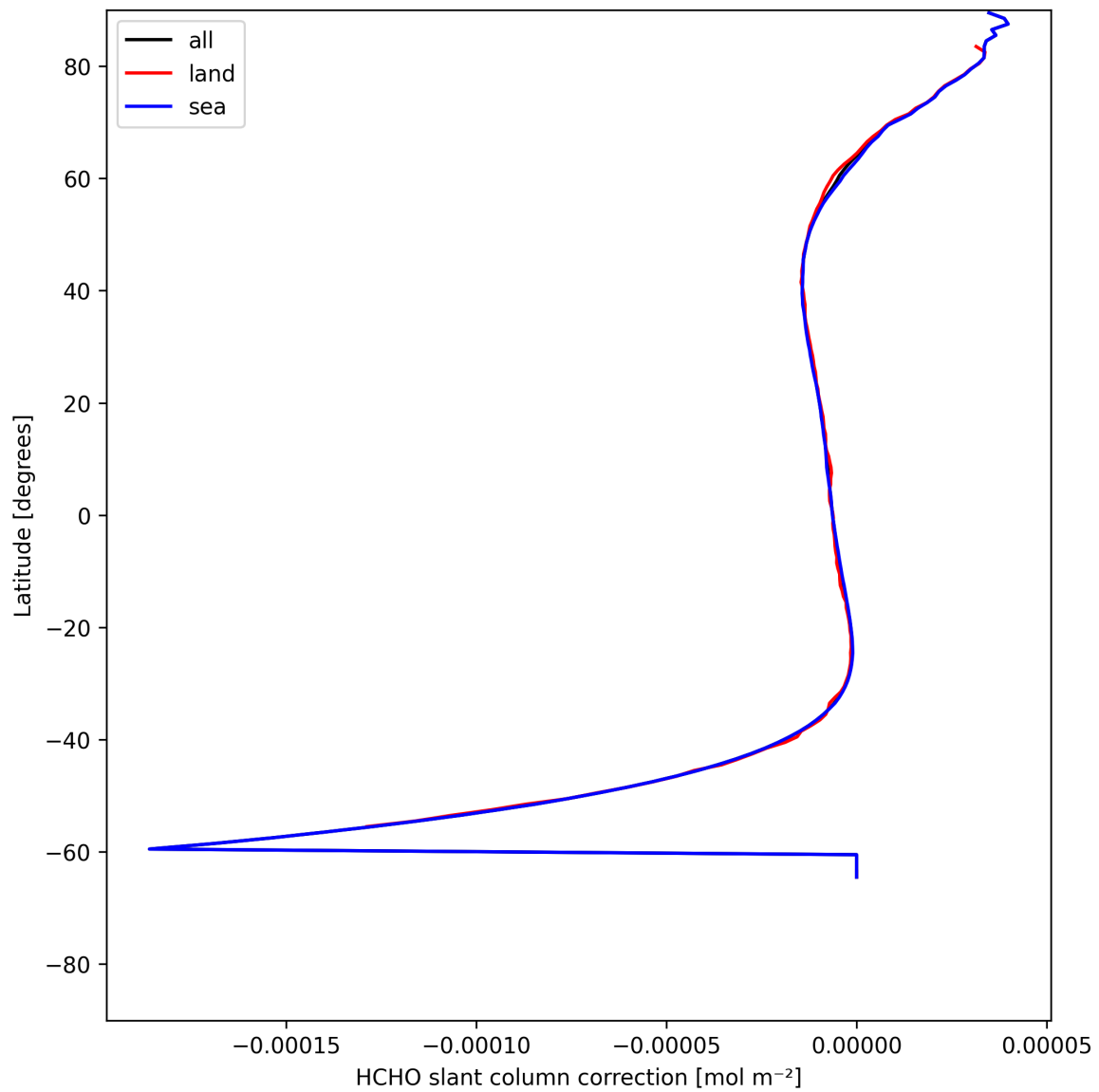
Figure 33: Zonal average of “HCHO slant column correction” for 2025-07-19 to 2025-07-21.
