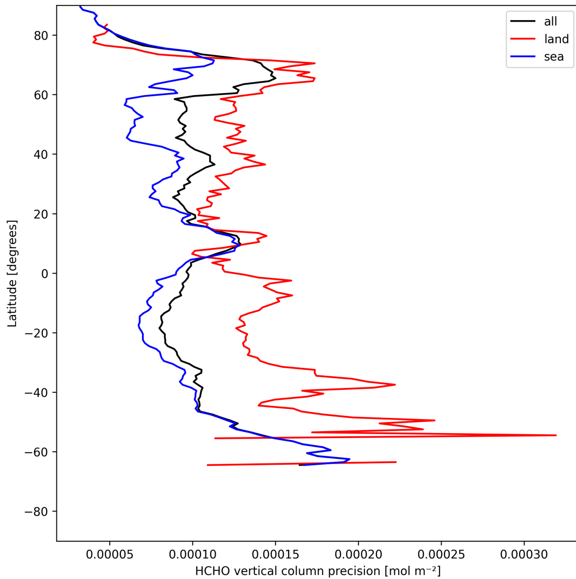
Figure 22: Zonal average of “HCHO vertical column precision” for 2025-07-19 to 2025-07-21.
