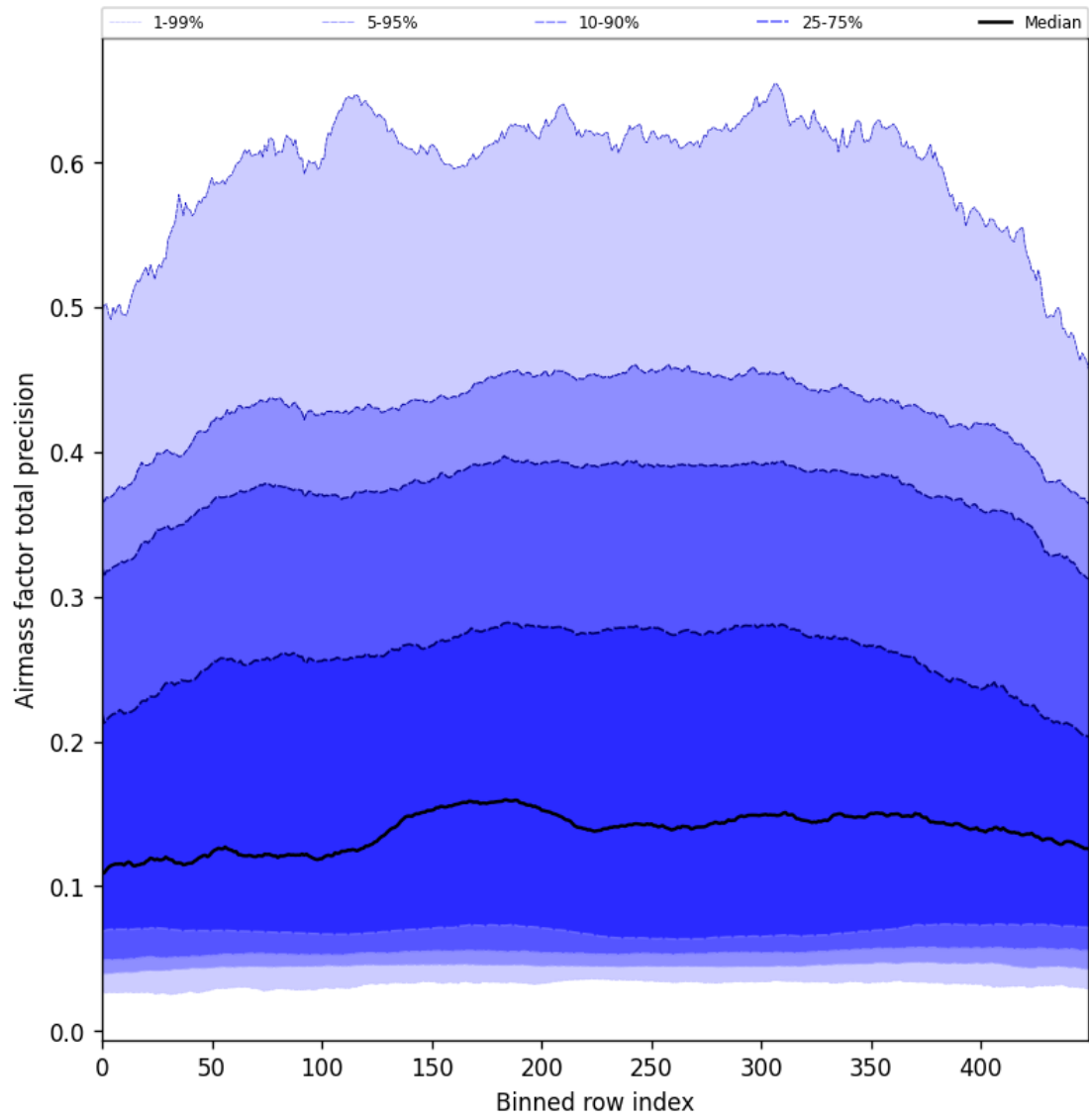
Figure 55: Along track statistics of “Airmass factor total precision” for 2025-07-19 to 2025-07-21
