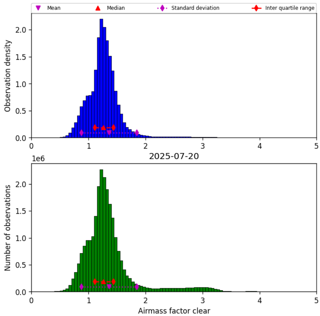
Figure 42: Histogram of “Airmass factor clear” for 2025-07-19 to 2025-07-21
