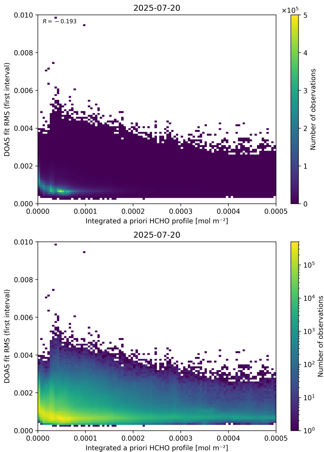
Figure 148: Scatter density plot of “Integrated a priori HCHO profile” against “DOAS fit RMS (first interval)” for 2025-07-19 to 2025-07-21.
