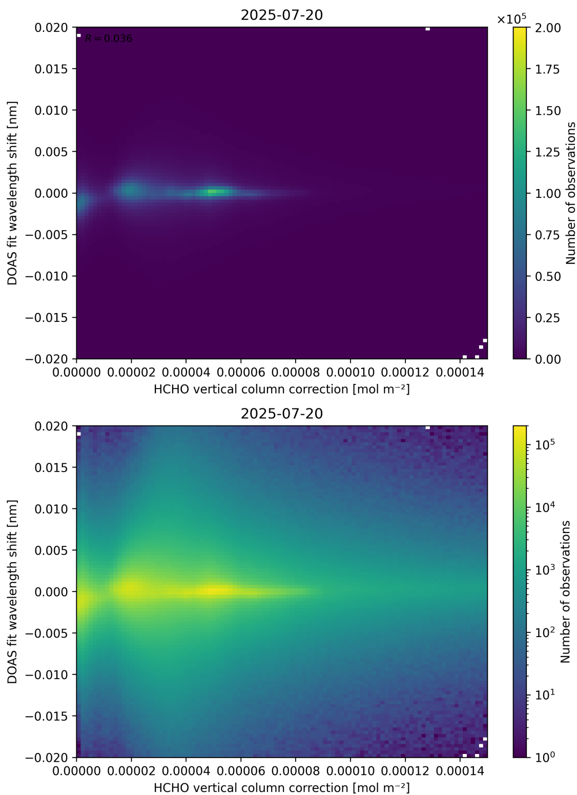
Figure 113: Scatter density plot of “HCHO vertical column correction” against “DOAS fit wavelength shift” for 2025-07-19 to 2025-07-21.
