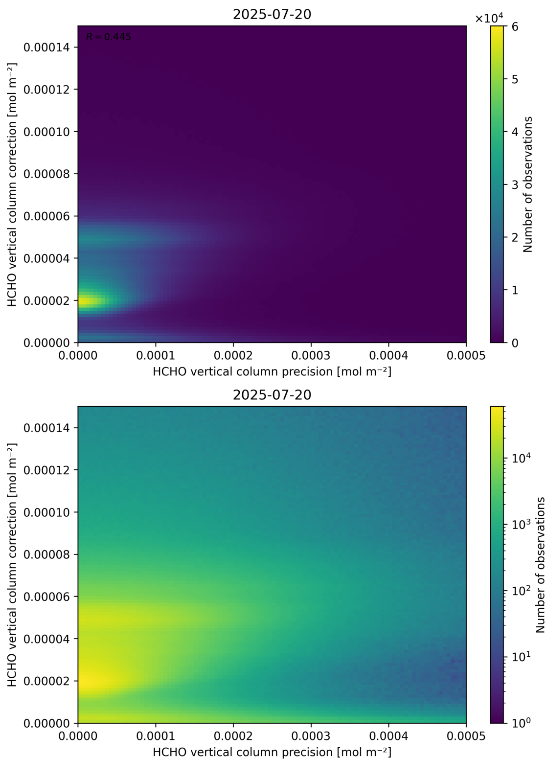
Figure 146: Scatter density plot of “HCHO vertical column precision” against “HCHO vertical column correction” for 2025-07-19 to 2025-07-21.
