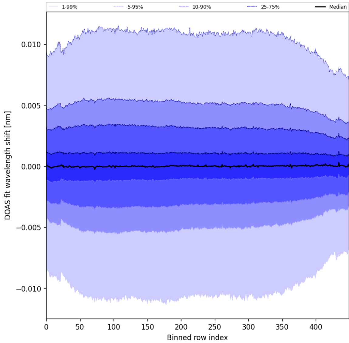
Figure 58: Along track statistics of “DOAS fit wavelength shift” for 2025-07-19 to 2025-07-21
