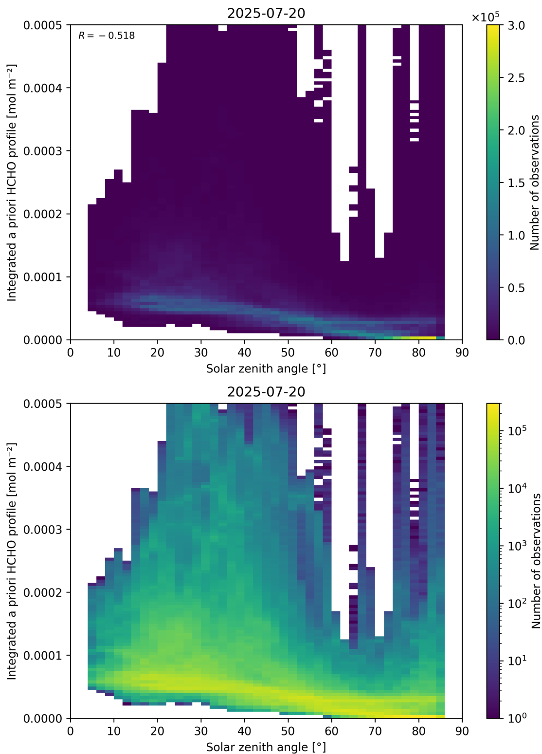
Figure 180: Scatter density plot of “Solar zenith angle” against “Integrated a priori HCHO profile” for 2025-07-19 to 2025-07-21.
