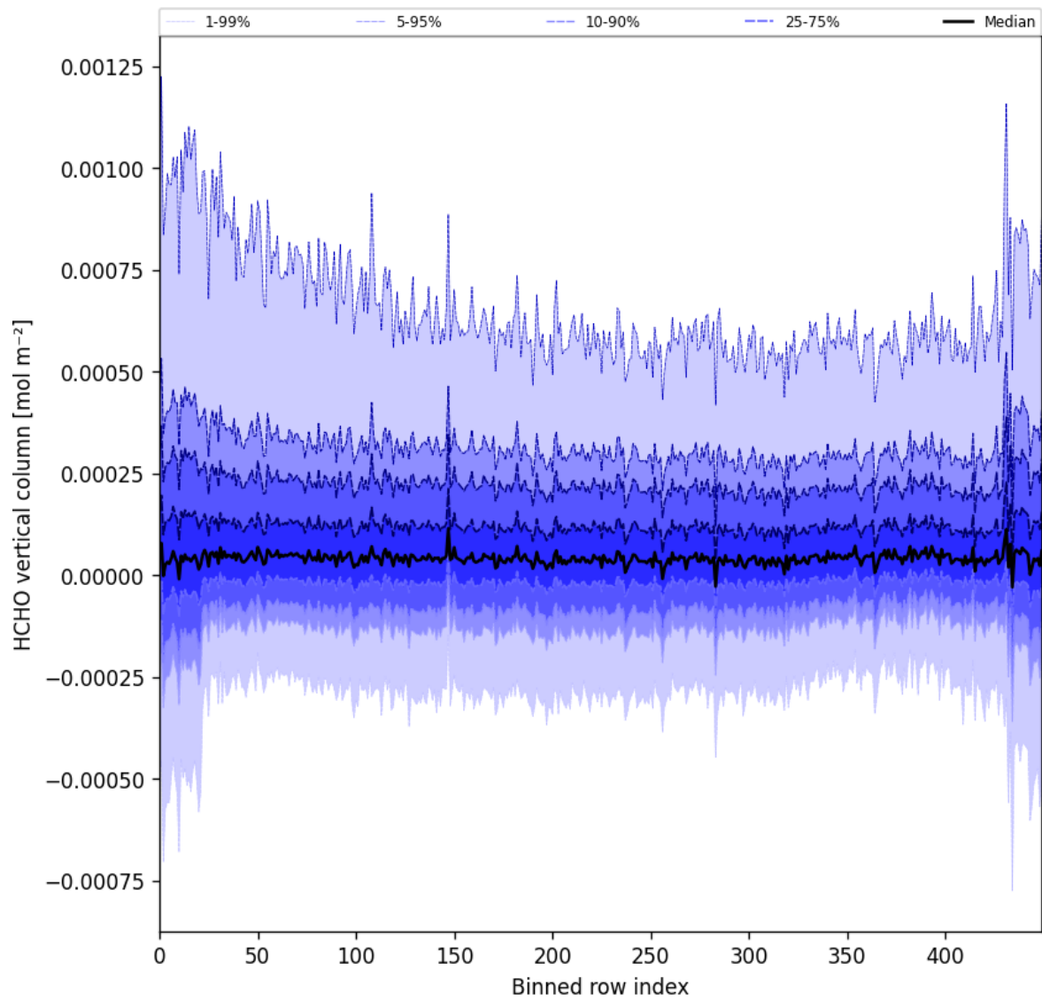
Figure 49: Along track statistics of “HCHO vertical column” for 2025-07-19 to 2025-07-21
