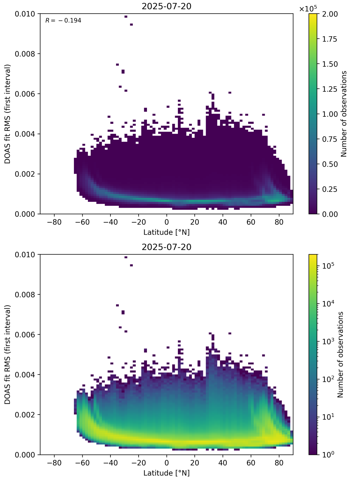
Figure 153: Scatter density plot of “Latitude” against “DOAS fit RMS (first interval)” for 2025-07-19 to 2025-07-21.
