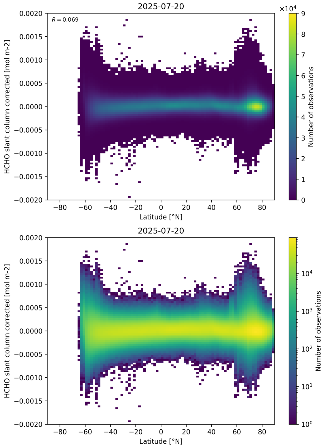
Figure 157: Scatter density plot of “Latitude” against “HCHO slant column corrected” for 2025-07-19 to 2025-07-21.
