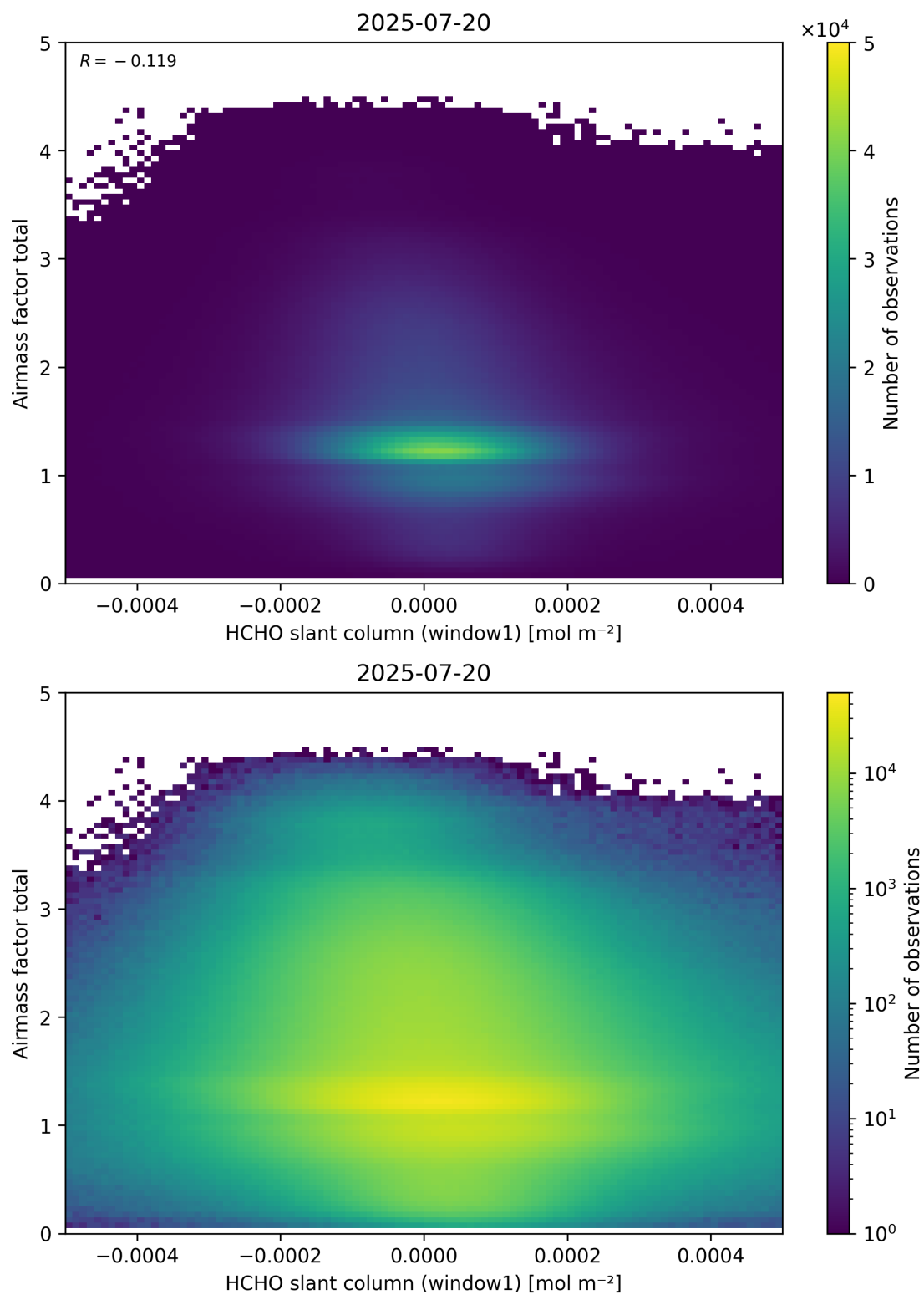
Figure 85: Scatter density plot of “HCHO slant column (window1)” against “Airmass factor total” for 2025-07-19 to 2025-07-21.
