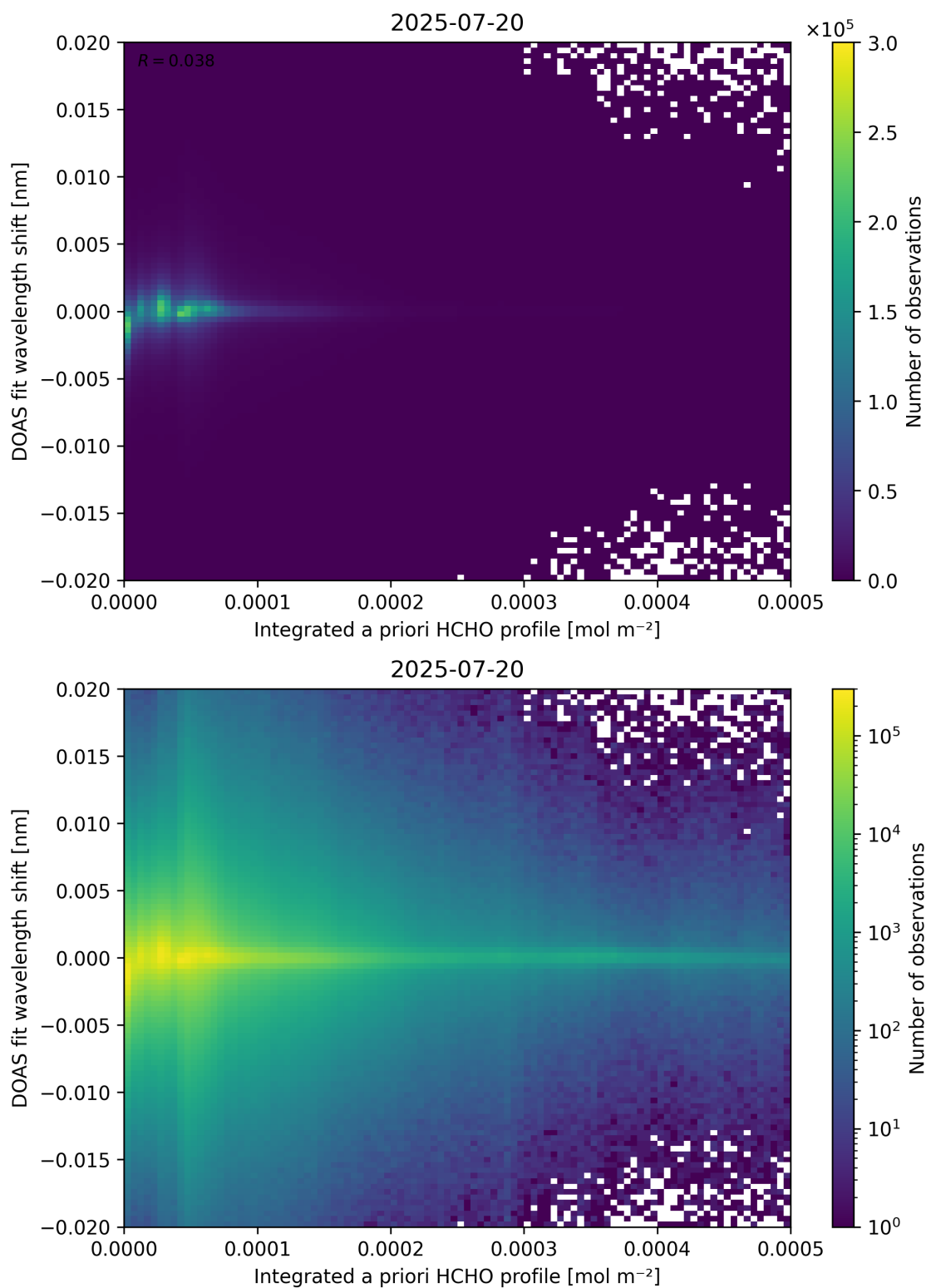
Figure 149: Scatter density plot of “Integrated a priori HCHO profile” against “DOAS fit wavelength shift” for 2025-07-19 to 2025-07-21.
