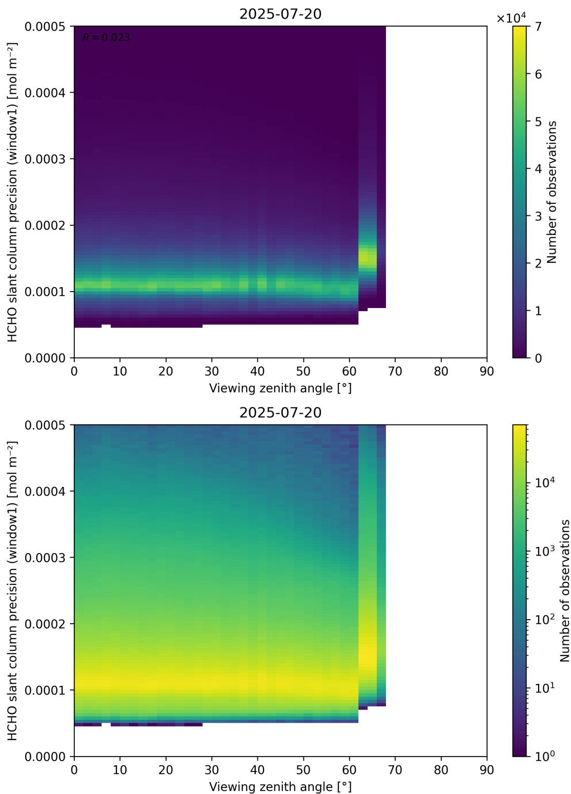
Figure 189: Scatter density plot of “Viewing zenith angle” against “HCHO slant column precision (window1)” for 2025-07-19 to 2025-07-21.
