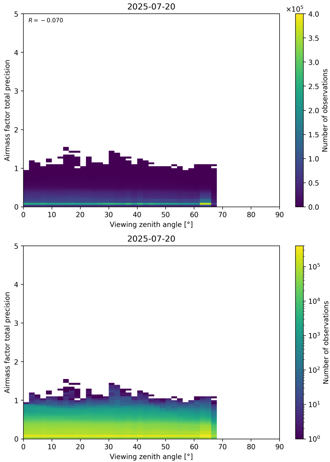
Figure 191: Scatter density plot of “Viewing zenith angle” against “Airmass factor total precision” for 2025-07-19 to 2025-07-21.
