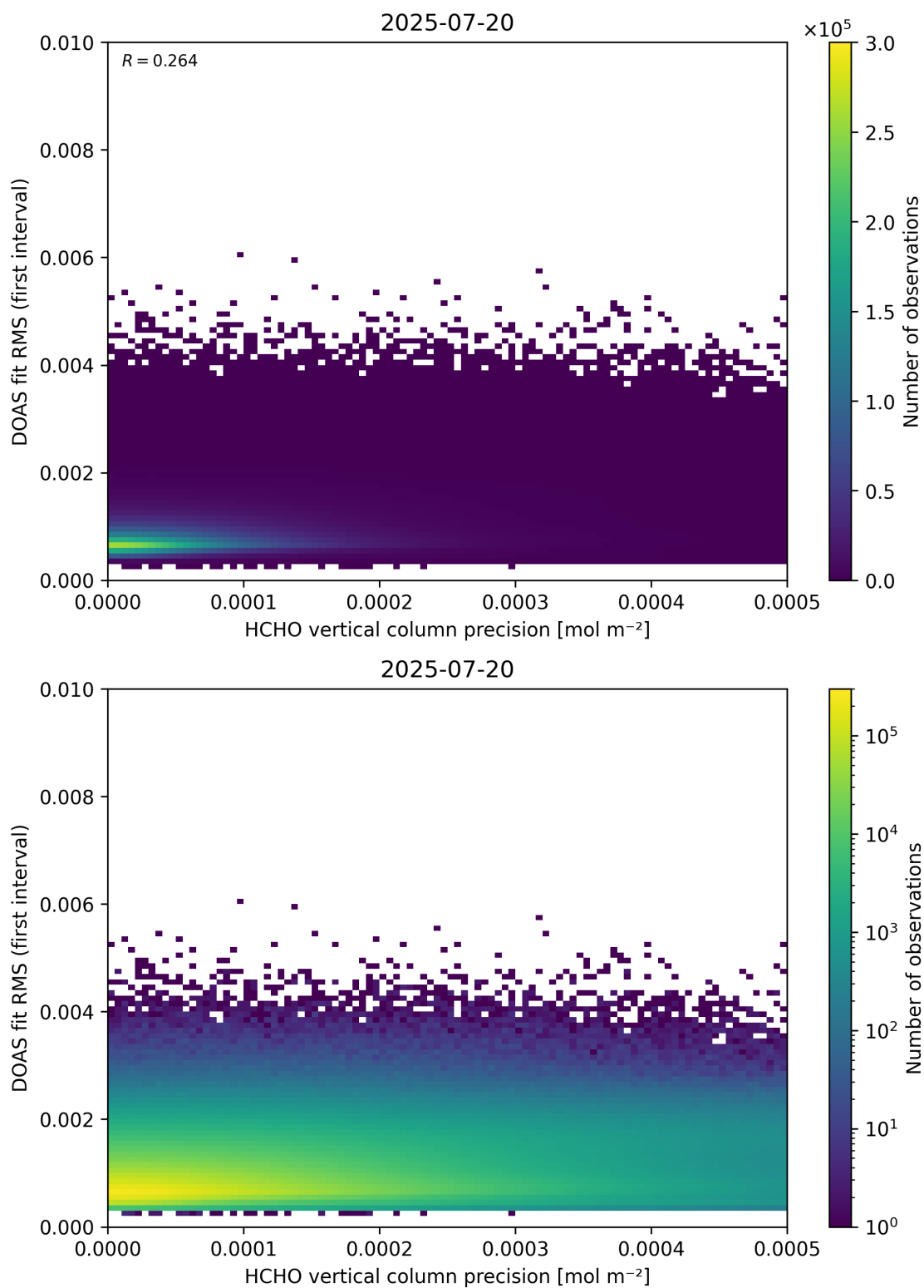
Figure 136: Scatter density plot of “HCHO vertical column precision” against “DOAS fit RMS (first interval)” for 2025-07-19 to 2025-07-21.
