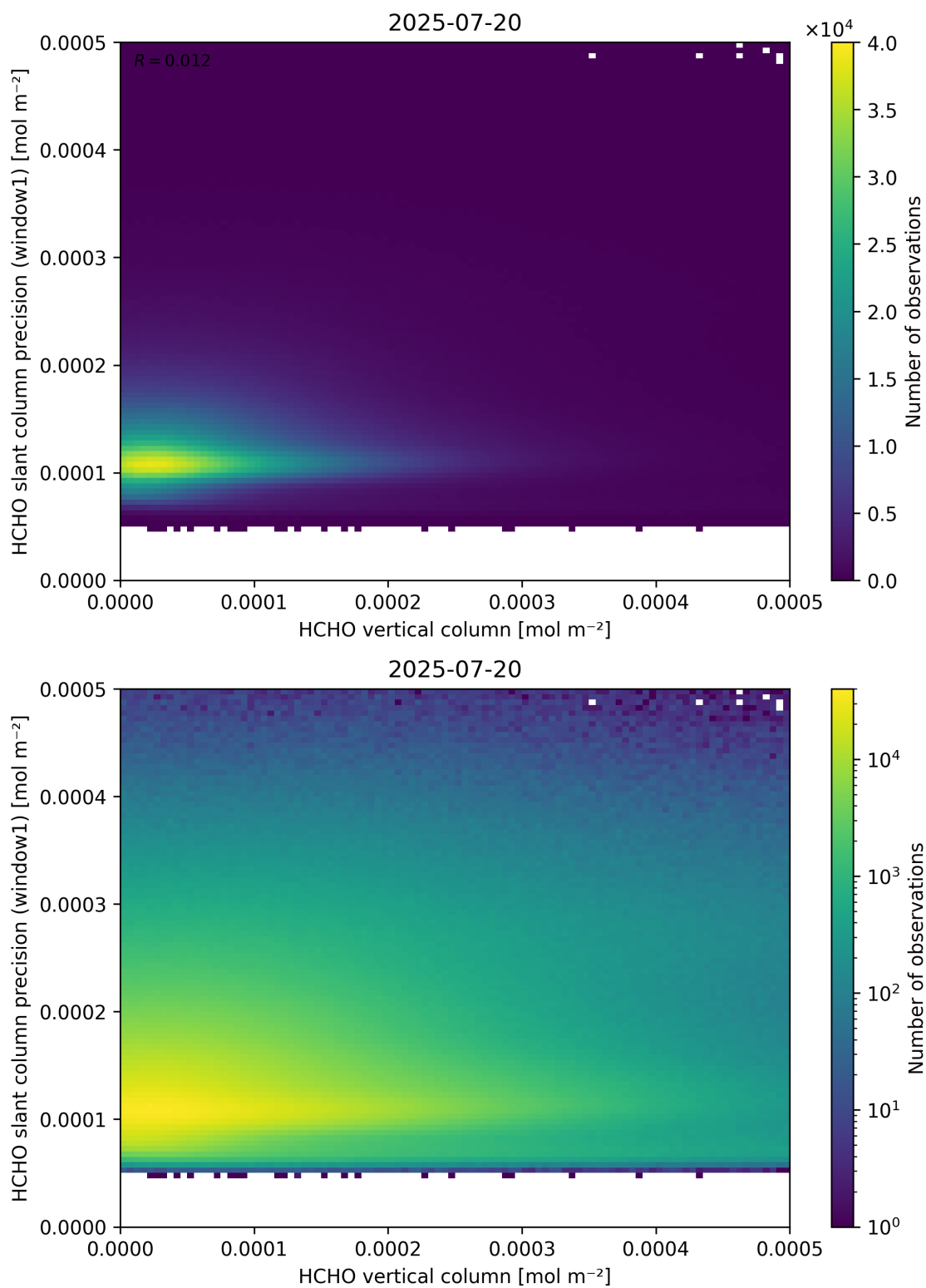
Figure 130: Scatter density plot of “HCHO vertical column” against “HCHO slant column precision (window1)” for 2025-07-19 to 2025-07-21.
