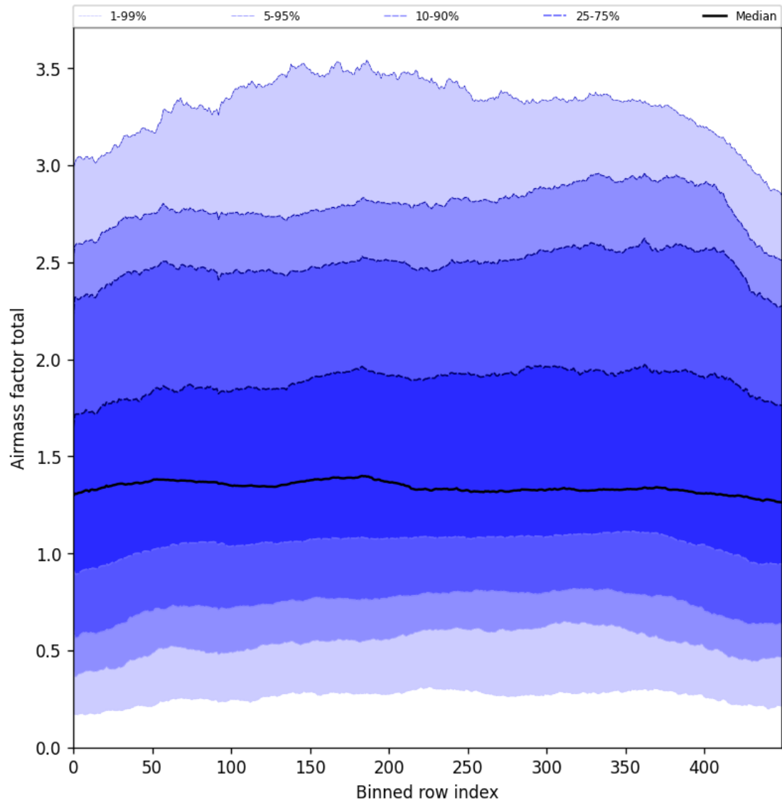
Figure 54: Along track statistics of “Airmass factor total” for 2025-07-19 to 2025-07-21
