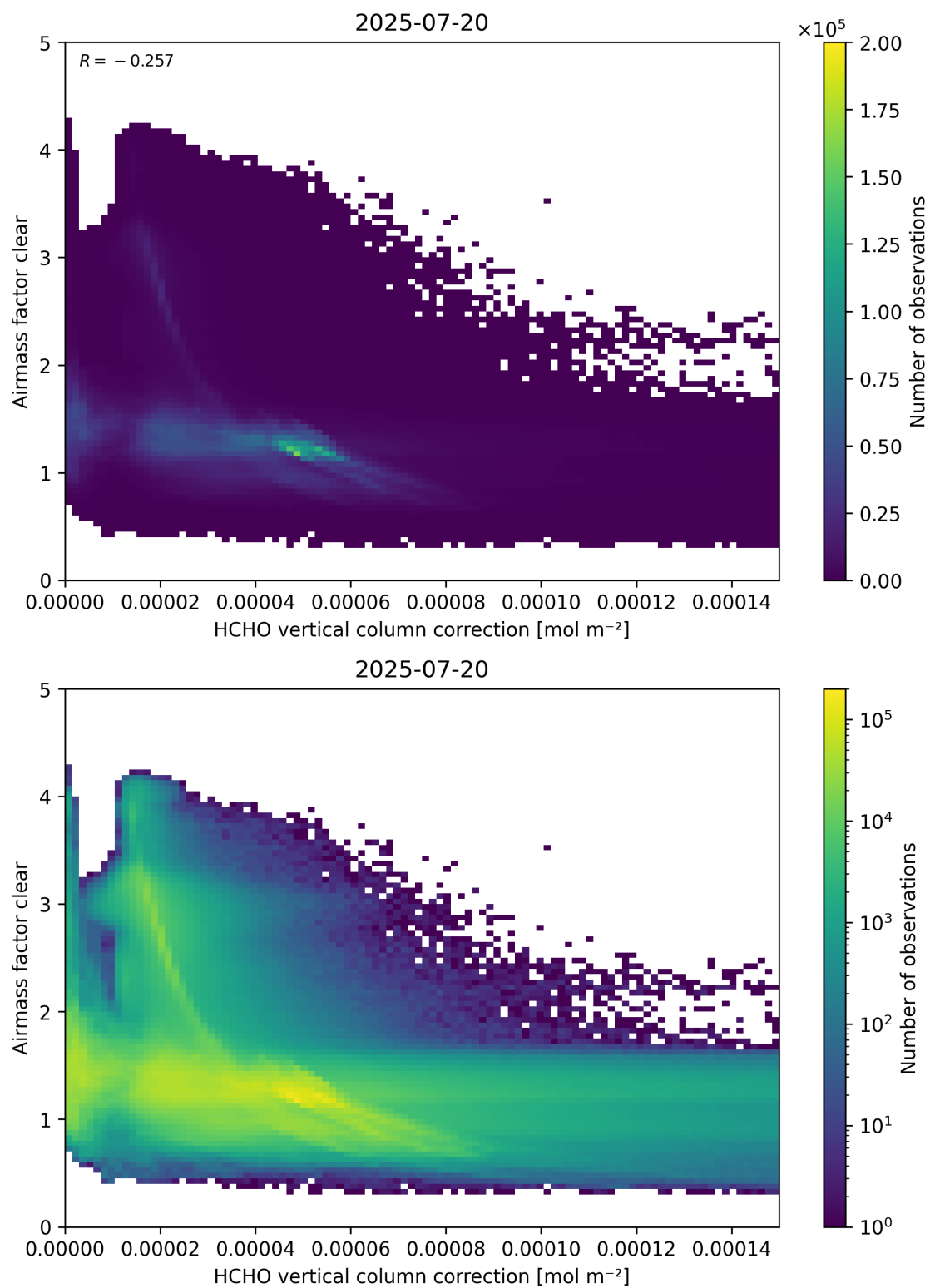
Figure 115: Scatter density plot of “HCHO vertical column correction” against “Airmass factor clear” for 2025-07-19 to 2025-07-21.
