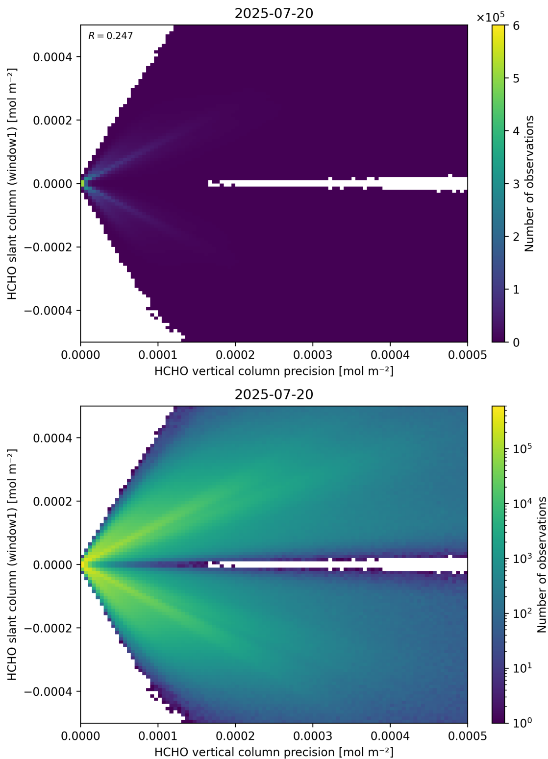
Figure 142: Scatter density plot of “HCHO vertical column precision” against “HCHO slant column (window1)” for 2025-07-19 to 2025-07-21.
