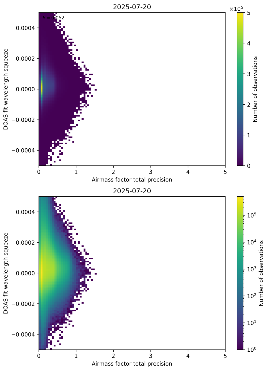
Figure 107: Scatter density plot of “Airmass factor total precision” against “DOAS fit wavelength squeeze” for 2025-07-19 to 2025-07-21.
