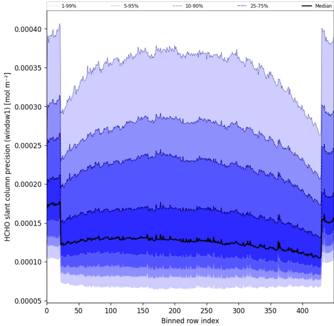
Figure 53: Along track statistics of “HCHO slant column precision (window1)” for 2025-07-19 to 2025-07-21
