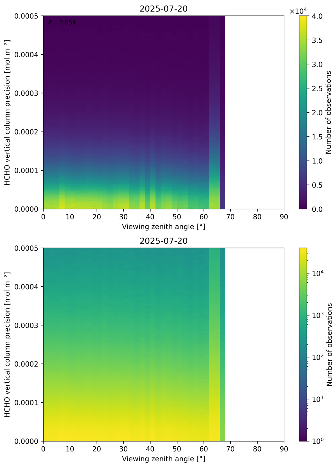
Figure 194: Scatter density plot of “Viewing zenith angle” against “HCHO vertical column precision” for 2025-07-19 to 2025-07-21.
