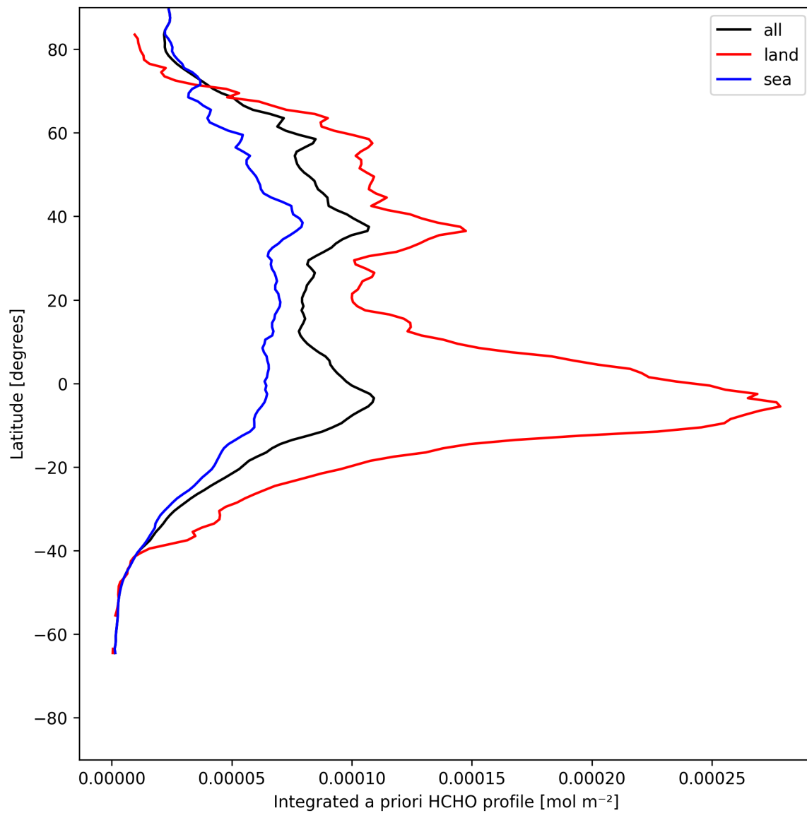
Figure 29: Zonal average of “Integrated a priori HCHO profile” for 2025-07-19 to 2025-07-21.
