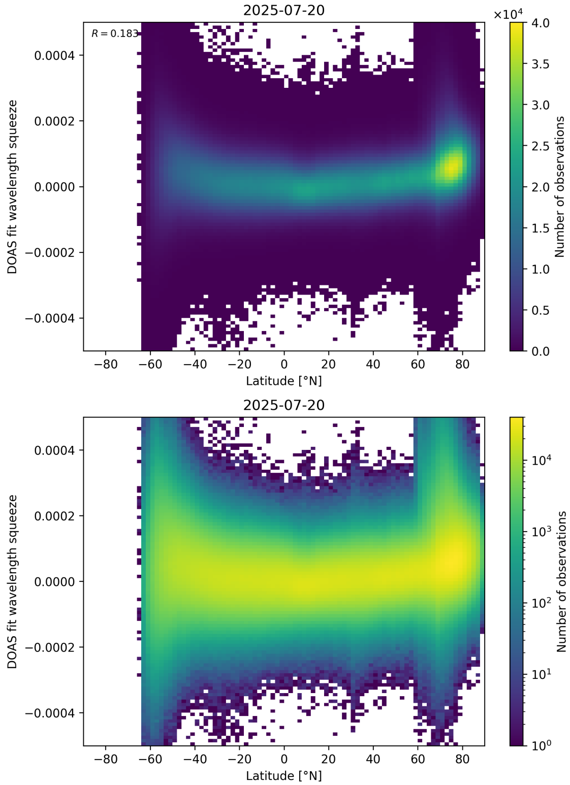
Figure 155: Scatter density plot of “Latitude” against “DOAS fit wavelength squeeze” for 2025-07-19 to 2025-07-21.
