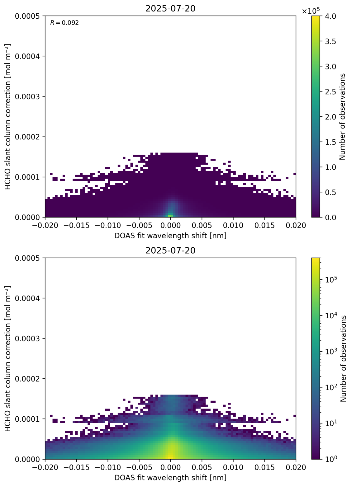
Figure 67: Scatter density plot of “DOAS fit wavelength shift” against “HCHO slant column correction” for 2025-07-19 to 2025-07-21.
