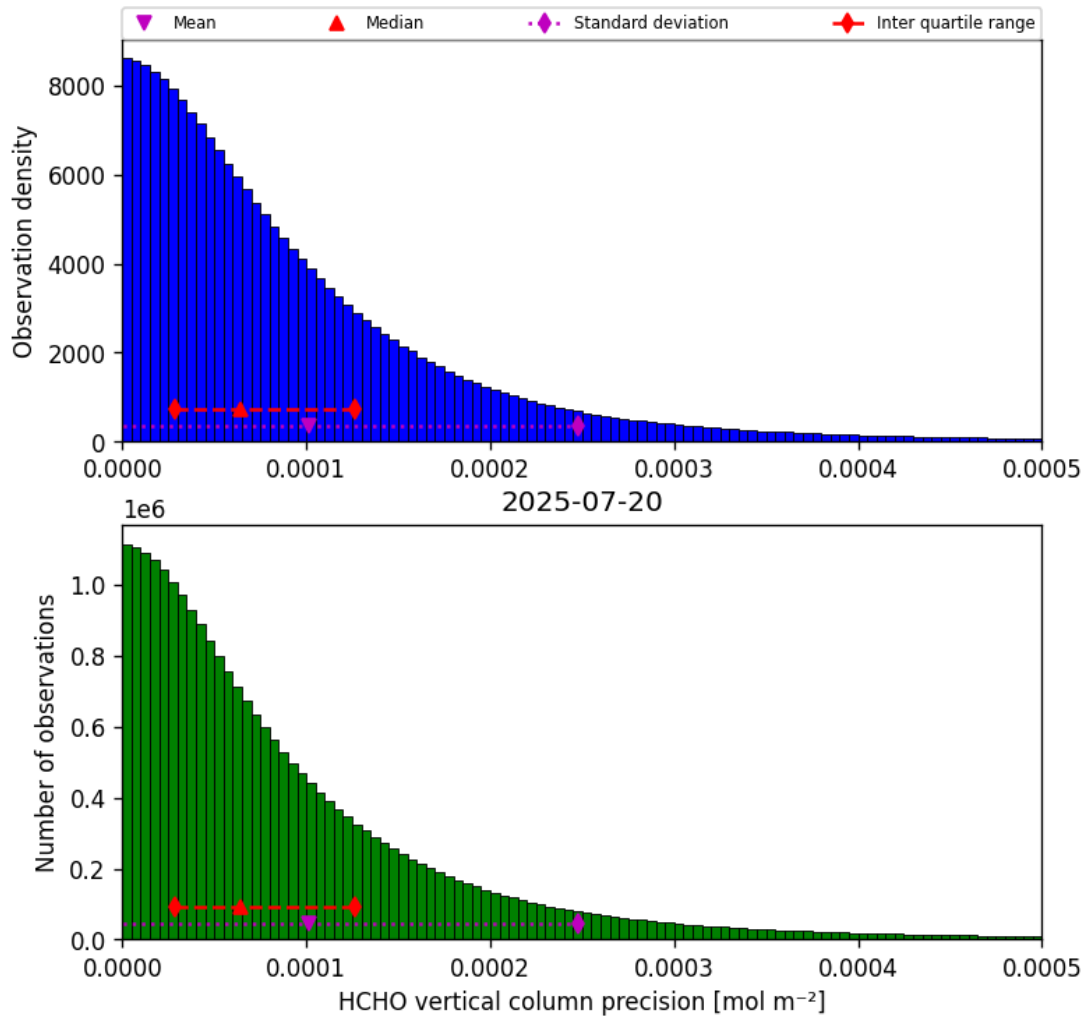
Figure 36: Histogram of “HCHO vertical column precision” for 2025-07-19 to 2025-07-21
