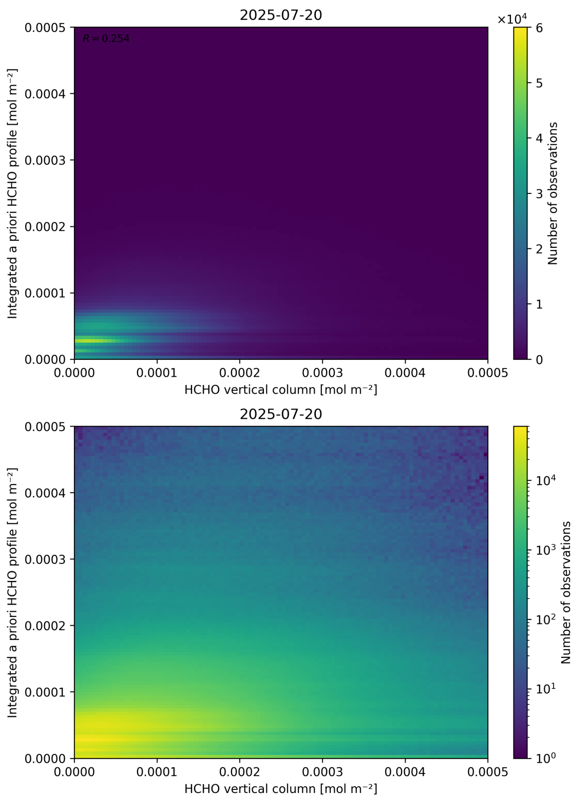
Figure 135: Scatter density plot of “HCHO vertical column” against “Integrated a priori HCHO profile” for 2025-07-19 to 2025-07-21.
