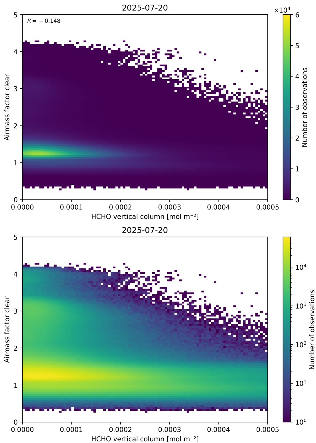
Figure 126: Scatter density plot of “HCHO vertical column” against “Airmass factor clear” for 2025-07-19 to 2025-07-21.
