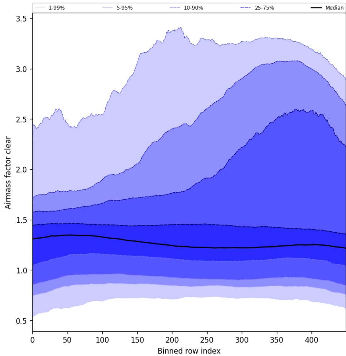
Figure 56: Along track statistics of “Air mass factor clear” for 2025-07-19 to 2025-07-21
