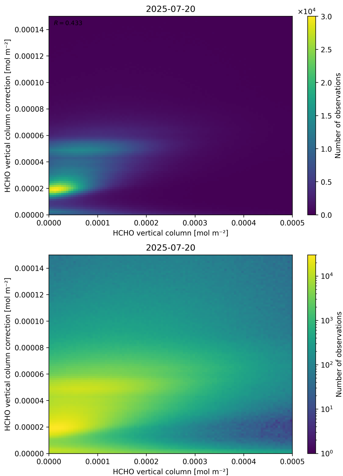
Figure 133: Scatter density plot of “HCHO vertical column” against “HCHO vertical column correction” for 2025-07-19 to 2025-07-21.
