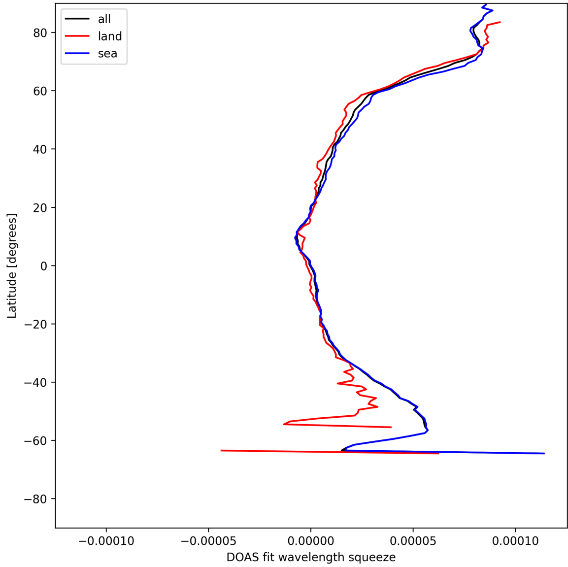
Figure 31: Zonal average of “DOAS fit wavelength squeeze” for 2025-07-19 to 2025-07-21.
