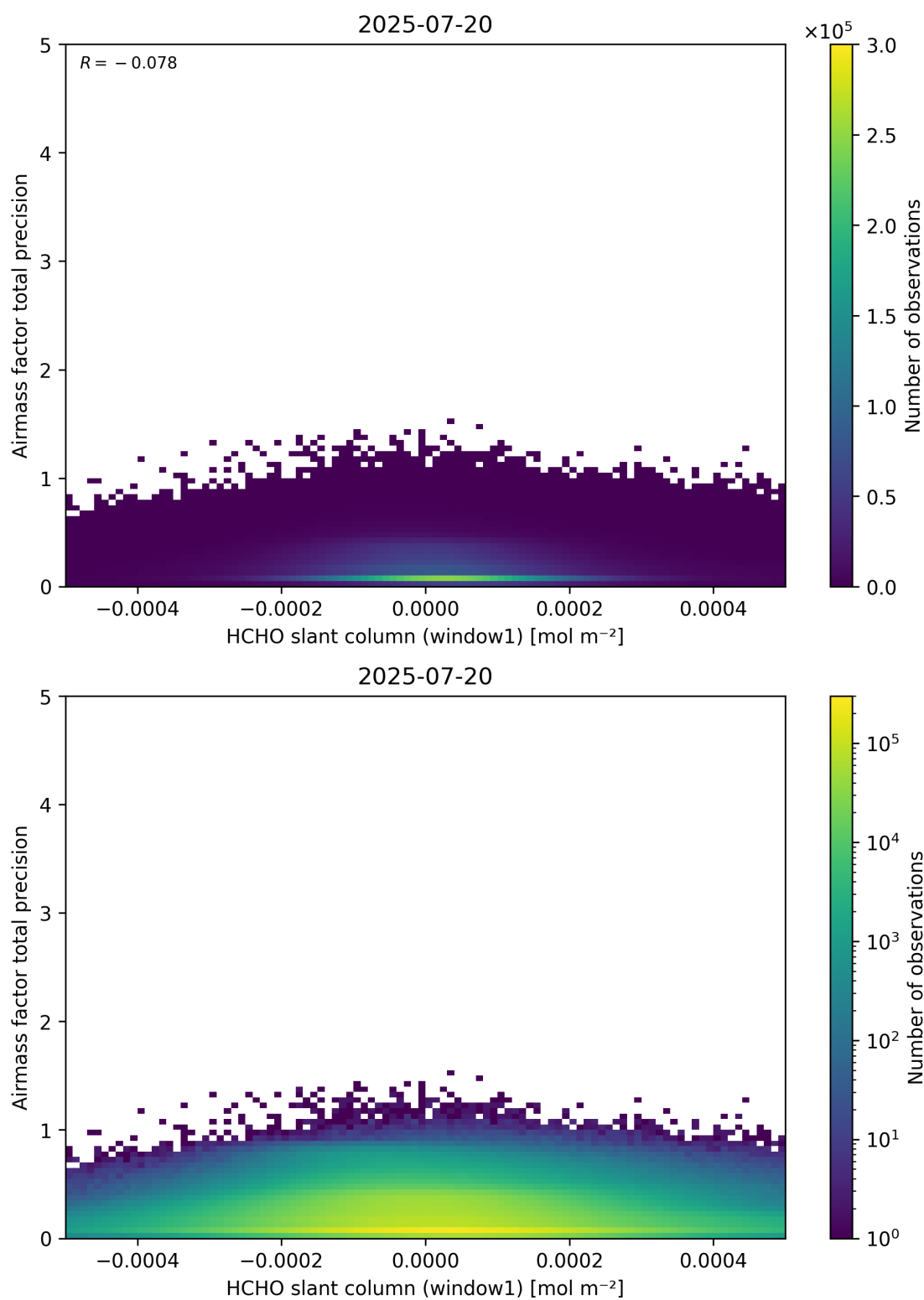
Figure 86: Scatter density plot of “HCHO slant column (window1)” against “Airmass factor total precision” for 2025-07-19 to 2025-07-21.
