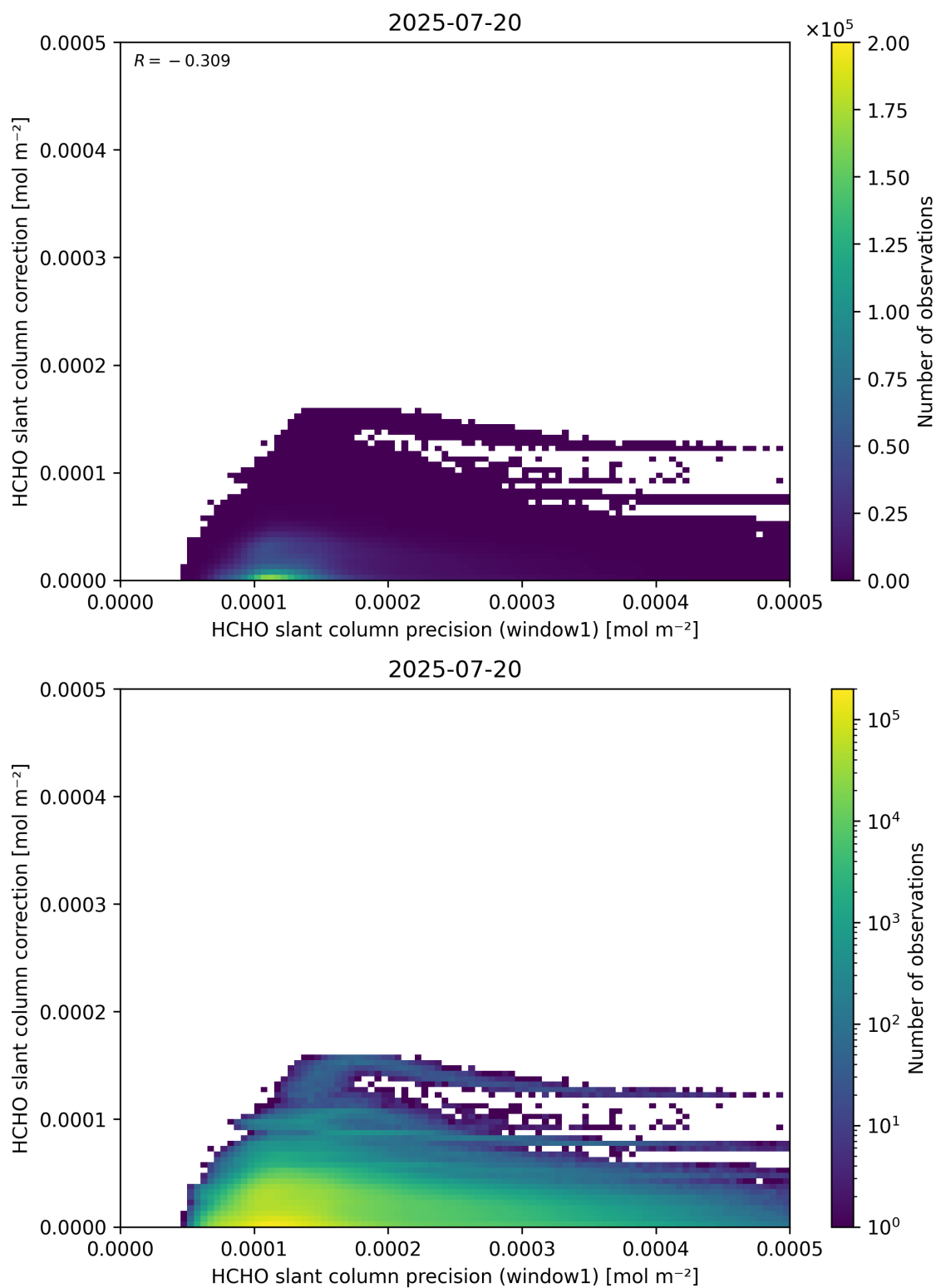
Figure 93: Scatter density plot of “HCHO slant column precision (window1)” against “HCHO slant column correction” for 2025-07-19 to 2025-07-21.
