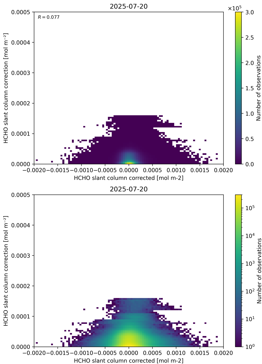
Figure 77: Scatter density plot of “HCHO slant column corrected” against “HCHO slant column correction” for 2025-07-19 to 2025-07-21.
