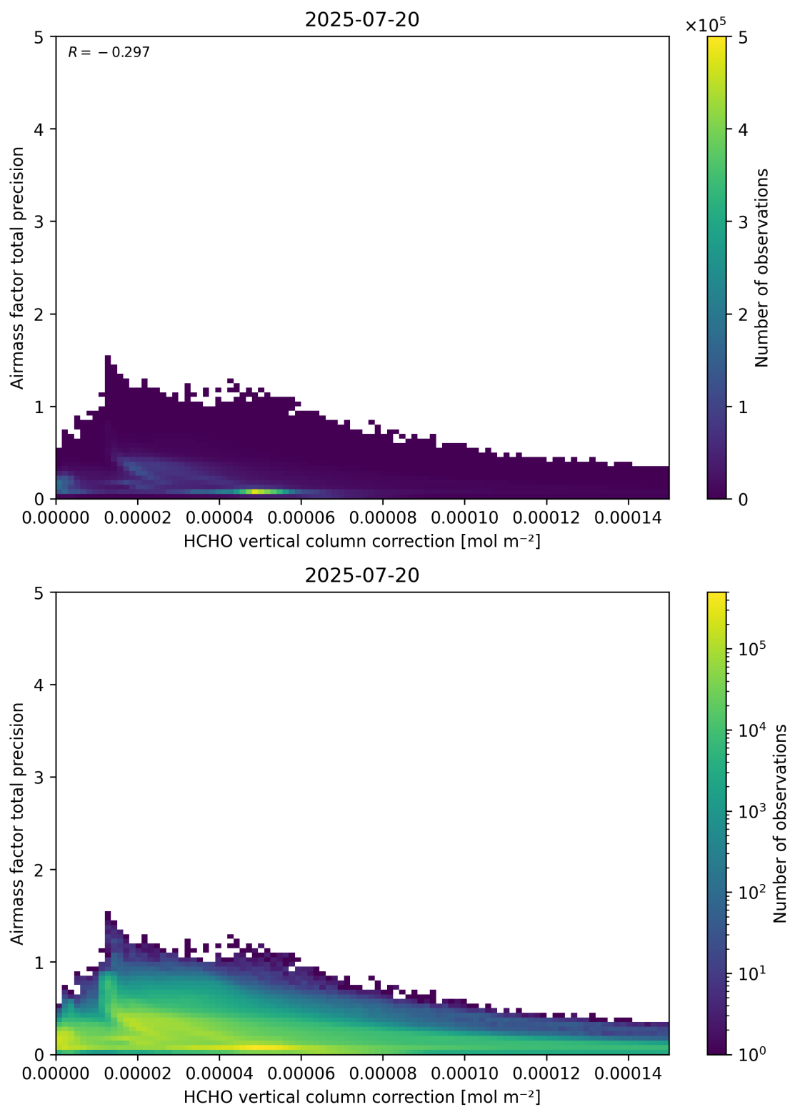
Figure 121: Scatter density plot of “HCHO vertical column correction” against “Airmass factor total precision” for 2025-07-19 to 2025-07-21.
