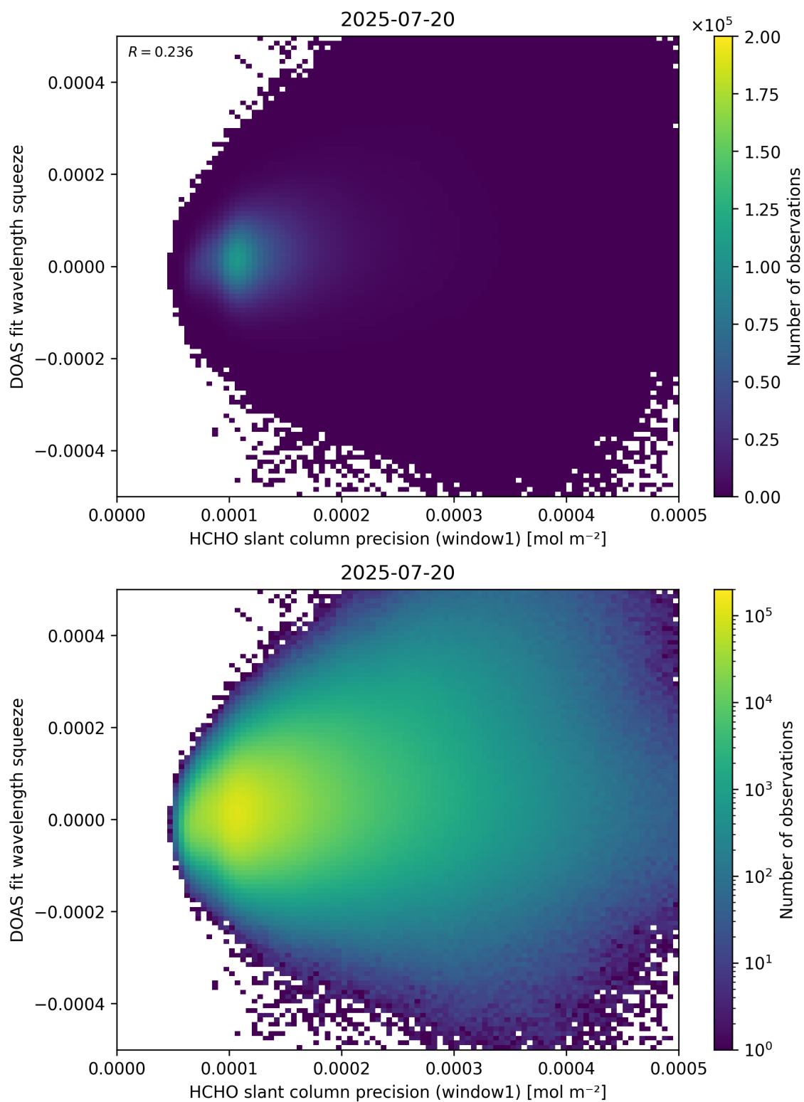
Figure 90: Scatter density plot of “HCHO slant column precision (window1)” against “DOAS fit wavelength squeeze” for 2025-07-19 to 2025-07-21.
