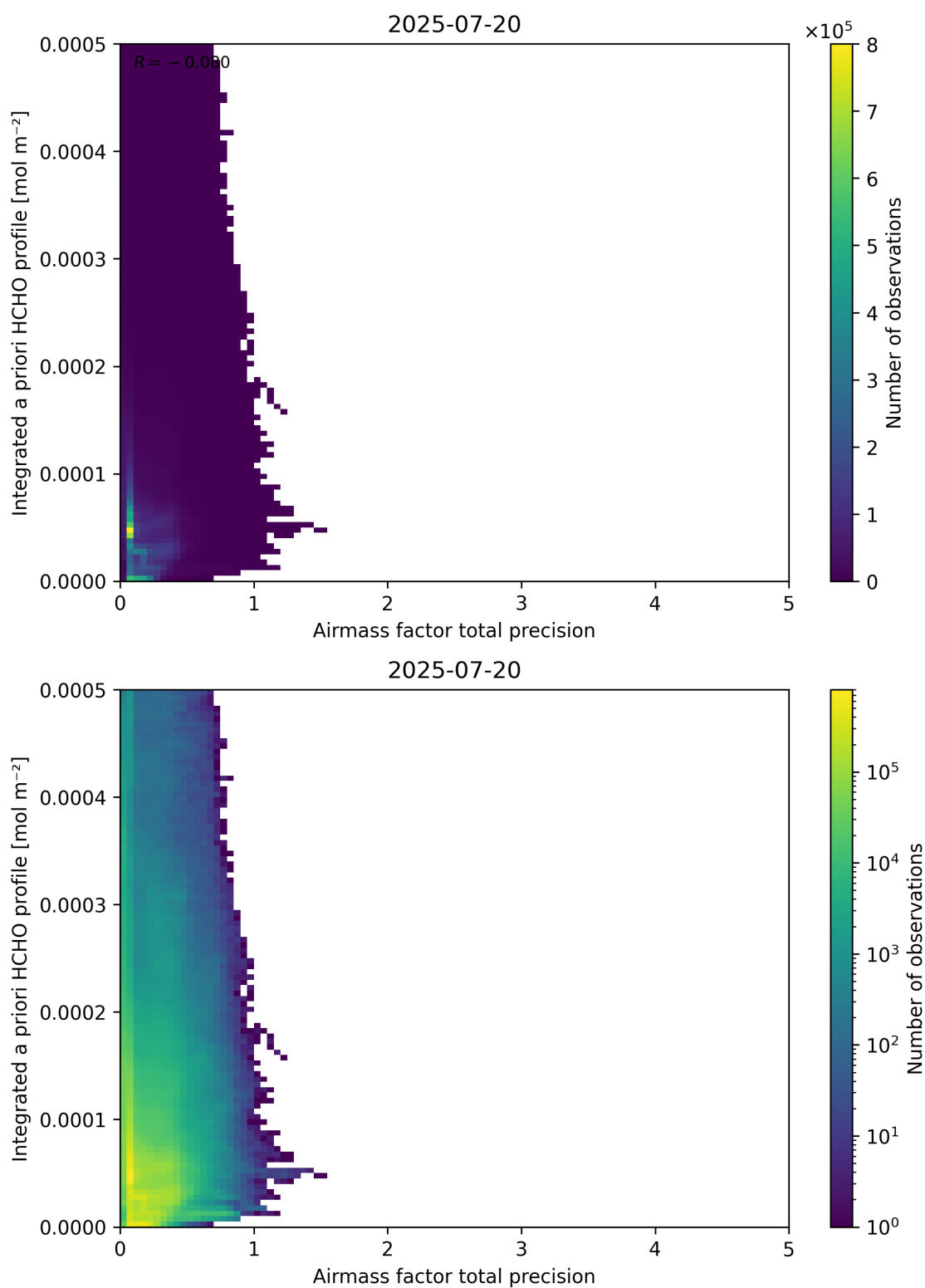
Figure 111: Scatter density plot of “Airmass factor total precision” against “Integrated a priori HCHO profile” for 2025-07-19 to 2025-07-21.
