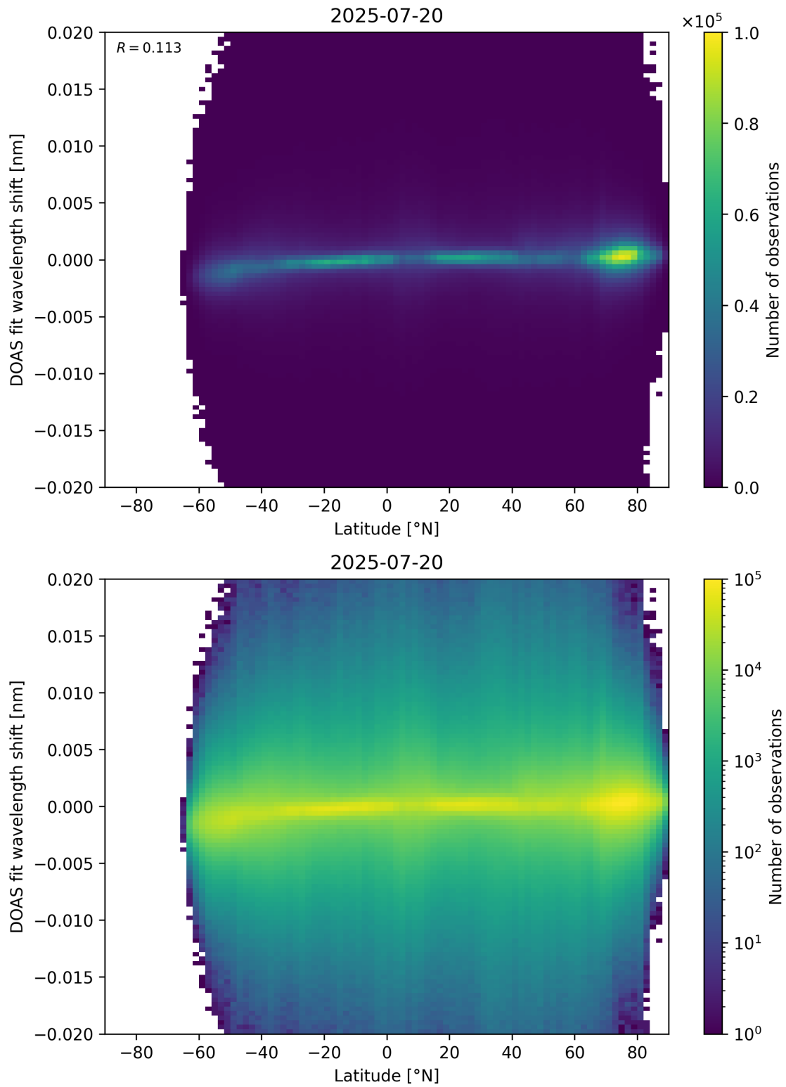
Figure 154: Scatter density plot of “Latitude” against “DOAS fit wavelength shift” for 2025-07-19 to 2025-07-21.
