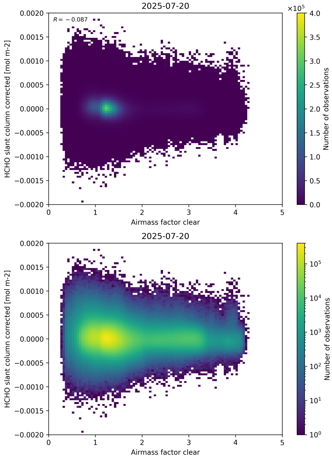
Figure 74: Scatter density plot of “Airmass factor clear” against “HCHO slant column corrected” for 2025-07-19 to 2025-07-21.
