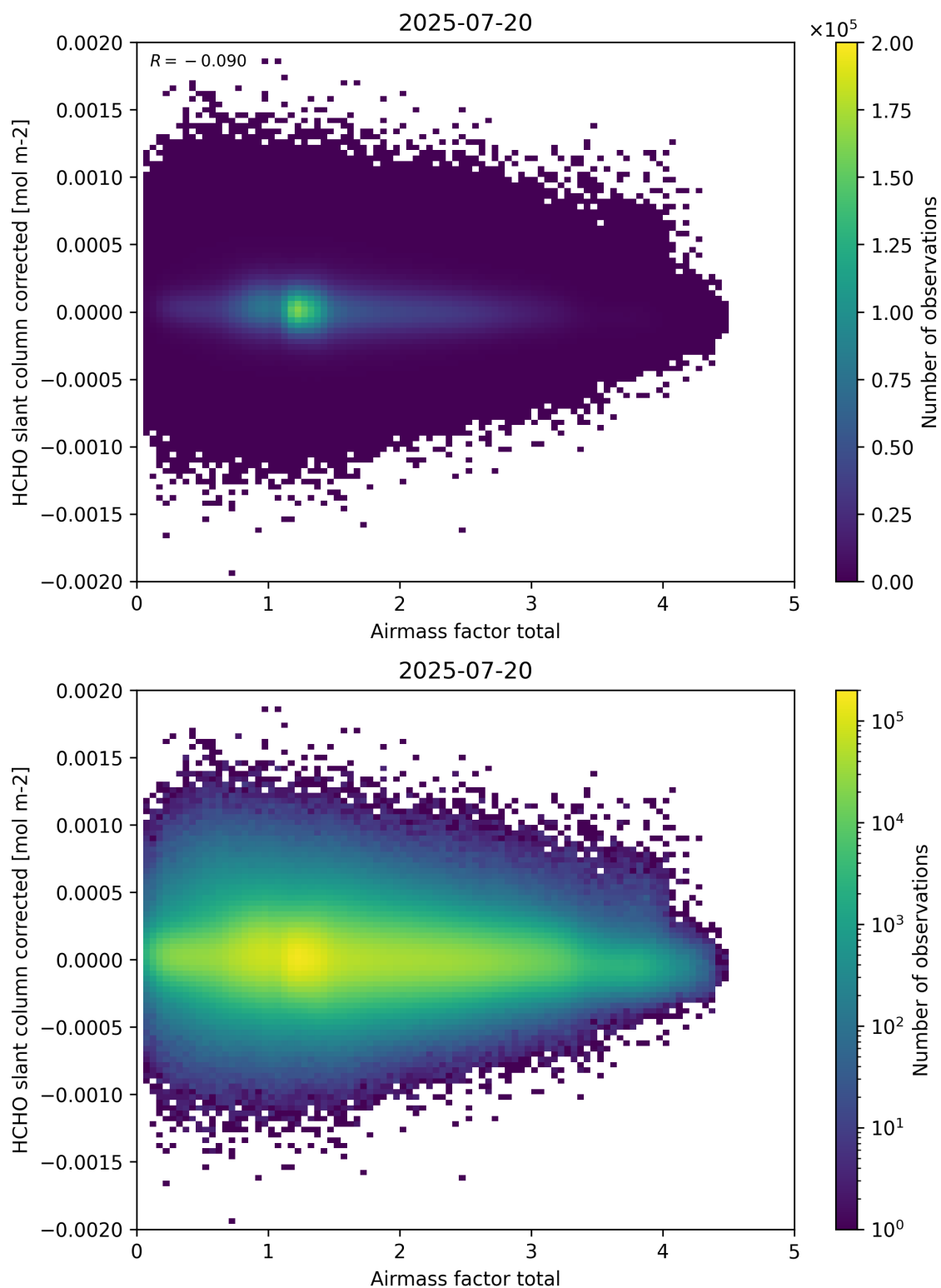
Figure 101: Scatter density plot of “Airmass factor total” against “HCHO slant column corrected” for 2025-07-19 to 2025-07-21.
