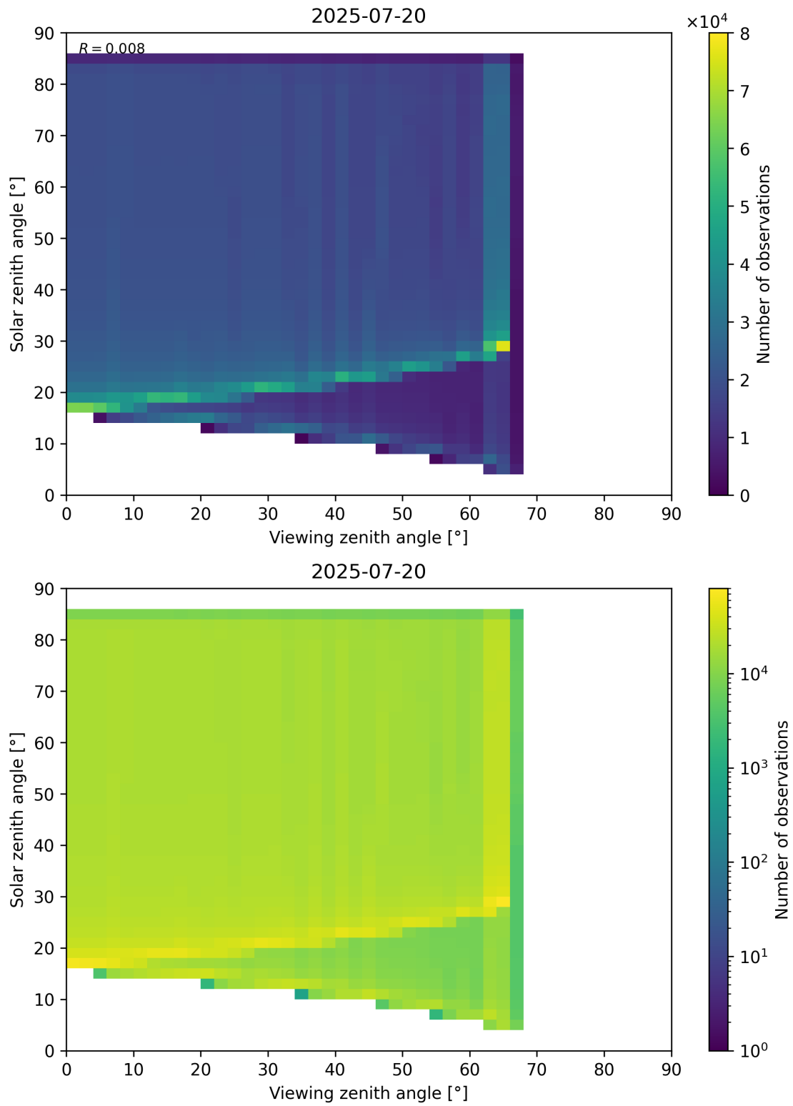
Figure 197: Scatter density plot of “Viewing zenith angle” against “Solar zenith angle” for 2025-07-19 to 2025-07-21.
