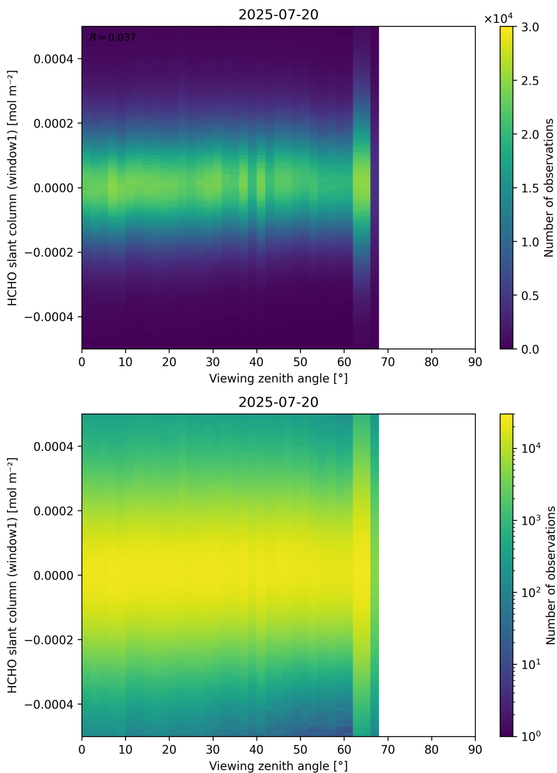
Figure 188: Scatter density plot of “Viewing zenith angle” against “HCHO slant column (window1)” for 2025-07-19 to 2025-07-21.
