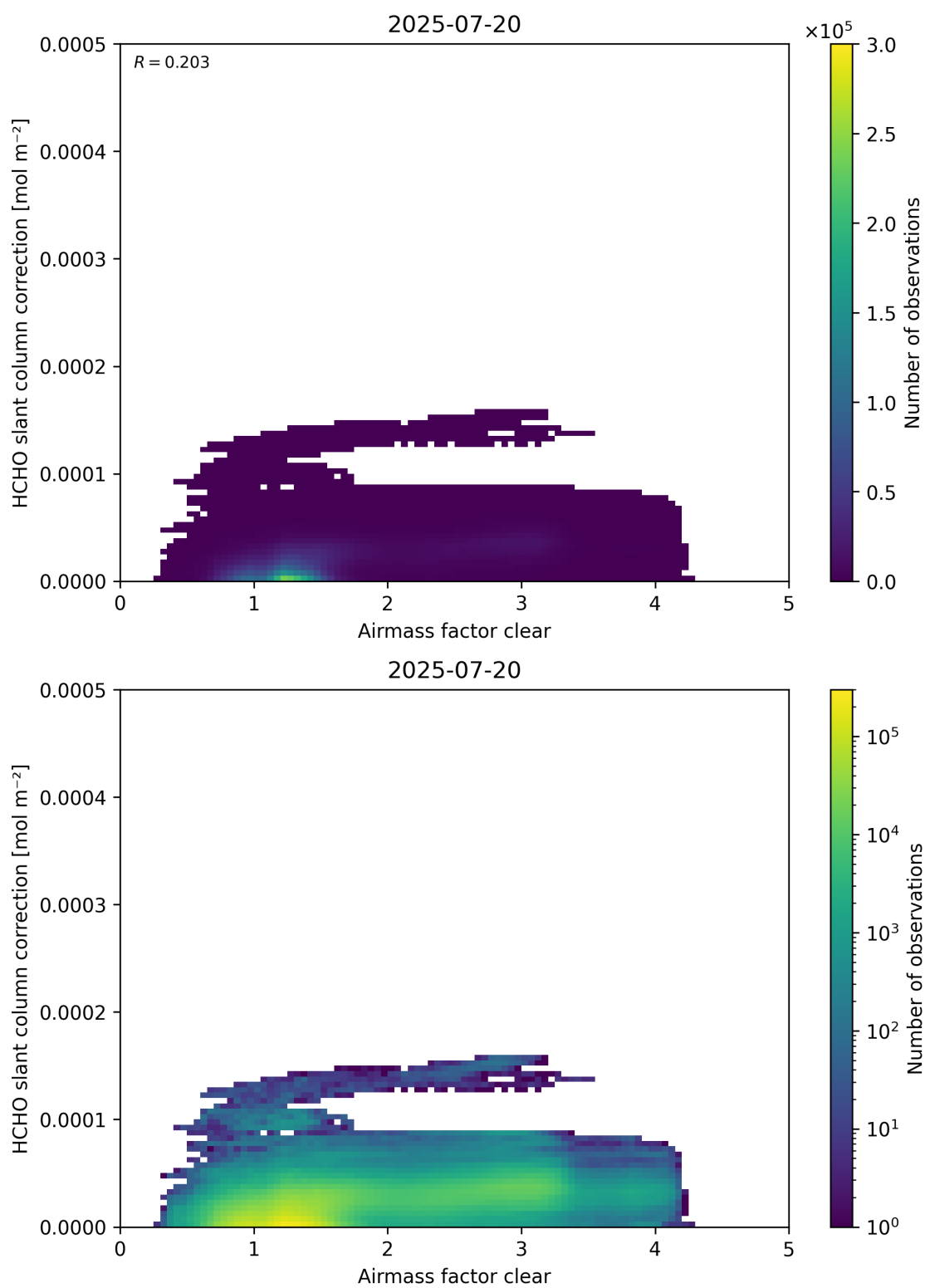
Figure 75: Scatter density plot of “Airmass factor clear” against “HCHO slant column correction” for 2025-07-19 to 2025-07-21.
