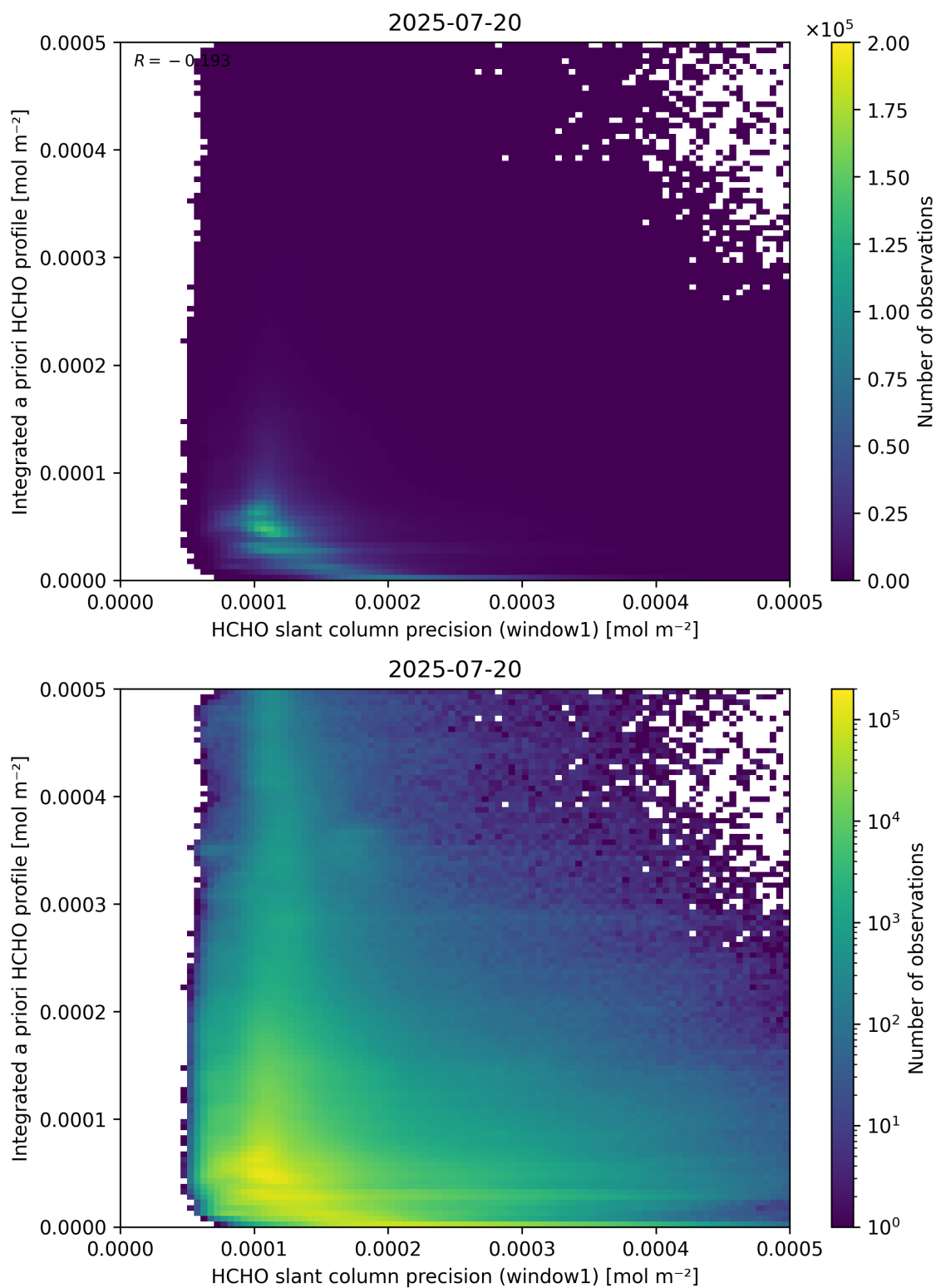
Figure 96: Scatter density plot of “HCHO slant column precision (window1)” against “Integrated a priori HCHO profile” for 2025-07-19 to 2025-07-21.
