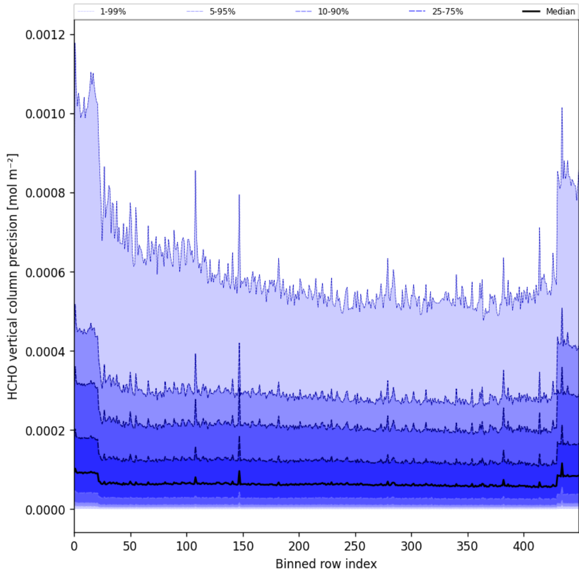
Figure 50: Along track statistics of “HCHO vertical column precision” for 2025-07-19 to 2025-07-21
