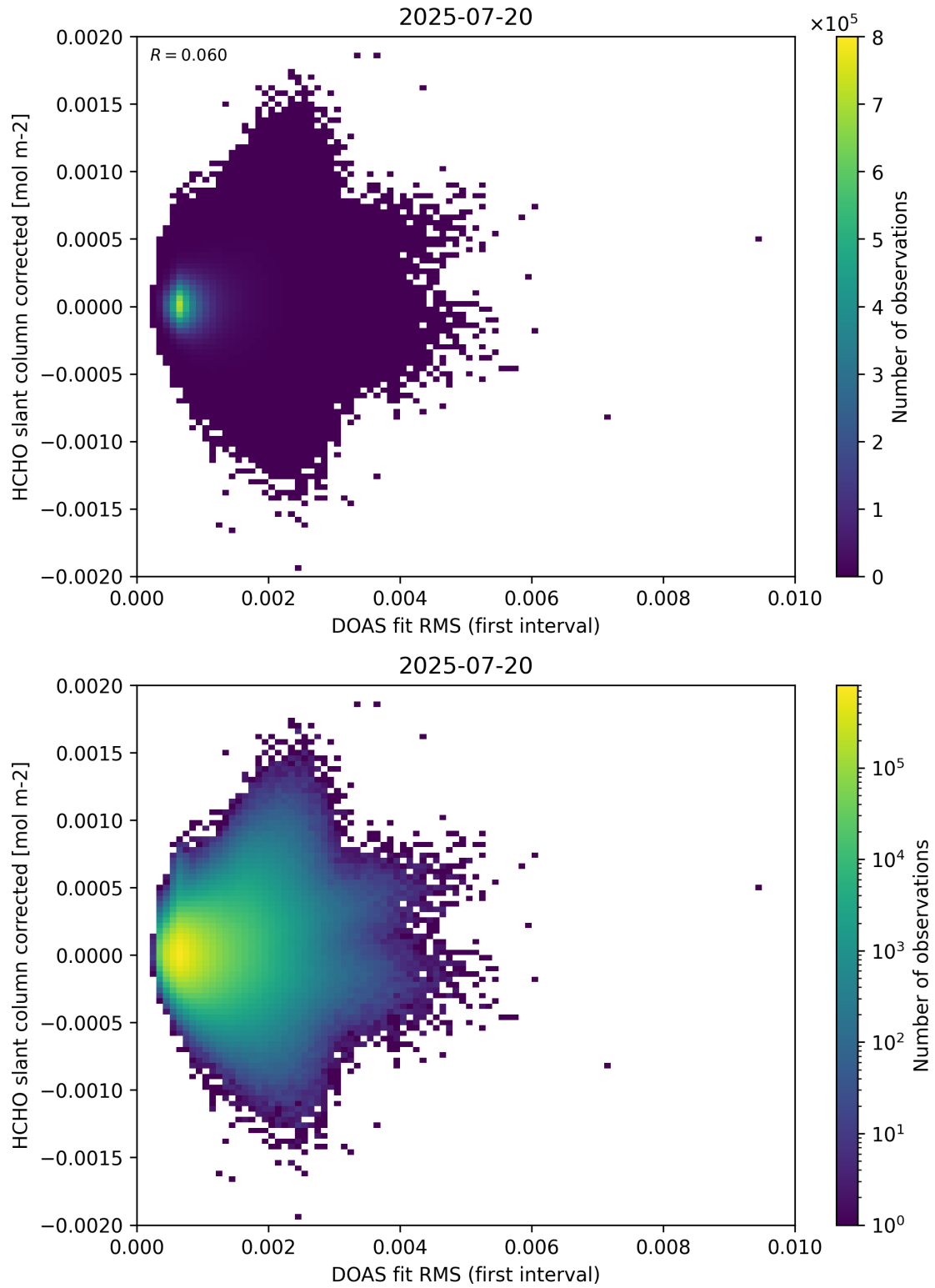
Figure 62: Scatter density plot of “DOAS fit RMS (first interval)” against “HCHO slant column corrected” for 2025-07-19 to 2025-07-21.
