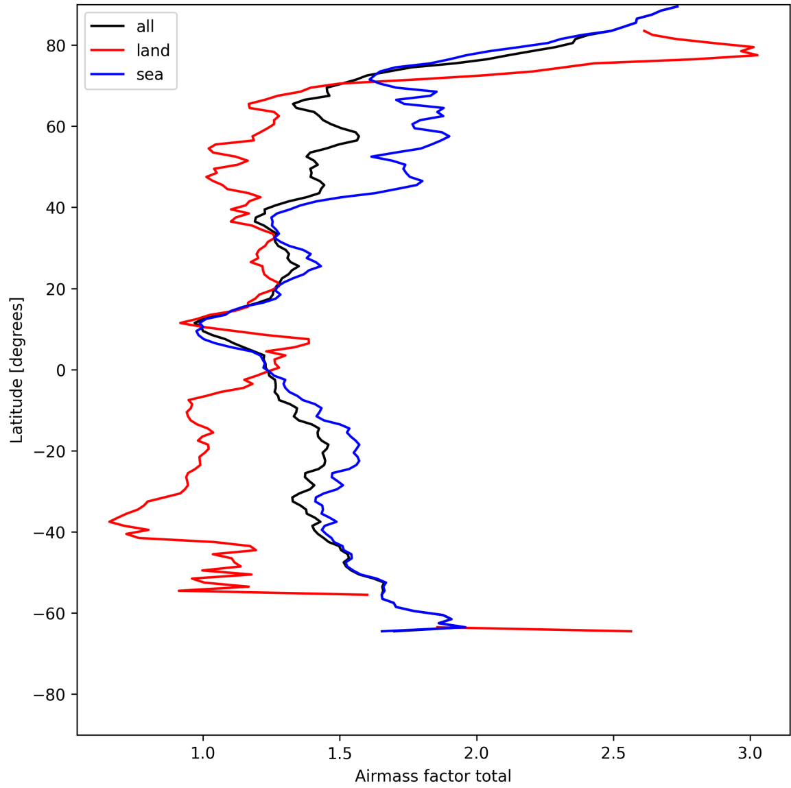
Figure 26: Zonal average of “Airmass factor total” for 2025-07-19 to 2025-07-21.
