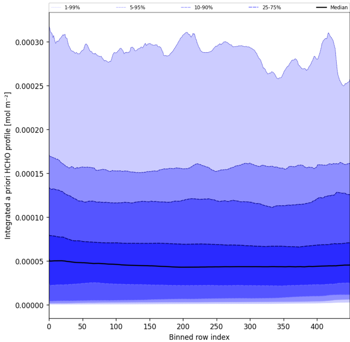
Figure 57: Along track statistics of “Integrated a priori HCHO profile” for 2025-07-19 to 2025-07-21
