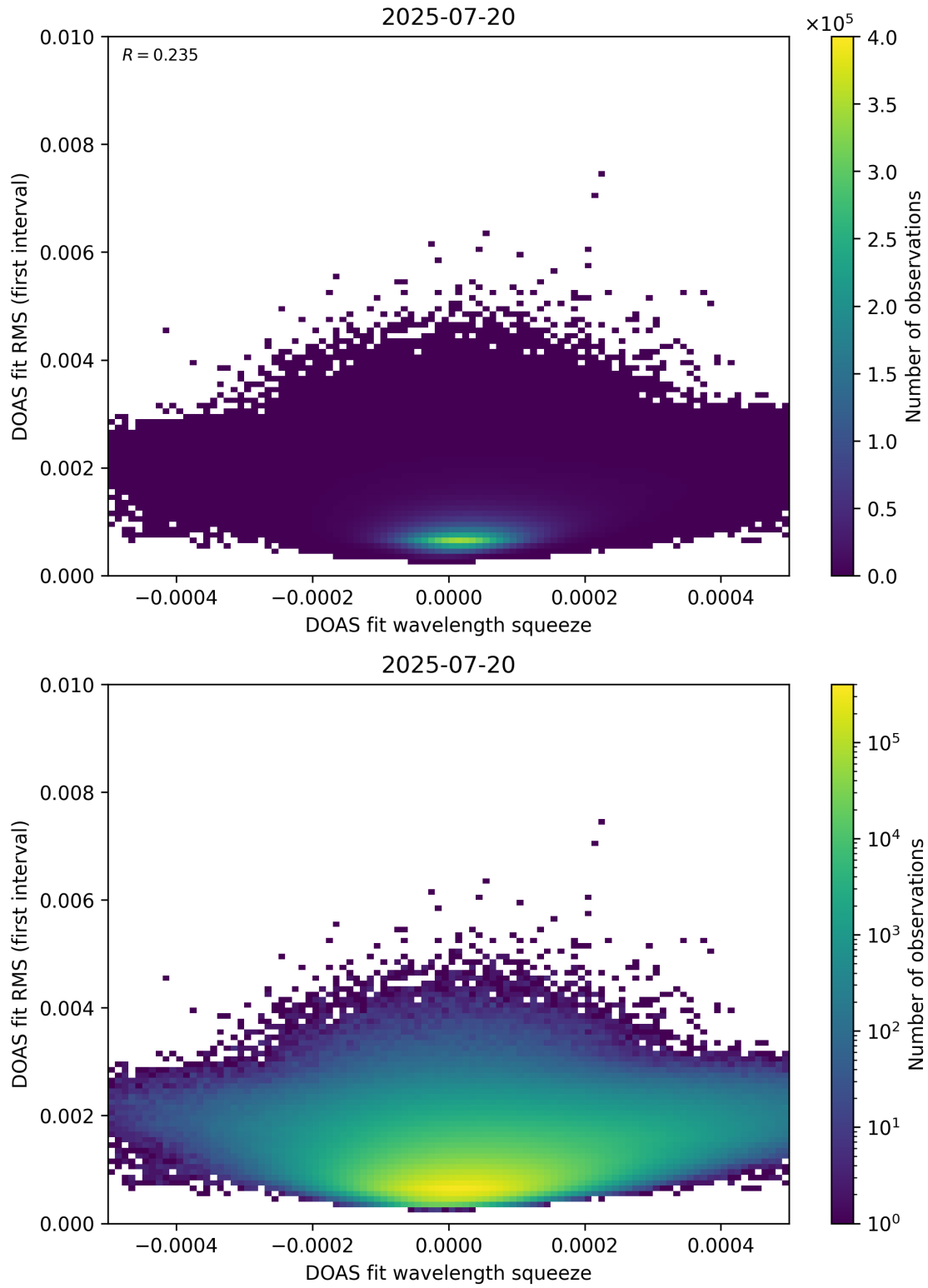
Figure 68: Scatter density plot of “DOAS fit wavelength squeeze” against “DOAS fit RMS (first interval)” for 2025-07-19 to 2025-07-21.
