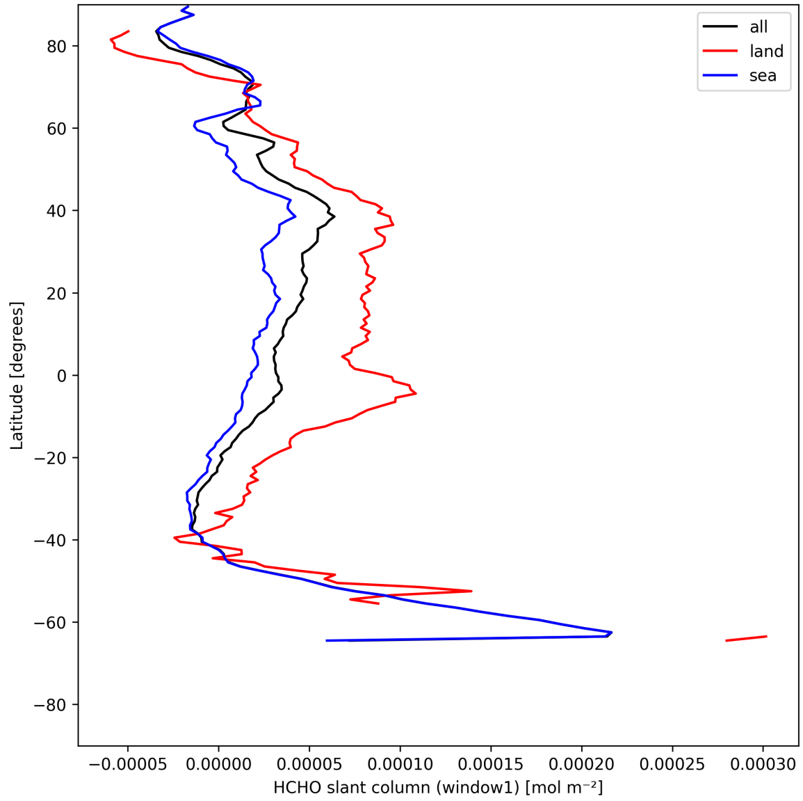
Figure 24: Zonal average of “HCHO slant column (window1)” for 2025-07-19 to 2025-07-21.
