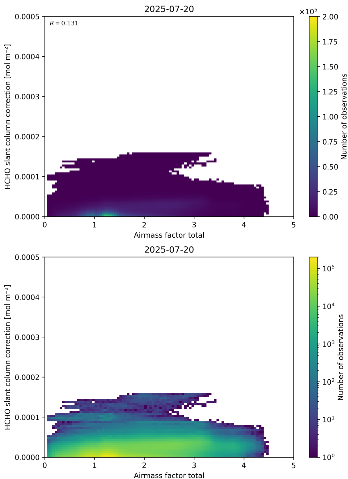
Figure 102: Scatter density plot of “Airmass factor total” against “HCHO slant column correction” for 2025-07-19 to 2025-07-21.
