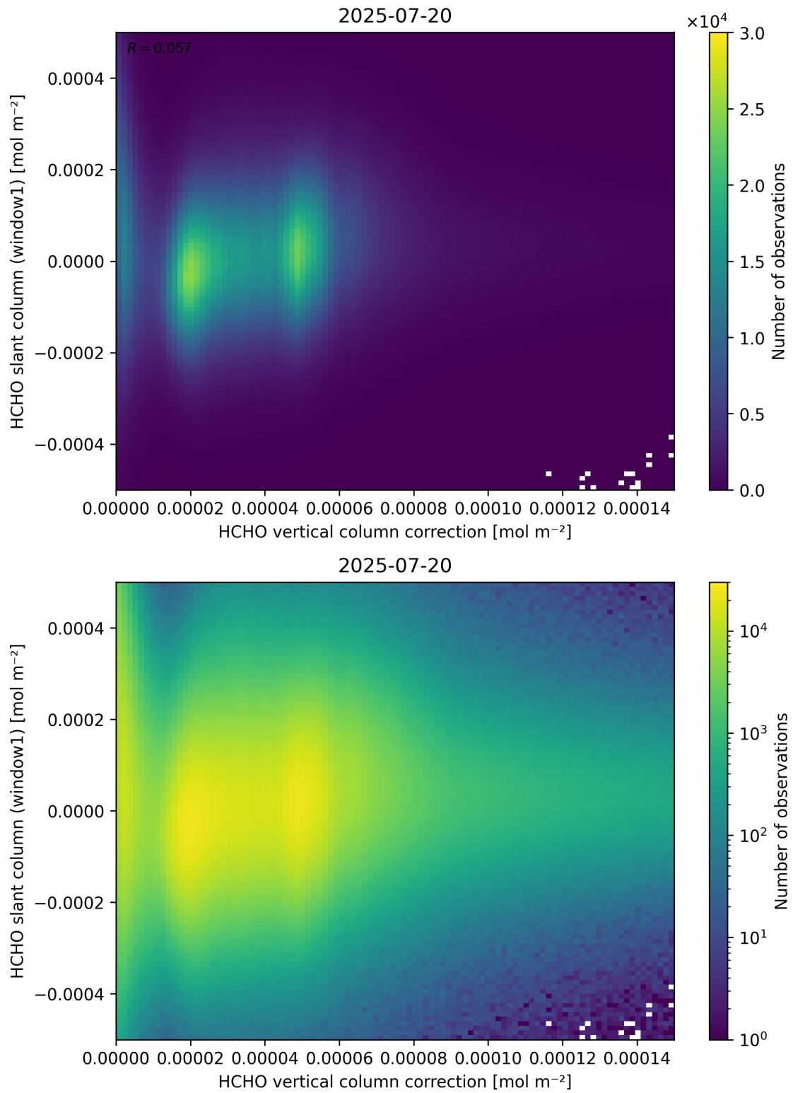
Figure 118: Scatter density plot of “HCHO vertical column correction” against “HCHO slant column (window1)” for 2025-07-19 to 2025-07-21.
