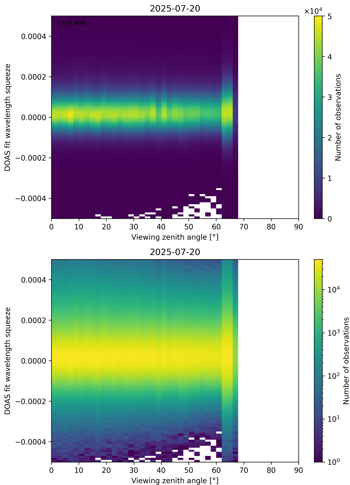
Figure 184: Scatter density plot of “Viewing zenith angle” against “DOAS fit wavelength squeeze” for 2025-07-19 to 2025-07-21.
