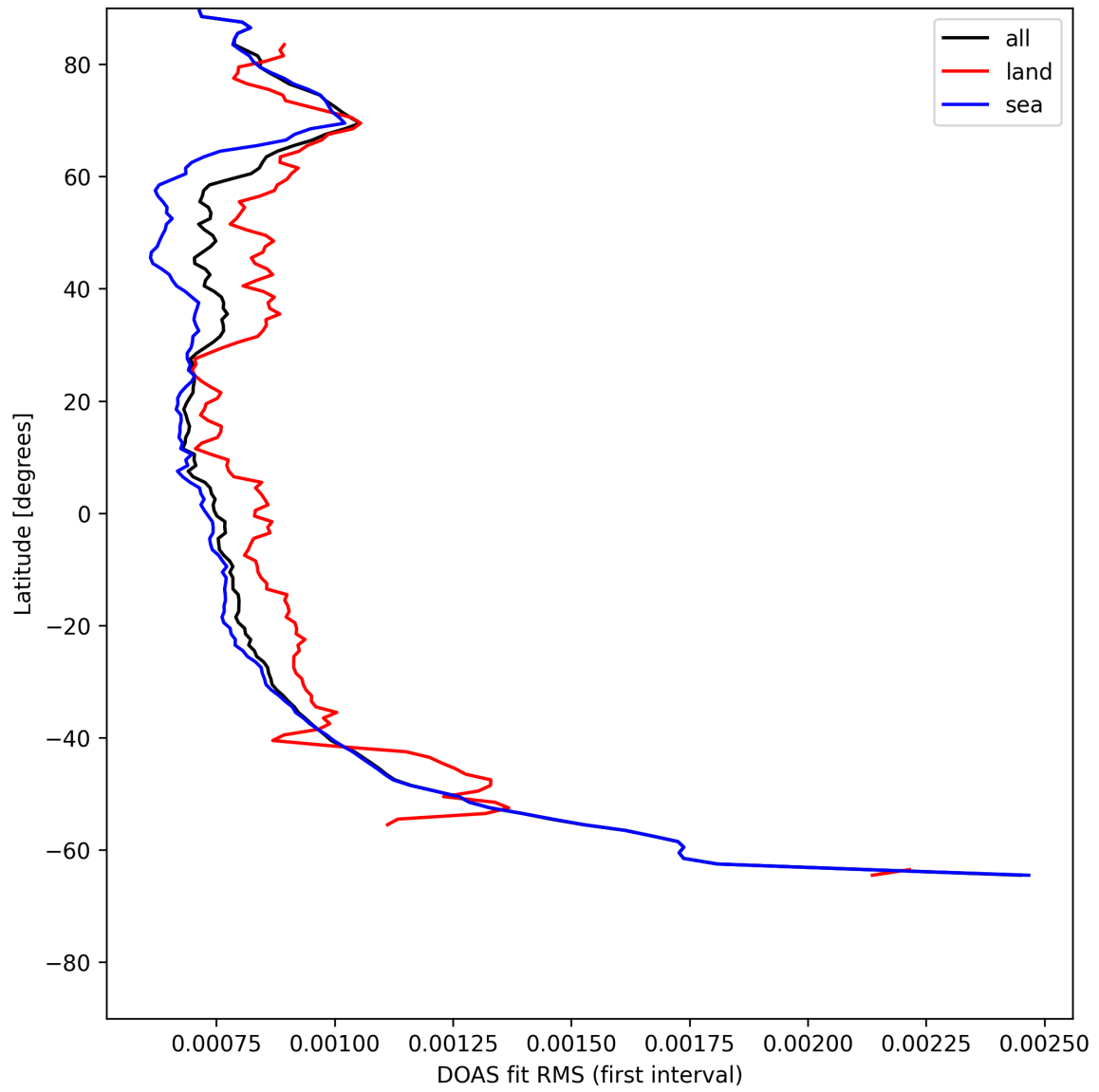
Figure 32: Zonal average of “DOAS fit RMS (first interval)” for 2025-07-19 to 2025-07-21.
