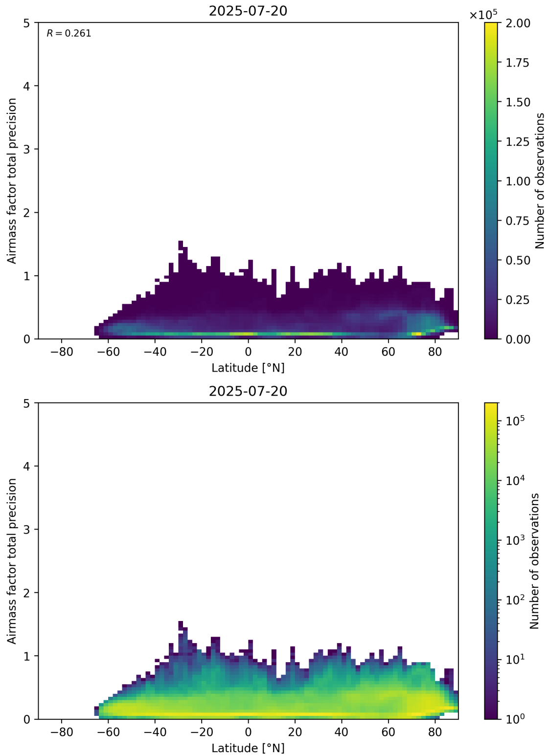
Figure 162: Scatter density plot of “Latitude” against “Airmass factor total precision” for 2025-07-19 to 2025-07-21.
