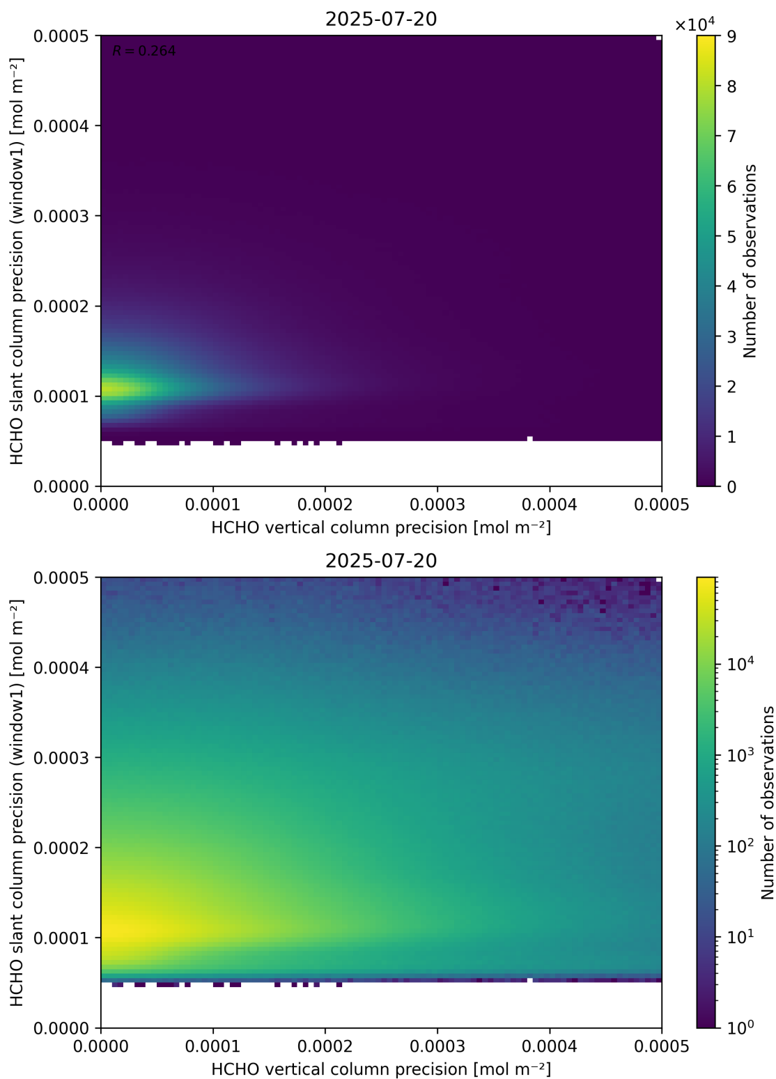
Figure 143: Scatter density plot of “HCHO vertical column precision” against “HCHO slant column precision (window1)” for 2025-07-19 to 2025-07-21.
