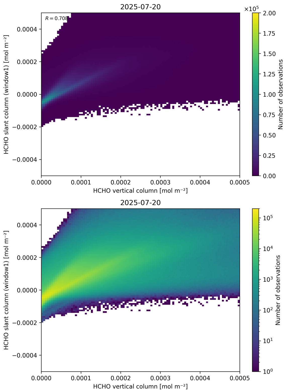
Figure 129: Scatter density plot of “HCHO vertical column” against “HCHO slant column (window1)” for 2025-07-19 to 2025-07-21.
