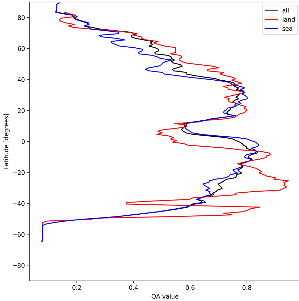
Figure 20: Zonal average of “QA value” for 2025-07-19 to 2025-07-21.
