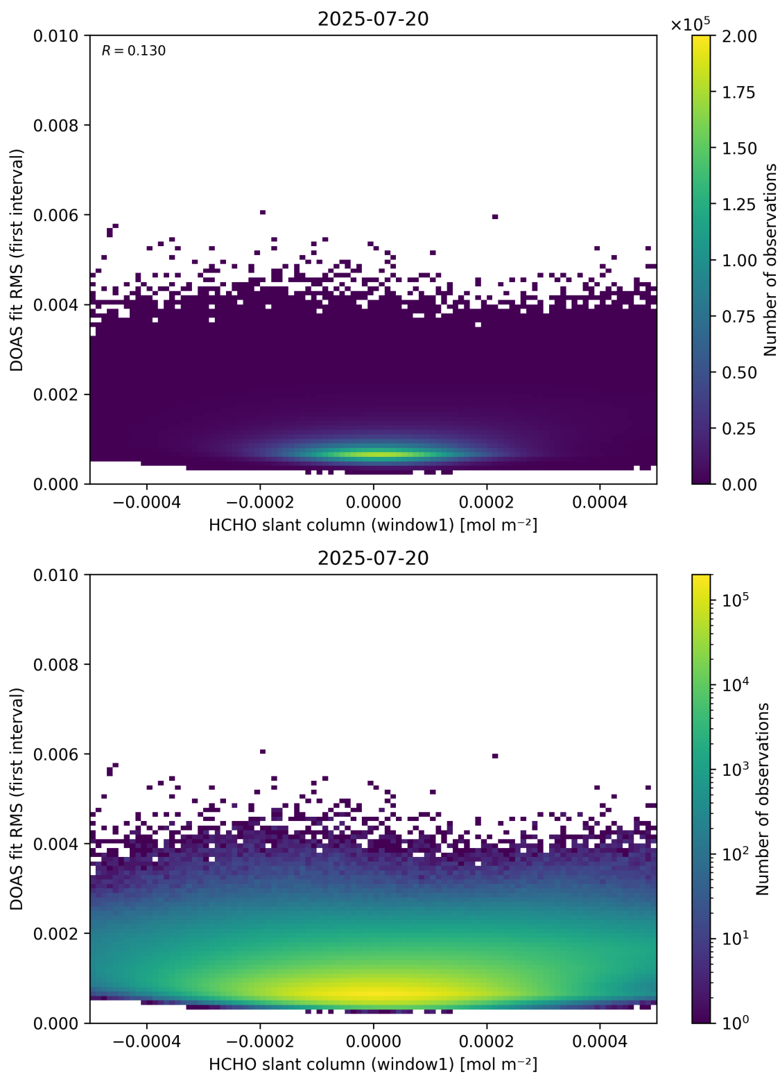
Figure 78: Scatter density plot of “HCHO slant column (window1)” against “DOAS fit RMS (first interval)” for 2025-07-19 to 2025-07-21.
