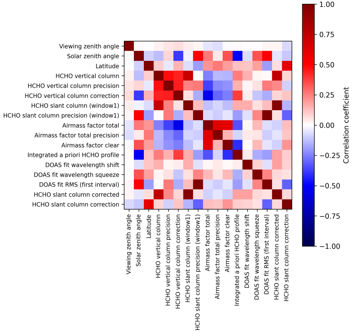
Figure 2: Map of correlation matrix for 2025-07-19 to 2025-07-21.
