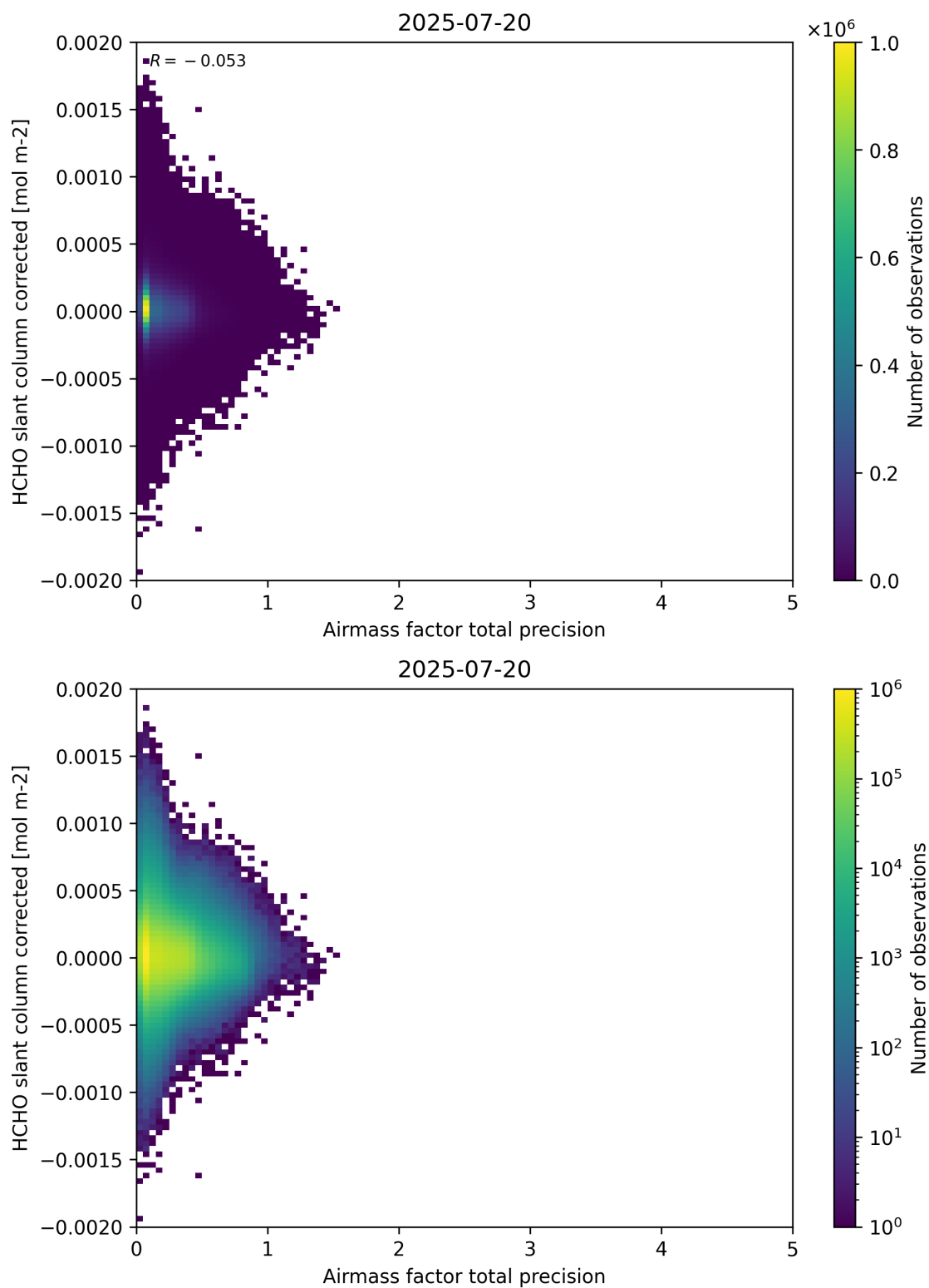
Figure 109: Scatter density plot of “Airmass factor total precision” against “HCHO slant column corrected” for 2025-07-19 to 2025-07-21.
