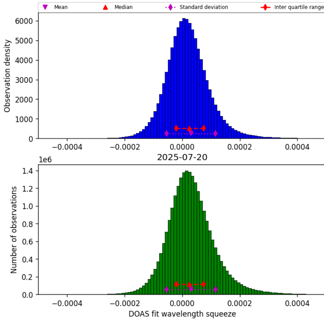
Figure 45: Histogram of “DOAS fit wavelength squeeze” for 2025-07-19 to 2025-07-21
