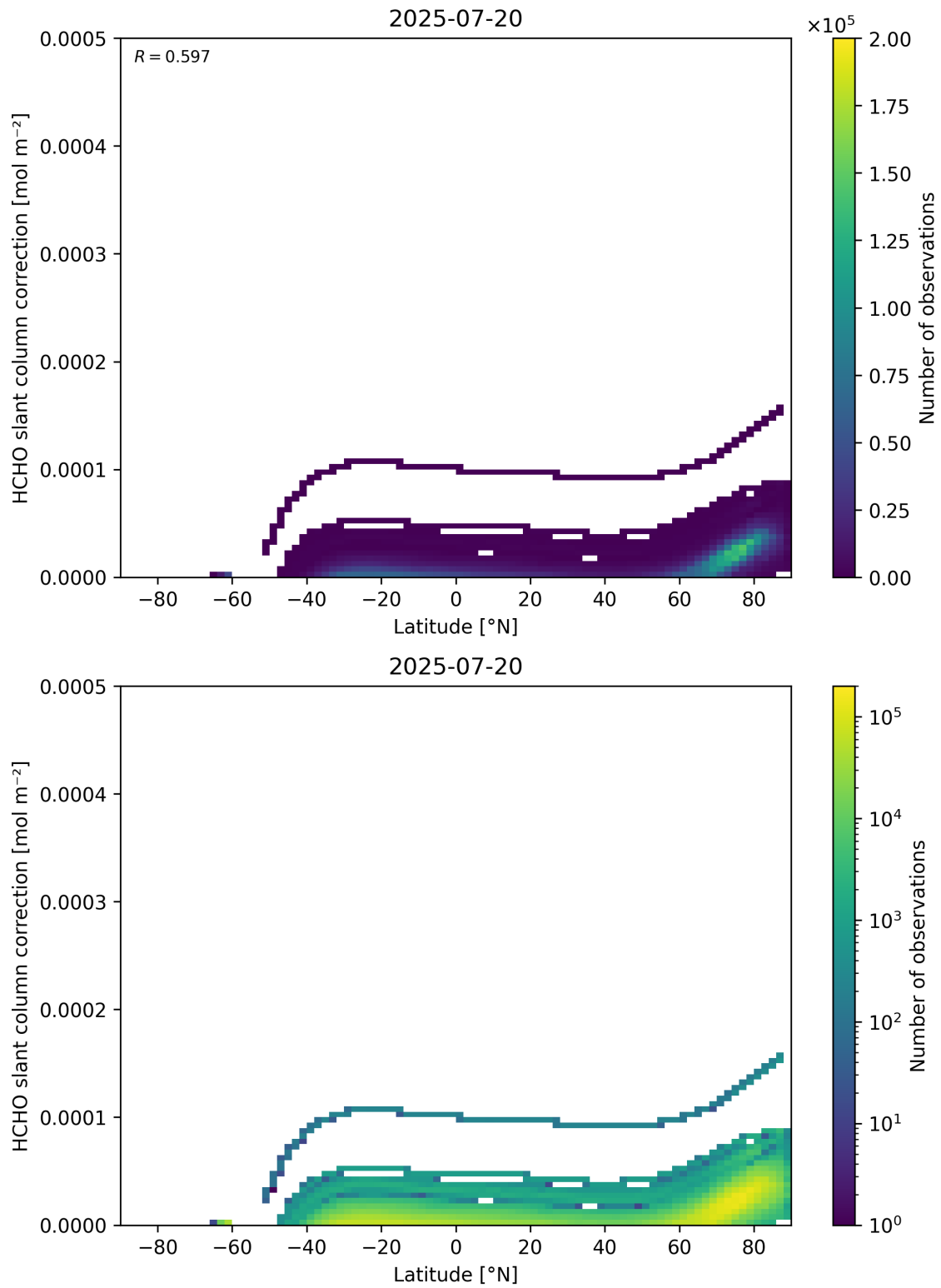
Figure 158: Scatter density plot of “Latitude” against “HCHO slant column correction” for 2025-07-19 to 2025-07-21.
