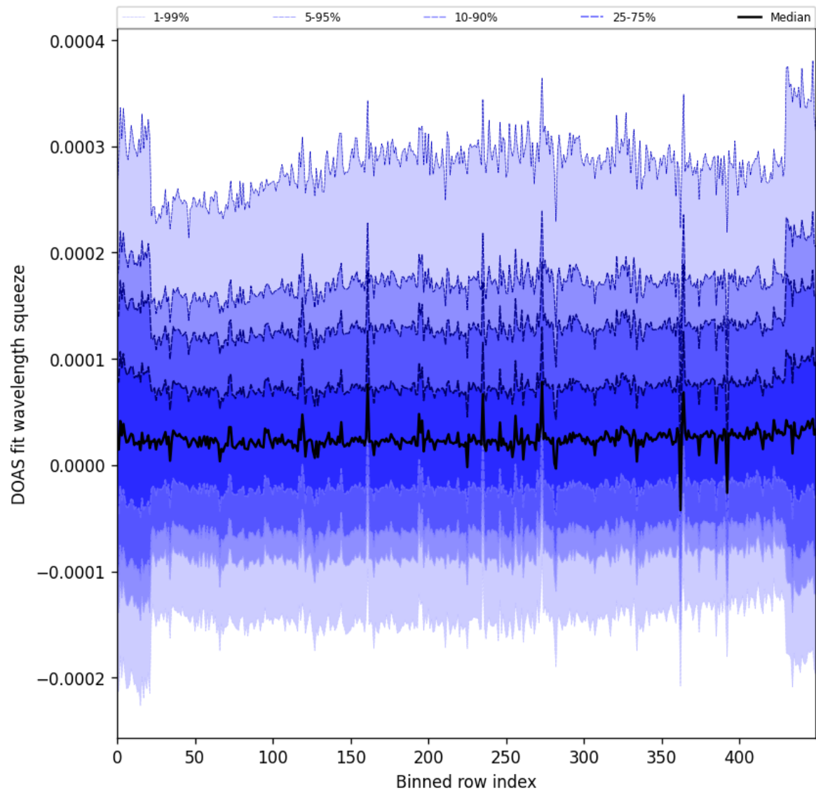
Figure 59: Along track statistics of “DOAS fit wavelength squeeze” for 2025-07-19 to 2025-07-21
