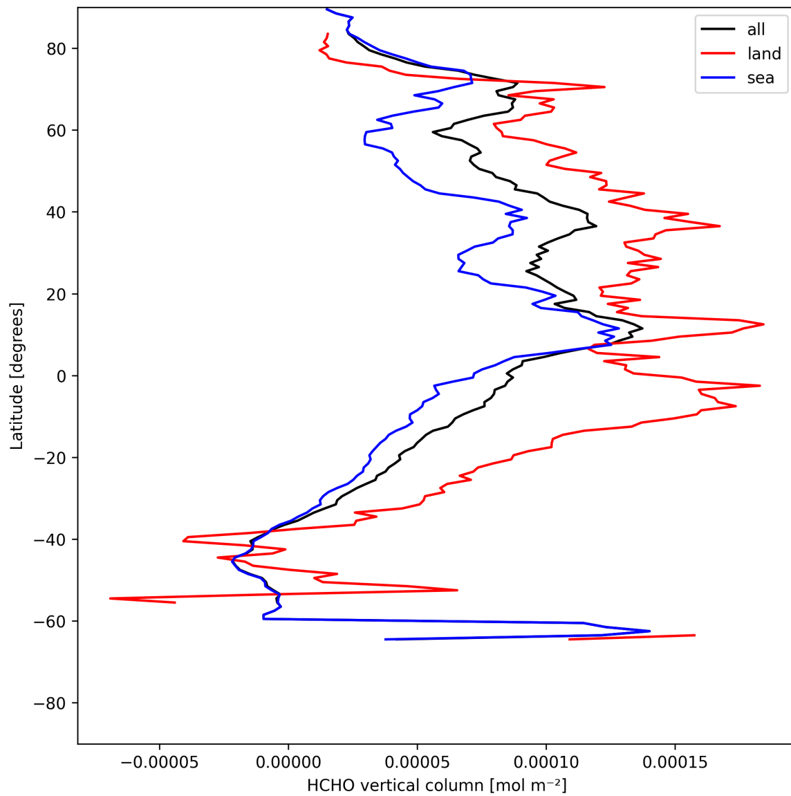
Figure 21: Zonal average of “HCHO vertical column” for 2025-07-19 to 2025-07-21.
