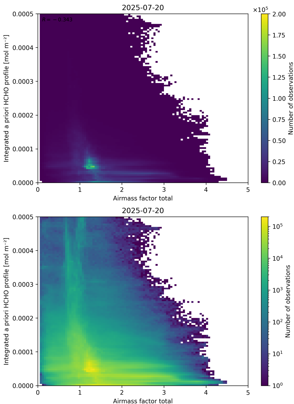
Figure 104: Scatter density plot of “Airmass factor total” against “Integrated a priori HCHO profile” for 2025-07-19 to 2025-07-21.
