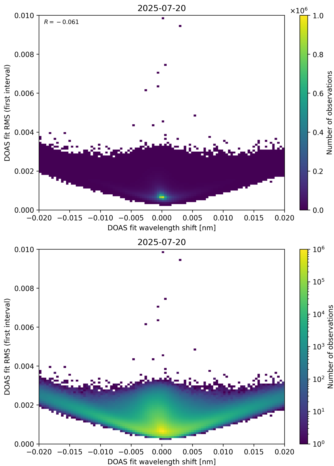
Figure 64: Scatter density plot of “DOAS fit wavelength shift” against “DOAS fit RMS (first interval)” for 2025-07-19 to 2025-07-21.
