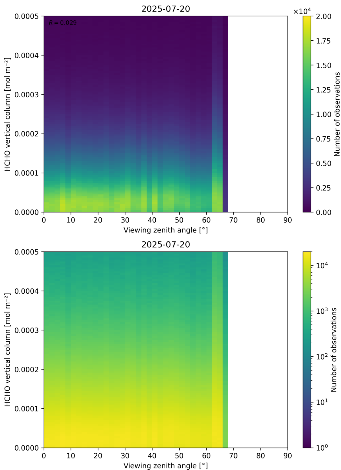
Figure 192: Scatter density plot of “Viewing zenith angle” against “HCHO vertical column” for 2025-07-19 to 2025-07-21.
