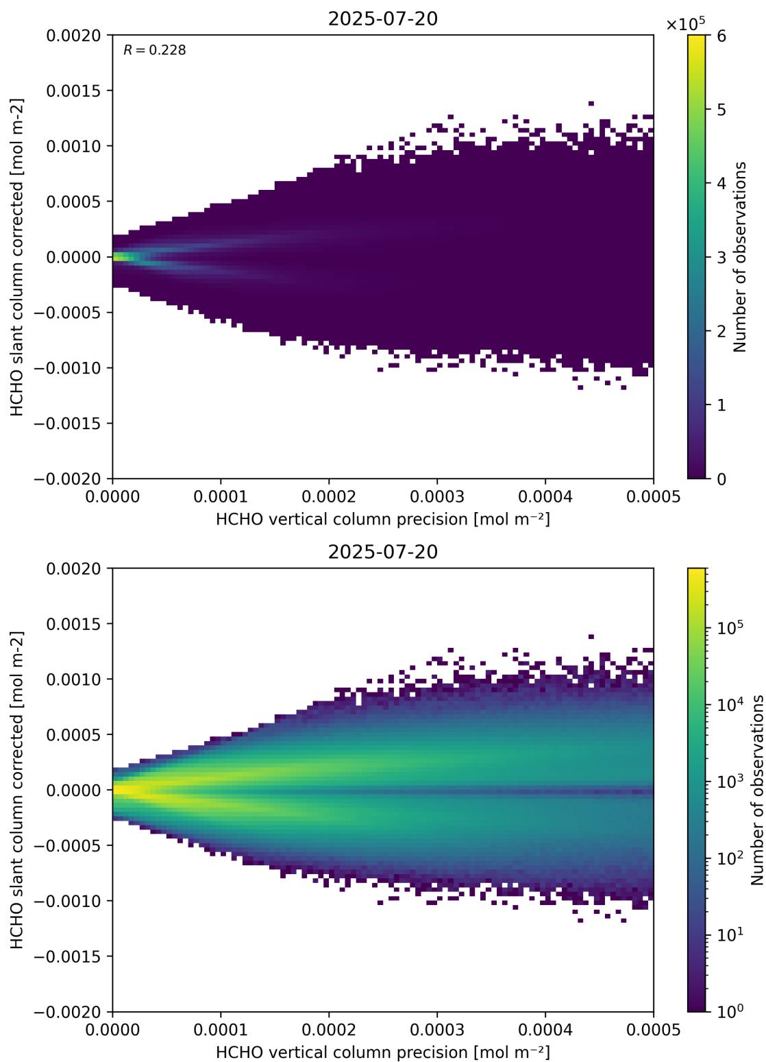
Figure 140: Scatter density plot of “HCHO vertical column precision” against “HCHO slant column corrected” for 2025-07-19 to 2025-07-21.
