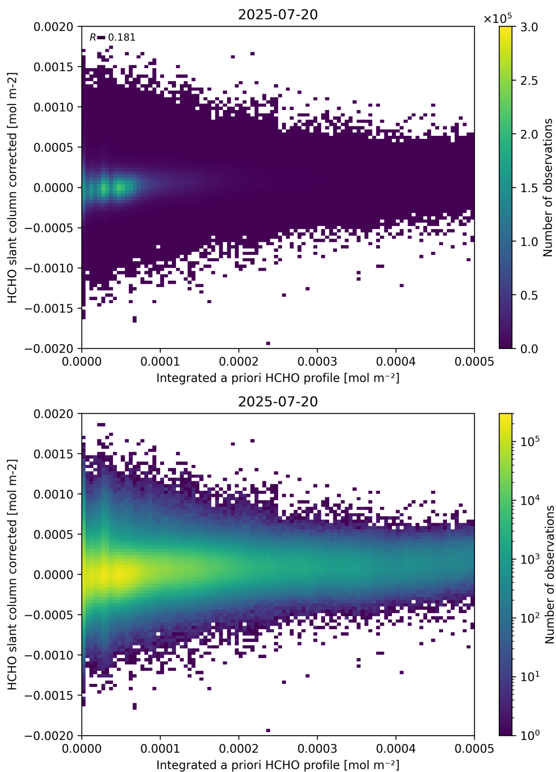
Figure 151: Scatter density plot of “Integrated a priori HCHO profile” against “HCHO slant column corrected” for 2025-07-19 to 2025-07-21.
