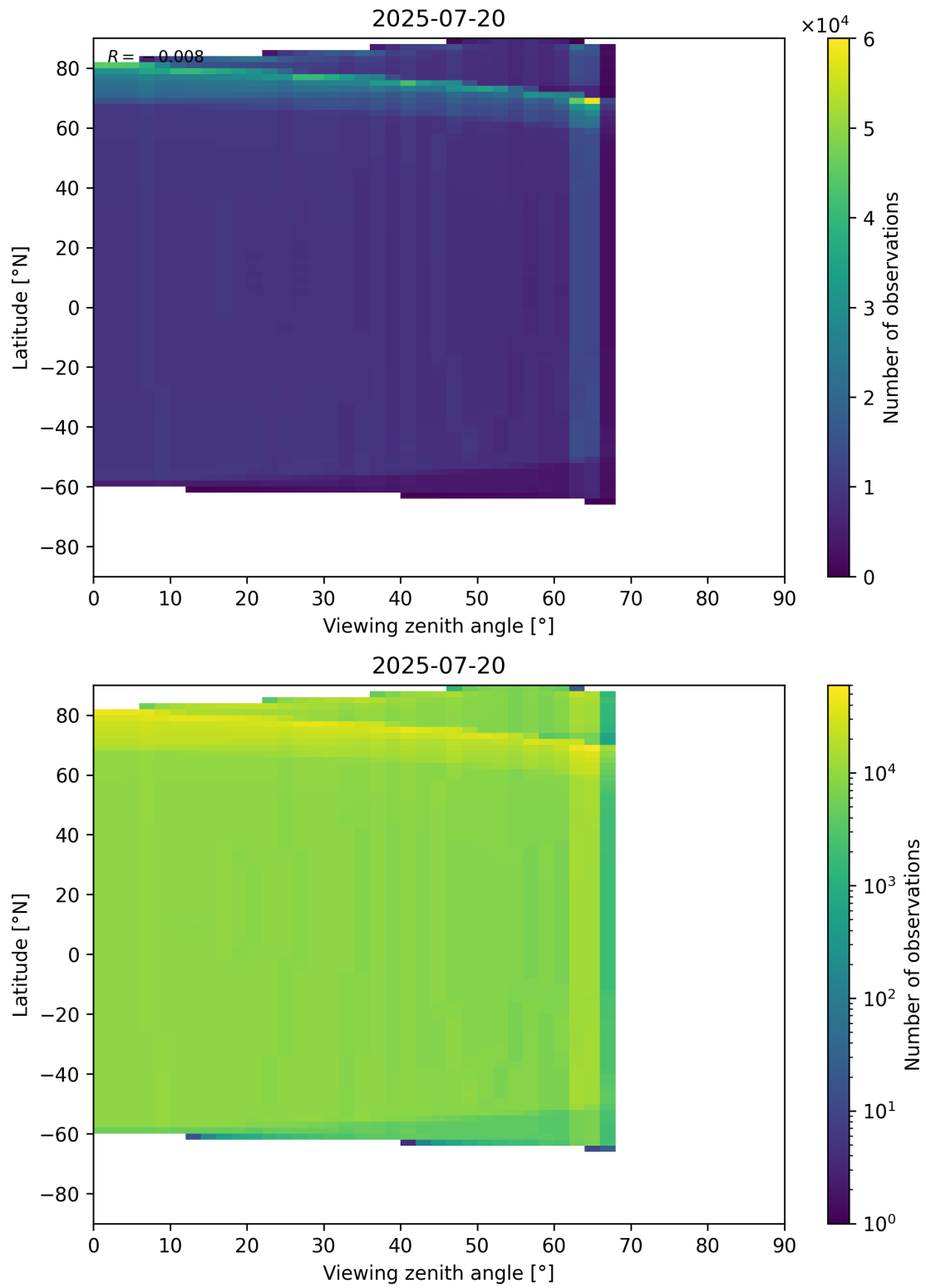
Figure 196: Scatter density plot of “Viewing zenith angle” against “Latitude” for 2025-07-19 to 2025-07-21.
