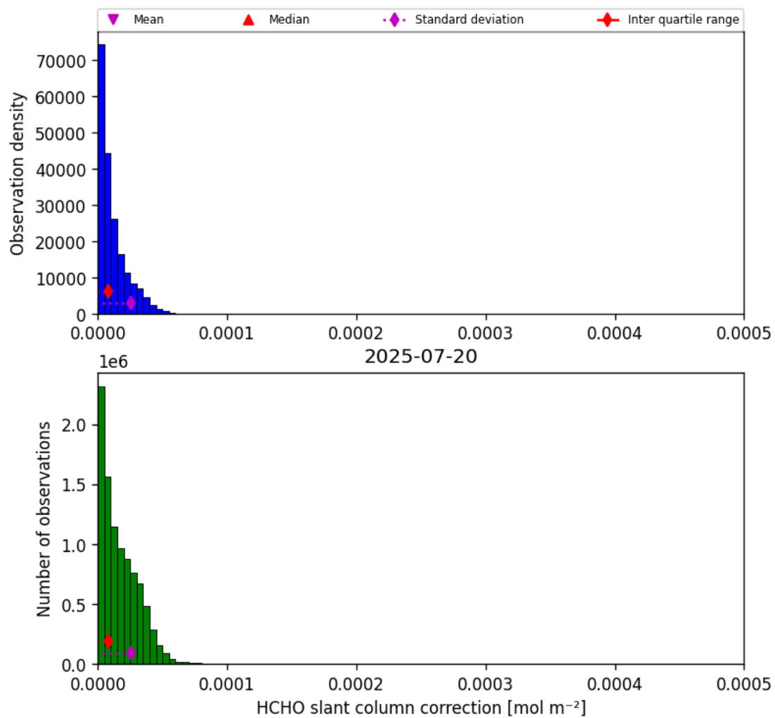
Figure 47: Histogram of “HCHO slant column correction” for 2025-07-19 to 2025-07-21
