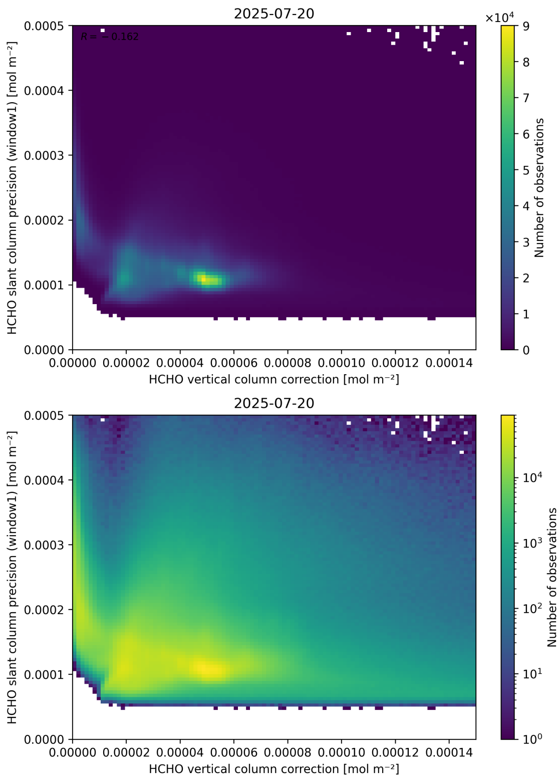
Figure 119: Scatter density plot of “HCHO vertical column correction” against “HCHO slant column precision (window1)” for 2025-07-19 to 2025-07-21.
