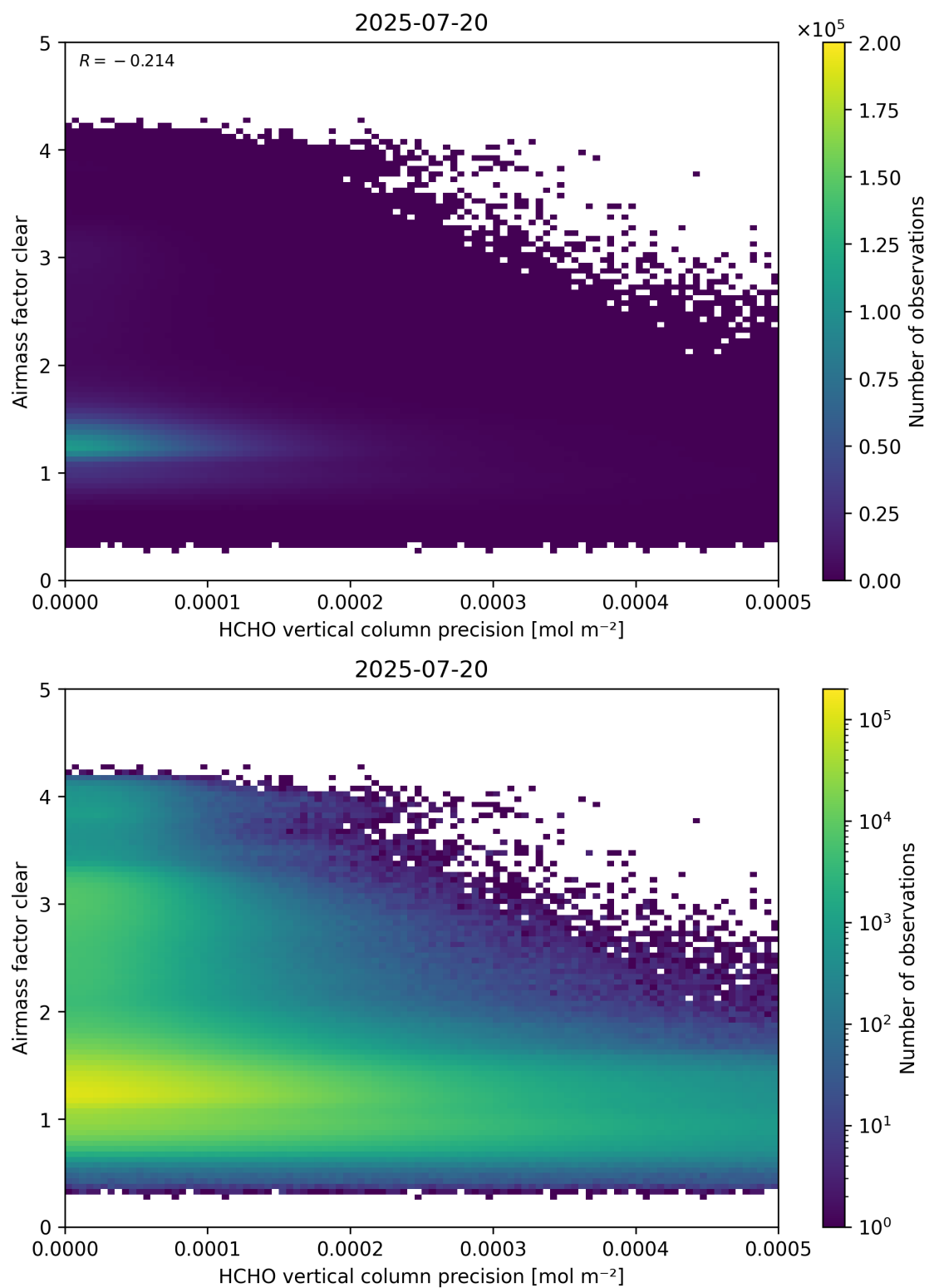
Figure 139: Scatter density plot of “HCHO vertical column precision” against “Airmass factor clear” for 2025-07-19 to 2025-07-21.
