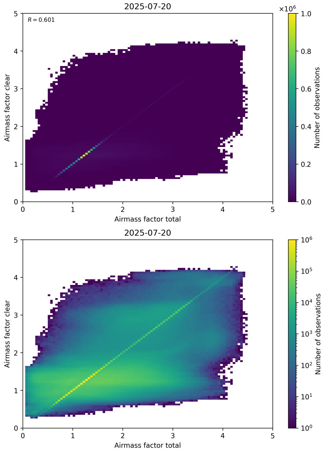
Figure 100: Scatter density plot of “Airmass factor total” against “Airmass factor clear” for 2025-07-19 to 2025-07-21.
