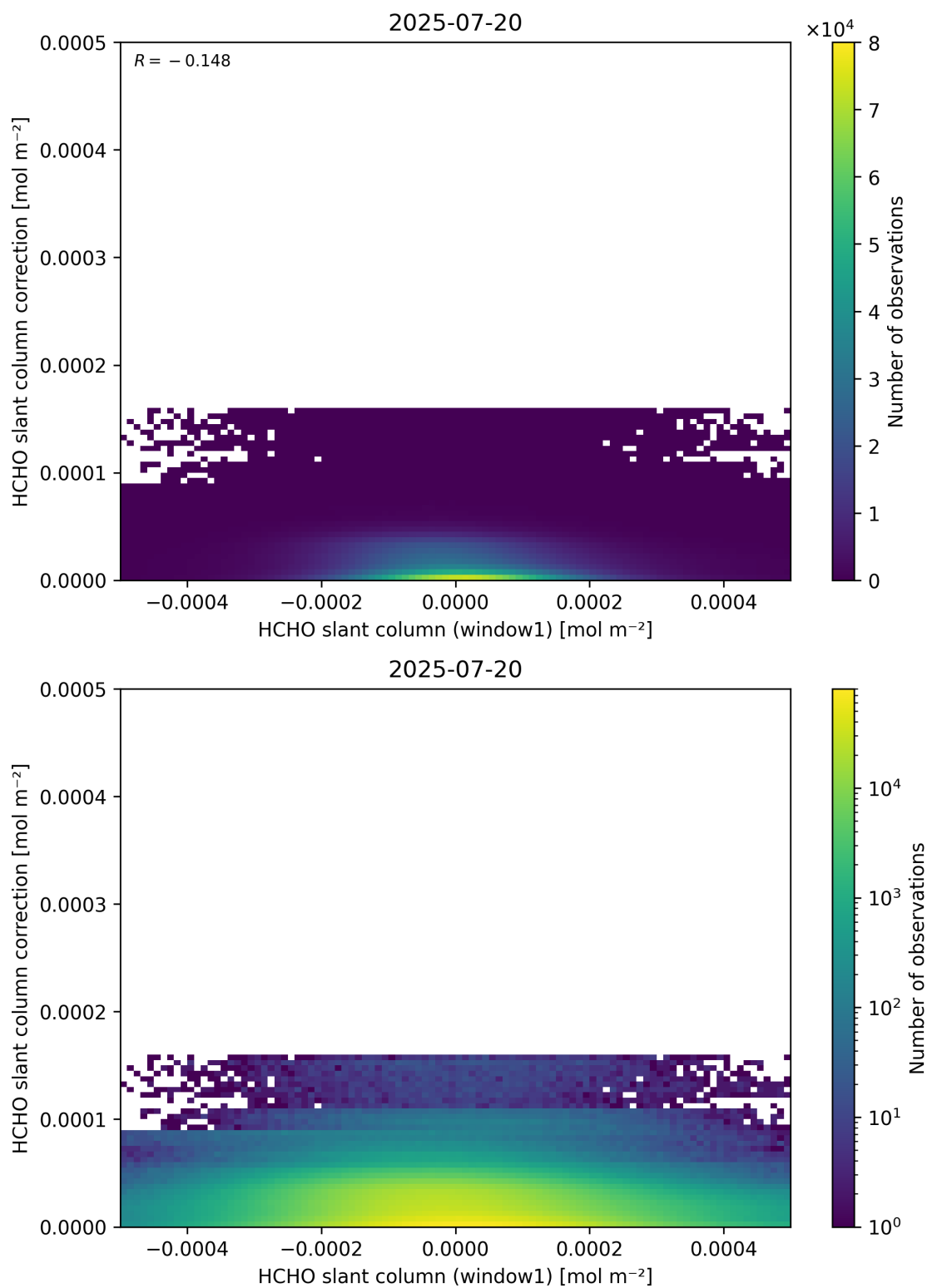
Figure 83: Scatter density plot of “HCHO slant column (window1)” against “HCHO slant column correction” for 2025-07-19 to 2025-07-21.
