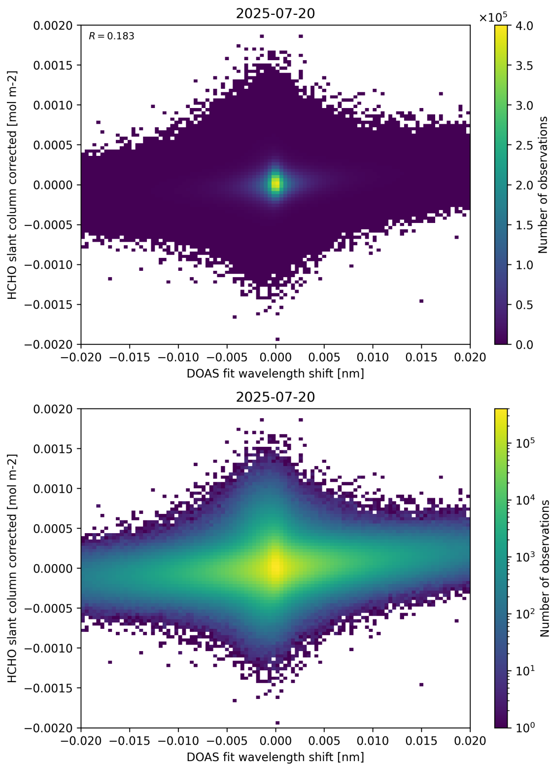
Figure 66: Scatter density plot of “DOAS fit wavelength shift” against “HCHO slant column corrected” for 2025-07-19 to 2025-07-21.
