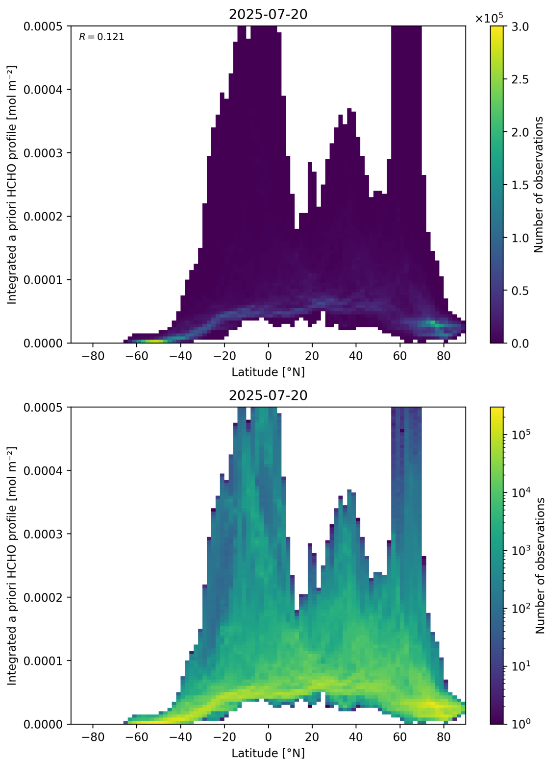
Figure 166: Scatter density plot of “Latitude” against “Integrated a priori HCHO profile” for 2025-07-19 to 2025-07-21.
