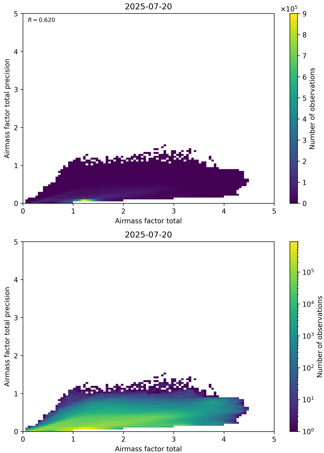
Figure 103: Scatter density plot of “Airmass factor total” against “Airmass factor total precision” for 2025-07-19 to 2025-07-21.
