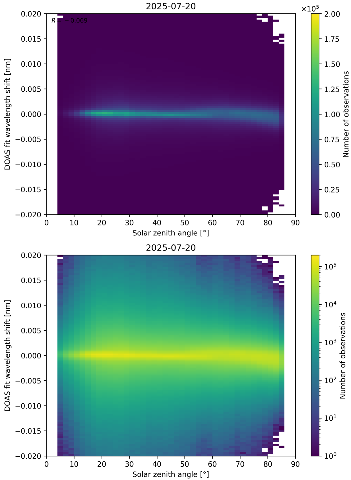
Figure 168: Scatter density plot of “Solar zenith angle” against “DOAS fit wavelength shift” for 2025-07-19 to 2025-07-21.
