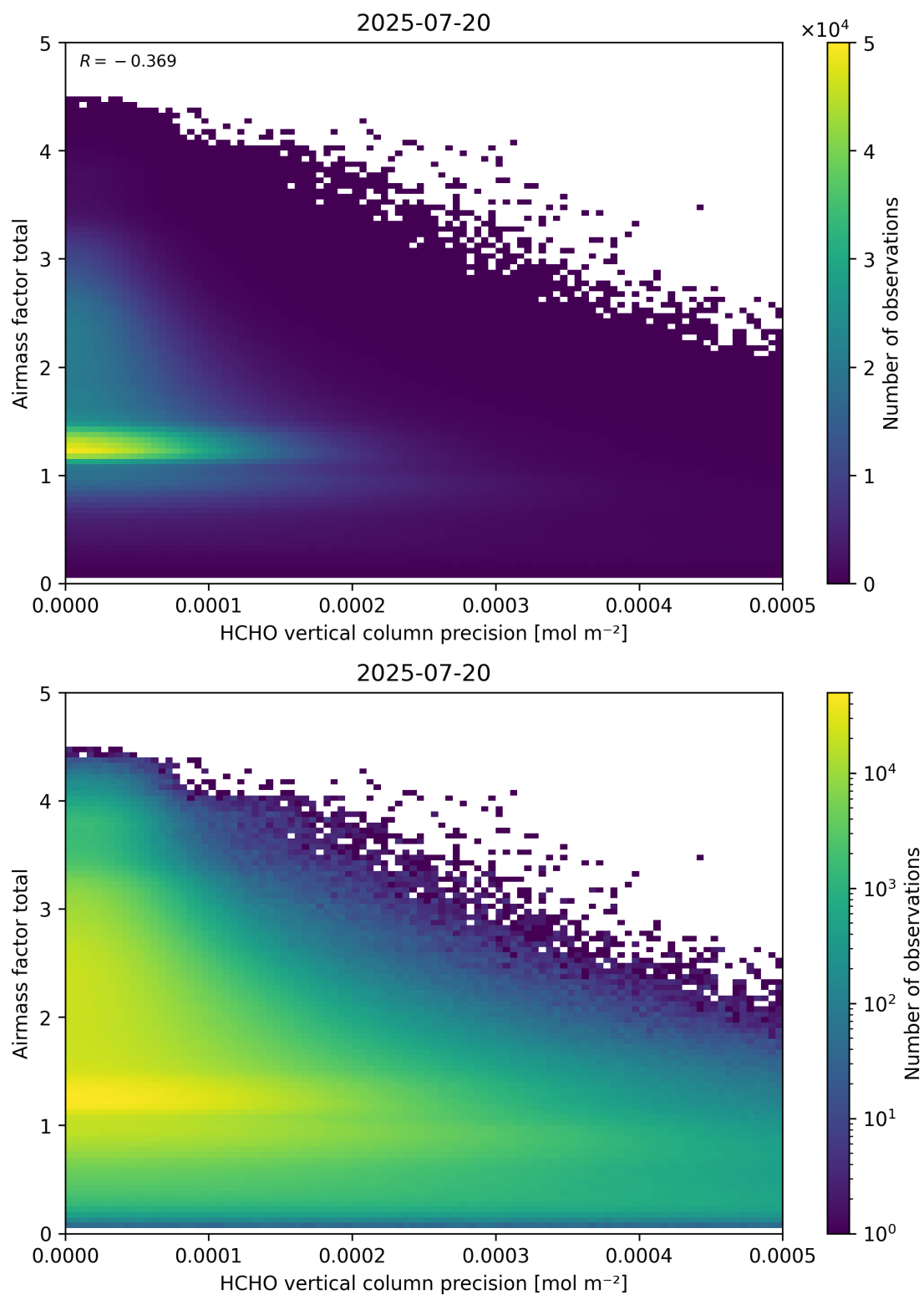
Figure 144: Scatter density plot of “HCHO vertical column precision” against “Airmass factor total” for 2025-07-19 to 2025-07-21.
