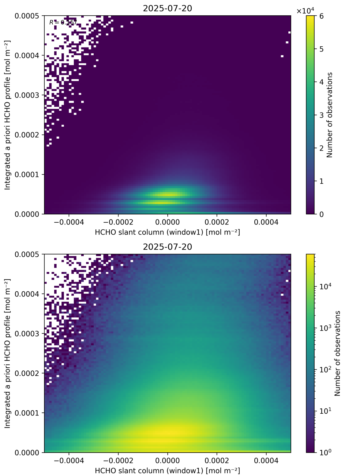
Figure 87: Scatter density plot of “HCHO slant column (window1)” against “Integrated a priori HCHO profile” for 2025-07-19 to 2025-07-21.
