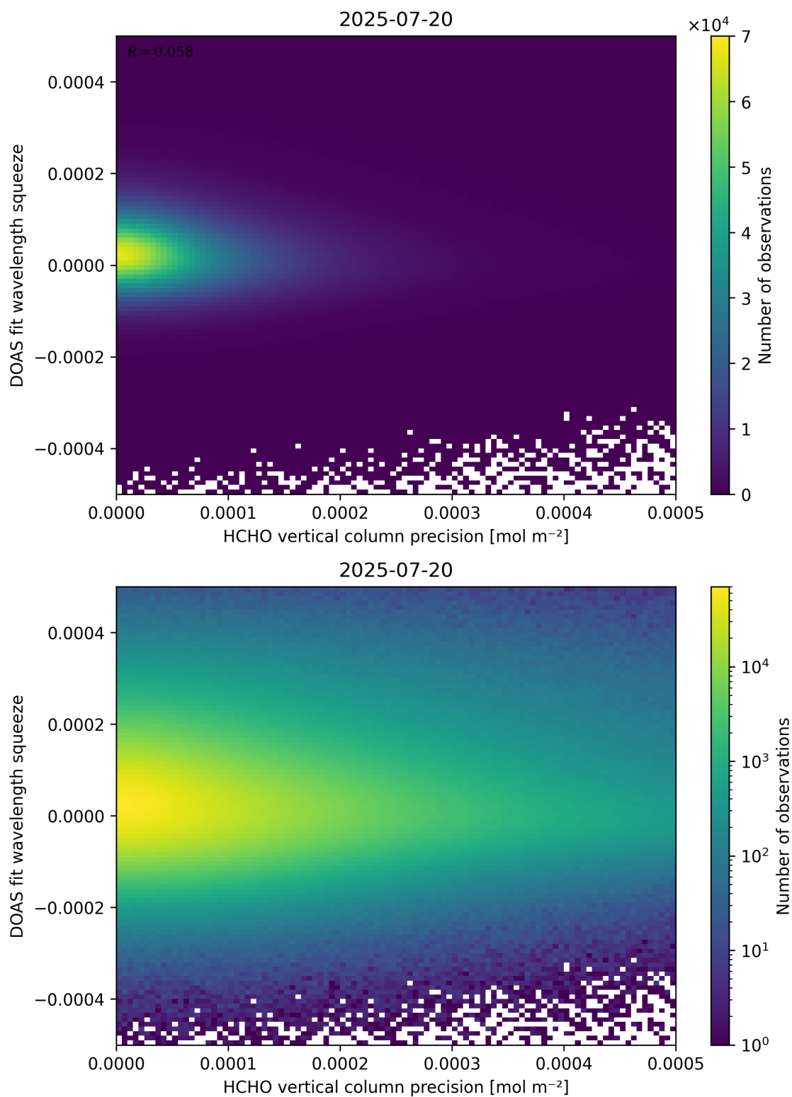
Figure 138: Scatter density plot of “HCHO vertical column precision” against “DOAS fit wavelength squeeze” for 2025-07-19 to 2025-07-21.
