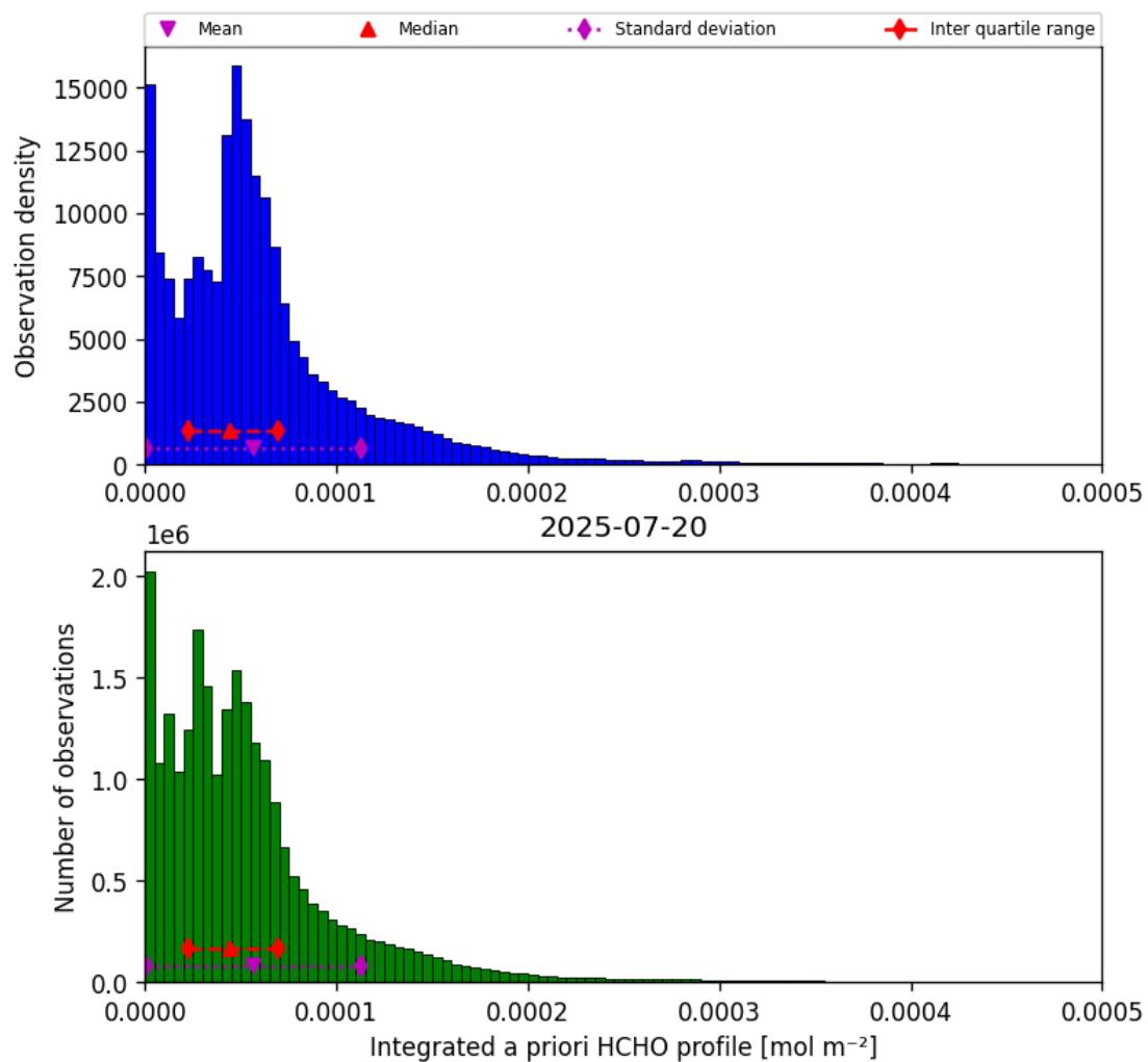
Figure 43: Histogram of “Integrated a priori HCHO profile” for 2025-07-19 to 2025-07-21
