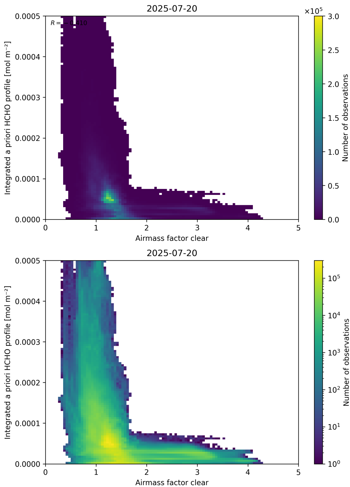
Figure 76: Scatter density plot of “Airmass factor clear” against “Integrated a priori HCHO profile” for 2025-07-19 to 2025-07-21.
