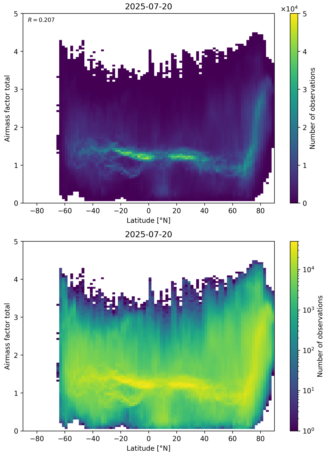
Figure 161: Scatter density plot of “Latitude” against “Airmass factor total” for 2025-07-19 to 2025-07-21.
