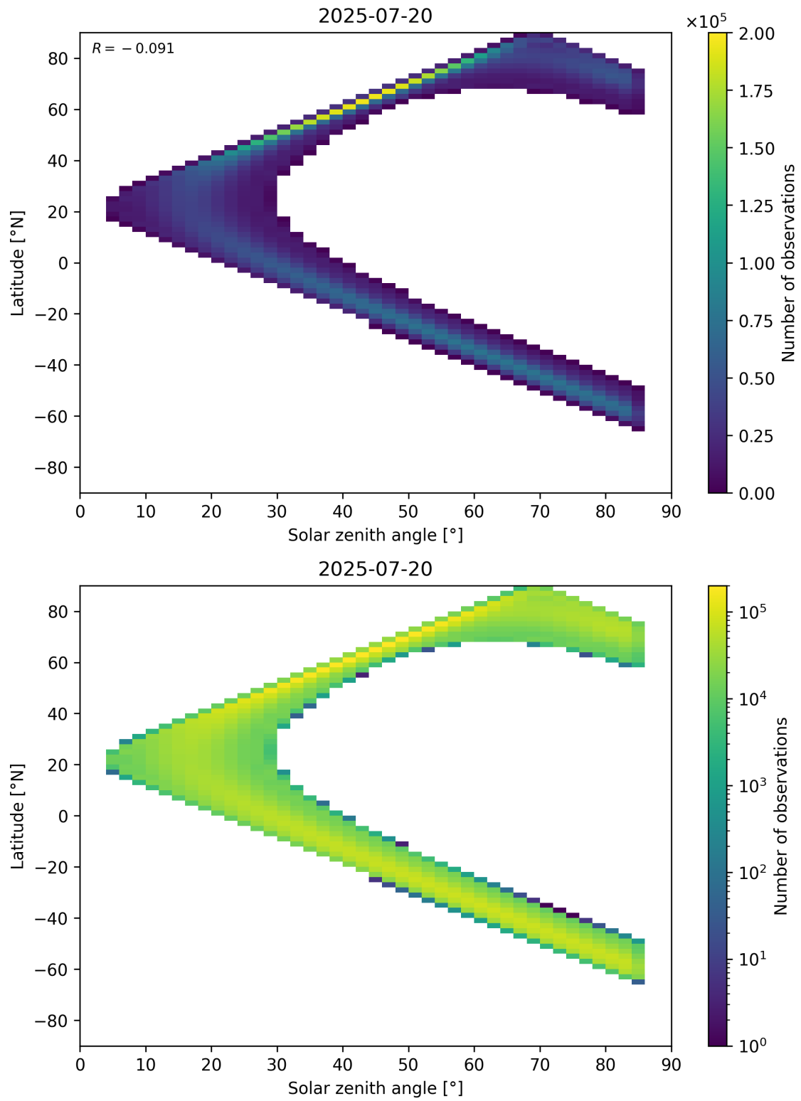
Figure 181: Scatter density plot of “Solar zenith angle” against “Latitude” for 2025-07-19 to 2025-07-21.
