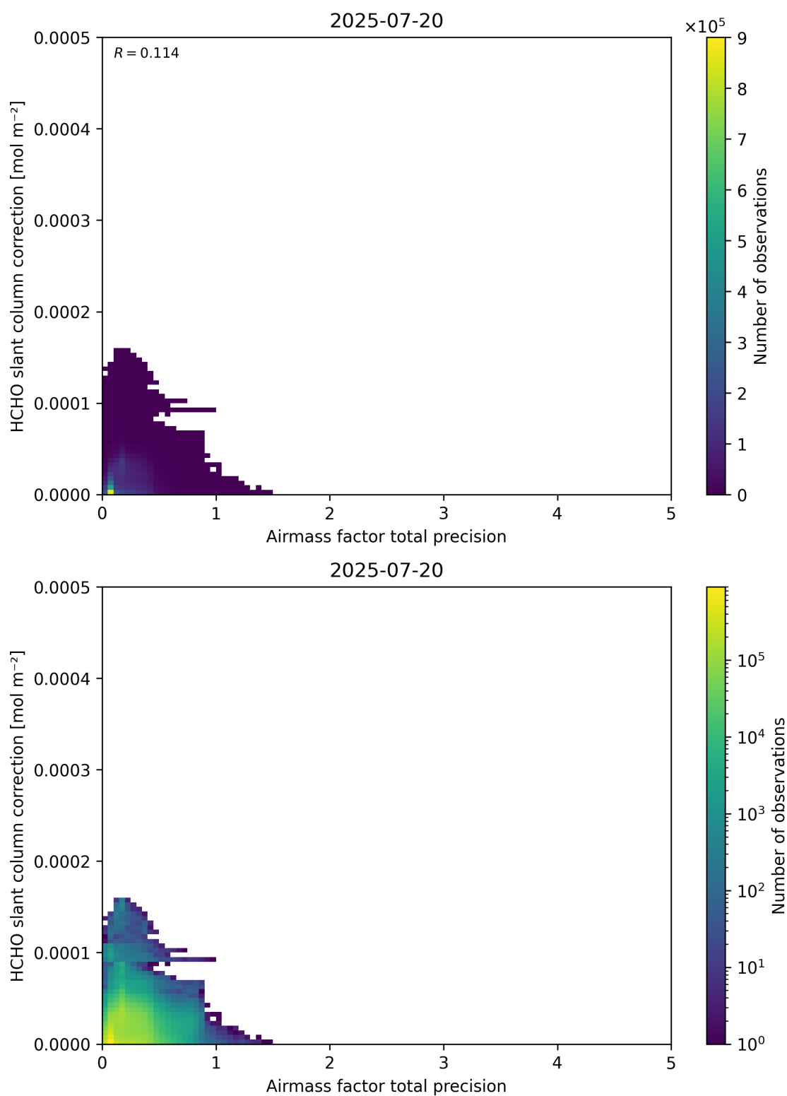
Figure 110: Scatter density plot of “Airmass factor total precision” against “HCHO slant column correction” for 2025-07-19 to 2025-07-21.
