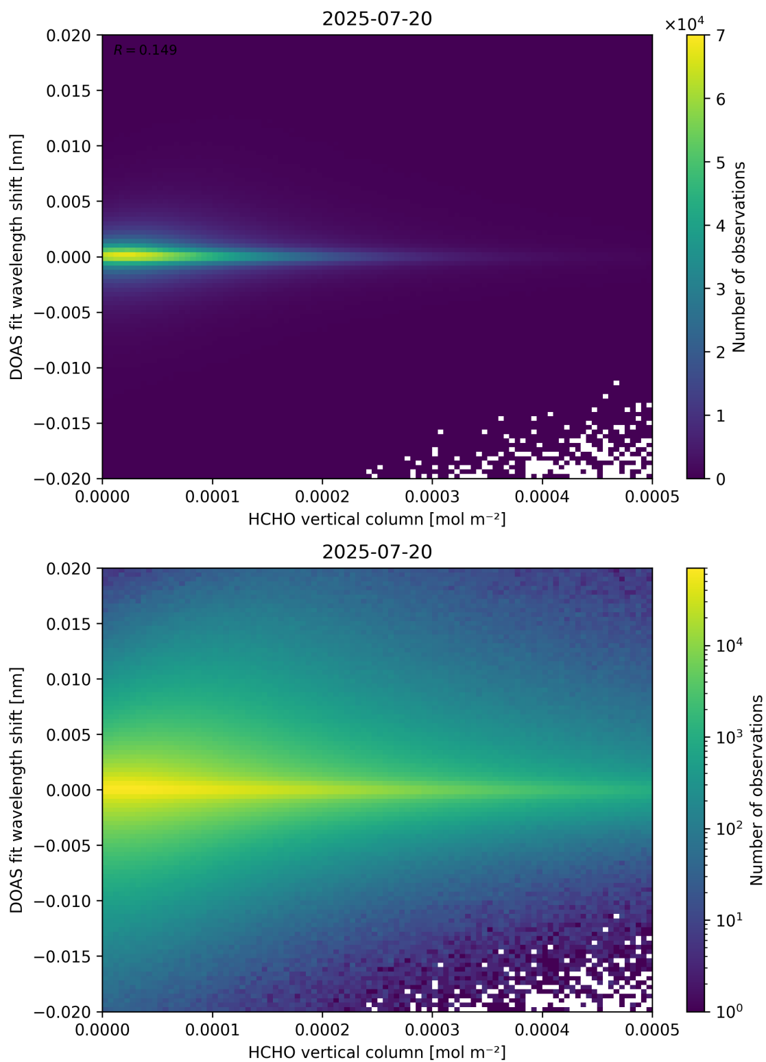
Figure 124: Scatter density plot of “HCHO vertical column” against “DOAS fit wavelength shift” for 2025-07-19 to 2025-07-21.
