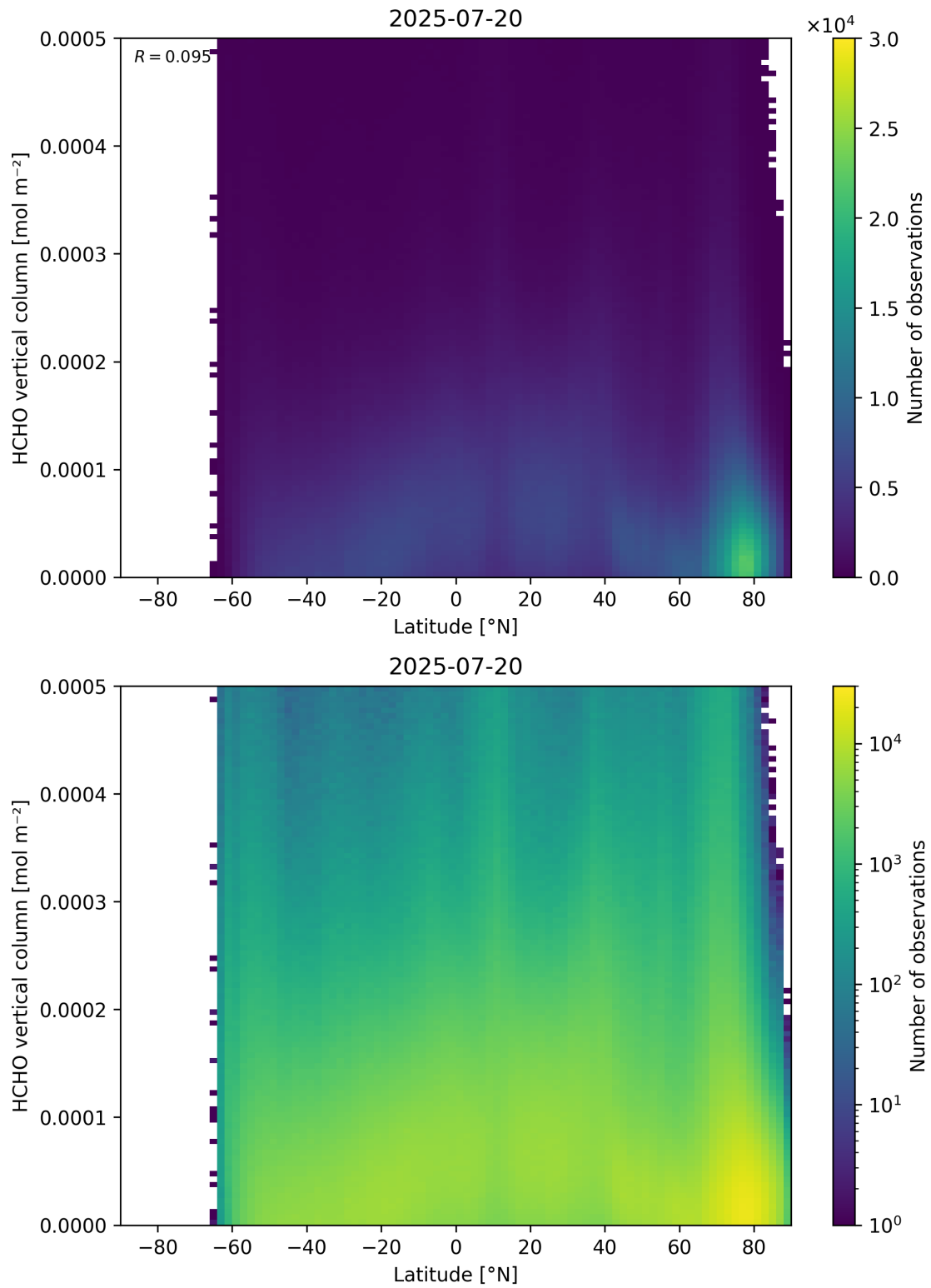
Figure 163: Scatter density plot of “Latitude” against “HCHO vertical column” for 2025-07-19 to 2025-07-21.
