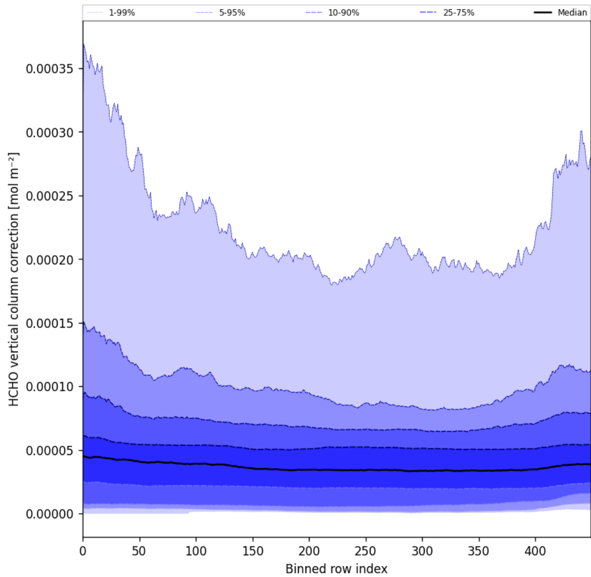
Figure 51: Along track statistics of "HCHO vertical column correction" for 2025-07-19 to 2025-07-21
