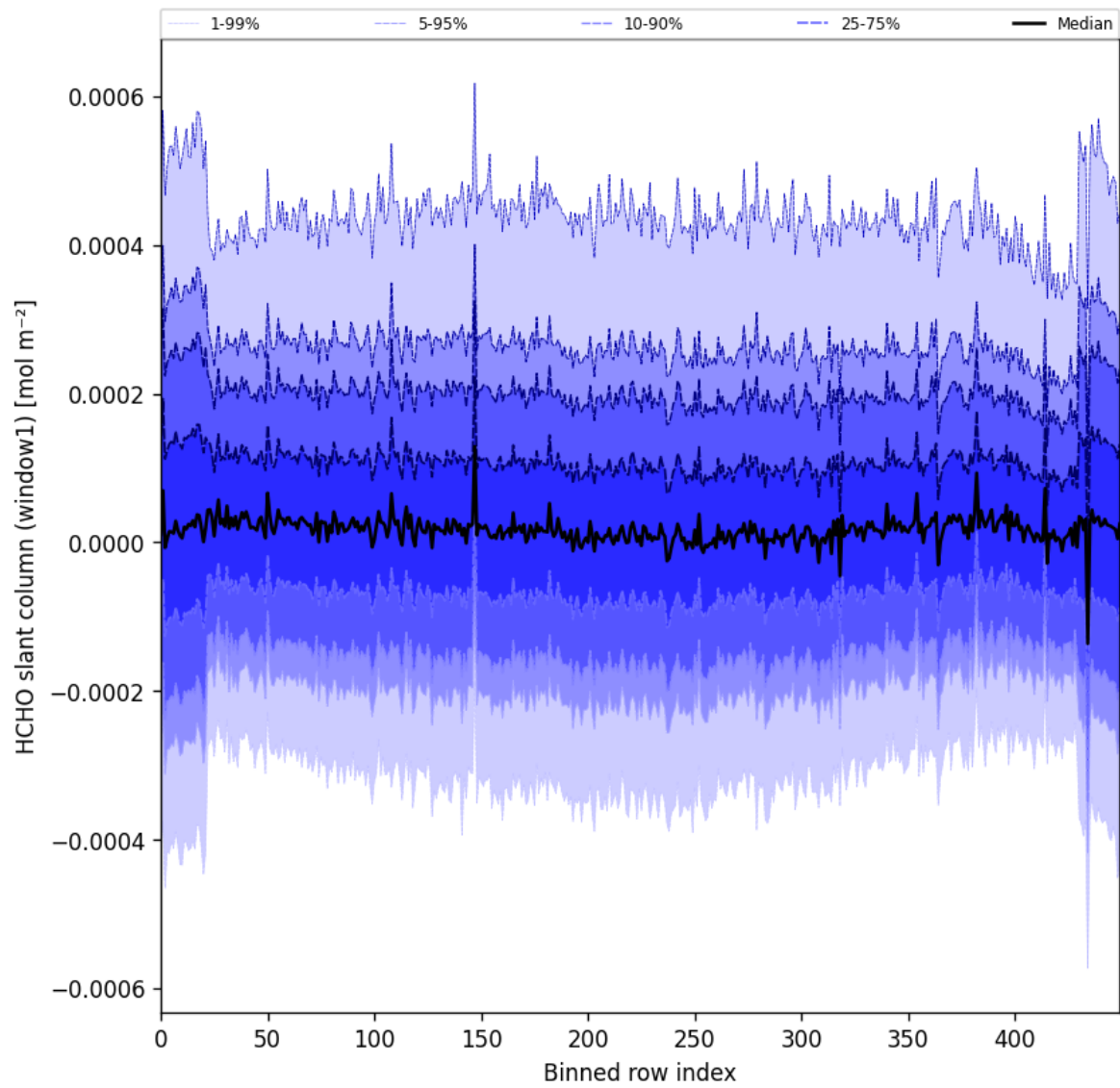
Figure 52: Along track statistics of “HCHO slant column (window1)” for 2025-07-19 to 2025-07-21
