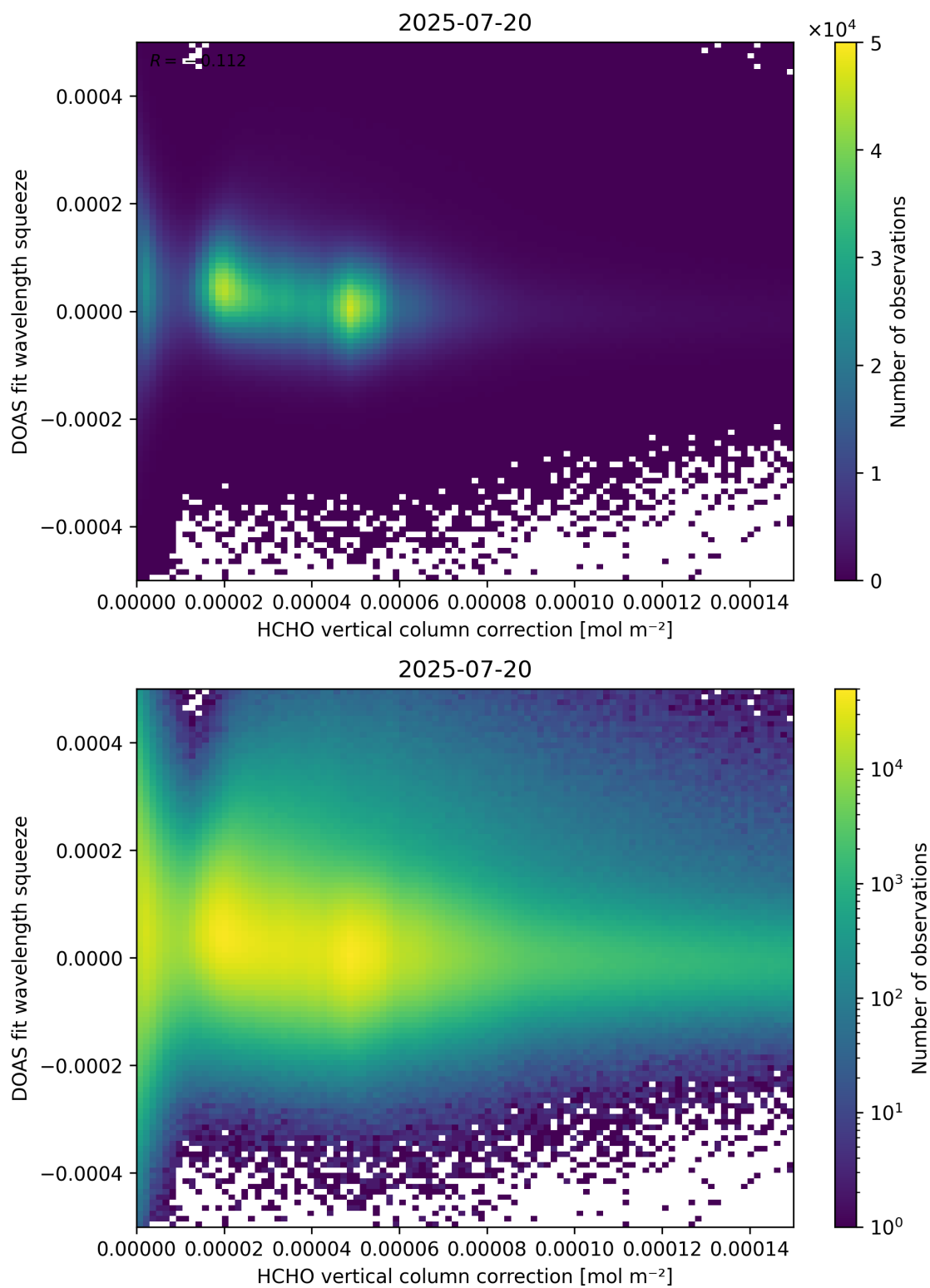
Figure 114: Scatter density plot of “HCHO vertical column correction” against “DOAS fit wavelength squeeze” for 2025-07-19 to 2025-07-21.
