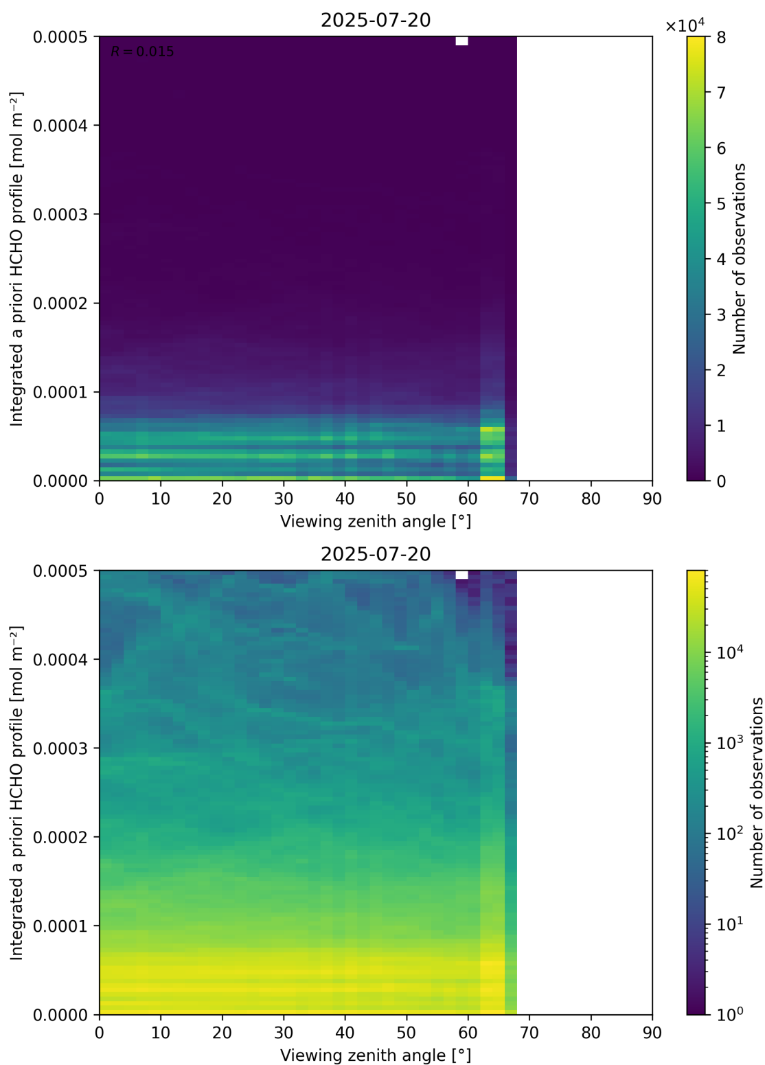
Figure 195: Scatter density plot of “Viewing zenith angle” against “Integrated a priori HCHO profile” for 2025-07-19 to 2025-07-21.
