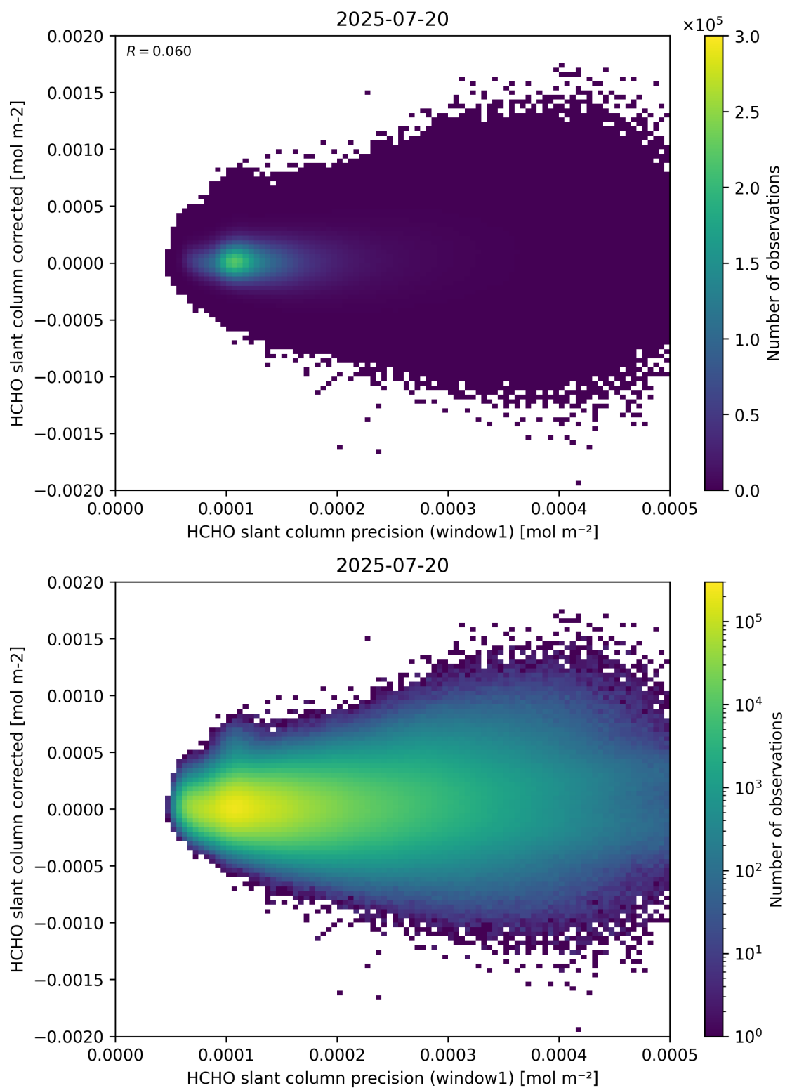
Figure 92: Scatter density plot of “HCHO slant column precision (window1)” against “HCHO slant column corrected” for 2025-07-19 to 2025-07-21.
