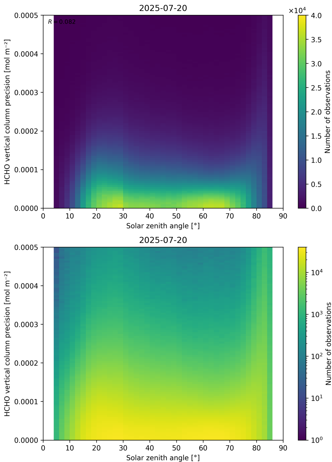
Figure 179: Scatter density plot of “Solar zenith angle” against “HCHO vertical column precision” for 2025-07-19 to 2025-07-21.
