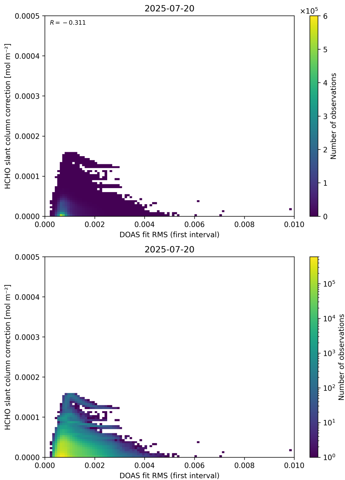
Figure 63: Scatter density plot of “DOAS fit RMS (first interval)” against “HCHO slant column correction” for 2025-07-19 to 2025-07-21.
