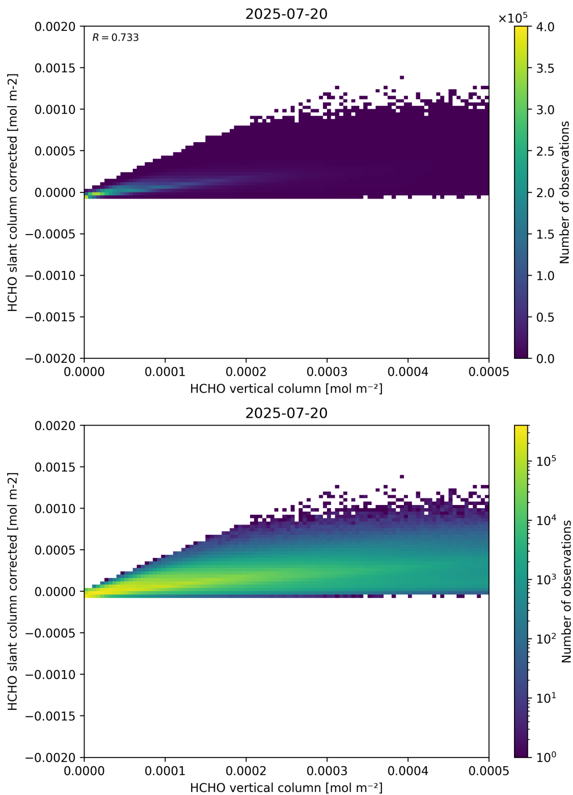
Figure 127: Scatter density plot of “HCHO vertical column” against “HCHO slant column corrected” for 2025-07-19 to 2025-07-21.
