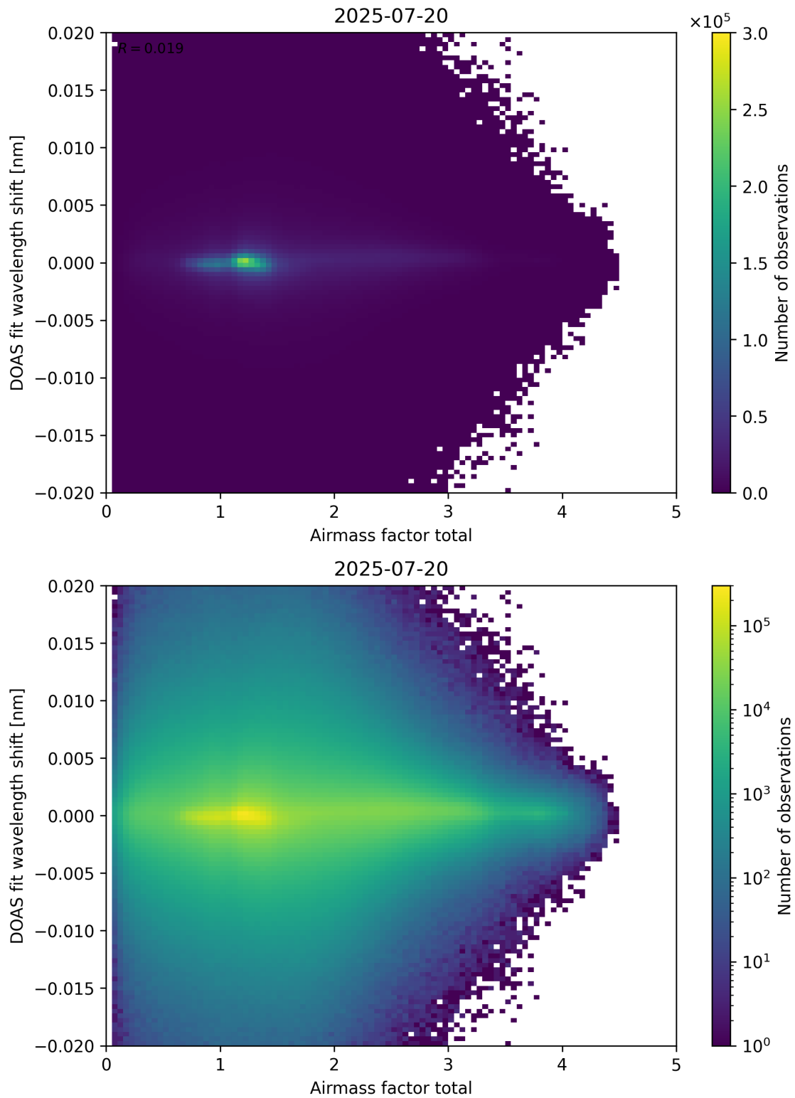
Figure 98: Scatter density plot of “Airmass factor total” against “DOAS fit wavelength shift” for 2025-07-19 to 2025-07-21.
