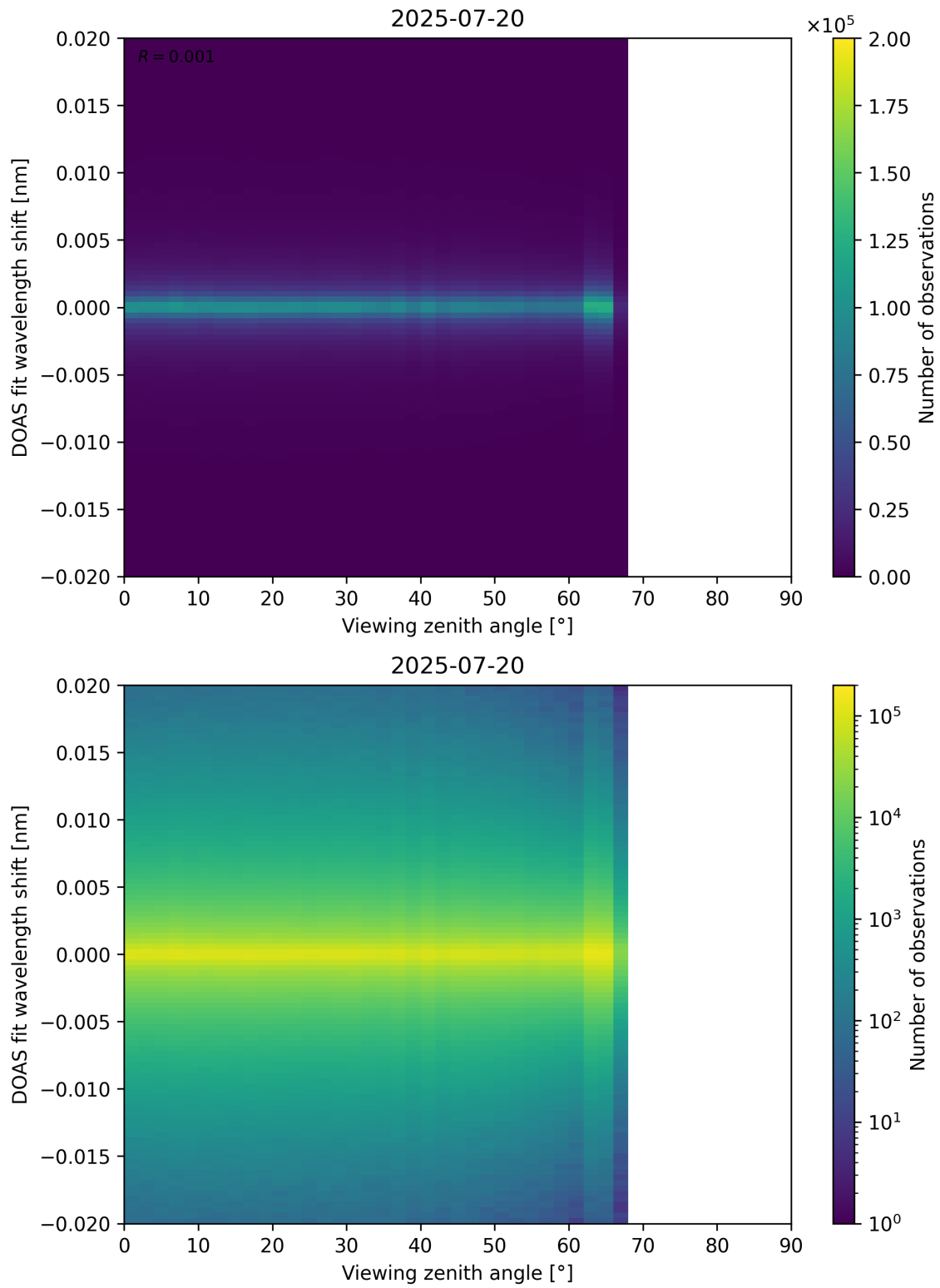
Figure 183: Scatter density plot of “Viewing zenith angle” against “DOAS fit wavelength shift” for 2025-07-19 to 2025-07-21.
