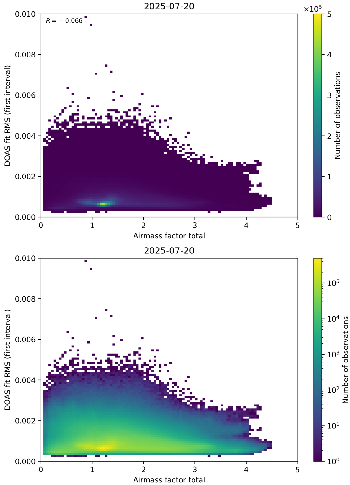
Figure 97: Scatter density plot of “Airmass factor total” against “DOAS fit RMS (first interval)” for 2025-07-19 to 2025-07-21.
