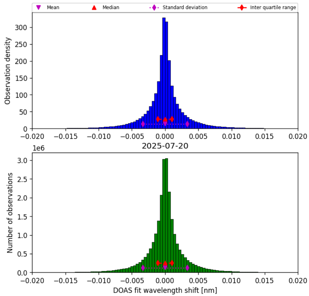
Figure 44: Histogram of “DOAS fit wavelength shift” for 2025-07-19 to 2025-07-21
