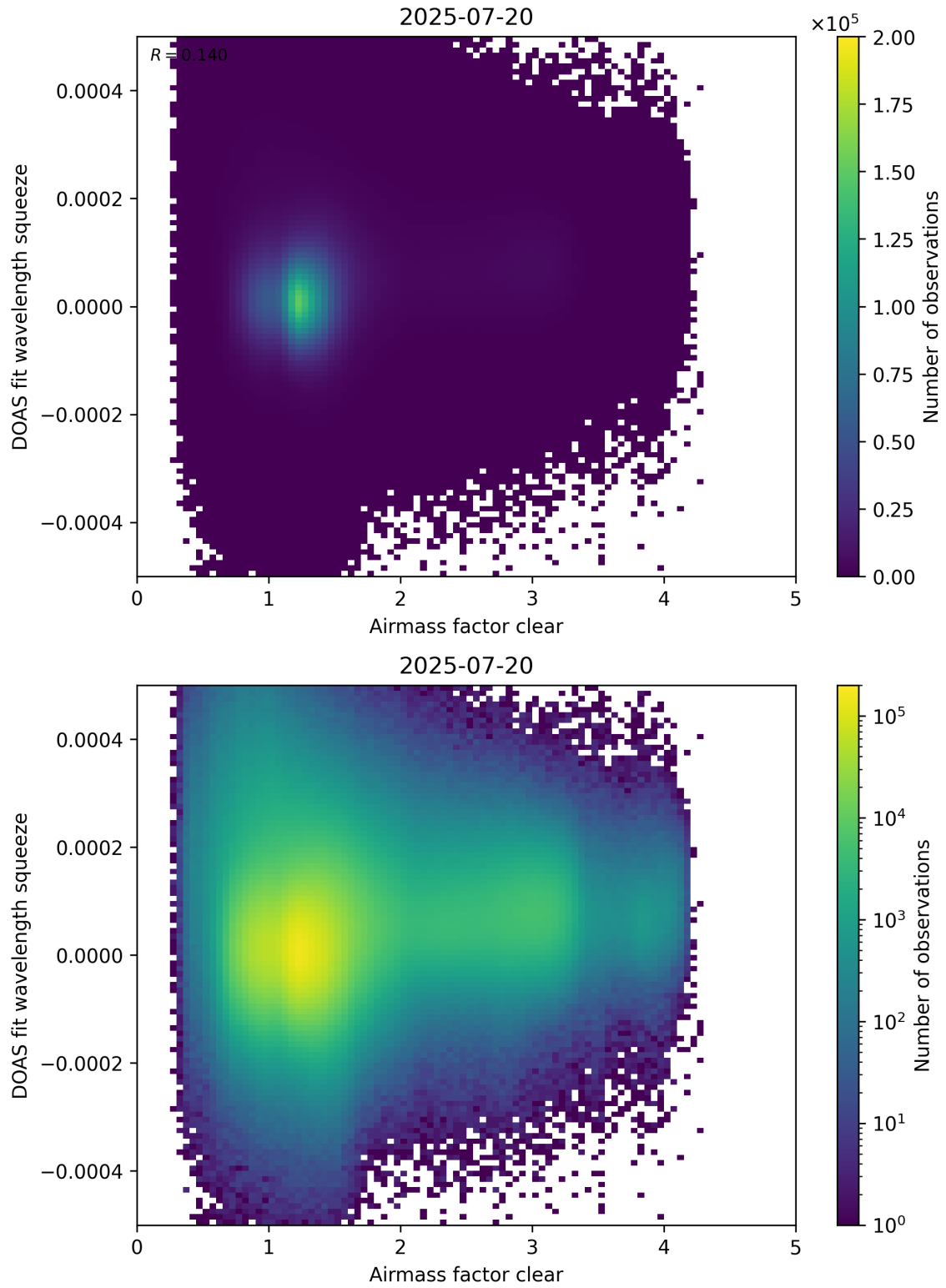
Figure 73: Scatter density plot of “Airmass factor clear” against “DOAS fit wavelength squeeze” for 2025-07-19 to 2025-07-21.
