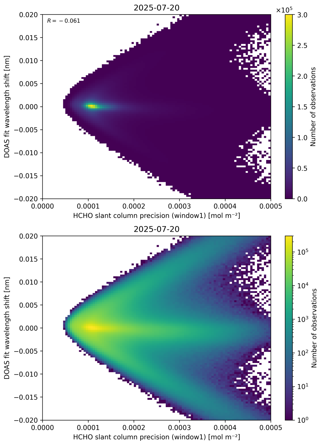
Figure 89: Scatter density plot of “HCHO slant column precision (window1)” against “DOAS fit wavelength shift” for 2025-07-19 to 2025-07-21.
