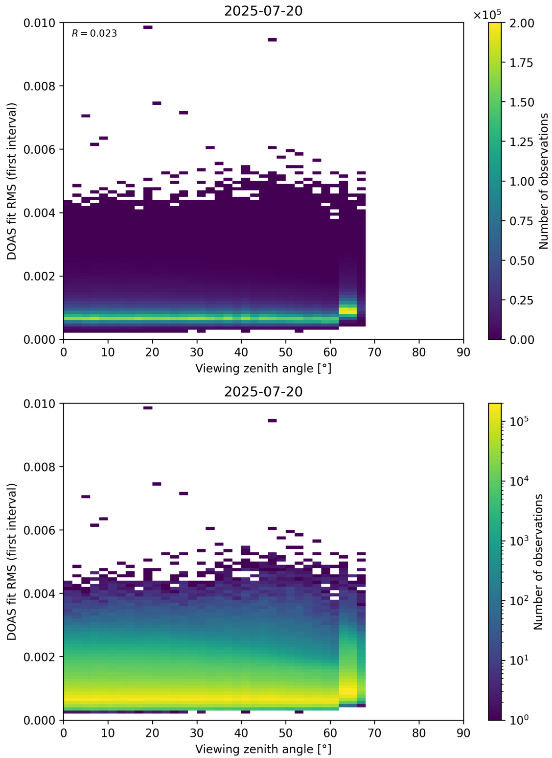
Figure 182: Scatter density plot of “Viewing zenith angle” against “DOAS fit RMS (first interval)” for 2025-07-19 to 2025-07-21.
