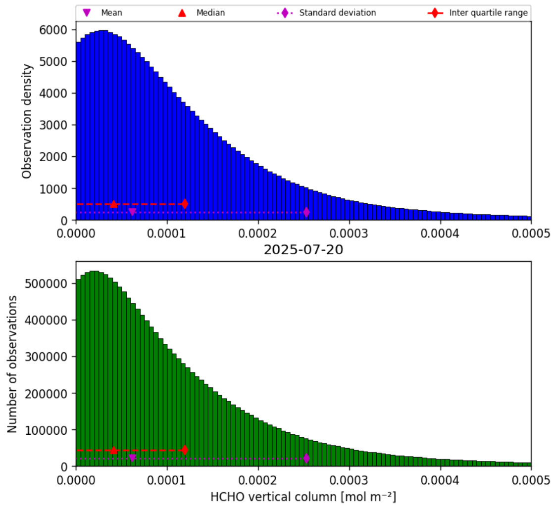
Figure 35: Histogram of “HCHO vertical column” for 2025-07-19 to 2025-07-21
