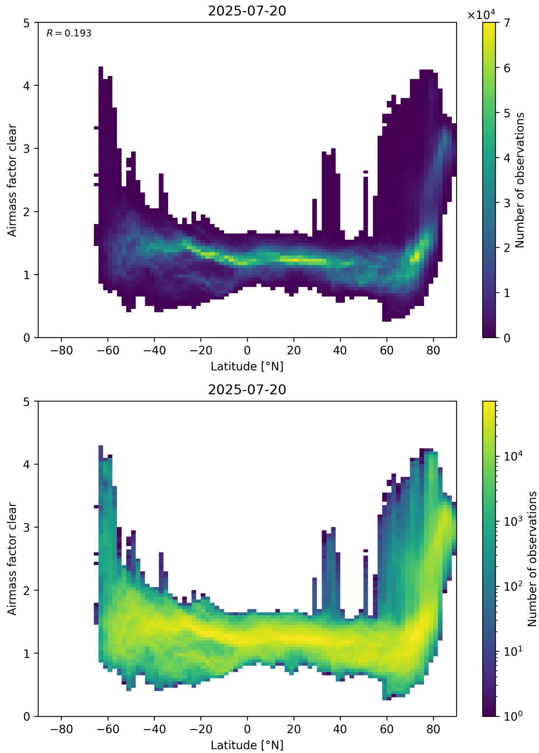
Figure 156: Scatter density plot of “Latitude” against “Airmass factor clear” for 2025-07-19 to 2025-07-21.
