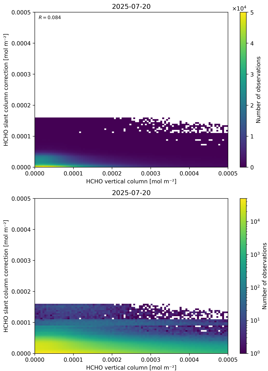
Figure 128: Scatter density plot of “HCHO vertical column” against “HCHO slant column correction” for 2025-07-19 to 2025-07-21.
