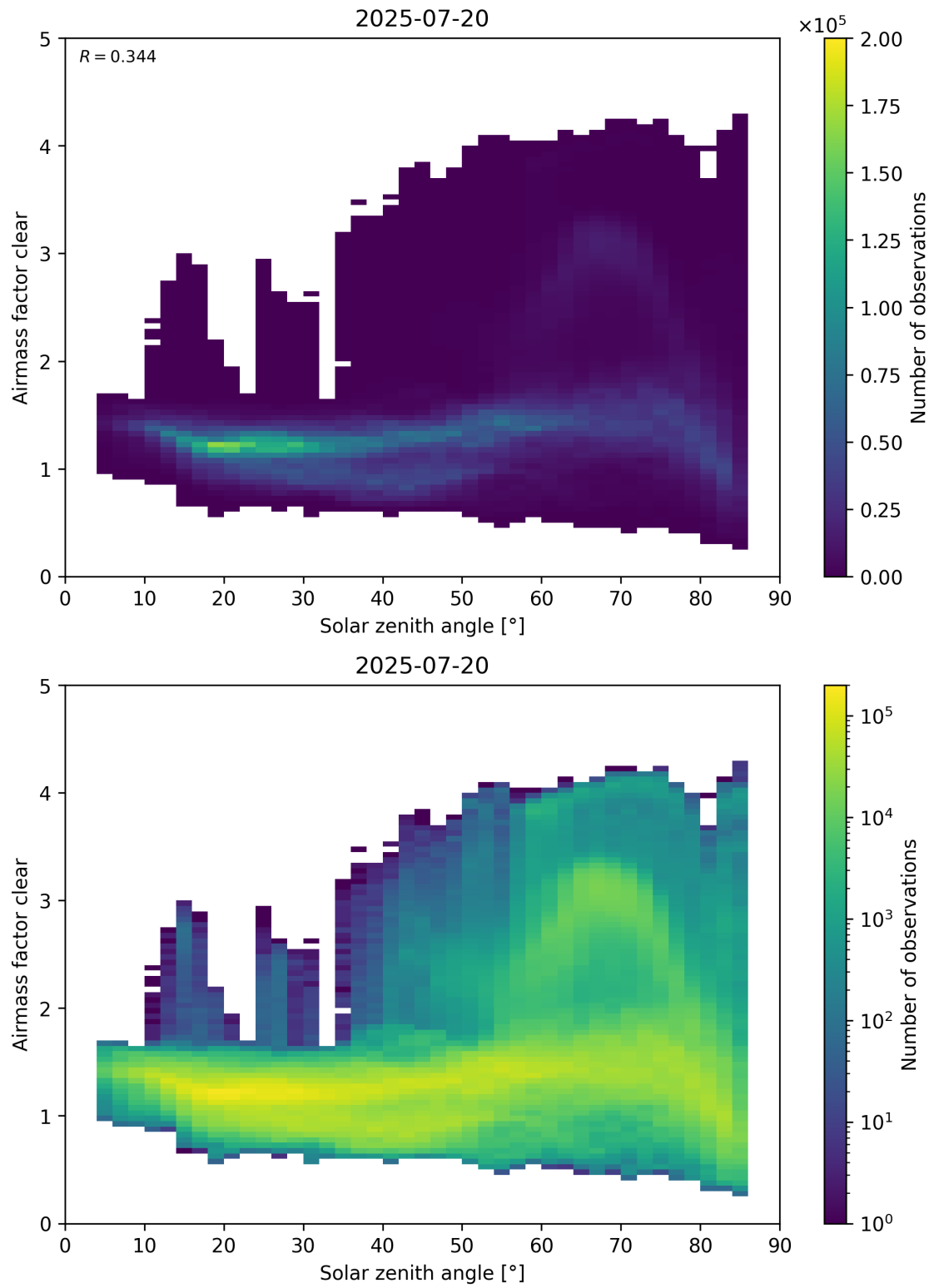
Figure 170: Scatter density plot of “Solar zenith angle” against “Airmass factor clear” for 2025-07-19 to 2025-07-21.
