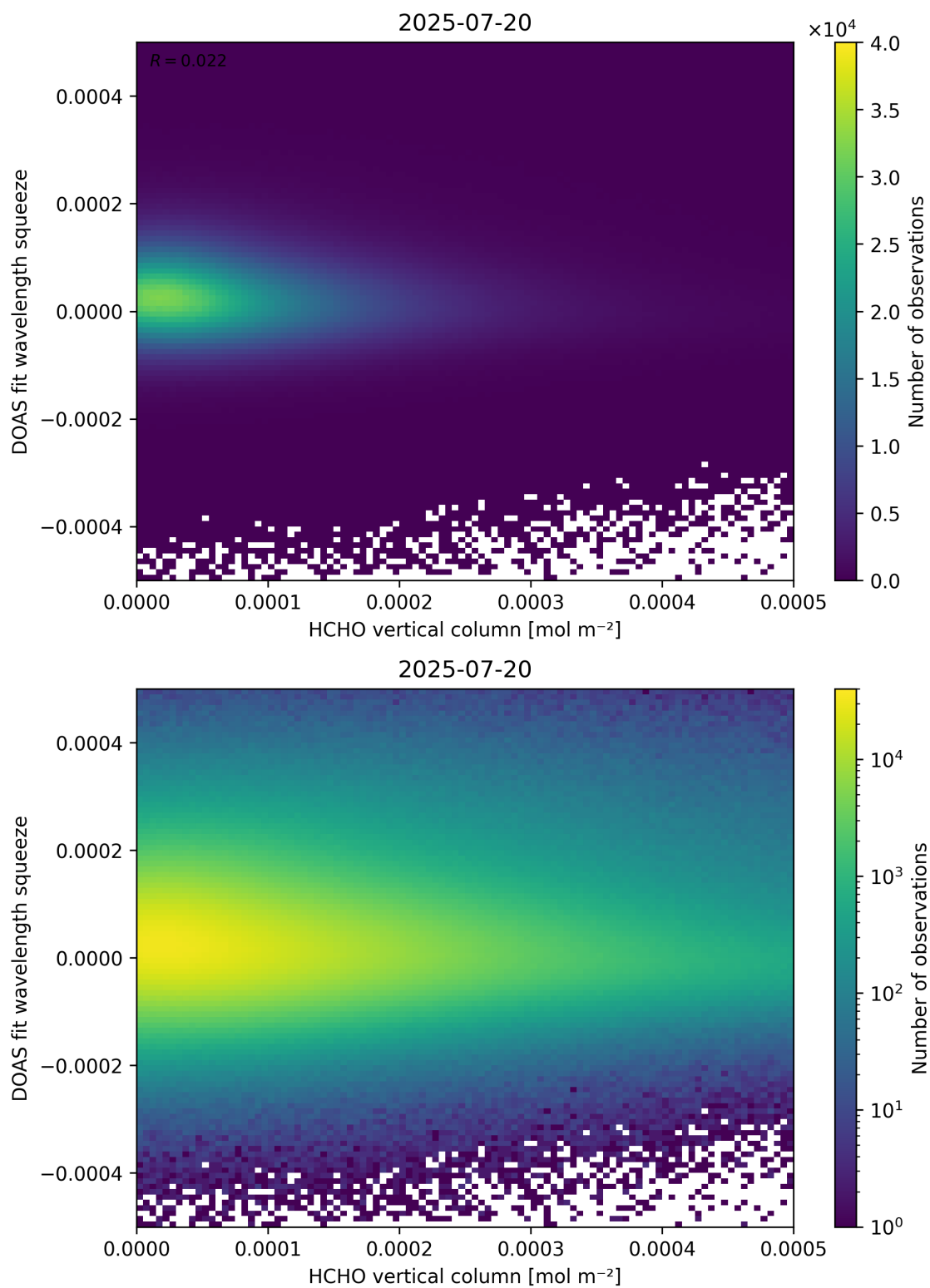
Figure 125: Scatter density plot of “HCHO vertical column” against “DOAS fit wavelength squeeze” for 2025-07-19 to 2025-07-21.
