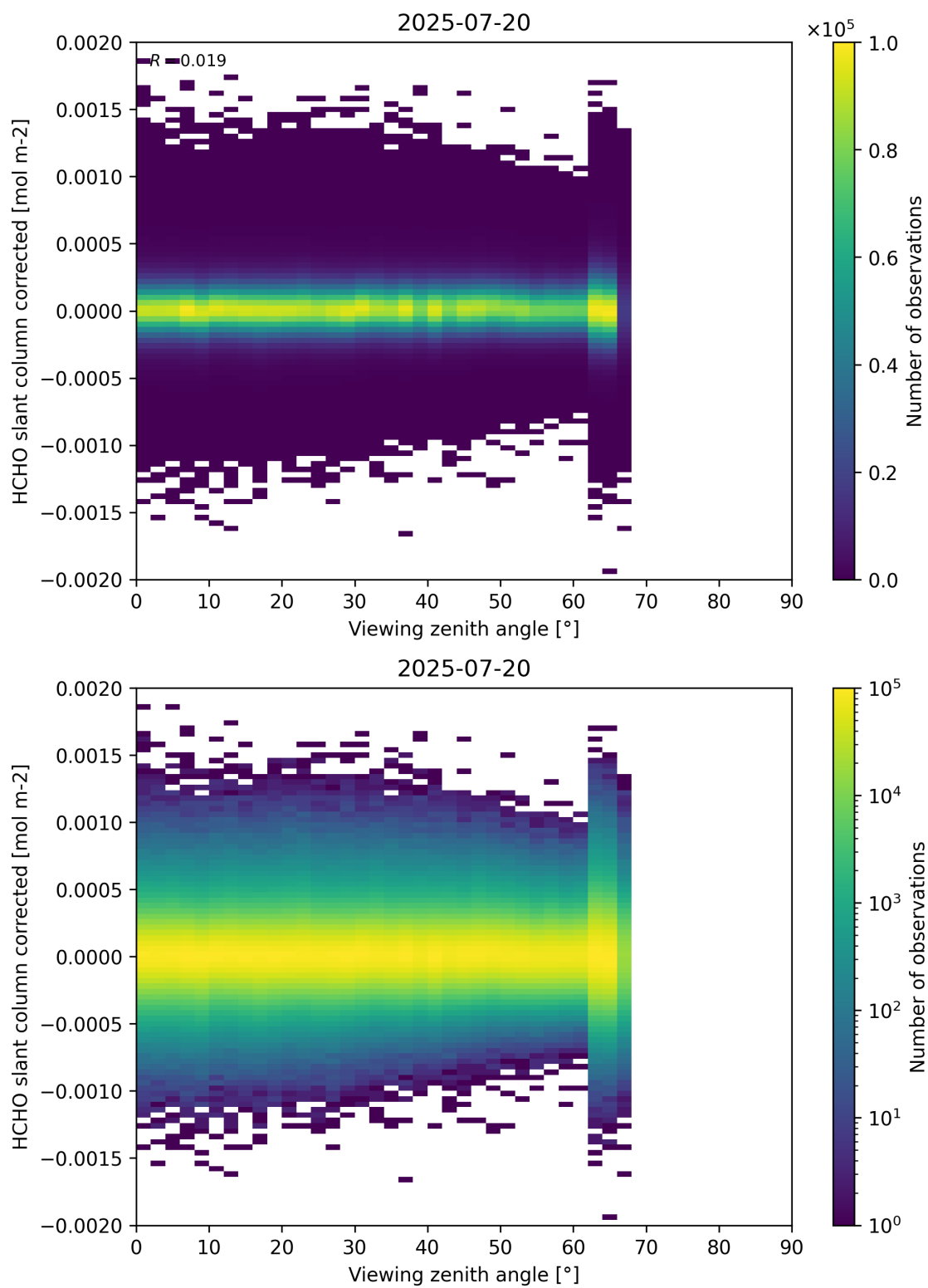
Figure 186: Scatter density plot of “Viewing zenith angle” against “HCHO slant column corrected” for 2025-07-19 to 2025-07-21.
