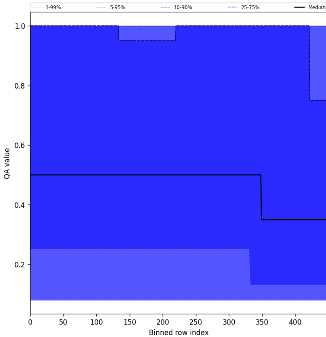
Figure 48: Along track statistics of “QA value” for 2025-07-19 to 2025-07-21
