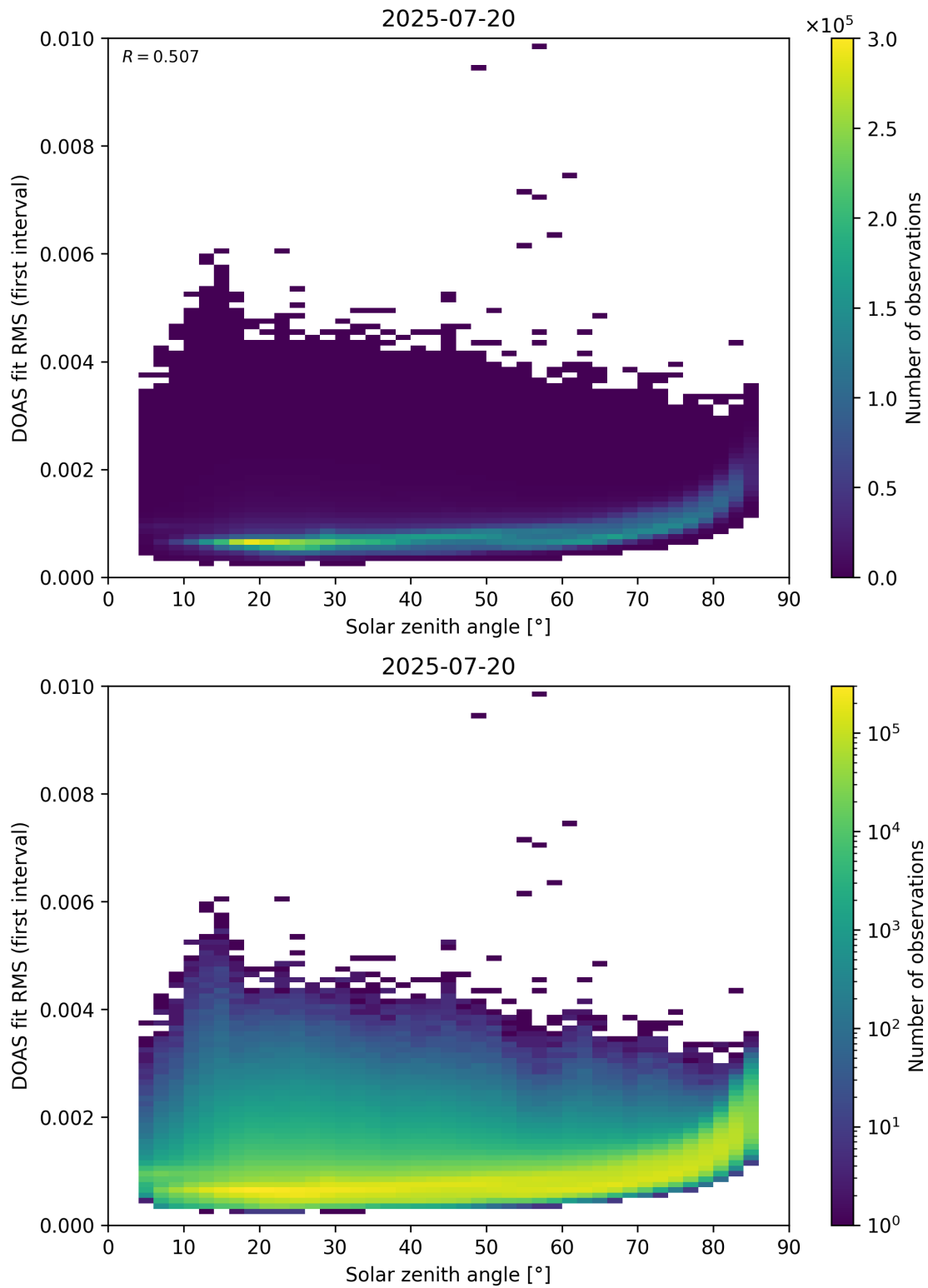
Figure 167: Scatter density plot of “Solar zenith angle” against “DOAS fit RMS (first interval)” for 2025-07-19 to 2025-07-21.
