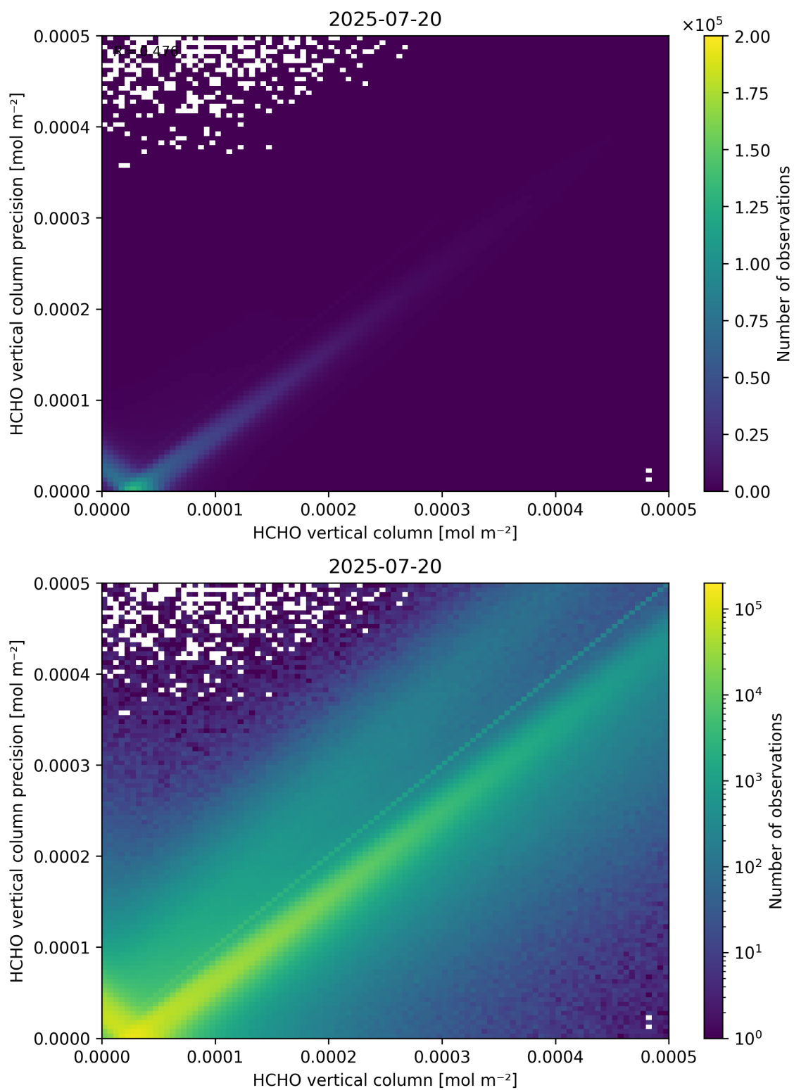
Figure 134: Scatter density plot of “HCHO vertical column” against “HCHO vertical column precision” for 2025-07-19 to 2025-07-21.
