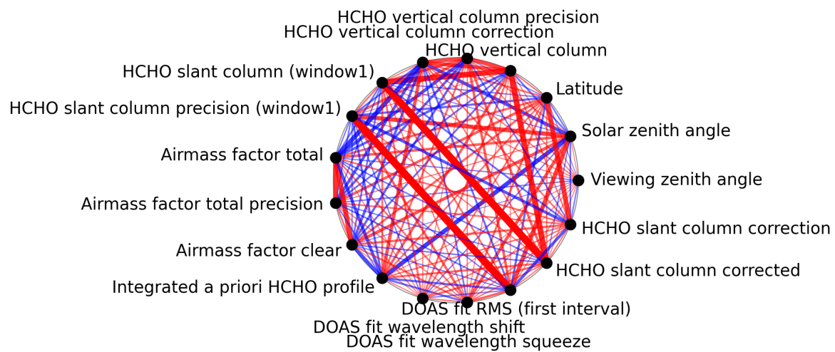
Figure 1: Map of correlation graph for 2025-07-19 to 2025-07-21.
