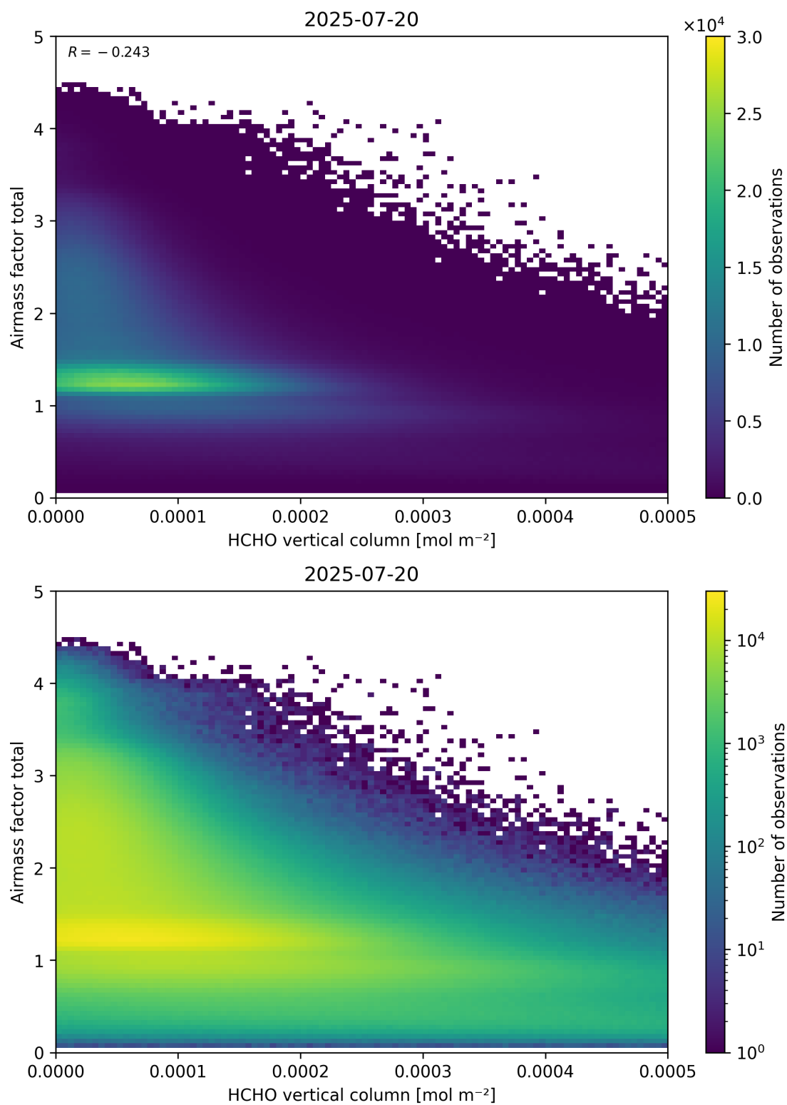
Figure 131: Scatter density plot of “HCHO vertical column” against “Airmass factor total” for 2025-07-19 to 2025-07-21.
