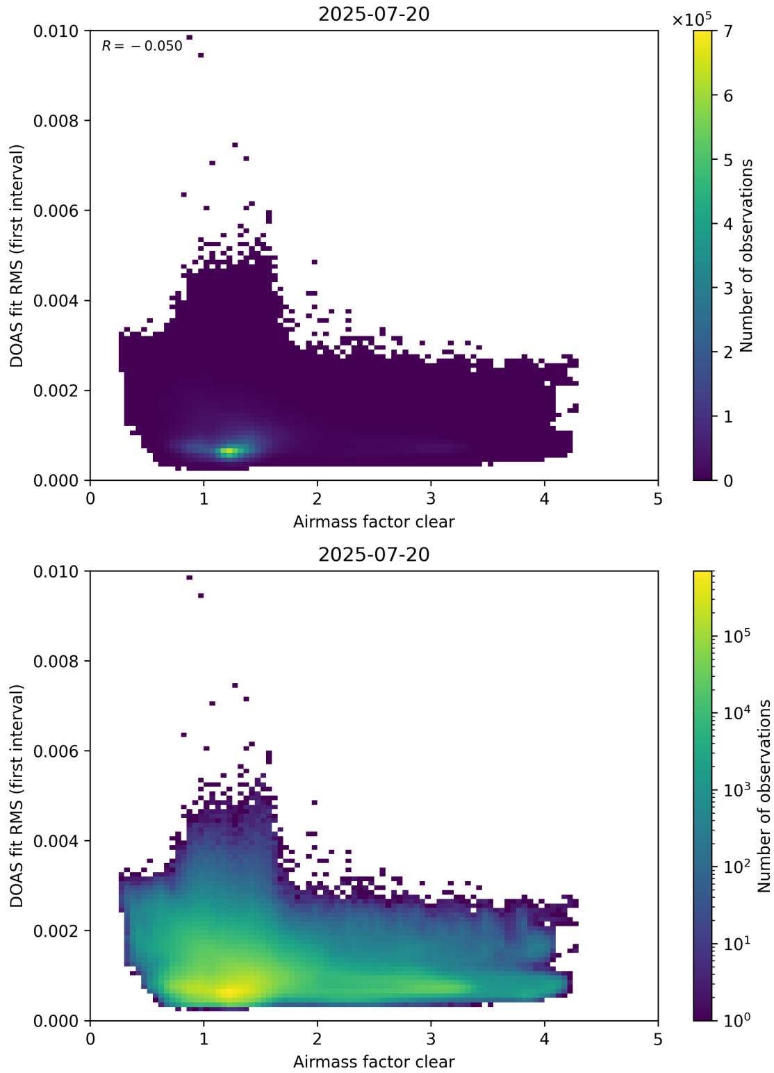
Figure 71: Scatter density plot of “Airmass factor clear” against “DOAS fit RMS (first interval)” for 2025-07-19 to 2025-07-21.
