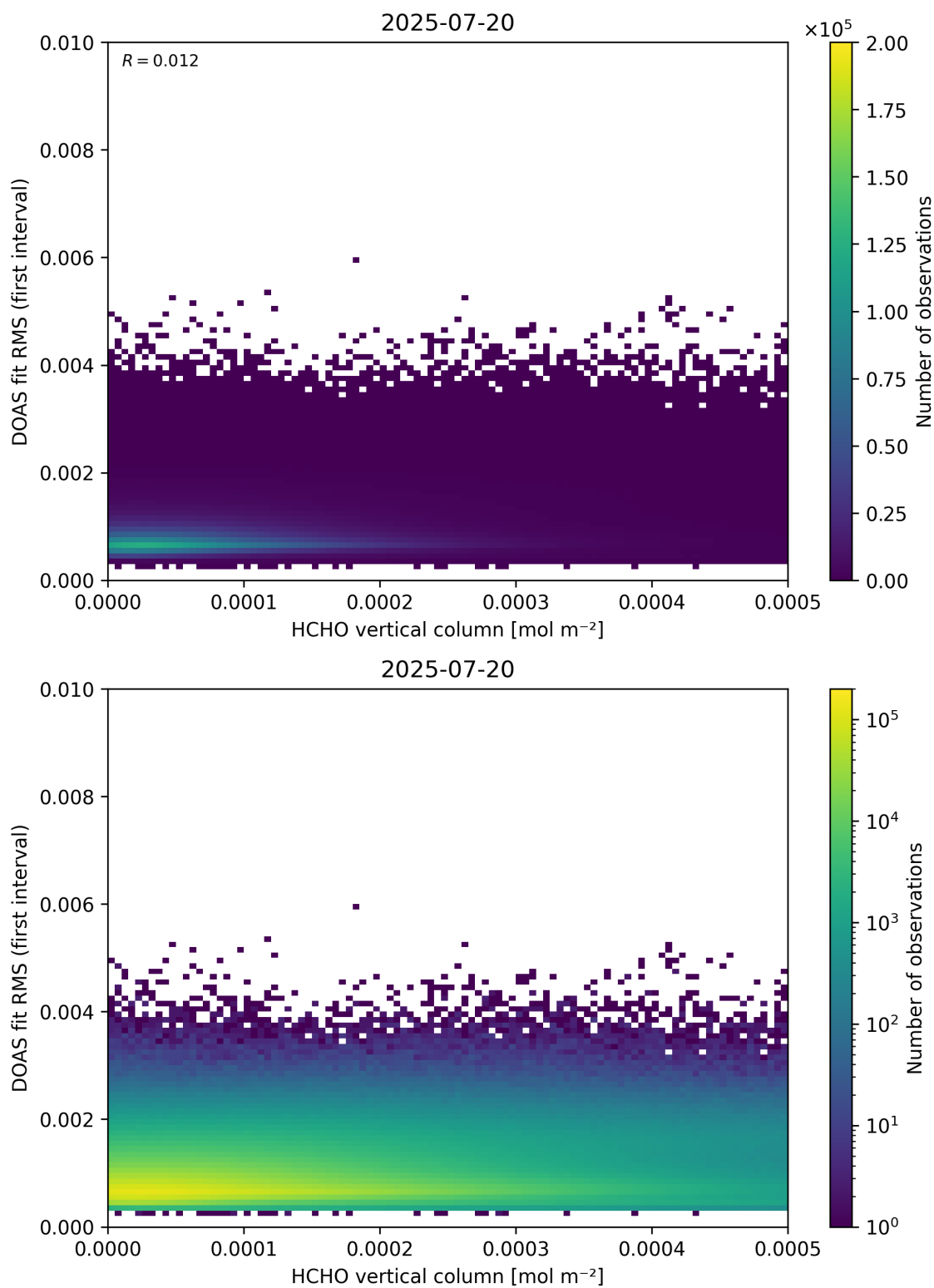
Figure 123: Scatter density plot of “HCHO vertical column” against “DOAS fit RMS (first interval)” for 2025-07-19 to 2025-07-21.
