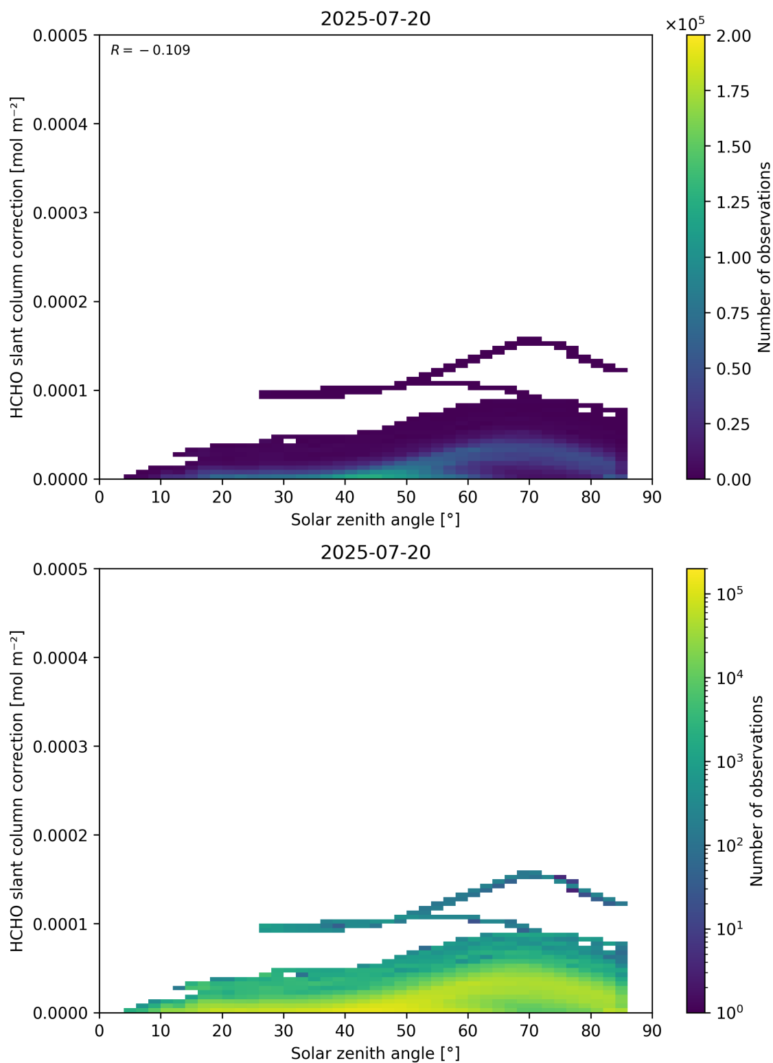
Figure 172: Scatter density plot of “Solar zenith angle” against “HCHO slant column correction” for 2025-07-19 to 2025-07-21.
