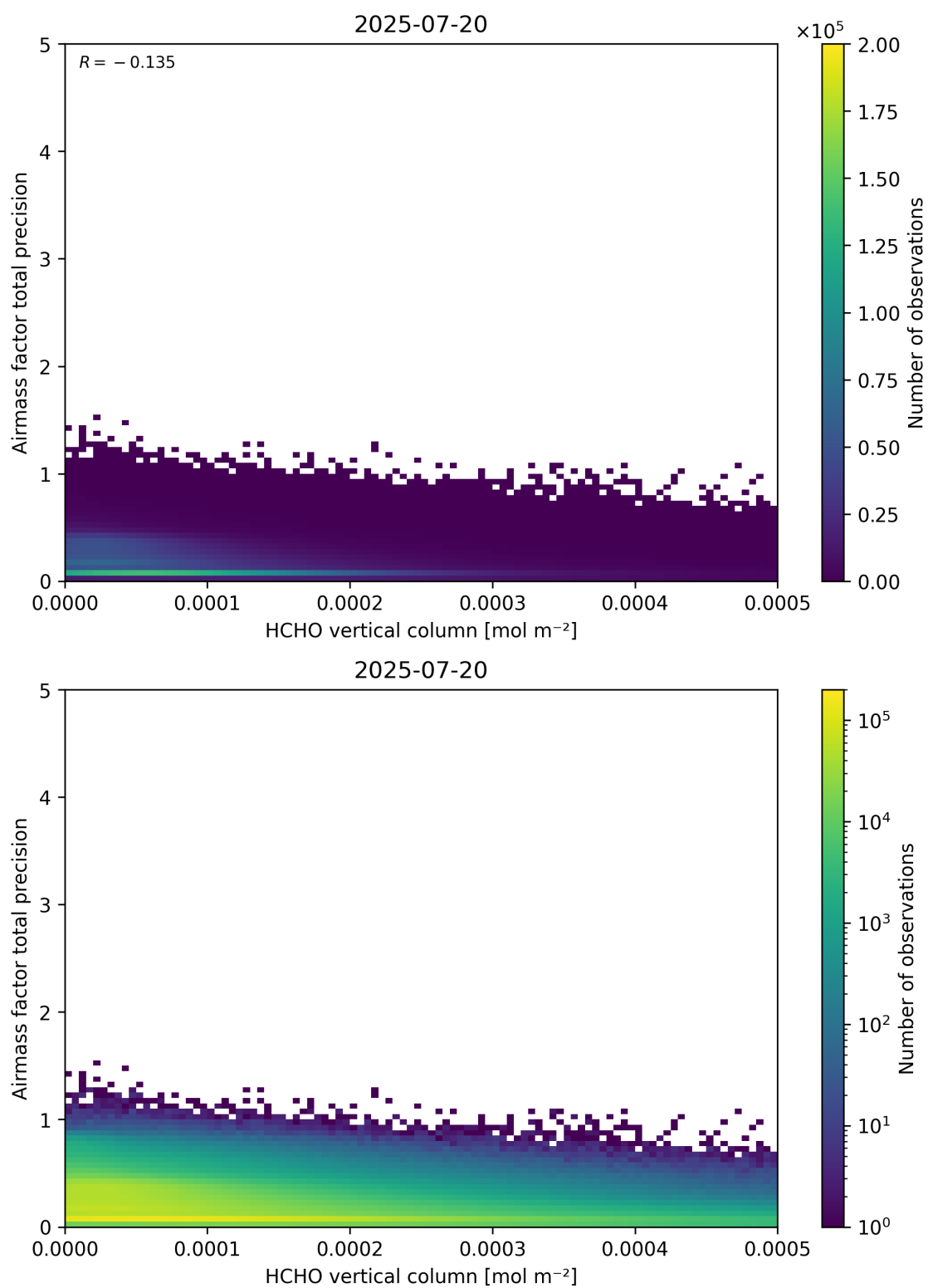
Figure 132: Scatter density plot of “HCHO vertical column” against “Airmass factor total precision” for 2025-07-19 to 2025-07-21.
