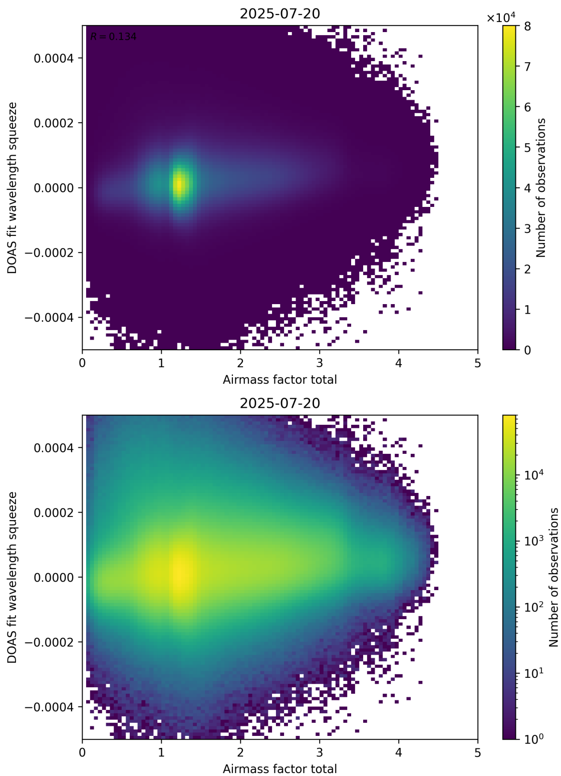
Figure 99: Scatter density plot of “Airmass factor total” against “DOAS fit wavelength squeeze” for 2025-07-19 to 2025-07-21.
