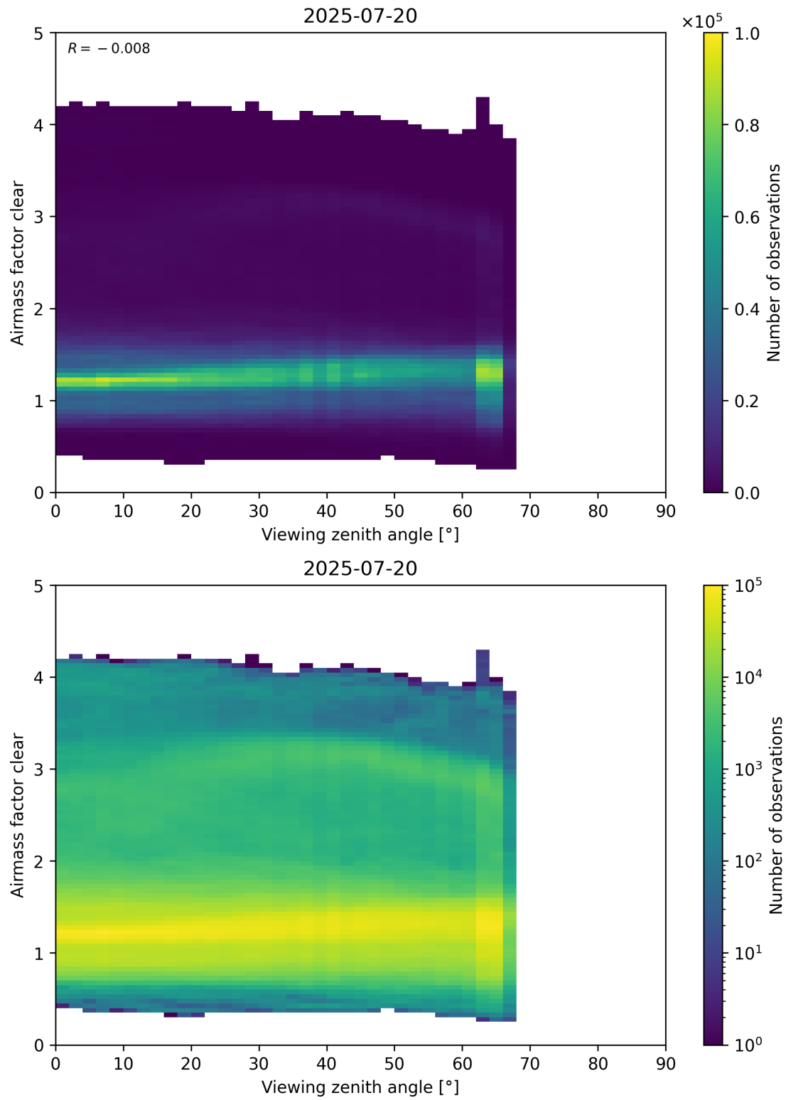
Figure 185: Scatter density plot of “Viewing zenith angle” against “Airmass factor clear” for 2025-07-19 to 2025-07-21.
