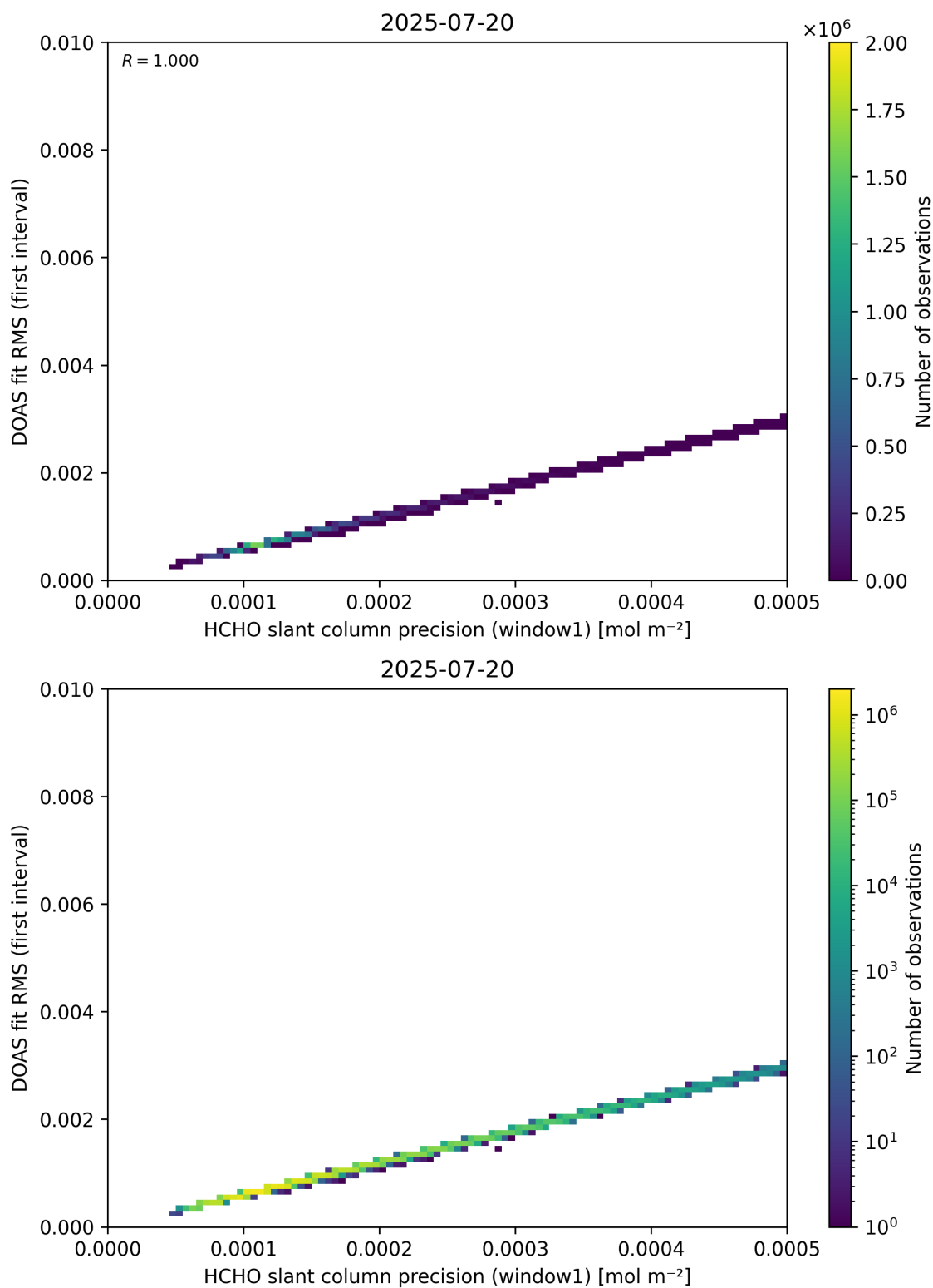
Figure 88: Scatter density plot of “HCHO slant column precision (window1)” against “DOAS fit RMS (first interval)” for 2025-07-19 to 2025-07-21.
