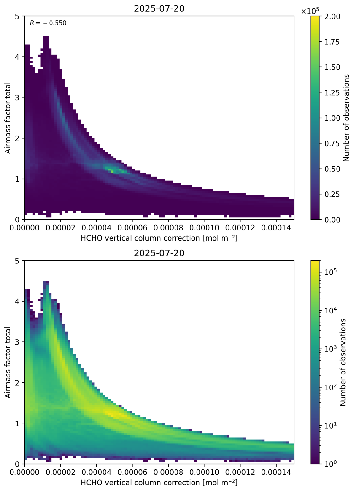
Figure 120: Scatter density plot of “HCHO vertical column correction” against “Airmass factor total” for 2025-07-19 to 2025-07-21.
