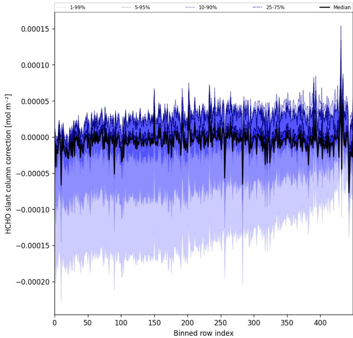
Figure 61: Along track statistics of “HCHO slant column correction” for 2025-07-19 to 2025-07-21
