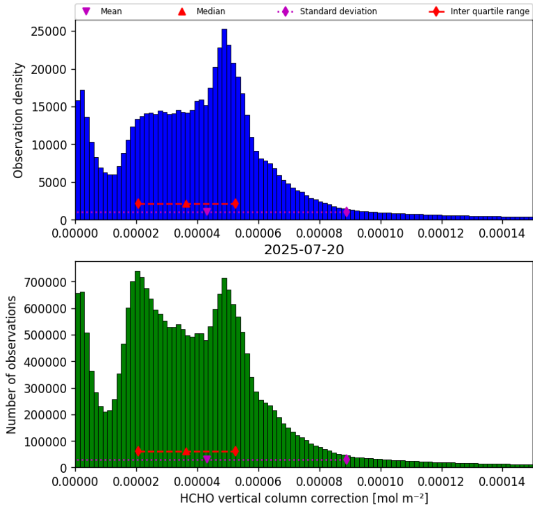
Figure 37: Histogram of “HCHO vertical column correction” for 2025-07-19 to 2025-07-21
