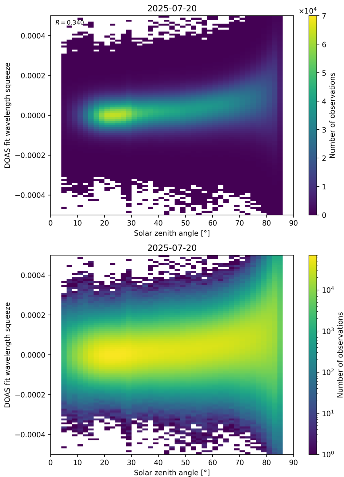
Figure 169: Scatter density plot of “Solar zenith angle” against “DOAS fit wavelength squeeze” for 2025-07-19 to 2025-07-21.
