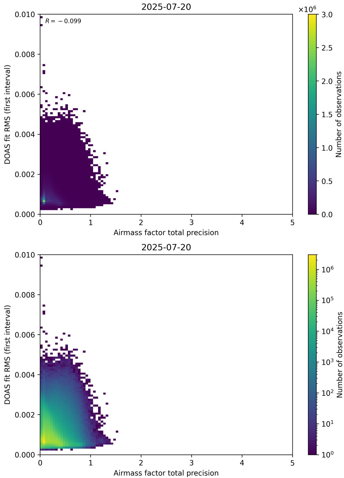
Figure 105: Scatter density plot of “Airmass factor total precision” against “DOAS fit RMS (first interval)” for 2025-07-19 to 2025-07-21.
