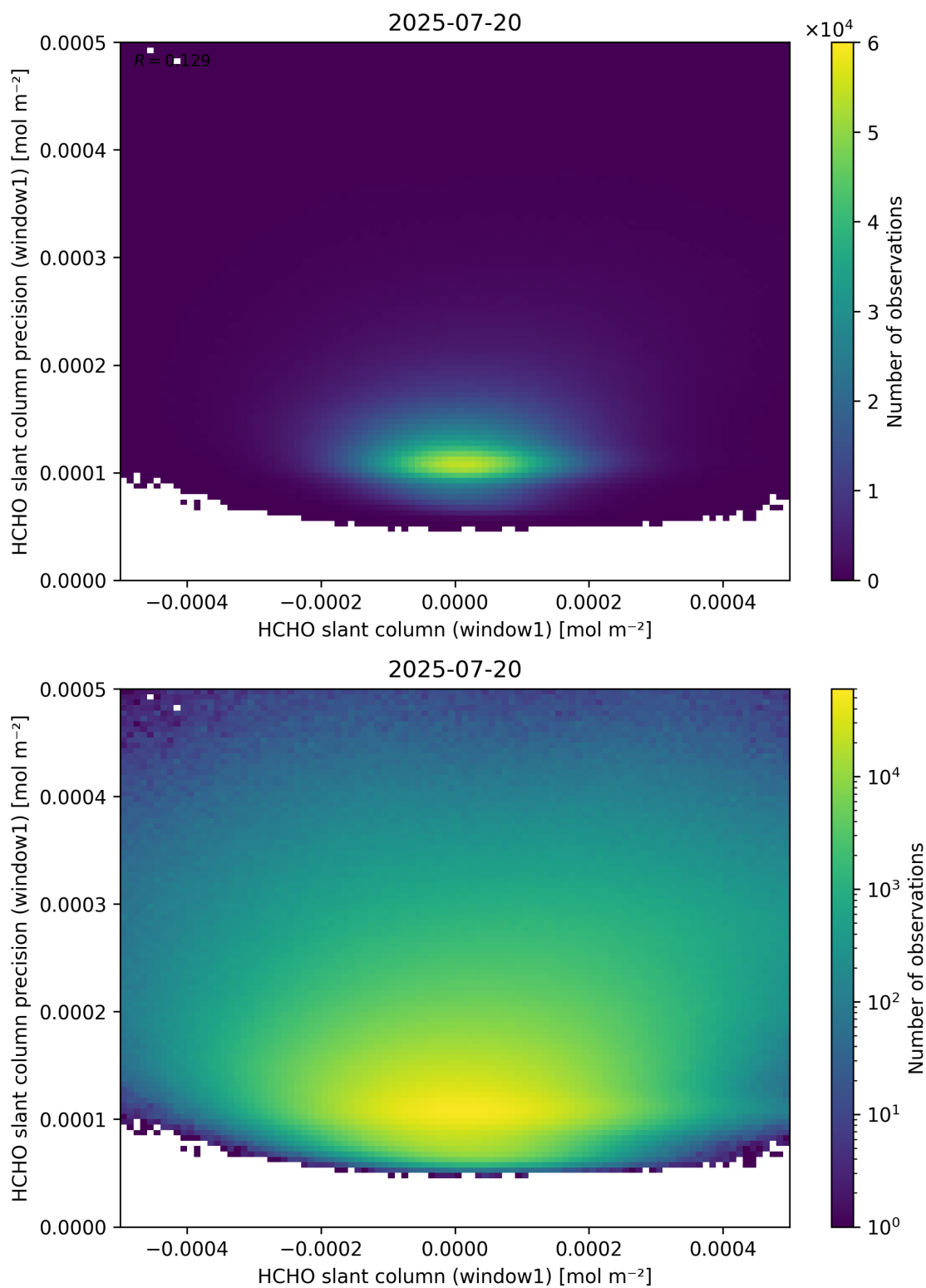
Figure 84: Scatter density plot of “HCHO slant column (window1)” against “HCHO slant column precision (window1)” for 2025-07-19 to 2025-07-21.
