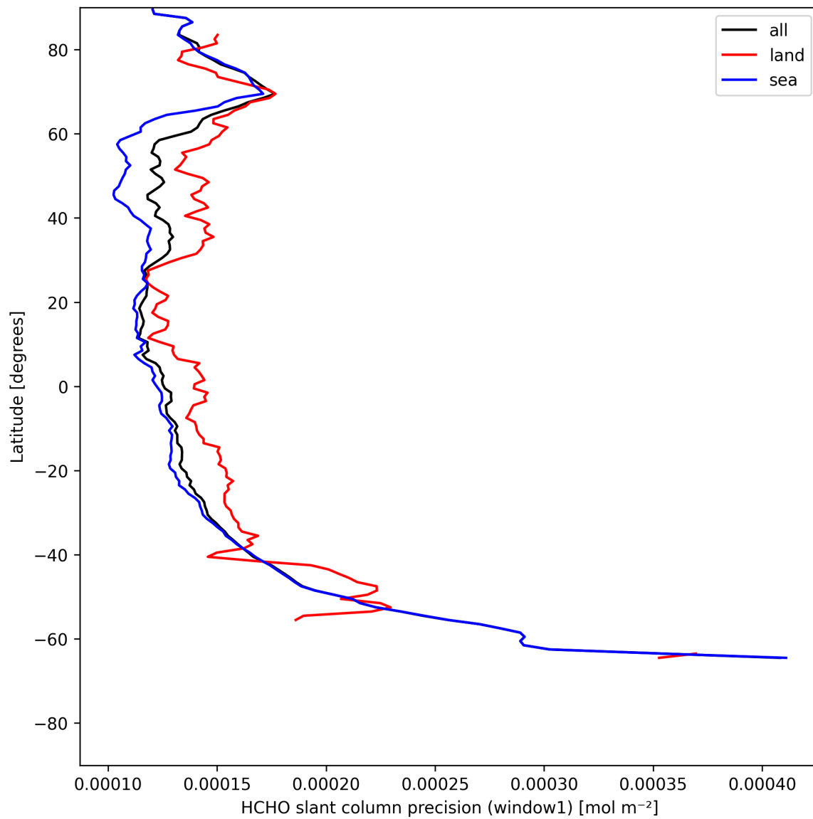
Figure 25: Zonal average of "HCHO slant column precision (window1)" for 2025-07-19 to 2025-07-21.
