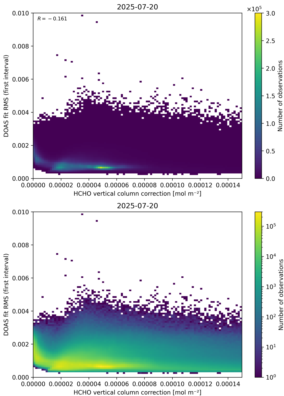
Figure 112: Scatter density plot of “HCHO vertical column correction” against “DOAS fit RMS (first interval)” for 2025-07-19 to 2025-07-21.
