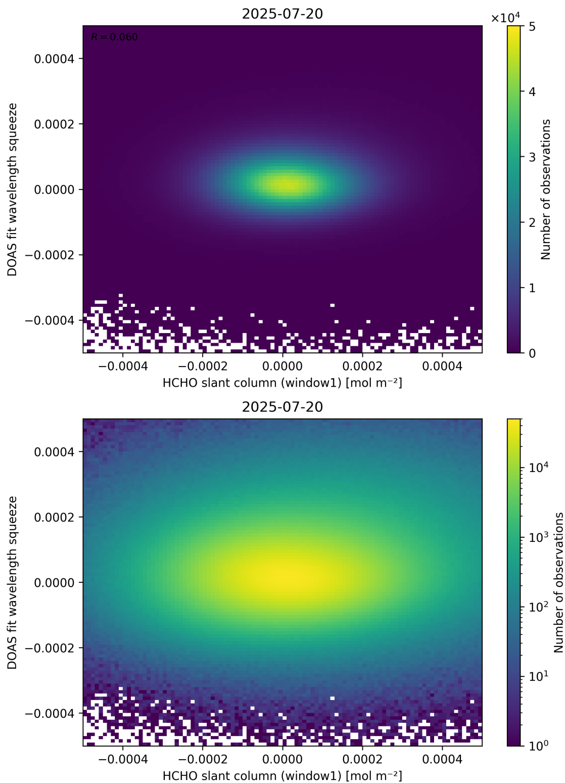
Figure 80: Scatter density plot of “HCHO slant column (window1)” against “DOAS fit wavelength squeeze” for 2025-07-19 to 2025-07-21.
