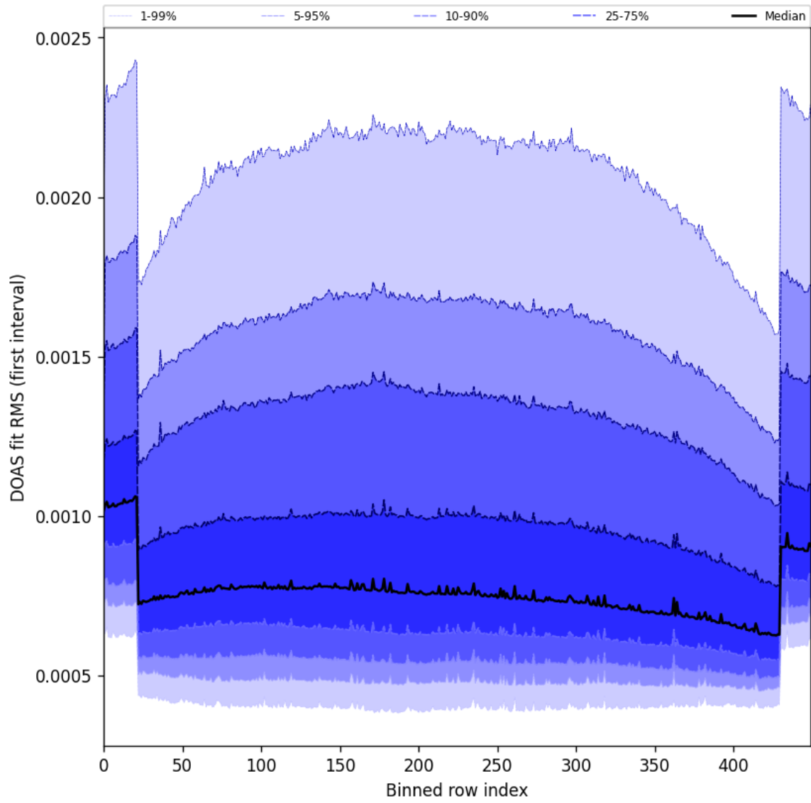
Figure 60: Along track statistics of “DOAS fit RMS (first interval)” for 2025-07-19 to 2025-07-21
