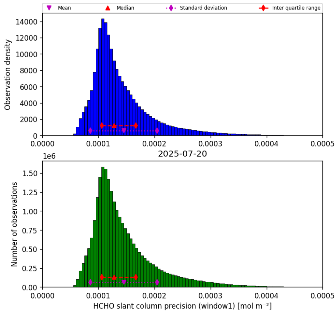
Figure 39: Histogram of “HCHO slant column precision (window1)” for 2025-07-19 to 2025-07-21
