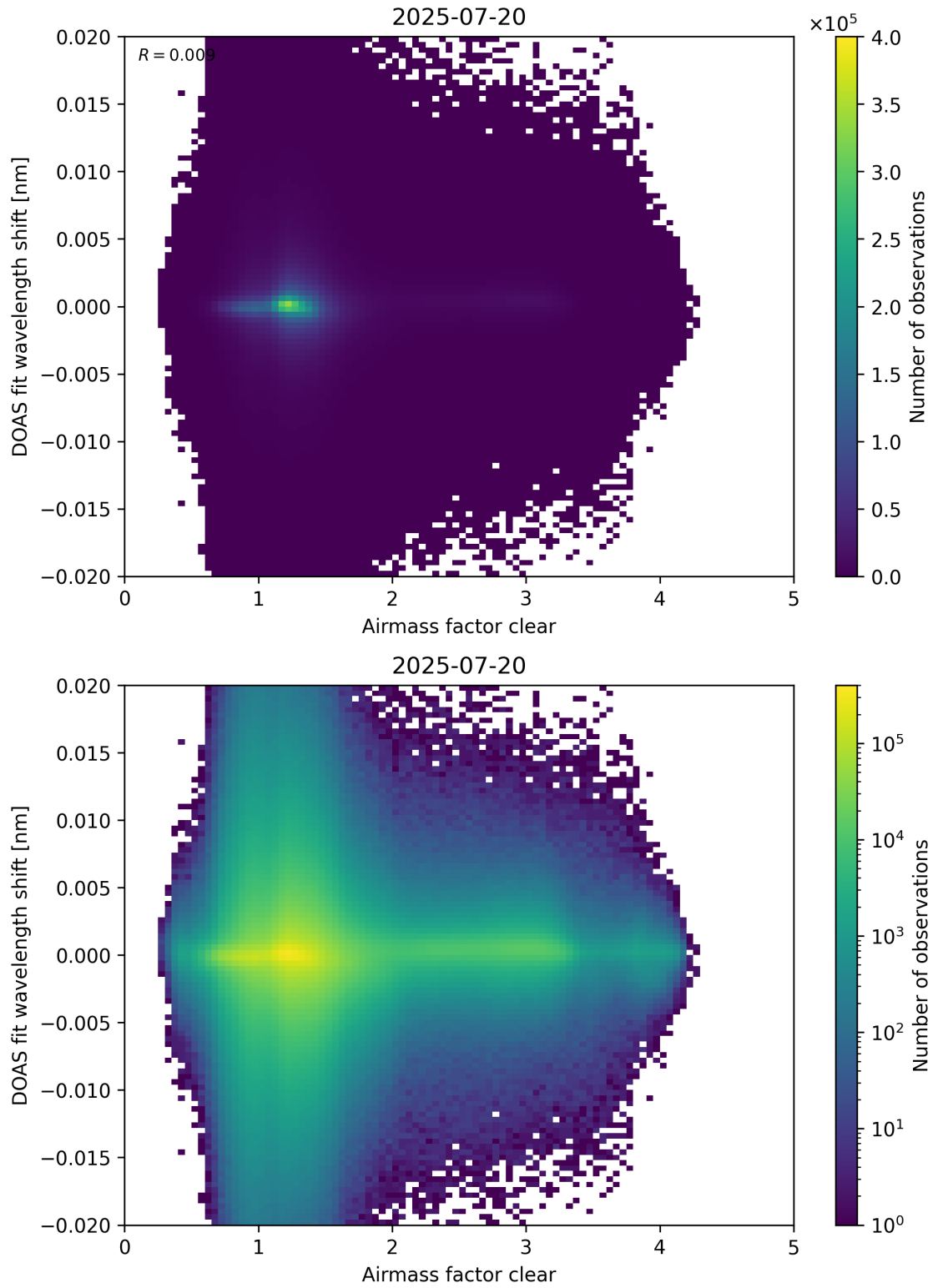
Figure 72: Scatter density plot of “Airmass factor clear” against “DOAS fit wavelength shift” for 2025-07-19 to 2025-07-21.
