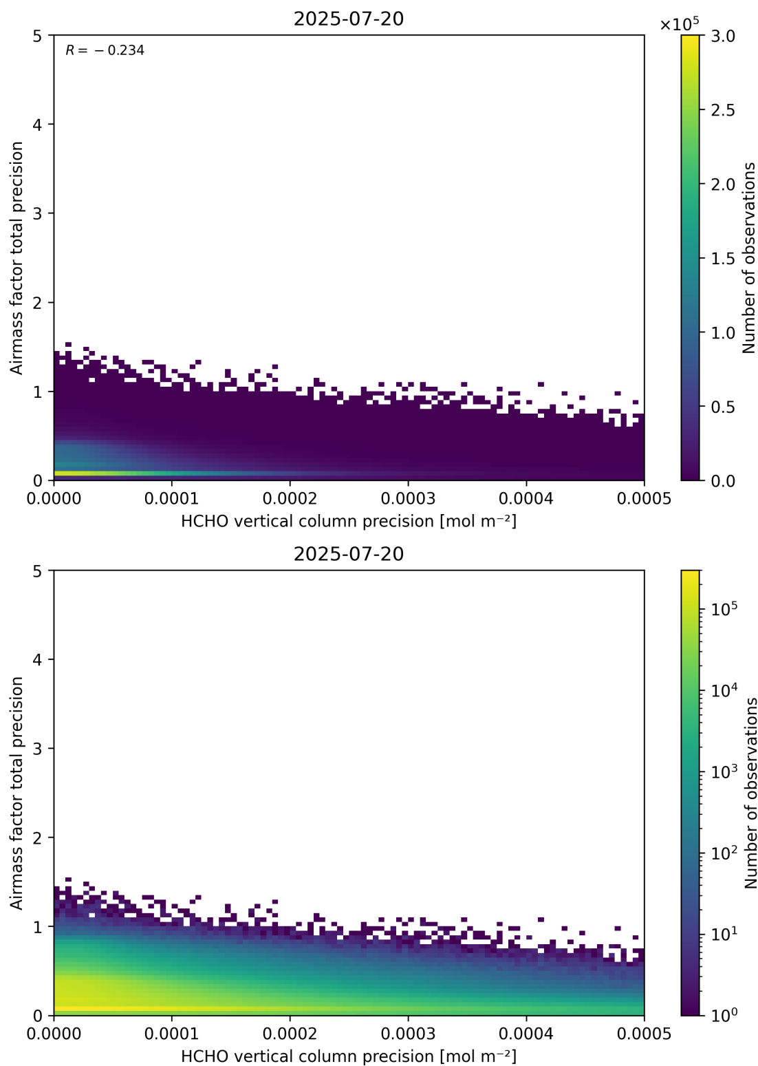
Figure 145: Scatter density plot of “HCHO vertical column precision” against “Airmass factor total precision” for 2025-07-19 to 2025-07-21.
