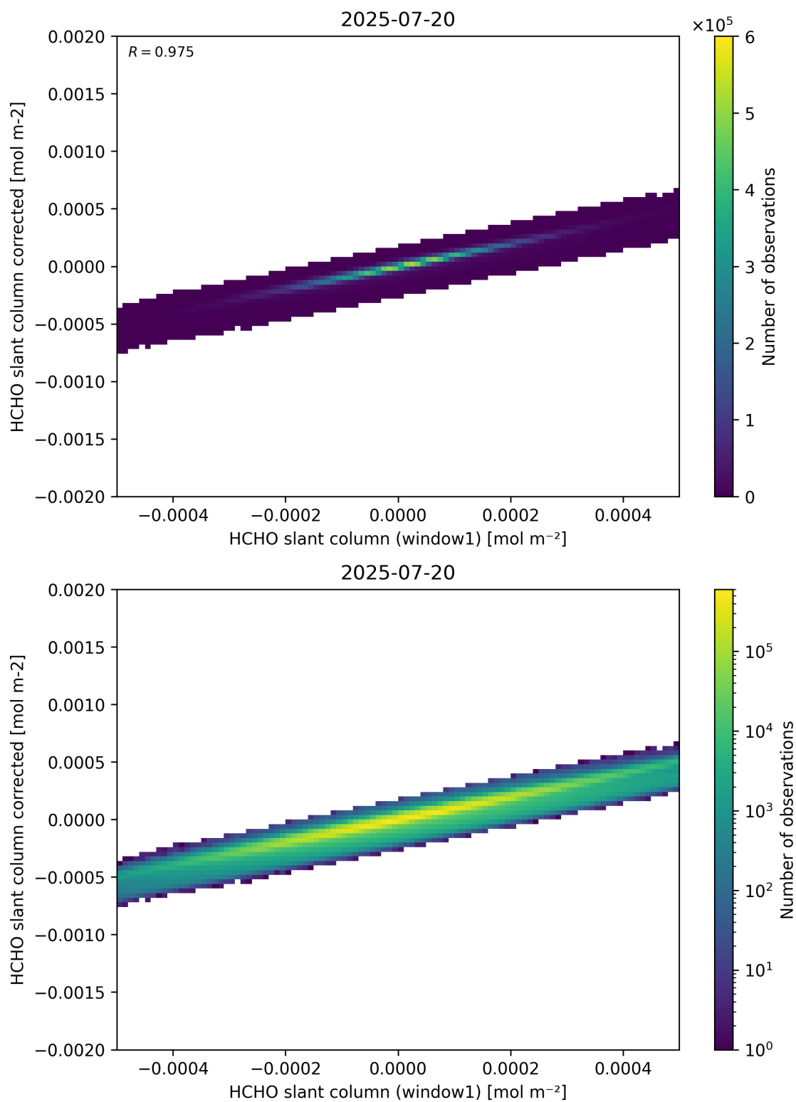
Figure 82: Scatter density plot of “HCHO slant column (window1)” against “HCHO slant column corrected” for 2025-07-19 to 2025-07-21.
