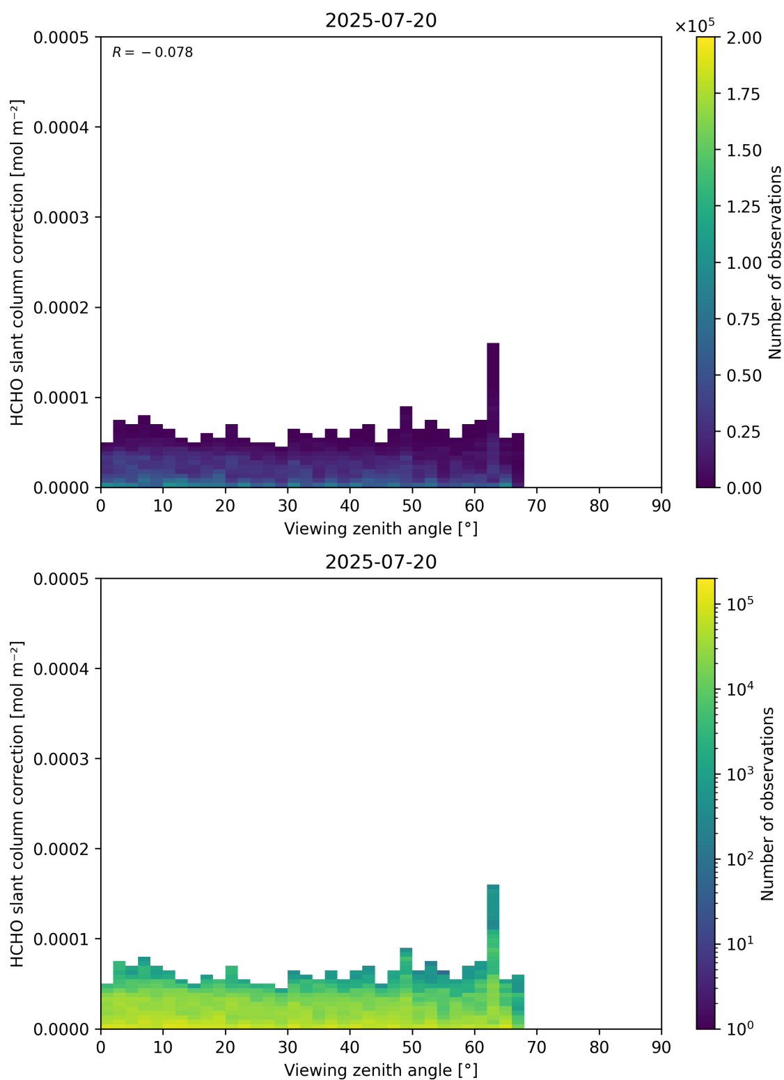
Figure 187: Scatter density plot of “Viewing zenith angle” against “HCHO slant column correction” for 2025-07-19 to 2025-07-21.
