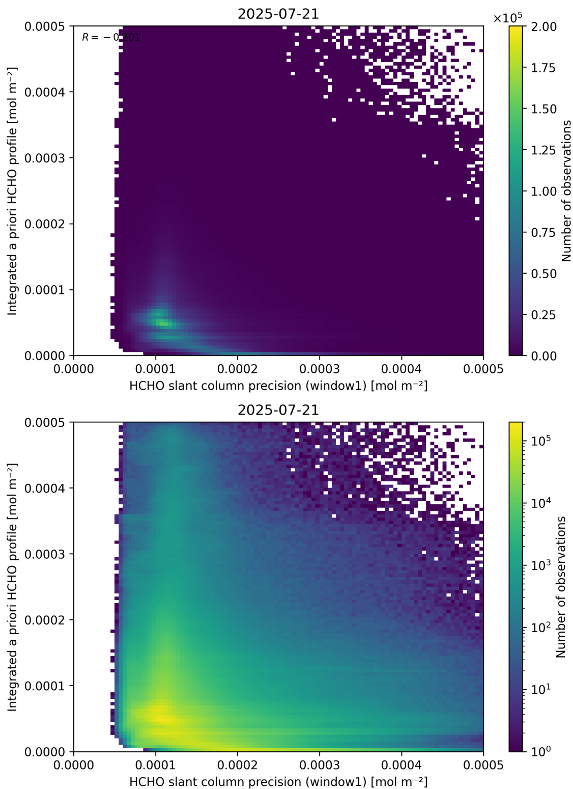
Figure 96: Scatter density plot of “HCHO slant column precision (window1)” against “Integrated a priori HCHO profile” for 2025-07-20 to 2025-07-22.
