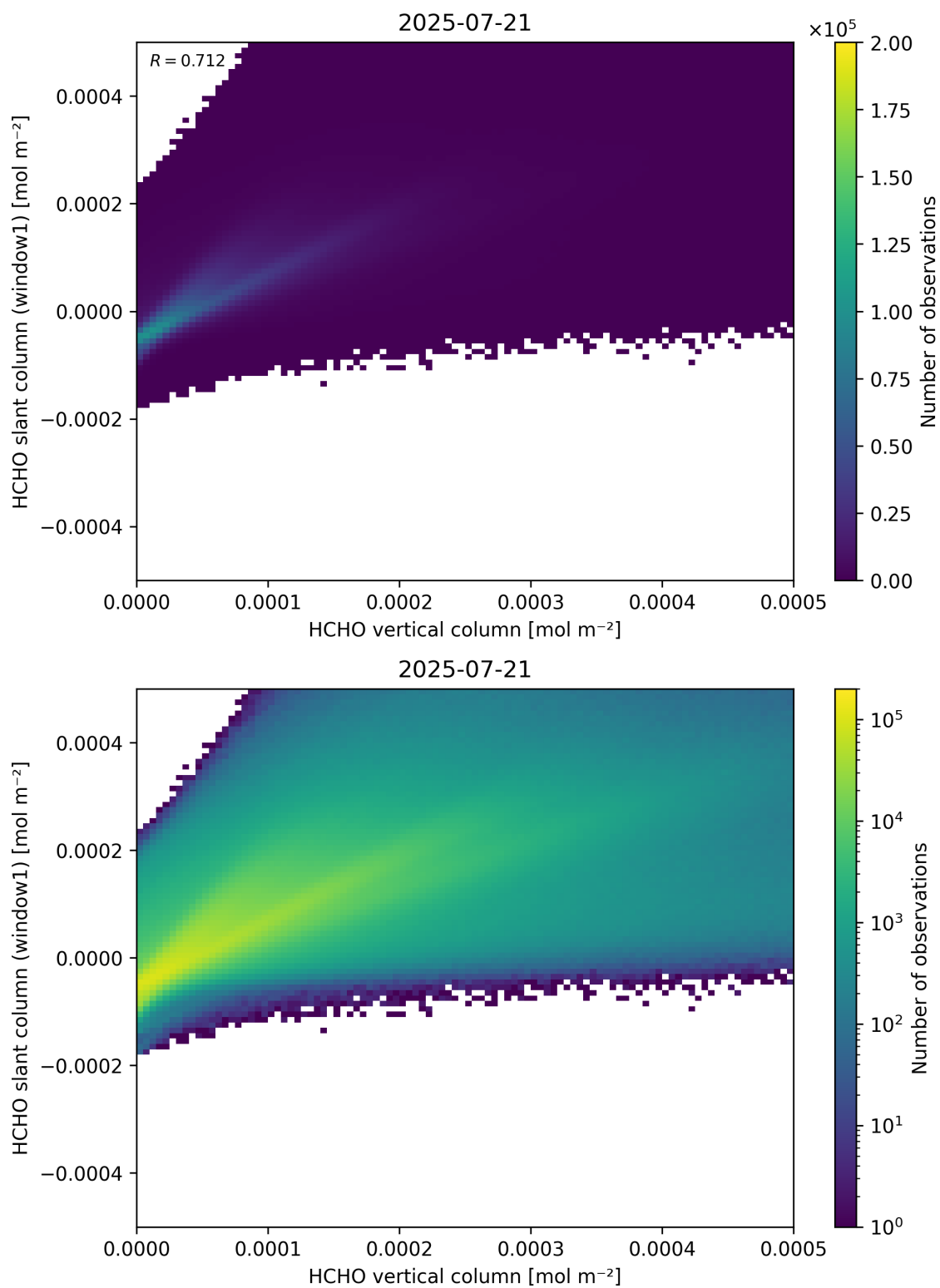
Figure 129: Scatter density plot of “HCHO vertical column” against “HCHO slant column (window1)” for 2025-07-20 to 2025-07-22.
