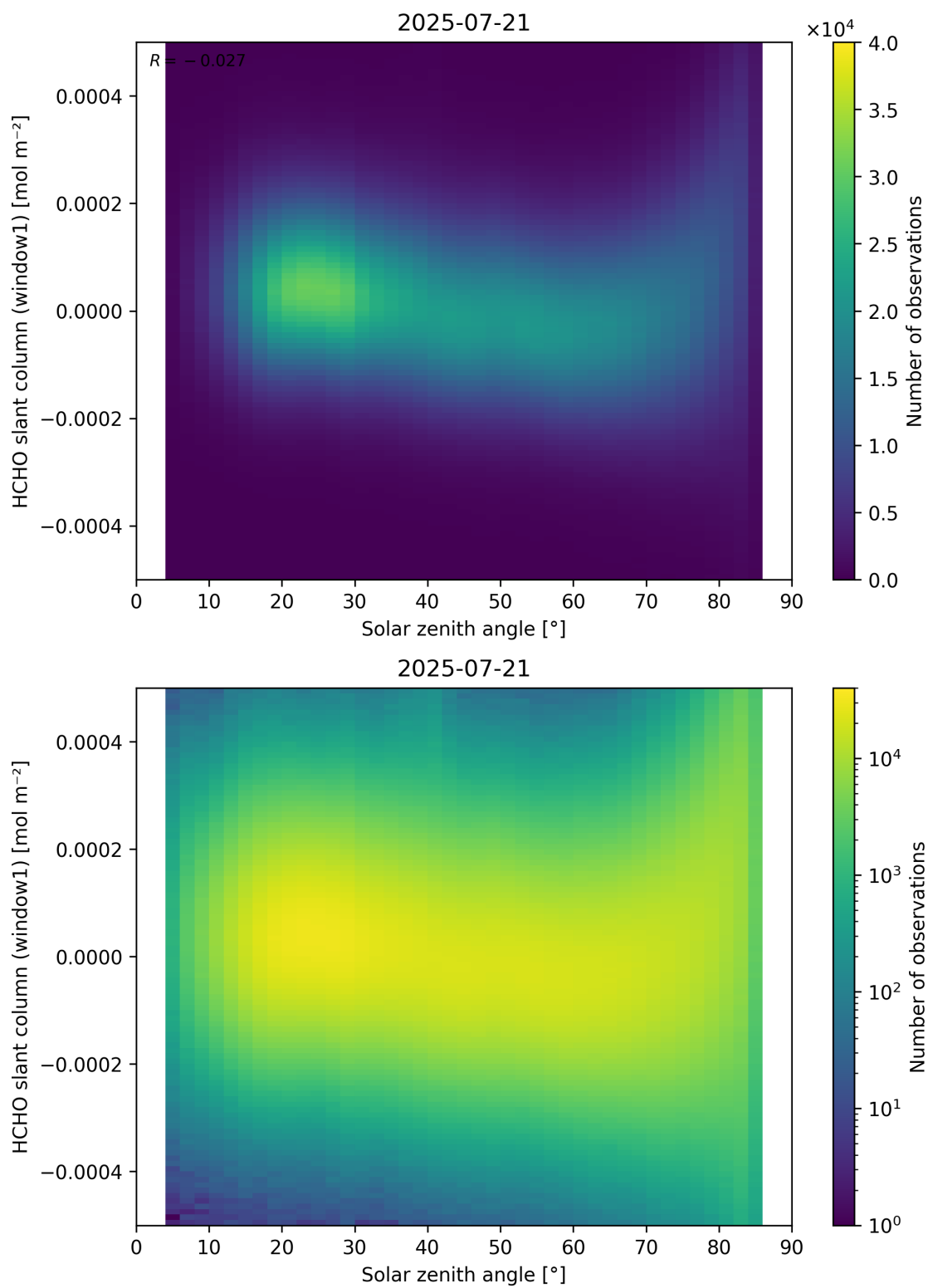
Figure 173: Scatter density plot of “Solar zenith angle” against “HCHO slant column (window1)” for 2025-07-20 to 2025-07-22.
