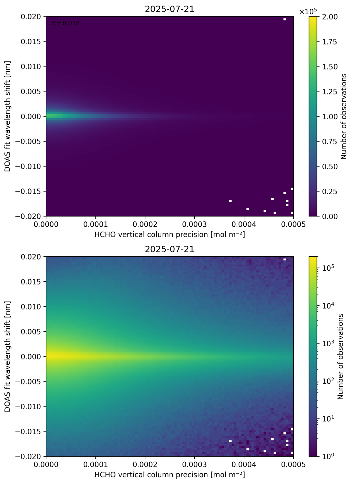
Figure 137: Scatter density plot of “HCHO vertical column precision” against “DOAS fit wavelength shift” for 2025-07-20 to 2025-07-22.
