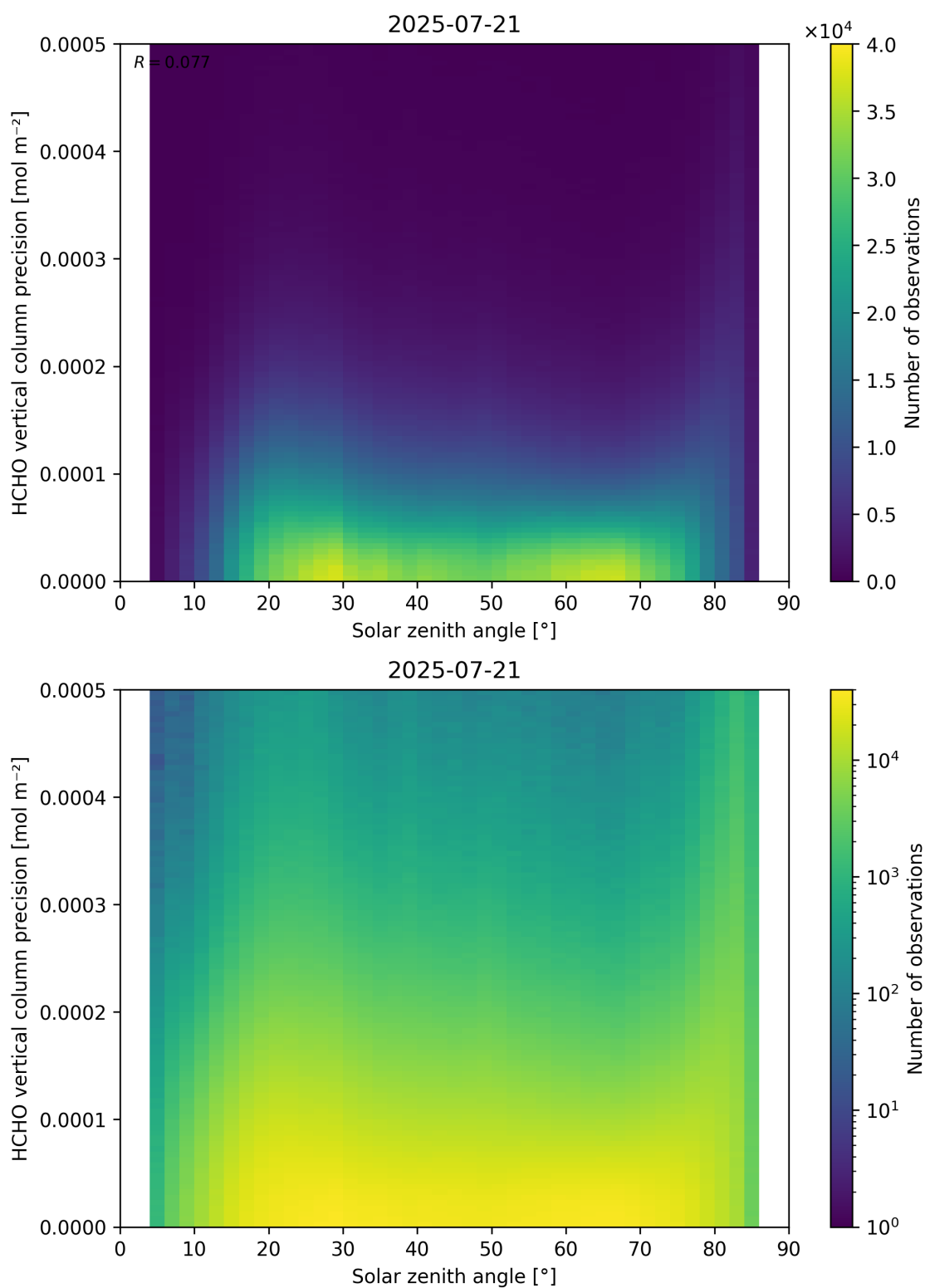
Figure 179: Scatter density plot of “Solar zenith angle” against “HCHO vertical column precision” for 2025-07-20 to 2025-07-22.
