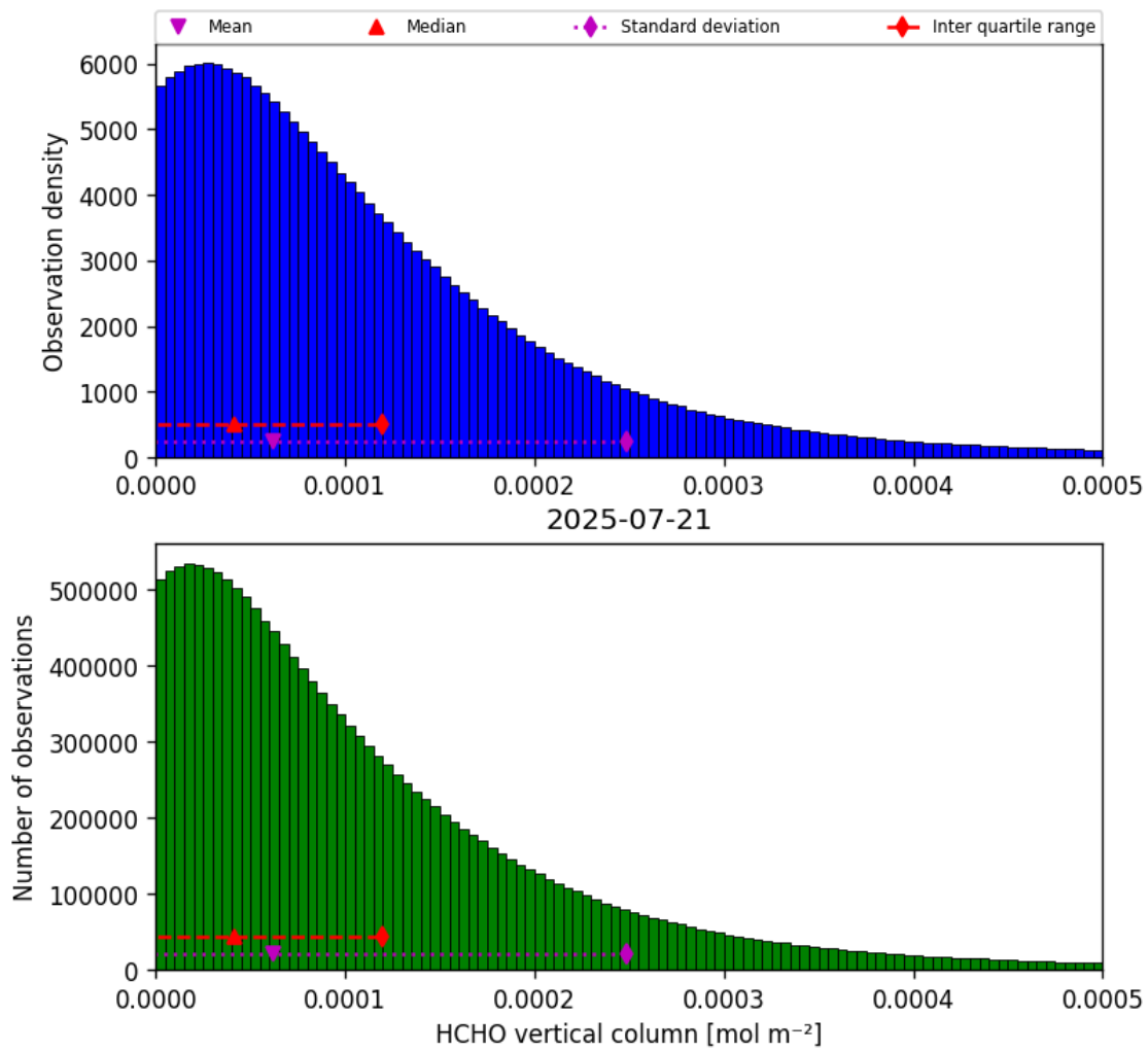
Figure 35: Histogram of “HCHO vertical column” for 2025-07-20 to 2025-07-22
