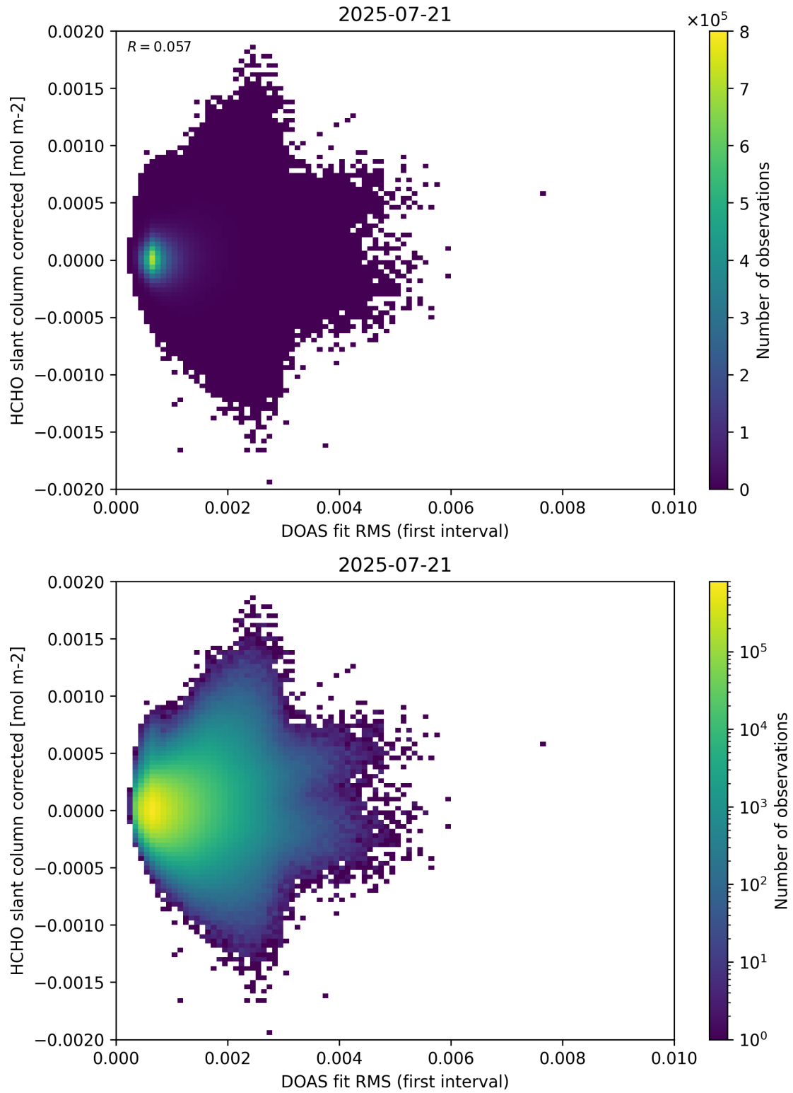
Figure 62: Scatter density plot of “DOAS fit RMS (first interval)” against “HCHO slant column corrected” for 2025-07-20 to 2025-07-22.
