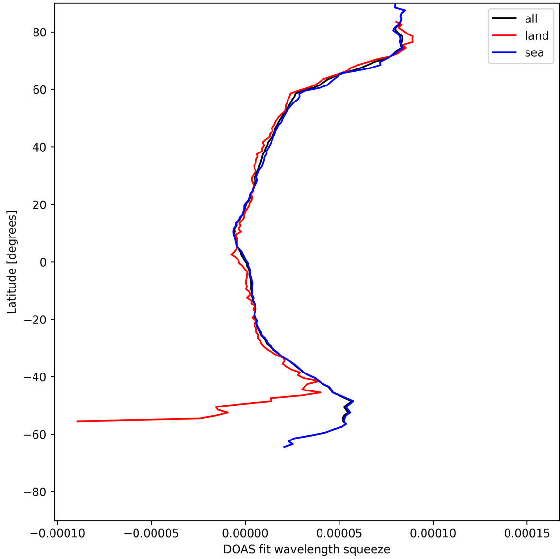
Figure 31: Zonal average of “DOAS fit wavelength squeeze” for 2025-07-20 to 2025-07-22.
