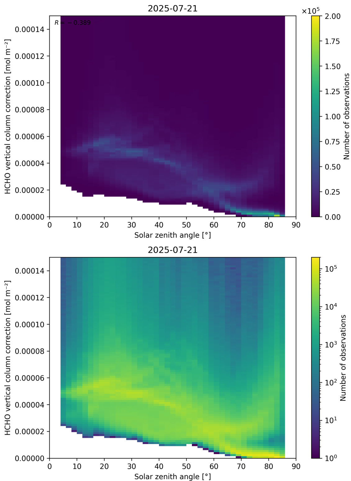
Figure 178: Scatter density plot of “Solar zenith angle” against “HCHO vertical column correction” for 2025-07-20 to 2025-07-22.
