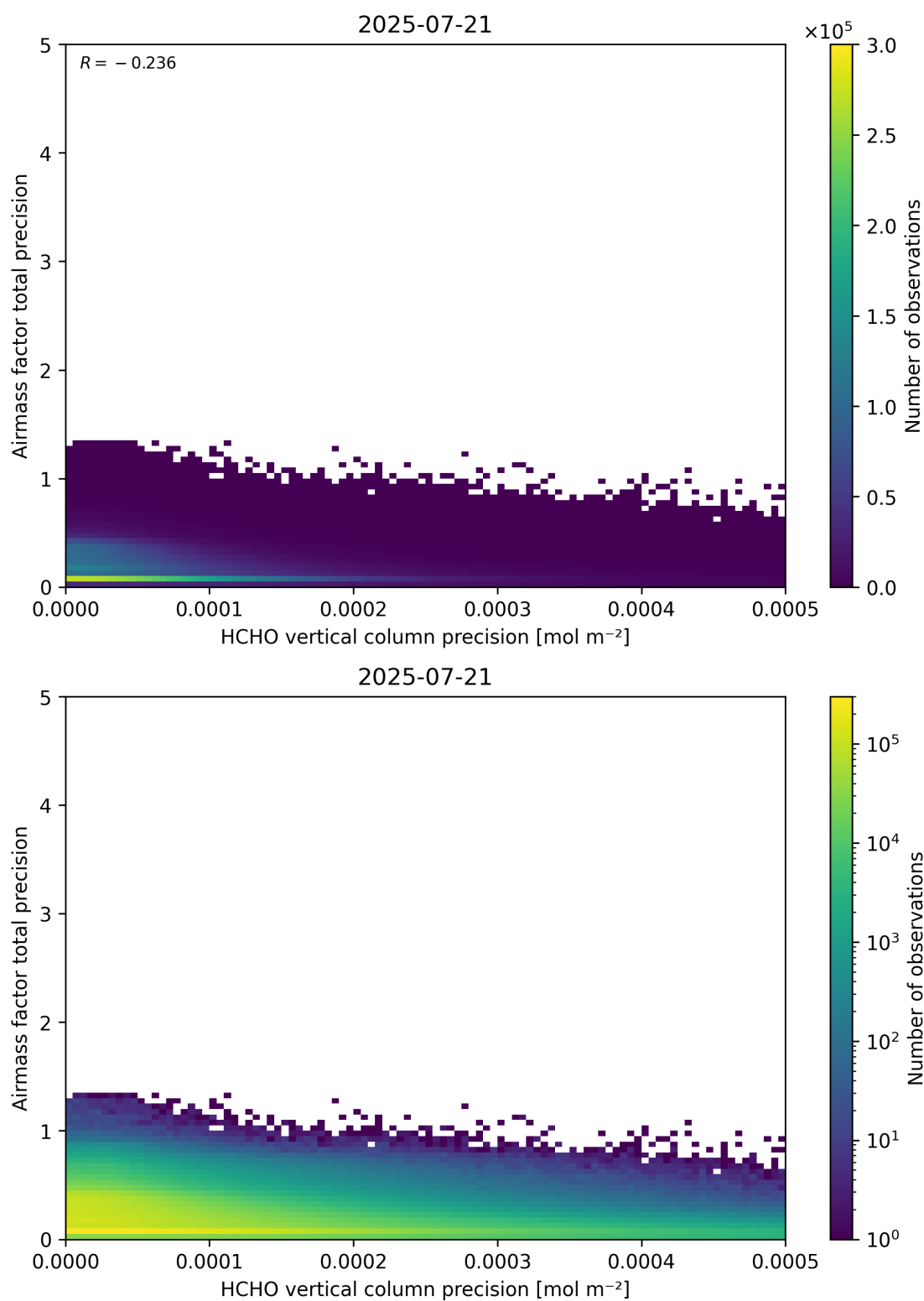
Figure 145: Scatter density plot of “HCHO vertical column precision” against “Airmass factor total precision” for 2025-07-20 to 2025-07-22.
