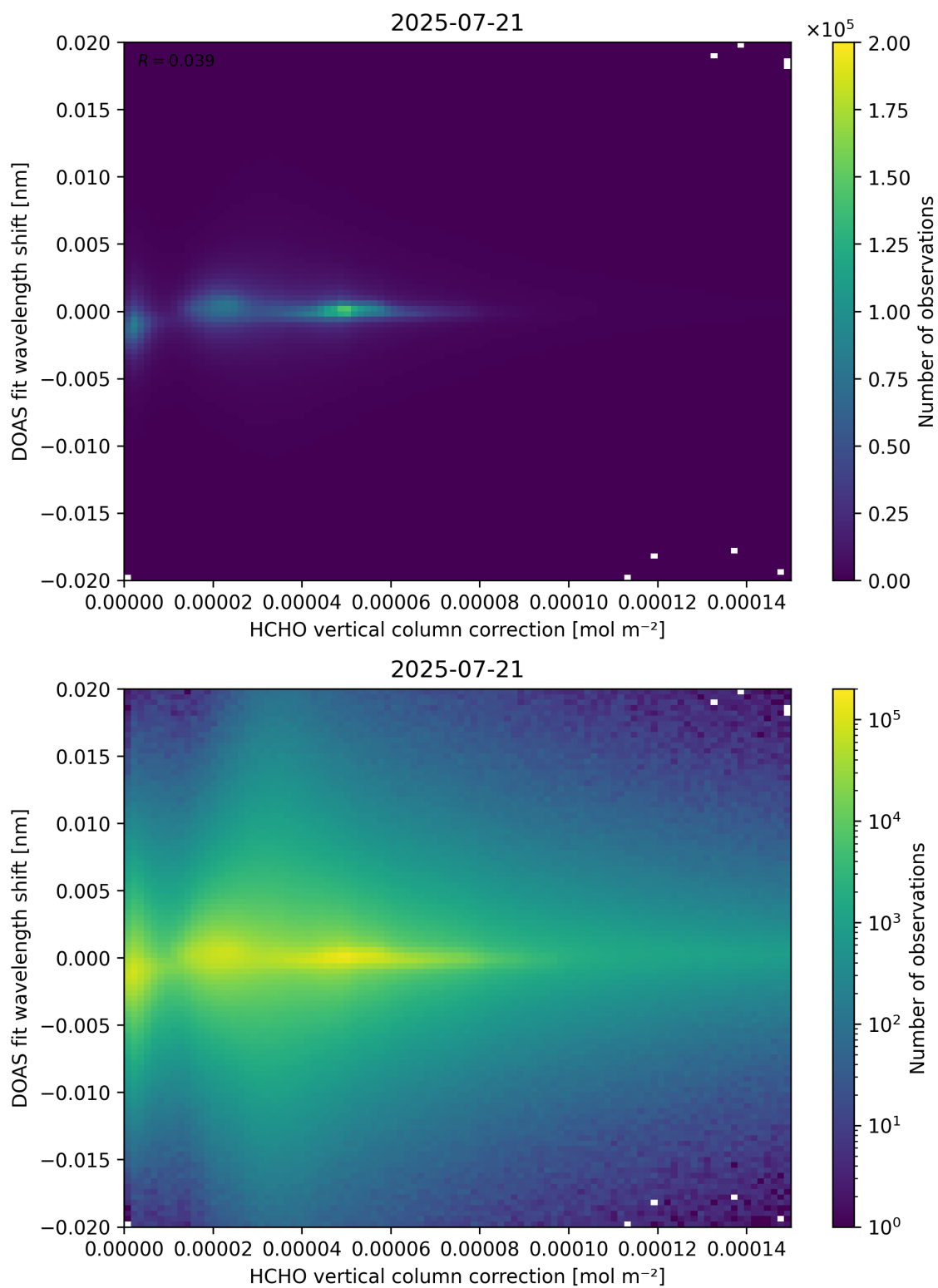
Figure 113: Scatter density plot of “HCHO vertical column correction” against “DOAS fit wavelength shift” for 2025-07-20 to 2025-07-22.
