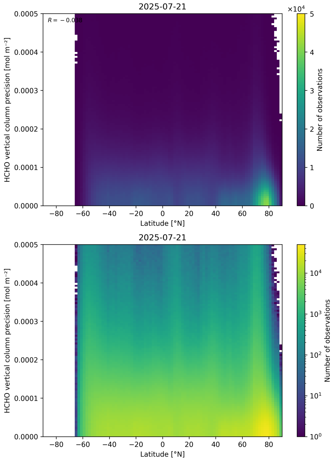
Figure 165: Scatter density plot of “Latitude” against “HCHO vertical column precision” for 2025-07-20 to 2025-07-22.
