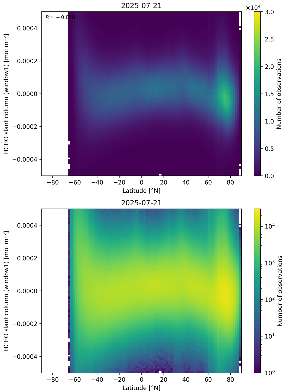
Figure 159: Scatter density plot of “Latitude” against “HCHO slant column (window1)” for 2025-07-20 to 2025-07-22.
