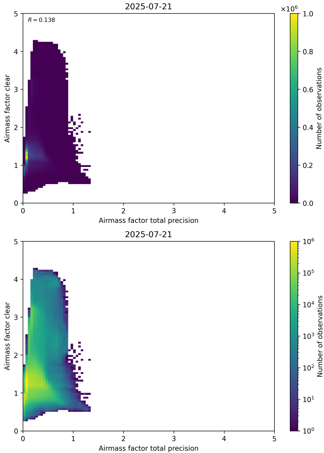
Figure 108: Scatter density plot of “Airmass factor total precision” against “Airmass factor clear” for 2025-07-20 to 2025-07-22.
