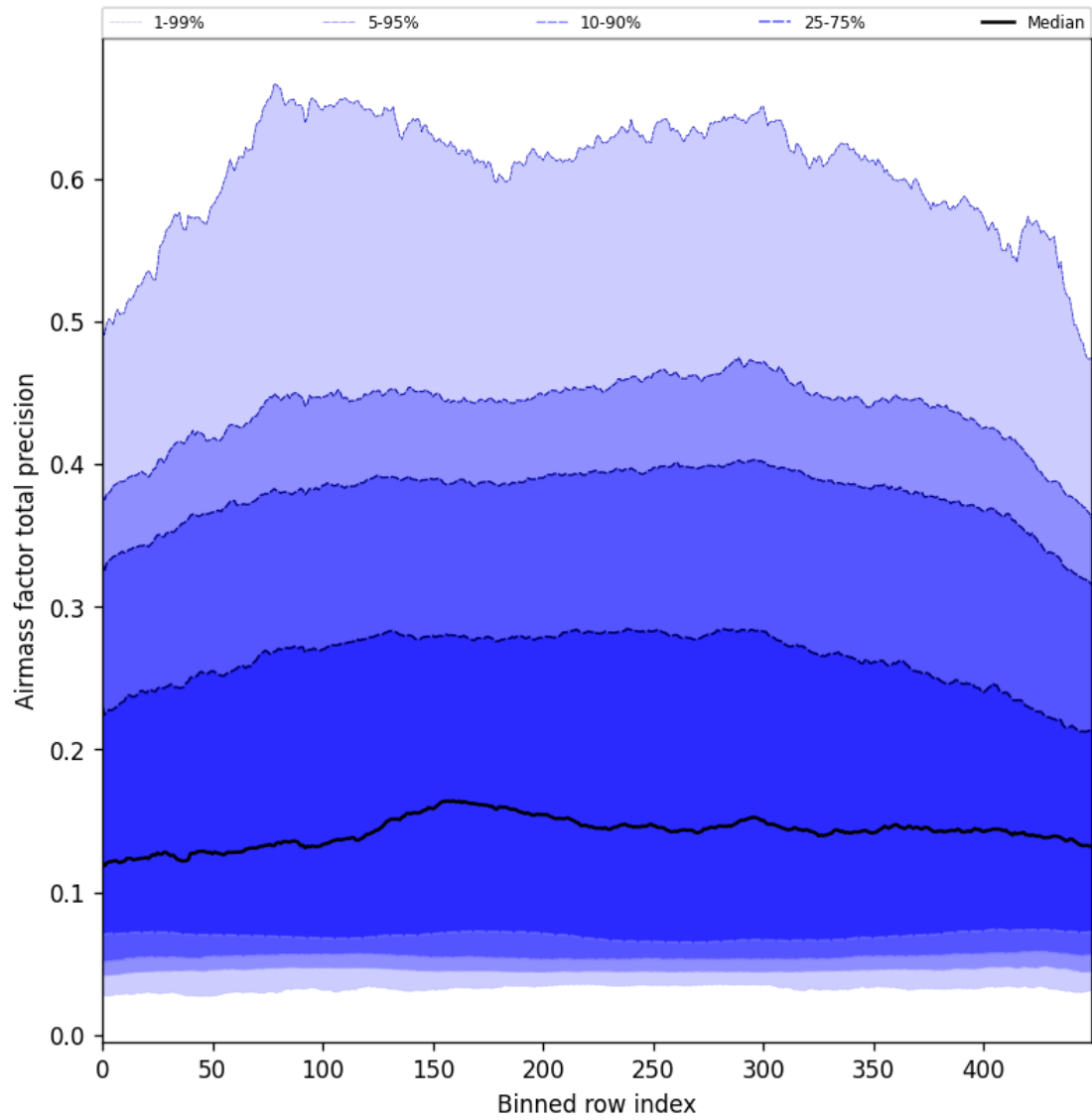
Figure 55: Along track statistics of “Airmass factor total precision” for 2025-07-20 to 2025-07-22
