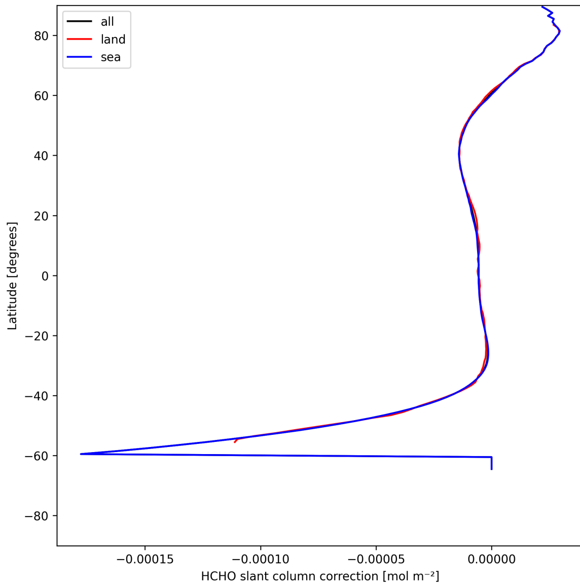
Figure 33: Zonal average of “HCHO slant column correction” for 2025-07-20 to 2025-07-22.
