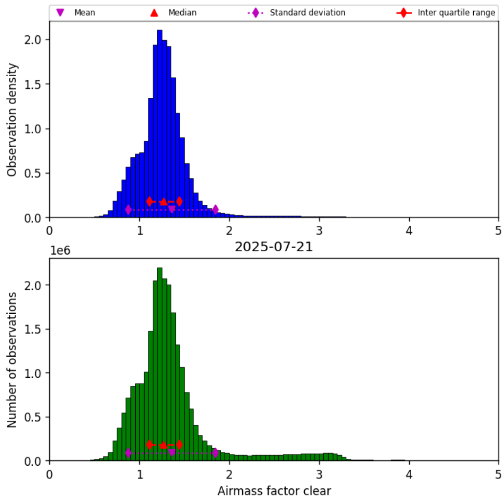
Figure 42: Histogram of “Airmass factor clear” for 2025-07-20 to 2025-07-22
