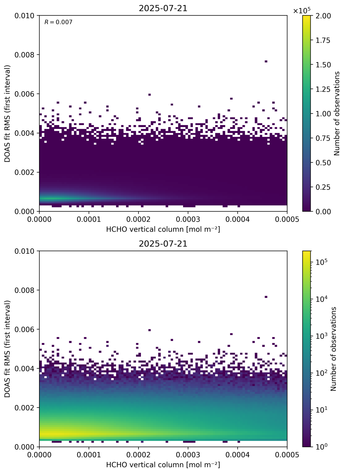
Figure 123: Scatter density plot of “HCHO vertical column” against “DOAS fit RMS (first interval)” for 2025-07-20 to 2025-07-22.
