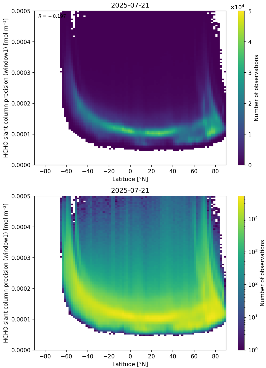
Figure 160: Scatter density plot of “Latitude” against “HCHO slant column precision (window1)” for 2025-07-20 to 2025-07-22.
