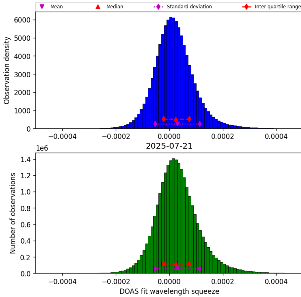
Figure 45: Histogram of “DOAS fit wavelength squeeze” for 2025-07-20 to 2025-07-22
