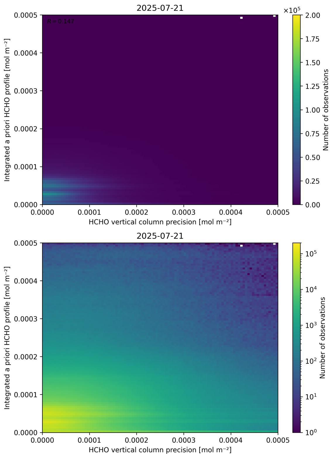
Figure 147: Scatter density plot of “HCHO vertical column precision” against “Integrated a priori HCHO profile” for 2025-07-20 to 2025-07-22.
