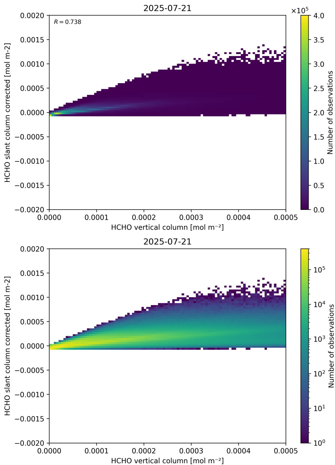
Figure 127: Scatter density plot of “HCHO vertical column” against “HCHO slant column corrected” for 2025-07-20 to 2025-07-22.
