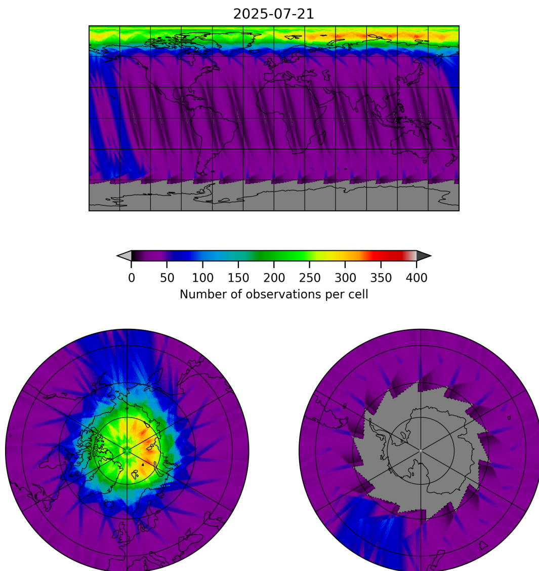
Figure 19: Map of the number of observations for 2025-07-20 to 2025-07-22
