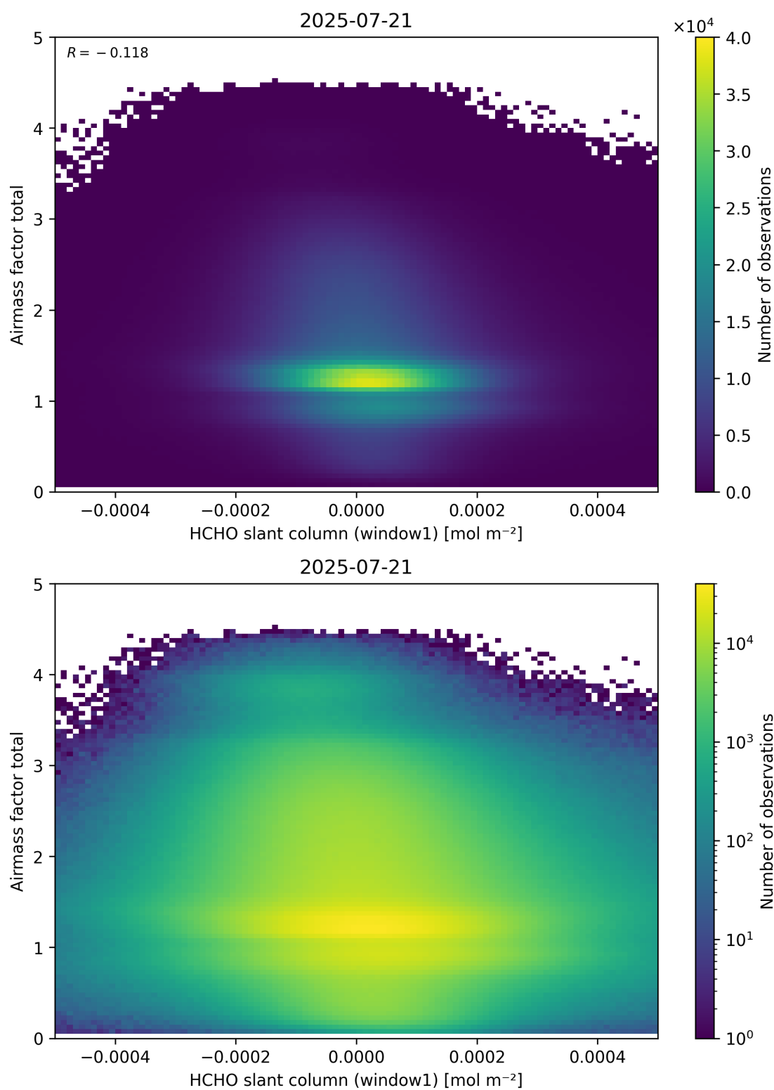
Figure 85: Scatter density plot of “HCHO slant column (window1)” against “Airmass factor total” for 2025-07-20 to 2025-07-22.
