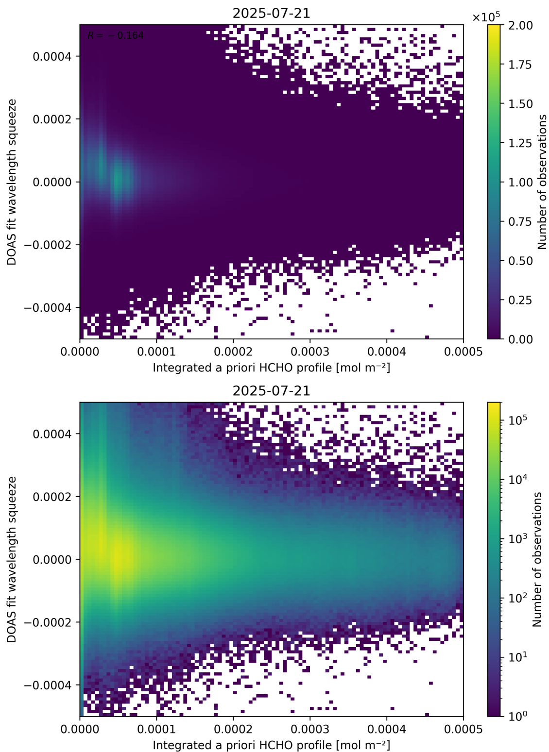
Figure 150: Scatter density plot of “Integrated a priori HCHO profile” against “DOAS fit wavelength squeeze” for 2025-07-20 to 2025-07-22.
