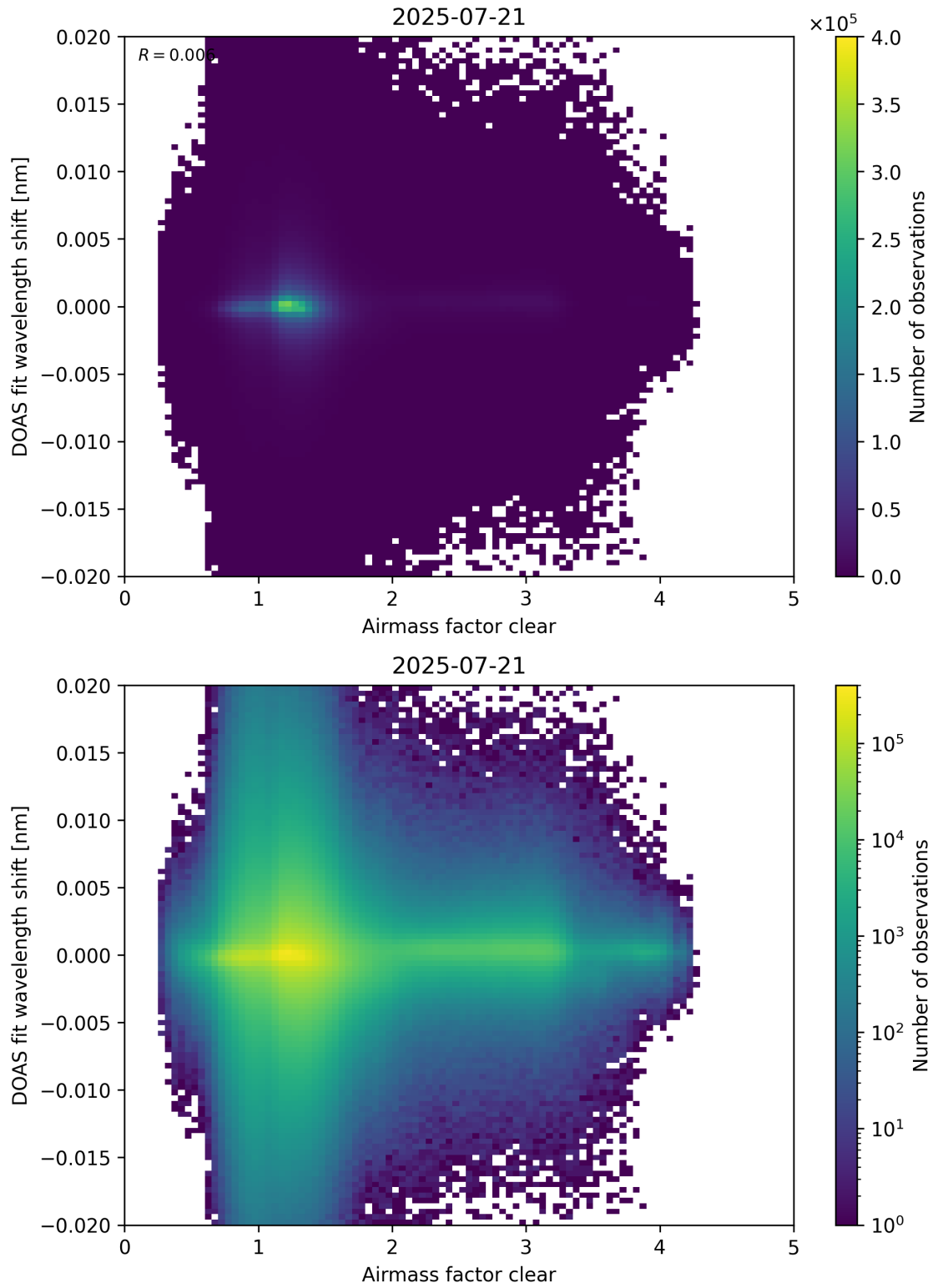
Figure 72: Scatter density plot of “Airmass factor clear” against “DOAS fit wavelength shift” for 2025-07-20 to 2025-07-22.
