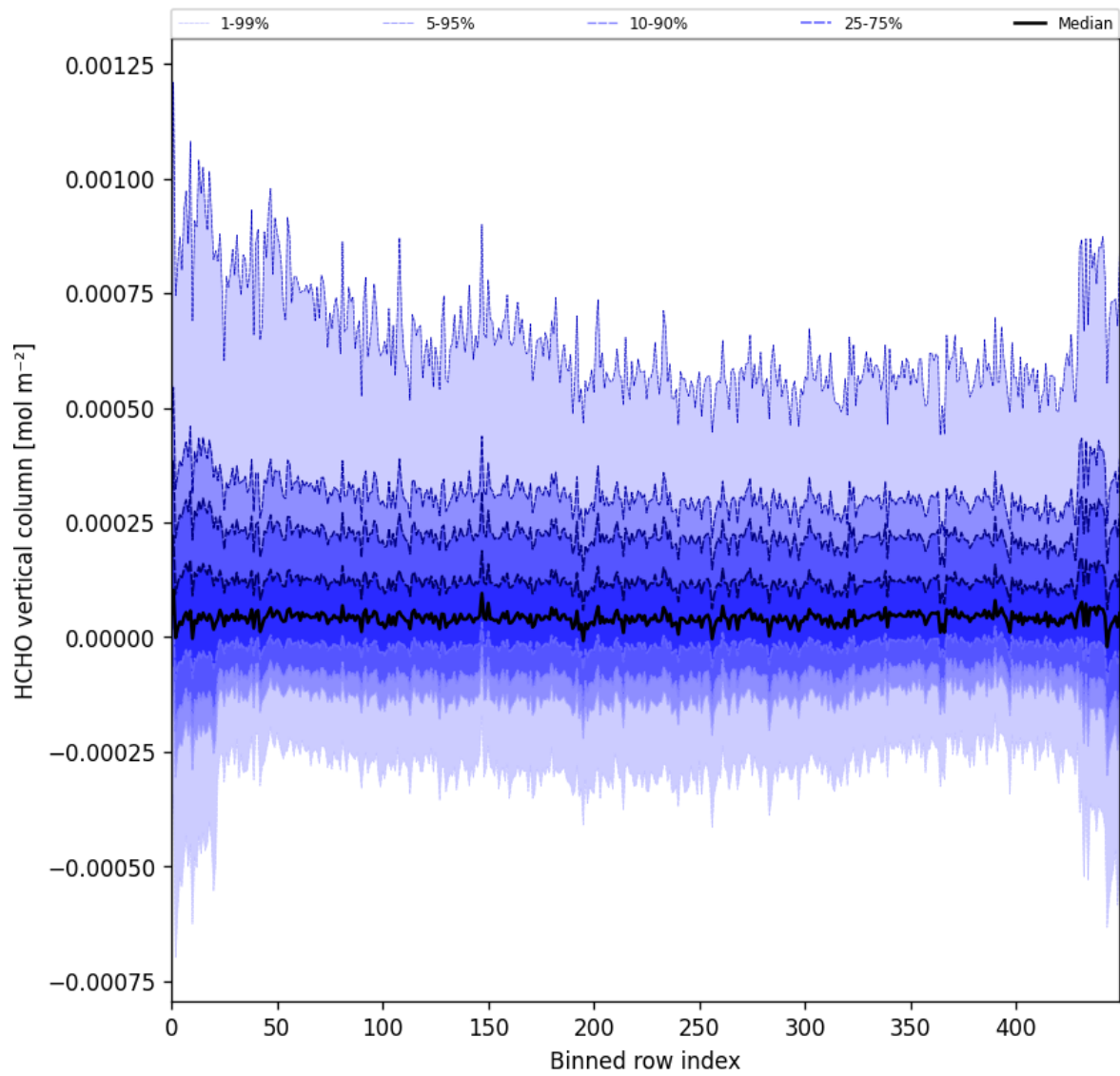
Figure 49: Along track statistics of “HCHO vertical column” for 2025-07-20 to 2025-07-22
