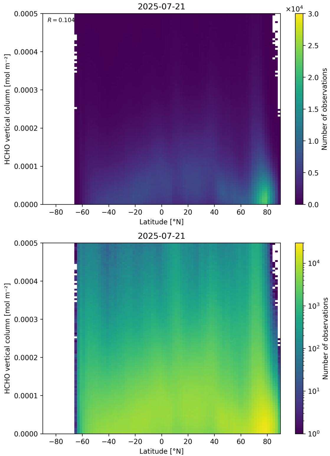
Figure 163: Scatter density plot of “Latitude” against “HCHO vertical column” for 2025-07-20 to 2025-07-22.
