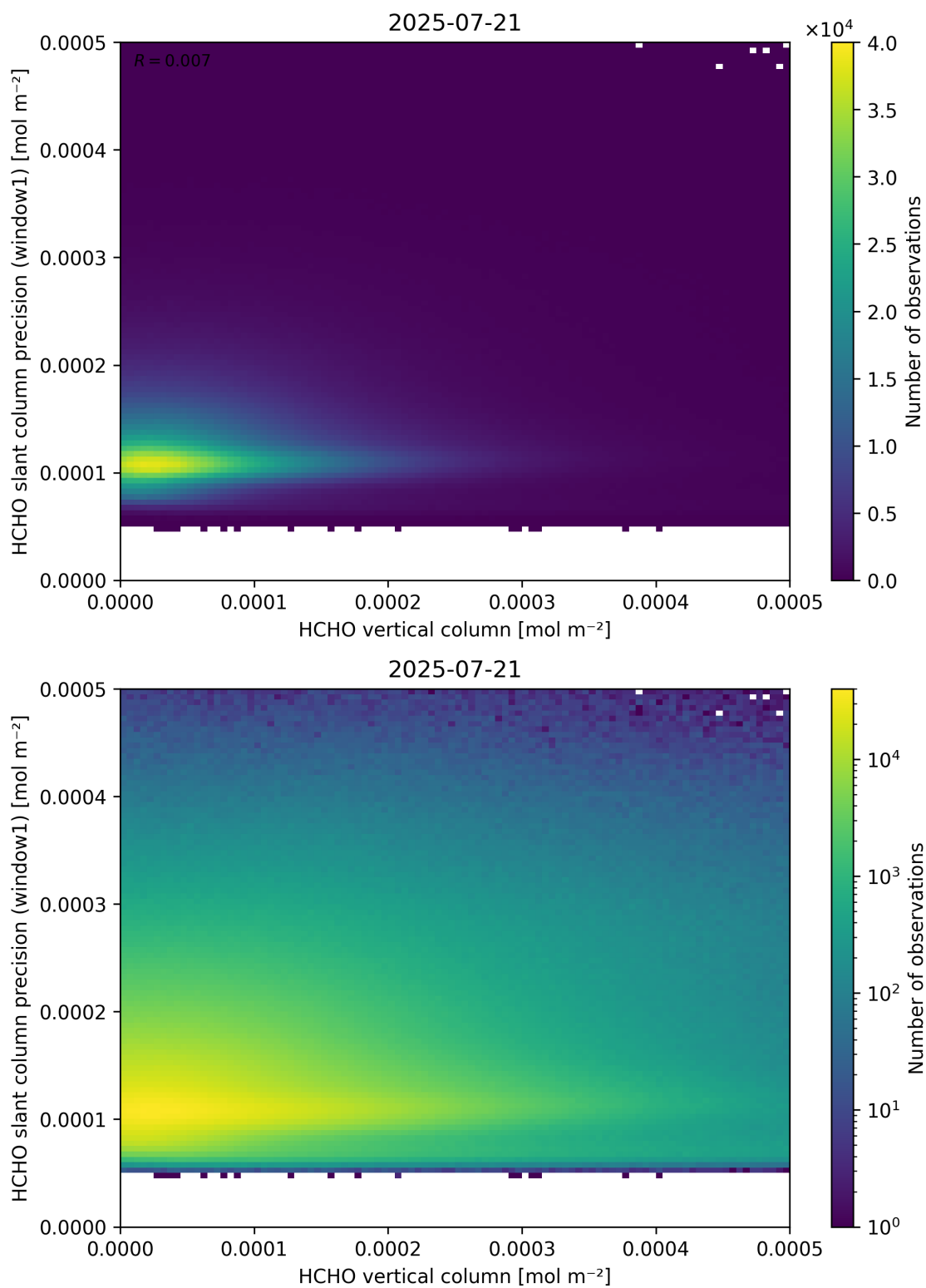
Figure 130: Scatter density plot of “HCHO vertical column” against “HCHO slant column precision (window1)” for 2025-07-20 to 2025-07-22.
