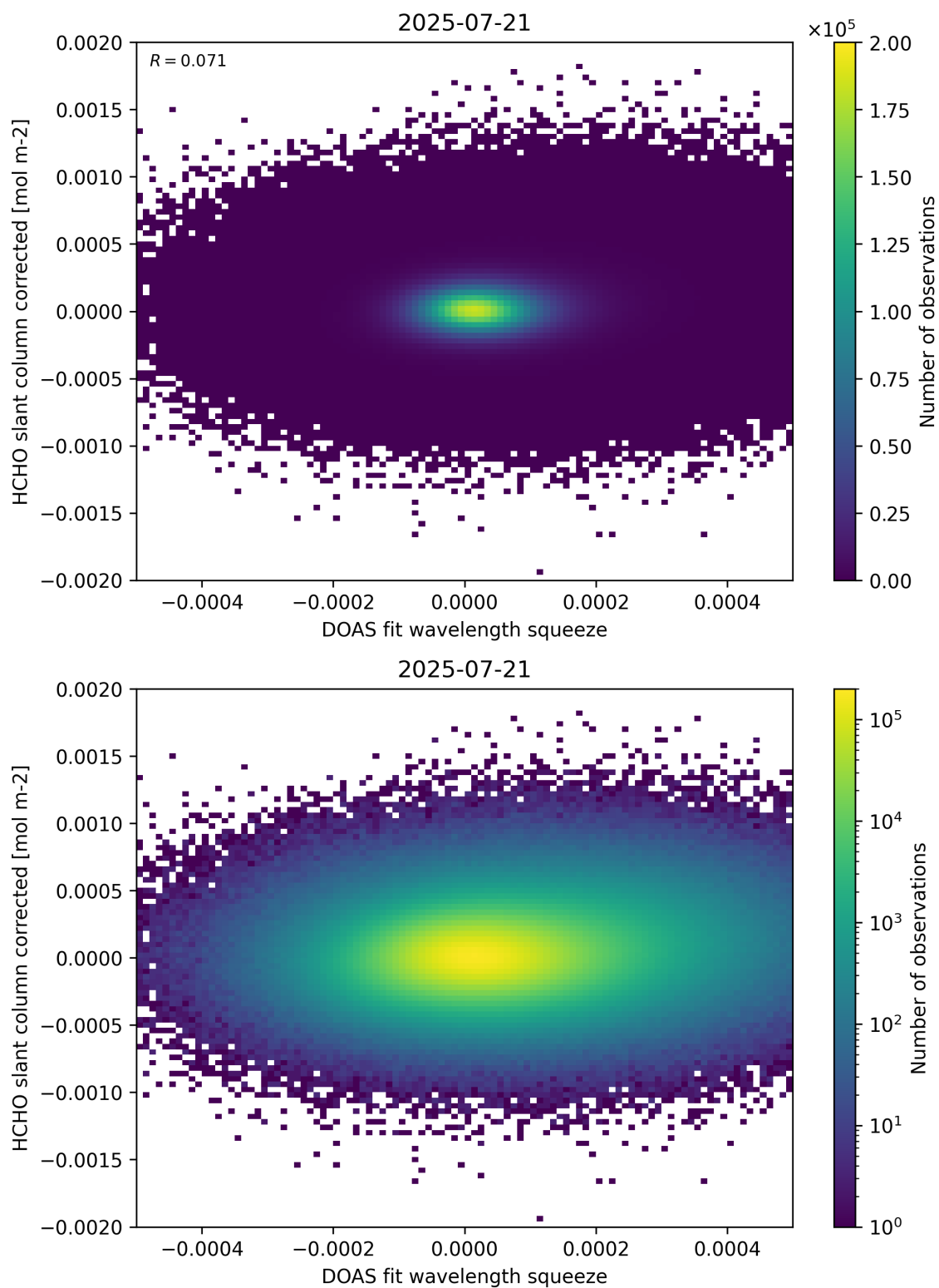
Figure 69: Scatter density plot of “DOAS fit wavelength squeeze” against “HCHO slant column corrected” for 2025-07-20 to 2025-07-22.
