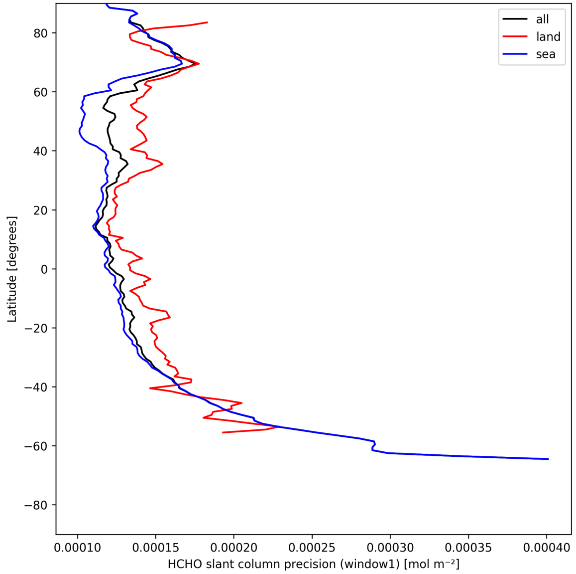
Figure 25: Zonal average of “HCHO slant column precision (window1)” for 2025-07-20 to 2025-07-22.
