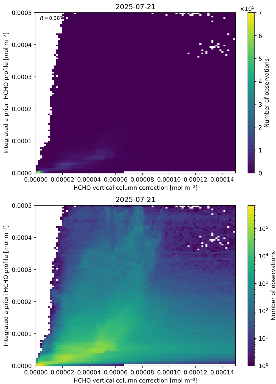
Figure 122: Scatter density plot of “HCHO vertical column correction” against “Integrated a priori HCHO profile” for 2025-07-20 to 2025-07-22.
