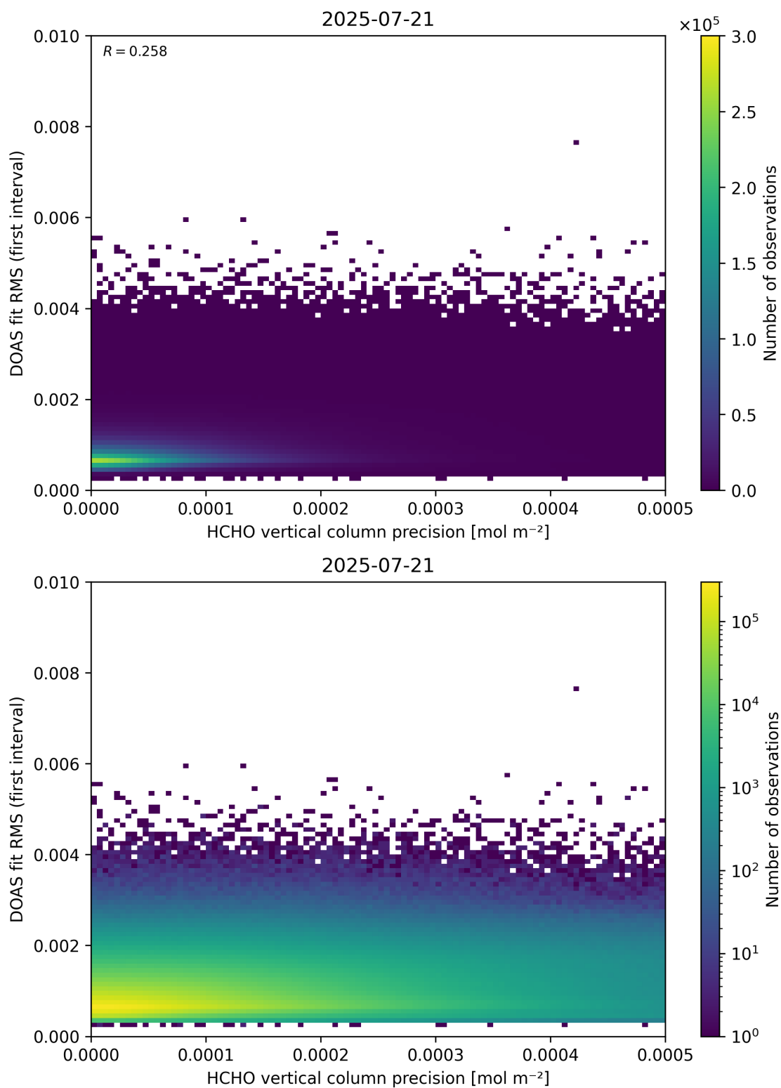
Figure 136: Scatter density plot of “HCHO vertical column precision” against “DOAS fit RMS (first interval)” for 2025-07-20 to 2025-07-22.
