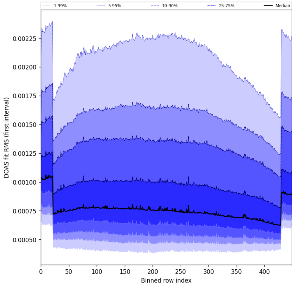
Figure 60: Along track statistics of “DOAS fit RMS (first interval)” for 2025-07-20 to 2025-07-22
