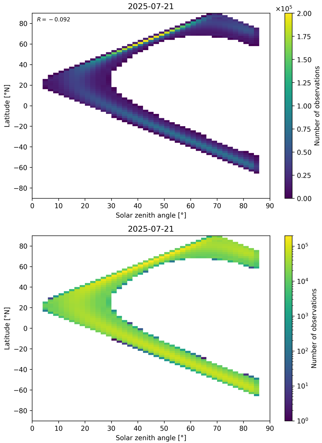
Figure 181: Scatter density plot of “Solar zenith angle” against “Latitude” for 2025-07-20 to 2025-07-22.
