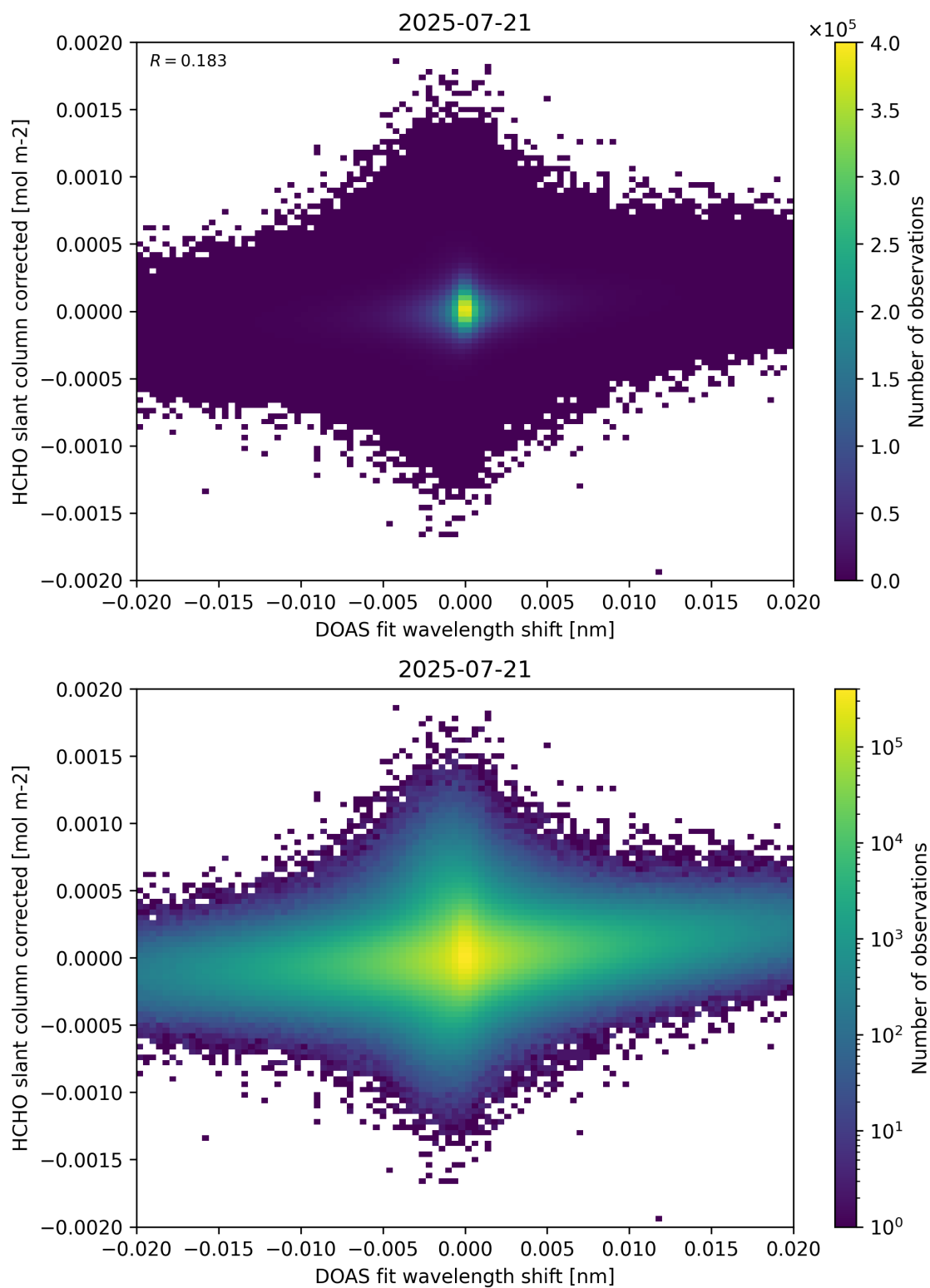
Figure 66: Scatter density plot of “DOAS fit wavelength shift” against “HCHO slant column corrected” for 2025-07-20 to 2025-07-22.
