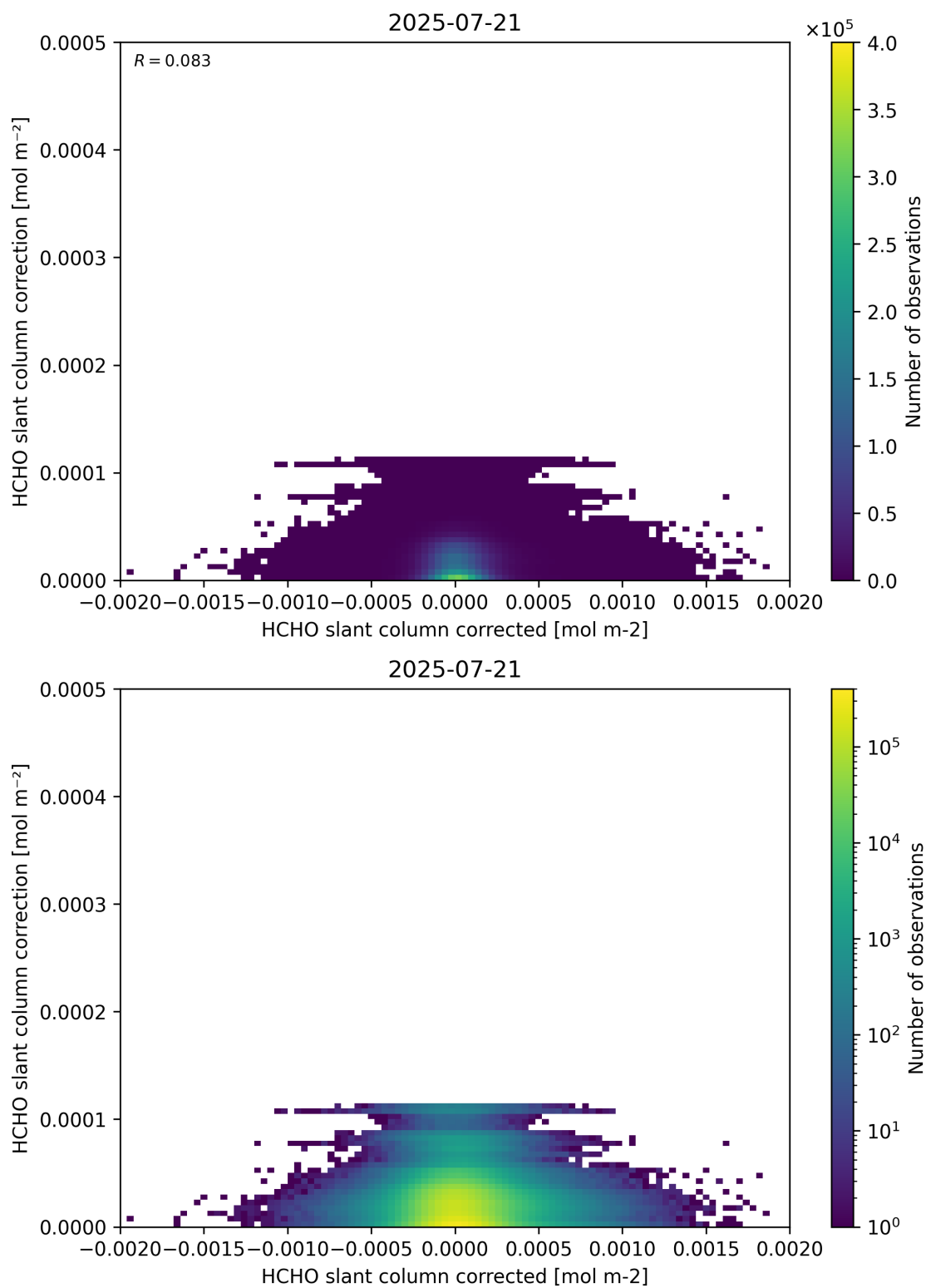
Figure 77: Scatter density plot of “HCHO slant column corrected” against “HCHO slant column correction” for 2025-07-20 to 2025-07-22.
