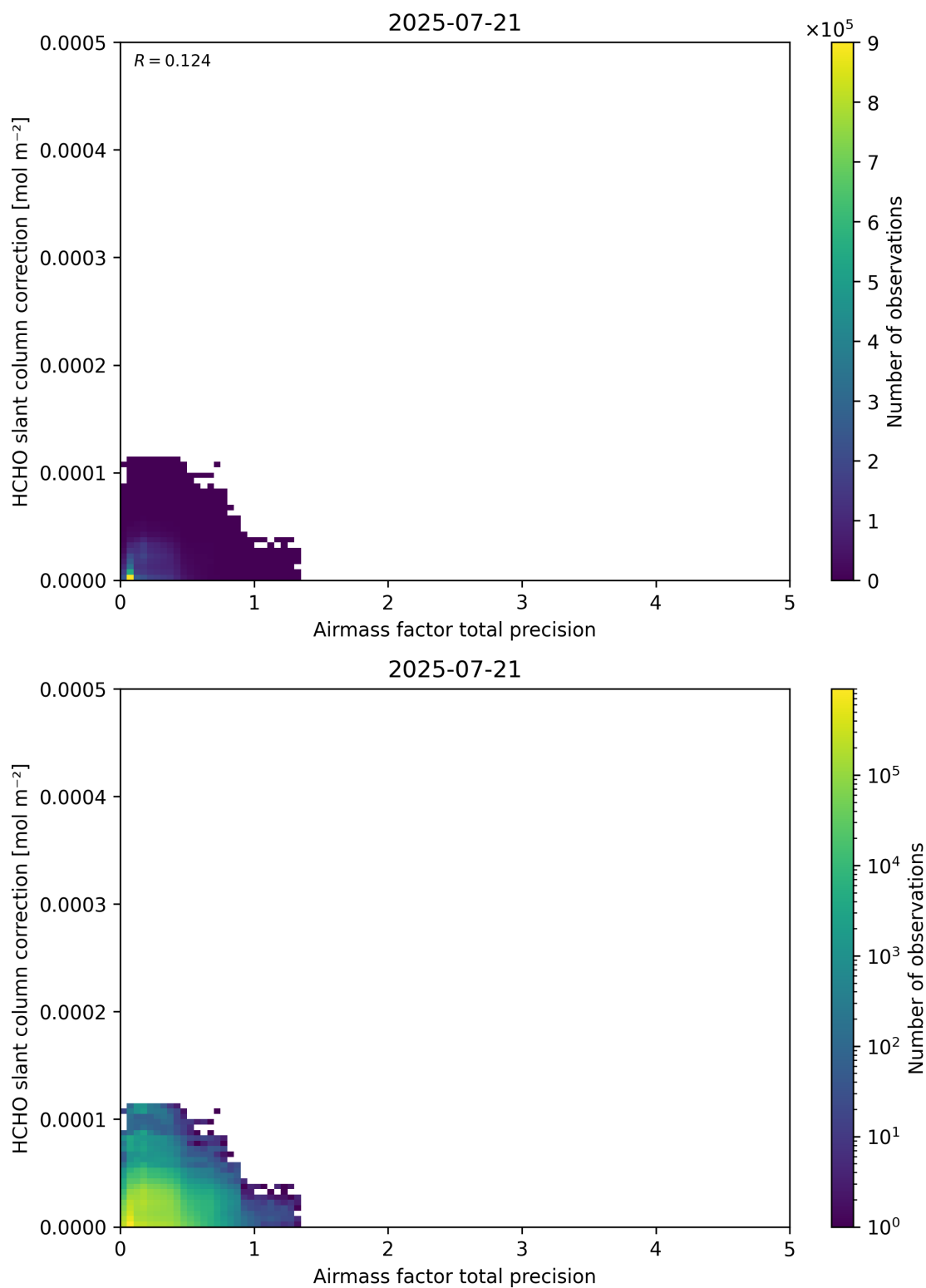
Figure 110: Scatter density plot of “Airmass factor total precision” against “HCHO slant column correction” for 2025-07-20 to 2025-07-22.
