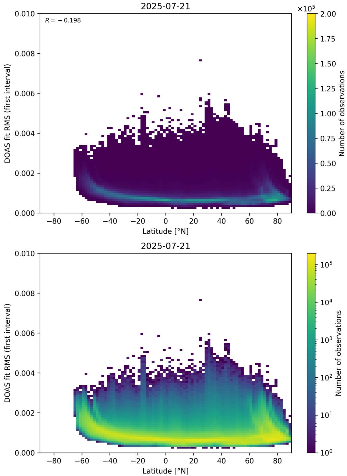
Figure 153: Scatter density plot of “Latitude” against “DOAS fit RMS (first interval)” for 2025-07-20 to 2025-07-22.
