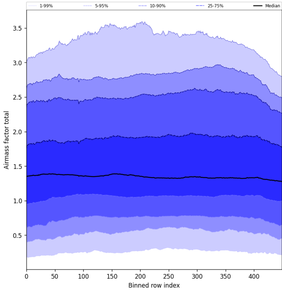
Figure 54: Along track statistics of “Airmass factor total” for 2025-07-20 to 2025-07-22
