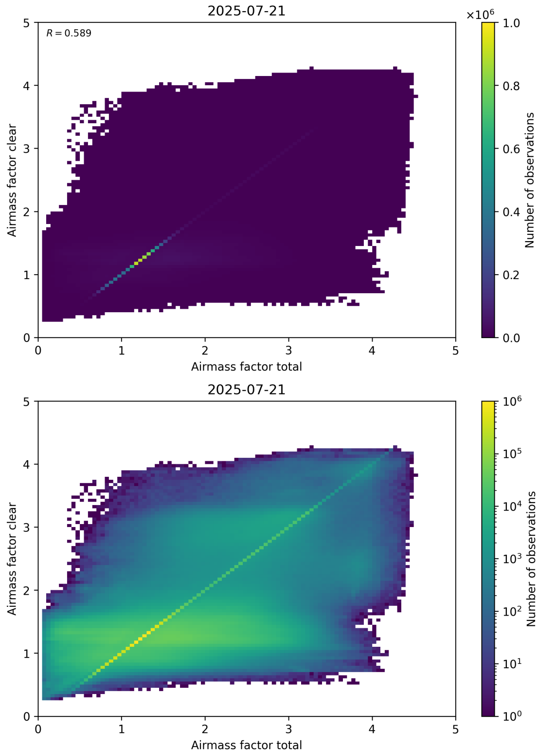
Figure 100: Scatter density plot of “Airmass factor total” against “Airmass factor clear” for 2025-07-20 to 2025-07-22.
