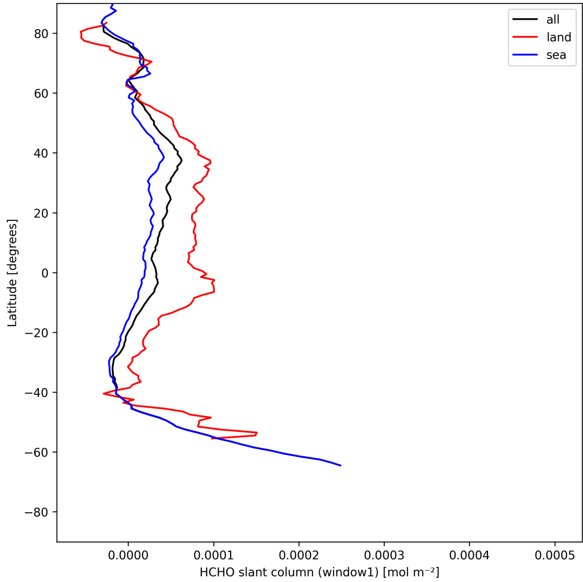
Figure 24: Zonal average of “HCHO slant column (window1)” for 2025-07-20 to 2025-07-22.
