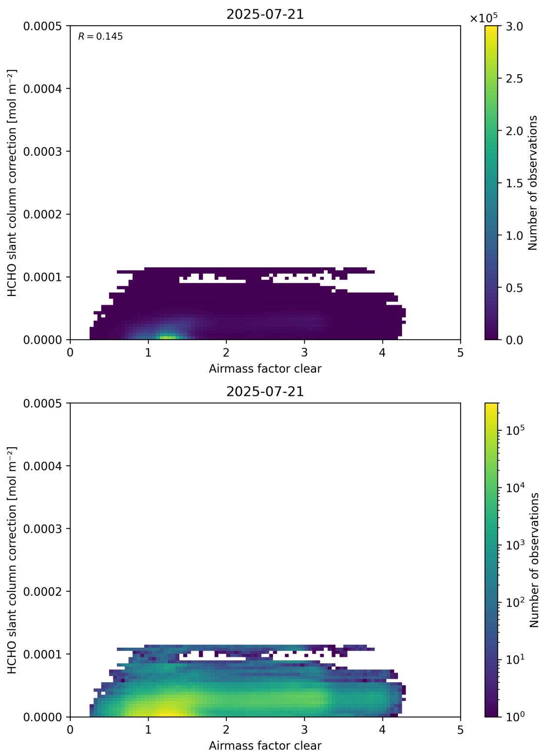
Figure 75: Scatter density plot of “Airmass factor clear” against “HCHO slant column correction” for 2025-07-20 to 2025-07-22.
