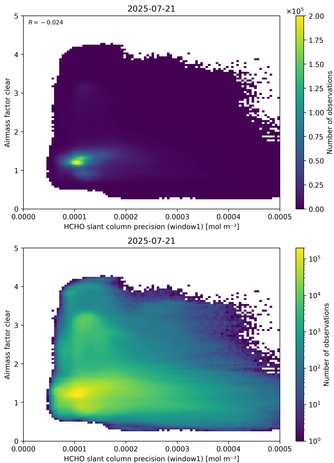
Figure 91: Scatter density plot of “HCHO slant column precision (window1)” against “Airmass factor clear” for 2025-07-20 to 2025-07-22.
