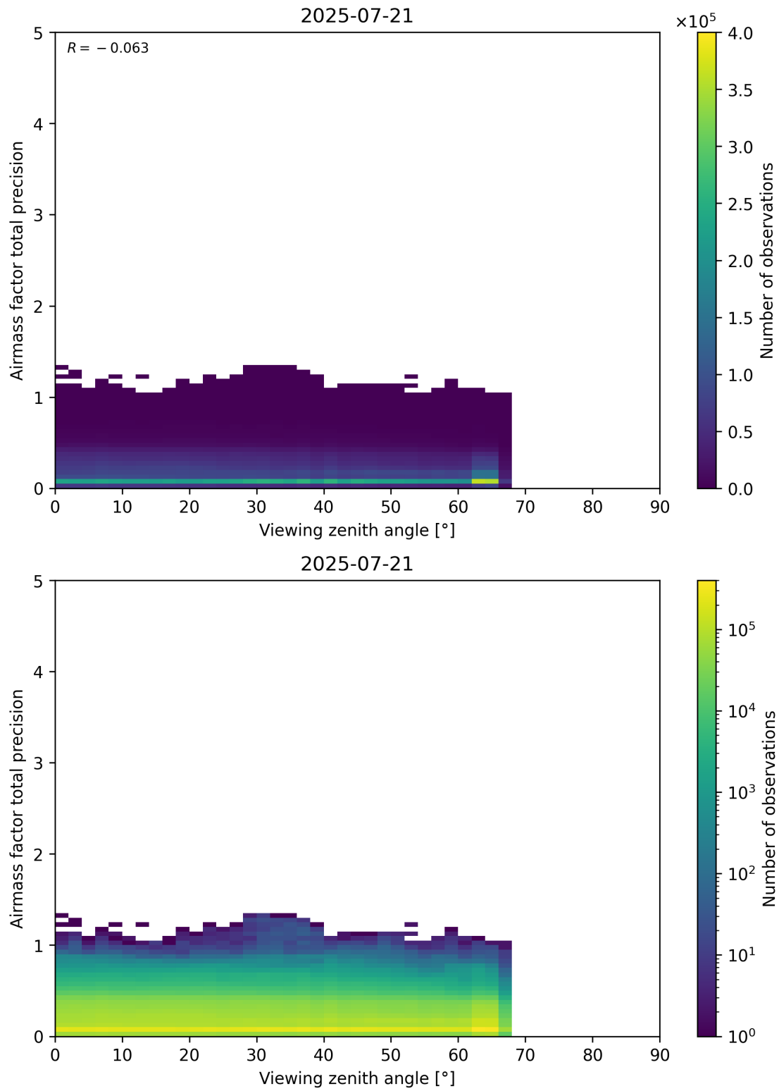
Figure 191: Scatter density plot of “Viewing zenith angle” against “Airmass factor total precision” for 2025-07-20 to 2025-07-22.
