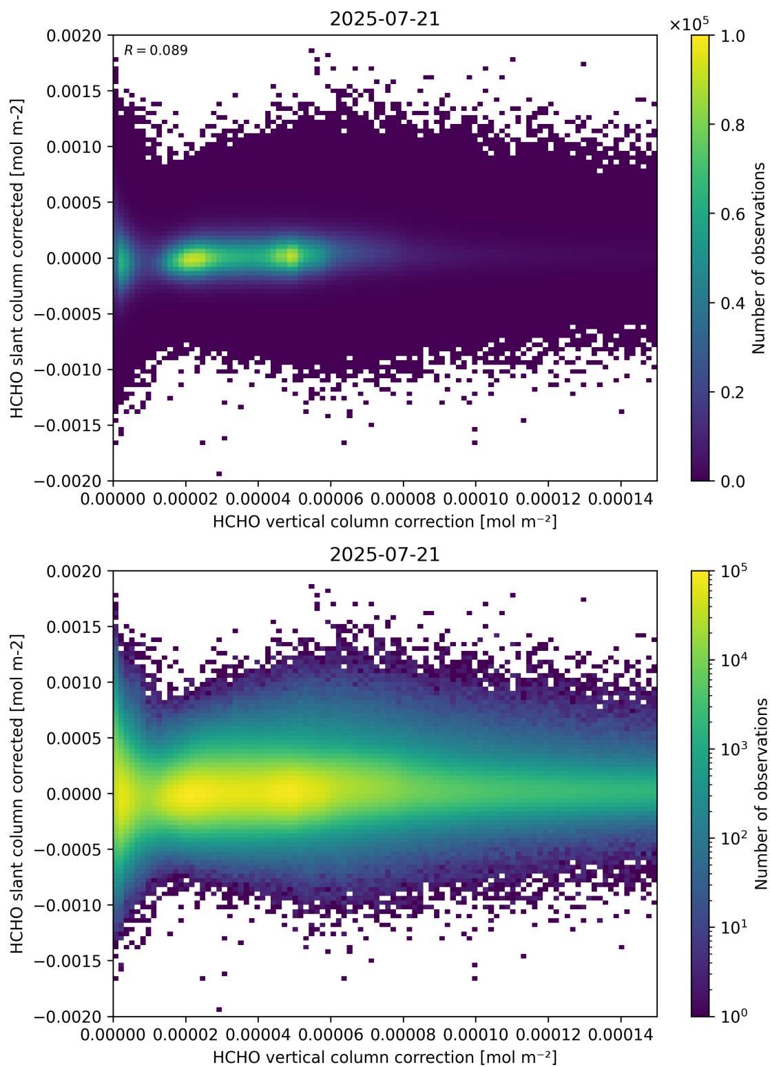
Figure 116: Scatter density plot of “HCHO vertical column correction” against “HCHO slant column corrected” for 2025-07-20 to 2025-07-22.
