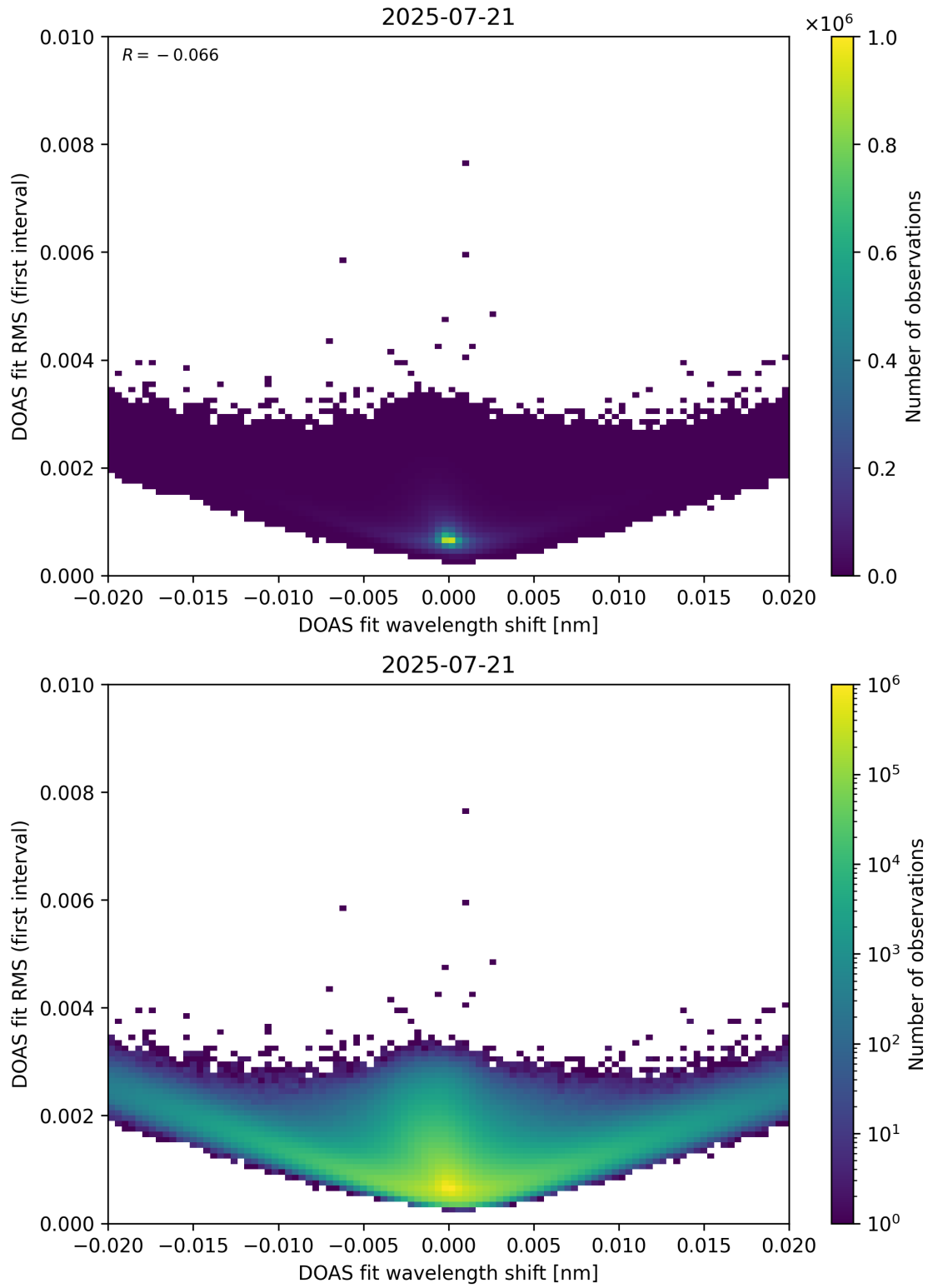
Figure 64: Scatter density plot of “DOAS fit wavelength shift” against “DOAS fit RMS (first interval)” for 2025-07-20 to 2025-07-22.
