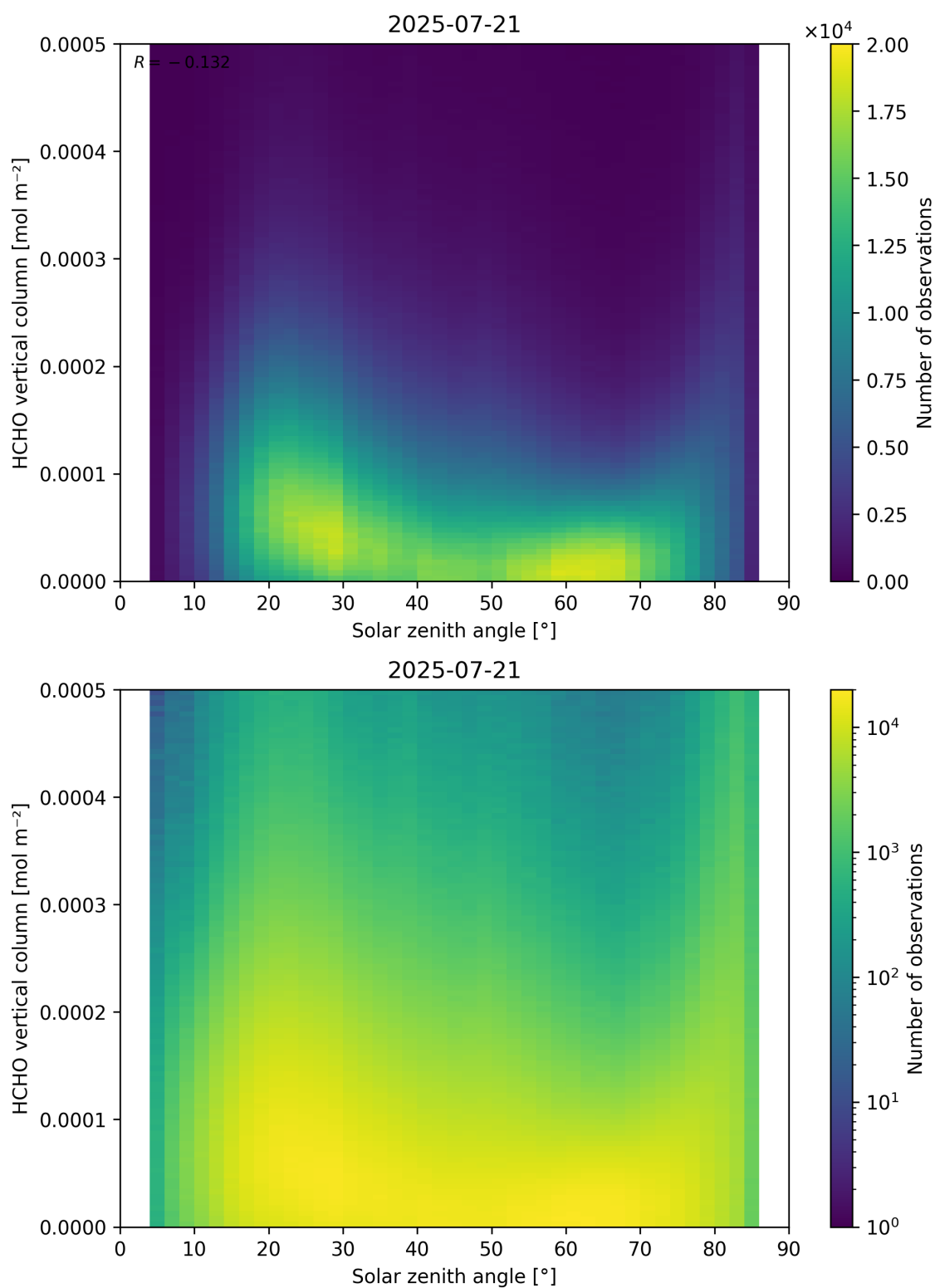
Figure 177: Scatter density plot of “Solar zenith angle” against “HCHO vertical column” for 2025-07-20 to 2025-07-22.
