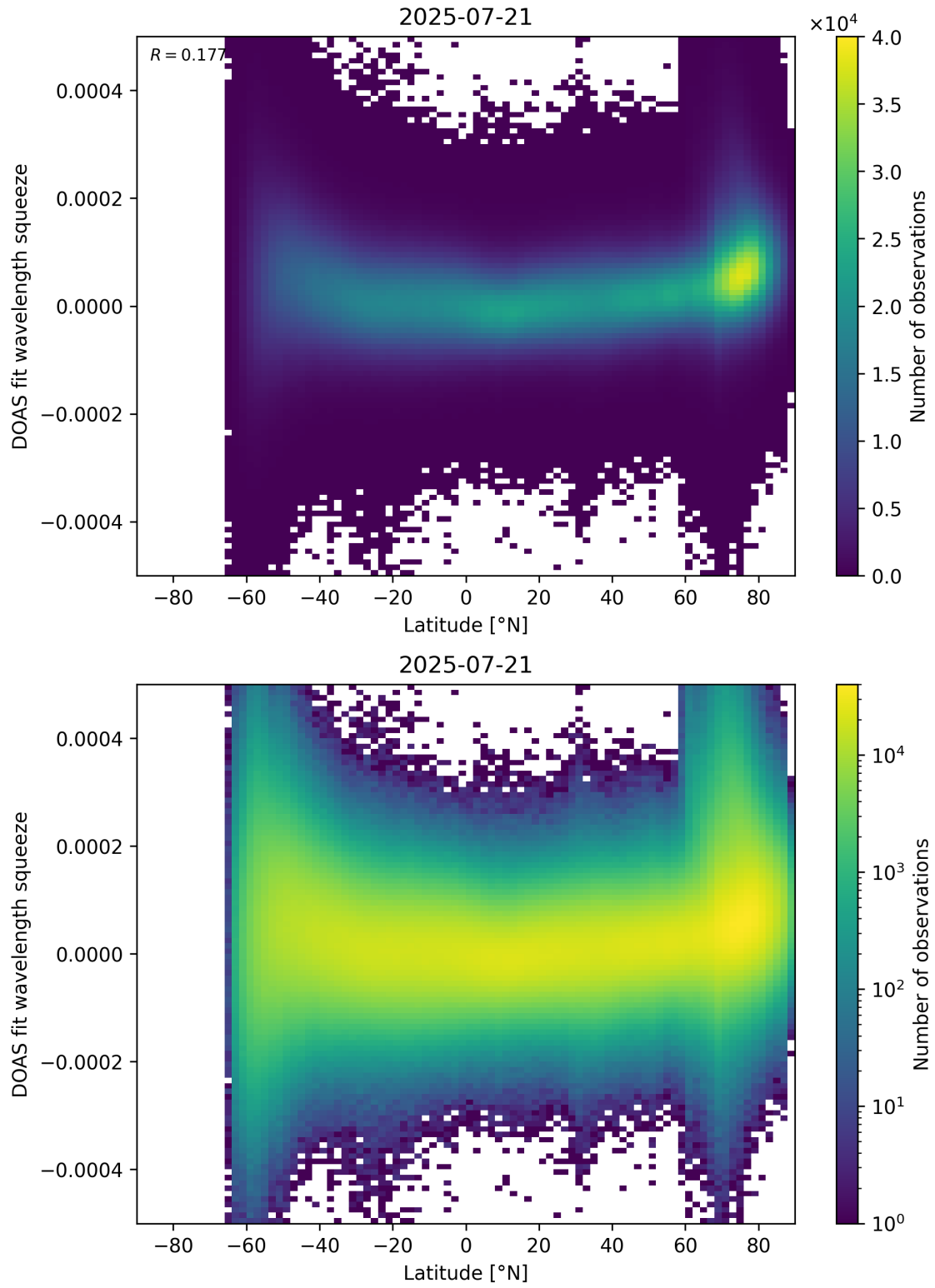
Figure 155: Scatter density plot of “Latitude” against “DOAS fit wavelength squeeze” for 2025-07-20 to 2025-07-22.
