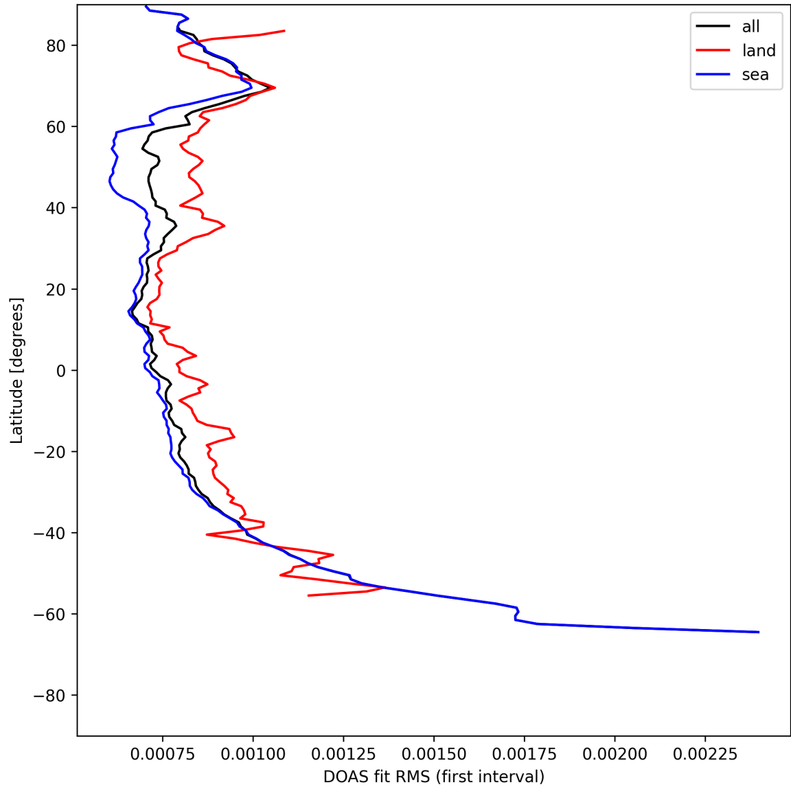
Figure 32: Zonal average of “DOAS fit RMS (first interval)” for 2025-07-20 to 2025-07-22.
