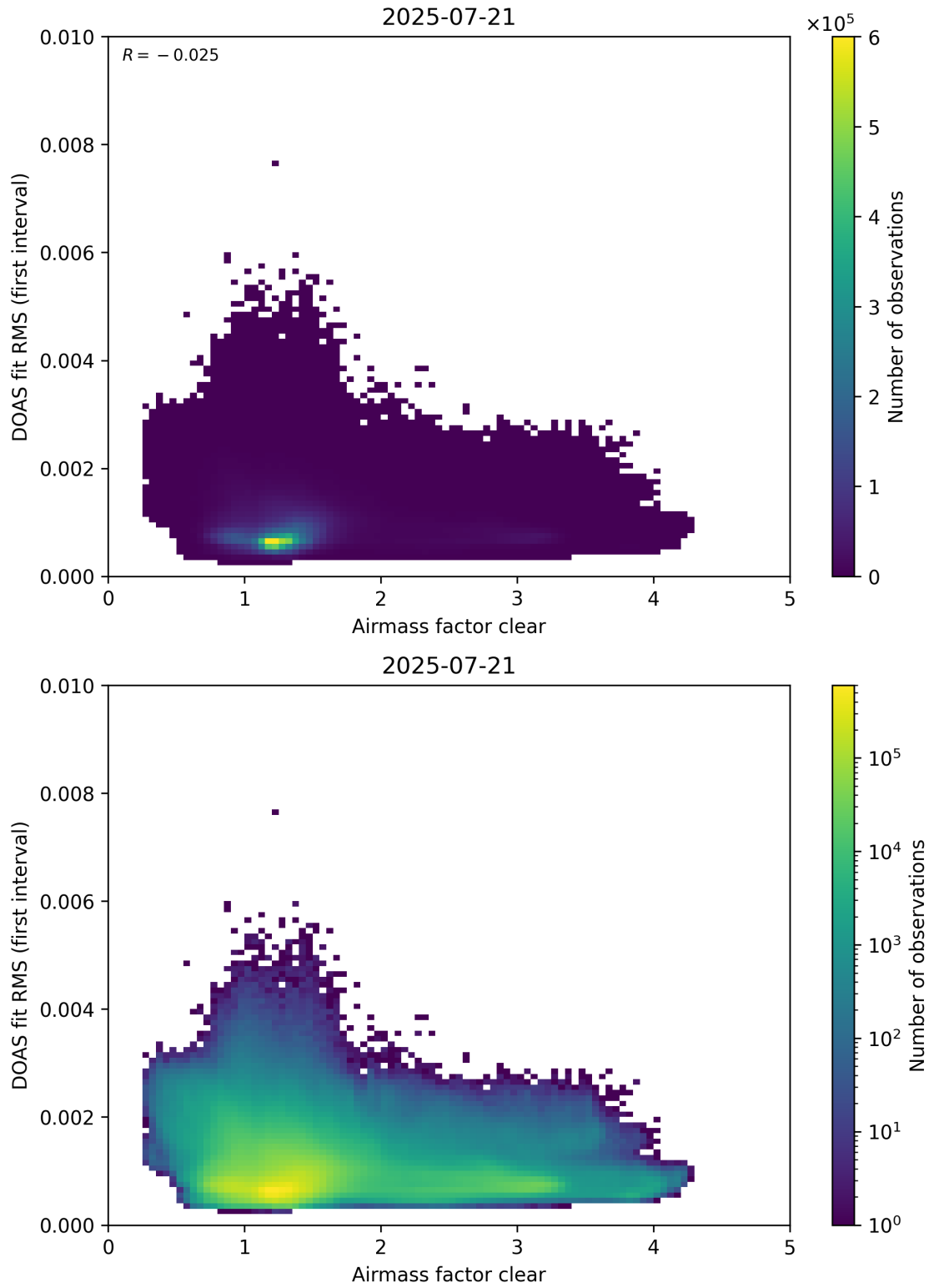
Figure 71: Scatter density plot of “Airmass factor clear” against “DOAS fit RMS (first interval)” for 2025-07-20 to 2025-07-22.
