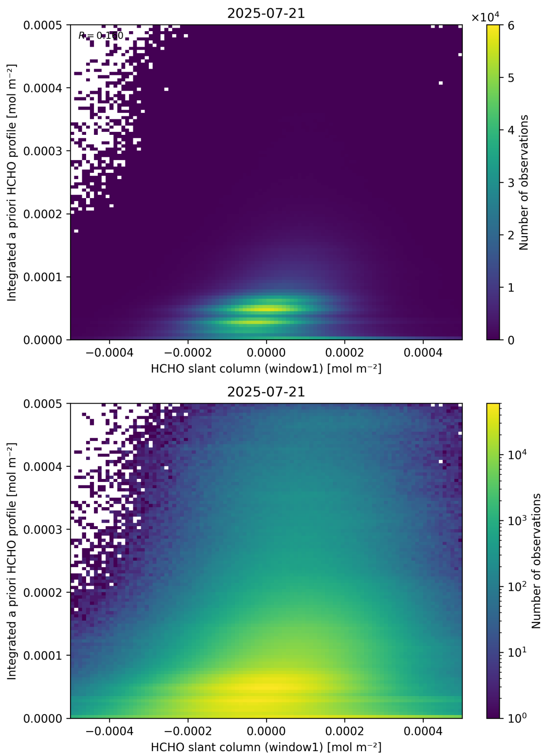
Figure 87: Scatter density plot of “HCHO slant column (window1)” against “Integrated a priori HCHO profile” for 2025-07-20 to 2025-07-22.
