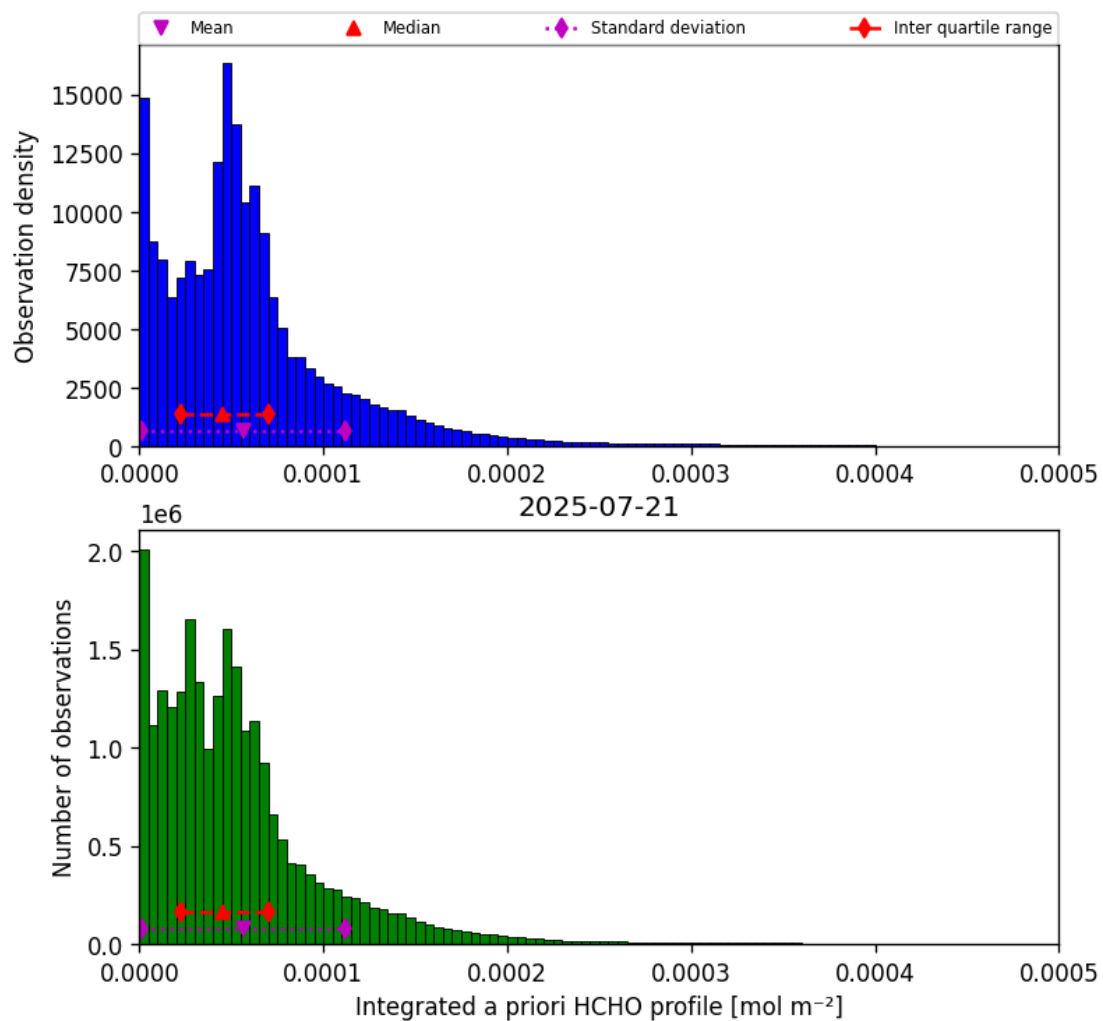
Figure 43: Histogram of “Integrated a priori HCHO profile” for 2025-07-20 to 2025-07-22
