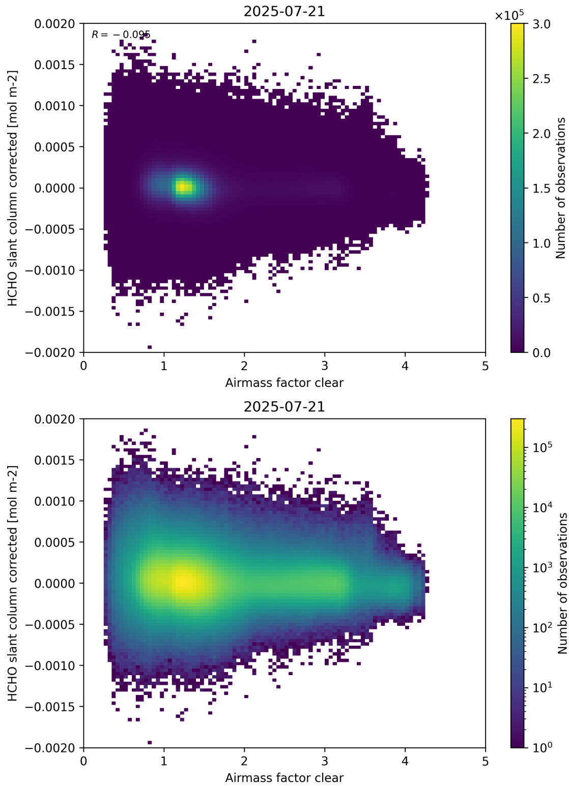
Figure 74: Scatter density plot of “Airmass factor clear” against “HCHO slant column corrected” for 2025-07-20 to 2025-07-22.
