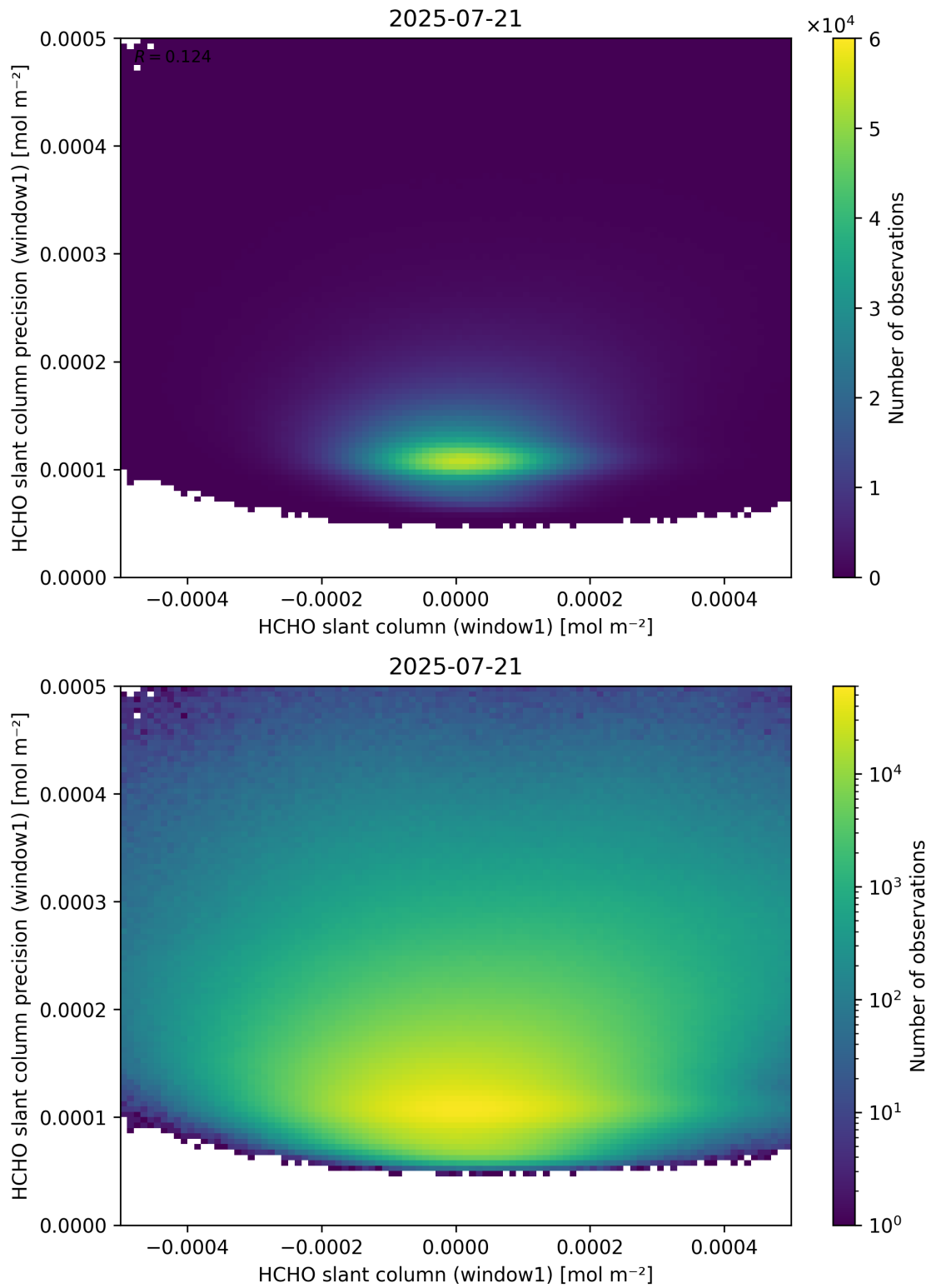
Figure 84: Scatter density plot of “HCHO slant column (window1)” against “HCHO slant column precision (window1)” for 2025-07-20 to 2025-07-22.
