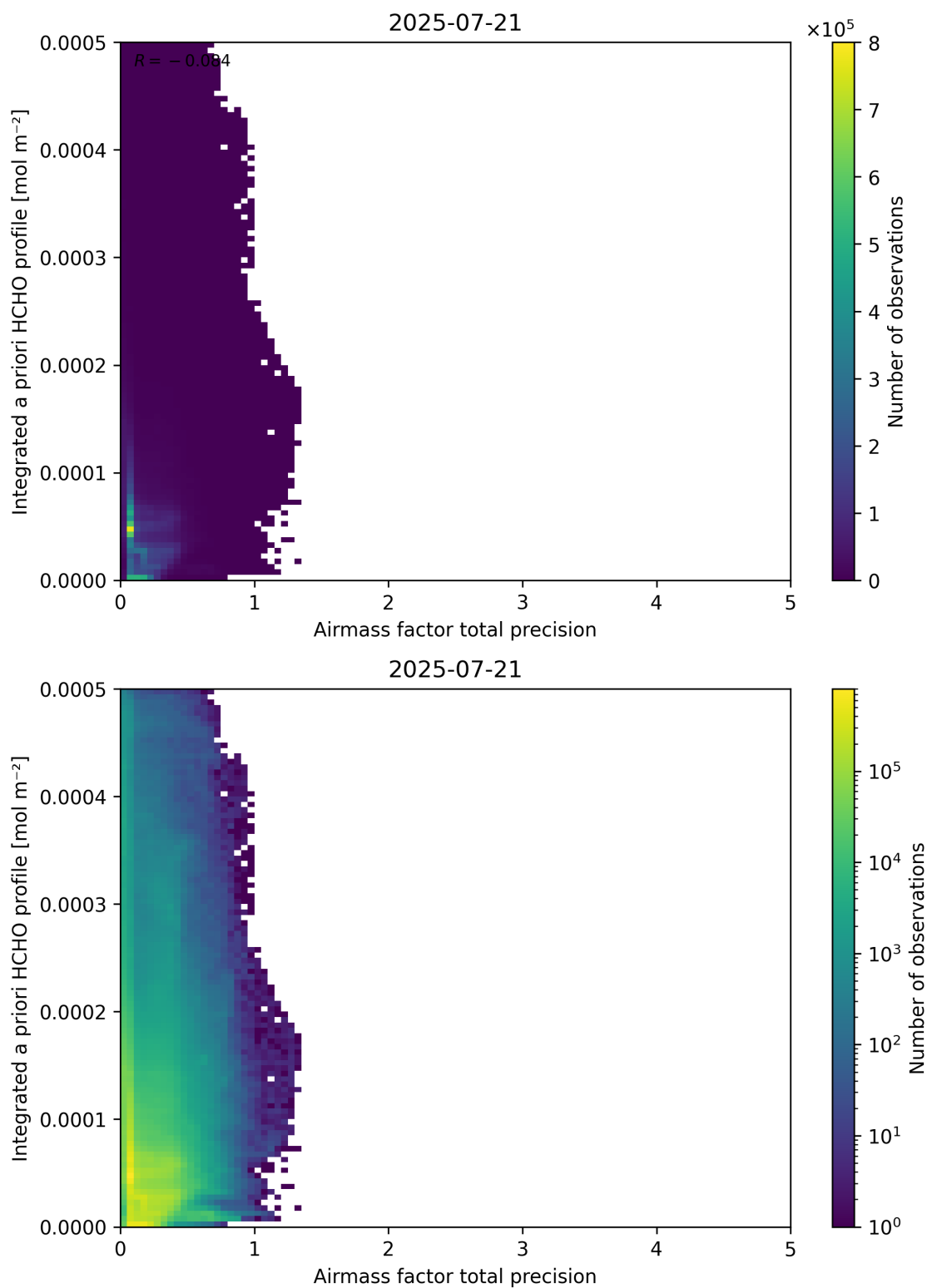
Figure 111: Scatter density plot of “Airmass factor total precision” against “Integrated a priori HCHO profile” for 2025-07-20 to 2025-07-22.
