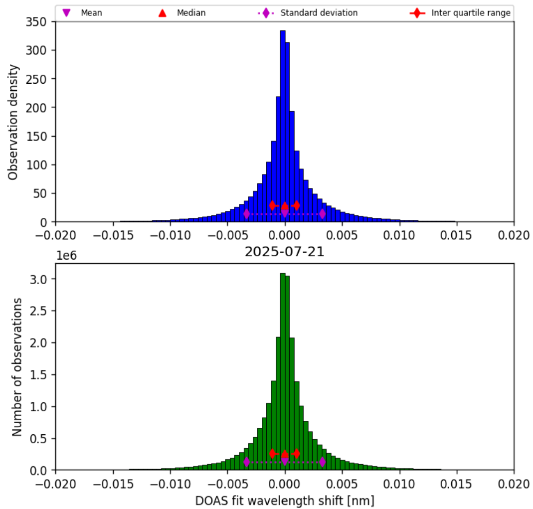
Figure 44: Histogram of “DOAS fit wavelength shift” for 2025-07-20 to 2025-07-22
