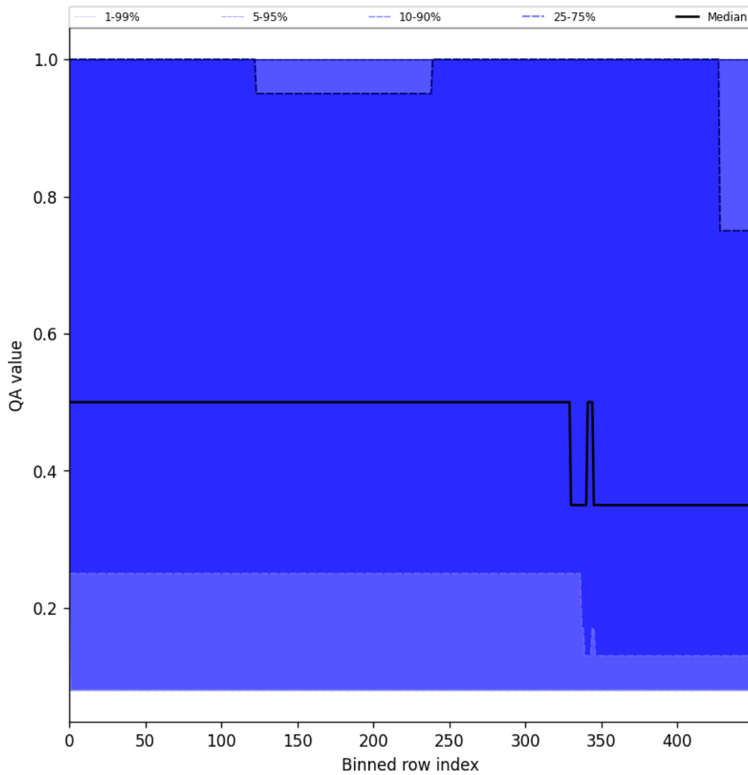
Figure 48: Along track statistics of “QA value” for 2025-07-20 to 2025-07-22
