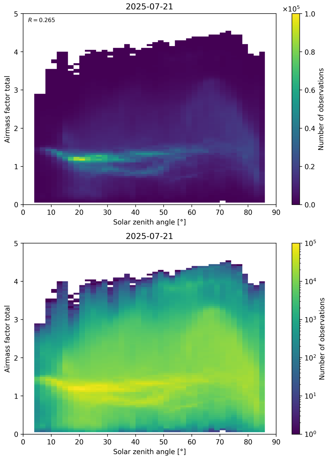
Figure 175: Scatter density plot of “Solar zenith angle” against “Airmass factor total” for 2025-07-20 to 2025-07-22.
