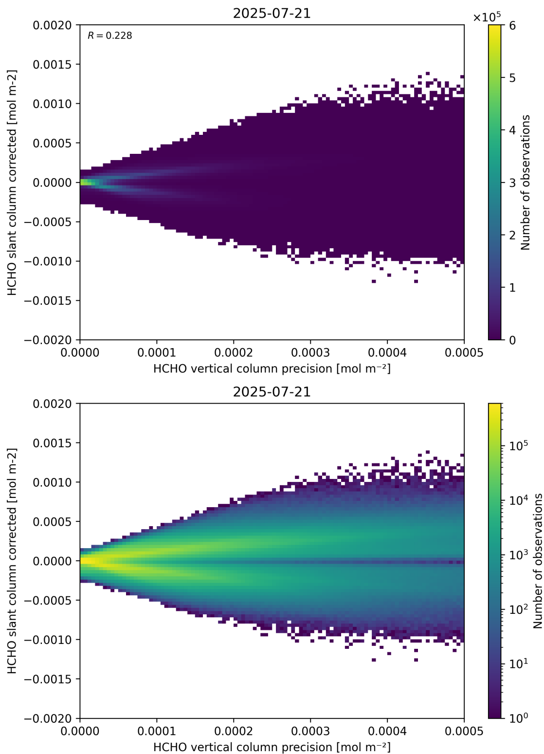
Figure 140: Scatter density plot of “HCHO vertical column precision” against “HCHO slant column corrected” for 2025-07-20 to 2025-07-22.
