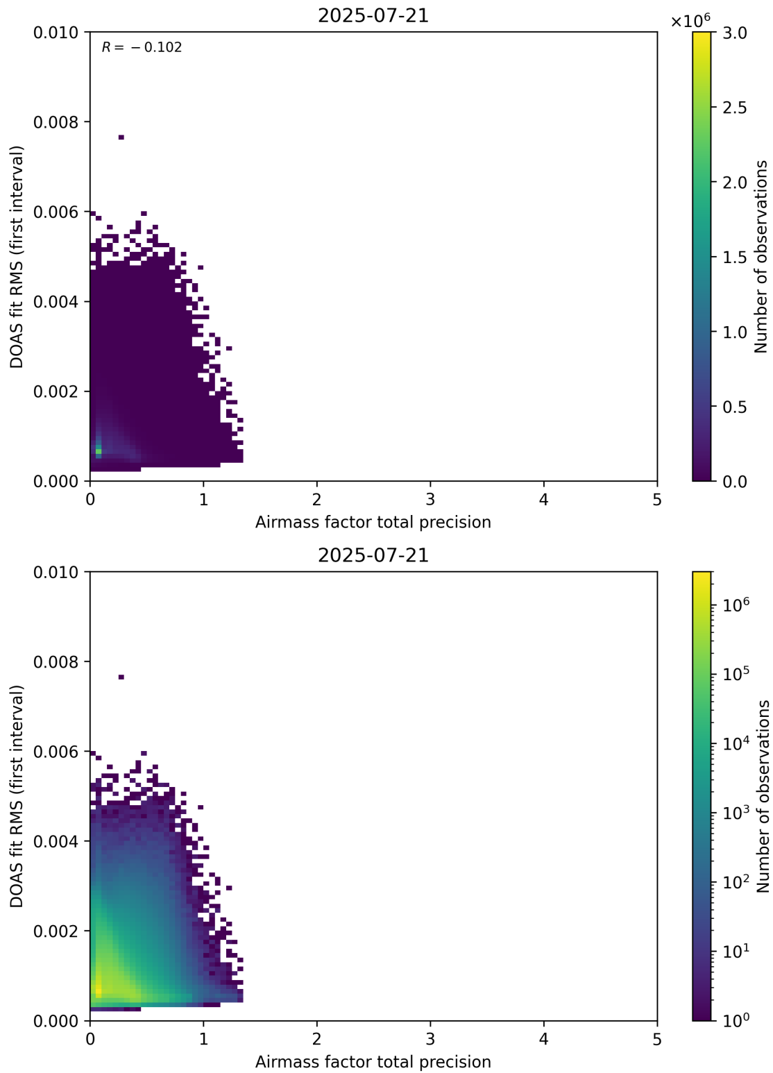
Figure 105: Scatter density plot of “Airmass factor total precision” against “DOAS fit RMS (first interval)” for 2025-07-20 to 2025-07-22.
