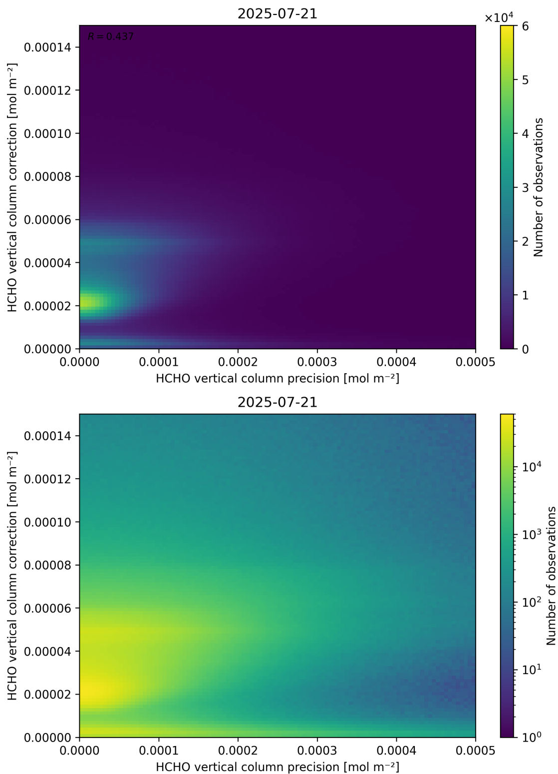
Figure 146: Scatter density plot of “HCHO vertical column precision” against “HCHO vertical column correction” for 2025-07-20 to 2025-07-22.
