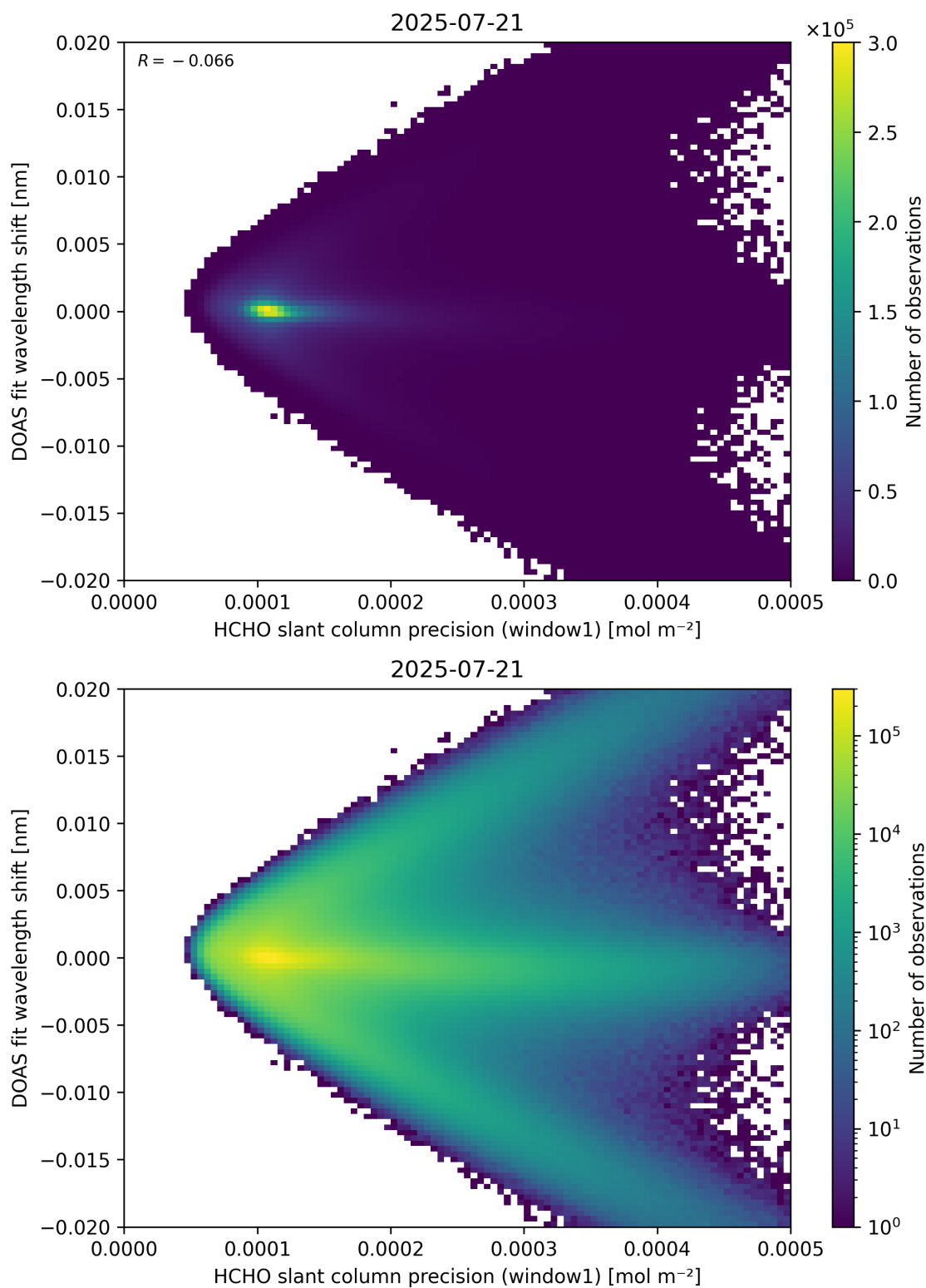
Figure 89: Scatter density plot of “HCHO slant column precision (window1)” against “DOAS fit wavelength shift” for 2025-07-20 to 2025-07-22.
