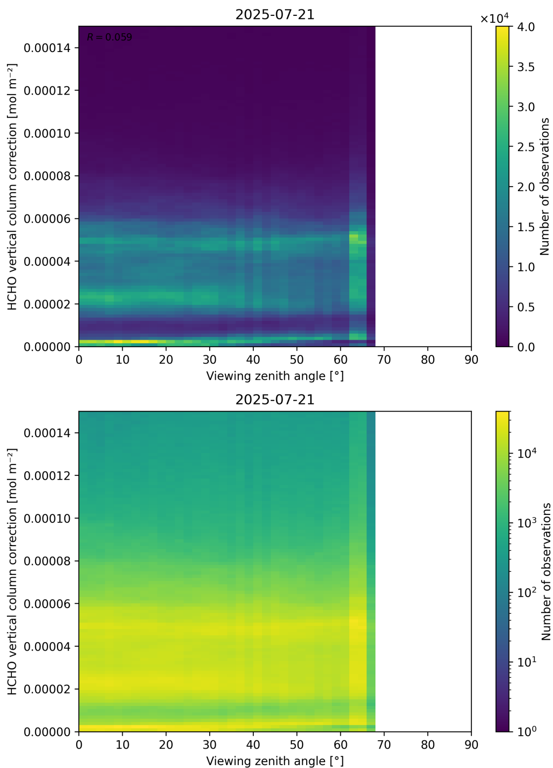
Figure 193: Scatter density plot of “Viewing zenith angle” against “HCHO vertical column correction” for 2025-07-20 to 2025-07-22.
