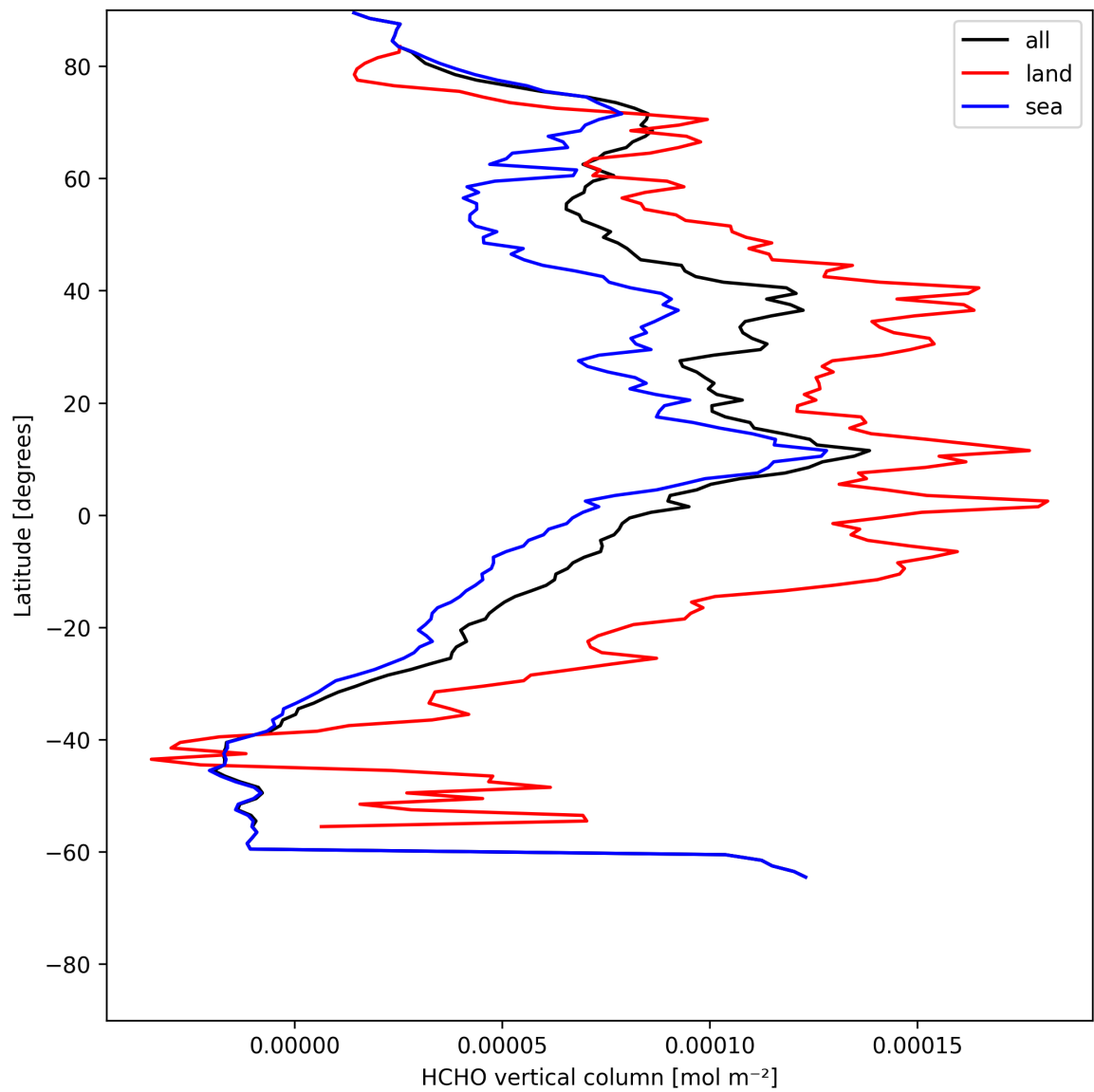
Figure 21: Zonal average of “HCHO vertical column” for 2025-07-20 to 2025-07-22.
