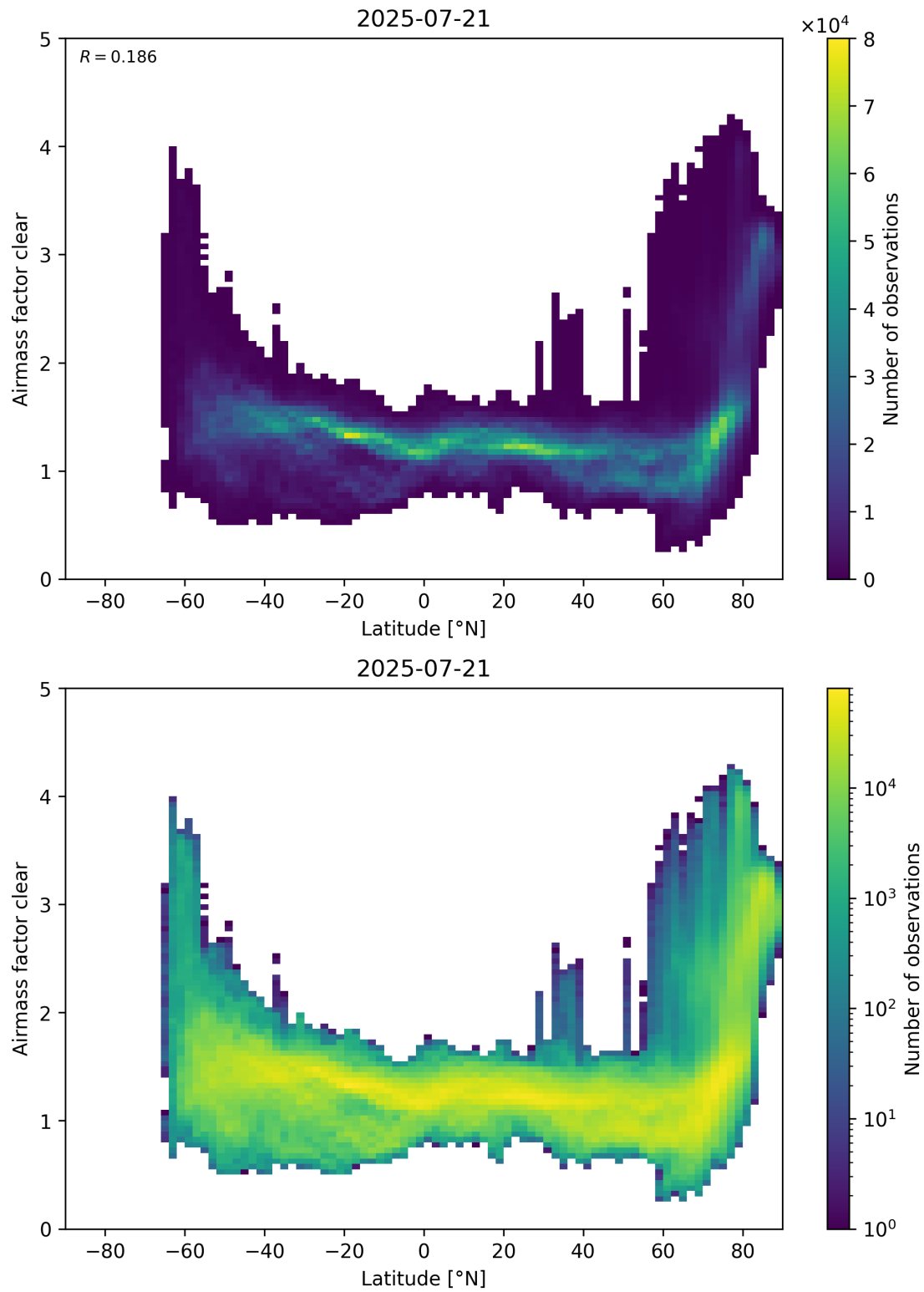
Figure 156: Scatter density plot of “Latitude” against “Airmass factor clear” for 2025-07-20 to 2025-07-22.
