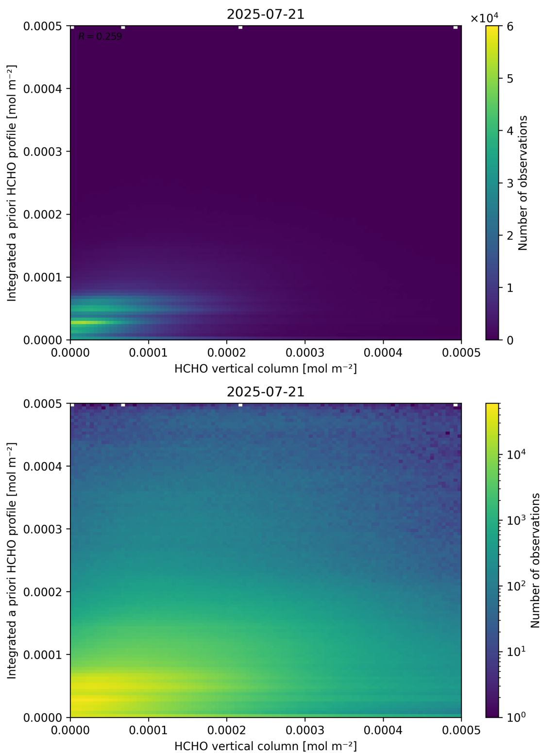
Figure 135: Scatter density plot of “HCHO vertical column” against “Integrated a priori HCHO profile” for 2025-07-20 to 2025-07-22.
