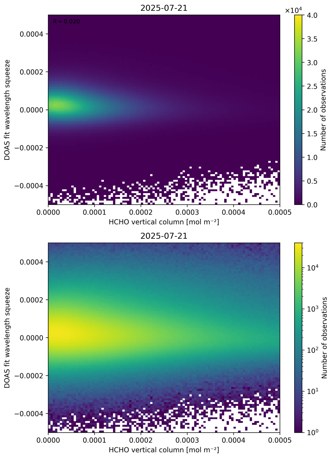
Figure 125: Scatter density plot of “HCHO vertical column” against “DOAS fit wavelength squeeze” for 2025-07-20 to 2025-07-22.
