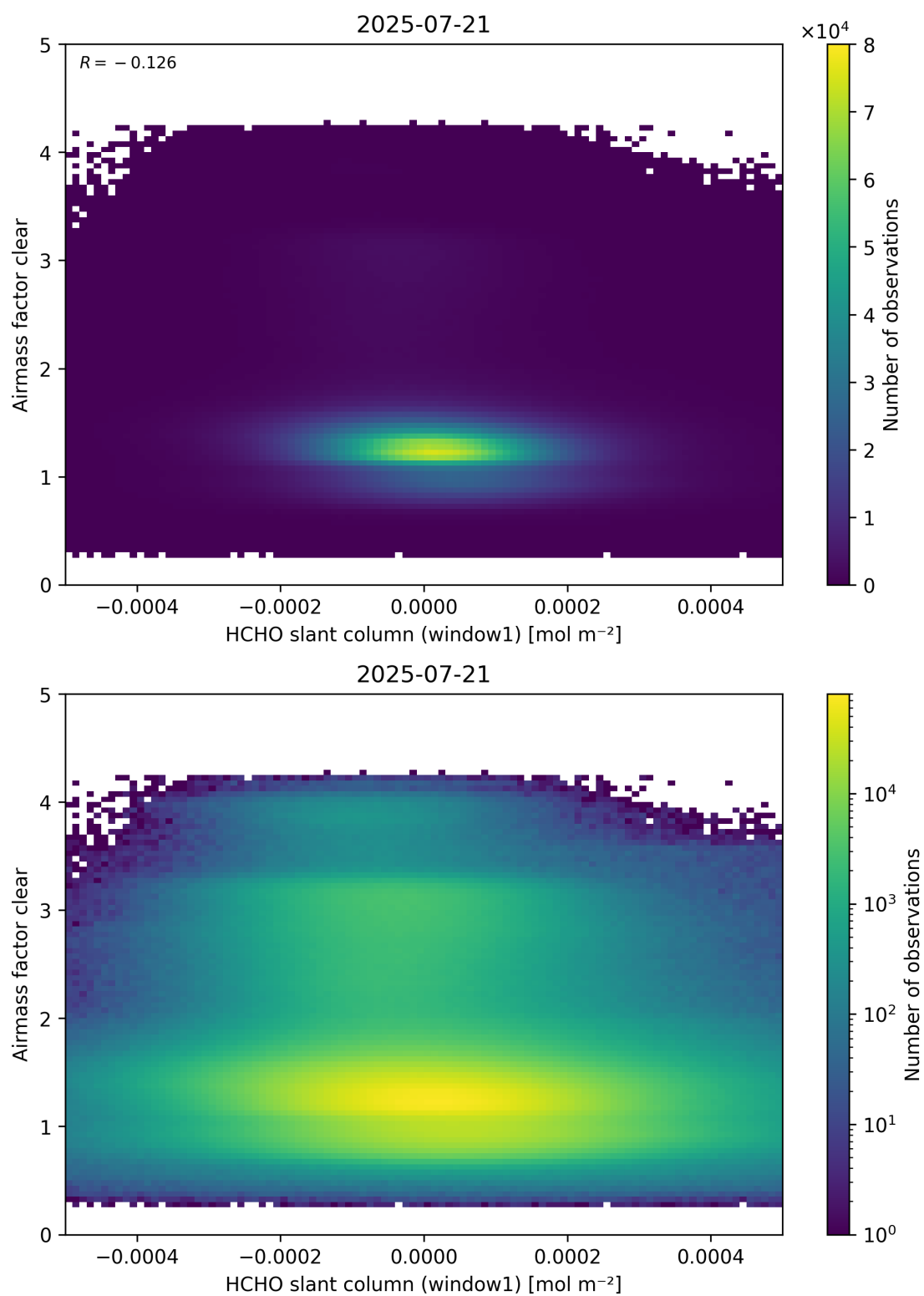
Figure 81: Scatter density plot of “HCHO slant column (window1)” against “Airmass factor clear” for 2025-07-20 to 2025-07-22.
