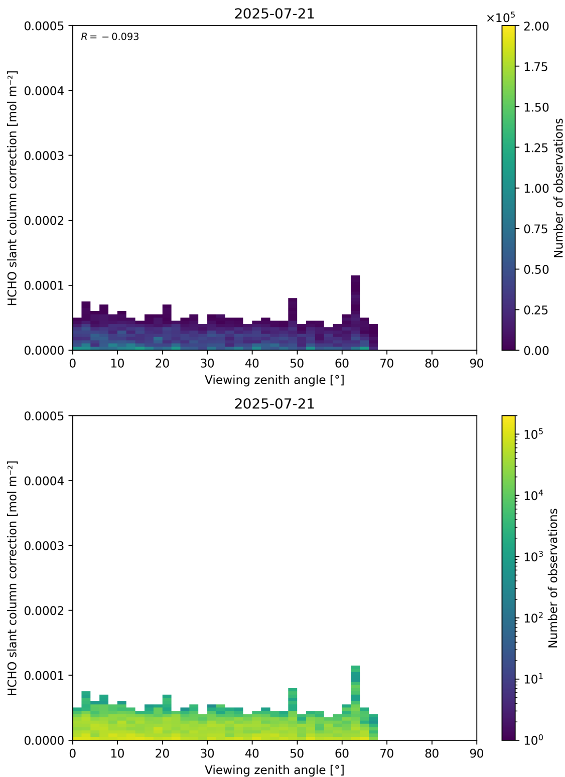
Figure 187: Scatter density plot of “Viewing zenith angle” against “HCHO slant column correction” for 2025-07-20 to 2025-07-22.
