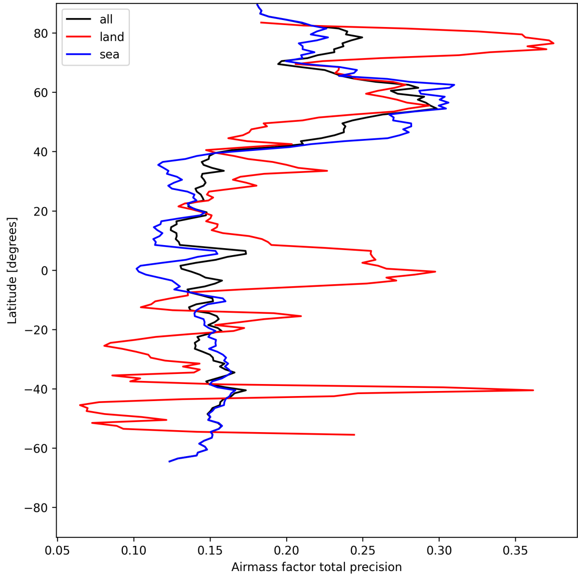
Figure 27: Zonal average of “Airmass factor total precision” for 2025-07-20 to 2025-07-22.
