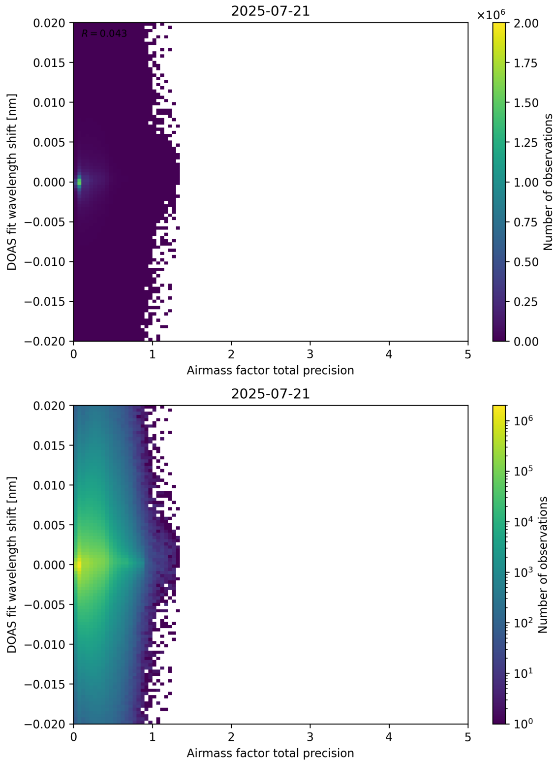
Figure 106: Scatter density plot of “Airmass factor total precision” against “DOAS fit wavelength shift” for 2025-07-20 to 2025-07-22.
