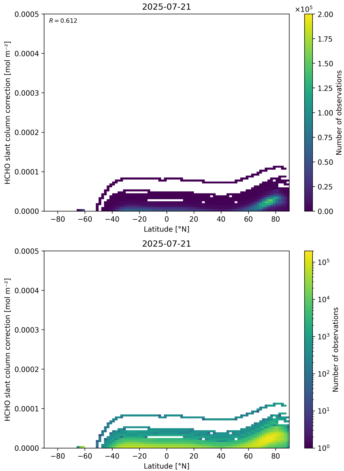
Figure 158: Scatter density plot of “Latitude” against “HCHO slant column correction” for 2025-07-20 to 2025-07-22.
