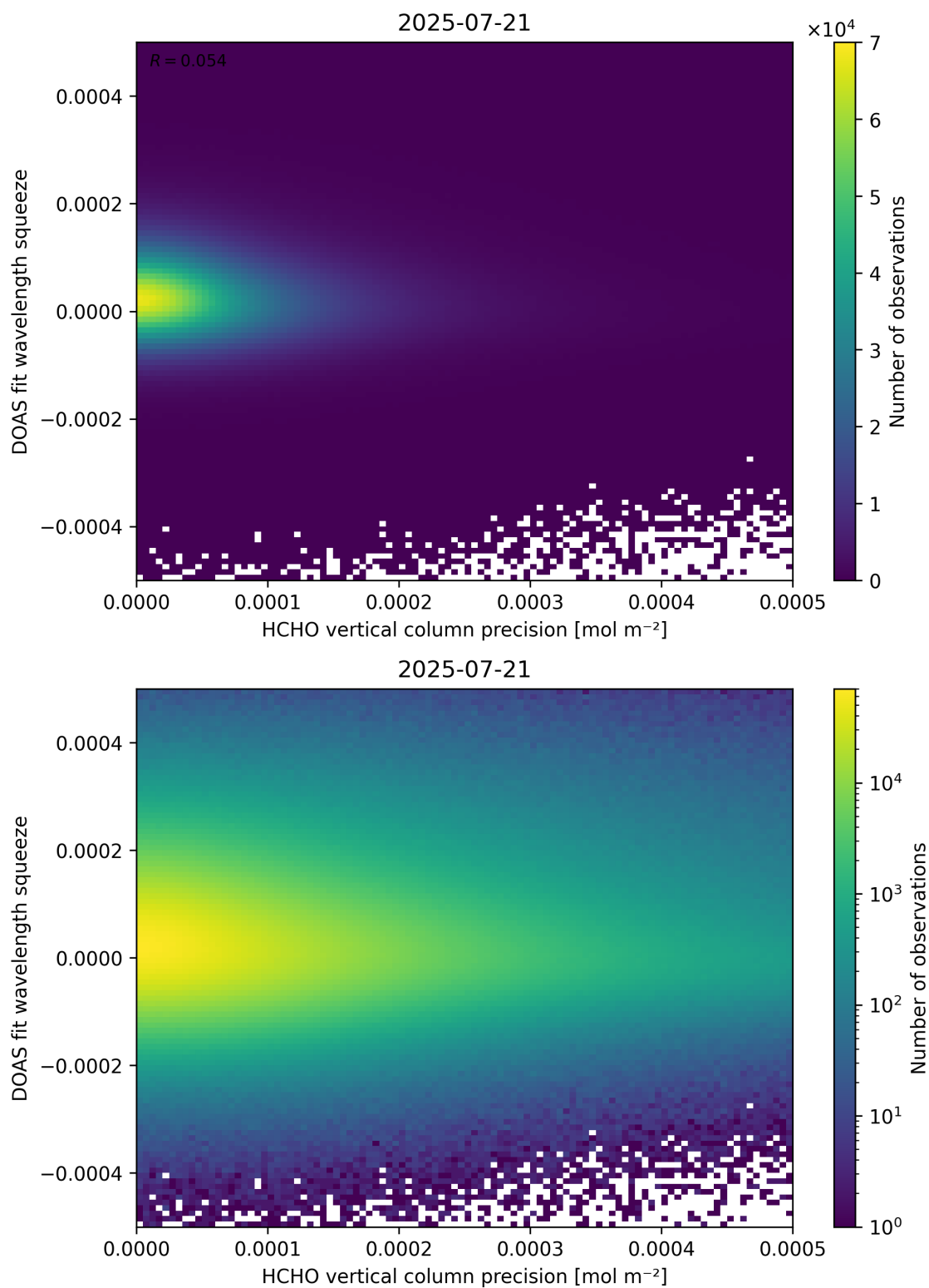
Figure 138: Scatter density plot of “HCHO vertical column precision” against “DOAS fit wavelength squeeze” for 2025-07-20 to 2025-07-22.
