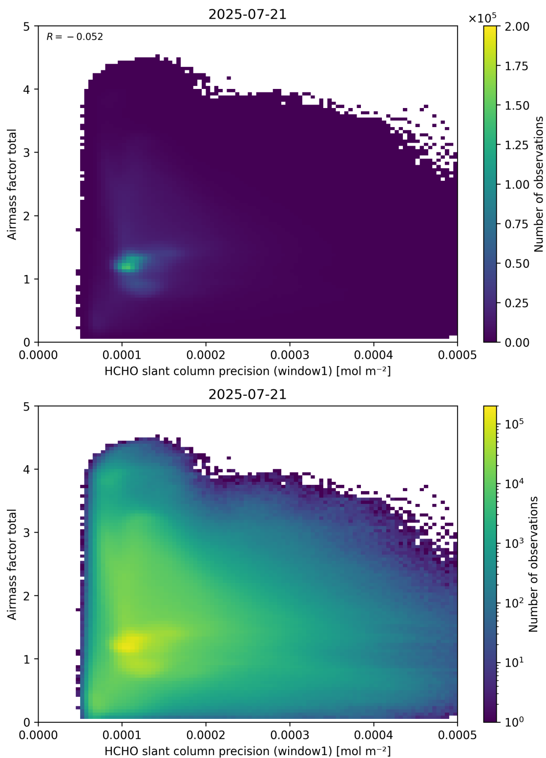
Figure 94: Scatter density plot of “HCHO slant column precision (window1)” against “Airmass factor total” for 2025-07-20 to 2025-07-22.
