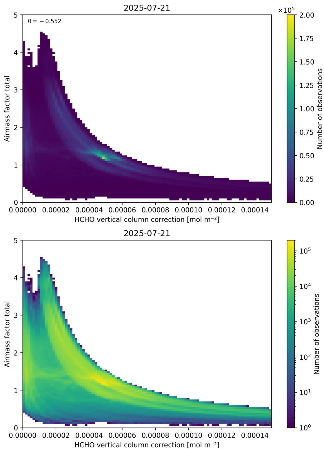
Figure 120: Scatter density plot of “HCHO vertical column correction” against “Airmass factor total” for 2025-07-20 to 2025-07-22.
