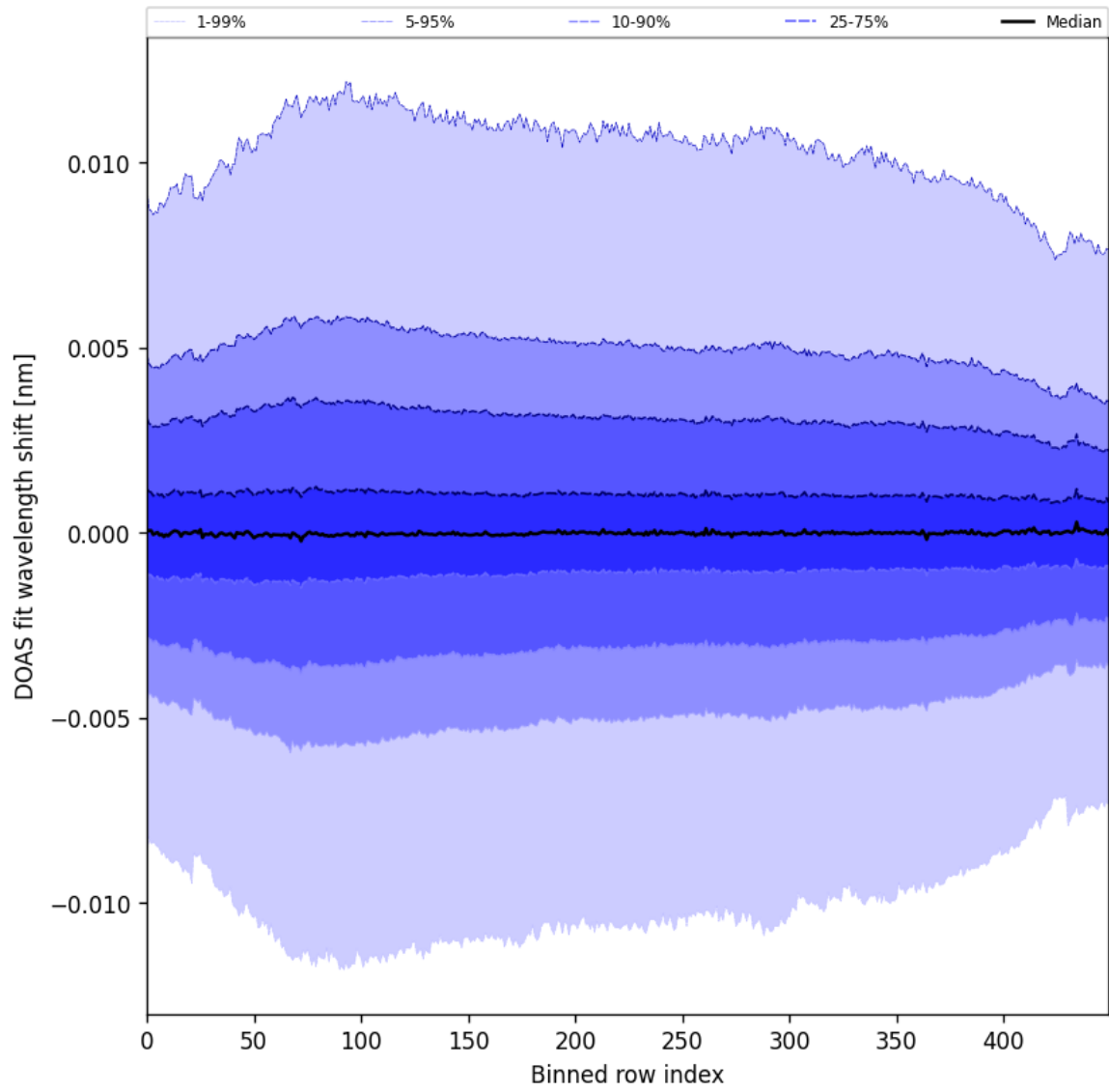
Figure 58: Along track statistics of “DOAS fit wavelength shift” for 2025-07-20 to 2025-07-22
