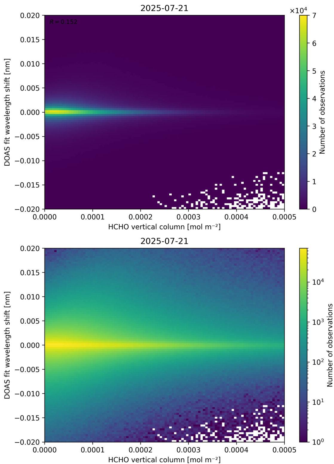
Figure 124: Scatter density plot of “HCHO vertical column” against “DOAS fit wavelength shift” for 2025-07-20 to 2025-07-22.
