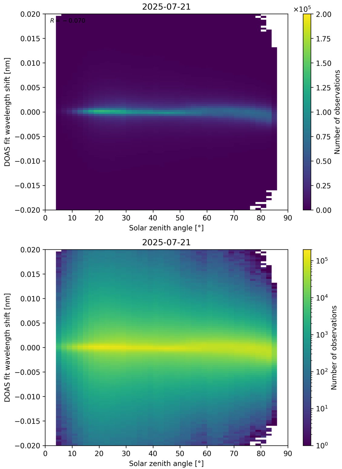
Figure 168: Scatter density plot of “Solar zenith angle” against “DOAS fit wavelength shift” for 2025-07-20 to 2025-07-22.
