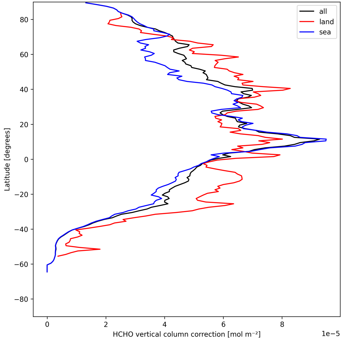
Figure 23: Zonal average of “HCHO vertical column correction” for 2025-07-20 to 2025-07-22.
