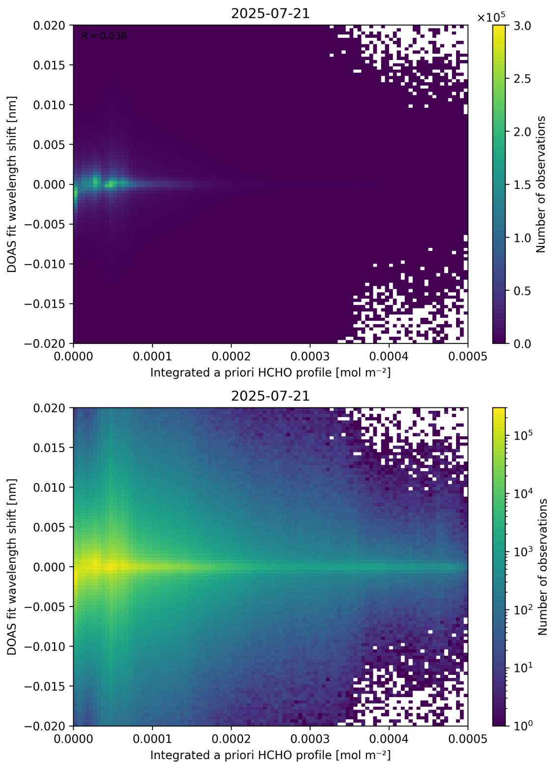
Figure 149: Scatter density plot of “Integrated a priori HCHO profile” against “DOAS fit wavelength shift” for 2025-07-20 to 2025-07-22.
