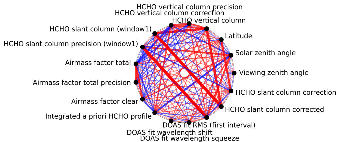
Figure 1: Map of correlation graph for 2025-07-20 to 2025-07-22.
