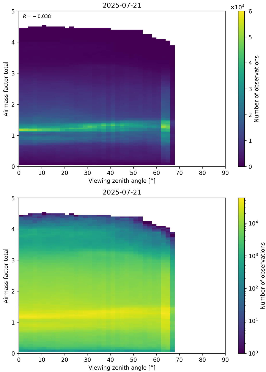
Figure 190: Scatter density plot of “Viewing zenith angle” against “Airmass factor total” for 2025-07-20 to 2025-07-22.
