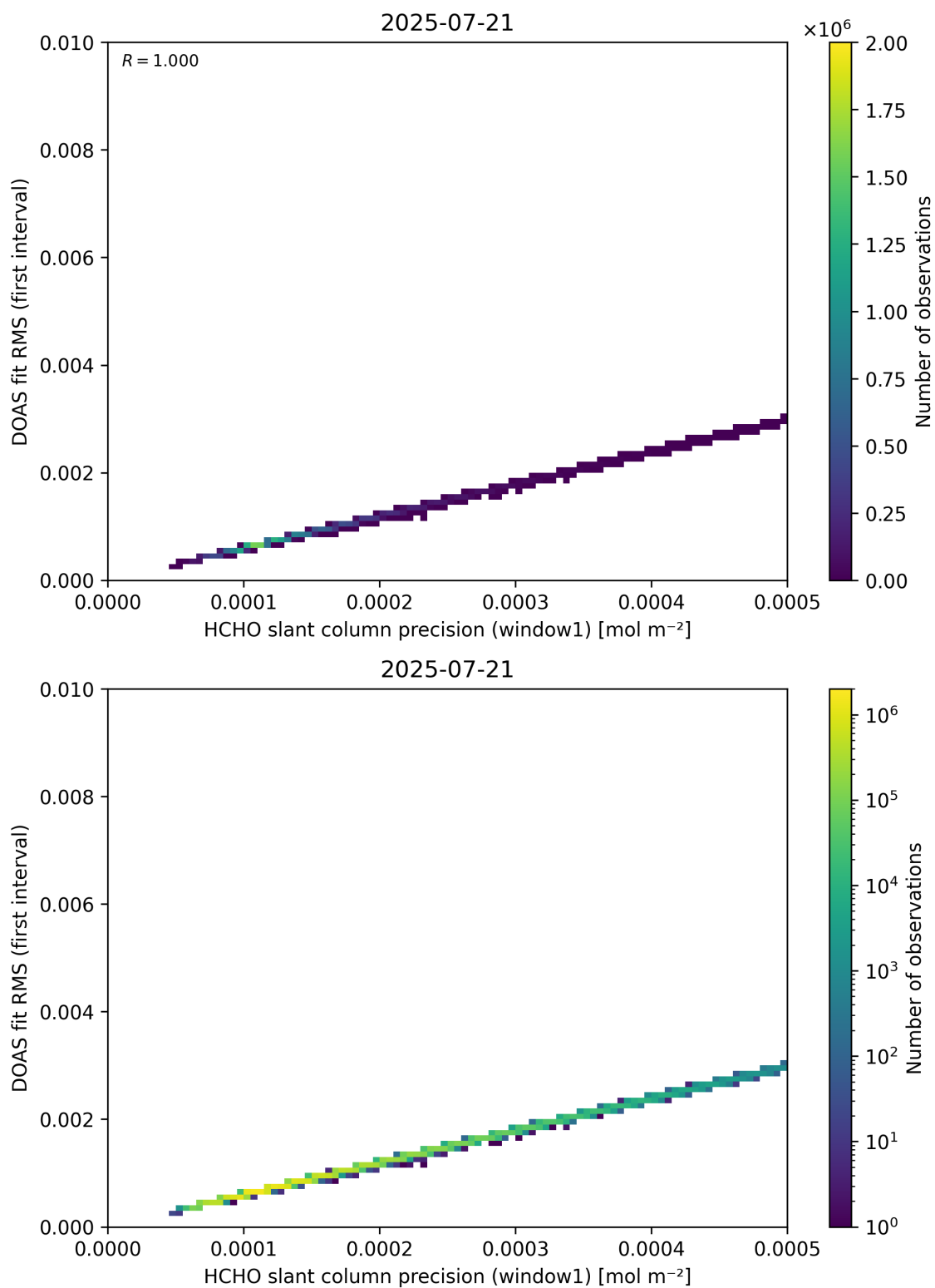
Figure 88: Scatter density plot of “HCHO slant column precision (window1)” against “DOAS fit RMS (first interval)” for 2025-07-20 to 2025-07-22.
