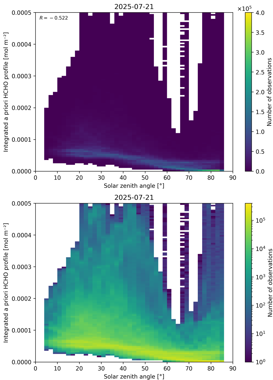
Figure 180: Scatter density plot of “Solar zenith angle” against “Integrated a priori HCHO profile” for 2025-07-20 to 2025-07-22.
