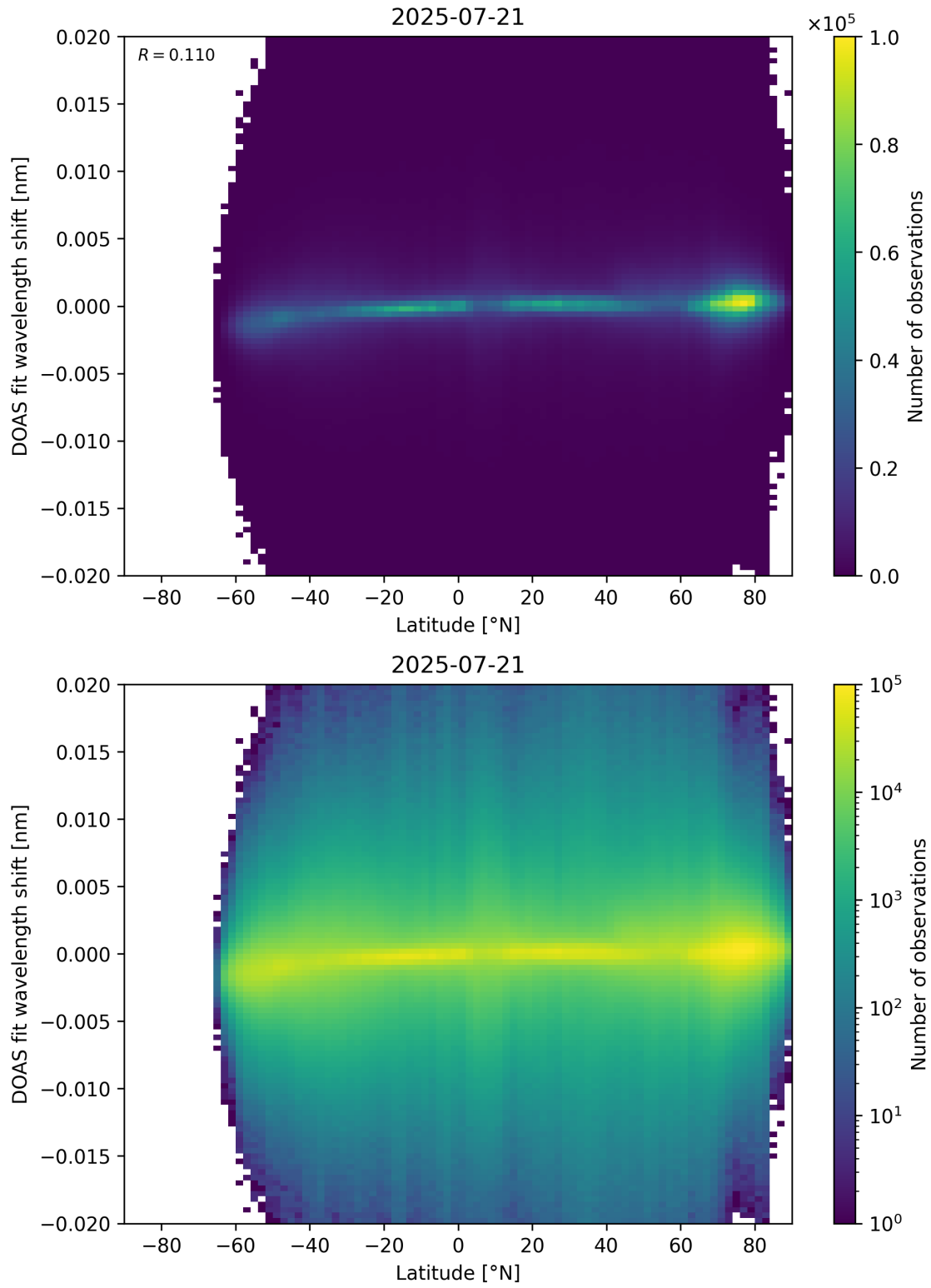
Figure 154: Scatter density plot of “Latitude” against “DOAS fit wavelength shift” for 2025-07-20 to 2025-07-22.
