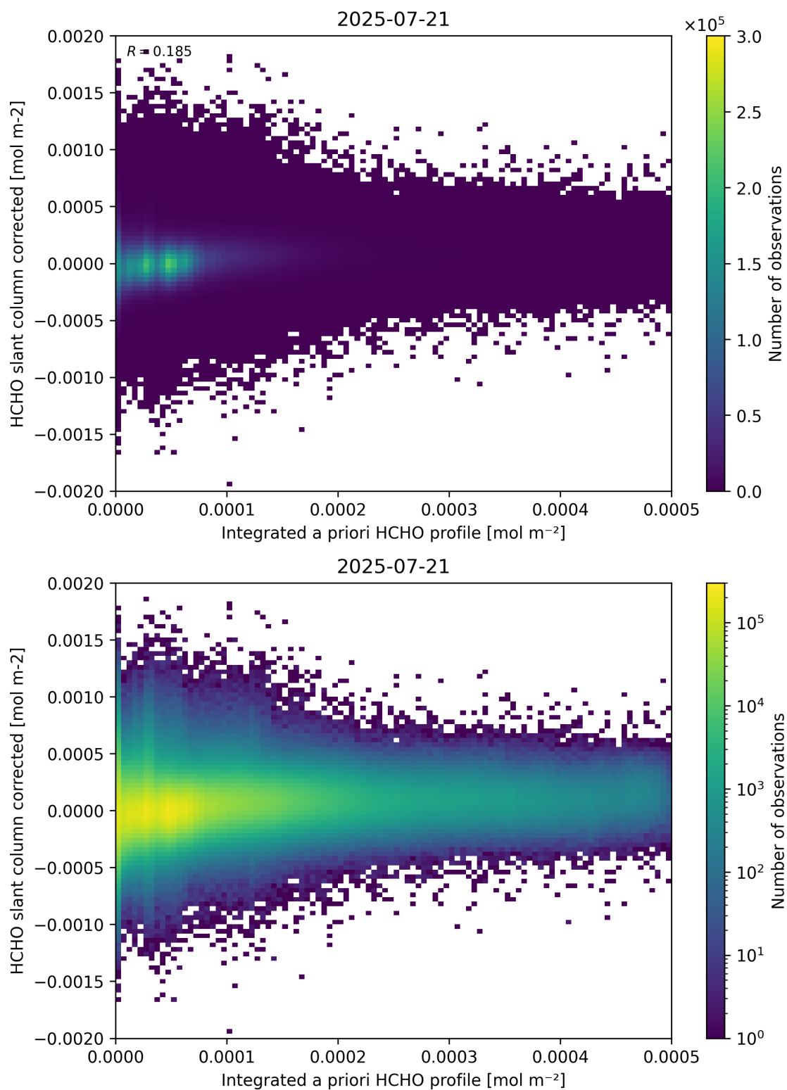
Figure 151: Scatter density plot of “Integrated a priori HCHO profile” against “HCHO slant column corrected” for 2025-07-20 to 2025-07-22.
