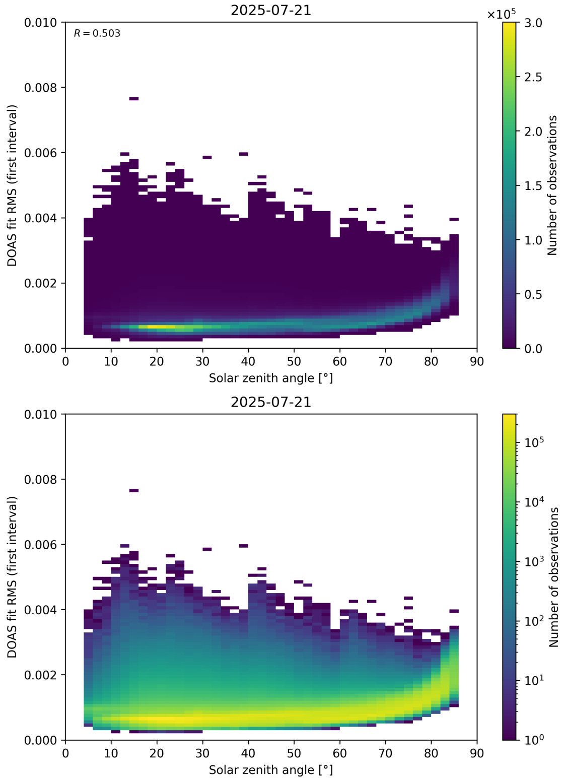
Figure 167: Scatter density plot of “Solar zenith angle” against “DOAS fit RMS (first interval)” for 2025-07-20 to 2025-07-22.
