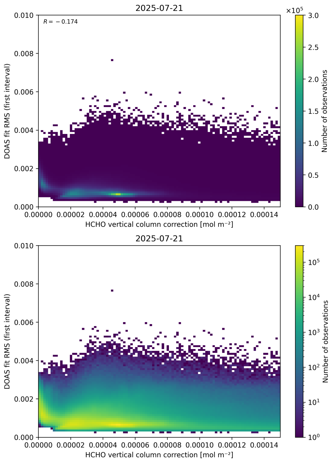
Figure 112: Scatter density plot of “HCHO vertical column correction” against “DOAS fit RMS (first interval)” for 2025-07-20 to 2025-07-22.
