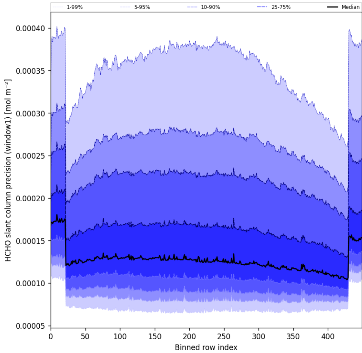
Figure 53: Along track statistics of “HCHO slant column precision (window1)” for 2025-07-20 to 2025-07-22
