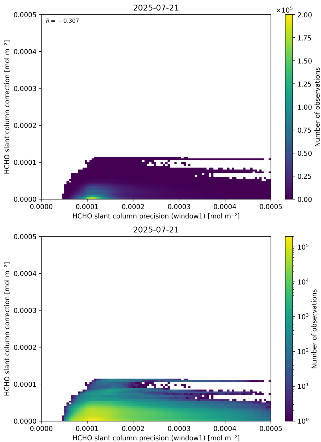
Figure 93: Scatter density plot of “HCHO slant column precision (window1)” against “HCHO slant column correction” for 2025-07-20 to 2025-07-22.
