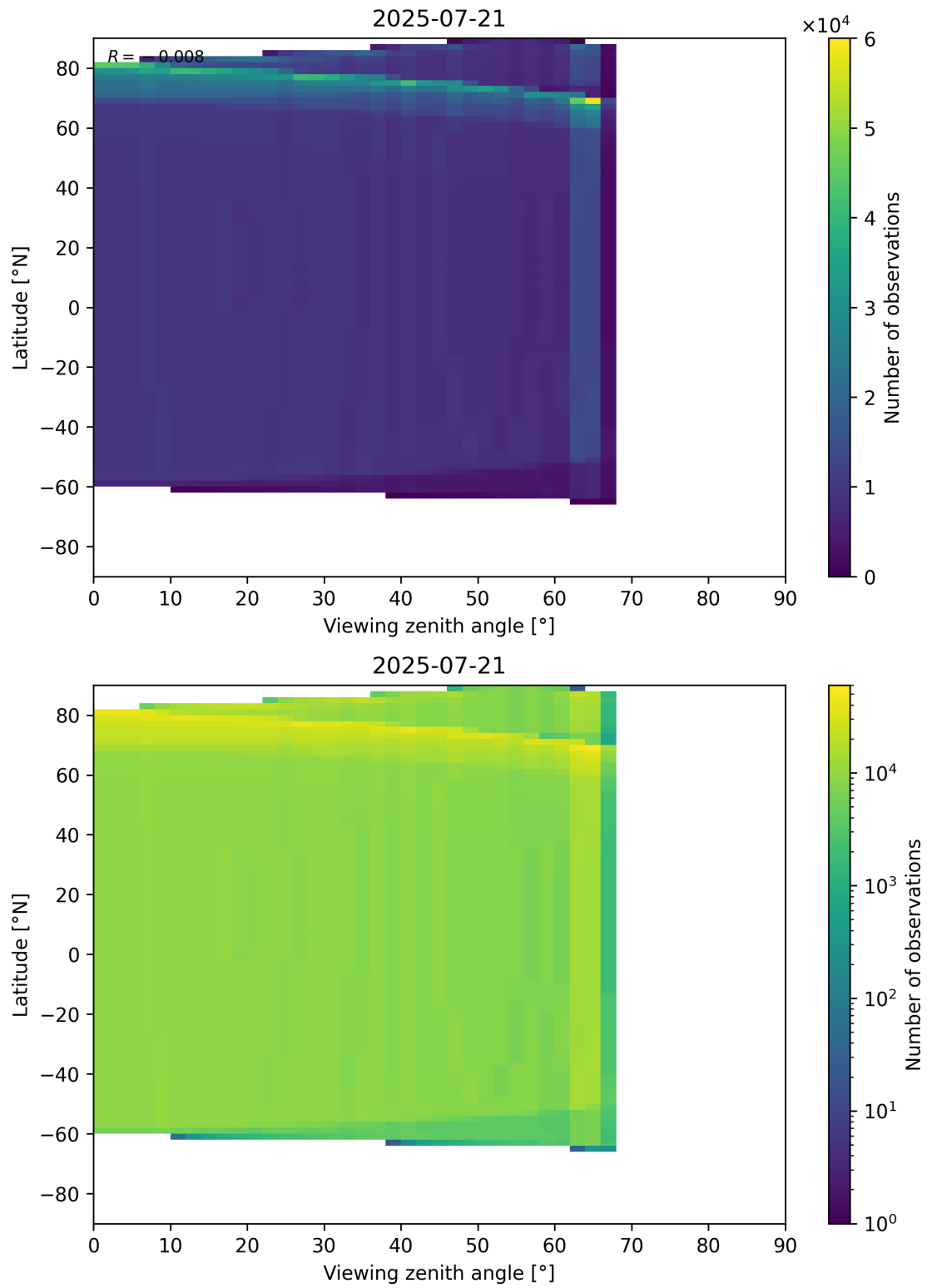
Figure 196: Scatter density plot of “Viewing zenith angle” against “Latitude” for 2025-07-20 to 2025-07-22.
