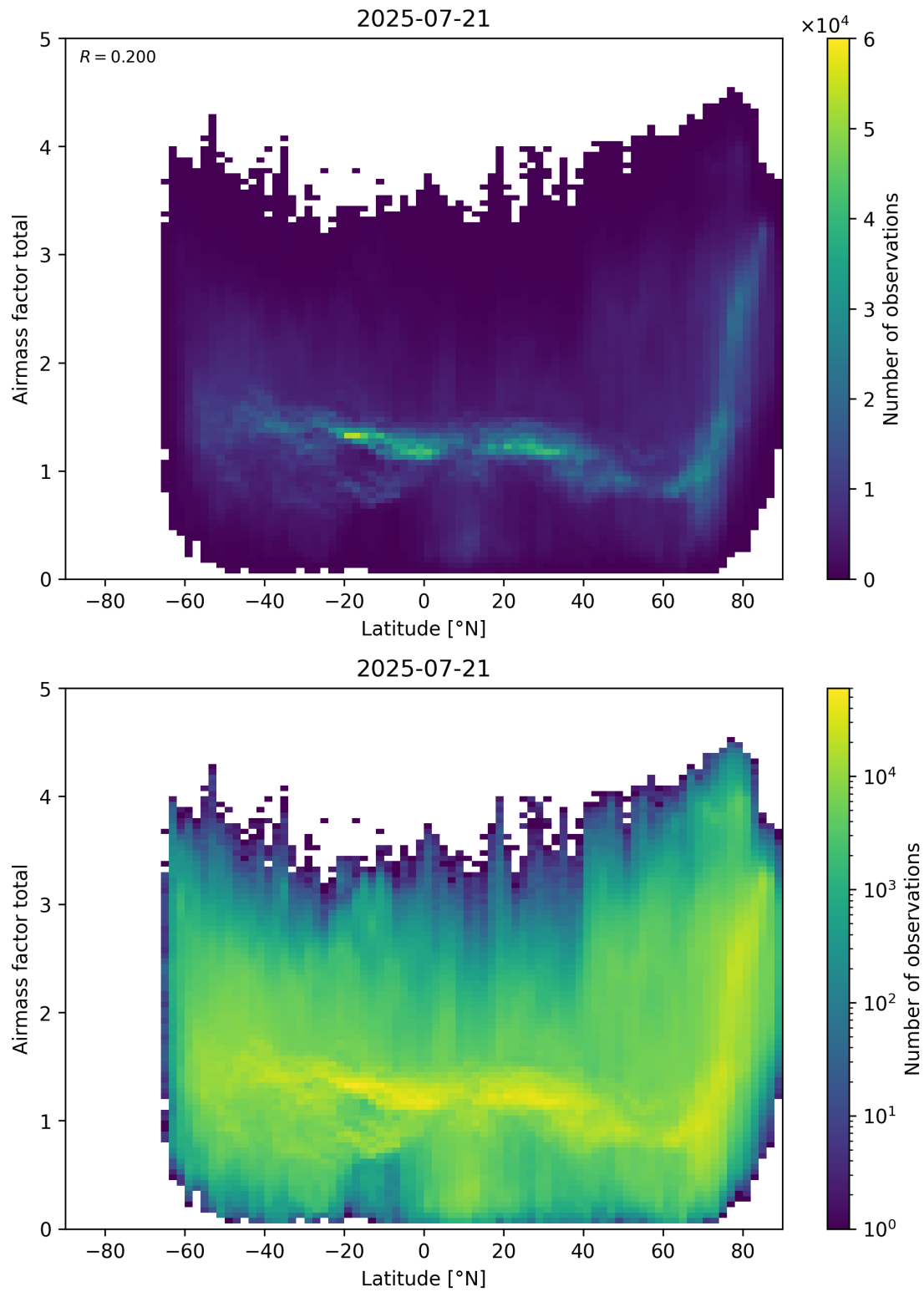
Figure 161: Scatter density plot of “Latitude” against “Airmass factor total” for 2025-07-20 to 2025-07-22.
