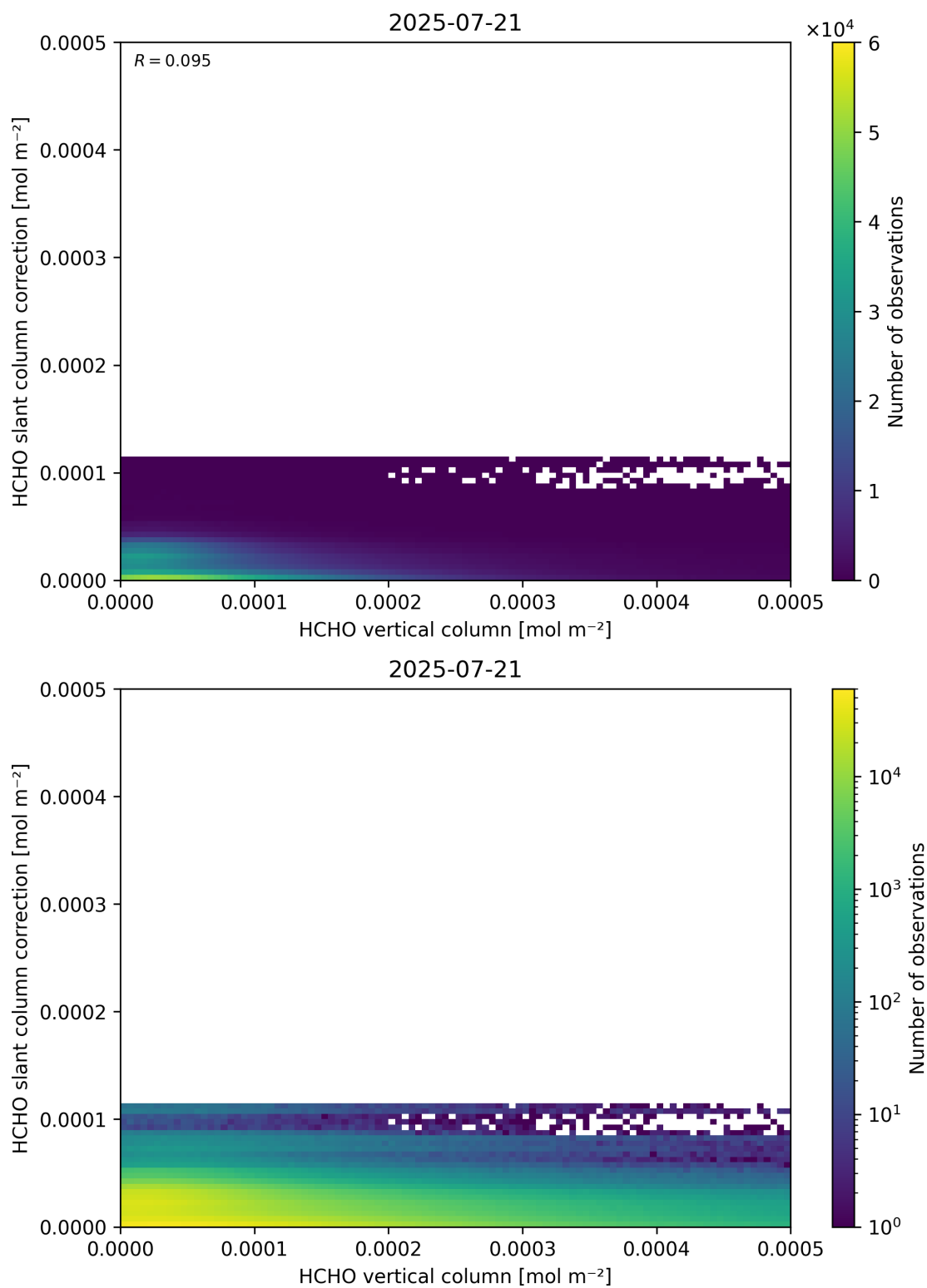
Figure 128: Scatter density plot of “HCHO vertical column” against “HCHO slant column correction” for 2025-07-20 to 2025-07-22.
