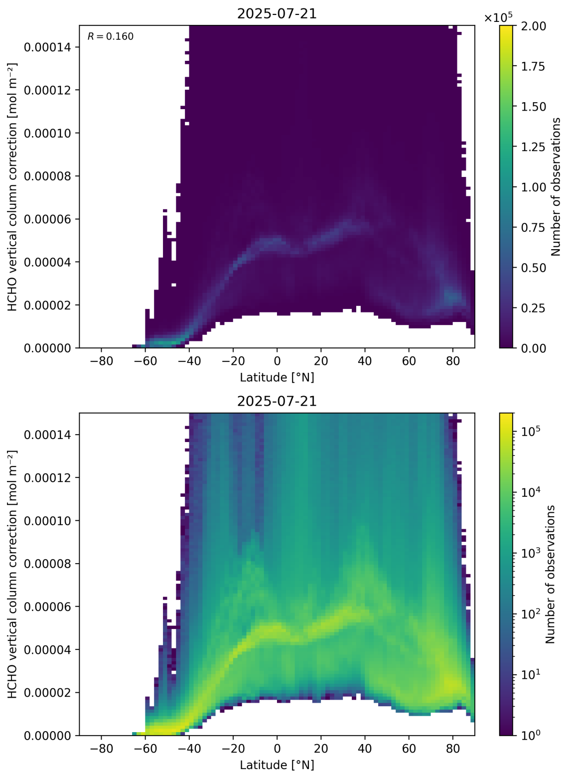
Figure 164: Scatter density plot of “Latitude” against “HCHO vertical column correction” for 2025-07-20 to 2025-07-22.
