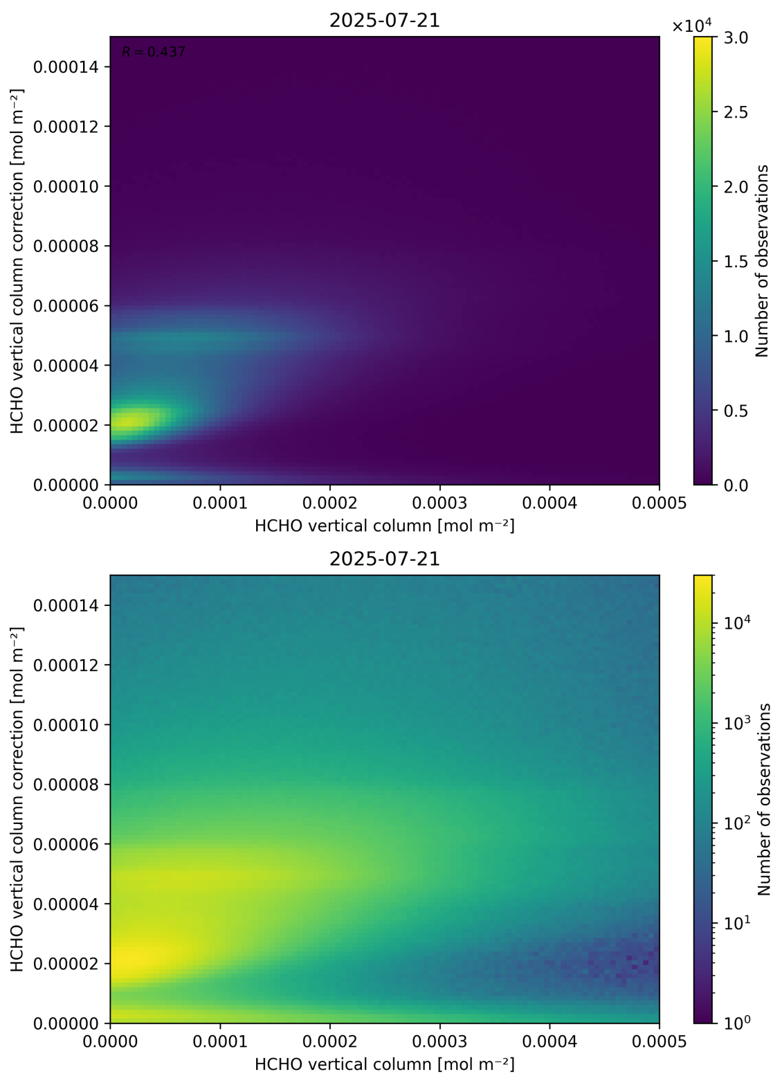
Figure 133: Scatter density plot of “HCHO vertical column” against “HCHO vertical column correction” for 2025-07-20 to 2025-07-22.
