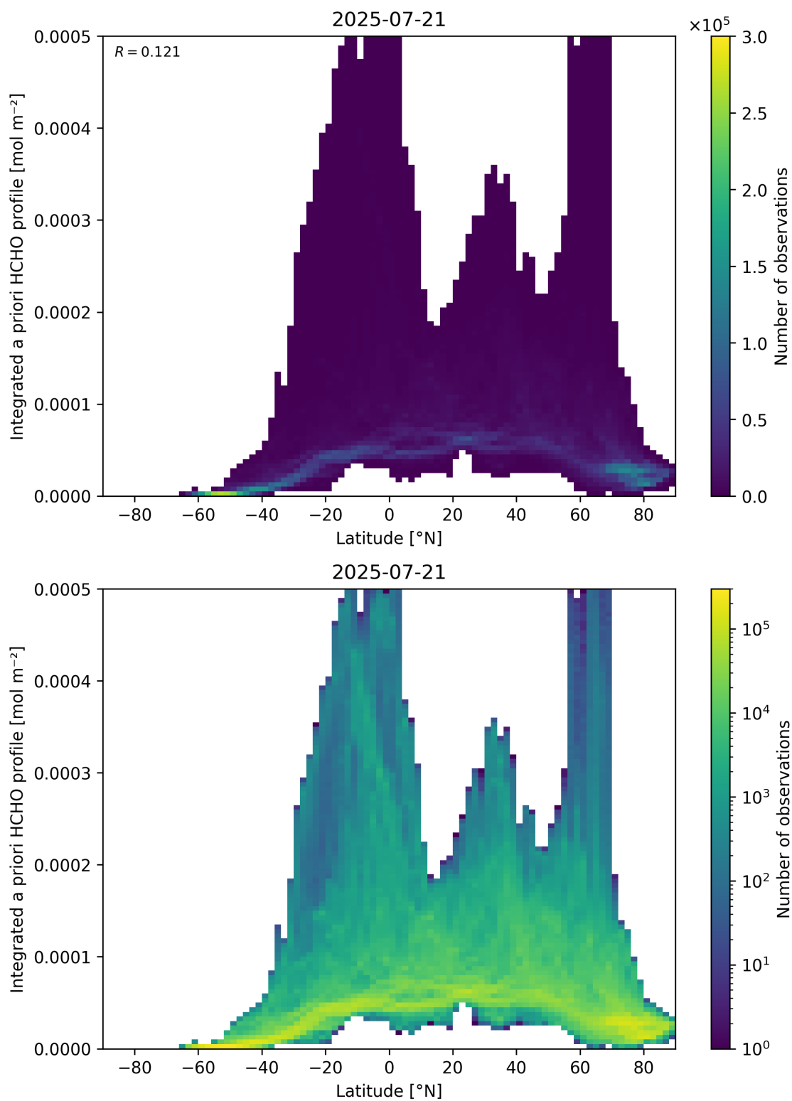
Figure 166: Scatter density plot of “Latitude” against “Integrated a priori HCHO profile” for 2025-07-20 to 2025-07-22.
