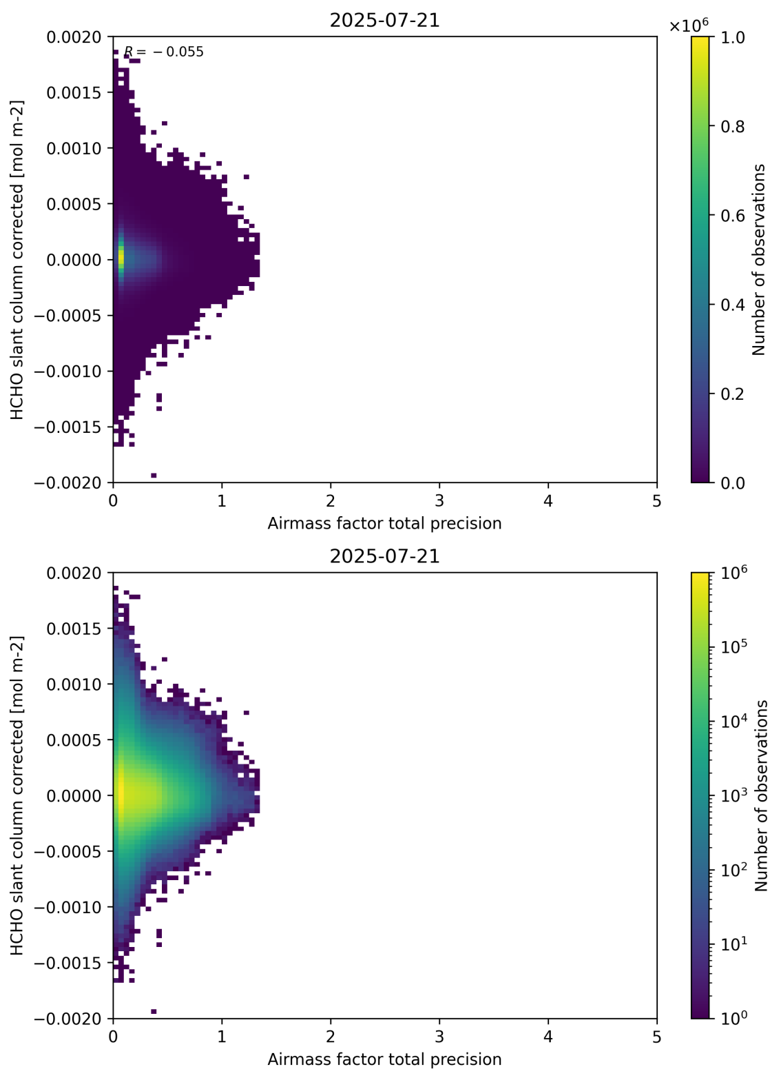
Figure 109: Scatter density plot of “Airmass factor total precision” against “HCHO slant column corrected” for 2025-07-20 to 2025-07-22.
