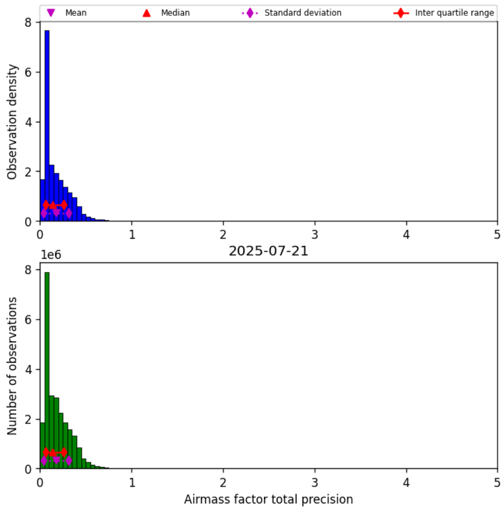
Figure 41: Histogram of “Airmass factor total precision” for 2025-07-20 to 2025-07-22
