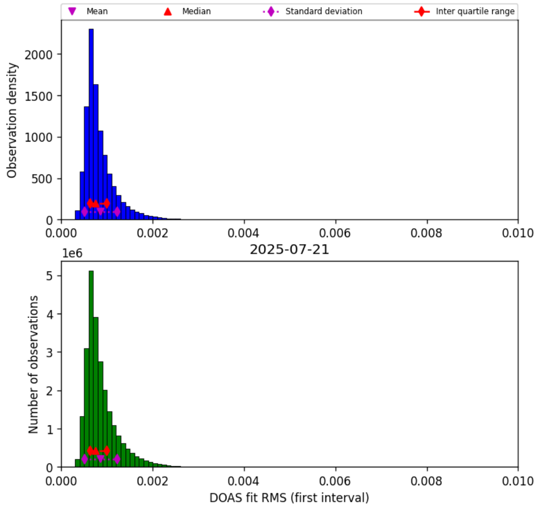
Figure 46: Histogram of “DOAS fit RMS (first interval)” for 2025-07-20 to 2025-07-22
