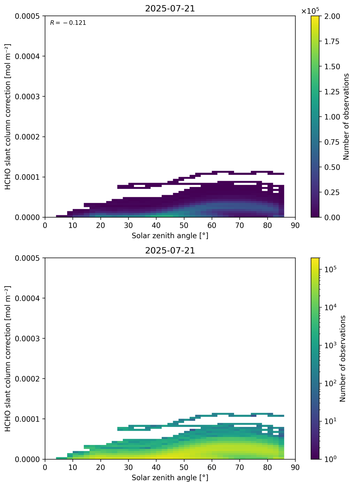
Figure 172: Scatter density plot of “Solar zenith angle” against “HCHO slant column correction” for 2025-07-20 to 2025-07-22.
