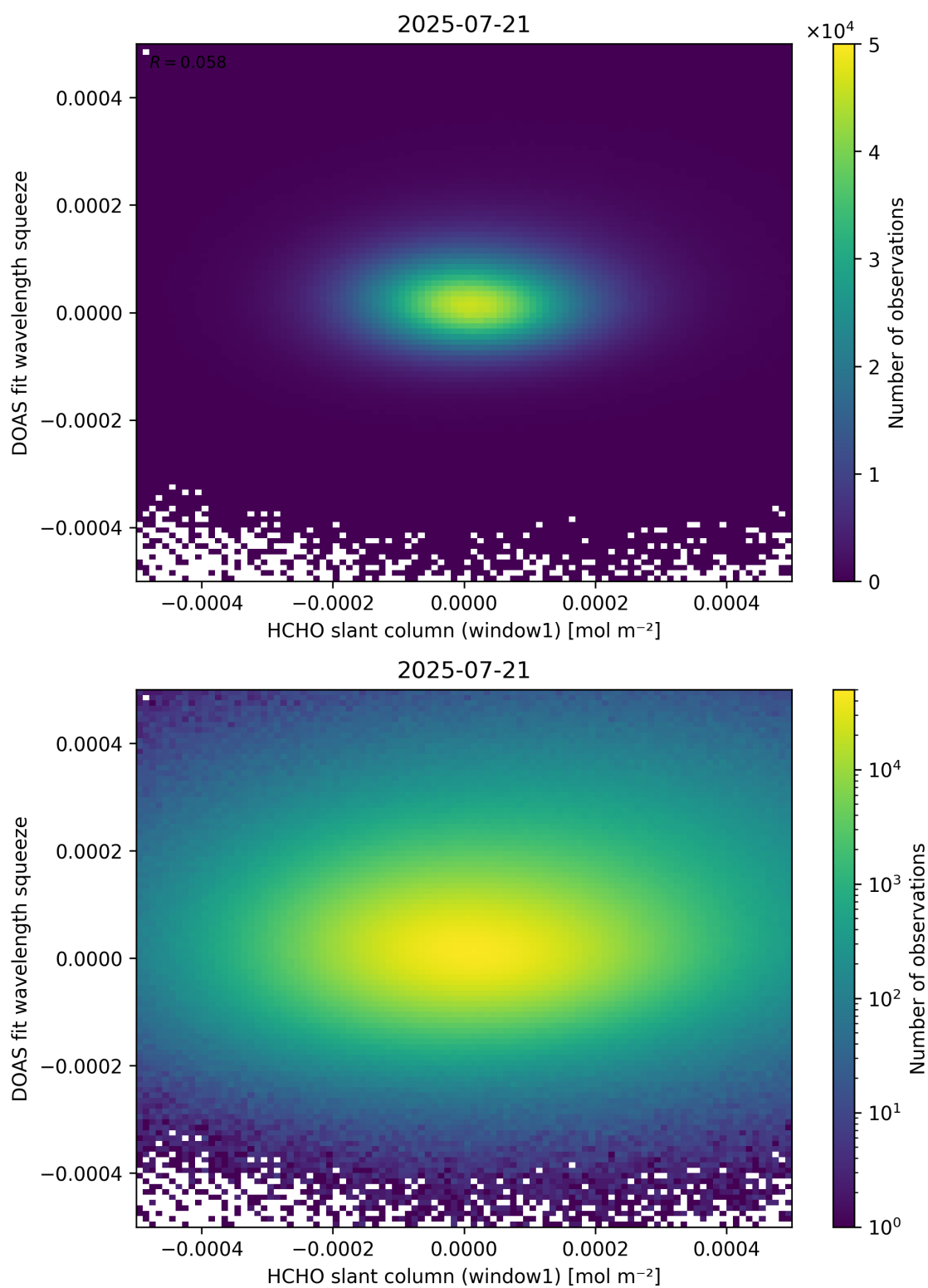
Figure 80: Scatter density plot of “HCHO slant column (window1)” against “DOAS fit wavelength squeeze” for 2025-07-20 to 2025-07-22.
