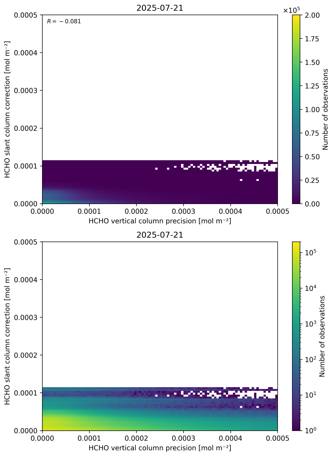
Figure 141: Scatter density plot of “HCHO vertical column precision” against “HCHO slant column correction” for 2025-07-20 to 2025-07-22.
