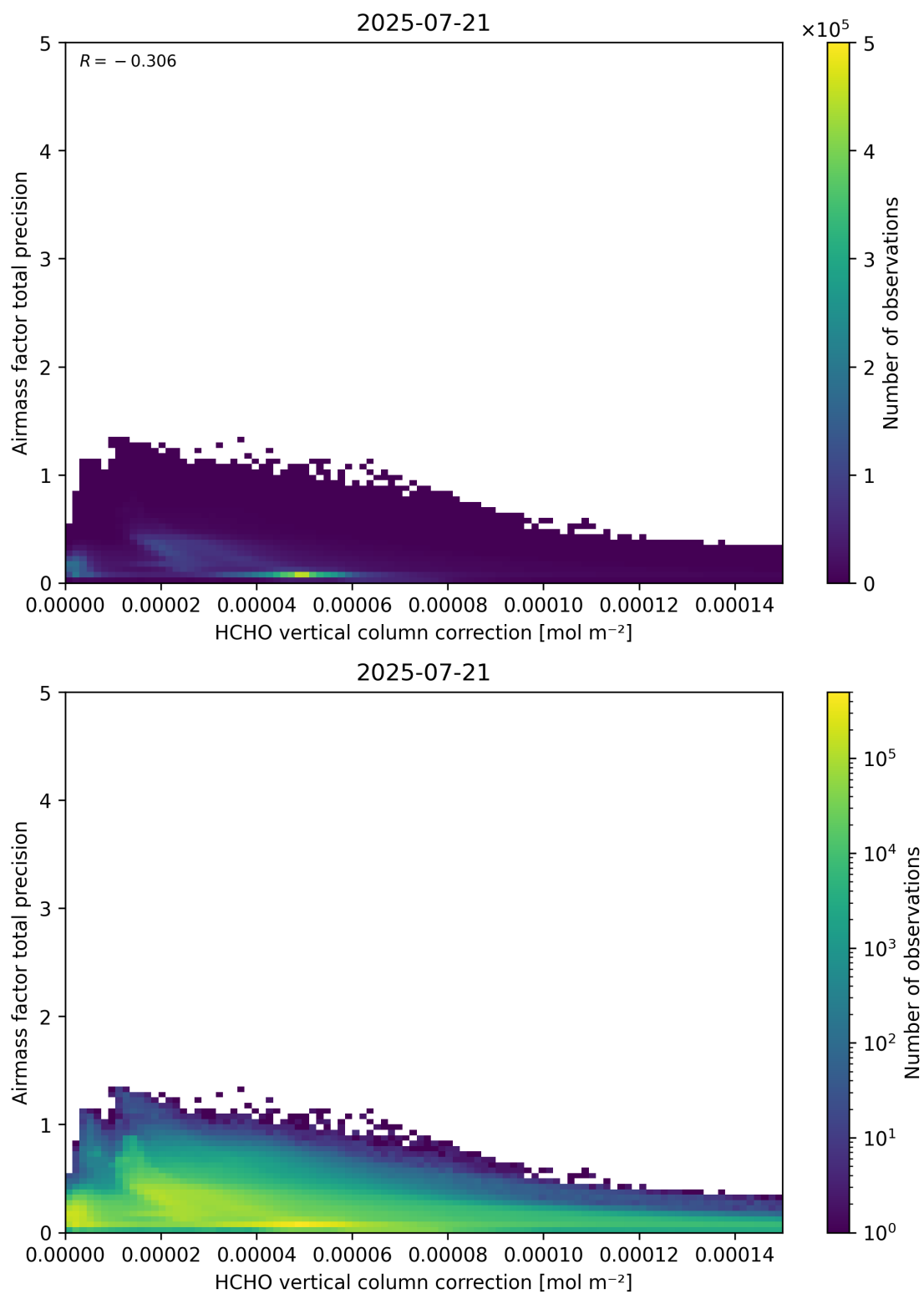
Figure 121: Scatter density plot of “HCHO vertical column correction” against “Airmass factor total precision” for 2025-07-20 to 2025-07-22.
