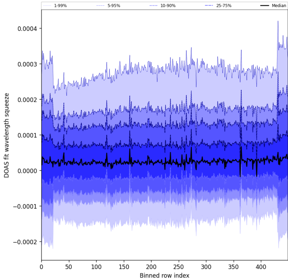
Figure 59: Along track statistics of “DOAS fit wavelength squeeze” for 2025-07-20 to 2025-07-22
