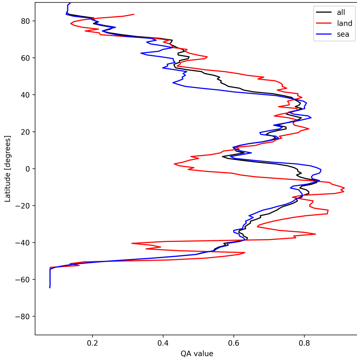
Figure 20: Zonal average of “QA value” for 2025-07-20 to 2025-07-22.
