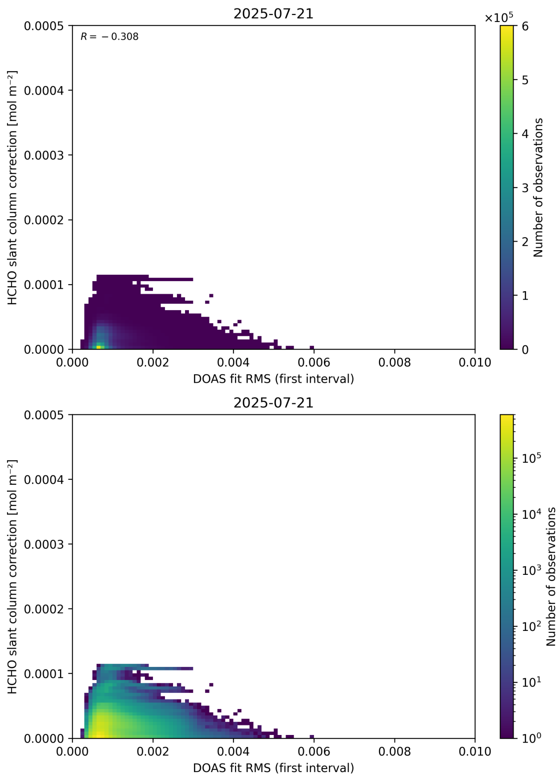
Figure 63: Scatter density plot of “DOAS fit RMS (first interval)” against “HCHO slant column correction” for 2025-07-20 to 2025-07-22.
