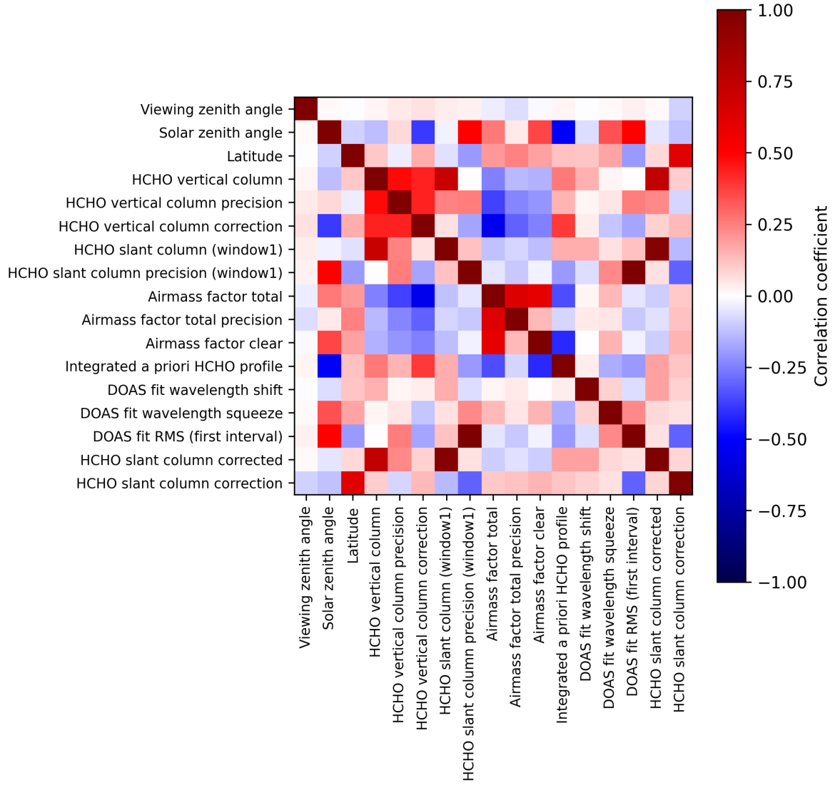
Figure 2: Map of correlation matrix for 2025-07-20 to 2025-07-22.
