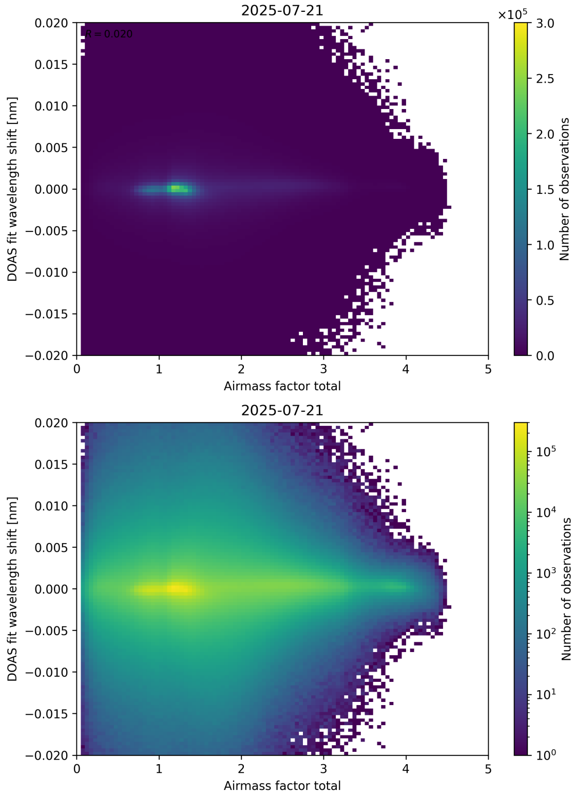
Figure 98: Scatter density plot of “Airmass factor total” against “DOAS fit wavelength shift” for 2025-07-20 to 2025-07-22.
