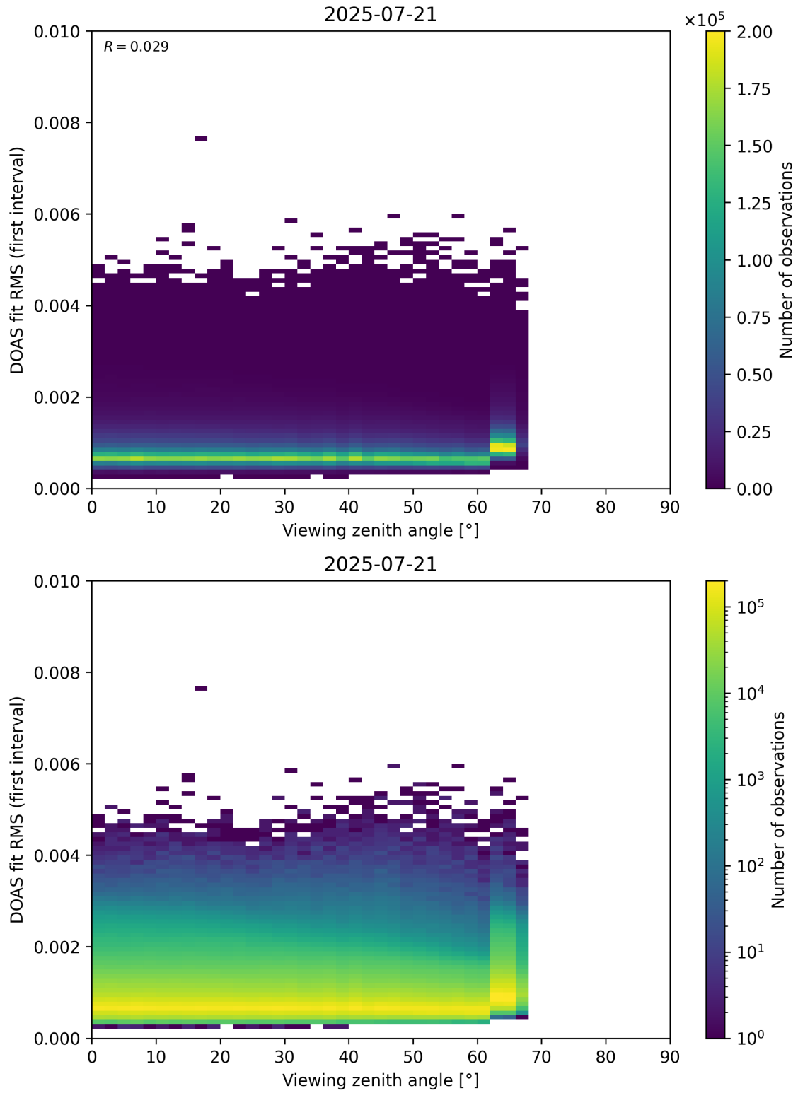
Figure 182: Scatter density plot of “Viewing zenith angle” against “DOAS fit RMS (first interval)” for 2025-07-20 to 2025-07-22.
