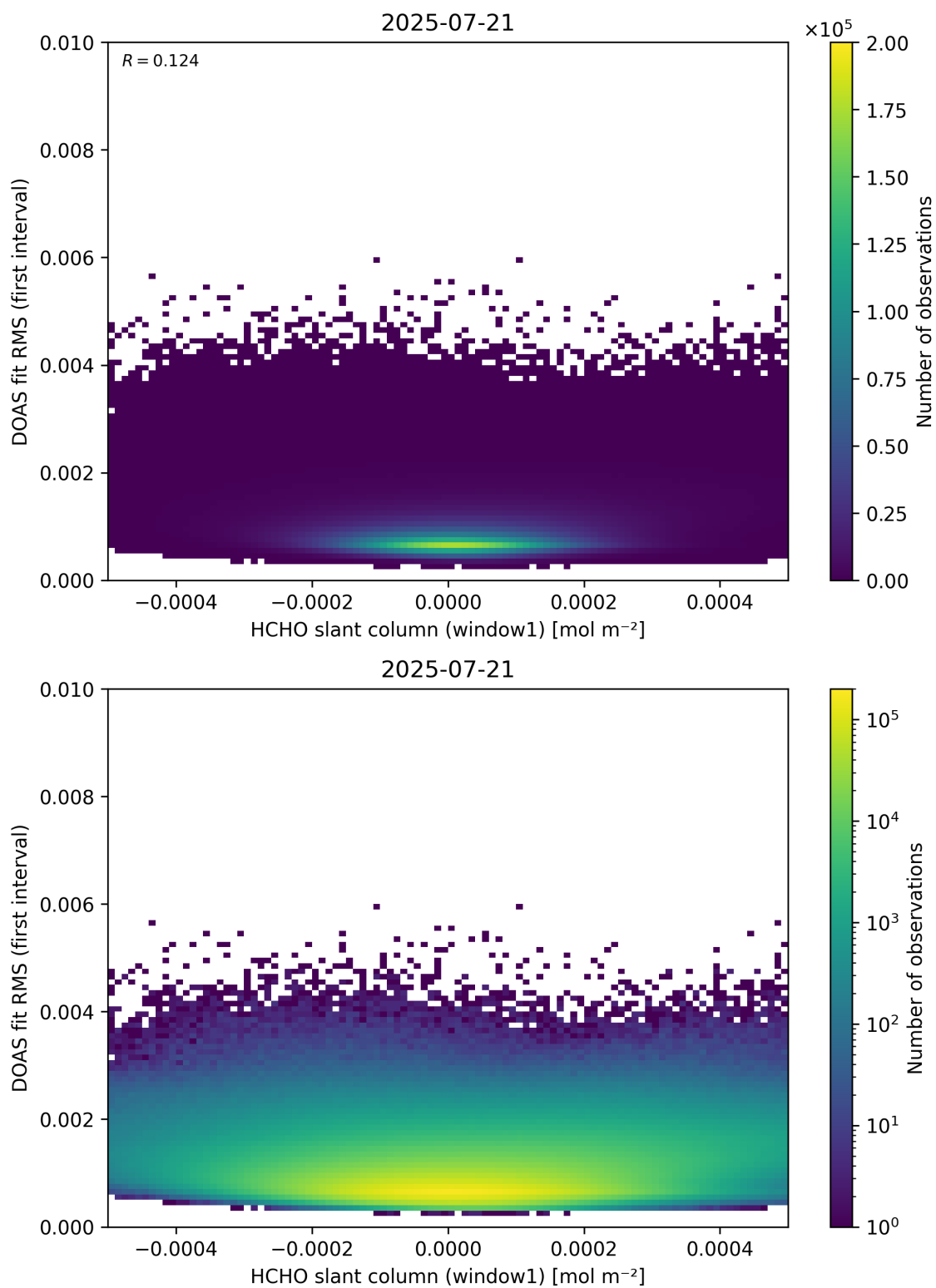
Figure 78: Scatter density plot of “HCHO slant column (window1)” against “DOAS fit RMS (first interval)” for 2025-07-20 to 2025-07-22.
