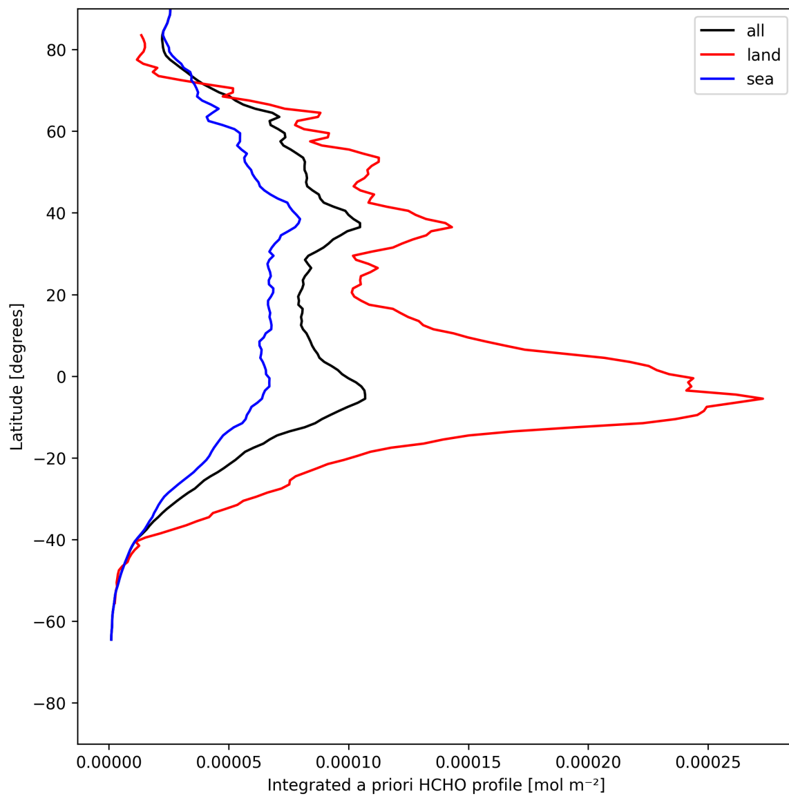
Figure 29: Zonal average of “Integrated a priori HCHO profile” for 2025-07-20 to 2025-07-22.
