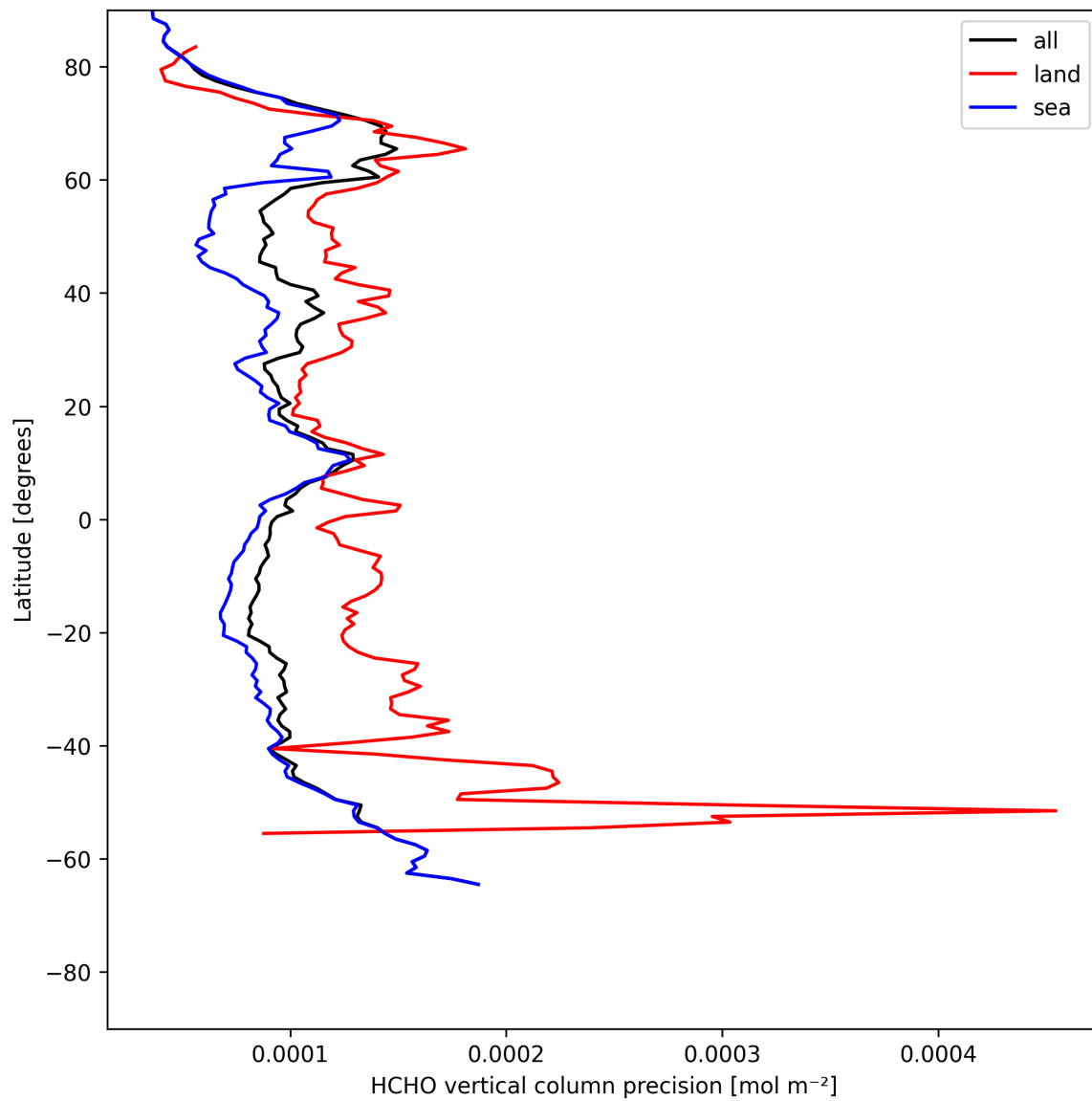
Figure 22: Zonal average of “HCHO vertical column precision” for 2025-07-20 to 2025-07-22.
