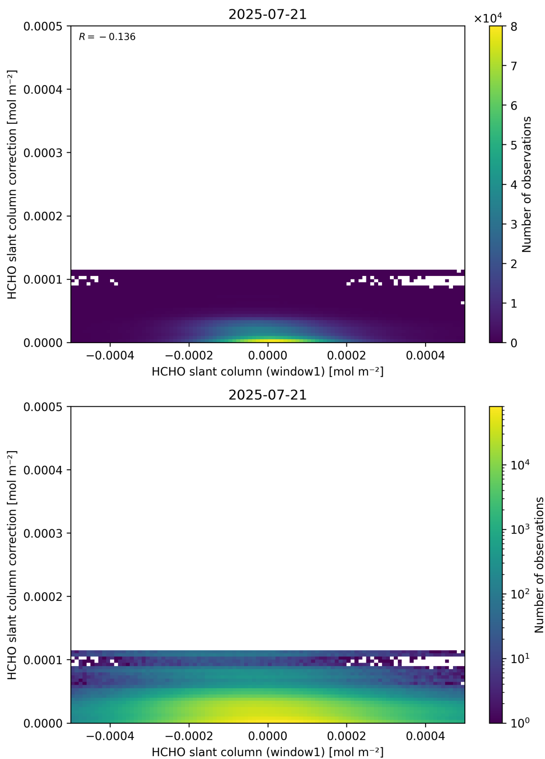
Figure 83: Scatter density plot of “HCHO slant column (window1)” against “HCHO slant column correction” for 2025-07-20 to 2025-07-22.
