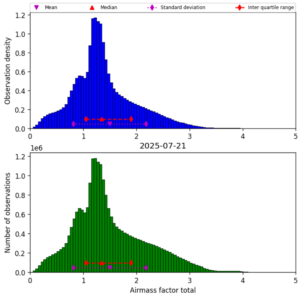
Figure 40: Histogram of “Airmass factor total” for 2025-07-20 to 2025-07-22
