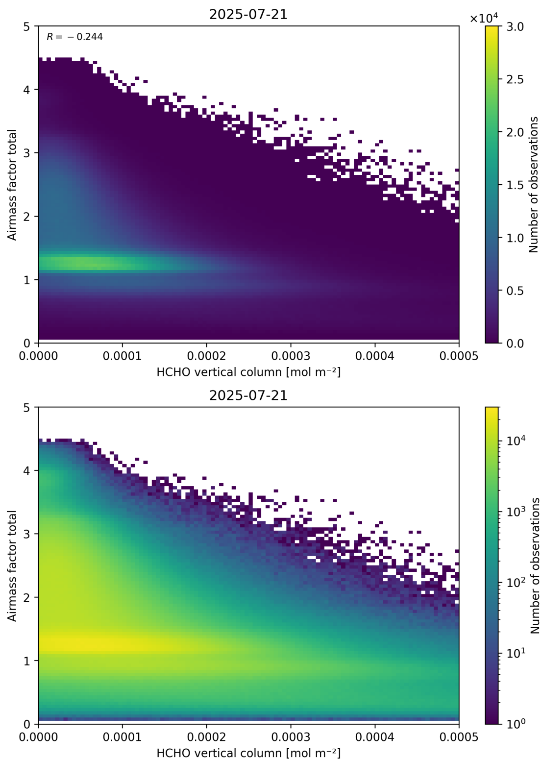
Figure 131: Scatter density plot of “HCHO vertical column” against “Airmass factor total” for 2025-07-20 to 2025-07-22.
