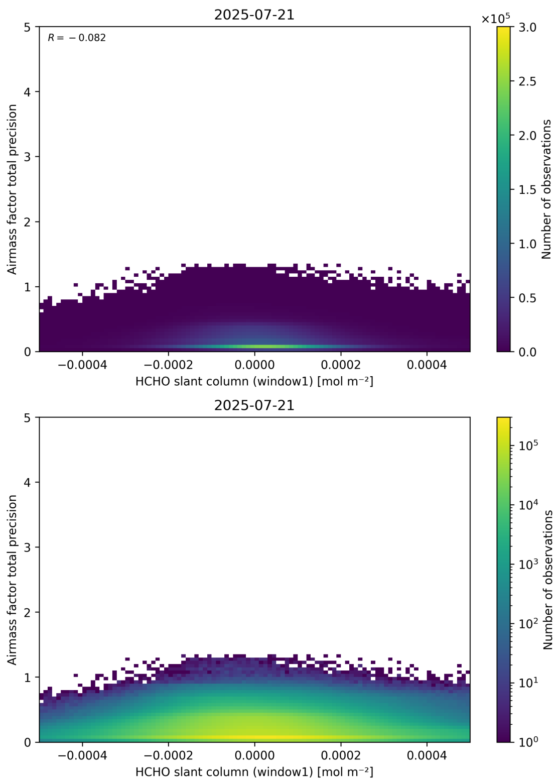
Figure 86: Scatter density plot of “HCHO slant column (window1)” against “Airmass factor total precision” for 2025-07-20 to 2025-07-22.
