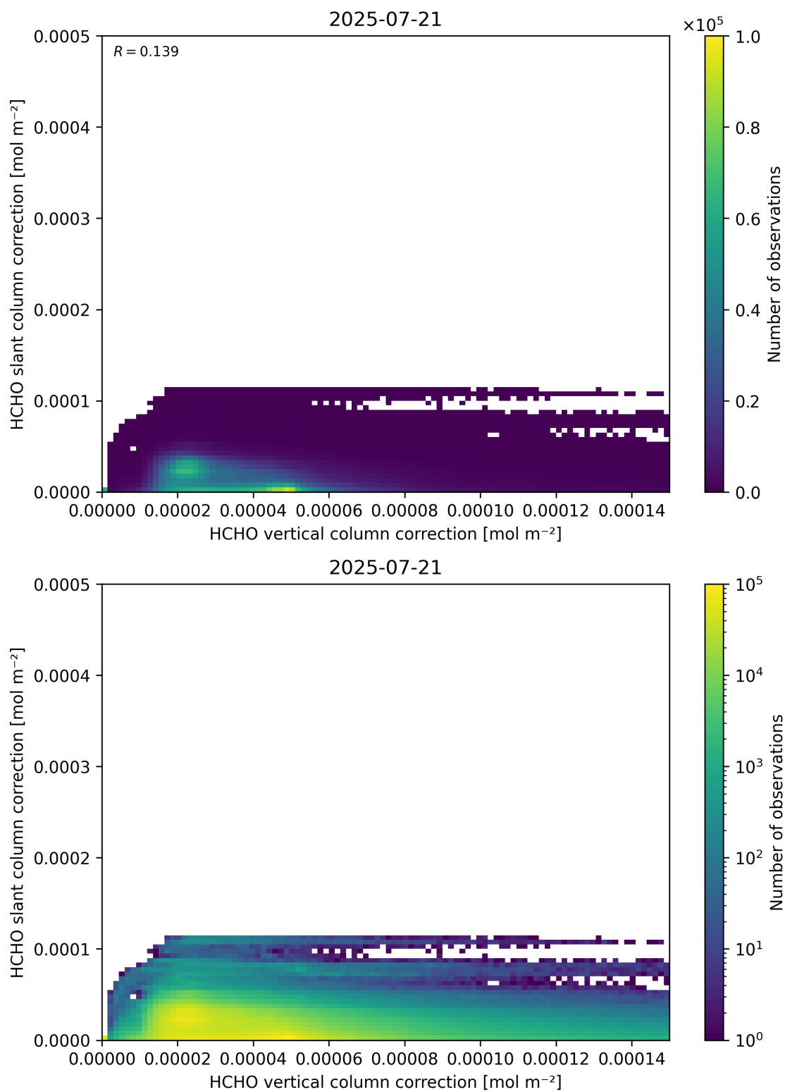
Figure 117: Scatter density plot of “HCHO vertical column correction” against “HCHO slant column correction” for 2025-07-20 to 2025-07-22.
