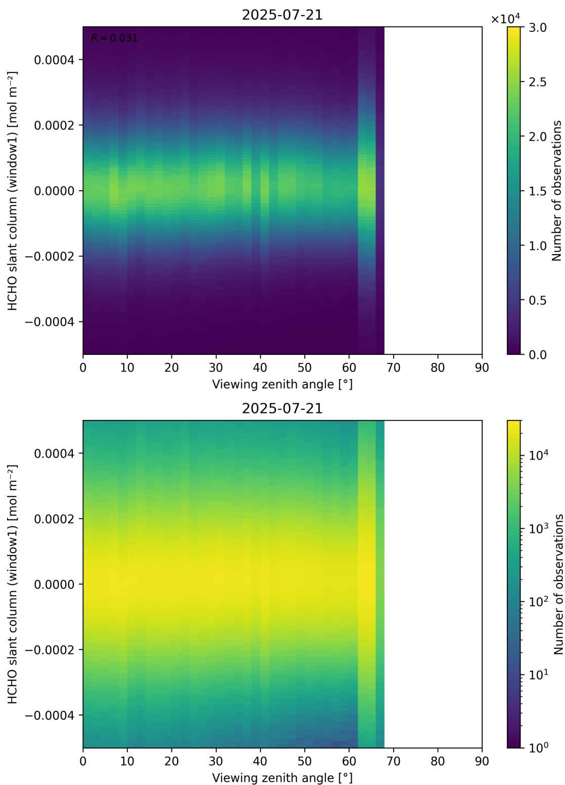
Figure 188: Scatter density plot of “Viewing zenith angle” against “HCHO slant column (window1)” for 2025-07-20 to 2025-07-22.
