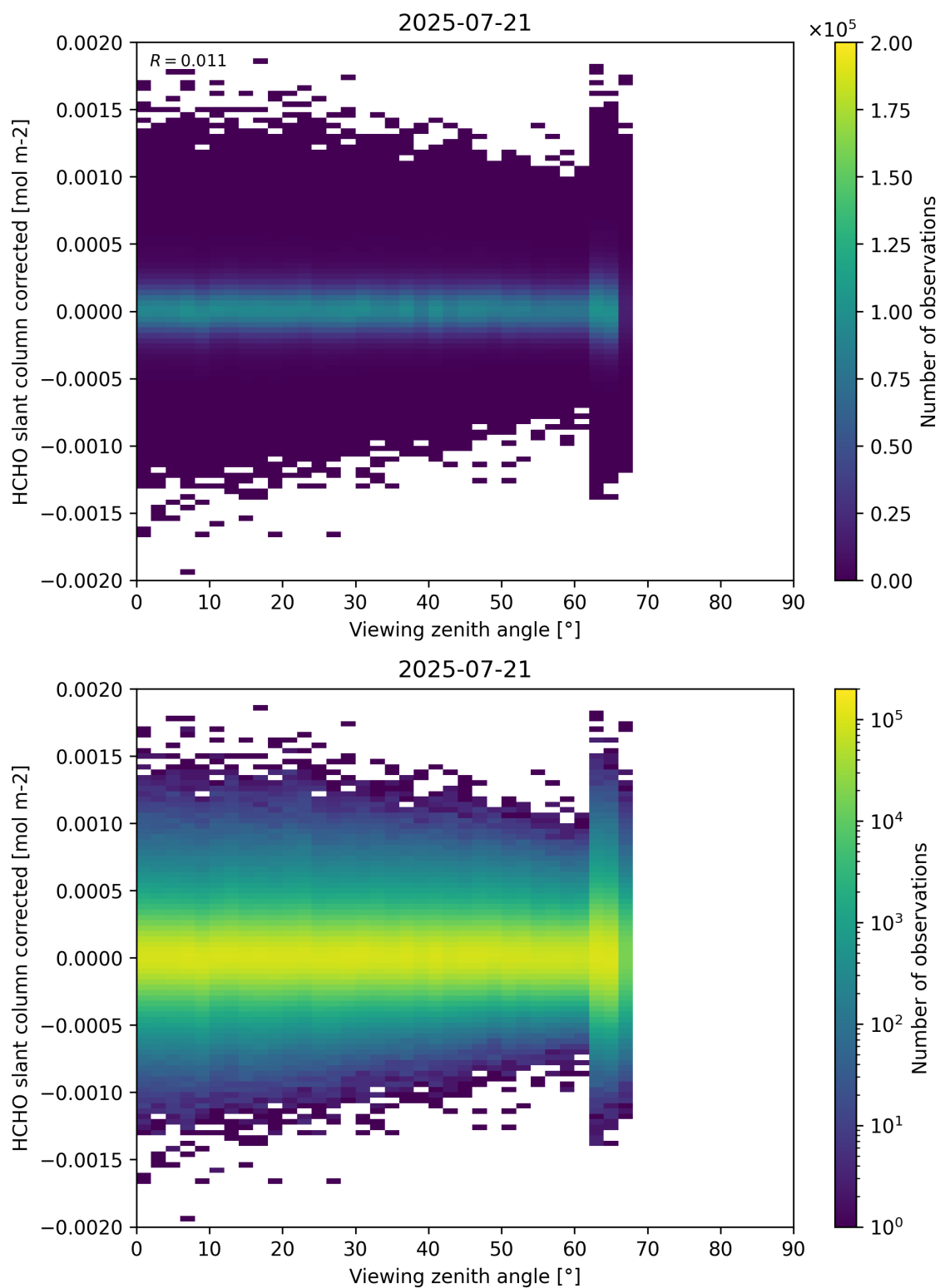
Figure 186: Scatter density plot of “Viewing zenith angle” against “HCHO slant column corrected” for 2025-07-20 to 2025-07-22.
