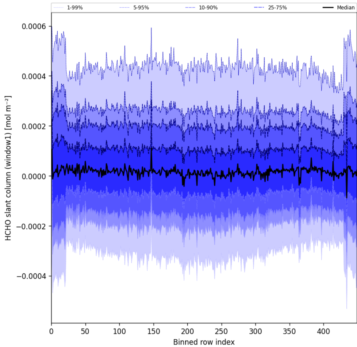
Figure 52: Along track statistics of “HCHO slant column (window1)” for 2025-07-20 to 2025-07-22
