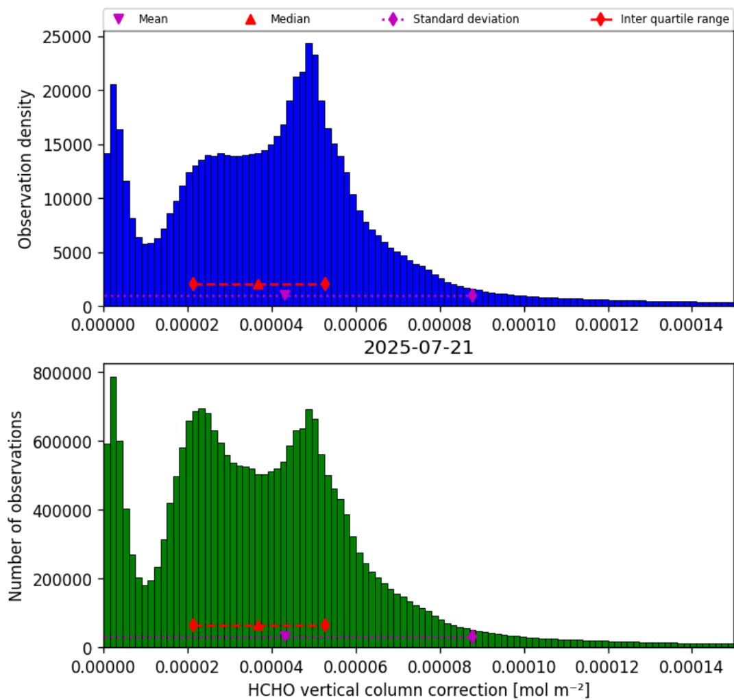
Figure 37: Histogram of “HCHO vertical column correction” for 2025-07-20 to 2025-07-22
