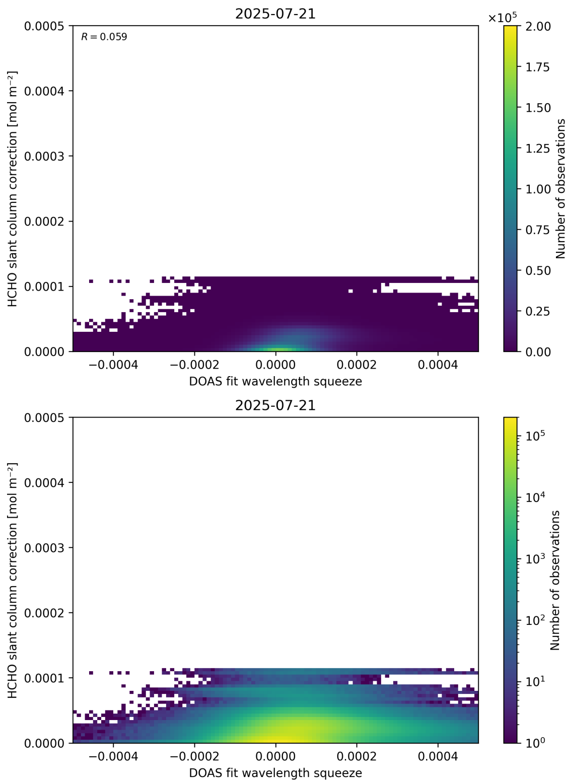
Figure 70: Scatter density plot of “DOAS fit wavelength squeeze” against “HCHO slant column correction” for 2025-07-20 to 2025-07-22.
