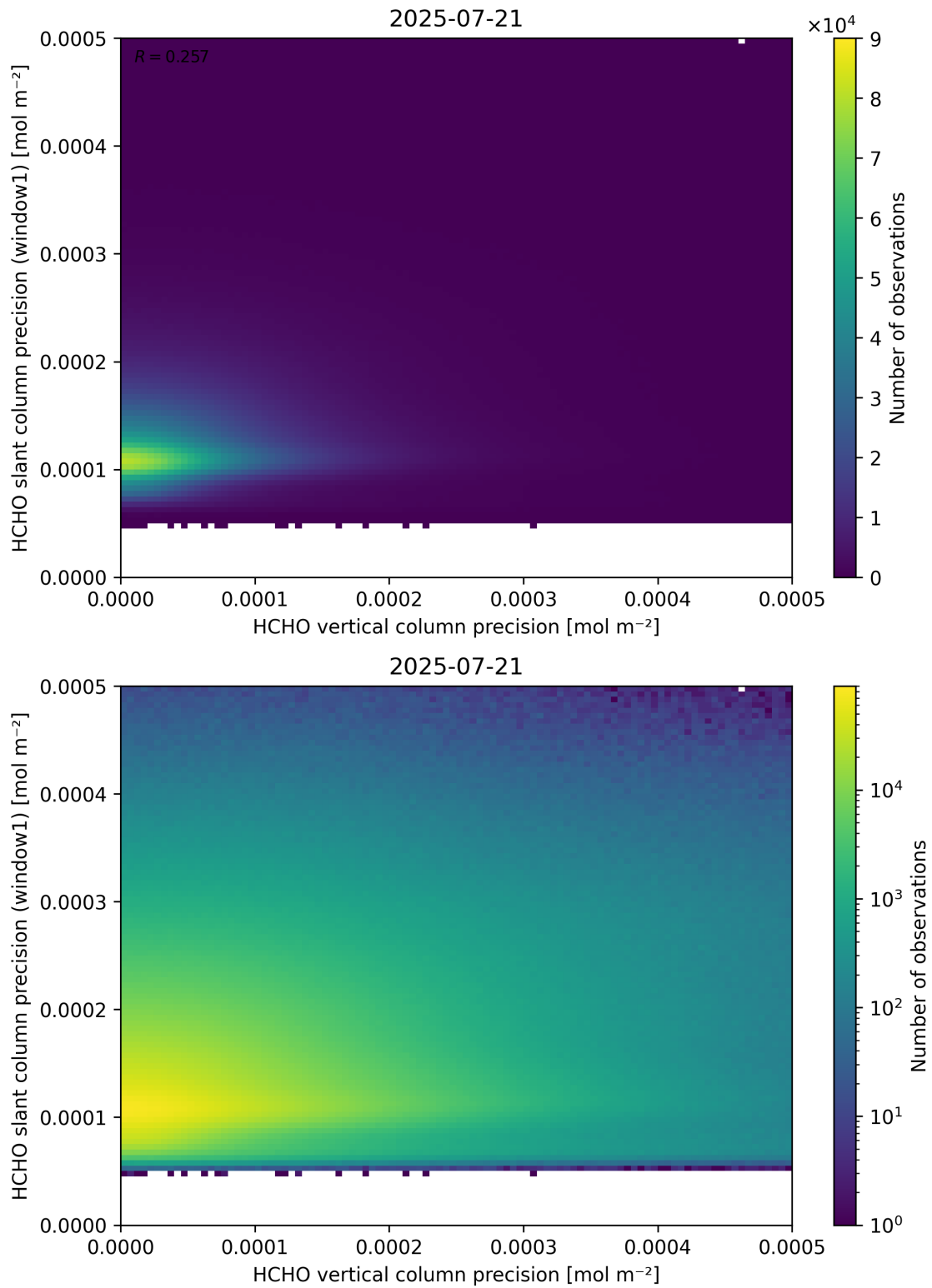
Figure 143: Scatter density plot of “HCHO vertical column precision” against “HCHO slant column precision (window1)” for 2025-07-20 to 2025-07-22.
