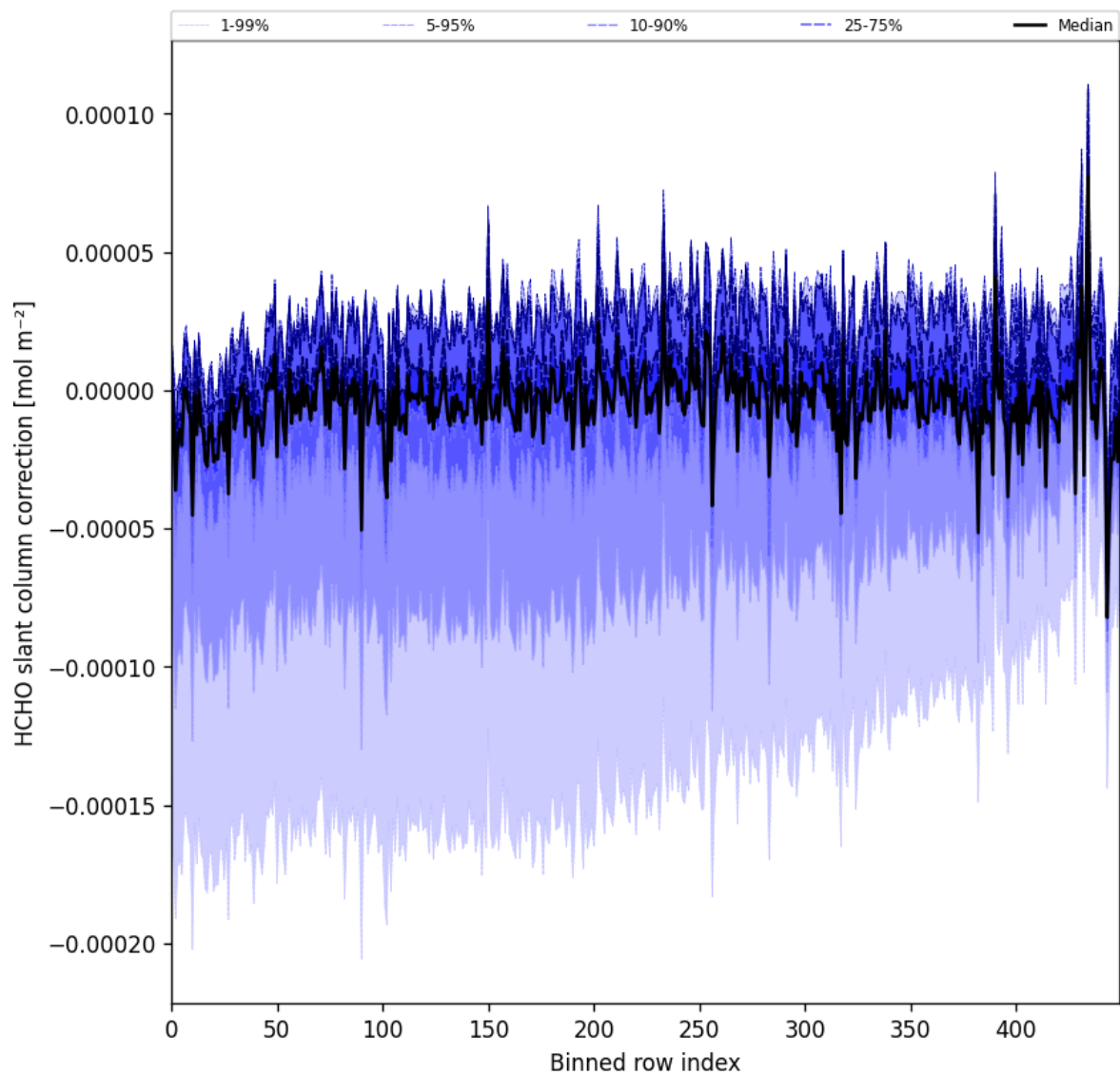
Figure 61: Along track statistics of “HCHO slant column correction” for 2025-07-20 to 2025-07-22
