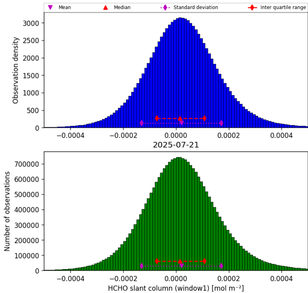
Figure 38: Histogram of “HCHO slant column (window1)” for 2025-07-20 to 2025-07-22
