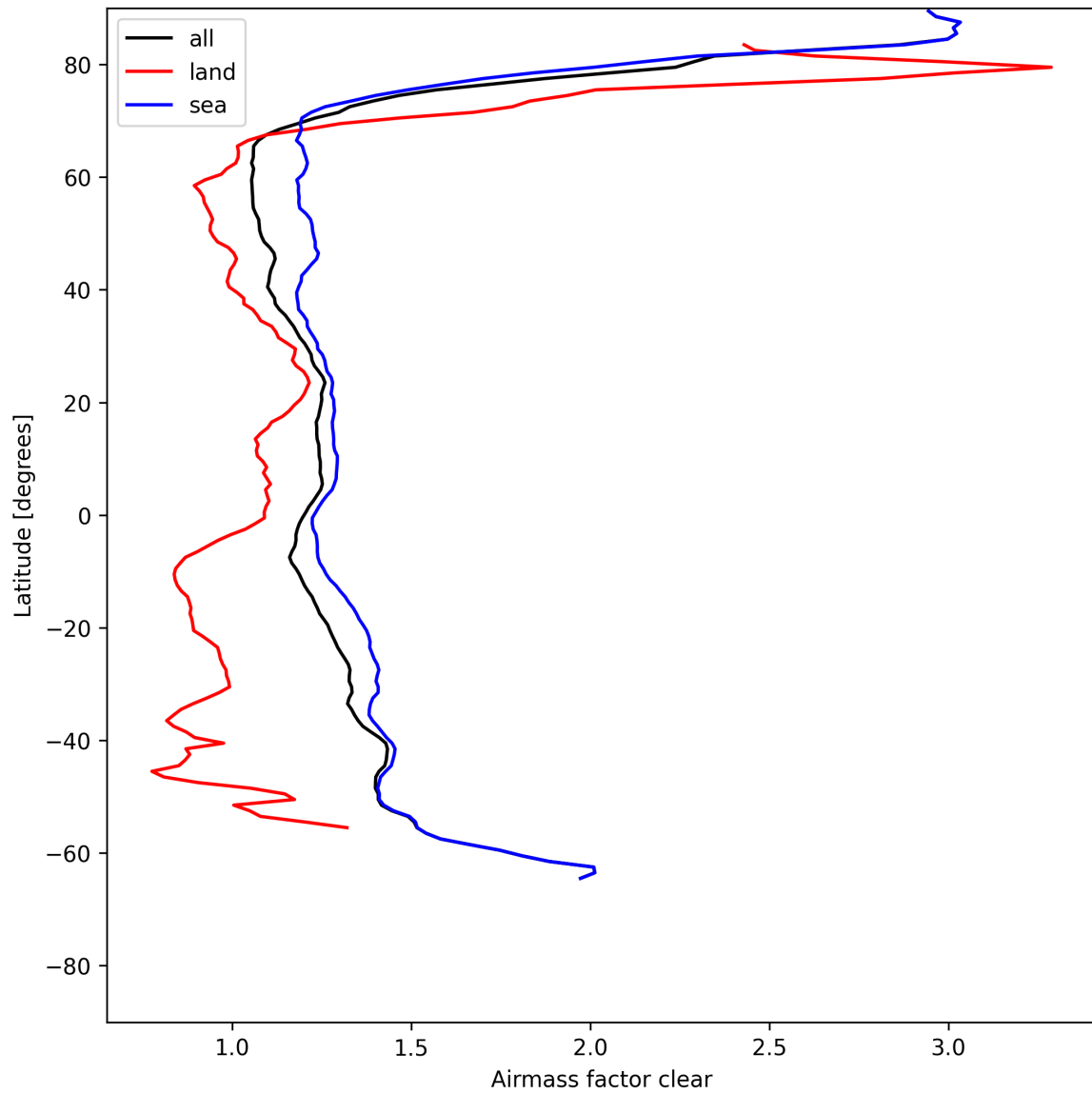
Figure 28: Zonal average of “Airmass factor clear” for 2025-07-20 to 2025-07-22.
