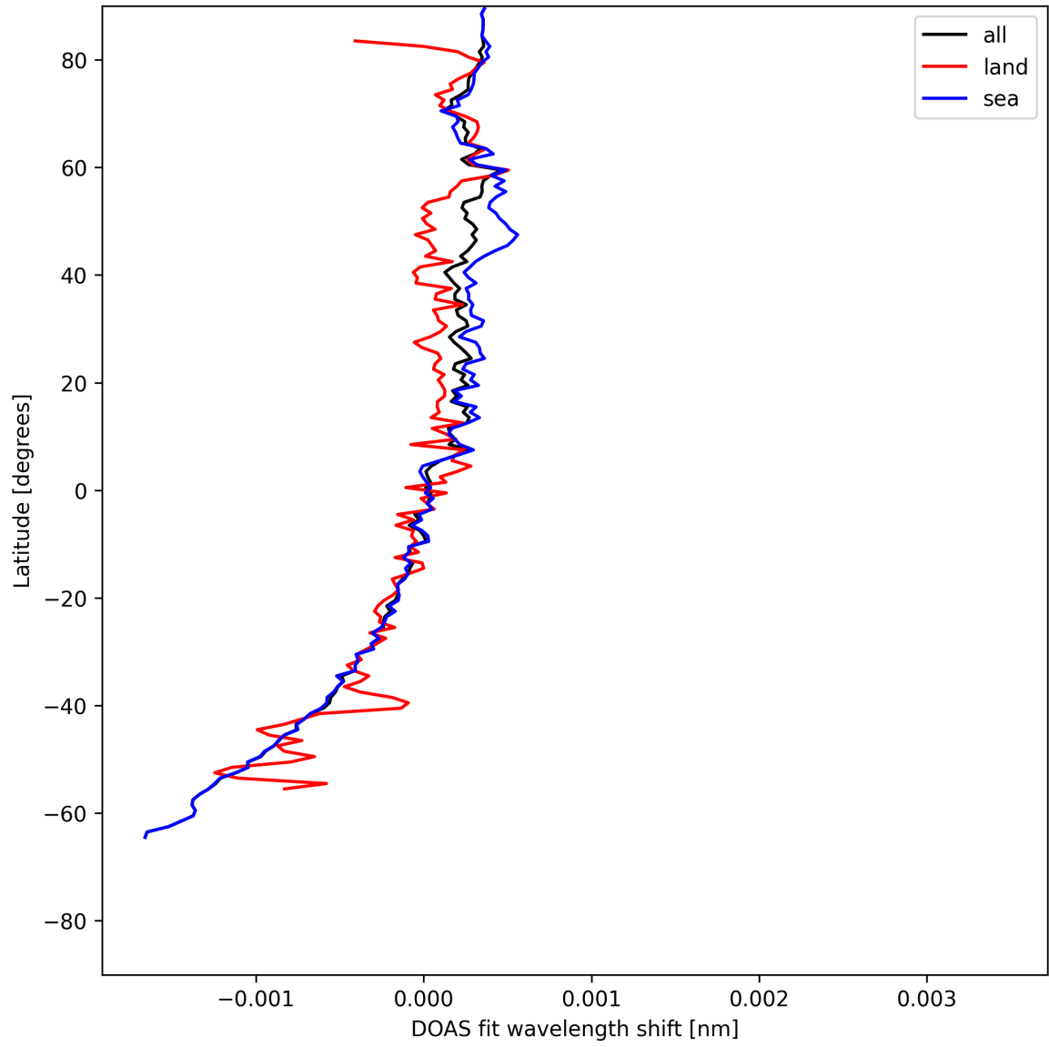
Figure 30: Zonal average of “DOAS fit wavelength shift” for 2025-07-20 to 2025-07-22.
