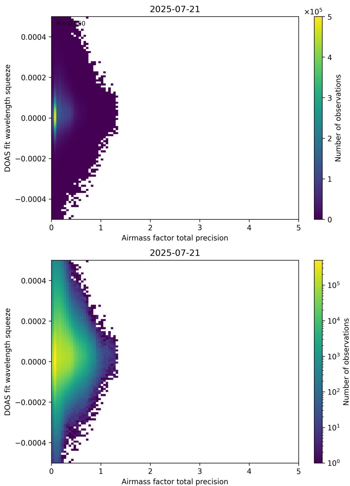
Figure 107: Scatter density plot of “Airmass factor total precision” against “DOAS fit wavelength squeeze” for 2025-07-20 to 2025-07-22.
