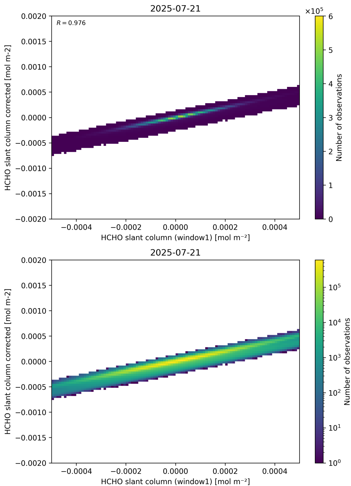
Figure 82: Scatter density plot of “HCHO slant column (window1)” against “HCHO slant column corrected” for 2025-07-20 to 2025-07-22.
