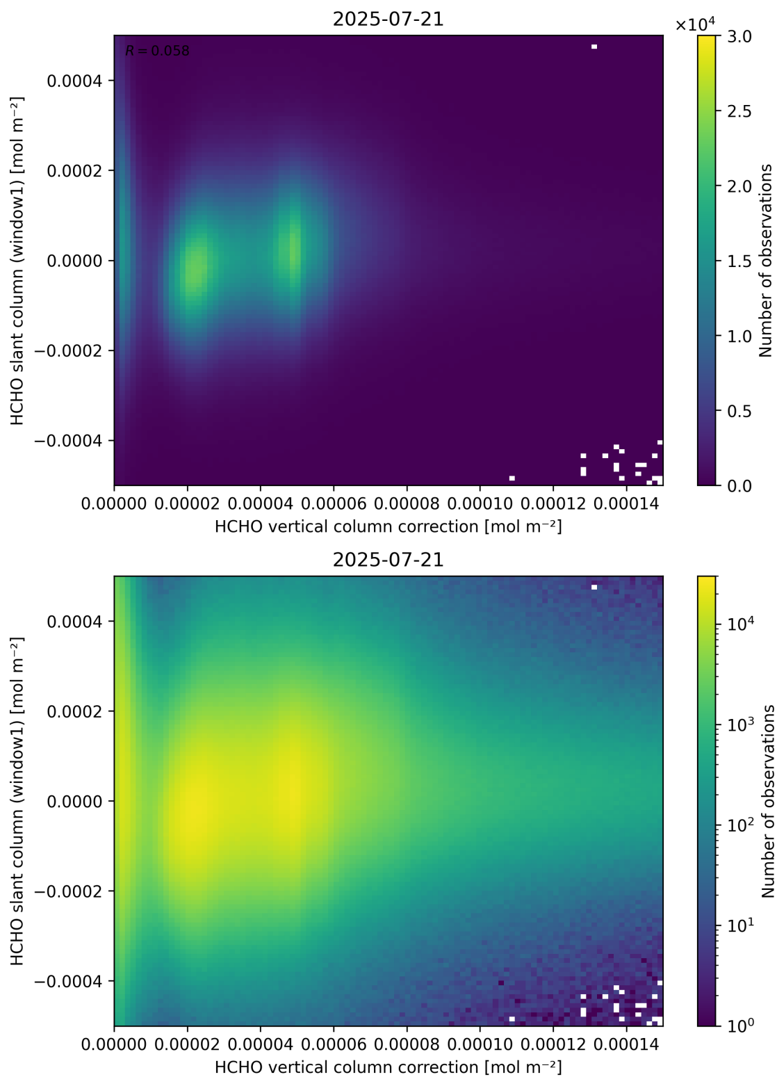
Figure 118: Scatter density plot of “HCHO vertical column correction” against “HCHO slant column (window1)” for 2025-07-20 to 2025-07-22.
