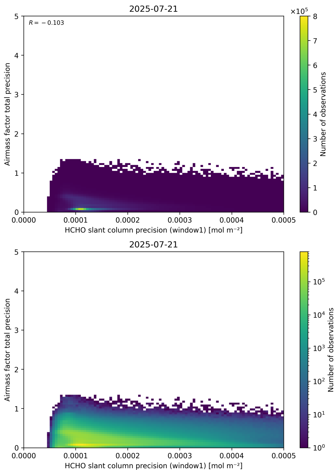
Figure 95: Scatter density plot of “HCHO slant column precision (window1)” against “Airmass factor total precision” for 2025-07-20 to 2025-07-22.
