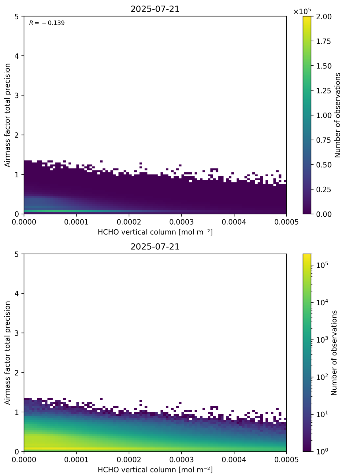
Figure 132: Scatter density plot of “HCHO vertical column” against “Airmass factor total precision” for 2025-07-20 to 2025-07-22.
