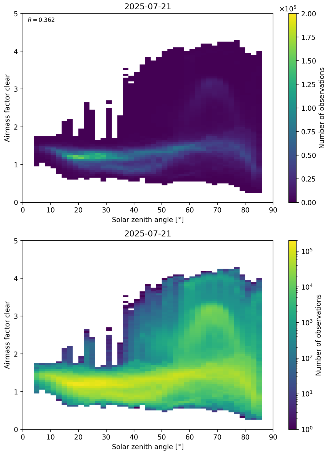
Figure 170: Scatter density plot of “Solar zenith angle” against “Airmass factor clear” for 2025-07-20 to 2025-07-22.
