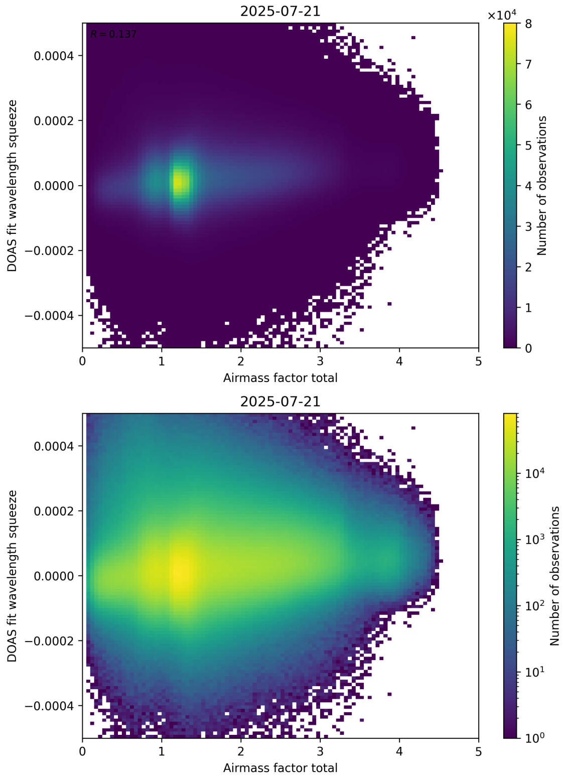
Figure 99: Scatter density plot of “Airmass factor total” against “DOAS fit wavelength squeeze” for 2025-07-20 to 2025-07-22.
