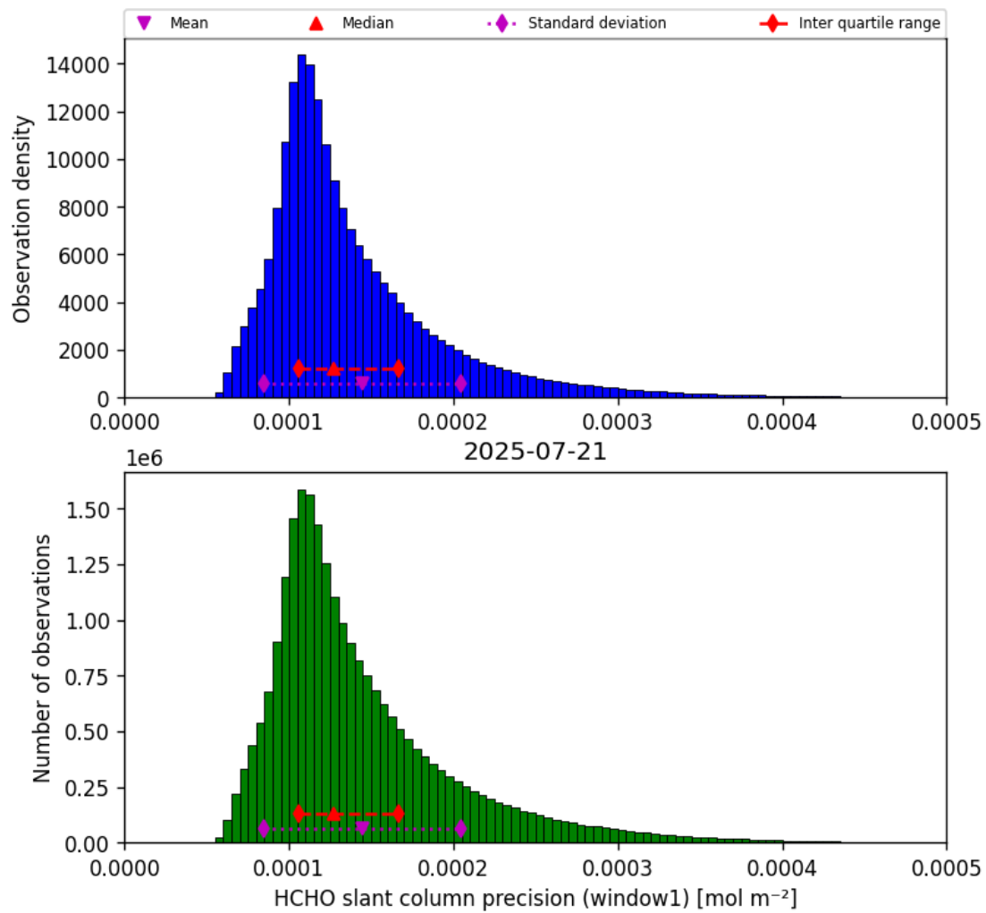
Figure 39: Histogram of “HCHO slant column precision (window1)” for 2025-07-20 to 2025-07-22
