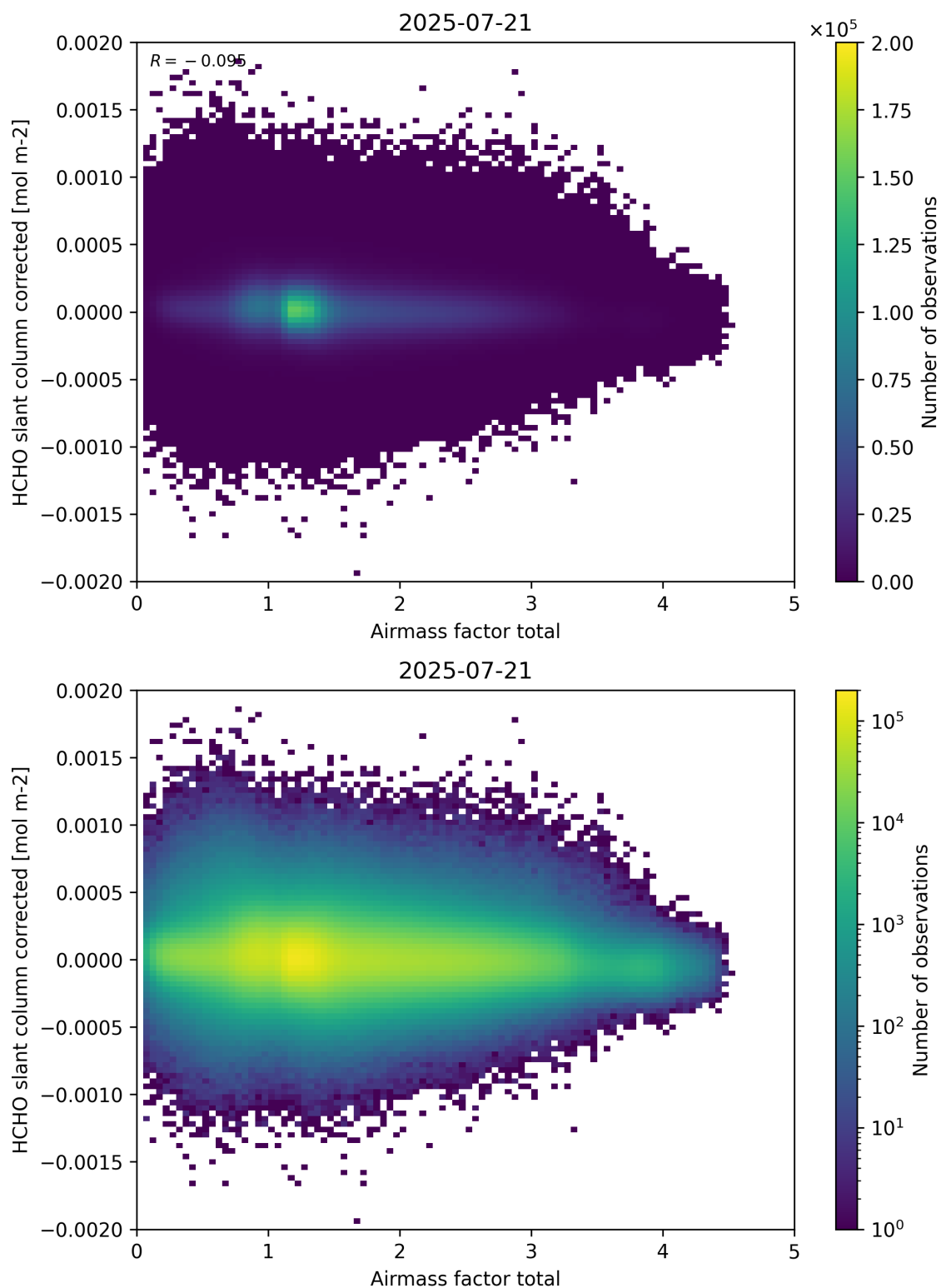
Figure 101: Scatter density plot of “Airmass factor total” against “HCHO slant column corrected” for 2025-07-20 to 2025-07-22.
