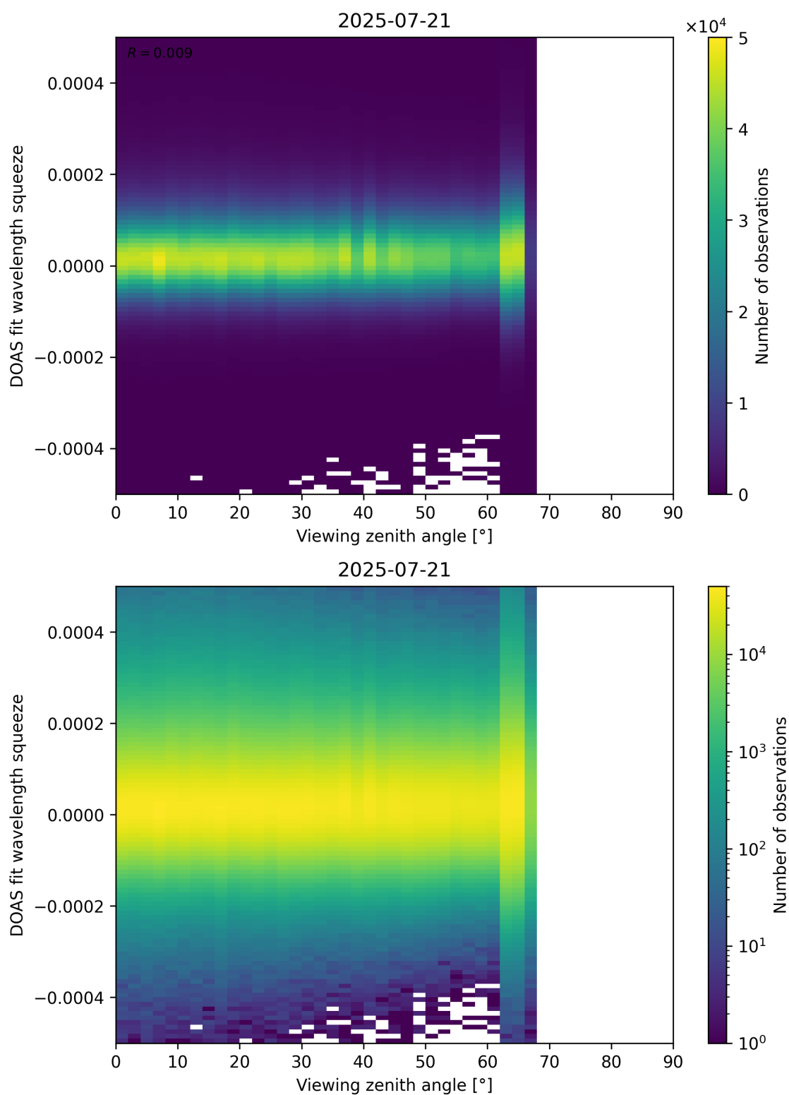
Figure 184: Scatter density plot of “Viewing zenith angle” against “DOAS fit wavelength squeeze” for 2025-07-20 to 2025-07-22.
