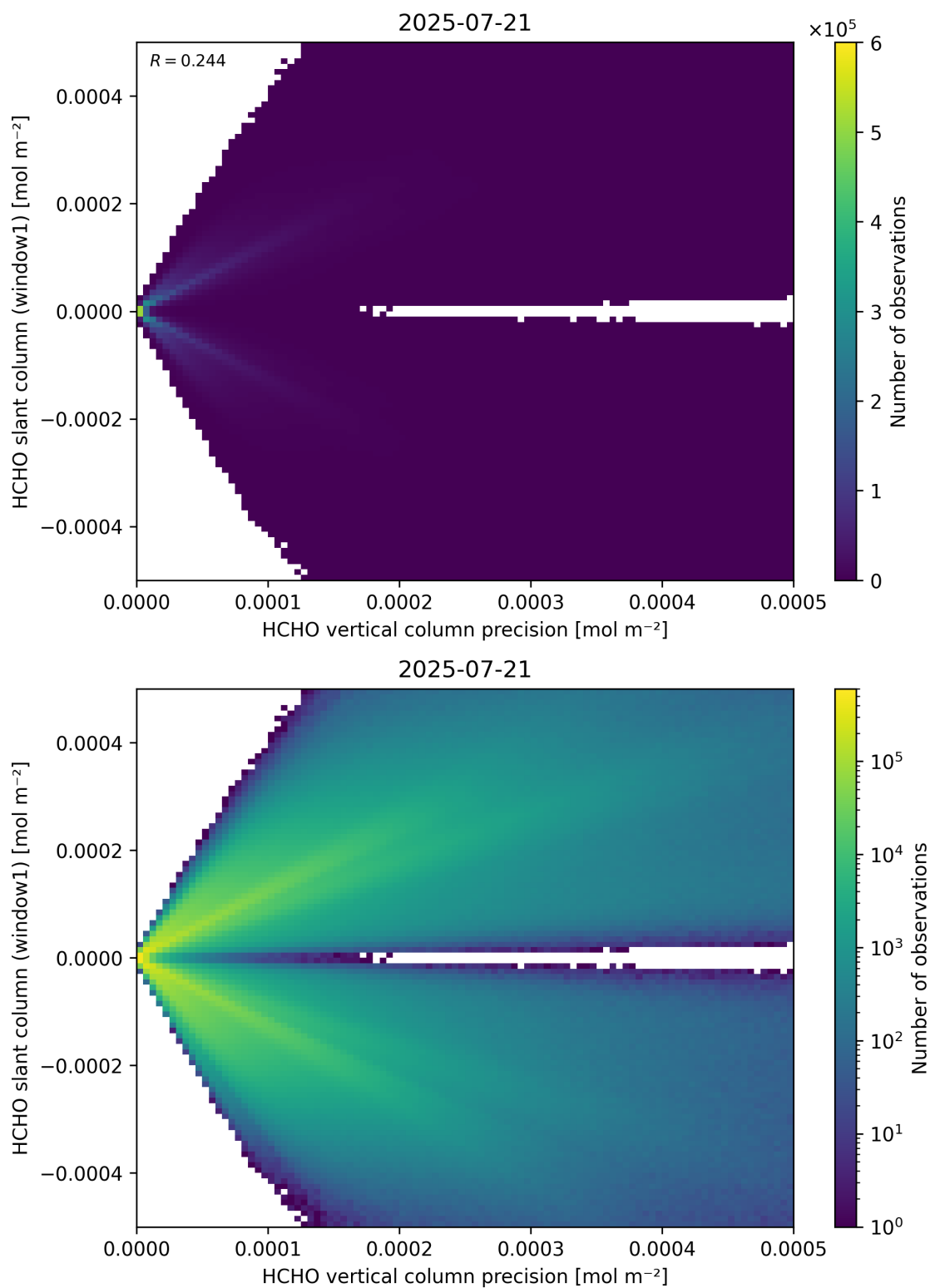
Figure 142: Scatter density plot of “HCHO vertical column precision” against “HCHO slant column (window1)” for 2025-07-20 to 2025-07-22.
