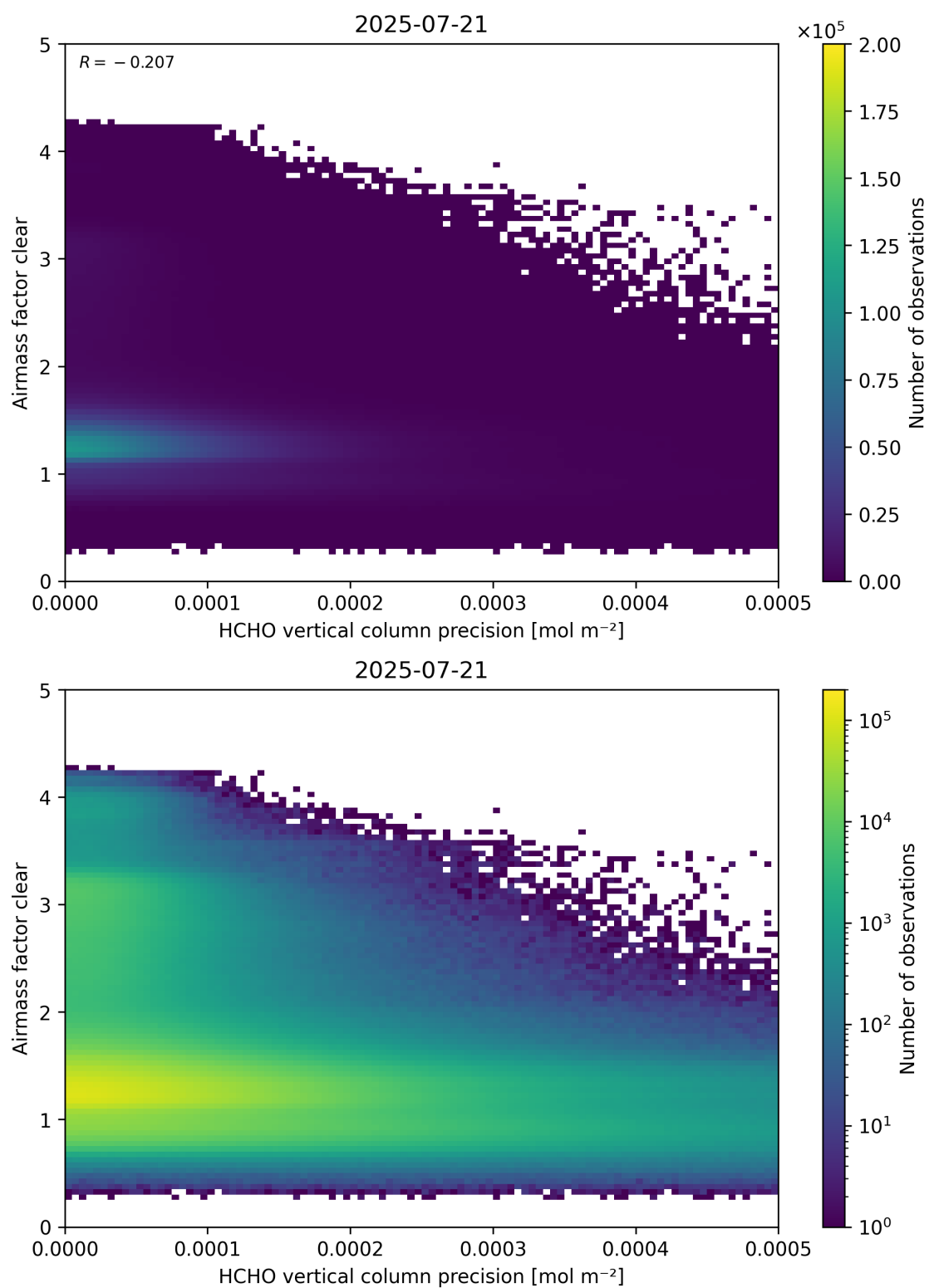
Figure 139: Scatter density plot of “HCHO vertical column precision” against “Airmass factor clear” for 2025-07-20 to 2025-07-22.
