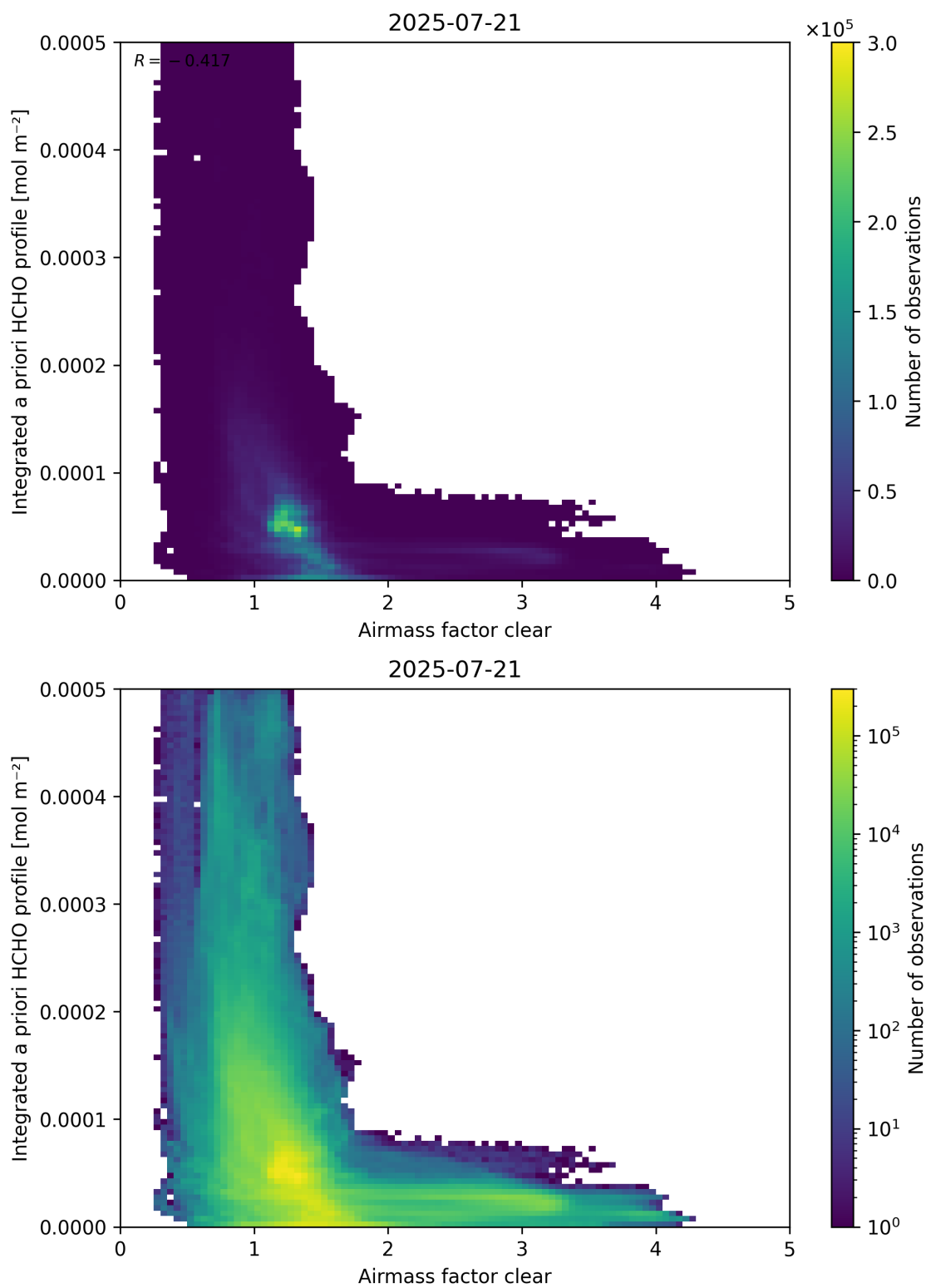
Figure 76: Scatter density plot of “Airmass factor clear” against “Integrated a priori HCHO profile” for 2025-07-20 to 2025-07-22.
