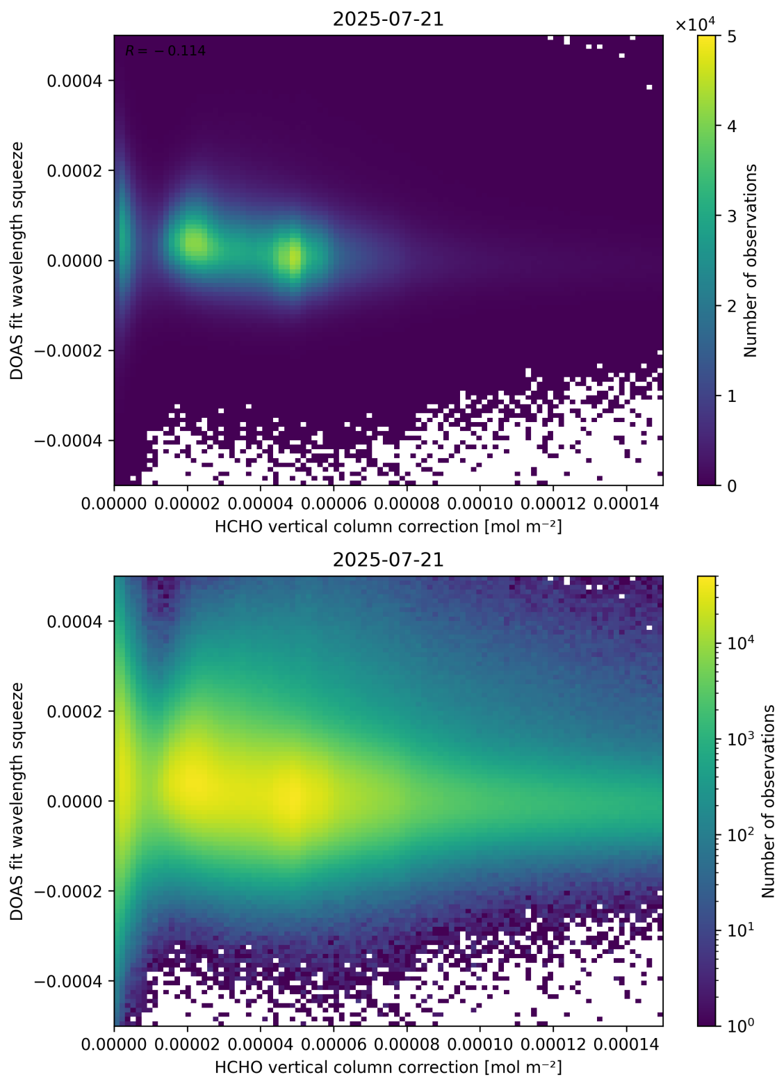
Figure 114: Scatter density plot of “HCHO vertical column correction” against “DOAS fit wavelength squeeze” for 2025-07-20 to 2025-07-22.
