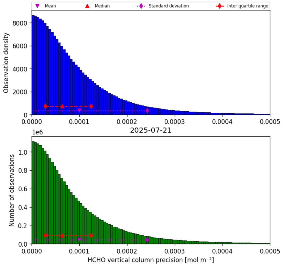
Figure 36: Histogram of “HCHO vertical column precision” for 2025-07-20 to 2025-07-22
