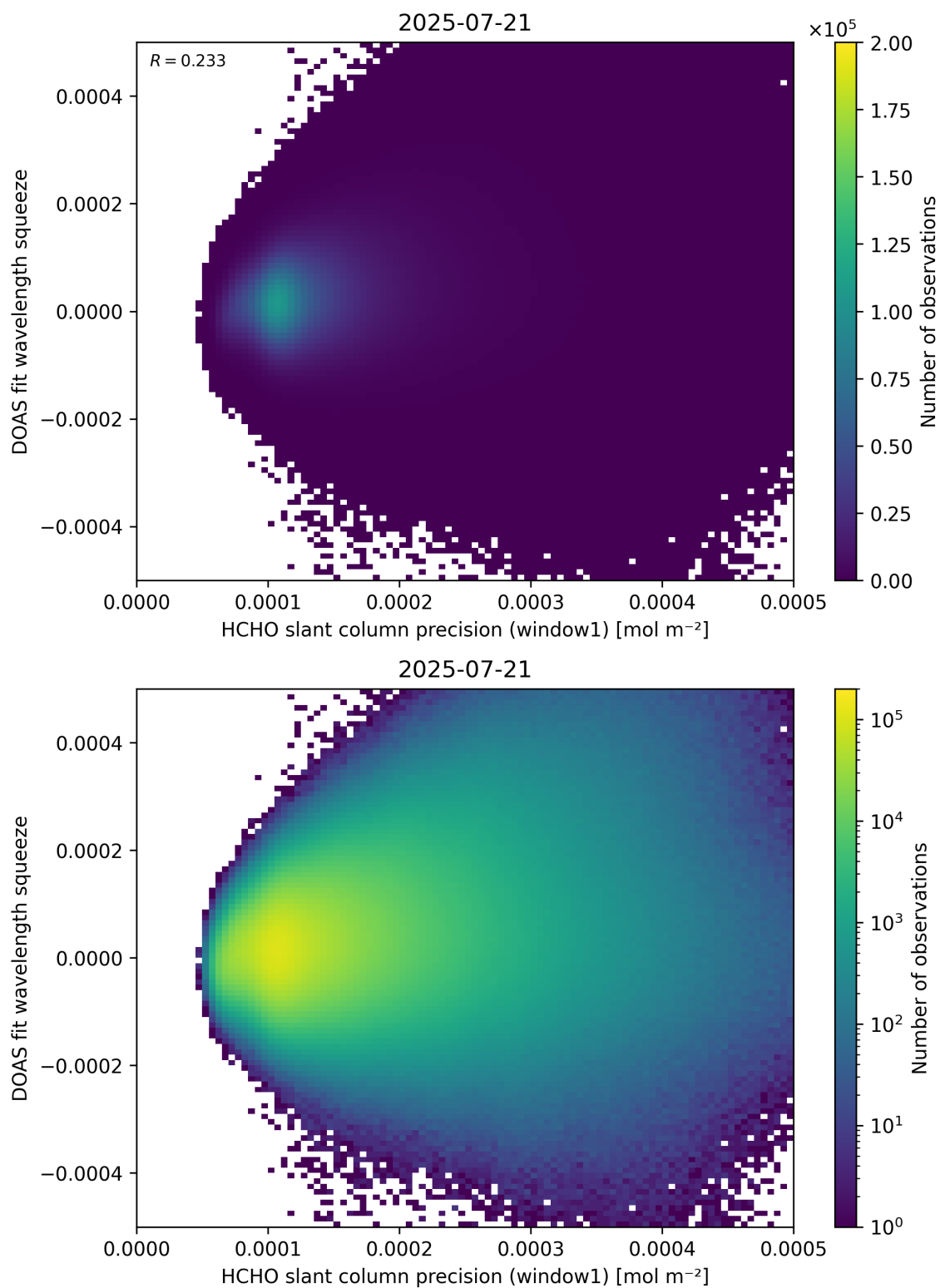
Figure 90: Scatter density plot of “HCHO slant column precision (window1)” against “DOAS fit wavelength squeeze” for 2025-07-20 to 2025-07-22.
