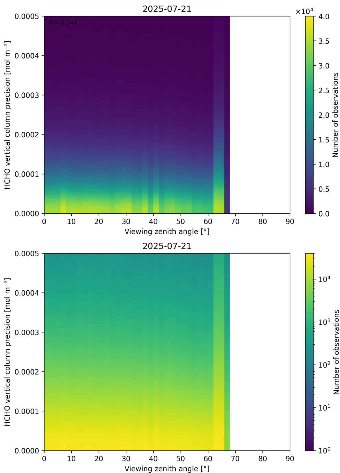
Figure 194: Scatter density plot of “Viewing zenith angle” against “HCHO vertical column precision” for 2025-07-20 to 2025-07-22.
