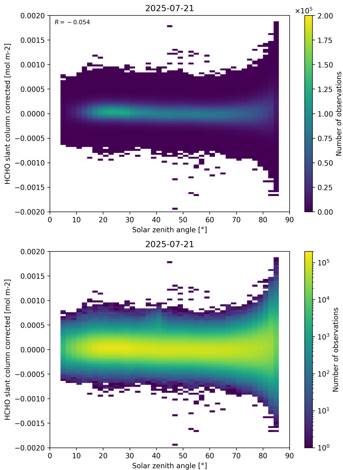
Figure 171: Scatter density plot of “Solar zenith angle” against “HCHO slant column corrected” for 2025-07-20 to 2025-07-22.
