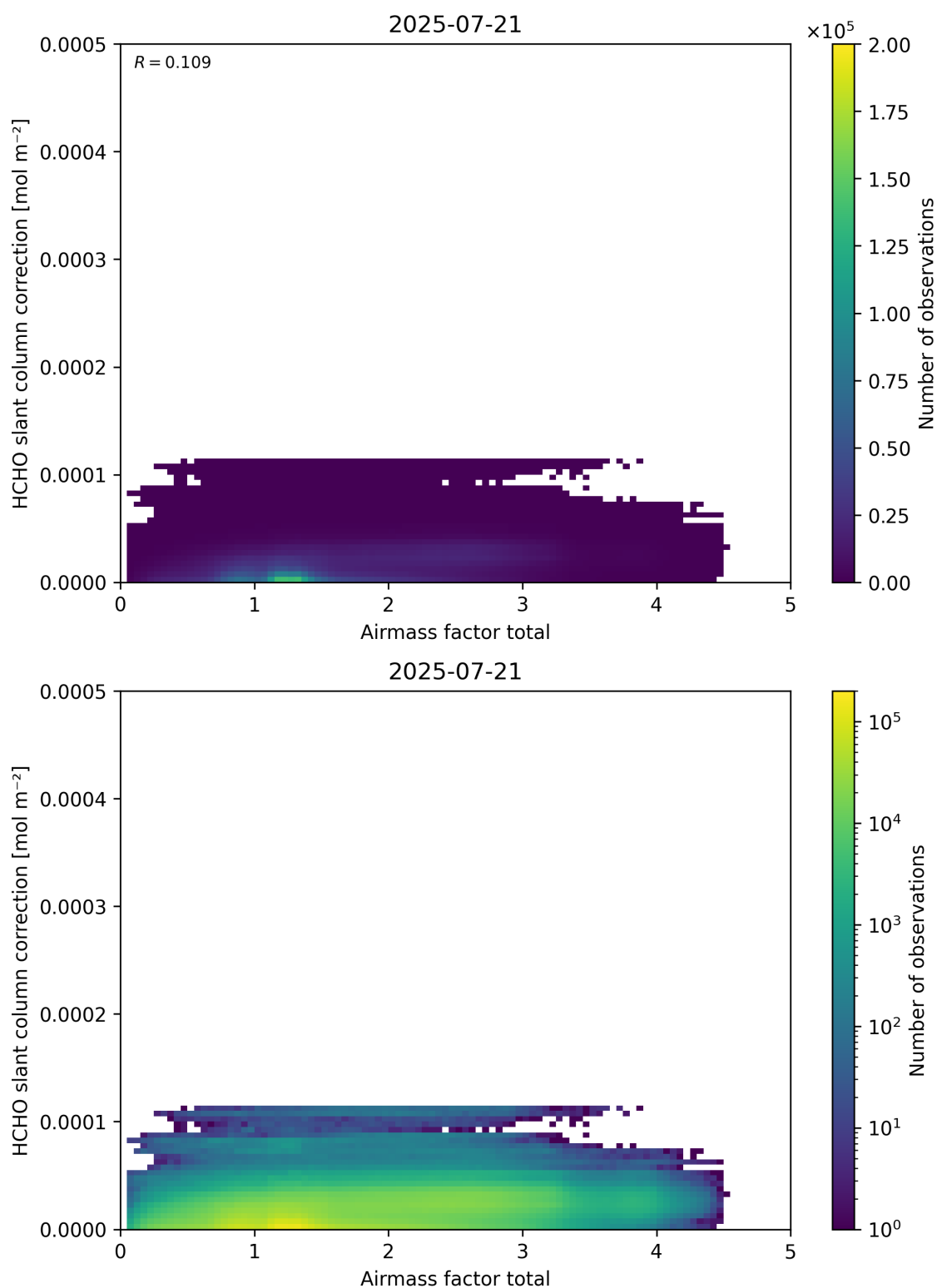
Figure 102: Scatter density plot of “Airmass factor total” against “HCHO slant column correction” for 2025-07-20 to 2025-07-22.
