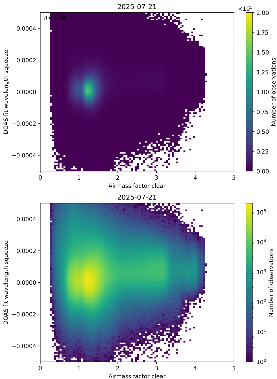
Figure 73: Scatter density plot of “Airmass factor clear” against “DOAS fit wavelength squeeze” for 2025-07-20 to 2025-07-22.
