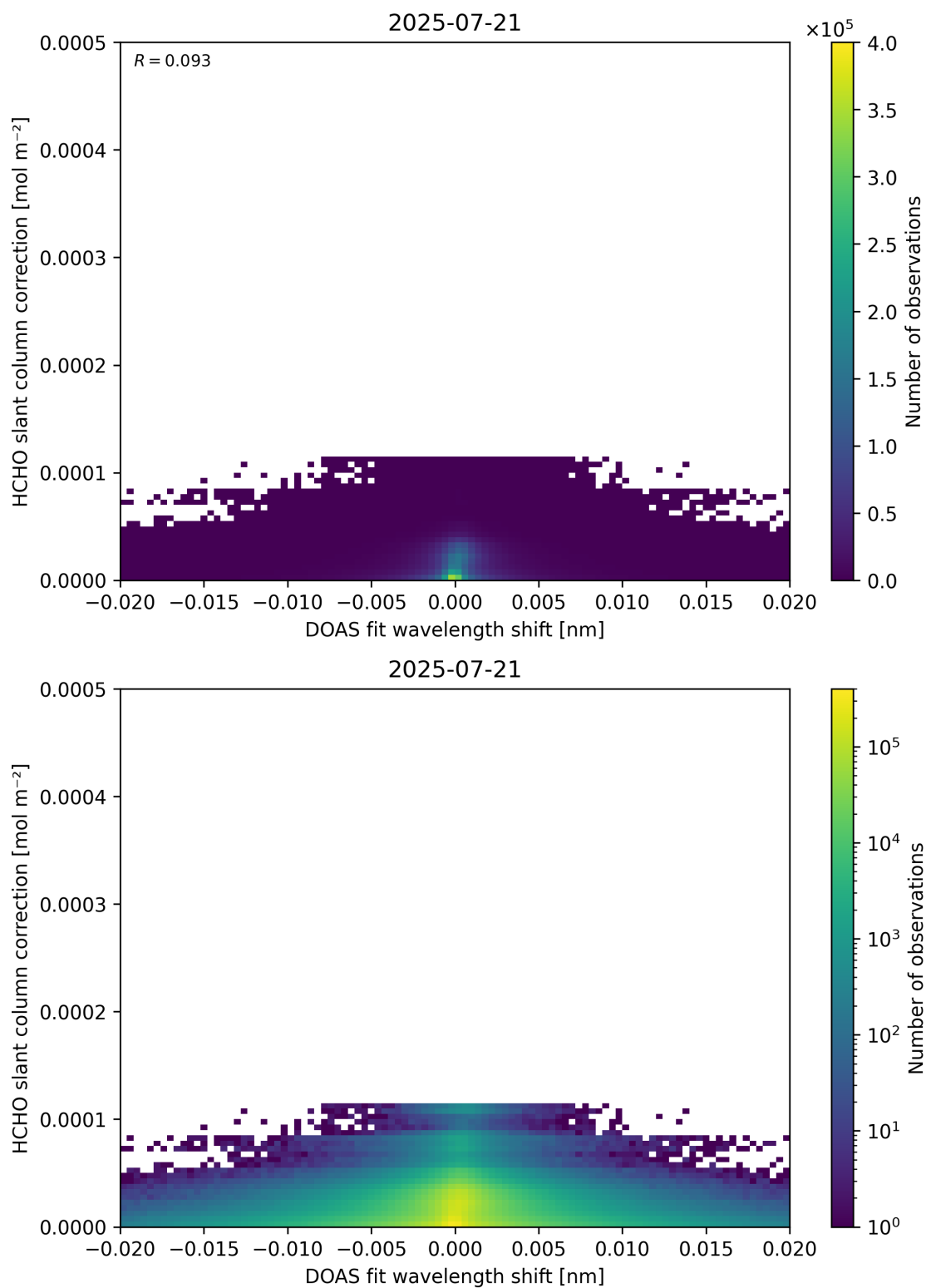
Figure 67: Scatter density plot of “DOAS fit wavelength shift” against “HCHO slant column correction” for 2025-07-20 to 2025-07-22.
