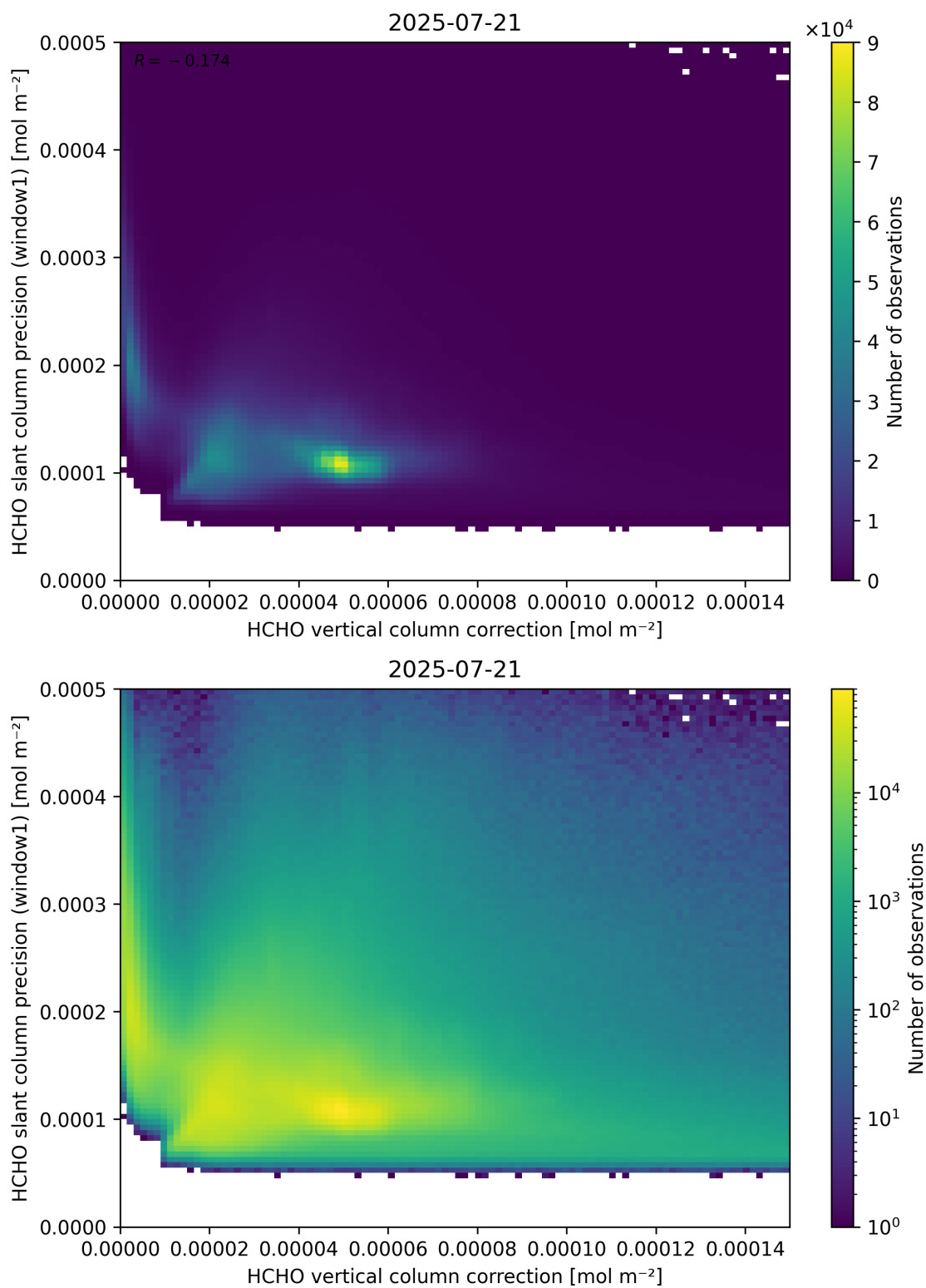
Figure 119: Scatter density plot of “HCHO vertical column correction” against “HCHO slant column precision (window1)” for 2025-07-20 to 2025-07-22.
