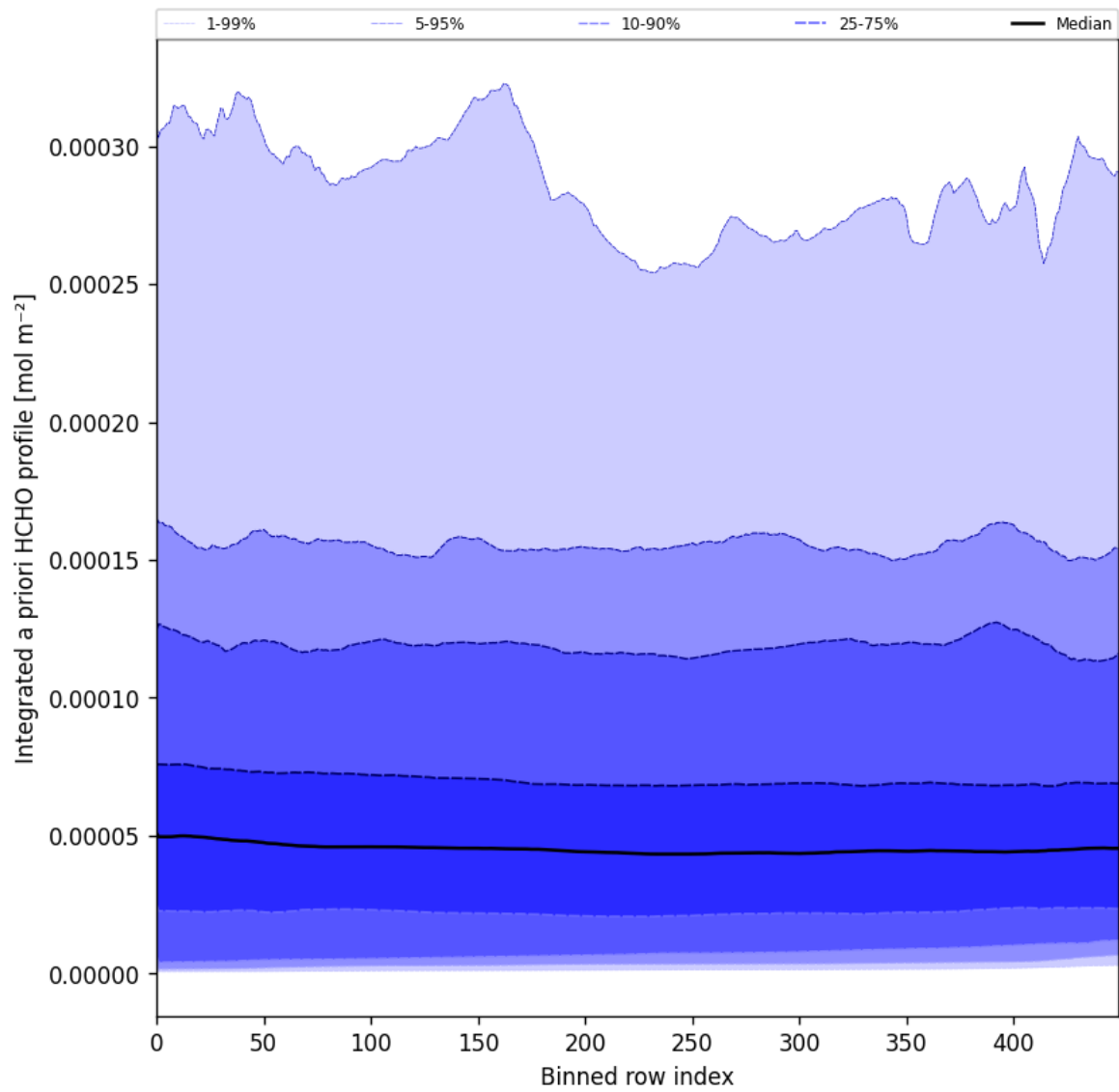
Figure 57: Along track statistics of “Integrated a priori HCHO profile” for 2025-07-20 to 2025-07-22
