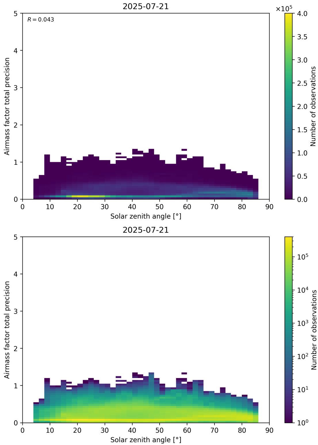
Figure 176: Scatter density plot of “Solar zenith angle” against “Airmass factor total precision” for 2025-07-20 to 2025-07-22.
