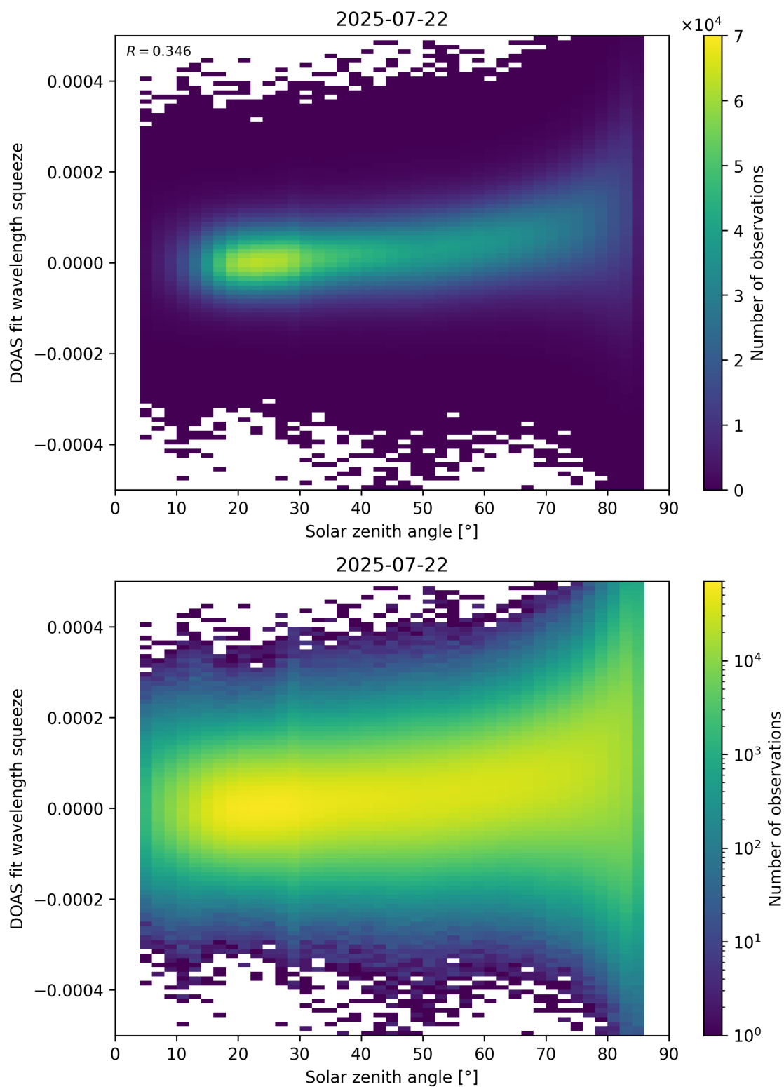
Figure 169: Scatter density plot of “Solar zenith angle” against “DOAS fit wavelength squeeze” for 2025-07-21 to 2025-07-23.
