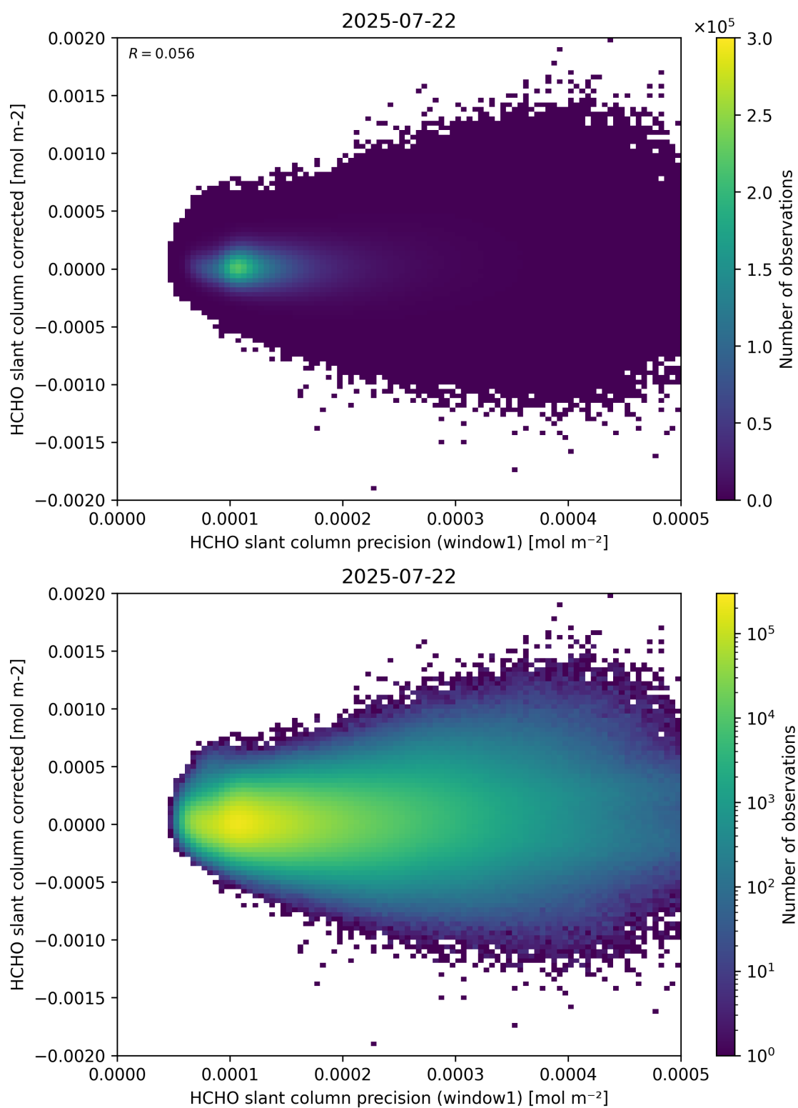
Figure 92: Scatter density plot of “HCHO slant column precision (window1)” against “HCHO slant column corrected” for 2025-07-21 to 2025-07-23.
