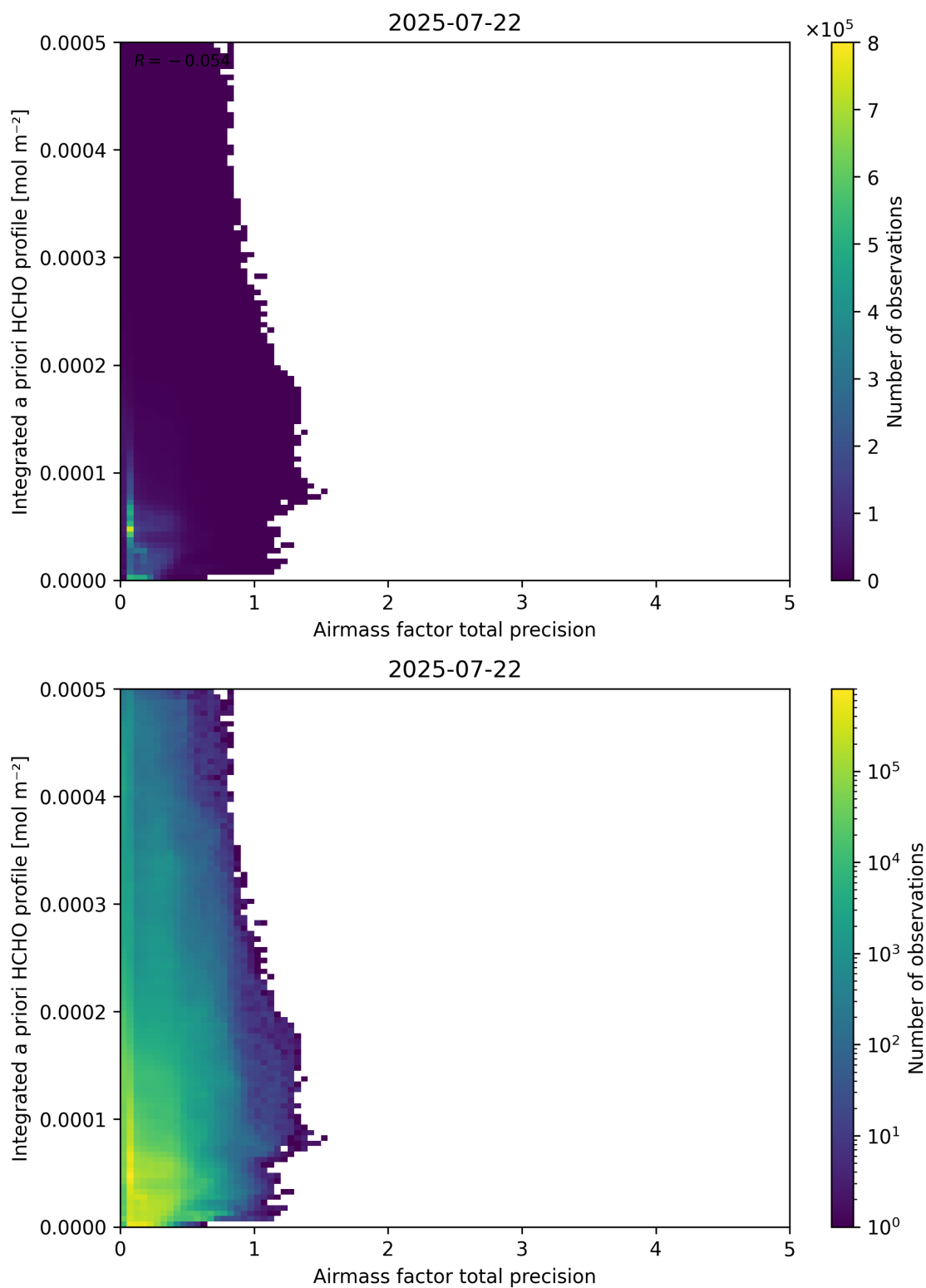
Figure 111: Scatter density plot of “Airmass factor total precision” against “Integrated a priori HCHO profile” for 2025-07-21 to 2025-07-23.
