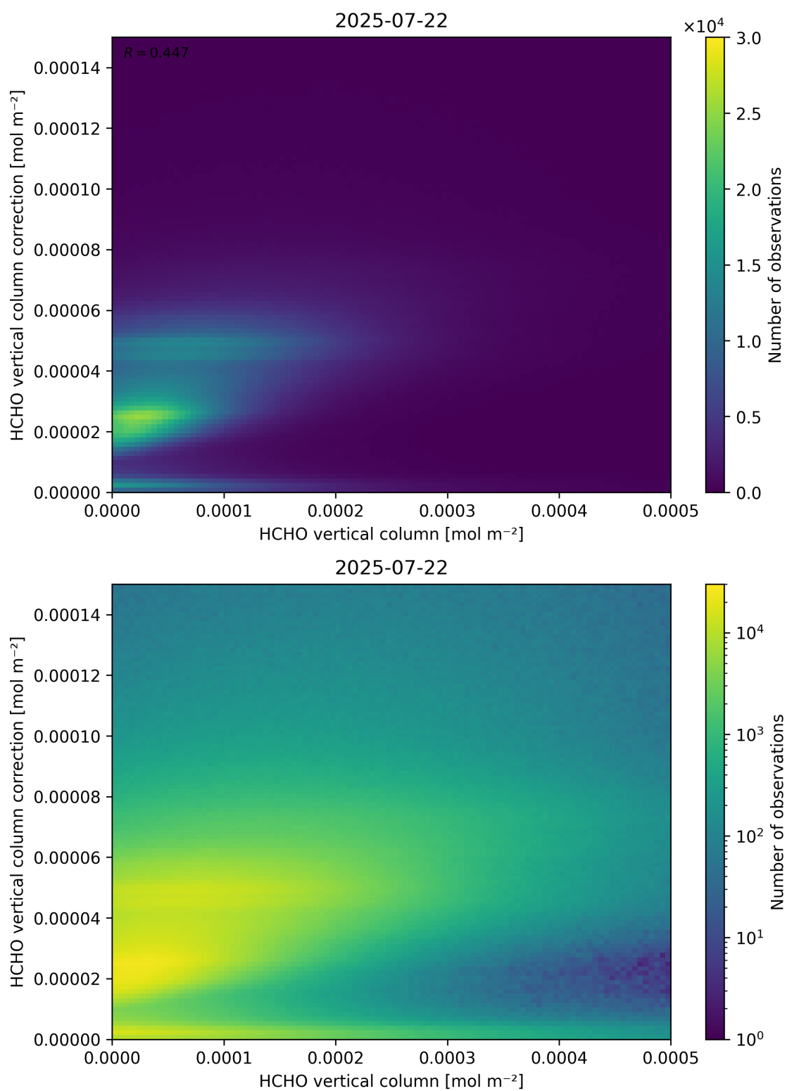
Figure 133: Scatter density plot of “HCHO vertical column” against “HCHO vertical column correction” for 2025-07-21 to 2025-07-23.
