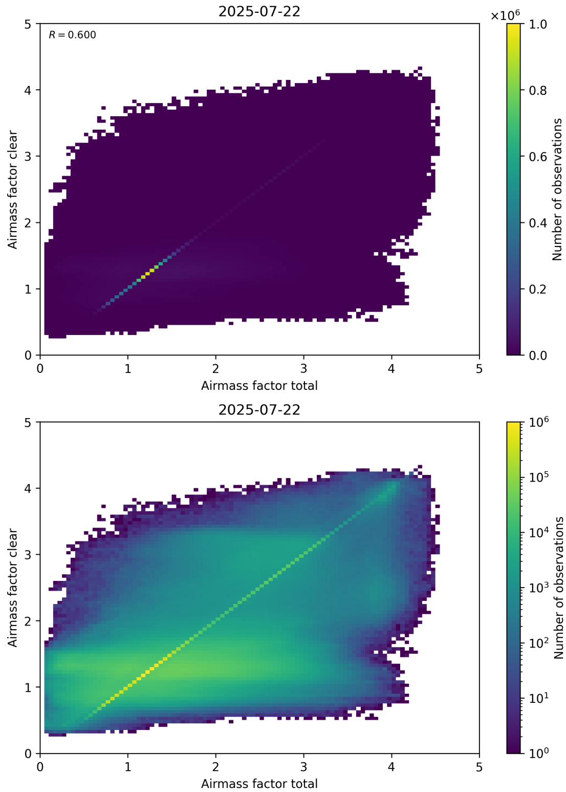
Figure 100: Scatter density plot of “Airmass factor total” against “Airmass factor clear” for 2025-07-21 to 2025-07-23.
