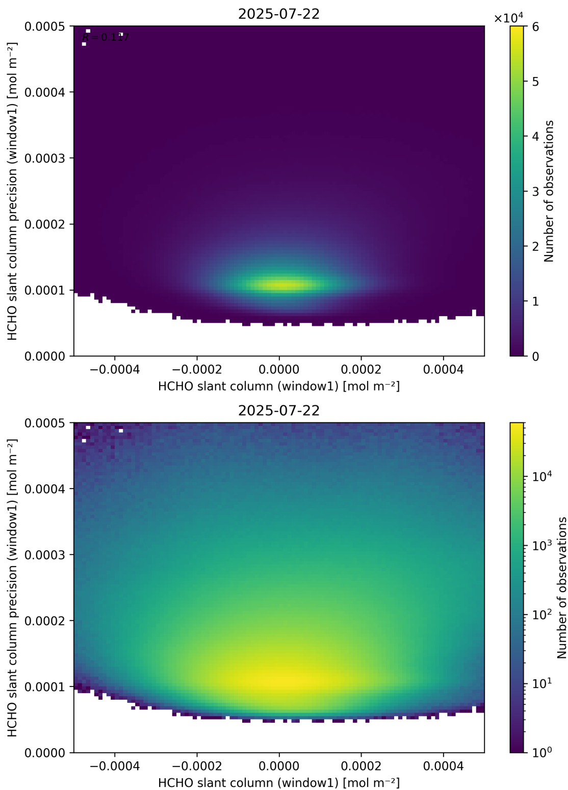
Figure 84: Scatter density plot of “HCHO slant column (window1)” against “HCHO slant column precision (window1)” for 2025-07-21 to 2025-07-23.
