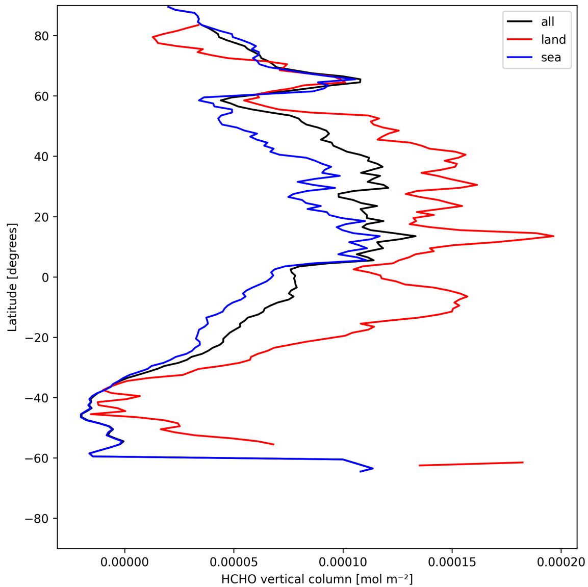
Figure 21: Zonal average of “HCHO vertical column” for 2025-07-21 to 2025-07-23.
