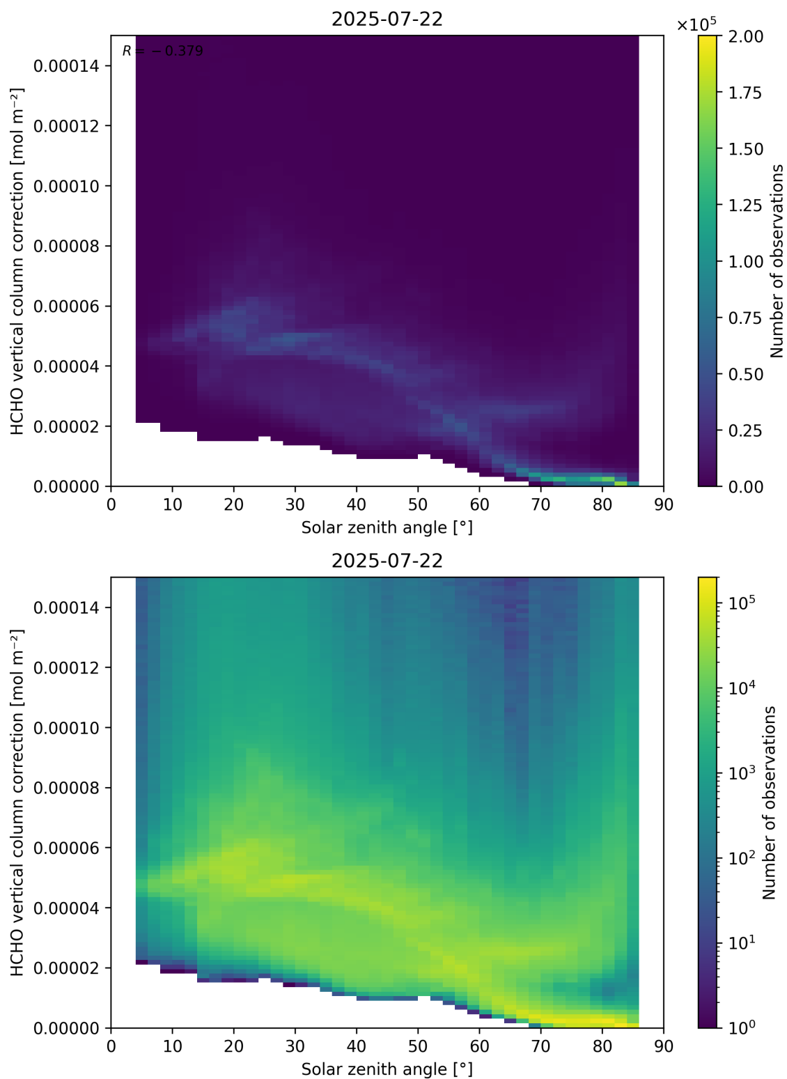
Figure 178: Scatter density plot of “Solar zenith angle” against “HCHO vertical column correction” for 2025-07-21 to 2025-07-23.
