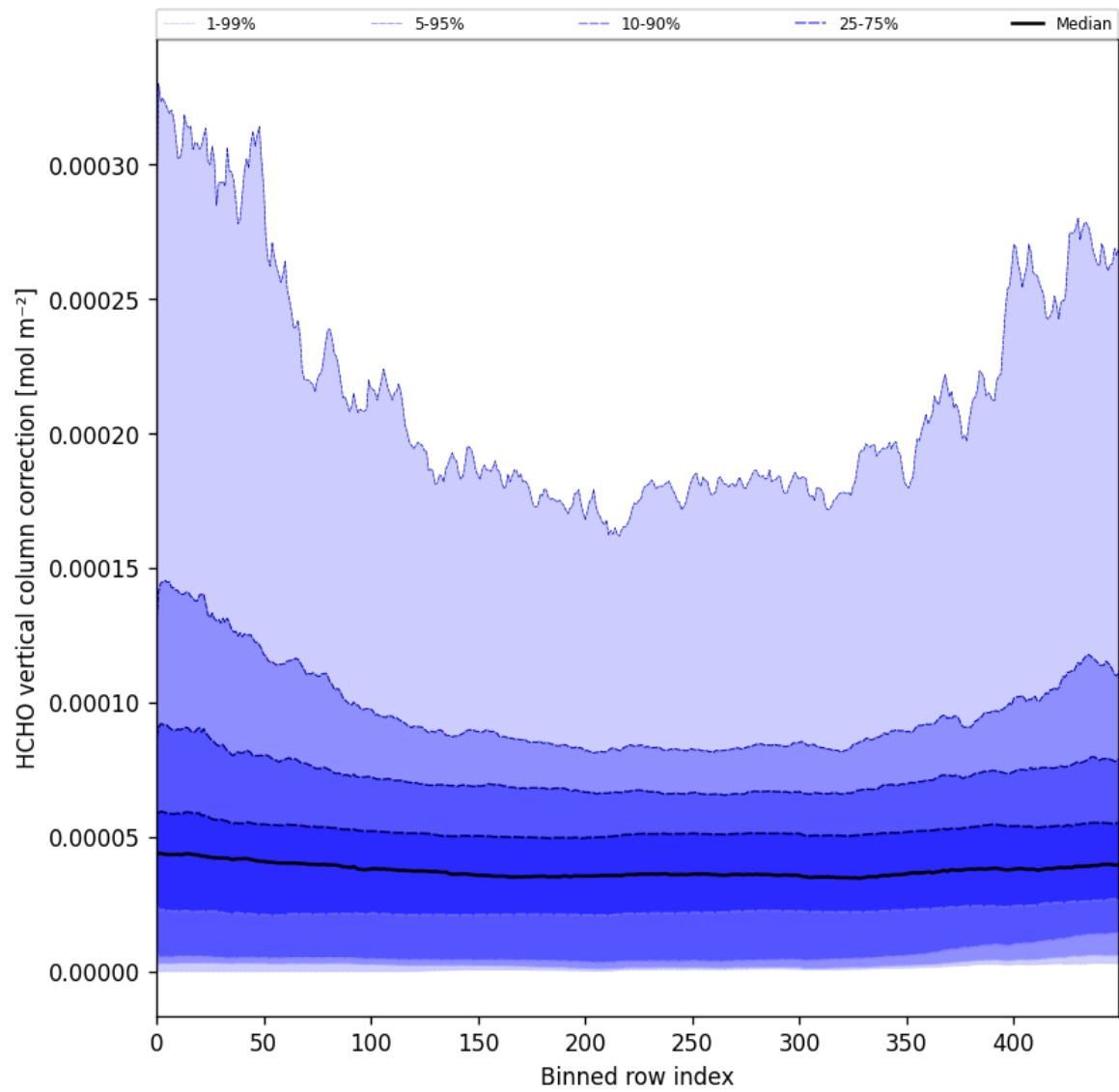
Figure 51: Along track statistics of “HCHO vertical column correction” for 2025-07-21 to 2025-07-23
