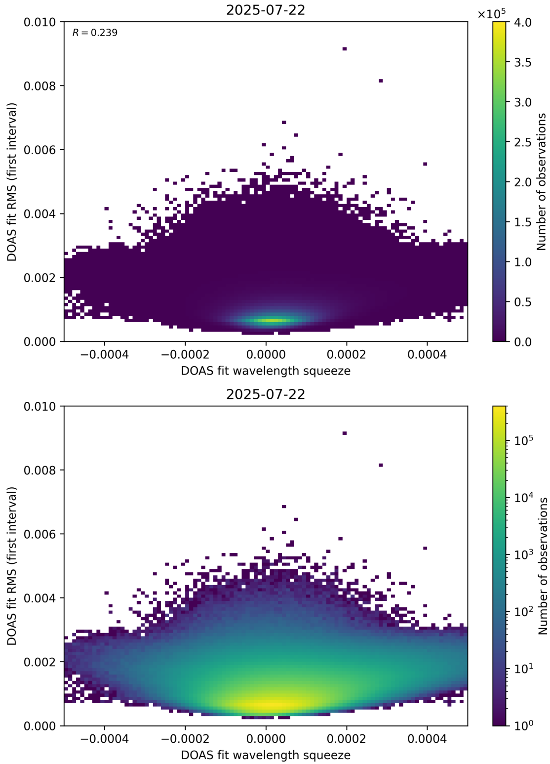
Figure 68: Scatter density plot of “DOAS fit wavelength squeeze” against “DOAS fit RMS (first interval)” for 2025-07-21 to 2025-07-23.
