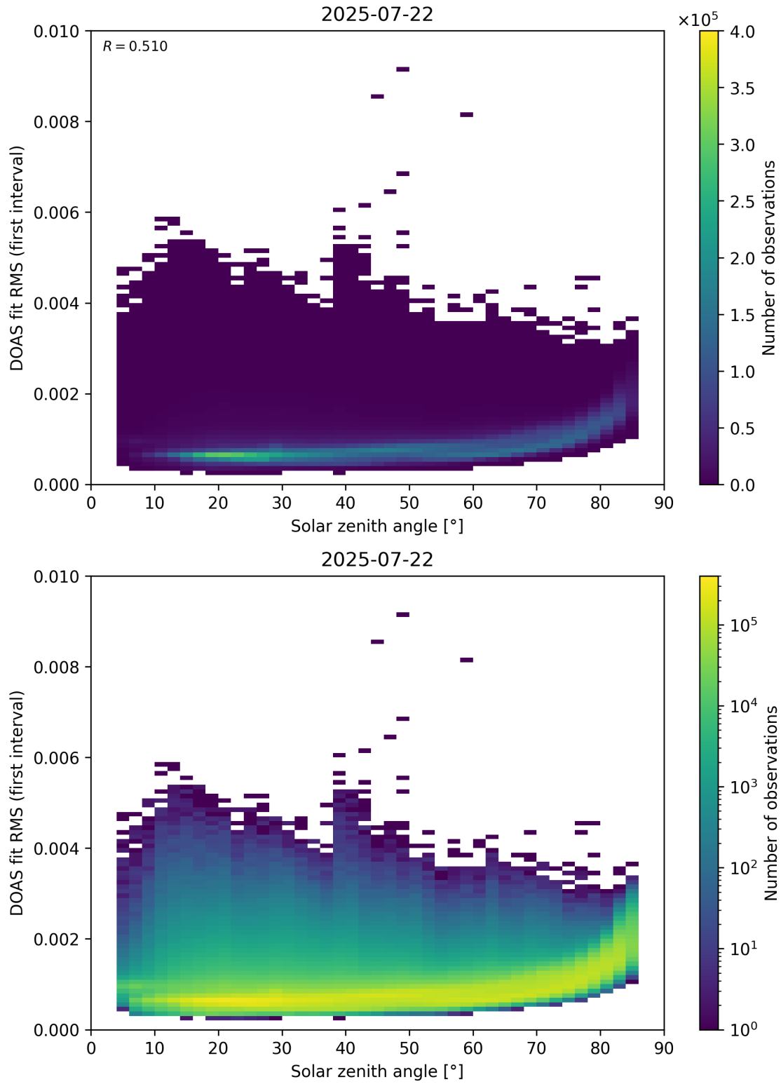
Figure 167: Scatter density plot of “Solar zenith angle” against “DOAS fit RMS (first interval)” for 2025-07-21 to 2025-07-23.
