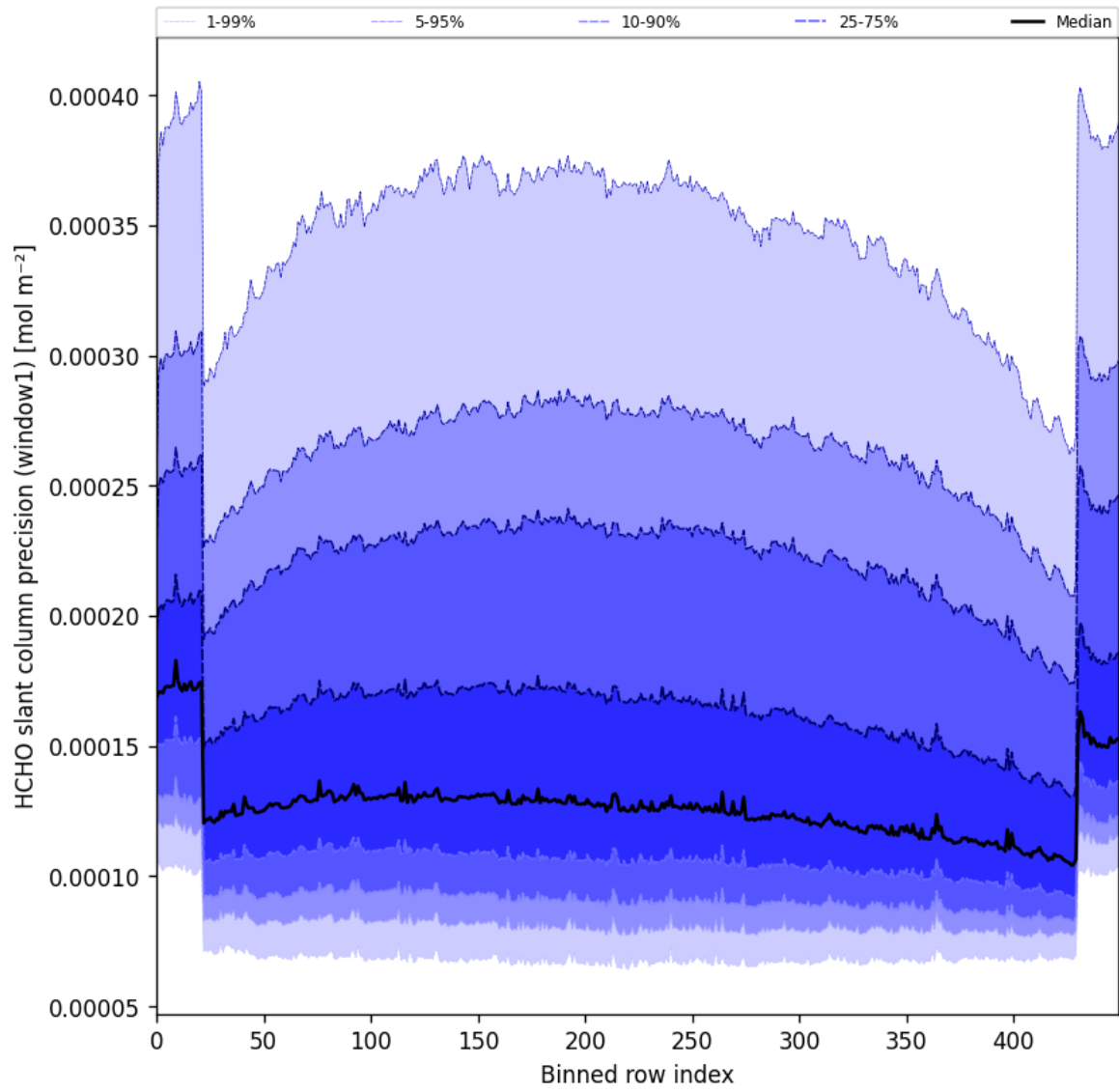
Figure 53: Along track statistics of “HCHO slant column precision (window1)” for 2025-07-21 to 2025-07-23
