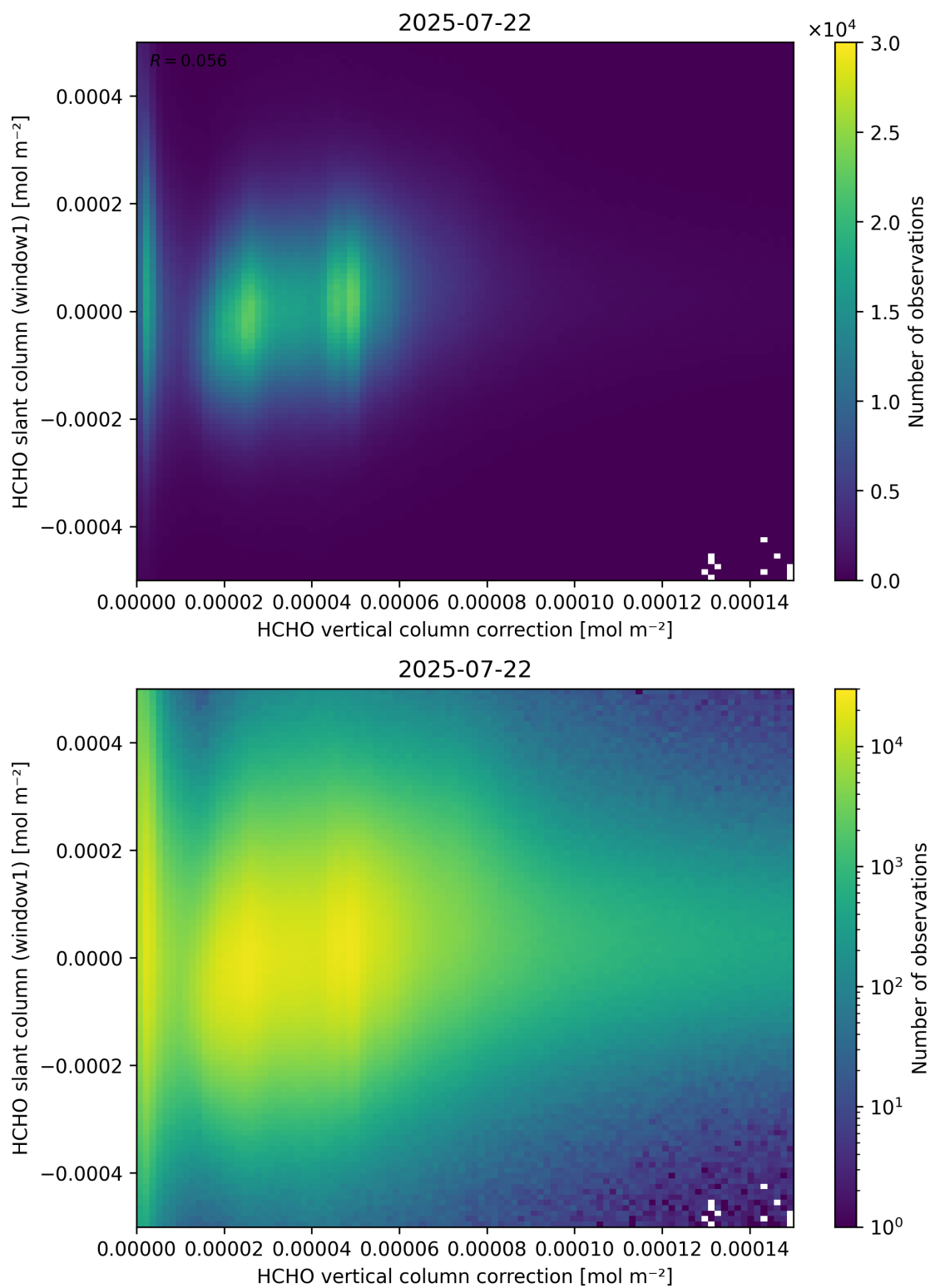
Figure 118: Scatter density plot of “HCHO vertical column correction” against “HCHO slant column (window1)” for 2025-07-21 to 2025-07-23.
