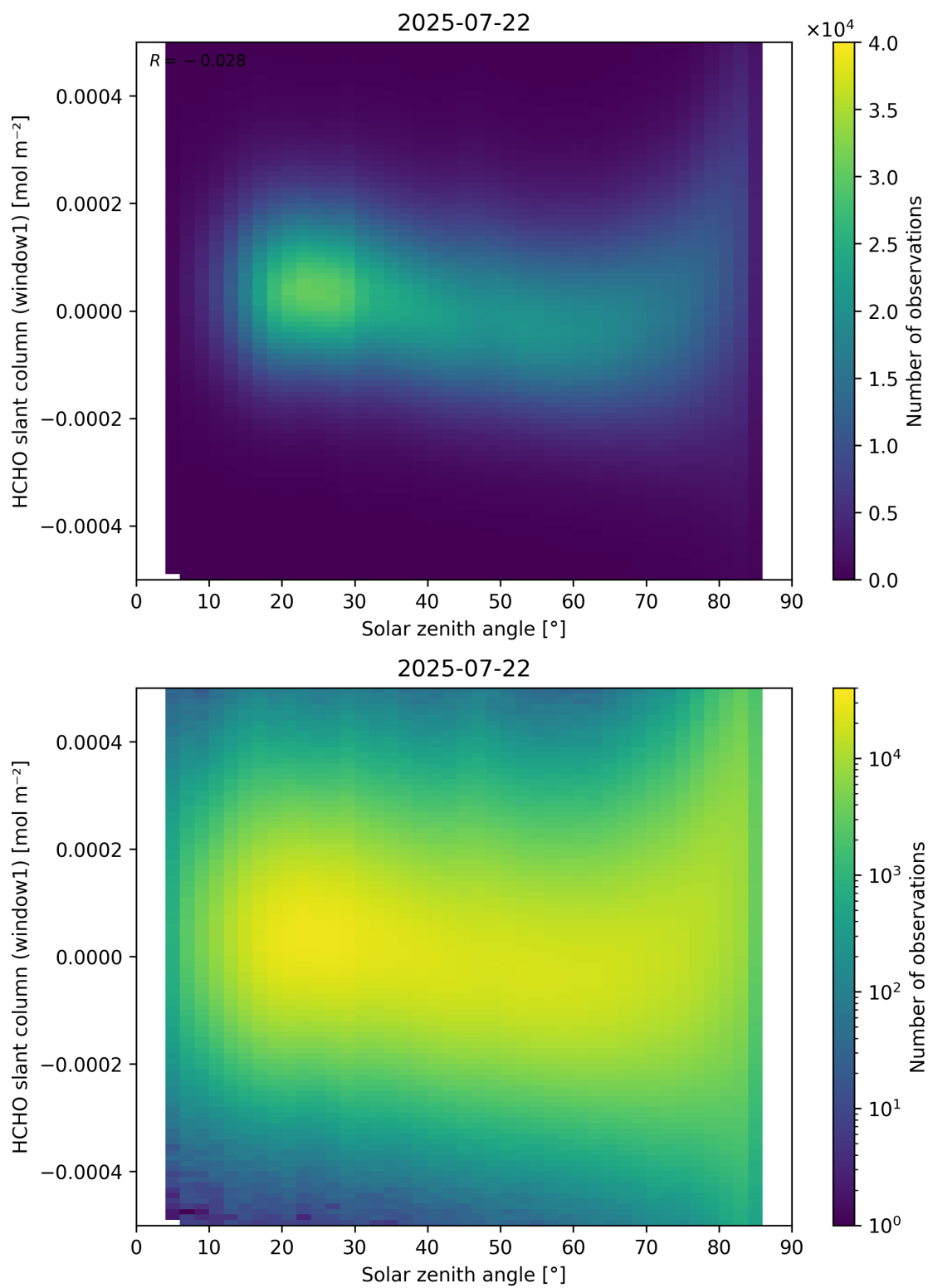
Figure 173: Scatter density plot of “Solar zenith angle” against “HCHO slant column (window1)” for 2025-07-21 to 2025-07-23.
