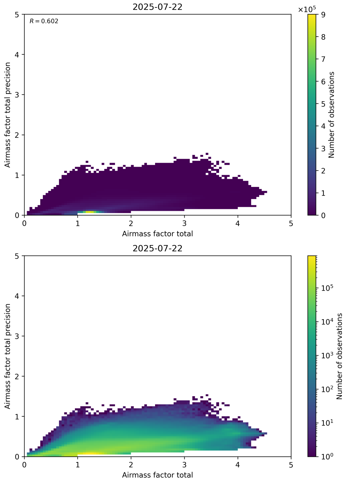
Figure 103: Scatter density plot of “Airmass factor total” against “Airmass factor total precision” for 2025-07-21 to 2025-07-23.
