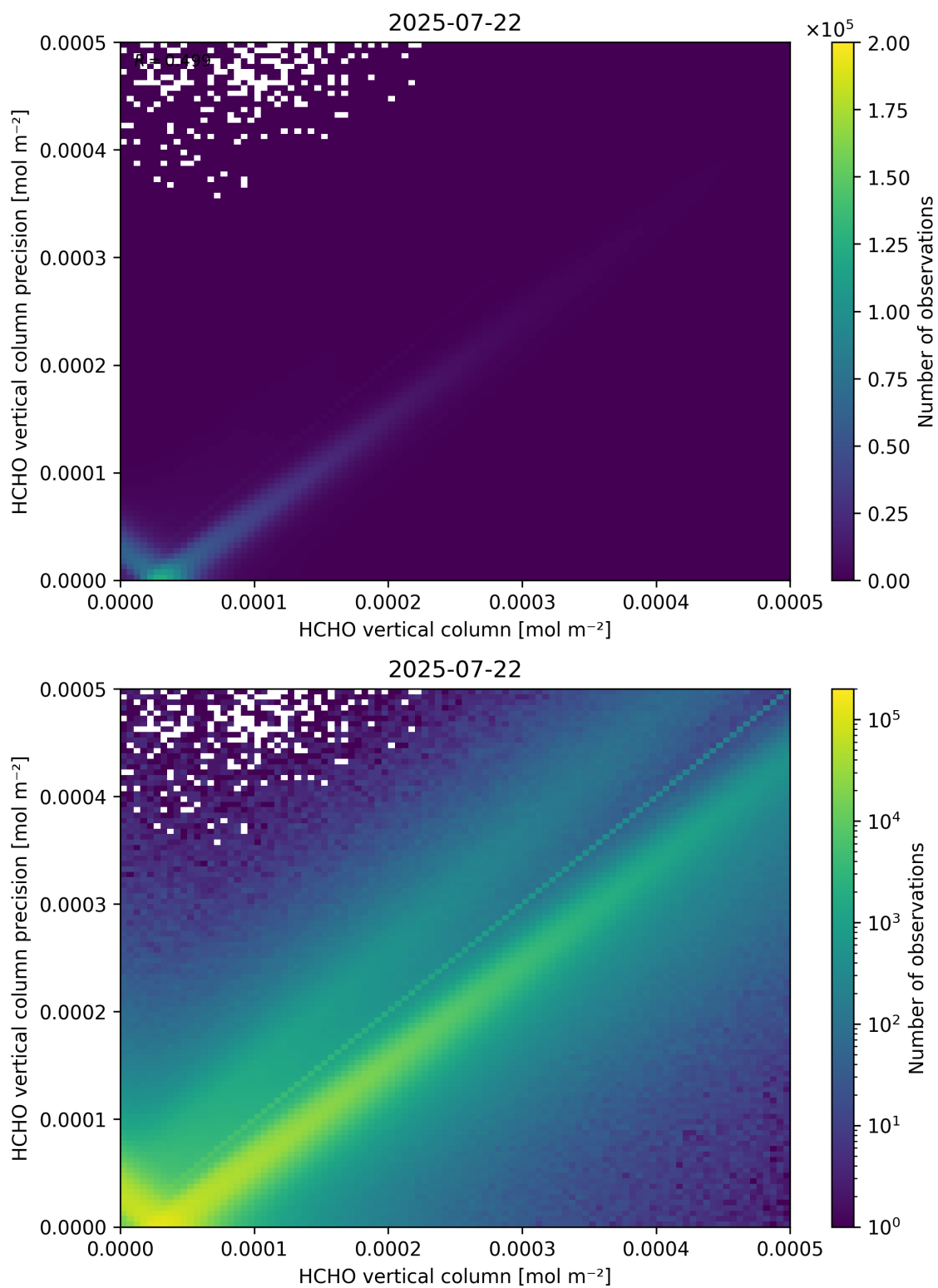
Figure 134: Scatter density plot of “HCHO vertical column” against “HCHO vertical column precision” for 2025-07-21 to 2025-07-23.
