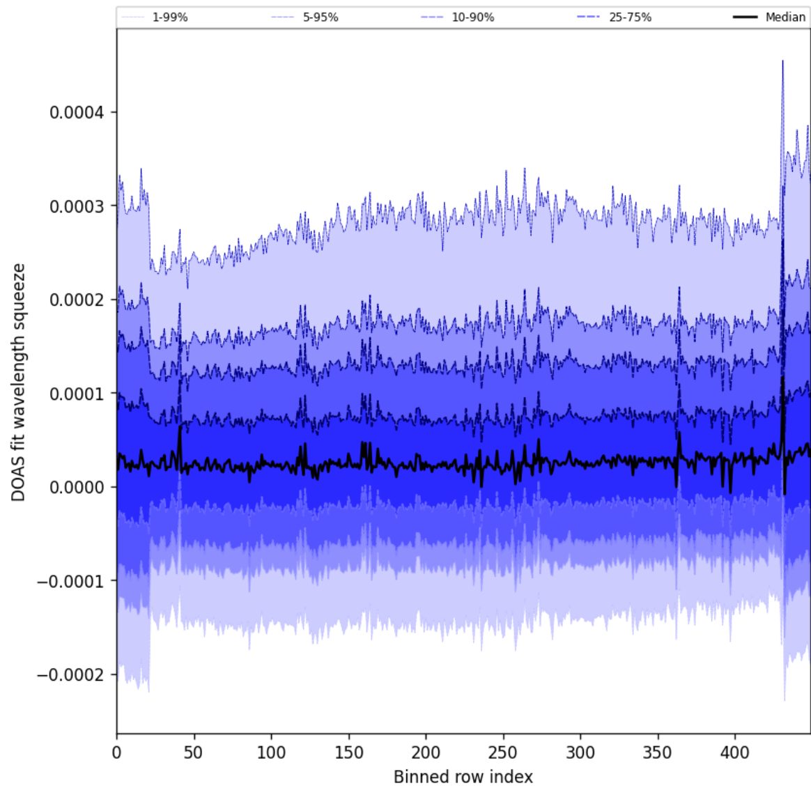
Figure 59: Along track statistics of “DOAS fit wavelength squeeze” for 2025-07-21 to 2025-07-23
