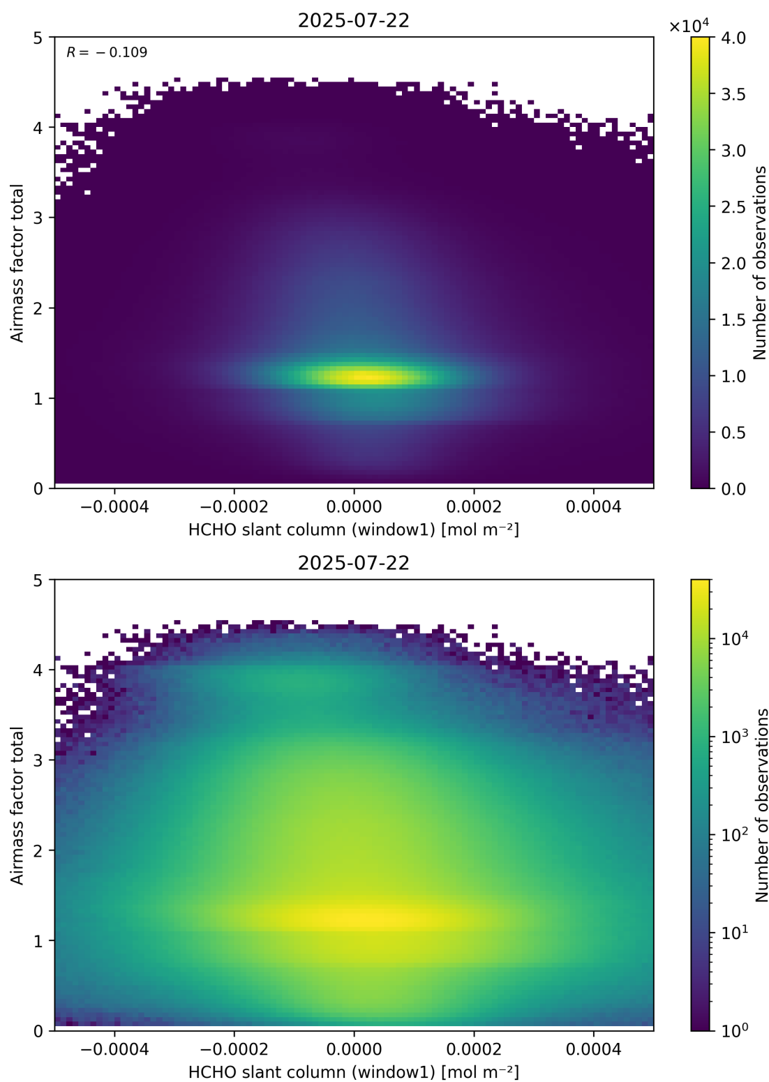
Figure 85: Scatter density plot of “HCHO slant column (window1)” against “Airmass factor total” for 2025-07-21 to 2025-07-23.
