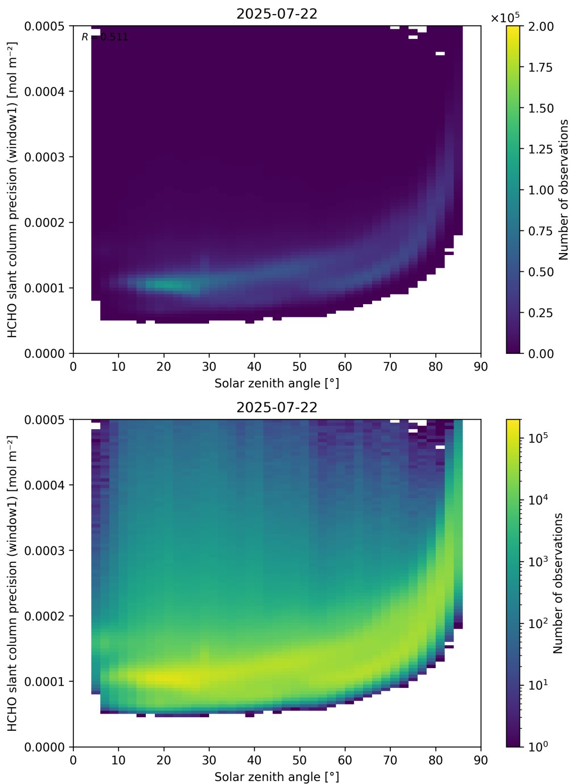
Figure 174: Scatter density plot of “Solar zenith angle” against “HCHO slant column precision (window1)” for 2025-07-21 to 2025-07-23.
