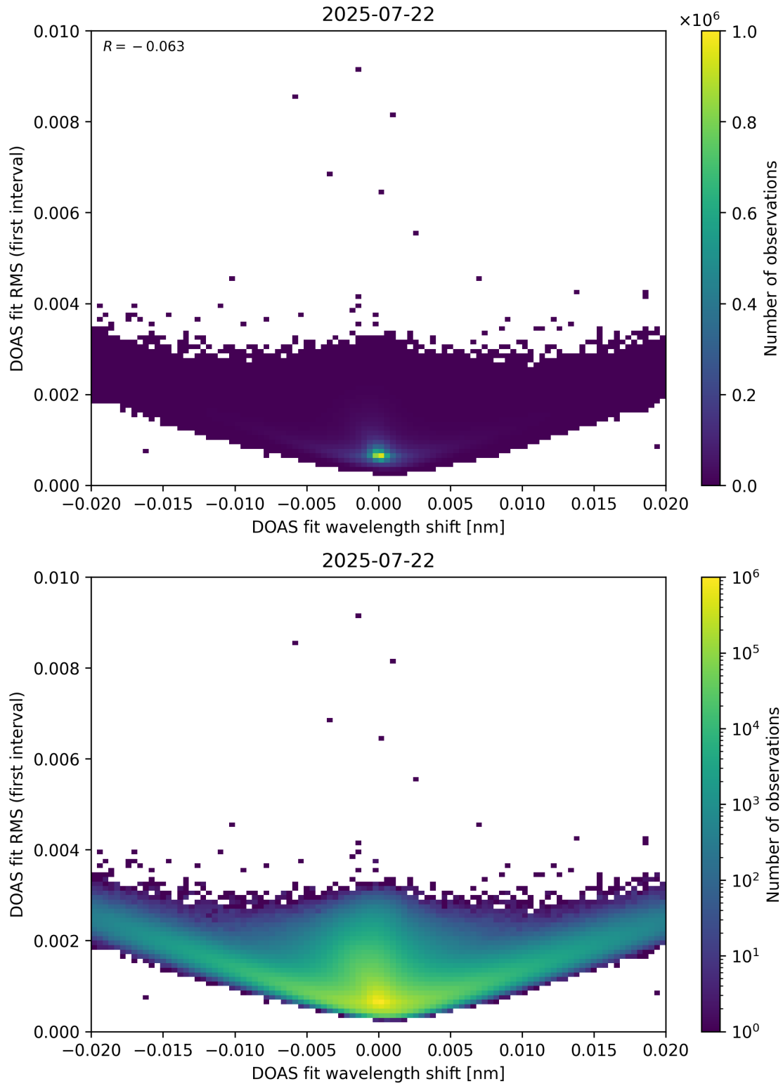
Figure 64: Scatter density plot of “DOAS fit wavelength shift” against “DOAS fit RMS (first interval)” for 2025-07-21 to 2025-07-23.
