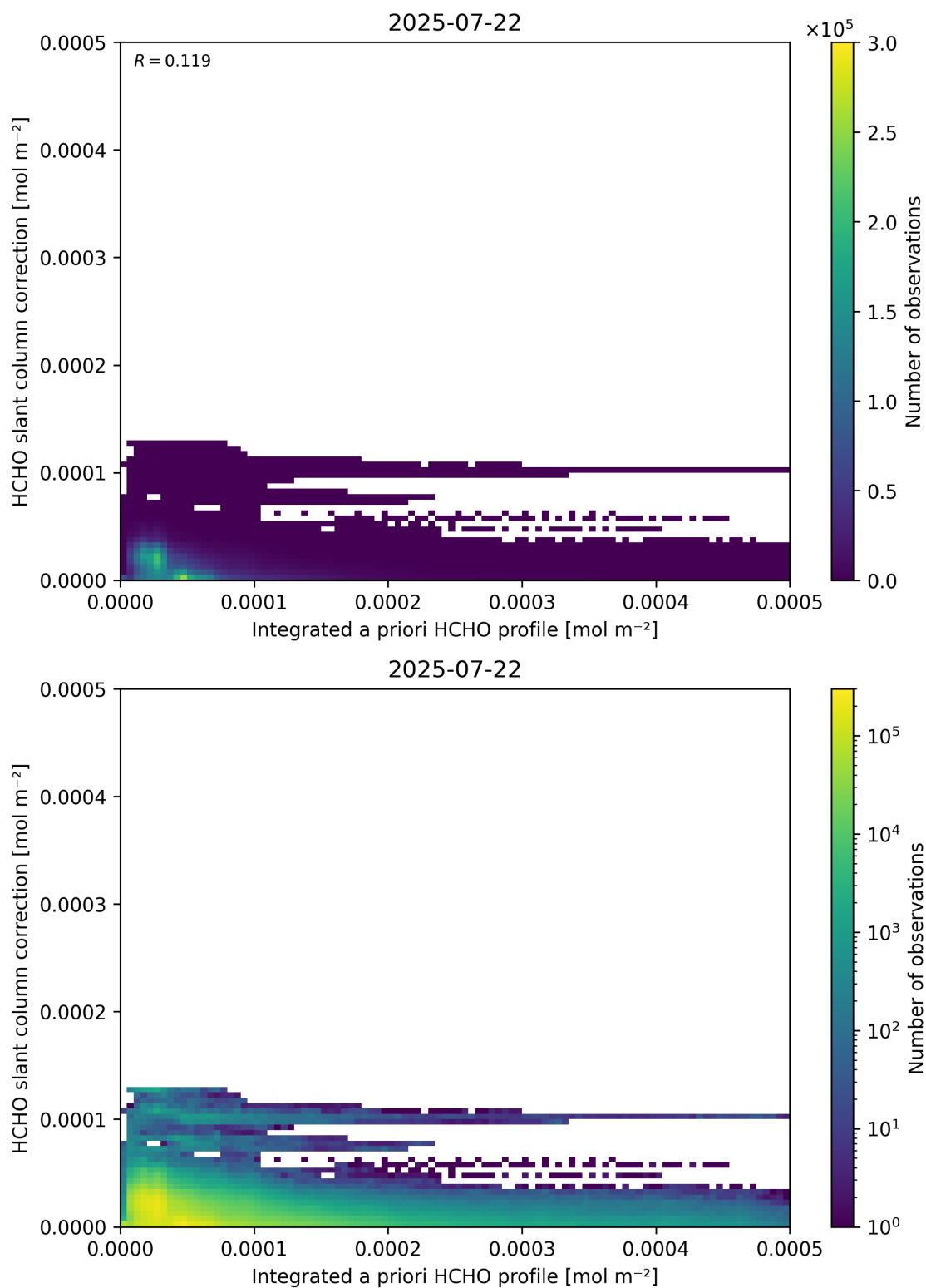
Figure 152: Scatter density plot of “Integrated a priori HCHO profile” against “HCHO slant column correction” for 2025-07-21 to 2025-07-23.
