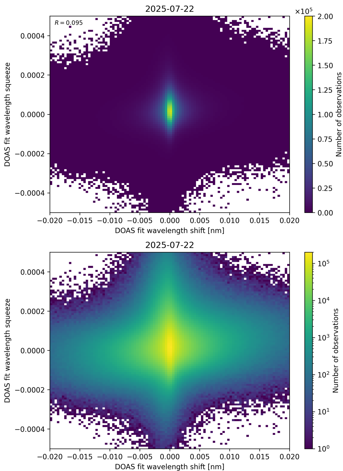
Figure 65: Scatter density plot of “DOAS fit wavelength shift” against “DOAS fit wavelength squeeze” for 2025-07-21 to 2025-07-23.
