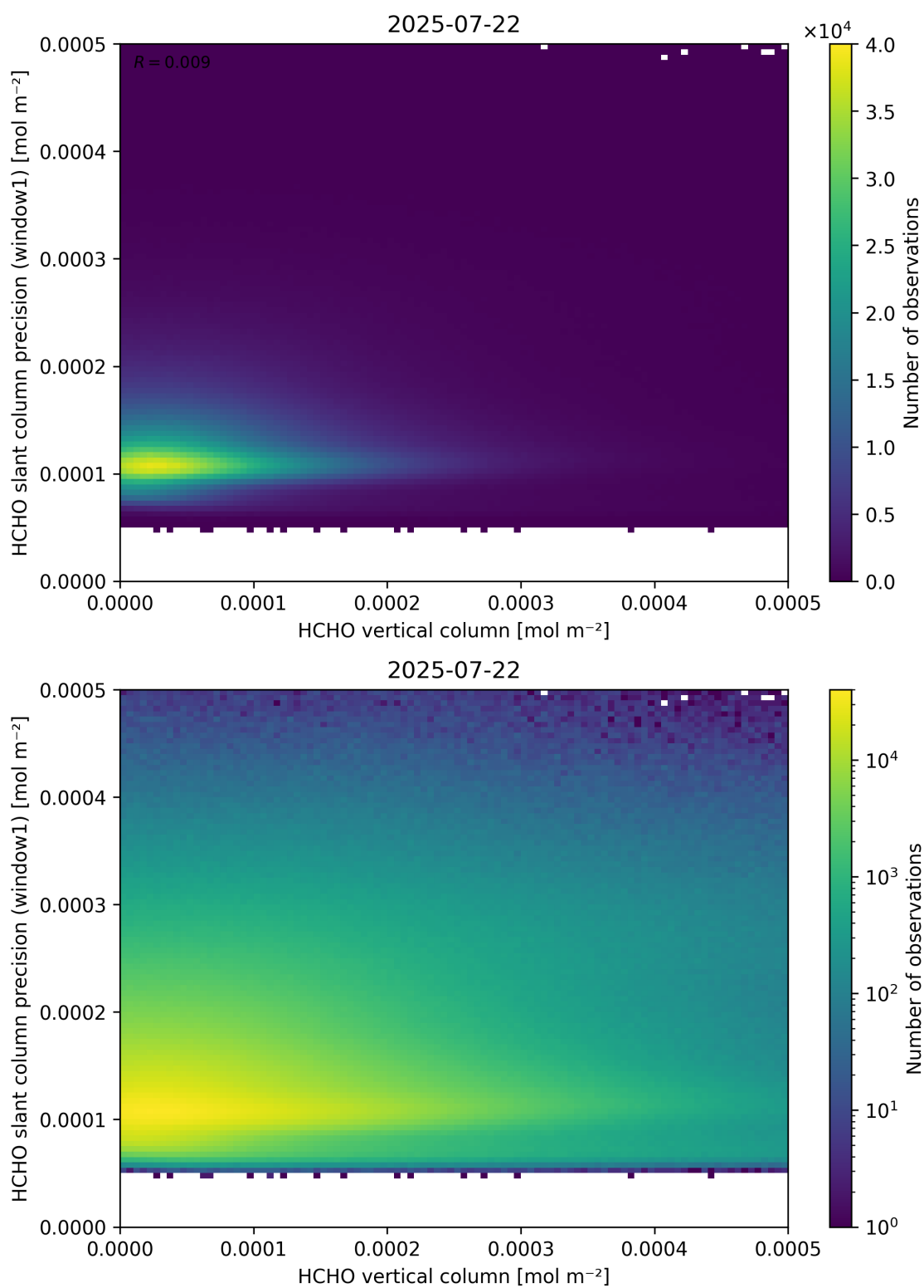
Figure 130: Scatter density plot of “HCHO vertical column” against “HCHO slant column precision (window1)” for 2025-07-21 to 2025-07-23.
