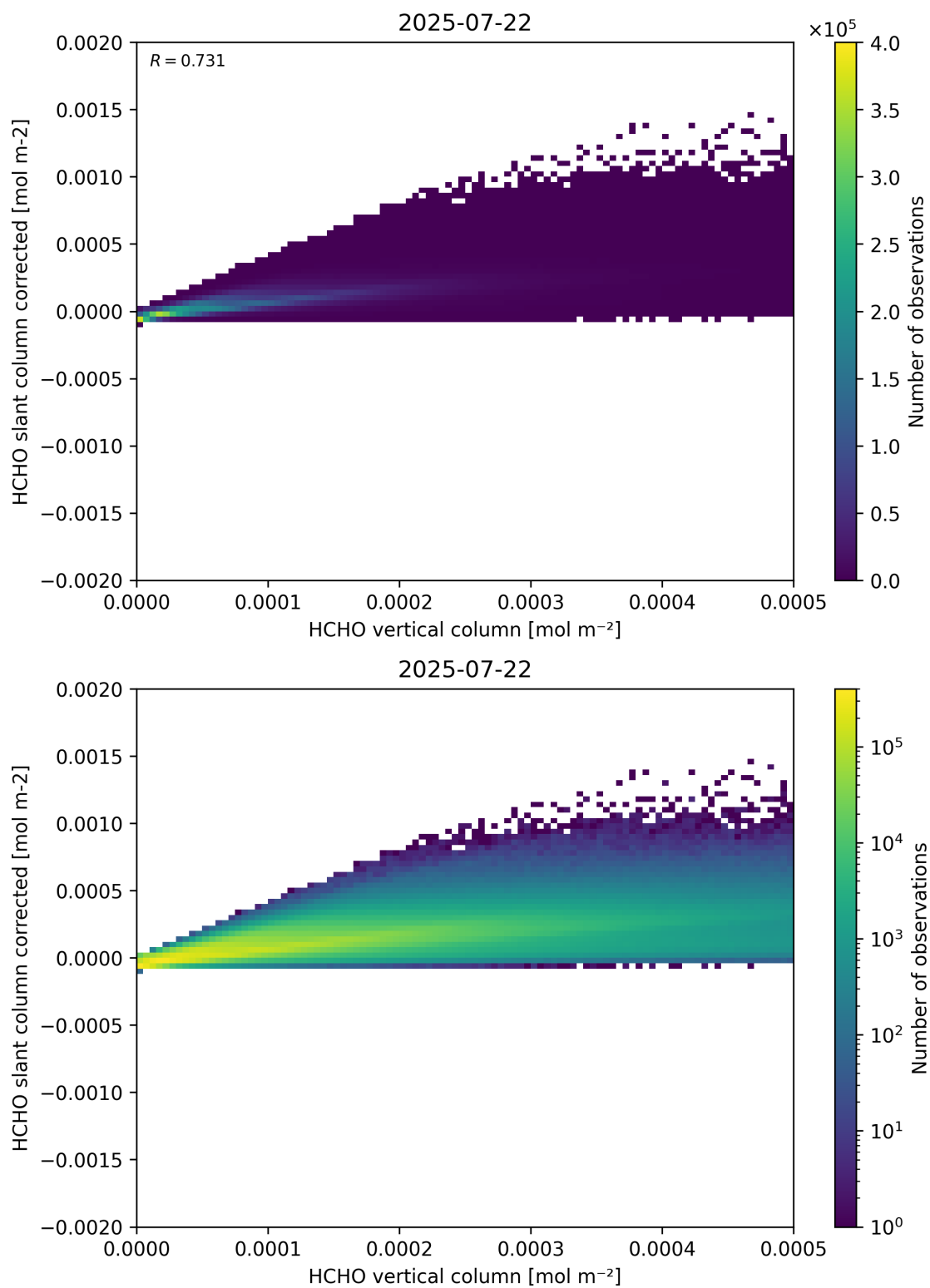
Figure 127: Scatter density plot of “HCHO vertical column” against “HCHO slant column corrected” for 2025-07-21 to 2025-07-23.
