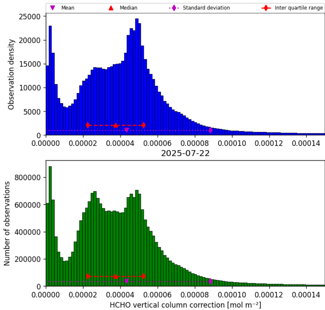
Figure 37: Histogram of “HCHO vertical column correction” for 2025-07-21 to 2025-07-23
