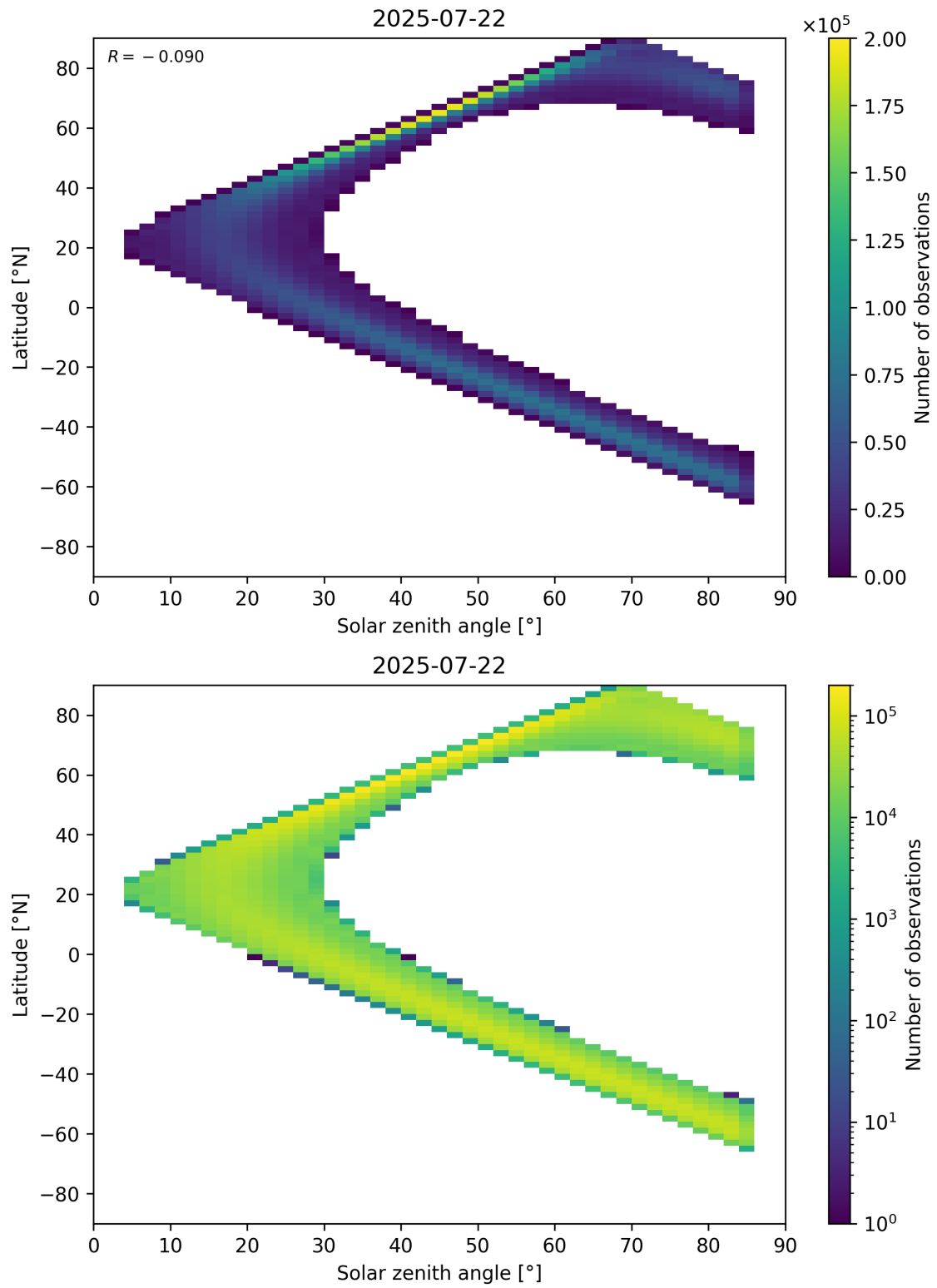
Figure 181: Scatter density plot of “Solar zenith angle” against “Latitude” for 2025-07-21 to 2025-07-23.
