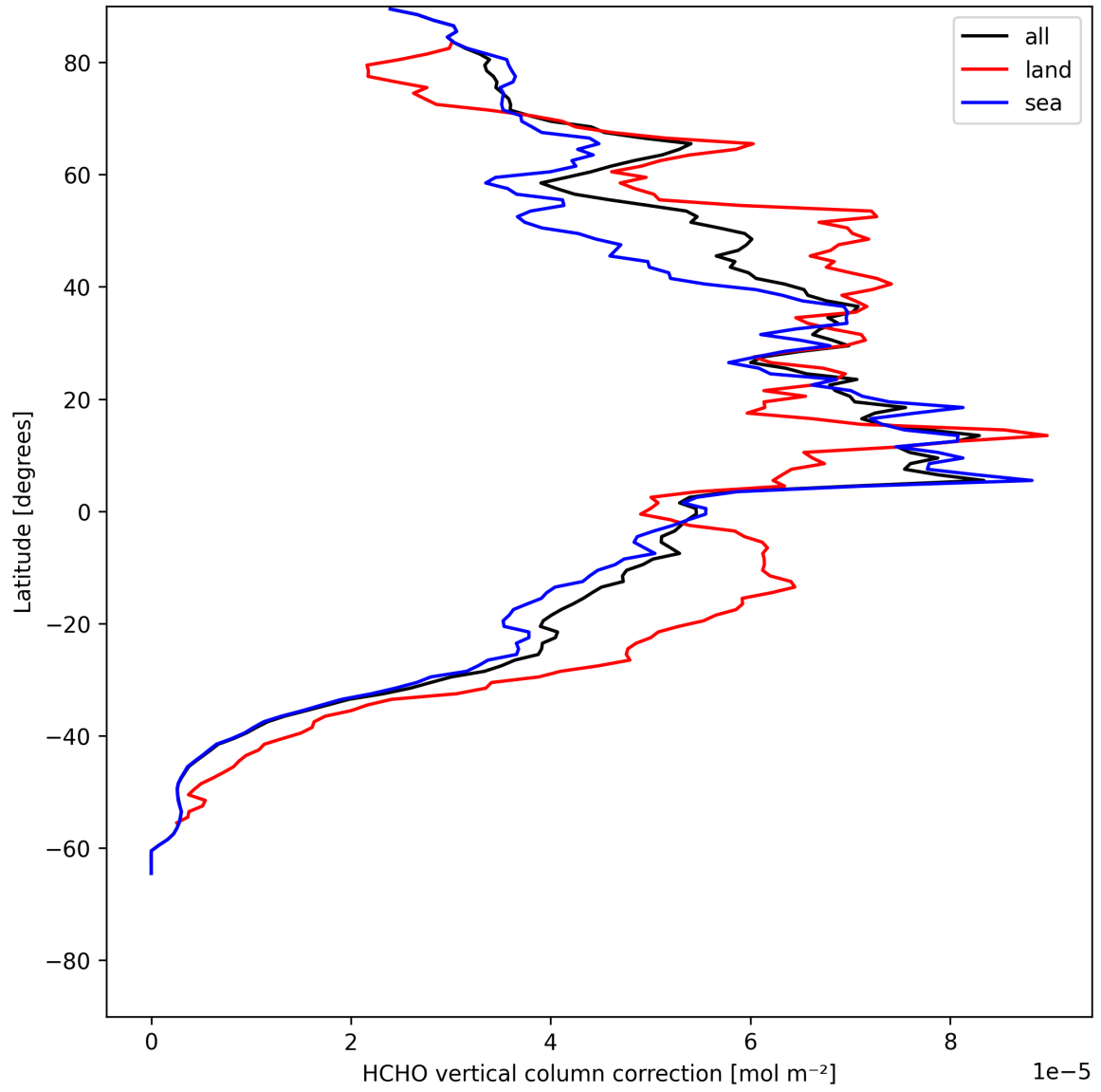
Figure 23: Zonal average of “HCHO vertical column correction” for 2025-07-21 to 2025-07-23.
