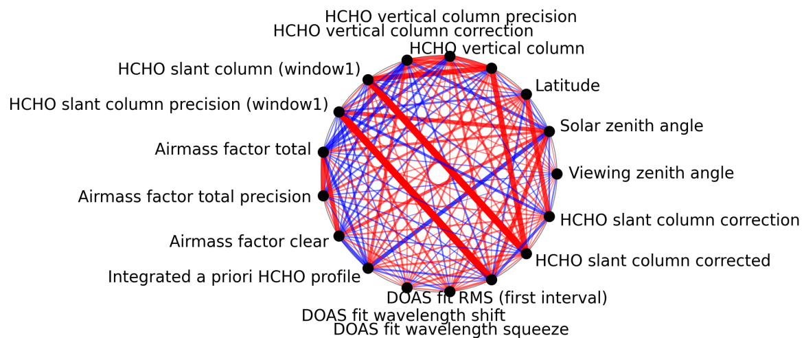
Figure 1: Map of correlation graph for 2025-07-21 to 2025-07-23.
