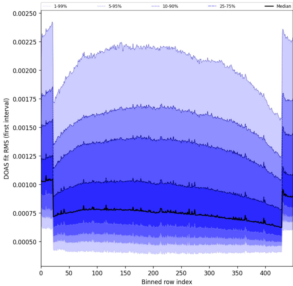
Figure 60: Along track statistics of “DOAS fit RMS (first interval)” for 2025-07-21 to 2025-07-23
