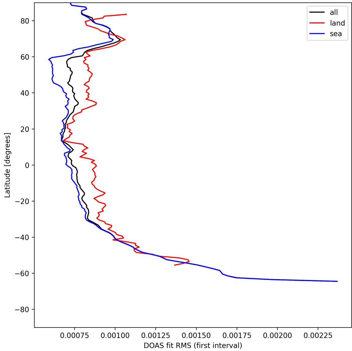
Figure 32: Zonal average of “DOAS fit RMS (first interval)” for 2025-07-21 to 2025-07-23.
