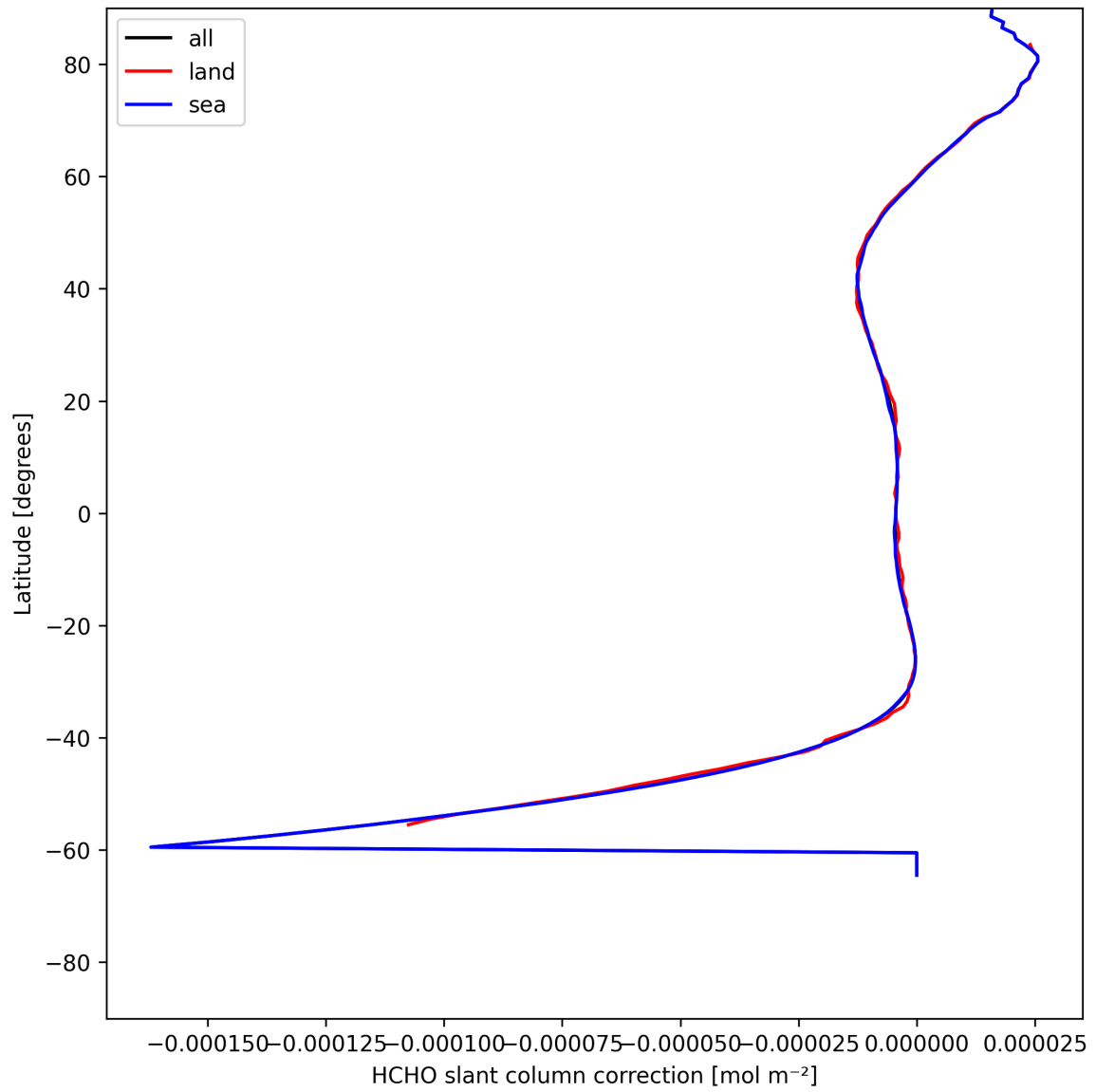
Figure 33: Zonal average of “HCHO slant column correction” for 2025-07-21 to 2025-07-23.
