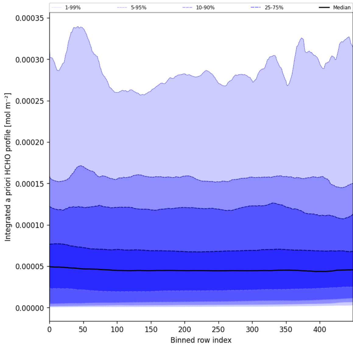
Figure 57: Along track statistics of “Integrated a priori HCHO profile” for 2025-07-21 to 2025-07-23
