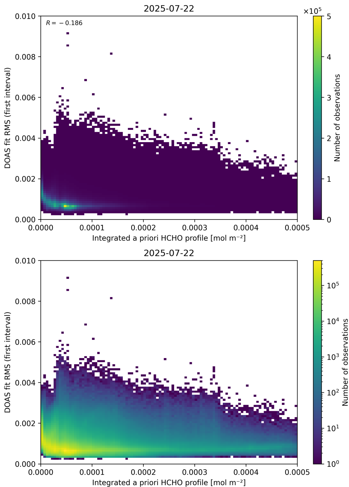
Figure 148: Scatter density plot of “Integrated a priori HCHO profile” against “DOAS fit RMS (first interval)” for 2025-07-21 to 2025-07-23.
