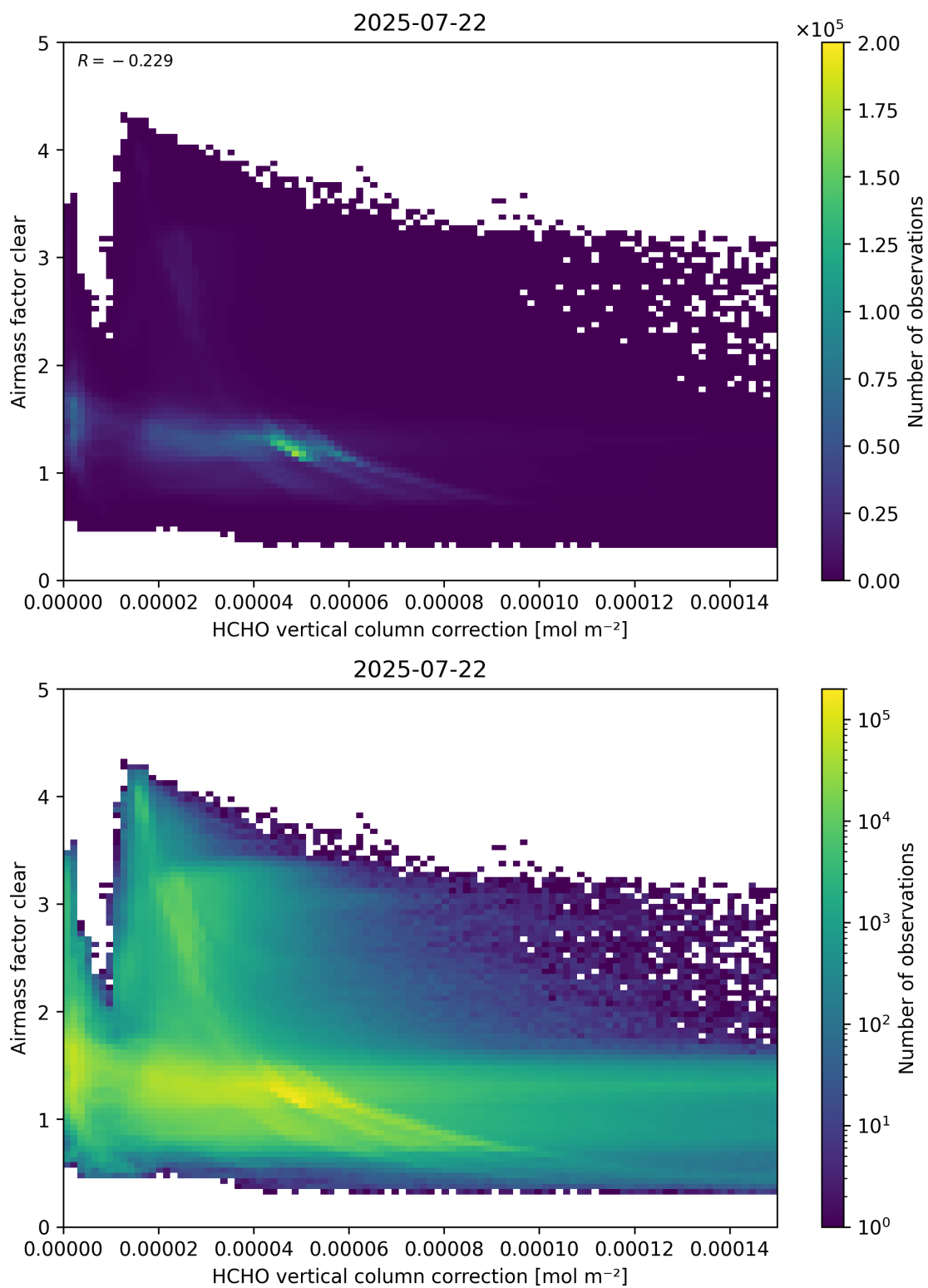
Figure 115: Scatter density plot of “HCHO vertical column correction” against “Airmass factor clear” for 2025-07-21 to 2025-07-23.
