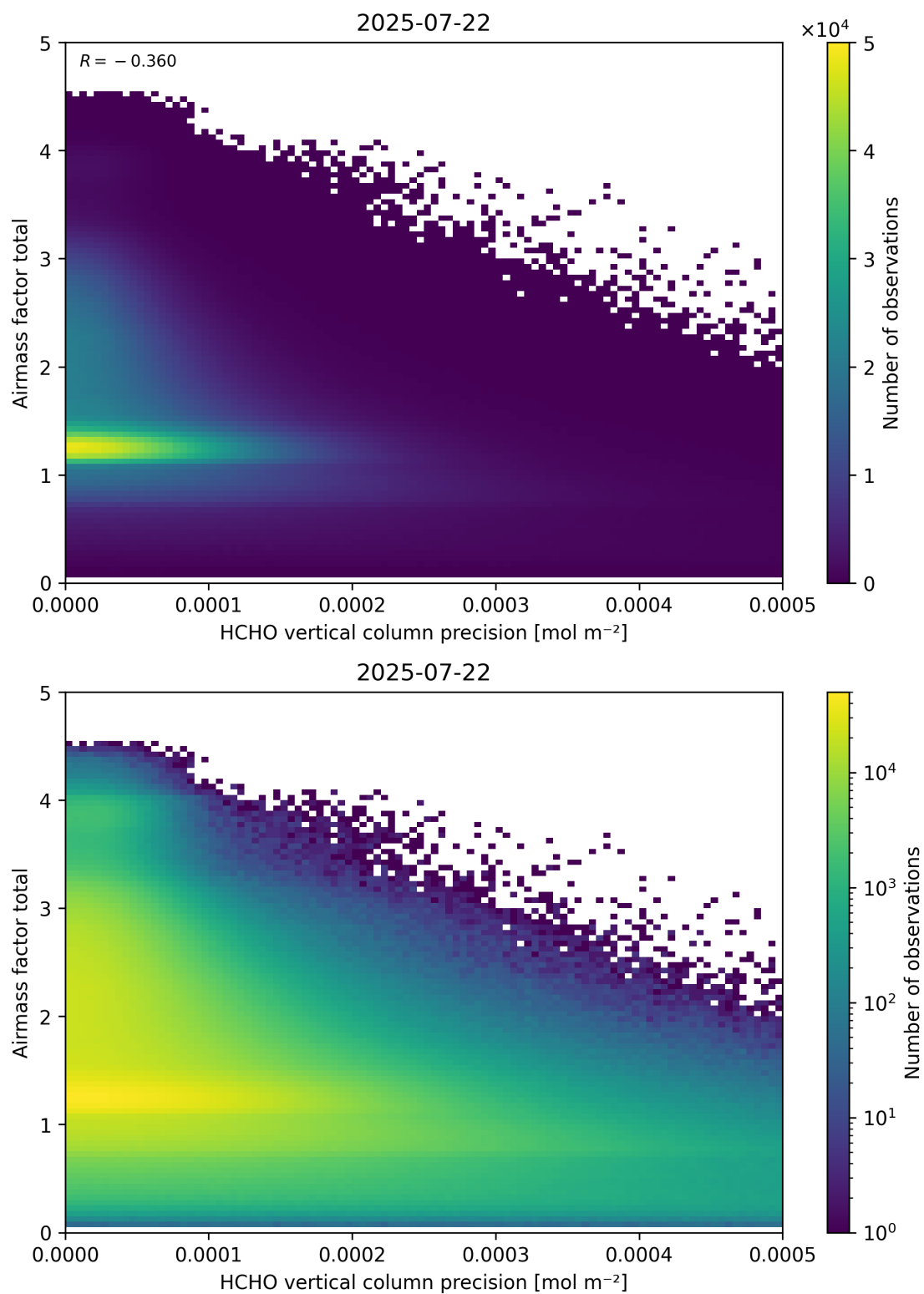
Figure 144: Scatter density plot of “HCHO vertical column precision” against “Airmass factor total” for 2025-07-21 to 2025-07-23.
