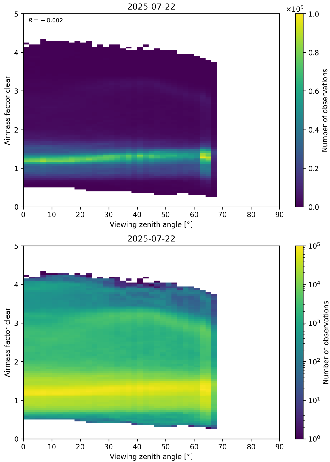
Figure 185: Scatter density plot of “Viewing zenith angle” against “Airmass factor clear” for 2025-07-21 to 2025-07-23.
