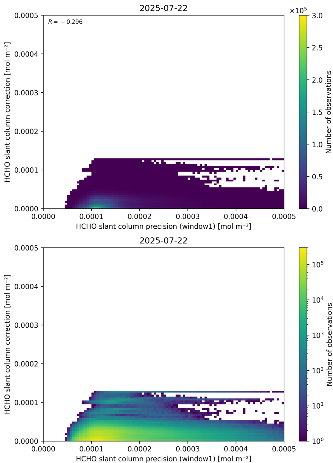
Figure 93: Scatter density plot of “HCHO slant column precision (window1)” against “HCHO slant column correction” for 2025-07-21 to 2025-07-23.
