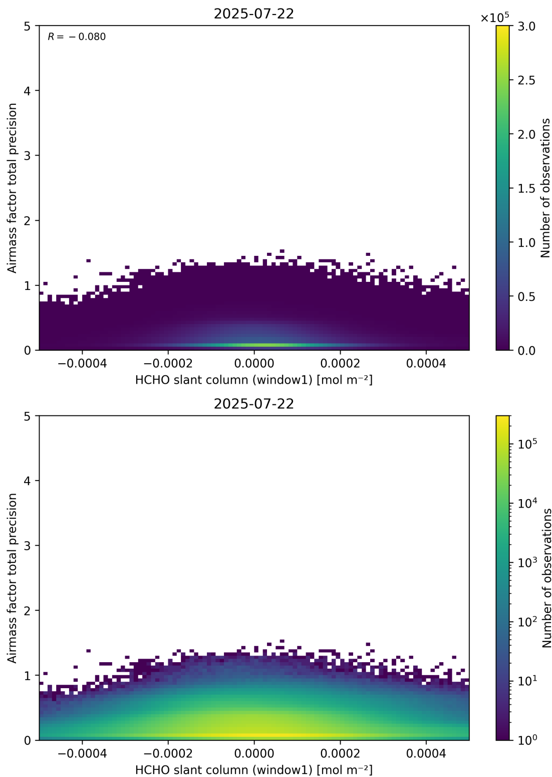
Figure 86: Scatter density plot of “HCHO slant column (window1)” against “Airmass factor total precision” for 2025-07-21 to 2025-07-23.
