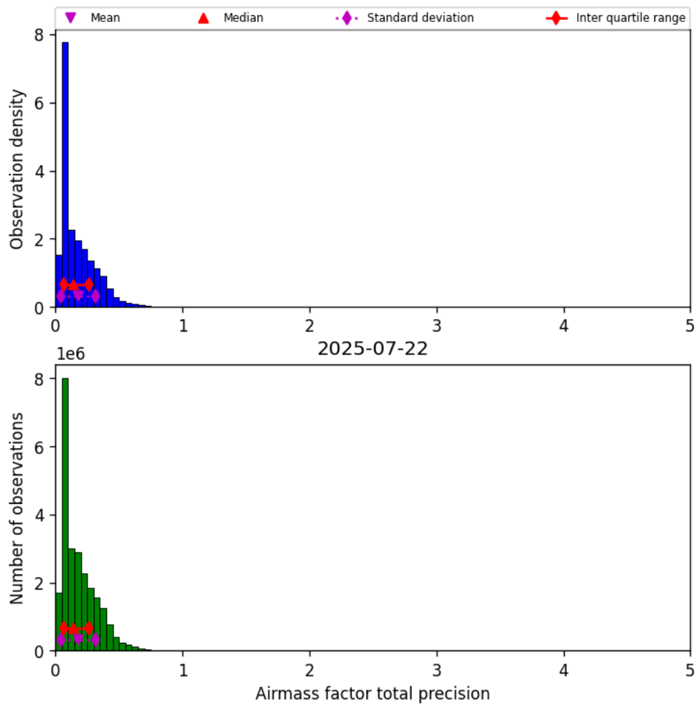
Figure 41: Histogram of “Airmass factor total precision” for 2025-07-21 to 2025-07-23
