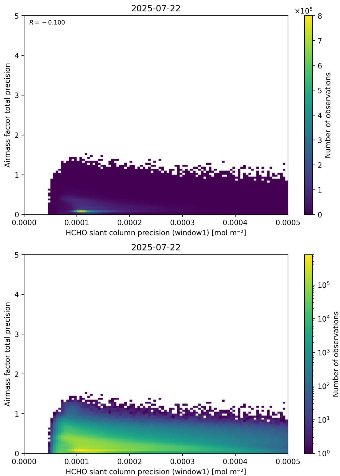
Figure 95: Scatter density plot of “HCHO slant column precision (window1)” against “Airmass factor total precision” for 2025-07-21 to 2025-07-23.
