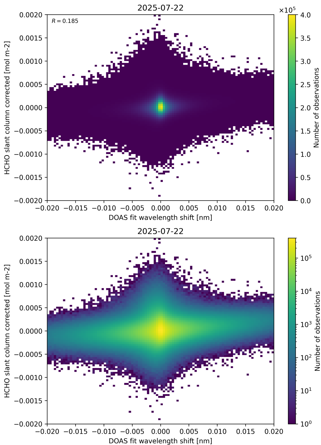
Figure 66: Scatter density plot of “DOAS fit wavelength shift” against “HCHO slant column corrected” for 2025-07-21 to 2025-07-23.
