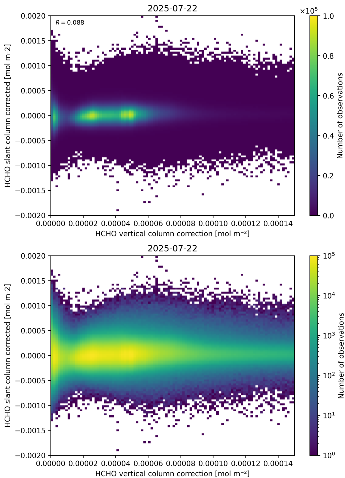
Figure 116: Scatter density plot of “HCHO vertical column correction” against “HCHO slant column corrected” for 2025-07-21 to 2025-07-23.
