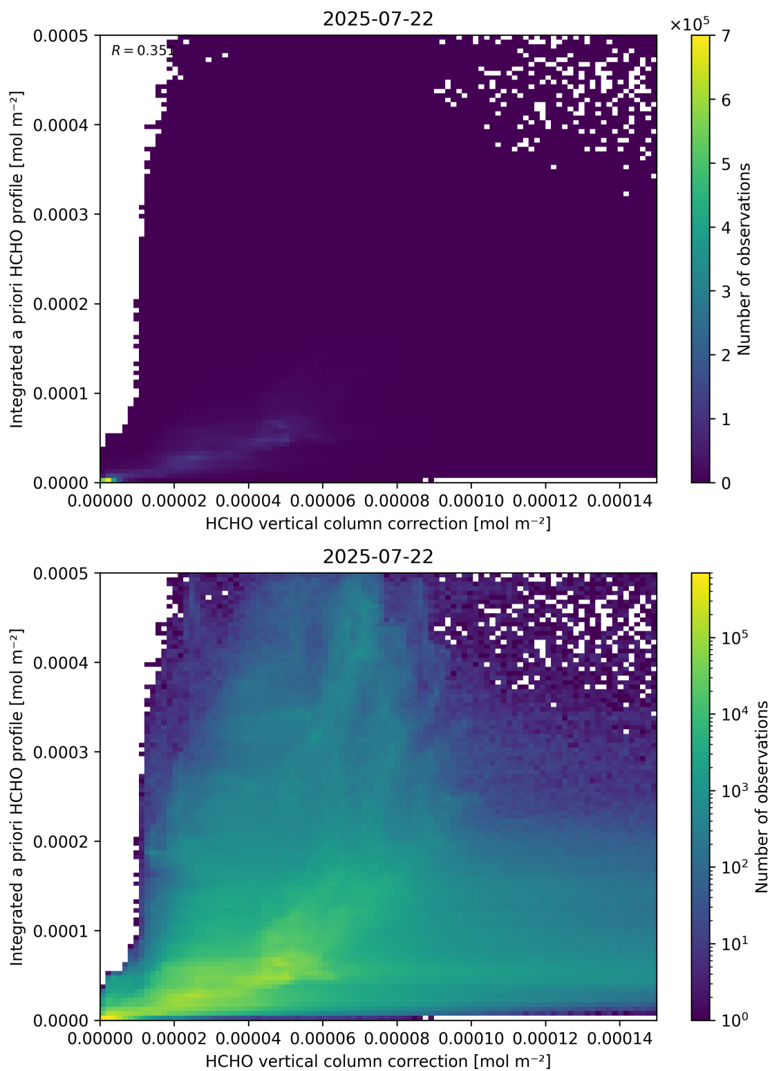
Figure 122: Scatter density plot of “HCHO vertical column correction” against “Integrated a priori HCHO profile” for 2025-07-21 to 2025-07-23.
