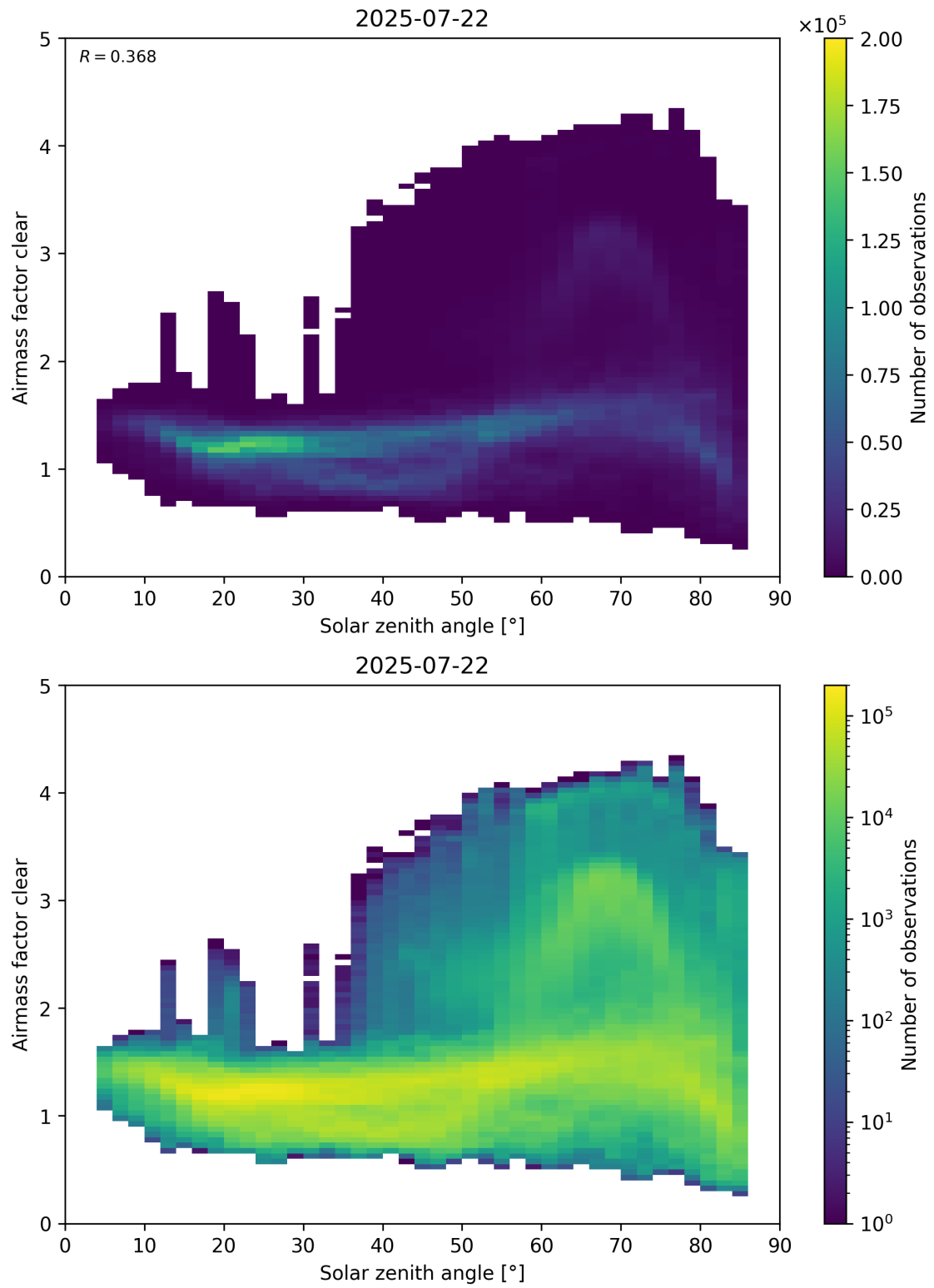
Figure 170: Scatter density plot of “Solar zenith angle” against “Airmass factor clear” for 2025-07-21 to 2025-07-23.
