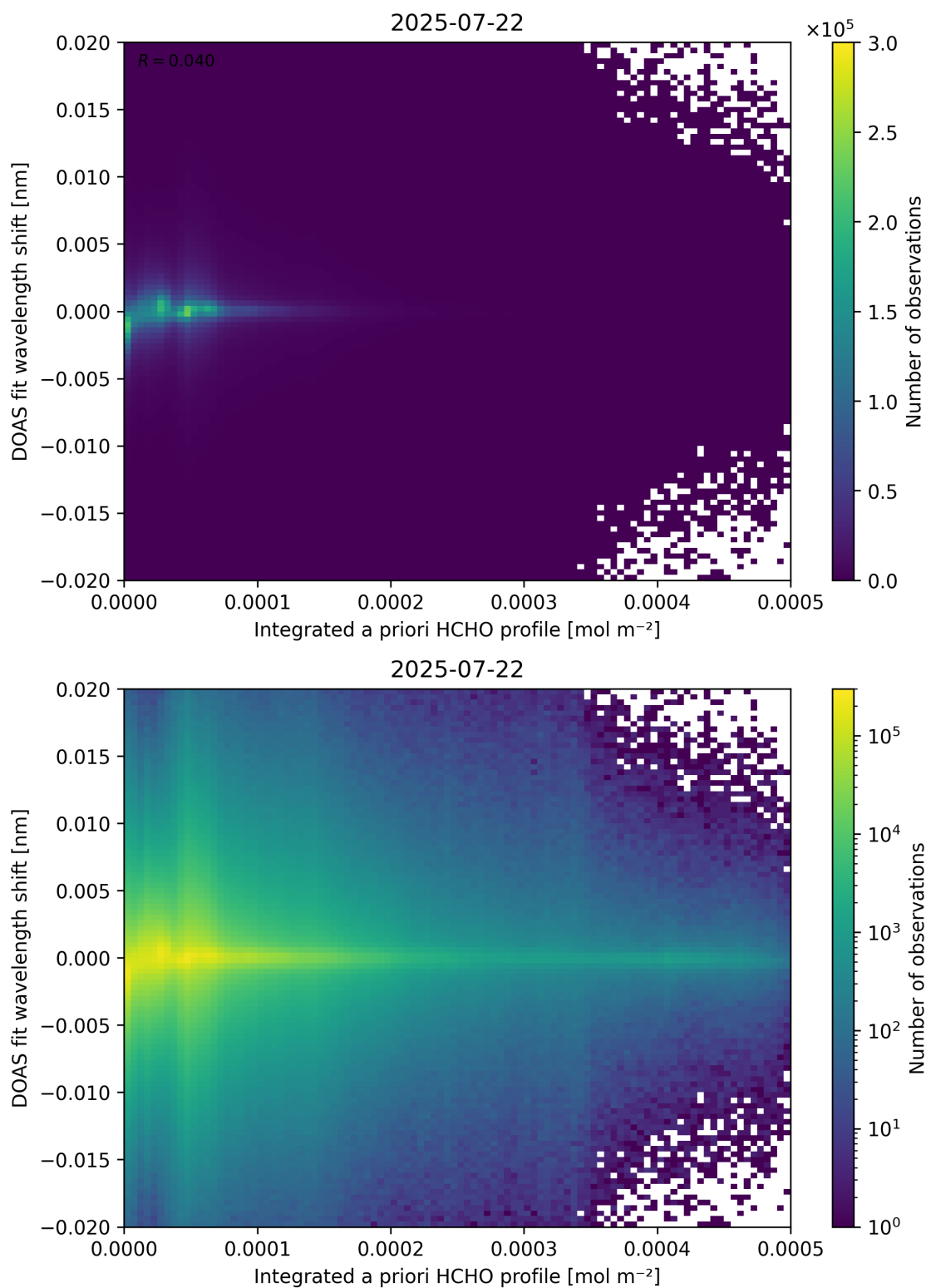
Figure 149: Scatter density plot of “Integrated a priori HCHO profile” against “DOAS fit wavelength shift” for 2025-07-21 to 2025-07-23.
