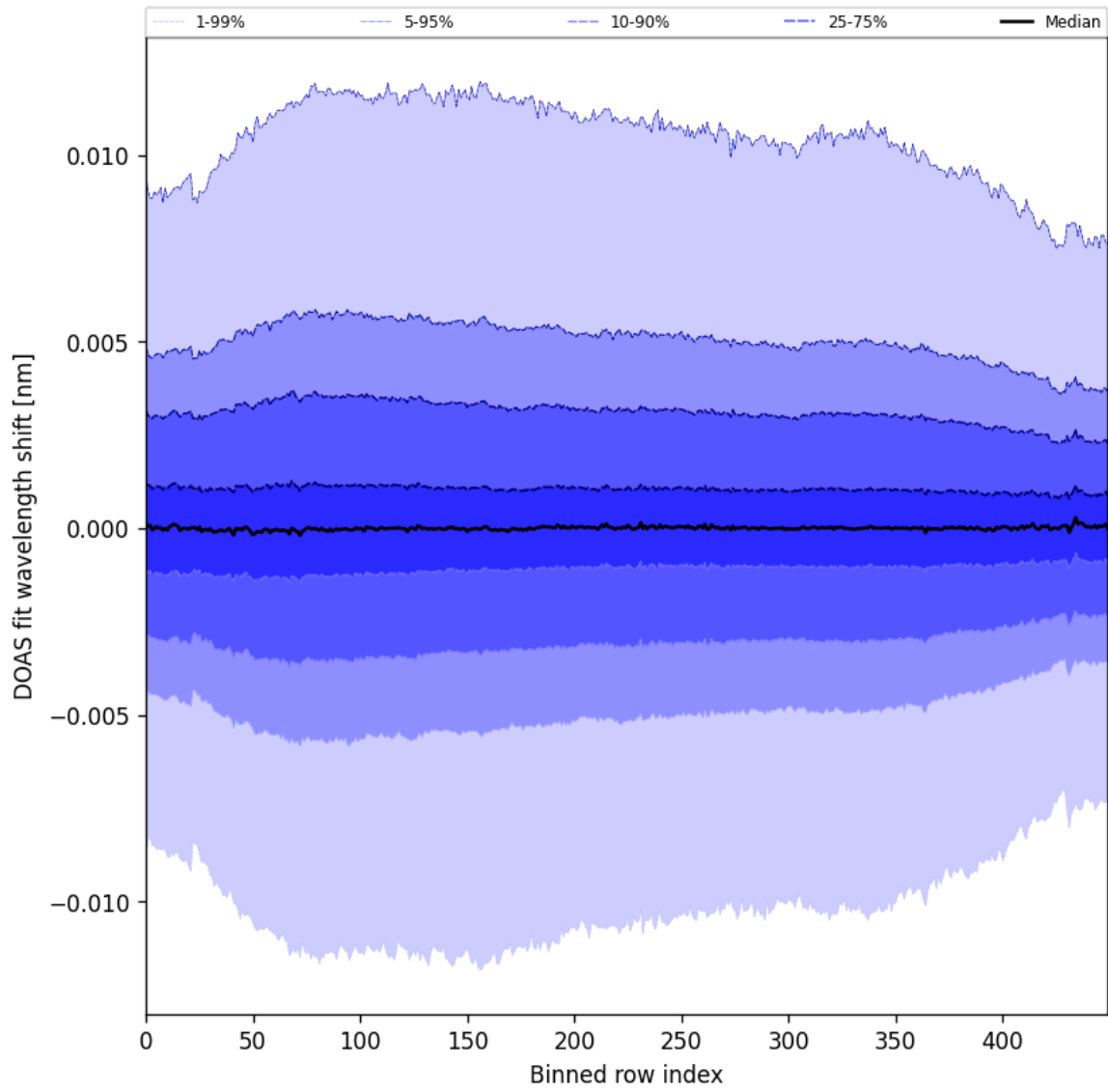
Figure 58: Along track statistics of “DOAS fit wavelength shift” for 2025-07-21 to 2025-07-23
