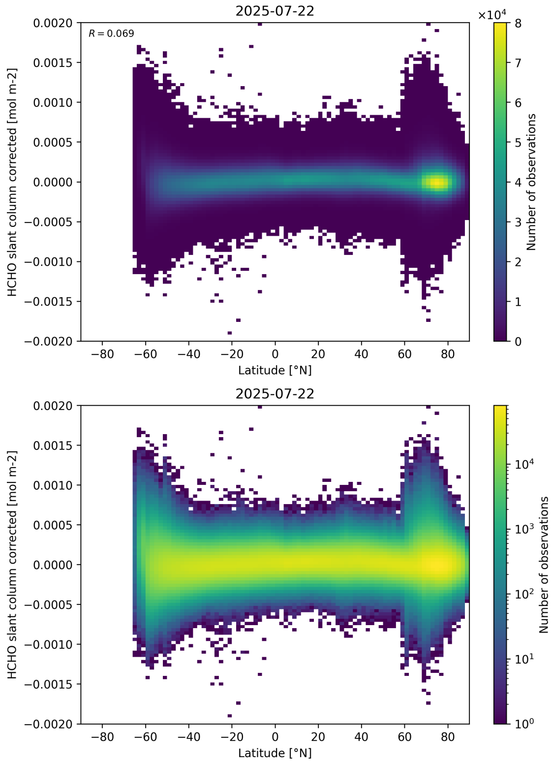
Figure 157: Scatter density plot of “Latitude” against “HCHO slant column corrected” for 2025-07-21 to 2025-07-23.
