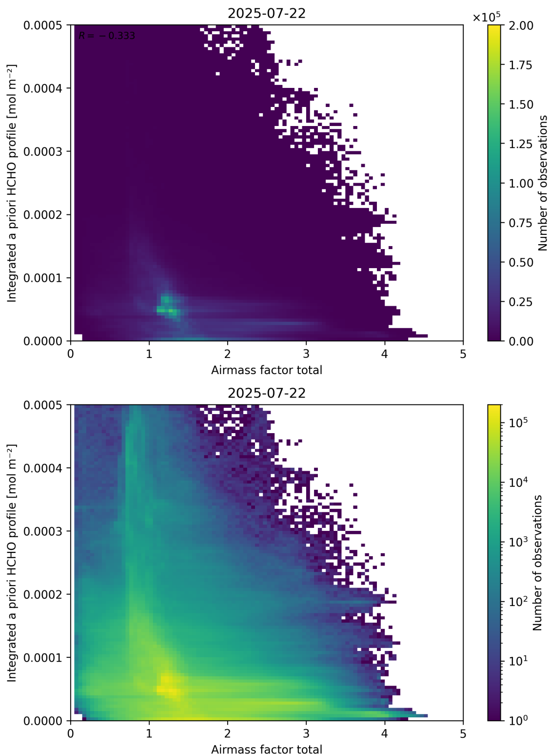
Figure 104: Scatter density plot of “Airmass factor total” against “Integrated a priori HCHO profile” for 2025-07-21 to 2025-07-23.
