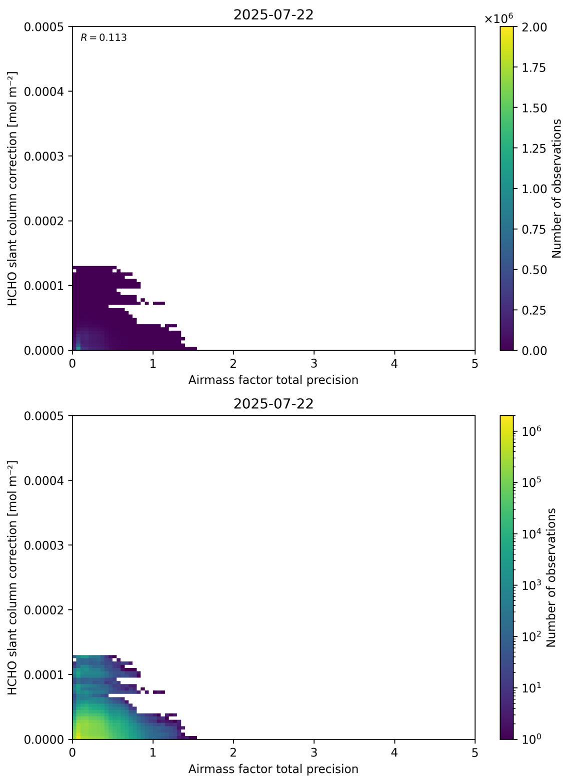
Figure 110: Scatter density plot of “Airmass factor total precision” against “HCHO slant column correction” for 2025-07-21 to 2025-07-23.
