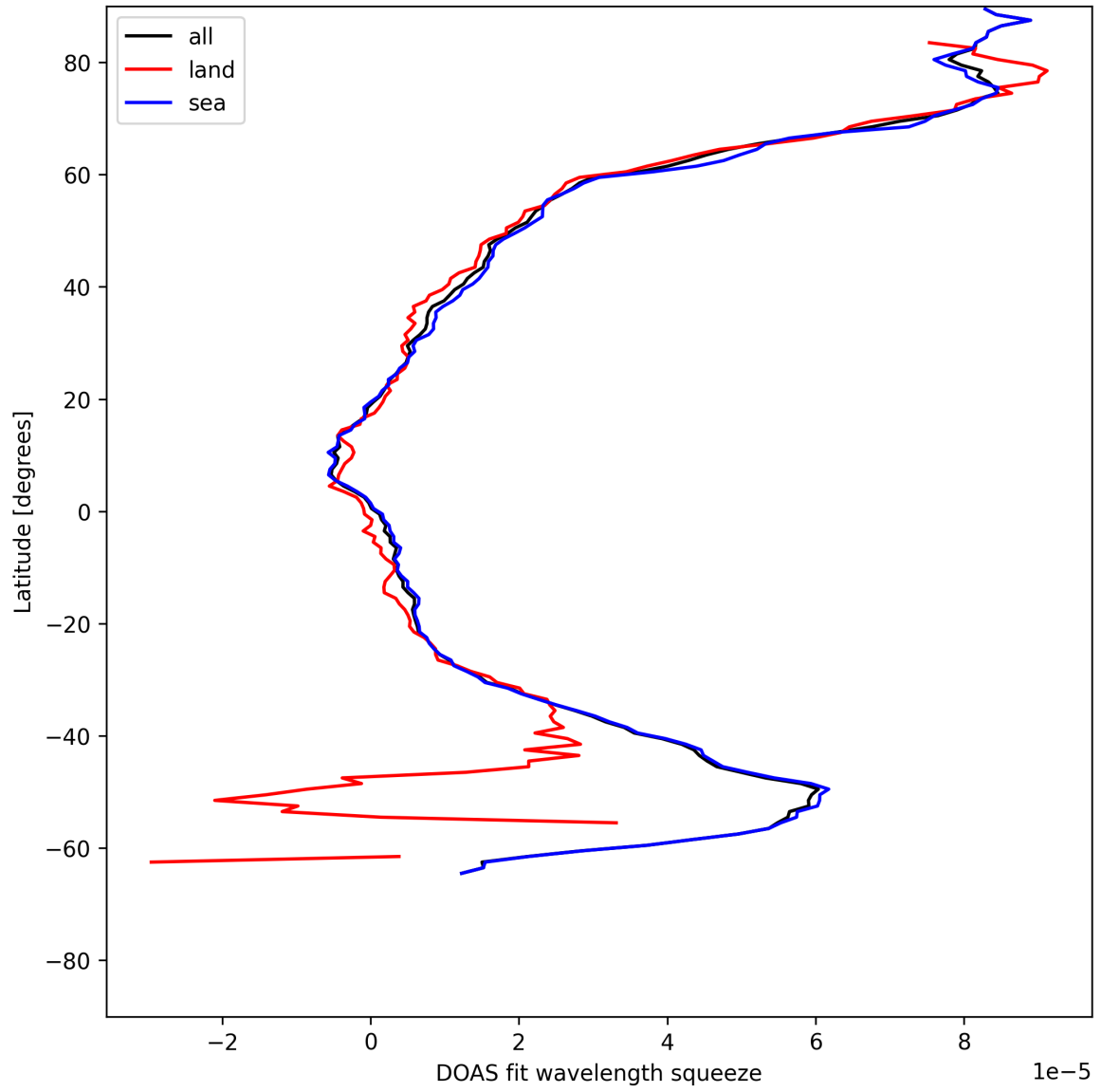
Figure 31: Zonal average of “DOAS fit wavelength squeeze” for 2025-07-21 to 2025-07-23.
