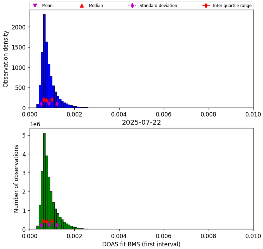
Figure 46: Histogram of “DOAS fit RMS (first interval)” for 2025-07-21 to 2025-07-23
