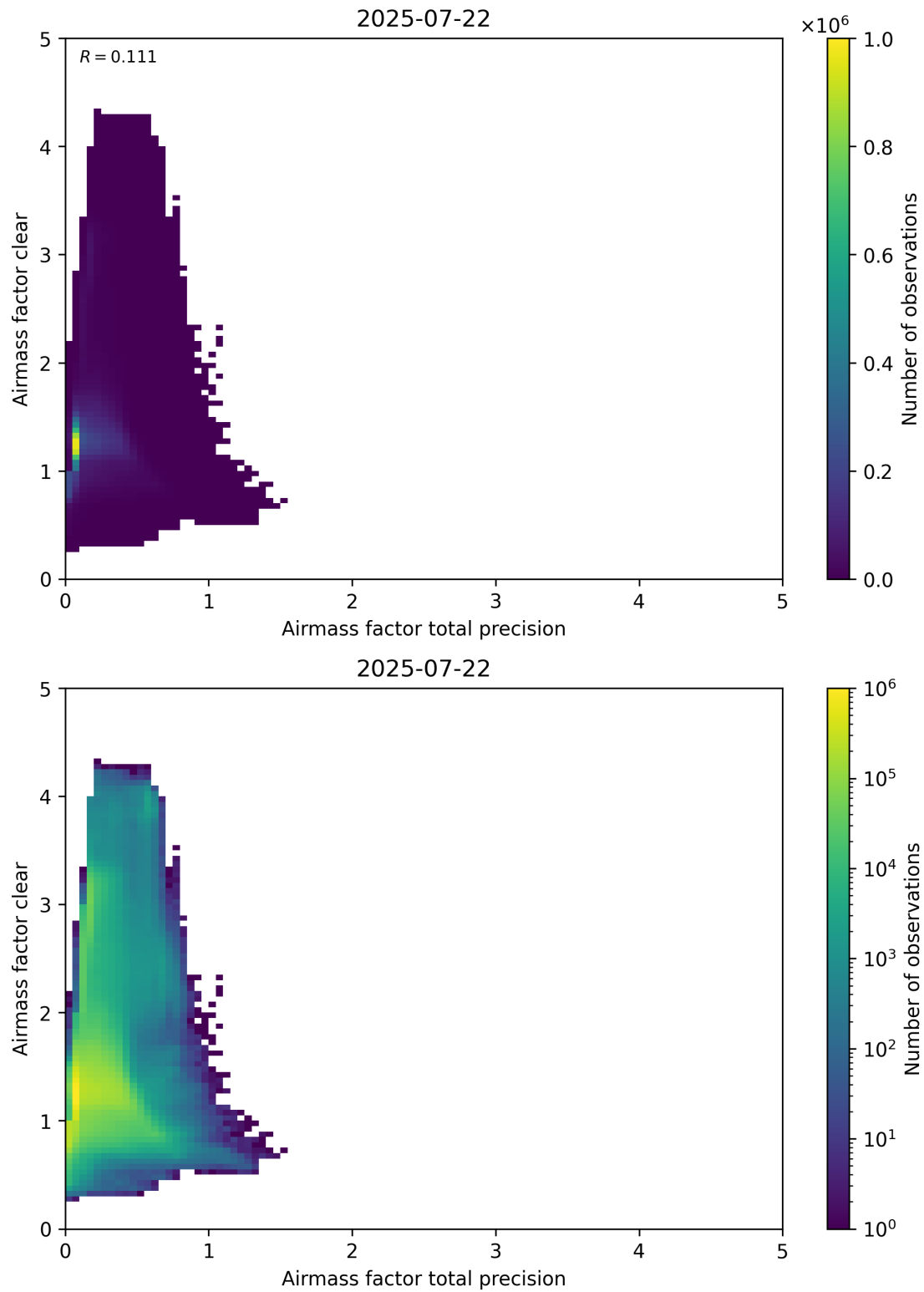
Figure 108: Scatter density plot of “Airmass factor total precision” against “Airmass factor clear” for 2025-07-21 to 2025-07-23.
