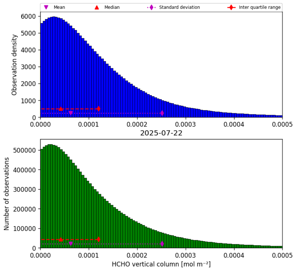
Figure 35: Histogram of “HCHO vertical column” for 2025-07-21 to 2025-07-23
