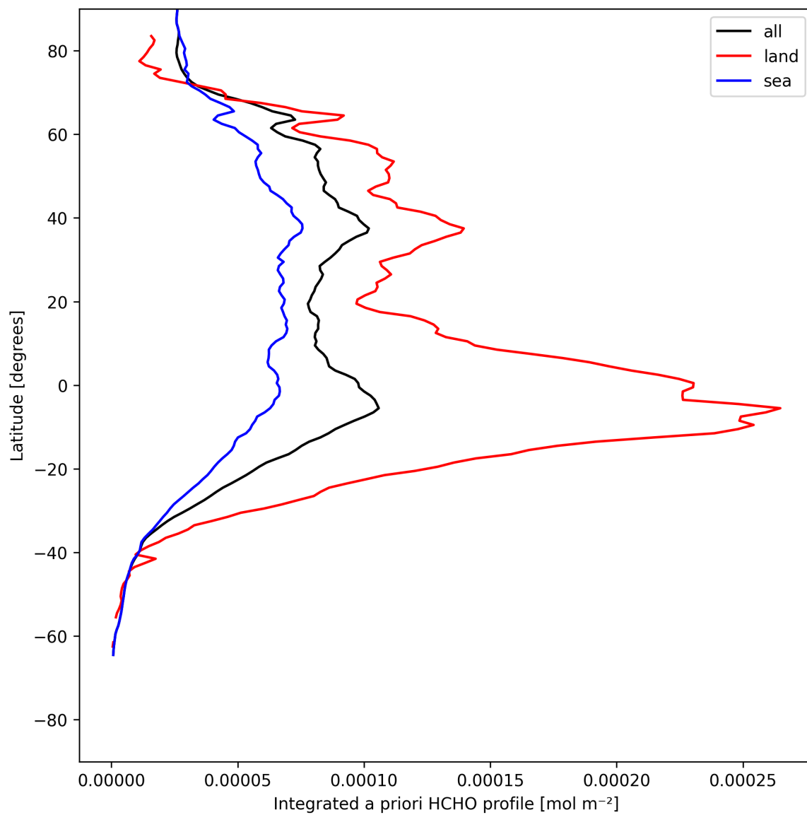
Figure 29: Zonal average of “Integrated a priori HCHO profile” for 2025-07-21 to 2025-07-23.
