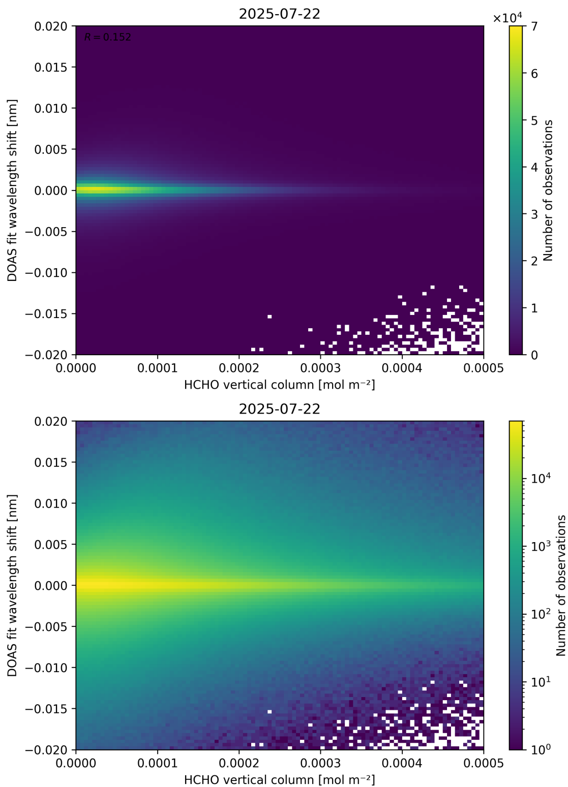
Figure 124: Scatter density plot of “HCHO vertical column” against “DOAS fit wavelength shift” for 2025-07-21 to 2025-07-23.
