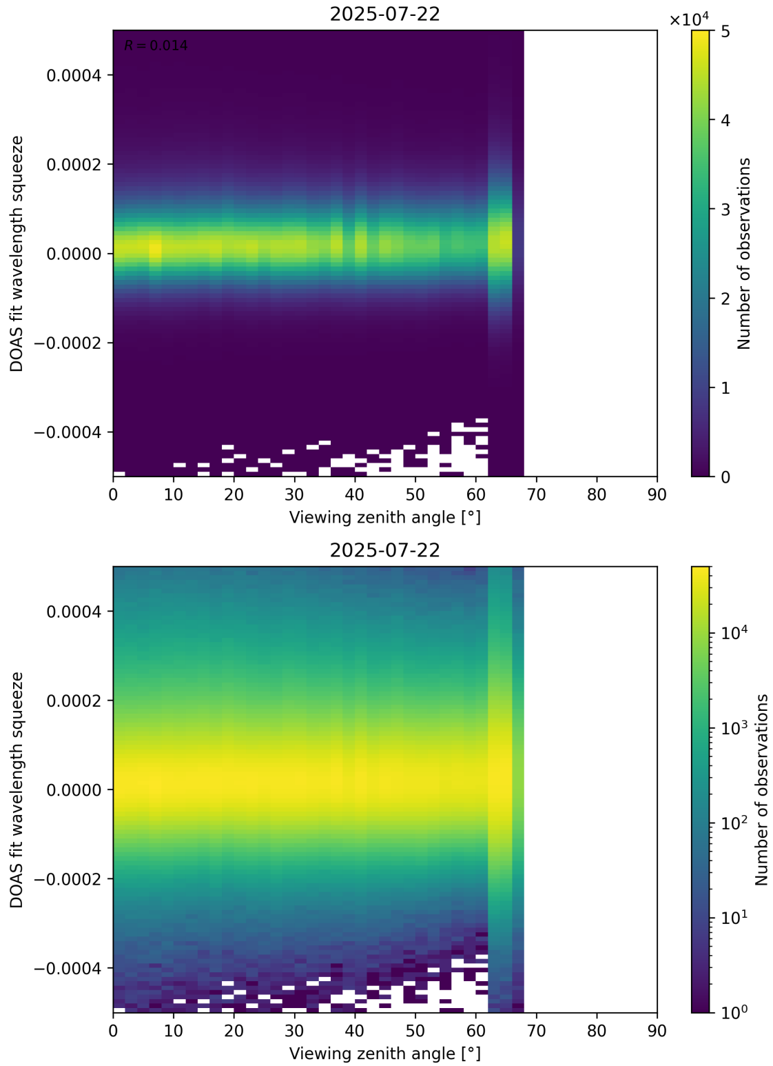
Figure 184: Scatter density plot of “Viewing zenith angle” against “DOAS fit wavelength squeeze” for 2025-07-21 to 2025-07-23.
