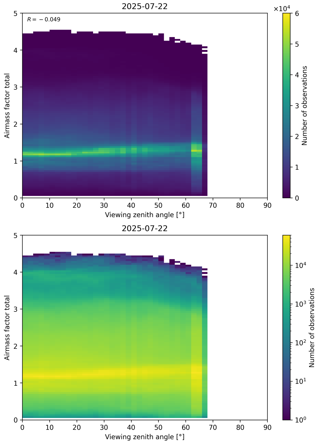
Figure 190: Scatter density plot of “Viewing zenith angle” against “Airmass factor total” for 2025-07-21 to 2025-07-23.
