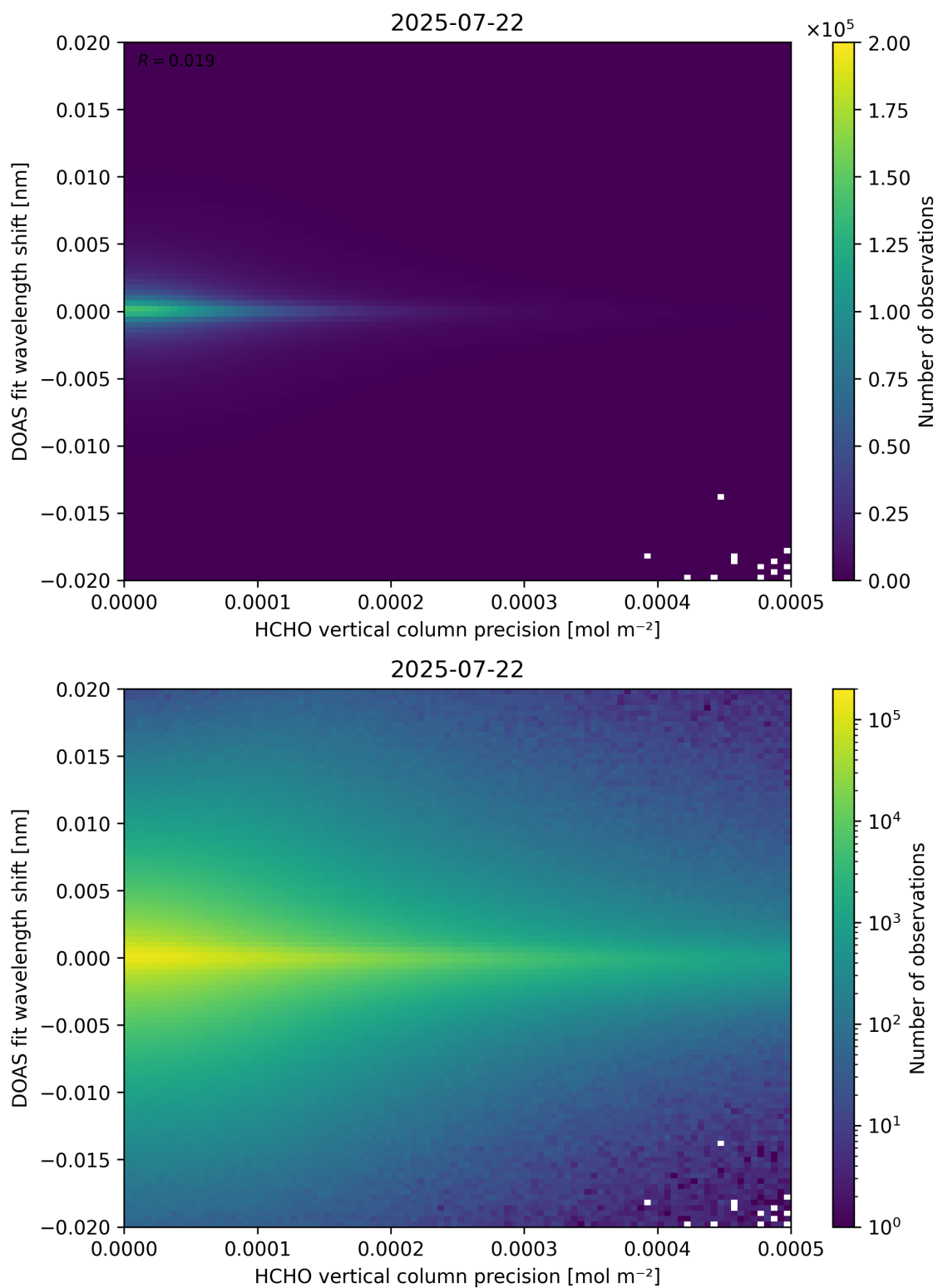
Figure 137: Scatter density plot of “HCHO vertical column precision” against “DOAS fit wavelength shift” for 2025-07-21 to 2025-07-23.
