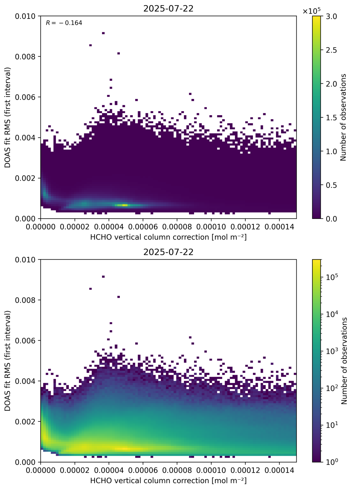
Figure 112: Scatter density plot of “HCHO vertical column correction” against “DOAS fit RMS (first interval)” for 2025-07-21 to 2025-07-23.
