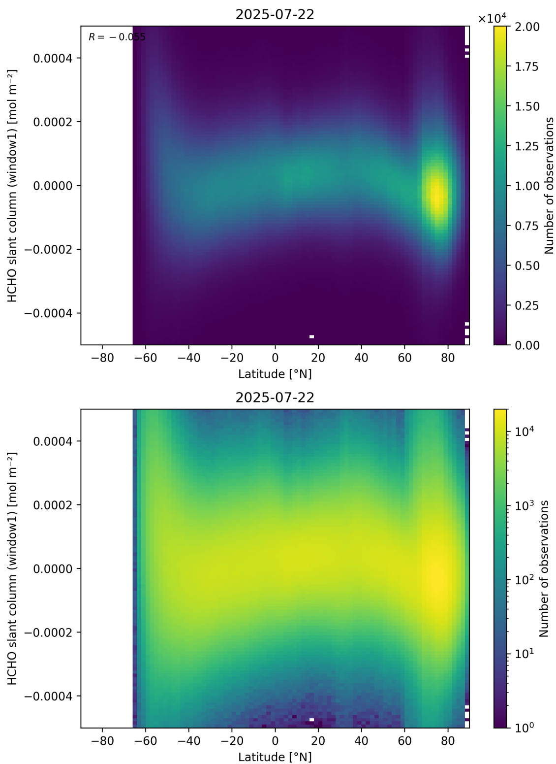
Figure 159: Scatter density plot of “Latitude” against “HCHO slant column (window1)” for 2025-07-21 to 2025-07-23.
