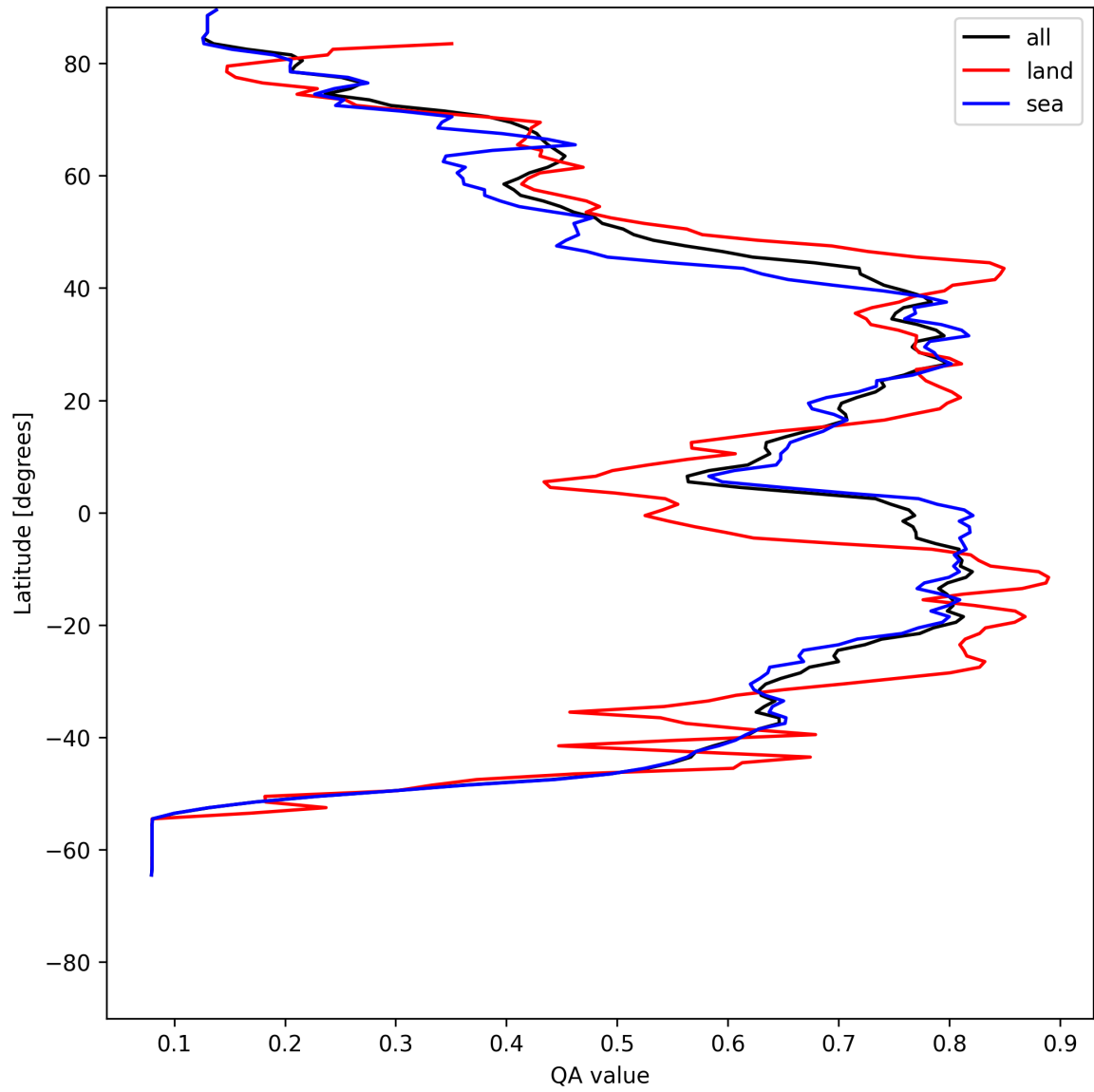
Figure 20: Zonal average of “QA value” for 2025-07-21 to 2025-07-23.
