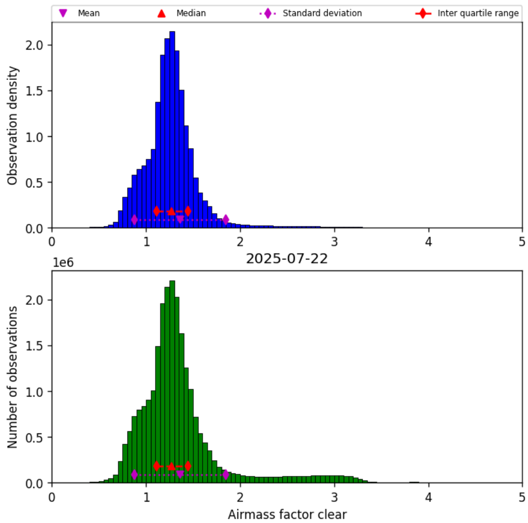
Figure 42: Histogram of “Airmass factor clear” for 2025-07-21 to 2025-07-23
