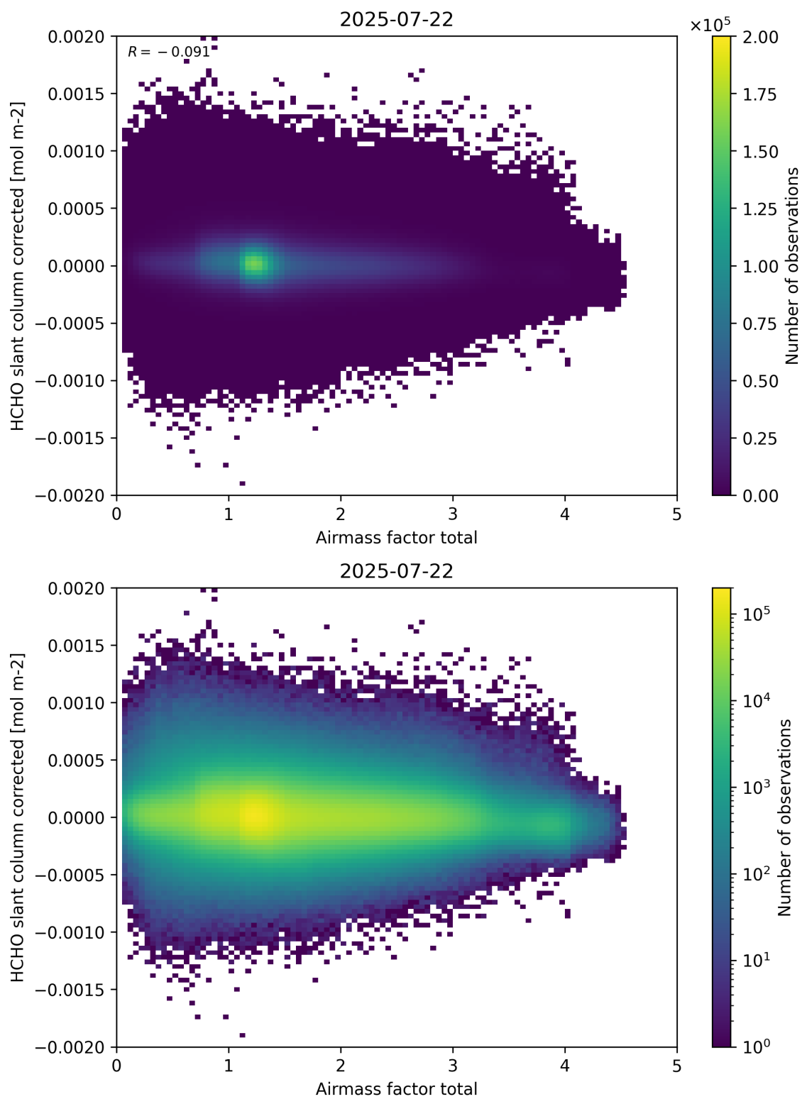
Figure 101: Scatter density plot of “Airmass factor total” against “HCHO slant column corrected” for 2025-07-21 to 2025-07-23.
