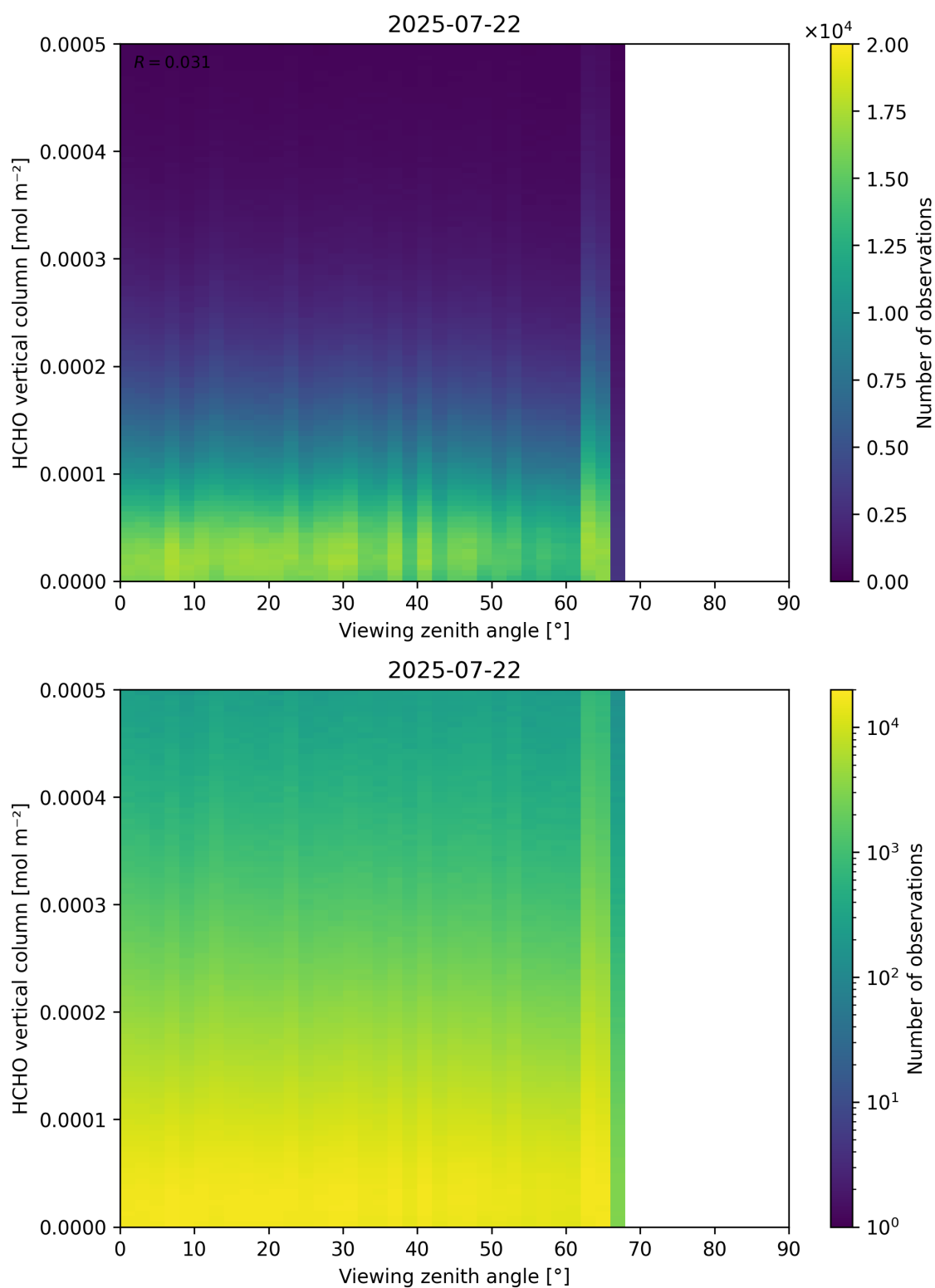
Figure 192: Scatter density plot of “Viewing zenith angle” against “HCHO vertical column” for 2025-07-21 to 2025-07-23.
