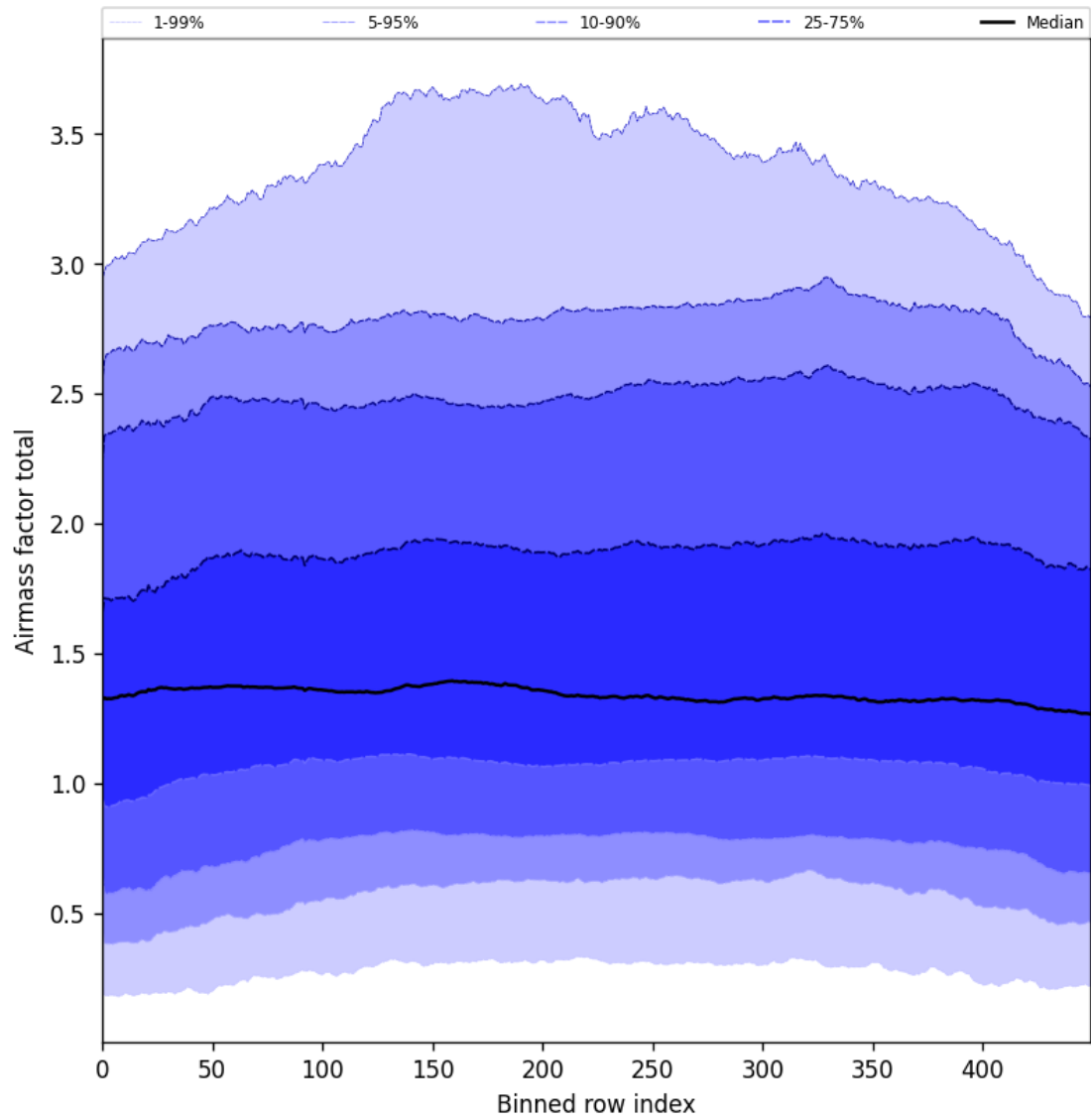
Figure 54: Along track statistics of “Airmass factor total” for 2025-07-21 to 2025-07-23
