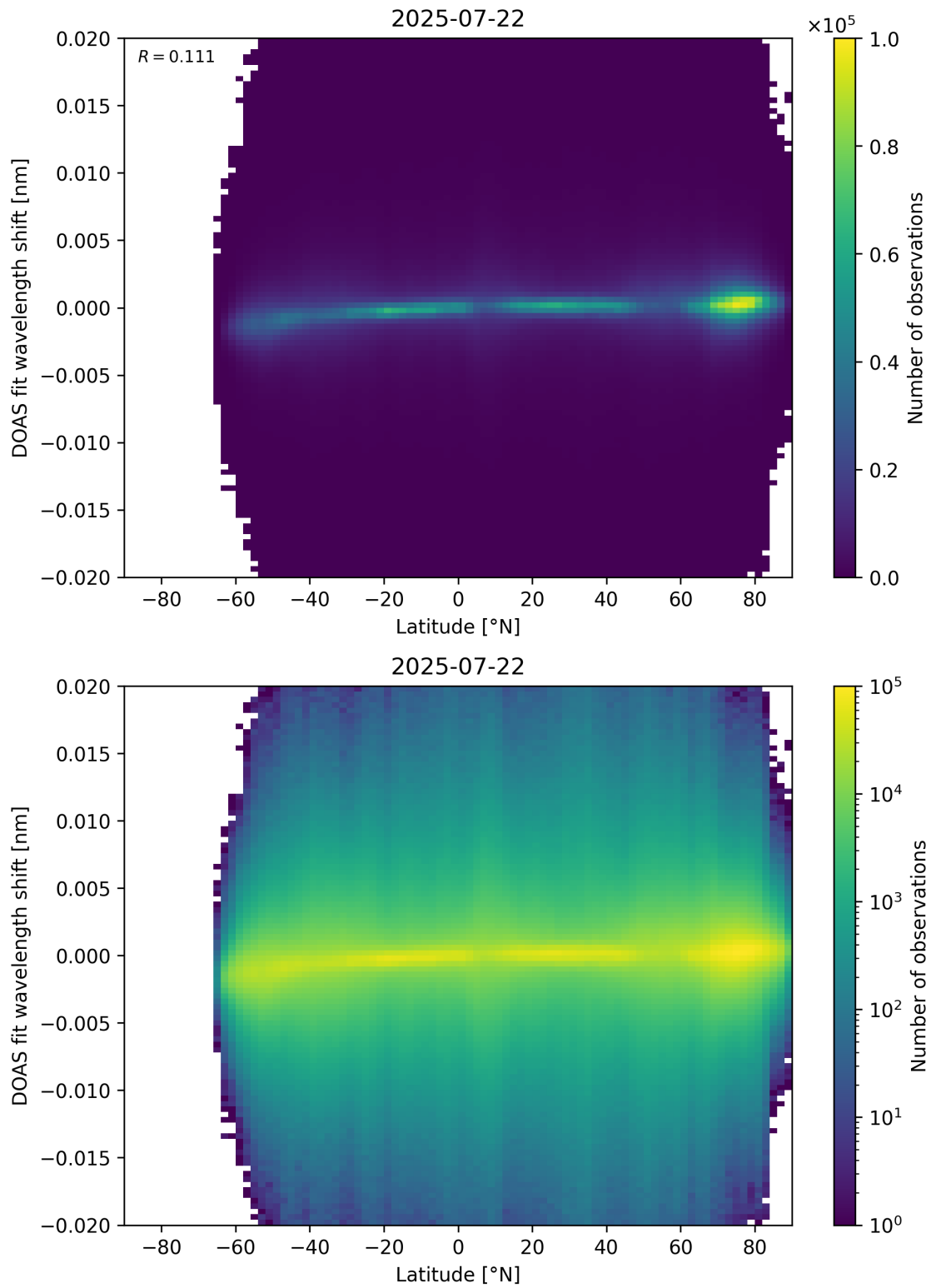
Figure 154: Scatter density plot of “Latitude” against “DOAS fit wavelength shift” for 2025-07-21 to 2025-07-23.
