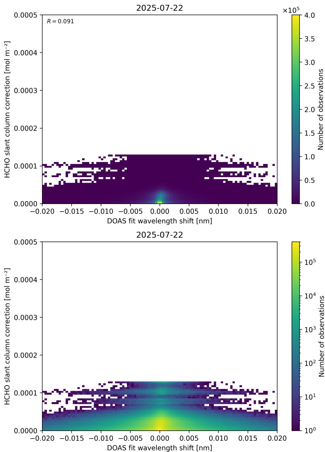
Figure 67: Scatter density plot of “DOAS fit wavelength shift” against “HCHO slant column correction” for 2025-07-21 to 2025-07-23.
