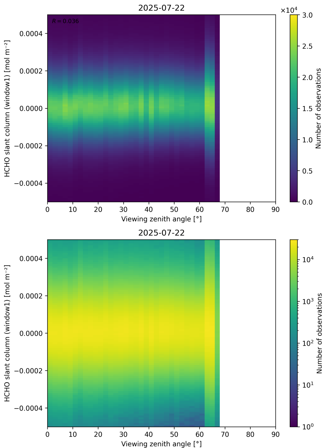
Figure 188: Scatter density plot of “Viewing zenith angle” against “HCHO slant column (window1)” for 2025-07-21 to 2025-07-23.
