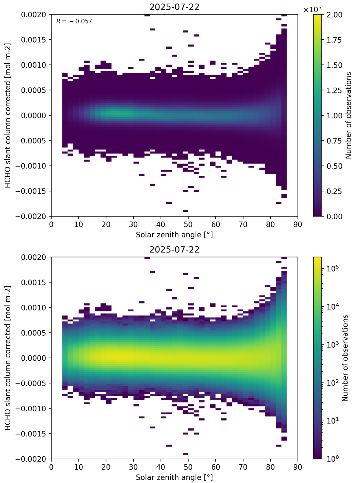
Figure 171: Scatter density plot of “Solar zenith angle” against “HCHO slant column corrected” for 2025-07-21 to 2025-07-23.
