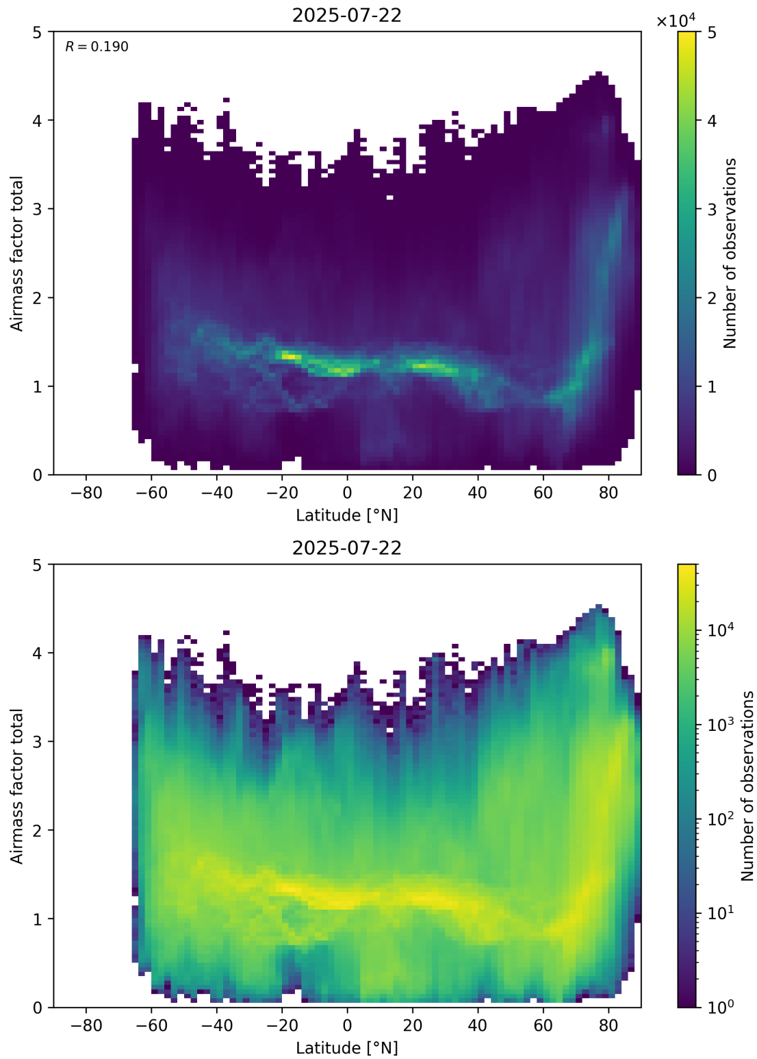
Figure 161: Scatter density plot of “Latitude” against “Airmass factor total” for 2025-07-21 to 2025-07-23.
