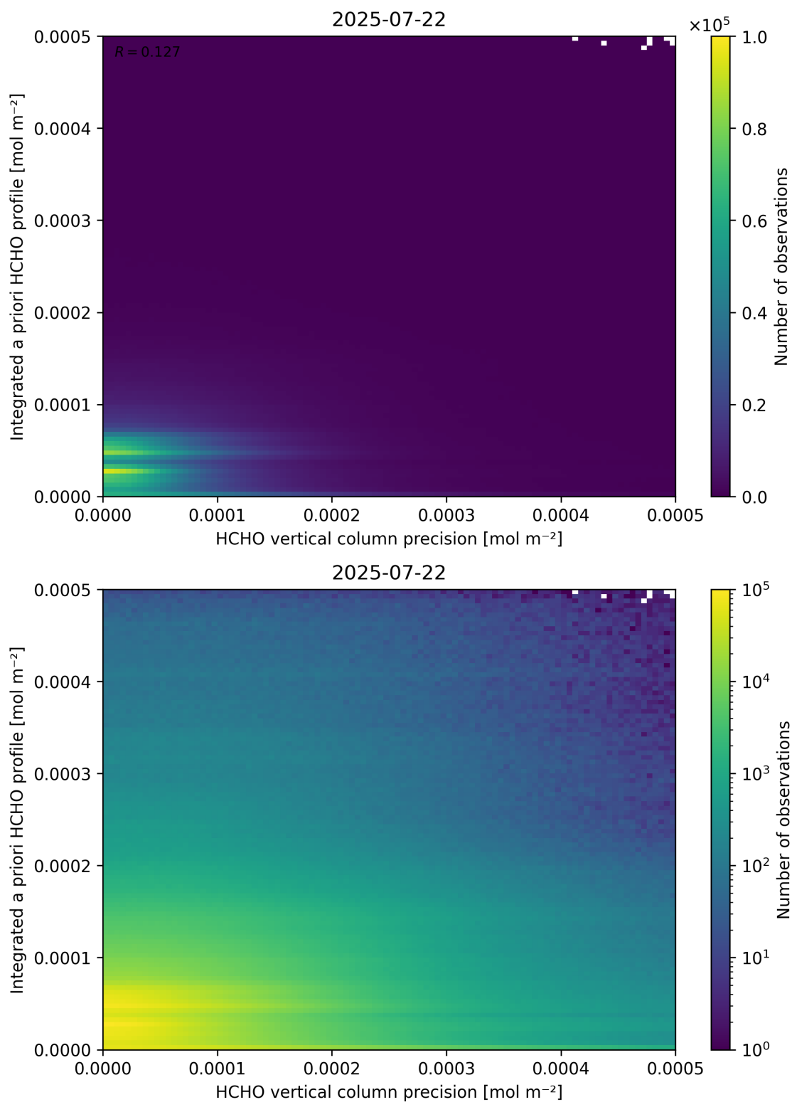
Figure 147: Scatter density plot of “HCHO vertical column precision” against “Integrated a priori HCHO profile” for 2025-07-21 to 2025-07-23.
