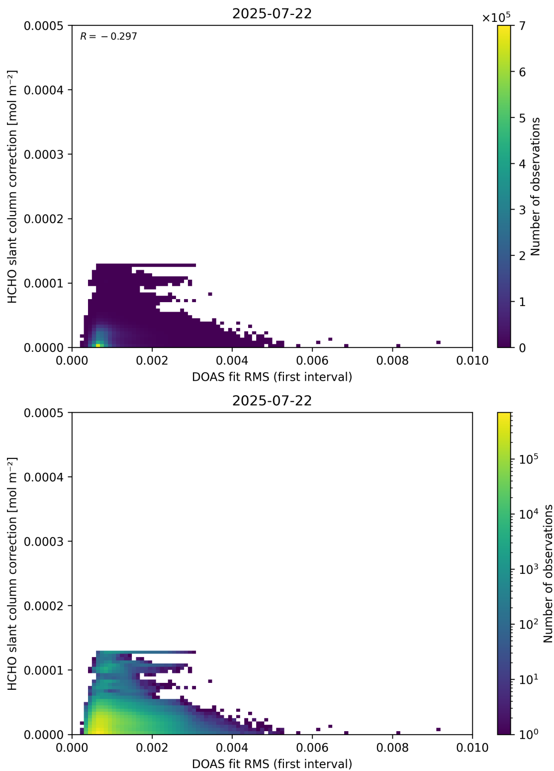
Figure 63: Scatter density plot of “DOAS fit RMS (first interval)” against “HCHO slant column correction” for 2025-07-21 to 2025-07-23.
