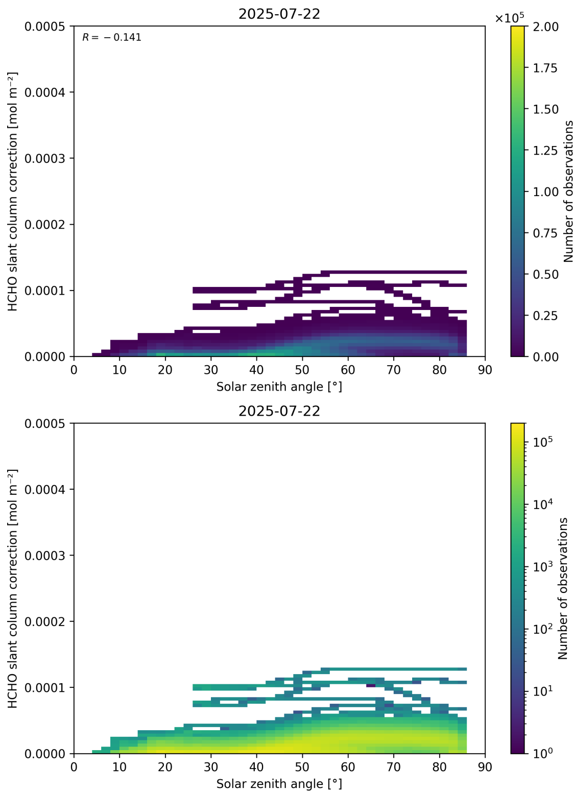
Figure 172: Scatter density plot of “Solar zenith angle” against “HCHO slant column correction” for 2025-07-21 to 2025-07-23.
