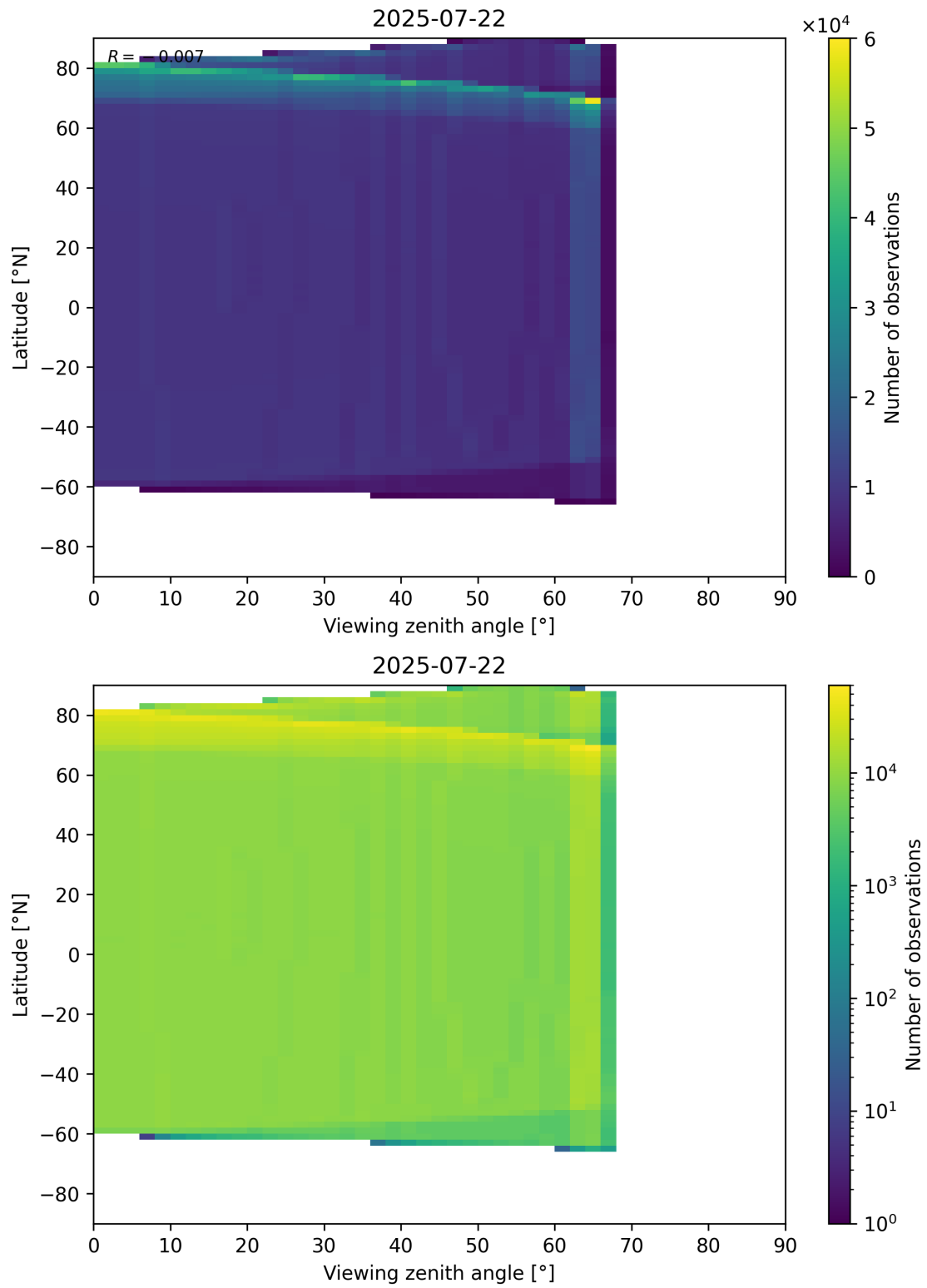
Figure 196: Scatter density plot of “Viewing zenith angle” against “Latitude” for 2025-07-21 to 2025-07-23.
