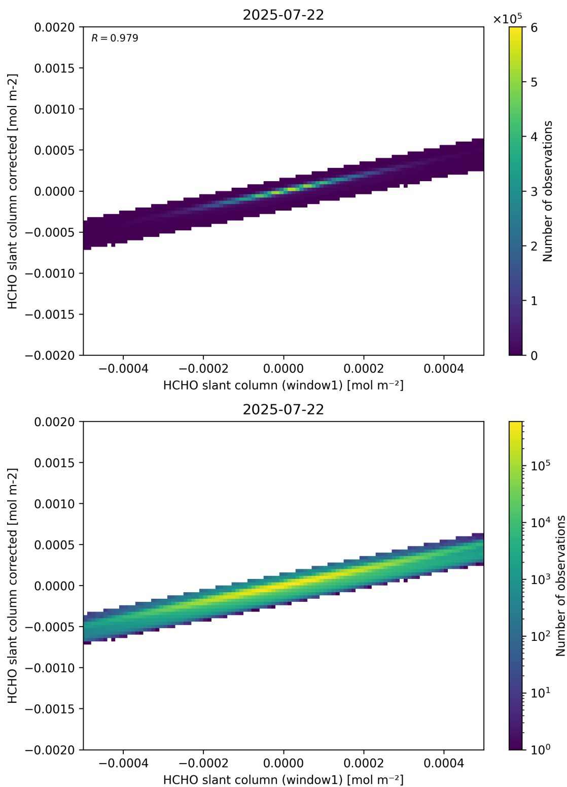
Figure 82: Scatter density plot of “HCHO slant column (window1)” against “HCHO slant column corrected” for 2025-07-21 to 2025-07-23.
