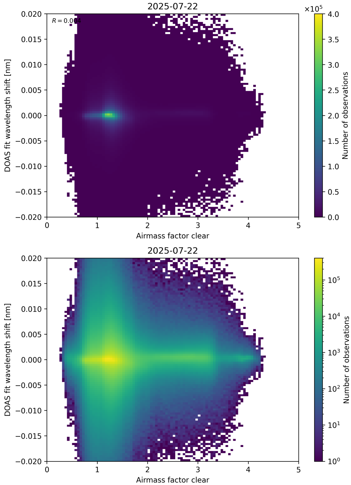
Figure 72: Scatter density plot of “Airmass factor clear” against “DOAS fit wavelength shift” for 2025-07-21 to 2025-07-23.
