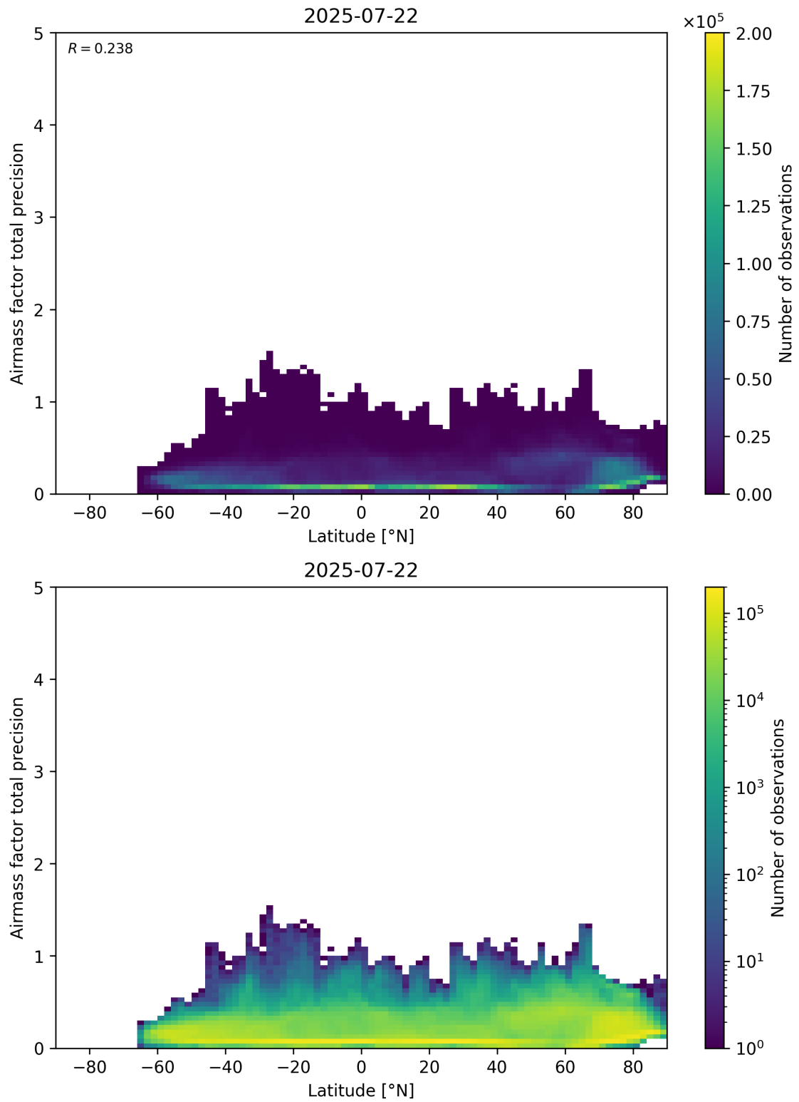
Figure 162: Scatter density plot of “Latitude” against “Airmass factor total precision” for 2025-07-21 to 2025-07-23.
