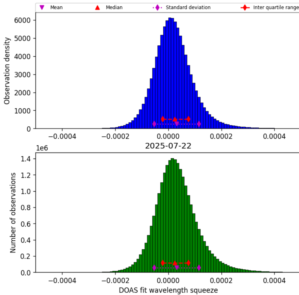
Figure 45: Histogram of “DOAS fit wavelength squeeze” for 2025-07-21 to 2025-07-23
