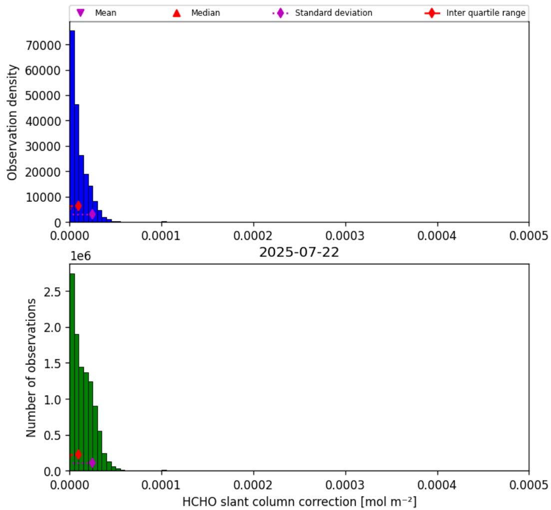
Figure 47: Histogram of “HCHO slant column correction” for 2025-07-21 to 2025-07-23
