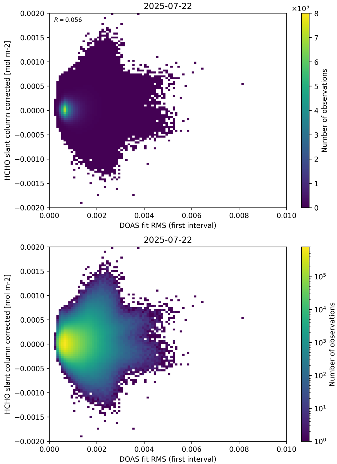
Figure 62: Scatter density plot of “DOAS fit RMS (first interval)” against “HCHO slant column corrected” for 2025-07-21 to 2025-07-23.
