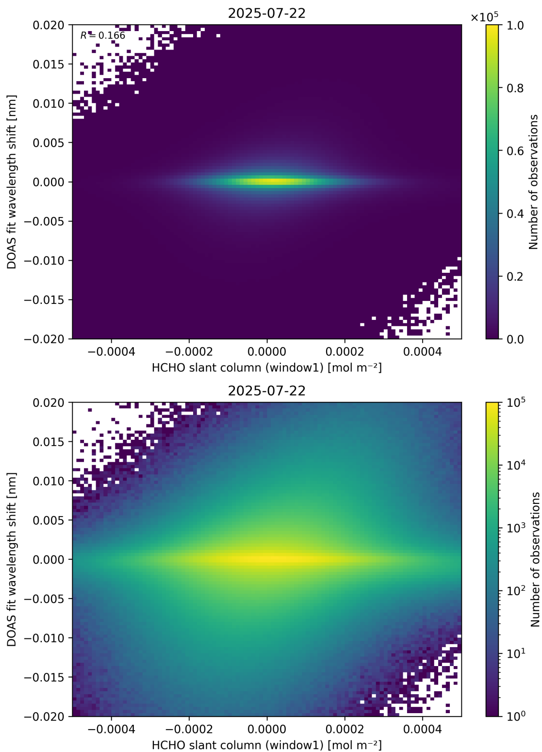
Figure 79: Scatter density plot of “HCHO slant column (window1)” against “DOAS fit wavelength shift” for 2025-07-21 to 2025-07-23.
