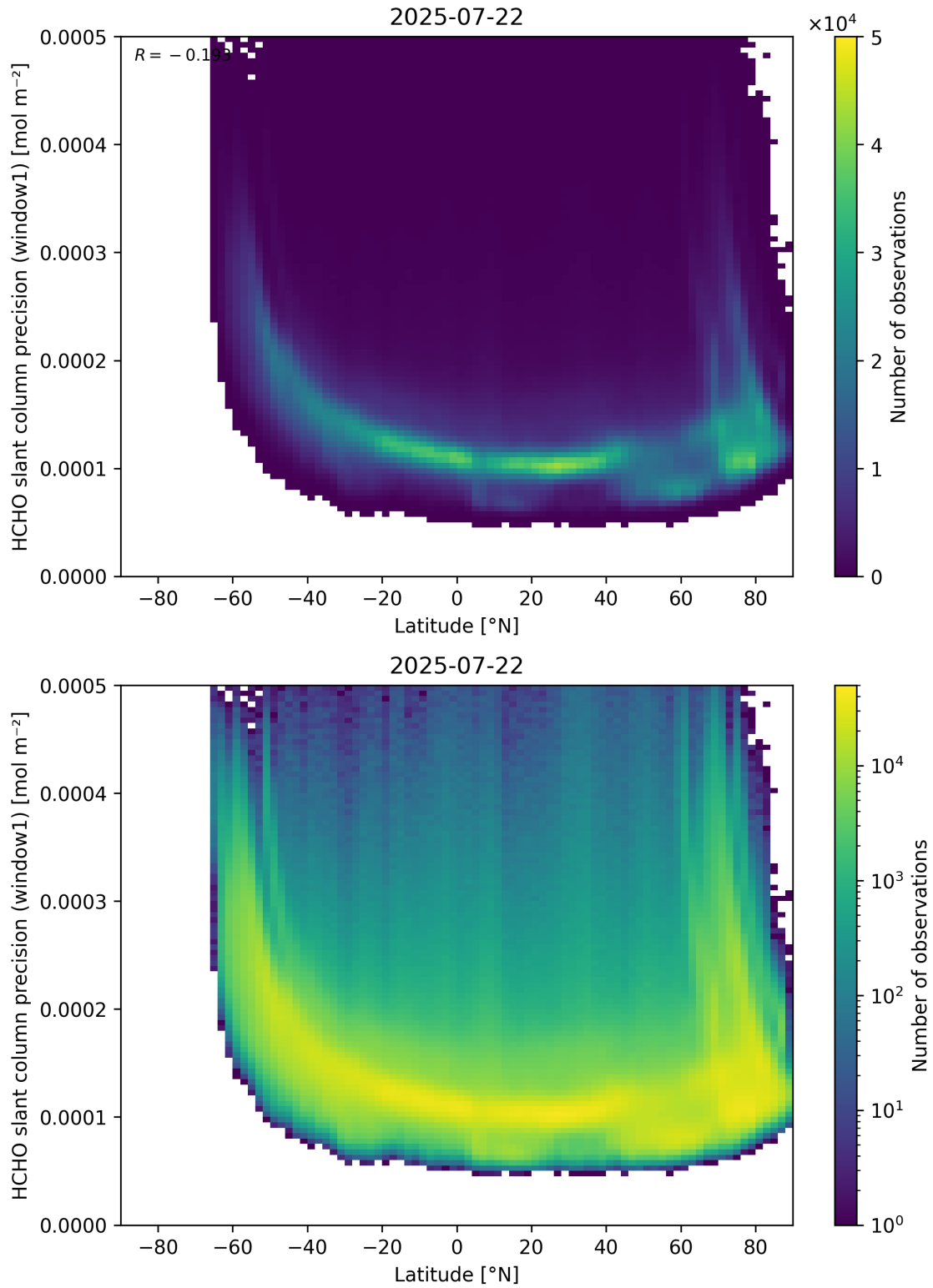
Figure 160: Scatter density plot of “Latitude” against “HCHO slant column precision (window1)” for 2025-07-21 to 2025-07-23.
