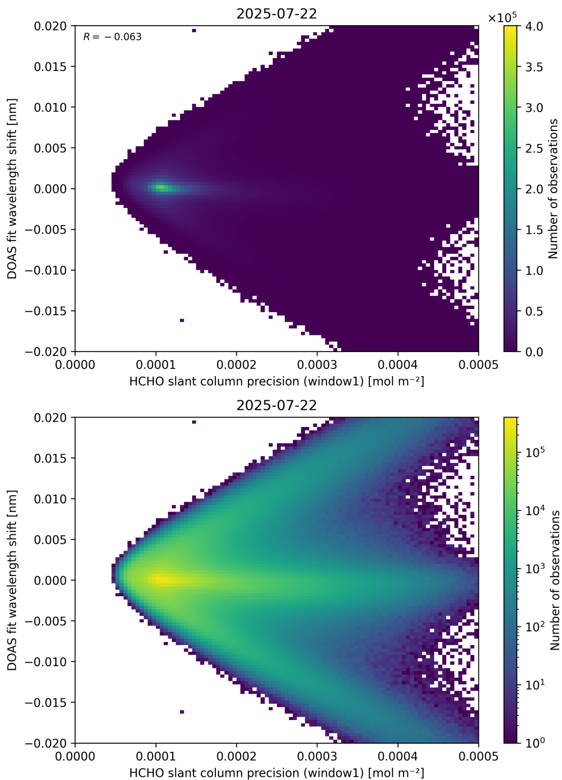
Figure 89: Scatter density plot of “HCHO slant column precision (window1)” against “DOAS fit wavelength shift” for 2025-07-21 to 2025-07-23.
