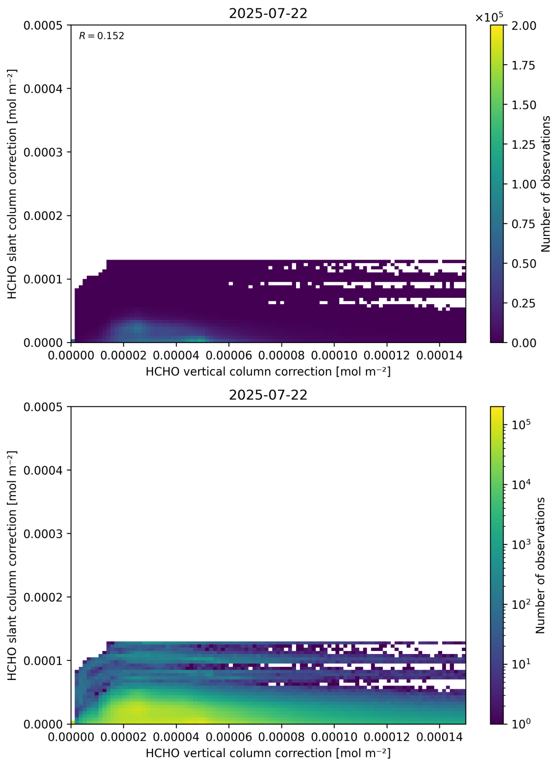
Figure 117: Scatter density plot of “HCHO vertical column correction” against “HCHO slant column correction” for 2025-07-21 to 2025-07-23.
