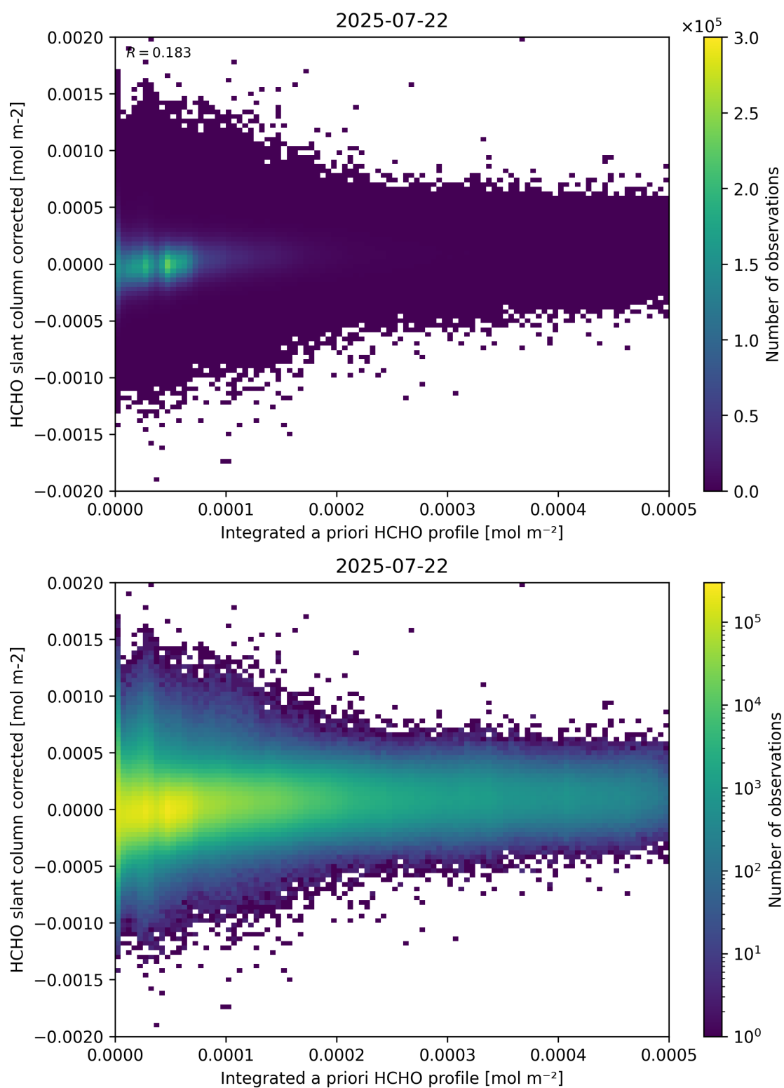
Figure 151: Scatter density plot of “Integrated a priori HCHO profile” against “HCHO slant column corrected” for 2025-07-21 to 2025-07-23.
