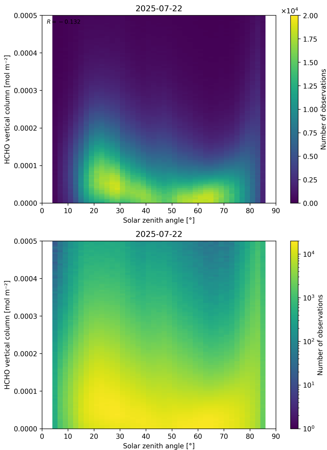
Figure 177: Scatter density plot of “Solar zenith angle” against “HCHO vertical column” for 2025-07-21 to 2025-07-23.
