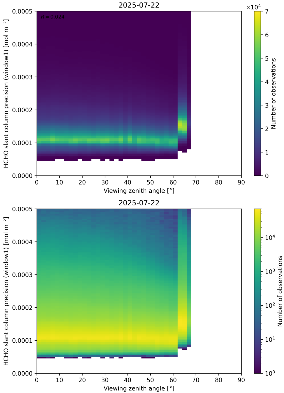
Figure 189: Scatter density plot of “Viewing zenith angle” against “HCHO slant column precision (window1)” for 2025-07-21 to 2025-07-23.
