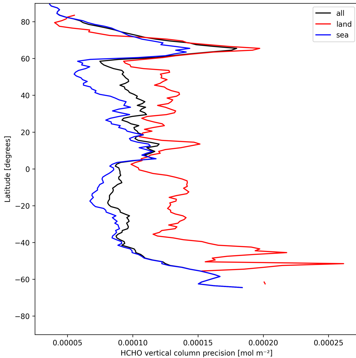
Figure 22: Zonal average of “HCHO vertical column precision” for 2025-07-21 to 2025-07-23.
