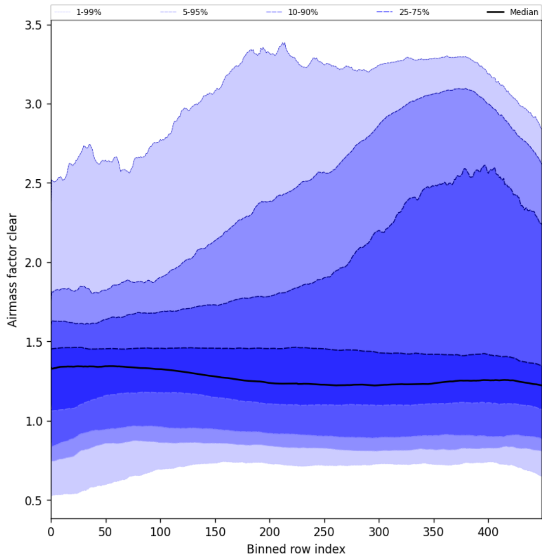
Figure 56: Along track statistics of “Airmass factor clear” for 2025-07-21 to 2025-07-23
