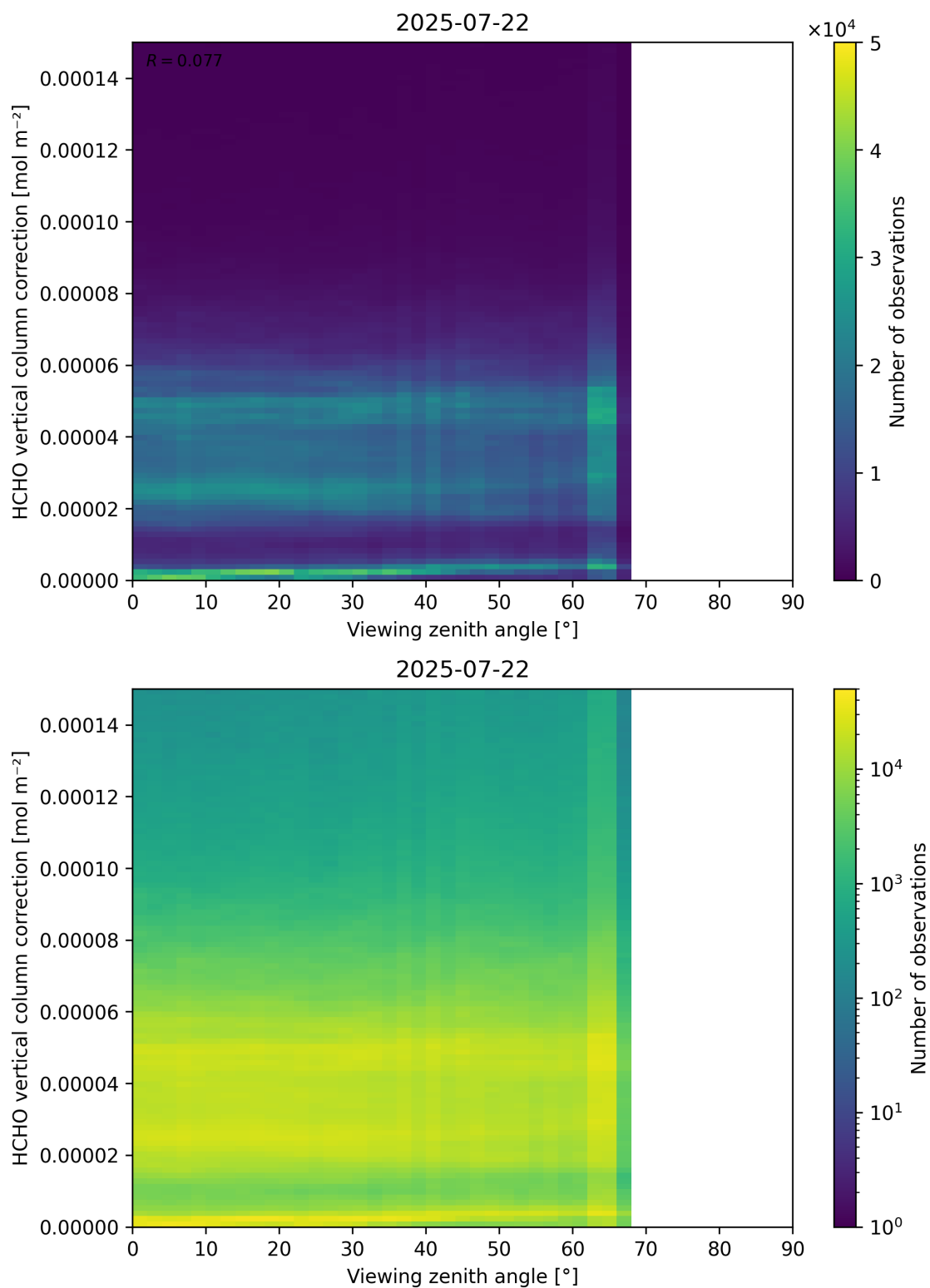
Figure 193: Scatter density plot of “Viewing zenith angle” against “HCHO vertical column correction” for 2025-07-21 to 2025-07-23.
