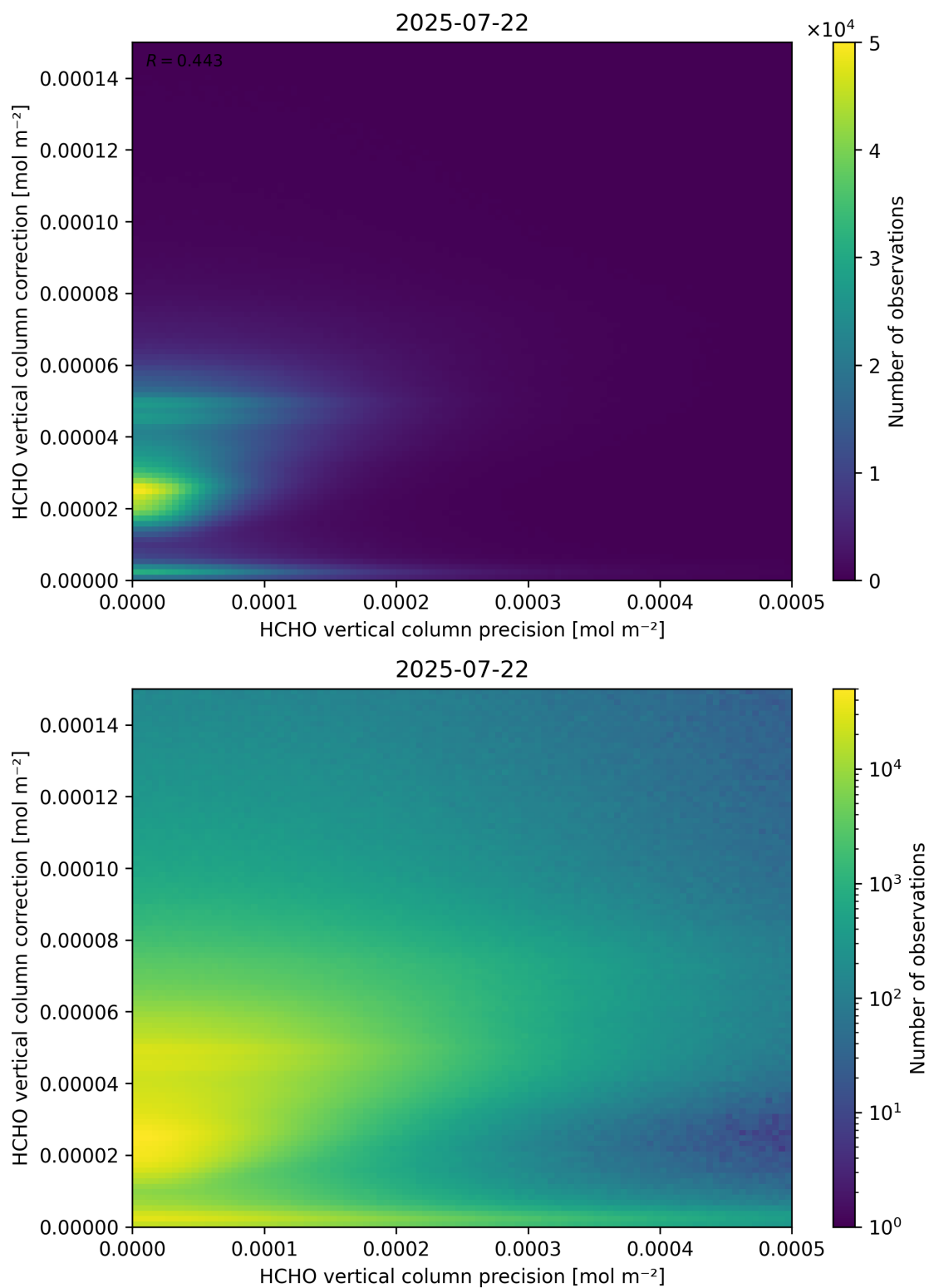
Figure 146: Scatter density plot of “HCHO vertical column precision” against “HCHO vertical column correction” for 2025-07-21 to 2025-07-23.
