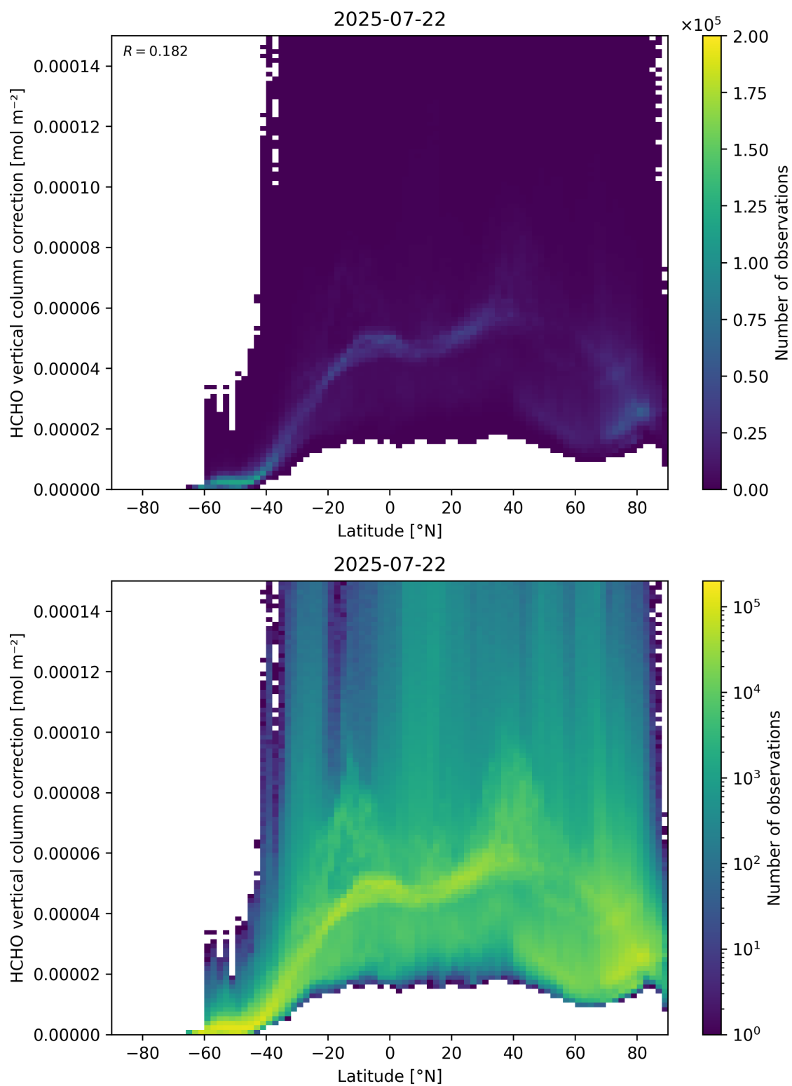
Figure 164: Scatter density plot of “Latitude” against “HCHO vertical column correction” for 2025-07-21 to 2025-07-23.
