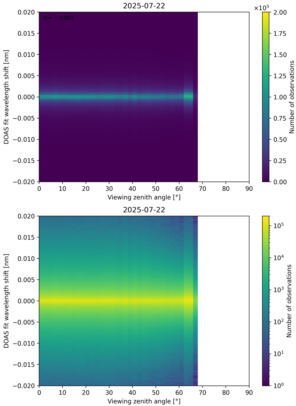
Figure 183: Scatter density plot of “Viewing zenith angle” against “DOAS fit wavelength shift” for 2025-07-21 to 2025-07-23.
