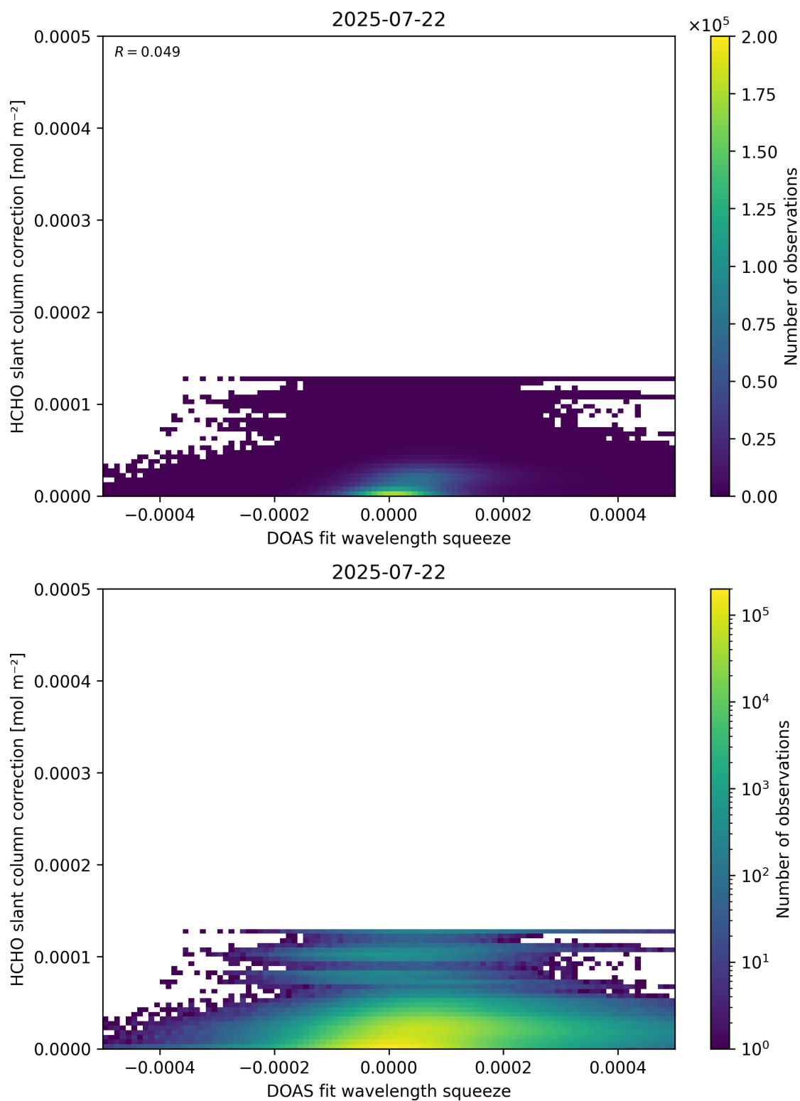
Figure 70: Scatter density plot of “DOAS fit wavelength squeeze” against “HCHO slant column correction” for 2025-07-21 to 2025-07-23.
