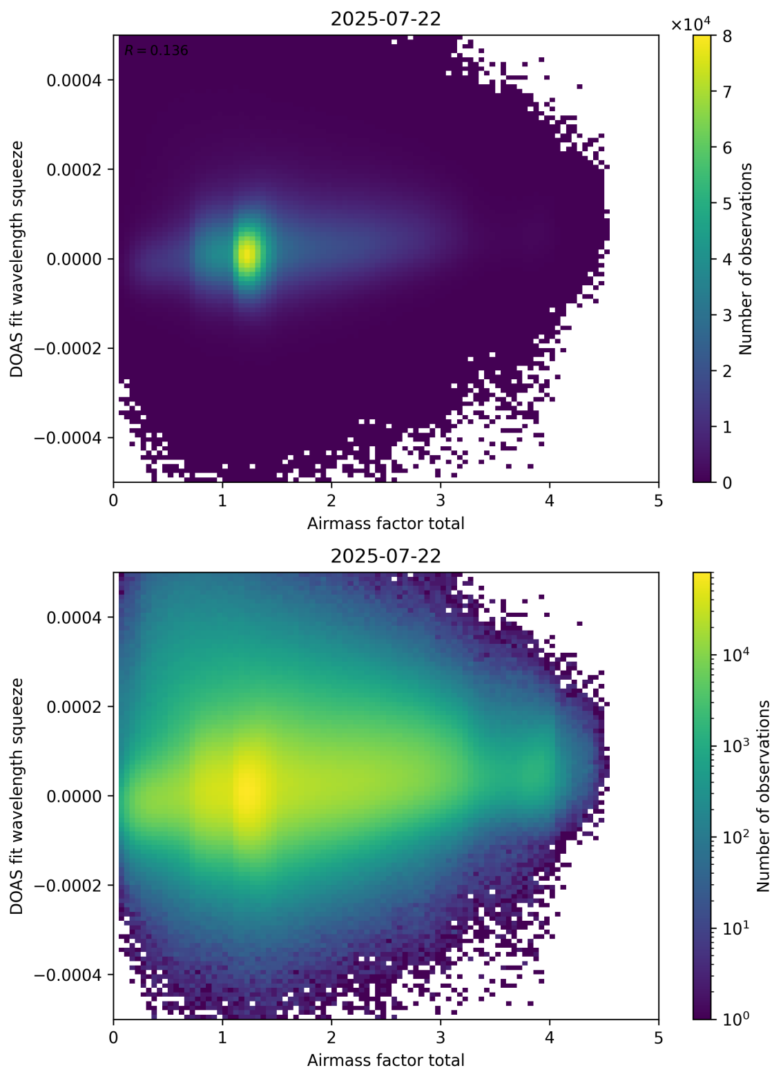
Figure 99: Scatter density plot of “Airmass factor total” against “DOAS fit wavelength squeeze” for 2025-07-21 to 2025-07-23.
