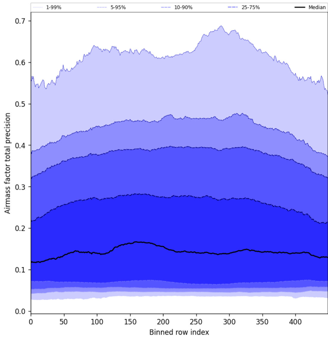
Figure 55: Along track statistics of “Airmass factor total precision” for 2025-07-21 to 2025-07-23
