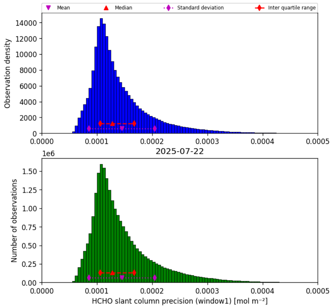
Figure 39: Histogram of “HCHO slant column precision (window1)” for 2025-07-21 to 2025-07-23
