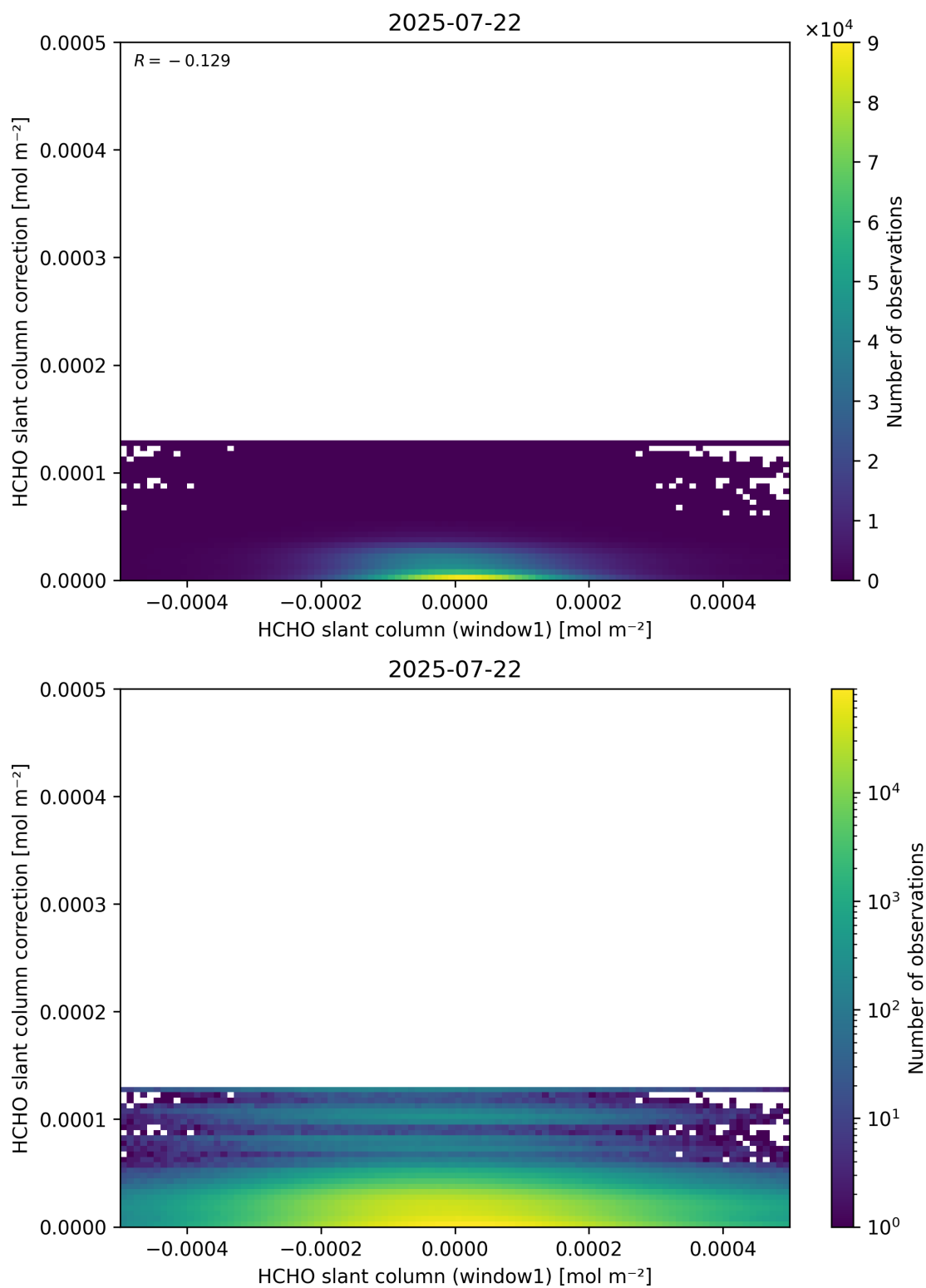
Figure 83: Scatter density plot of “HCHO slant column (window1)” against “HCHO slant column correction” for 2025-07-21 to 2025-07-23.
