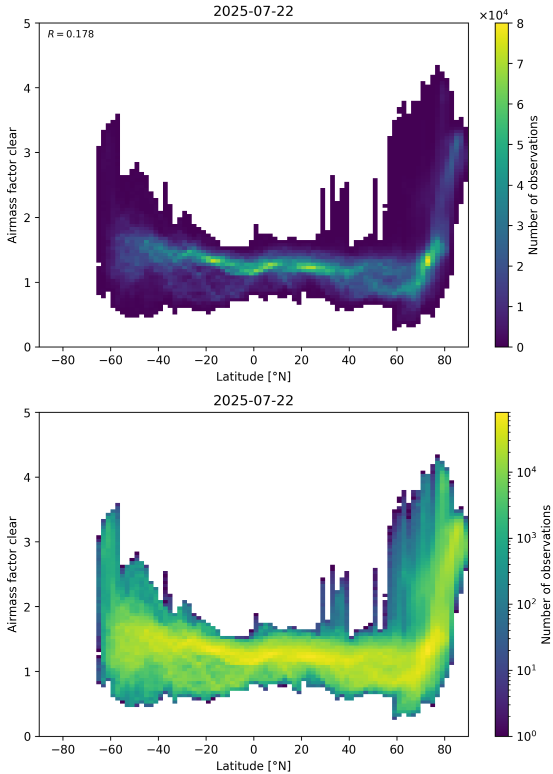
Figure 156: Scatter density plot of “Latitude” against “Airmass factor clear” for 2025-07-21 to 2025-07-23.
