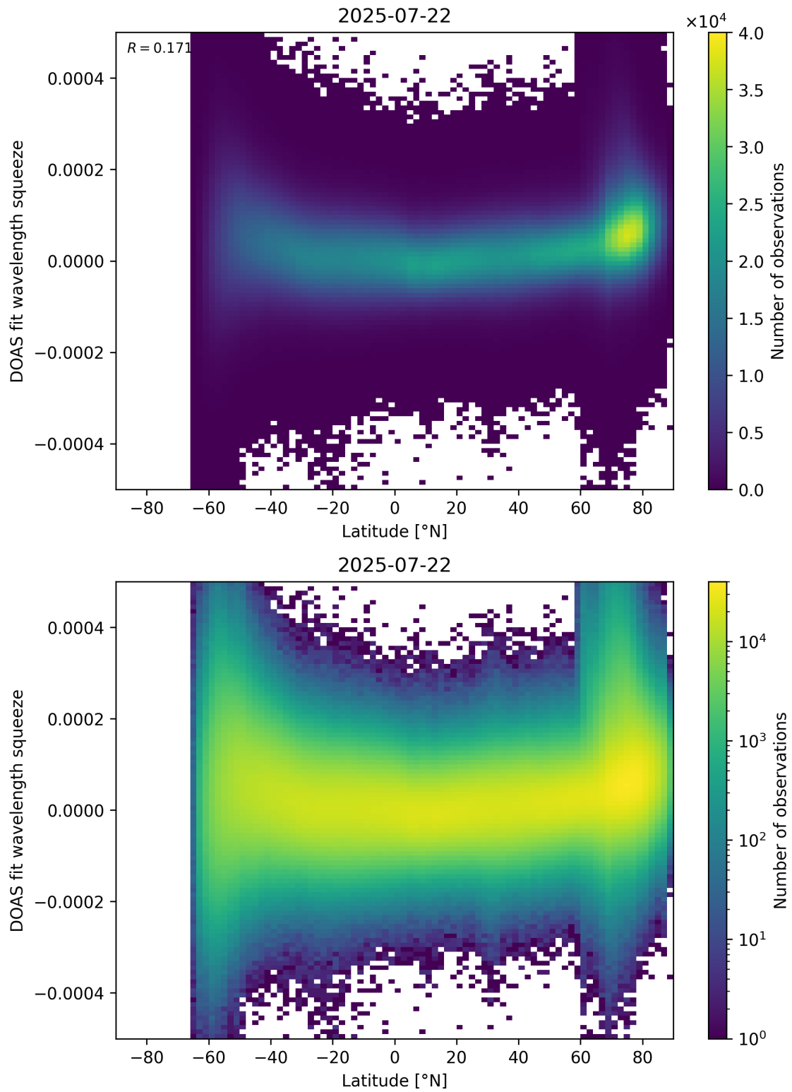
Figure 155: Scatter density plot of “Latitude” against “DOAS fit wavelength squeeze” for 2025-07-21 to 2025-07-23.
