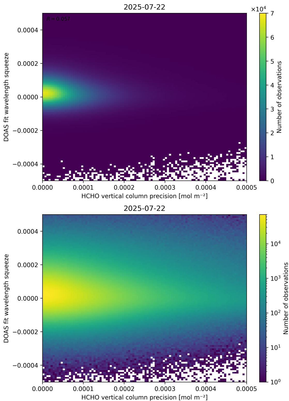
Figure 138: Scatter density plot of “HCHO vertical column precision” against “DOAS fit wavelength squeeze” for 2025-07-21 to 2025-07-23.
