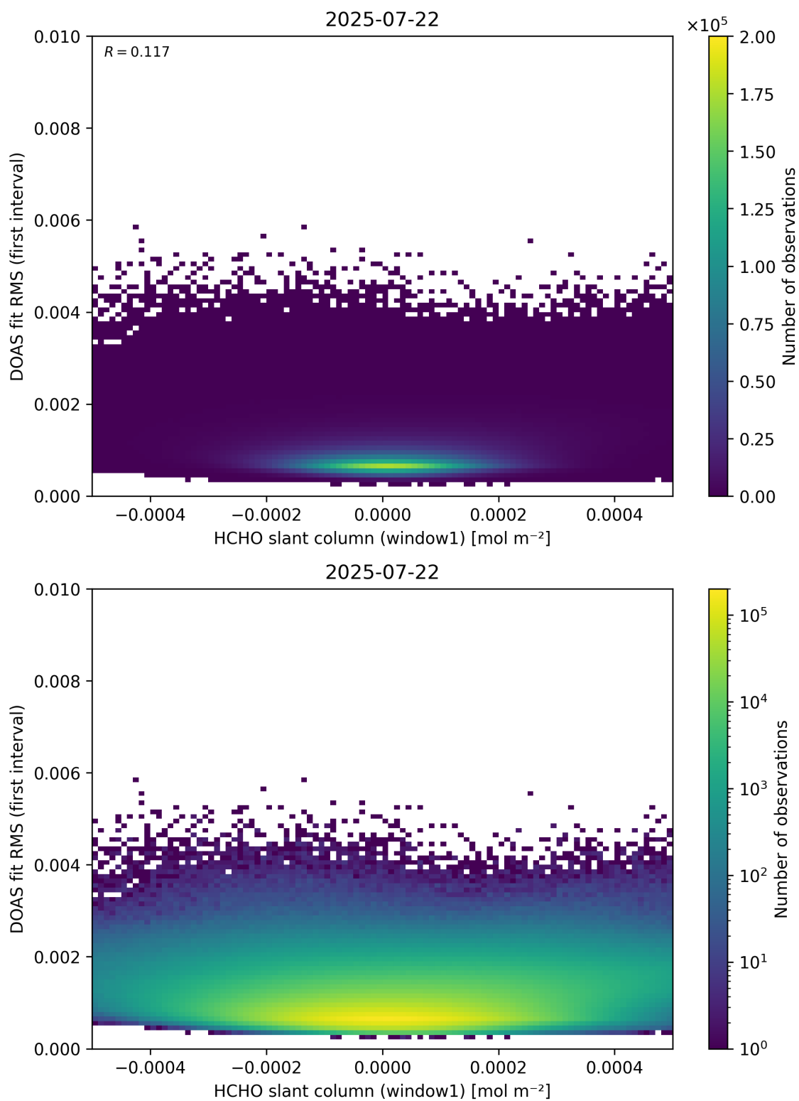
Figure 78: Scatter density plot of “HCHO slant column (window1)” against “DOAS fit RMS (first interval)” for 2025-07-21 to 2025-07-23.
