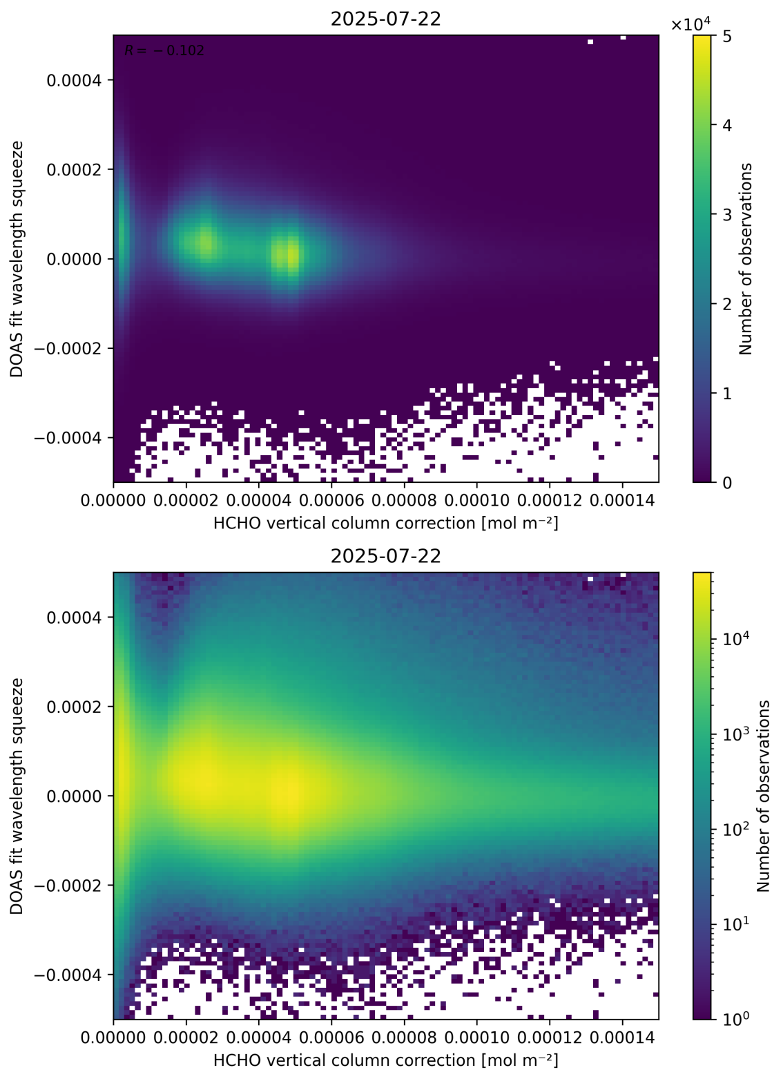
Figure 114: Scatter density plot of “HCHO vertical column correction” against “DOAS fit wavelength squeeze” for 2025-07-21 to 2025-07-23.
