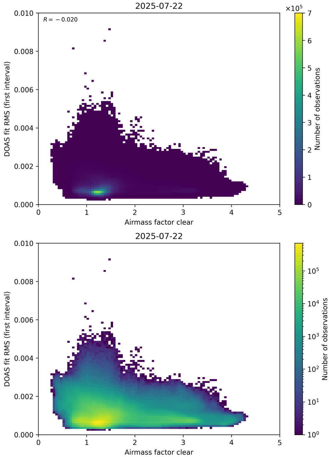
Figure 71: Scatter density plot of “Airmass factor clear” against “DOAS fit RMS (first interval)” for 2025-07-21 to 2025-07-23.
