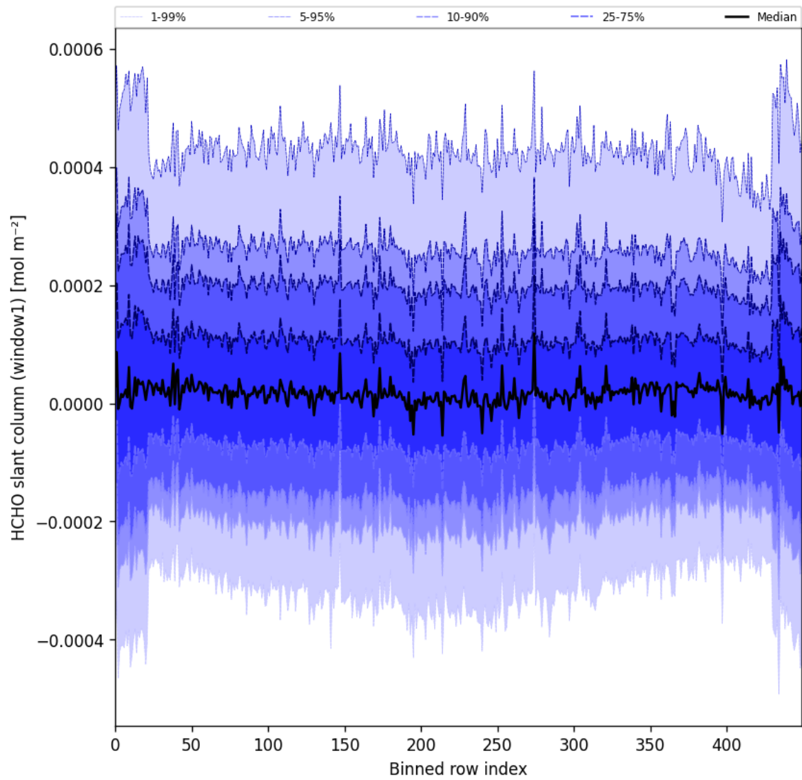
Figure 52: Along track statistics of “HCHO slant column (window1)” for 2025-07-21 to 2025-07-23
