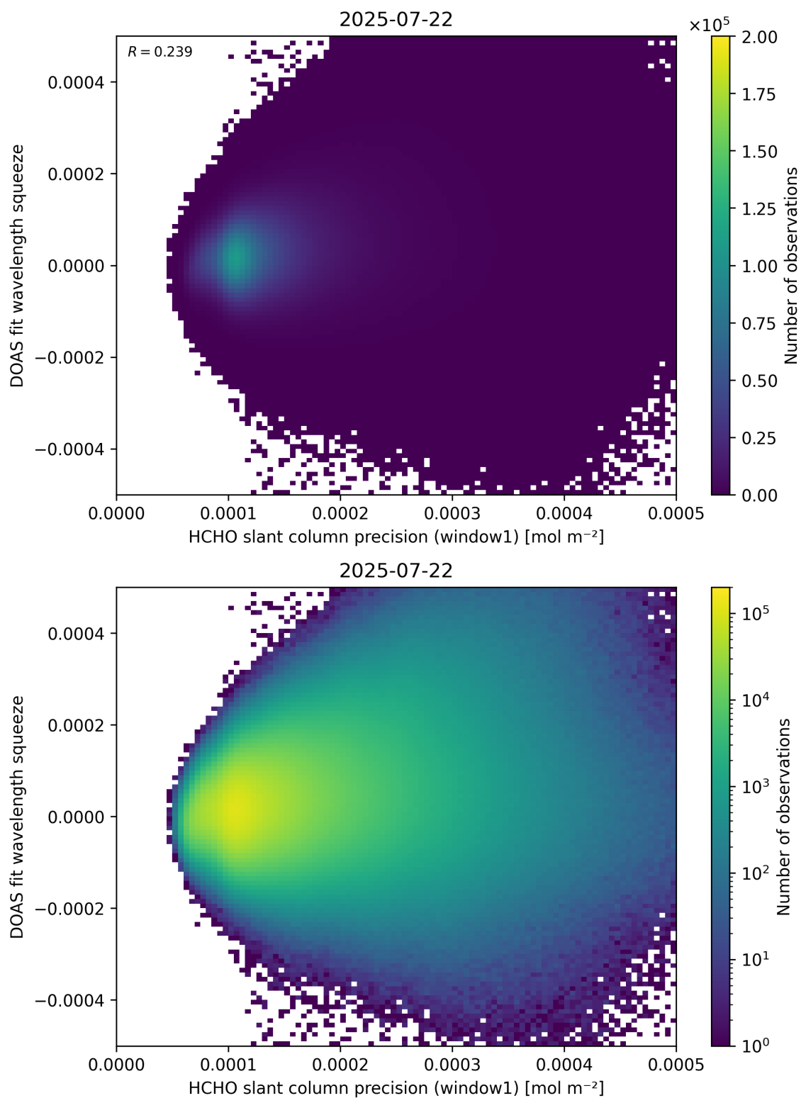
Figure 90: Scatter density plot of “HCHO slant column precision (window1)” against “DOAS fit wavelength squeeze” for 2025-07-21 to 2025-07-23.
