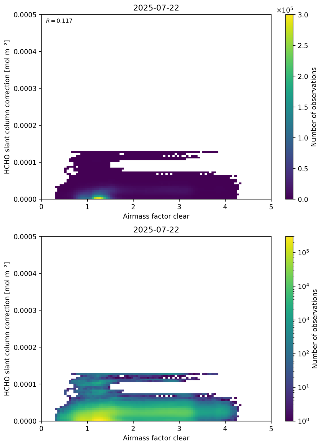
Figure 75: Scatter density plot of “Airmass factor clear” against “HCHO slant column correction” for 2025-07-21 to 2025-07-23.
