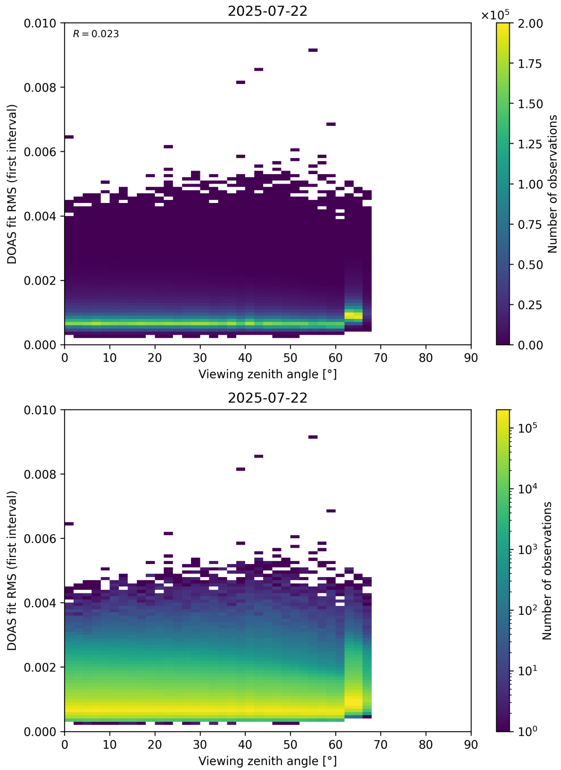
Figure 182: Scatter density plot of “Viewing zenith angle” against “DOAS fit RMS (first interval)” for 2025-07-21 to 2025-07-23.
