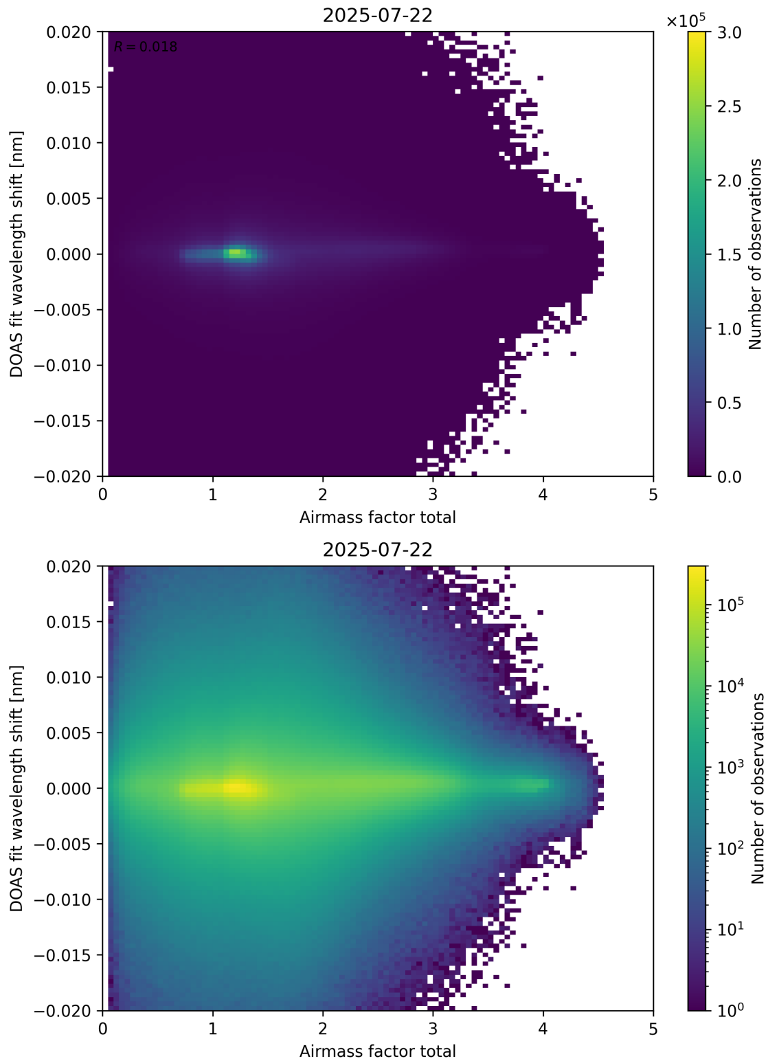
Figure 98: Scatter density plot of “Airmass factor total” against “DOAS fit wavelength shift” for 2025-07-21 to 2025-07-23.
