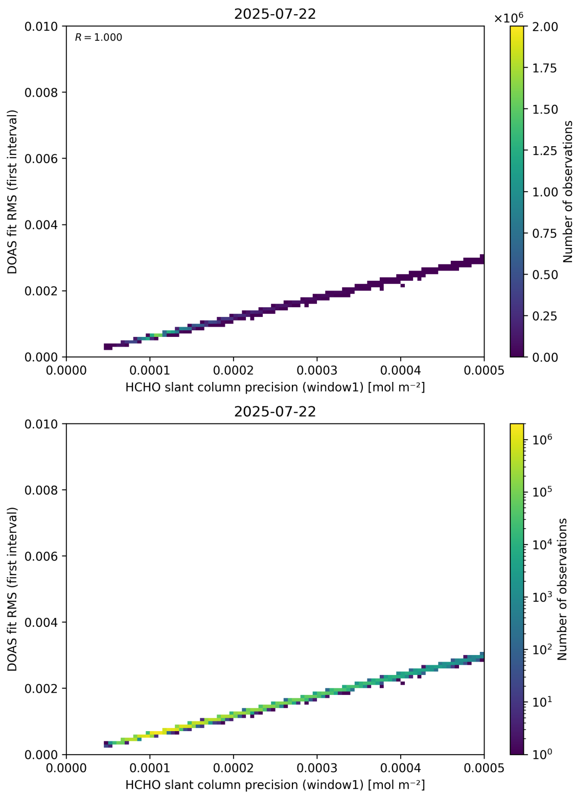
Figure 88: Scatter density plot of “HCHO slant column precision (window1)” against “DOAS fit RMS (first interval)” for 2025-07-21 to 2025-07-23.
