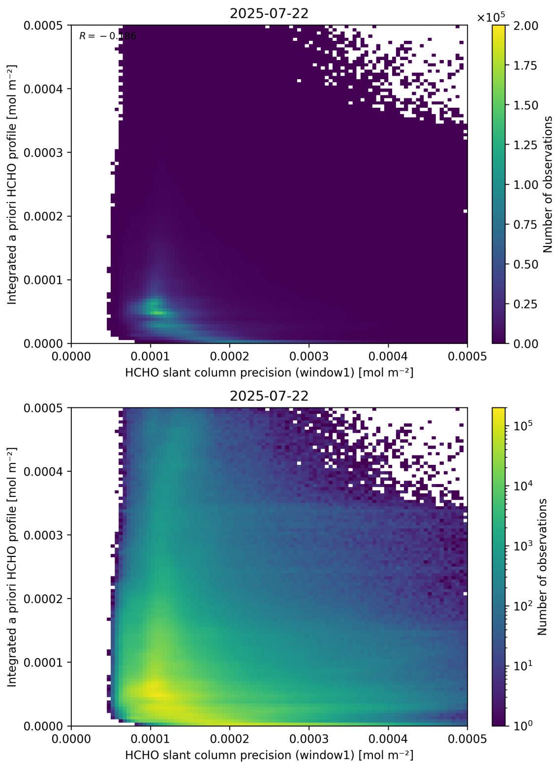
Figure 96: Scatter density plot of “HCHO slant column precision (window1)” against “Integrated a priori HCHO profile” for 2025-07-21 to 2025-07-23.
