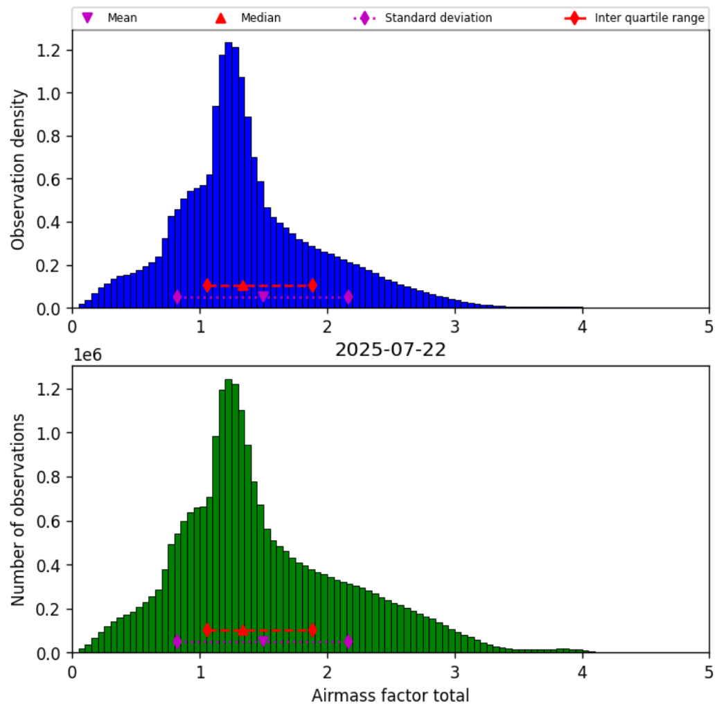
Figure 40: Histogram of “Airmass factor total” for 2025-07-21 to 2025-07-23
