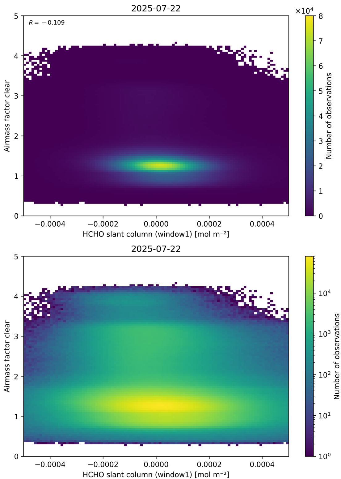
Figure 81: Scatter density plot of “HCHO slant column (window1)” against “Airmass factor clear” for 2025-07-21 to 2025-07-23.
