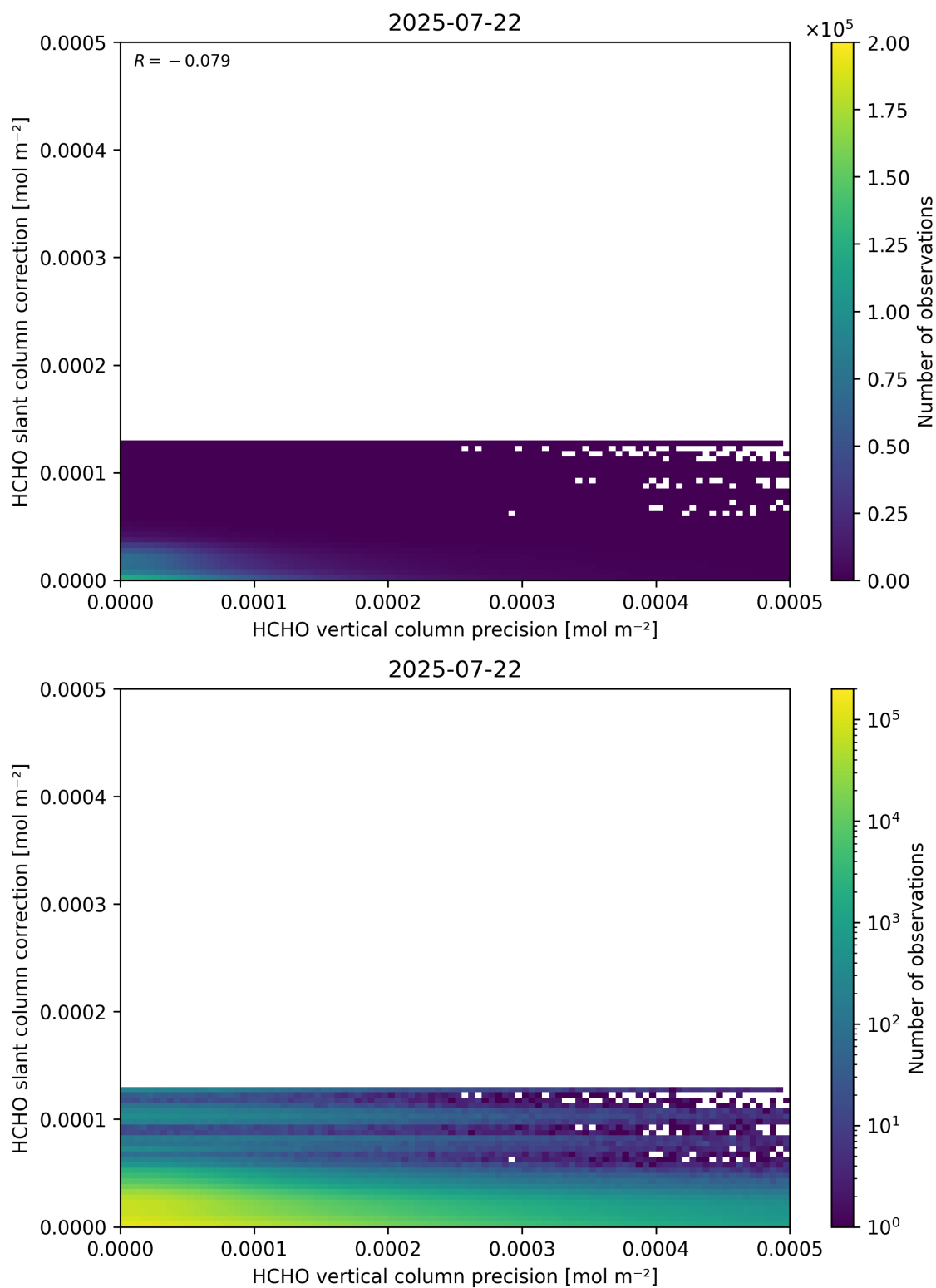
Figure 141: Scatter density plot of “HCHO vertical column precision” against “HCHO slant column correction” for 2025-07-21 to 2025-07-23.
