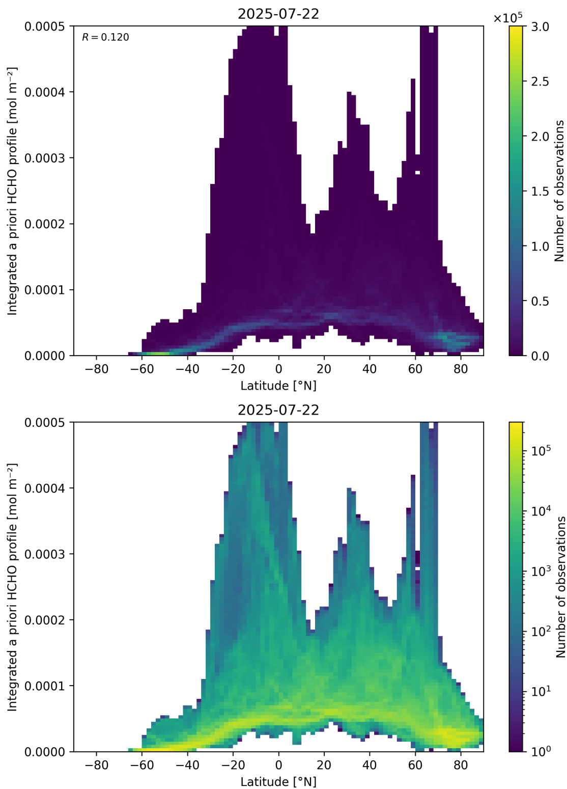
Figure 166: Scatter density plot of “Latitude” against “Integrated a priori HCHO profile” for 2025-07-21 to 2025-07-23.
