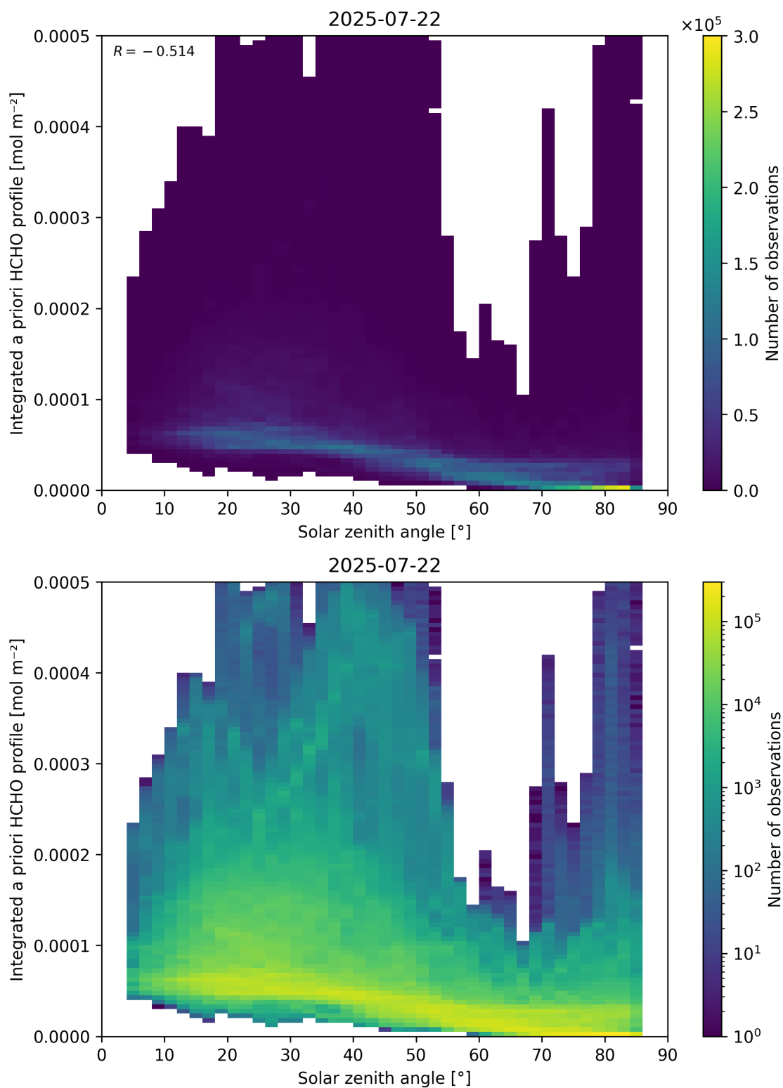
Figure 180: Scatter density plot of “Solar zenith angle” against “Integrated a priori HCHO profile” for 2025-07-21 to 2025-07-23.
