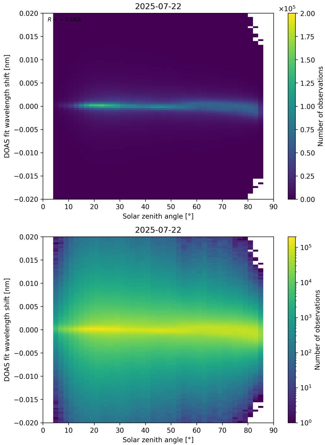
Figure 168: Scatter density plot of “Solar zenith angle” against “DOAS fit wavelength shift” for 2025-07-21 to 2025-07-23.
