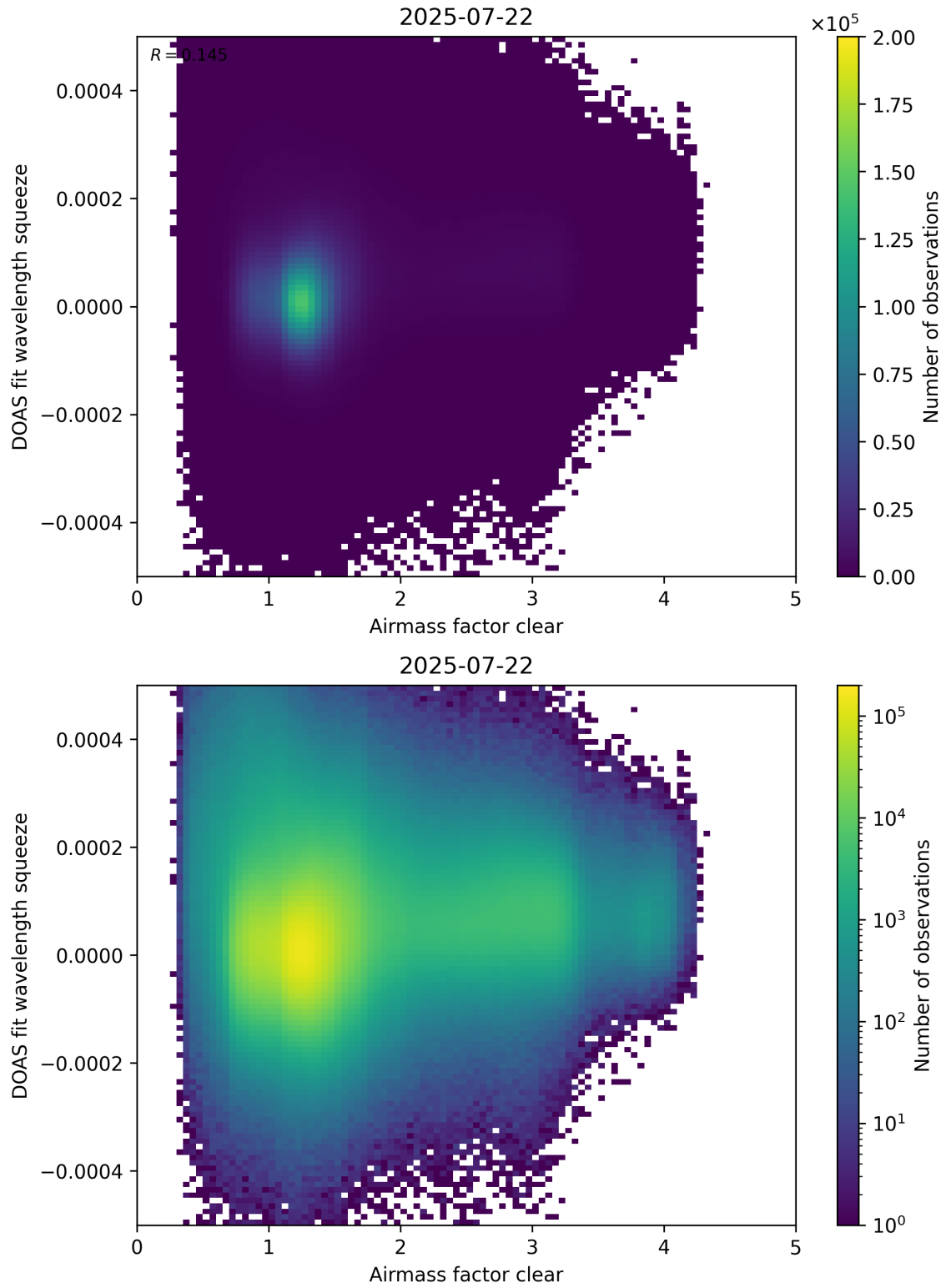
Figure 73: Scatter density plot of “Airmass factor clear” against “DOAS fit wavelength squeeze” for 2025-07-21 to 2025-07-23.
