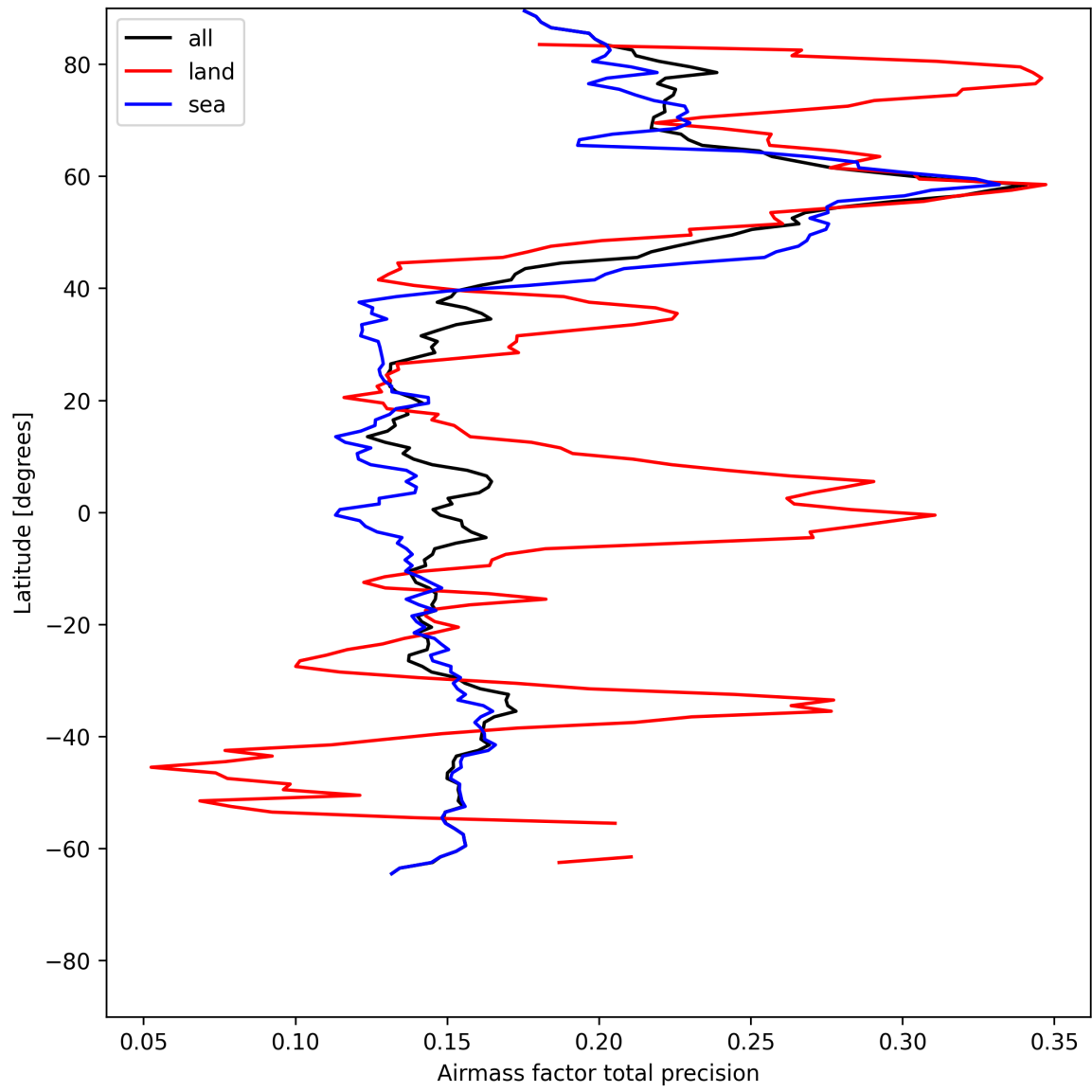
Figure 27: Zonal average of “Airmass factor total precision” for 2025-07-21 to 2025-07-23.
