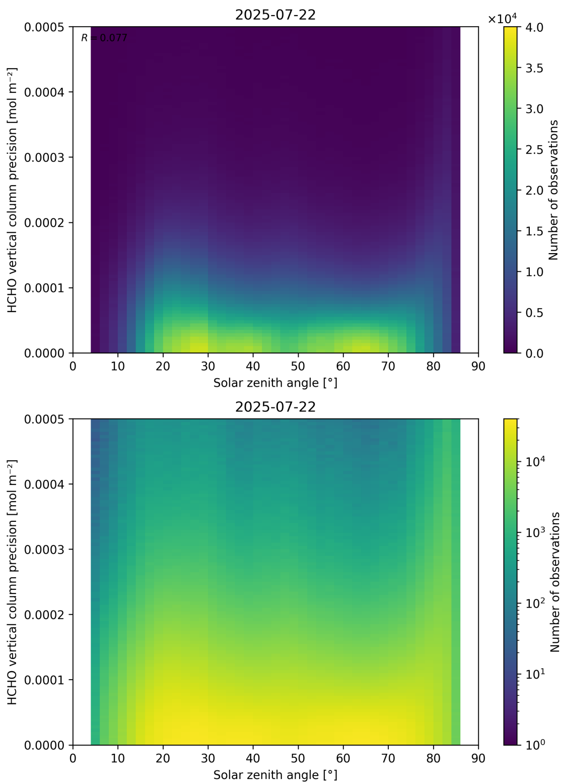
Figure 179: Scatter density plot of “Solar zenith angle” against “HCHO vertical column precision” for 2025-07-21 to 2025-07-23.
