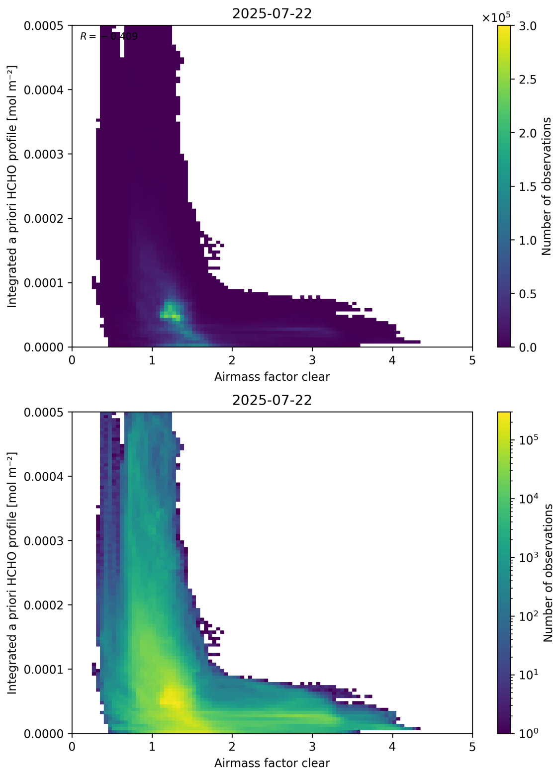
Figure 76: Scatter density plot of “Airmass factor clear” against “Integrated a priori HCHO profile” for 2025-07-21 to 2025-07-23.
