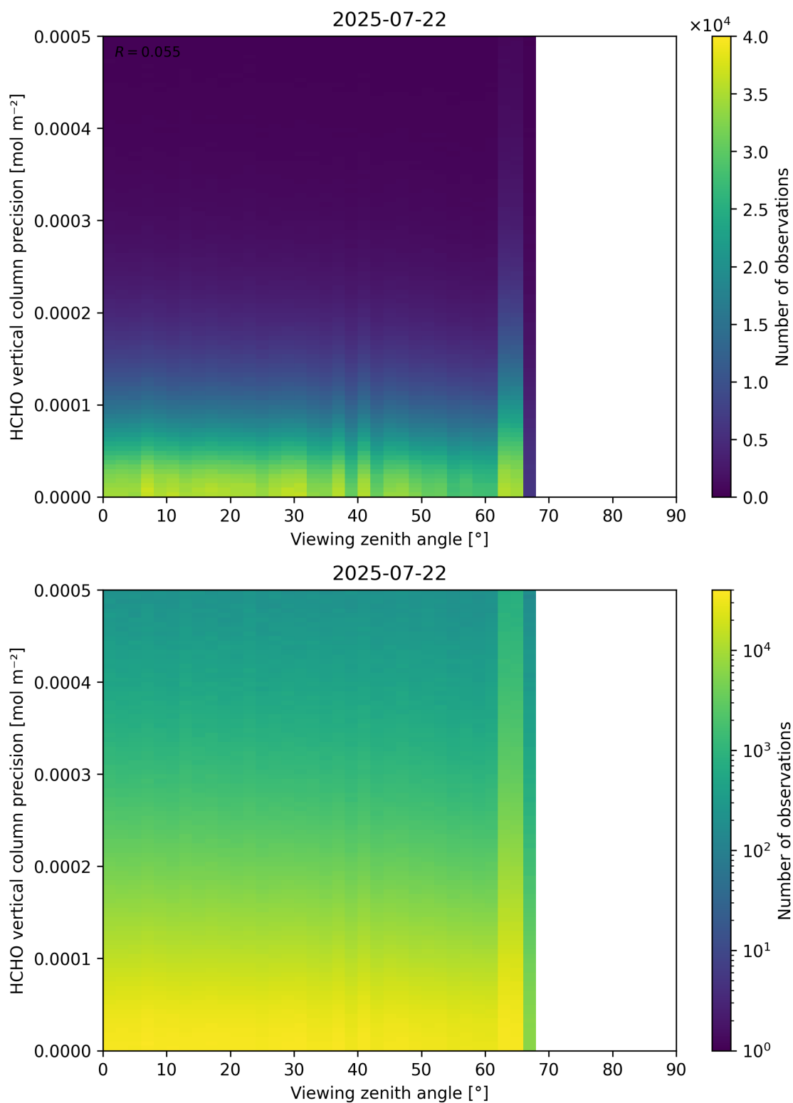
Figure 194: Scatter density plot of “Viewing zenith angle” against “HCHO vertical column precision” for 2025-07-21 to 2025-07-23.
