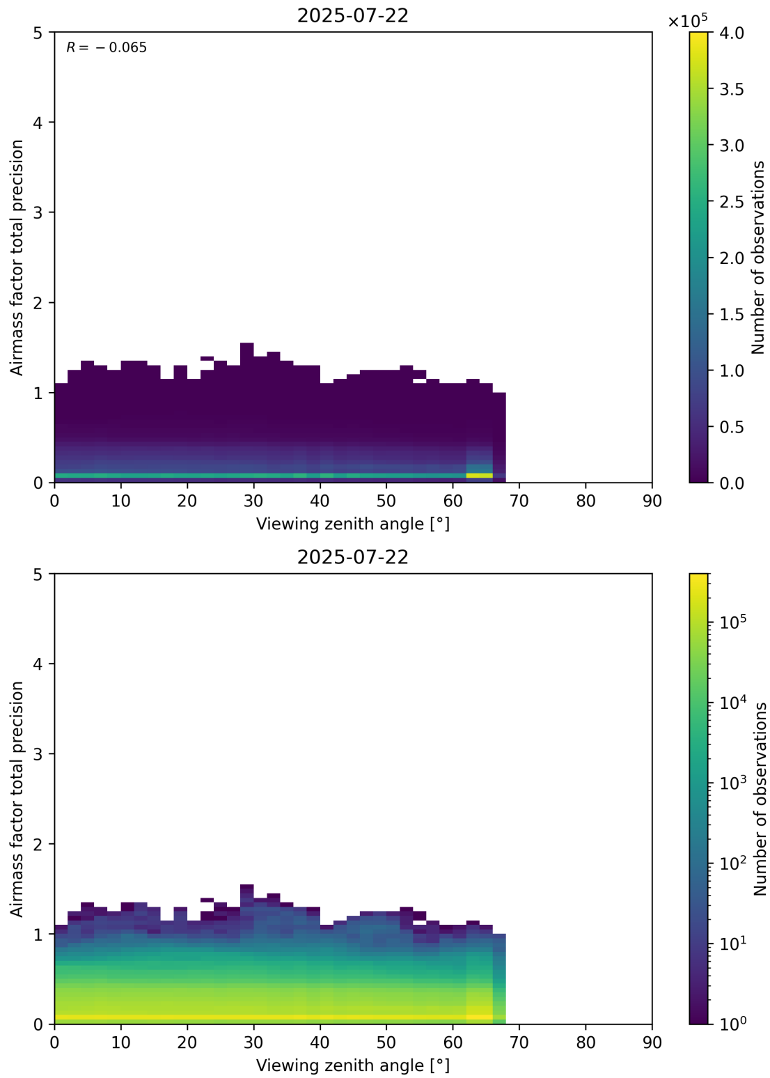
Figure 191: Scatter density plot of “Viewing zenith angle” against “Airmass factor total precision” for 2025-07-21 to 2025-07-23.
