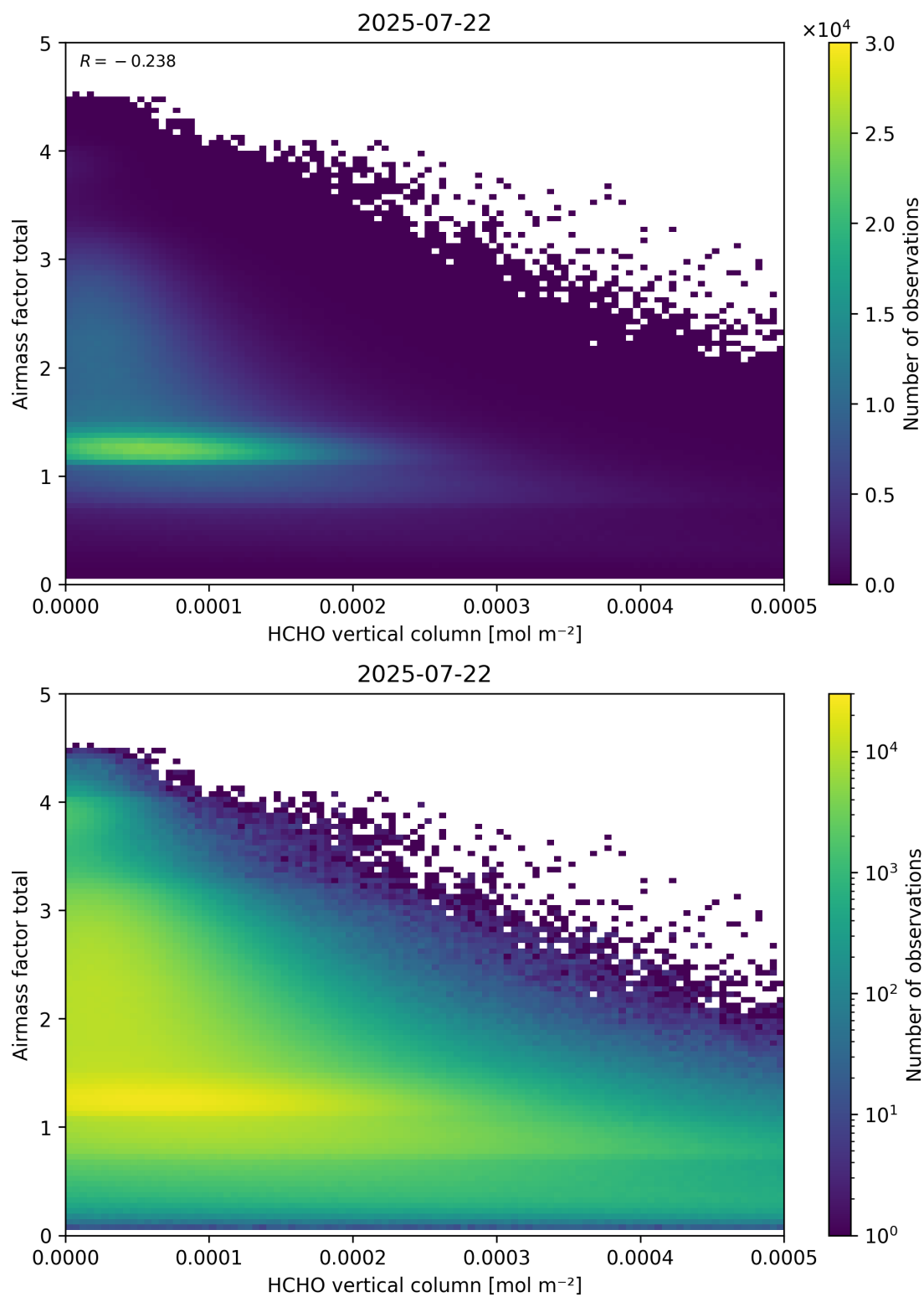
Figure 131: Scatter density plot of “HCHO vertical column” against “Airmass factor total” for 2025-07-21 to 2025-07-23.
