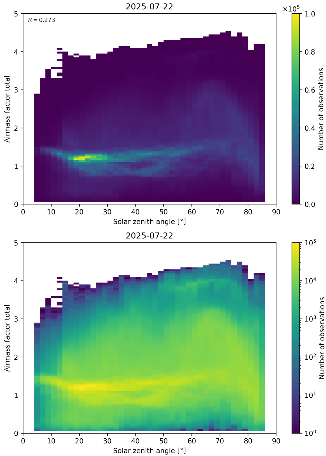
Figure 175: Scatter density plot of “Solar zenith angle” against “Airmass factor total” for 2025-07-21 to 2025-07-23.
