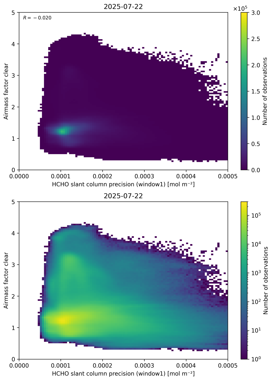
Figure 91: Scatter density plot of “HCHO slant column precision (window1)” against “Airmass factor clear” for 2025-07-21 to 2025-07-23.
