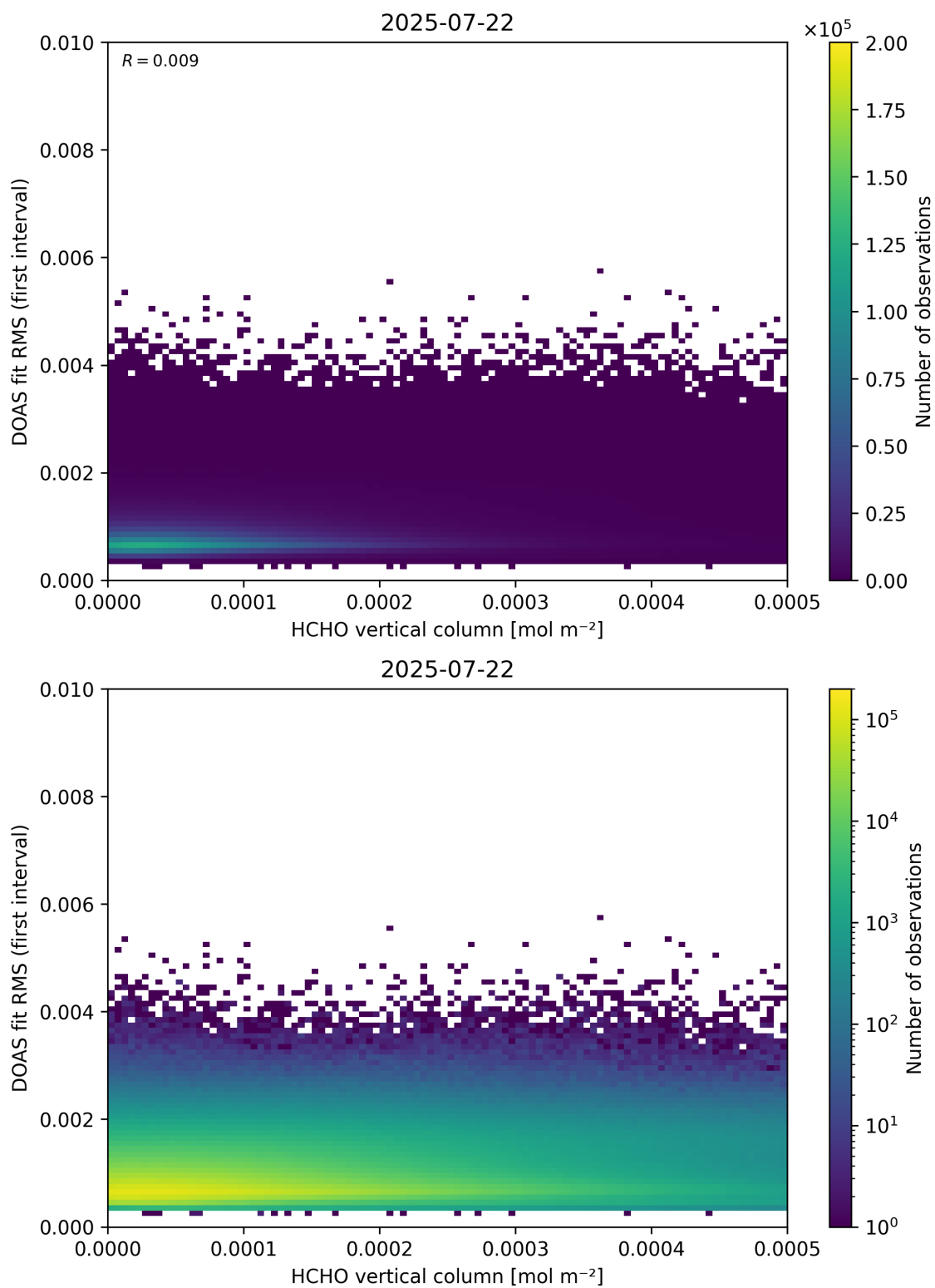
Figure 123: Scatter density plot of “HCHO vertical column” against “DOAS fit RMS (first interval)” for 2025-07-21 to 2025-07-23.
