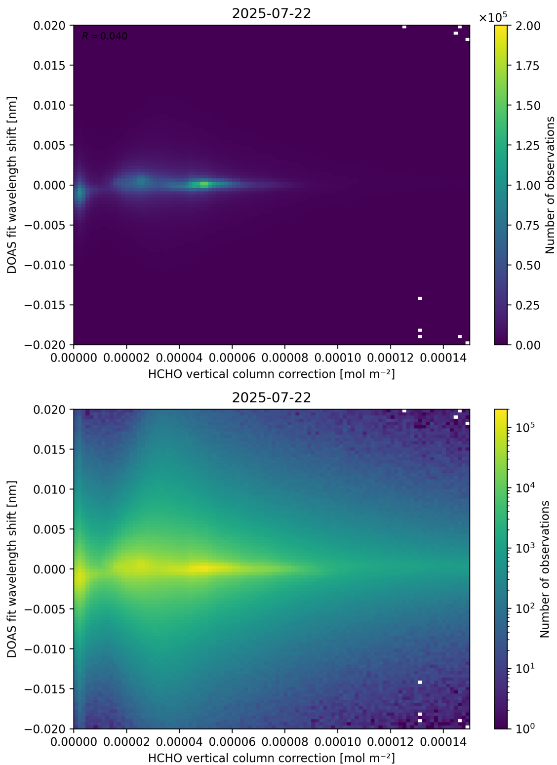
Figure 113: Scatter density plot of “HCHO vertical column correction” against “DOAS fit wavelength shift” for 2025-07-21 to 2025-07-23.
