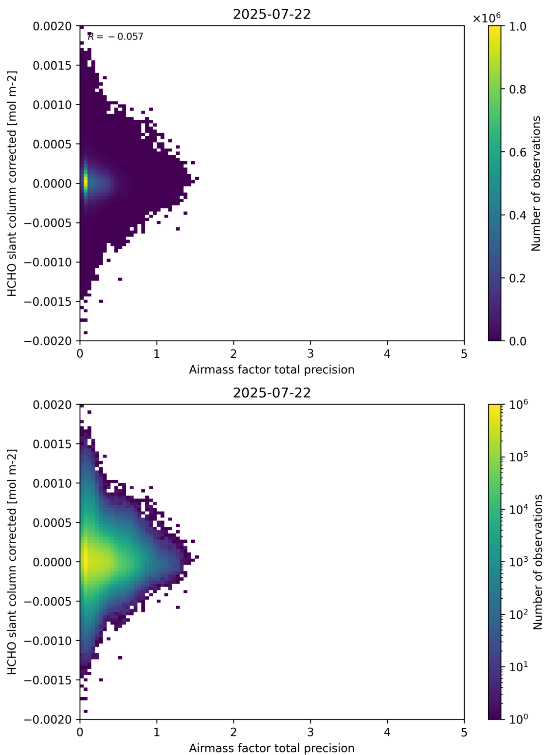
Figure 109: Scatter density plot of “Airmass factor total precision” against “HCHO slant column corrected” for 2025-07-21 to 2025-07-23.
