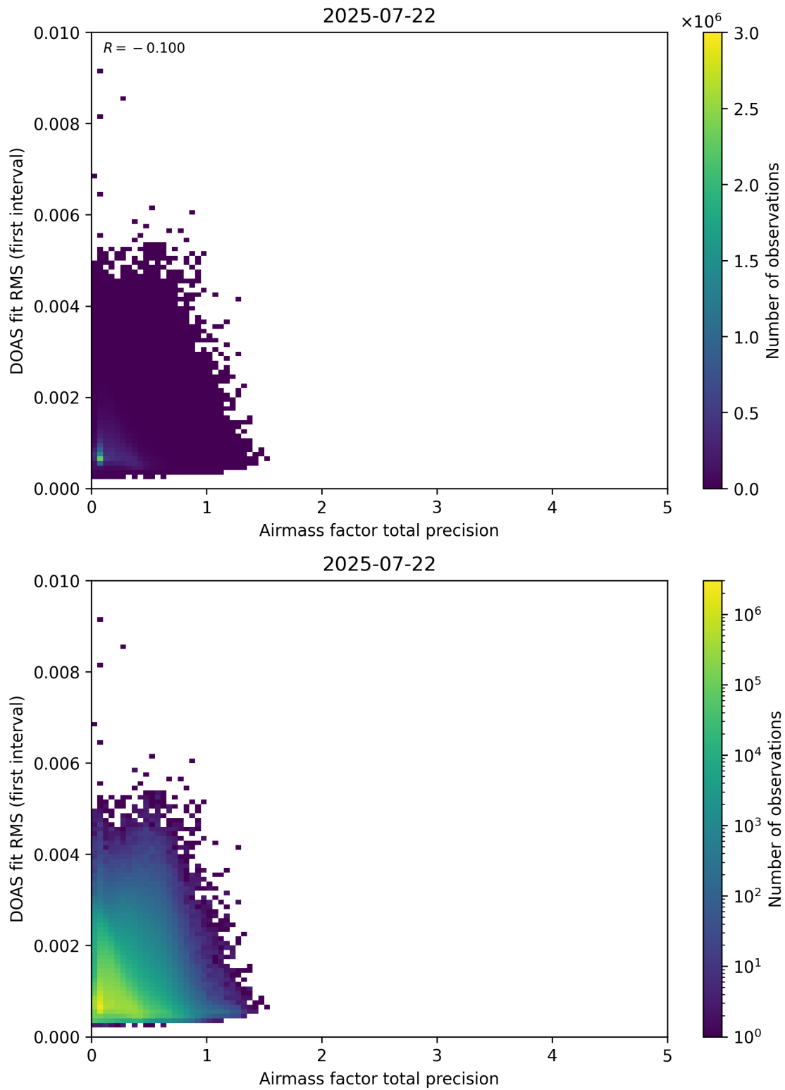
Figure 105: Scatter density plot of “Airmass factor total precision” against “DOAS fit RMS (first interval)” for 2025-07-21 to 2025-07-23.
