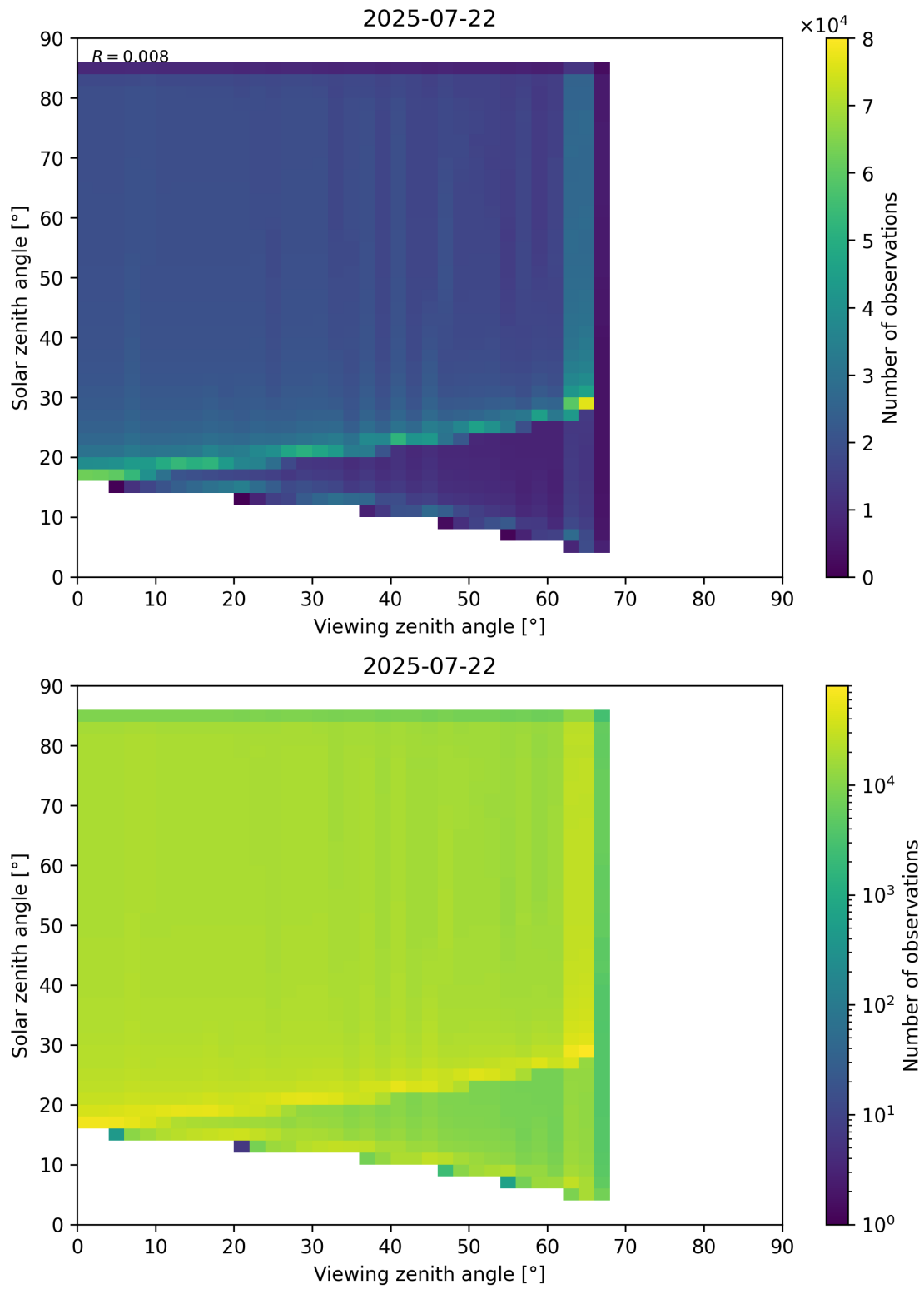
Figure 197: Scatter density plot of “Viewing zenith angle” against “Solar zenith angle” for 2025-07-21 to 2025-07-23.
