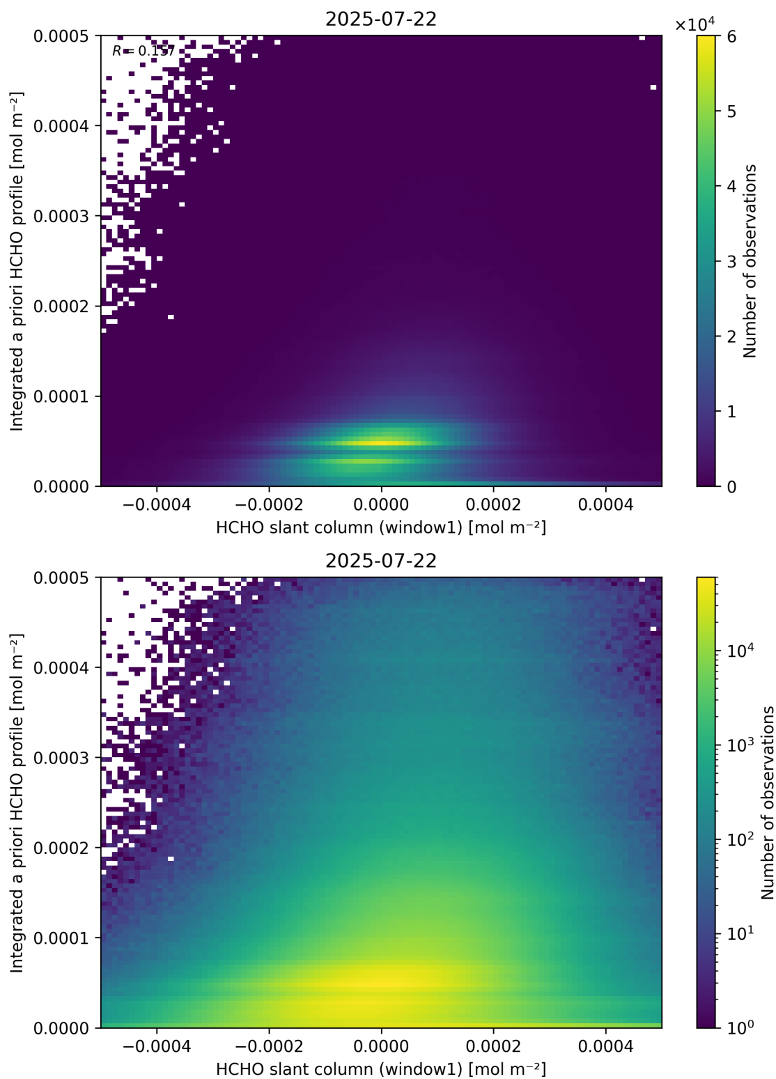
Figure 87: Scatter density plot of “HCHO slant column (window1)” against “Integrated a priori HCHO profile” for 2025-07-21 to 2025-07-23.
