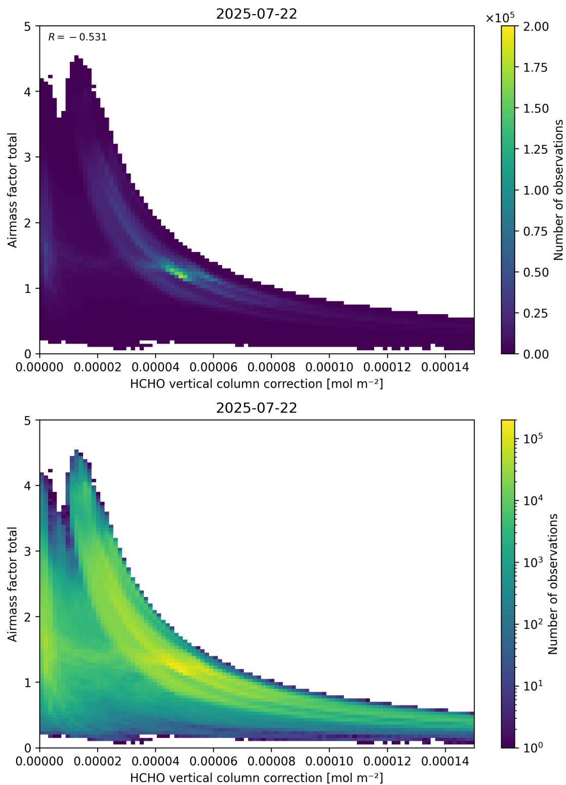
Figure 120: Scatter density plot of “HCHO vertical column correction” against “Airmass factor total” for 2025-07-21 to 2025-07-23.
