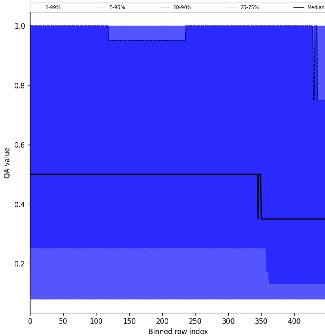
Figure 48: Along track statistics of “QA value” for 2025-07-21 to 2025-07-23
