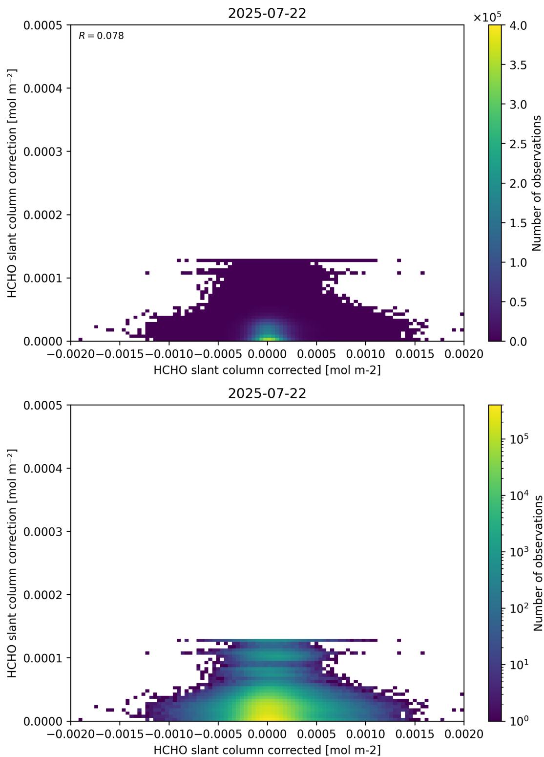
Figure 77: Scatter density plot of “HCHO slant column corrected” against “HCHO slant column correction” for 2025-07-21 to 2025-07-23.
