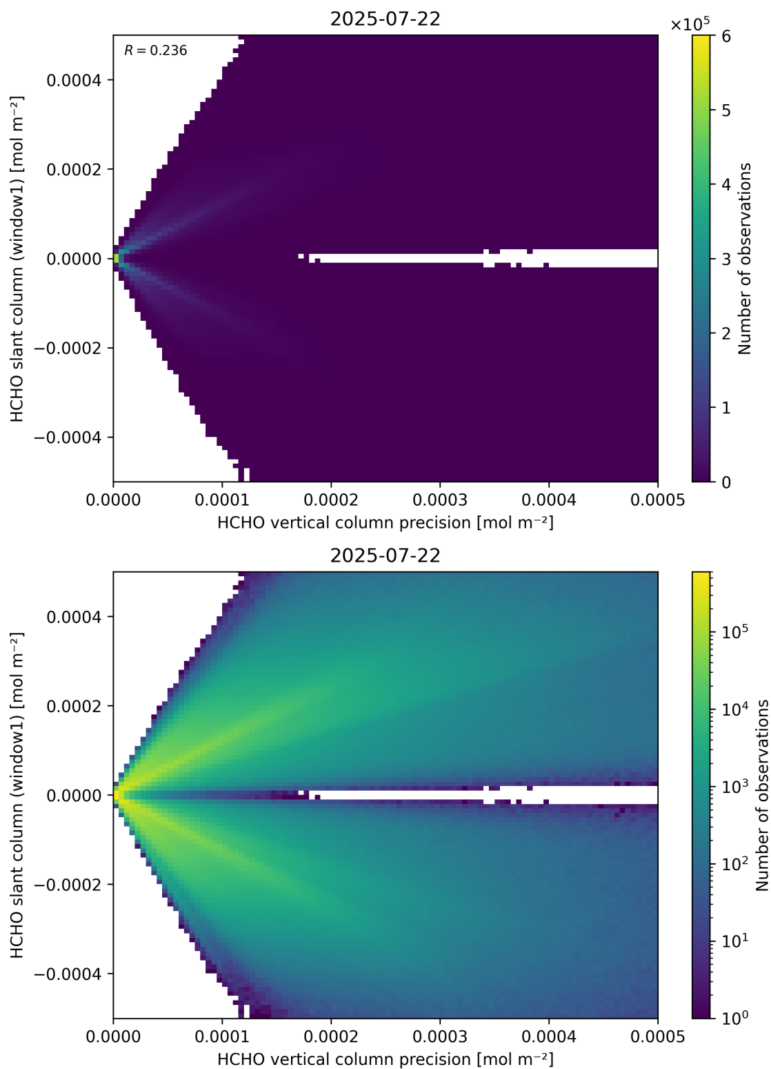
Figure 142: Scatter density plot of “HCHO vertical column precision” against “HCHO slant column (window1)” for 2025-07-21 to 2025-07-23.
