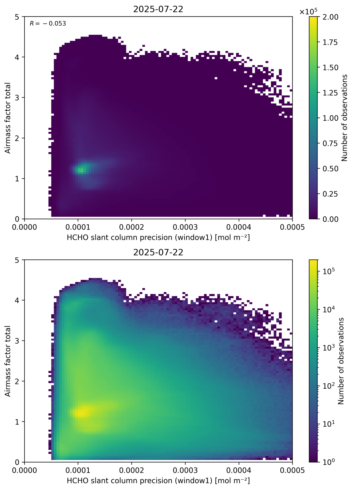
Figure 94: Scatter density plot of “HCHO slant column precision (window1)” against “Airmass factor total” for 2025-07-21 to 2025-07-23.
