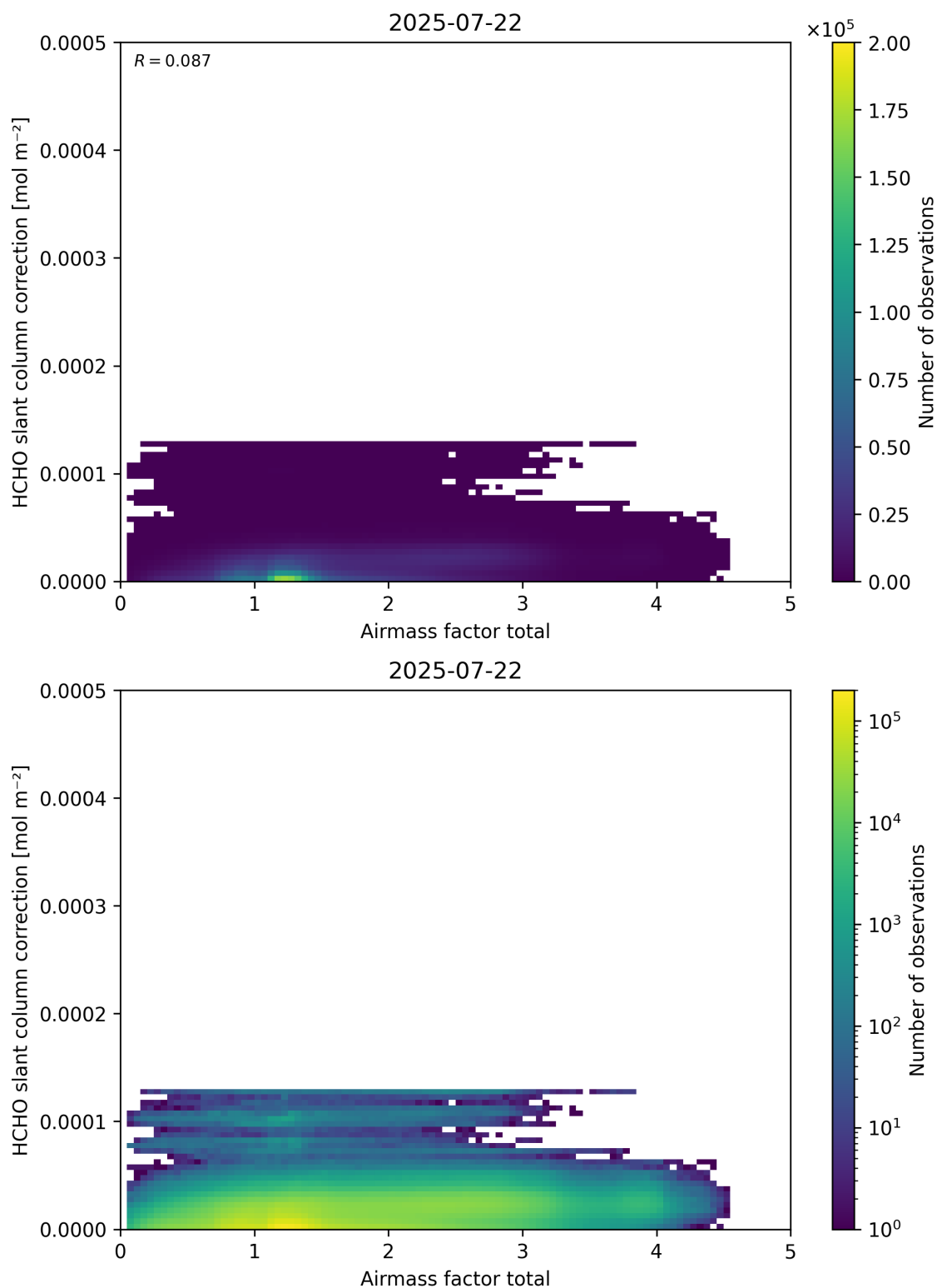
Figure 102: Scatter density plot of “Airmass factor total” against “HCHO slant column correction” for 2025-07-21 to 2025-07-23.
