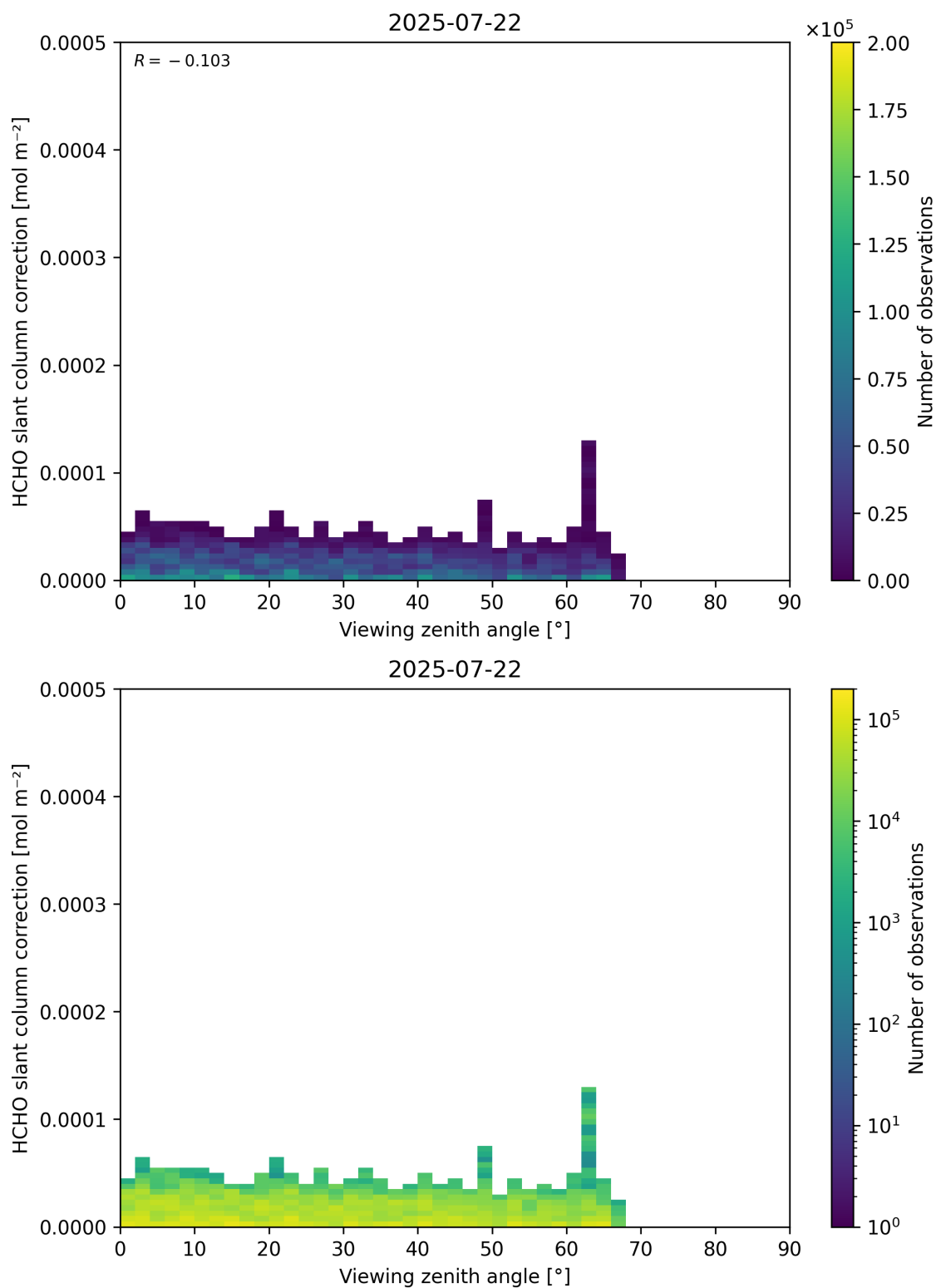
Figure 187: Scatter density plot of “Viewing zenith angle” against “HCHO slant column correction” for 2025-07-21 to 2025-07-23.
