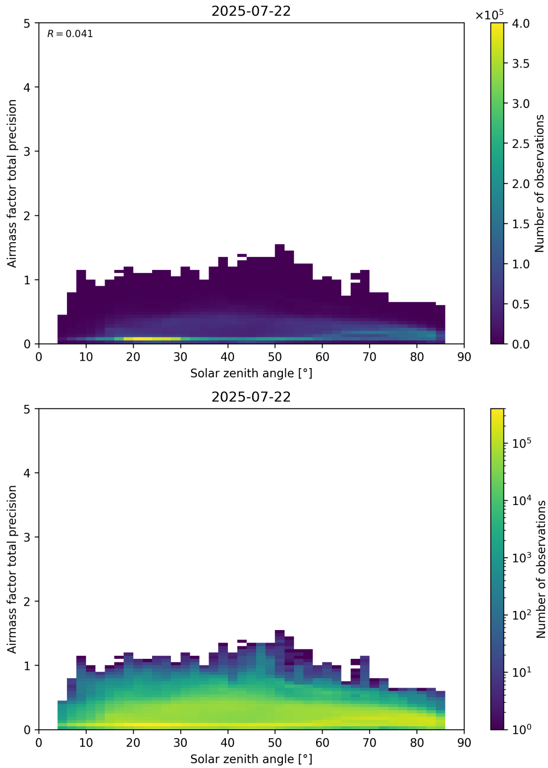
Figure 176: Scatter density plot of “Solar zenith angle” against “Airmass factor total precision” for 2025-07-21 to 2025-07-23.
