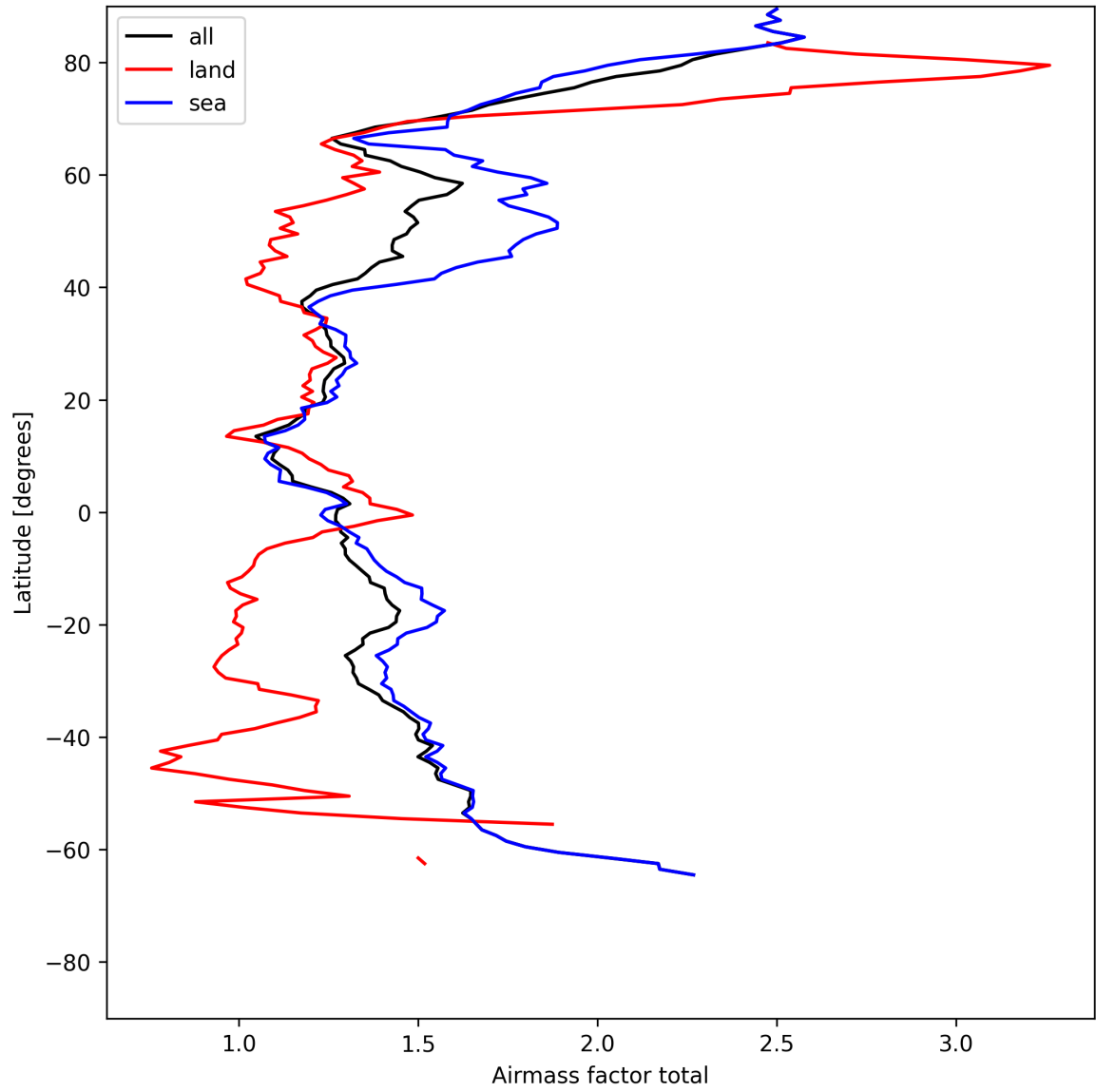
Figure 26: Zonal average of “Airmass factor total” for 2025-07-21 to 2025-07-23.
