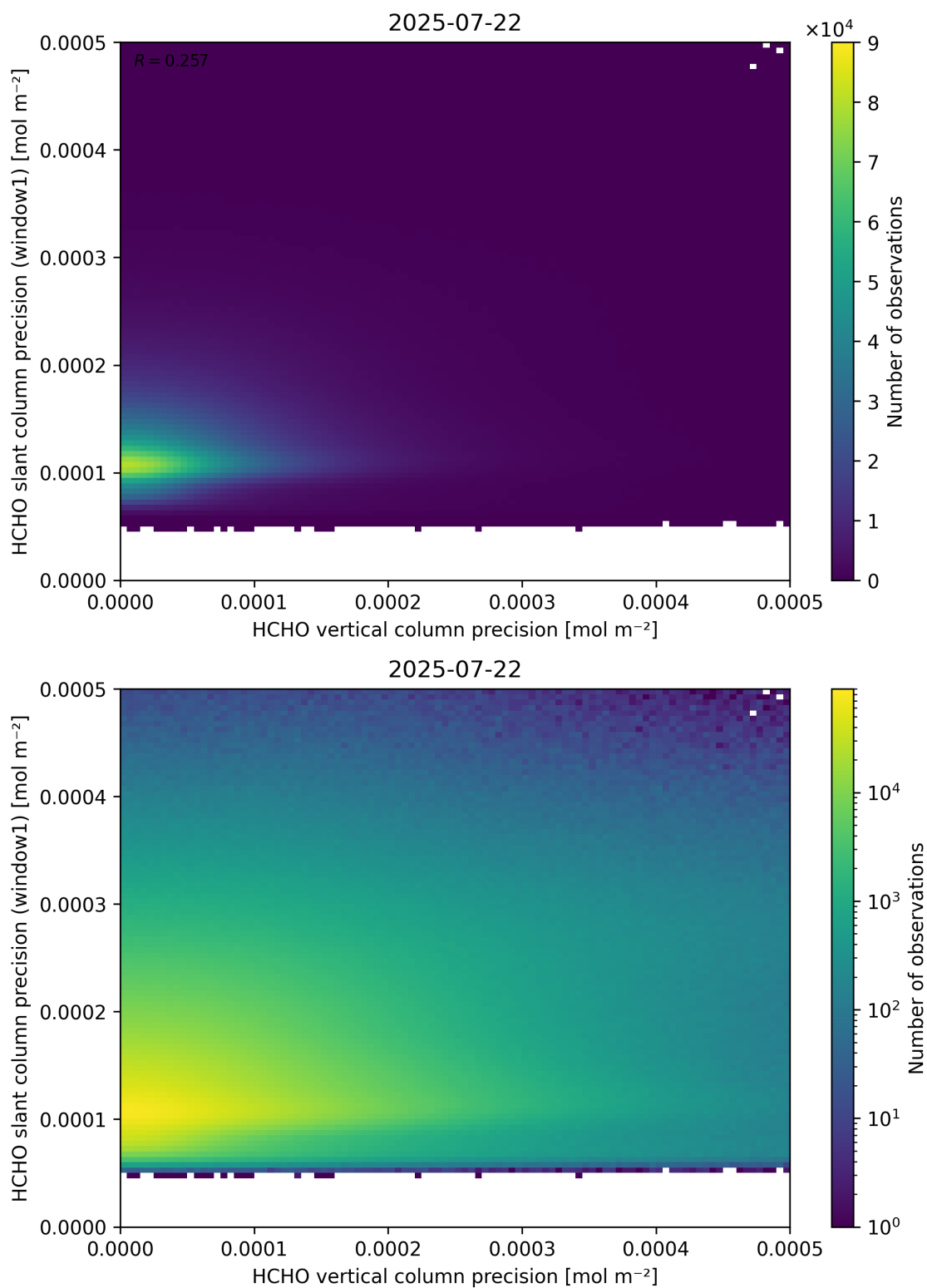
Figure 143: Scatter density plot of “HCHO vertical column precision” against “HCHO slant column precision (window1)” for 2025-07-21 to 2025-07-23.
