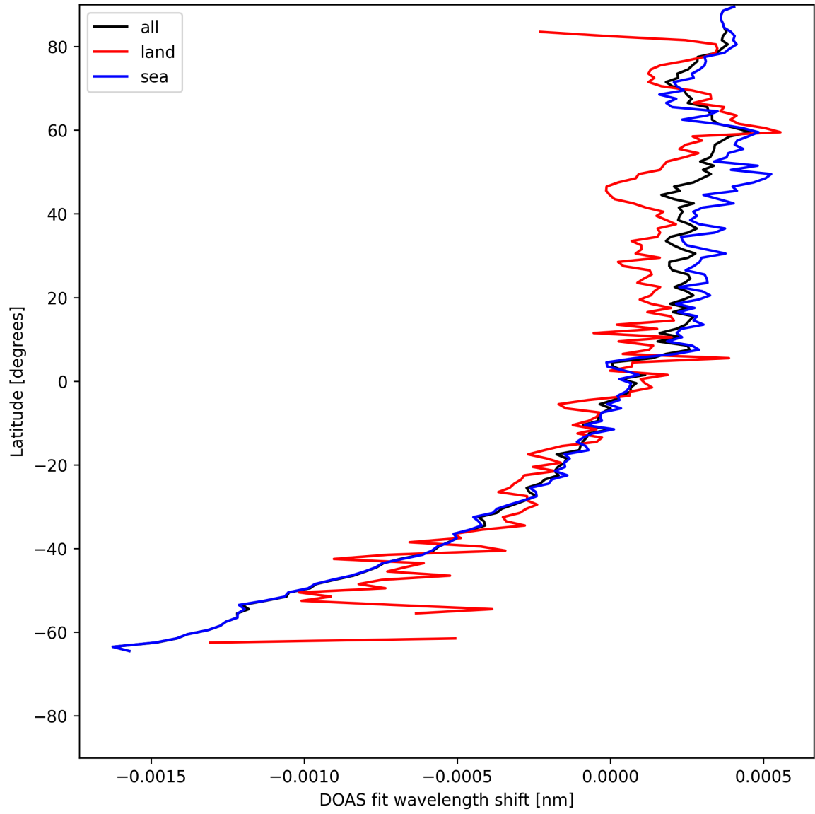
Figure 30: Zonal average of “DOAS fit wavelength shift” for 2025-07-21 to 2025-07-23.
