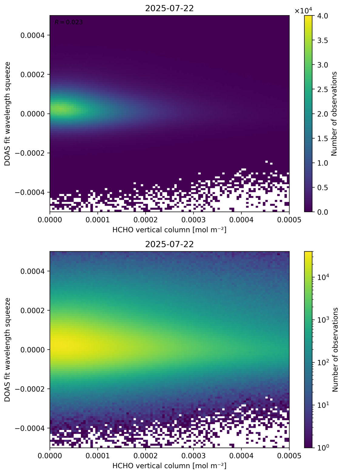
Figure 125: Scatter density plot of “HCHO vertical column” against “DOAS fit wavelength squeeze” for 2025-07-21 to 2025-07-23.
