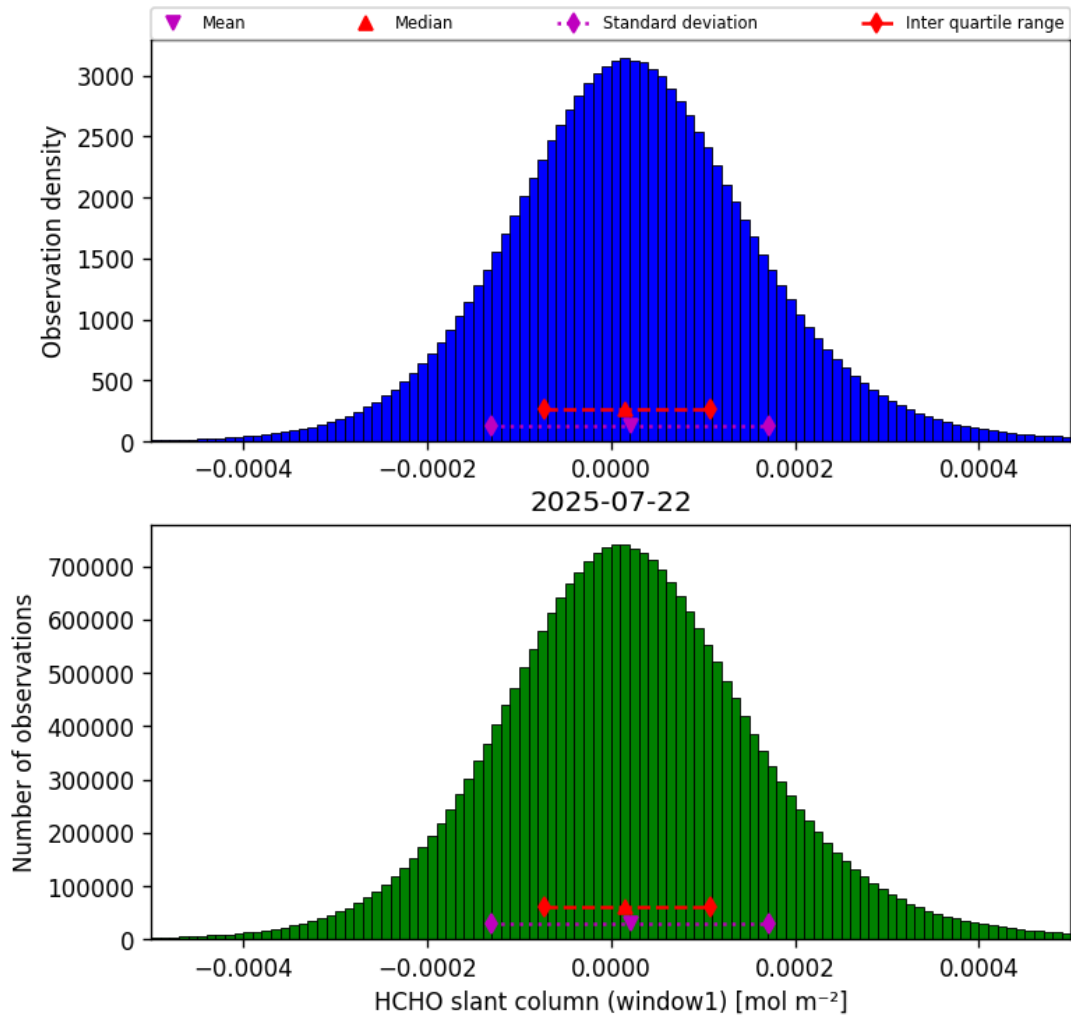
Figure 38: Histogram of “HCHO slant column (window1)” for 2025-07-21 to 2025-07-23
