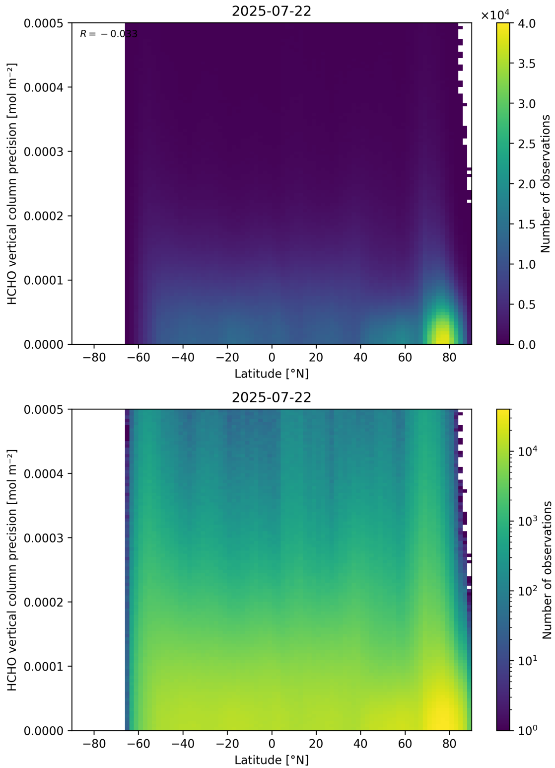
Figure 165: Scatter density plot of “Latitude” against “HCHO vertical column precision” for 2025-07-21 to 2025-07-23.
