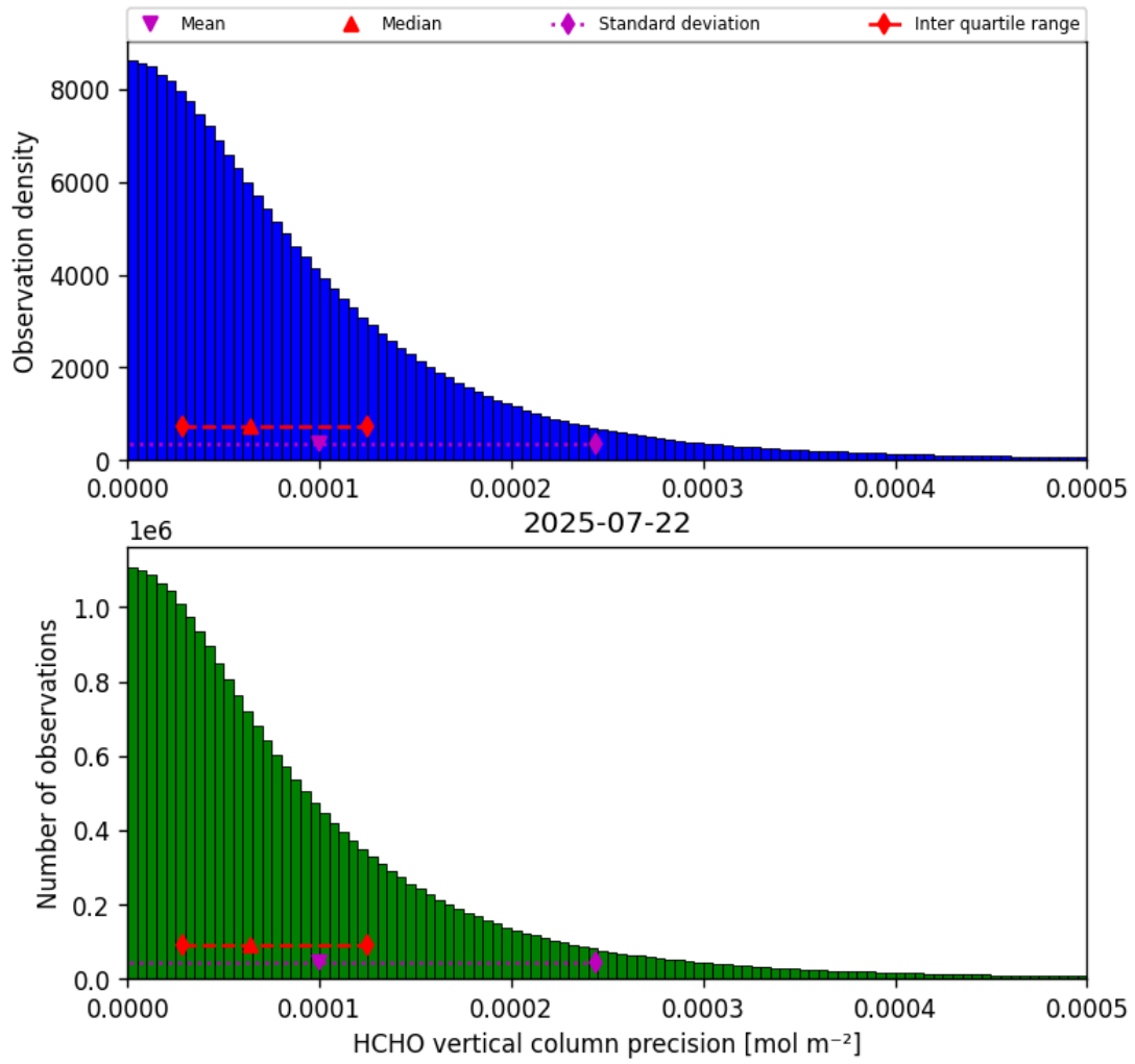
Figure 36: Histogram of “HCHO vertical column precision” for 2025-07-21 to 2025-07-23
