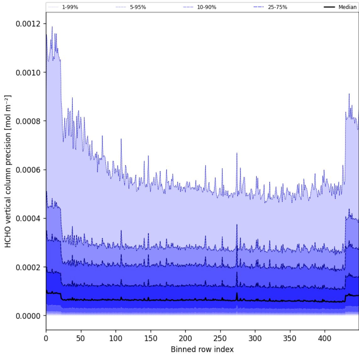
Figure 50: Along track statistics of “HCHO vertical column precision” for 2025-07-21 to 2025-07-23
