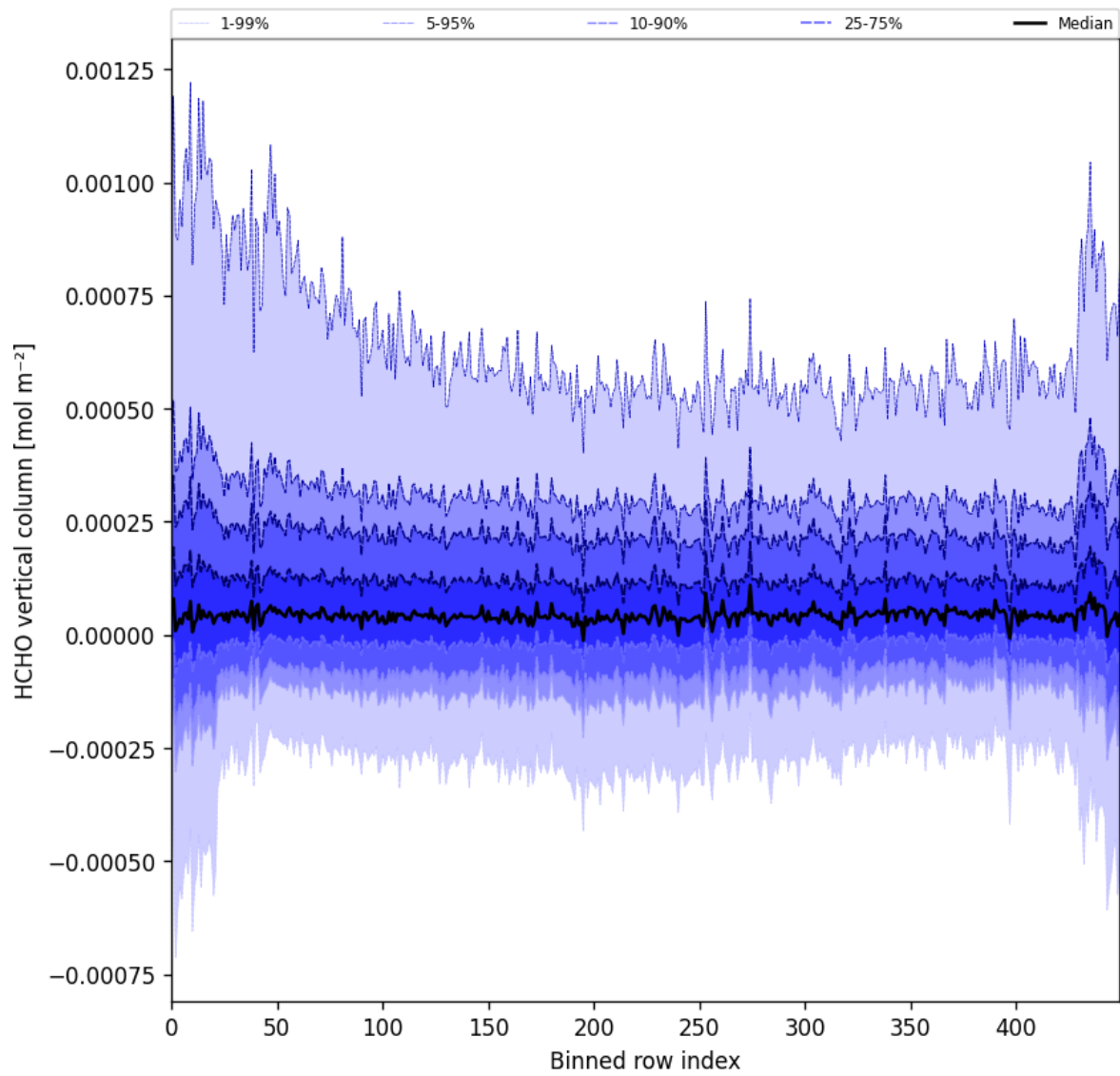
Figure 49: Along track statistics of “HCHO vertical column” for 2025-07-21 to 2025-07-23
