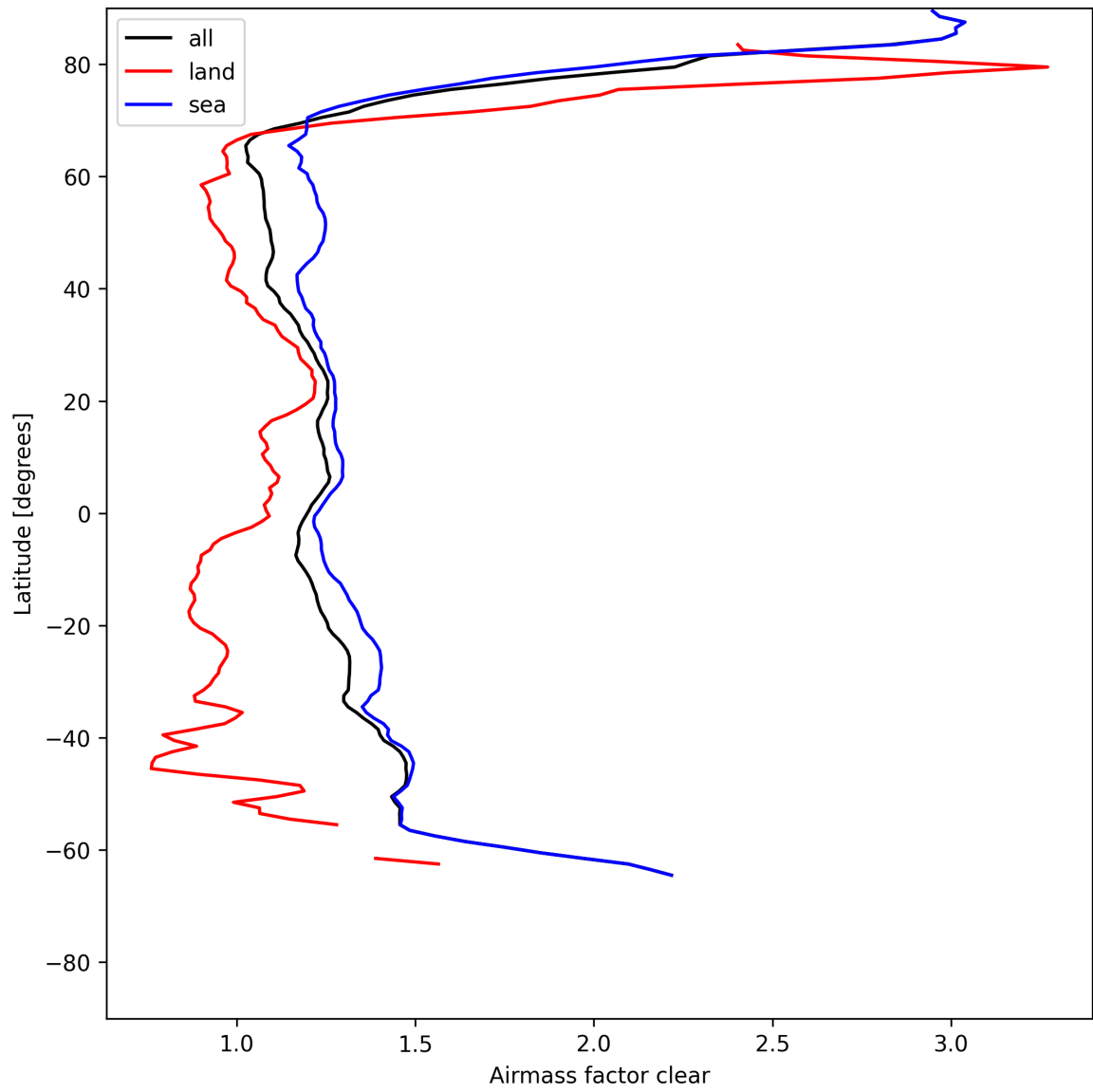
Figure 28: Zonal average of “Airmass factor clear” for 2025-07-21 to 2025-07-23.
