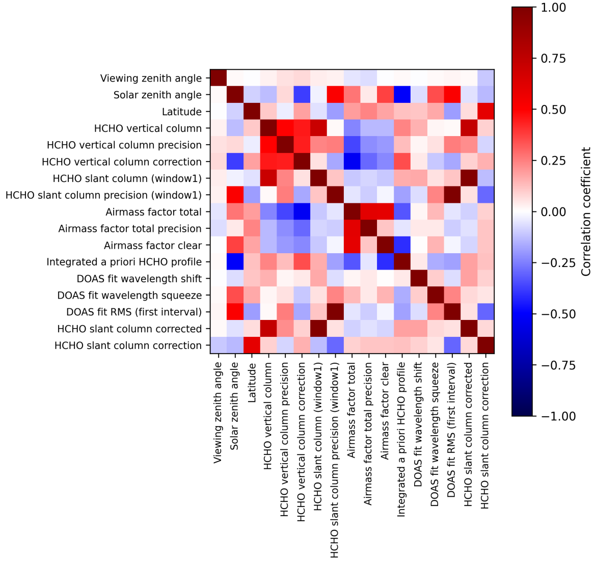
Figure 2: Map of correlation matrix for 2025-07-21 to 2025-07-23.
