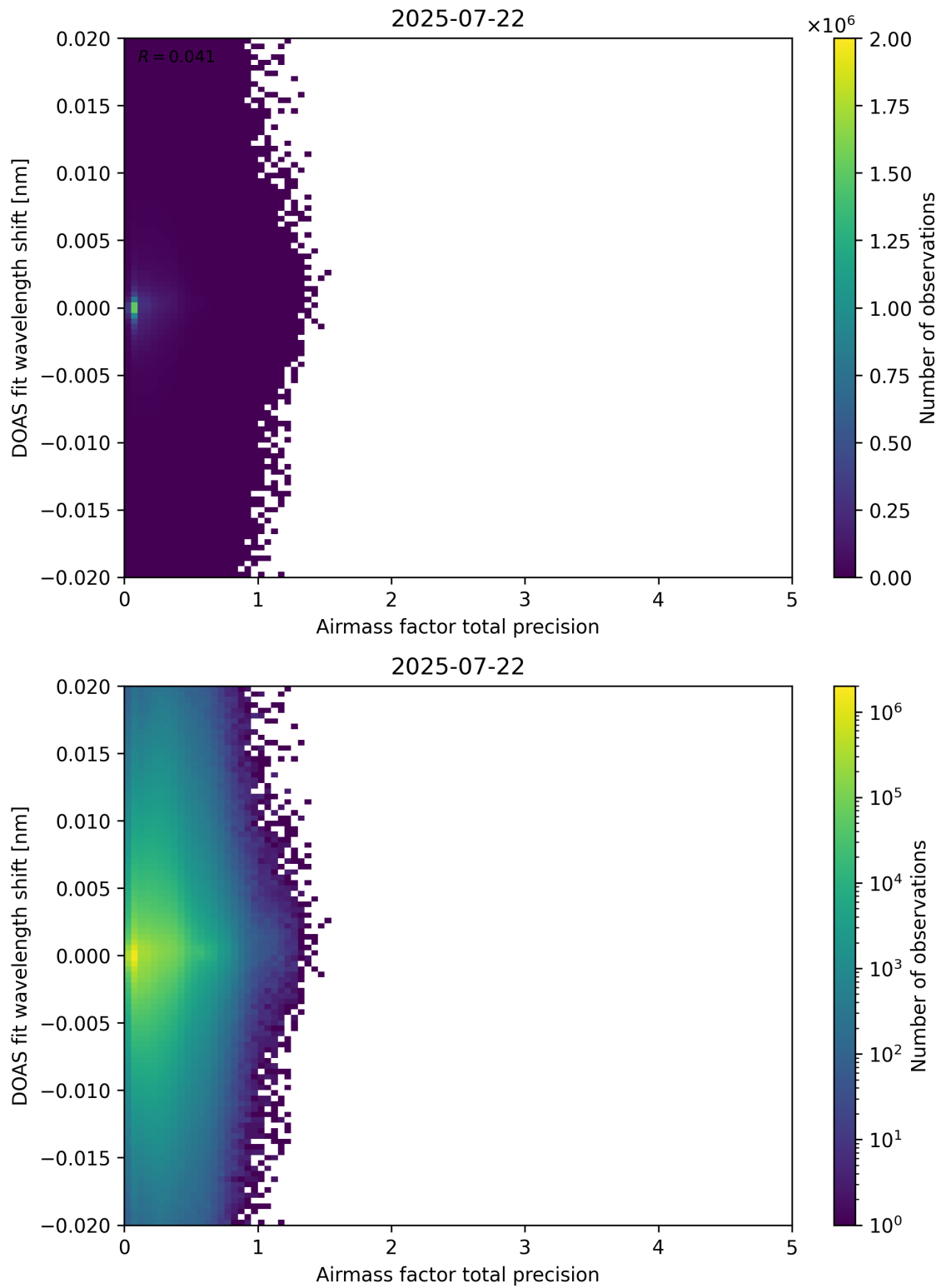
Figure 106: Scatter density plot of “Airmass factor total precision” against “DOAS fit wavelength shift” for 2025-07-21 to 2025-07-23.
