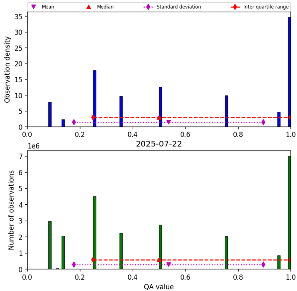
Figure 34: Histogram of “QA value” for 2025-07-21 to 2025-07-23
