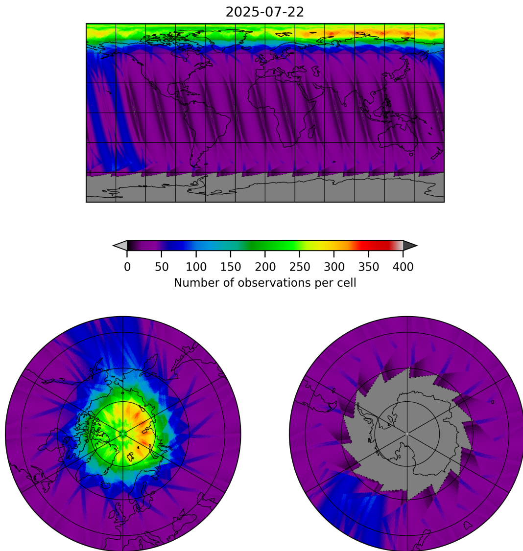
Figure 19: Map of the number of observations for 2025-07-21 to 2025-07-23
