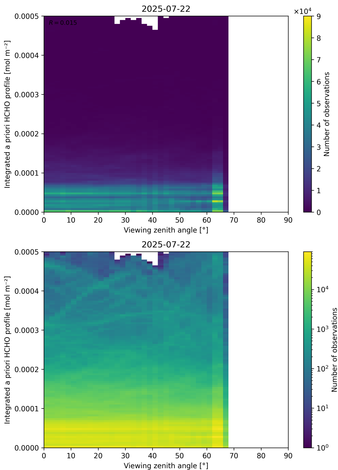
Figure 195: Scatter density plot of “Viewing zenith angle” against “Integrated a priori HCHO profile” for 2025-07-21 to 2025-07-23.
