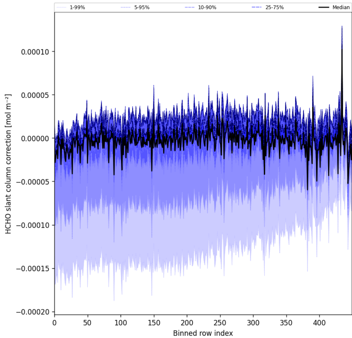
Figure 61: Along track statistics of “HCHO slant column correction” for 2025-07-21 to 2025-07-23
