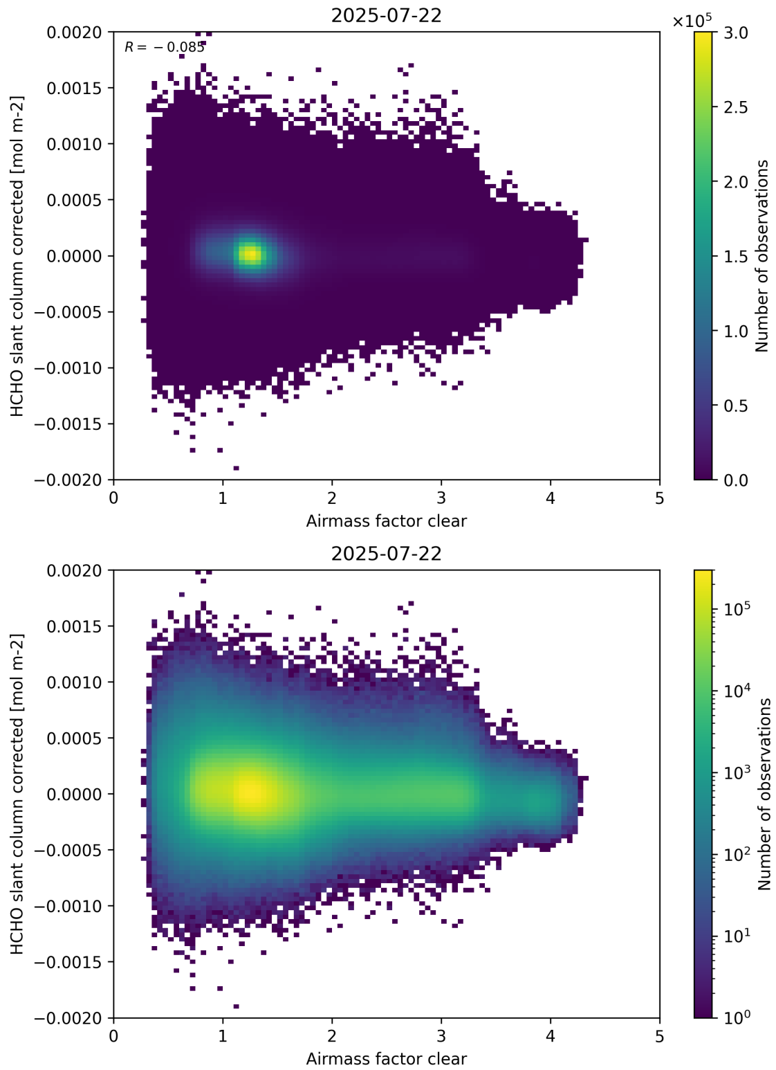
Figure 74: Scatter density plot of “Airmass factor clear” against “HCHO slant column corrected” for 2025-07-21 to 2025-07-23.
