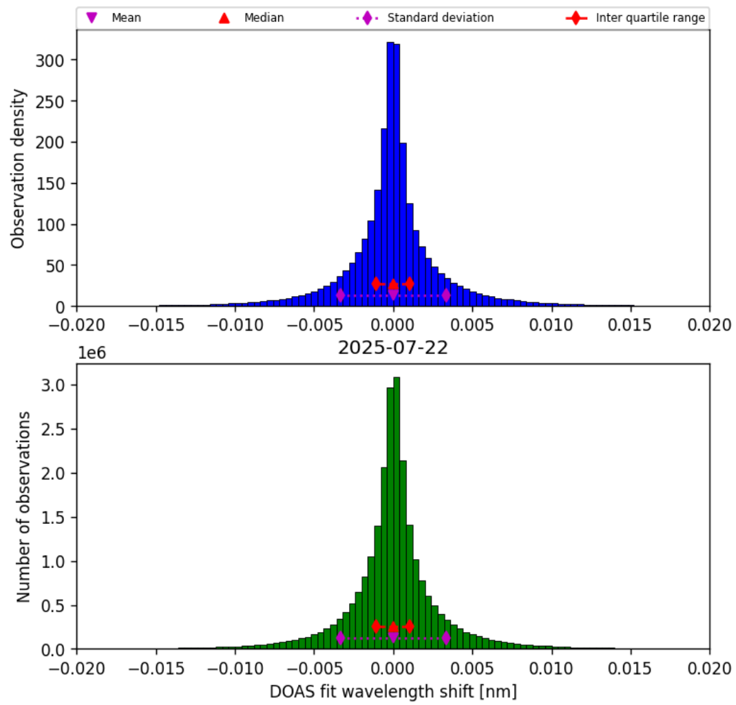
Figure 44: Histogram of “DOAS fit wavelength shift” for 2025-07-21 to 2025-07-23
