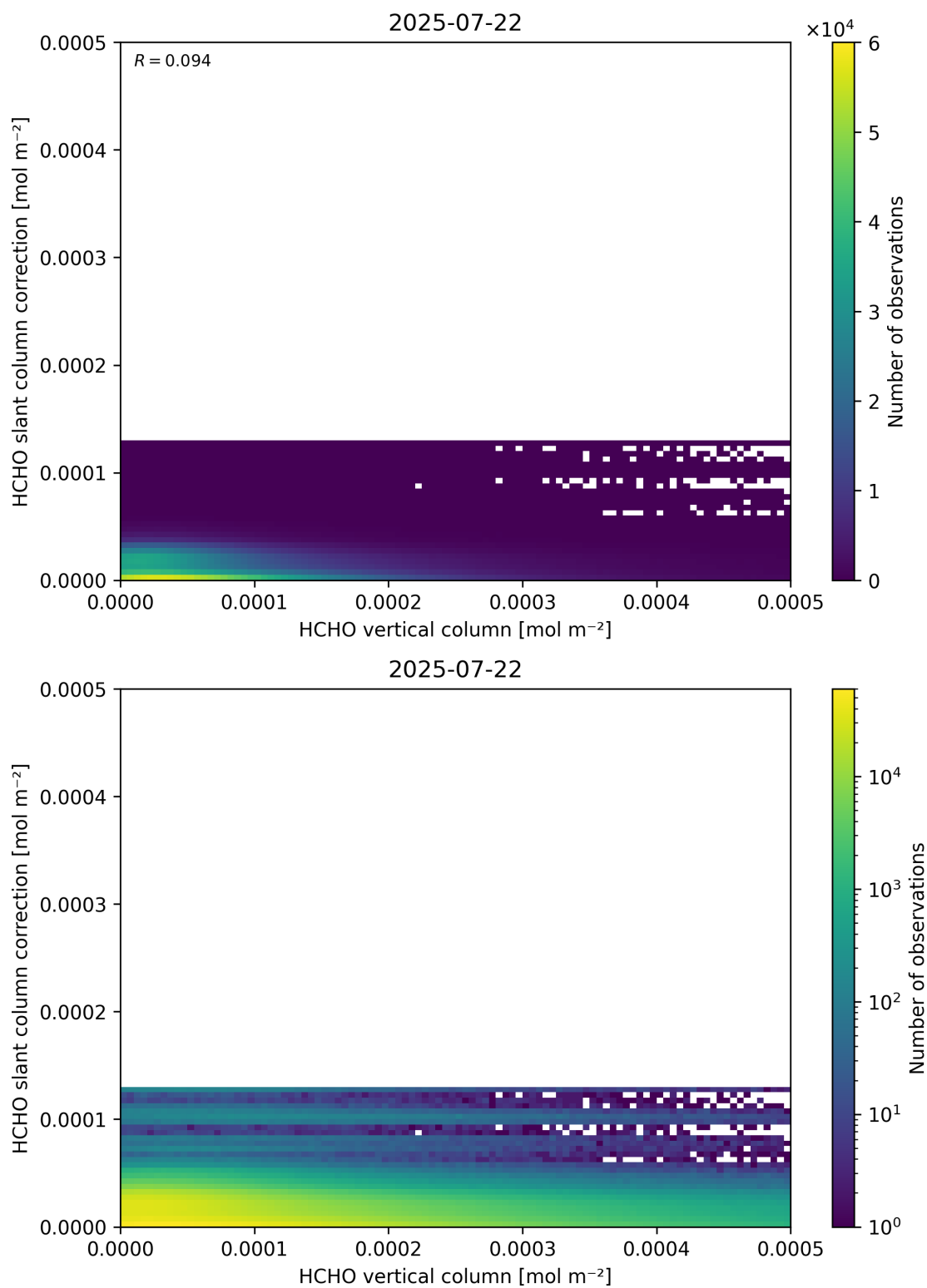
Figure 128: Scatter density plot of “HCHO vertical column” against “HCHO slant column correction” for 2025-07-21 to 2025-07-23.
