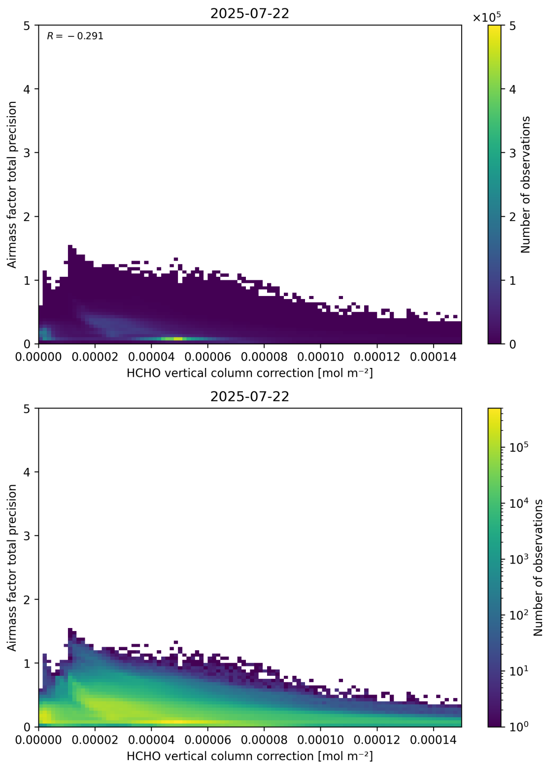
Figure 121: Scatter density plot of “HCHO vertical column correction” against “Airmass factor total precision” for 2025-07-21 to 2025-07-23.
