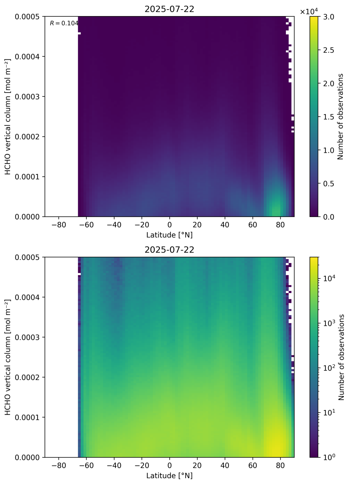
Figure 163: Scatter density plot of “Latitude” against “HCHO vertical column” for 2025-07-21 to 2025-07-23.
