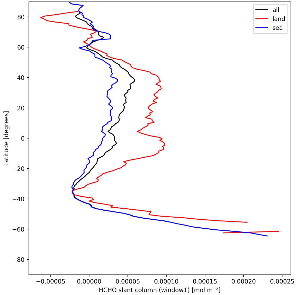
Figure 24: Zonal average of “HCHO slant column (window1)” for 2025-07-21 to 2025-07-23.
