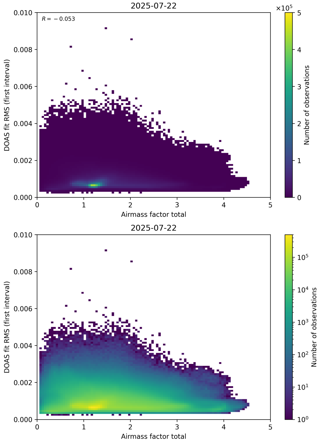
Figure 97: Scatter density plot of “Airmass factor total” against “DOAS fit RMS (first interval)” for 2025-07-21 to 2025-07-23.
