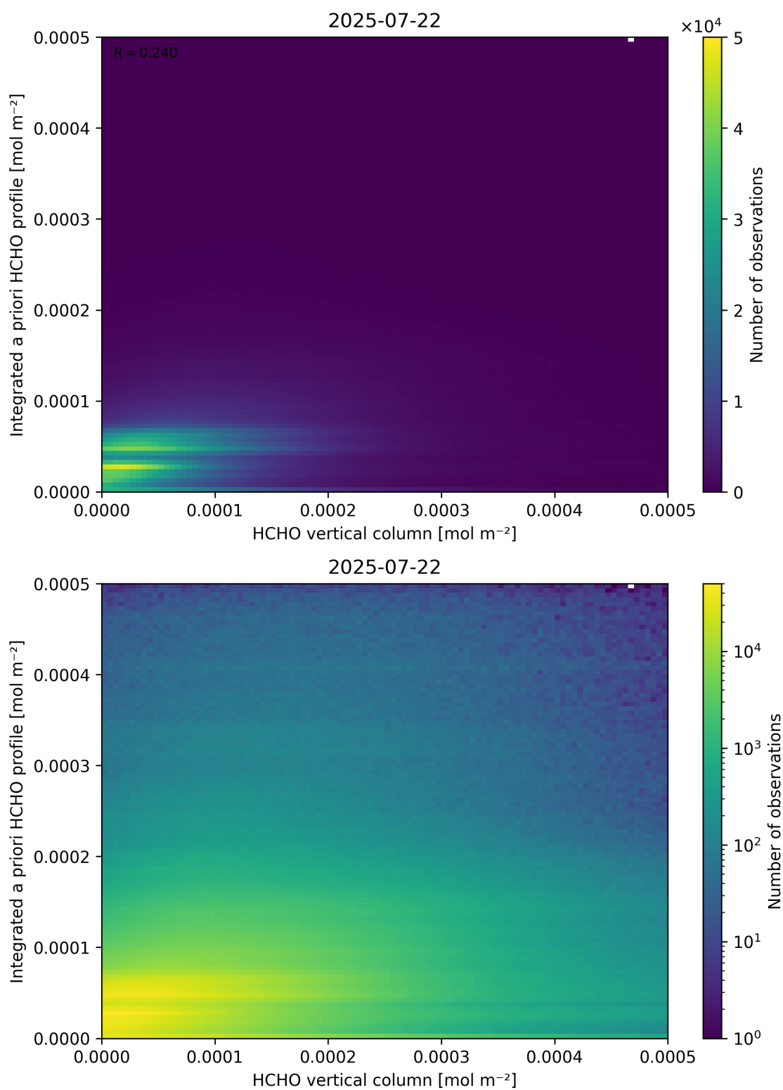
Figure 135: Scatter density plot of “HCHO vertical column” against “Integrated a priori HCHO profile” for 2025-07-21 to 2025-07-23.
