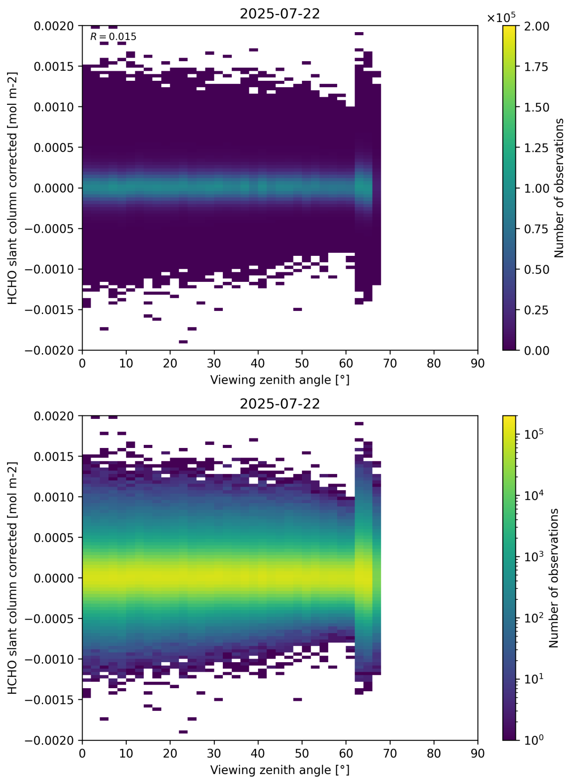
Figure 186: Scatter density plot of “Viewing zenith angle” against “HCHO slant column corrected” for 2025-07-21 to 2025-07-23.
