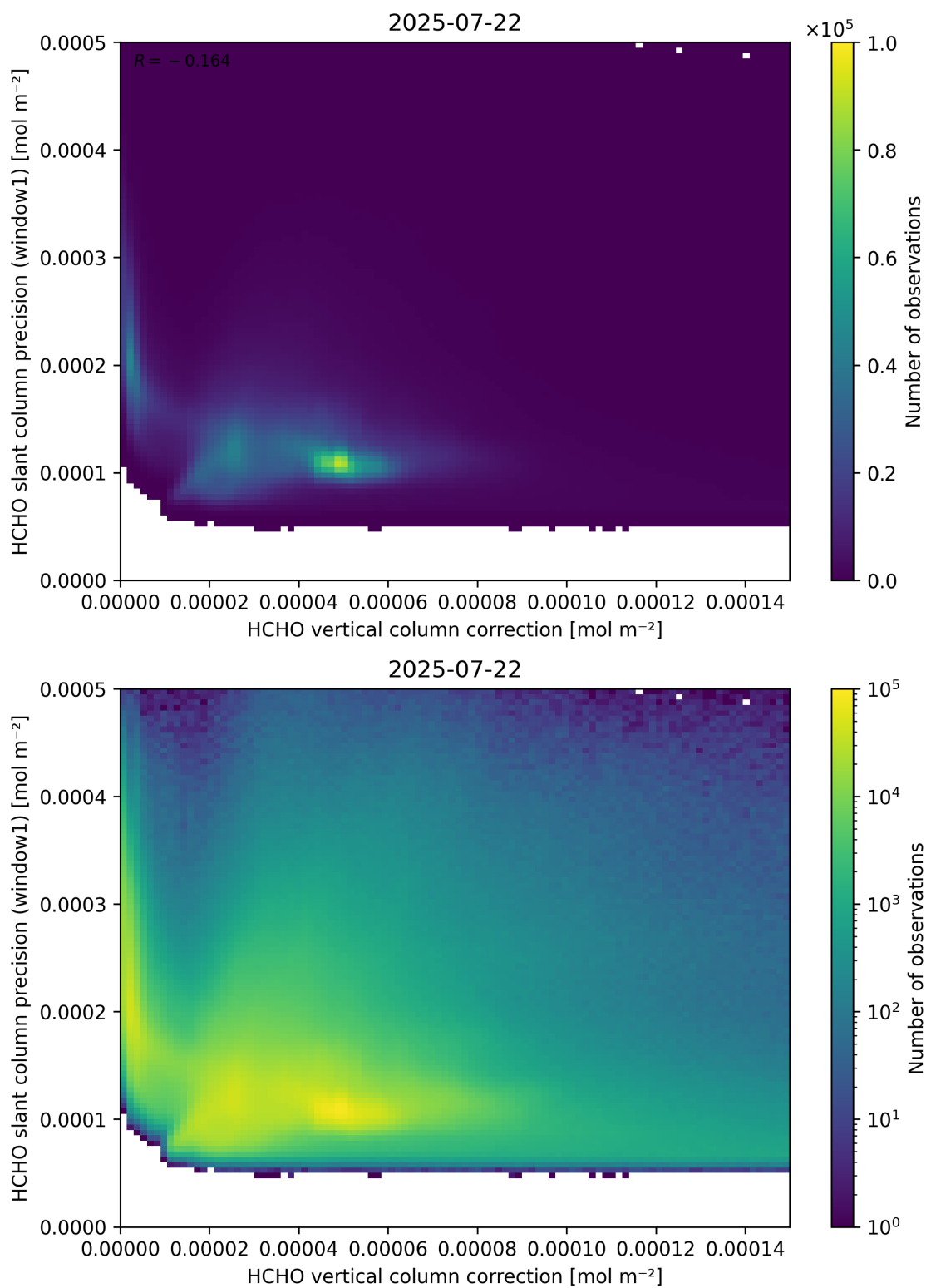
Figure 119: Scatter density plot of “HCHO vertical column correction” against “HCHO slant column precision (window1)” for 2025-07-21 to 2025-07-23.
