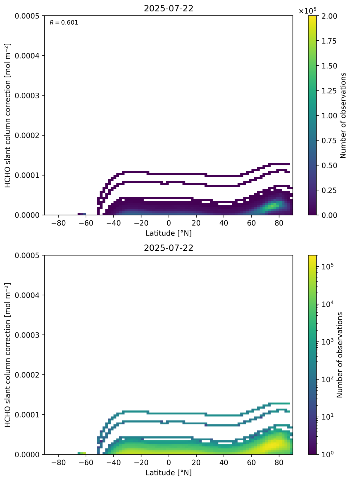
Figure 158: Scatter density plot of “Latitude” against “HCHO slant column correction” for 2025-07-21 to 2025-07-23.
