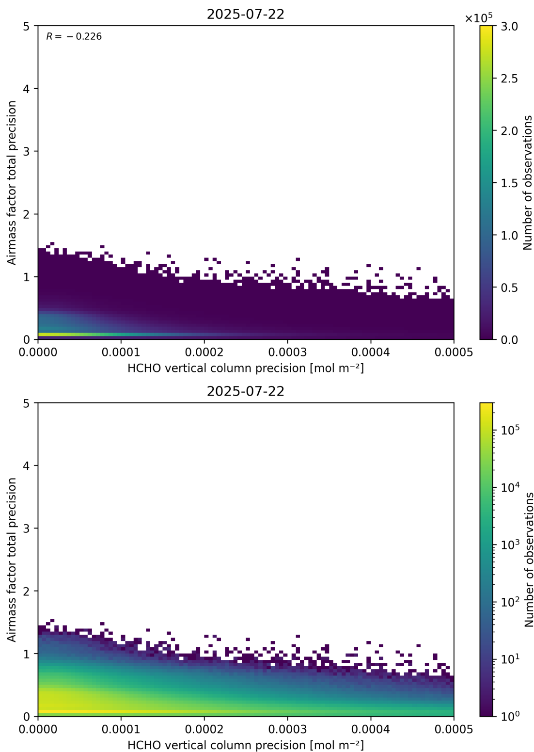
Figure 145: Scatter density plot of “HCHO vertical column precision” against “Airmass factor total precision” for 2025-07-21 to 2025-07-23.
