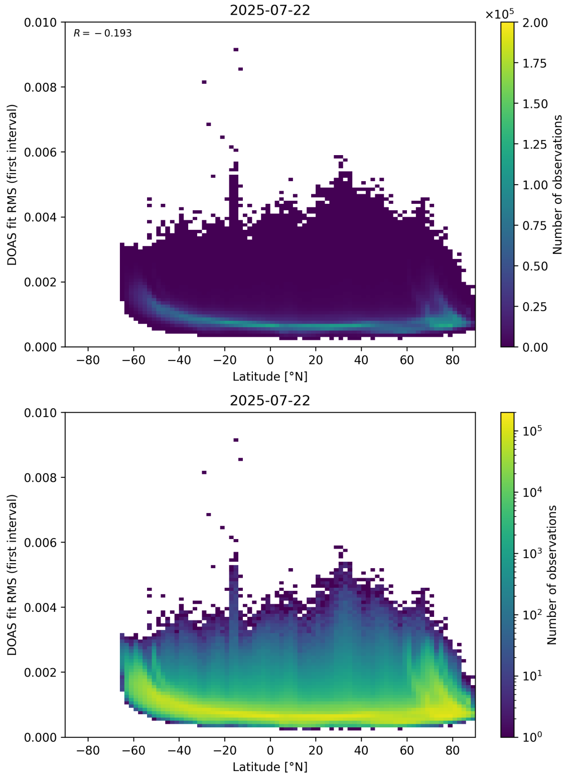
Figure 153: Scatter density plot of “Latitude” against “DOAS fit RMS (first interval)” for 2025-07-21 to 2025-07-23.
