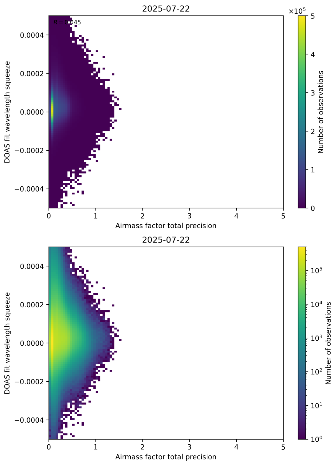
Figure 107: Scatter density plot of “Airmass factor total precision” against “DOAS fit wavelength squeeze” for 2025-07-21 to 2025-07-23.
