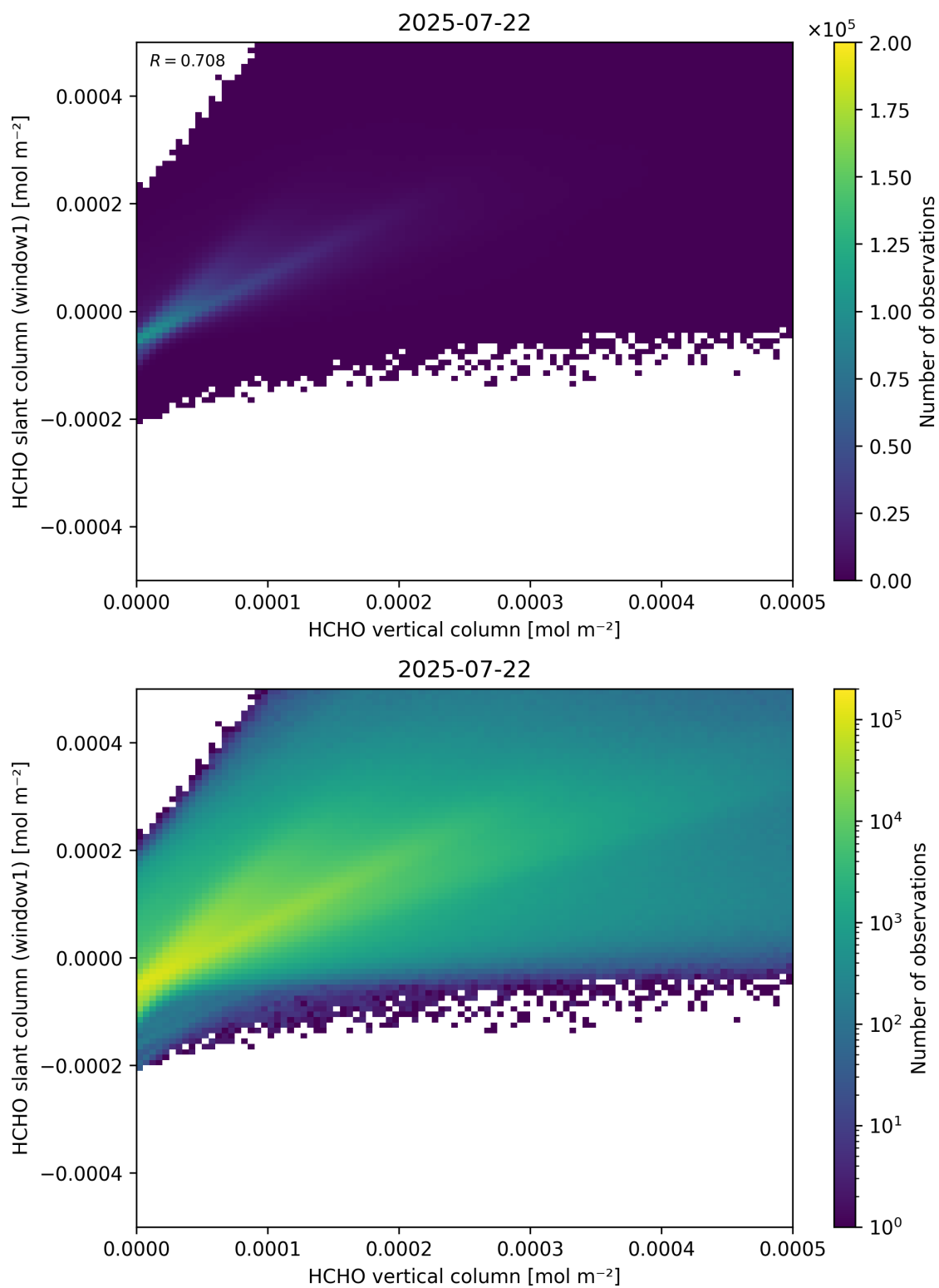
Figure 129: Scatter density plot of “HCHO vertical column” against “HCHO slant column (window1)” for 2025-07-21 to 2025-07-23.
