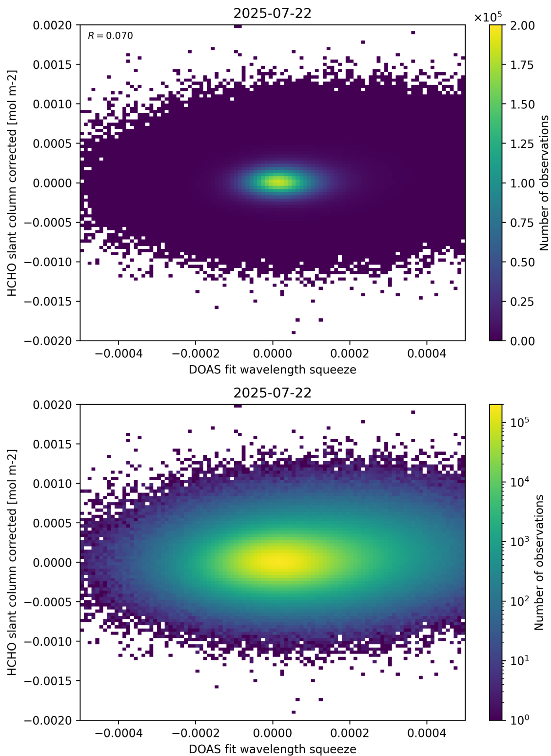
Figure 69: Scatter density plot of “DOAS fit wavelength squeeze” against “HCHO slant column corrected” for 2025-07-21 to 2025-07-23.
