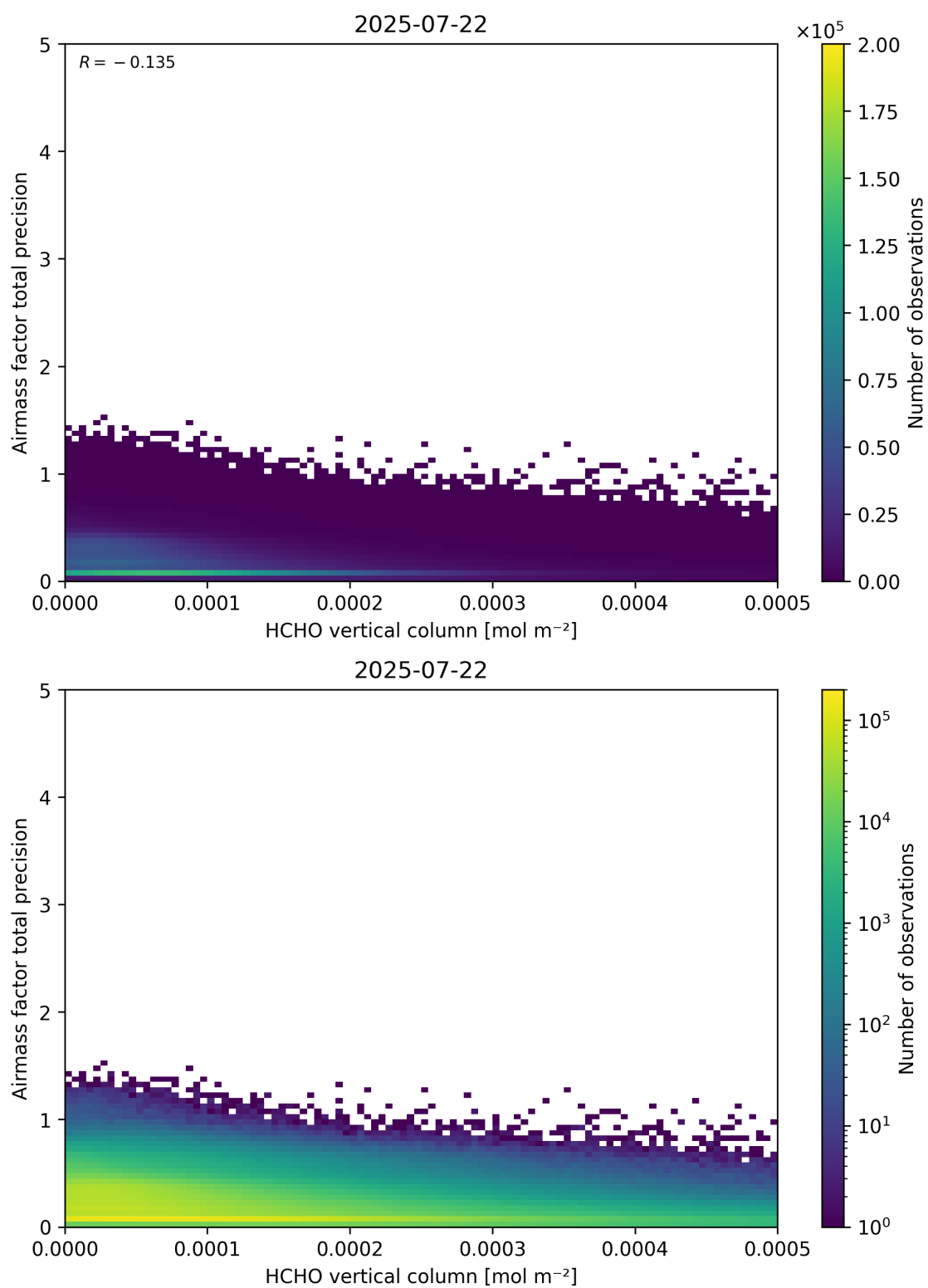
Figure 132: Scatter density plot of “HCHO vertical column” against “Airmass factor total precision” for 2025-07-21 to 2025-07-23.
