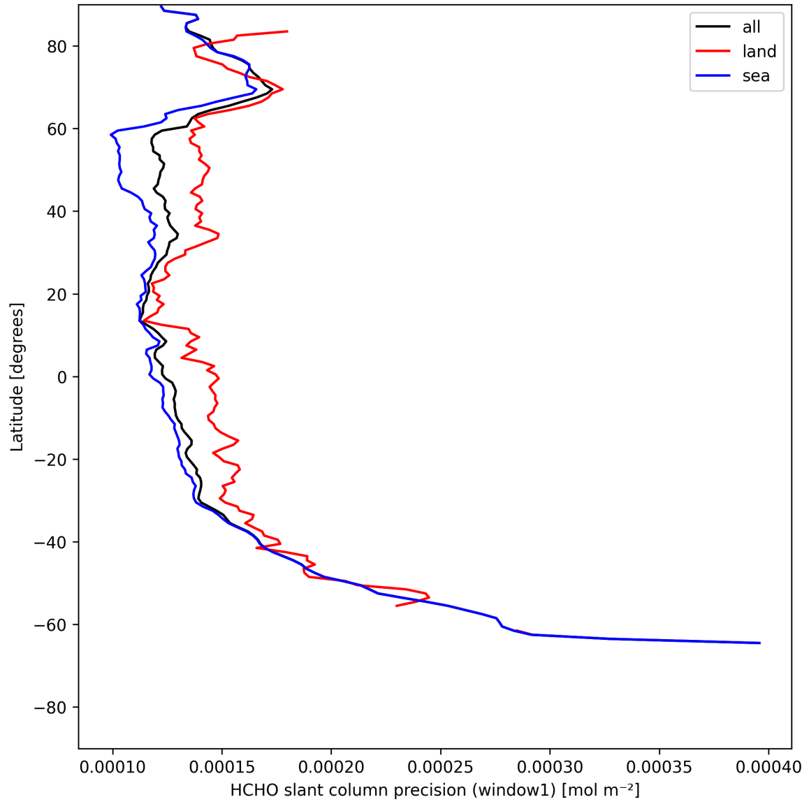
Figure 25: Zonal average of “HCHO slant column precision (window1)” for 2025-07-21 to 2025-07-23.
