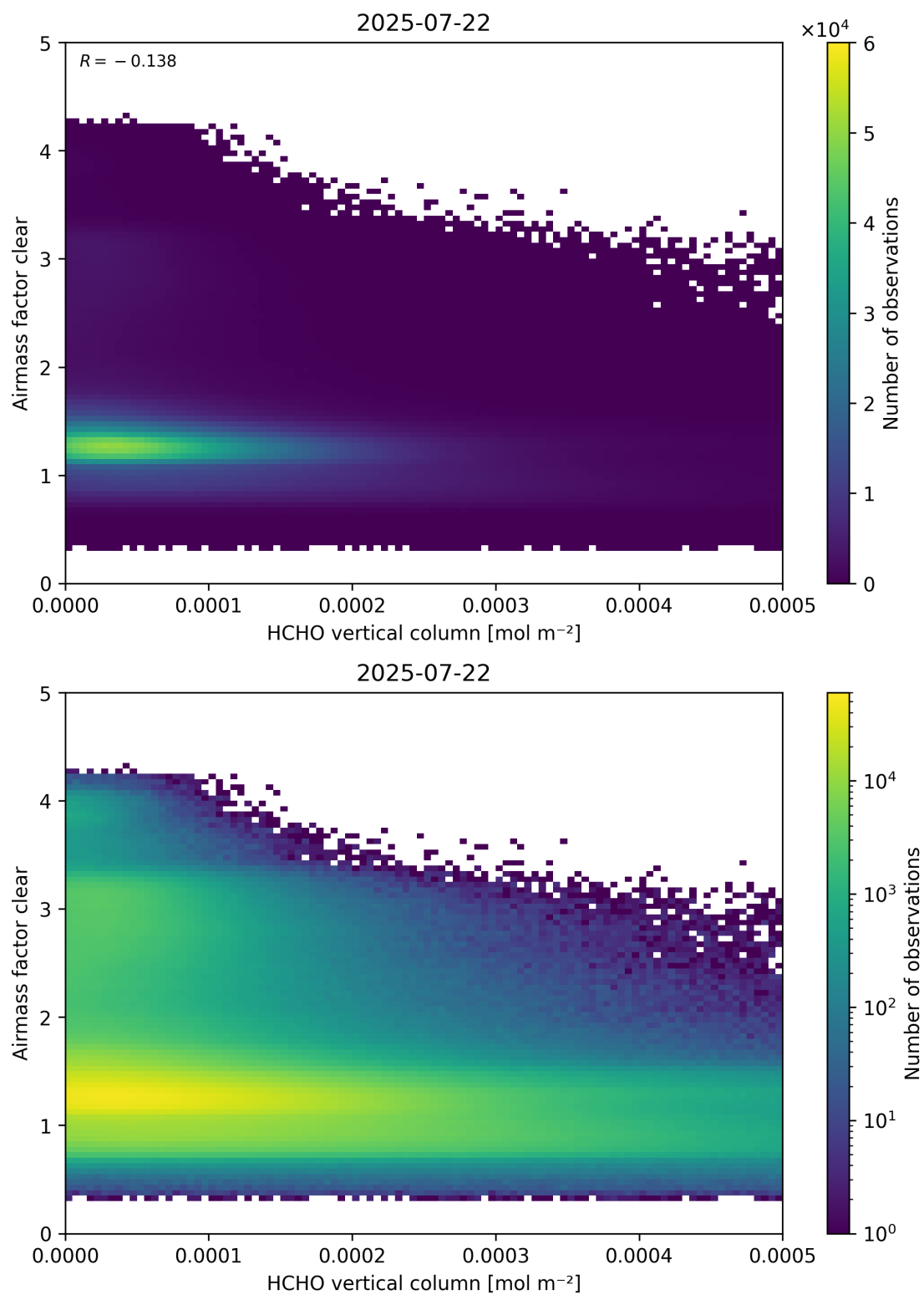
Figure 126: Scatter density plot of “HCHO vertical column” against “Airmass factor clear” for 2025-07-21 to 2025-07-23.
