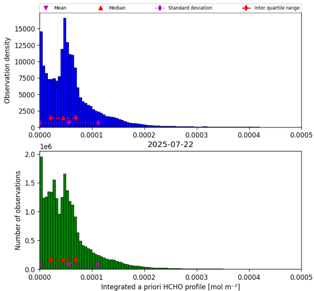
Figure 43: Histogram of “Integrated a priori HCHO profile” for 2025-07-21 to 2025-07-23
