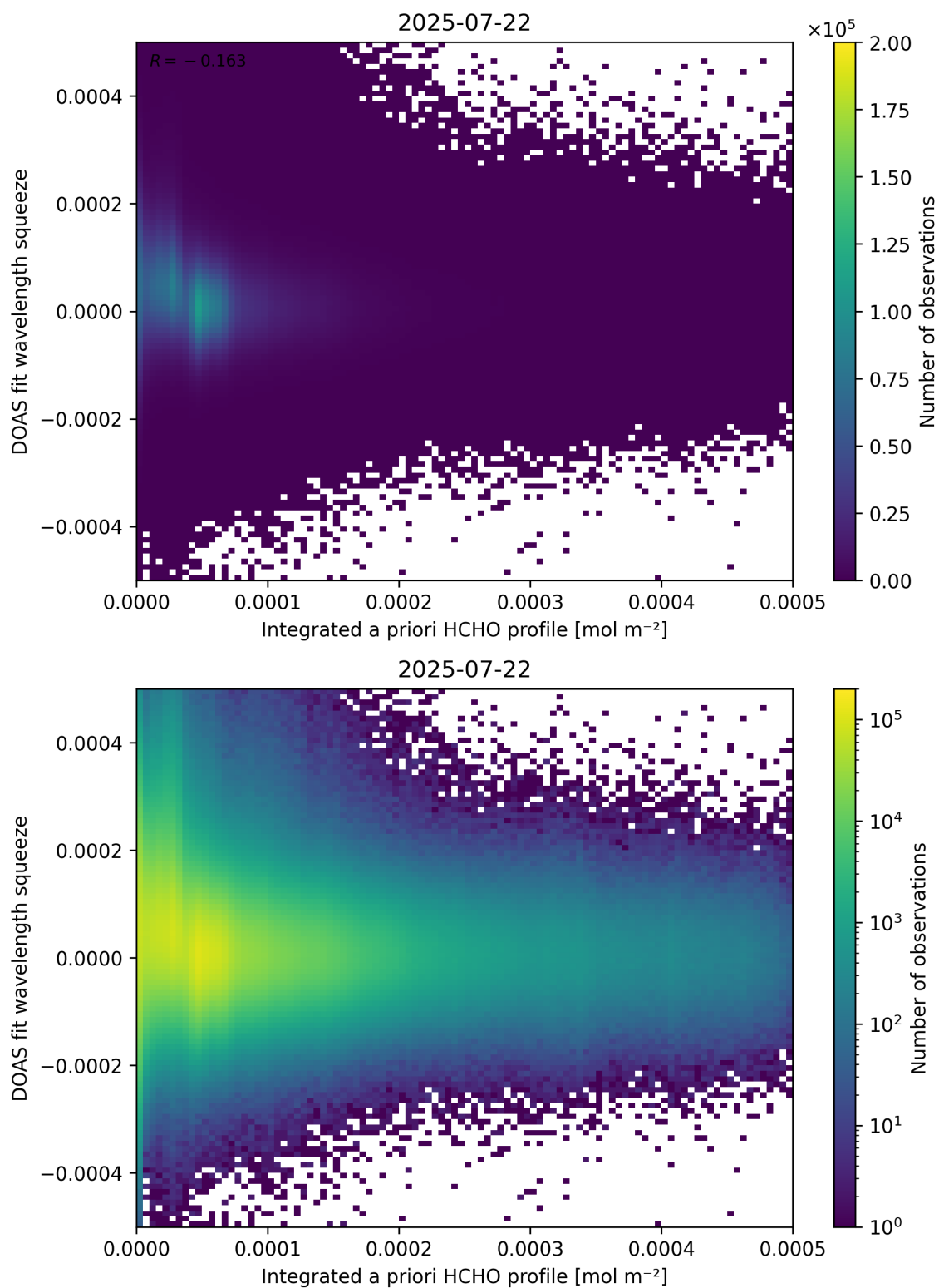
Figure 150: Scatter density plot of “Integrated a priori HCHO profile” against “DOAS fit wavelength squeeze” for 2025-07-21 to 2025-07-23.
