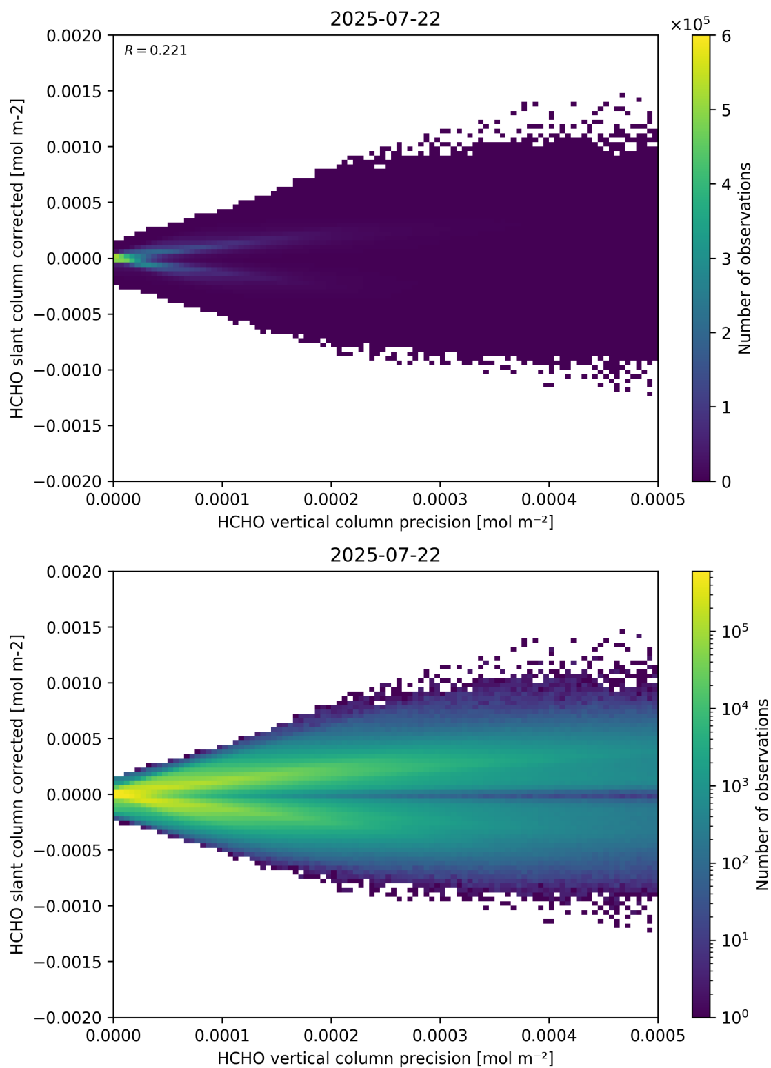
Figure 140: Scatter density plot of “HCHO vertical column precision” against “HCHO slant column corrected” for 2025-07-21 to 2025-07-23.
