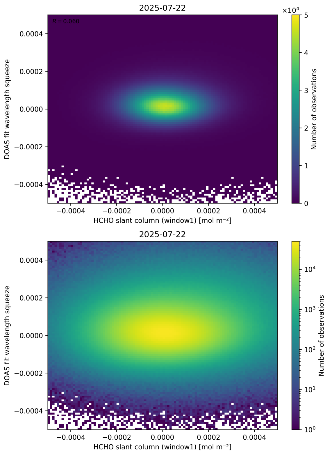
Figure 80: Scatter density plot of “HCHO slant column (window1)” against “DOAS fit wavelength squeeze” for 2025-07-21 to 2025-07-23.
