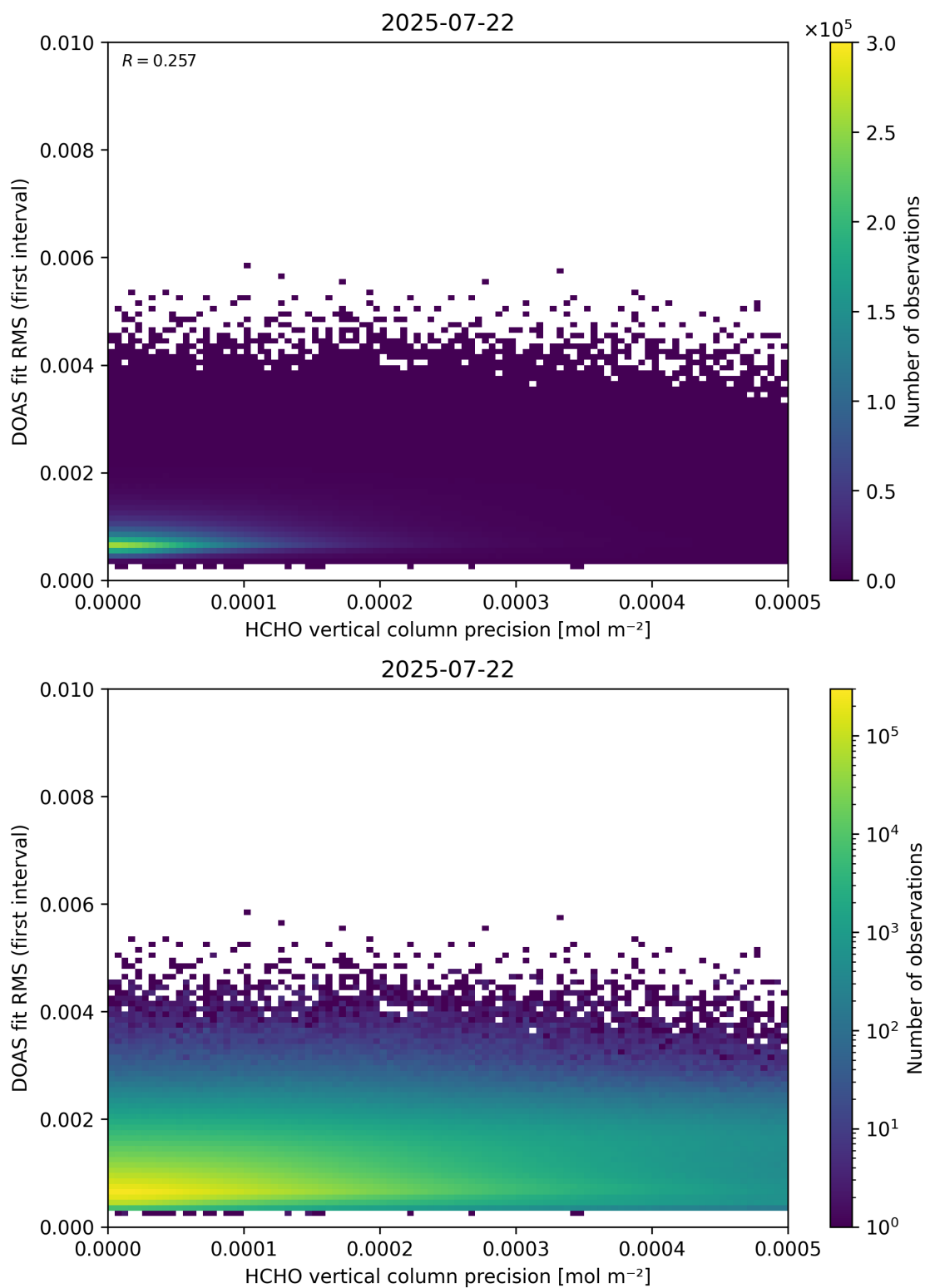
Figure 136: Scatter density plot of “HCHO vertical column precision” against “DOAS fit RMS (first interval)” for 2025-07-21 to 2025-07-23.
