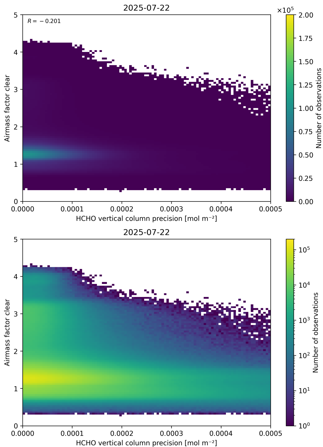
Figure 139: Scatter density plot of “HCHO vertical column precision” against “Airmass factor clear” for 2025-07-21 to 2025-07-23.
