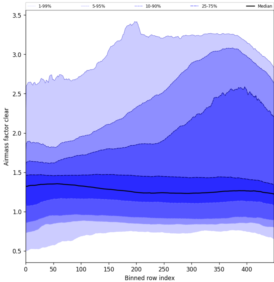
Figure 56: Along track statistics of “Airmass factor clear” for 2025-07-22 to 2025-07-24
