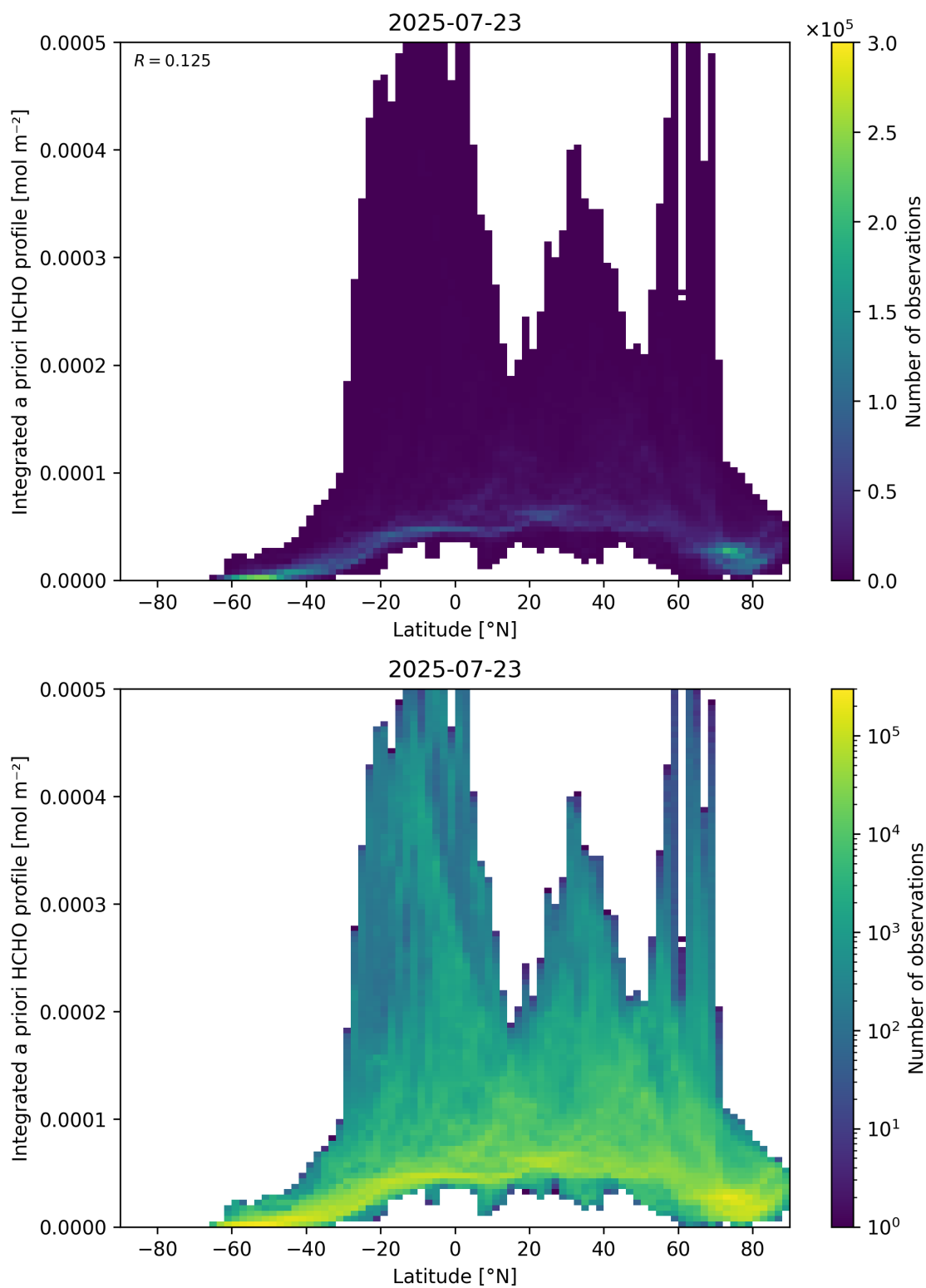
Figure 166: Scatter density plot of “Latitude” against “Integrated a priori HCHO profile” for 2025-07-22 to 2025-07-24.
