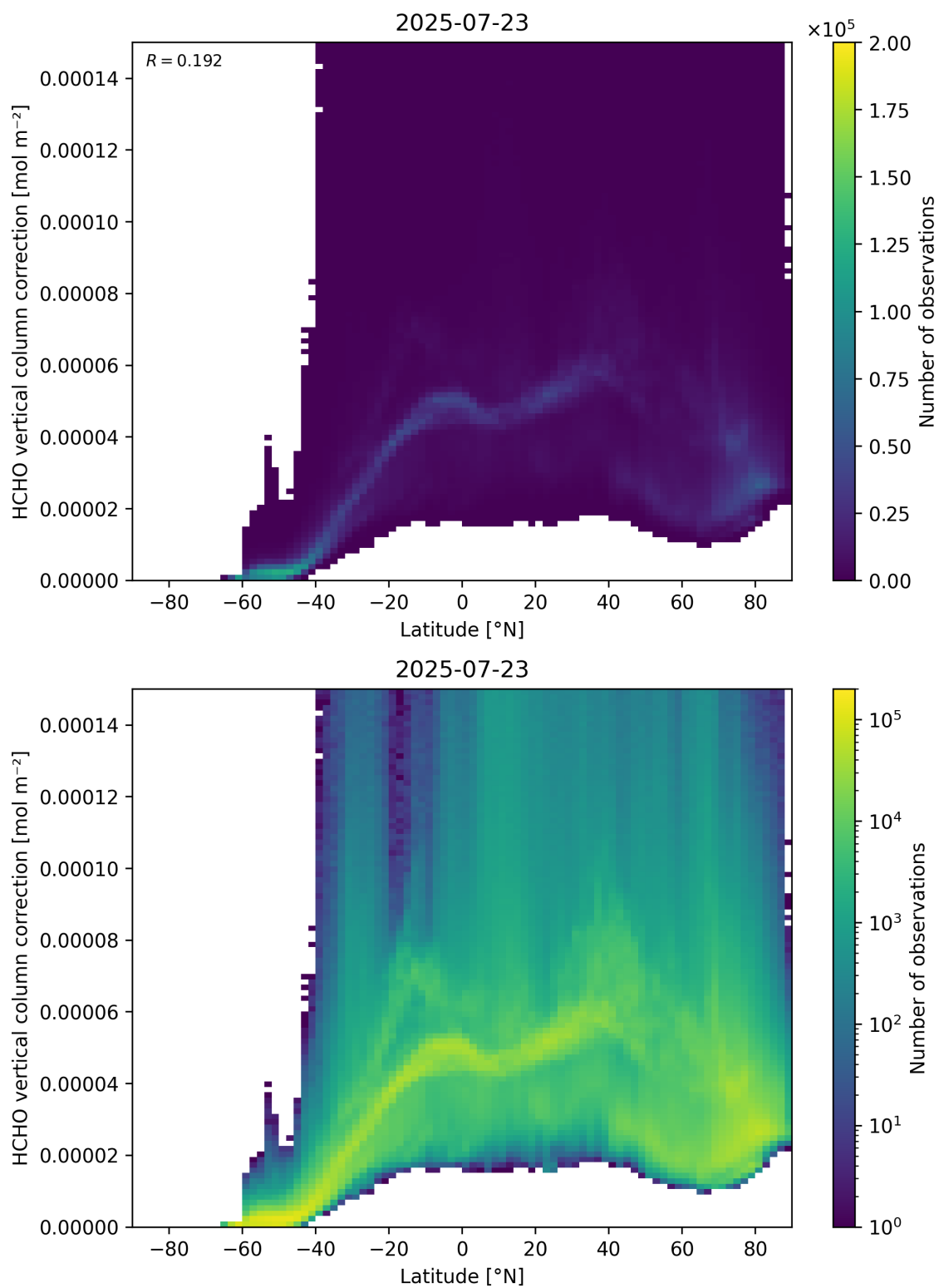
Figure 164: Scatter density plot of “Latitude” against “HCHO vertical column correction” for 2025-07-22 to 2025-07-24.
