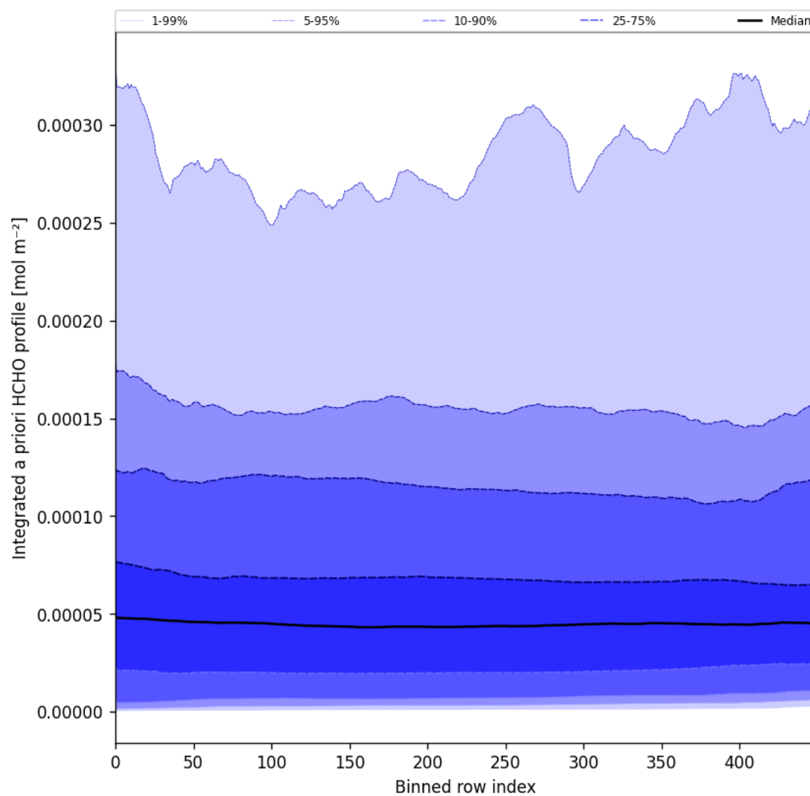
Figure 57: Along track statistics of "Integrated a priori HCHO profile" for 2025-07-22 to 2025-07-24
