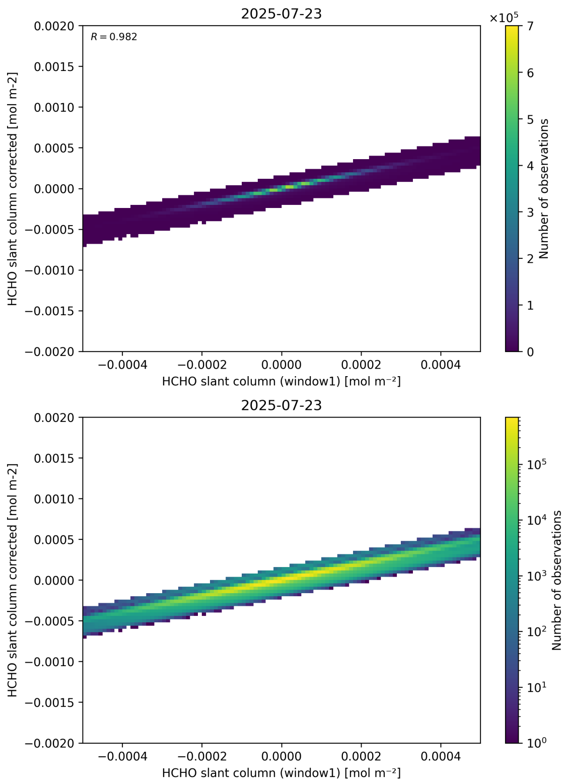
Figure 82: Scatter density plot of “HCHO slant column (window1)” against “HCHO slant column corrected” for 2025-07-22 to 2025-07-24.
