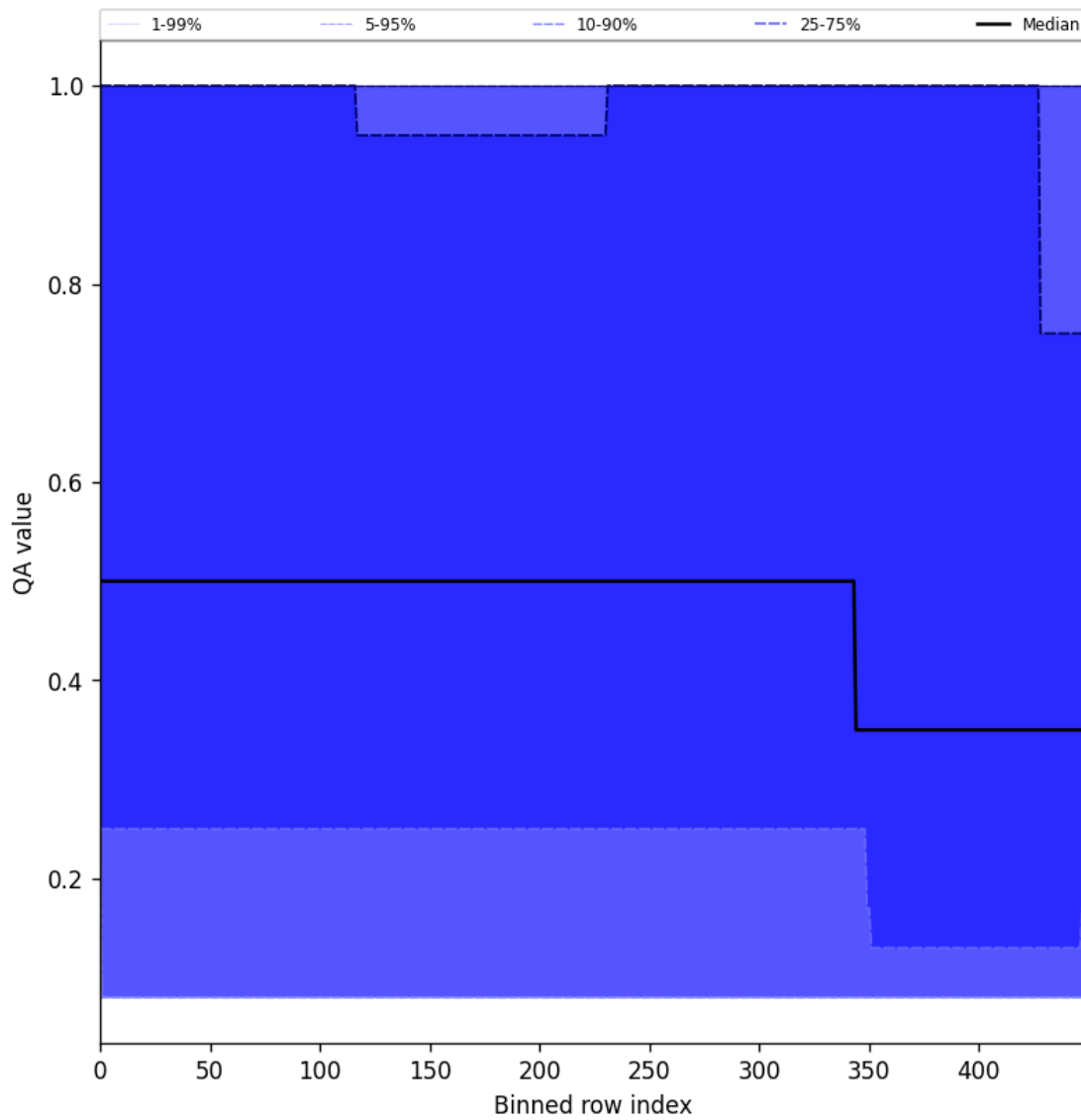
Figure 48: Along track statistics of “QA value” for 2025-07-22 to 2025-07-24
