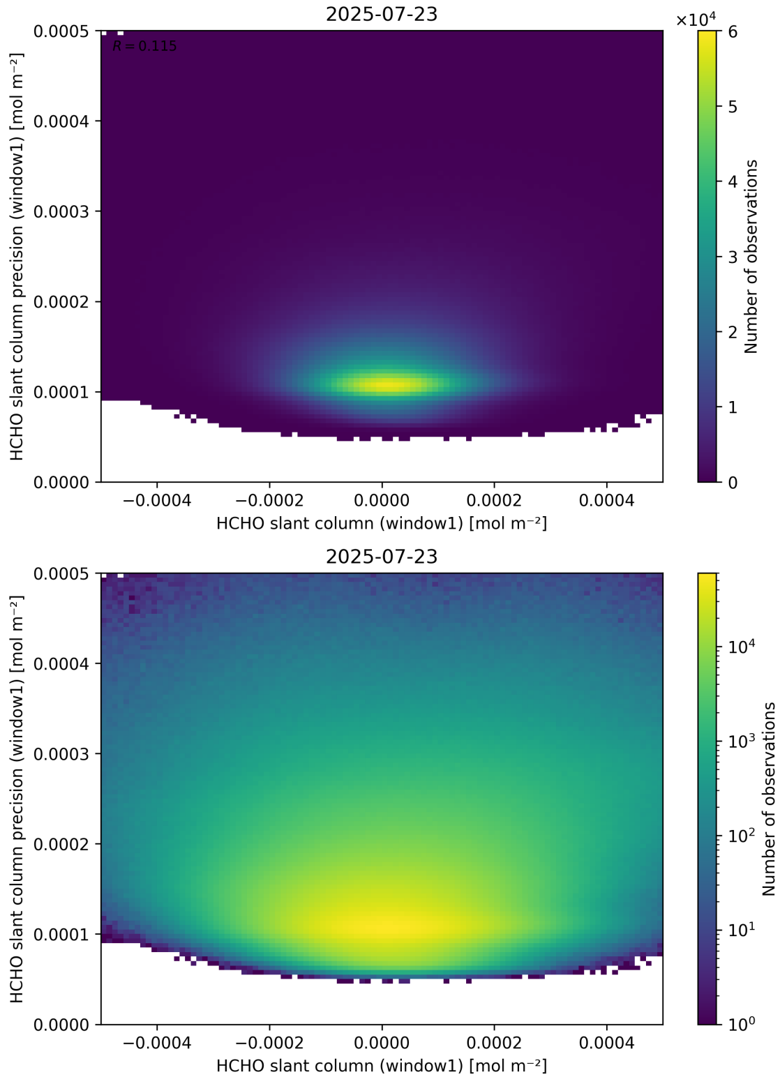
Figure 84: Scatter density plot of “HCHO slant column (window1)” against “HCHO slant column precision (window1)” for 2025-07-22 to 2025-07-24.
