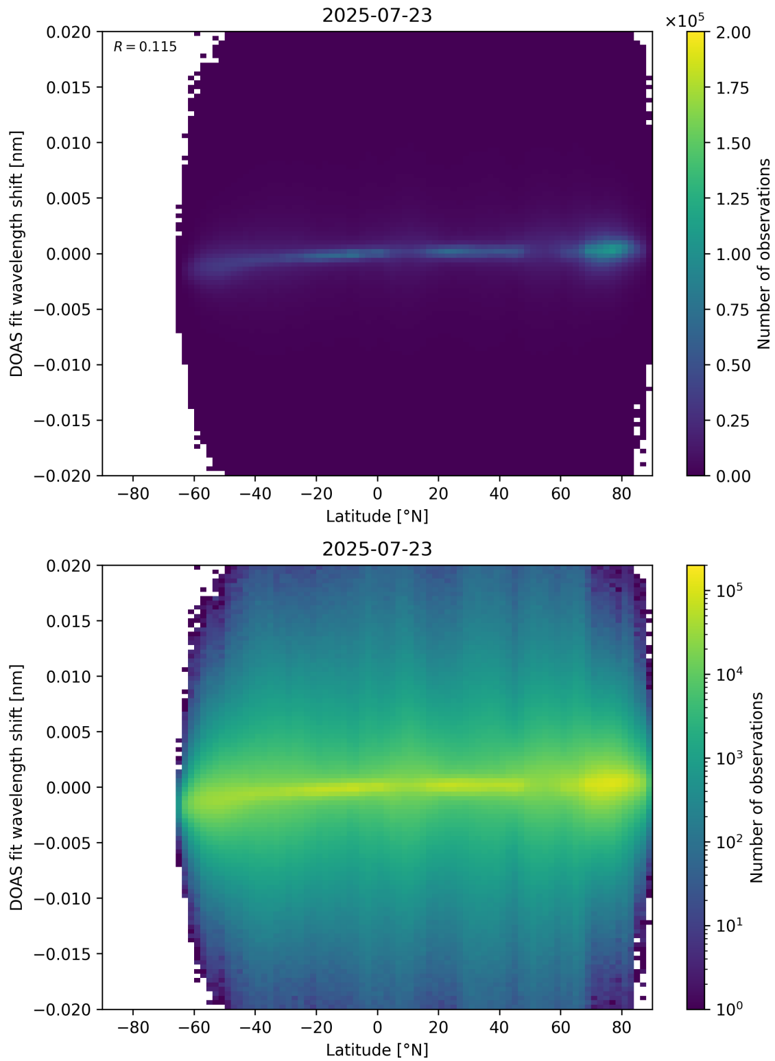
Figure 154: Scatter density plot of “Latitude” against “DOAS fit wavelength shift” for 2025-07-22 to 2025-07-24.
