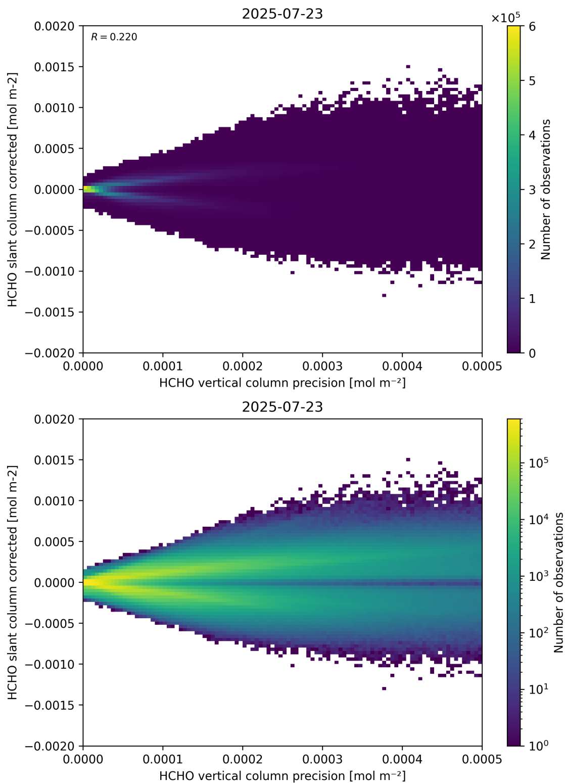
Figure 140: Scatter density plot of “HCHO vertical column precision” against “HCHO slant column corrected” for 2025-07-22 to 2025-07-24.
