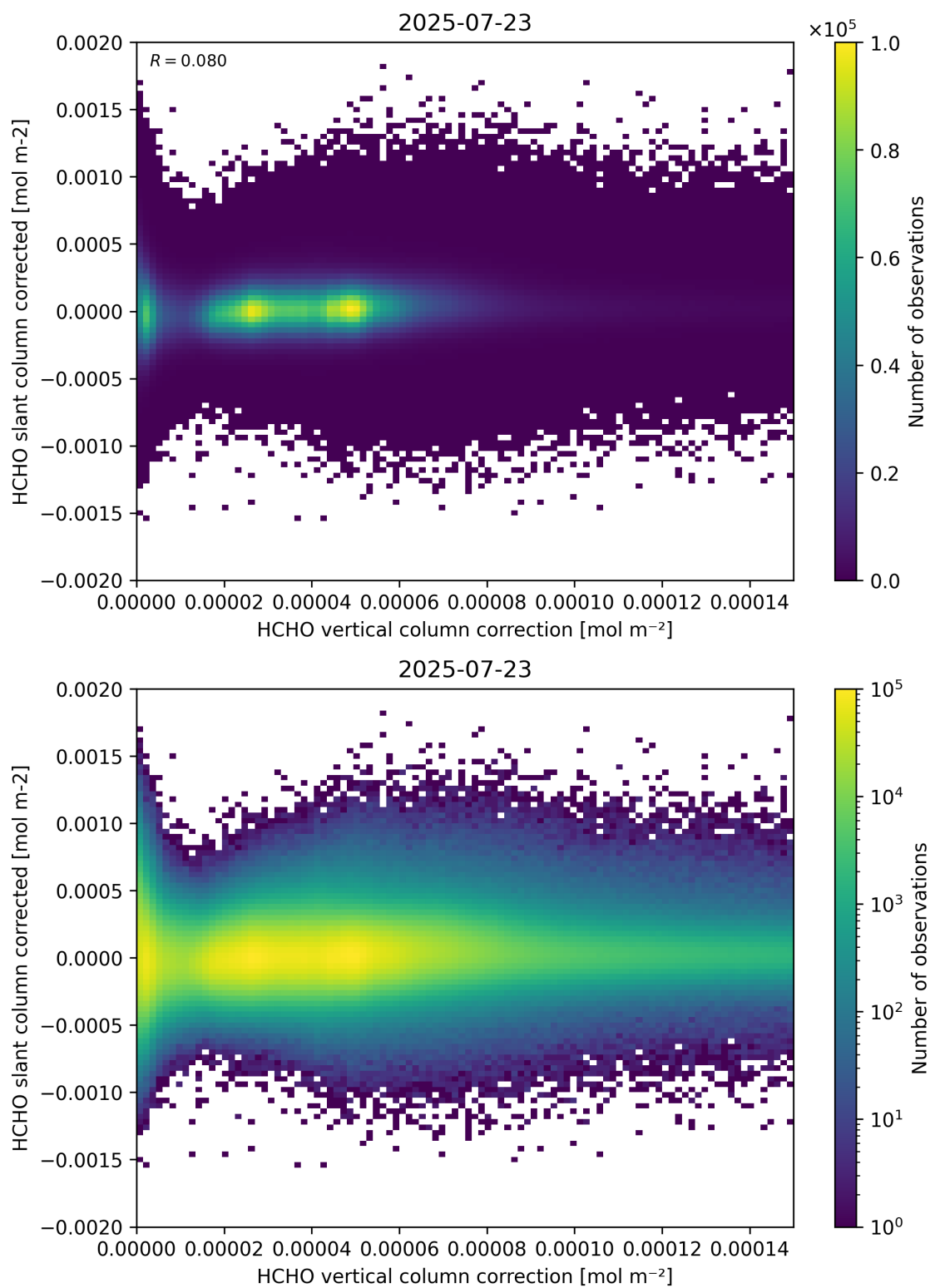
Figure 116: Scatter density plot of “HCHO vertical column correction” against “HCHO slant column corrected” for 2025-07-22 to 2025-07-24.
