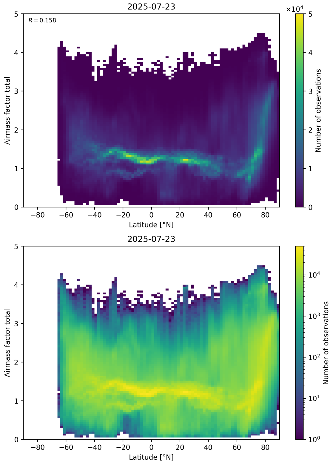
Figure 161: Scatter density plot of “Latitude” against “Airmass factor total” for 2025-07-22 to 2025-07-24.
