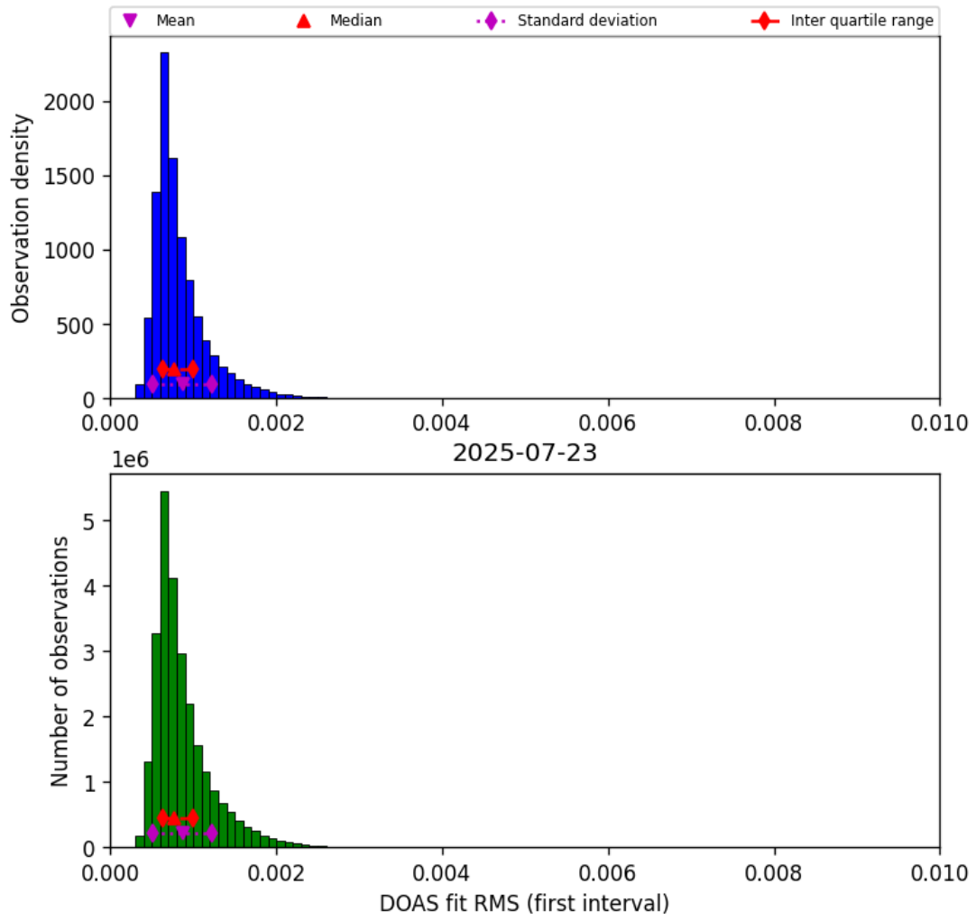
Figure 46: Histogram of “DOAS fit RMS (first interval)” for 2025-07-22 to 2025-07-24
