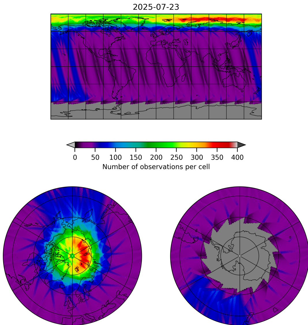
Figure 19: Map of the number of observations for 2025-07-22 to 2025-07-24
