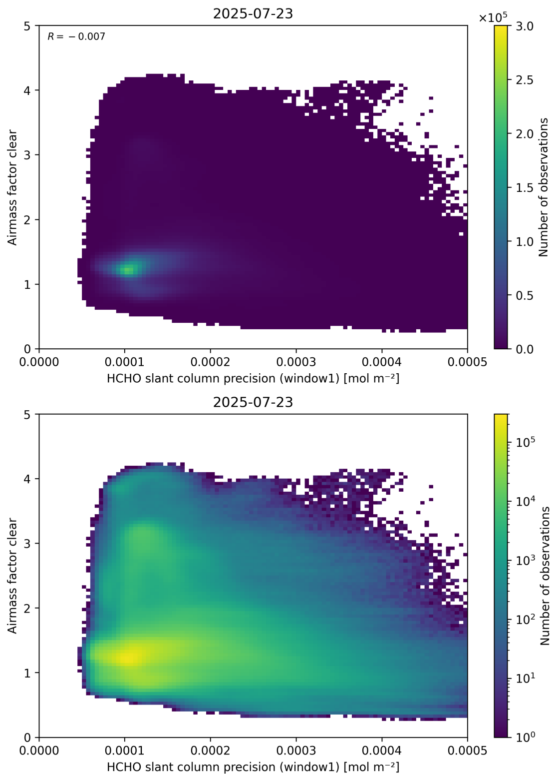
Figure 91: Scatter density plot of “HCHO slant column precision (window1)” against “Airmass factor clear” for 2025-07-22 to 2025-07-24.
