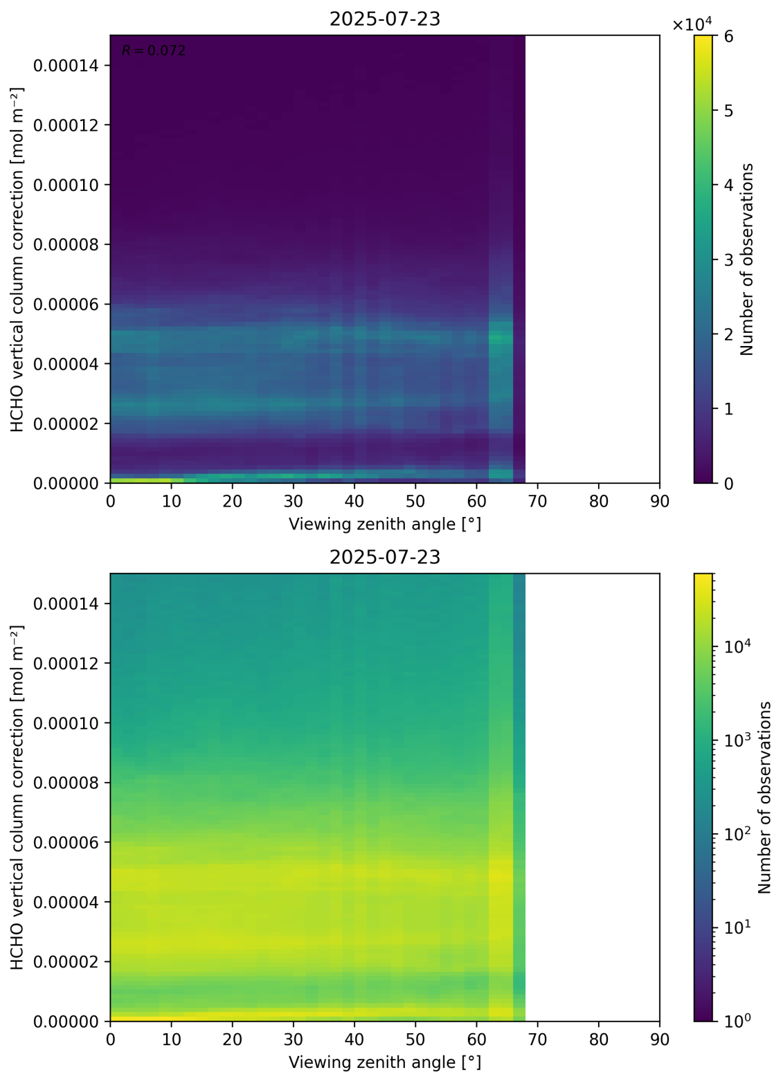
Figure 193: Scatter density plot of “Viewing zenith angle” against “HCHO vertical column correction” for 2025-07-22 to 2025-07-24.
