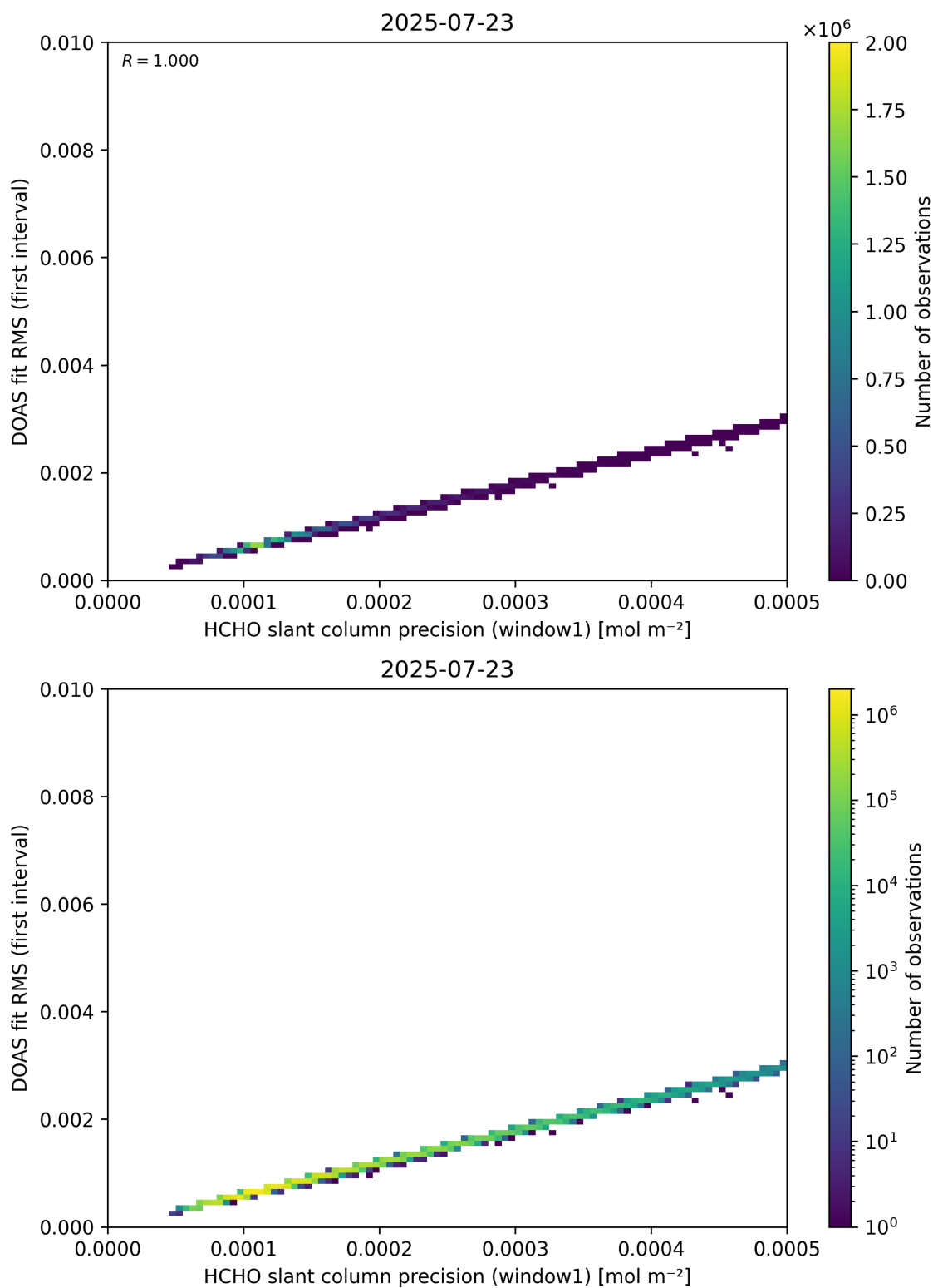
Figure 88: Scatter density plot of “HCHO slant column precision (window1)” against “DOAS fit RMS (first interval)” for 2025-07-22 to 2025-07-24.
