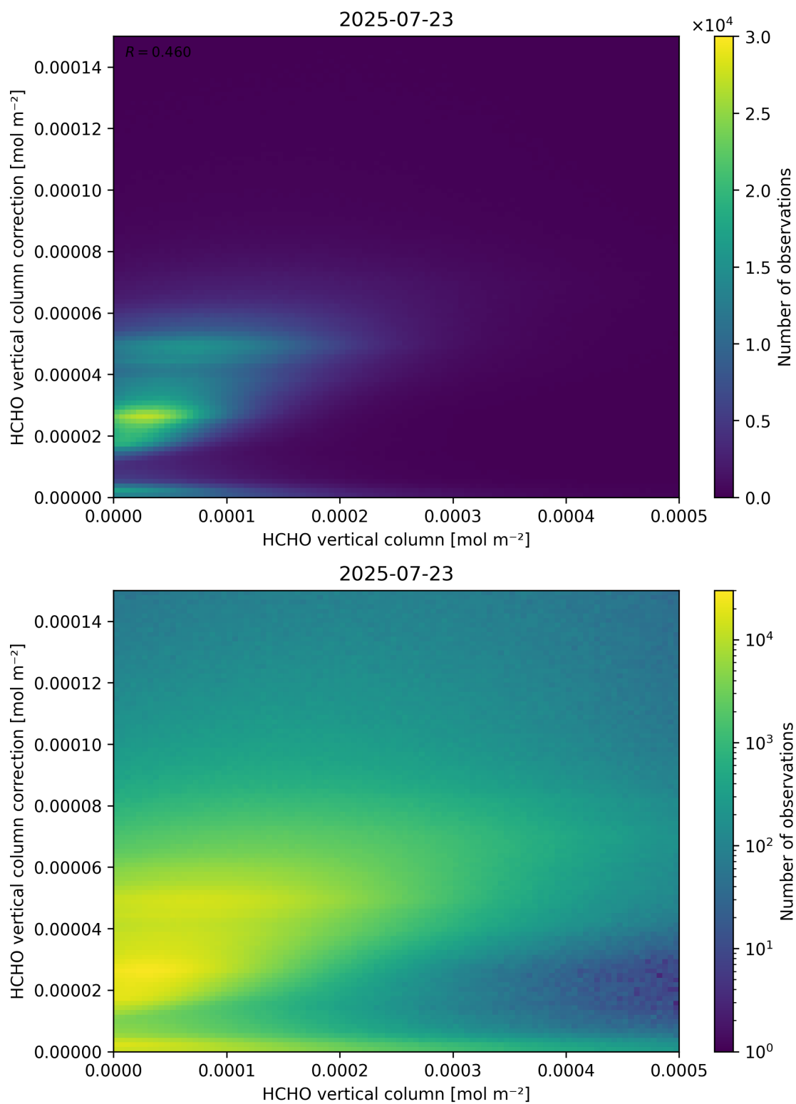
Figure 133: Scatter density plot of “HCHO vertical column” against “HCHO vertical column correction” for 2025-07-22 to 2025-07-24.
