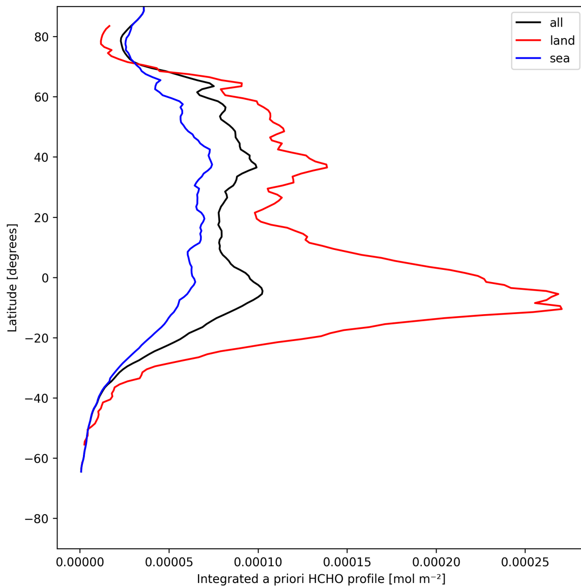
Figure 29: Zonal average of “Integrated a priori HCHO profile” for 2025-07-22 to 2025-07-24.
