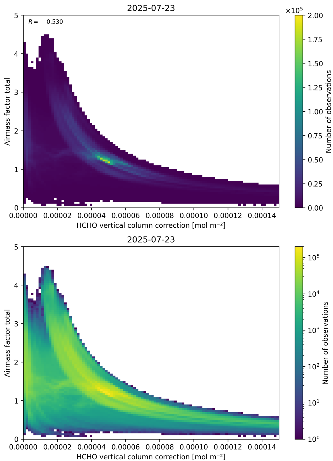
Figure 120: Scatter density plot of “HCHO vertical column correction” against “Airmass factor total” for 2025-07-22 to 2025-07-24.
