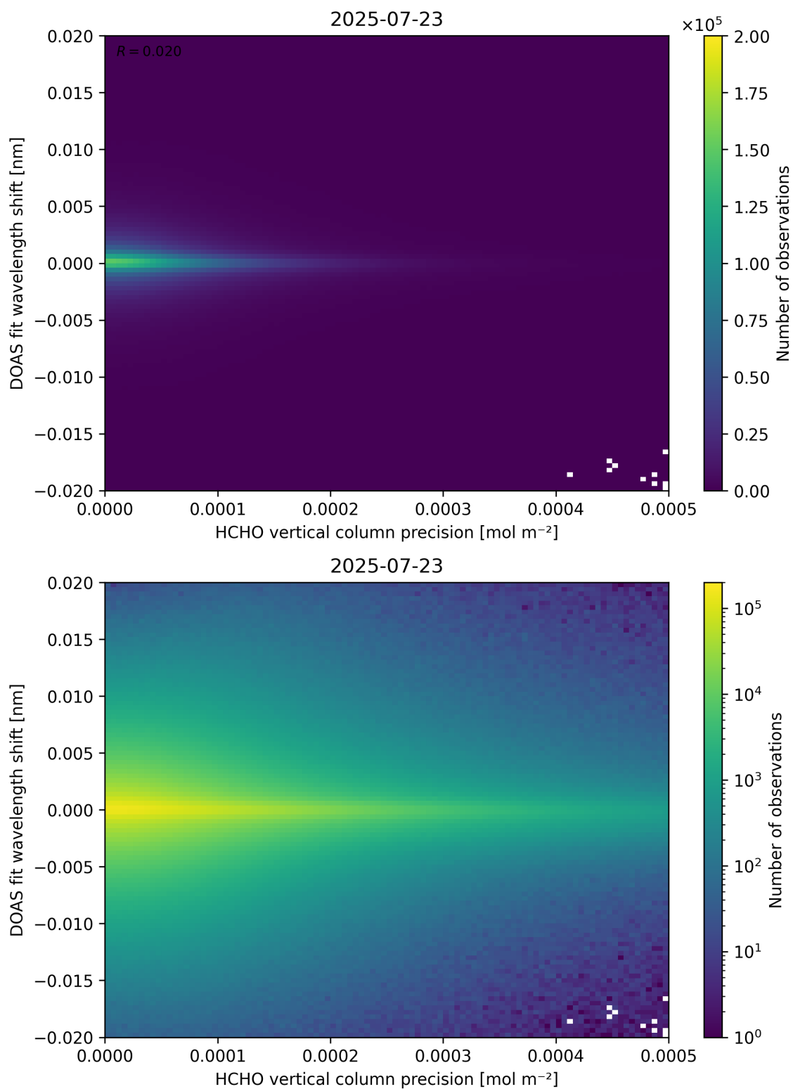
Figure 137: Scatter density plot of “HCHO vertical column precision” against “DOAS fit wavelength shift” for 2025-07-22 to 2025-07-24.
