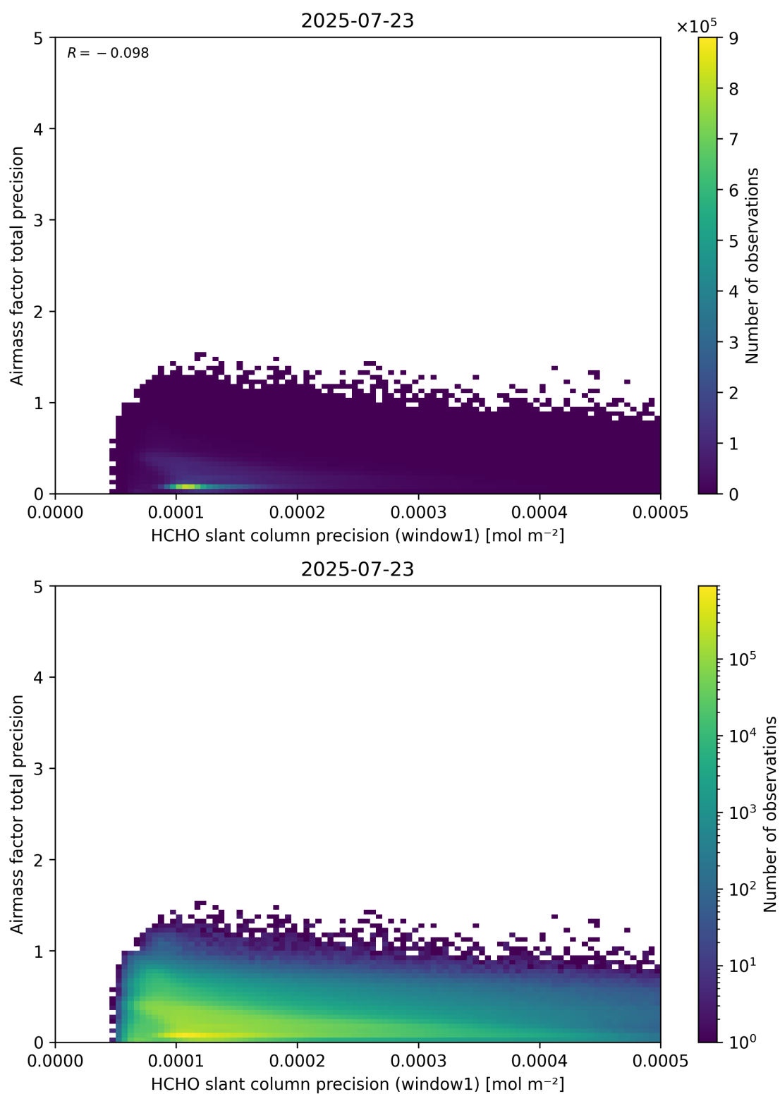
Figure 95: Scatter density plot of “HCHO slant column precision (window1)” against “Airmass factor total precision” for 2025-07-22 to 2025-07-24.
