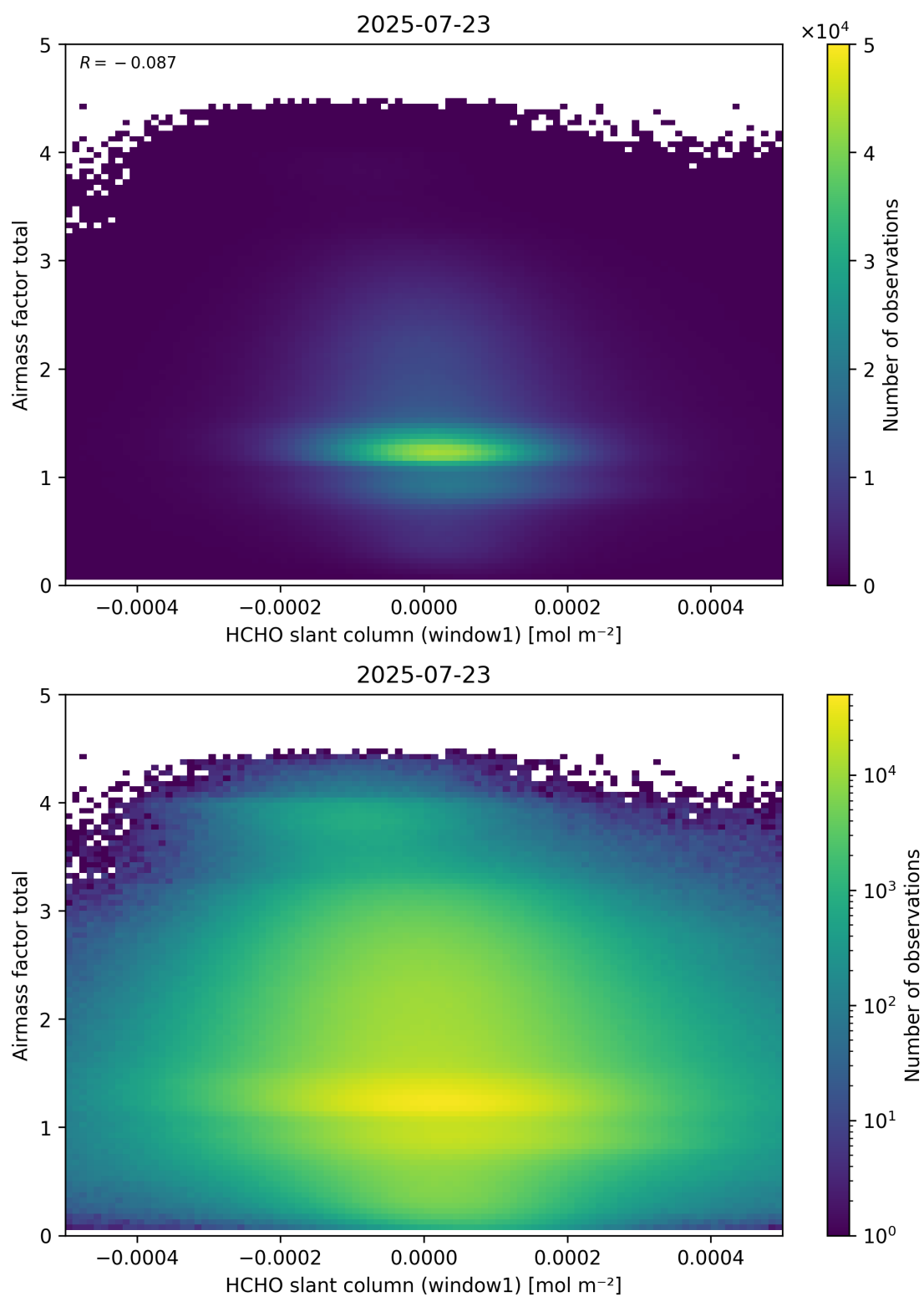
Figure 85: Scatter density plot of “HCHO slant column (window1)” against “Airmass factor total” for 2025-07-22 to 2025-07-24.
