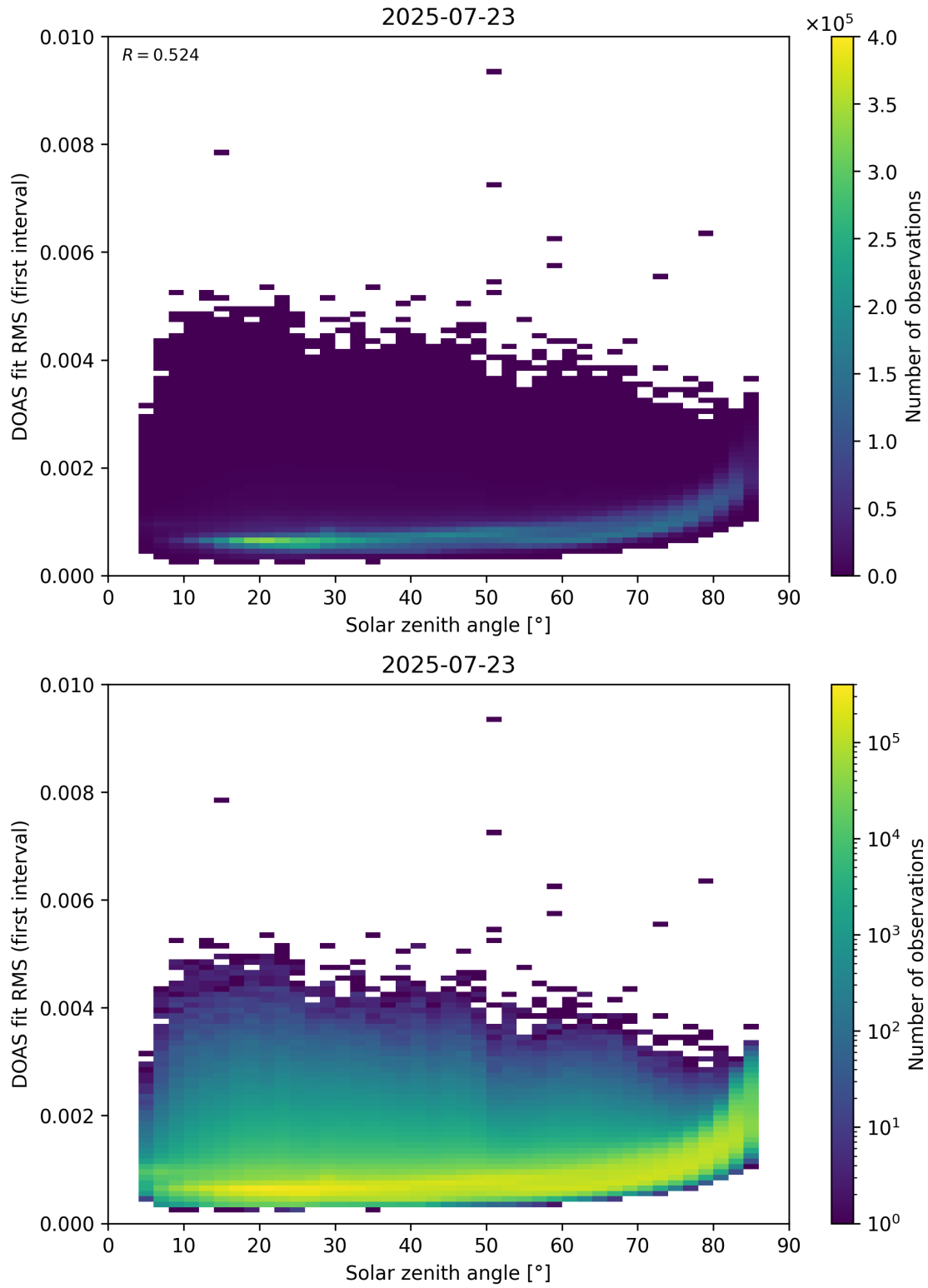
Figure 167: Scatter density plot of “Solar zenith angle” against “DOAS fit RMS (first interval)” for 2025-07-22 to 2025-07-24.
