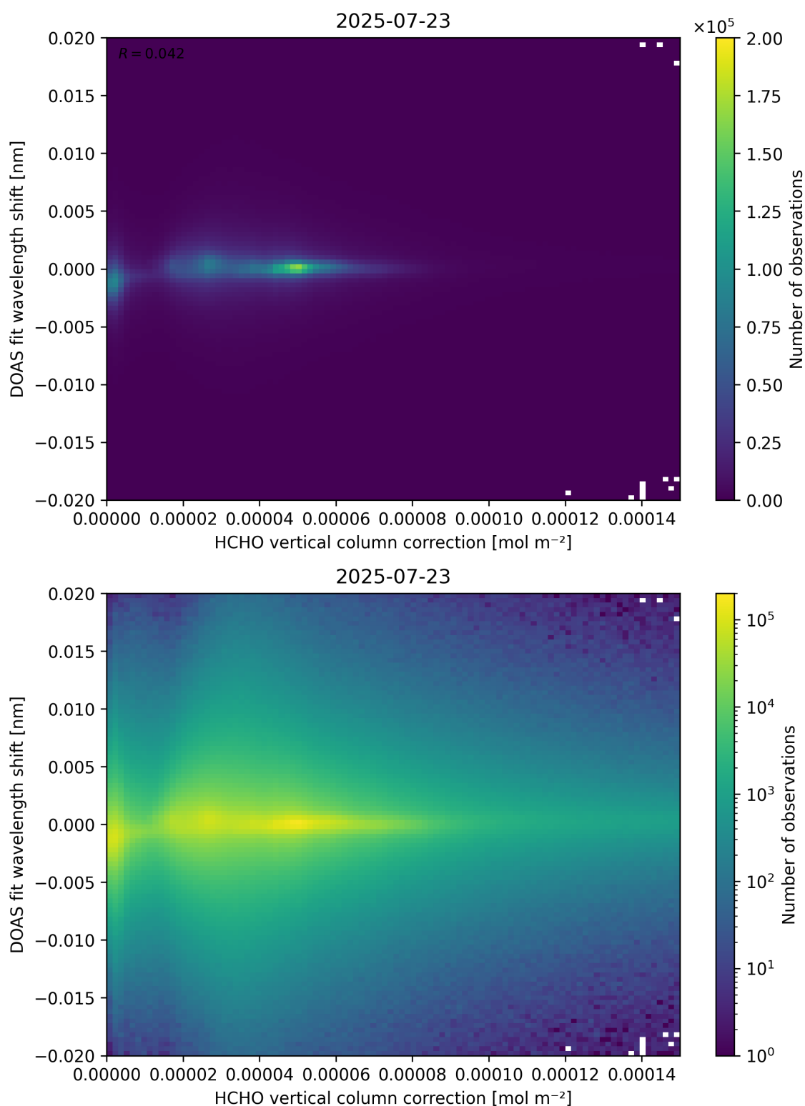
Figure 113: Scatter density plot of “HCHO vertical column correction” against “DOAS fit wavelength shift” for 2025-07-22 to 2025-07-24.
