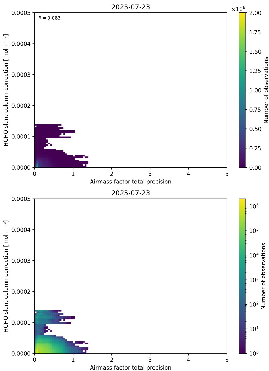
Figure 110: Scatter density plot of “Airmass factor total precision” against “HCHO slant column correction” for 2025-07-22 to 2025-07-24.
