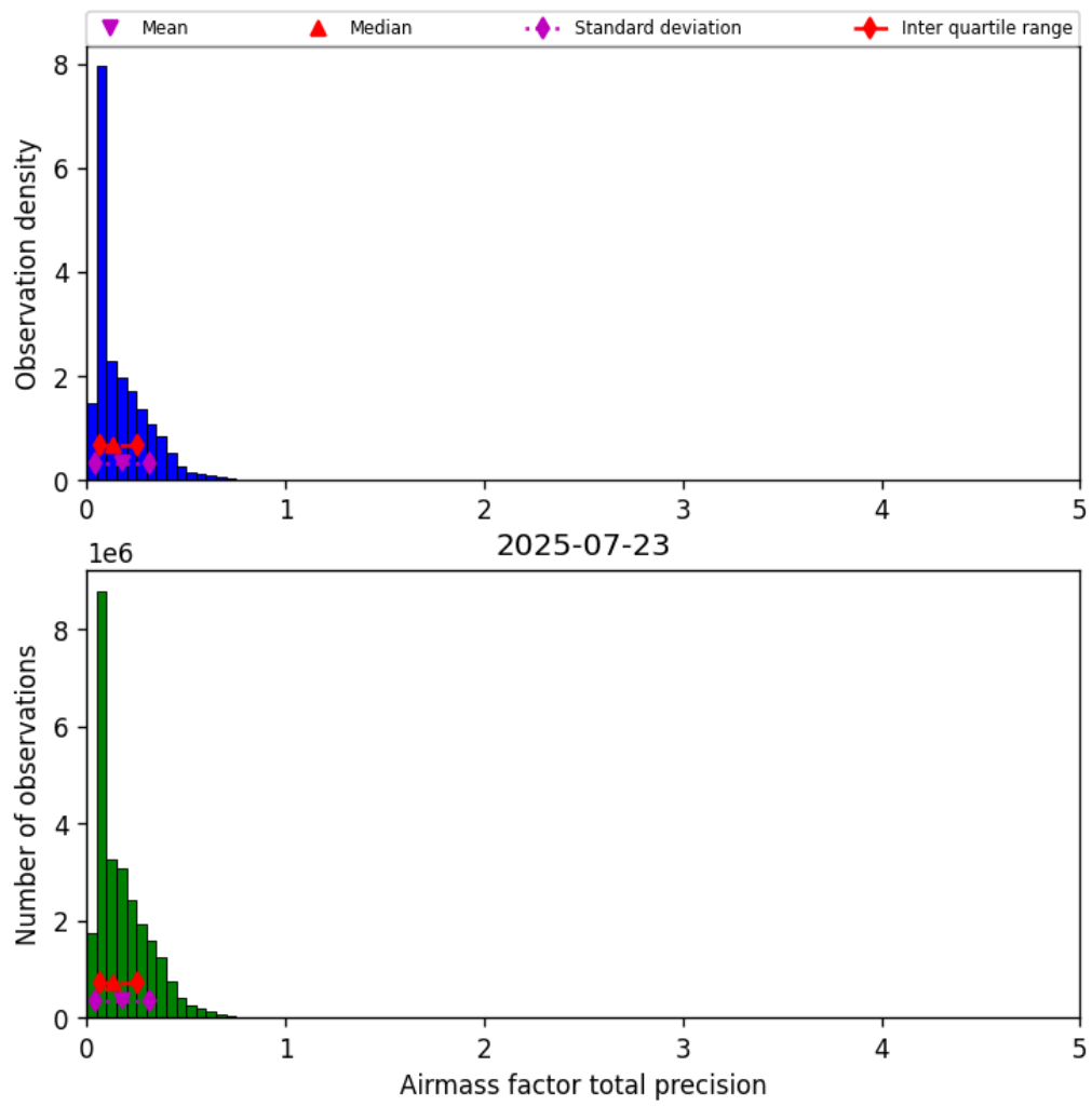
Figure 41: Histogram of “Airmass factor total precision” for 2025-07-22 to 2025-07-24
