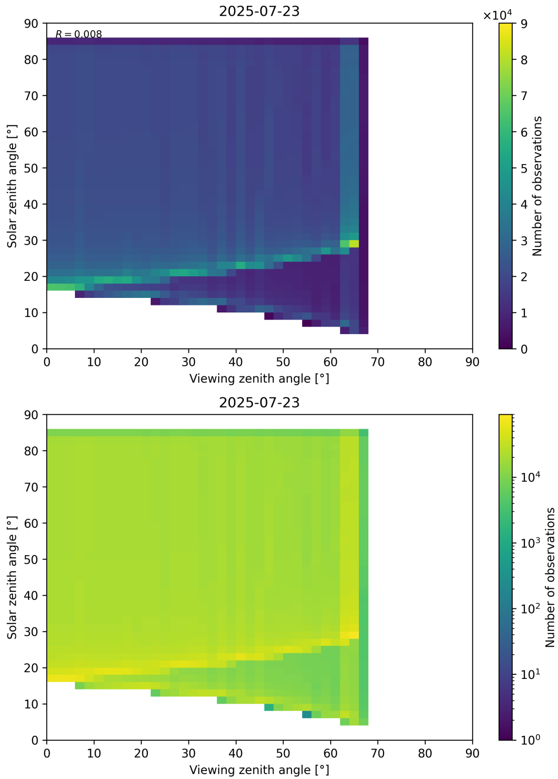
Figure 197: Scatter density plot of “Viewing zenith angle” against “Solar zenith angle” for 2025-07-22 to 2025-07-24.
