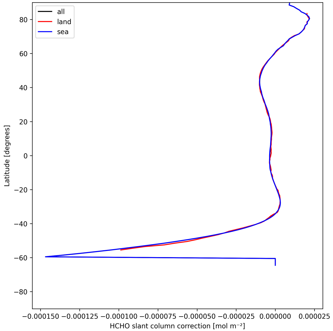
Figure 33: Zonal average of “HCHO slant column correction” for 2025-07-22 to 2025-07-24.
