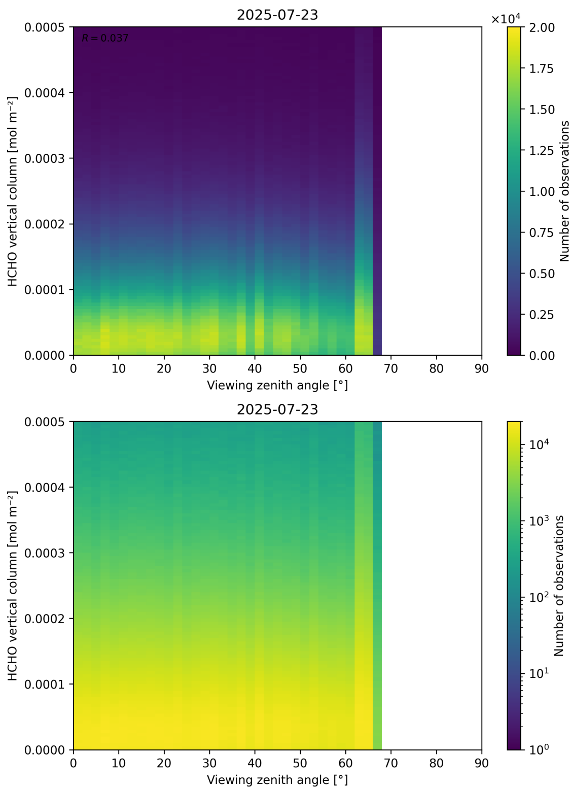
Figure 192: Scatter density plot of “Viewing zenith angle” against “HCHO vertical column” for 2025-07-22 to 2025-07-24.
