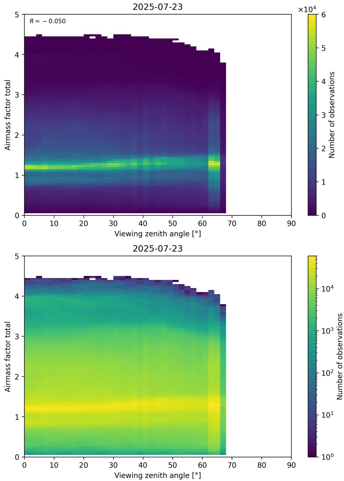
Figure 190: Scatter density plot of “Viewing zenith angle” against “Airmass factor total” for 2025-07-22 to 2025-07-24.
