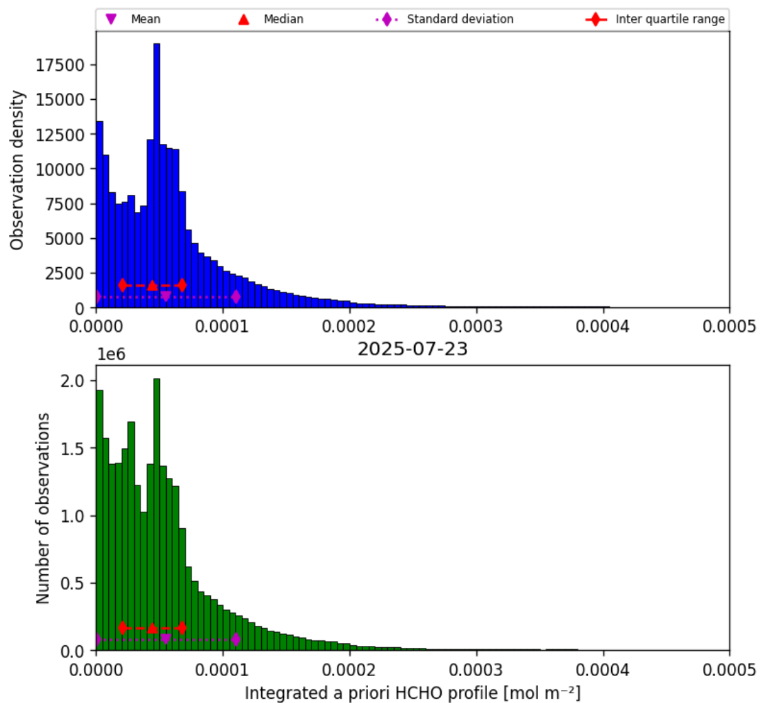
Figure 43: Histogram of “Integrated a priori HCHO profile” for 2025-07-22 to 2025-07-24
