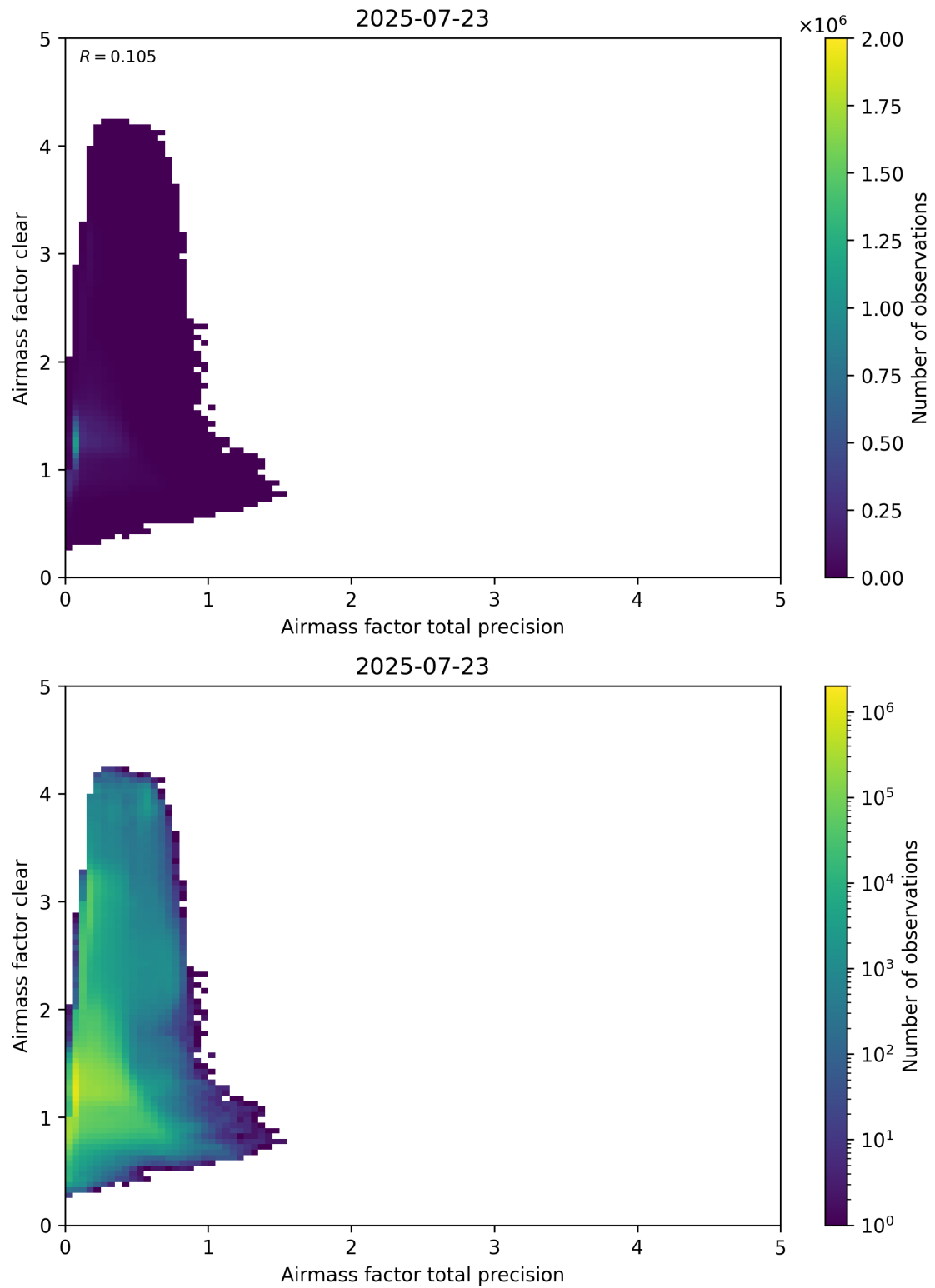
Figure 108: Scatter density plot of “Airmass factor total precision” against “Airmass factor clear” for 2025-07-22 to 2025-07-24.
