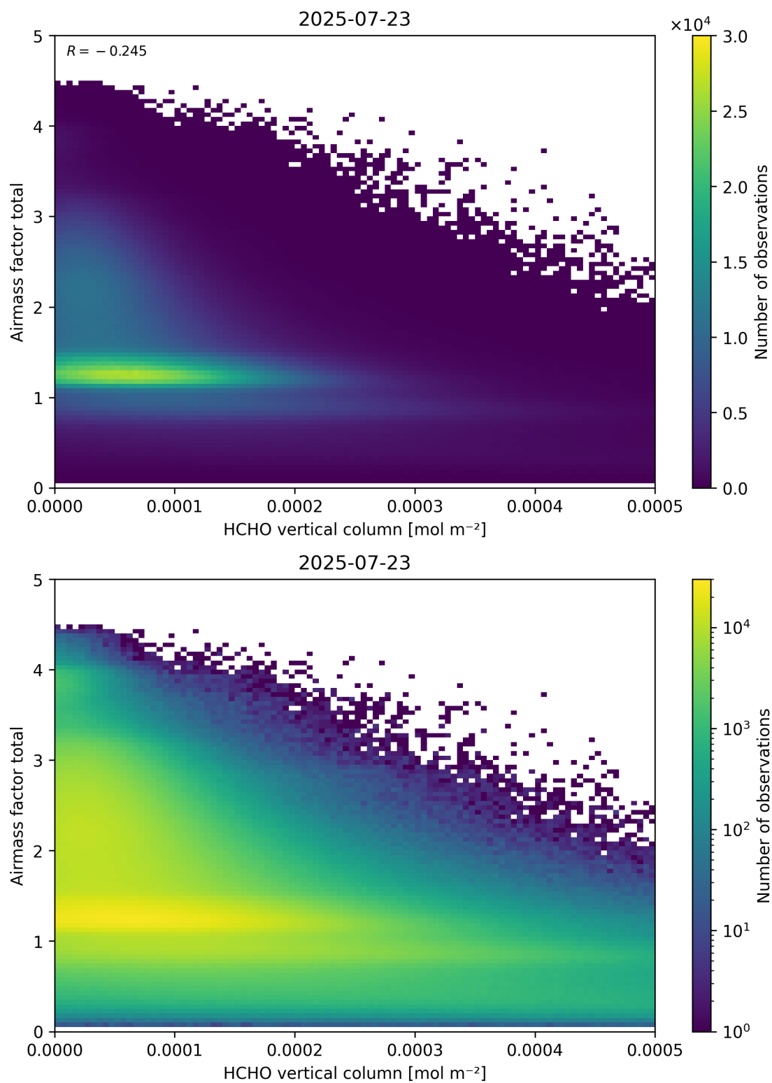
Figure 131: Scatter density plot of “HCHO vertical column” against “Airmass factor total” for 2025-07-22 to 2025-07-24.
