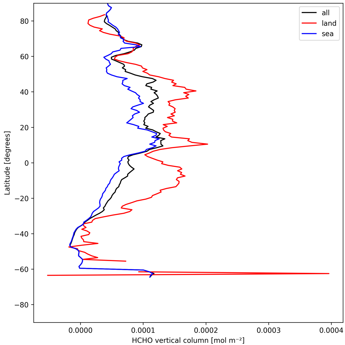
Figure 21: Zonal average of “HCHO vertical column” for 2025-07-22 to 2025-07-24.
