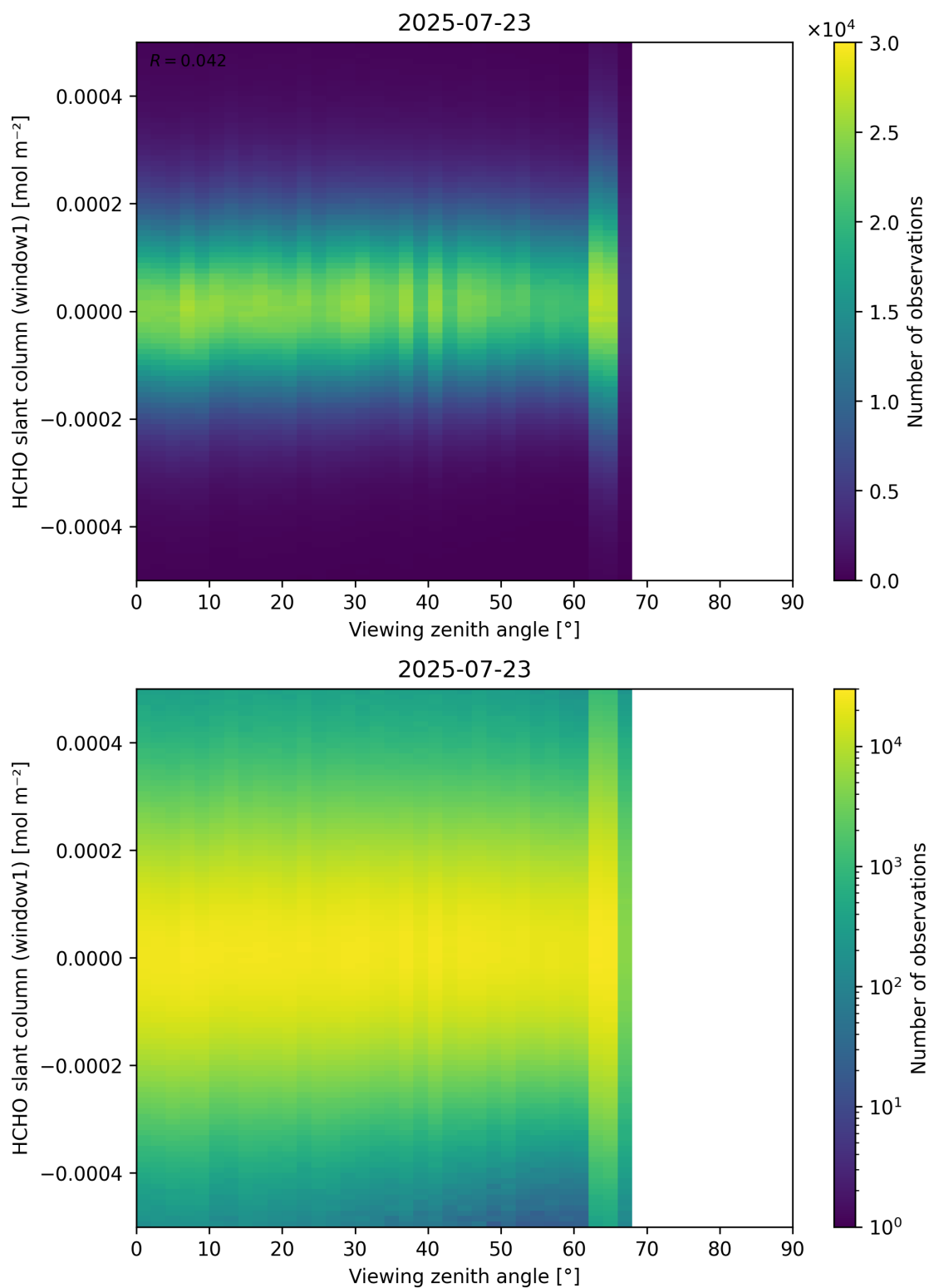
Figure 188: Scatter density plot of “Viewing zenith angle” against “HCHO slant column (window1)” for 2025-07-22 to 2025-07-24.
