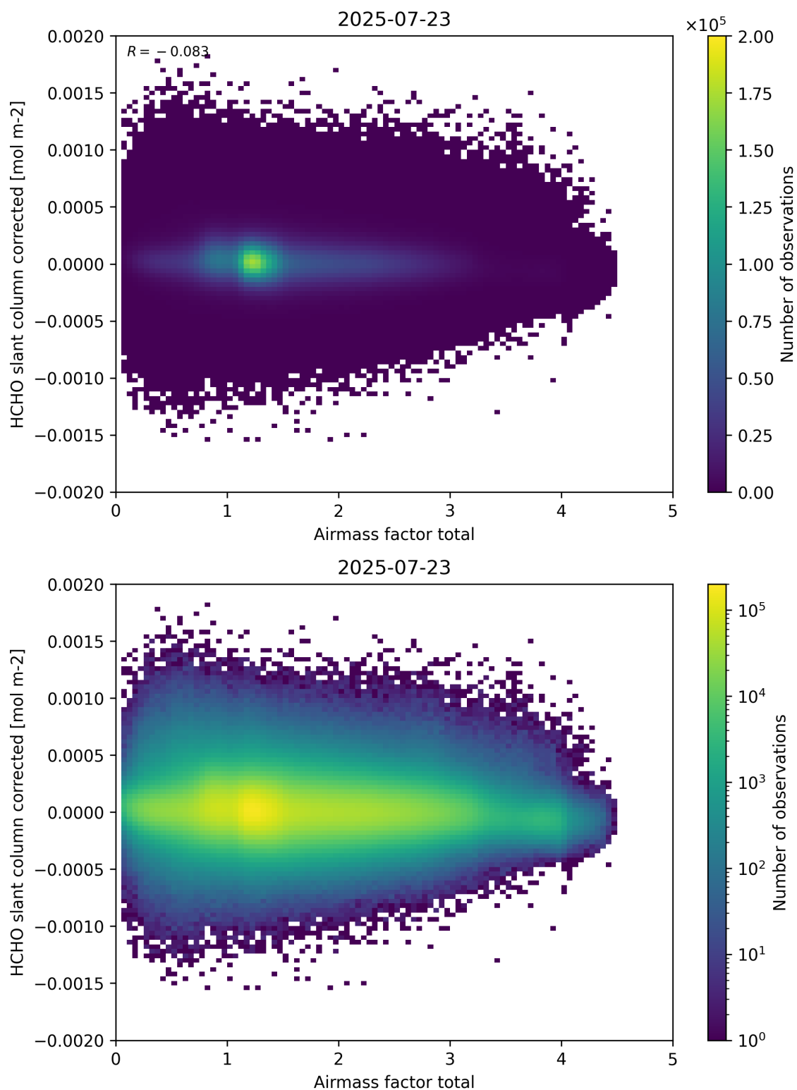
Figure 101: Scatter density plot of “Airmass factor total” against “HCHO slant column corrected” for 2025-07-22 to 2025-07-24.
