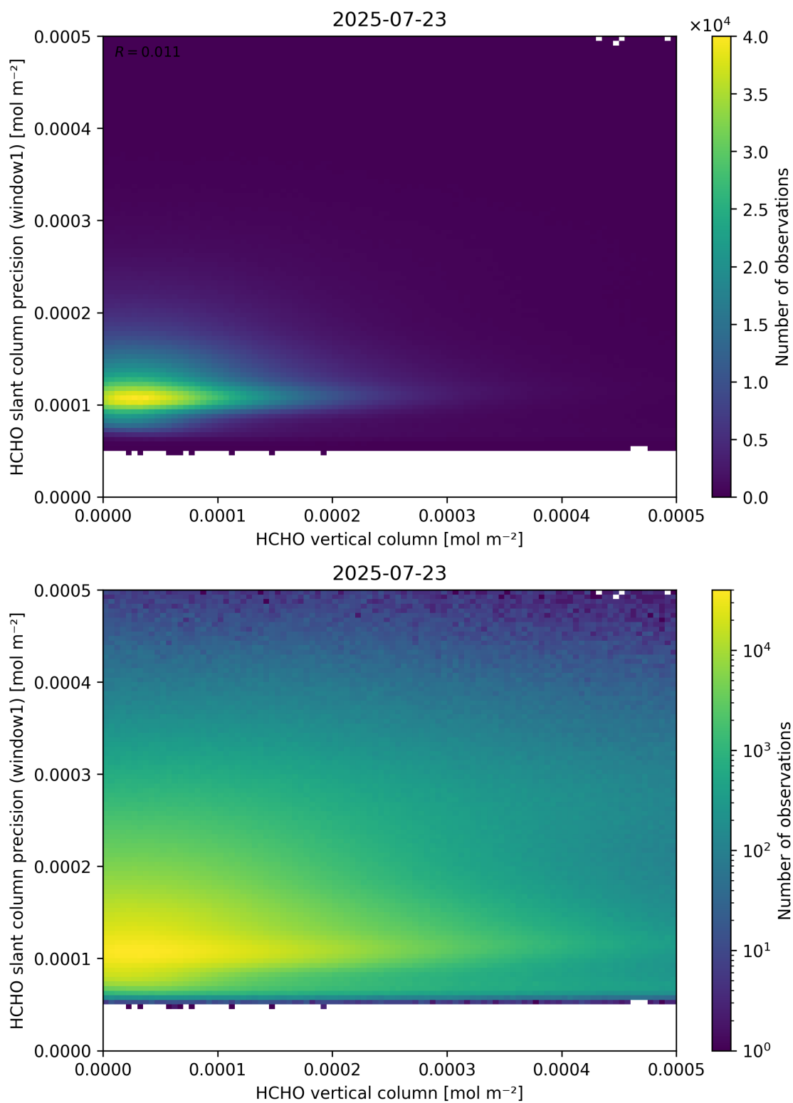
Figure 130: Scatter density plot of “HCHO vertical column” against “HCHO slant column precision (window1)” for 2025-07-22 to 2025-07-24.
