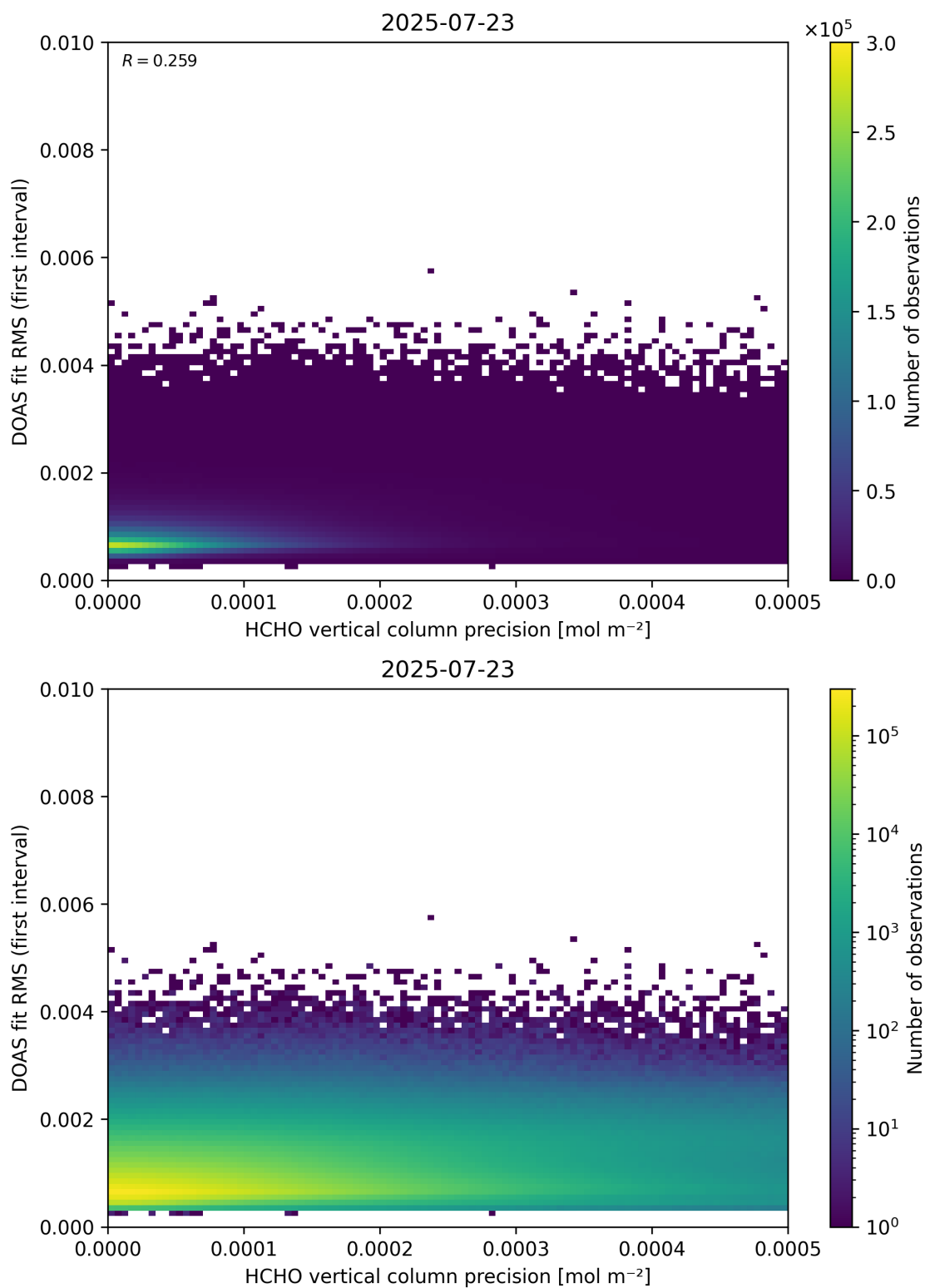
Figure 136: Scatter density plot of “HCHO vertical column precision” against “DOAS fit RMS (first interval)” for 2025-07-22 to 2025-07-24.
