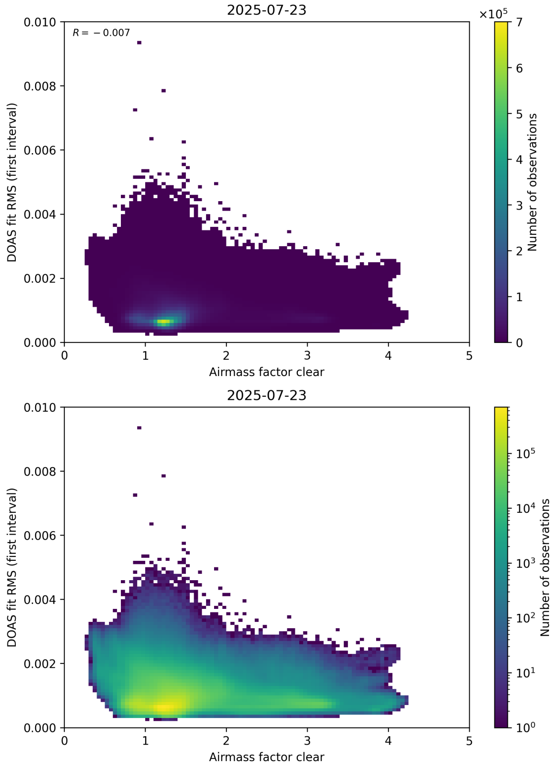
Figure 71: Scatter density plot of “Airmass factor clear” against “DOAS fit RMS (first interval)” for 2025-07-22 to 2025-07-24.
