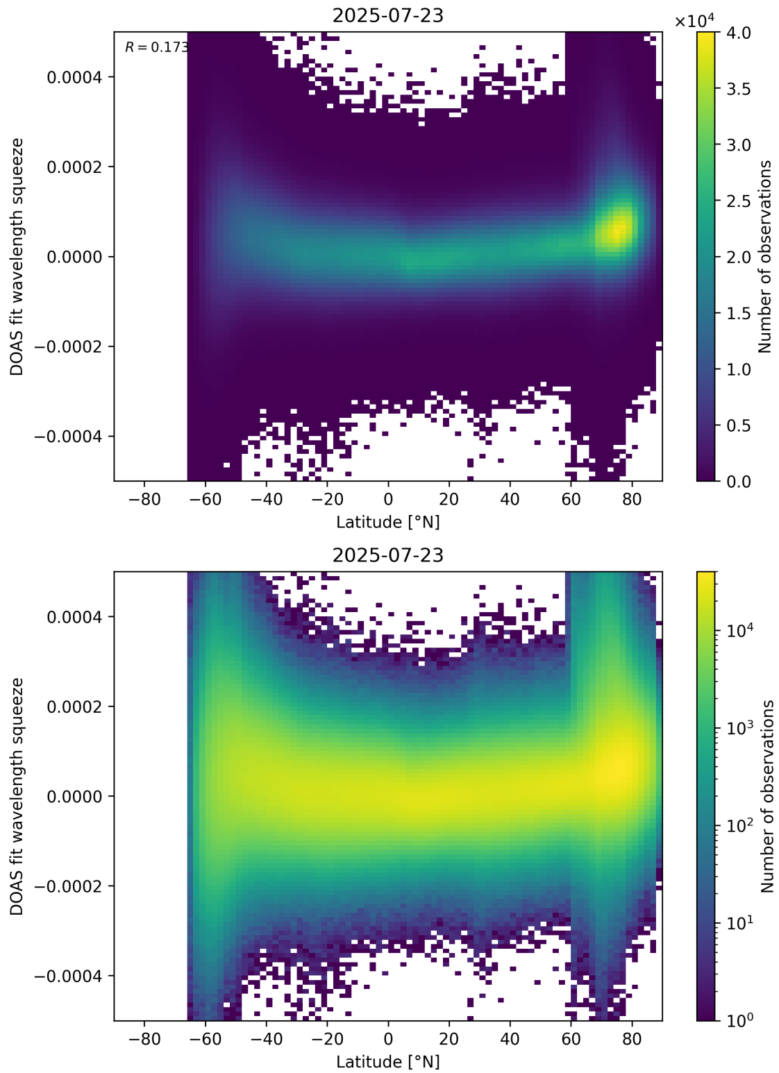
Figure 155: Scatter density plot of “Latitude” against “DOAS fit wavelength squeeze” for 2025-07-22 to 2025-07-24.
