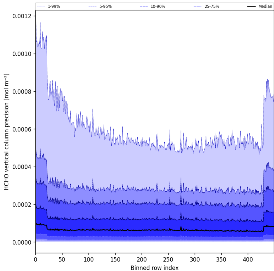
Figure 50: Along track statistics of “HCHO vertical column precision” for 2025-07-22 to 2025-07-24
