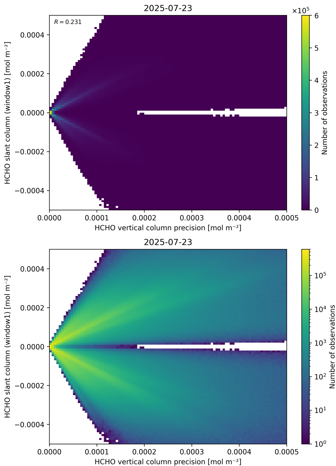
Figure 142: Scatter density plot of “HCHO vertical column precision” against “HCHO slant column (window1)” for 2025-07-22 to 2025-07-24.
