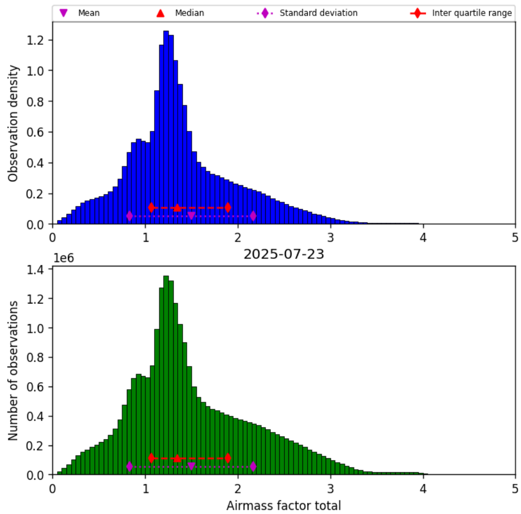
Figure 40: Histogram of “Airmass factor total” for 2025-07-22 to 2025-07-24
