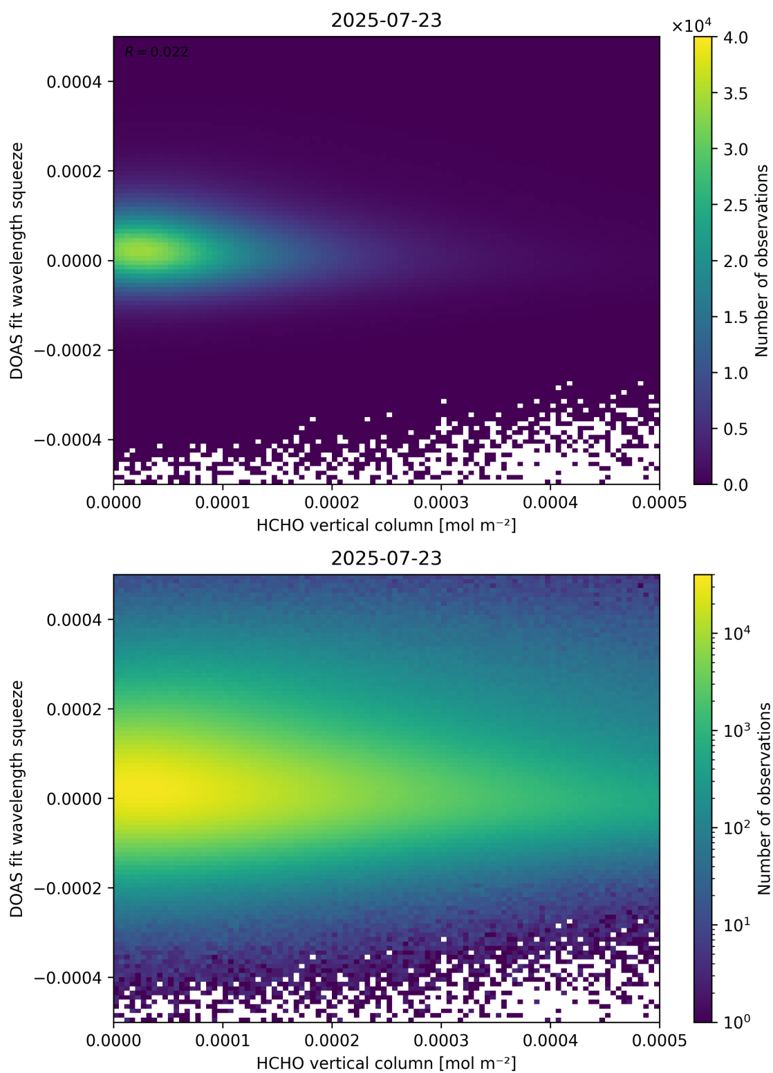
Figure 125: Scatter density plot of “HCHO vertical column” against “DOAS fit wavelength squeeze” for 2025-07-22 to 2025-07-24.
