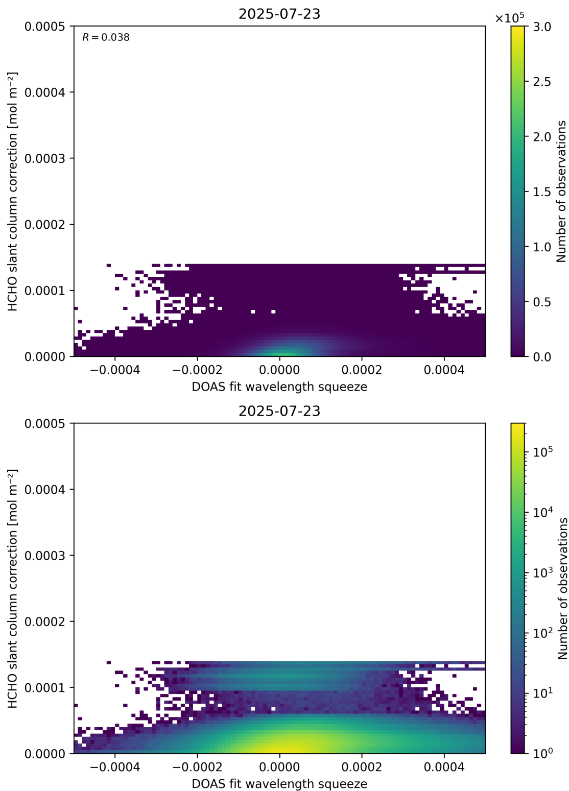
Figure 70: Scatter density plot of “DOAS fit wavelength squeeze” against “HCHO slant column correction” for 2025-07-22 to 2025-07-24.
