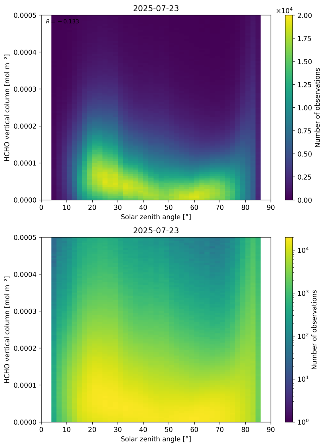
Figure 177: Scatter density plot of “Solar zenith angle” against “HCHO vertical column” for 2025-07-22 to 2025-07-24.
