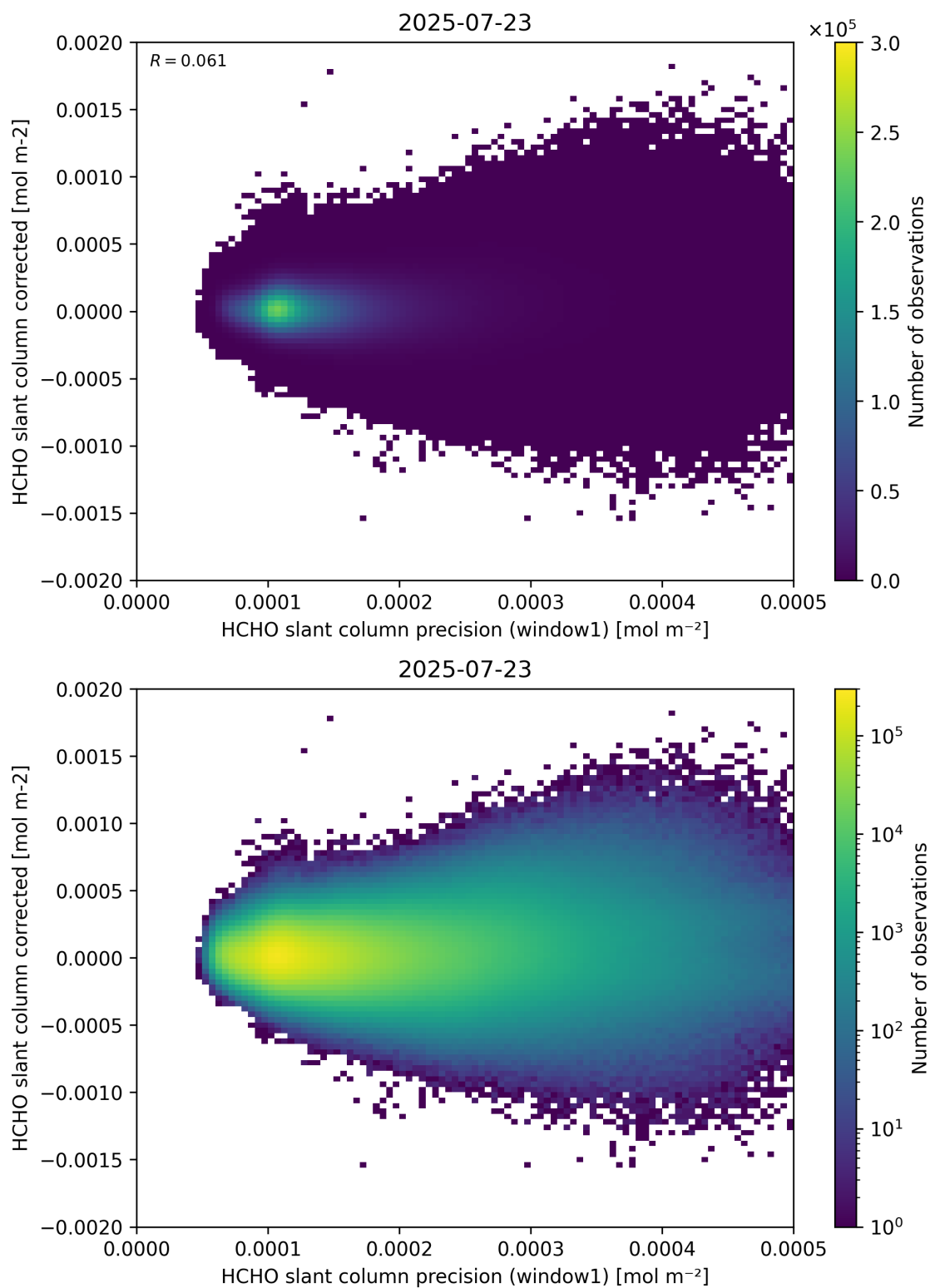
Figure 92: Scatter density plot of “HCHO slant column precision (window1)” against “HCHO slant column corrected” for 2025-07-22 to 2025-07-24.
