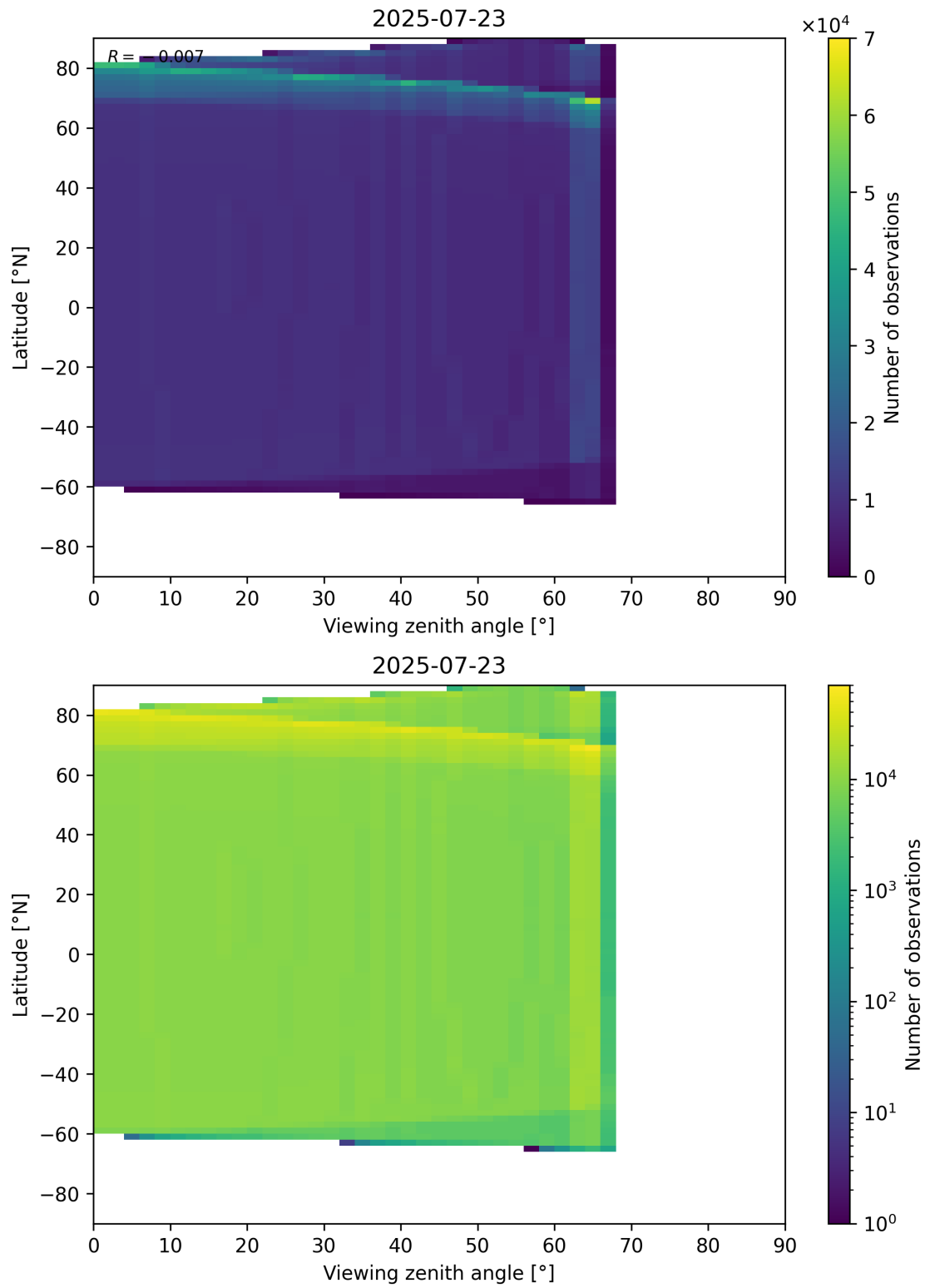
Figure 196: Scatter density plot of “Viewing zenith angle” against “Latitude” for 2025-07-22 to 2025-07-24.
