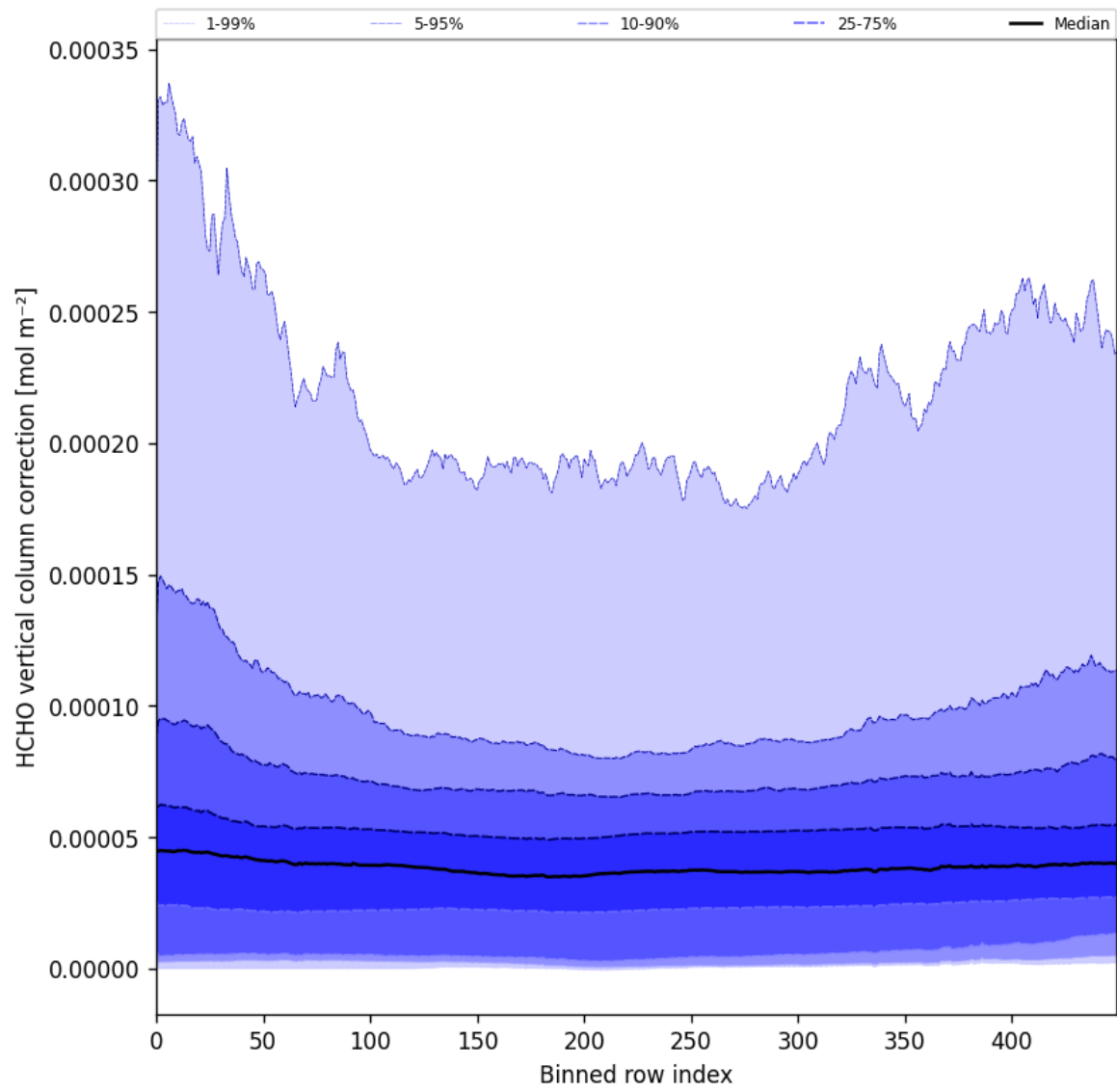
Figure 51: Along track statistics of “HCHO vertical column correction” for 2025-07-22 to 2025-07-24
