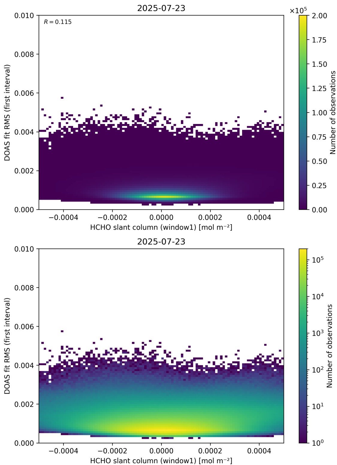
Figure 78: Scatter density plot of “HCHO slant column (window1)” against “DOAS fit RMS (first interval)” for 2025-07-22 to 2025-07-24.
