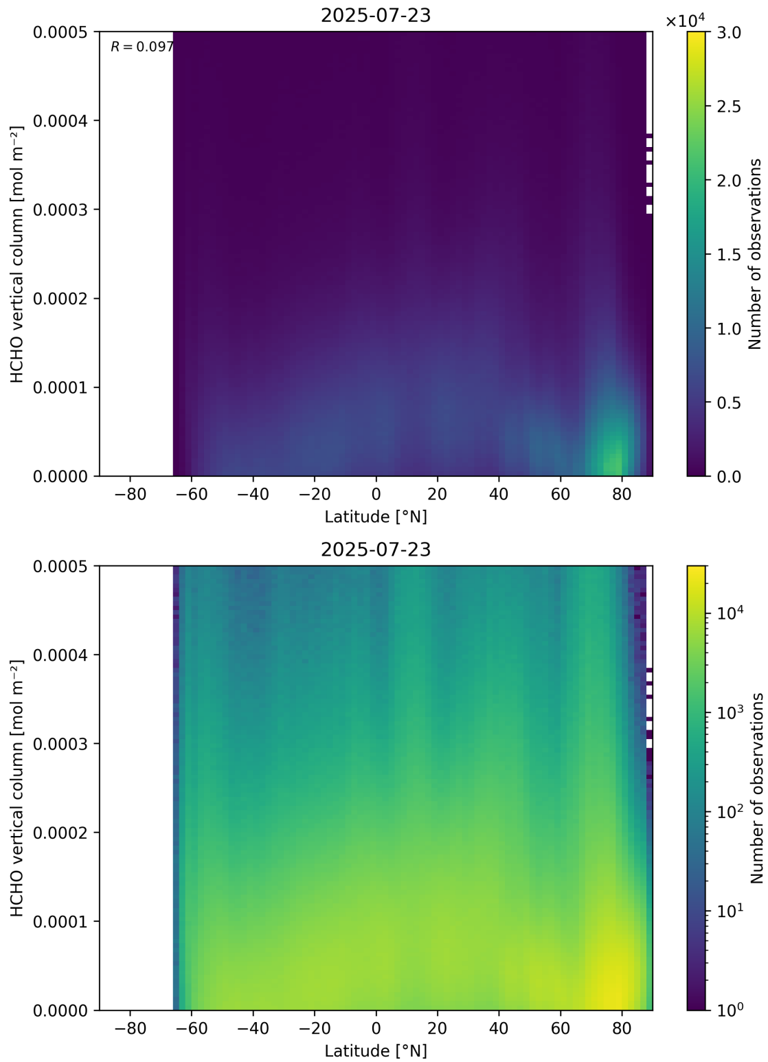
Figure 163: Scatter density plot of “Latitude” against “HCHO vertical column” for 2025-07-22 to 2025-07-24.
