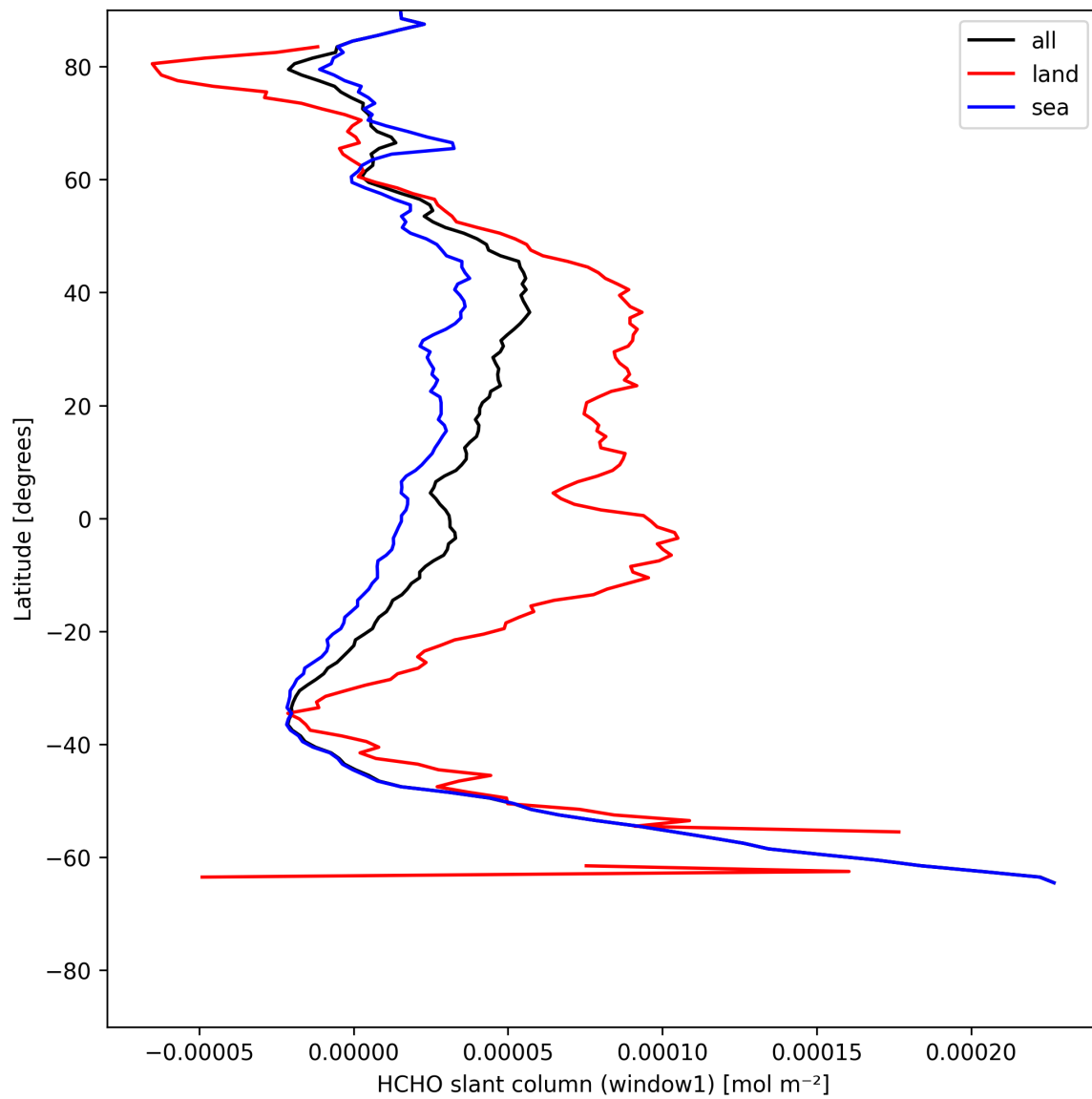
Figure 24: Zonal average of “HCHO slant column (window1)” for 2025-07-22 to 2025-07-24.
