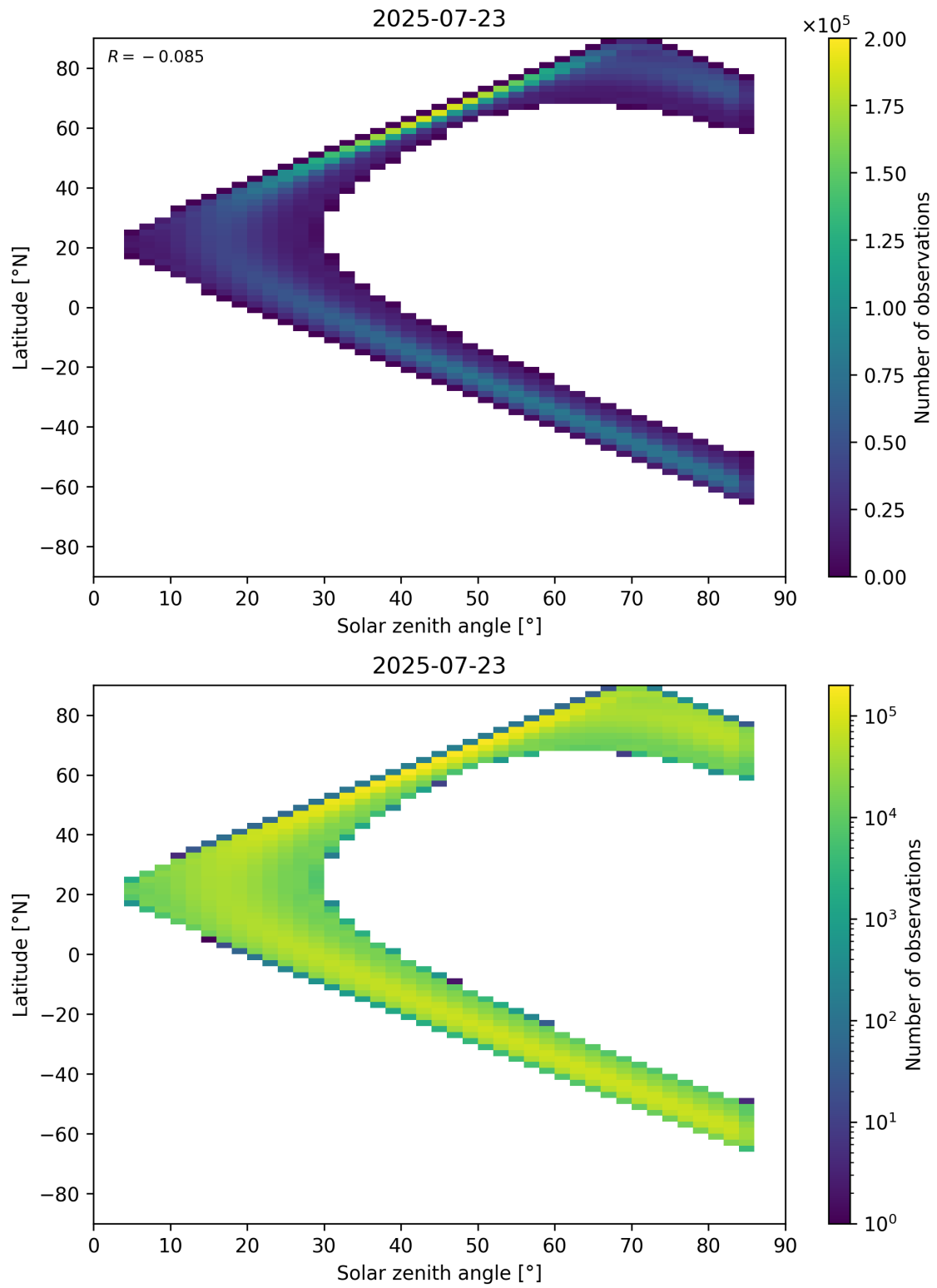
Figure 181: Scatter density plot of “Solar zenith angle” against “Latitude” for 2025-07-22 to 2025-07-24.
