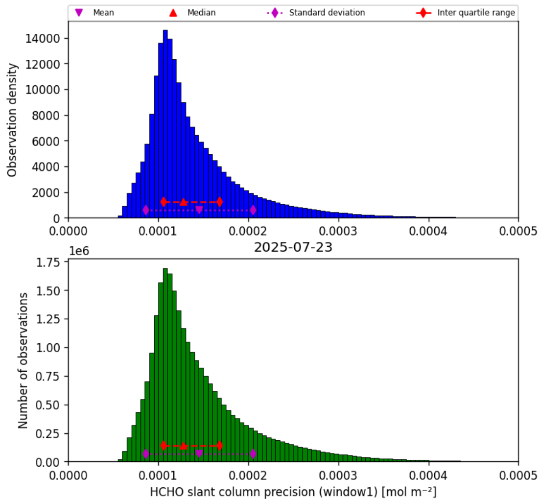
Figure 39: Histogram of “HCHO slant column precision (window1)” for 2025-07-22 to 2025-07-24
