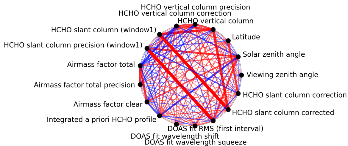
Figure 1: Map of correlation graph for 2025-07-22 to 2025-07-24.
