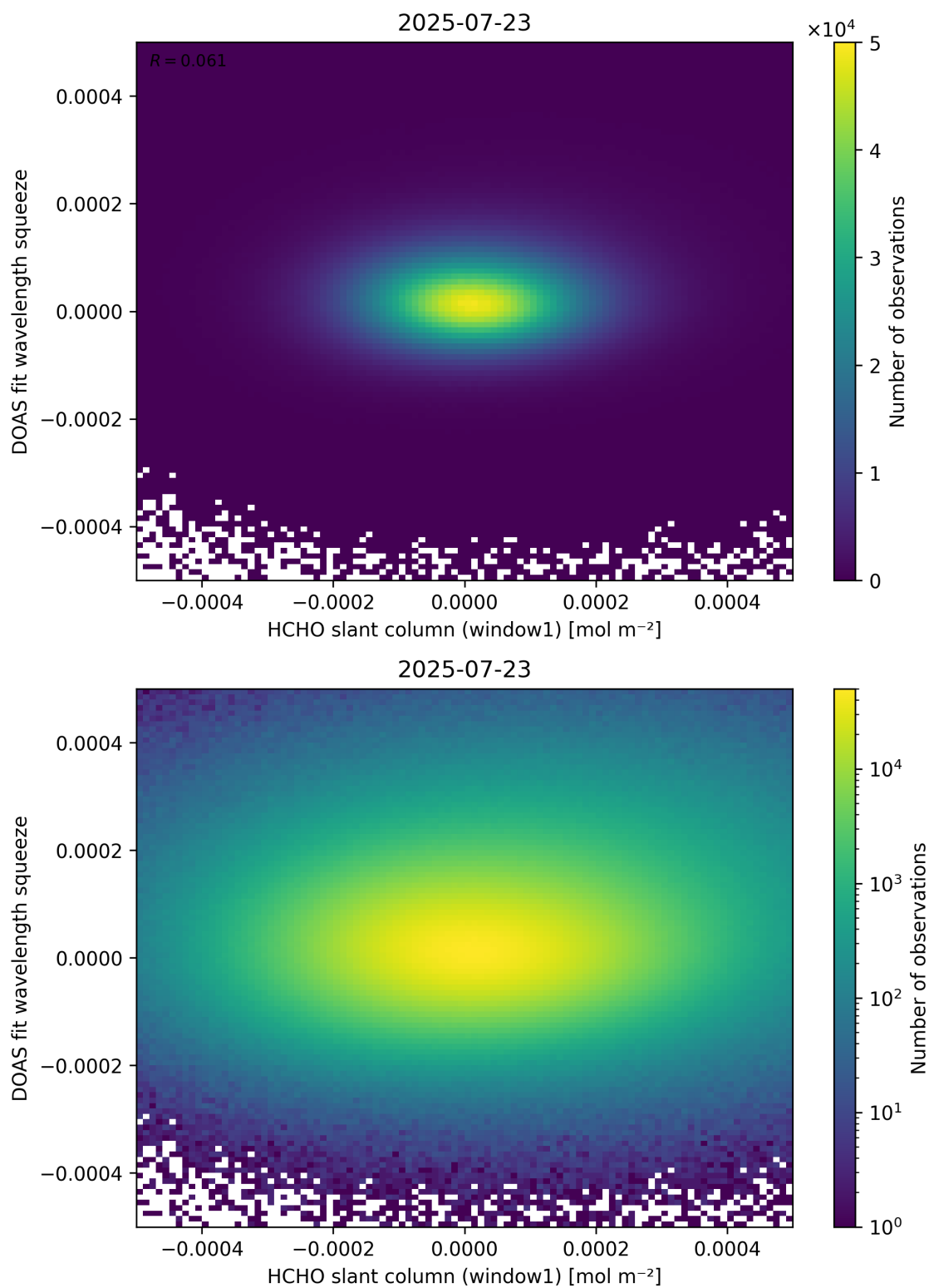
Figure 80: Scatter density plot of “HCHO slant column (window1)” against “DOAS fit wavelength squeeze” for 2025-07-22 to 2025-07-24.
