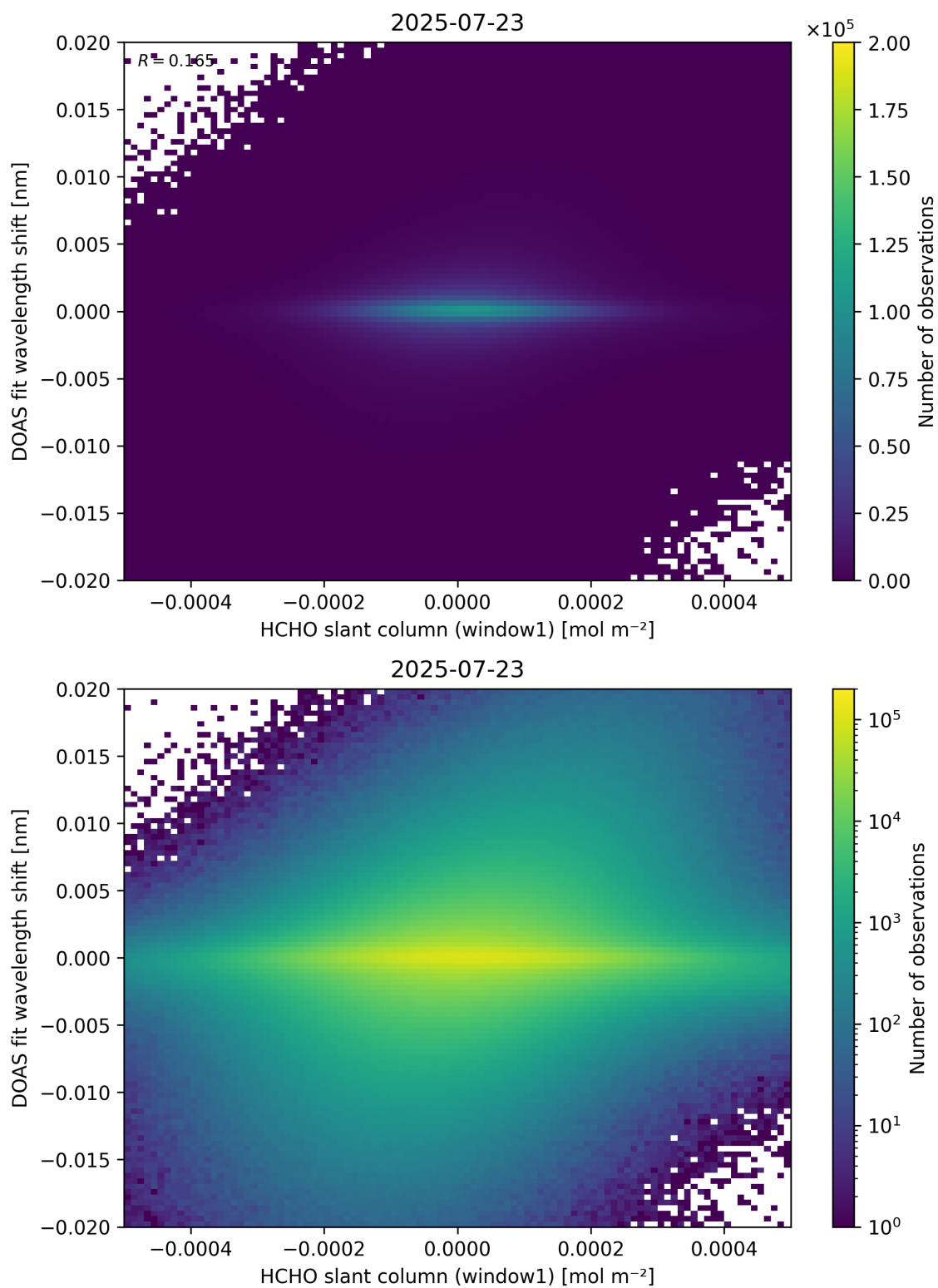
Figure 79: Scatter density plot of “HCHO slant column (window1)” against “DOAS fit wavelength shift” for 2025-07-22 to 2025-07-24.
