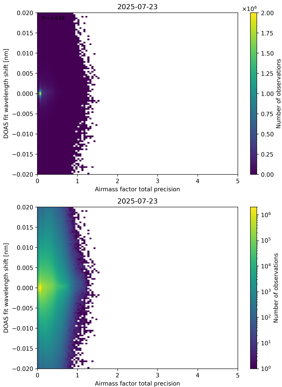
Figure 106: Scatter density plot of “Airmass factor total precision” against “DOAS fit wavelength shift” for 2025-07-22 to 2025-07-24.
