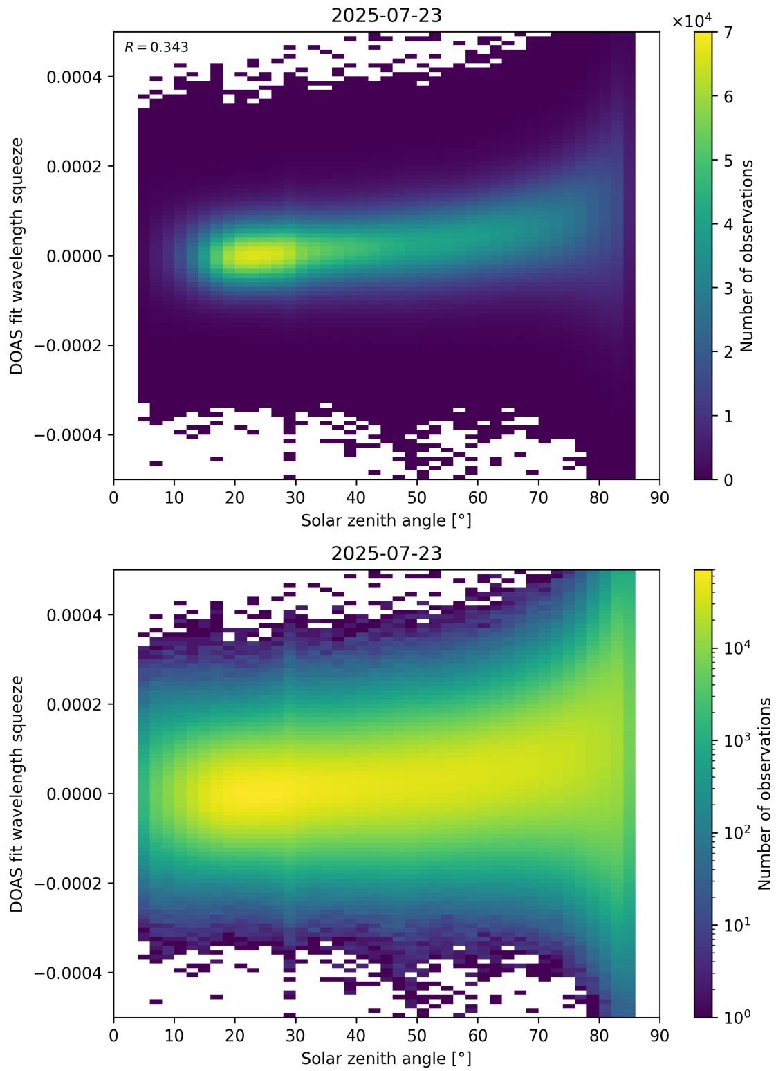
Figure 169: Scatter density plot of “Solar zenith angle” against “DOAS fit wavelength squeeze” for 2025-07-22 to 2025-07-24.
