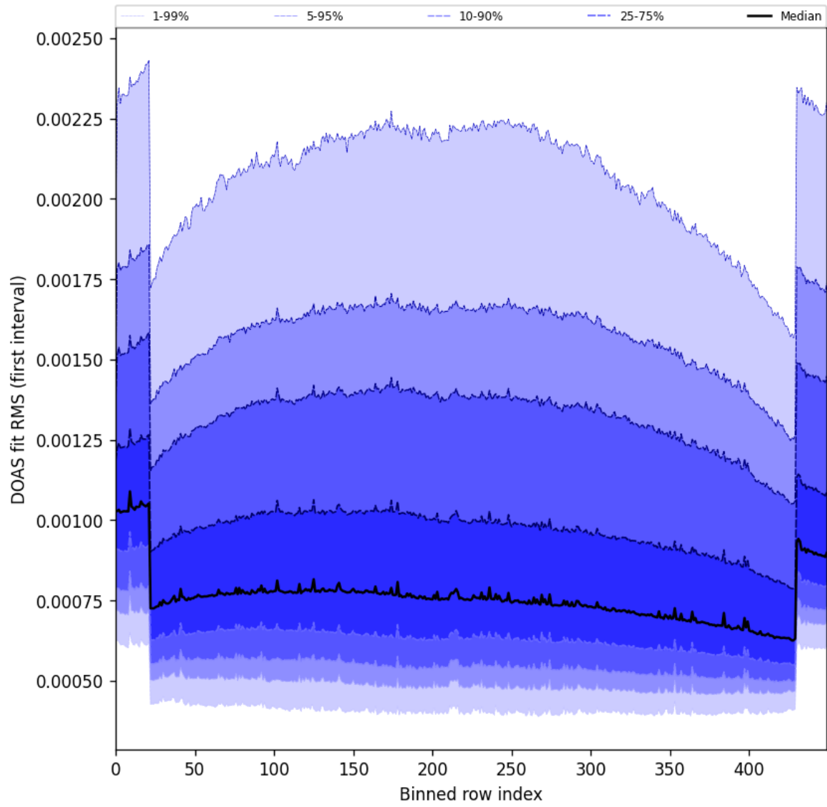
Figure 60: Along track statistics of “DOAS fit RMS (first interval)” for 2025-07-22 to 2025-07-24
