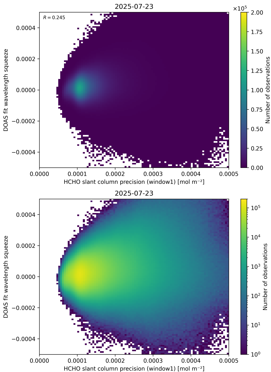
Figure 90: Scatter density plot of “HCHO slant column precision (window1)” against “DOAS fit wavelength squeeze” for 2025-07-22 to 2025-07-24.
