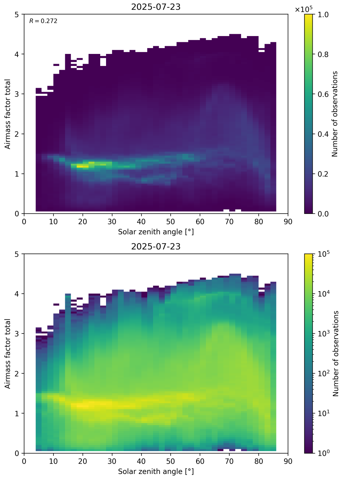
Figure 175: Scatter density plot of “Solar zenith angle” against “Airmass factor total” for 2025-07-22 to 2025-07-24.
