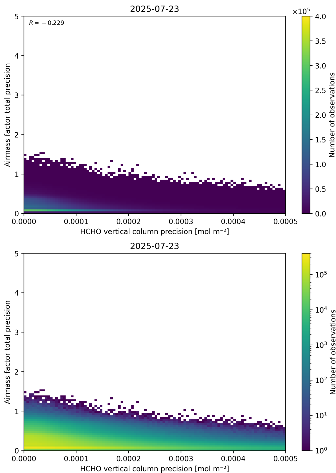
Figure 145: Scatter density plot of “HCHO vertical column precision” against “Airmass factor total precision” for 2025-07-22 to 2025-07-24.
