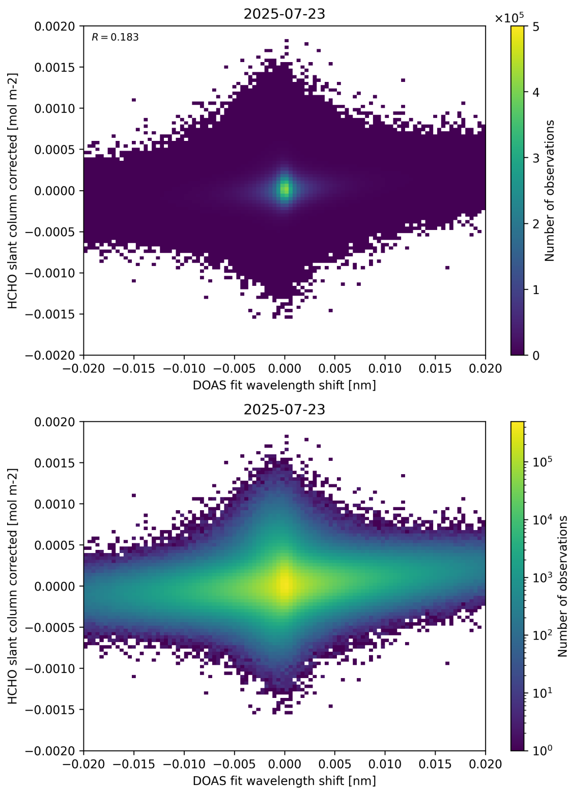
Figure 66: Scatter density plot of “DOAS fit wavelength shift” against “HCHO slant column corrected” for 2025-07-22 to 2025-07-24.
