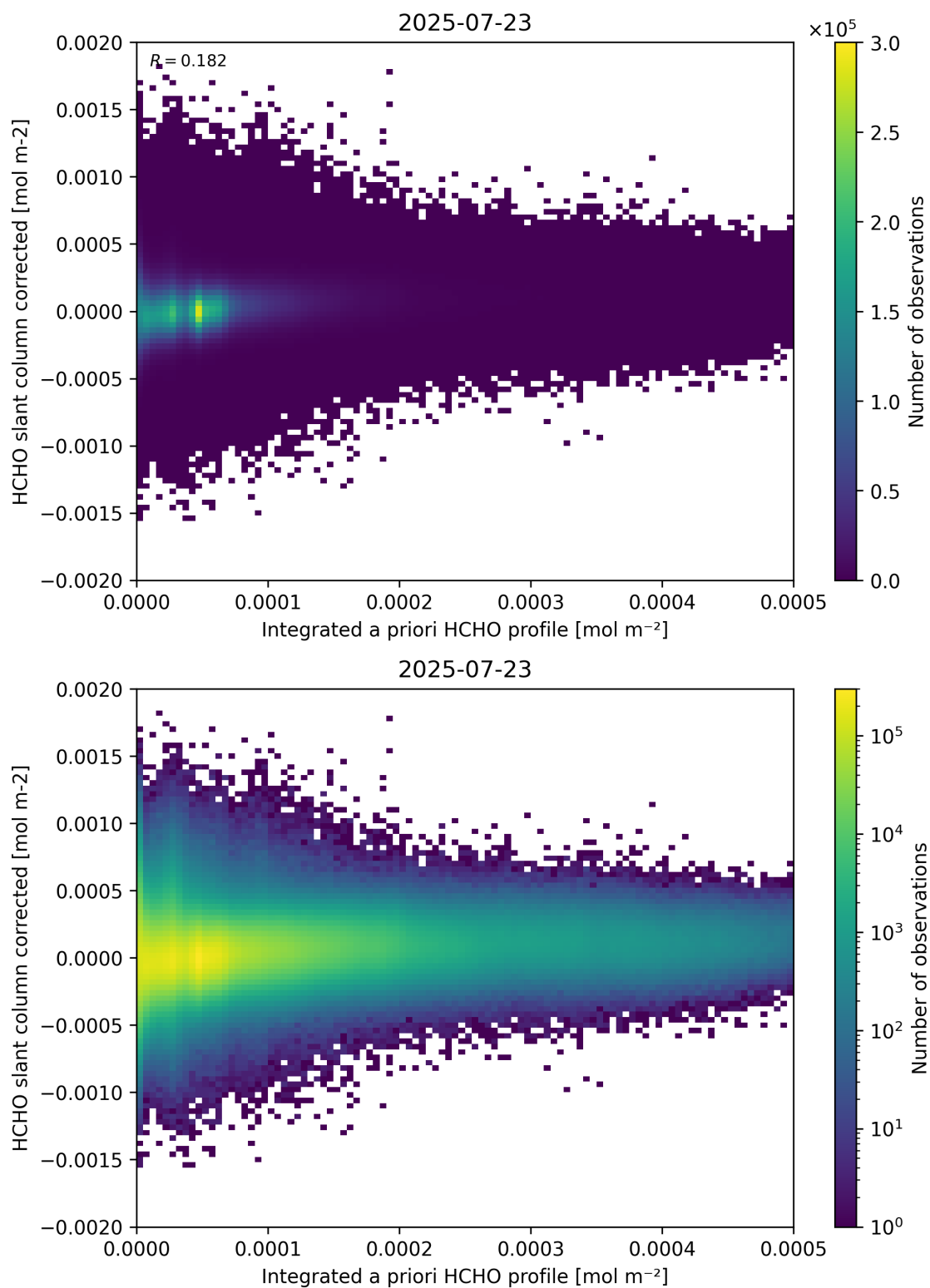
Figure 151: Scatter density plot of “Integrated a priori HCHO profile” against “HCHO slant column corrected” for 2025-07-22 to 2025-07-24.
