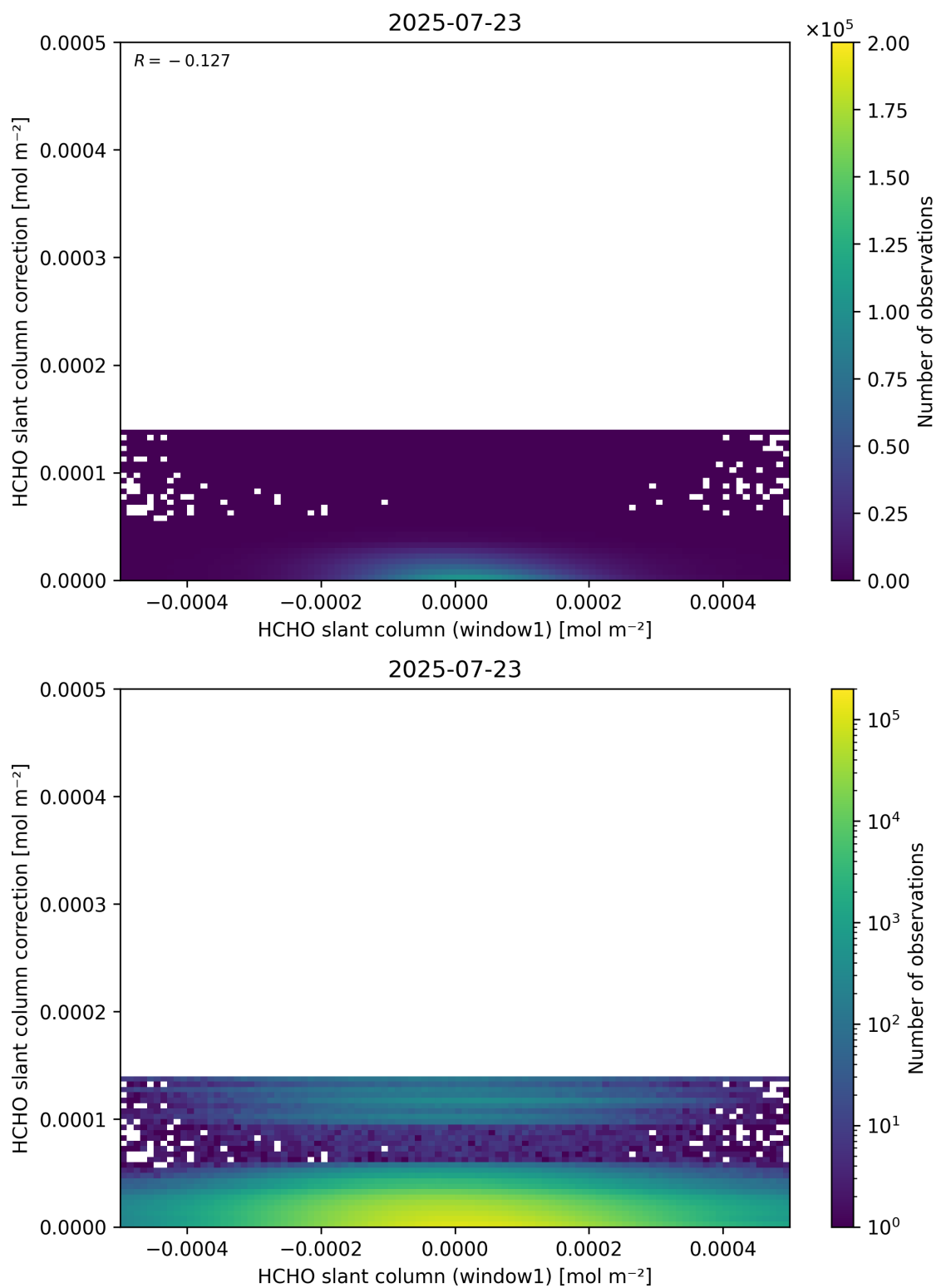
Figure 83: Scatter density plot of “HCHO slant column (window1)” against “HCHO slant column correction” for 2025-07-22 to 2025-07-24.
