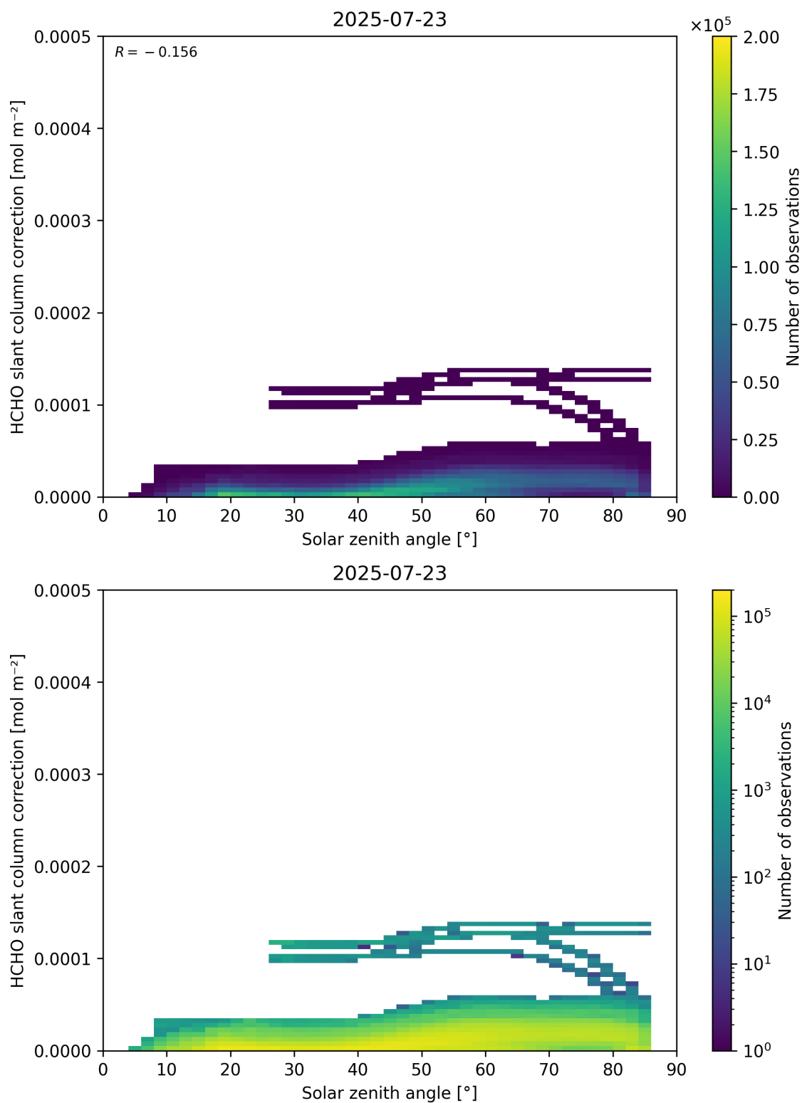
Figure 172: Scatter density plot of “Solar zenith angle” against “HCHO slant column correction” for 2025-07-22 to 2025-07-24.
