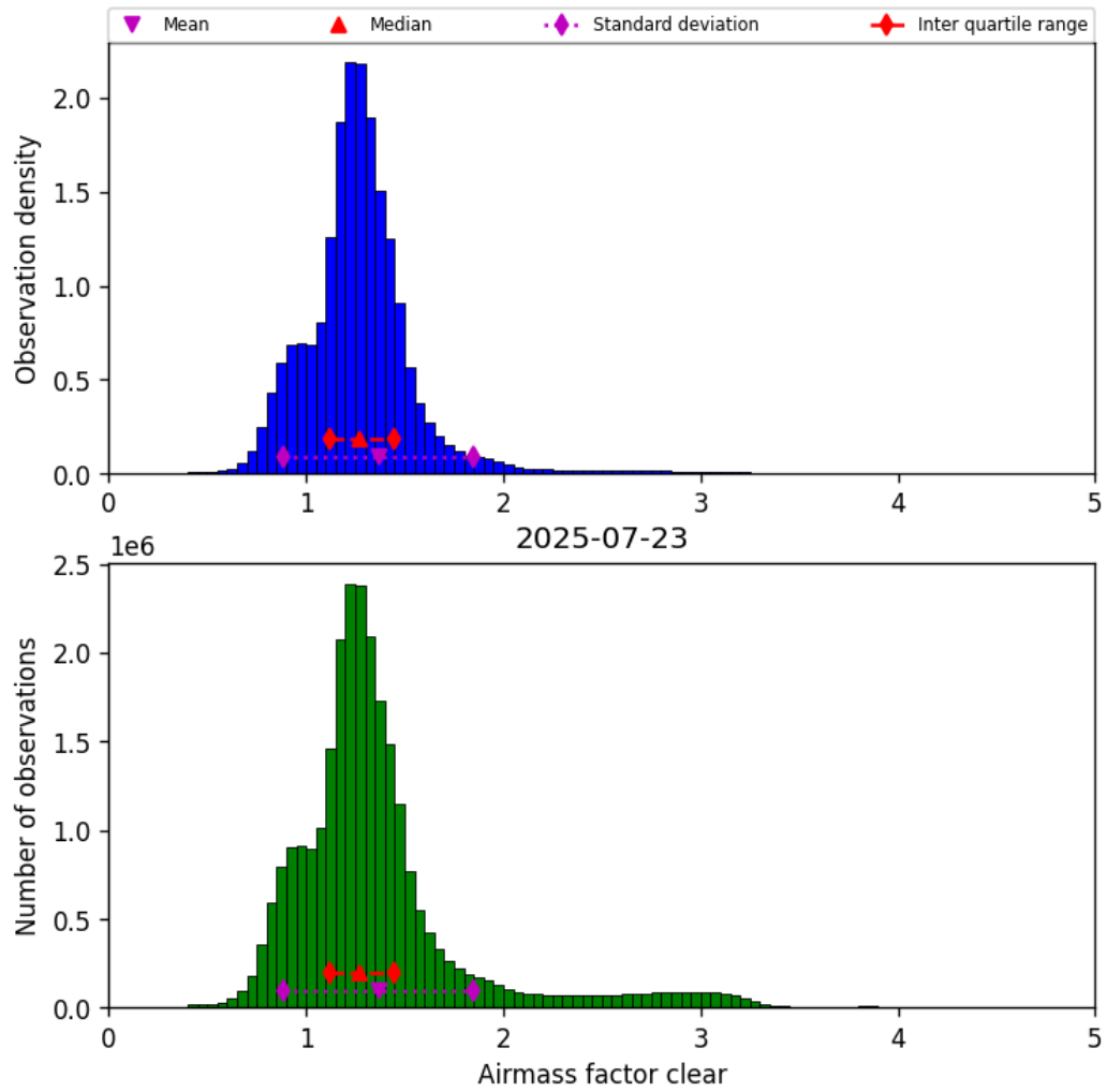
Figure 42: Histogram of “Airmass factor clear” for 2025-07-22 to 2025-07-24
