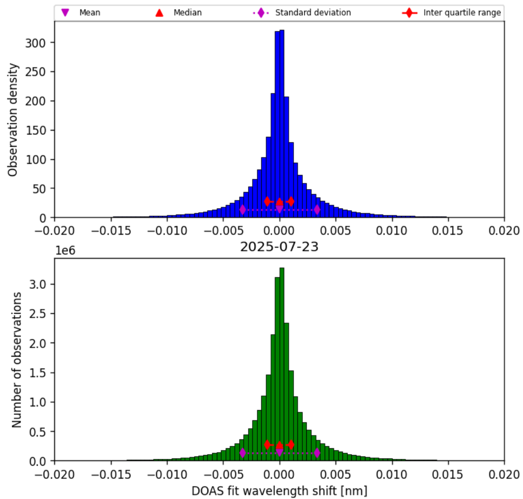
Figure 44: Histogram of “DOAS fit wavelength shift” for 2025-07-22 to 2025-07-24
