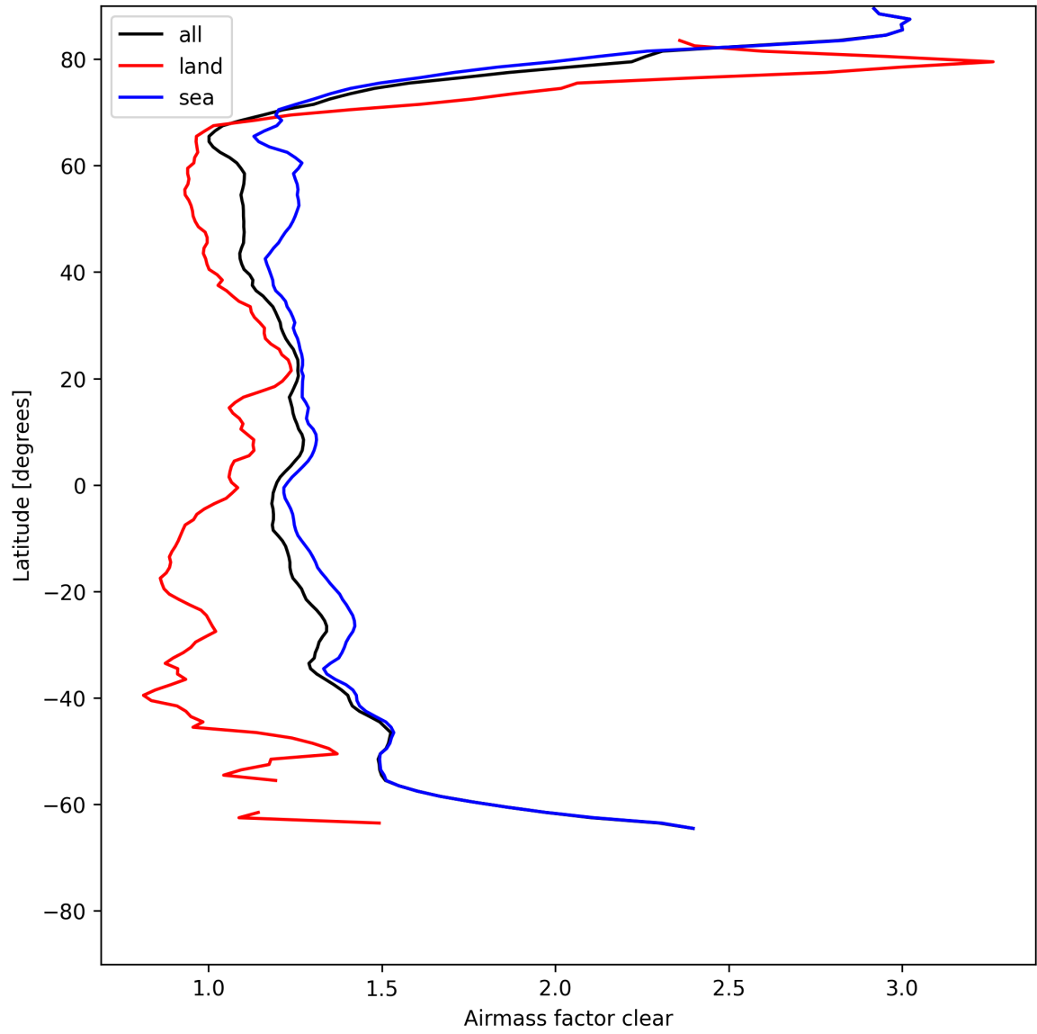
Figure 28: Zonal average of “Airmass factor clear” for 2025-07-22 to 2025-07-24.
