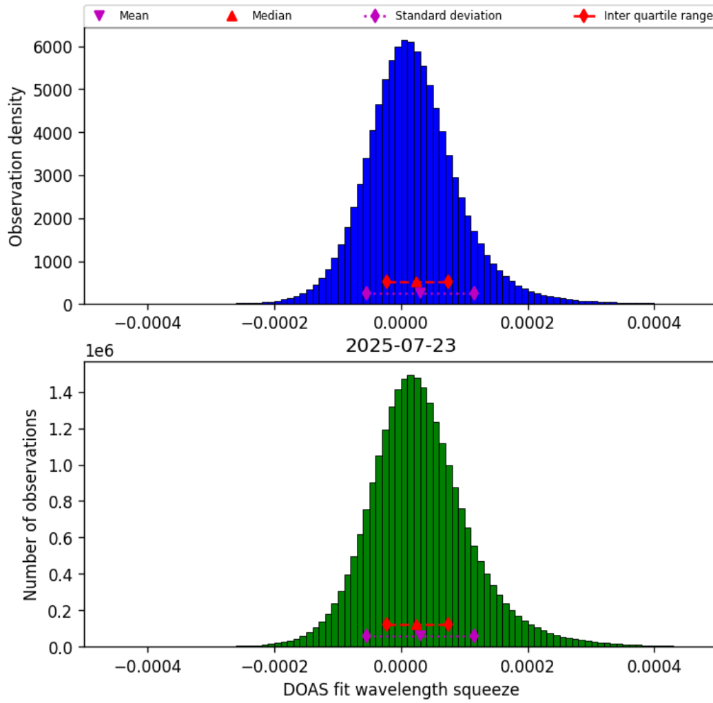
Figure 45: Histogram of “DOAS fit wavelength squeeze” for 2025-07-22 to 2025-07-24
