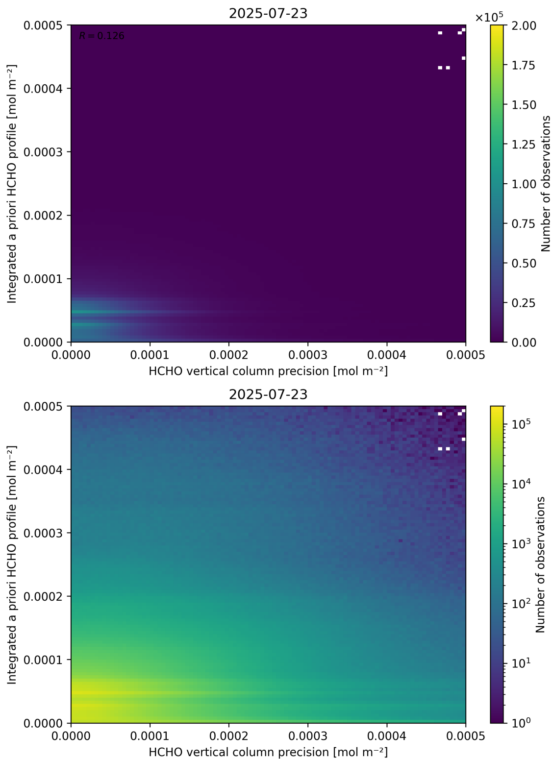
Figure 147: Scatter density plot of “HCHO vertical column precision” against “Integrated a priori HCHO profile” for 2025-07-22 to 2025-07-24.
