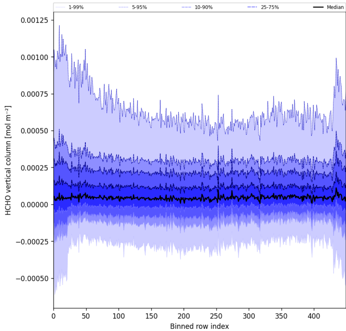
Figure 49: Along track statistics of “HCHO vertical column” for 2025-07-22 to 2025-07-24
