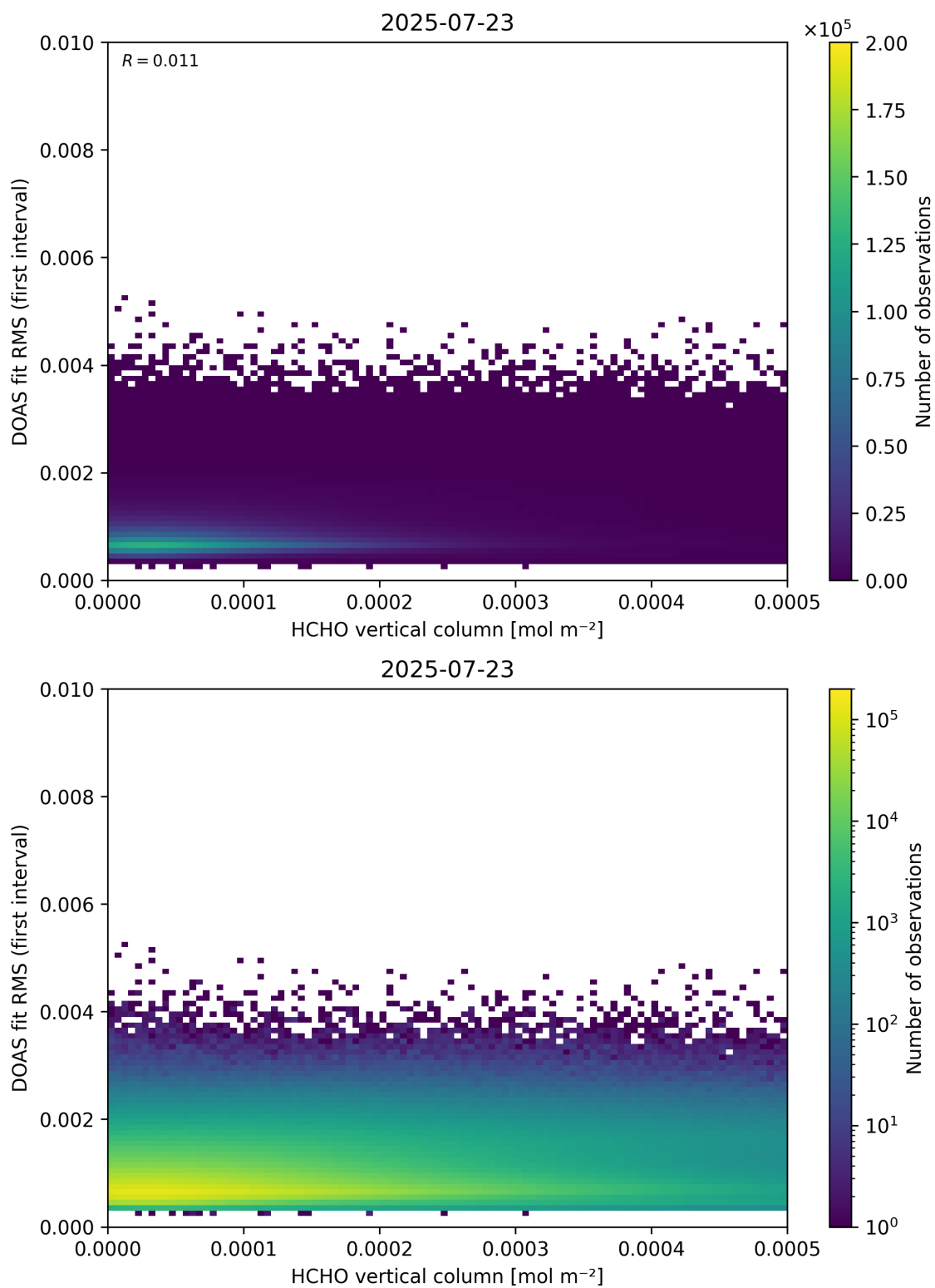
Figure 123: Scatter density plot of “HCHO vertical column” against “DOAS fit RMS (first interval)” for 2025-07-22 to 2025-07-24.
