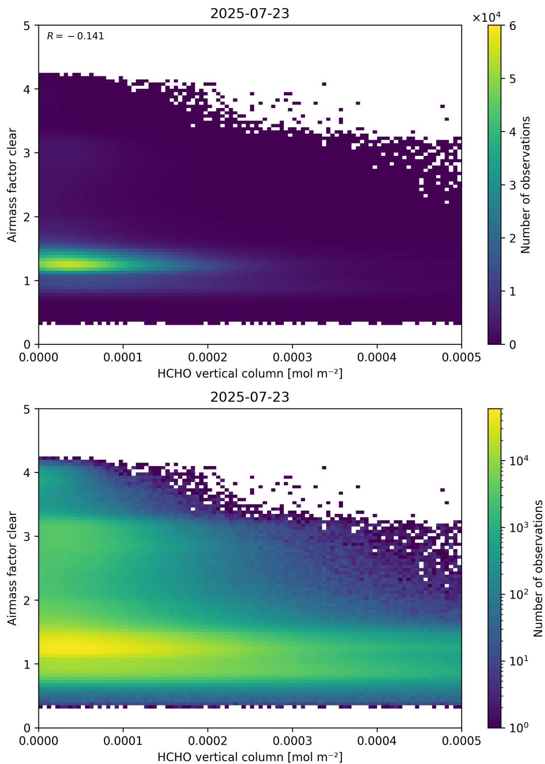
Figure 126: Scatter density plot of “HCHO vertical column” against “Airmass factor clear” for 2025-07-22 to 2025-07-24.
