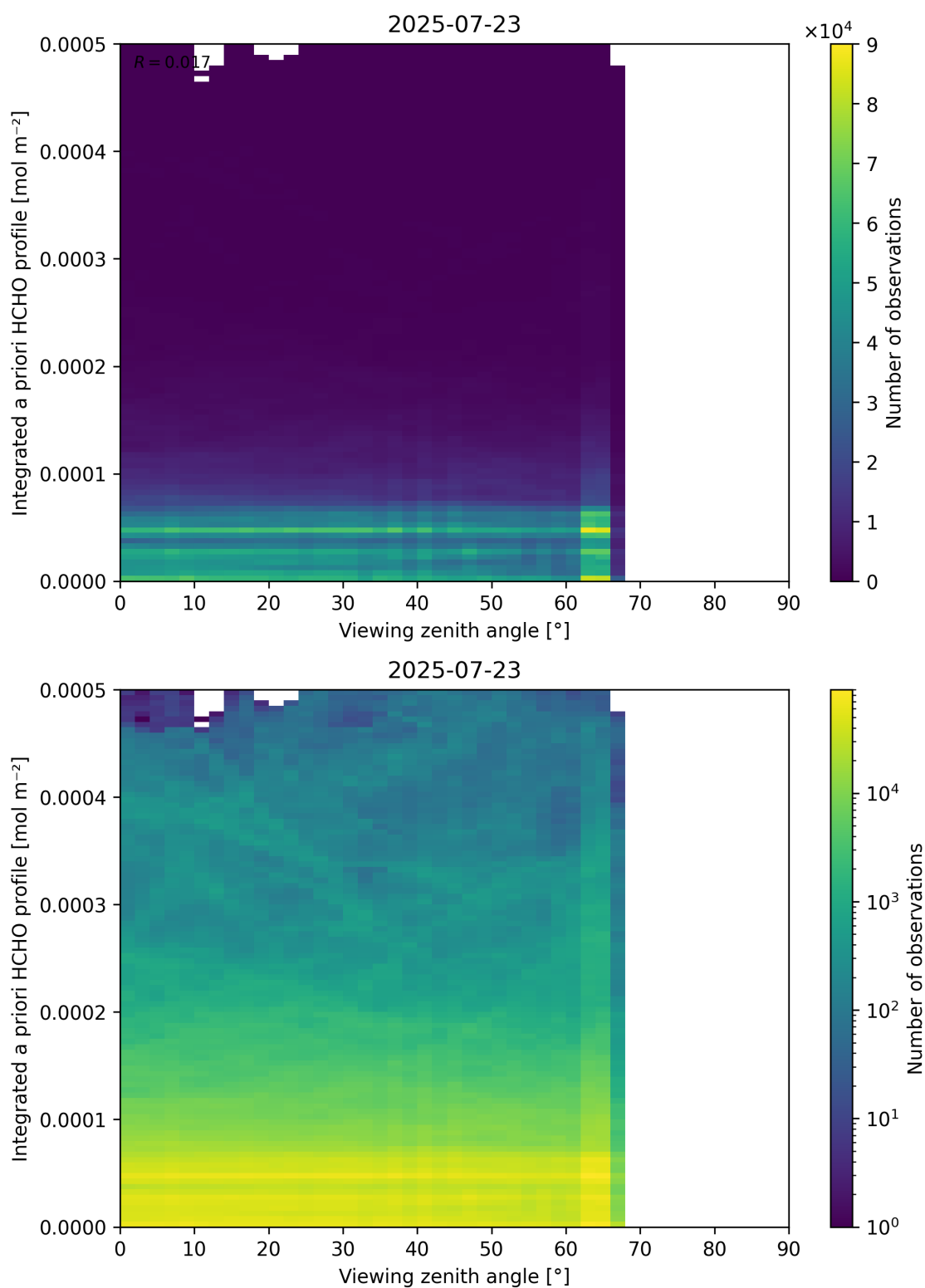
Figure 195: Scatter density plot of “Viewing zenith angle” against “Integrated a priori HCHO profile” for 2025-07-22 to 2025-07-24.
