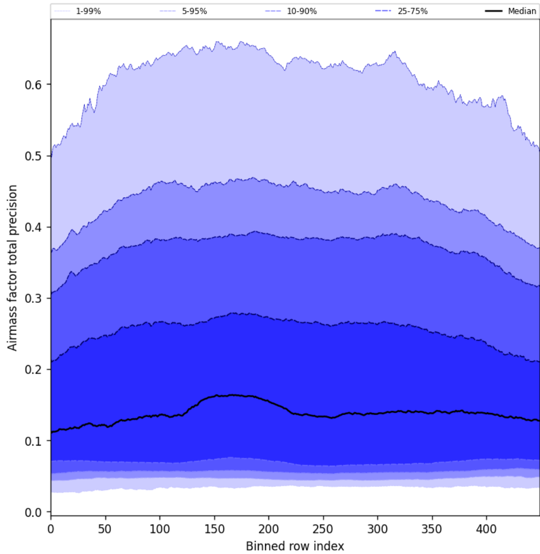
Figure 55: Along track statistics of “Airmass factor total precision” for 2025-07-22 to 2025-07-24
