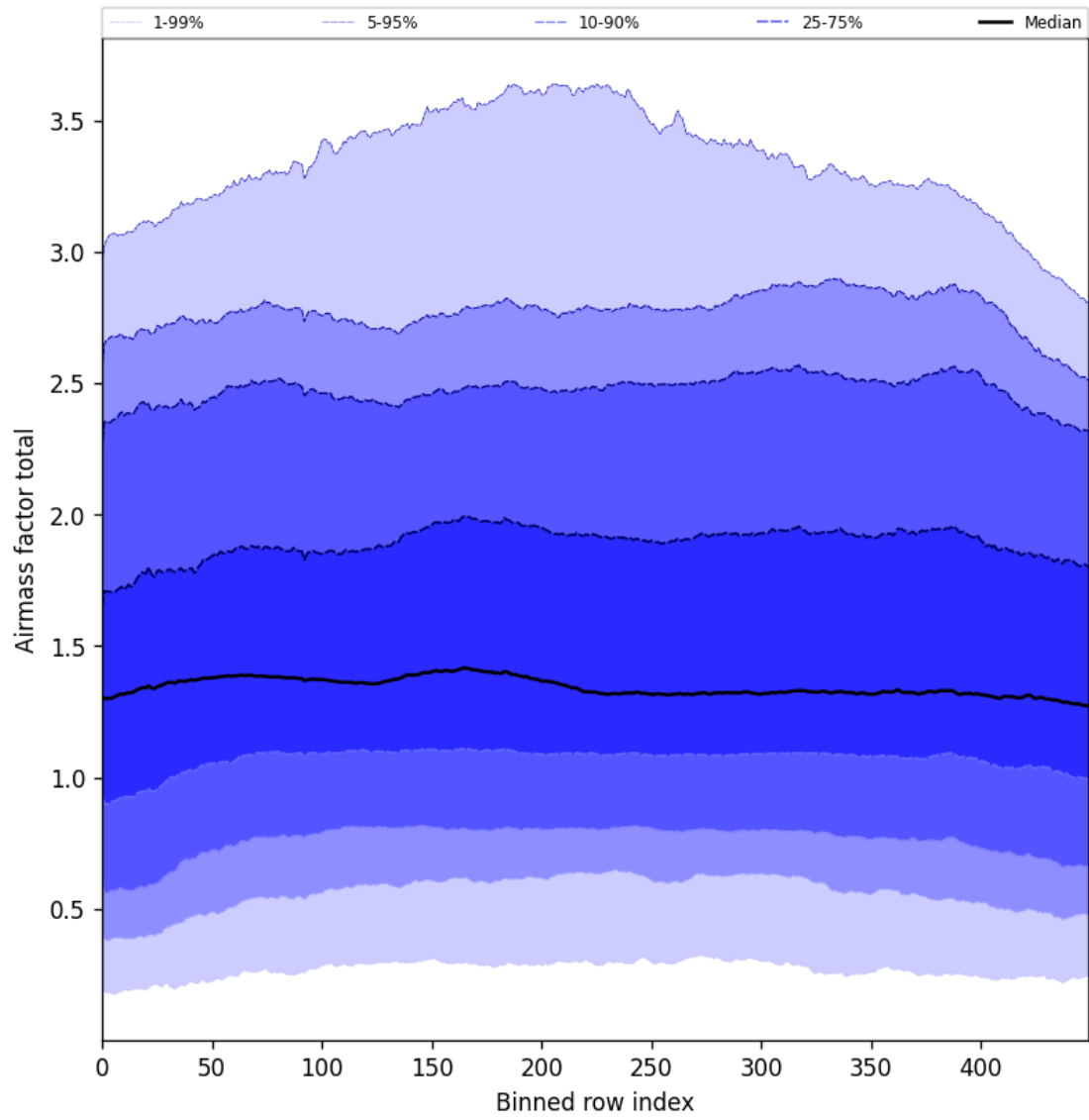
Figure 54: Along track statistics of “Airmass factor total” for 2025-07-22 to 2025-07-24
