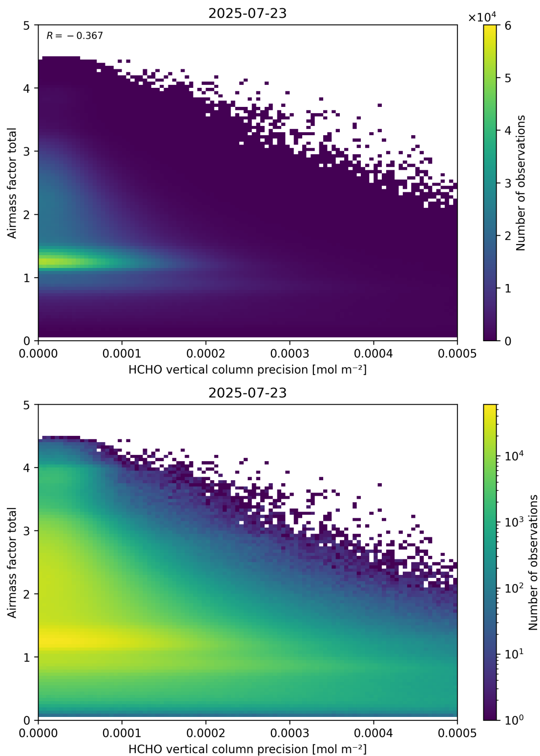
Figure 144: Scatter density plot of “HCHO vertical column precision” against “Airmass factor total” for 2025-07-22 to 2025-07-24.
