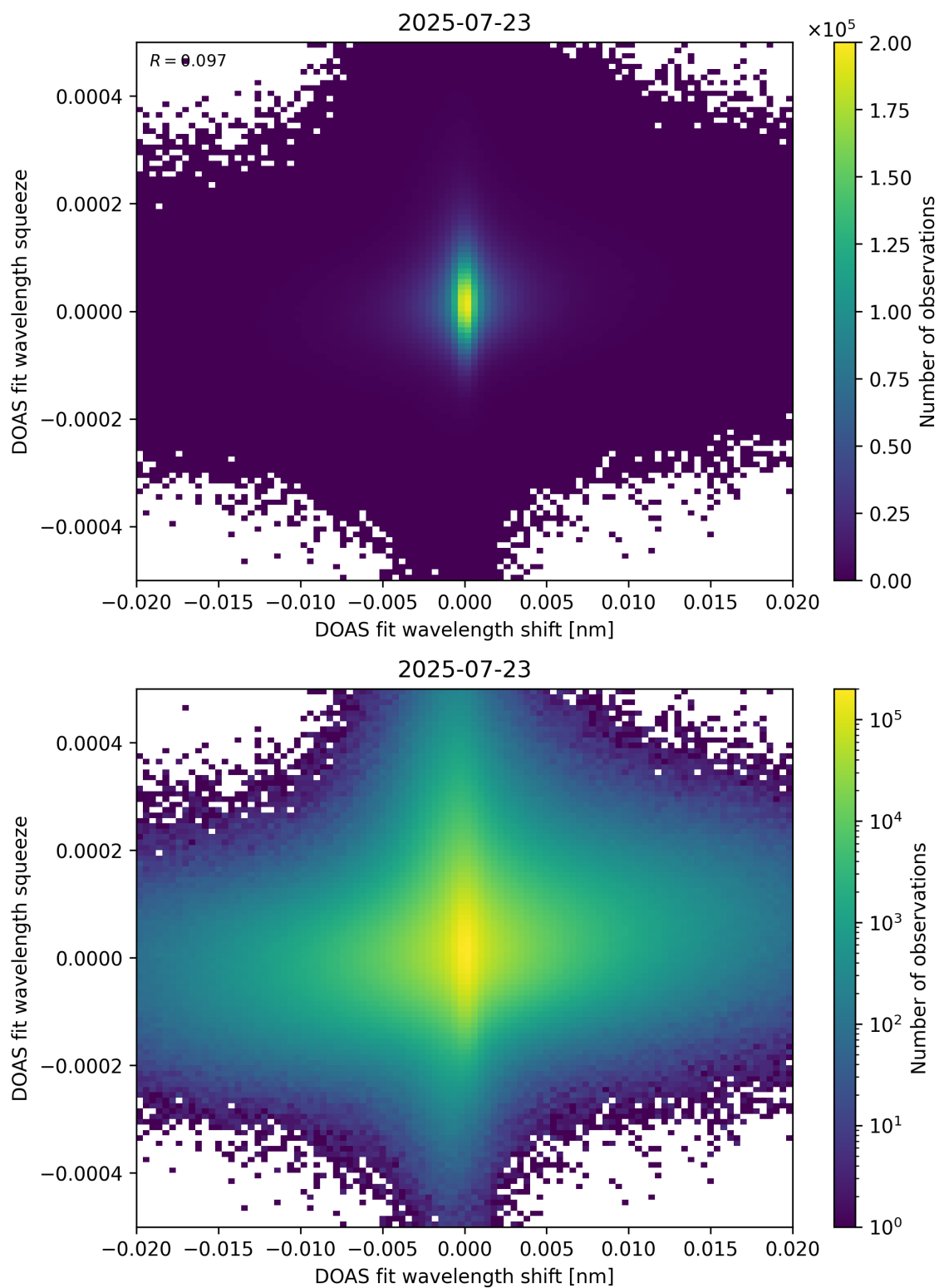
Figure 65: Scatter density plot of “DOAS fit wavelength shift” against “DOAS fit wavelength squeeze” for 2025-07-22 to 2025-07-24.
