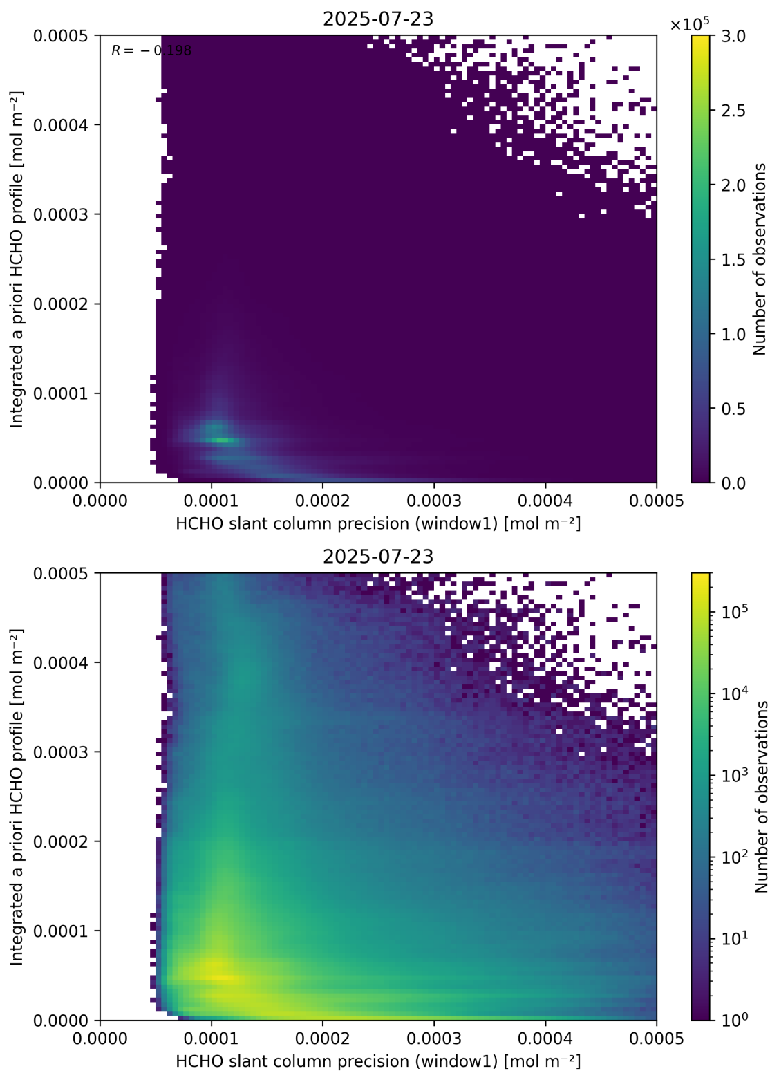
Figure 96: Scatter density plot of “HCHO slant column precision (window1)” against “Integrated a priori HCHO profile” for 2025-07-22 to 2025-07-24.
