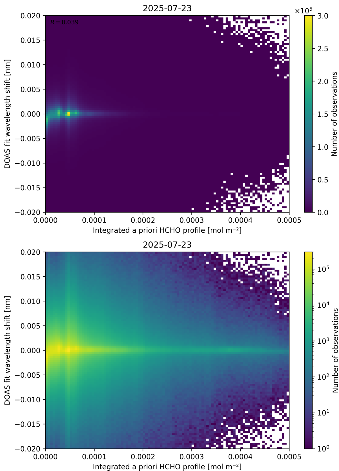
Figure 149: Scatter density plot of “Integrated a priori HCHO profile” against “DOAS fit wavelength shift” for 2025-07-22 to 2025-07-24.
