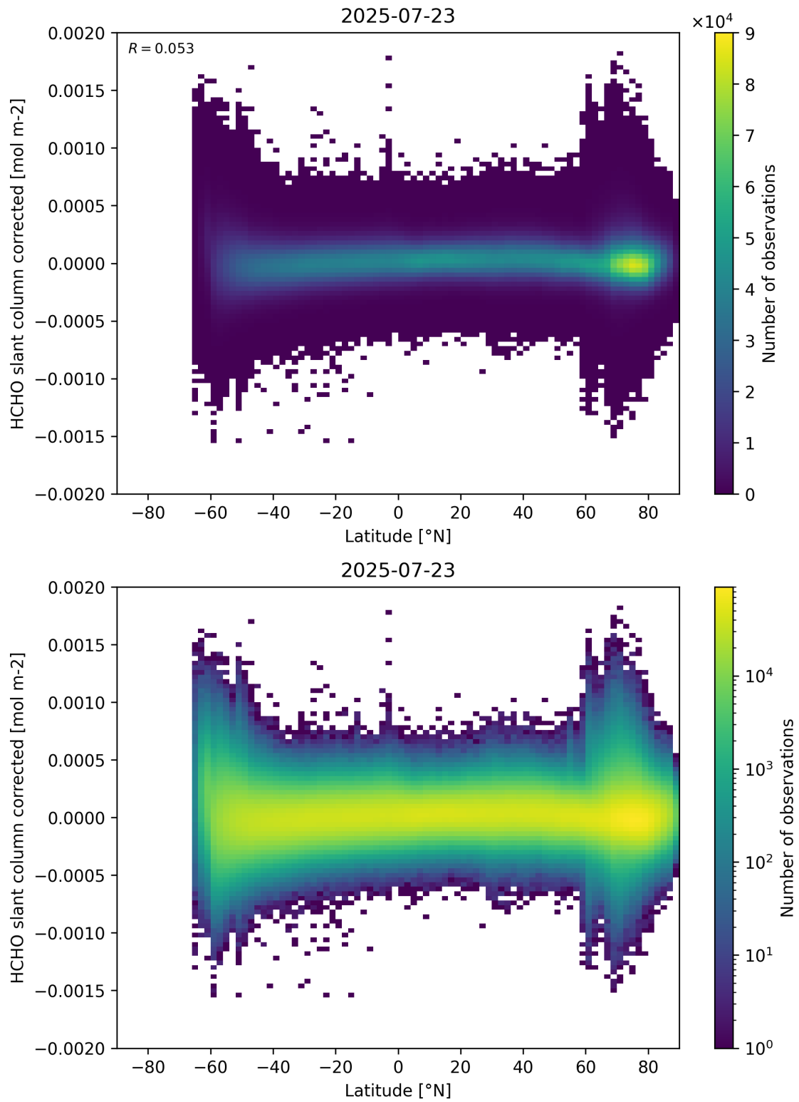
Figure 157: Scatter density plot of “Latitude” against “HCHO slant column corrected” for 2025-07-22 to 2025-07-24.
