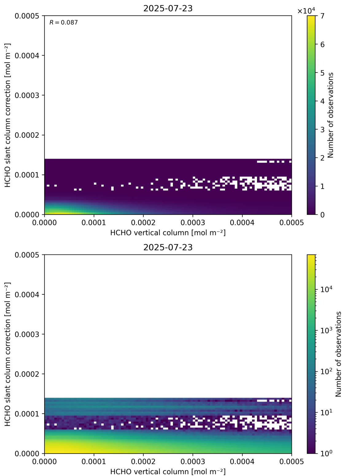
Figure 128: Scatter density plot of “HCHO vertical column” against “HCHO slant column correction” for 2025-07-22 to 2025-07-24.
