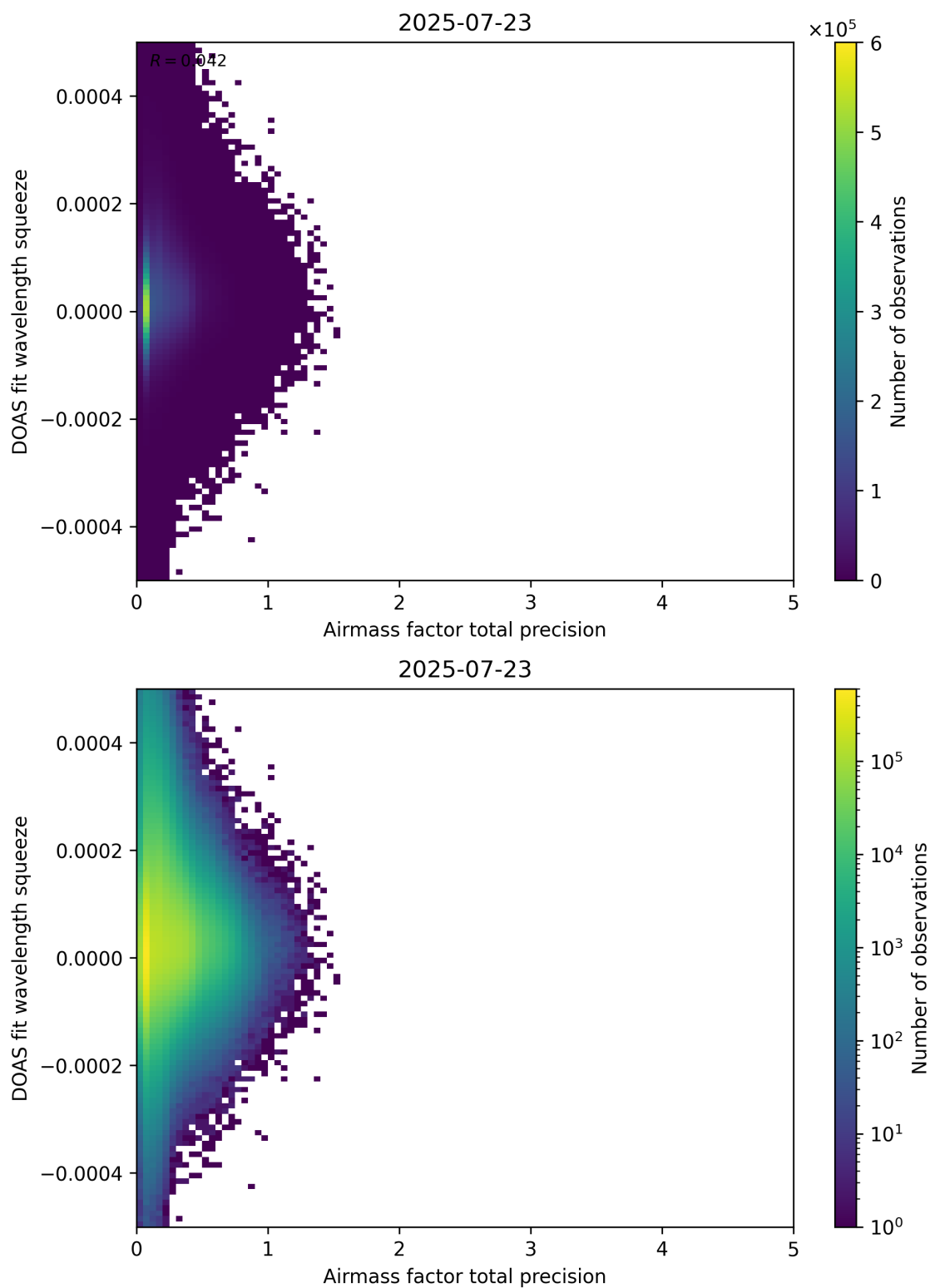
Figure 107: Scatter density plot of “Airmass factor total precision” against “DOAS fit wavelength squeeze” for 2025-07-22 to 2025-07-24.
