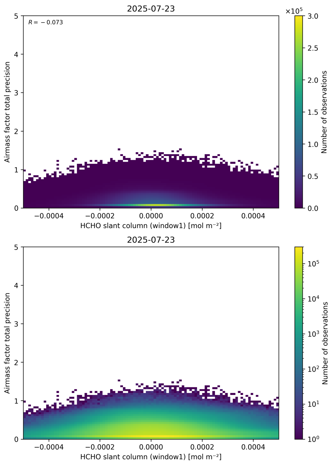
Figure 86: Scatter density plot of “HCHO slant column (window1)” against “Airmass factor total precision” for 2025-07-22 to 2025-07-24.
