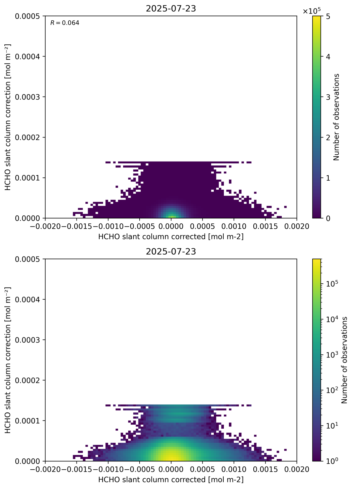
Figure 77: Scatter density plot of “HCHO slant column corrected” against “HCHO slant column correction” for 2025-07-22 to 2025-07-24.
