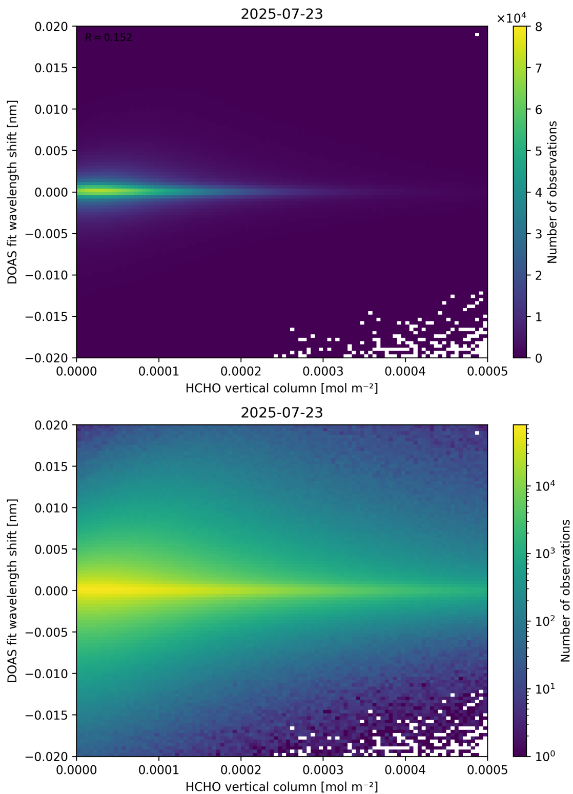
Figure 124: Scatter density plot of “HCHO vertical column” against “DOAS fit wavelength shift” for 2025-07-22 to 2025-07-24.
