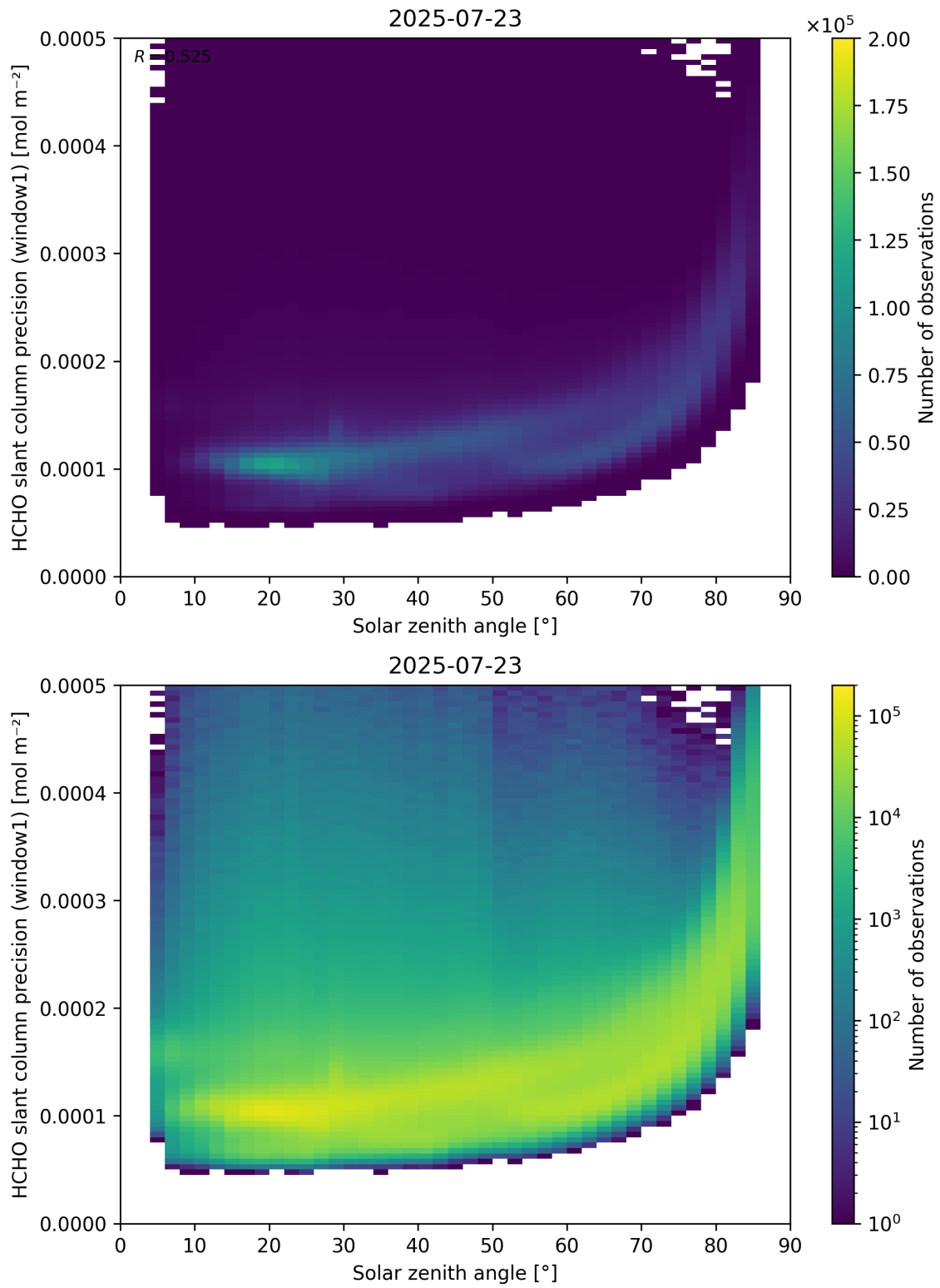
Figure 174: Scatter density plot of “Solar zenith angle” against “HCHO slant column precision (window1)” for 2025-07-22 to 2025-07-24.
