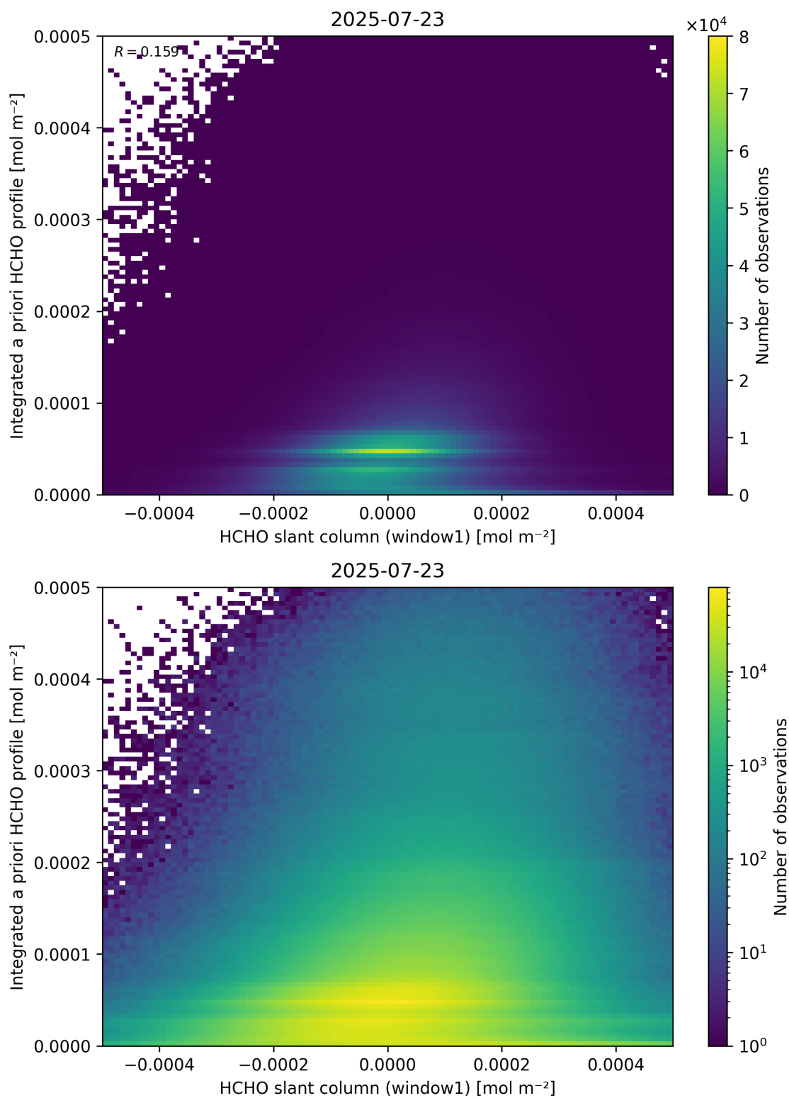
Figure 87: Scatter density plot of “HCHO slant column (window1)” against “Integrated a priori HCHO profile” for 2025-07-22 to 2025-07-24.
