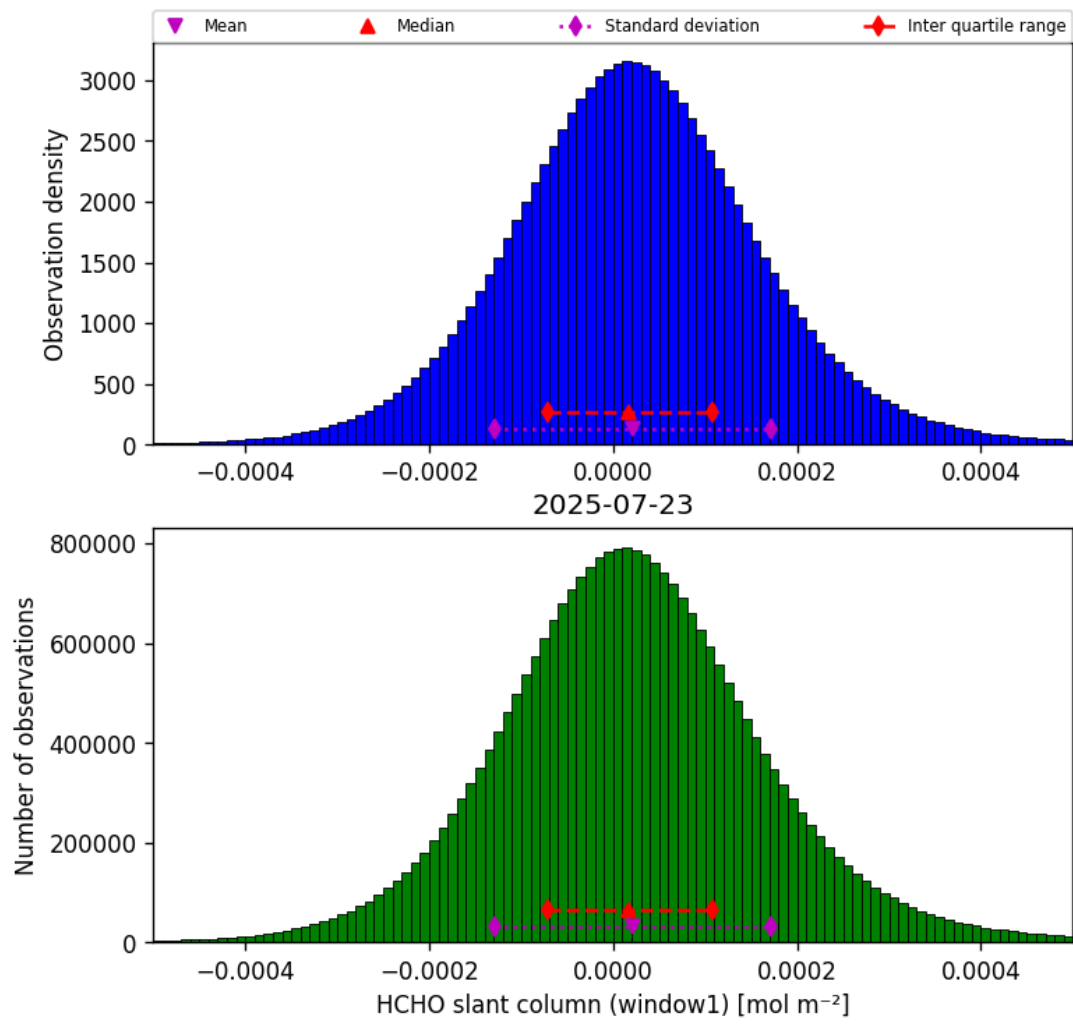
Figure 38: Histogram of “HCHO slant column (window1)” for 2025-07-22 to 2025-07-24
