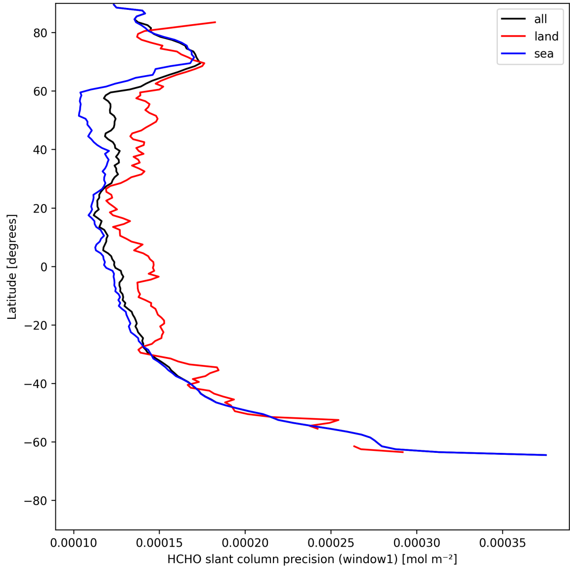
Figure 25: Zonal average of “HCHO slant column precision (window1)” for 2025-07-22 to 2025-07-24.
