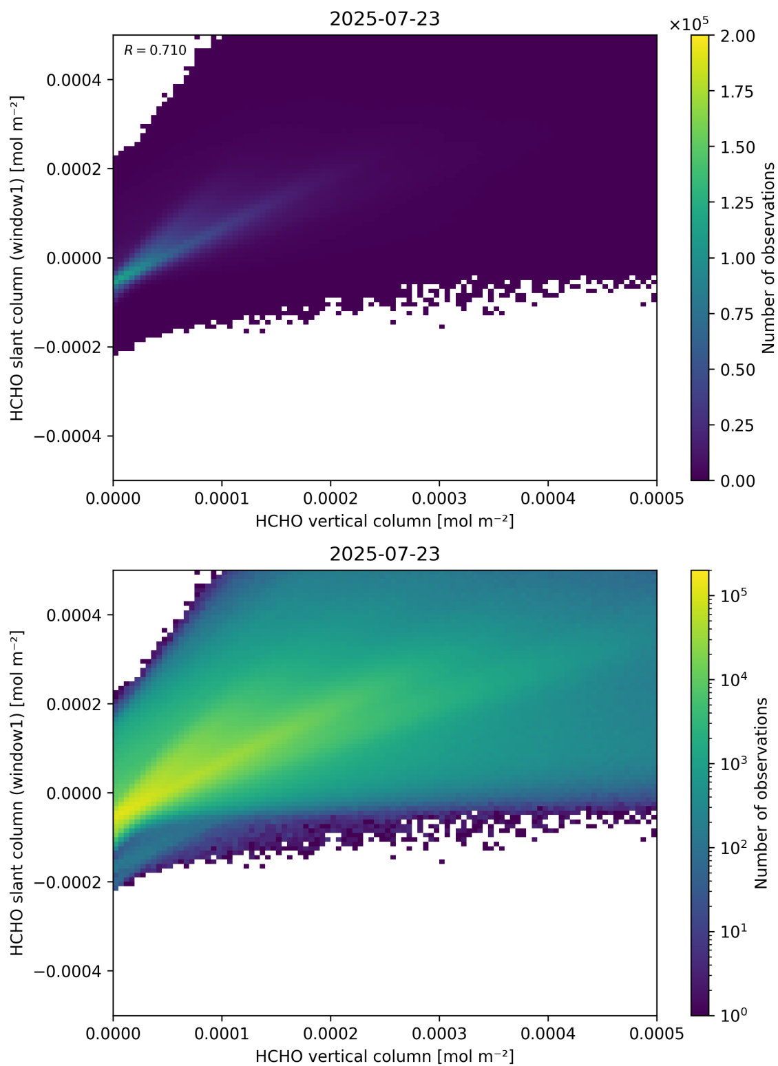
Figure 129: Scatter density plot of “HCHO vertical column” against “HCHO slant column (window1)” for 2025-07-22 to 2025-07-24.
