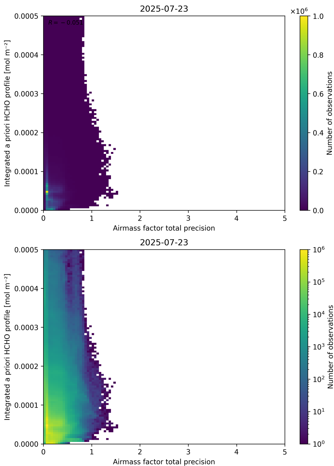
Figure 111: Scatter density plot of “Airmass factor total precision” against “Integrated a priori HCHO profile” for 2025-07-22 to 2025-07-24.
