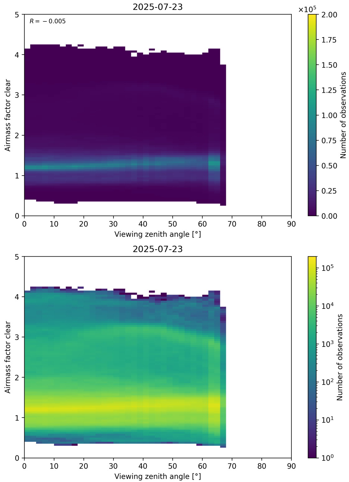
Figure 185: Scatter density plot of “Viewing zenith angle” against “Airmass factor clear” for 2025-07-22 to 2025-07-24.
