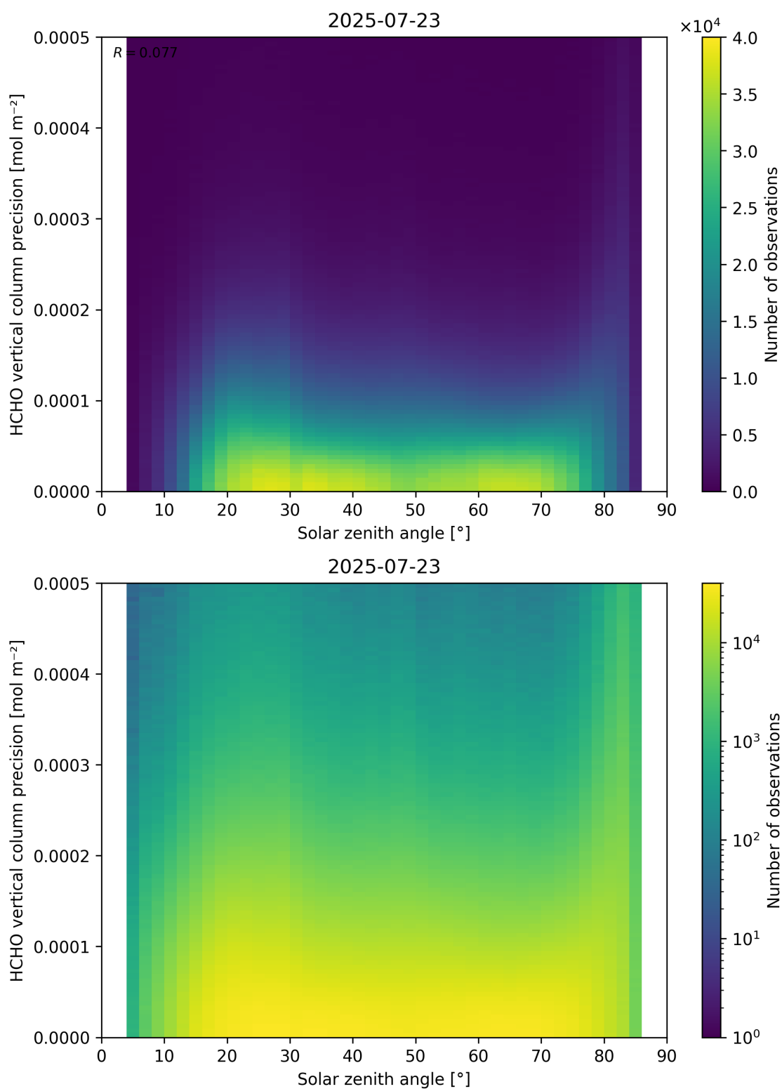
Figure 179: Scatter density plot of “Solar zenith angle” against “HCHO vertical column precision” for 2025-07-22 to 2025-07-24.
