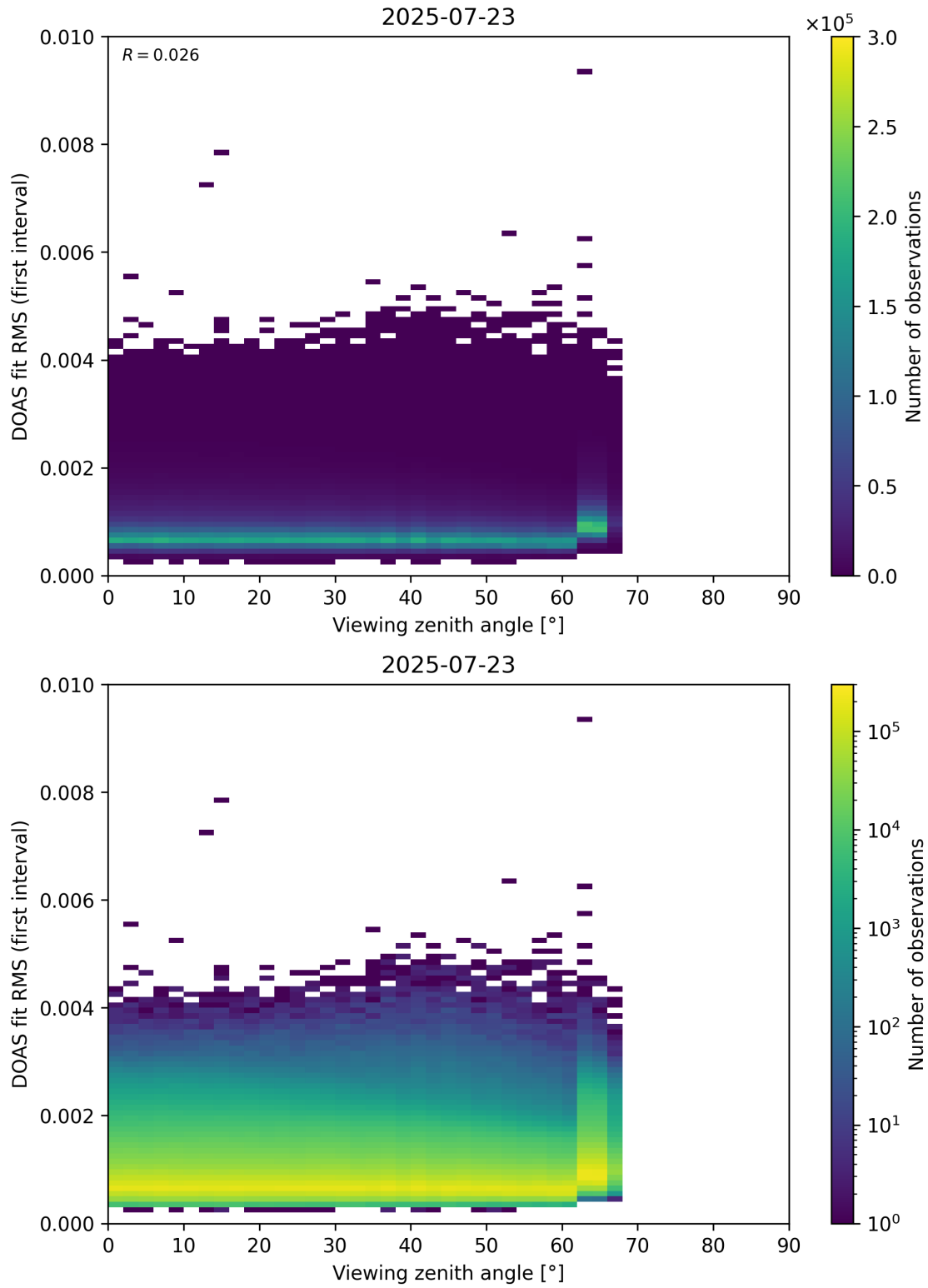
Figure 182: Scatter density plot of “Viewing zenith angle” against “DOAS fit RMS (first interval)” for 2025-07-22 to 2025-07-24.
