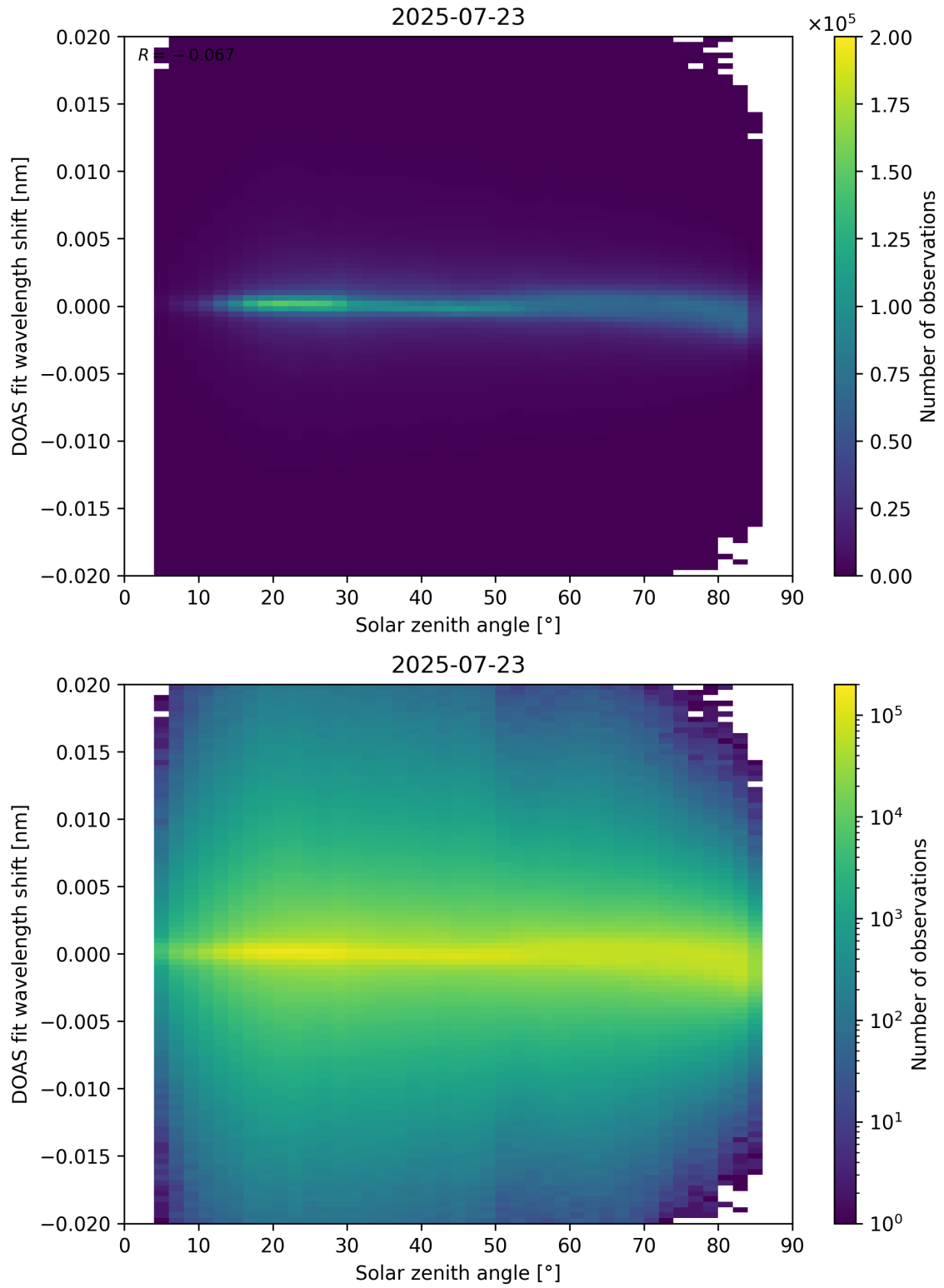
Figure 168: Scatter density plot of “Solar zenith angle” against “DOAS fit wavelength shift” for 2025-07-22 to 2025-07-24.
