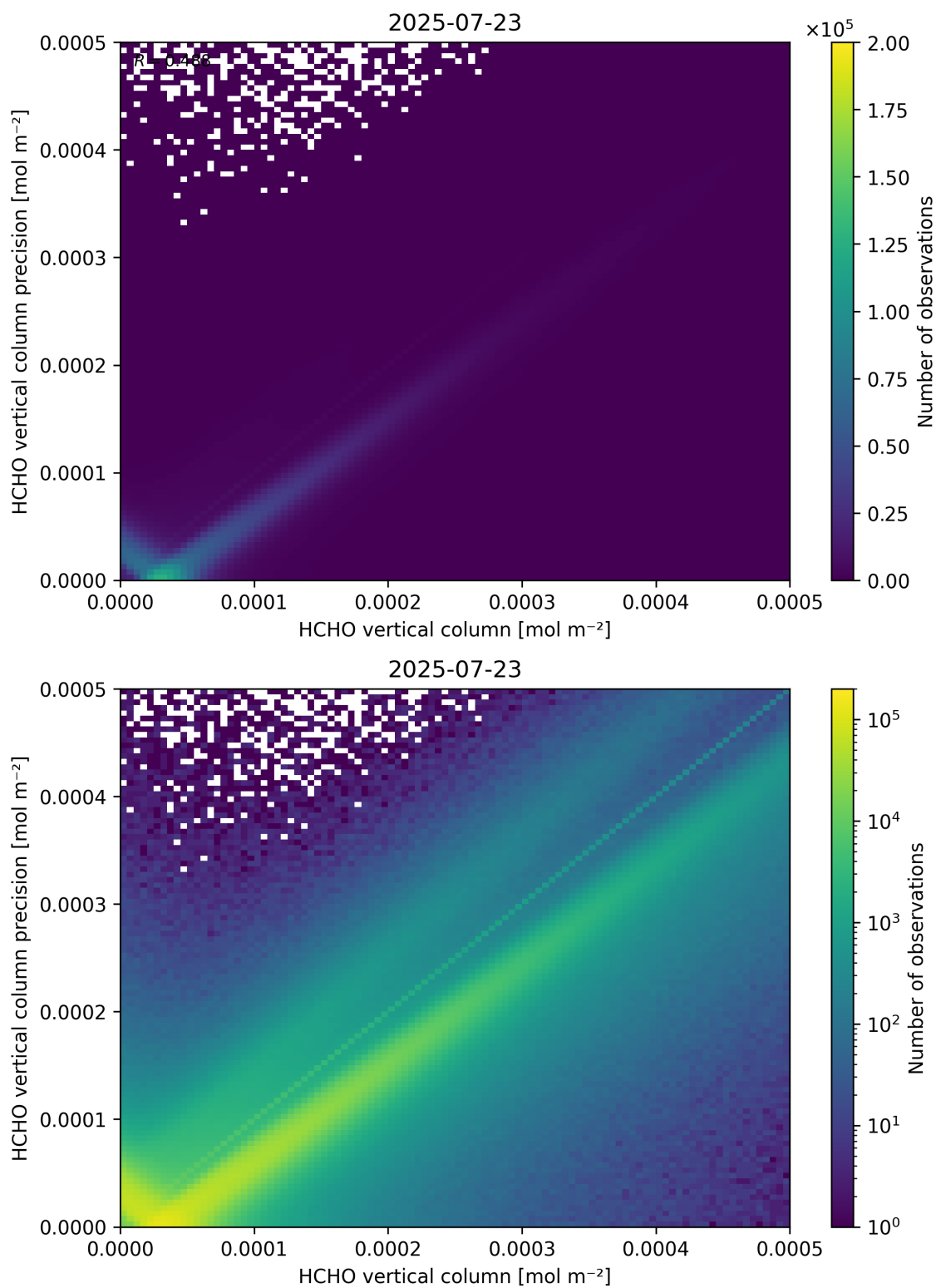
Figure 134: Scatter density plot of “HCHO vertical column” against “HCHO vertical column precision” for 2025-07-22 to 2025-07-24.
