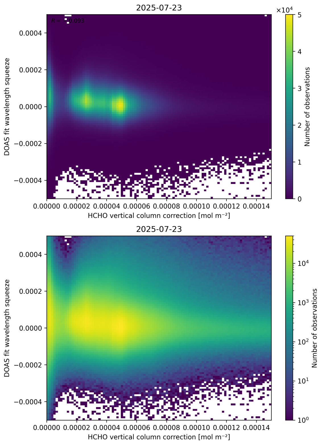
Figure 114: Scatter density plot of “HCHO vertical column correction” against “DOAS fit wavelength squeeze” for 2025-07-22 to 2025-07-24.
