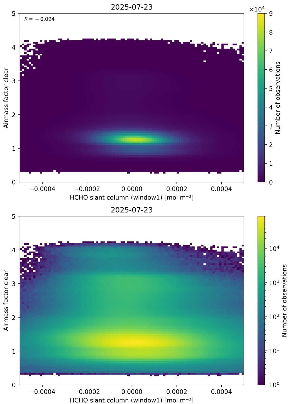
Figure 81: Scatter density plot of “HCHO slant column (window1)” against “Airmass factor clear” for 2025-07-22 to 2025-07-24.
