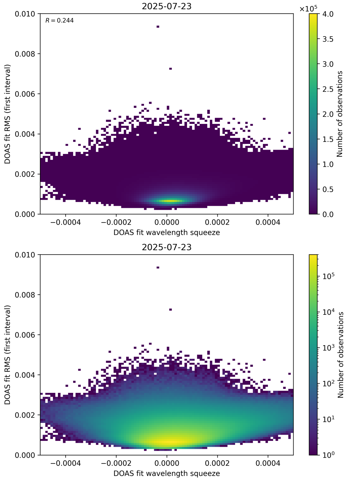
Figure 68: Scatter density plot of “DOAS fit wavelength squeeze” against “DOAS fit RMS (first interval)” for 2025-07-22 to 2025-07-24.
