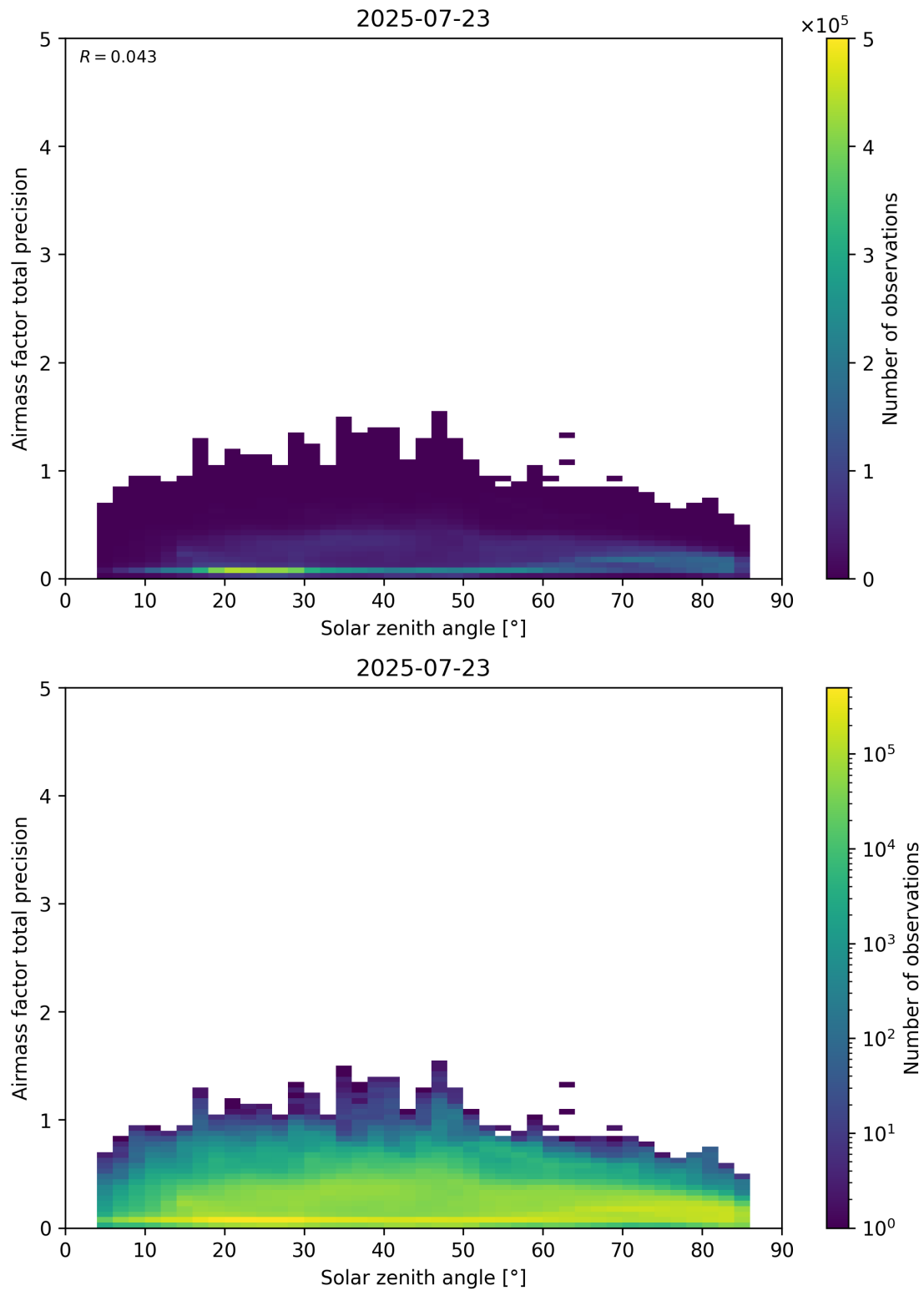
Figure 176: Scatter density plot of “Solar zenith angle” against “Airmass factor total precision” for 2025-07-22 to 2025-07-24.
