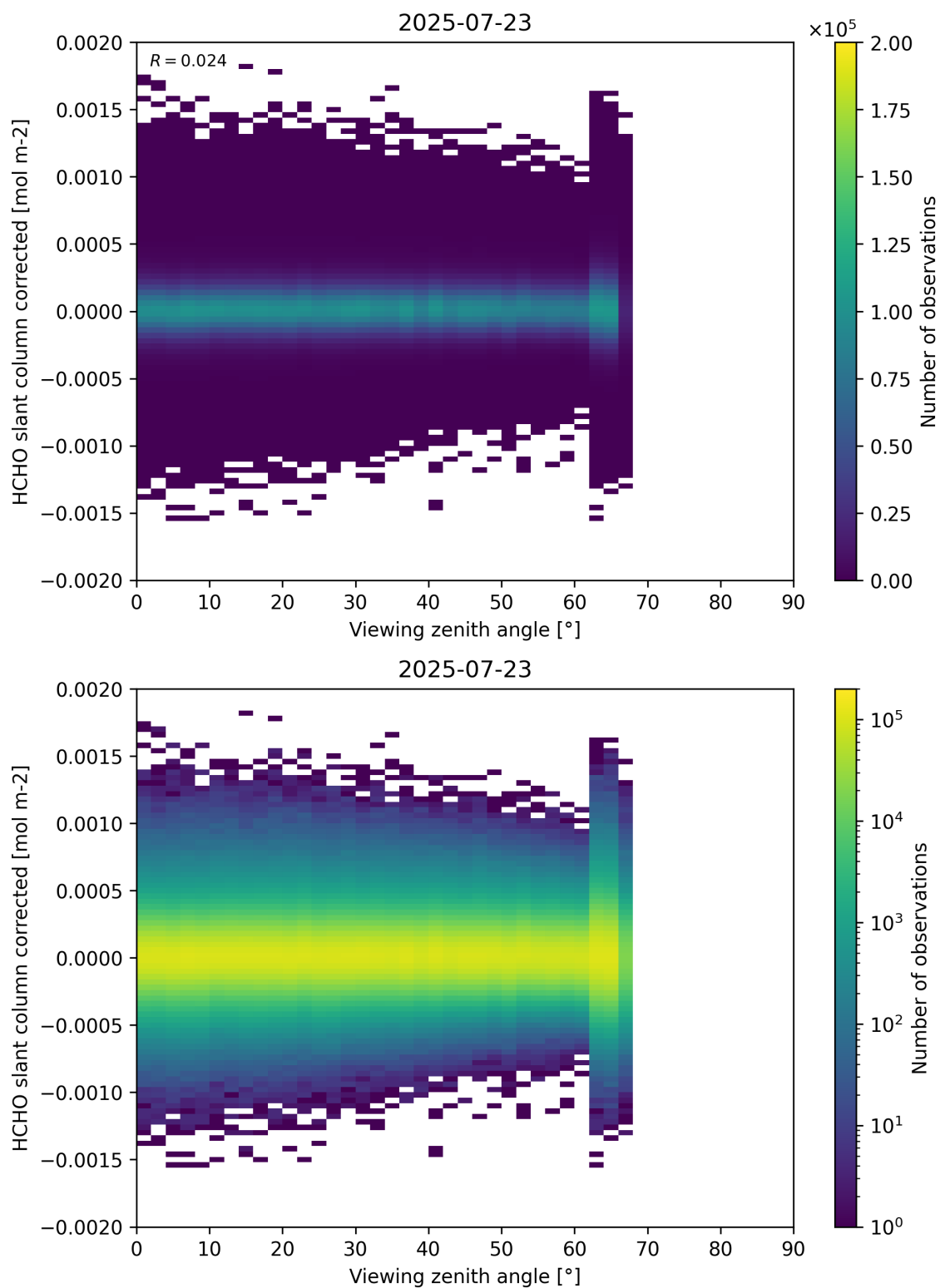
Figure 186: Scatter density plot of “Viewing zenith angle” against “HCHO slant column corrected” for 2025-07-22 to 2025-07-24.
