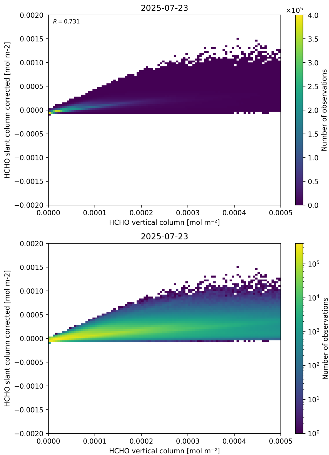
Figure 127: Scatter density plot of “HCHO vertical column” against “HCHO slant column corrected” for 2025-07-22 to 2025-07-24.
