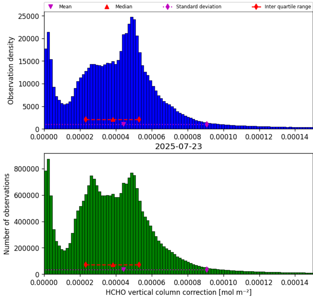
Figure 37: Histogram of “HCHO vertical column correction” for 2025-07-22 to 2025-07-24
