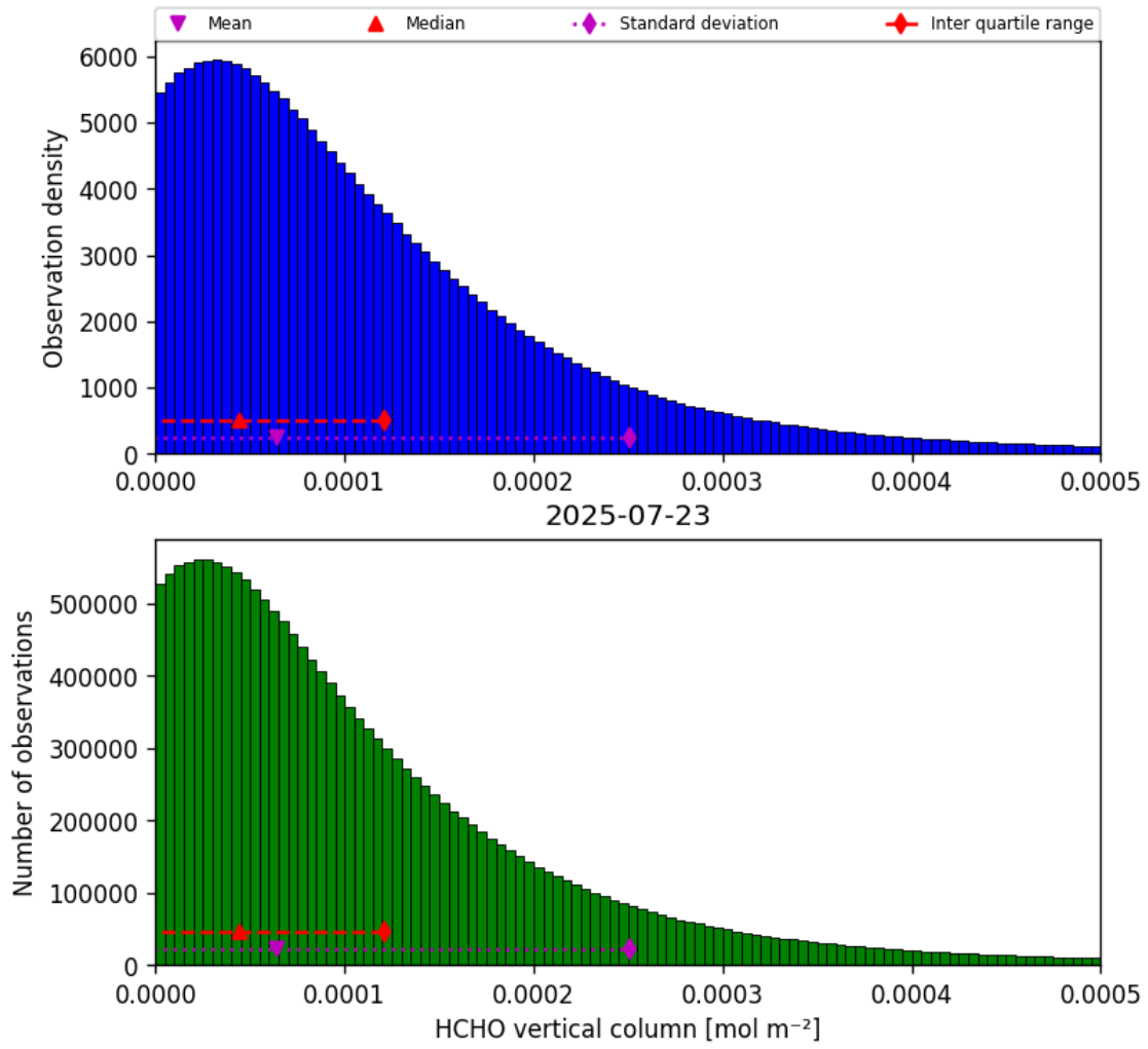
Figure 35: Histogram of “HCHO vertical column” for 2025-07-22 to 2025-07-24
