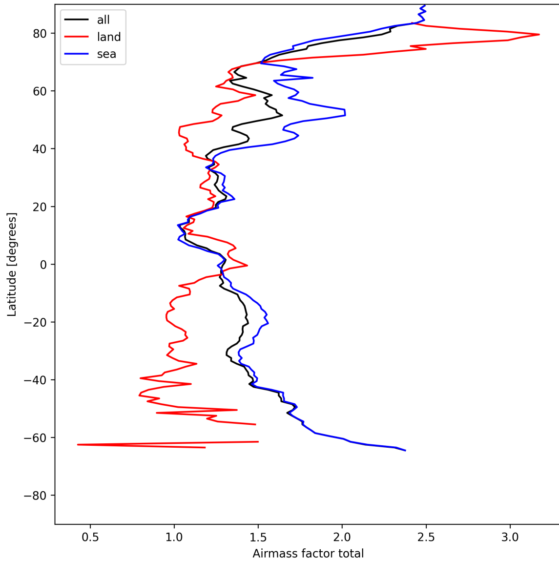
Figure 26: Zonal average of “Airmass factor total” for 2025-07-22 to 2025-07-24.
