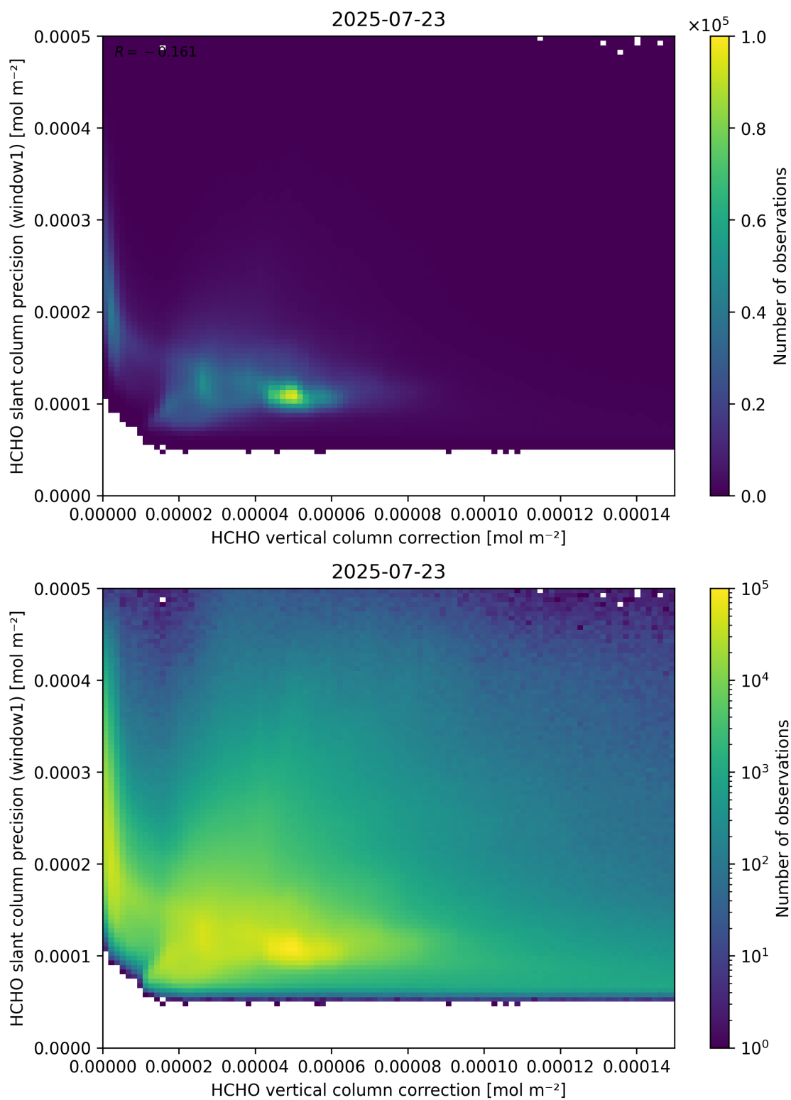
Figure 119: Scatter density plot of “HCHO vertical column correction” against “HCHO slant column precision (window1)” for 2025-07-22 to 2025-07-24.
