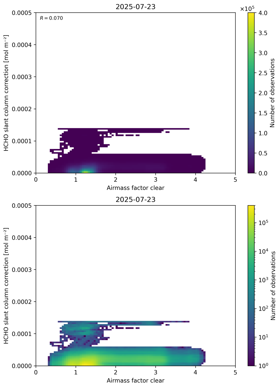
Figure 75: Scatter density plot of “Airmass factor clear” against “HCHO slant column correction” for 2025-07-22 to 2025-07-24.
