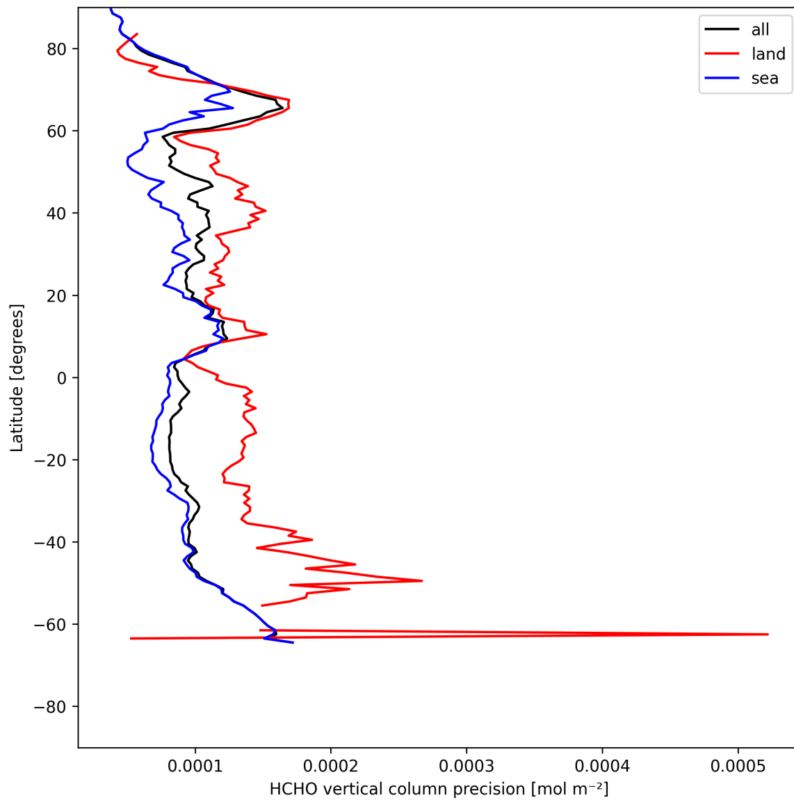
Figure 22: Zonal average of “HCHO vertical column precision” for 2025-07-22 to 2025-07-24.
