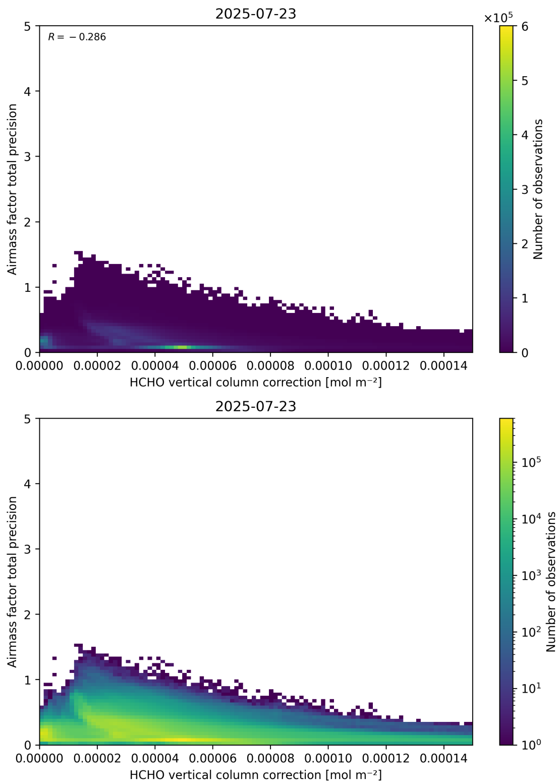
Figure 121: Scatter density plot of “HCHO vertical column correction” against “Airmass factor total precision” for 2025-07-22 to 2025-07-24.
