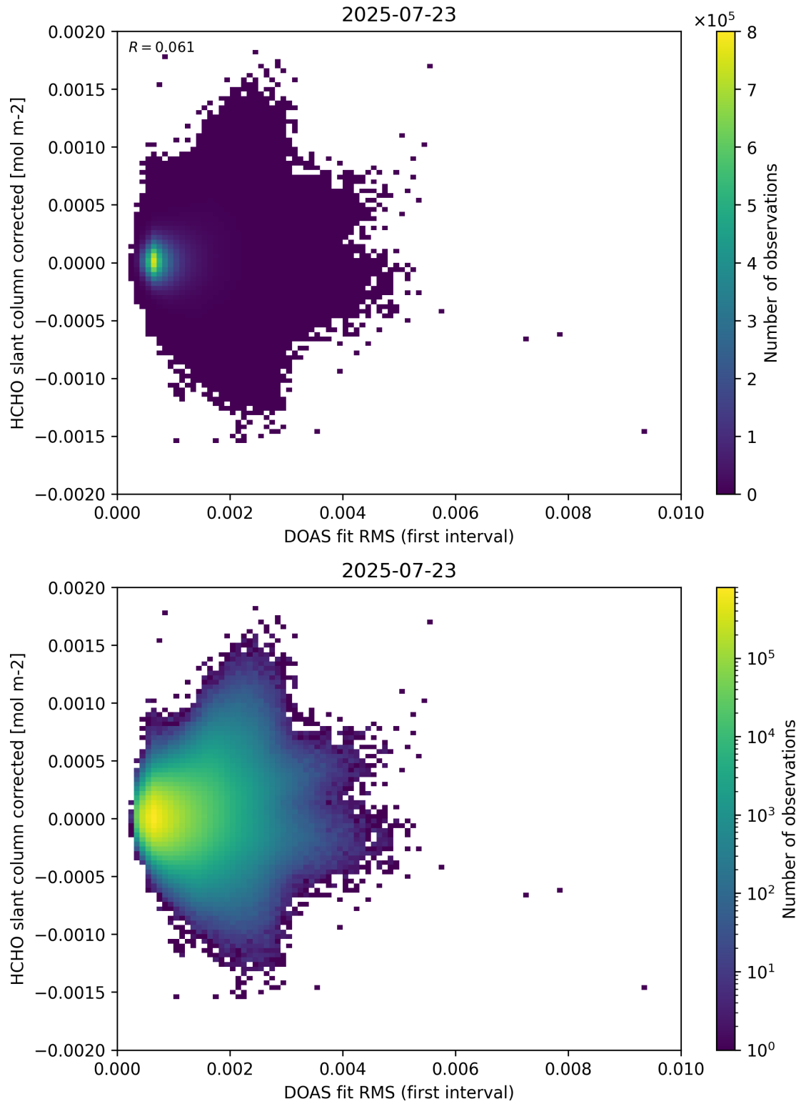
Figure 62: Scatter density plot of “DOAS fit RMS (first interval)” against “HCHO slant column corrected” for 2025-07-22 to 2025-07-24.
