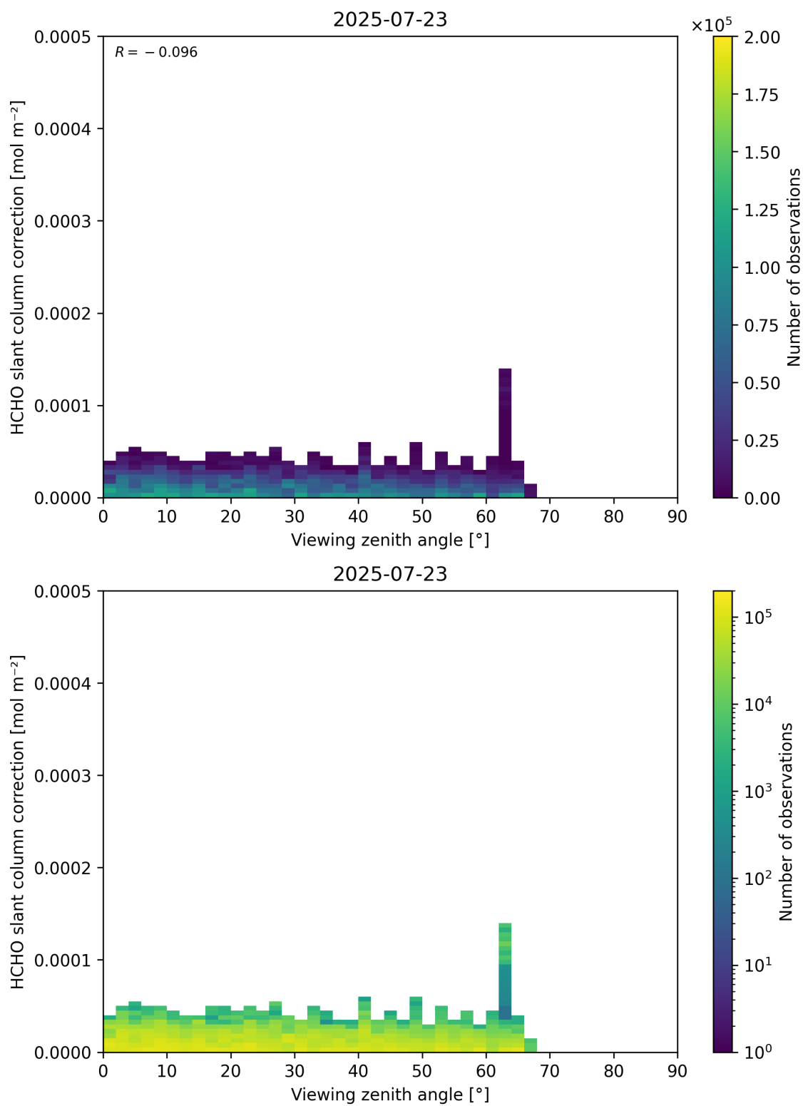
Figure 187: Scatter density plot of “Viewing zenith angle” against “HCHO slant column correction” for 2025-07-22 to 2025-07-24.
