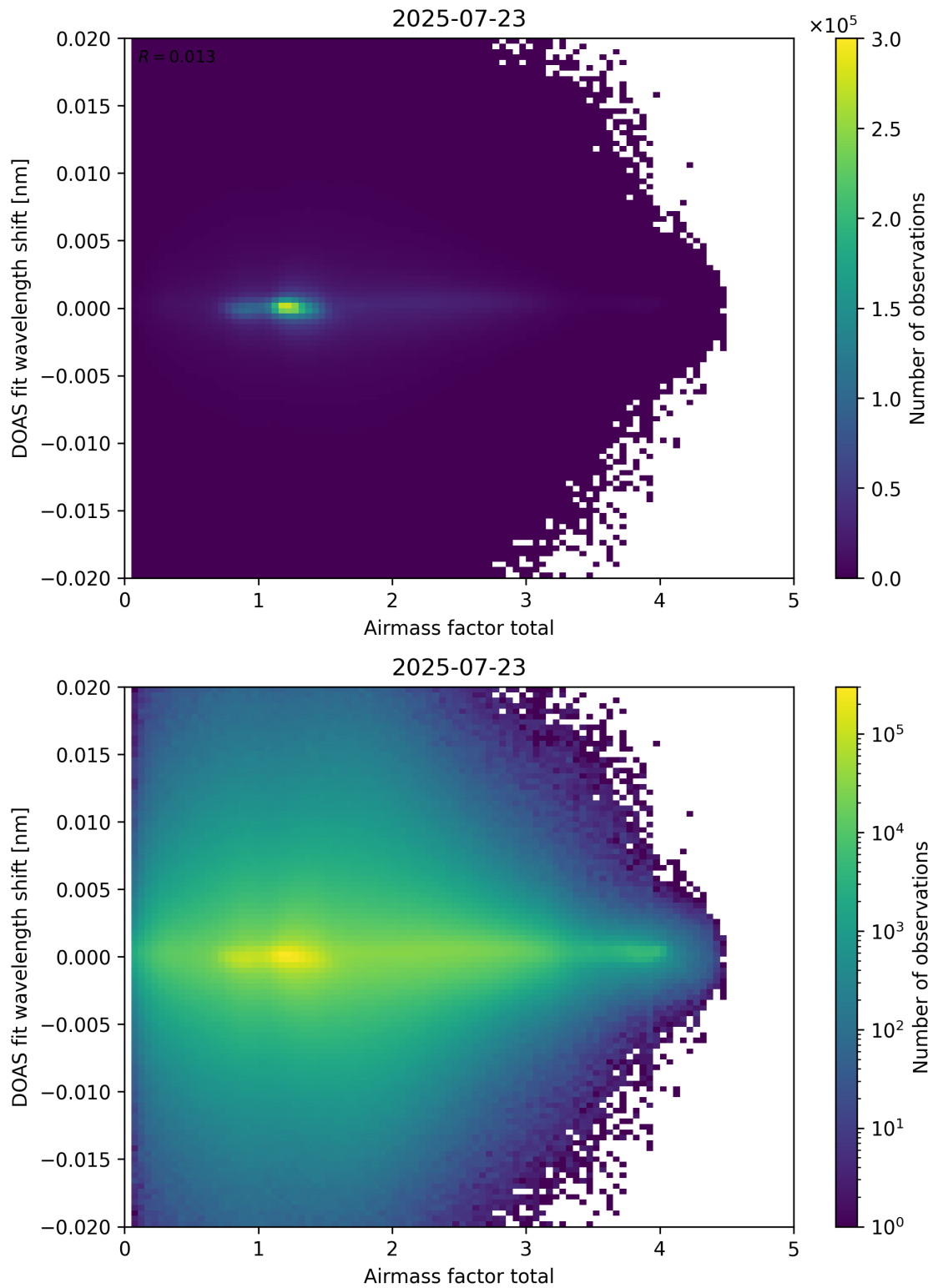
Figure 98: Scatter density plot of “Airmass factor total” against “DOAS fit wavelength shift” for 2025-07-22 to 2025-07-24.
