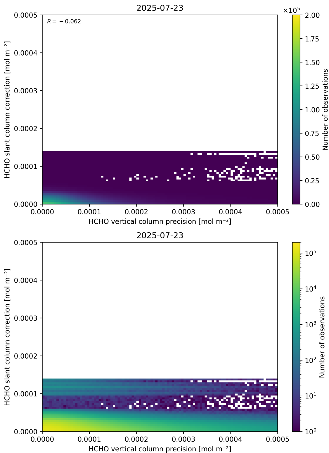
Figure 141: Scatter density plot of “HCHO vertical column precision” against “HCHO slant column correction” for 2025-07-22 to 2025-07-24.
