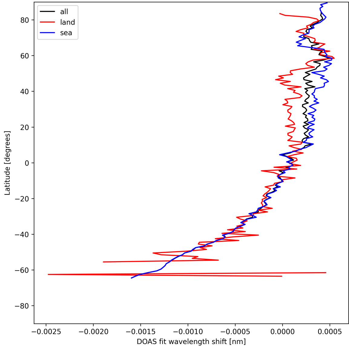
Figure 30: Zonal average of “DOAS fit wavelength shift” for 2025-07-22 to 2025-07-24.
