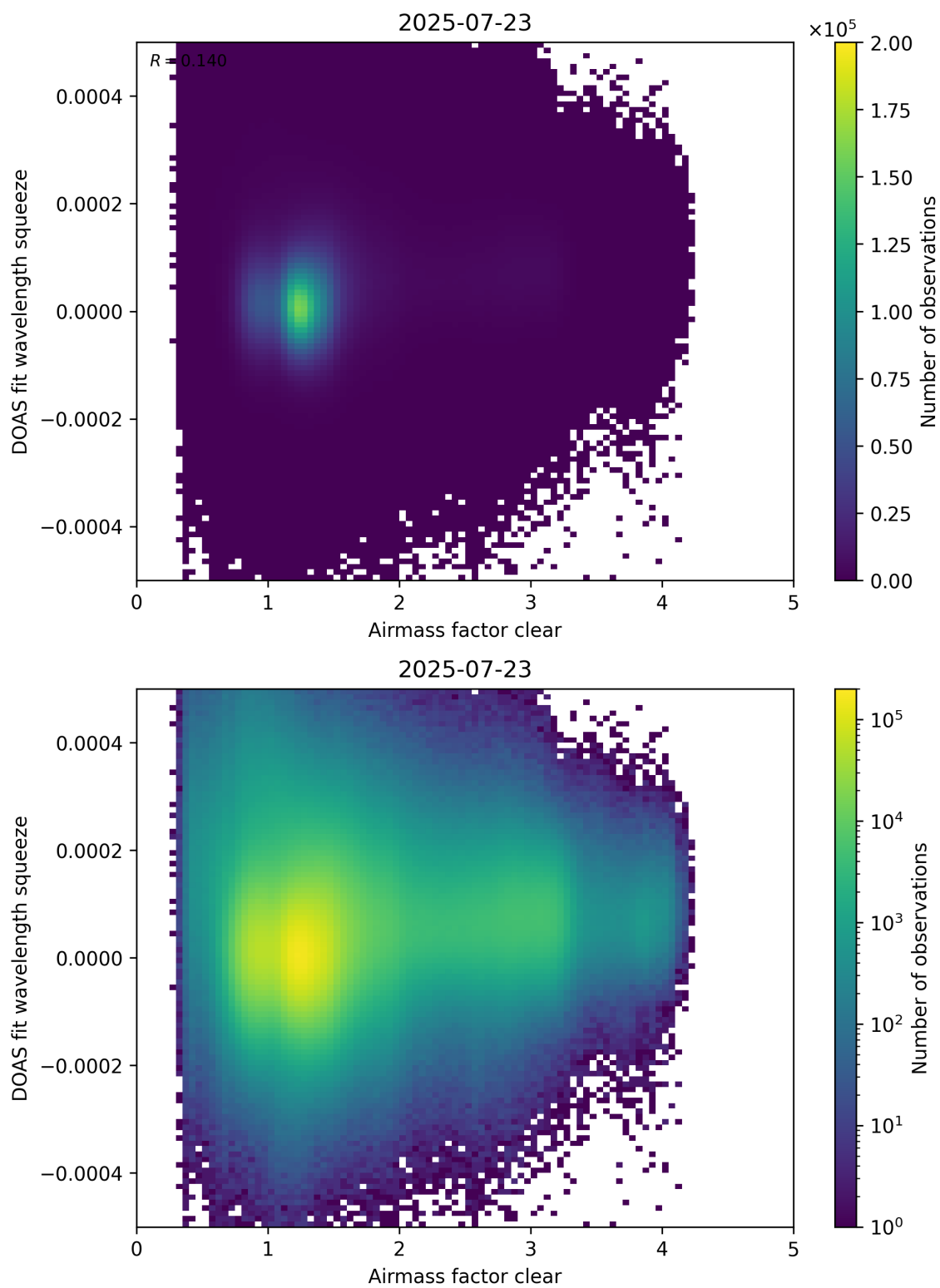
Figure 73: Scatter density plot of “Airmass factor clear” against “DOAS fit wavelength squeeze” for 2025-07-22 to 2025-07-24.
