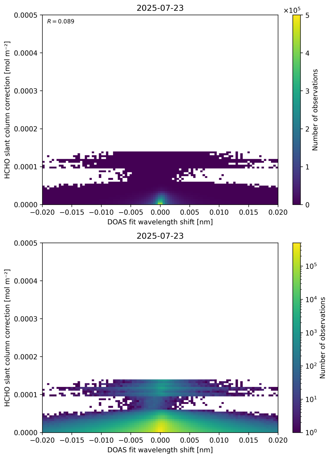
Figure 67: Scatter density plot of “DOAS fit wavelength shift” against “HCHO slant column correction” for 2025-07-22 to 2025-07-24.
