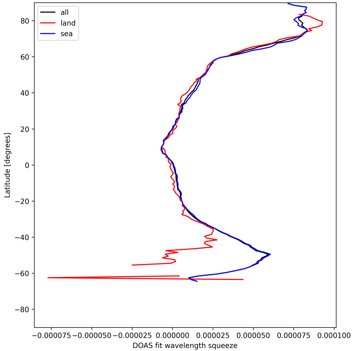
Figure 31: Zonal average of “DOAS fit wavelength squeeze” for 2025-07-22 to 2025-07-24.
