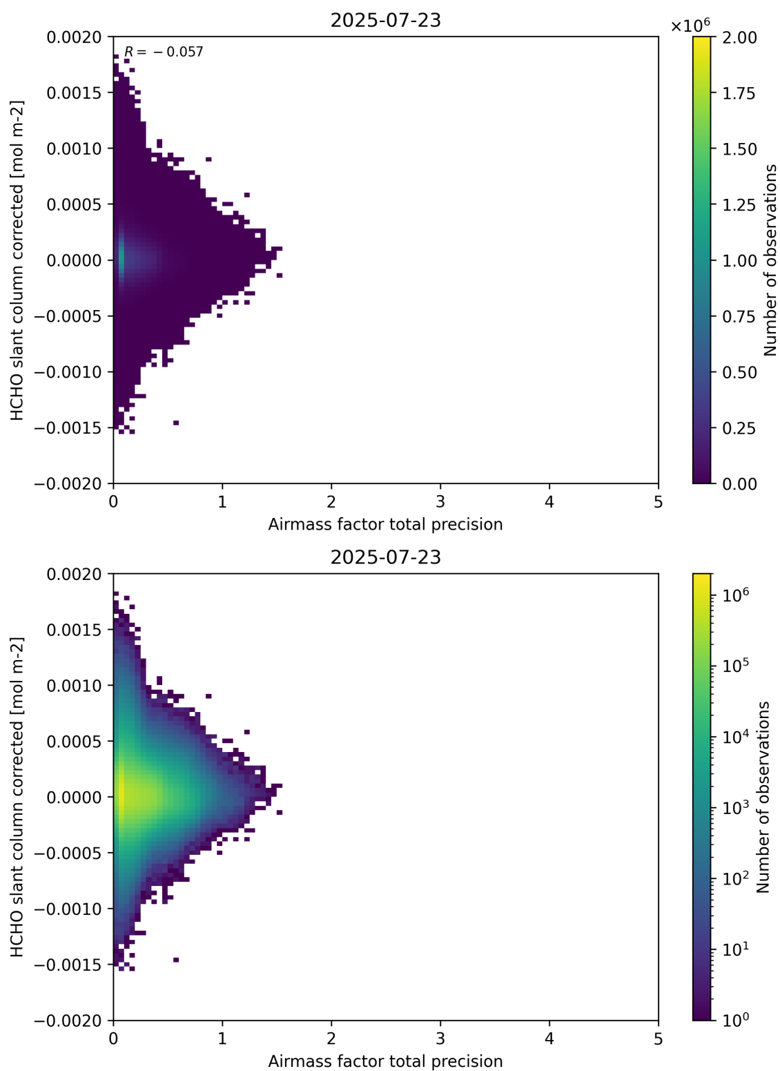
Figure 109: Scatter density plot of “Airmass factor total precision” against “HCHO slant column corrected” for 2025-07-22 to 2025-07-24.
