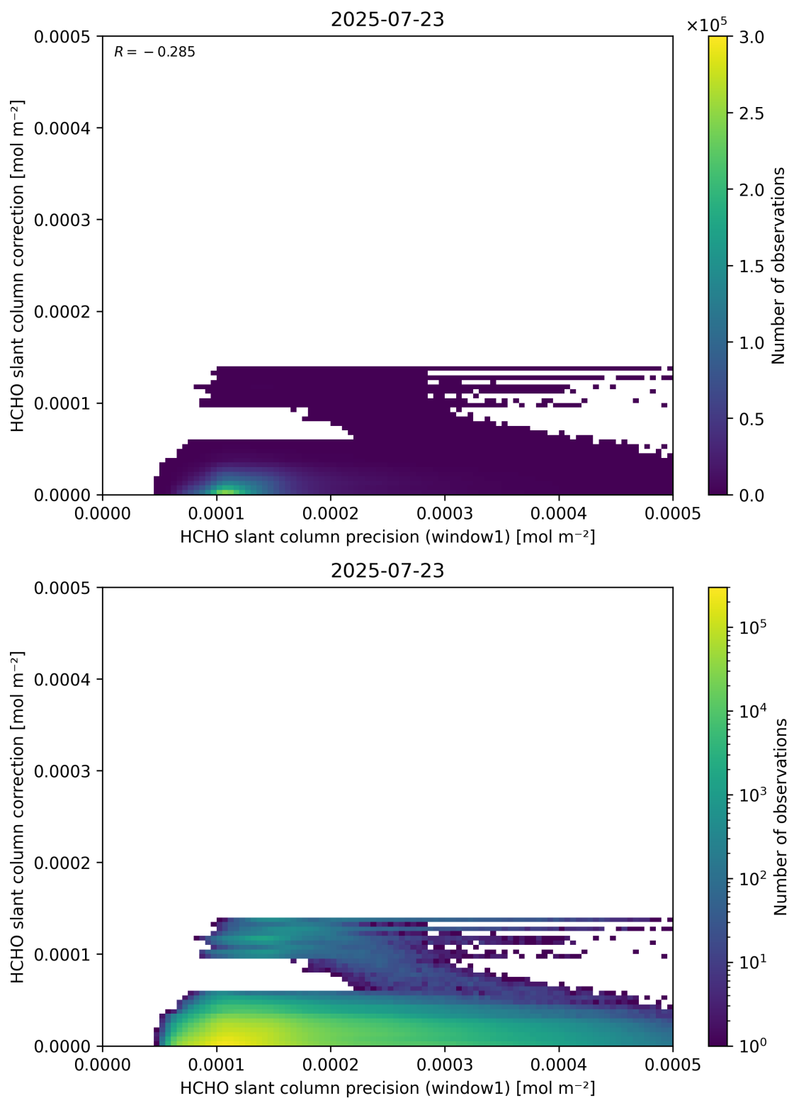
Figure 93: Scatter density plot of “HCHO slant column precision (window1)” against “HCHO slant column correction” for 2025-07-22 to 2025-07-24.
