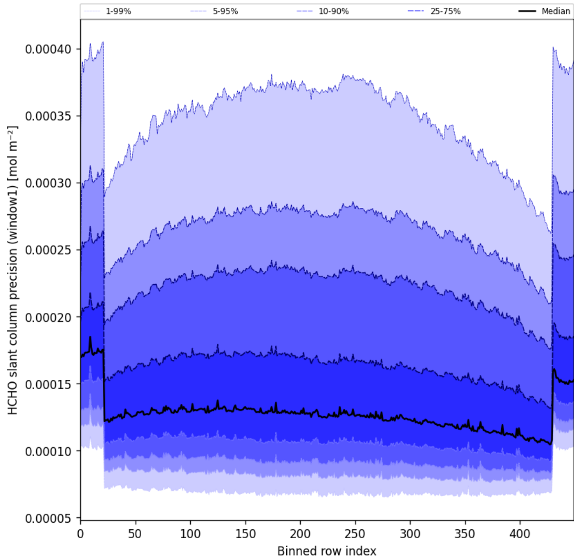
Figure 53: Along track statistics of “HCHO slant column precision (window1)” for 2025-07-22 to 2025-07-24
