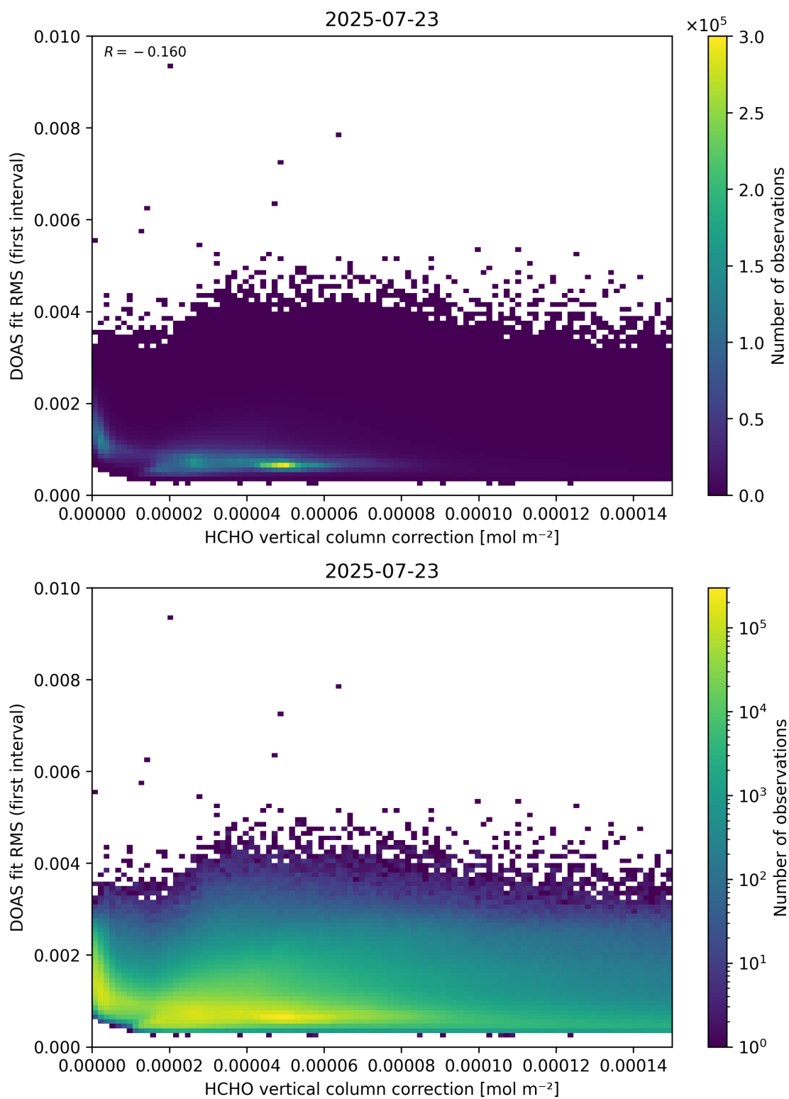
Figure 112: Scatter density plot of “HCHO vertical column correction” against “DOAS fit RMS (first interval)” for 2025-07-22 to 2025-07-24.
