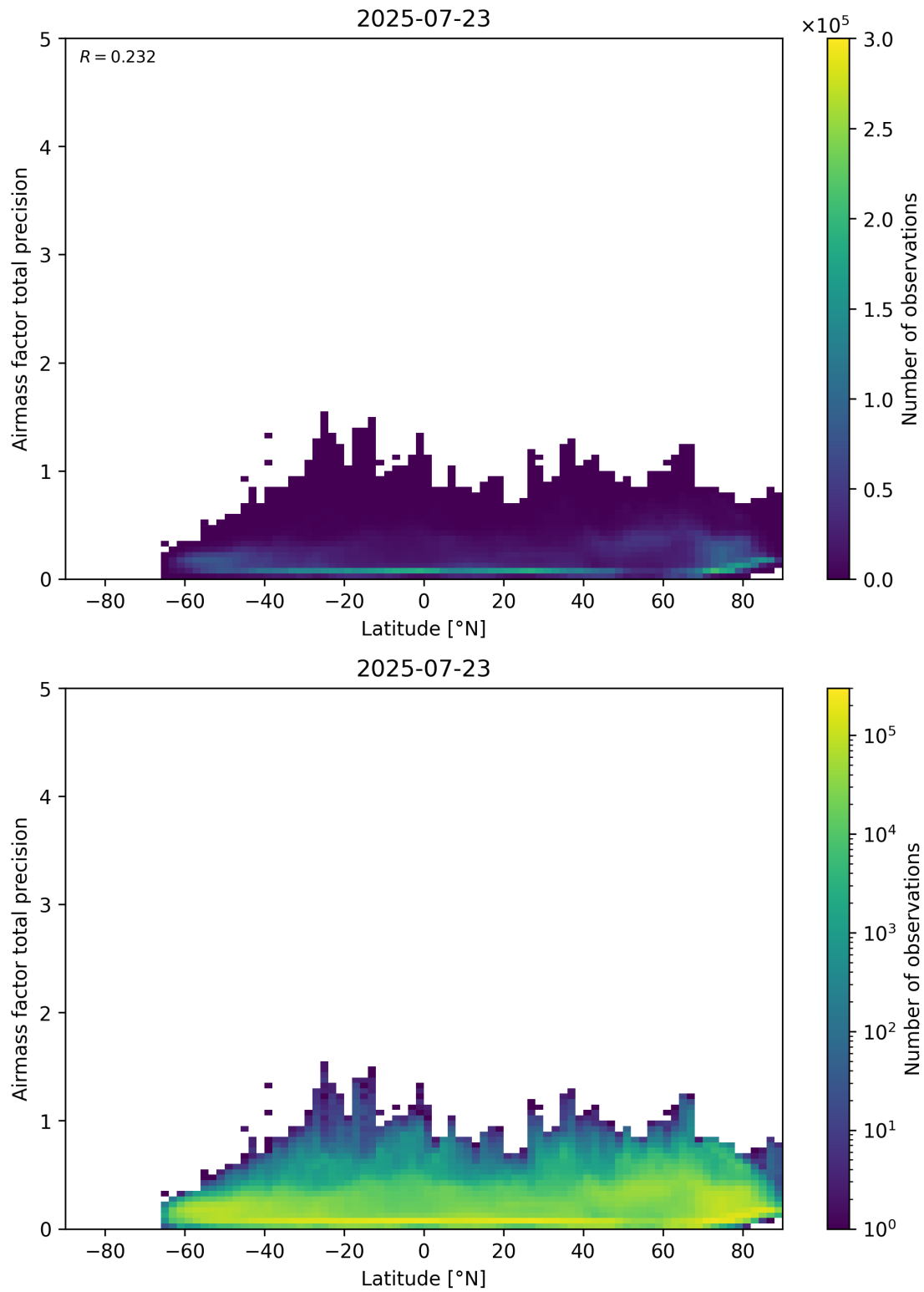
Figure 162: Scatter density plot of “Latitude” against “Airmass factor total precision” for 2025-07-22 to 2025-07-24.
