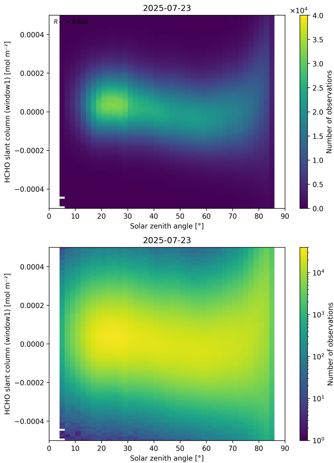
Figure 173: Scatter density plot of “Solar zenith angle” against “HCHO slant column (window1)” for 2025-07-22 to 2025-07-24.
