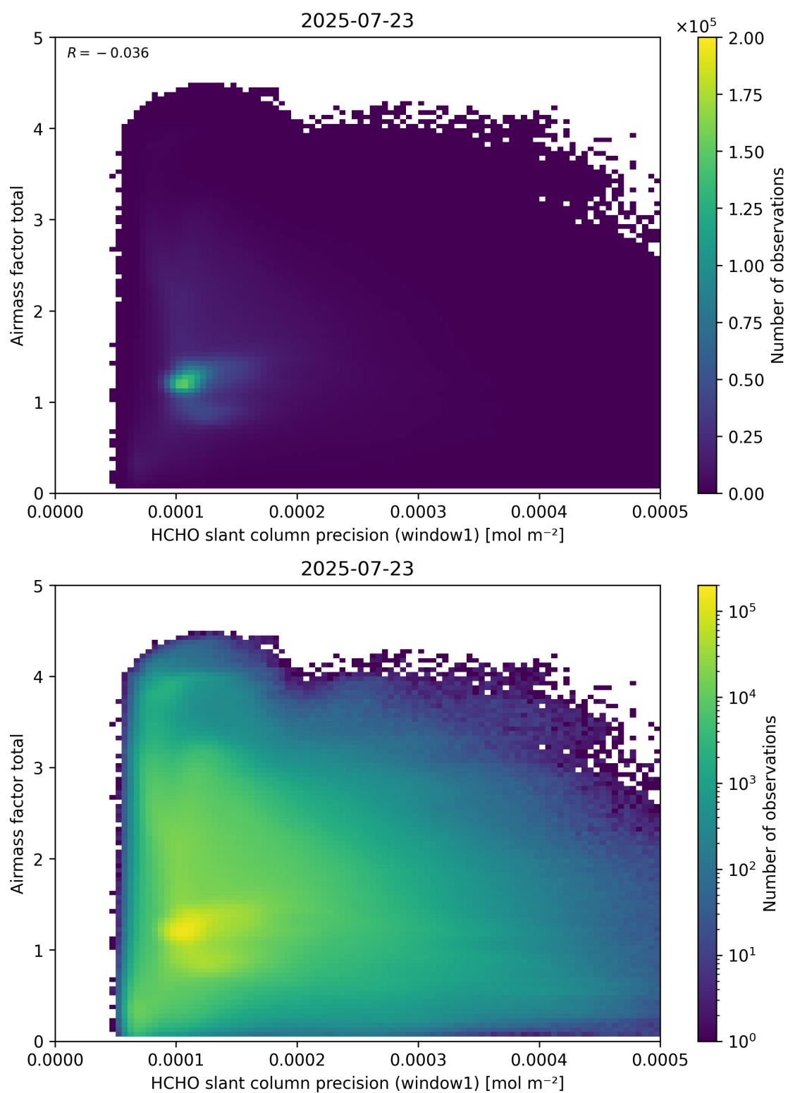
Figure 94: Scatter density plot of “HCHO slant column precision (window1)” against “Airmass factor total” for 2025-07-22 to 2025-07-24.
