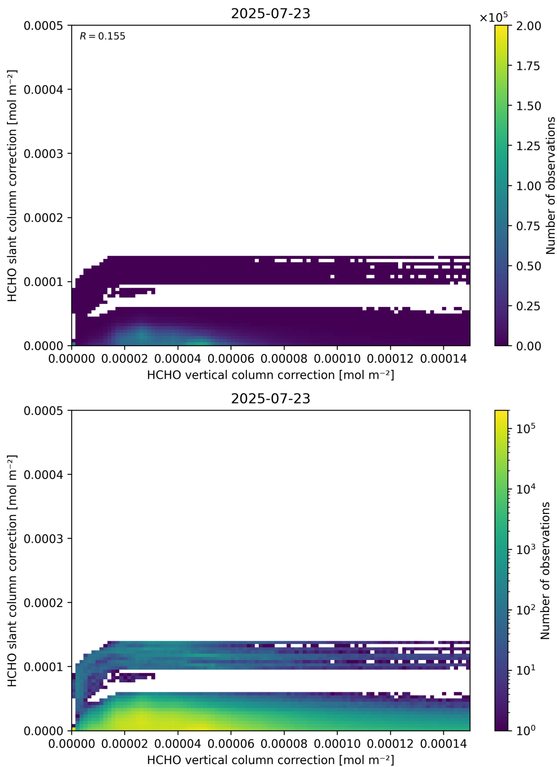
Figure 117: Scatter density plot of “HCHO vertical column correction” against “HCHO slant column correction” for 2025-07-22 to 2025-07-24.
