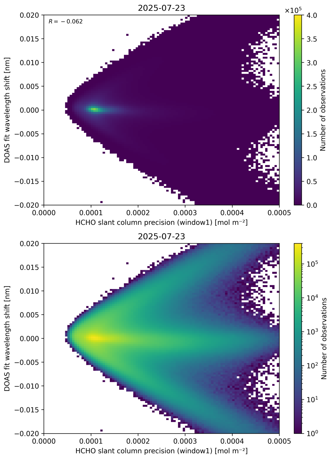
Figure 89: Scatter density plot of “HCHO slant column precision (window1)” against “DOAS fit wavelength shift” for 2025-07-22 to 2025-07-24.
