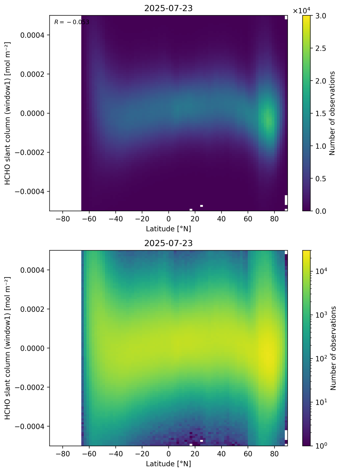
Figure 159: Scatter density plot of “Latitude” against “HCHO slant column (window1)” for 2025-07-22 to 2025-07-24.
