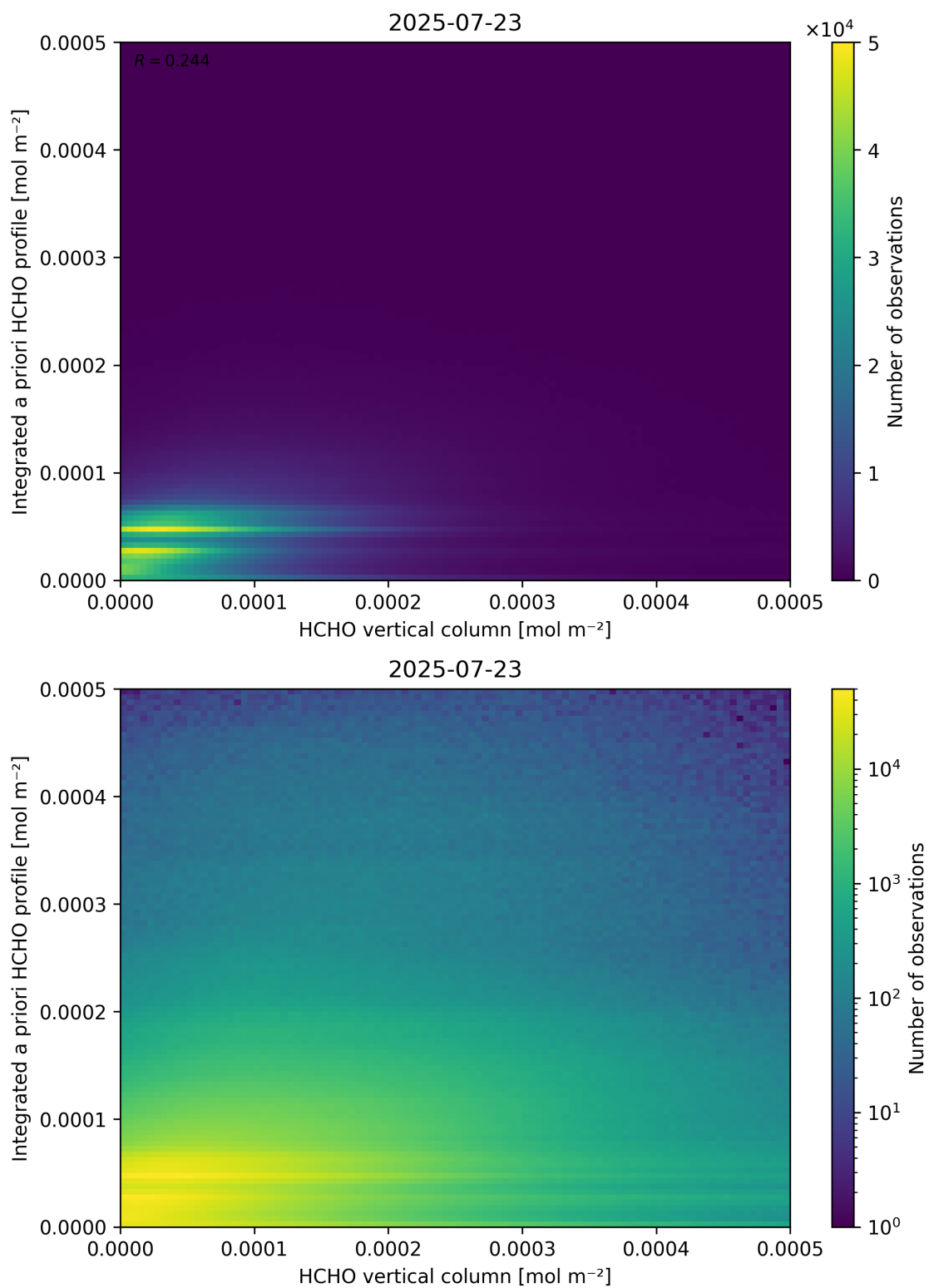
Figure 135: Scatter density plot of “HCHO vertical column” against “Integrated a priori HCHO profile” for 2025-07-22 to 2025-07-24.
