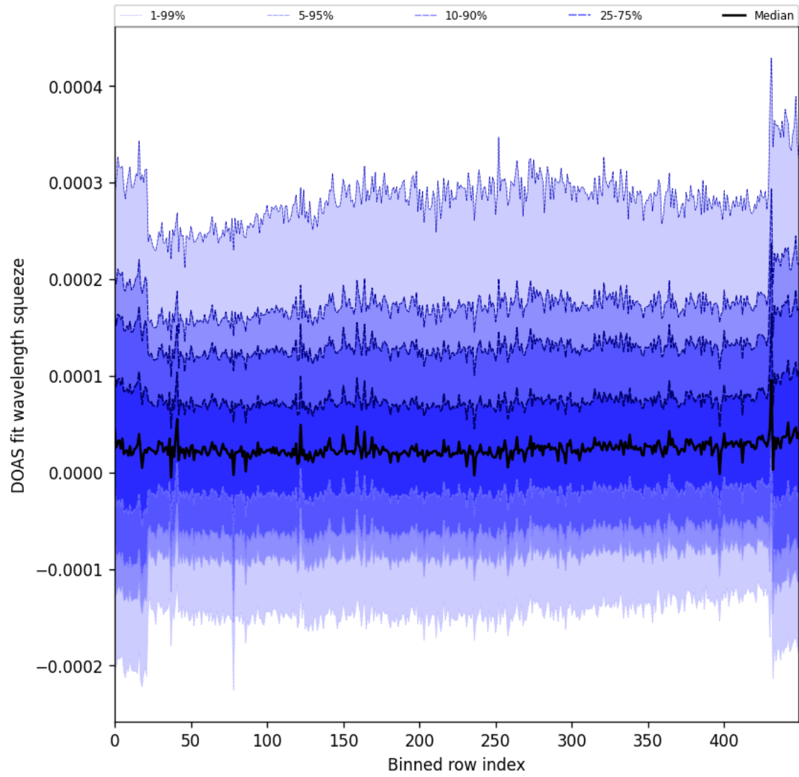
Figure 59: Along track statistics of “DOAS fit wavelength squeeze” for 2025-07-22 to 2025-07-24
