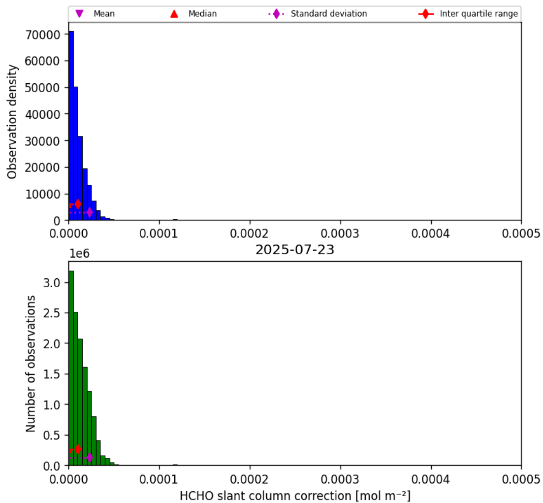
Figure 47: Histogram of “HCHO slant column correction” for 2025-07-22 to 2025-07-24
