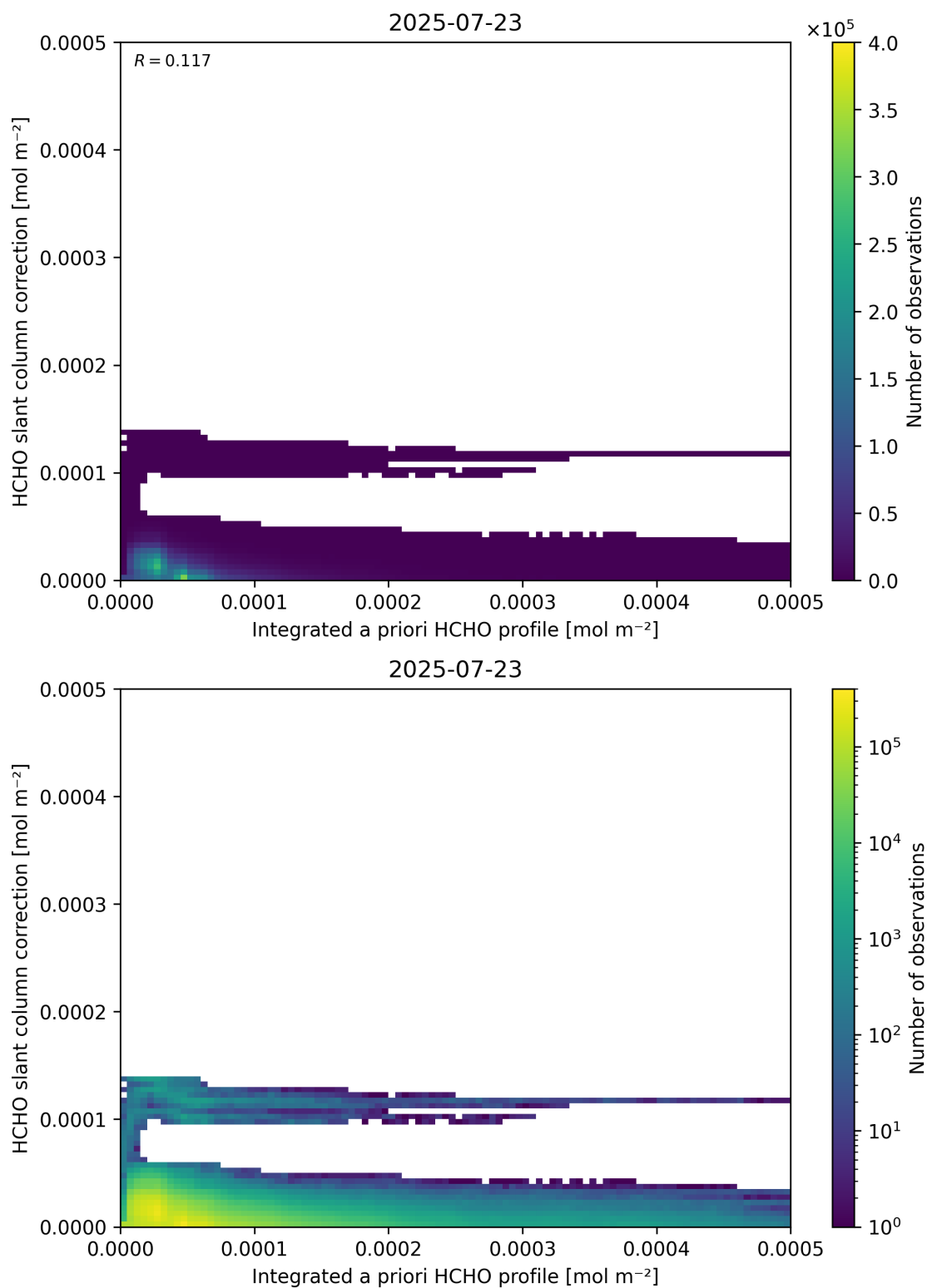
Figure 152: Scatter density plot of “Integrated a priori HCHO profile” against “HCHO slant column correction” for 2025-07-22 to 2025-07-24.
