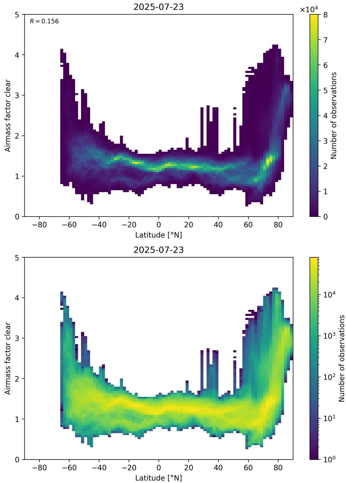
Figure 156: Scatter density plot of “Latitude” against “Airmass factor clear” for 2025-07-22 to 2025-07-24.
