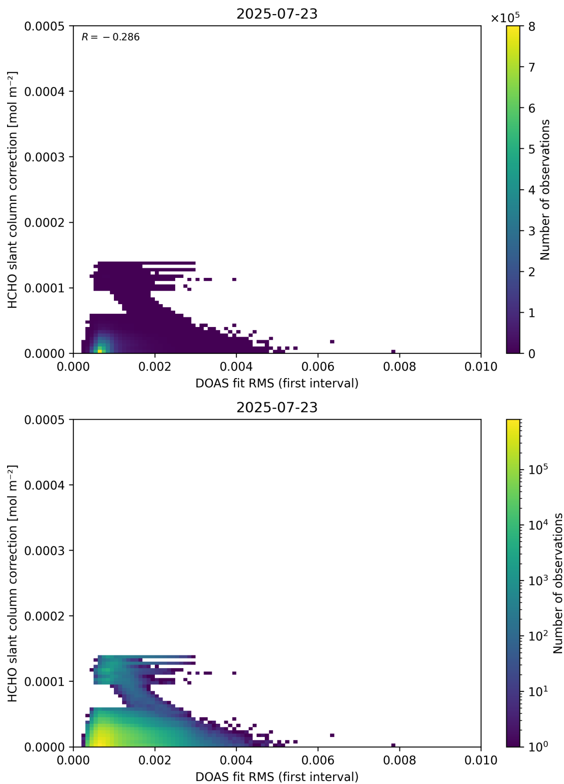
Figure 63: Scatter density plot of “DOAS fit RMS (first interval)” against “HCHO slant column correction” for 2025-07-22 to 2025-07-24.
