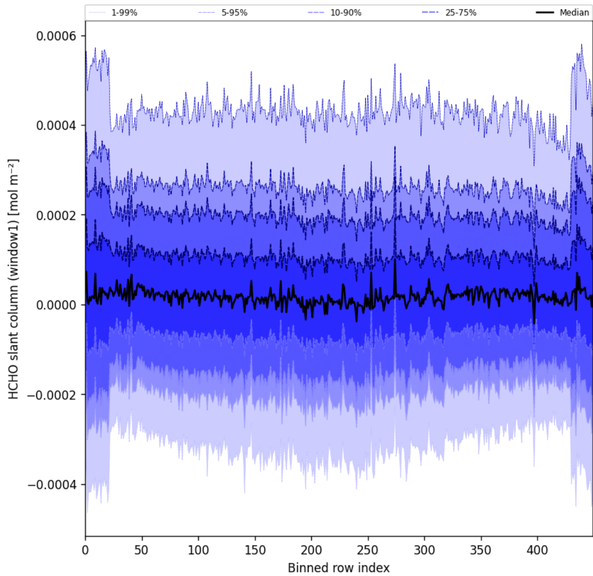
Figure 52: Along track statistics of “HCHO slant column (window1)” for 2025-07-22 to 2025-07-24
