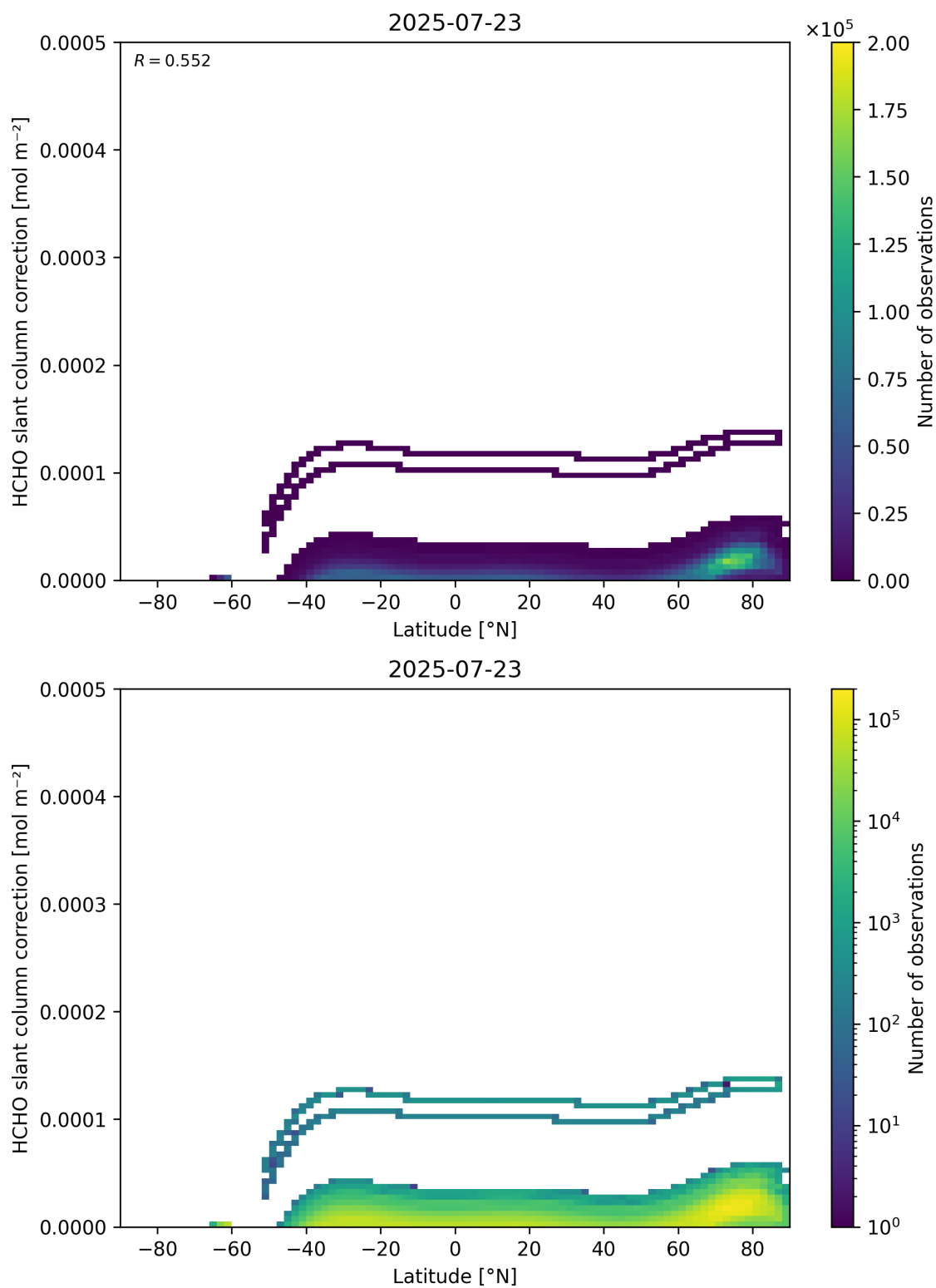
Figure 158: Scatter density plot of “Latitude” against “HCHO slant column correction” for 2025-07-22 to 2025-07-24.
