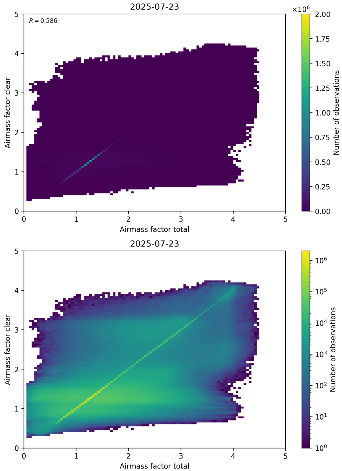
Figure 100: Scatter density plot of “Airmass factor total” against “Airmass factor clear” for 2025-07-22 to 2025-07-24.
