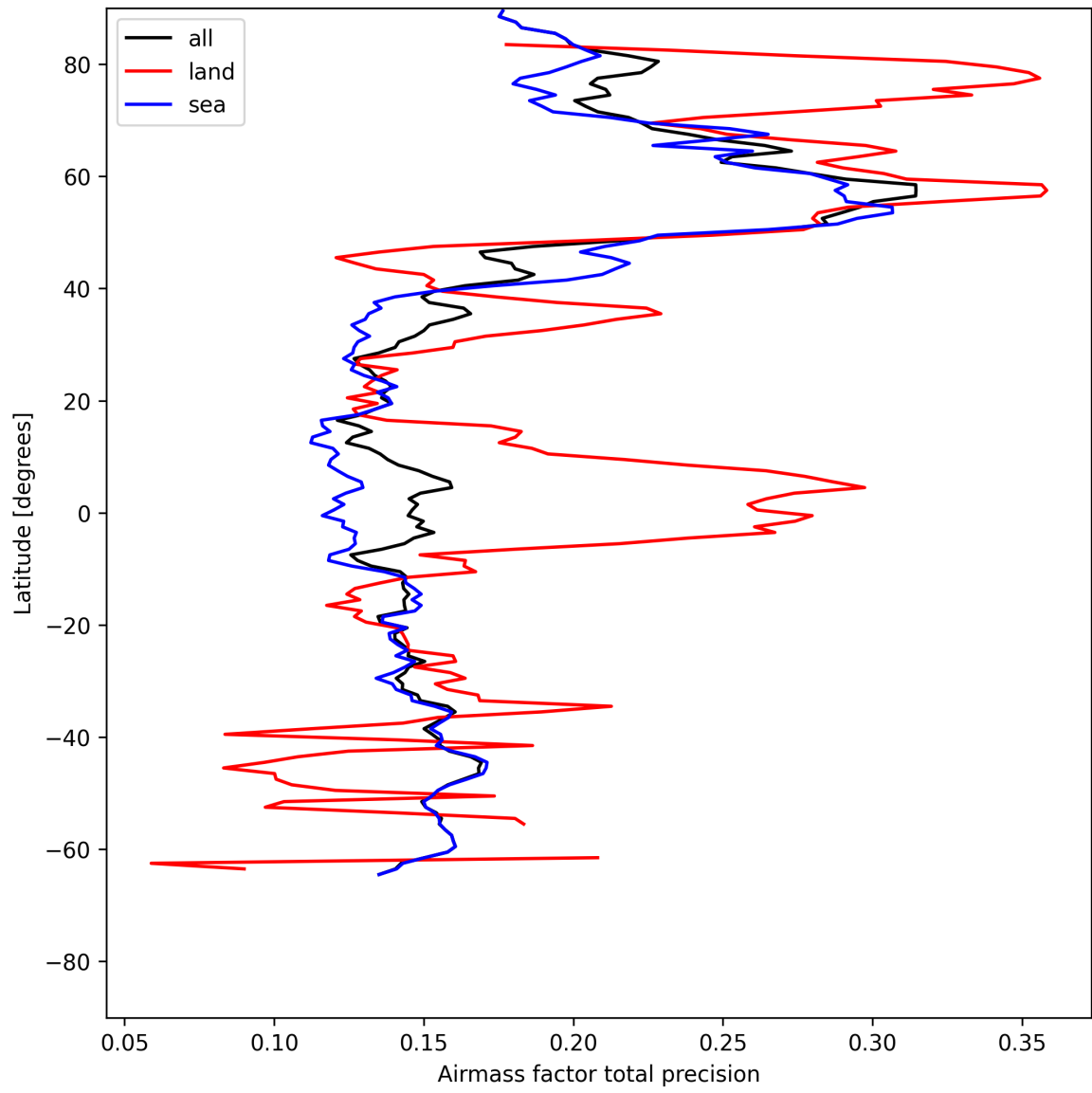
Figure 27: Zonal average of “Airmass factor total precision” for 2025-07-22 to 2025-07-24.
