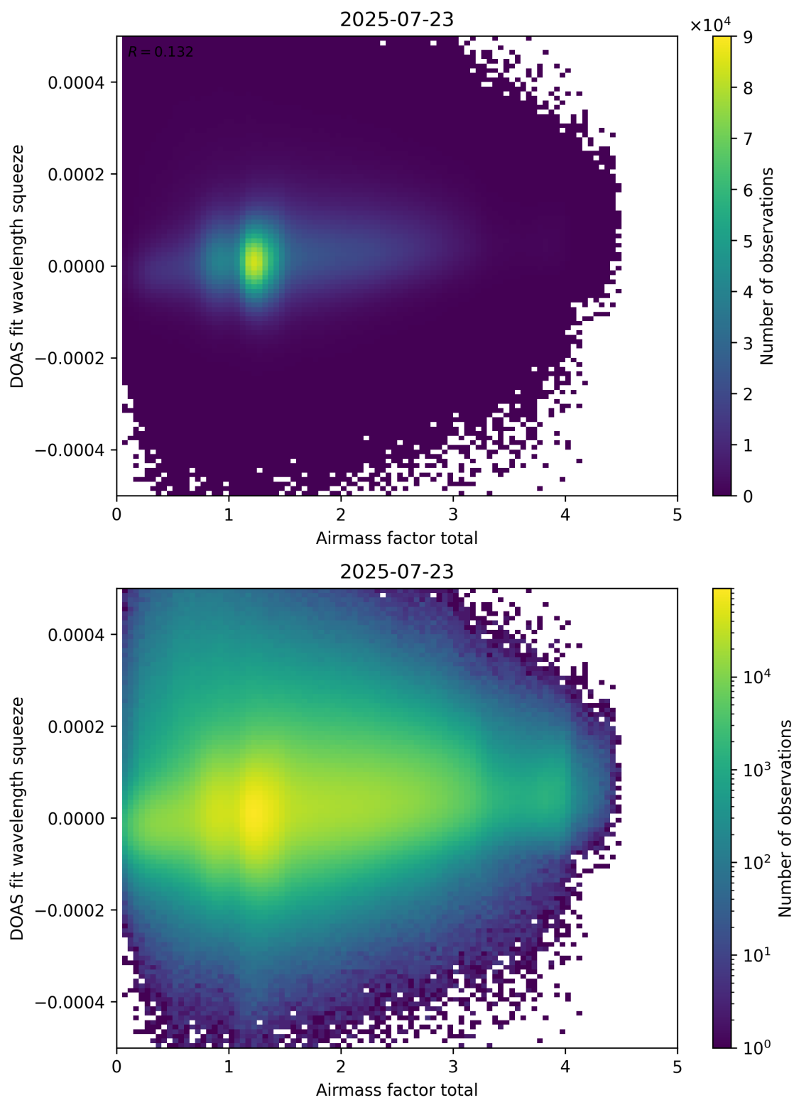
Figure 99: Scatter density plot of “Airmass factor total” against “DOAS fit wavelength squeeze” for 2025-07-22 to 2025-07-24.
