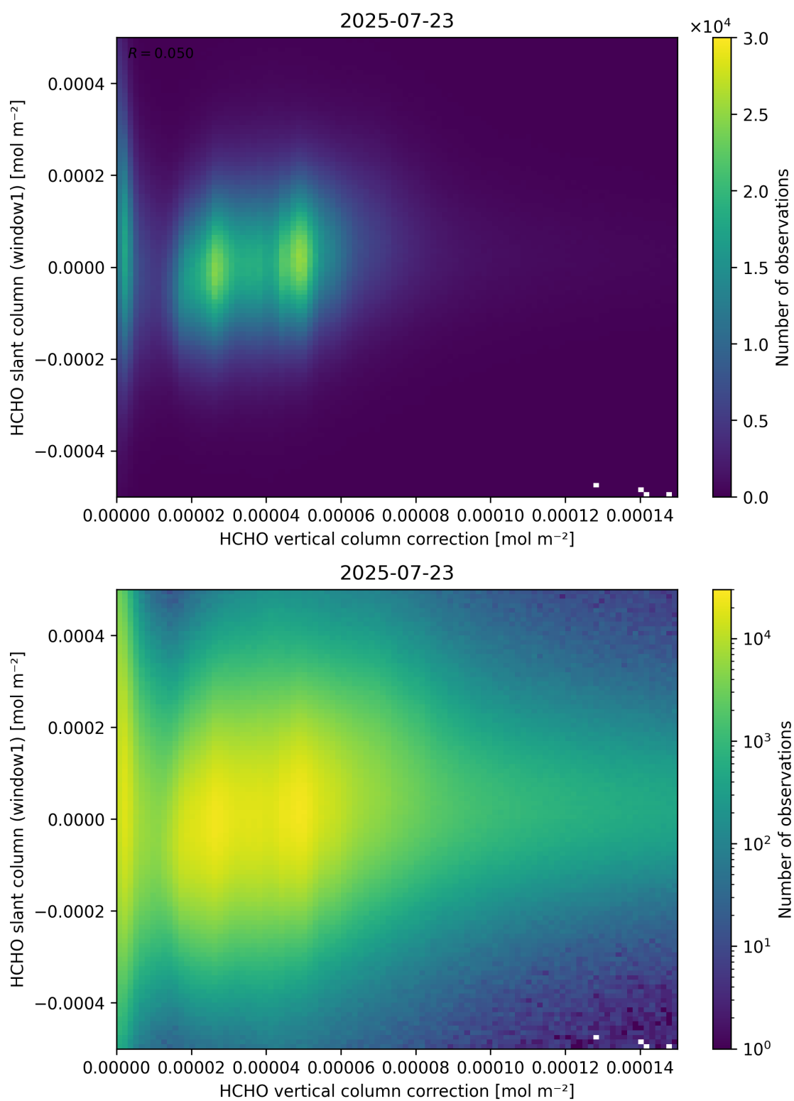
Figure 118: Scatter density plot of “HCHO vertical column correction” against “HCHO slant column (window1)” for 2025-07-22 to 2025-07-24.
