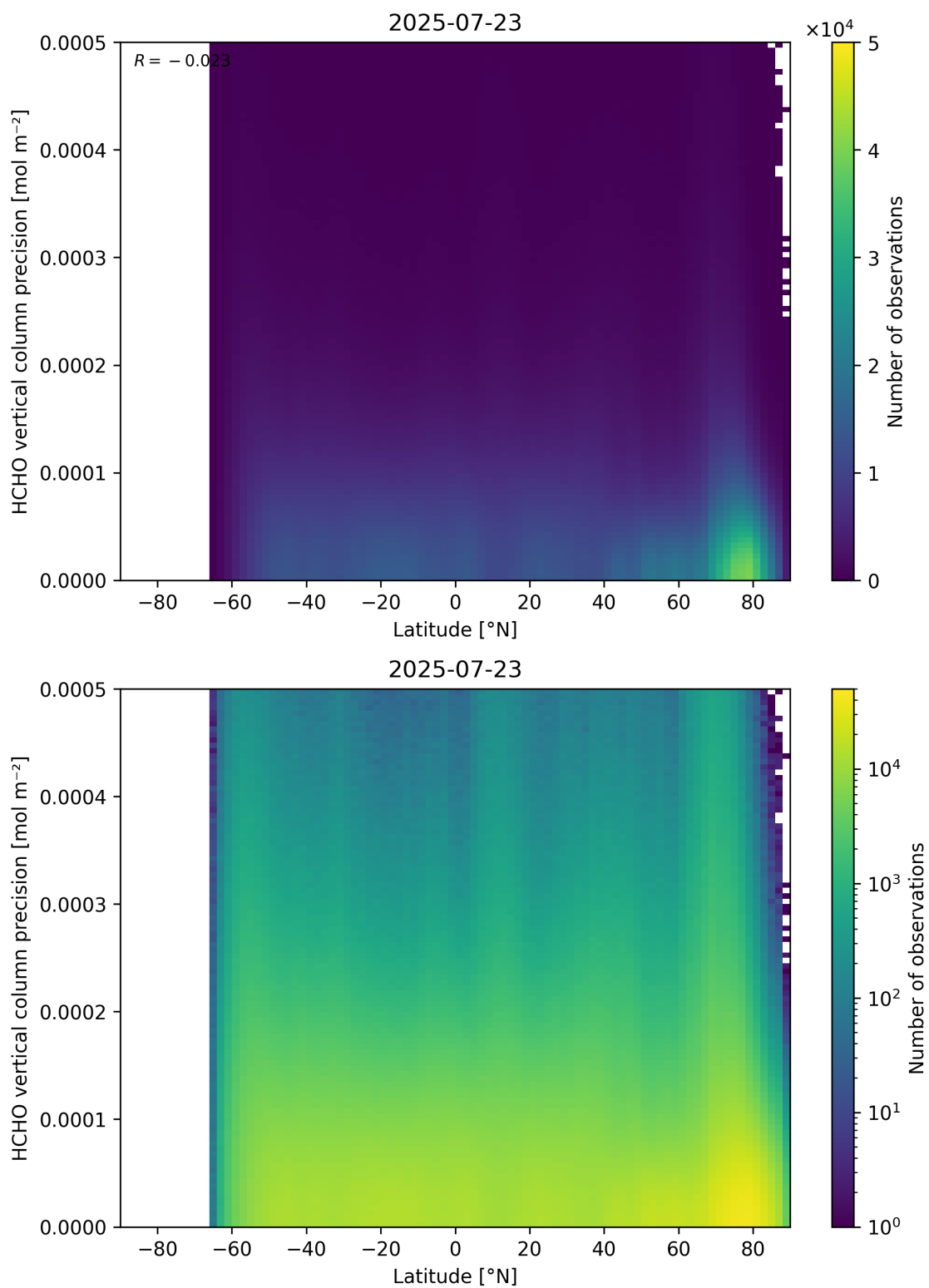
Figure 165: Scatter density plot of “Latitude” against “HCHO vertical column precision” for 2025-07-22 to 2025-07-24.
