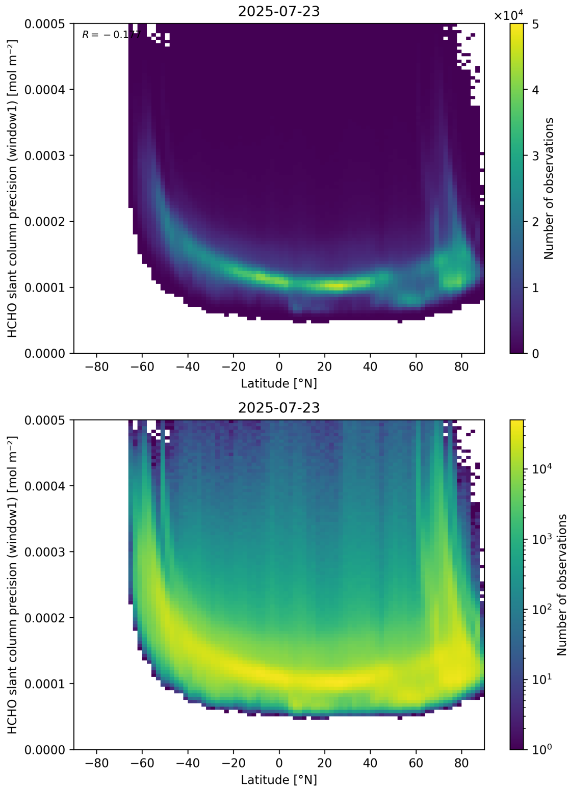
Figure 160: Scatter density plot of “Latitude” against “HCHO slant column precision (window1)” for 2025-07-22 to 2025-07-24.
