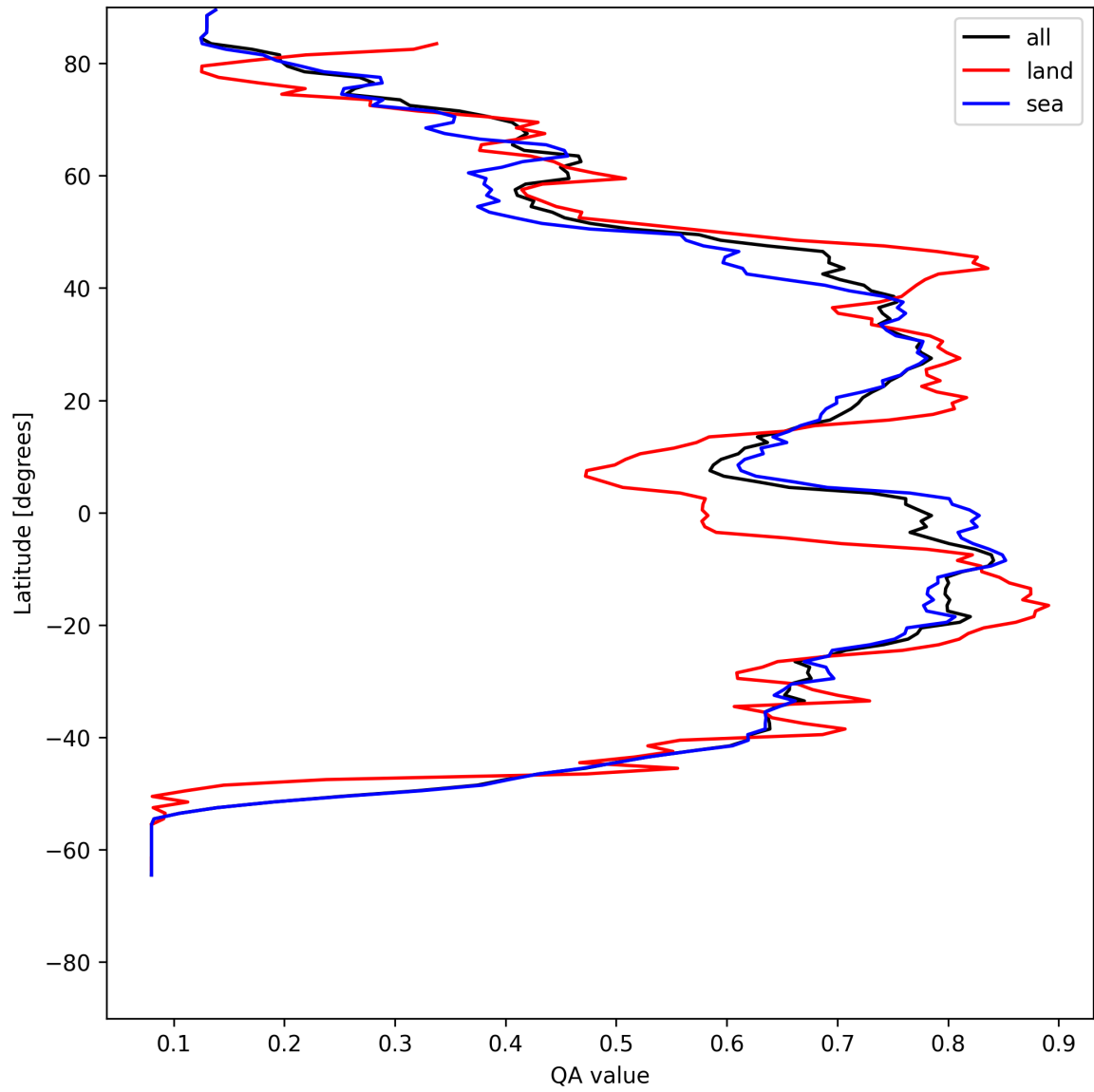
Figure 20: Zonal average of “QA value” for 2025-07-22 to 2025-07-24.
