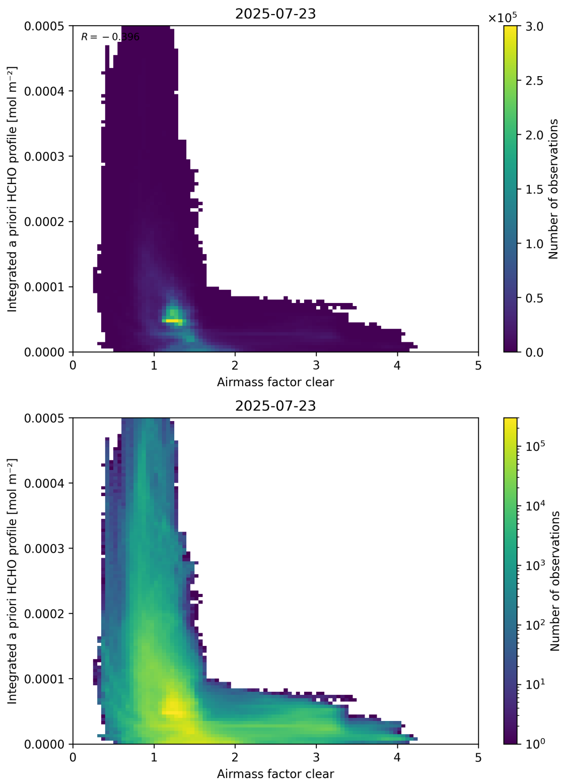
Figure 76: Scatter density plot of “Airmass factor clear” against “Integrated a priori HCHO profile” for 2025-07-22 to 2025-07-24.
