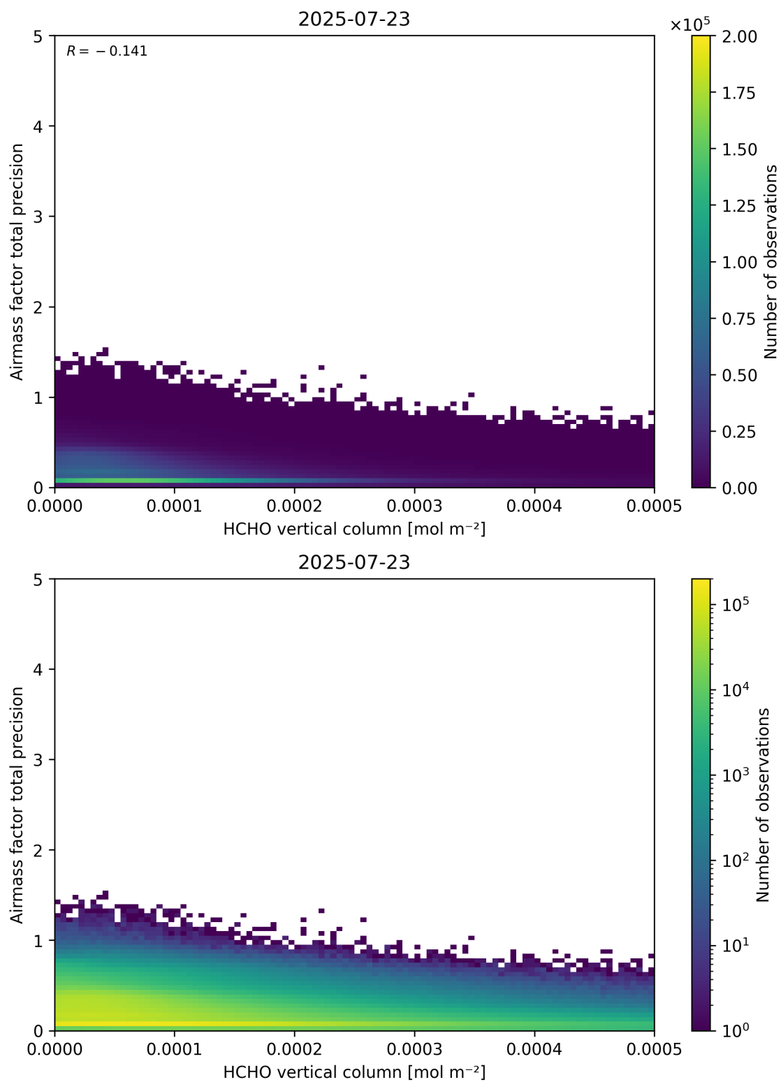
Figure 132: Scatter density plot of “HCHO vertical column” against “Airmass factor total precision” for 2025-07-22 to 2025-07-24.
