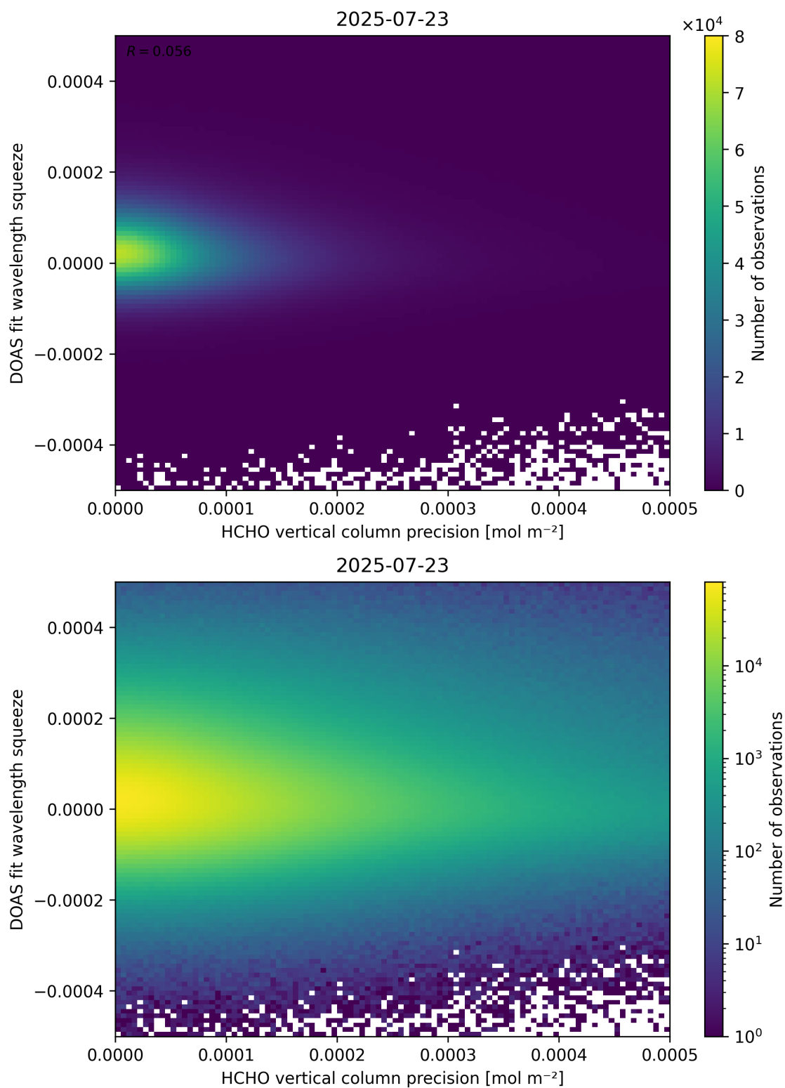
Figure 138: Scatter density plot of “HCHO vertical column precision” against “DOAS fit wavelength squeeze” for 2025-07-22 to 2025-07-24.
