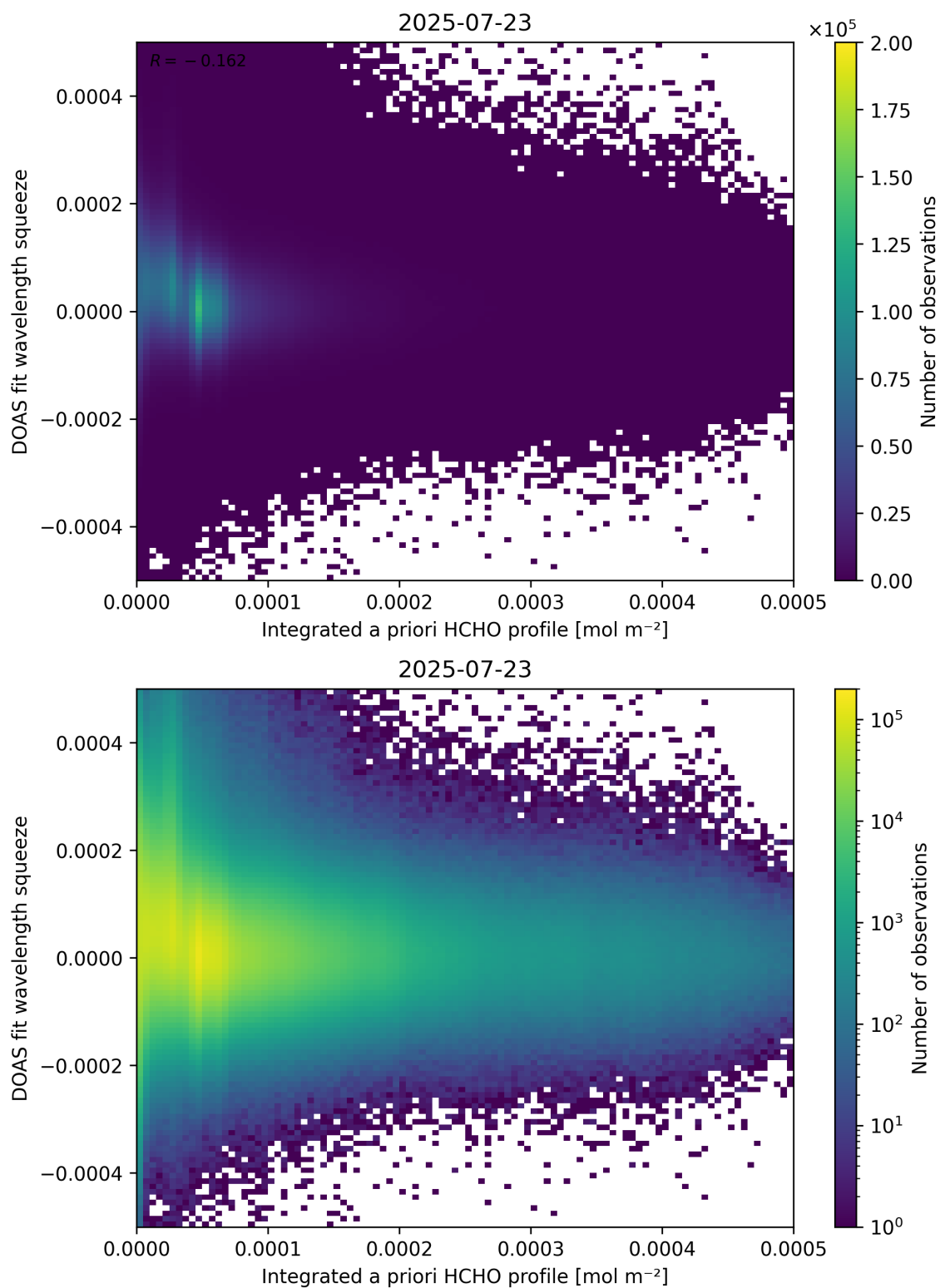
Figure 150: Scatter density plot of “Integrated a priori HCHO profile” against “DOAS fit wavelength squeeze” for 2025-07-22 to 2025-07-24.
