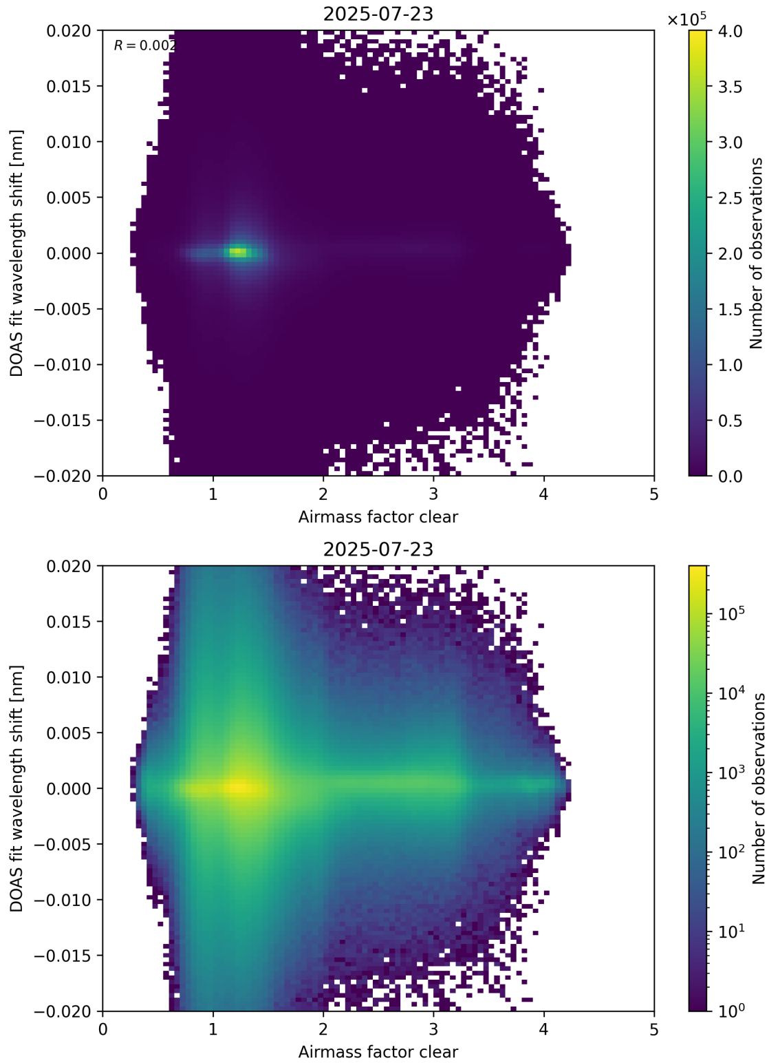
Figure 72: Scatter density plot of “Airmass factor clear” against “DOAS fit wavelength shift” for 2025-07-22 to 2025-07-24.
