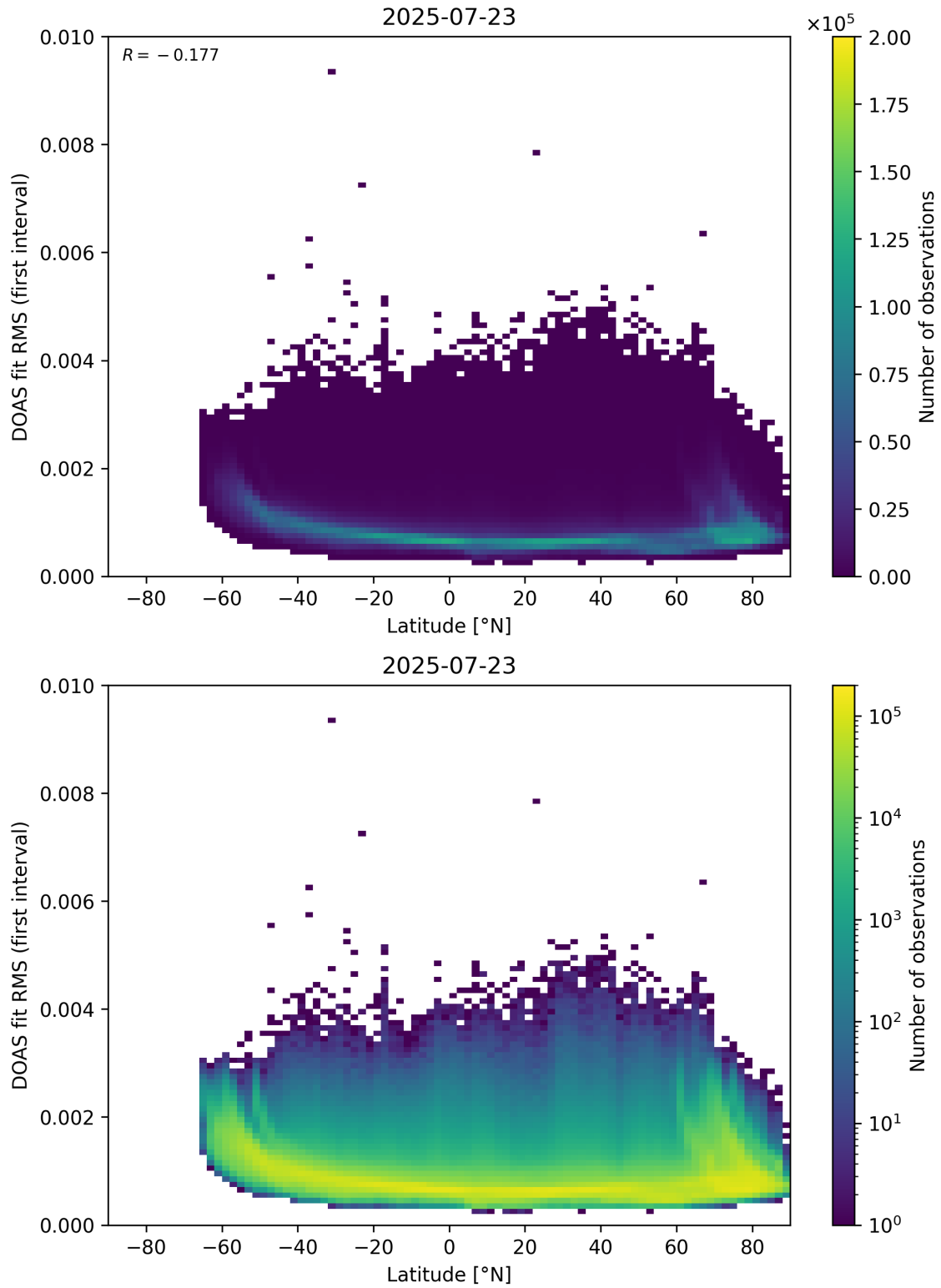
Figure 153: Scatter density plot of “Latitude” against “DOAS fit RMS (first interval)” for 2025-07-22 to 2025-07-24.
