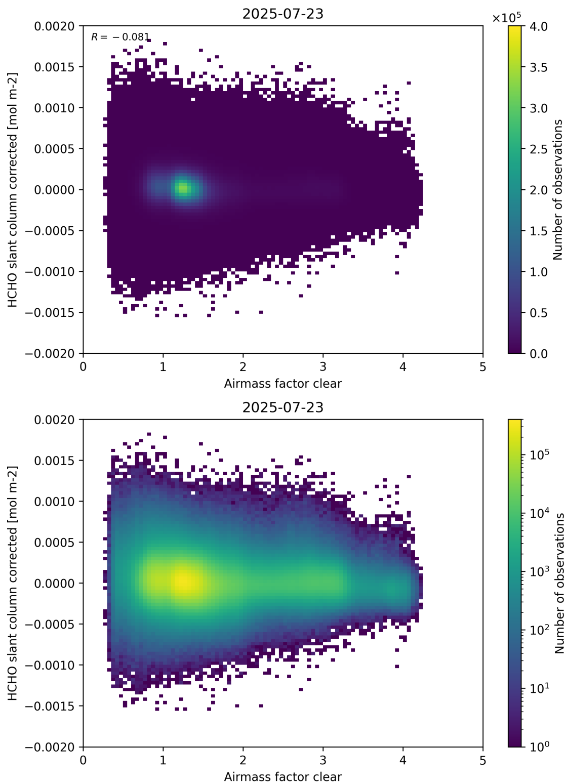
Figure 74: Scatter density plot of “Airmass factor clear” against “HCHO slant column corrected” for 2025-07-22 to 2025-07-24.
