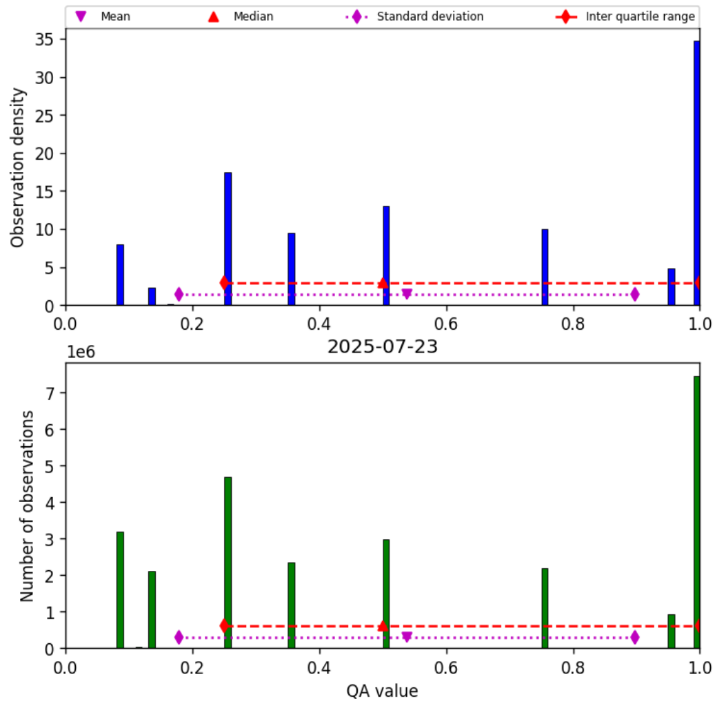
Figure 34: Histogram of “QA value” for 2025-07-22 to 2025-07-24
