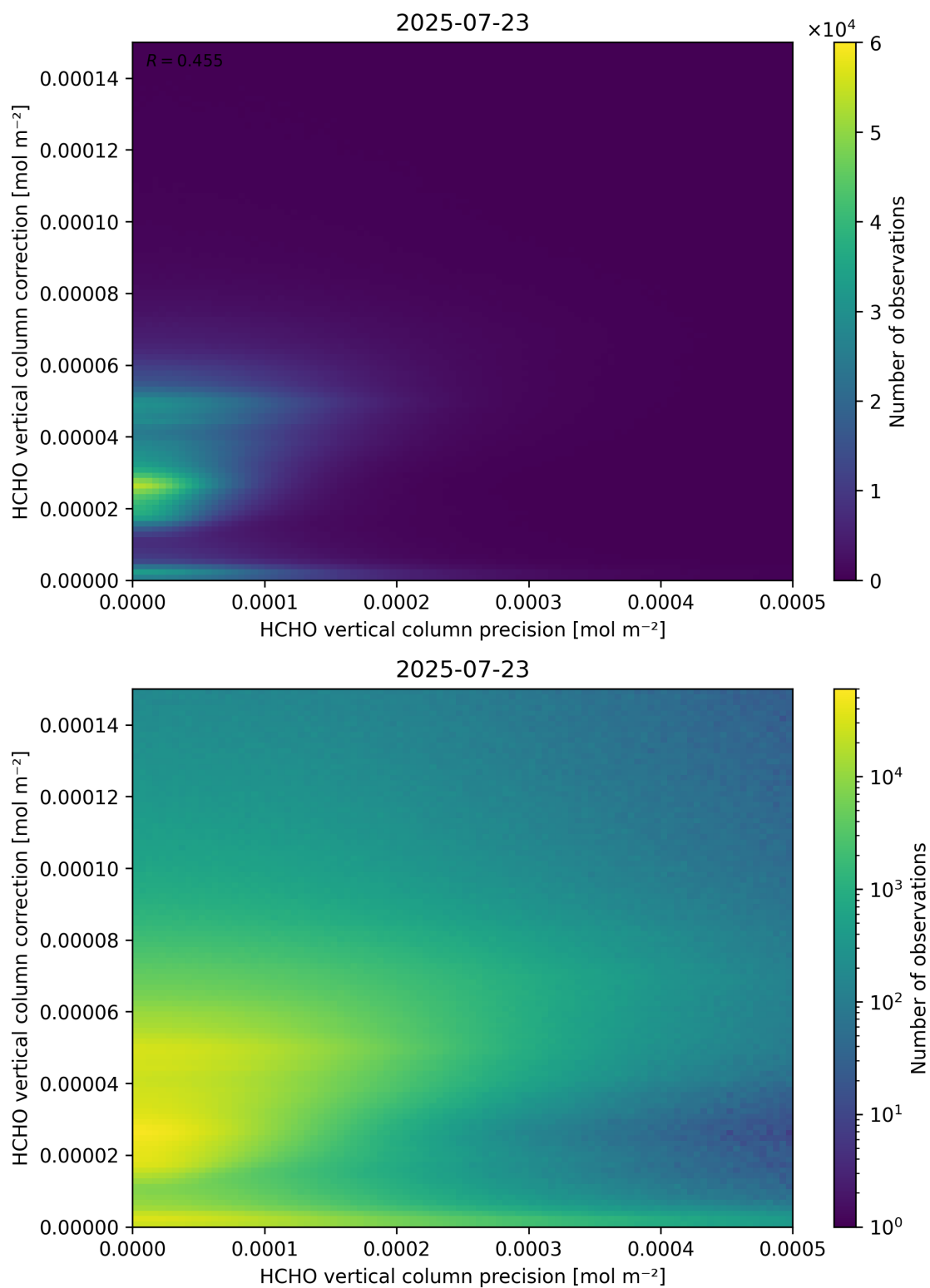
Figure 146: Scatter density plot of “HCHO vertical column precision” against “HCHO vertical column correction” for 2025-07-22 to 2025-07-24.
