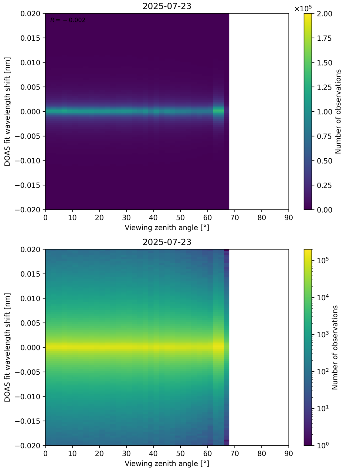
Figure 183: Scatter density plot of “Viewing zenith angle” against “DOAS fit wavelength shift” for 2025-07-22 to 2025-07-24.
