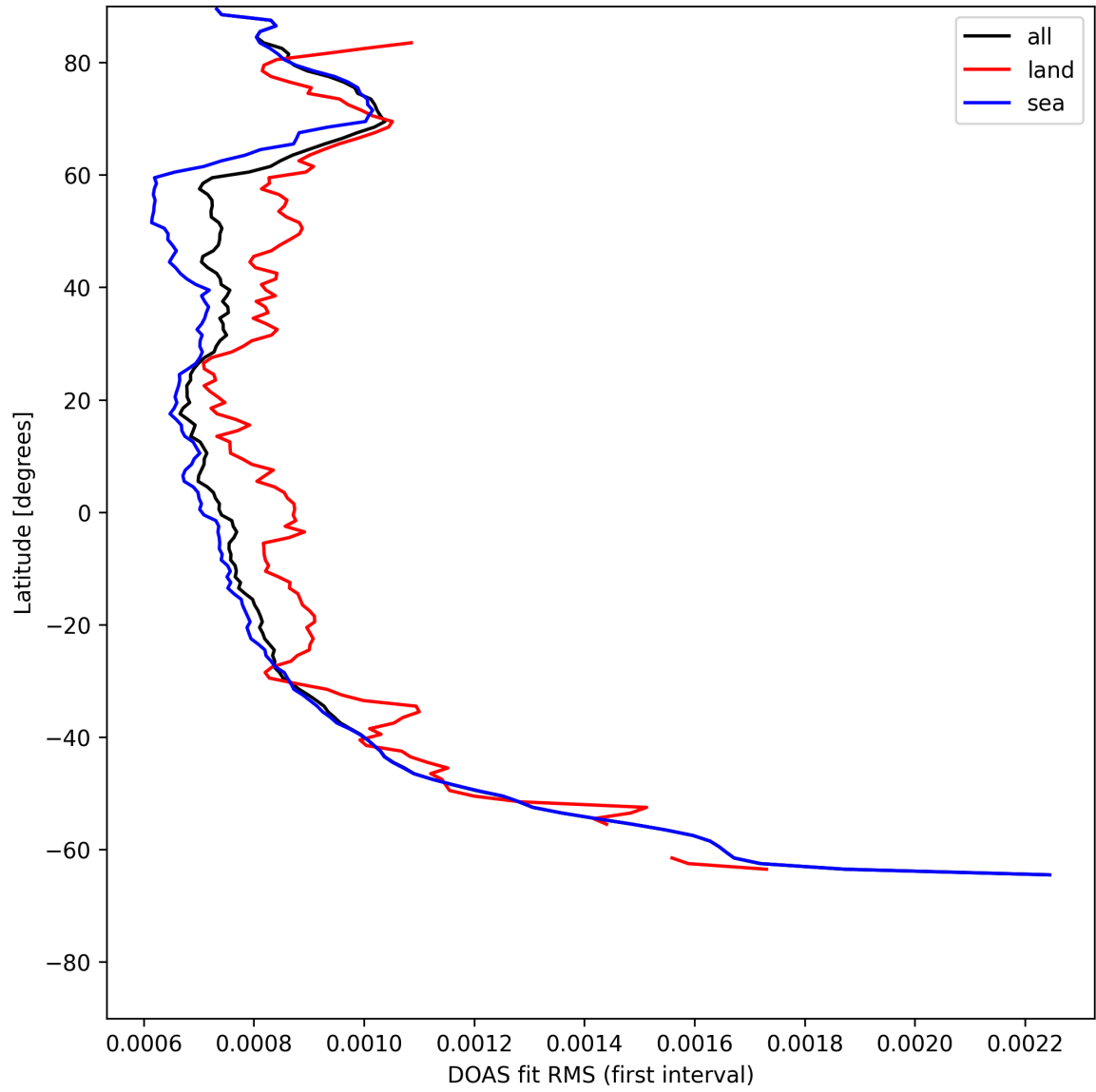
Figure 32: Zonal average of "DOAS fit RMS (first interval)" for 2025-07-22 to 2025-07-24.
