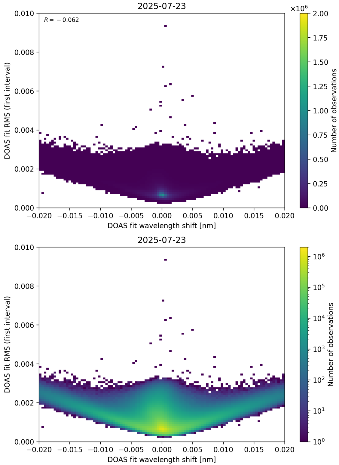
Figure 64: Scatter density plot of “DOAS fit wavelength shift” against “DOAS fit RMS (first interval)” for 2025-07-22 to 2025-07-24.
