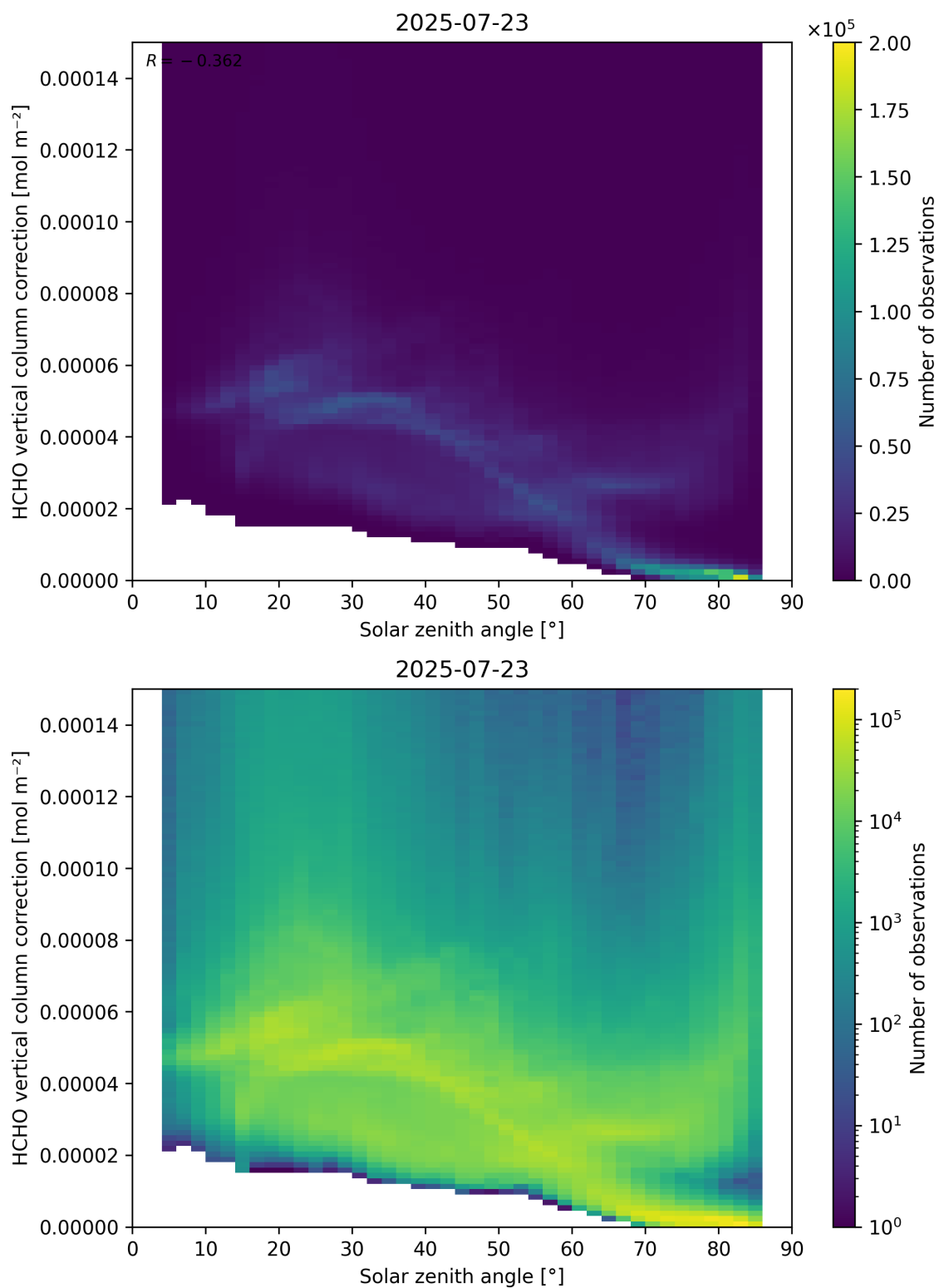
Figure 178: Scatter density plot of “Solar zenith angle” against “HCHO vertical column correction” for 2025-07-22 to 2025-07-24.
