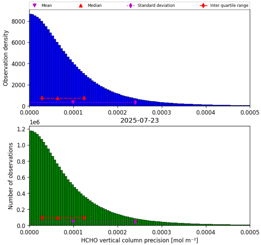
Figure 36: Histogram of “HCHO vertical column precision” for 2025-07-22 to 2025-07-24
