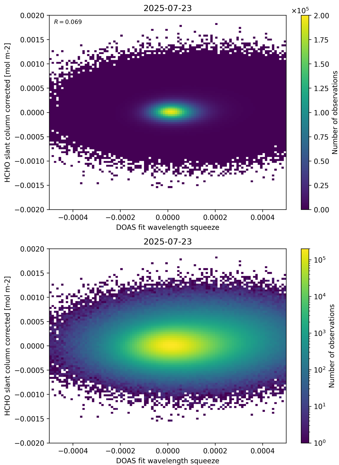
Figure 69: Scatter density plot of “DOAS fit wavelength squeeze” against “HCHO slant column corrected” for 2025-07-22 to 2025-07-24.
