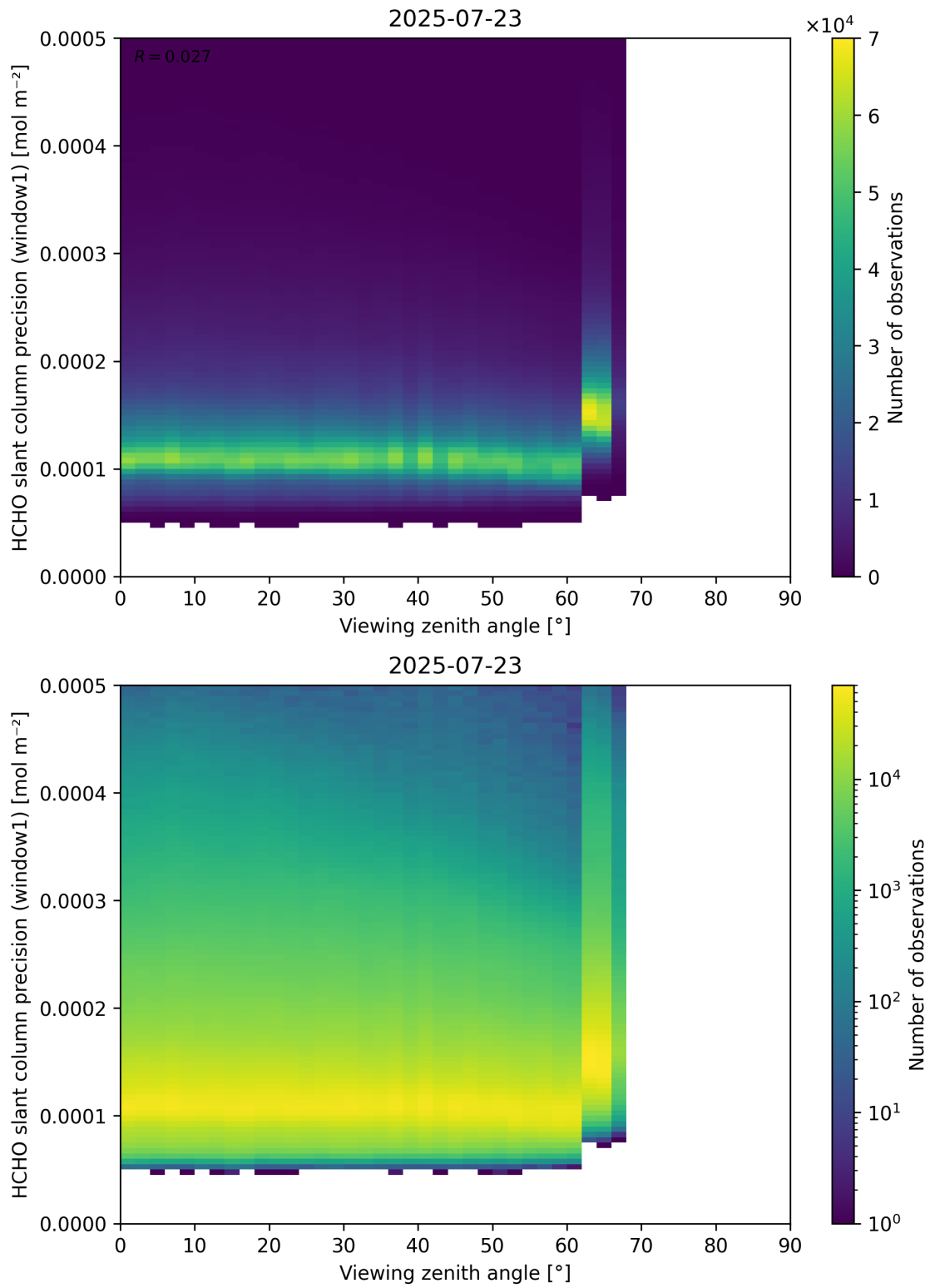
Figure 189: Scatter density plot of “Viewing zenith angle” against “HCHO slant column precision (window1)” for 2025-07-22 to 2025-07-24.
