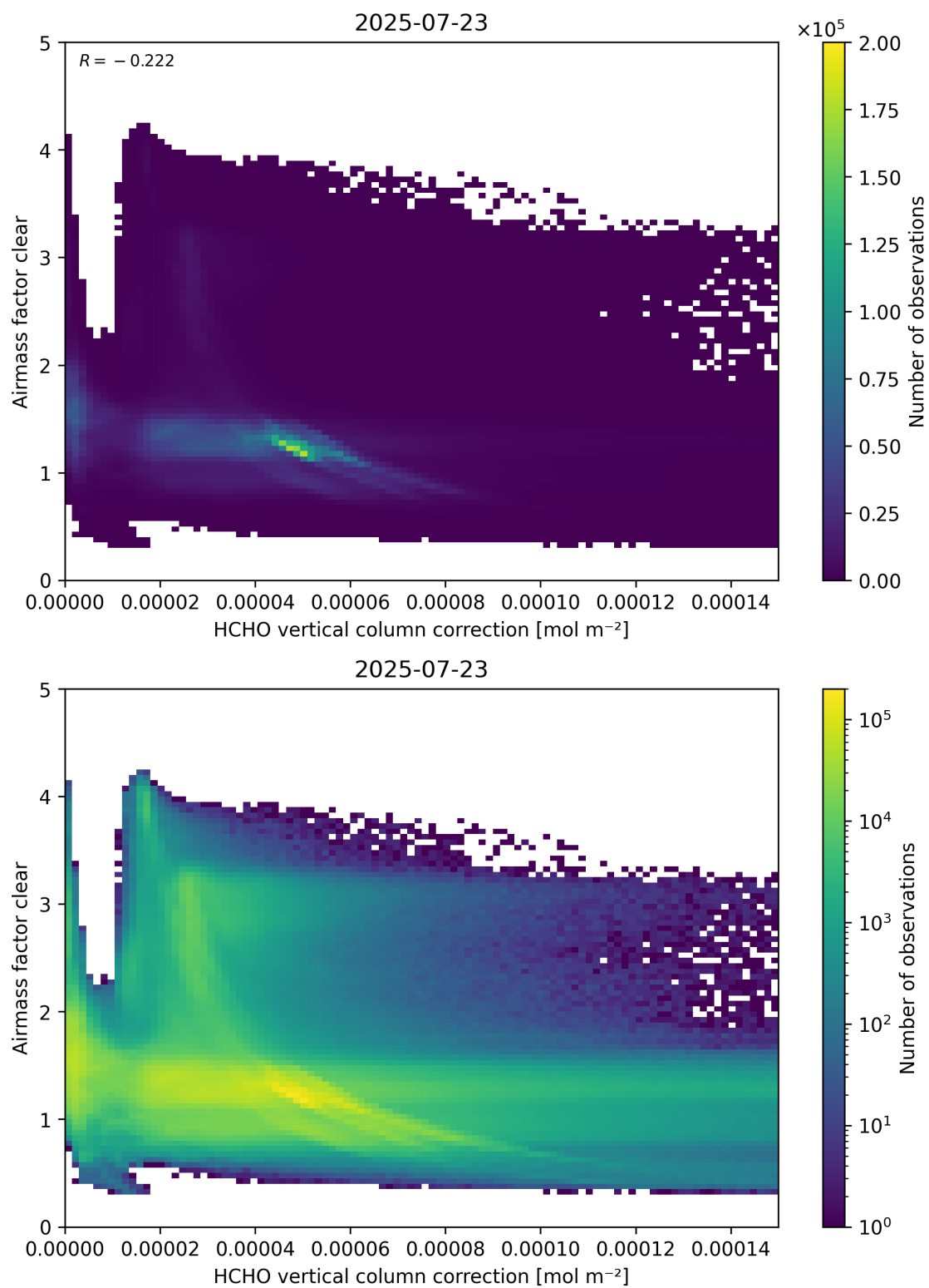
Figure 115: Scatter density plot of “HCHO vertical column correction” against “Airmass factor clear” for 2025-07-22 to 2025-07-24.
