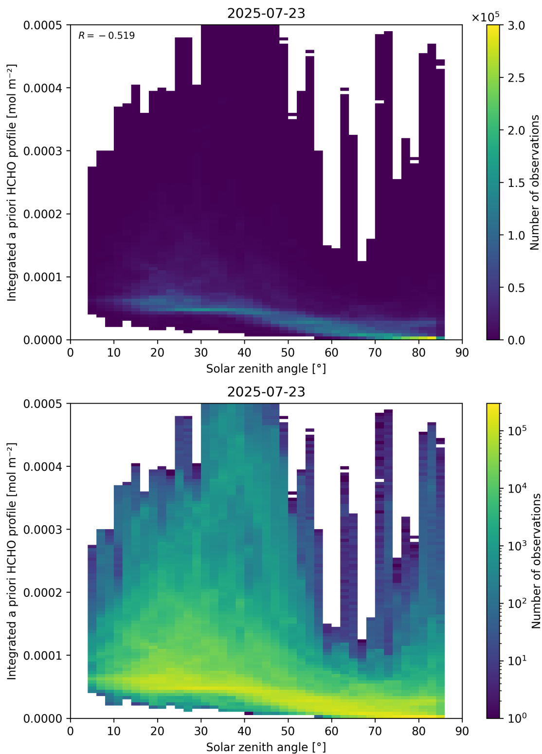
Figure 180: Scatter density plot of “Solar zenith angle” against “Integrated a priori HCHO profile” for 2025-07-22 to 2025-07-24.
