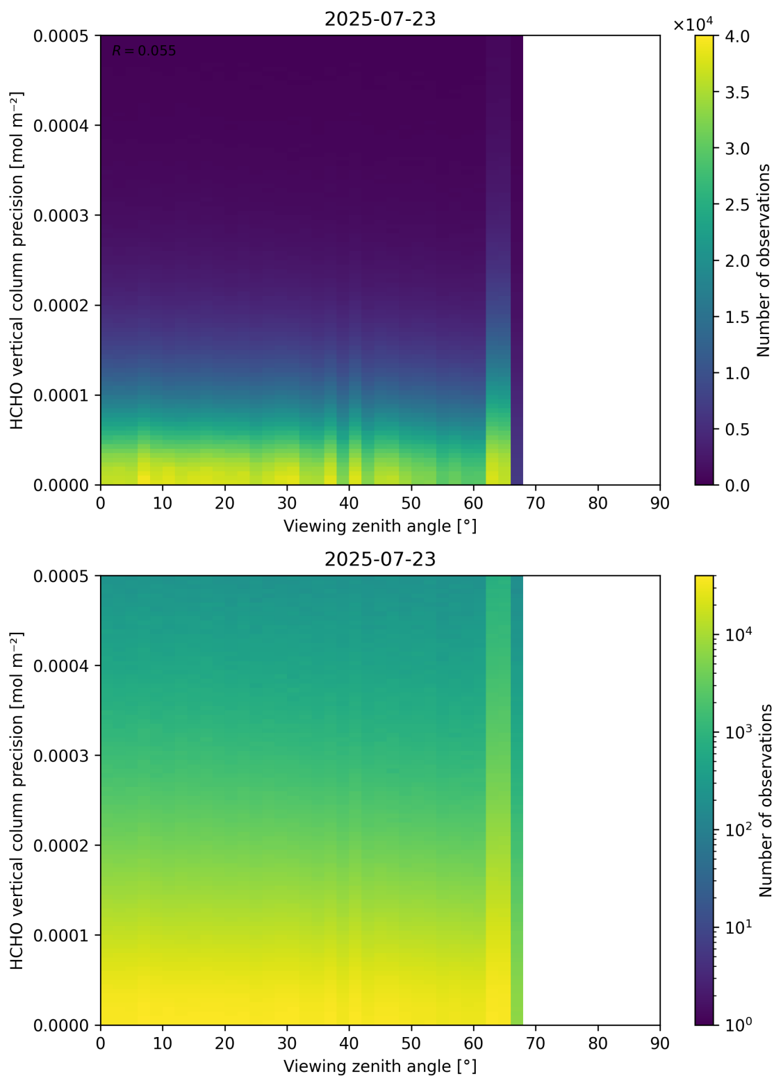
Figure 194: Scatter density plot of “Viewing zenith angle” against “HCHO vertical column precision” for 2025-07-22 to 2025-07-24.
