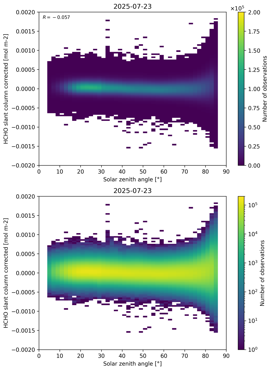
Figure 171: Scatter density plot of “Solar zenith angle” against “HCHO slant column corrected” for 2025-07-22 to 2025-07-24.
