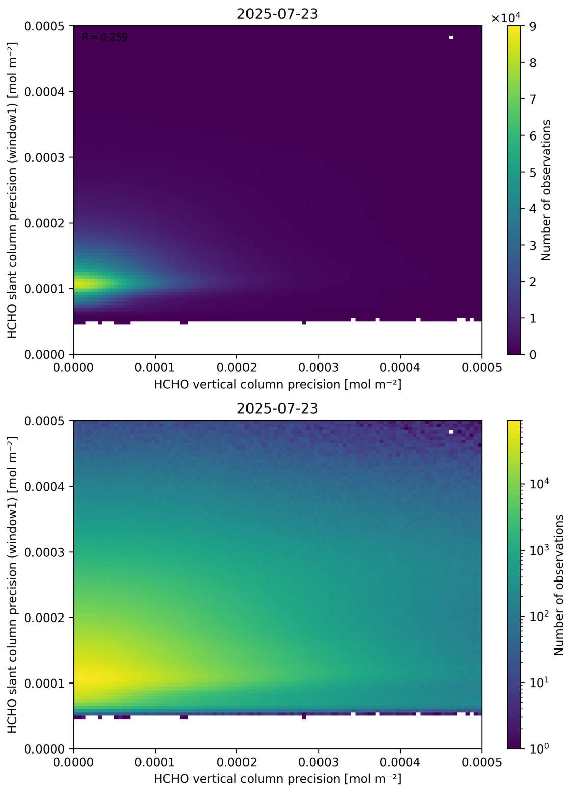
Figure 143: Scatter density plot of “HCHO vertical column precision” against “HCHO slant column precision (window1)” for 2025-07-22 to 2025-07-24.
