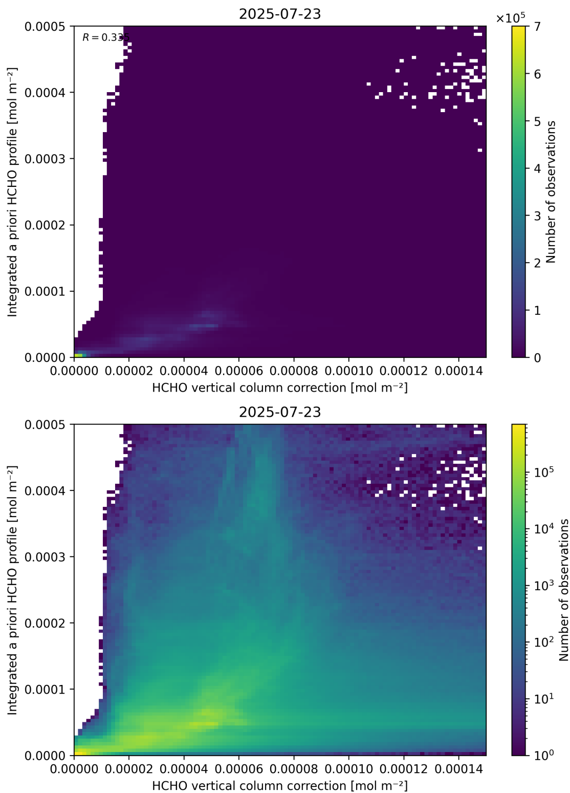
Figure 122: Scatter density plot of “HCHO vertical column correction” against “Integrated a priori HCHO profile” for 2025-07-22 to 2025-07-24.
