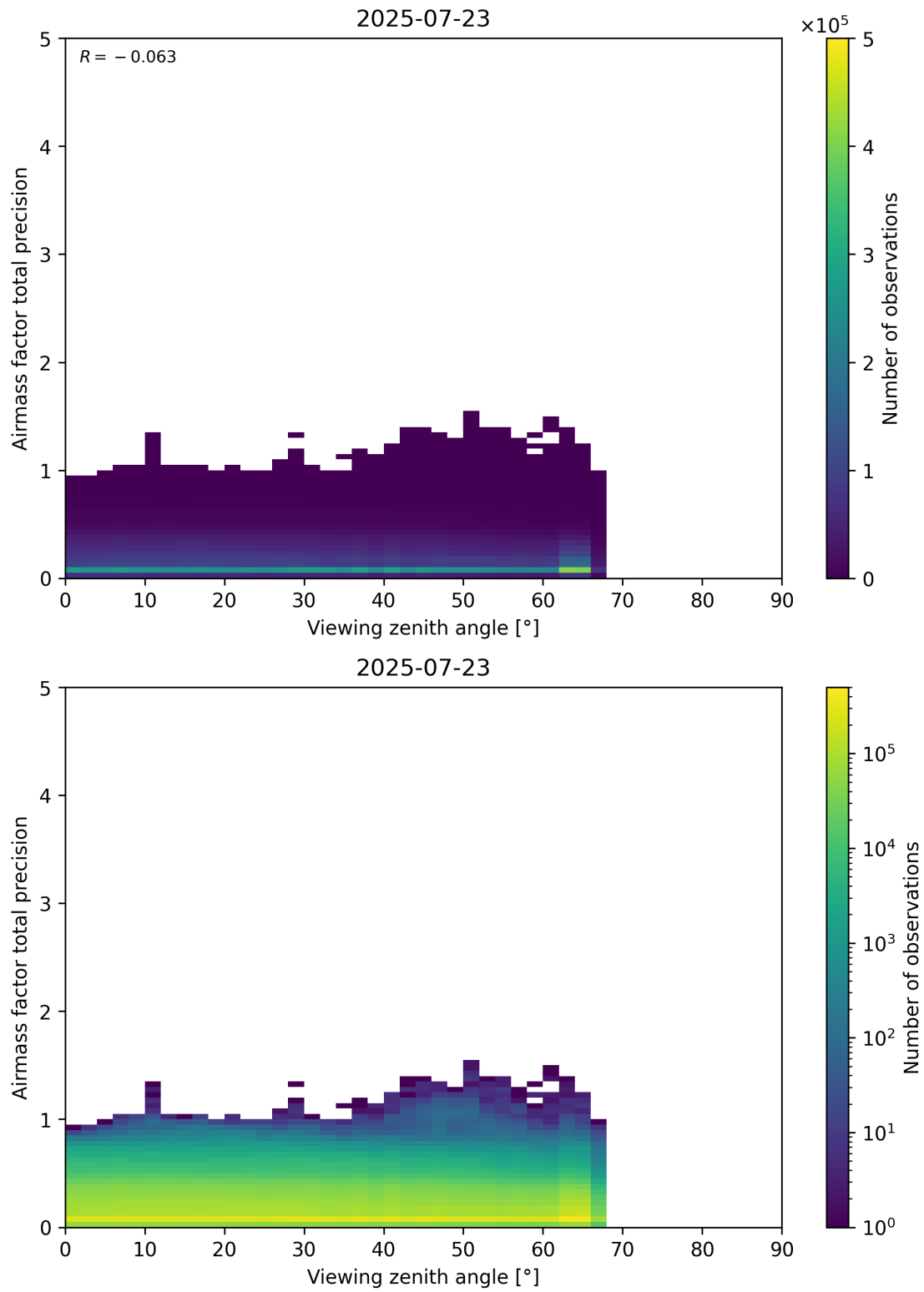
Figure 191: Scatter density plot of “Viewing zenith angle” against “Airmass factor total precision” for 2025-07-22 to 2025-07-24.
