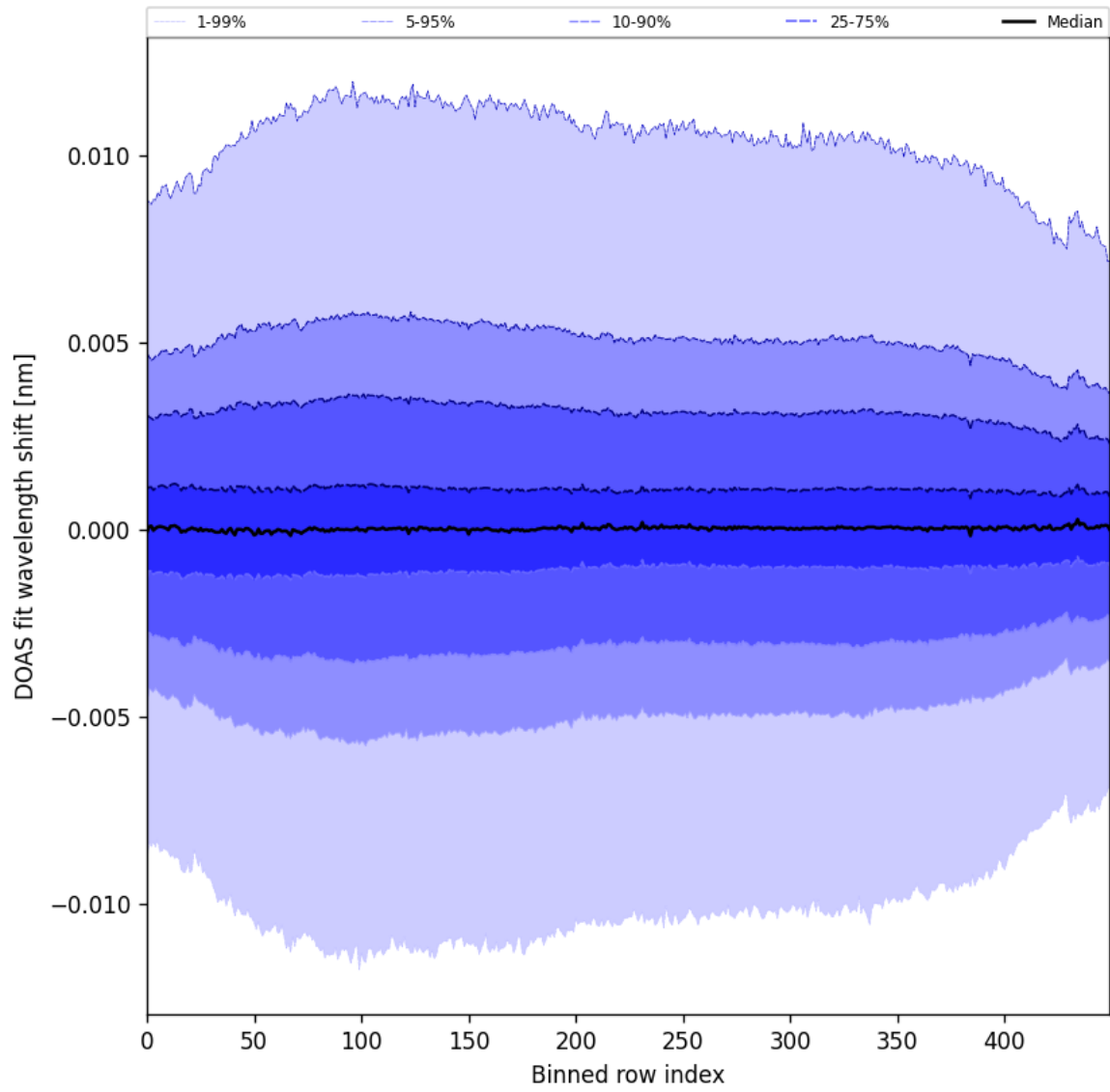
Figure 58: Along track statistics of “DOAS fit wavelength shift” for 2025-07-22 to 2025-07-24
