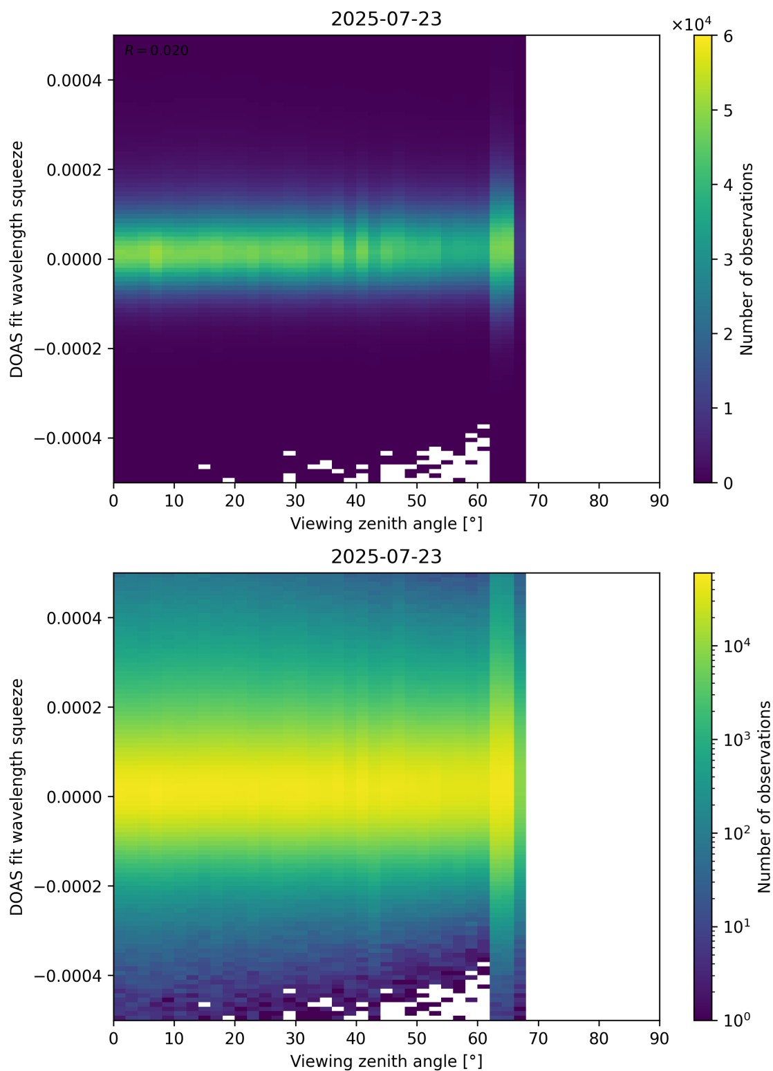
Figure 184: Scatter density plot of “Viewing zenith angle” against “DOAS fit wavelength squeeze” for 2025-07-22 to 2025-07-24.
