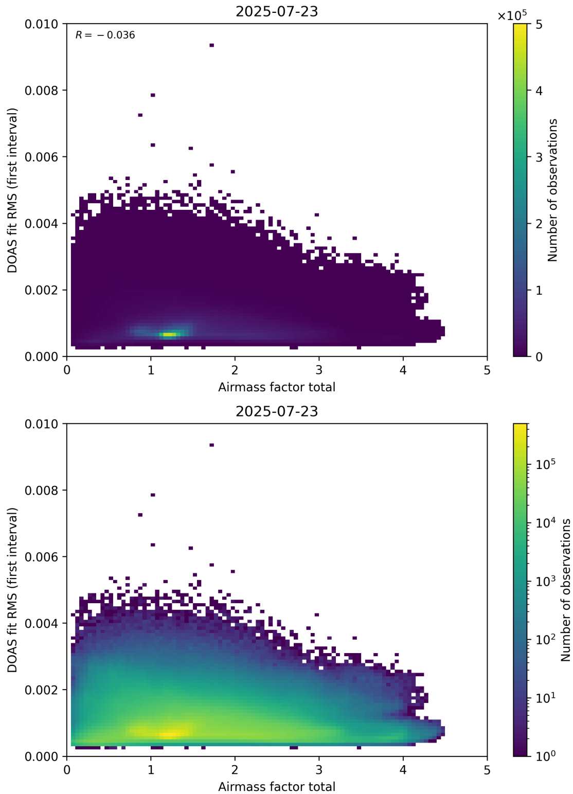
Figure 97: Scatter density plot of “Airmass factor total” against “DOAS fit RMS (first interval)” for 2025-07-22 to 2025-07-24.
