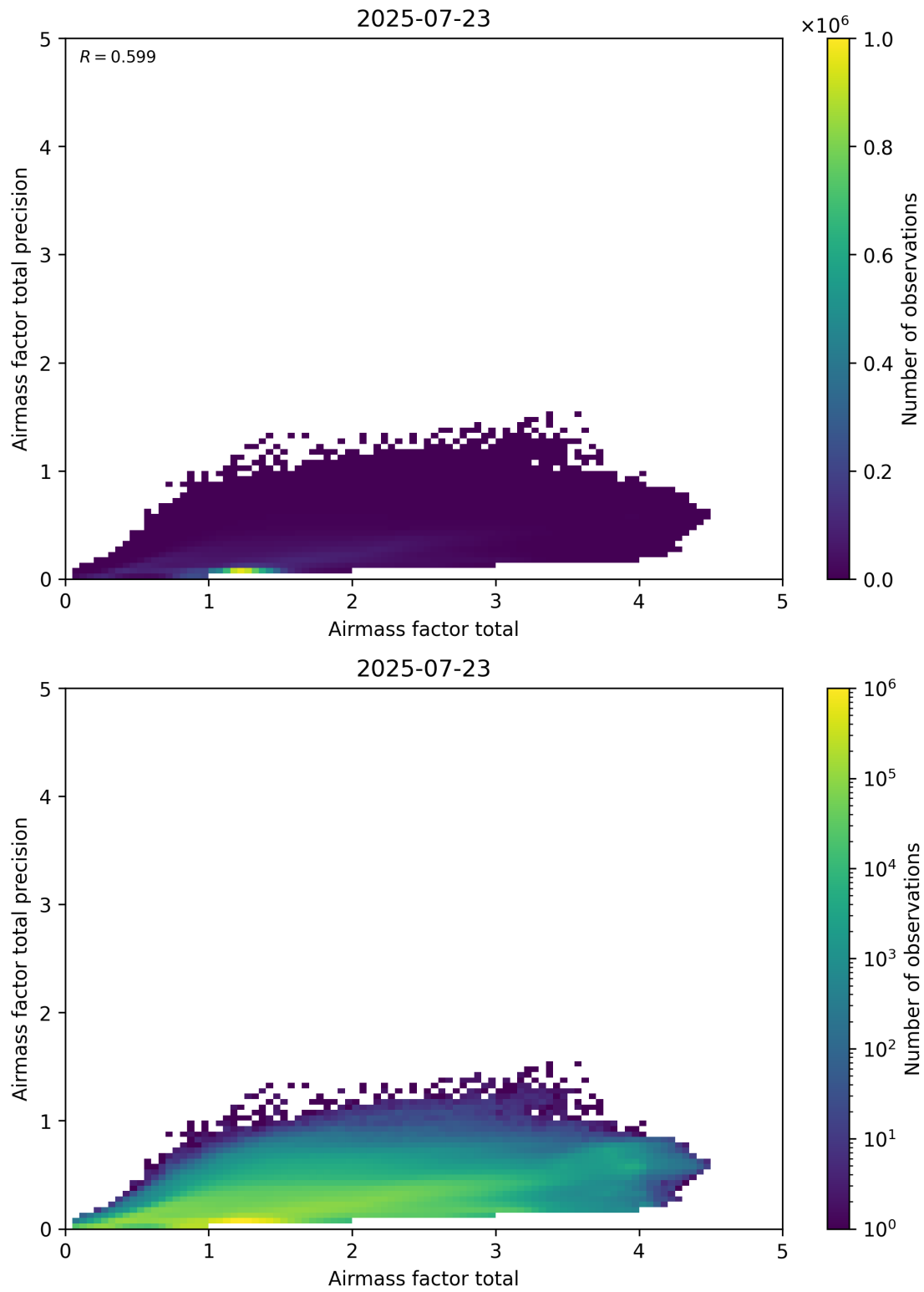
Figure 103: Scatter density plot of “Airmass factor total” against “Airmass factor total precision” for 2025-07-22 to 2025-07-24.
