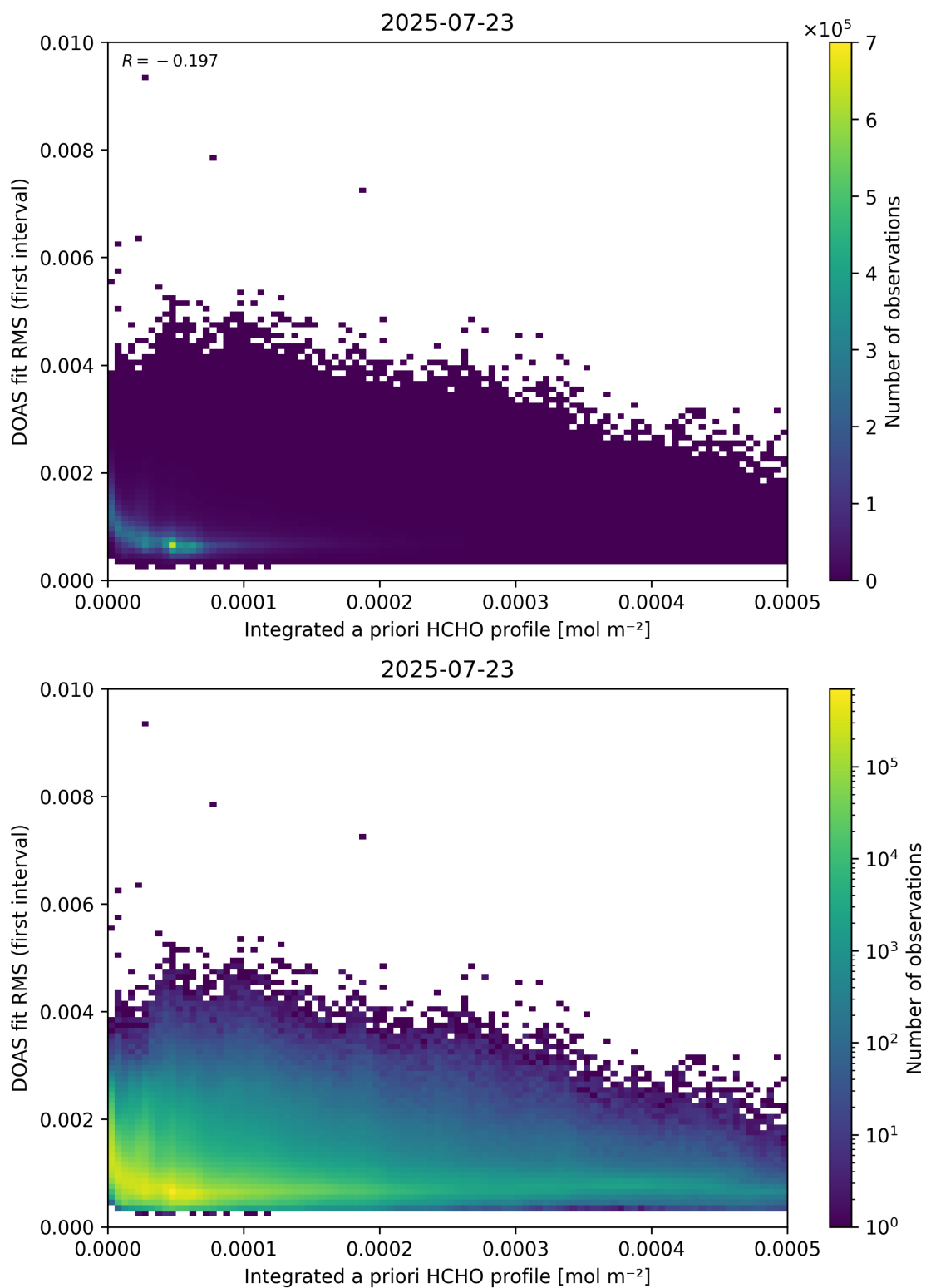
Figure 148: Scatter density plot of “Integrated a priori HCHO profile” against “DOAS fit RMS (first interval)” for 2025-07-22 to 2025-07-24.
