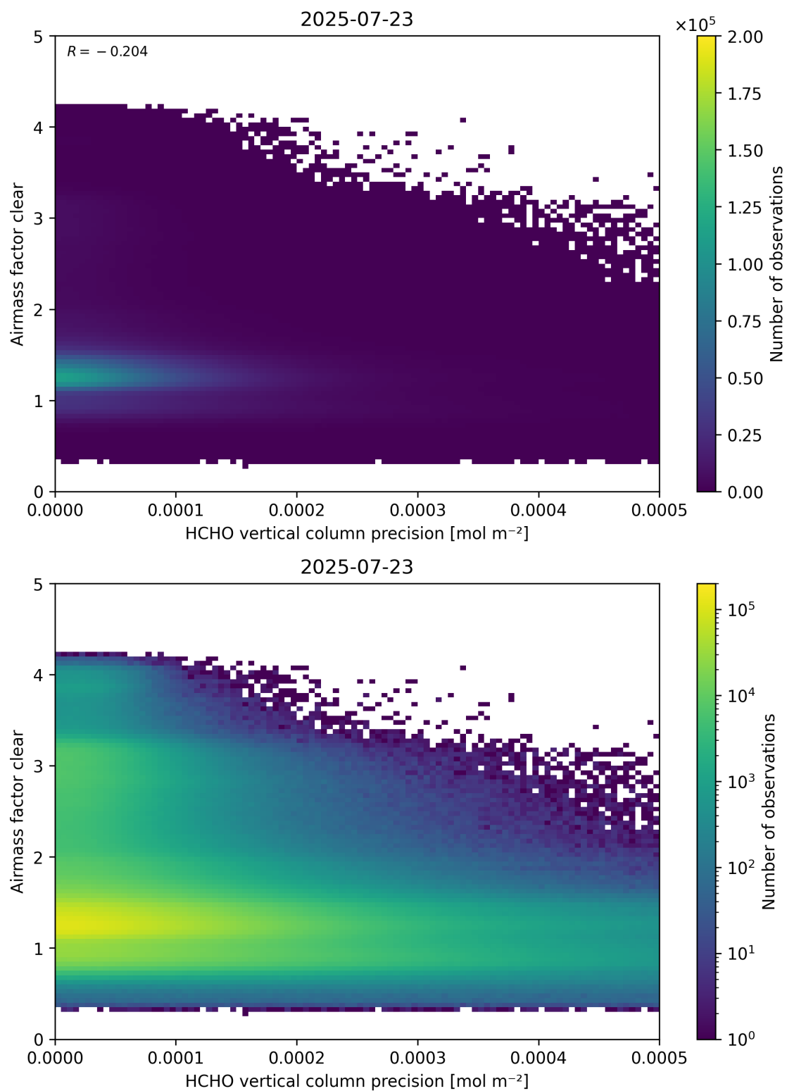
Figure 139: Scatter density plot of “HCHO vertical column precision” against “Airmass factor clear” for 2025-07-22 to 2025-07-24.
