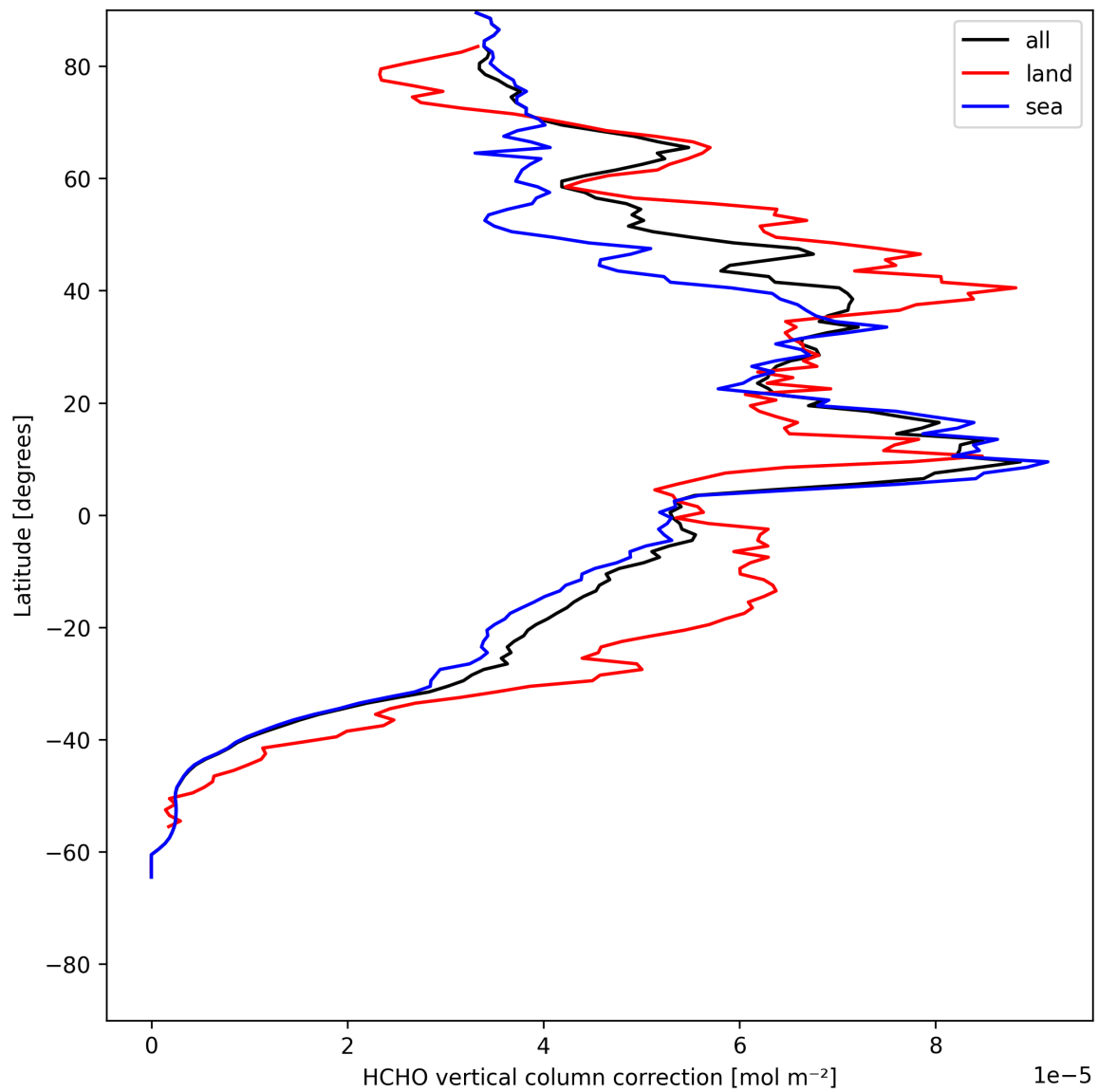
Figure 23: Zonal average of “HCHO vertical column correction” for 2025-07-22 to 2025-07-24.
