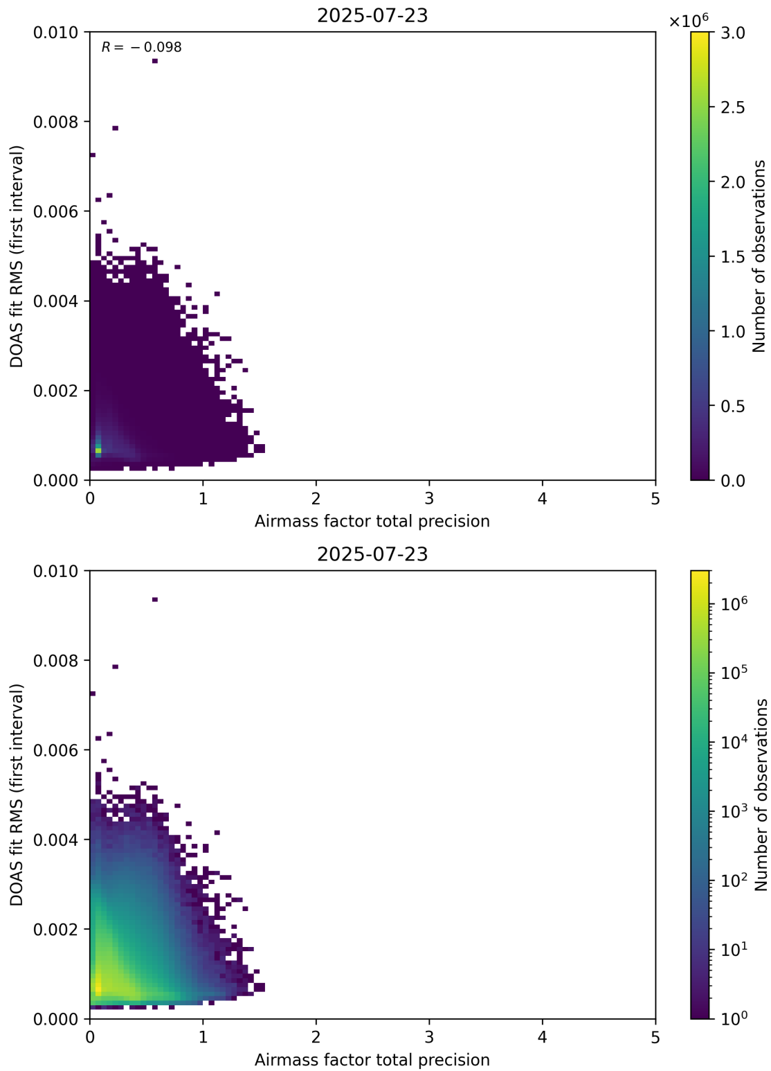
Figure 105: Scatter density plot of “Airmass factor total precision” against “DOAS fit RMS (first interval)” for 2025-07-22 to 2025-07-24.
