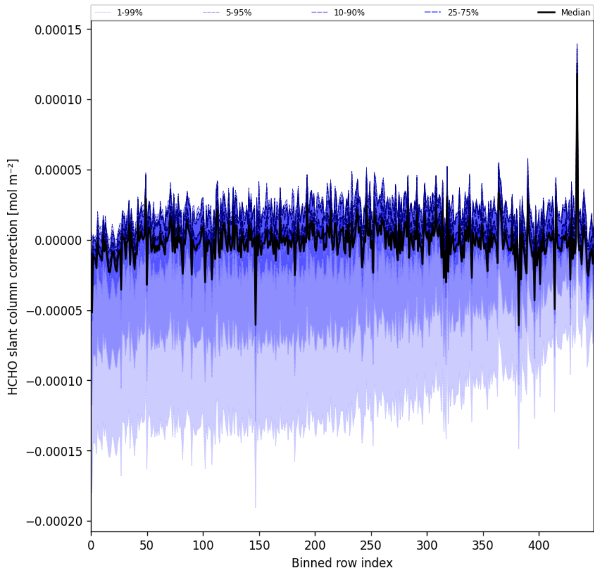
Figure 61: Along track statistics of “HCHO slant column correction” for 2025-07-22 to 2025-07-24
