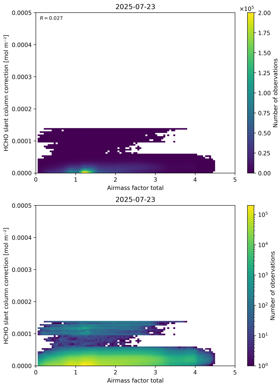
Figure 102: Scatter density plot of “Airmass factor total” against “HCHO slant column correction” for 2025-07-22 to 2025-07-24.
