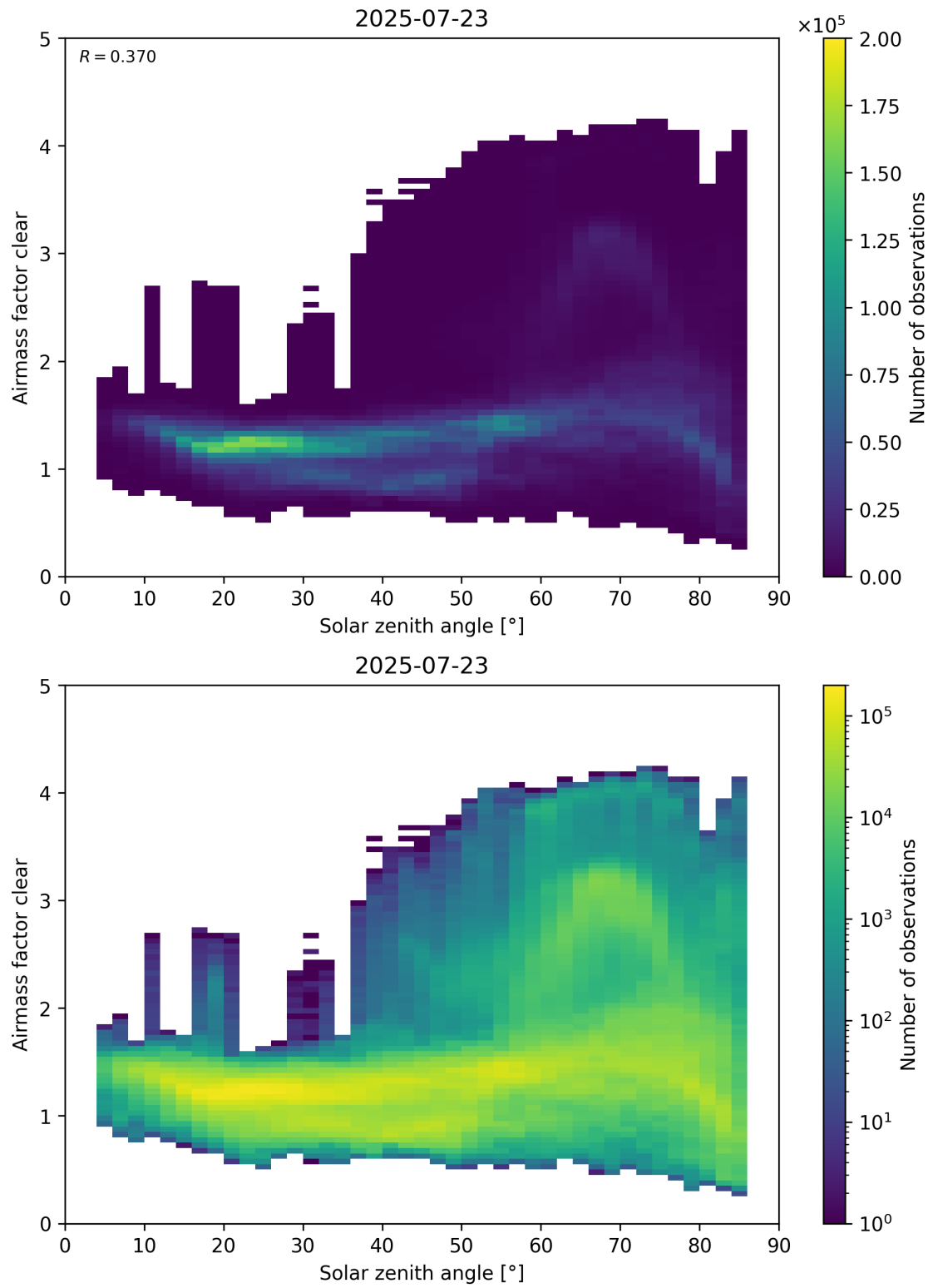
Figure 170: Scatter density plot of “Solar zenith angle” against “Airmass factor clear” for 2025-07-22 to 2025-07-24.
