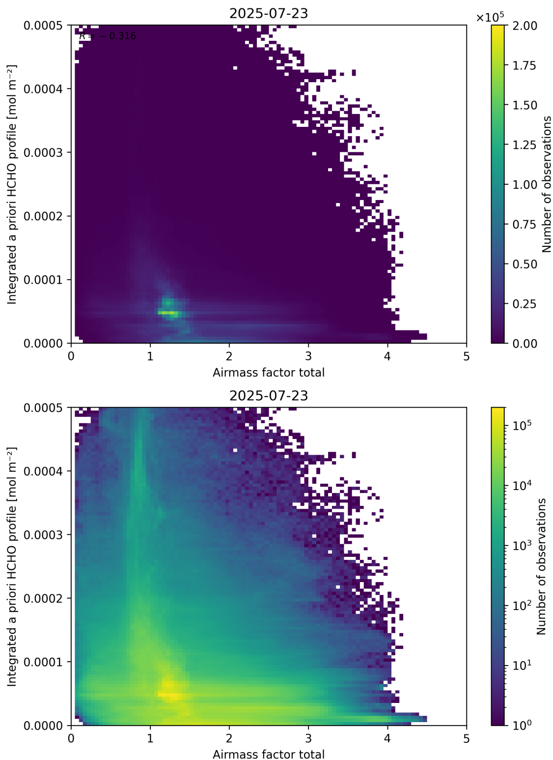
Figure 104: Scatter density plot of “Airmass factor total” against “Integrated a priori HCHO profile” for 2025-07-22 to 2025-07-24.
