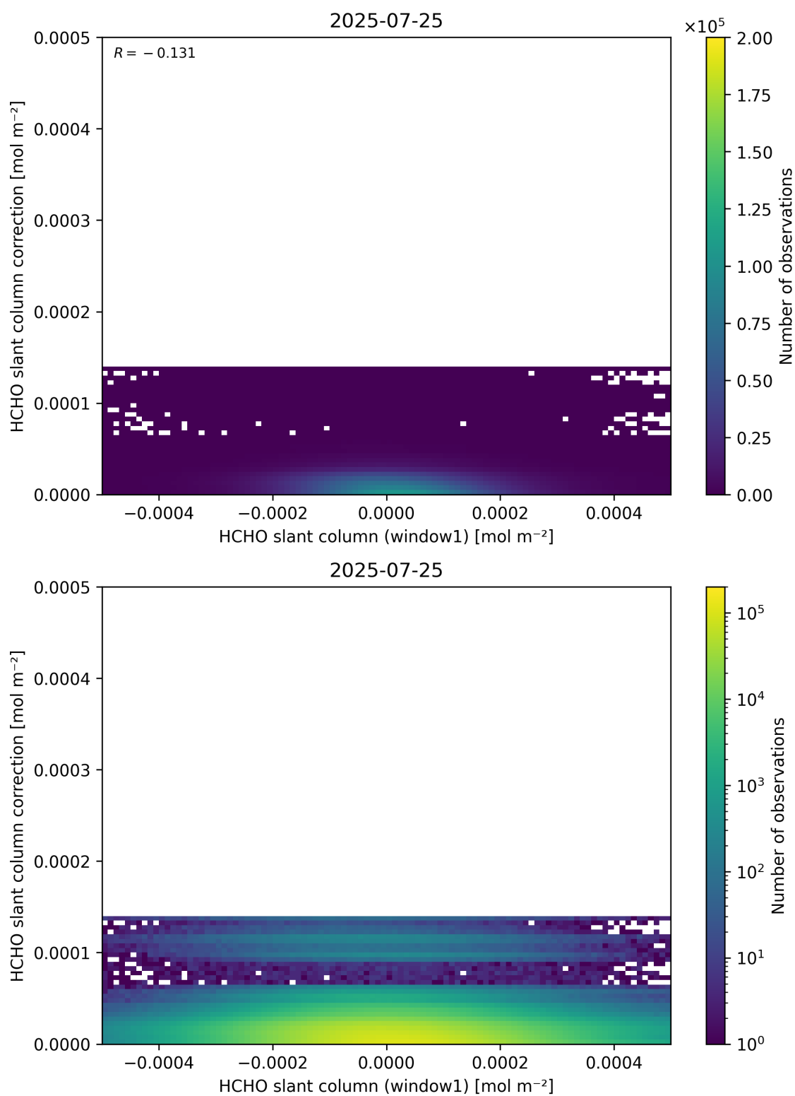
Figure 83: Scatter density plot of “HCHO slant column (window1)” against “HCHO slant column correction” for 2025-07-24 to 2025-07-26.
