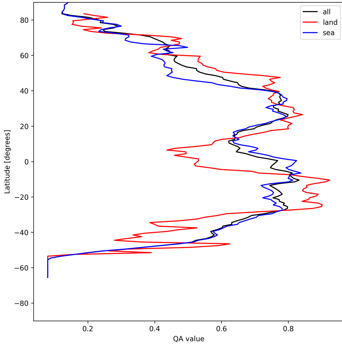
Figure 20: Zonal average of “QA value” for 2025-07-24 to 2025-07-26.
