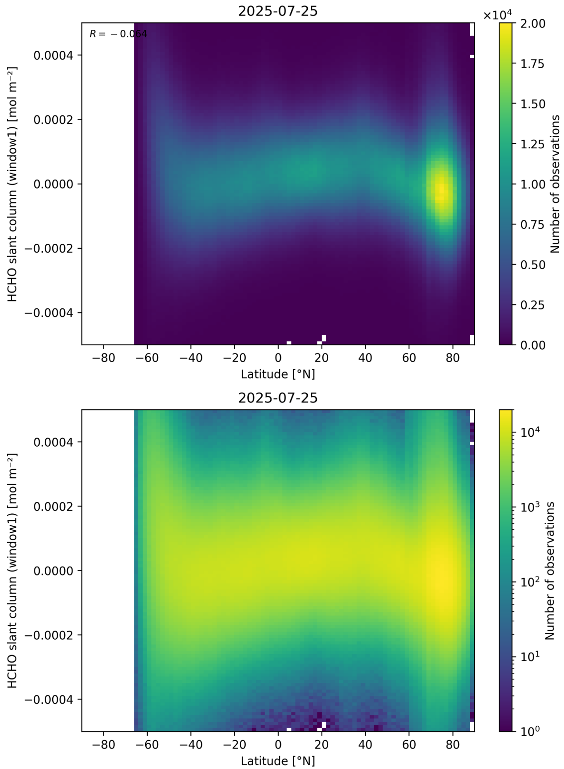
Figure 159: Scatter density plot of “Latitude” against “HCHO slant column (window1)” for 2025-07-24 to 2025-07-26.
