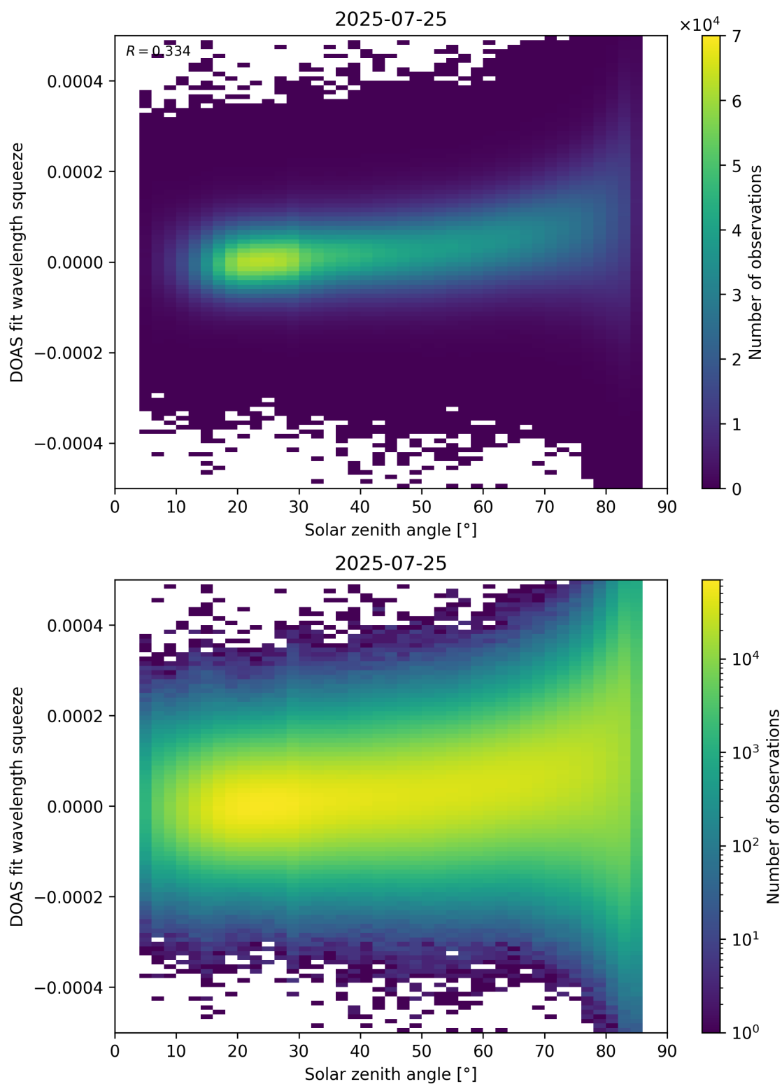
Figure 169: Scatter density plot of “Solar zenith angle” against “DOAS fit wavelength squeeze” for 2025-07-24 to 2025-07-26.
