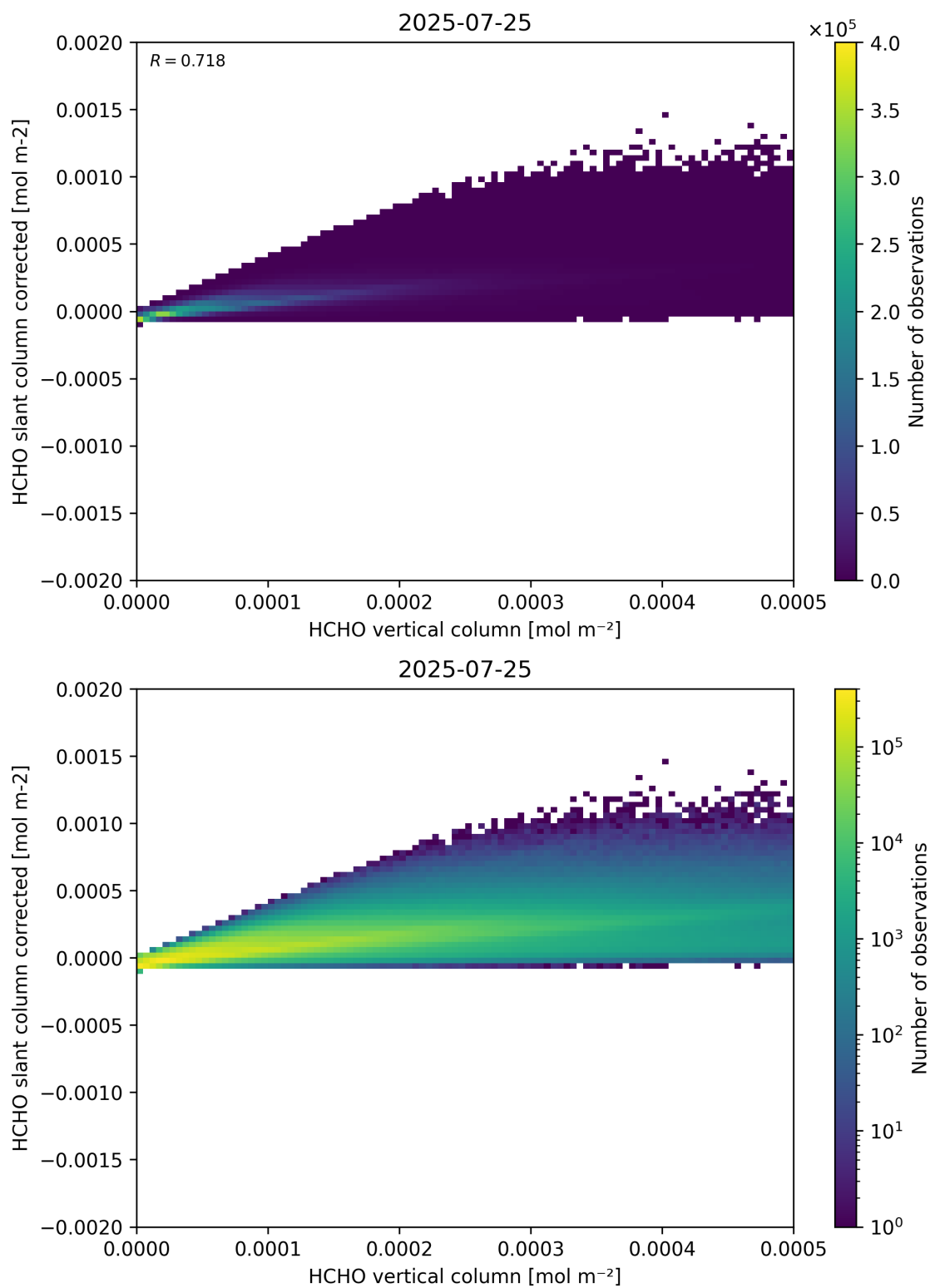
Figure 127: Scatter density plot of “HCHO vertical column” against “HCHO slant column corrected” for 2025-07-24 to 2025-07-26.
