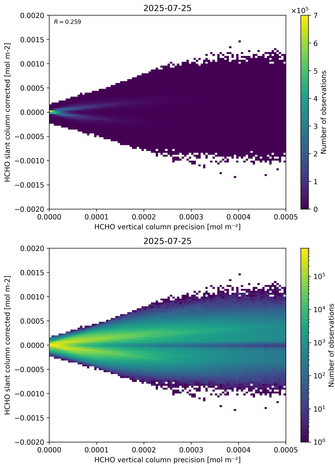
Figure 140: Scatter density plot of “HCHO vertical column precision” against “HCHO slant column corrected” for 2025-07-24 to 2025-07-26.
