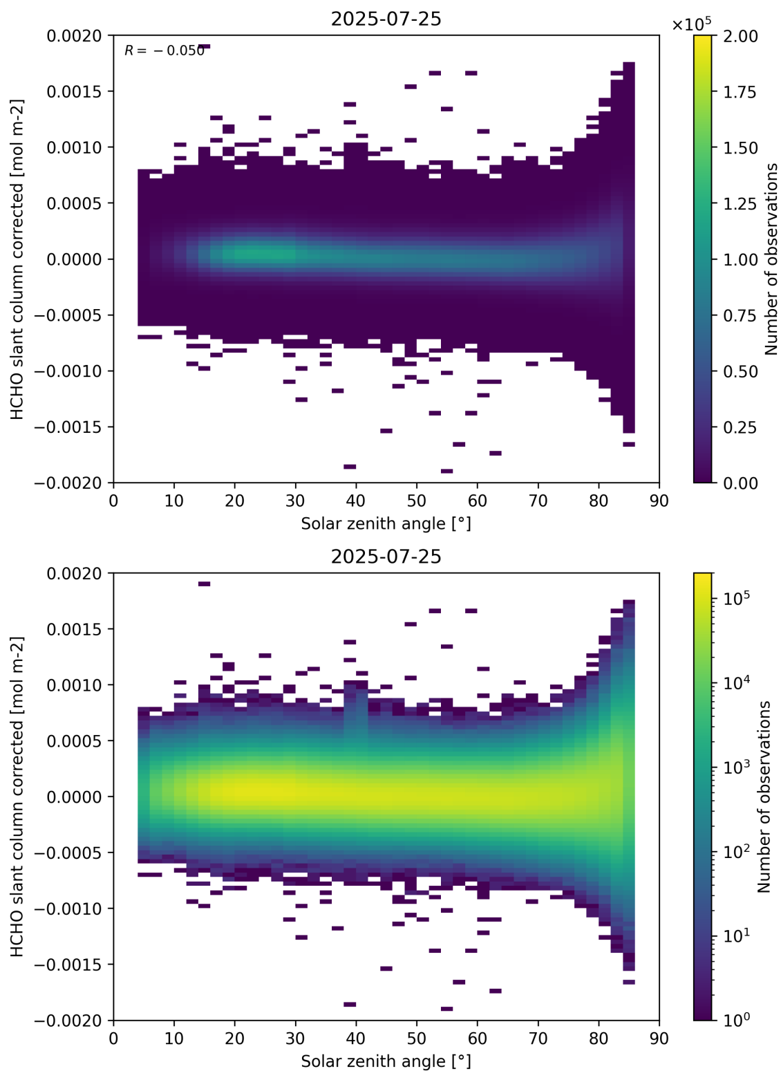
Figure 171: Scatter density plot of “Solar zenith angle” against “HCHO slant column corrected” for 2025-07-24 to 2025-07-26.
