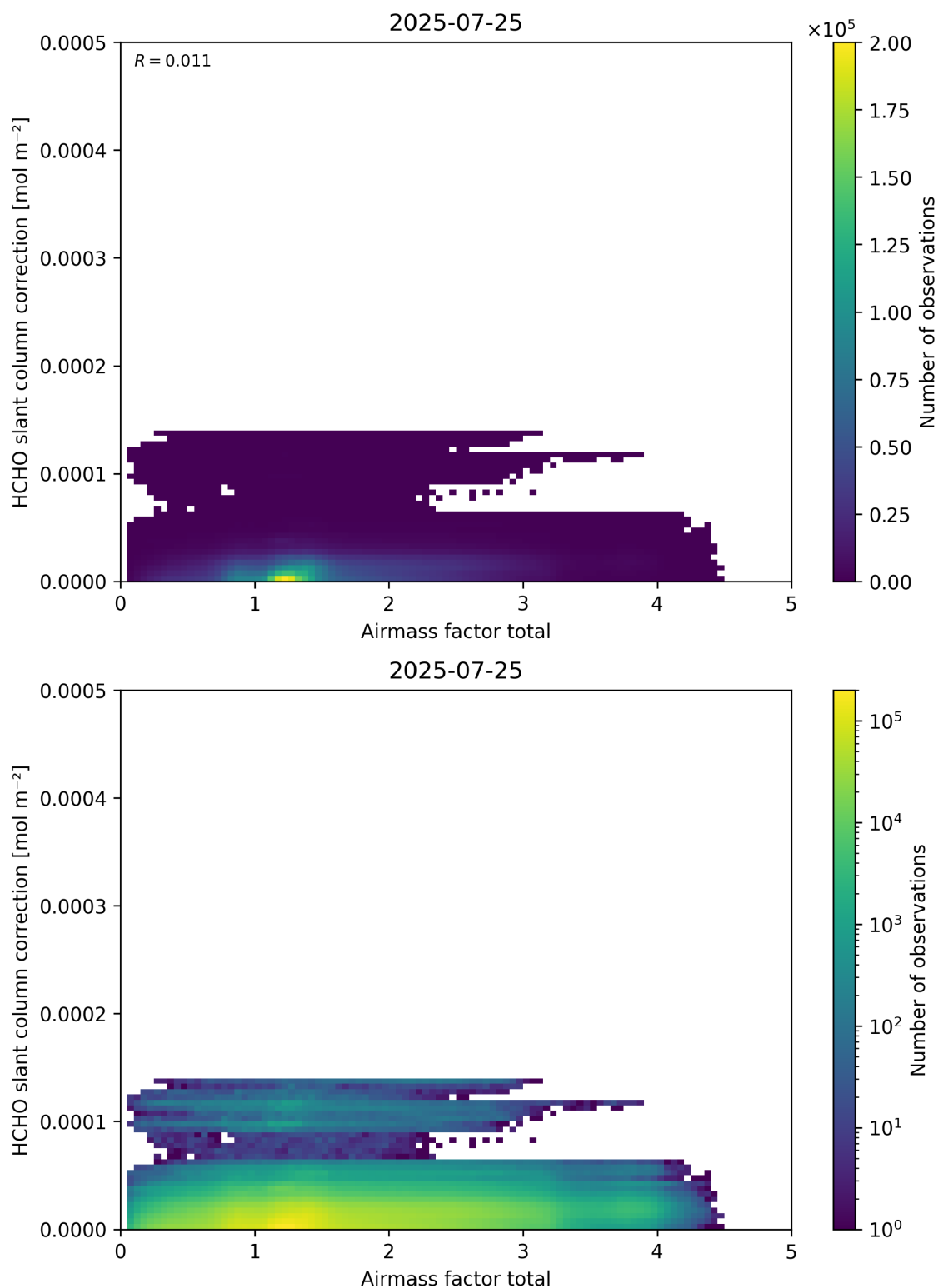
Figure 102: Scatter density plot of “Airmass factor total” against “HCHO slant column correction” for 2025-07-24 to 2025-07-26.
