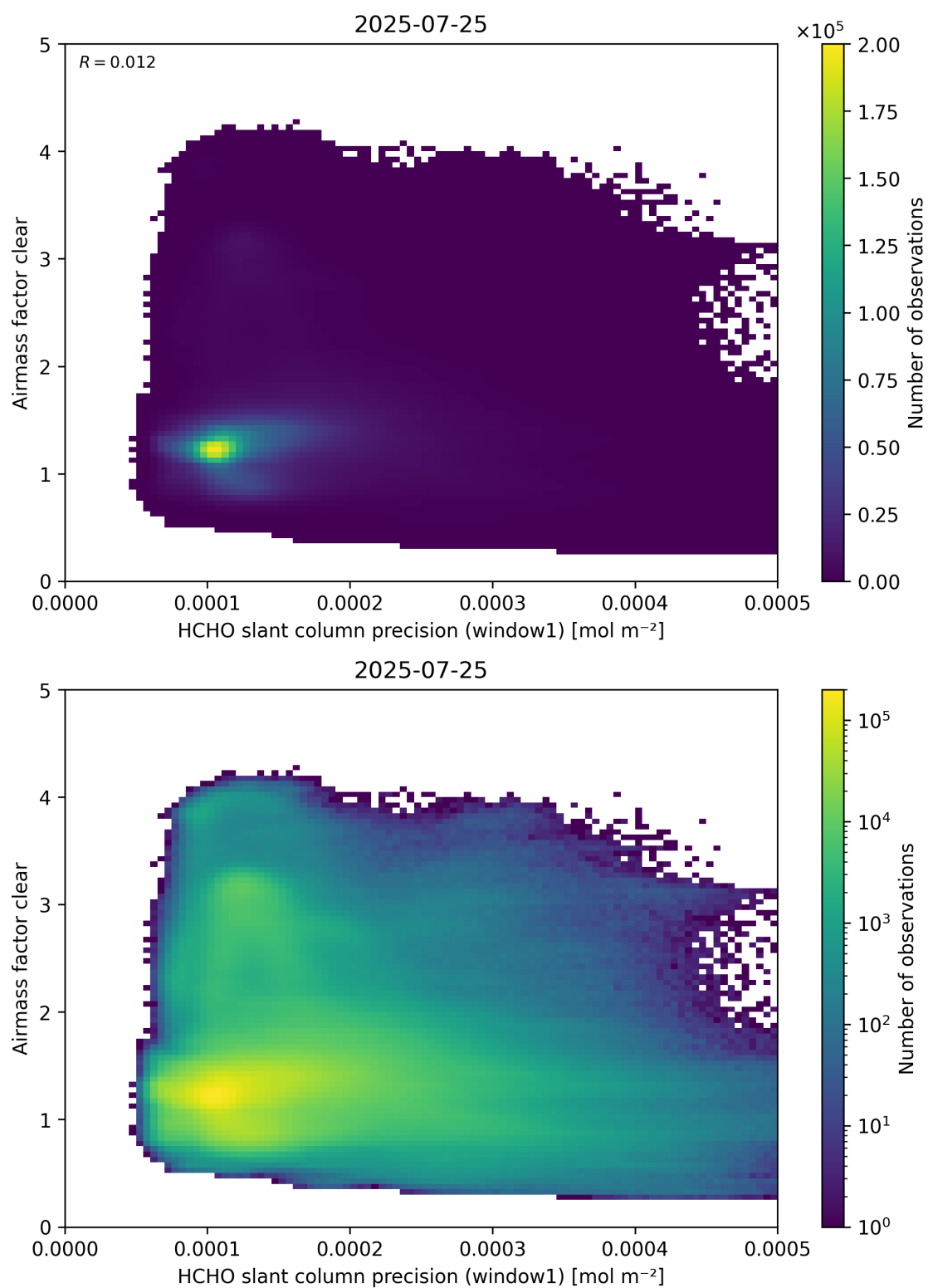
Figure 91: Scatter density plot of “HCHO slant column precision (window1)” against “Airmass factor clear” for 2025-07-24 to 2025-07-26.
