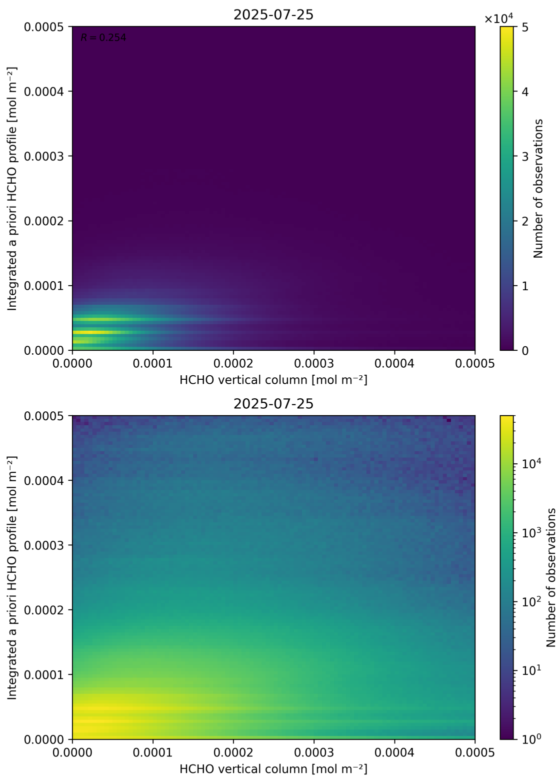
Figure 135: Scatter density plot of “HCHO vertical column” against “Integrated a priori HCHO profile” for 2025-07-24 to 2025-07-26.
