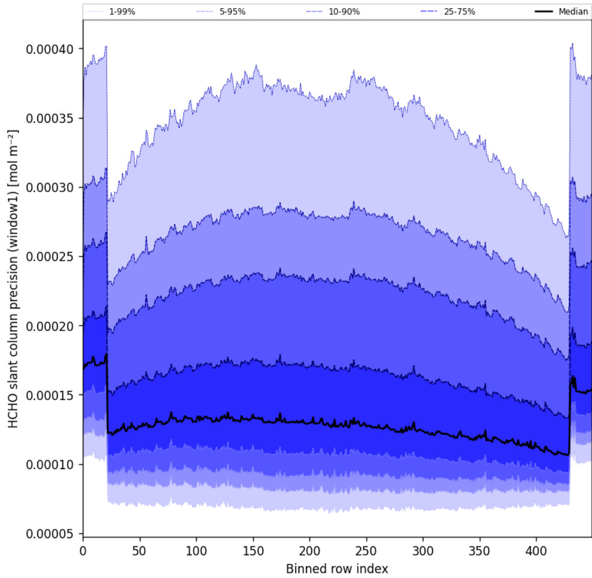
Figure 53: Along track statistics of “HCHO slant column precision (window1)” for 2025-07-24 to 2025-07-26
