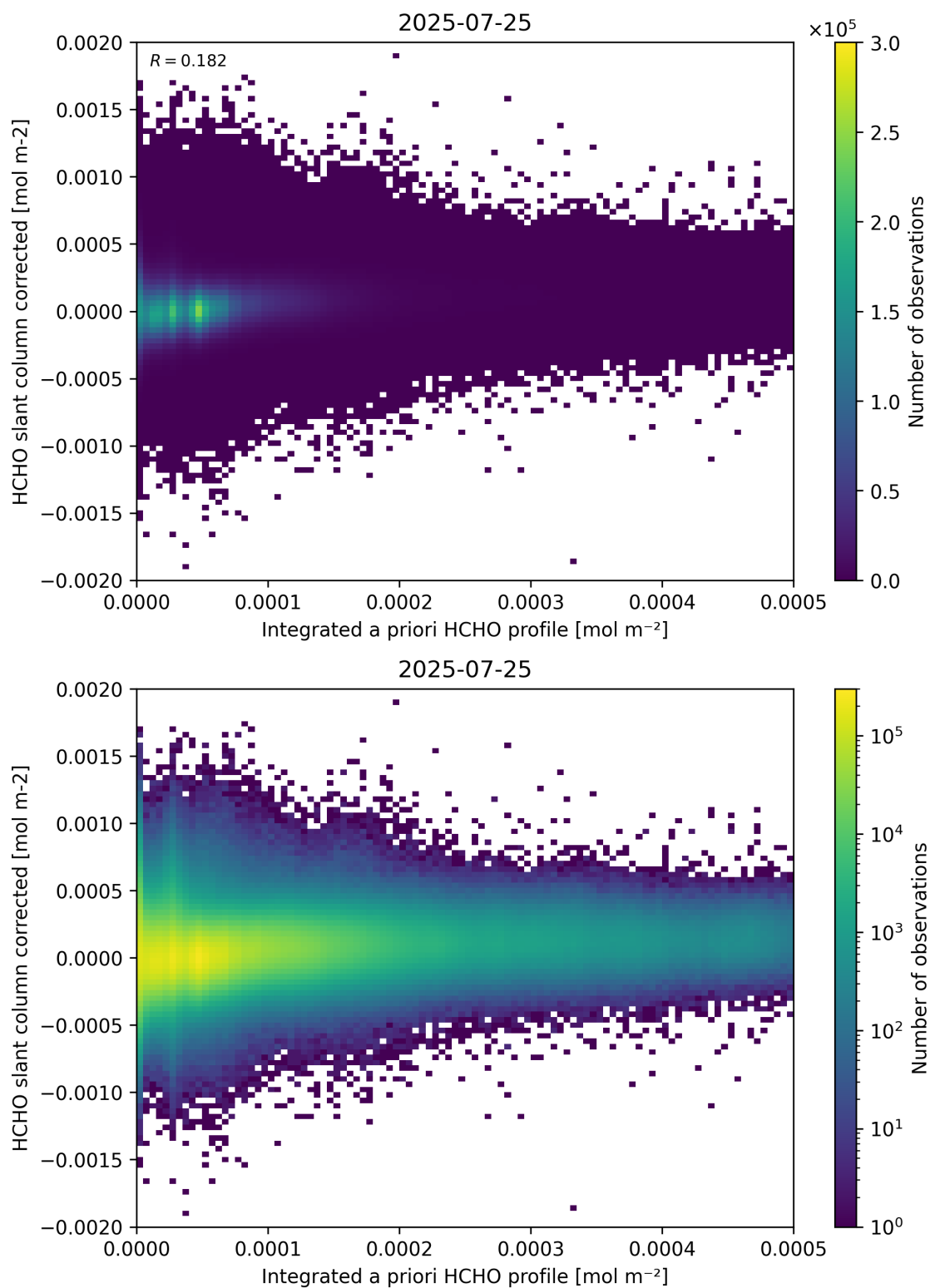
Figure 151: Scatter density plot of “Integrated a priori HCHO profile” against “HCHO slant column corrected” for 2025-07-24 to 2025-07-26.
