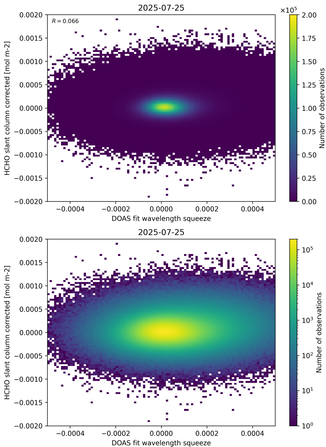
Figure 69: Scatter density plot of “DOAS fit wavelength squeeze” against “HCHO slant column corrected” for 2025-07-24 to 2025-07-26.
