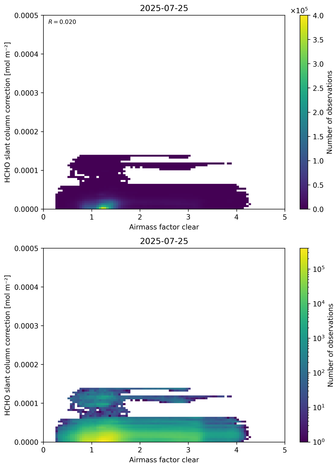
Figure 75: Scatter density plot of “Airmass factor clear” against “HCHO slant column correction” for 2025-07-24 to 2025-07-26.
