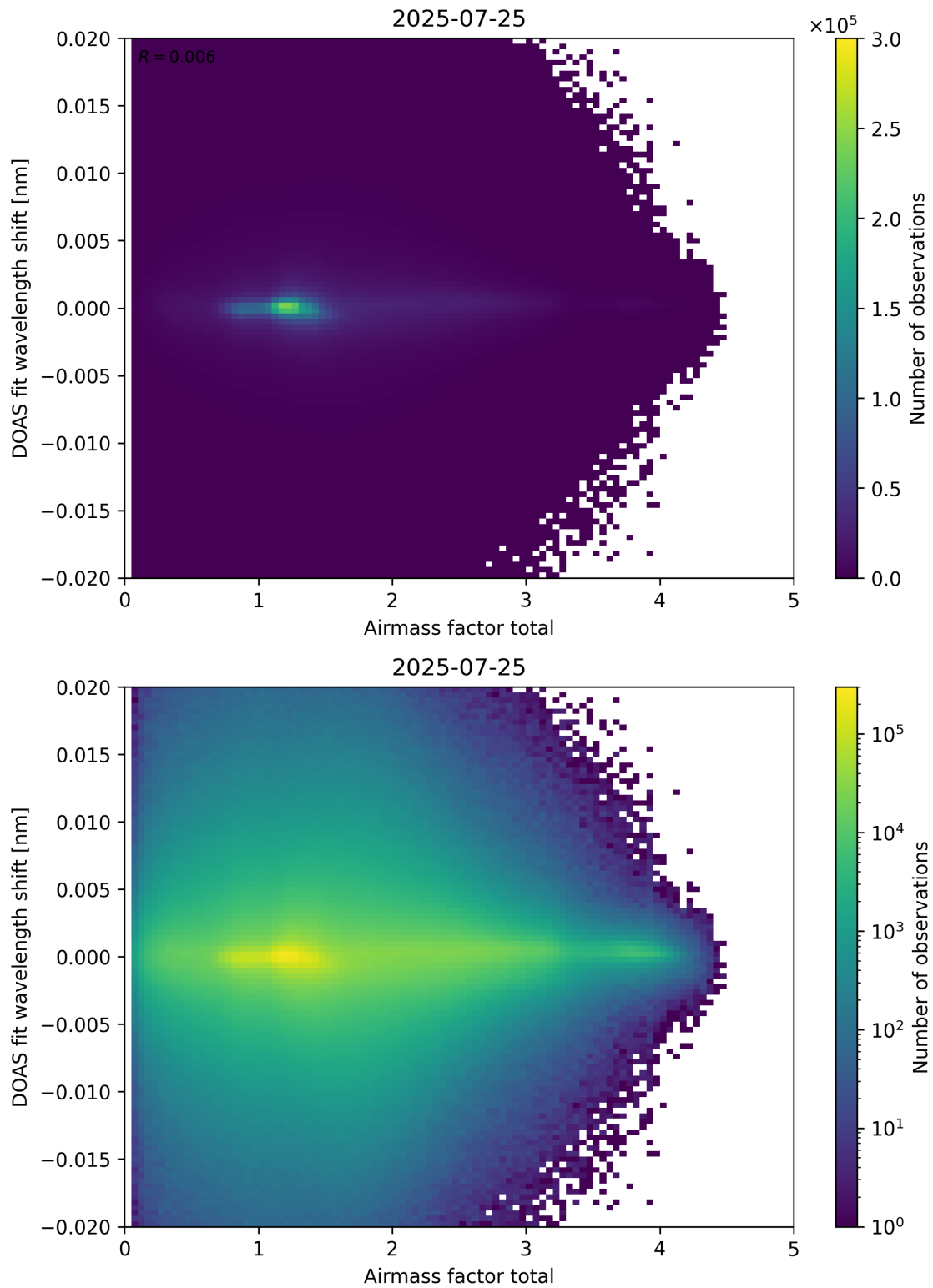
Figure 98: Scatter density plot of “Airmass factor total” against “DOAS fit wavelength shift” for 2025-07-24 to 2025-07-26.
