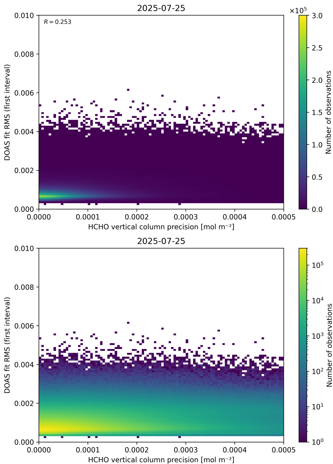
Figure 136: Scatter density plot of “HCHO vertical column precision” against “DOAS fit RMS (first interval)” for 2025-07-24 to 2025-07-26.
