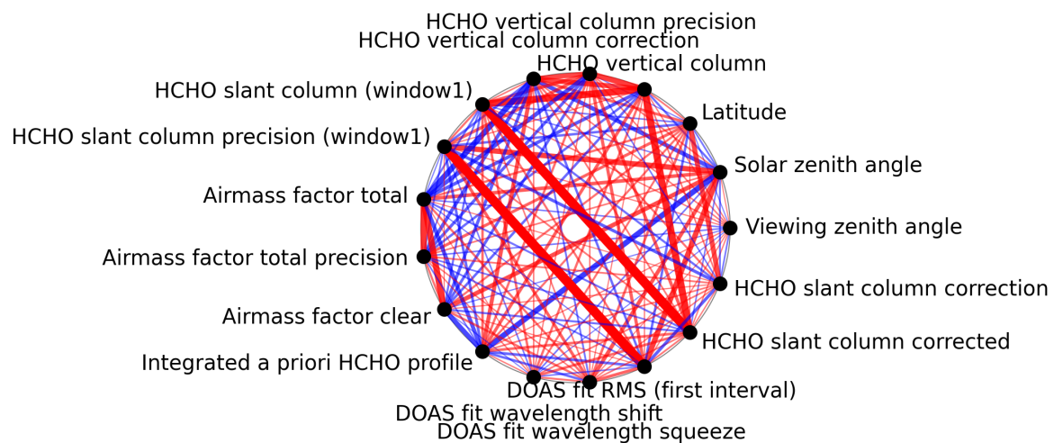
Figure 1: Map of correlation graph for 2025-07-24 to 2025-07-26.
