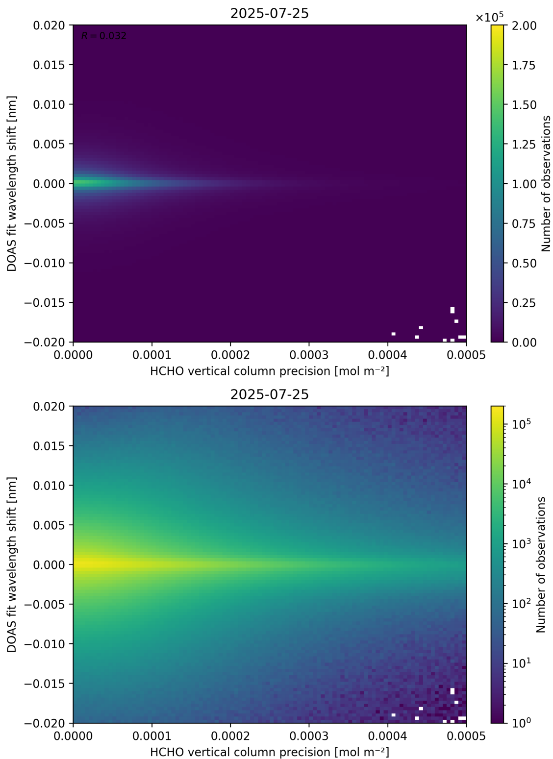
Figure 137: Scatter density plot of “HCHO vertical column precision” against “DOAS fit wavelength shift” for 2025-07-24 to 2025-07-26.
