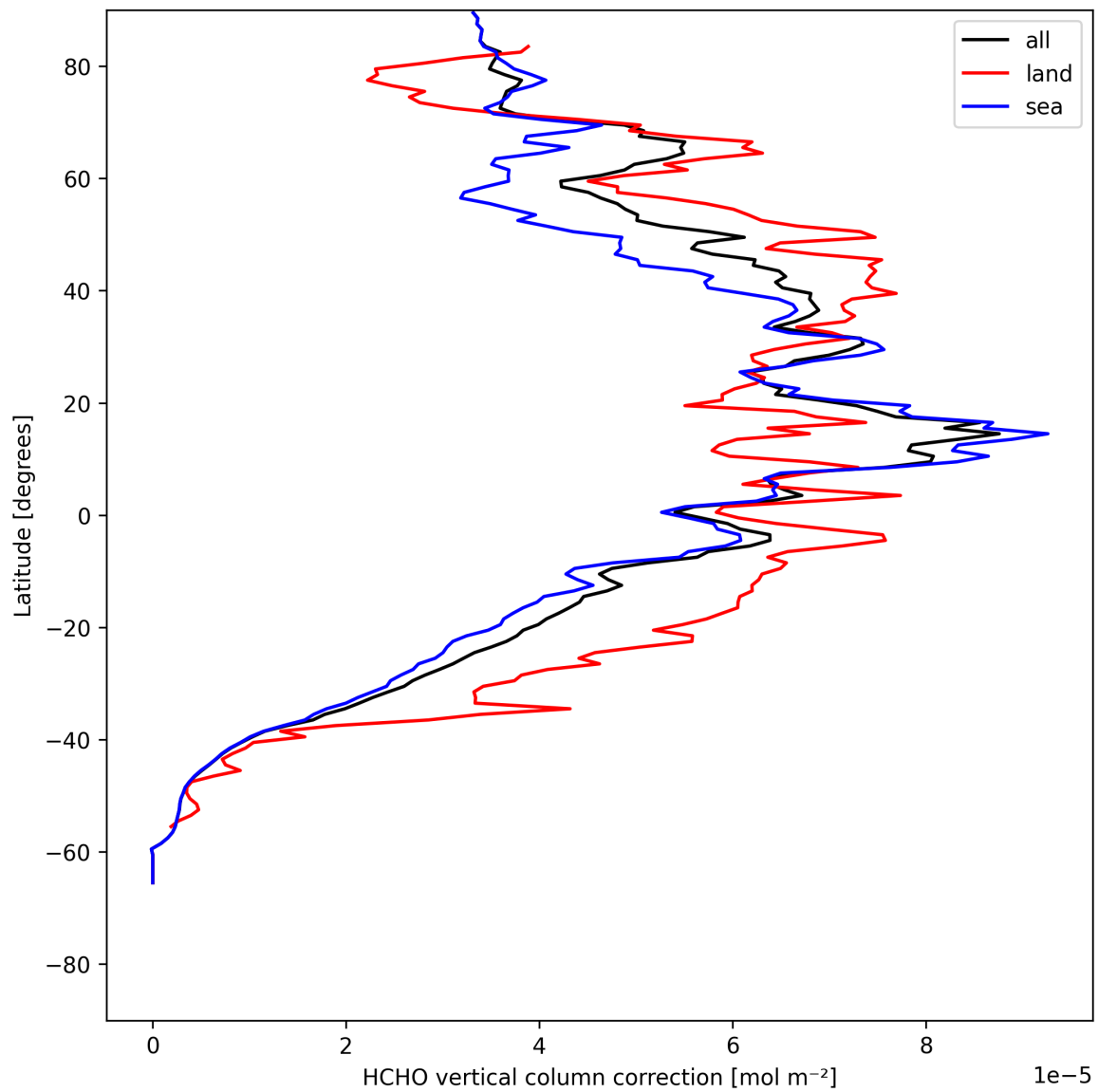
Figure 23: Zonal average of “HCHO vertical column correction” for 2025-07-24 to 2025-07-26.
