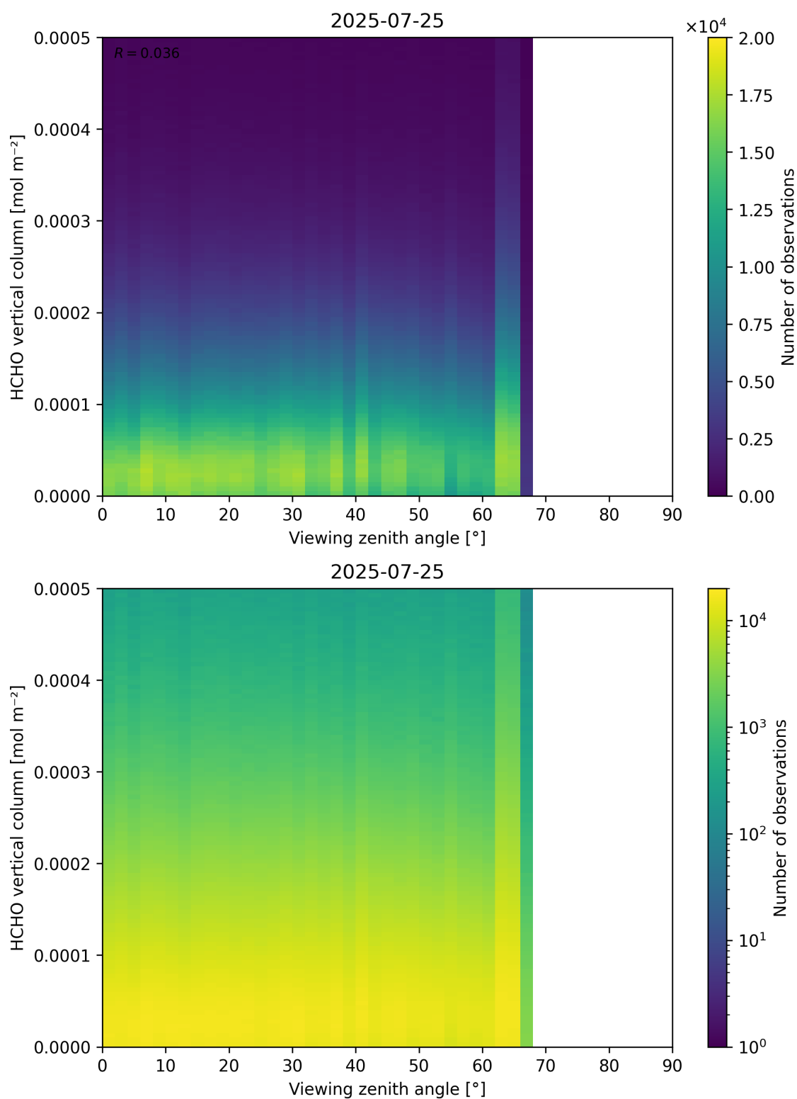
Figure 192: Scatter density plot of “Viewing zenith angle” against “HCHO vertical column” for 2025-07-24 to 2025-07-26.
