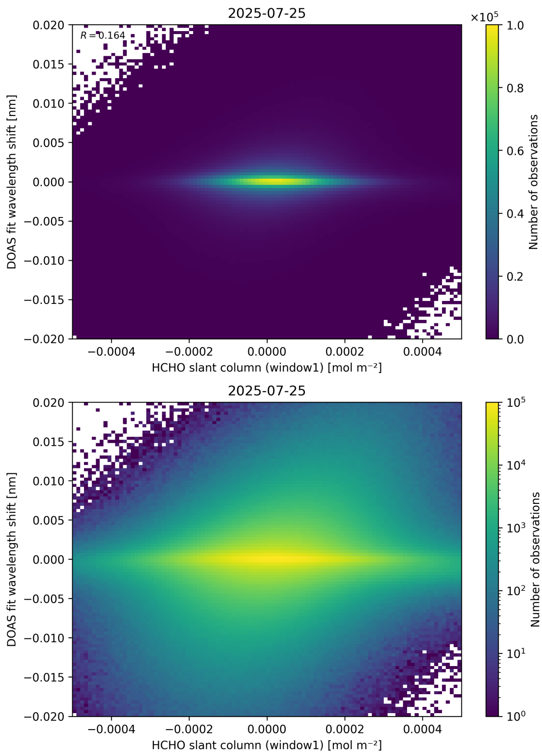
Figure 79: Scatter density plot of “HCHO slant column (window1)” against “DOAS fit wavelength shift” for 2025-07-24 to 2025-07-26.
