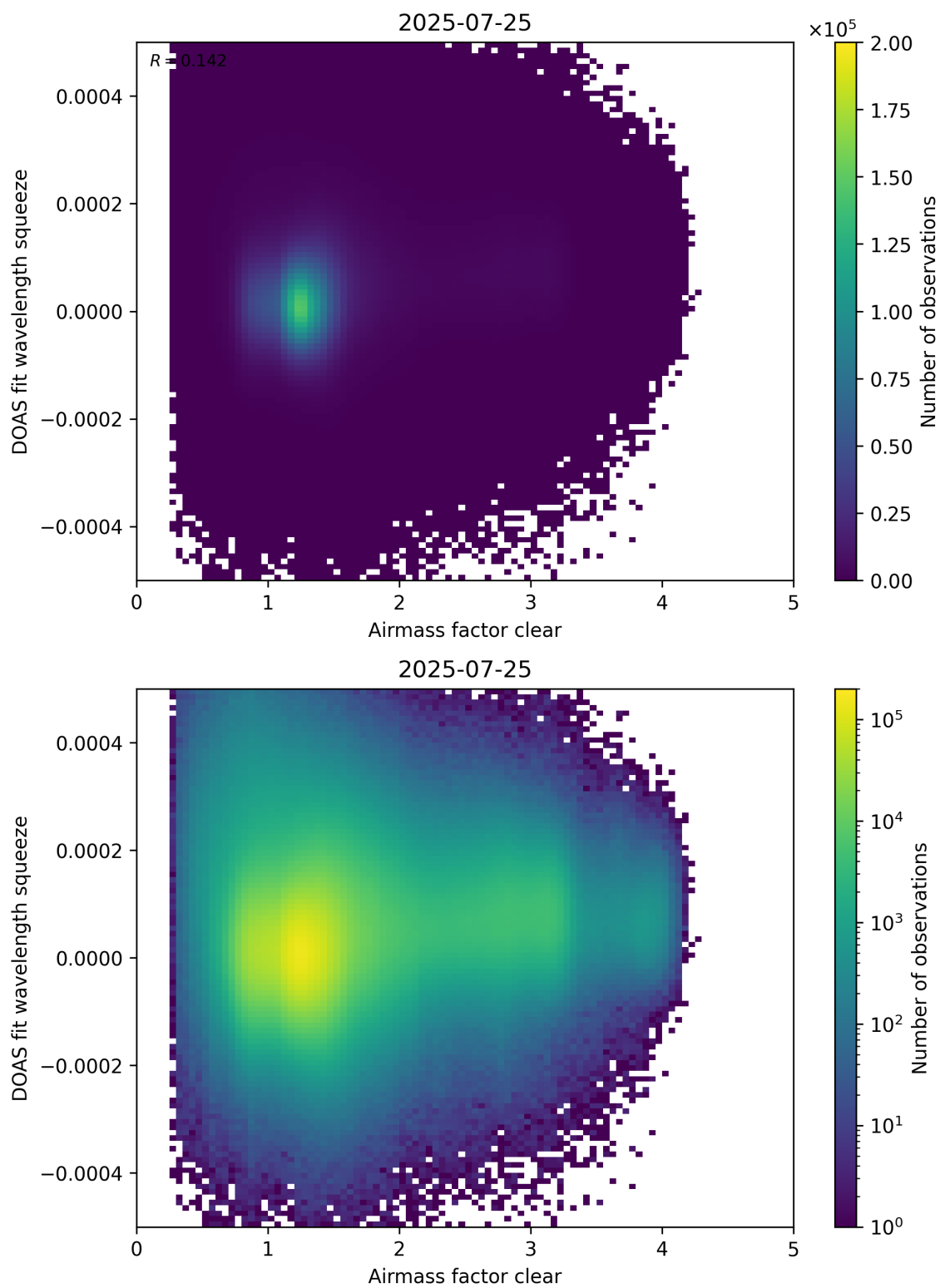
Figure 73: Scatter density plot of “Airmass factor clear” against “DOAS fit wavelength squeeze” for 2025-07-24 to 2025-07-26.
