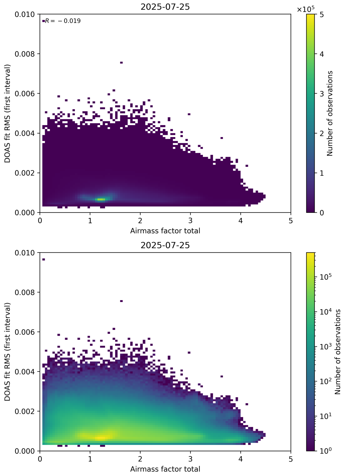
Figure 97: Scatter density plot of “Airmass factor total” against “DOAS fit RMS (first interval)” for 2025-07-24 to 2025-07-26.
