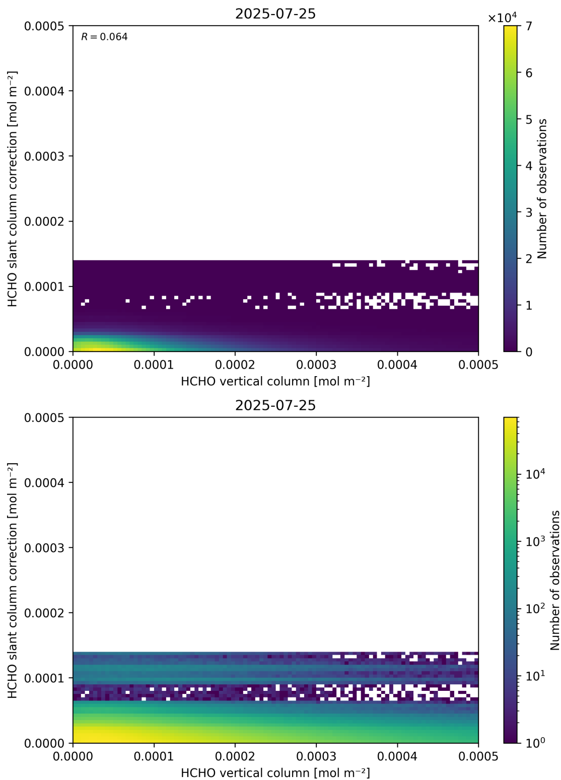
Figure 128: Scatter density plot of “HCHO vertical column” against “HCHO slant column correction” for 2025-07-24 to 2025-07-26.
