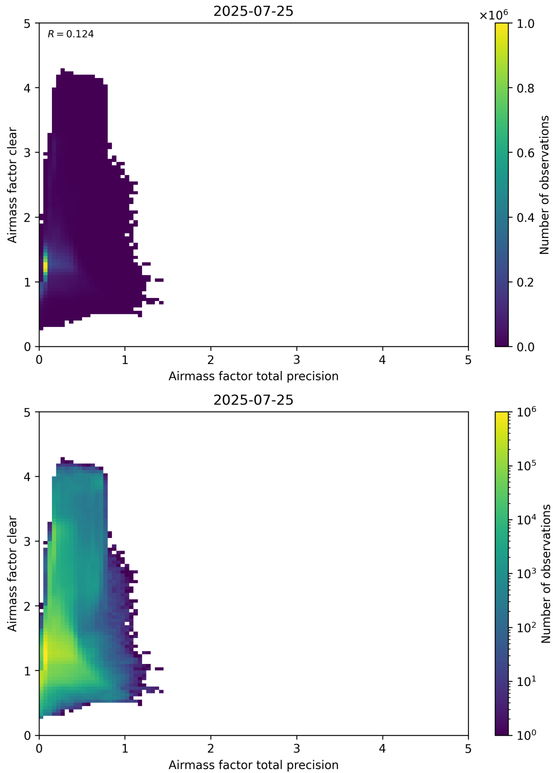
Figure 108: Scatter density plot of “Airmass factor total precision” against “Airmass factor clear” for 2025-07-24 to 2025-07-26.
