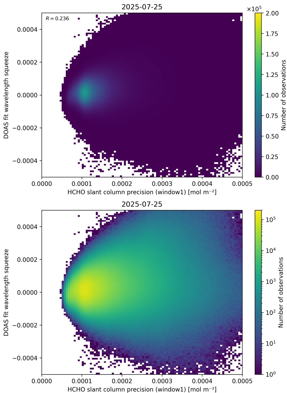
Figure 90: Scatter density plot of “HCHO slant column precision (window1)” against “DOAS fit wavelength squeeze” for 2025-07-24 to 2025-07-26.
