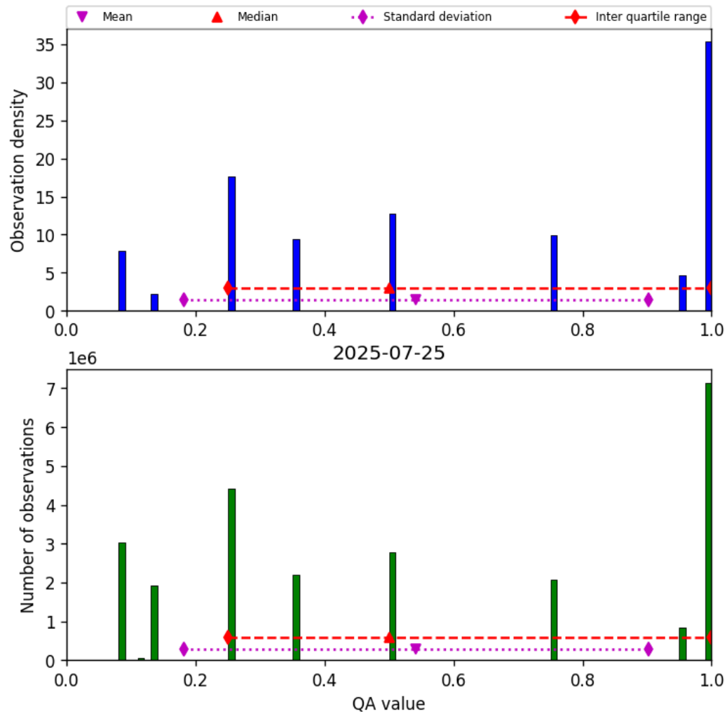
Figure 34: Histogram of “QA value” for 2025-07-24 to 2025-07-26
