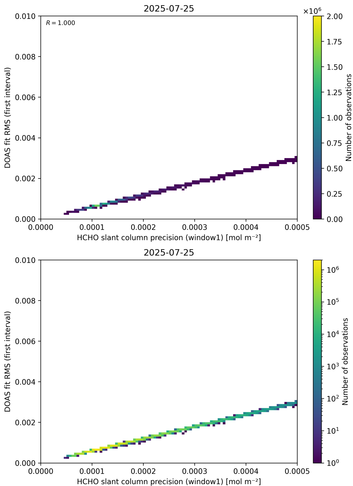
Figure 88: Scatter density plot of “HCHO slant column precision (window1)” against “DOAS fit RMS (first interval)” for 2025-07-24 to 2025-07-26.
