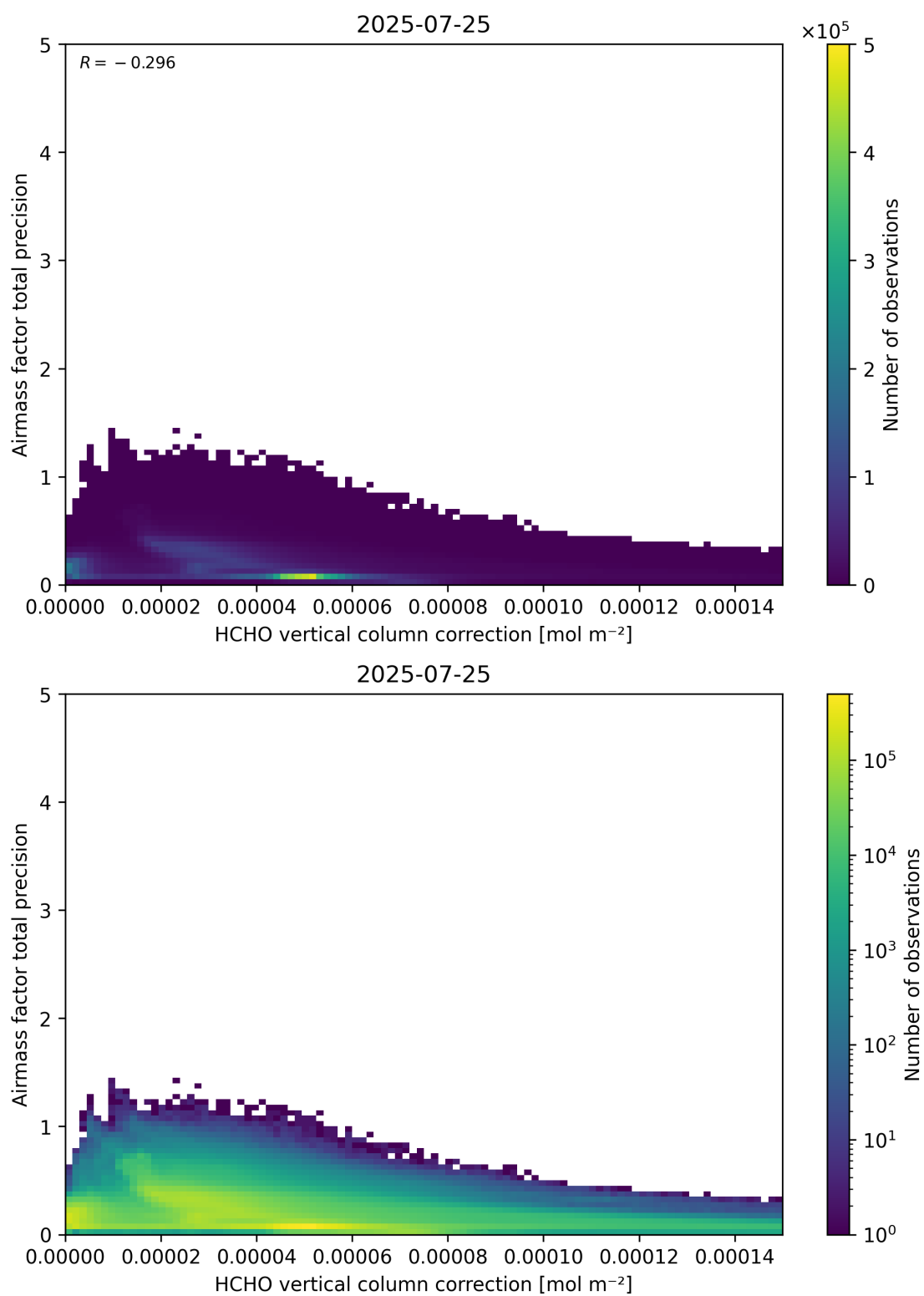
Figure 121: Scatter density plot of “HCHO vertical column correction” against “Airmass factor total precision” for 2025-07-24 to 2025-07-26.
