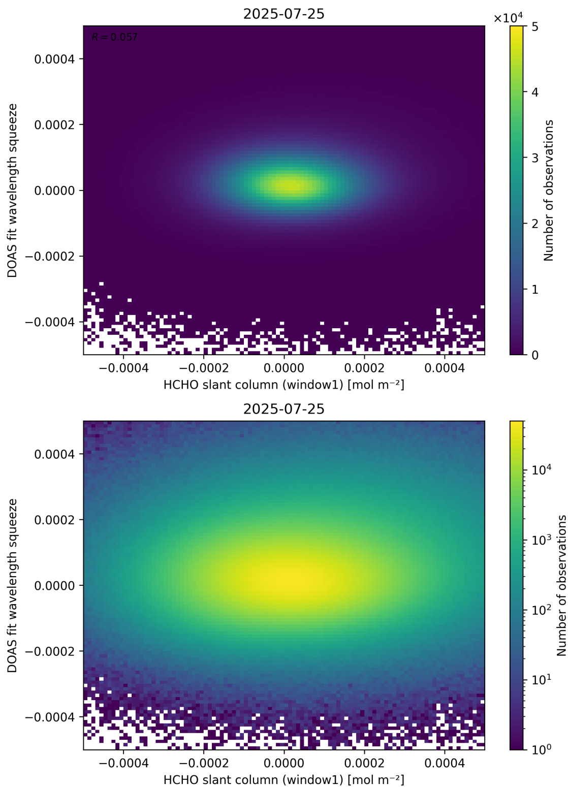
Figure 80: Scatter density plot of “HCHO slant column (window1)” against “DOAS fit wavelength squeeze” for 2025-07-24 to 2025-07-26.
