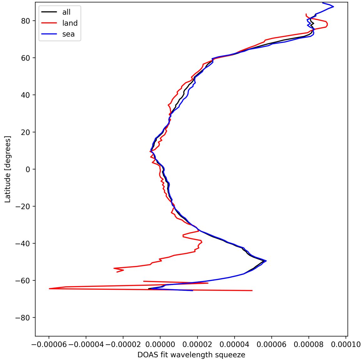
Figure 31: Zonal average of “DOAS fit wavelength squeeze” for 2025-07-24 to 2025-07-26.
