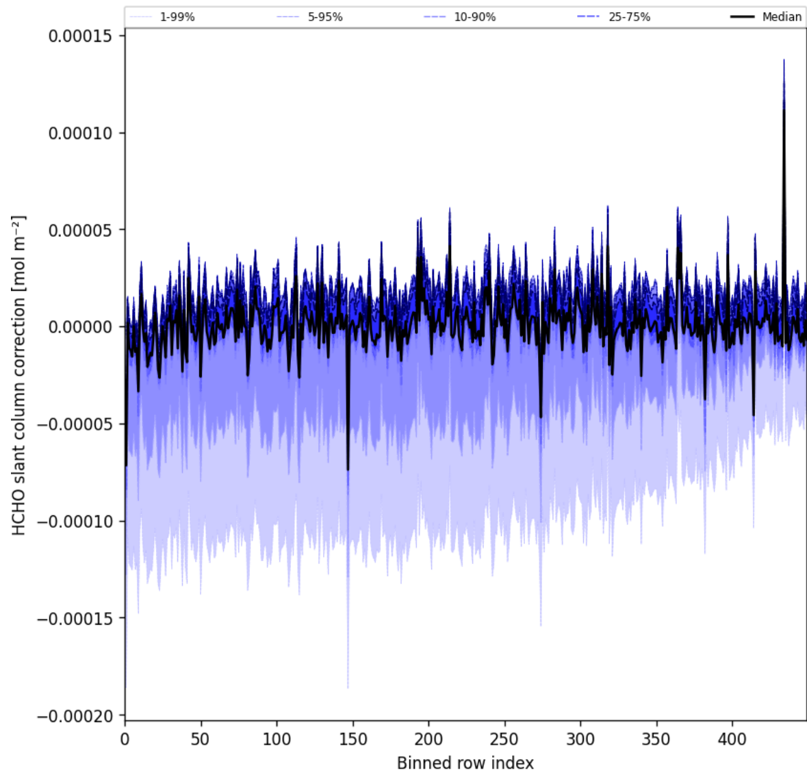
Figure 61: Along track statistics of “HCHO slant column correction” for 2025-07-24 to 2025-07-26
