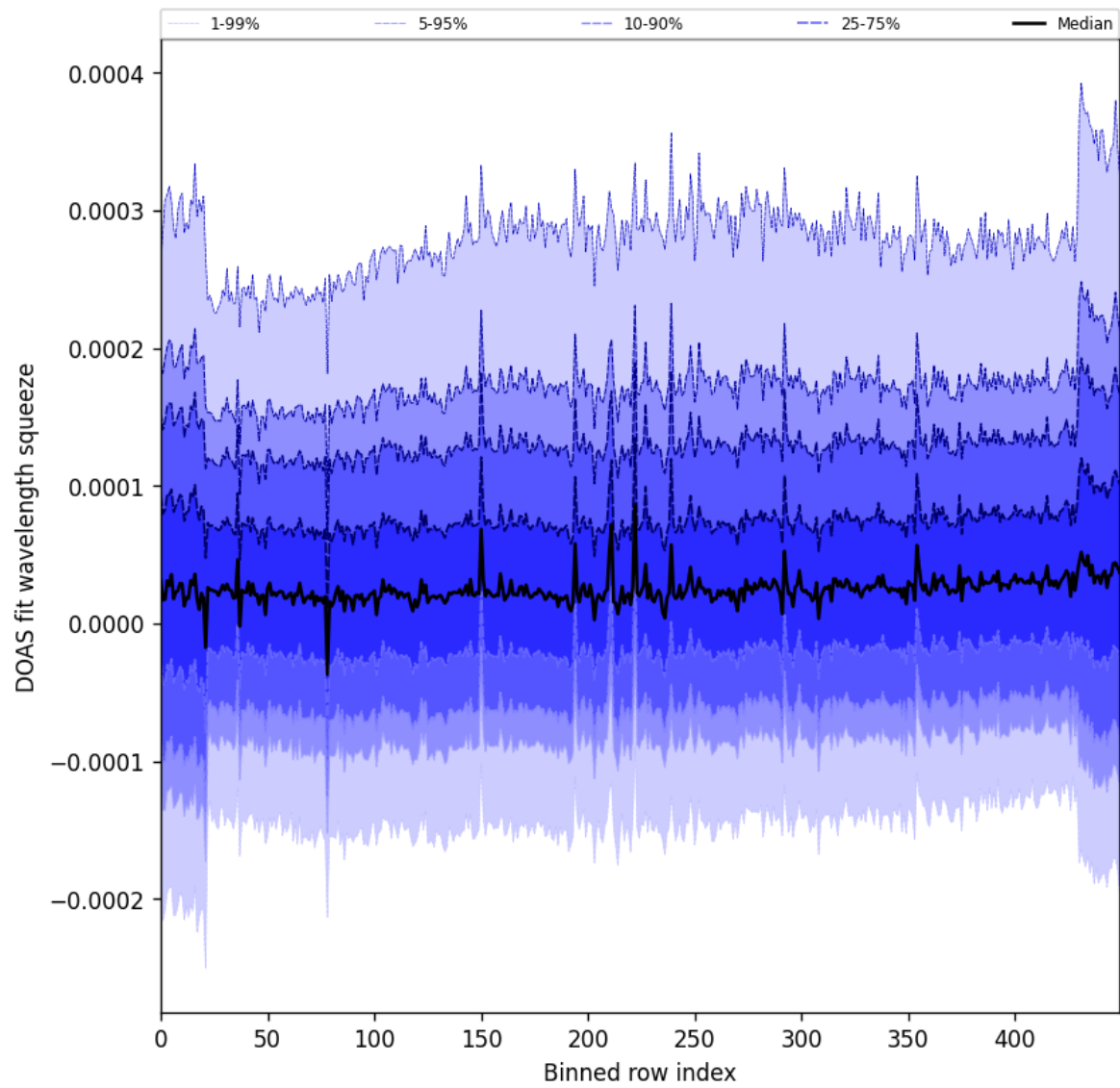
Figure 59: Along track statistics of “DOAS fit wavelength squeeze” for 2025-07-24 to 2025-07-26
