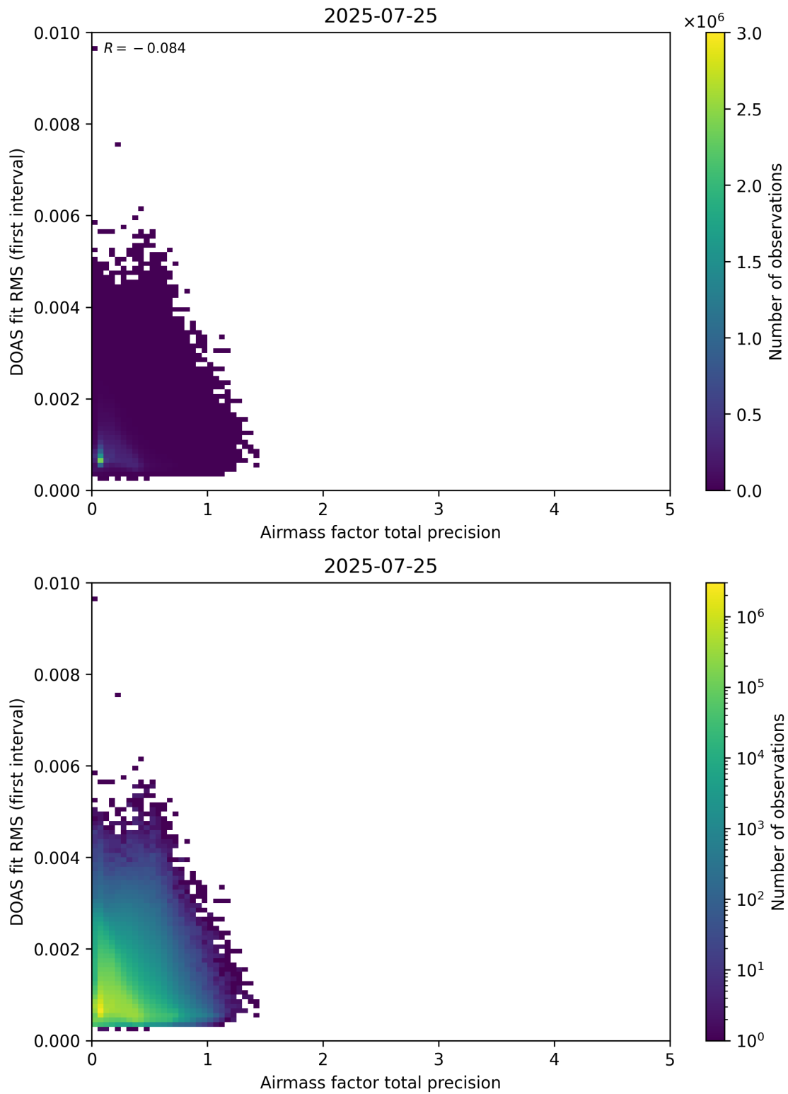
Figure 105: Scatter density plot of “Airmass factor total precision” against “DOAS fit RMS (first interval)” for 2025-07-24 to 2025-07-26.
