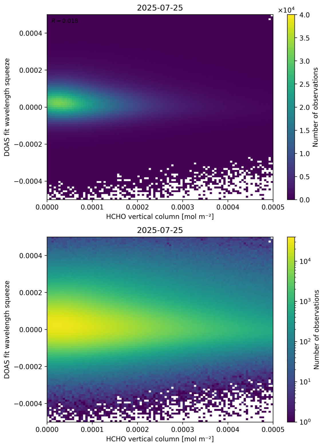
Figure 125: Scatter density plot of “HCHO vertical column” against “DOAS fit wavelength squeeze” for 2025-07-24 to 2025-07-26.
