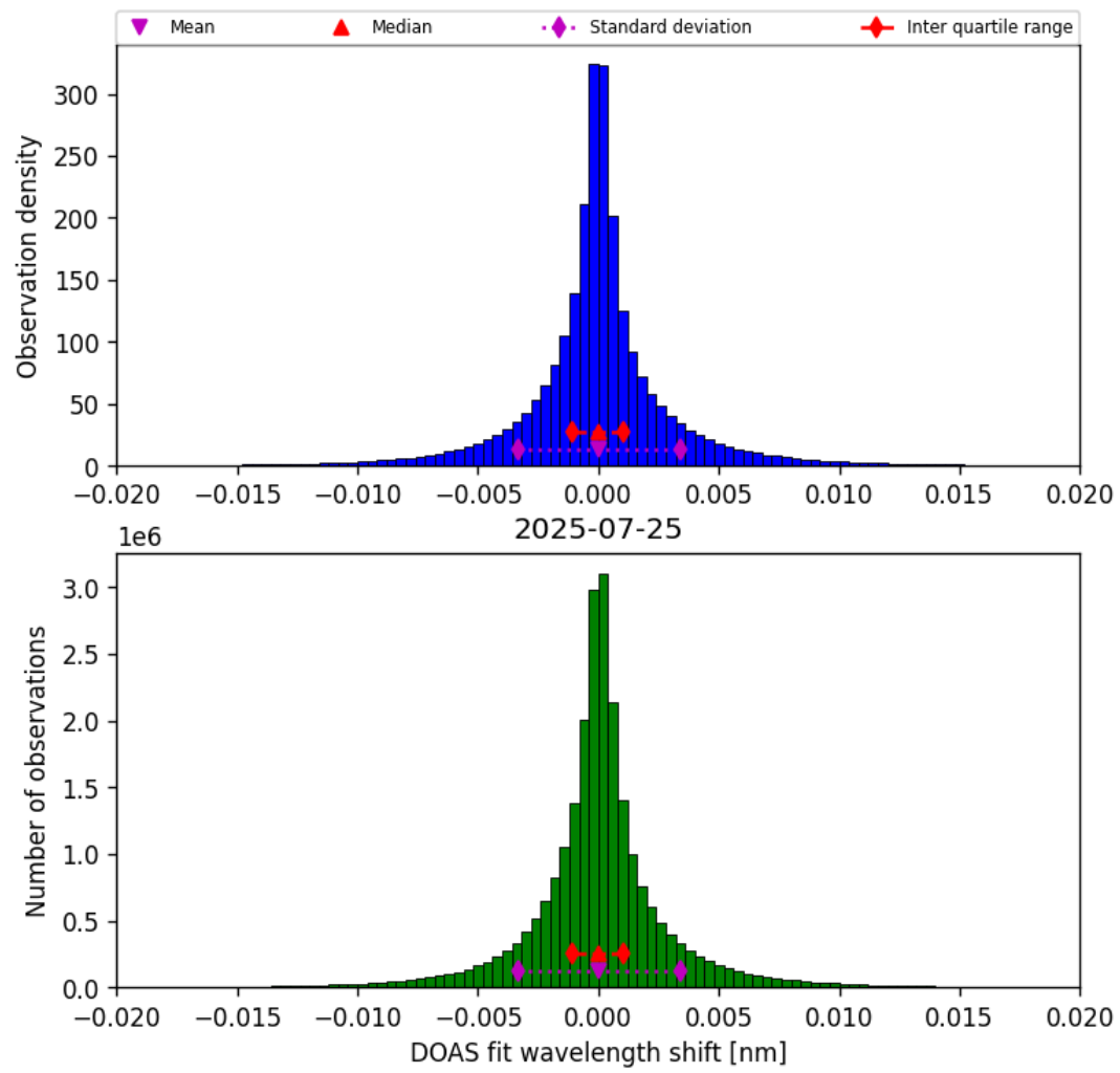
Figure 44: Histogram of “DOAS fit wavelength shift” for 2025-07-24 to 2025-07-26
