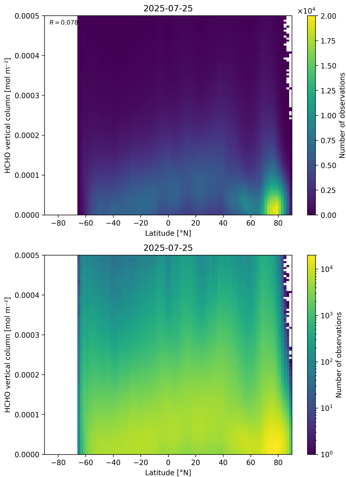
Figure 163: Scatter density plot of “Latitude” against “HCHO vertical column” for 2025-07-24 to 2025-07-26.
