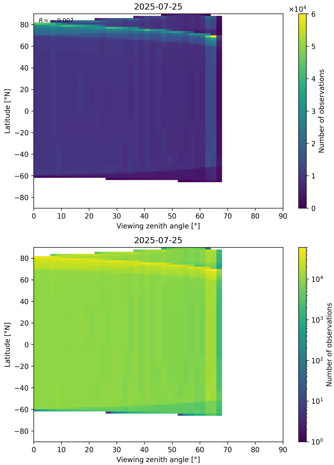
Figure 196: Scatter density plot of “Viewing zenith angle” against “Latitude” for 2025-07-24 to 2025-07-26.
