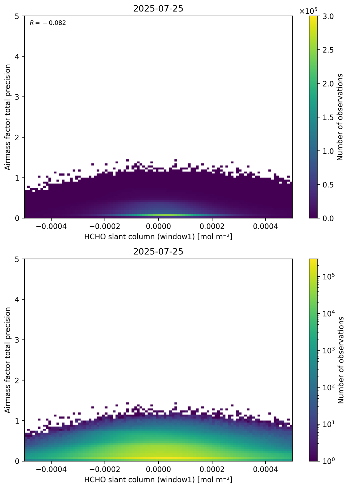
Figure 86: Scatter density plot of “HCHO slant column (window1)” against “Airmass factor total precision” for 2025-07-24 to 2025-07-26.
