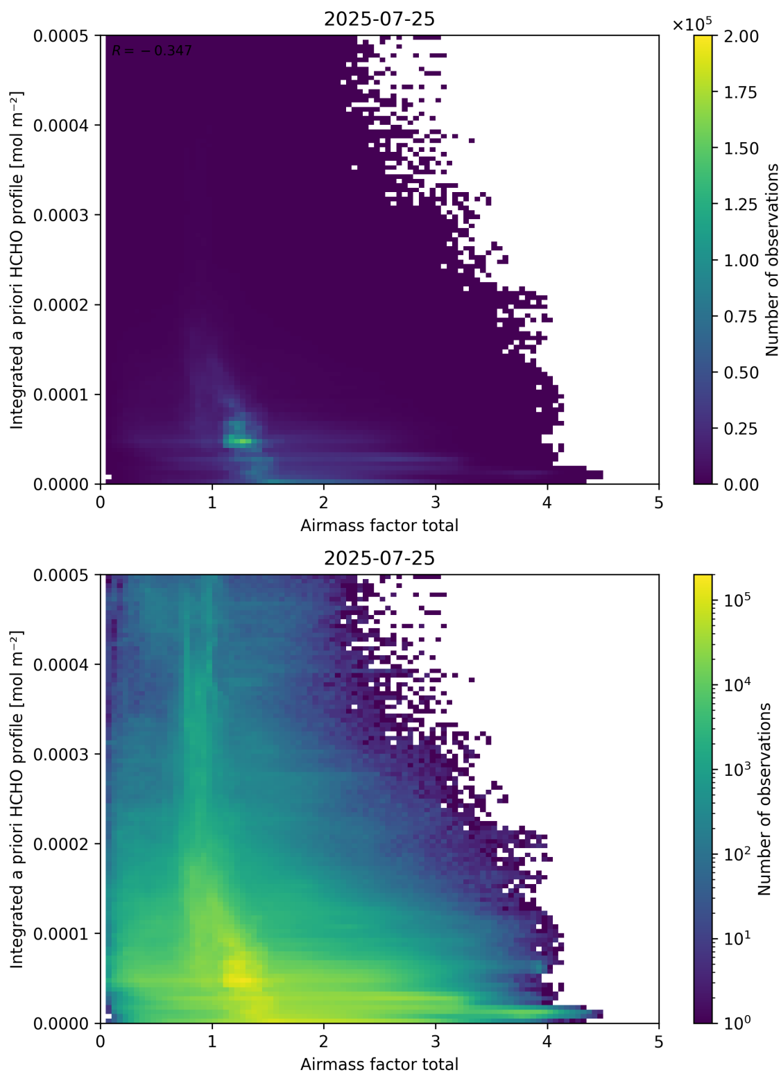
Figure 104: Scatter density plot of “Airmass factor total” against “Integrated a priori HCHO profile” for 2025-07-24 to 2025-07-26.
