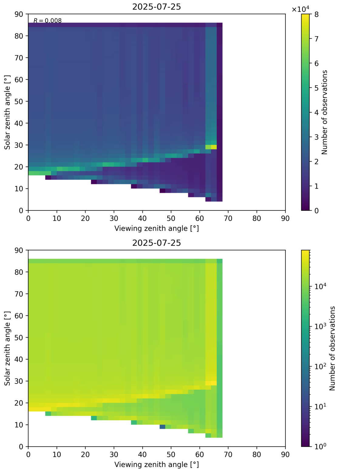
Figure 197: Scatter density plot of “Viewing zenith angle” against “Solar zenith angle” for 2025-07-24 to 2025-07-26.
