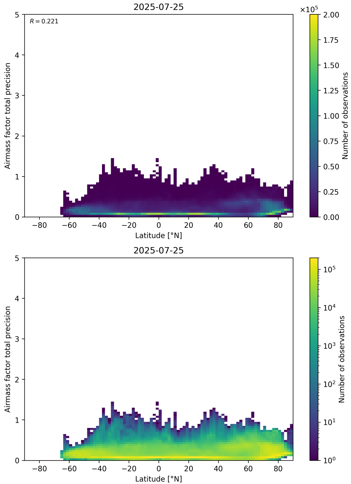
Figure 162: Scatter density plot of “Latitude” against “Airmass factor total precision” for 2025-07-24 to 2025-07-26.
