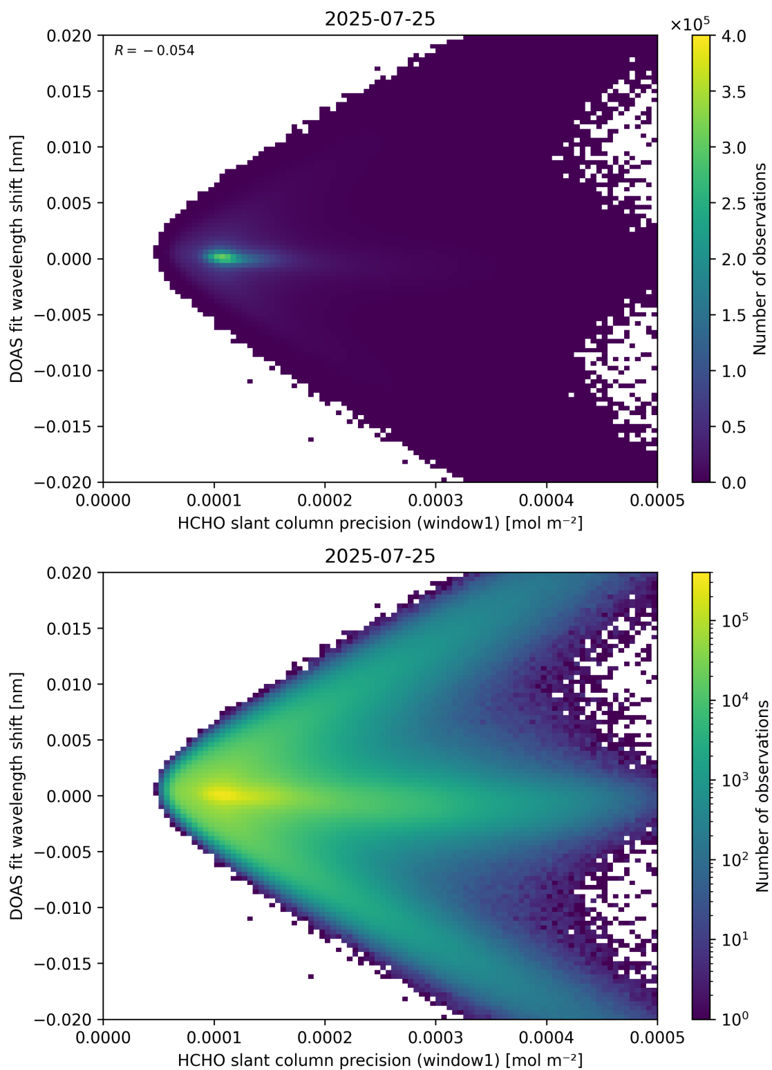
Figure 89: Scatter density plot of “HCHO slant column precision (window1)” against “DOAS fit wavelength shift” for 2025-07-24 to 2025-07-26.
