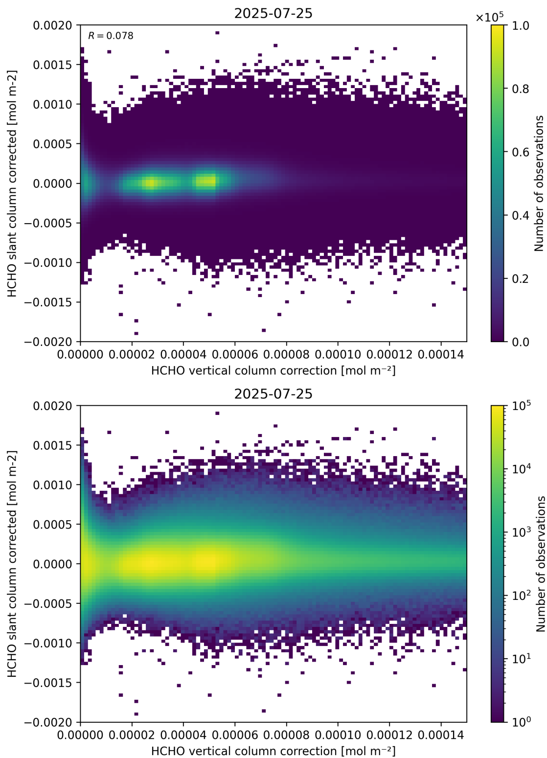
Figure 116: Scatter density plot of “HCHO vertical column correction” against “HCHO slant column corrected” for 2025-07-24 to 2025-07-26.
