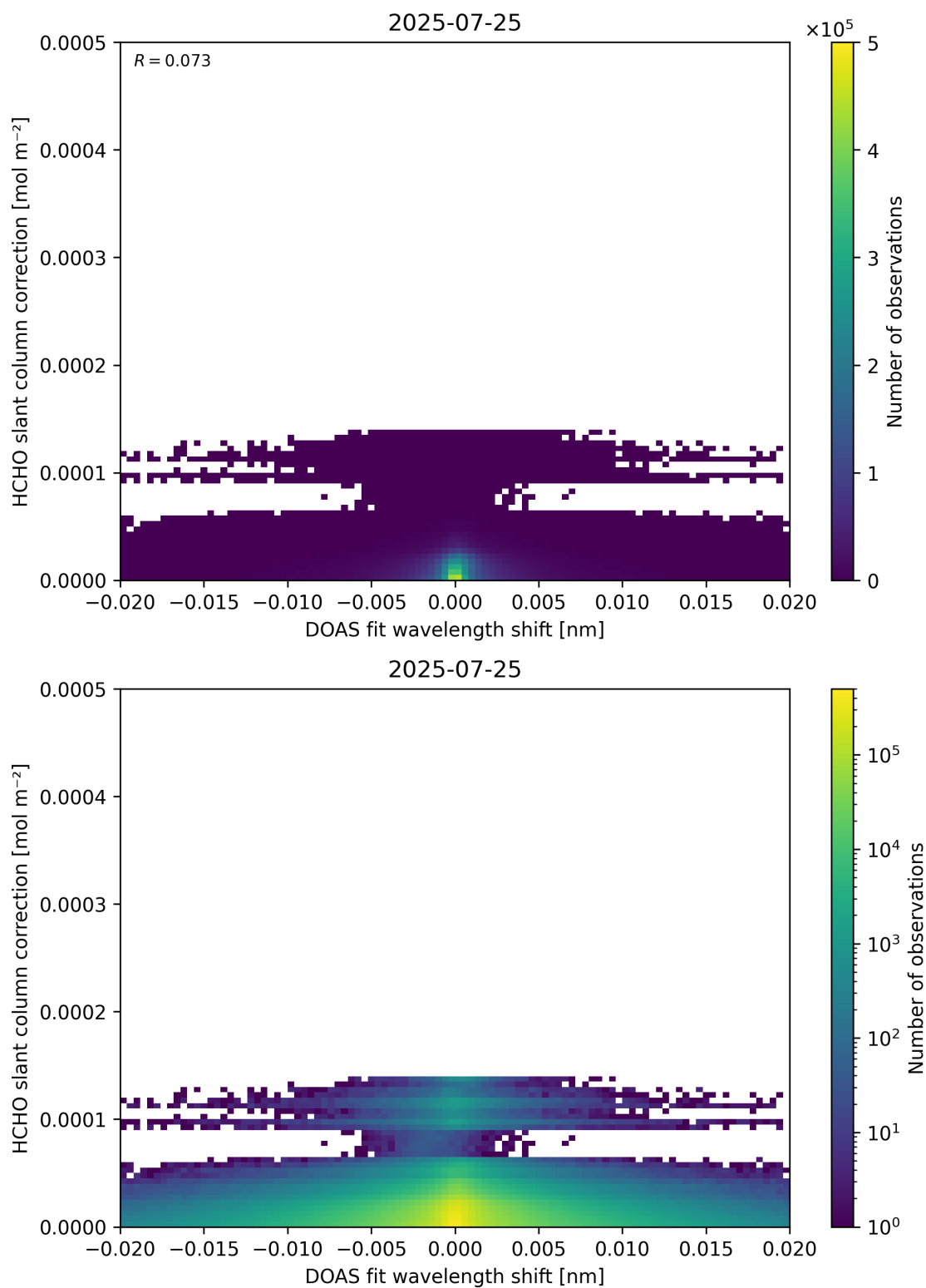
Figure 67: Scatter density plot of “DOAS fit wavelength shift” against “HCHO slant column correction” for 2025-07-24 to 2025-07-26.
