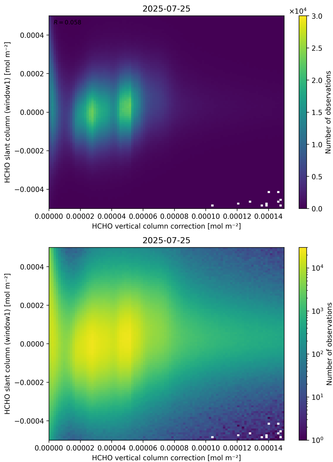
Figure 118: Scatter density plot of “HCHO vertical column correction” against “HCHO slant column (window1)” for 2025-07-24 to 2025-07-26.
