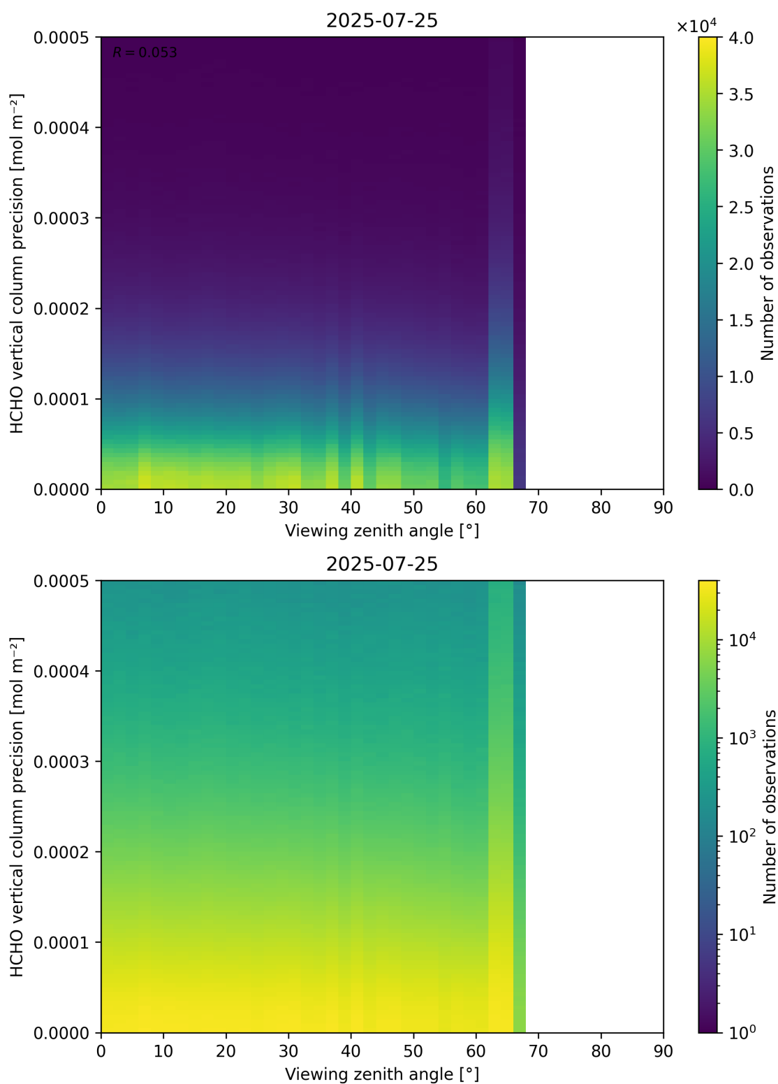
Figure 194: Scatter density plot of “Viewing zenith angle” against “HCHO vertical column precision” for 2025-07-24 to 2025-07-26.
