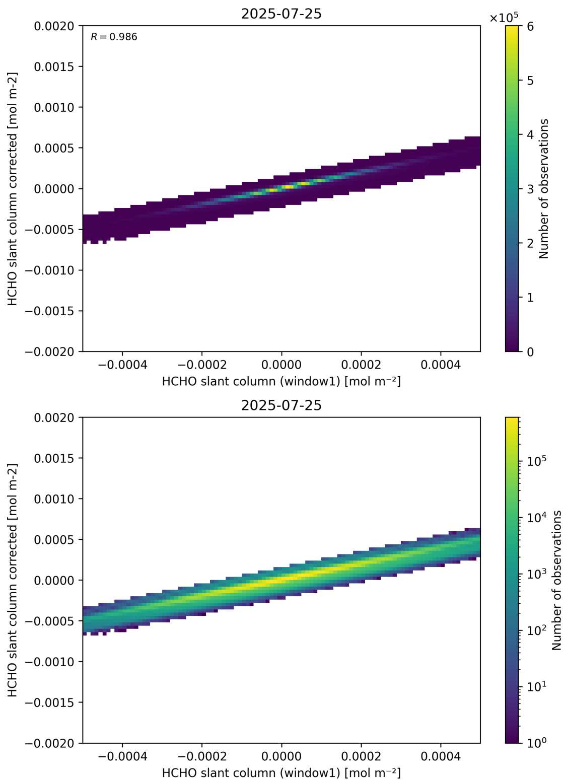
Figure 82: Scatter density plot of “HCHO slant column (window1)” against “HCHO slant column corrected” for 2025-07-24 to 2025-07-26.
