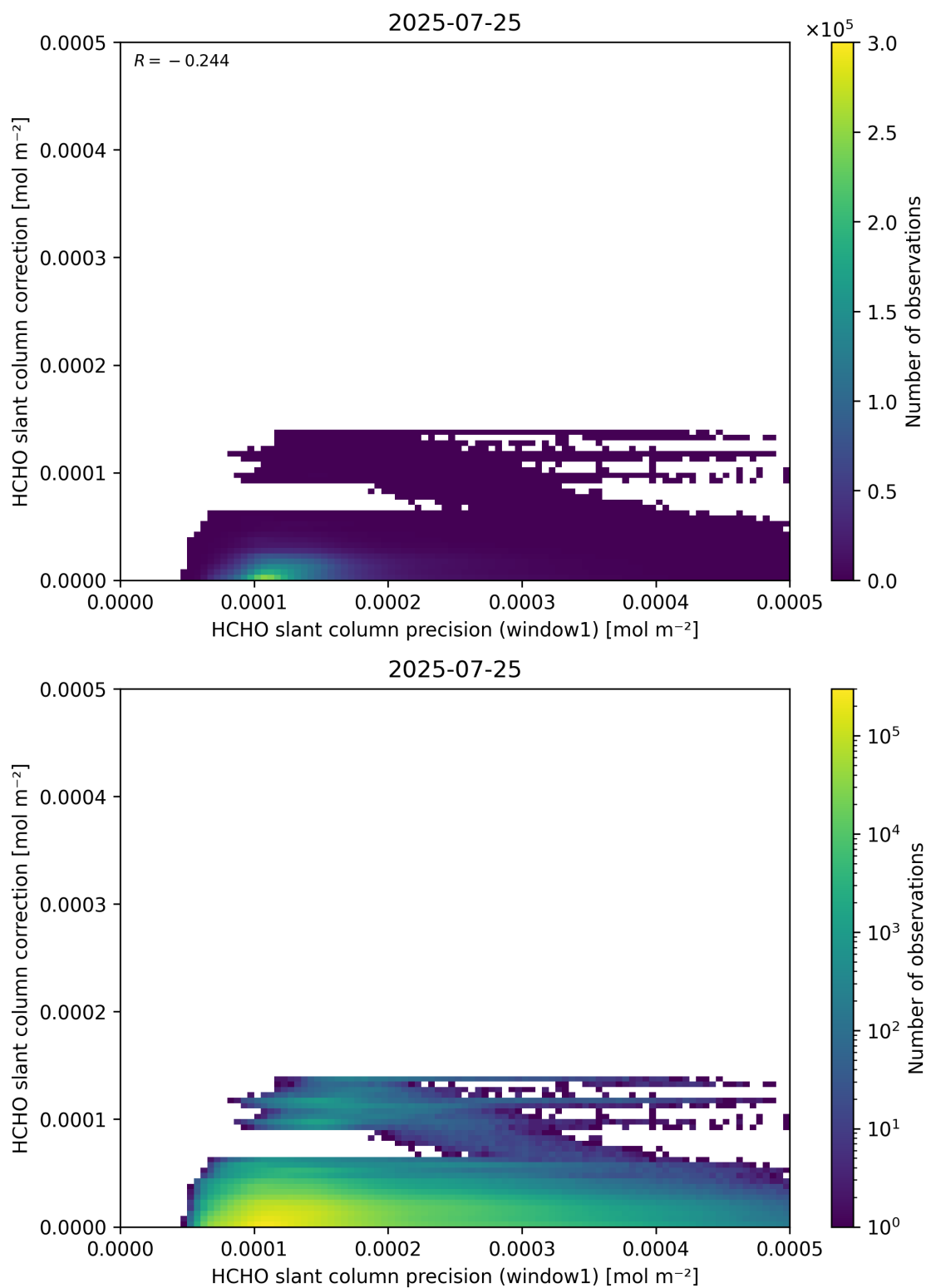
Figure 93: Scatter density plot of “HCHO slant column precision (window1)” against “HCHO slant column correction” for 2025-07-24 to 2025-07-26.
