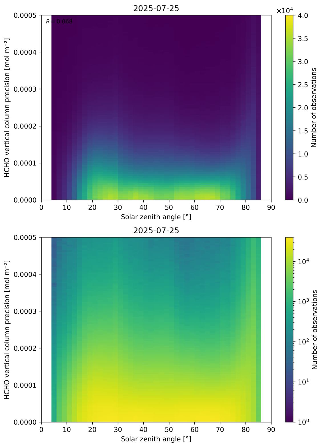
Figure 179: Scatter density plot of “Solar zenith angle” against “HCHO vertical column precision” for 2025-07-24 to 2025-07-26.
