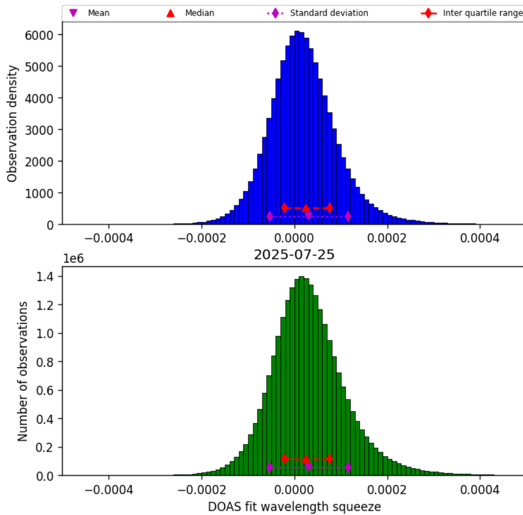
Figure 45: Histogram of “DOAS fit wavelength squeeze” for 2025-07-24 to 2025-07-26
