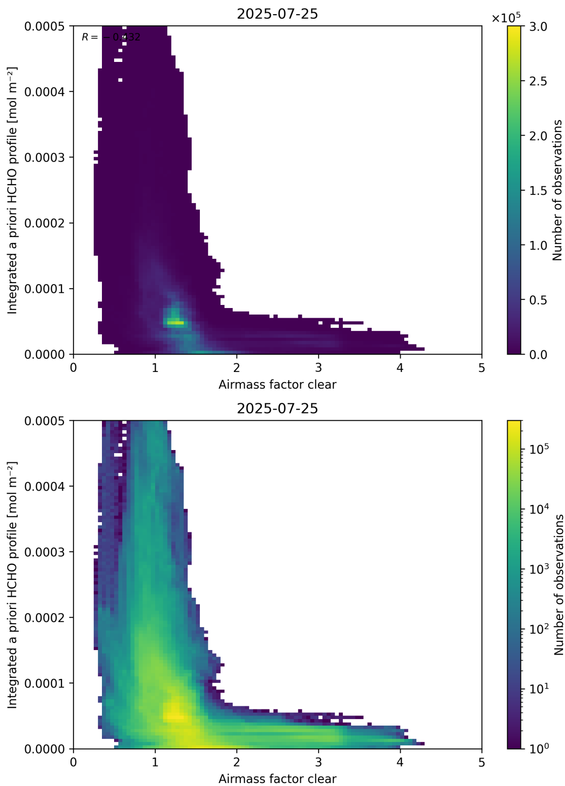
Figure 76: Scatter density plot of “Airmass factor clear” against “Integrated a priori HCHO profile” for 2025-07-24 to 2025-07-26.
