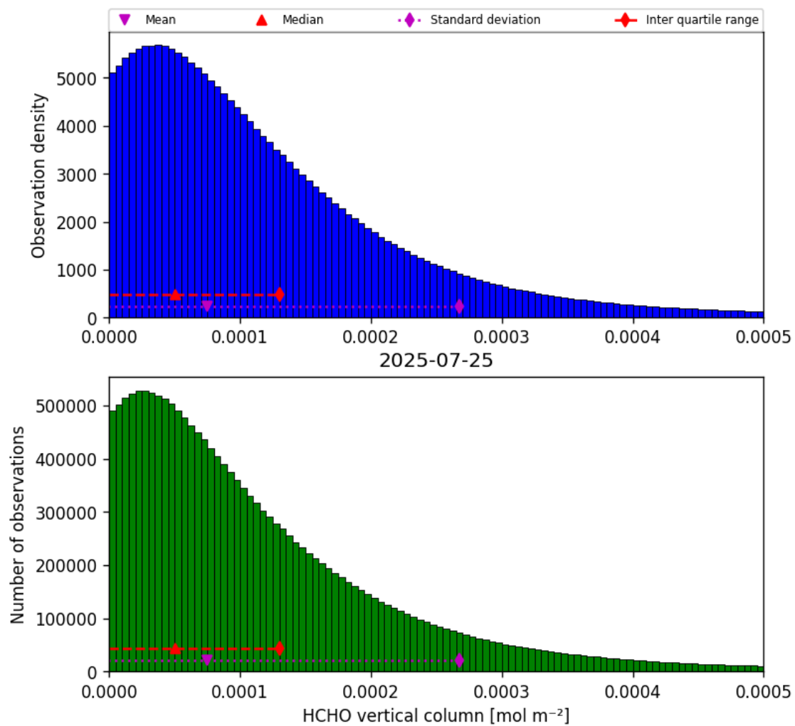
Figure 35: Histogram of “HCHO vertical column” for 2025-07-24 to 2025-07-26
