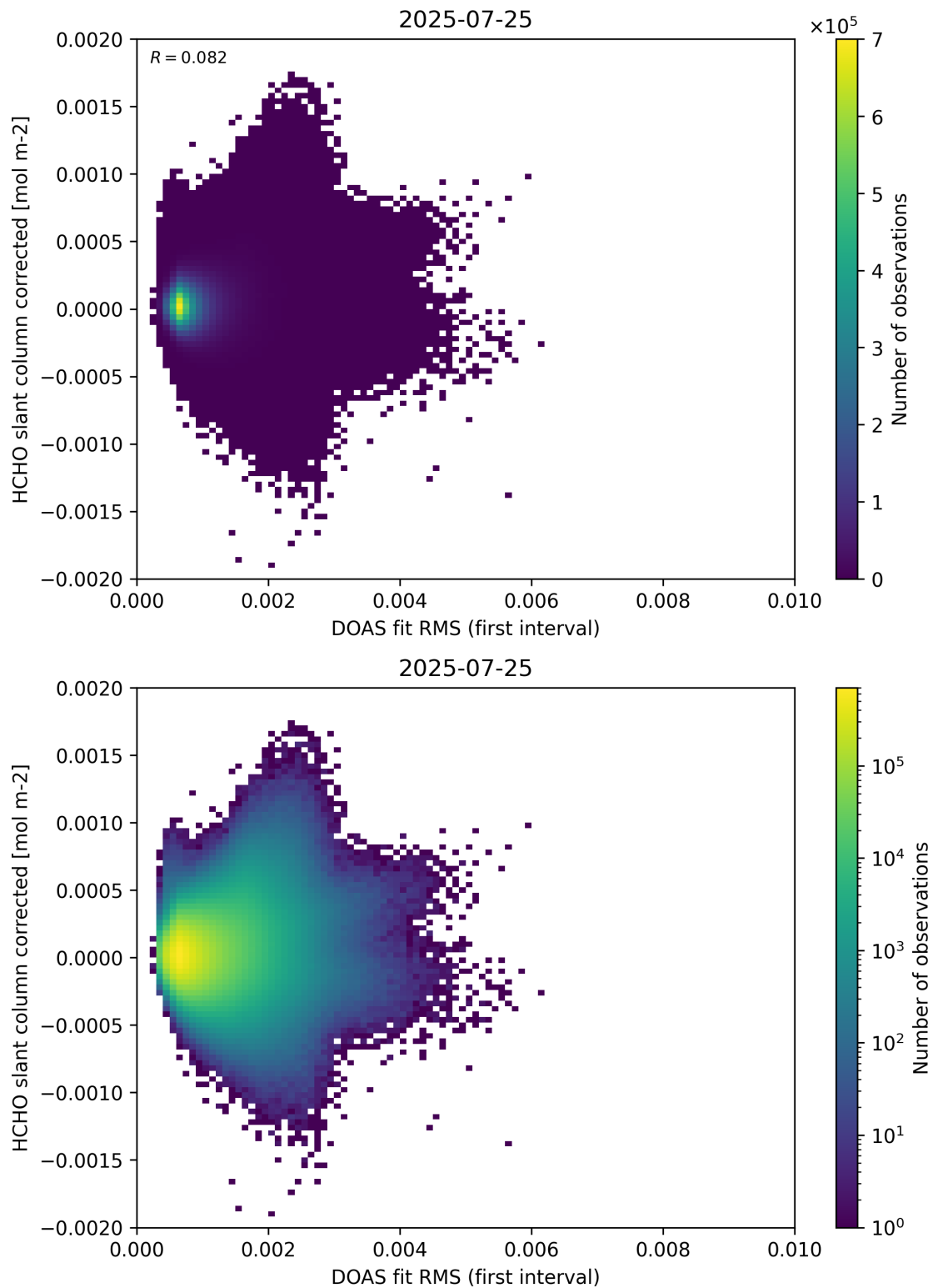
Figure 62: Scatter density plot of “DOAS fit RMS (first interval)” against “HCHO slant column corrected” for 2025-07-24 to 2025-07-26.
