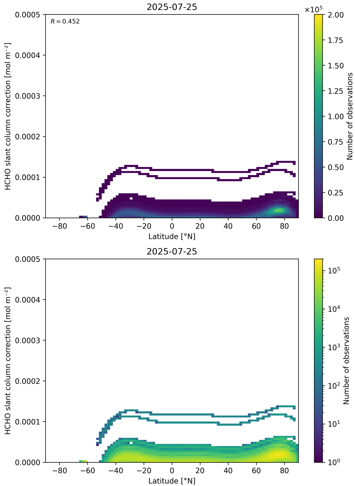
Figure 158: Scatter density plot of “Latitude” against “HCHO slant column correction” for 2025-07-24 to 2025-07-26.
