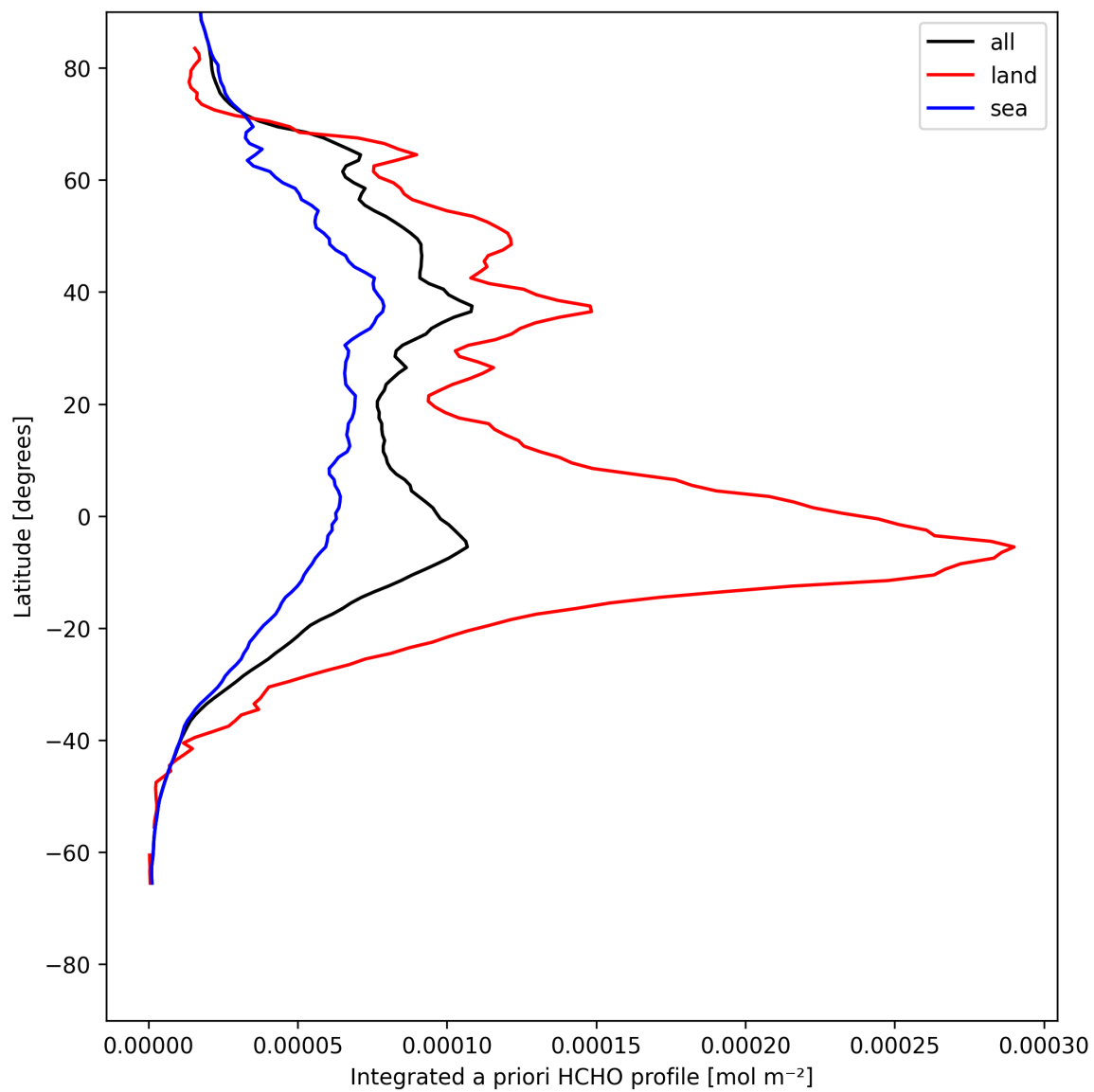
Figure 29: Zonal average of “Integrated a priori HCHO profile” for 2025-07-24 to 2025-07-26.
