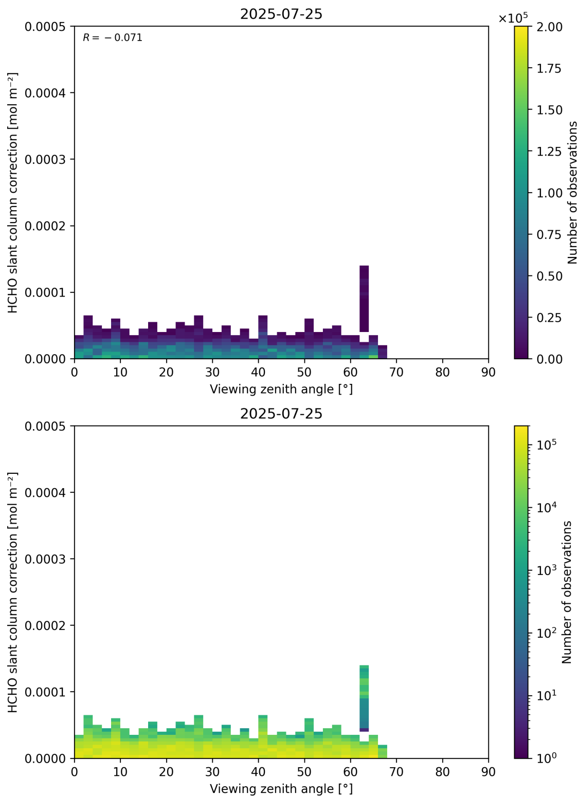
Figure 187: Scatter density plot of “Viewing zenith angle” against “HCHO slant column correction” for 2025-07-24 to 2025-07-26.
