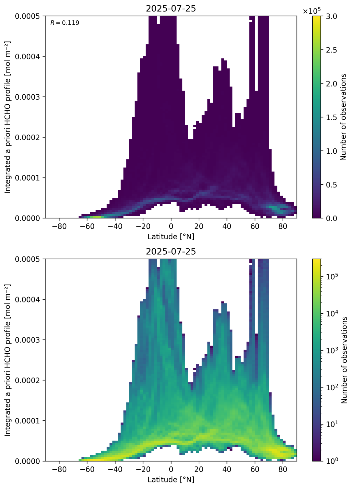
Figure 166: Scatter density plot of “Latitude” against “Integrated a priori HCHO profile” for 2025-07-24 to 2025-07-26.
