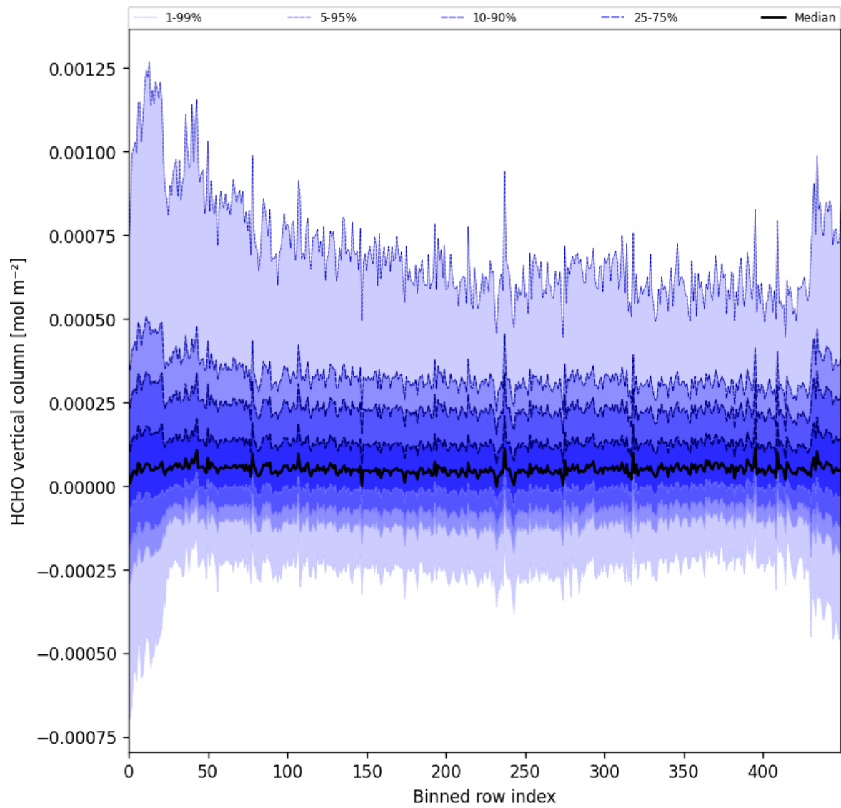
Figure 49: Along track statistics of “HCHO vertical column” for 2025-07-24 to 2025-07-26
