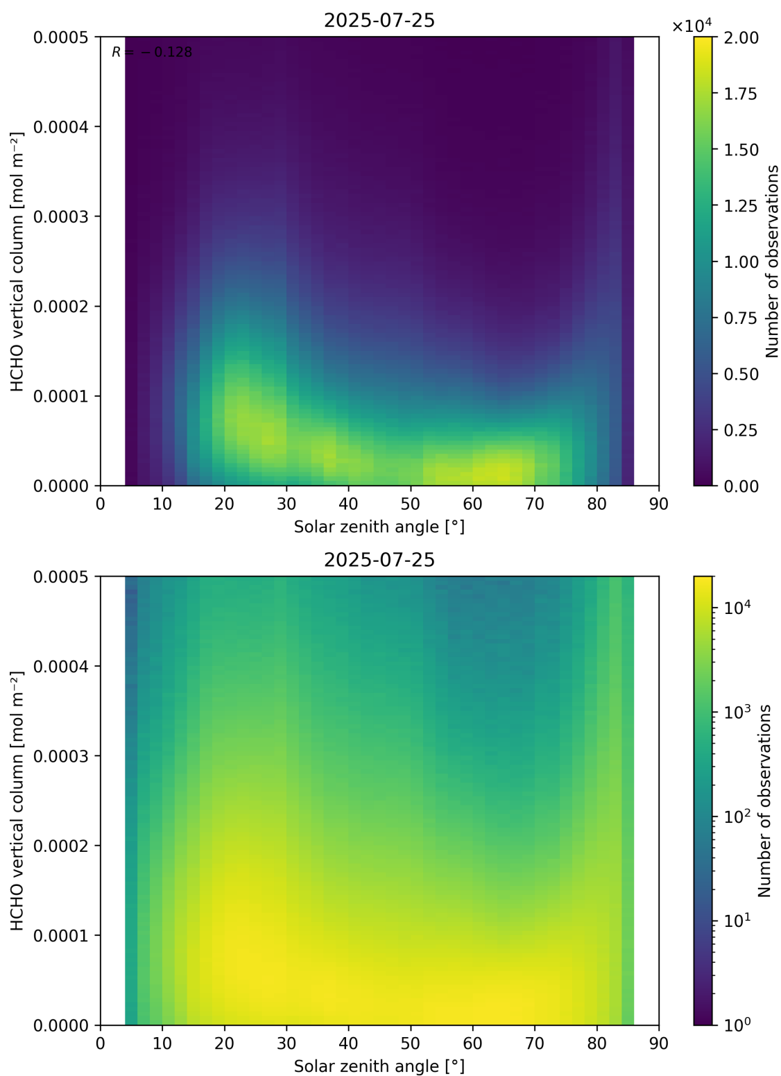
Figure 177: Scatter density plot of “Solar zenith angle” against “HCHO vertical column” for 2025-07-24 to 2025-07-26.
