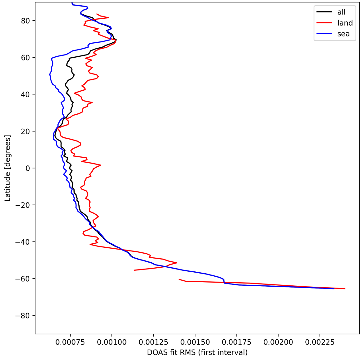
Figure 32: Zonal average of "DOAS fit RMS (first interval)" for 2025-07-24 to 2025-07-26.
