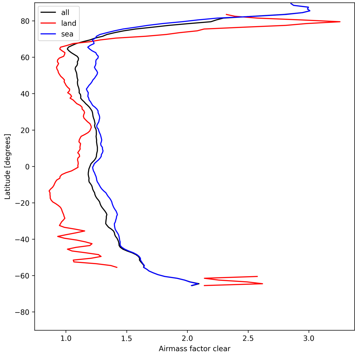
Figure 28: Zonal average of “Airmass factor clear” for 2025-07-24 to 2025-07-26.
