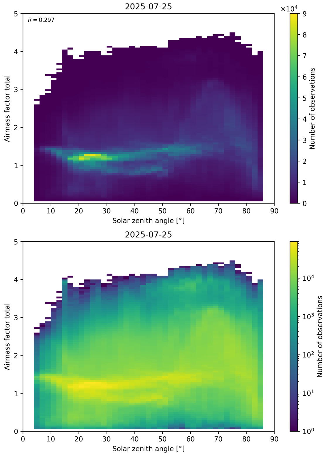
Figure 175: Scatter density plot of “Solar zenith angle” against “Airmass factor total” for 2025-07-24 to 2025-07-26.
