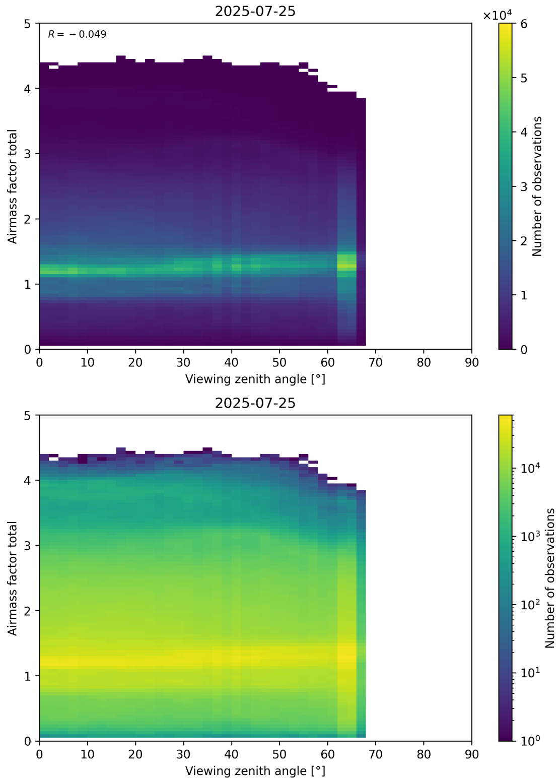
Figure 190: Scatter density plot of “Viewing zenith angle” against “Airmass factor total” for 2025-07-24 to 2025-07-26.
