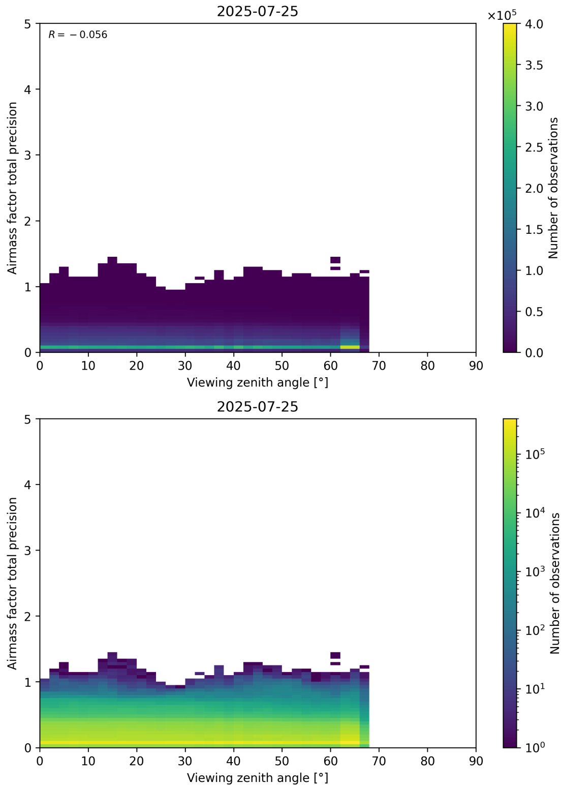
Figure 191: Scatter density plot of “Viewing zenith angle” against “Airmass factor total precision” for 2025-07-24 to 2025-07-26.
