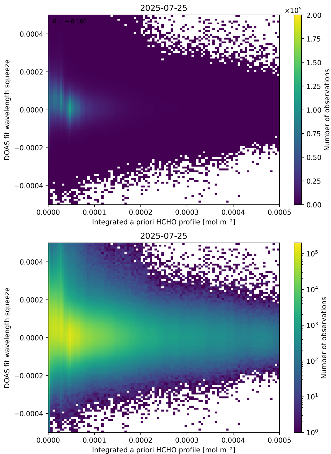
Figure 150: Scatter density plot of “Integrated a priori HCHO profile” against “DOAS fit wavelength squeeze” for 2025-07-24 to 2025-07-26.
