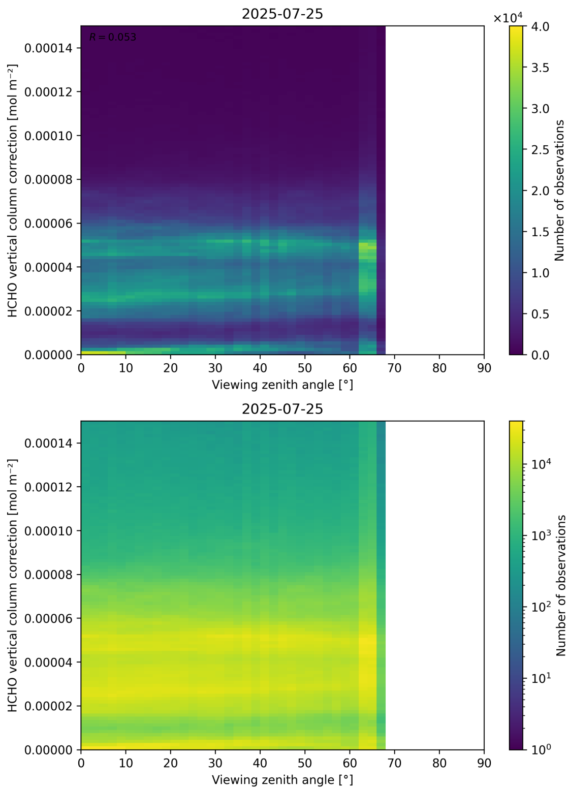
Figure 193: Scatter density plot of “Viewing zenith angle” against “HCHO vertical column correction” for 2025-07-24 to 2025-07-26.
