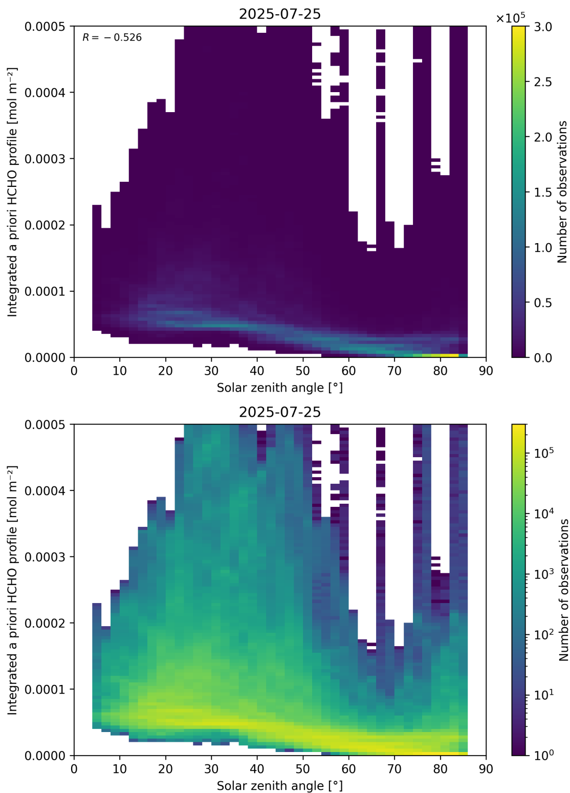
Figure 180: Scatter density plot of “Solar zenith angle” against “Integrated a priori HCHO profile” for 2025-07-24 to 2025-07-26.
