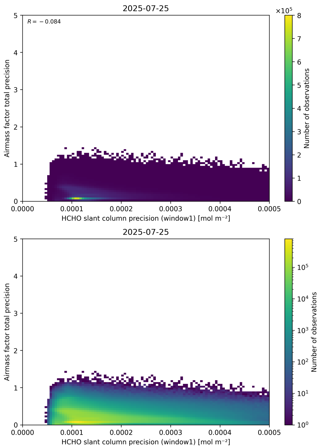
Figure 95: Scatter density plot of “HCHO slant column precision (window1)” against “Airmass factor total precision” for 2025-07-24 to 2025-07-26.
