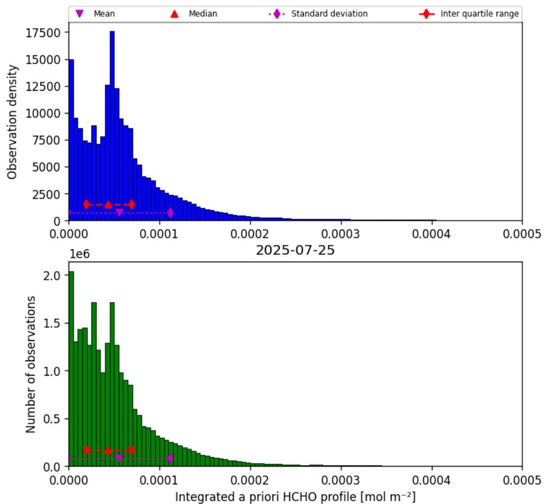
Figure 43: Histogram of “Integrated a priori HCHO profile” for 2025-07-24 to 2025-07-26
