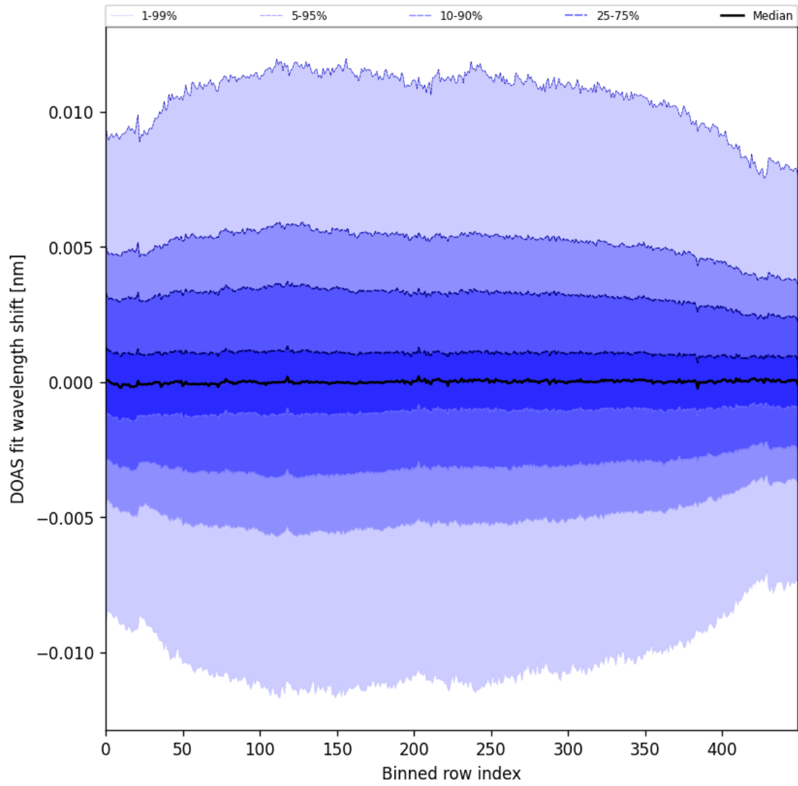
Figure 58: Along track statistics of “DOAS fit wavelength shift” for 2025-07-24 to 2025-07-26
