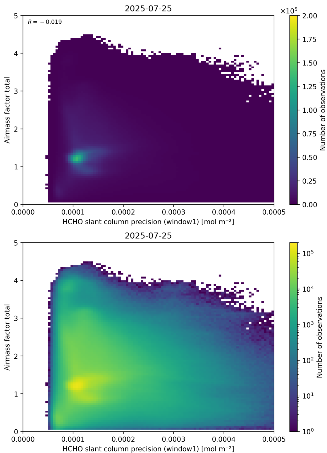
Figure 94: Scatter density plot of “HCHO slant column precision (window1)” against “Airmass factor total” for 2025-07-24 to 2025-07-26.
