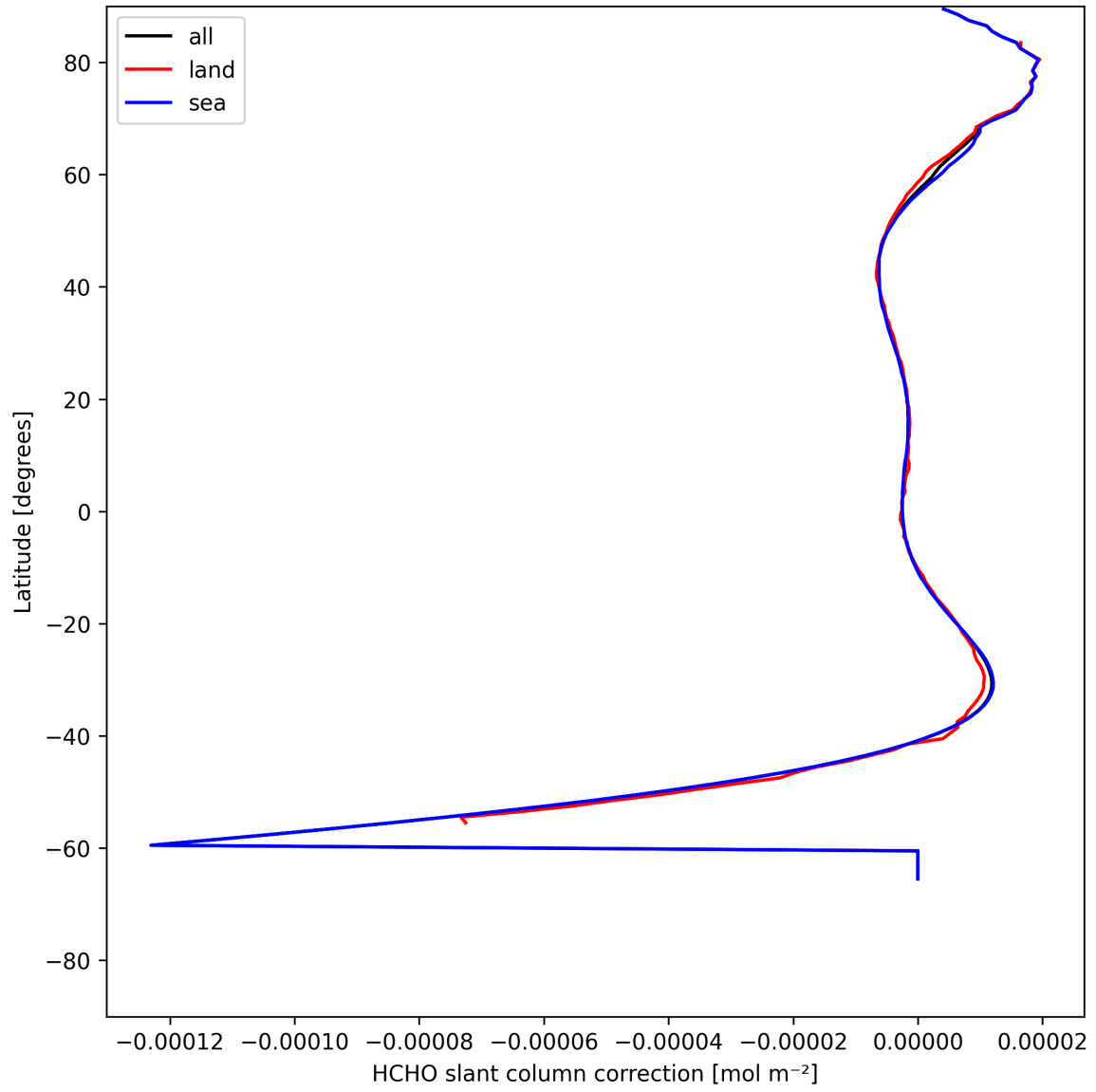
Figure 33: Zonal average of “HCHO slant column correction” for 2025-07-24 to 2025-07-26.
