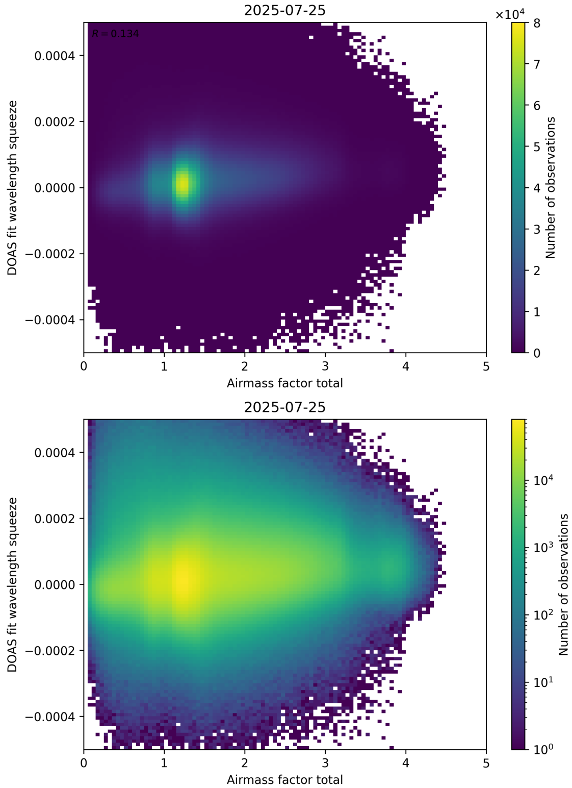
Figure 99: Scatter density plot of “Airmass factor total” against “DOAS fit wavelength squeeze” for 2025-07-24 to 2025-07-26.
