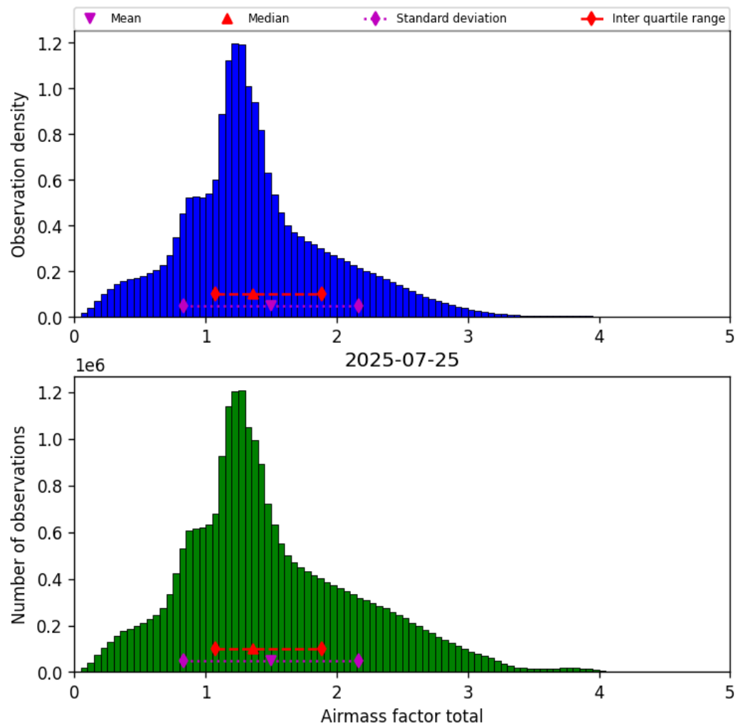
Figure 40: Histogram of “Airmass factor total” for 2025-07-24 to 2025-07-26
