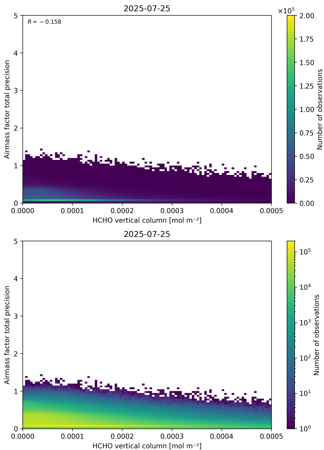
Figure 132: Scatter density plot of “HCHO vertical column” against “Airmass factor total precision” for 2025-07-24 to 2025-07-26.
