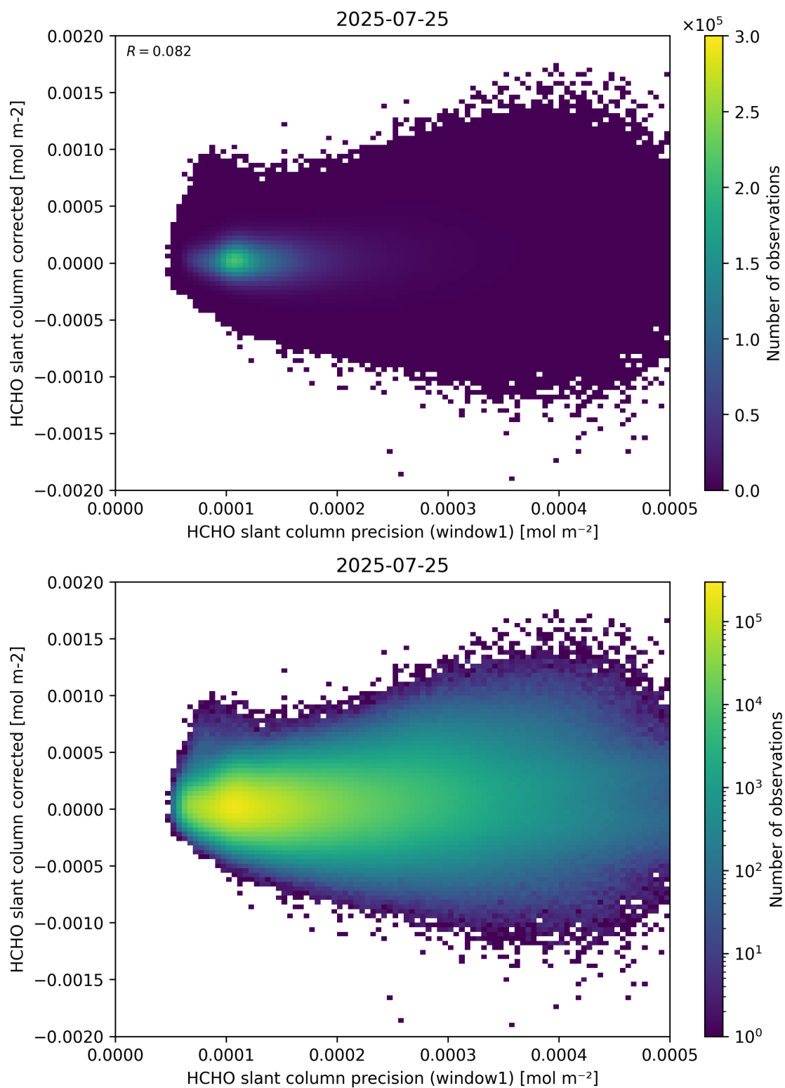
Figure 92: Scatter density plot of “HCHO slant column precision (window1)” against “HCHO slant column corrected” for 2025-07-24 to 2025-07-26.
