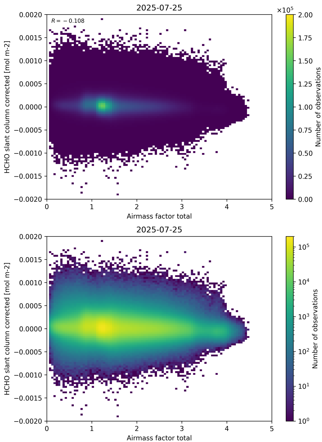
Figure 101: Scatter density plot of “Airmass factor total” against “HCHO slant column corrected” for 2025-07-24 to 2025-07-26.
