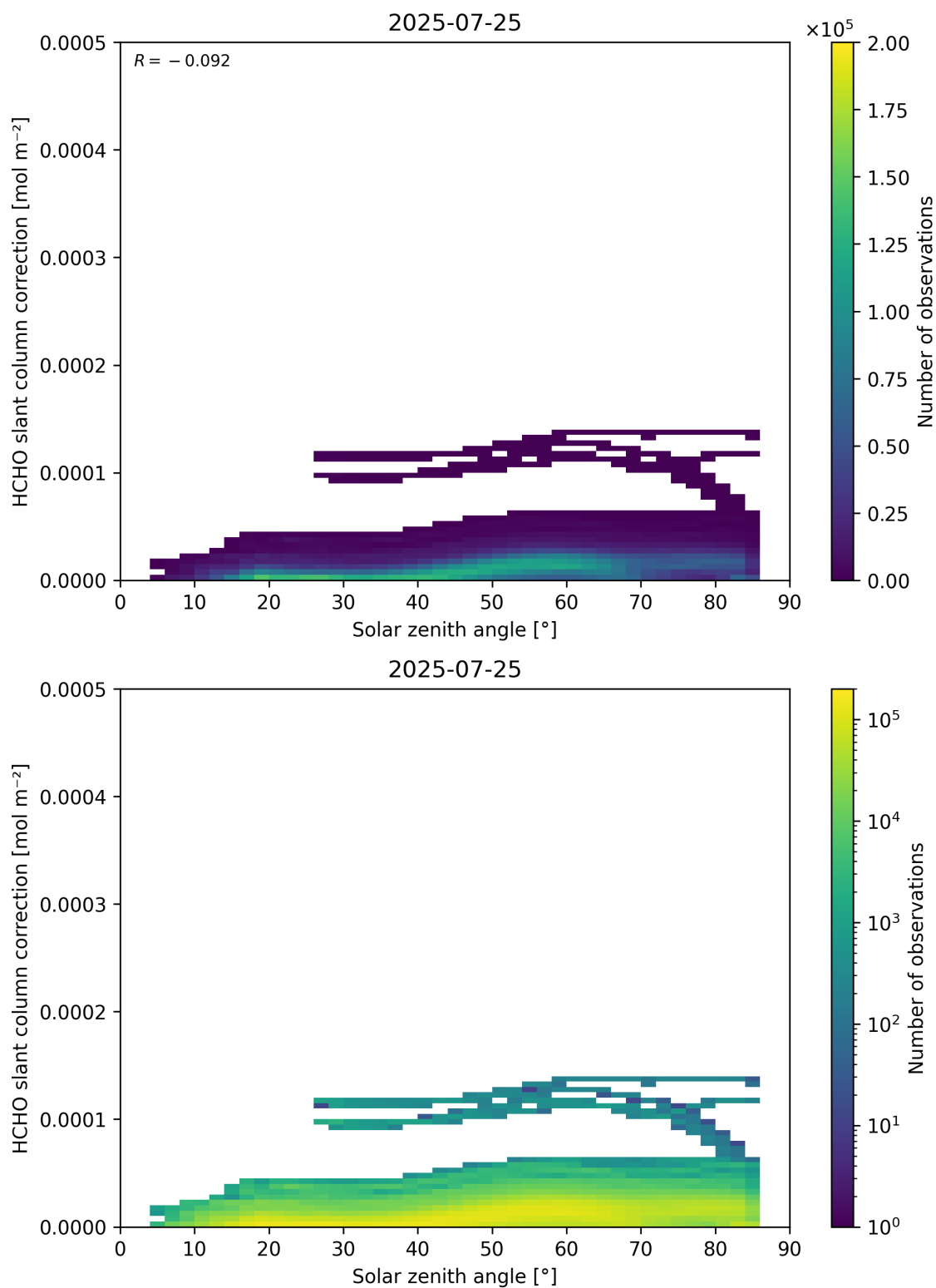
Figure 172: Scatter density plot of “Solar zenith angle” against “HCHO slant column correction” for 2025-07-24 to 2025-07-26.
