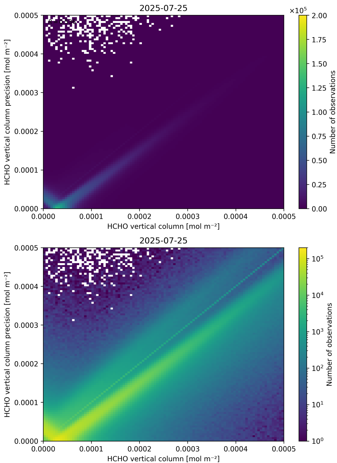
Figure 134: Scatter density plot of “HCHO vertical column” against “HCHO vertical column precision” for 2025-07-24 to 2025-07-26.
