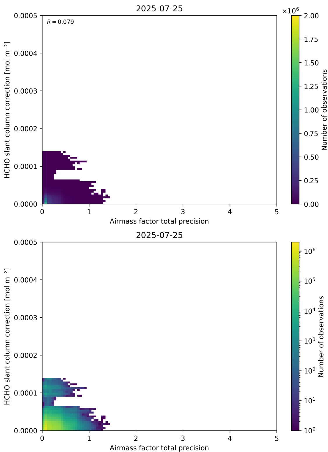
Figure 110: Scatter density plot of “Airmass factor total precision” against “HCHO slant column correction” for 2025-07-24 to 2025-07-26.
