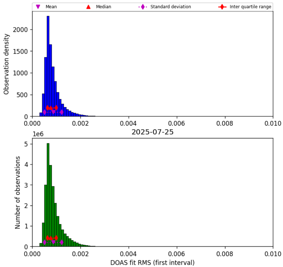
Figure 46: Histogram of “DOAS fit RMS (first interval)” for 2025-07-24 to 2025-07-26
