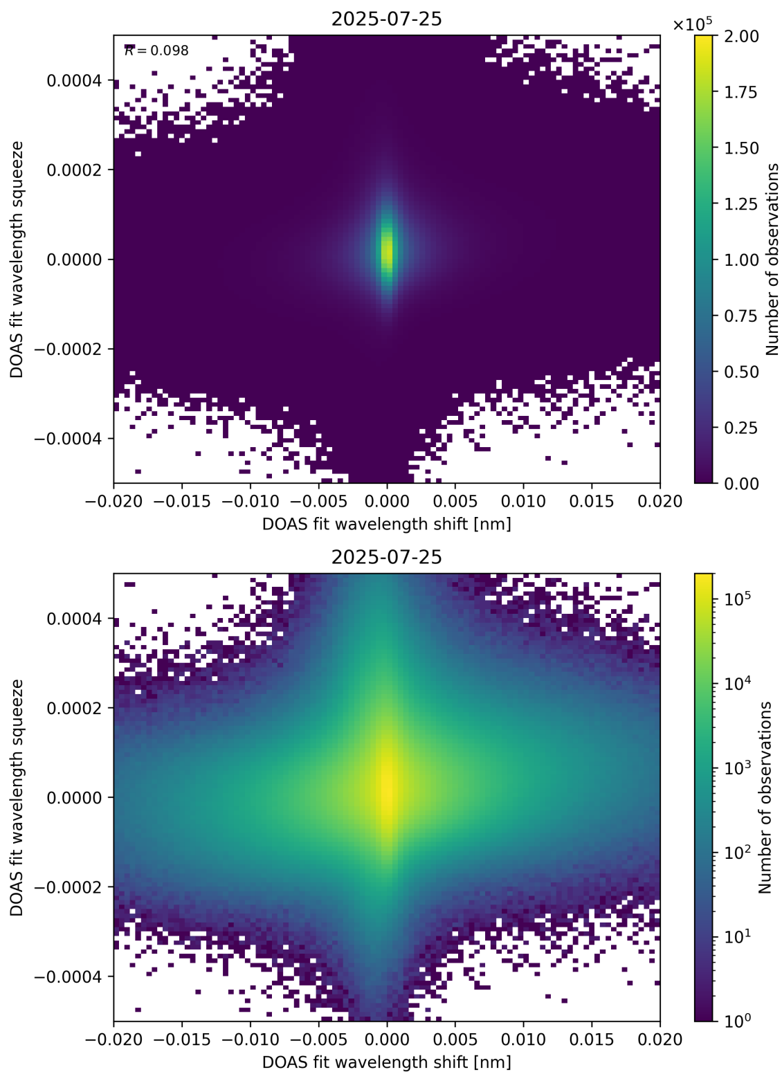
Figure 65: Scatter density plot of “DOAS fit wavelength shift” against “DOAS fit wavelength squeeze” for 2025-07-24 to 2025-07-26.
