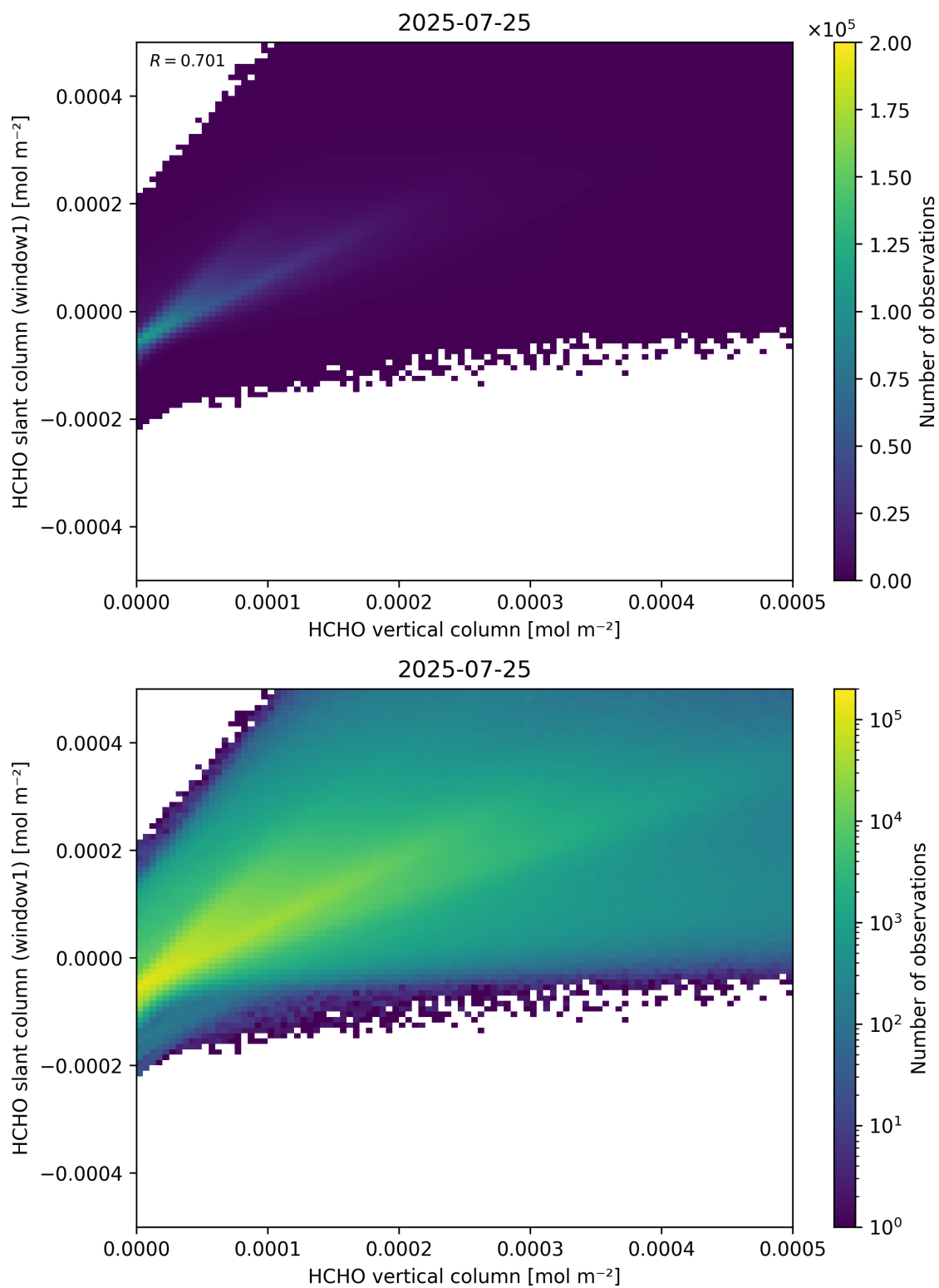
Figure 129: Scatter density plot of “HCHO vertical column” against “HCHO slant column (window1)” for 2025-07-24 to 2025-07-26.
