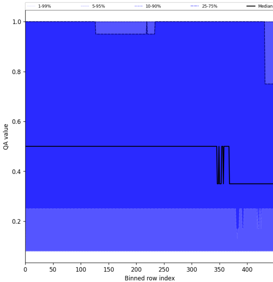
Figure 48: Along track statistics of “QA value” for 2025-07-24 to 2025-07-26
