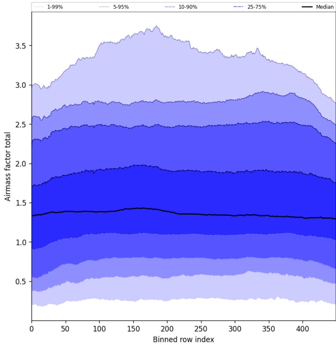
Figure 54: Along track statistics of “Airmass factor total” for 2025-07-24 to 2025-07-26
