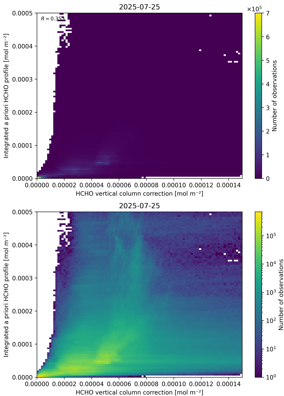
Figure 122: Scatter density plot of “HCHO vertical column correction” against “Integrated a priori HCHO profile” for 2025-07-24 to 2025-07-26.
