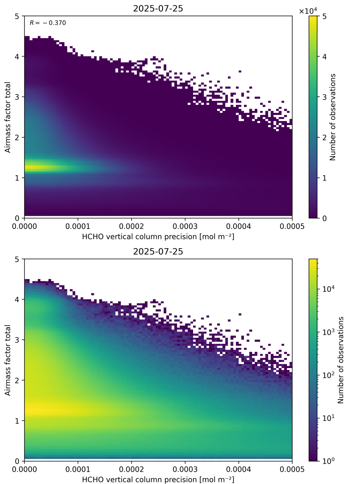
Figure 144: Scatter density plot of “HCHO vertical column precision” against “Airmass factor total” for 2025-07-24 to 2025-07-26.
