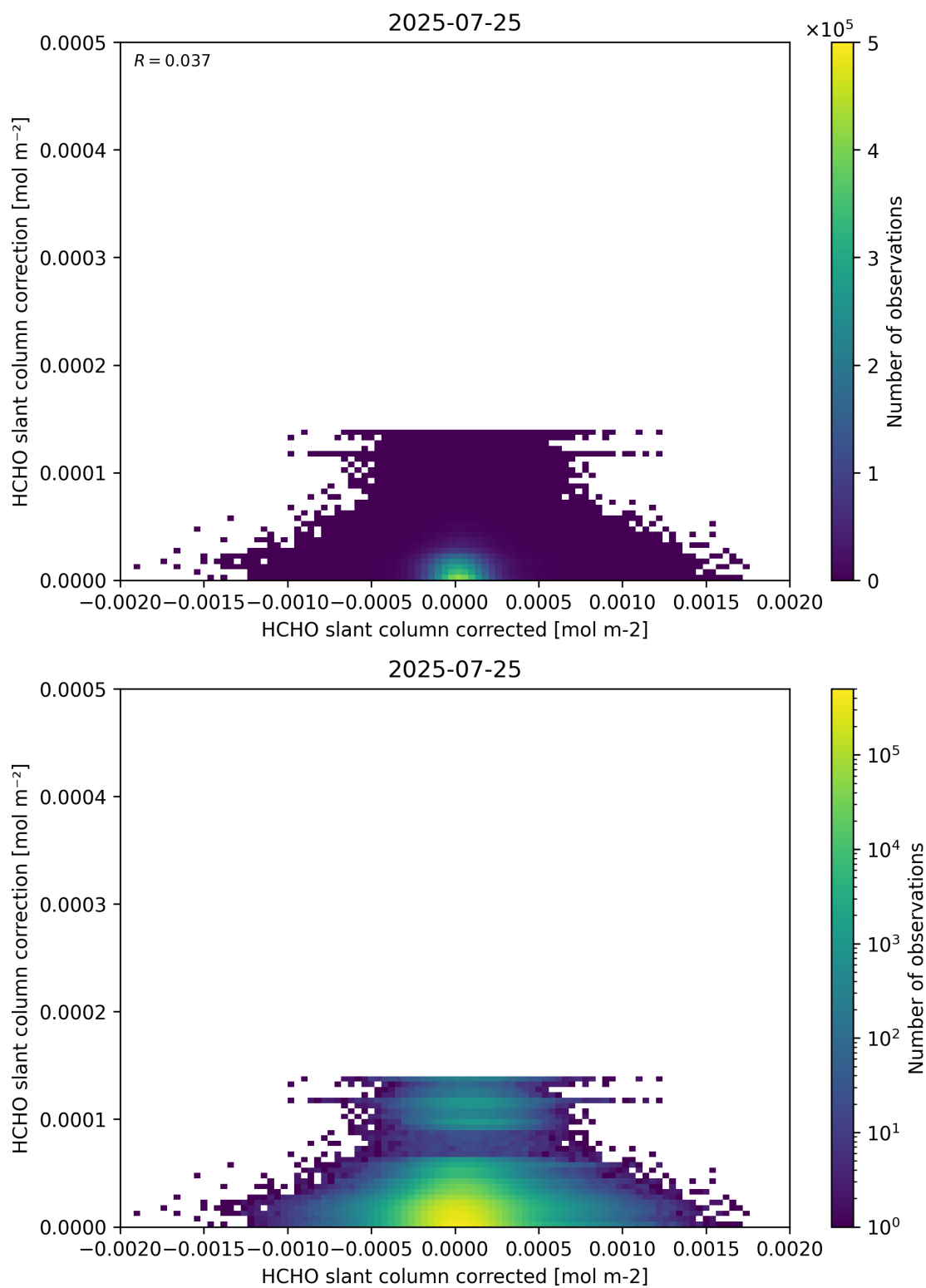
Figure 77: Scatter density plot of “HCHO slant column corrected” against “HCHO slant column correction” for 2025-07-24 to 2025-07-26.
