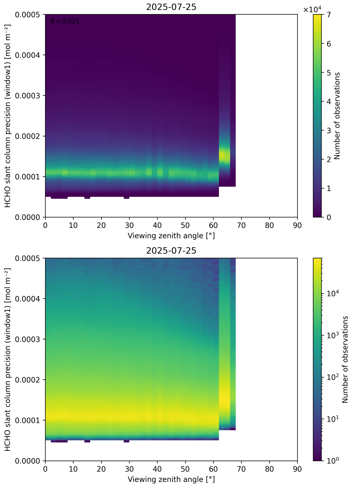
Figure 189: Scatter density plot of “Viewing zenith angle” against “HCHO slant column precision (window1)” for 2025-07-24 to 2025-07-26.
