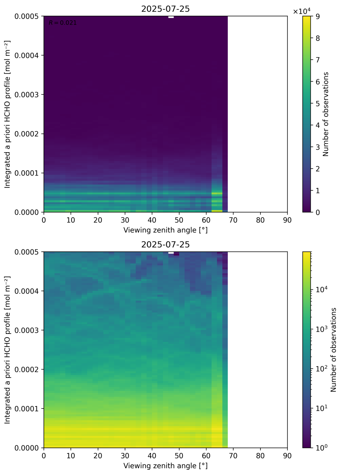
Figure 195: Scatter density plot of “Viewing zenith angle” against “Integrated a priori HCHO profile” for 2025-07-24 to 2025-07-26.
