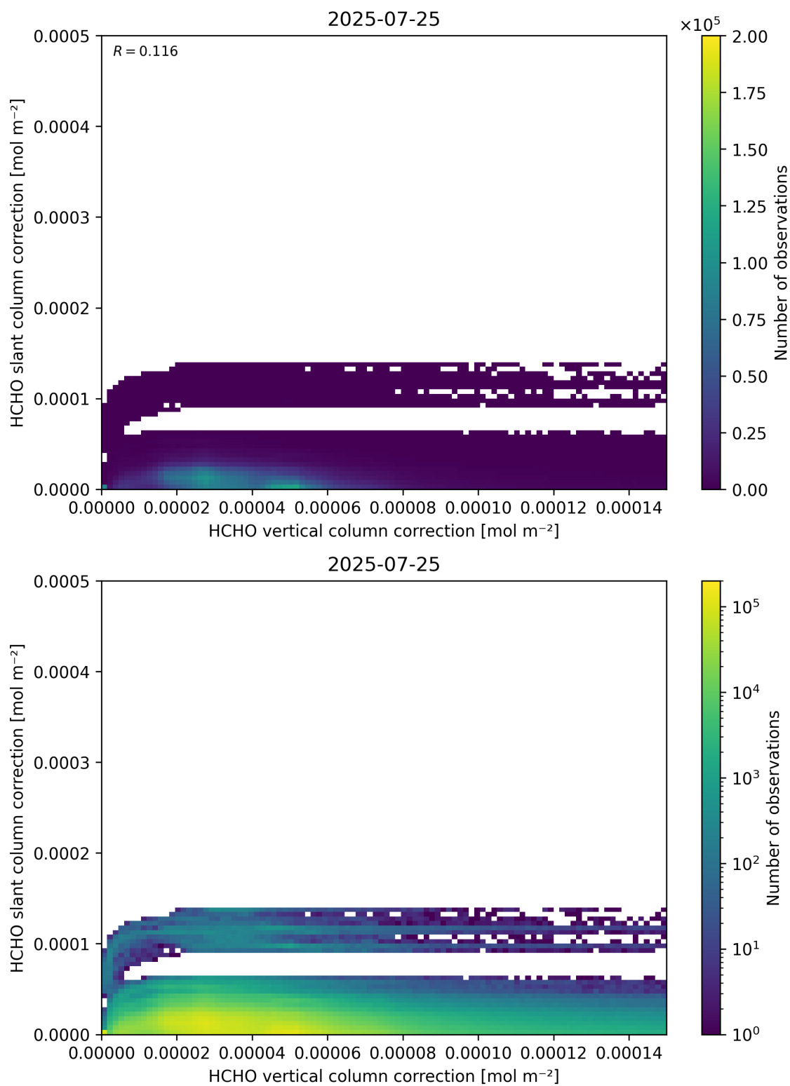
Figure 117: Scatter density plot of “HCHO vertical column correction” against “HCHO slant column correction” for 2025-07-24 to 2025-07-26.
