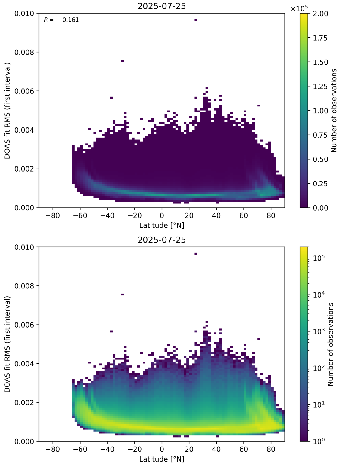
Figure 153: Scatter density plot of “Latitude” against “DOAS fit RMS (first interval)” for 2025-07-24 to 2025-07-26.
