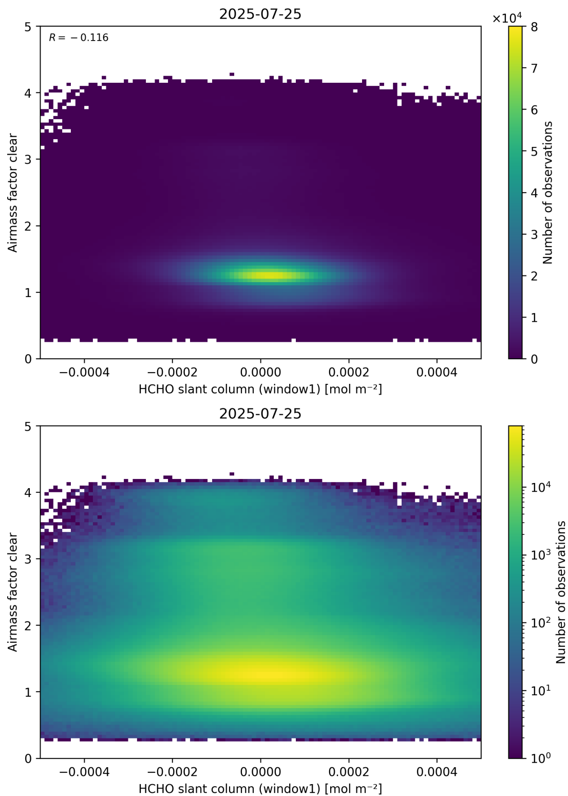
Figure 81: Scatter density plot of “HCHO slant column (window1)” against “Airmass factor clear” for 2025-07-24 to 2025-07-26.
