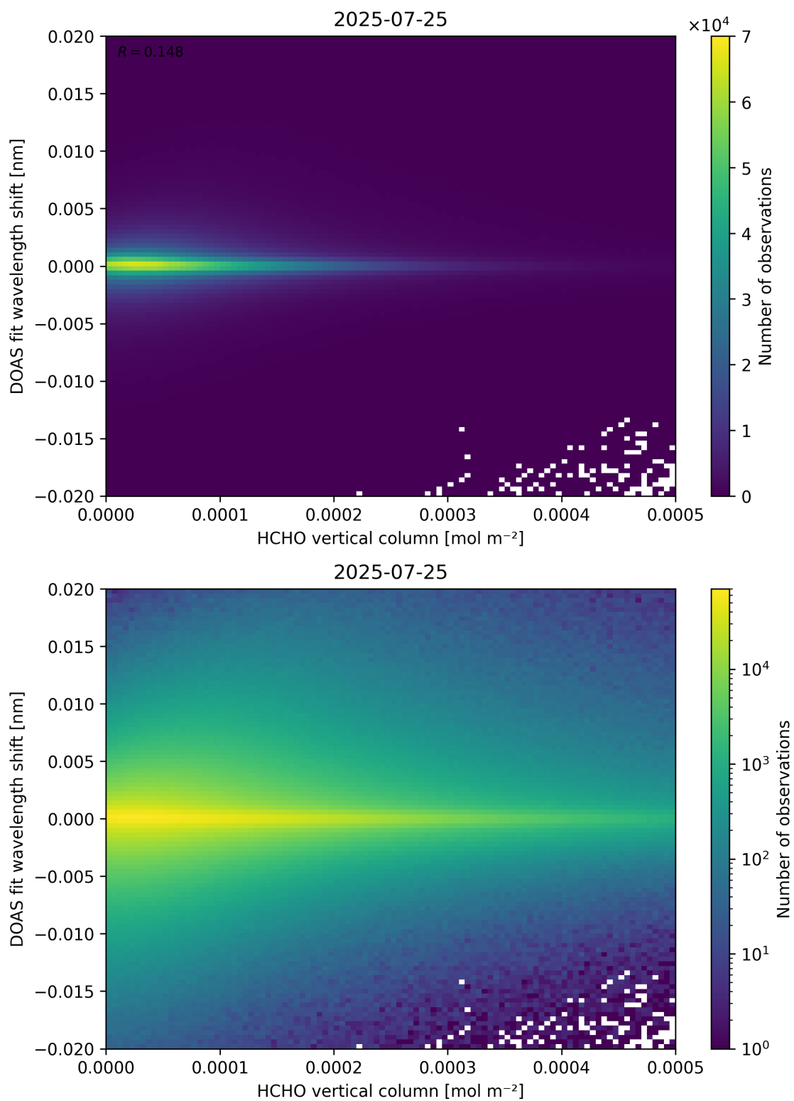
Figure 124: Scatter density plot of “HCHO vertical column” against “DOAS fit wavelength shift” for 2025-07-24 to 2025-07-26.
