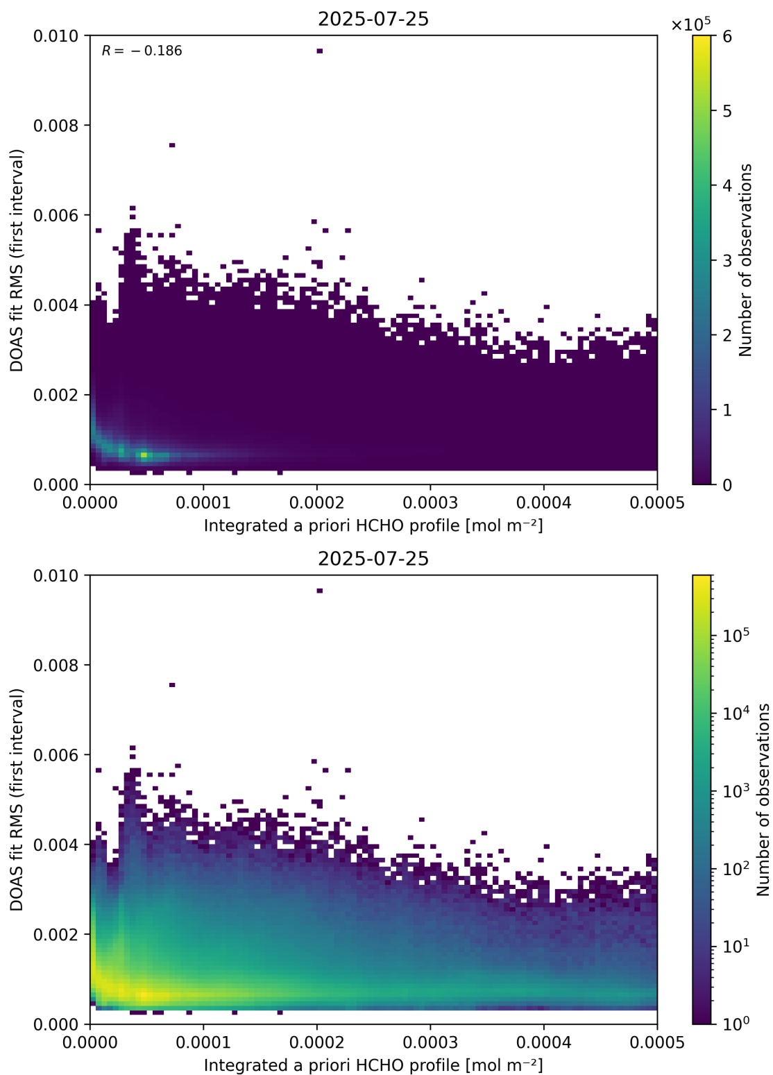
Figure 148: Scatter density plot of “Integrated a priori HCHO profile” against “DOAS fit RMS (first interval)” for 2025-07-24 to 2025-07-26.
