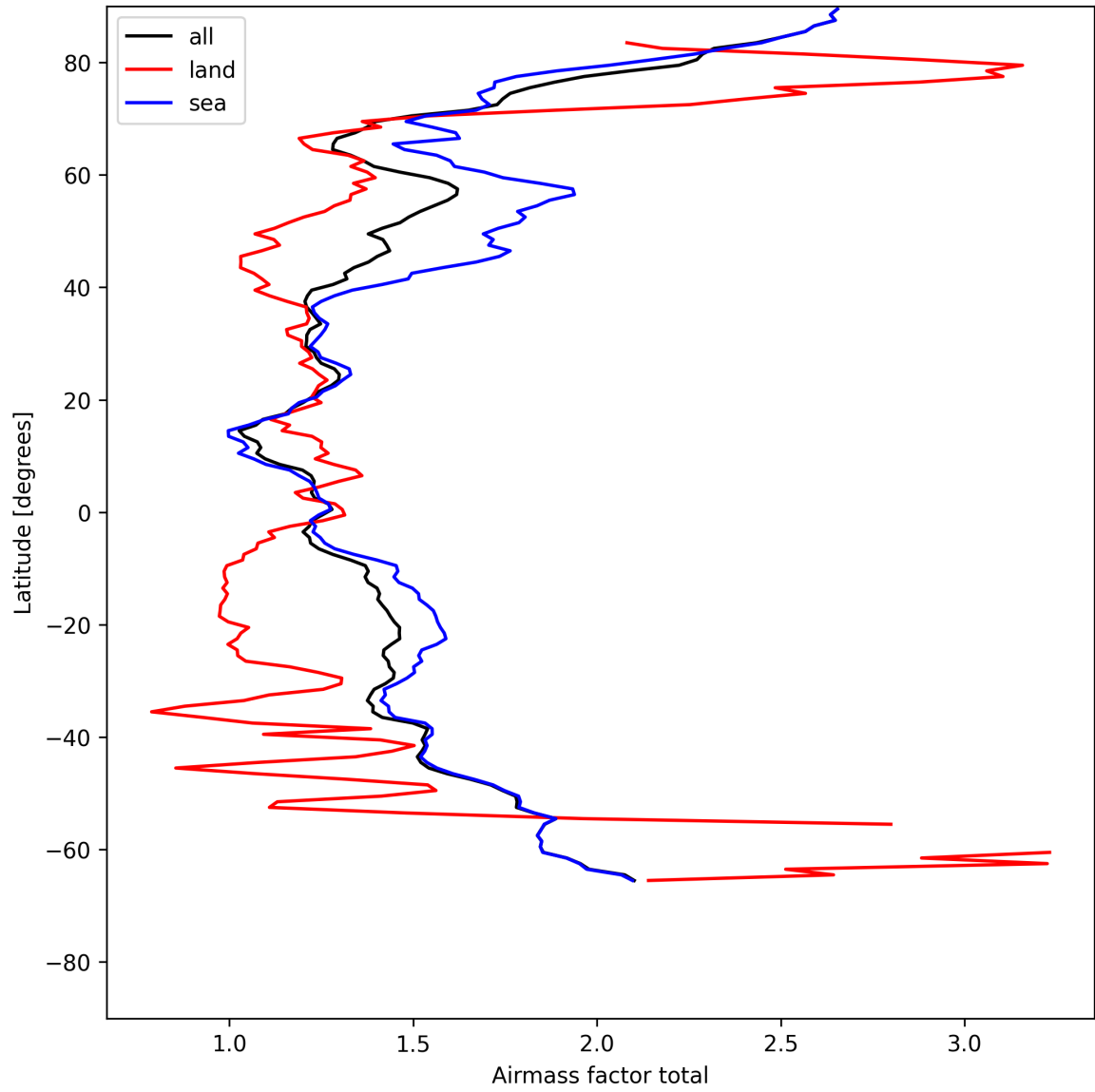
Figure 26: Zonal average of “Airmass factor total” for 2025-07-24 to 2025-07-26.
