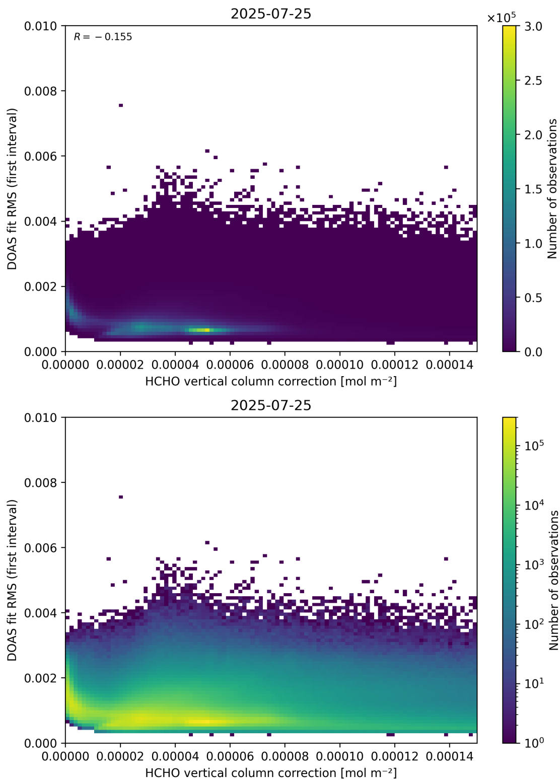
Figure 112: Scatter density plot of “HCHO vertical column correction” against “DOAS fit RMS (first interval)” for 2025-07-24 to 2025-07-26.
