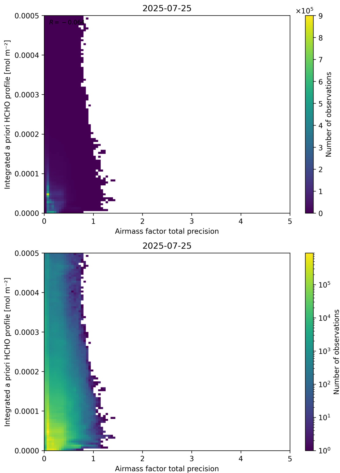
Figure 111: Scatter density plot of “Airmass factor total precision” against “Integrated a priori HCHO profile” for 2025-07-24 to 2025-07-26.
