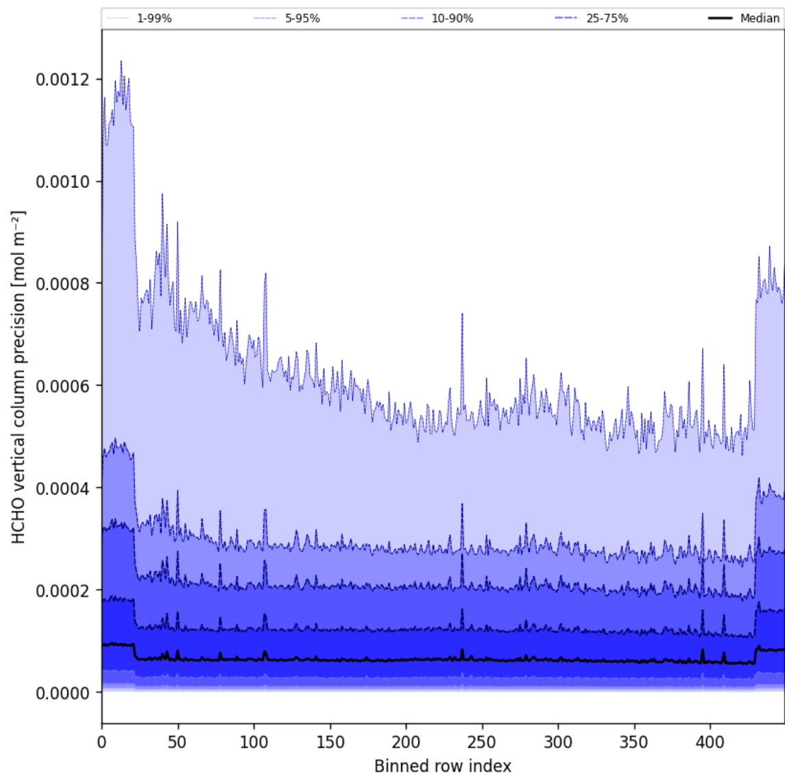
Figure 50: Along track statistics of “HCHO vertical column precision” for 2025-07-24 to 2025-07-26
