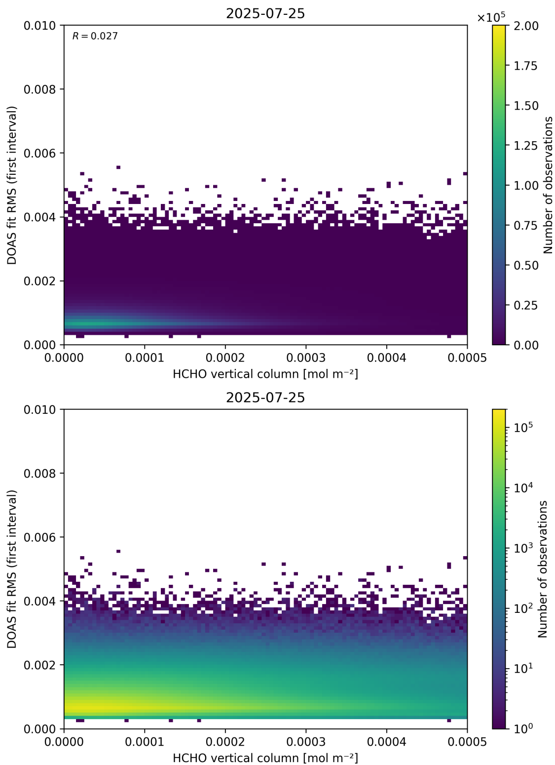
Figure 123: Scatter density plot of “HCHO vertical column” against “DOAS fit RMS (first interval)” for 2025-07-24 to 2025-07-26.
