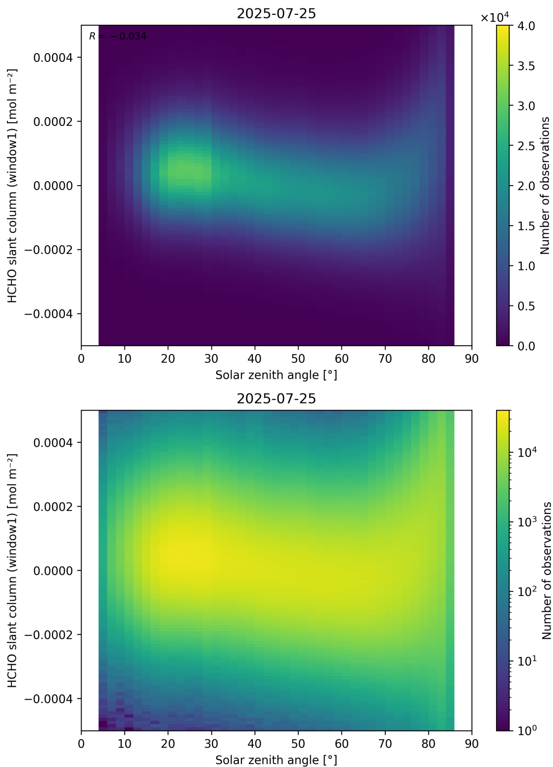
Figure 173: Scatter density plot of “Solar zenith angle” against “HCHO slant column (window1)” for 2025-07-24 to 2025-07-26.
