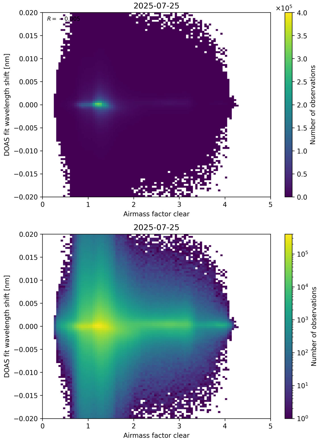
Figure 72: Scatter density plot of “Airmass factor clear” against “DOAS fit wavelength shift” for 2025-07-24 to 2025-07-26.
