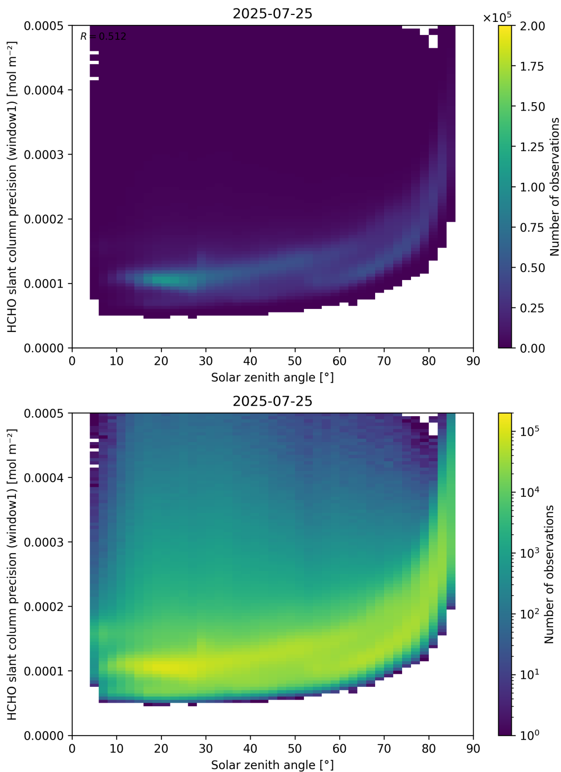
Figure 174: Scatter density plot of “Solar zenith angle” against “HCHO slant column precision (window1)” for 2025-07-24 to 2025-07-26.
