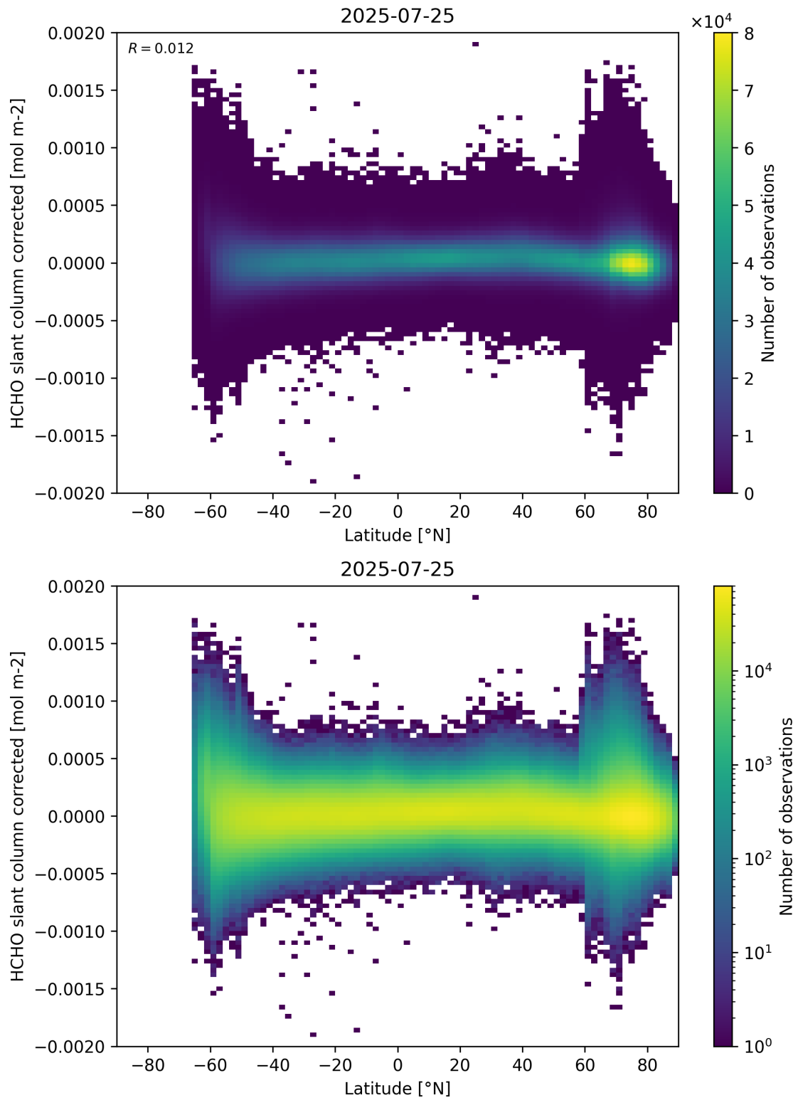
Figure 157: Scatter density plot of “Latitude” against “HCHO slant column corrected” for 2025-07-24 to 2025-07-26.
