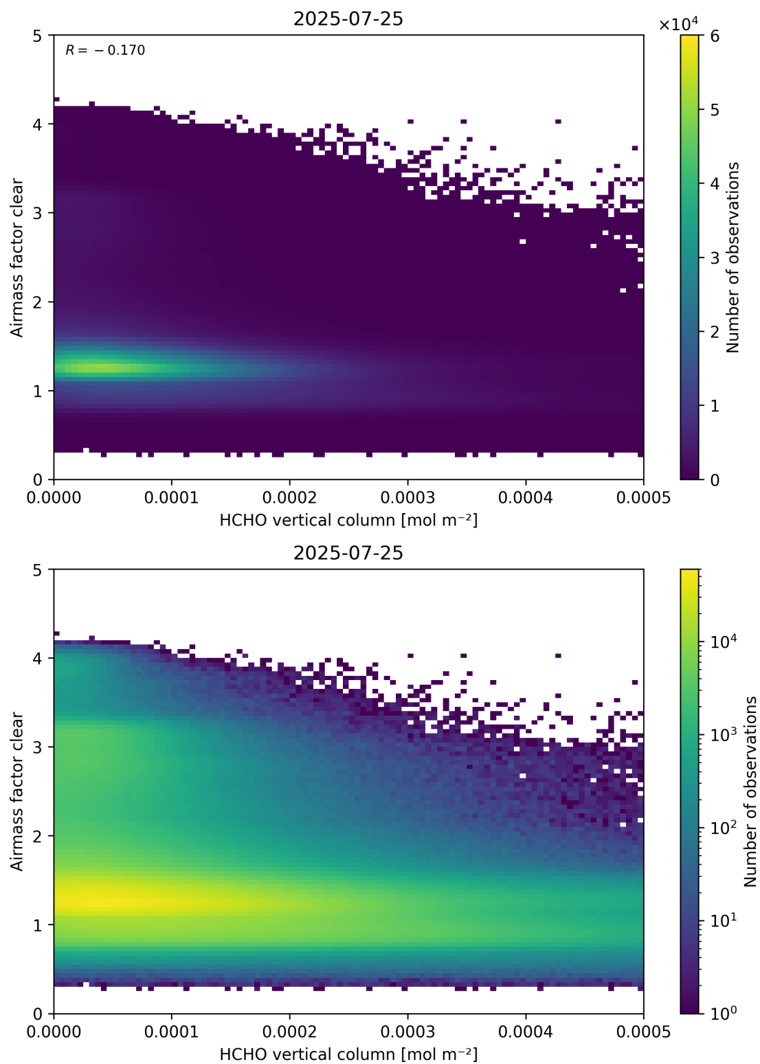
Figure 126: Scatter density plot of “HCHO vertical column” against “Airmass factor clear” for 2025-07-24 to 2025-07-26.
