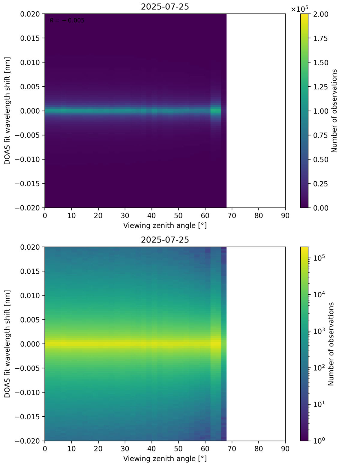
Figure 183: Scatter density plot of “Viewing zenith angle” against “DOAS fit wavelength shift” for 2025-07-24 to 2025-07-26.
