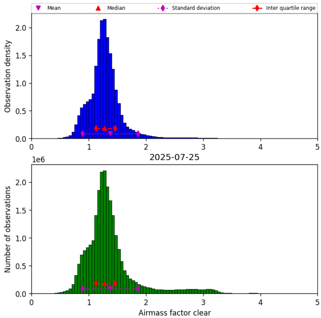
Figure 42: Histogram of “Airmass factor clear” for 2025-07-24 to 2025-07-26
