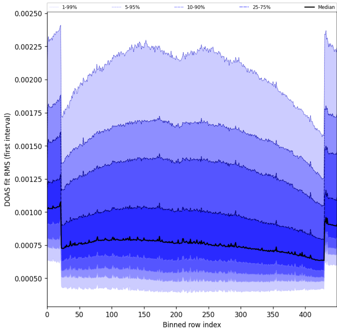
Figure 60: Along track statistics of “DOAS fit RMS (first interval)” for 2025-07-24 to 2025-07-26
