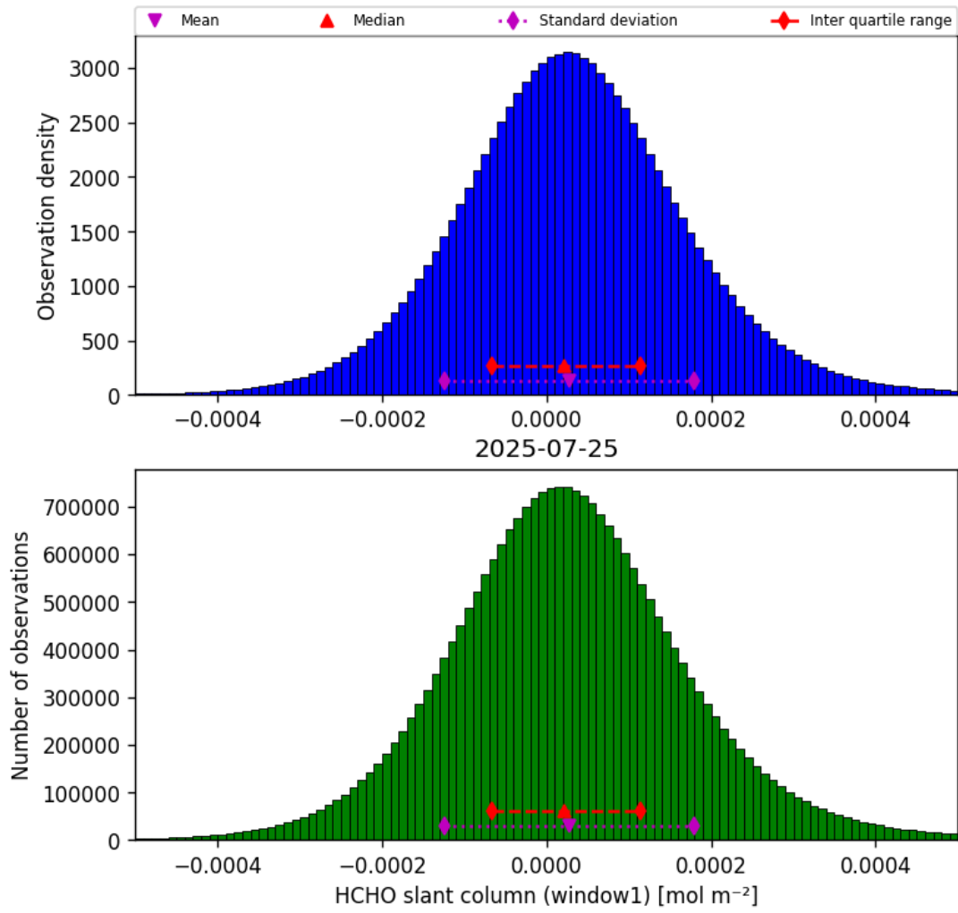
Figure 38: Histogram of “HCHO slant column (window1)” for 2025-07-24 to 2025-07-26
