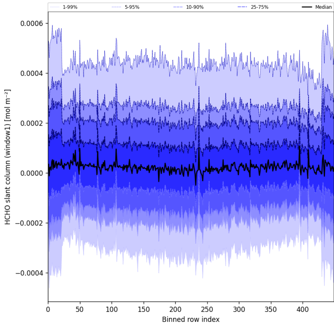
Figure 52: Along track statistics of “HCHO slant column (window1)” for 2025-07-24 to 2025-07-26
