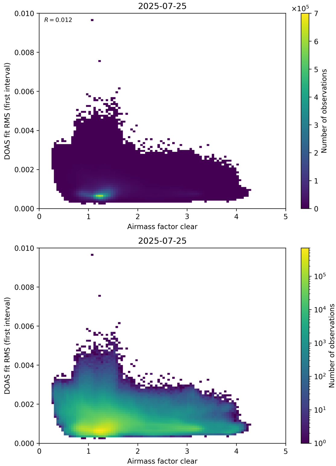
Figure 71: Scatter density plot of “Airmass factor clear” against “DOAS fit RMS (first interval)” for 2025-07-24 to 2025-07-26.
