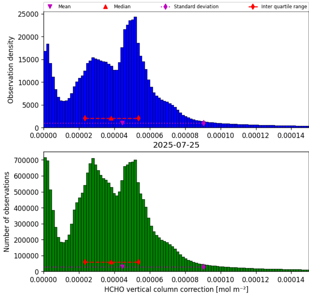
Figure 37: Histogram of “HCHO vertical column correction” for 2025-07-24 to 2025-07-26
