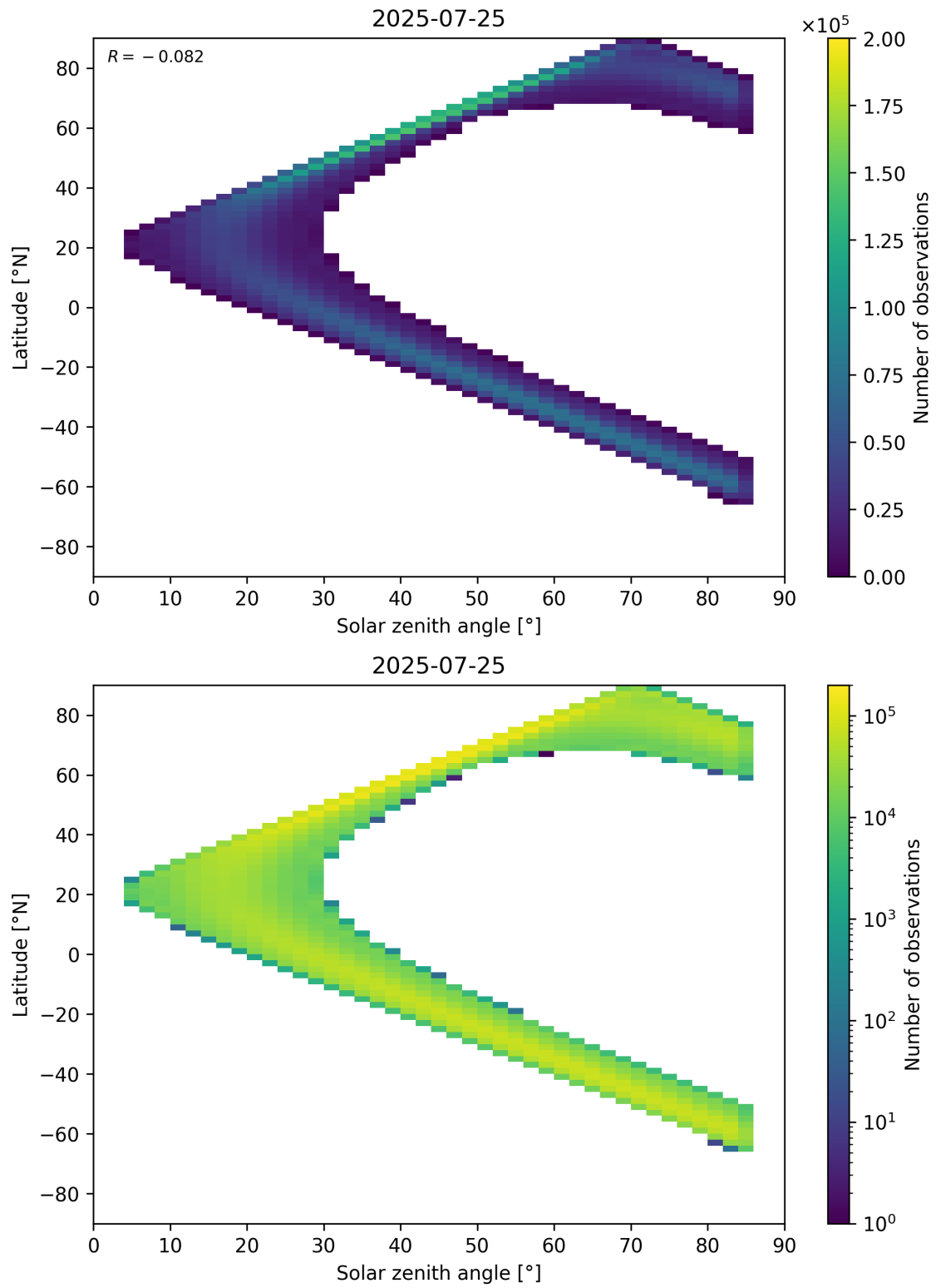
Figure 181: Scatter density plot of “Solar zenith angle” against “Latitude” for 2025-07-24 to 2025-07-26.
