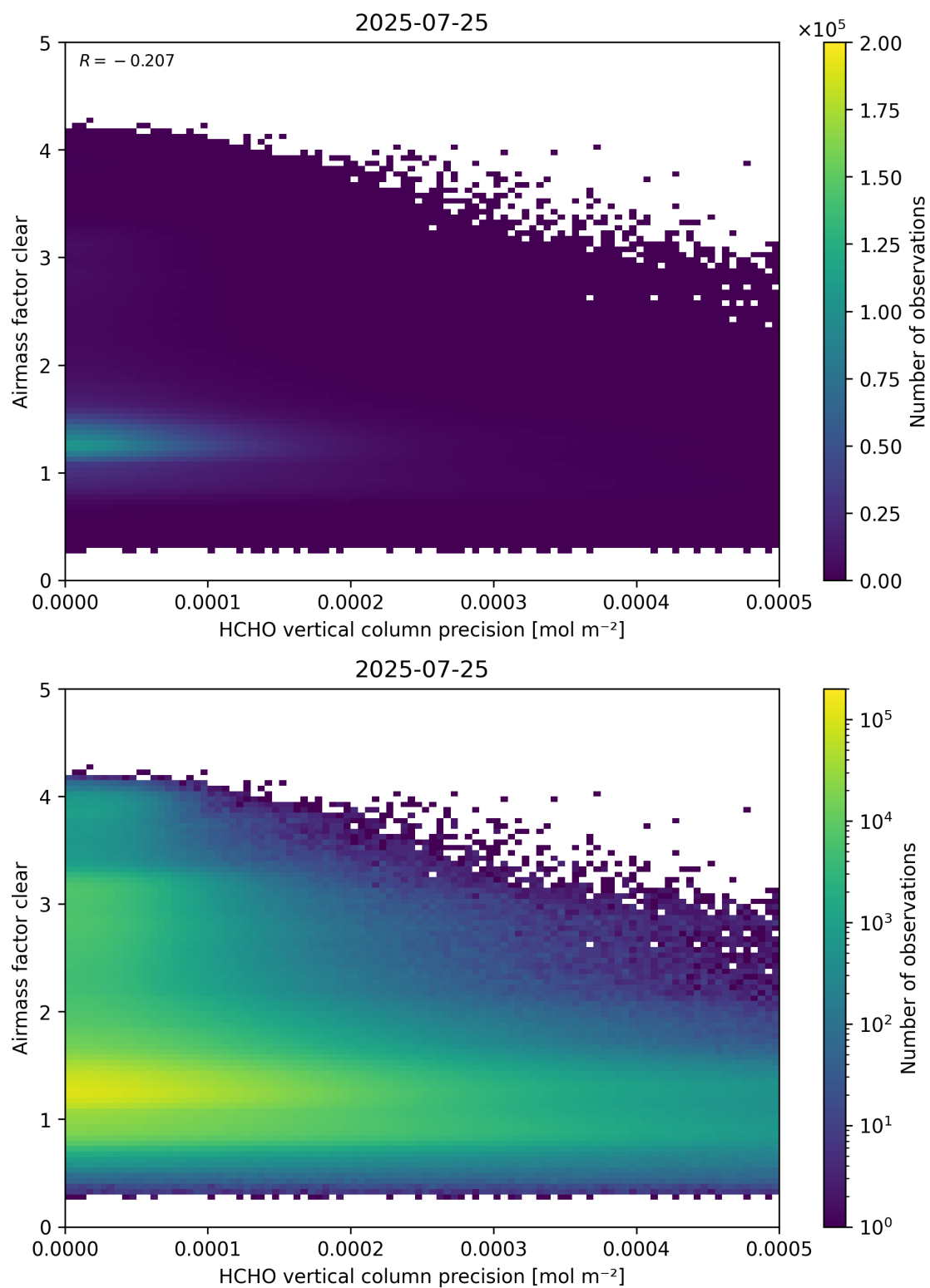
Figure 139: Scatter density plot of “HCHO vertical column precision” against “Airmass factor clear” for 2025-07-24 to 2025-07-26.
