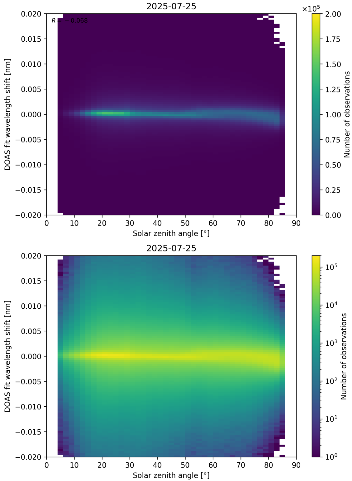
Figure 168: Scatter density plot of “Solar zenith angle” against “DOAS fit wavelength shift” for 2025-07-24 to 2025-07-26.
