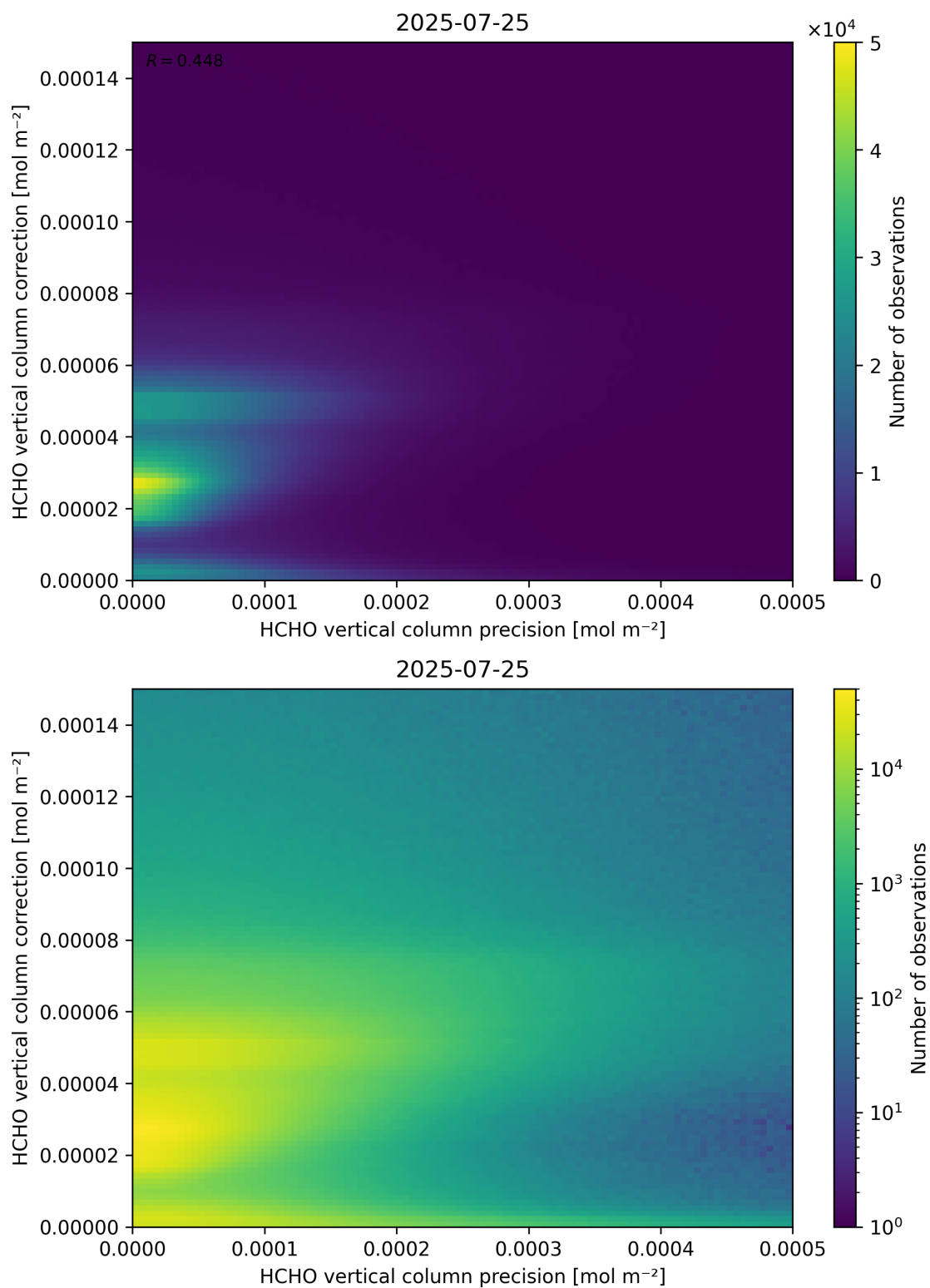
Figure 146: Scatter density plot of “HCHO vertical column precision” against “HCHO vertical column correction” for 2025-07-24 to 2025-07-26.
