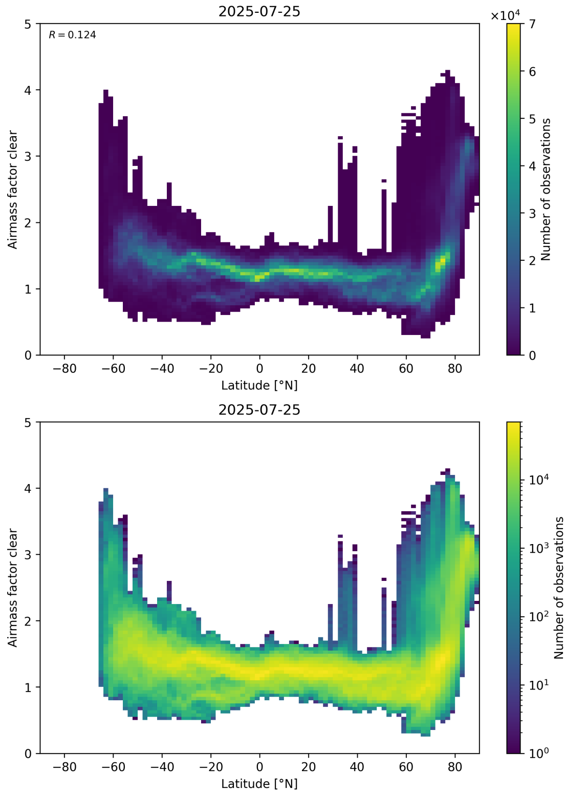
Figure 156: Scatter density plot of “Latitude” against “Airmass factor clear” for 2025-07-24 to 2025-07-26.
