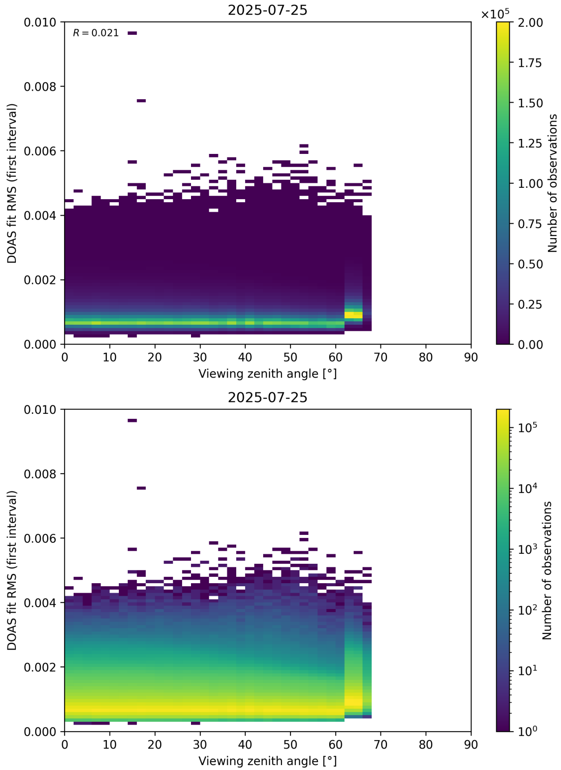
Figure 182: Scatter density plot of “Viewing zenith angle” against “DOAS fit RMS (first interval)” for 2025-07-24 to 2025-07-26.
