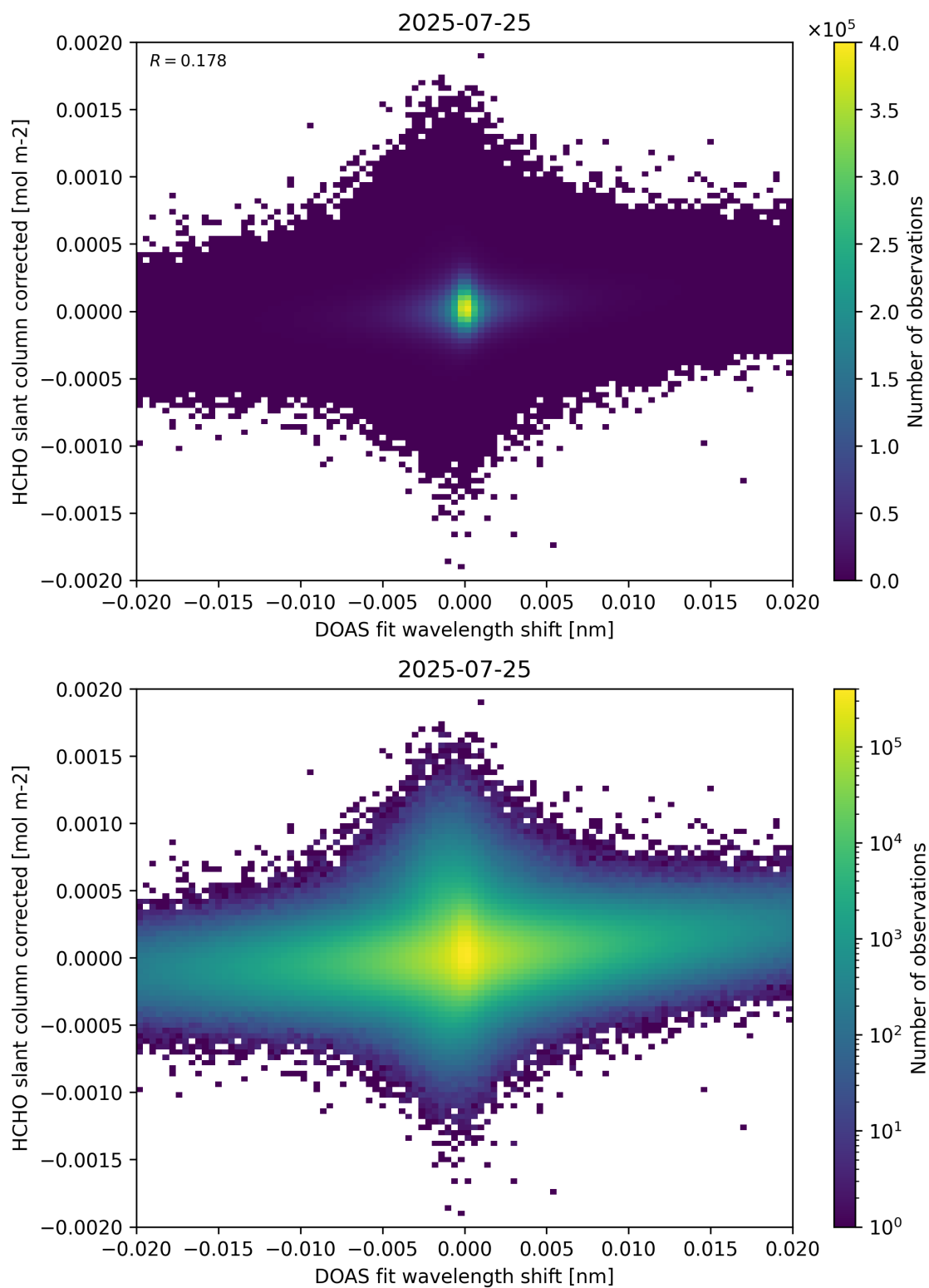
Figure 66: Scatter density plot of “DOAS fit wavelength shift” against “HCHO slant column corrected” for 2025-07-24 to 2025-07-26.
