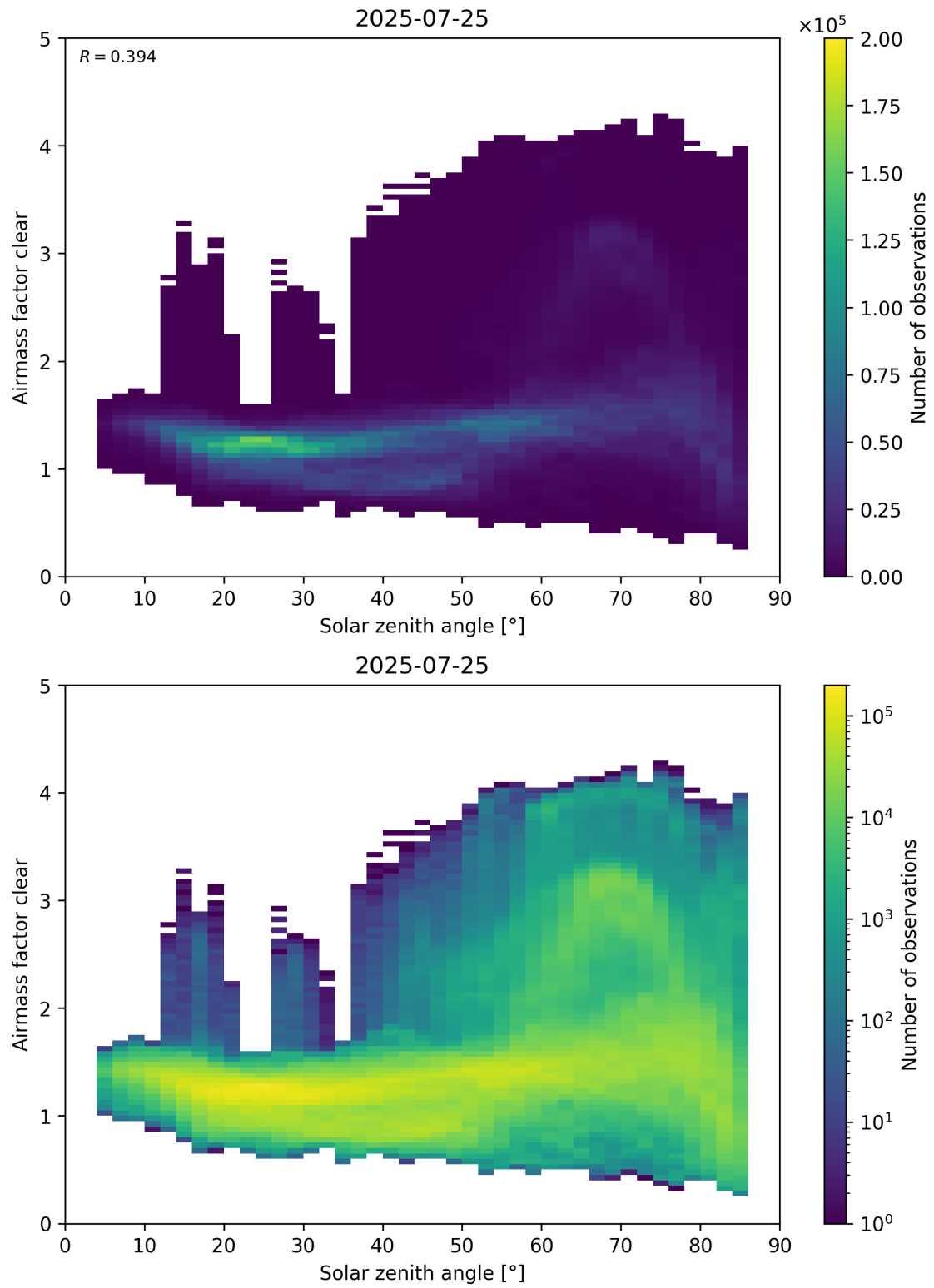
Figure 170: Scatter density plot of “Solar zenith angle” against “Airmass factor clear” for 2025-07-24 to 2025-07-26.
