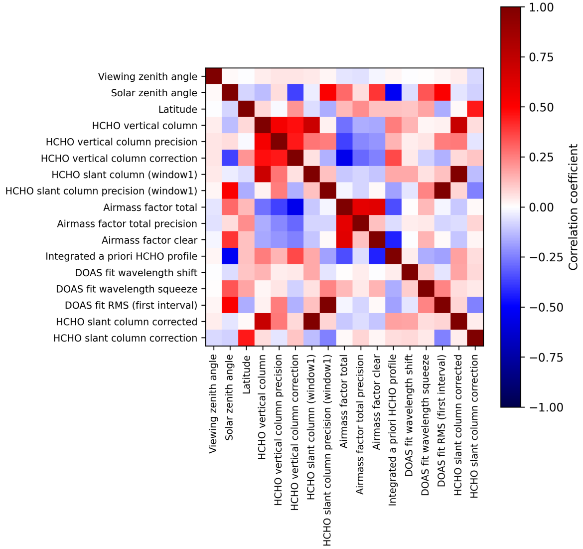
Figure 2: Map of correlation matrix for 2025-07-24 to 2025-07-26.
