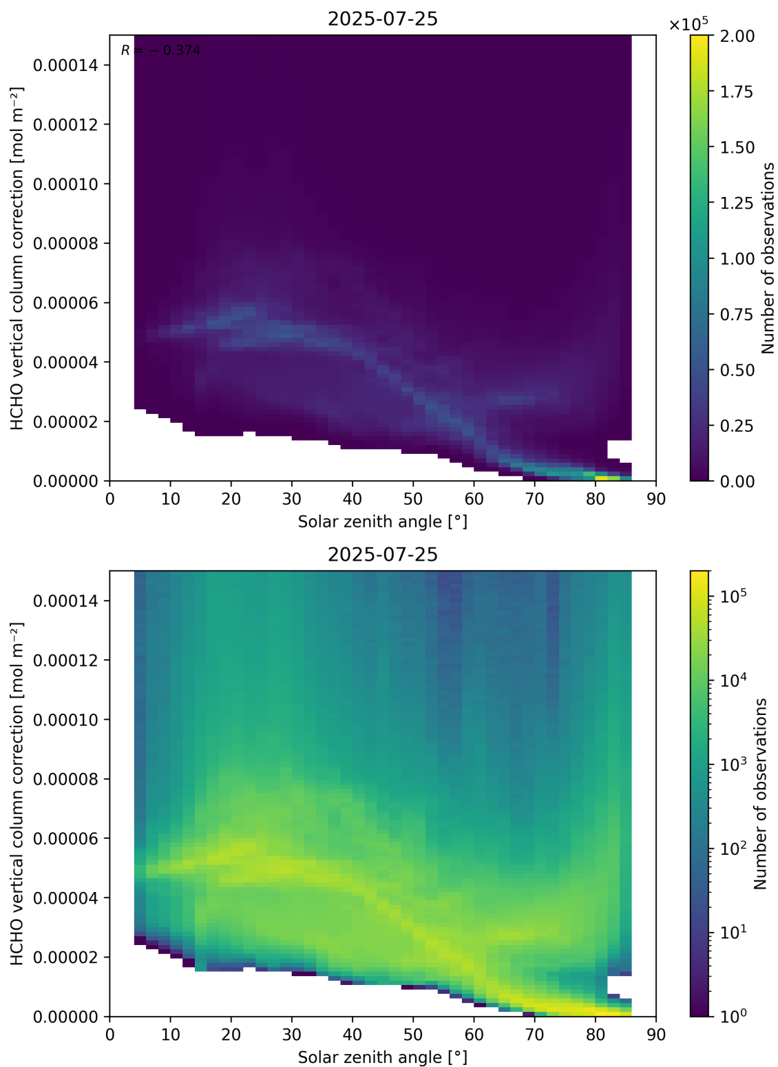
Figure 178: Scatter density plot of “Solar zenith angle” against “HCHO vertical column correction” for 2025-07-24 to 2025-07-26.
