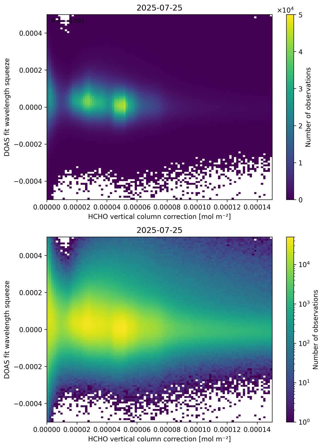
Figure 114: Scatter density plot of “HCHO vertical column correction” against “DOAS fit wavelength squeeze” for 2025-07-24 to 2025-07-26.
