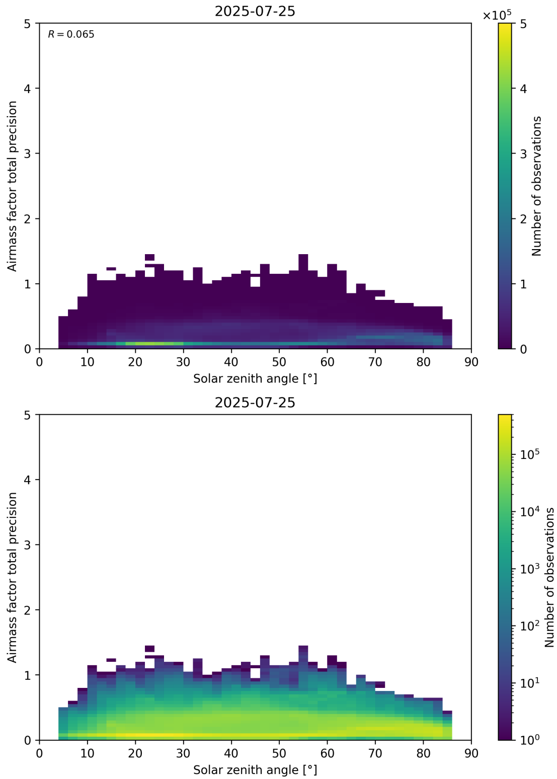
Figure 176: Scatter density plot of “Solar zenith angle” against “Airmass factor total precision” for 2025-07-24 to 2025-07-26.
