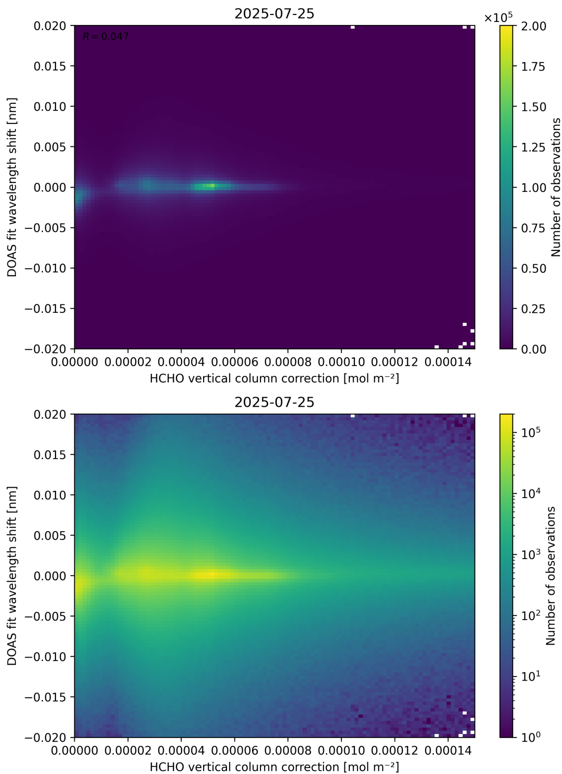
Figure 113: Scatter density plot of “HCHO vertical column correction” against “DOAS fit wavelength shift” for 2025-07-24 to 2025-07-26.
