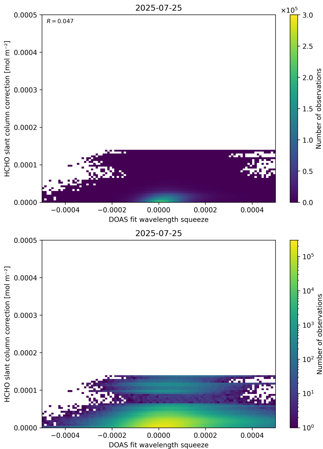
Figure 70: Scatter density plot of “DOAS fit wavelength squeeze” against “HCHO slant column correction” for 2025-07-24 to 2025-07-26.
