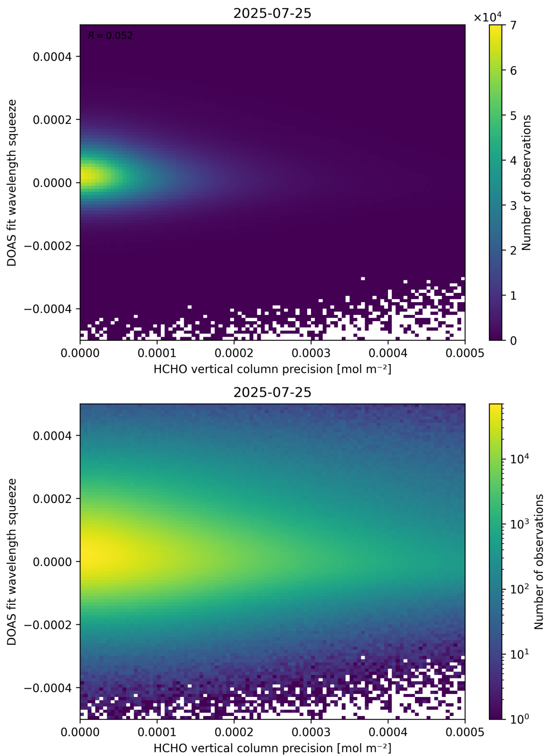
Figure 138: Scatter density plot of “HCHO vertical column precision” against “DOAS fit wavelength squeeze” for 2025-07-24 to 2025-07-26.
