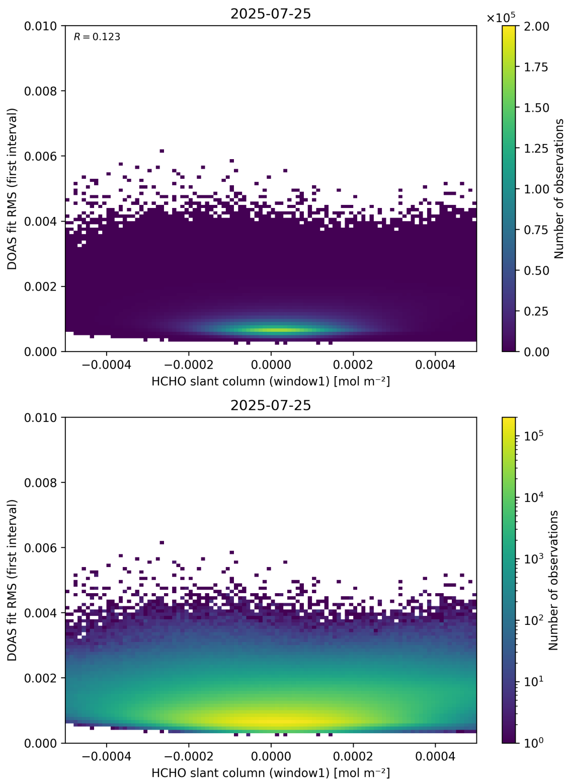
Figure 78: Scatter density plot of “HCHO slant column (window1)” against “DOAS fit RMS (first interval)” for 2025-07-24 to 2025-07-26.
