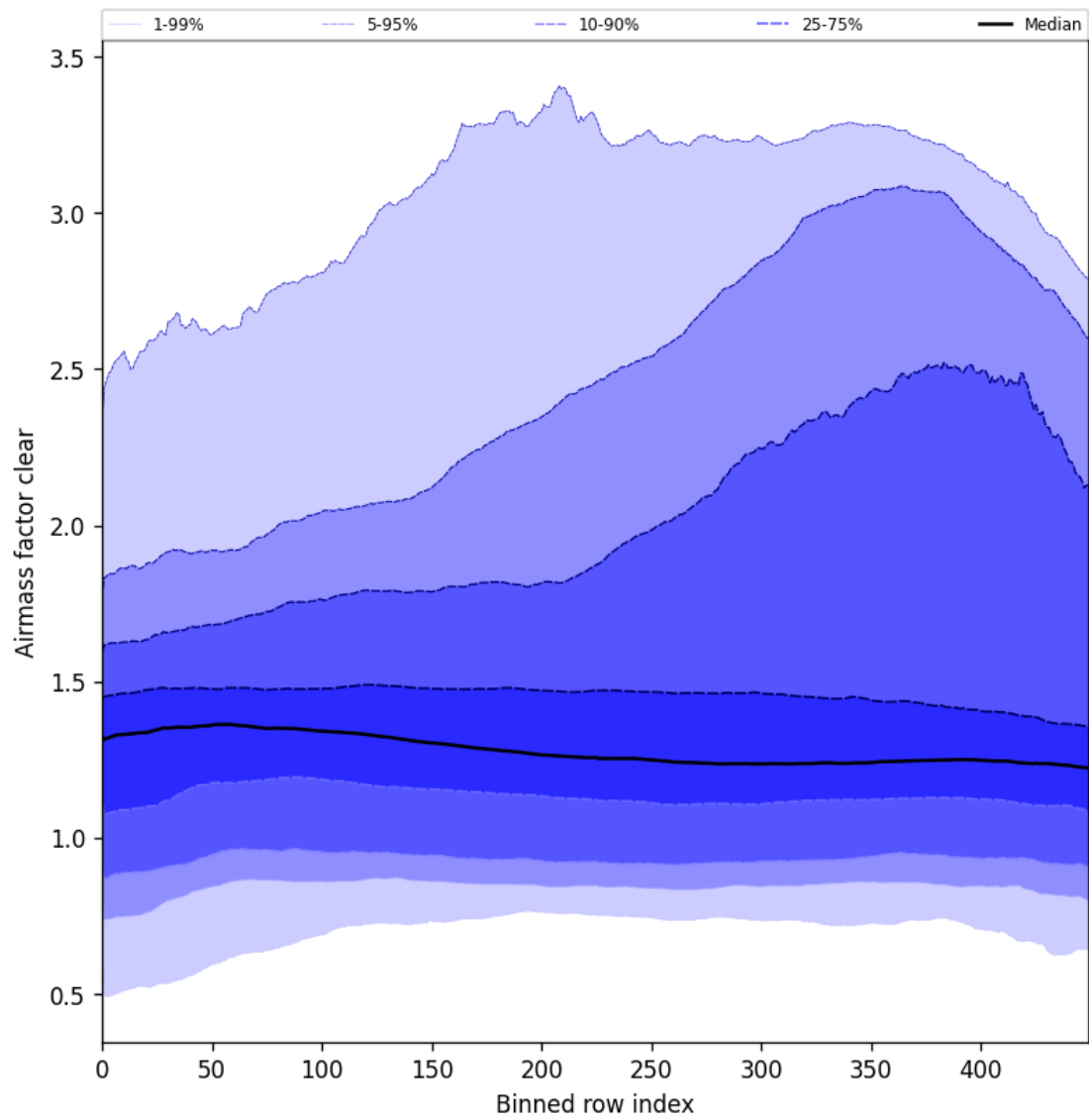
Figure 56: Along track statistics of “Airmass factor clear” for 2025-07-24 to 2025-07-26
