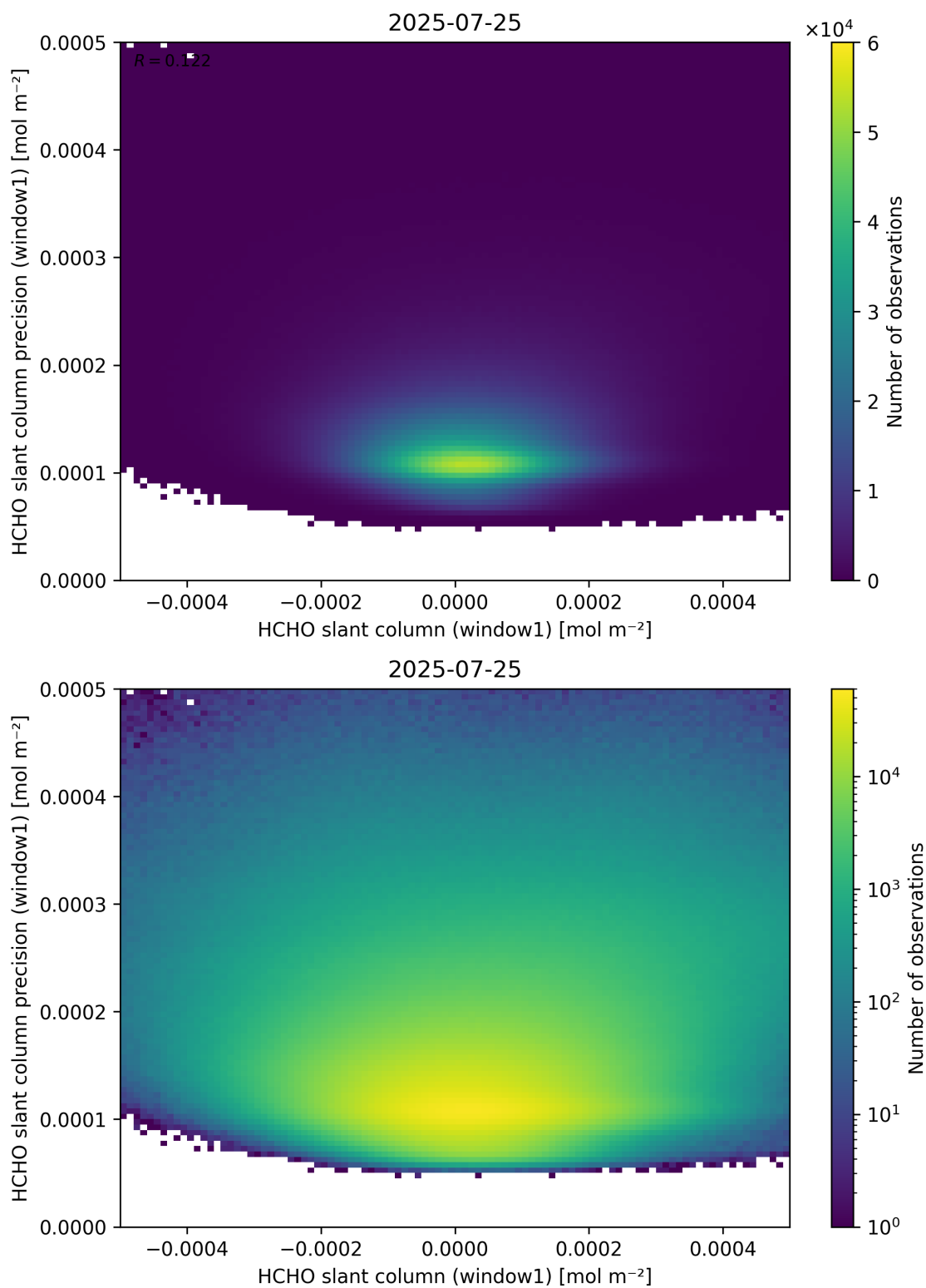
Figure 84: Scatter density plot of “HCHO slant column (window1)” against “HCHO slant column precision (window1)” for 2025-07-24 to 2025-07-26.
