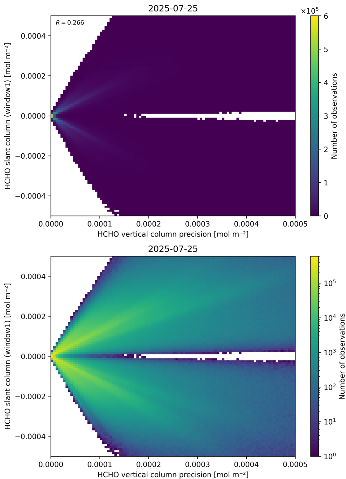
Figure 142: Scatter density plot of “HCHO vertical column precision” against “HCHO slant column (window1)” for 2025-07-24 to 2025-07-26.
