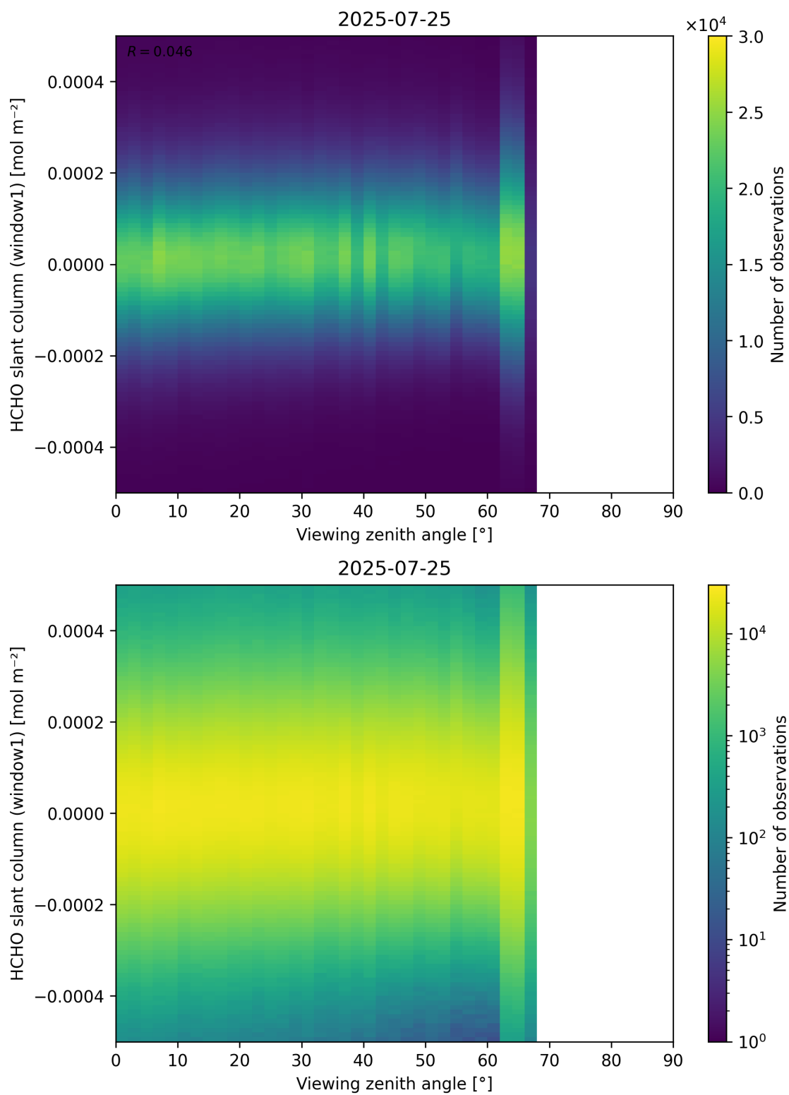
Figure 188: Scatter density plot of “Viewing zenith angle” against “HCHO slant column (window1)” for 2025-07-24 to 2025-07-26.
