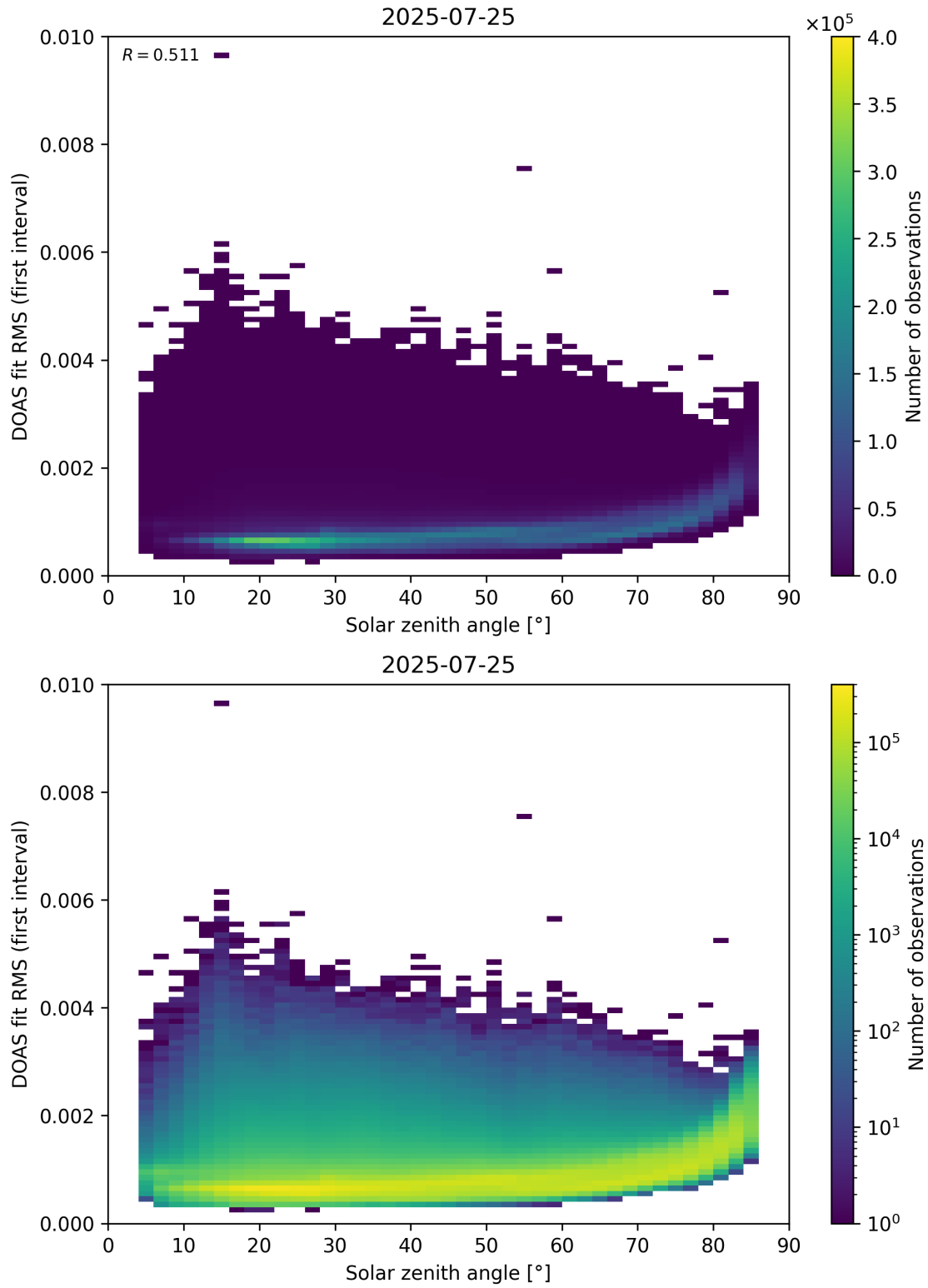
Figure 167: Scatter density plot of “Solar zenith angle” against “DOAS fit RMS (first interval)” for 2025-07-24 to 2025-07-26.
