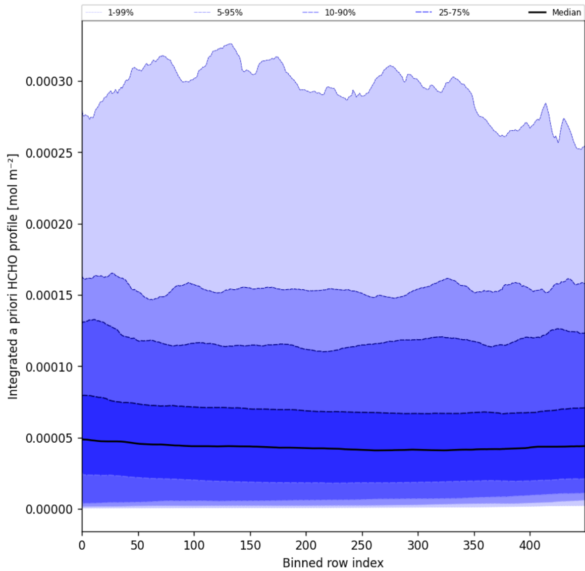
Figure 57: Along track statistics of "Integrated a priori HCHO profile" for 2025-07-24 to 2025-07-26
