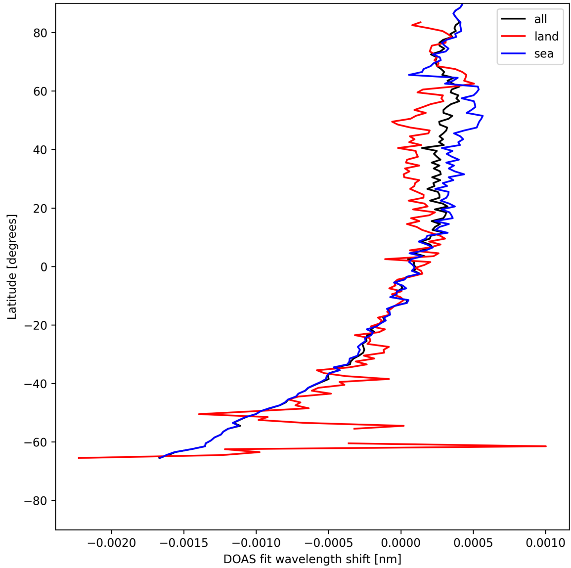
Figure 30: Zonal average of “DOAS fit wavelength shift” for 2025-07-24 to 2025-07-26.
