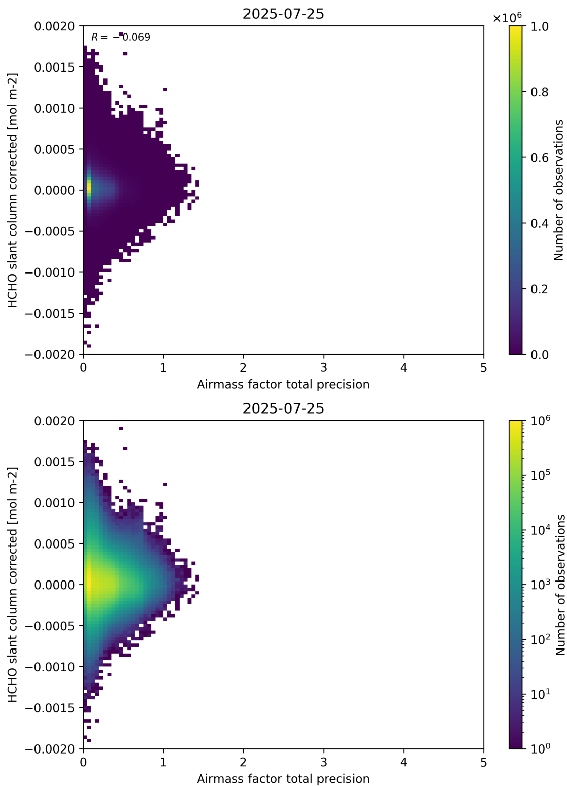
Figure 109: Scatter density plot of “Airmass factor total precision” against “HCHO slant column corrected” for 2025-07-24 to 2025-07-26.
