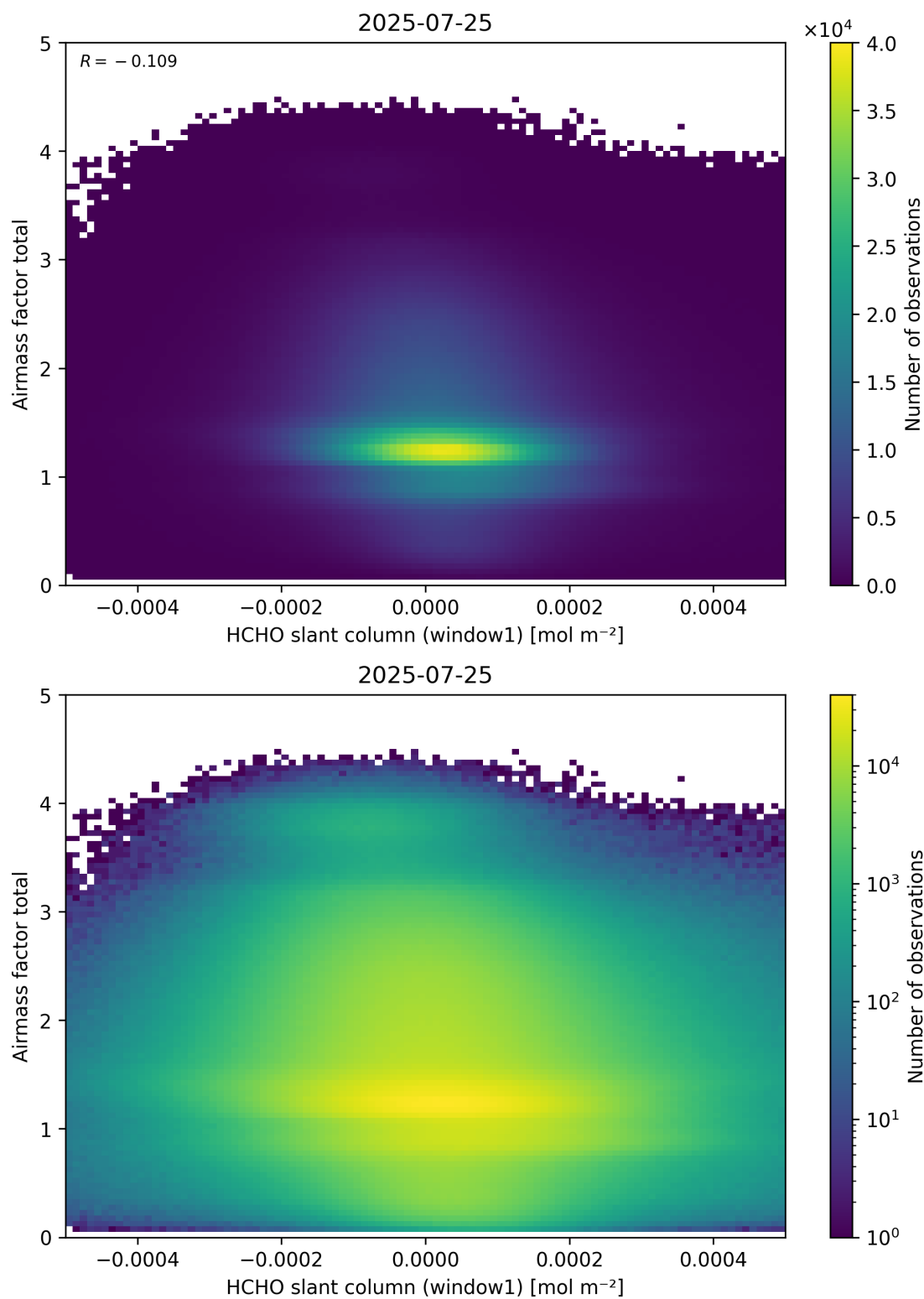
Figure 85: Scatter density plot of “HCHO slant column (window1)” against “Airmass factor total” for 2025-07-24 to 2025-07-26.
