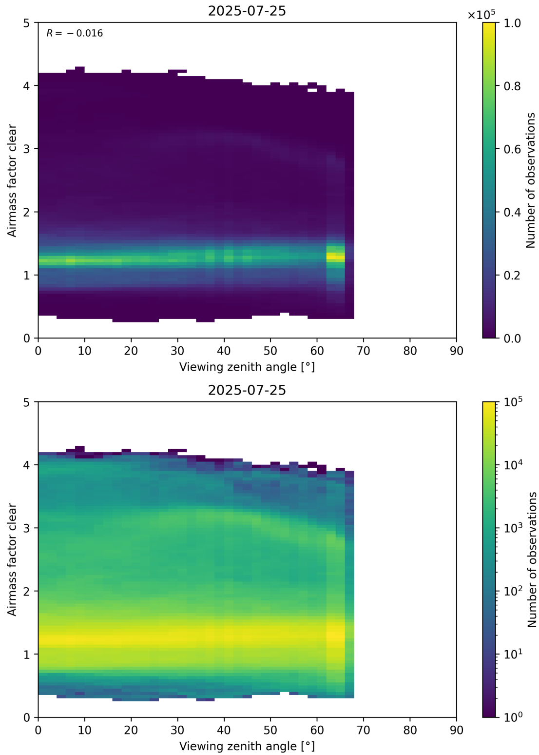
Figure 185: Scatter density plot of “Viewing zenith angle” against “Airmass factor clear” for 2025-07-24 to 2025-07-26.
