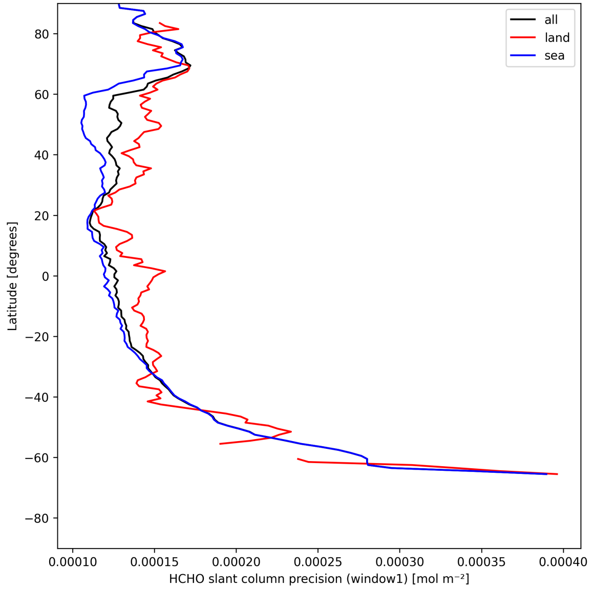
Figure 25: Zonal average of “HCHO slant column precision (window1)” for 2025-07-24 to 2025-07-26.
