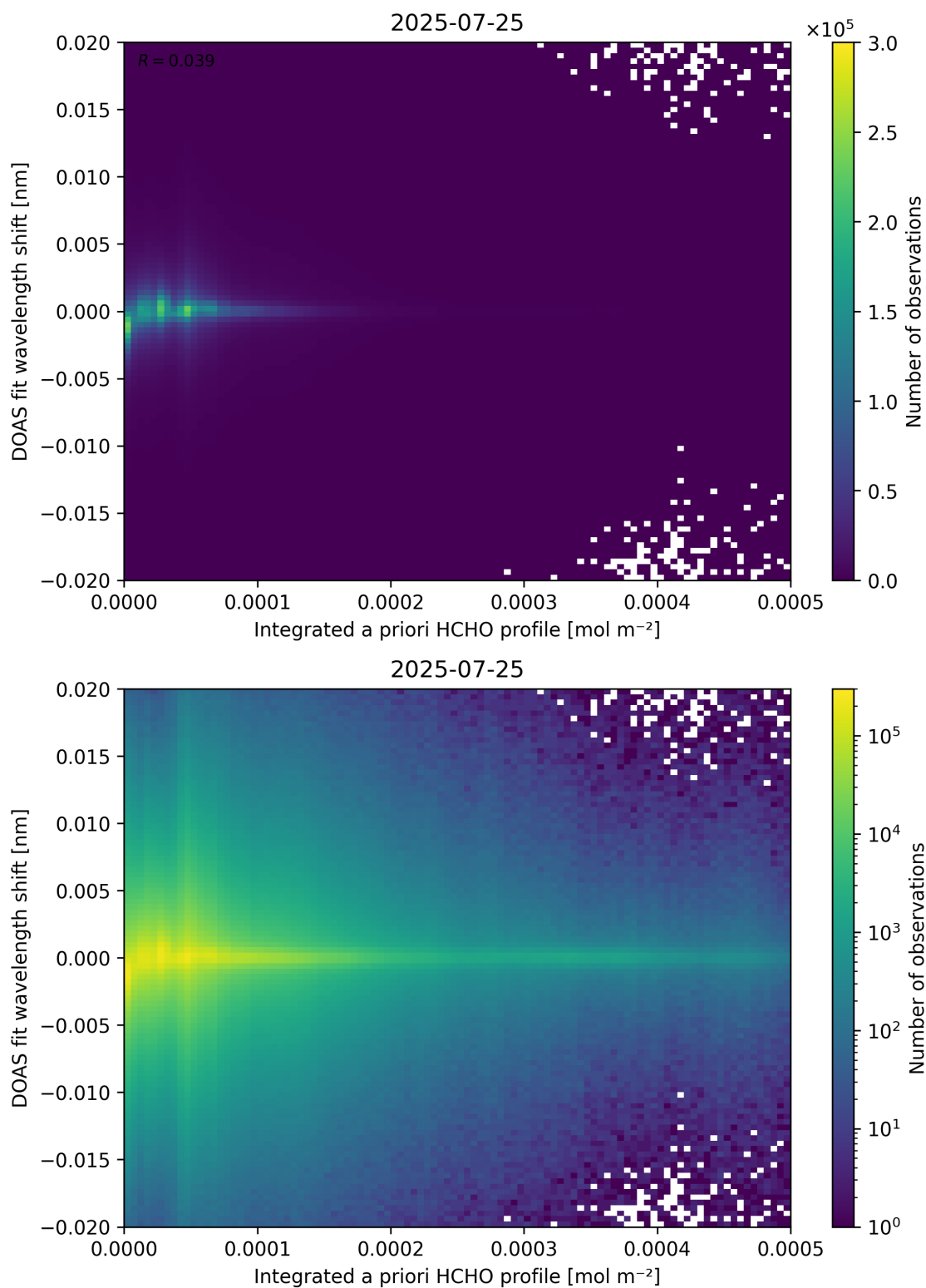
Figure 149: Scatter density plot of “Integrated a priori HCHO profile” against “DOAS fit wavelength shift” for 2025-07-24 to 2025-07-26.
