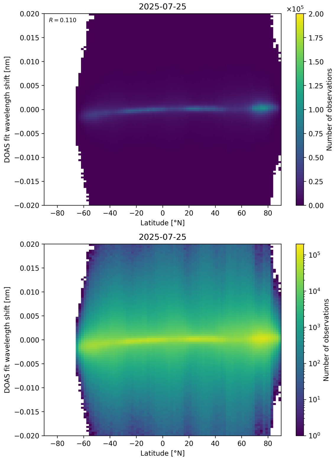
Figure 154: Scatter density plot of “Latitude” against “DOAS fit wavelength shift” for 2025-07-24 to 2025-07-26.
