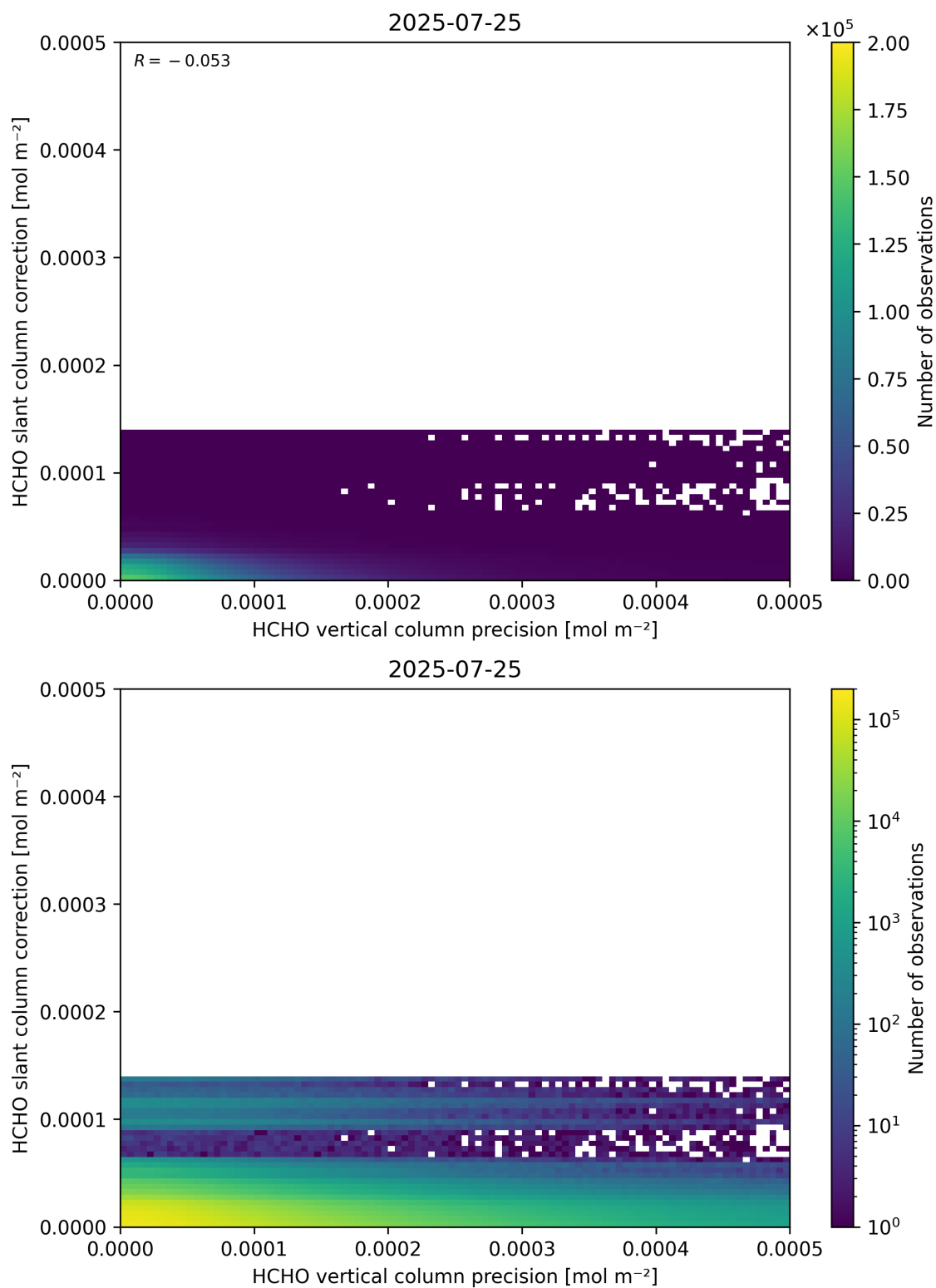
Figure 141: Scatter density plot of “HCHO vertical column precision” against “HCHO slant column correction” for 2025-07-24 to 2025-07-26.
