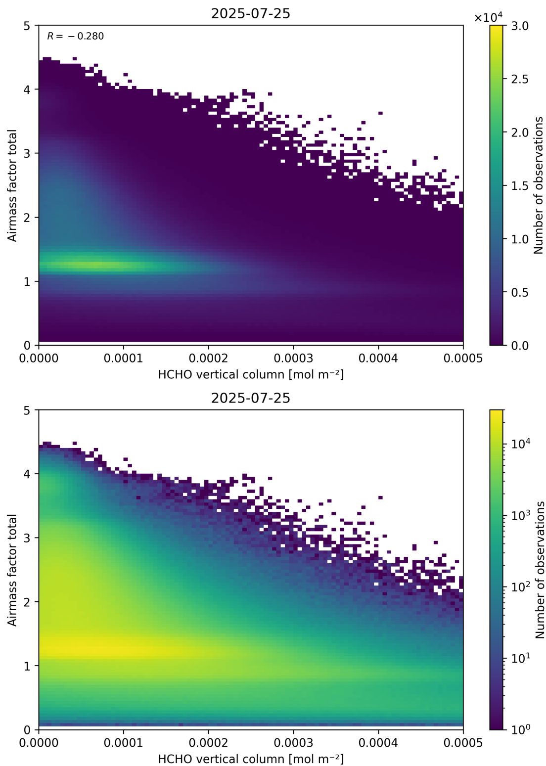
Figure 131: Scatter density plot of “HCHO vertical column” against “Airmass factor total” for 2025-07-24 to 2025-07-26.
