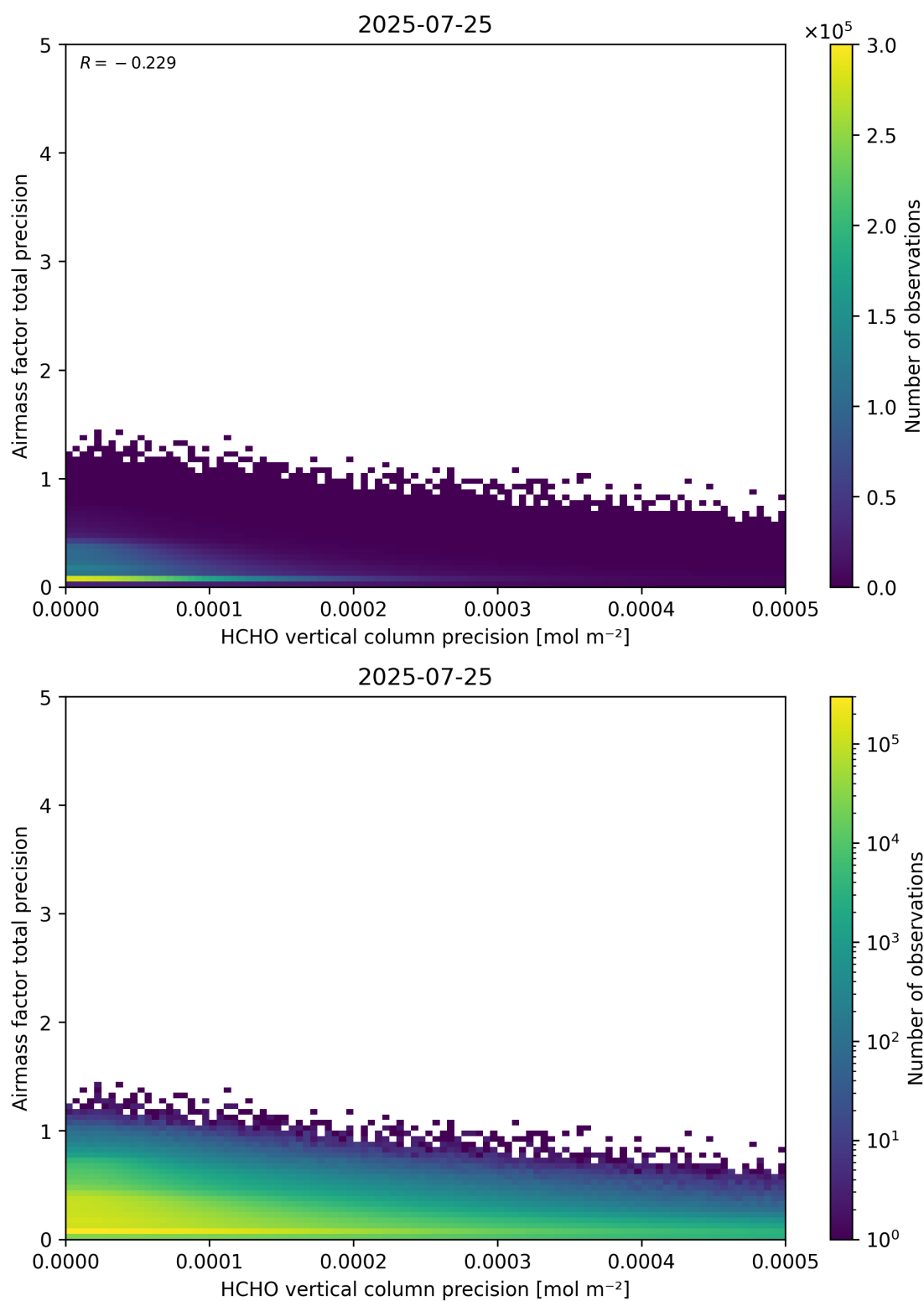
Figure 145: Scatter density plot of “HCHO vertical column precision” against “Airmass factor total precision” for 2025-07-24 to 2025-07-26.
