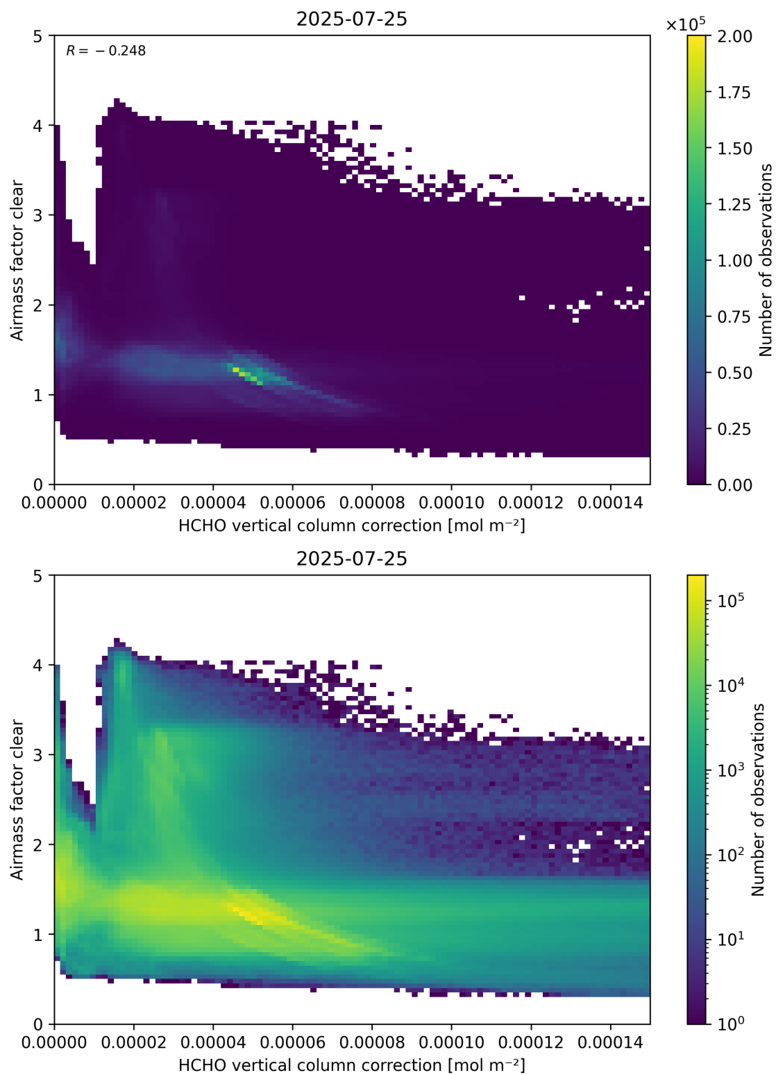
Figure 115: Scatter density plot of “HCHO vertical column correction” against “Airmass factor clear” for 2025-07-24 to 2025-07-26.
