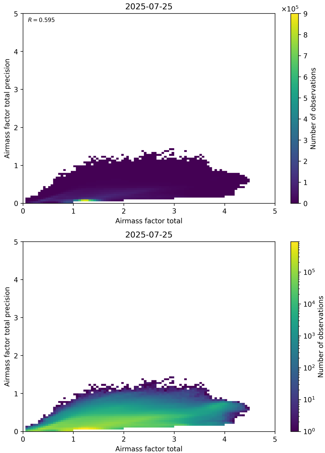
Figure 103: Scatter density plot of “Airmass factor total” against “Airmass factor total precision” for 2025-07-24 to 2025-07-26.
