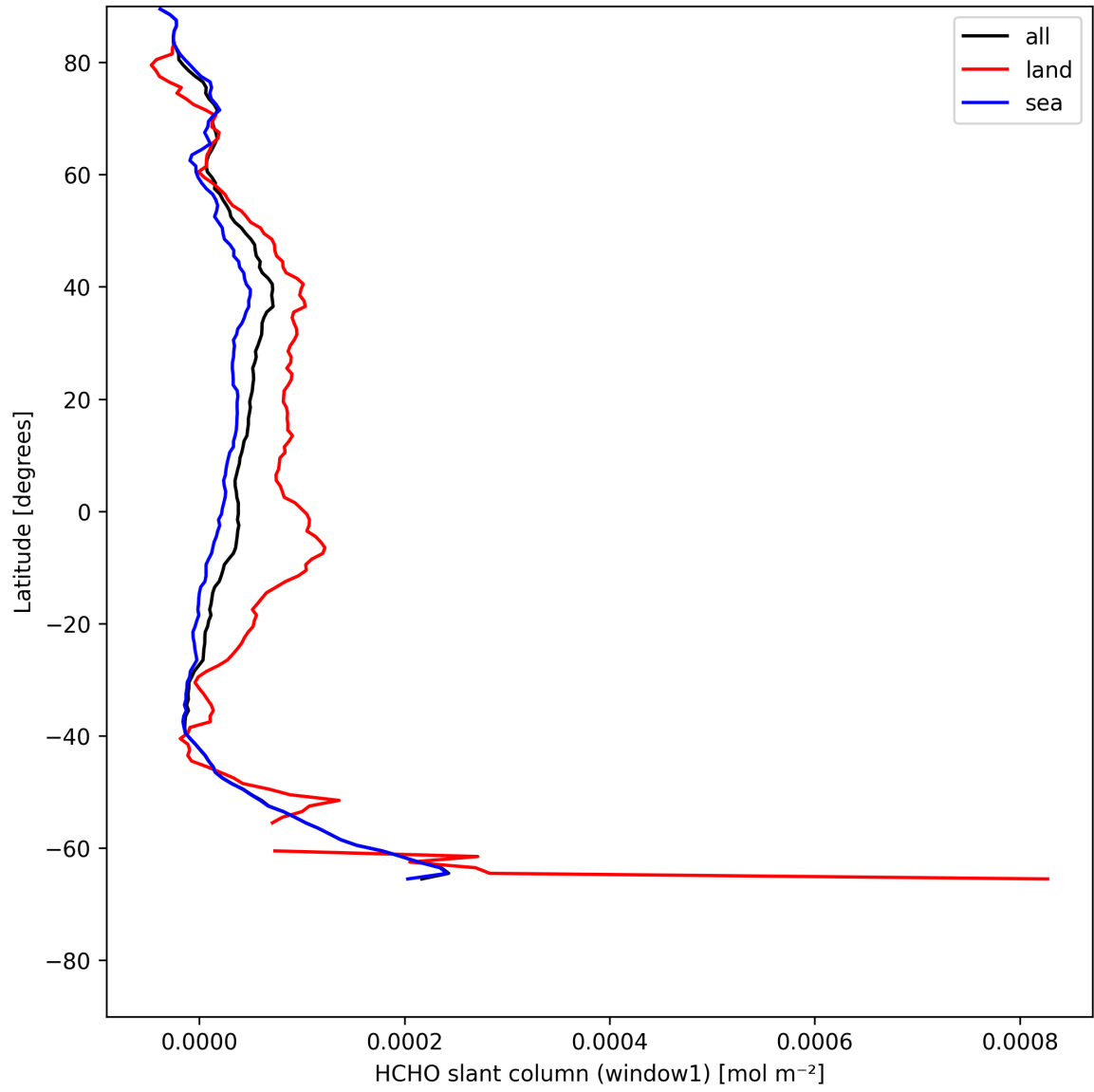
Figure 24: Zonal average of “HCHO slant column (window1)” for 2025-07-24 to 2025-07-26.
