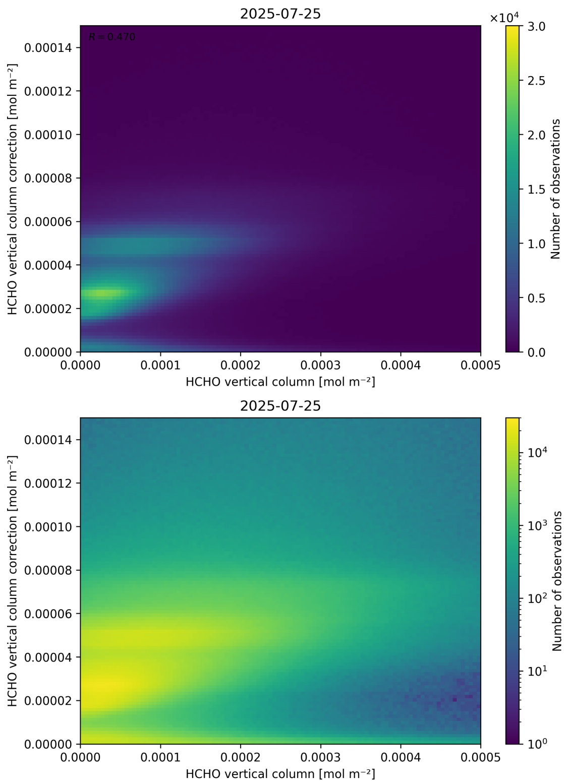
Figure 133: Scatter density plot of “HCHO vertical column” against “HCHO vertical column correction” for 2025-07-24 to 2025-07-26.
