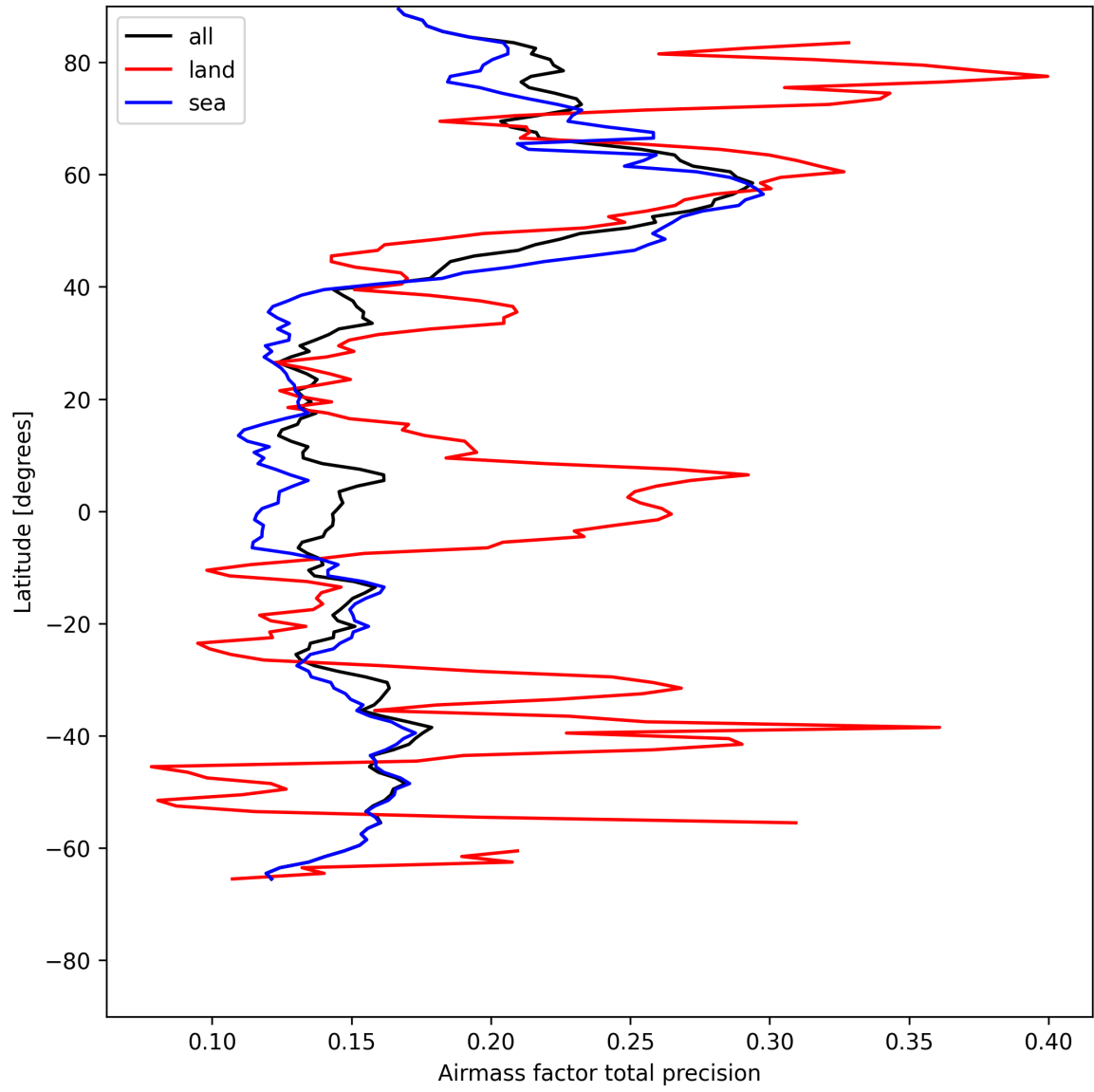
Figure 27: Zonal average of “Airmass factor total precision” for 2025-07-24 to 2025-07-26.
