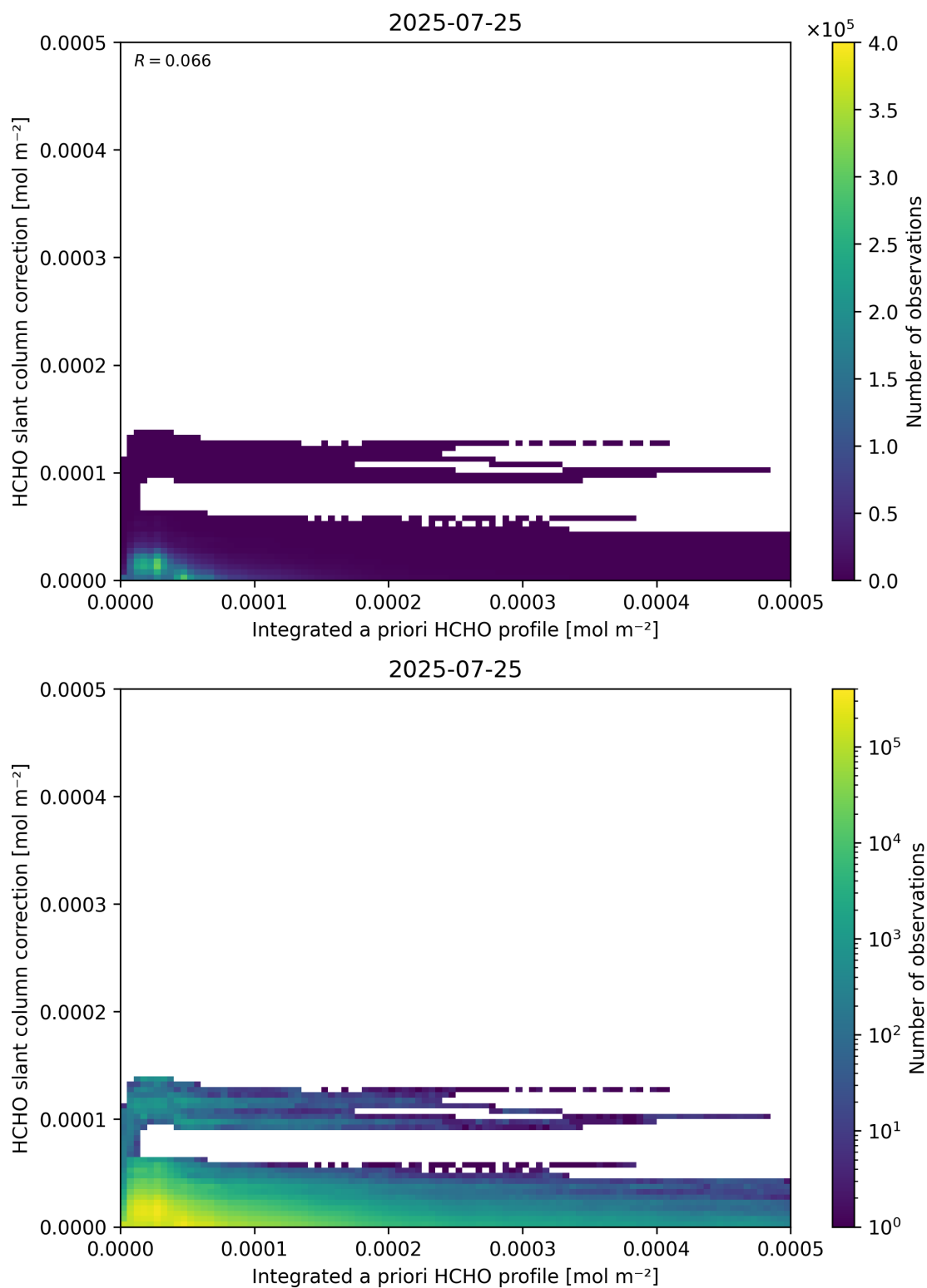
Figure 152: Scatter density plot of “Integrated a priori HCHO profile” against “HCHO slant column correction” for 2025-07-24 to 2025-07-26.
