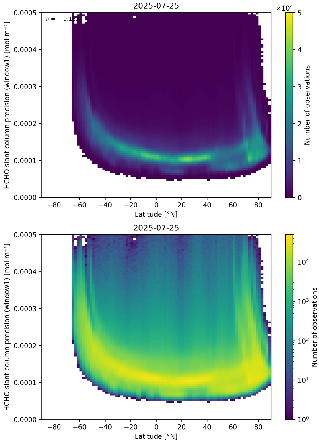
Figure 160: Scatter density plot of “Latitude” against “HCHO slant column precision (window1)” for 2025-07-24 to 2025-07-26.
