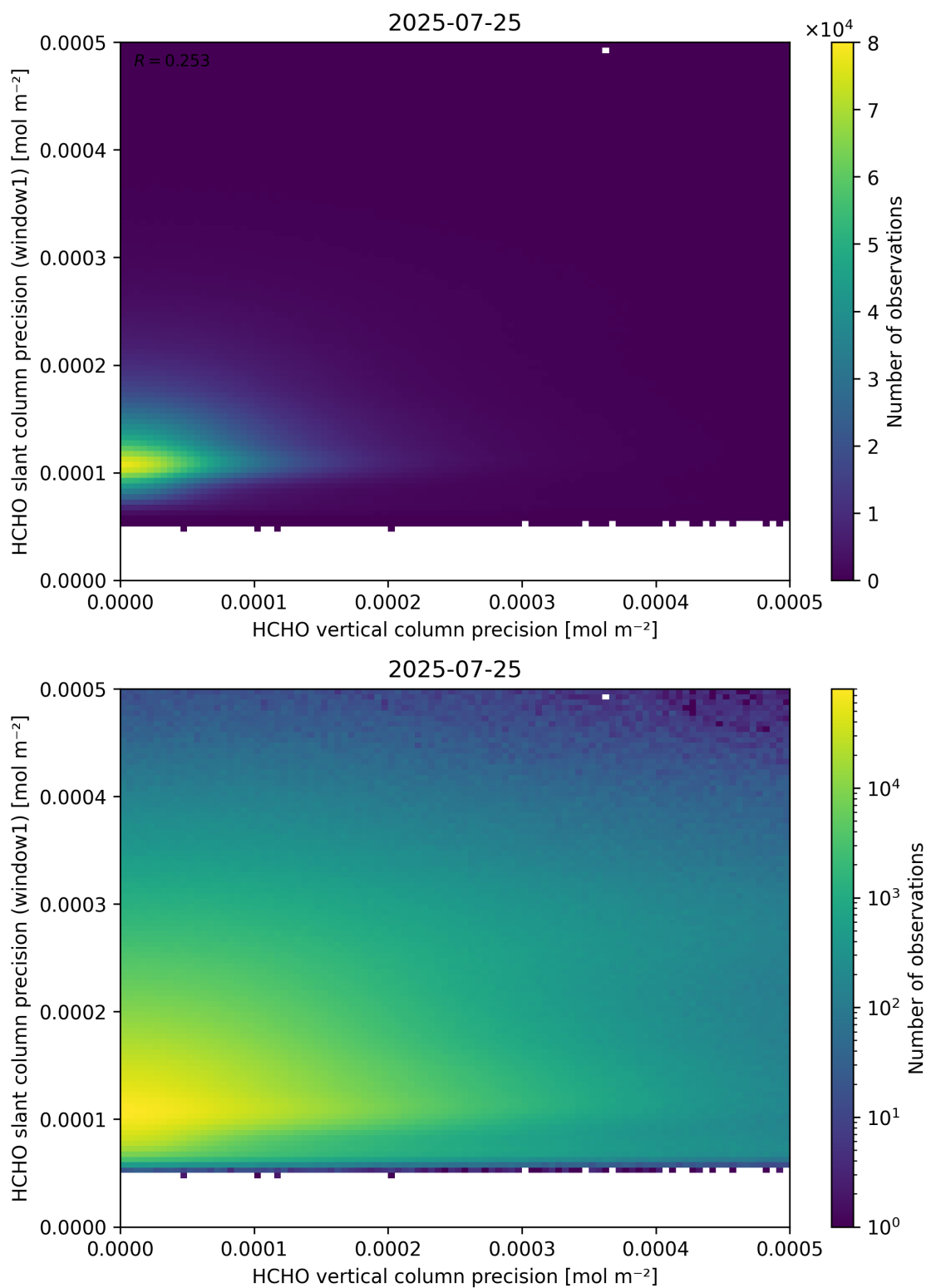
Figure 143: Scatter density plot of “HCHO vertical column precision” against “HCHO slant column precision (window1)” for 2025-07-24 to 2025-07-26.
