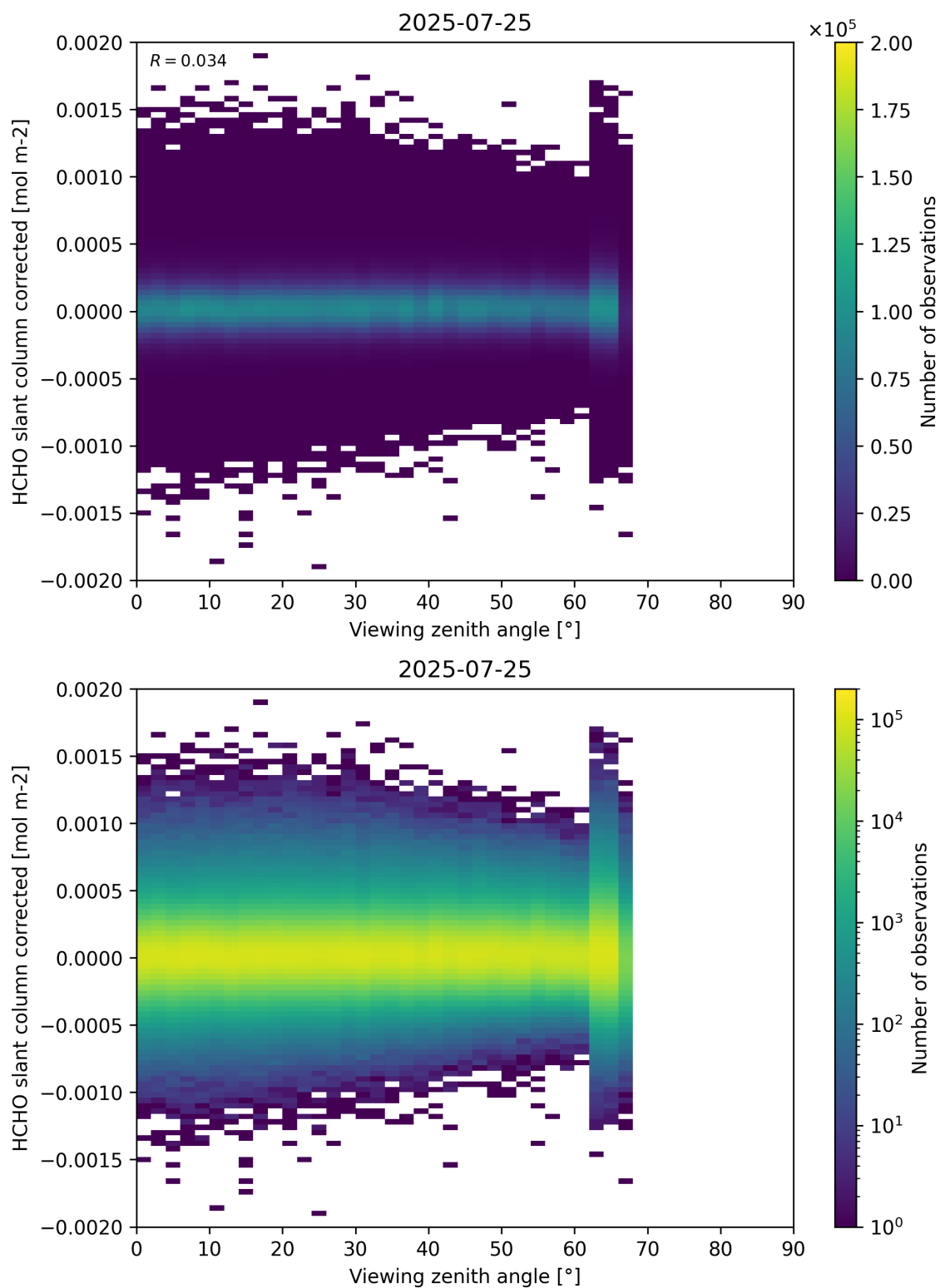
Figure 186: Scatter density plot of “Viewing zenith angle” against “HCHO slant column corrected” for 2025-07-24 to 2025-07-26.
