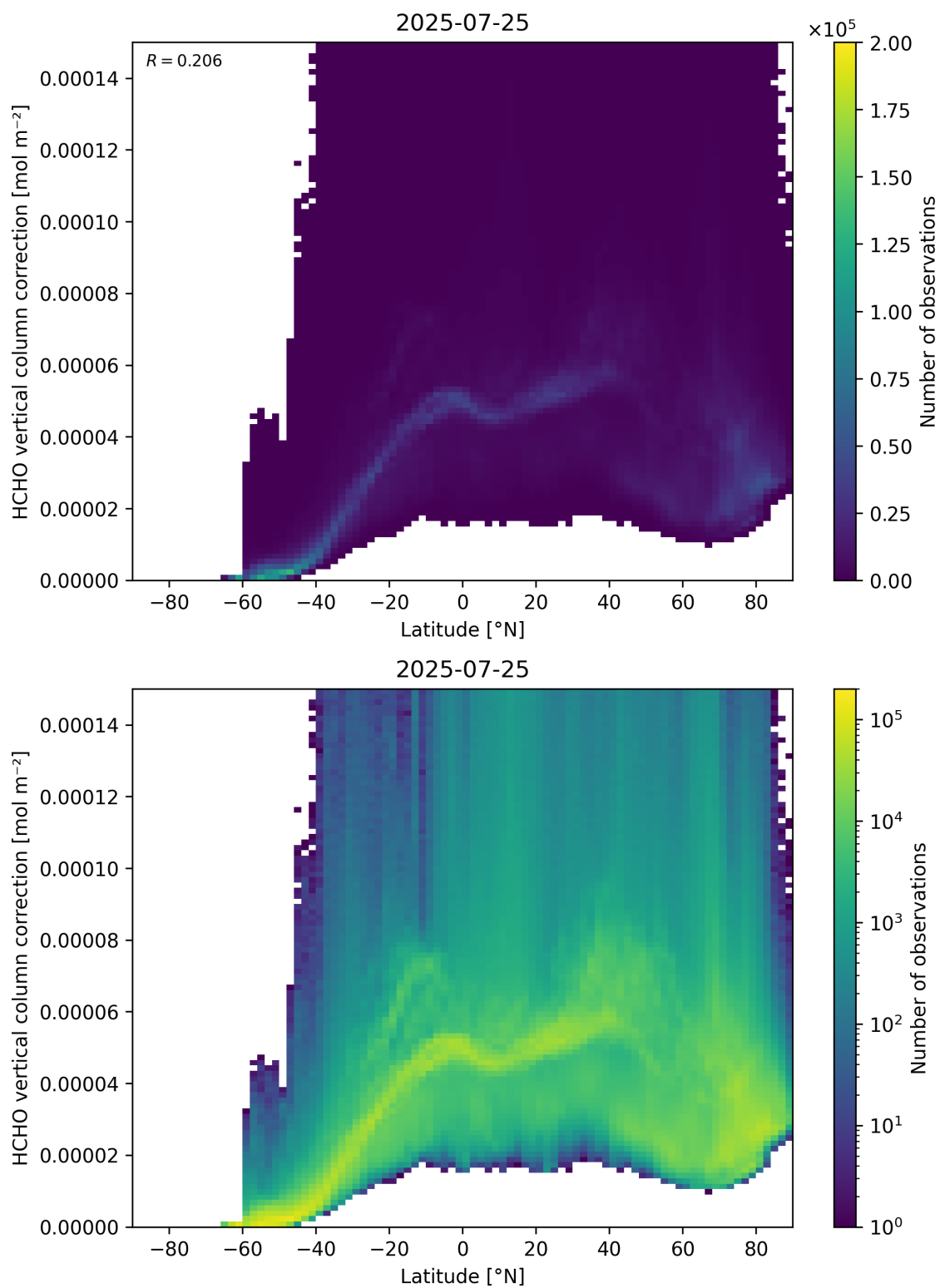
Figure 164: Scatter density plot of “Latitude” against “HCHO vertical column correction” for 2025-07-24 to 2025-07-26.
