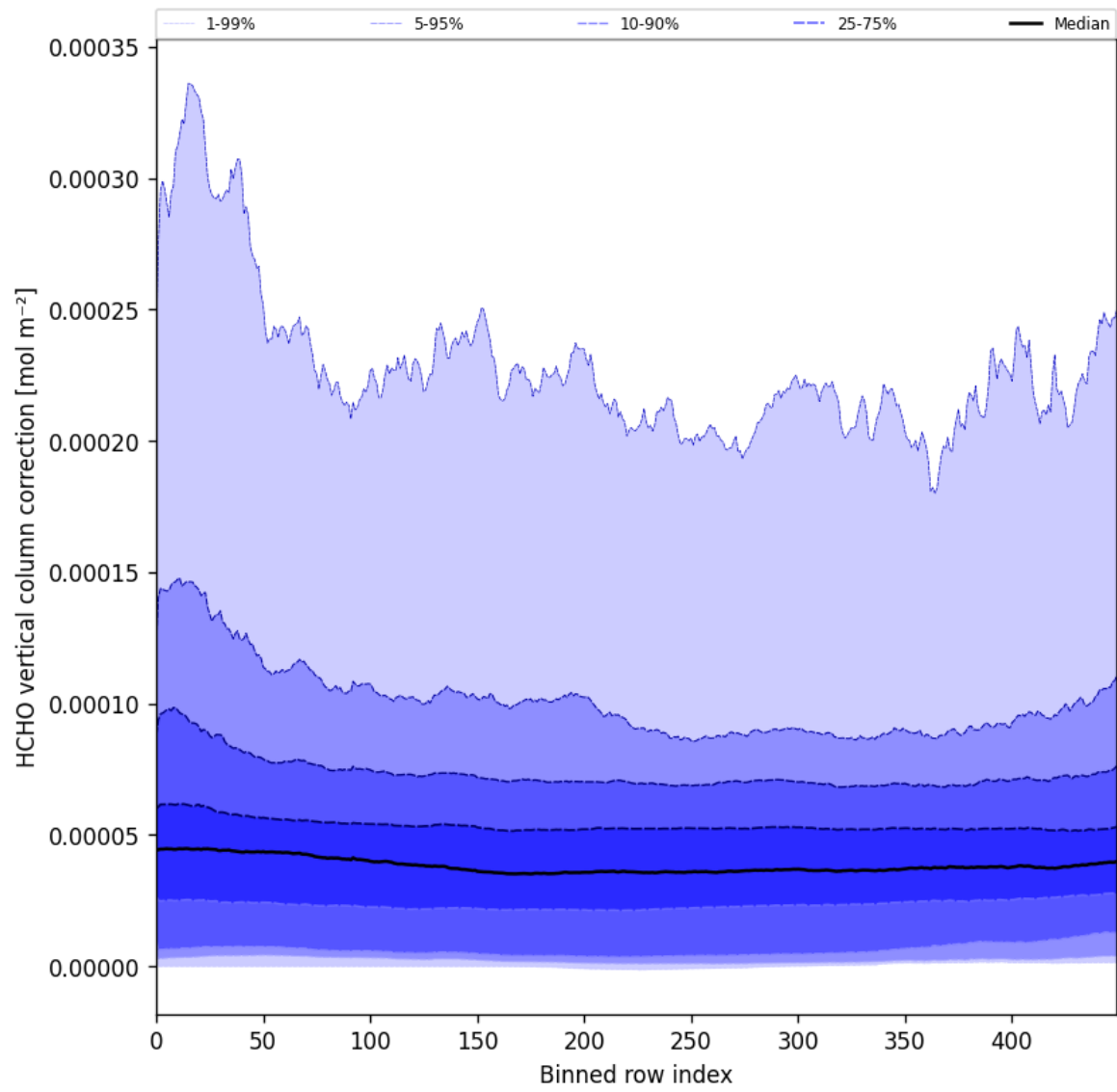
Figure 51: Along track statistics of “HCHO vertical column correction” for 2025-07-24 to 2025-07-26
