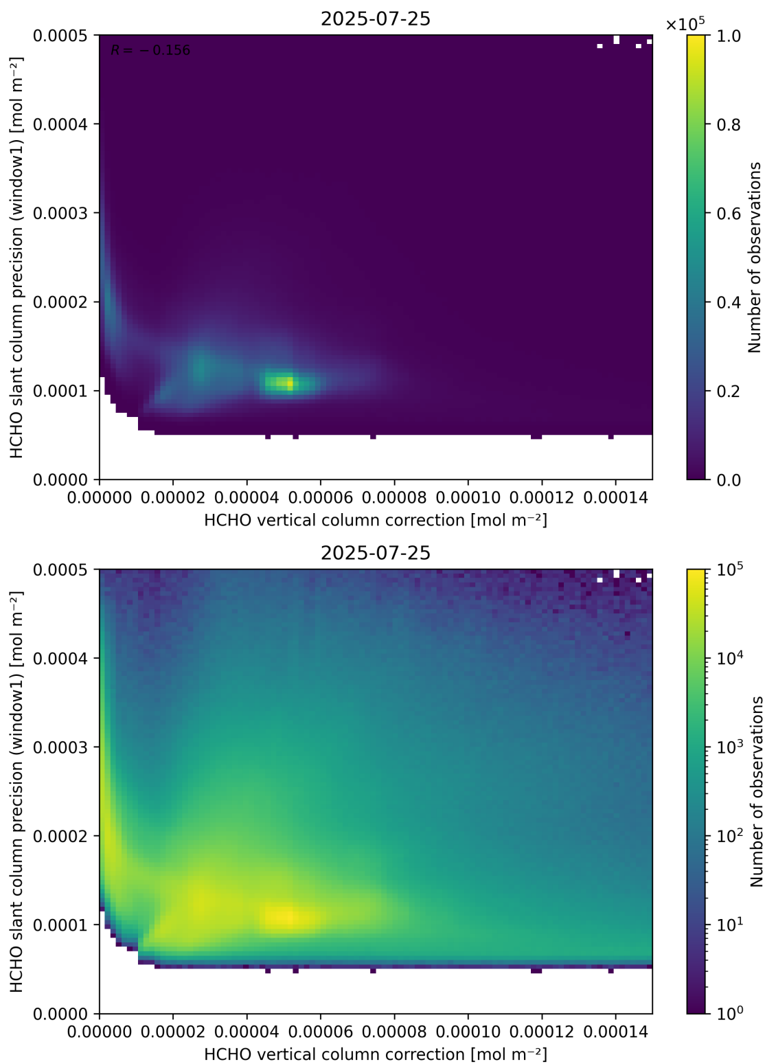
Figure 119: Scatter density plot of “HCHO vertical column correction” against “HCHO slant column precision (window1)” for 2025-07-24 to 2025-07-26.
