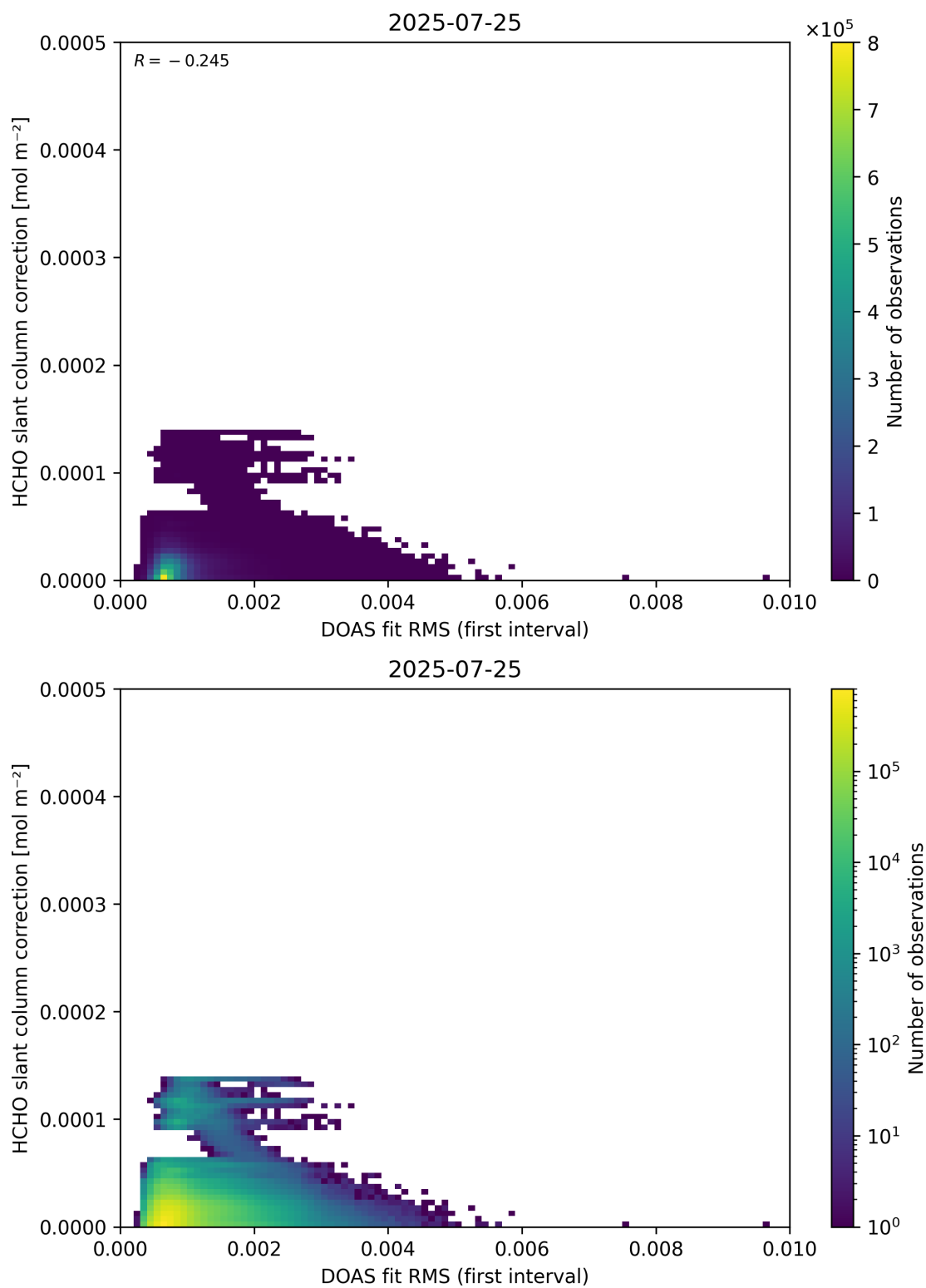
Figure 63: Scatter density plot of “DOAS fit RMS (first interval)” against “HCHO slant column correction” for 2025-07-24 to 2025-07-26.
