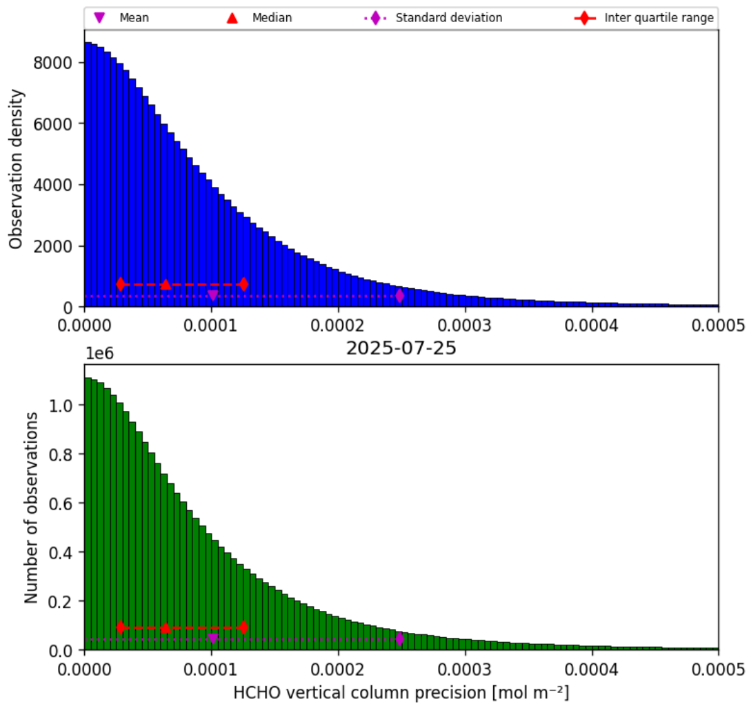
Figure 36: Histogram of “HCHO vertical column precision” for 2025-07-24 to 2025-07-26
