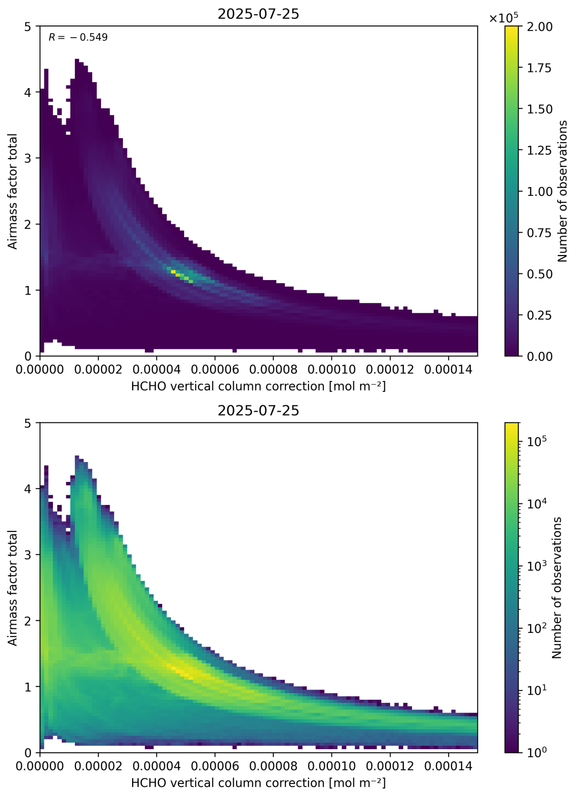
Figure 120: Scatter density plot of “HCHO vertical column correction” against “Airmass factor total” for 2025-07-24 to 2025-07-26.
