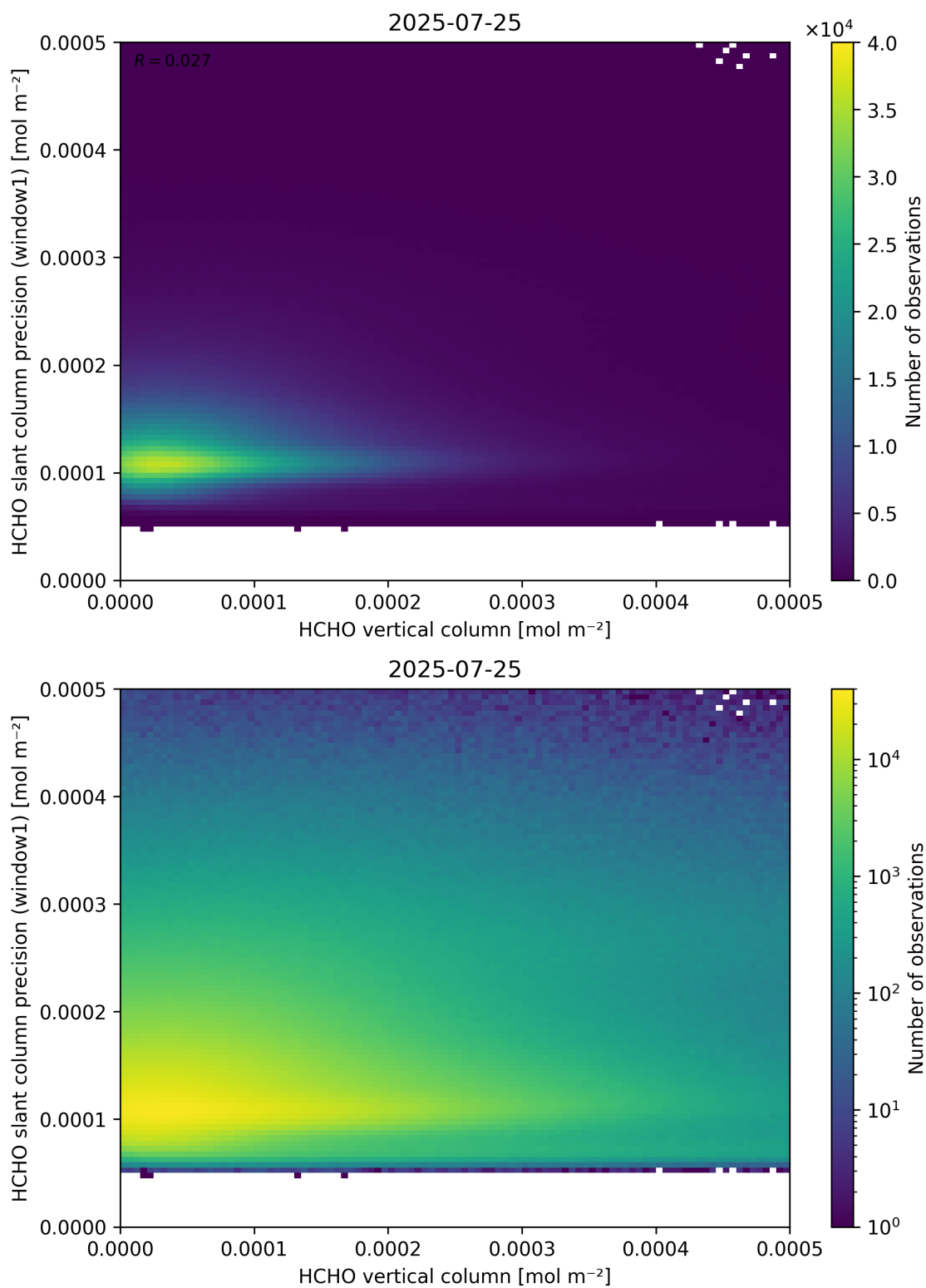
Figure 130: Scatter density plot of “HCHO vertical column” against “HCHO slant column precision (window1)” for 2025-07-24 to 2025-07-26.
