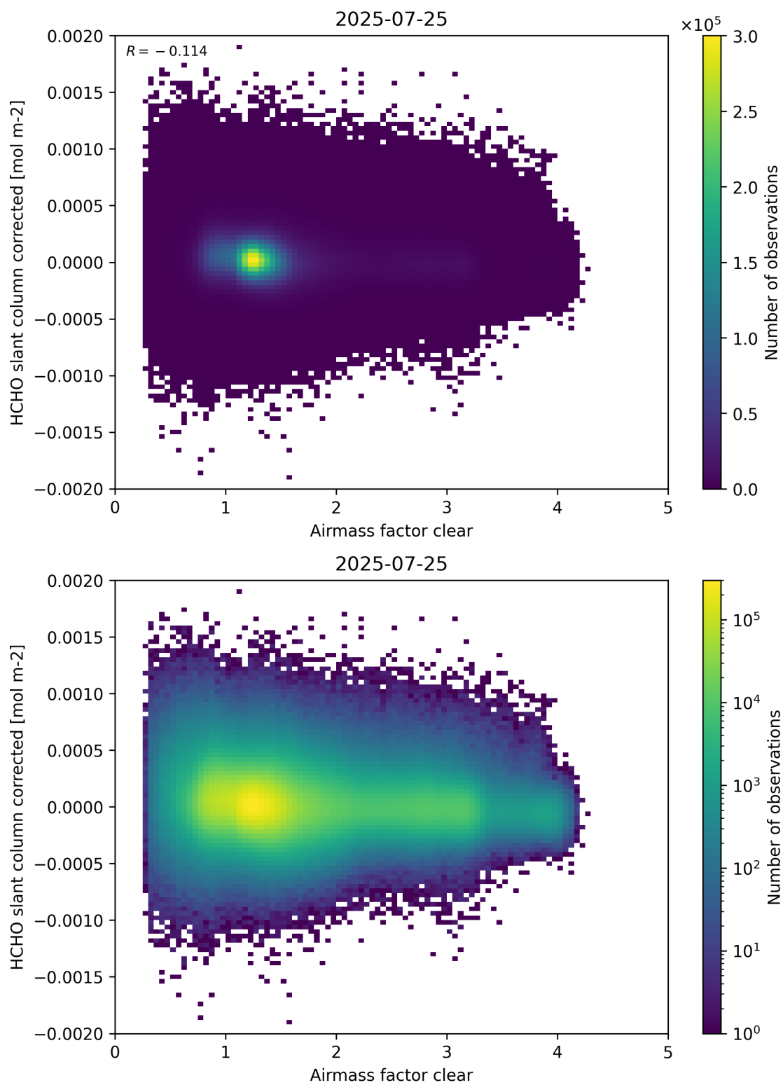
Figure 74: Scatter density plot of “Airmass factor clear” against “HCHO slant column corrected” for 2025-07-24 to 2025-07-26.
