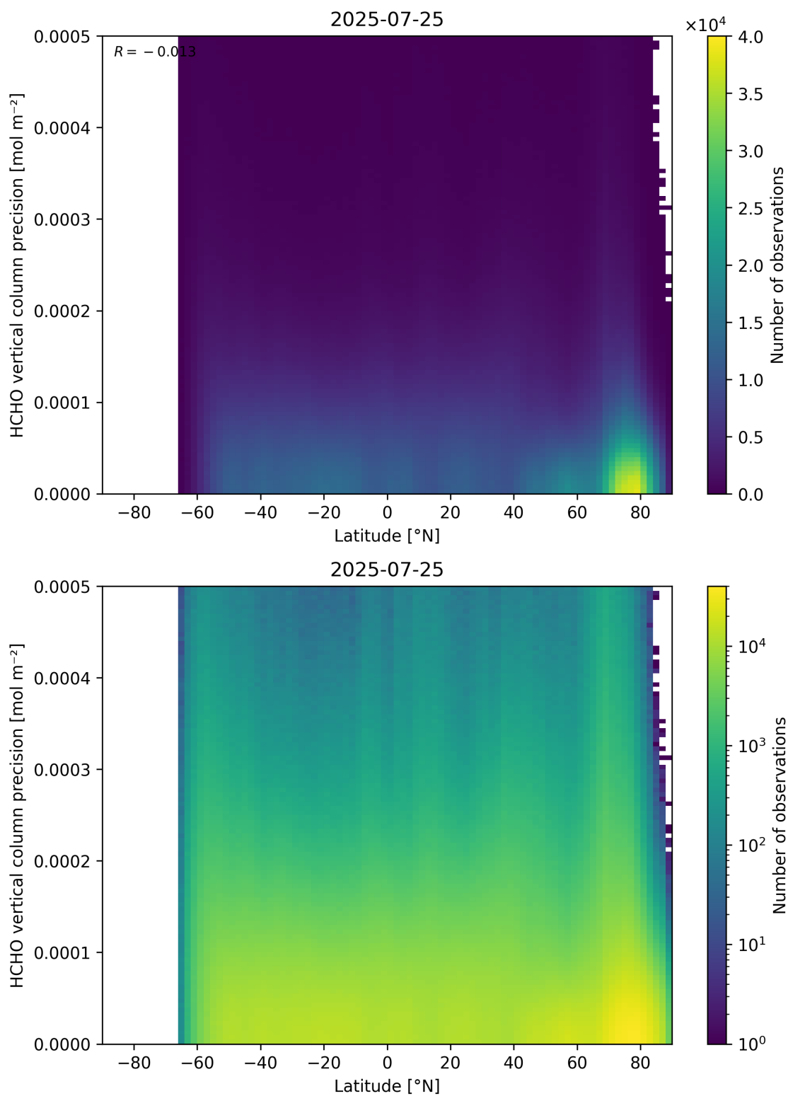
Figure 165: Scatter density plot of “Latitude” against “HCHO vertical column precision” for 2025-07-24 to 2025-07-26.
