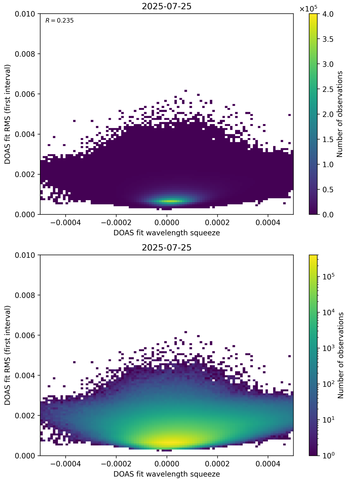
Figure 68: Scatter density plot of “DOAS fit wavelength squeeze” against “DOAS fit RMS (first interval)” for 2025-07-24 to 2025-07-26.
