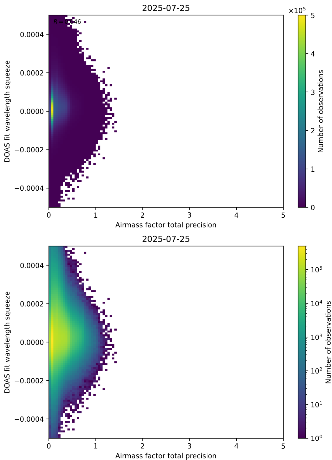
Figure 107: Scatter density plot of “Airmass factor total precision” against “DOAS fit wavelength squeeze” for 2025-07-24 to 2025-07-26.
