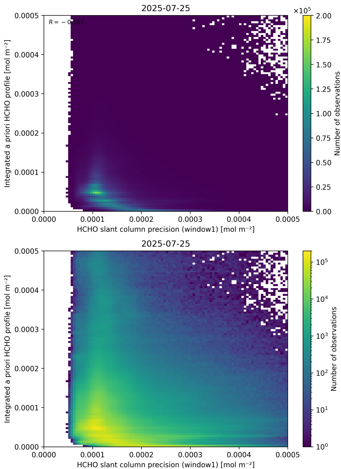
Figure 96: Scatter density plot of “HCHO slant column precision (window1)” against “Integrated a priori HCHO profile” for 2025-07-24 to 2025-07-26.
