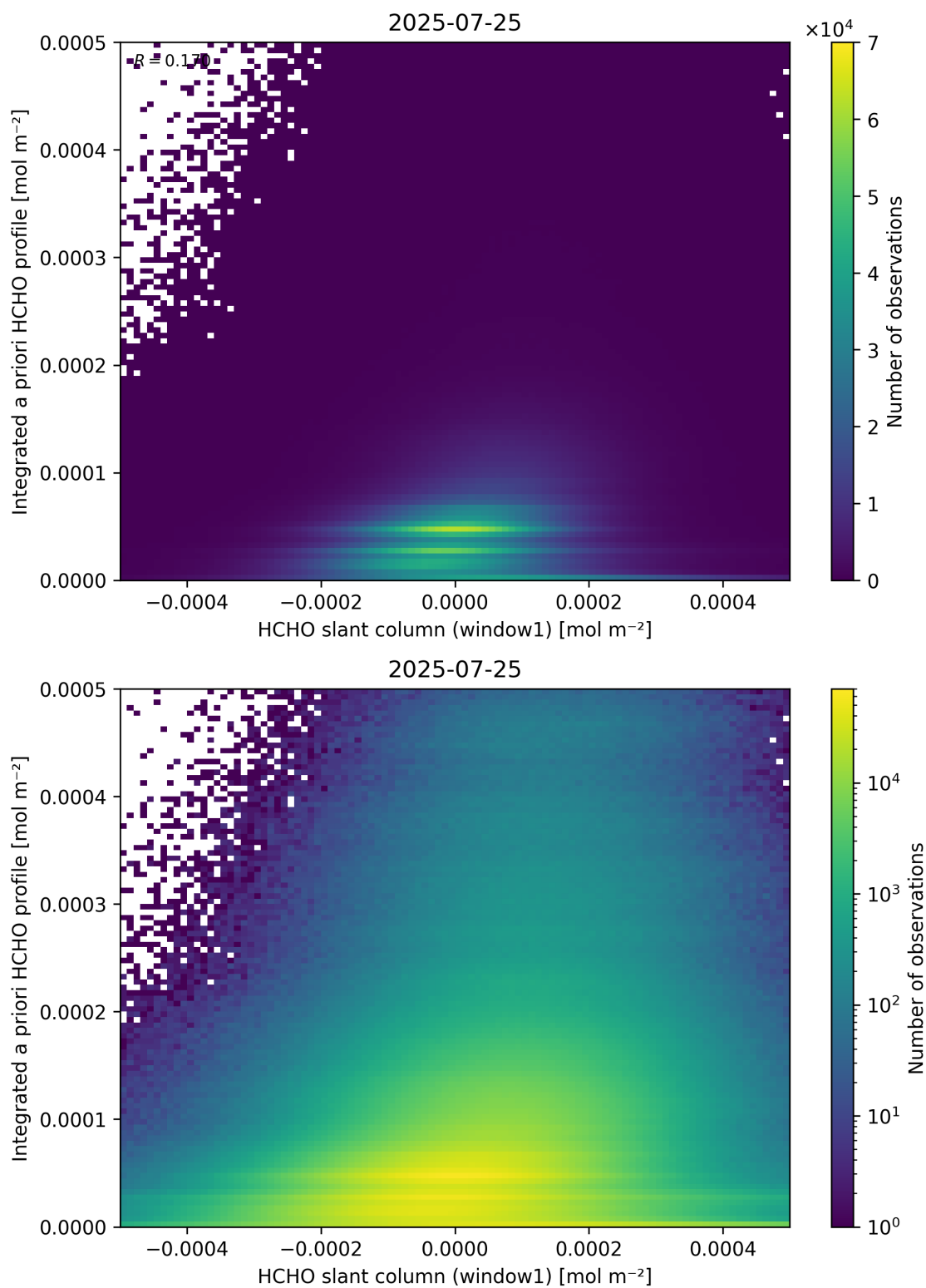
Figure 87: Scatter density plot of “HCHO slant column (window1)” against “Integrated a priori HCHO profile” for 2025-07-24 to 2025-07-26.
