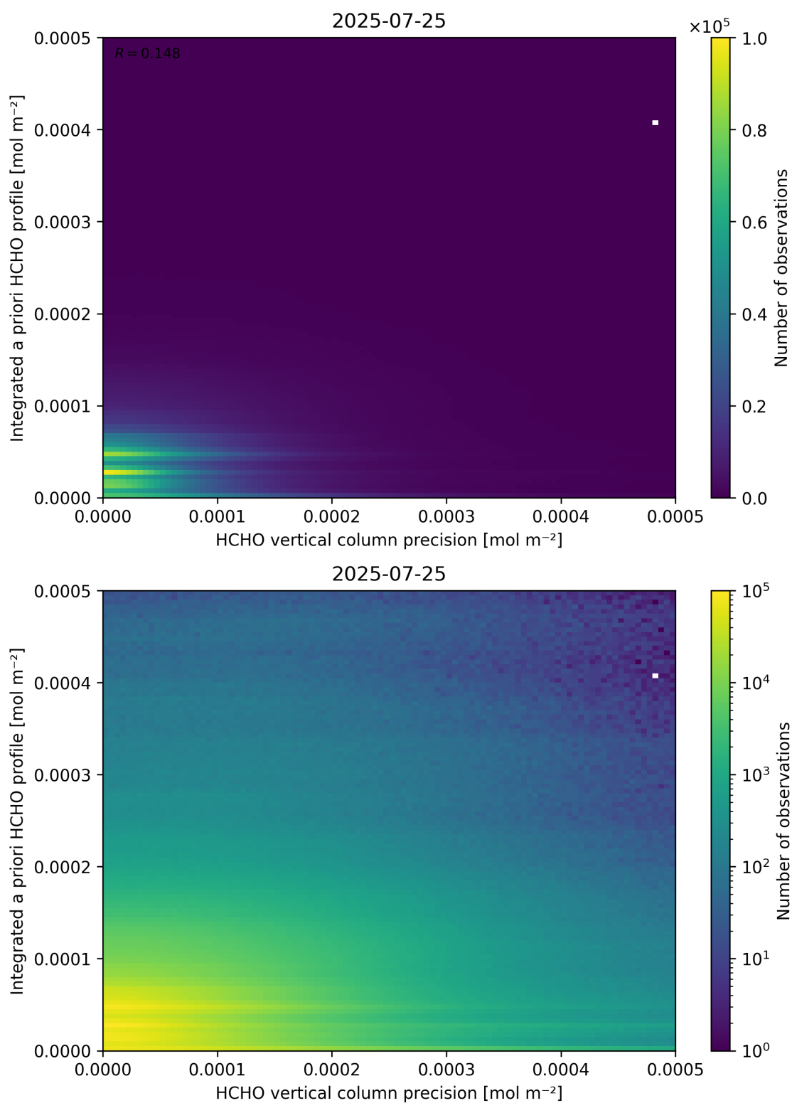
Figure 147: Scatter density plot of “HCHO vertical column precision” against “Integrated a priori HCHO profile” for 2025-07-24 to 2025-07-26.
