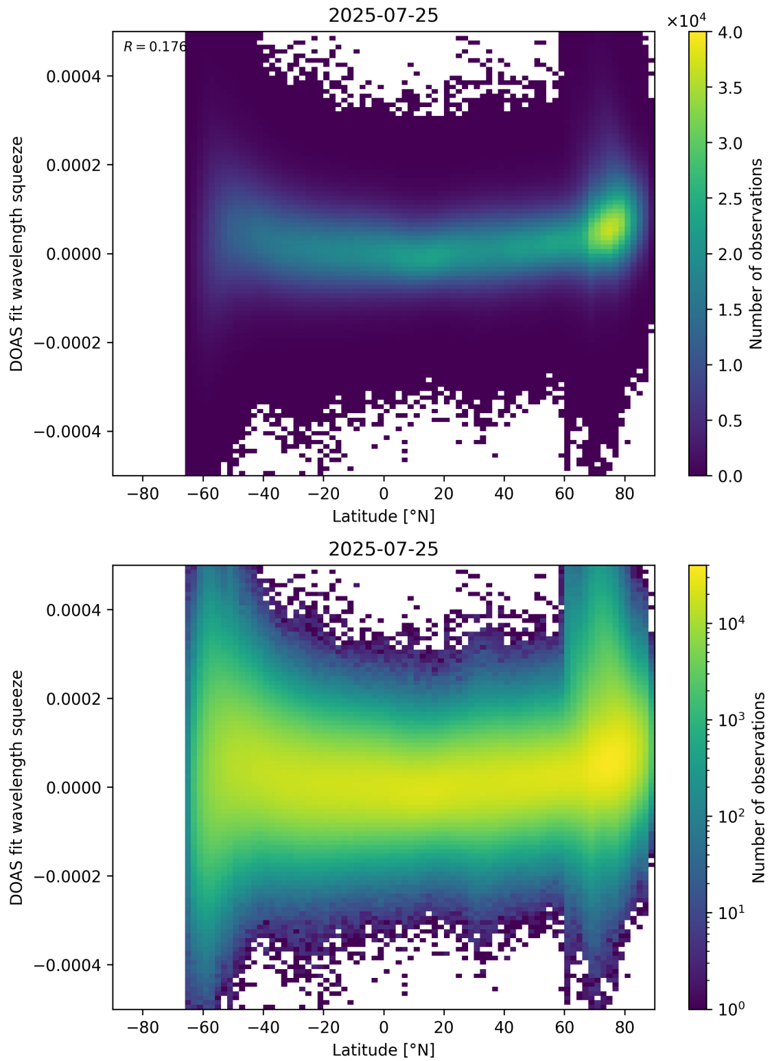
Figure 155: Scatter density plot of “Latitude” against “DOAS fit wavelength squeeze” for 2025-07-24 to 2025-07-26.
