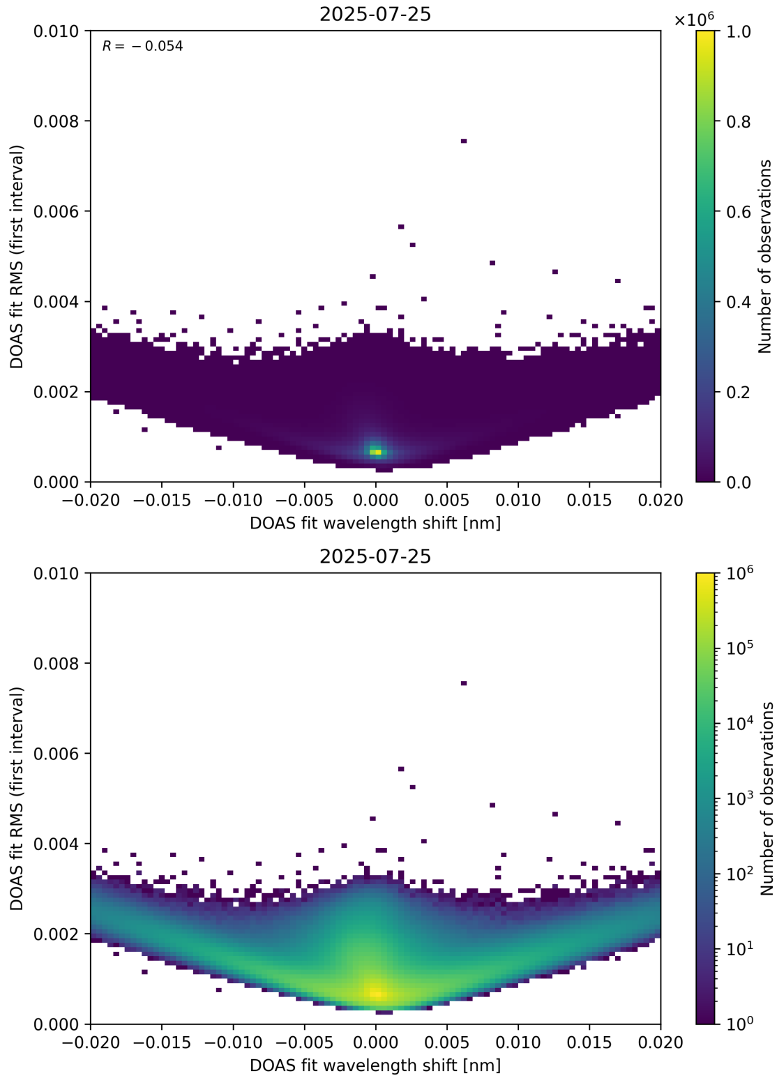
Figure 64: Scatter density plot of “DOAS fit wavelength shift” against “DOAS fit RMS (first interval)” for 2025-07-24 to 2025-07-26.
