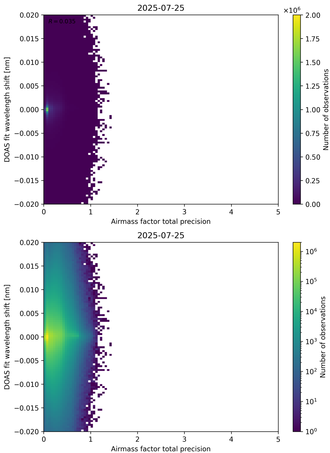
Figure 106: Scatter density plot of “Airmass factor total precision” against “DOAS fit wavelength shift” for 2025-07-24 to 2025-07-26.
