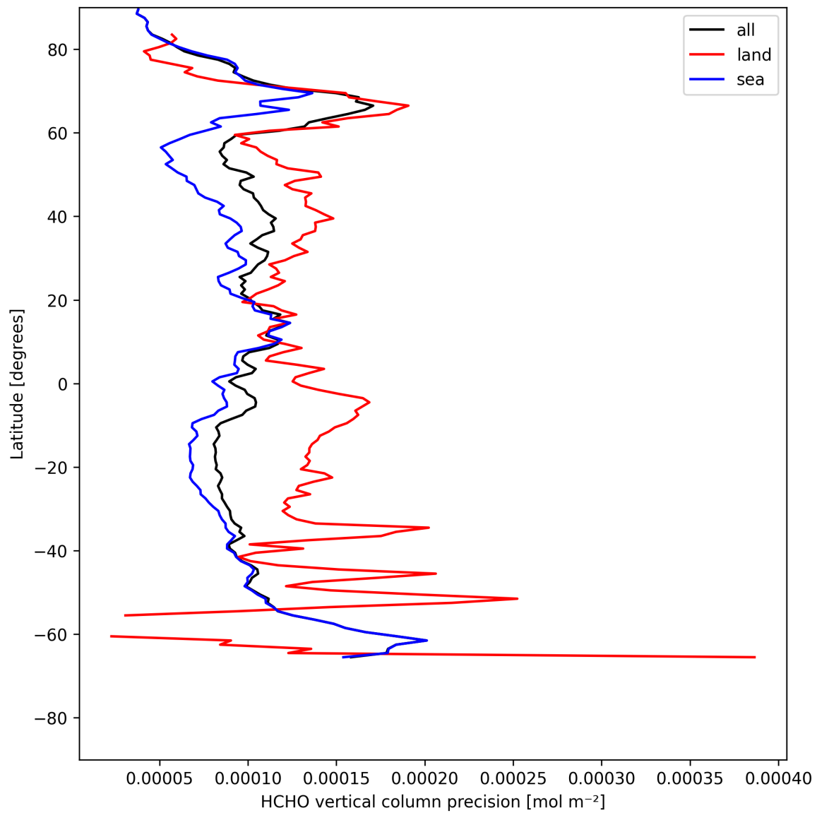
Figure 22: Zonal average of “HCHO vertical column precision” for 2025-07-24 to 2025-07-26.
