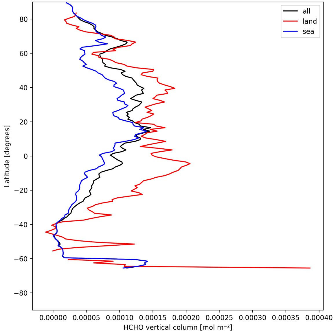
Figure 21: Zonal average of “HCHO vertical column” for 2025-07-24 to 2025-07-26.
