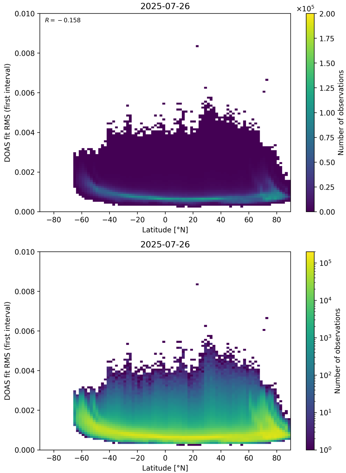
Figure 153: Scatter density plot of “Latitude” against “DOAS fit RMS (first interval)” for 2025-07-25 to 2025-07-27.
