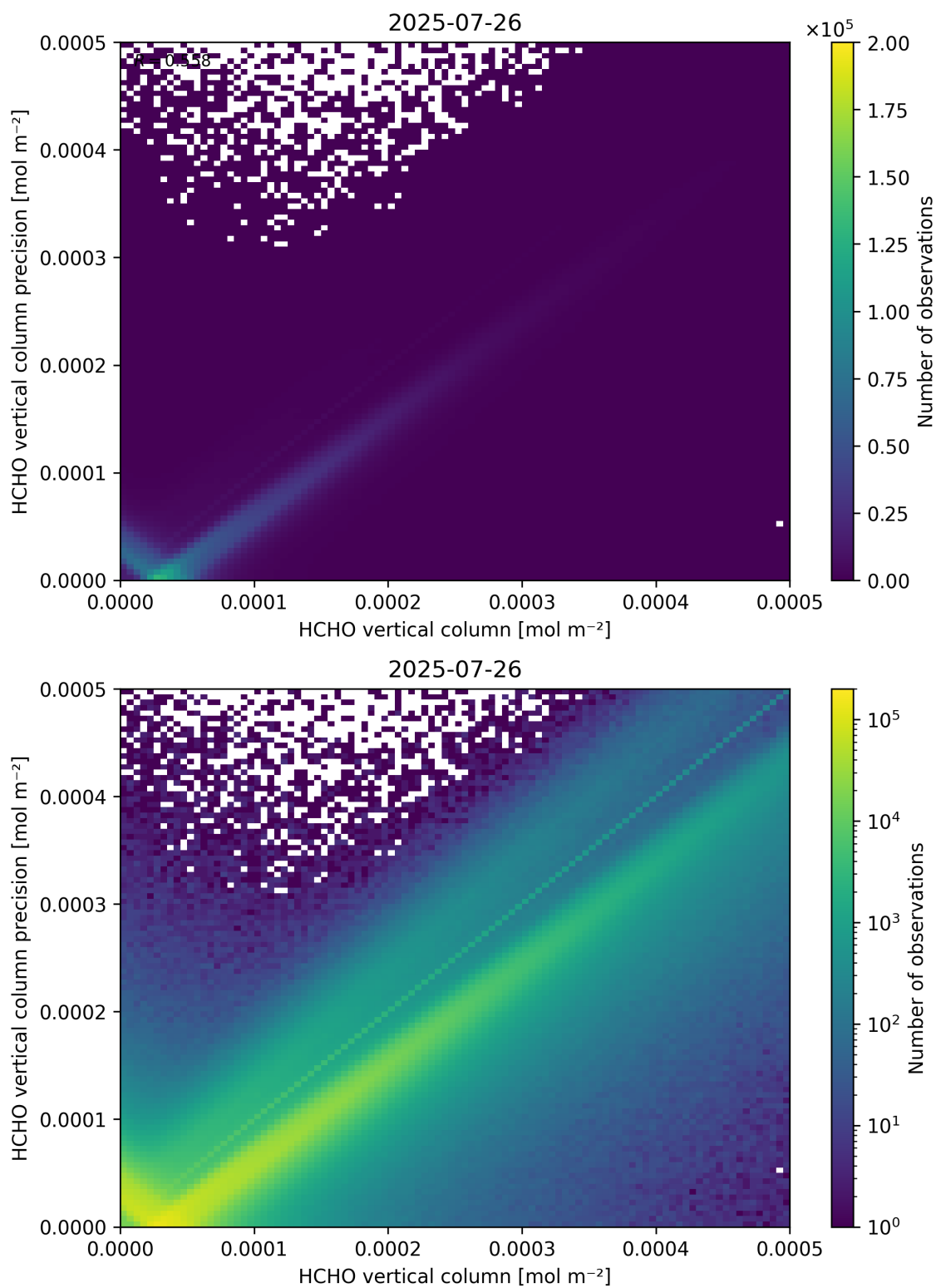
Figure 134: Scatter density plot of “HCHO vertical column” against “HCHO vertical column precision” for 2025-07-25 to 2025-07-27.
