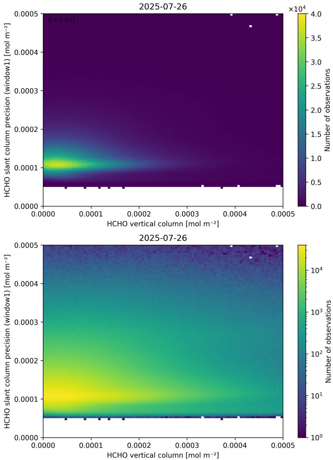
Figure 130: Scatter density plot of “HCHO vertical column” against “HCHO slant column precision (window1)” for 2025-07-25 to 2025-07-27.
