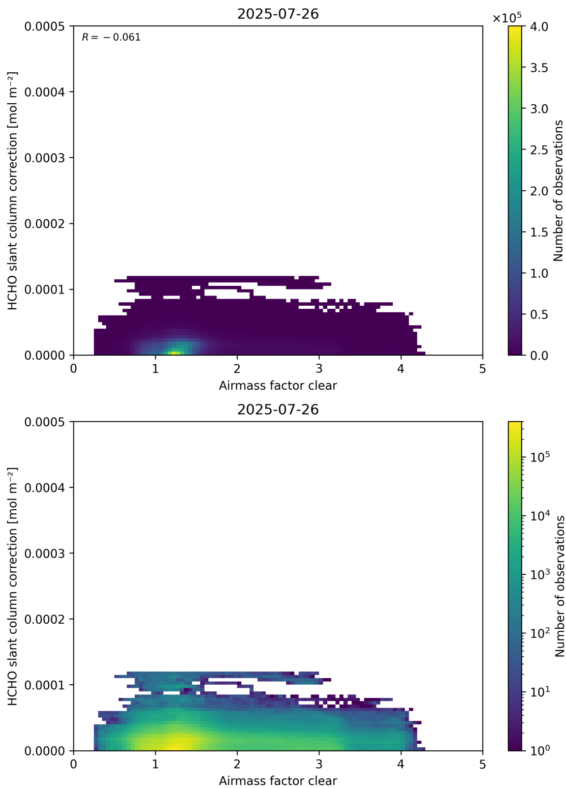
Figure 75: Scatter density plot of “Airmass factor clear” against “HCHO slant column correction” for 2025-07-25 to 2025-07-27.
