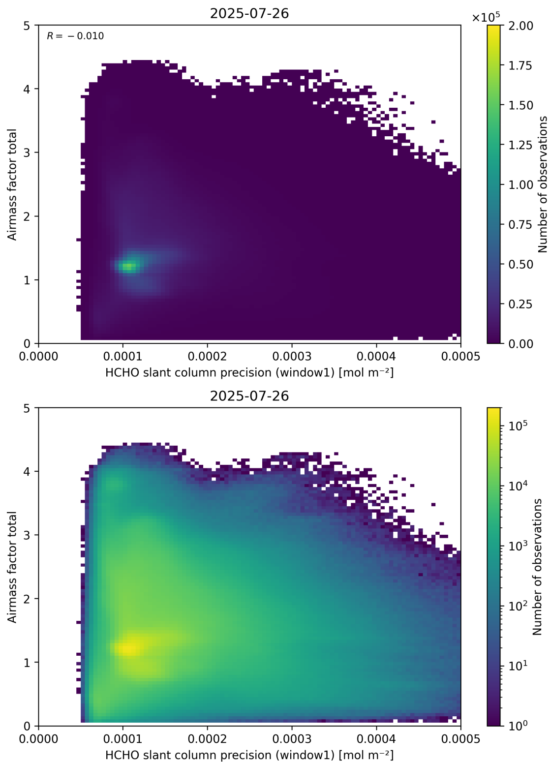
Figure 94: Scatter density plot of “HCHO slant column precision (window1)” against “Airmass factor total” for 2025-07-25 to 2025-07-27.
