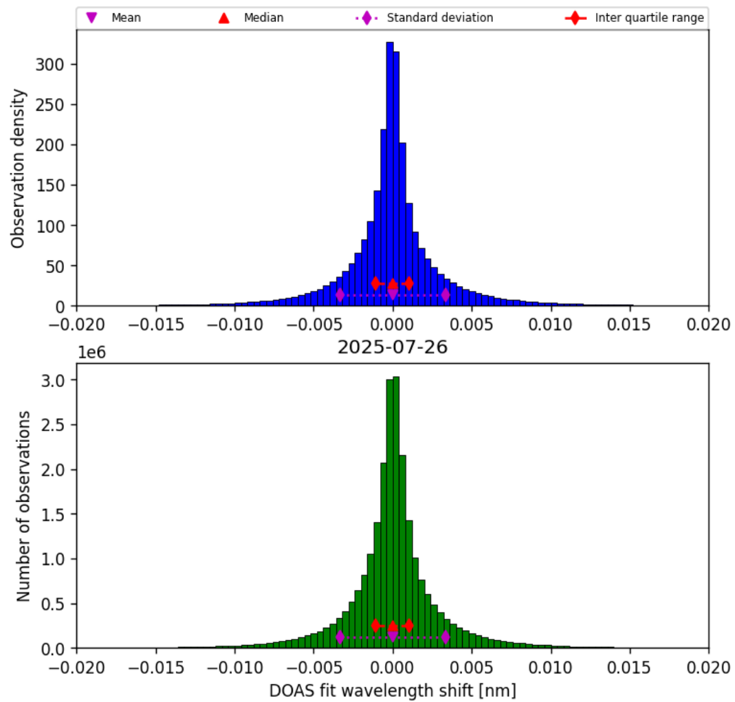
Figure 44: Histogram of “DOAS fit wavelength shift” for 2025-07-25 to 2025-07-27
