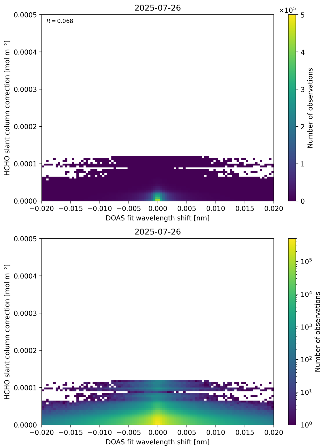
Figure 67: Scatter density plot of “DOAS fit wavelength shift” against “HCHO slant column correction” for 2025-07-25 to 2025-07-27.
