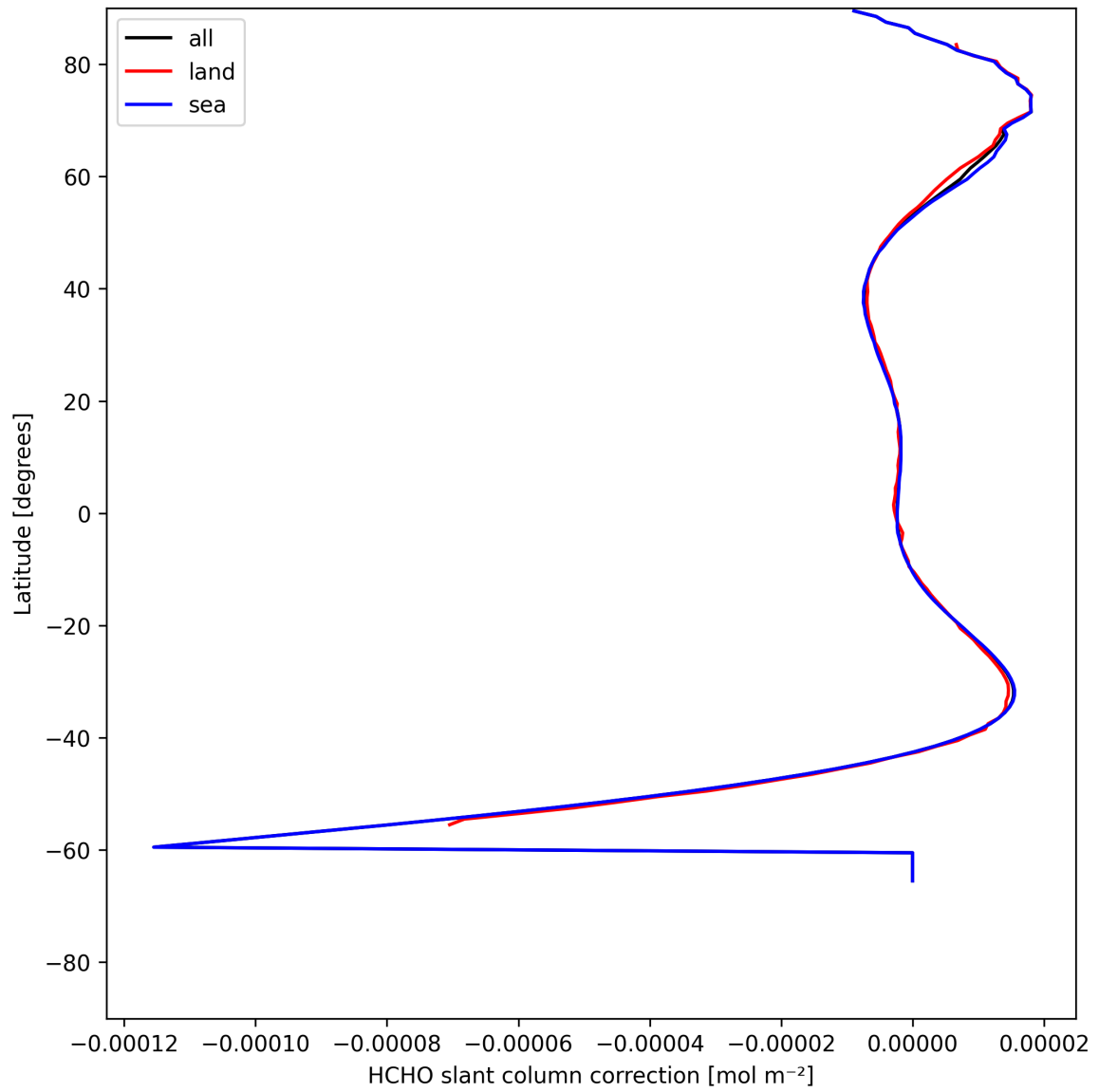
Figure 33: Zonal average of “HCHO slant column correction” for 2025-07-25 to 2025-07-27.
