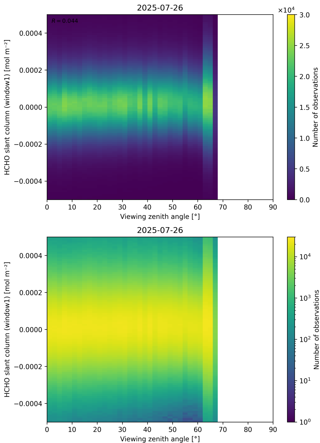
Figure 188: Scatter density plot of “Viewing zenith angle” against “HCHO slant column (window1)” for 2025-07-25 to 2025-07-27.
