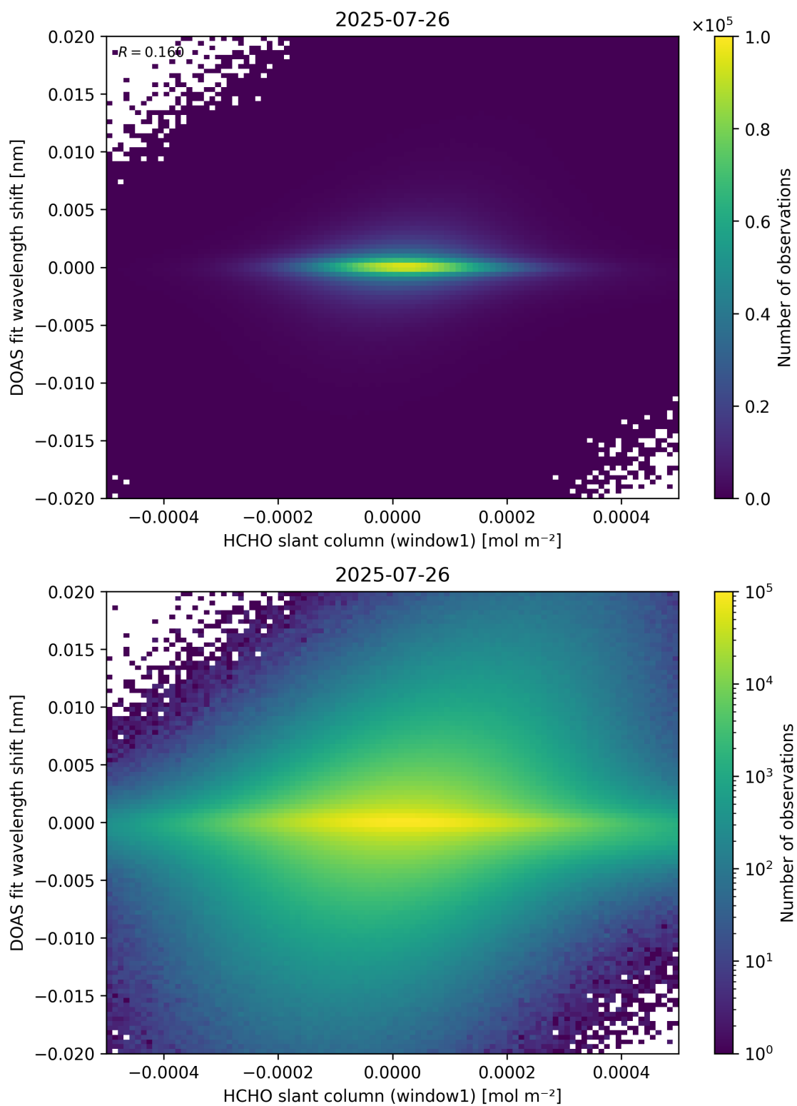
Figure 79: Scatter density plot of “HCHO slant column (window1)” against “DOAS fit wavelength shift” for 2025-07-25 to 2025-07-27.
