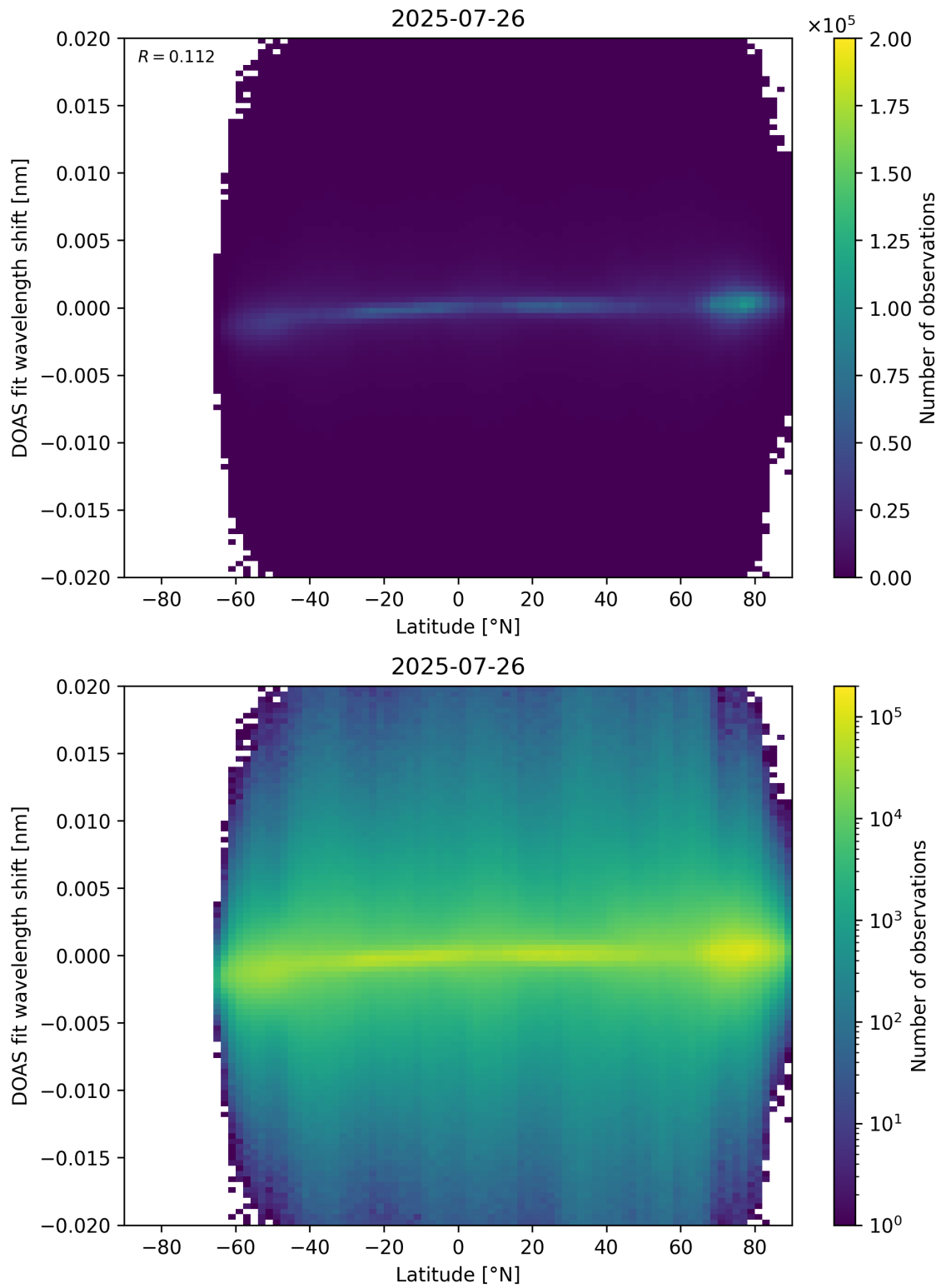
Figure 154: Scatter density plot of “Latitude” against “DOAS fit wavelength shift” for 2025-07-25 to 2025-07-27.
