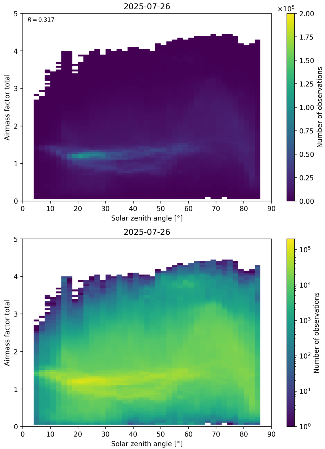
Figure 175: Scatter density plot of “Solar zenith angle” against “Airmass factor total” for 2025-07-25 to 2025-07-27.
