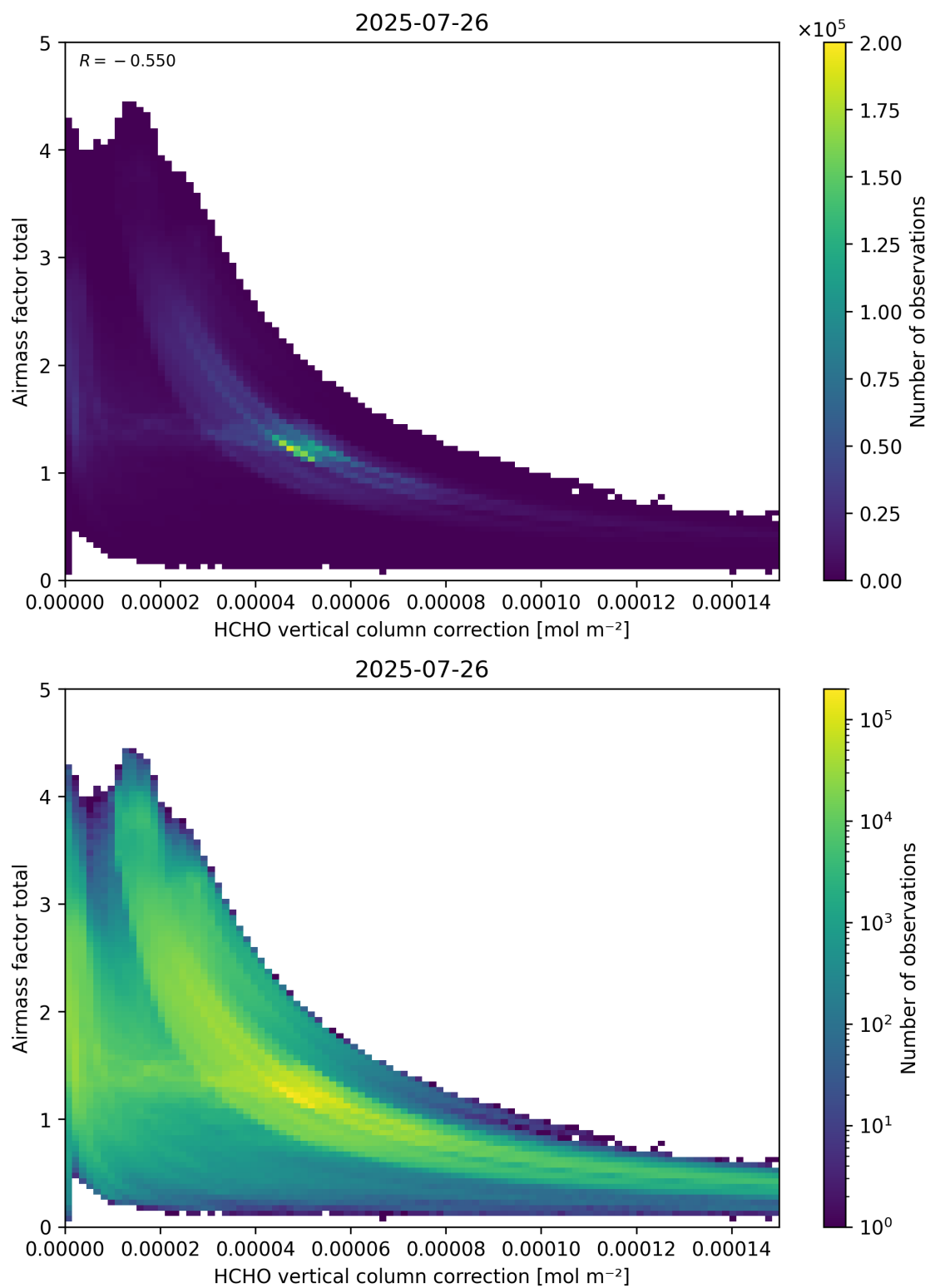
Figure 120: Scatter density plot of “HCHO vertical column correction” against “Airmass factor total” for 2025-07-25 to 2025-07-27.
