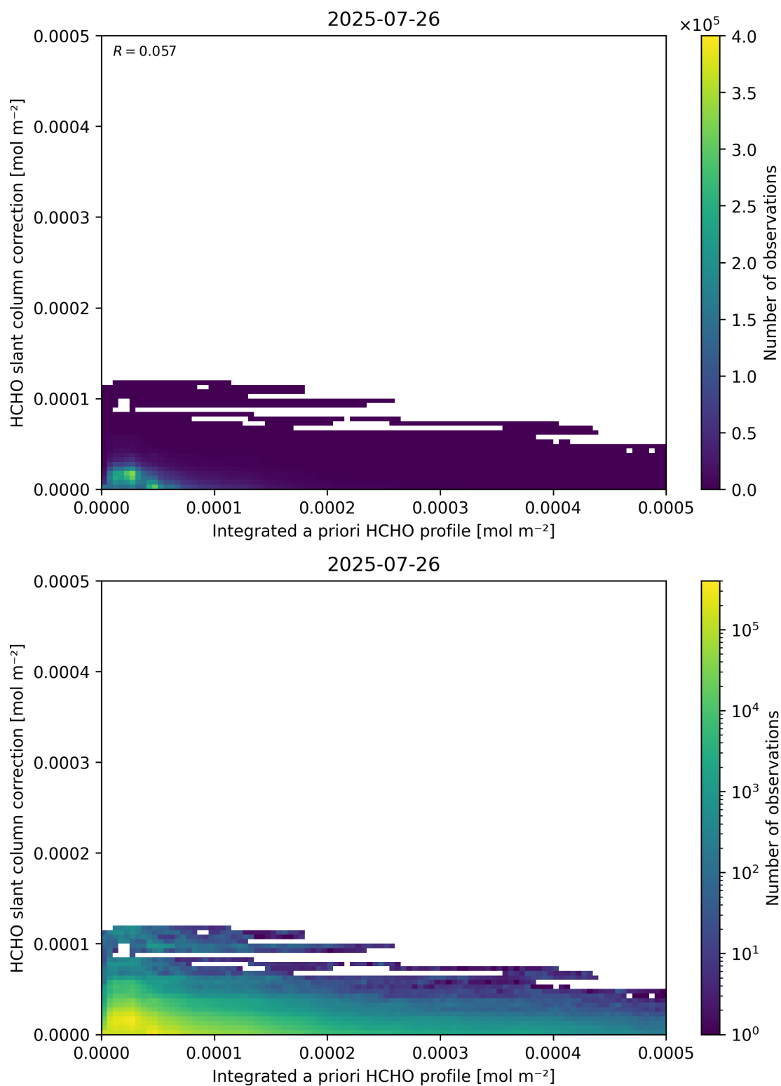
Figure 152: Scatter density plot of “Integrated a priori HCHO profile” against “HCHO slant column correction” for 2025-07-25 to 2025-07-27.
