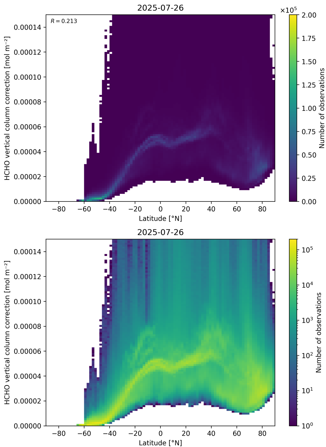
Figure 164: Scatter density plot of “Latitude” against “HCHO vertical column correction” for 2025-07-25 to 2025-07-27.
