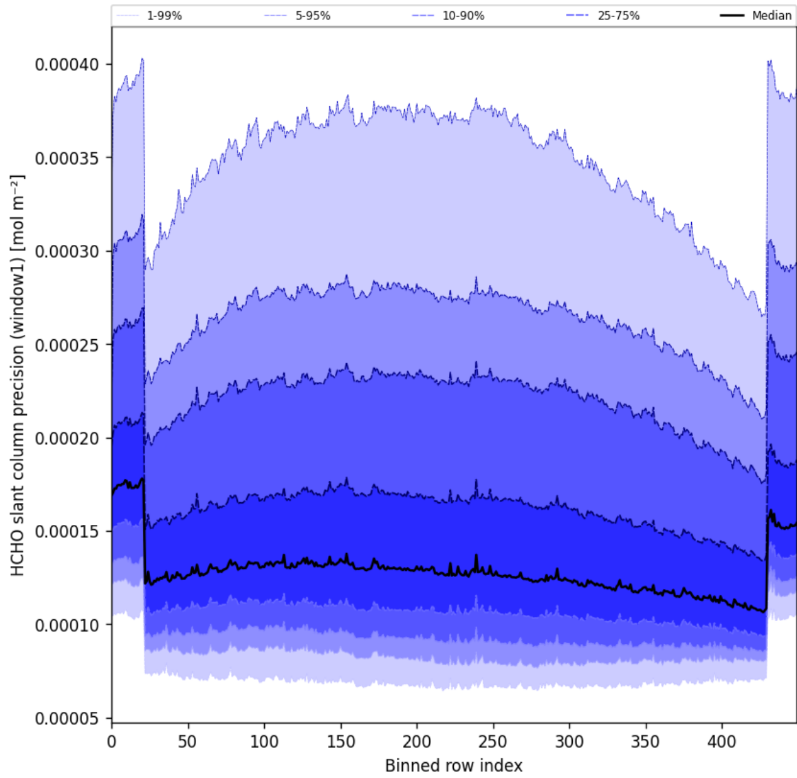
Figure 53: Along track statistics of “HCHO slant column precision (window1)” for 2025-07-25 to 2025-07-27
