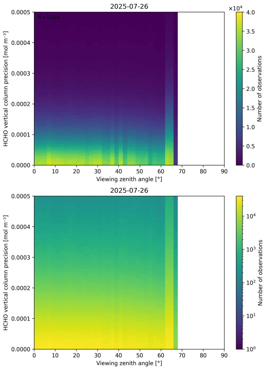
Figure 194: Scatter density plot of “Viewing zenith angle” against “HCHO vertical column precision” for 2025-07-25 to 2025-07-27.
