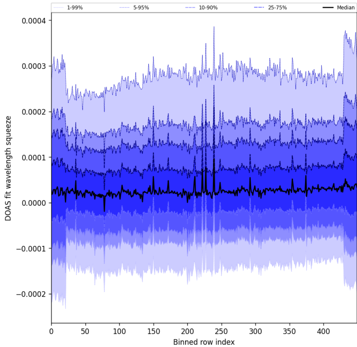
Figure 59: Along track statistics of “DOAS fit wavelength squeeze” for 2025-07-25 to 2025-07-27
