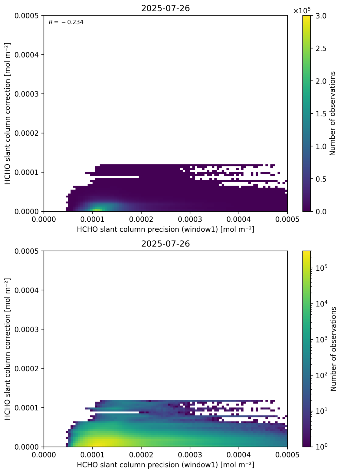
Figure 93: Scatter density plot of “HCHO slant column precision (window1)” against “HCHO slant column correction” for 2025-07-25 to 2025-07-27.
