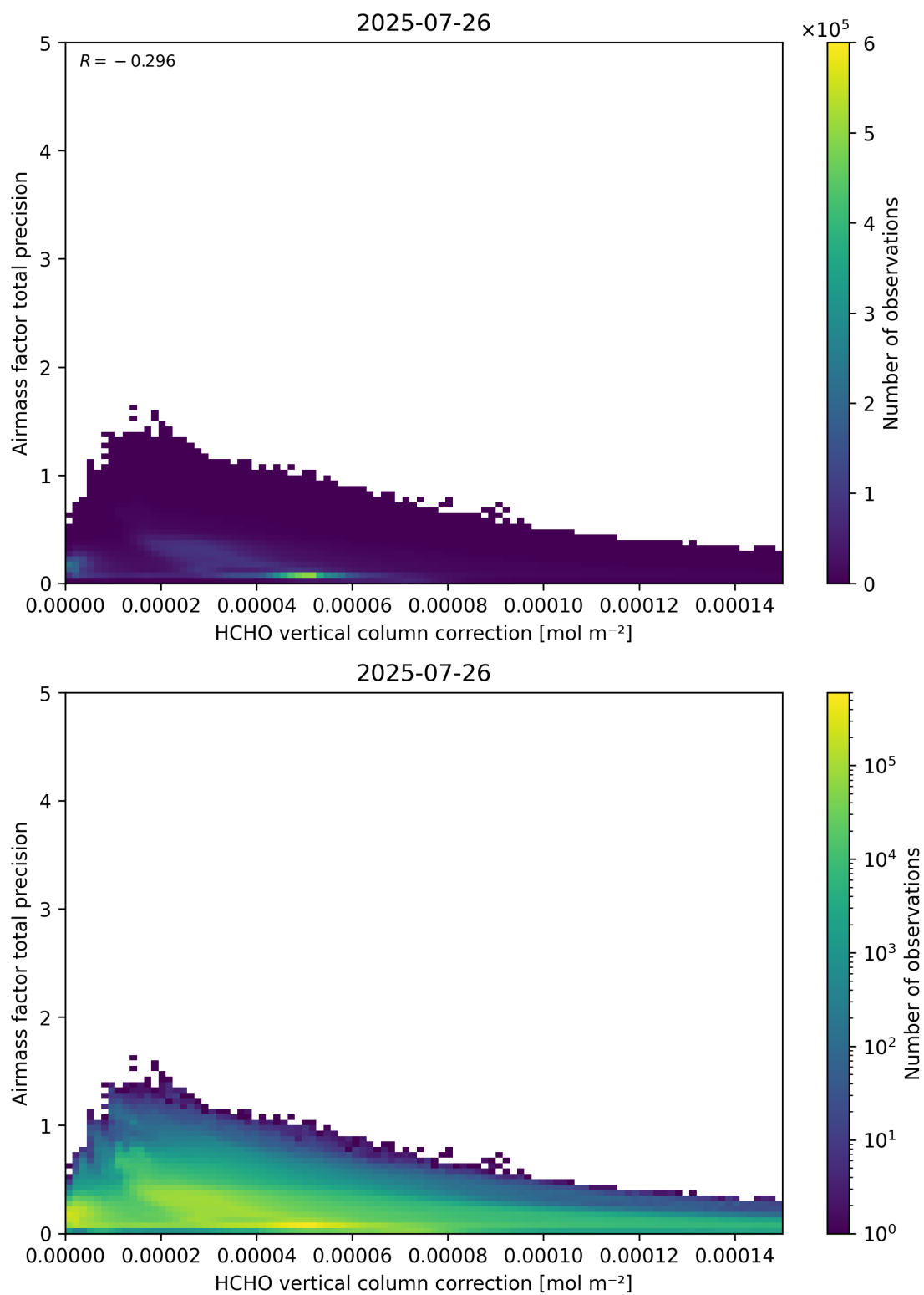
Figure 121: Scatter density plot of “HCHO vertical column correction” against “Airmass factor total precision” for 2025-07-25 to 2025-07-27.
