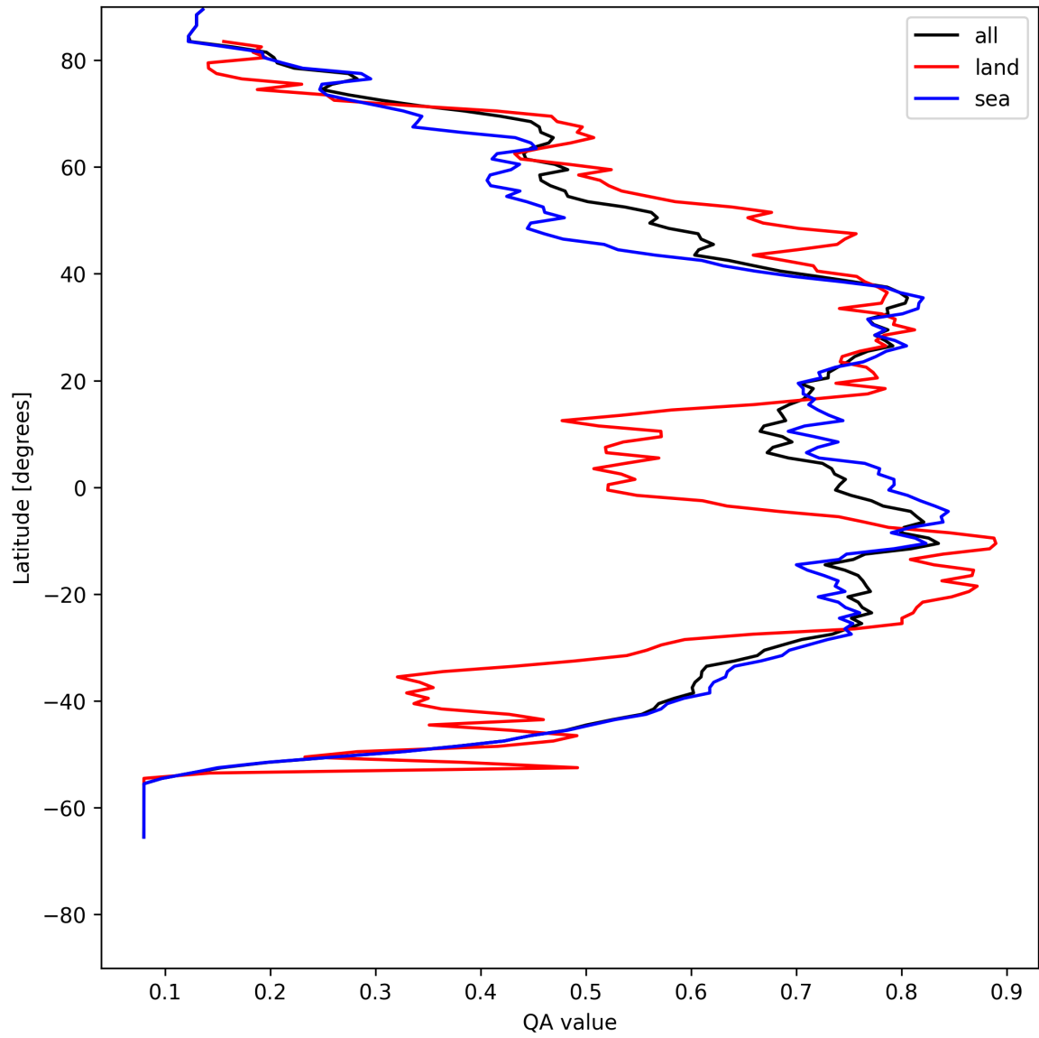
Figure 20: Zonal average of “QA value” for 2025-07-25 to 2025-07-27.
