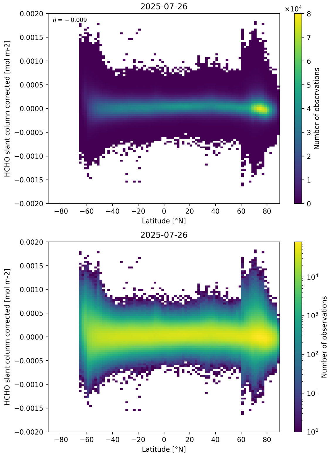
Figure 157: Scatter density plot of “Latitude” against “HCHO slant column corrected” for 2025-07-25 to 2025-07-27.
