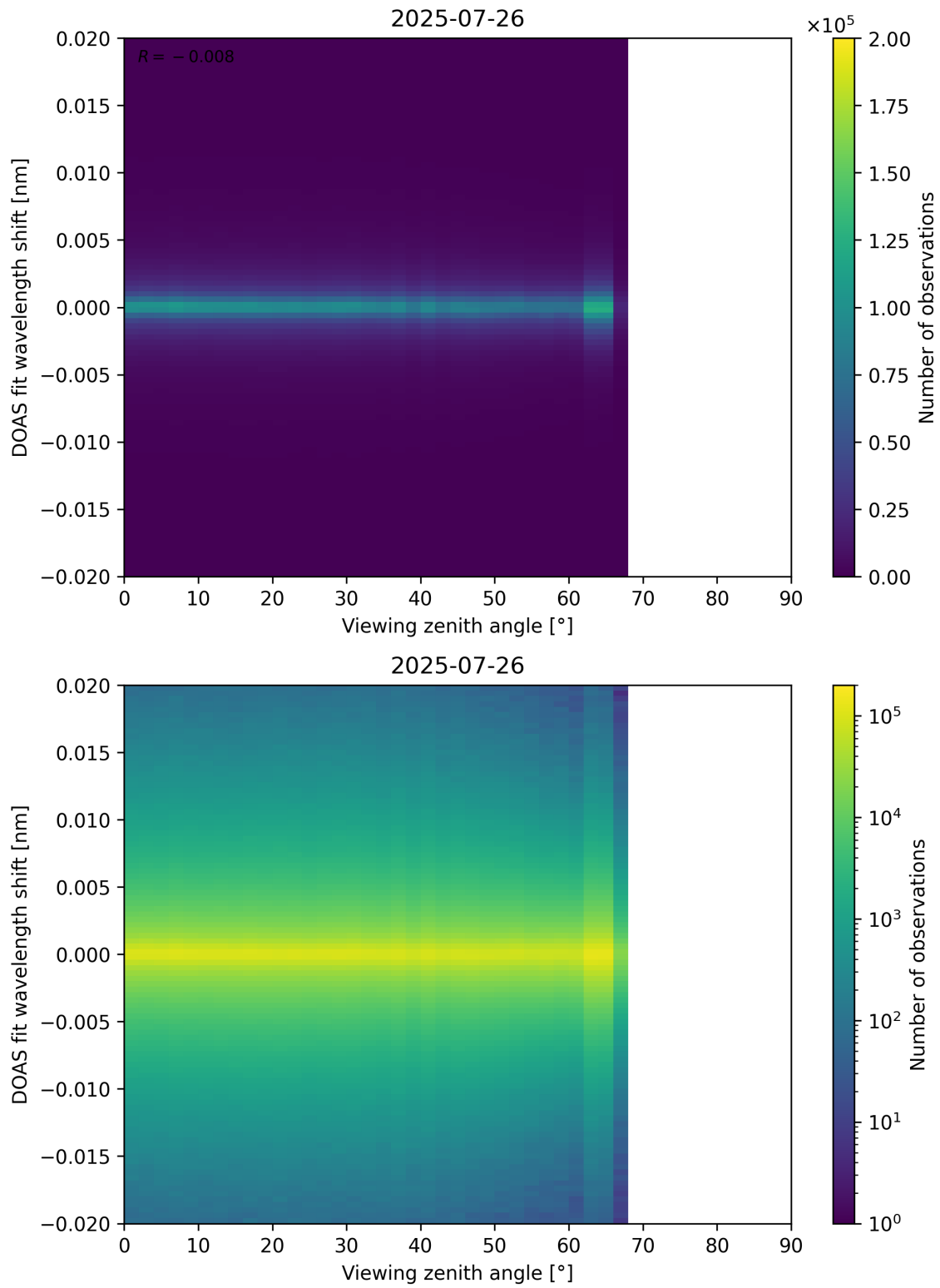
Figure 183: Scatter density plot of “Viewing zenith angle” against “DOAS fit wavelength shift” for 2025-07-25 to 2025-07-27.
