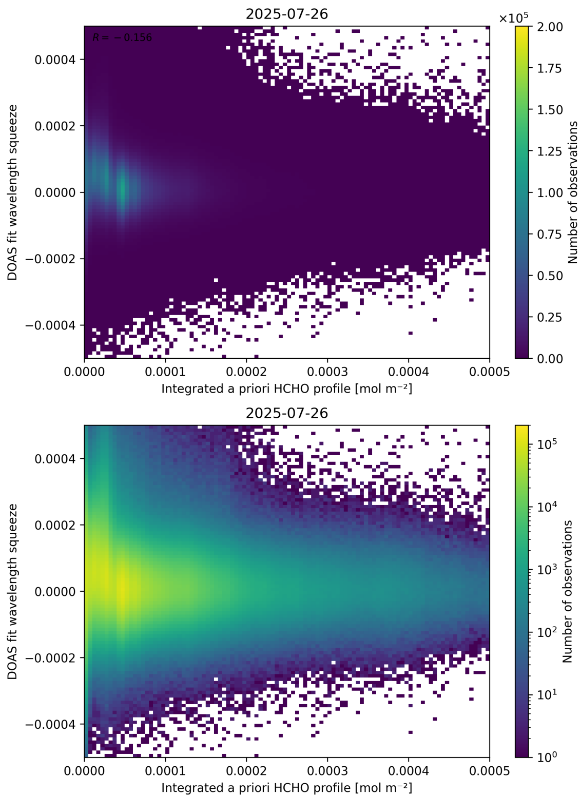
Figure 150: Scatter density plot of “Integrated a priori HCHO profile” against “DOAS fit wavelength squeeze” for 2025-07-25 to 2025-07-27.
