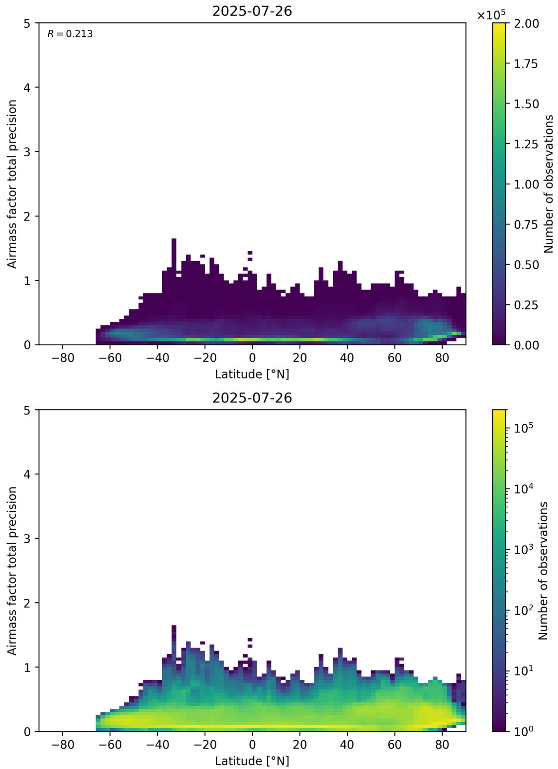
Figure 162: Scatter density plot of “Latitude” against “Airmass factor total precision” for 2025-07-25 to 2025-07-27.
