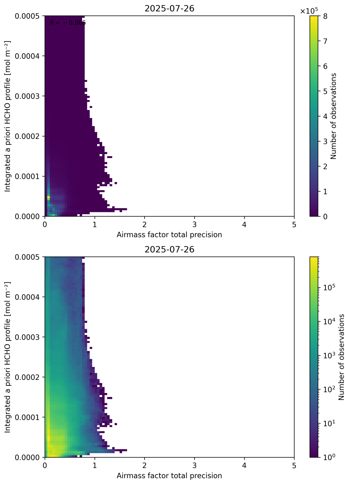
Figure 111: Scatter density plot of “Airmass factor total precision” against “Integrated a priori HCHO profile” for 2025-07-25 to 2025-07-27.
