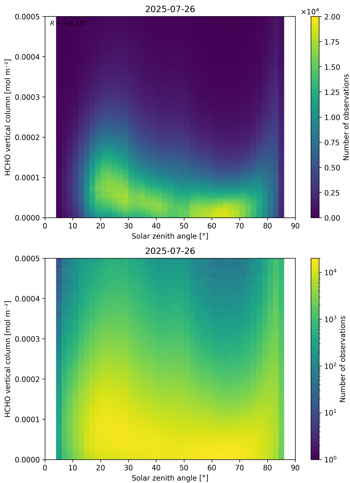
Figure 177: Scatter density plot of “Solar zenith angle” against “HCHO vertical column” for 2025-07-25 to 2025-07-27.
