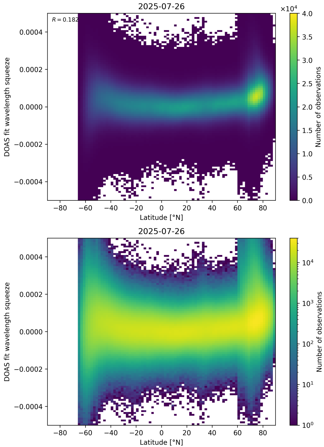
Figure 155: Scatter density plot of “Latitude” against “DOAS fit wavelength squeeze” for 2025-07-25 to 2025-07-27.
