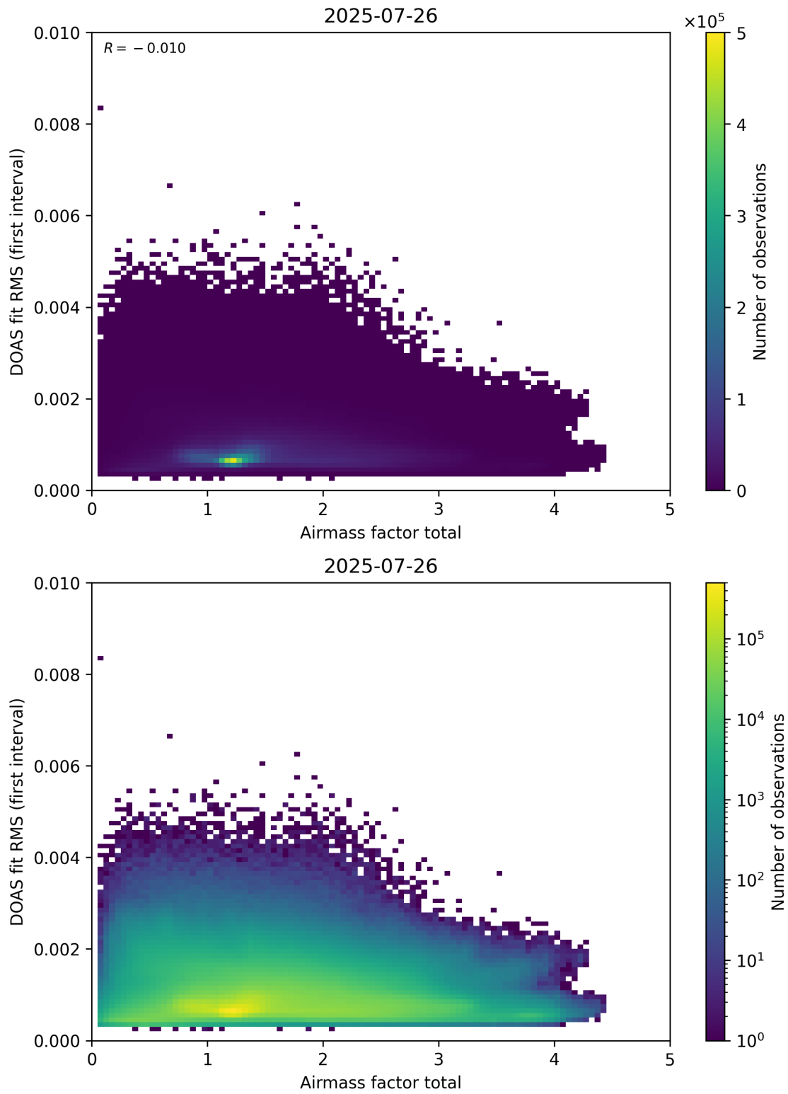
Figure 97: Scatter density plot of “Airmass factor total” against “DOAS fit RMS (first interval)” for 2025-07-25 to 2025-07-27.
