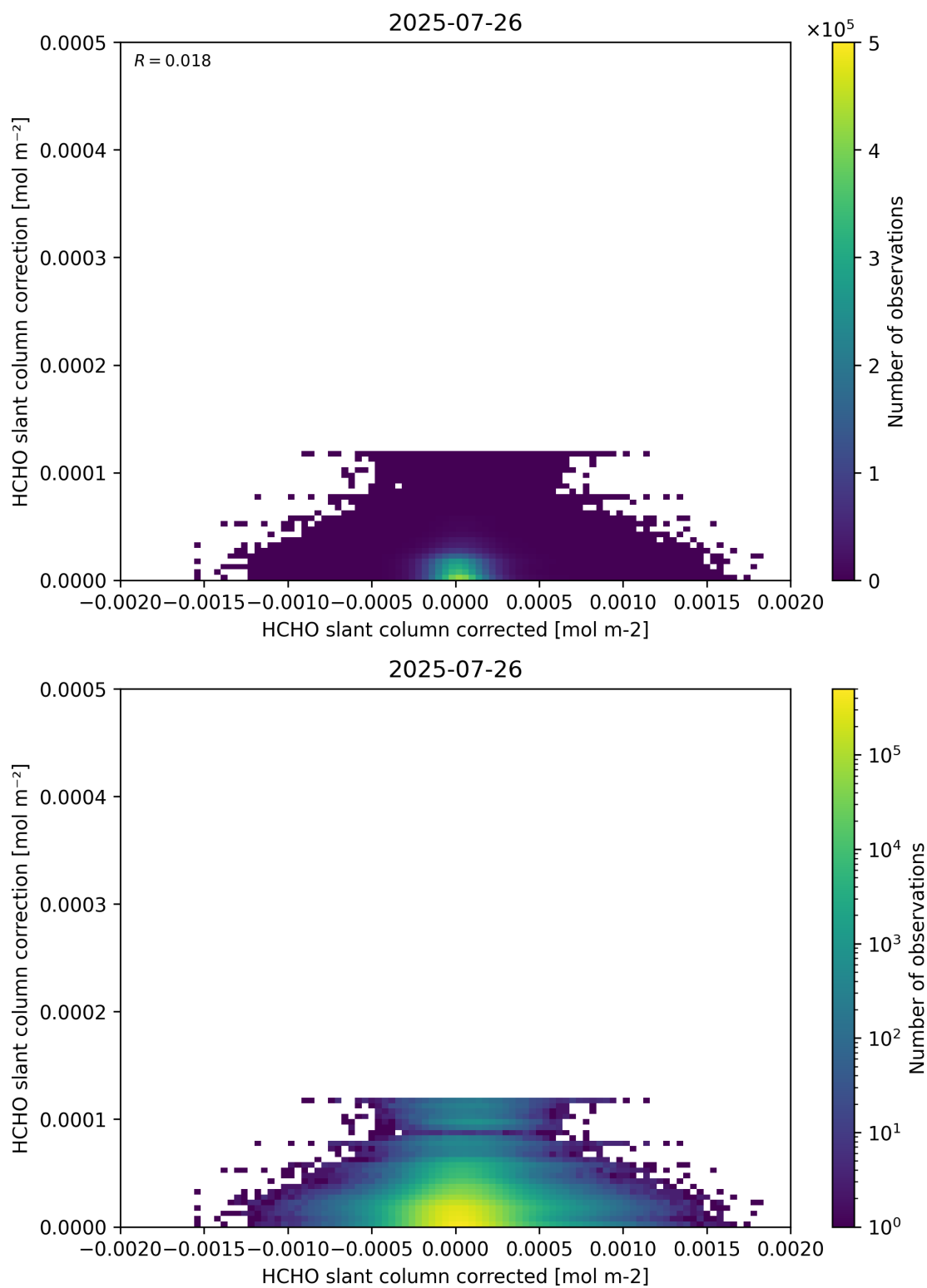
Figure 77: Scatter density plot of “HCHO slant column corrected” against “HCHO slant column correction” for 2025-07-25 to 2025-07-27.
