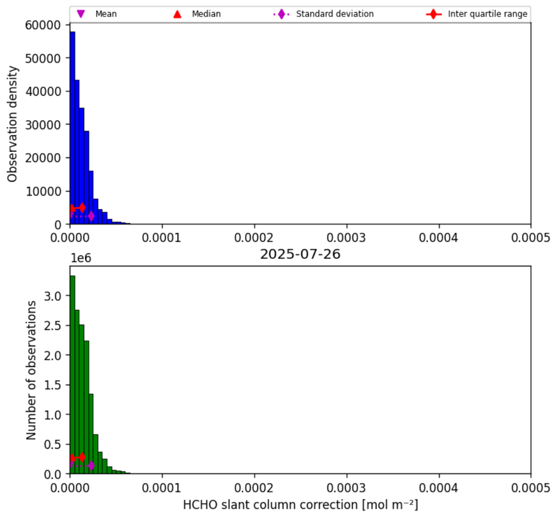
Figure 47: Histogram of “HCHO slant column correction” for 2025-07-25 to 2025-07-27
