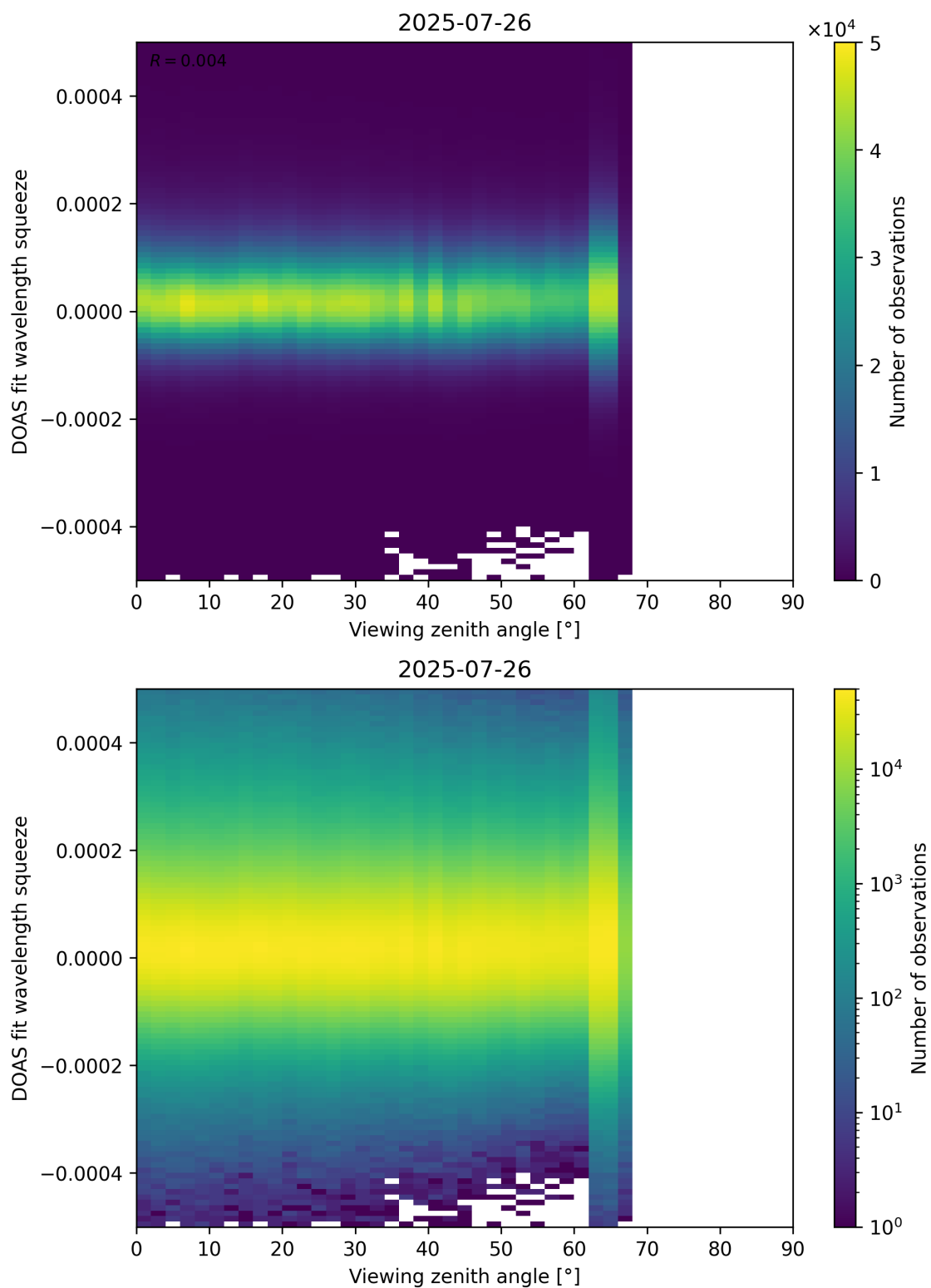
Figure 184: Scatter density plot of “Viewing zenith angle” against “DOAS fit wavelength squeeze” for 2025-07-25 to 2025-07-27.
