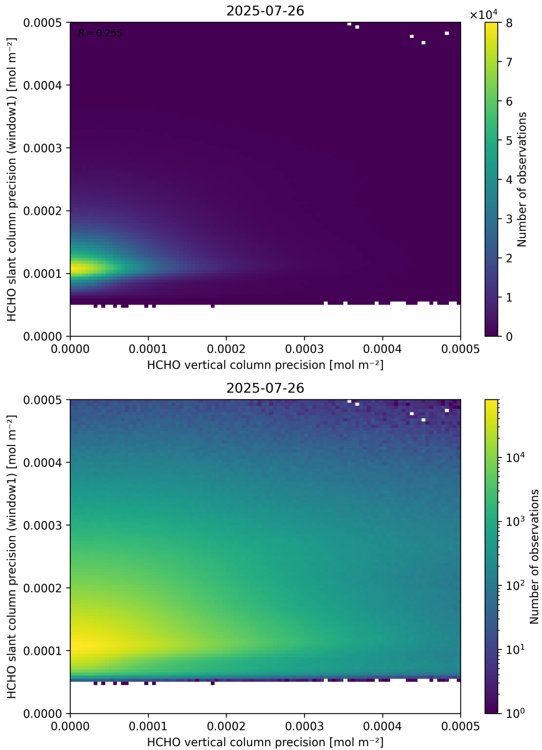
Figure 143: Scatter density plot of “HCHO vertical column precision” against “HCHO slant column precision (window1)” for 2025-07-25 to 2025-07-27.
