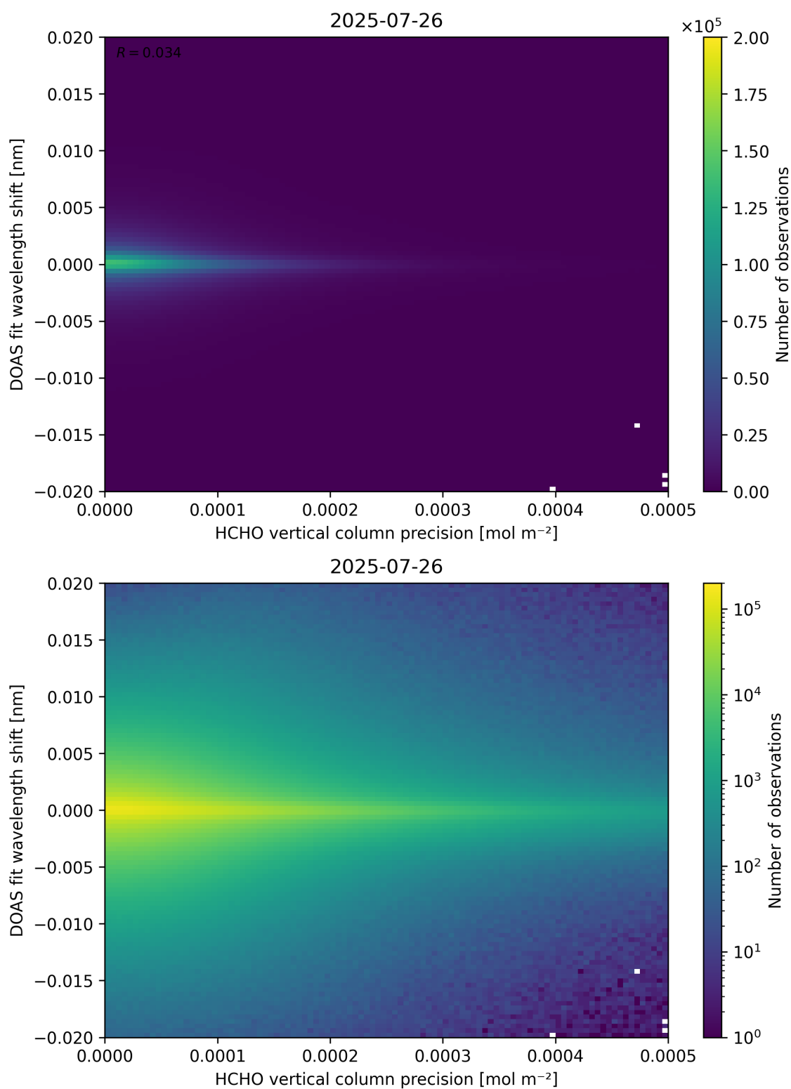
Figure 137: Scatter density plot of “HCHO vertical column precision” against “DOAS fit wavelength shift” for 2025-07-25 to 2025-07-27.
