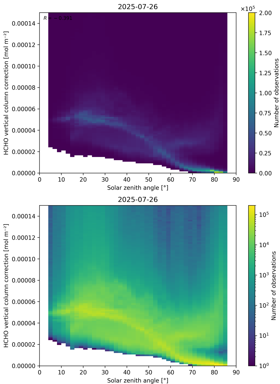
Figure 178: Scatter density plot of “Solar zenith angle” against “HCHO vertical column correction” for 2025-07-25 to 2025-07-27.
