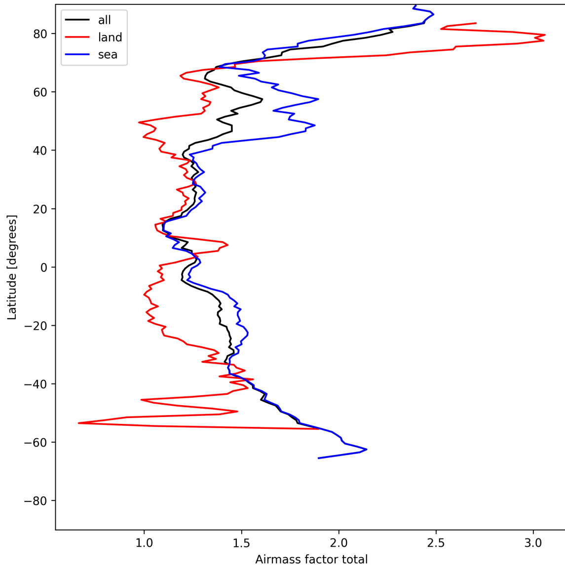
Figure 26: Zonal average of “Airmass factor total” for 2025-07-25 to 2025-07-27.
