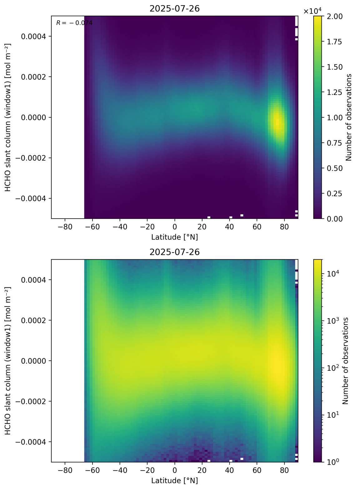
Figure 159: Scatter density plot of “Latitude” against “HCHO slant column (window1)” for 2025-07-25 to 2025-07-27.
