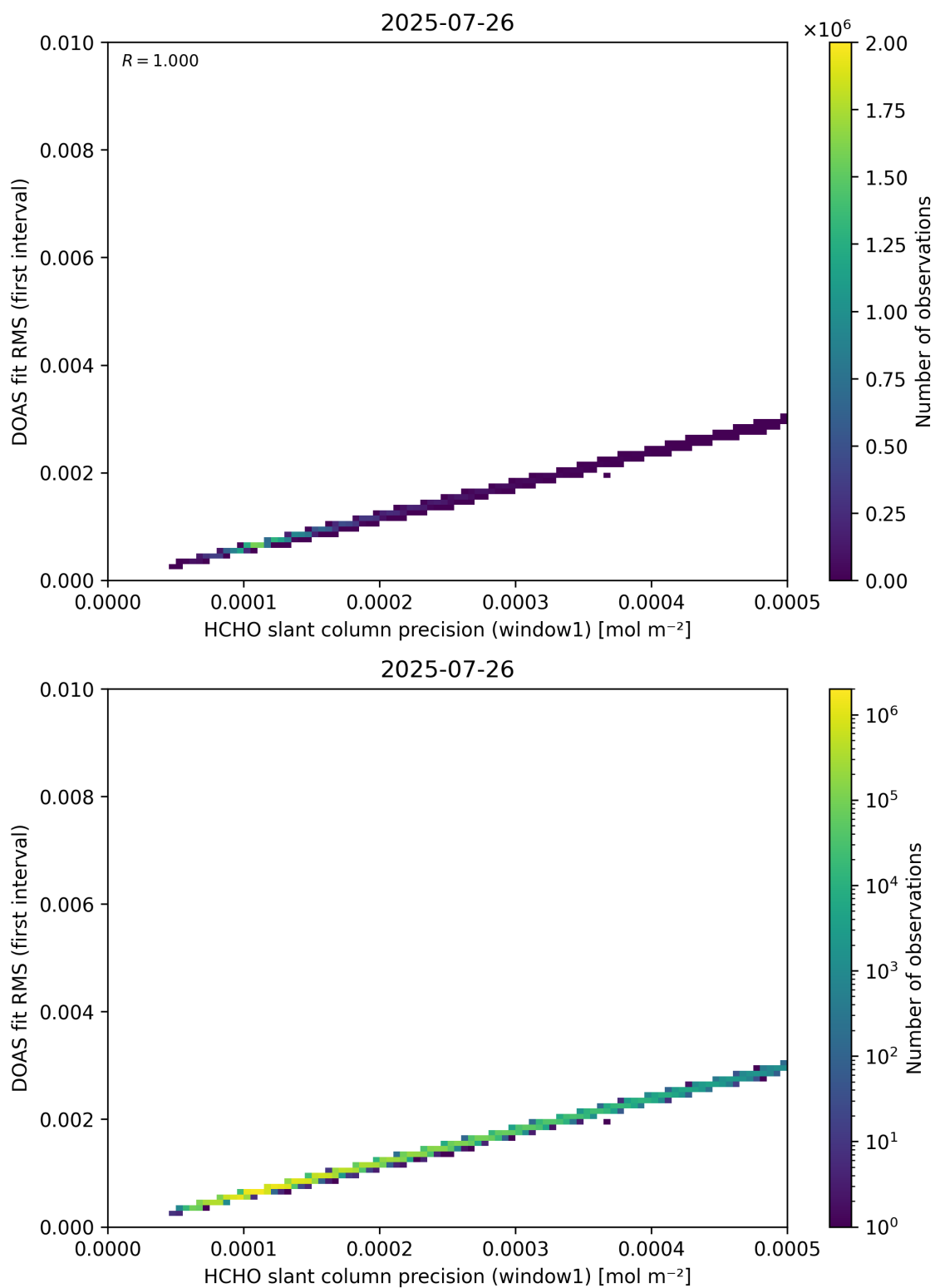
Figure 88: Scatter density plot of “HCHO slant column precision (window1)” against “DOAS fit RMS (first interval)” for 2025-07-25 to 2025-07-27.
