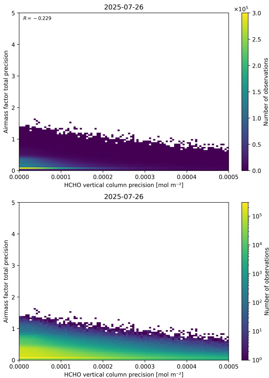
Figure 145: Scatter density plot of “HCHO vertical column precision” against “Airmass factor total precision” for 2025-07-25 to 2025-07-27.
