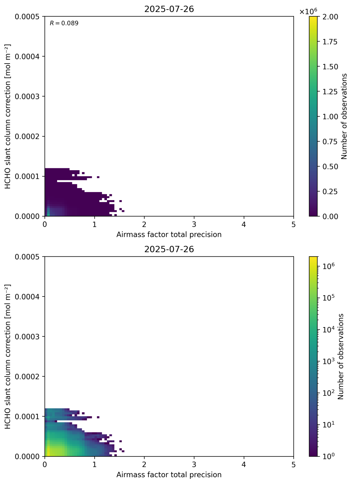
Figure 110: Scatter density plot of “Airmass factor total precision” against “HCHO slant column correction” for 2025-07-25 to 2025-07-27.
