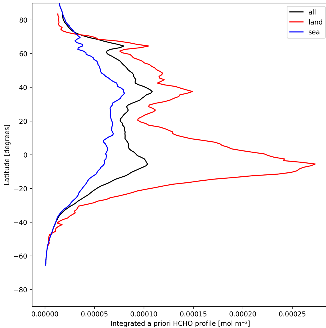
Figure 29: Zonal average of “Integrated a priori HCHO profile” for 2025-07-25 to 2025-07-27.
