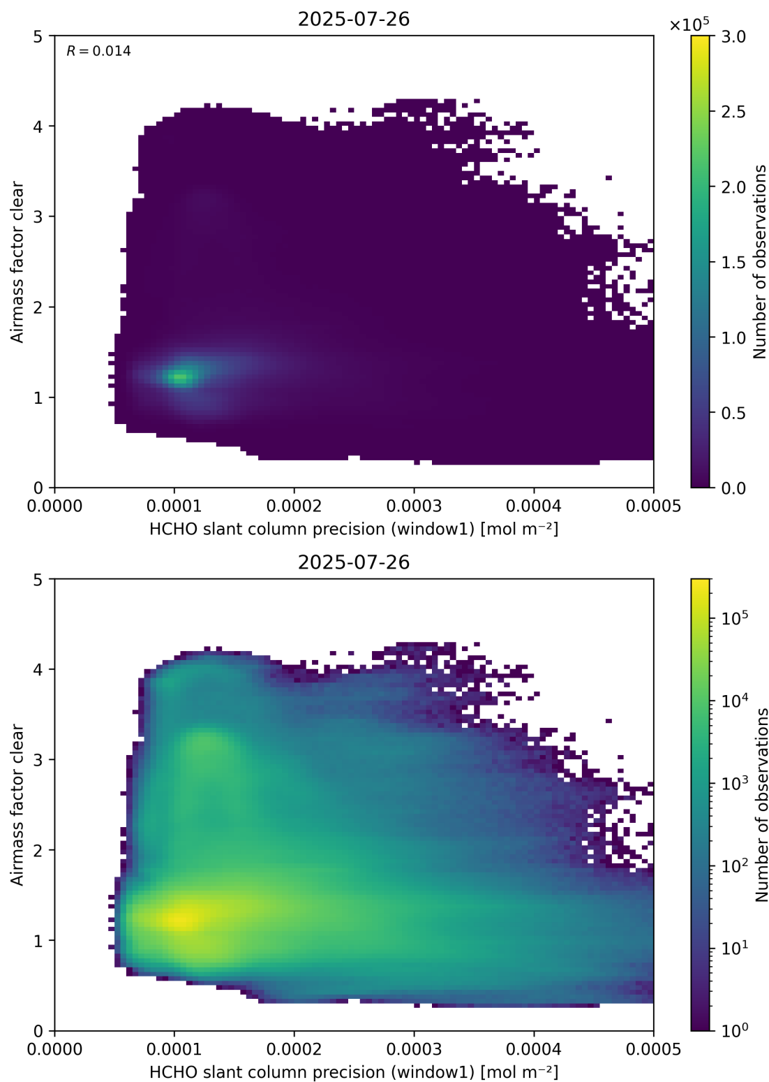
Figure 91: Scatter density plot of “HCHO slant column precision (window1)” against “Airmass factor clear” for 2025-07-25 to 2025-07-27.
