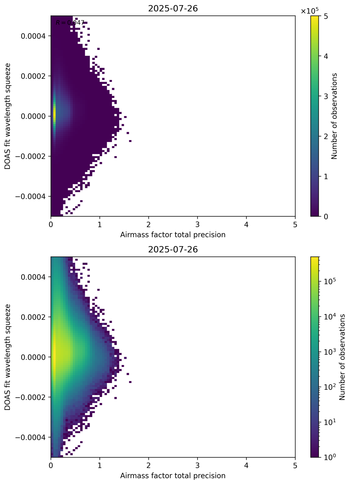
Figure 107: Scatter density plot of “Airmass factor total precision” against “DOAS fit wavelength squeeze” for 2025-07-25 to 2025-07-27.
