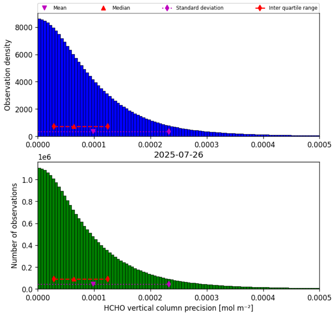
Figure 36: Histogram of “HCHO vertical column precision” for 2025-07-25 to 2025-07-27
