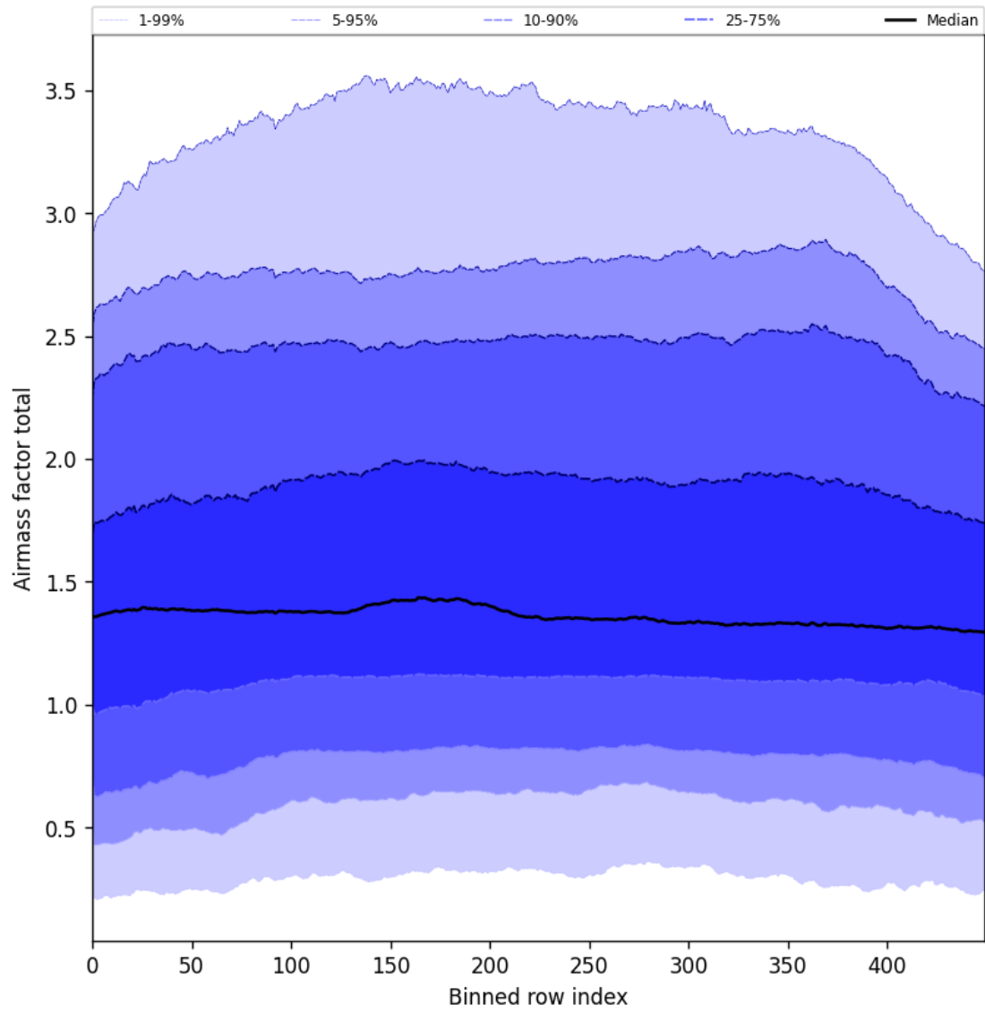
Figure 54: Along track statistics of “Airmass factor total” for 2025-07-25 to 2025-07-27
