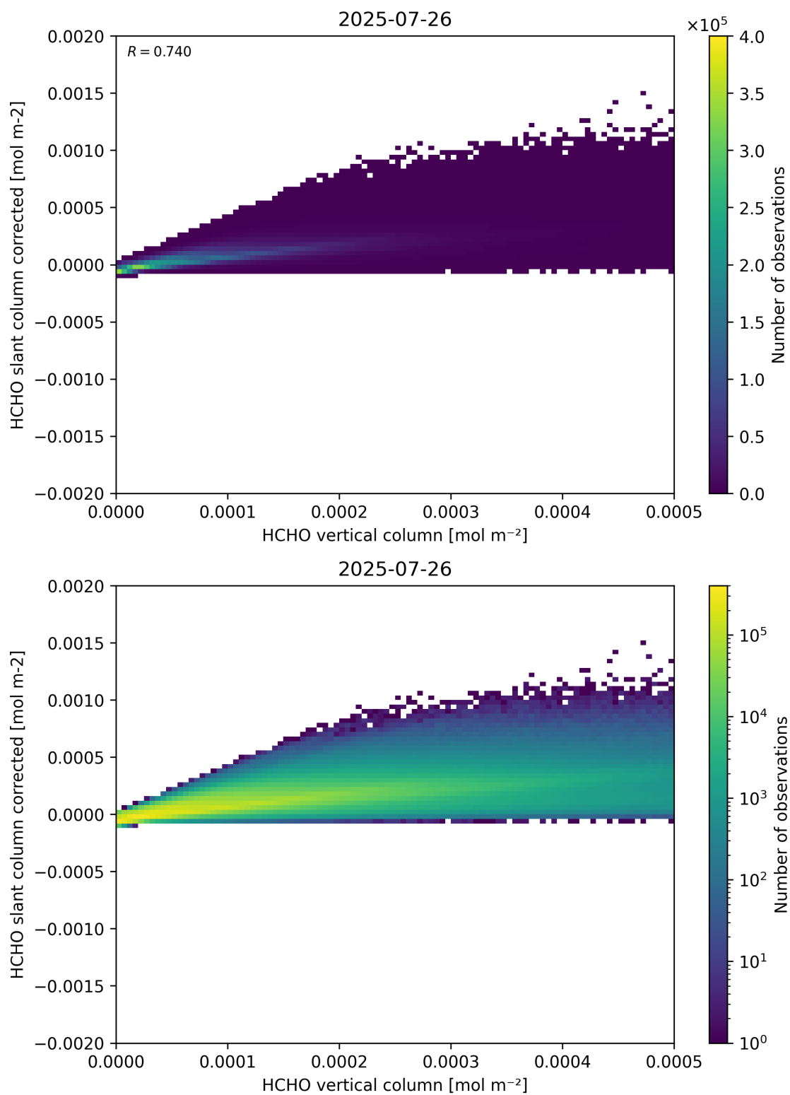
Figure 127: Scatter density plot of “HCHO vertical column” against “HCHO slant column corrected” for 2025-07-25 to 2025-07-27.
