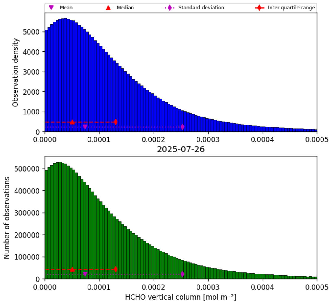
Figure 35: Histogram of “HCHO vertical column” for 2025-07-25 to 2025-07-27
