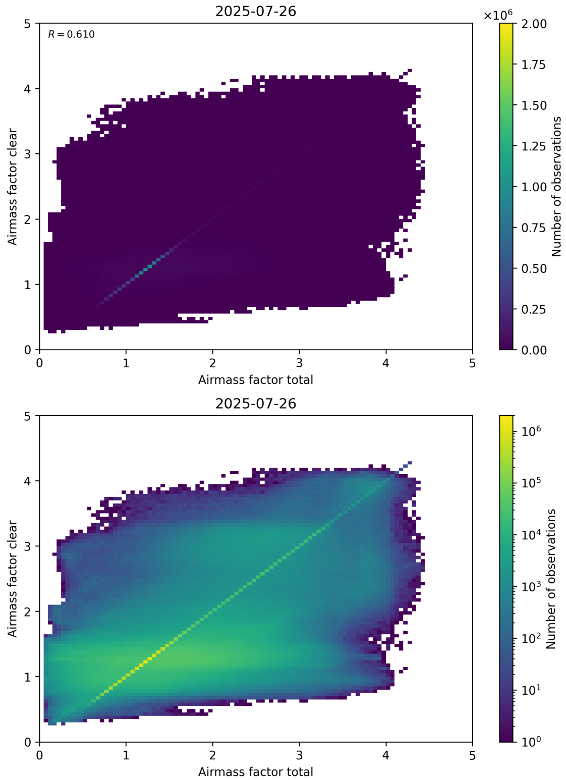
Figure 100: Scatter density plot of “Airmass factor total” against “Airmass factor clear” for 2025-07-25 to 2025-07-27.
