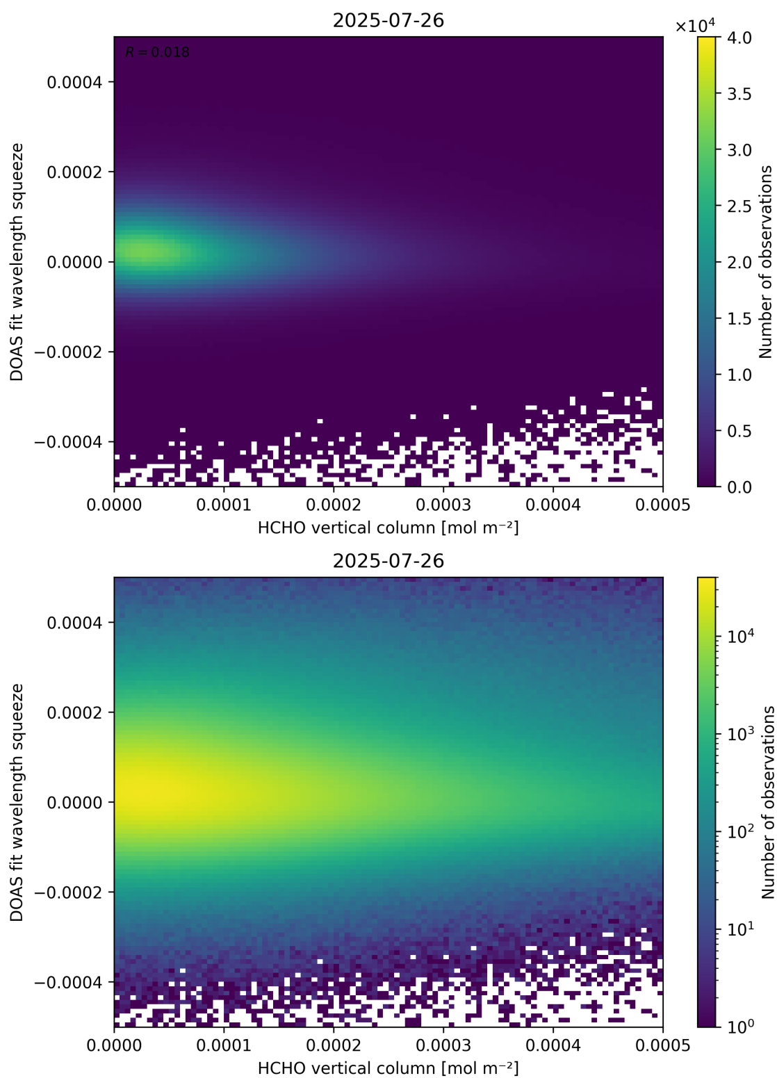
Figure 125: Scatter density plot of “HCHO vertical column” against “DOAS fit wavelength squeeze” for 2025-07-25 to 2025-07-27.
