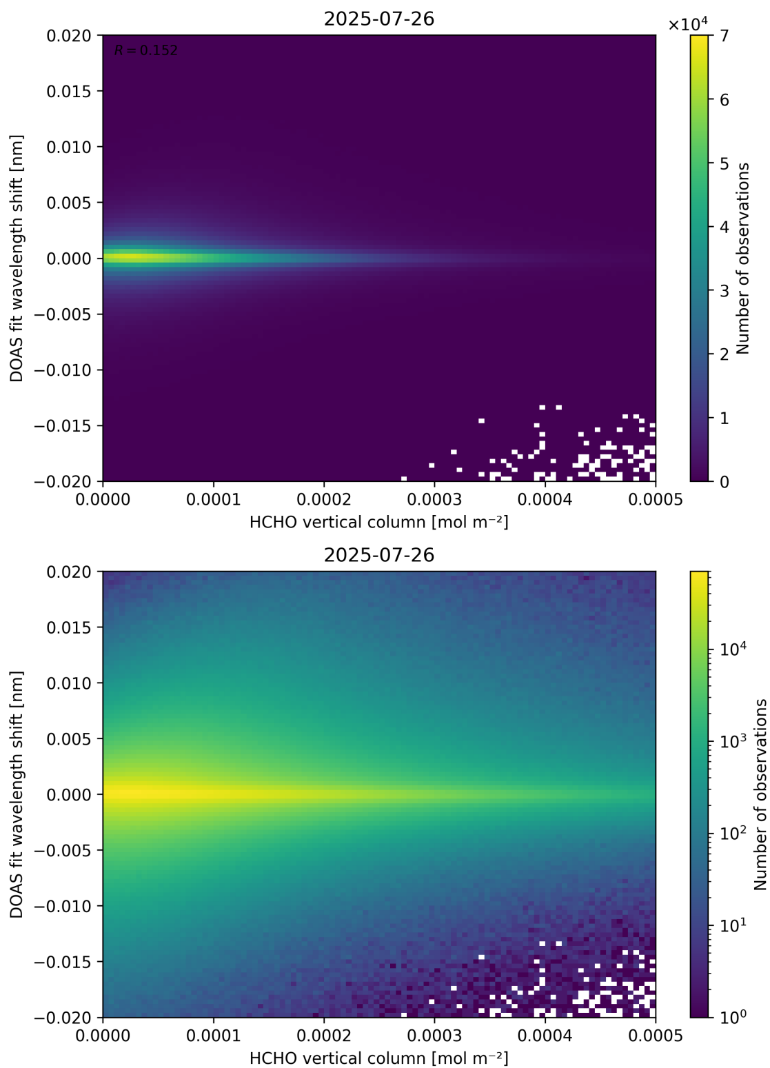
Figure 124: Scatter density plot of “HCHO vertical column” against “DOAS fit wavelength shift” for 2025-07-25 to 2025-07-27.
