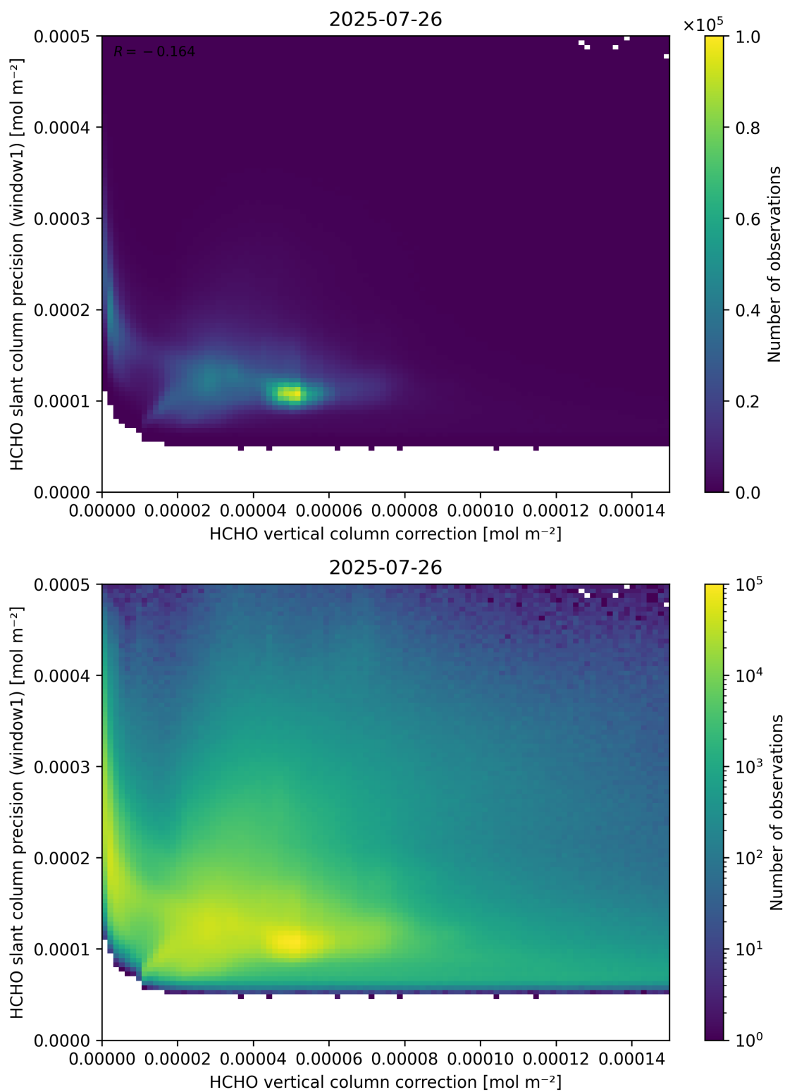
Figure 119: Scatter density plot of “HCHO vertical column correction” against “HCHO slant column precision (window1)” for 2025-07-25 to 2025-07-27.
