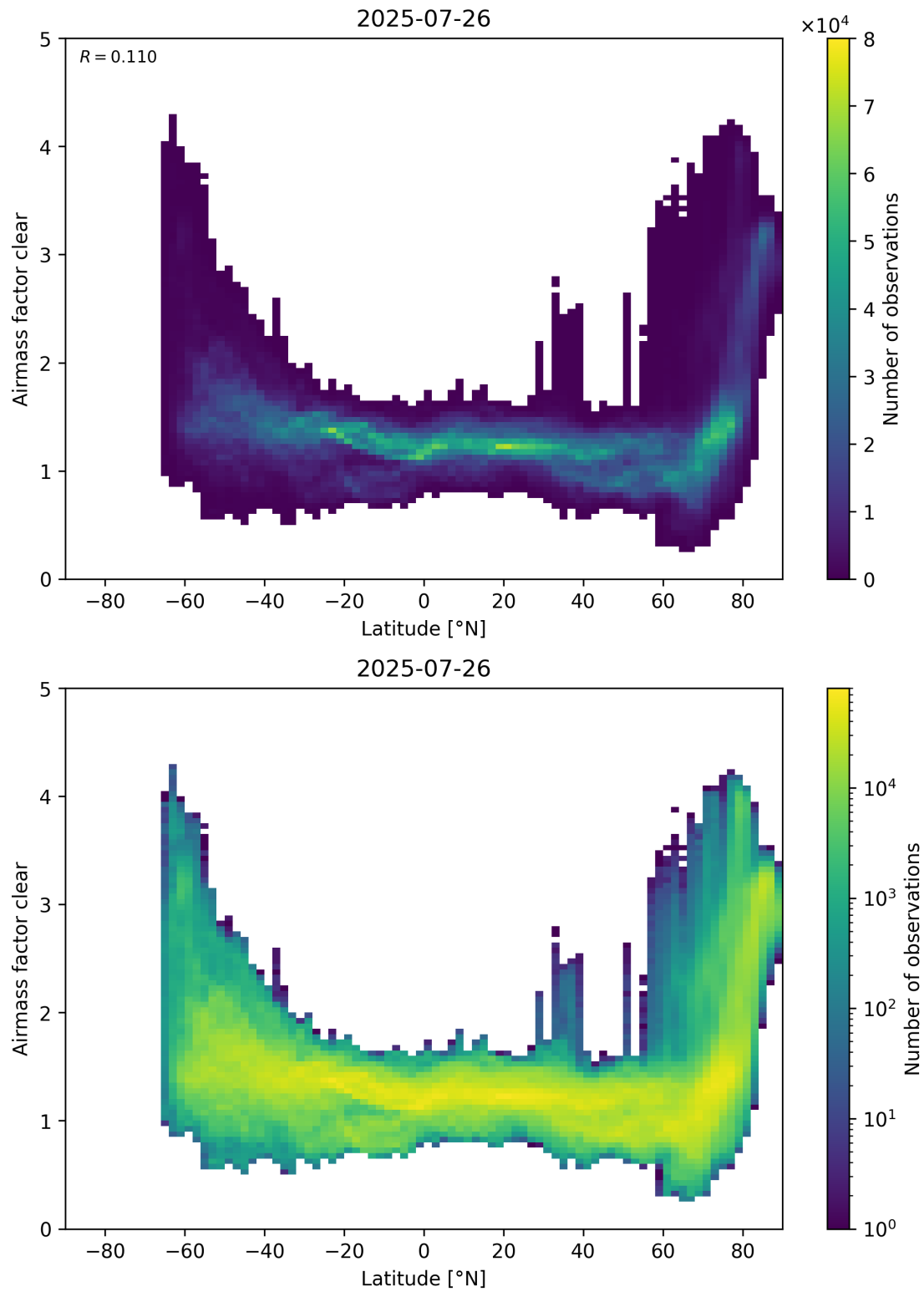
Figure 156: Scatter density plot of “Latitude” against “Airmass factor clear” for 2025-07-25 to 2025-07-27.
