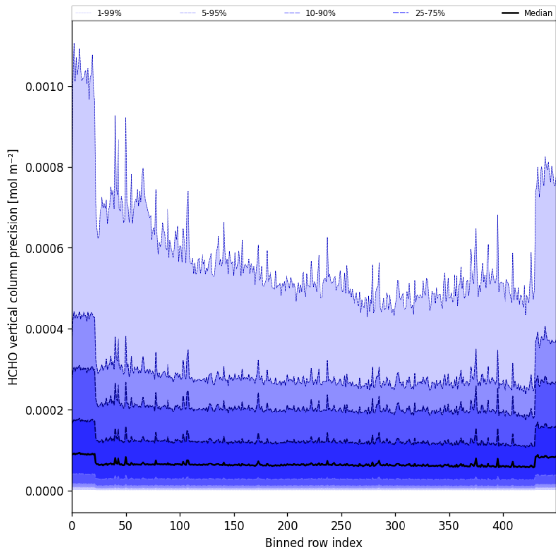
Figure 50: Along track statistics of “HCHO vertical column precision” for 2025-07-25 to 2025-07-27
