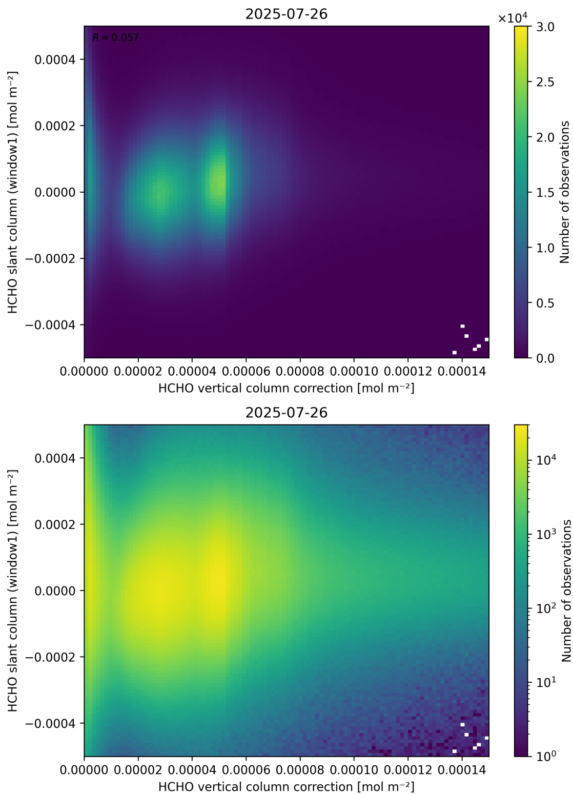
Figure 118: Scatter density plot of “HCHO vertical column correction” against “HCHO slant column (window1)” for 2025-07-25 to 2025-07-27.
