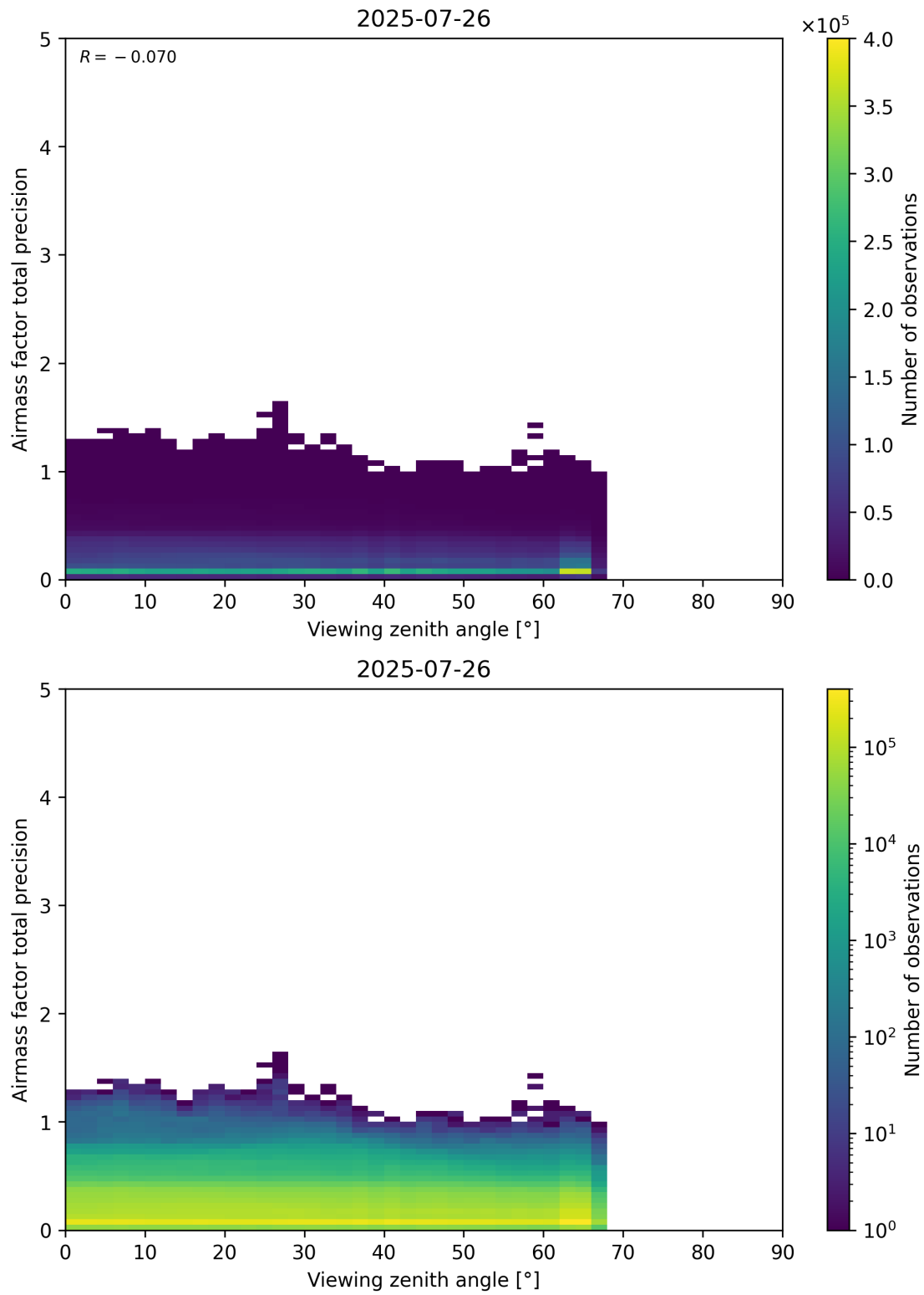
Figure 191: Scatter density plot of “Viewing zenith angle” against “Airmass factor total precision” for 2025-07-25 to 2025-07-27.
