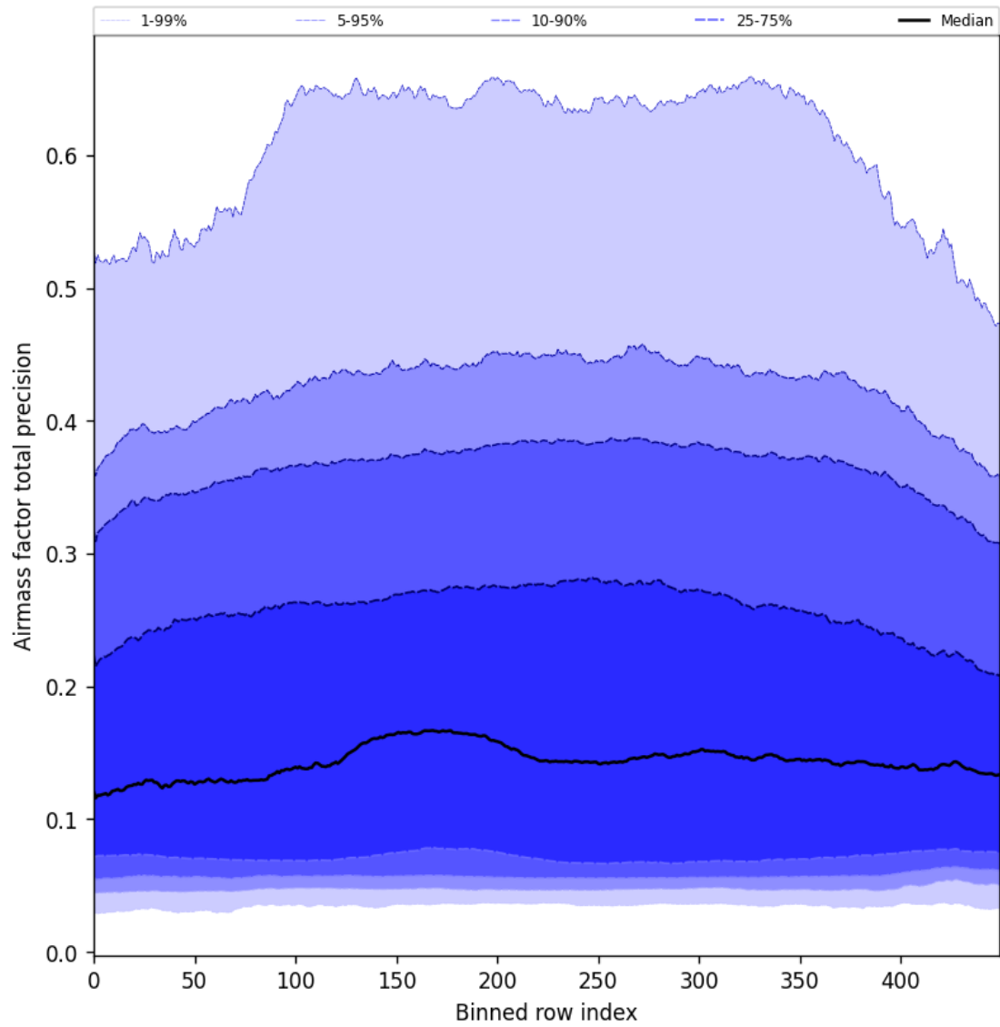
Figure 55: Along track statistics of “Airmass factor total precision” for 2025-07-25 to 2025-07-27
