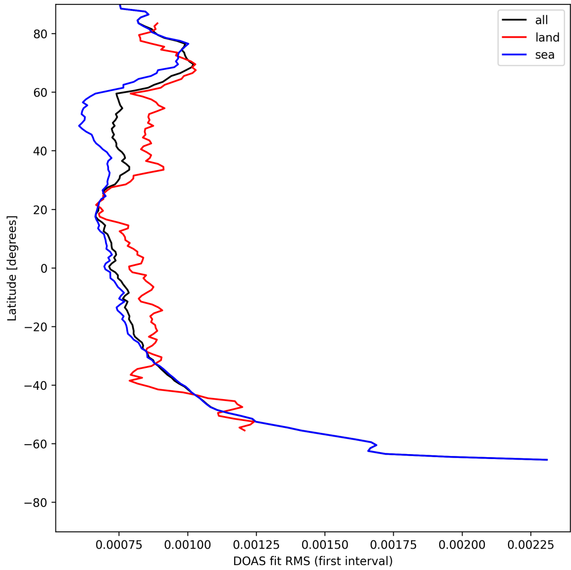
Figure 32: Zonal average of "DOAS fit RMS (first interval)" for 2025-07-25 to 2025-07-27.
