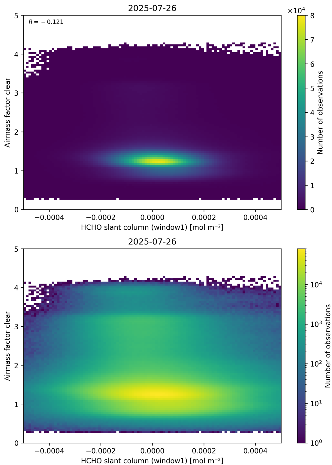
Figure 81: Scatter density plot of “HCHO slant column (window1)” against “Airmass factor clear” for 2025-07-25 to 2025-07-27.
