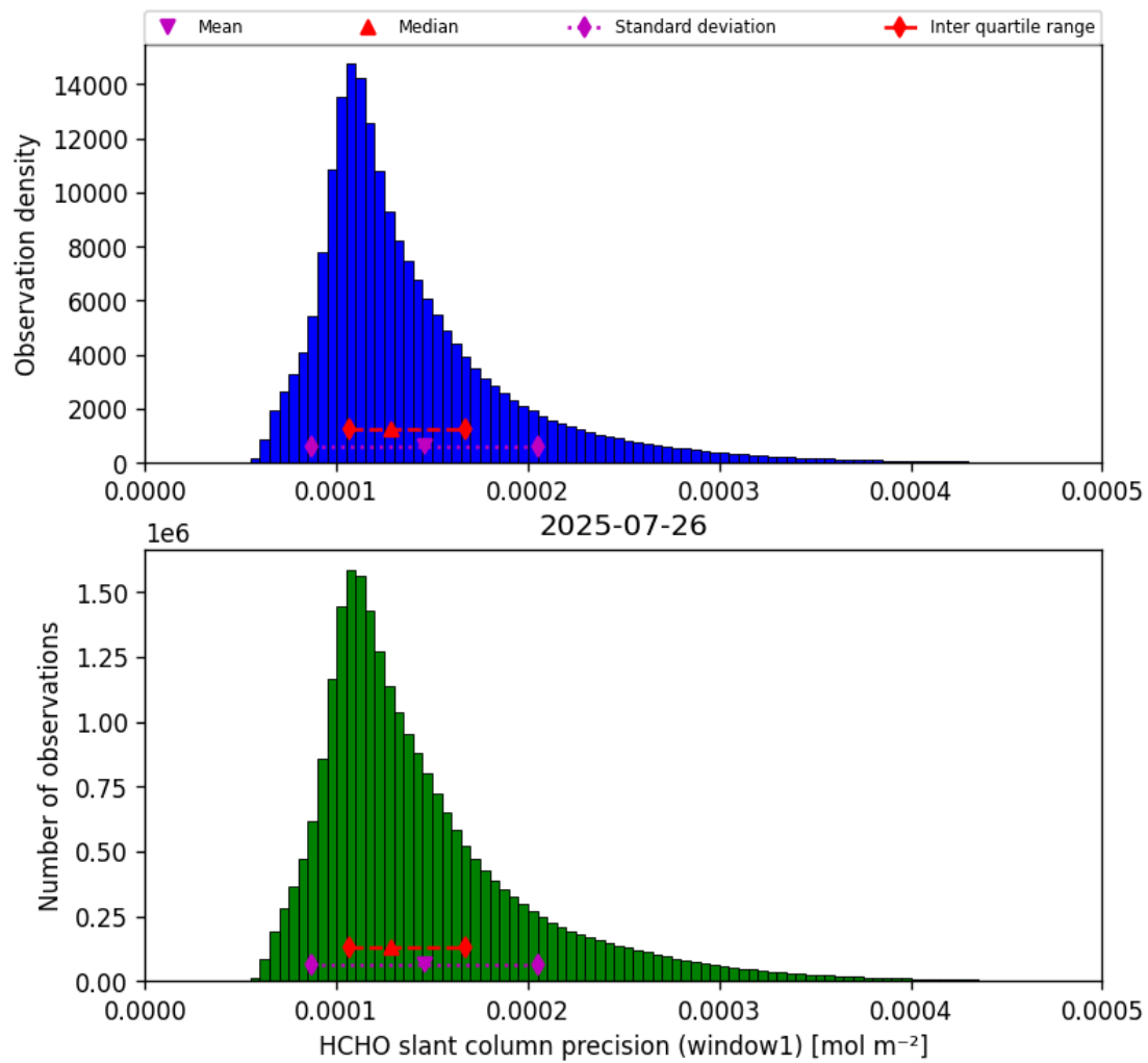
Figure 39: Histogram of “HCHO slant column precision (window1)” for 2025-07-25 to 2025-07-27
