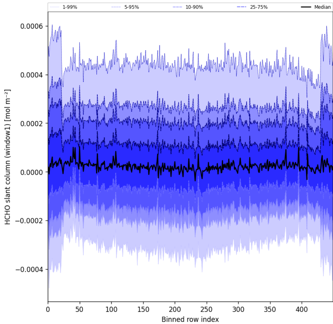
Figure 52: Along track statistics of “HCHO slant column (window1)” for 2025-07-25 to 2025-07-27
