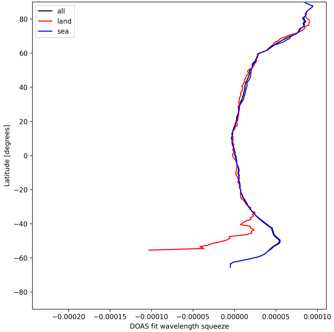
Figure 31: Zonal average of “DOAS fit wavelength squeeze” for 2025-07-25 to 2025-07-27.
