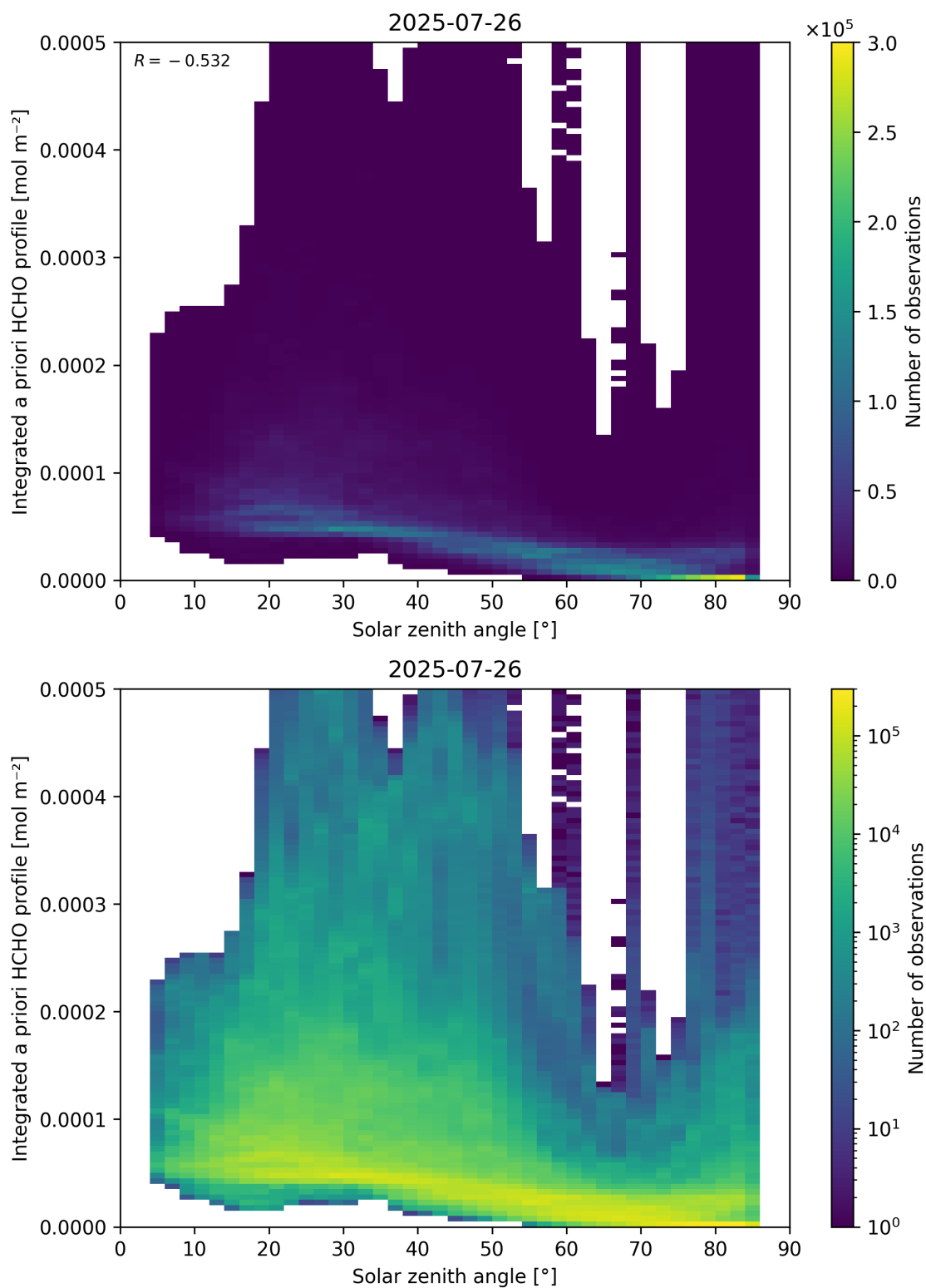
Figure 180: Scatter density plot of “Solar zenith angle” against “Integrated a priori HCHO profile” for 2025-07-25 to 2025-07-27.
