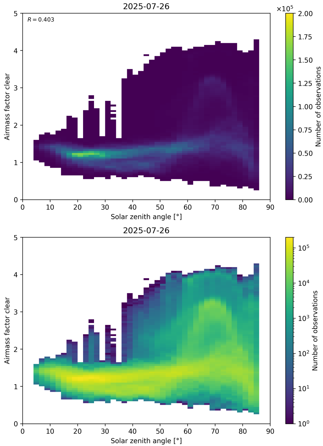
Figure 170: Scatter density plot of “Solar zenith angle” against “Airmass factor clear” for 2025-07-25 to 2025-07-27.
