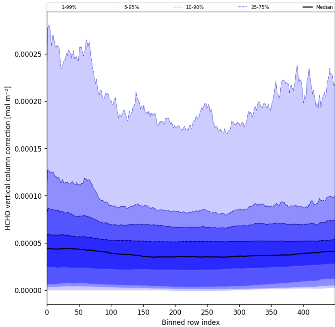
Figure 51: Along track statistics of “HCHO vertical column correction” for 2025-07-25 to 2025-07-27
