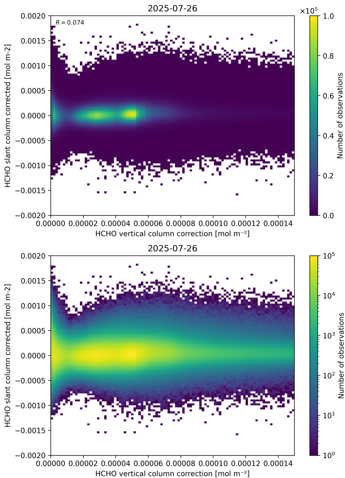
Figure 116: Scatter density plot of “HCHO vertical column correction” against “HCHO slant column corrected” for 2025-07-25 to 2025-07-27.
