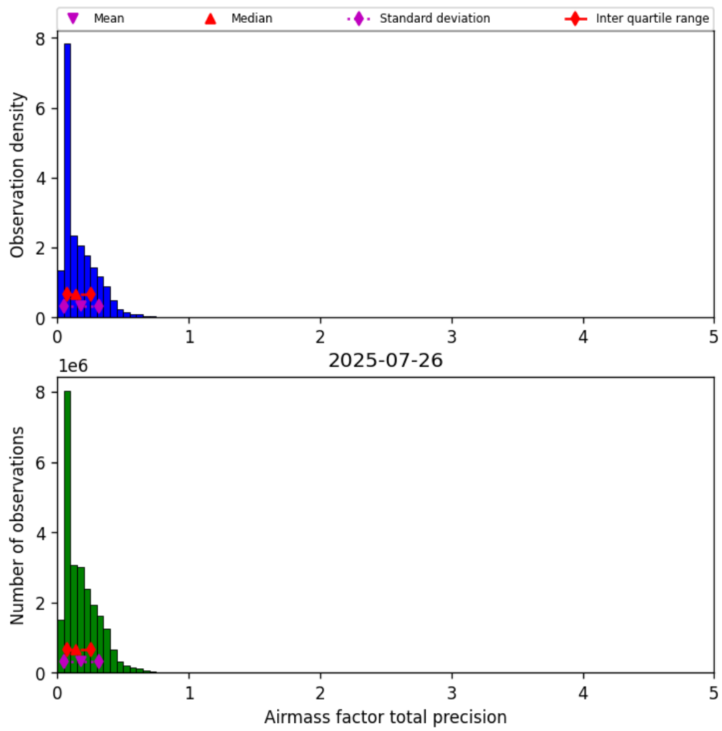
Figure 41: Histogram of “Airmass factor total precision” for 2025-07-25 to 2025-07-27
