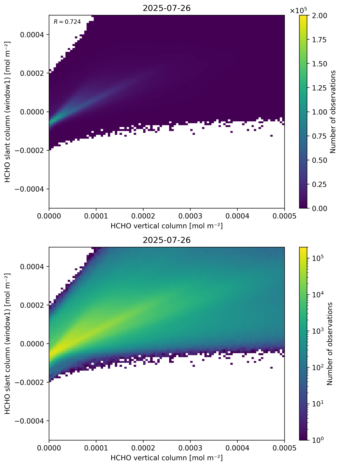
Figure 129: Scatter density plot of “HCHO vertical column” against “HCHO slant column (window1)” for 2025-07-25 to 2025-07-27.
