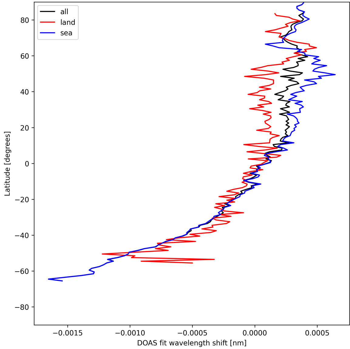
Figure 30: Zonal average of “DOAS fit wavelength shift” for 2025-07-25 to 2025-07-27.
