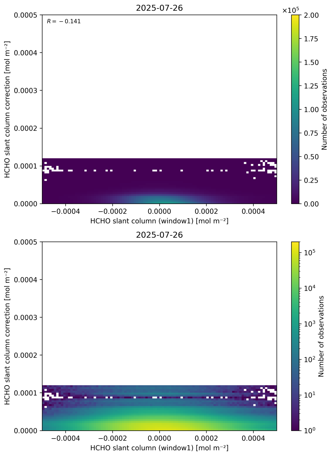
Figure 83: Scatter density plot of “HCHO slant column (window1)” against “HCHO slant column correction” for 2025-07-25 to 2025-07-27.
