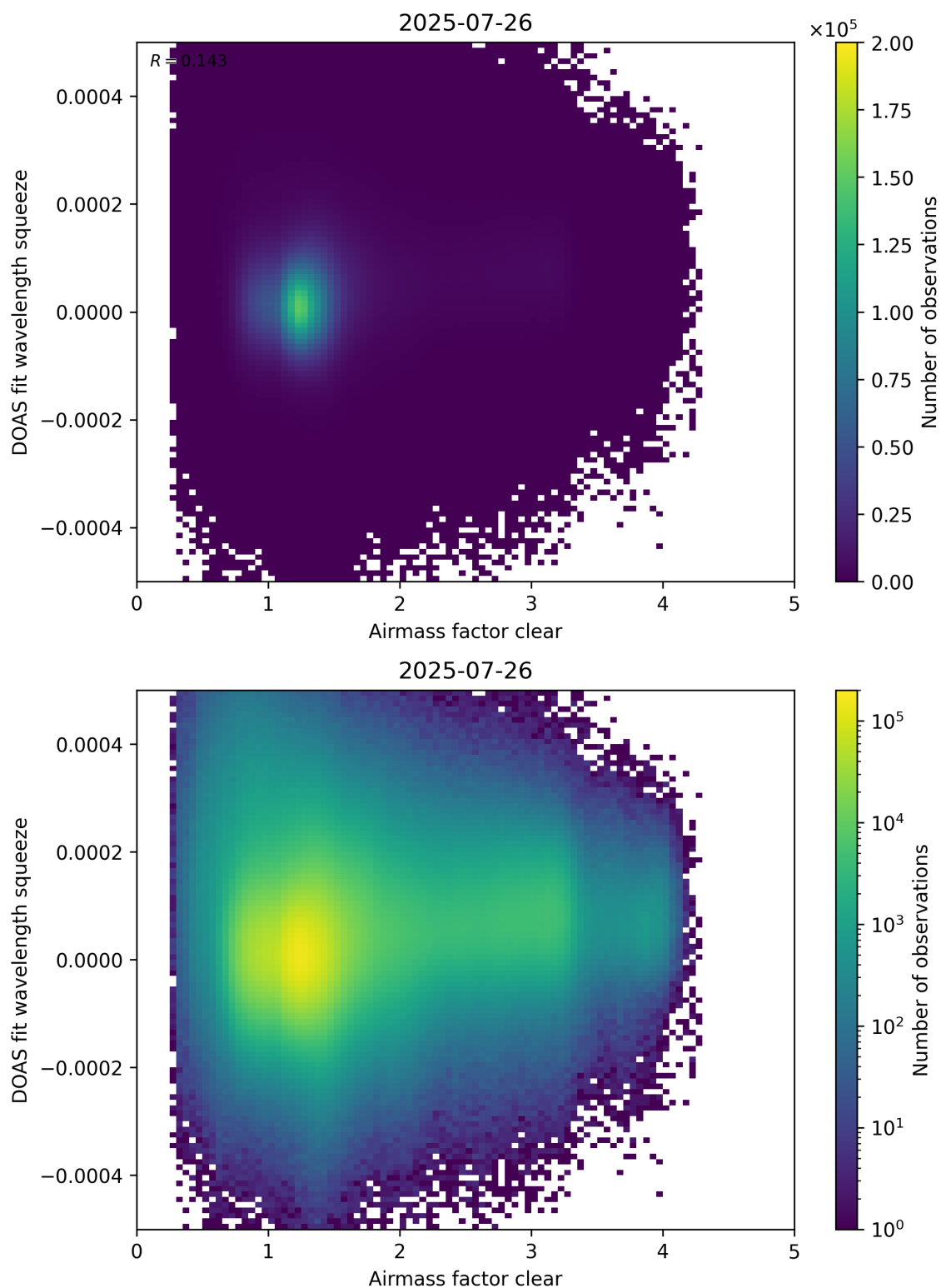
Figure 73: Scatter density plot of “Airmass factor clear” against “DOAS fit wavelength squeeze” for 2025-07-25 to 2025-07-27.
