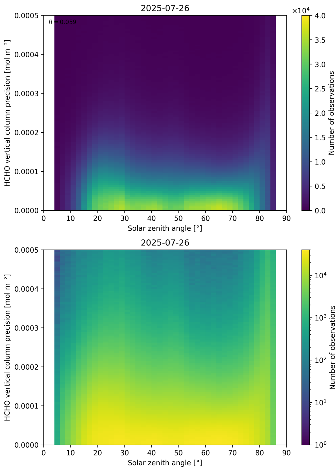
Figure 179: Scatter density plot of “Solar zenith angle” against “HCHO vertical column precision” for 2025-07-25 to 2025-07-27.
