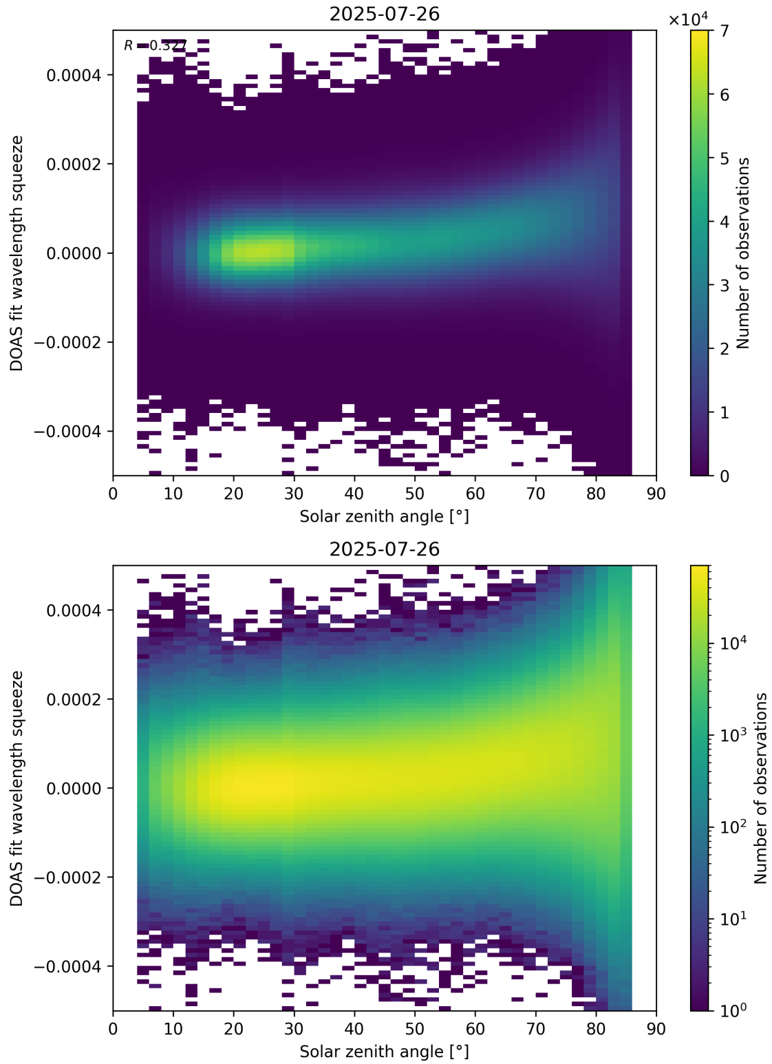
Figure 169: Scatter density plot of “Solar zenith angle” against “DOAS fit wavelength squeeze” for 2025-07-25 to 2025-07-27.
