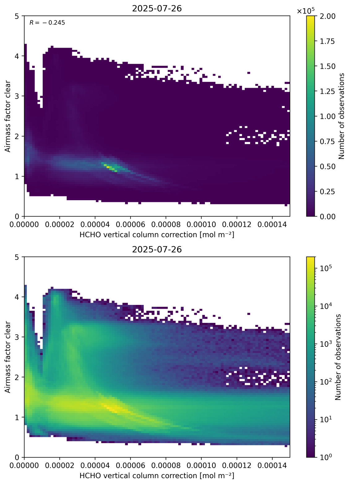
Figure 115: Scatter density plot of “HCHO vertical column correction” against “Airmass factor clear” for 2025-07-25 to 2025-07-27.
