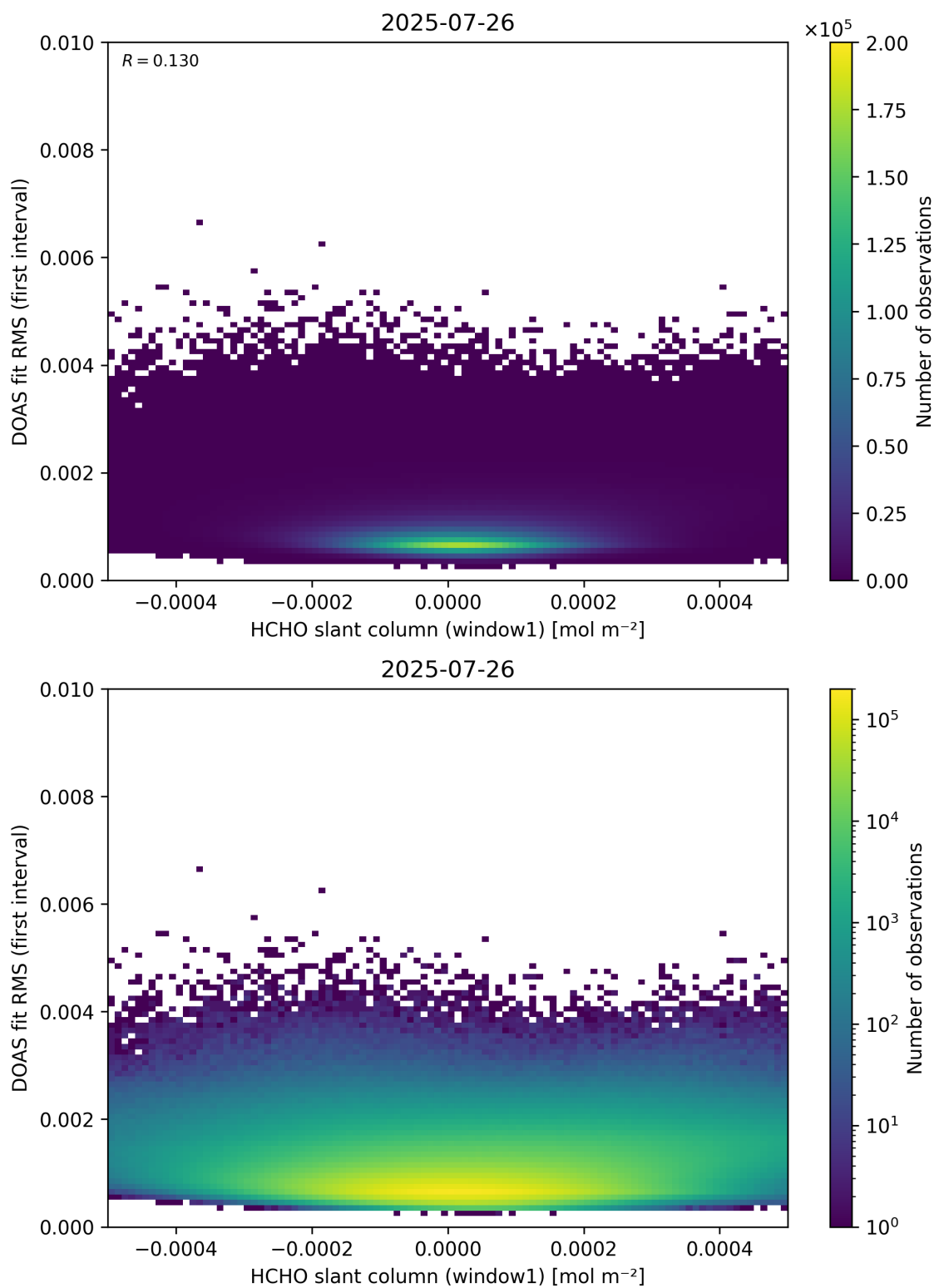
Figure 78: Scatter density plot of “HCHO slant column (window1)” against “DOAS fit RMS (first interval)” for 2025-07-25 to 2025-07-27.
