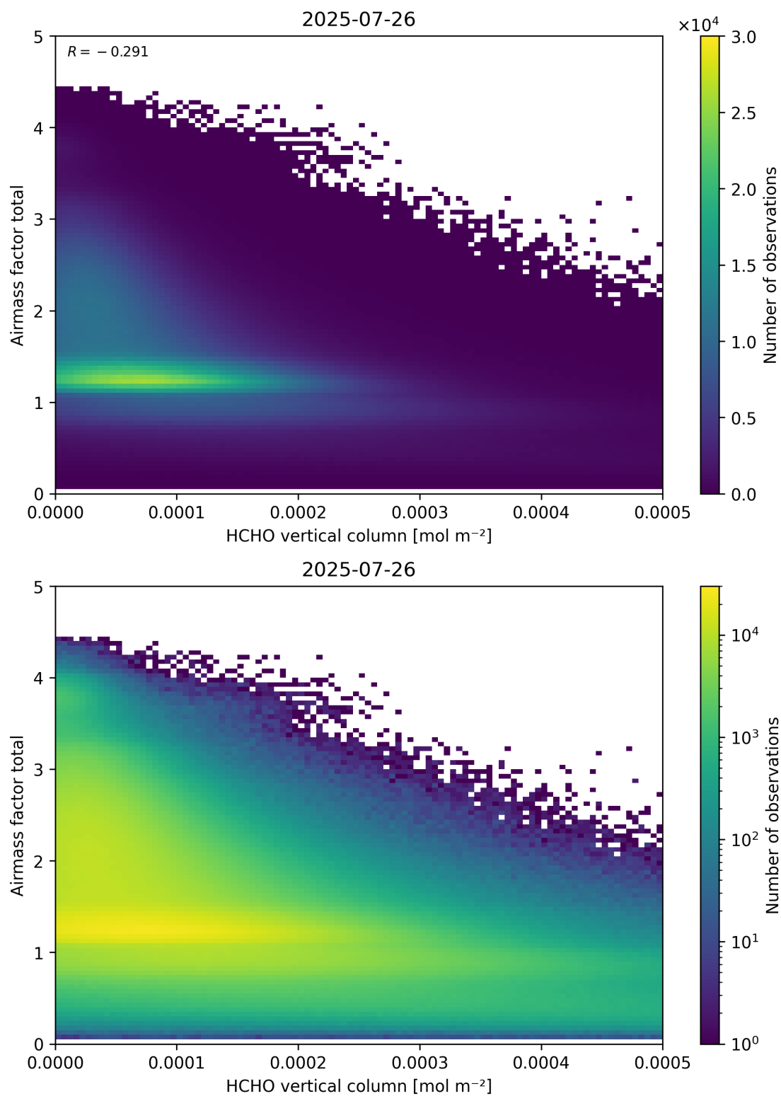
Figure 131: Scatter density plot of “HCHO vertical column” against “Airmass factor total” for 2025-07-25 to 2025-07-27.
