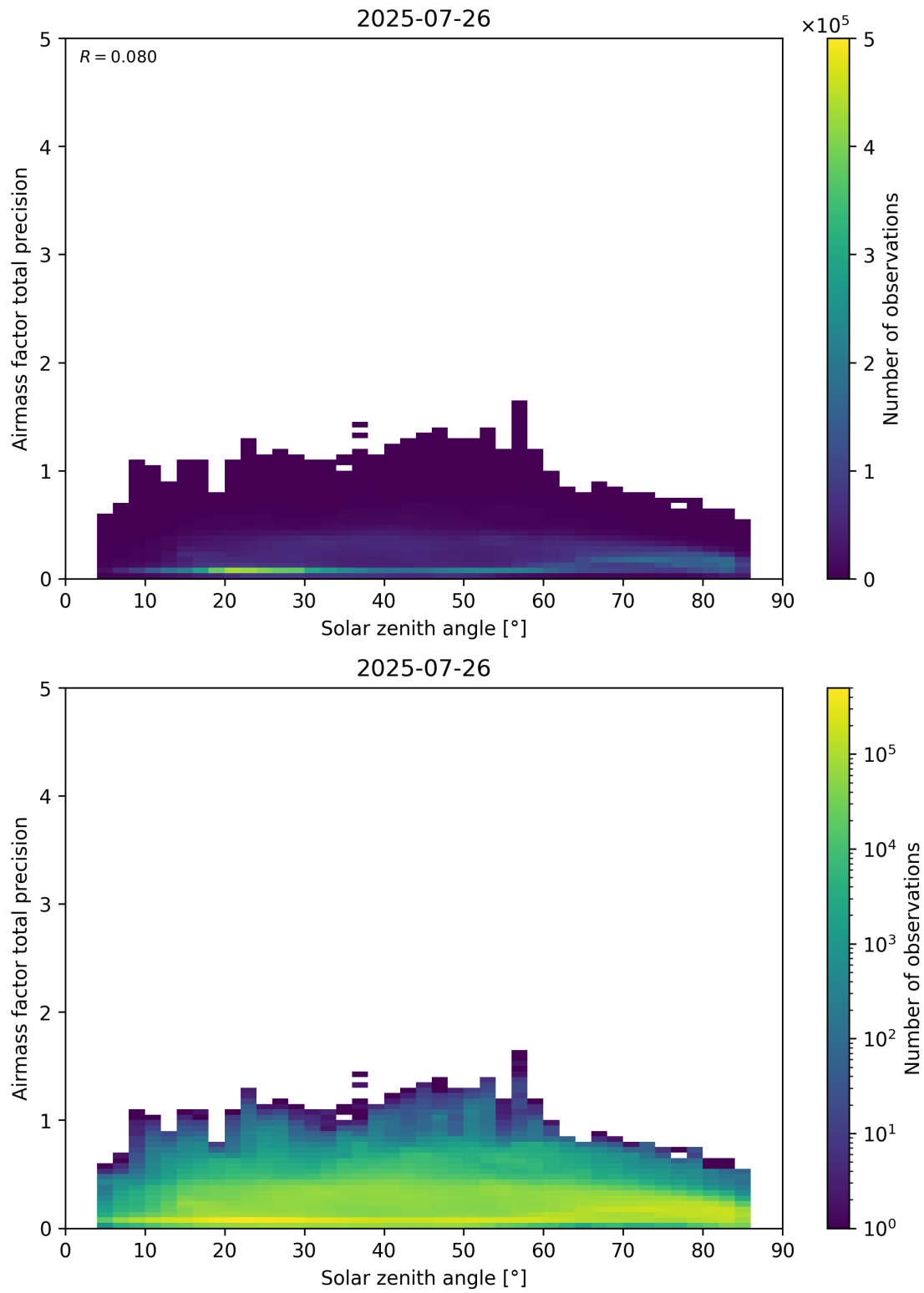
Figure 176: Scatter density plot of “Solar zenith angle” against “Airmass factor total precision” for 2025-07-25 to 2025-07-27.
