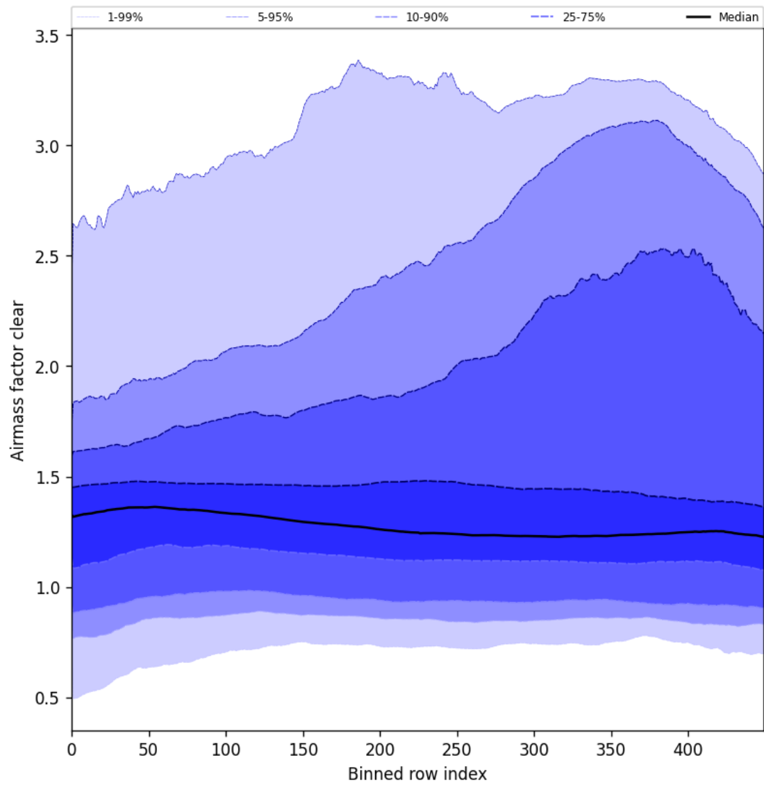
Figure 56: Along track statistics of “Air mass factor clear” for 2025-07-25 to 2025-07-27
