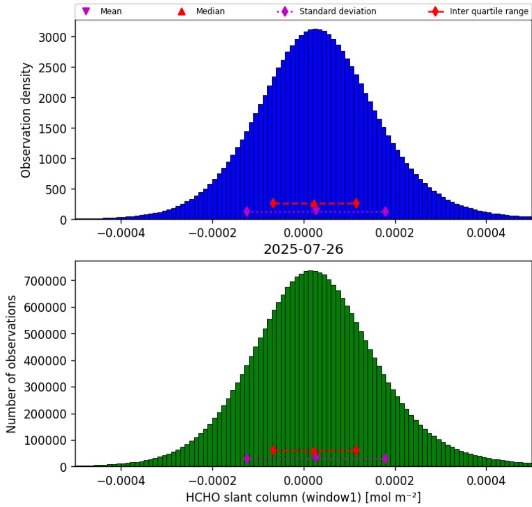
Figure 38: Histogram of “HCHO slant column (window1)” for 2025-07-25 to 2025-07-27
