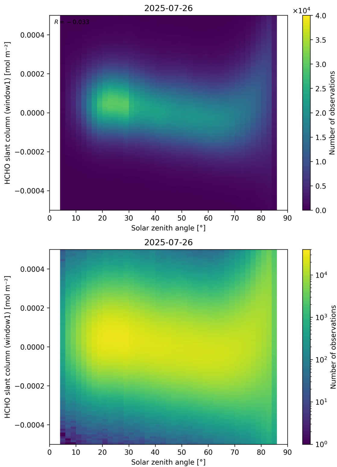
Figure 173: Scatter density plot of “Solar zenith angle” against “HCHO slant column (window1)” for 2025-07-25 to 2025-07-27.
