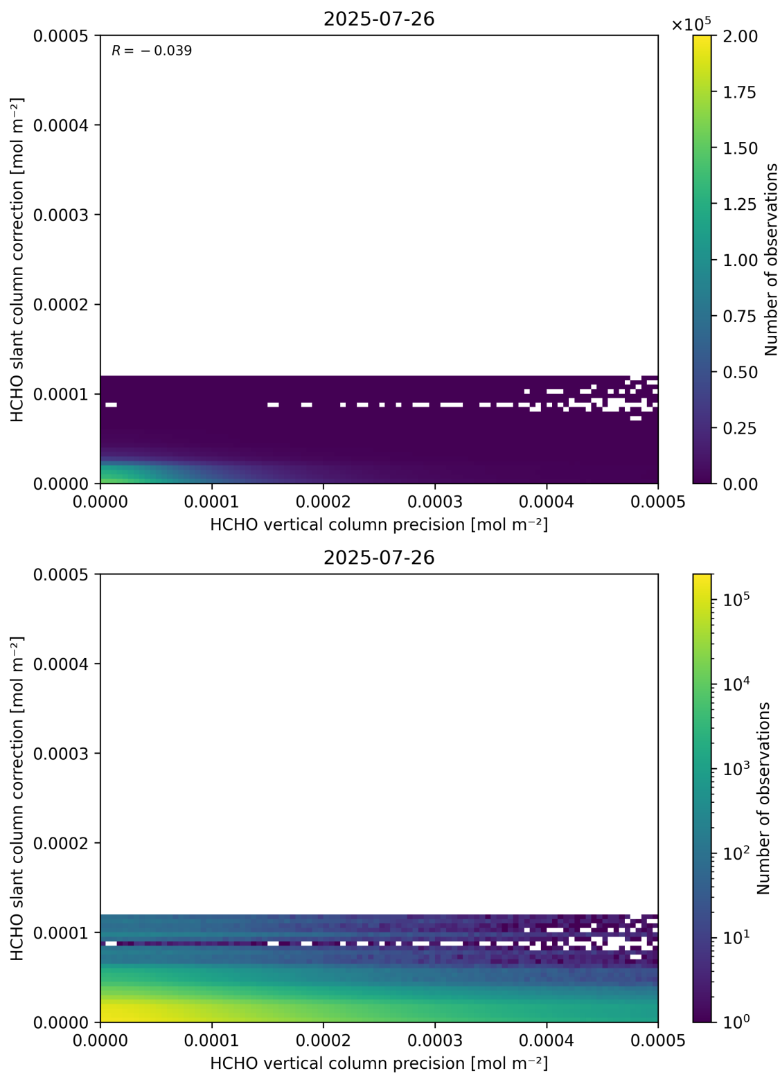
Figure 141: Scatter density plot of “HCHO vertical column precision” against “HCHO slant column correction” for 2025-07-25 to 2025-07-27.
