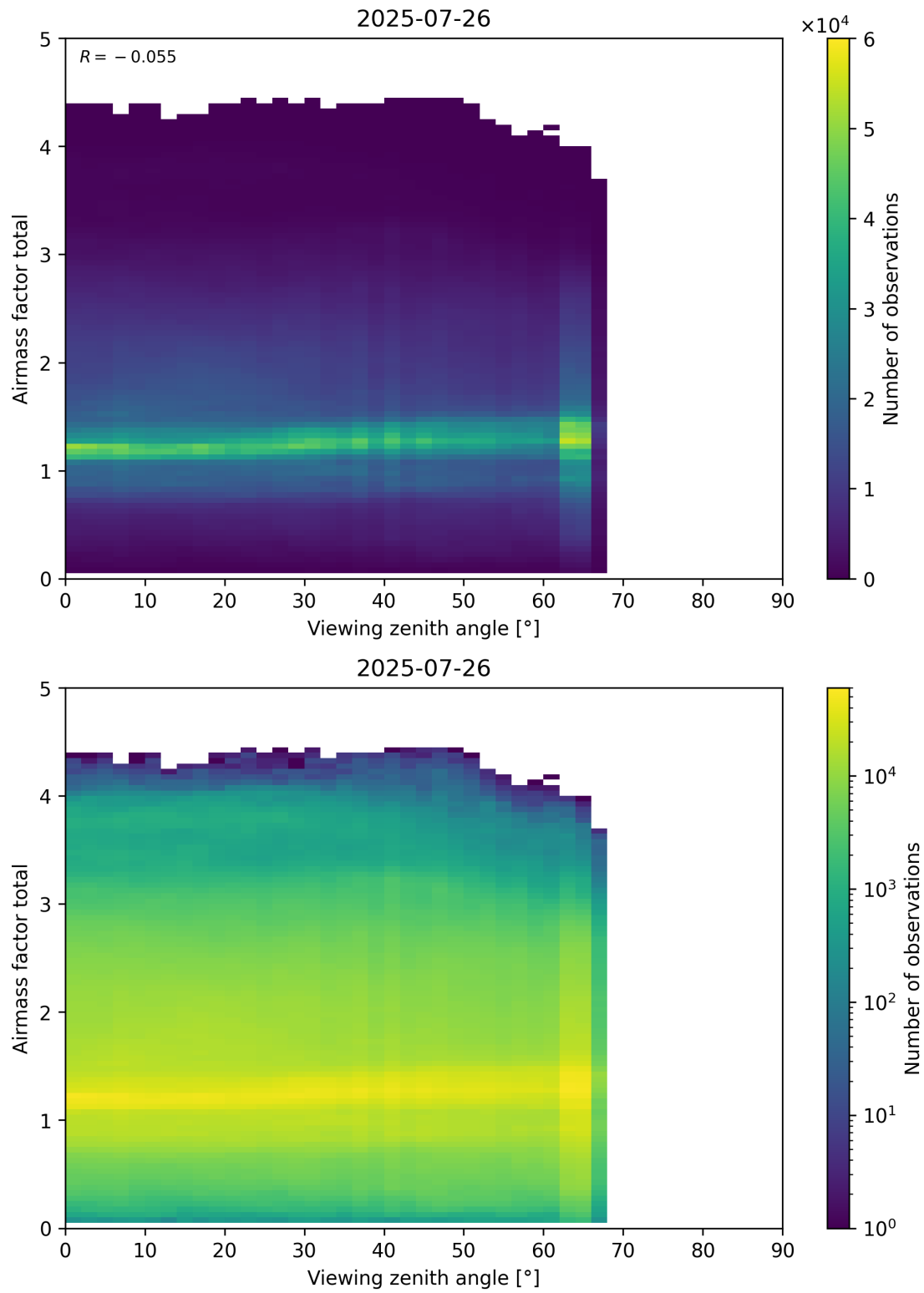
Figure 190: Scatter density plot of “Viewing zenith angle” against “Airmass factor total” for 2025-07-25 to 2025-07-27.
