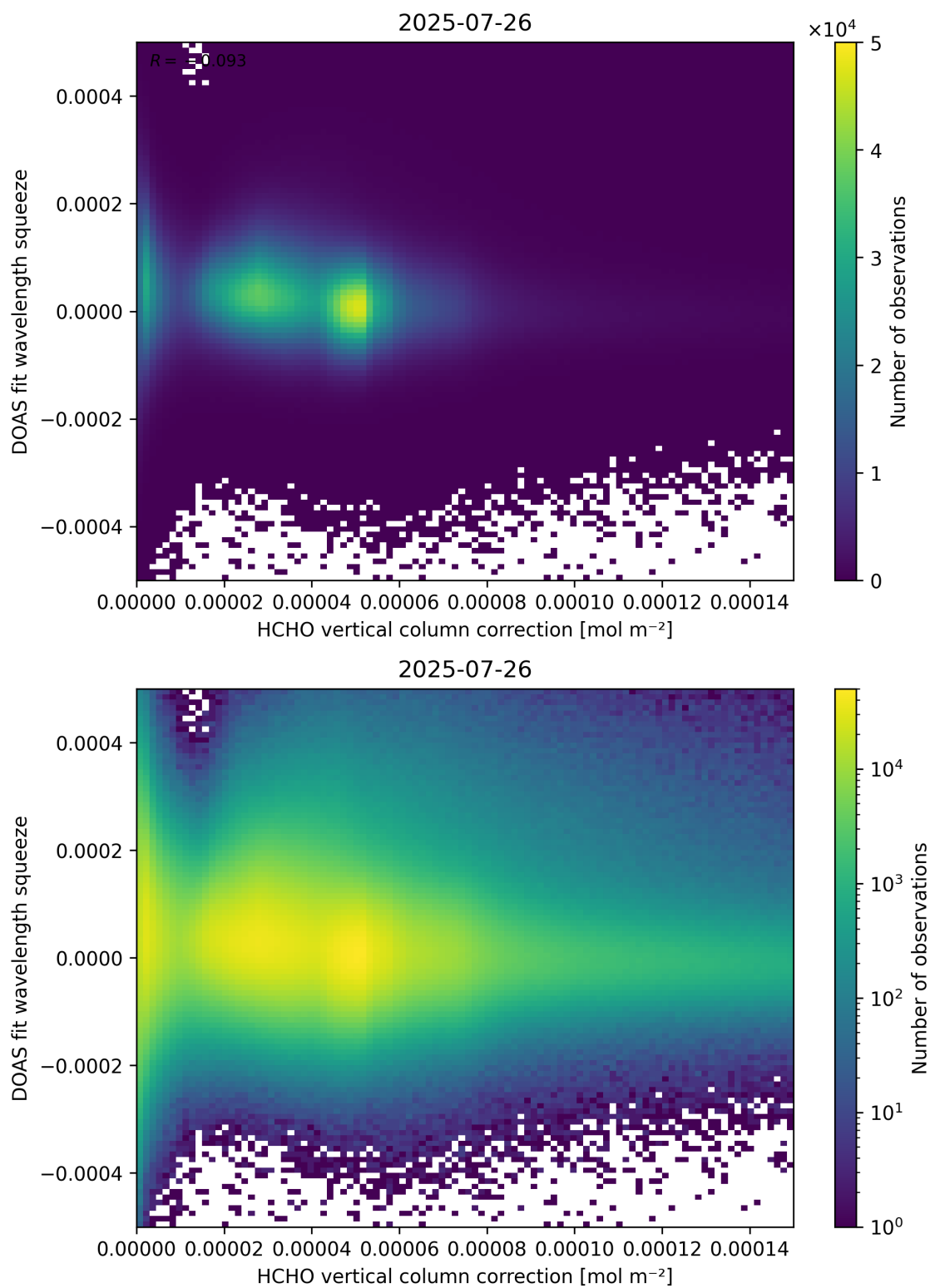
Figure 114: Scatter density plot of “HCHO vertical column correction” against “DOAS fit wavelength squeeze” for 2025-07-25 to 2025-07-27.
