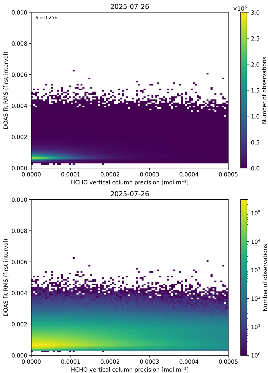
Figure 136: Scatter density plot of “HCHO vertical column precision” against “DOAS fit RMS (first interval)” for 2025-07-25 to 2025-07-27.
