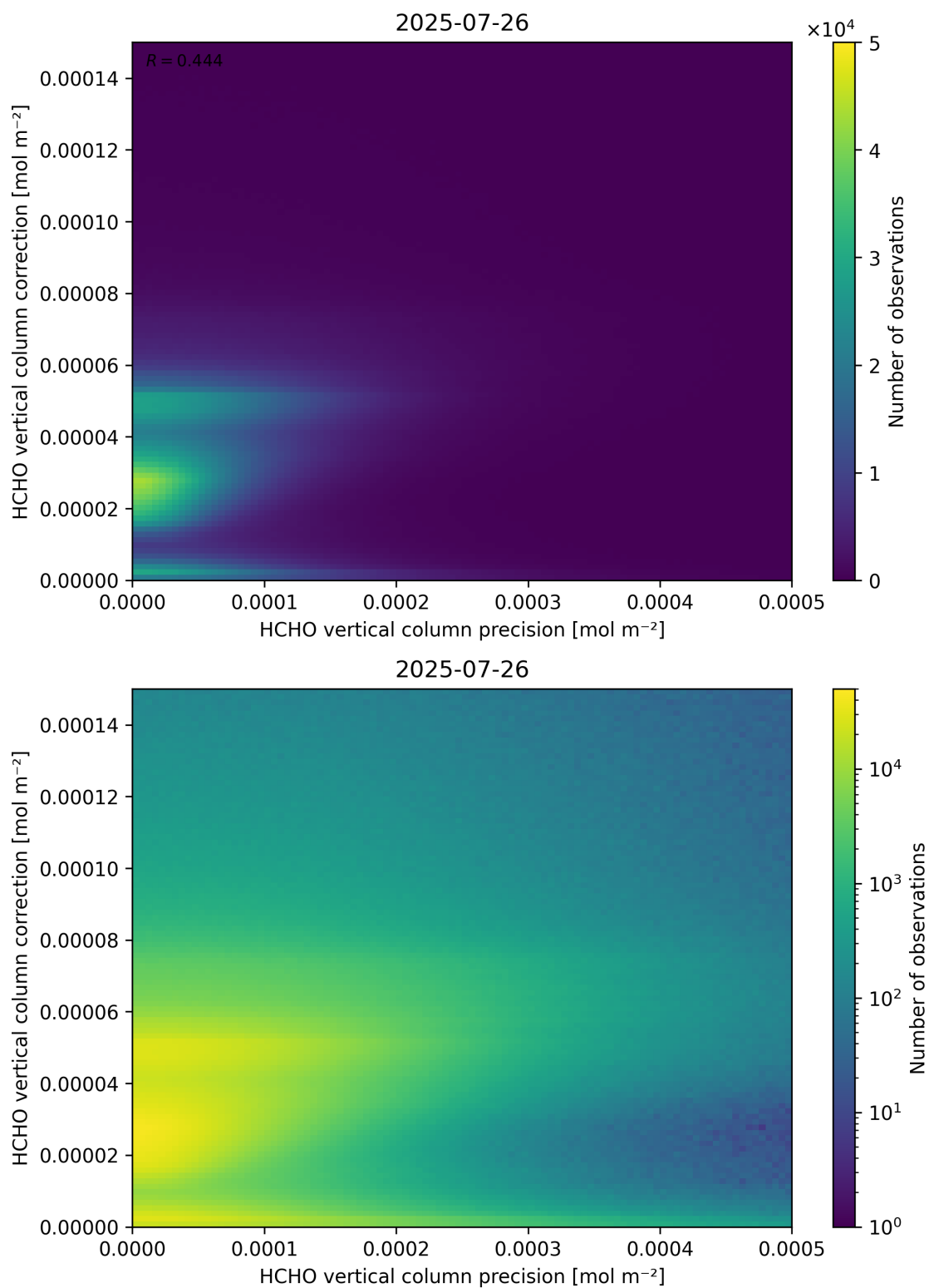
Figure 146: Scatter density plot of “HCHO vertical column precision” against “HCHO vertical column correction” for 2025-07-25 to 2025-07-27.
