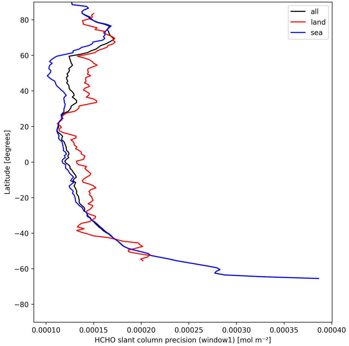
Figure 25: Zonal average of “HCHO slant column precision (window1)” for 2025-07-25 to 2025-07-27.
