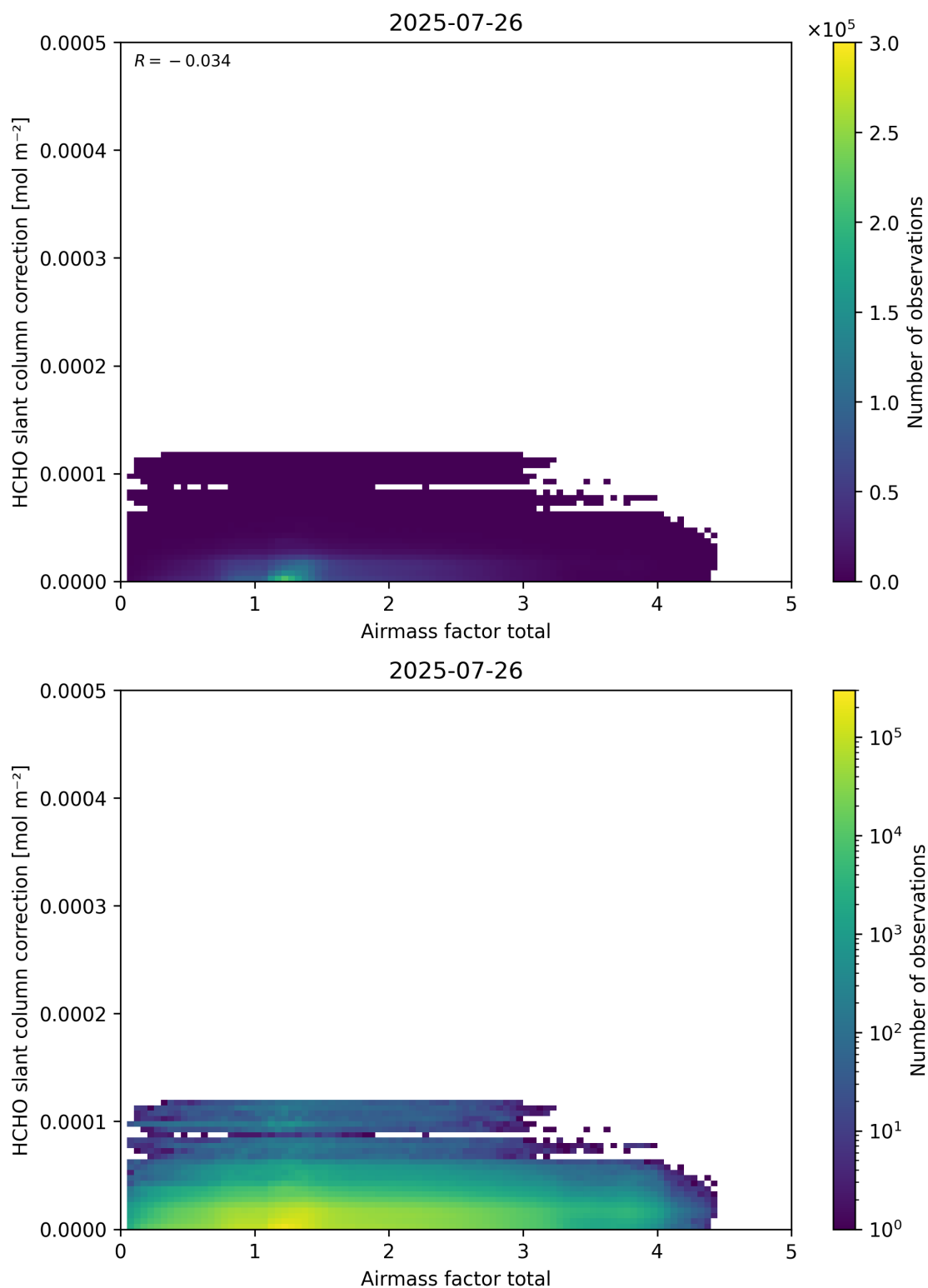
Figure 102: Scatter density plot of “Airmass factor total” against “HCHO slant column correction” for 2025-07-25 to 2025-07-27.
