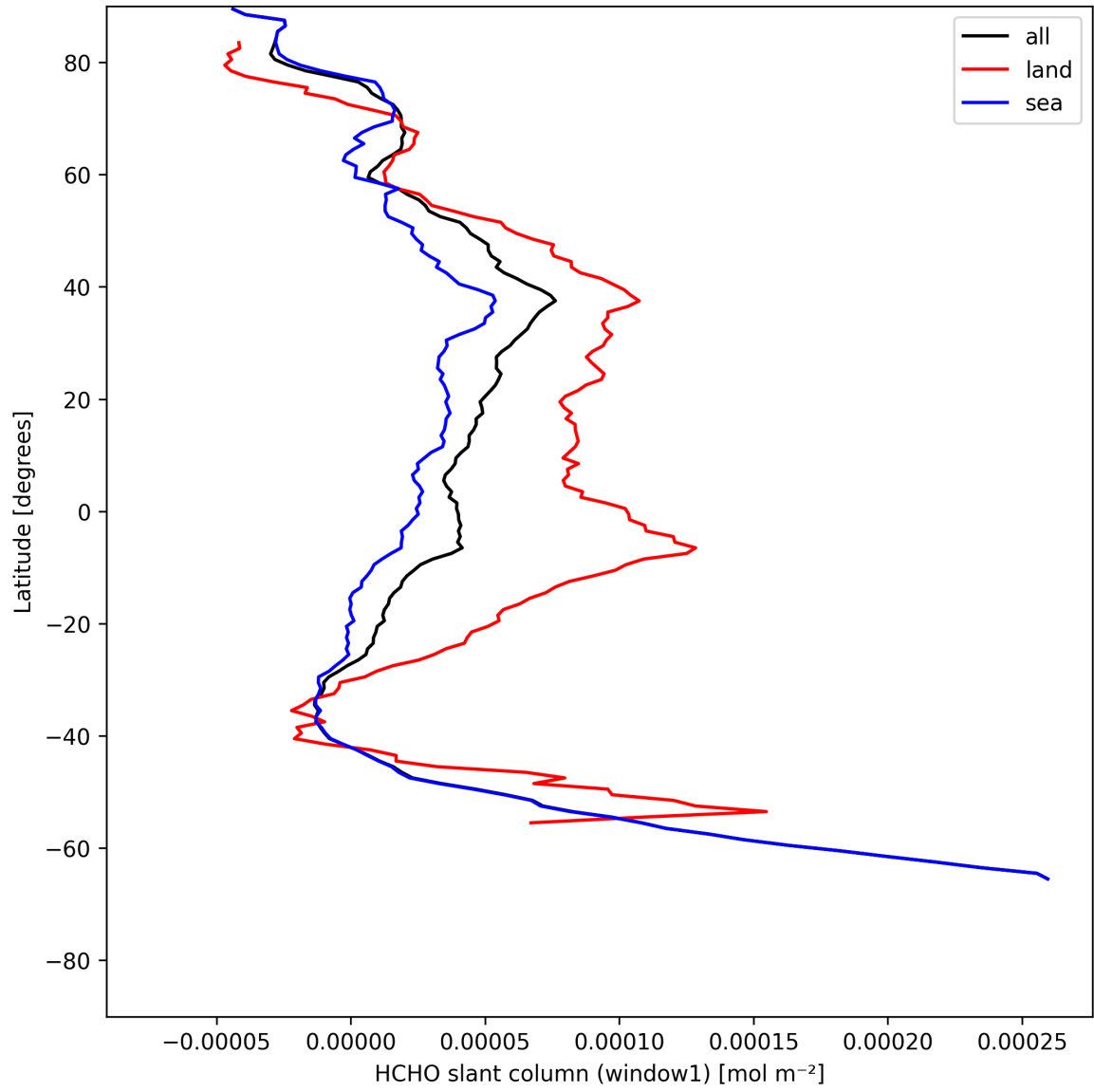
Figure 24: Zonal average of “HCHO slant column (window1)” for 2025-07-25 to 2025-07-27.
