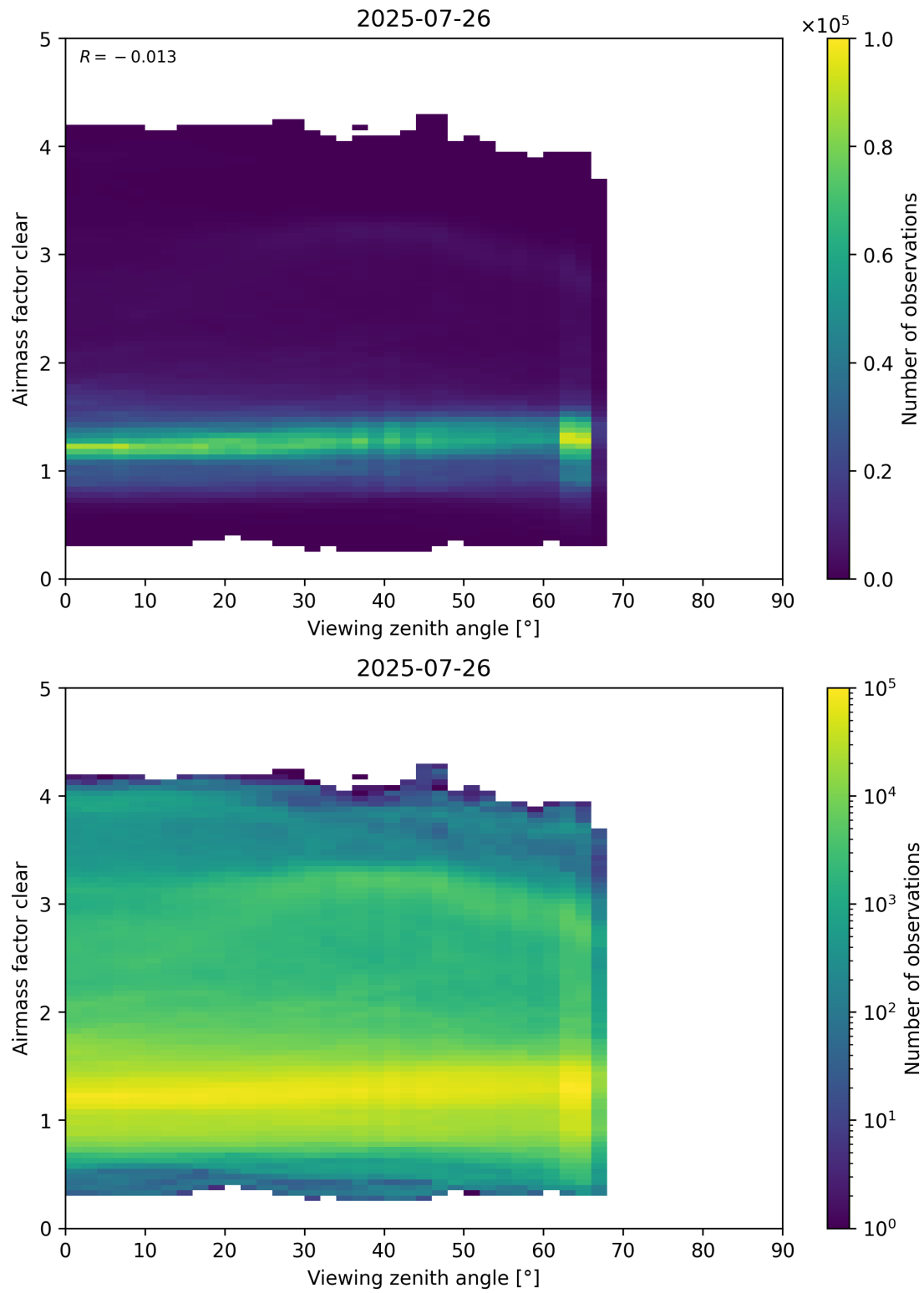
Figure 185: Scatter density plot of “Viewing zenith angle” against “Airmass factor clear” for 2025-07-25 to 2025-07-27.
