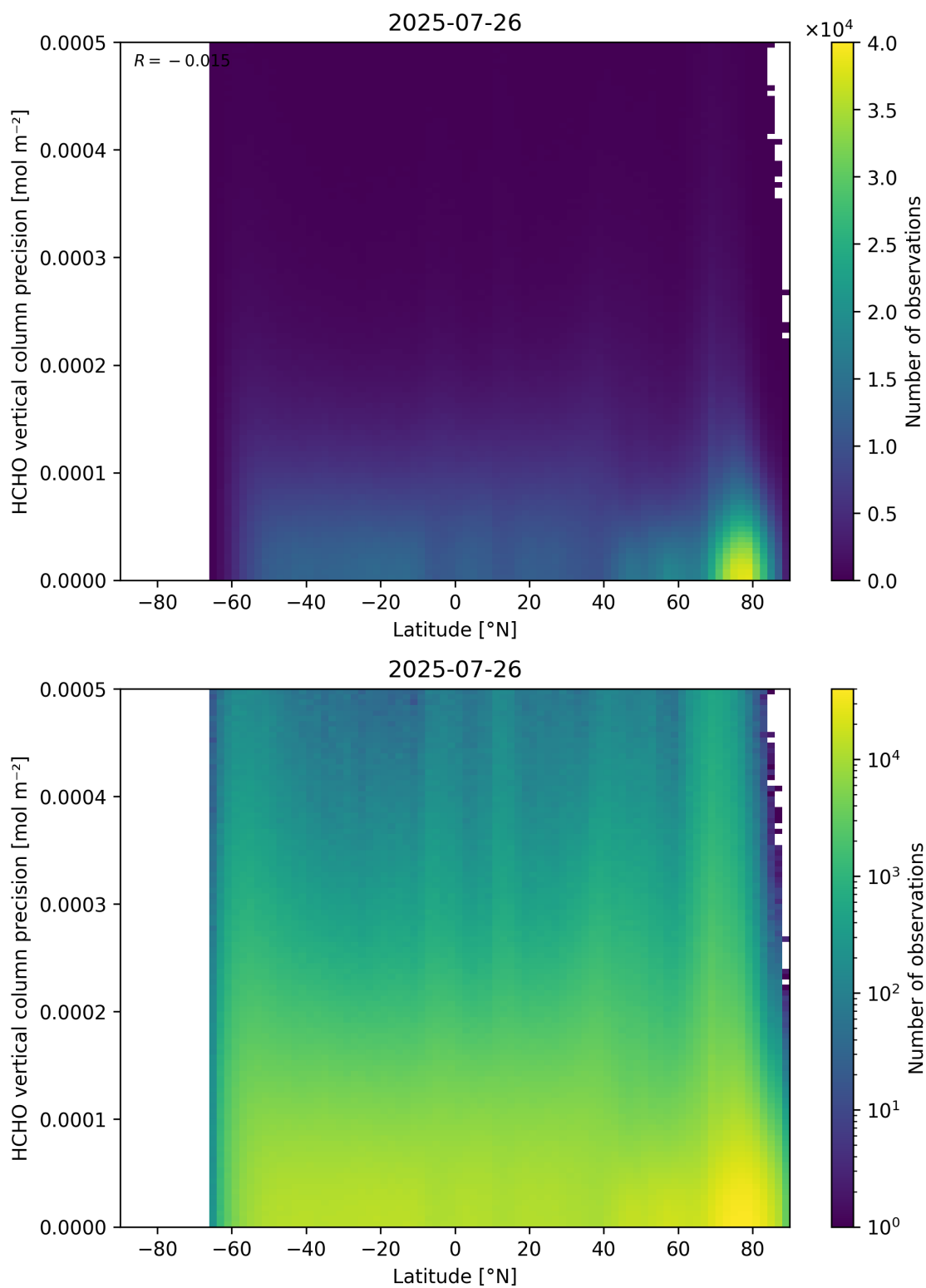
Figure 165: Scatter density plot of “Latitude” against “HCHO vertical column precision” for 2025-07-25 to 2025-07-27.
