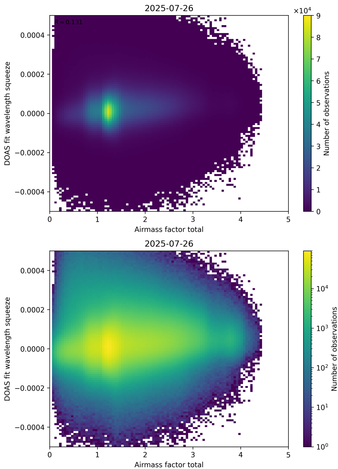
Figure 99: Scatter density plot of “Airmass factor total” against “DOAS fit wavelength squeeze” for 2025-07-25 to 2025-07-27.
