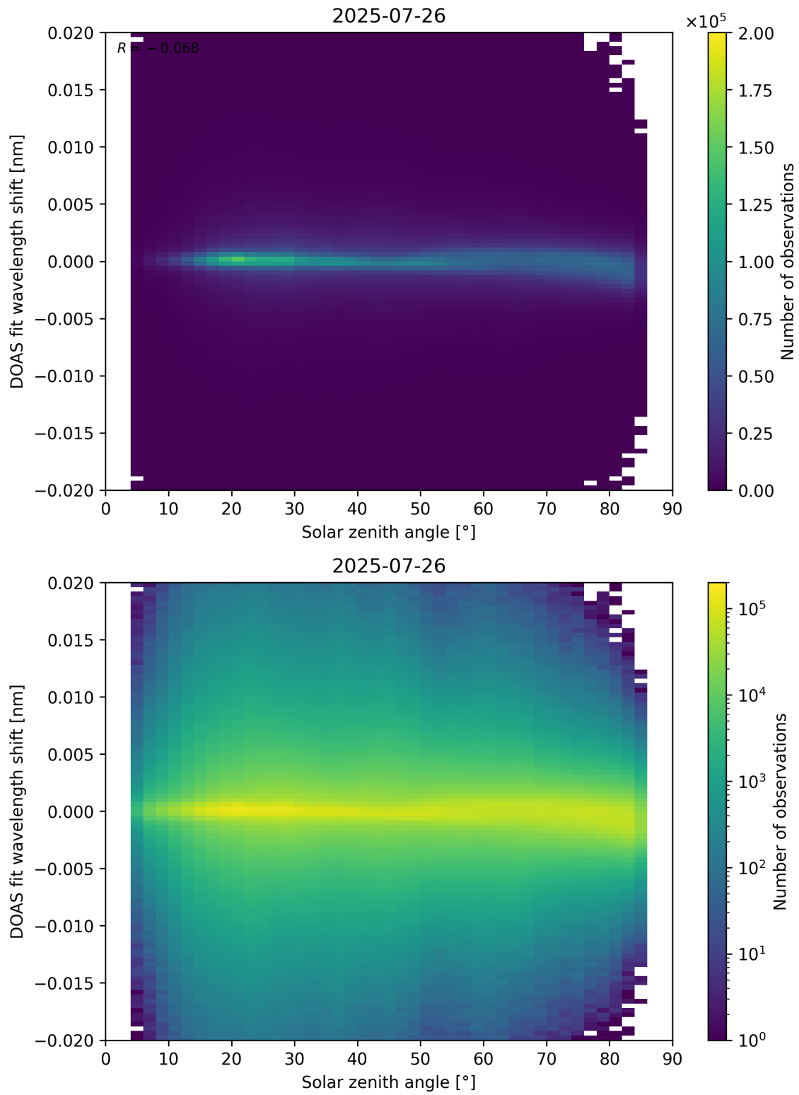
Figure 168: Scatter density plot of “Solar zenith angle” against “DOAS fit wavelength shift” for 2025-07-25 to 2025-07-27.
