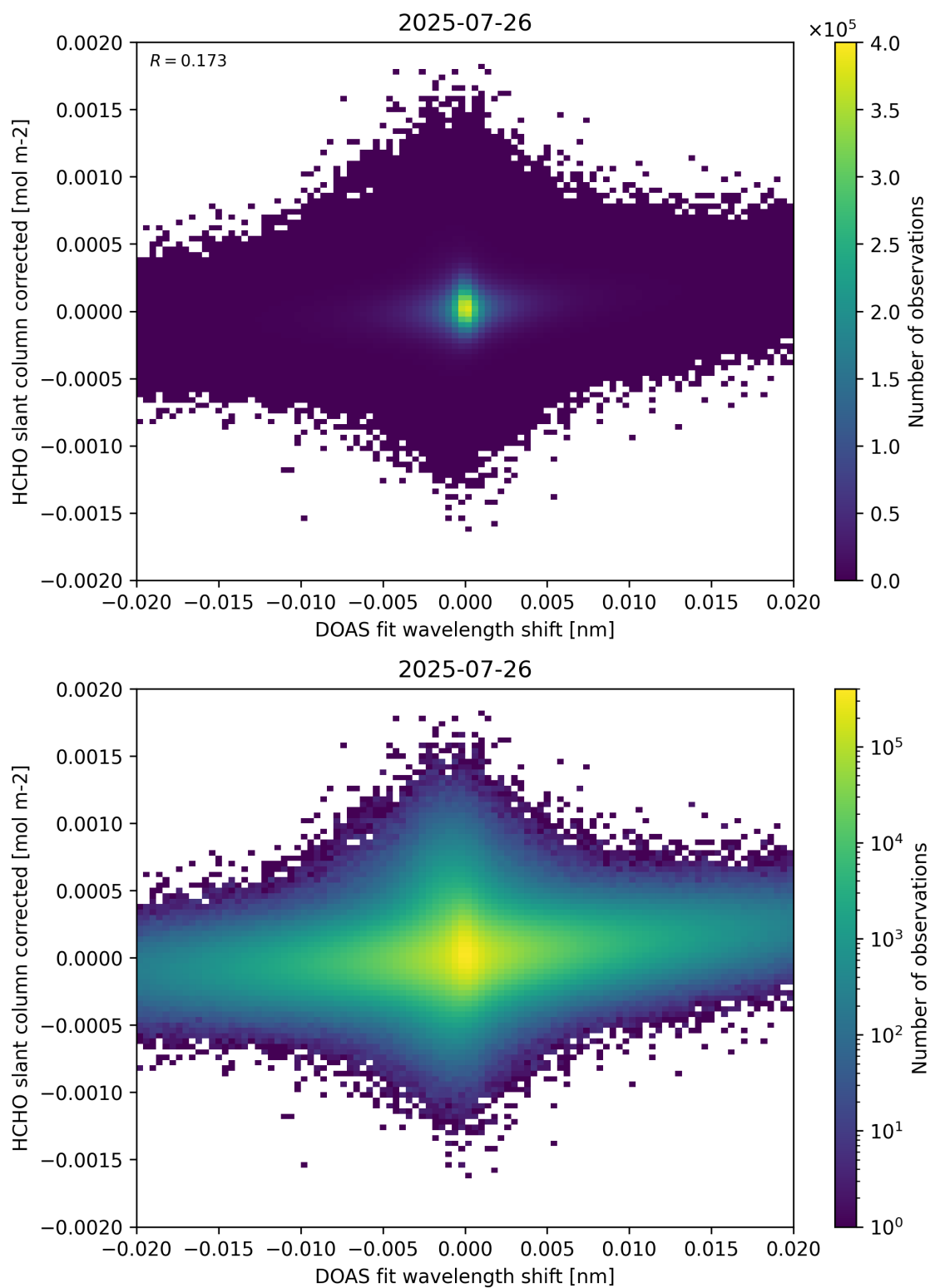
Figure 66: Scatter density plot of “DOAS fit wavelength shift” against “HCHO slant column corrected” for 2025-07-25 to 2025-07-27.
