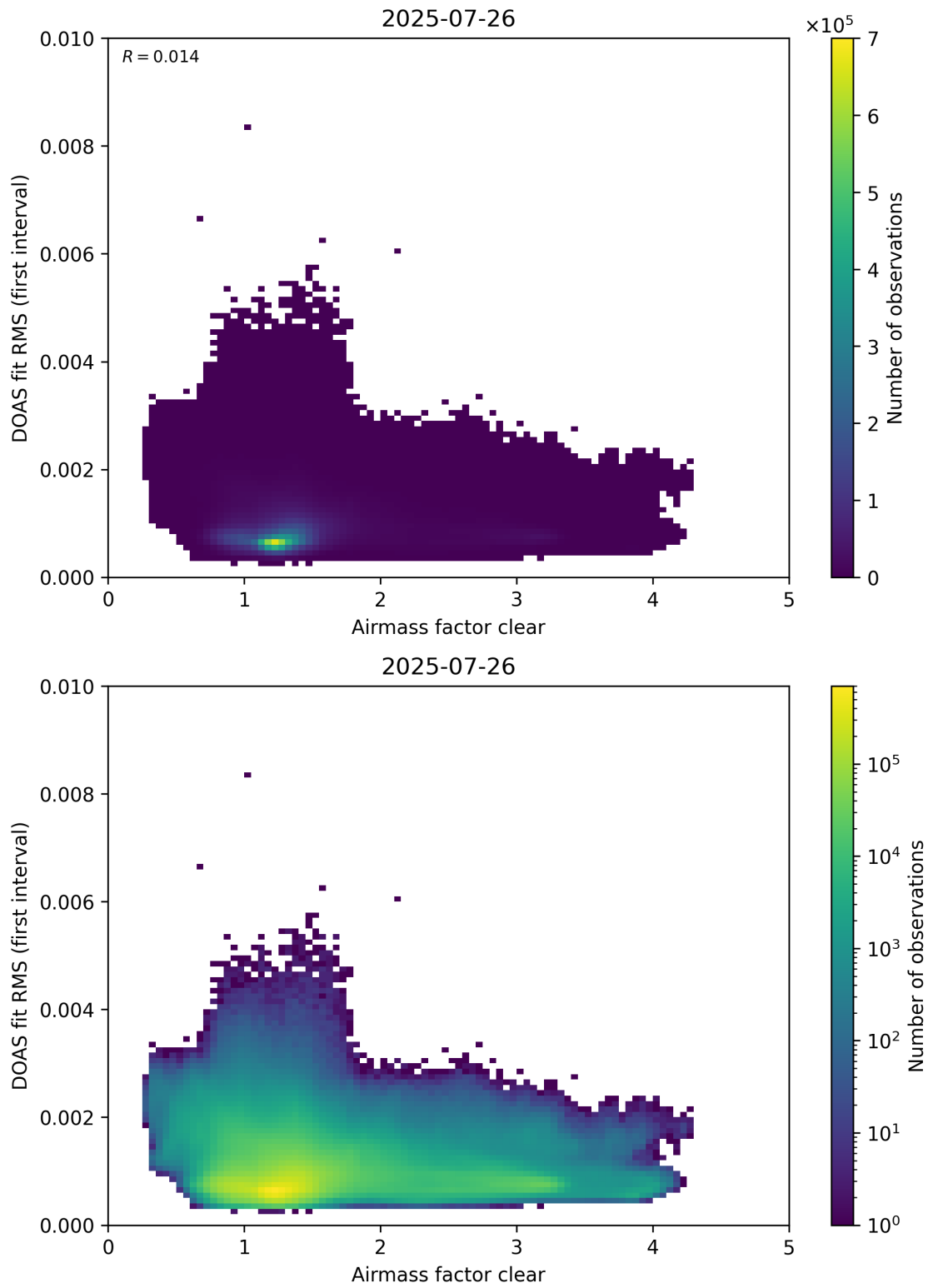
Figure 71: Scatter density plot of “Airmass factor clear” against “DOAS fit RMS (first interval)” for 2025-07-25 to 2025-07-27.
