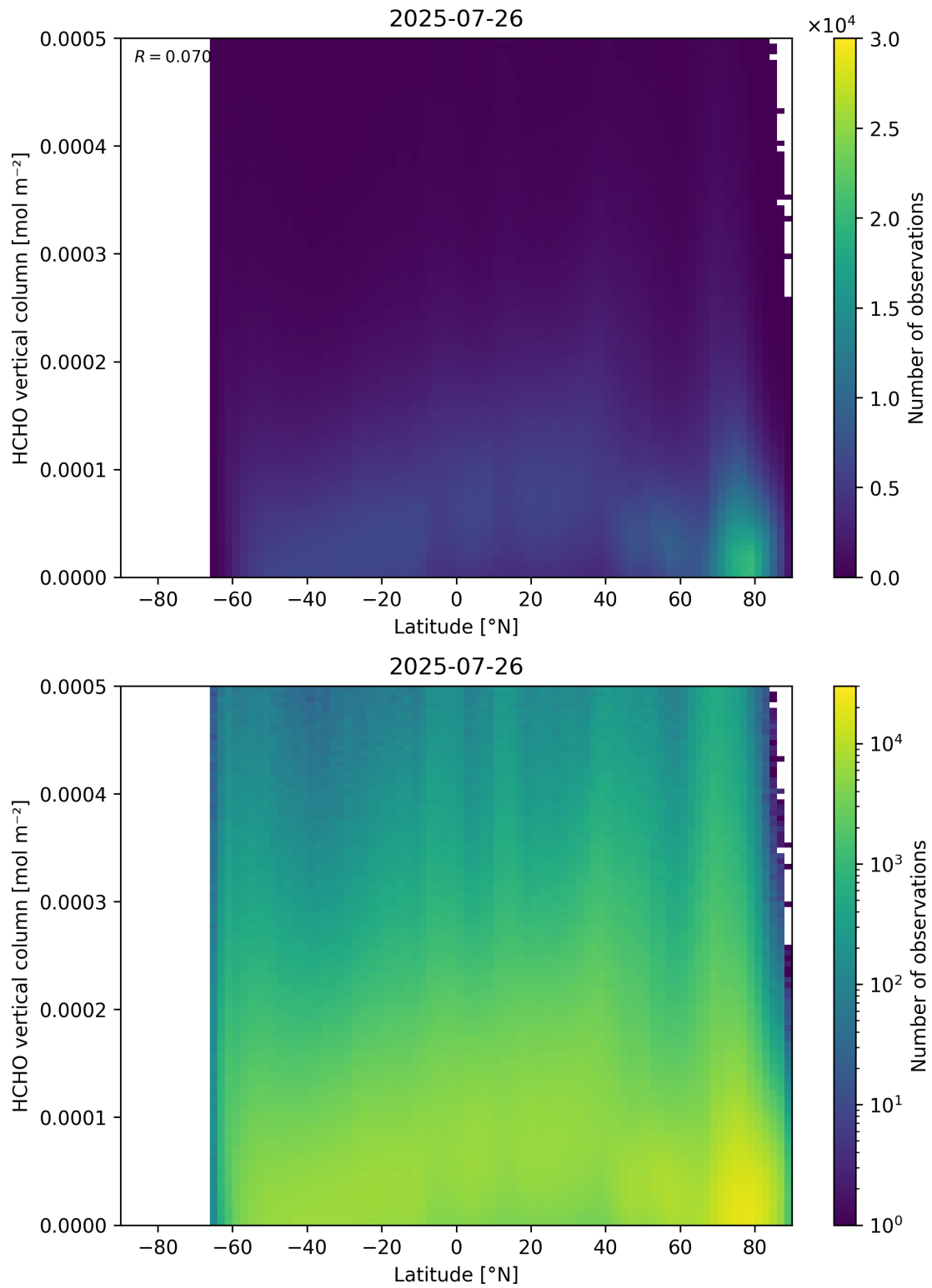
Figure 163: Scatter density plot of “Latitude” against “HCHO vertical column” for 2025-07-25 to 2025-07-27.
