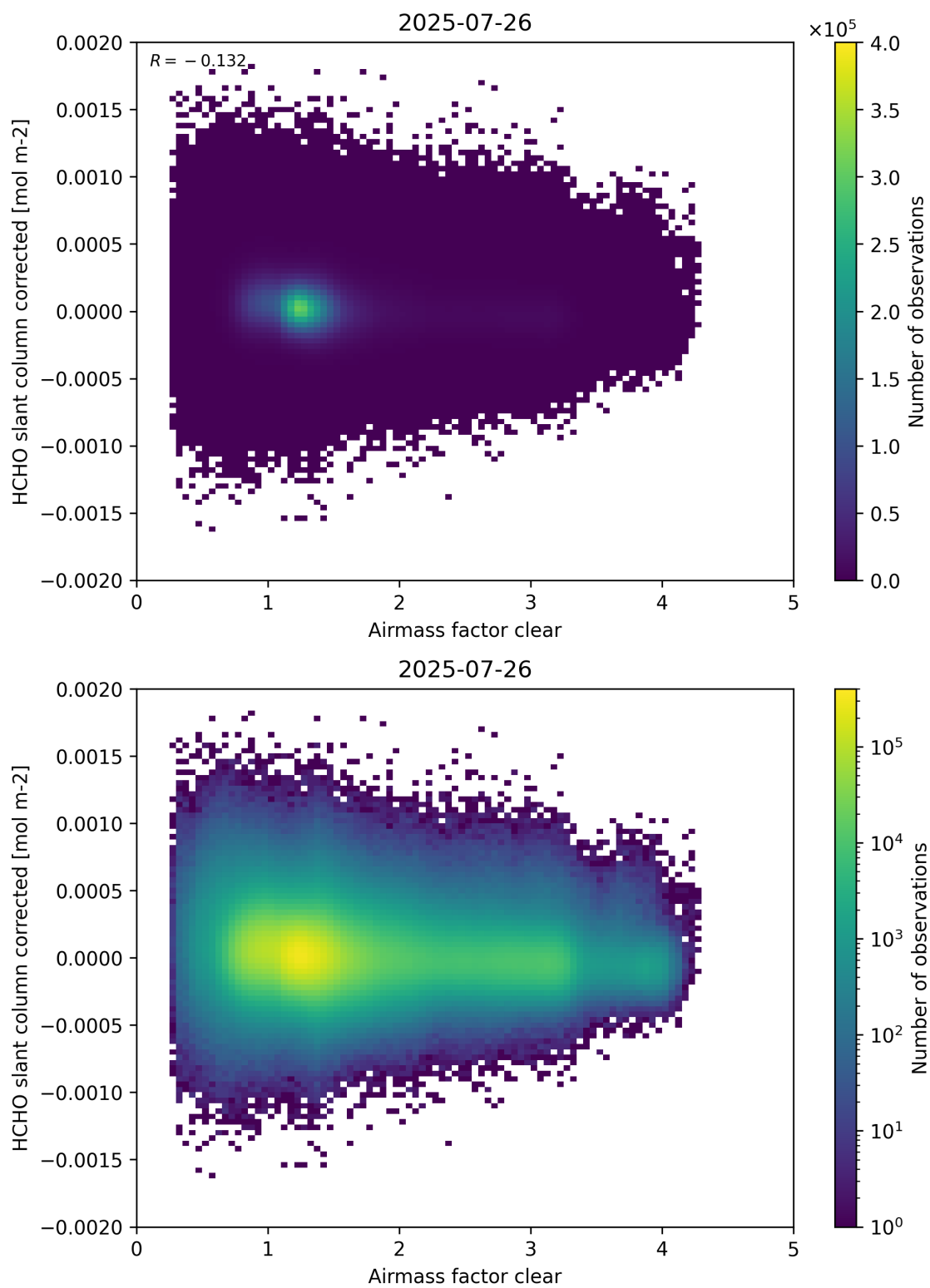
Figure 74: Scatter density plot of “Airmass factor clear” against “HCHO slant column corrected” for 2025-07-25 to 2025-07-27.
