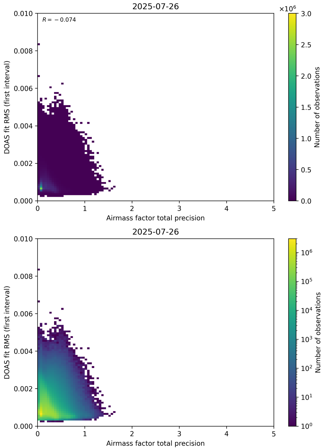
Figure 105: Scatter density plot of “Airmass factor total precision” against “DOAS fit RMS (first interval)” for 2025-07-25 to 2025-07-27.
