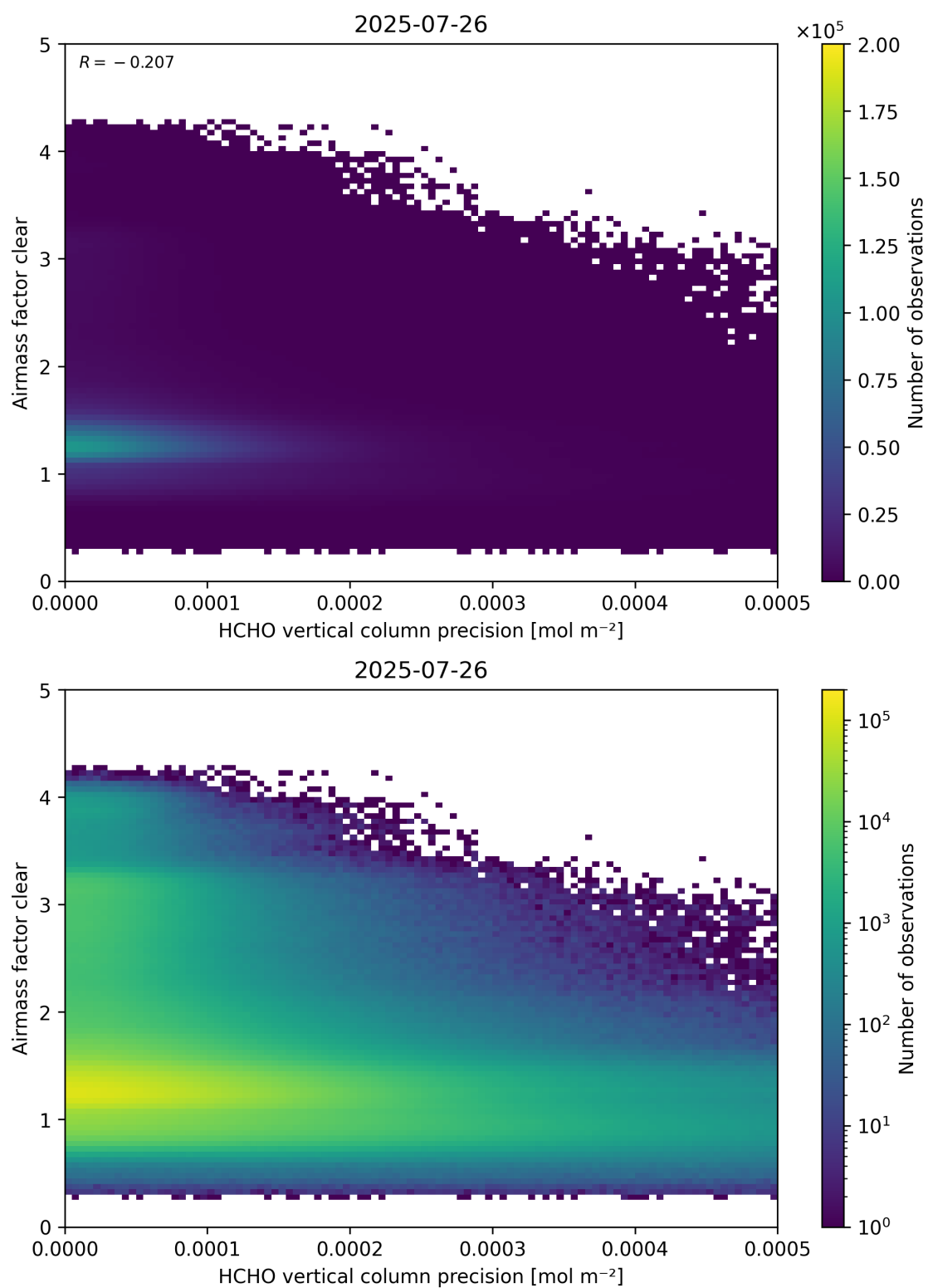
Figure 139: Scatter density plot of “HCHO vertical column precision” against “Airmass factor clear” for 2025-07-25 to 2025-07-27.
