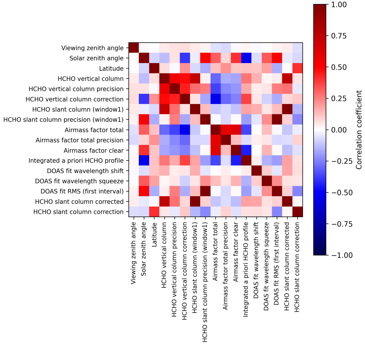
Figure 2: Map of correlation matrix for 2025-07-25 to 2025-07-27.
