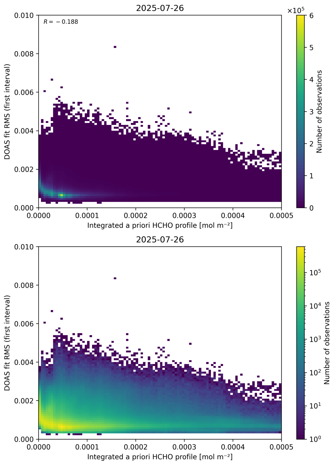
Figure 148: Scatter density plot of “Integrated a priori HCHO profile” against “DOAS fit RMS (first interval)” for 2025-07-25 to 2025-07-27.
