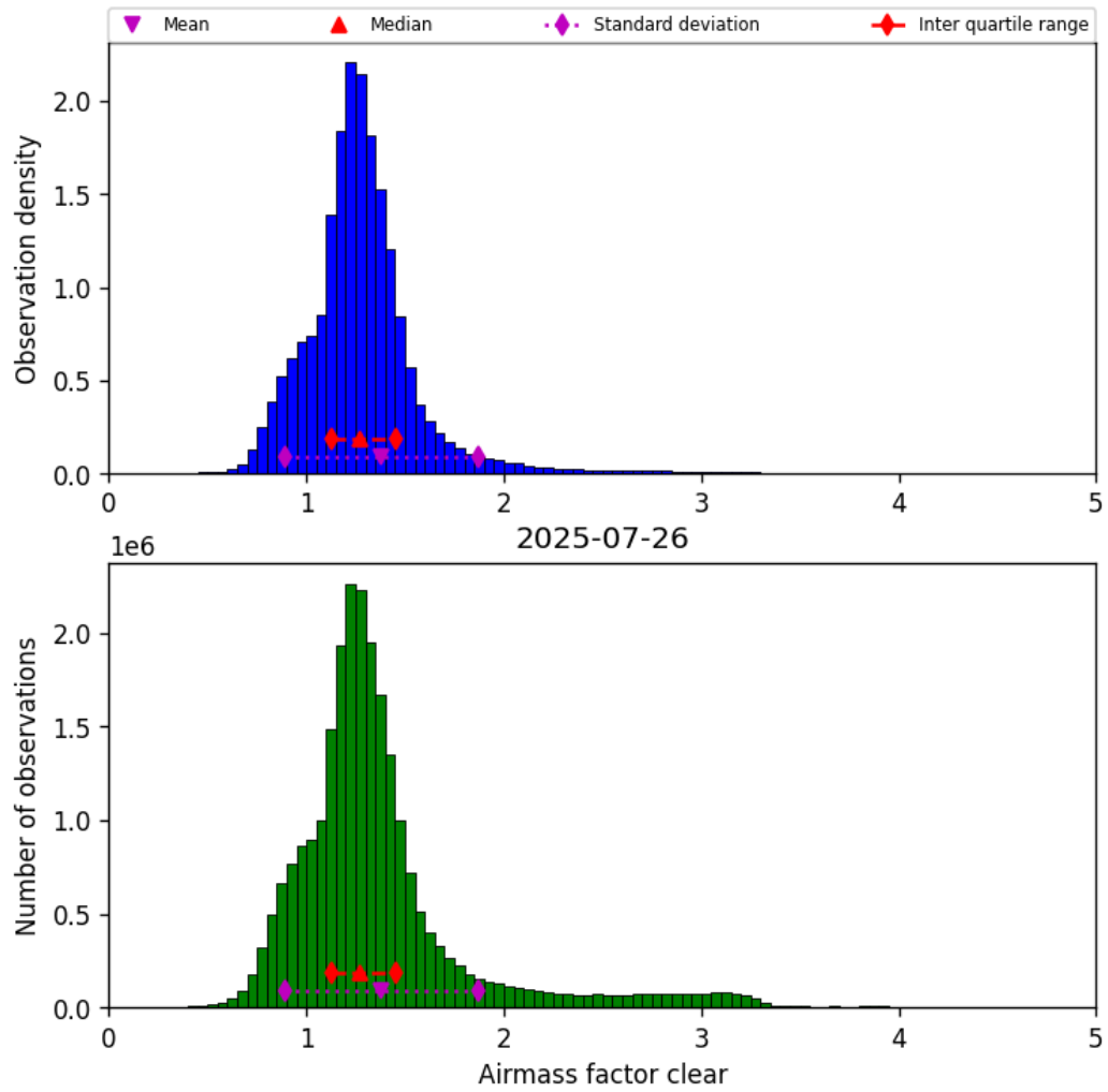
Figure 42: Histogram of “Airmass factor clear” for 2025-07-25 to 2025-07-27
