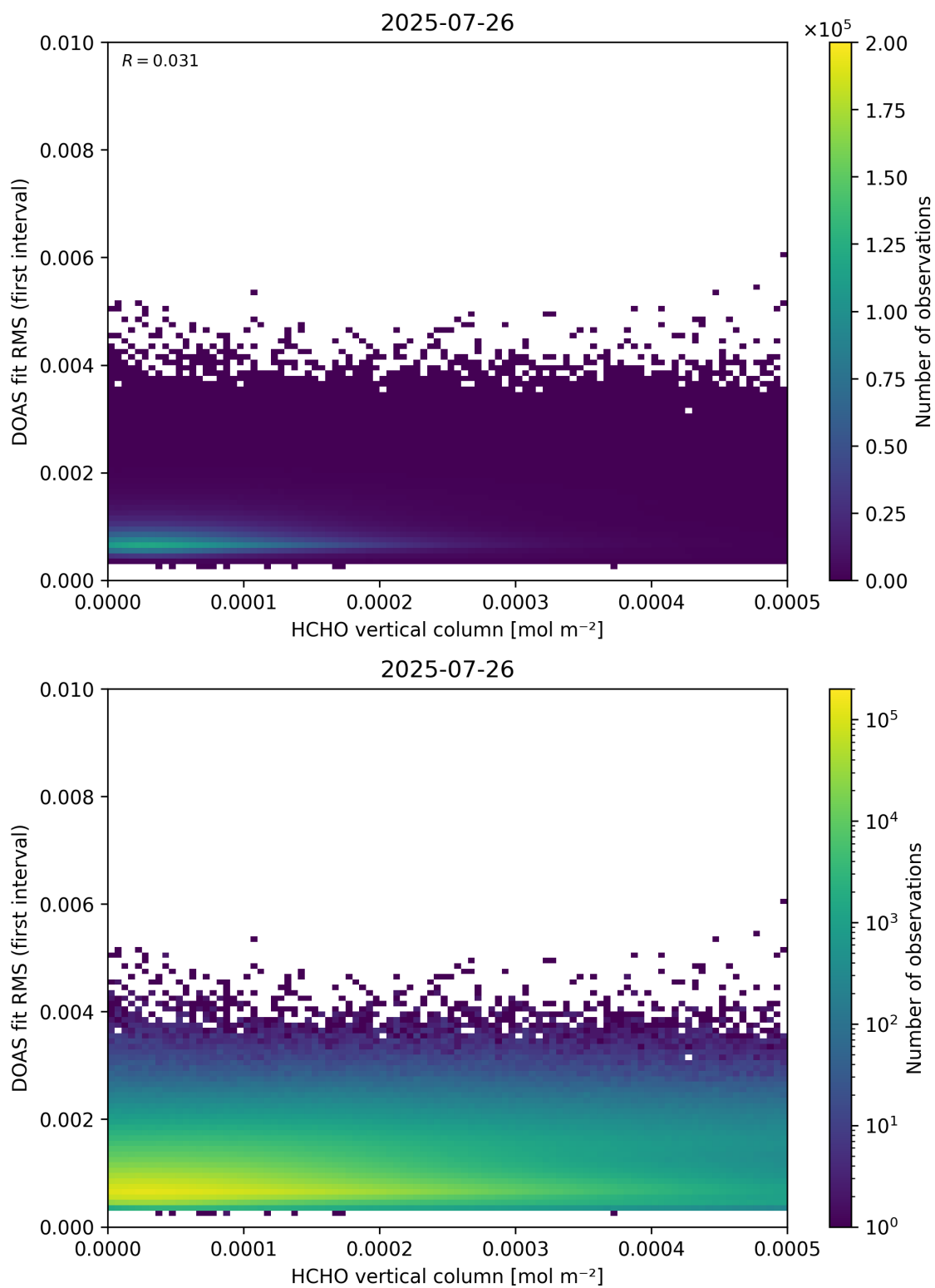
Figure 123: Scatter density plot of “HCHO vertical column” against “DOAS fit RMS (first interval)” for 2025-07-25 to 2025-07-27.
