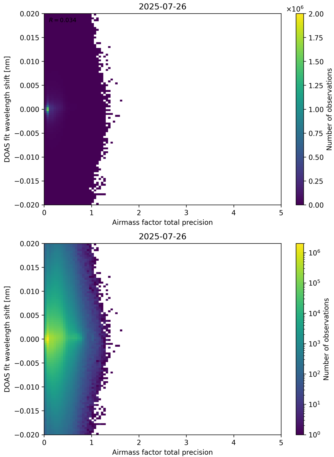
Figure 106: Scatter density plot of “Airmass factor total precision” against “DOAS fit wavelength shift” for 2025-07-25 to 2025-07-27.
