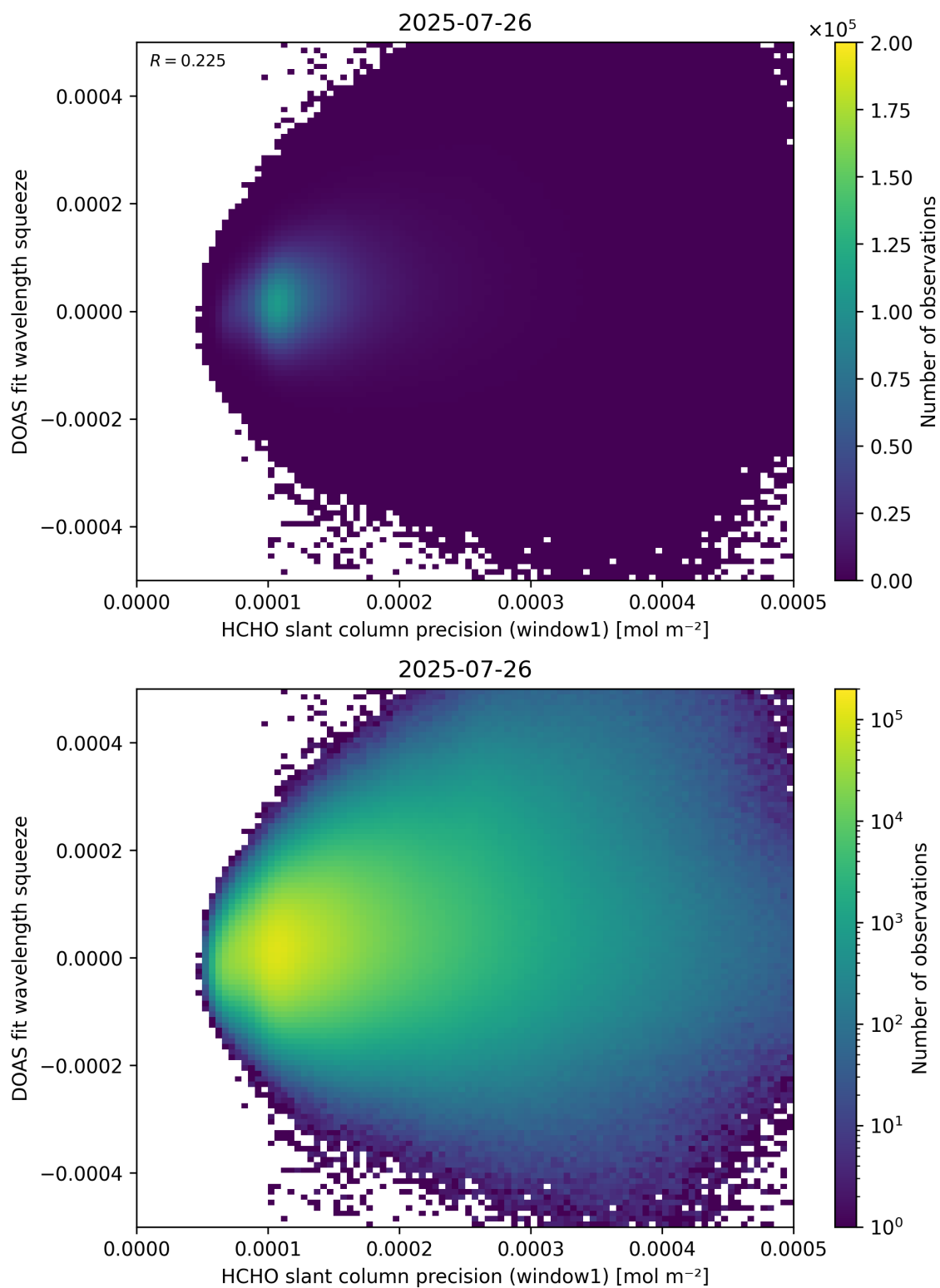
Figure 90: Scatter density plot of “HCHO slant column precision (window1)” against “DOAS fit wavelength squeeze” for 2025-07-25 to 2025-07-27.
