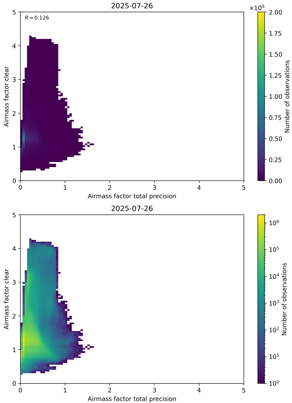
Figure 108: Scatter density plot of “Airmass factor total precision” against “Airmass factor clear” for 2025-07-25 to 2025-07-27.
