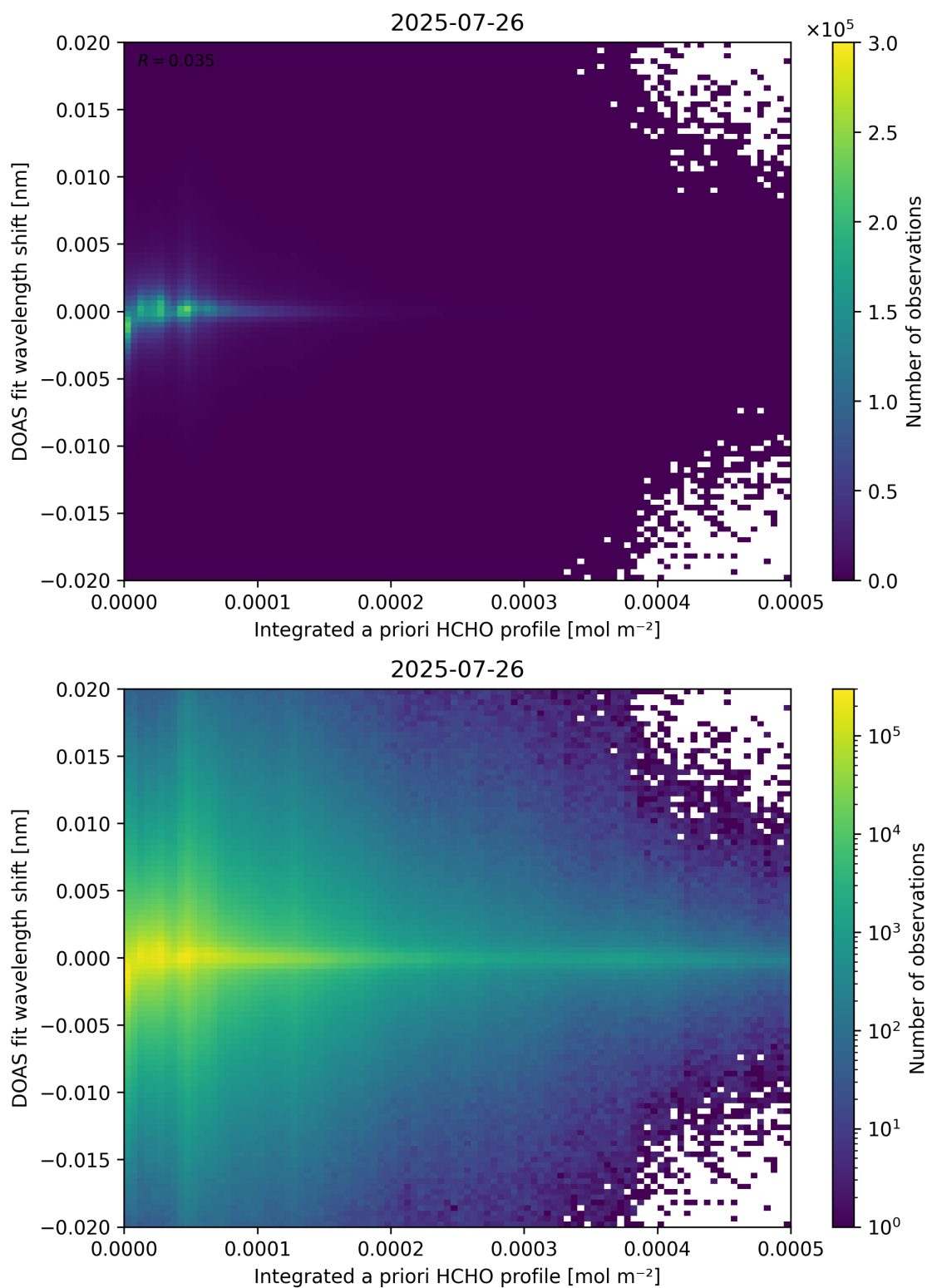
Figure 149: Scatter density plot of “Integrated a priori HCHO profile” against “DOAS fit wavelength shift” for 2025-07-25 to 2025-07-27.
