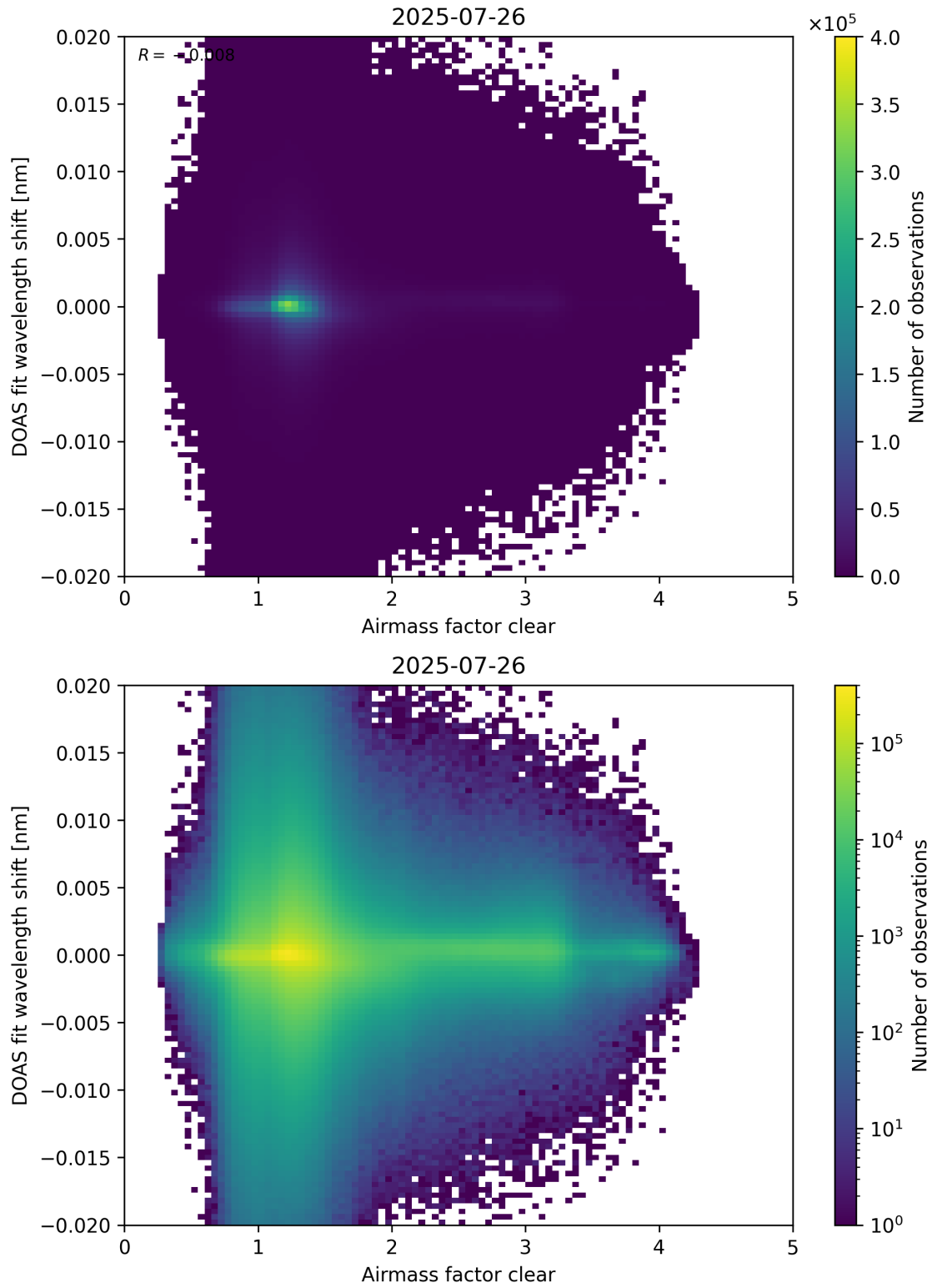
Figure 72: Scatter density plot of “Airmass factor clear” against “DOAS fit wavelength shift” for 2025-07-25 to 2025-07-27.
