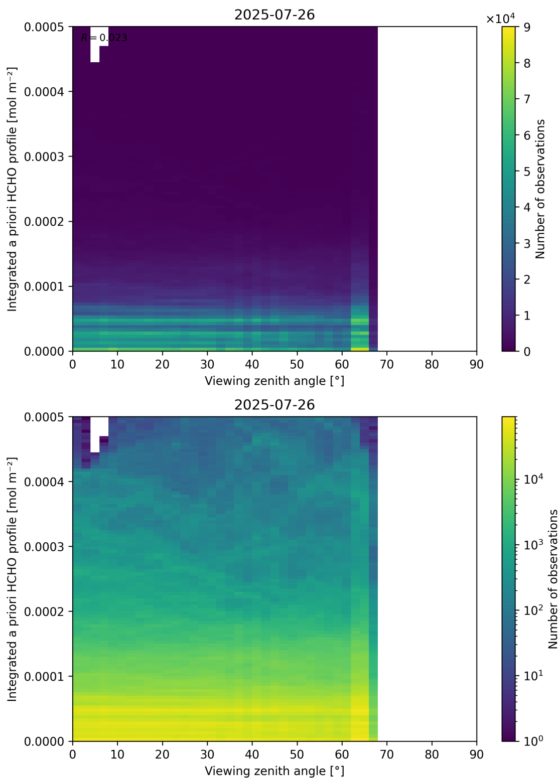
Figure 195: Scatter density plot of “Viewing zenith angle” against “Integrated a priori HCHO profile” for 2025-07-25 to 2025-07-27.
