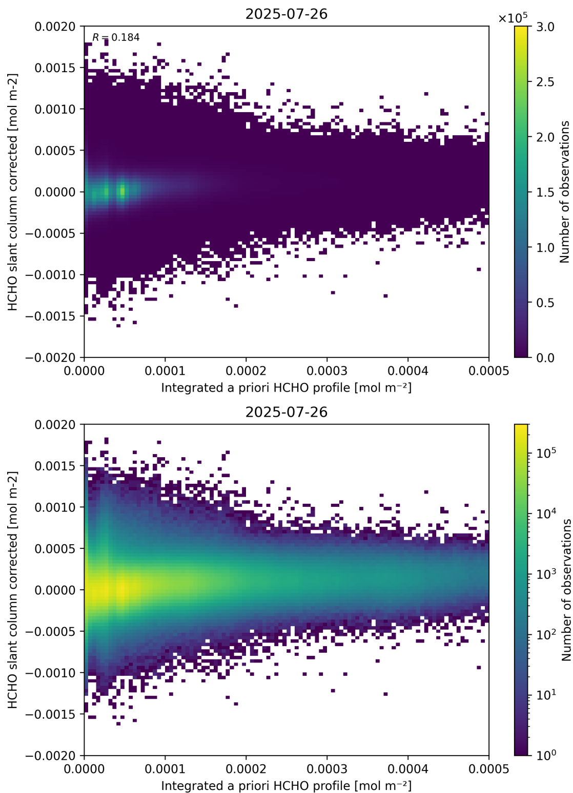
Figure 151: Scatter density plot of “Integrated a priori HCHO profile” against “HCHO slant column corrected” for 2025-07-25 to 2025-07-27.
