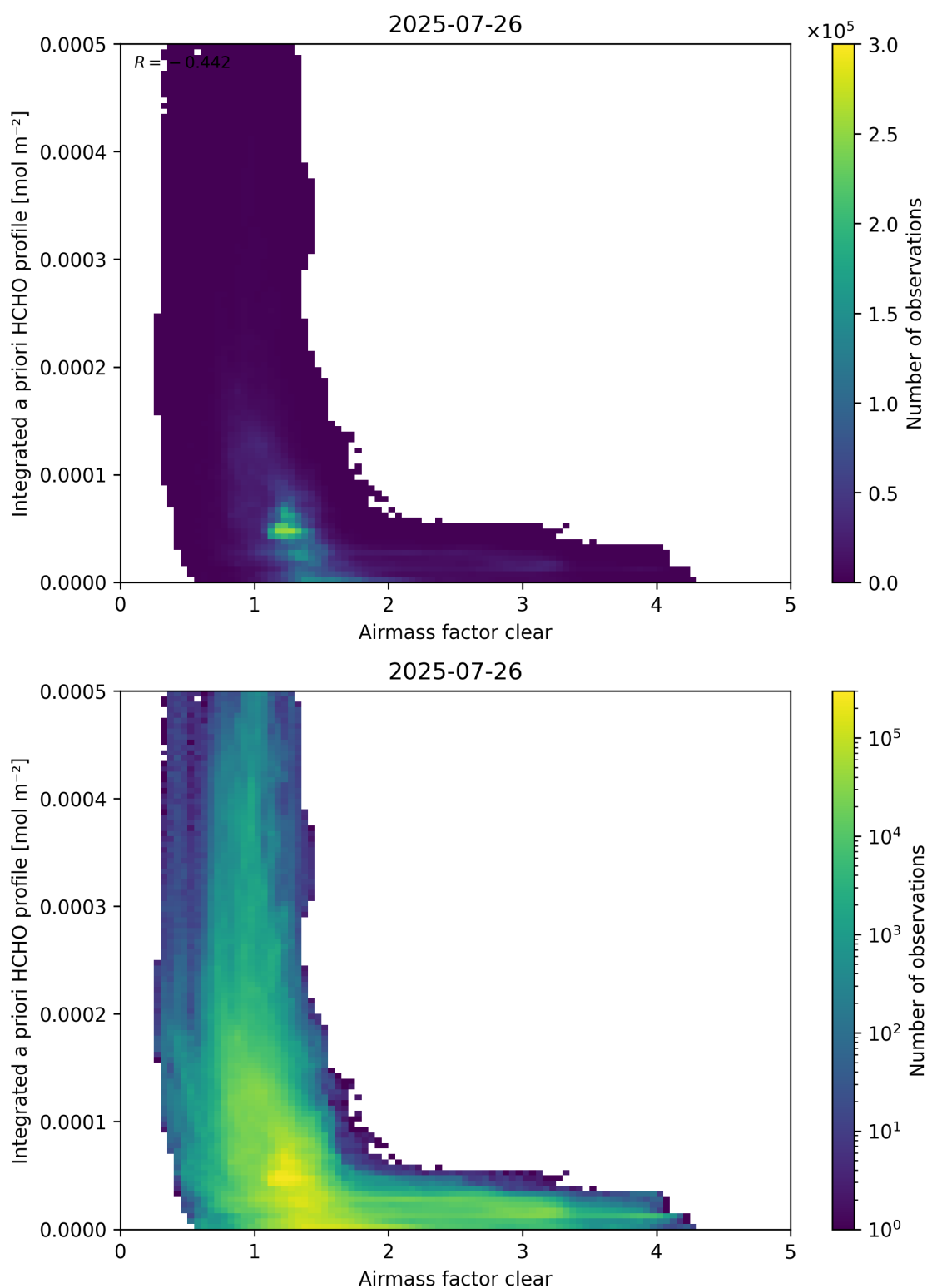
Figure 76: Scatter density plot of “Airmass factor clear” against “Integrated a priori HCHO profile” for 2025-07-25 to 2025-07-27.
