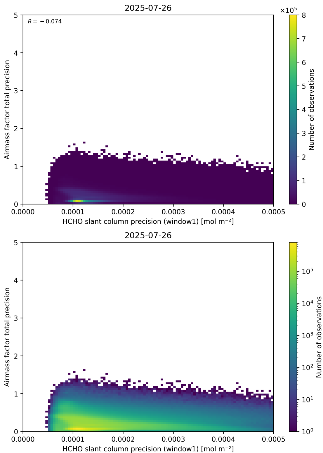
Figure 95: Scatter density plot of “HCHO slant column precision (window1)” against “Airmass factor total precision” for 2025-07-25 to 2025-07-27.
