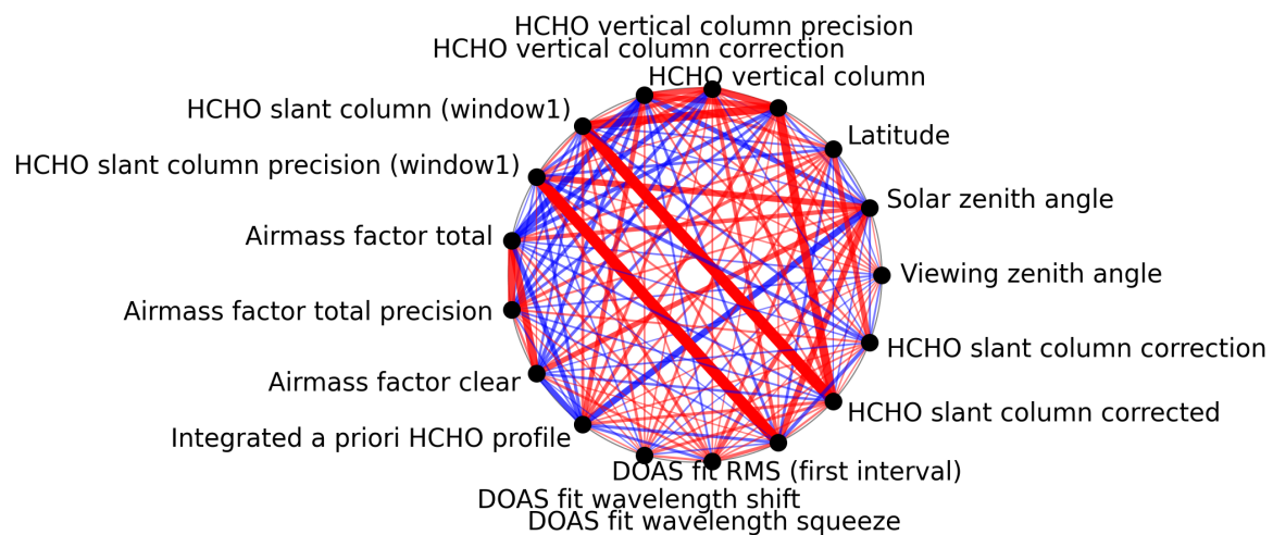
Figure 1: Map of correlation graph for 2025-07-25 to 2025-07-27.
