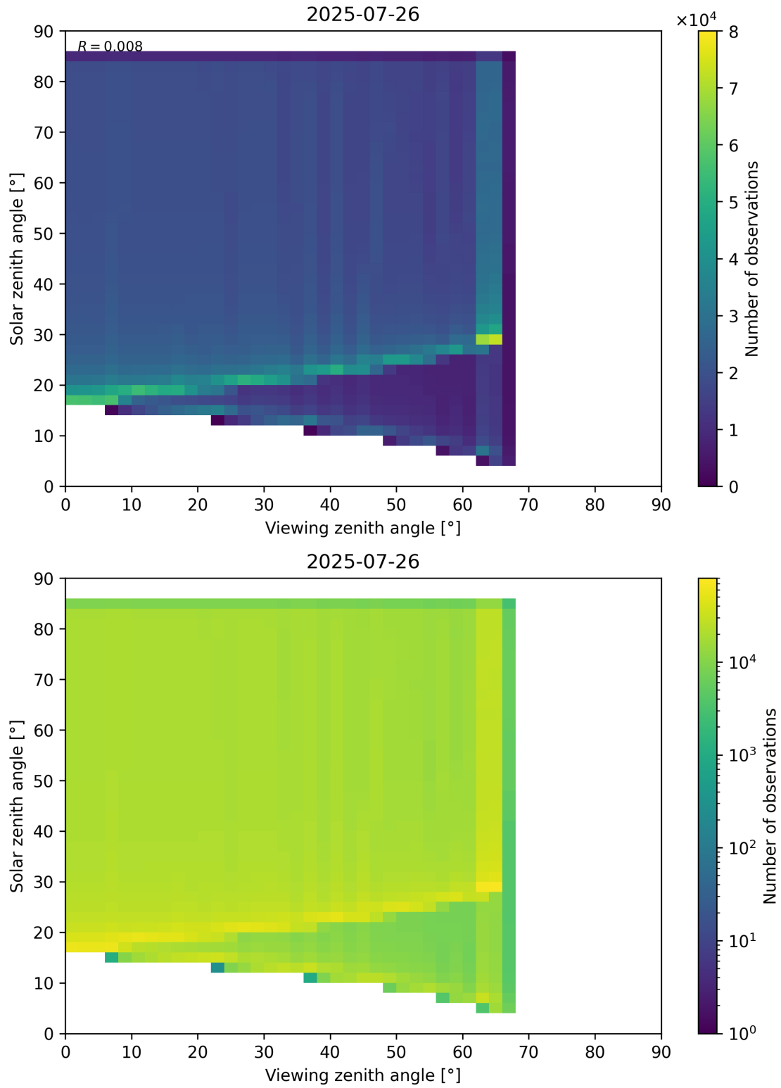
Figure 197: Scatter density plot of “Viewing zenith angle” against “Solar zenith angle” for 2025-07-25 to 2025-07-27.
