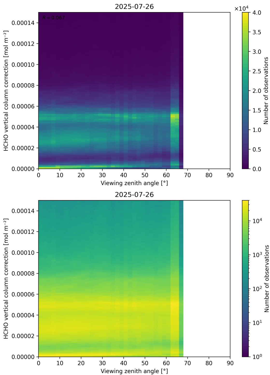
Figure 193: Scatter density plot of “Viewing zenith angle” against “HCHO vertical column correction” for 2025-07-25 to 2025-07-27.
