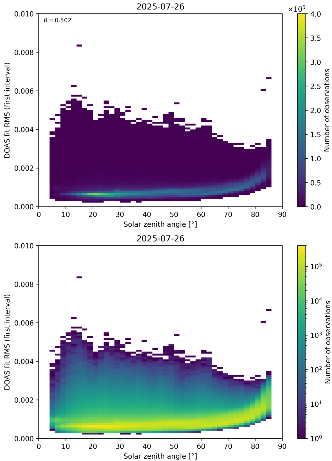
Figure 167: Scatter density plot of “Solar zenith angle” against “DOAS fit RMS (first interval)” for 2025-07-25 to 2025-07-27.
