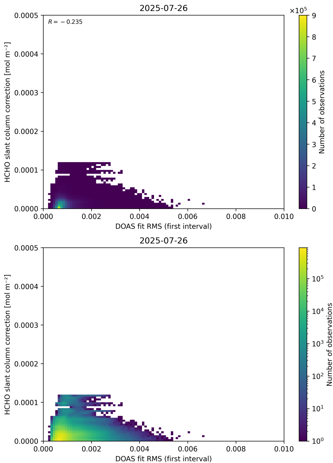
Figure 63: Scatter density plot of “DOAS fit RMS (first interval)” against “HCHO slant column correction” for 2025-07-25 to 2025-07-27.
