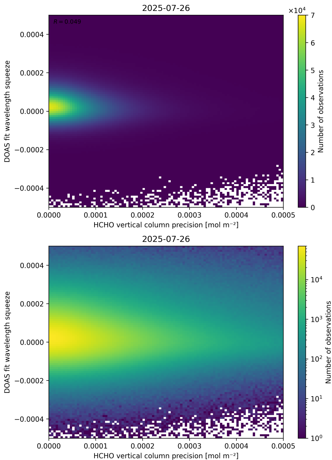
Figure 138: Scatter density plot of “HCHO vertical column precision” against “DOAS fit wavelength squeeze” for 2025-07-25 to 2025-07-27.
