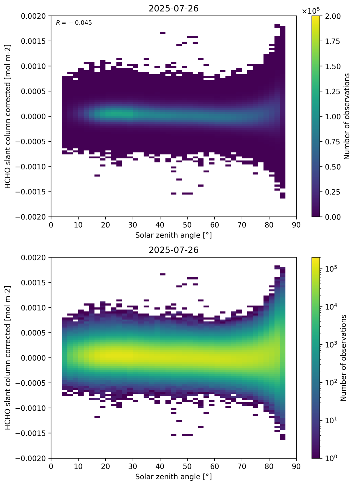
Figure 171: Scatter density plot of “Solar zenith angle” against “HCHO slant column corrected” for 2025-07-25 to 2025-07-27.
