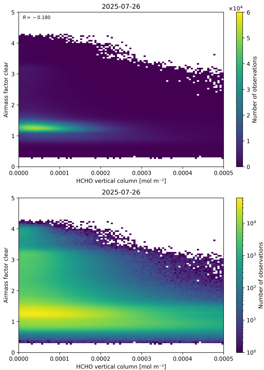
Figure 126: Scatter density plot of “HCHO vertical column” against “Airmass factor clear” for 2025-07-25 to 2025-07-27.
