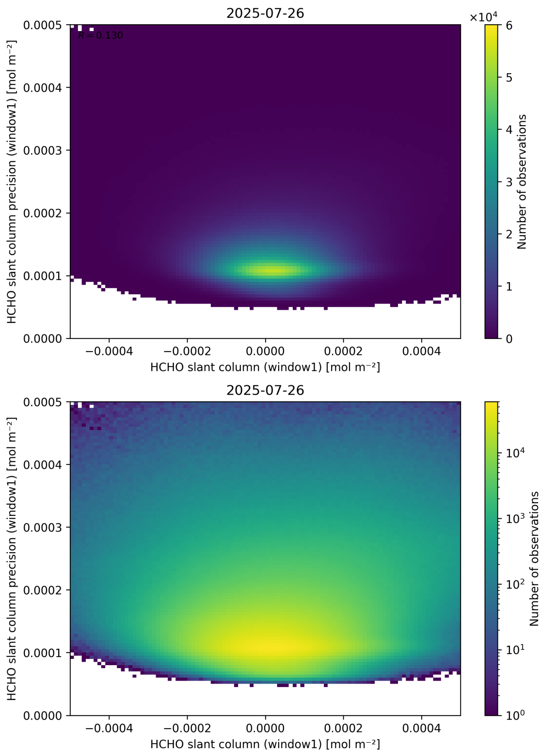
Figure 84: Scatter density plot of “HCHO slant column (window1)” against “HCHO slant column precision (window1)” for 2025-07-25 to 2025-07-27.
