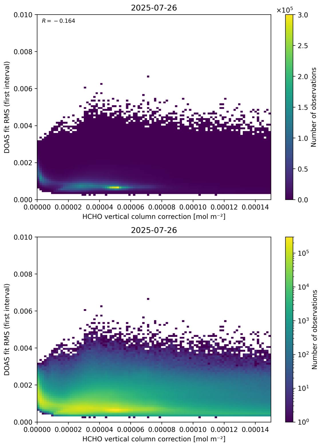
Figure 112: Scatter density plot of “HCHO vertical column correction” against “DOAS fit RMS (first interval)” for 2025-07-25 to 2025-07-27.
