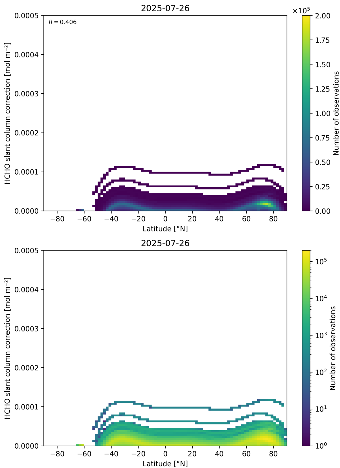
Figure 158: Scatter density plot of “Latitude” against “HCHO slant column correction” for 2025-07-25 to 2025-07-27.
