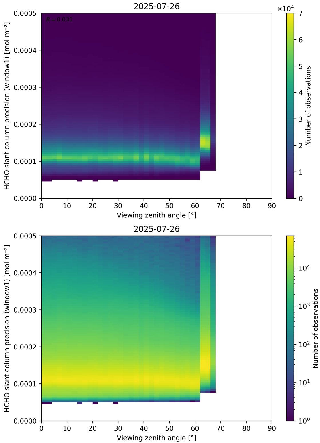
Figure 189: Scatter density plot of “Viewing zenith angle” against “HCHO slant column precision (window1)” for 2025-07-25 to 2025-07-27.
