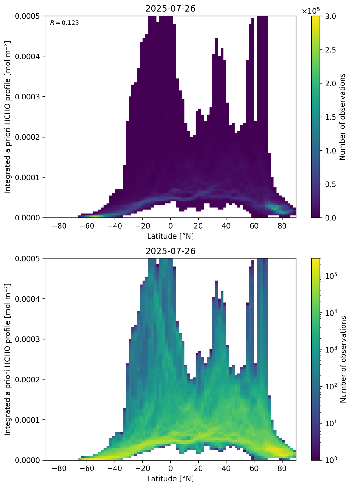
Figure 166: Scatter density plot of “Latitude” against “Integrated a priori HCHO profile” for 2025-07-25 to 2025-07-27.
