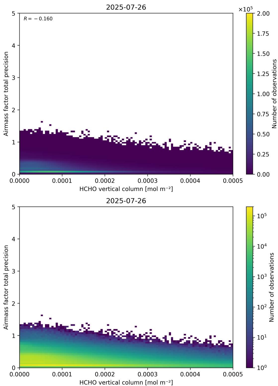
Figure 132: Scatter density plot of “HCHO vertical column” against “Airmass factor total precision” for 2025-07-25 to 2025-07-27.
