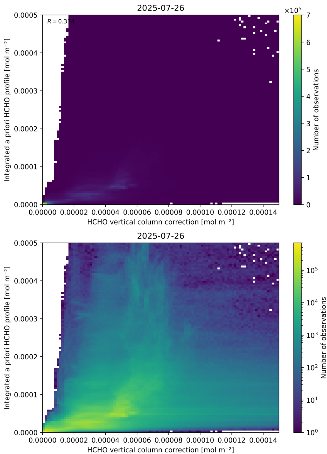
Figure 122: Scatter density plot of “HCHO vertical column correction” against “Integrated a priori HCHO profile” for 2025-07-25 to 2025-07-27.
