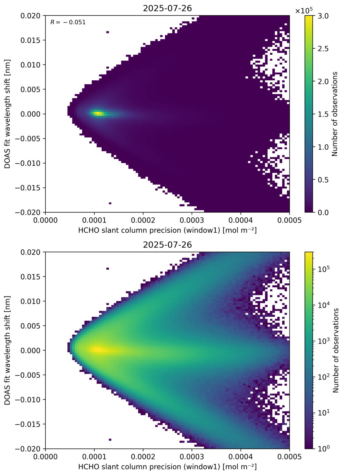
Figure 89: Scatter density plot of “HCHO slant column precision (window1)” against “DOAS fit wavelength shift” for 2025-07-25 to 2025-07-27.
