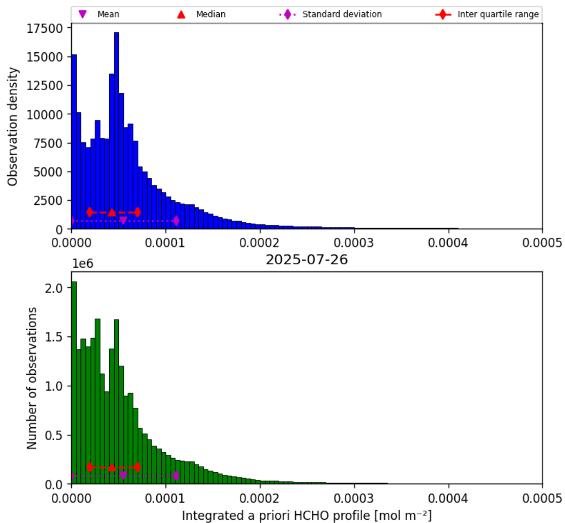
Figure 43: Histogram of “Integrated a priori HCHO profile” for 2025-07-25 to 2025-07-27
