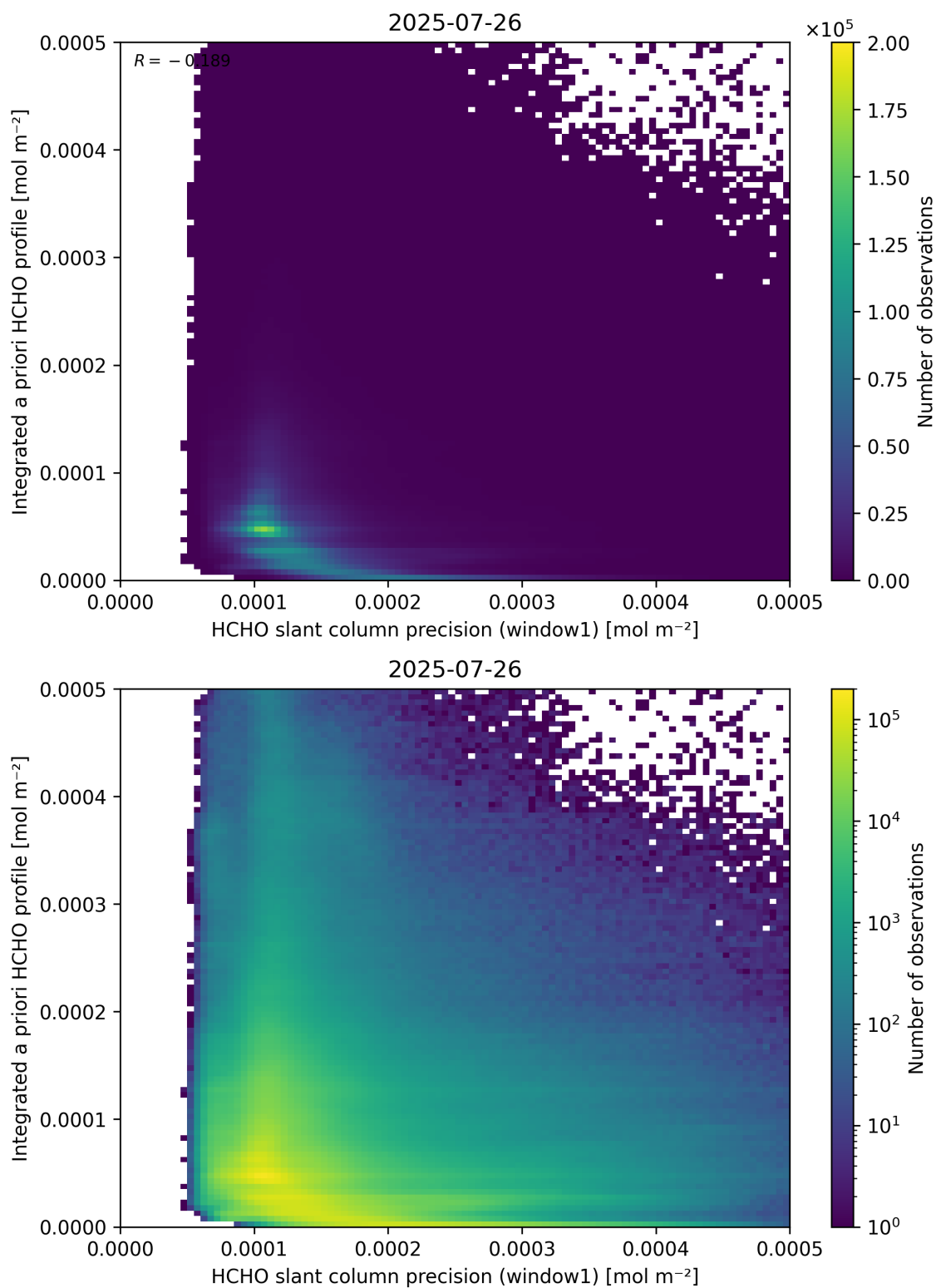
Figure 96: Scatter density plot of “HCHO slant column precision (window1)” against “Integrated a priori HCHO profile” for 2025-07-25 to 2025-07-27.
