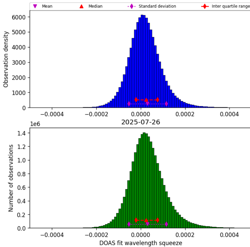
Figure 45: Histogram of “DOAS fit wavelength squeeze” for 2025-07-25 to 2025-07-27
