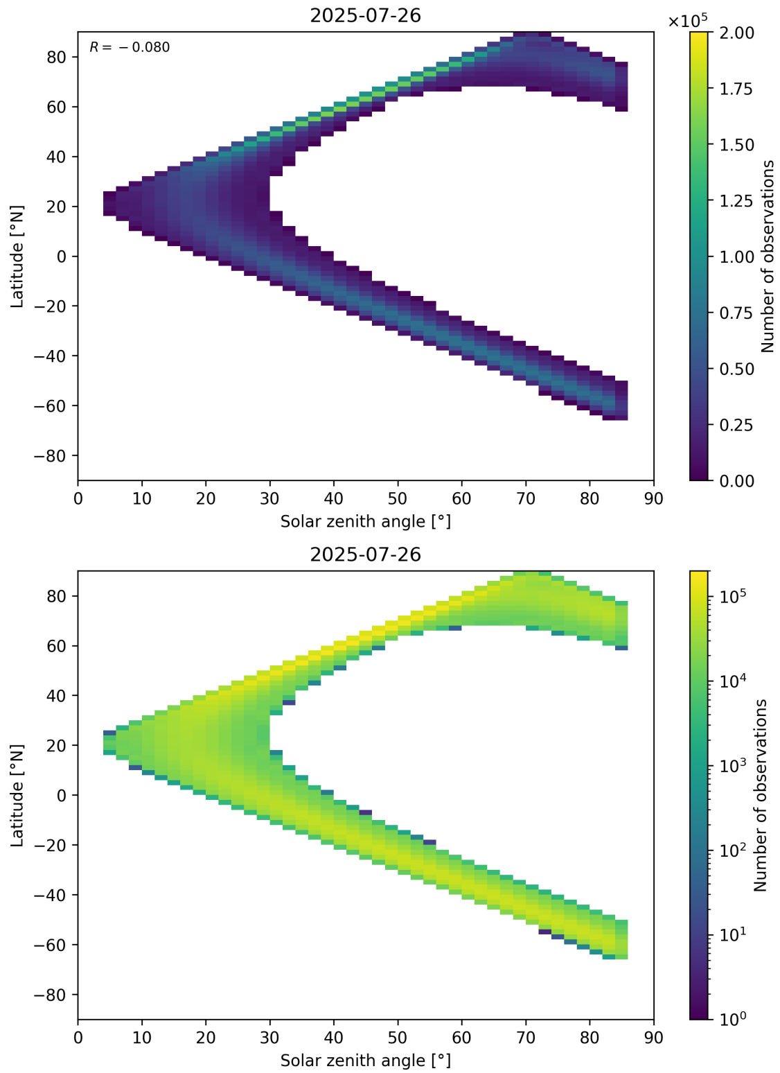
Figure 181: Scatter density plot of “Solar zenith angle” against “Latitude” for 2025-07-25 to 2025-07-27.
