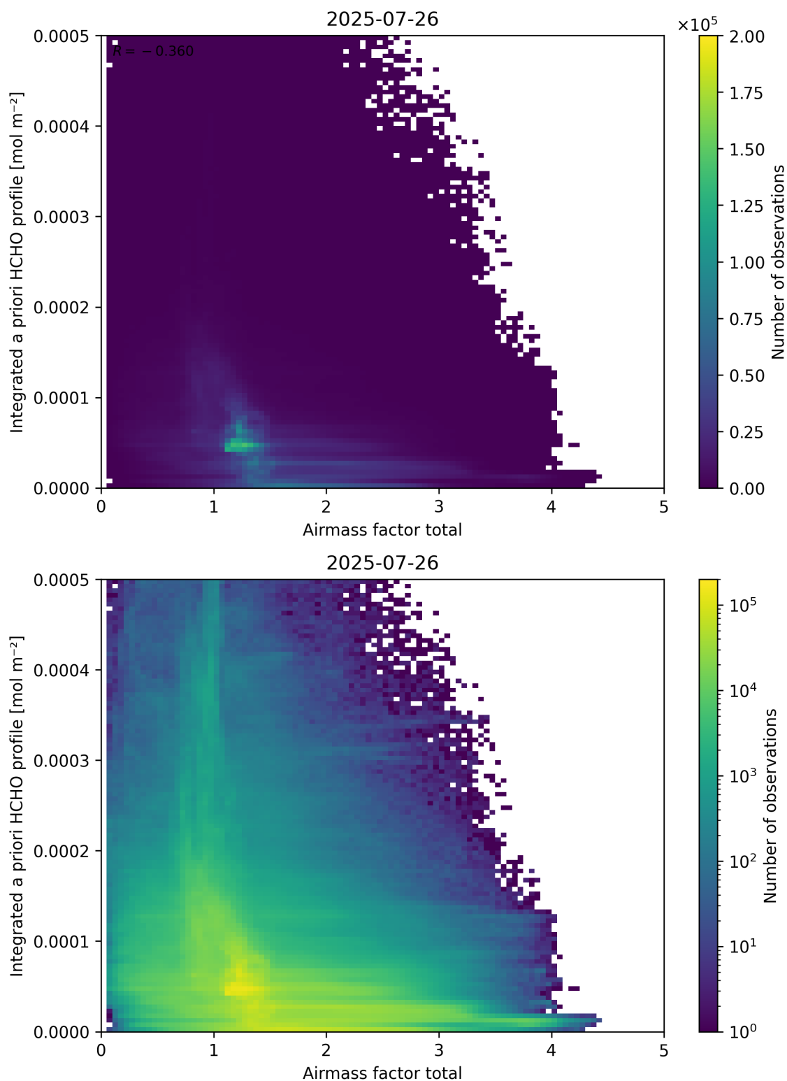
Figure 104: Scatter density plot of “Airmass factor total” against “Integrated a priori HCHO profile” for 2025-07-25 to 2025-07-27.
