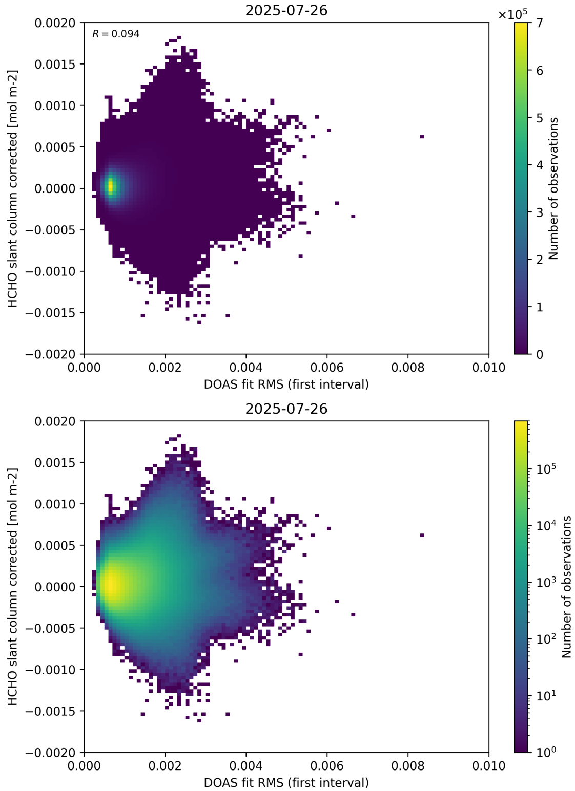
Figure 62: Scatter density plot of “DOAS fit RMS (first interval)” against “HCHO slant column corrected” for 2025-07-25 to 2025-07-27.
