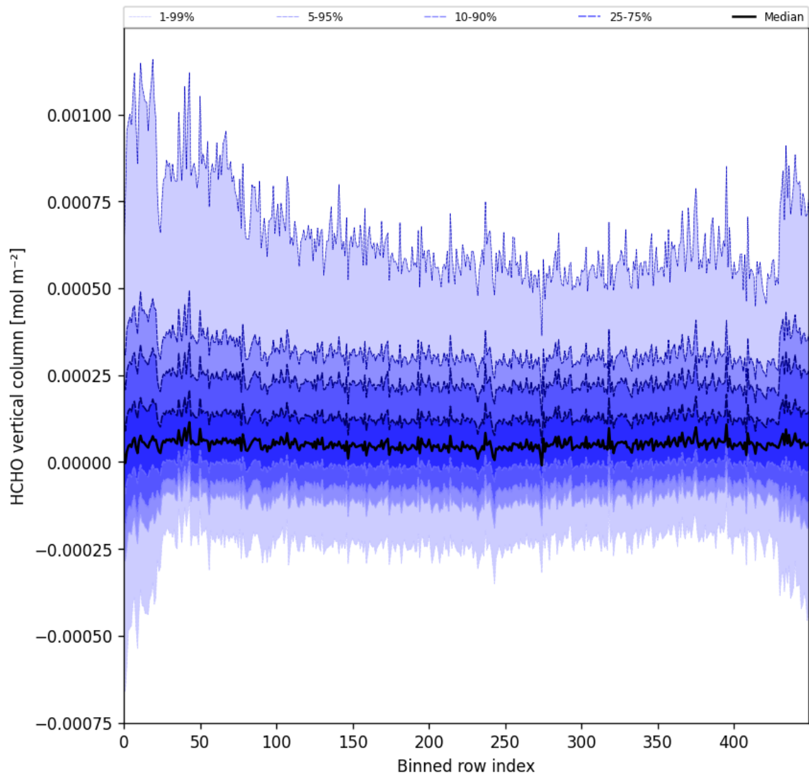
Figure 49: Along track statistics of “HCHO vertical column” for 2025-07-25 to 2025-07-27
