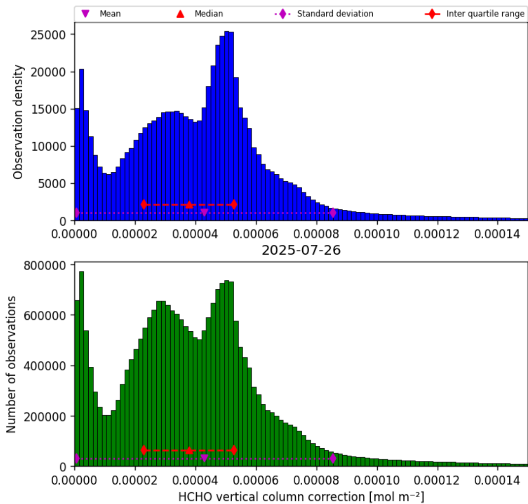
Figure 37: Histogram of “HCHO vertical column correction” for 2025-07-25 to 2025-07-27
