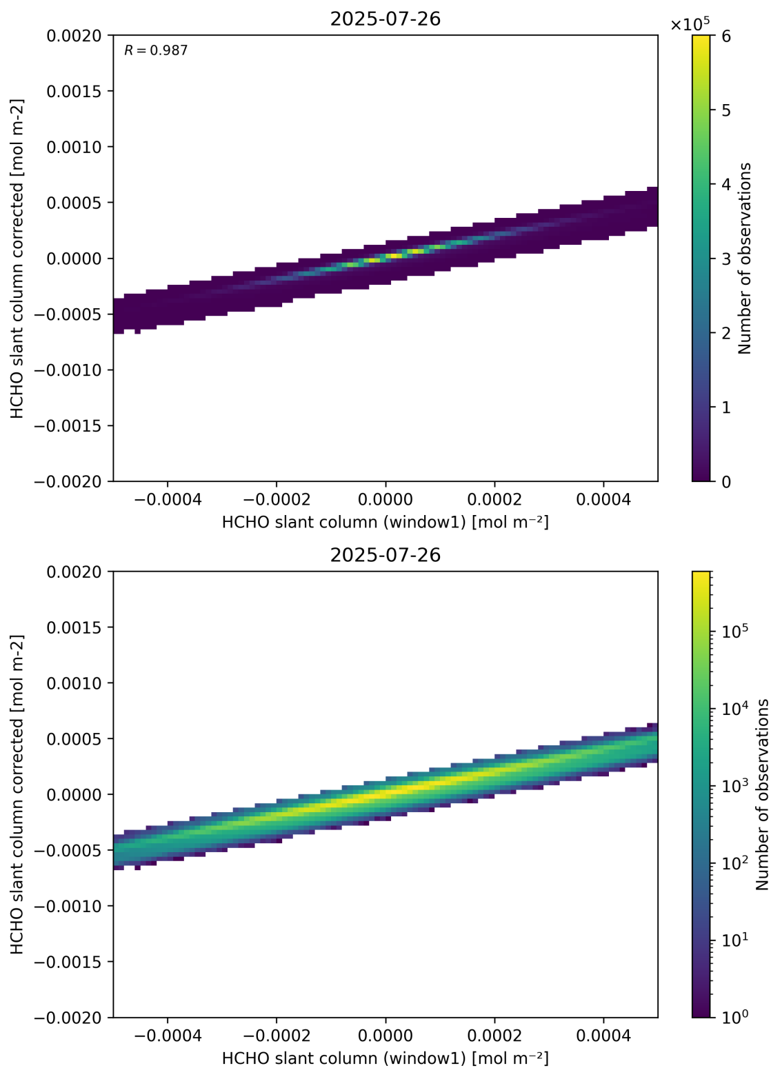
Figure 82: Scatter density plot of “HCHO slant column (window1)” against “HCHO slant column corrected” for 2025-07-25 to 2025-07-27.
