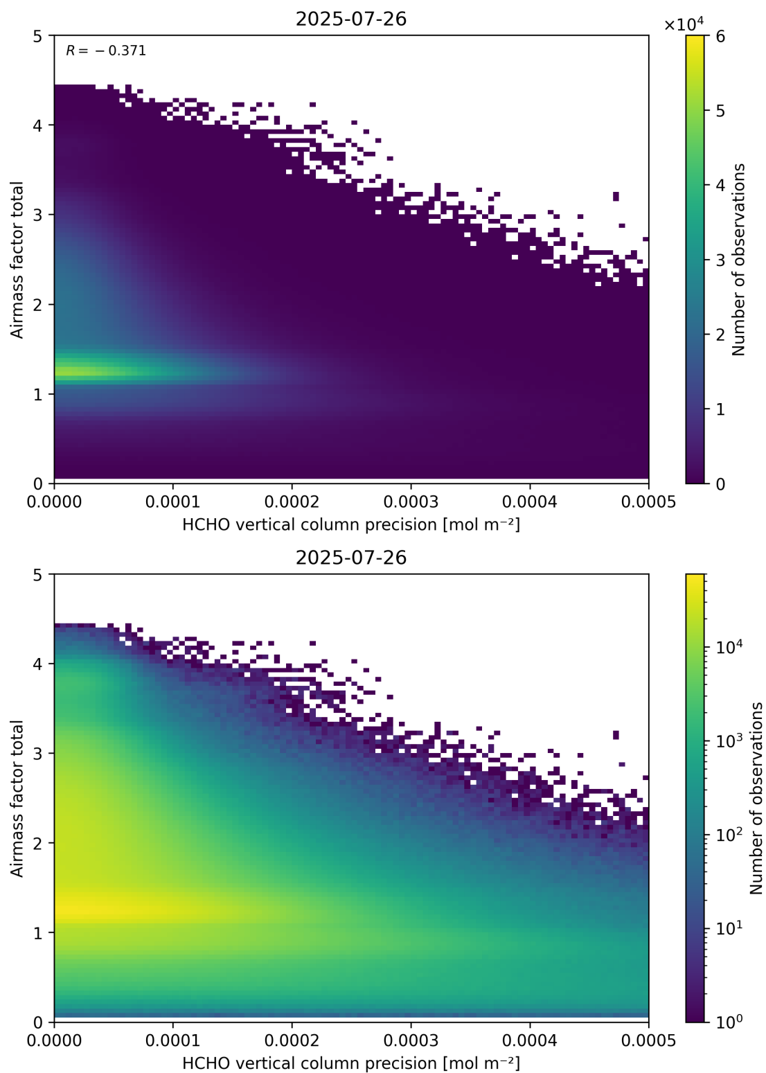
Figure 144: Scatter density plot of “HCHO vertical column precision” against “Airmass factor total” for 2025-07-25 to 2025-07-27.
