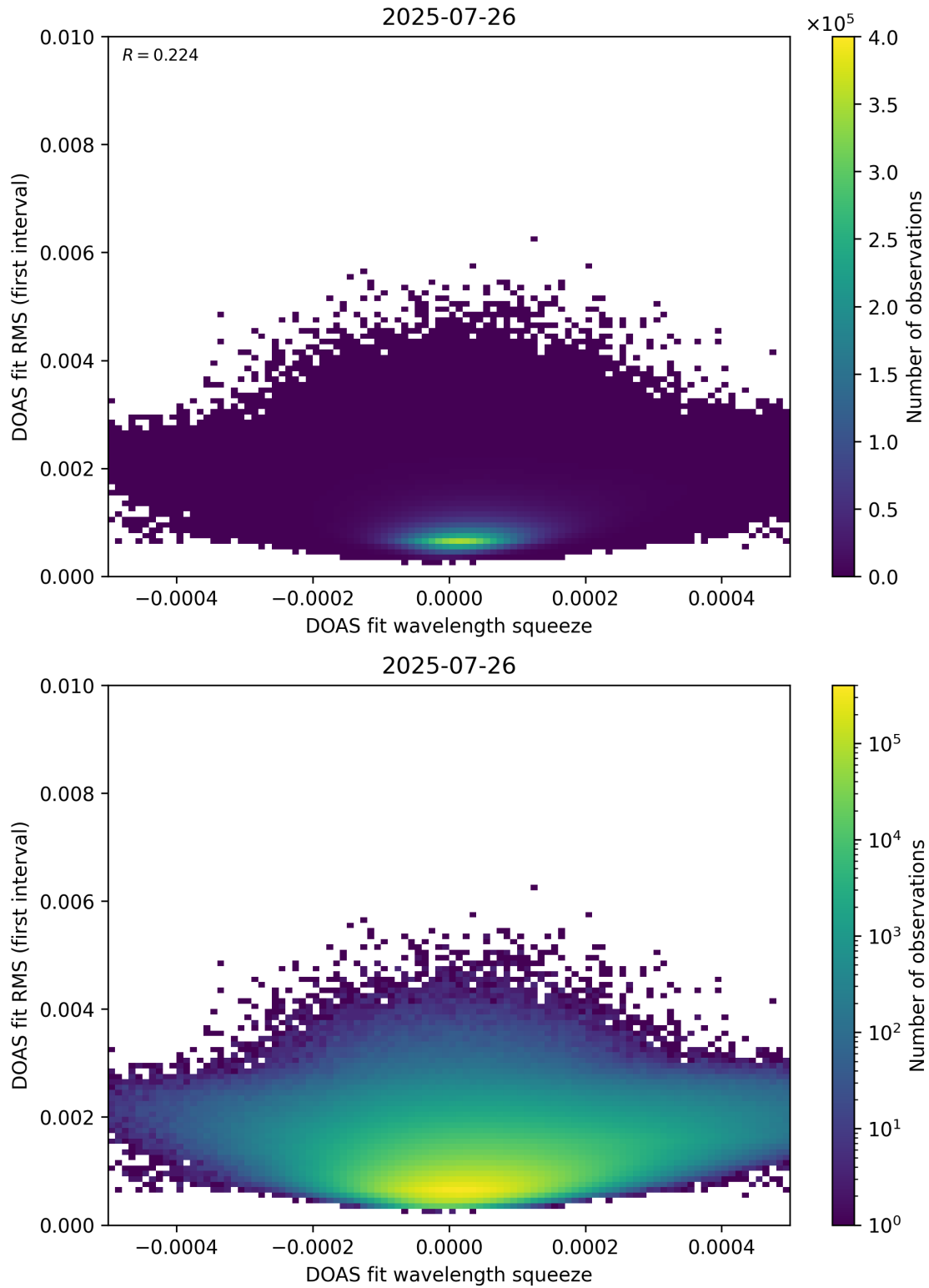
Figure 68: Scatter density plot of “DOAS fit wavelength squeeze” against “DOAS fit RMS (first interval)” for 2025-07-25 to 2025-07-27.
