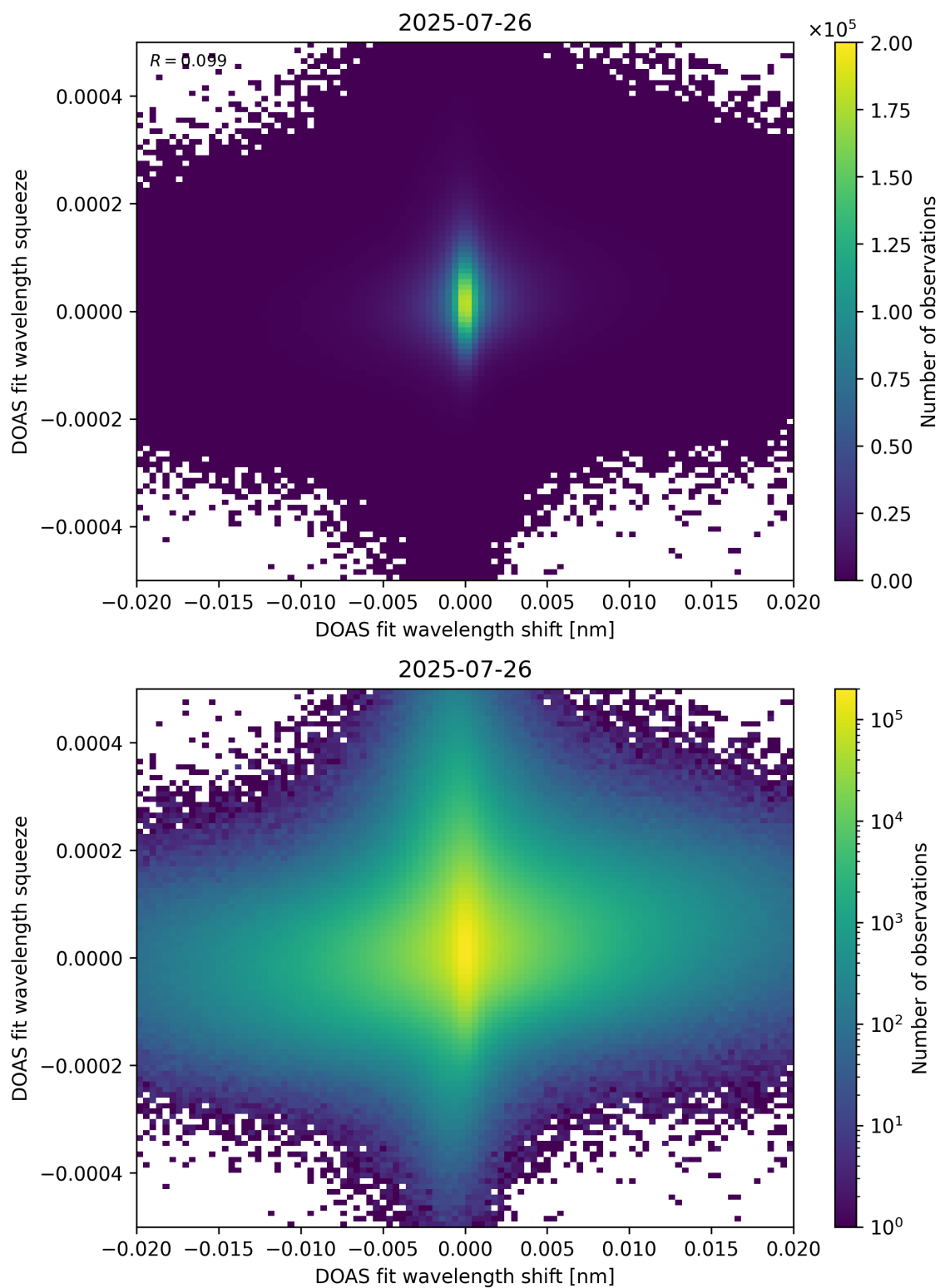
Figure 65: Scatter density plot of “DOAS fit wavelength shift” against “DOAS fit wavelength squeeze” for 2025-07-25 to 2025-07-27.
