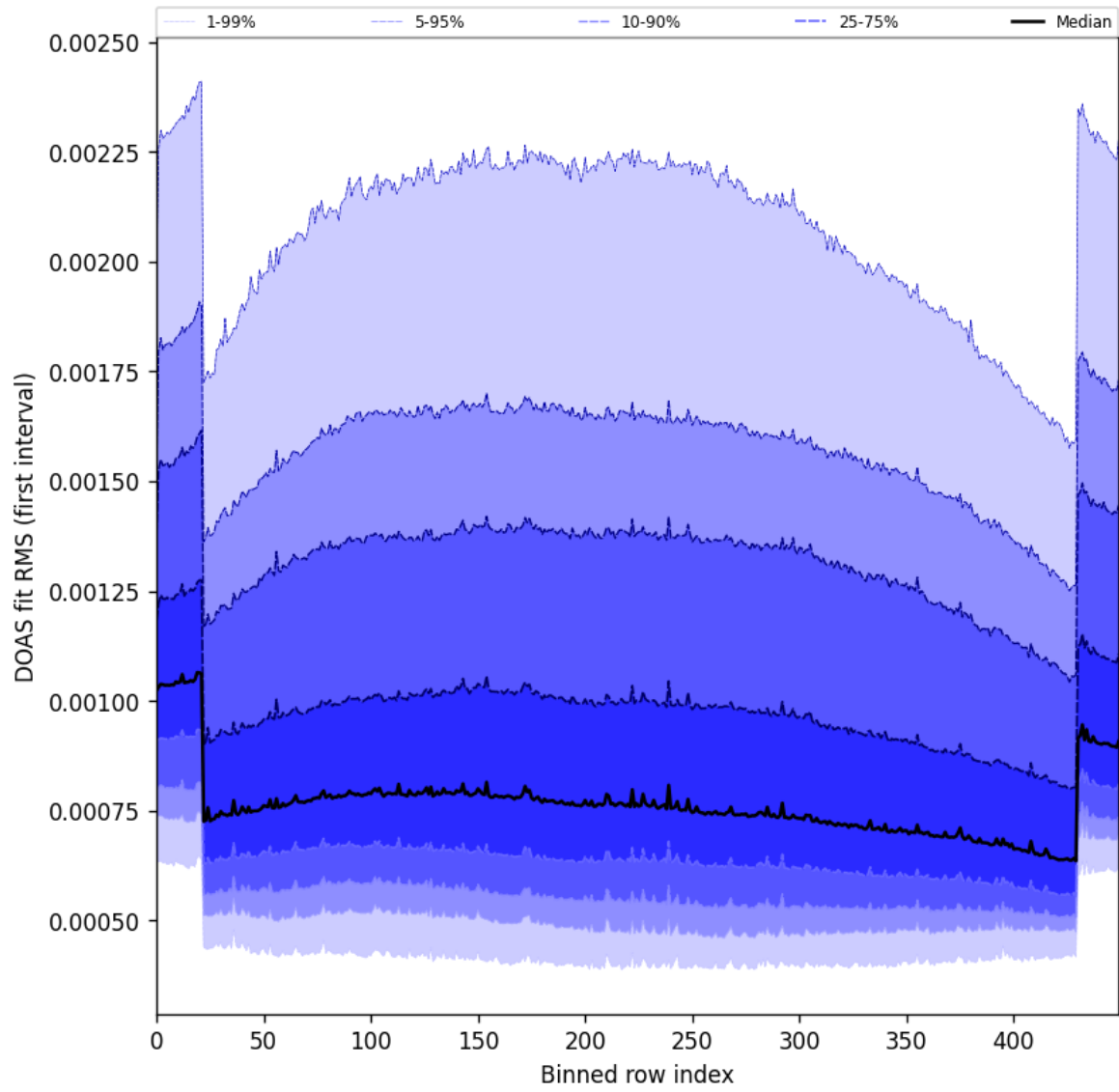
Figure 60: Along track statistics of “DOAS fit RMS (first interval)” for 2025-07-25 to 2025-07-27
