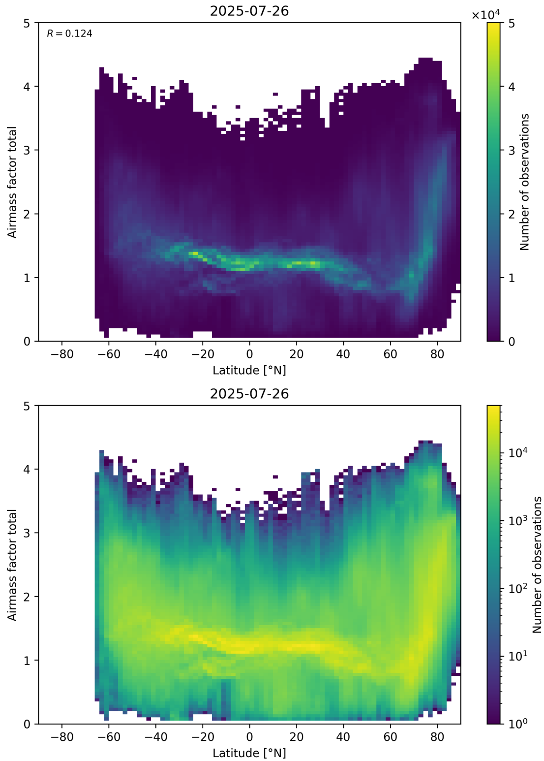
Figure 161: Scatter density plot of “Latitude” against “Airmass factor total” for 2025-07-25 to 2025-07-27.
