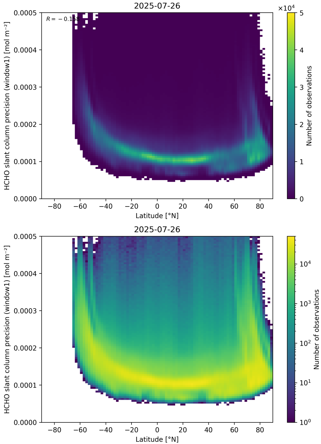
Figure 160: Scatter density plot of “Latitude” against “HCHO slant column precision (window1)” for 2025-07-25 to 2025-07-27.
