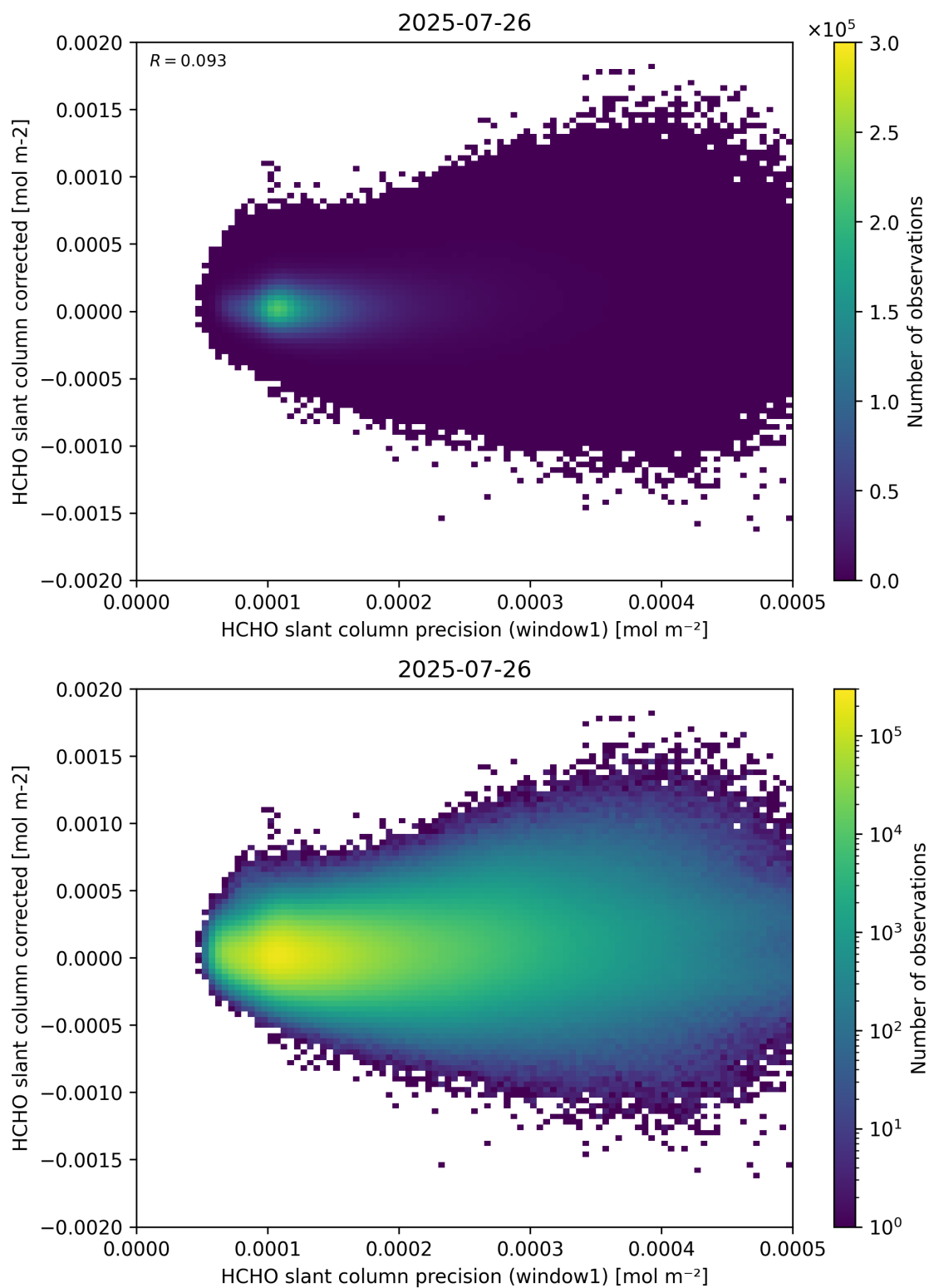
Figure 92: Scatter density plot of “HCHO slant column precision (window1)” against “HCHO slant column corrected” for 2025-07-25 to 2025-07-27.
