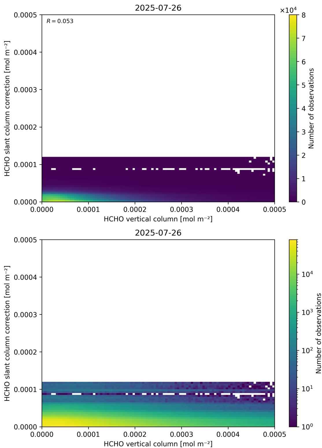
Figure 128: Scatter density plot of “HCHO vertical column” against “HCHO slant column correction” for 2025-07-25 to 2025-07-27.
