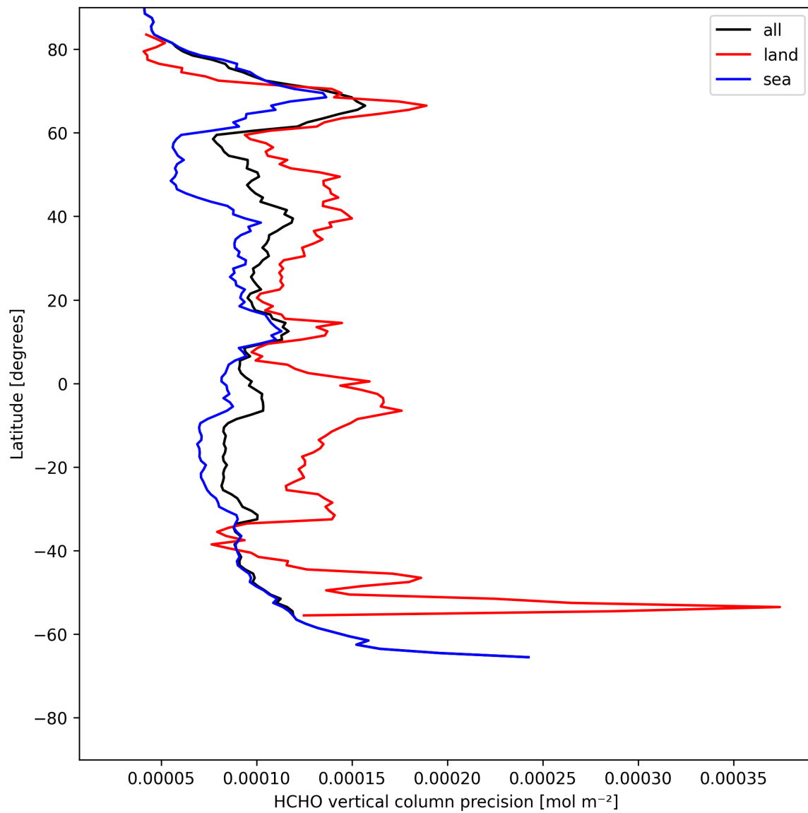
Figure 22: Zonal average of “HCHO vertical column precision” for 2025-07-25 to 2025-07-27.
