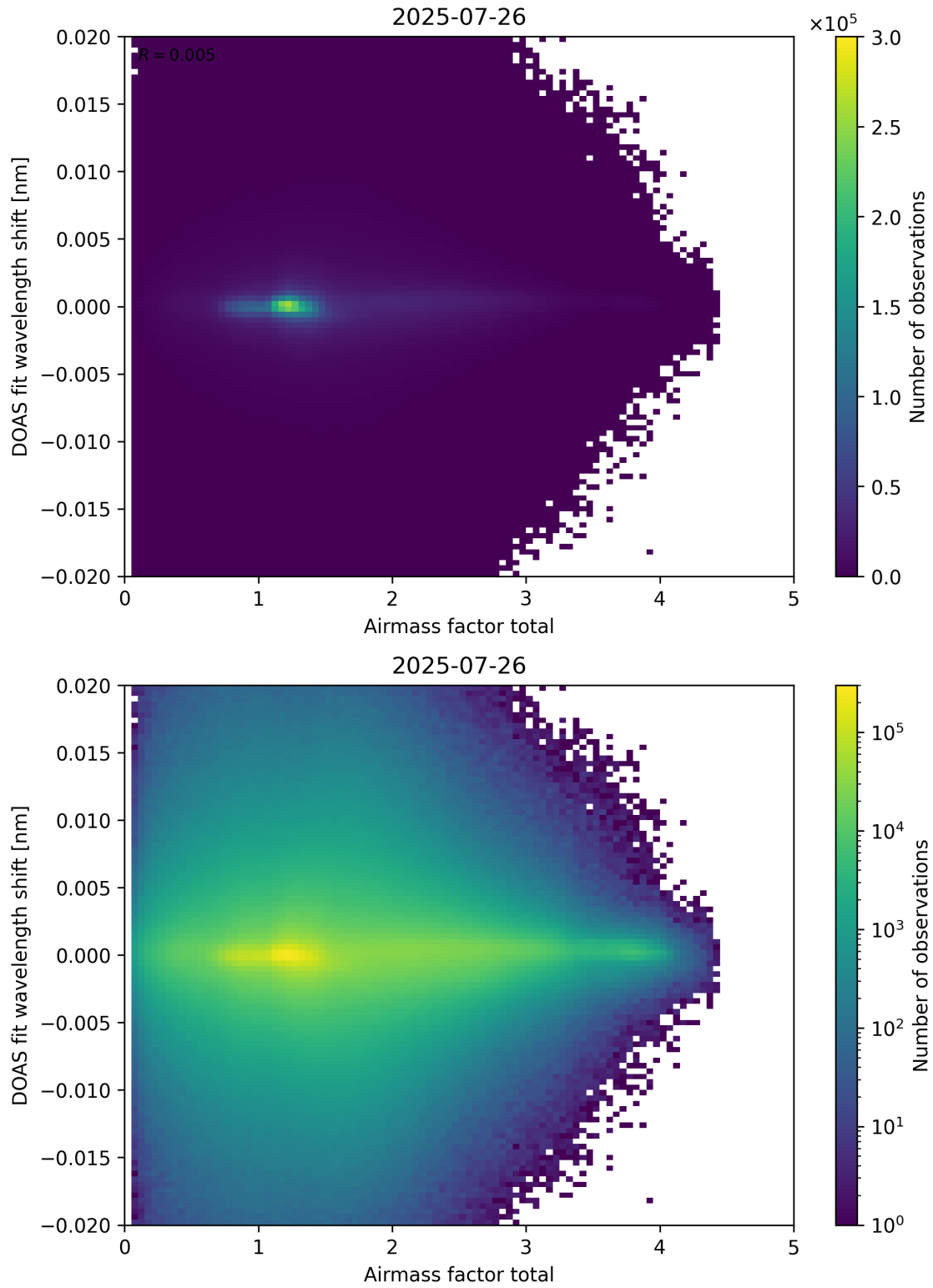
Figure 98: Scatter density plot of “Airmass factor total” against “DOAS fit wavelength shift” for 2025-07-25 to 2025-07-27.
