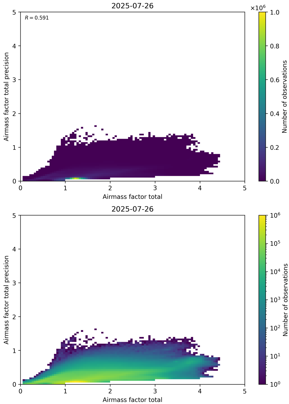
Figure 103: Scatter density plot of “Airmass factor total” against “Airmass factor total precision” for 2025-07-25 to 2025-07-27.
