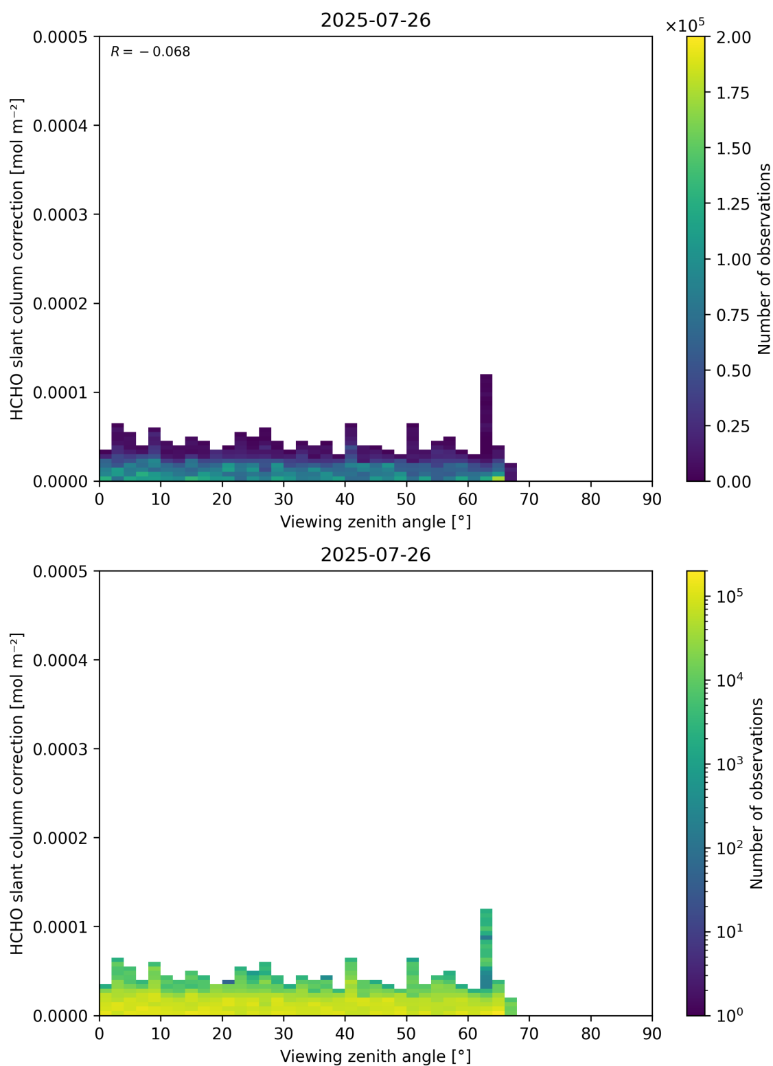
Figure 187: Scatter density plot of “Viewing zenith angle” against “HCHO slant column correction” for 2025-07-25 to 2025-07-27.
