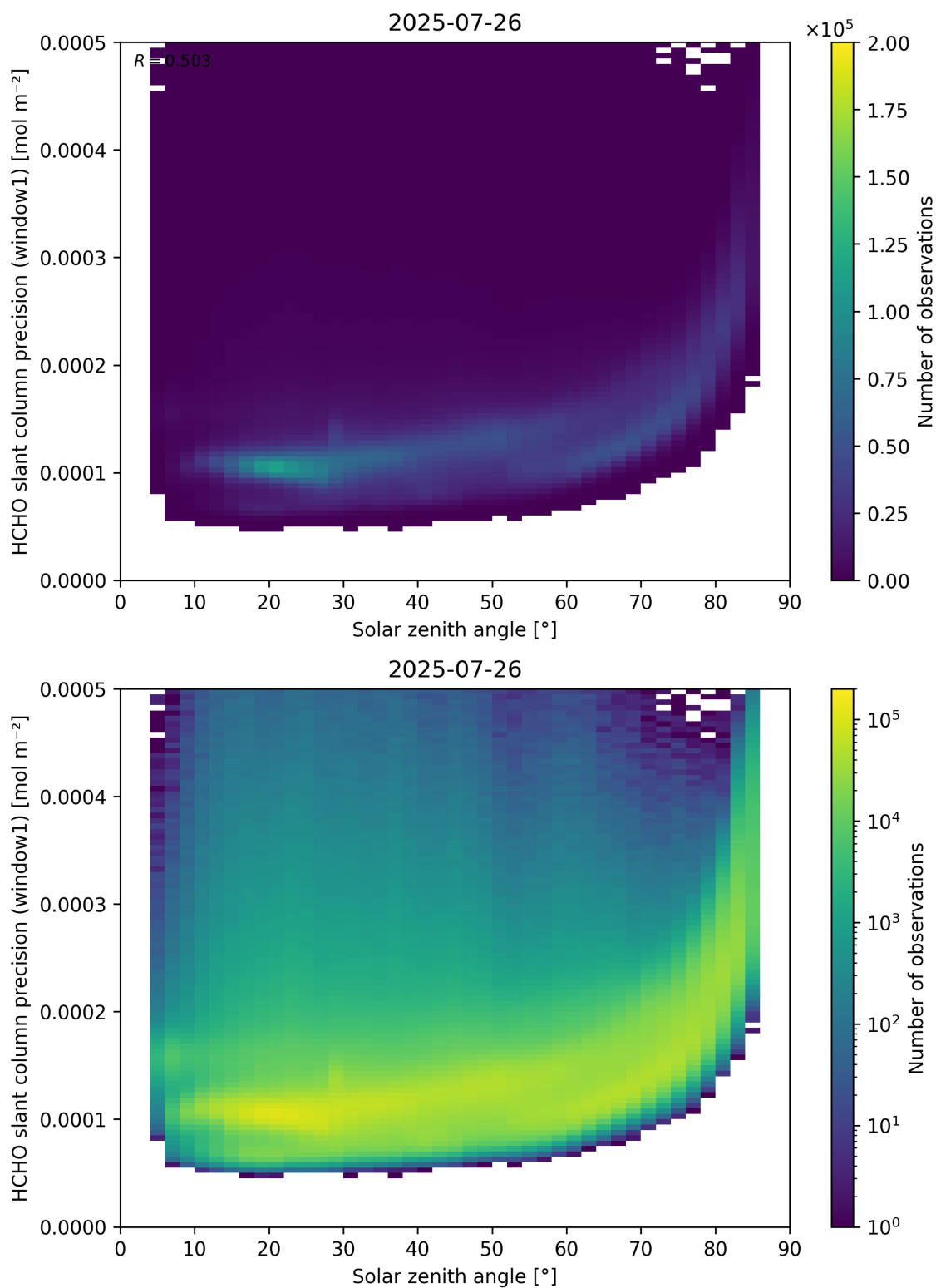
Figure 174: Scatter density plot of “Solar zenith angle” against “HCHO slant column precision (window1)” for 2025-07-25 to 2025-07-27.
