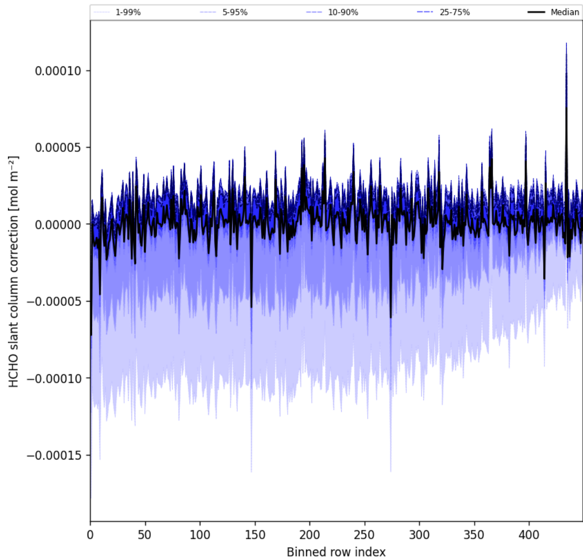
Figure 61: Along track statistics of “HCHO slant column correction” for 2025-07-25 to 2025-07-27
