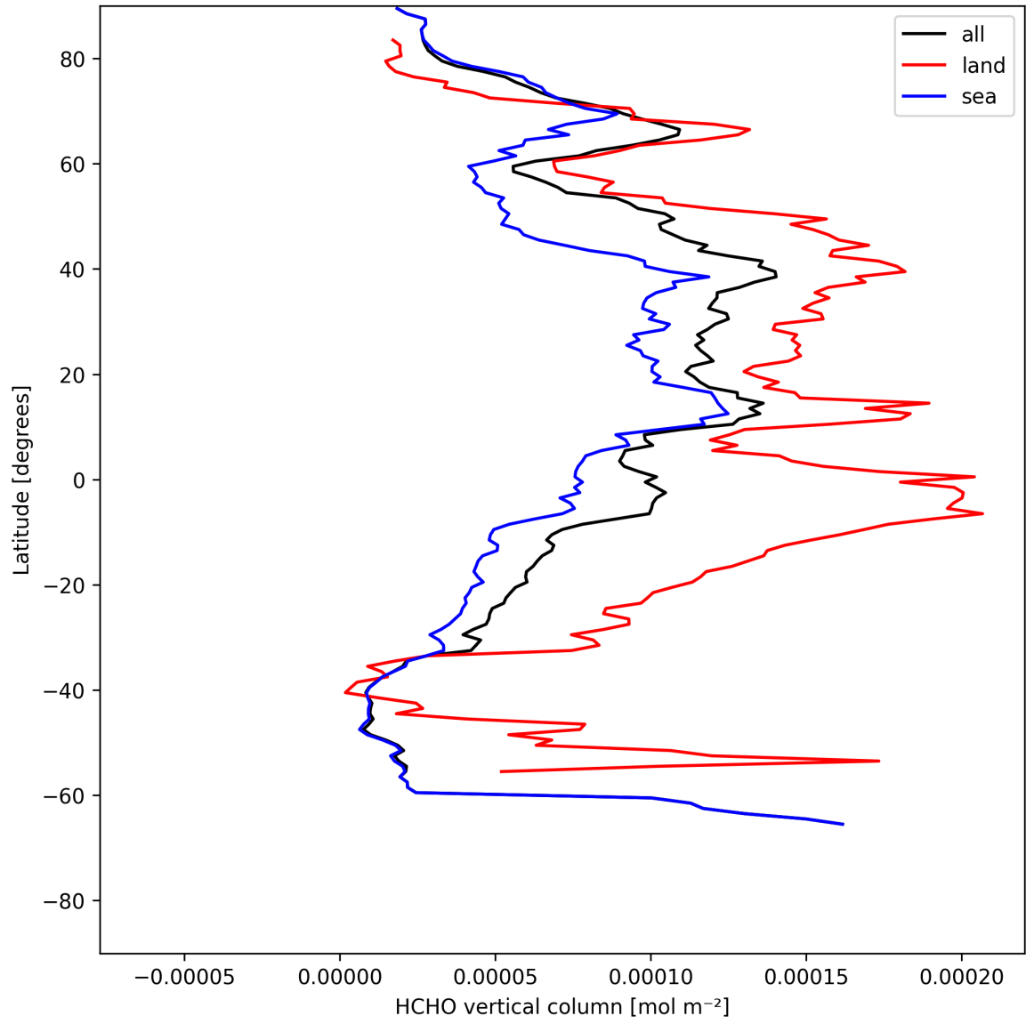
Figure 21: Zonal average of “HCHO vertical column” for 2025-07-25 to 2025-07-27.
