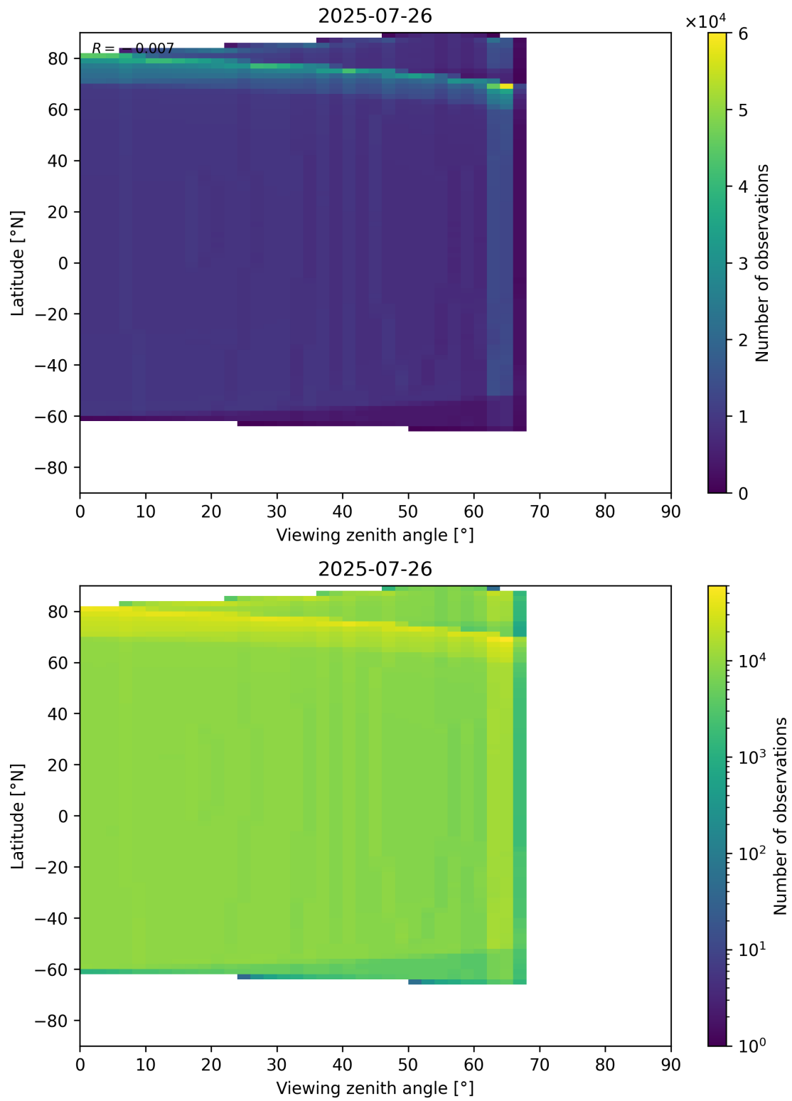
Figure 196: Scatter density plot of “Viewing zenith angle” against “Latitude” for 2025-07-25 to 2025-07-27.
