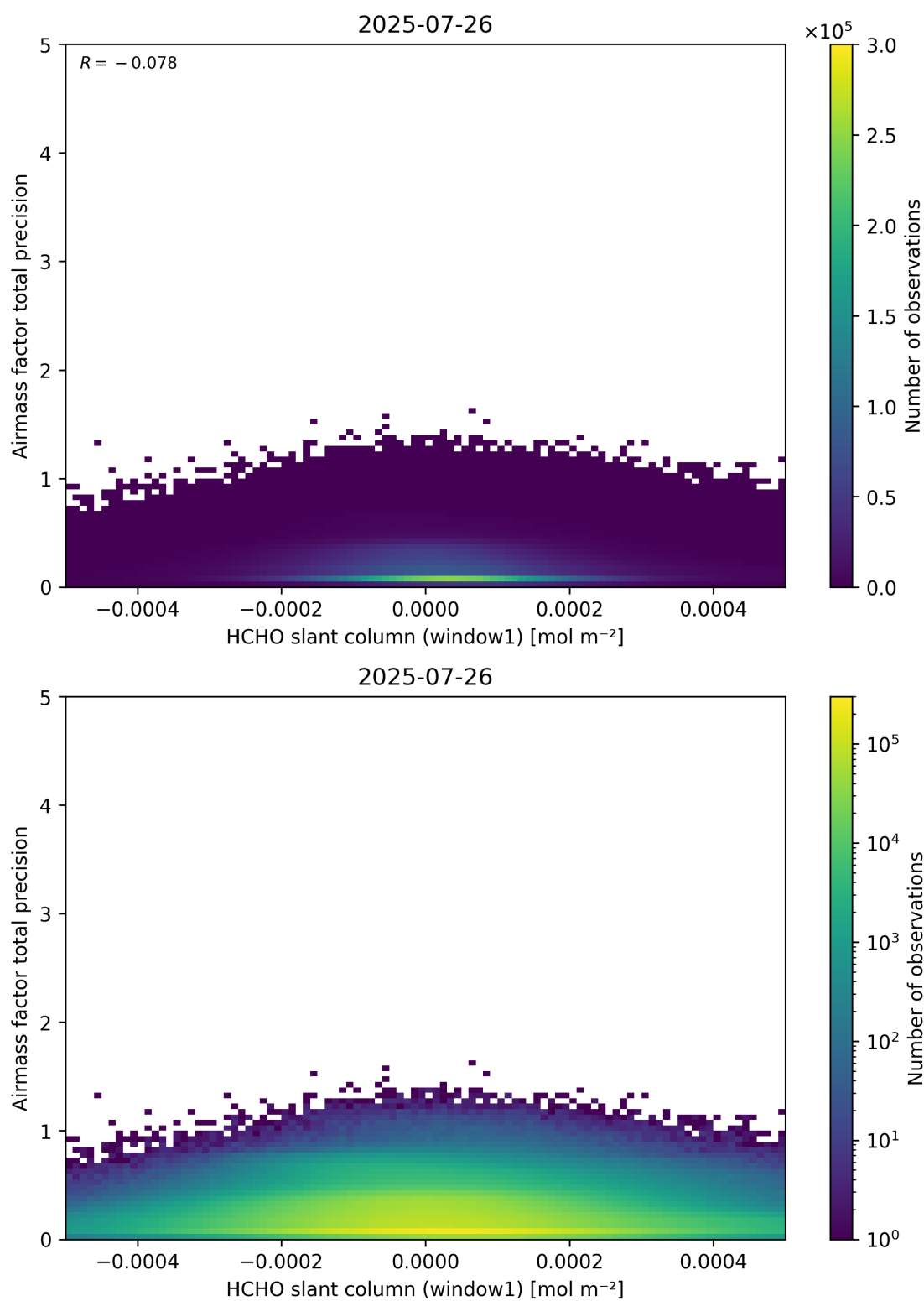
Figure 86: Scatter density plot of “HCHO slant column (window1)” against “Airmass factor total precision” for 2025-07-25 to 2025-07-27.
