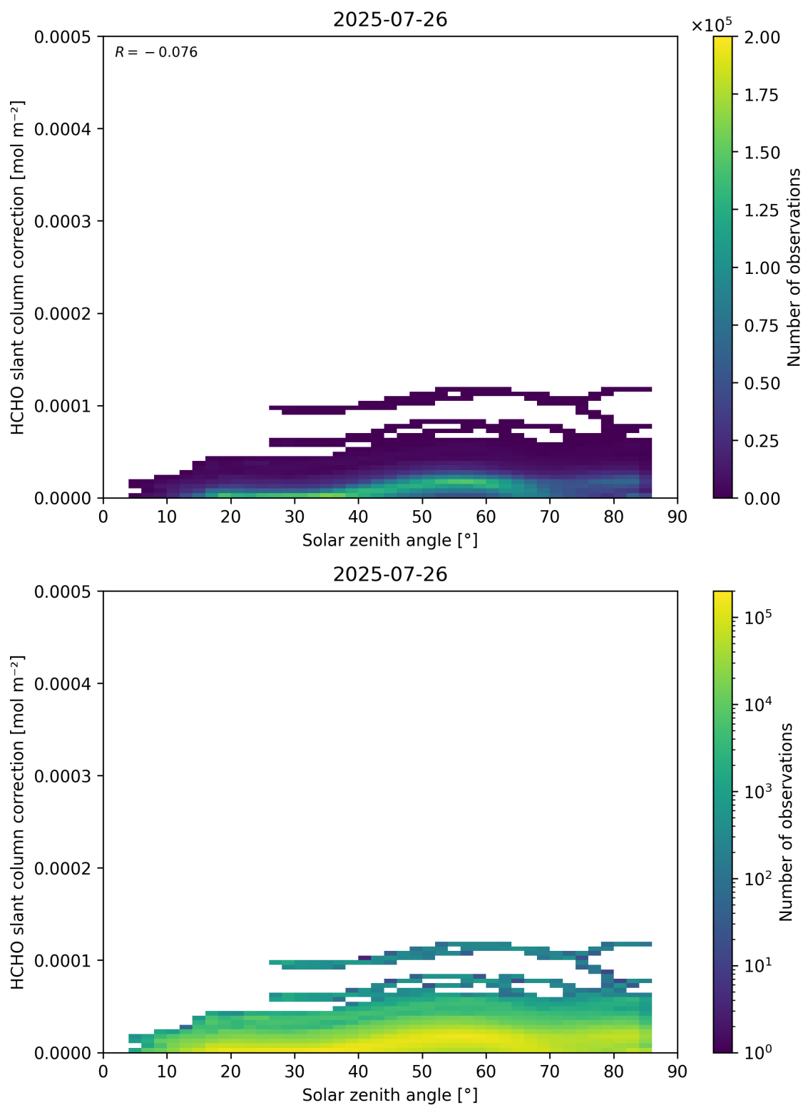
Figure 172: Scatter density plot of “Solar zenith angle” against “HCHO slant column correction” for 2025-07-25 to 2025-07-27.
