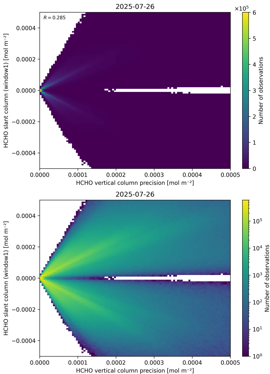
Figure 142: Scatter density plot of “HCHO vertical column precision” against “HCHO slant column (window1)” for 2025-07-25 to 2025-07-27.
