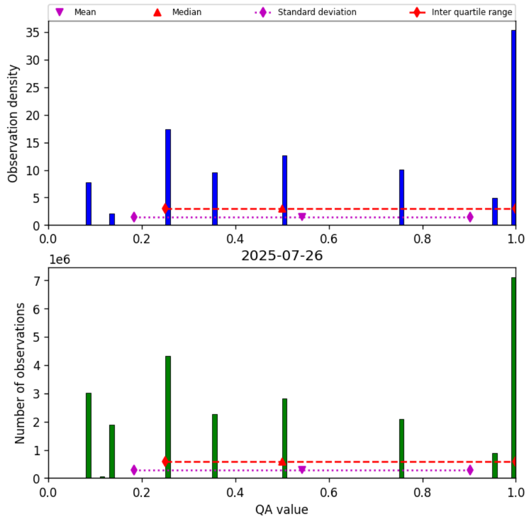
Figure 34: Histogram of “QA value” for 2025-07-25 to 2025-07-27
