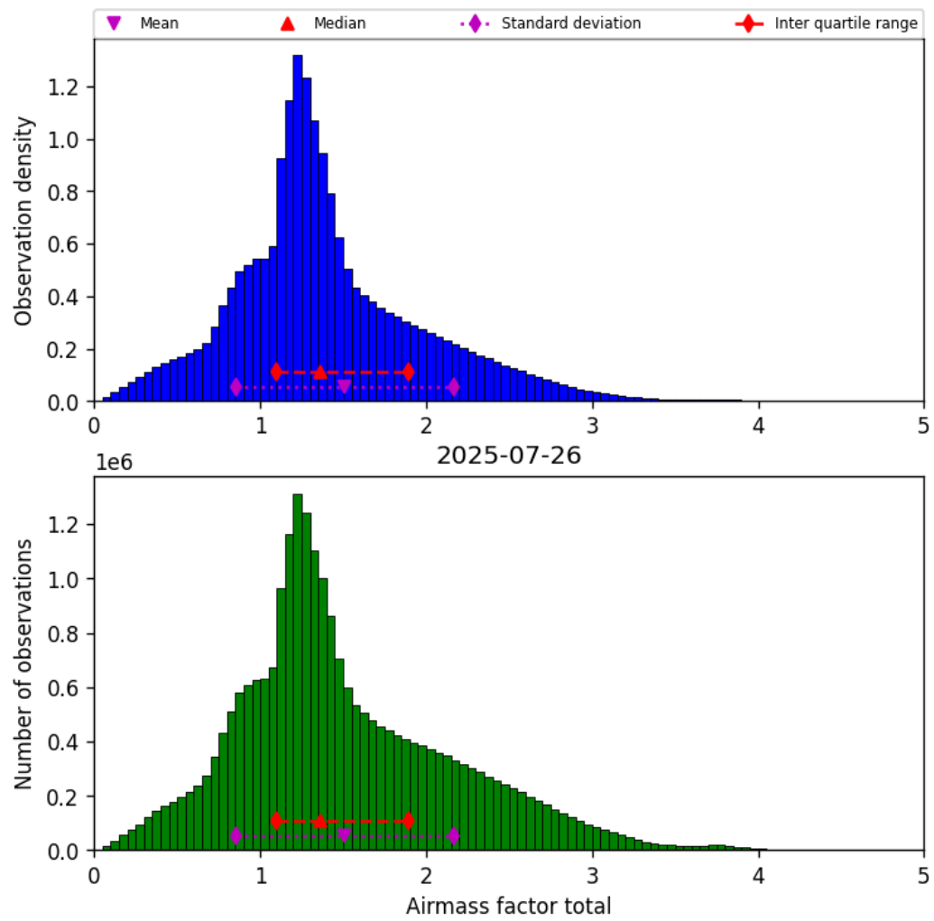
Figure 40: Histogram of “Airmass factor total” for 2025-07-25 to 2025-07-27
