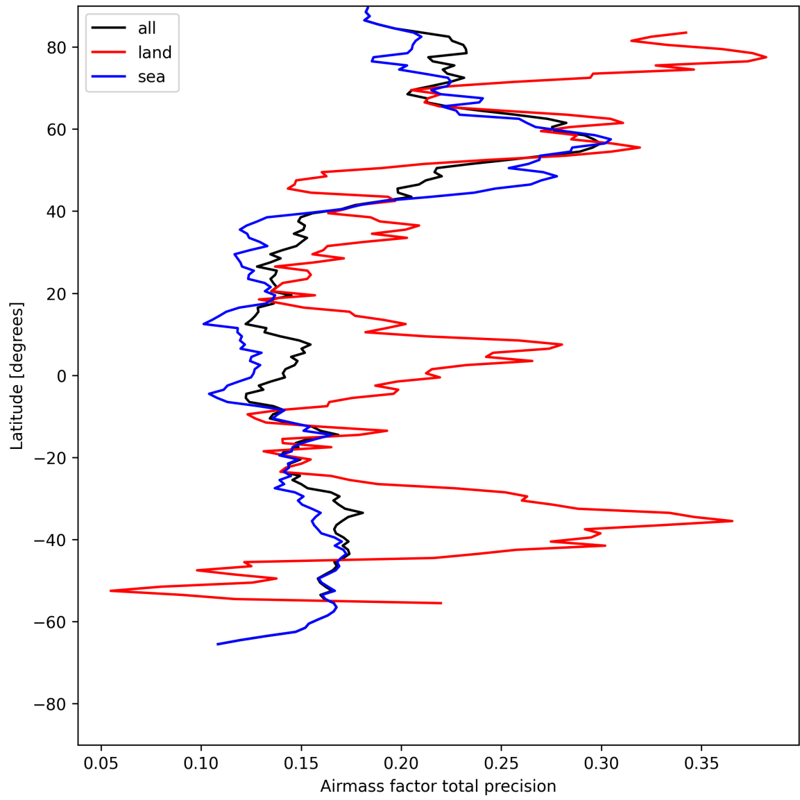
Figure 27: Zonal average of “Airmass factor total precision” for 2025-07-25 to 2025-07-27.
