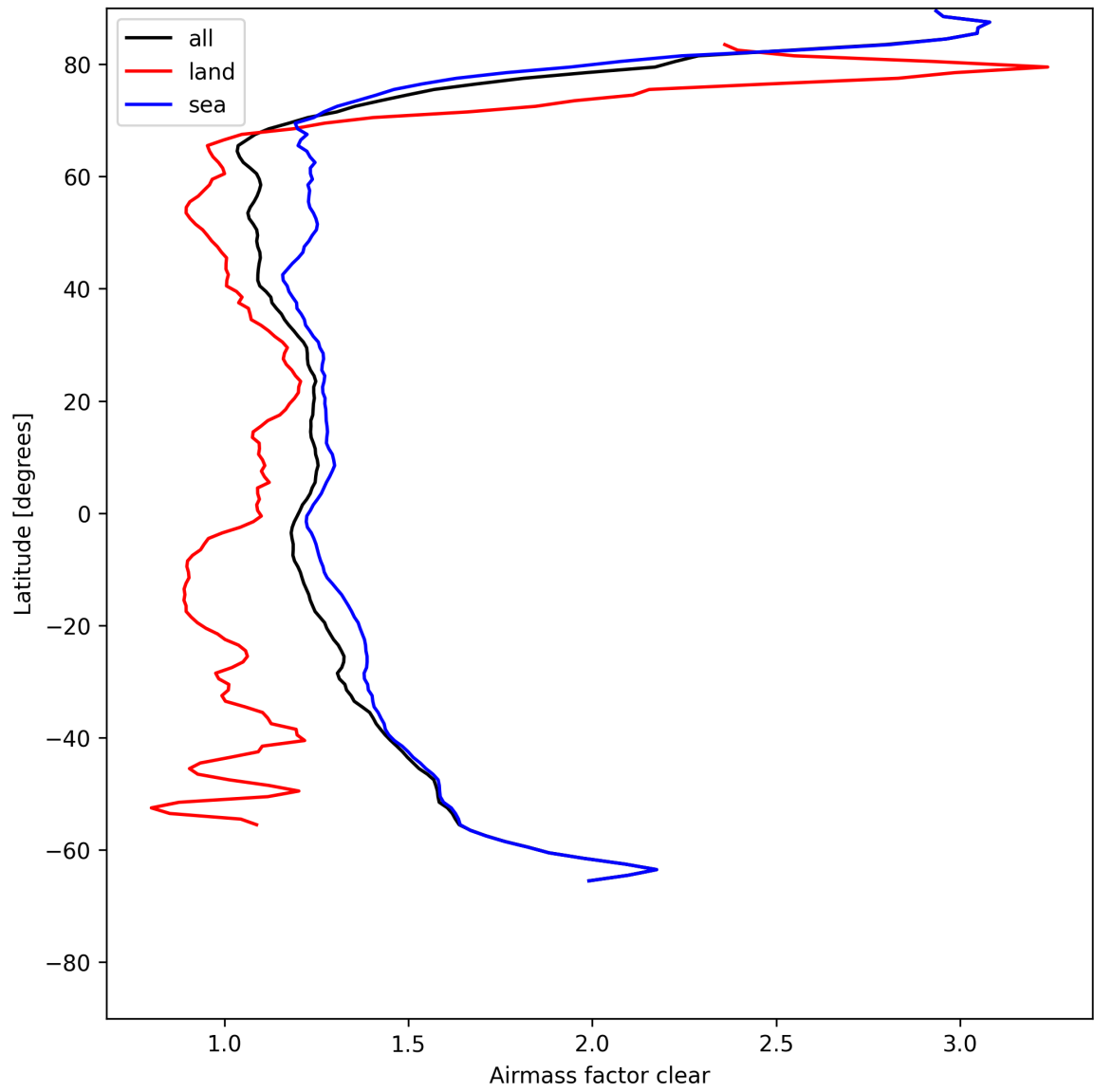
Figure 28: Zonal average of “Airmass factor clear” for 2025-07-25 to 2025-07-27.
