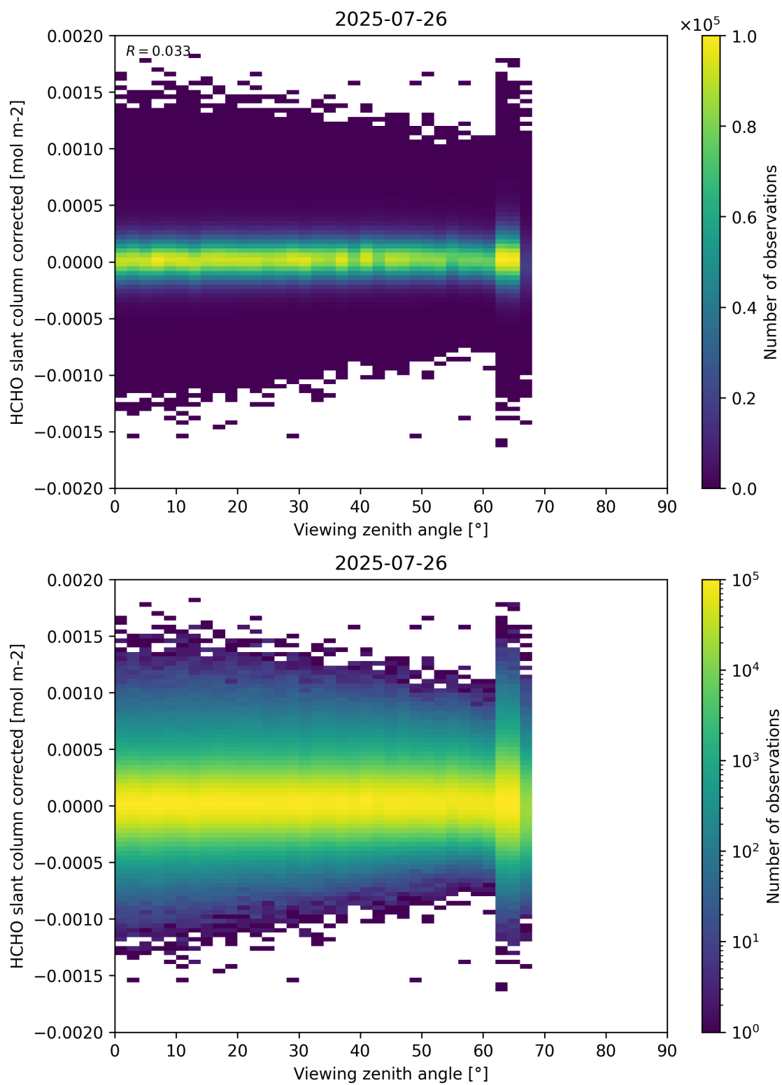
Figure 186: Scatter density plot of “Viewing zenith angle” against “HCHO slant column corrected” for 2025-07-25 to 2025-07-27.
