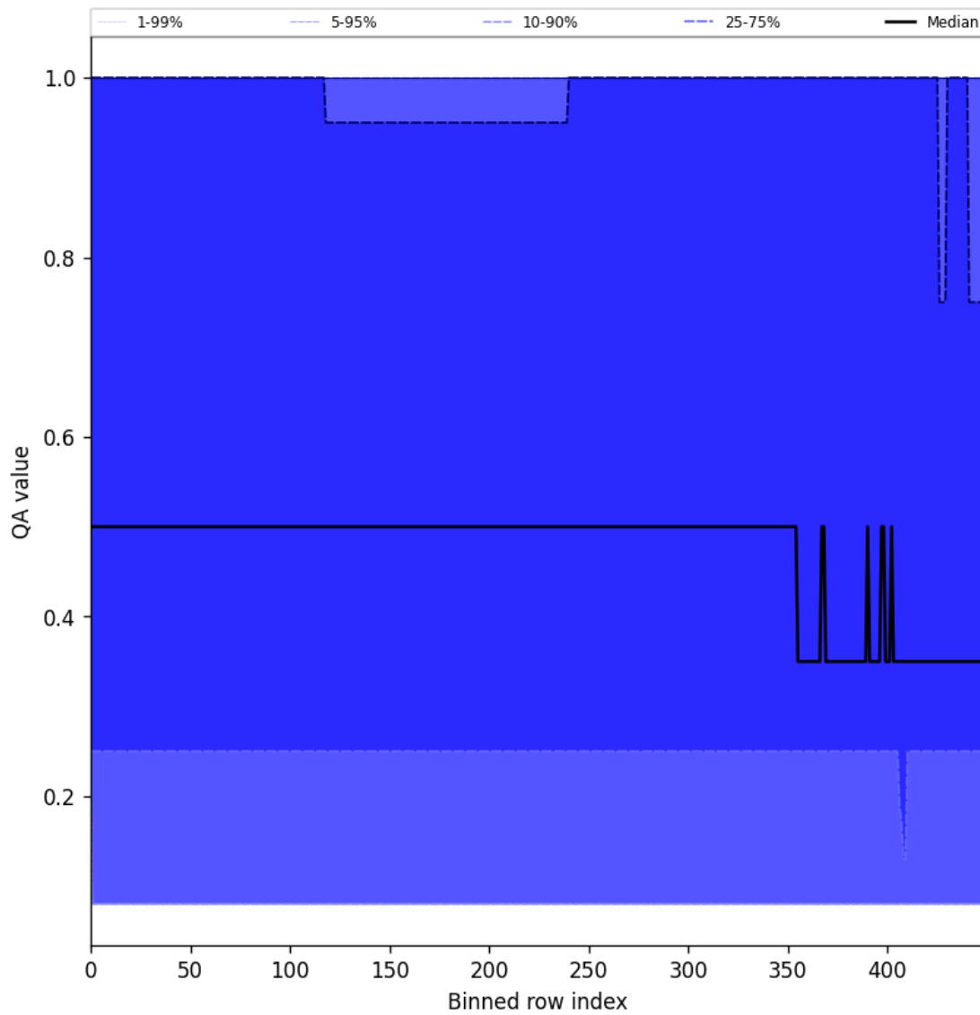
Figure 48: Along track statistics of “QA value” for 2025-07-25 to 2025-07-27
