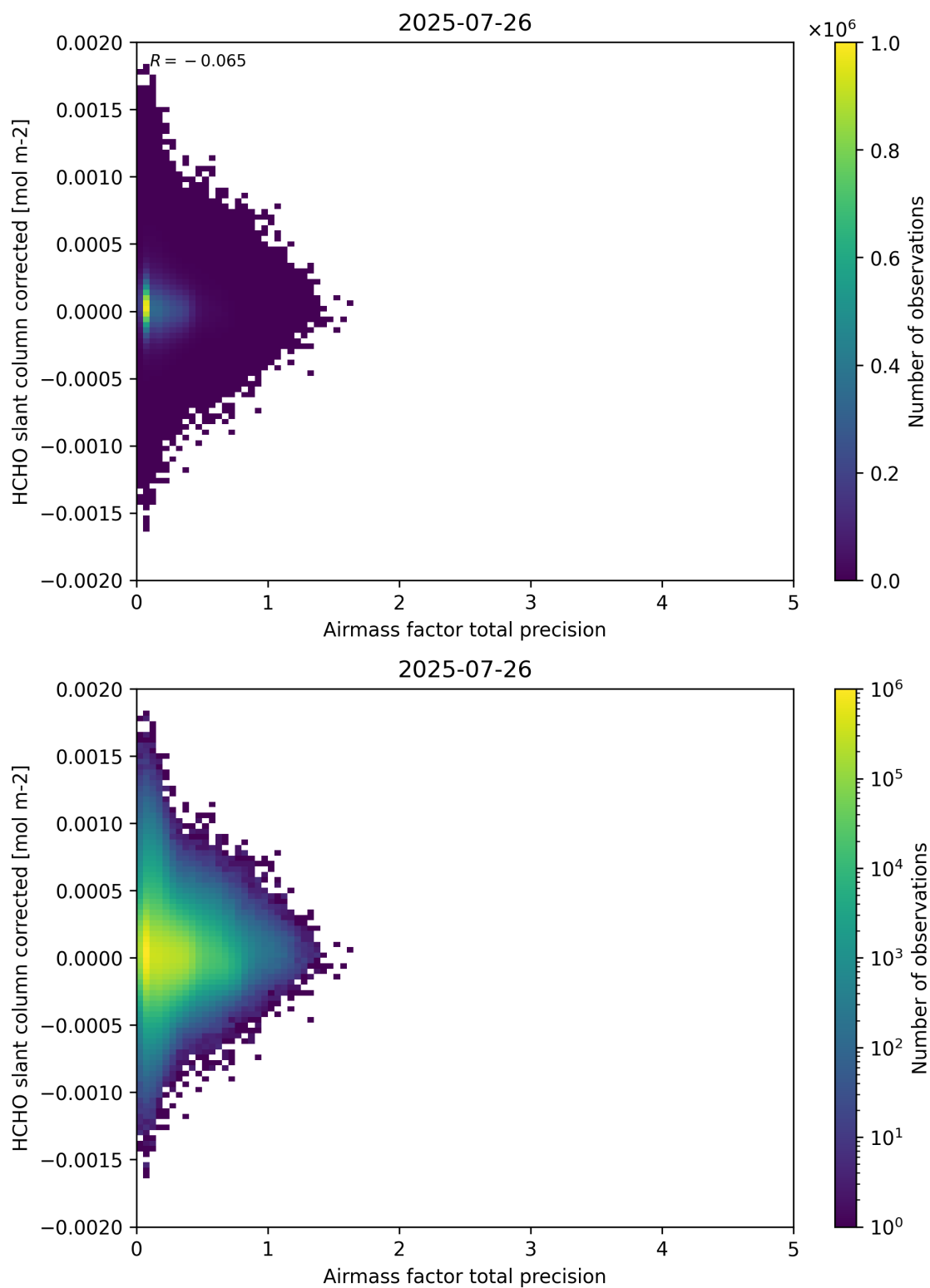
Figure 109: Scatter density plot of “Airmass factor total precision” against “HCHO slant column corrected” for 2025-07-25 to 2025-07-27.
