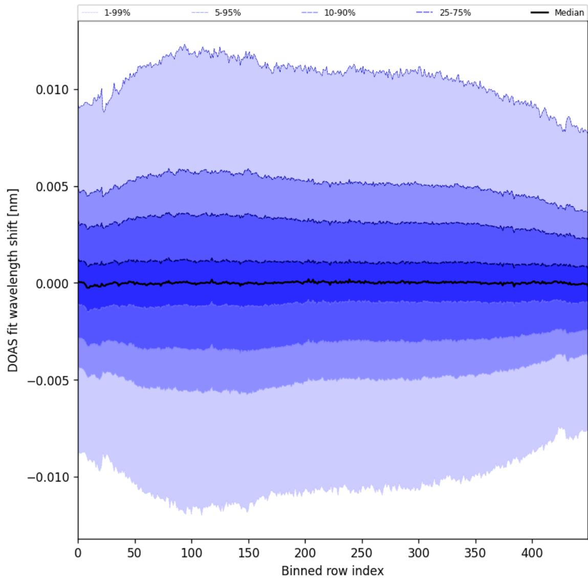
Figure 58: Along track statistics of “DOAS fit wavelength shift” for 2025-07-25 to 2025-07-27
