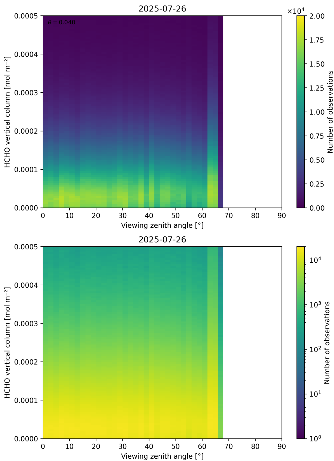
Figure 192: Scatter density plot of “Viewing zenith angle” against “HCHO vertical column” for 2025-07-25 to 2025-07-27.
