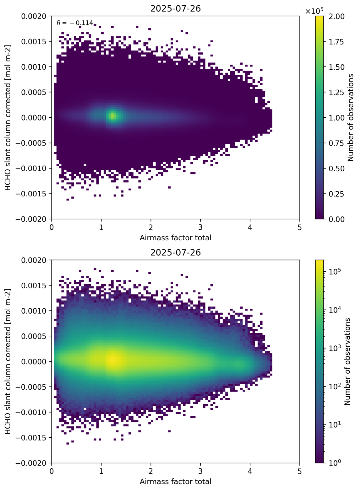
Figure 101: Scatter density plot of “Airmass factor total” against “HCHO slant column corrected” for 2025-07-25 to 2025-07-27.
