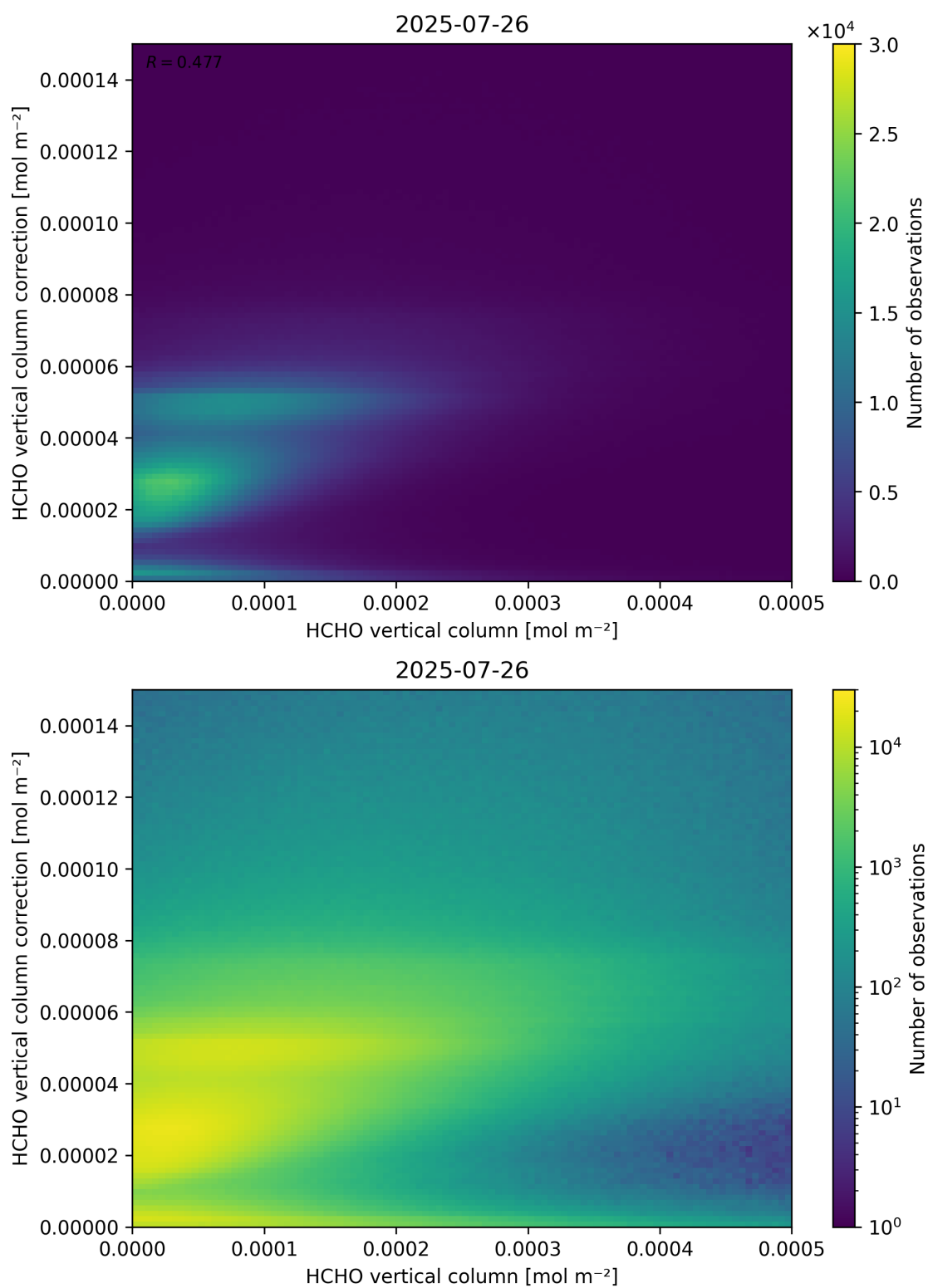
Figure 133: Scatter density plot of “HCHO vertical column” against “HCHO vertical column correction” for 2025-07-25 to 2025-07-27.
