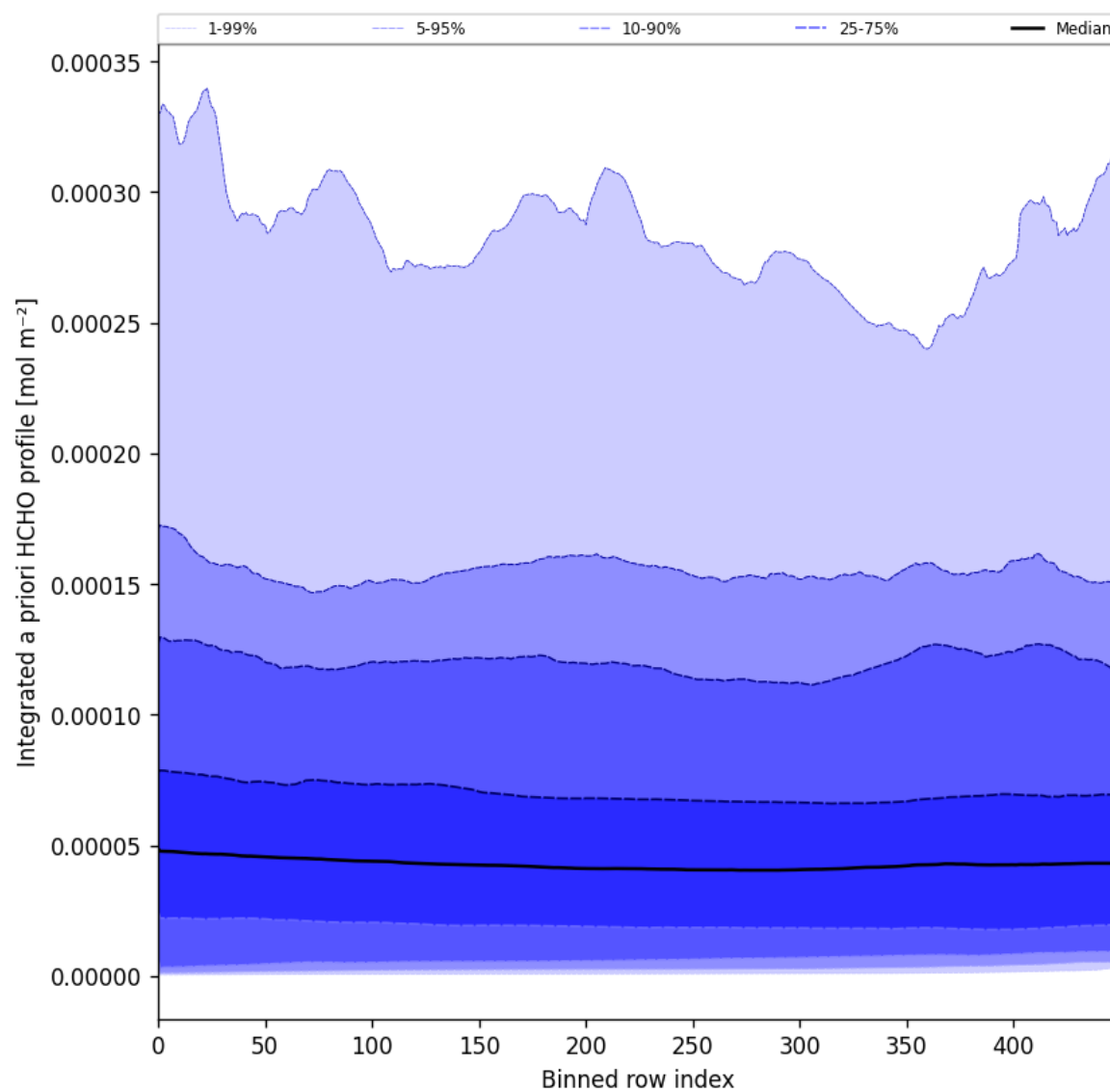
Figure 57: Along track statistics of “Integrated a priori HCHO profile” for 2025-07-25 to 2025-07-27
