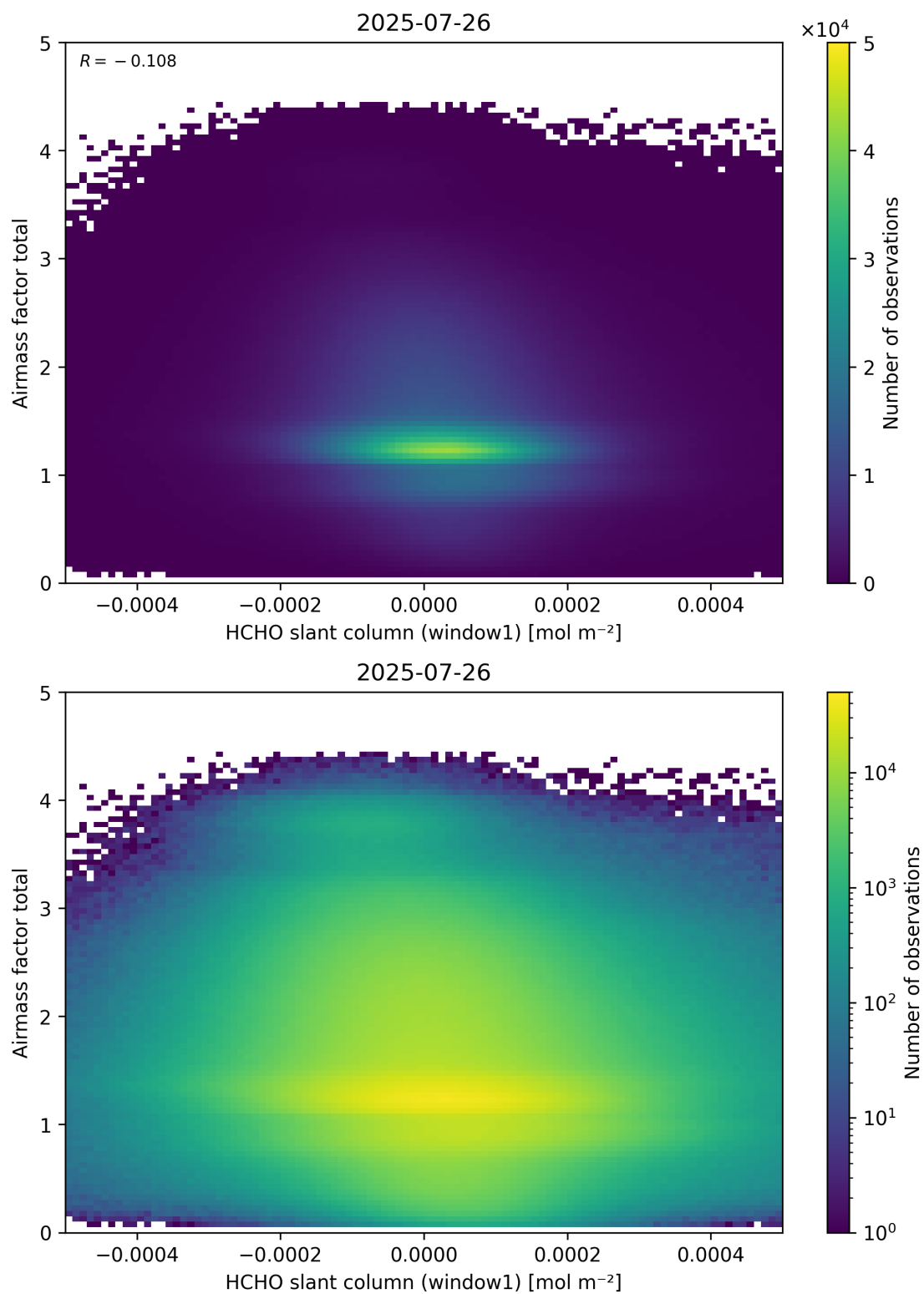
Figure 85: Scatter density plot of “HCHO slant column (window1)” against “Airmass factor total” for 2025-07-25 to 2025-07-27.
