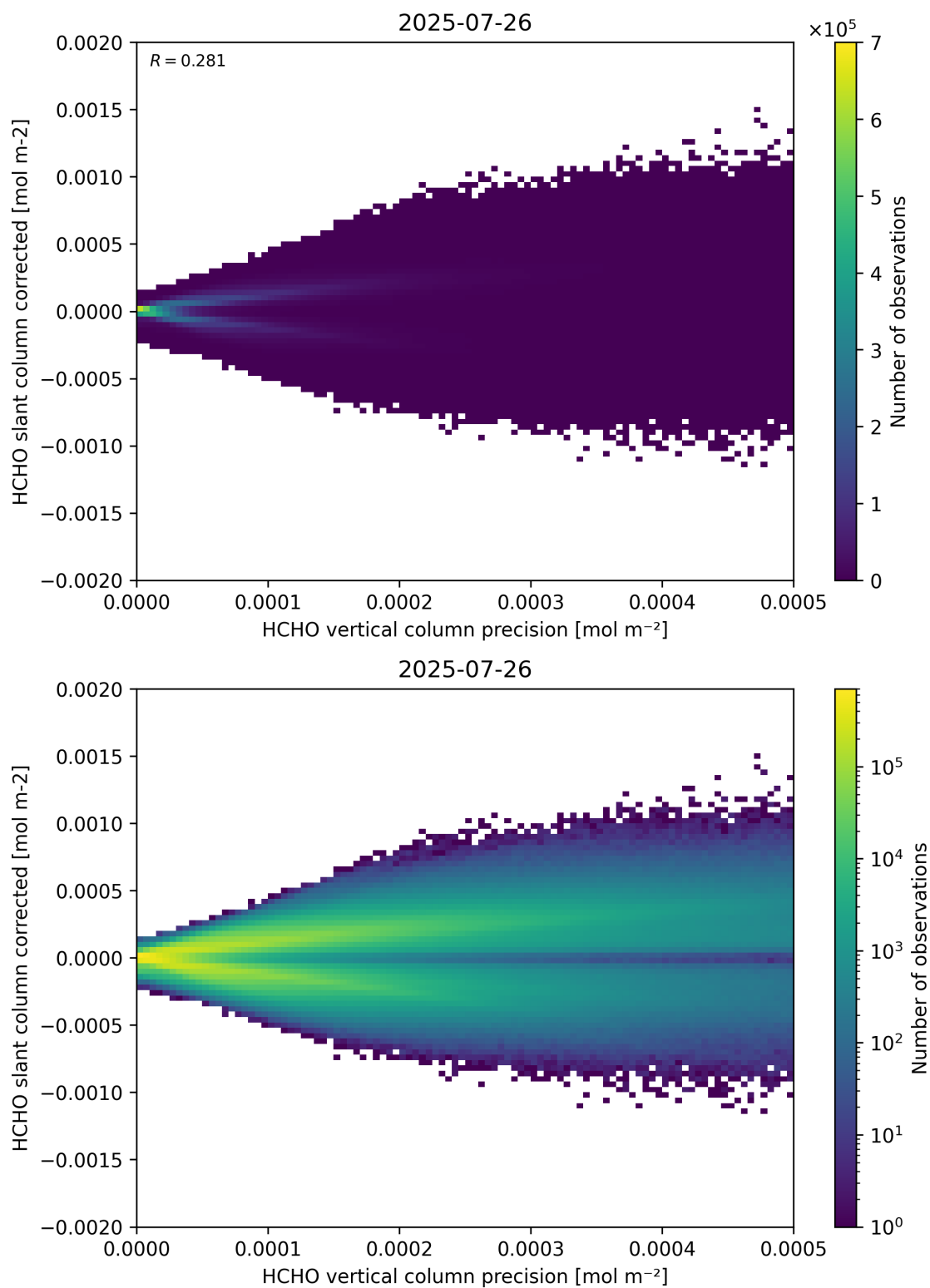
Figure 140: Scatter density plot of “HCHO vertical column precision” against “HCHO slant column corrected” for 2025-07-25 to 2025-07-27.
