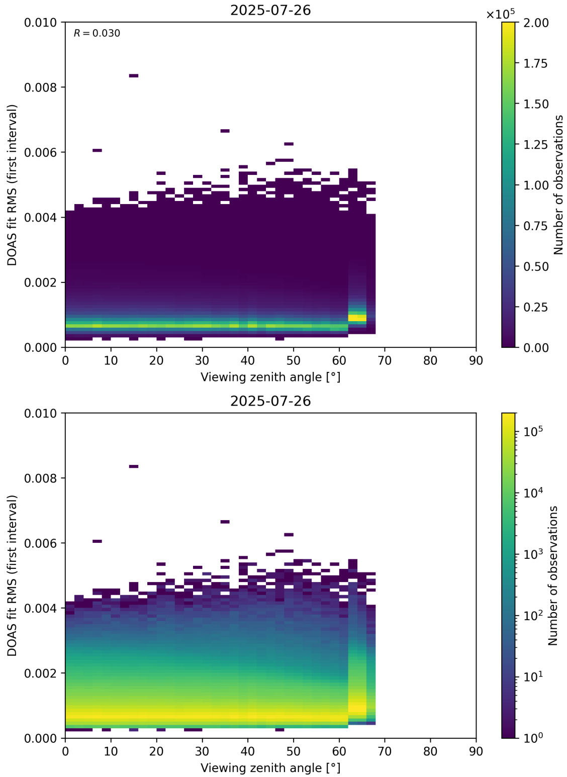
Figure 182: Scatter density plot of “Viewing zenith angle” against “DOAS fit RMS (first interval)” for 2025-07-25 to 2025-07-27.
