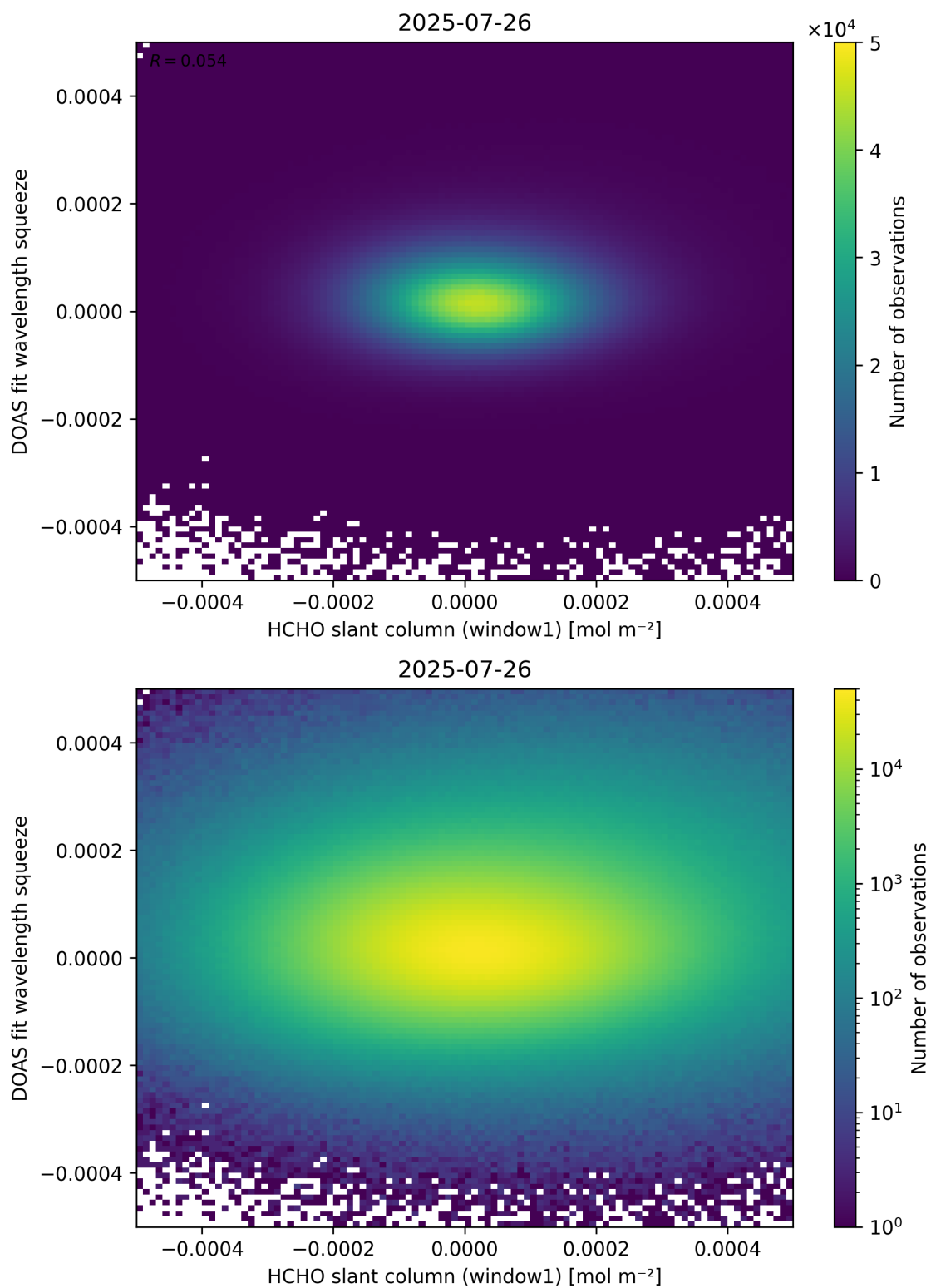
Figure 80: Scatter density plot of “HCHO slant column (window1)” against “DOAS fit wavelength squeeze” for 2025-07-25 to 2025-07-27.
