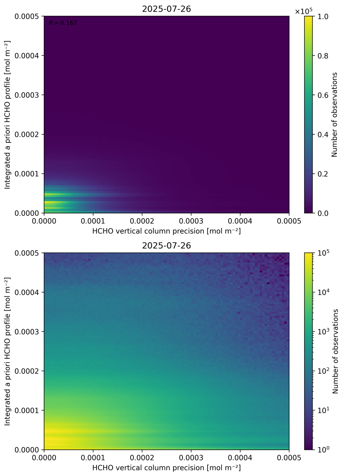
Figure 147: Scatter density plot of “HCHO vertical column precision” against “Integrated a priori HCHO profile” for 2025-07-25 to 2025-07-27.
