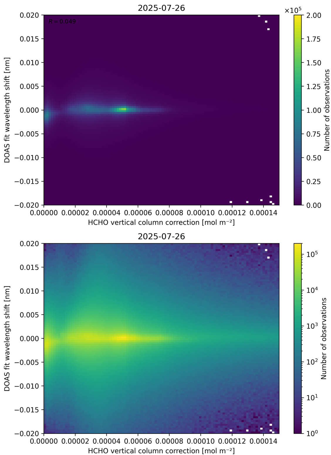
Figure 113: Scatter density plot of “HCHO vertical column correction” against “DOAS fit wavelength shift” for 2025-07-25 to 2025-07-27.
