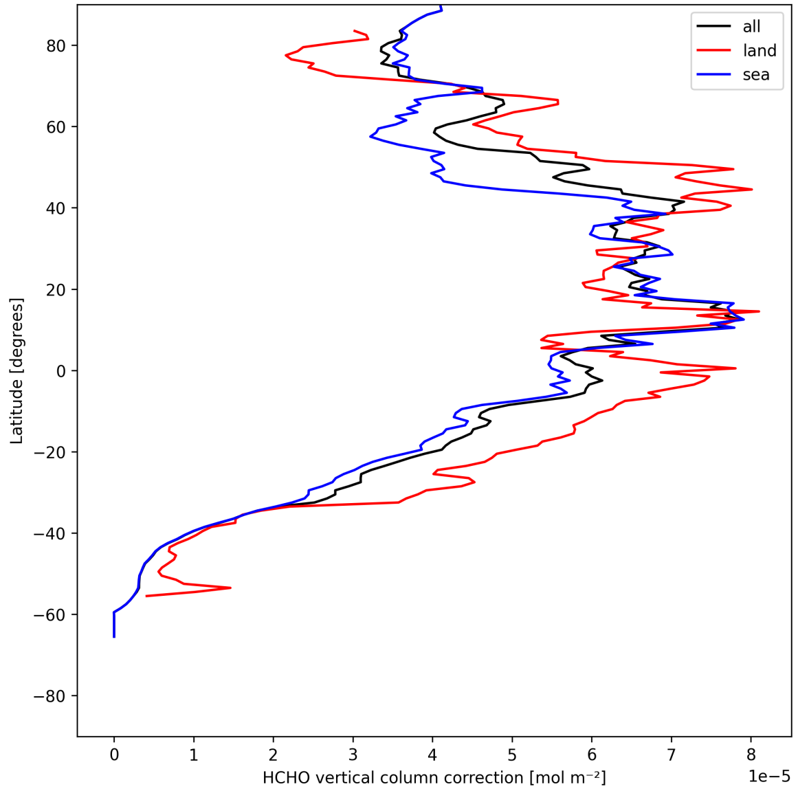
Figure 23: Zonal average of “HCHO vertical column correction” for 2025-07-25 to 2025-07-27.
