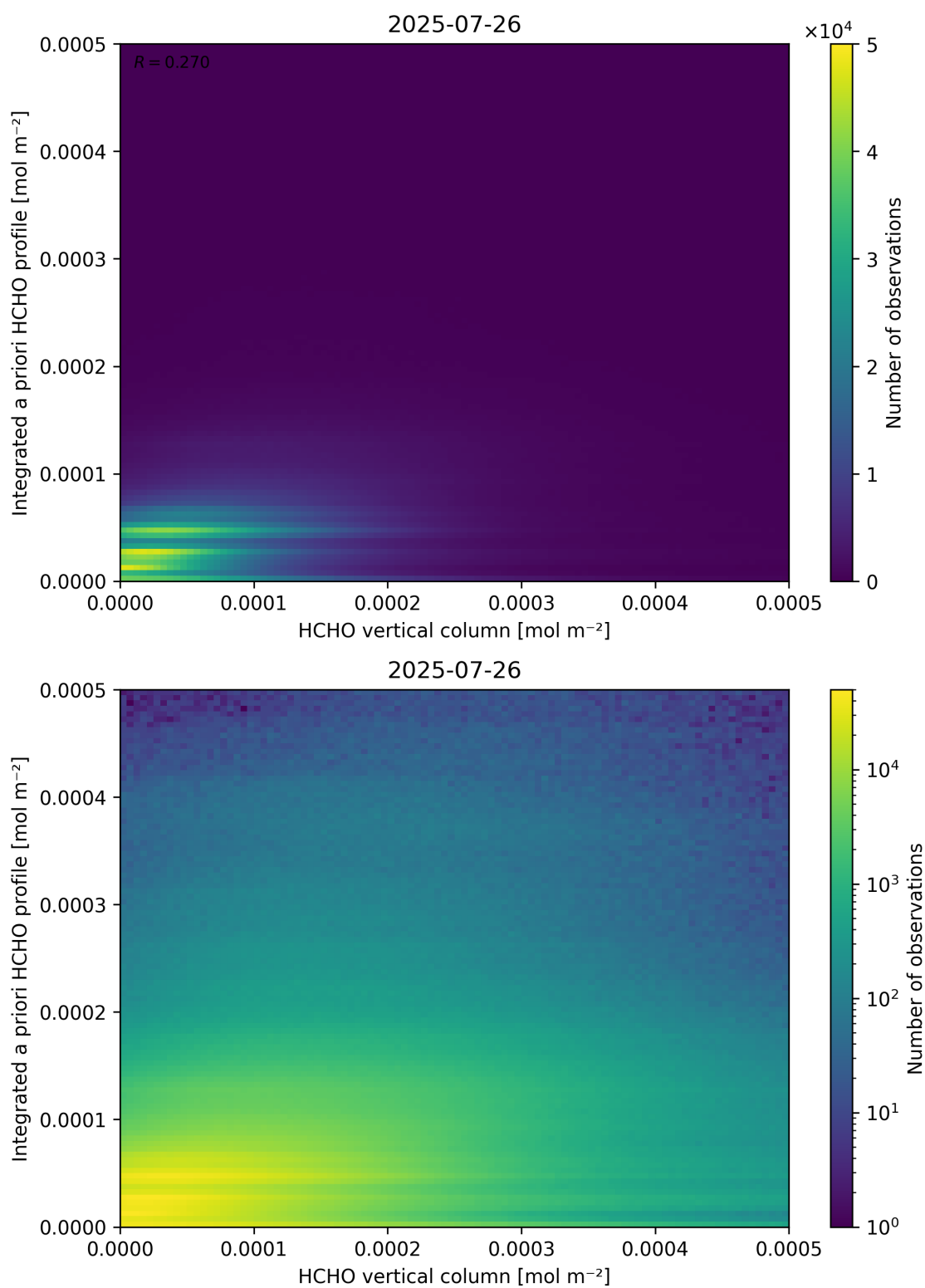
Figure 135: Scatter density plot of “HCHO vertical column” against “Integrated a priori HCHO profile” for 2025-07-25 to 2025-07-27.
