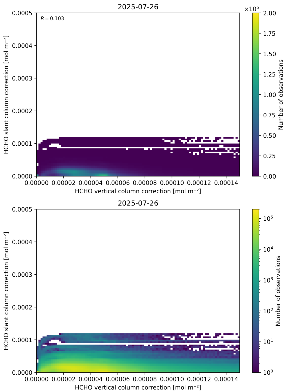
Figure 117: Scatter density plot of “HCHO vertical column correction” against “HCHO slant column correction” for 2025-07-25 to 2025-07-27.
