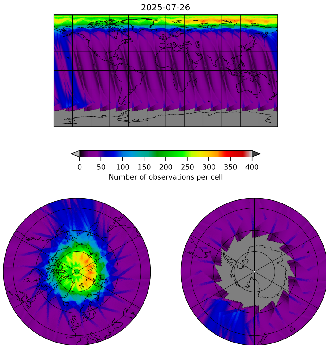
Figure 19: Map of the number of observations for 2025-07-25 to 2025-07-27
