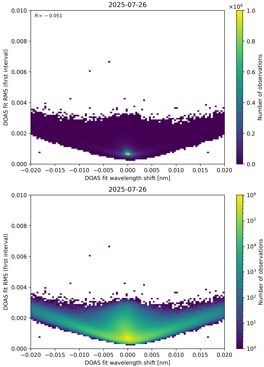
Figure 64: Scatter density plot of “DOAS fit wavelength shift” against “DOAS fit RMS (first interval)” for 2025-07-25 to 2025-07-27.
