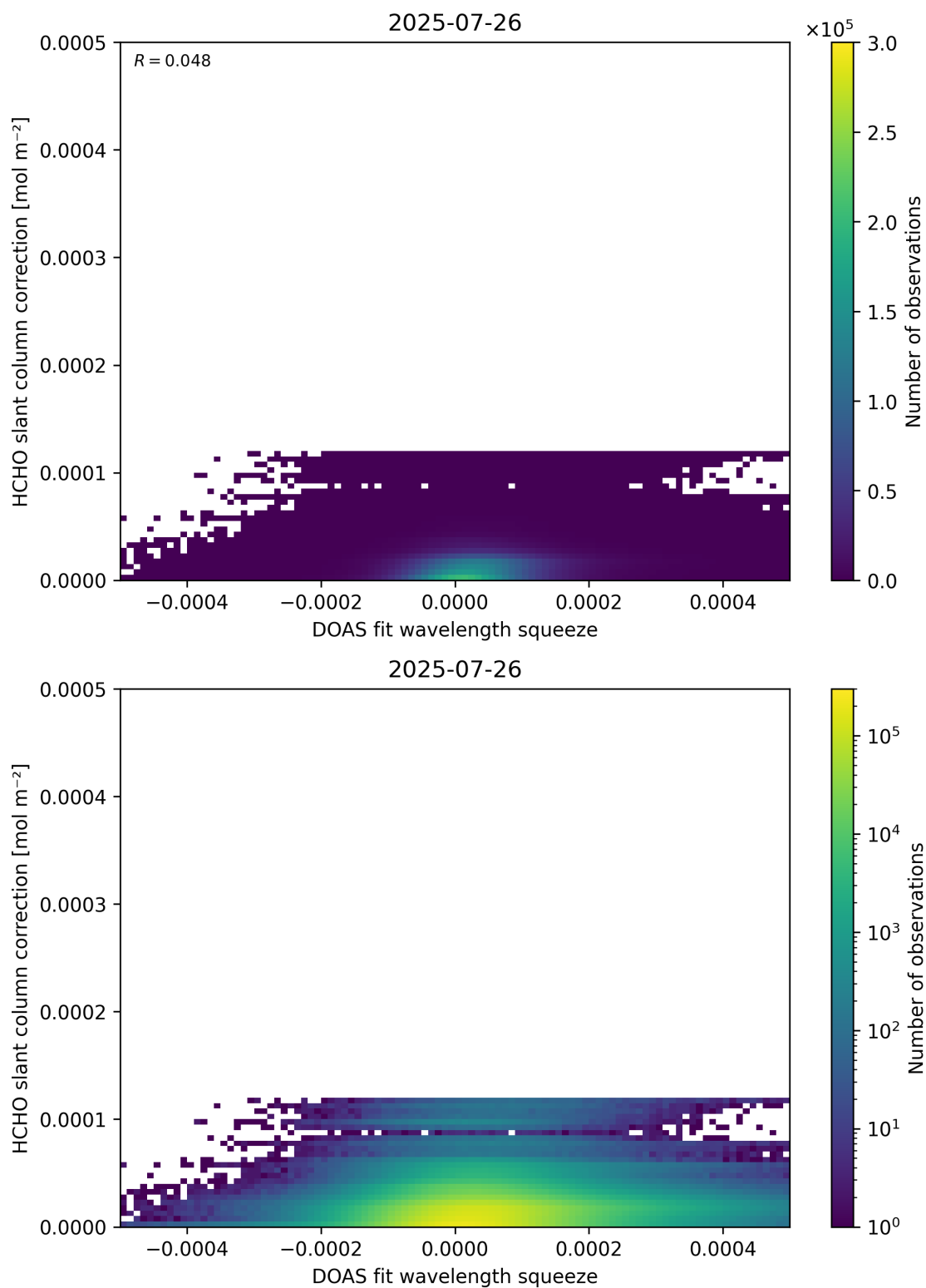
Figure 70: Scatter density plot of “DOAS fit wavelength squeeze” against “HCHO slant column correction” for 2025-07-25 to 2025-07-27.
