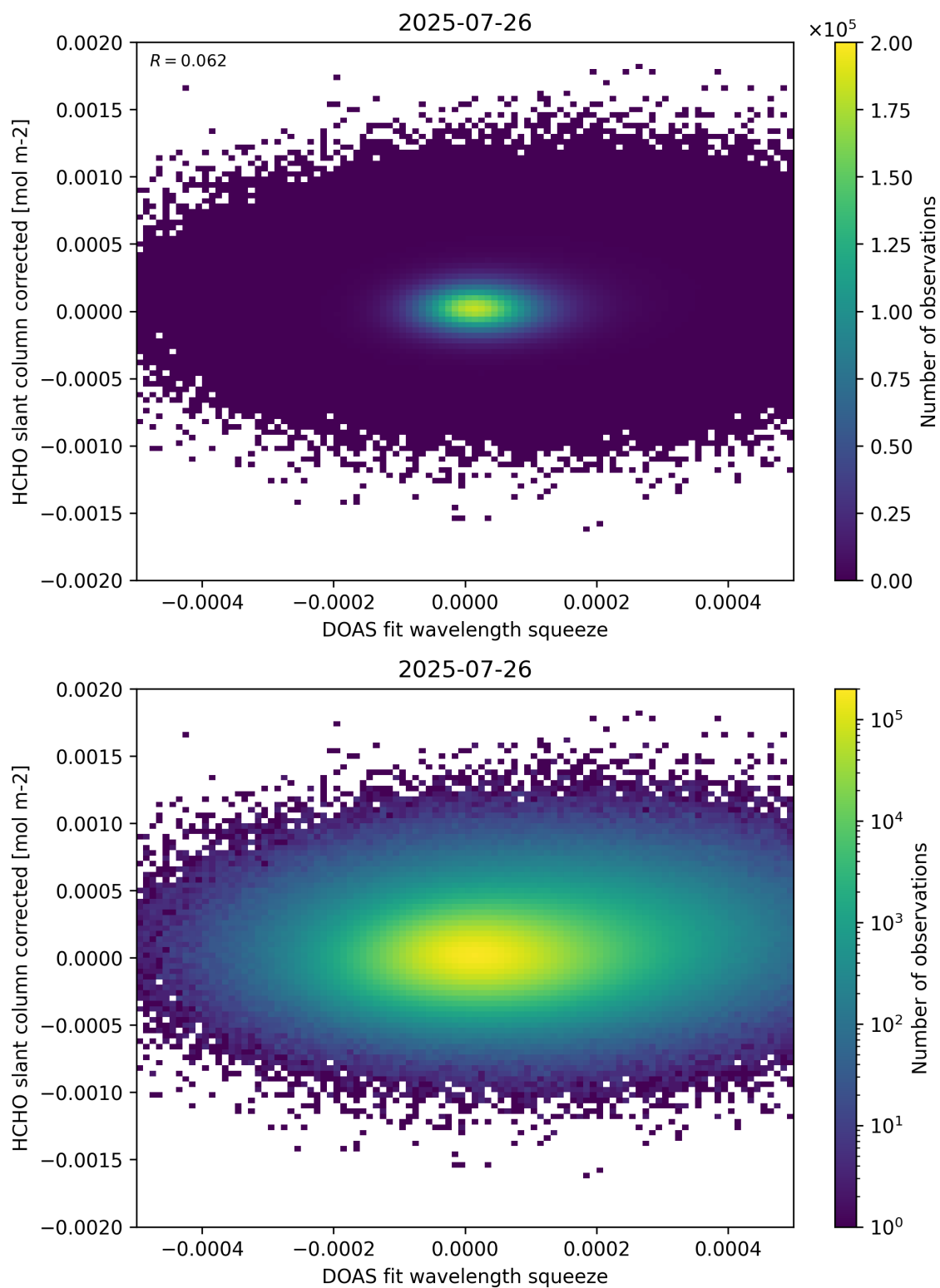
Figure 69: Scatter density plot of “DOAS fit wavelength squeeze” against “HCHO slant column corrected” for 2025-07-25 to 2025-07-27.
