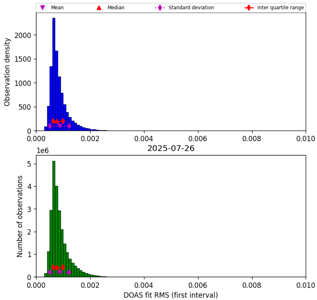
Figure 46: Histogram of “DOAS fit RMS (first interval)” for 2025-07-25 to 2025-07-27
