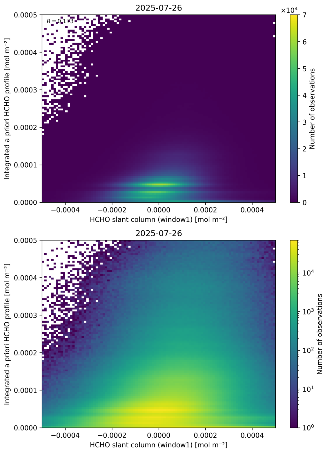
Figure 87: Scatter density plot of “HCHO slant column (window1)” against “Integrated a priori HCHO profile” for 2025-07-25 to 2025-07-27.
