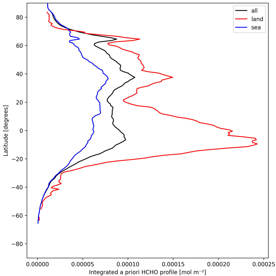
Figure 29: Zonal average of “Integrated a priori HCHO profile” for 2025-07-26 to 2025-07-28.
