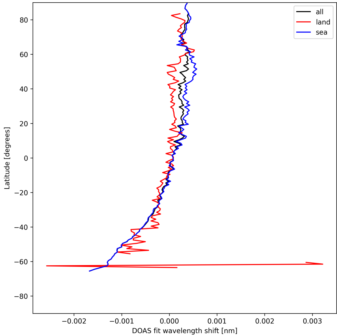
Figure 30: Zonal average of "DOAS fit wavelength shift" for 2025-07-26 to 2025-07-28.
