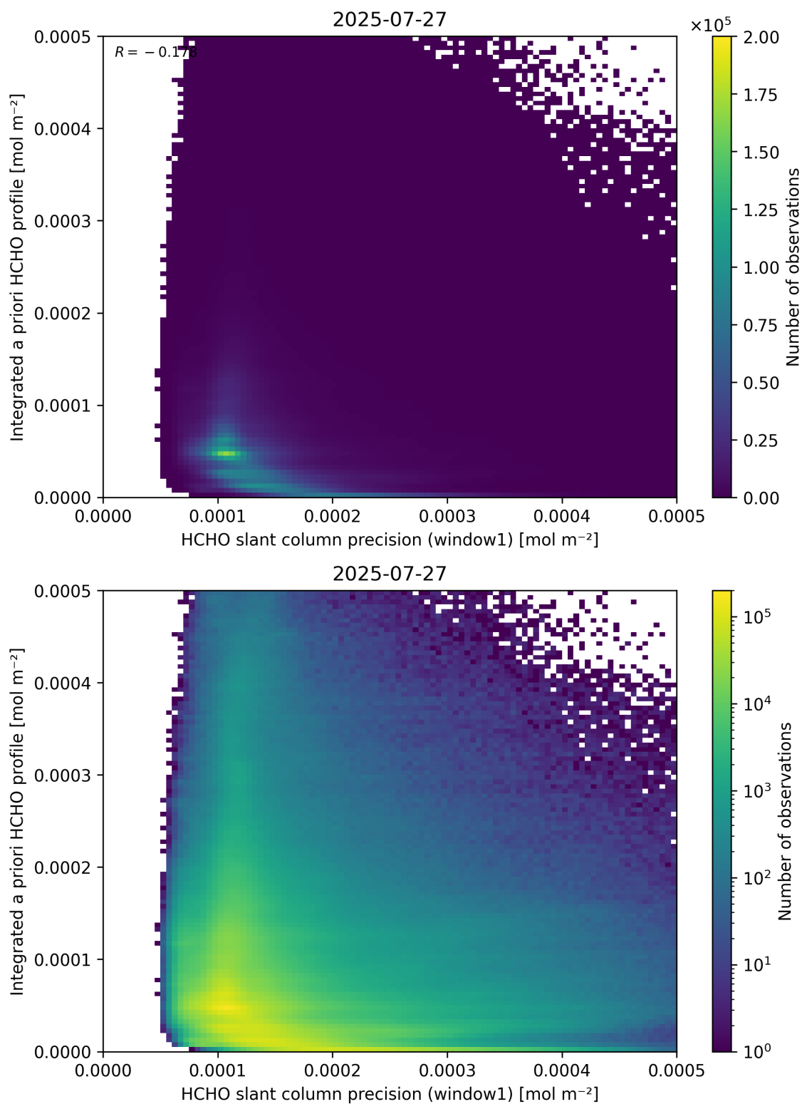
Figure 96: Scatter density plot of “HCHO slant column precision (window1)” against “Integrated a priori HCHO profile” for 2025-07-26 to 2025-07-28.
