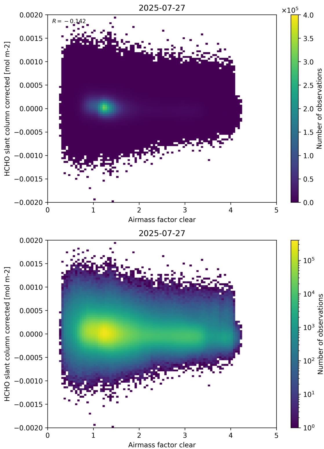
Figure 74: Scatter density plot of “Airmass factor clear” against “HCHO slant column corrected” for 2025-07-26 to 2025-07-28.
