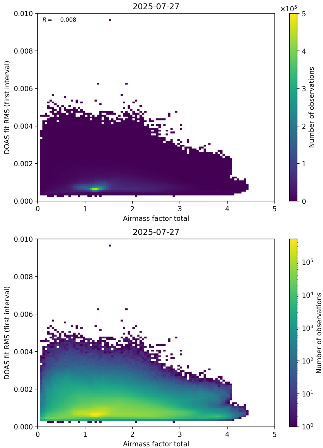
Figure 97: Scatter density plot of “Airmass factor total” against “DOAS fit RMS (first interval)” for 2025-07-26 to 2025-07-28.
