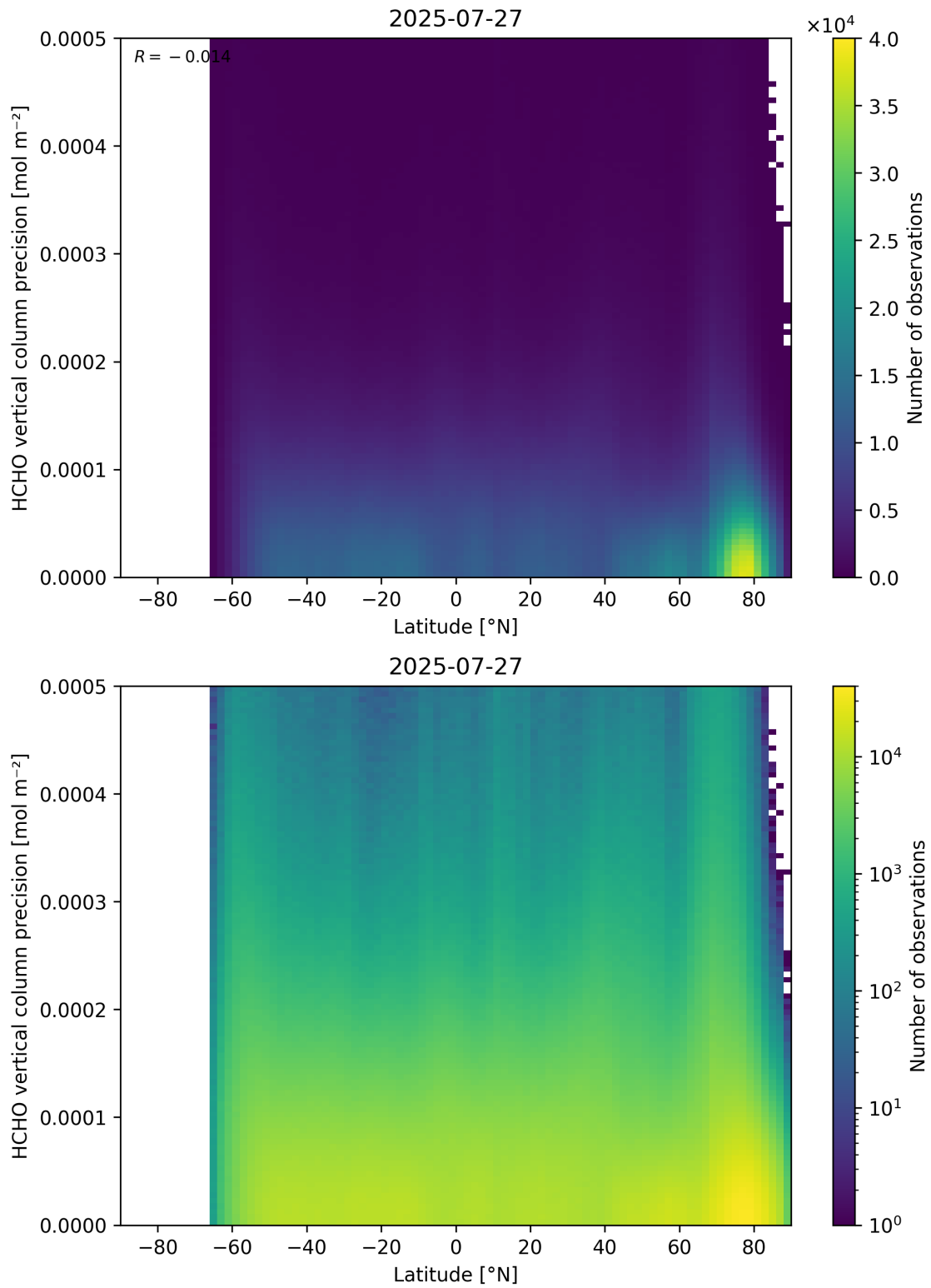
Figure 165: Scatter density plot of “Latitude” against “HCHO vertical column precision” for 2025-07-26 to 2025-07-28.
