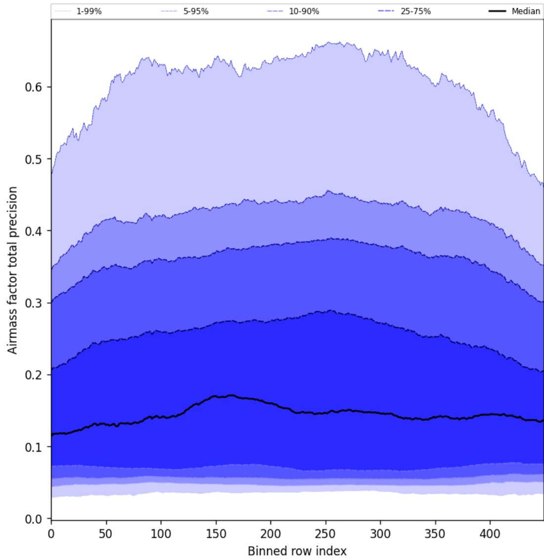
Figure 55: Along track statistics of “Airmass factor total precision” for 2025-07-26 to 2025-07-28
