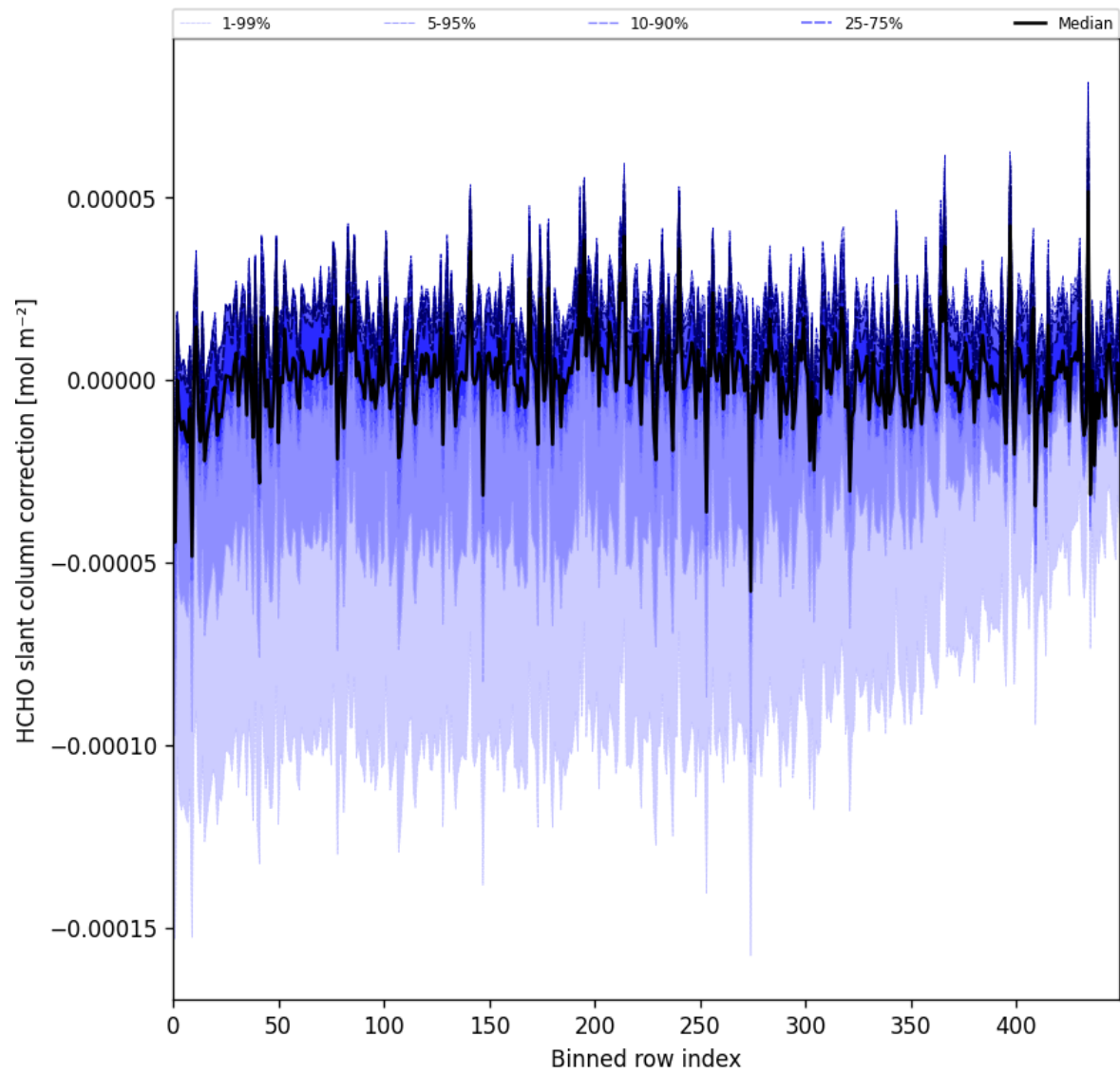
Figure 61: Along track statistics of “HCHO slant column correction” for 2025-07-26 to 2025-07-28
