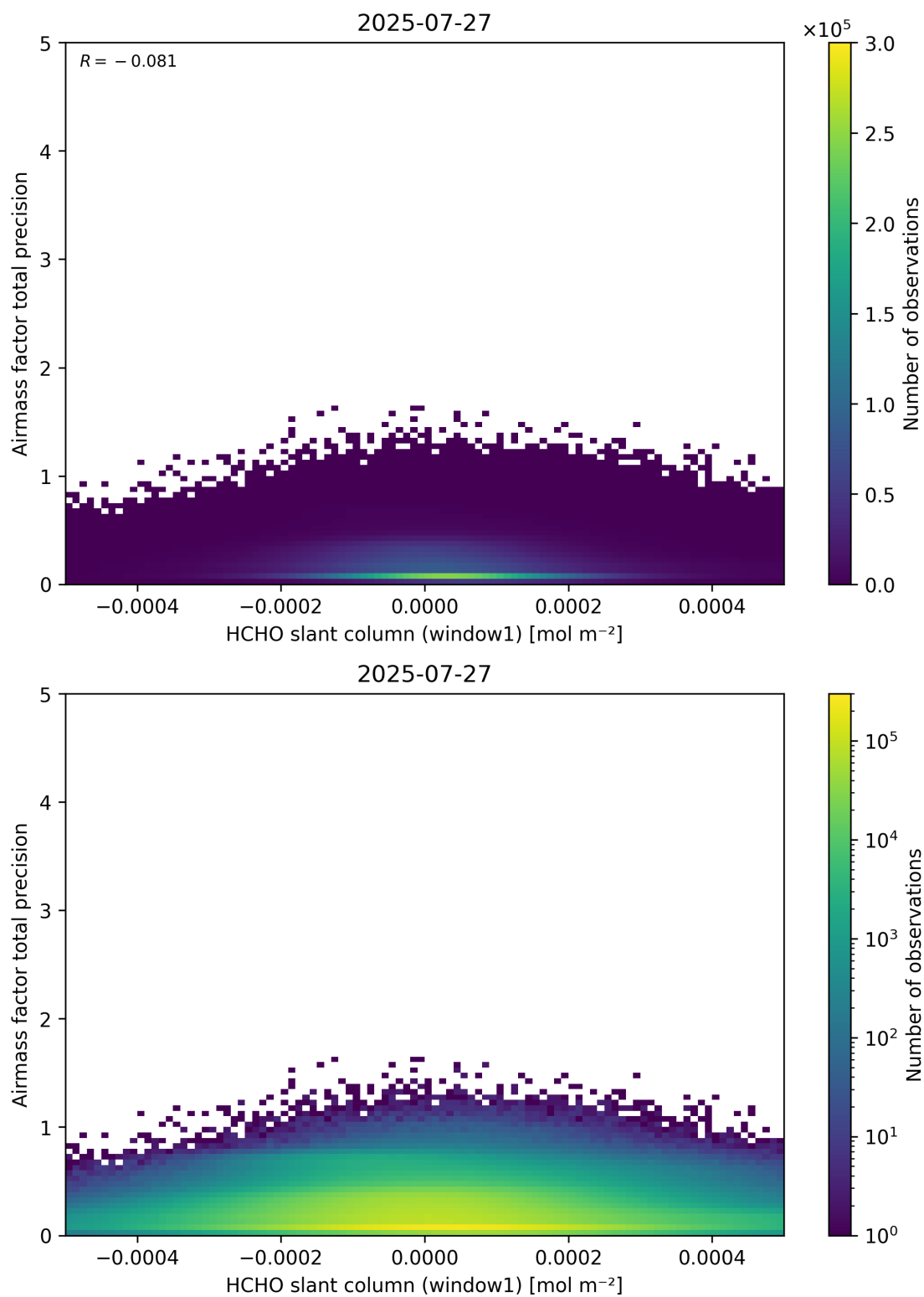
Figure 86: Scatter density plot of “HCHO slant column (window1)” against “Airmass factor total precision” for 2025-07-26 to 2025-07-28.
