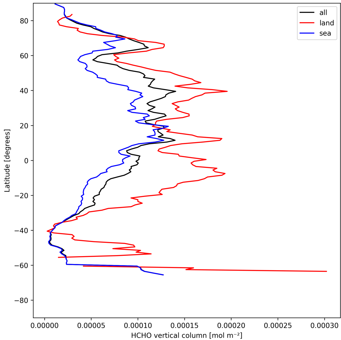
Figure 21: Zonal average of “HCHO vertical column” for 2025-07-26 to 2025-07-28.
