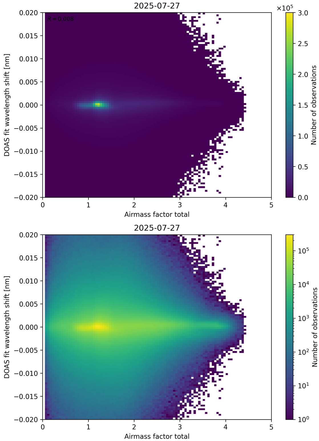
Figure 98: Scatter density plot of “Airmass factor total” against “DOAS fit wavelength shift” for 2025-07-26 to 2025-07-28.
