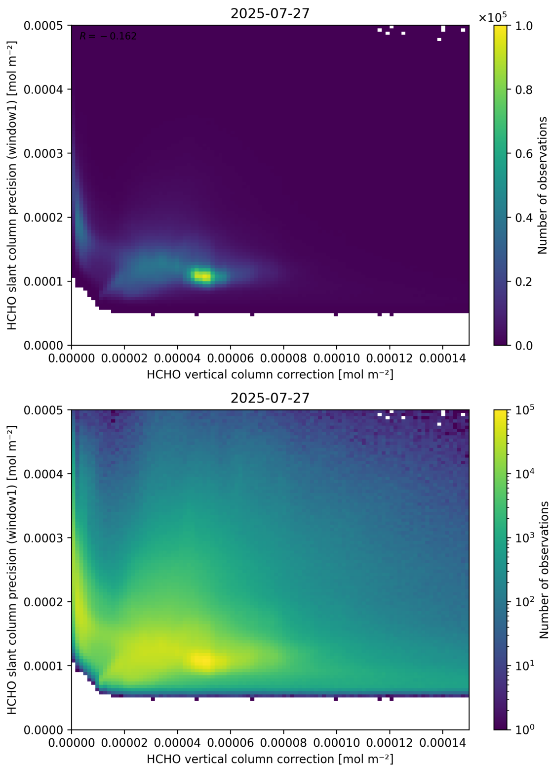
Figure 119: Scatter density plot of “HCHO vertical column correction” against “HCHO slant column precision (window1)” for 2025-07-26 to 2025-07-28.
