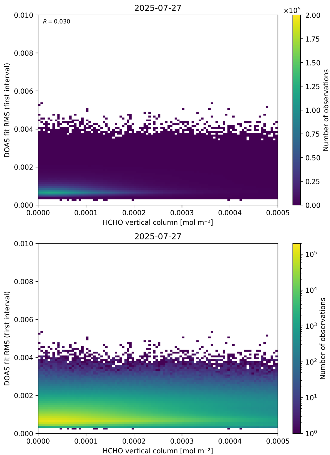
Figure 123: Scatter density plot of “HCHO vertical column” against “DOAS fit RMS (first interval)” for 2025-07-26 to 2025-07-28.
