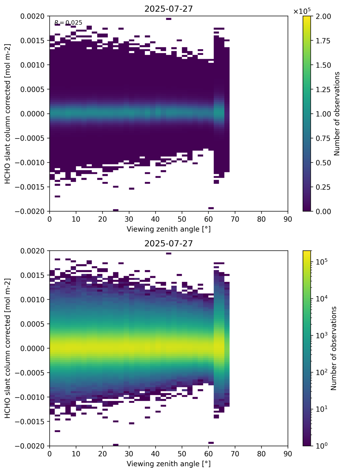
Figure 186: Scatter density plot of “Viewing zenith angle” against “HCHO slant column corrected” for 2025-07-26 to 2025-07-28.
