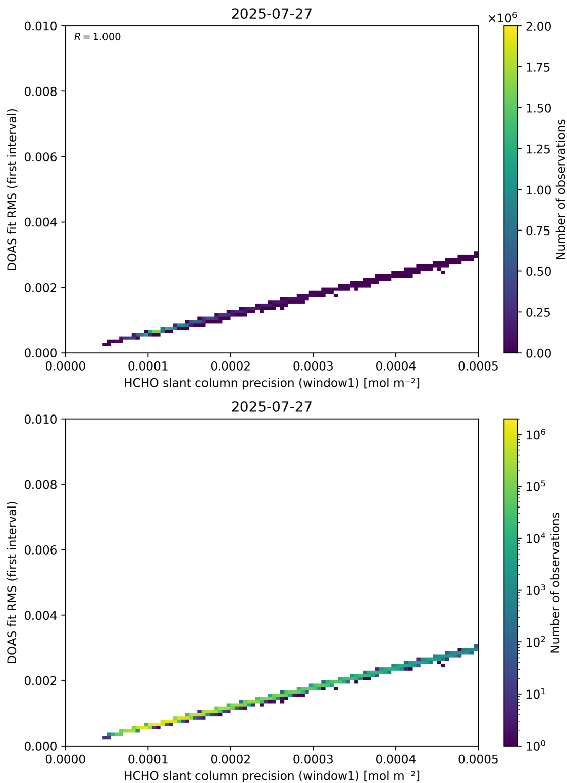
Figure 88: Scatter density plot of “HCHO slant column precision (window1)” against “DOAS fit RMS (first interval)” for 2025-07-26 to 2025-07-28.
