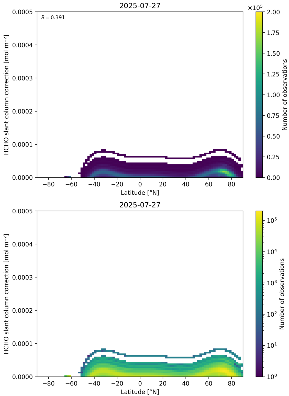
Figure 158: Scatter density plot of “Latitude” against “HCHO slant column correction” for 2025-07-26 to 2025-07-28.
