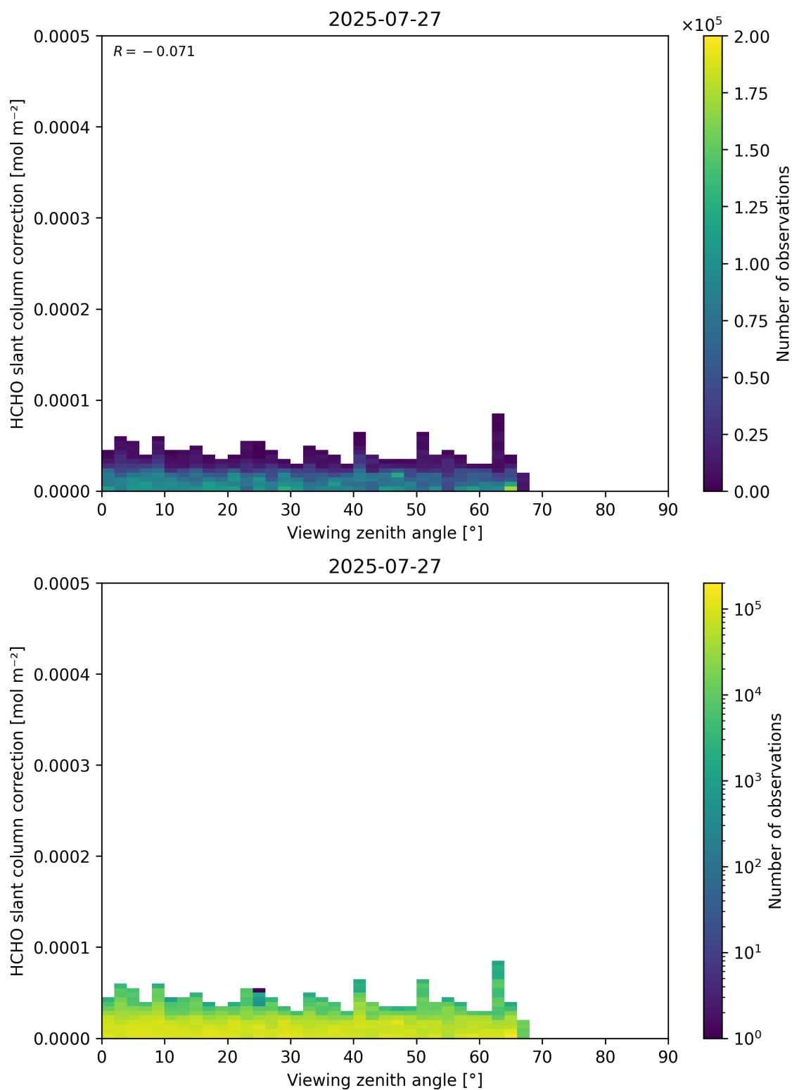
Figure 187: Scatter density plot of “Viewing zenith angle” against “HCHO slant column correction” for 2025-07-26 to 2025-07-28.
