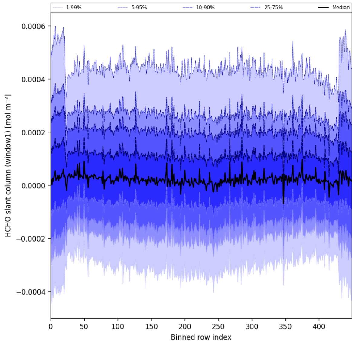
Figure 52: Along track statistics of “HCHO slant column (window1)” for 2025-07-26 to 2025-07-28
