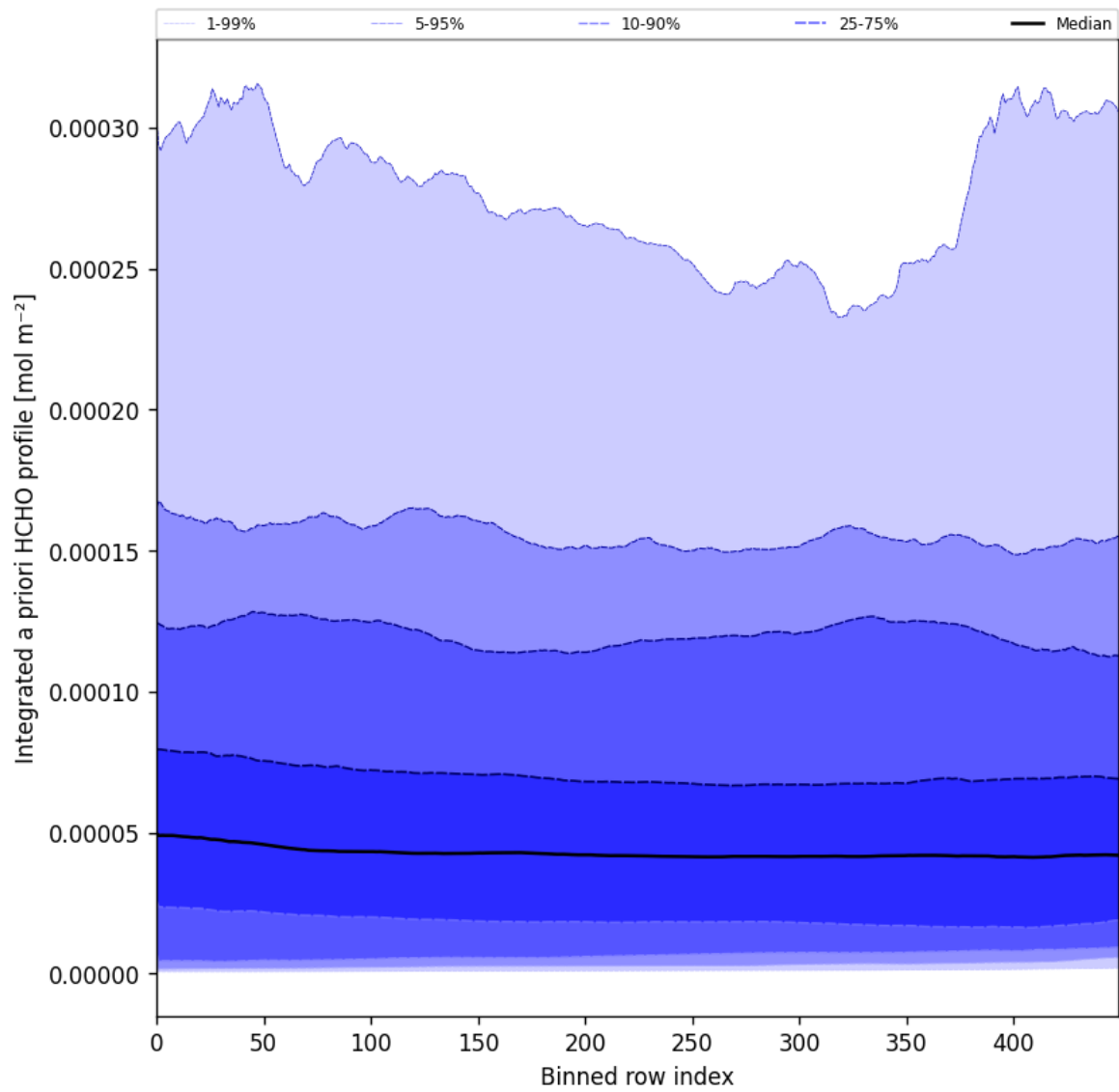
Figure 57: Along track statistics of “Integrated a priori HCHO profile” for 2025-07-26 to 2025-07-28
