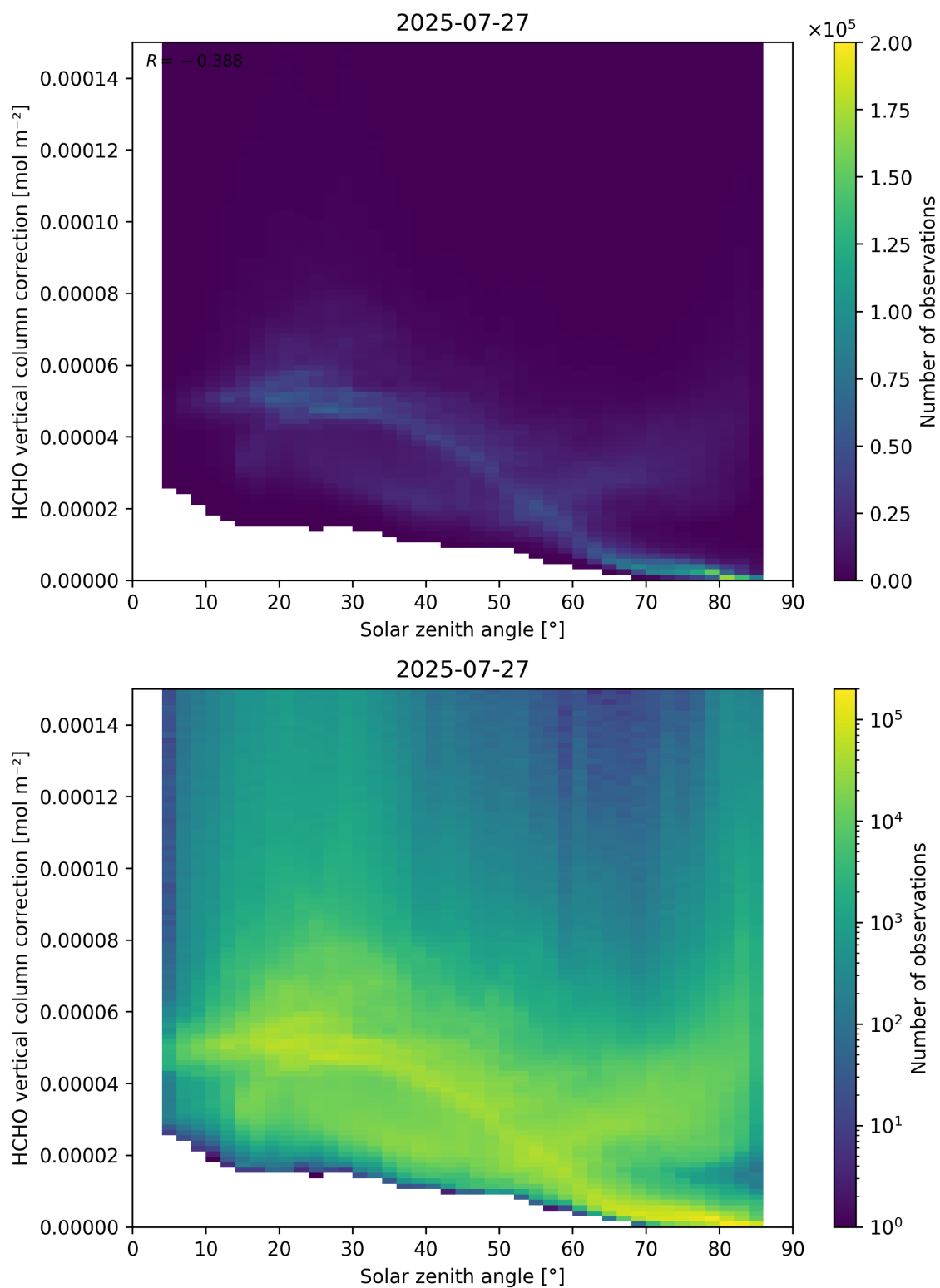
Figure 178: Scatter density plot of “Solar zenith angle” against “HCHO vertical column correction” for 2025-07-26 to 2025-07-28.
