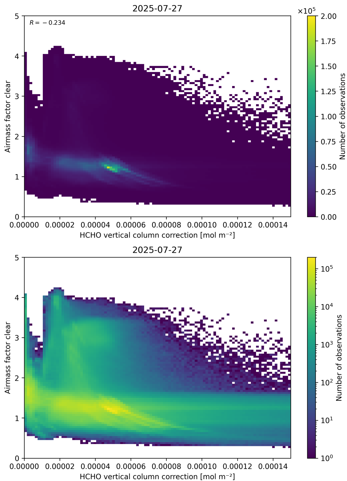
Figure 115: Scatter density plot of “HCHO vertical column correction” against “Airmass factor clear” for 2025-07-26 to 2025-07-28.
