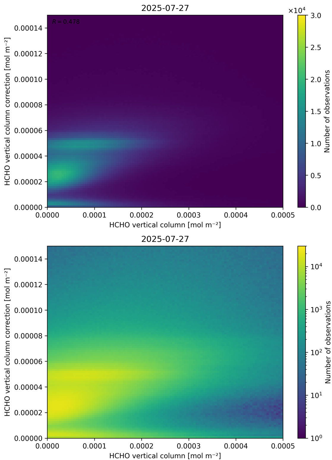
Figure 133: Scatter density plot of “HCHO vertical column” against “HCHO vertical column correction” for 2025-07-26 to 2025-07-28.
