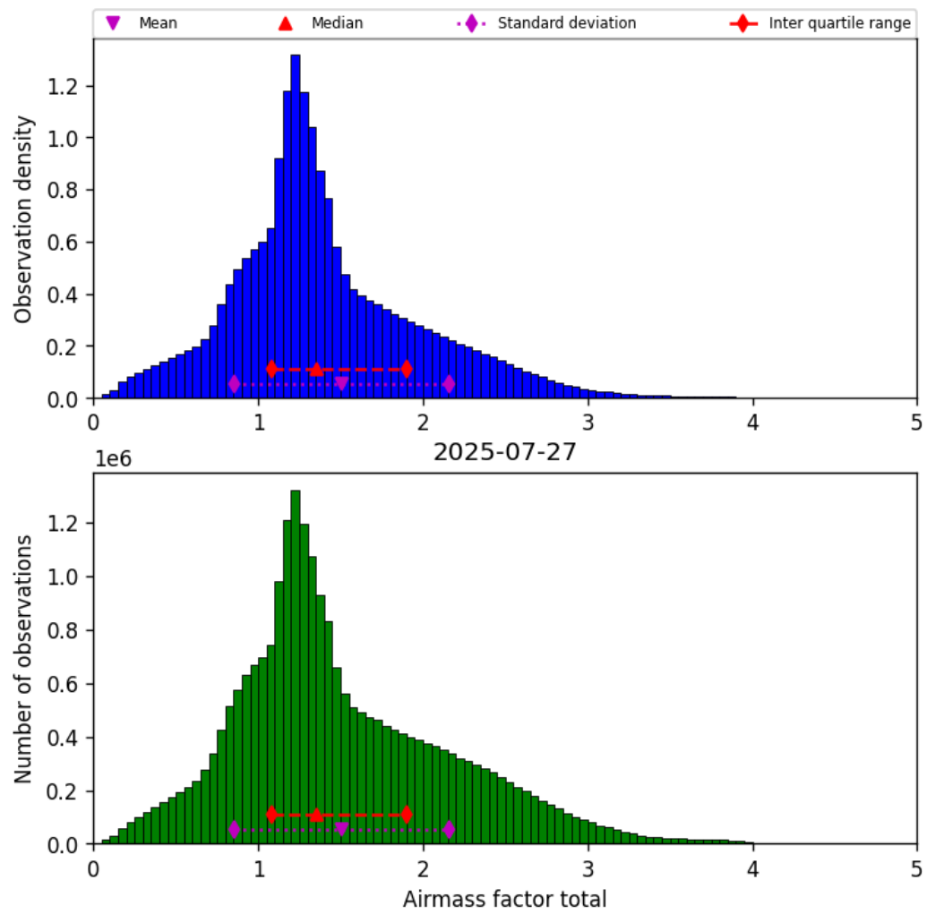
Figure 40: Histogram of “Airmass factor total” for 2025-07-26 to 2025-07-28
