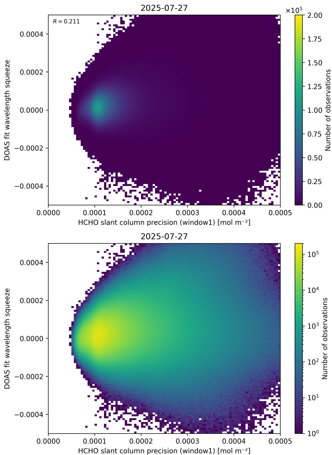
Figure 90: Scatter density plot of “HCHO slant column precision (window1)” against “DOAS fit wavelength squeeze” for 2025-07-26 to 2025-07-28.
