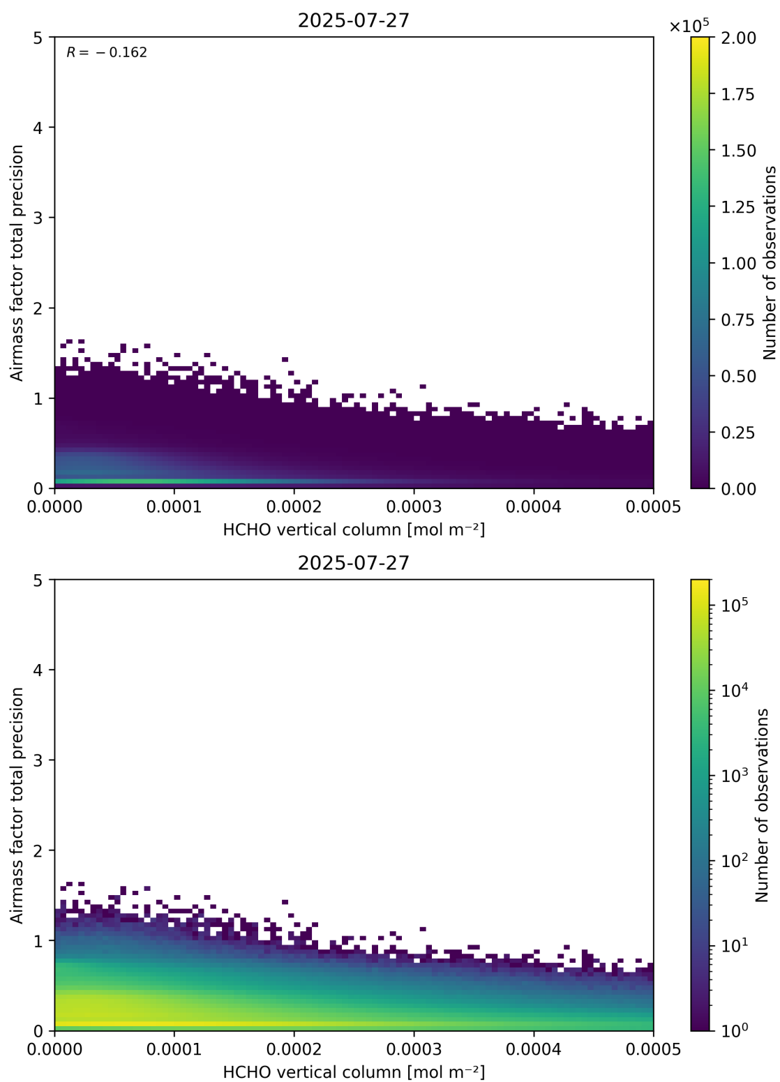
Figure 132: Scatter density plot of “HCHO vertical column” against “Airmass factor total precision” for 2025-07-26 to 2025-07-28.
