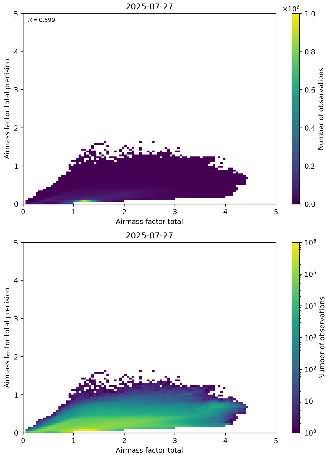
Figure 103: Scatter density plot of “Airmass factor total” against “Airmass factor total precision” for 2025-07-26 to 2025-07-28.
