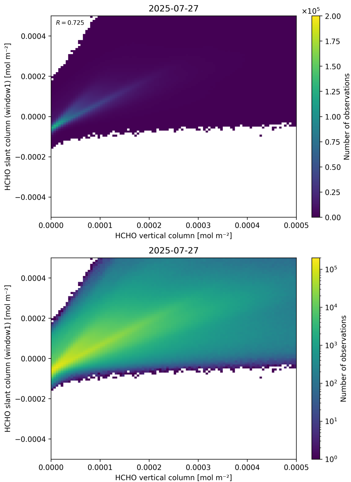
Figure 129: Scatter density plot of “HCHO vertical column” against “HCHO slant column (window1)” for 2025-07-26 to 2025-07-28.
