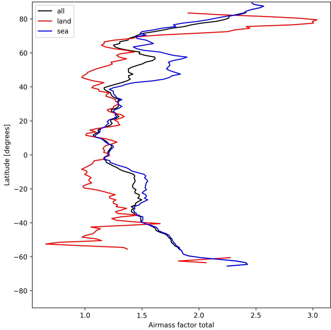
Figure 26: Zonal average of “Airmass factor total” for 2025-07-26 to 2025-07-28.
