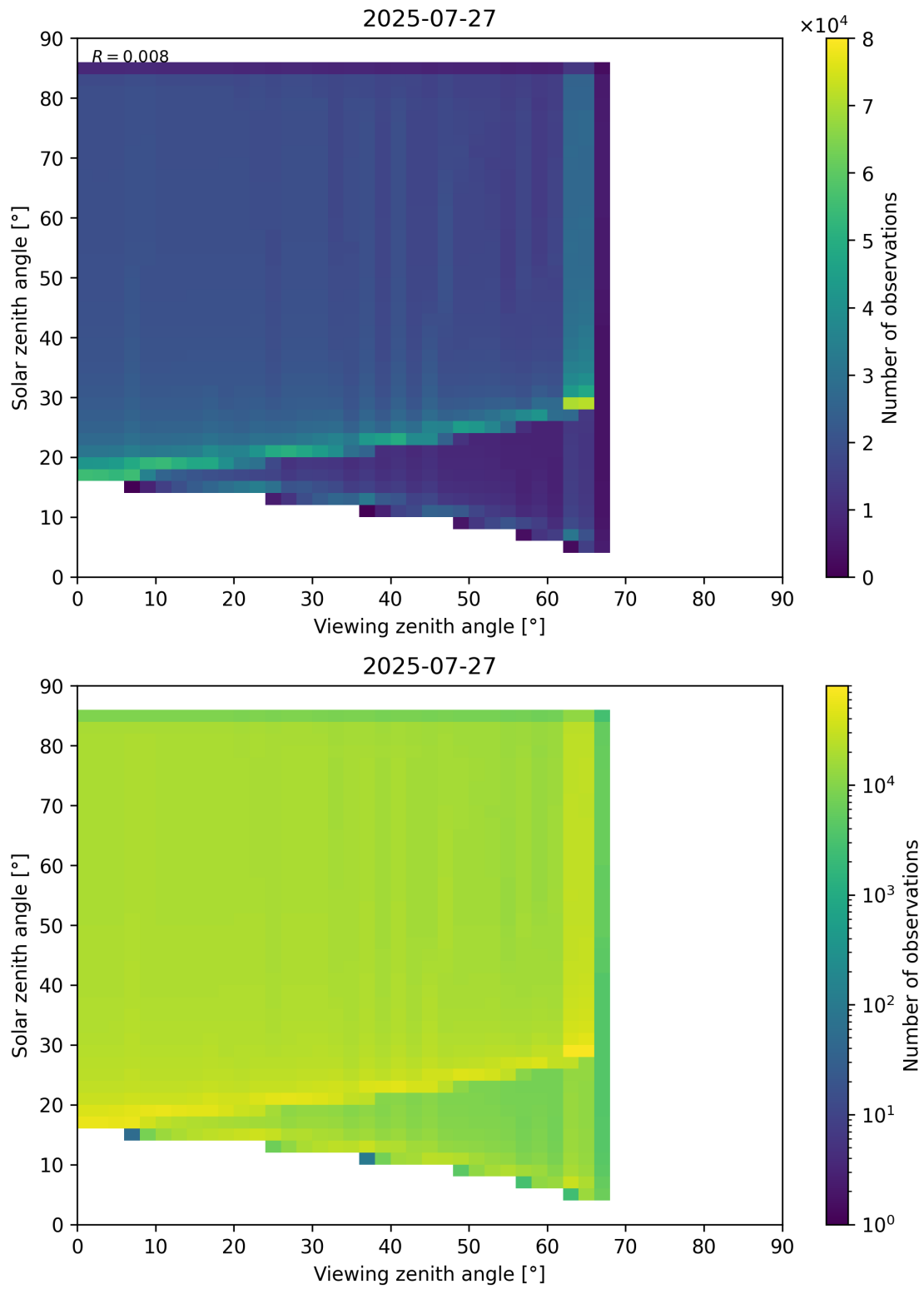
Figure 197: Scatter density plot of “Viewing zenith angle” against “Solar zenith angle” for 2025-07-26 to 2025-07-28.
