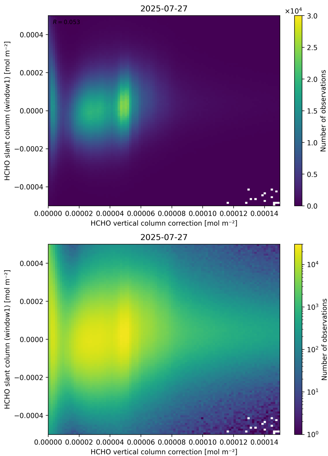
Figure 118: Scatter density plot of “HCHO vertical column correction” against “HCHO slant column (window1)” for 2025-07-26 to 2025-07-28.
