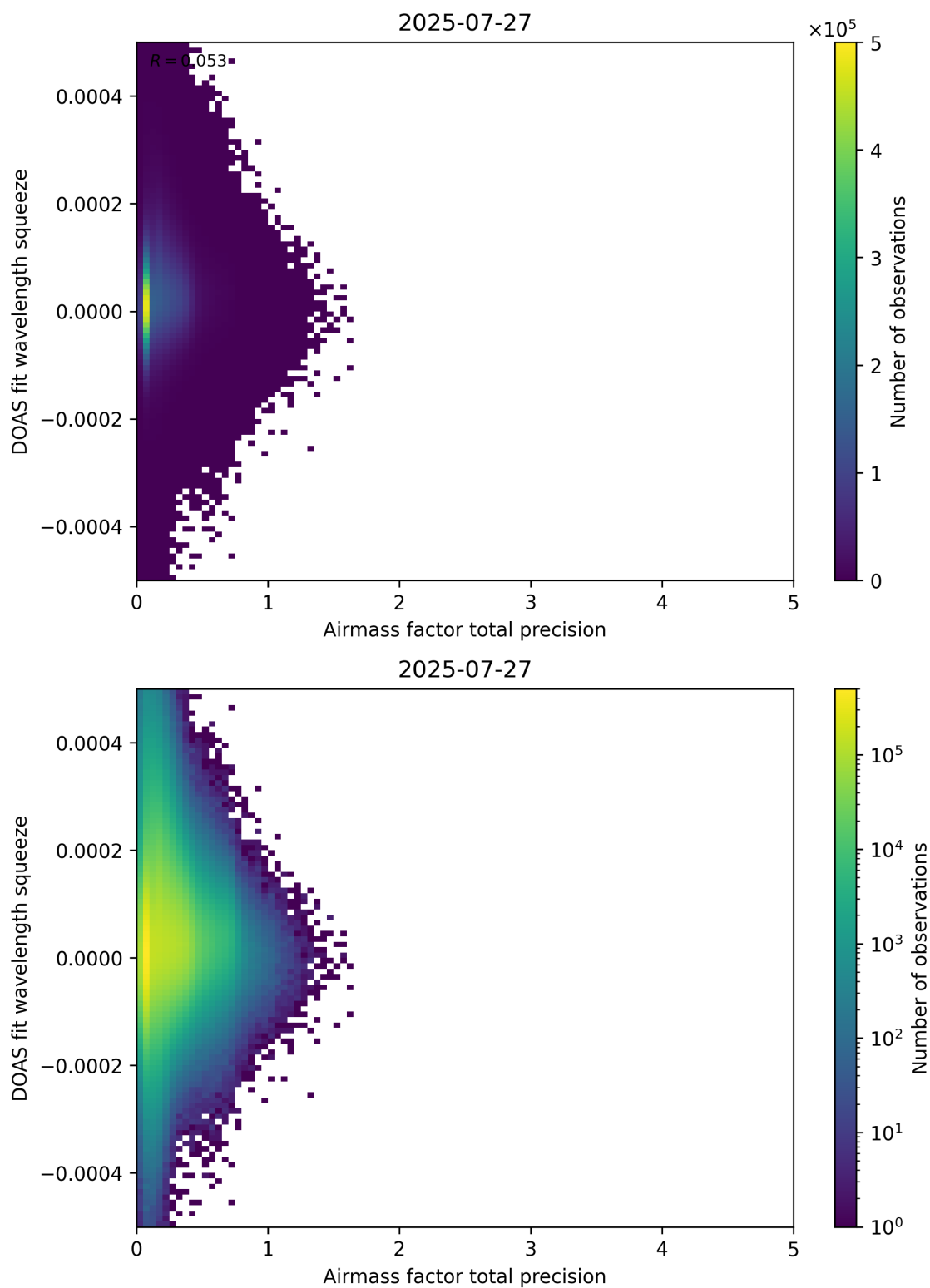
Figure 107: Scatter density plot of “Airmass factor total precision” against “DOAS fit wavelength squeeze” for 2025-07-26 to 2025-07-28.
