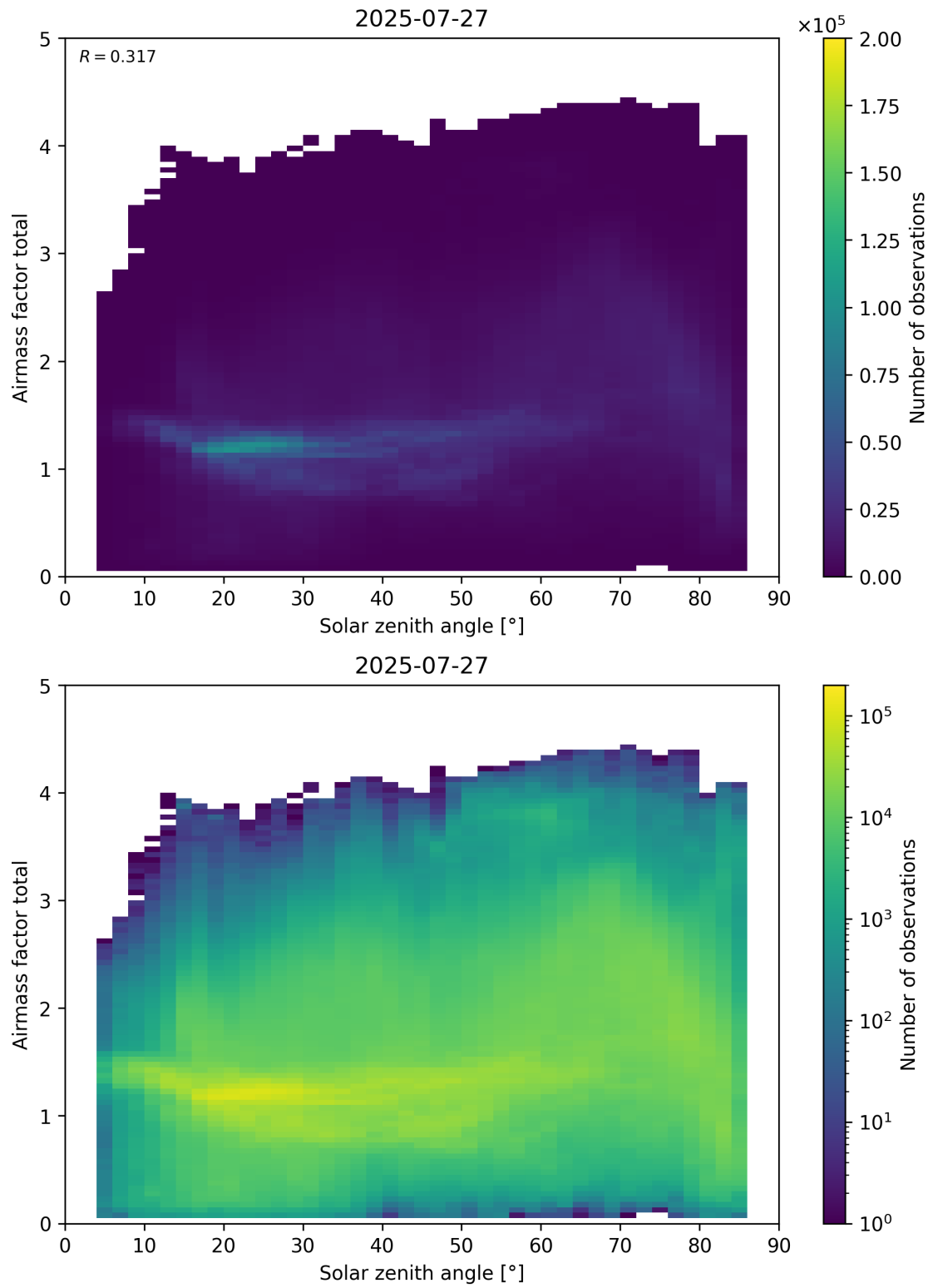
Figure 175: Scatter density plot of “Solar zenith angle” against “Airmass factor total” for 2025-07-26 to 2025-07-28.
