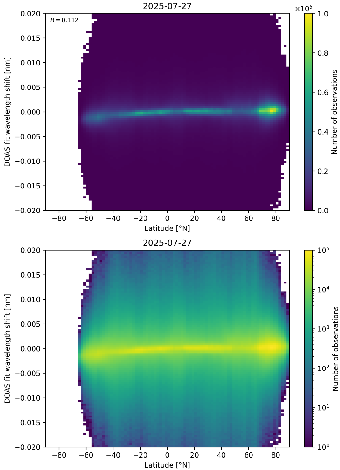
Figure 154: Scatter density plot of “Latitude” against “DOAS fit wavelength shift” for 2025-07-26 to 2025-07-28.
