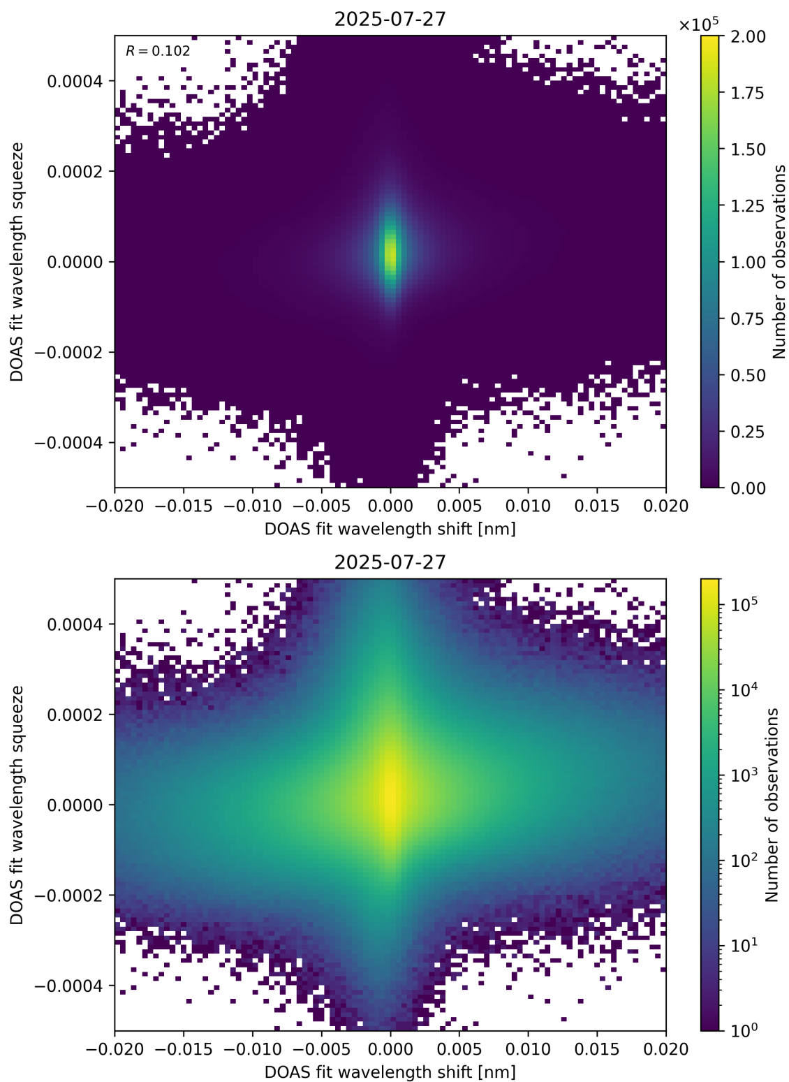
Figure 65: Scatter density plot of “DOAS fit wavelength shift” against “DOAS fit wavelength squeeze” for 2025-07-26 to 2025-07-28.
