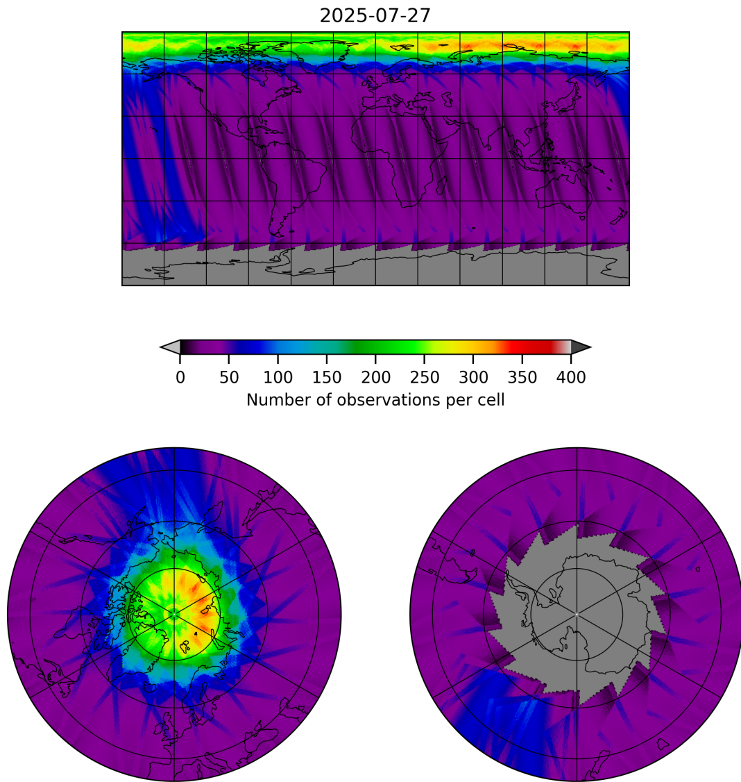
Figure 19: Map of the number of observations for 2025-07-26 to 2025-07-28
