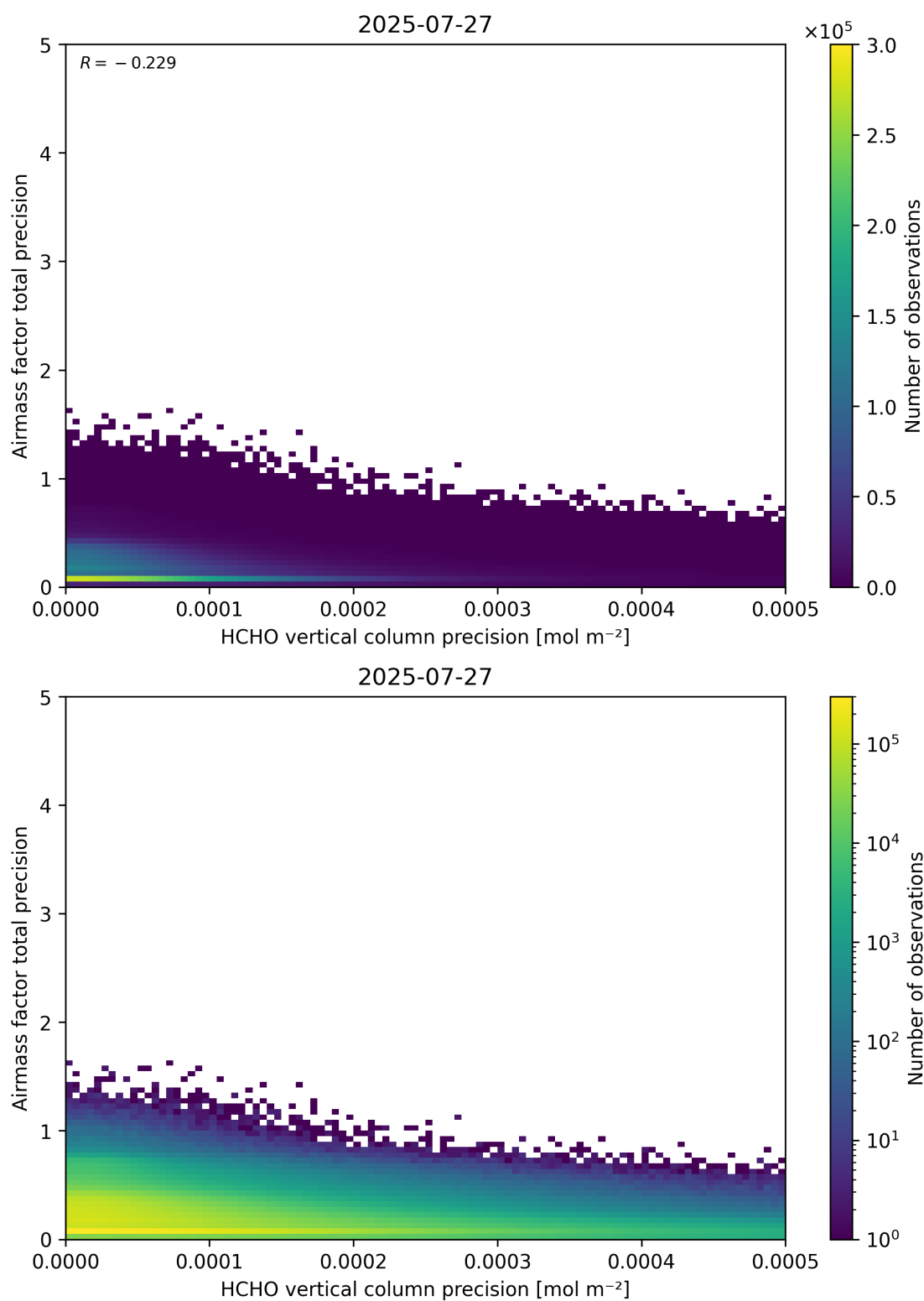
Figure 145: Scatter density plot of “HCHO vertical column precision” against “Airmass factor total precision” for 2025-07-26 to 2025-07-28.
