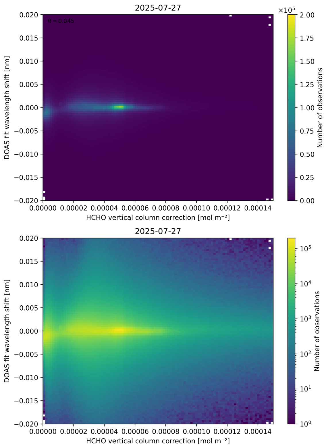
Figure 113: Scatter density plot of “HCHO vertical column correction” against “DOAS fit wavelength shift” for 2025-07-26 to 2025-07-28.
