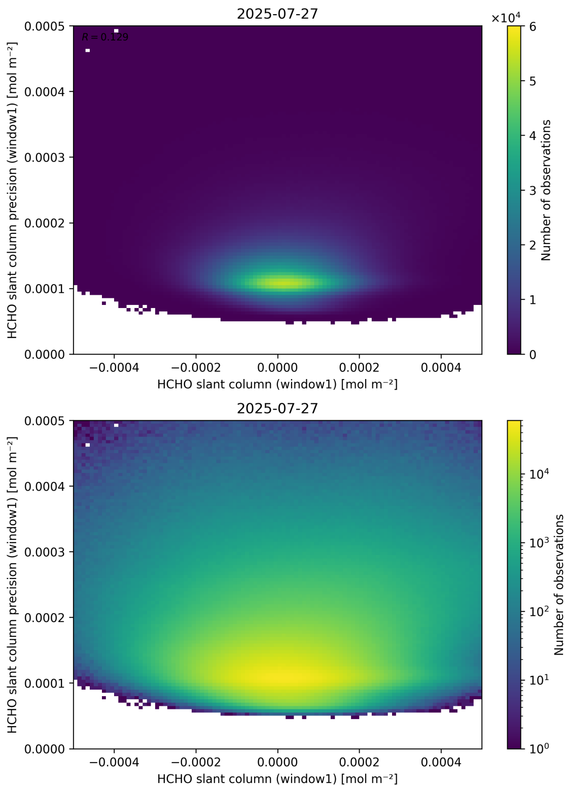
Figure 84: Scatter density plot of “HCHO slant column (window1)” against “HCHO slant column precision (window1)” for 2025-07-26 to 2025-07-28.
