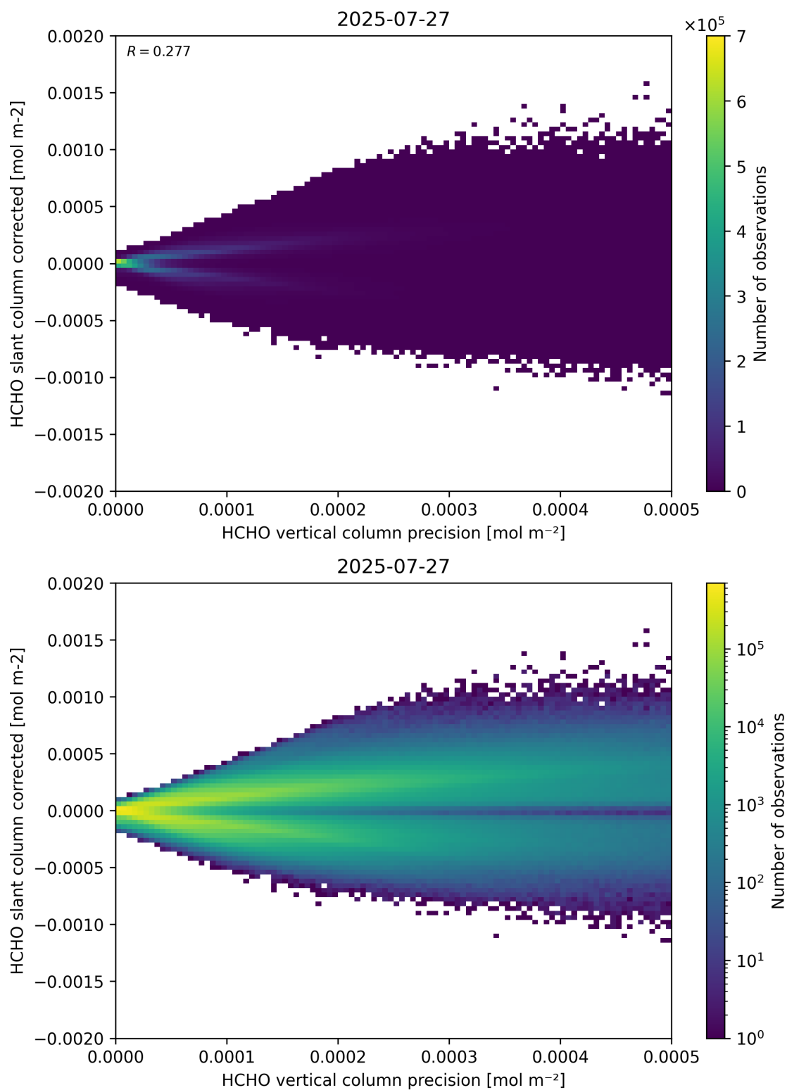
Figure 140: Scatter density plot of “HCHO vertical column precision” against “HCHO slant column corrected” for 2025-07-26 to 2025-07-28.
