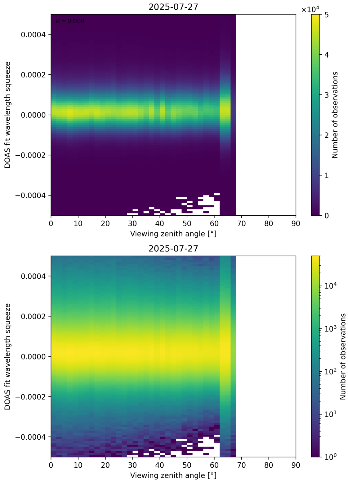
Figure 184: Scatter density plot of “Viewing zenith angle” against “DOAS fit wavelength squeeze” for 2025-07-26 to 2025-07-28.
