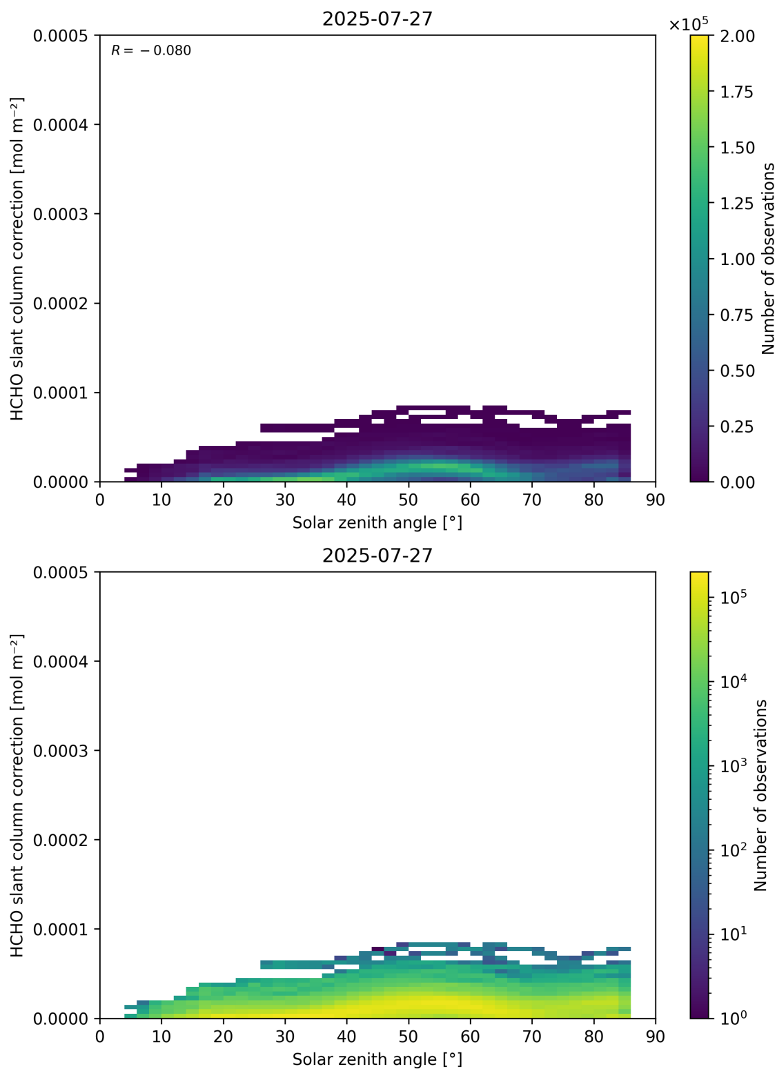
Figure 172: Scatter density plot of “Solar zenith angle” against “HCHO slant column correction” for 2025-07-26 to 2025-07-28.
