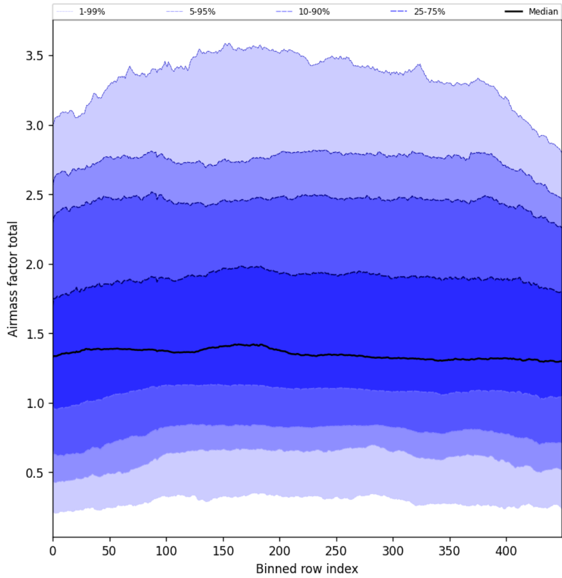
Figure 54: Along track statistics of “Airmass factor total” for 2025-07-26 to 2025-07-28
