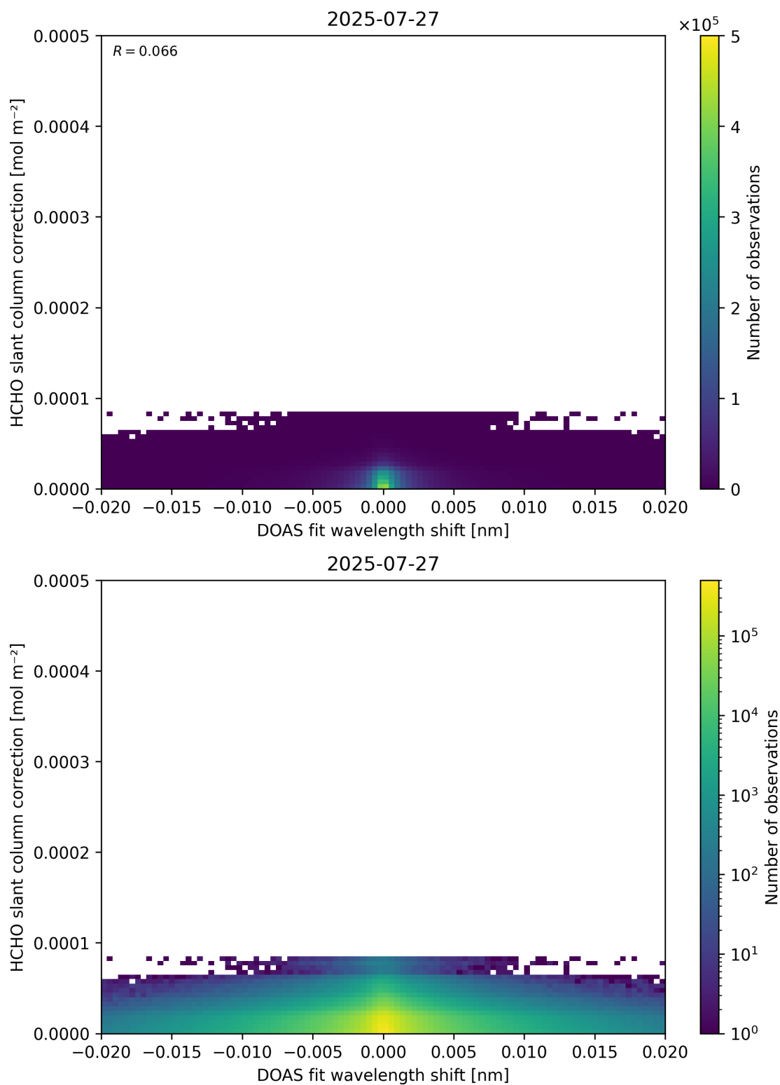
Figure 67: Scatter density plot of “DOAS fit wavelength shift” against “HCHO slant column correction” for 2025-07-26 to 2025-07-28.
