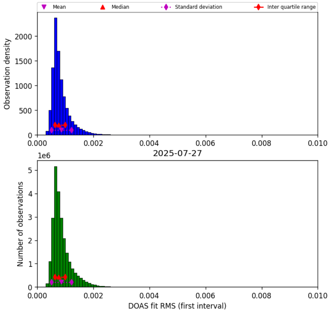
Figure 46: Histogram of “DOAS fit RMS (first interval)” for 2025-07-26 to 2025-07-28
