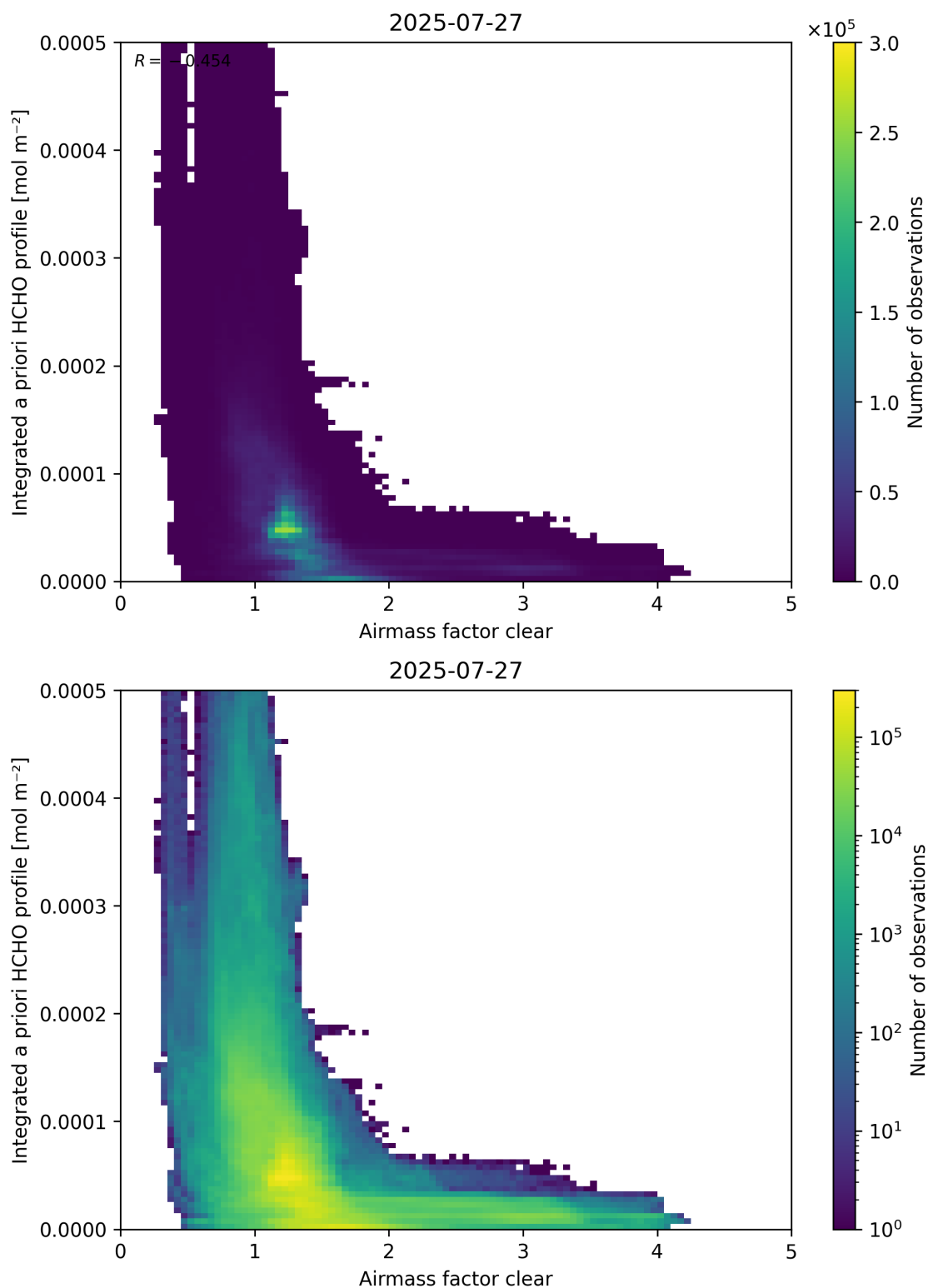
Figure 76: Scatter density plot of “Airmass factor clear” against “Integrated a priori HCHO profile” for 2025-07-26 to 2025-07-28.
