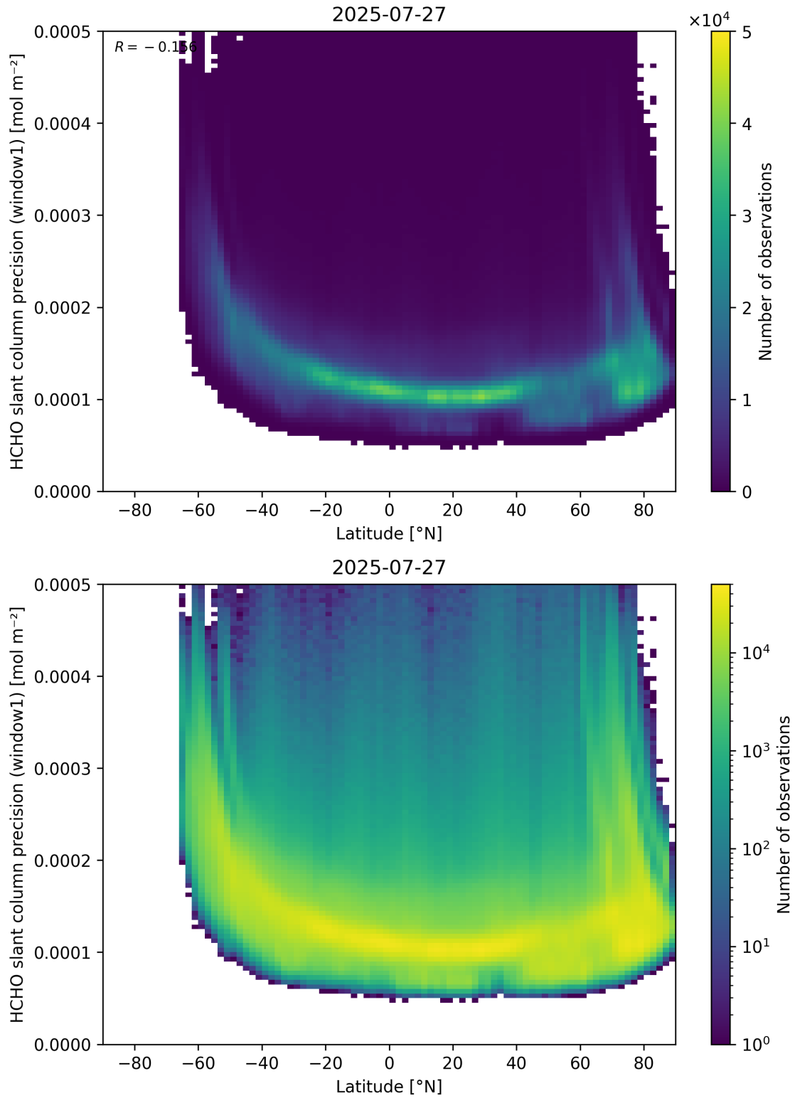
Figure 160: Scatter density plot of “Latitude” against “HCHO slant column precision (window1)” for 2025-07-26 to 2025-07-28.
