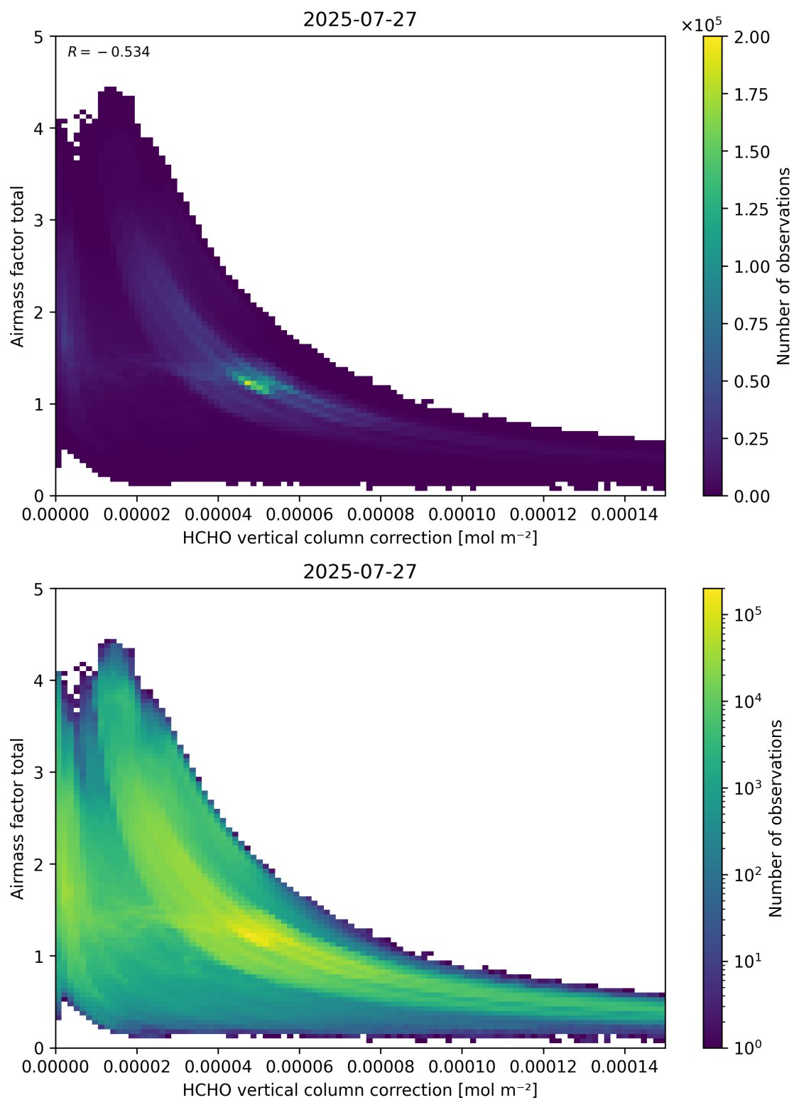
Figure 120: Scatter density plot of “HCHO vertical column correction” against “Airmass factor total” for 2025-07-26 to 2025-07-28.
