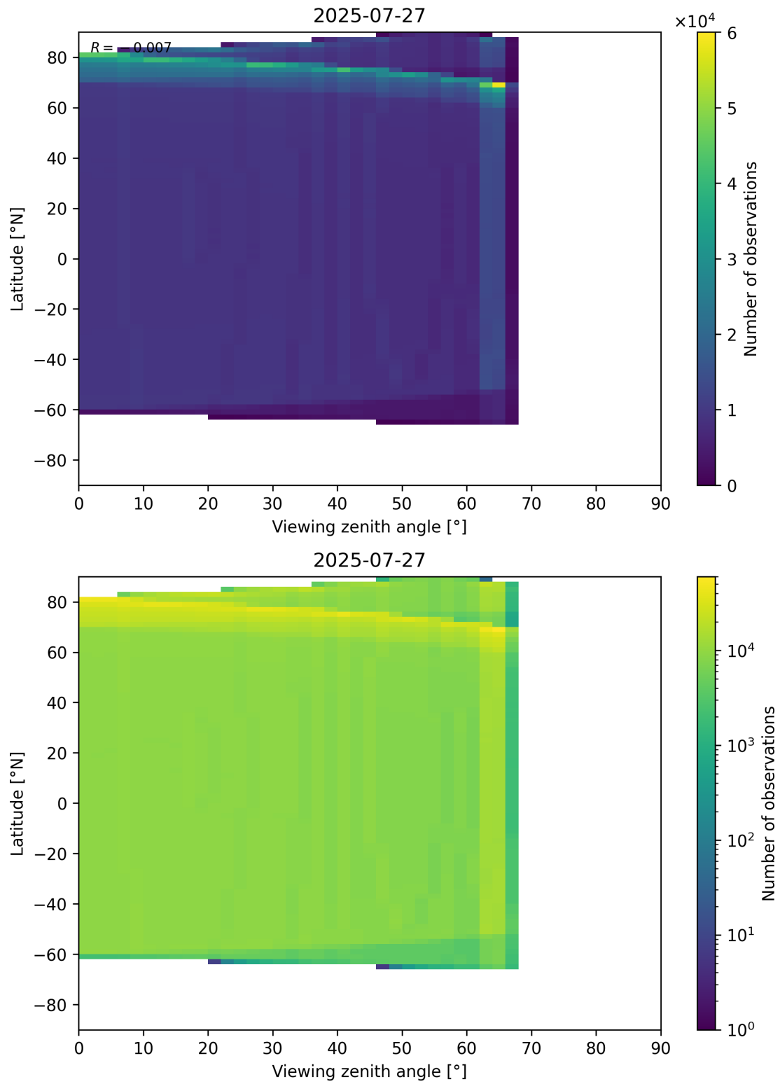
Figure 196: Scatter density plot of “Viewing zenith angle” against “Latitude” for 2025-07-26 to 2025-07-28.
