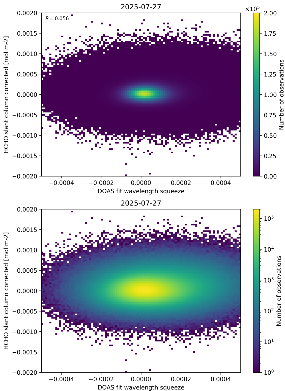
Figure 69: Scatter density plot of “DOAS fit wavelength squeeze” against “HCHO slant column corrected” for 2025-07-26 to 2025-07-28.
