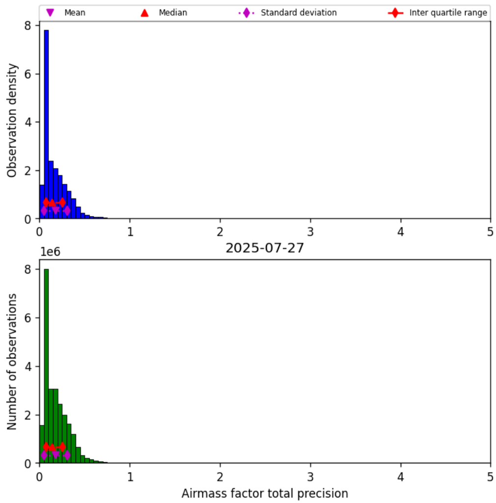
Figure 41: Histogram of “Airmass factor total precision” for 2025-07-26 to 2025-07-28
