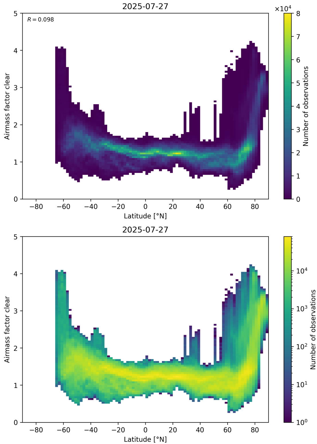
Figure 156: Scatter density plot of “Latitude” against “Airmass factor clear” for 2025-07-26 to 2025-07-28.
