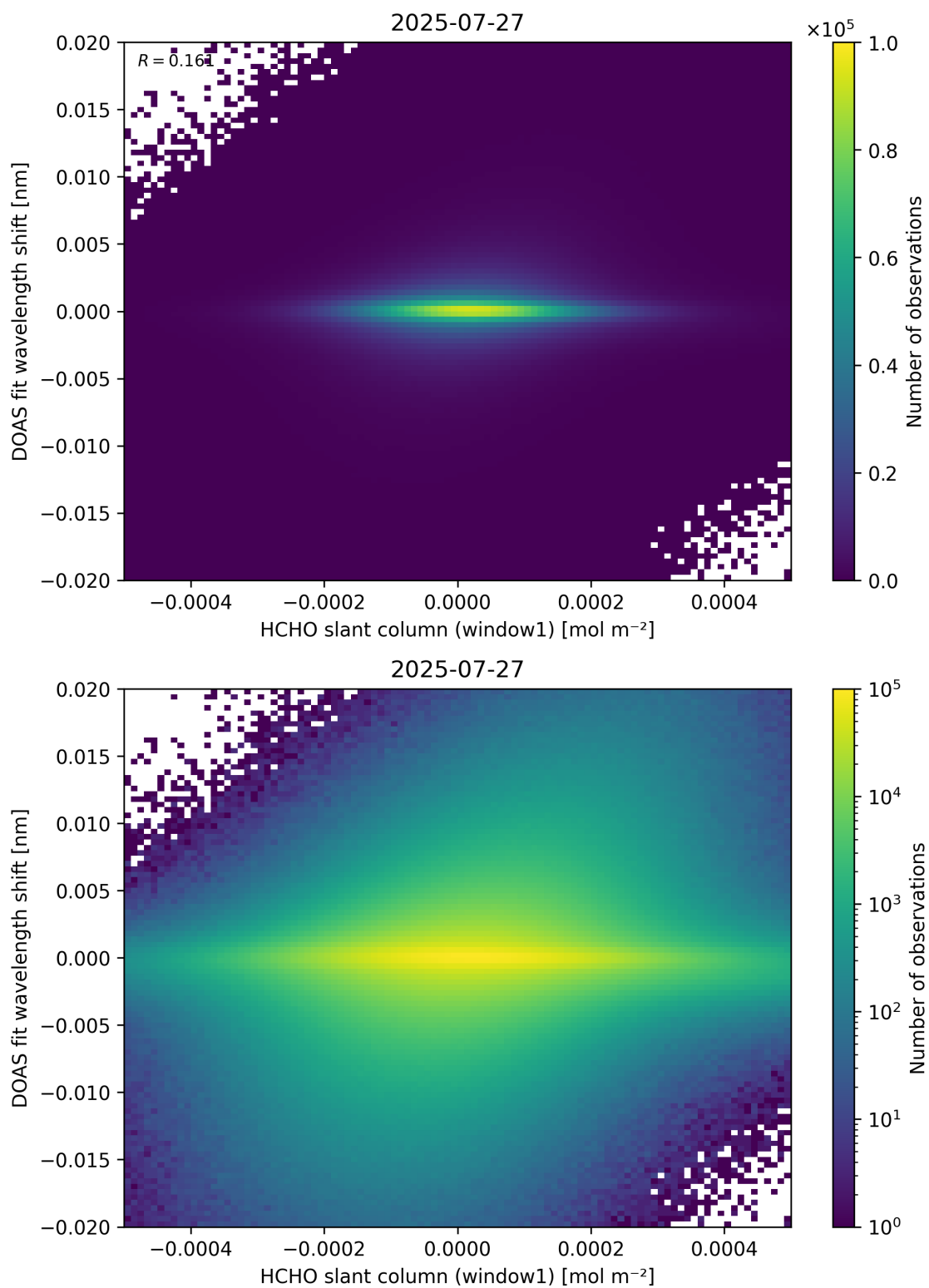
Figure 79: Scatter density plot of “HCHO slant column (window1)” against “DOAS fit wavelength shift” for 2025-07-26 to 2025-07-28.
