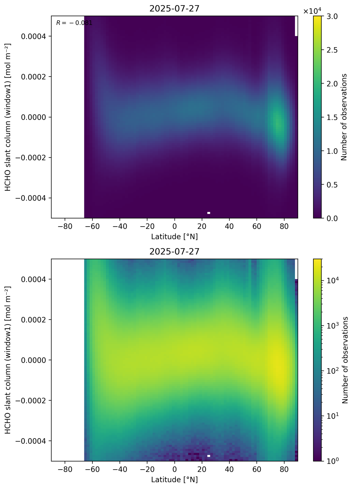
Figure 159: Scatter density plot of “Latitude” against “HCHO slant column (window1)” for 2025-07-26 to 2025-07-28.
