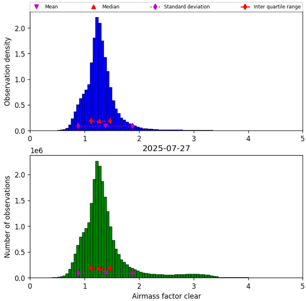
Figure 42: Histogram of “Airmass factor clear” for 2025-07-26 to 2025-07-28
