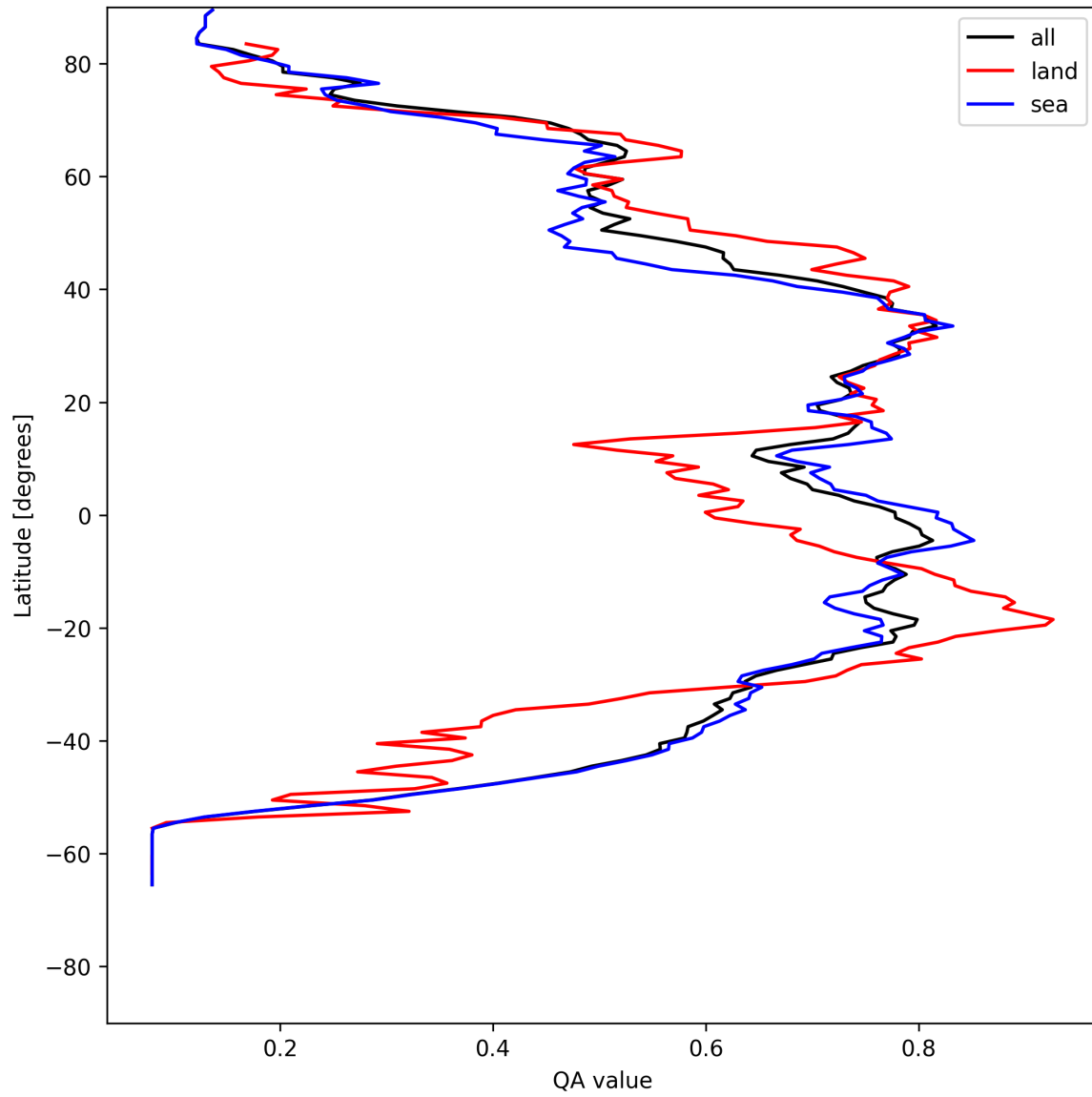
Figure 20: Zonal average of “QA value” for 2025-07-26 to 2025-07-28.
