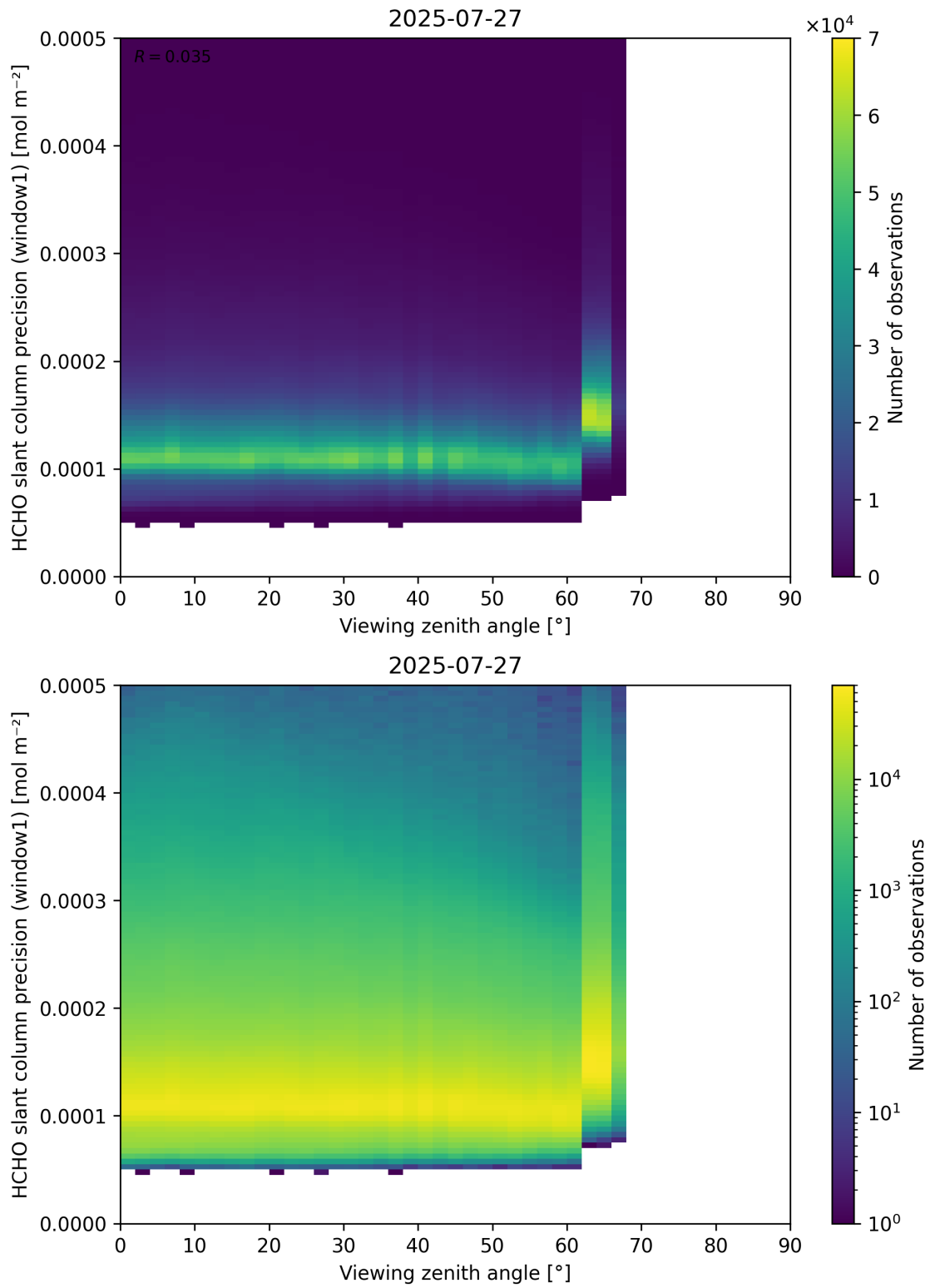
Figure 189: Scatter density plot of “Viewing zenith angle” against “HCHO slant column precision (window1)” for 2025-07-26 to 2025-07-28.
