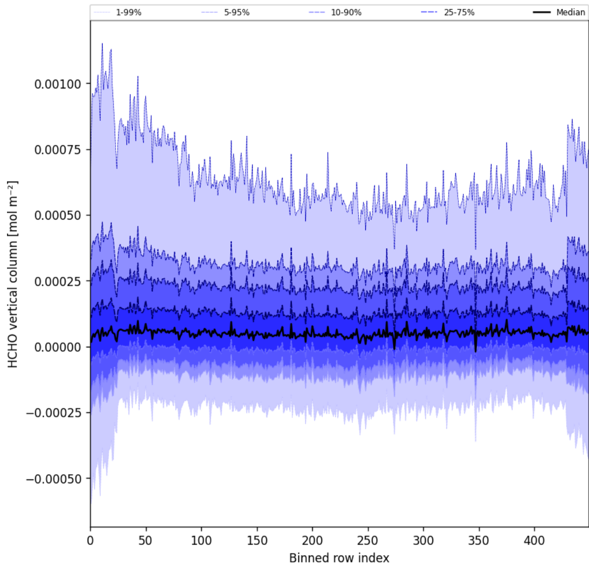
Figure 49: Along track statistics of “HCHO vertical column” for 2025-07-26 to 2025-07-28
