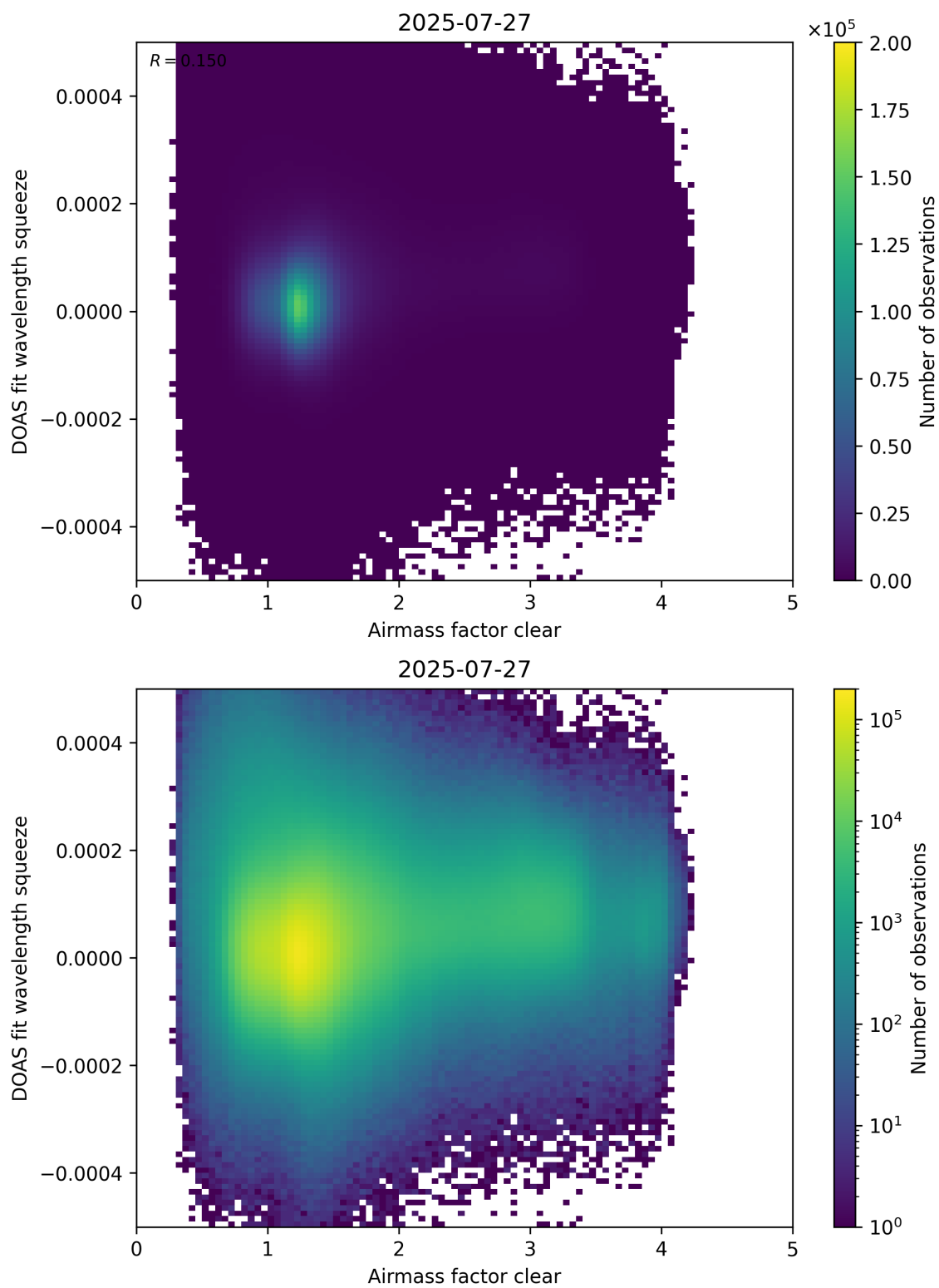
Figure 73: Scatter density plot of “Airmass factor clear” against “DOAS fit wavelength squeeze” for 2025-07-26 to 2025-07-28.
