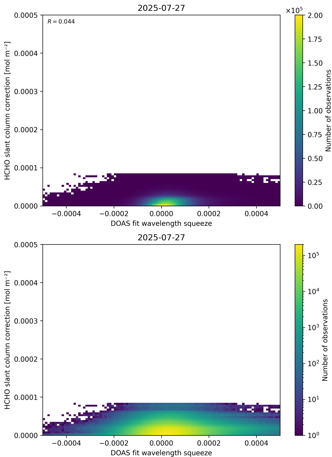
Figure 70: Scatter density plot of “DOAS fit wavelength squeeze” against “HCHO slant column correction” for 2025-07-26 to 2025-07-28.
