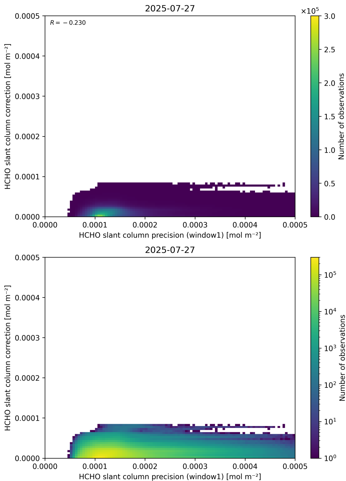
Figure 93: Scatter density plot of “HCHO slant column precision (window1)” against “HCHO slant column correction” for 2025-07-26 to 2025-07-28.
