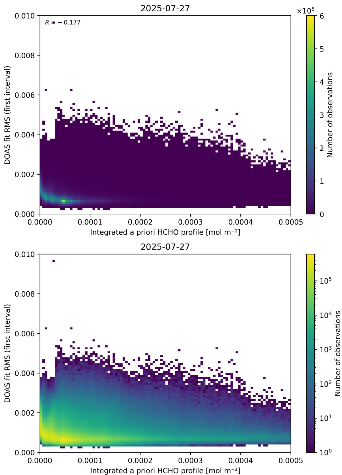
Figure 148: Scatter density plot of “Integrated a priori HCHO profile” against “DOAS fit RMS (first interval)” for 2025-07-26 to 2025-07-28.
