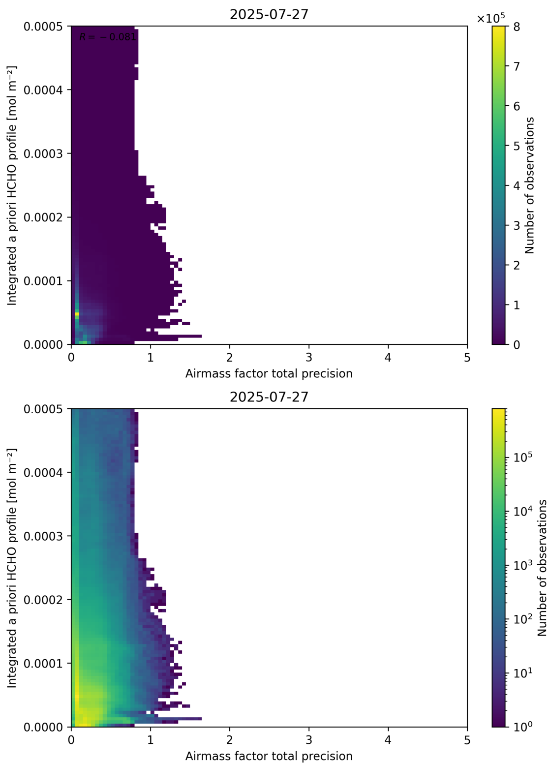
Figure 111: Scatter density plot of “Airmass factor total precision” against “Integrated a priori HCHO profile” for 2025-07-26 to 2025-07-28.
