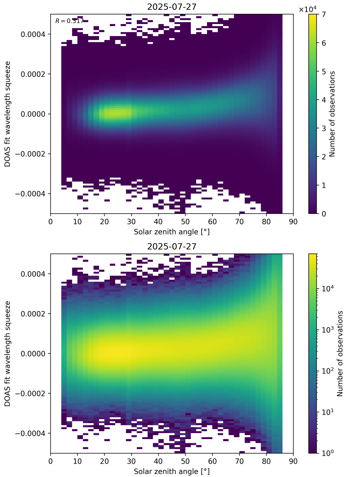
Figure 169: Scatter density plot of “Solar zenith angle” against “DOAS fit wavelength squeeze” for 2025-07-26 to 2025-07-28.
