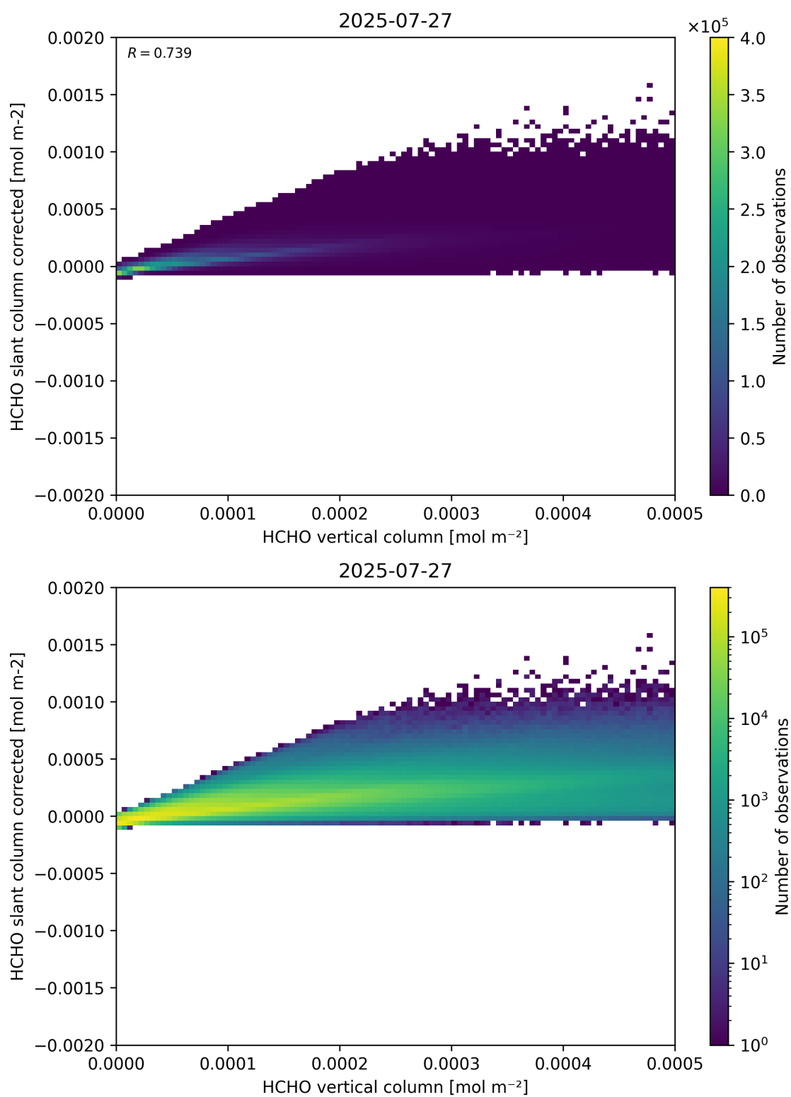
Figure 127: Scatter density plot of “HCHO vertical column” against “HCHO slant column corrected” for 2025-07-26 to 2025-07-28.
