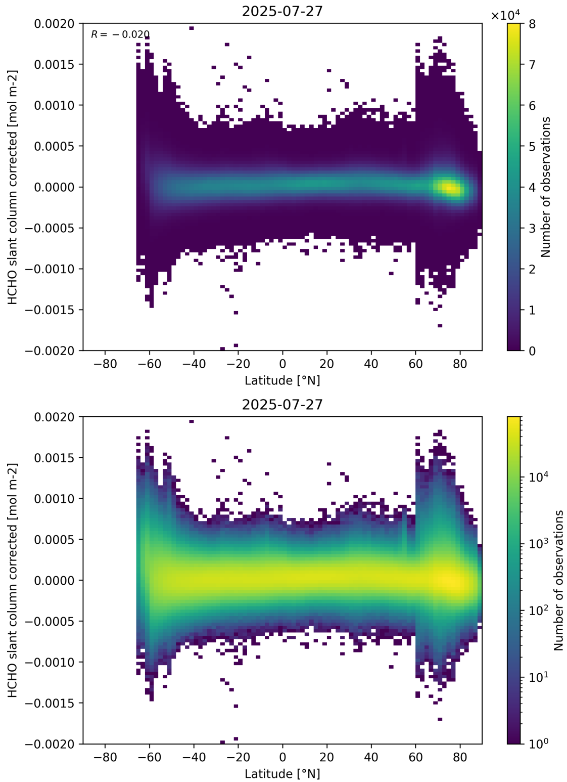
Figure 157: Scatter density plot of “Latitude” against “HCHO slant column corrected” for 2025-07-26 to 2025-07-28.
