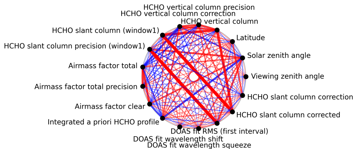
Figure 1: Map of correlation graph for 2025-07-26 to 2025-07-28.
