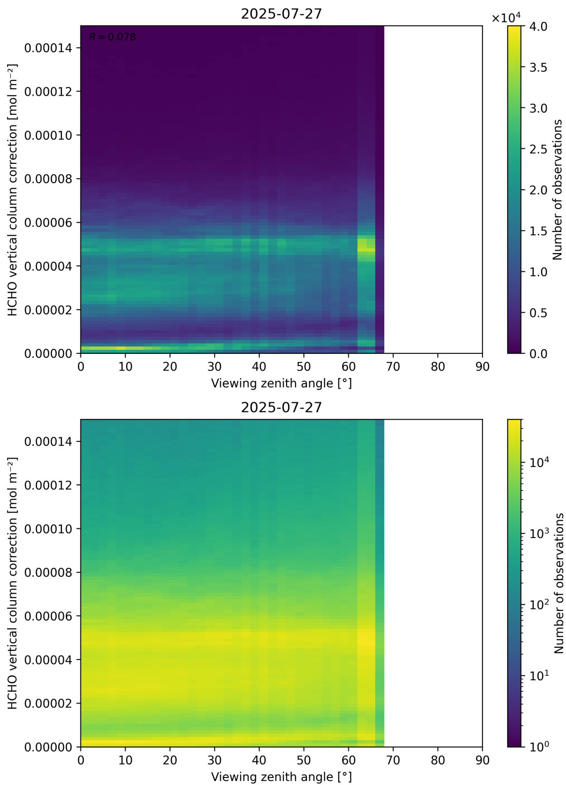
Figure 193: Scatter density plot of “Viewing zenith angle” against “HCHO vertical column correction” for 2025-07-26 to 2025-07-28.
