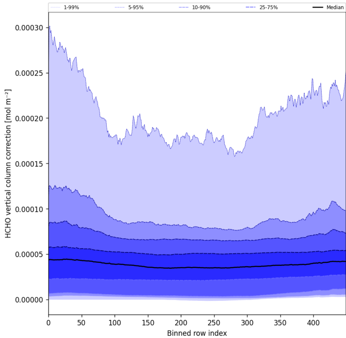
Figure 51: Along track statistics of “HCHO vertical column correction” for 2025-07-26 to 2025-07-28
