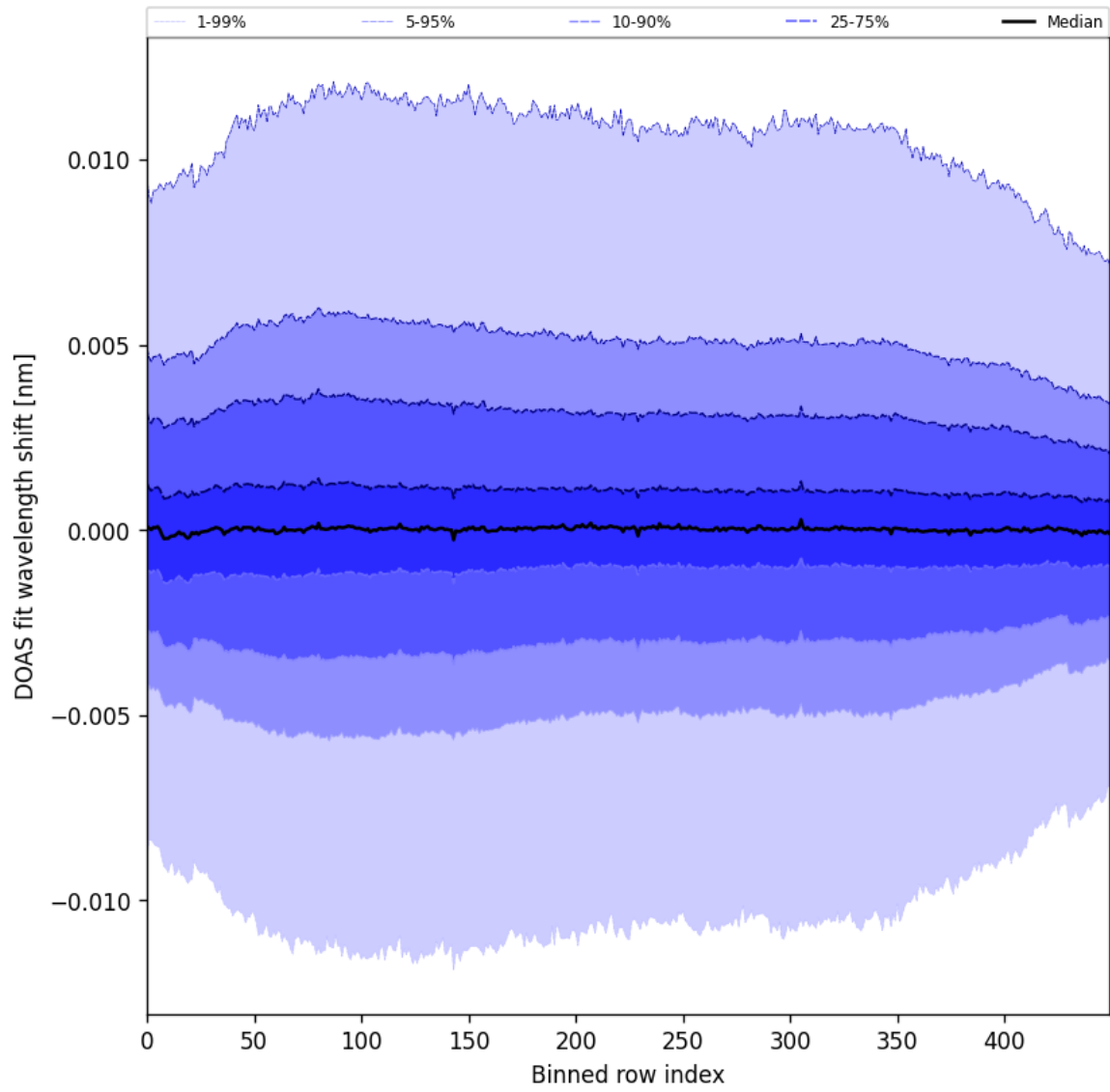
Figure 58: Along track statistics of “DOAS fit wavelength shift” for 2025-07-26 to 2025-07-28
