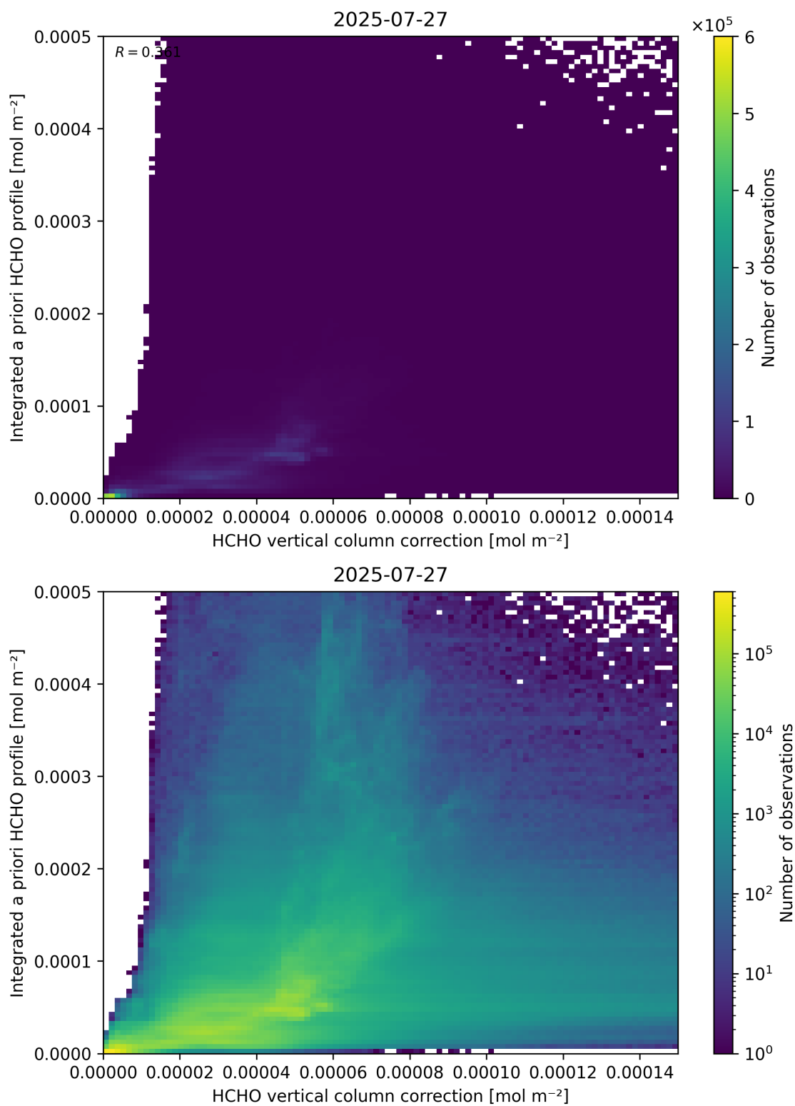
Figure 122: Scatter density plot of “HCHO vertical column correction” against “Integrated a priori HCHO profile” for 2025-07-26 to 2025-07-28.
