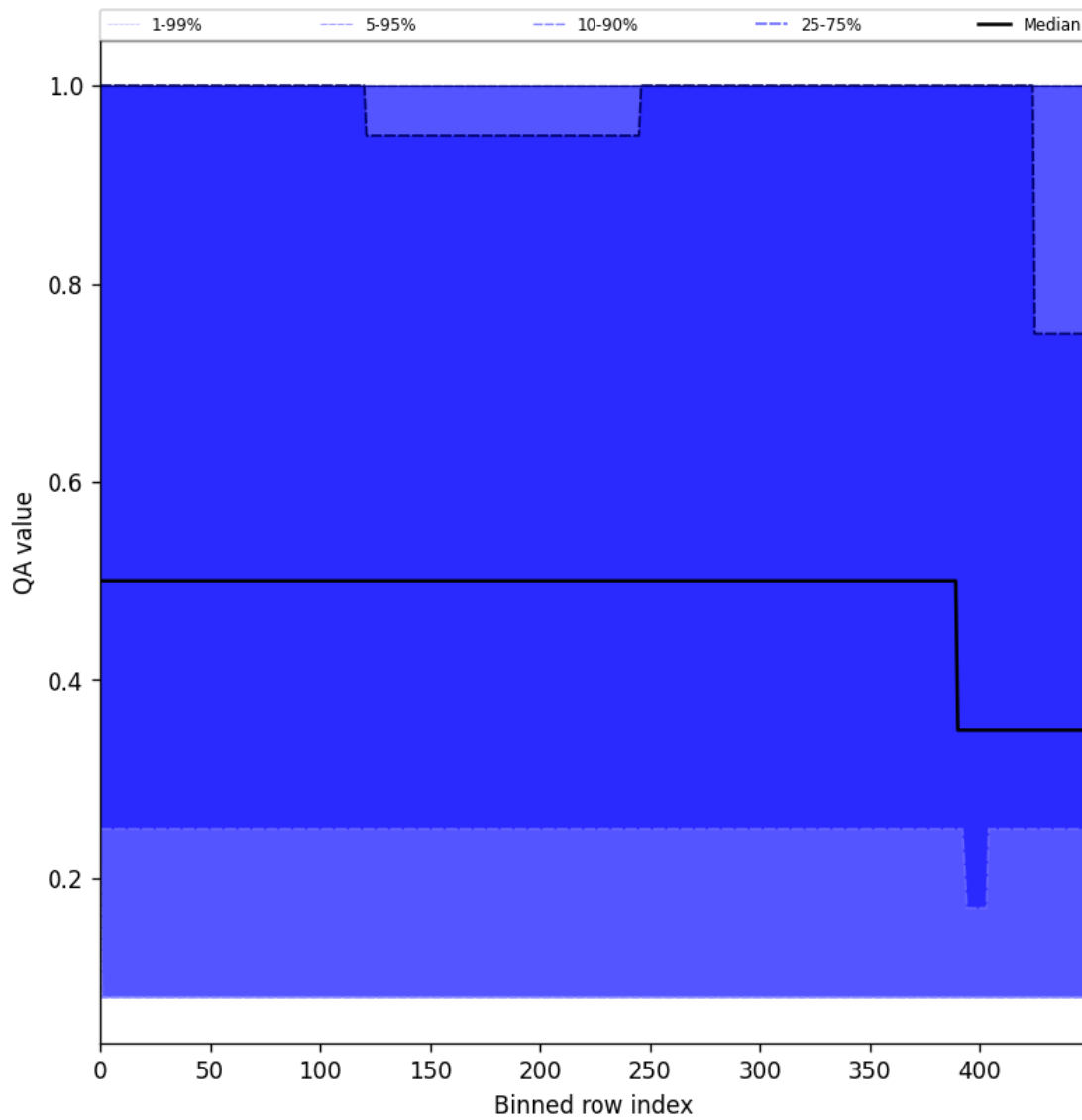
Figure 48: Along track statistics of “QA value” for 2025-07-26 to 2025-07-28
