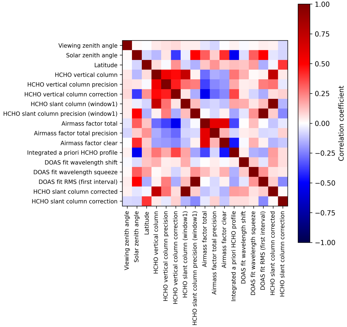
Figure 2: Map of correlation matrix for 2025-07-26 to 2025-07-28.
