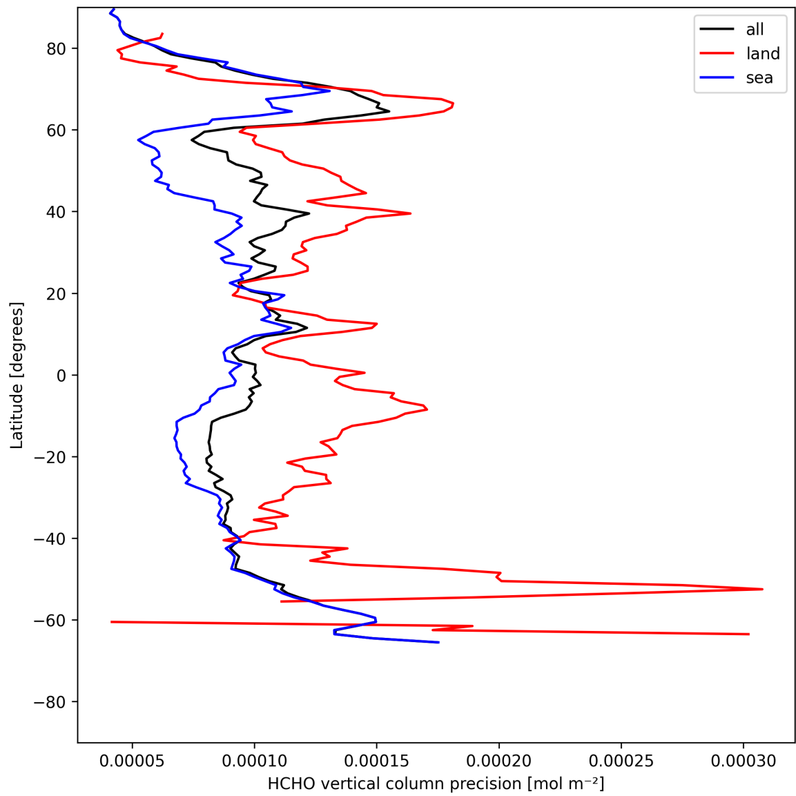
Figure 22: Zonal average of “HCHO vertical column precision” for 2025-07-26 to 2025-07-28.
