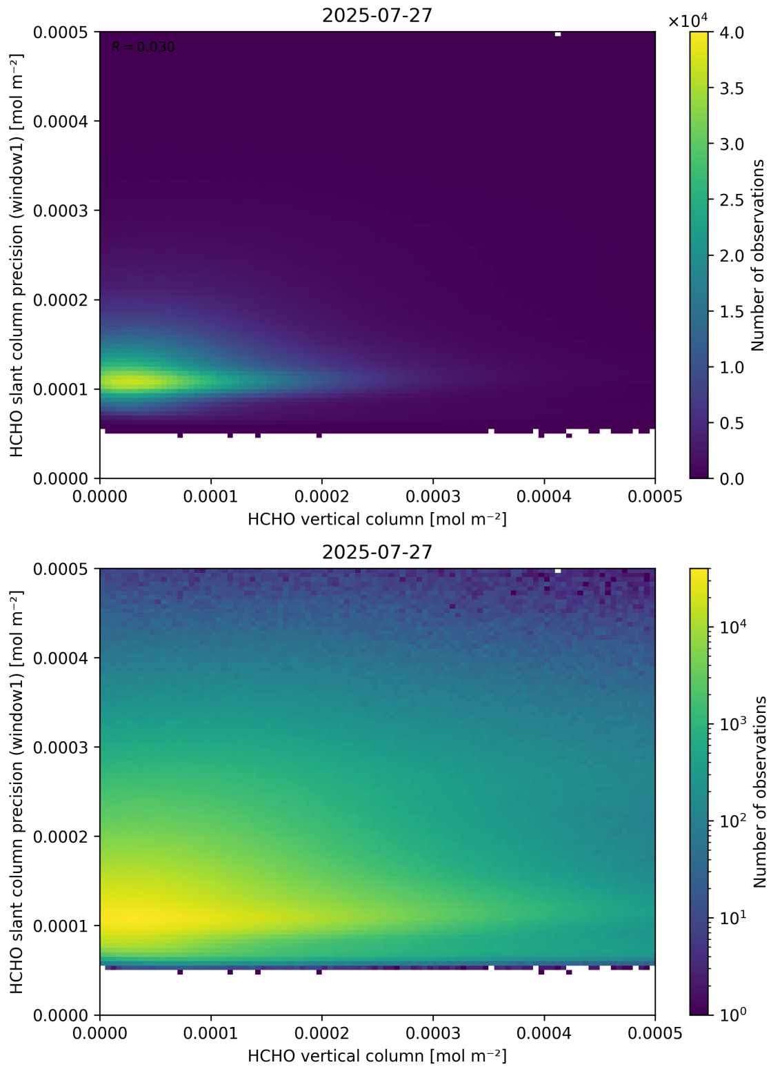
Figure 130: Scatter density plot of “HCHO vertical column” against “HCHO slant column precision (window1)” for 2025-07-26 to 2025-07-28.
