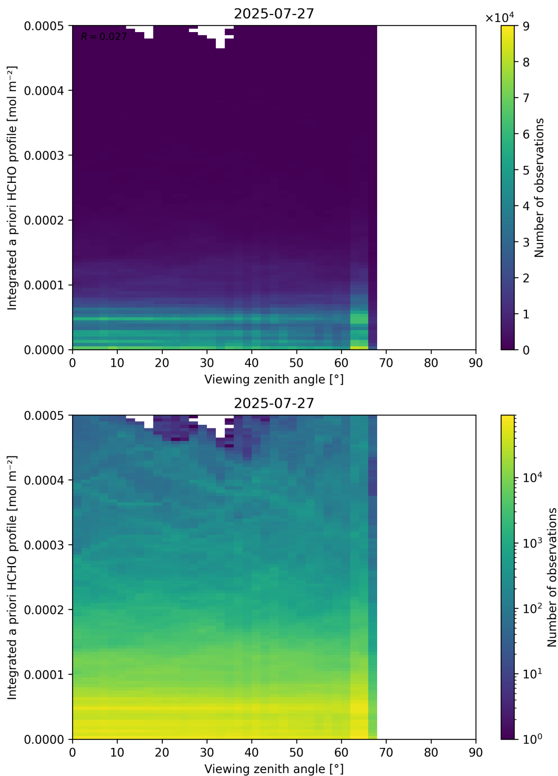
Figure 195: Scatter density plot of “Viewing zenith angle” against “Integrated a priori HCHO profile” for 2025-07-26 to 2025-07-28.
