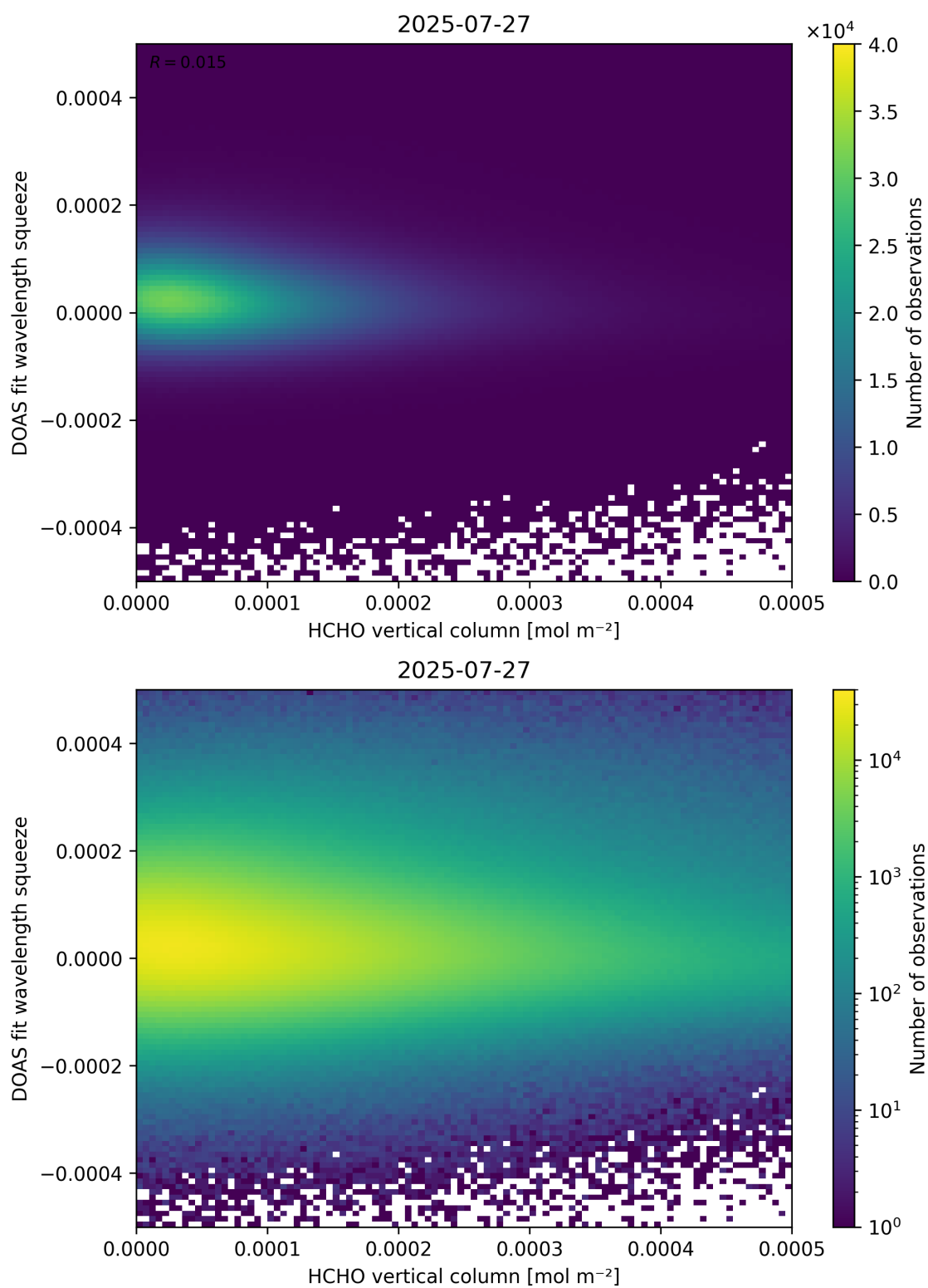
Figure 125: Scatter density plot of “HCHO vertical column” against “DOAS fit wavelength squeeze” for 2025-07-26 to 2025-07-28.
