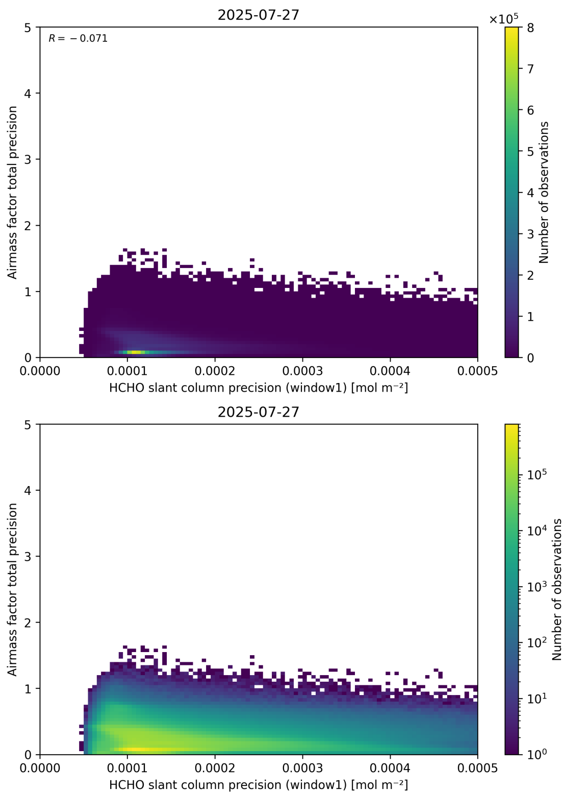
Figure 95: Scatter density plot of “HCHO slant column precision (window1)” against “Airmass factor total precision” for 2025-07-26 to 2025-07-28.
