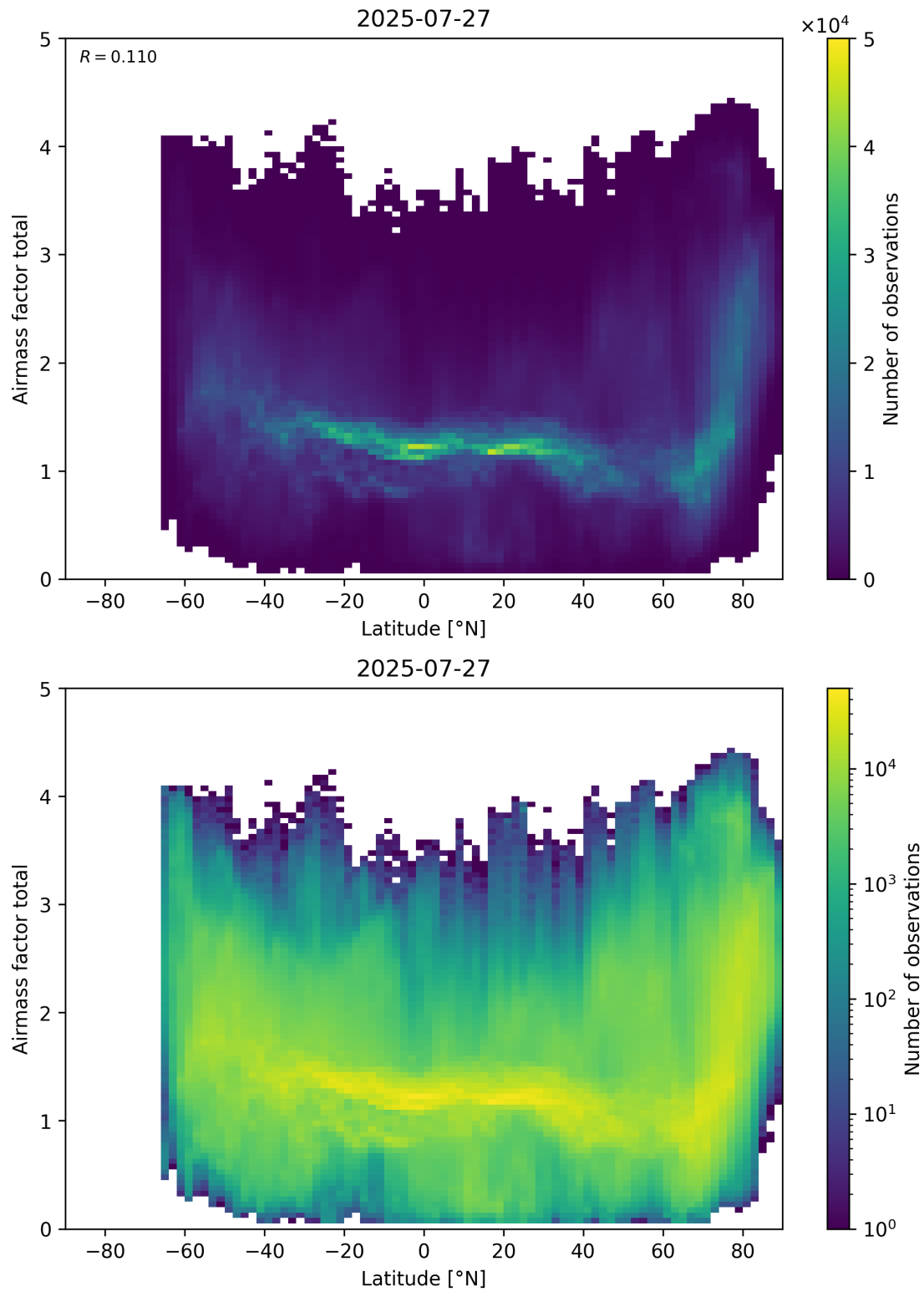
Figure 161: Scatter density plot of “Latitude” against “Airmass factor total” for 2025-07-26 to 2025-07-28.
