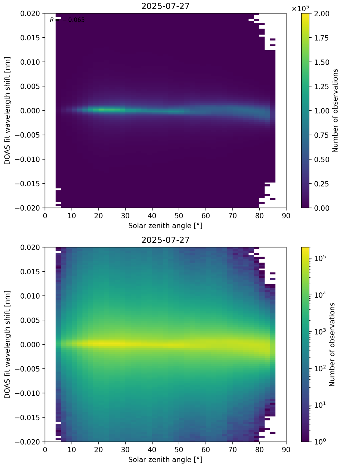
Figure 168: Scatter density plot of “Solar zenith angle” against “DOAS fit wavelength shift” for 2025-07-26 to 2025-07-28.
