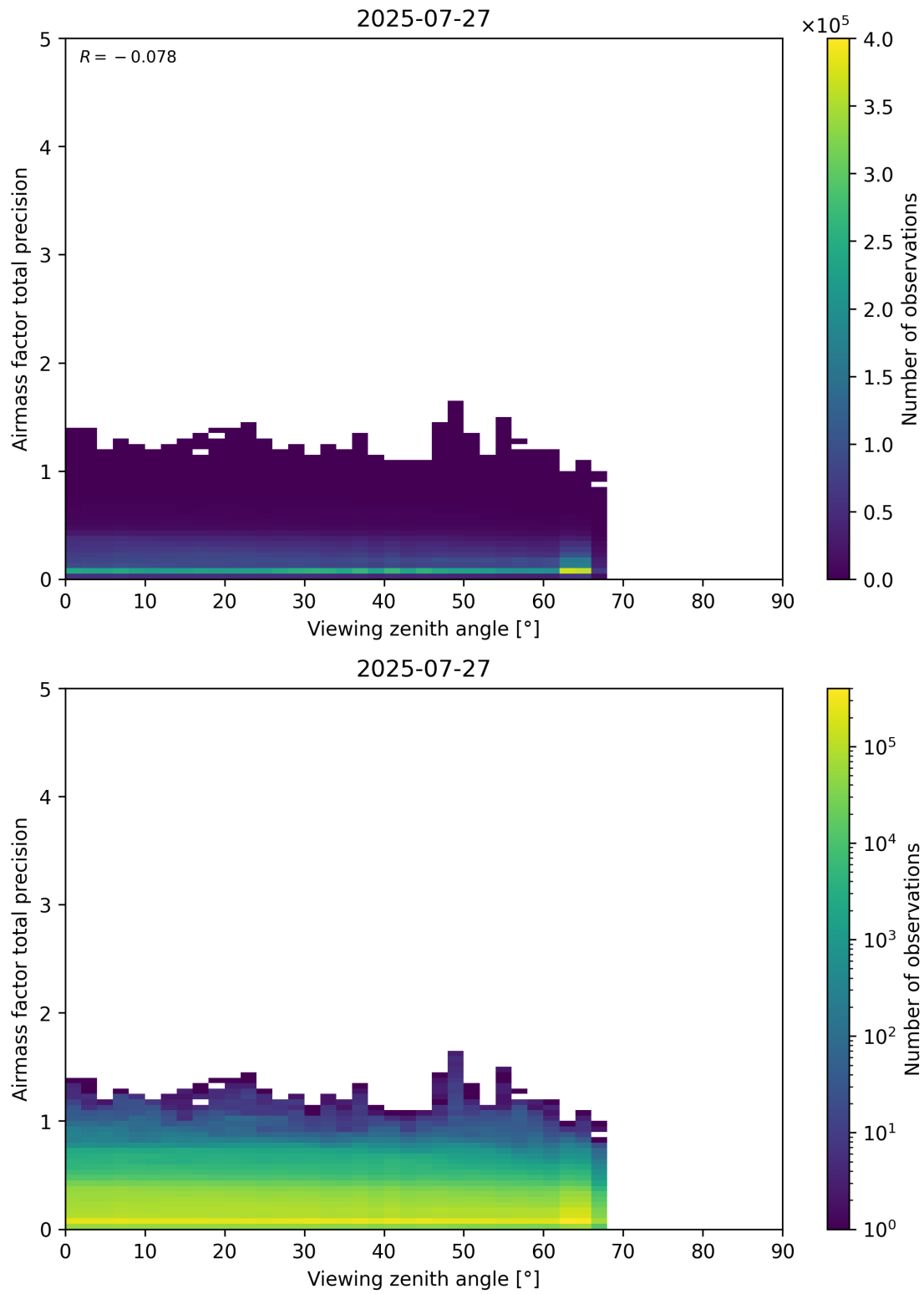
Figure 191: Scatter density plot of “Viewing zenith angle” against “Airmass factor total precision” for 2025-07-26 to 2025-07-28.
