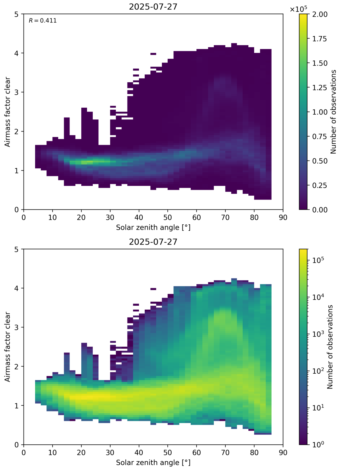
Figure 170: Scatter density plot of “Solar zenith angle” against “Airmass factor clear” for 2025-07-26 to 2025-07-28.
