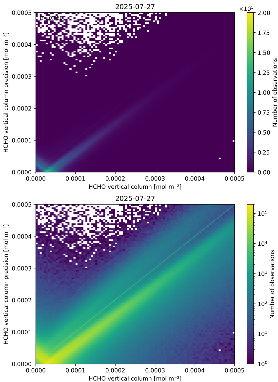
Figure 134: Scatter density plot of “HCHO vertical column” against “HCHO vertical column precision” for 2025-07-26 to 2025-07-28.
