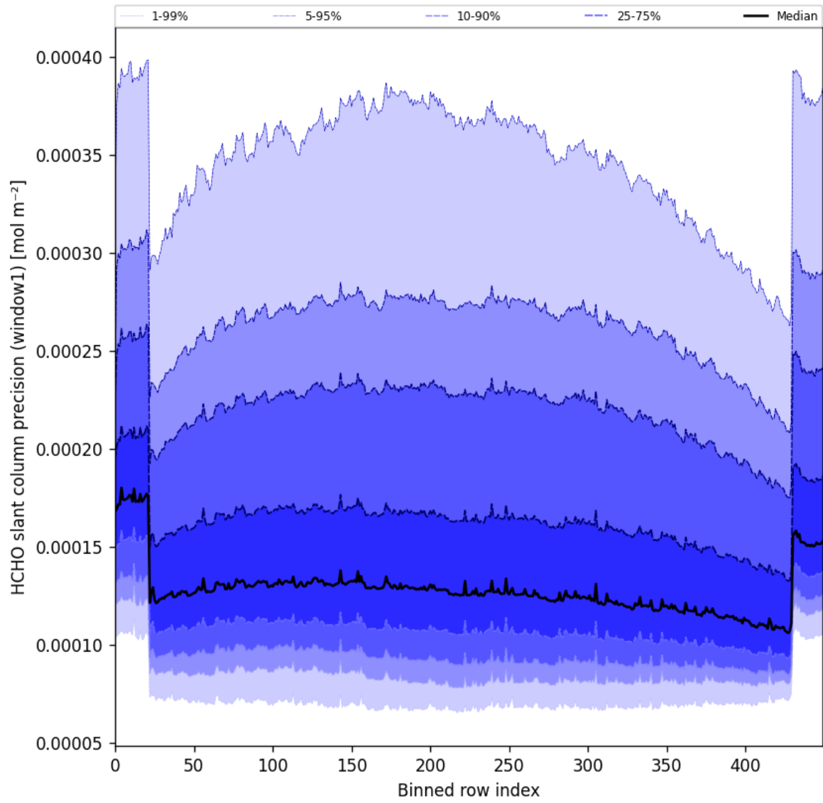
Figure 53: Along track statistics of “HCHO slant column precision (window1)” for 2025-07-26 to 2025-07-28
