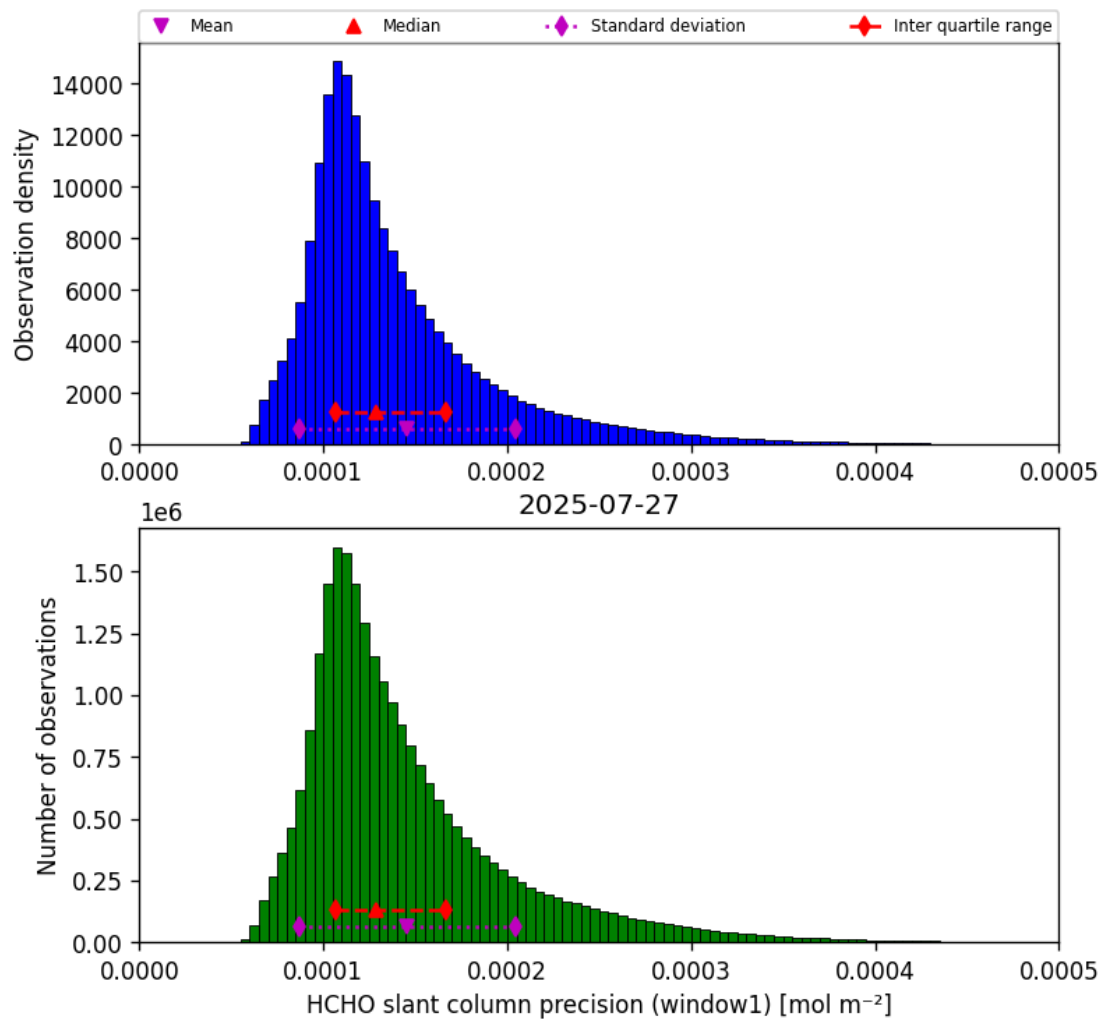
Figure 39: Histogram of “HCHO slant column precision (window1)” for 2025-07-26 to 2025-07-28
