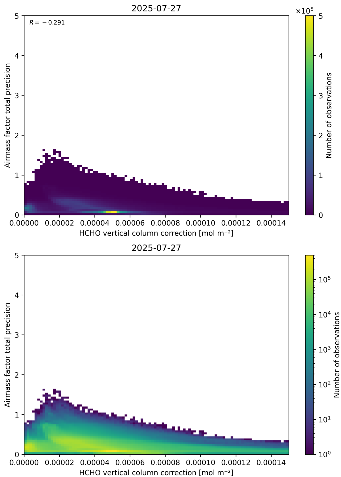
Figure 121: Scatter density plot of “HCHO vertical column correction” against “Airmass factor total precision” for 2025-07-26 to 2025-07-28.
