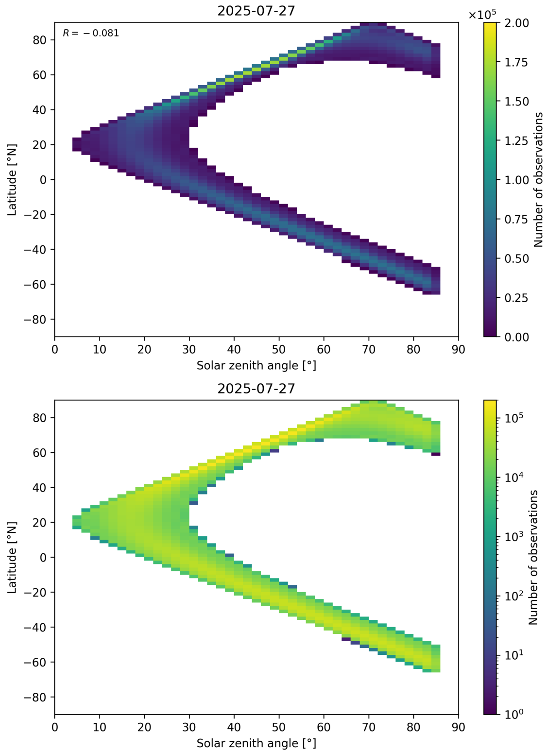
Figure 181: Scatter density plot of “Solar zenith angle” against “Latitude” for 2025-07-26 to 2025-07-28.
