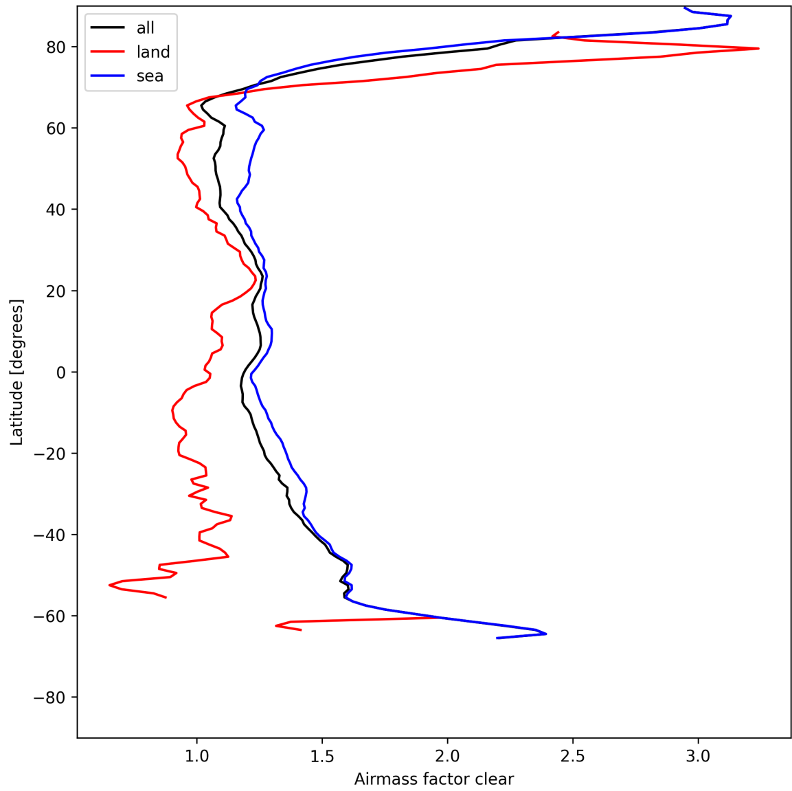
Figure 28: Zonal average of “Airmass factor clear” for 2025-07-26 to 2025-07-28.
