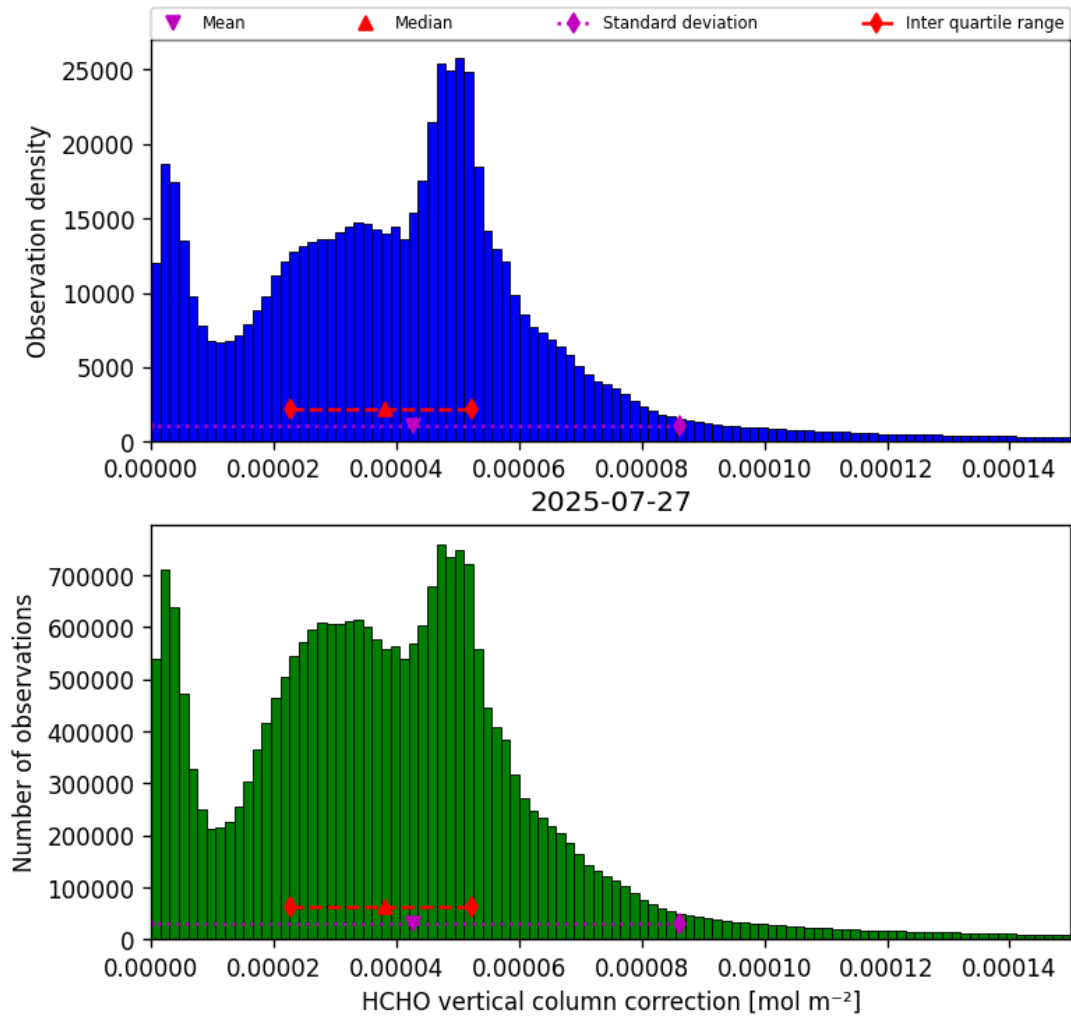
Figure 37: Histogram of “HCHO vertical column correction” for 2025-07-26 to 2025-07-28
