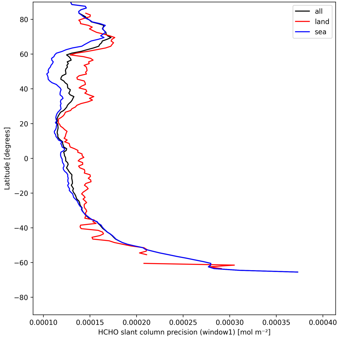
Figure 25: Zonal average of “HCHO slant column precision (window1)” for 2025-07-26 to 2025-07-28.
