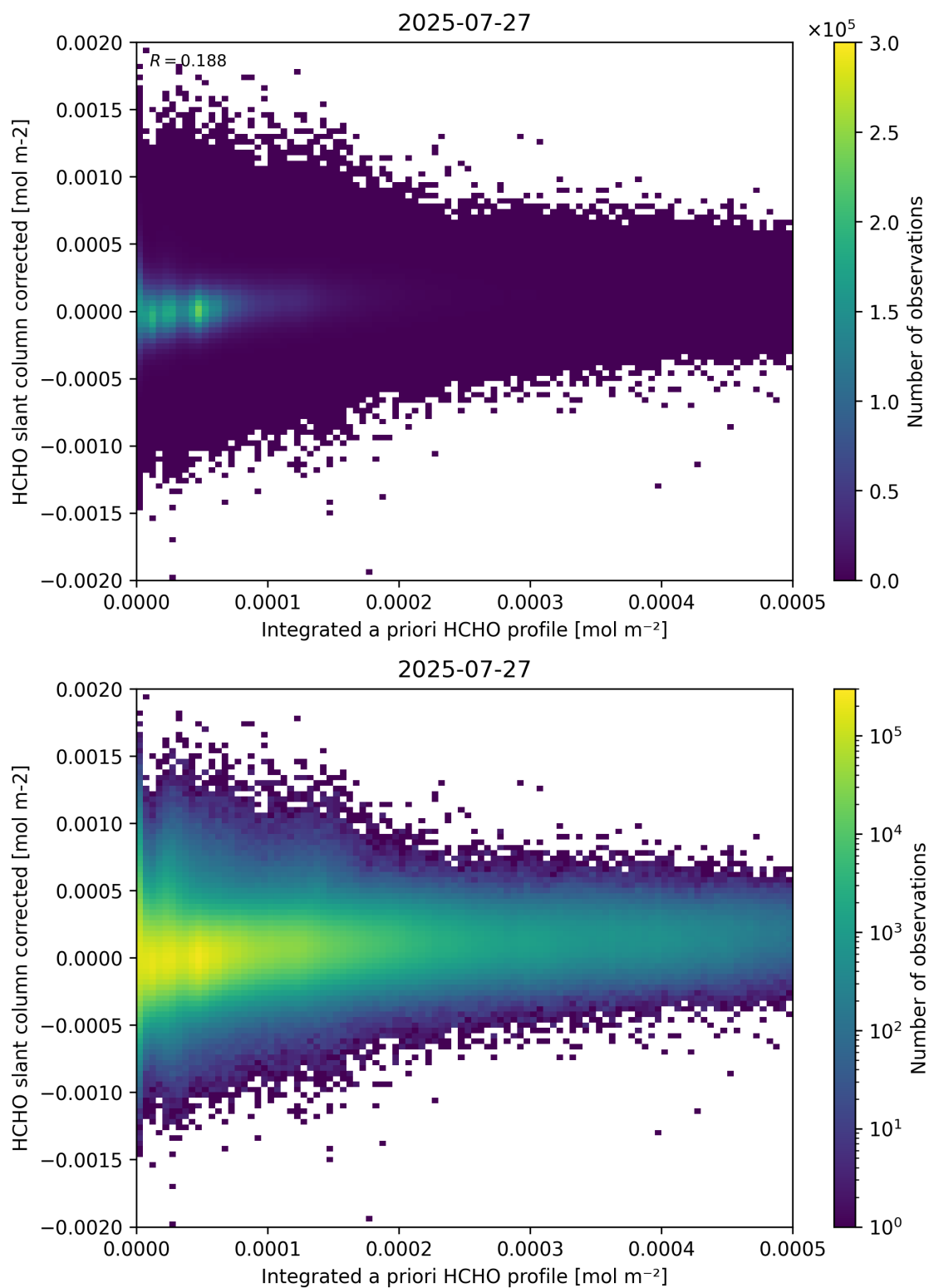
Figure 151: Scatter density plot of “Integrated a priori HCHO profile” against “HCHO slant column corrected” for 2025-07-26 to 2025-07-28.
