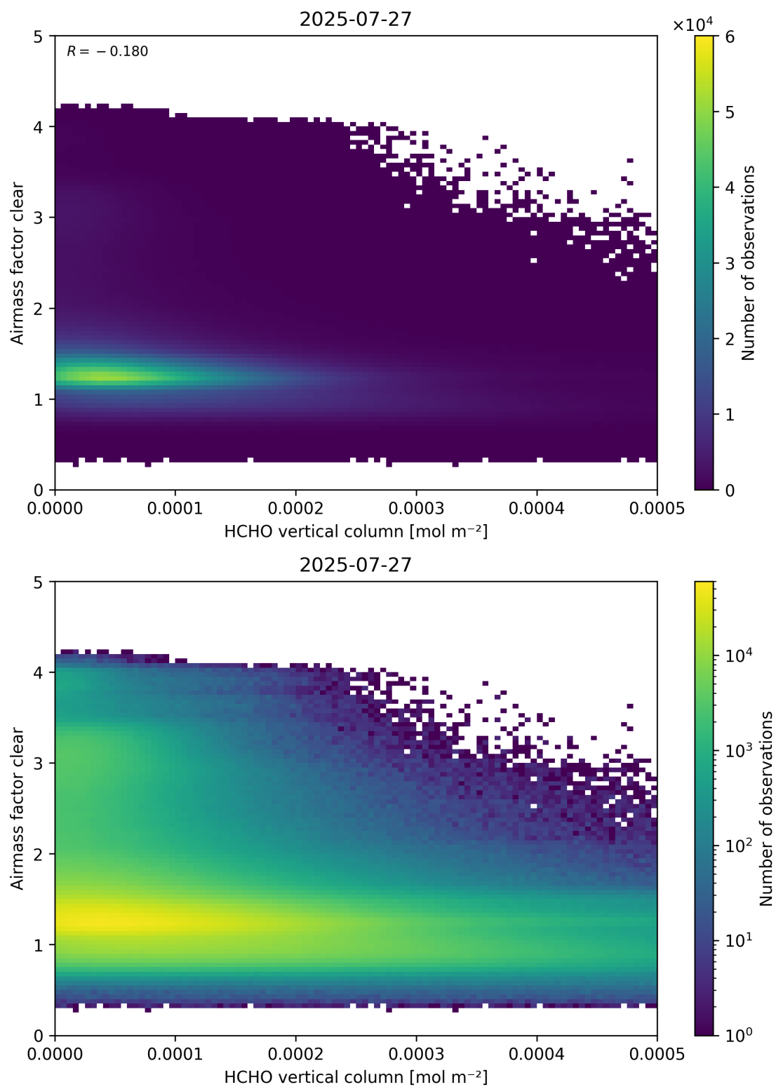
Figure 126: Scatter density plot of “HCHO vertical column” against “Airmass factor clear” for 2025-07-26 to 2025-07-28.
