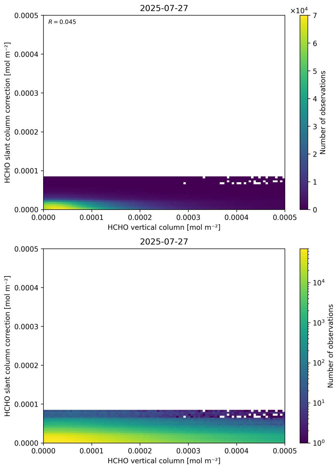
Figure 128: Scatter density plot of “HCHO vertical column” against “HCHO slant column correction” for 2025-07-26 to 2025-07-28.
