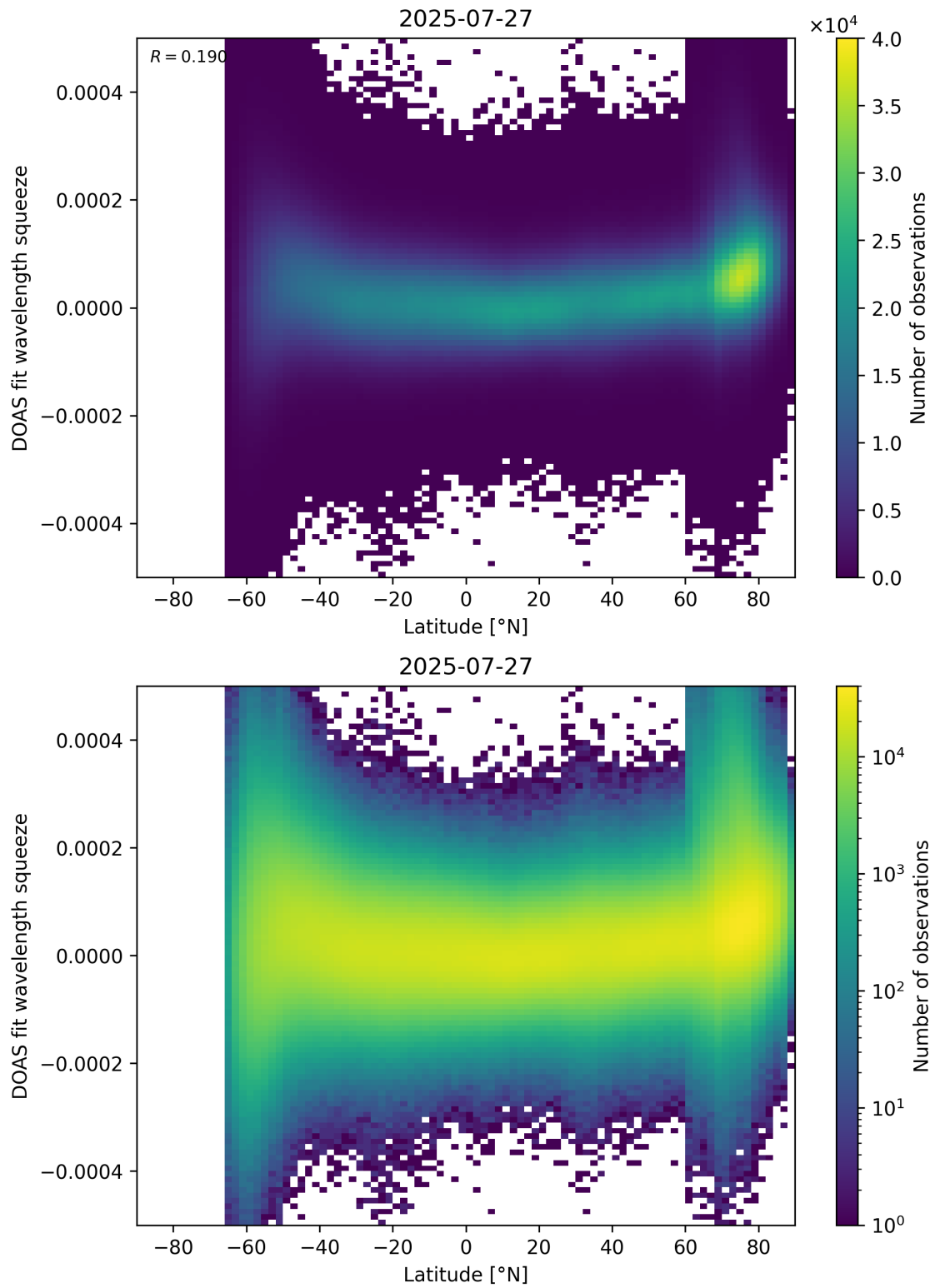
Figure 155: Scatter density plot of “Latitude” against “DOAS fit wavelength squeeze” for 2025-07-26 to 2025-07-28.
