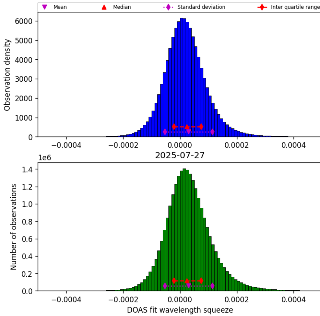
Figure 45: Histogram of “DOAS fit wavelength squeeze” for 2025-07-26 to 2025-07-28
