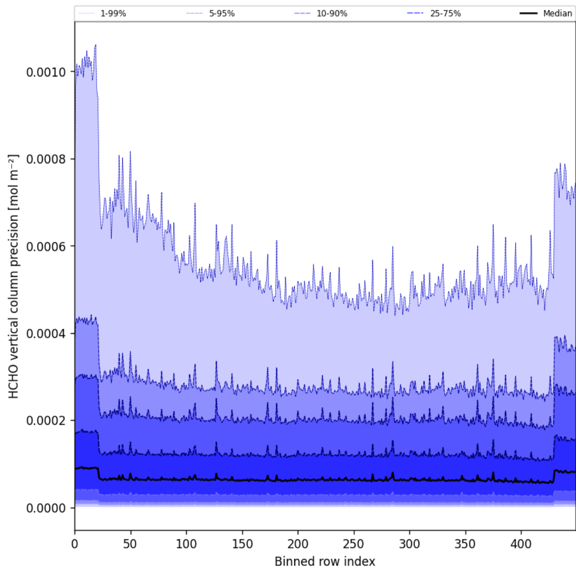
Figure 50: Along track statistics of “HCHO vertical column precision” for 2025-07-26 to 2025-07-28
