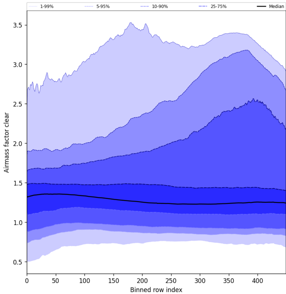
Figure 56: Along track statistics of “Air mass factor clear” for 2025-07-26 to 2025-07-28
