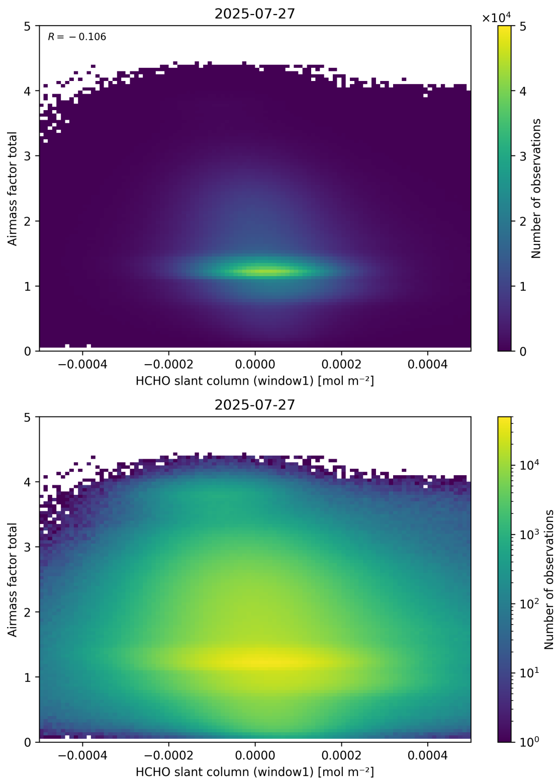
Figure 85: Scatter density plot of “HCHO slant column (window1)” against “Airmass factor total” for 2025-07-26 to 2025-07-28.
