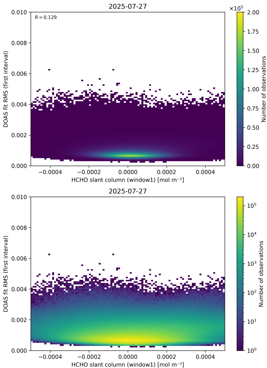
Figure 78: Scatter density plot of “HCHO slant column (window1)” against “DOAS fit RMS (first interval)” for 2025-07-26 to 2025-07-28.
