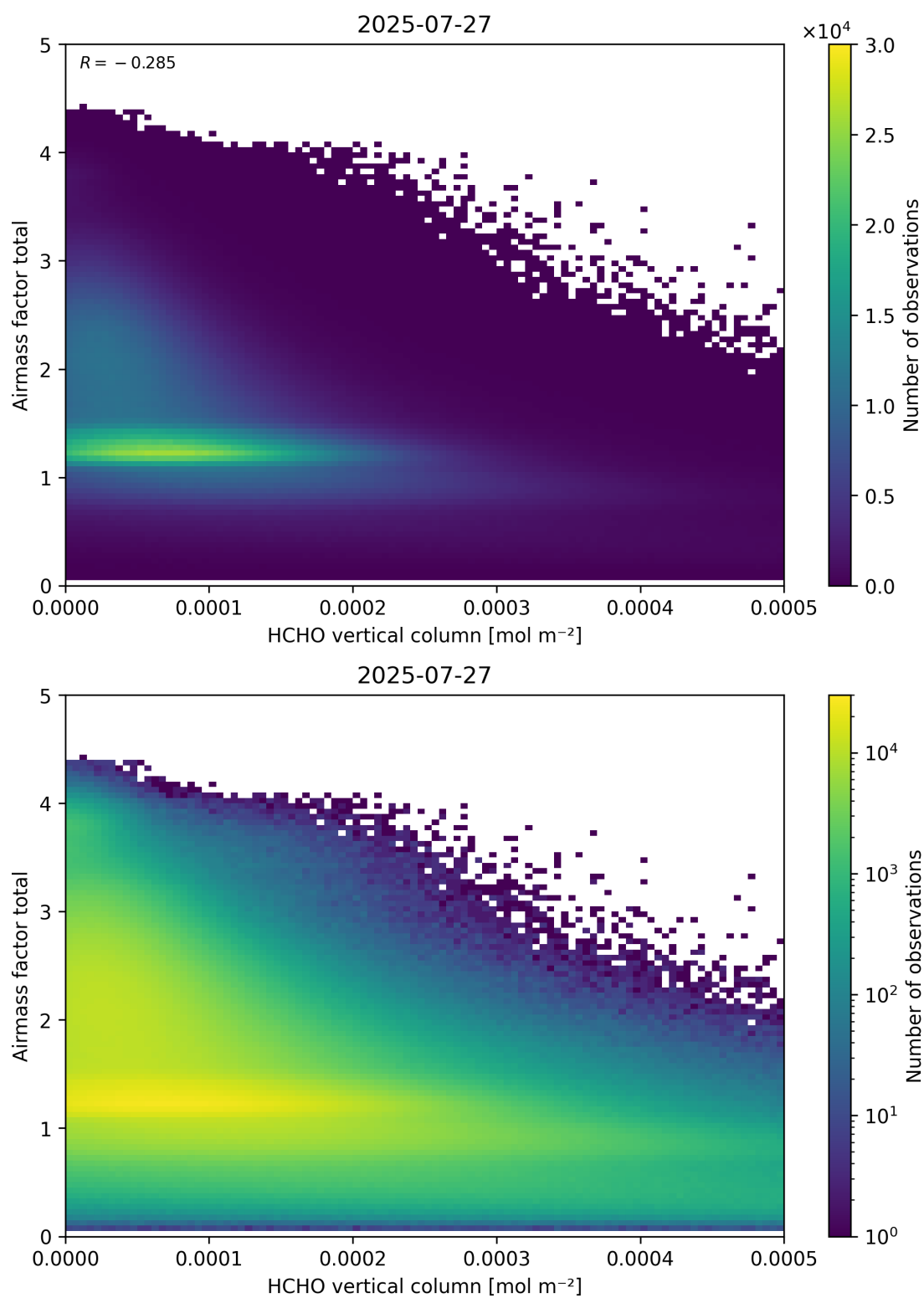
Figure 131: Scatter density plot of “HCHO vertical column” against “Airmass factor total” for 2025-07-26 to 2025-07-28.
