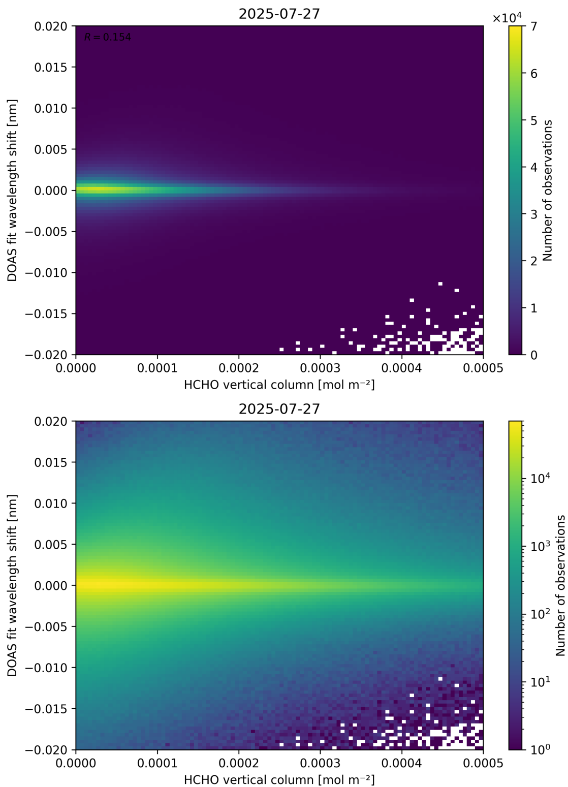
Figure 124: Scatter density plot of “HCHO vertical column” against “DOAS fit wavelength shift” for 2025-07-26 to 2025-07-28.
