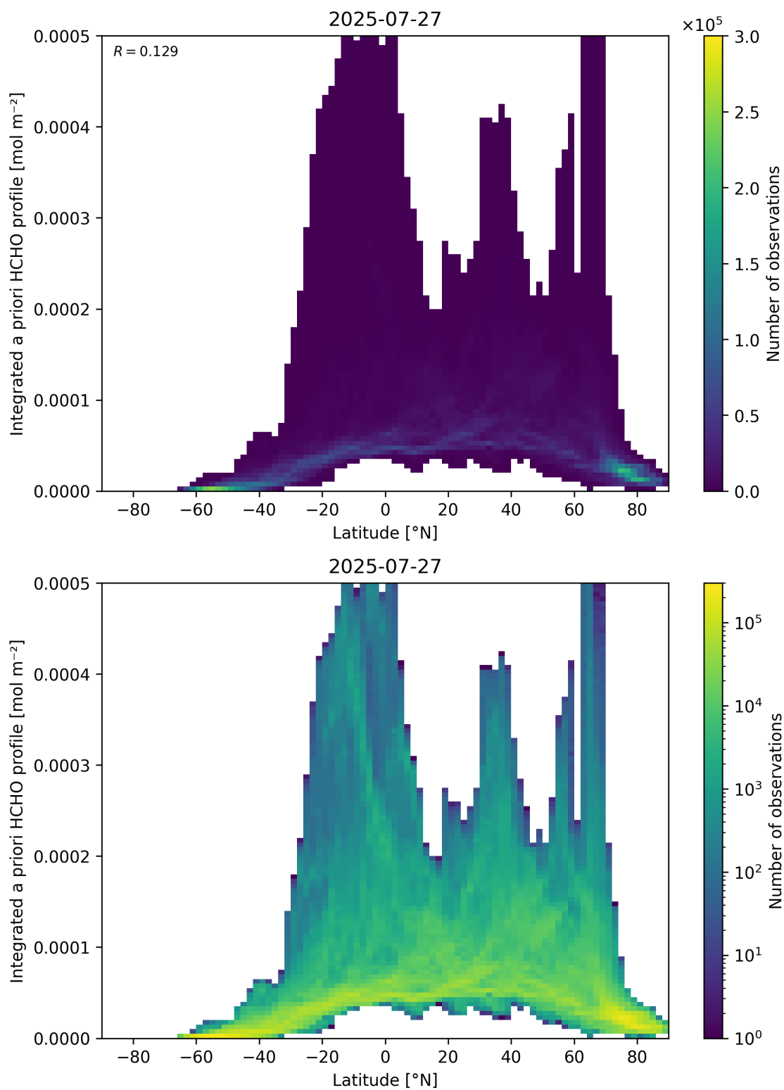
Figure 166: Scatter density plot of “Latitude” against “Integrated a priori HCHO profile” for 2025-07-26 to 2025-07-28.
