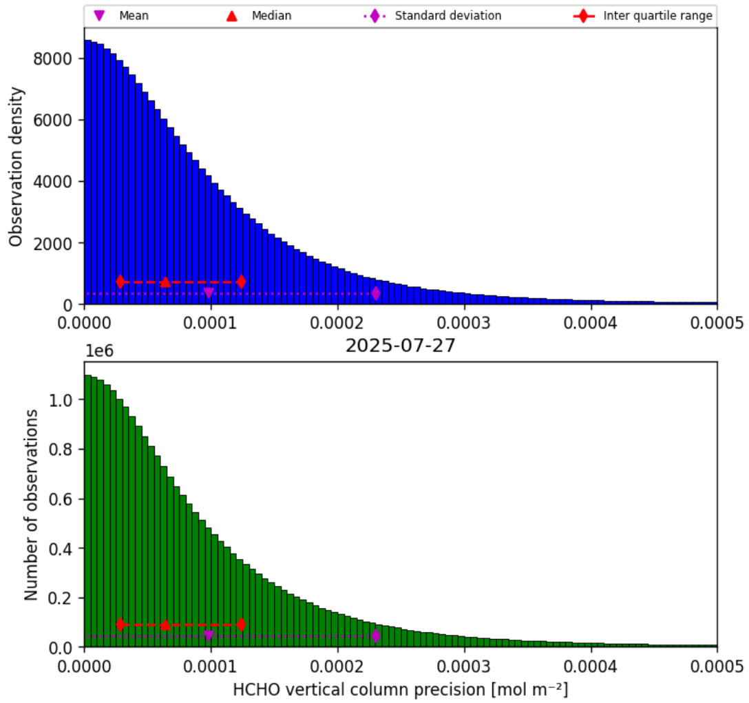
Figure 36: Histogram of “HCHO vertical column precision” for 2025-07-26 to 2025-07-28
