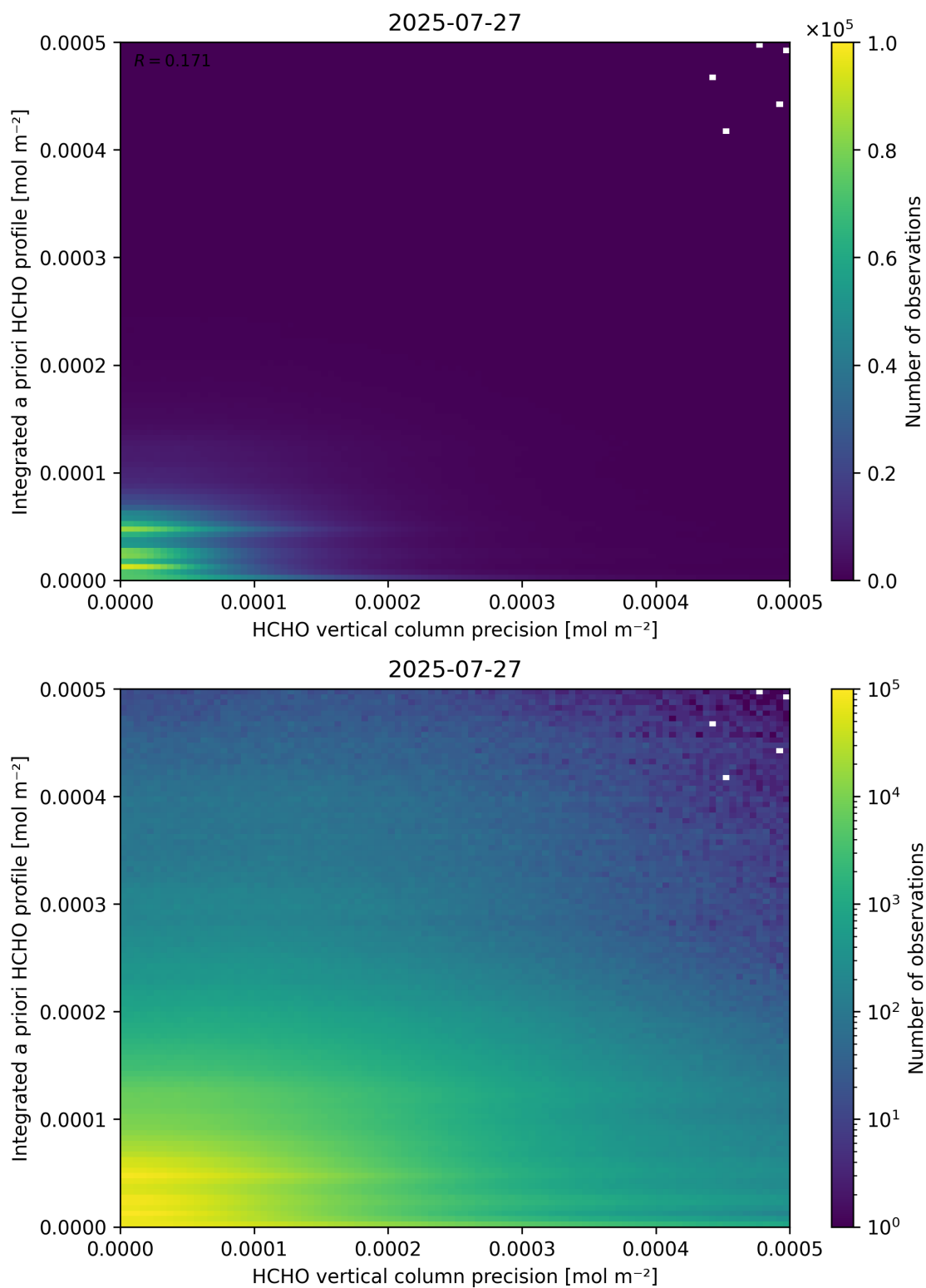
Figure 147: Scatter density plot of “HCHO vertical column precision” against “Integrated a priori HCHO profile” for 2025-07-26 to 2025-07-28.
