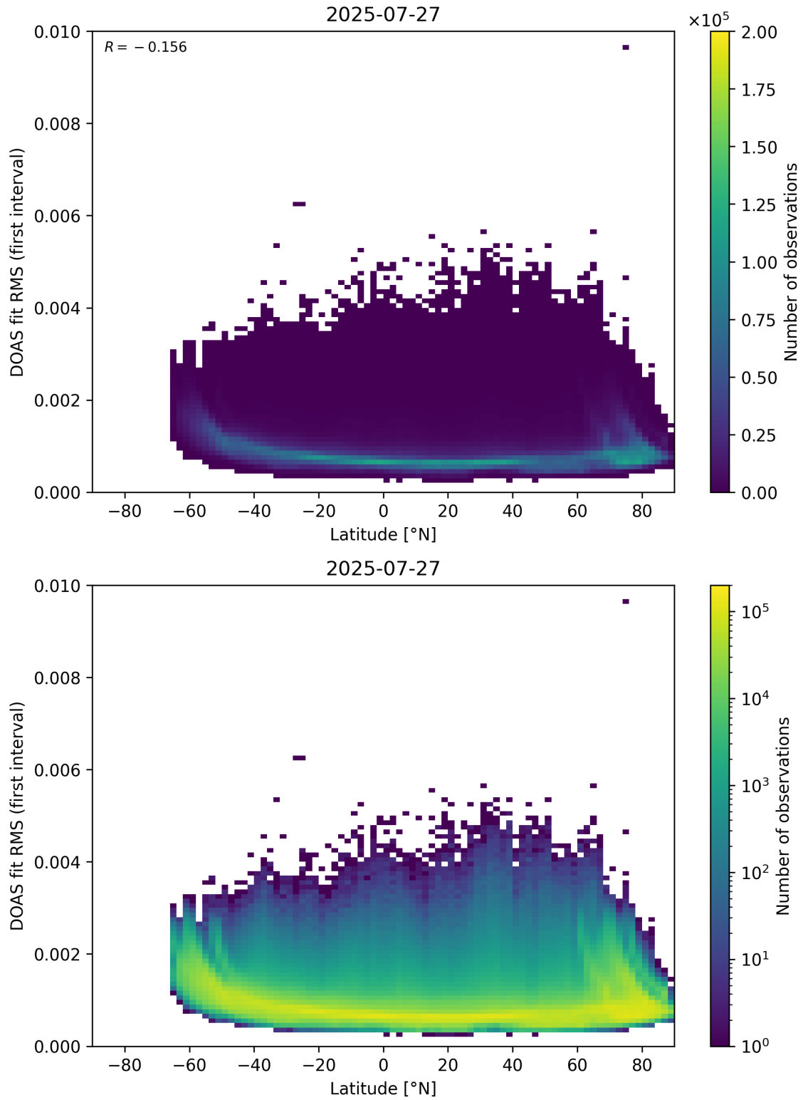
Figure 153: Scatter density plot of “Latitude” against “DOAS fit RMS (first interval)” for 2025-07-26 to 2025-07-28.
