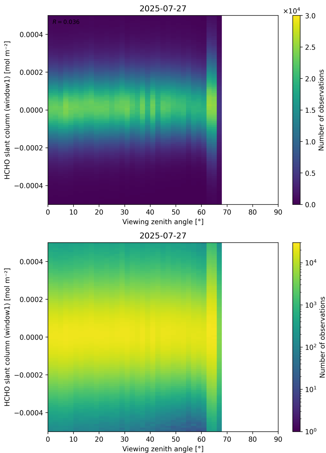
Figure 188: Scatter density plot of “Viewing zenith angle” against “HCHO slant column (window1)” for 2025-07-26 to 2025-07-28.
