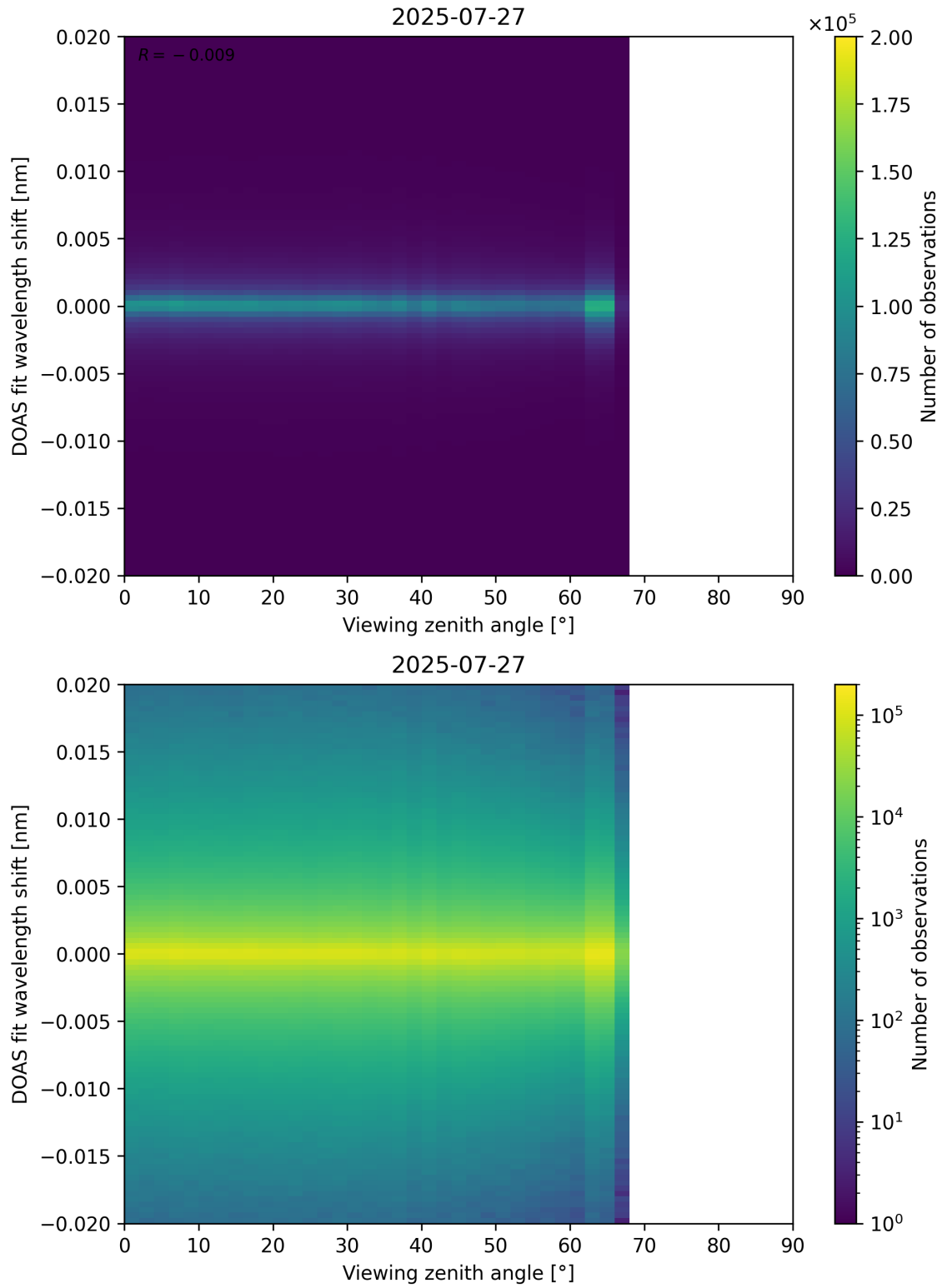
Figure 183: Scatter density plot of “Viewing zenith angle” against “DOAS fit wavelength shift” for 2025-07-26 to 2025-07-28.
