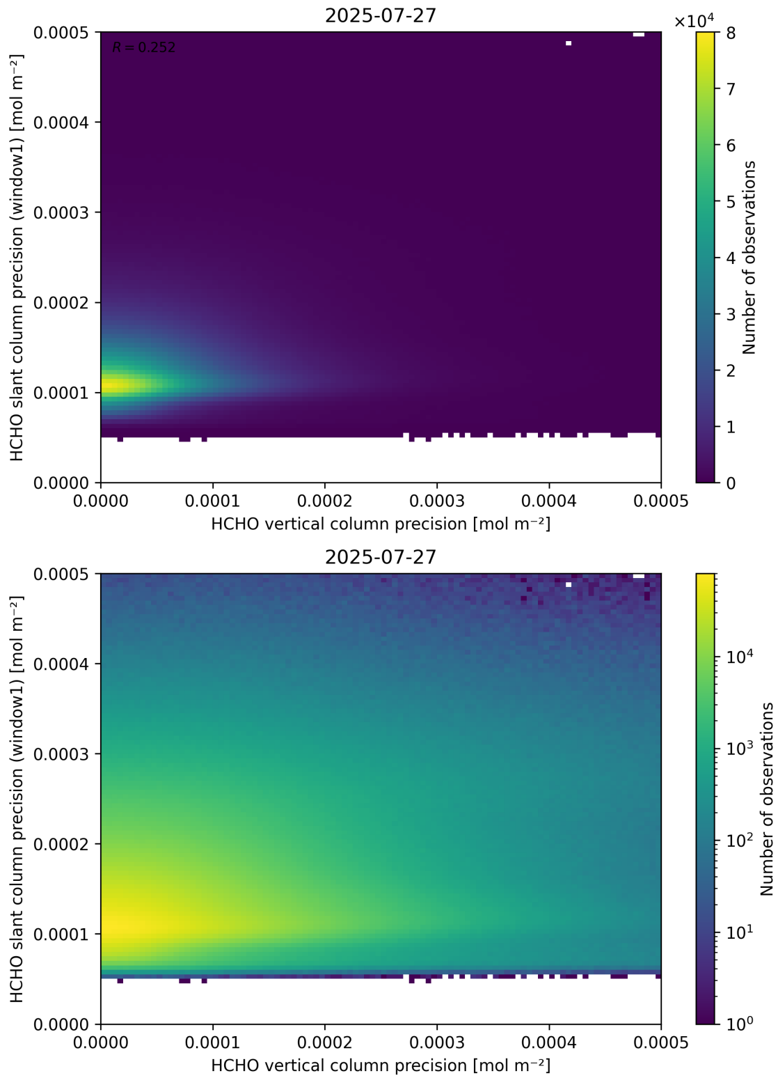
Figure 143: Scatter density plot of “HCHO vertical column precision” against “HCHO slant column precision (window1)” for 2025-07-26 to 2025-07-28.
