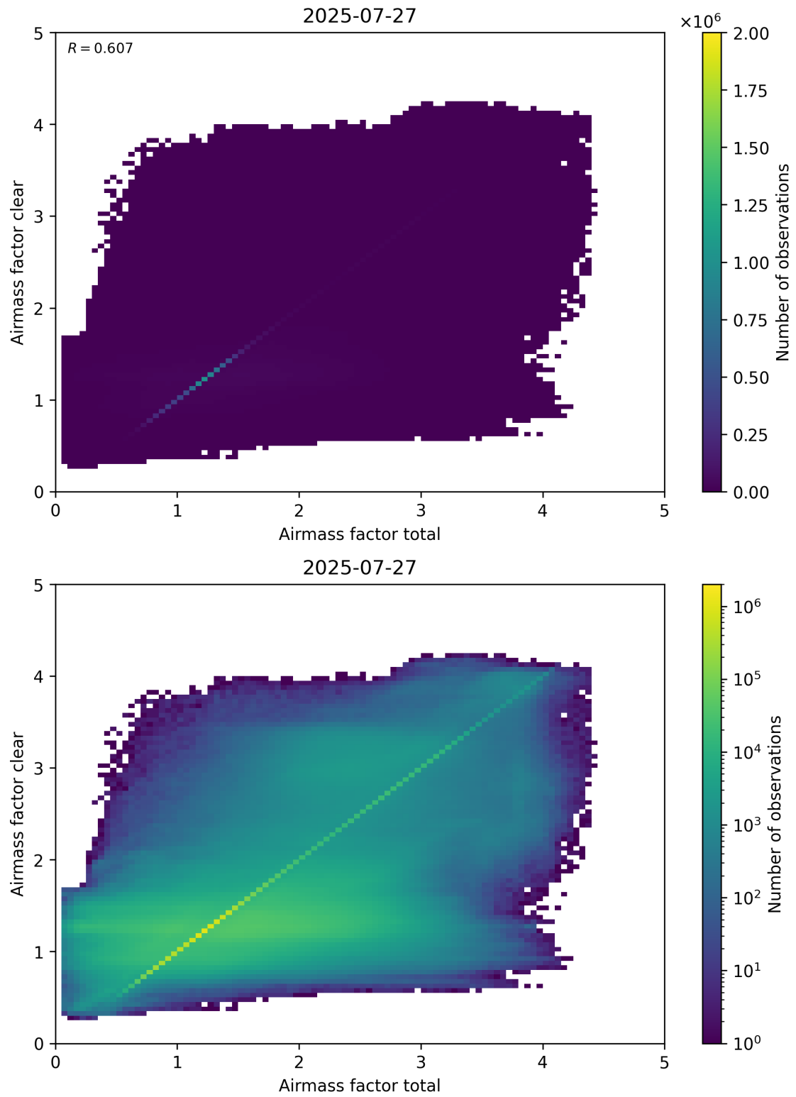
Figure 100: Scatter density plot of “Airmass factor total” against “Airmass factor clear” for 2025-07-26 to 2025-07-28.
