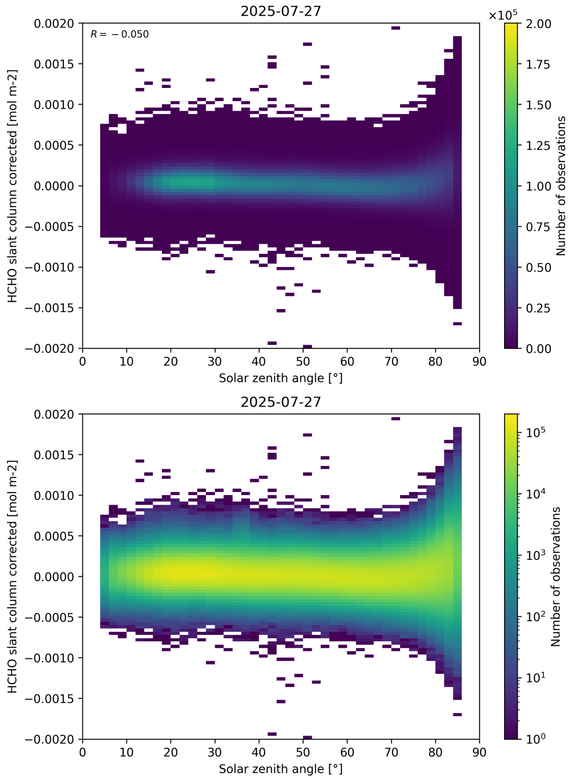
Figure 171: Scatter density plot of “Solar zenith angle” against “HCHO slant column corrected” for 2025-07-26 to 2025-07-28.
