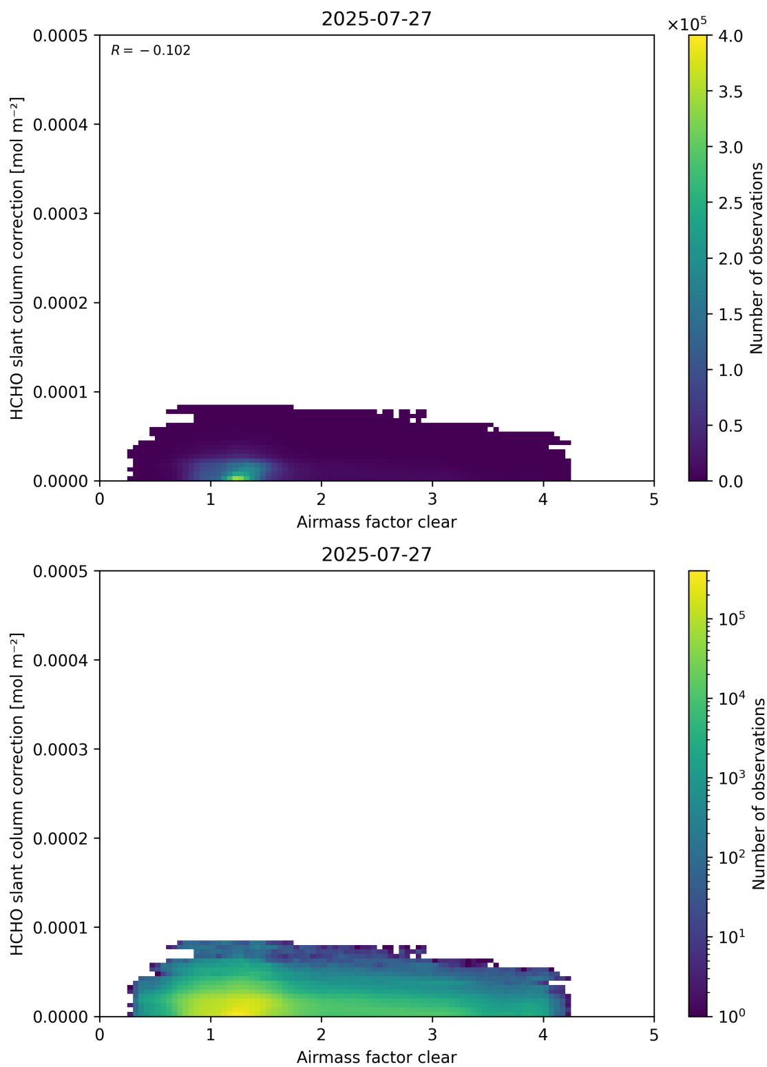
Figure 75: Scatter density plot of “Airmass factor clear” against “HCHO slant column correction” for 2025-07-26 to 2025-07-28.
