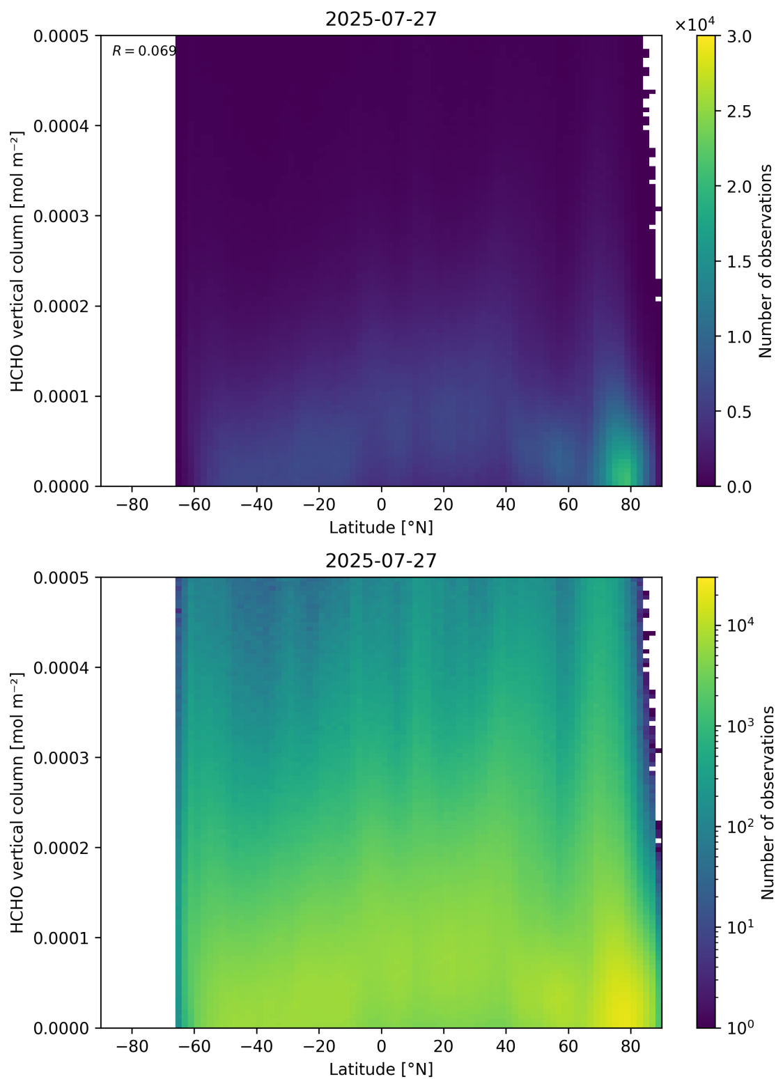
Figure 163: Scatter density plot of “Latitude” against “HCHO vertical column” for 2025-07-26 to 2025-07-28.
