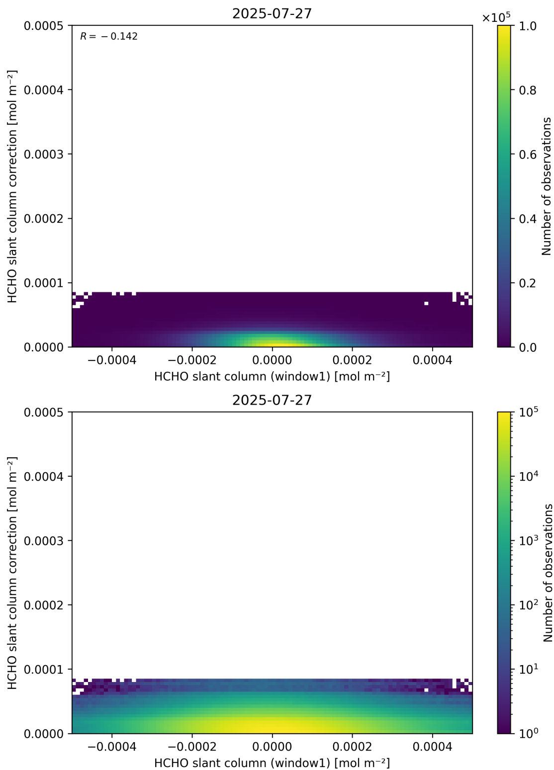
Figure 83: Scatter density plot of “HCHO slant column (window1)” against “HCHO slant column correction” for 2025-07-26 to 2025-07-28.
