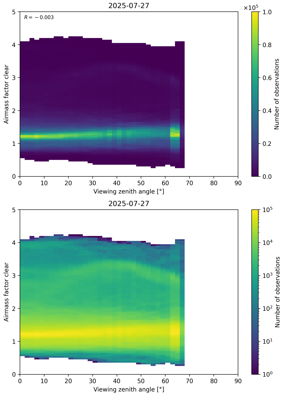
Figure 185: Scatter density plot of “Viewing zenith angle” against “Airmass factor clear” for 2025-07-26 to 2025-07-28.
