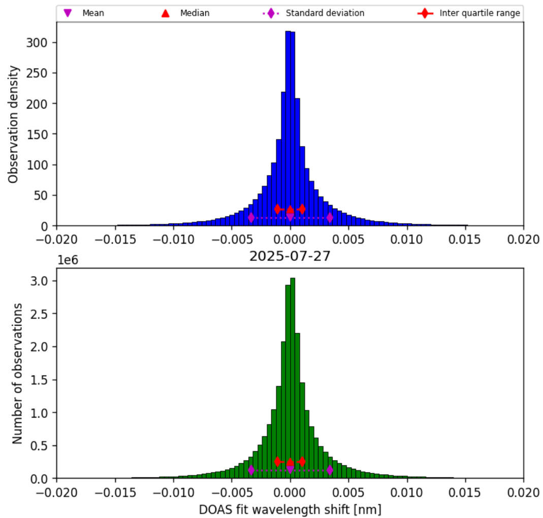
Figure 44: Histogram of “DOAS fit wavelength shift” for 2025-07-26 to 2025-07-28
