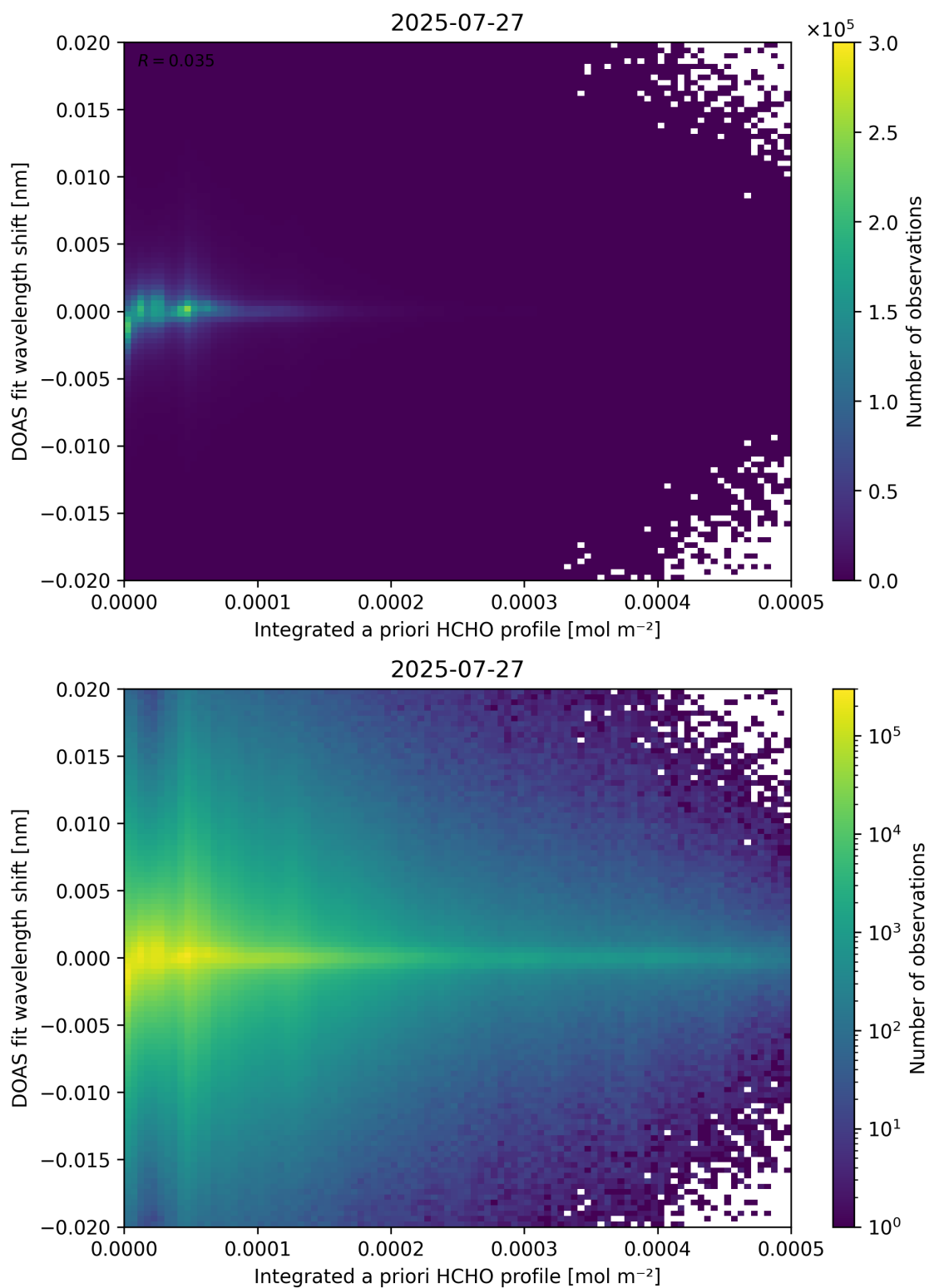
Figure 149: Scatter density plot of “Integrated a priori HCHO profile” against “DOAS fit wavelength shift” for 2025-07-26 to 2025-07-28.
