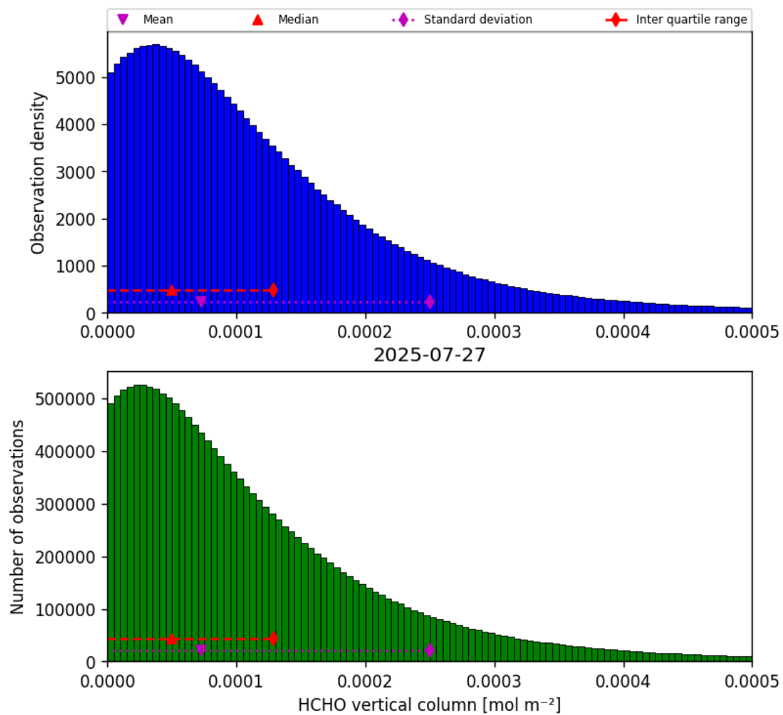
Figure 35: Histogram of “HCHO vertical column” for 2025-07-26 to 2025-07-28
