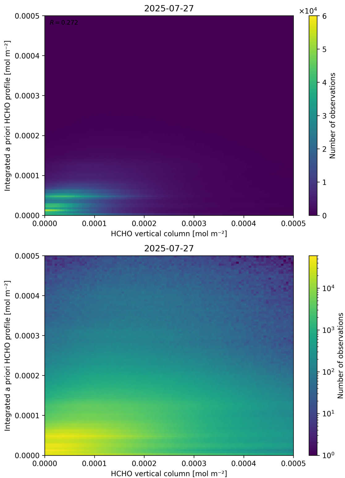
Figure 135: Scatter density plot of “HCHO vertical column” against “Integrated a priori HCHO profile” for 2025-07-26 to 2025-07-28.
