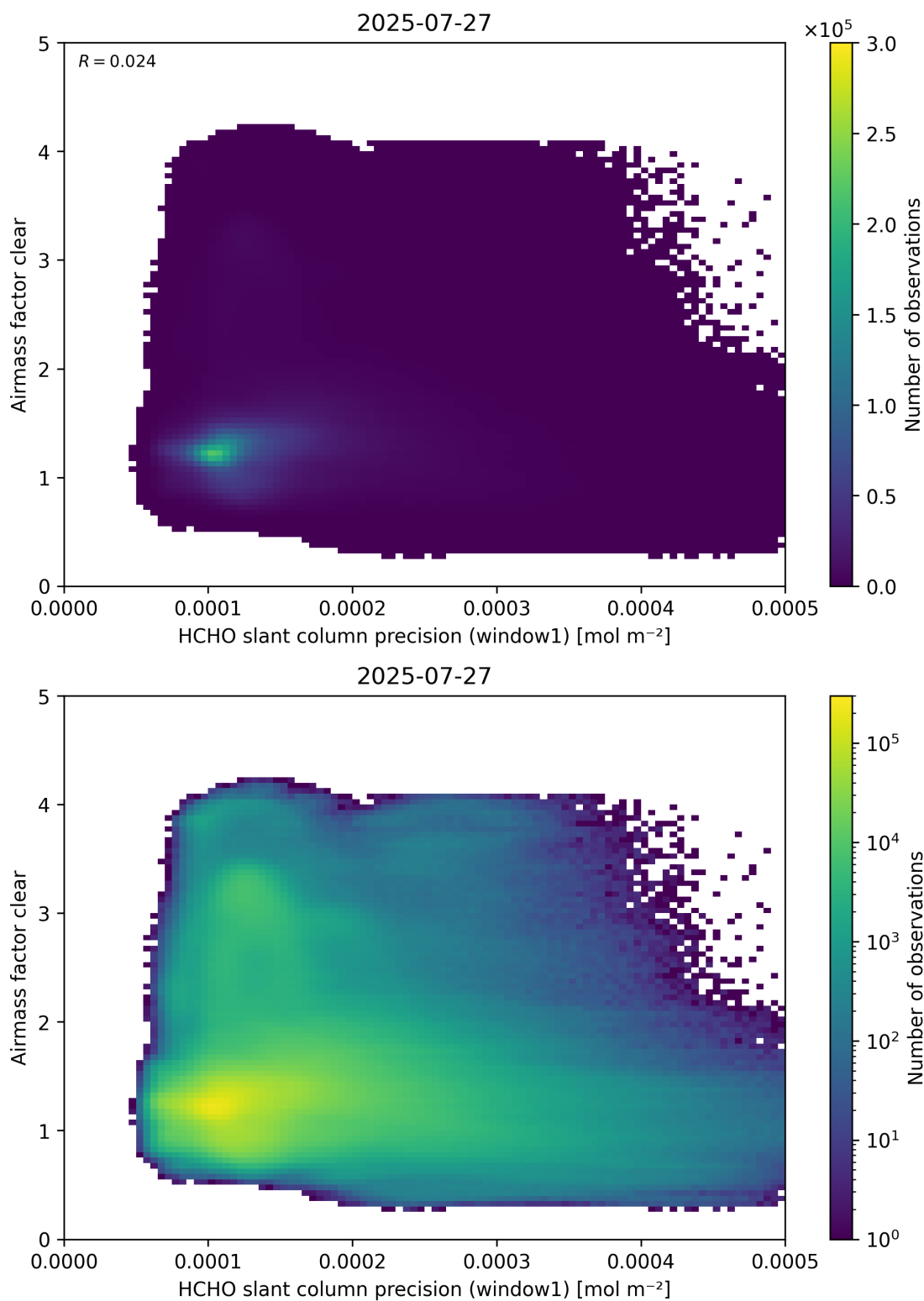
Figure 91: Scatter density plot of “HCHO slant column precision (window1)” against “Airmass factor clear” for 2025-07-26 to 2025-07-28.
