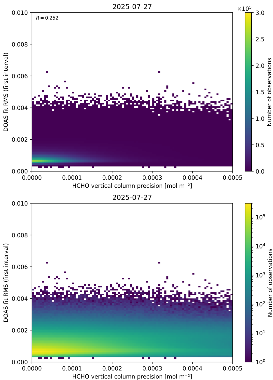
Figure 136: Scatter density plot of “HCHO vertical column precision” against “DOAS fit RMS (first interval)” for 2025-07-26 to 2025-07-28.
