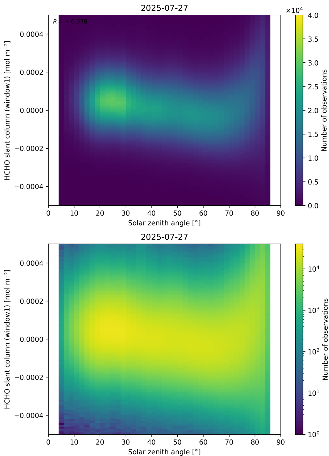
Figure 173: Scatter density plot of “Solar zenith angle” against “HCHO slant column (window1)” for 2025-07-26 to 2025-07-28.
