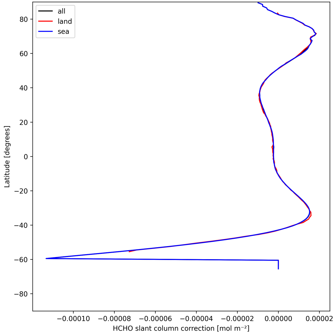
Figure 33: Zonal average of “HCHO slant column correction” for 2025-07-26 to 2025-07-28.
