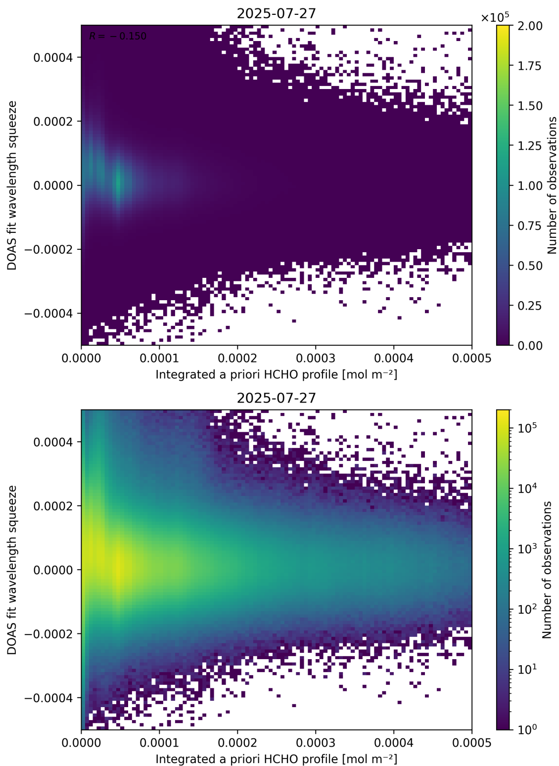
Figure 150: Scatter density plot of “Integrated a priori HCHO profile” against “DOAS fit wavelength squeeze” for 2025-07-26 to 2025-07-28.
