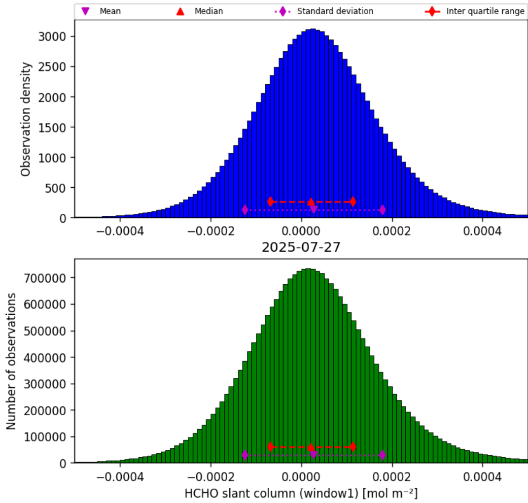
Figure 38: Histogram of “HCHO slant column (window1)” for 2025-07-26 to 2025-07-28
