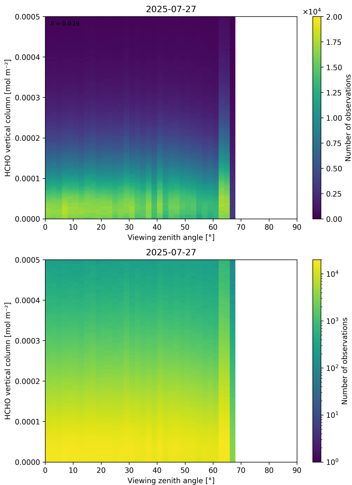
Figure 192: Scatter density plot of “Viewing zenith angle” against “HCHO vertical column” for 2025-07-26 to 2025-07-28.
