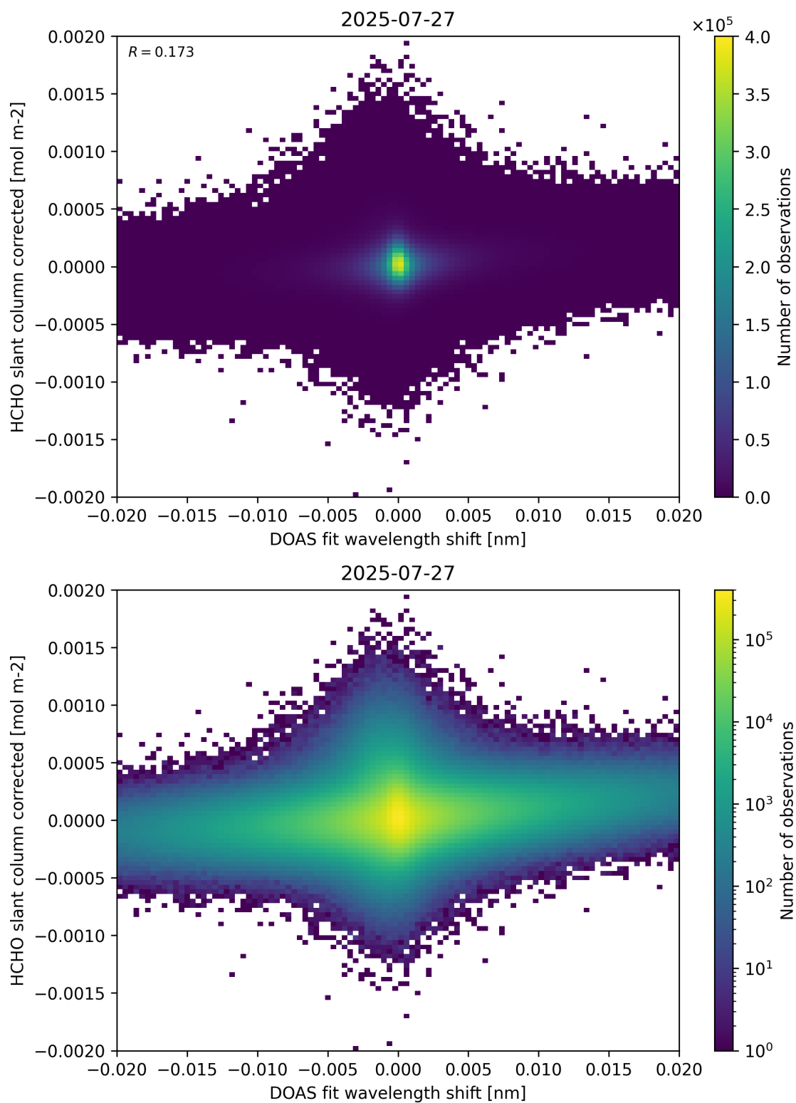
Figure 66: Scatter density plot of “DOAS fit wavelength shift” against “HCHO slant column corrected” for 2025-07-26 to 2025-07-28.
