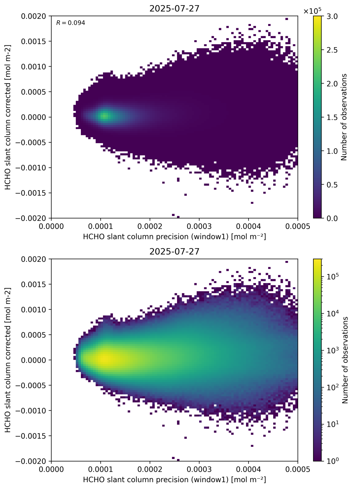
Figure 92: Scatter density plot of “HCHO slant column precision (window1)” against “HCHO slant column corrected” for 2025-07-26 to 2025-07-28.
