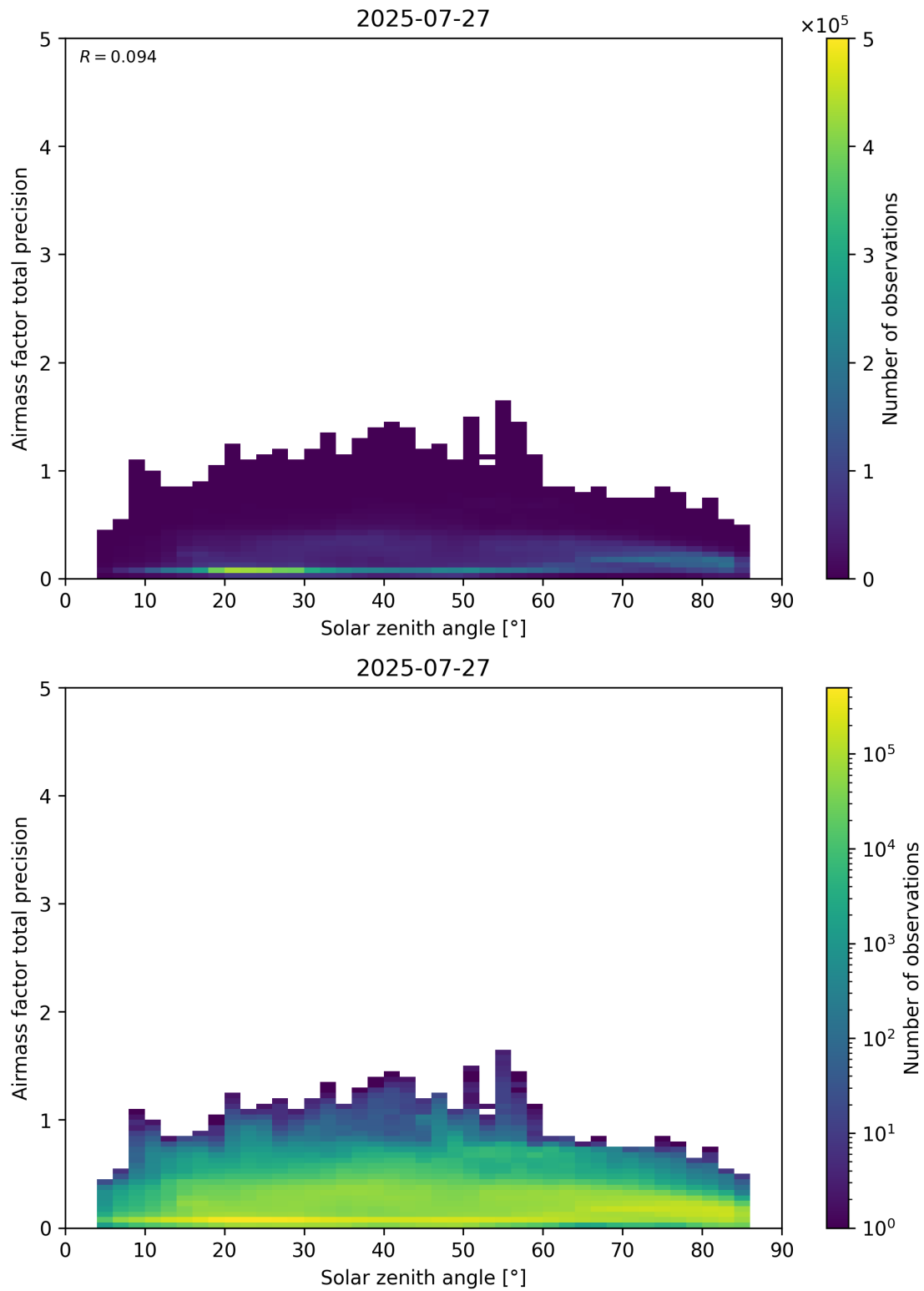
Figure 176: Scatter density plot of “Solar zenith angle” against “Airmass factor total precision” for 2025-07-26 to 2025-07-28.
