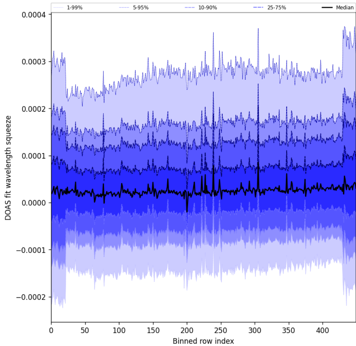
Figure 59: Along track statistics of “DOAS fit wavelength squeeze” for 2025-07-26 to 2025-07-28
