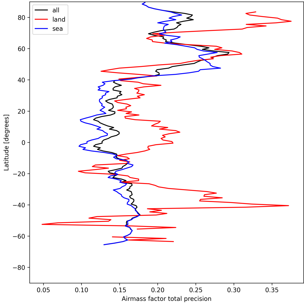
Figure 27: Zonal average of “Airmass factor total precision” for 2025-07-26 to 2025-07-28.
