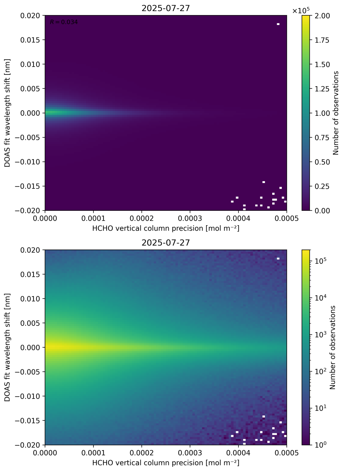
Figure 137: Scatter density plot of “HCHO vertical column precision” against “DOAS fit wavelength shift” for 2025-07-26 to 2025-07-28.
