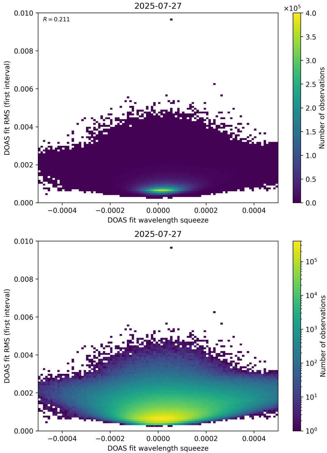
Figure 68: Scatter density plot of “DOAS fit wavelength squeeze” against “DOAS fit RMS (first interval)” for 2025-07-26 to 2025-07-28.
