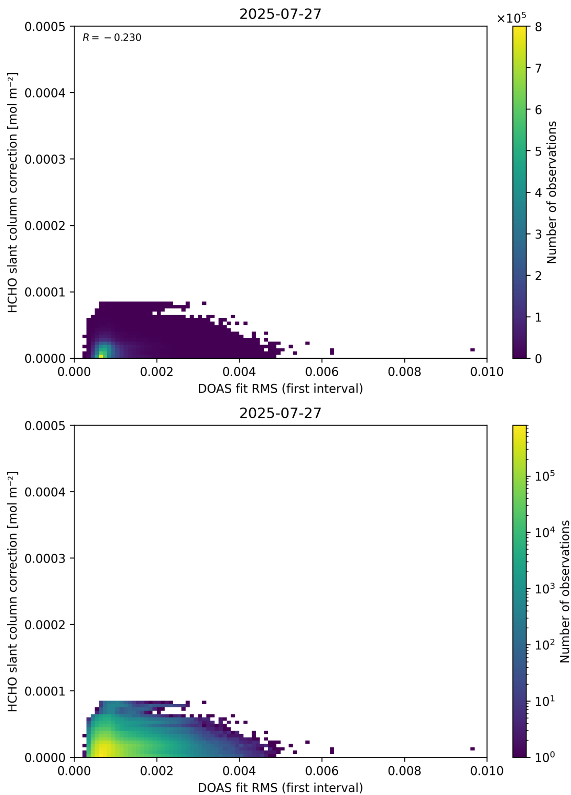
Figure 63: Scatter density plot of “DOAS fit RMS (first interval)” against “HCHO slant column correction” for 2025-07-26 to 2025-07-28.
