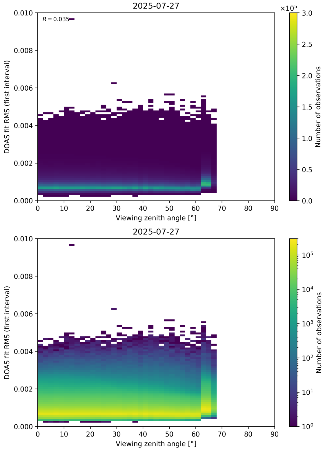
Figure 182: Scatter density plot of “Viewing zenith angle” against “DOAS fit RMS (first interval)” for 2025-07-26 to 2025-07-28.
