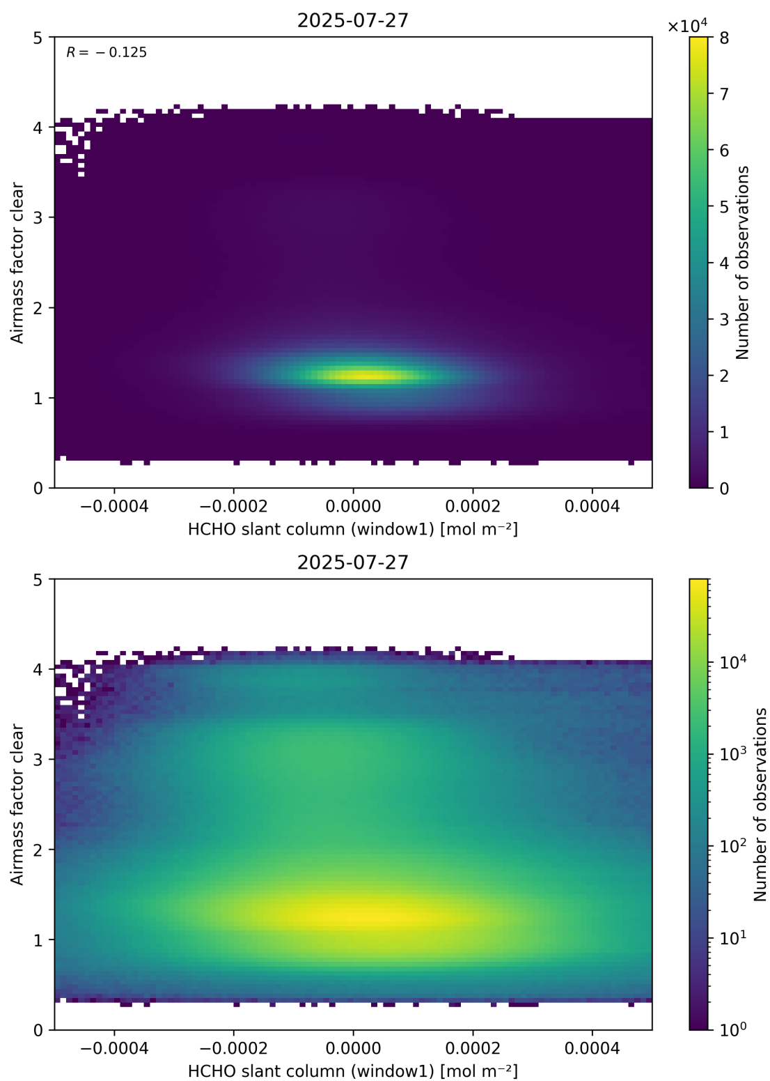
Figure 81: Scatter density plot of “HCHO slant column (window1)” against “Airmass factor clear” for 2025-07-26 to 2025-07-28.
