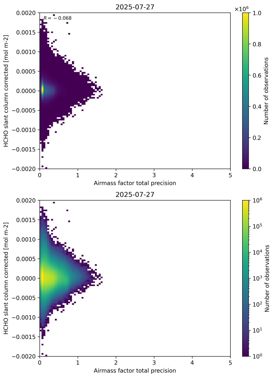
Figure 109: Scatter density plot of “Airmass factor total precision” against “HCHO slant column corrected” for 2025-07-26 to 2025-07-28.
