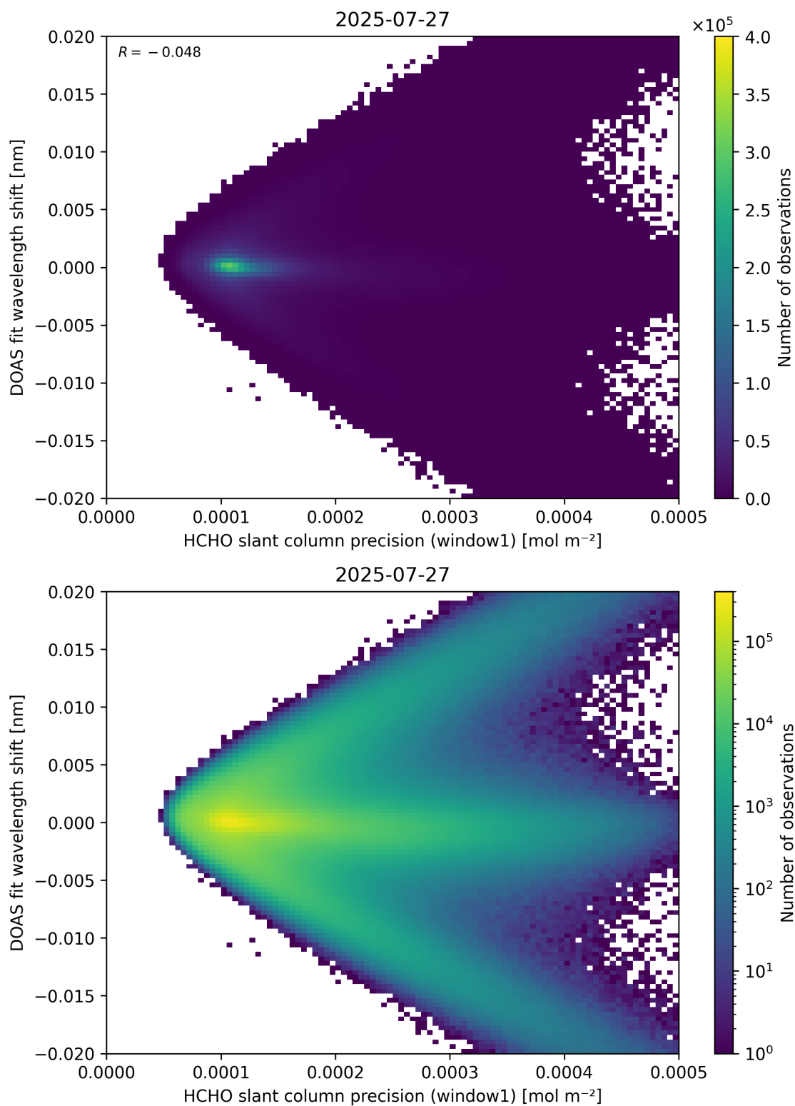
Figure 89: Scatter density plot of “HCHO slant column precision (window1)” against “DOAS fit wavelength shift” for 2025-07-26 to 2025-07-28.
