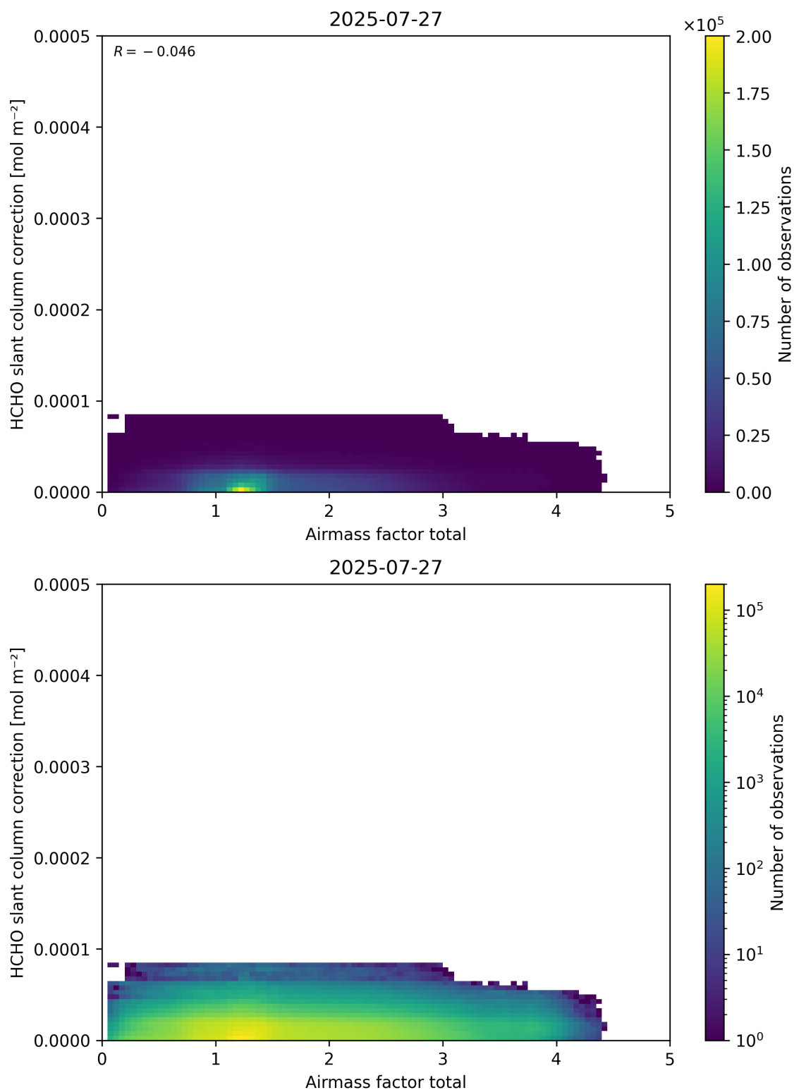
Figure 102: Scatter density plot of “Airmass factor total” against “HCHO slant column correction” for 2025-07-26 to 2025-07-28.
