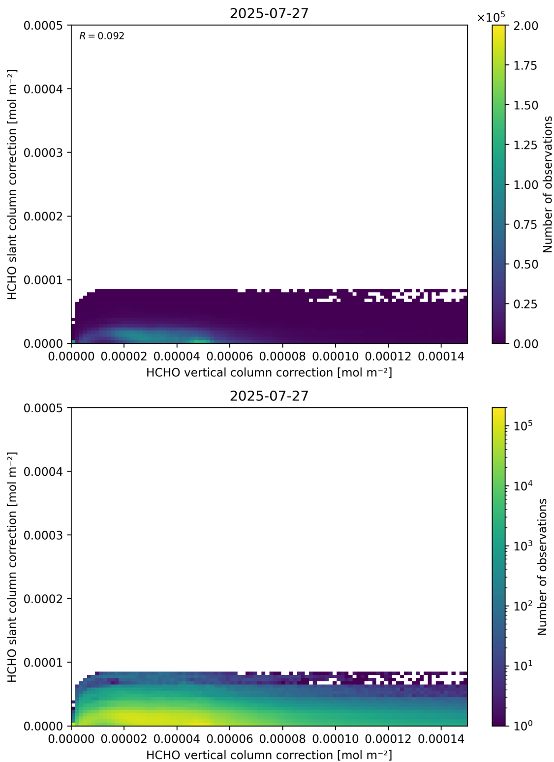
Figure 117: Scatter density plot of “HCHO vertical column correction” against “HCHO slant column correction” for 2025-07-26 to 2025-07-28.
