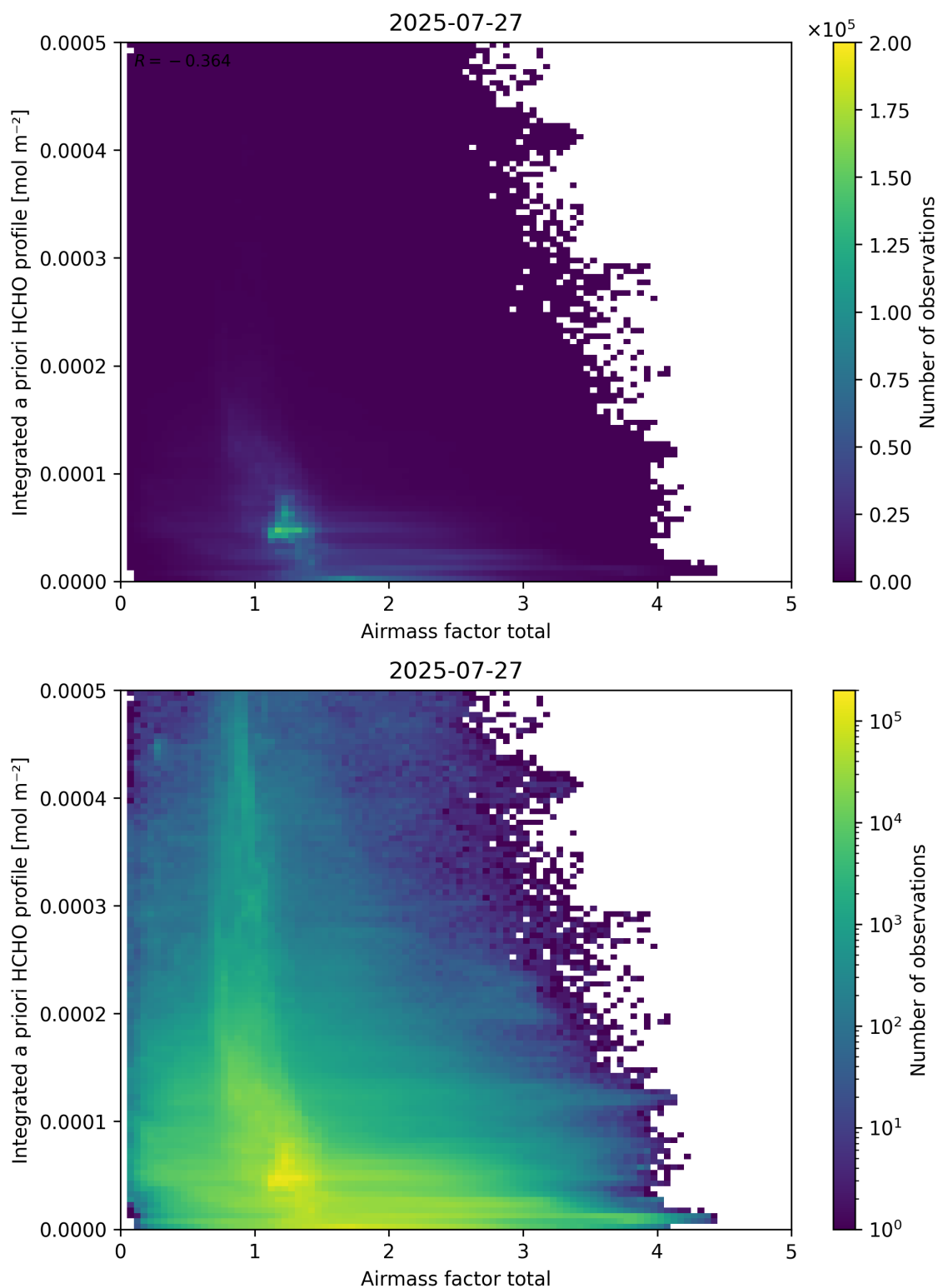
Figure 104: Scatter density plot of “Airmass factor total” against “Integrated a priori HCHO profile” for 2025-07-26 to 2025-07-28.
