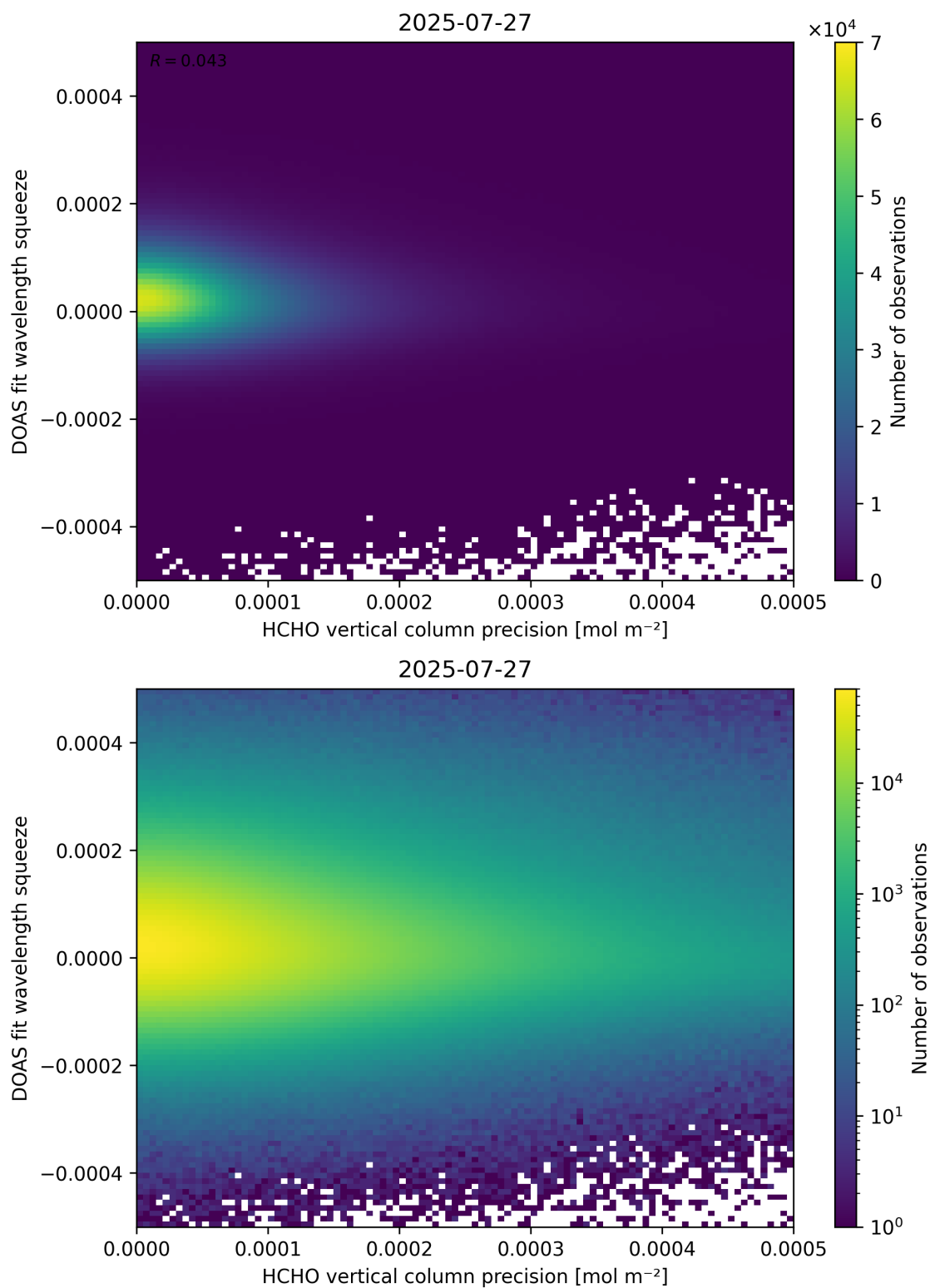
Figure 138: Scatter density plot of “HCHO vertical column precision” against “DOAS fit wavelength squeeze” for 2025-07-26 to 2025-07-28.
