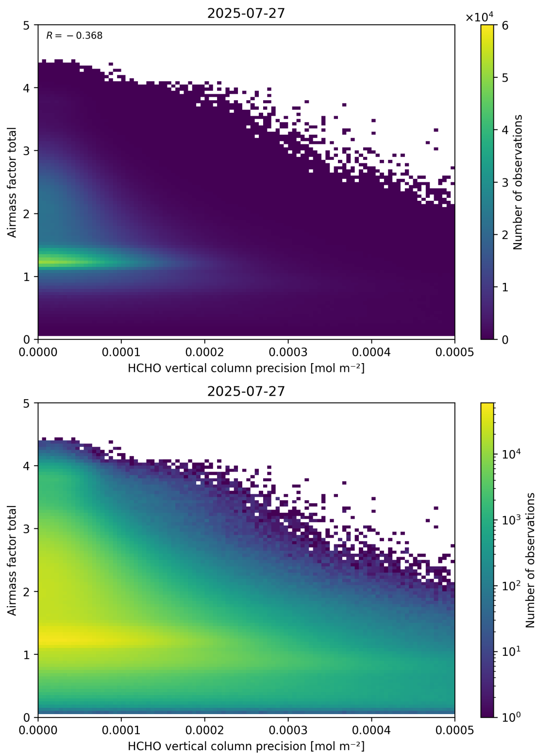
Figure 144: Scatter density plot of “HCHO vertical column precision” against “Airmass factor total” for 2025-07-26 to 2025-07-28.
