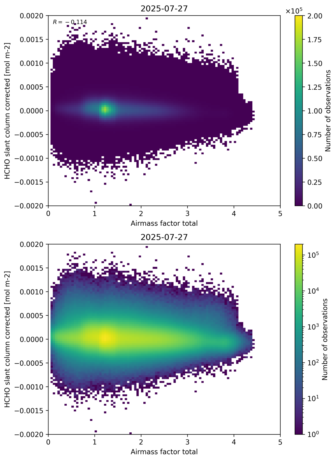
Figure 101: Scatter density plot of “Airmass factor total” against “HCHO slant column corrected” for 2025-07-26 to 2025-07-28.
