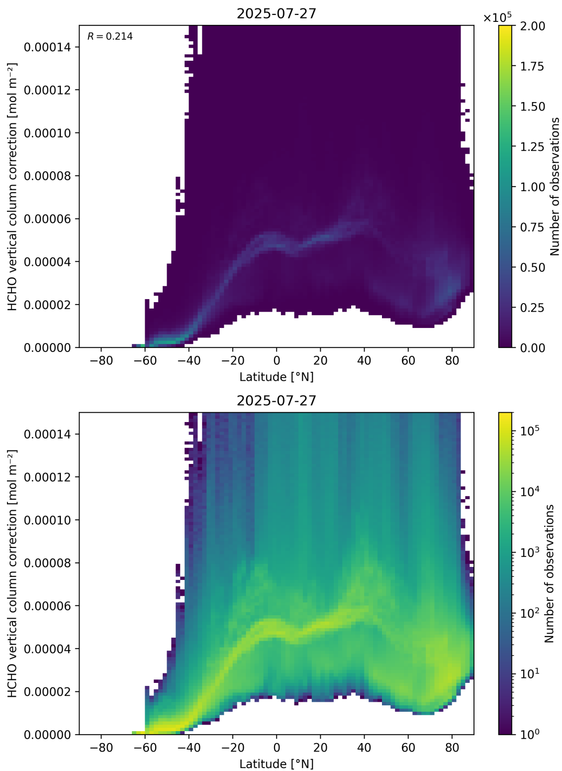
Figure 164: Scatter density plot of “Latitude” against “HCHO vertical column correction” for 2025-07-26 to 2025-07-28.
