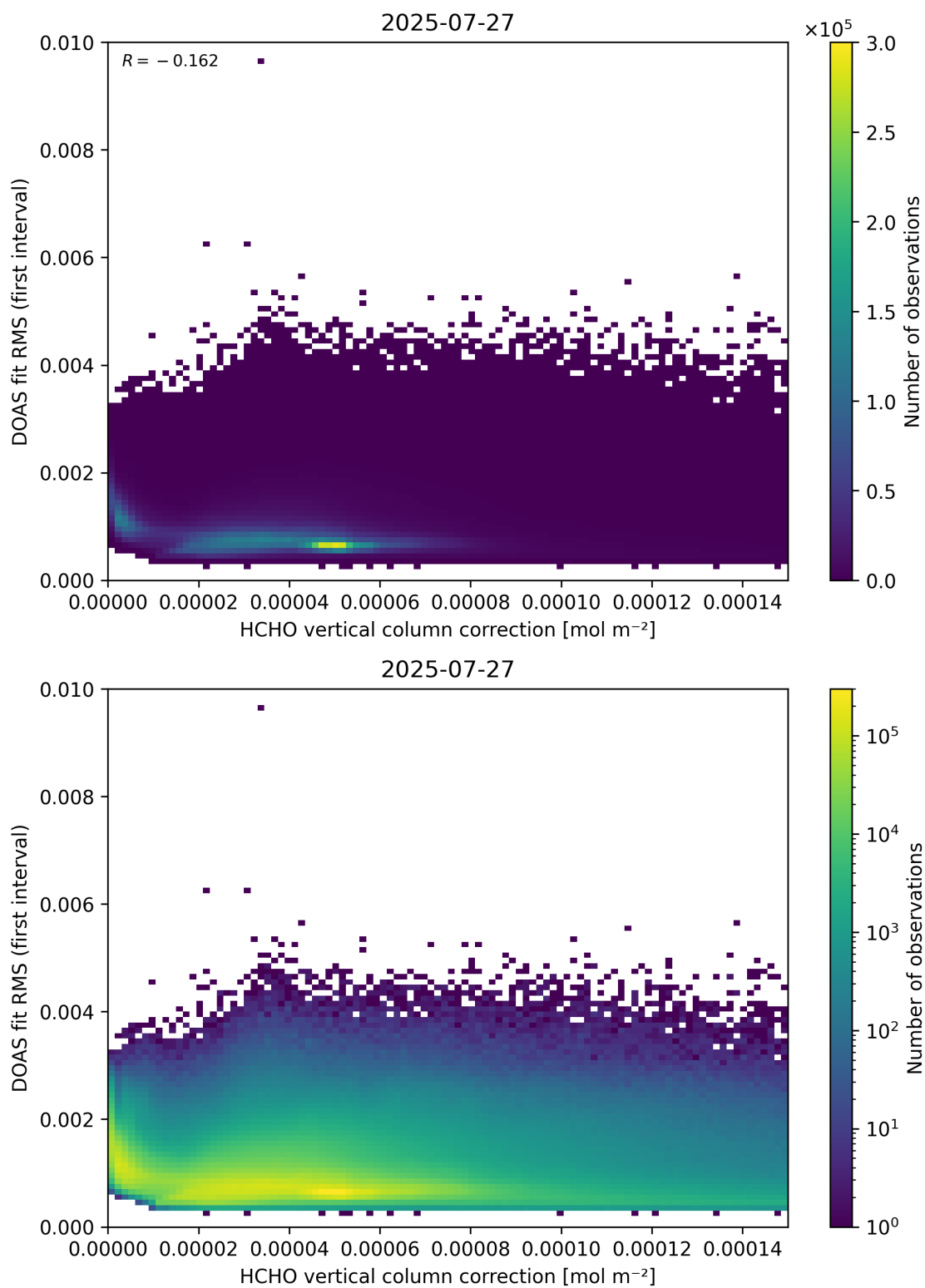
Figure 112: Scatter density plot of “HCHO vertical column correction” against “DOAS fit RMS (first interval)” for 2025-07-26 to 2025-07-28.
