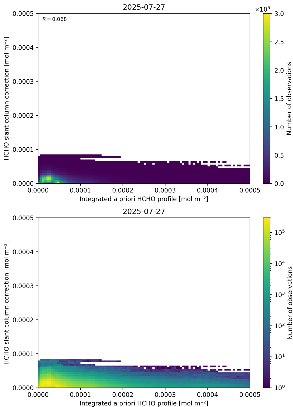
Figure 152: Scatter density plot of “Integrated a priori HCHO profile” against “HCHO slant column correction” for 2025-07-26 to 2025-07-28.
