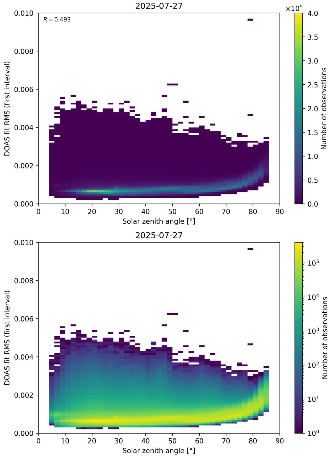
Figure 167: Scatter density plot of “Solar zenith angle” against “DOAS fit RMS (first interval)” for 2025-07-26 to 2025-07-28.
