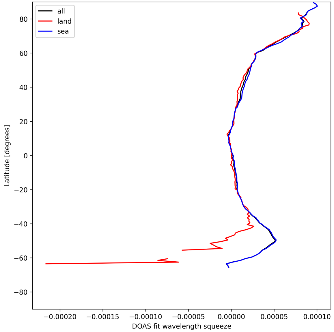
Figure 31: Zonal average of “DOAS fit wavelength squeeze” for 2025-07-26 to 2025-07-28.
