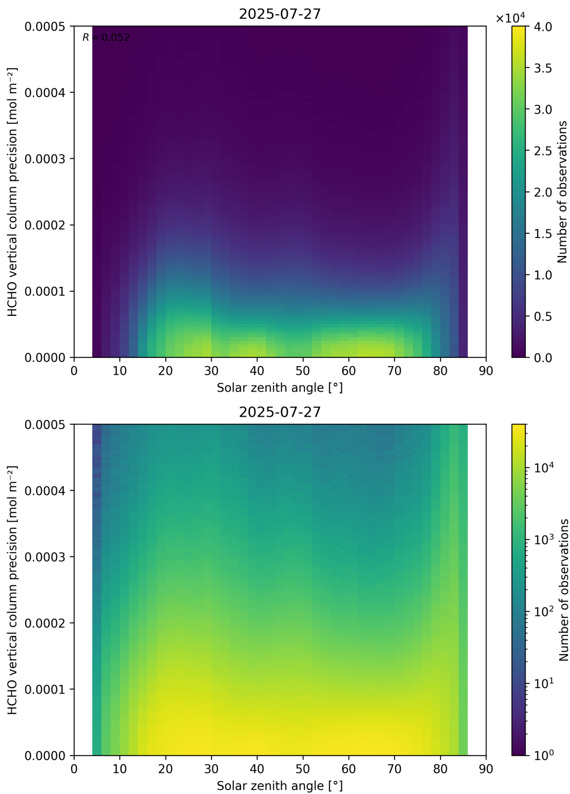
Figure 179: Scatter density plot of “Solar zenith angle” against “HCHO vertical column precision” for 2025-07-26 to 2025-07-28.
