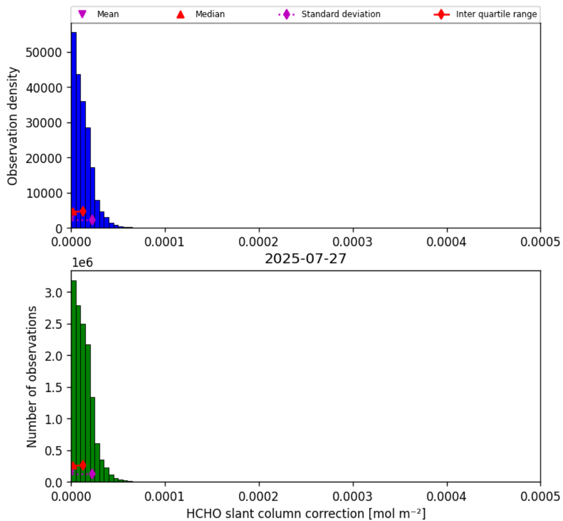
Figure 47: Histogram of “HCHO slant column correction” for 2025-07-26 to 2025-07-28
