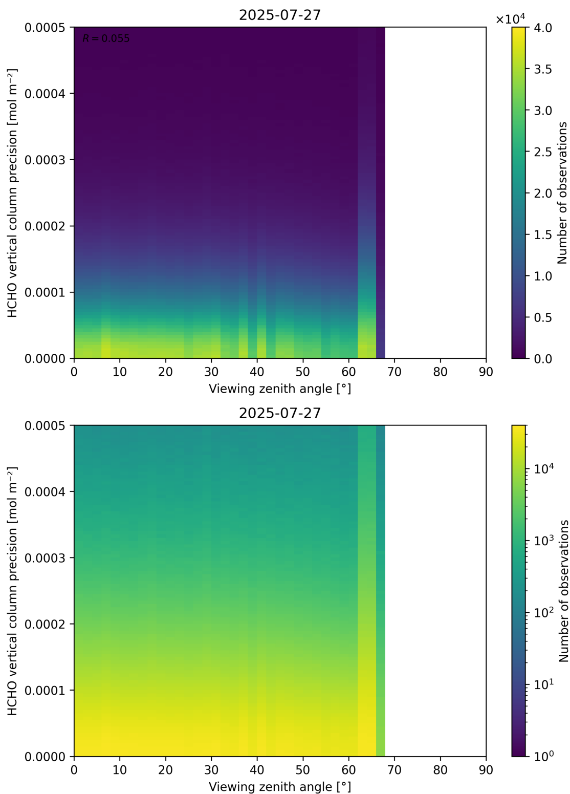
Figure 194: Scatter density plot of “Viewing zenith angle” against “HCHO vertical column precision” for 2025-07-26 to 2025-07-28.
