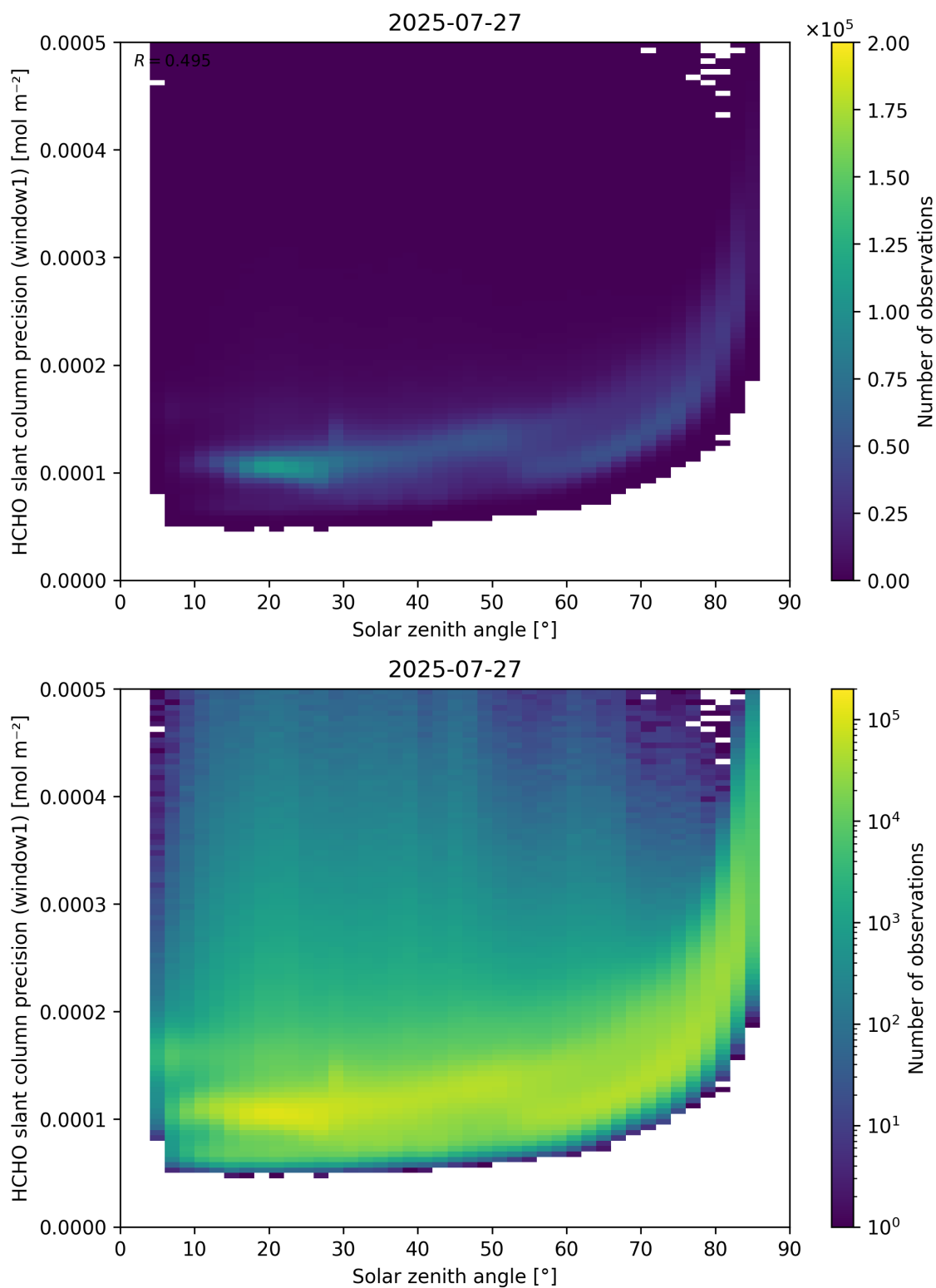
Figure 174: Scatter density plot of “Solar zenith angle” against “HCHO slant column precision (window1)” for 2025-07-26 to 2025-07-28.
