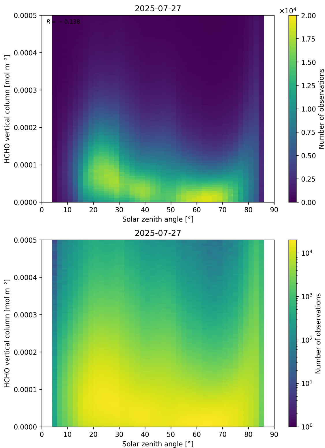
Figure 177: Scatter density plot of “Solar zenith angle” against “HCHO vertical column” for 2025-07-26 to 2025-07-28.
