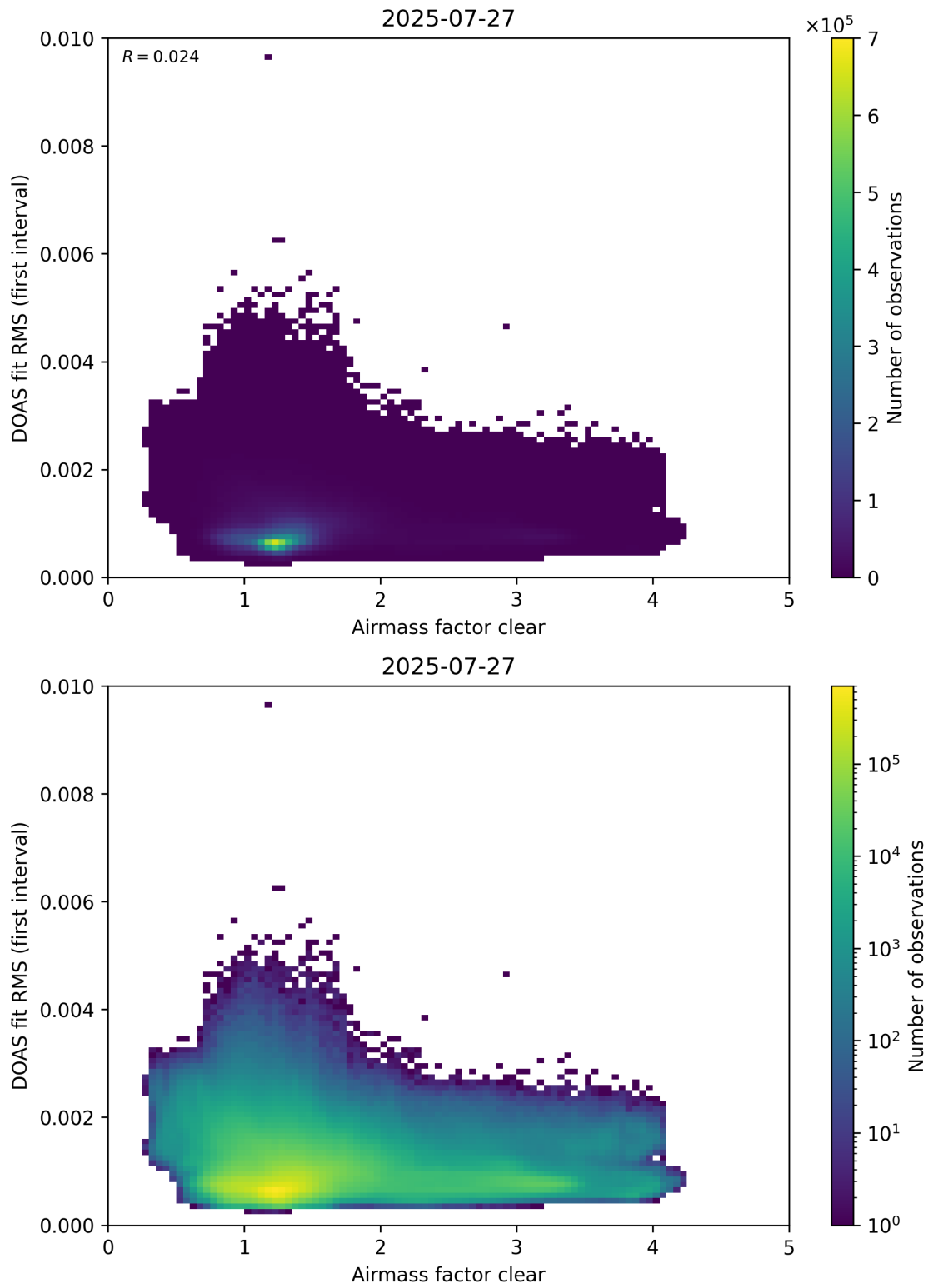
Figure 71: Scatter density plot of “Airmass factor clear” against “DOAS fit RMS (first interval)” for 2025-07-26 to 2025-07-28.
