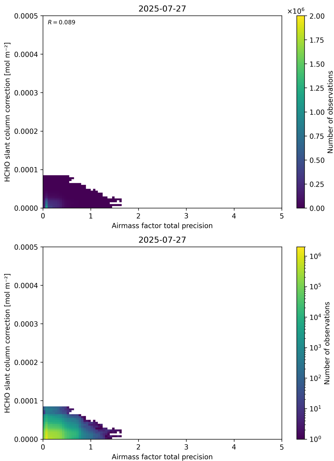
Figure 110: Scatter density plot of “Airmass factor total precision” against “HCHO slant column correction” for 2025-07-26 to 2025-07-28.
