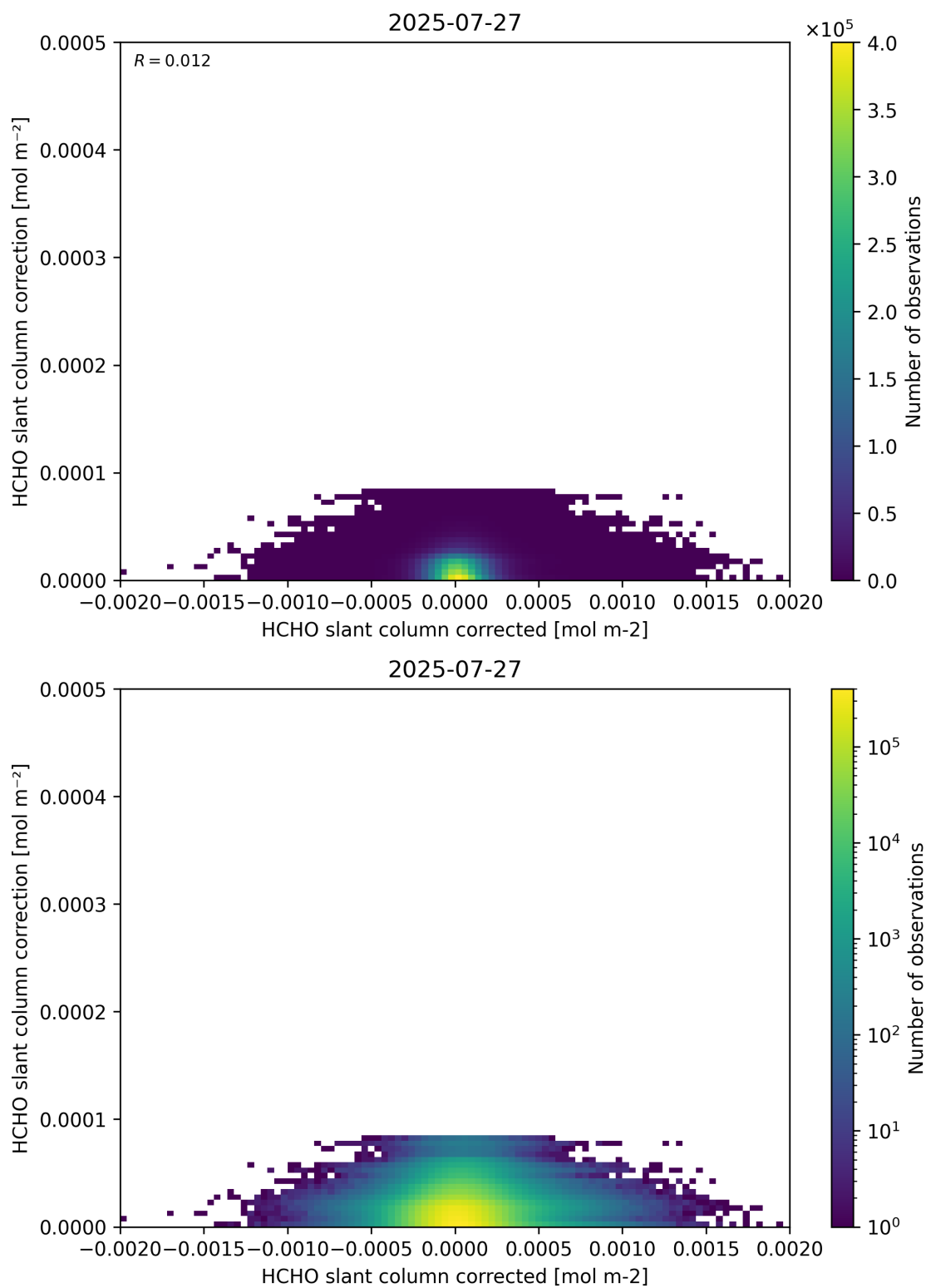
Figure 77: Scatter density plot of “HCHO slant column corrected” against “HCHO slant column correction” for 2025-07-26 to 2025-07-28.
