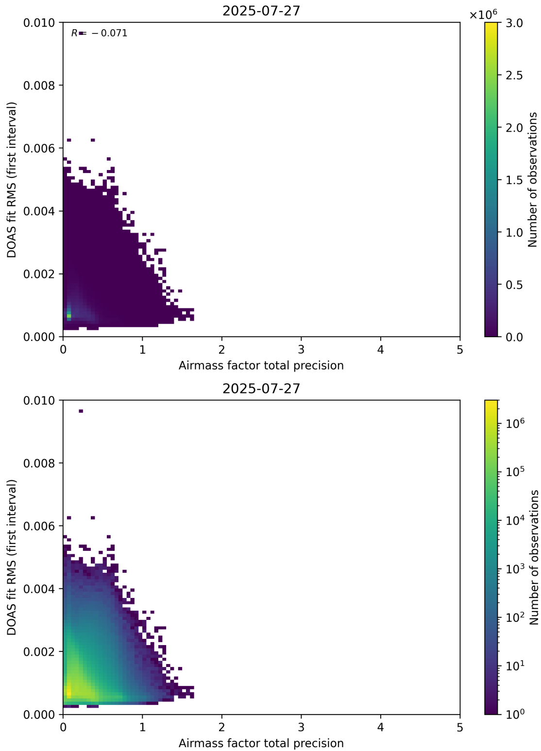
Figure 105: Scatter density plot of “Airmass factor total precision” against “DOAS fit RMS (first interval)” for 2025-07-26 to 2025-07-28.
