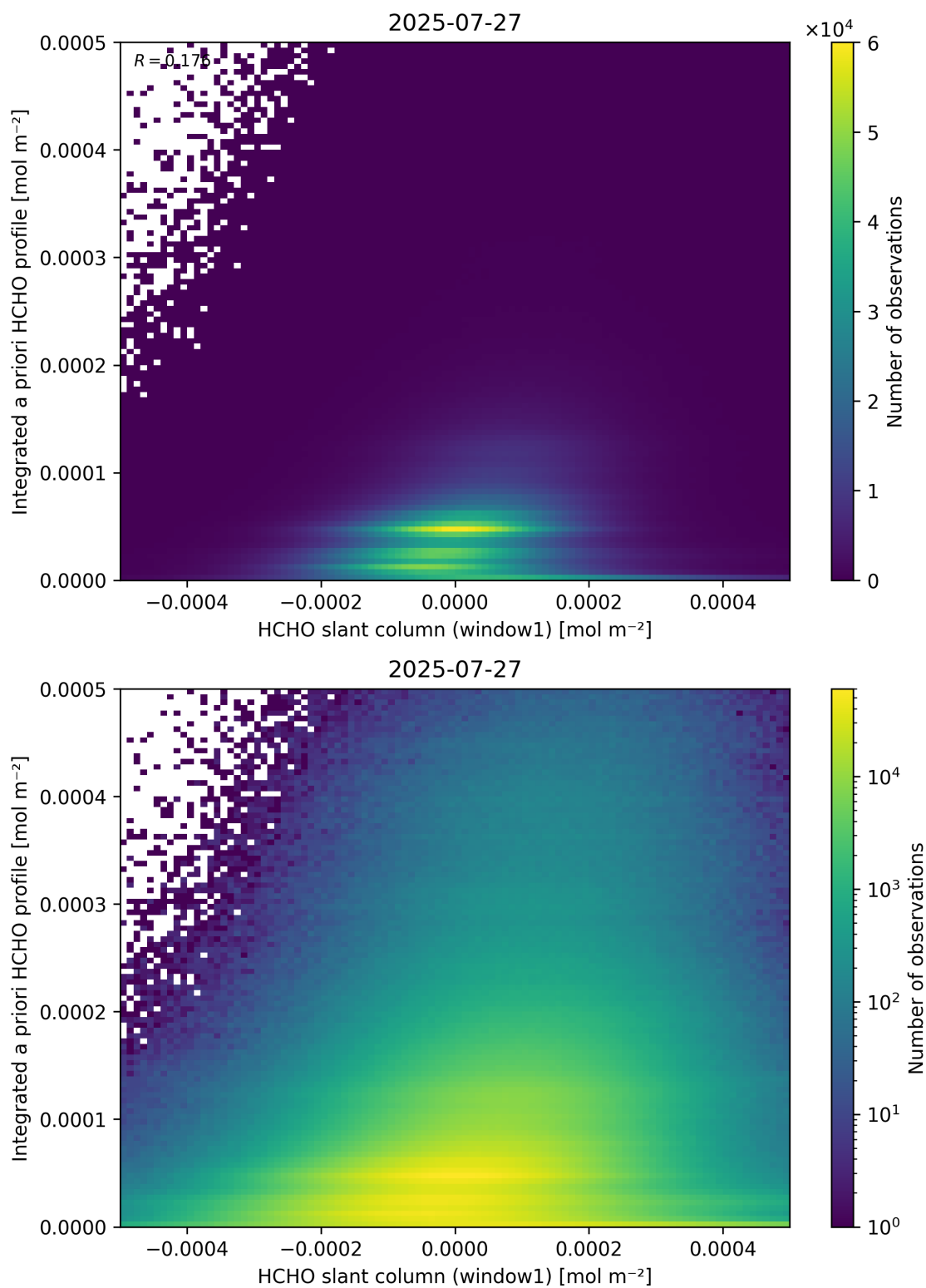
Figure 87: Scatter density plot of “HCHO slant column (window1)” against “Integrated a priori HCHO profile” for 2025-07-26 to 2025-07-28.
