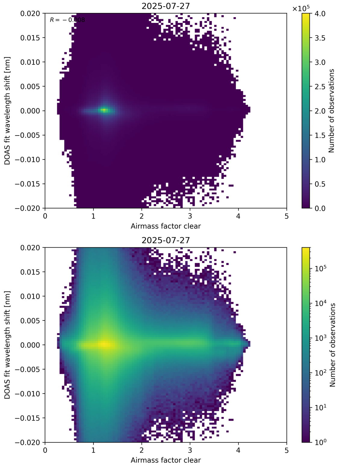
Figure 72: Scatter density plot of “Airmass factor clear” against “DOAS fit wavelength shift” for 2025-07-26 to 2025-07-28.
