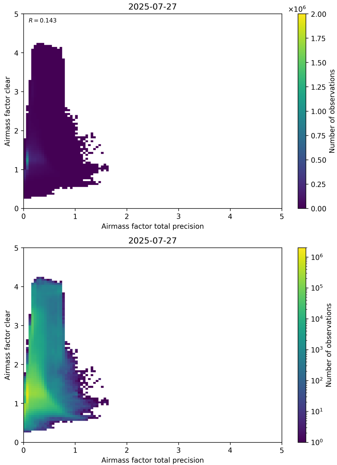
Figure 108: Scatter density plot of “Airmass factor total precision” against “Airmass factor clear” for 2025-07-26 to 2025-07-28.
