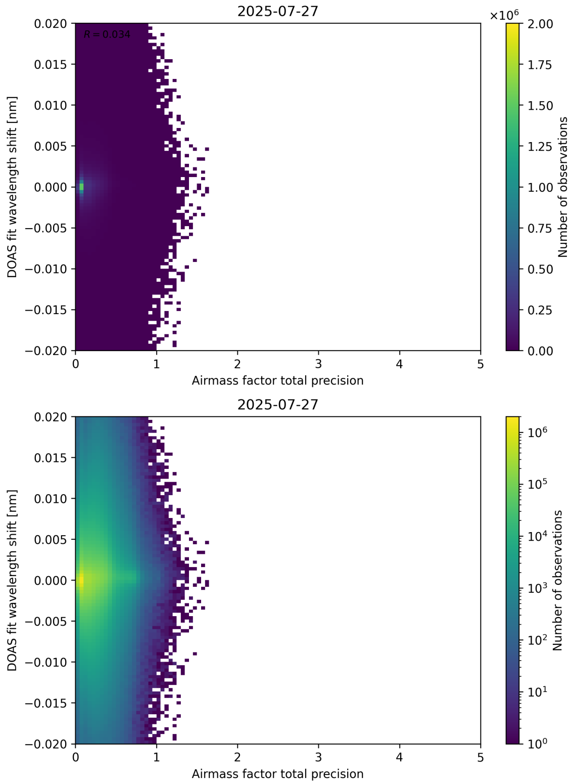
Figure 106: Scatter density plot of “Airmass factor total precision” against “DOAS fit wavelength shift” for 2025-07-26 to 2025-07-28.
