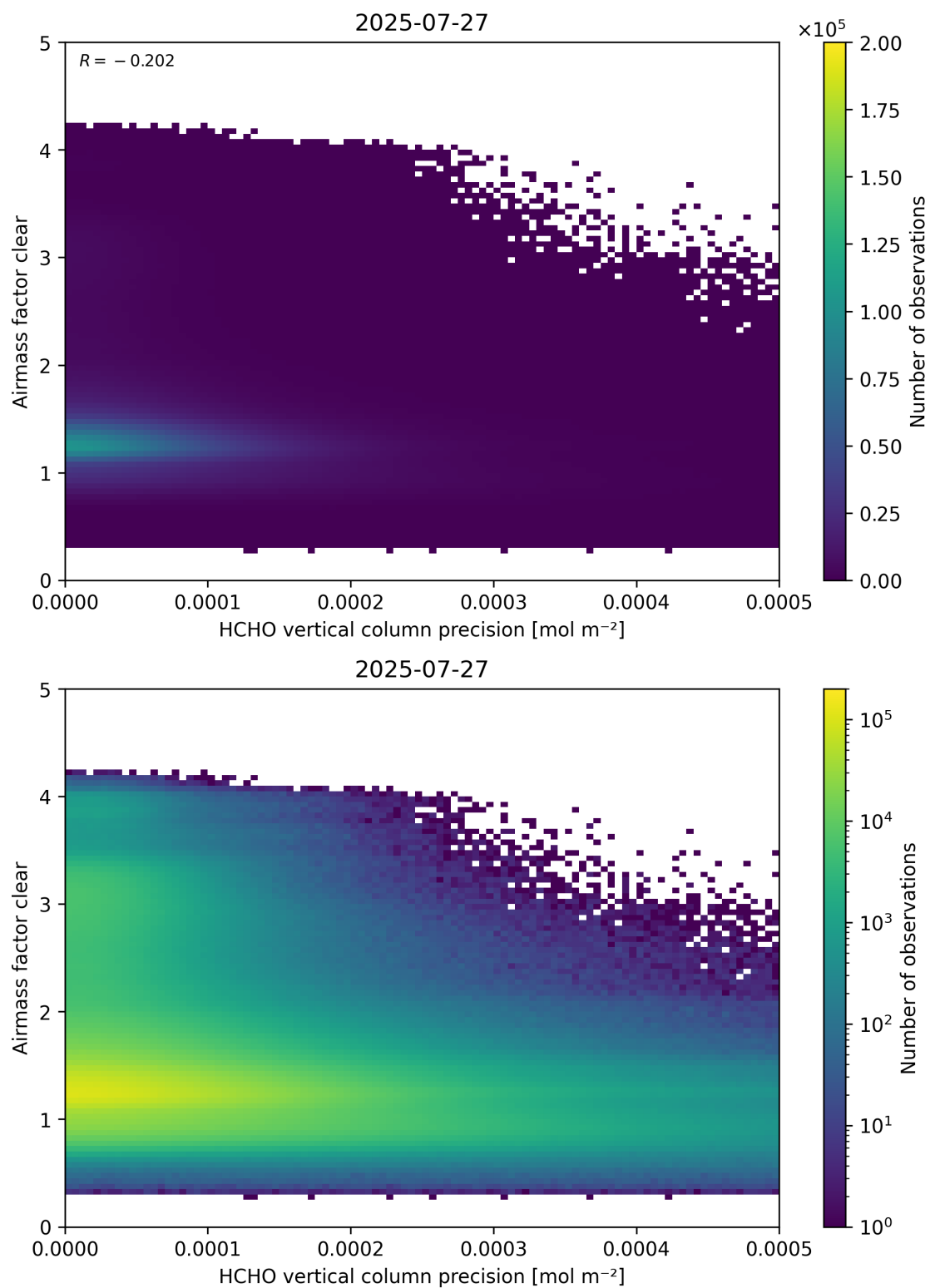
Figure 139: Scatter density plot of “HCHO vertical column precision” against “Airmass factor clear” for 2025-07-26 to 2025-07-28.
