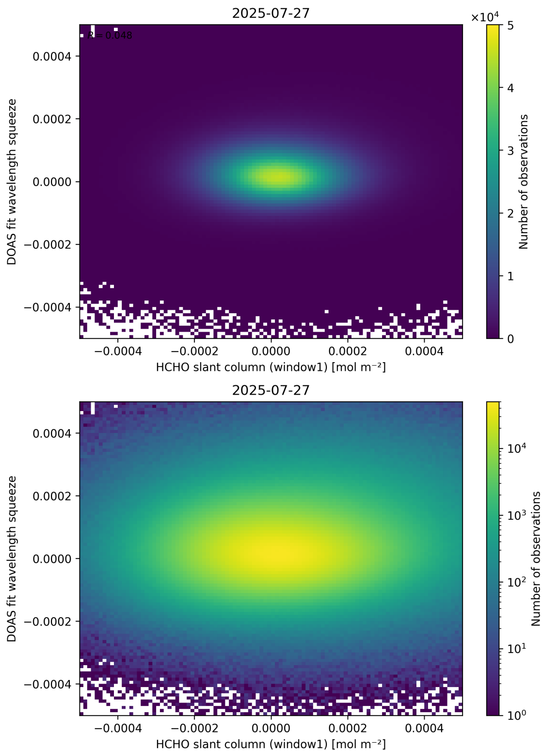
Figure 80: Scatter density plot of “HCHO slant column (window1)” against “DOAS fit wavelength squeeze” for 2025-07-26 to 2025-07-28.
