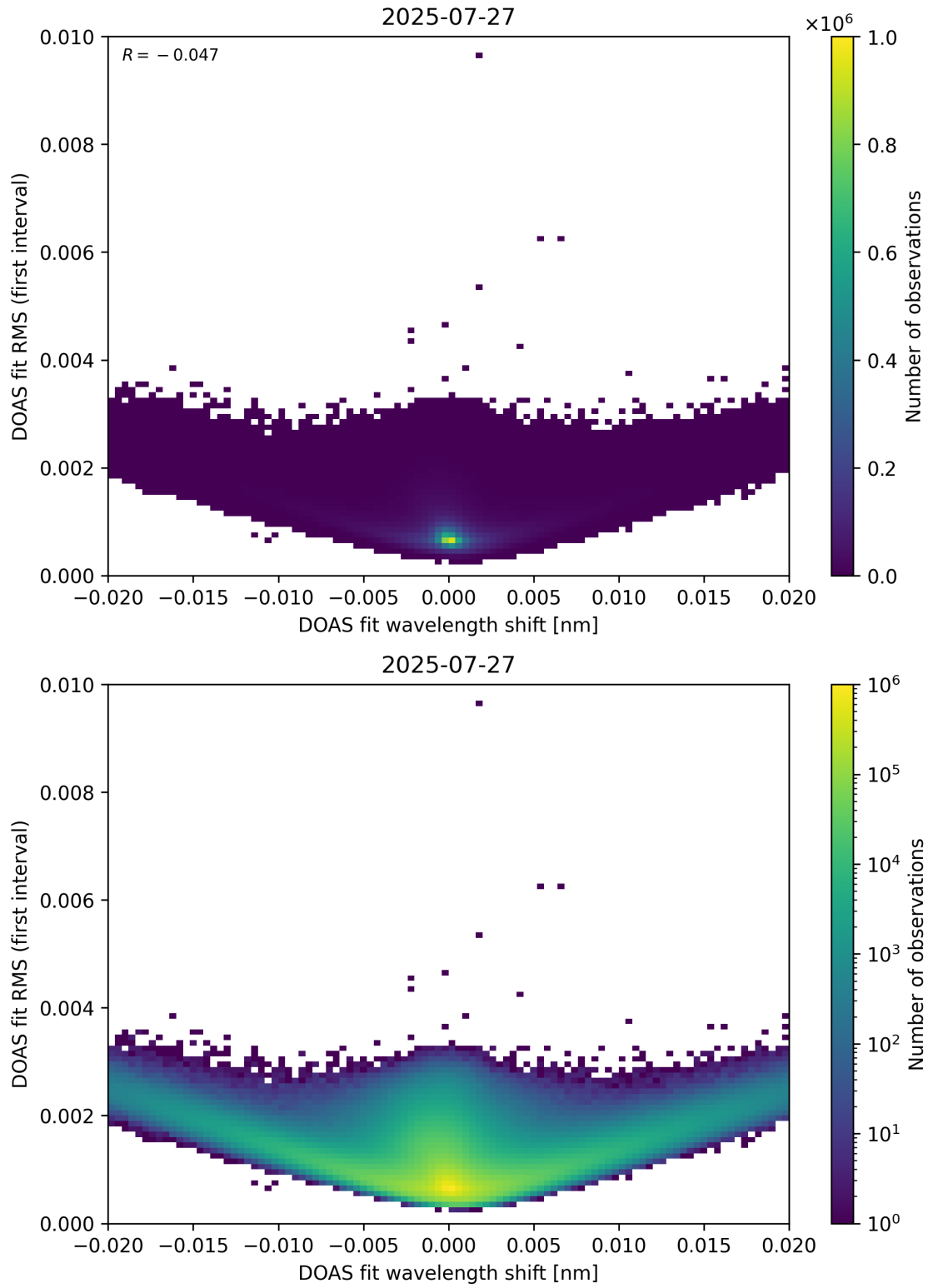
Figure 64: Scatter density plot of “DOAS fit wavelength shift” against “DOAS fit RMS (first interval)” for 2025-07-26 to 2025-07-28.
