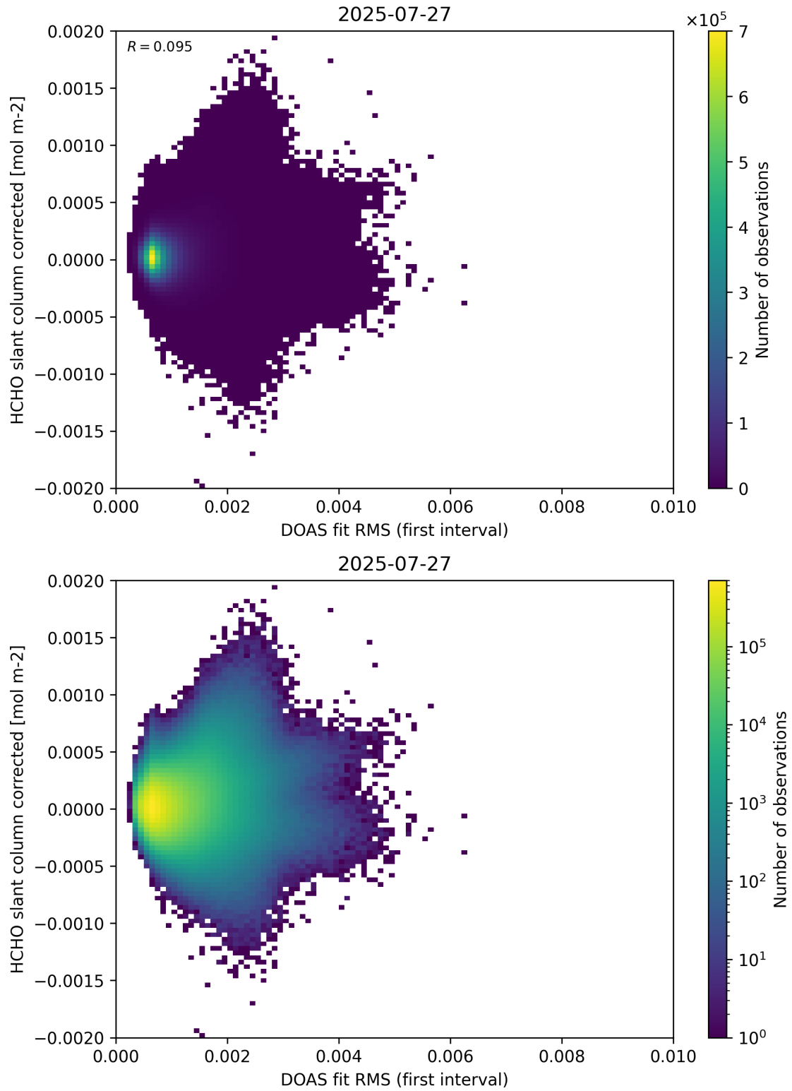
Figure 62: Scatter density plot of “DOAS fit RMS (first interval)” against “HCHO slant column corrected” for 2025-07-26 to 2025-07-28.
