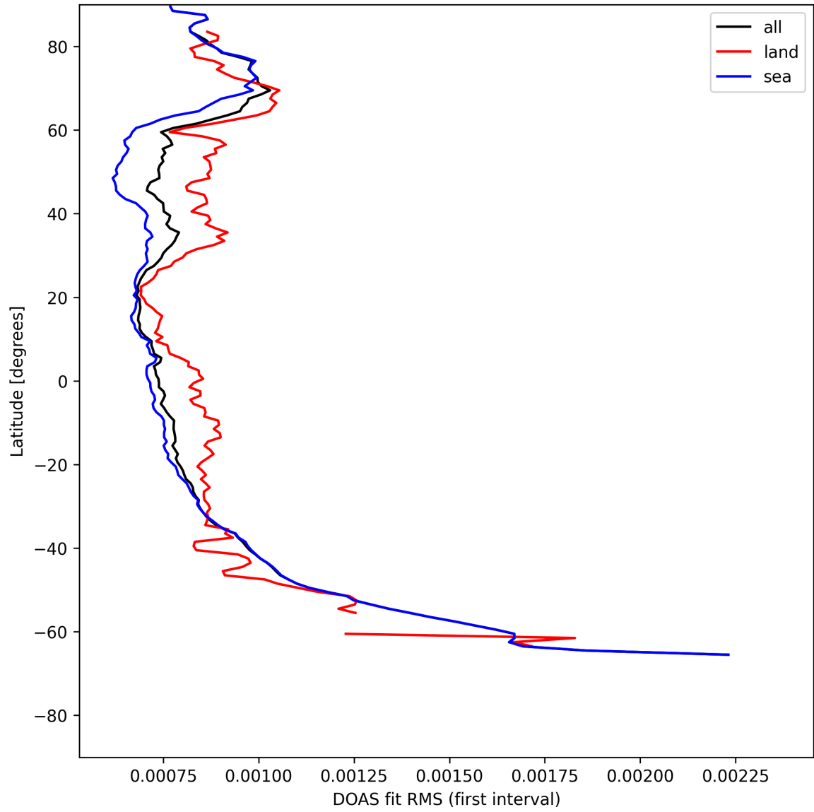
Figure 32: Zonal average of "DOAS fit RMS (first interval)" for 2025-07-26 to 2025-07-28.
