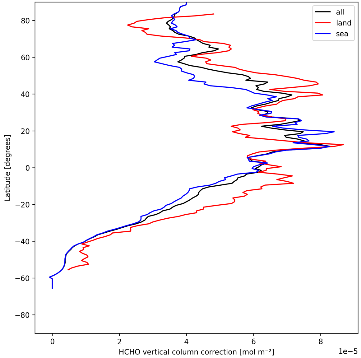
Figure 23: Zonal average of “HCHO vertical column correction” for 2025-07-26 to 2025-07-28.
