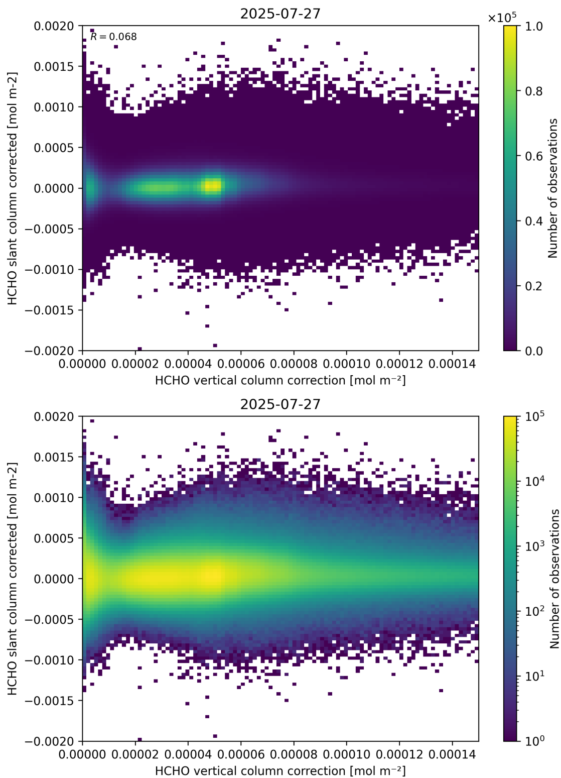
Figure 116: Scatter density plot of “HCHO vertical column correction” against “HCHO slant column corrected” for 2025-07-26 to 2025-07-28.
