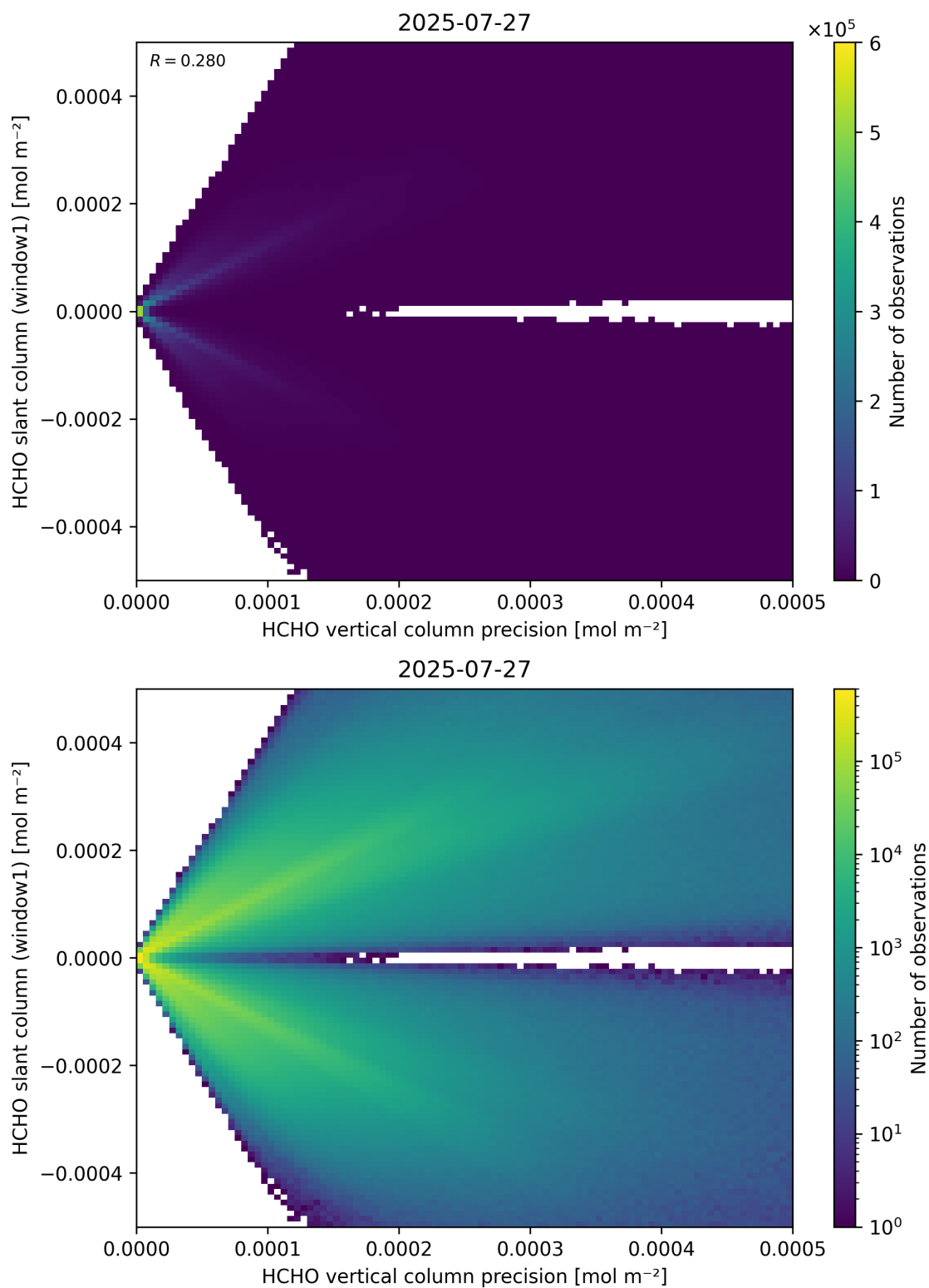
Figure 142: Scatter density plot of “HCHO vertical column precision” against “HCHO slant column (window1)” for 2025-07-26 to 2025-07-28.
