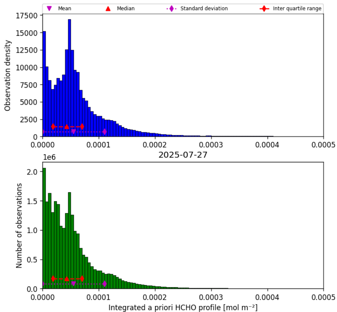
Figure 43: Histogram of “Integrated a priori HCHO profile” for 2025-07-26 to 2025-07-28
