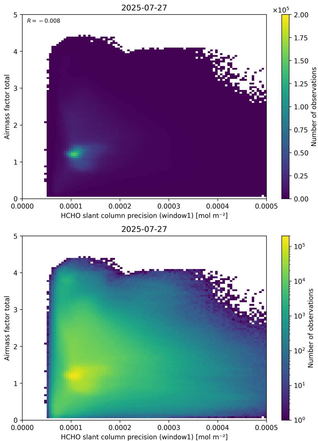
Figure 94: Scatter density plot of “HCHO slant column precision (window1)” against “Airmass factor total” for 2025-07-26 to 2025-07-28.
