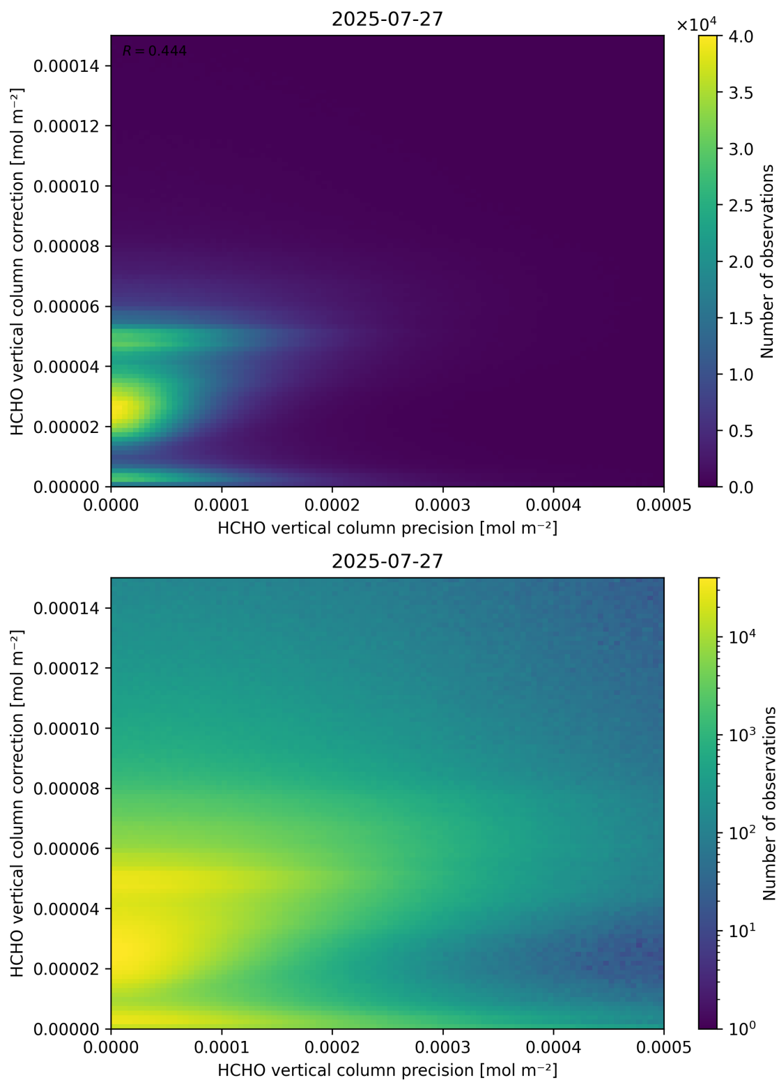
Figure 146: Scatter density plot of “HCHO vertical column precision” against “HCHO vertical column correction” for 2025-07-26 to 2025-07-28.
