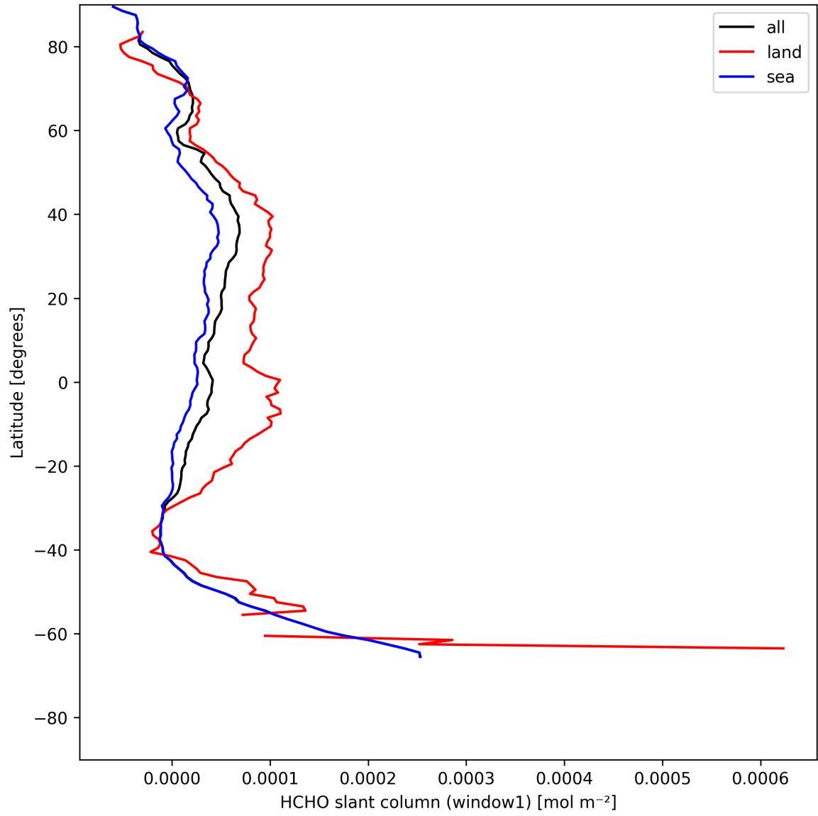
Figure 24: Zonal average of “HCHO slant column (window1)” for 2025-07-26 to 2025-07-28.
