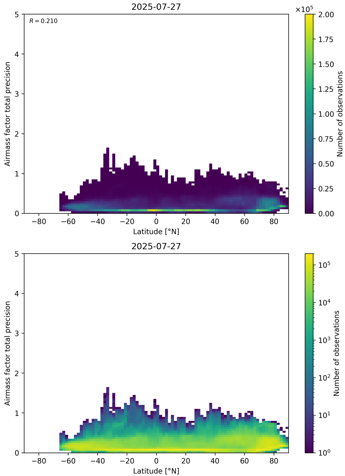
Figure 162: Scatter density plot of “Latitude” against “Airmass factor total precision” for 2025-07-26 to 2025-07-28.
