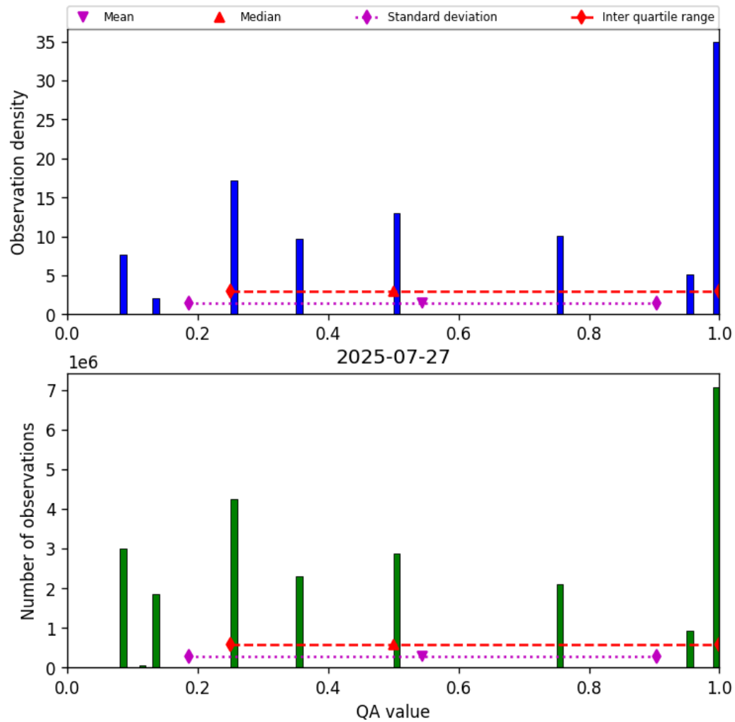
Figure 34: Histogram of “QA value” for 2025-07-26 to 2025-07-28
