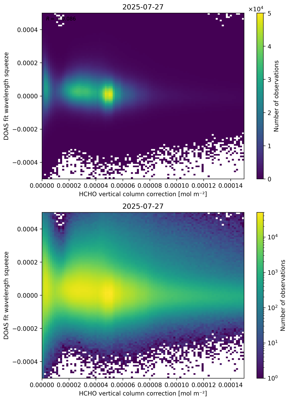
Figure 114: Scatter density plot of “HCHO vertical column correction” against “DOAS fit wavelength squeeze” for 2025-07-26 to 2025-07-28.
