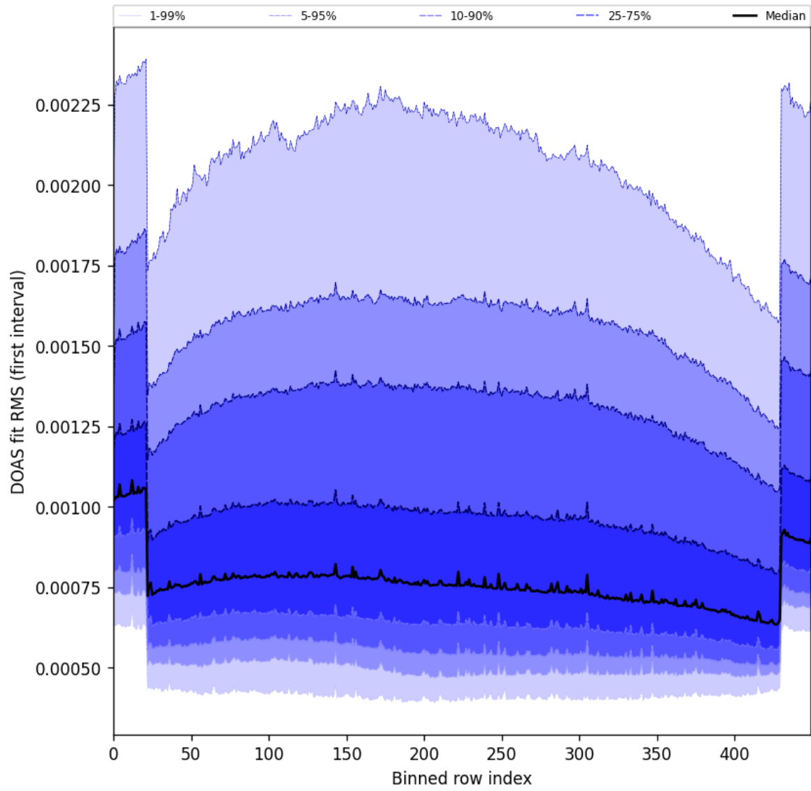
Figure 60: Along track statistics of “DOAS fit RMS (first interval)” for 2025-07-26 to 2025-07-28
