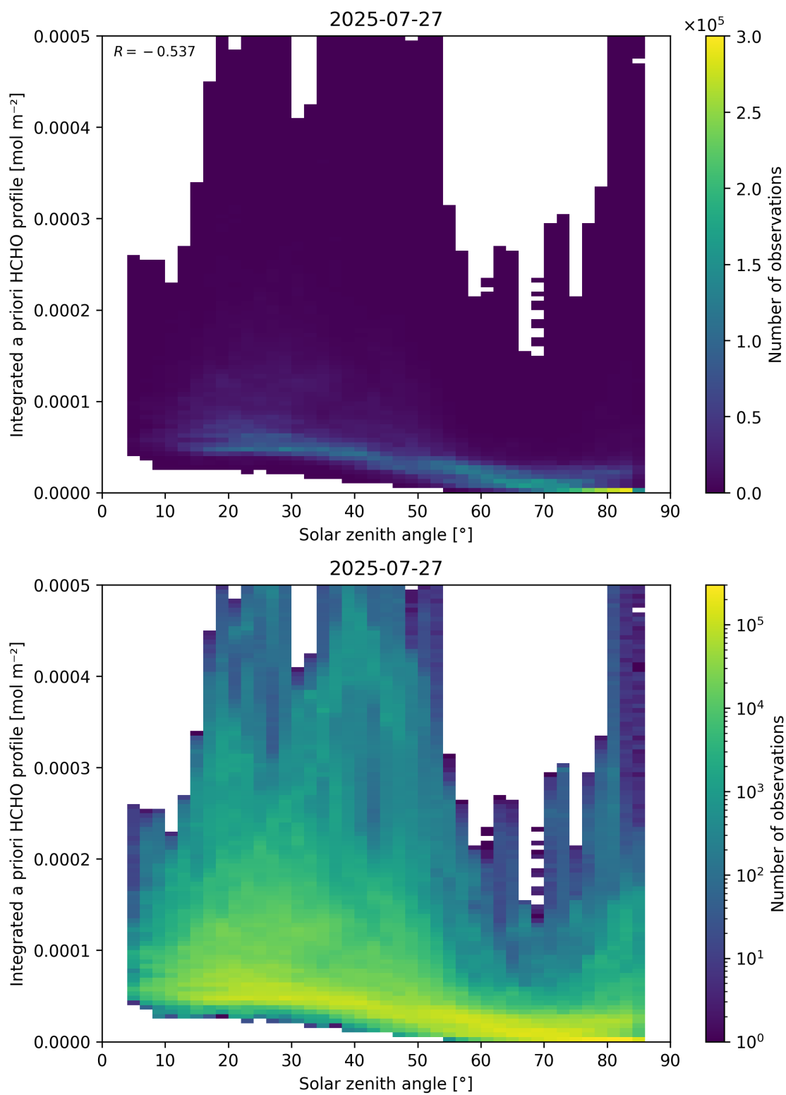
Figure 180: Scatter density plot of “Solar zenith angle” against “Integrated a priori HCHO profile” for 2025-07-26 to 2025-07-28.
