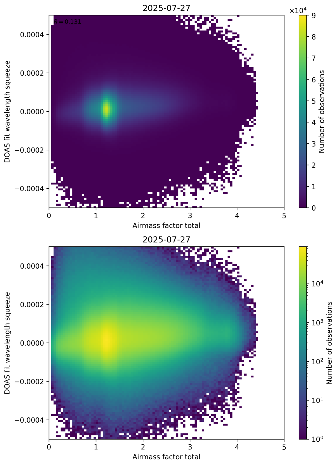
Figure 99: Scatter density plot of “Airmass factor total” against “DOAS fit wavelength squeeze” for 2025-07-26 to 2025-07-28.
