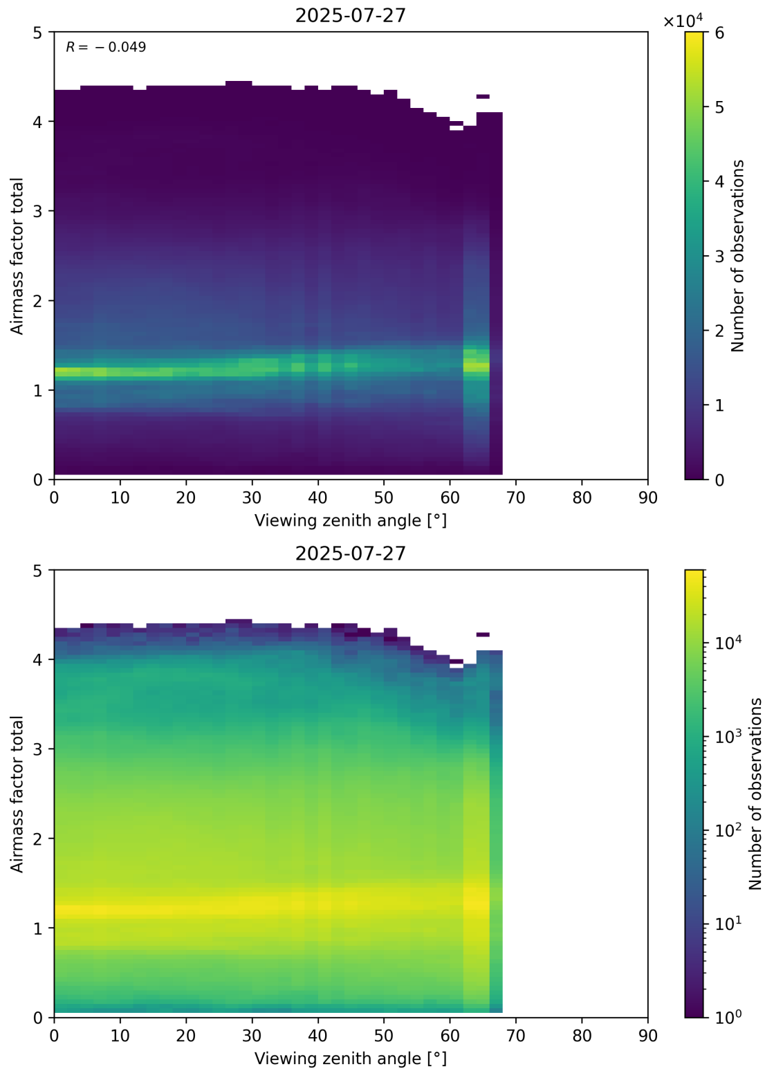
Figure 190: Scatter density plot of “Viewing zenith angle” against “Airmass factor total” for 2025-07-26 to 2025-07-28.
