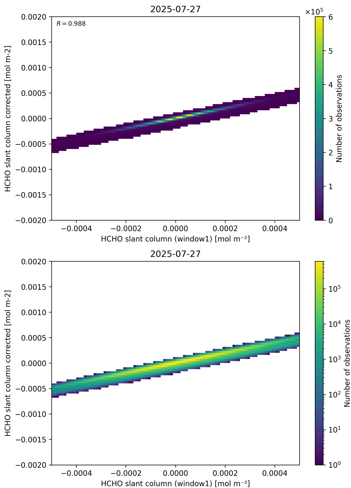
Figure 82: Scatter density plot of “HCHO slant column (window1)” against “HCHO slant column corrected” for 2025-07-26 to 2025-07-28.
