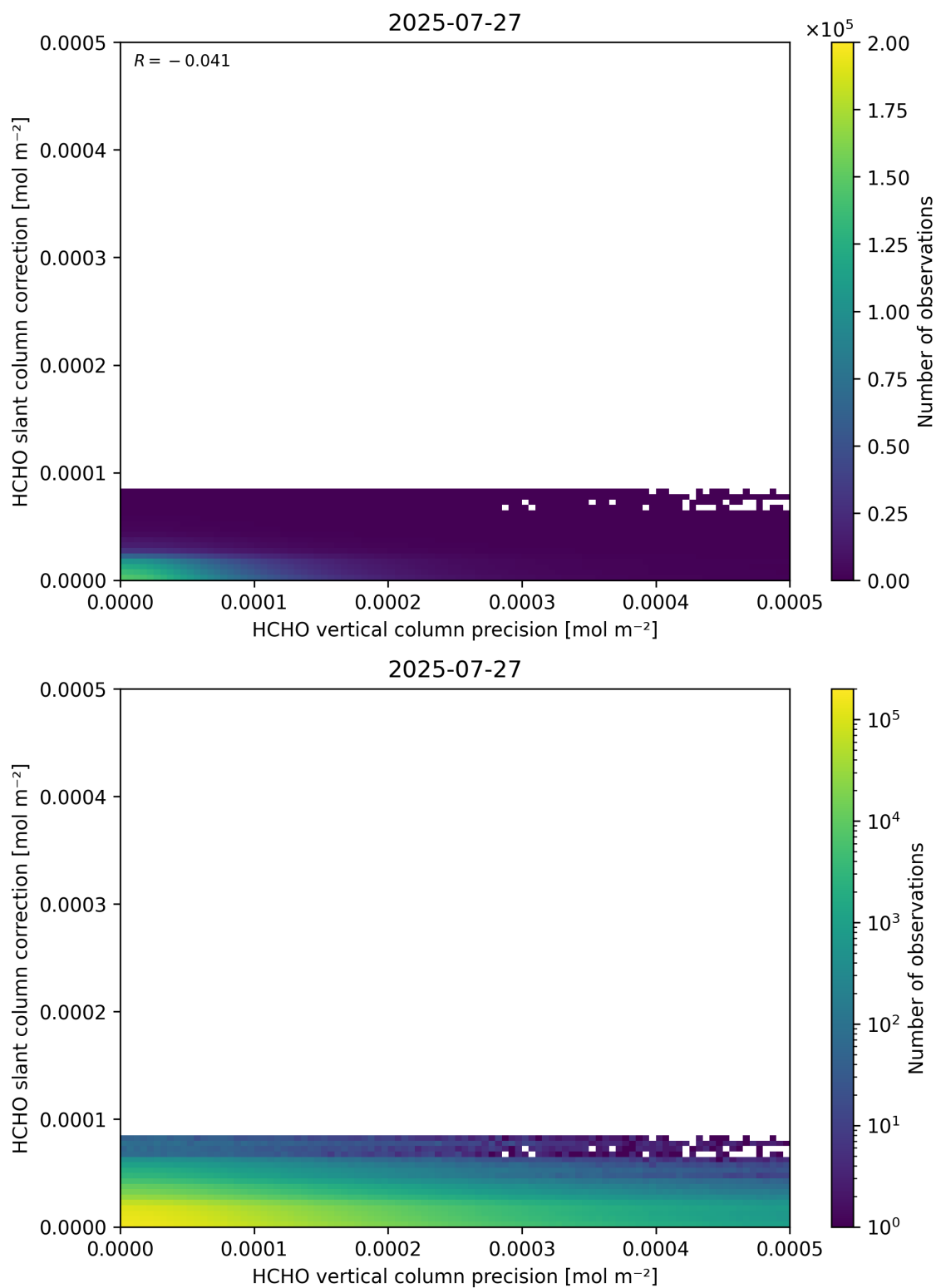
Figure 141: Scatter density plot of “HCHO vertical column precision” against “HCHO slant column correction” for 2025-07-26 to 2025-07-28.
