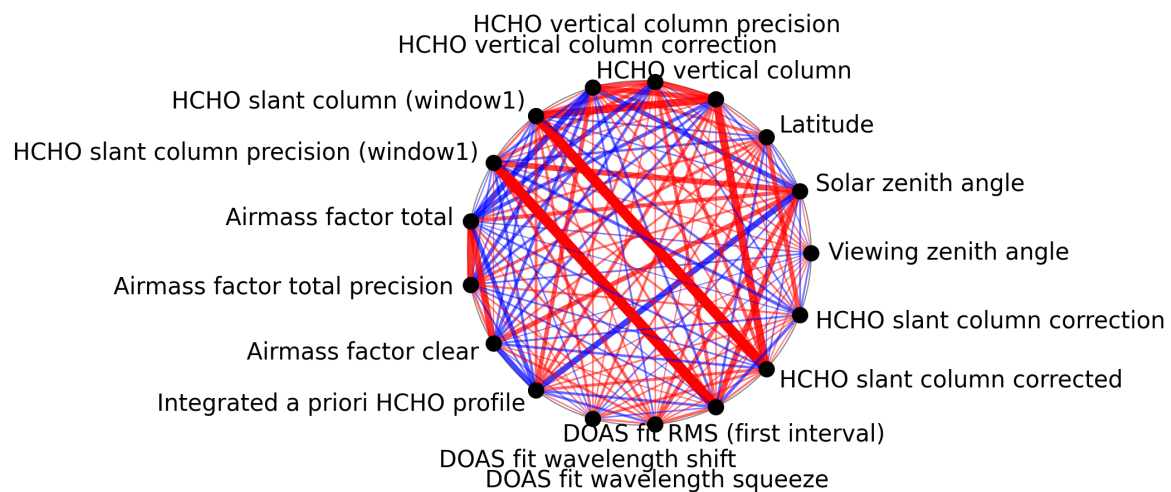
Figure 1: Map of correlation graph for 2025-07-27 to 2025-07-29.
