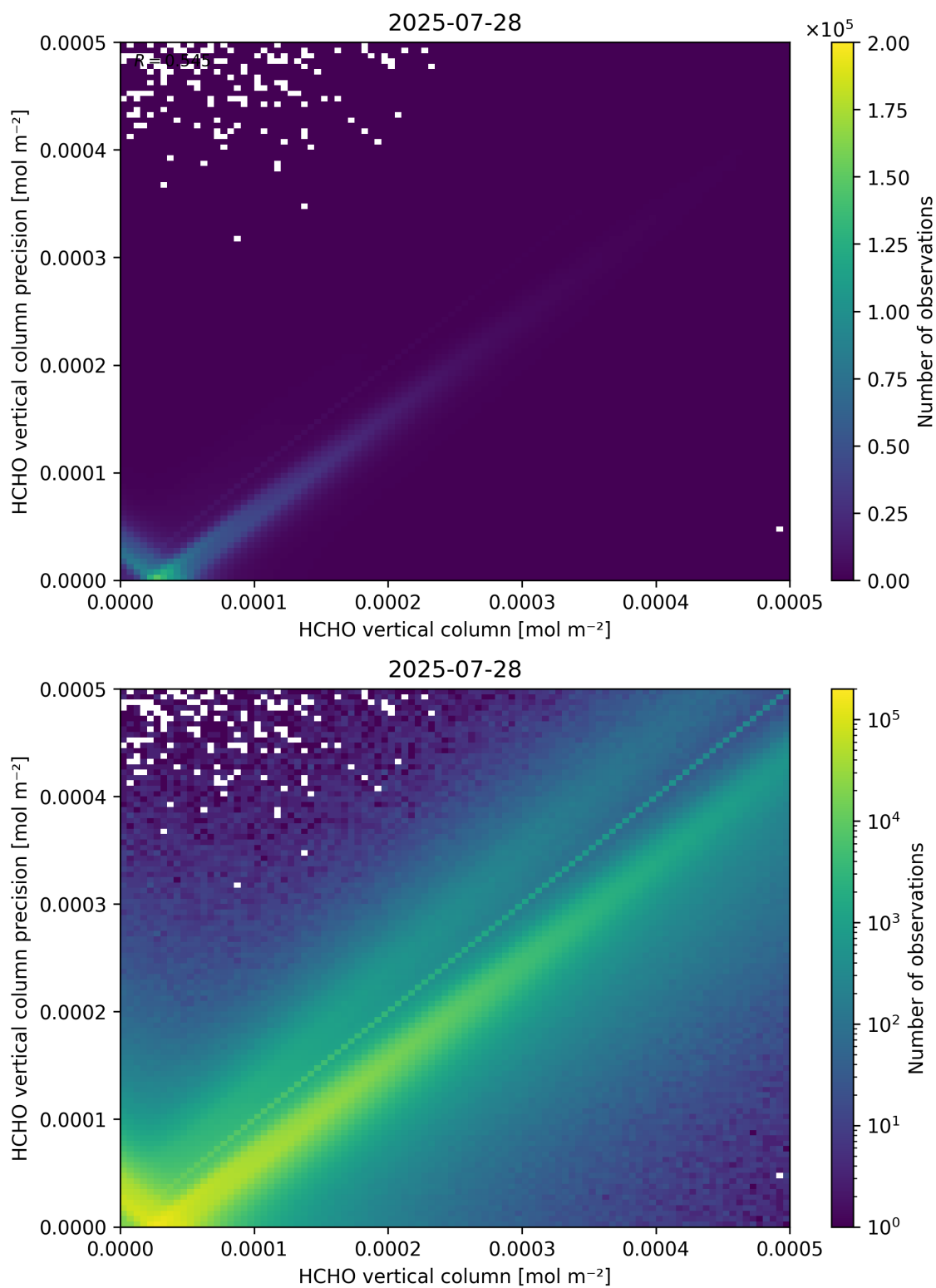
Figure 134: Scatter density plot of “HCHO vertical column” against “HCHO vertical column precision” for 2025-07-27 to 2025-07-29.
