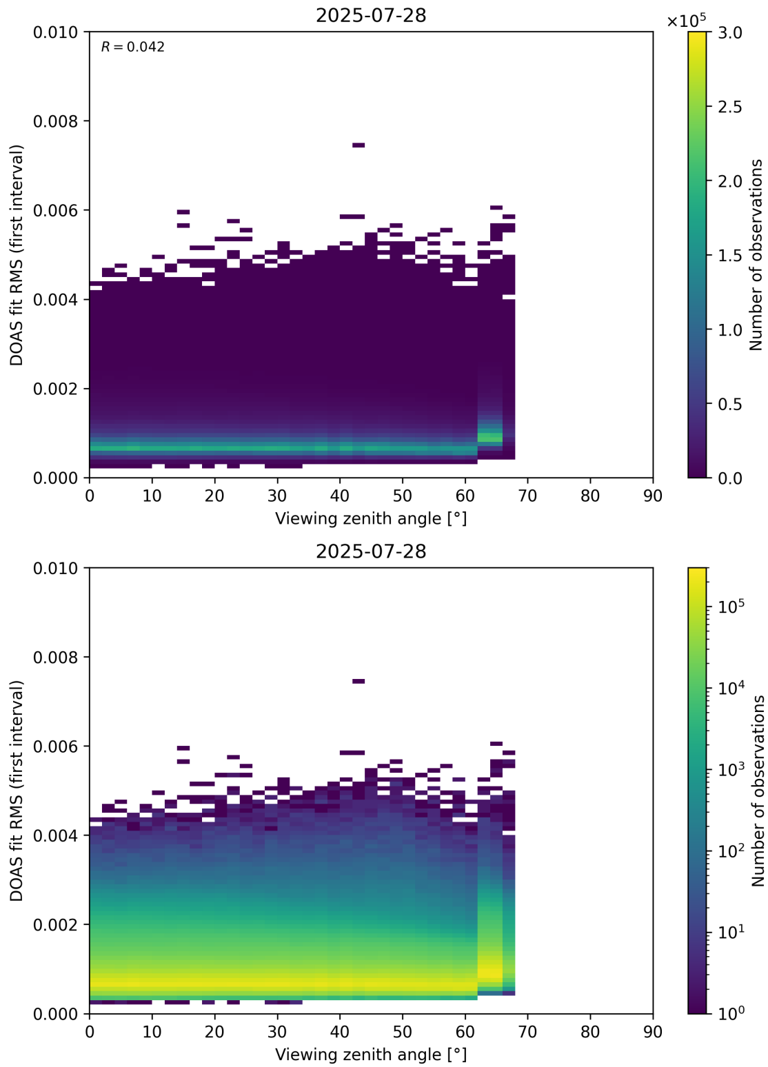
Figure 182: Scatter density plot of “Viewing zenith angle” against “DOAS fit RMS (first interval)” for 2025-07-27 to 2025-07-29.
