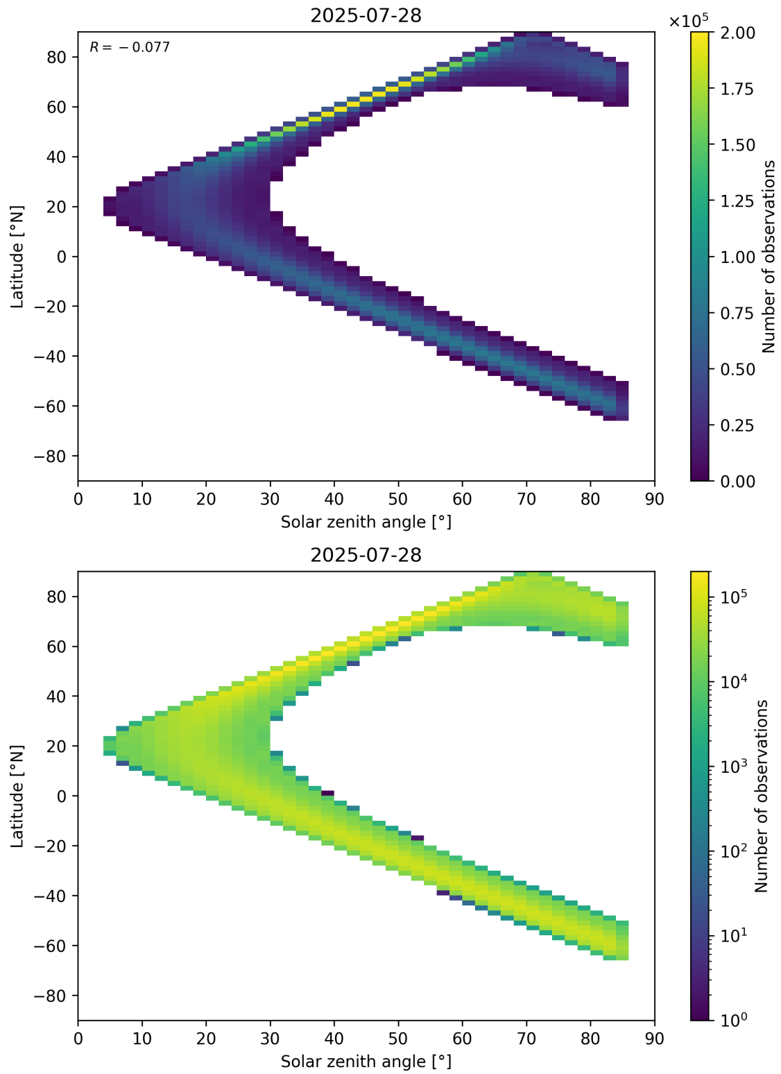
Figure 181: Scatter density plot of “Solar zenith angle” against “Latitude” for 2025-07-27 to 2025-07-29.
