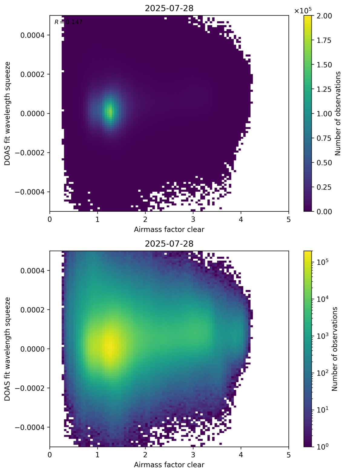
Figure 73: Scatter density plot of “Airmass factor clear” against “DOAS fit wavelength squeeze” for 2025-07-27 to 2025-07-29.
