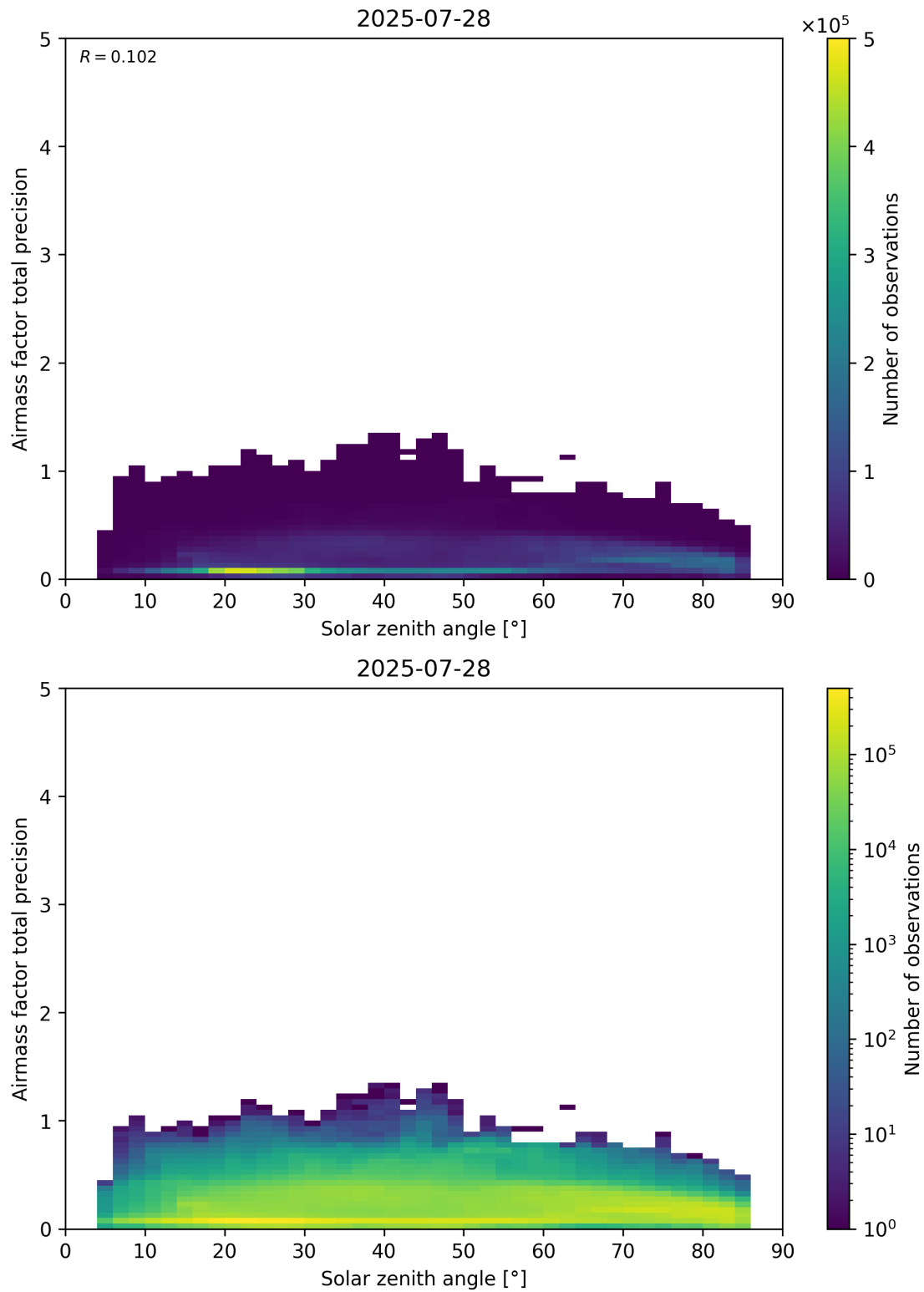
Figure 176: Scatter density plot of “Solar zenith angle” against “Airmass factor total precision” for 2025-07-27 to 2025-07-29.
