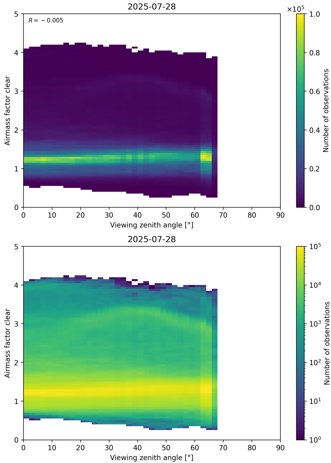
Figure 185: Scatter density plot of “Viewing zenith angle” against “Airmass factor clear” for 2025-07-27 to 2025-07-29.
