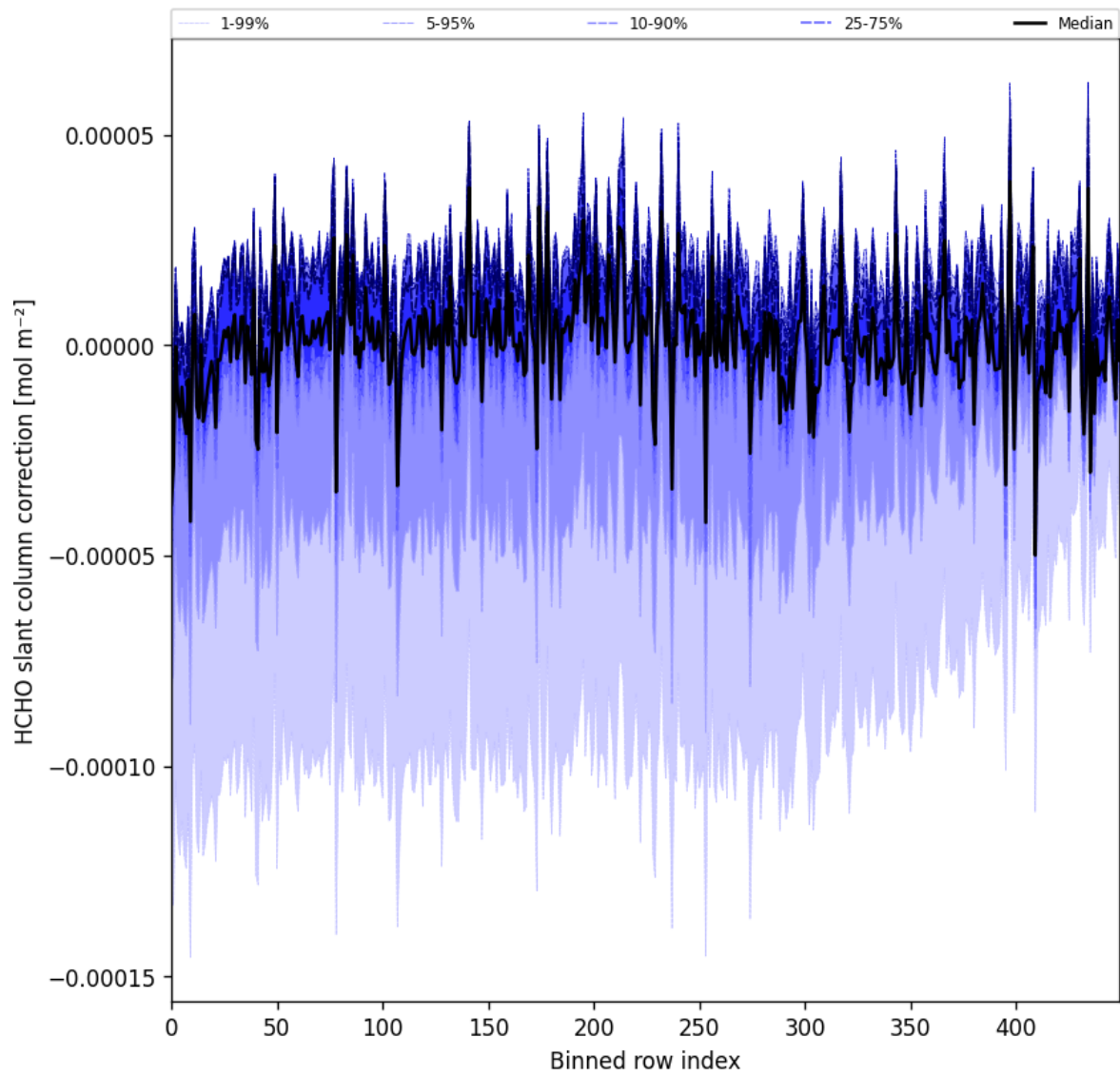
Figure 61: Along track statistics of “HCHO slant column correction” for 2025-07-27 to 2025-07-29
