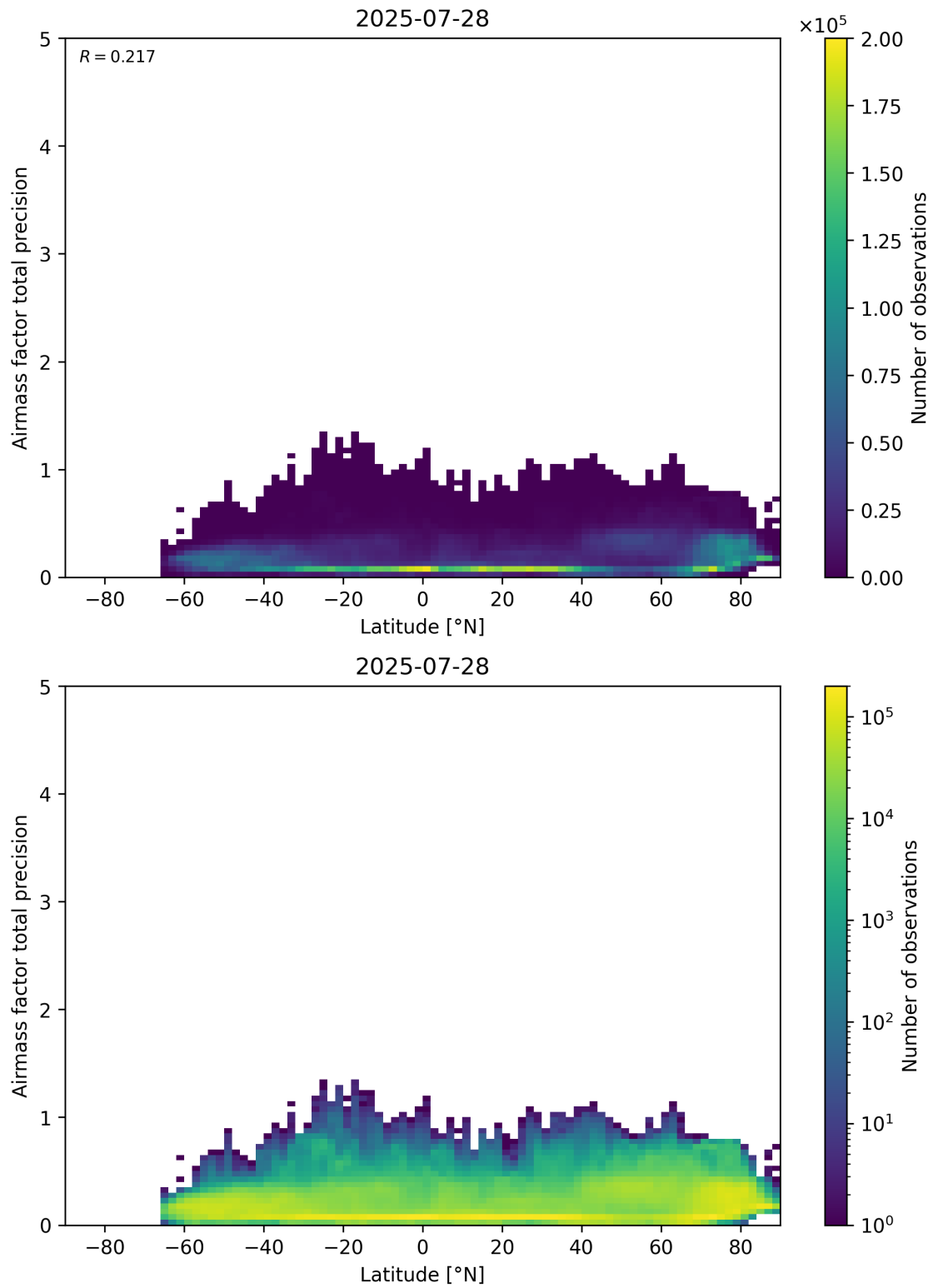
Figure 162: Scatter density plot of “Latitude” against “Airmass factor total precision” for 2025-07-27 to 2025-07-29.
