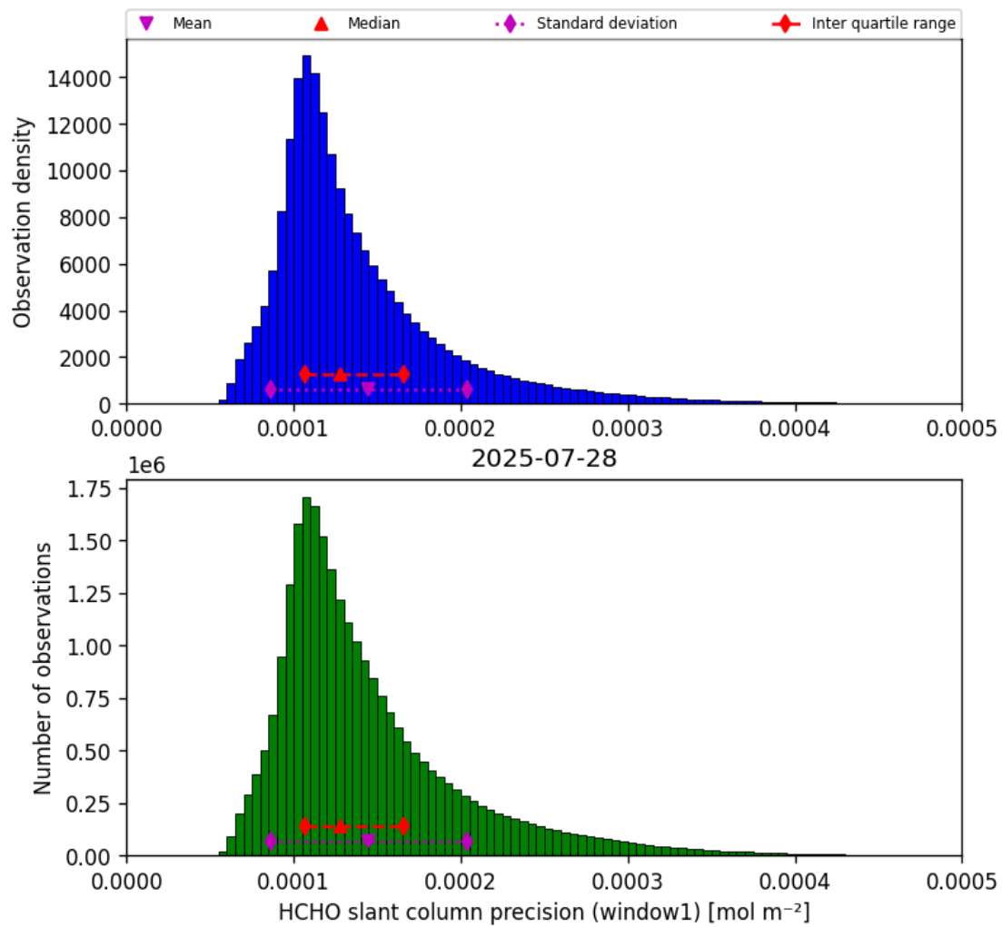
Figure 39: Histogram of “HCHO slant column precision (window1)” for 2025-07-27 to 2025-07-29
