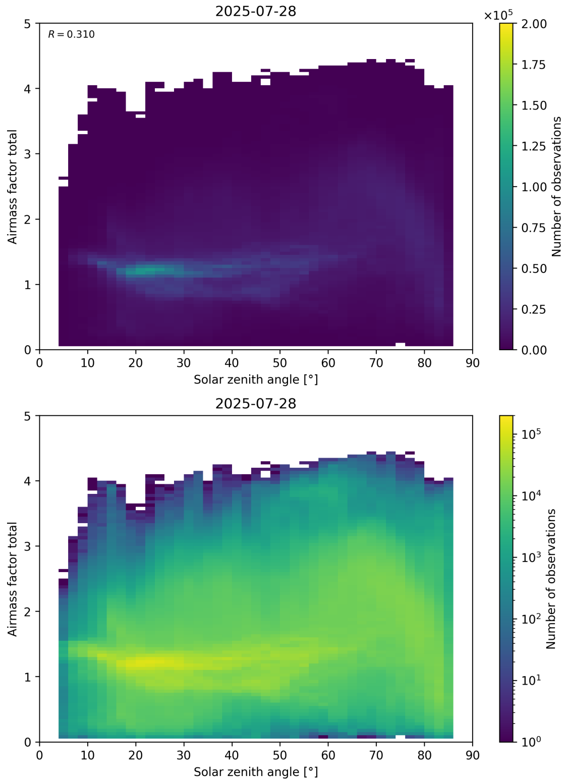
Figure 175: Scatter density plot of “Solar zenith angle” against “Airmass factor total” for 2025-07-27 to 2025-07-29.
