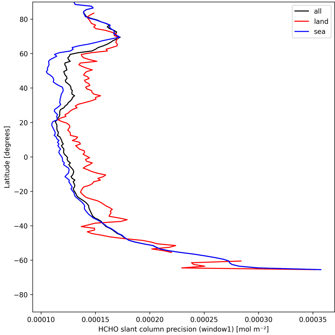
Figure 25: Zonal average of “HCHO slant column precision (window1)” for 2025-07-27 to 2025-07-29.
