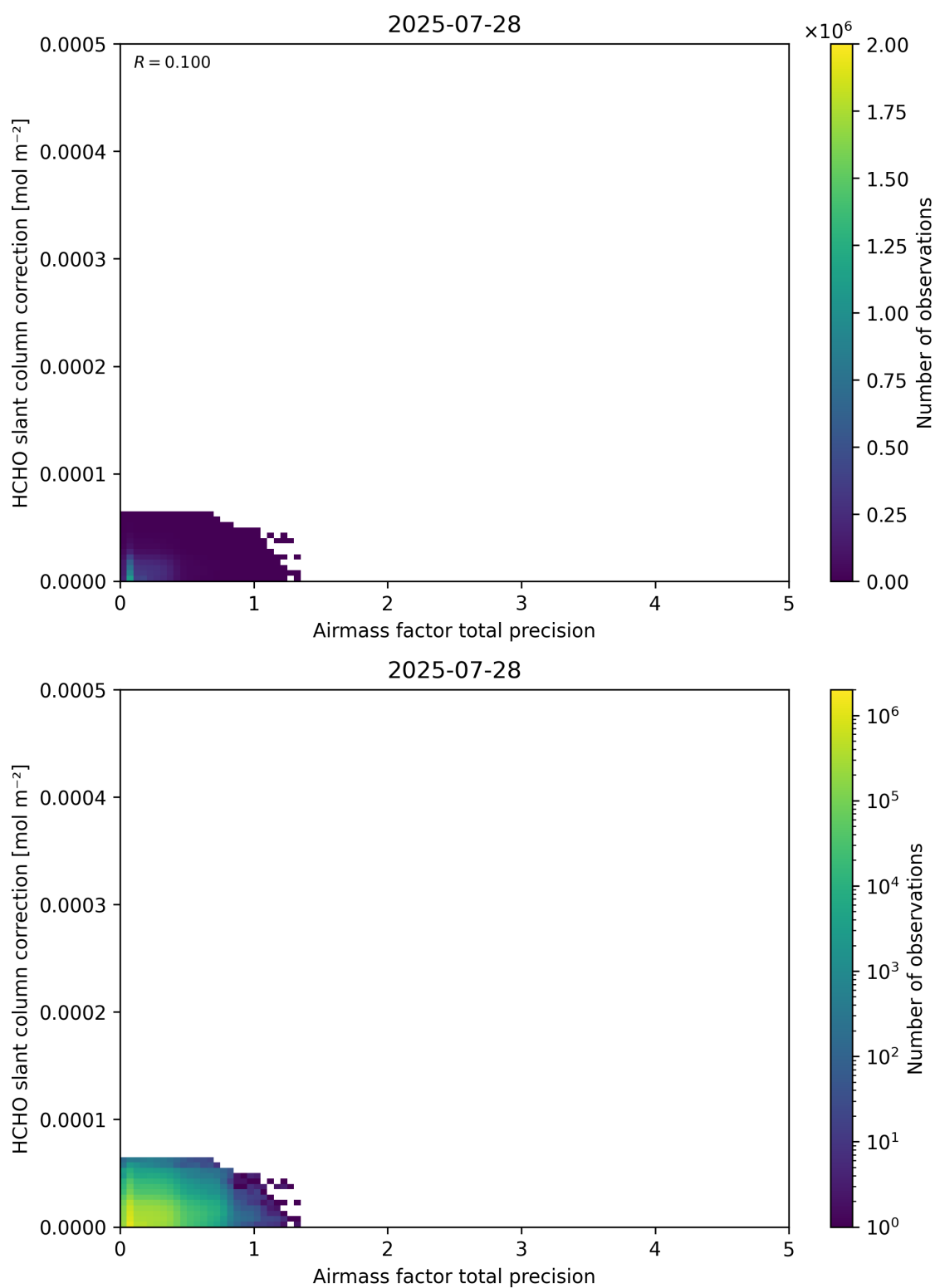
Figure 110: Scatter density plot of “Airmass factor total precision” against “HCHO slant column correction” for 2025-07-27 to 2025-07-29.
