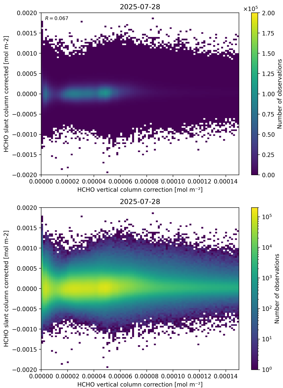
Figure 116: Scatter density plot of “HCHO vertical column correction” against “HCHO slant column corrected” for 2025-07-27 to 2025-07-29.
