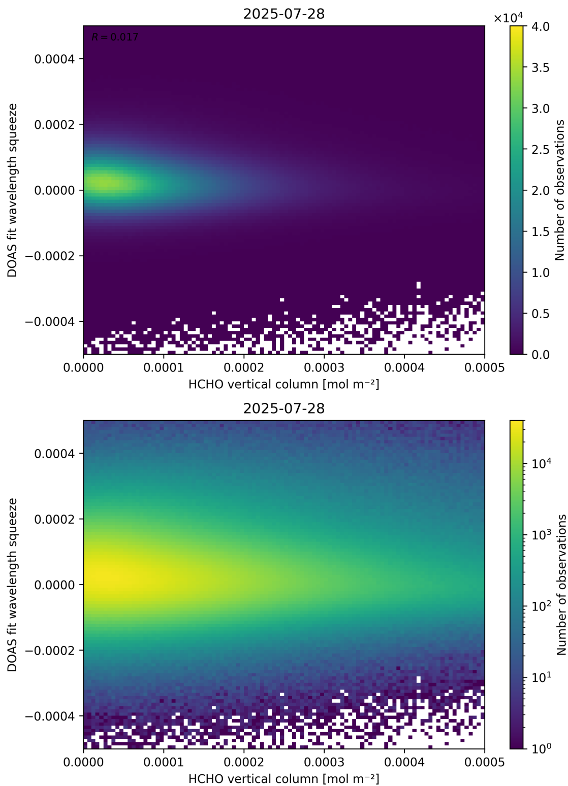
Figure 125: Scatter density plot of “HCHO vertical column” against “DOAS fit wavelength squeeze” for 2025-07-27 to 2025-07-29.
