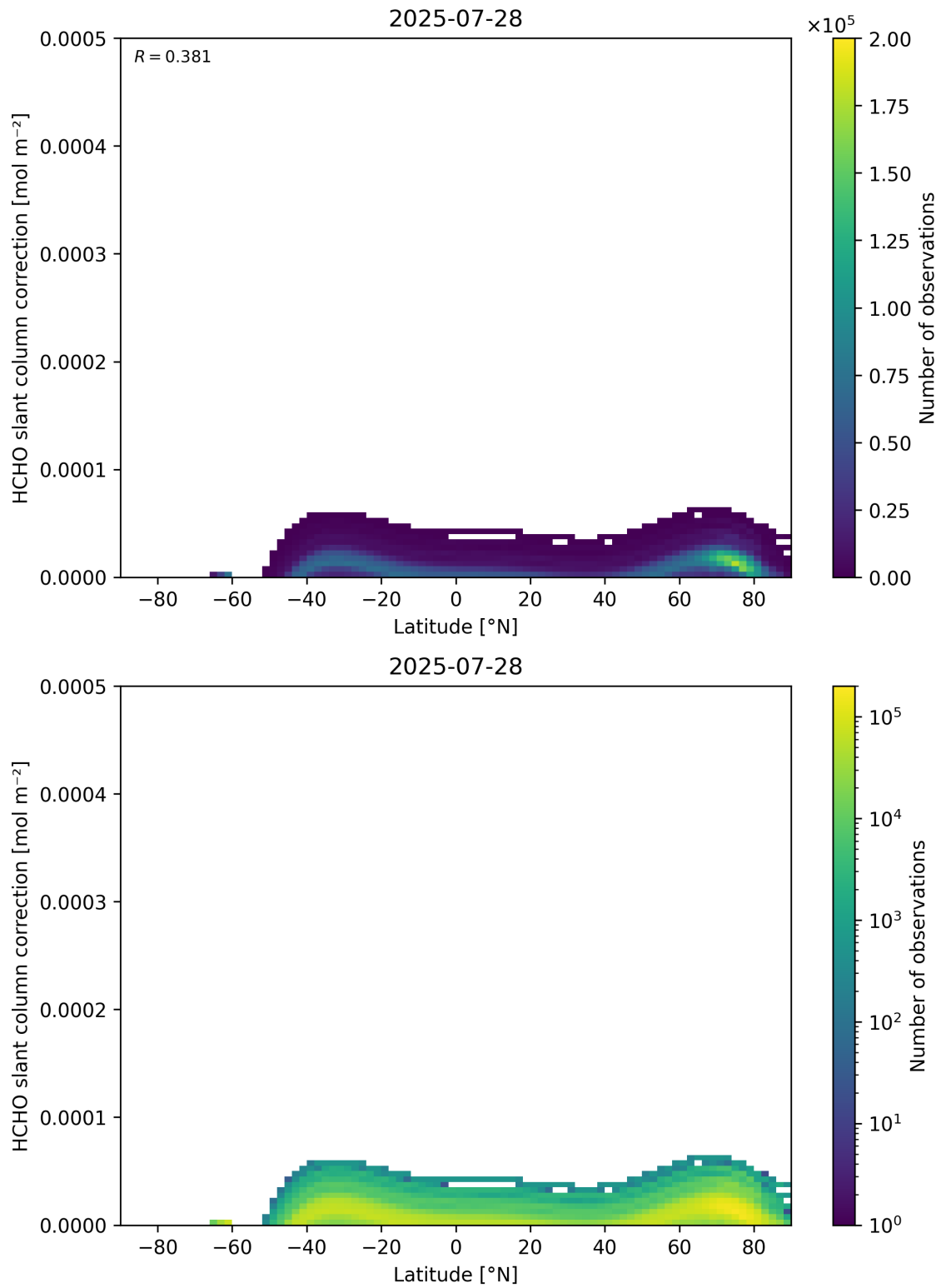
Figure 158: Scatter density plot of “Latitude” against “HCHO slant column correction” for 2025-07-27 to 2025-07-29.
