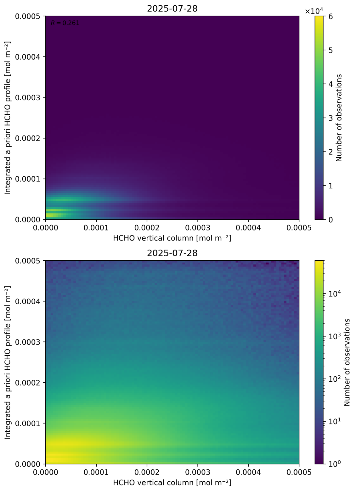
Figure 135: Scatter density plot of “HCHO vertical column” against “Integrated a priori HCHO profile” for 2025-07-27 to 2025-07-29.
