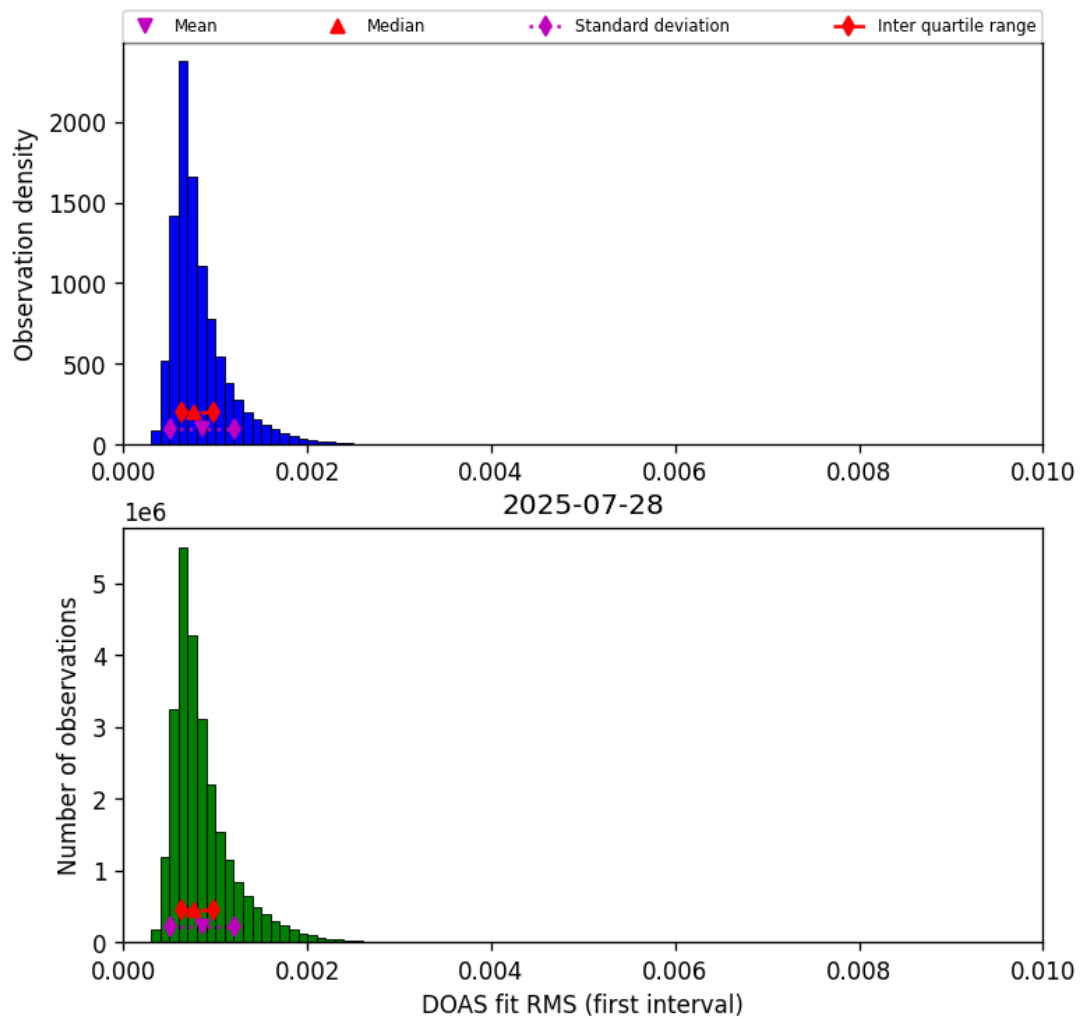
Figure 46: Histogram of “DOAS fit RMS (first interval)” for 2025-07-27 to 2025-07-29
