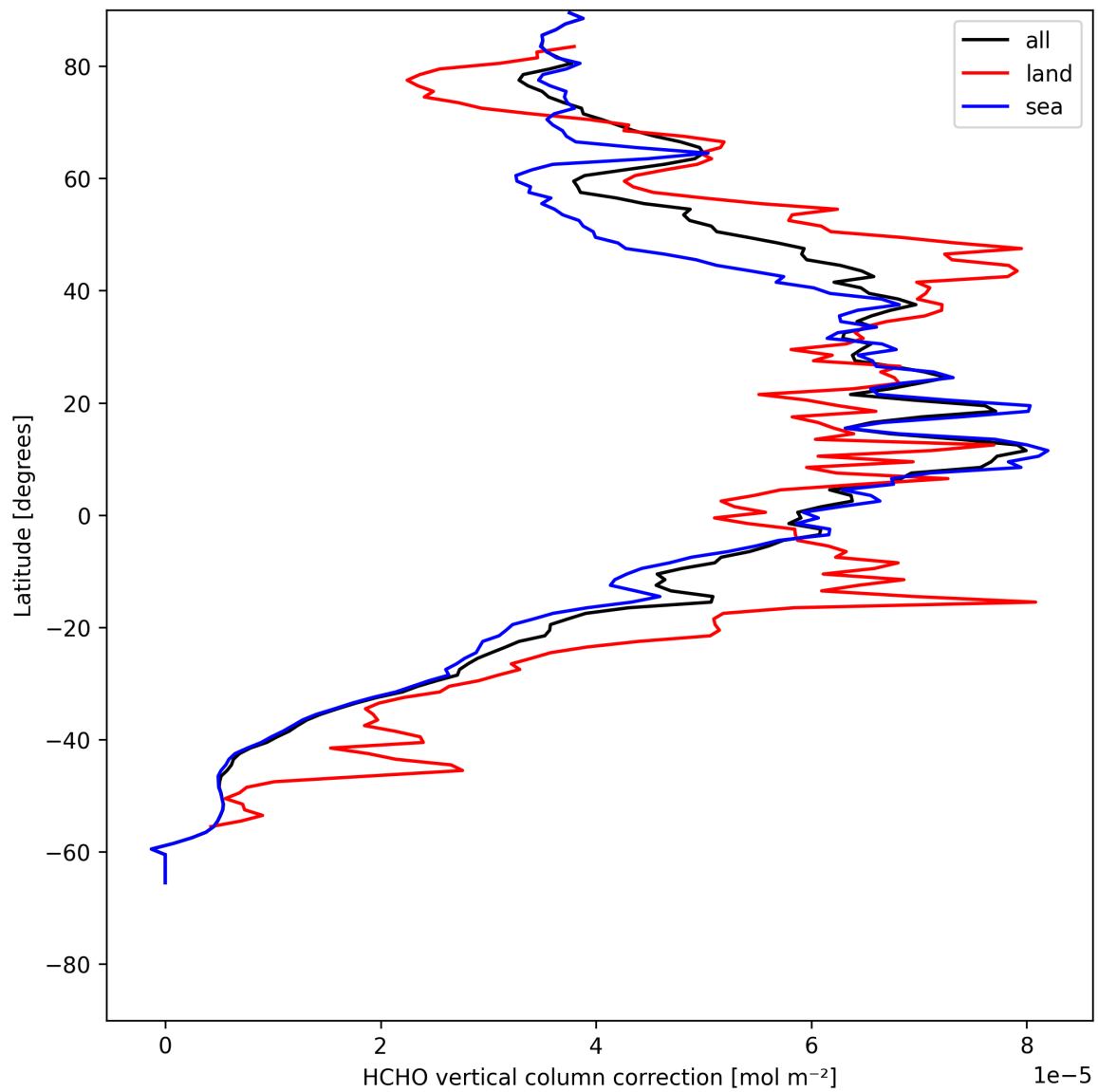
Figure 23: Zonal average of “HCHO vertical column correction” for 2025-07-27 to 2025-07-29.
