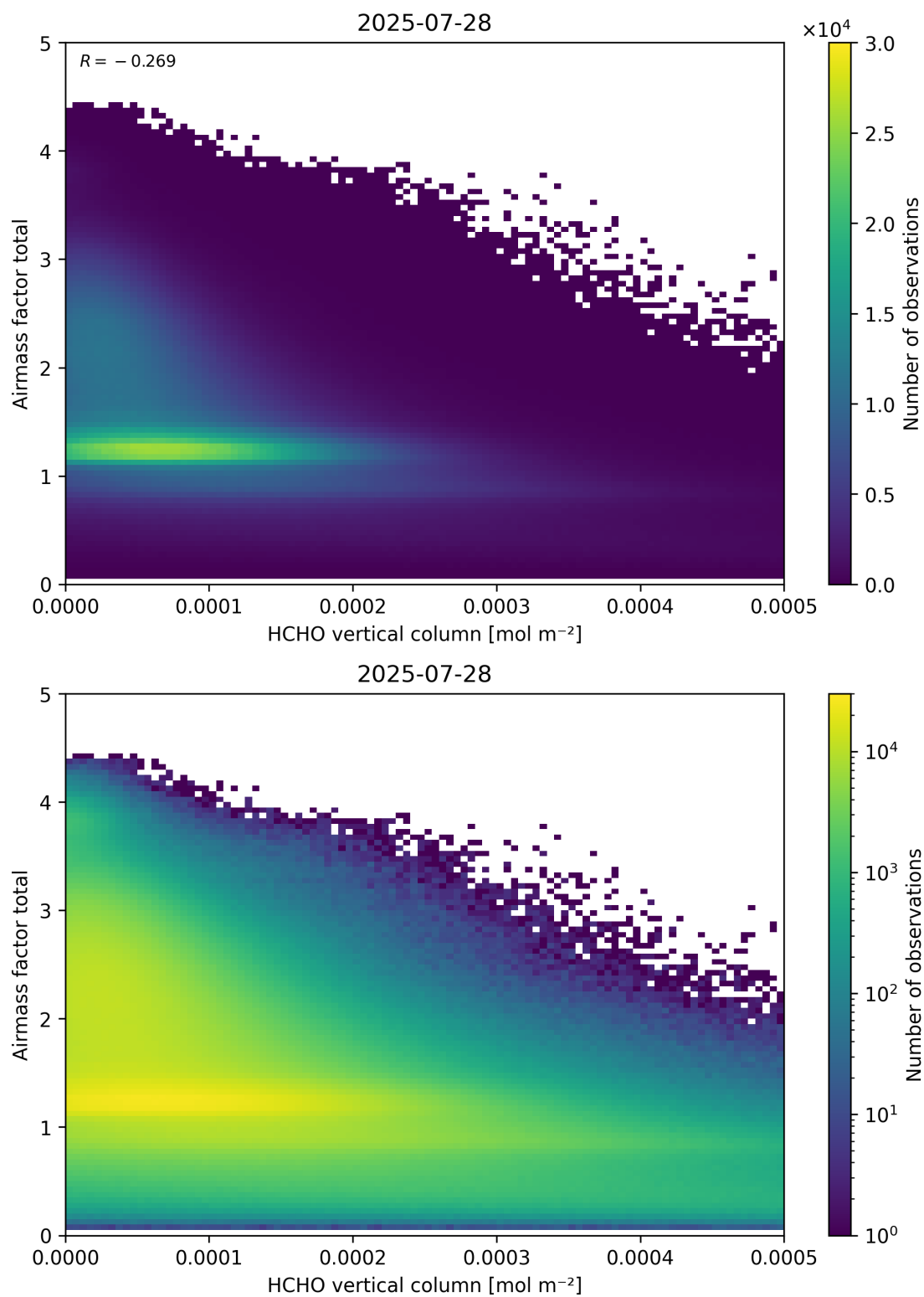
Figure 131: Scatter density plot of “HCHO vertical column” against “Airmass factor total” for 2025-07-27 to 2025-07-29.
