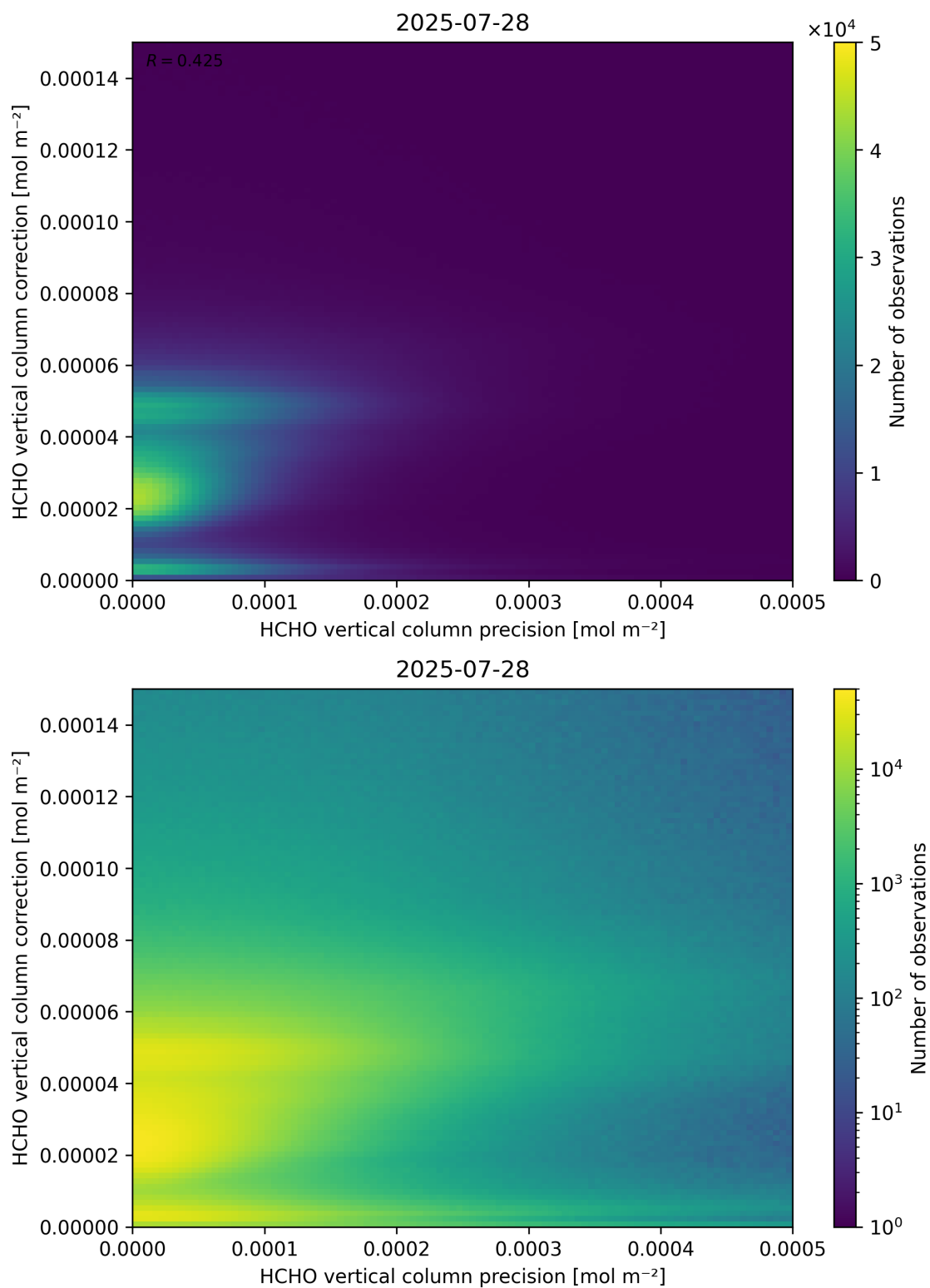
Figure 146: Scatter density plot of “HCHO vertical column precision” against “HCHO vertical column correction” for 2025-07-27 to 2025-07-29.
