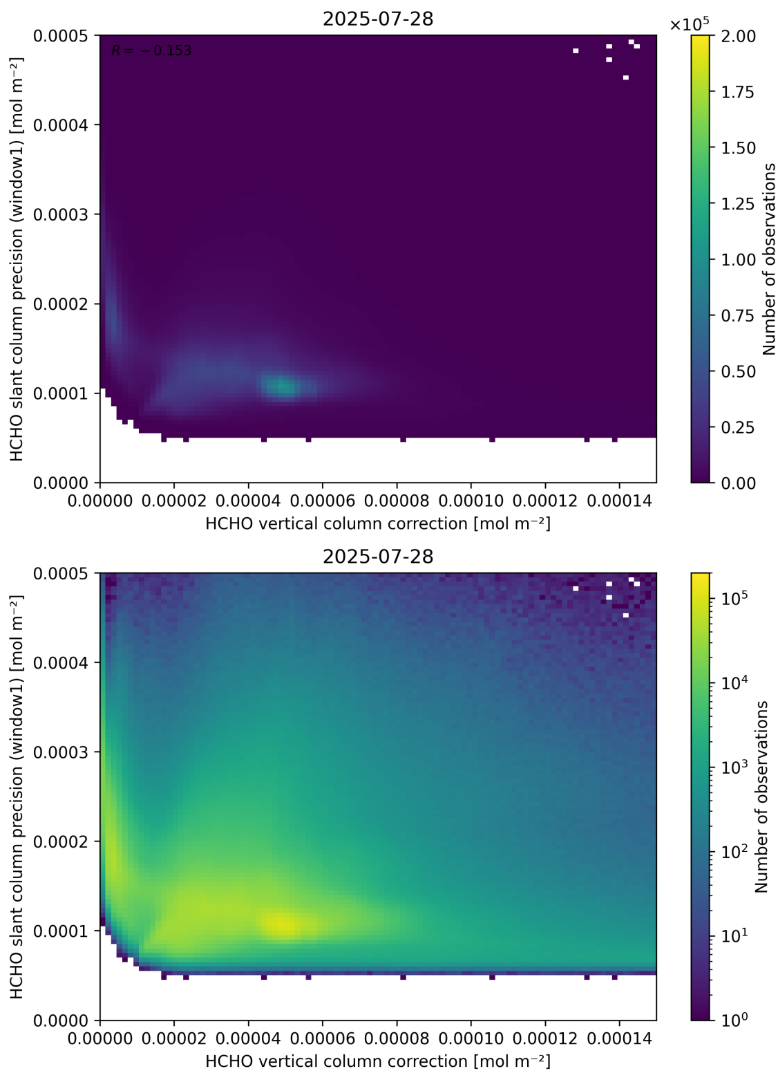
Figure 119: Scatter density plot of “HCHO vertical column correction” against “HCHO slant column precision (window1)” for 2025-07-27 to 2025-07-29.
