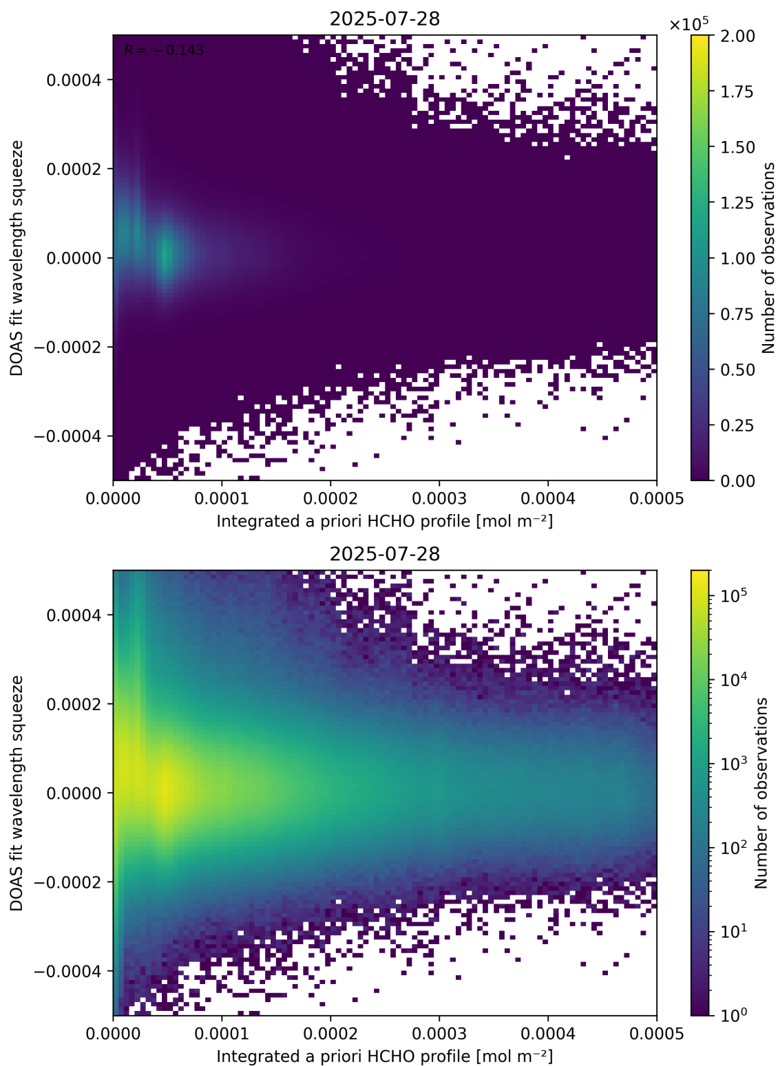
Figure 150: Scatter density plot of “Integrated a priori HCHO profile” against “DOAS fit wavelength squeeze” for 2025-07-27 to 2025-07-29.
