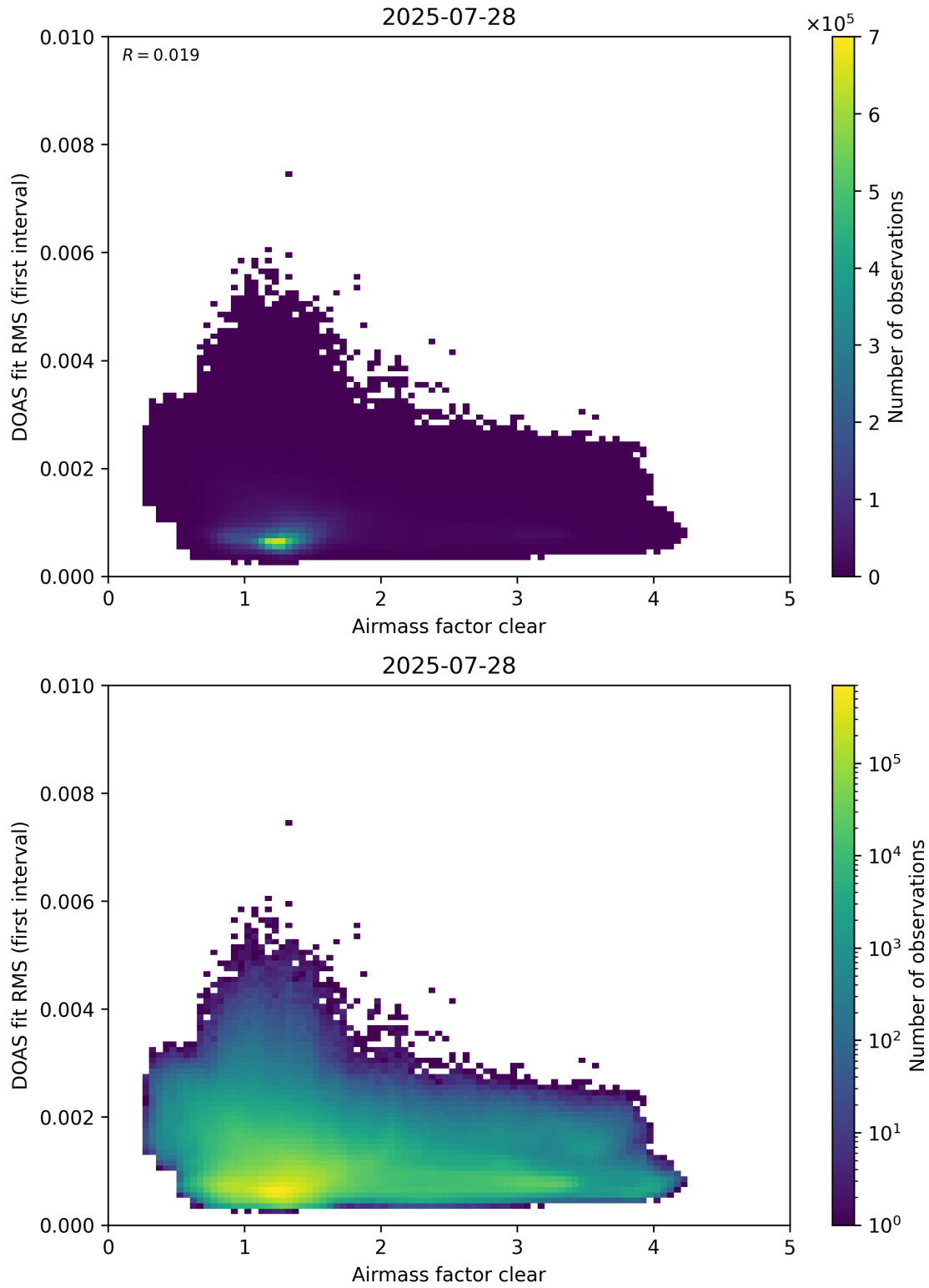
Figure 71: Scatter density plot of “Airmass factor clear” against “DOAS fit RMS (first interval)” for 2025-07-27 to 2025-07-29.
