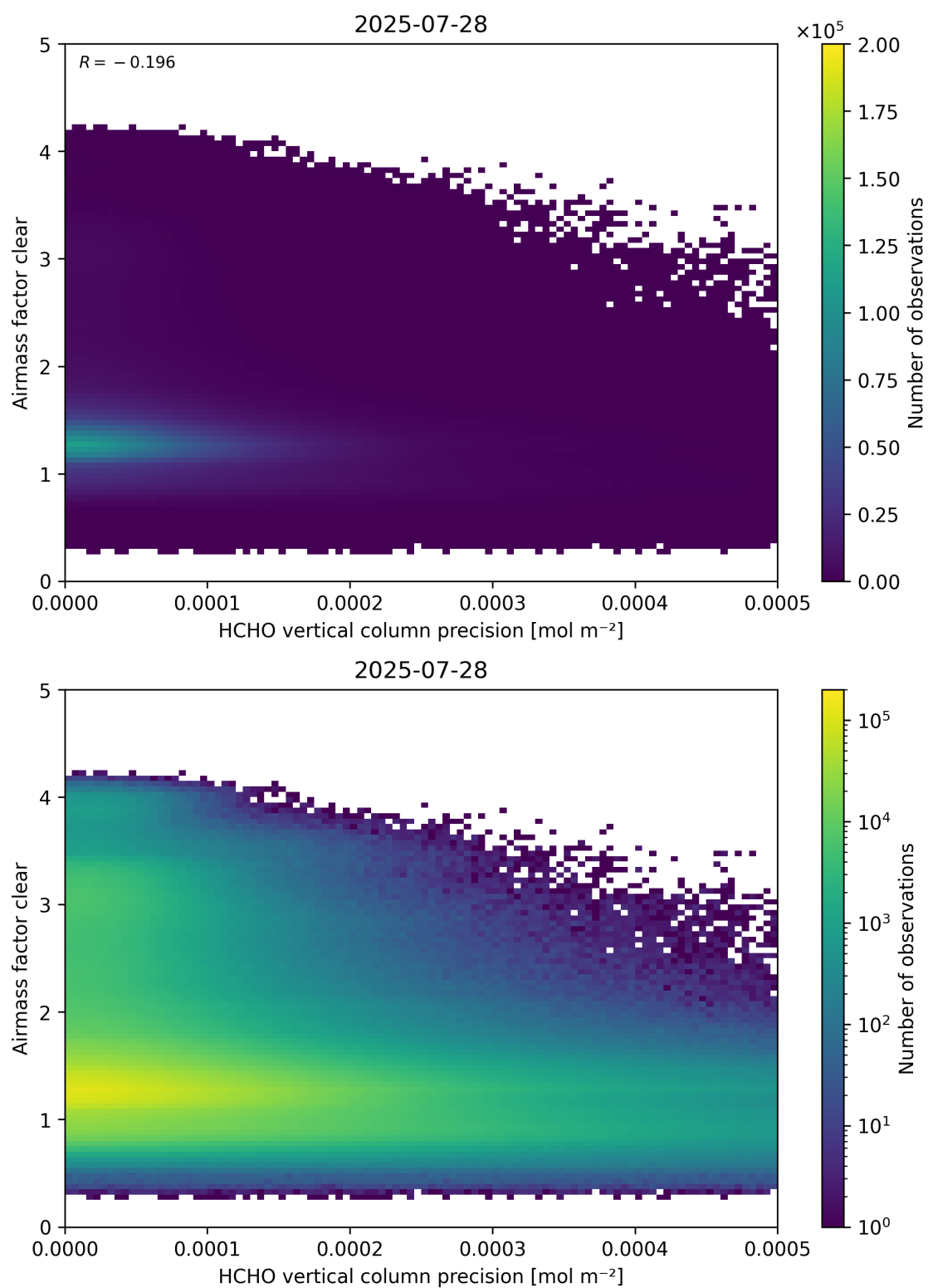
Figure 139: Scatter density plot of “HCHO vertical column precision” against “Airmass factor clear” for 2025-07-27 to 2025-07-29.
