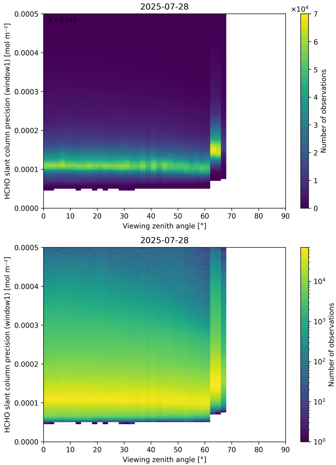
Figure 189: Scatter density plot of “Viewing zenith angle” against “HCHO slant column precision (window1)” for 2025-07-27 to 2025-07-29.
