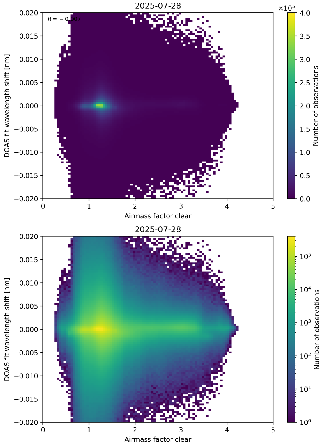
Figure 72: Scatter density plot of “Airmass factor clear” against “DOAS fit wavelength shift” for 2025-07-27 to 2025-07-29.
