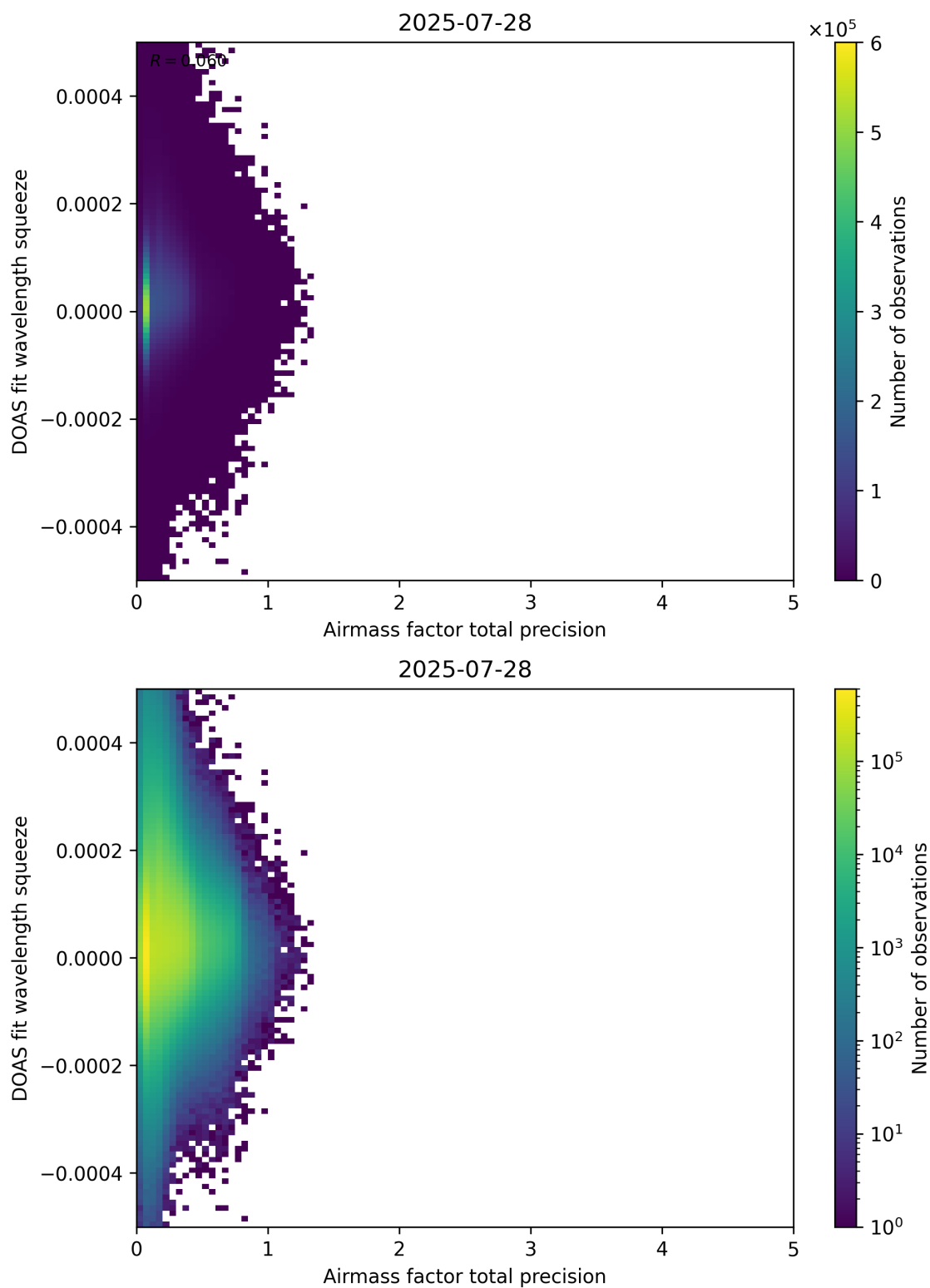
Figure 107: Scatter density plot of “Airmass factor total precision” against “DOAS fit wavelength squeeze” for 2025-07-27 to 2025-07-29.
