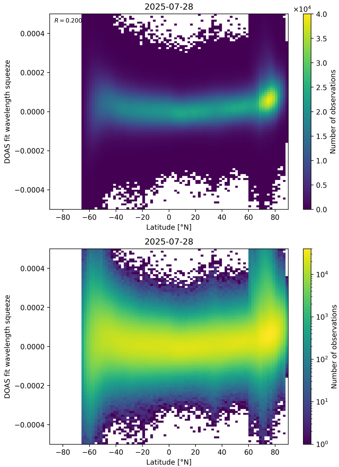
Figure 155: Scatter density plot of “Latitude” against “DOAS fit wavelength squeeze” for 2025-07-27 to 2025-07-29.
