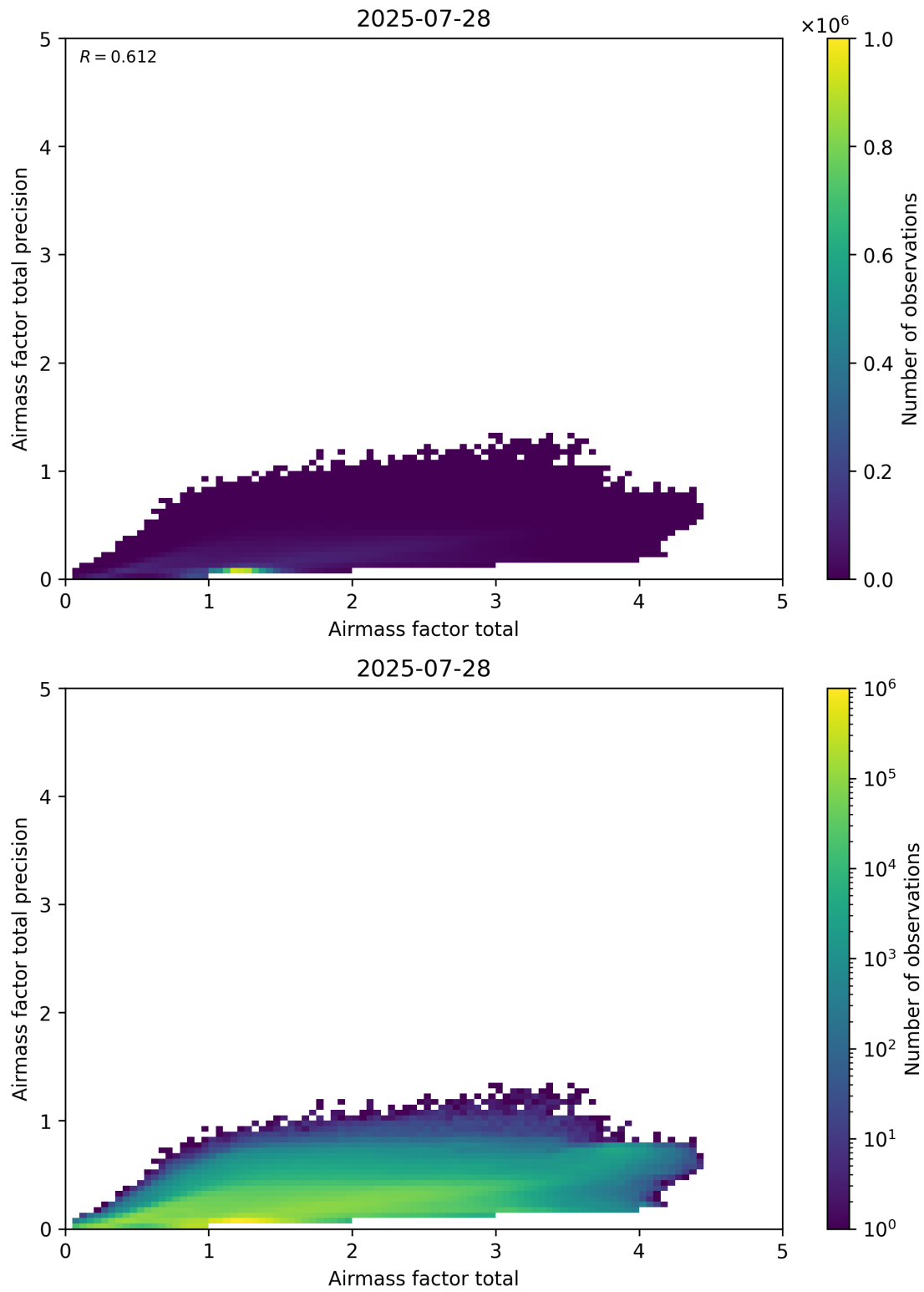
Figure 103: Scatter density plot of “Airmass factor total” against “Airmass factor total precision” for 2025-07-27 to 2025-07-29.
