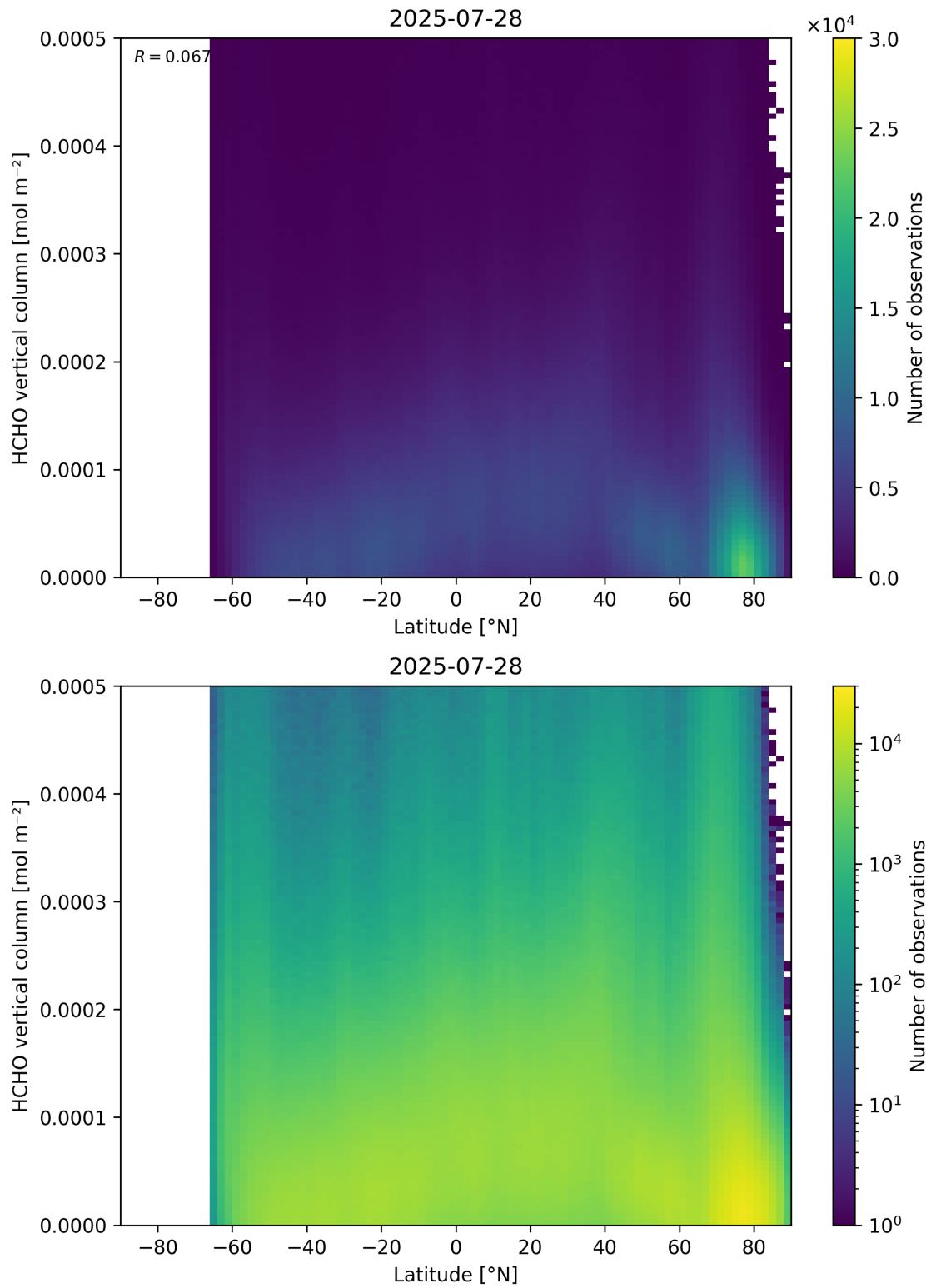
Figure 163: Scatter density plot of “Latitude” against “HCHO vertical column” for 2025-07-27 to 2025-07-29.
