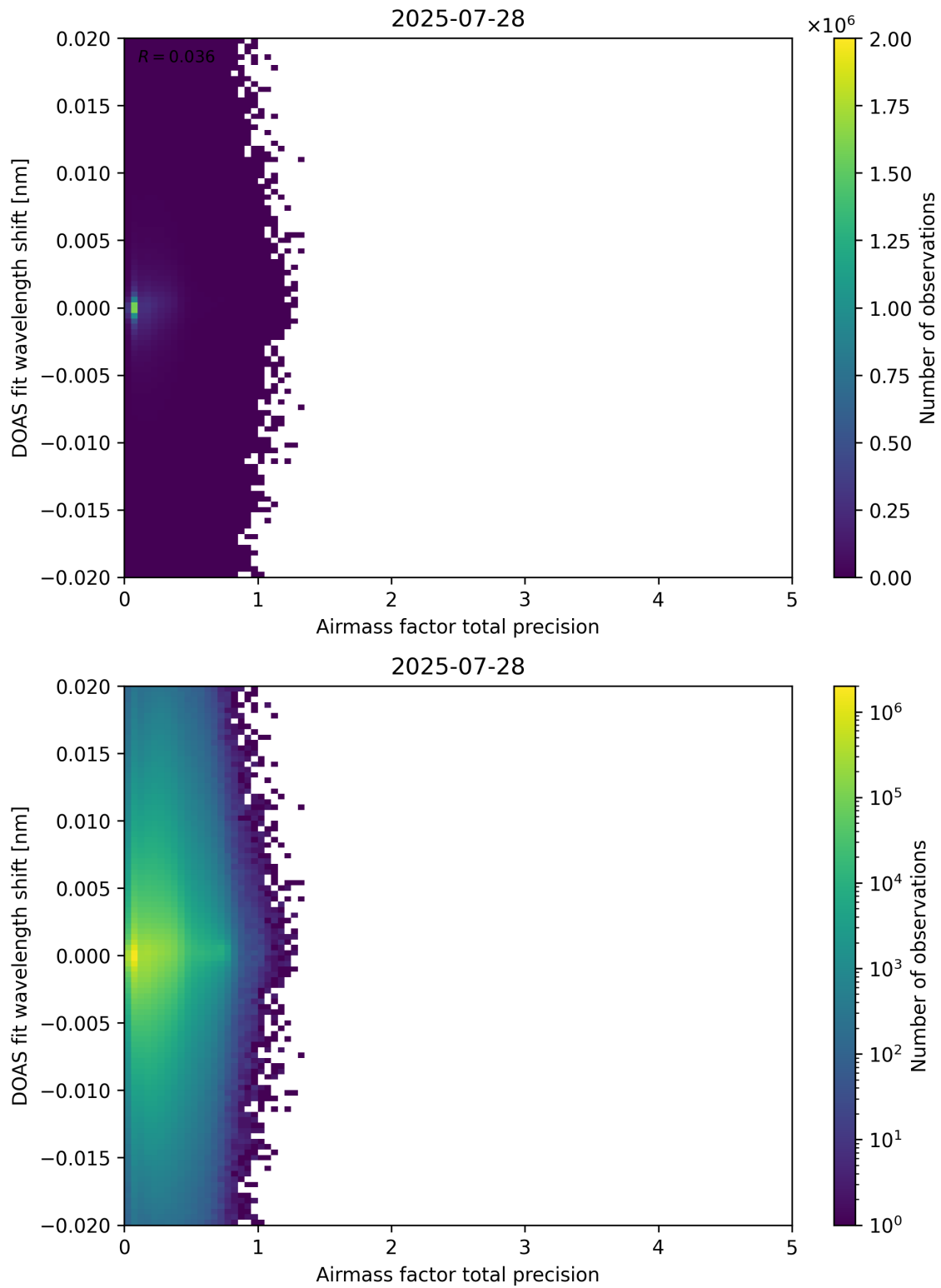
Figure 106: Scatter density plot of “Airmass factor total precision” against “DOAS fit wavelength shift” for 2025-07-27 to 2025-07-29.
