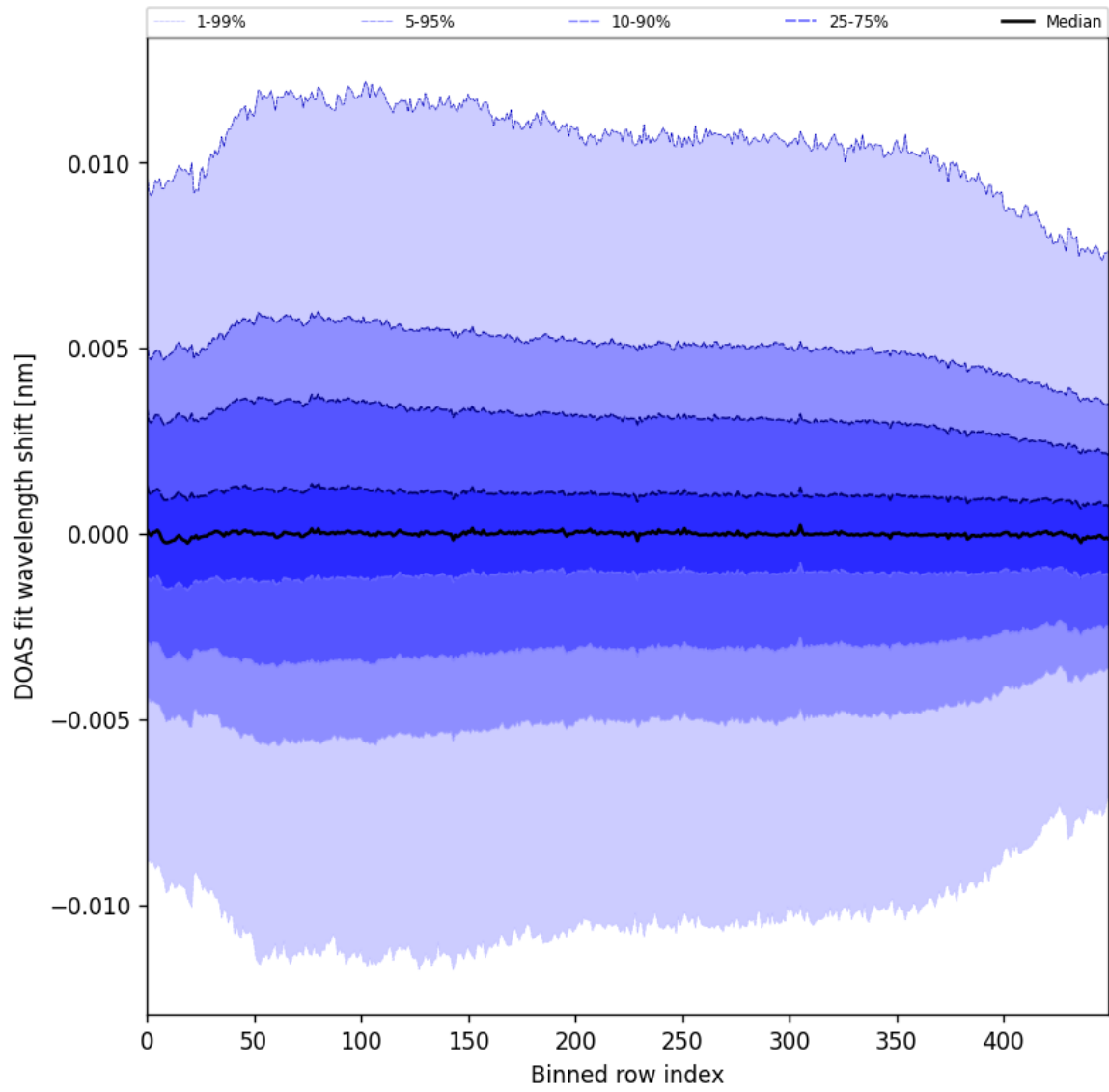
Figure 58: Along track statistics of “DOAS fit wavelength shift” for 2025-07-27 to 2025-07-29
