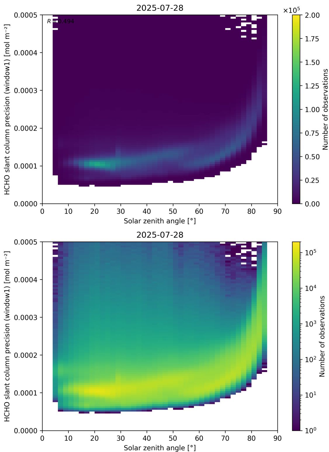
Figure 174: Scatter density plot of “Solar zenith angle” against “HCHO slant column precision (window1)” for 2025-07-27 to 2025-07-29.
