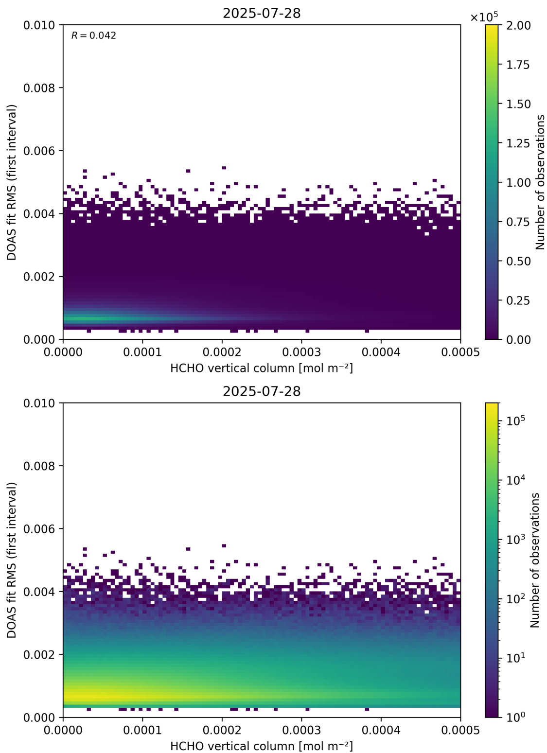
Figure 123: Scatter density plot of “HCHO vertical column” against “DOAS fit RMS (first interval)” for 2025-07-27 to 2025-07-29.
