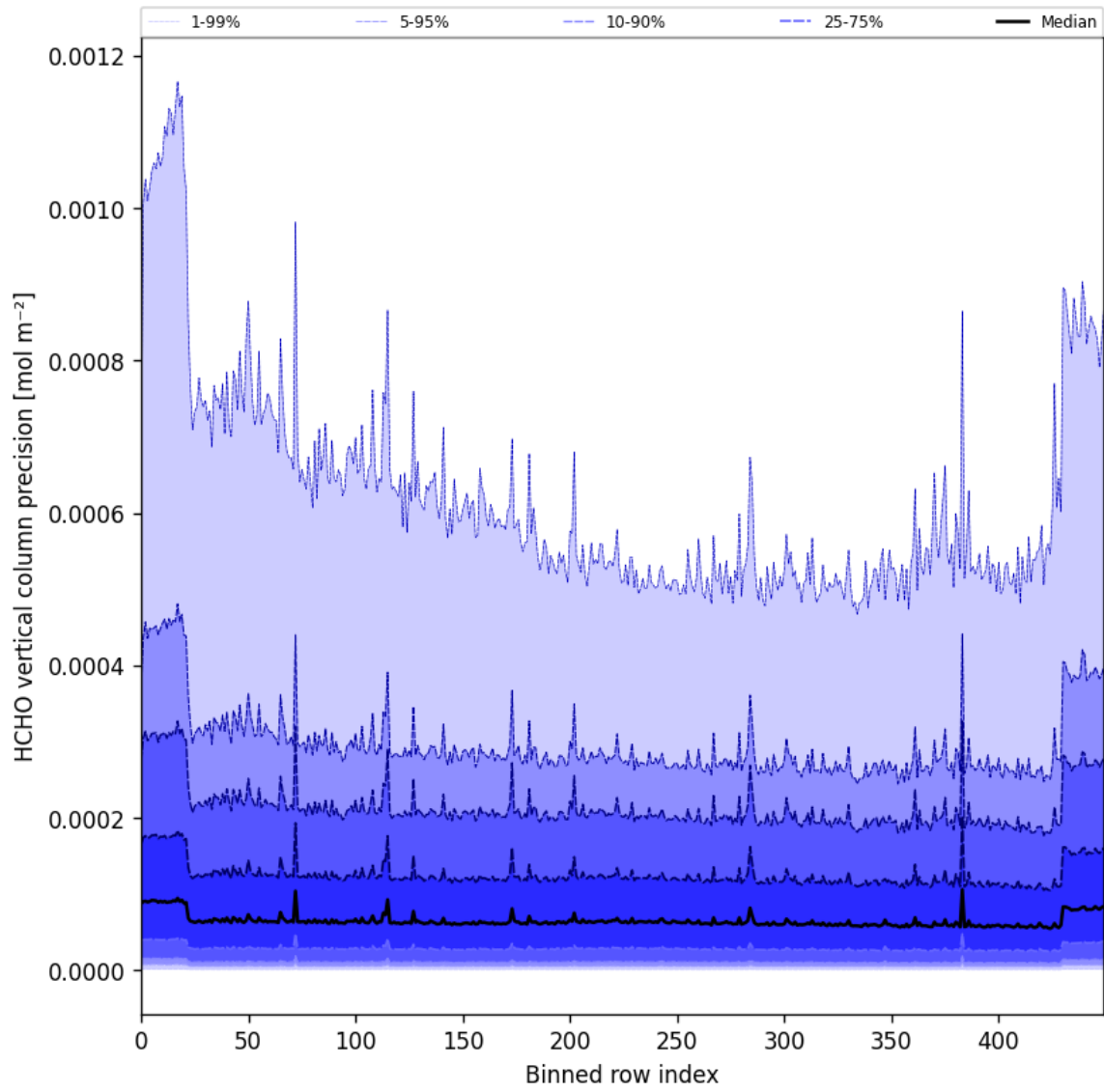
Figure 50: Along track statistics of “HCHO vertical column precision” for 2025-07-27 to 2025-07-29
