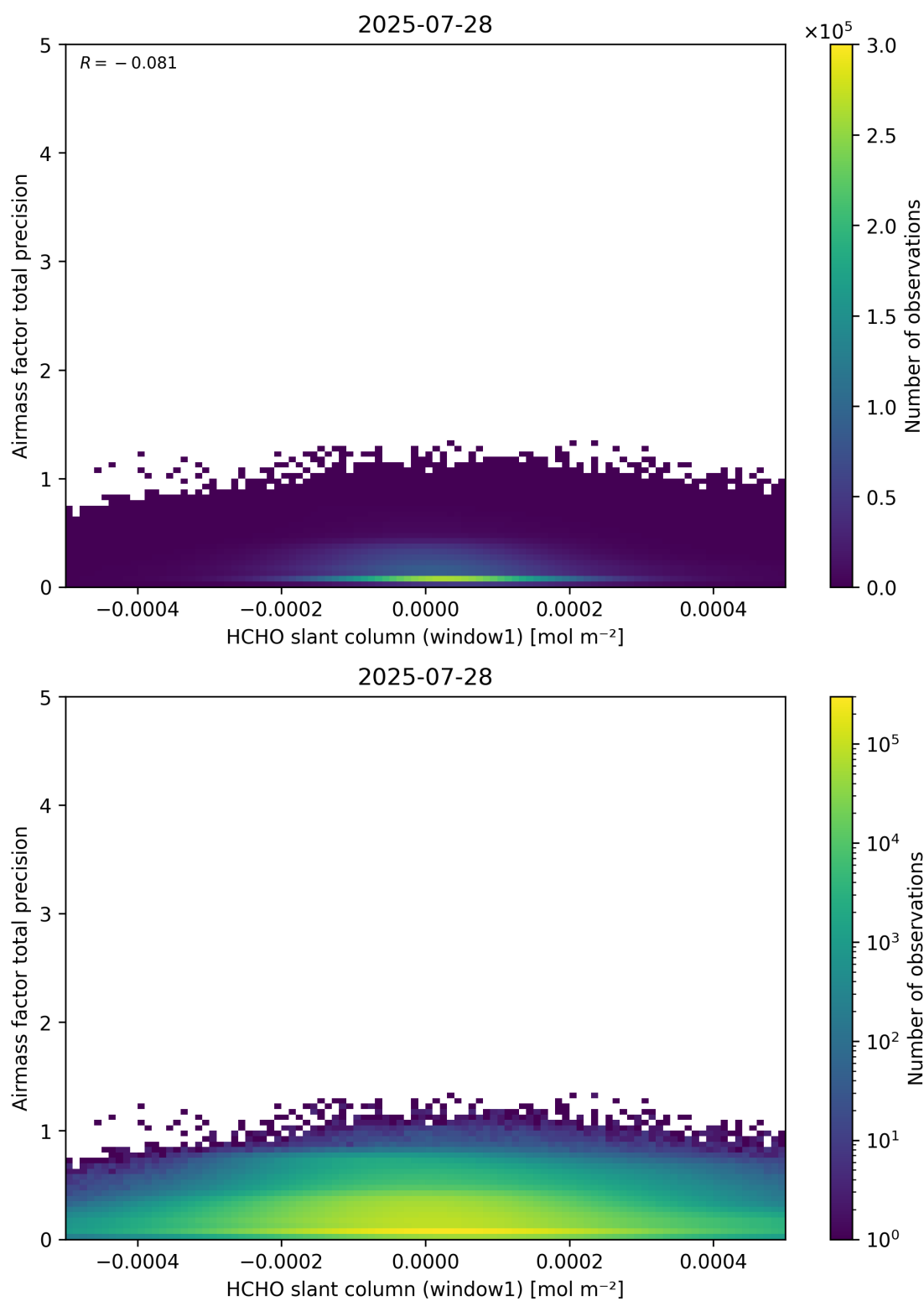
Figure 86: Scatter density plot of “HCHO slant column (window1)” against “Airmass factor total precision” for 2025-07-27 to 2025-07-29.
