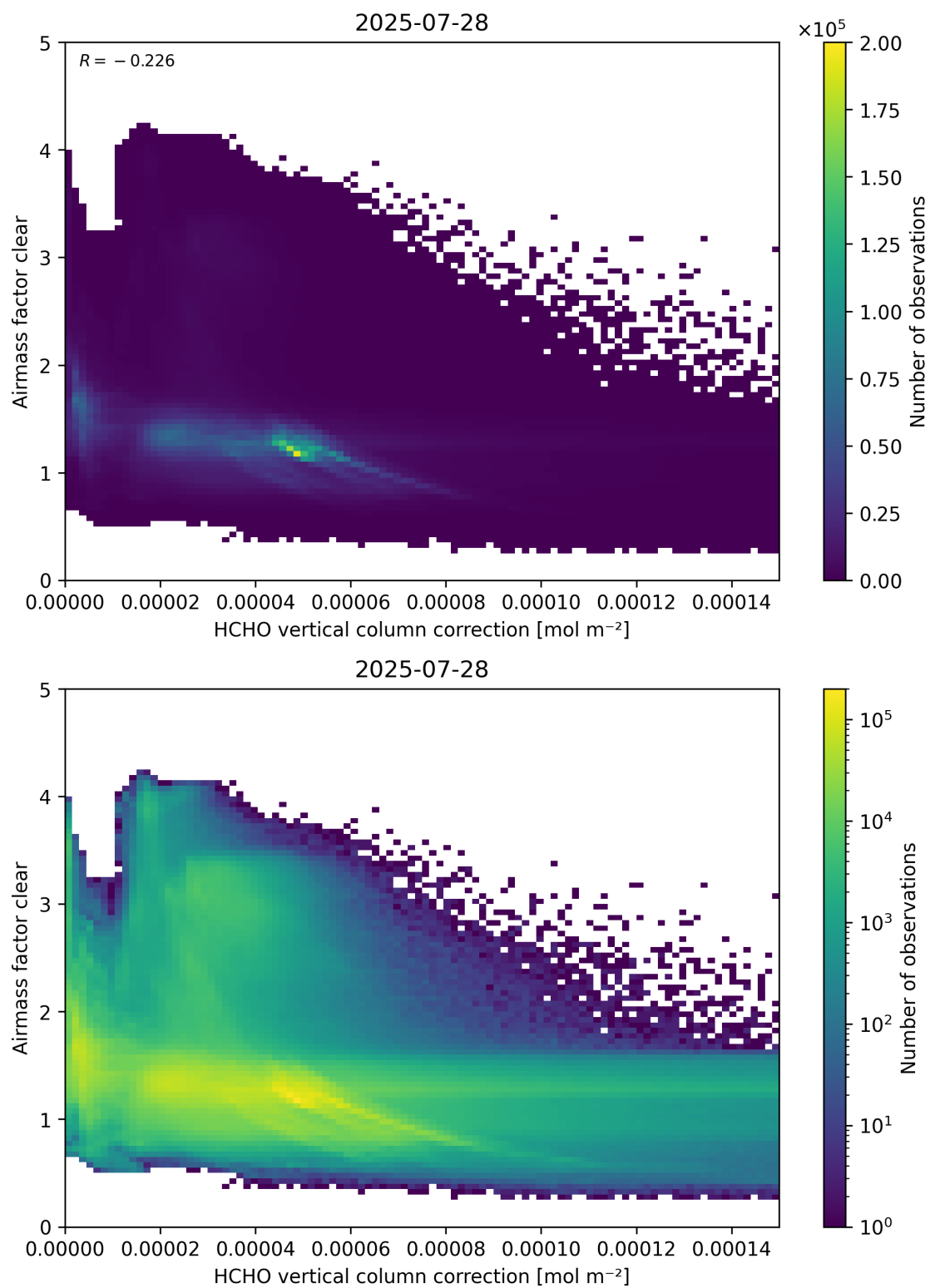
Figure 115: Scatter density plot of “HCHO vertical column correction” against “Airmass factor clear” for 2025-07-27 to 2025-07-29.
