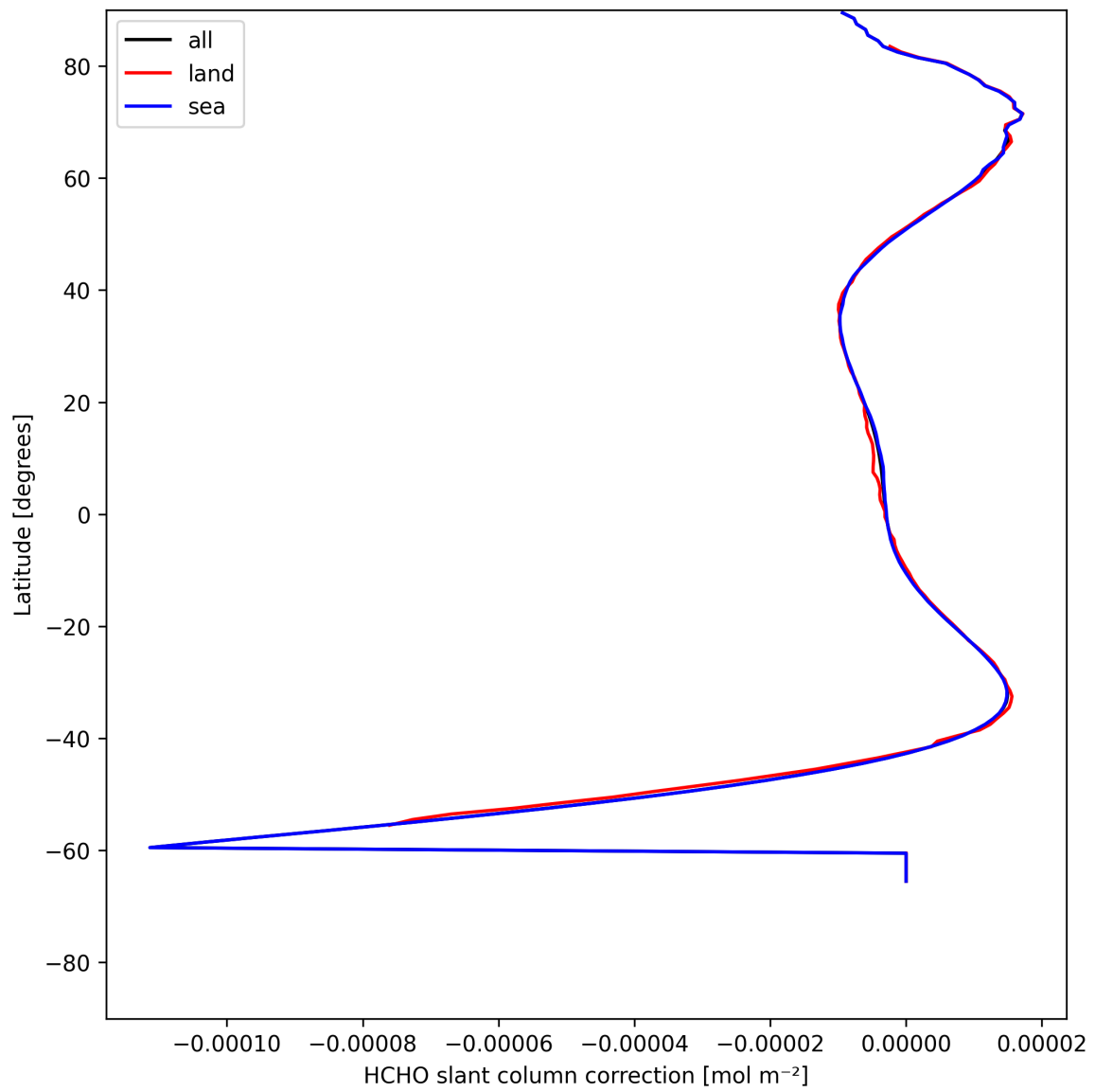
Figure 33: Zonal average of “HCHO slant column correction” for 2025-07-27 to 2025-07-29.
