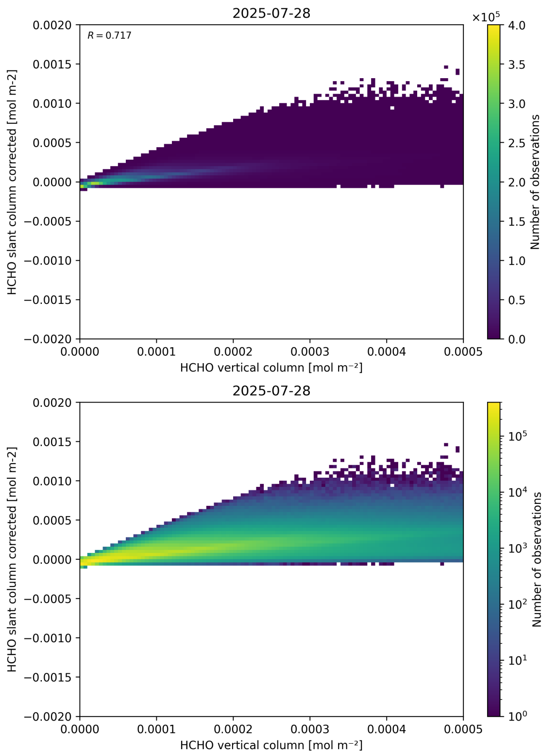
Figure 127: Scatter density plot of “HCHO vertical column” against “HCHO slant column corrected” for 2025-07-27 to 2025-07-29.
