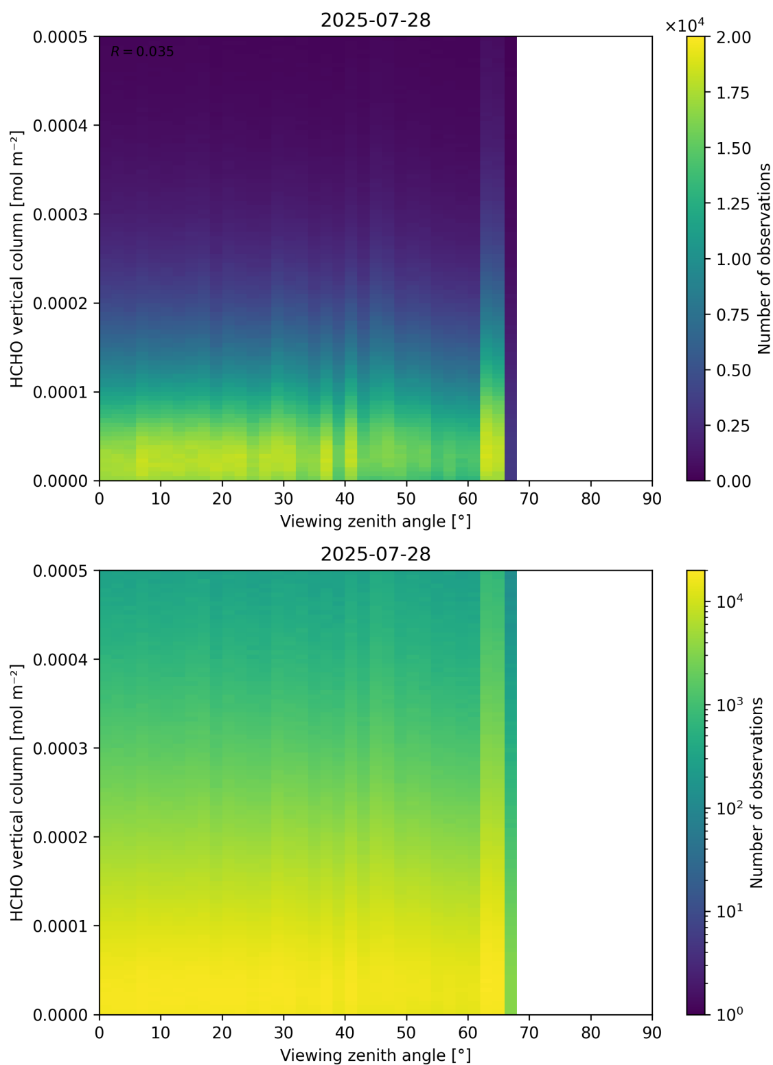
Figure 192: Scatter density plot of “Viewing zenith angle” against “HCHO vertical column” for 2025-07-27 to 2025-07-29.
