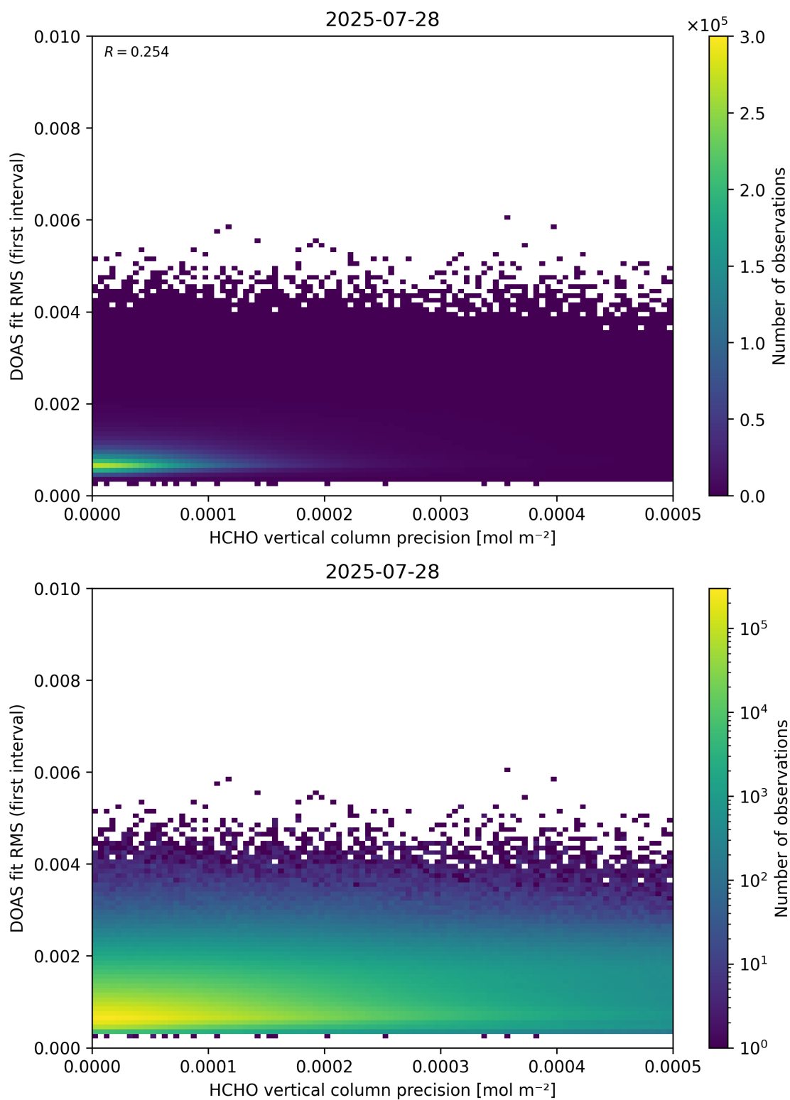
Figure 136: Scatter density plot of “HCHO vertical column precision” against “DOAS fit RMS (first interval)” for 2025-07-27 to 2025-07-29.
