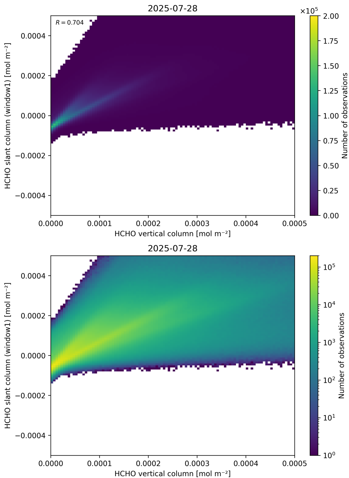
Figure 129: Scatter density plot of “HCHO vertical column” against “HCHO slant column (window1)” for 2025-07-27 to 2025-07-29.
