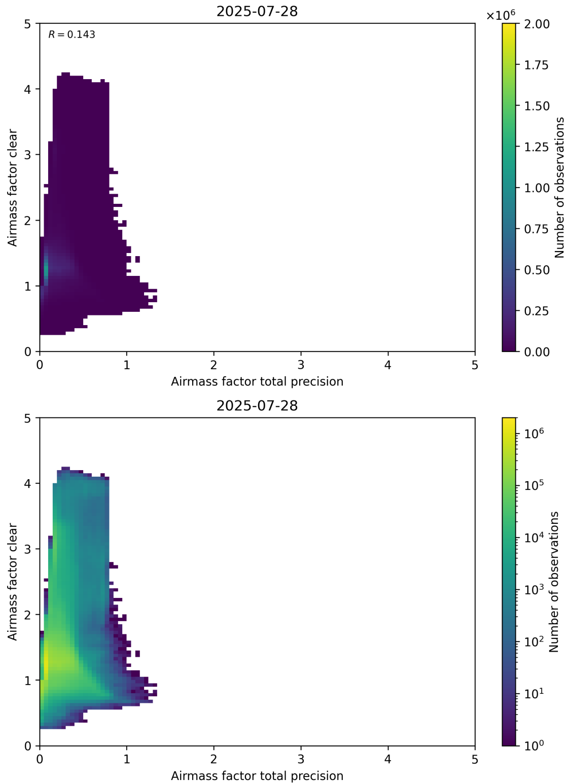
Figure 108: Scatter density plot of “Airmass factor total precision” against “Airmass factor clear” for 2025-07-27 to 2025-07-29.
