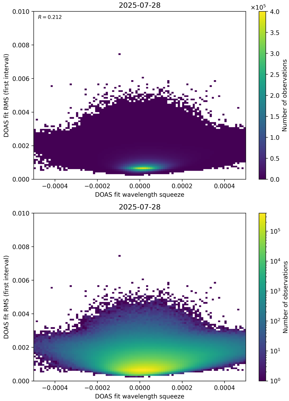
Figure 68: Scatter density plot of “DOAS fit wavelength squeeze” against “DOAS fit RMS (first interval)” for 2025-07-27 to 2025-07-29.
