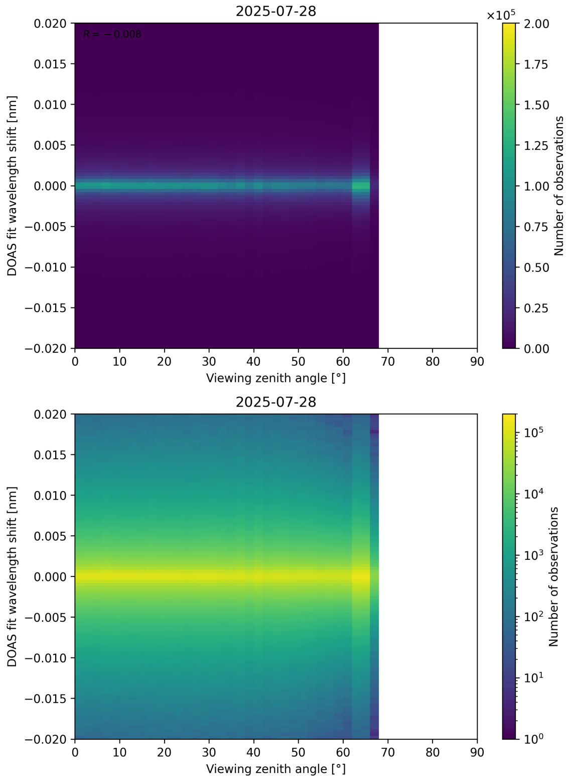
Figure 183: Scatter density plot of “Viewing zenith angle” against “DOAS fit wavelength shift” for 2025-07-27 to 2025-07-29.
