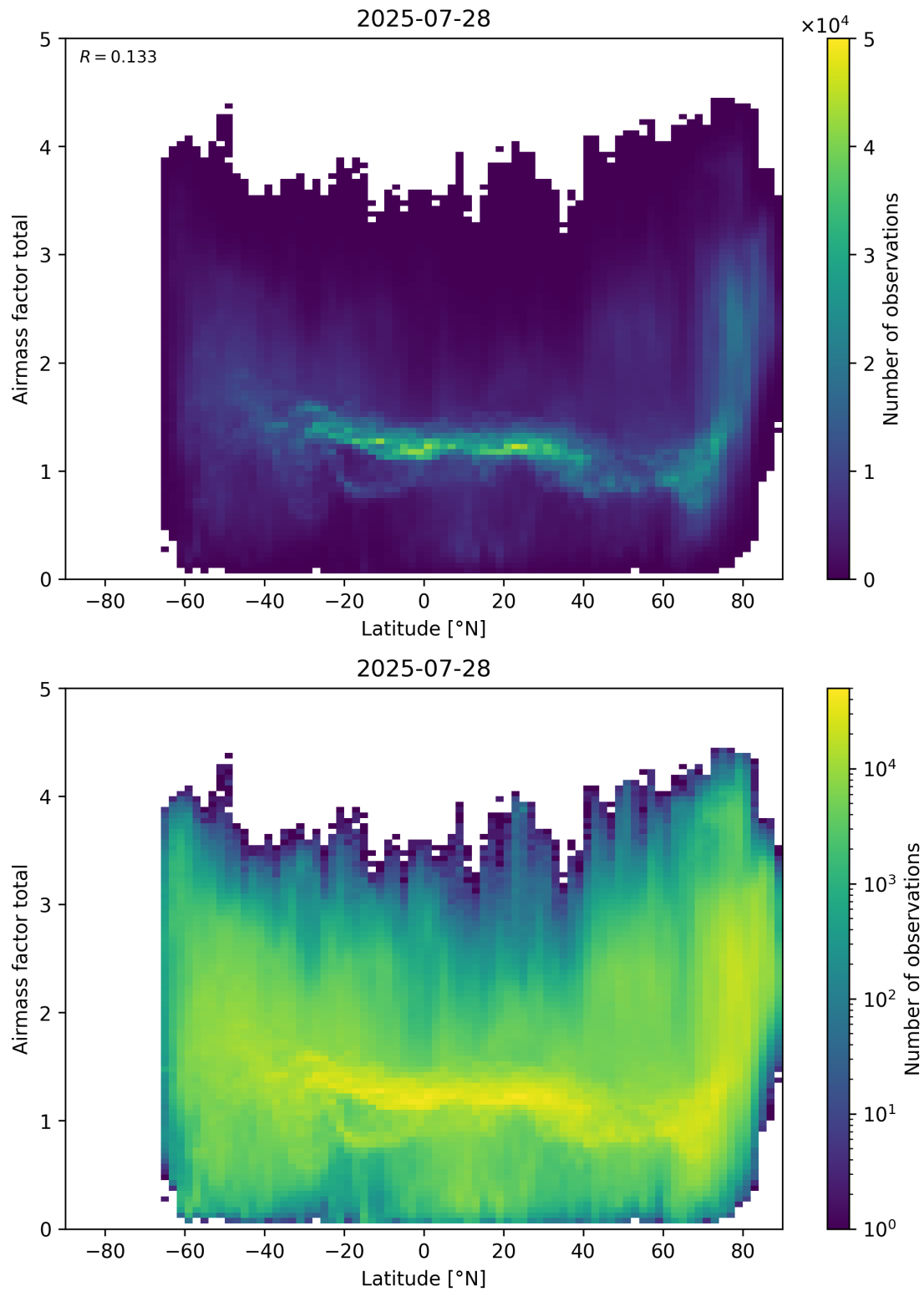
Figure 161: Scatter density plot of “Latitude” against “Airmass factor total” for 2025-07-27 to 2025-07-29.
