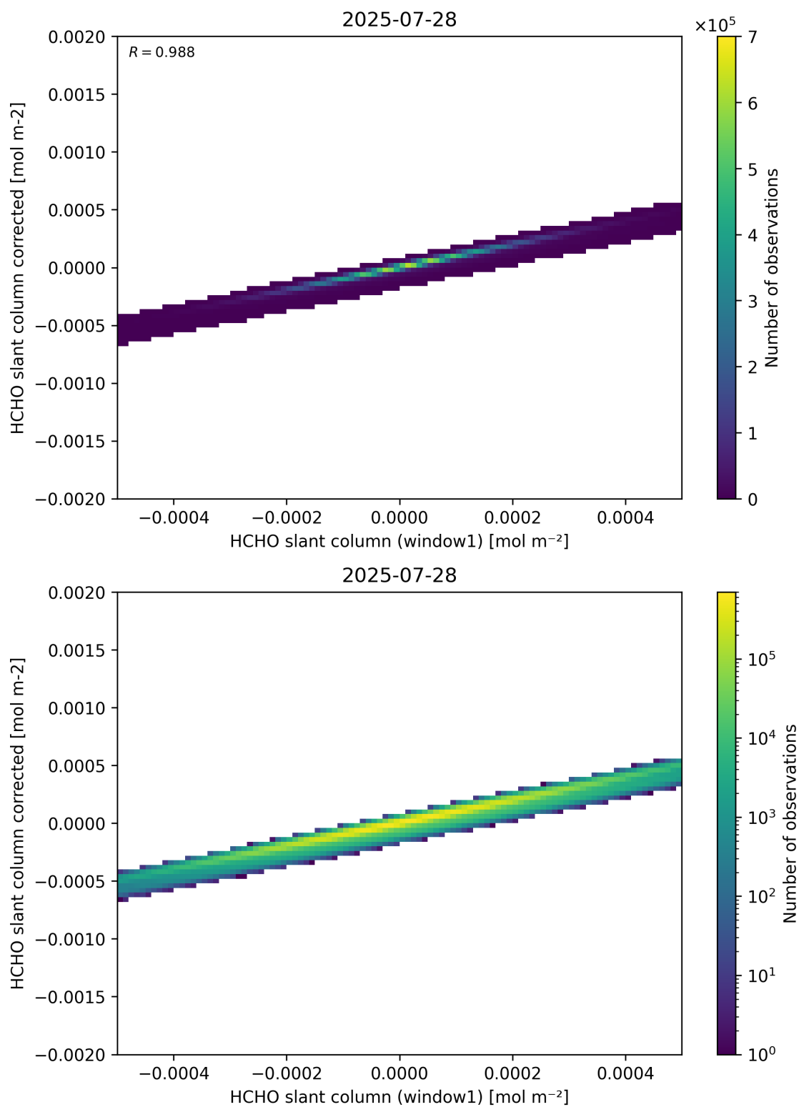
Figure 82: Scatter density plot of “HCHO slant column (window1)” against “HCHO slant column corrected” for 2025-07-27 to 2025-07-29.
