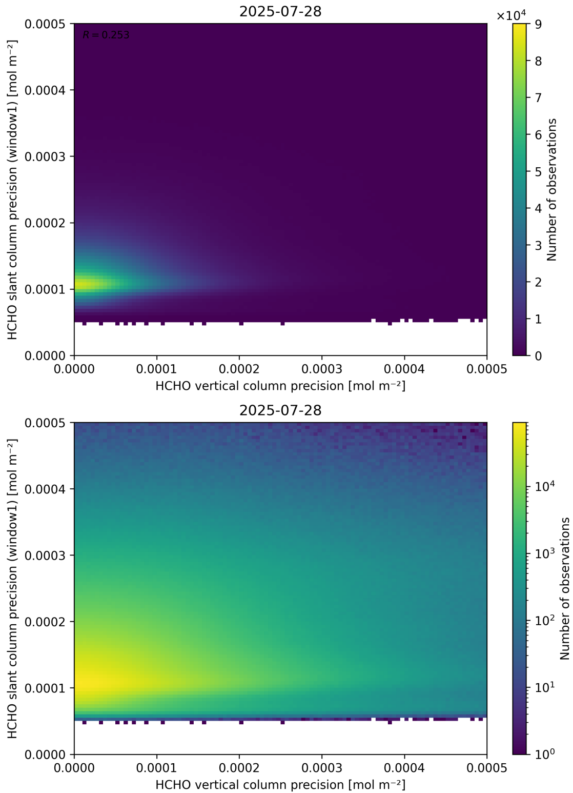
Figure 143: Scatter density plot of “HCHO vertical column precision” against “HCHO slant column precision (window1)” for 2025-07-27 to 2025-07-29.
