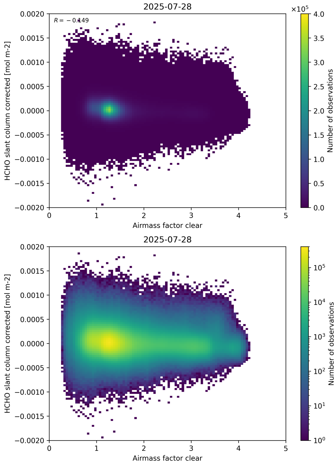
Figure 74: Scatter density plot of “Airmass factor clear” against “HCHO slant column corrected” for 2025-07-27 to 2025-07-29.
