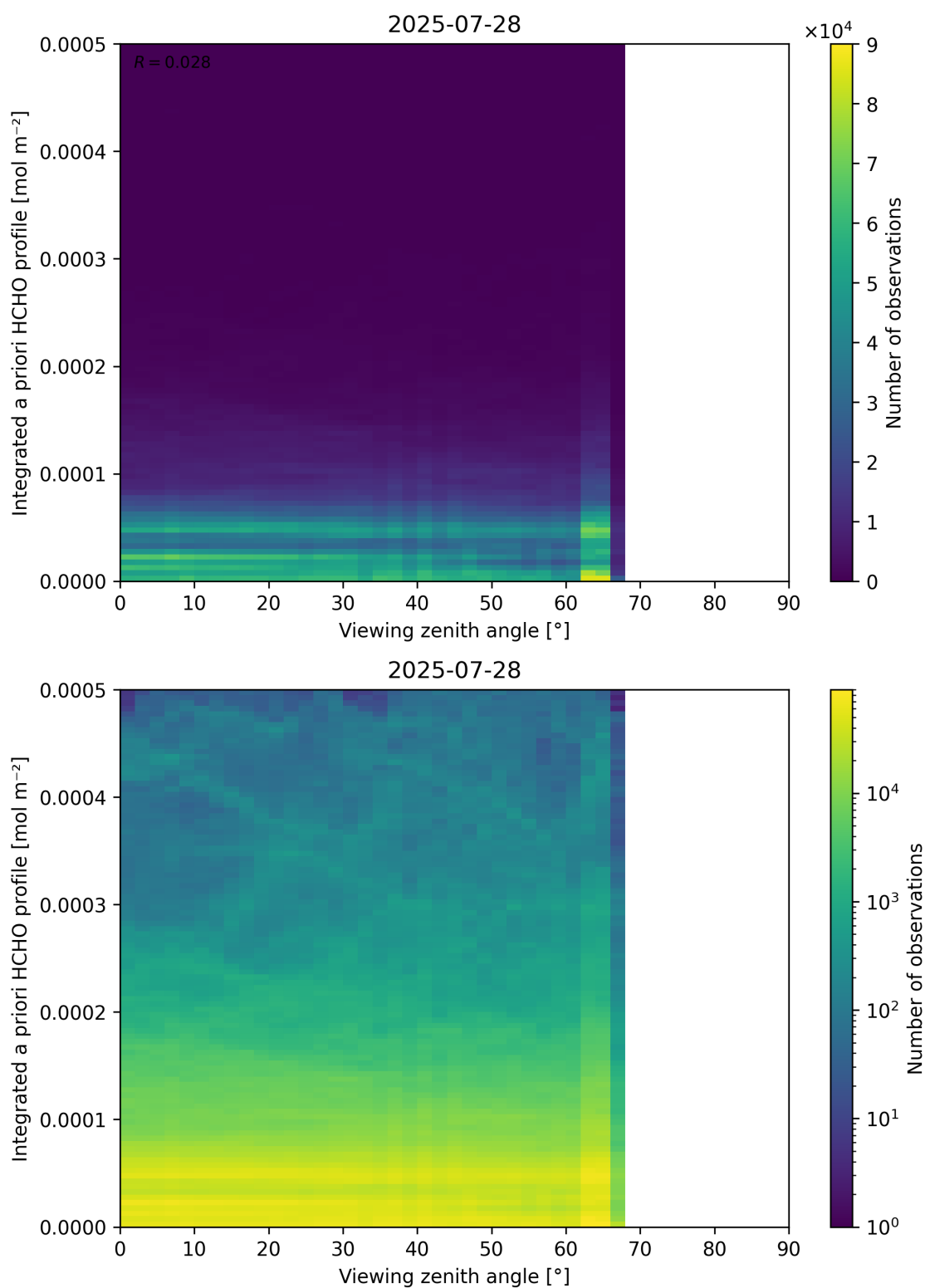
Figure 195: Scatter density plot of “Viewing zenith angle” against “Integrated a priori HCHO profile” for 2025-07-27 to 2025-07-29.
