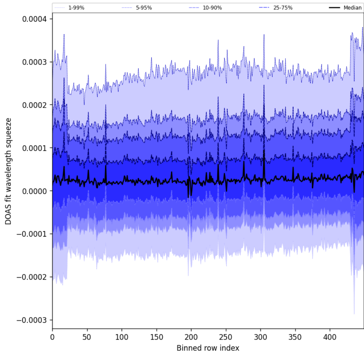
Figure 59: Along track statistics of “DOAS fit wavelength squeeze” for 2025-07-27 to 2025-07-29
