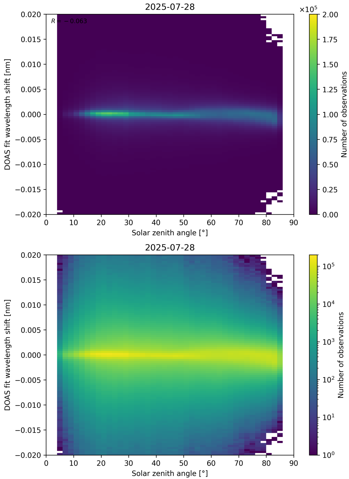
Figure 168: Scatter density plot of “Solar zenith angle” against “DOAS fit wavelength shift” for 2025-07-27 to 2025-07-29.
