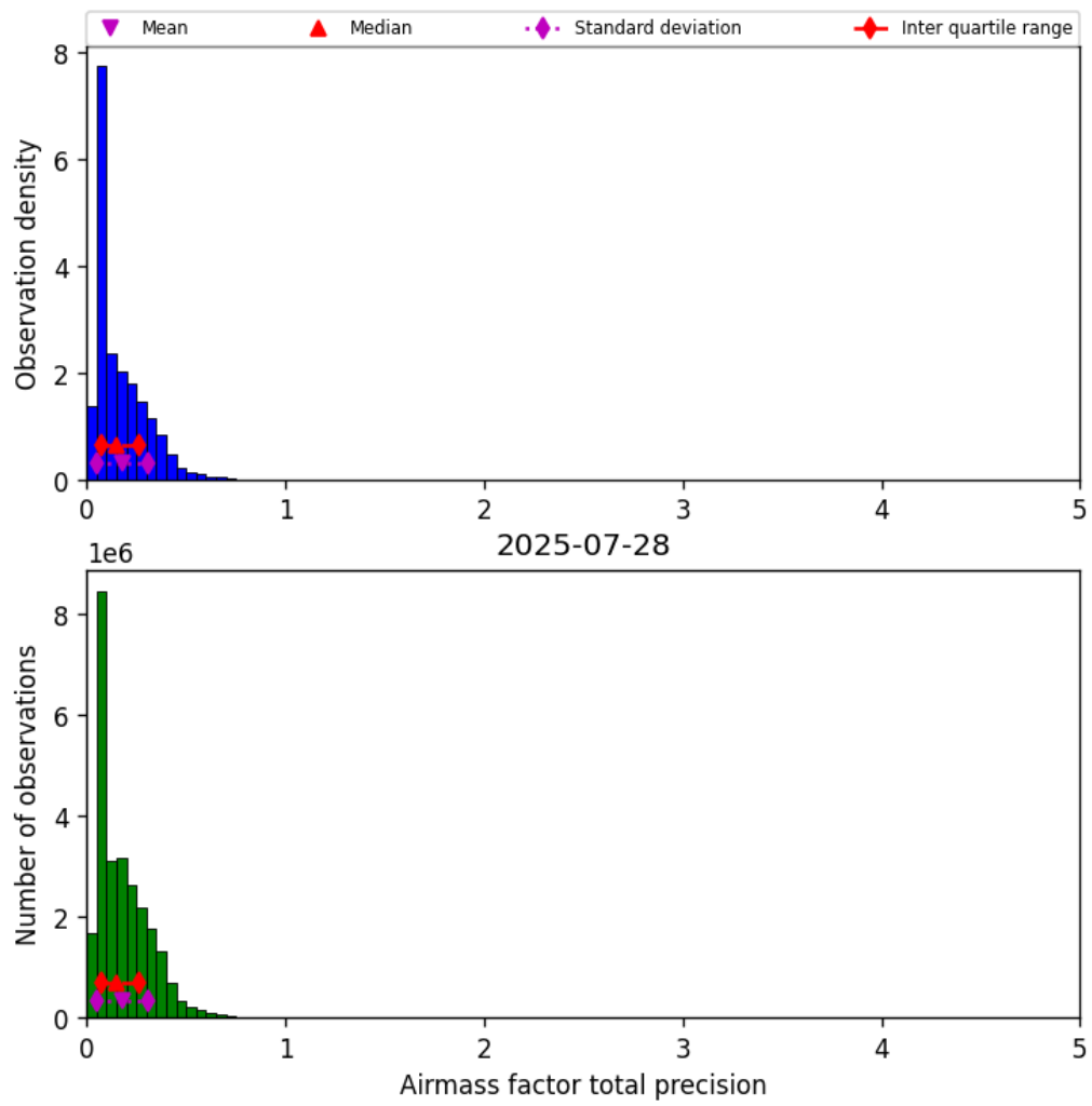
Figure 41: Histogram of “Airmass factor total precision” for 2025-07-27 to 2025-07-29
