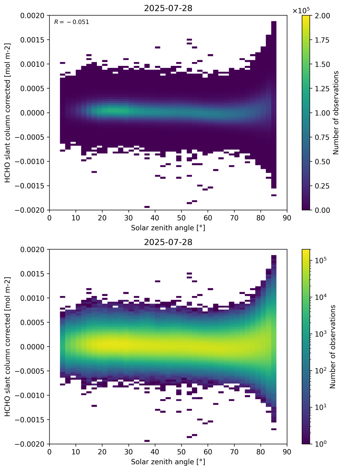
Figure 171: Scatter density plot of “Solar zenith angle” against “HCHO slant column corrected” for 2025-07-27 to 2025-07-29.
