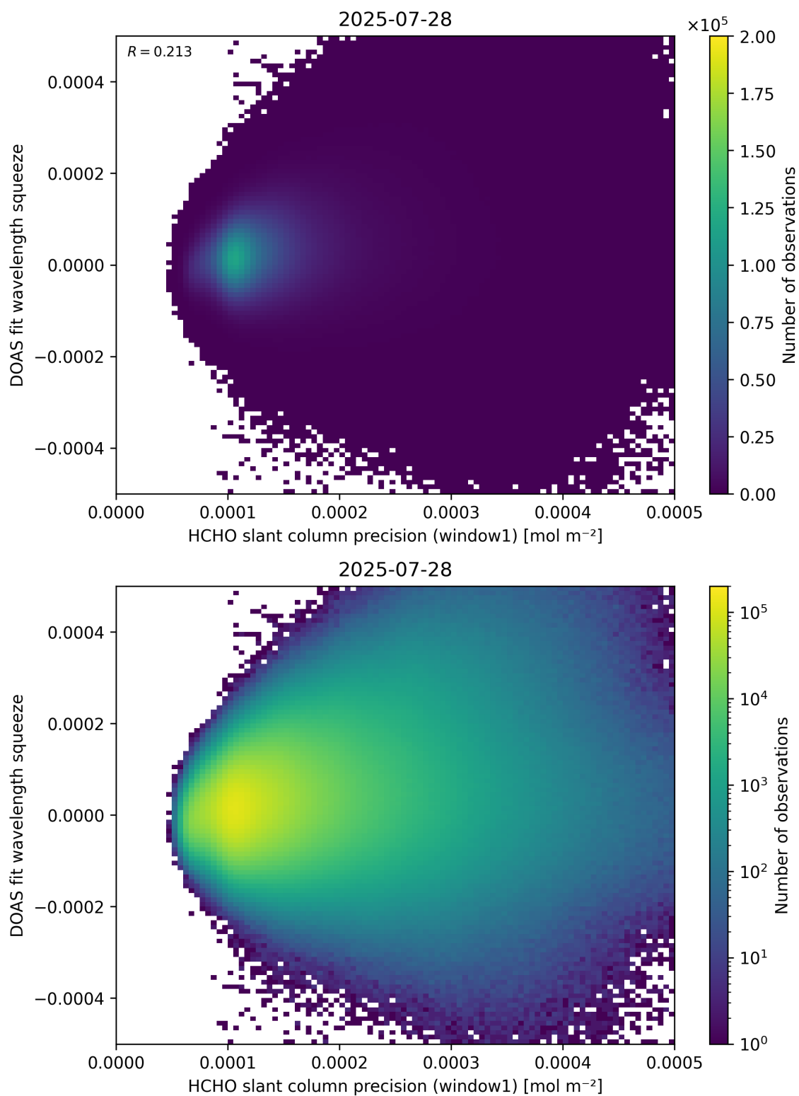
Figure 90: Scatter density plot of “HCHO slant column precision (window1)” against “DOAS fit wavelength squeeze” for 2025-07-27 to 2025-07-29.
