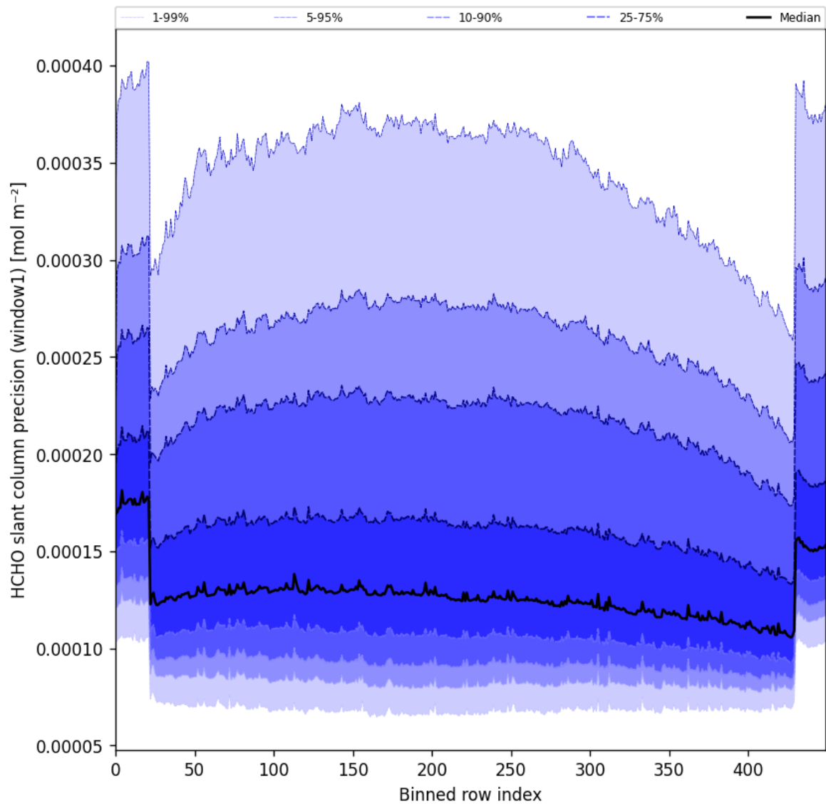
Figure 53: Along track statistics of “HCHO slant column precision (window1)” for 2025-07-27 to 2025-07-29
