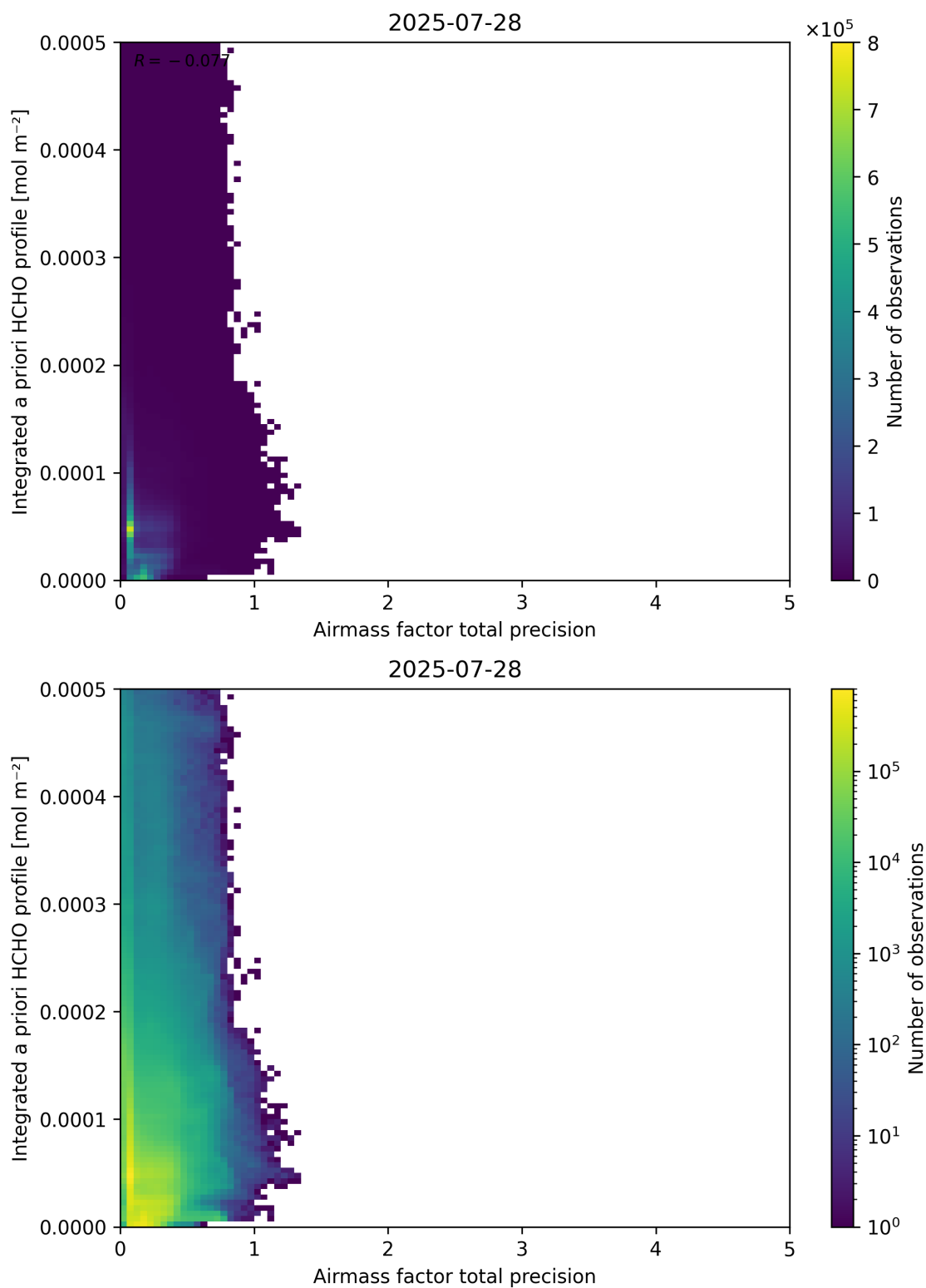
Figure 111: Scatter density plot of “Airmass factor total precision” against “Integrated a priori HCHO profile” for 2025-07-27 to 2025-07-29.
