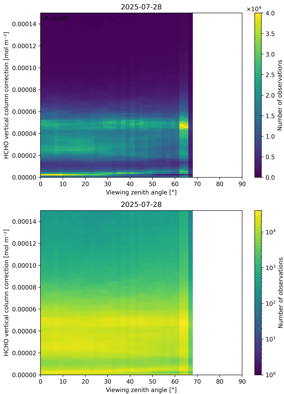
Figure 193: Scatter density plot of “Viewing zenith angle” against “HCHO vertical column correction” for 2025-07-27 to 2025-07-29.
