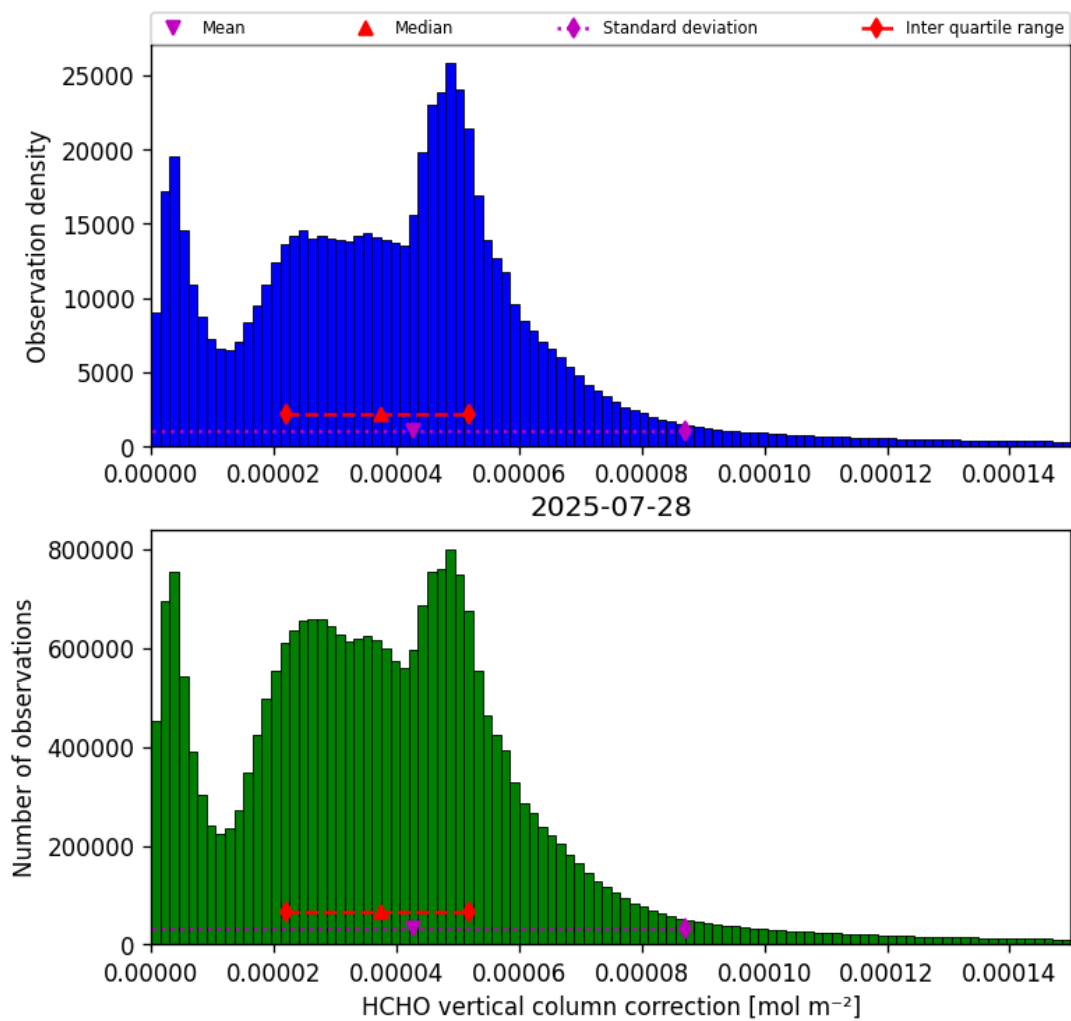
Figure 37: Histogram of “HCHO vertical column correction” for 2025-07-27 to 2025-07-29
