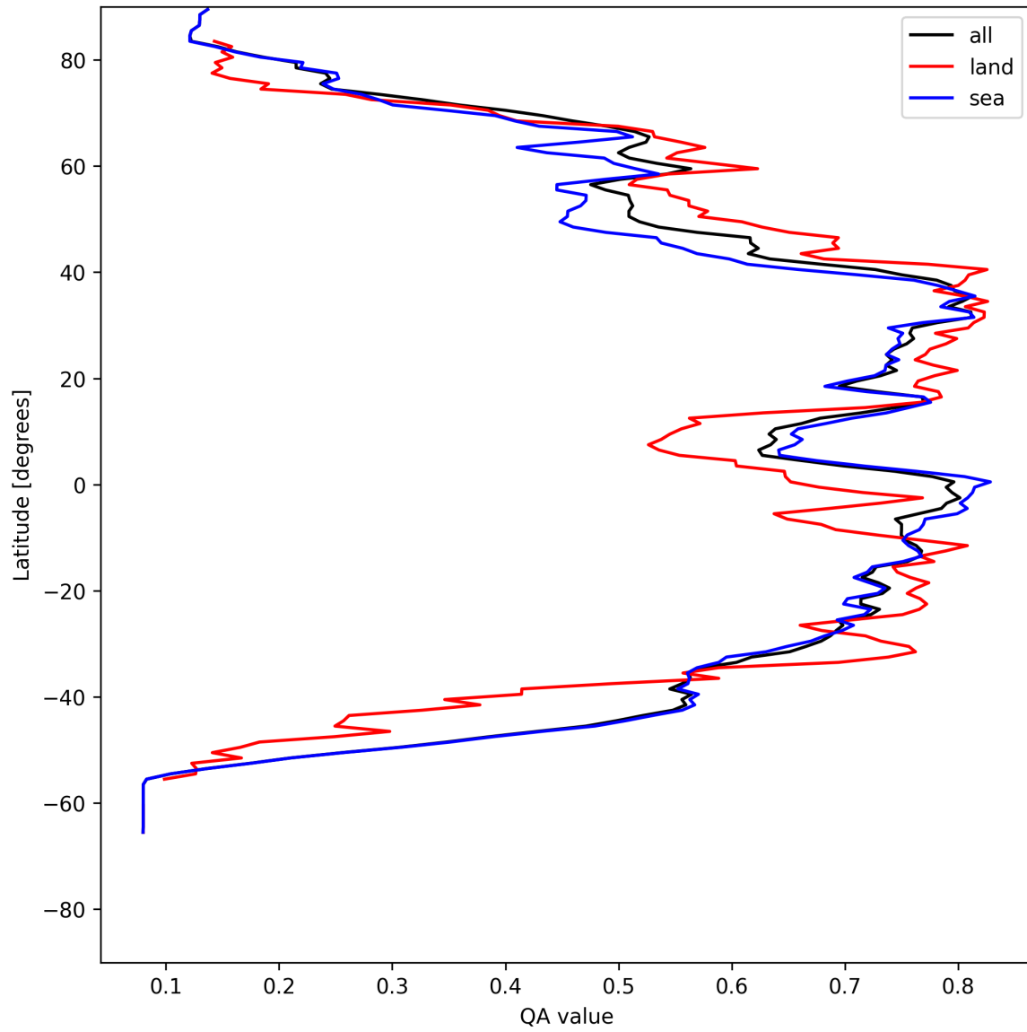
Figure 20: Zonal average of “QA value” for 2025-07-27 to 2025-07-29.
