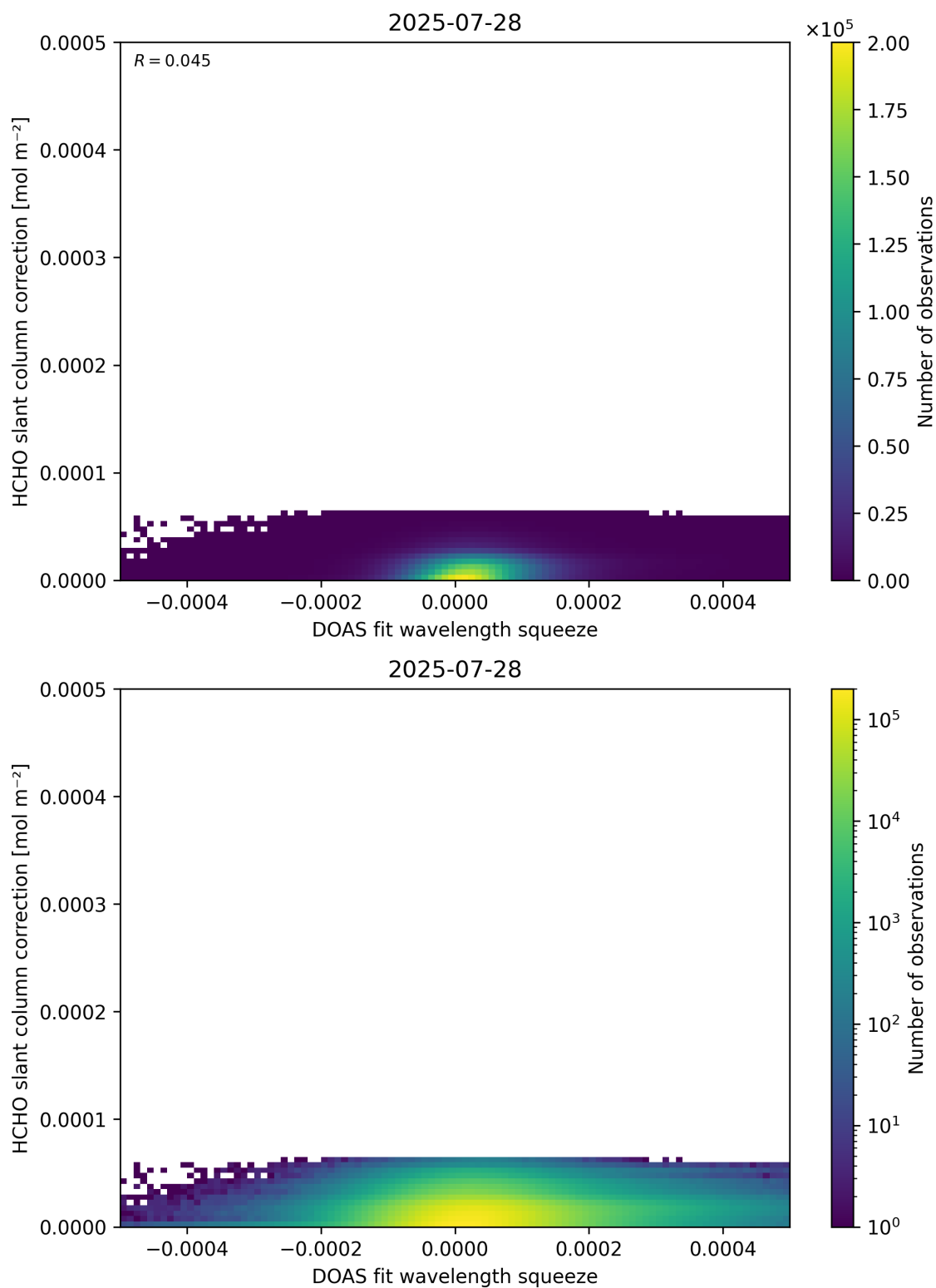
Figure 70: Scatter density plot of “DOAS fit wavelength squeeze” against “HCHO slant column correction” for 2025-07-27 to 2025-07-29.
