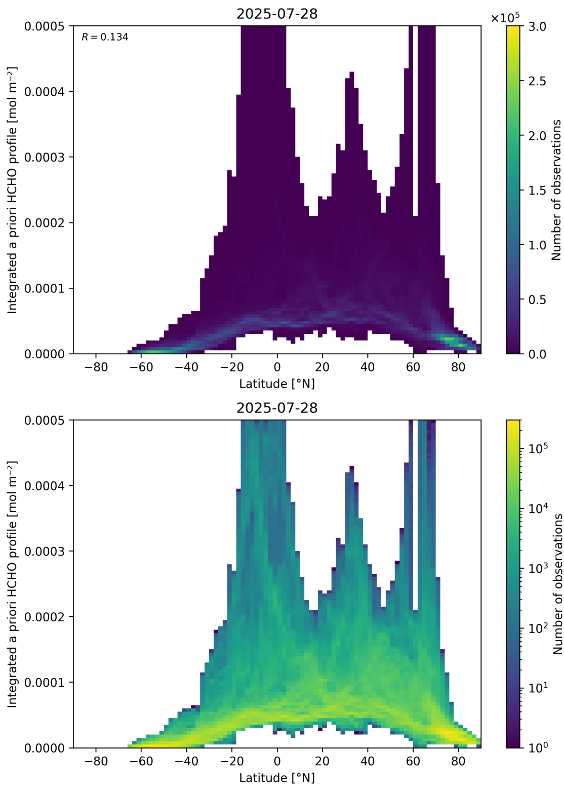
Figure 166: Scatter density plot of “Latitude” against “Integrated a priori HCHO profile” for 2025-07-27 to 2025-07-29.
