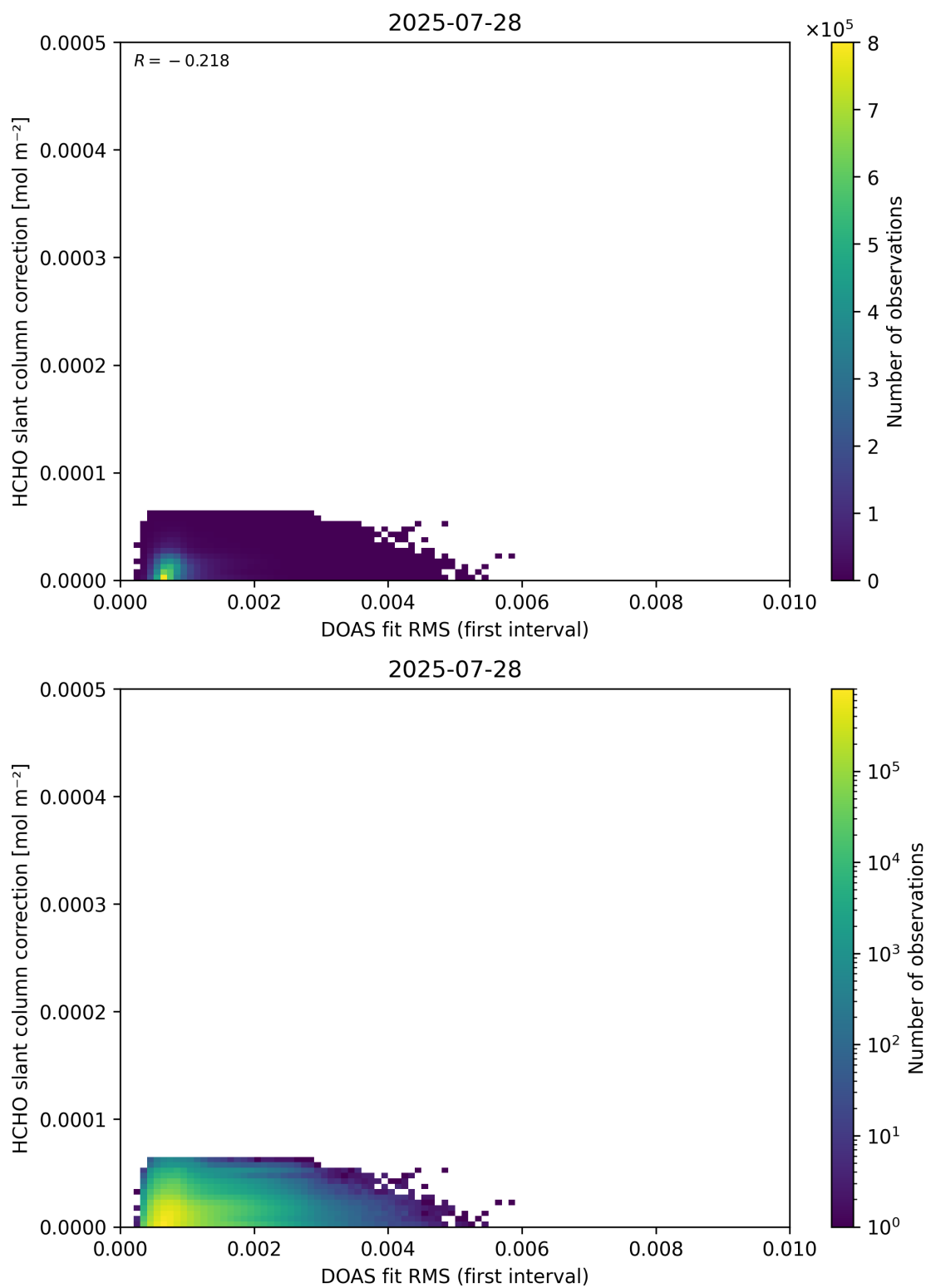
Figure 63: Scatter density plot of “DOAS fit RMS (first interval)” against “HCHO slant column correction” for 2025-07-27 to 2025-07-29.
