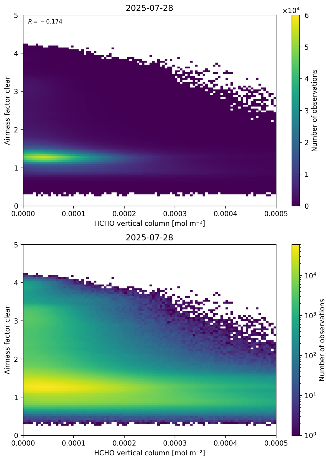
Figure 126: Scatter density plot of “HCHO vertical column” against “Airmass factor clear” for 2025-07-27 to 2025-07-29.
