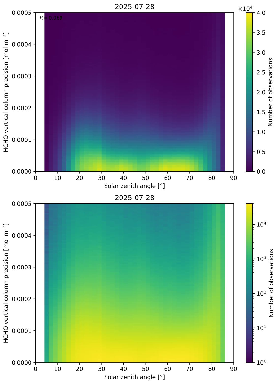
Figure 179: Scatter density plot of “Solar zenith angle” against “HCHO vertical column precision” for 2025-07-27 to 2025-07-29.
