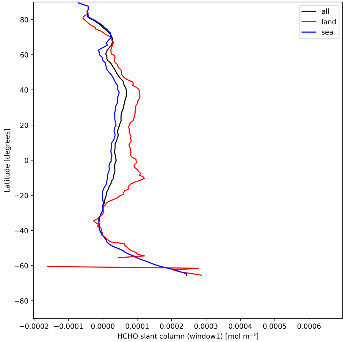
Figure 24: Zonal average of “HCHO slant column (window1)” for 2025-07-27 to 2025-07-29.
