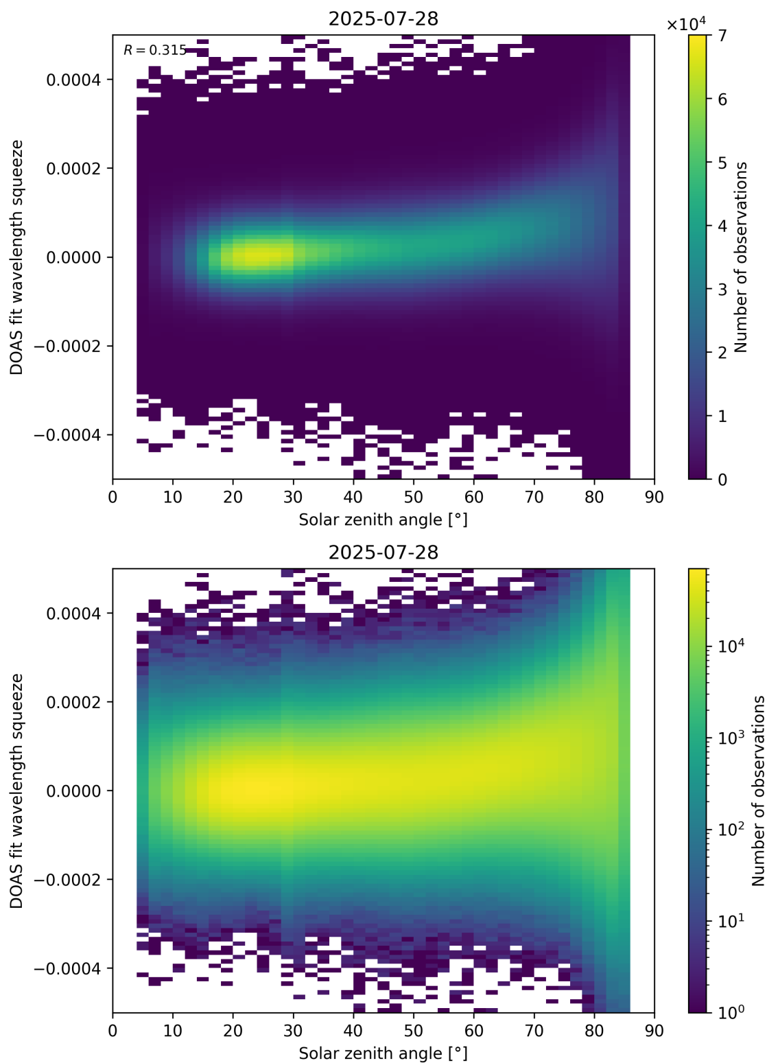
Figure 169: Scatter density plot of “Solar zenith angle” against “DOAS fit wavelength squeeze” for 2025-07-27 to 2025-07-29.
