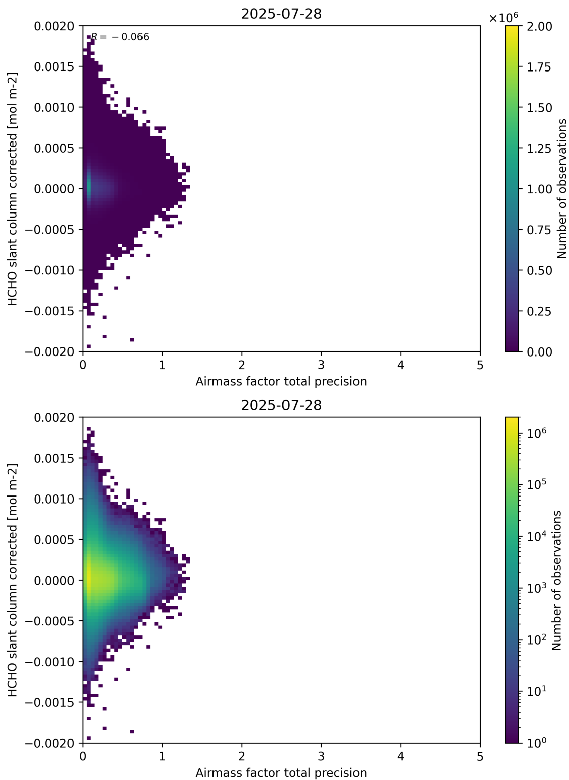
Figure 109: Scatter density plot of “Airmass factor total precision” against “HCHO slant column corrected” for 2025-07-27 to 2025-07-29.
