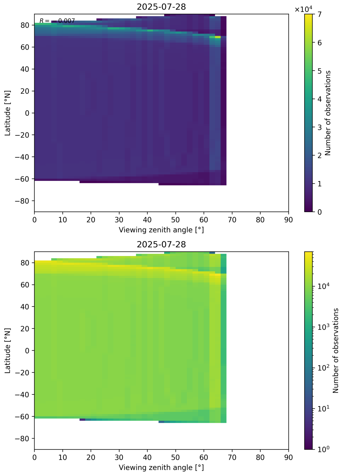
Figure 196: Scatter density plot of “Viewing zenith angle” against “Latitude” for 2025-07-27 to 2025-07-29.
