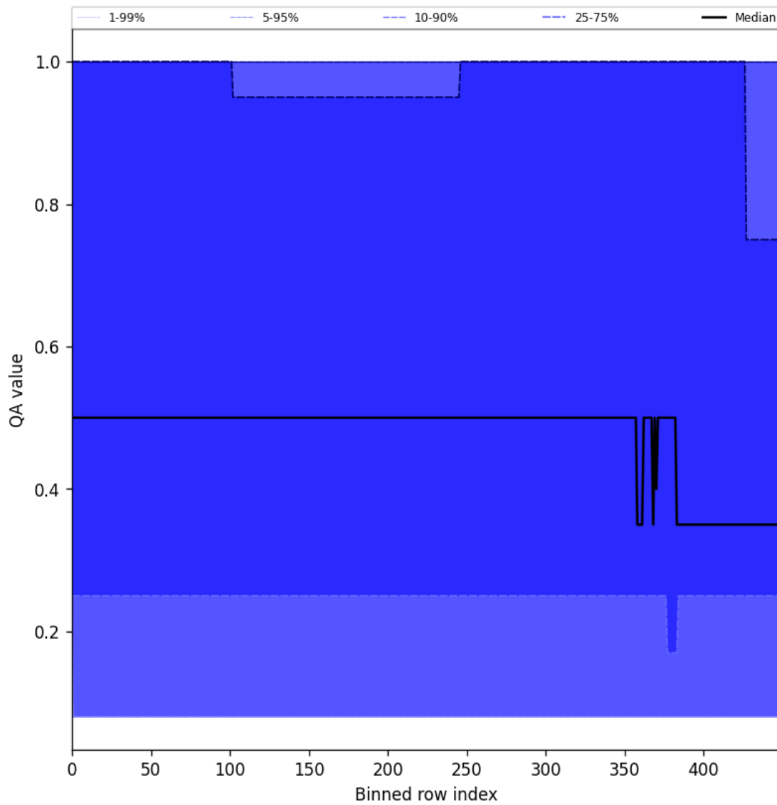
Figure 48: Along track statistics of “QA value” for 2025-07-27 to 2025-07-29
