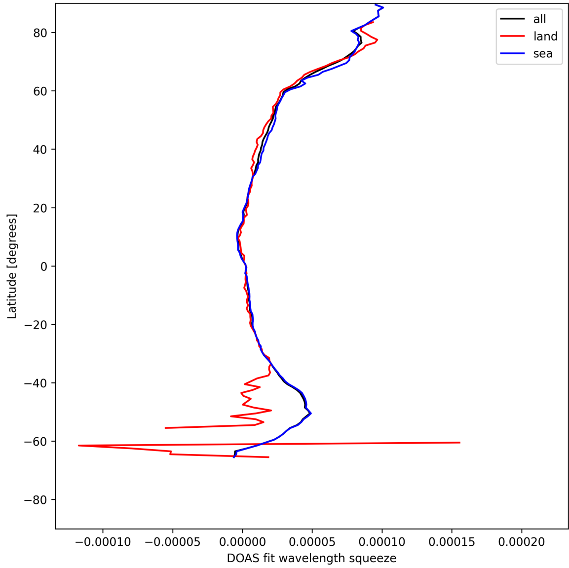
Figure 31: Zonal average of “DOAS fit wavelength squeeze” for 2025-07-27 to 2025-07-29.
