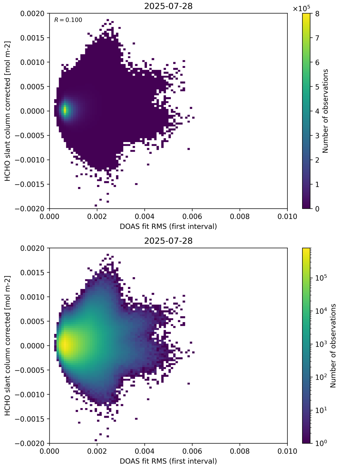
Figure 62: Scatter density plot of “DOAS fit RMS (first interval)” against “HCHO slant column corrected” for 2025-07-27 to 2025-07-29.
