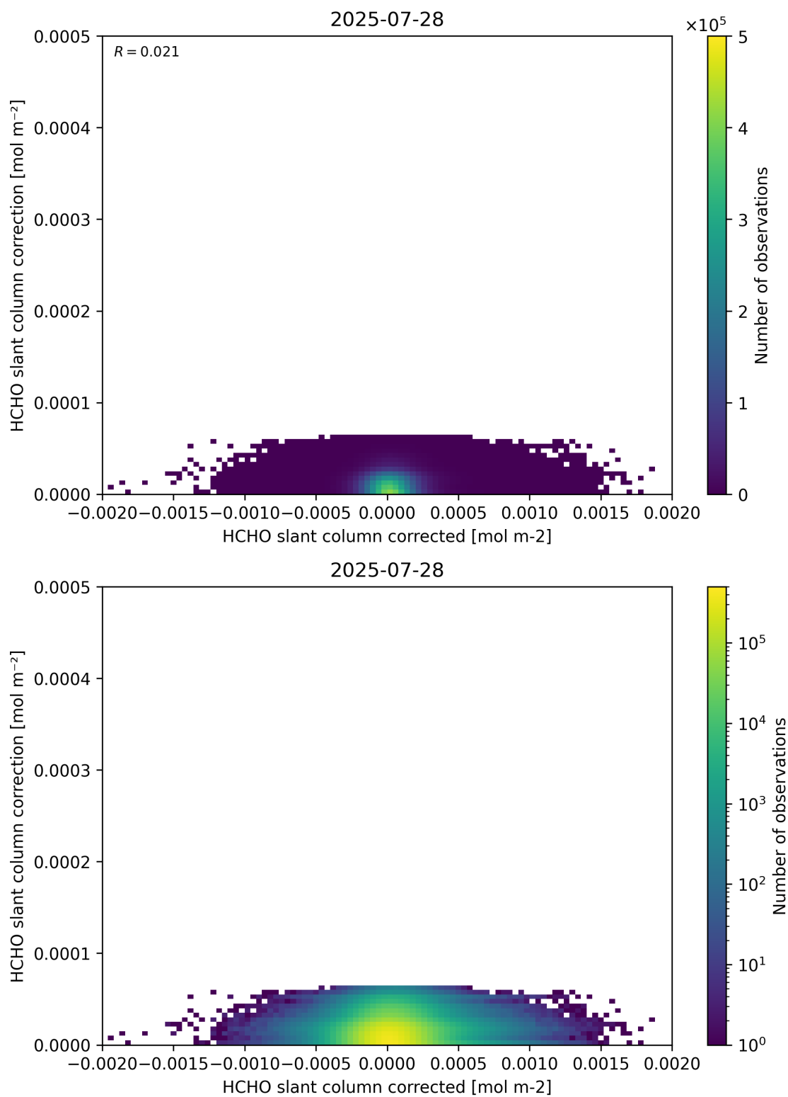
Figure 77: Scatter density plot of “HCHO slant column corrected” against “HCHO slant column correction” for 2025-07-27 to 2025-07-29.
