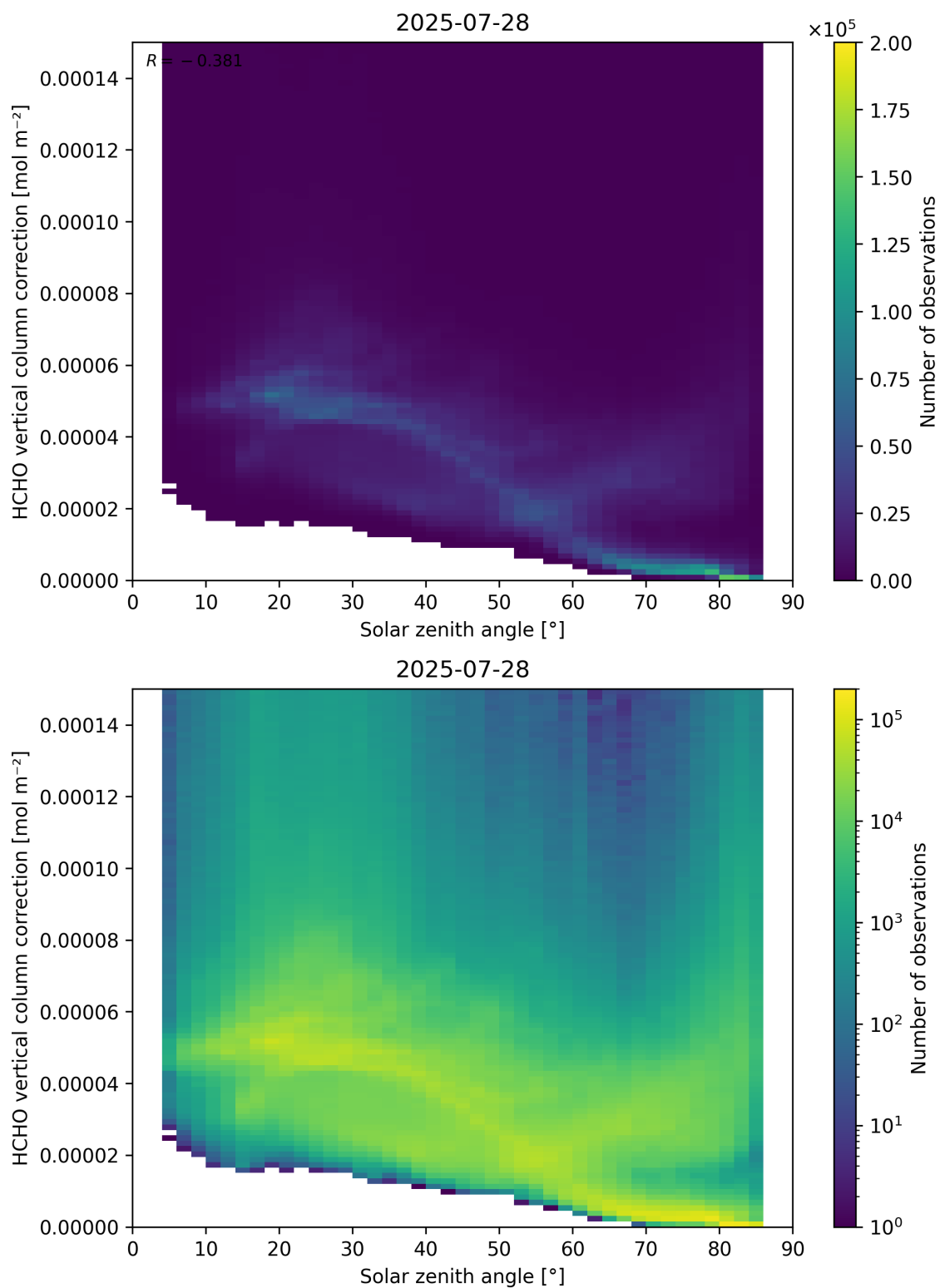
Figure 178: Scatter density plot of “Solar zenith angle” against “HCHO vertical column correction” for 2025-07-27 to 2025-07-29.
