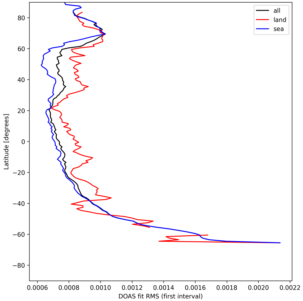
Figure 32: Zonal average of "DOAS fit RMS (first interval)" for 2025-07-27 to 2025-07-29.
