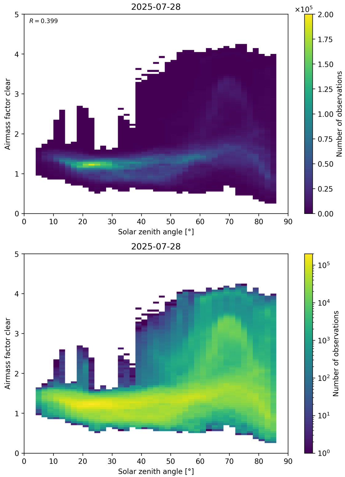
Figure 170: Scatter density plot of “Solar zenith angle” against “Airmass factor clear” for 2025-07-27 to 2025-07-29.
