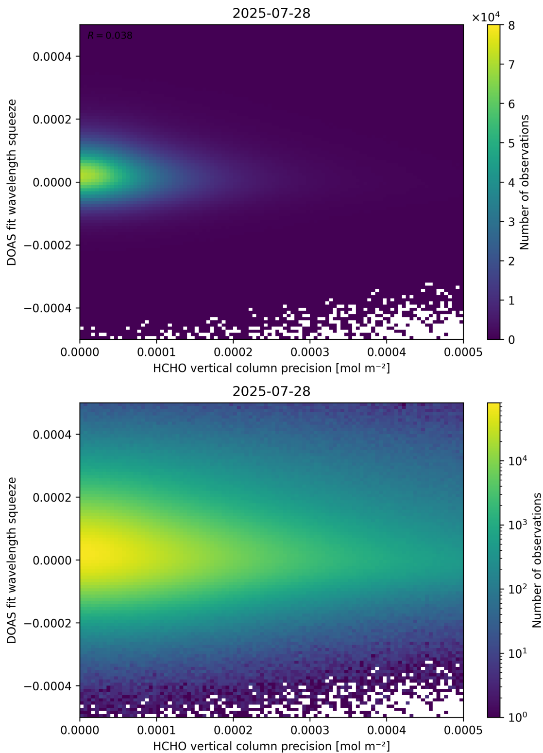
Figure 138: Scatter density plot of “HCHO vertical column precision” against “DOAS fit wavelength squeeze” for 2025-07-27 to 2025-07-29.
