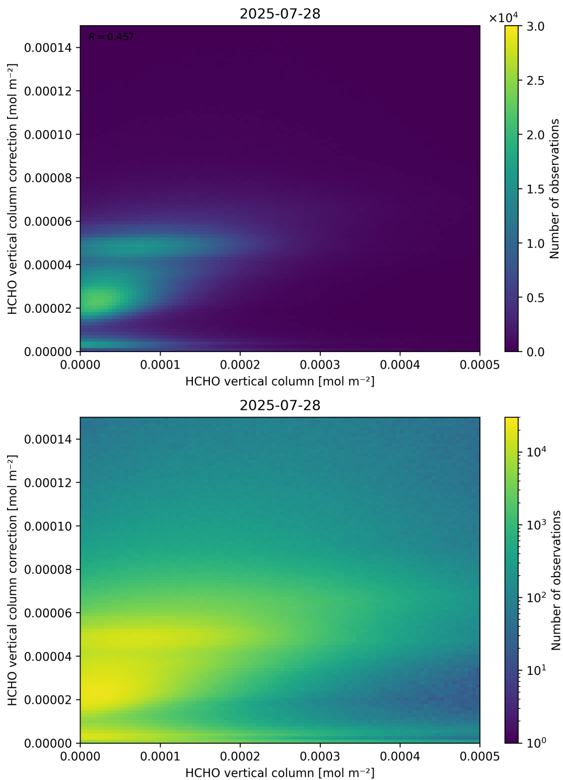
Figure 133: Scatter density plot of “HCHO vertical column” against “HCHO vertical column correction” for 2025-07-27 to 2025-07-29.
