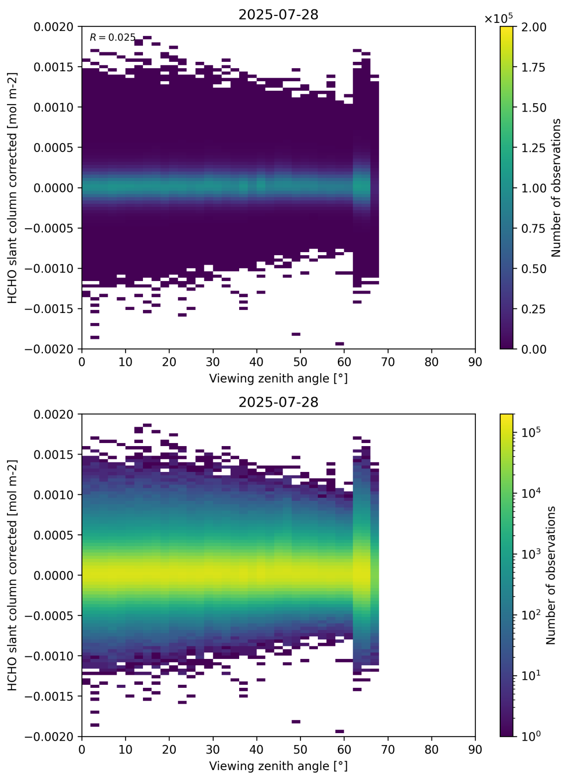
Figure 186: Scatter density plot of “Viewing zenith angle” against “HCHO slant column corrected” for 2025-07-27 to 2025-07-29.
