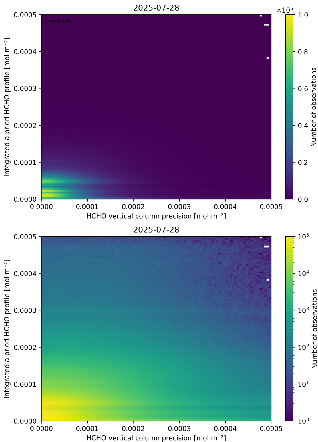
Figure 147: Scatter density plot of “HCHO vertical column precision” against “Integrated a priori HCHO profile” for 2025-07-27 to 2025-07-29.
