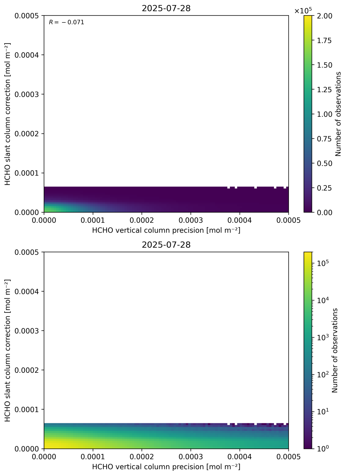
Figure 141: Scatter density plot of “HCHO vertical column precision” against “HCHO slant column correction” for 2025-07-27 to 2025-07-29.
