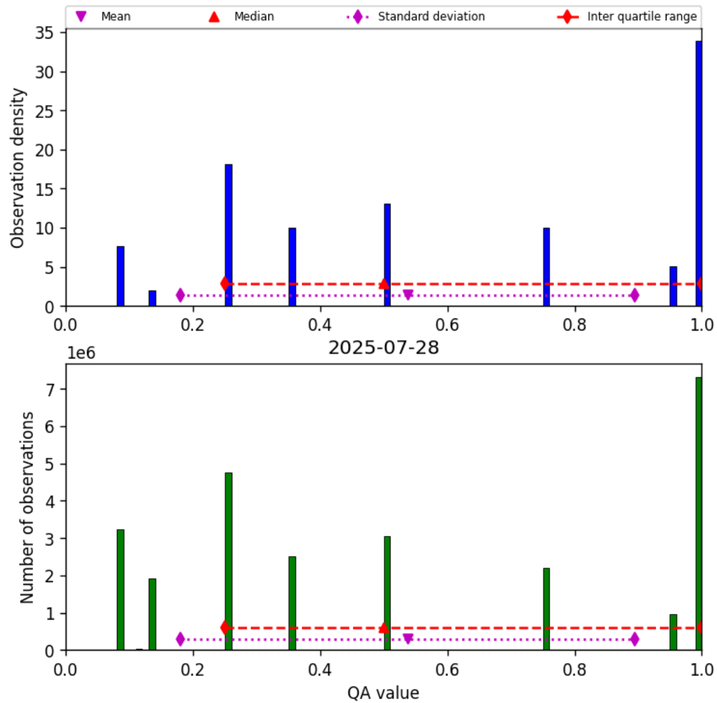
Figure 34: Histogram of “QA value” for 2025-07-27 to 2025-07-29
