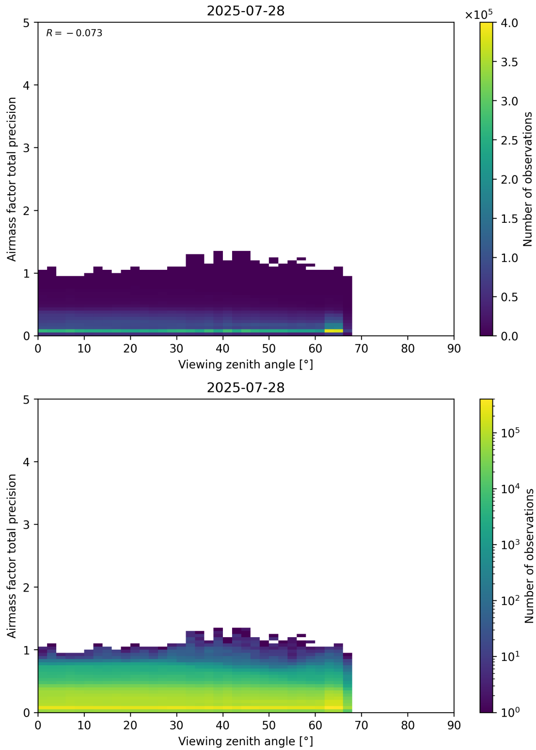
Figure 191: Scatter density plot of “Viewing zenith angle” against “Airmass factor total precision” for 2025-07-27 to 2025-07-29.
