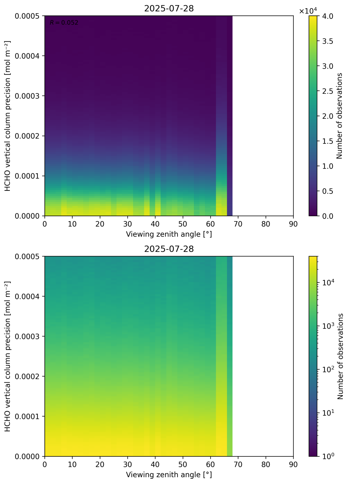
Figure 194: Scatter density plot of “Viewing zenith angle” against “HCHO vertical column precision” for 2025-07-27 to 2025-07-29.
