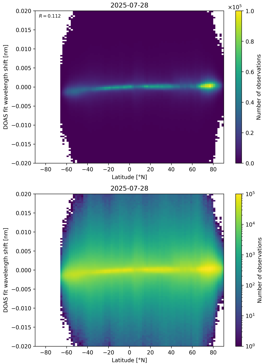
Figure 154: Scatter density plot of “Latitude” against “DOAS fit wavelength shift” for 2025-07-27 to 2025-07-29.
