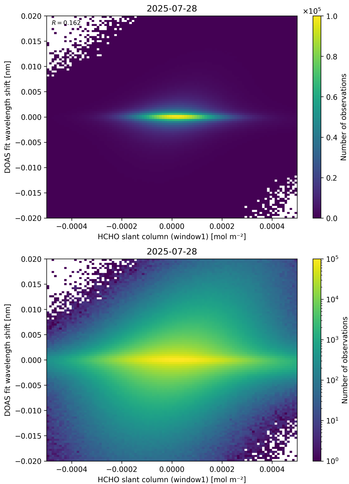
Figure 79: Scatter density plot of “HCHO slant column (window1)” against “DOAS fit wavelength shift” for 2025-07-27 to 2025-07-29.
