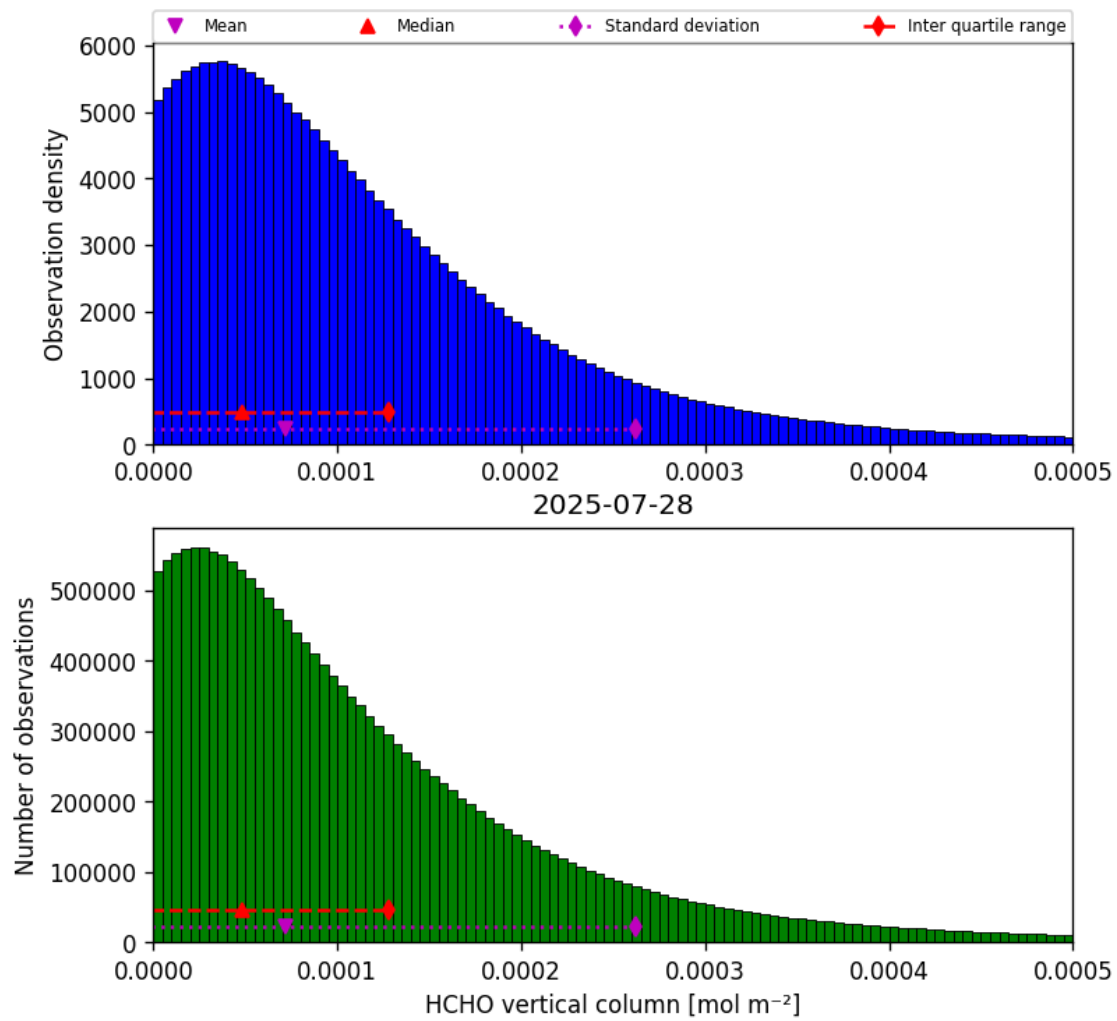
Figure 35: Histogram of “HCHO vertical column” for 2025-07-27 to 2025-07-29
