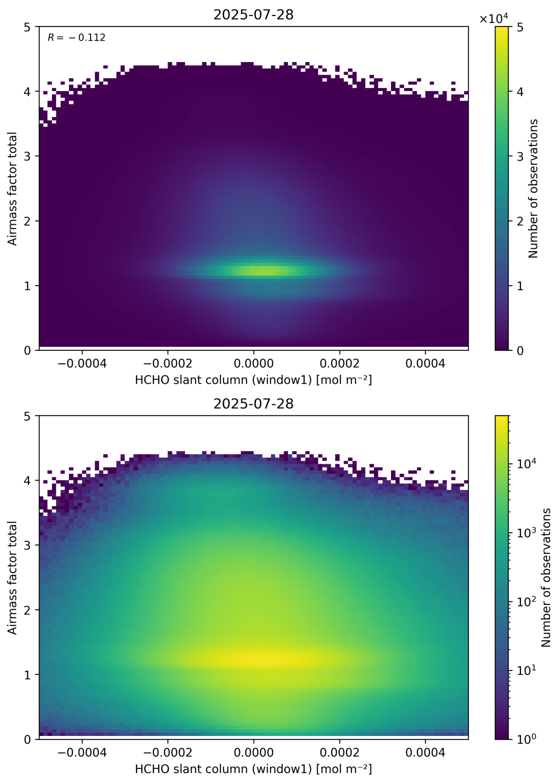
Figure 85: Scatter density plot of “HCHO slant column (window1)” against “Airmass factor total” for 2025-07-27 to 2025-07-29.
