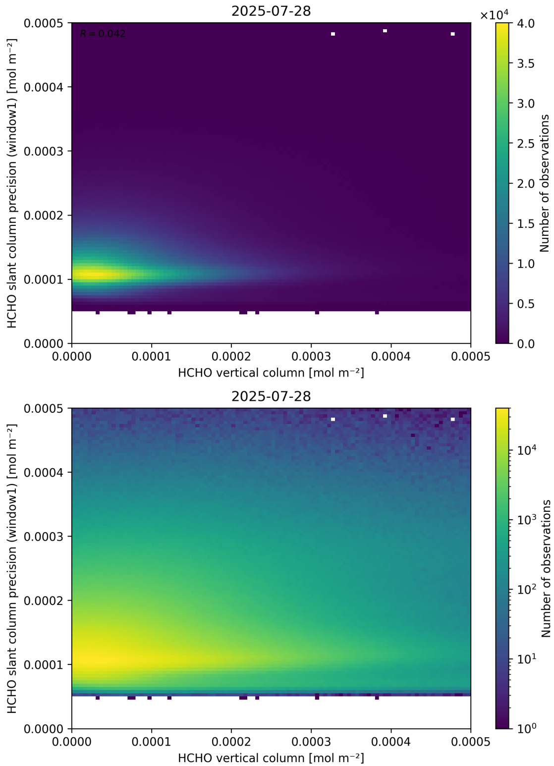
Figure 130: Scatter density plot of “HCHO vertical column” against “HCHO slant column precision (window1)” for 2025-07-27 to 2025-07-29.
