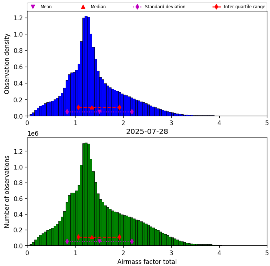
Figure 40: Histogram of “Airmass factor total” for 2025-07-27 to 2025-07-29
