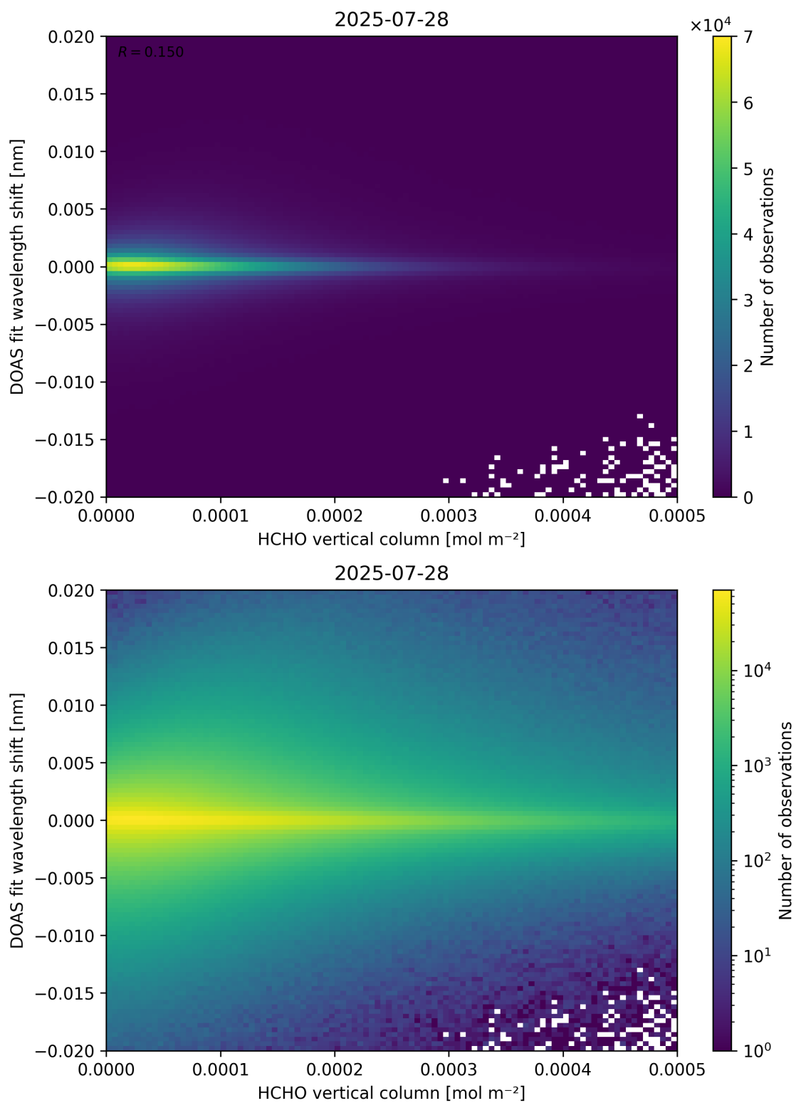
Figure 124: Scatter density plot of “HCHO vertical column” against “DOAS fit wavelength shift” for 2025-07-27 to 2025-07-29.
