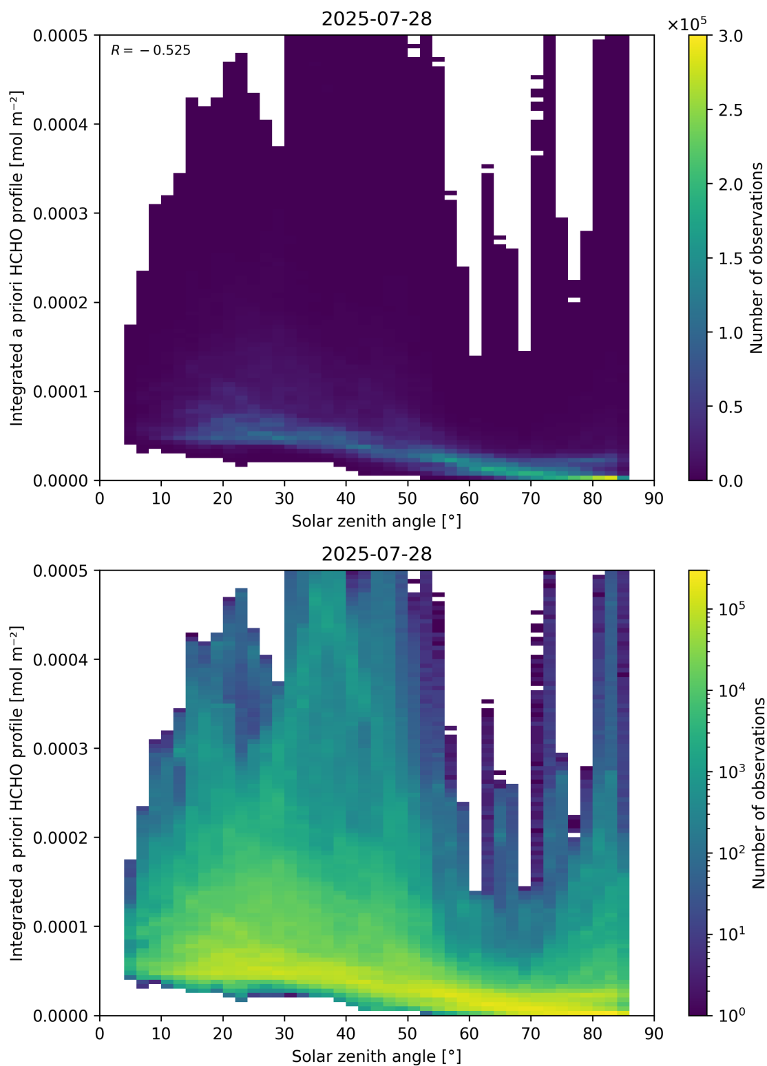
Figure 180: Scatter density plot of “Solar zenith angle” against “Integrated a priori HCHO profile” for 2025-07-27 to 2025-07-29.
