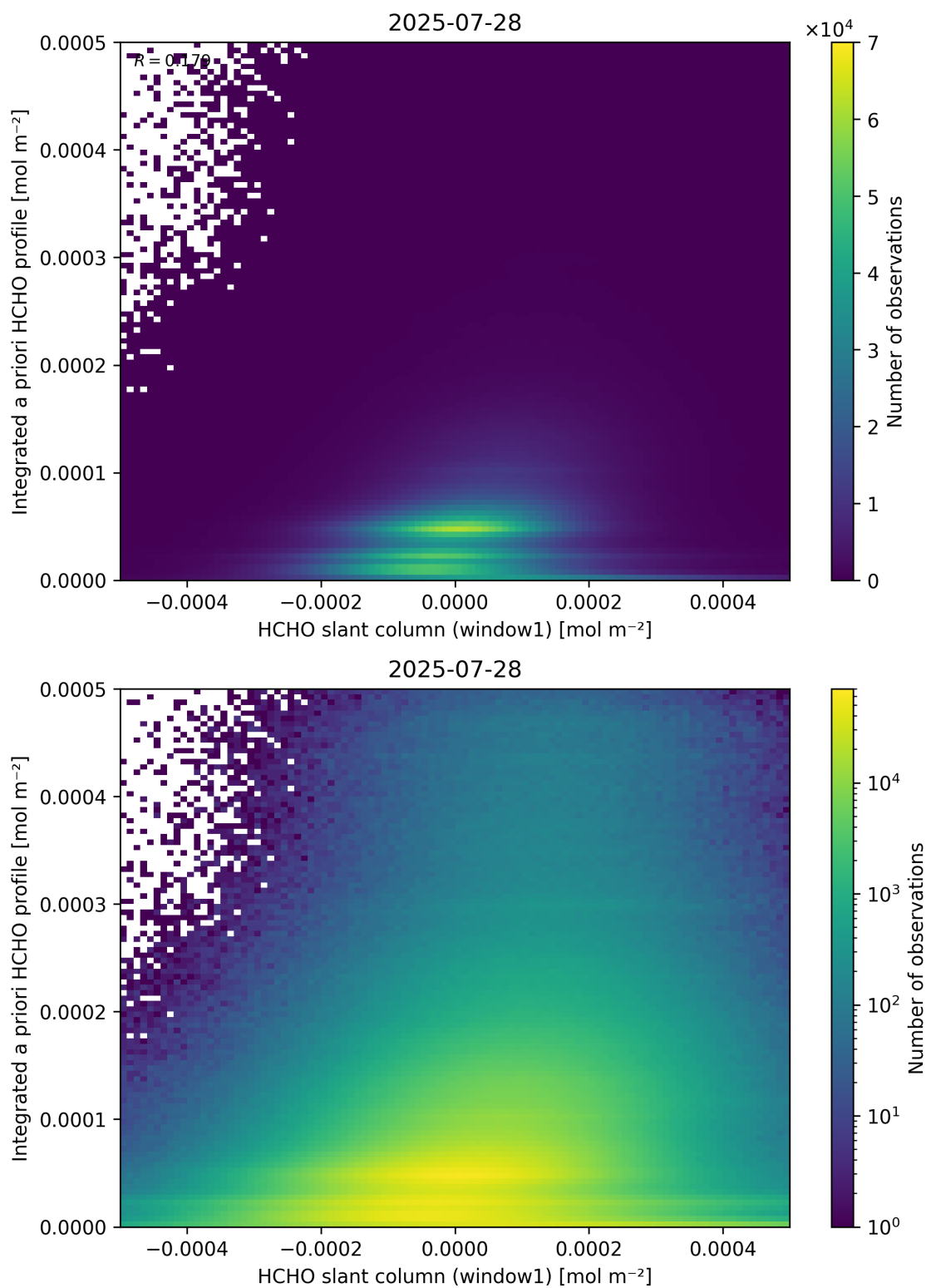
Figure 87: Scatter density plot of “HCHO slant column (window1)” against “Integrated a priori HCHO profile” for 2025-07-27 to 2025-07-29.
