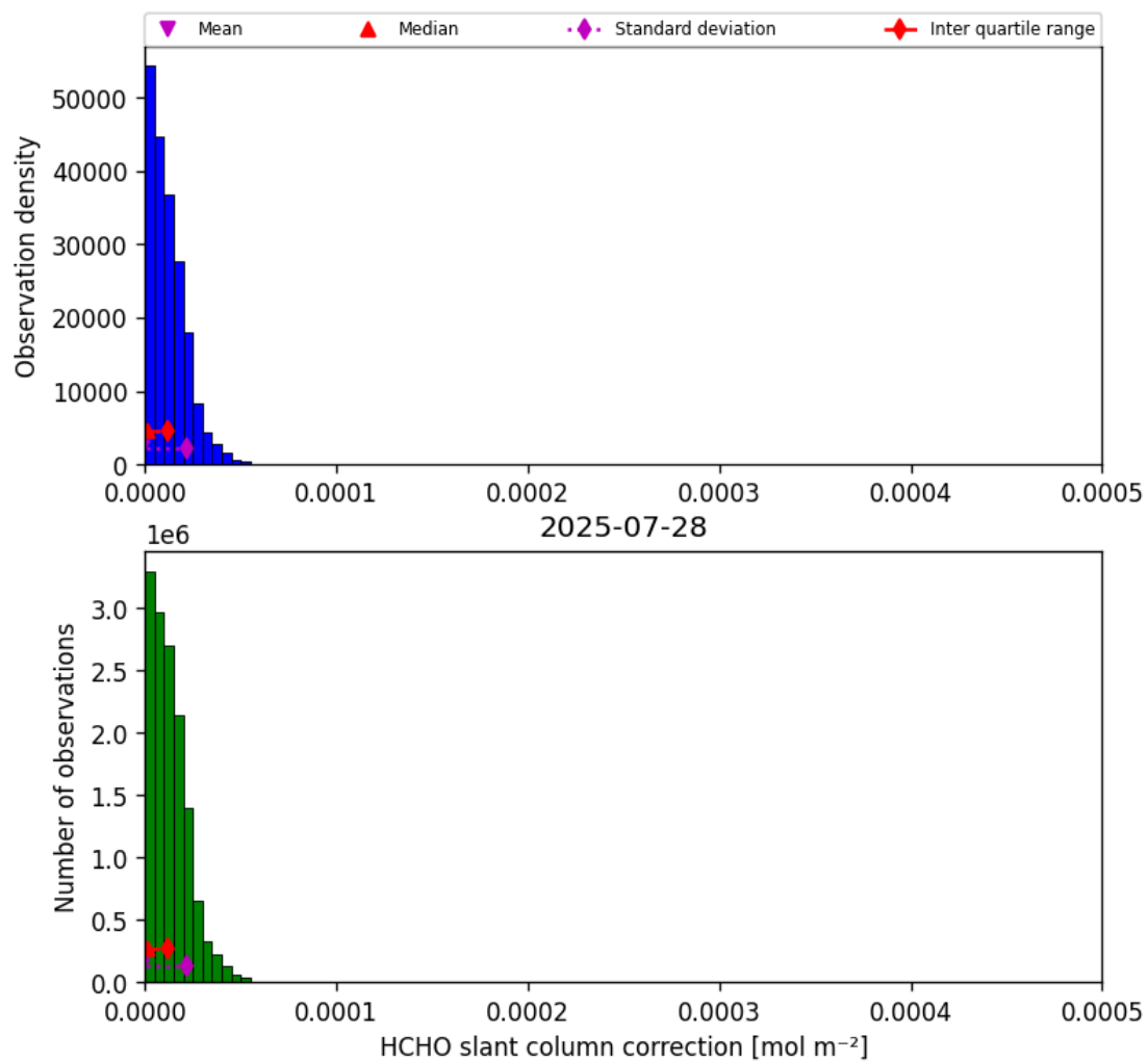
Figure 47: Histogram of “HCHO slant column correction” for 2025-07-27 to 2025-07-29
