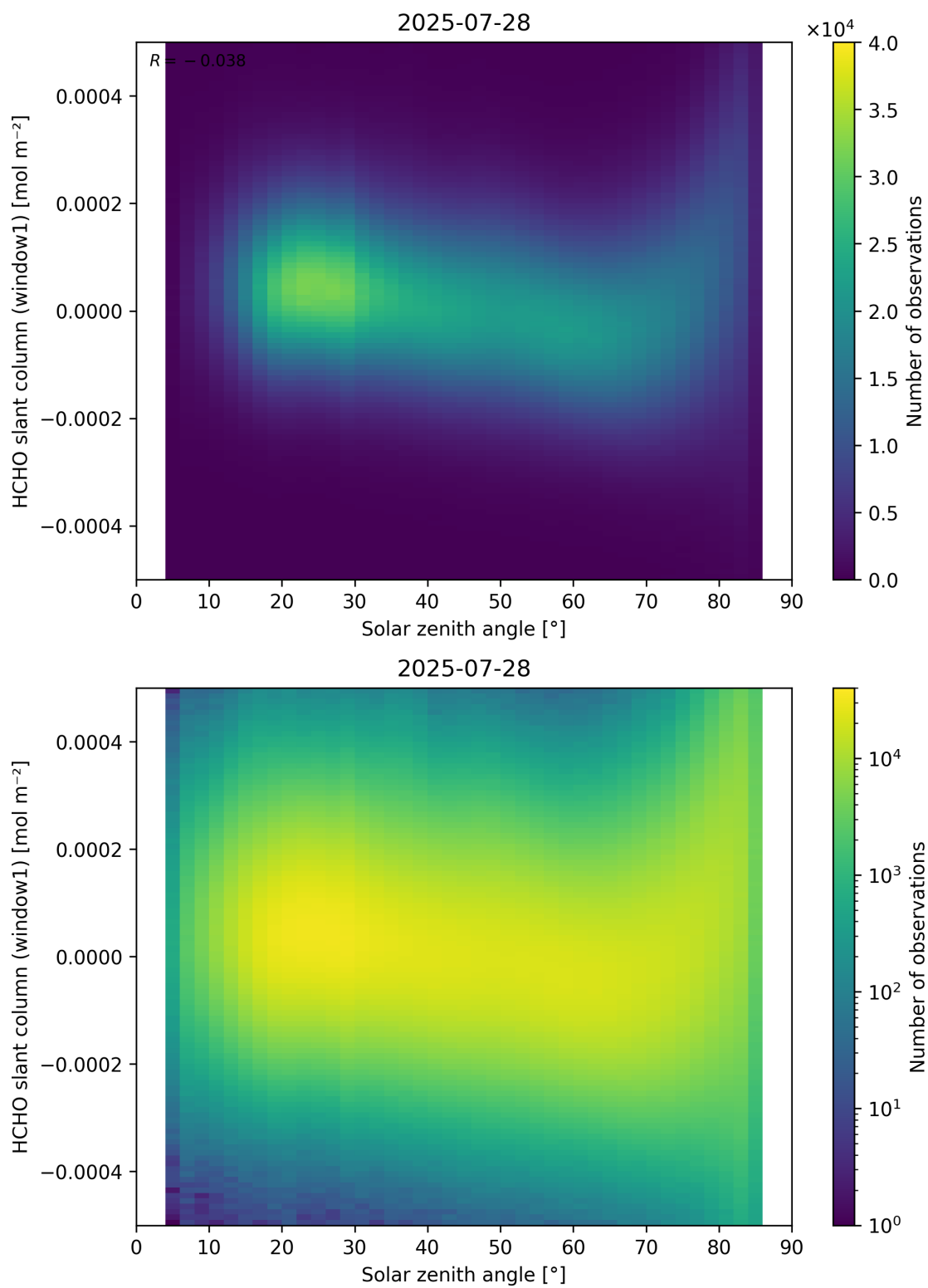
Figure 173: Scatter density plot of “Solar zenith angle” against “HCHO slant column (window1)” for 2025-07-27 to 2025-07-29.
