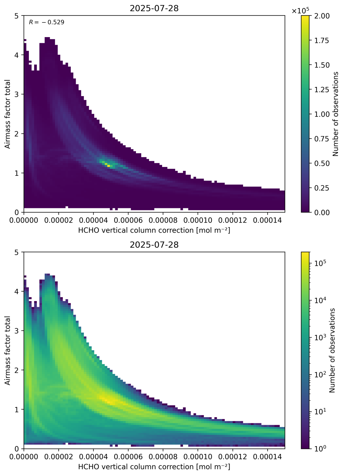
Figure 120: Scatter density plot of “HCHO vertical column correction” against “Airmass factor total” for 2025-07-27 to 2025-07-29.
