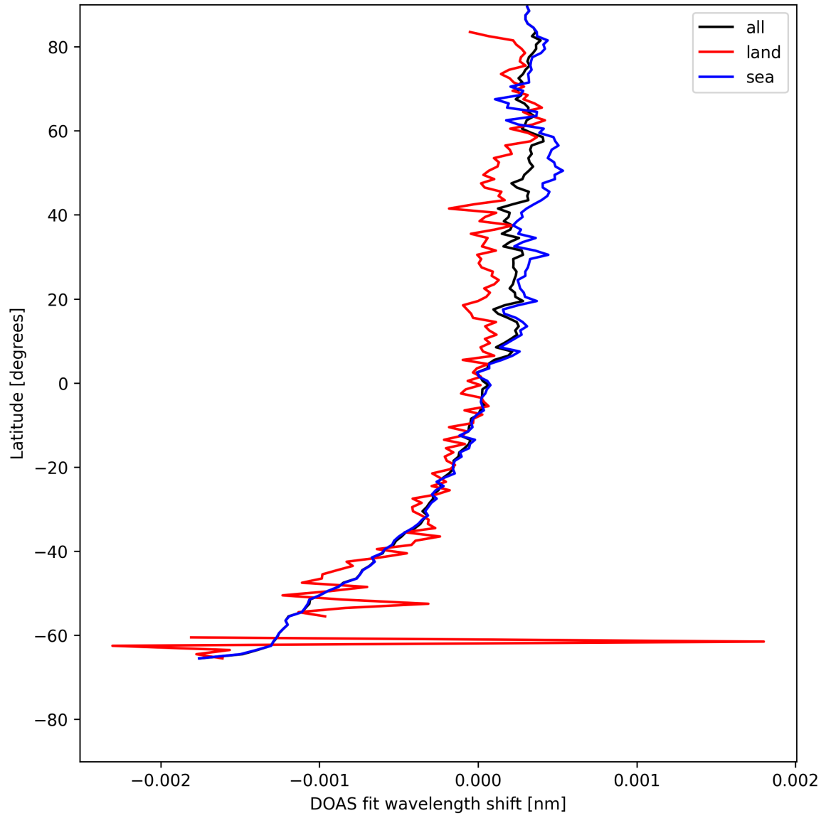
Figure 30: Zonal average of “DOAS fit wavelength shift” for 2025-07-27 to 2025-07-29.
