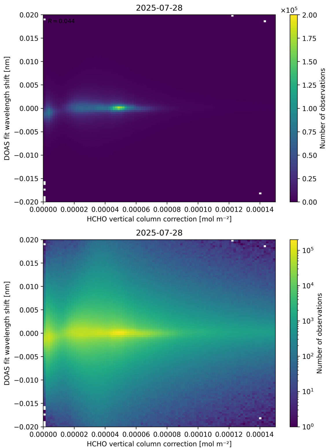
Figure 113: Scatter density plot of “HCHO vertical column correction” against “DOAS fit wavelength shift” for 2025-07-27 to 2025-07-29.
