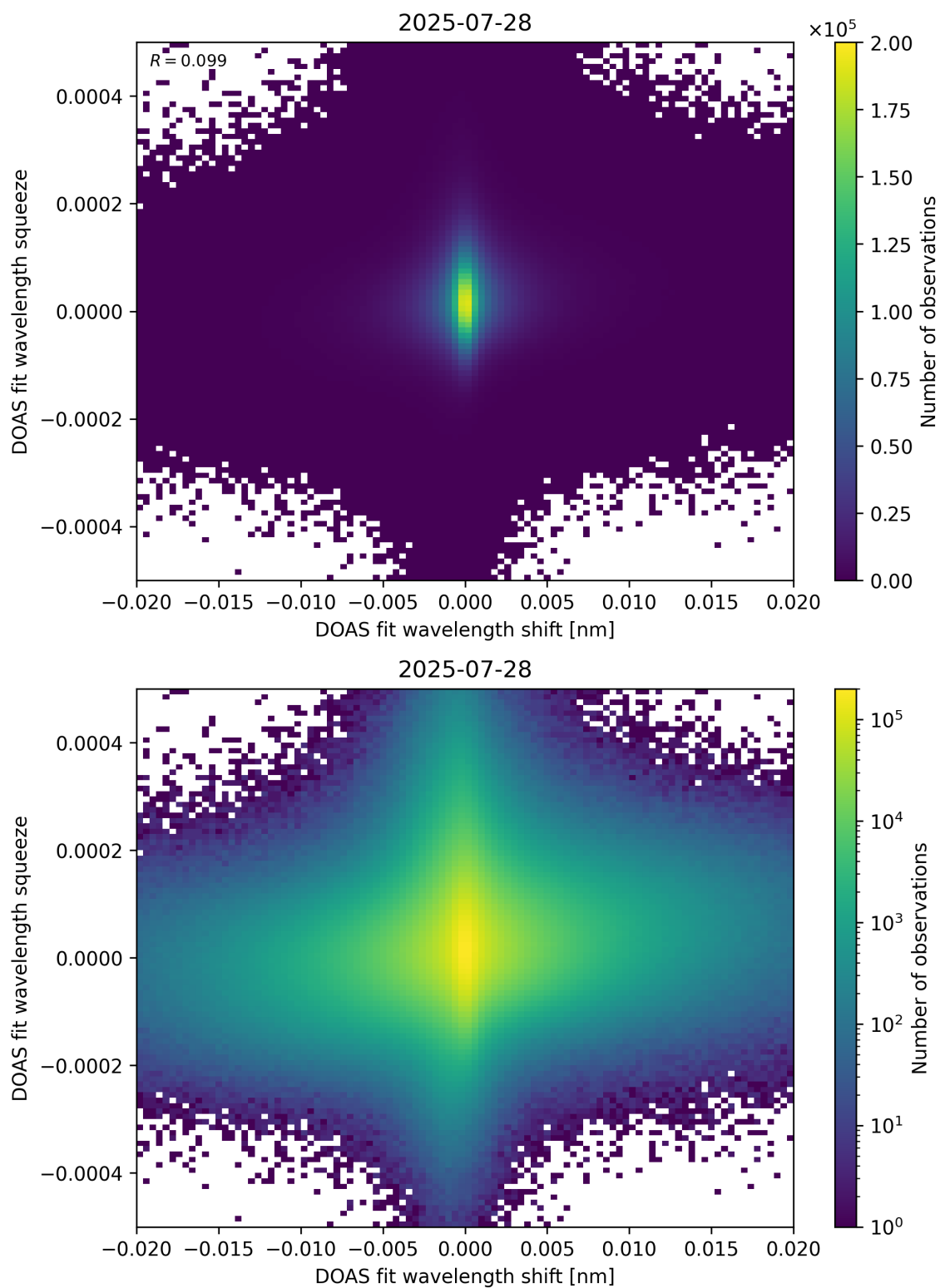
Figure 65: Scatter density plot of “DOAS fit wavelength shift” against “DOAS fit wavelength squeeze” for 2025-07-27 to 2025-07-29.
