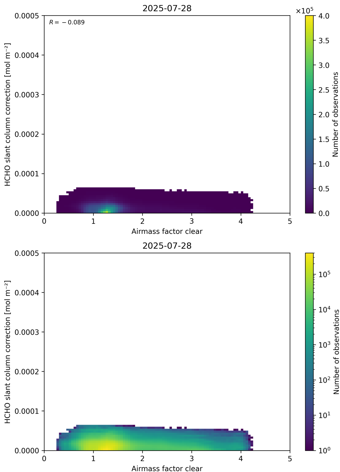
Figure 75: Scatter density plot of “Airmass factor clear” against “HCHO slant column correction” for 2025-07-27 to 2025-07-29.
