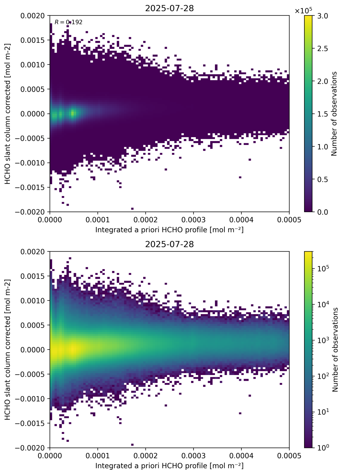
Figure 151: Scatter density plot of “Integrated a priori HCHO profile” against “HCHO slant column corrected” for 2025-07-27 to 2025-07-29.
