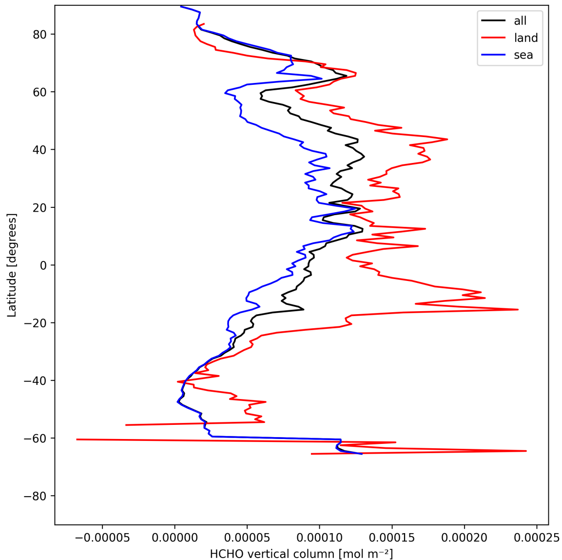
Figure 21: Zonal average of “HCHO vertical column” for 2025-07-27 to 2025-07-29.
