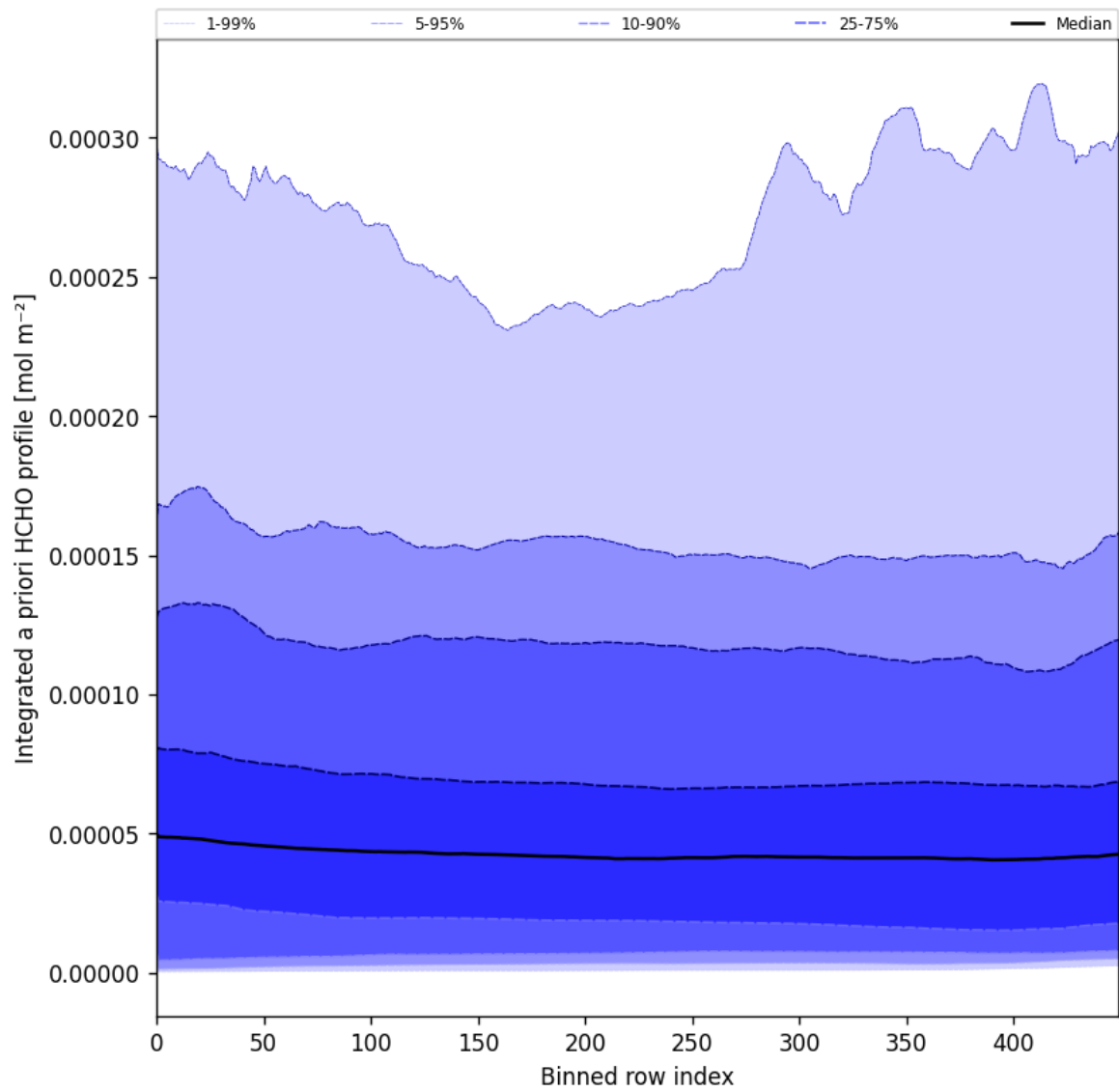
Figure 57: Along track statistics of "Integrated a priori HCHO profile" for 2025-07-27 to 2025-07-29
