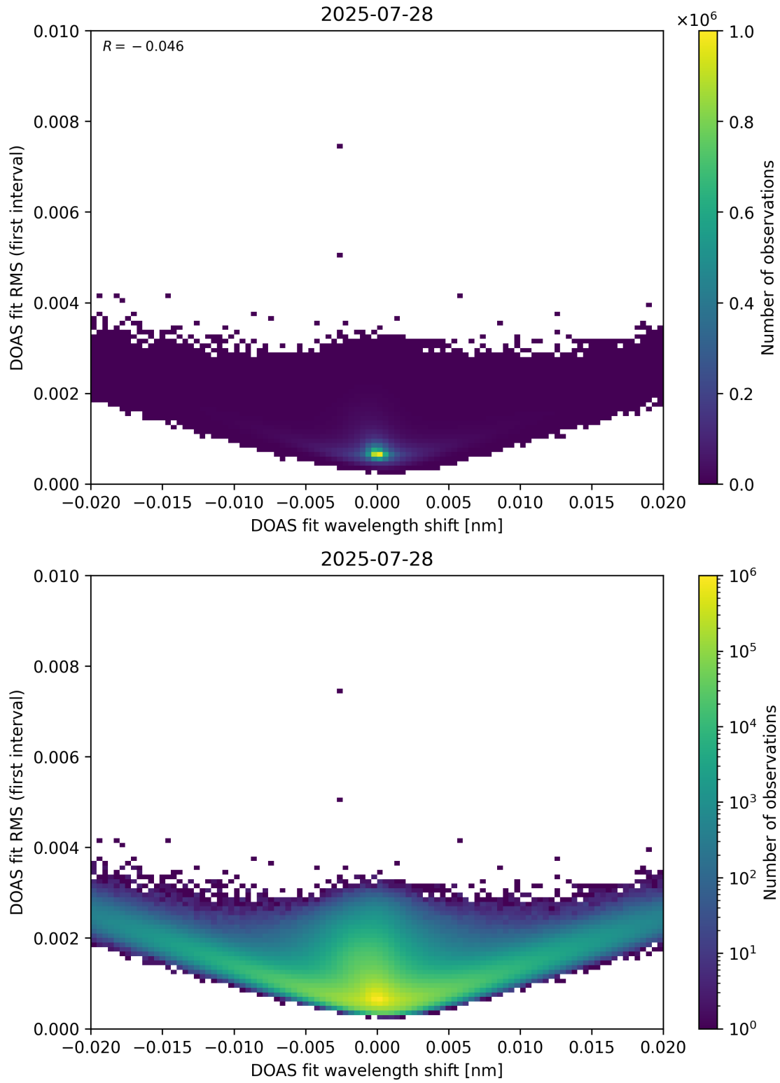
Figure 64: Scatter density plot of “DOAS fit wavelength shift” against “DOAS fit RMS (first interval)” for 2025-07-27 to 2025-07-29.
