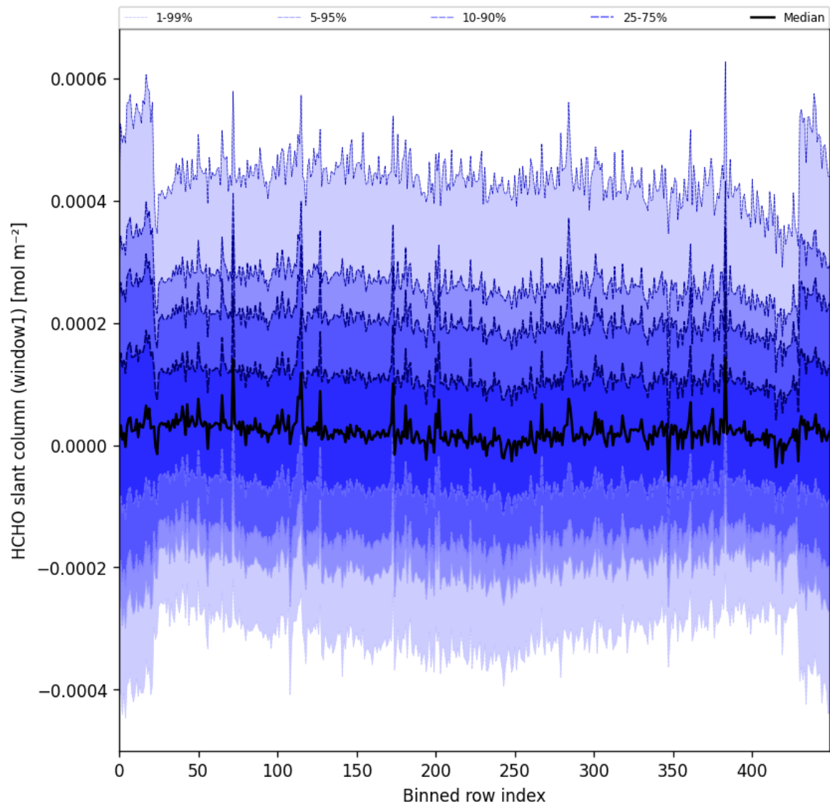
Figure 52: Along track statistics of “HCHO slant column (window1)” for 2025-07-27 to 2025-07-29
