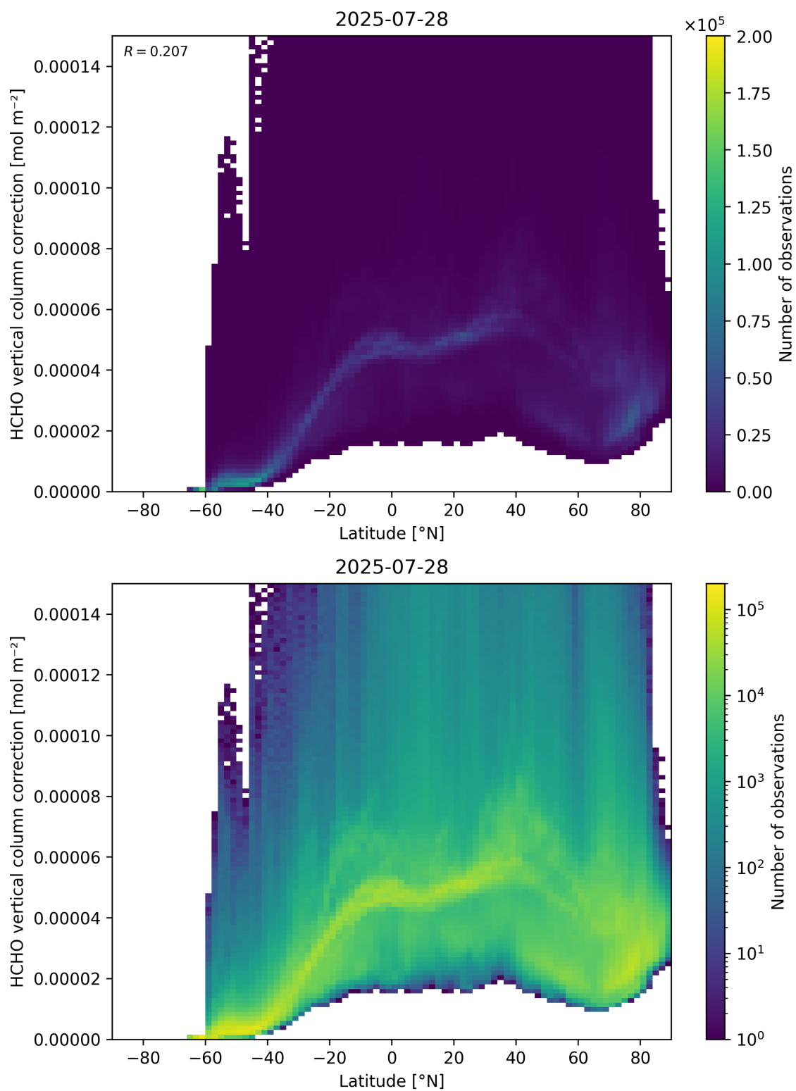
Figure 164: Scatter density plot of “Latitude” against “HCHO vertical column correction” for 2025-07-27 to 2025-07-29.
