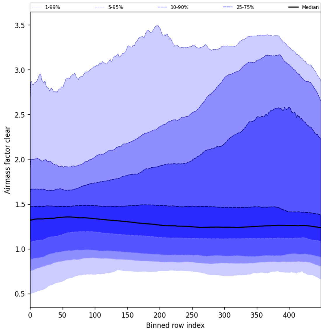
Figure 56: Along track statistics of “Airmass factor clear” for 2025-07-27 to 2025-07-29
