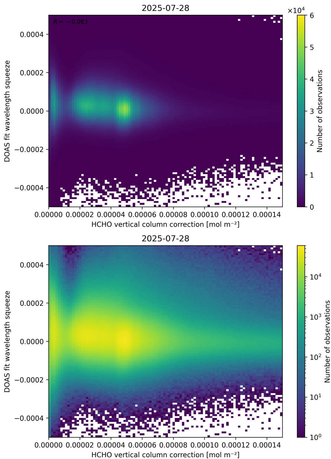
Figure 114: Scatter density plot of “HCHO vertical column correction” against “DOAS fit wavelength squeeze” for 2025-07-27 to 2025-07-29.
