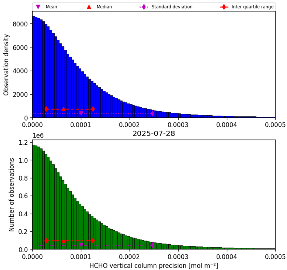
Figure 36: Histogram of “HCHO vertical column precision” for 2025-07-27 to 2025-07-29
