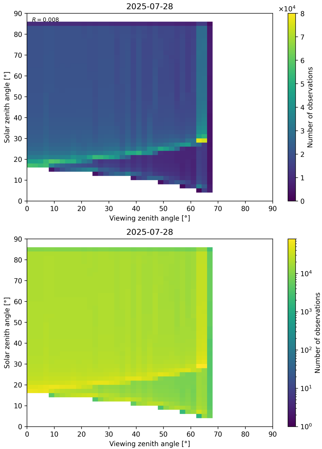
Figure 197: Scatter density plot of “Viewing zenith angle” against “Solar zenith angle” for 2025-07-27 to 2025-07-29.
