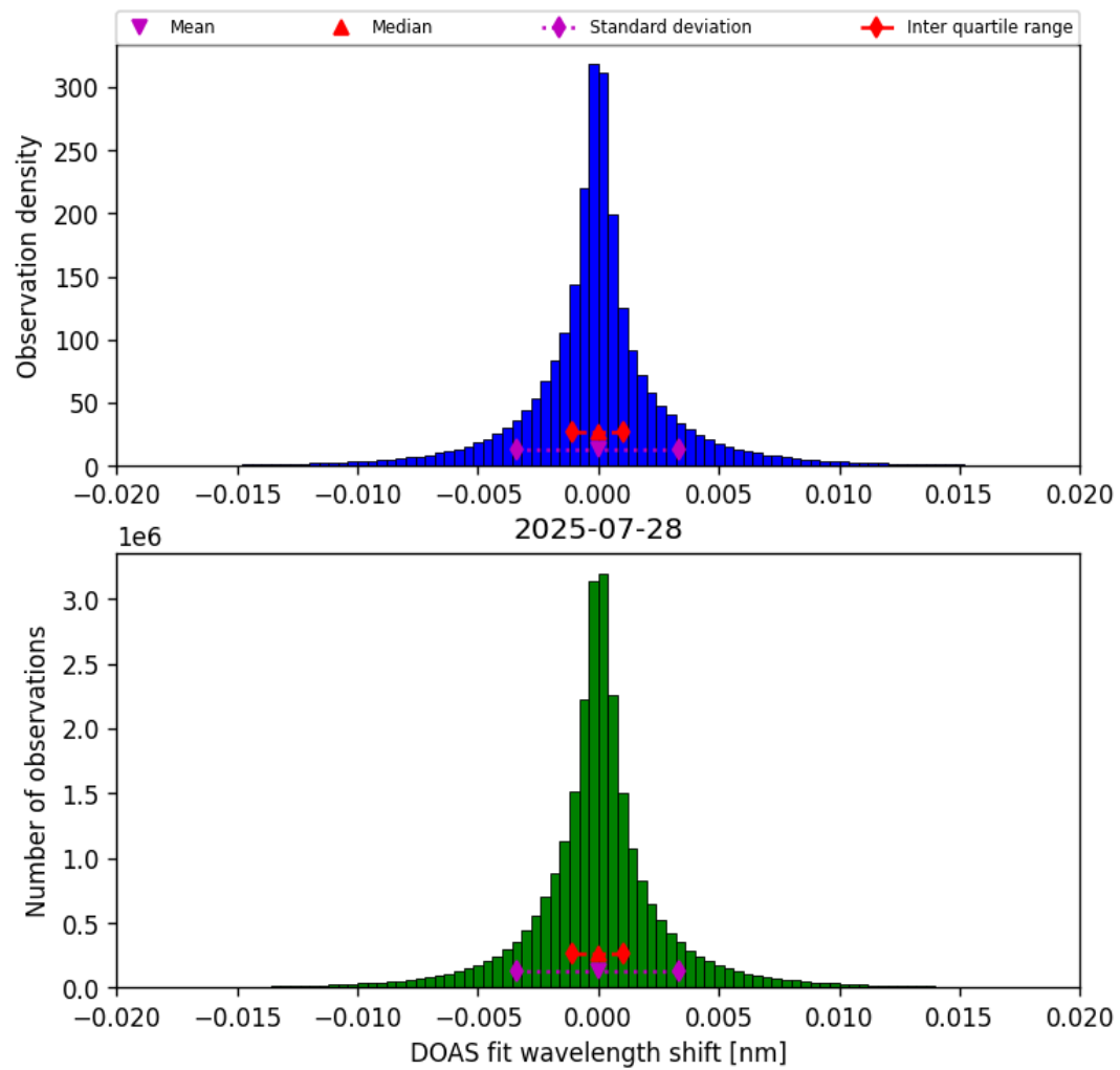
Figure 44: Histogram of “DOAS fit wavelength shift” for 2025-07-27 to 2025-07-29
