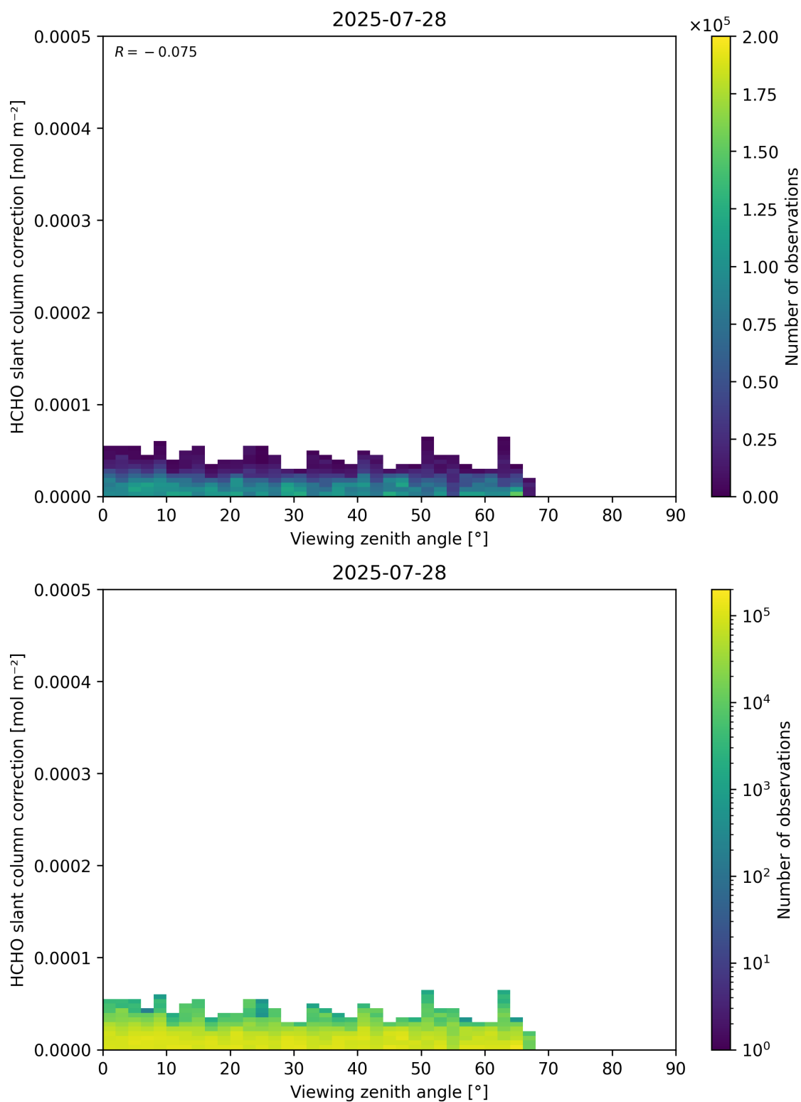
Figure 187: Scatter density plot of “Viewing zenith angle” against “HCHO slant column correction” for 2025-07-27 to 2025-07-29.
