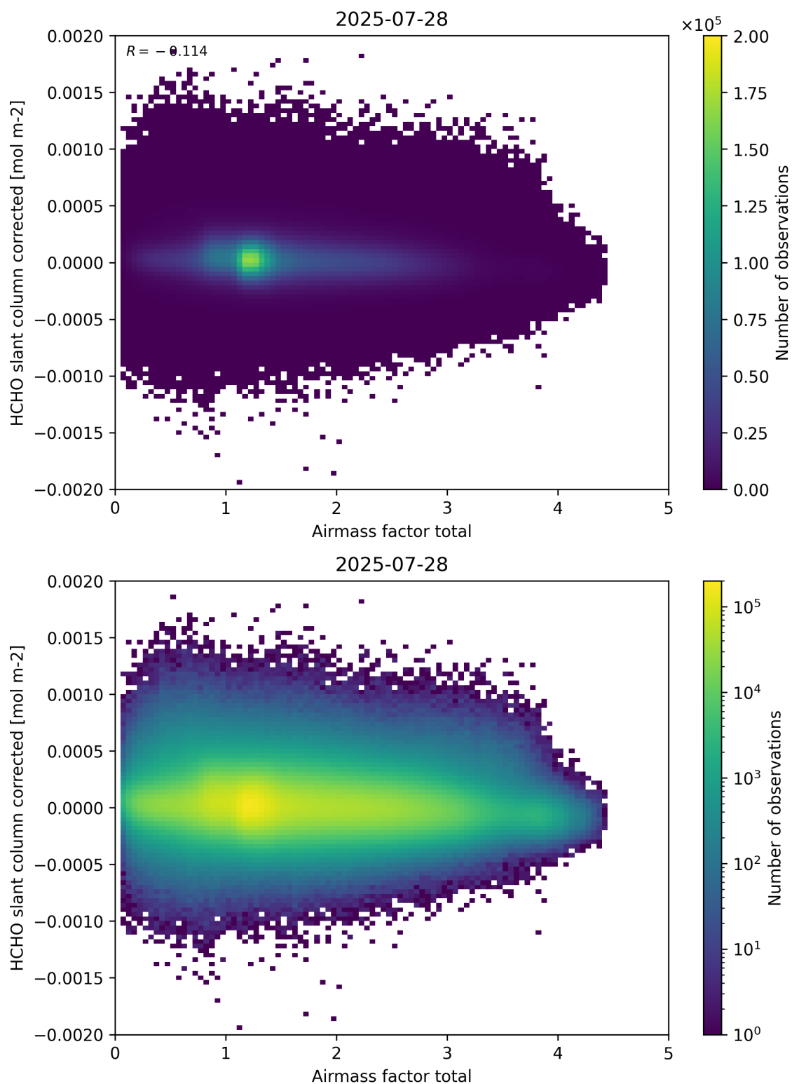
Figure 101: Scatter density plot of “Airmass factor total” against “HCHO slant column corrected” for 2025-07-27 to 2025-07-29.
