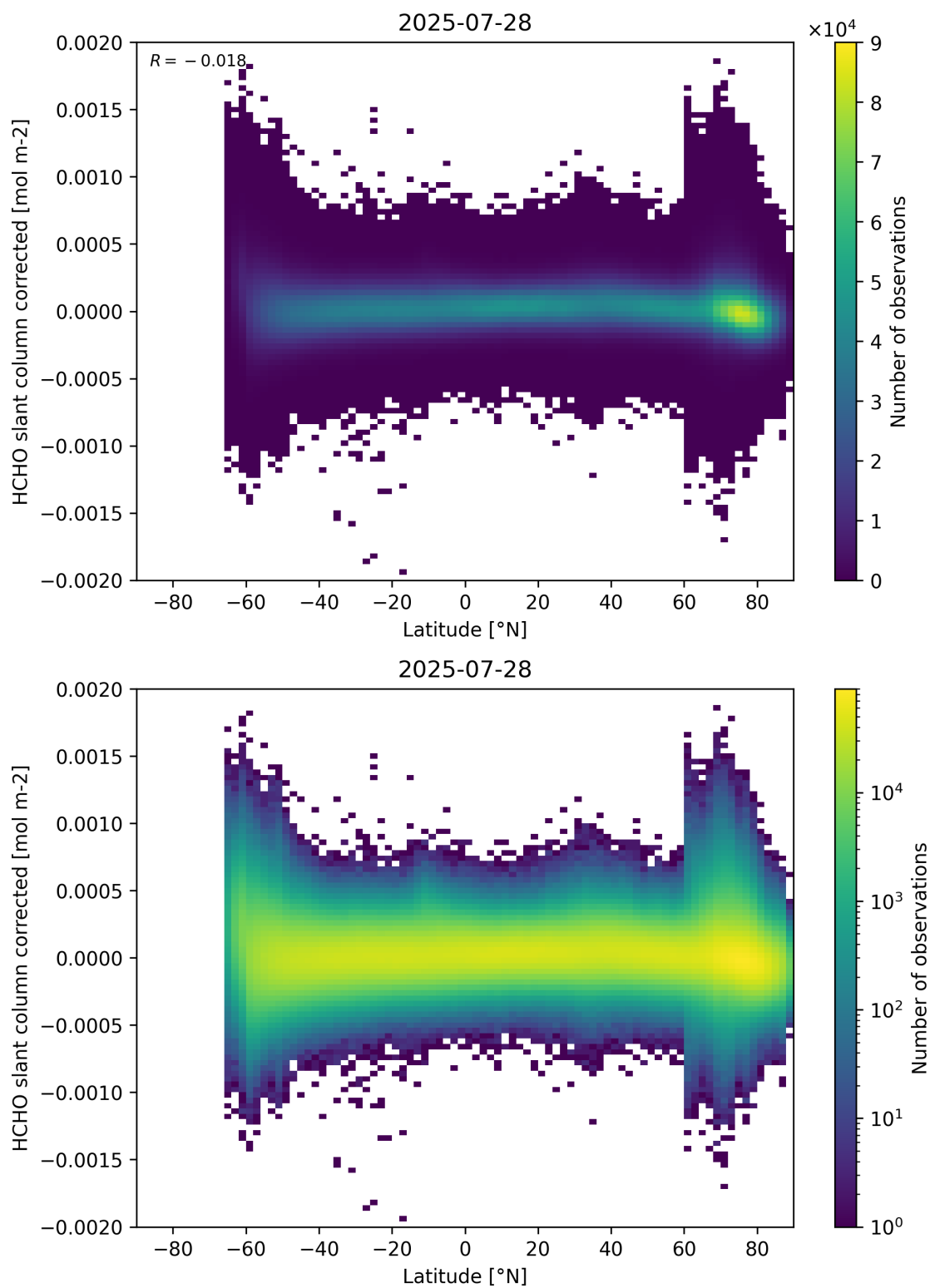
Figure 157: Scatter density plot of “Latitude” against “HCHO slant column corrected” for 2025-07-27 to 2025-07-29.
