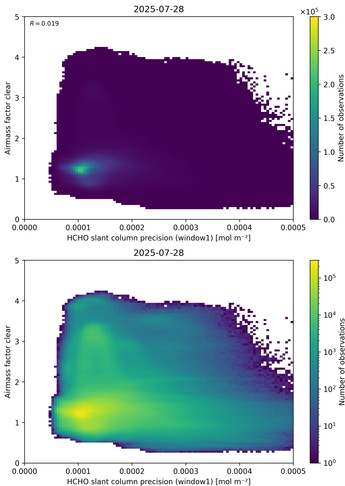
Figure 91: Scatter density plot of “HCHO slant column precision (window1)” against “Airmass factor clear” for 2025-07-27 to 2025-07-29.
