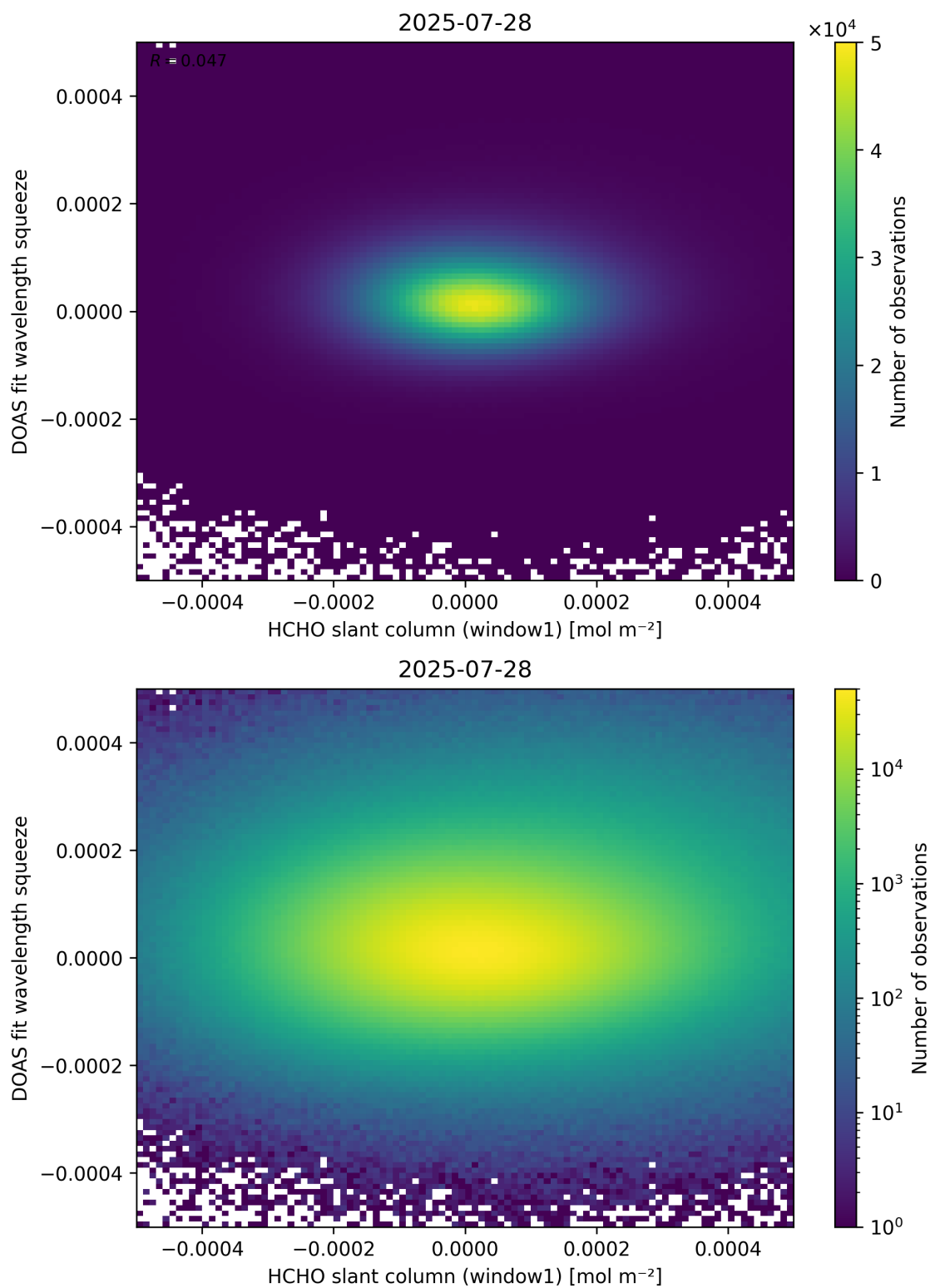
Figure 80: Scatter density plot of “HCHO slant column (window1)” against “DOAS fit wavelength squeeze” for 2025-07-27 to 2025-07-29.
