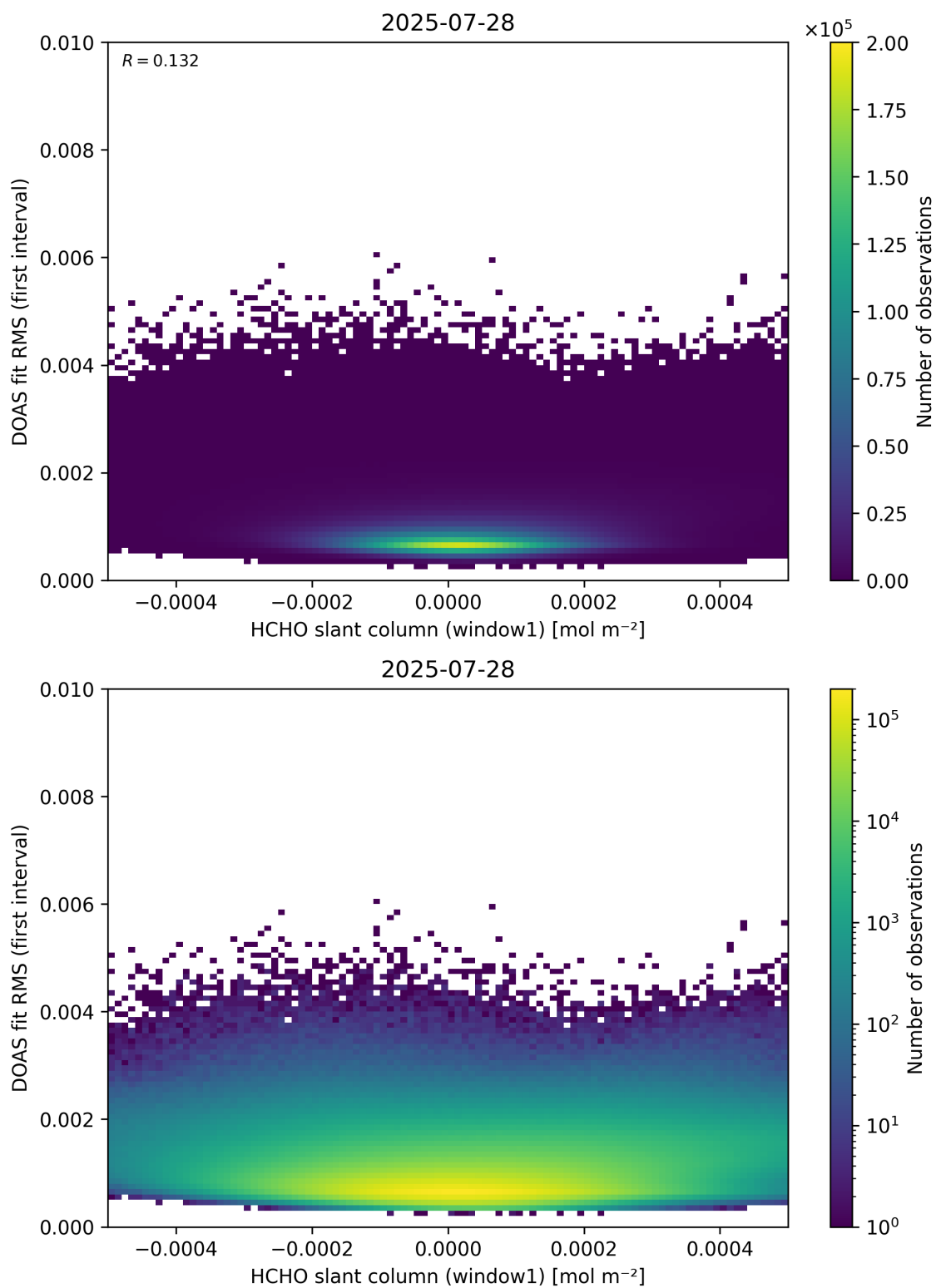
Figure 78: Scatter density plot of “HCHO slant column (window1)” against “DOAS fit RMS (first interval)” for 2025-07-27 to 2025-07-29.
