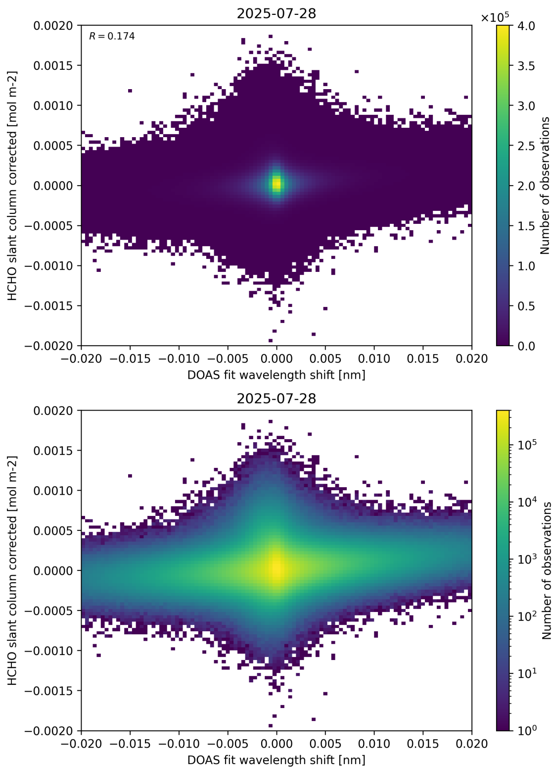
Figure 66: Scatter density plot of “DOAS fit wavelength shift” against “HCHO slant column corrected” for 2025-07-27 to 2025-07-29.
