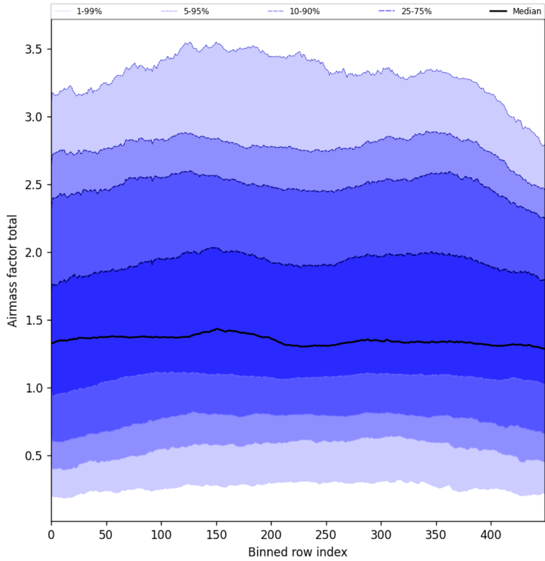
Figure 54: Along track statistics of “Airmass factor total” for 2025-07-27 to 2025-07-29
