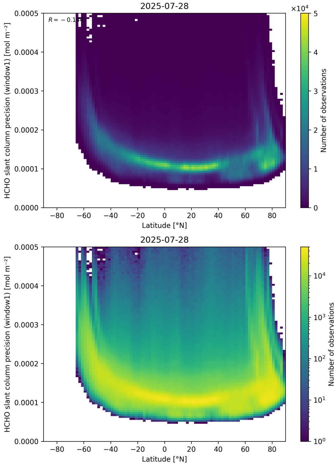
Figure 160: Scatter density plot of “Latitude” against “HCHO slant column precision (window1)” for 2025-07-27 to 2025-07-29.
