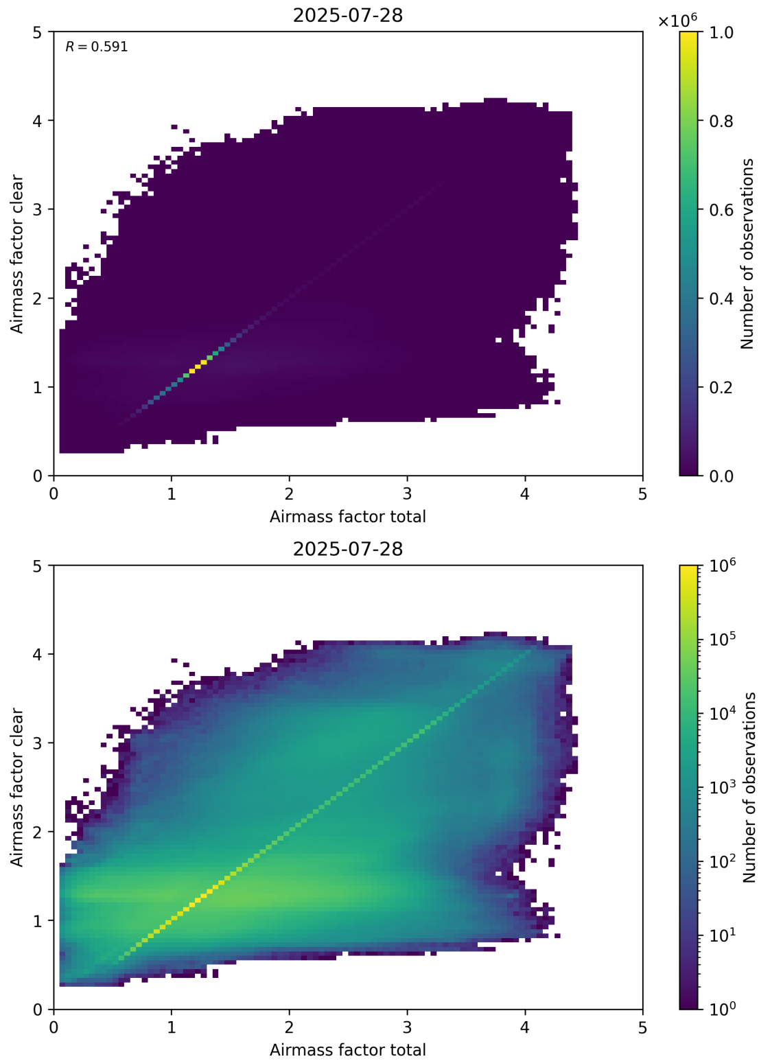
Figure 100: Scatter density plot of “Airmass factor total” against “Airmass factor clear” for 2025-07-27 to 2025-07-29.
