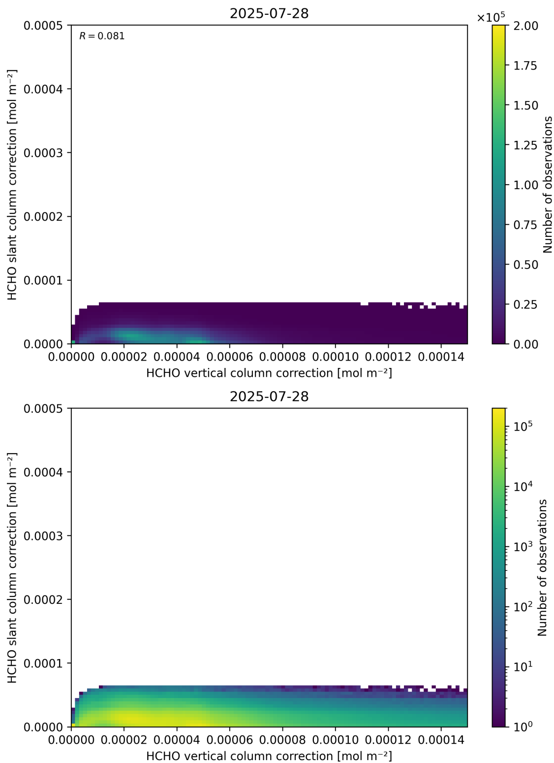
Figure 117: Scatter density plot of “HCHO vertical column correction” against “HCHO slant column correction” for 2025-07-27 to 2025-07-29.
