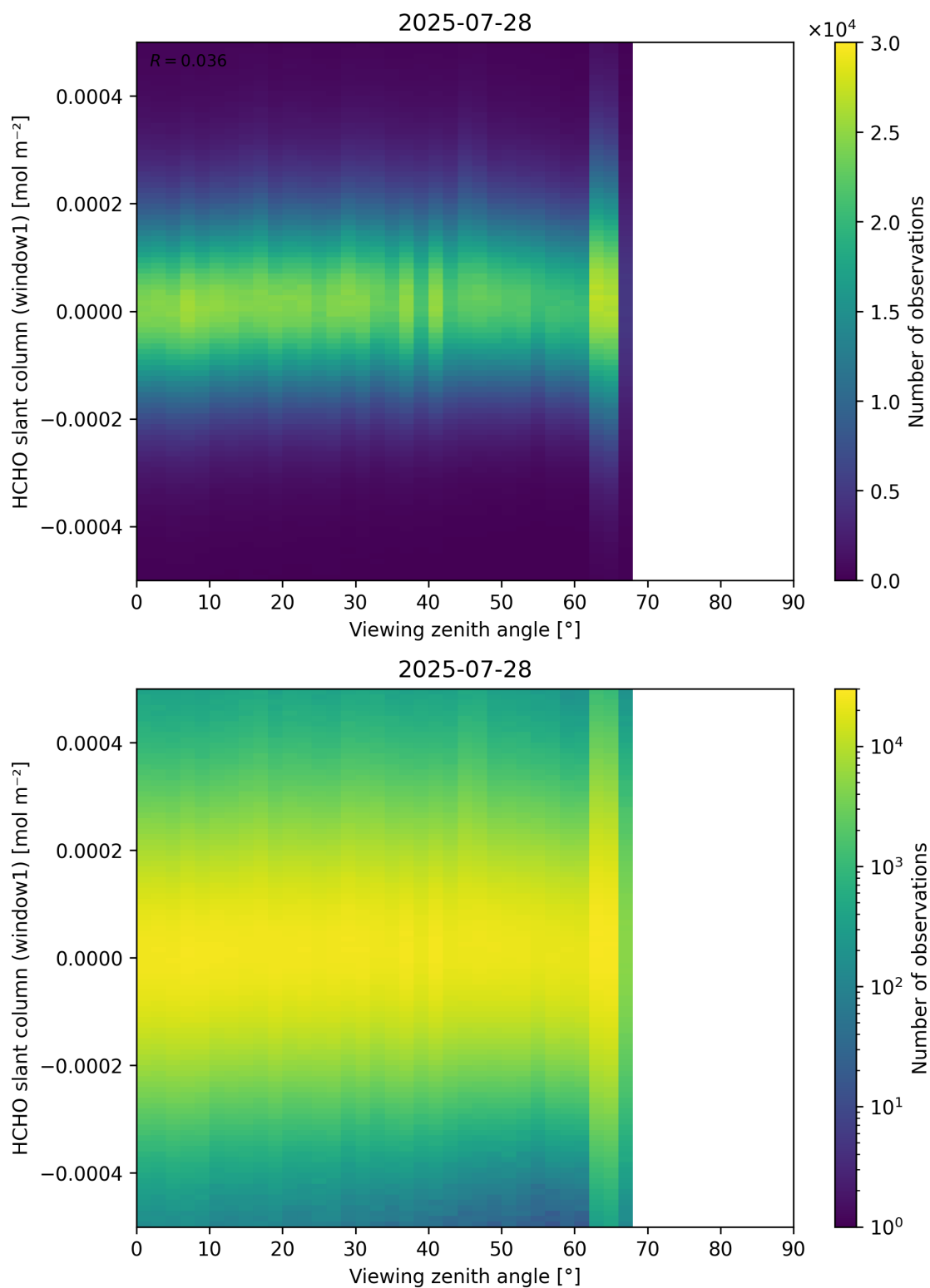
Figure 188: Scatter density plot of “Viewing zenith angle” against “HCHO slant column (window1)” for 2025-07-27 to 2025-07-29.
