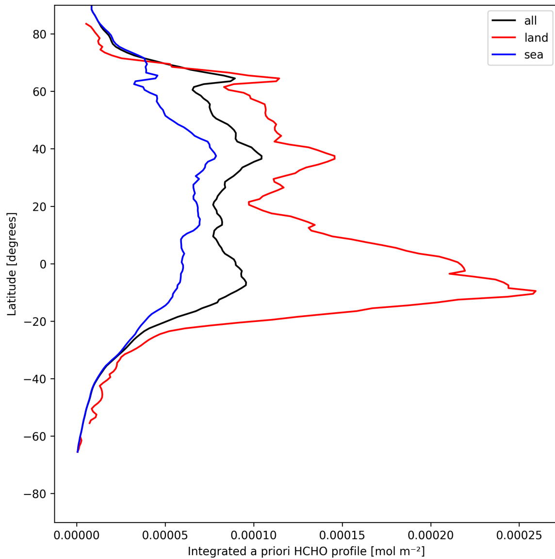
Figure 29: Zonal average of “Integrated a priori HCHO profile” for 2025-07-27 to 2025-07-29.
