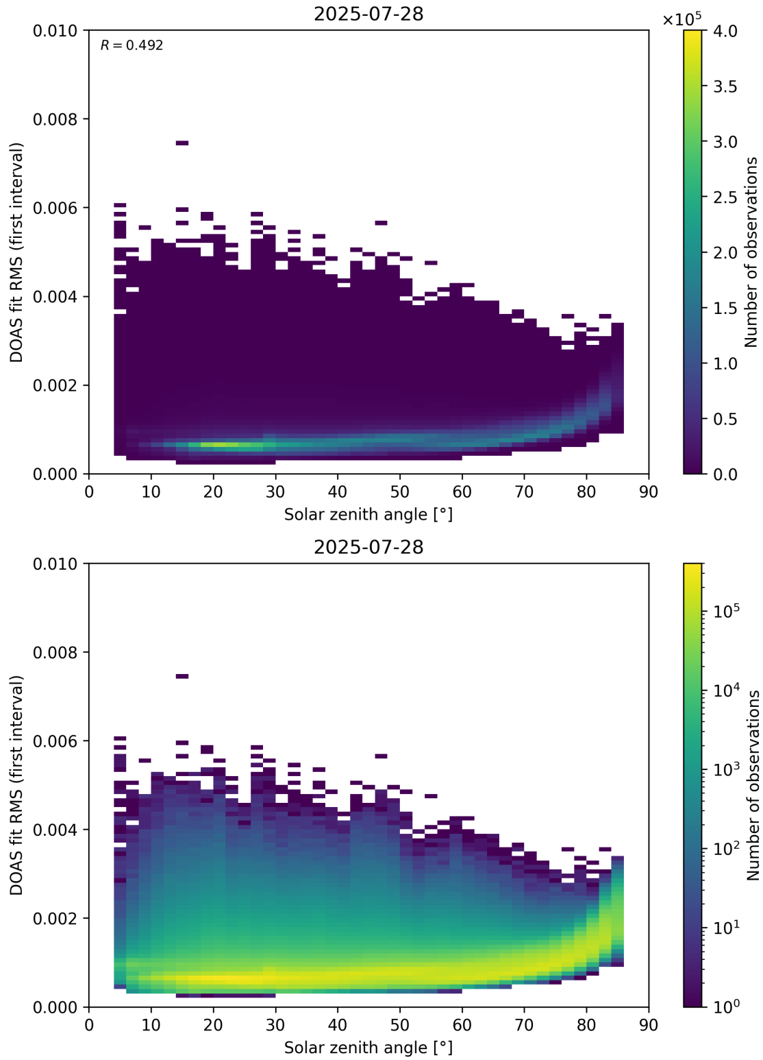
Figure 167: Scatter density plot of “Solar zenith angle” against “DOAS fit RMS (first interval)” for 2025-07-27 to 2025-07-29.
