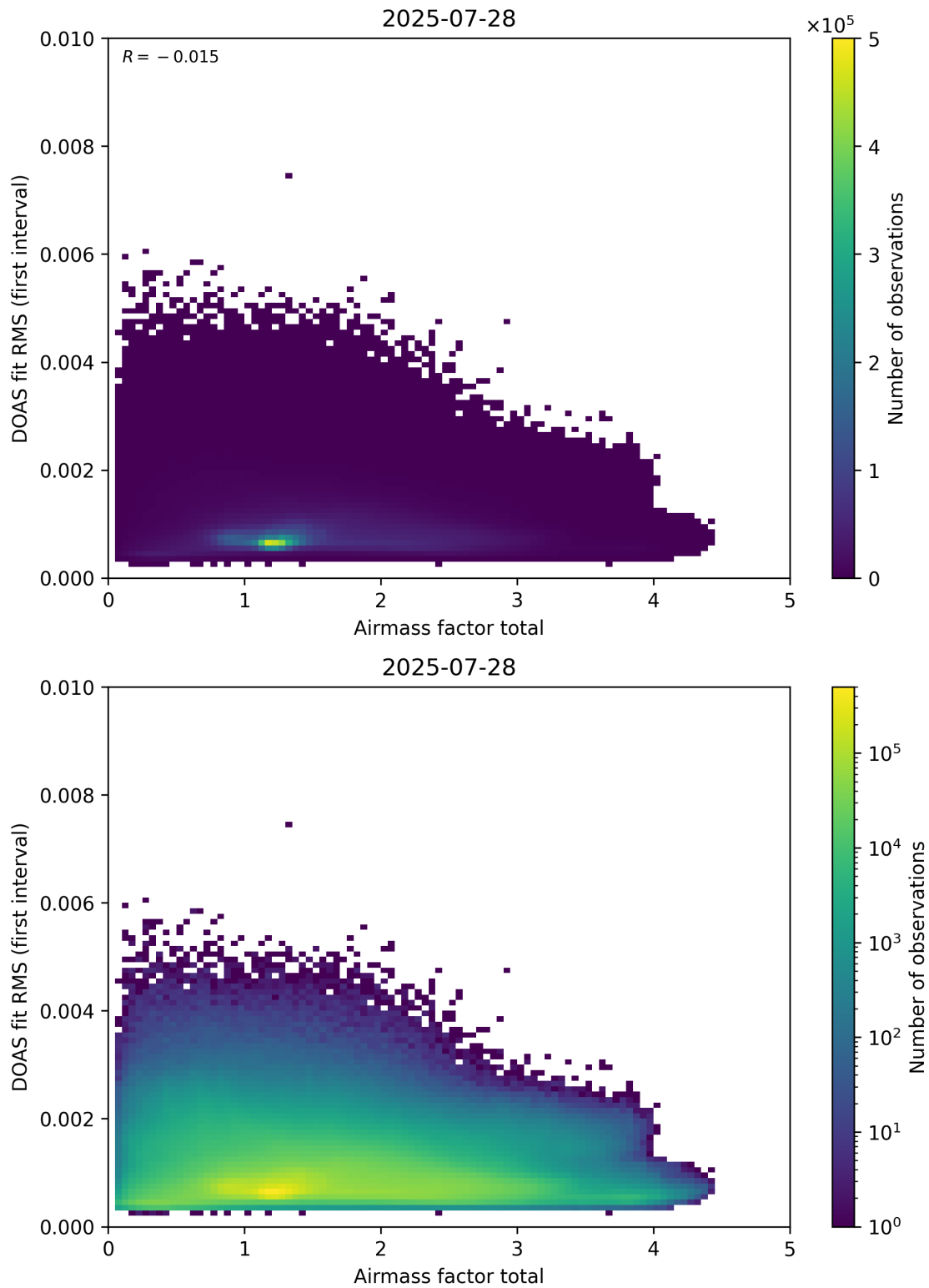
Figure 97: Scatter density plot of “Airmass factor total” against “DOAS fit RMS (first interval)” for 2025-07-27 to 2025-07-29.
