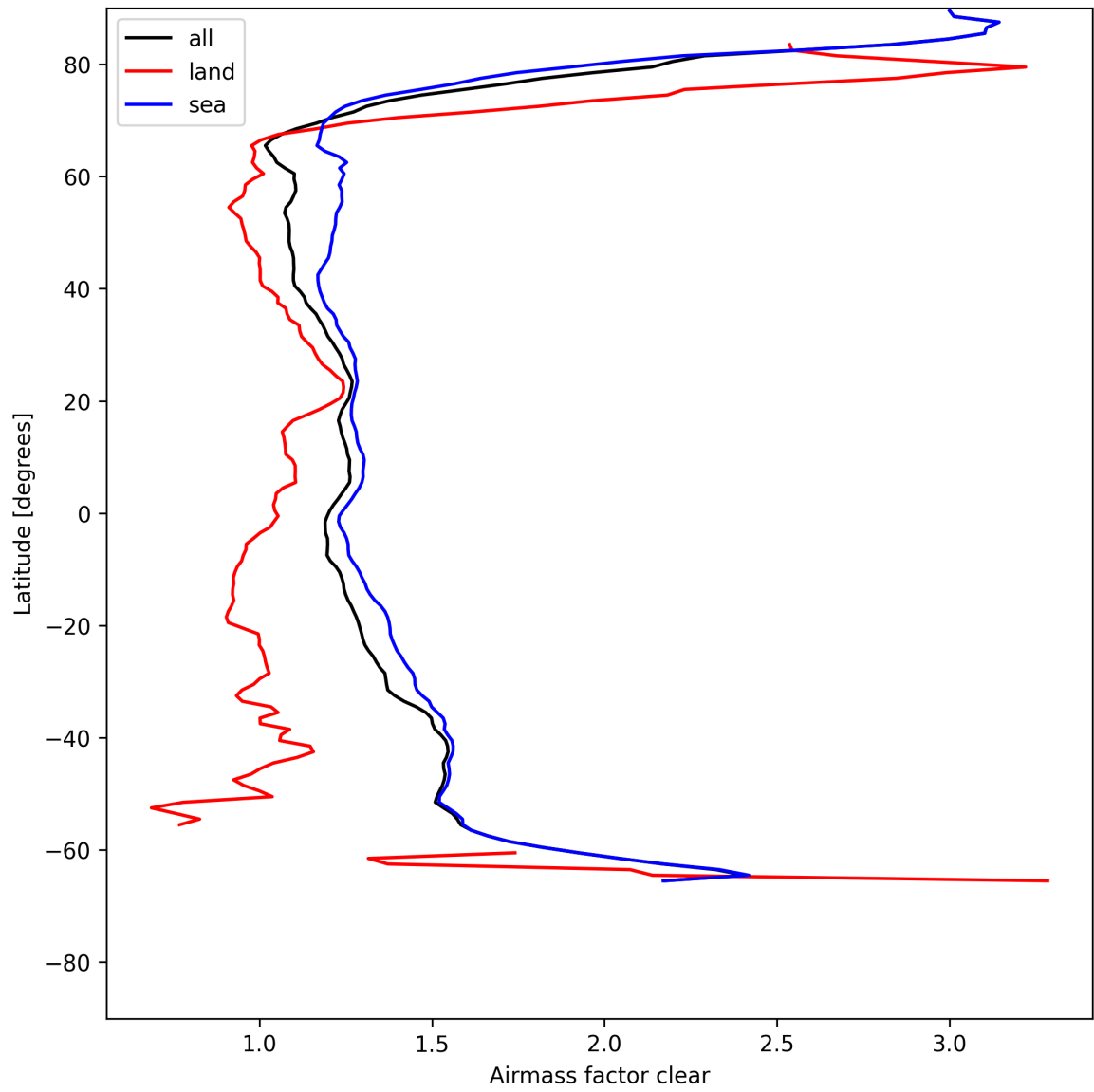
Figure 28: Zonal average of “Airmass factor clear” for 2025-07-27 to 2025-07-29.
