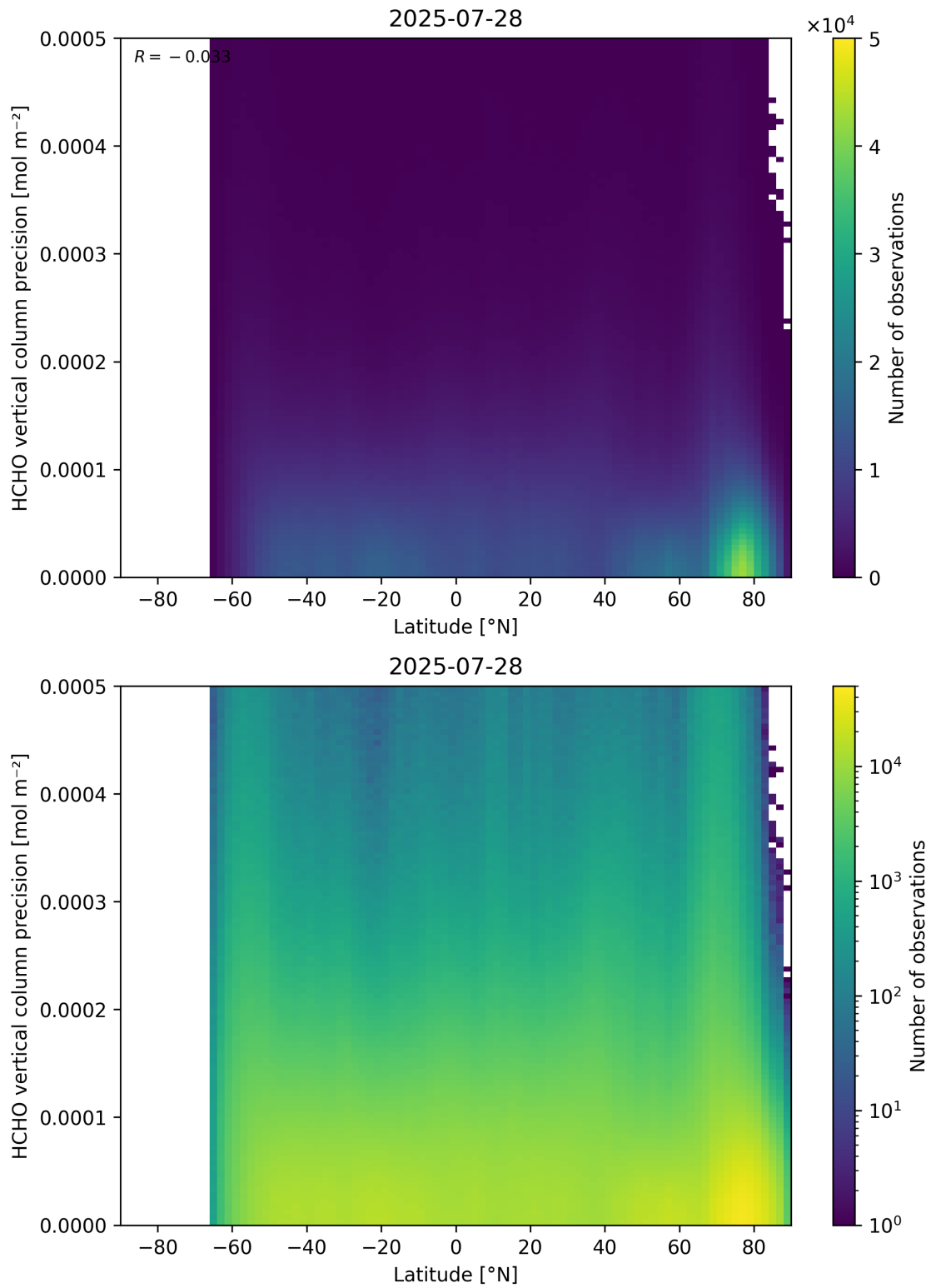
Figure 165: Scatter density plot of “Latitude” against “HCHO vertical column precision” for 2025-07-27 to 2025-07-29.
