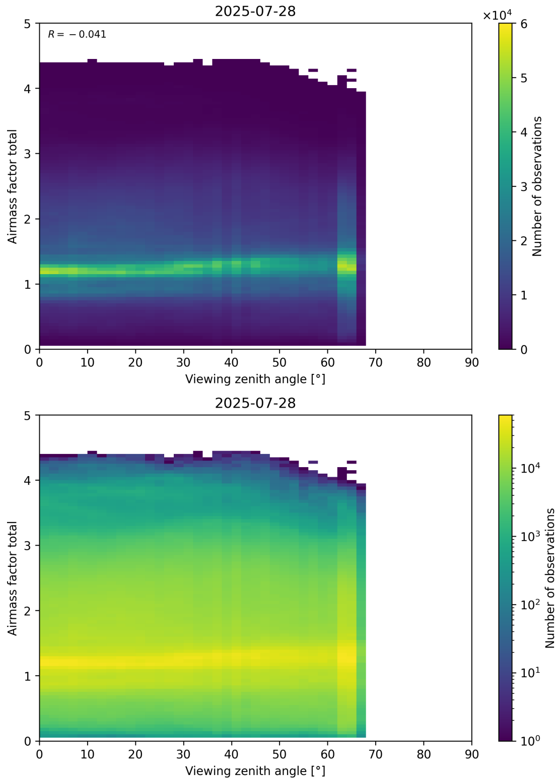
Figure 190: Scatter density plot of “Viewing zenith angle” against “Airmass factor total” for 2025-07-27 to 2025-07-29.
