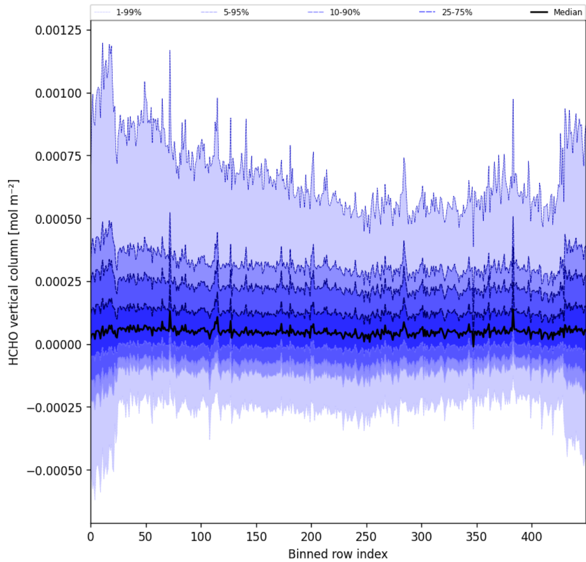
Figure 49: Along track statistics of “HCHO vertical column” for 2025-07-27 to 2025-07-29
