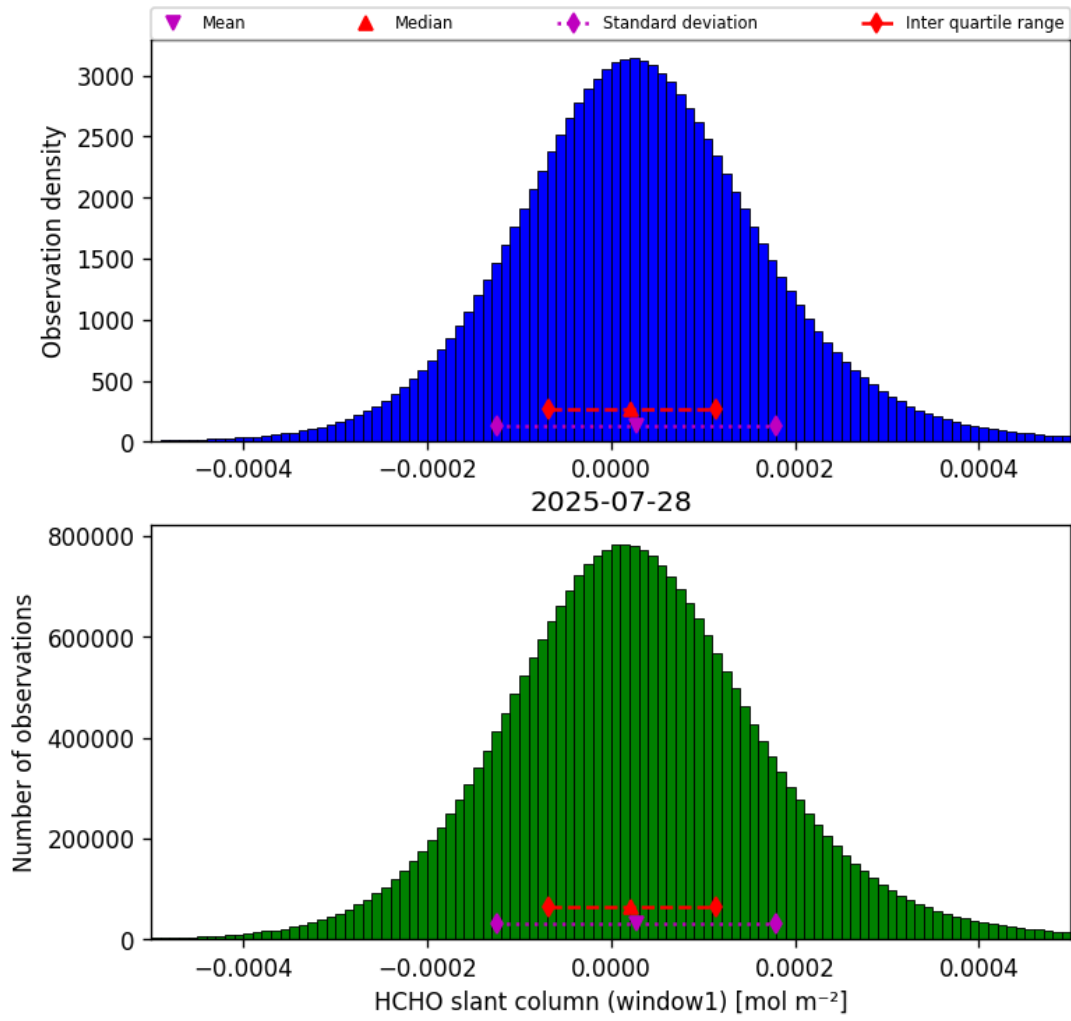
Figure 38: Histogram of “HCHO slant column (window1)” for 2025-07-27 to 2025-07-29
