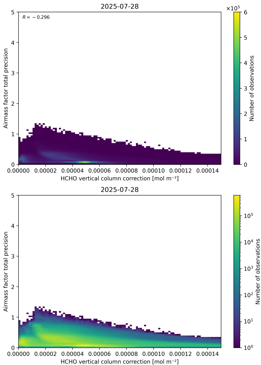
Figure 121: Scatter density plot of “HCHO vertical column correction” against “Airmass factor total precision” for 2025-07-27 to 2025-07-29.
