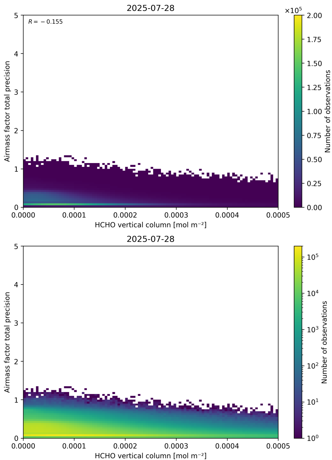
Figure 132: Scatter density plot of “HCHO vertical column” against “Airmass factor total precision” for 2025-07-27 to 2025-07-29.
