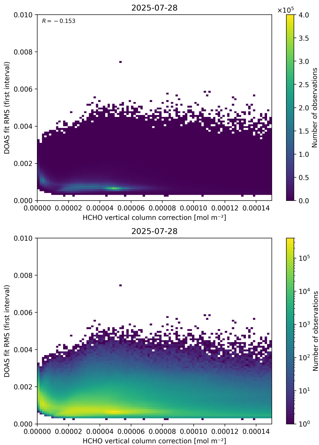
Figure 112: Scatter density plot of “HCHO vertical column correction” against “DOAS fit RMS (first interval)” for 2025-07-27 to 2025-07-29.
