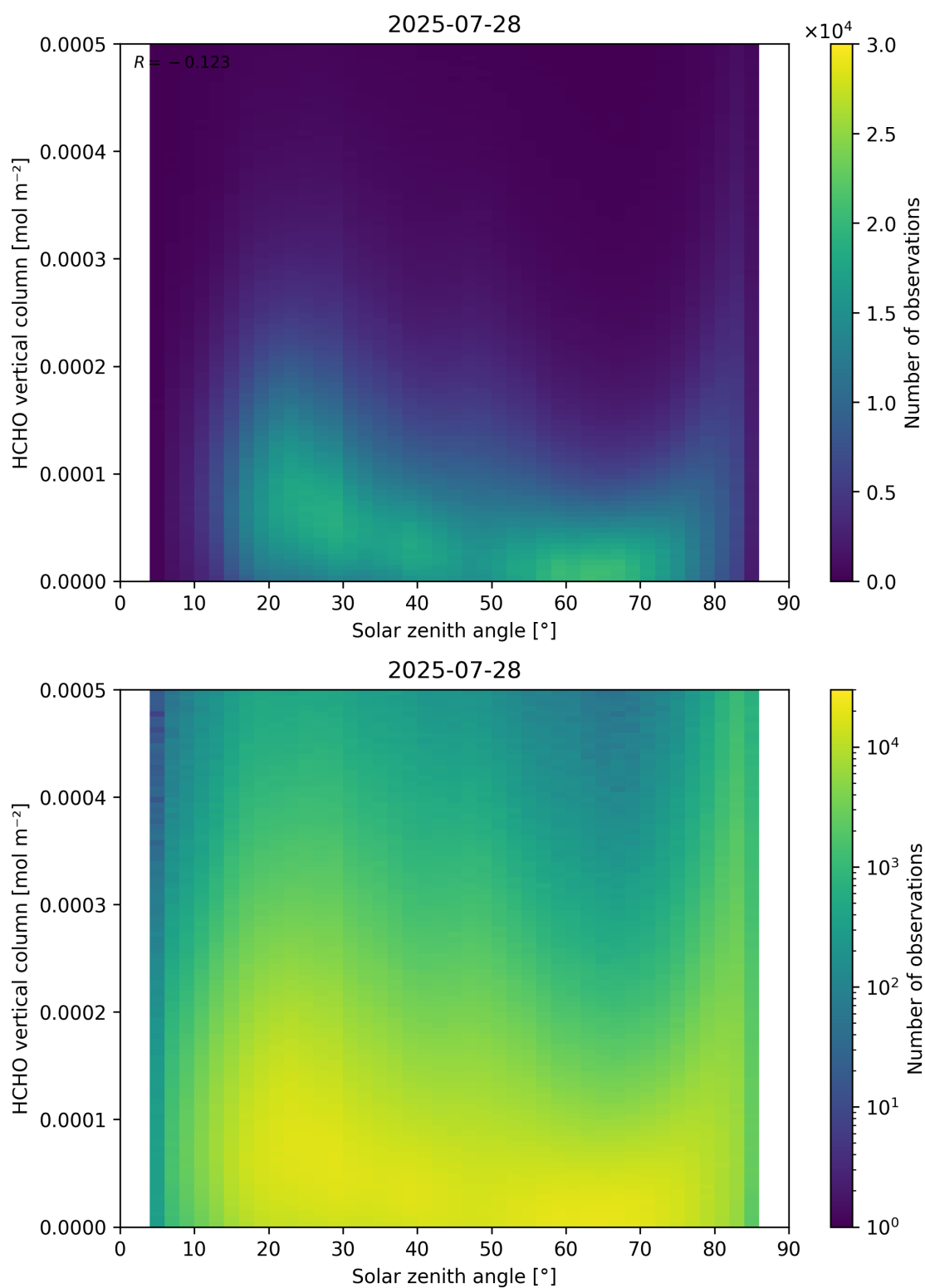
Figure 177: Scatter density plot of “Solar zenith angle” against “HCHO vertical column” for 2025-07-27 to 2025-07-29.
