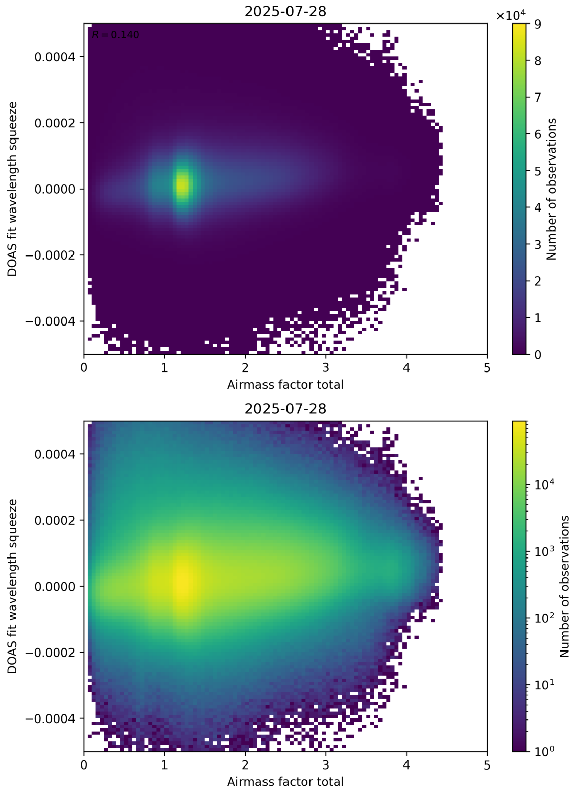
Figure 99: Scatter density plot of “Airmass factor total” against “DOAS fit wavelength squeeze” for 2025-07-27 to 2025-07-29.
