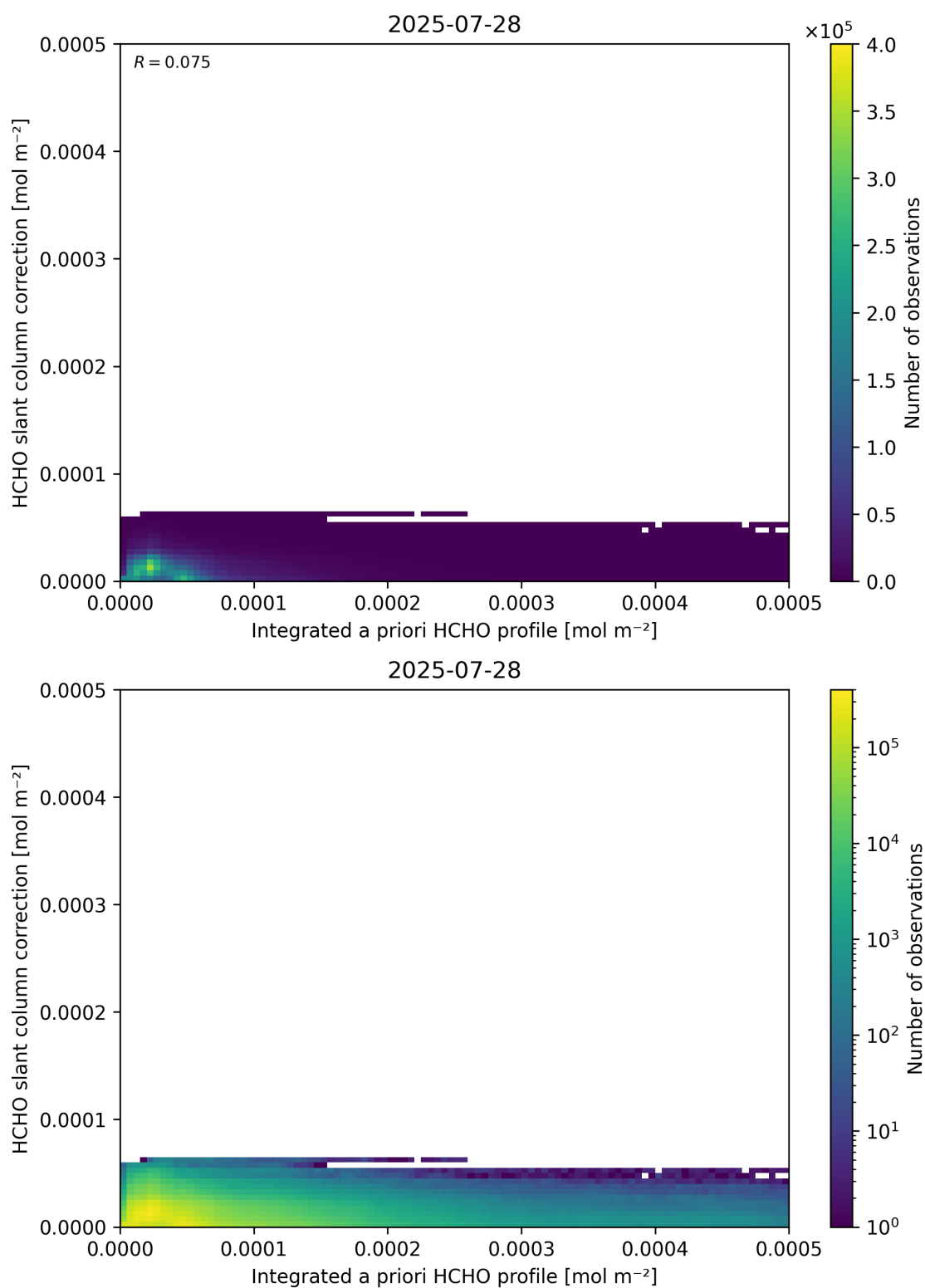
Figure 152: Scatter density plot of “Integrated a priori HCHO profile” against “HCHO slant column correction” for 2025-07-27 to 2025-07-29.
