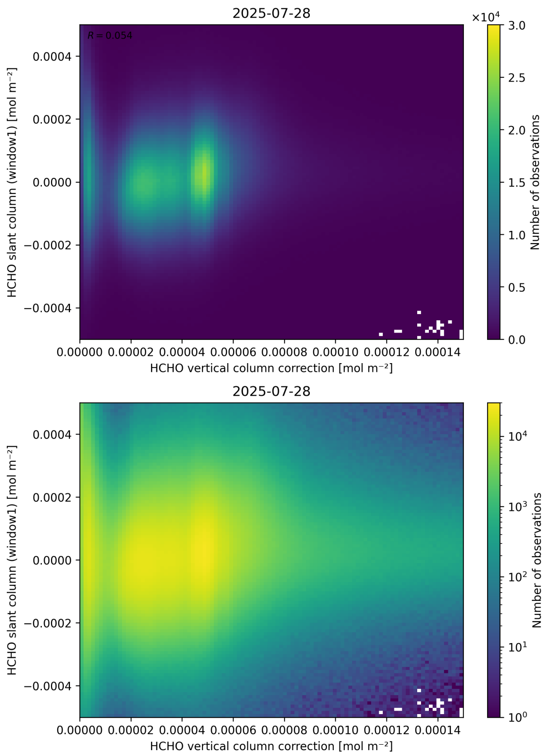
Figure 118: Scatter density plot of “HCHO vertical column correction” against “HCHO slant column (window1)” for 2025-07-27 to 2025-07-29.
