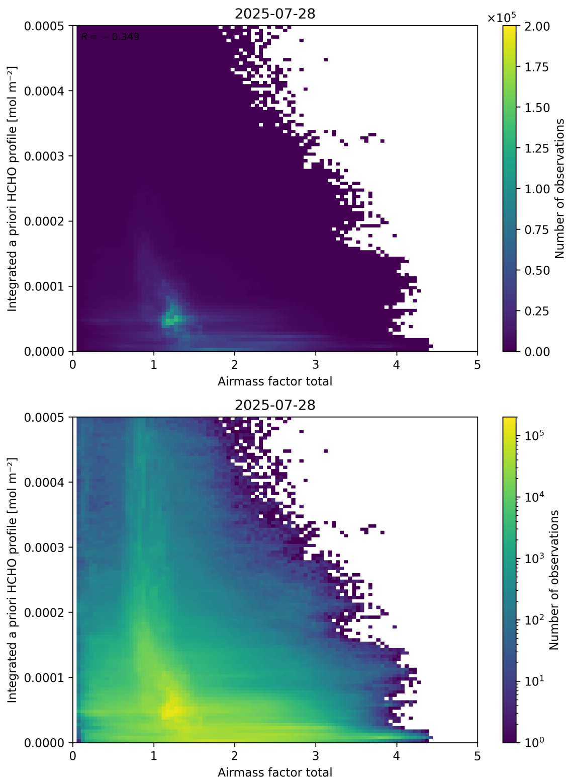
Figure 104: Scatter density plot of “Airmass factor total” against “Integrated a priori HCHO profile” for 2025-07-27 to 2025-07-29.
