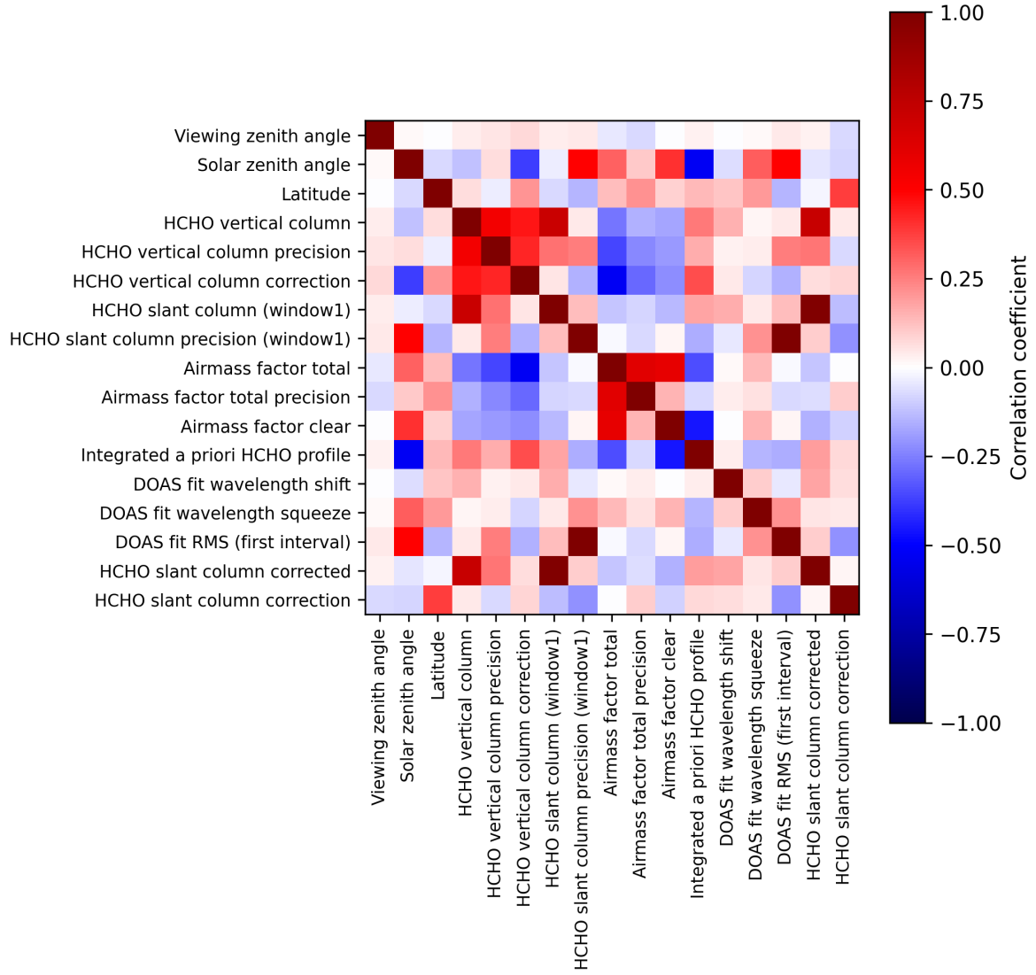
Figure 2: Map of correlation matrix for 2025-07-27 to 2025-07-29.
