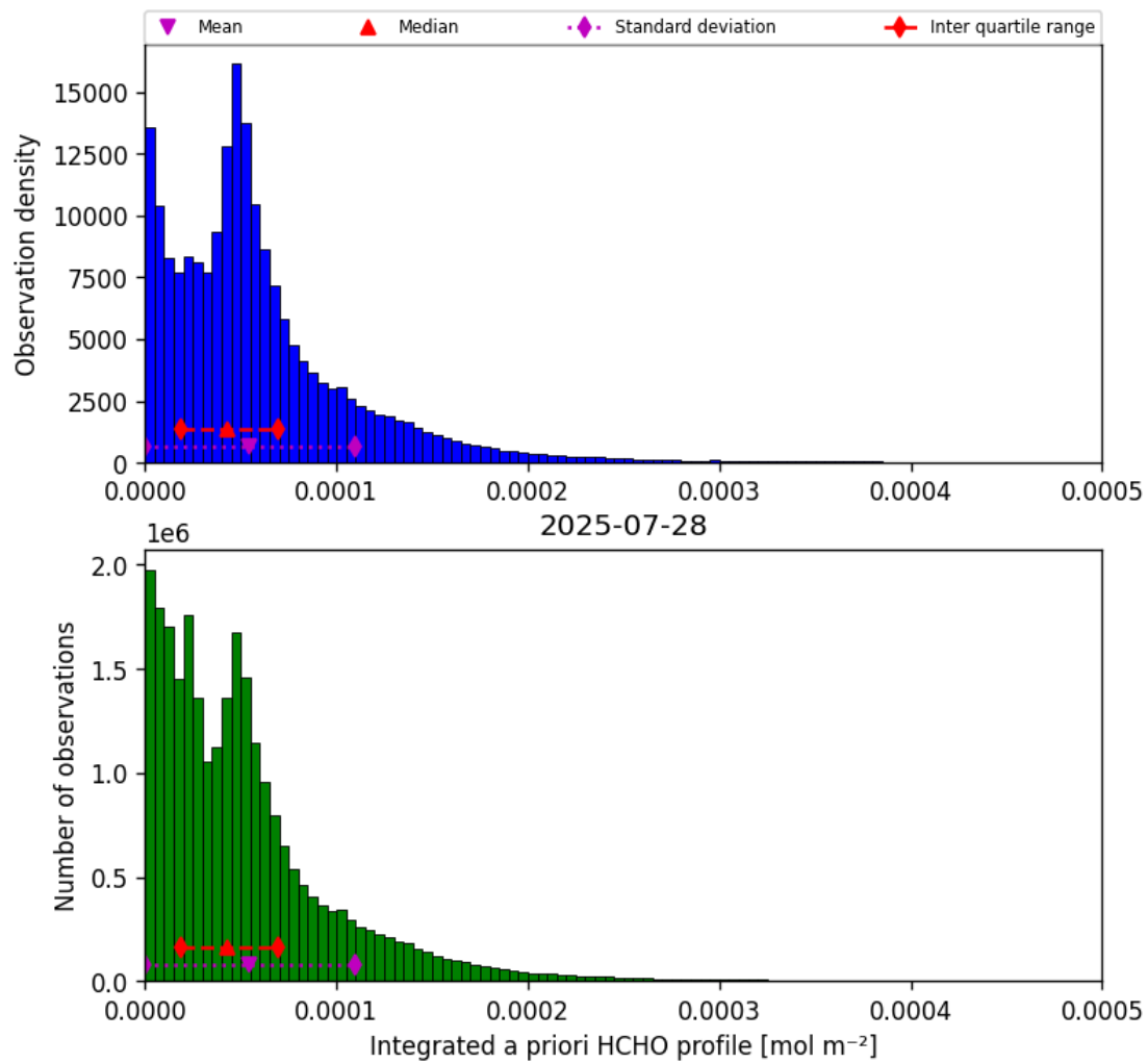
Figure 43: Histogram of “Integrated a priori HCHO profile” for 2025-07-27 to 2025-07-29
