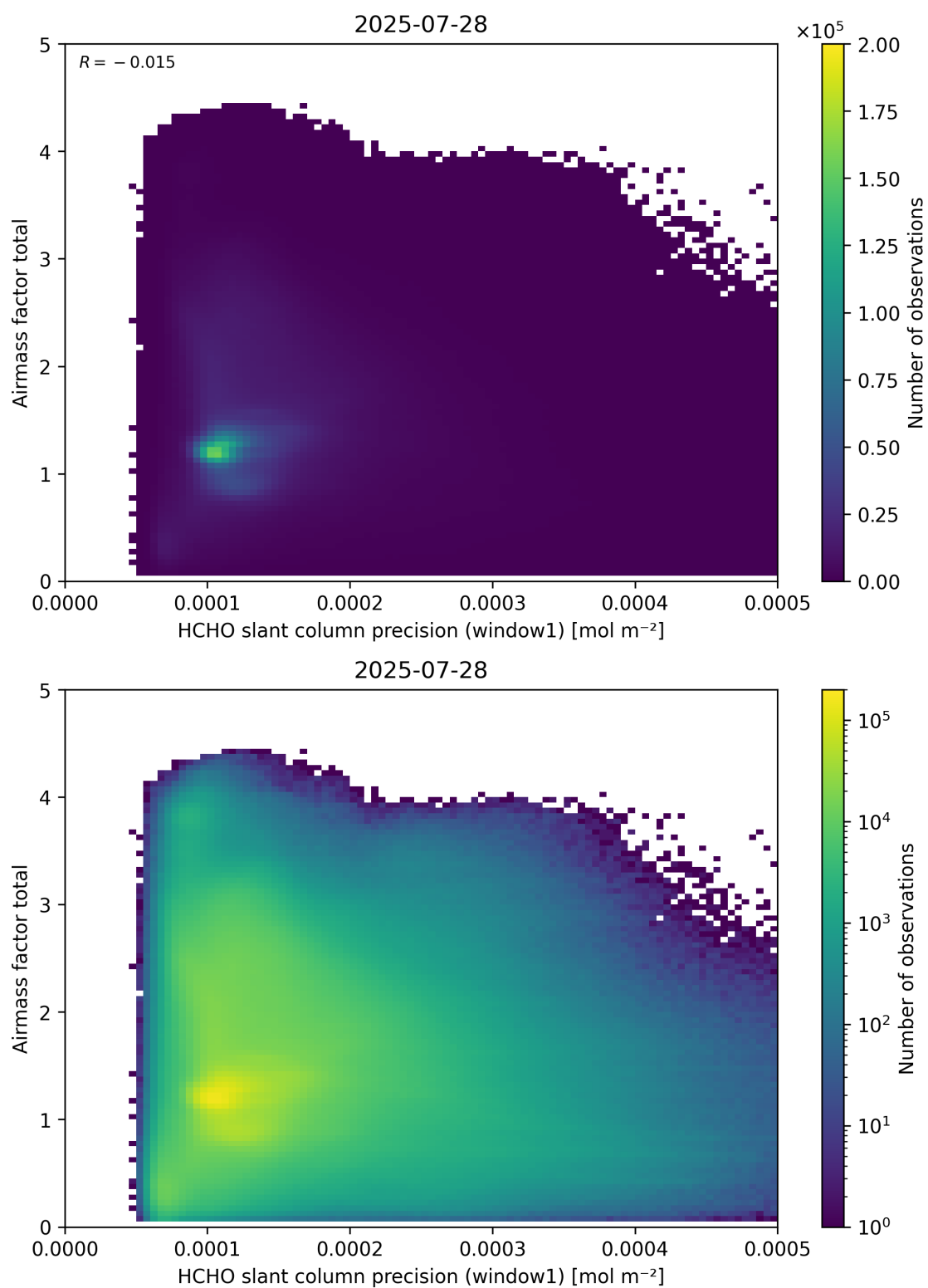
Figure 94: Scatter density plot of “HCHO slant column precision (window1)” against “Airmass factor total” for 2025-07-27 to 2025-07-29.
