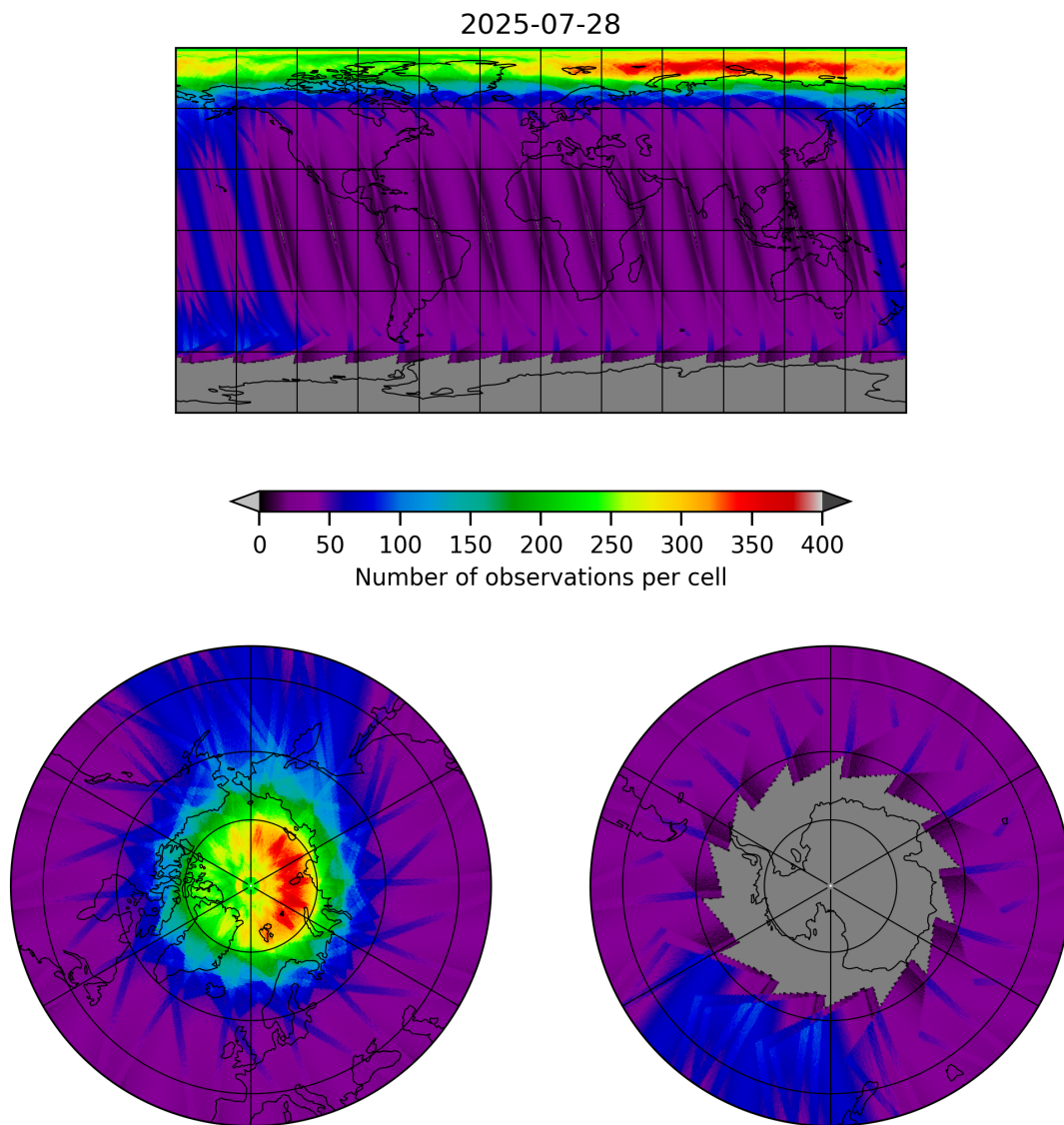
Figure 19: Map of the number of observations for 2025-07-27 to 2025-07-29
