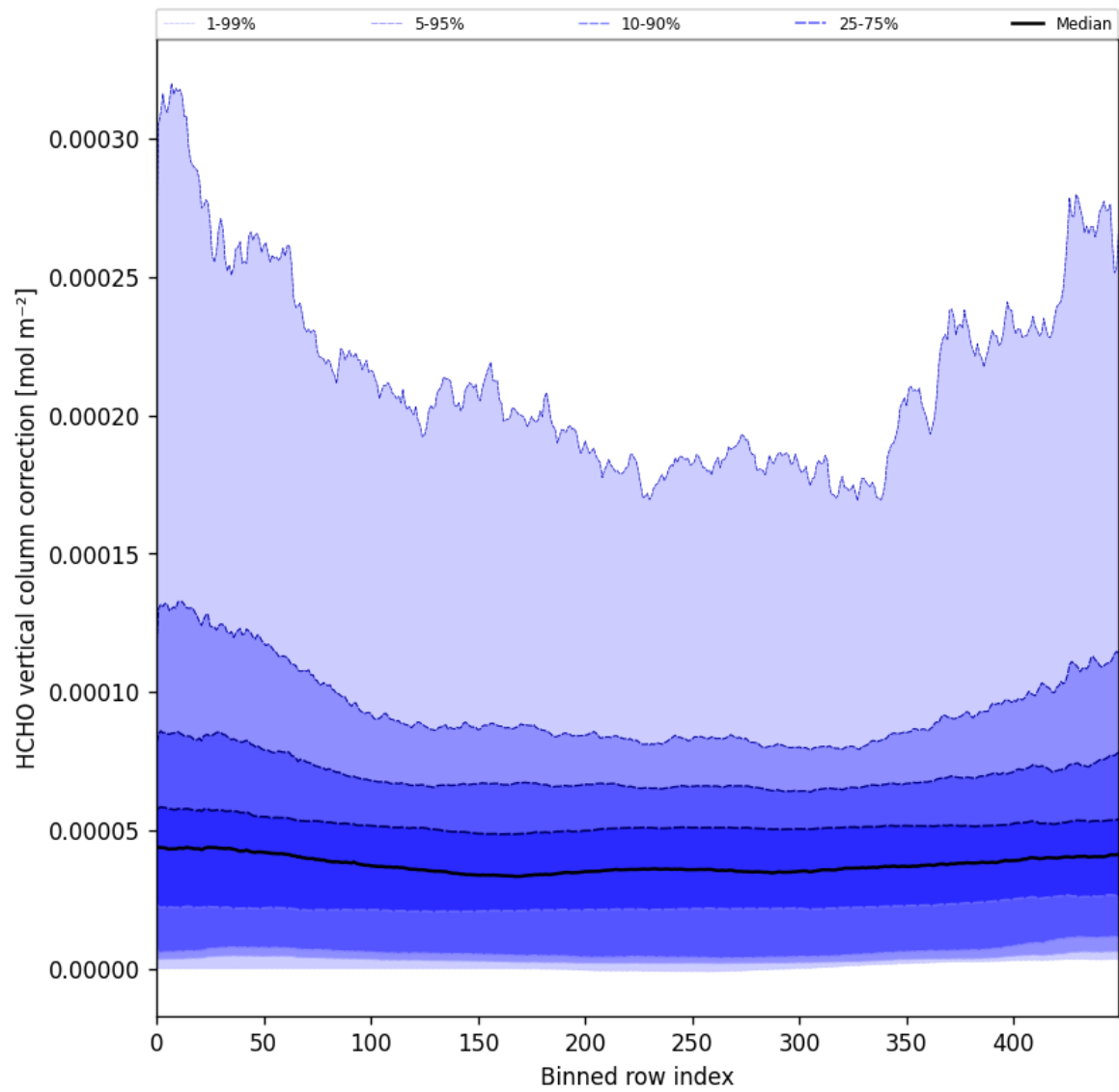
Figure 51: Along track statistics of “HCHO vertical column correction” for 2025-07-27 to 2025-07-29
