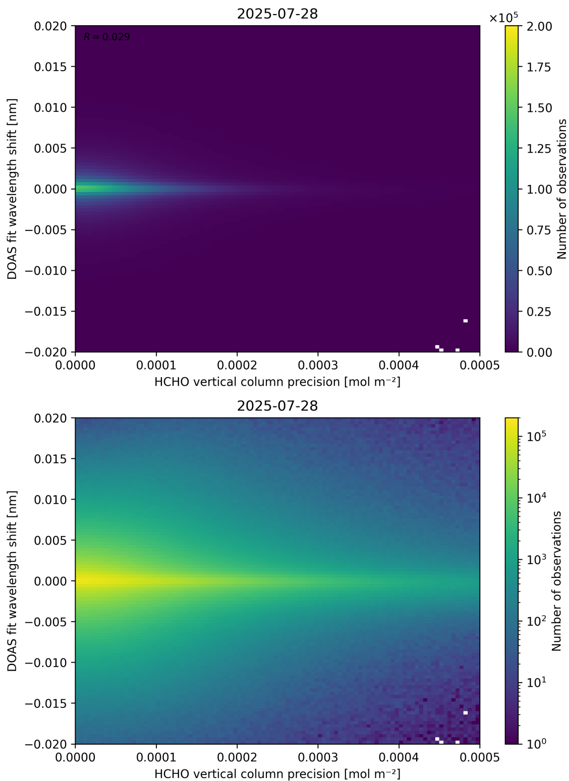
Figure 137: Scatter density plot of “HCHO vertical column precision” against “DOAS fit wavelength shift” for 2025-07-27 to 2025-07-29.
