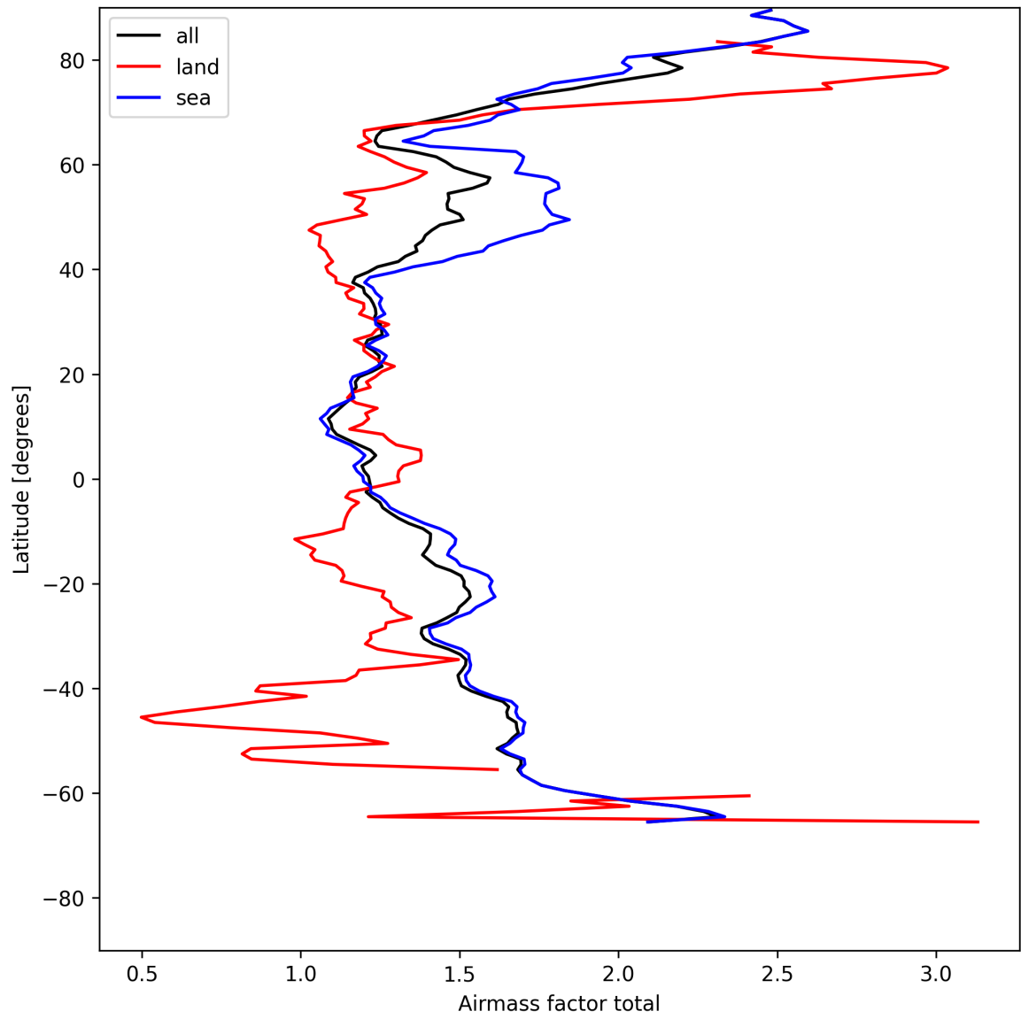
Figure 26: Zonal average of “Airmass factor total” for 2025-07-27 to 2025-07-29.
