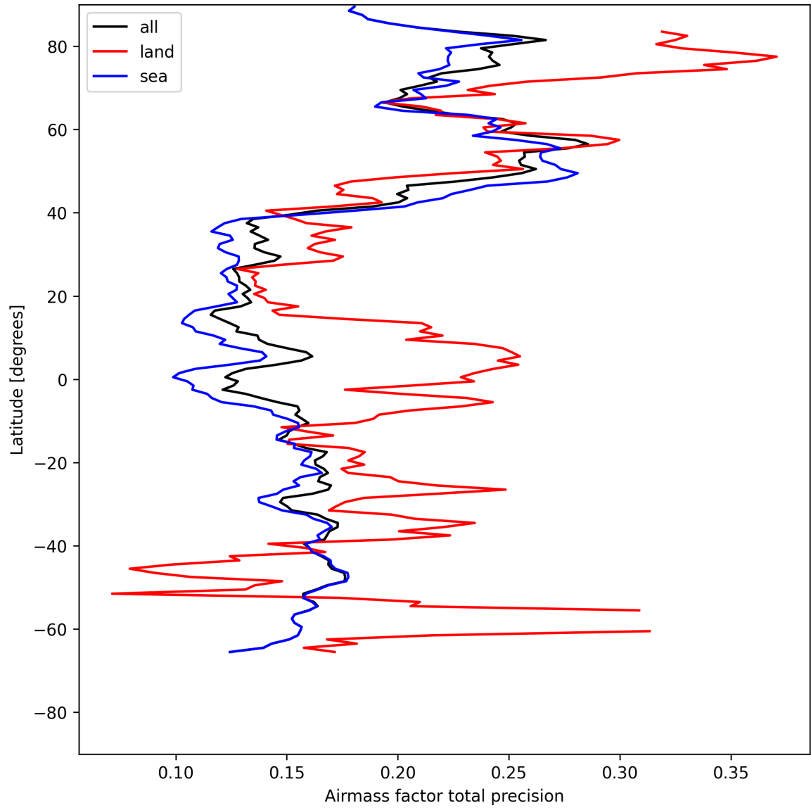
Figure 27: Zonal average of “Airmass factor total precision” for 2025-07-27 to 2025-07-29.
