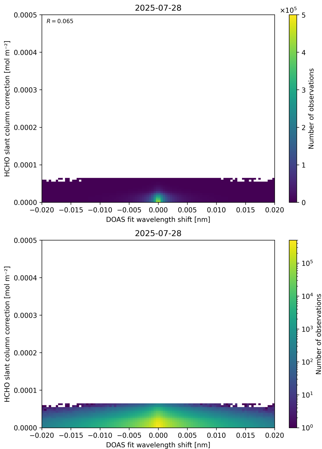
Figure 67: Scatter density plot of “DOAS fit wavelength shift” against “HCHO slant column correction” for 2025-07-27 to 2025-07-29.
