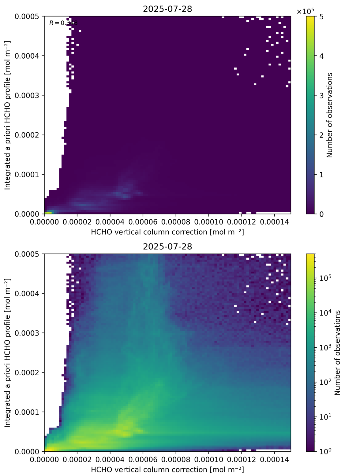
Figure 122: Scatter density plot of “HCHO vertical column correction” against “Integrated a priori HCHO profile” for 2025-07-27 to 2025-07-29.
