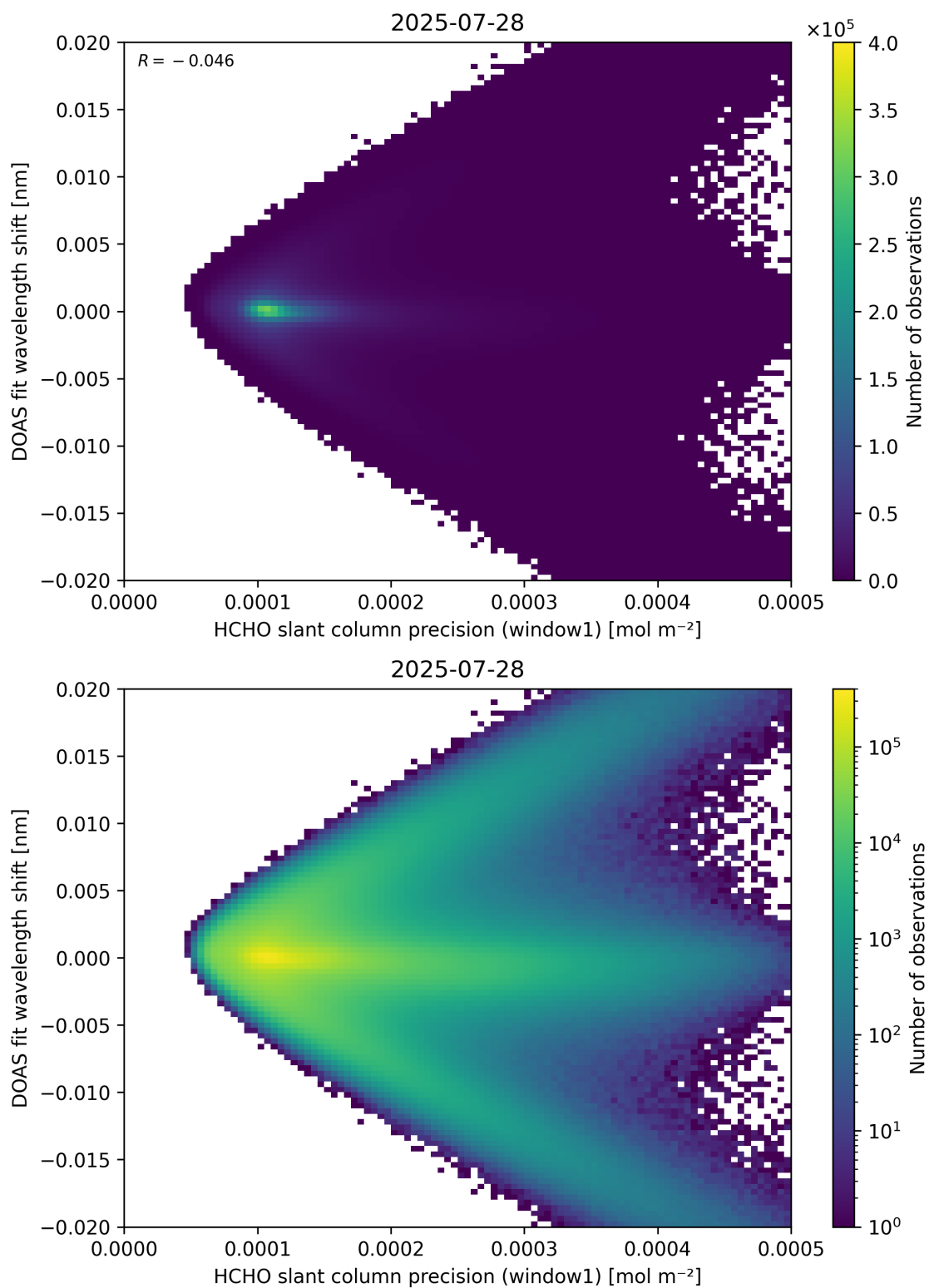
Figure 89: Scatter density plot of “HCHO slant column precision (window1)” against “DOAS fit wavelength shift” for 2025-07-27 to 2025-07-29.
