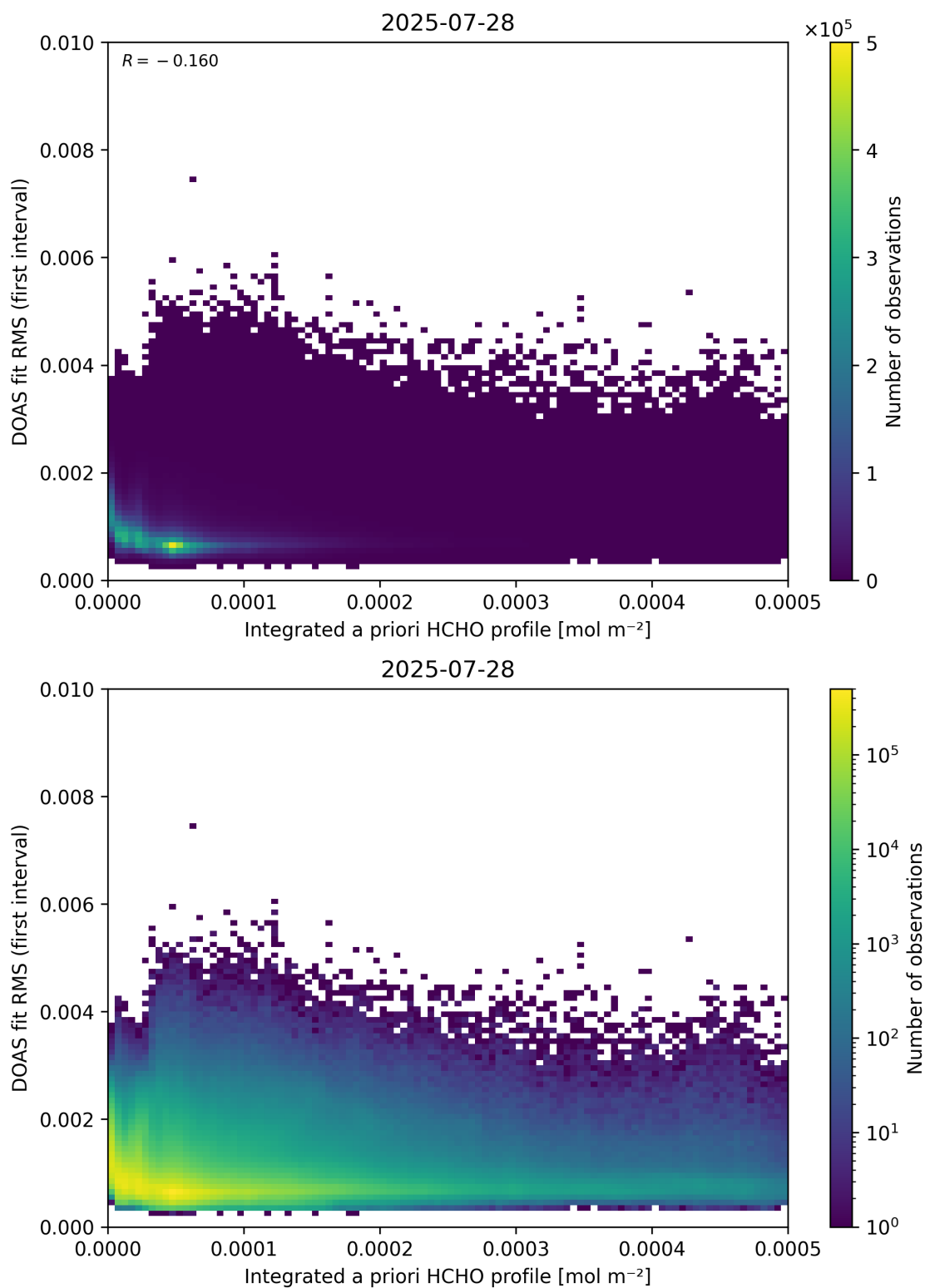
Figure 148: Scatter density plot of “Integrated a priori HCHO profile” against “DOAS fit RMS (first interval)” for 2025-07-27 to 2025-07-29.
