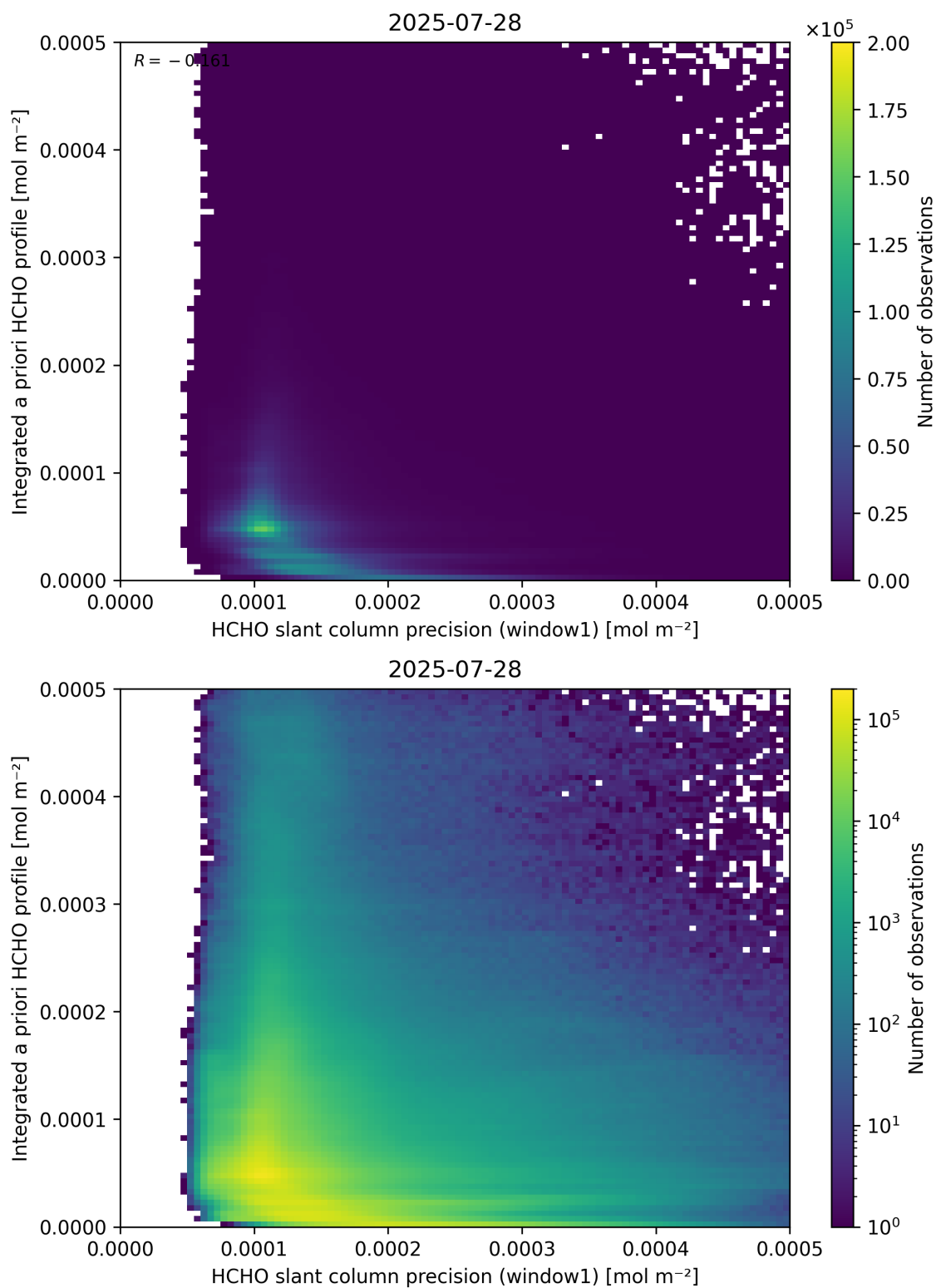
Figure 96: Scatter density plot of “HCHO slant column precision (window1)” against “Integrated a priori HCHO profile” for 2025-07-27 to 2025-07-29.
