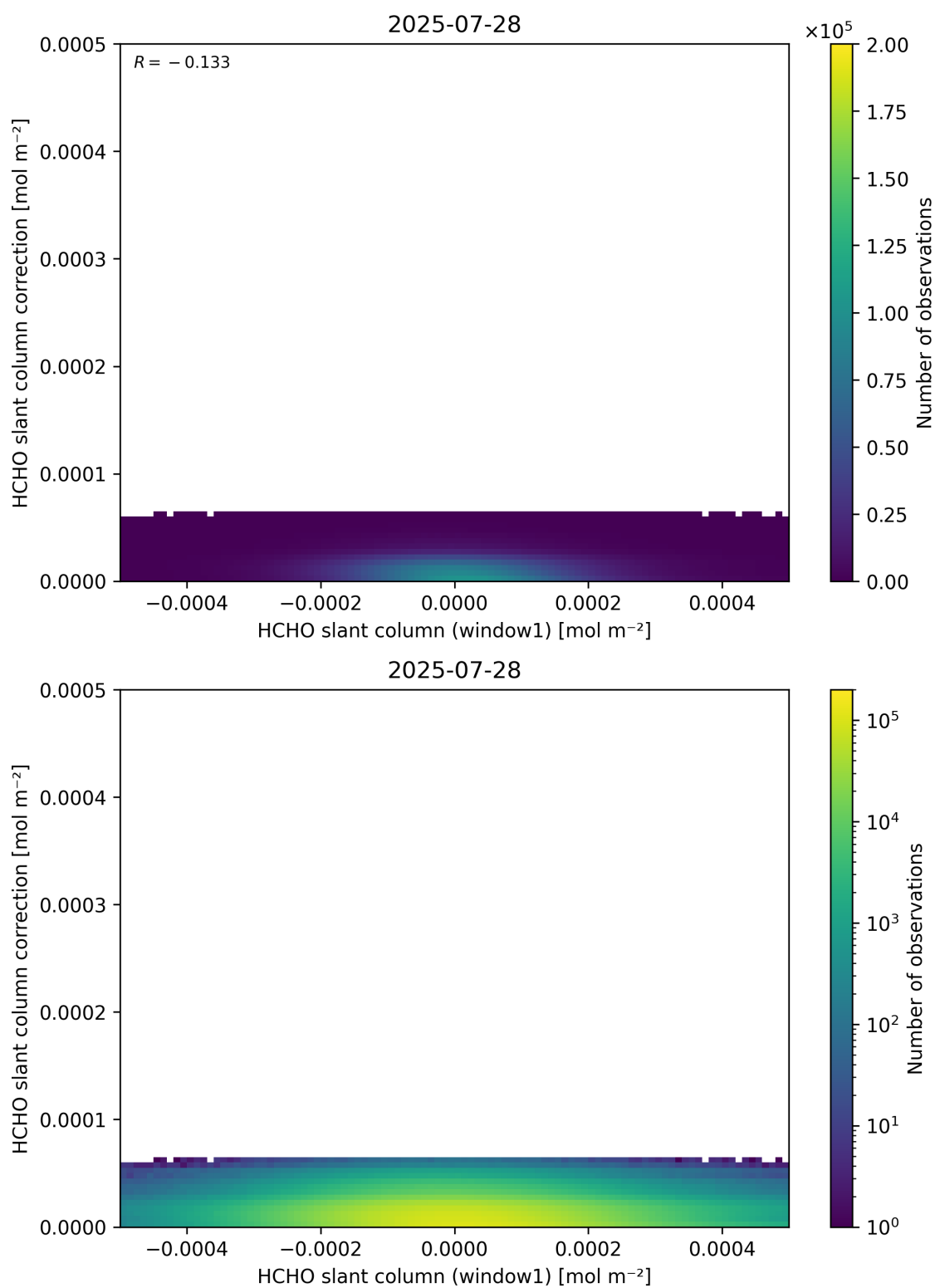
Figure 83: Scatter density plot of “HCHO slant column (window1)” against “HCHO slant column correction” for 2025-07-27 to 2025-07-29.
