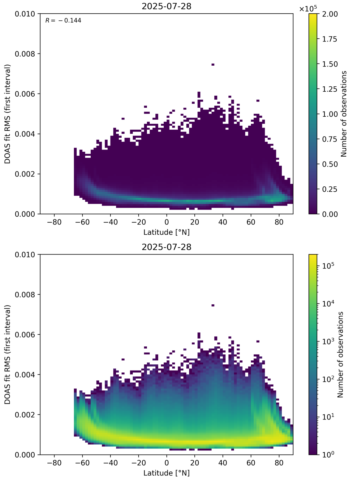
Figure 153: Scatter density plot of “Latitude” against “DOAS fit RMS (first interval)” for 2025-07-27 to 2025-07-29.
