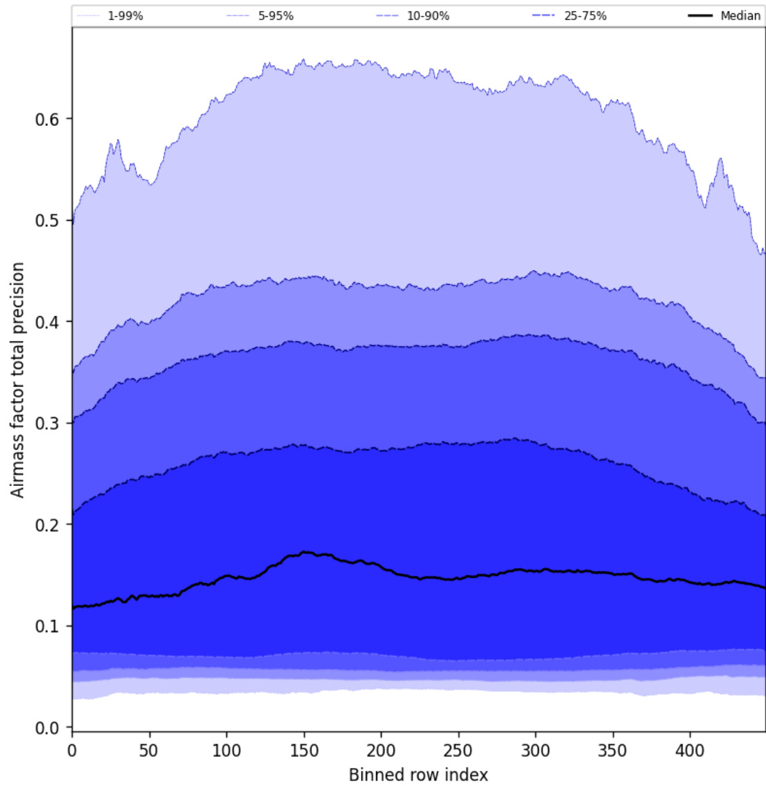
Figure 55: Along track statistics of “Airmass factor total precision” for 2025-07-27 to 2025-07-29
