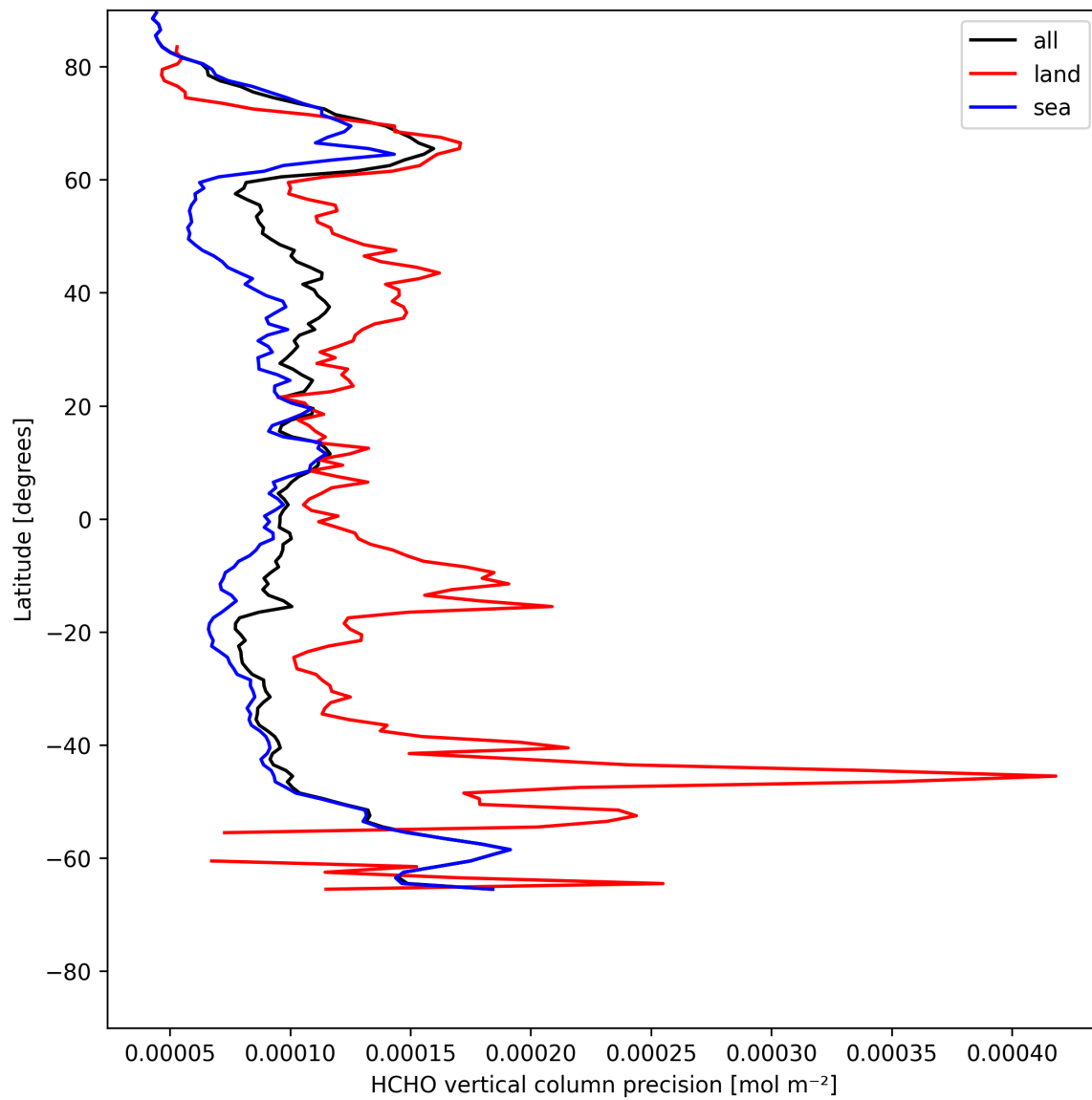
Figure 22: Zonal average of “HCHO vertical column precision” for 2025-07-27 to 2025-07-29.
