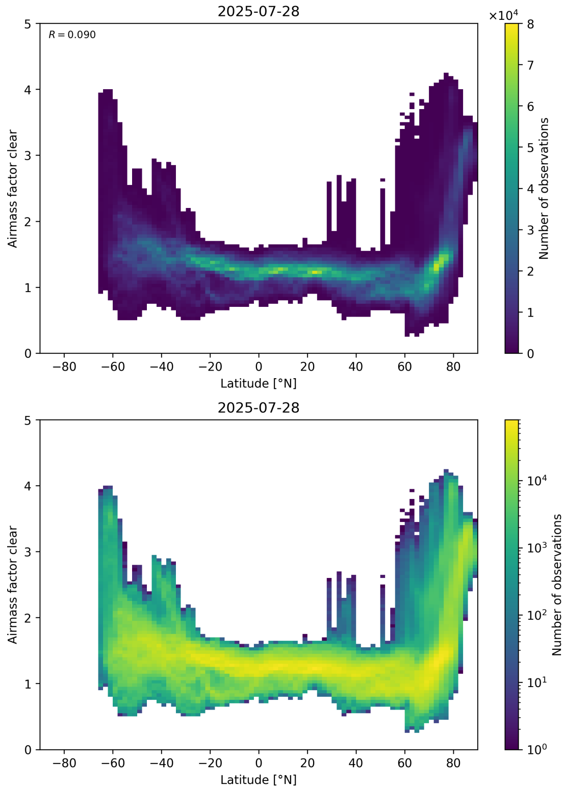
Figure 156: Scatter density plot of “Latitude” against “Airmass factor clear” for 2025-07-27 to 2025-07-29.
