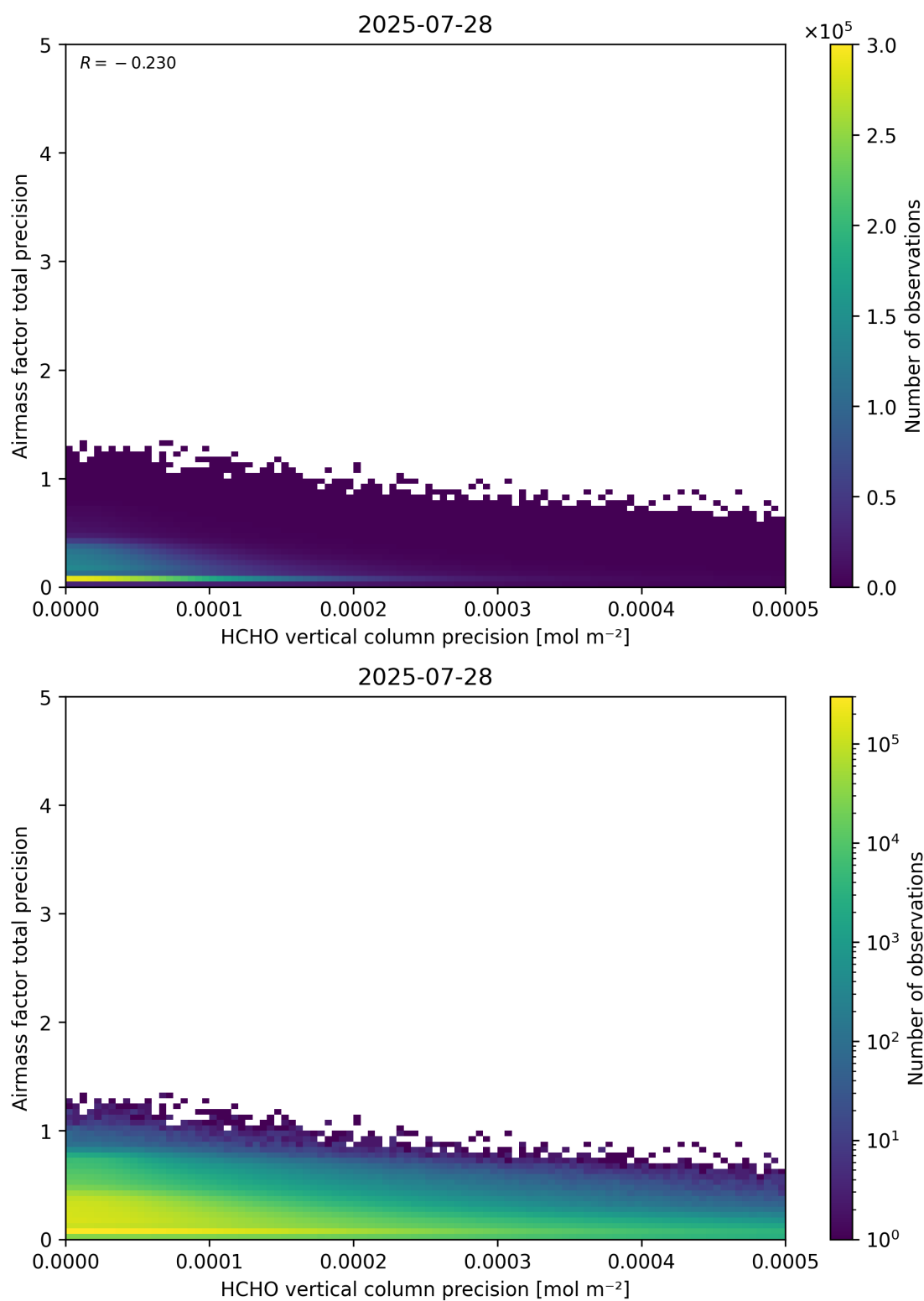
Figure 145: Scatter density plot of “HCHO vertical column precision” against “Airmass factor total precision” for 2025-07-27 to 2025-07-29.
