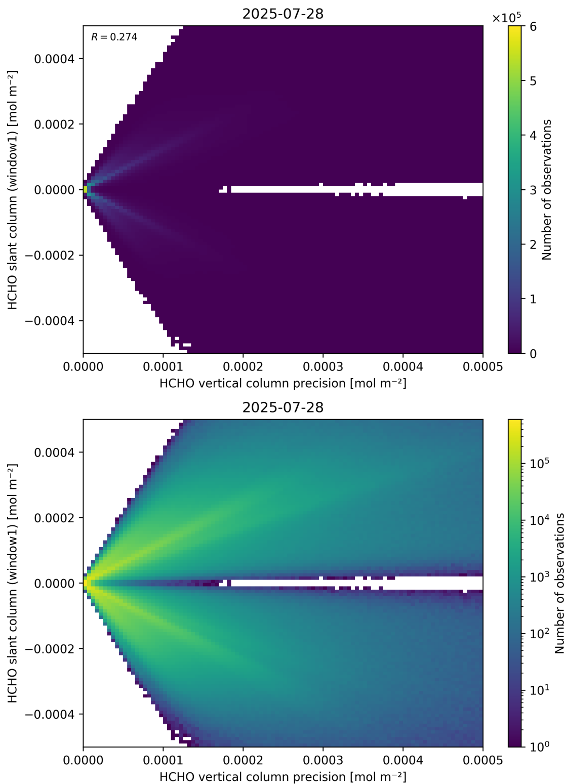
Figure 142: Scatter density plot of “HCHO vertical column precision” against “HCHO slant column (window1)” for 2025-07-27 to 2025-07-29.
