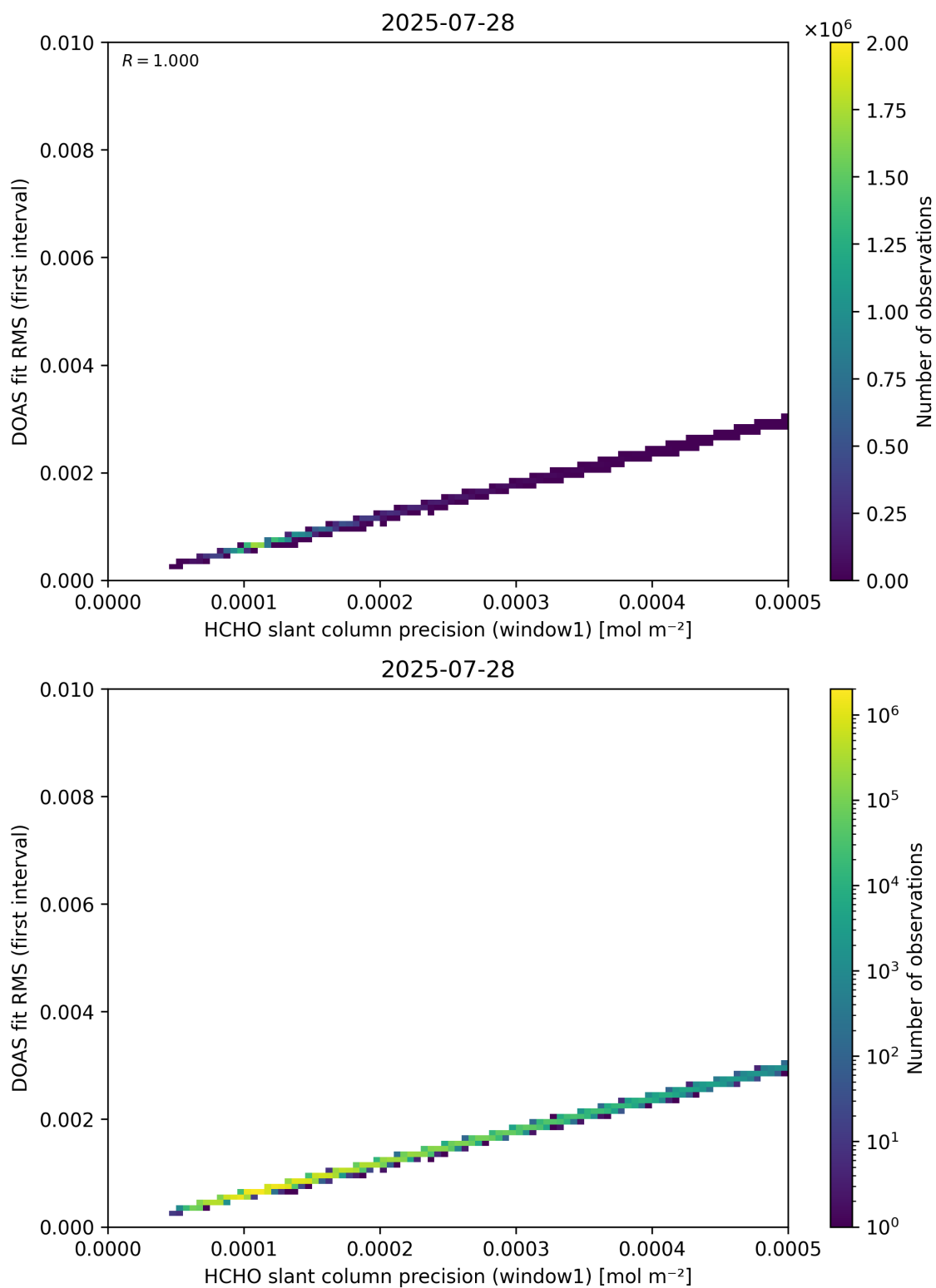
Figure 88: Scatter density plot of “HCHO slant column precision (window1)” against “DOAS fit RMS (first interval)” for 2025-07-27 to 2025-07-29.
