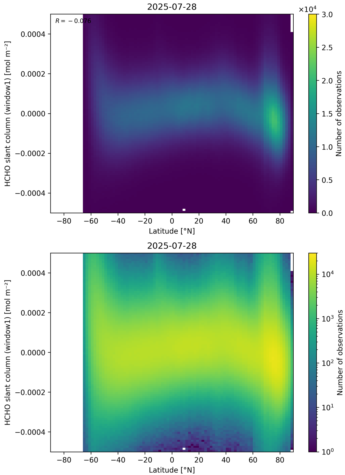
Figure 159: Scatter density plot of “Latitude” against “HCHO slant column (window1)” for 2025-07-27 to 2025-07-29.
