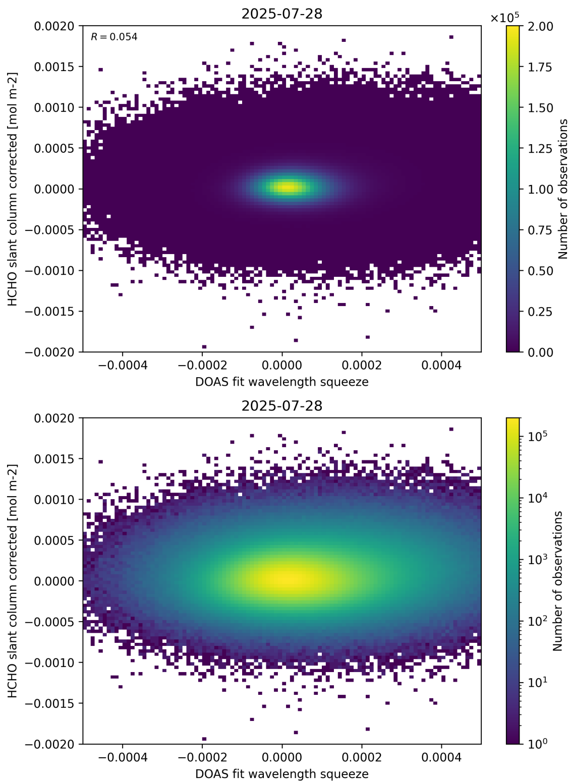
Figure 69: Scatter density plot of “DOAS fit wavelength squeeze” against “HCHO slant column corrected” for 2025-07-27 to 2025-07-29.
