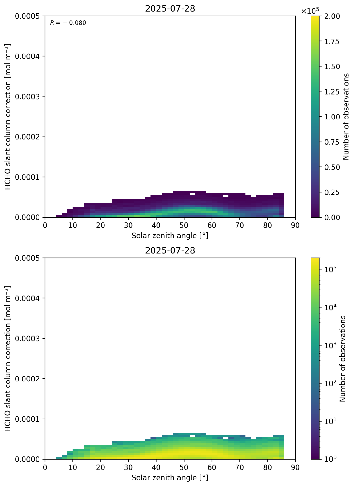
Figure 172: Scatter density plot of “Solar zenith angle” against “HCHO slant column correction” for 2025-07-27 to 2025-07-29.
