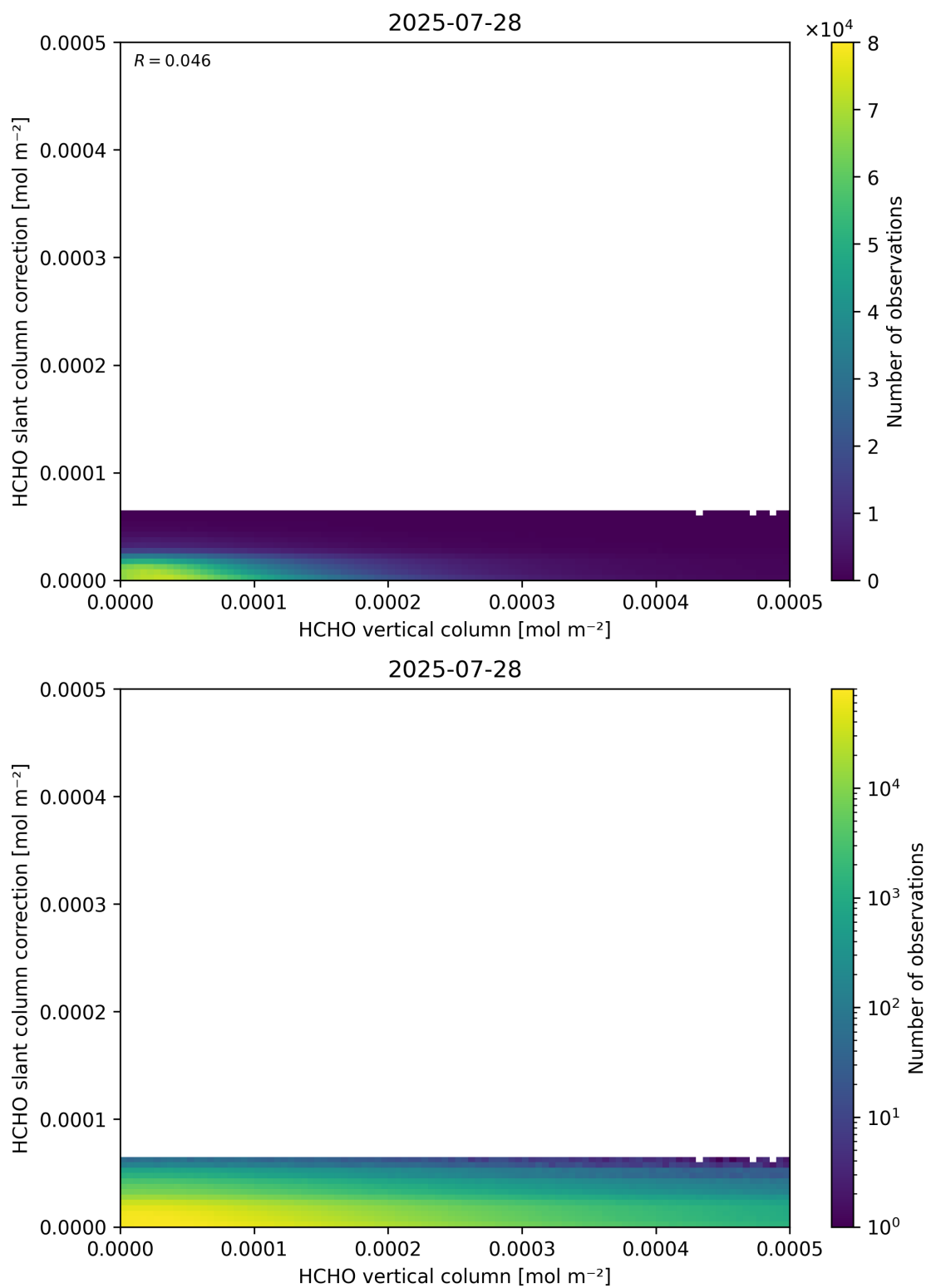
Figure 128: Scatter density plot of “HCHO vertical column” against “HCHO slant column correction” for 2025-07-27 to 2025-07-29.
