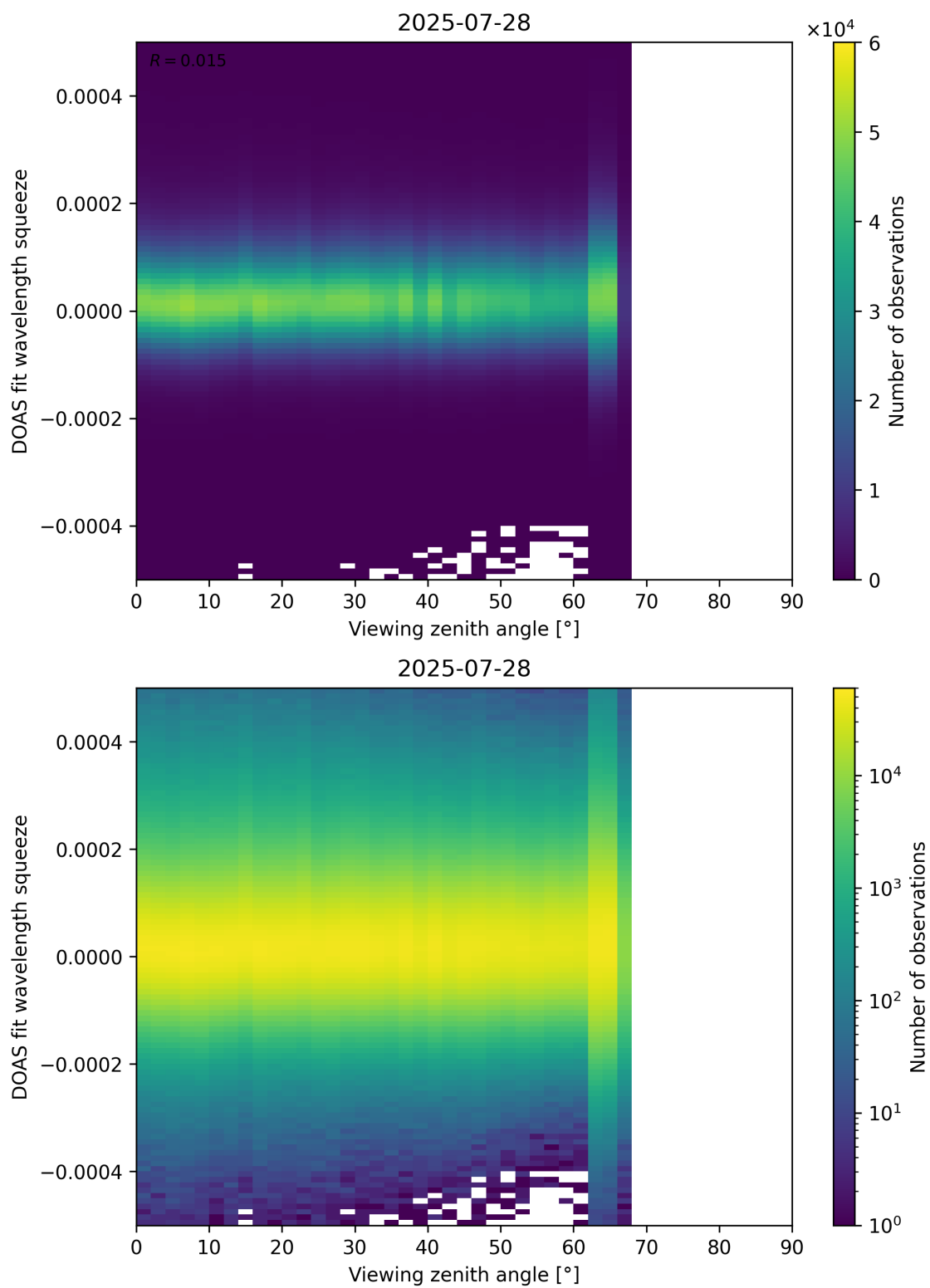
Figure 184: Scatter density plot of “Viewing zenith angle” against “DOAS fit wavelength squeeze” for 2025-07-27 to 2025-07-29.
