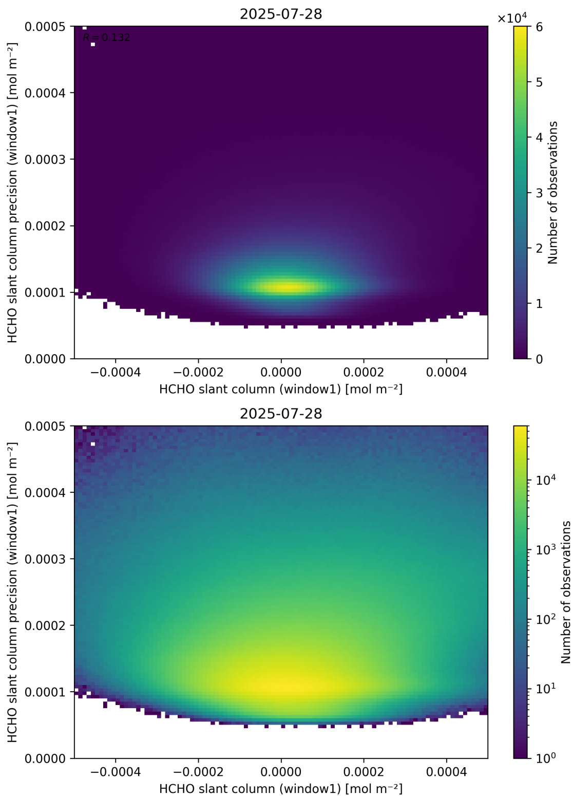
Figure 84: Scatter density plot of “HCHO slant column (window1)” against “HCHO slant column precision (window1)” for 2025-07-27 to 2025-07-29.
