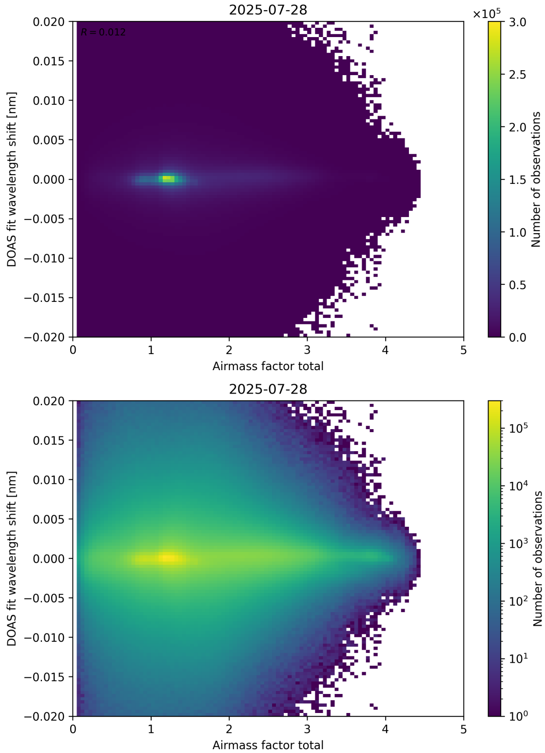
Figure 98: Scatter density plot of “Airmass factor total” against “DOAS fit wavelength shift” for 2025-07-27 to 2025-07-29.
