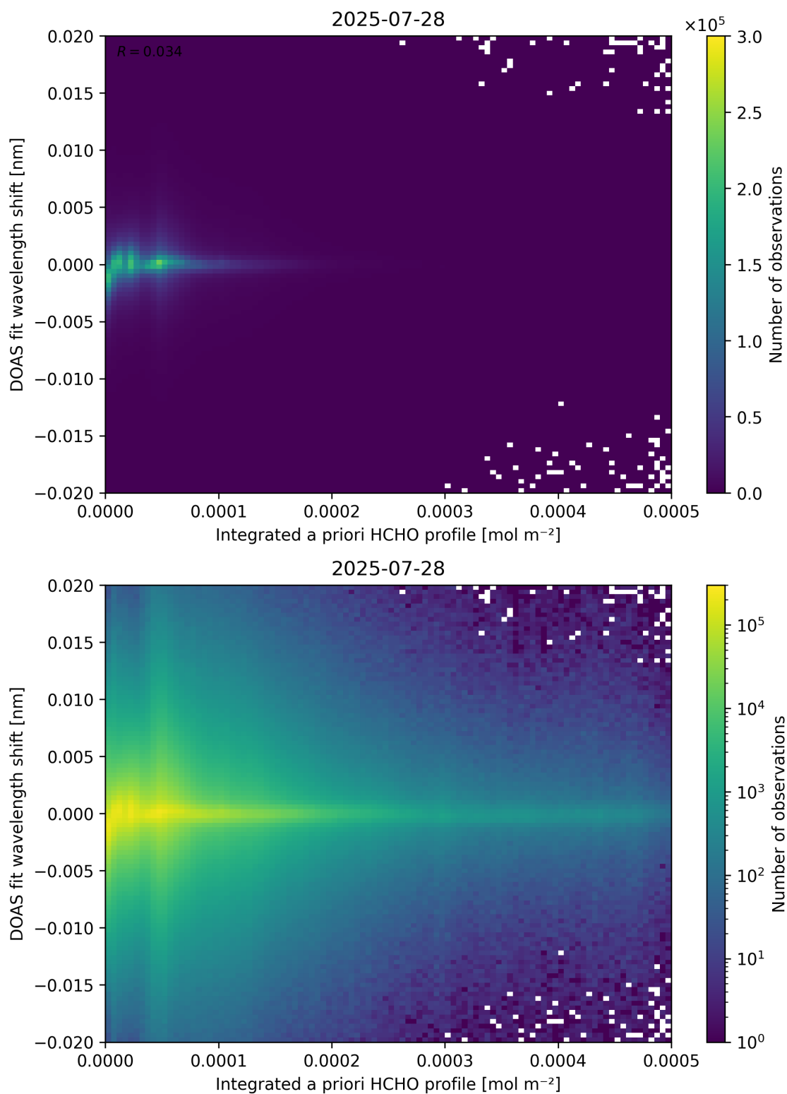
Figure 149: Scatter density plot of “Integrated a priori HCHO profile” against “DOAS fit wavelength shift” for 2025-07-27 to 2025-07-29.
