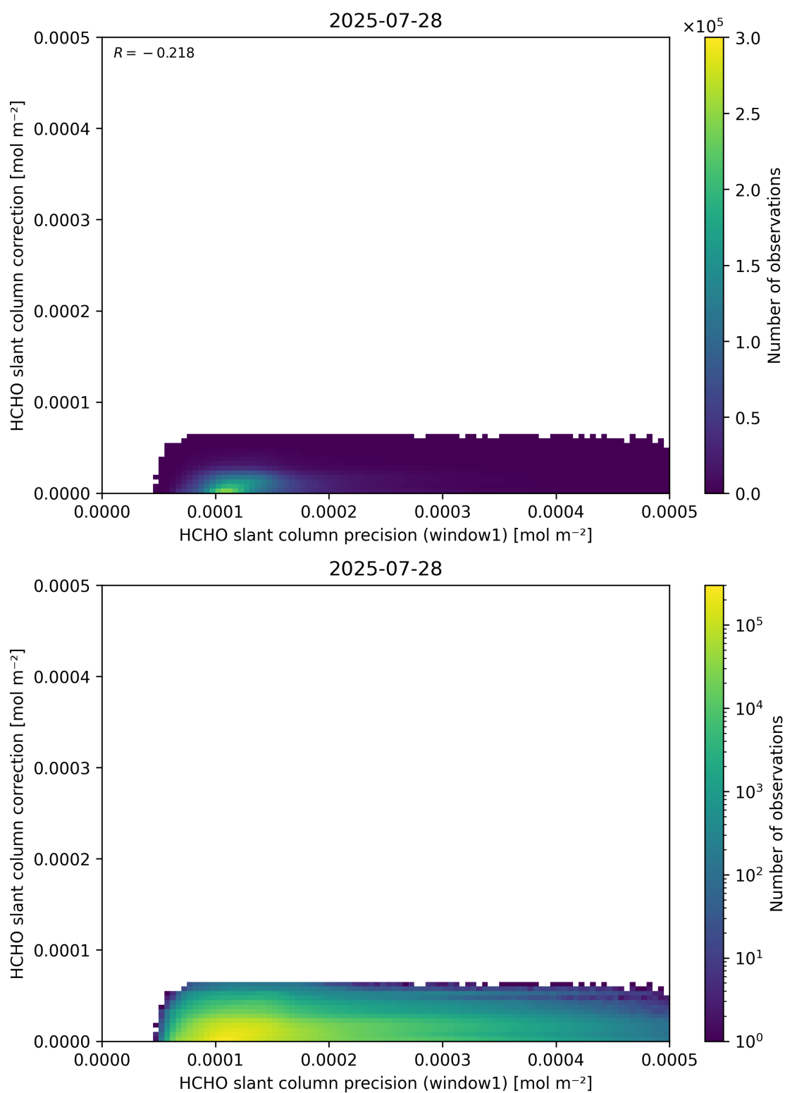
Figure 93: Scatter density plot of “HCHO slant column precision (window1)” against “HCHO slant column correction” for 2025-07-27 to 2025-07-29.
