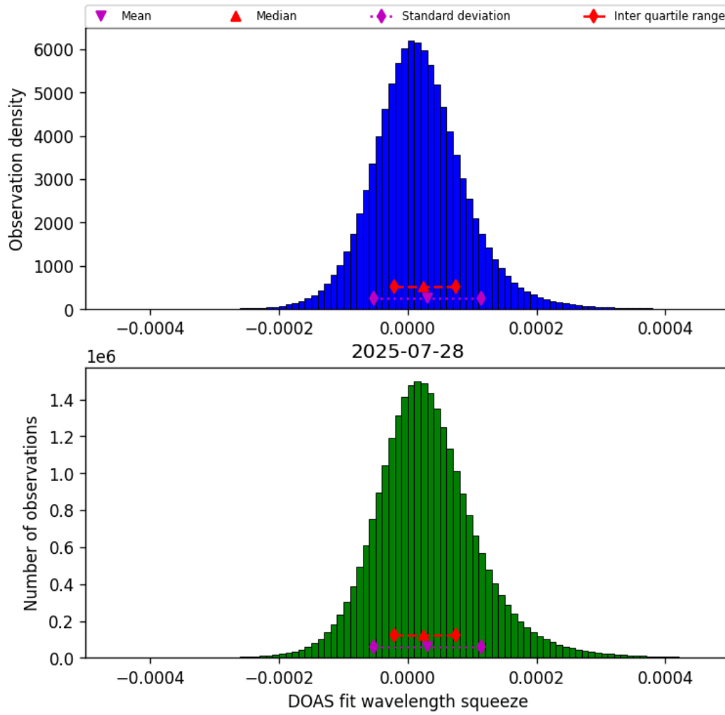
Figure 45: Histogram of “DOAS fit wavelength squeeze” for 2025-07-27 to 2025-07-29
