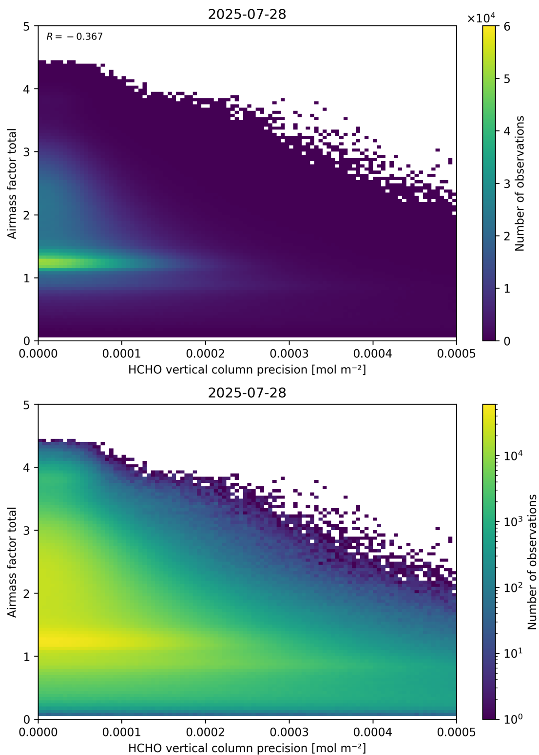
Figure 144: Scatter density plot of “HCHO vertical column precision” against “Airmass factor total” for 2025-07-27 to 2025-07-29.
