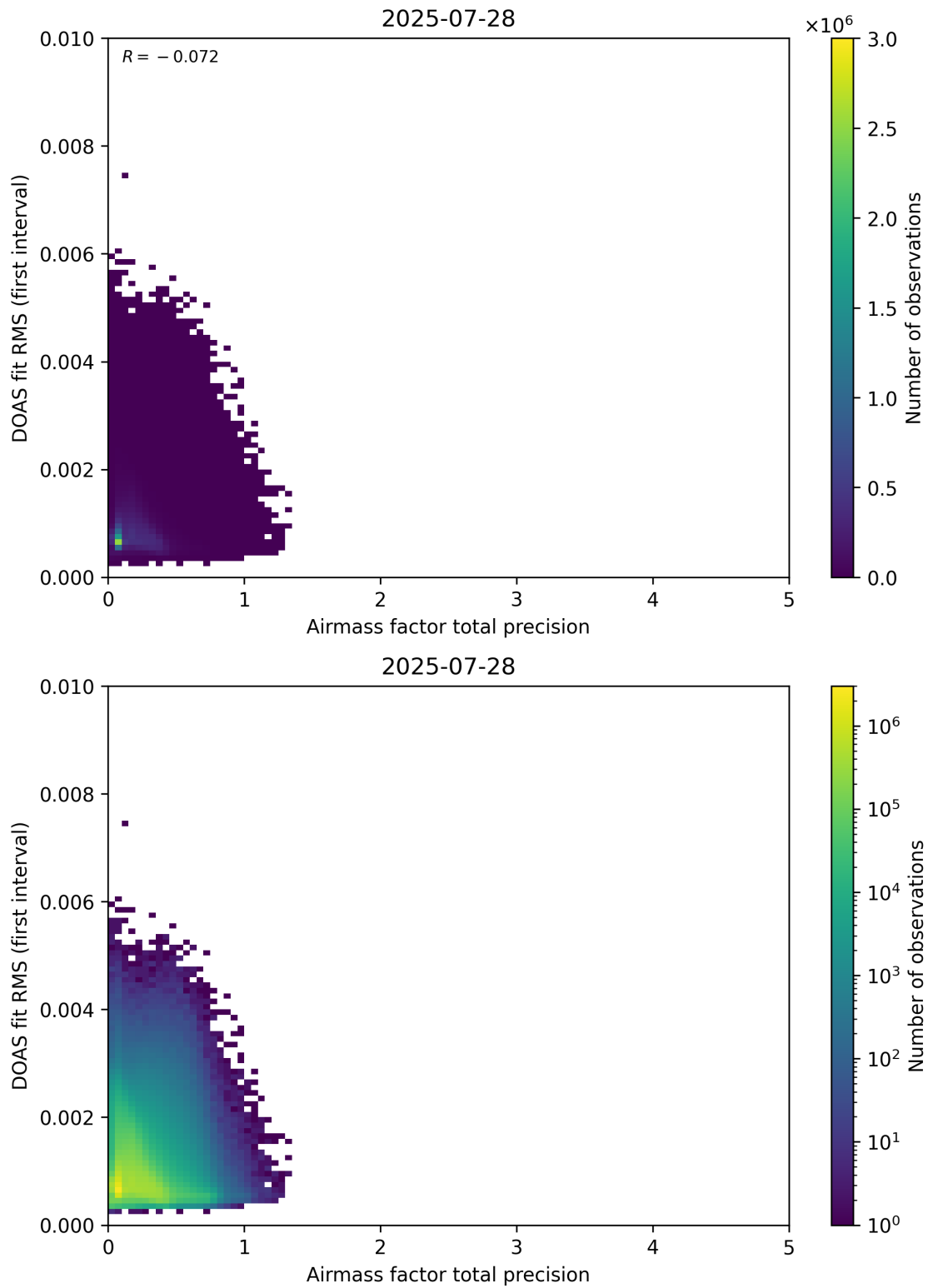
Figure 105: Scatter density plot of “Airmass factor total precision” against “DOAS fit RMS (first interval)” for 2025-07-27 to 2025-07-29.
