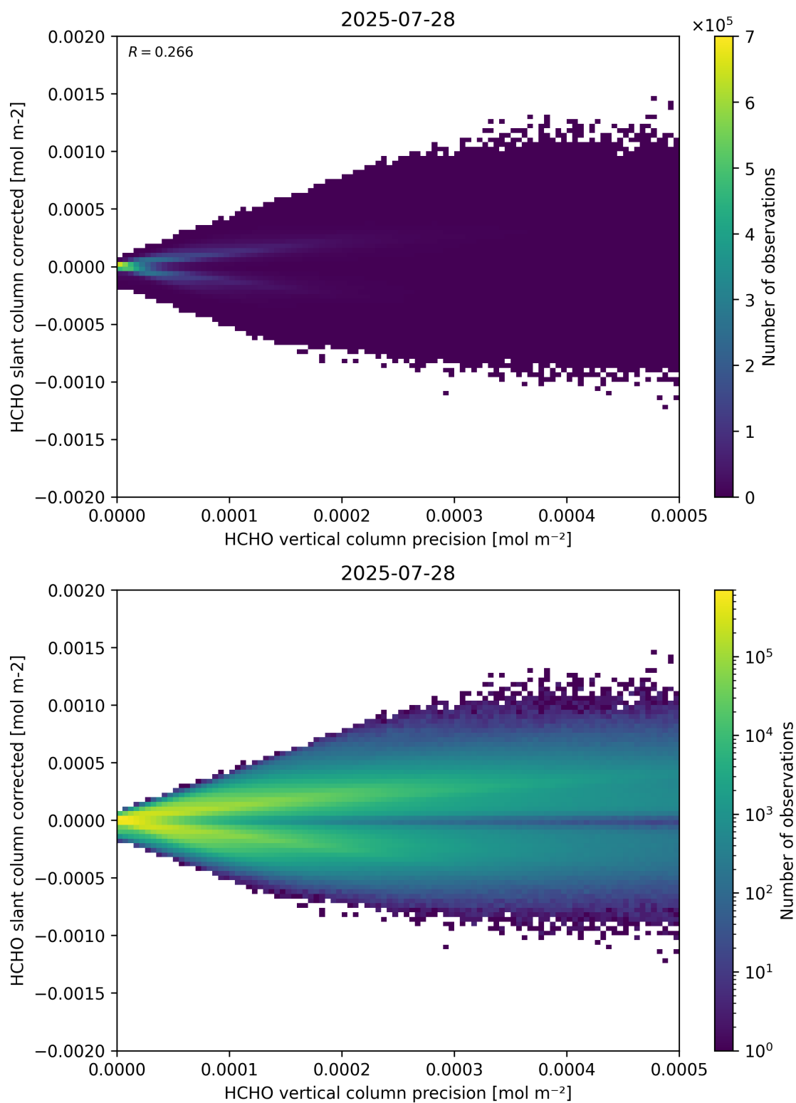
Figure 140: Scatter density plot of “HCHO vertical column precision” against “HCHO slant column corrected” for 2025-07-27 to 2025-07-29.
