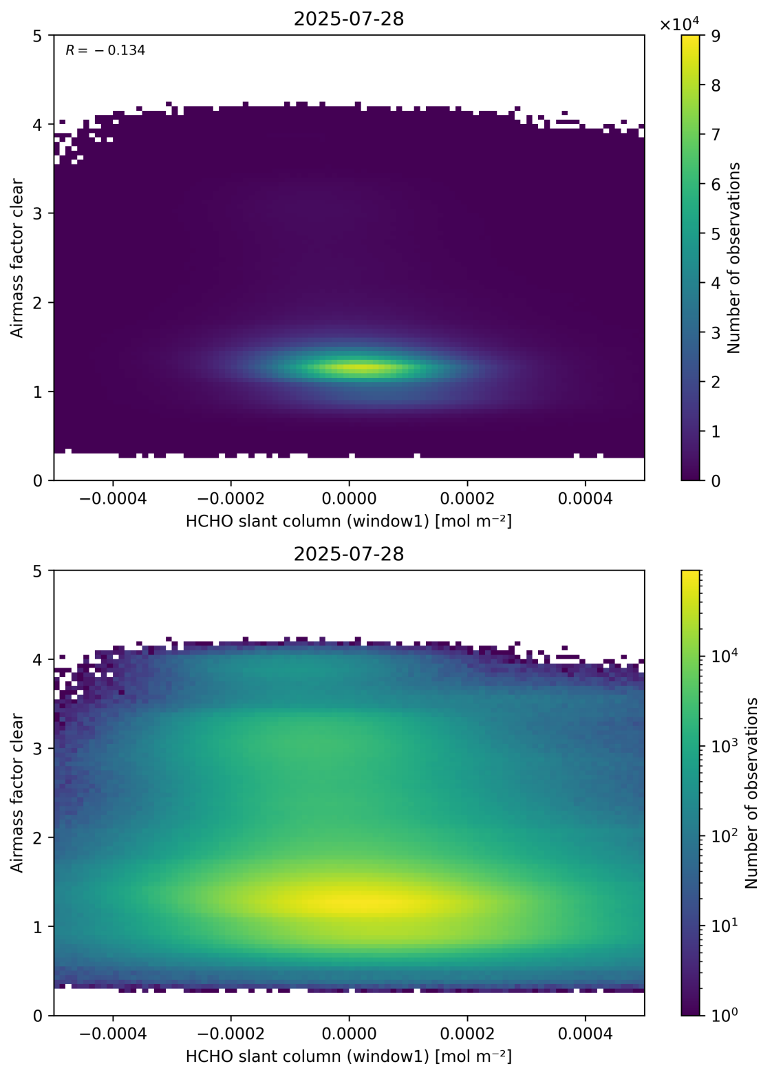
Figure 81: Scatter density plot of “HCHO slant column (window1)” against “Airmass factor clear” for 2025-07-27 to 2025-07-29.
