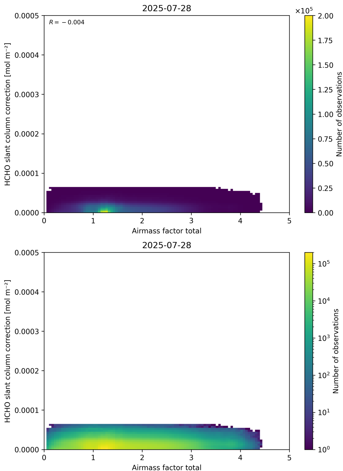
Figure 102: Scatter density plot of “Airmass factor total” against “HCHO slant column correction” for 2025-07-27 to 2025-07-29.
