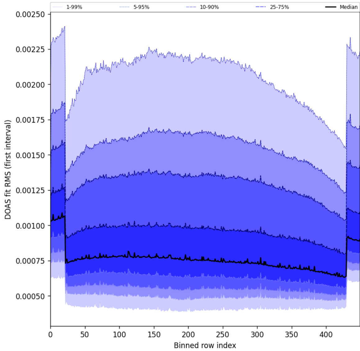
Figure 60: Along track statistics of “DOAS fit RMS (first interval)” for 2025-07-27 to 2025-07-29
