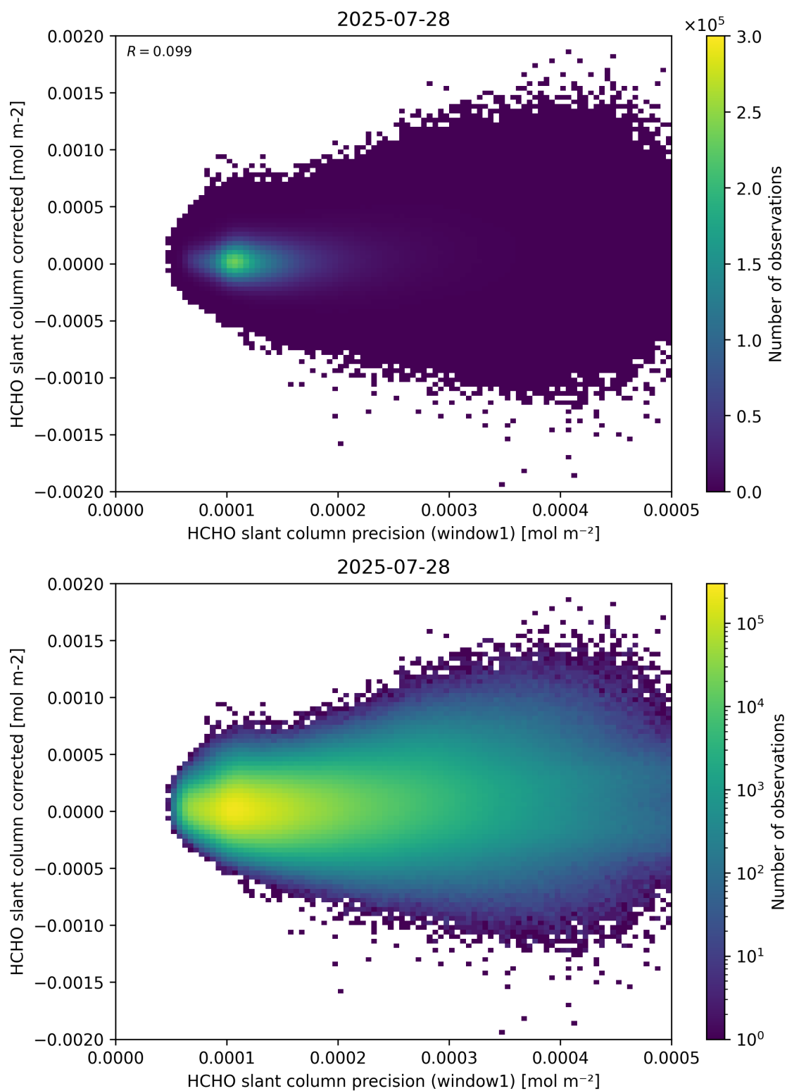
Figure 92: Scatter density plot of “HCHO slant column precision (window1)” against “HCHO slant column corrected” for 2025-07-27 to 2025-07-29.
