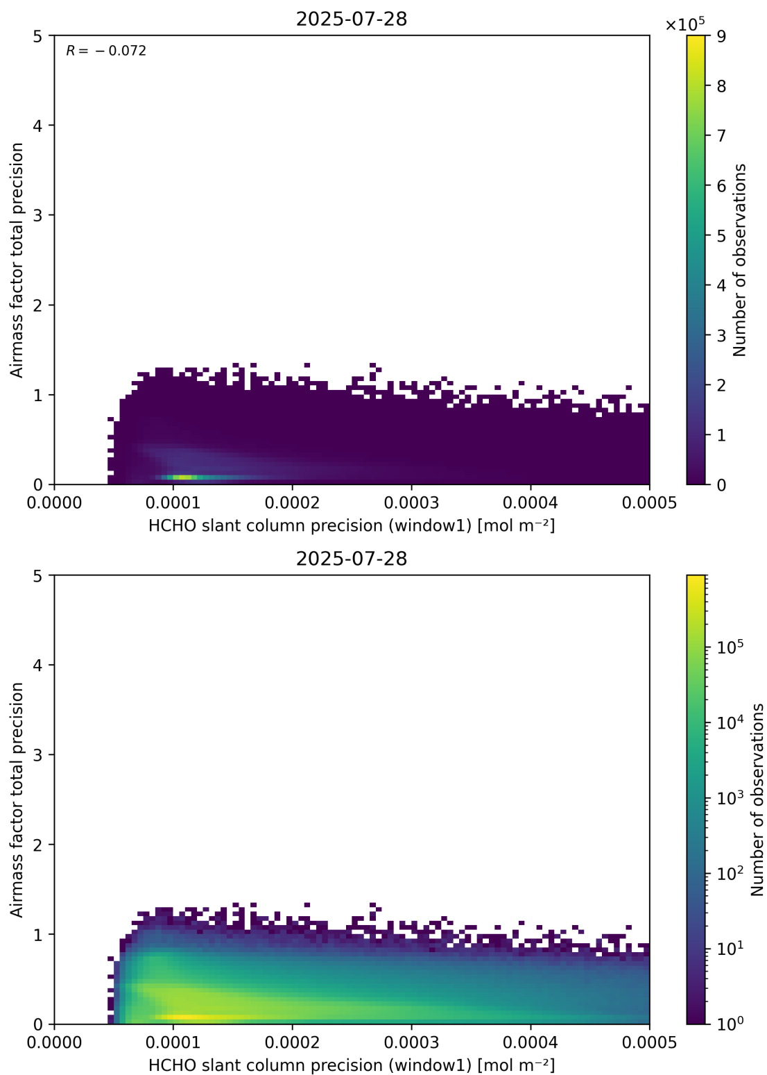
Figure 95: Scatter density plot of “HCHO slant column precision (window1)” against “Airmass factor total precision” for 2025-07-27 to 2025-07-29.
