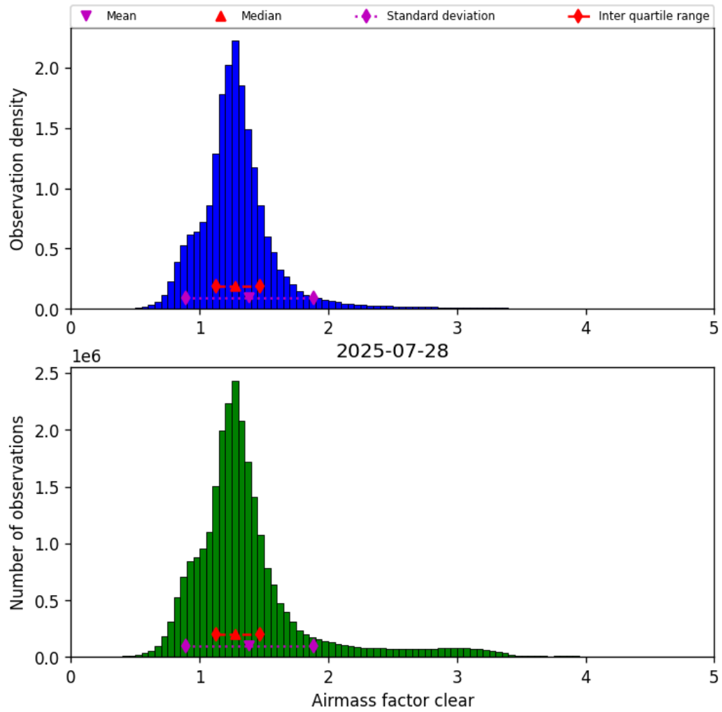
Figure 42: Histogram of “Airmass factor clear” for 2025-07-27 to 2025-07-29
