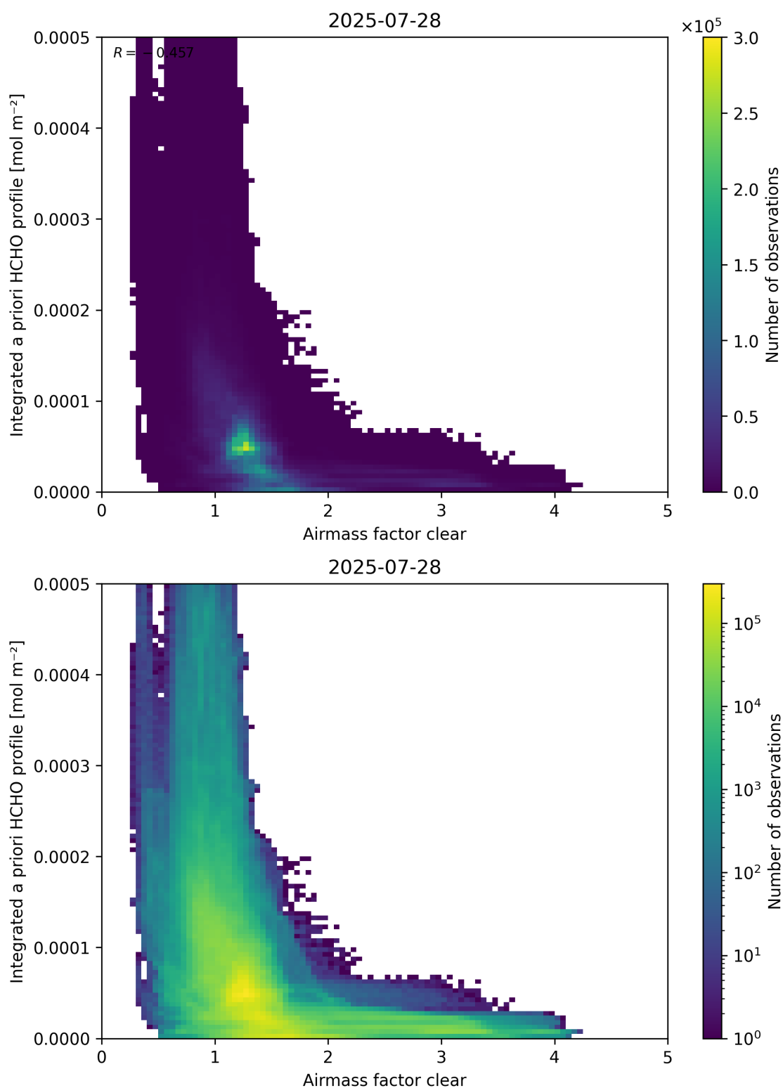
Figure 76: Scatter density plot of “Airmass factor clear” against “Integrated a priori HCHO profile” for 2025-07-27 to 2025-07-29.
