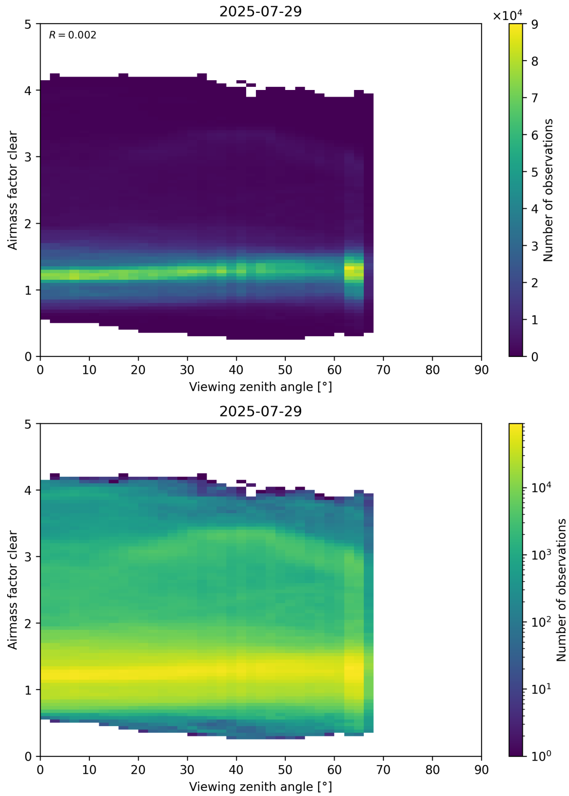
Figure 185: Scatter density plot of “Viewing zenith angle” against “Airmass factor clear” for 2025-07-29 to 2025-07-30.
