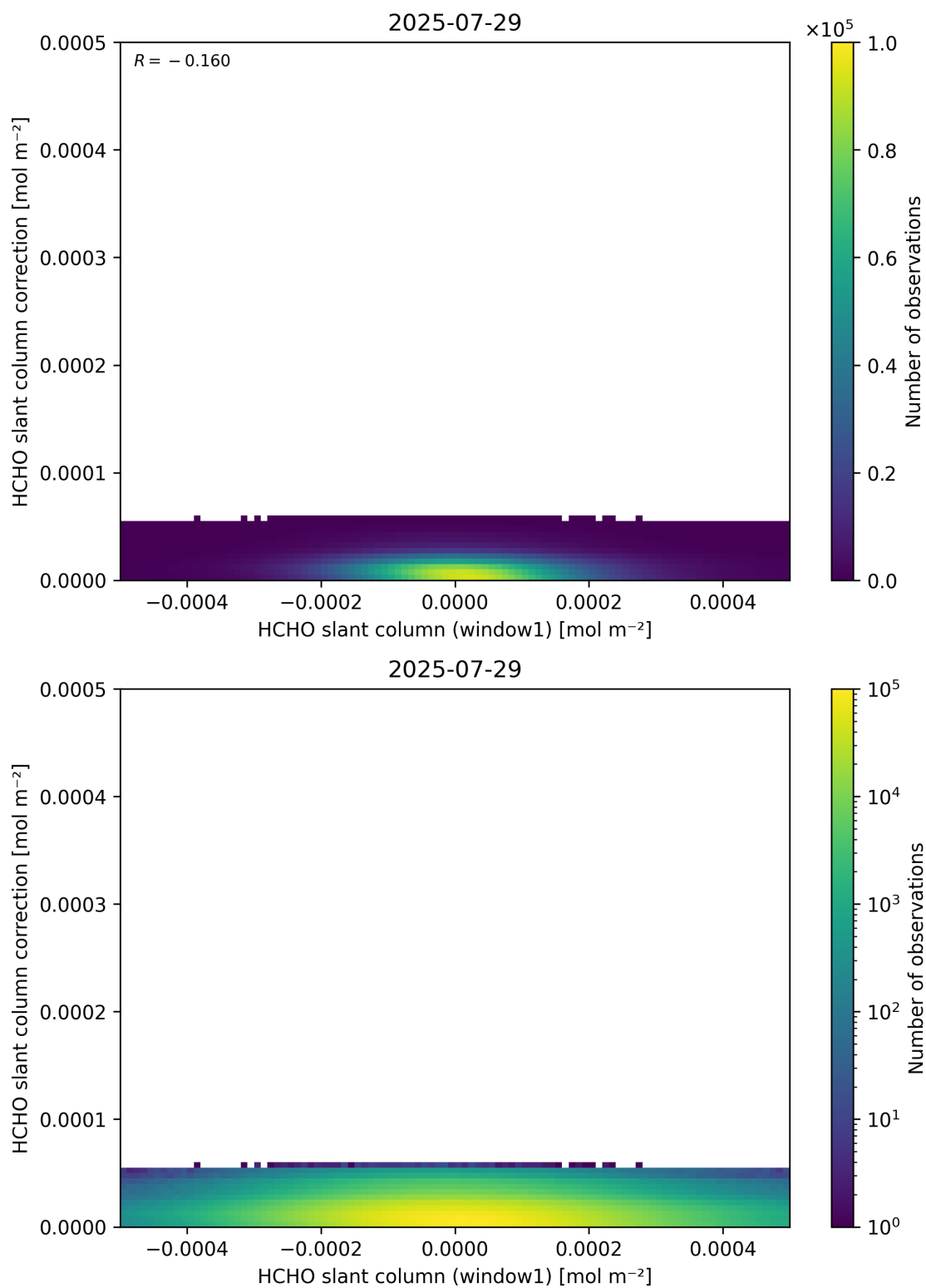
Figure 83: Scatter density plot of “HCHO slant column (window1)” against “HCHO slant column correction” for 2025-07-29 to 2025-07-30.
