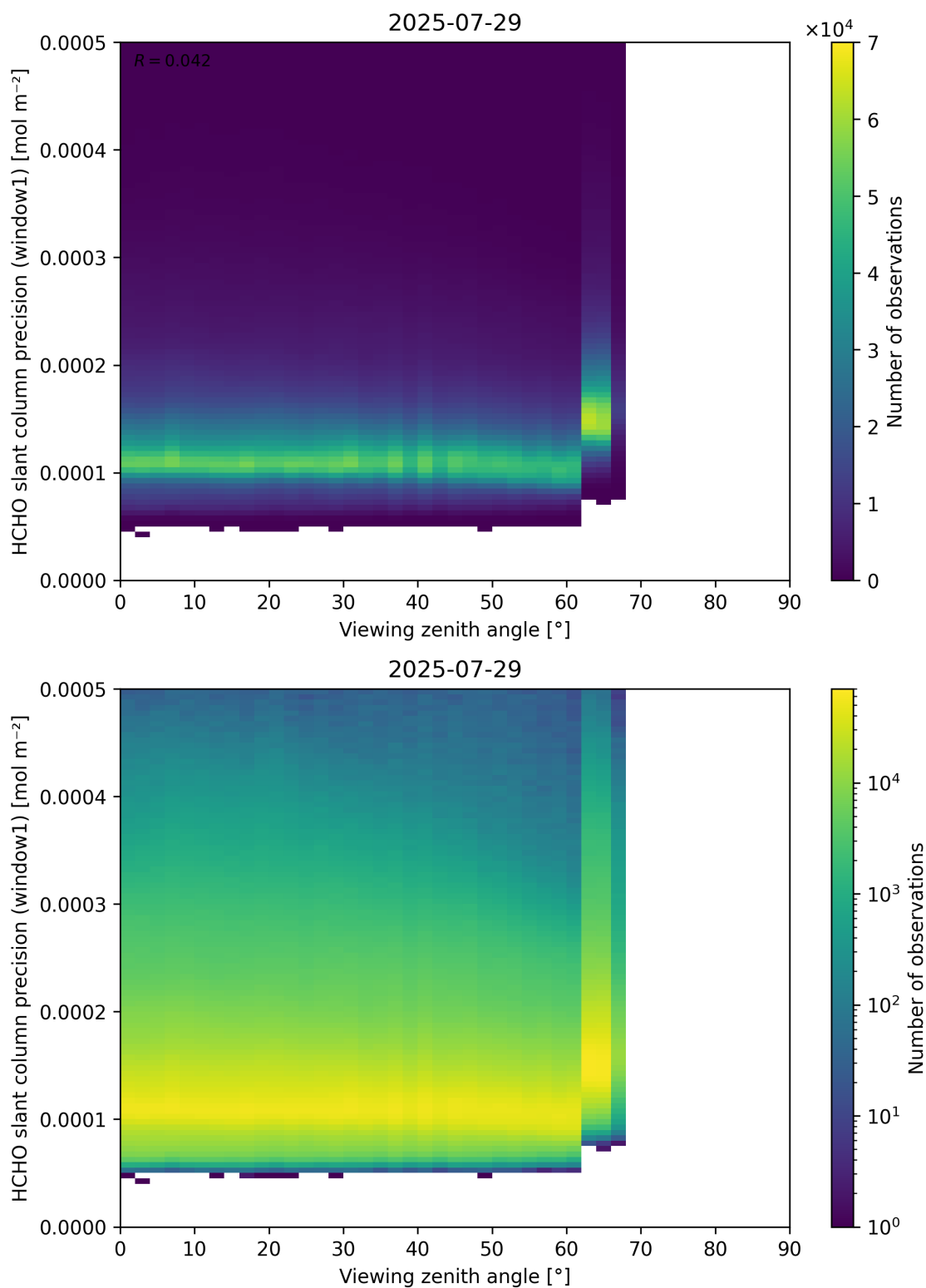
Figure 189: Scatter density plot of “Viewing zenith angle” against “HCHO slant column precision (window1)” for 2025-07-29 to 2025-07-30.
