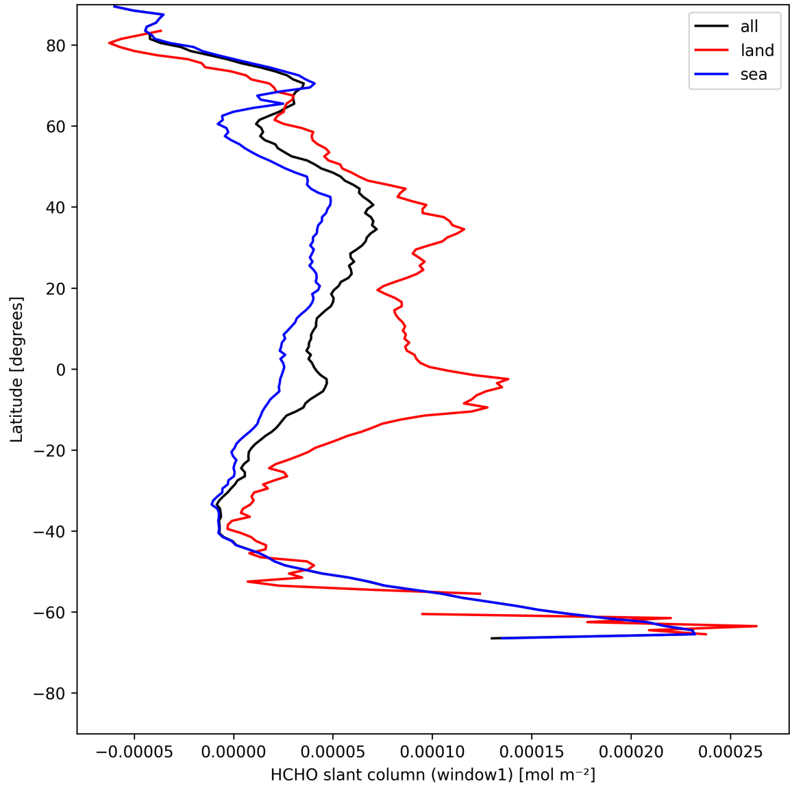
Figure 24: Zonal average of “HCHO slant column (window1)” for 2025-07-29 to 2025-07-30.
