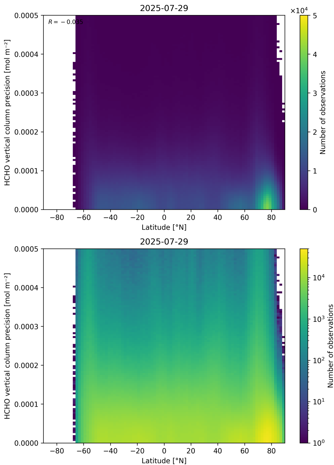
Figure 165: Scatter density plot of “Latitude” against “HCHO vertical column precision” for 2025-07-29 to 2025-07-30.
