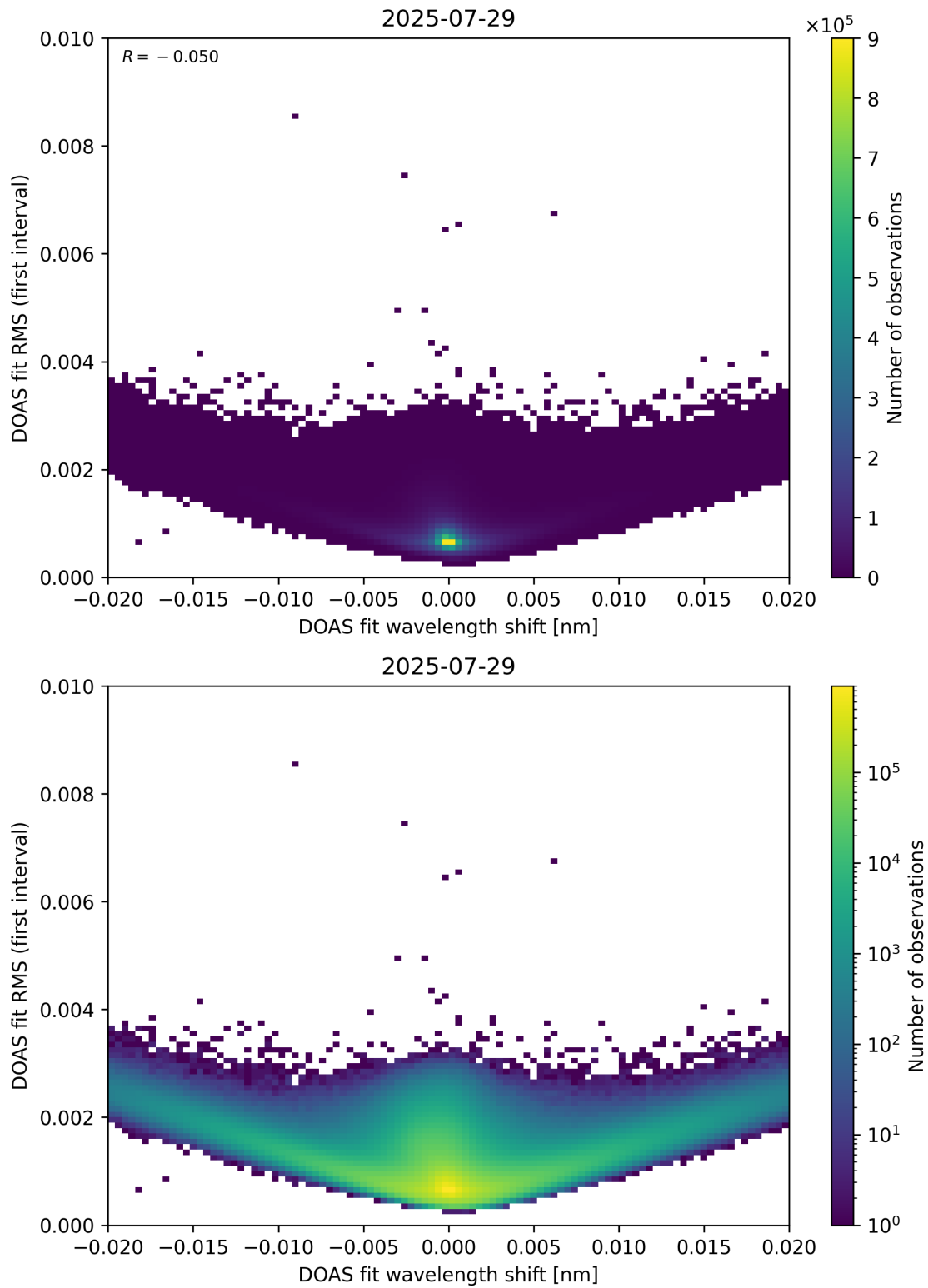
Figure 64: Scatter density plot of “DOAS fit wavelength shift” against “DOAS fit RMS (first interval)” for 2025-07-29 to 2025-07-30.
