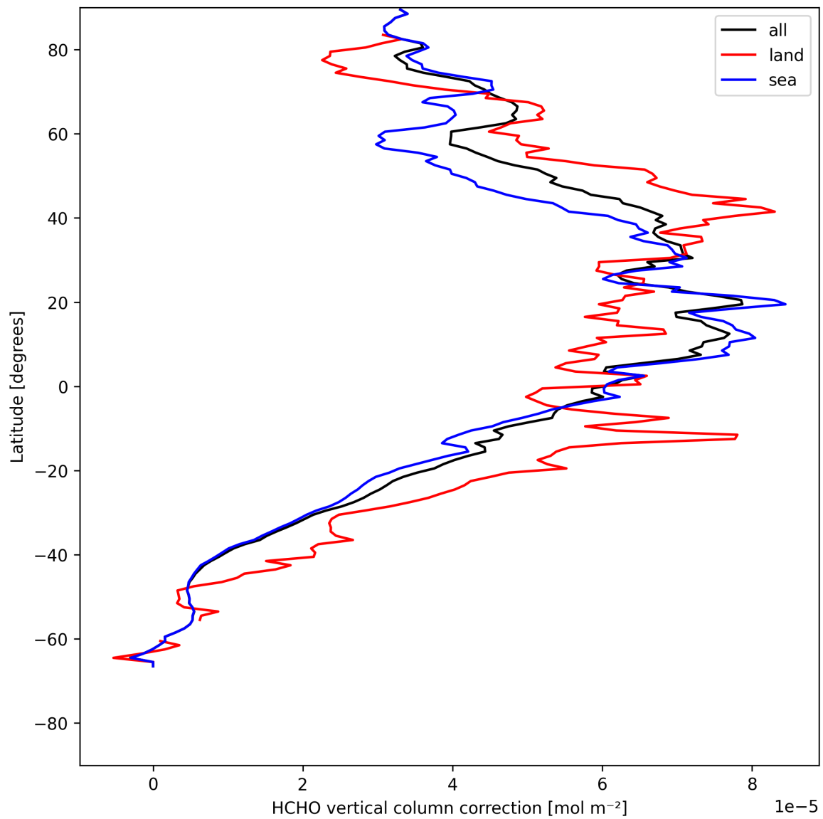
Figure 23: Zonal average of “HCHO vertical column correction” for 2025-07-29 to 2025-07-30.
