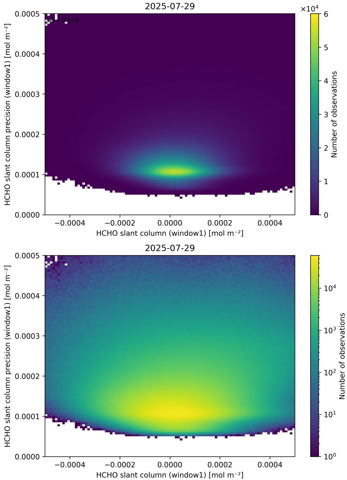
Figure 84: Scatter density plot of “HCHO slant column (window1)” against “HCHO slant column precision (window1)” for 2025-07-29 to 2025-07-30.
