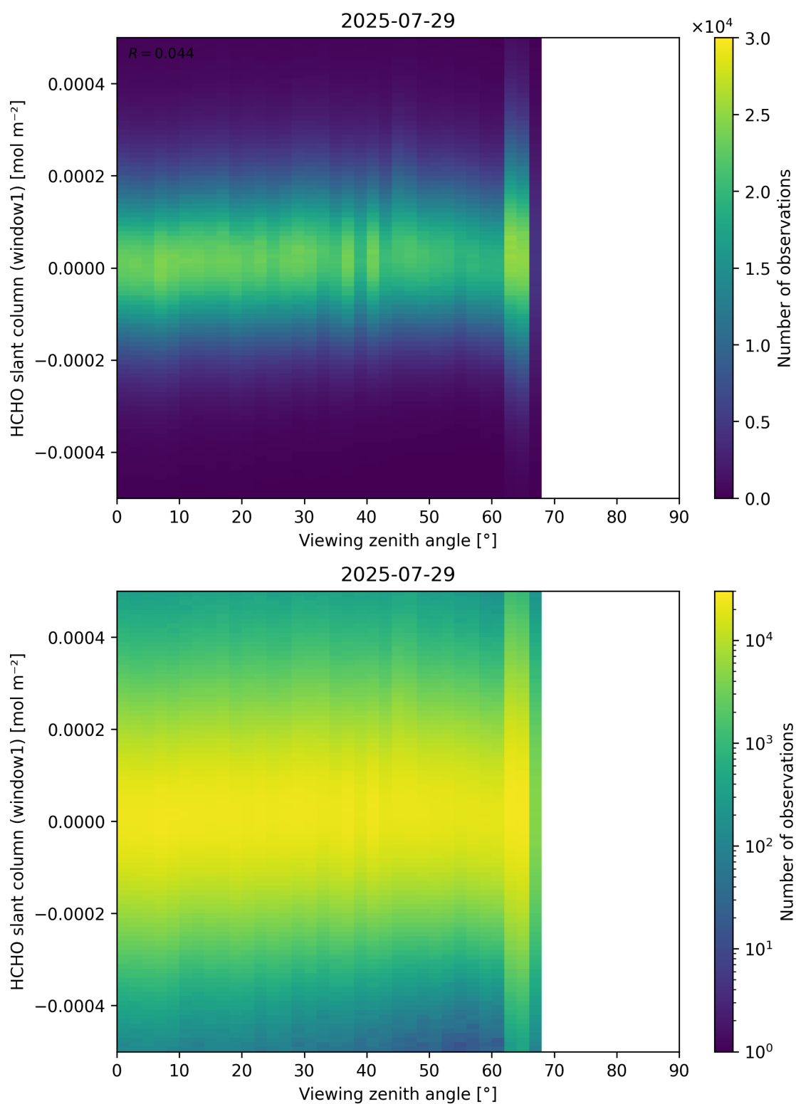
Figure 188: Scatter density plot of “Viewing zenith angle” against “HCHO slant column (window1)” for 2025-07-29 to 2025-07-30.
