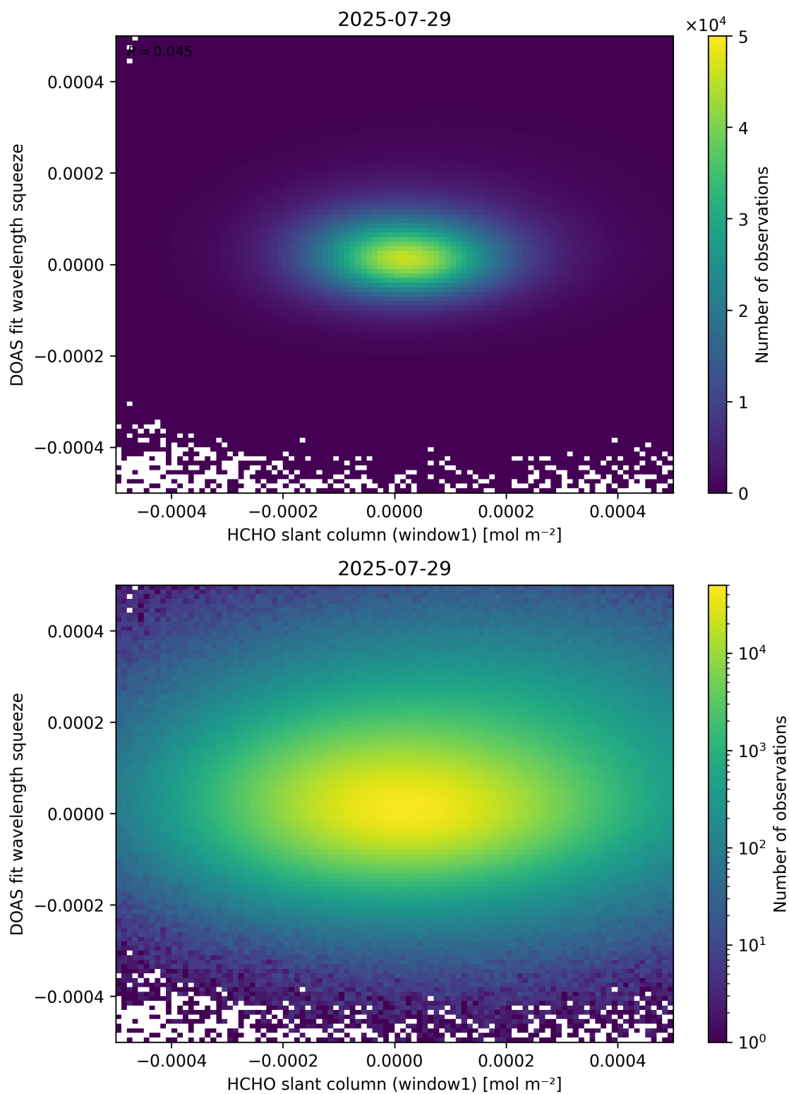
Figure 80: Scatter density plot of “HCHO slant column (window1)” against “DOAS fit wavelength squeeze” for 2025-07-29 to 2025-07-30.
