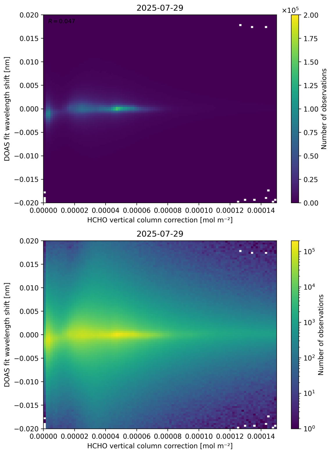
Figure 113: Scatter density plot of “HCHO vertical column correction” against “DOAS fit wavelength shift” for 2025-07-29 to 2025-07-30.
