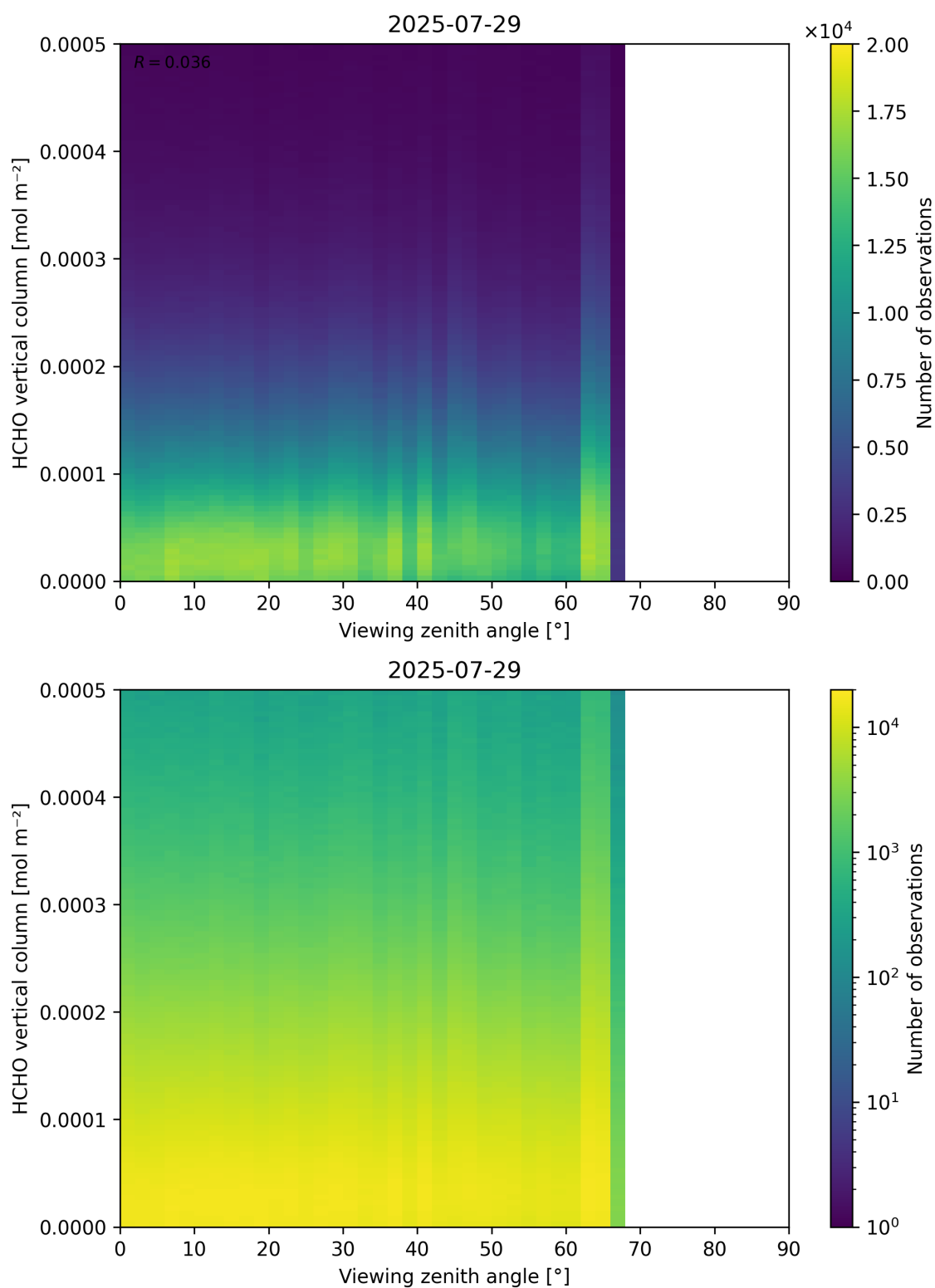
Figure 192: Scatter density plot of “Viewing zenith angle” against “HCHO vertical column” for 2025-07-29 to 2025-07-30.
