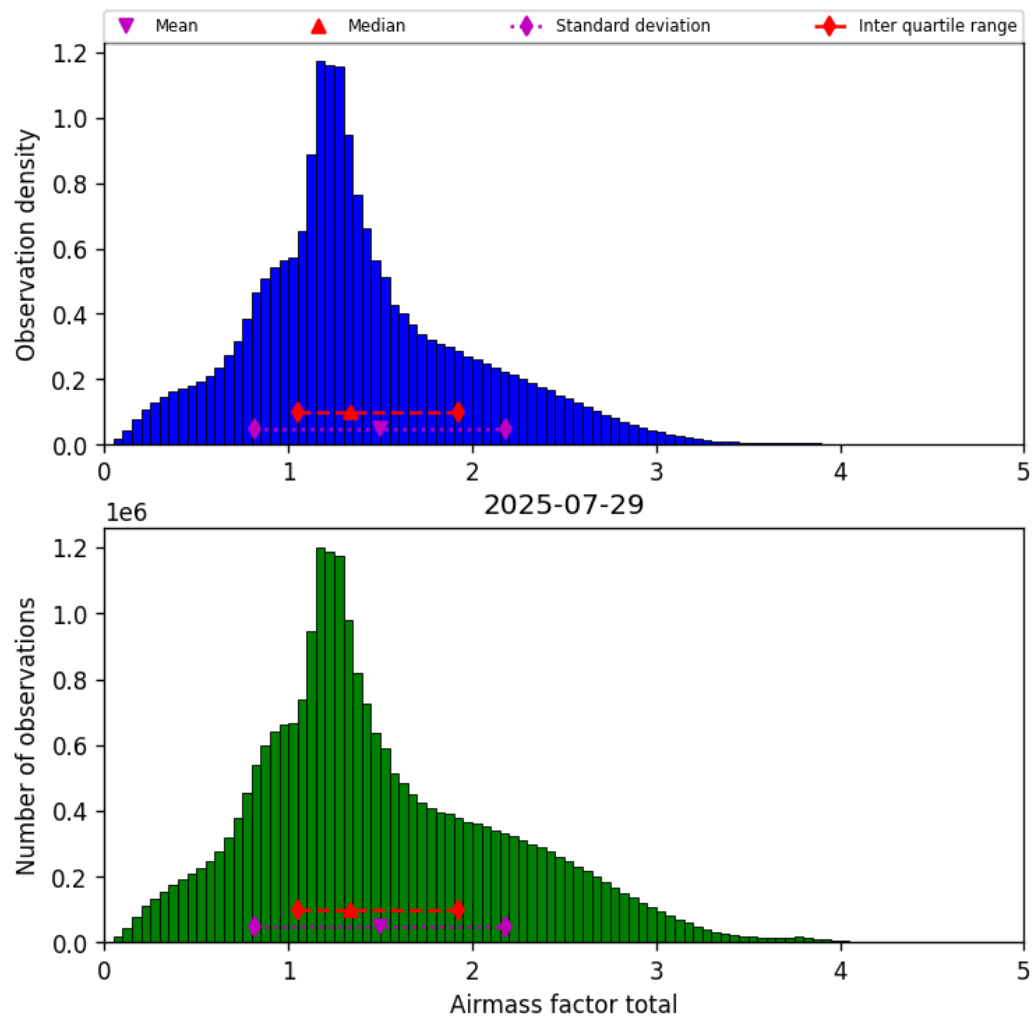
Figure 40: Histogram of “Airmass factor total” for 2025-07-29 to 2025-07-30
