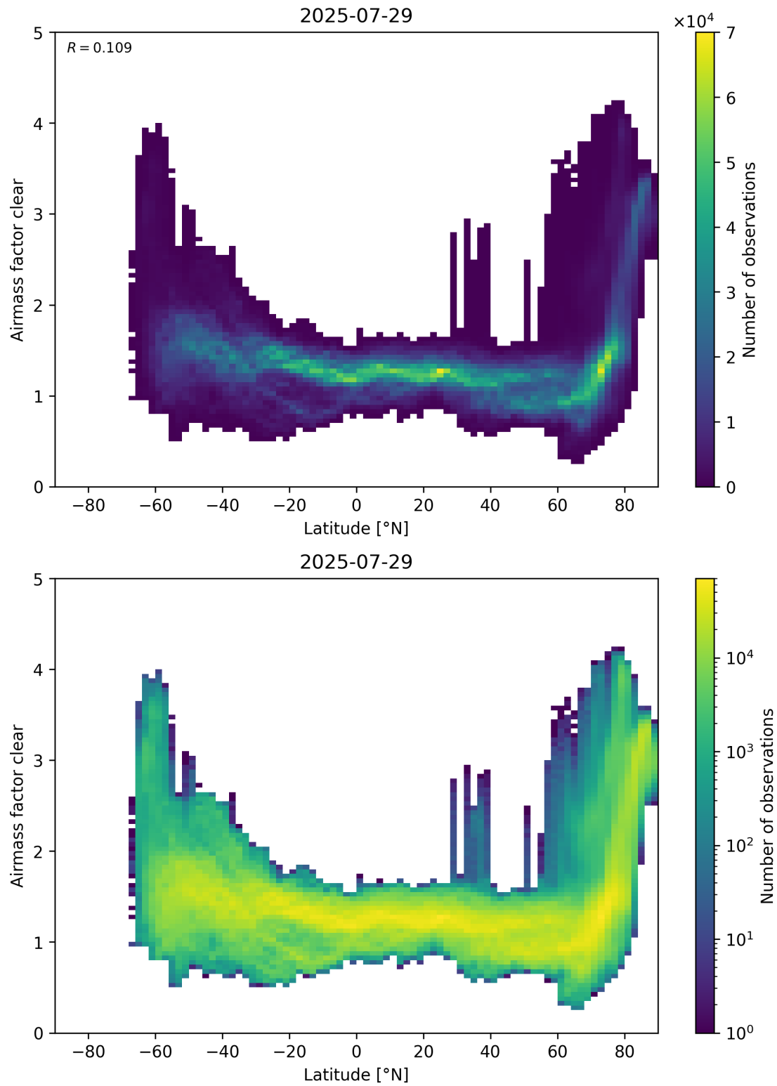
Figure 156: Scatter density plot of “Latitude” against “Airmass factor clear” for 2025-07-29 to 2025-07-30.
