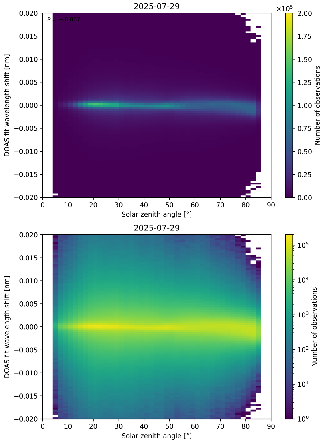
Figure 168: Scatter density plot of “Solar zenith angle” against “DOAS fit wavelength shift” for 2025-07-29 to 2025-07-30.
