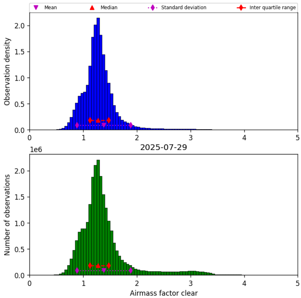
Figure 42: Histogram of “Airmass factor clear” for 2025-07-29 to 2025-07-30
