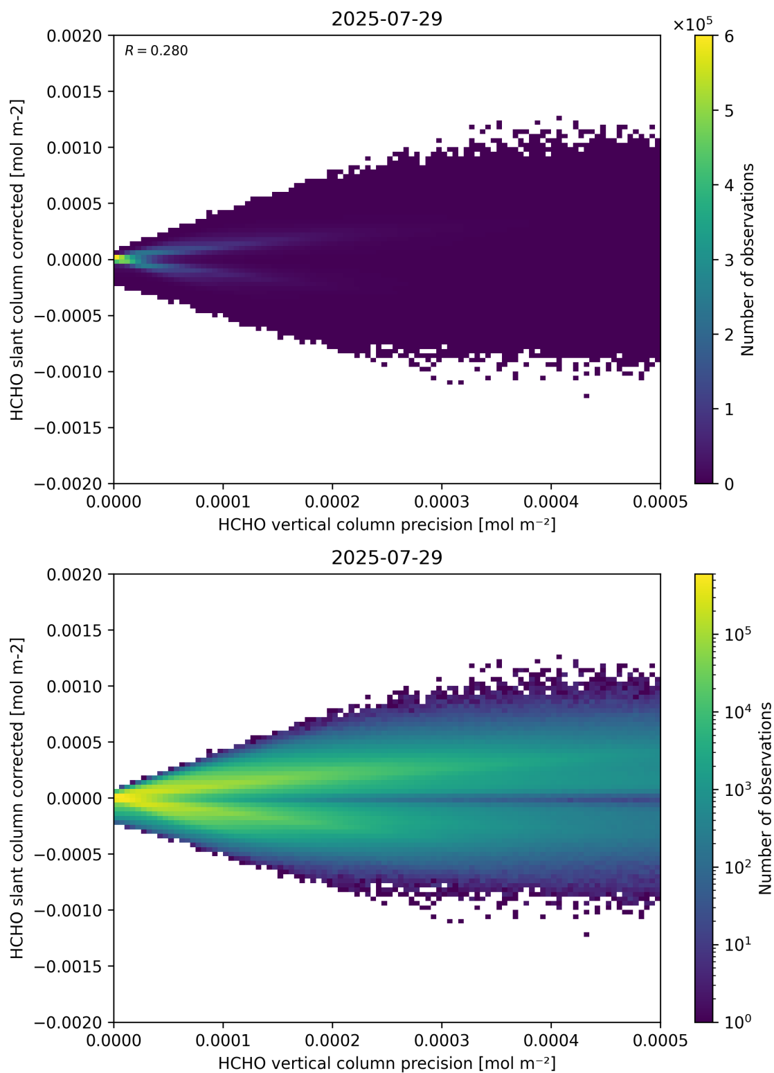
Figure 140: Scatter density plot of “HCHO vertical column precision” against “HCHO slant column corrected” for 2025-07-29 to 2025-07-30.
