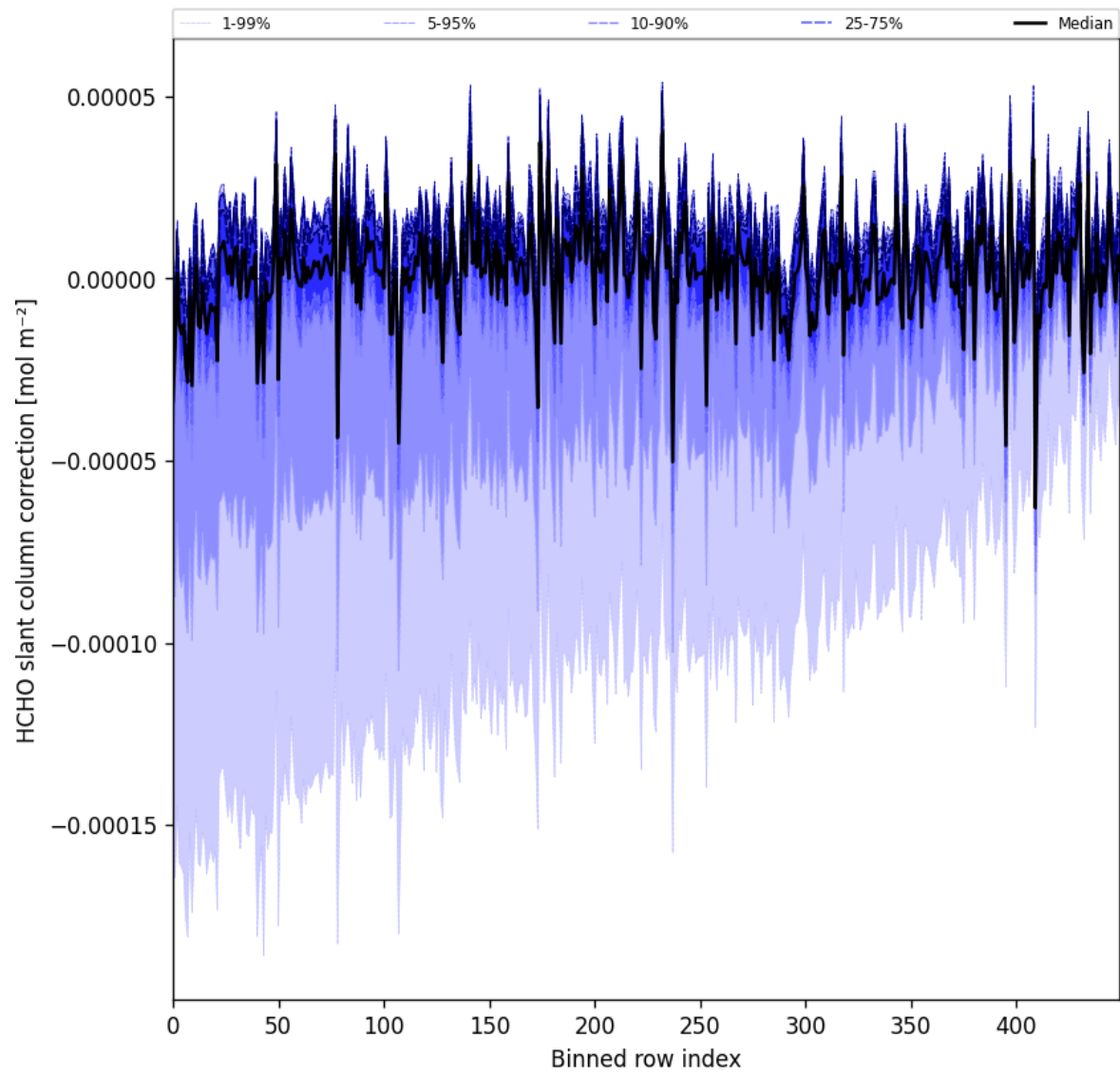
Figure 61: Along track statistics of “HCHO slant column correction” for 2025-07-29 to 2025-07-30
