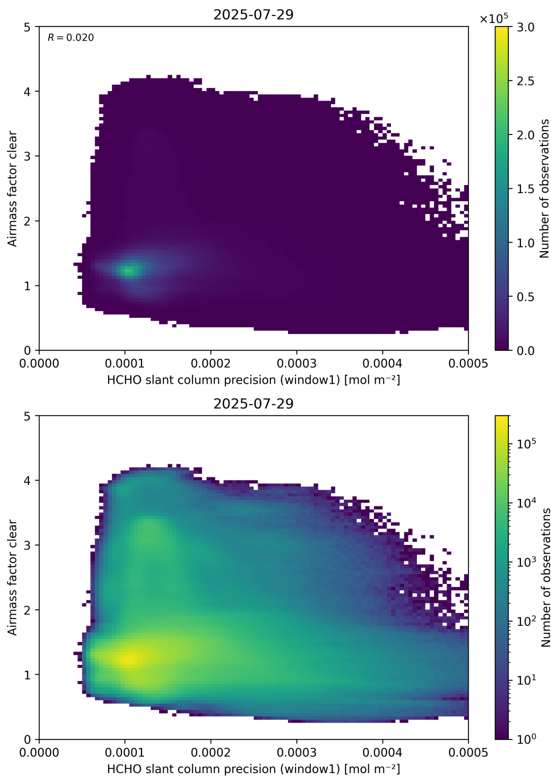
Figure 91: Scatter density plot of “HCHO slant column precision (window1)” against “Airmass factor clear” for 2025-07-29 to 2025-07-30.
