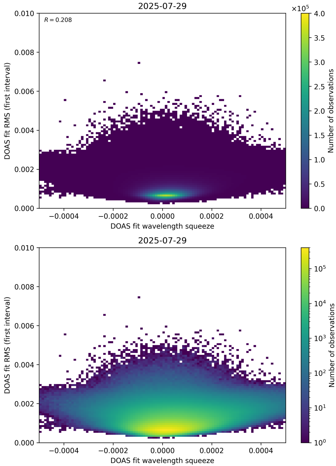
Figure 68: Scatter density plot of “DOAS fit wavelength squeeze” against “DOAS fit RMS (first interval)” for 2025-07-29 to 2025-07-30.
