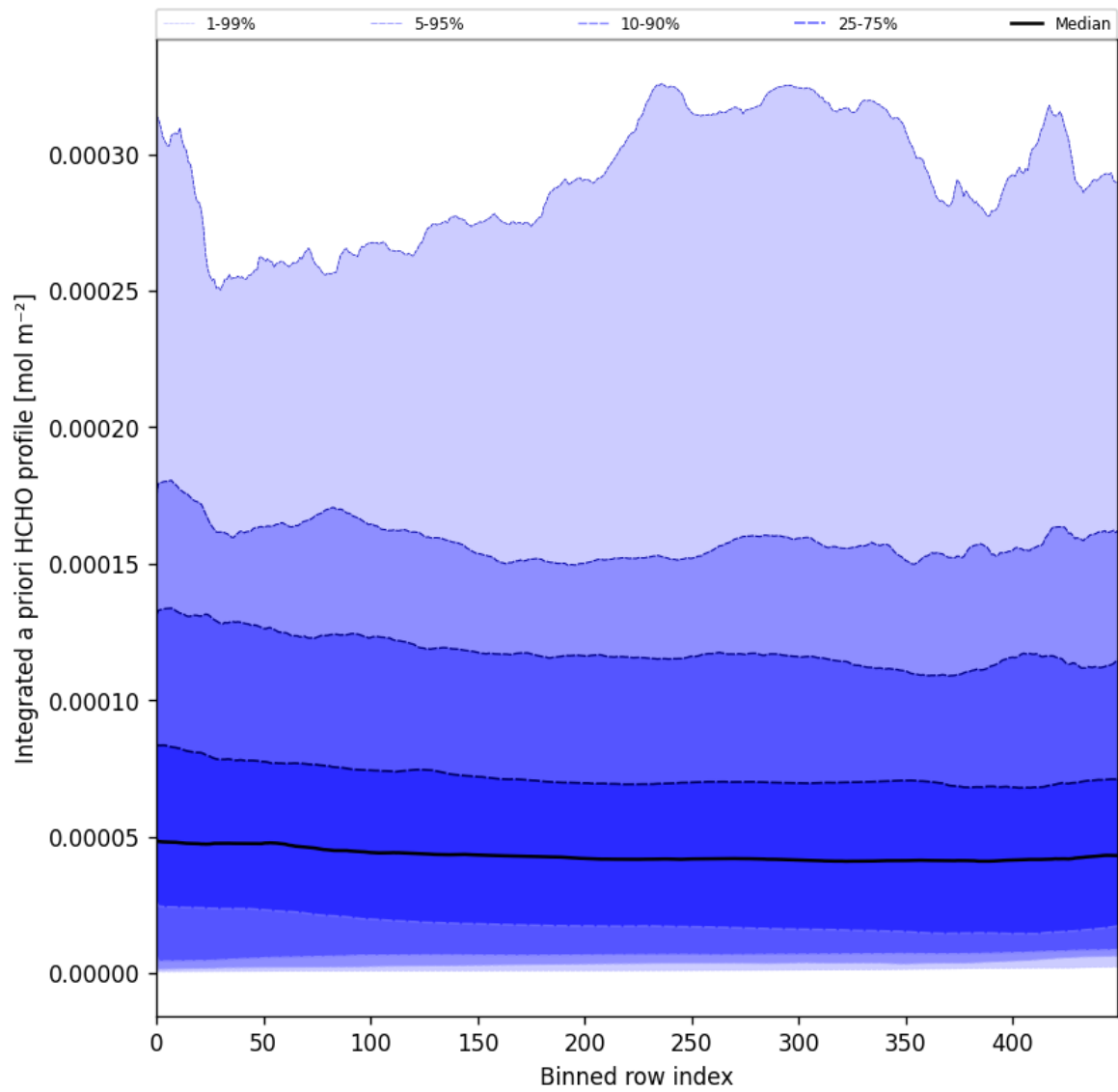
Figure 57: Along track statistics of “Integrated a priori HCHO profile” for 2025-07-29 to 2025-07-30
