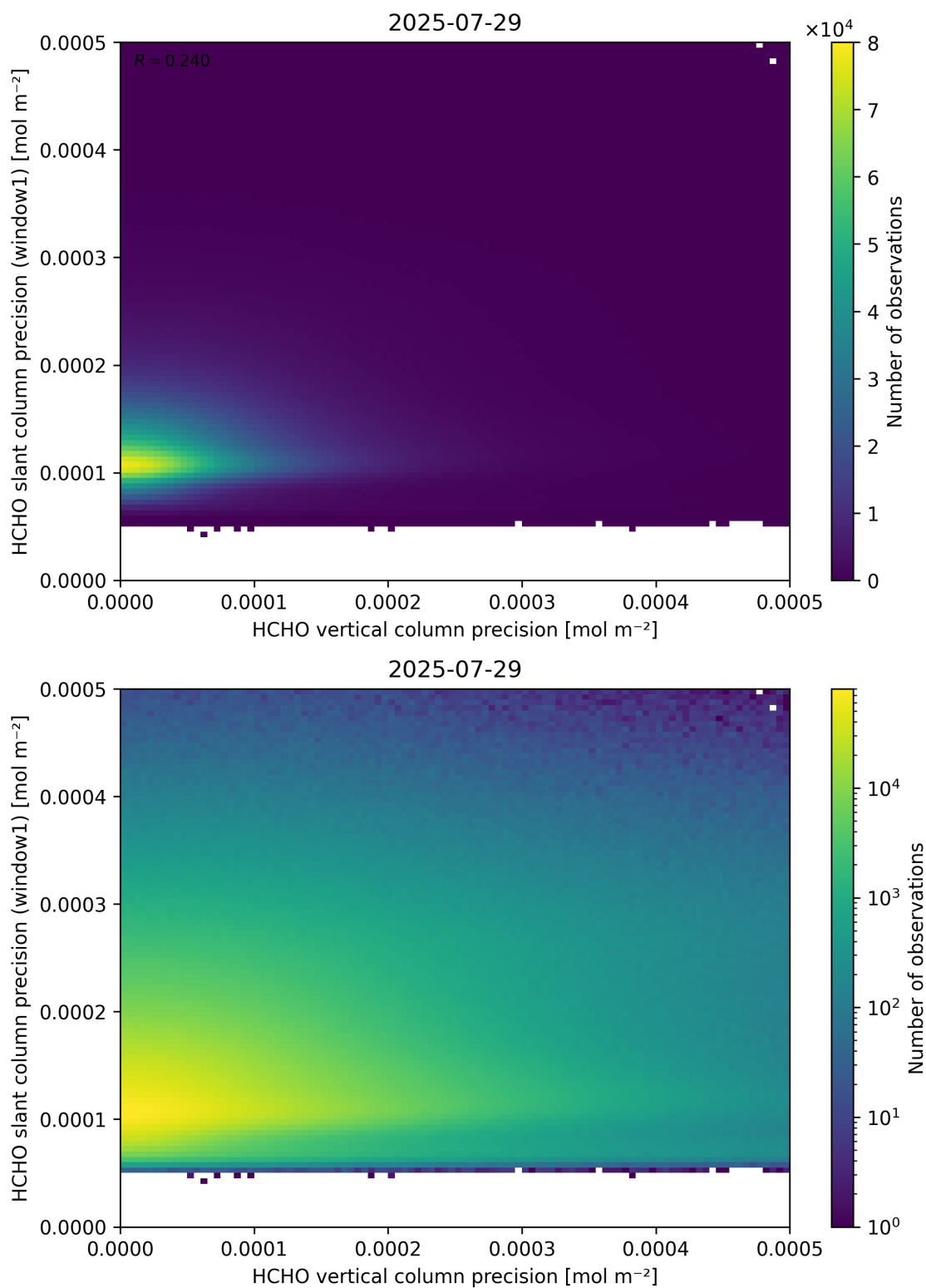
Figure 143: Scatter density plot of “HCHO vertical column precision” against “HCHO slant column precision (window1)” for 2025-07-29 to 2025-07-30.
