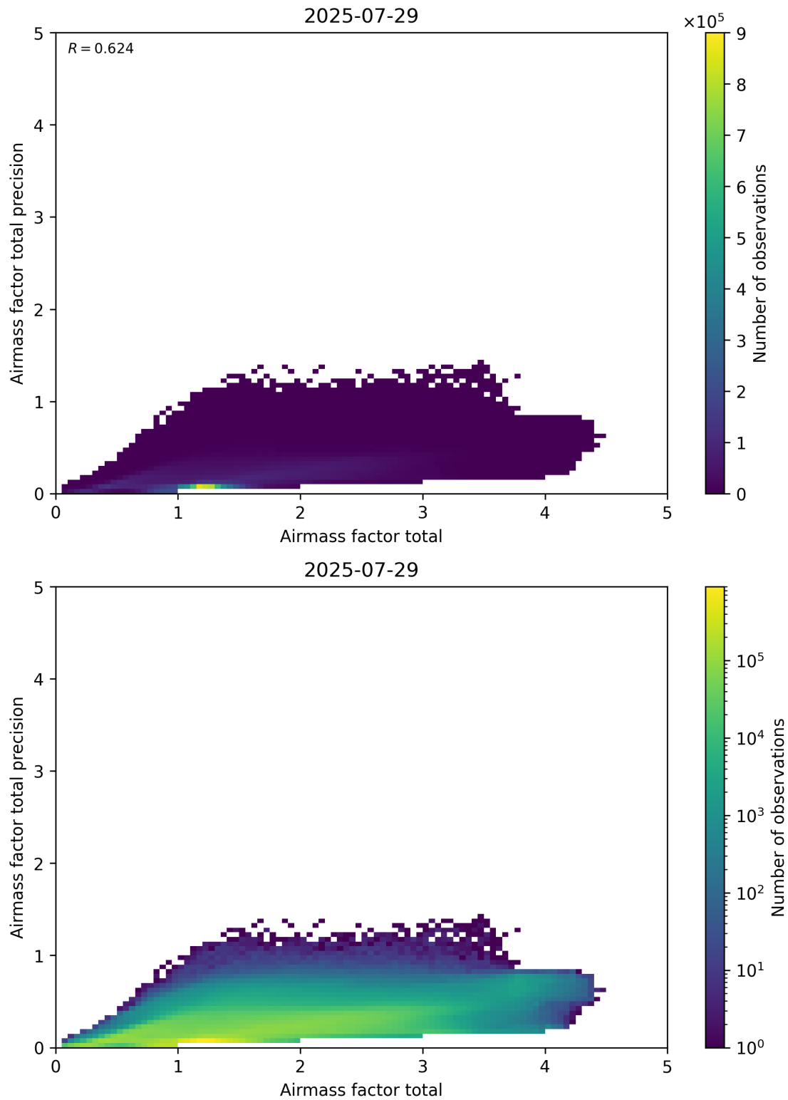
Figure 103: Scatter density plot of “Airmass factor total” against “Airmass factor total precision” for 2025-07-29 to 2025-07-30.
