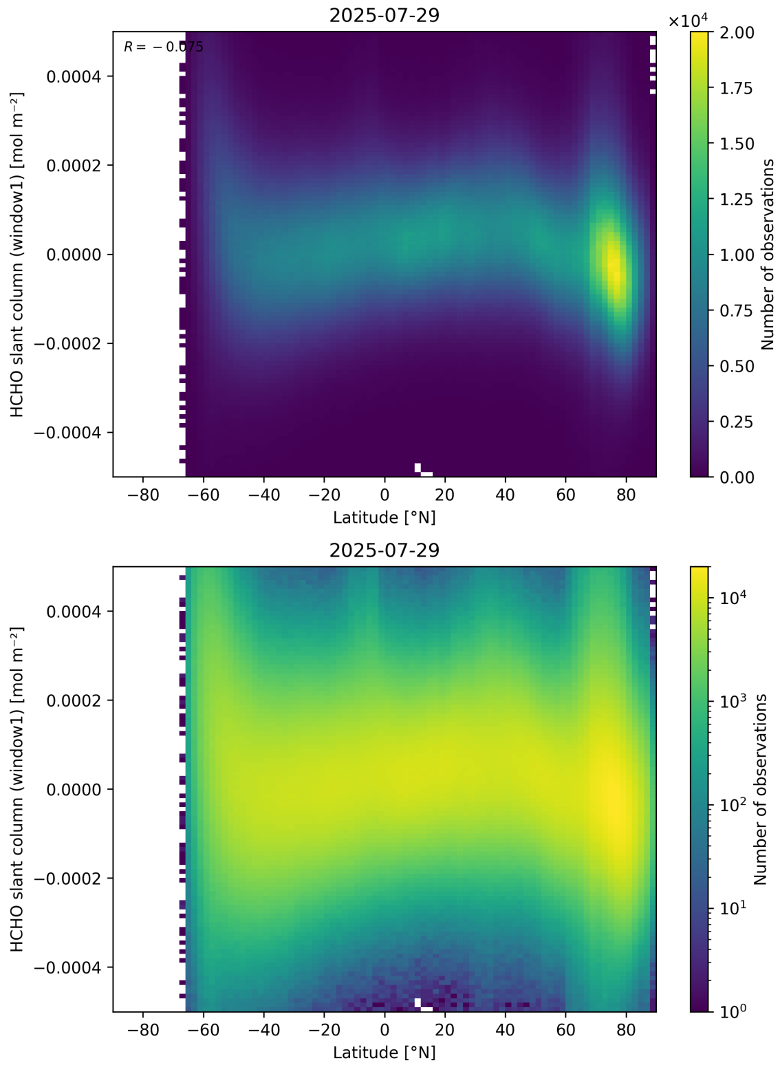
Figure 159: Scatter density plot of “Latitude” against “HCHO slant column (window1)” for 2025-07-29 to 2025-07-30.
