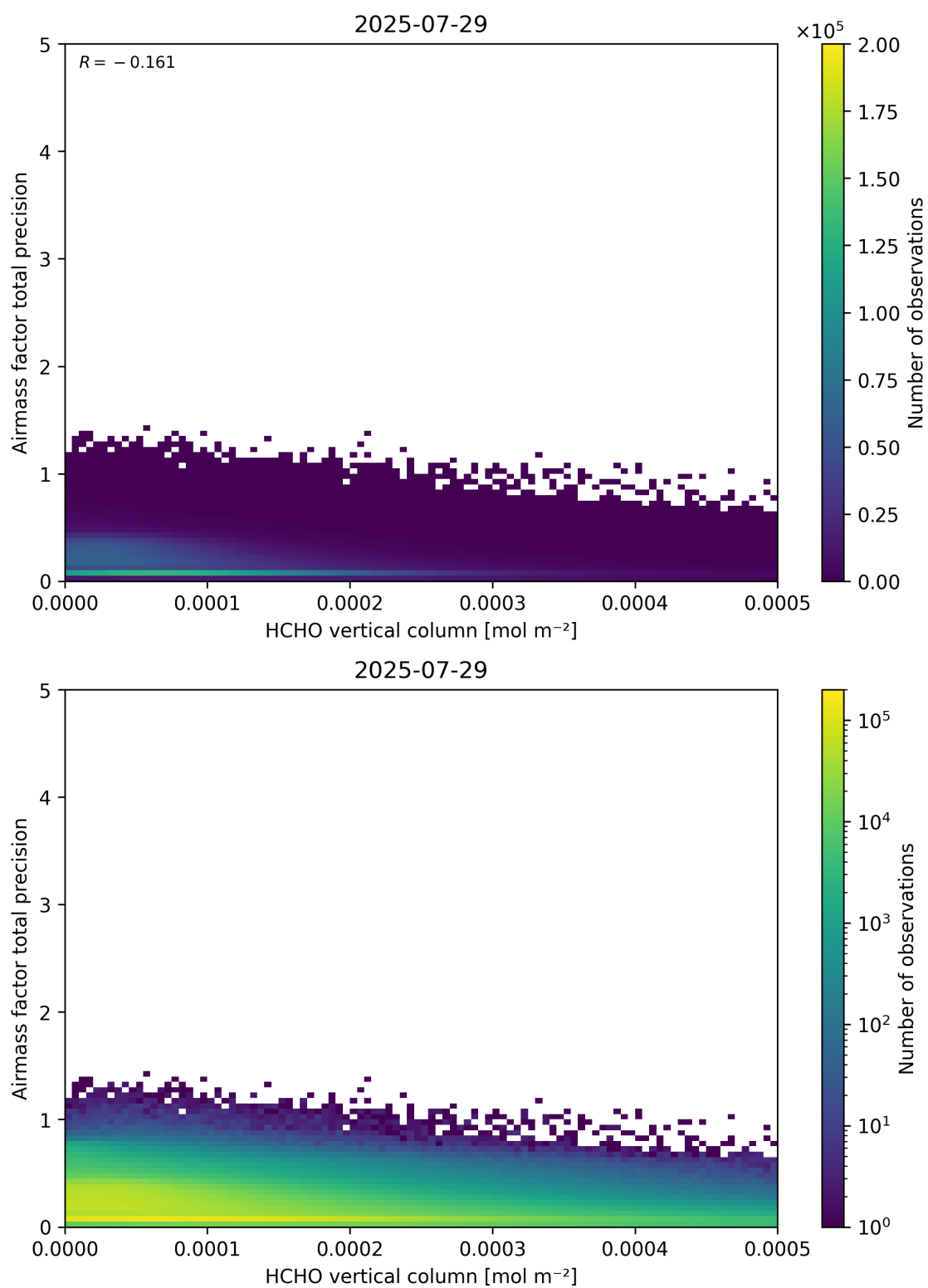
Figure 132: Scatter density plot of “HCHO vertical column” against “Airmass factor total precision” for 2025-07-29 to 2025-07-30.
