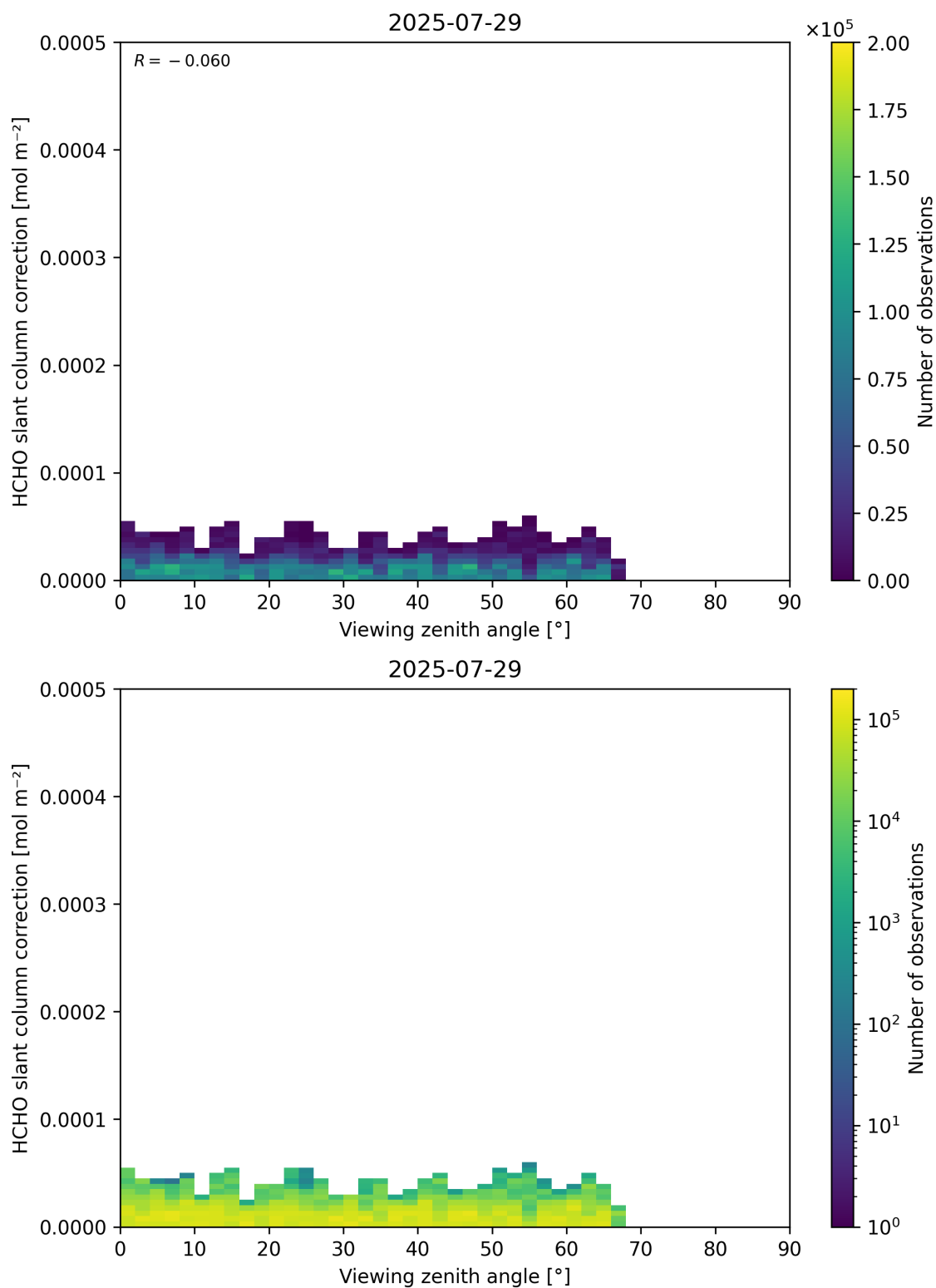
Figure 187: Scatter density plot of “Viewing zenith angle” against “HCHO slant column correction” for 2025-07-29 to 2025-07-30.
