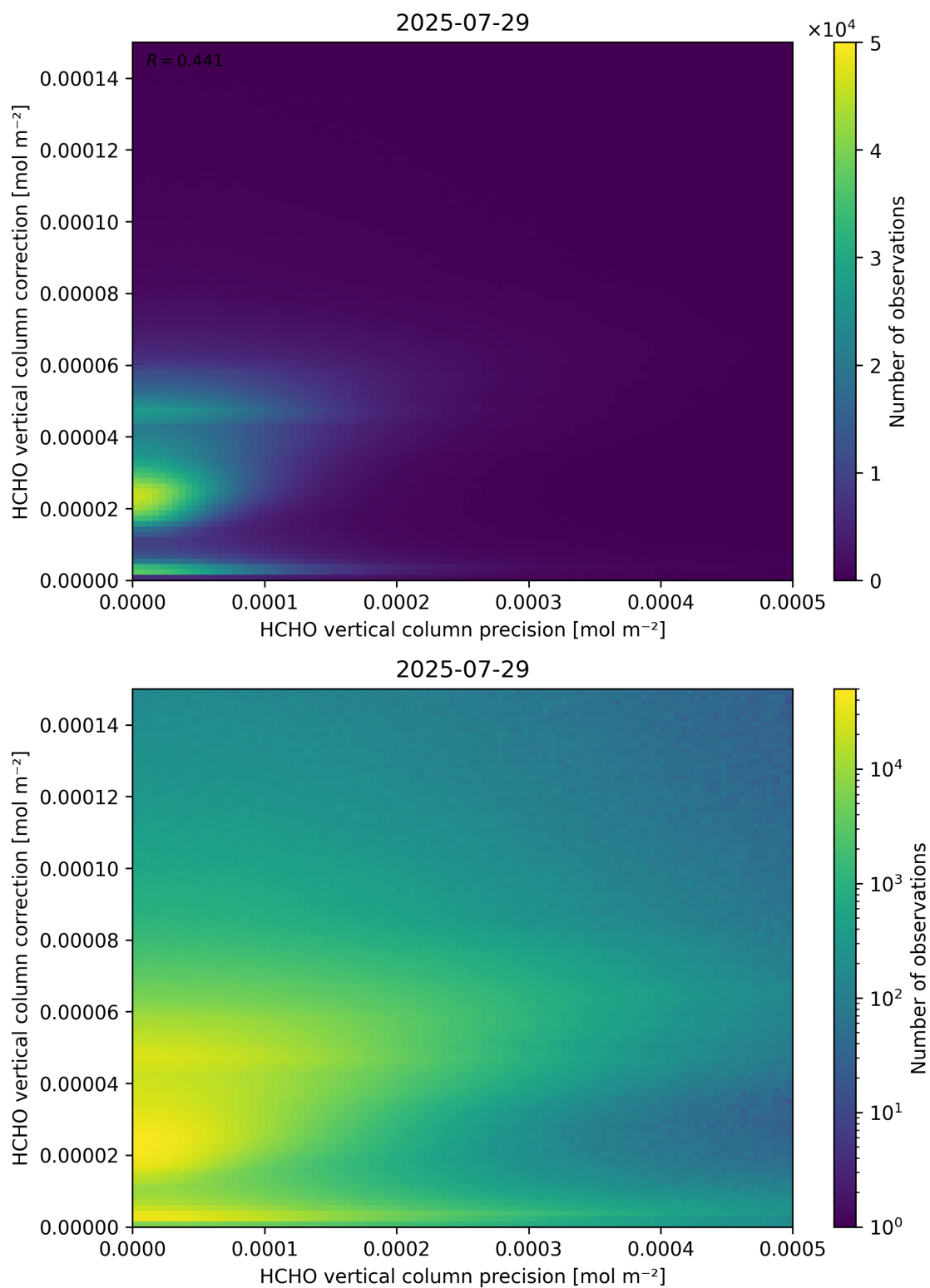
Figure 146: Scatter density plot of “HCHO vertical column precision” against “HCHO vertical column correction” for 2025-07-29 to 2025-07-30.
