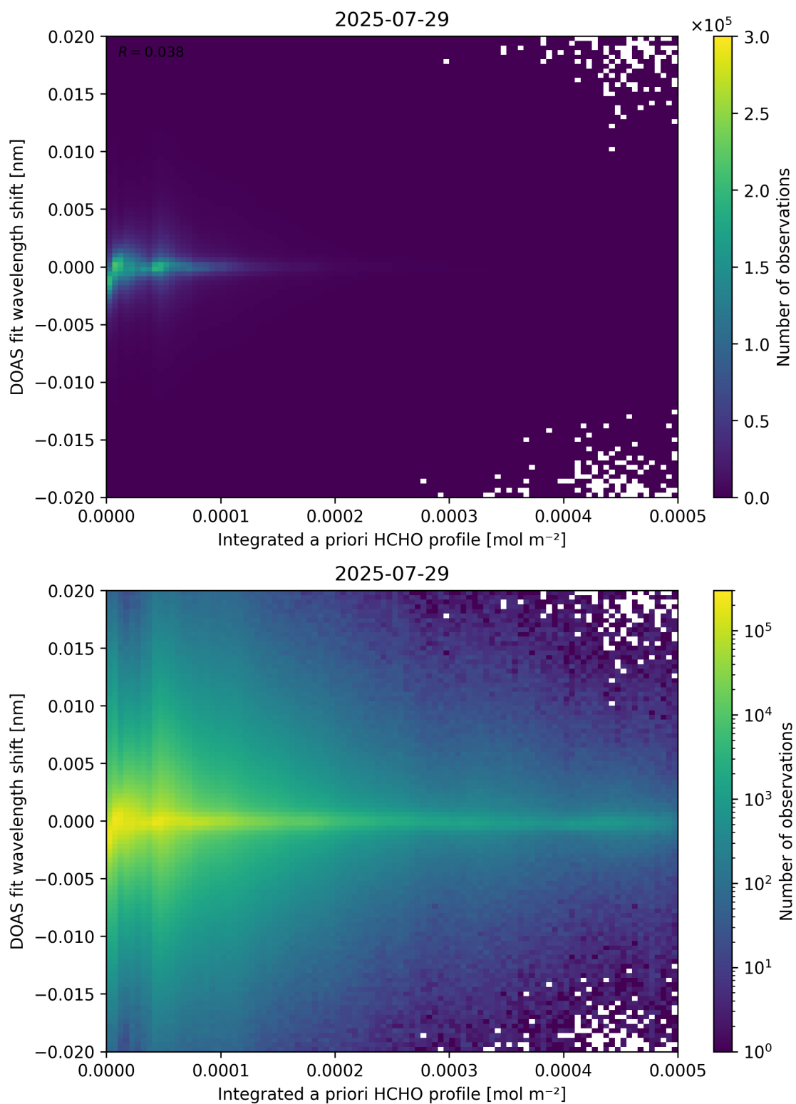
Figure 149: Scatter density plot of “Integrated a priori HCHO profile” against “DOAS fit wavelength shift” for 2025-07-29 to 2025-07-30.
