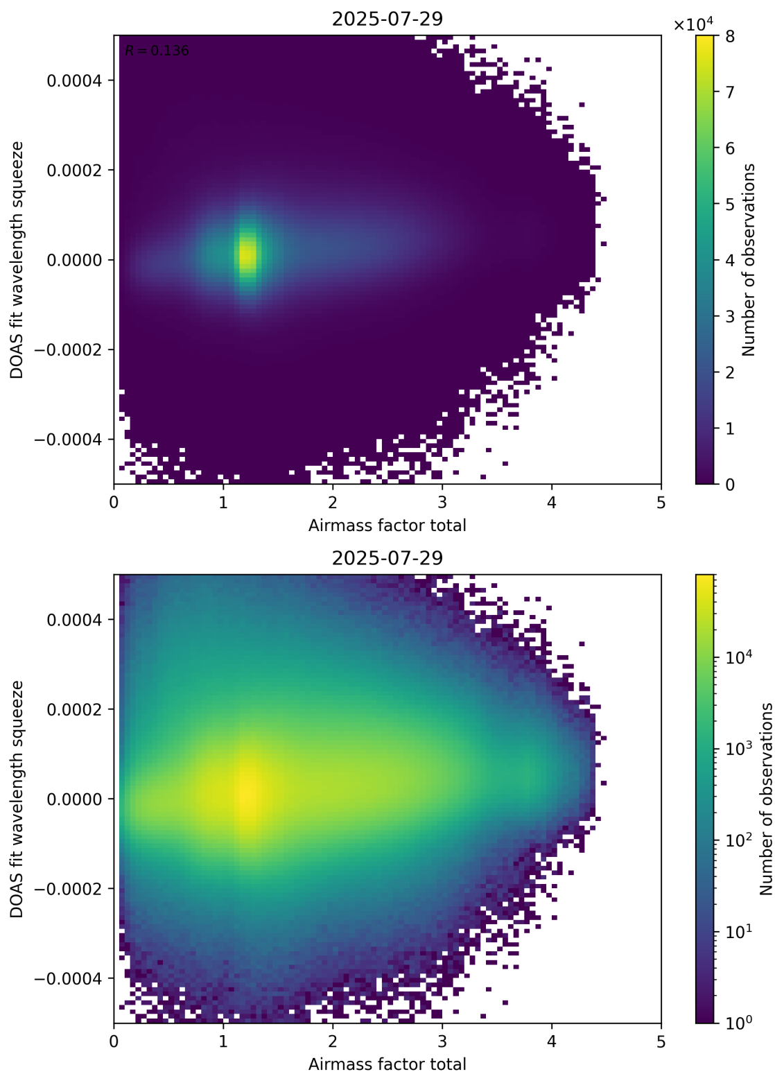
Figure 99: Scatter density plot of “Airmass factor total” against “DOAS fit wavelength squeeze” for 2025-07-29 to 2025-07-30.
