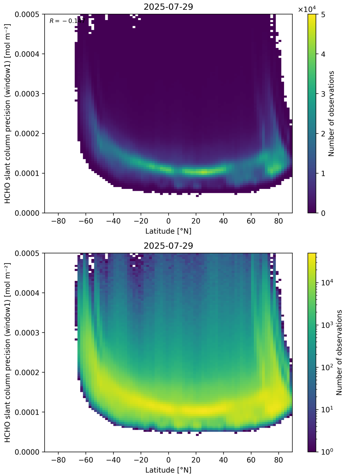
Figure 160: Scatter density plot of “Latitude” against “HCHO slant column precision (window1)” for 2025-07-29 to 2025-07-30.
