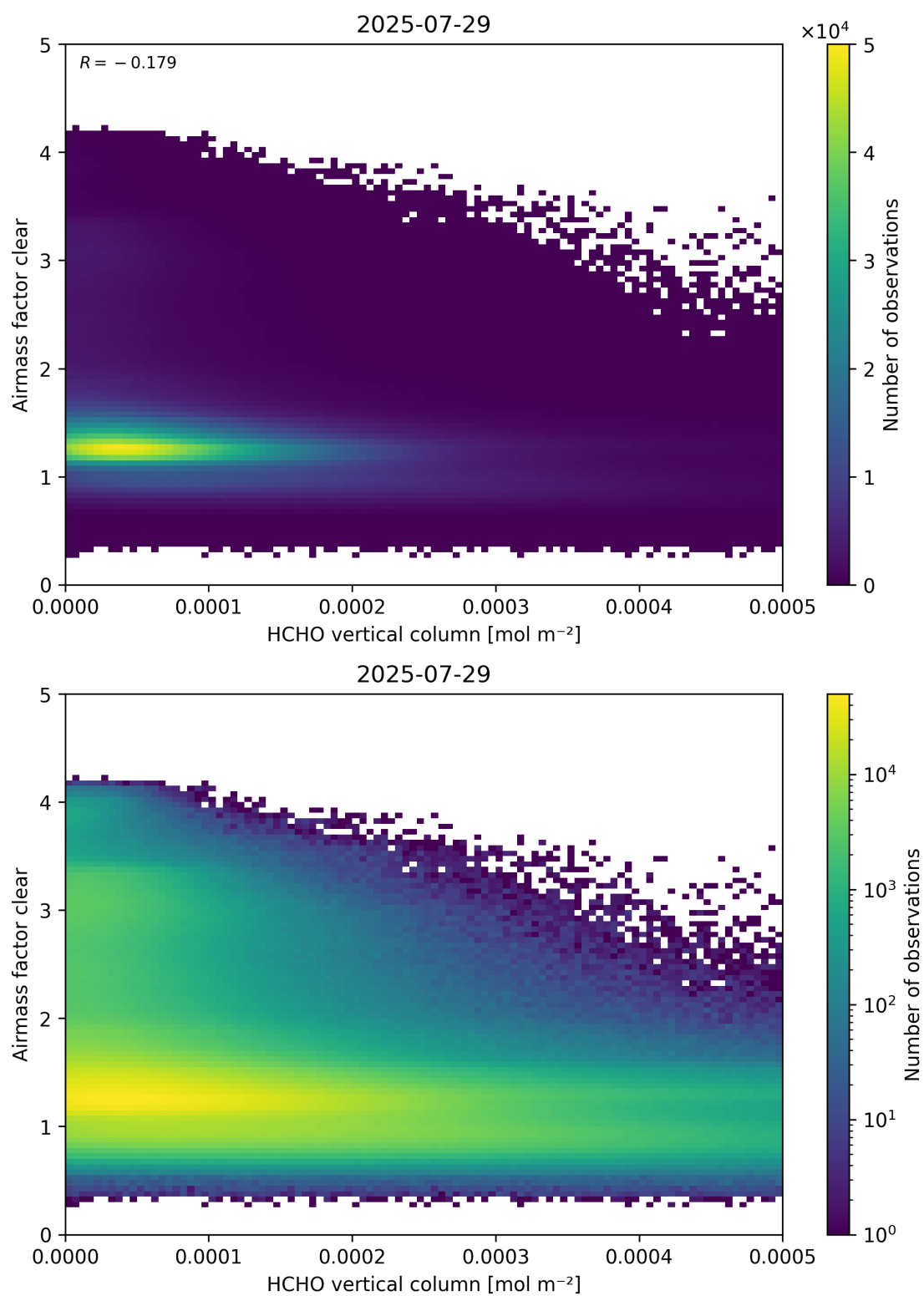
Figure 126: Scatter density plot of “HCHO vertical column” against “Airmass factor clear” for 2025-07-29 to 2025-07-30.
