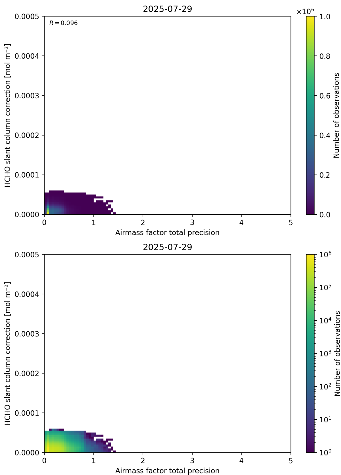
Figure 110: Scatter density plot of “Airmass factor total precision” against “HCHO slant column correction” for 2025-07-29 to 2025-07-30.
