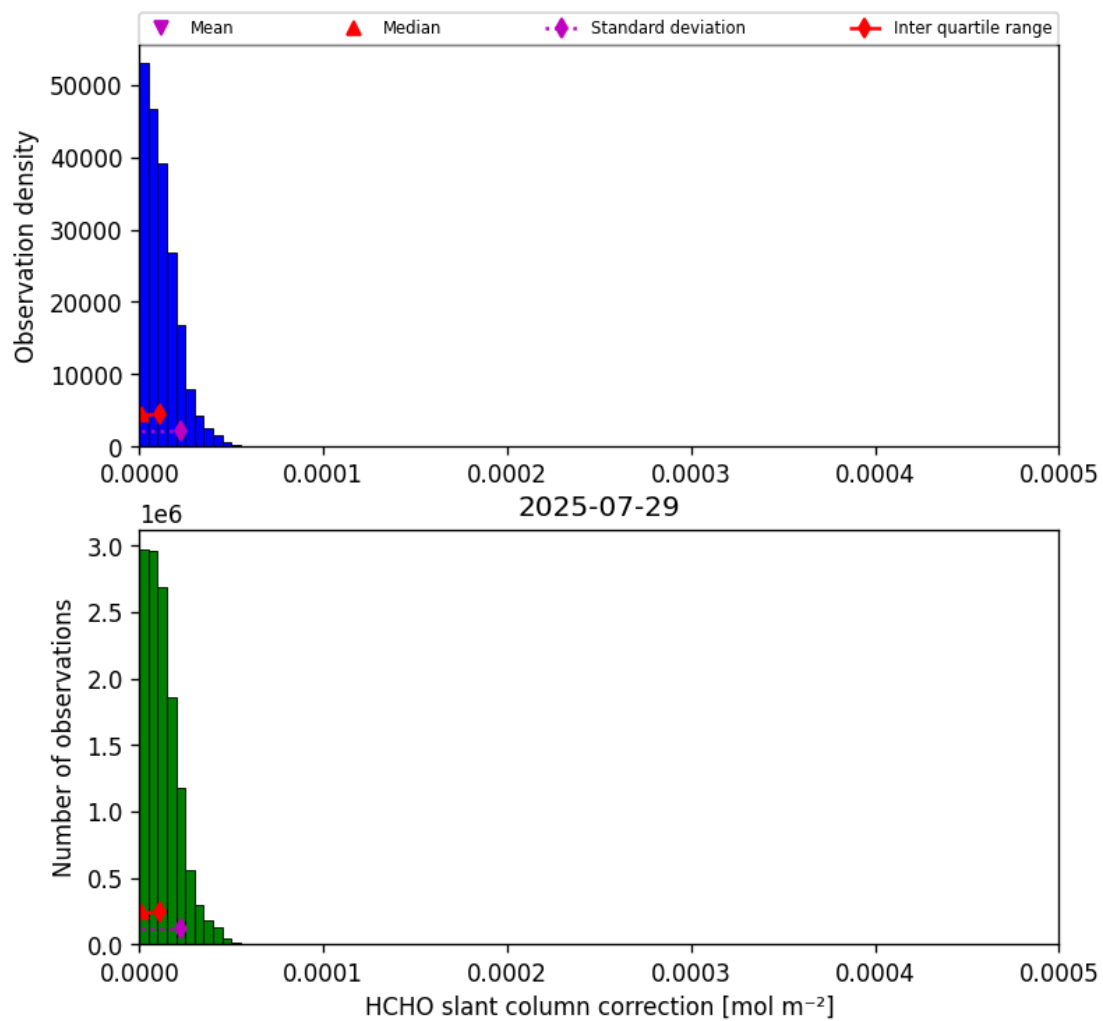
Figure 47: Histogram of “HCHO slant column correction” for 2025-07-29 to 2025-07-30
