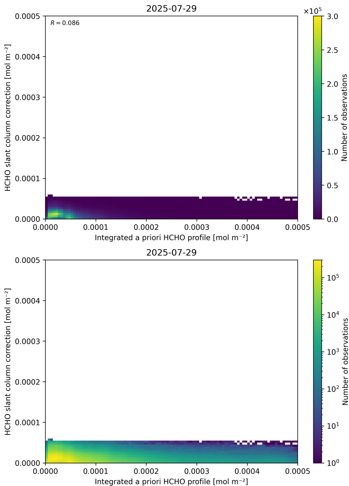
Figure 152: Scatter density plot of “Integrated a priori HCHO profile” against “HCHO slant column correction” for 2025-07-29 to 2025-07-30.
