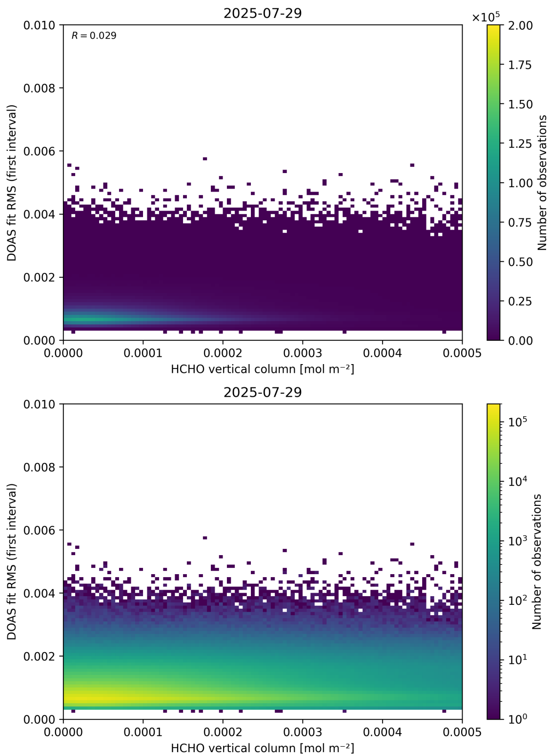
Figure 123: Scatter density plot of “HCHO vertical column” against “DOAS fit RMS (first interval)” for 2025-07-29 to 2025-07-30.
