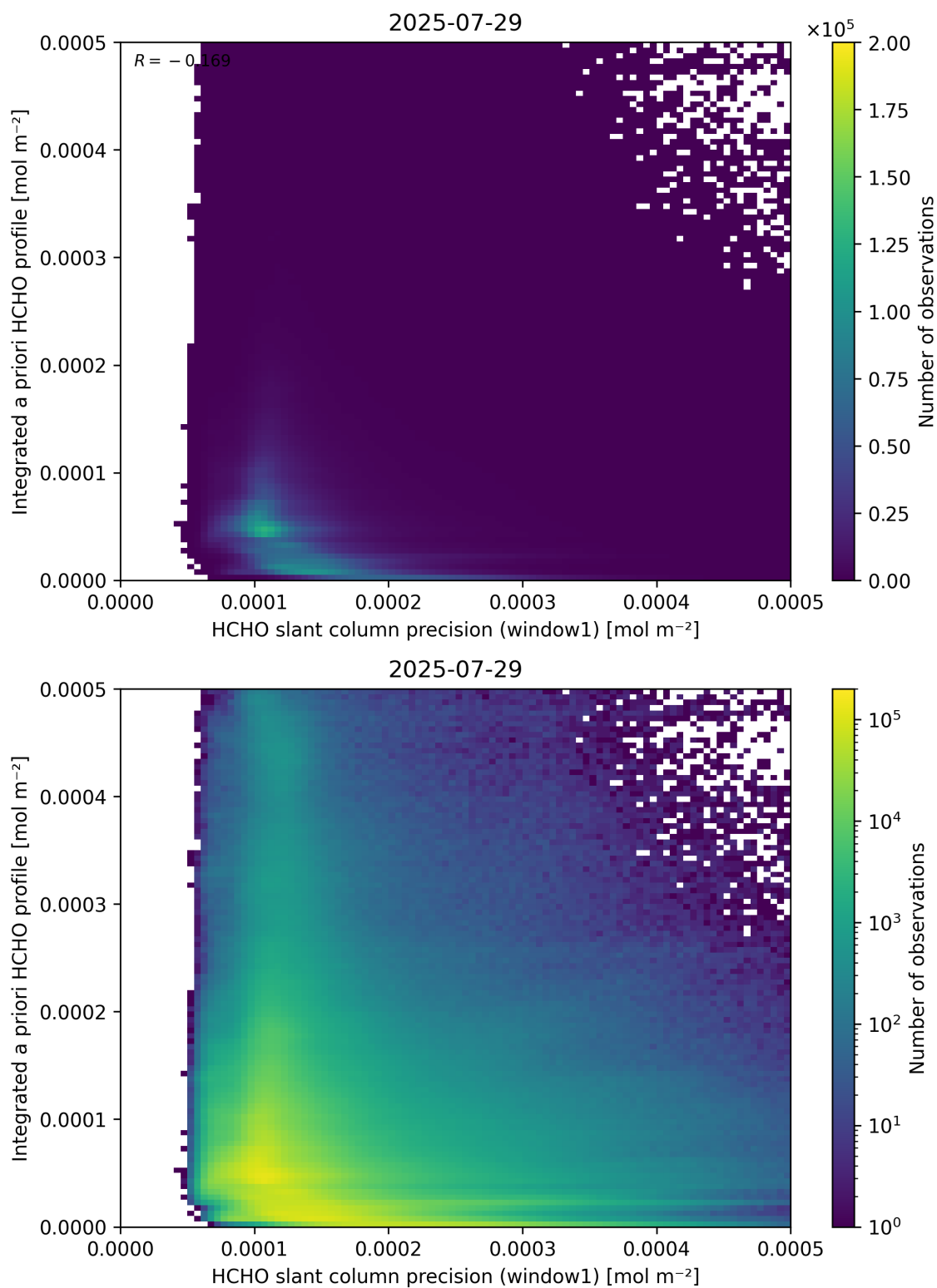
Figure 96: Scatter density plot of “HCHO slant column precision (window1)” against “Integrated a priori HCHO profile” for 2025-07-29 to 2025-07-30.
