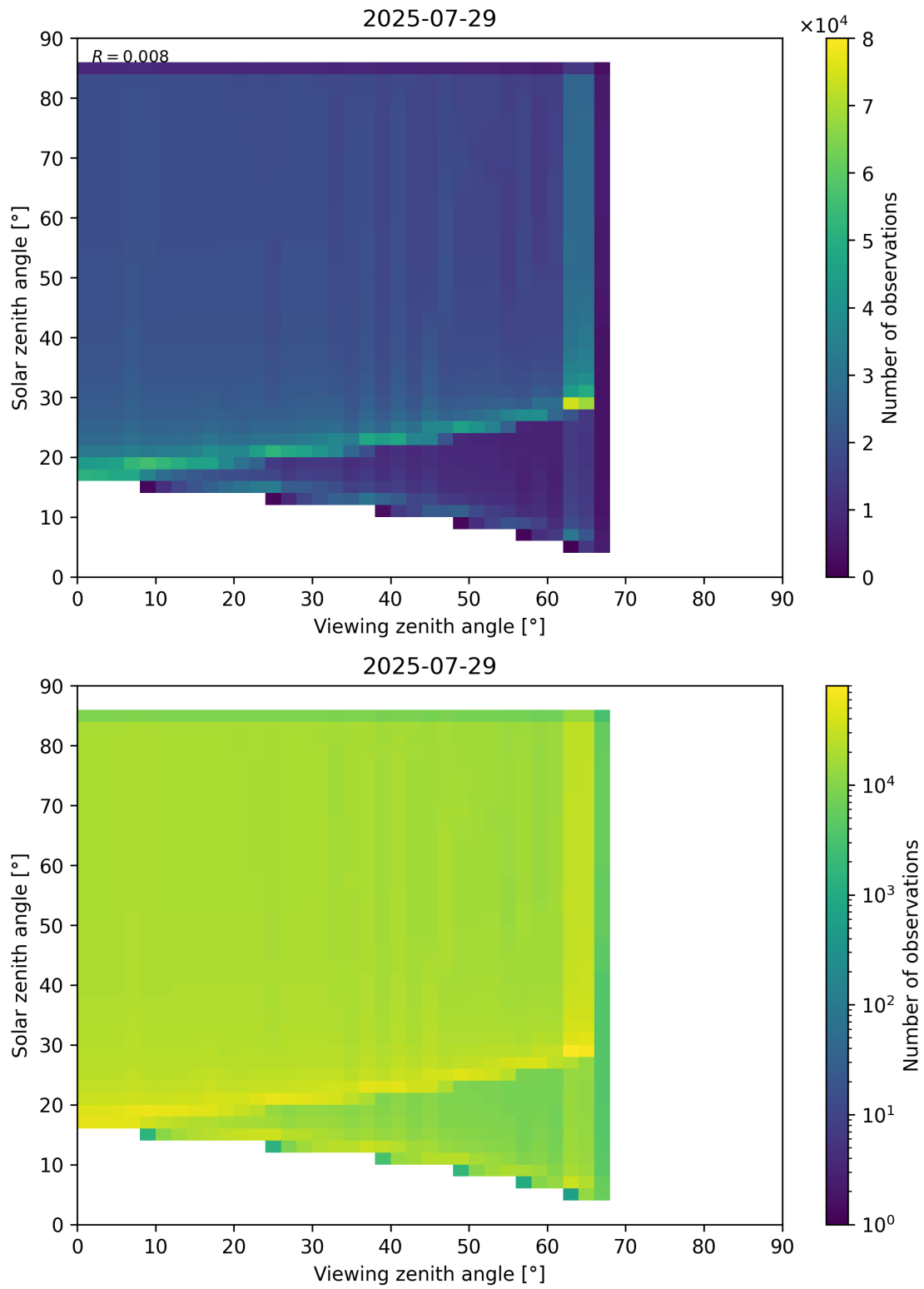
Figure 197: Scatter density plot of “Viewing zenith angle” against “Solar zenith angle” for 2025-07-29 to 2025-07-30.
