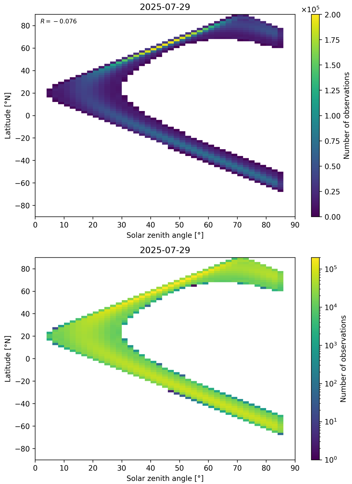
Figure 181: Scatter density plot of “Solar zenith angle” against “Latitude” for 2025-07-29 to 2025-07-30.
