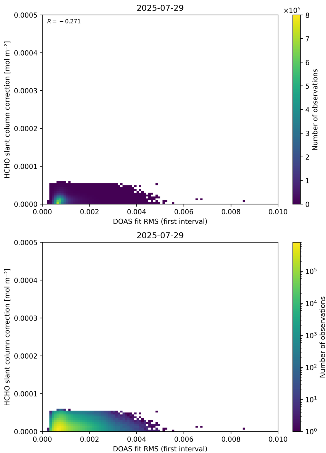
Figure 63: Scatter density plot of “DOAS fit RMS (first interval)” against “HCHO slant column correction” for 2025-07-29 to 2025-07-30.
