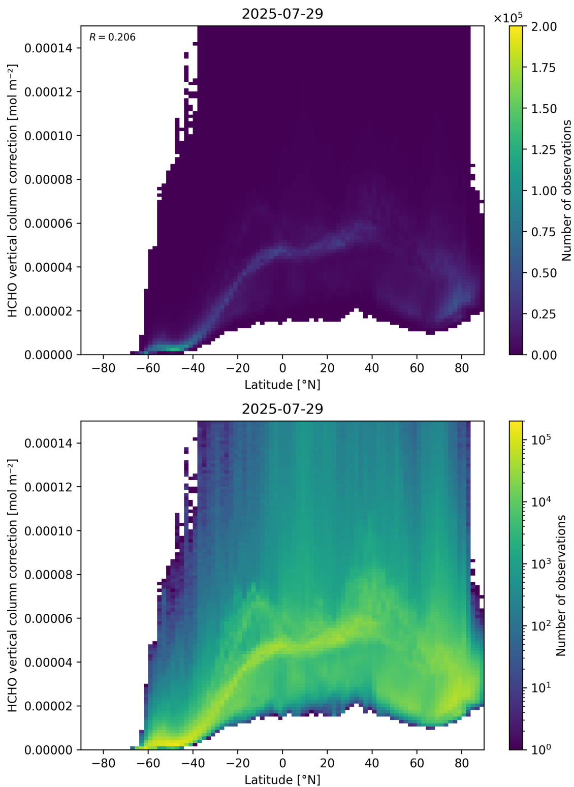
Figure 164: Scatter density plot of “Latitude” against “HCHO vertical column correction” for 2025-07-29 to 2025-07-30.
