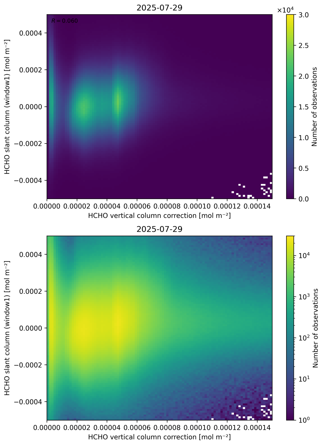
Figure 118: Scatter density plot of “HCHO vertical column correction” against “HCHO slant column (window1)” for 2025-07-29 to 2025-07-30.
