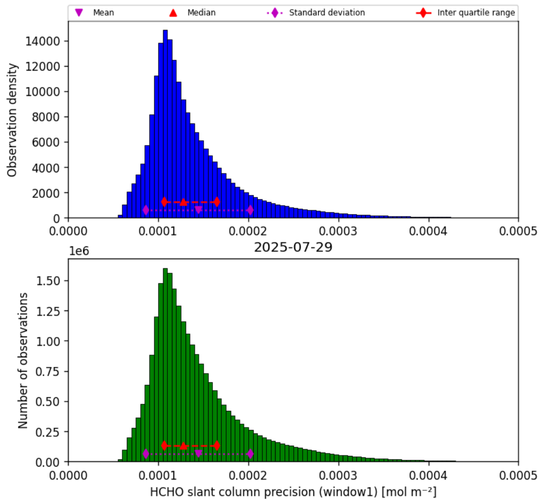
Figure 39: Histogram of “HCHO slant column precision (window1)” for 2025-07-29 to 2025-07-30
