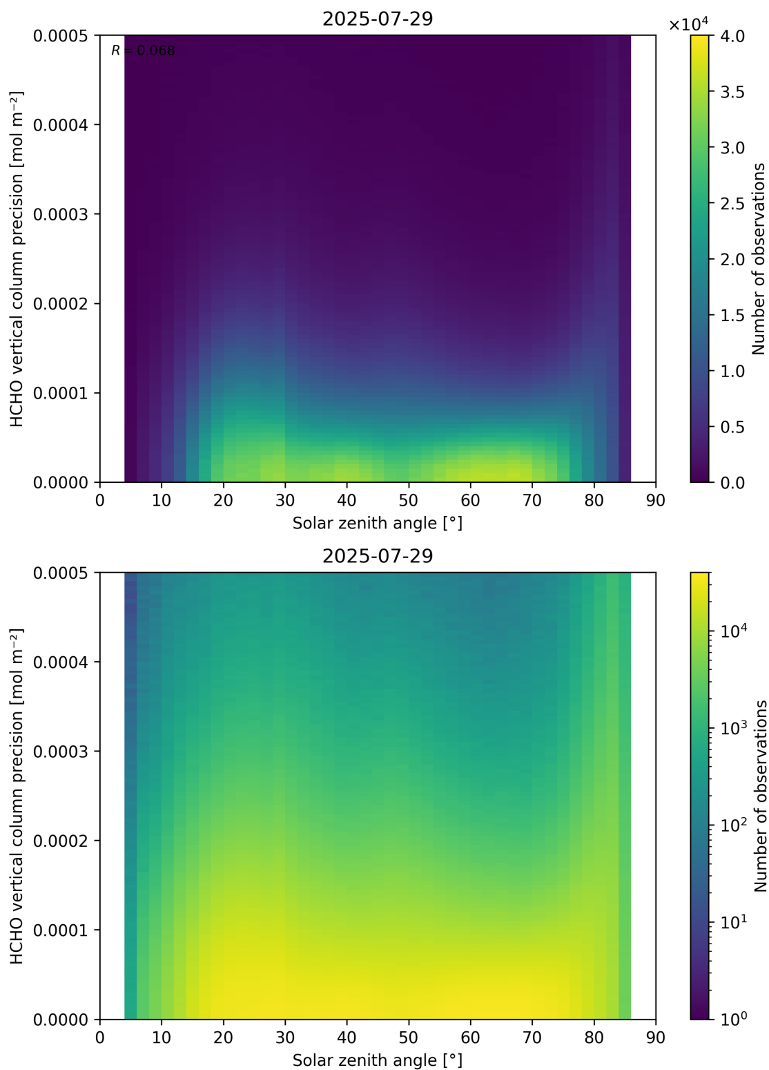
Figure 179: Scatter density plot of “Solar zenith angle” against “HCHO vertical column precision” for 2025-07-29 to 2025-07-30.
