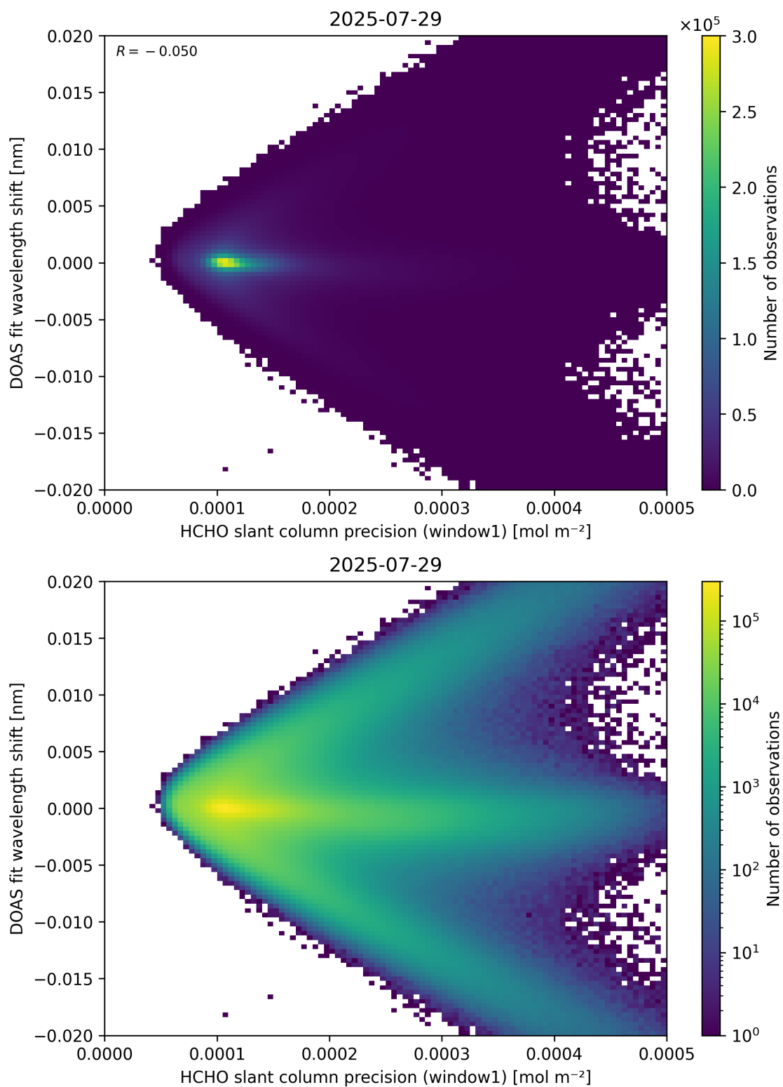
Figure 89: Scatter density plot of “HCHO slant column precision (window1)” against “DOAS fit wavelength shift” for 2025-07-29 to 2025-07-30.
