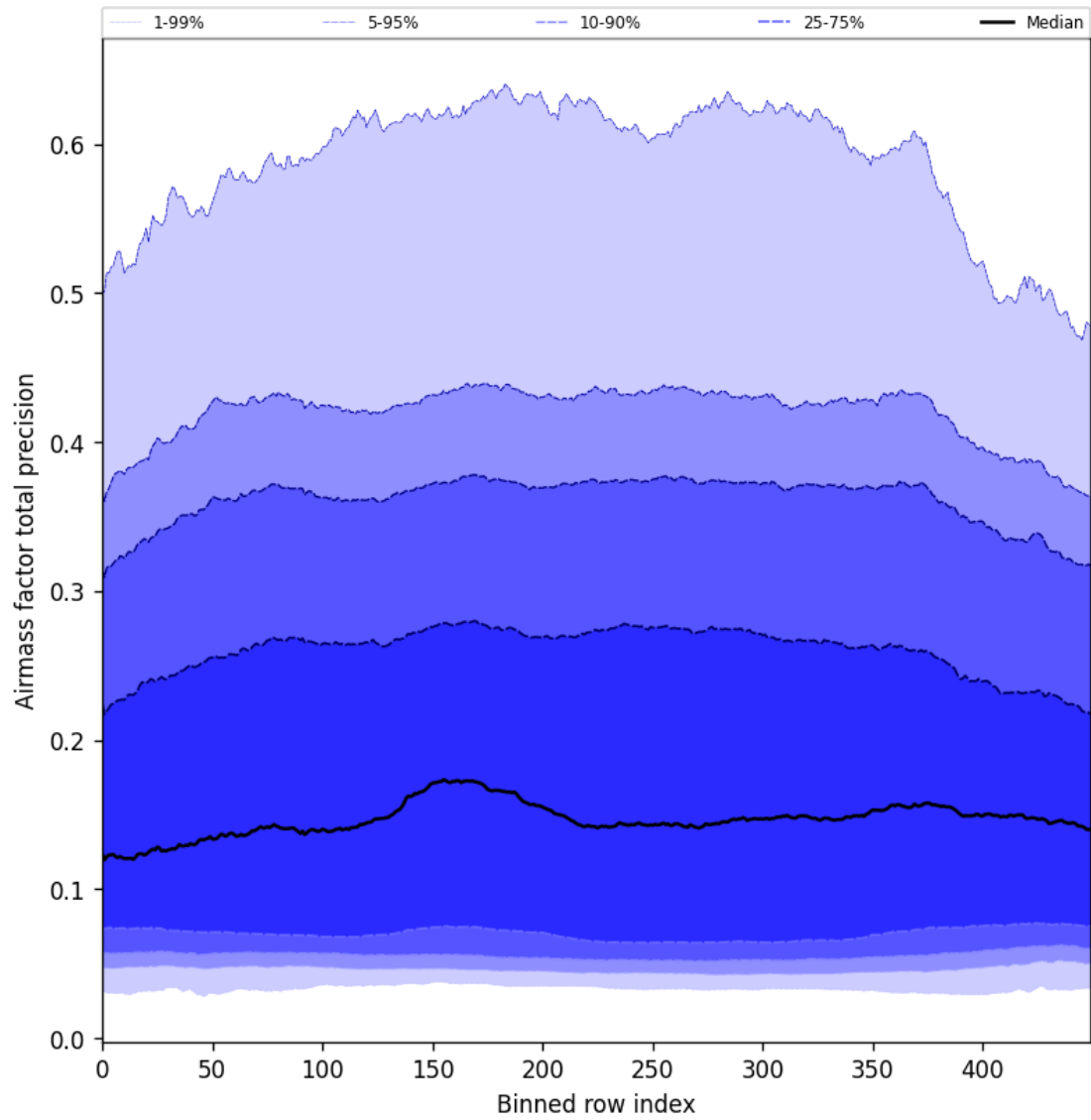
Figure 55: Along track statistics of “Airmass factor total precision” for 2025-07-29 to 2025-07-30
