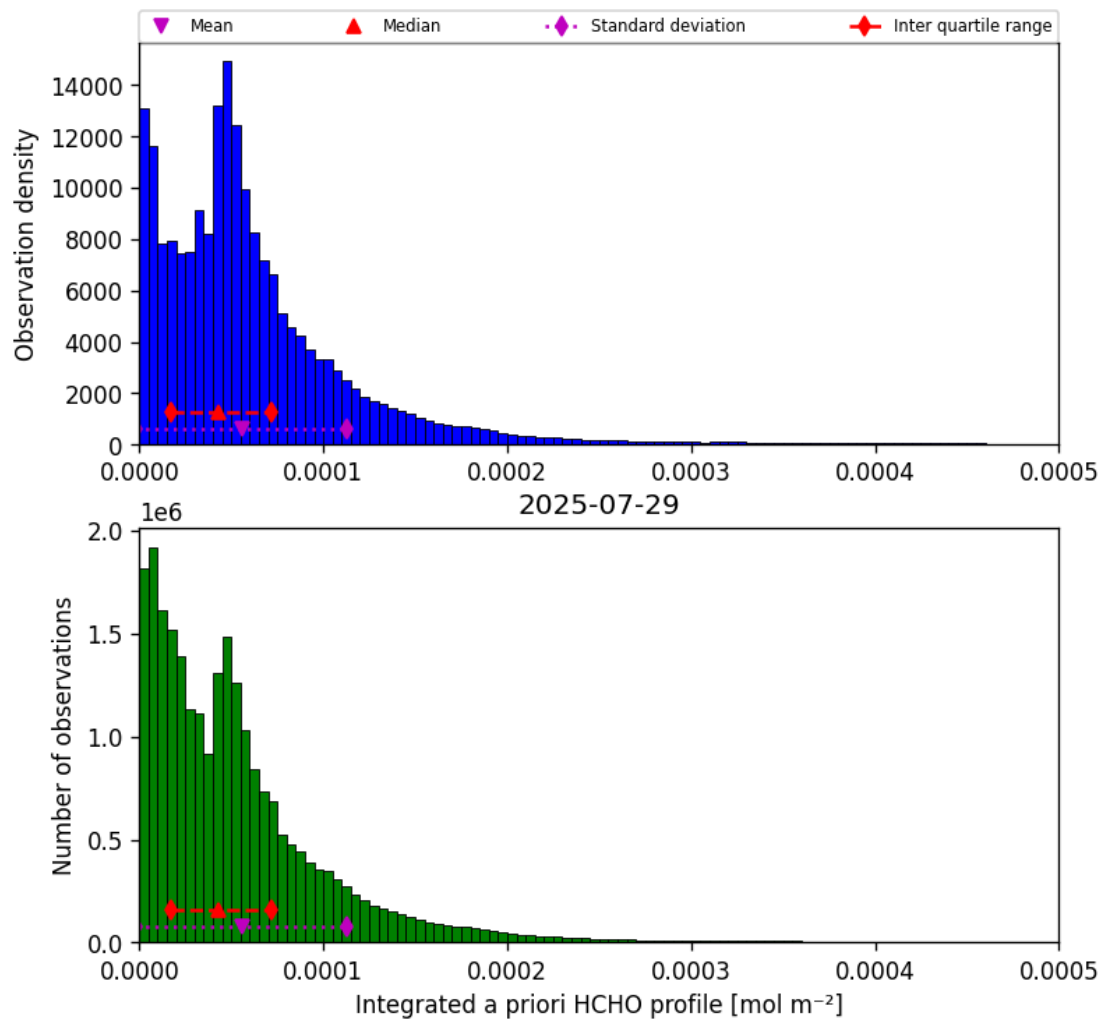
Figure 43: Histogram of “Integrated a priori HCHO profile” for 2025-07-29 to 2025-07-30
