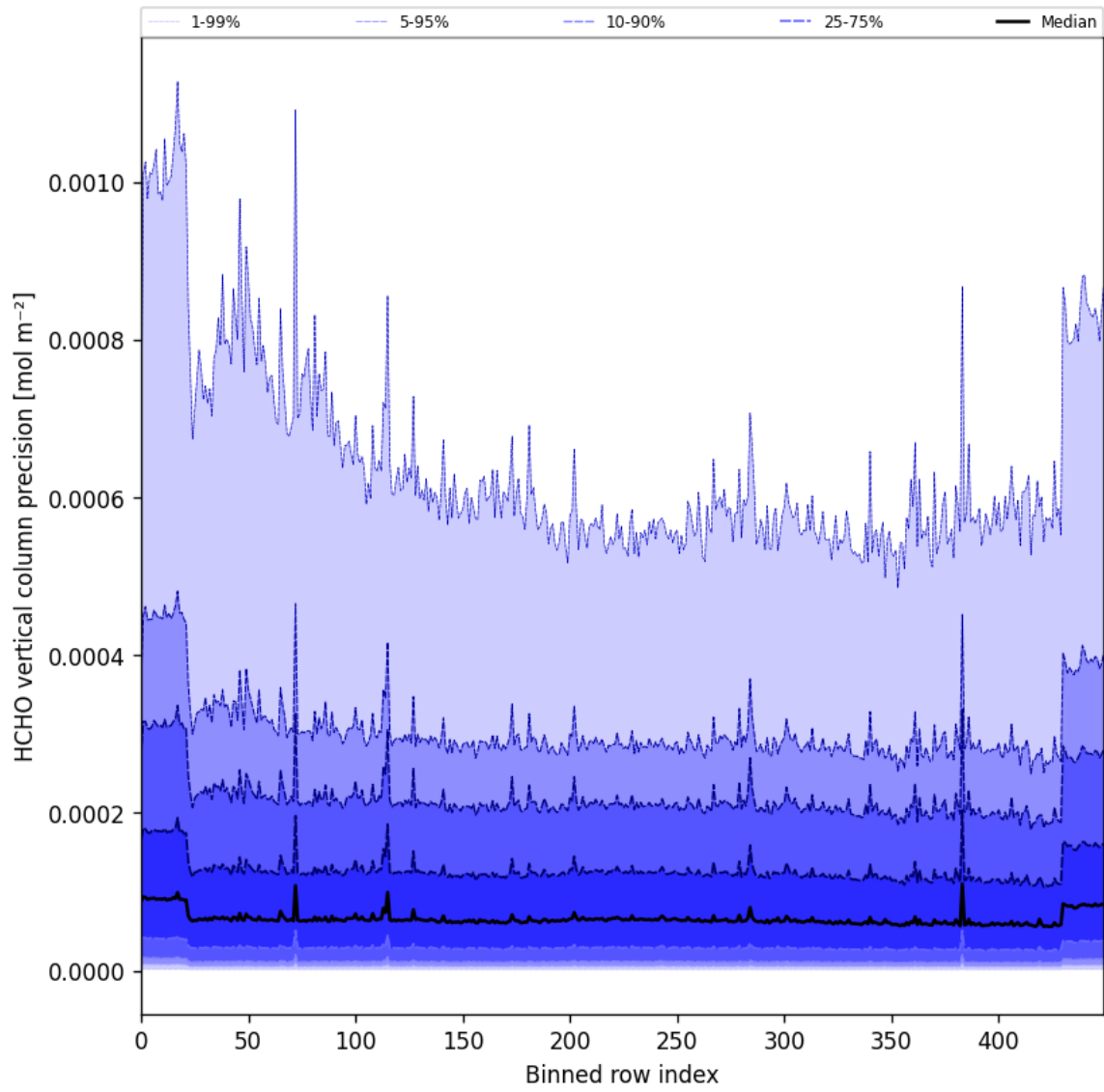
Figure 50: Along track statistics of “HCHO vertical column precision” for 2025-07-29 to 2025-07-30
