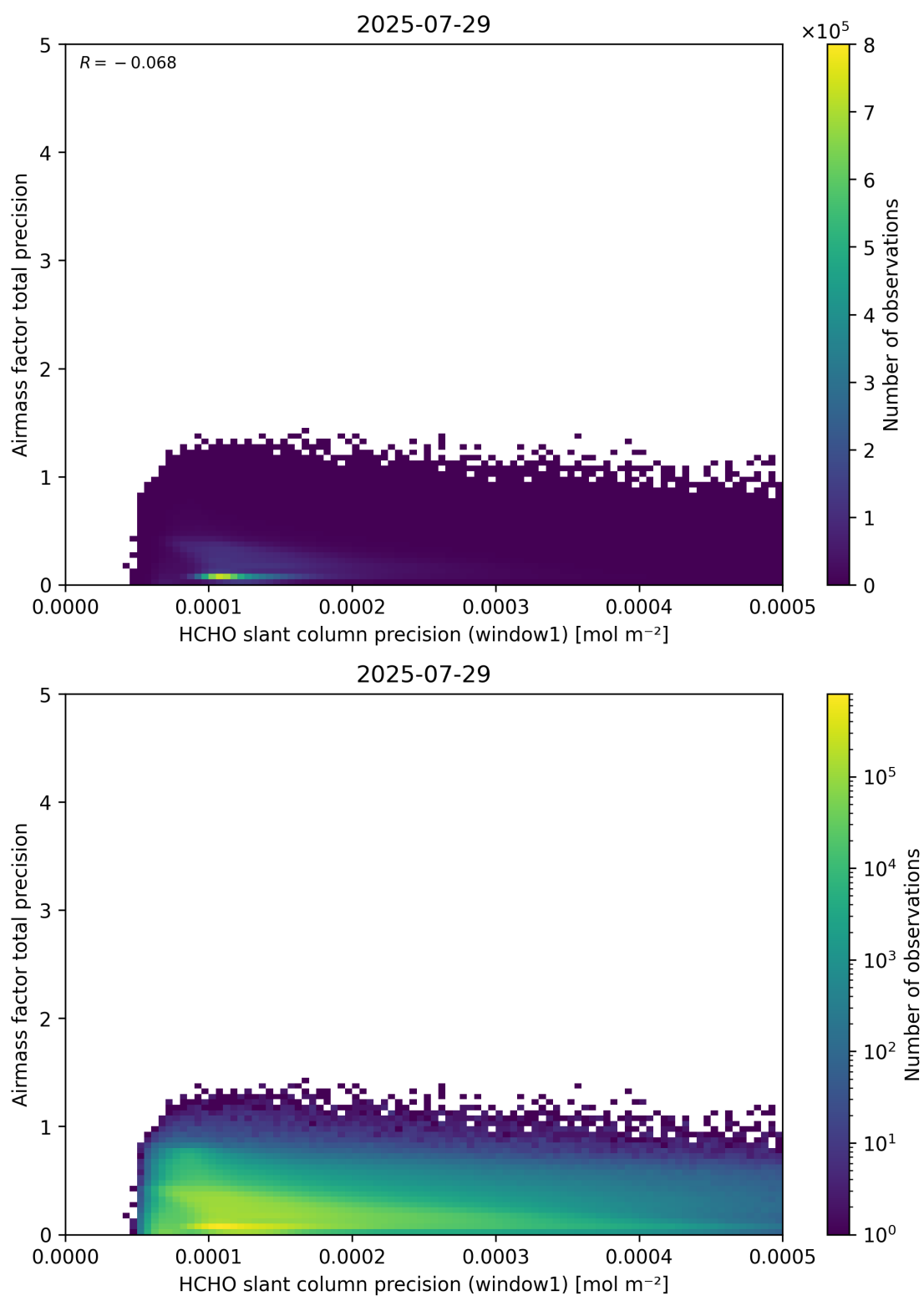
Figure 95: Scatter density plot of “HCHO slant column precision (window1)” against “Airmass factor total precision” for 2025-07-29 to 2025-07-30.
