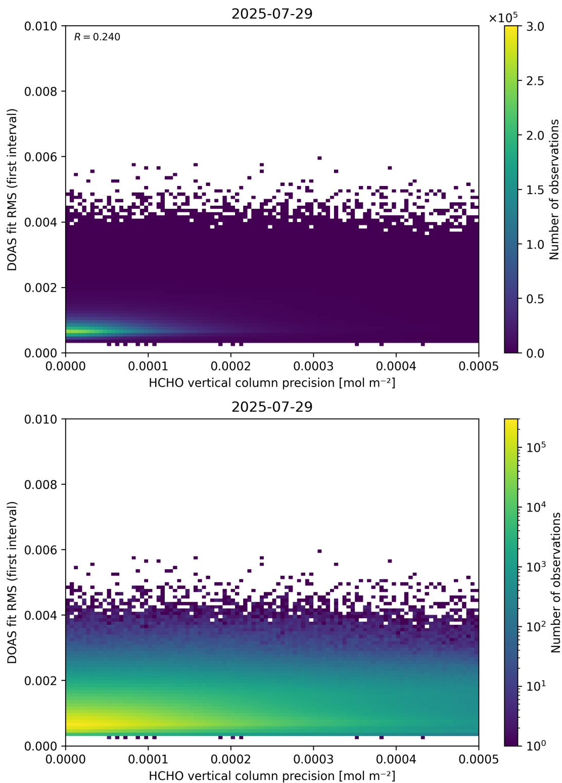
Figure 136: Scatter density plot of “HCHO vertical column precision” against “DOAS fit RMS (first interval)” for 2025-07-29 to 2025-07-30.
