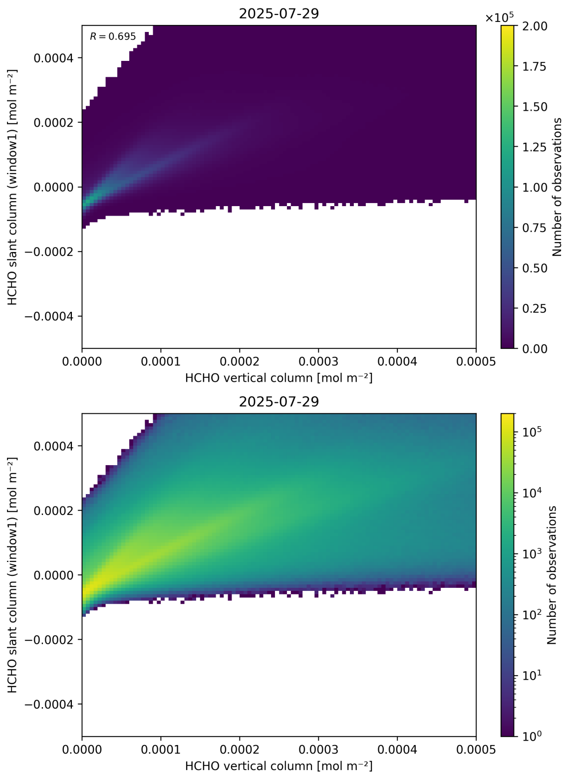
Figure 129: Scatter density plot of “HCHO vertical column” against “HCHO slant column (window1)” for 2025-07-29 to 2025-07-30.
