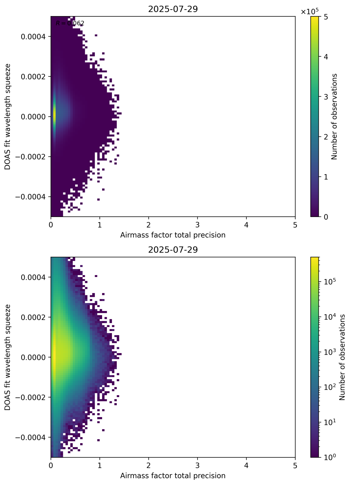
Figure 107: Scatter density plot of “Airmass factor total precision” against “DOAS fit wavelength squeeze” for 2025-07-29 to 2025-07-30.
