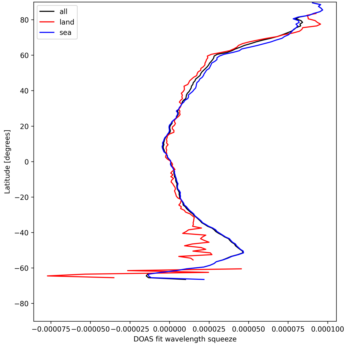
Figure 31: Zonal average of “DOAS fit wavelength squeeze” for 2025-07-29 to 2025-07-30.
