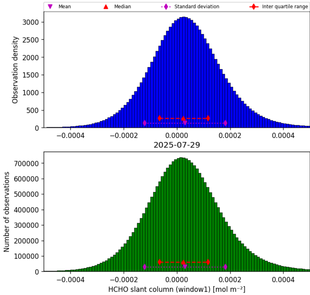
Figure 38: Histogram of “HCHO slant column (window1)” for 2025-07-29 to 2025-07-30
