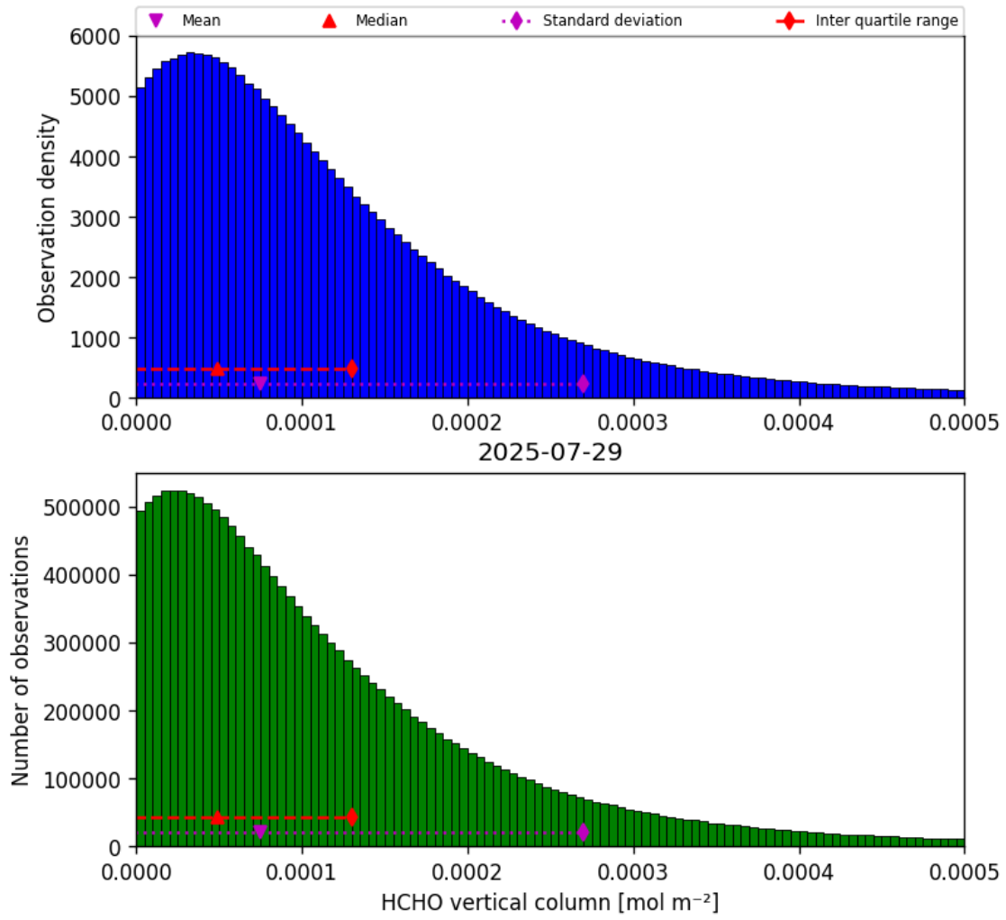
Figure 35: Histogram of “HCHO vertical column” for 2025-07-29 to 2025-07-30
