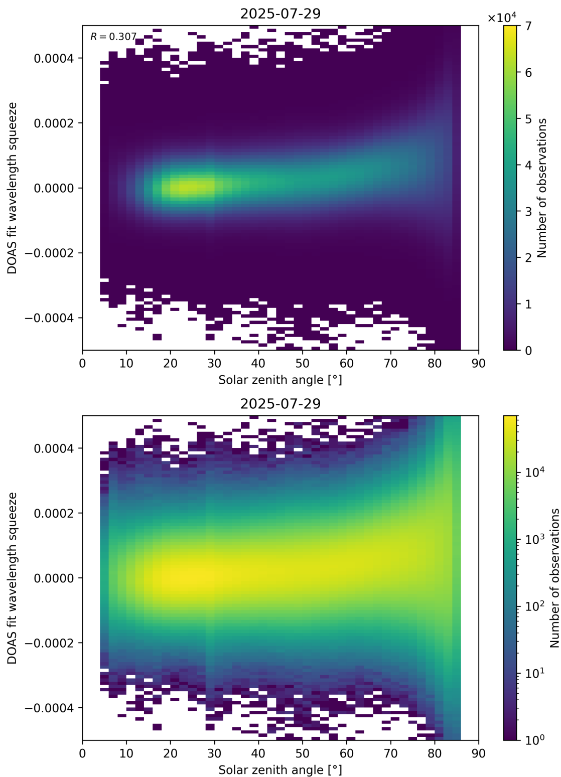
Figure 169: Scatter density plot of “Solar zenith angle” against “DOAS fit wavelength squeeze” for 2025-07-29 to 2025-07-30.
