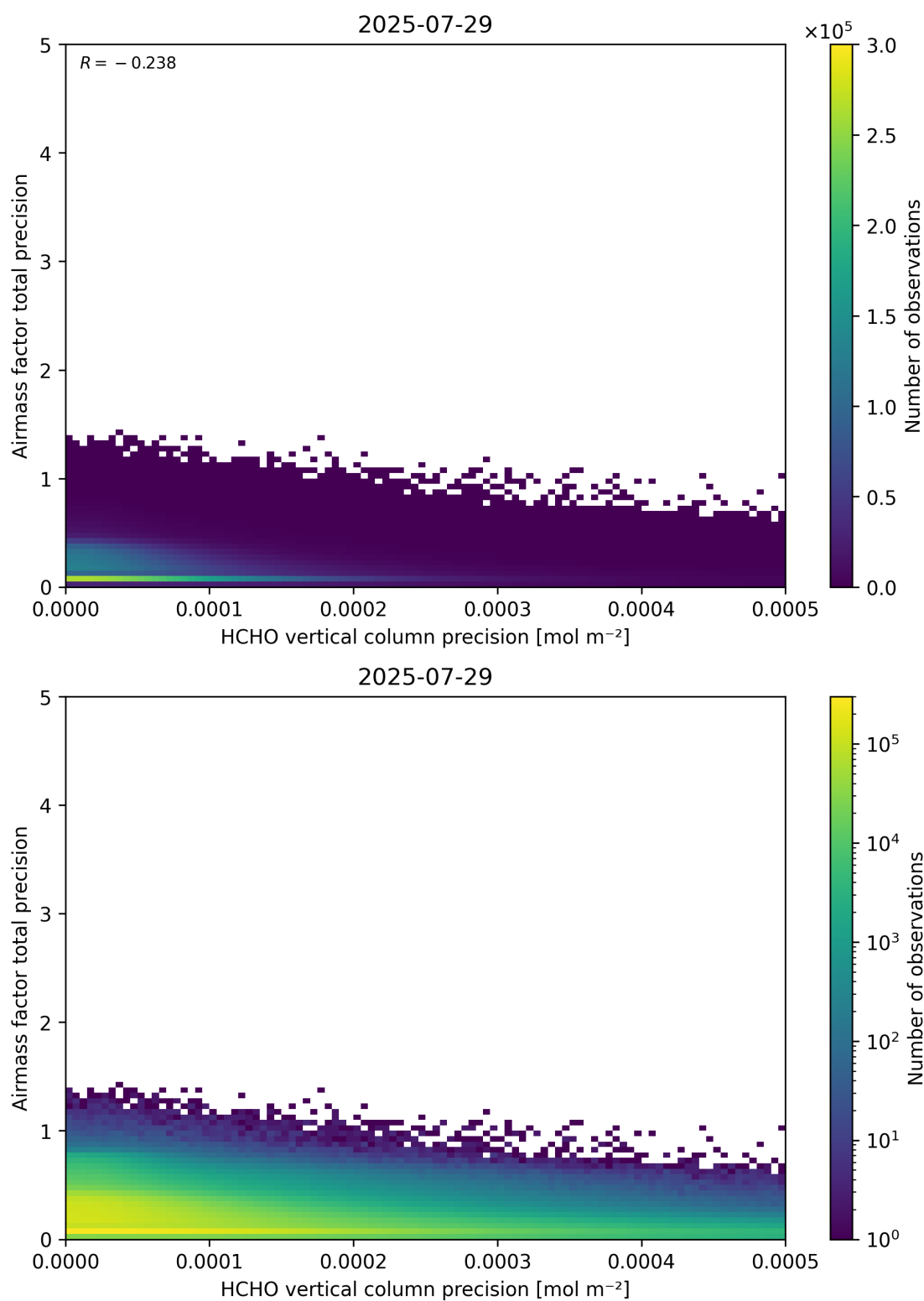
Figure 145: Scatter density plot of “HCHO vertical column precision” against “Airmass factor total precision” for 2025-07-29 to 2025-07-30.
