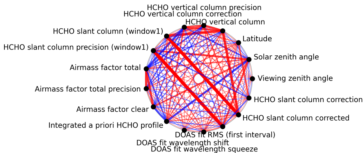
Figure 1: Map of correlation graph for 2025-07-29 to 2025-07-30.
