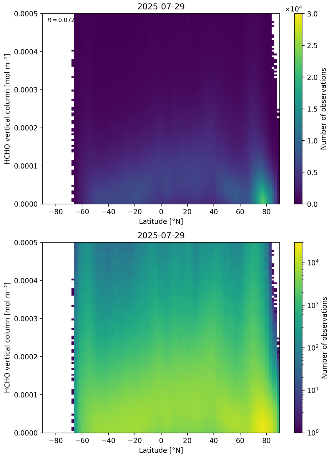
Figure 163: Scatter density plot of “Latitude” against “HCHO vertical column” for 2025-07-29 to 2025-07-30.
