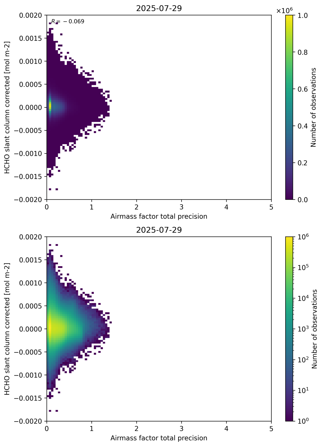
Figure 109: Scatter density plot of “Airmass factor total precision” against “HCHO slant column corrected” for 2025-07-29 to 2025-07-30.
