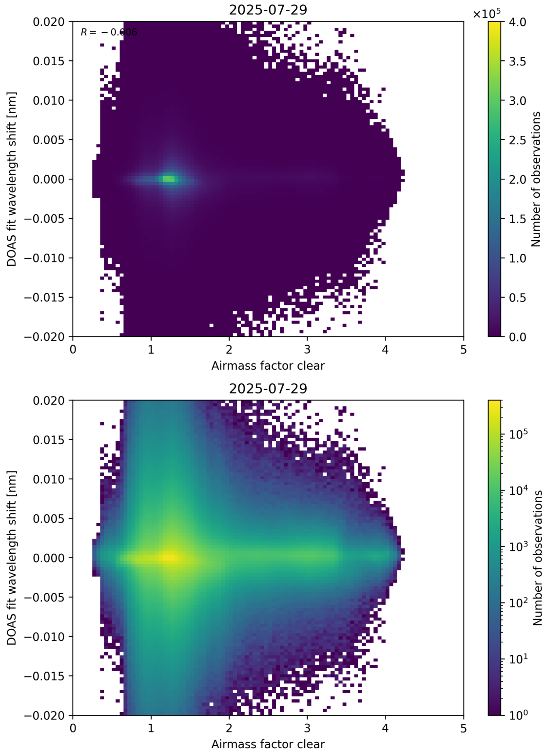
Figure 72: Scatter density plot of “Airmass factor clear” against “DOAS fit wavelength shift” for 2025-07-29 to 2025-07-30.
