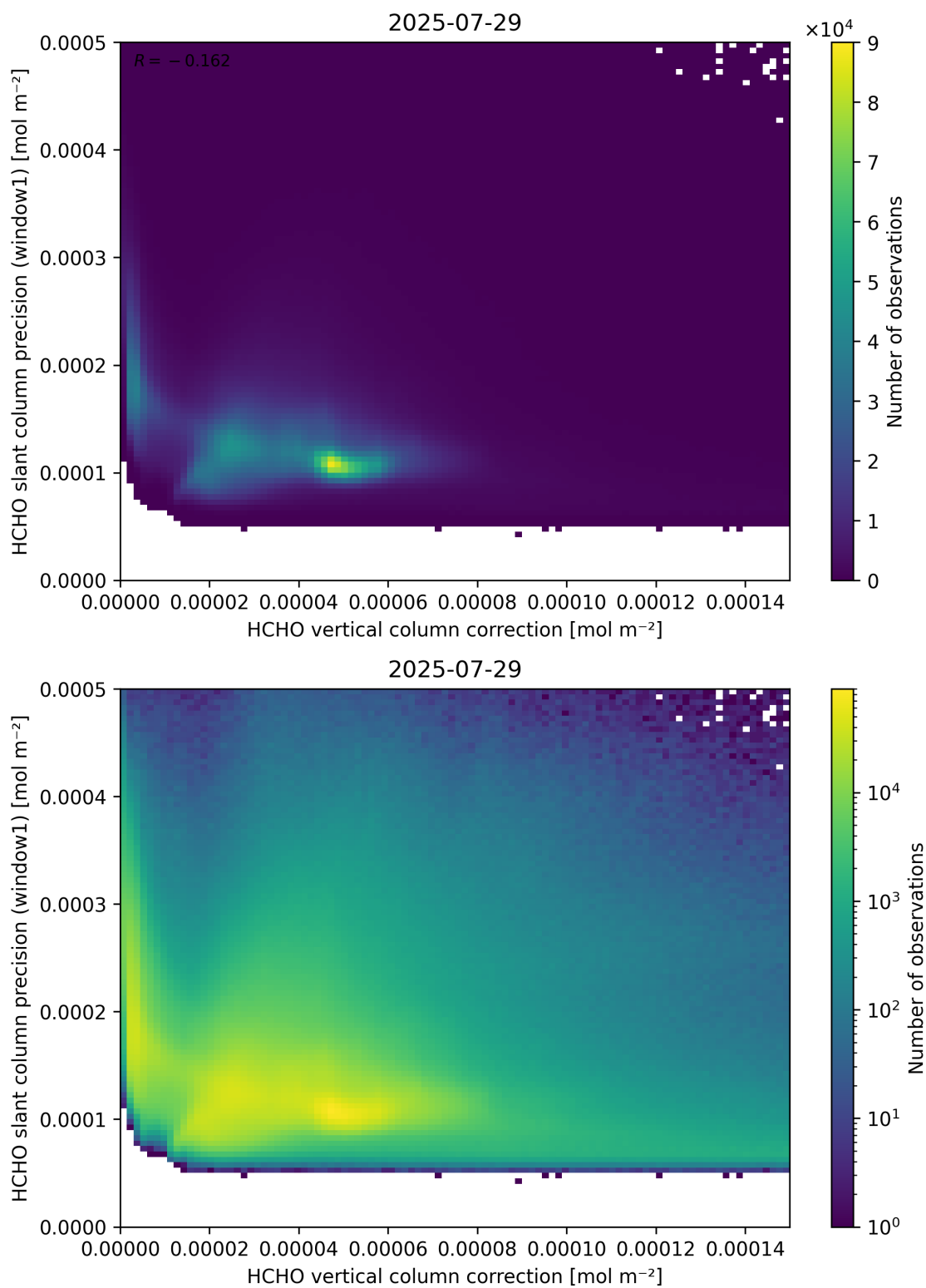
Figure 119: Scatter density plot of “HCHO vertical column correction” against “HCHO slant column precision (window1)” for 2025-07-29 to 2025-07-30.
