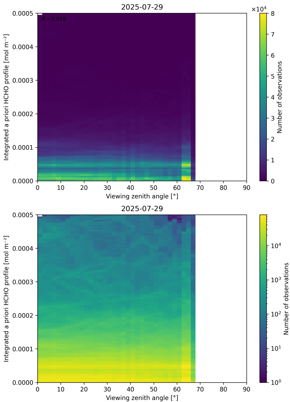
Figure 195: Scatter density plot of “Viewing zenith angle” against “Integrated a priori HCHO profile” for 2025-07-29 to 2025-07-30.
