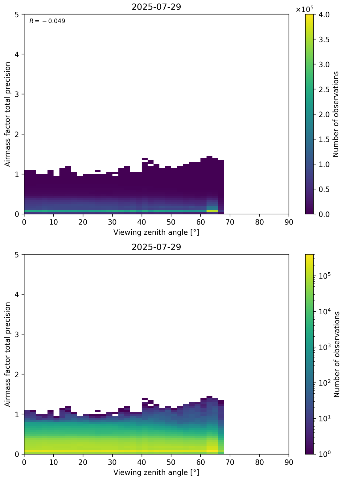
Figure 191: Scatter density plot of “Viewing zenith angle” against “Airmass factor total precision” for 2025-07-29 to 2025-07-30.
