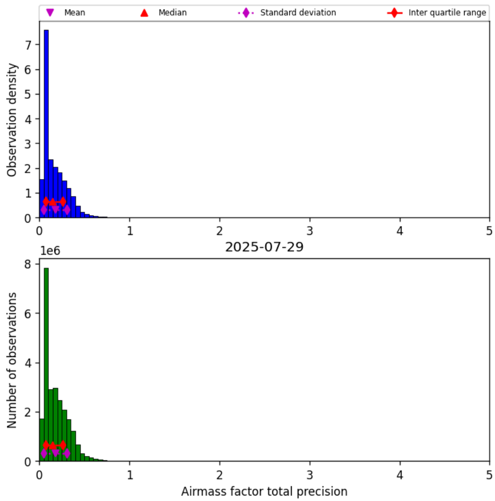
Figure 41: Histogram of “Airmass factor total precision” for 2025-07-29 to 2025-07-30
