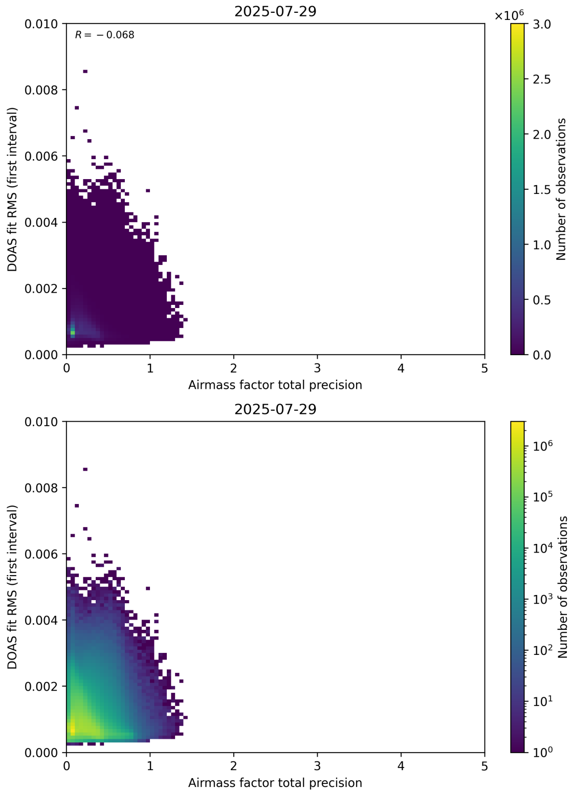
Figure 105: Scatter density plot of “Airmass factor total precision” against “DOAS fit RMS (first interval)” for 2025-07-29 to 2025-07-30.
