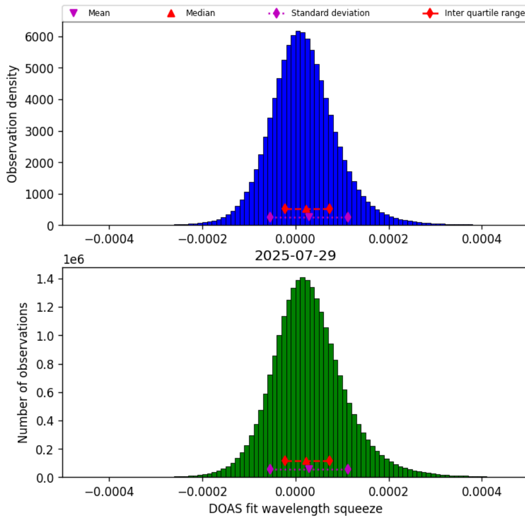
Figure 45: Histogram of “DOAS fit wavelength squeeze” for 2025-07-29 to 2025-07-30
