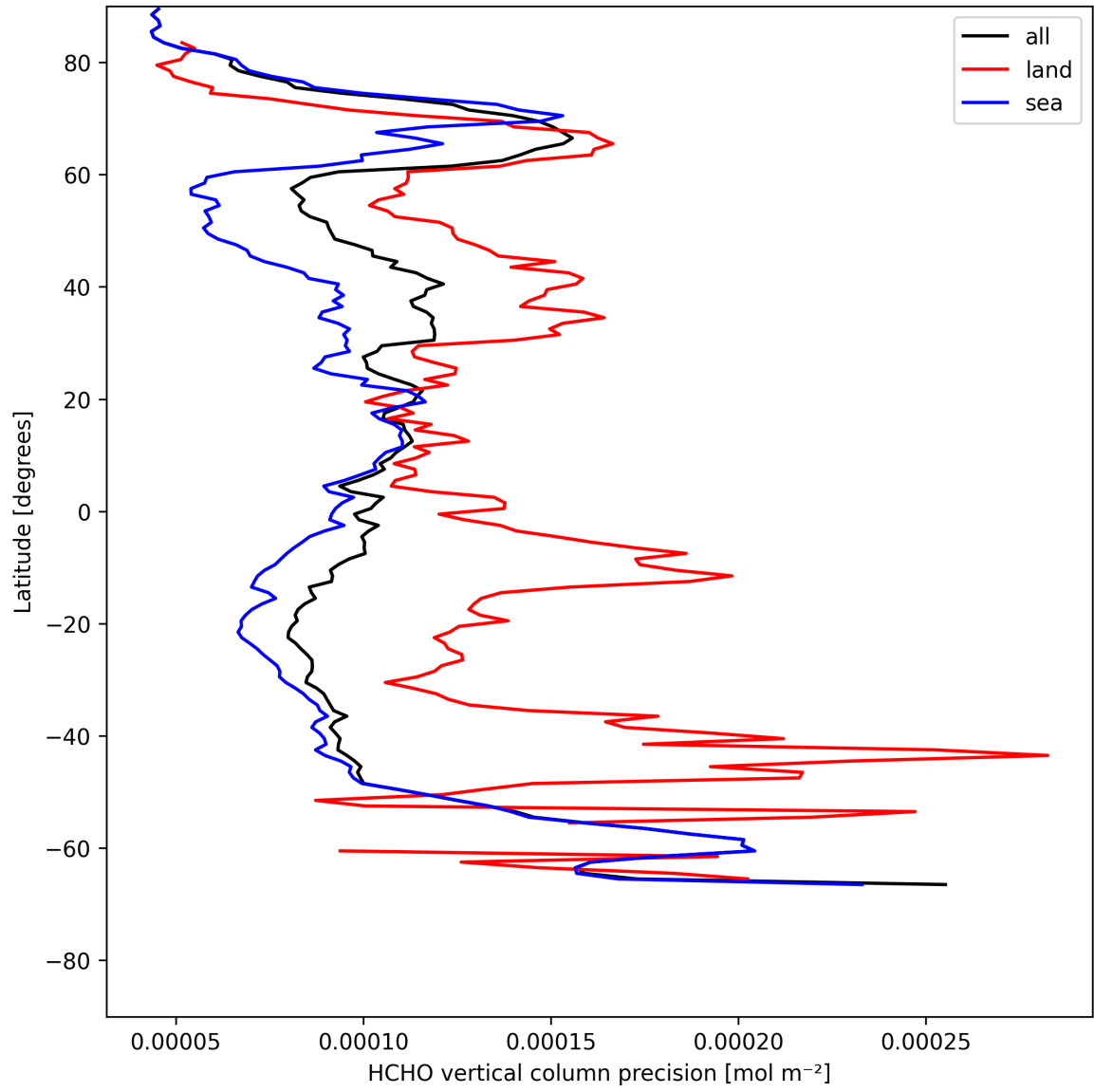
Figure 22: Zonal average of “HCHO vertical column precision” for 2025-07-29 to 2025-07-30.
