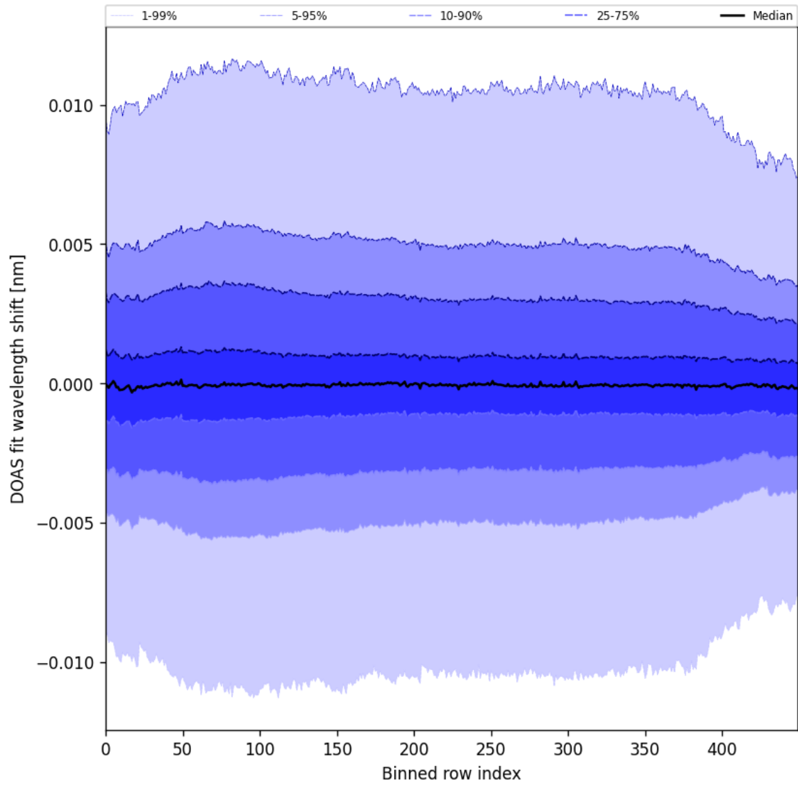
Figure 58: Along track statistics of “DOAS fit wavelength shift” for 2025-07-29 to 2025-07-30
