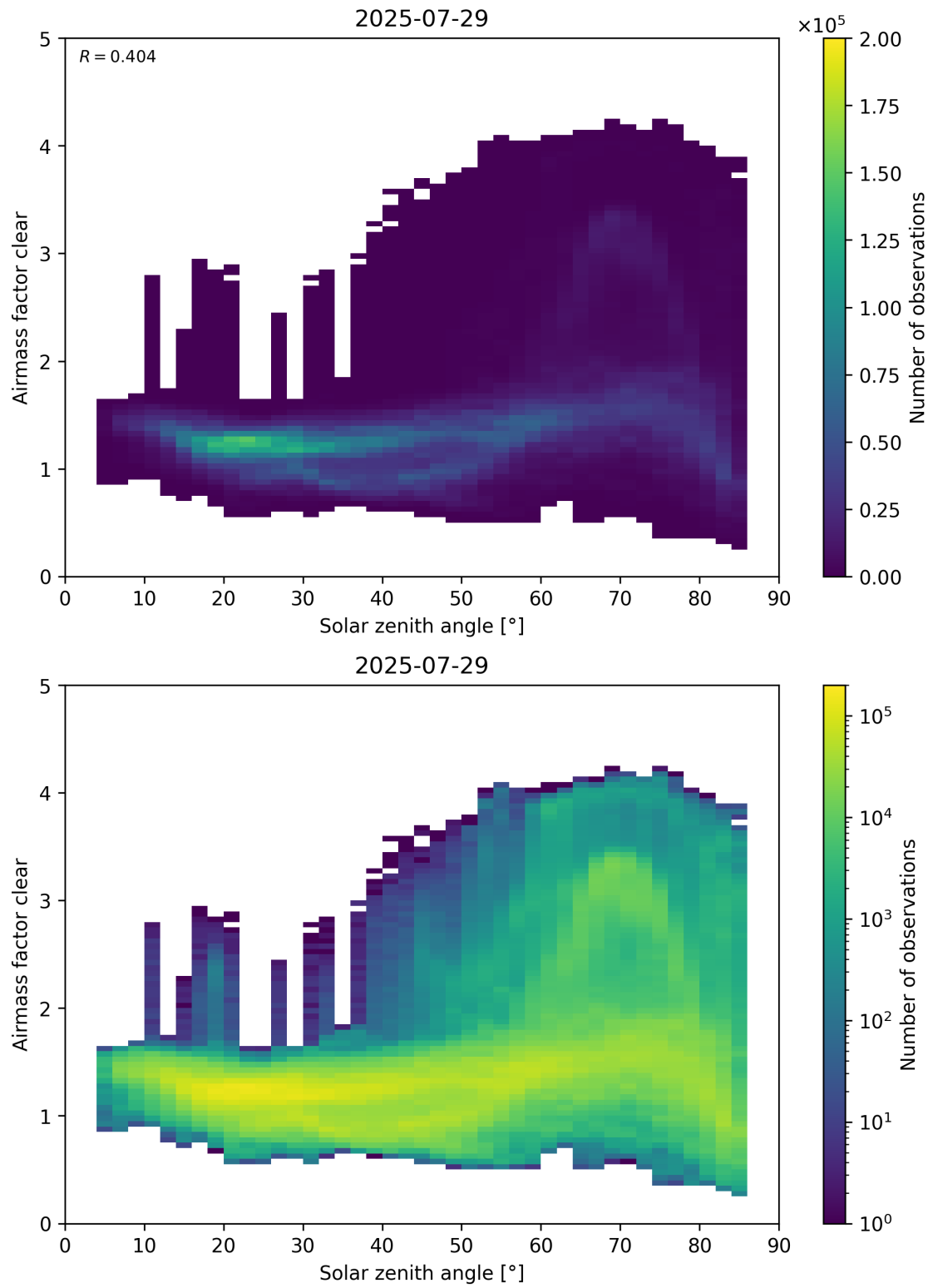
Figure 170: Scatter density plot of “Solar zenith angle” against “Airmass factor clear” for 2025-07-29 to 2025-07-30.
