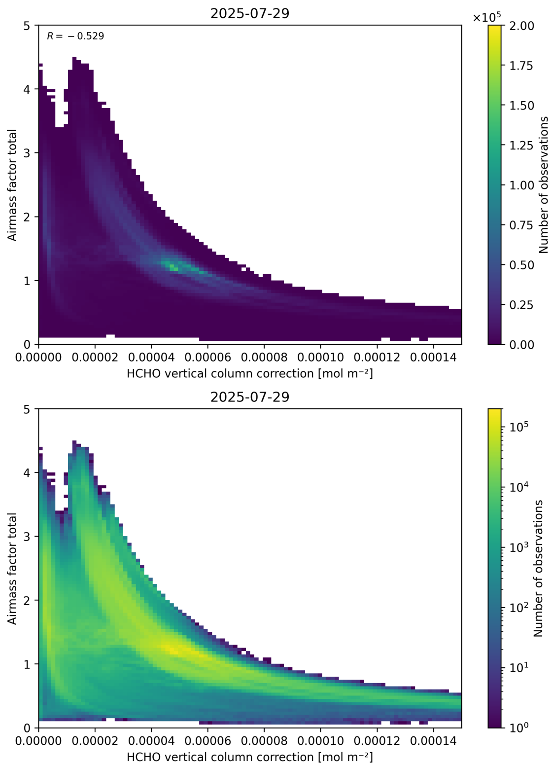
Figure 120: Scatter density plot of “HCHO vertical column correction” against “Airmass factor total” for 2025-07-29 to 2025-07-30.
