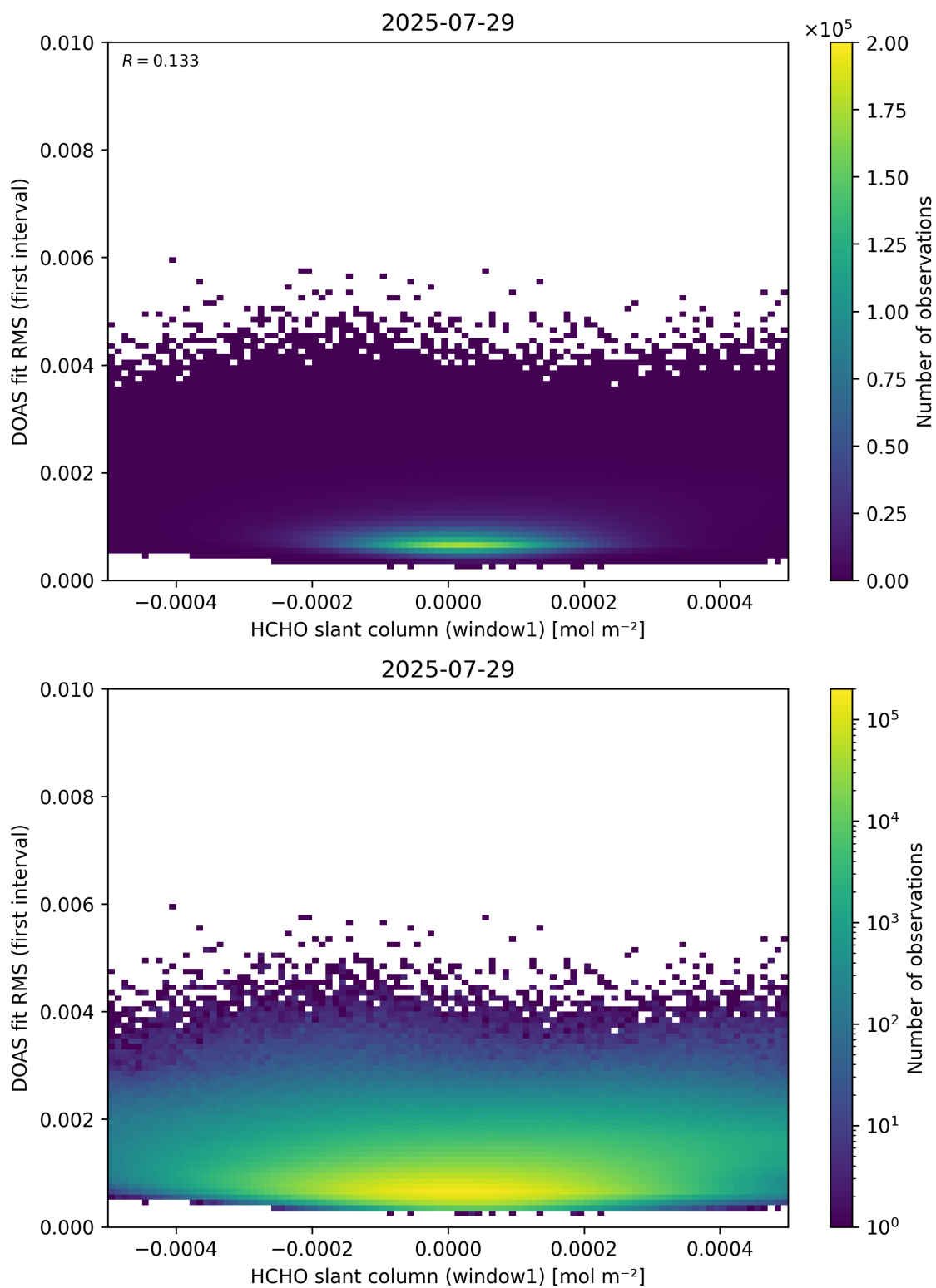
Figure 78: Scatter density plot of “HCHO slant column (window1)” against “DOAS fit RMS (first interval)” for 2025-07-29 to 2025-07-30.
