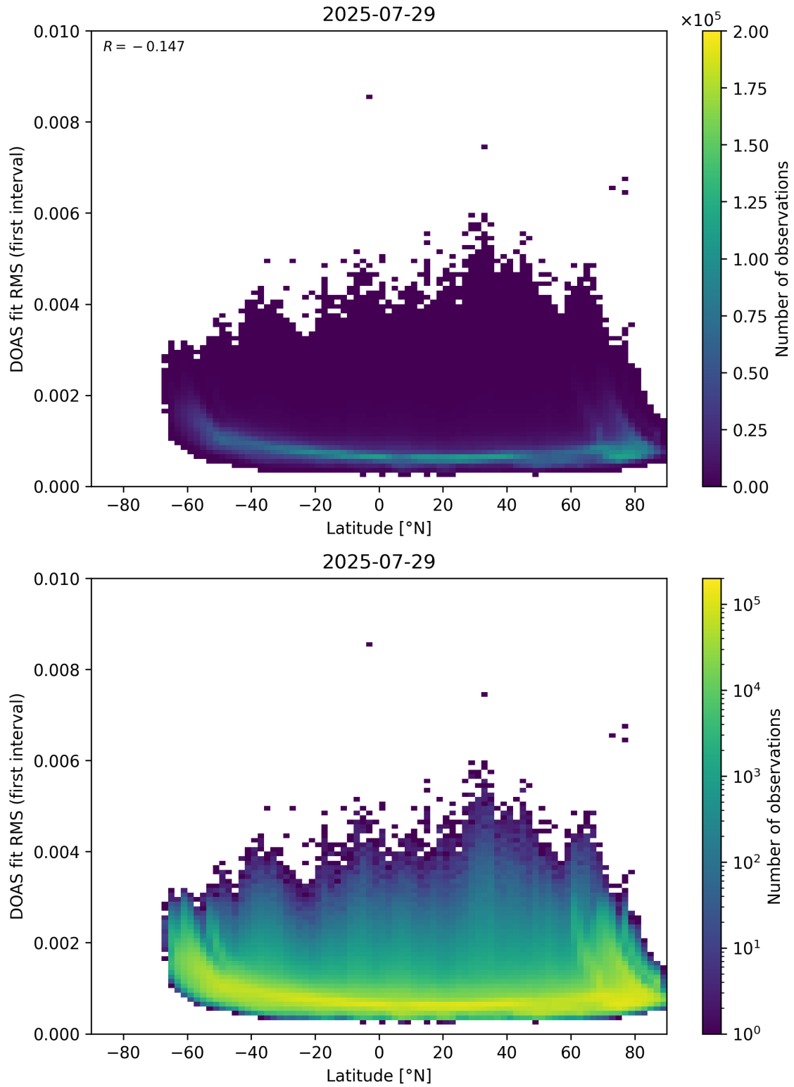
Figure 153: Scatter density plot of “Latitude” against “DOAS fit RMS (first interval)” for 2025-07-29 to 2025-07-30.
