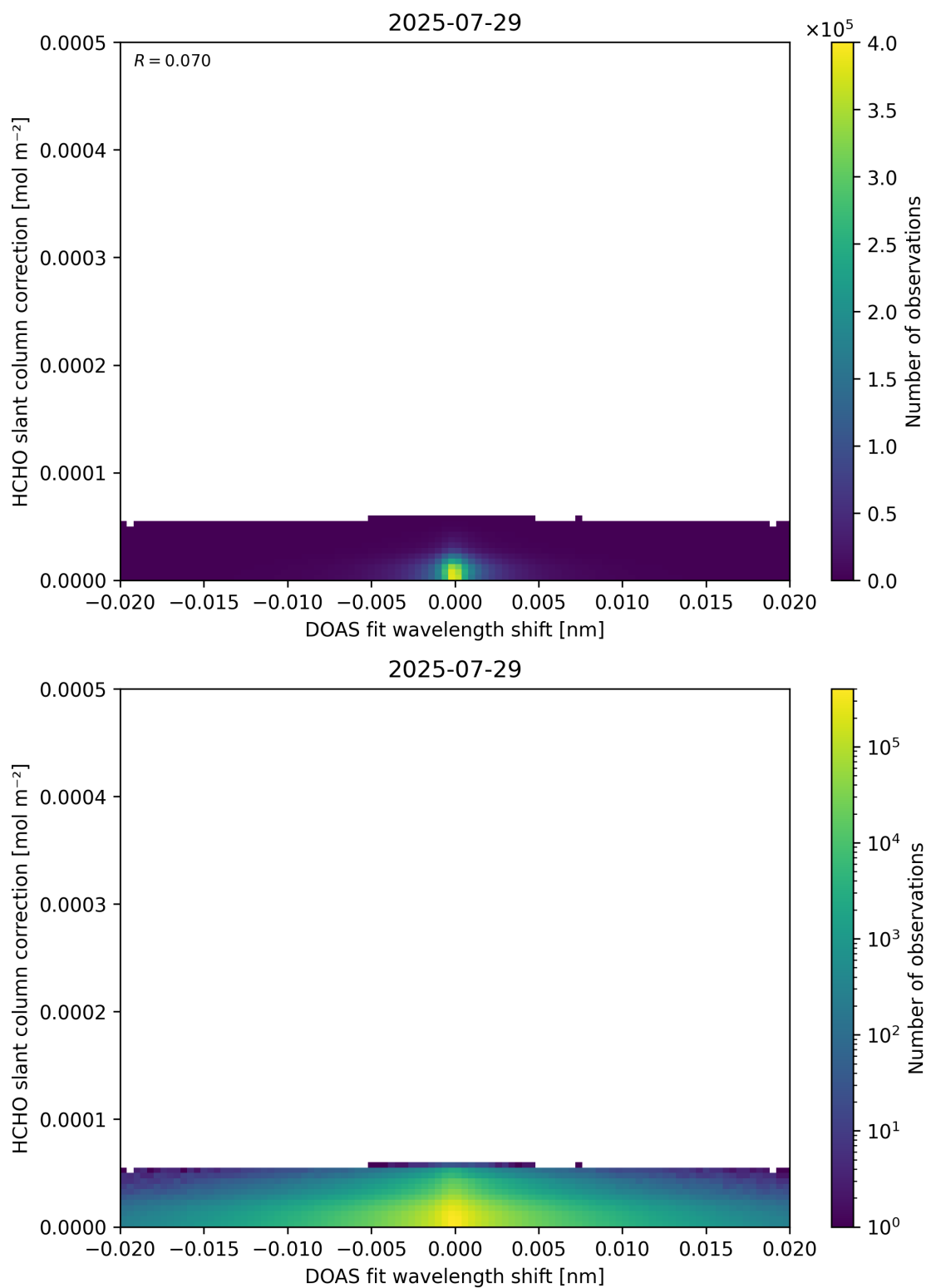
Figure 67: Scatter density plot of “DOAS fit wavelength shift” against “HCHO slant column correction” for 2025-07-29 to 2025-07-30.
