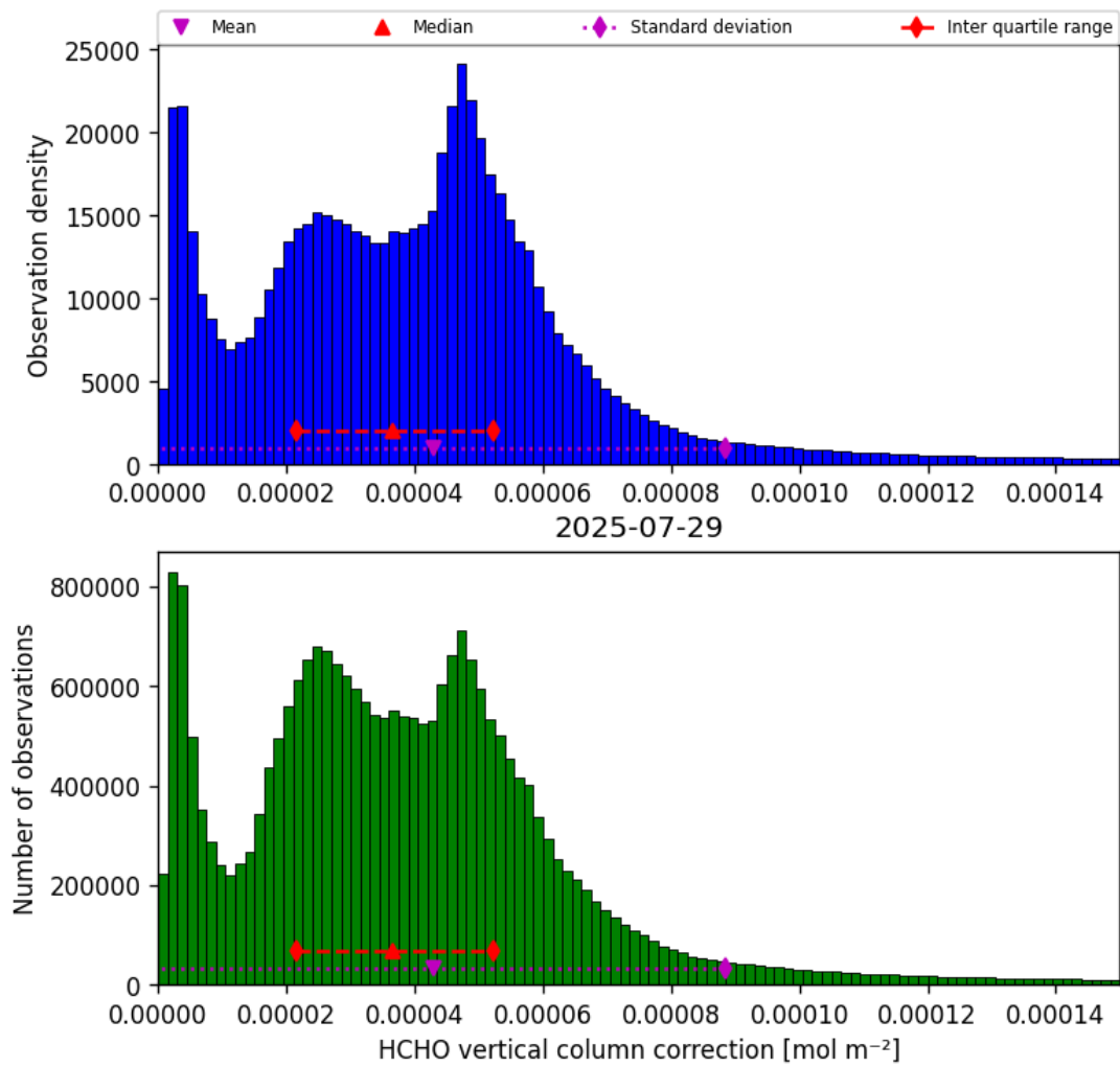
Figure 37: Histogram of “HCHO vertical column correction” for 2025-07-29 to 2025-07-30
