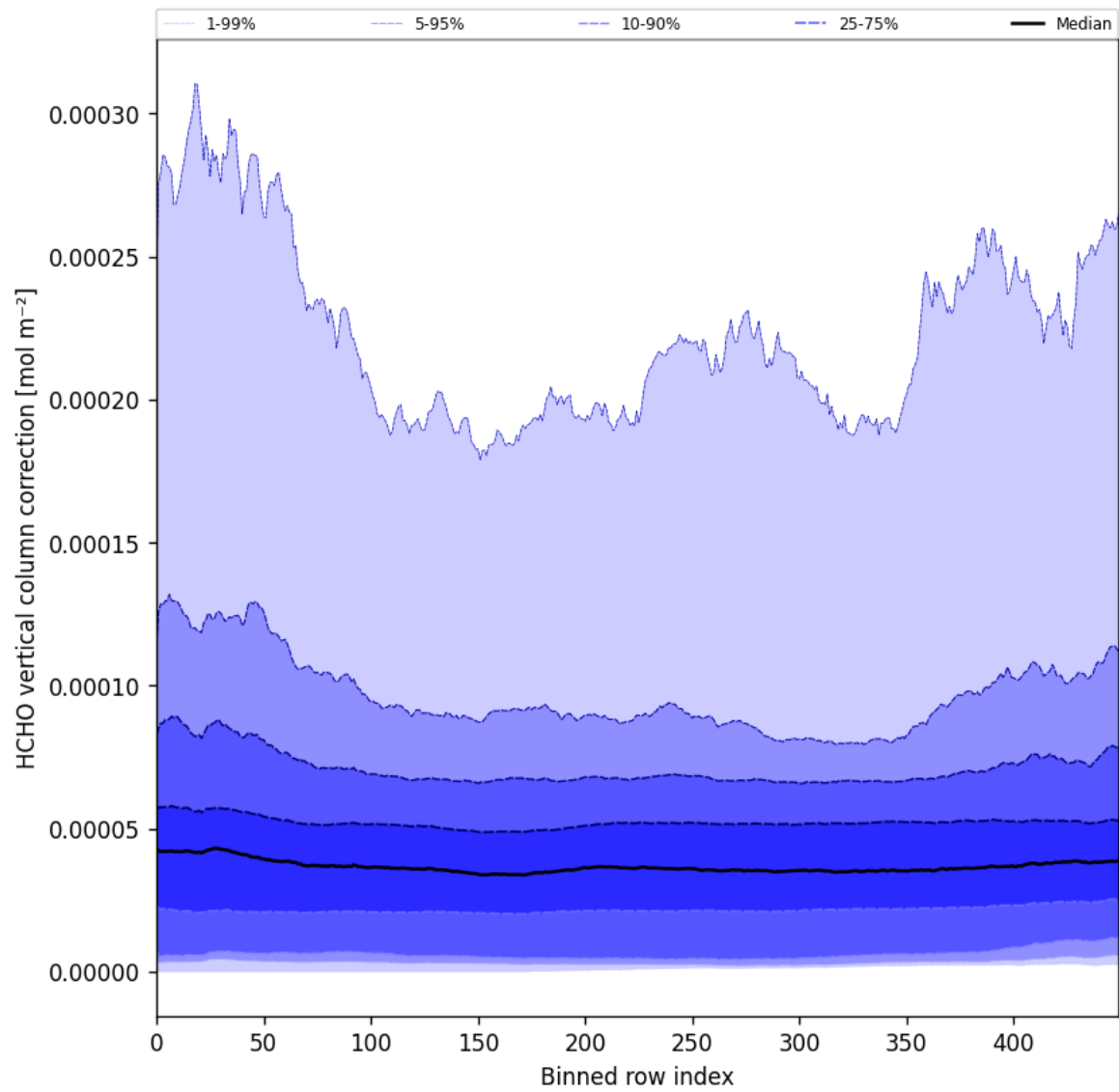
Figure 51: Along track statistics of “HCHO vertical column correction” for 2025-07-29 to 2025-07-30
