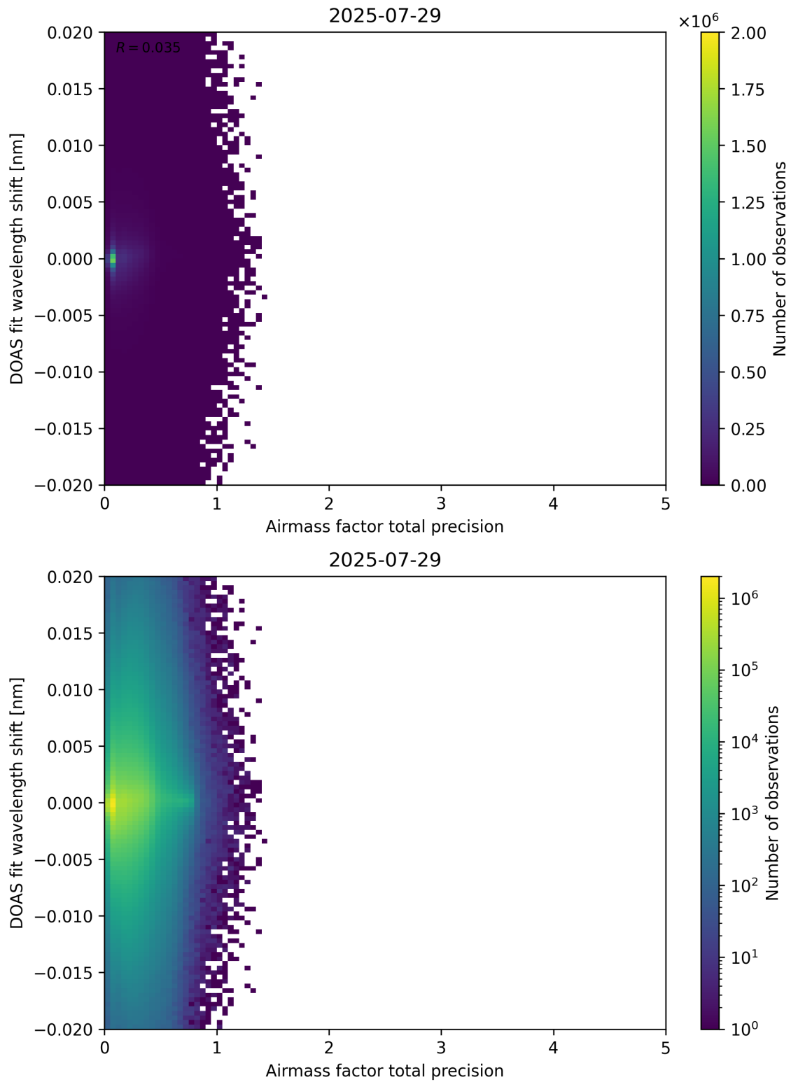
Figure 106: Scatter density plot of “Airmass factor total precision” against “DOAS fit wavelength shift” for 2025-07-29 to 2025-07-30.
