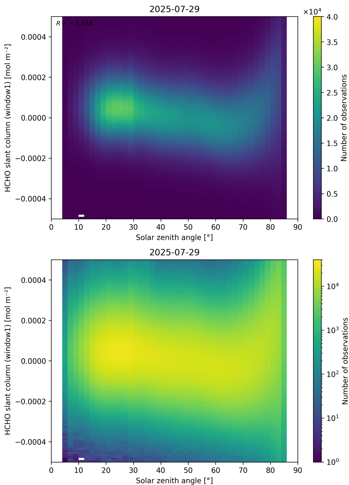
Figure 173: Scatter density plot of “Solar zenith angle” against “HCHO slant column (window1)” for 2025-07-29 to 2025-07-30.
