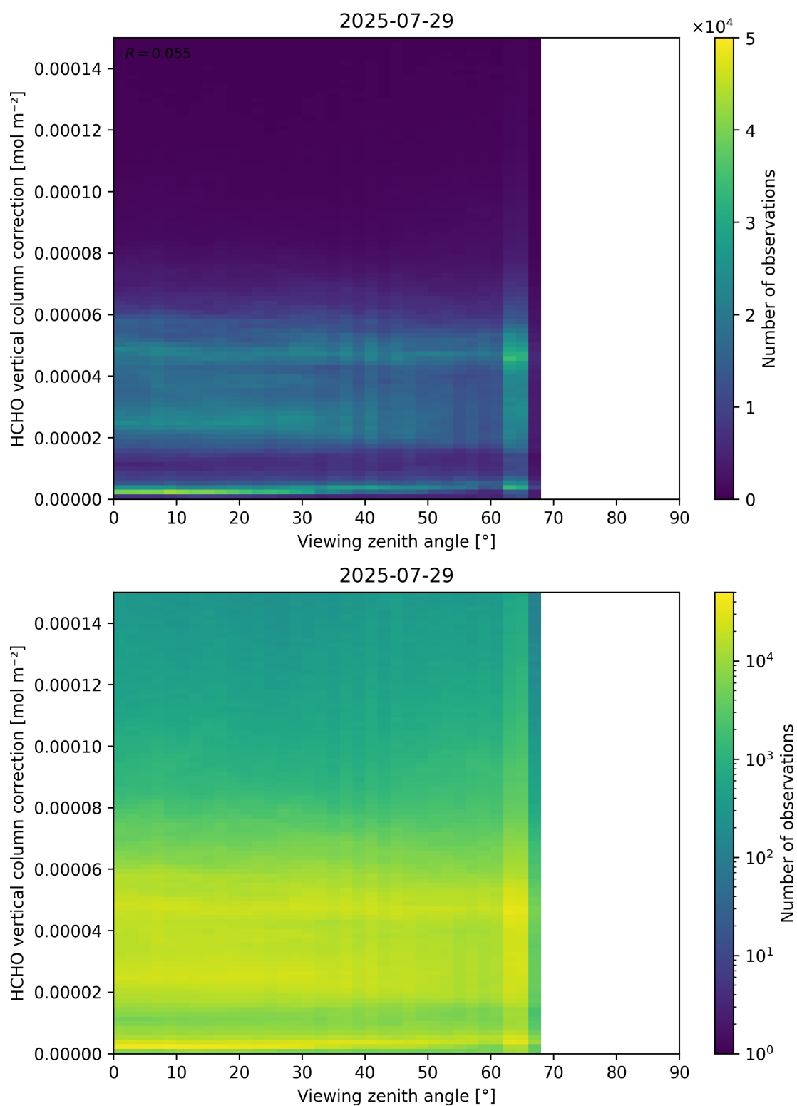
Figure 193: Scatter density plot of “Viewing zenith angle” against “HCHO vertical column correction” for 2025-07-29 to 2025-07-30.
