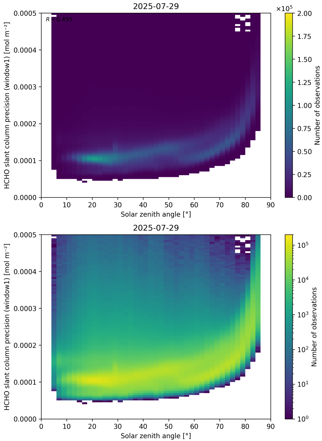
Figure 174: Scatter density plot of “Solar zenith angle” against “HCHO slant column precision (window1)” for 2025-07-29 to 2025-07-30.
