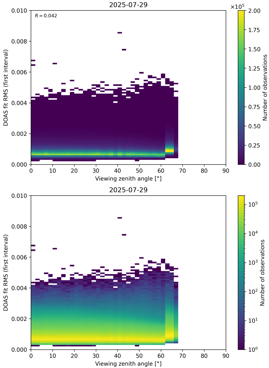
Figure 182: Scatter density plot of “Viewing zenith angle” against “DOAS fit RMS (first interval)” for 2025-07-29 to 2025-07-30.
