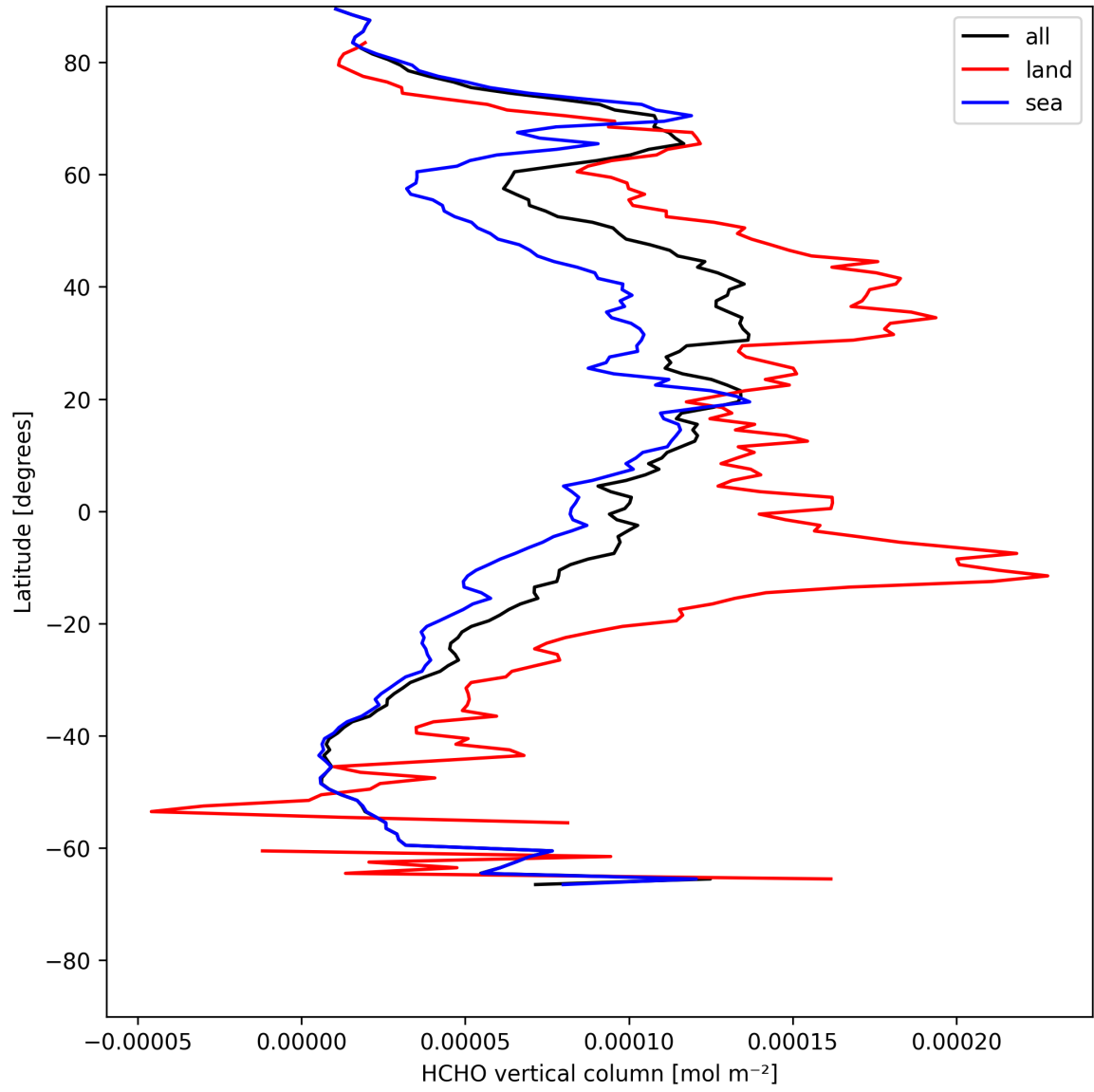
Figure 21: Zonal average of “HCHO vertical column” for 2025-07-29 to 2025-07-30.
