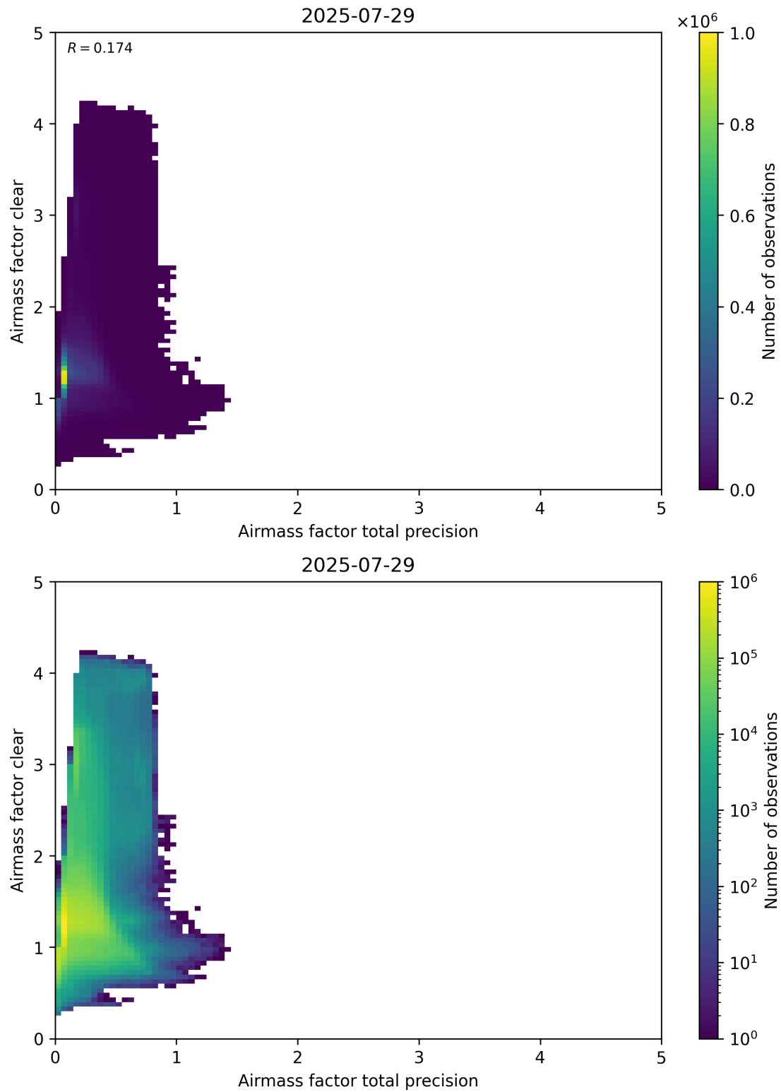
Figure 108: Scatter density plot of “Airmass factor total precision” against “Airmass factor clear” for 2025-07-29 to 2025-07-30.
