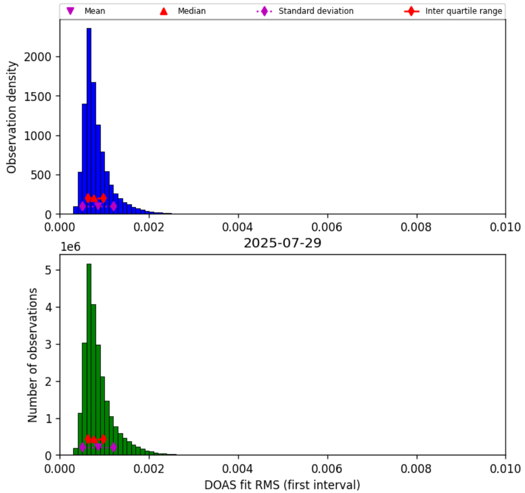
Figure 46: Histogram of “DOAS fit RMS (first interval)” for 2025-07-29 to 2025-07-30
