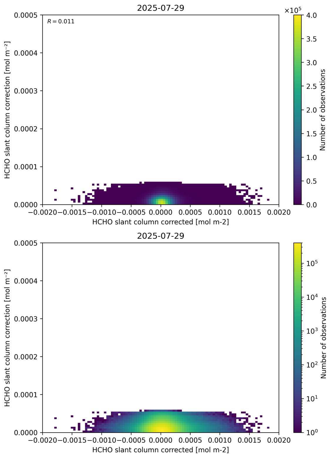
Figure 77: Scatter density plot of “HCHO slant column corrected” against “HCHO slant column correction” for 2025-07-29 to 2025-07-30.
