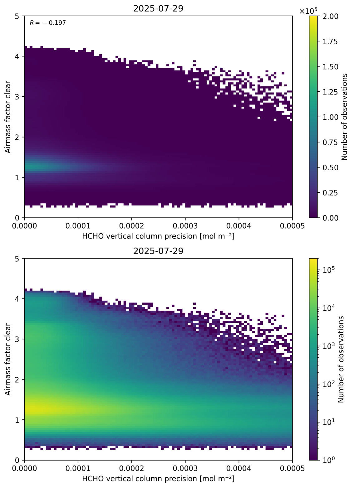
Figure 139: Scatter density plot of “HCHO vertical column precision” against “Airmass factor clear” for 2025-07-29 to 2025-07-30.
