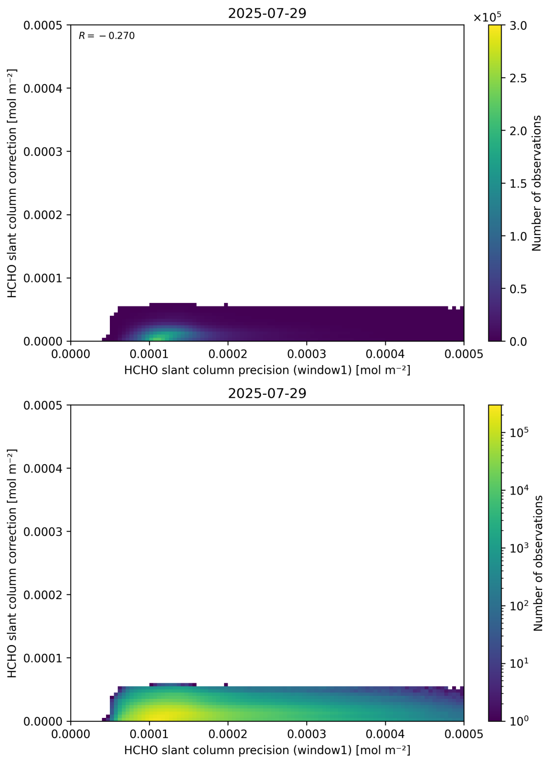
Figure 93: Scatter density plot of “HCHO slant column precision (window1)” against “HCHO slant column correction” for 2025-07-29 to 2025-07-30.
