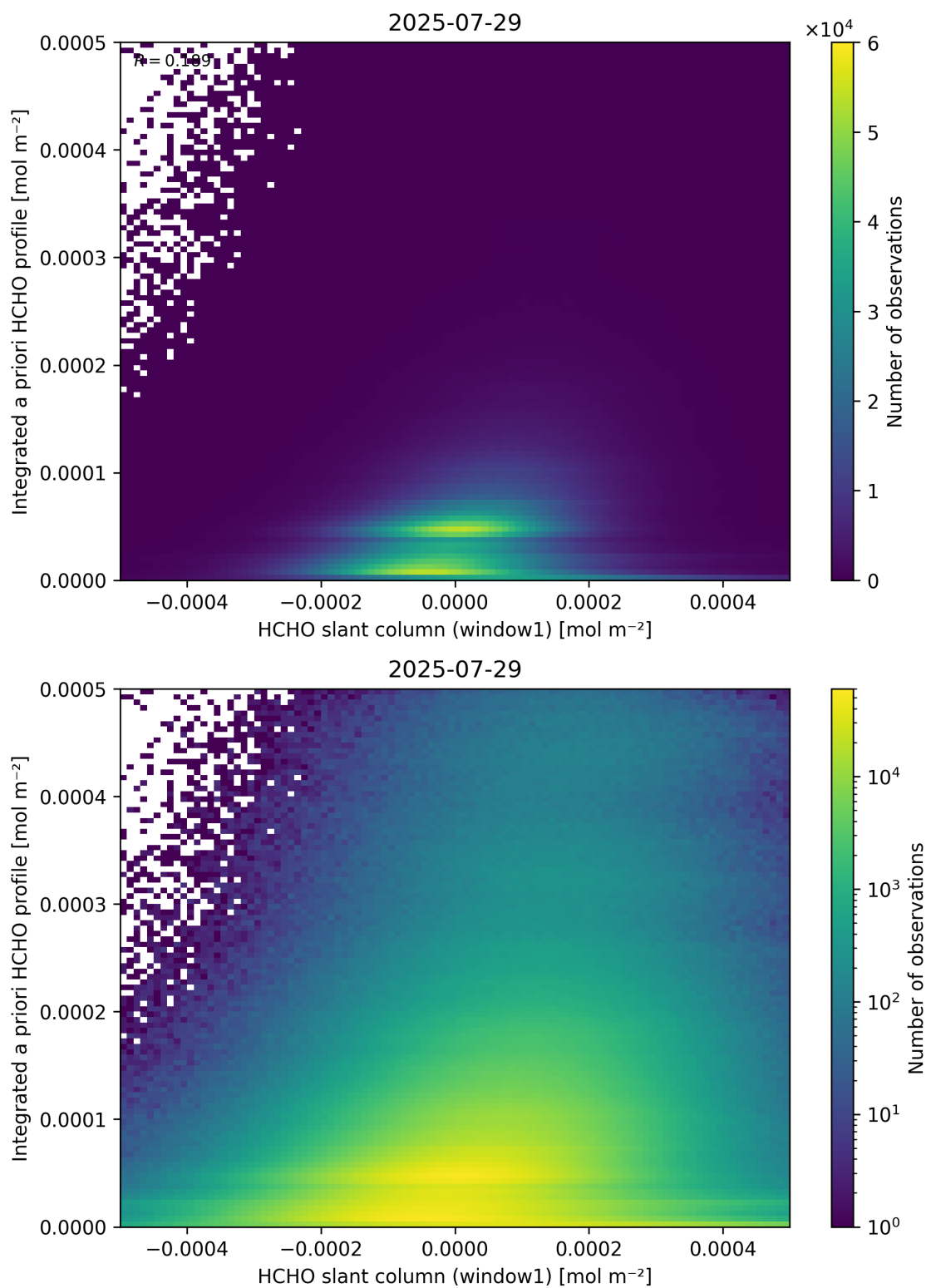
Figure 87: Scatter density plot of “HCHO slant column (window1)” against “Integrated a priori HCHO profile” for 2025-07-29 to 2025-07-30.
