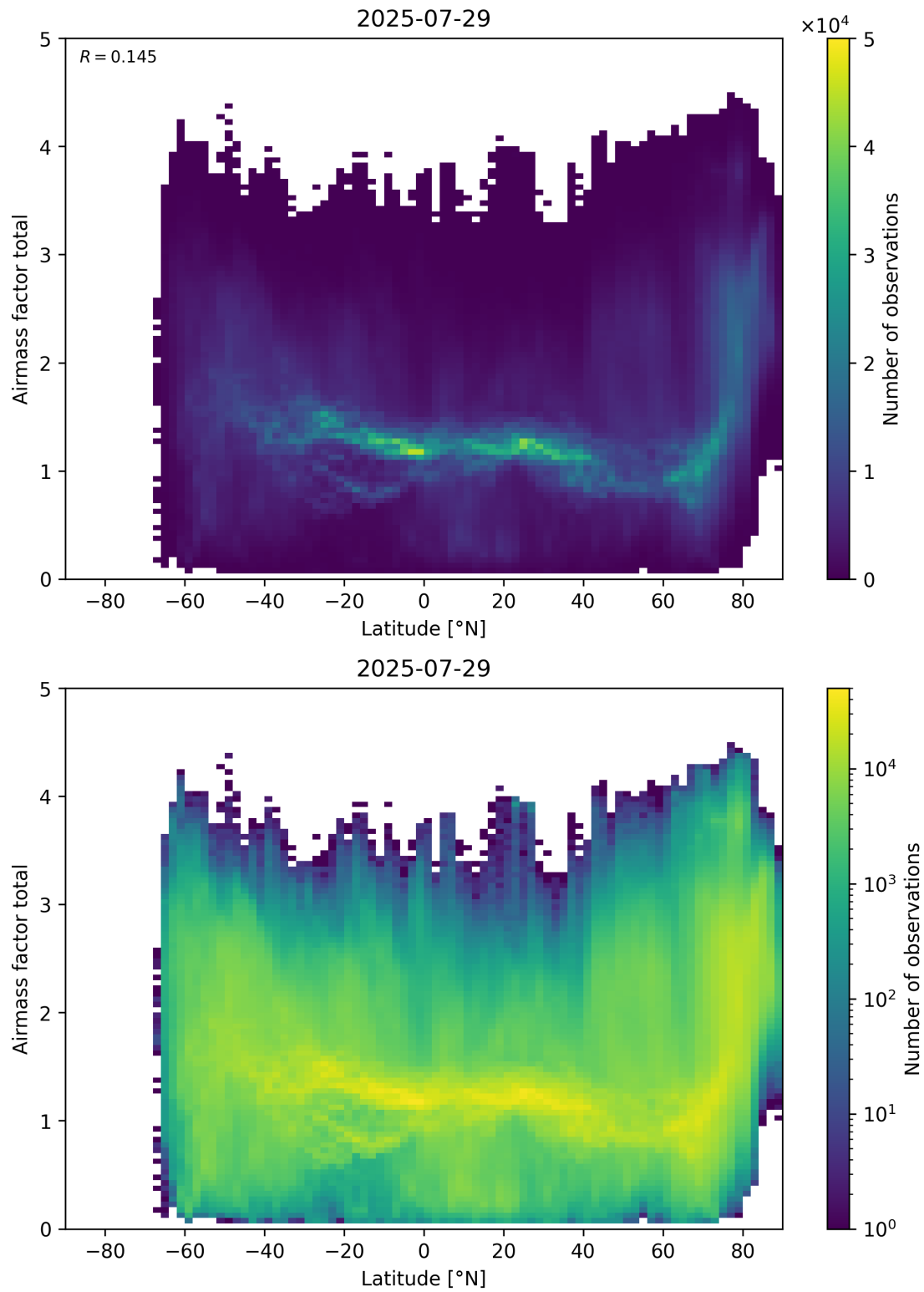
Figure 161: Scatter density plot of “Latitude” against “Airmass factor total” for 2025-07-29 to 2025-07-30.
