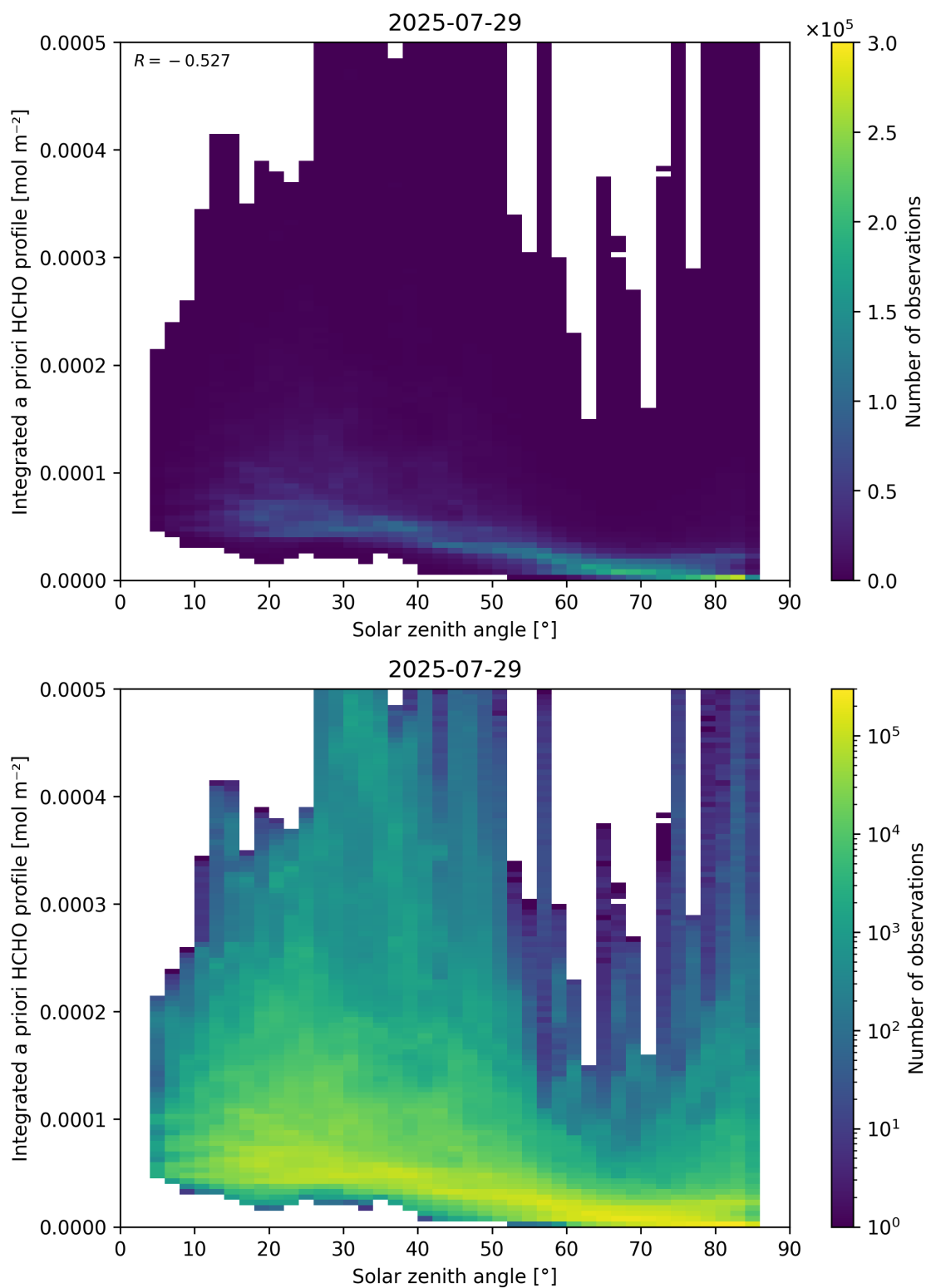
Figure 180: Scatter density plot of “Solar zenith angle” against “Integrated a priori HCHO profile” for 2025-07-29 to 2025-07-30.
