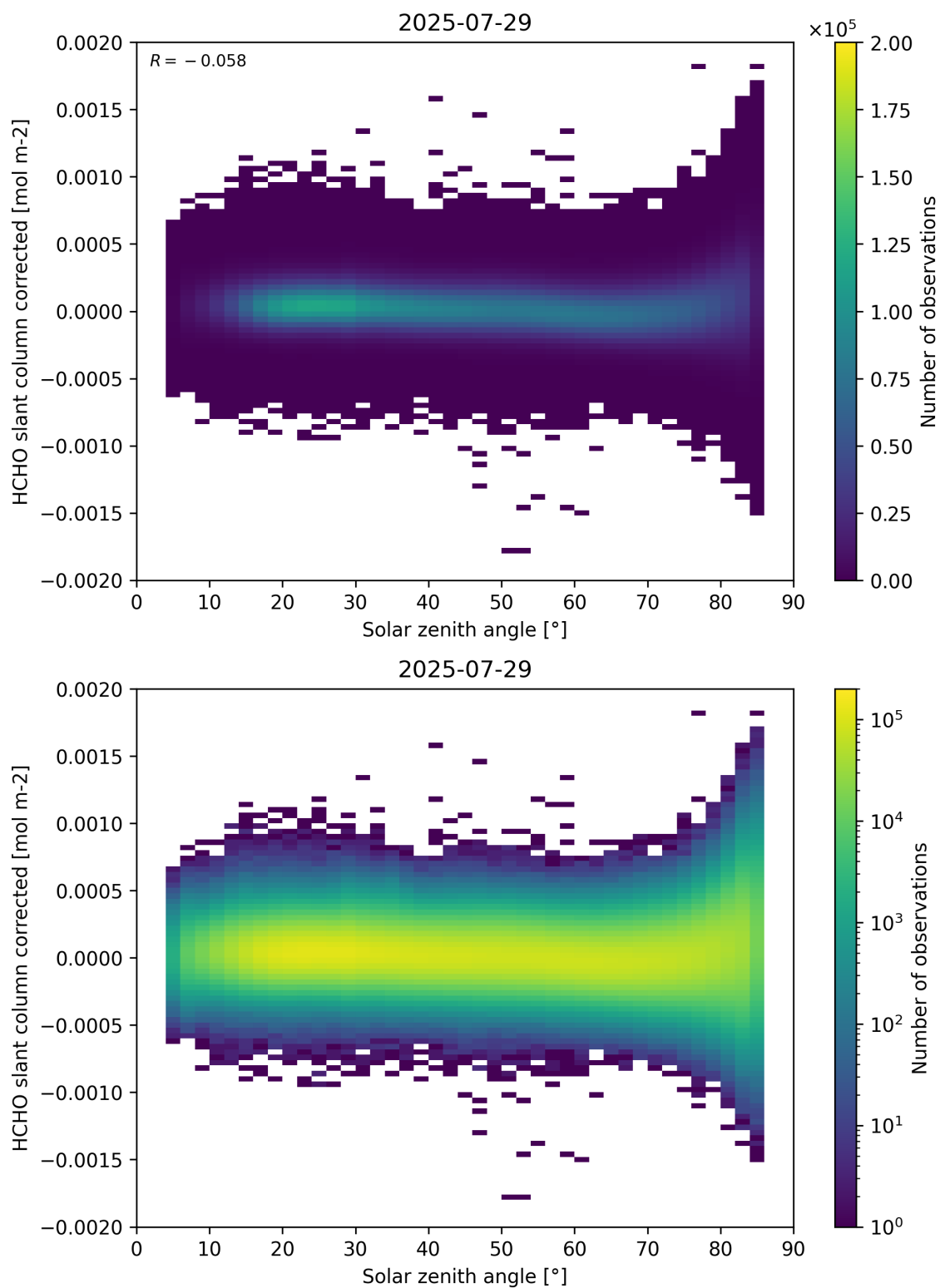
Figure 171: Scatter density plot of “Solar zenith angle” against “HCHO slant column corrected” for 2025-07-29 to 2025-07-30.
