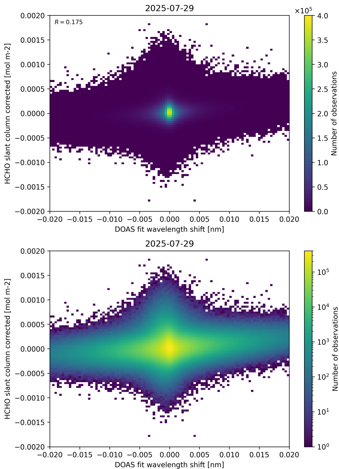
Figure 66: Scatter density plot of “DOAS fit wavelength shift” against “HCHO slant column corrected” for 2025-07-29 to 2025-07-30.
