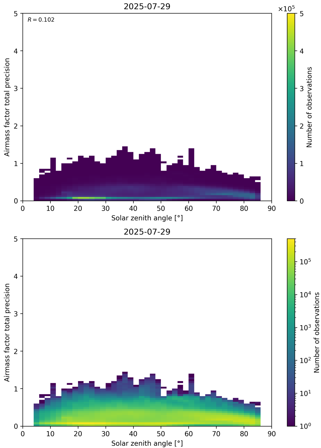
Figure 176: Scatter density plot of “Solar zenith angle” against “Airmass factor total precision” for 2025-07-29 to 2025-07-30.
