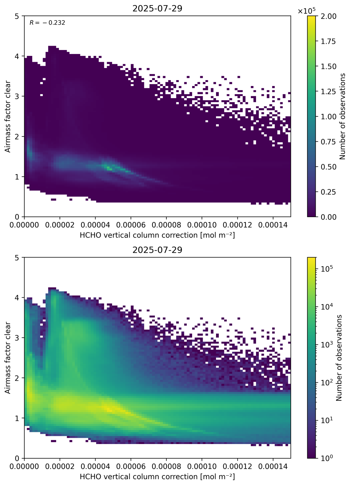
Figure 115: Scatter density plot of “HCHO vertical column correction” against “Airmass factor clear” for 2025-07-29 to 2025-07-30.
