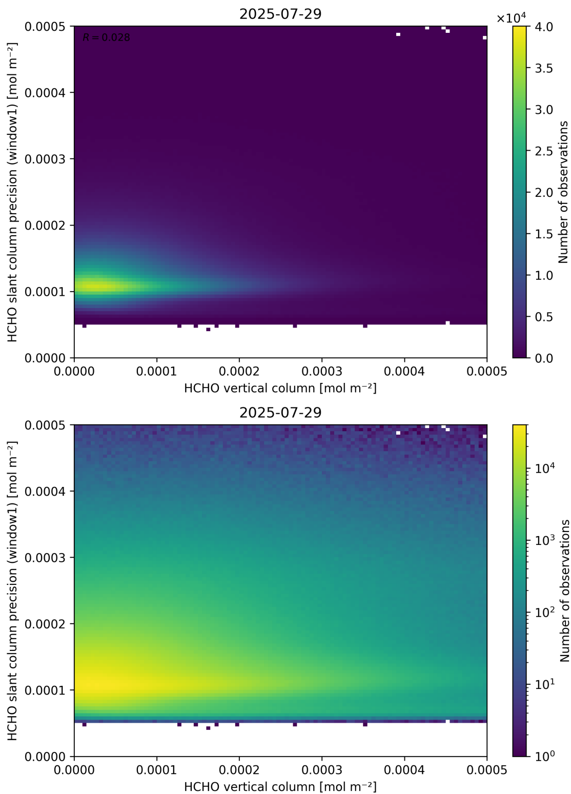
Figure 130: Scatter density plot of “HCHO vertical column” against “HCHO slant column precision (window1)” for 2025-07-29 to 2025-07-30.
