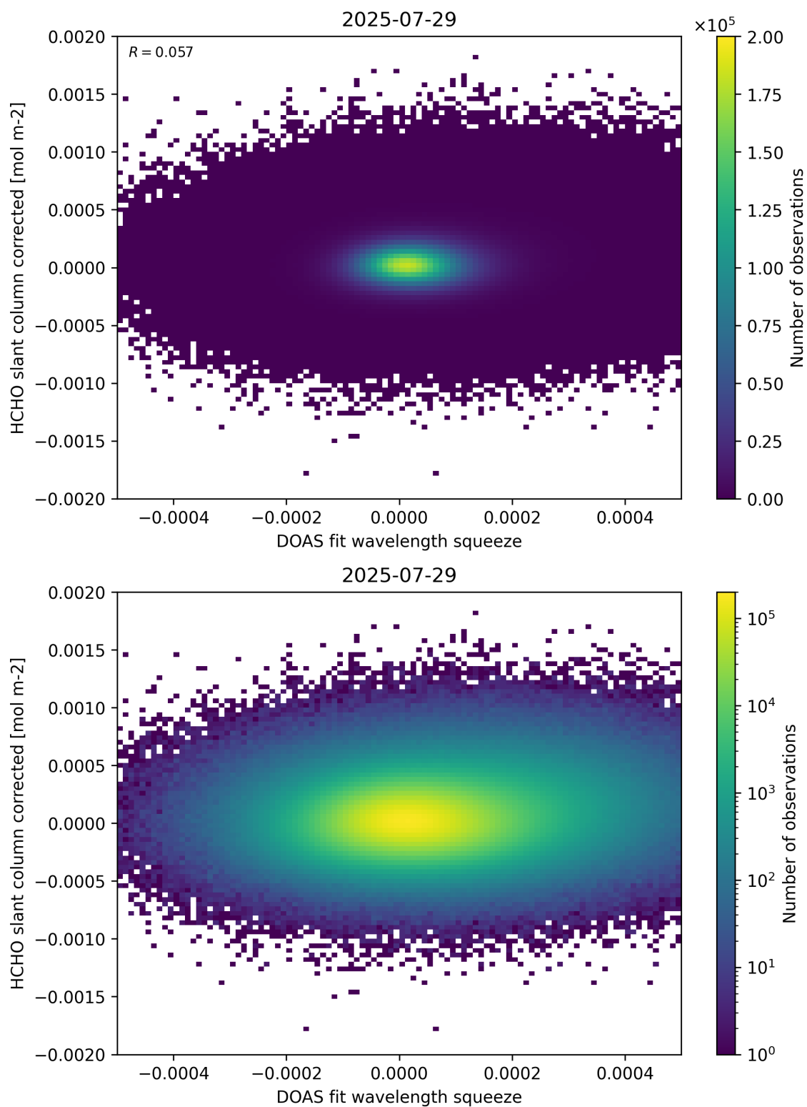
Figure 69: Scatter density plot of “DOAS fit wavelength squeeze” against “HCHO slant column corrected” for 2025-07-29 to 2025-07-30.
