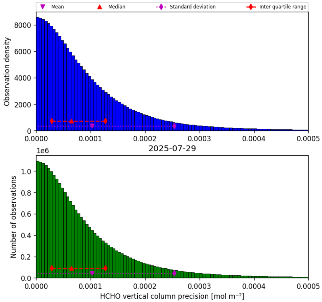
Figure 36: Histogram of “HCHO vertical column precision” for 2025-07-29 to 2025-07-30
