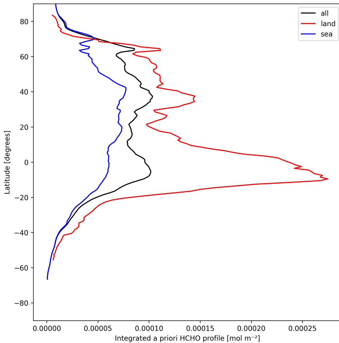
Figure 29: Zonal average of “Integrated a priori HCHO profile” for 2025-07-29 to 2025-07-30.
