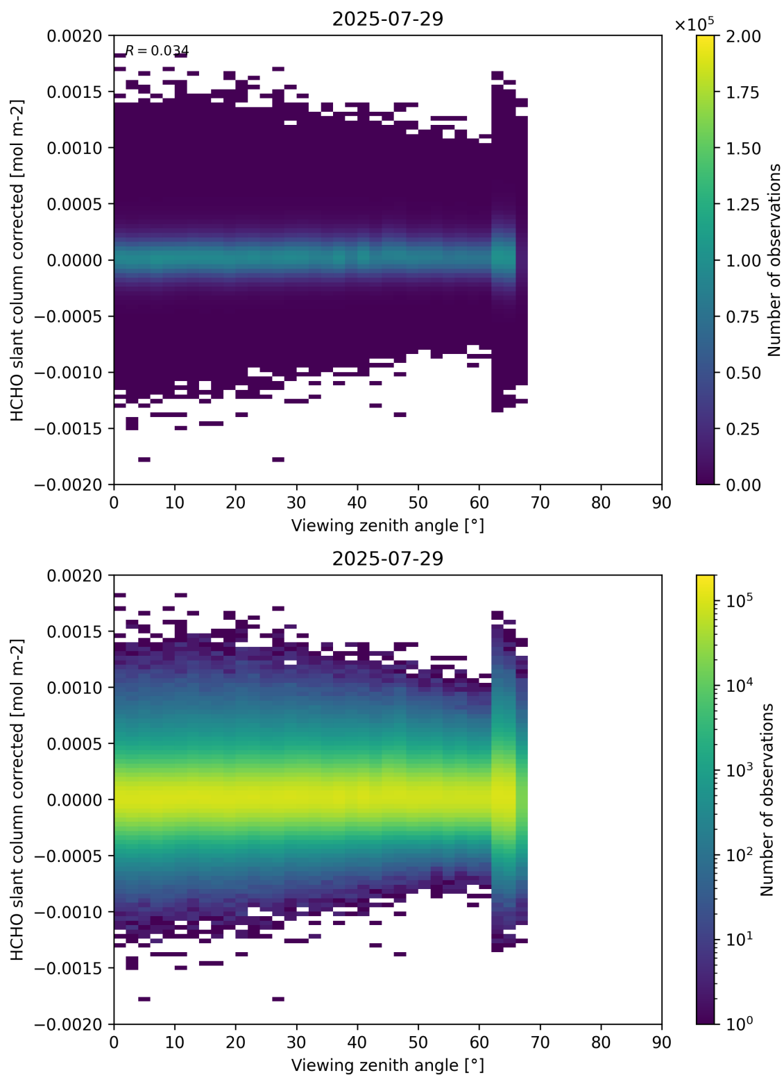
Figure 186: Scatter density plot of “Viewing zenith angle” against “HCHO slant column corrected” for 2025-07-29 to 2025-07-30.
