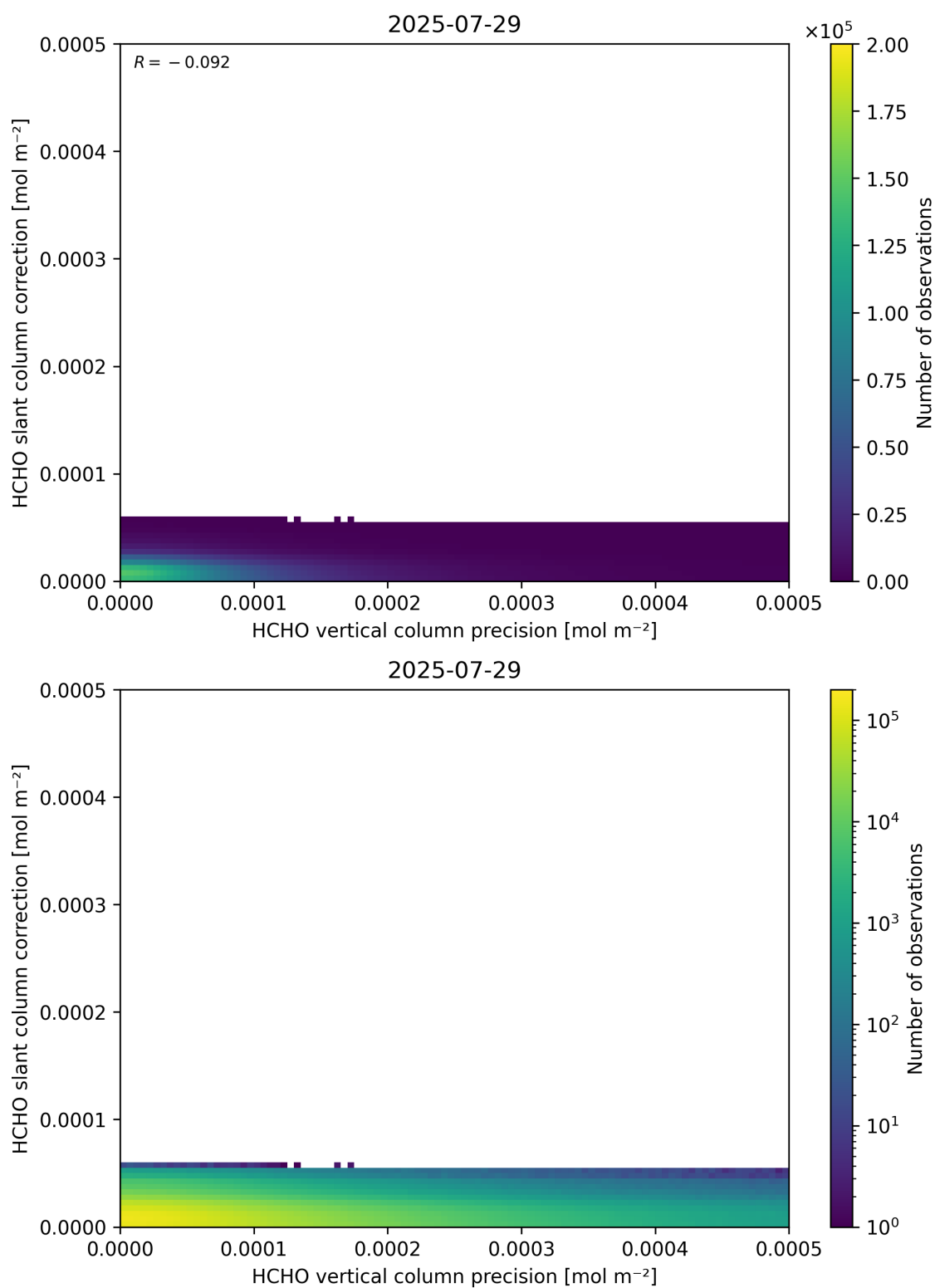
Figure 141: Scatter density plot of “HCHO vertical column precision” against “HCHO slant column correction” for 2025-07-29 to 2025-07-30.
