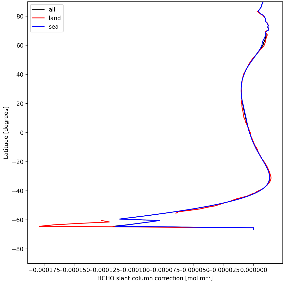
Figure 33: Zonal average of “HCHO slant column correction” for 2025-07-29 to 2025-07-30.
