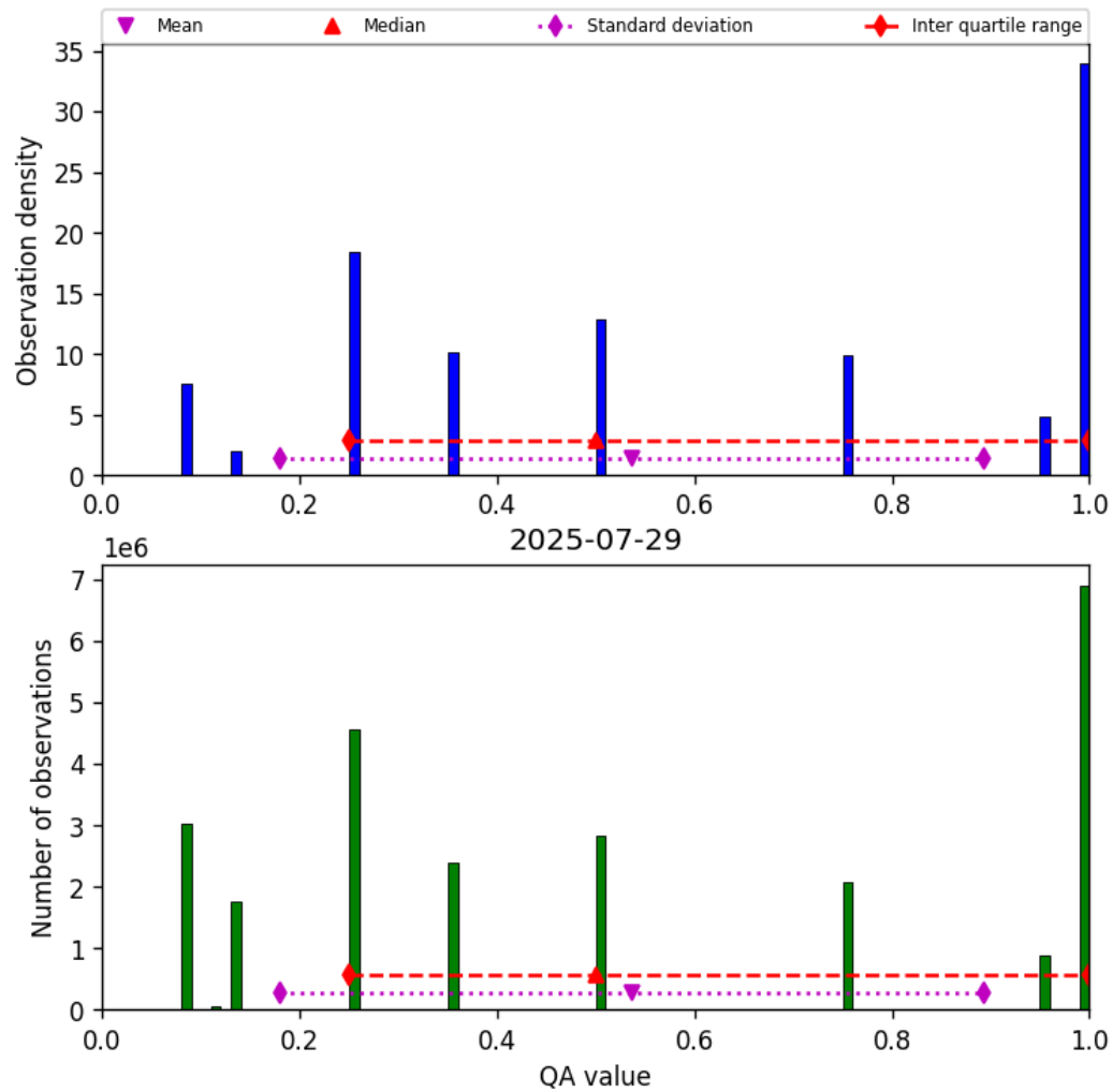
Figure 34: Histogram of “QA value” for 2025-07-29 to 2025-07-30
