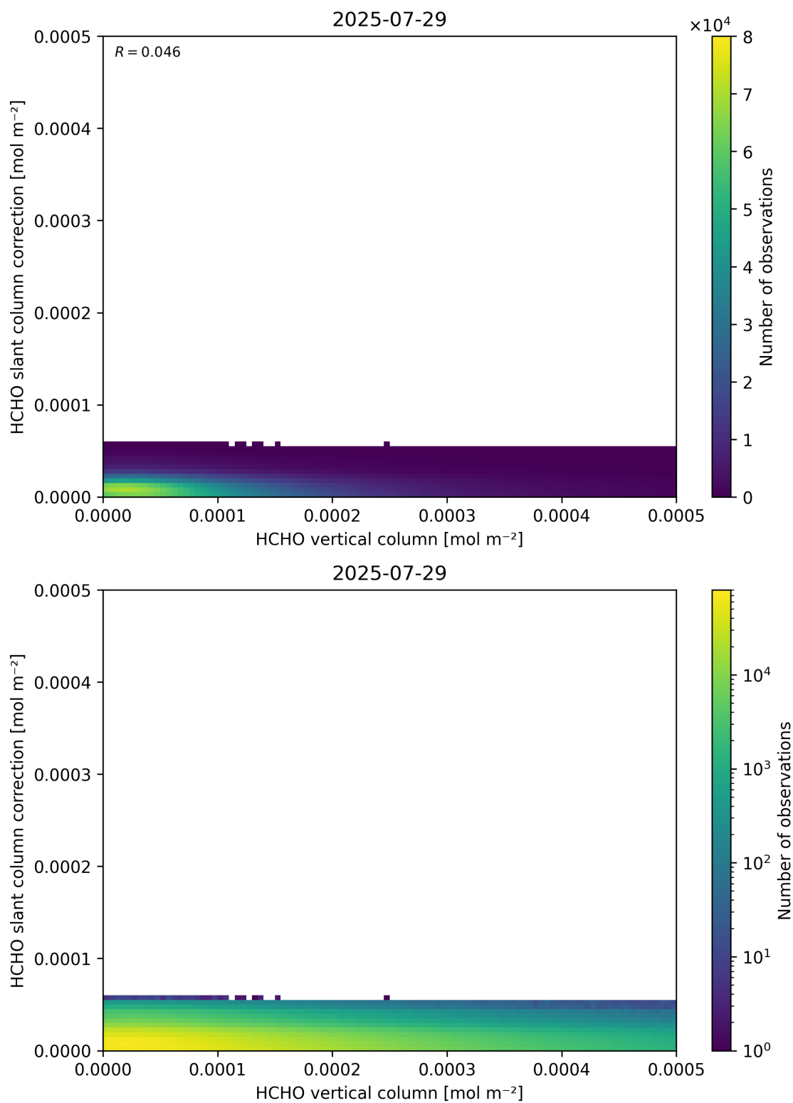
Figure 128: Scatter density plot of “HCHO vertical column” against “HCHO slant column correction” for 2025-07-29 to 2025-07-30.
