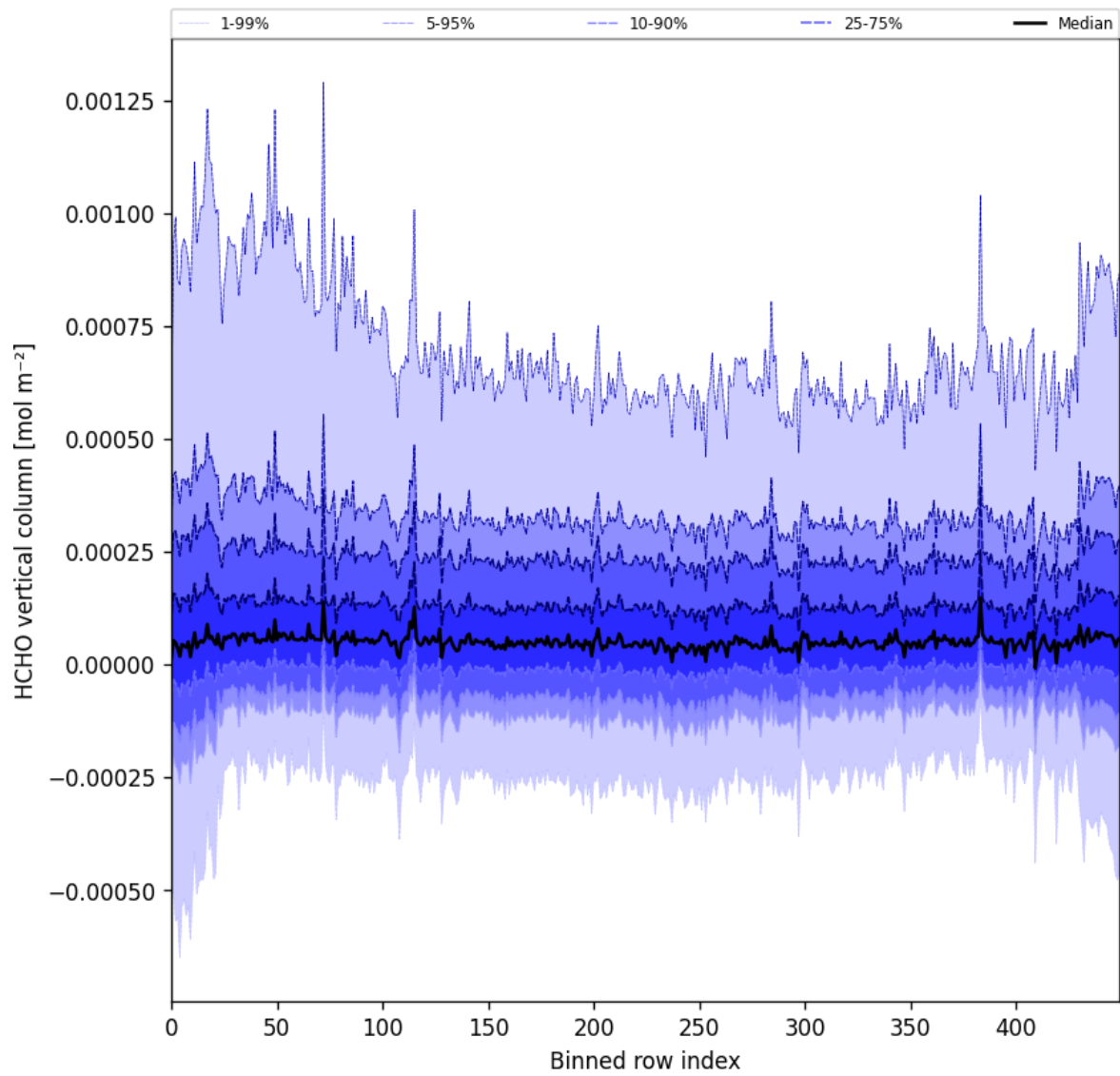
Figure 49: Along track statistics of “HCHO vertical column” for 2025-07-29 to 2025-07-30
