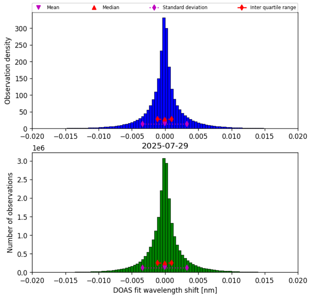
Figure 44: Histogram of “DOAS fit wavelength shift” for 2025-07-29 to 2025-07-30
