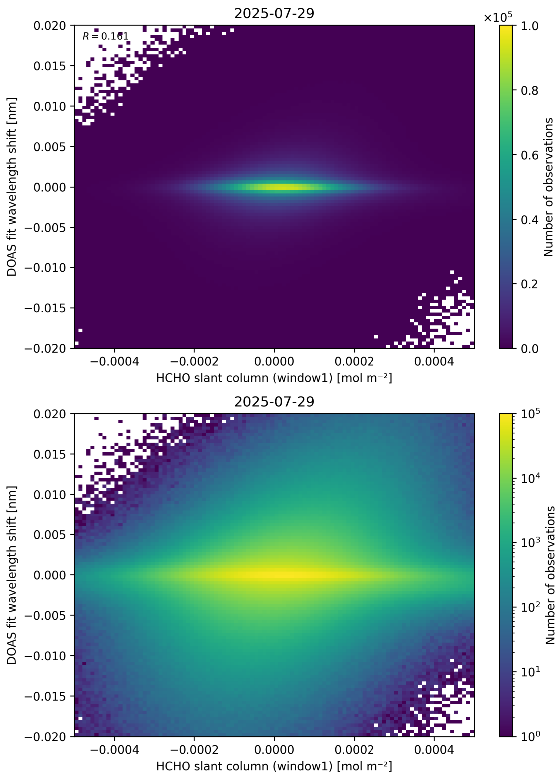
Figure 79: Scatter density plot of “HCHO slant column (window1)” against “DOAS fit wavelength shift” for 2025-07-29 to 2025-07-30.
