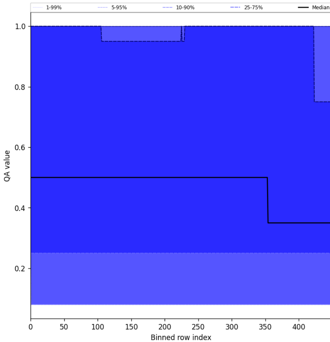
Figure 48: Along track statistics of “QA value” for 2025-07-29 to 2025-07-30
