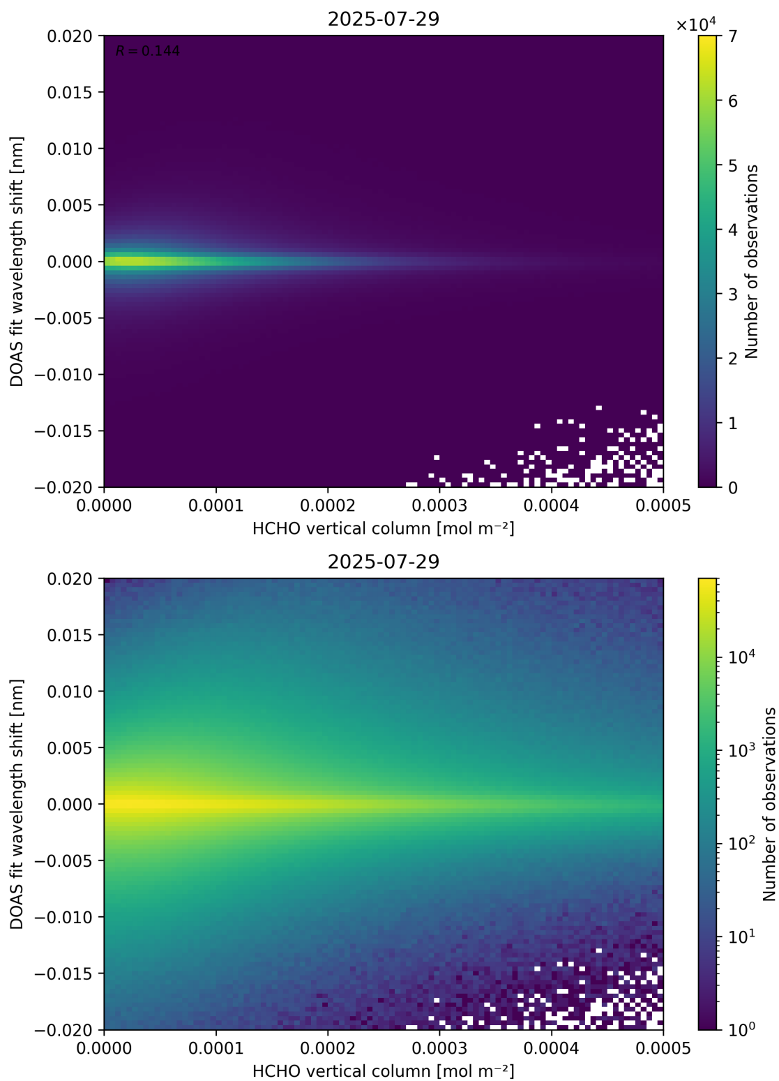
Figure 124: Scatter density plot of “HCHO vertical column” against “DOAS fit wavelength shift” for 2025-07-29 to 2025-07-30.
