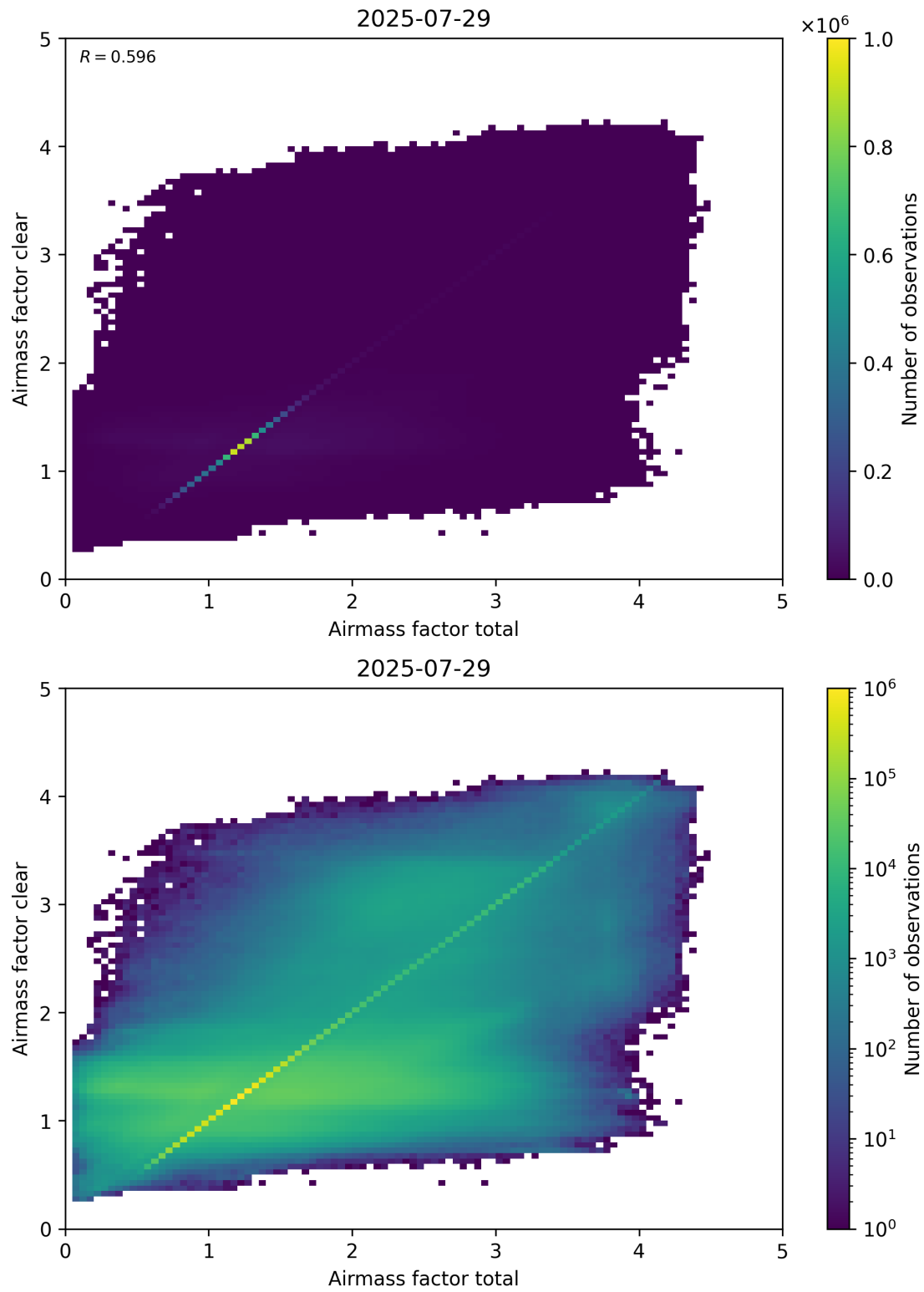
Figure 100: Scatter density plot of “Airmass factor total” against “Airmass factor clear” for 2025-07-29 to 2025-07-30.
