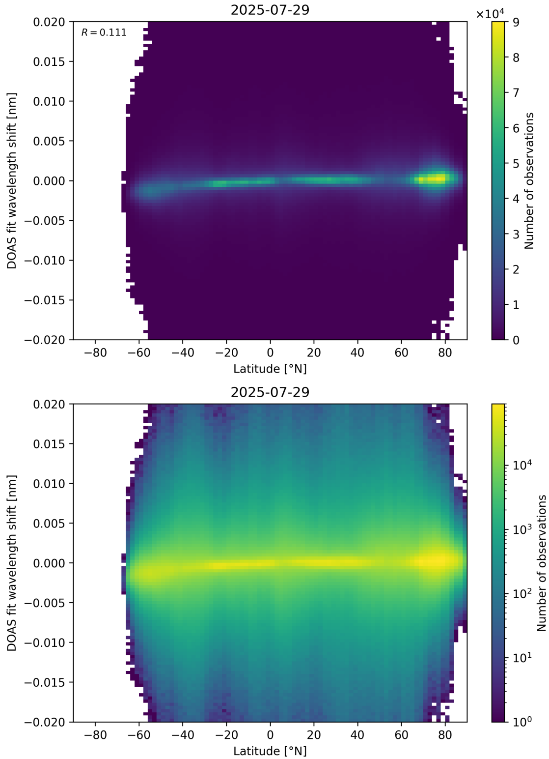
Figure 154: Scatter density plot of “Latitude” against “DOAS fit wavelength shift” for 2025-07-29 to 2025-07-30.
