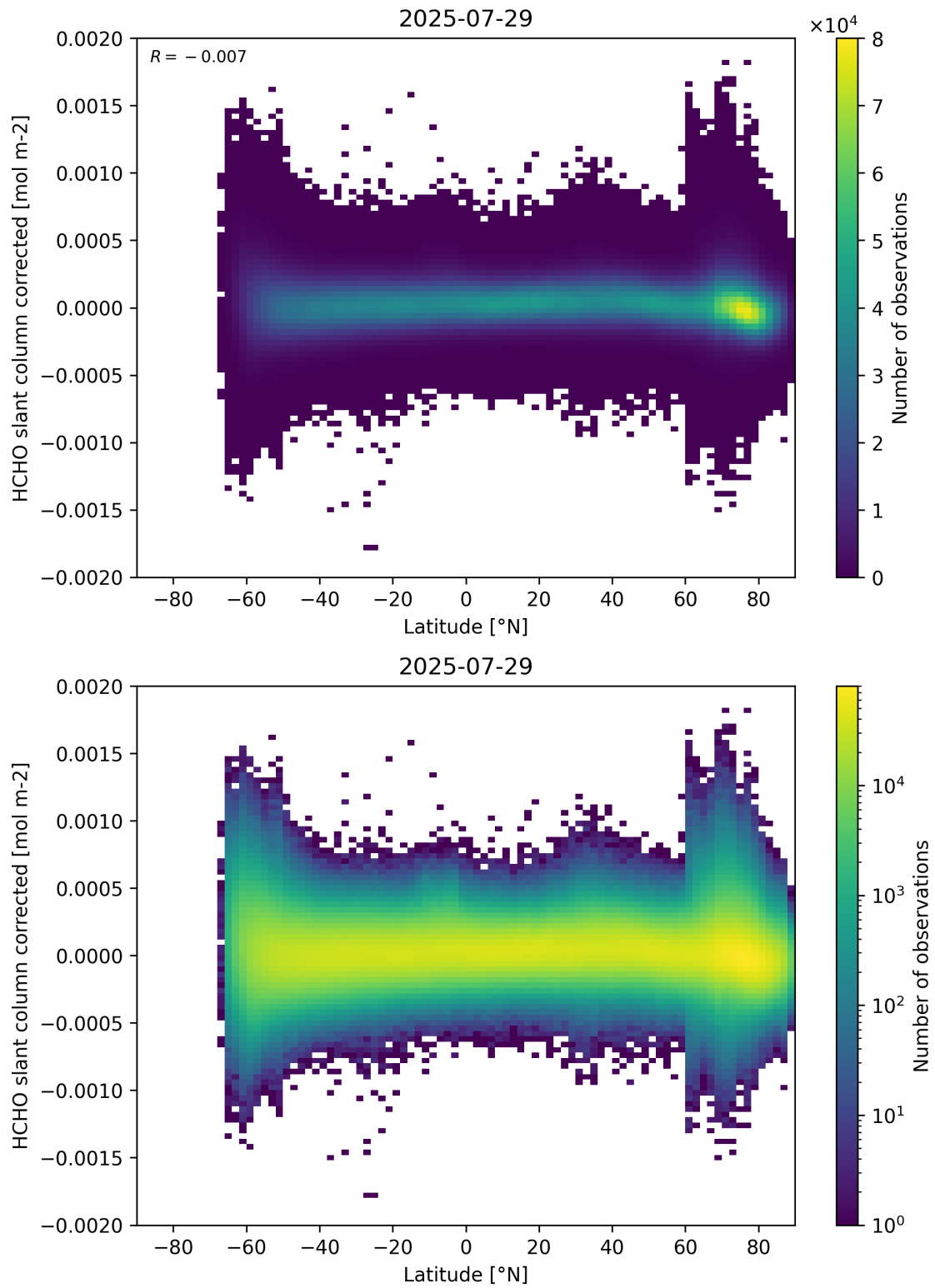
Figure 157: Scatter density plot of “Latitude” against “HCHO slant column corrected” for 2025-07-29 to 2025-07-30.
