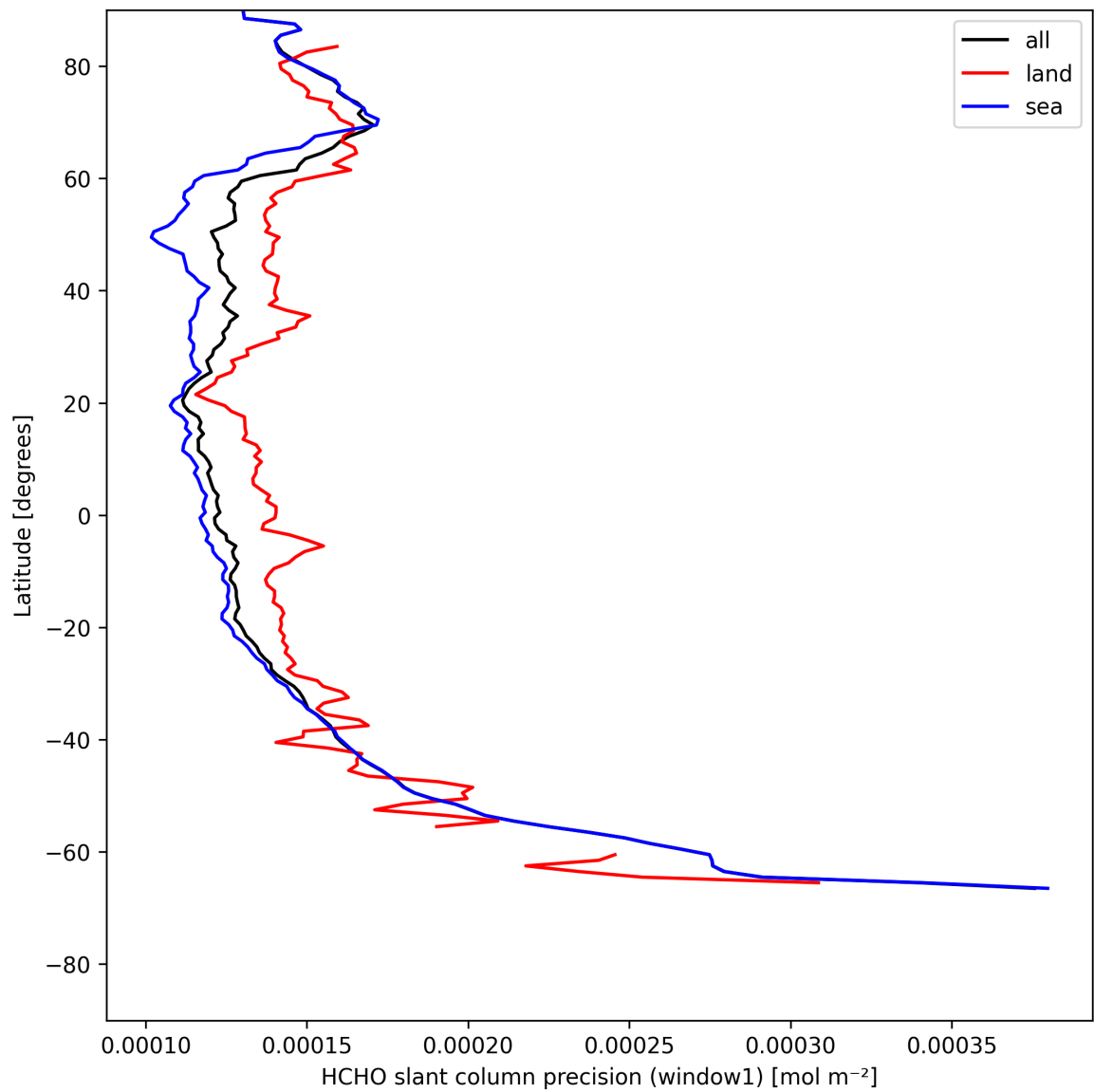
Figure 25: Zonal average of “HCHO slant column precision (window1)” for 2025-07-29 to 2025-07-30.
