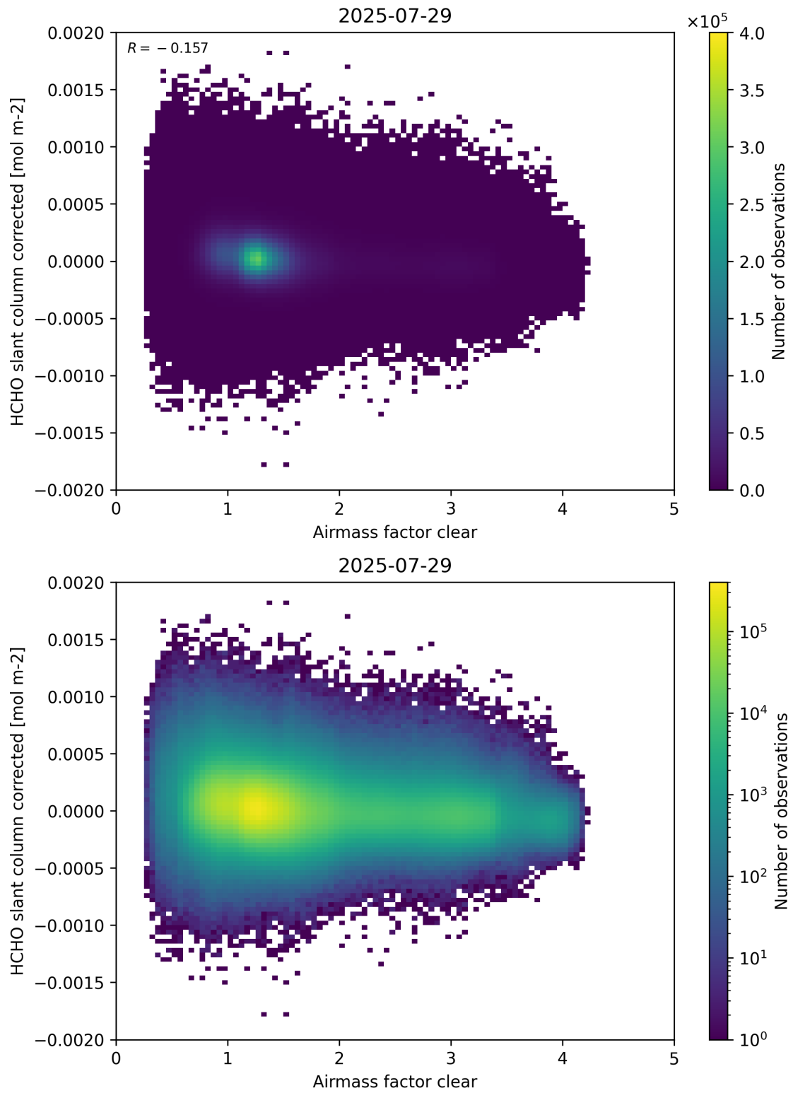
Figure 74: Scatter density plot of “Airmass factor clear” against “HCHO slant column corrected” for 2025-07-29 to 2025-07-30.
