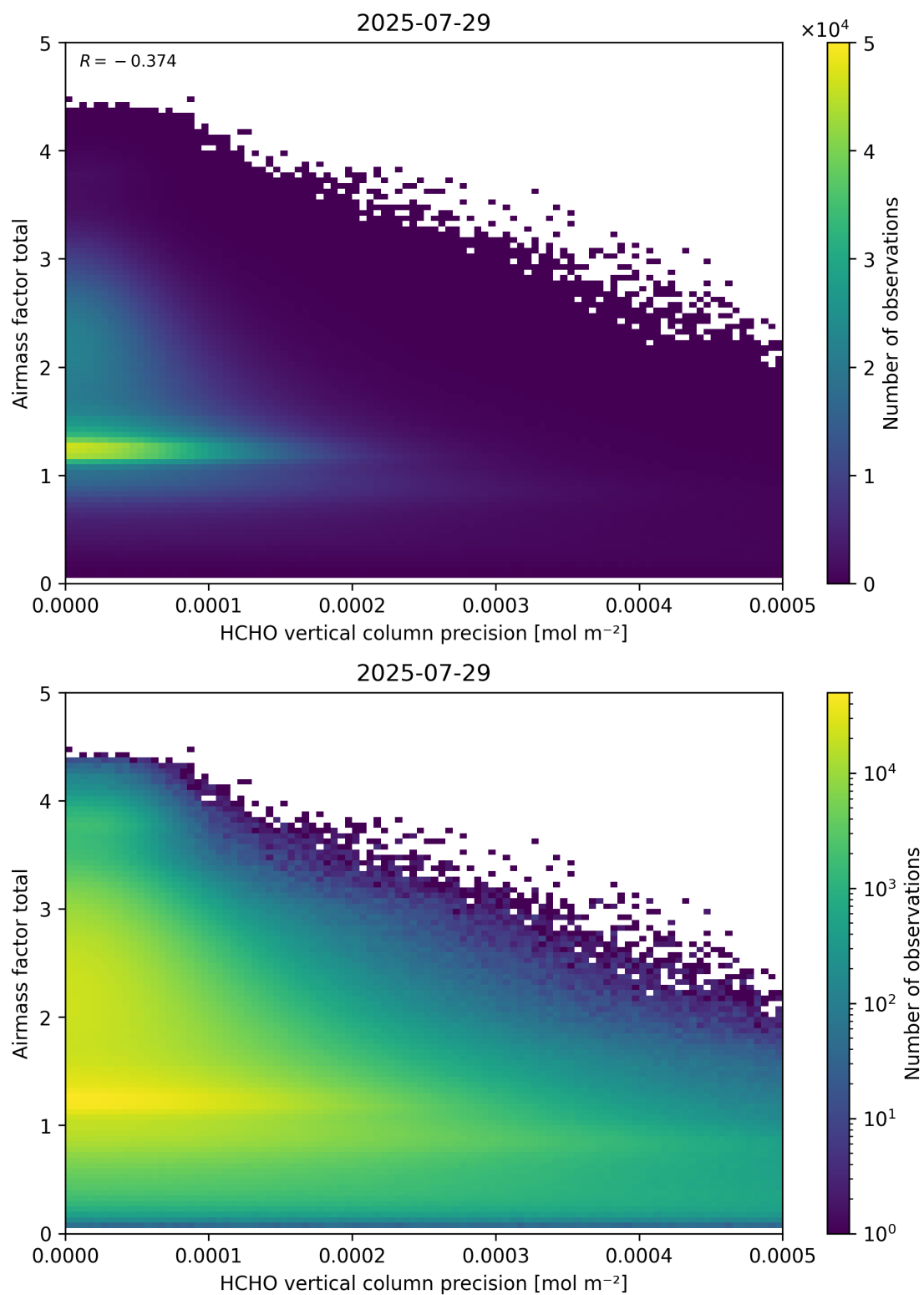
Figure 144: Scatter density plot of “HCHO vertical column precision” against “Airmass factor total” for 2025-07-29 to 2025-07-30.
