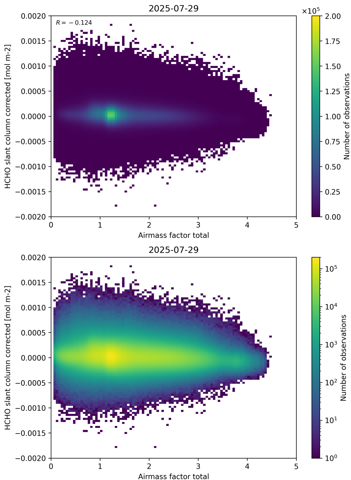
Figure 101: Scatter density plot of “Airmass factor total” against “HCHO slant column corrected” for 2025-07-29 to 2025-07-30.
