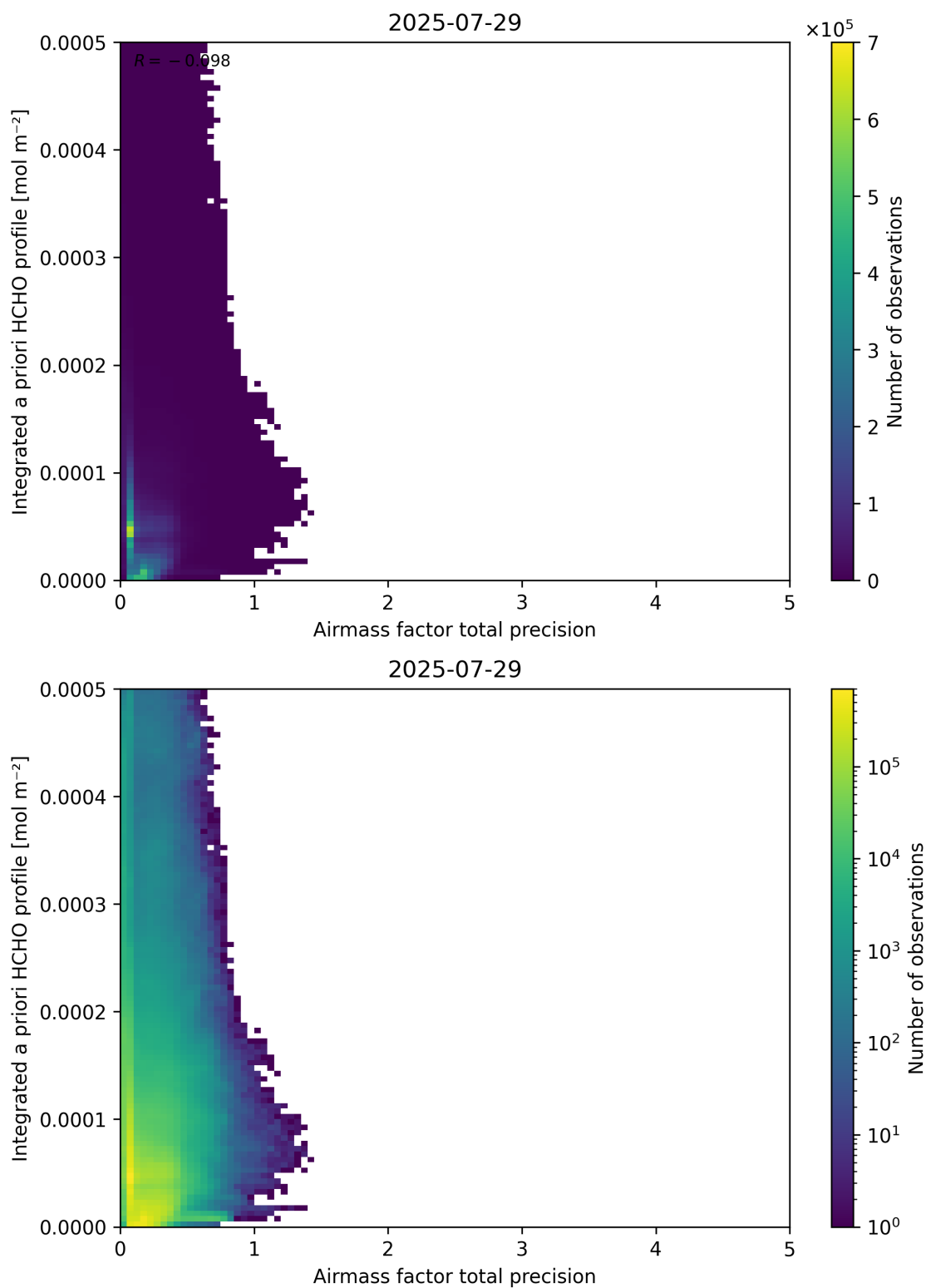
Figure 111: Scatter density plot of “Airmass factor total precision” against “Integrated a priori HCHO profile” for 2025-07-29 to 2025-07-30.
