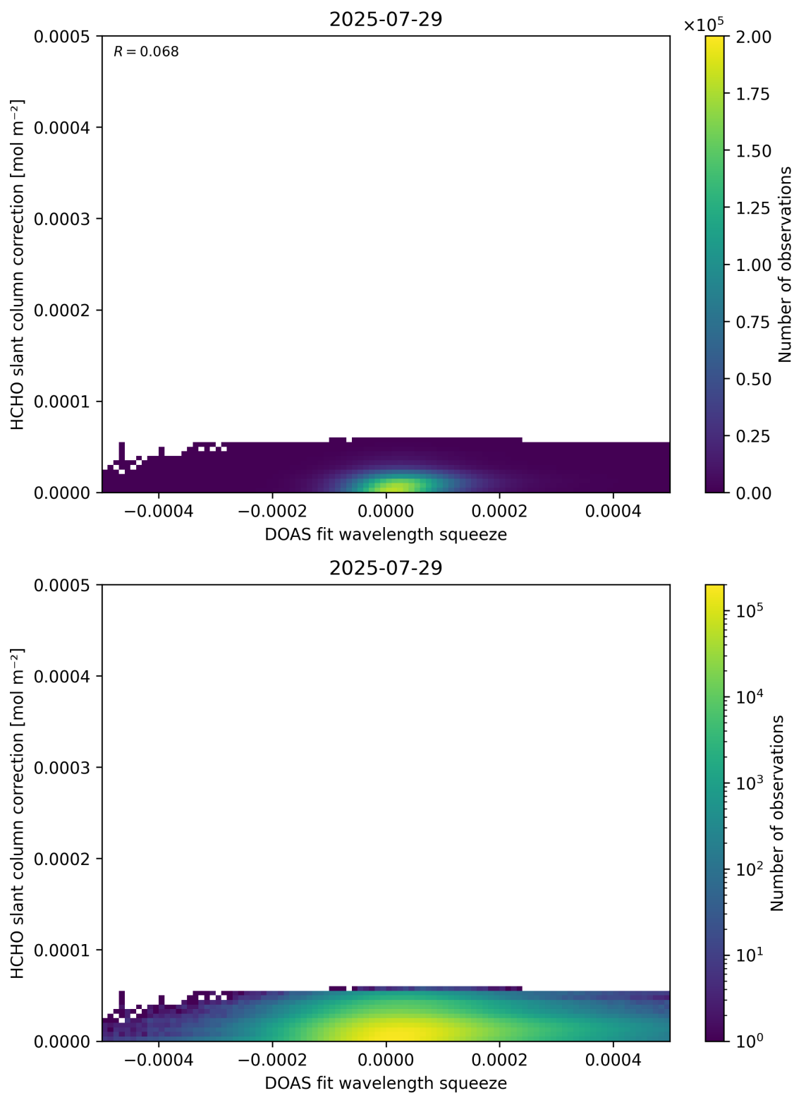
Figure 70: Scatter density plot of “DOAS fit wavelength squeeze” against “HCHO slant column correction” for 2025-07-29 to 2025-07-30.
