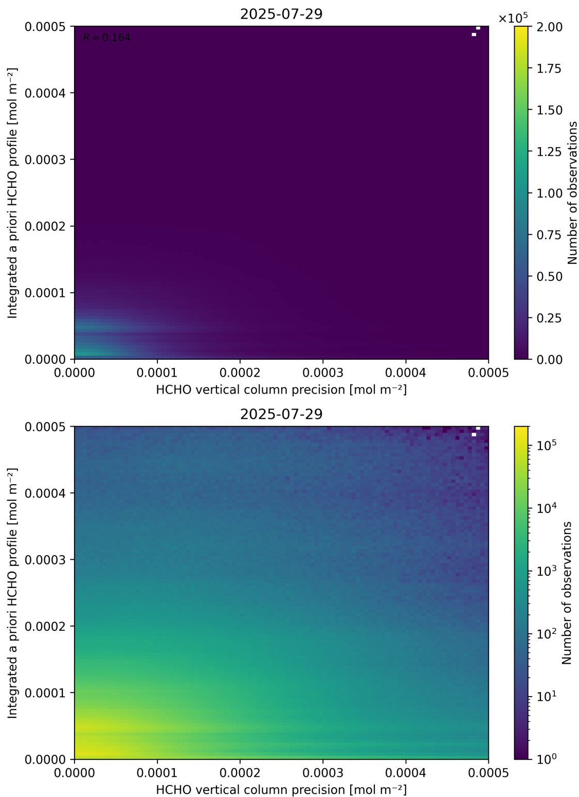
Figure 147: Scatter density plot of “HCHO vertical column precision” against “Integrated a priori HCHO profile” for 2025-07-29 to 2025-07-30.
