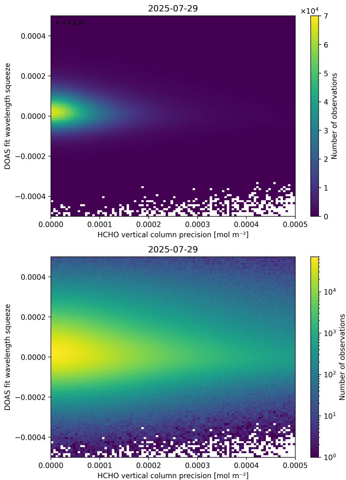
Figure 138: Scatter density plot of “HCHO vertical column precision” against “DOAS fit wavelength squeeze” for 2025-07-29 to 2025-07-30.
