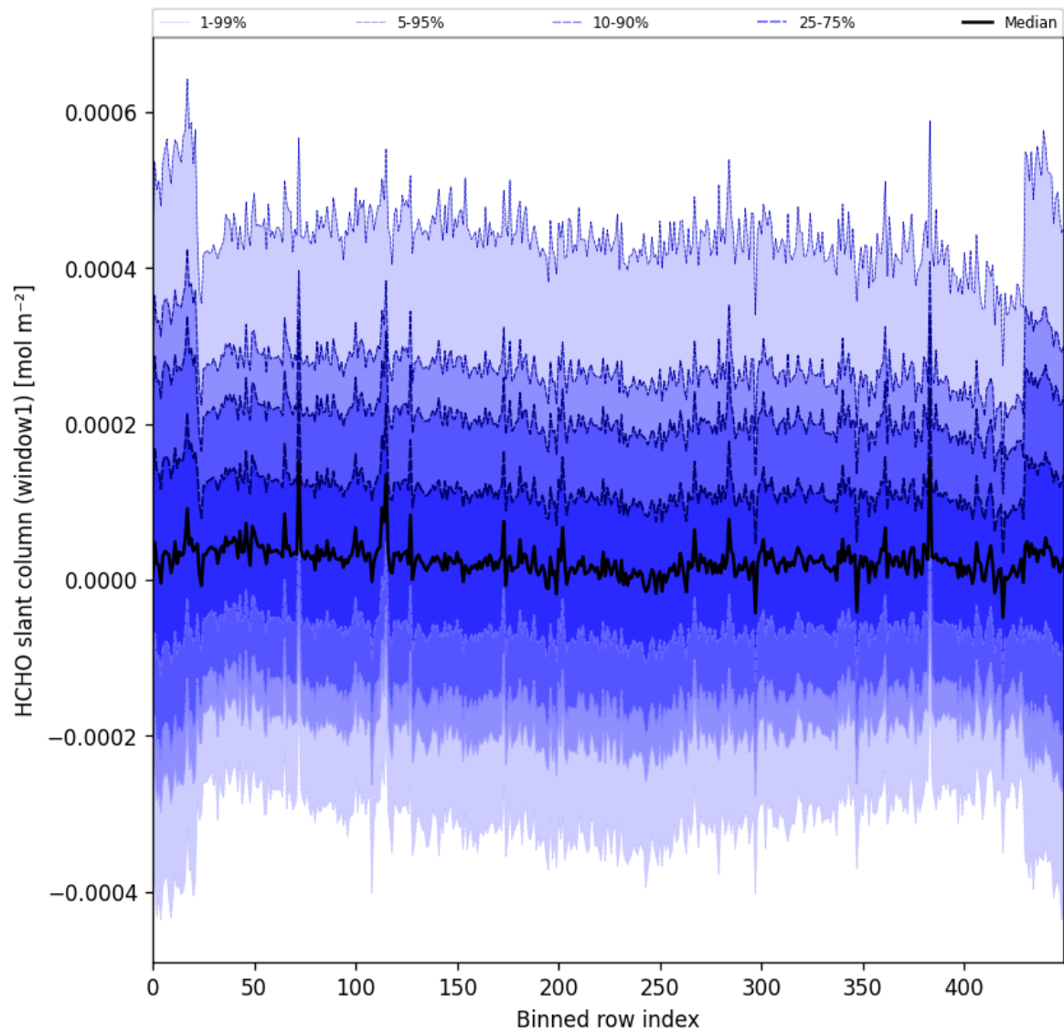
Figure 52: Along track statistics of “HCHO slant column (window1)” for 2025-07-29 to 2025-07-30
