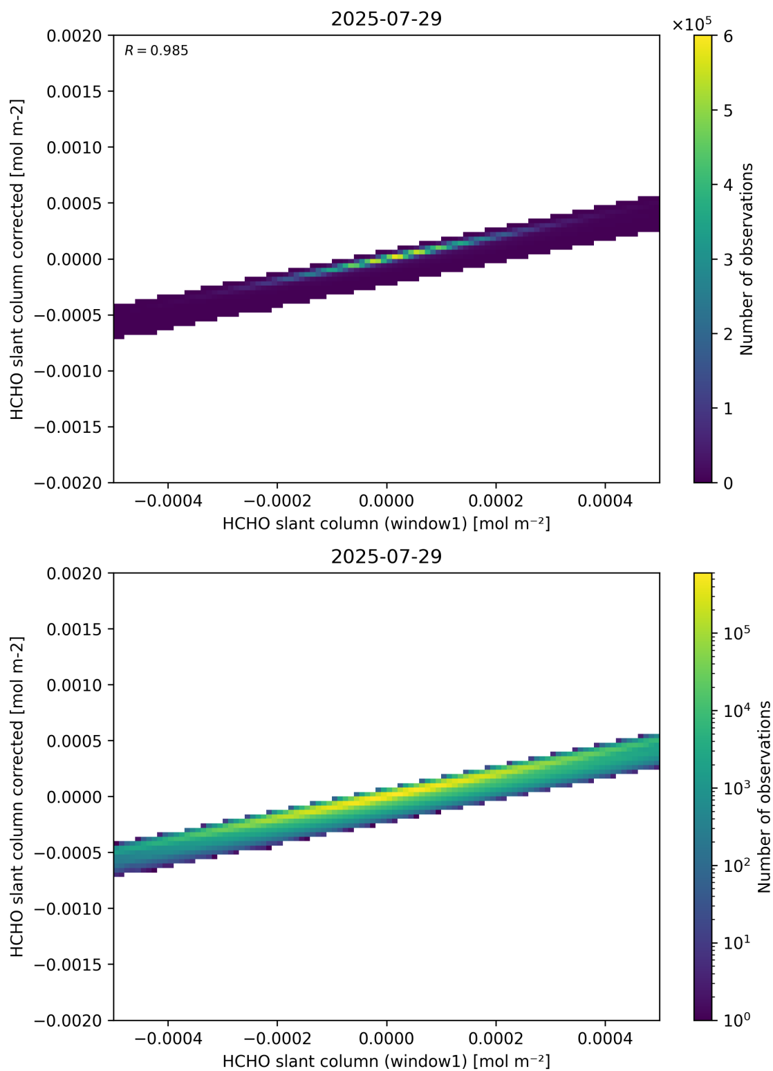
Figure 82: Scatter density plot of “HCHO slant column (window1)” against “HCHO slant column corrected” for 2025-07-29 to 2025-07-30.
