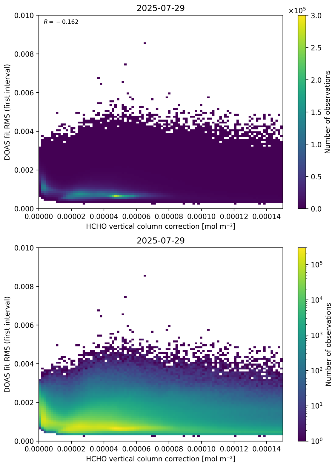
Figure 112: Scatter density plot of “HCHO vertical column correction” against “DOAS fit RMS (first interval)” for 2025-07-29 to 2025-07-30.
