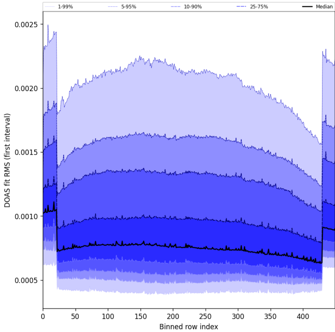
Figure 60: Along track statistics of “DOAS fit RMS (first interval)” for 2025-07-29 to 2025-07-30
