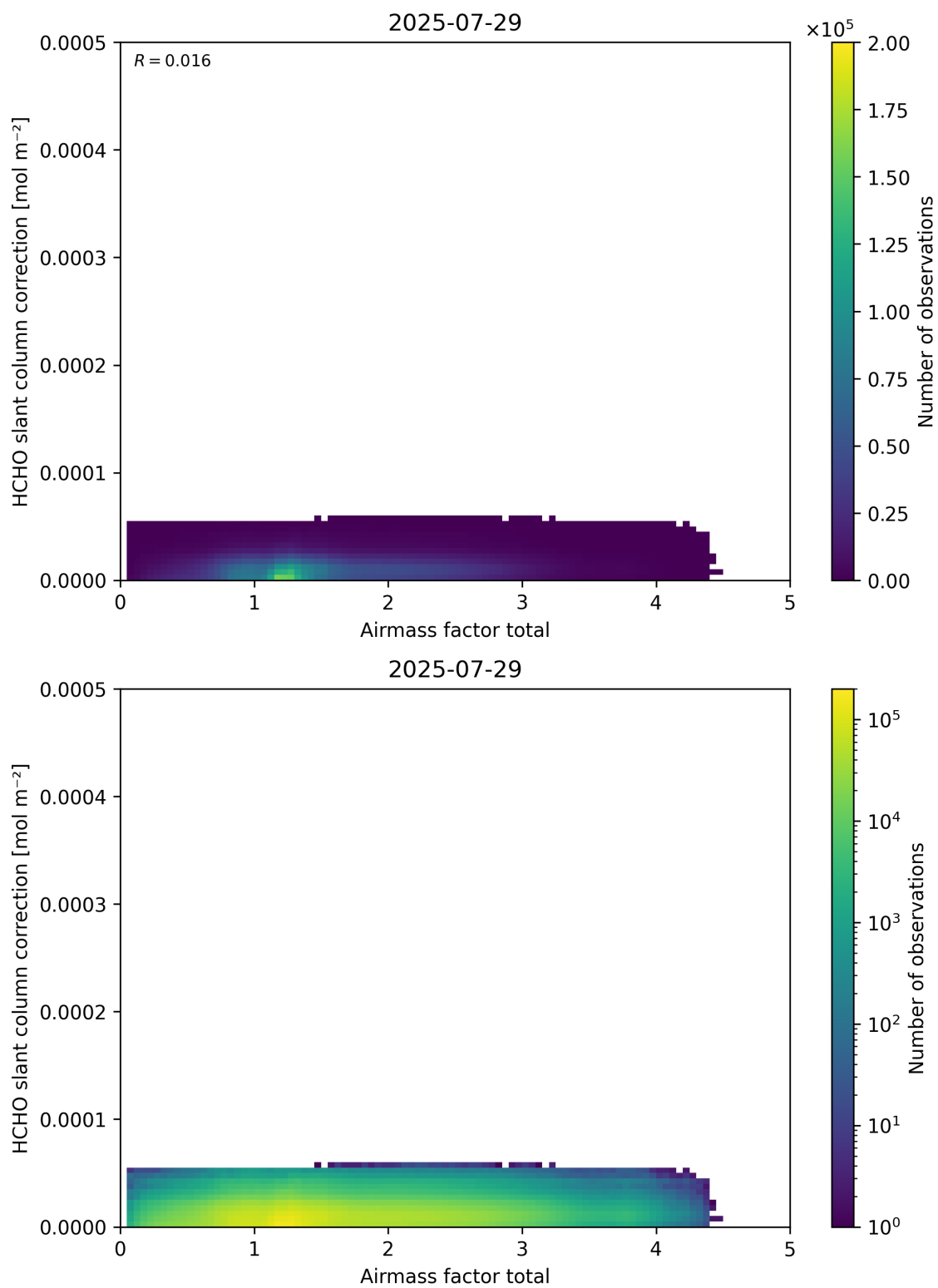
Figure 102: Scatter density plot of “Airmass factor total” against “HCHO slant column correction” for 2025-07-29 to 2025-07-30.
