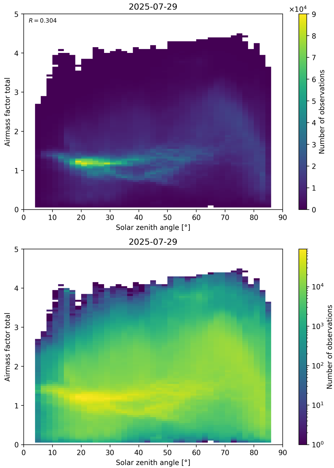
Figure 175: Scatter density plot of “Solar zenith angle” against “Airmass factor total” for 2025-07-29 to 2025-07-30.
