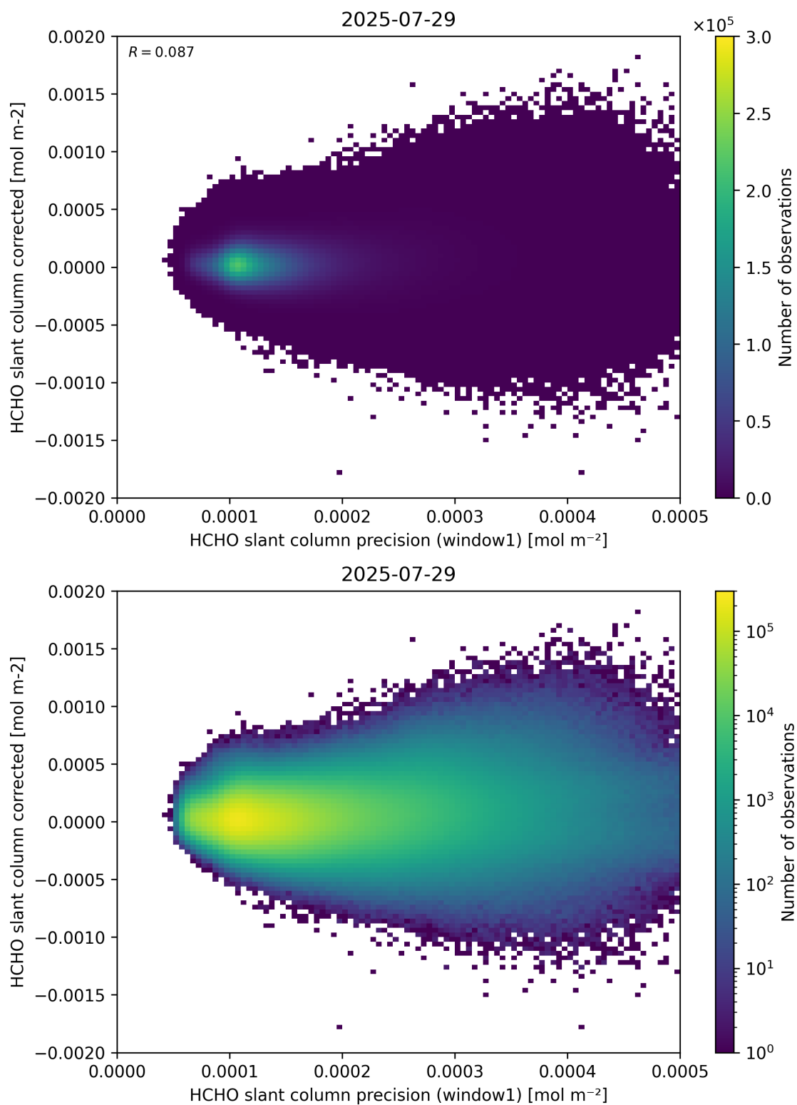
Figure 92: Scatter density plot of “HCHO slant column precision (window1)” against “HCHO slant column corrected” for 2025-07-29 to 2025-07-30.
