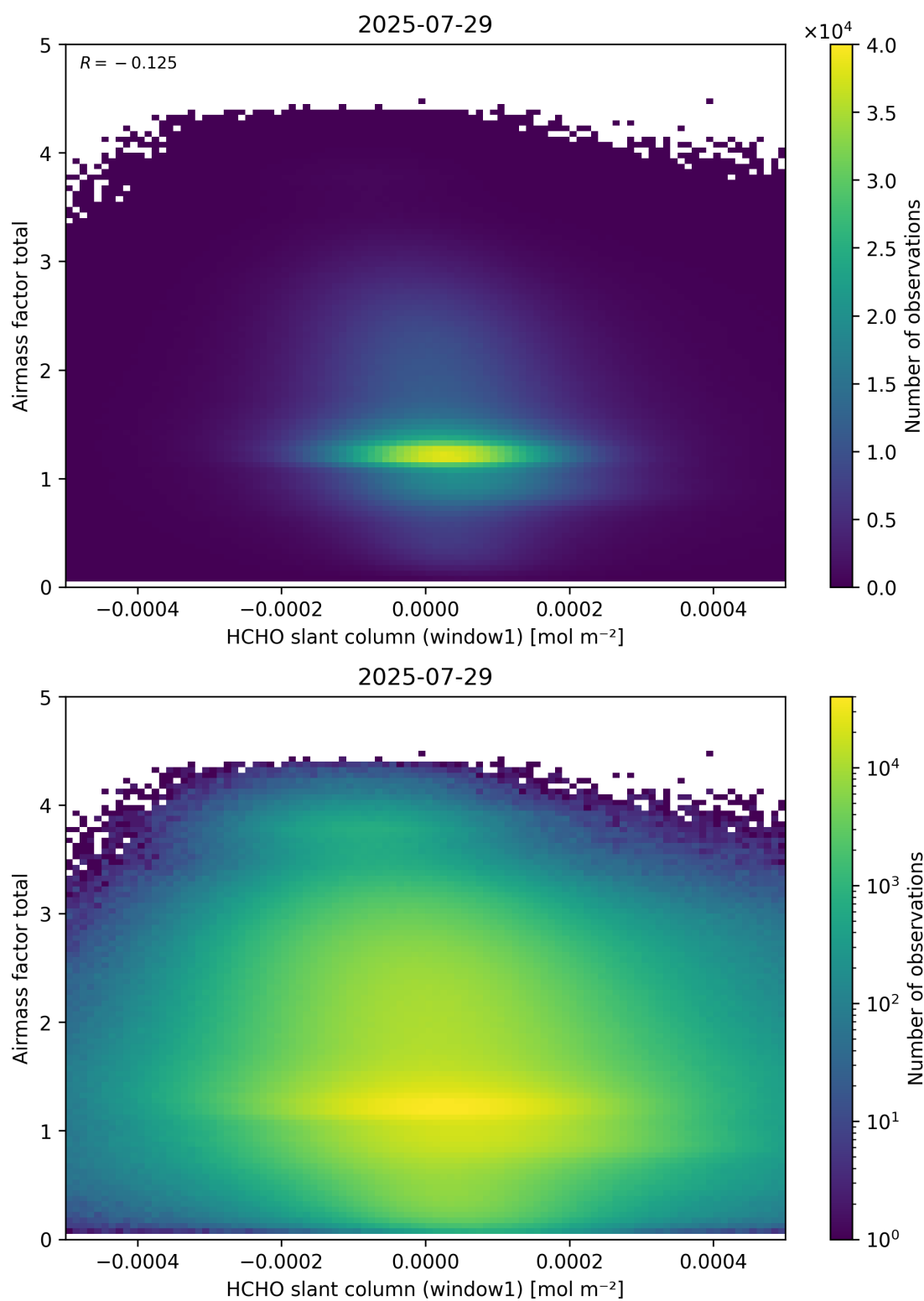
Figure 85: Scatter density plot of “HCHO slant column (window1)” against “Airmass factor total” for 2025-07-29 to 2025-07-30.
