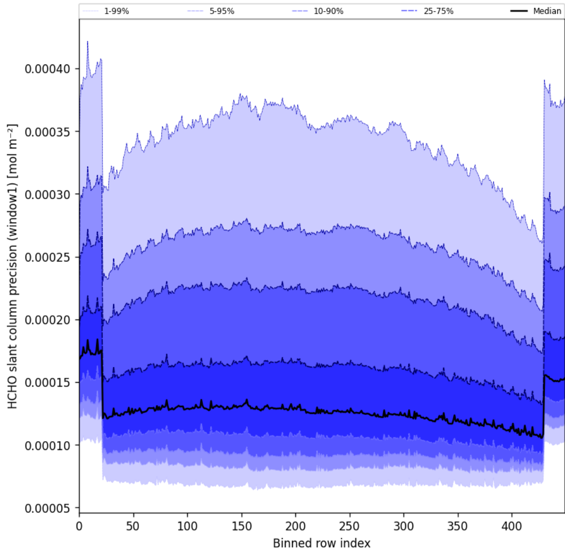
Figure 53: Along track statistics of “HCHO slant column precision (window1)” for 2025-07-29 to 2025-07-30
