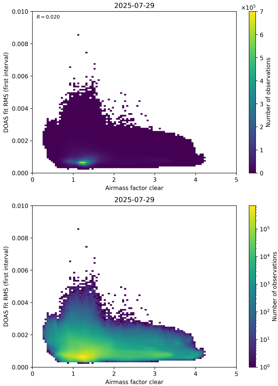
Figure 71: Scatter density plot of “Airmass factor clear” against “DOAS fit RMS (first interval)” for 2025-07-29 to 2025-07-30.
