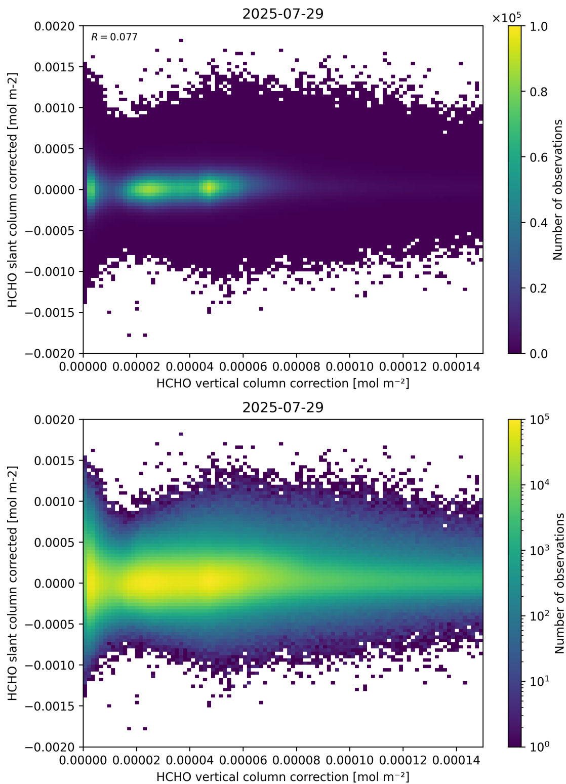
Figure 116: Scatter density plot of “HCHO vertical column correction” against “HCHO slant column corrected” for 2025-07-29 to 2025-07-30.
