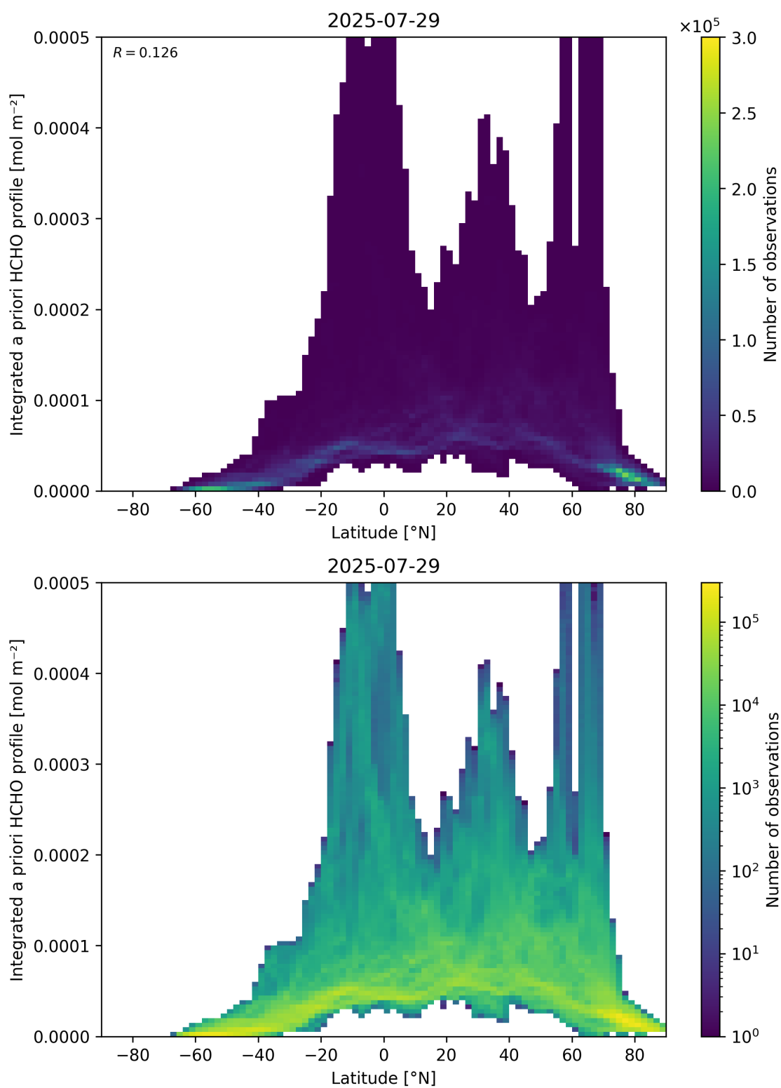
Figure 166: Scatter density plot of “Latitude” against “Integrated a priori HCHO profile” for 2025-07-29 to 2025-07-30.
