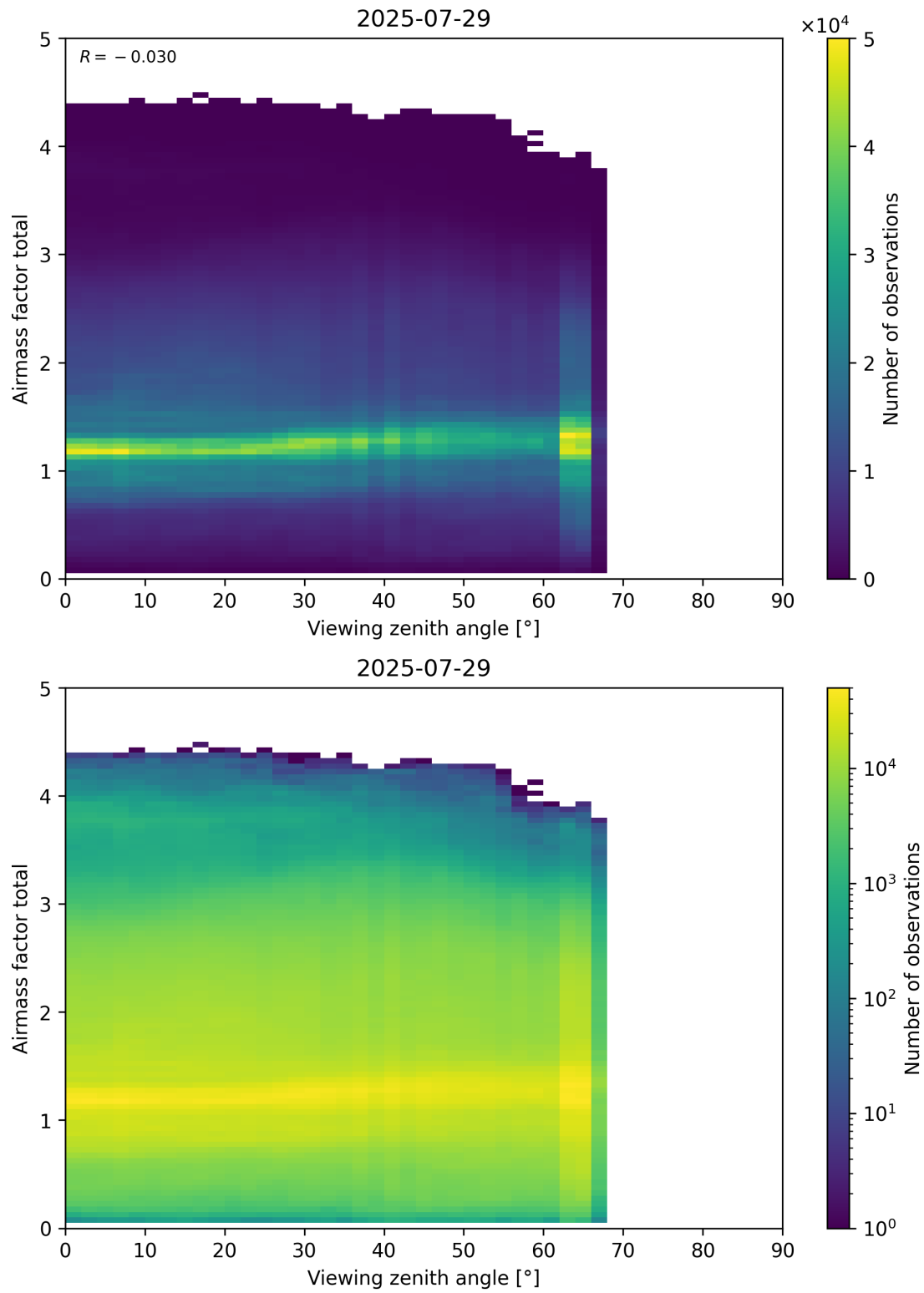
Figure 190: Scatter density plot of “Viewing zenith angle” against “Airmass factor total” for 2025-07-29 to 2025-07-30.
