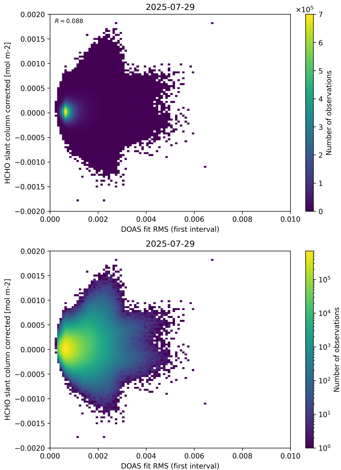
Figure 62: Scatter density plot of “DOAS fit RMS (first interval)” against “HCHO slant column corrected” for 2025-07-29 to 2025-07-30.
