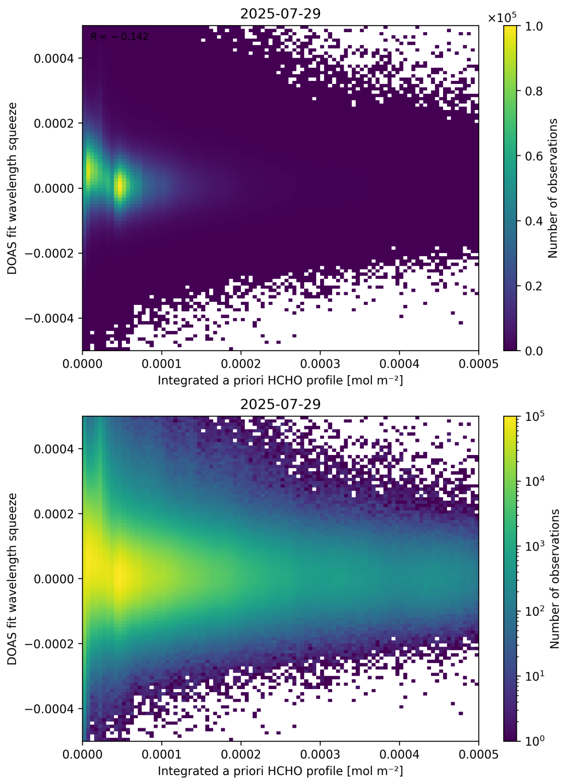
Figure 150: Scatter density plot of “Integrated a priori HCHO profile” against “DOAS fit wavelength squeeze” for 2025-07-29 to 2025-07-30.
