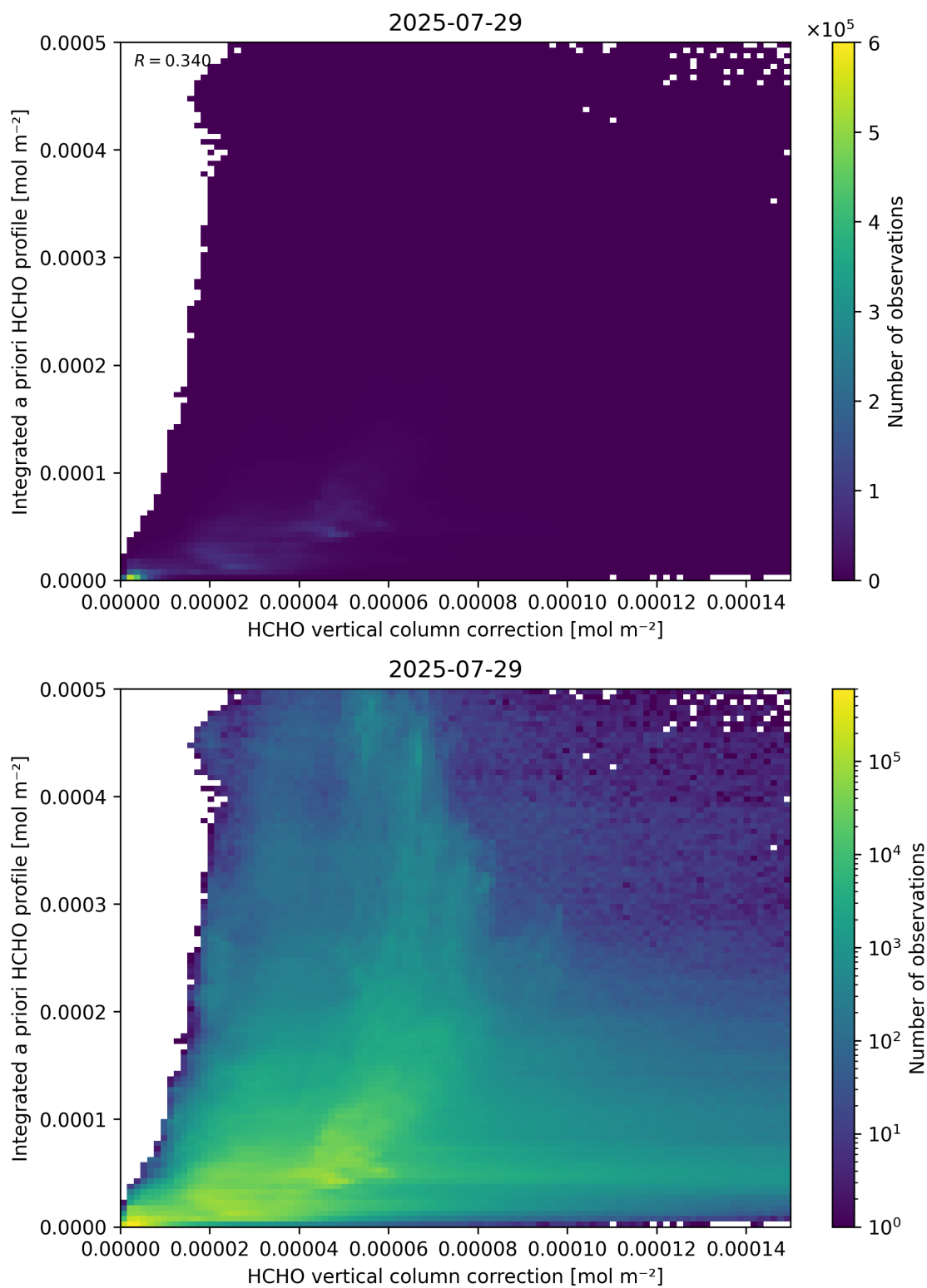
Figure 122: Scatter density plot of “HCHO vertical column correction” against “Integrated a priori HCHO profile” for 2025-07-29 to 2025-07-30.
