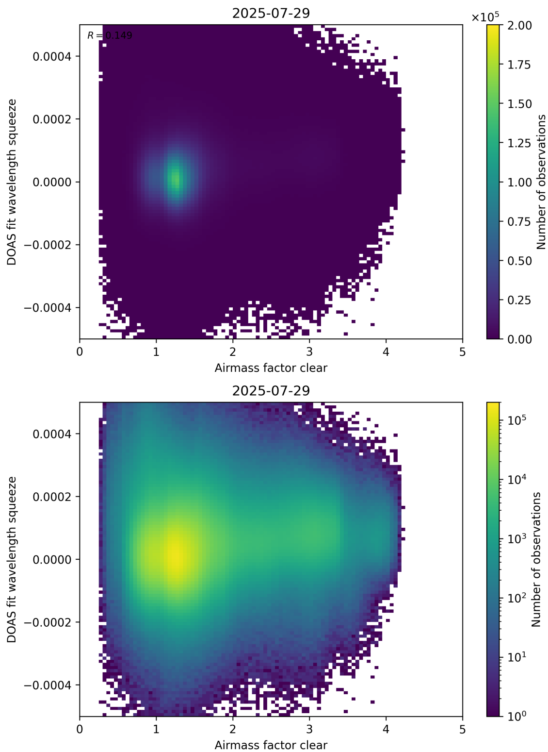
Figure 73: Scatter density plot of “Airmass factor clear” against “DOAS fit wavelength squeeze” for 2025-07-29 to 2025-07-30.
