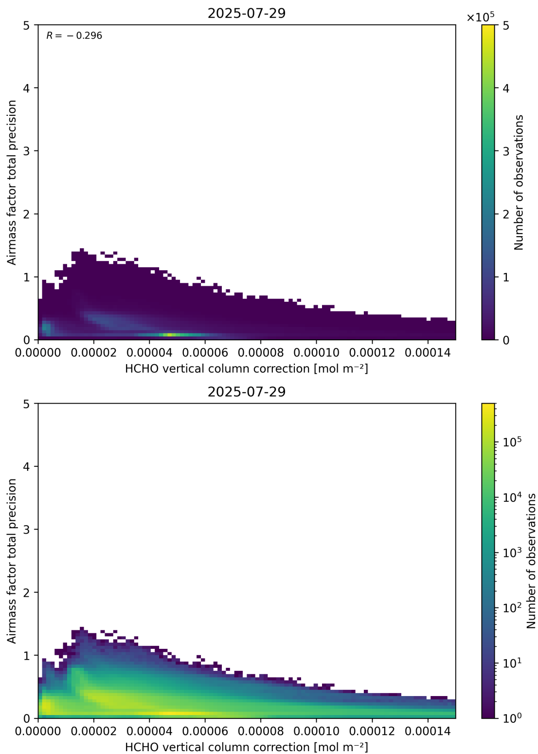
Figure 121: Scatter density plot of “HCHO vertical column correction” against “Airmass factor total precision” for 2025-07-29 to 2025-07-30.
