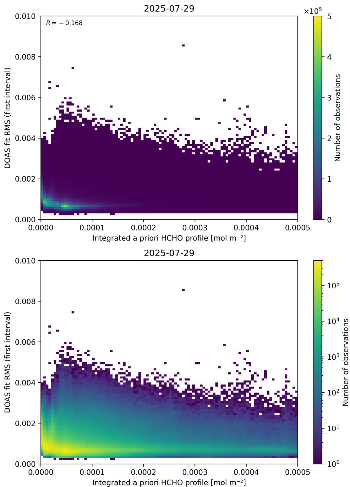
Figure 148: Scatter density plot of “Integrated a priori HCHO profile” against “DOAS fit RMS (first interval)” for 2025-07-29 to 2025-07-30.
