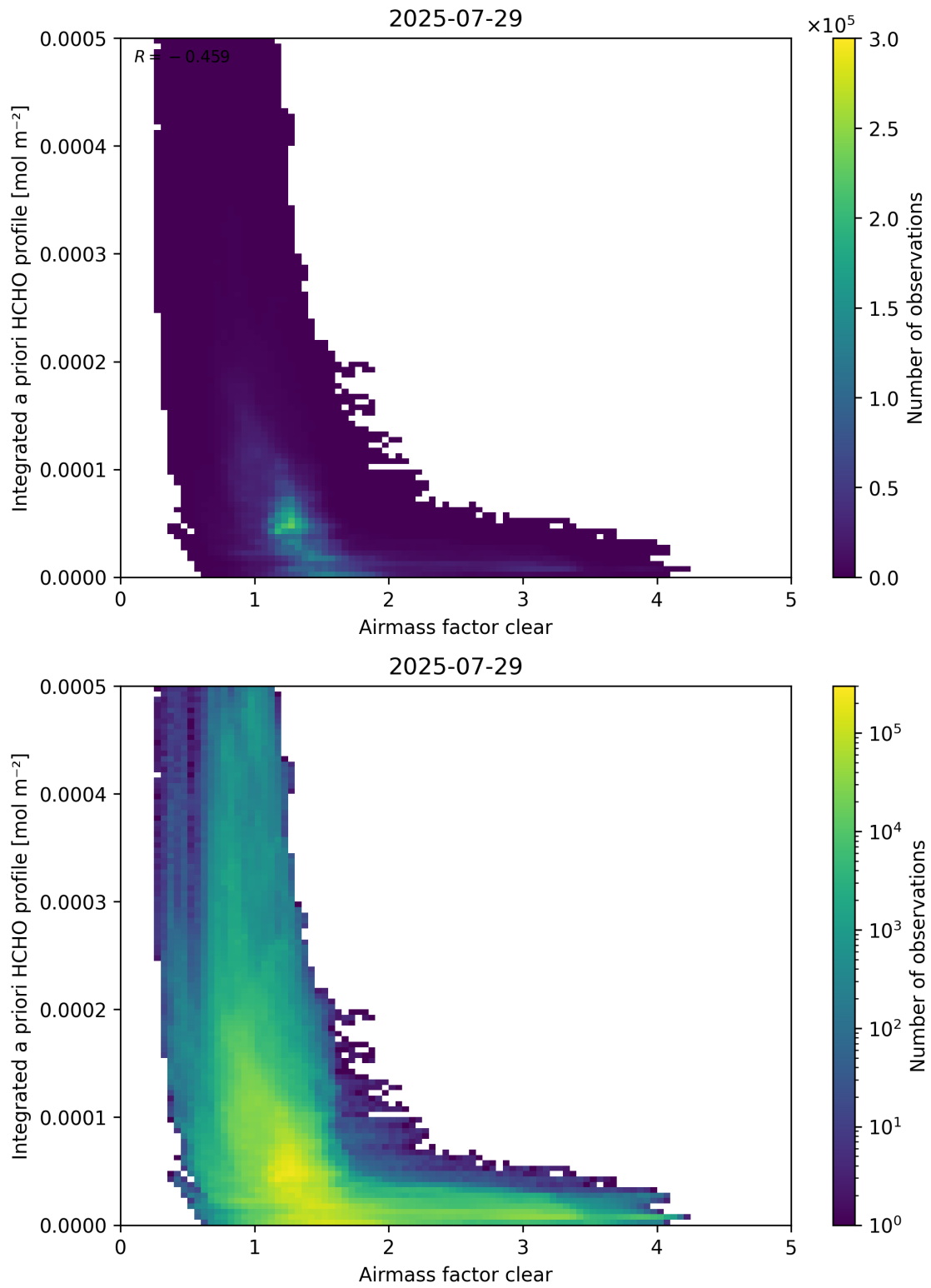
Figure 76: Scatter density plot of “Airmass factor clear” against “Integrated a priori HCHO profile” for 2025-07-29 to 2025-07-30.
