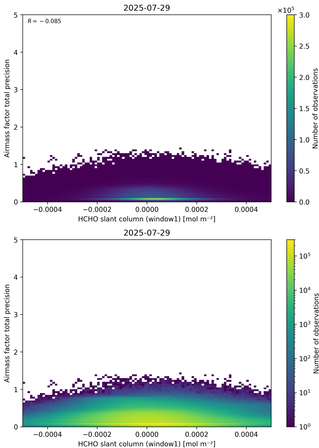
Figure 86: Scatter density plot of “HCHO slant column (window1)” against “Airmass factor total precision” for 2025-07-29 to 2025-07-30.
