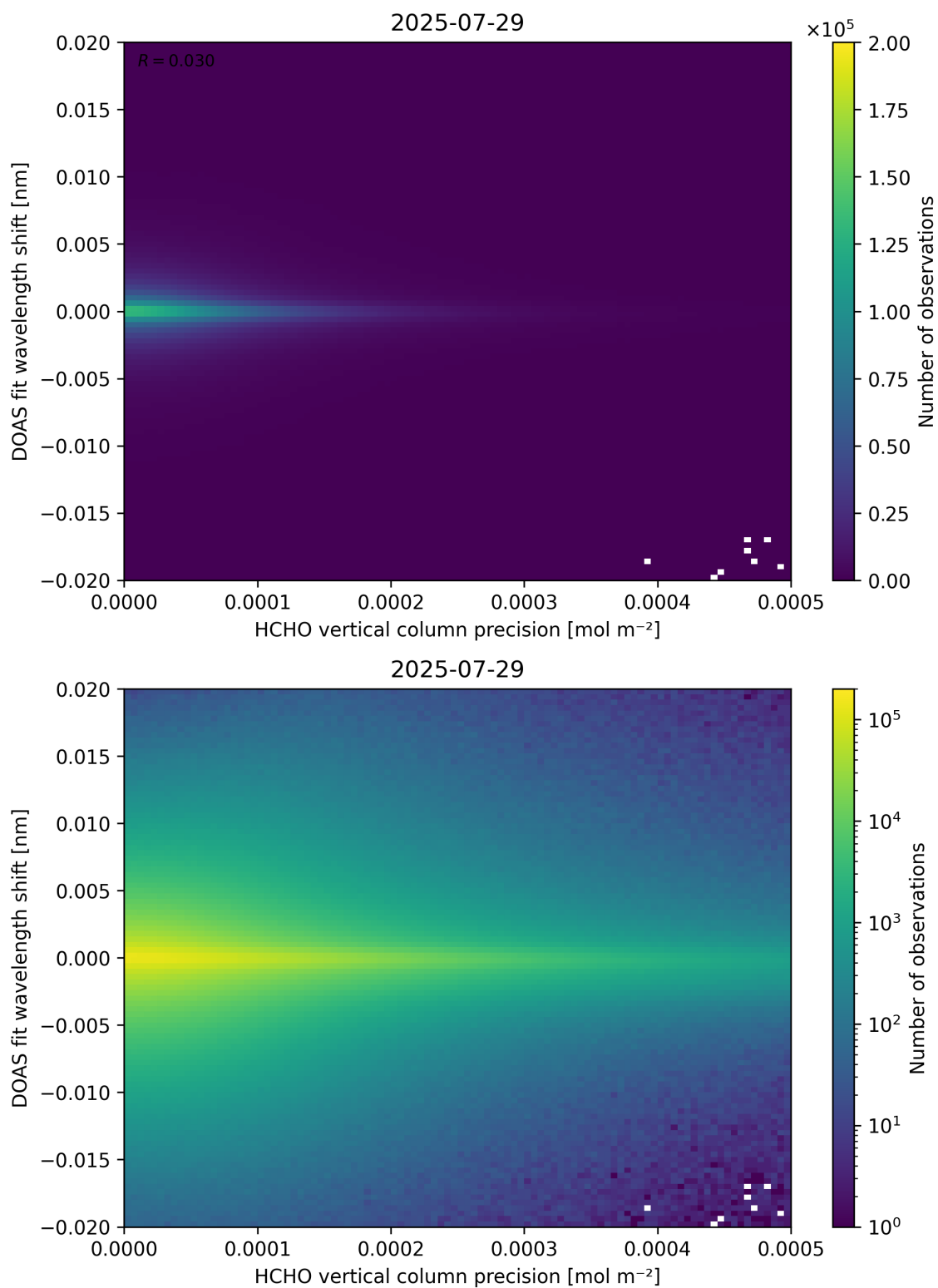
Figure 137: Scatter density plot of “HCHO vertical column precision” against “DOAS fit wavelength shift” for 2025-07-29 to 2025-07-30.
