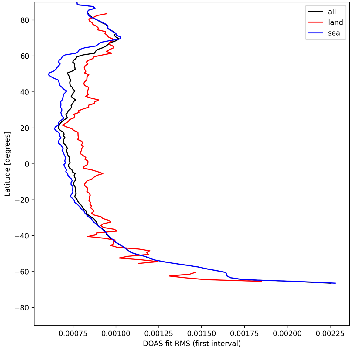
Figure 32: Zonal average of “DOAS fit RMS (first interval)” for 2025-07-29 to 2025-07-30.
