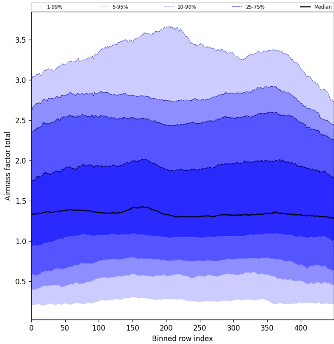
Figure 54: Along track statistics of “Airmass factor total” for 2025-07-29 to 2025-07-30
