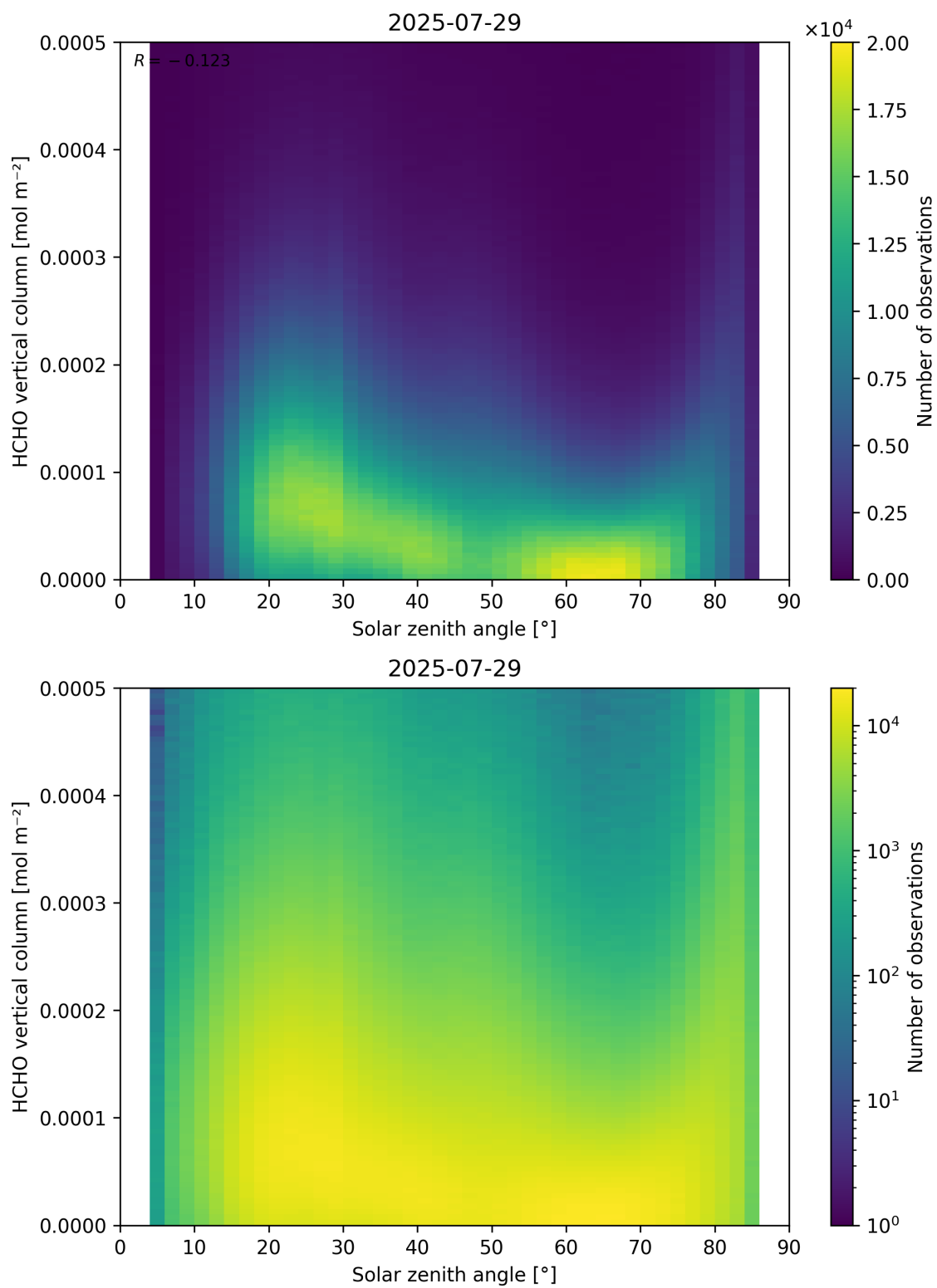
Figure 177: Scatter density plot of “Solar zenith angle” against “HCHO vertical column” for 2025-07-29 to 2025-07-30.
