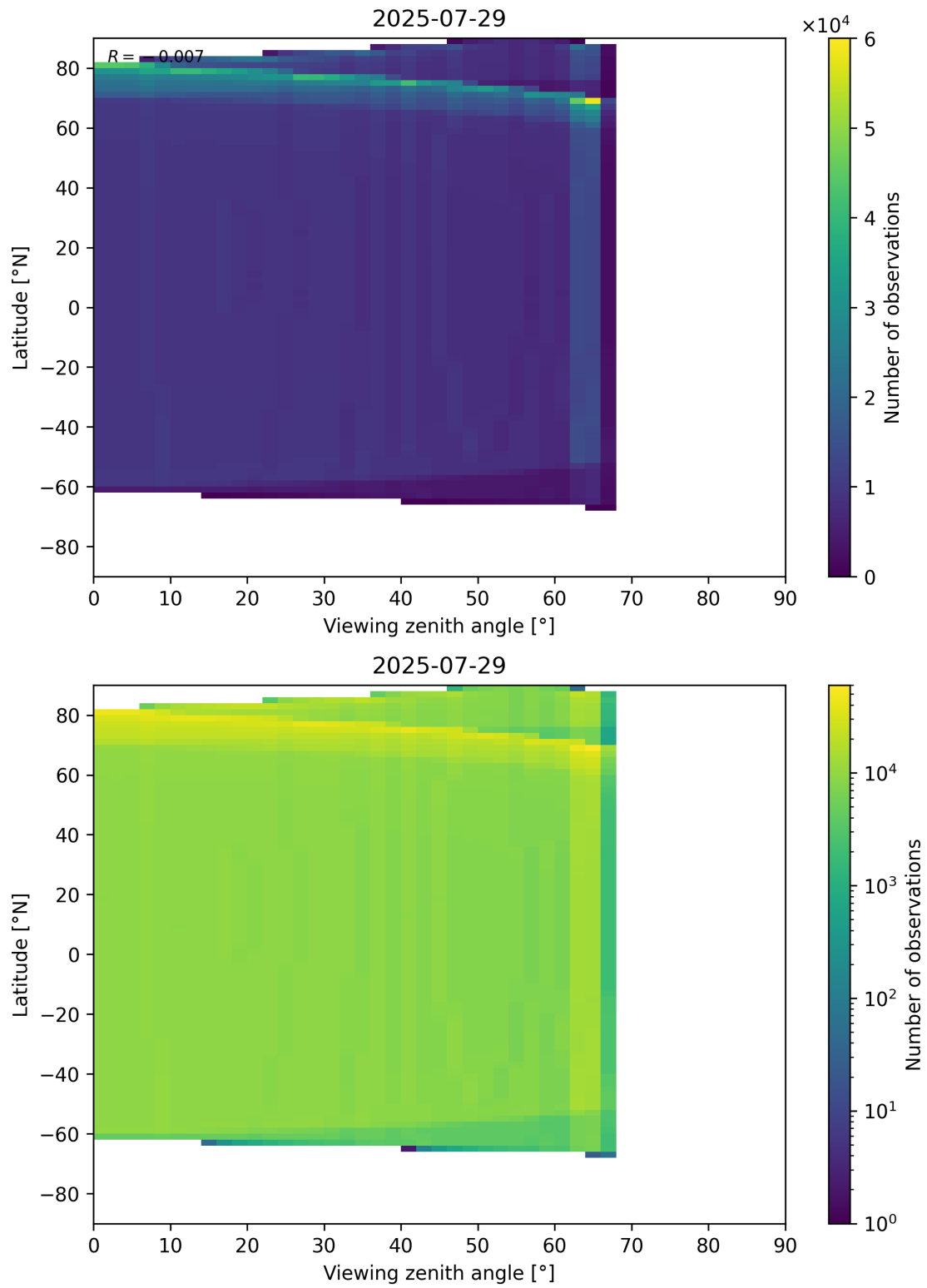
Figure 196: Scatter density plot of “Viewing zenith angle” against “Latitude” for 2025-07-29 to 2025-07-30.
