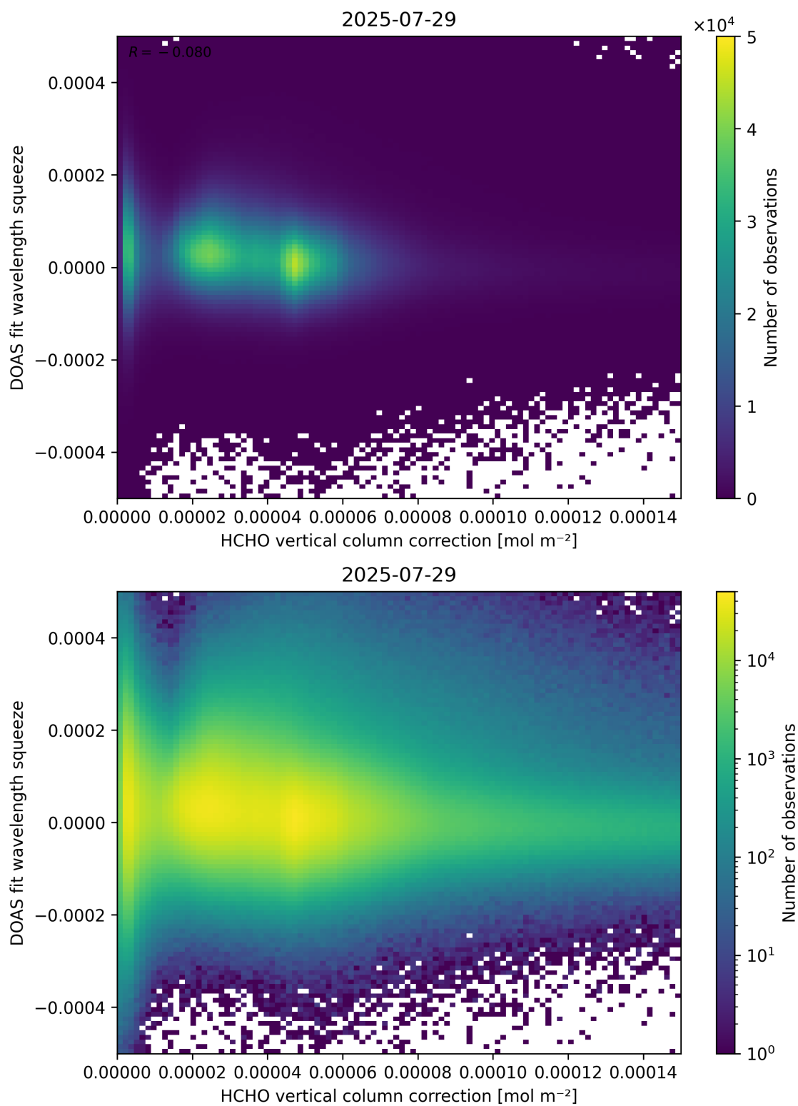
Figure 114: Scatter density plot of “HCHO vertical column correction” against “DOAS fit wavelength squeeze” for 2025-07-29 to 2025-07-30.
