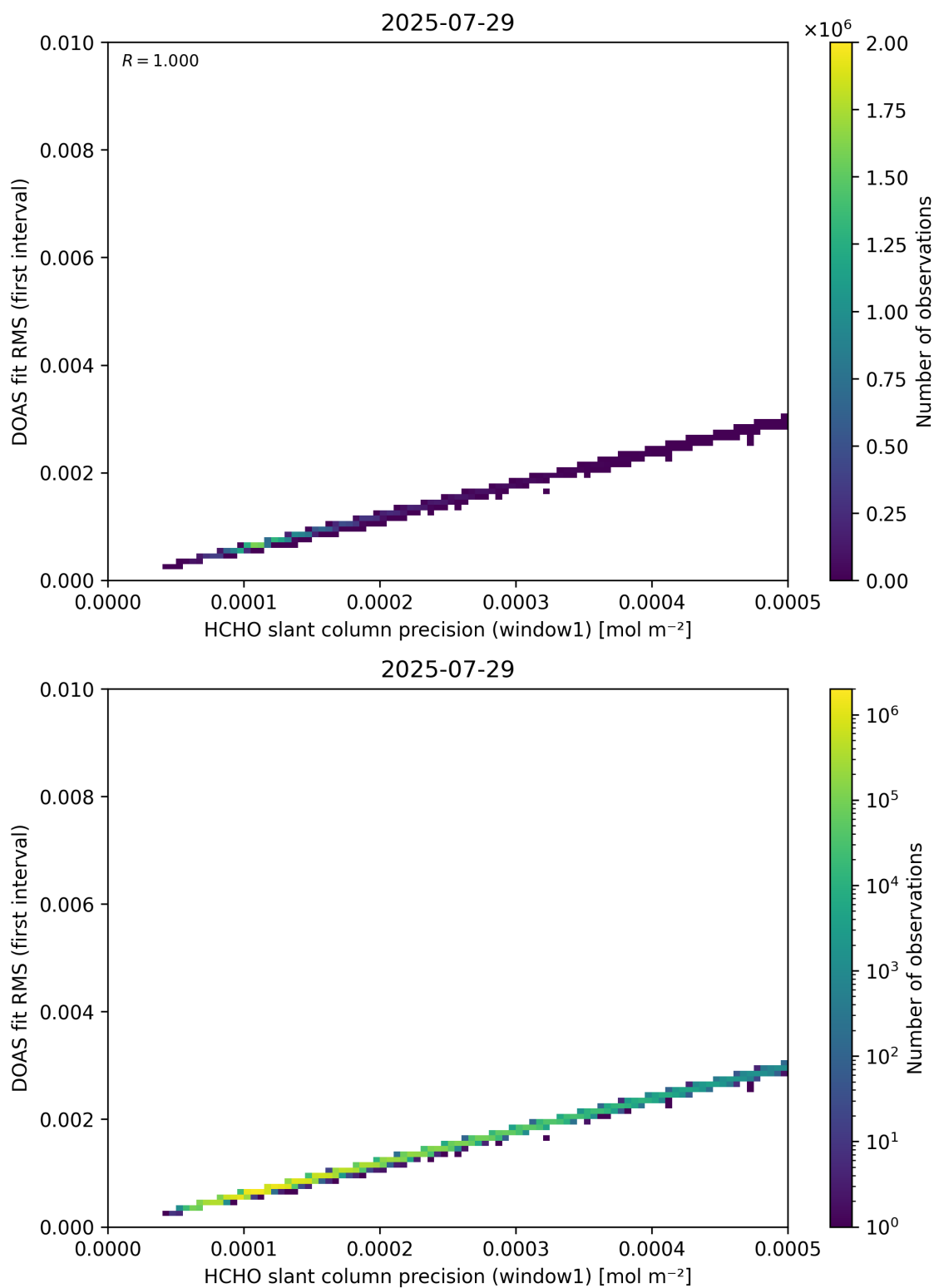
Figure 88: Scatter density plot of “HCHO slant column precision (window1)” against “DOAS fit RMS (first interval)” for 2025-07-29 to 2025-07-30.
