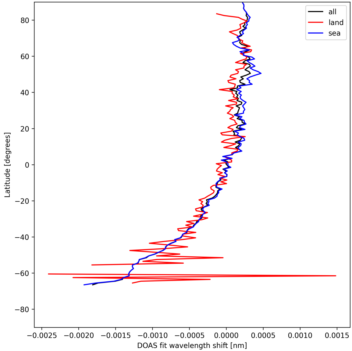
Figure 30: Zonal average of “DOAS fit wavelength shift” for 2025-07-29 to 2025-07-30.
