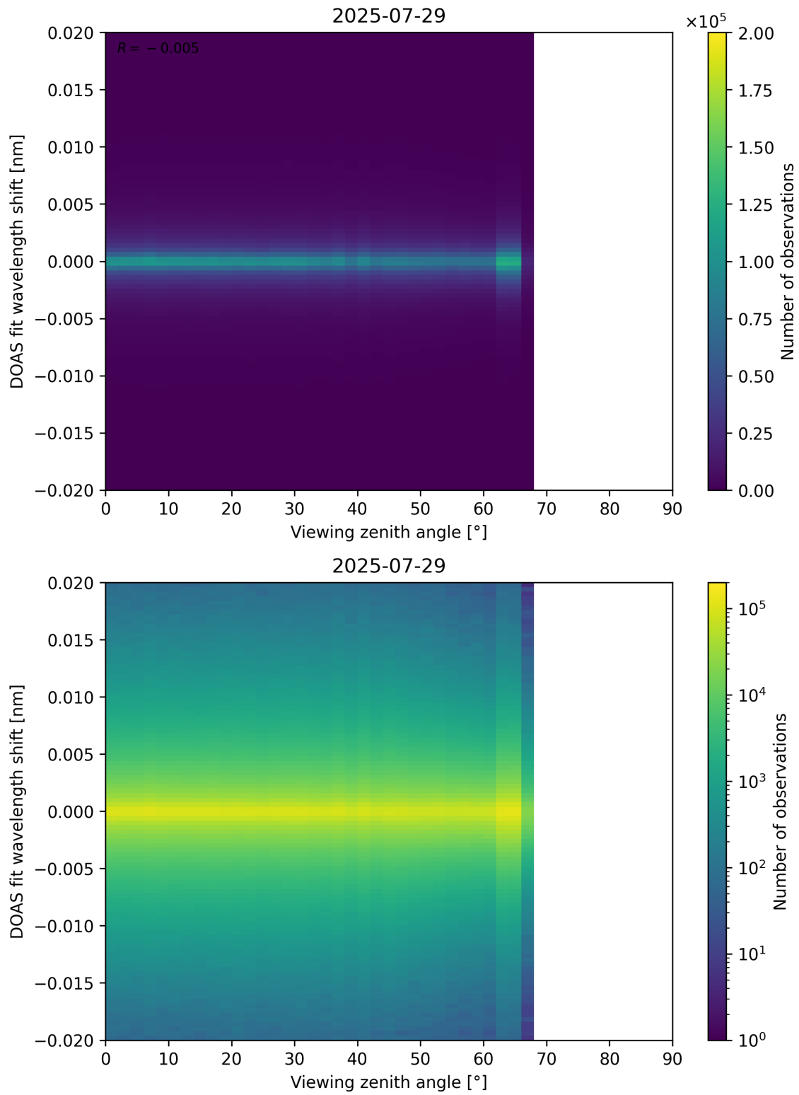
Figure 183: Scatter density plot of “Viewing zenith angle” against “DOAS fit wavelength shift” for 2025-07-29 to 2025-07-30.
