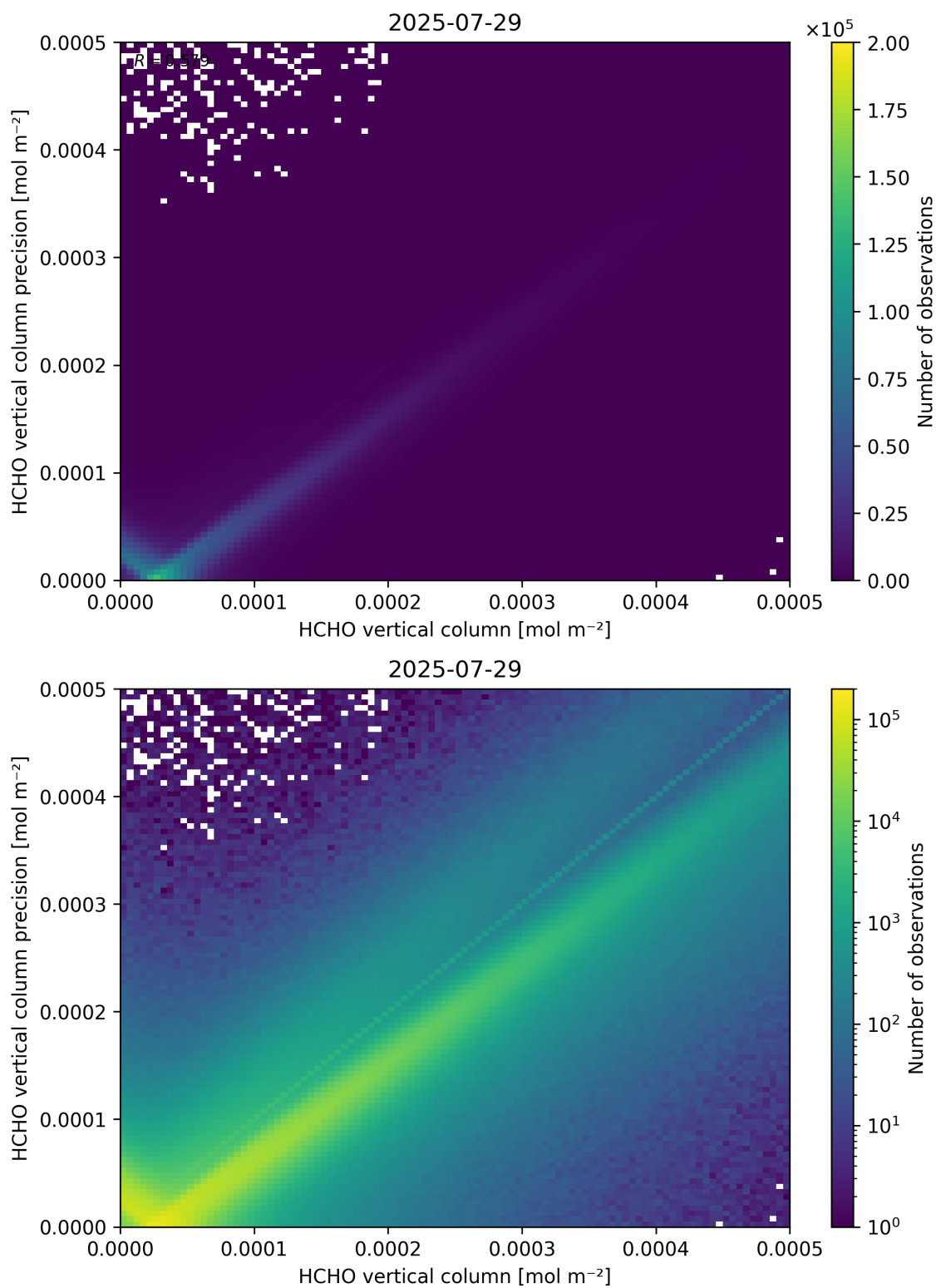
Figure 134: Scatter density plot of “HCHO vertical column” against “HCHO vertical column precision” for 2025-07-29 to 2025-07-30.
