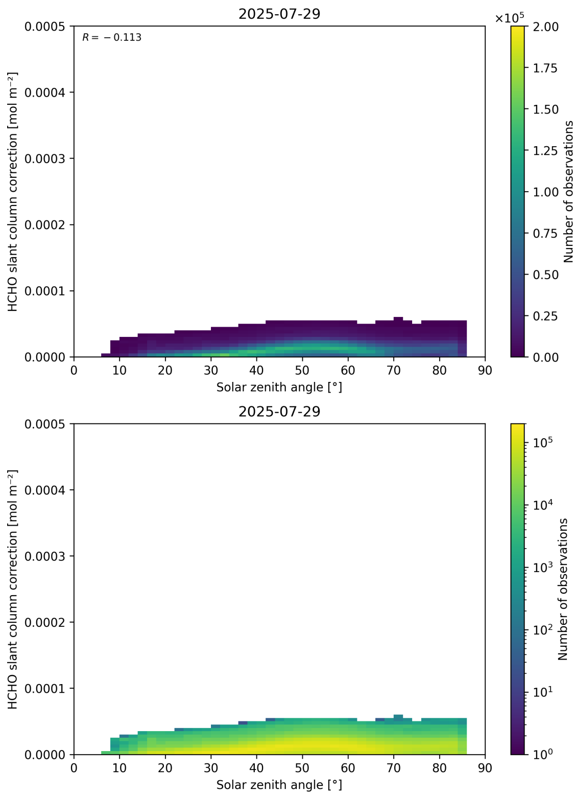
Figure 172: Scatter density plot of “Solar zenith angle” against “HCHO slant column correction” for 2025-07-29 to 2025-07-30.
