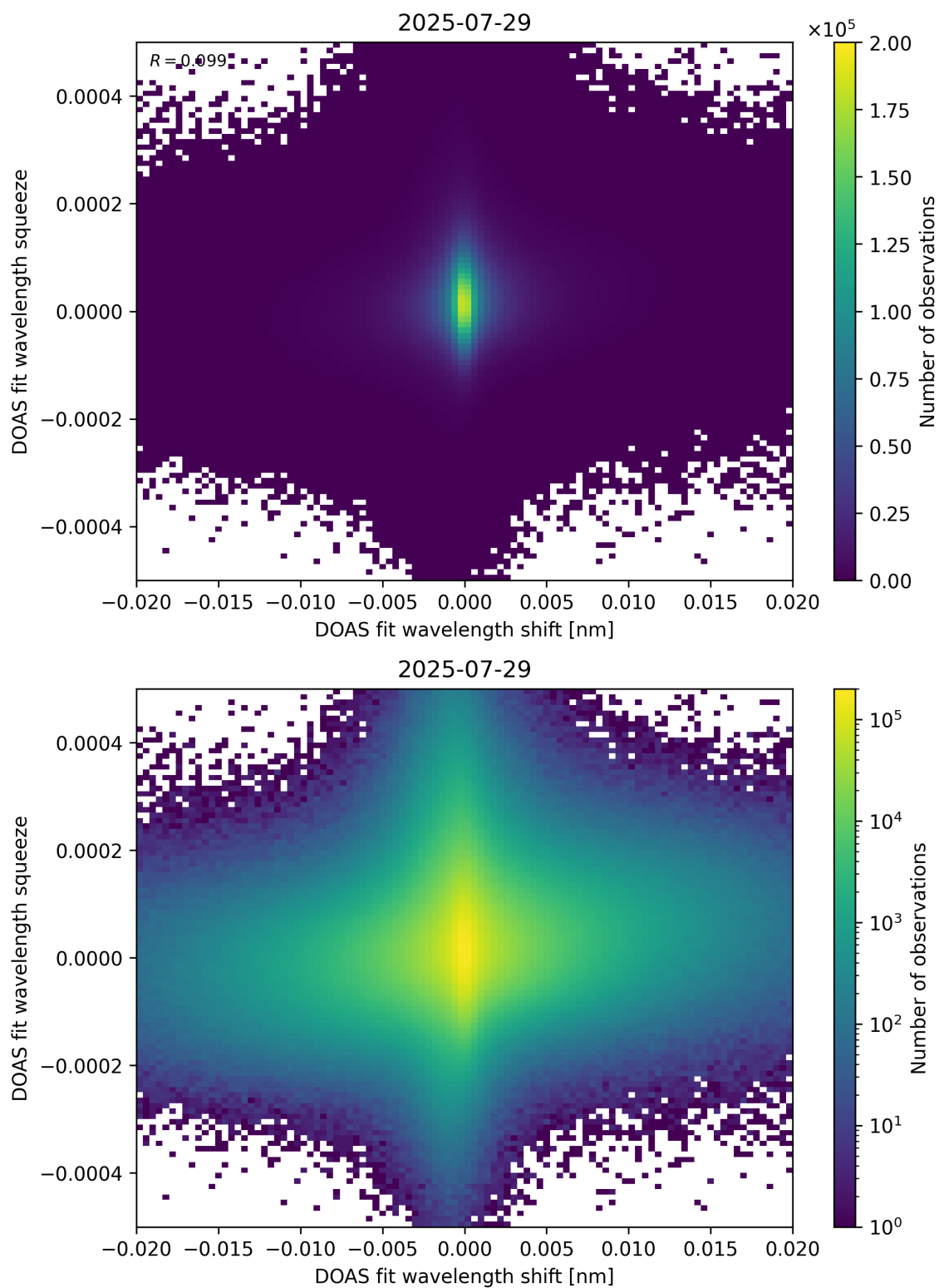
Figure 65: Scatter density plot of “DOAS fit wavelength shift” against “DOAS fit wavelength squeeze” for 2025-07-29 to 2025-07-30.
