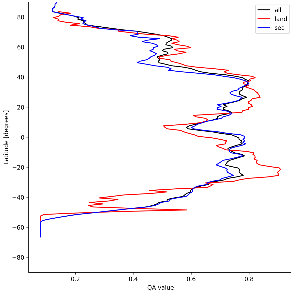
Figure 20: Zonal average of “QA value” for 2025-07-29 to 2025-07-30.
