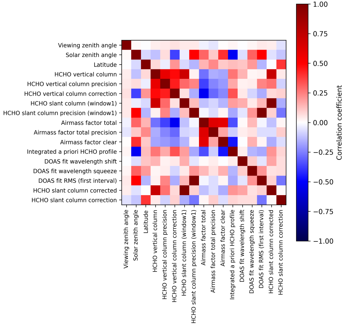
Figure 2: Map of correlation matrix for 2025-07-29 to 2025-07-30.
