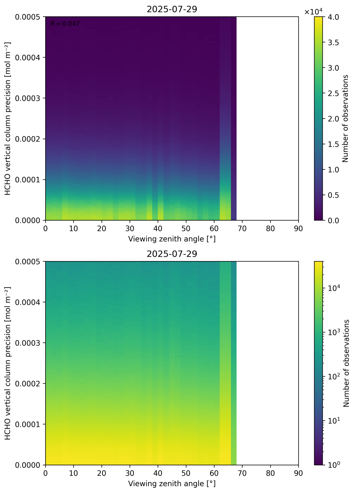
Figure 194: Scatter density plot of “Viewing zenith angle” against “HCHO vertical column precision” for 2025-07-29 to 2025-07-30.
