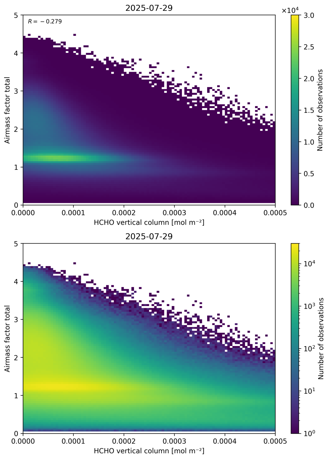
Figure 131: Scatter density plot of “HCHO vertical column” against “Airmass factor total” for 2025-07-29 to 2025-07-30.
