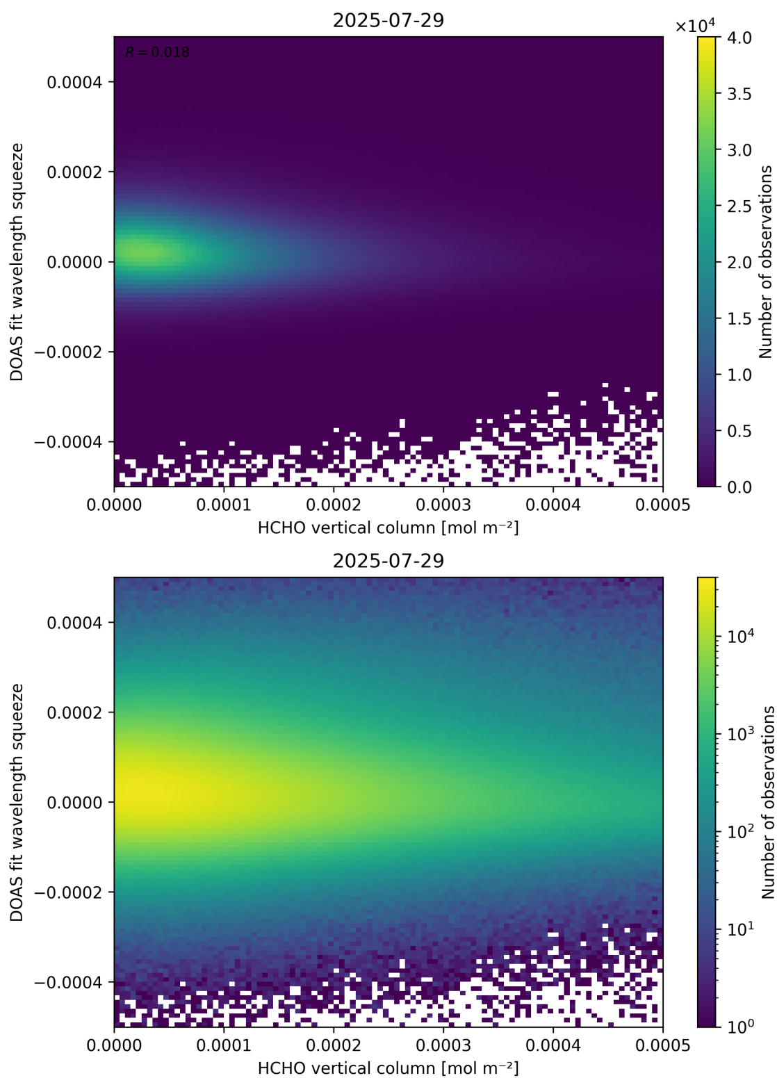
Figure 125: Scatter density plot of “HCHO vertical column” against “DOAS fit wavelength squeeze” for 2025-07-29 to 2025-07-30.
