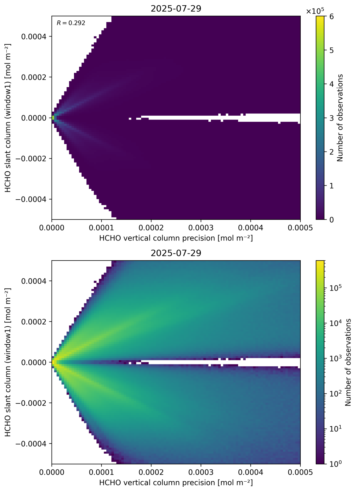
Figure 142: Scatter density plot of “HCHO vertical column precision” against “HCHO slant column (window1)” for 2025-07-29 to 2025-07-30.
