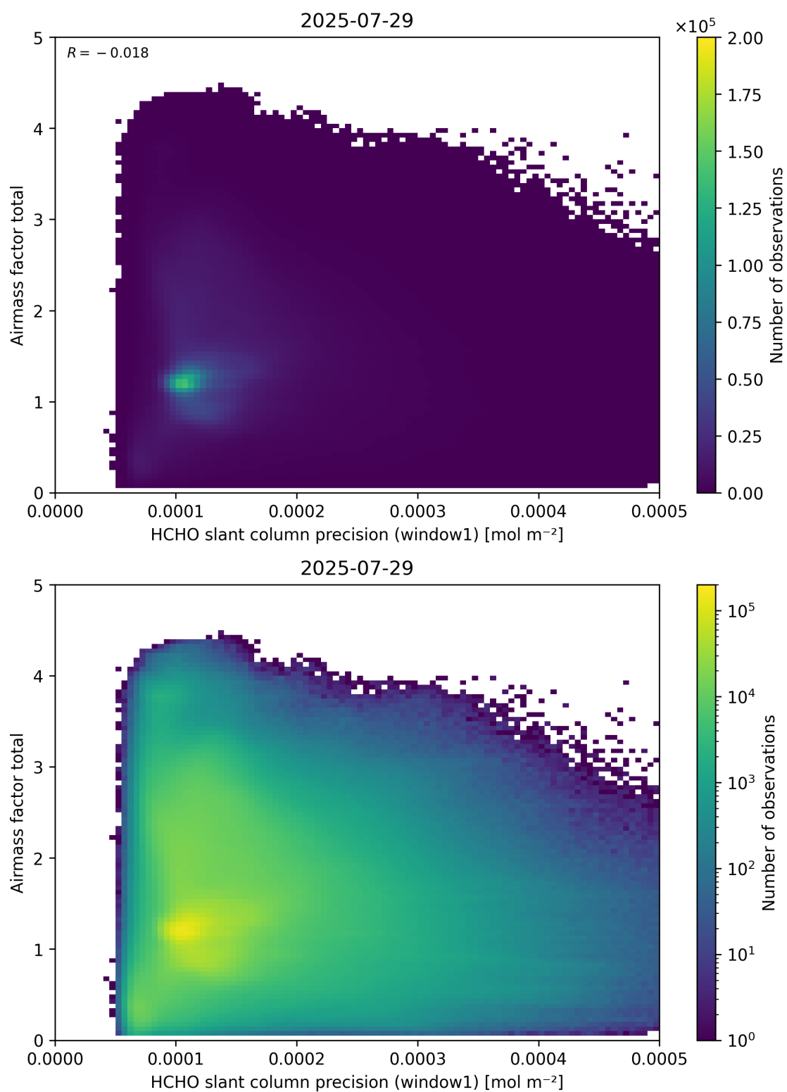
Figure 94: Scatter density plot of “HCHO slant column precision (window1)” against “Airmass factor total” for 2025-07-29 to 2025-07-30.
