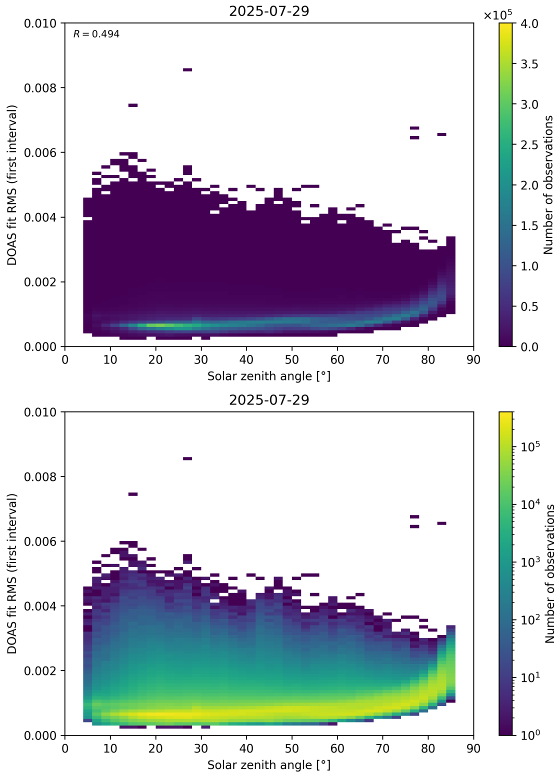
Figure 167: Scatter density plot of “Solar zenith angle” against “DOAS fit RMS (first interval)” for 2025-07-29 to 2025-07-30.
