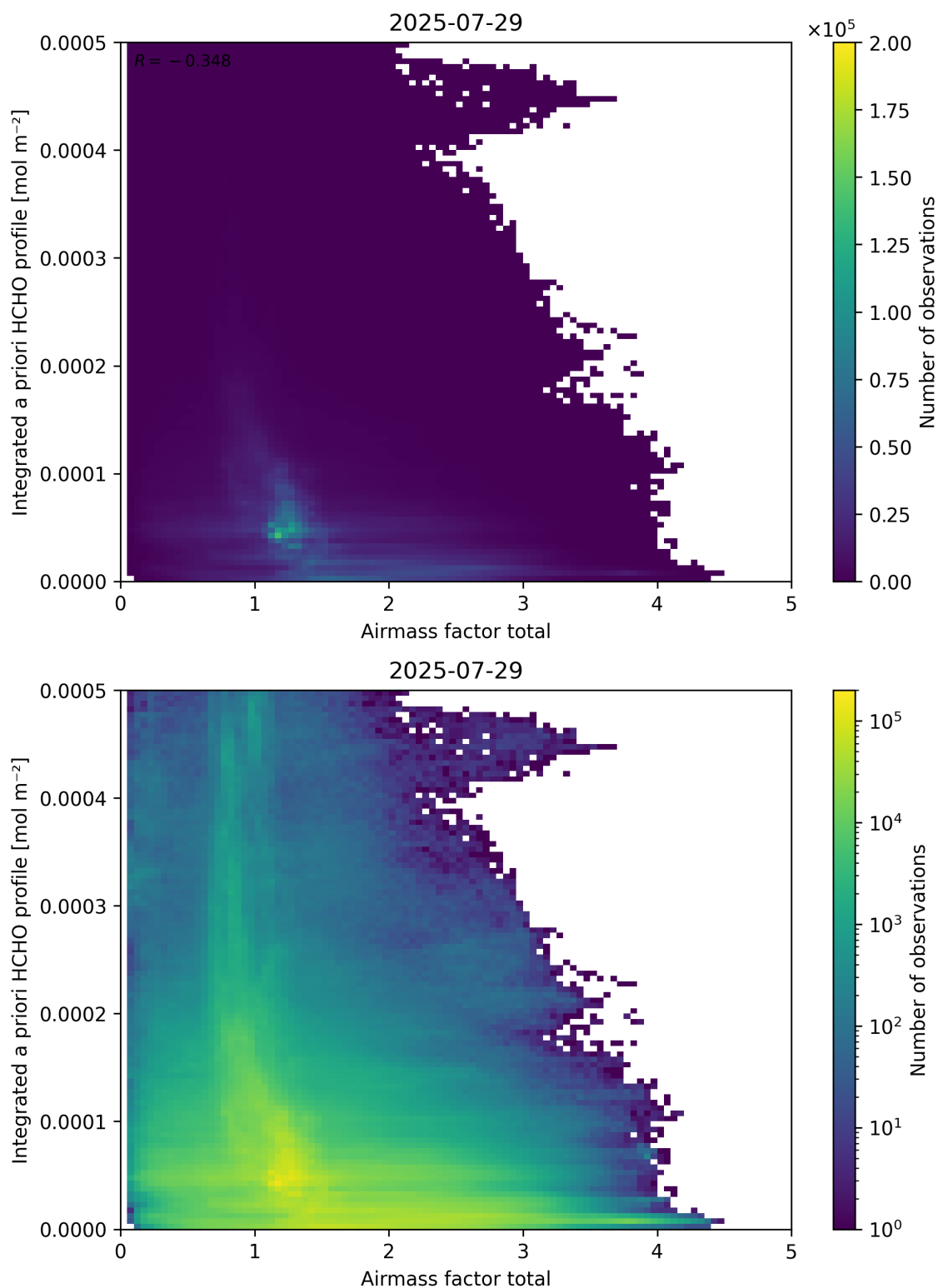
Figure 104: Scatter density plot of “Airmass factor total” against “Integrated a priori HCHO profile” for 2025-07-29 to 2025-07-30.
