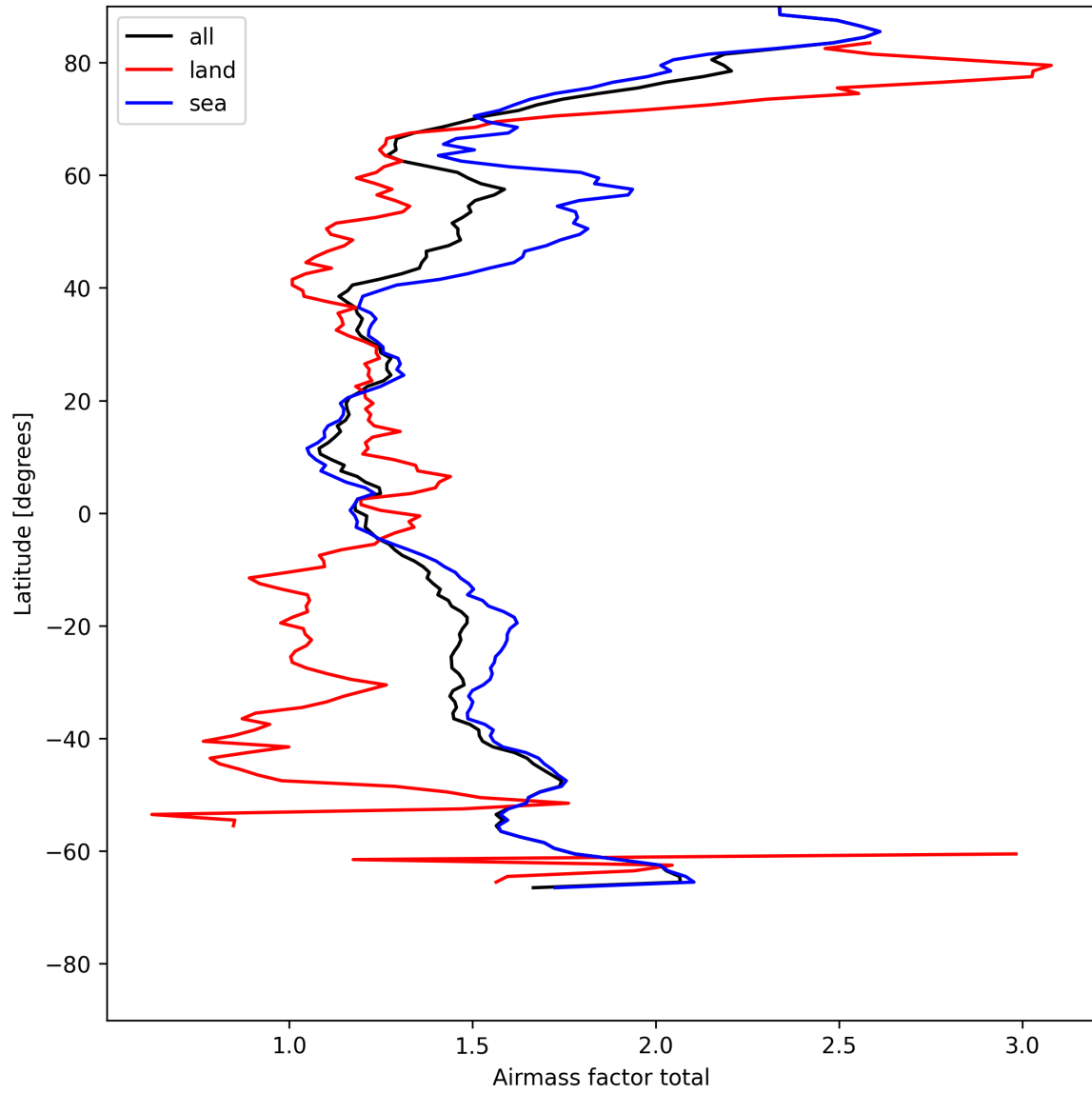
Figure 26: Zonal average of “Airmass factor total” for 2025-07-29 to 2025-07-30.
