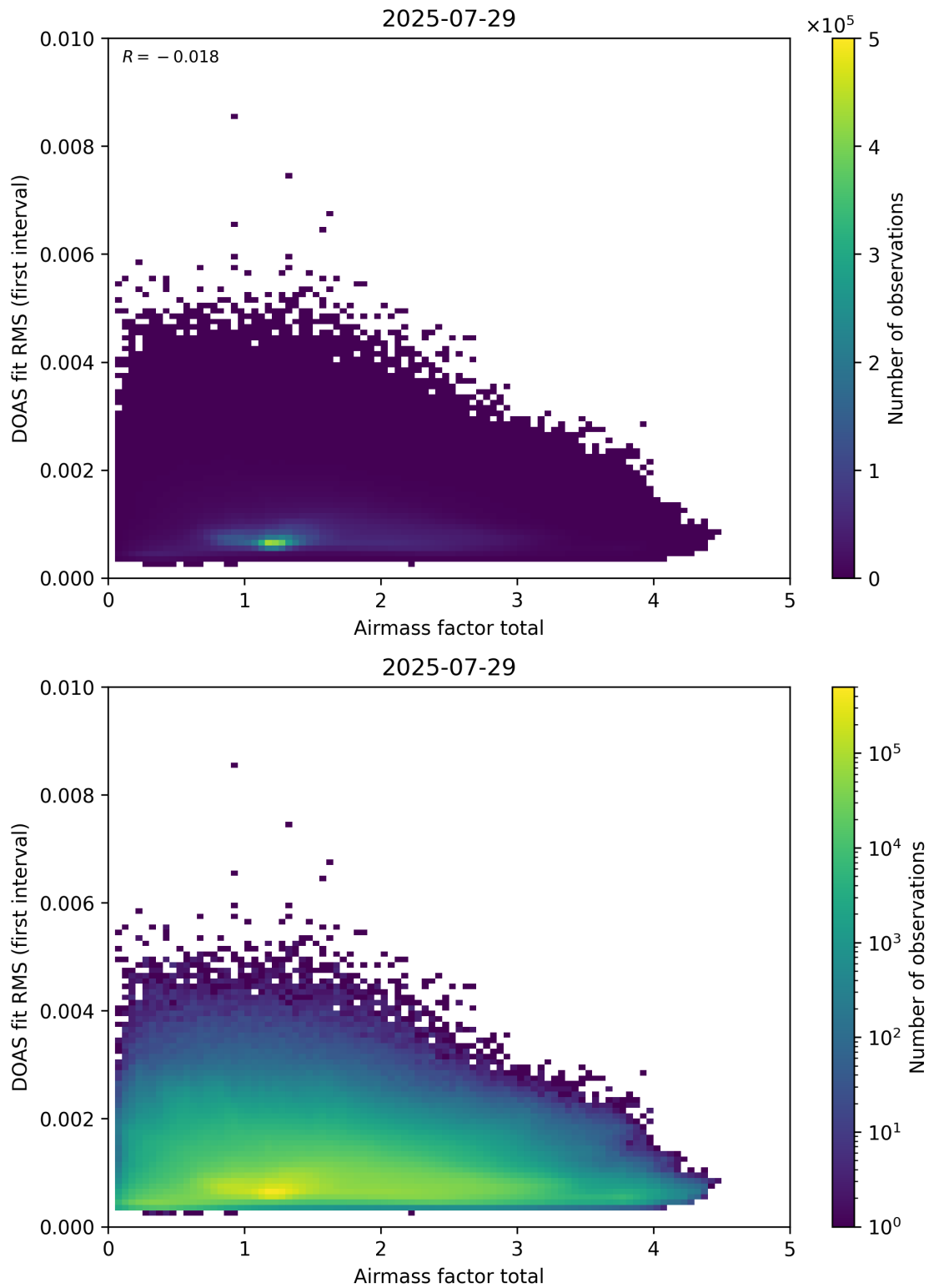
Figure 97: Scatter density plot of “Airmass factor total” against “DOAS fit RMS (first interval)” for 2025-07-29 to 2025-07-30.
