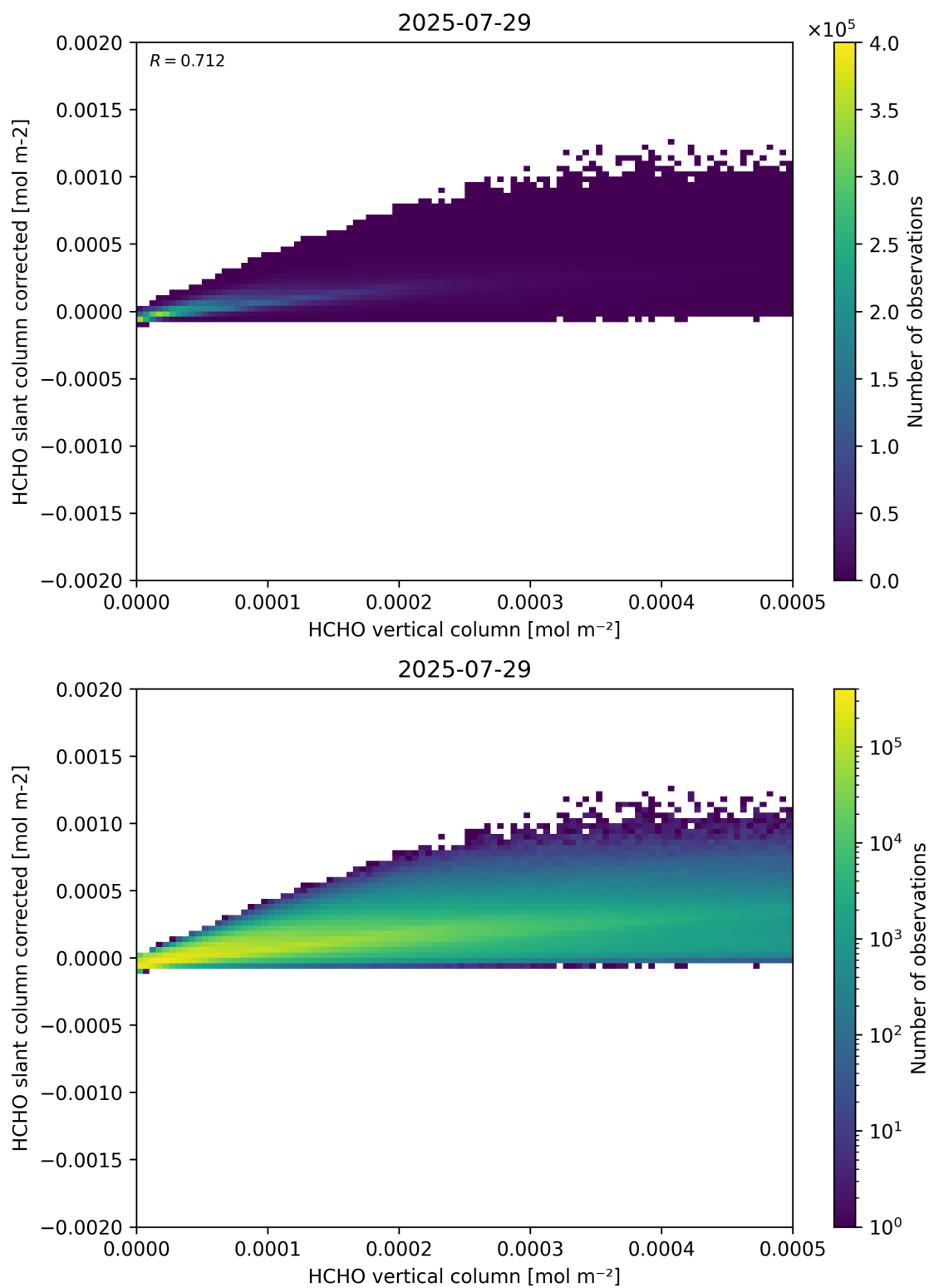
Figure 127: Scatter density plot of “HCHO vertical column” against “HCHO slant column corrected” for 2025-07-29 to 2025-07-30.
