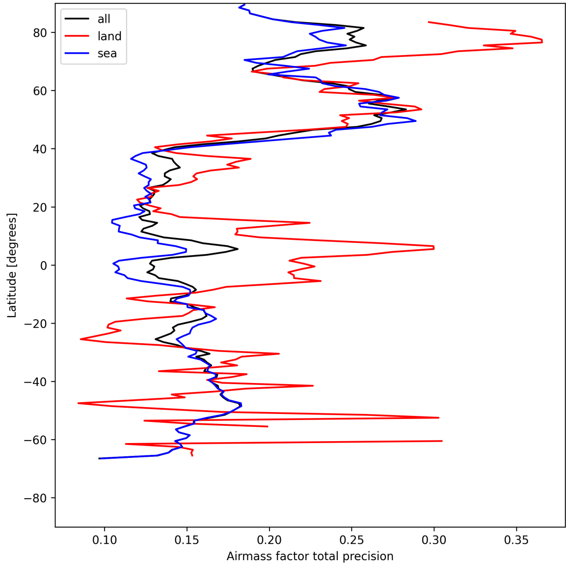
Figure 27: Zonal average of “Airmass factor total precision” for 2025-07-29 to 2025-07-30.
