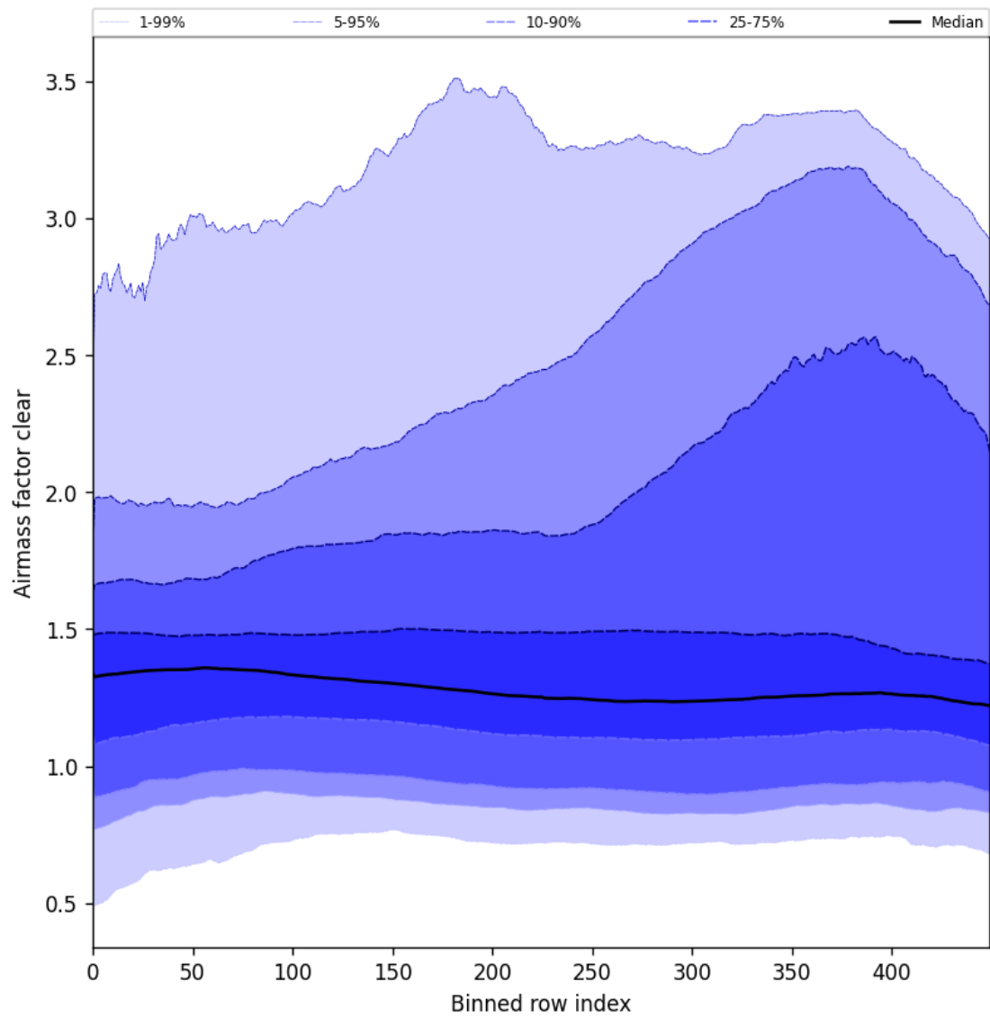
Figure 56: Along track statistics of “Airmass factor clear” for 2025-07-29 to 2025-07-30
