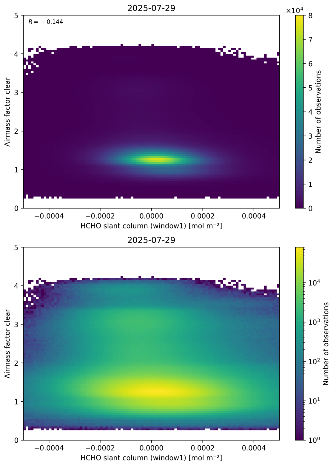
Figure 81: Scatter density plot of “HCHO slant column (window1)” against “Airmass factor clear” for 2025-07-29 to 2025-07-30.
