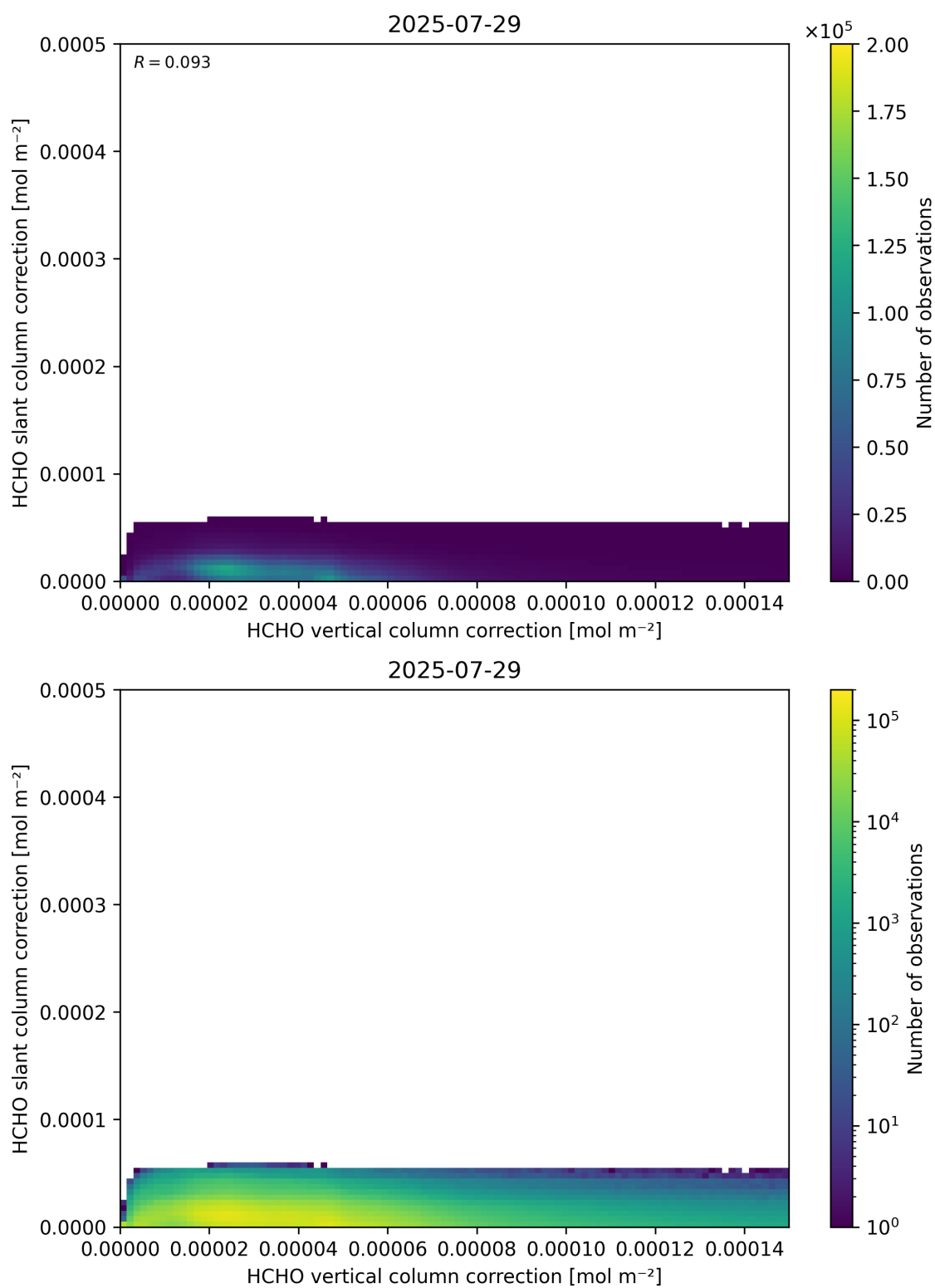
Figure 117: Scatter density plot of “HCHO vertical column correction” against “HCHO slant column correction” for 2025-07-29 to 2025-07-30.
