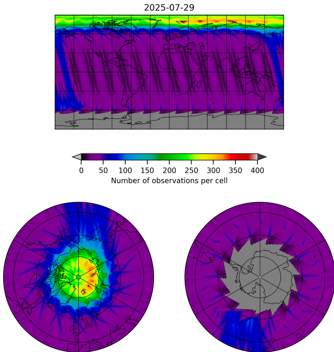
Figure 19: Map of the number of observations for 2025-07-29 to 2025-07-30
