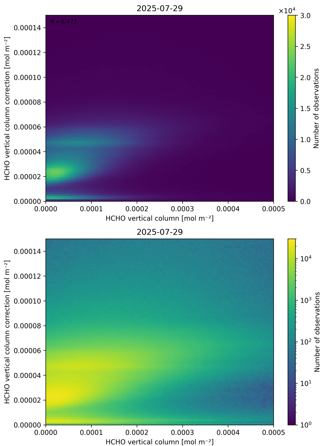
Figure 133: Scatter density plot of “HCHO vertical column” against “HCHO vertical column correction” for 2025-07-29 to 2025-07-30.
