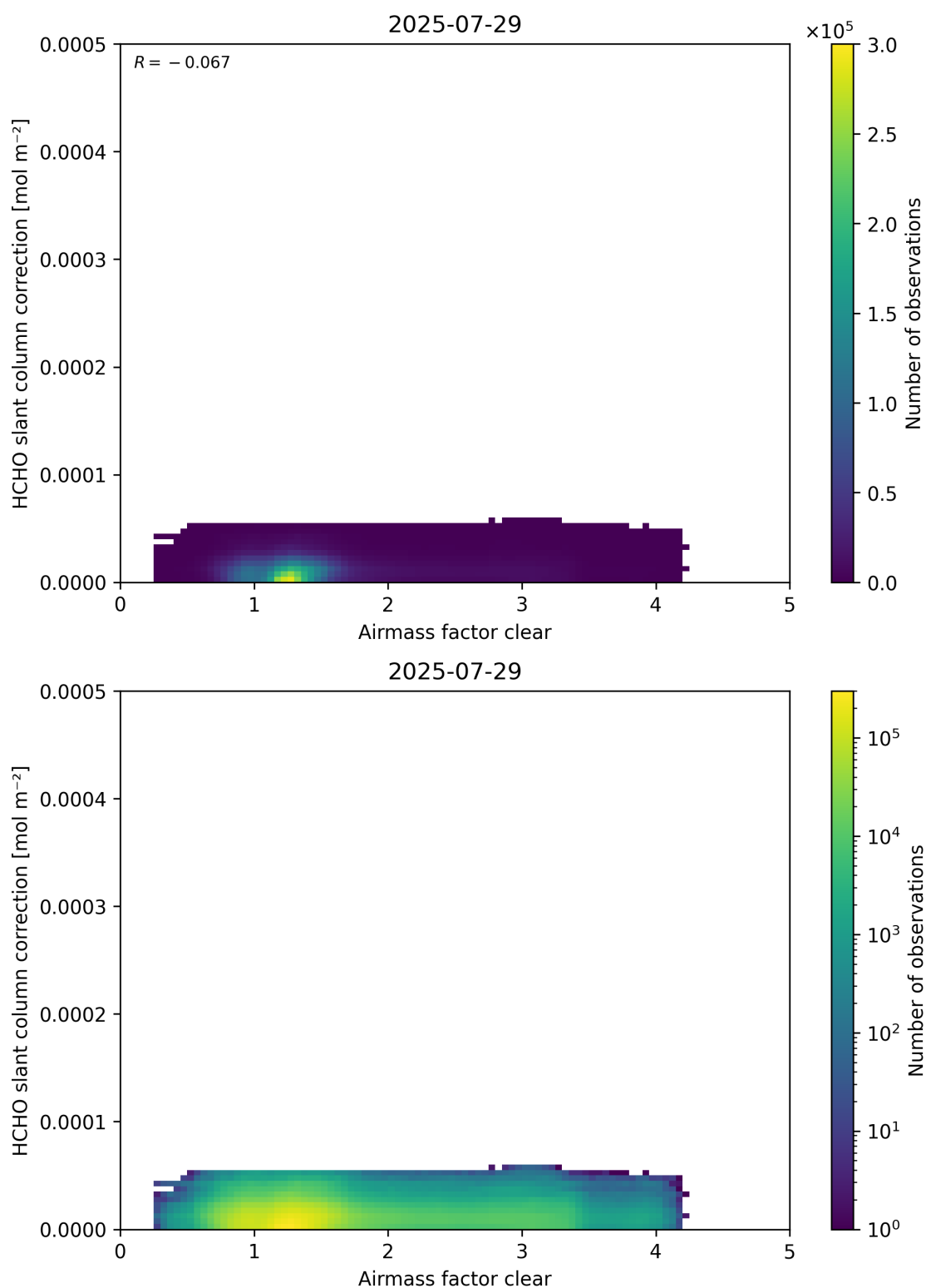
Figure 75: Scatter density plot of “Airmass factor clear” against “HCHO slant column correction” for 2025-07-29 to 2025-07-30.
