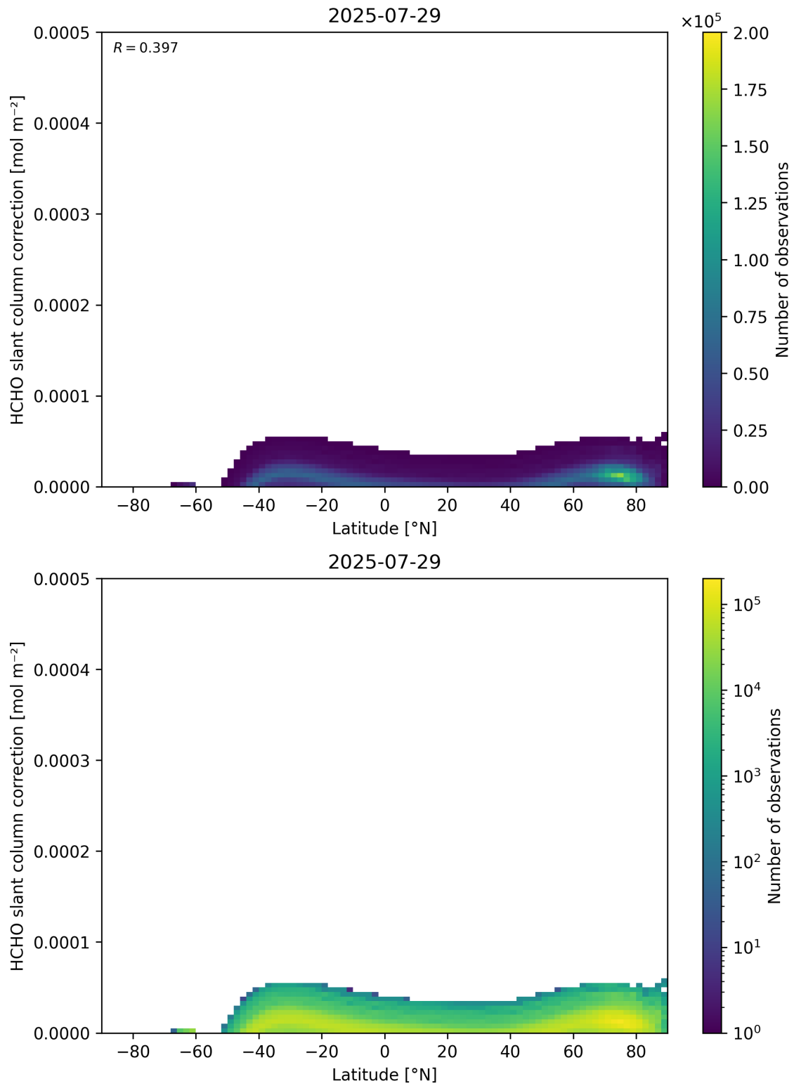
Figure 158: Scatter density plot of “Latitude” against “HCHO slant column correction” for 2025-07-29 to 2025-07-30.
