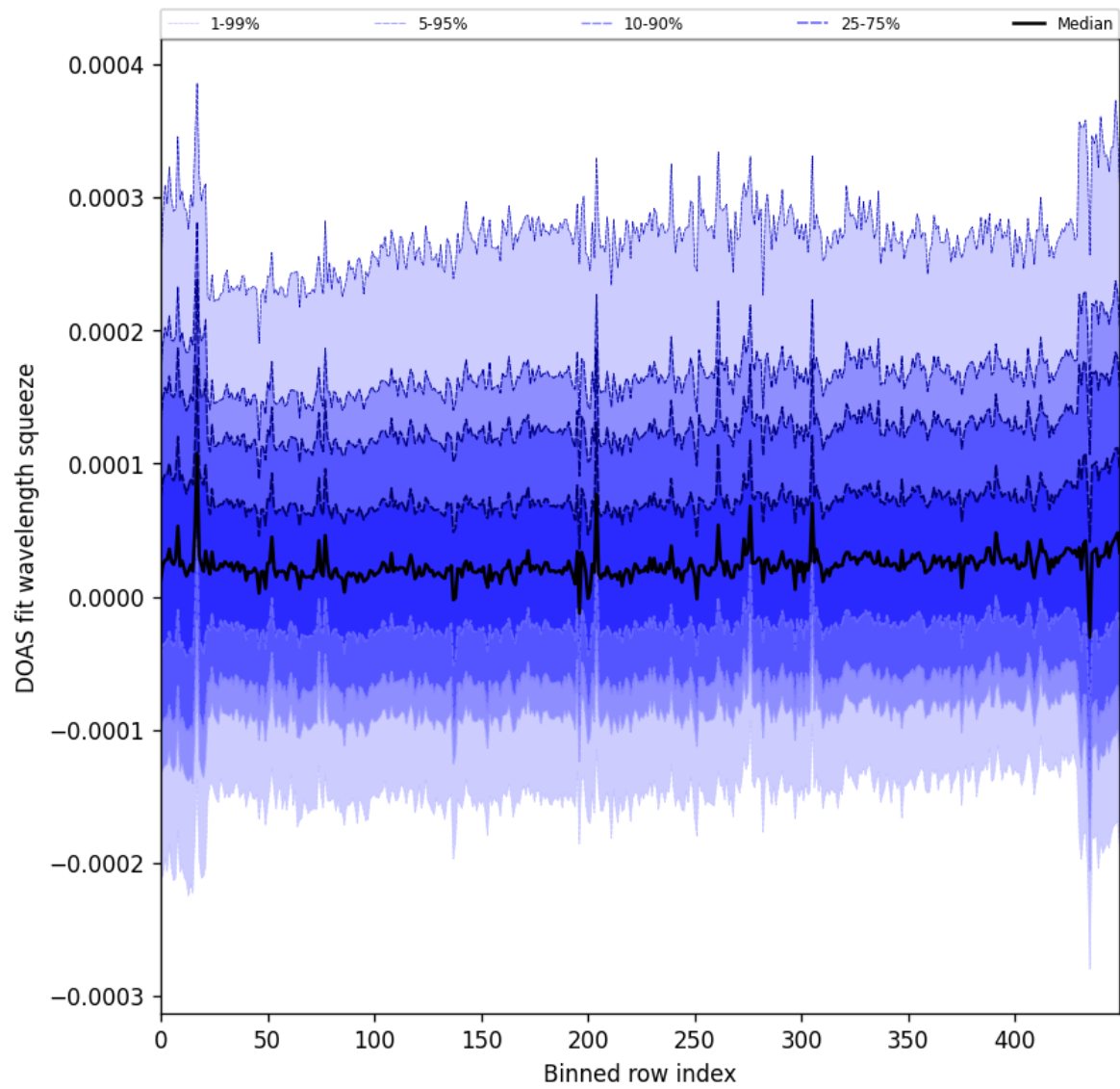
Figure 59: Along track statistics of “DOAS fit wavelength squeeze” for 2025-07-29 to 2025-07-30
