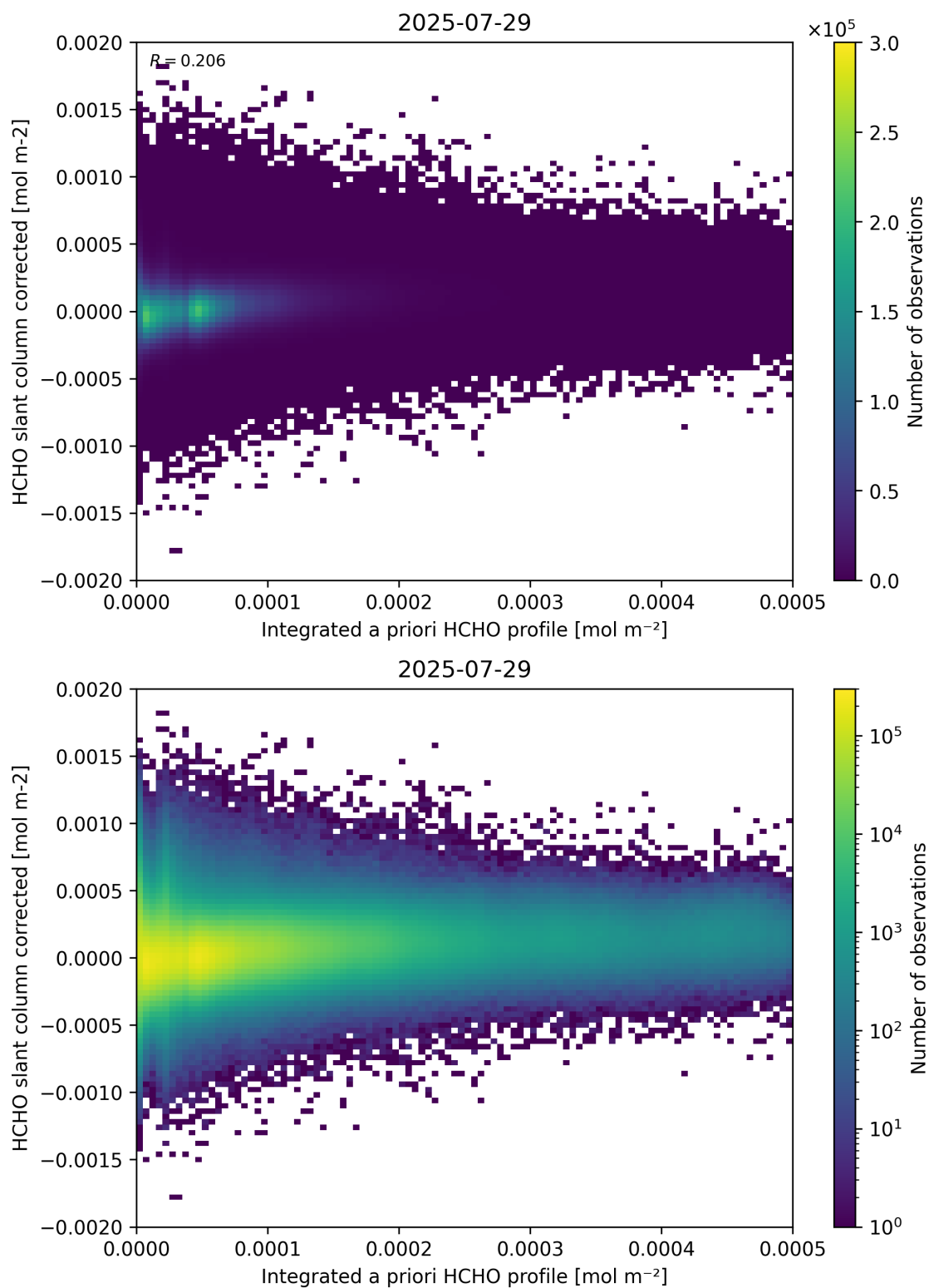
Figure 151: Scatter density plot of “Integrated a priori HCHO profile” against “HCHO slant column corrected” for 2025-07-29 to 2025-07-30.
