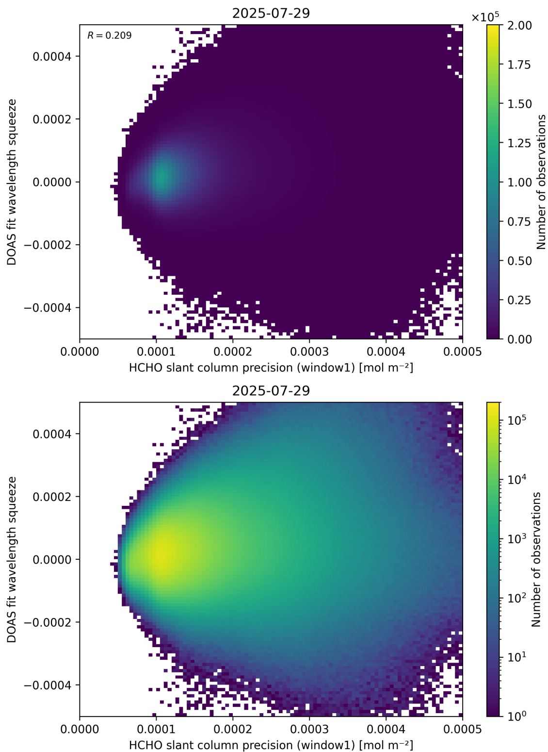
Figure 90: Scatter density plot of “HCHO slant column precision (window1)” against “DOAS fit wavelength squeeze” for 2025-07-29 to 2025-07-30.
