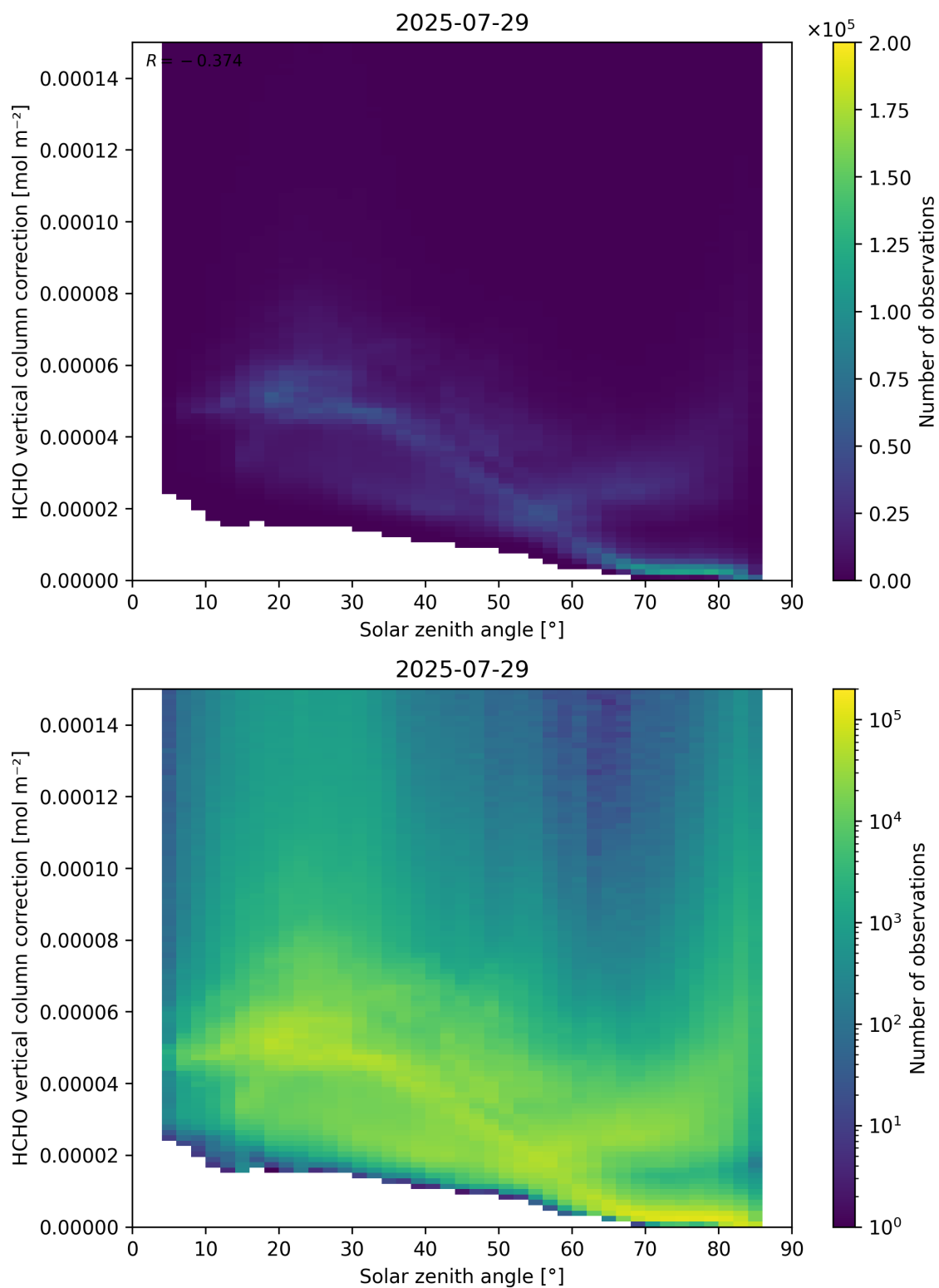
Figure 178: Scatter density plot of “Solar zenith angle” against “HCHO vertical column correction” for 2025-07-29 to 2025-07-30.
