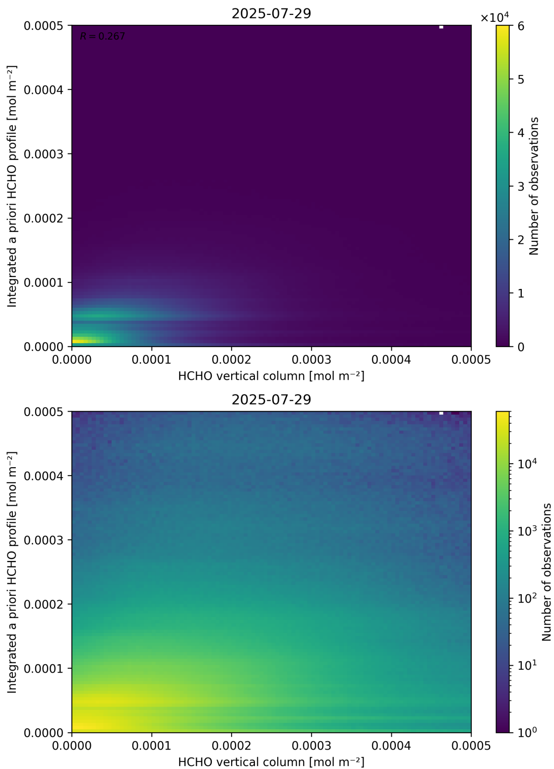
Figure 135: Scatter density plot of “HCHO vertical column” against “Integrated a priori HCHO profile” for 2025-07-29 to 2025-07-30.
