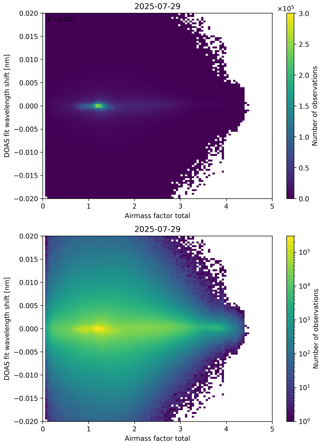
Figure 98: Scatter density plot of “Airmass factor total” against “DOAS fit wavelength shift” for 2025-07-29 to 2025-07-30.
