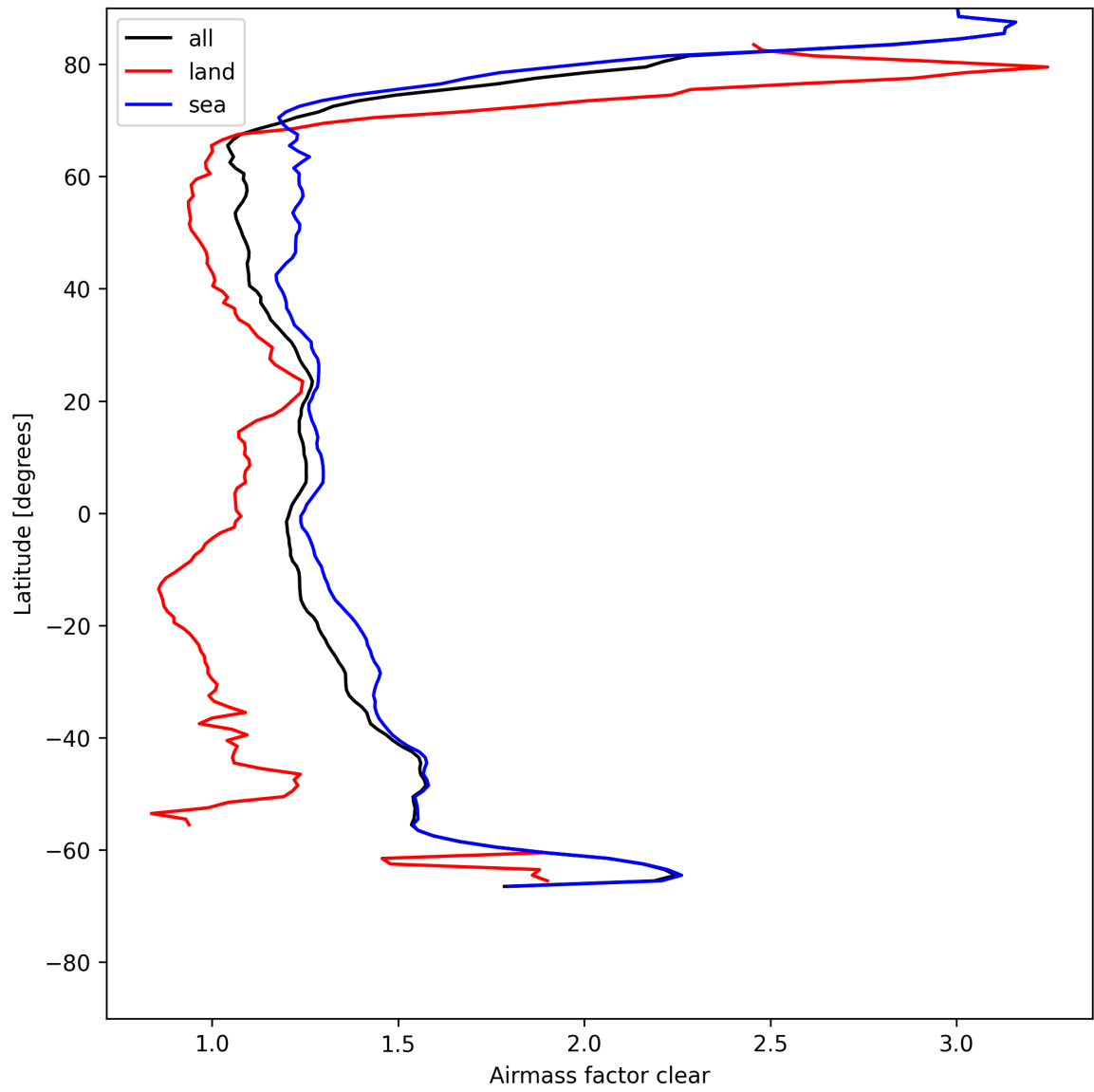
Figure 28: Zonal average of “Airmass factor clear” for 2025-07-29 to 2025-07-30.
