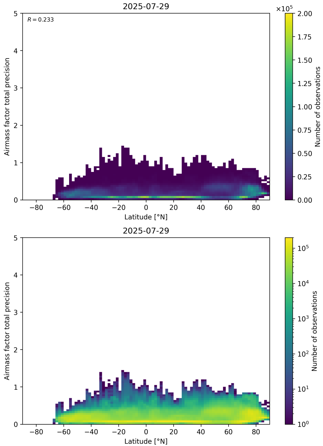
Figure 162: Scatter density plot of “Latitude” against “Airmass factor total precision” for 2025-07-29 to 2025-07-30.
