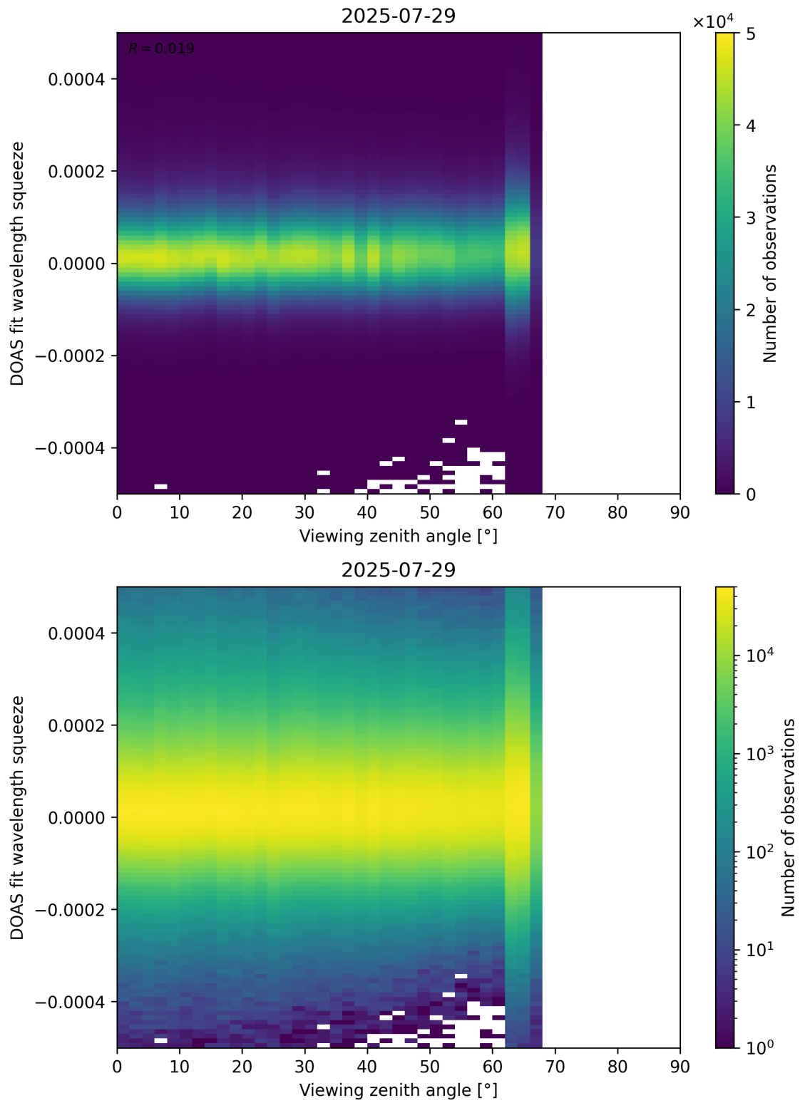
Figure 184: Scatter density plot of “Viewing zenith angle” against “DOAS fit wavelength squeeze” for 2025-07-29 to 2025-07-30.
