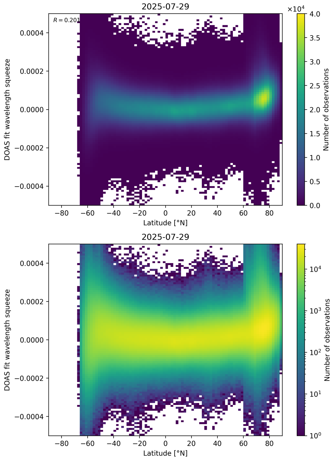
Figure 155: Scatter density plot of “Latitude” against “DOAS fit wavelength squeeze” for 2025-07-29 to 2025-07-30.
