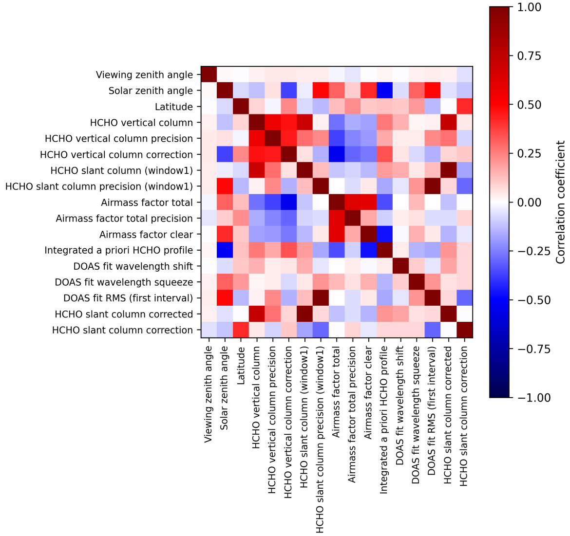
Figure 2: Map of correlation matrix for 2025-07-29 to 2025-07-31.
