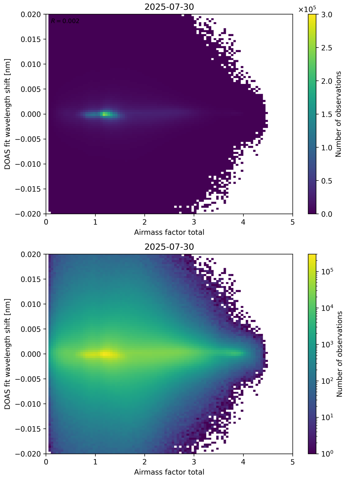
Figure 98: Scatter density plot of “Airmass factor total” against “DOAS fit wavelength shift” for 2025-07-29 to 2025-07-31.
