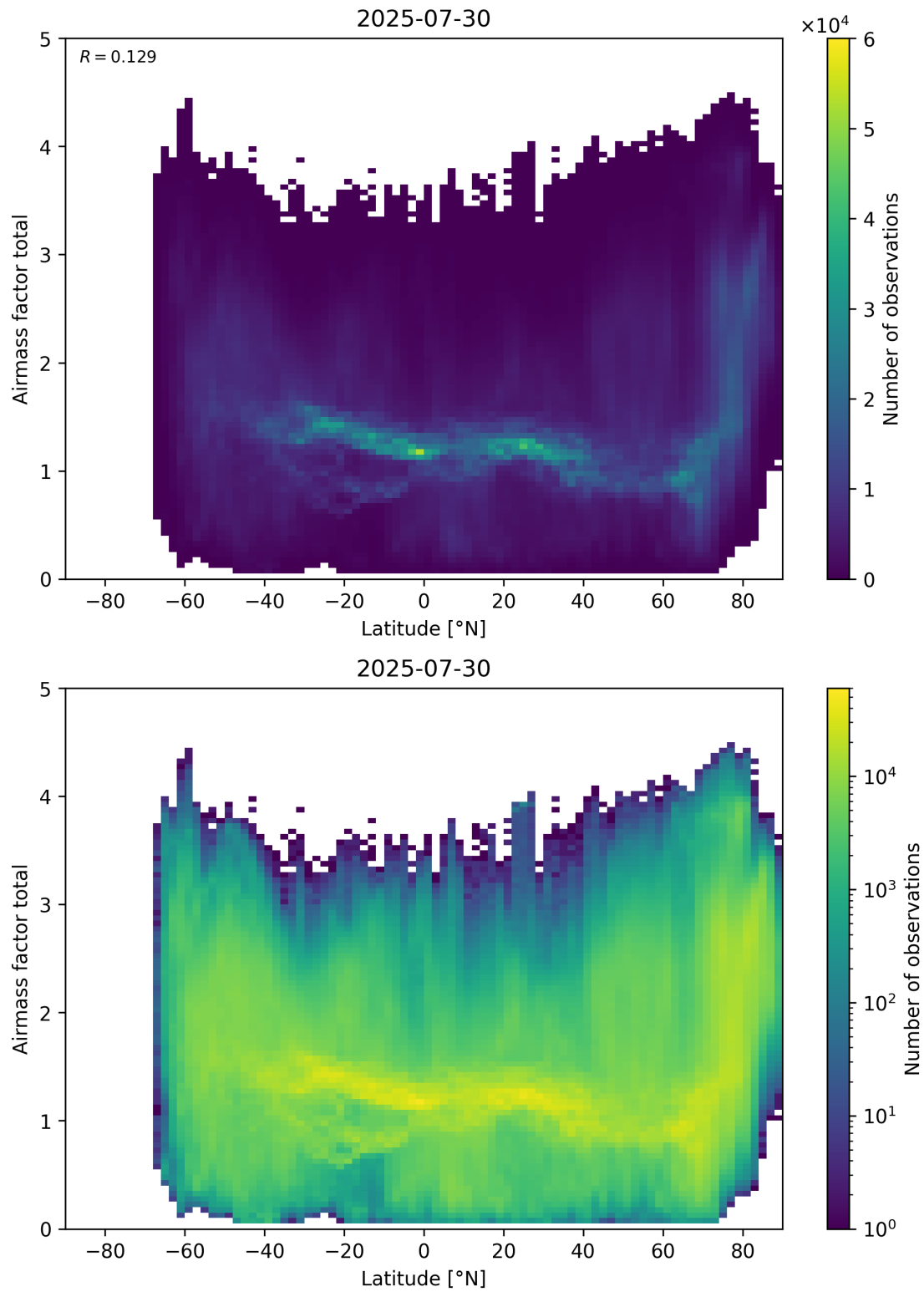
Figure 161: Scatter density plot of “Latitude” against “Airmass factor total” for 2025-07-29 to 2025-07-31.
