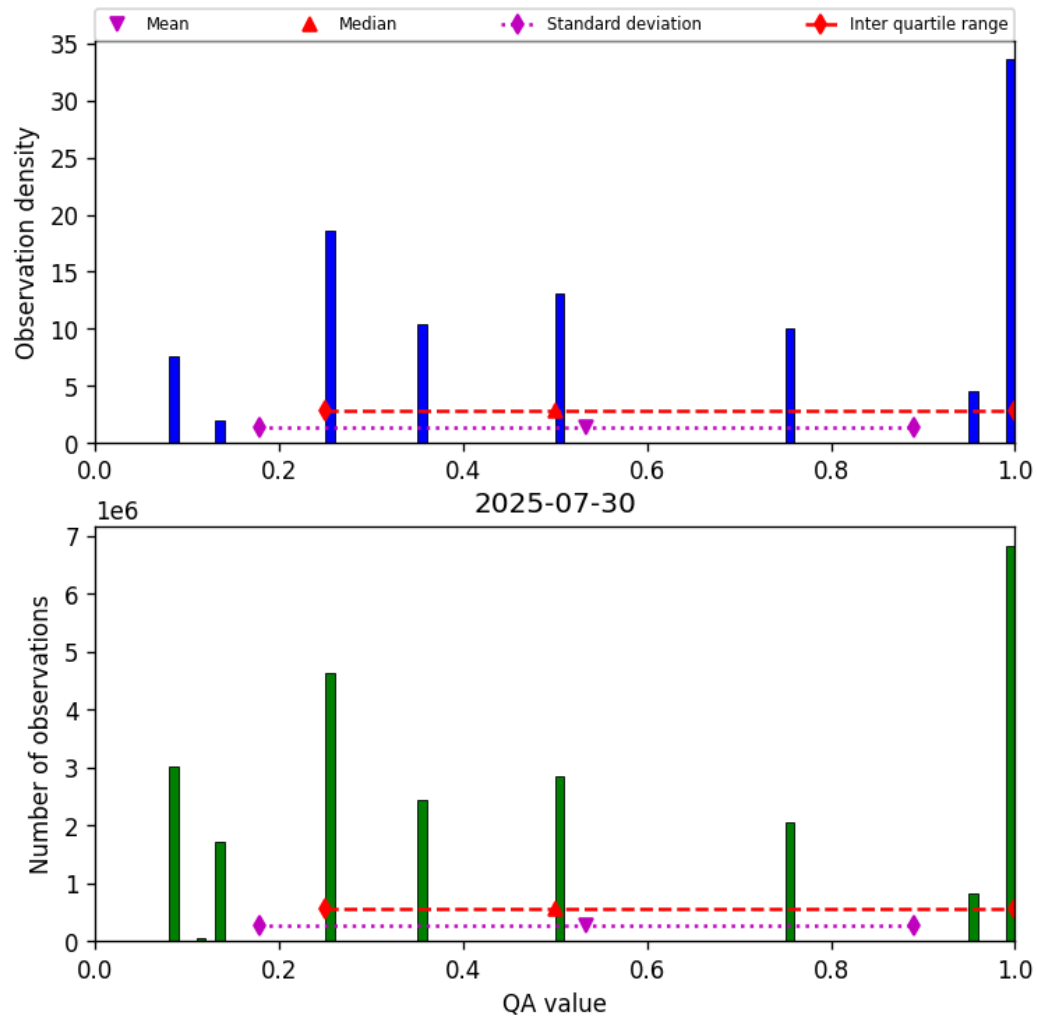
Figure 34: Histogram of “QA value” for 2025-07-29 to 2025-07-31
