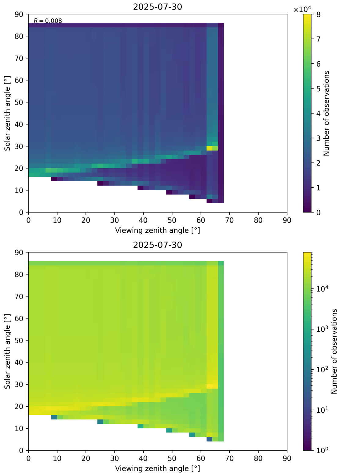
Figure 197: Scatter density plot of “Viewing zenith angle” against “Solar zenith angle” for 2025-07-29 to 2025-07-31.
