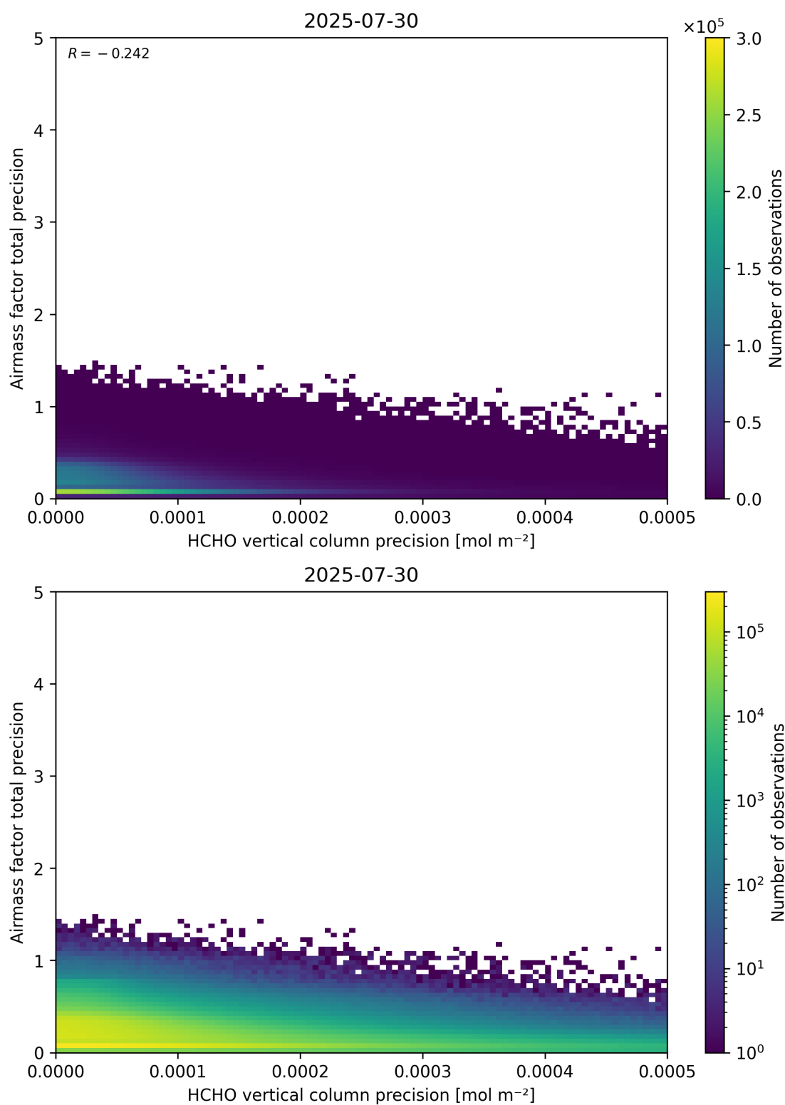
Figure 145: Scatter density plot of “HCHO vertical column precision” against “Airmass factor total precision” for 2025-07-29 to 2025-07-31.
