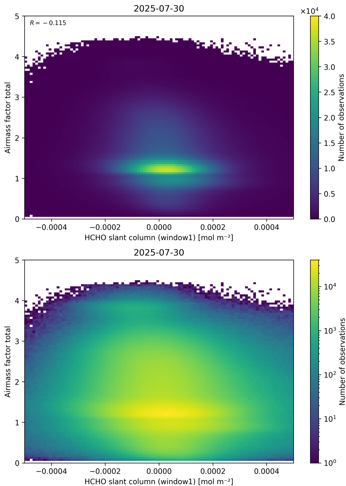
Figure 85: Scatter density plot of “HCHO slant column (window1)” against “Airmass factor total” for 2025-07-29 to 2025-07-31.
