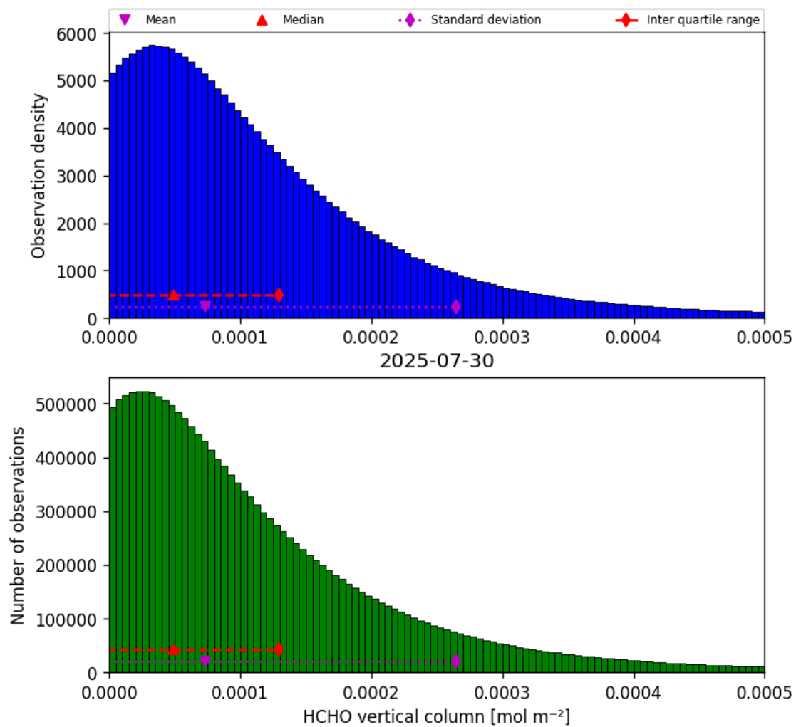
Figure 35: Histogram of “HCHO vertical column” for 2025-07-29 to 2025-07-31
