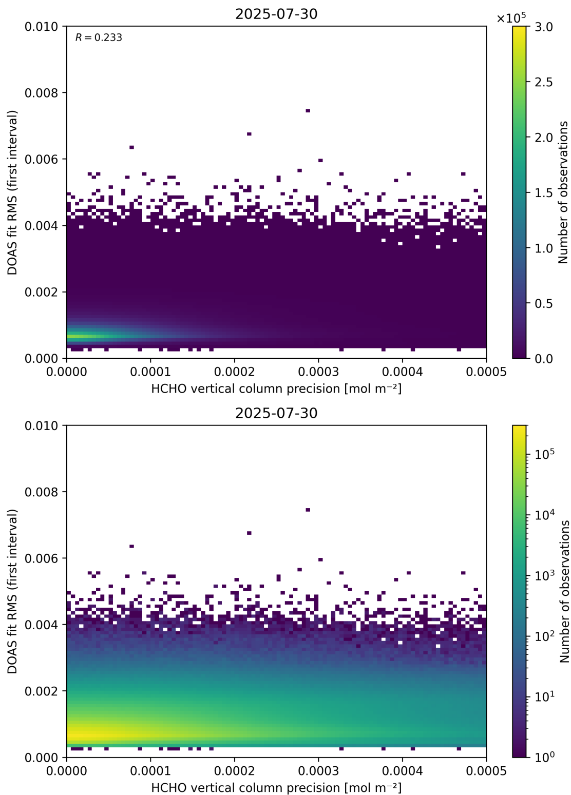
Figure 136: Scatter density plot of “HCHO vertical column precision” against “DOAS fit RMS (first interval)” for 2025-07-29 to 2025-07-31.
