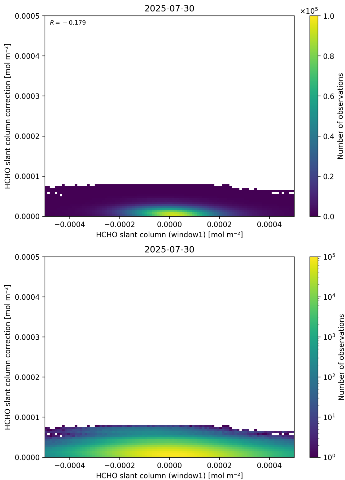
Figure 83: Scatter density plot of “HCHO slant column (window1)” against “HCHO slant column correction” for 2025-07-29 to 2025-07-31.
