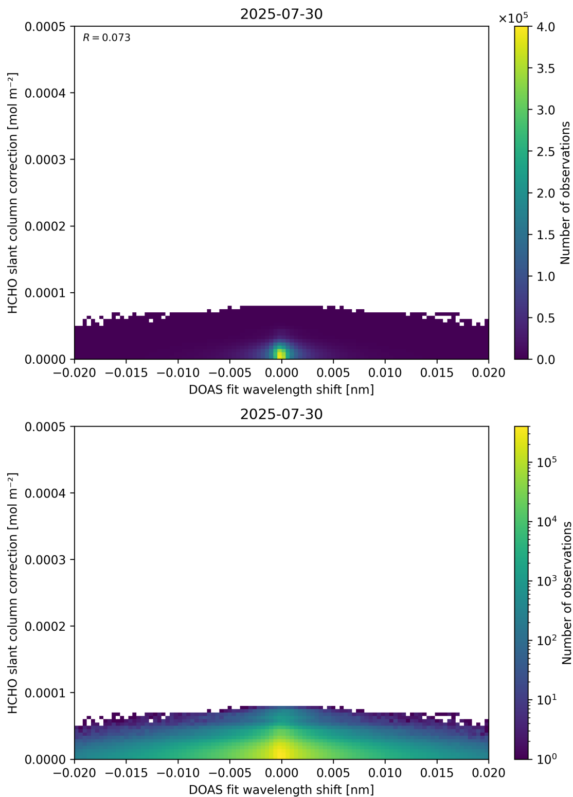
Figure 67: Scatter density plot of “DOAS fit wavelength shift” against “HCHO slant column correction” for 2025-07-29 to 2025-07-31.
