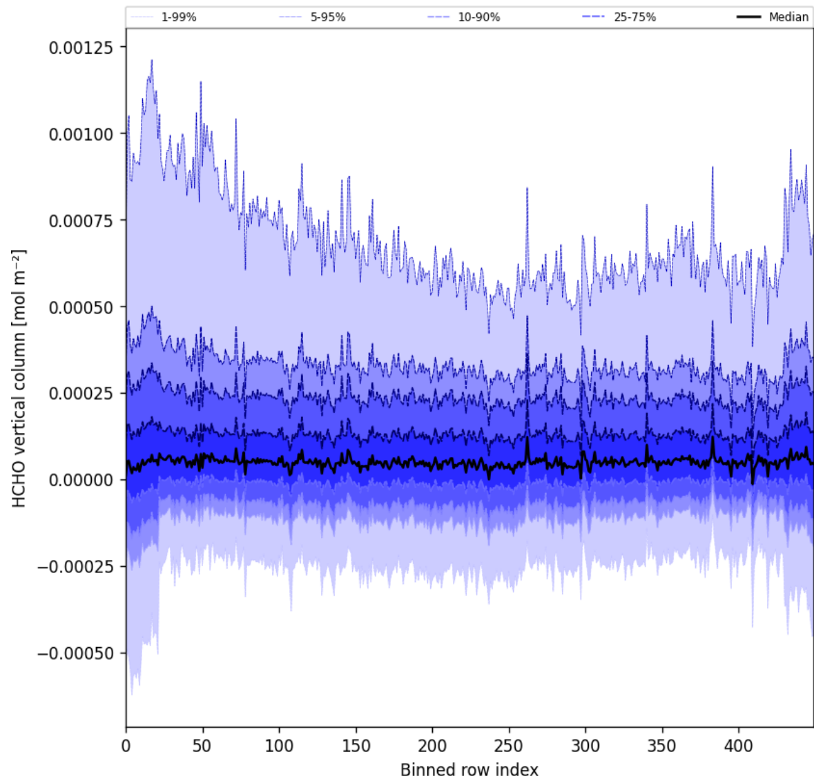
Figure 49: Along track statistics of “HCHO vertical column” for 2025-07-29 to 2025-07-31
