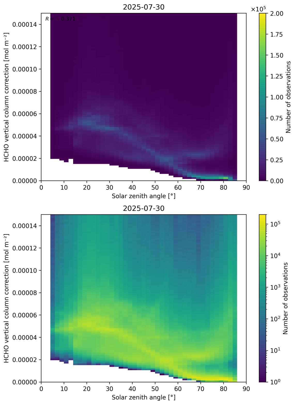
Figure 178: Scatter density plot of “Solar zenith angle” against “HCHO vertical column correction” for 2025-07-29 to 2025-07-31.
