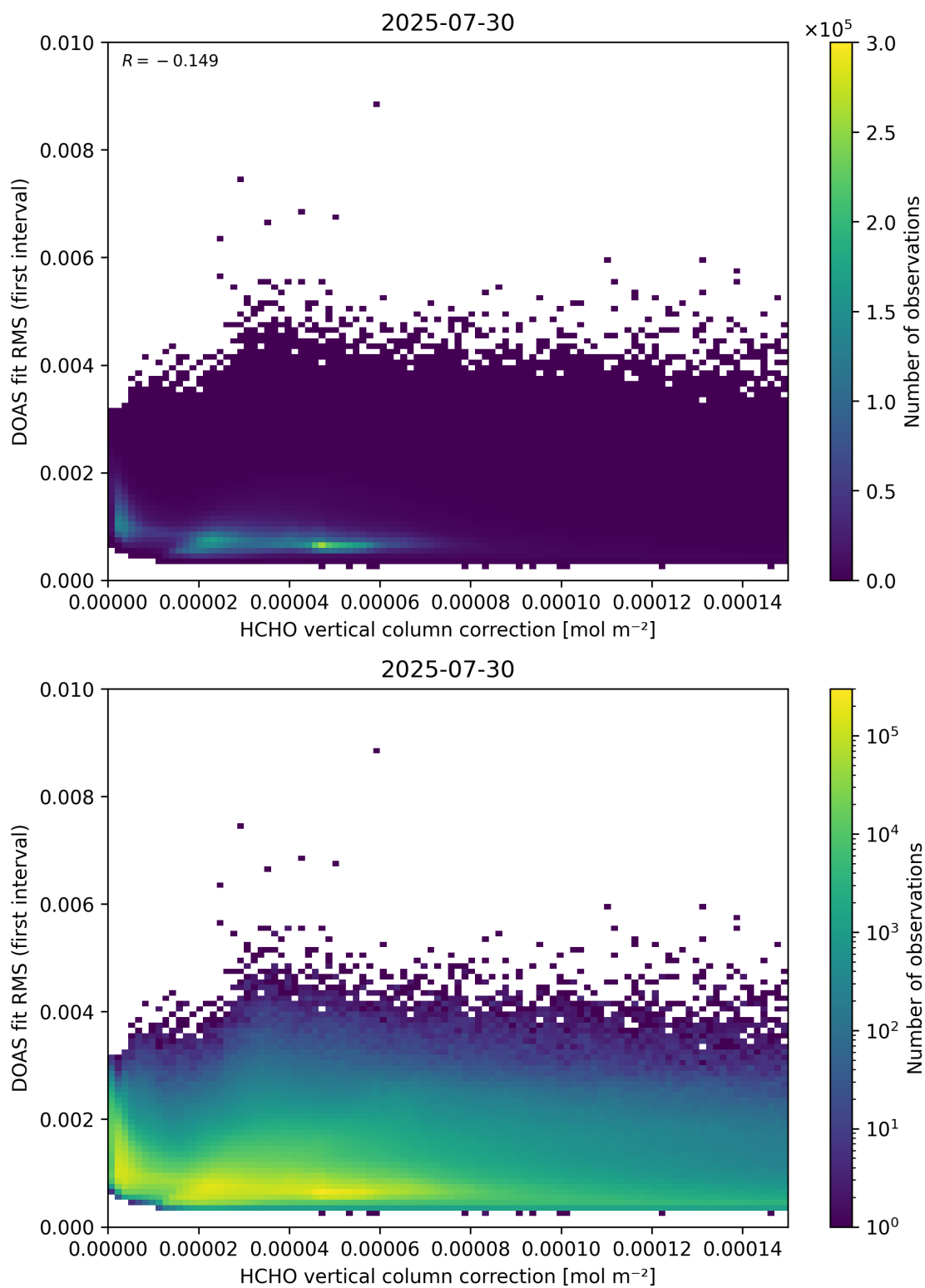
Figure 112: Scatter density plot of “HCHO vertical column correction” against “DOAS fit RMS (first interval)” for 2025-07-29 to 2025-07-31.
