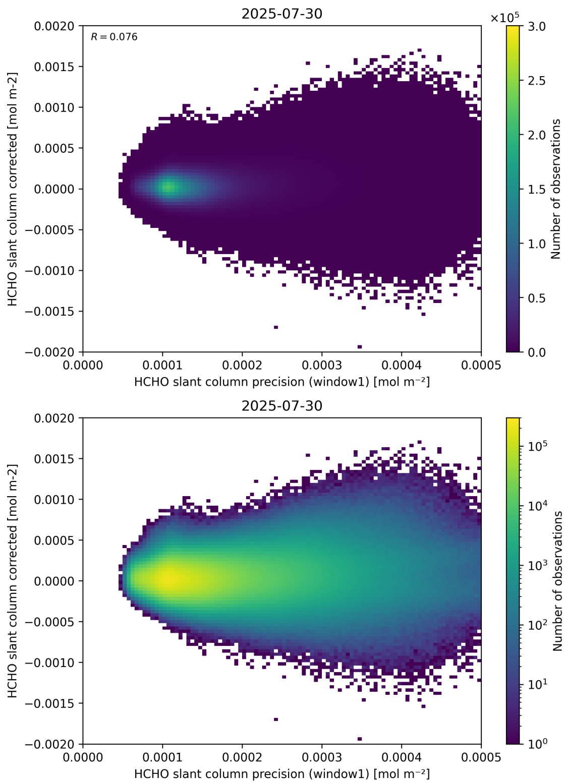
Figure 92: Scatter density plot of “HCHO slant column precision (window1)” against “HCHO slant column corrected” for 2025-07-29 to 2025-07-31.
