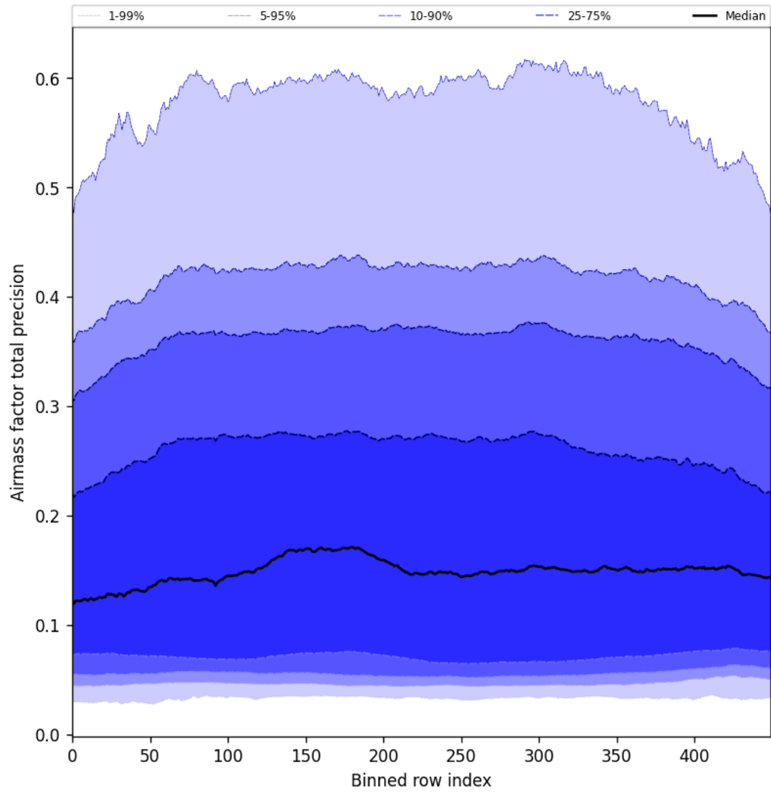
Figure 55: Along track statistics of “Airmass factor total precision” for 2025-07-29 to 2025-07-31
