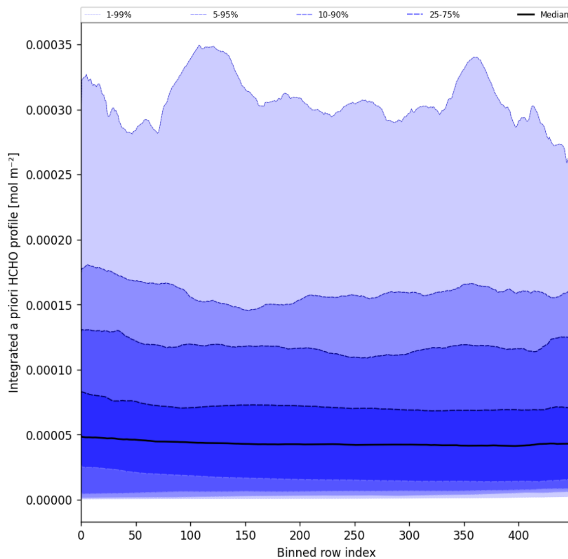
Figure 57: Along track statistics of “Integrated a priori HCHO profile” for 2025-07-29 to 2025-07-31
