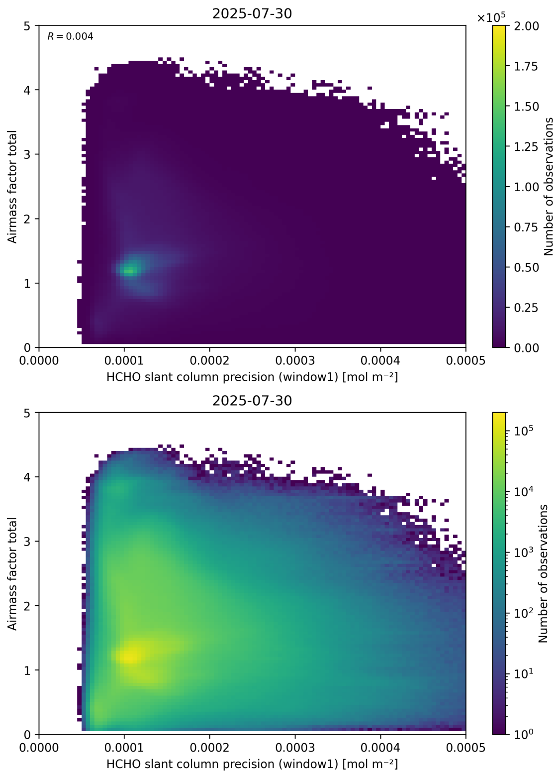
Figure 94: Scatter density plot of “HCHO slant column precision (window1)” against “Airmass factor total” for 2025-07-29 to 2025-07-31.
