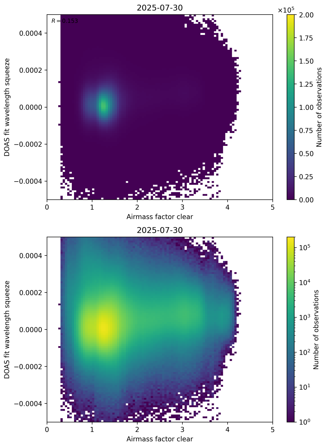
Figure 73: Scatter density plot of “Airmass factor clear” against “DOAS fit wavelength squeeze” for 2025-07-29 to 2025-07-31.
