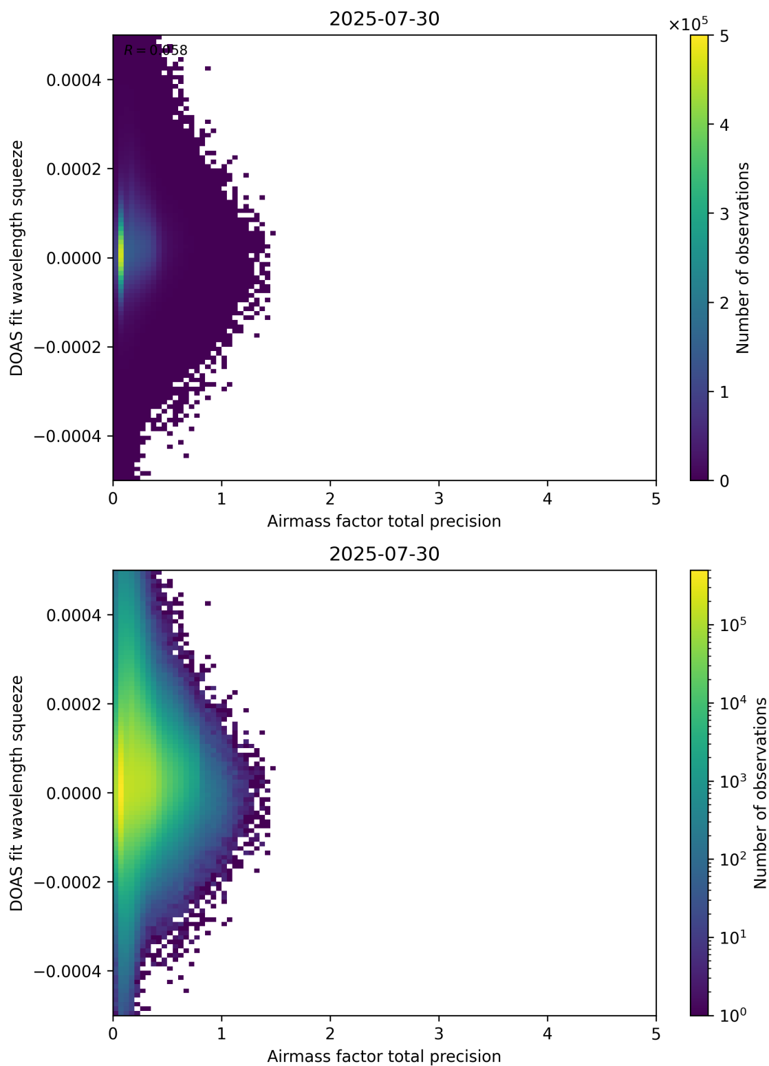
Figure 107: Scatter density plot of “Airmass factor total precision” against “DOAS fit wavelength squeeze” for 2025-07-29 to 2025-07-31.
