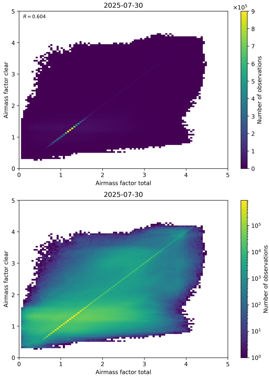
Figure 100: Scatter density plot of “Airmass factor total” against “Airmass factor clear” for 2025-07-29 to 2025-07-31.
