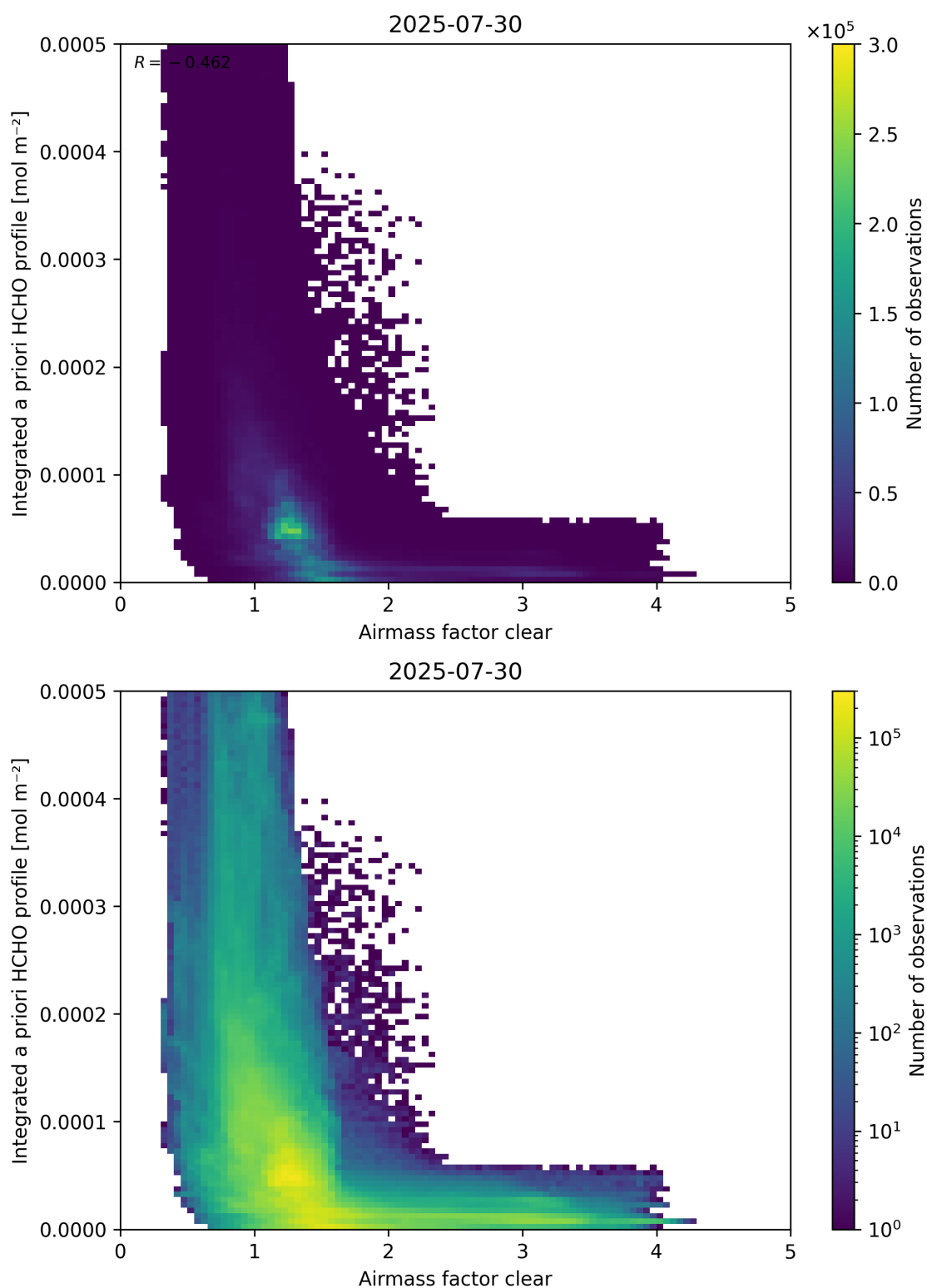
Figure 76: Scatter density plot of “Airmass factor clear” against “Integrated a priori HCHO profile” for 2025-07-29 to 2025-07-31.
