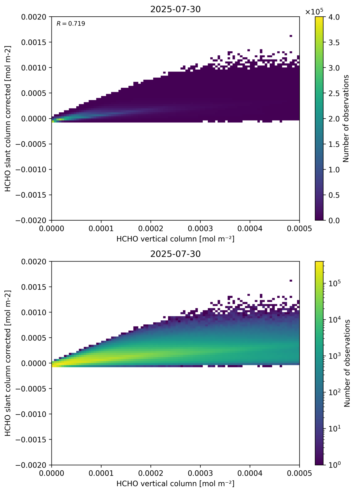
Figure 127: Scatter density plot of “HCHO vertical column” against “HCHO slant column corrected” for 2025-07-29 to 2025-07-31.
