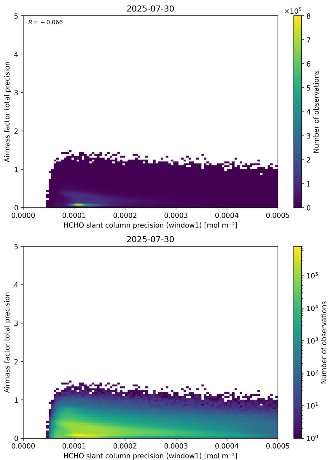
Figure 95: Scatter density plot of “HCHO slant column precision (window1)” against “Airmass factor total precision” for 2025-07-29 to 2025-07-31.
