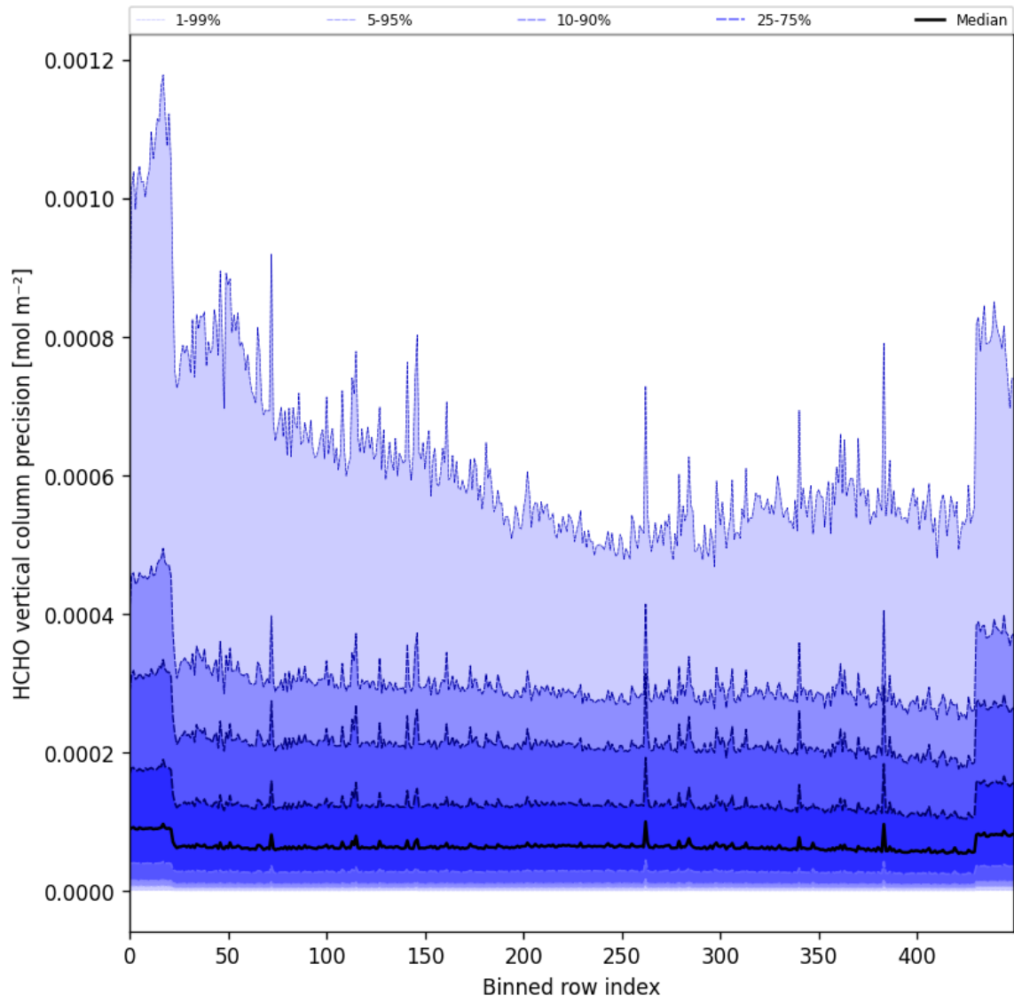
Figure 50: Along track statistics of “HCHO vertical column precision” for 2025-07-29 to 2025-07-31
