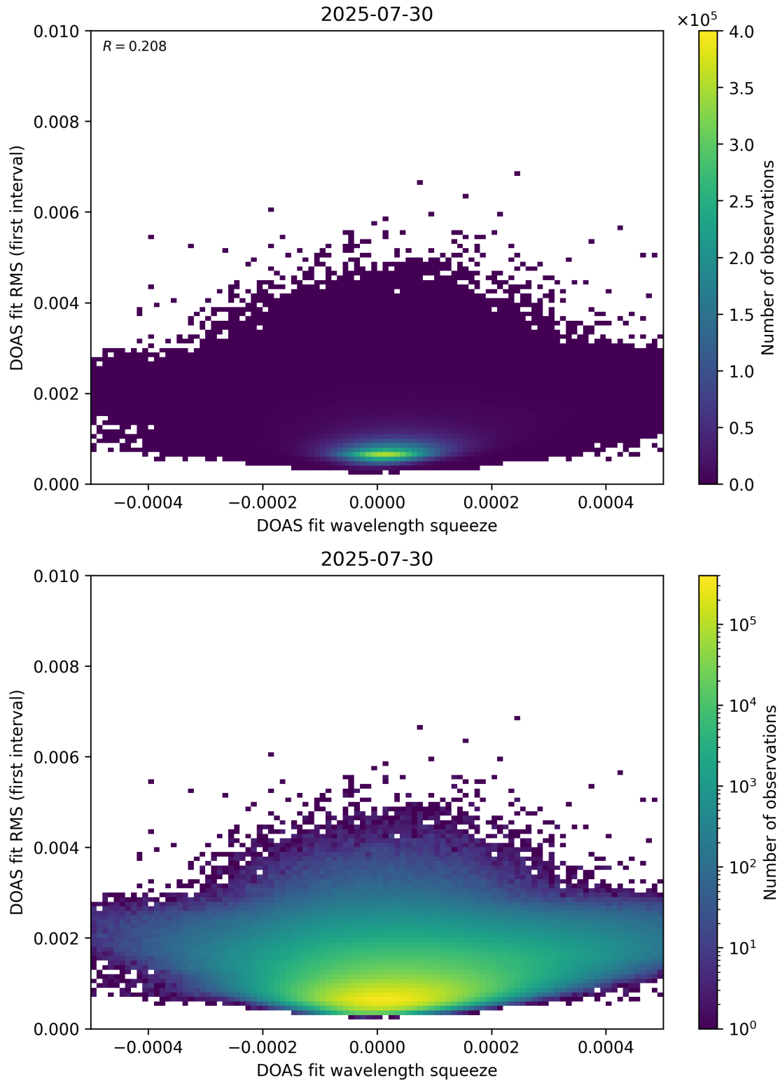
Figure 68: Scatter density plot of “DOAS fit wavelength squeeze” against “DOAS fit RMS (first interval)” for 2025-07-29 to 2025-07-31.
