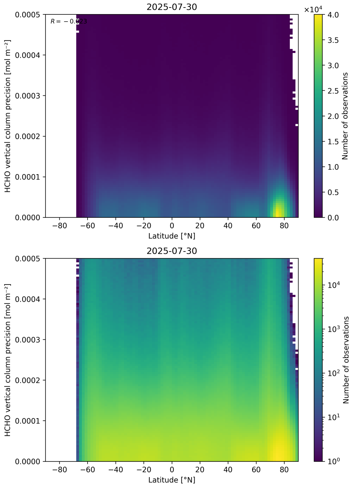
Figure 165: Scatter density plot of “Latitude” against “HCHO vertical column precision” for 2025-07-29 to 2025-07-31.
