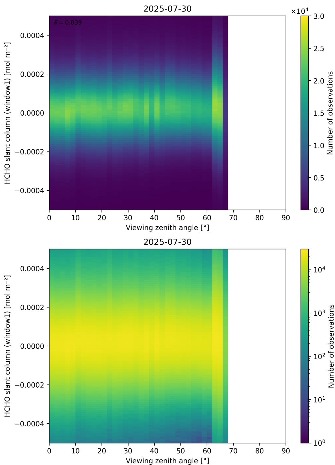
Figure 188: Scatter density plot of “Viewing zenith angle” against “HCHO slant column (window1)” for 2025-07-29 to 2025-07-31.
