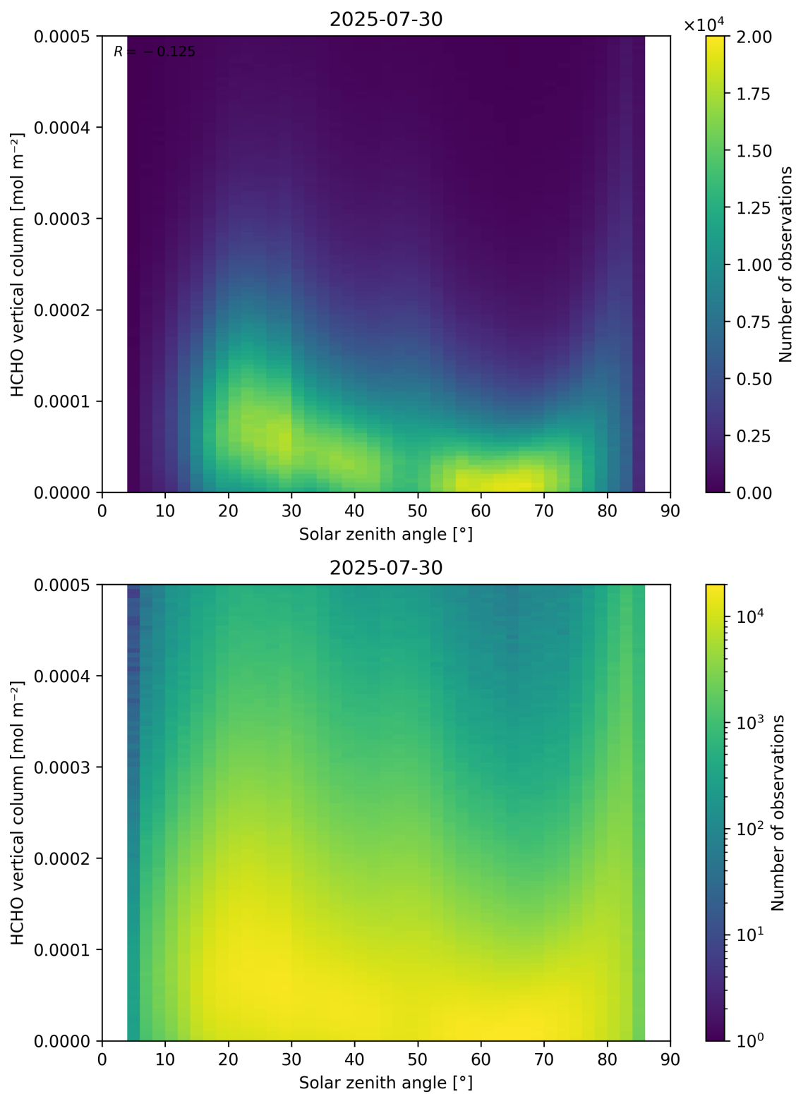
Figure 177: Scatter density plot of “Solar zenith angle” against “HCHO vertical column” for 2025-07-29 to 2025-07-31.
