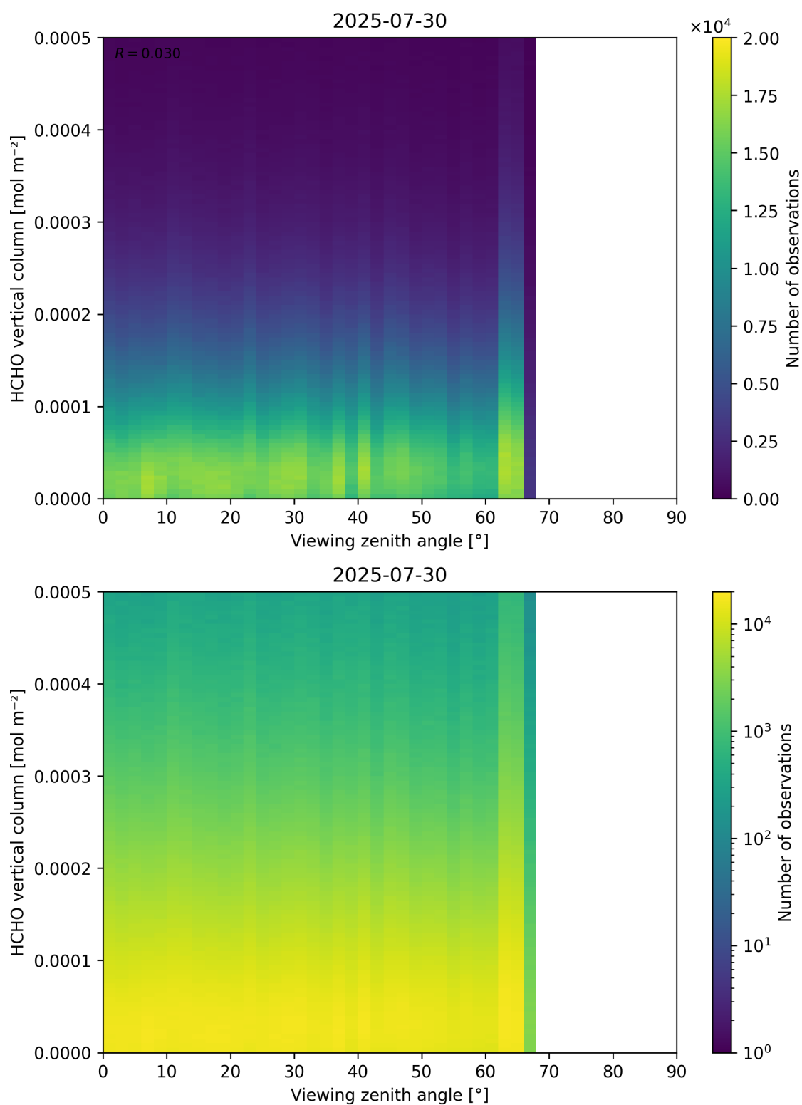
Figure 192: Scatter density plot of “Viewing zenith angle” against “HCHO vertical column” for 2025-07-29 to 2025-07-31.
