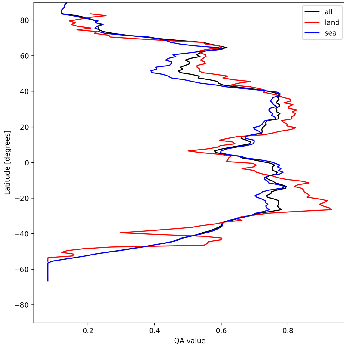
Figure 20: Zonal average of “QA value” for 2025-07-29 to 2025-07-31.
