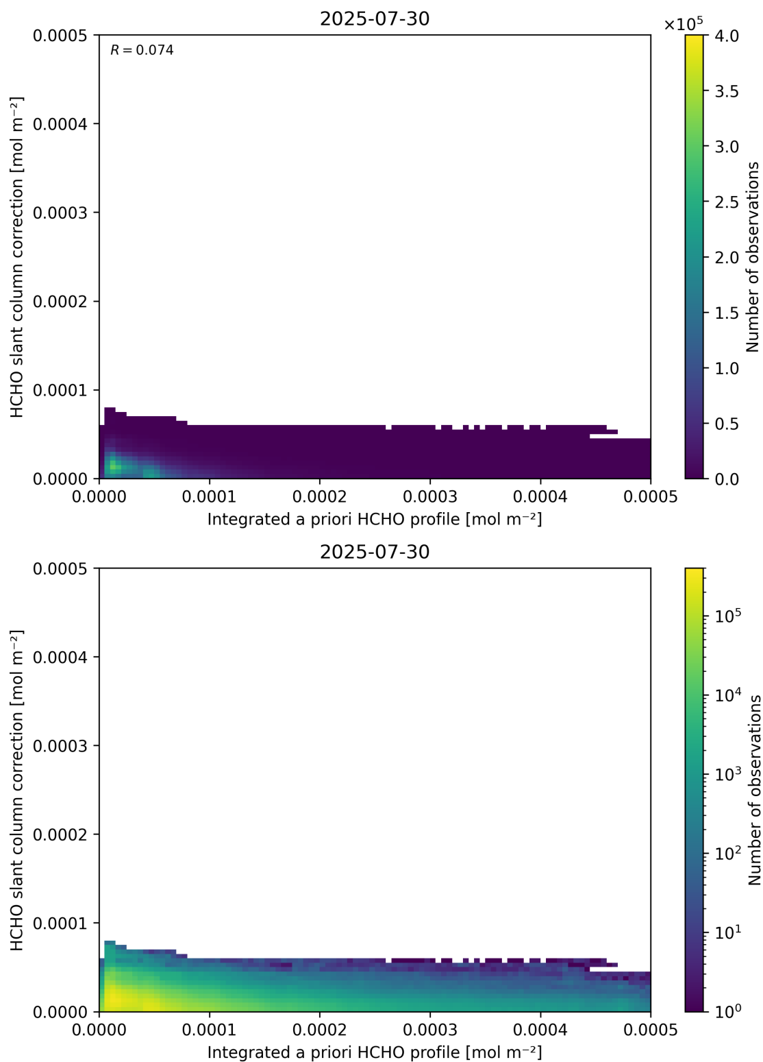
Figure 152: Scatter density plot of “Integrated a priori HCHO profile” against “HCHO slant column correction” for 2025-07-29 to 2025-07-31.
