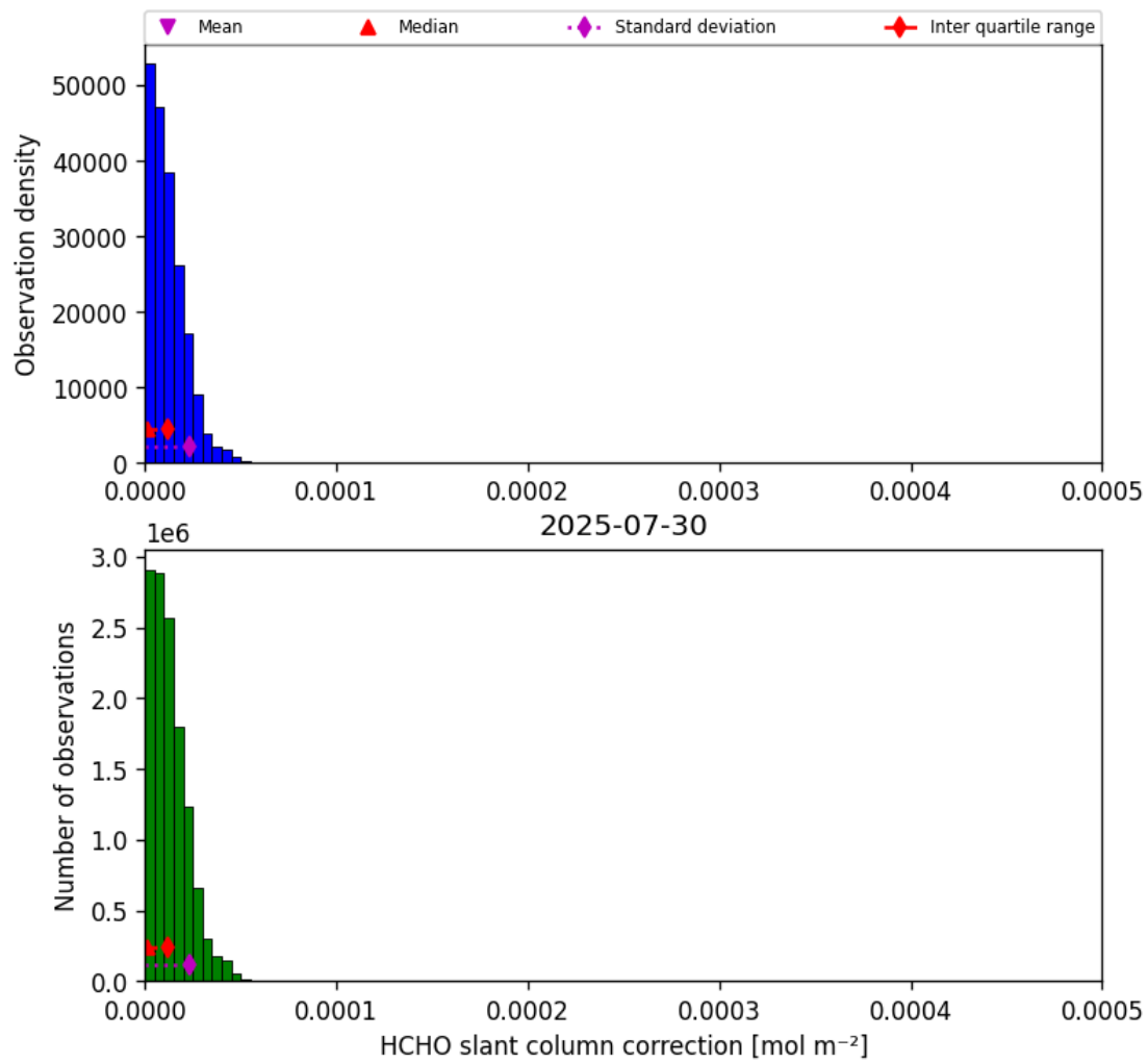
Figure 47: Histogram of “HCHO slant column correction” for 2025-07-29 to 2025-07-31
