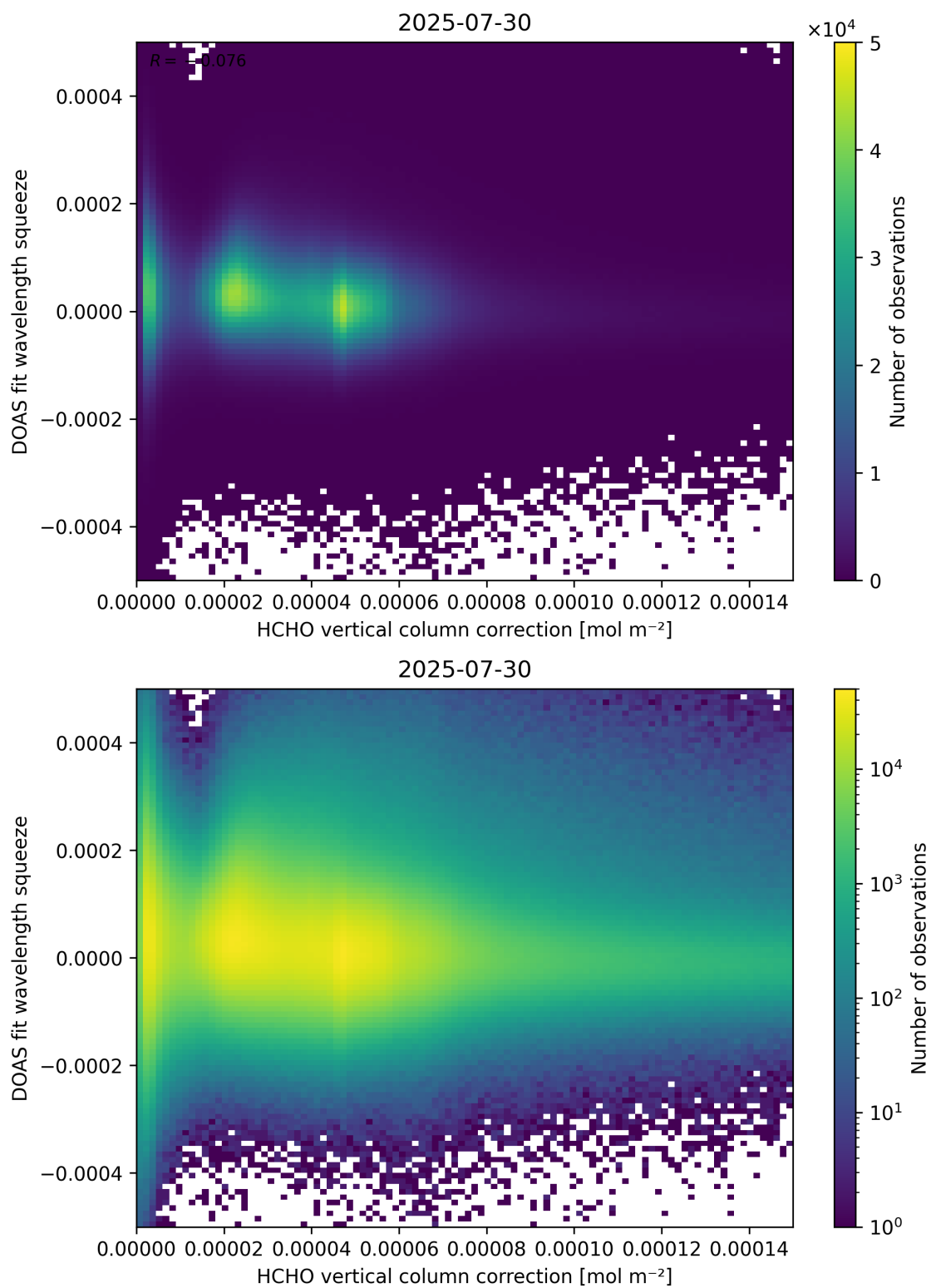
Figure 114: Scatter density plot of “HCHO vertical column correction” against “DOAS fit wavelength squeeze” for 2025-07-29 to 2025-07-31.
