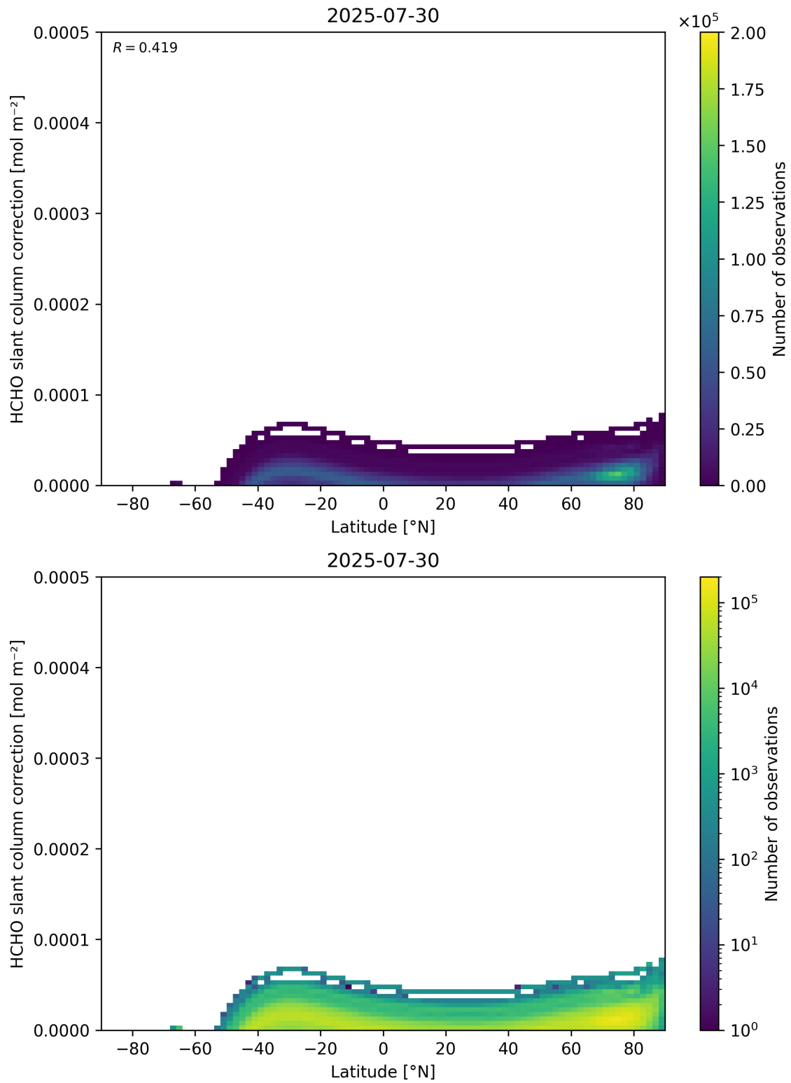
Figure 158: Scatter density plot of “Latitude” against “HCHO slant column correction” for 2025-07-29 to 2025-07-31.
