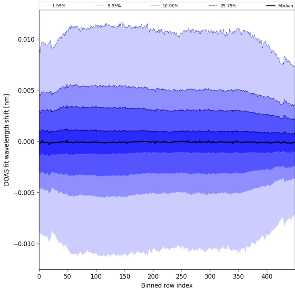
Figure 58: Along track statistics of “DOAS fit wavelength shift” for 2025-07-29 to 2025-07-31
