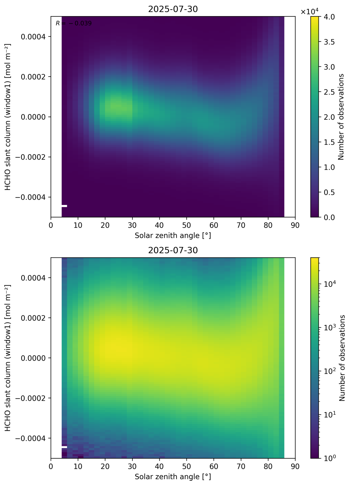
Figure 173: Scatter density plot of “Solar zenith angle” against “HCHO slant column (window1)” for 2025-07-29 to 2025-07-31.
