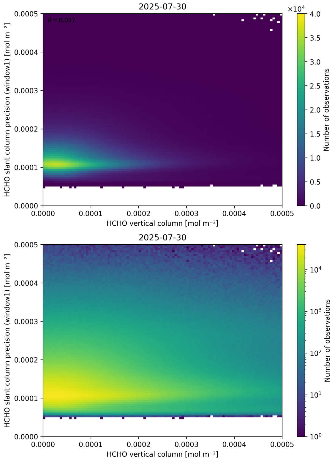
Figure 130: Scatter density plot of “HCHO vertical column” against “HCHO slant column precision (window1)” for 2025-07-29 to 2025-07-31.
