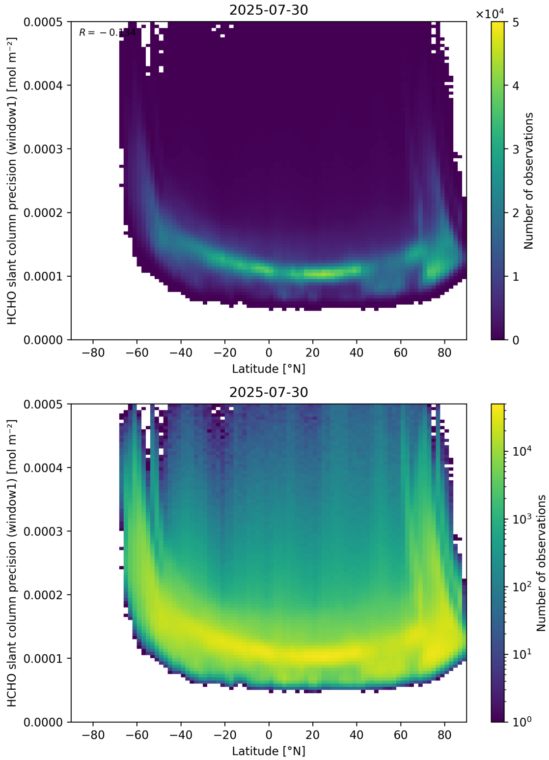
Figure 160: Scatter density plot of “Latitude” against “HCHO slant column precision (window1)” for 2025-07-29 to 2025-07-31.
