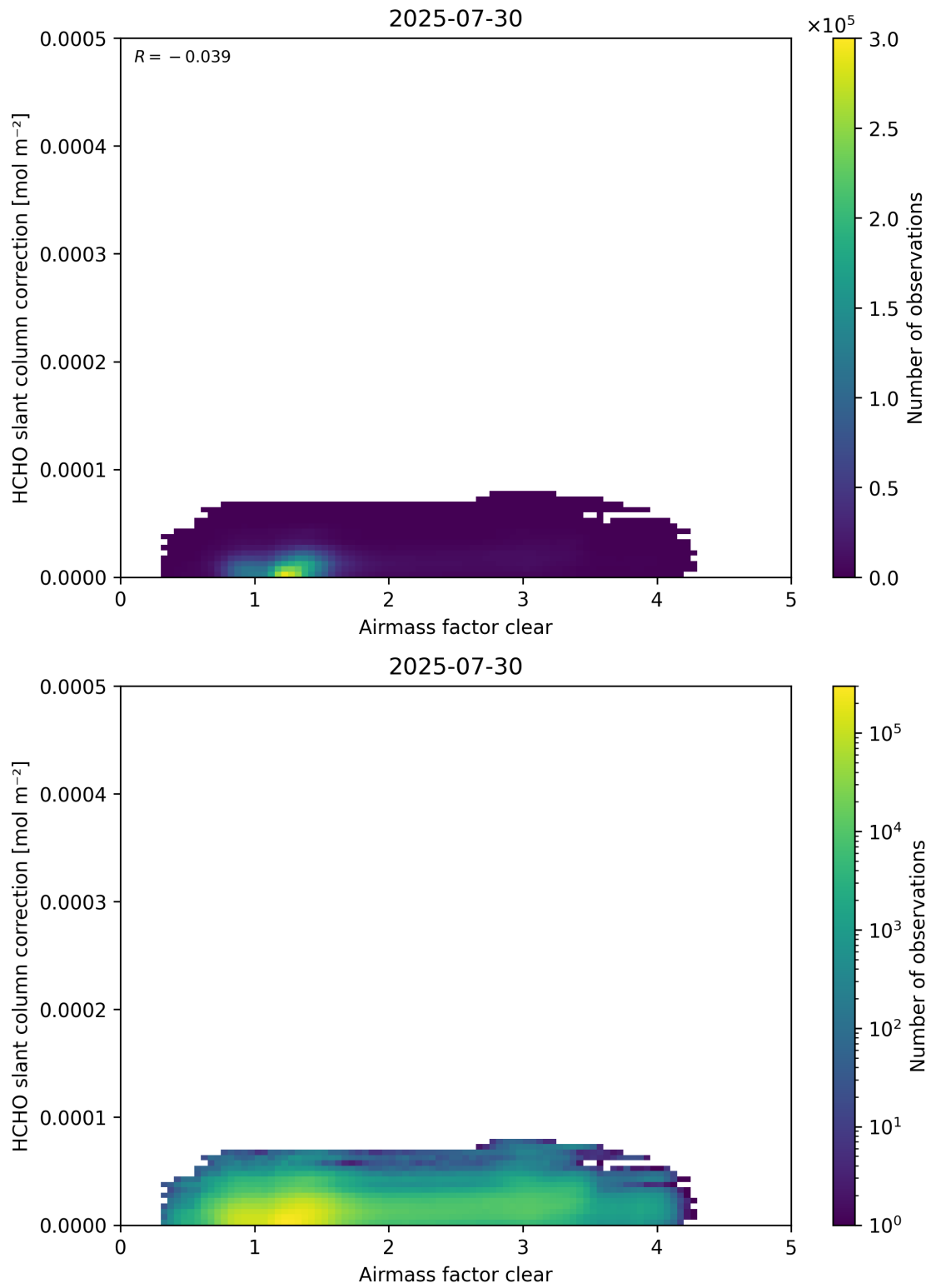
Figure 75: Scatter density plot of “Airmass factor clear” against “HCHO slant column correction” for 2025-07-29 to 2025-07-31.
