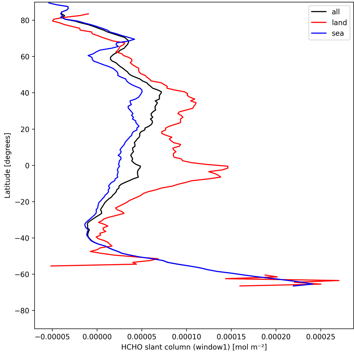
Figure 24: Zonal average of “HCHO slant column (window1)” for 2025-07-29 to 2025-07-31.
