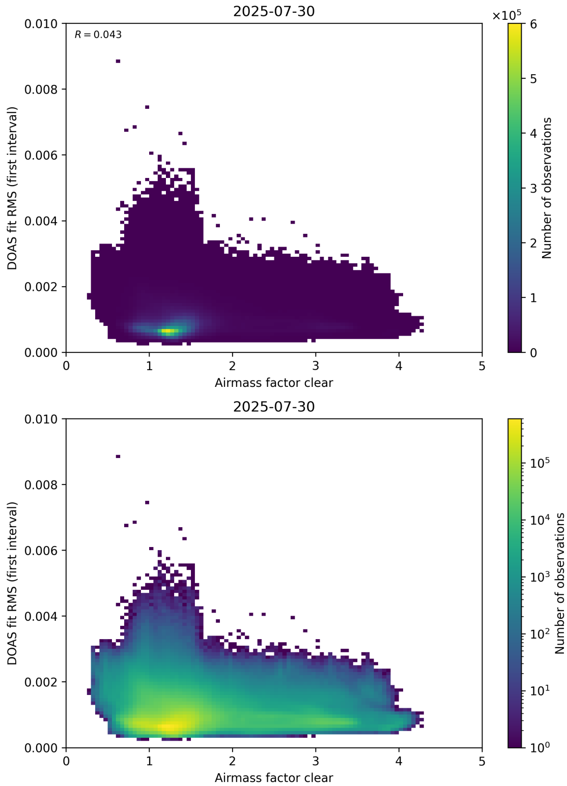
Figure 71: Scatter density plot of “Airmass factor clear” against “DOAS fit RMS (first interval)” for 2025-07-29 to 2025-07-31.
