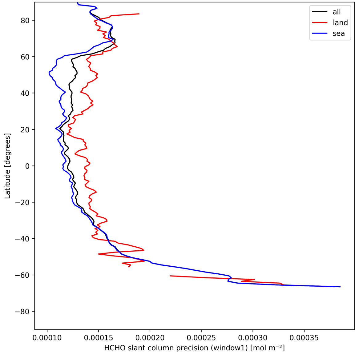
Figure 25: Zonal average of "HCHO slant column precision (window1)" for 2025-07-29 to 2025-07-31.
