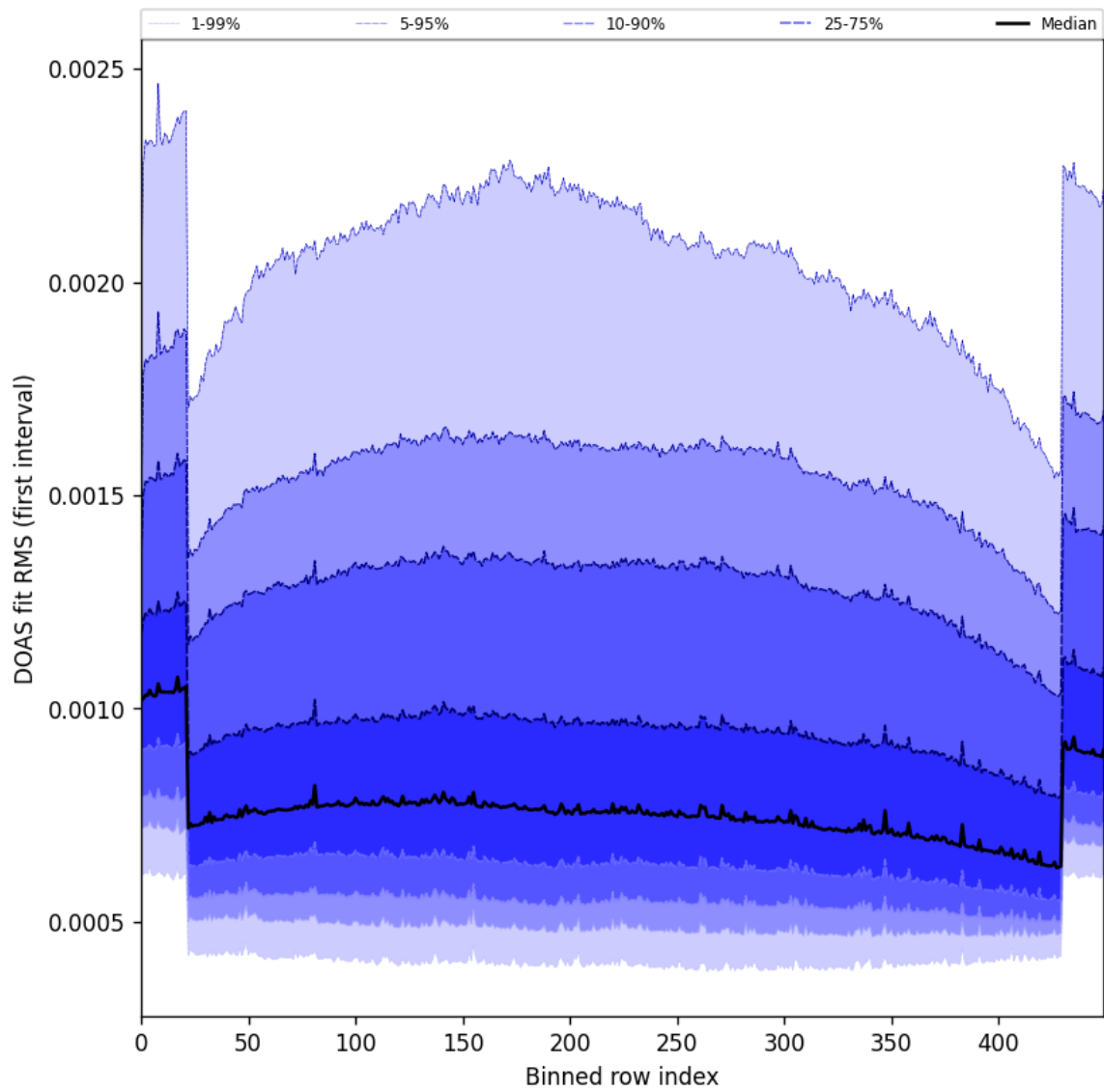
Figure 60: Along track statistics of “DOAS fit RMS (first interval)” for 2025-07-29 to 2025-07-31
