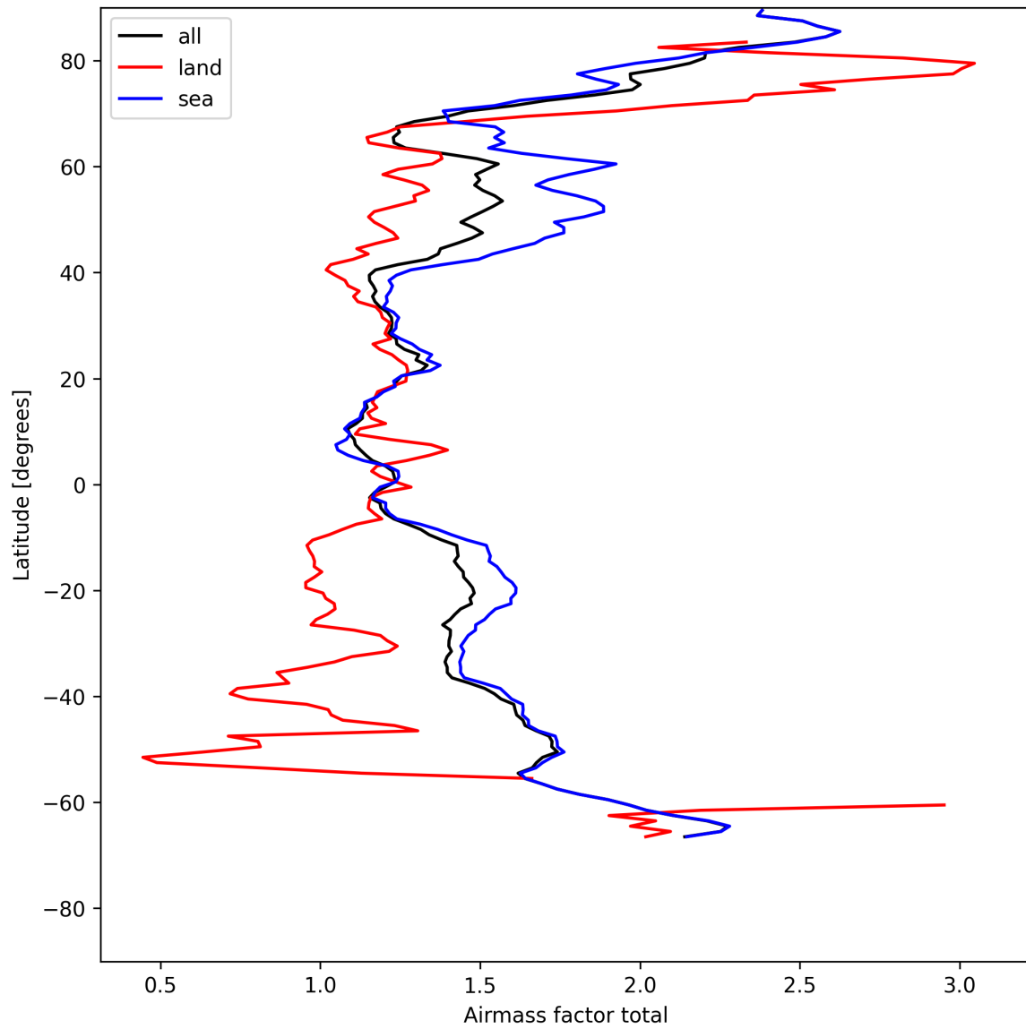
Figure 26: Zonal average of “Airmass factor total” for 2025-07-29 to 2025-07-31.
