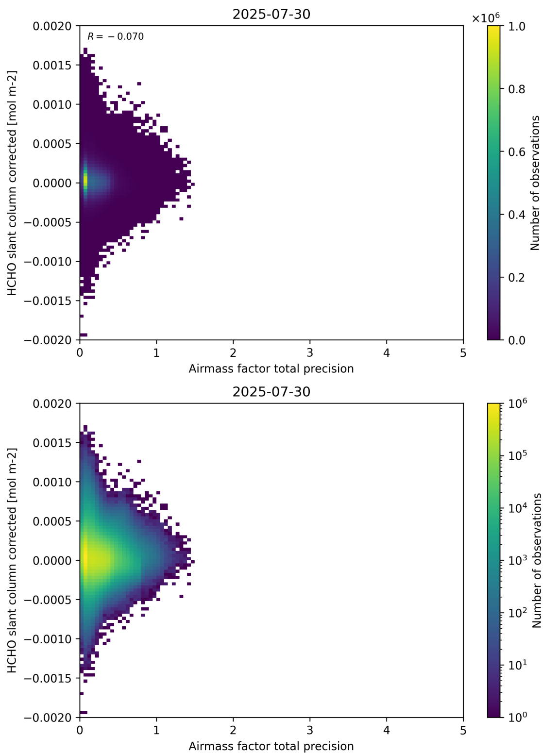
Figure 109: Scatter density plot of “Airmass factor total precision” against “HCHO slant column corrected” for 2025-07-29 to 2025-07-31.
