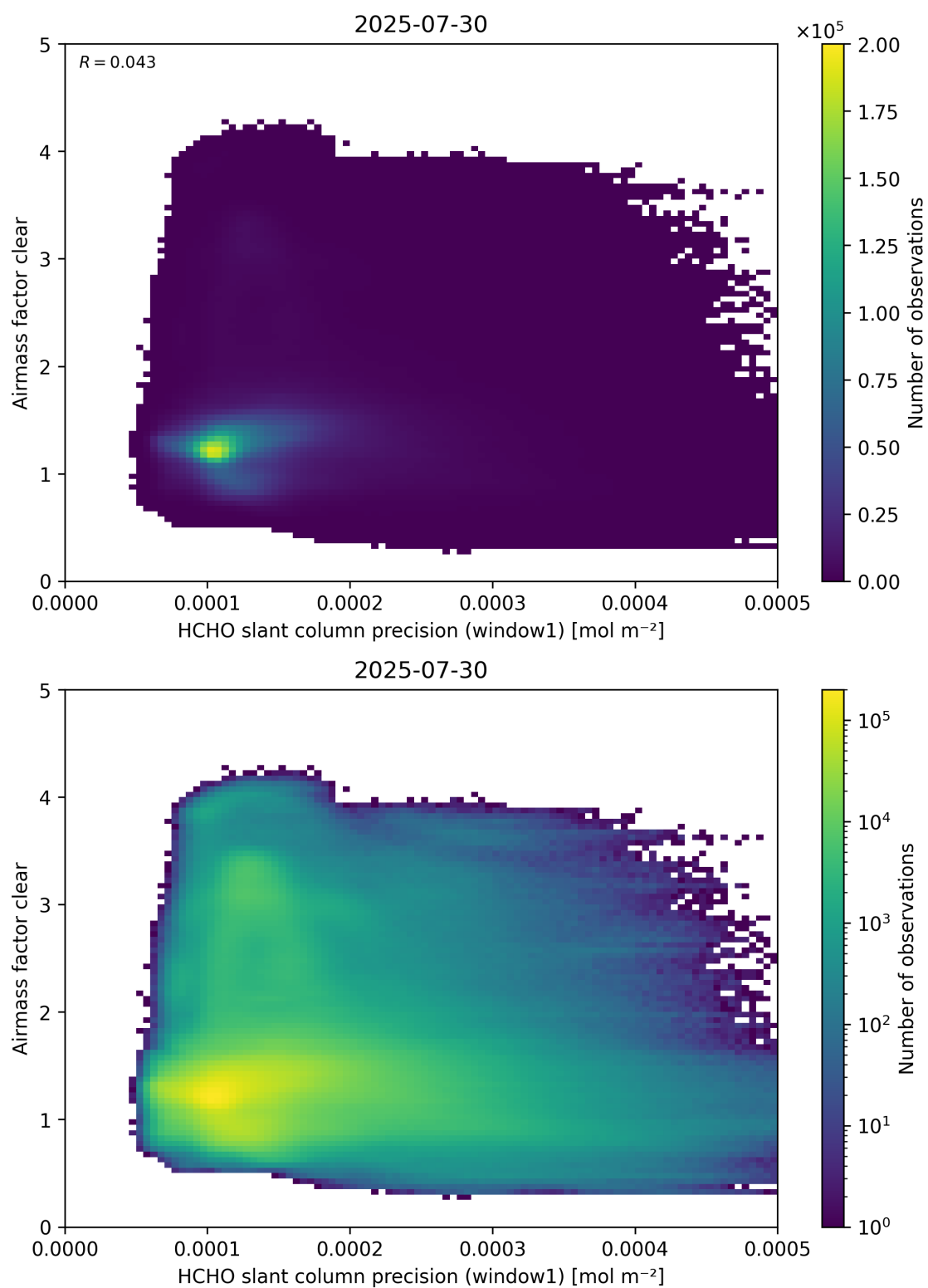
Figure 91: Scatter density plot of “HCHO slant column precision (window1)” against “Airmass factor clear” for 2025-07-29 to 2025-07-31.
