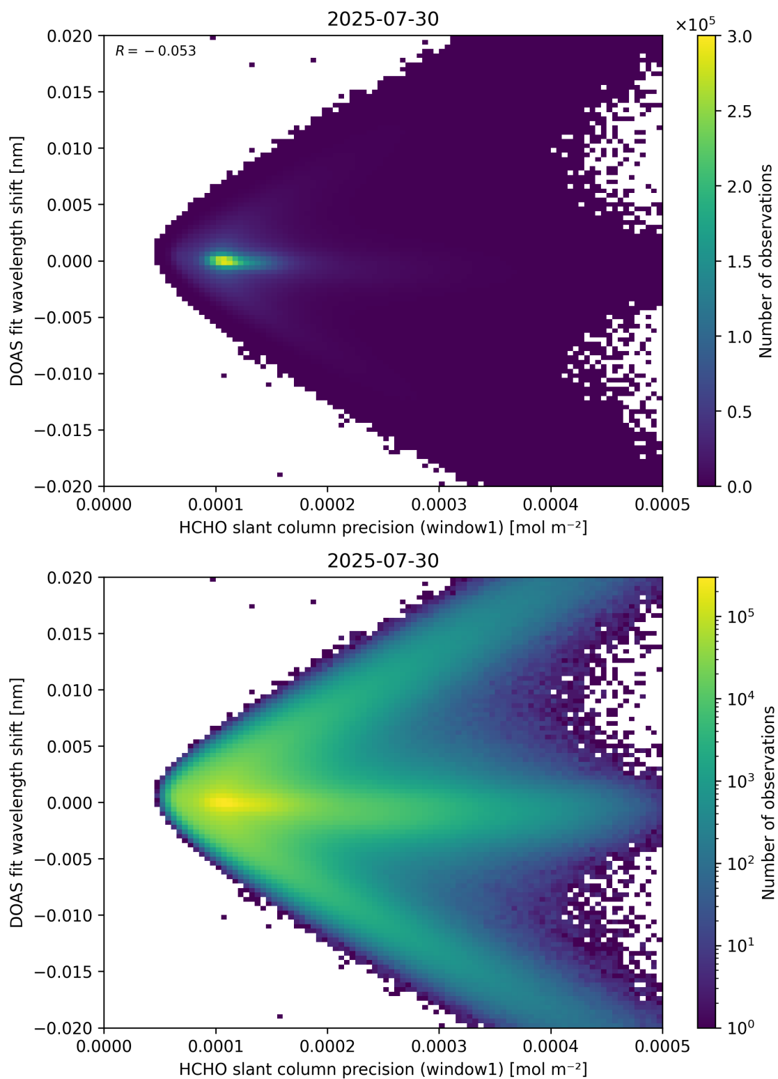
Figure 89: Scatter density plot of “HCHO slant column precision (window1)” against “DOAS fit wavelength shift” for 2025-07-29 to 2025-07-31.
