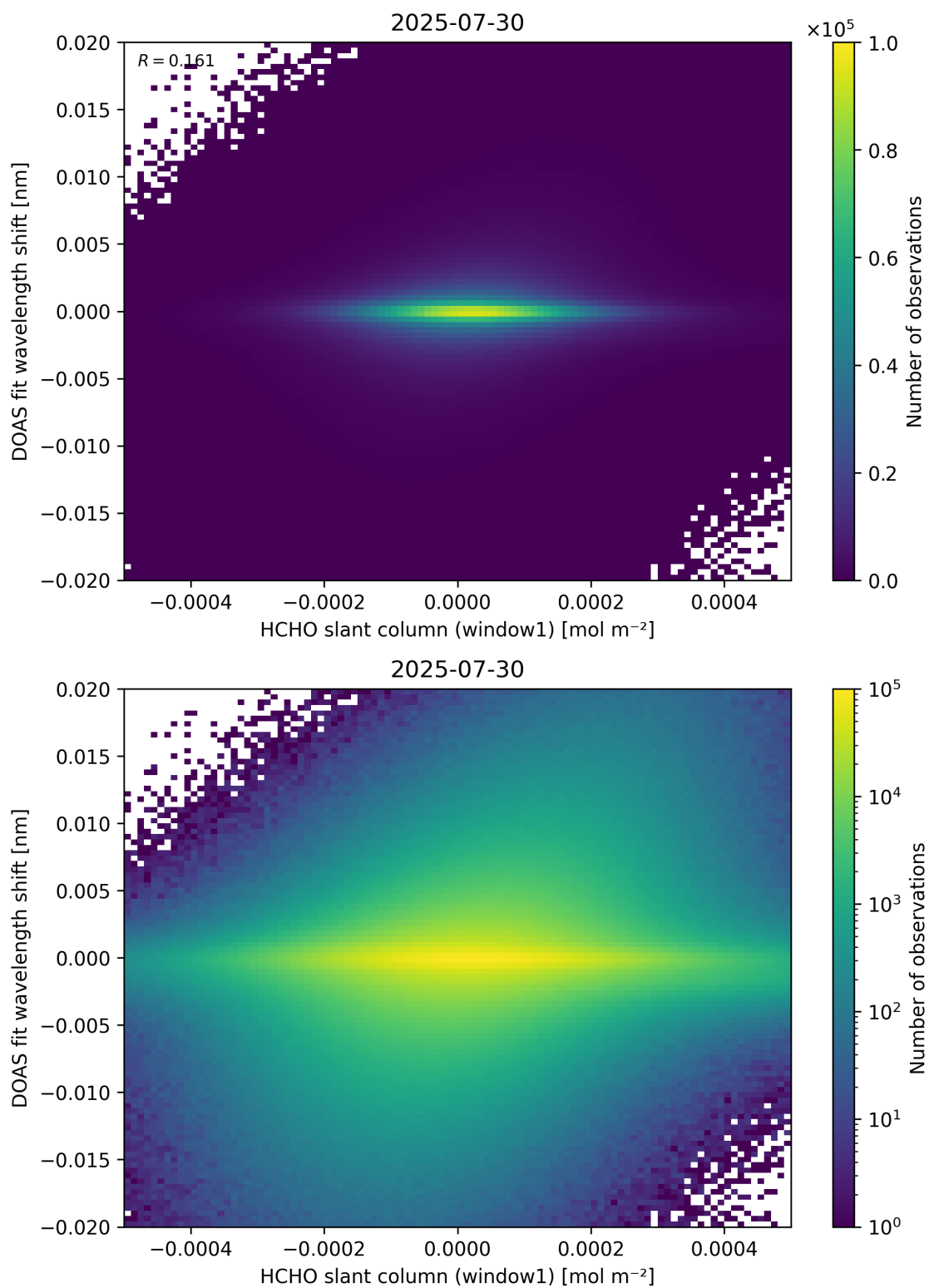
Figure 79: Scatter density plot of “HCHO slant column (window1)” against “DOAS fit wavelength shift” for 2025-07-29 to 2025-07-31.
