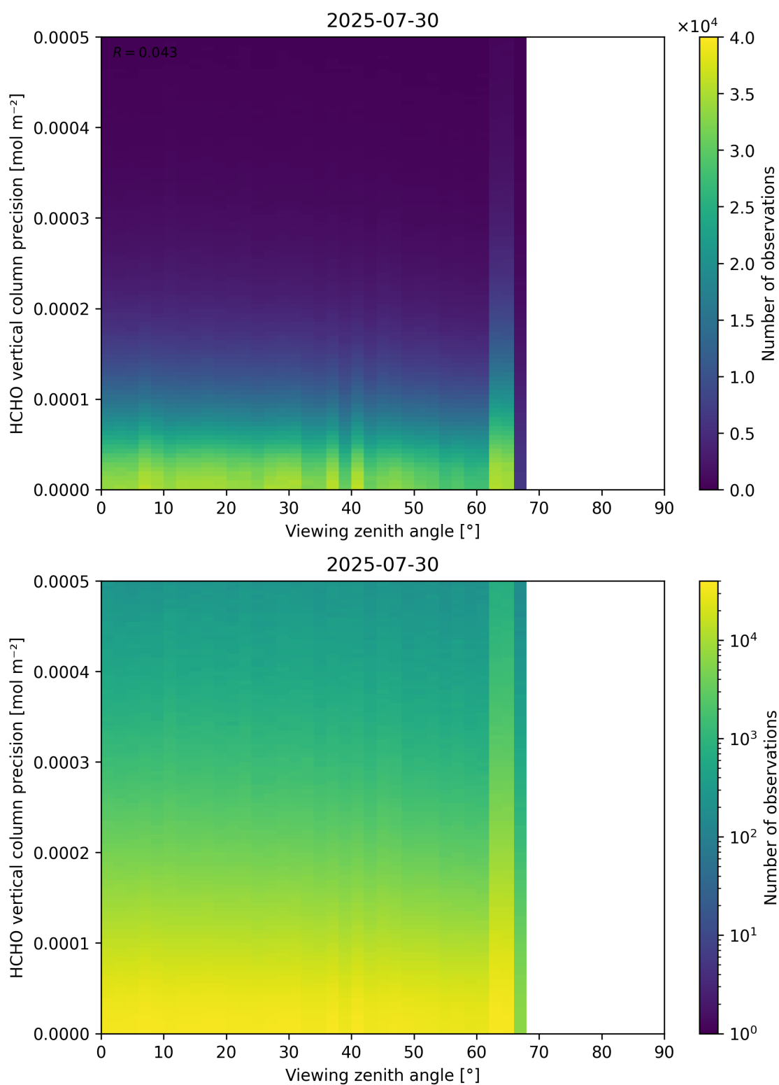
Figure 194: Scatter density plot of “Viewing zenith angle” against “HCHO vertical column precision” for 2025-07-29 to 2025-07-31.
