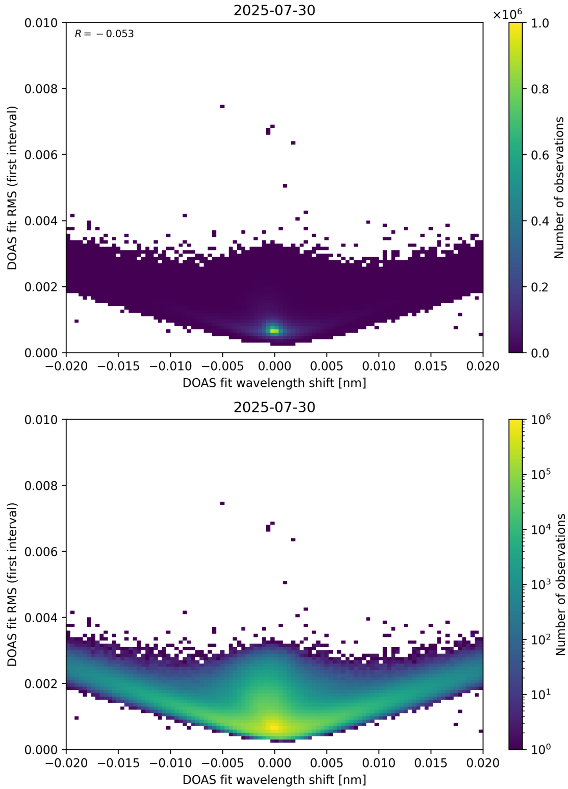
Figure 64: Scatter density plot of “DOAS fit wavelength shift” against “DOAS fit RMS (first interval)” for 2025-07-29 to 2025-07-31.
