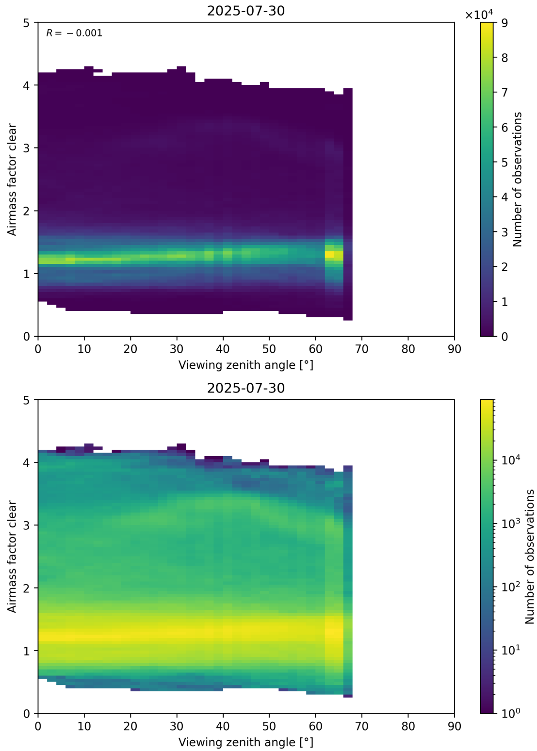
Figure 185: Scatter density plot of “Viewing zenith angle” against “Airmass factor clear” for 2025-07-29 to 2025-07-31.
