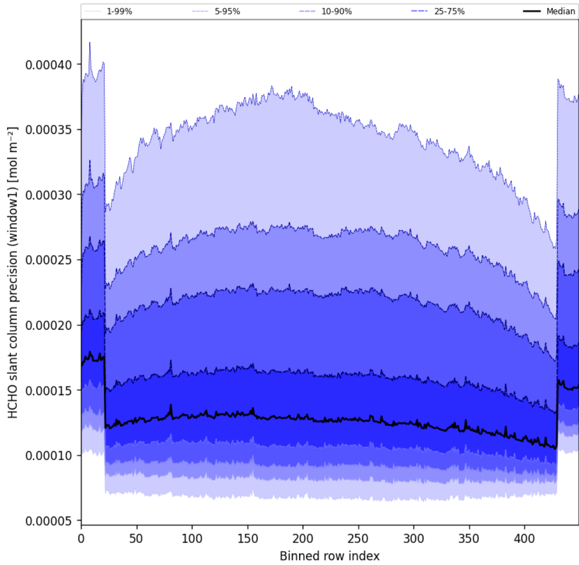
Figure 53: Along track statistics of “HCHO slant column precision (window1)” for 2025-07-29 to 2025-07-31
