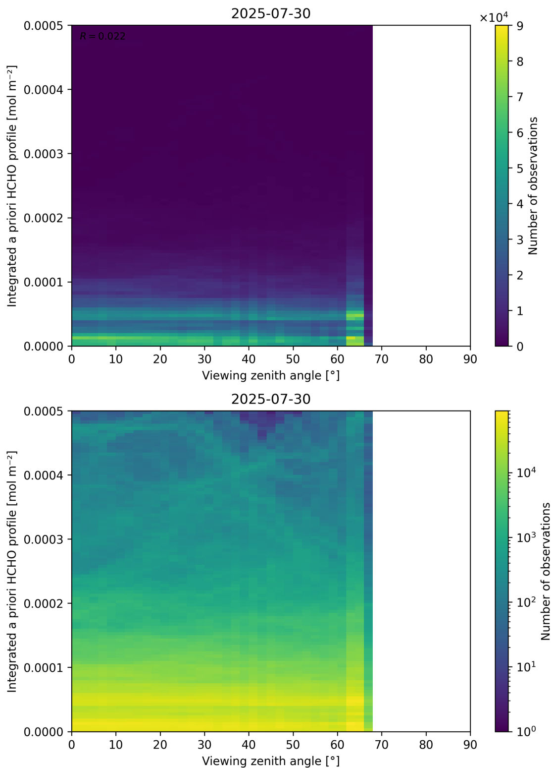
Figure 195: Scatter density plot of “Viewing zenith angle” against “Integrated a priori HCHO profile” for 2025-07-29 to 2025-07-31.
