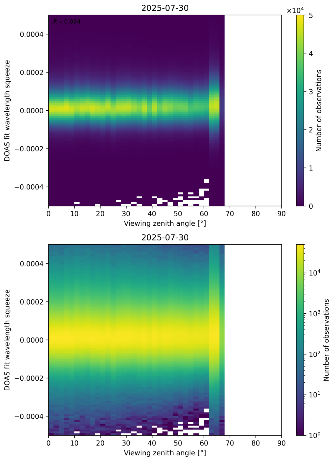
Figure 184: Scatter density plot of “Viewing zenith angle” against “DOAS fit wavelength squeeze” for 2025-07-29 to 2025-07-31.
