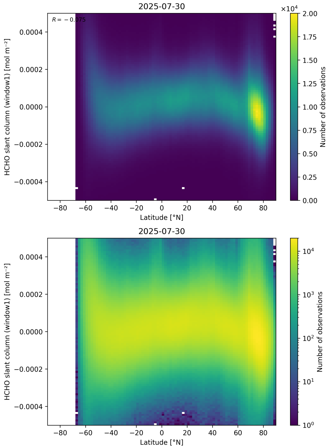
Figure 159: Scatter density plot of “Latitude” against “HCHO slant column (window1)” for 2025-07-29 to 2025-07-31.
