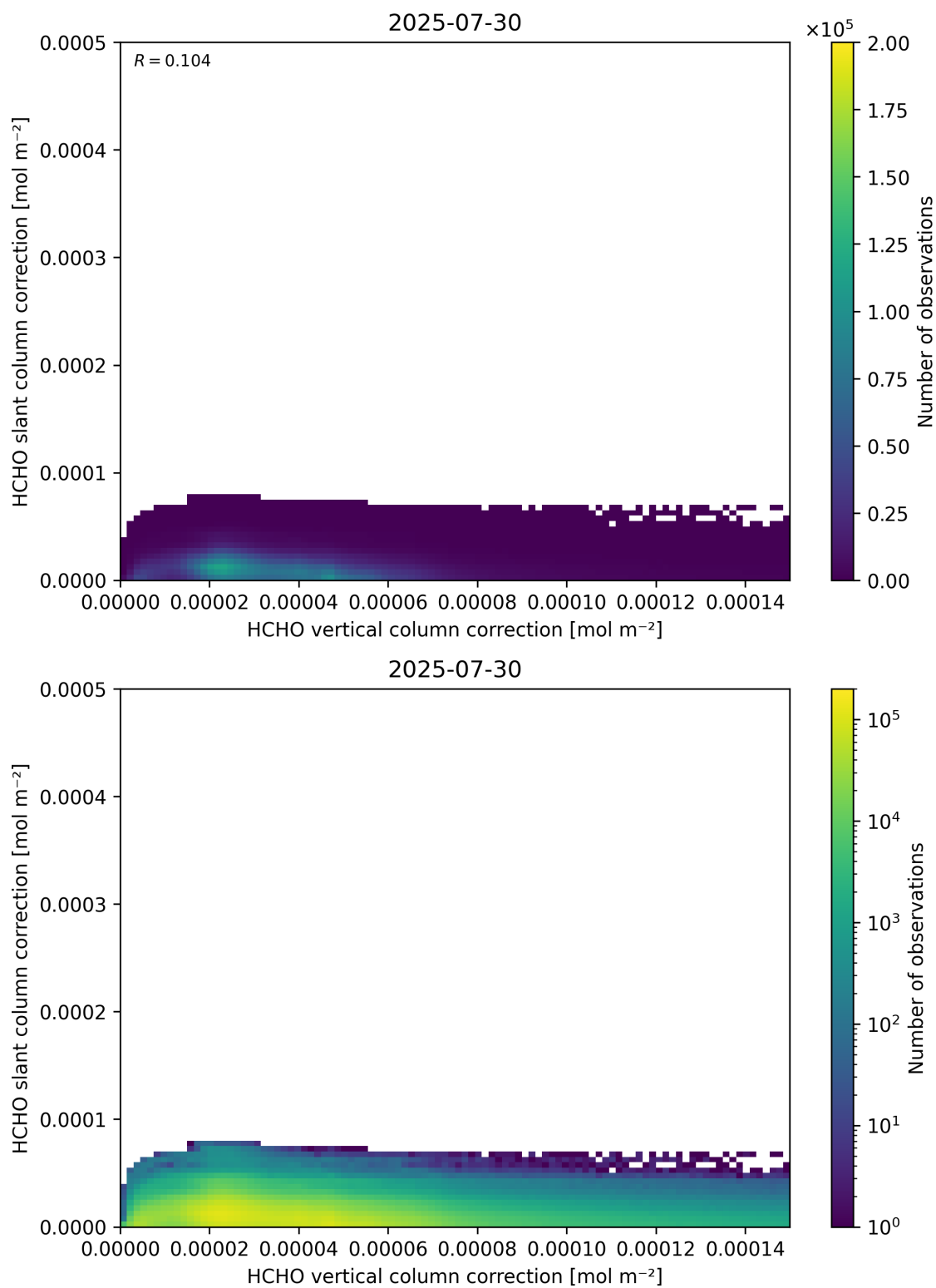
Figure 117: Scatter density plot of “HCHO vertical column correction” against “HCHO slant column correction” for 2025-07-29 to 2025-07-31.
