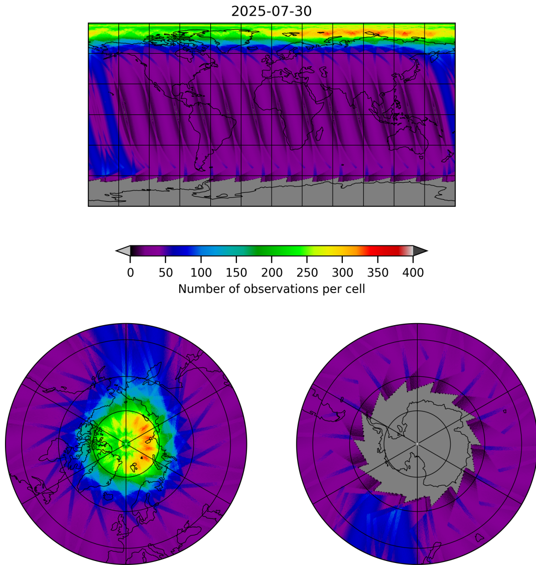
Figure 19: Map of the number of observations for 2025-07-29 to 2025-07-31
