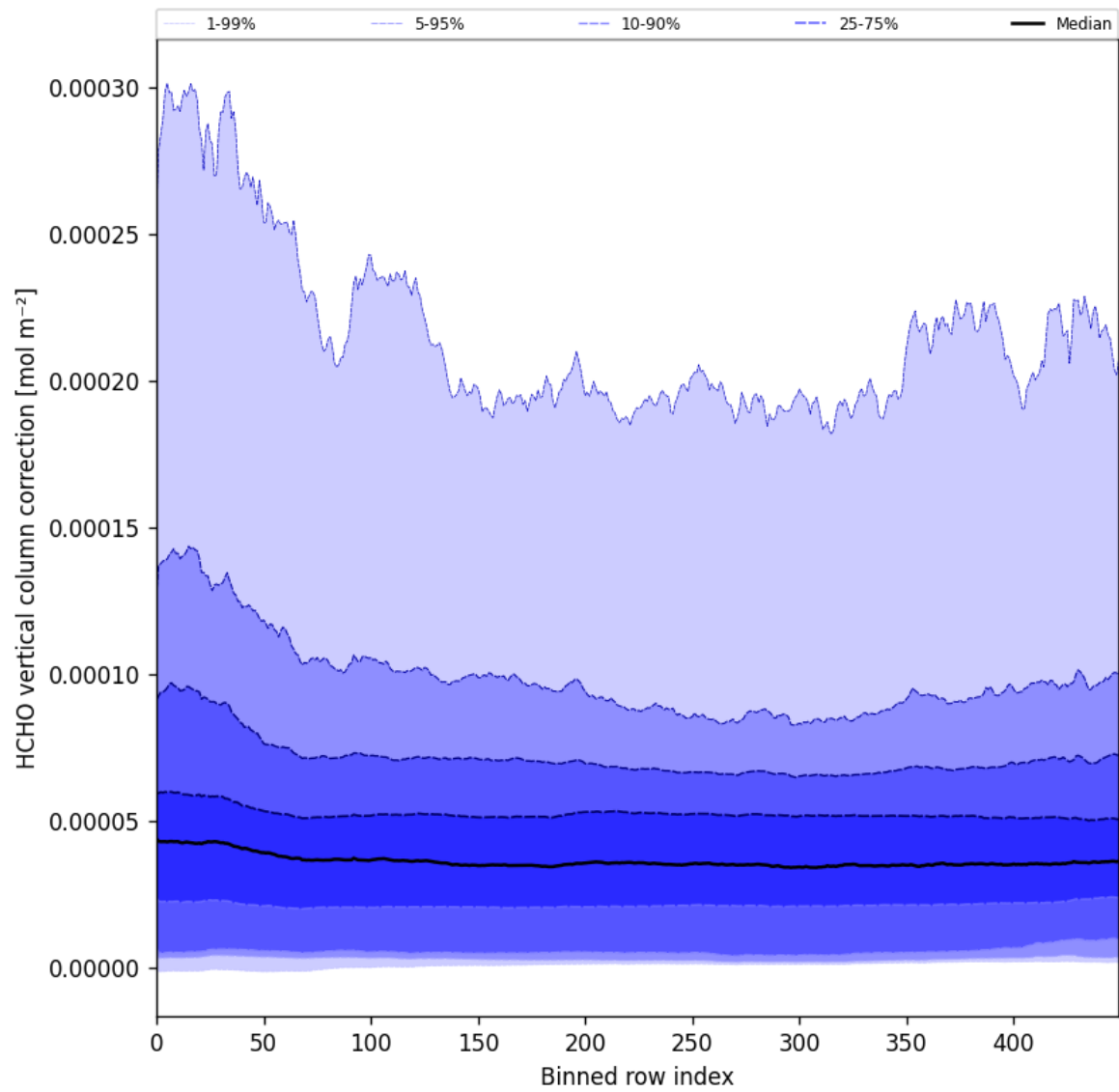
Figure 51: Along track statistics of “HCHO vertical column correction” for 2025-07-29 to 2025-07-31
