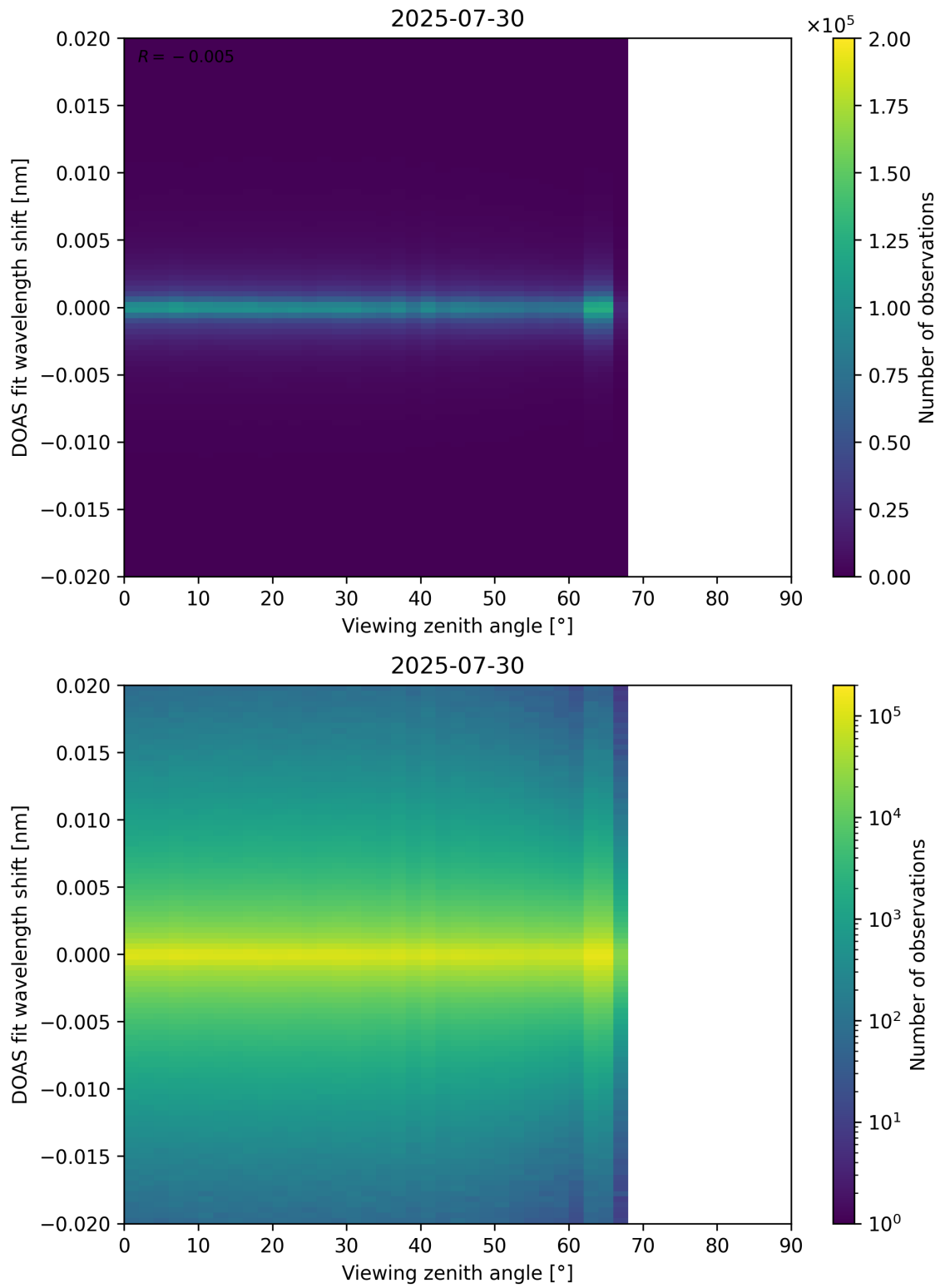
Figure 183: Scatter density plot of “Viewing zenith angle” against “DOAS fit wavelength shift” for 2025-07-29 to 2025-07-31.
