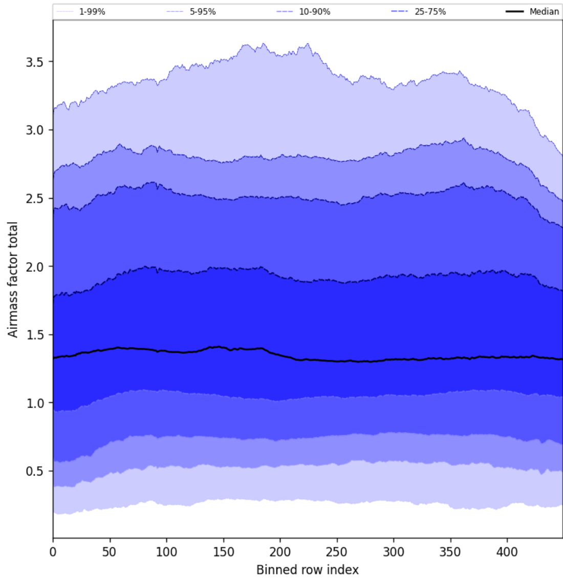
Figure 54: Along track statistics of “Airmass factor total” for 2025-07-29 to 2025-07-31
