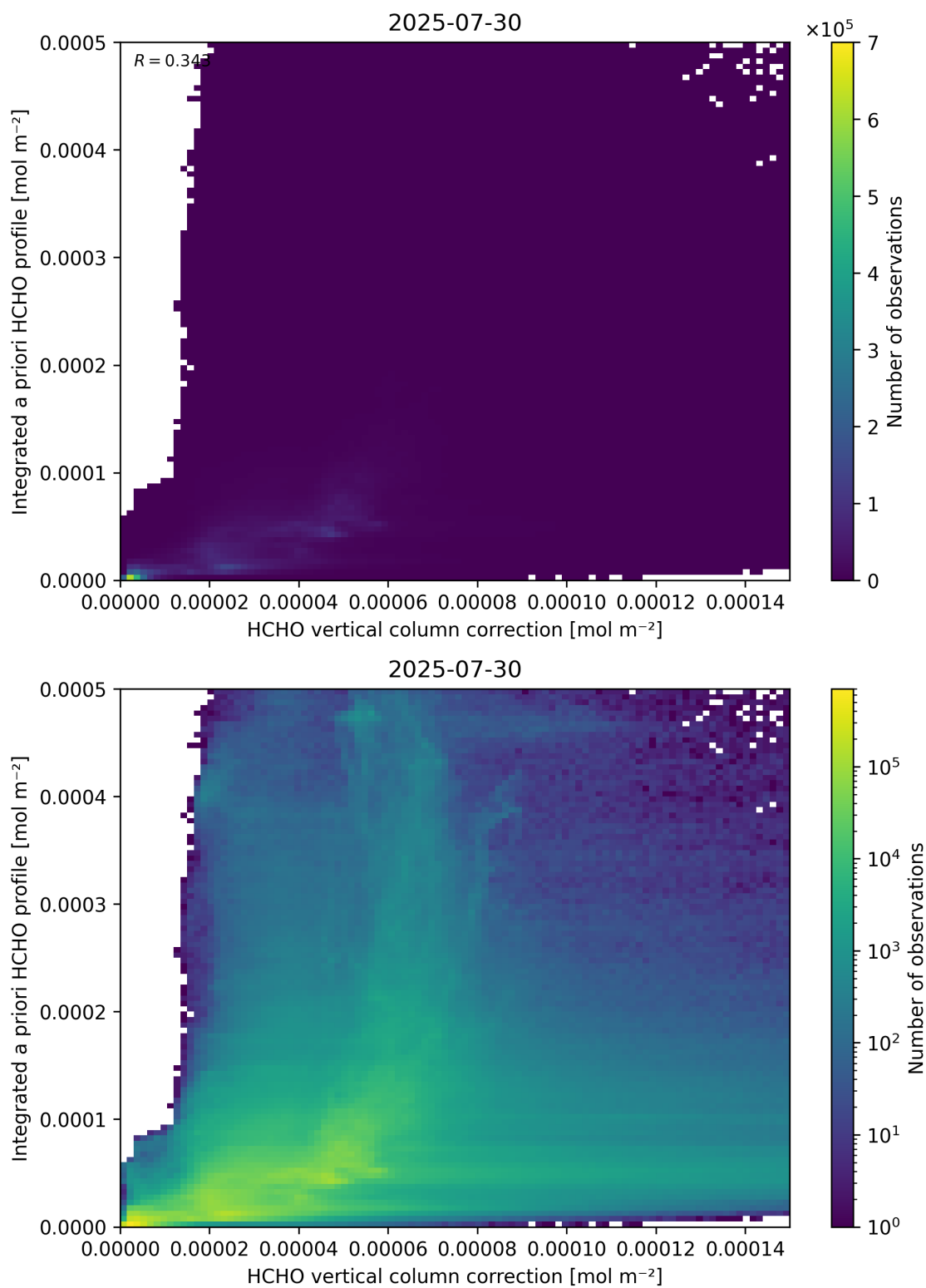
Figure 122: Scatter density plot of “HCHO vertical column correction” against “Integrated a priori HCHO profile” for 2025-07-29 to 2025-07-31.
