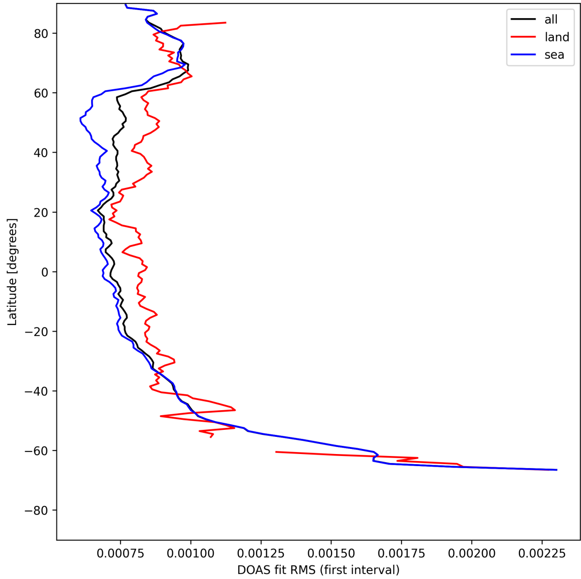
Figure 32: Zonal average of "DOAS fit RMS (first interval)" for 2025-07-29 to 2025-07-31.
