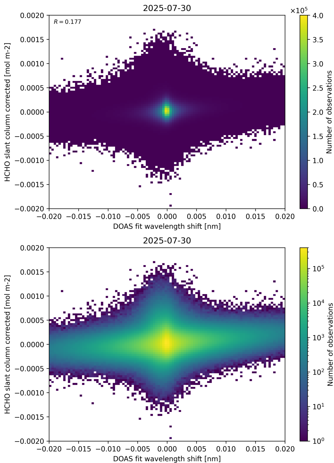
Figure 66: Scatter density plot of “DOAS fit wavelength shift” against “HCHO slant column corrected” for 2025-07-29 to 2025-07-31.
