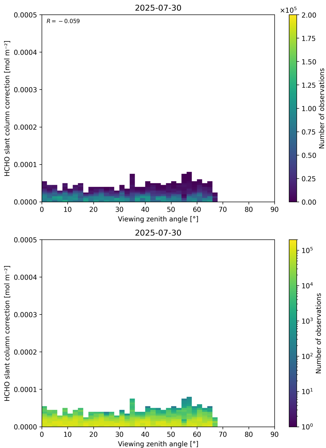
Figure 187: Scatter density plot of “Viewing zenith angle” against “HCHO slant column correction” for 2025-07-29 to 2025-07-31.
