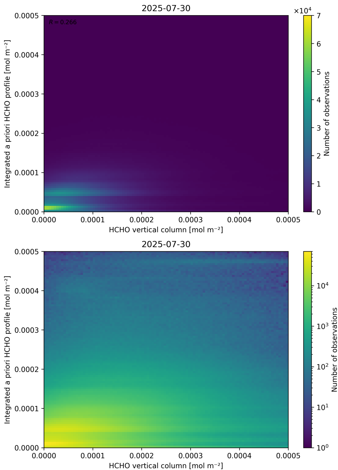
Figure 135: Scatter density plot of “HCHO vertical column” against “Integrated a priori HCHO profile” for 2025-07-29 to 2025-07-31.
