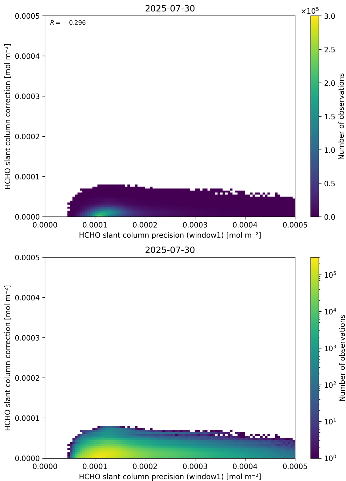
Figure 93: Scatter density plot of “HCHO slant column precision (window1)” against “HCHO slant column correction” for 2025-07-29 to 2025-07-31.
