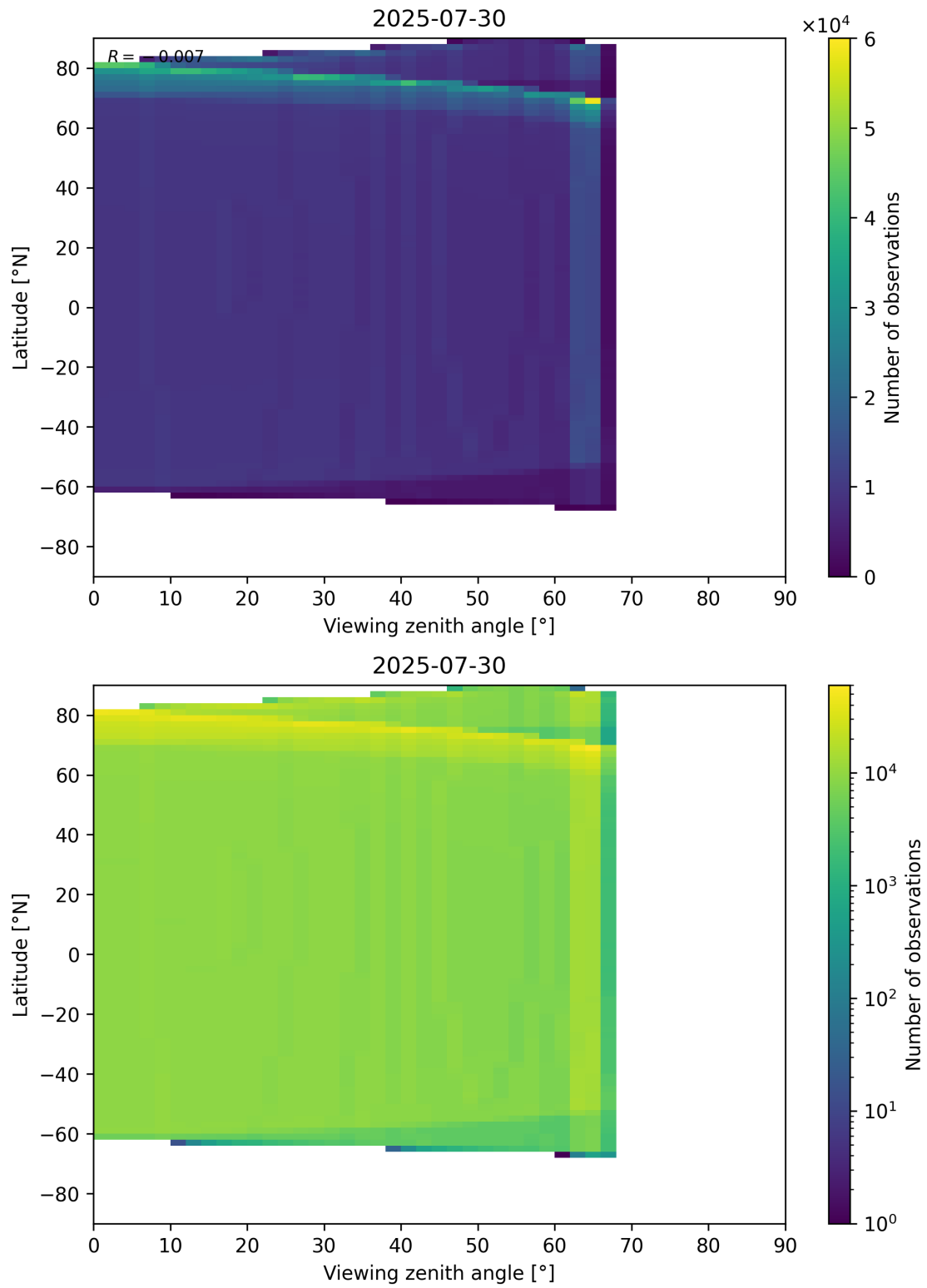
Figure 196: Scatter density plot of “Viewing zenith angle” against “Latitude” for 2025-07-29 to 2025-07-31.
