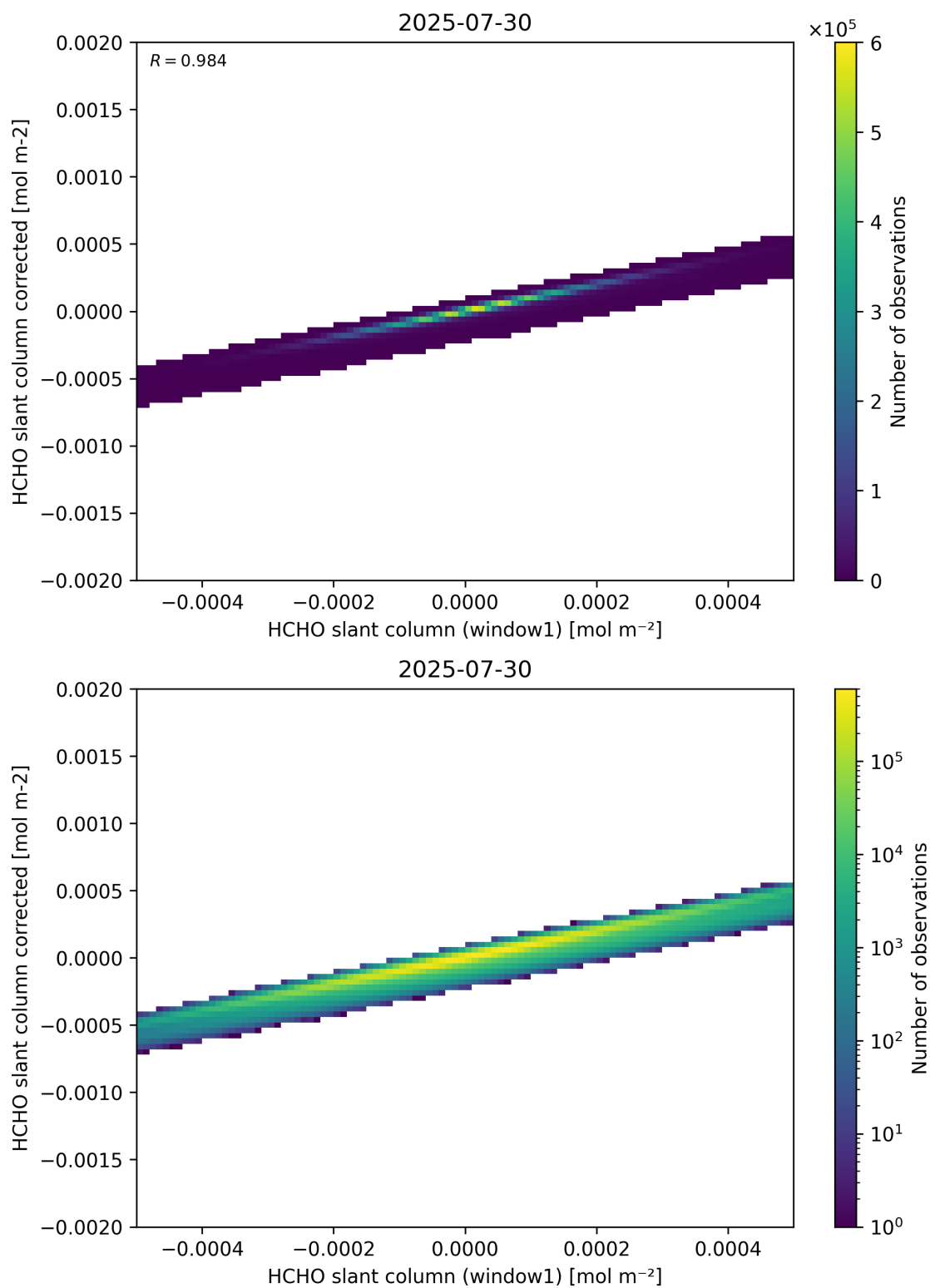
Figure 82: Scatter density plot of “HCHO slant column (window1)” against “HCHO slant column corrected” for 2025-07-29 to 2025-07-31.
