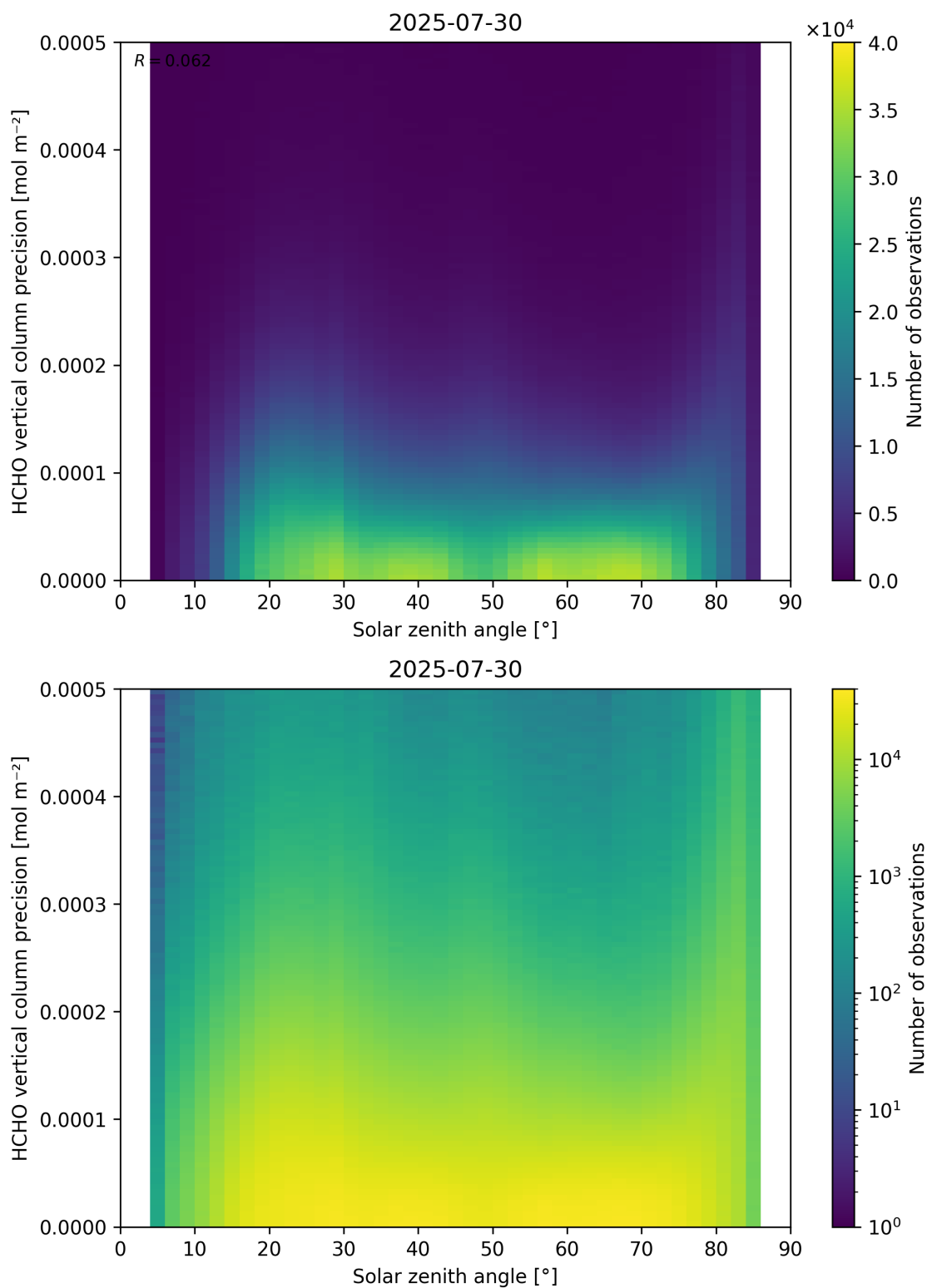
Figure 179: Scatter density plot of “Solar zenith angle” against “HCHO vertical column precision” for 2025-07-29 to 2025-07-31.
