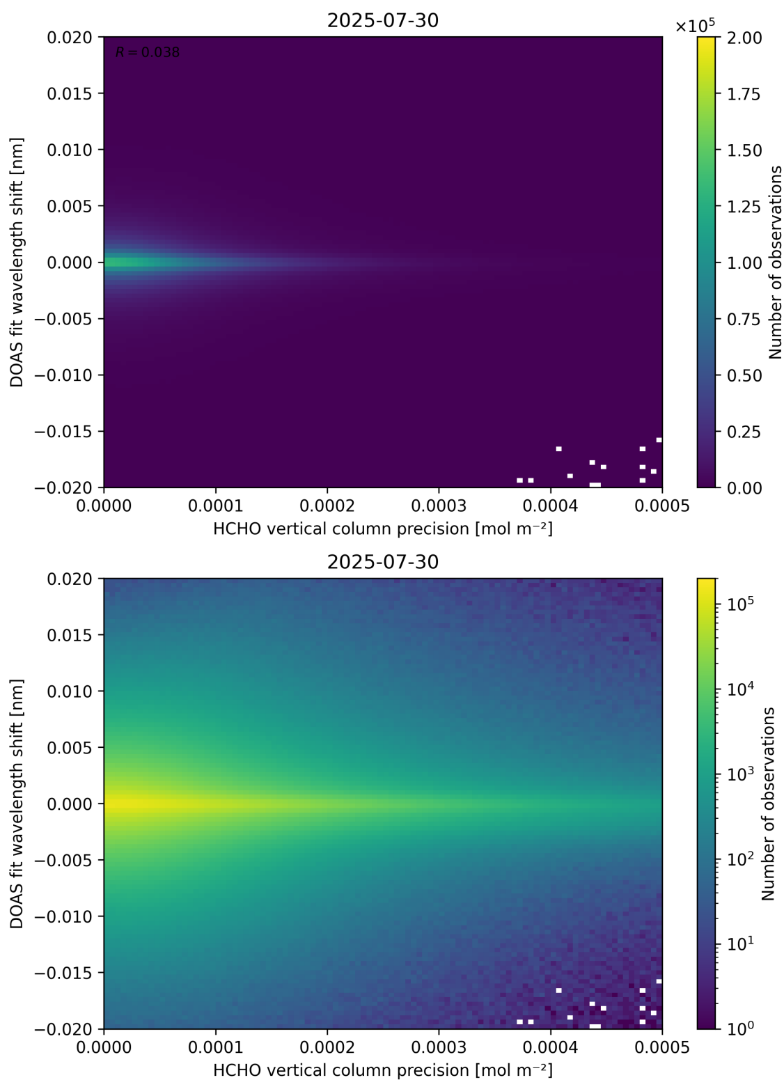
Figure 137: Scatter density plot of “HCHO vertical column precision” against “DOAS fit wavelength shift” for 2025-07-29 to 2025-07-31.
