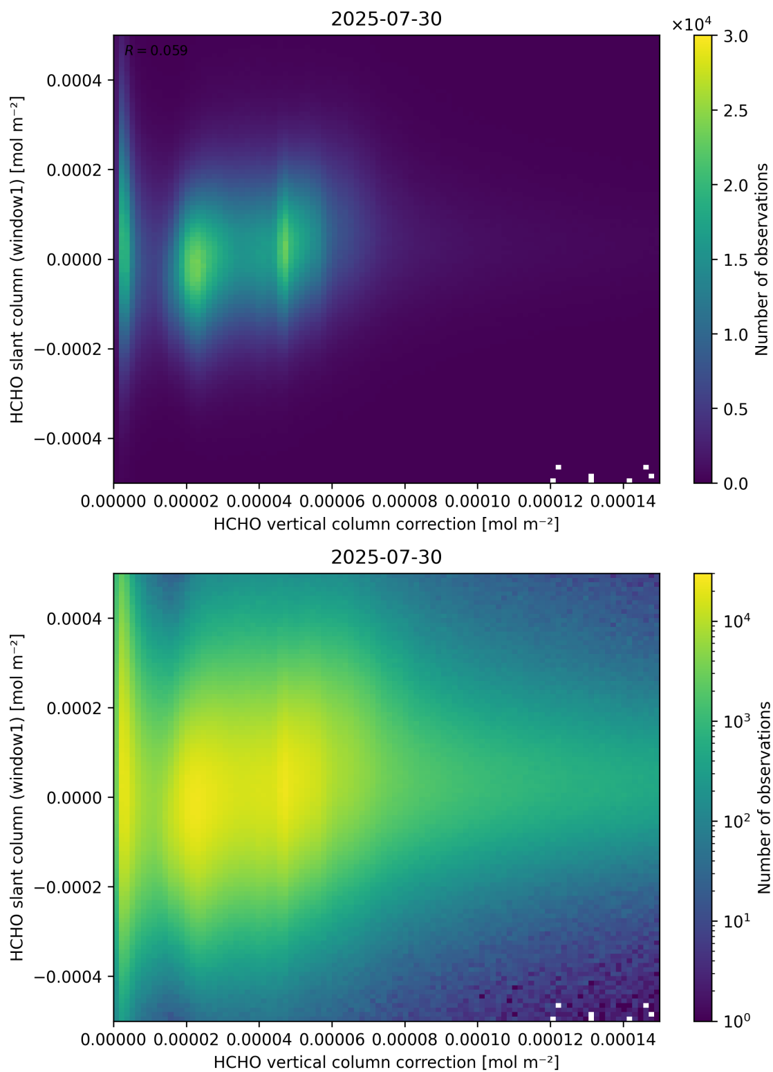
Figure 118: Scatter density plot of “HCHO vertical column correction” against “HCHO slant column (window1)” for 2025-07-29 to 2025-07-31.
