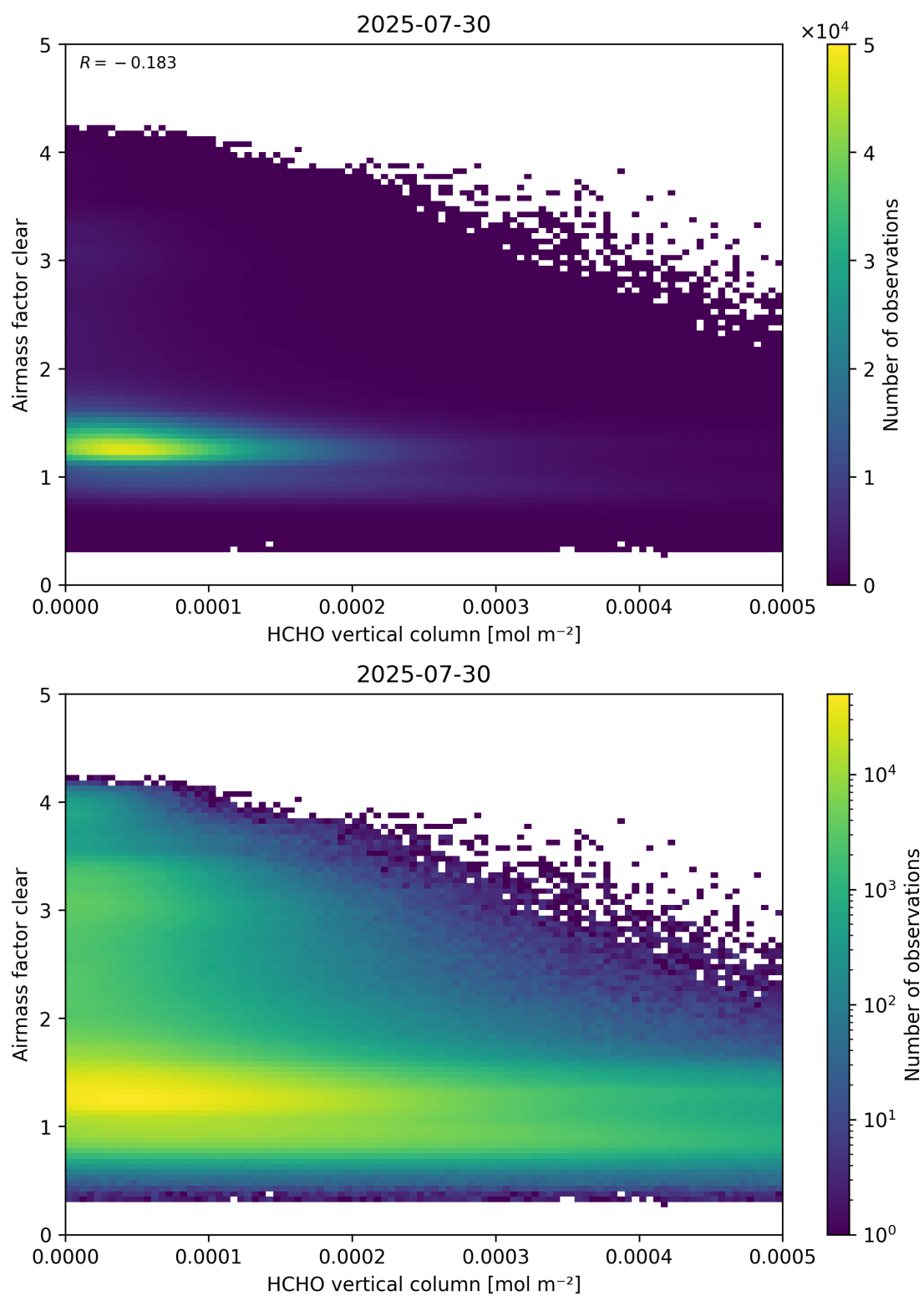
Figure 126: Scatter density plot of “HCHO vertical column” against “Airmass factor clear” for 2025-07-29 to 2025-07-31.
