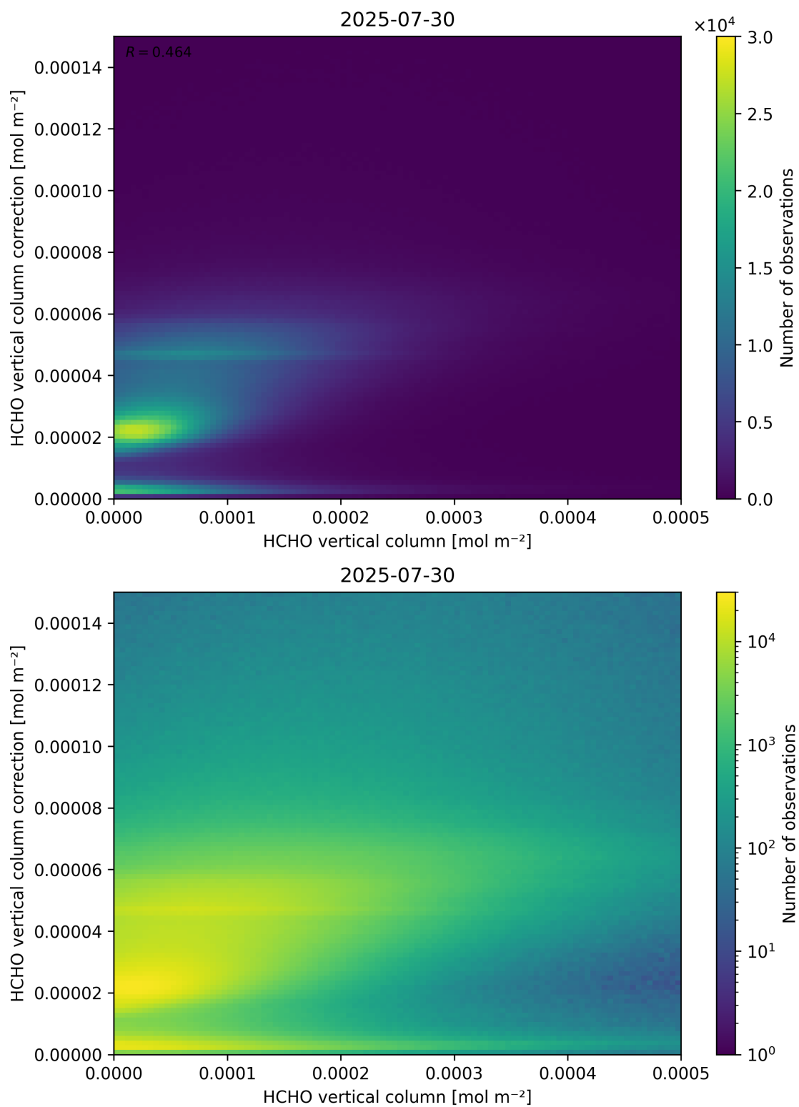
Figure 133: Scatter density plot of “HCHO vertical column” against “HCHO vertical column correction” for 2025-07-29 to 2025-07-31.
