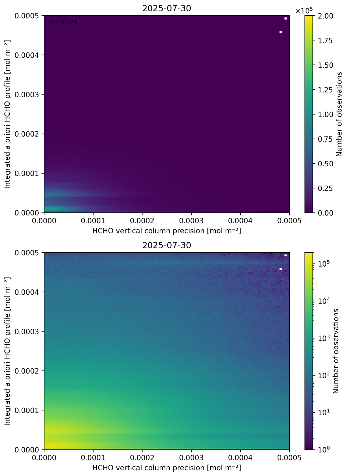
Figure 147: Scatter density plot of “HCHO vertical column precision” against “Integrated a priori HCHO profile” for 2025-07-29 to 2025-07-31.
