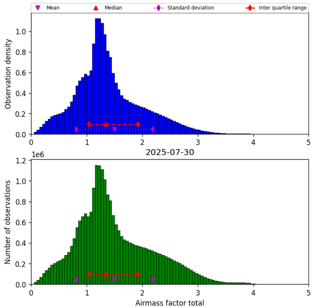
Figure 40: Histogram of “Airmass factor total” for 2025-07-29 to 2025-07-31
