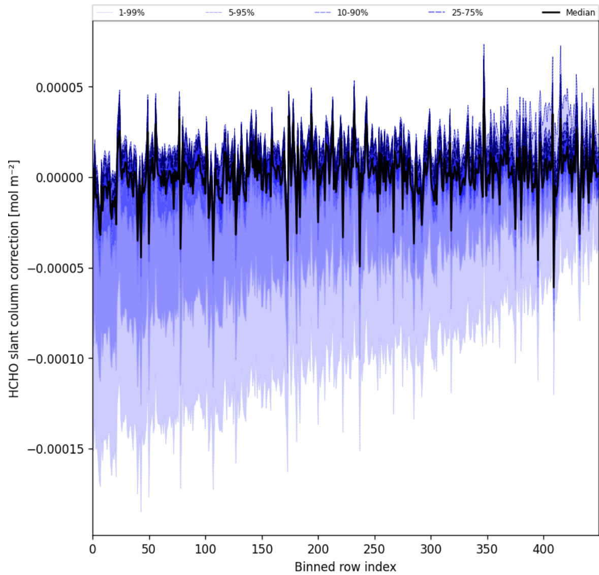
Figure 61: Along track statistics of “HCHO slant column correction” for 2025-07-29 to 2025-07-31
