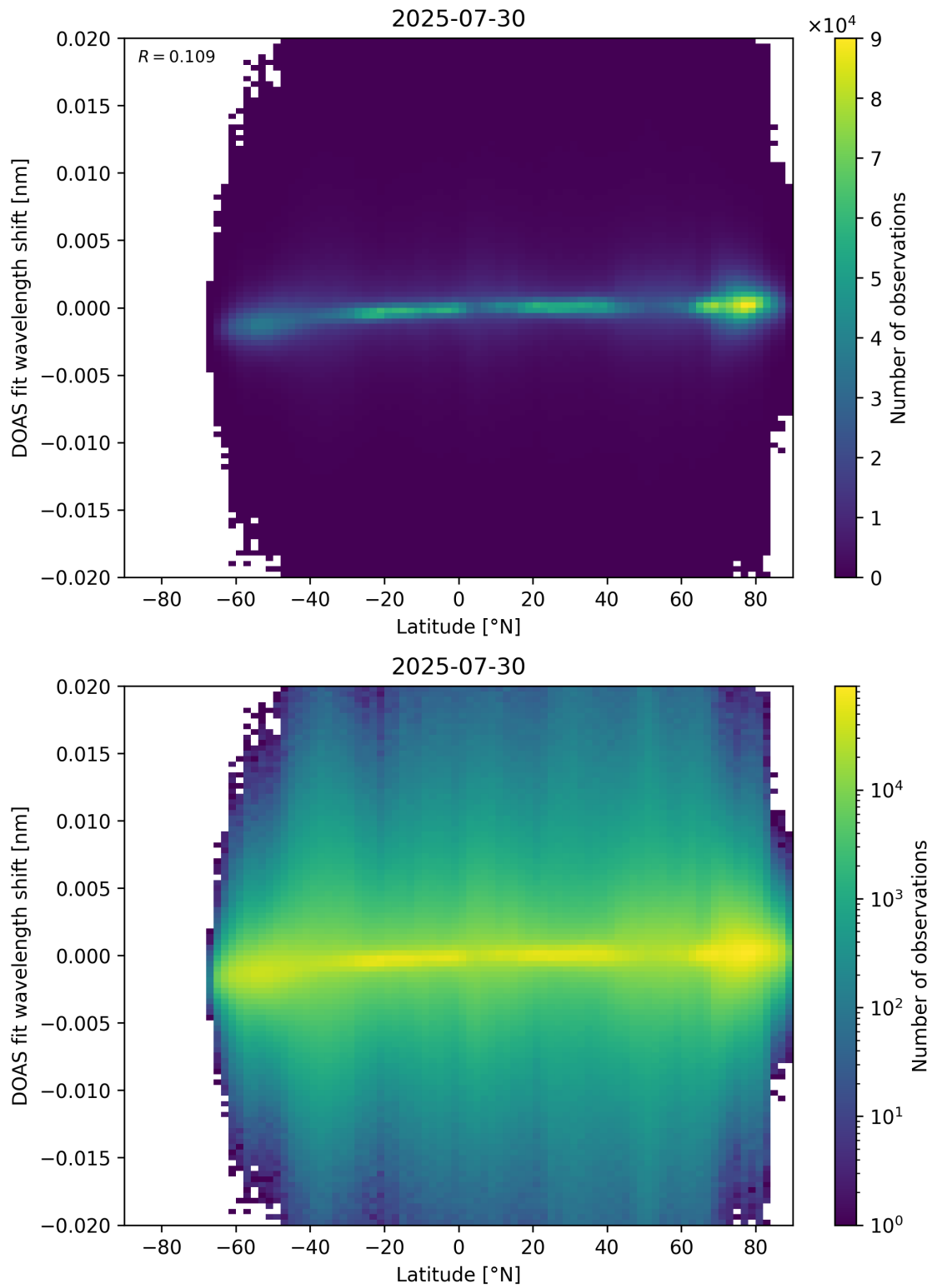
Figure 154: Scatter density plot of “Latitude” against “DOAS fit wavelength shift” for 2025-07-29 to 2025-07-31.
