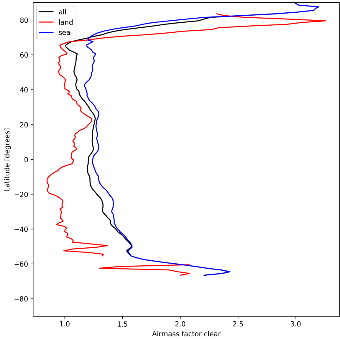
Figure 28: Zonal average of “Airmass factor clear” for 2025-07-29 to 2025-07-31.
