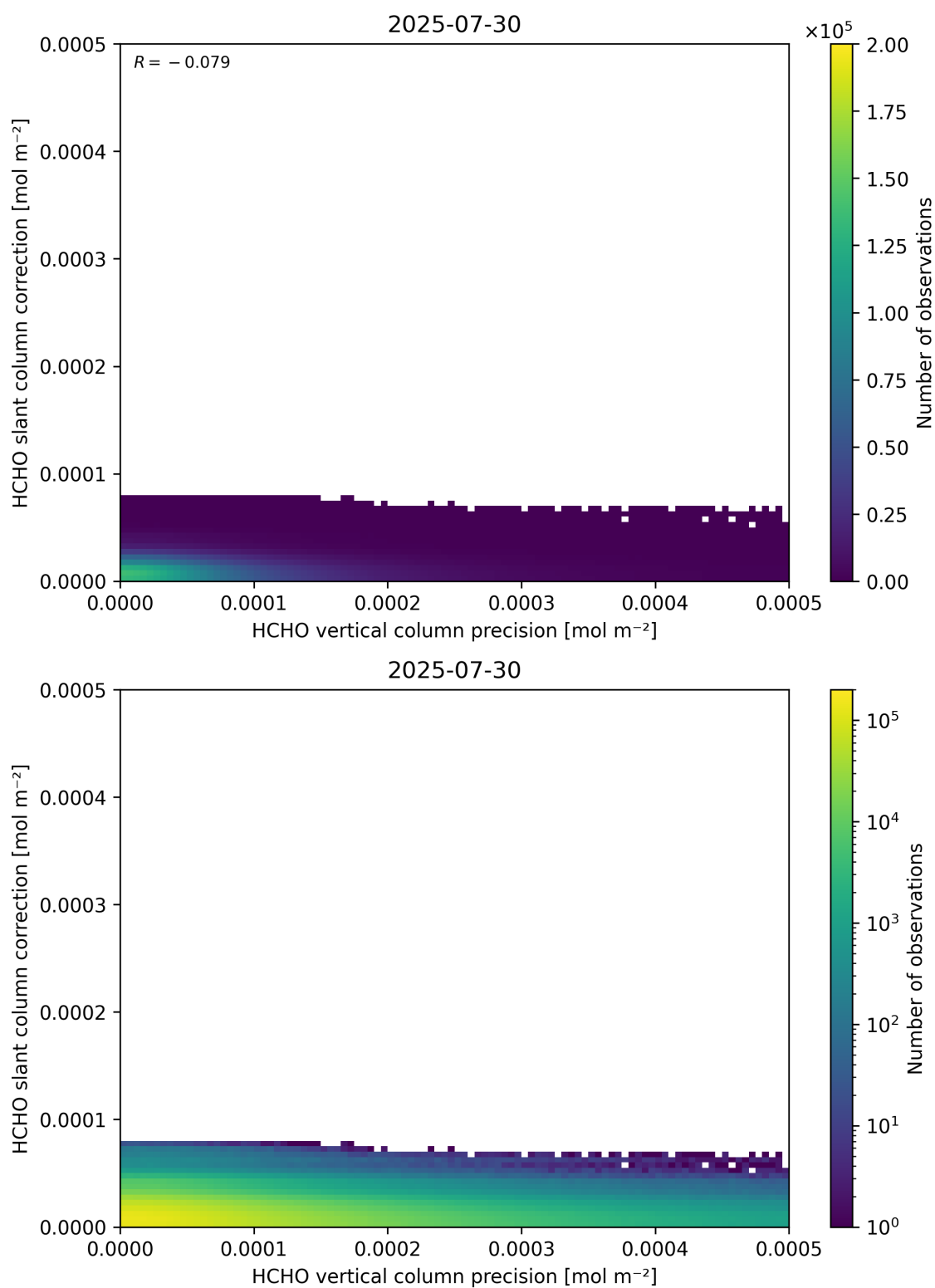
Figure 141: Scatter density plot of “HCHO vertical column precision” against “HCHO slant column correction” for 2025-07-29 to 2025-07-31.
