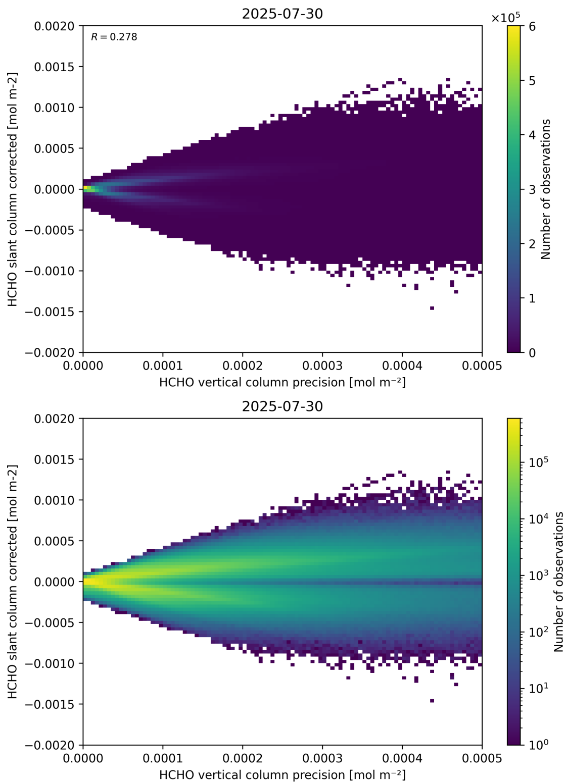
Figure 140: Scatter density plot of “HCHO vertical column precision” against “HCHO slant column corrected” for 2025-07-29 to 2025-07-31.
