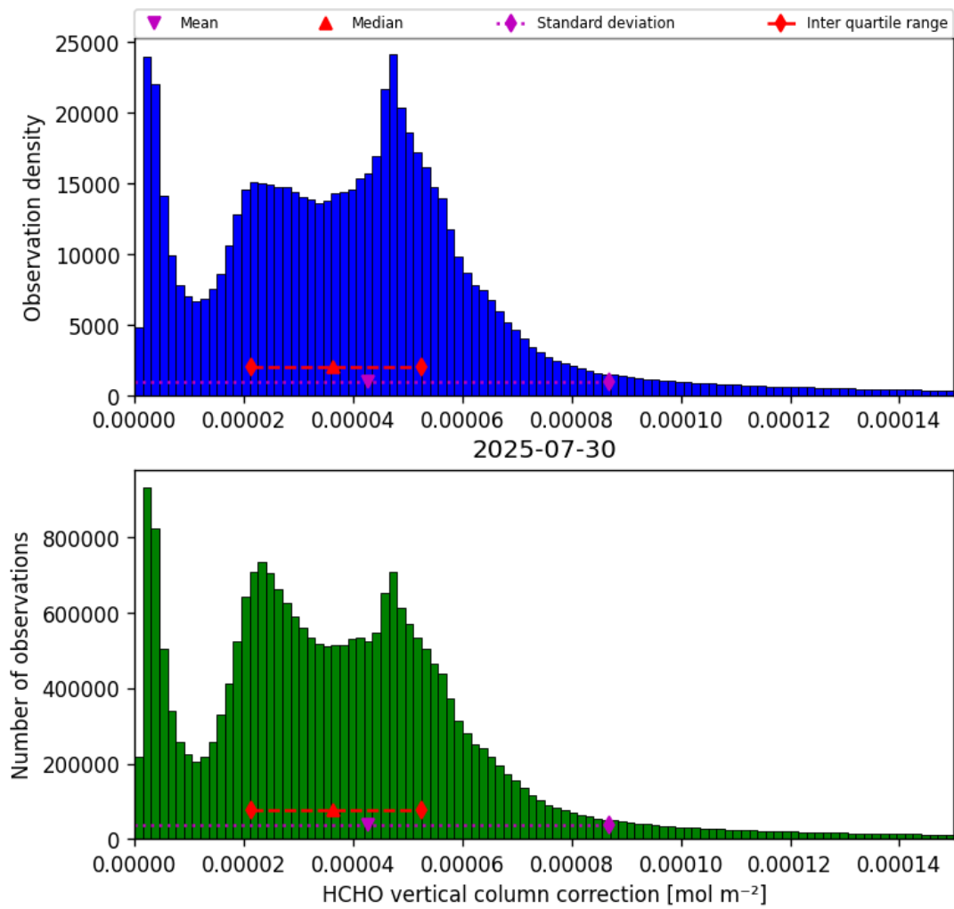
Figure 37: Histogram of “HCHO vertical column correction” for 2025-07-29 to 2025-07-31
