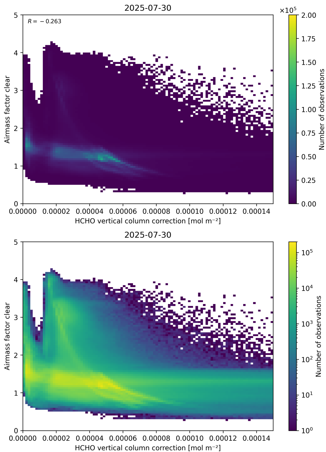
Figure 115: Scatter density plot of “HCHO vertical column correction” against “Airmass factor clear” for 2025-07-29 to 2025-07-31.
