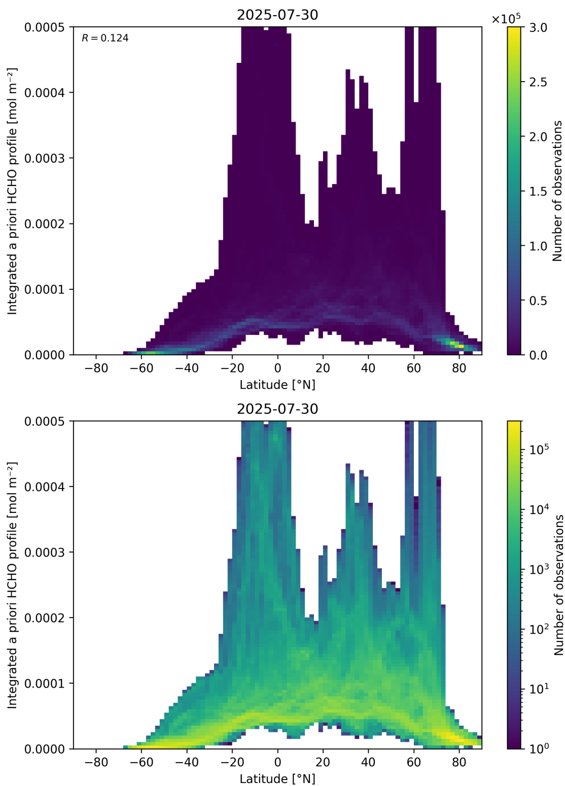
Figure 166: Scatter density plot of “Latitude” against “Integrated a priori HCHO profile” for 2025-07-29 to 2025-07-31.
