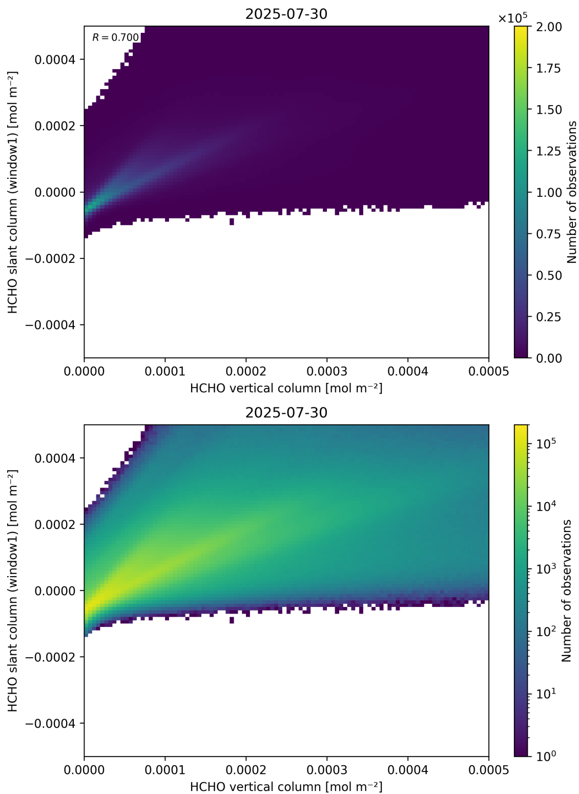
Figure 129: Scatter density plot of “HCHO vertical column” against “HCHO slant column (window1)” for 2025-07-29 to 2025-07-31.
