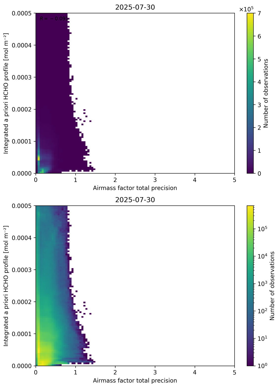
Figure 111: Scatter density plot of “Airmass factor total precision” against “Integrated a priori HCHO profile” for 2025-07-29 to 2025-07-31.
