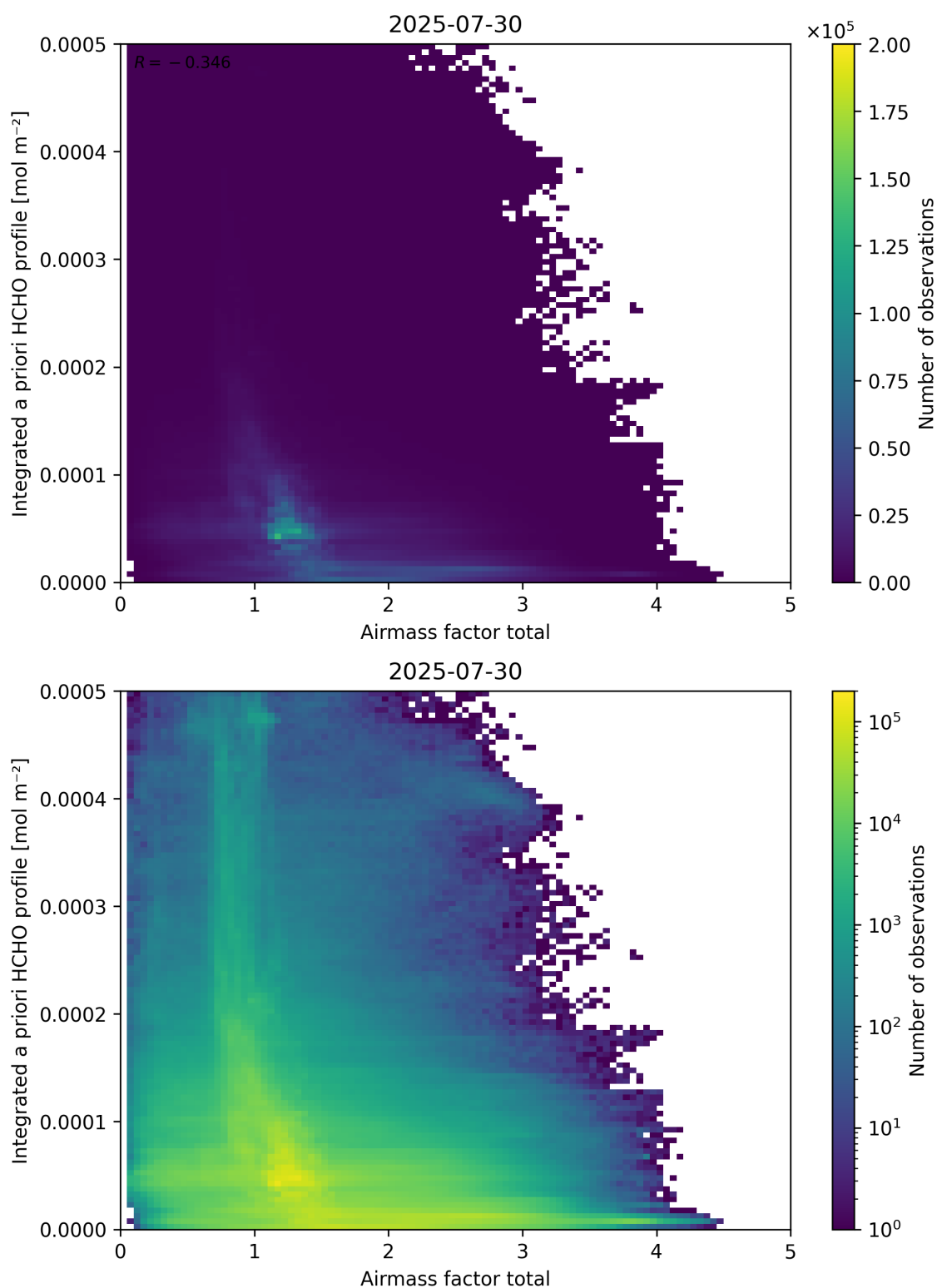
Figure 104: Scatter density plot of “Airmass factor total” against “Integrated a priori HCHO profile” for 2025-07-29 to 2025-07-31.
