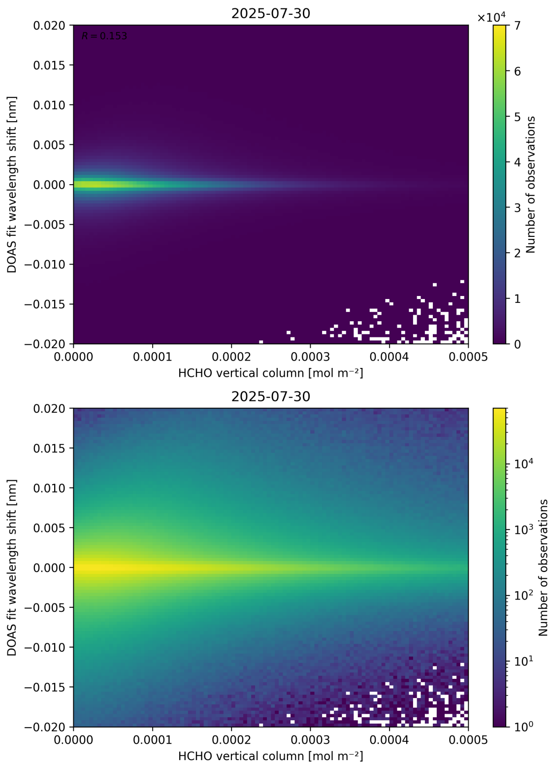
Figure 124: Scatter density plot of “HCHO vertical column” against “DOAS fit wavelength shift” for 2025-07-29 to 2025-07-31.
