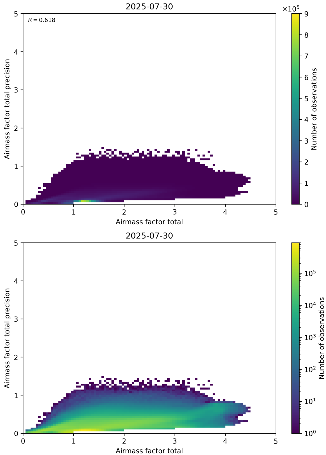
Figure 103: Scatter density plot of “Airmass factor total” against “Airmass factor total precision” for 2025-07-29 to 2025-07-31.
