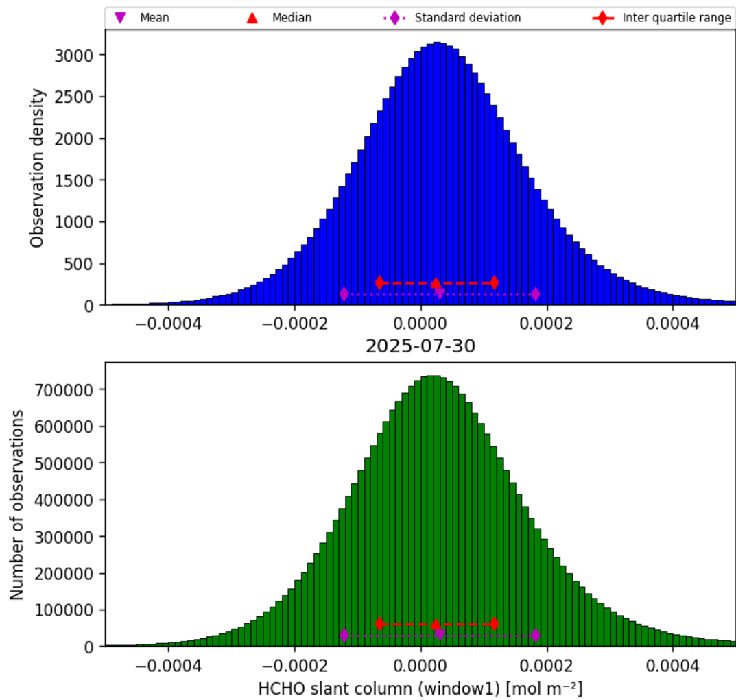
Figure 38: Histogram of “HCHO slant column (window1)” for 2025-07-29 to 2025-07-31
