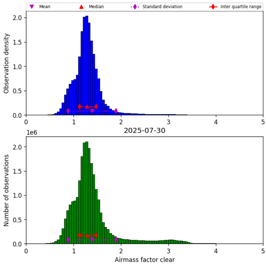
Figure 42: Histogram of “Airmass factor clear” for 2025-07-29 to 2025-07-31
