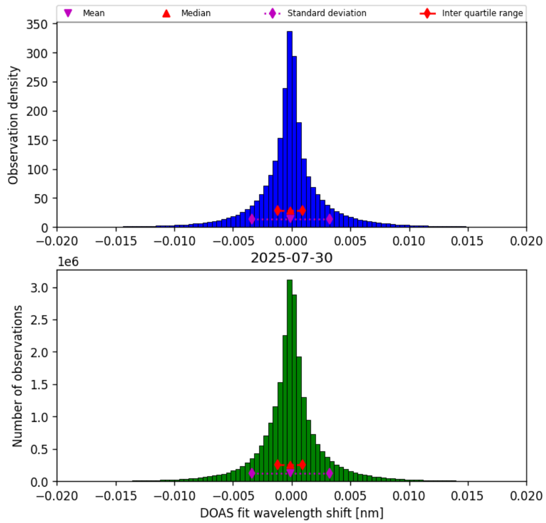
Figure 44: Histogram of “DOAS fit wavelength shift” for 2025-07-29 to 2025-07-31
