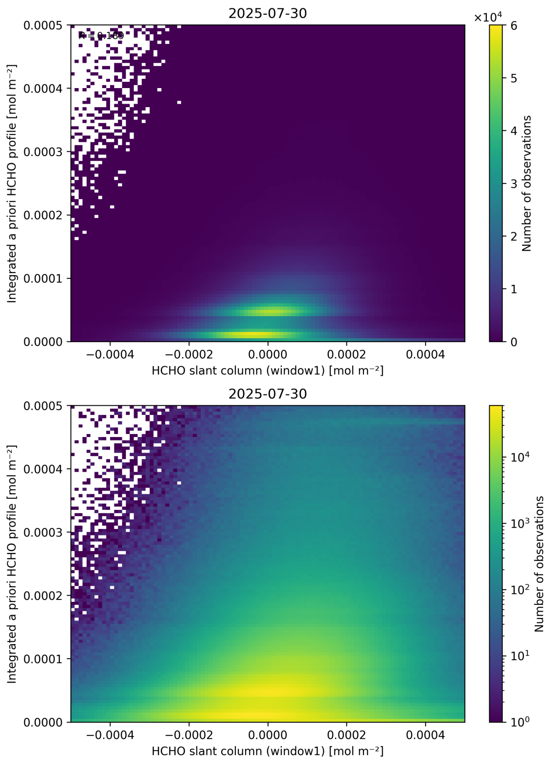
Figure 87: Scatter density plot of “HCHO slant column (window1)” against “Integrated a priori HCHO profile” for 2025-07-29 to 2025-07-31.
