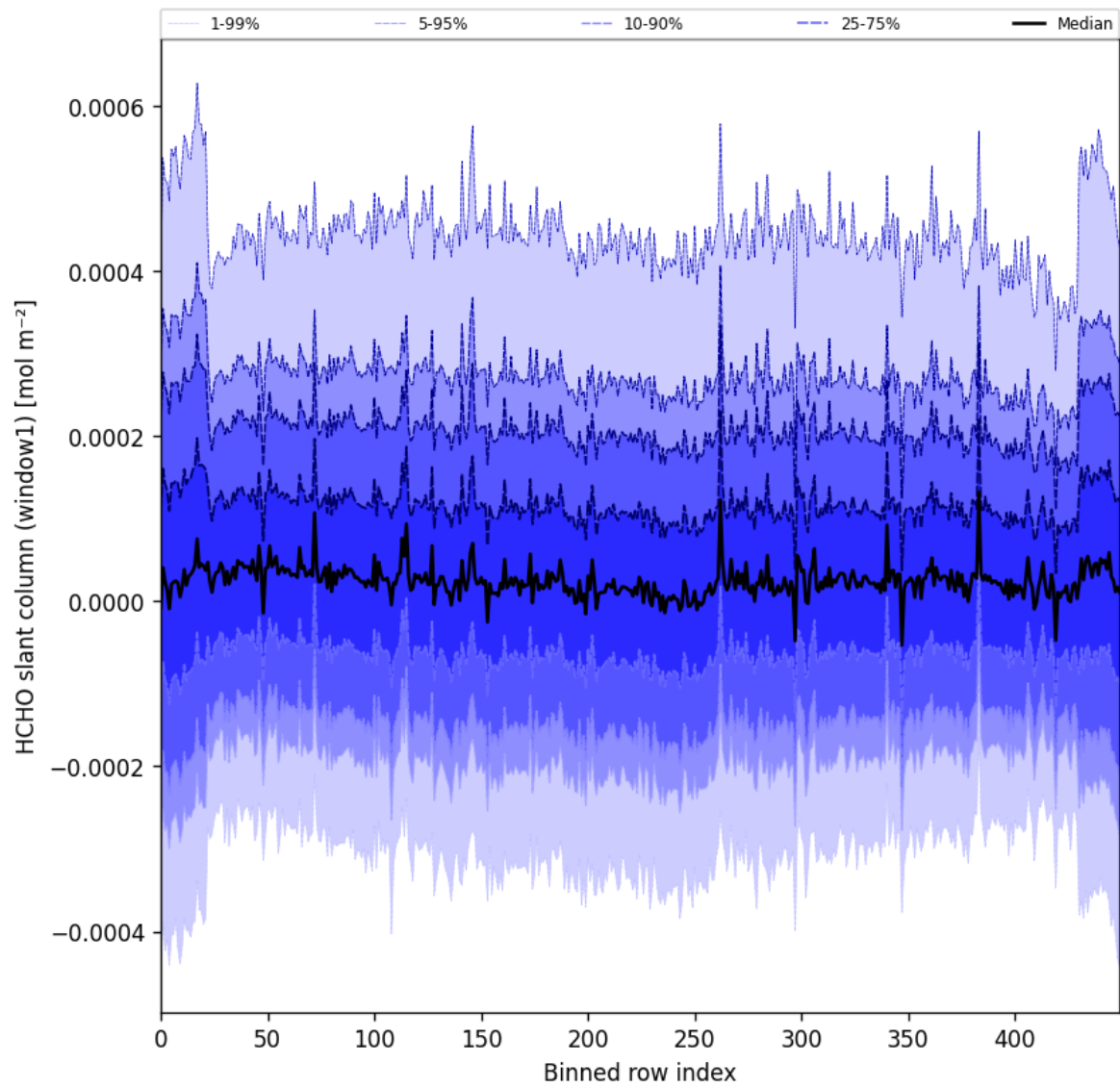
Figure 52: Along track statistics of “HCHO slant column (window1)” for 2025-07-29 to 2025-07-31
