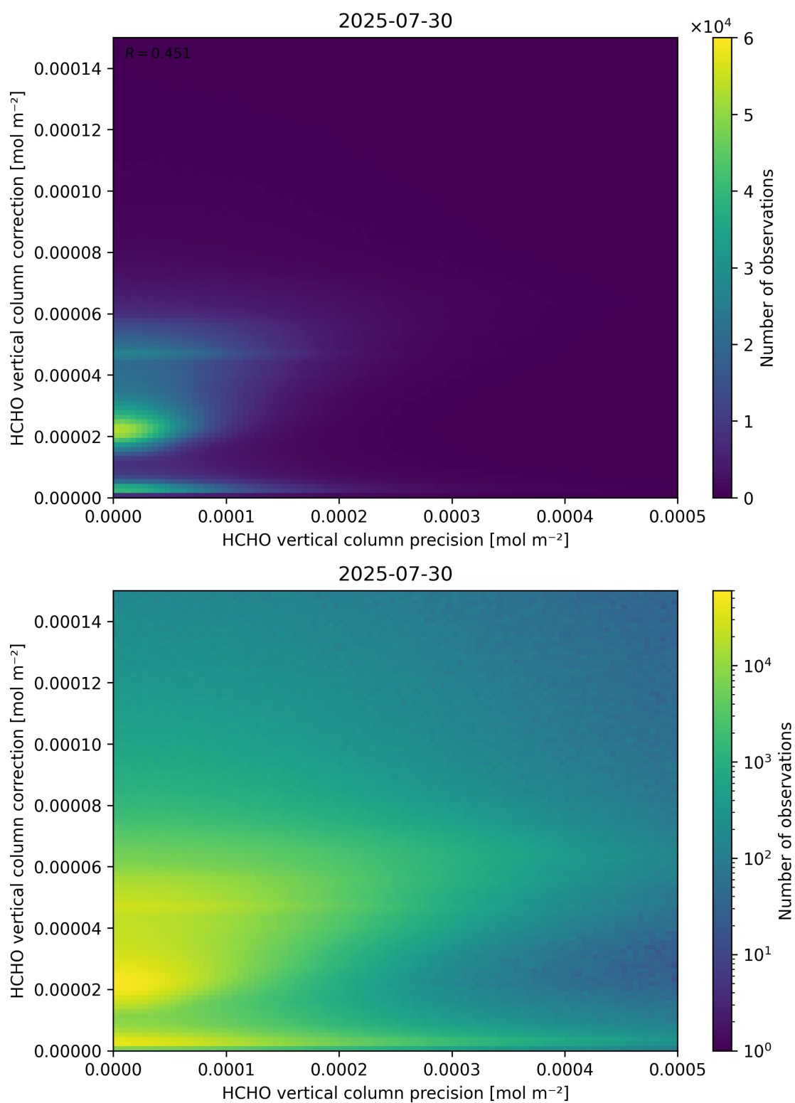
Figure 146: Scatter density plot of “HCHO vertical column precision” against “HCHO vertical column correction” for 2025-07-29 to 2025-07-31.
