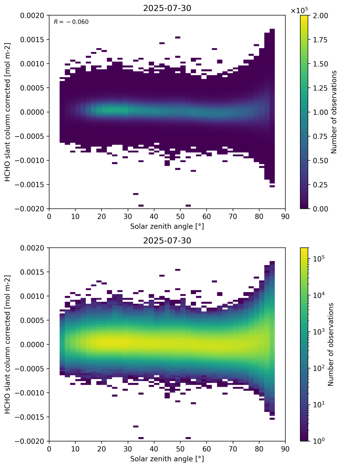
Figure 171: Scatter density plot of “Solar zenith angle” against “HCHO slant column corrected” for 2025-07-29 to 2025-07-31.
