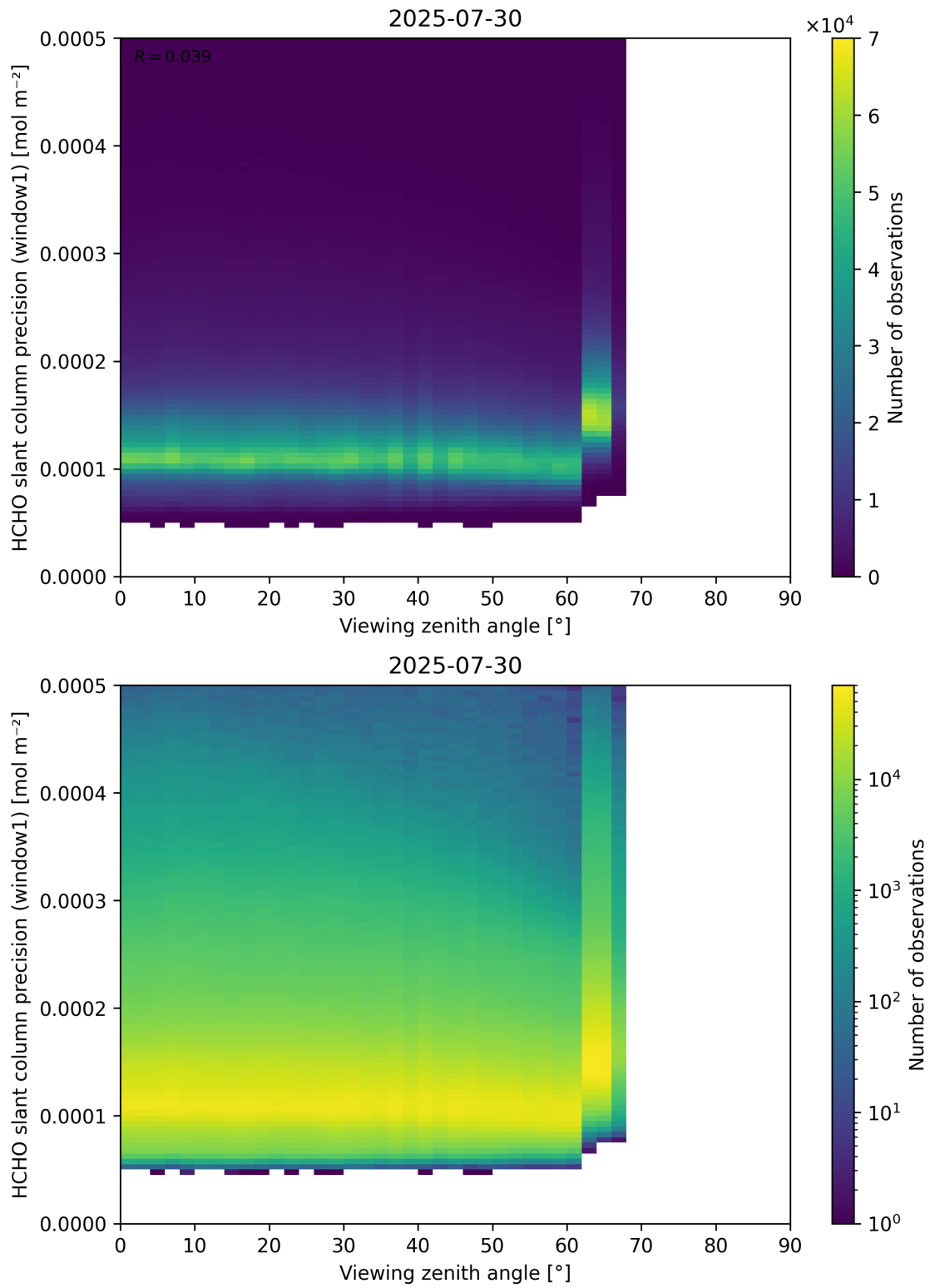
Figure 189: Scatter density plot of “Viewing zenith angle” against “HCHO slant column precision (window1)” for 2025-07-29 to 2025-07-31.
