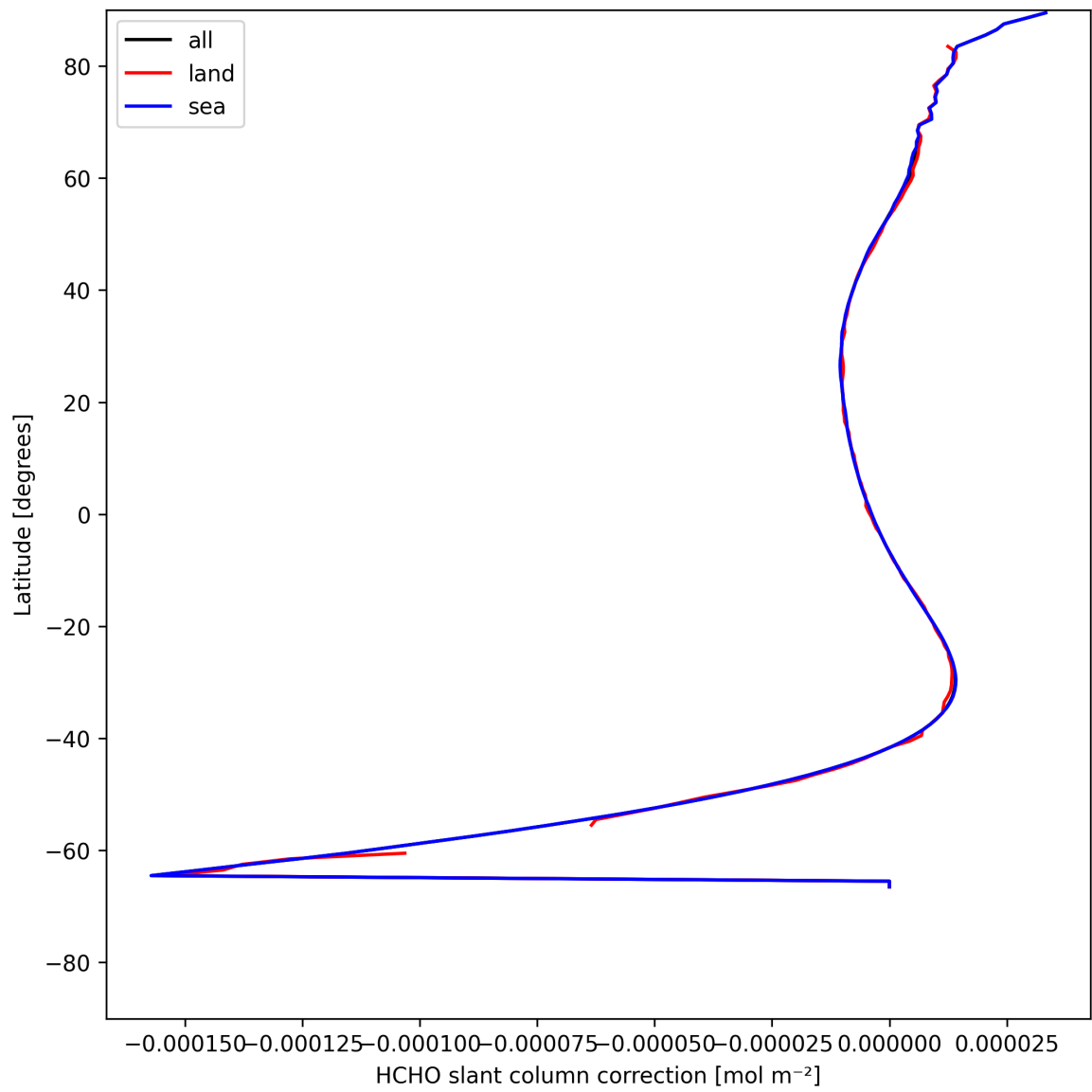
Figure 33: Zonal average of “HCHO slant column correction” for 2025-07-29 to 2025-07-31.
