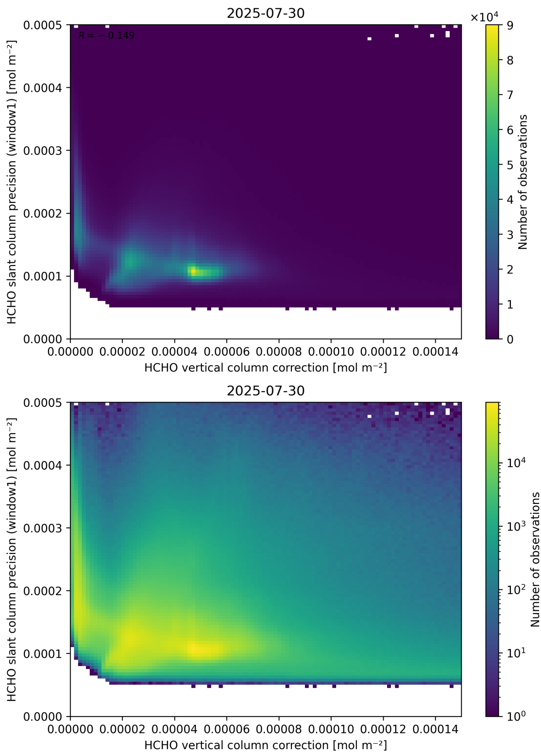
Figure 119: Scatter density plot of “HCHO vertical column correction” against “HCHO slant column precision (window1)” for 2025-07-29 to 2025-07-31.
