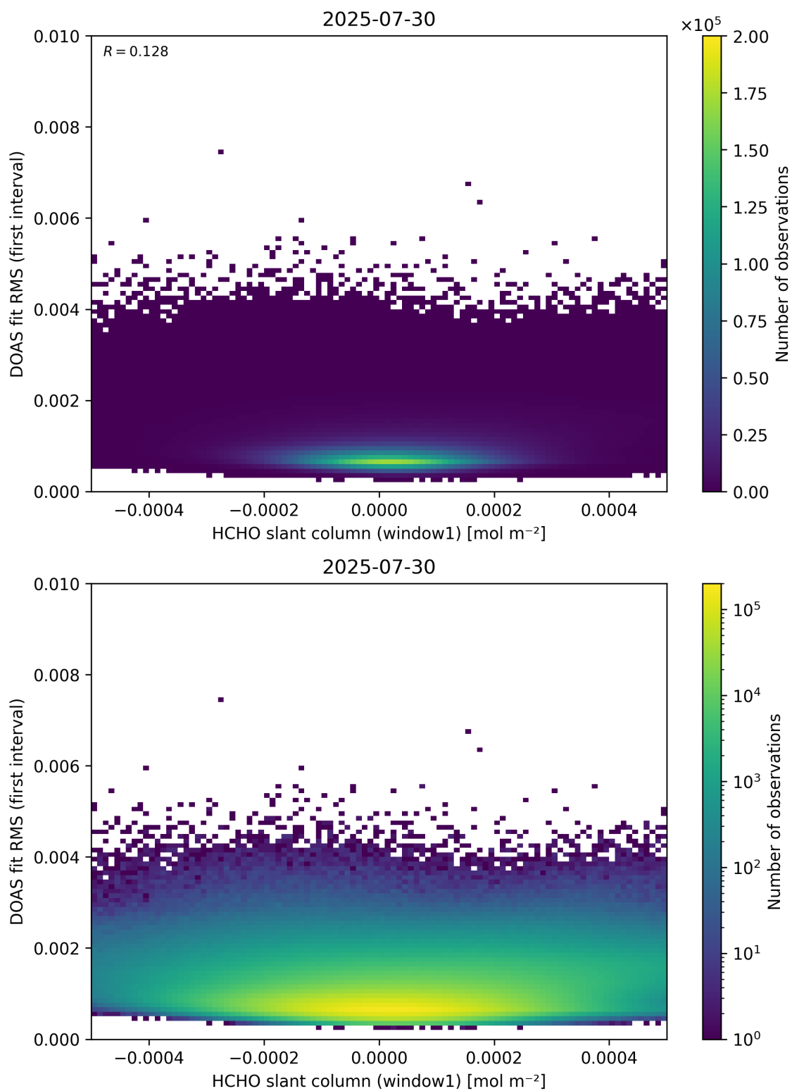
Figure 78: Scatter density plot of “HCHO slant column (window1)” against “DOAS fit RMS (first interval)” for 2025-07-29 to 2025-07-31.
