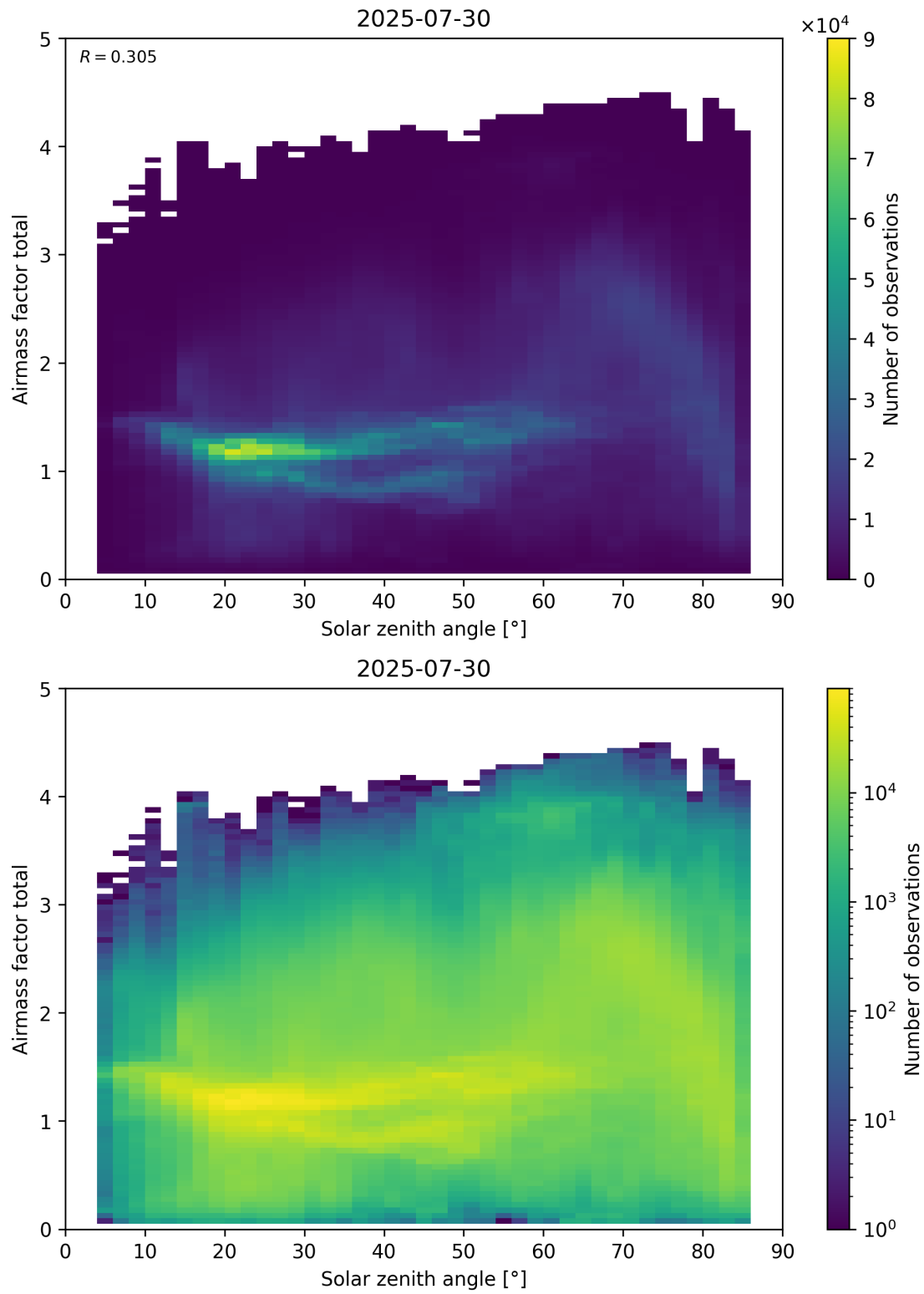
Figure 175: Scatter density plot of “Solar zenith angle” against “Airmass factor total” for 2025-07-29 to 2025-07-31.
