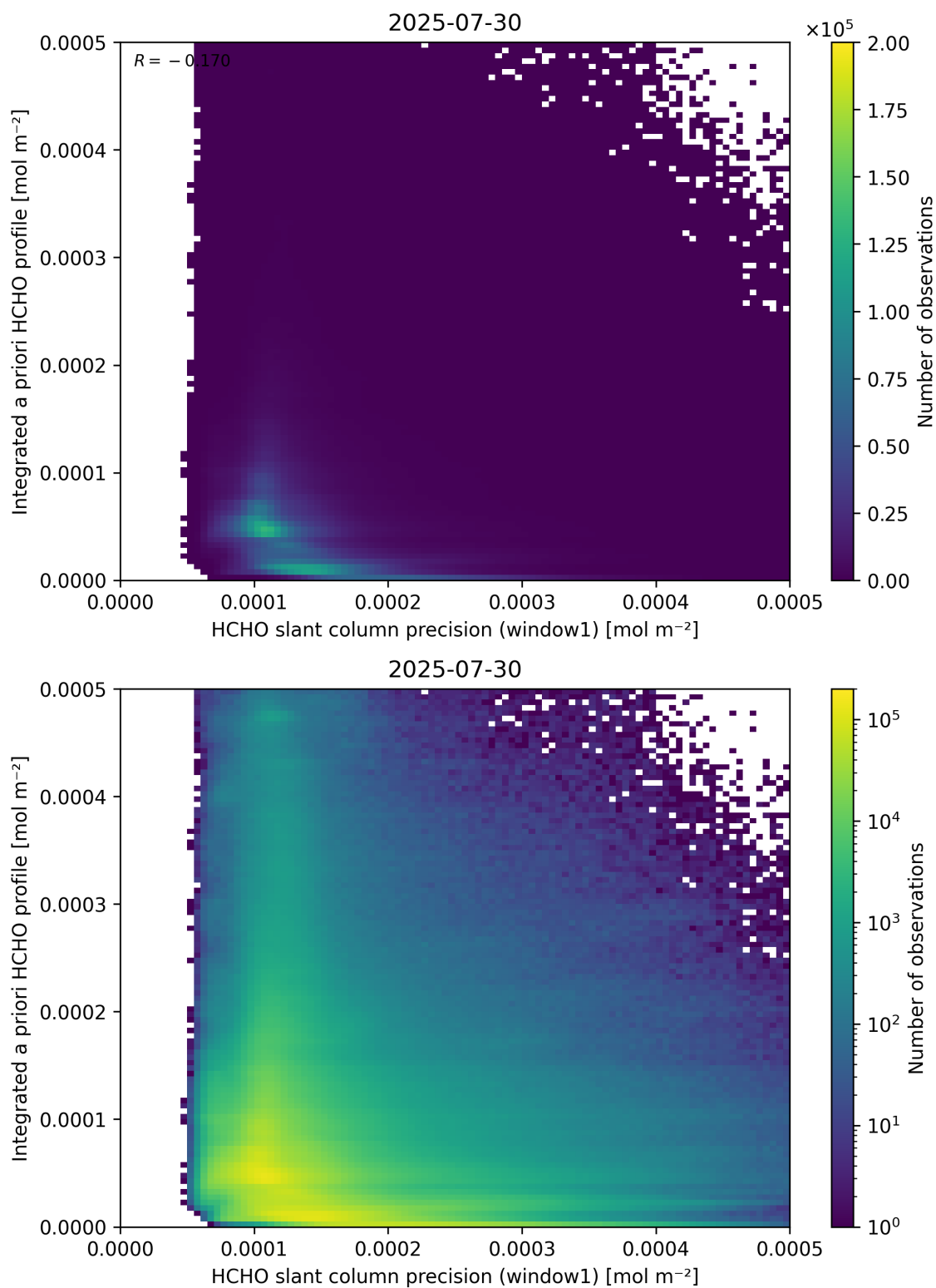
Figure 96: Scatter density plot of “HCHO slant column precision (window1)” against “Integrated a priori HCHO profile” for 2025-07-29 to 2025-07-31.
