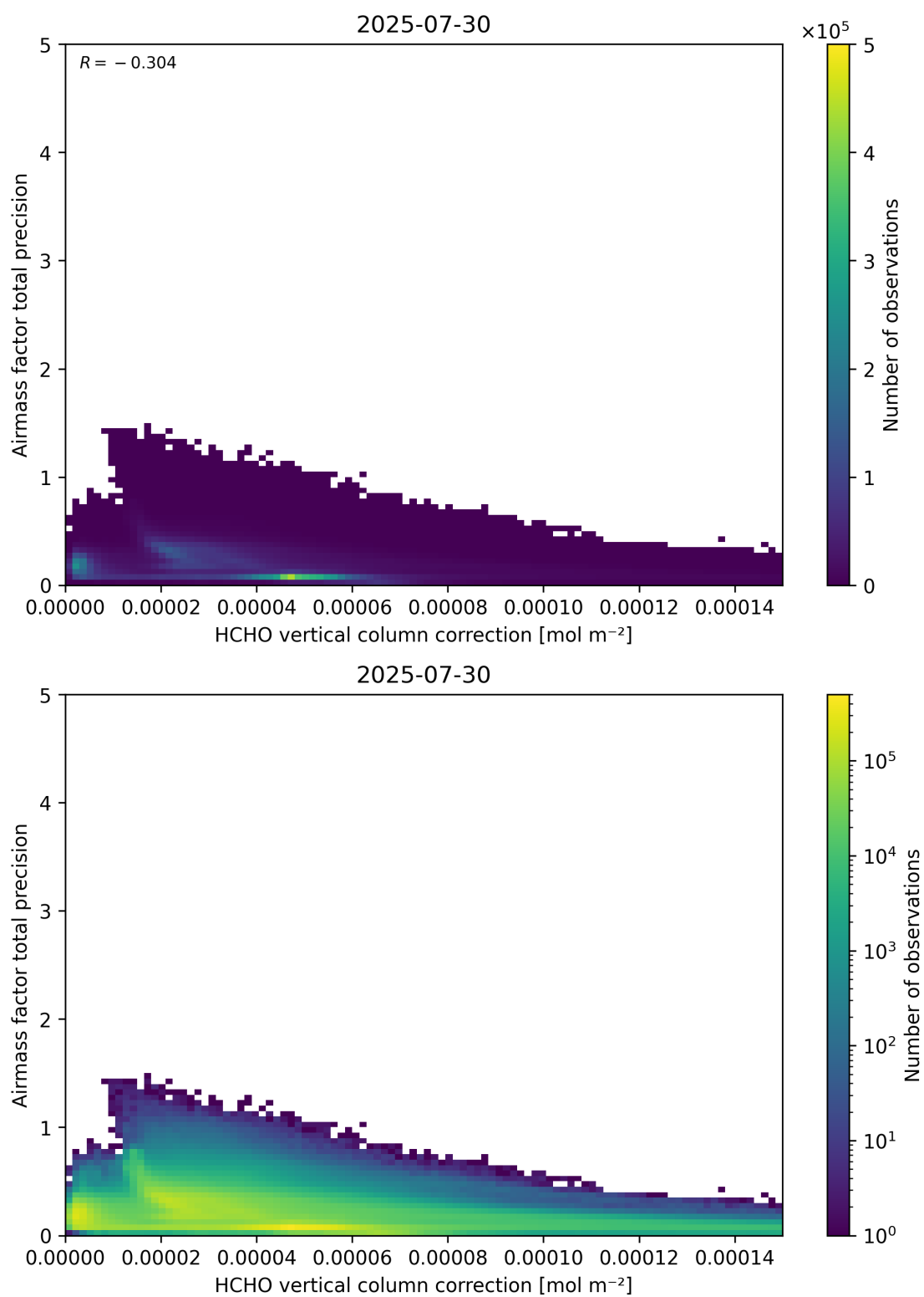
Figure 121: Scatter density plot of “HCHO vertical column correction” against “Airmass factor total precision” for 2025-07-29 to 2025-07-31.
