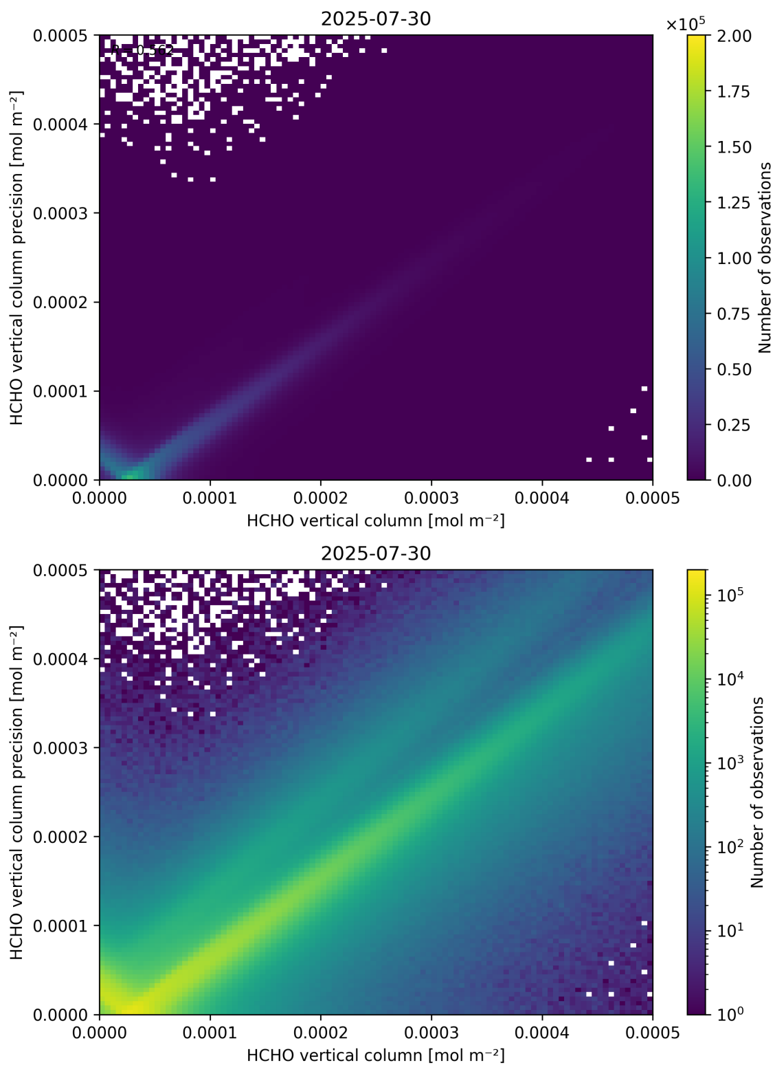
Figure 134: Scatter density plot of “HCHO vertical column” against “HCHO vertical column precision” for 2025-07-29 to 2025-07-31.
