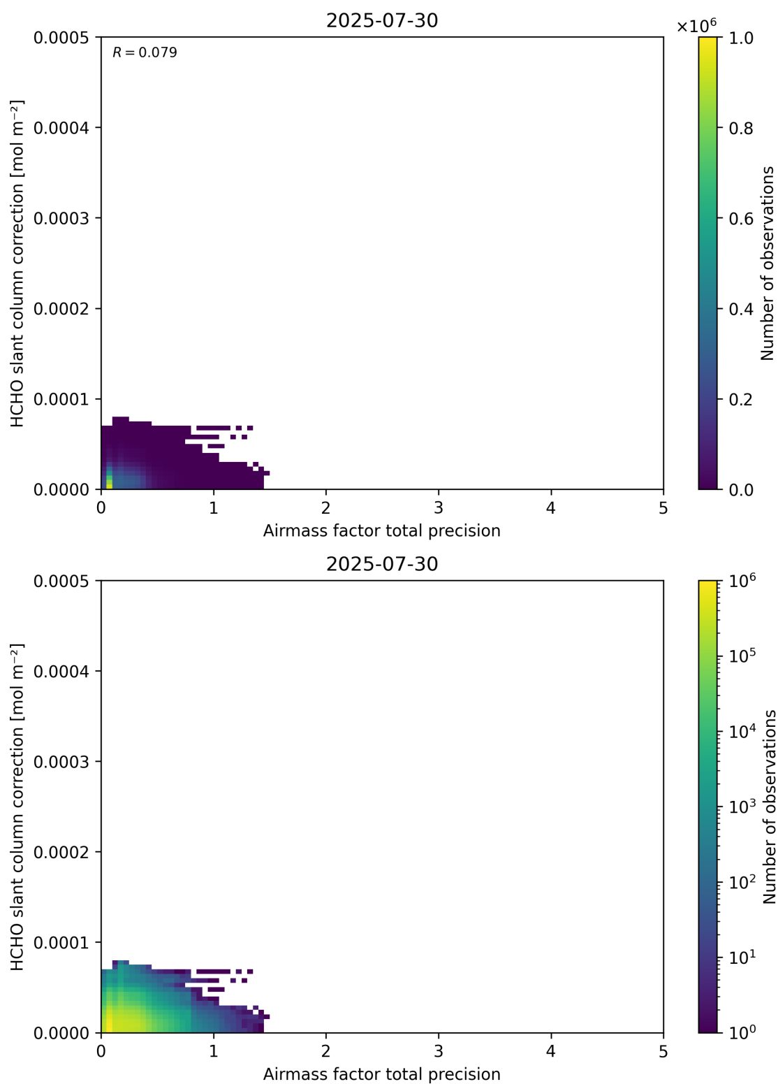
Figure 110: Scatter density plot of “Airmass factor total precision” against “HCHO slant column correction” for 2025-07-29 to 2025-07-31.
