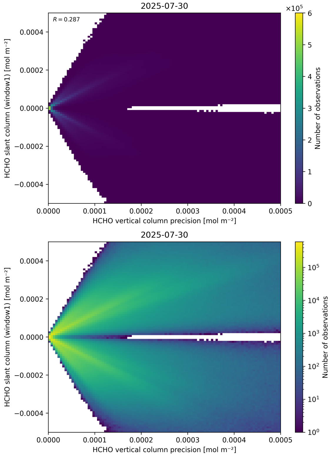
Figure 142: Scatter density plot of “HCHO vertical column precision” against “HCHO slant column (window1)” for 2025-07-29 to 2025-07-31.
