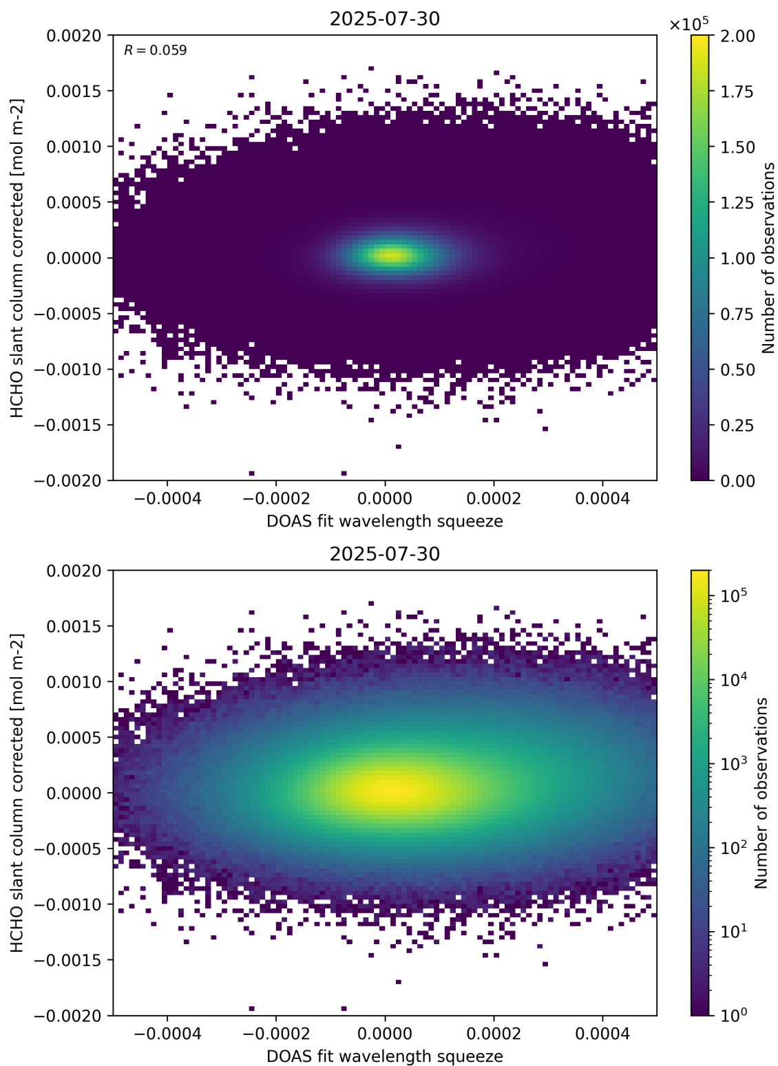
Figure 69: Scatter density plot of “DOAS fit wavelength squeeze” against “HCHO slant column corrected” for 2025-07-29 to 2025-07-31.
