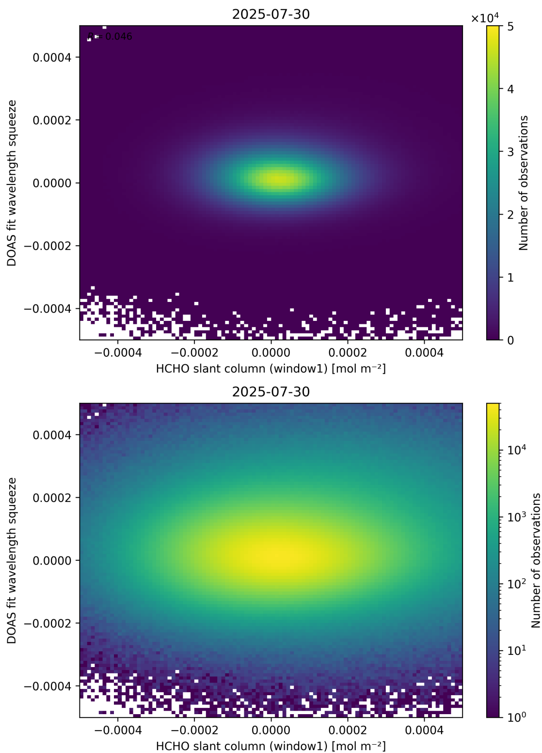
Figure 80: Scatter density plot of “HCHO slant column (window1)” against “DOAS fit wavelength squeeze” for 2025-07-29 to 2025-07-31.
