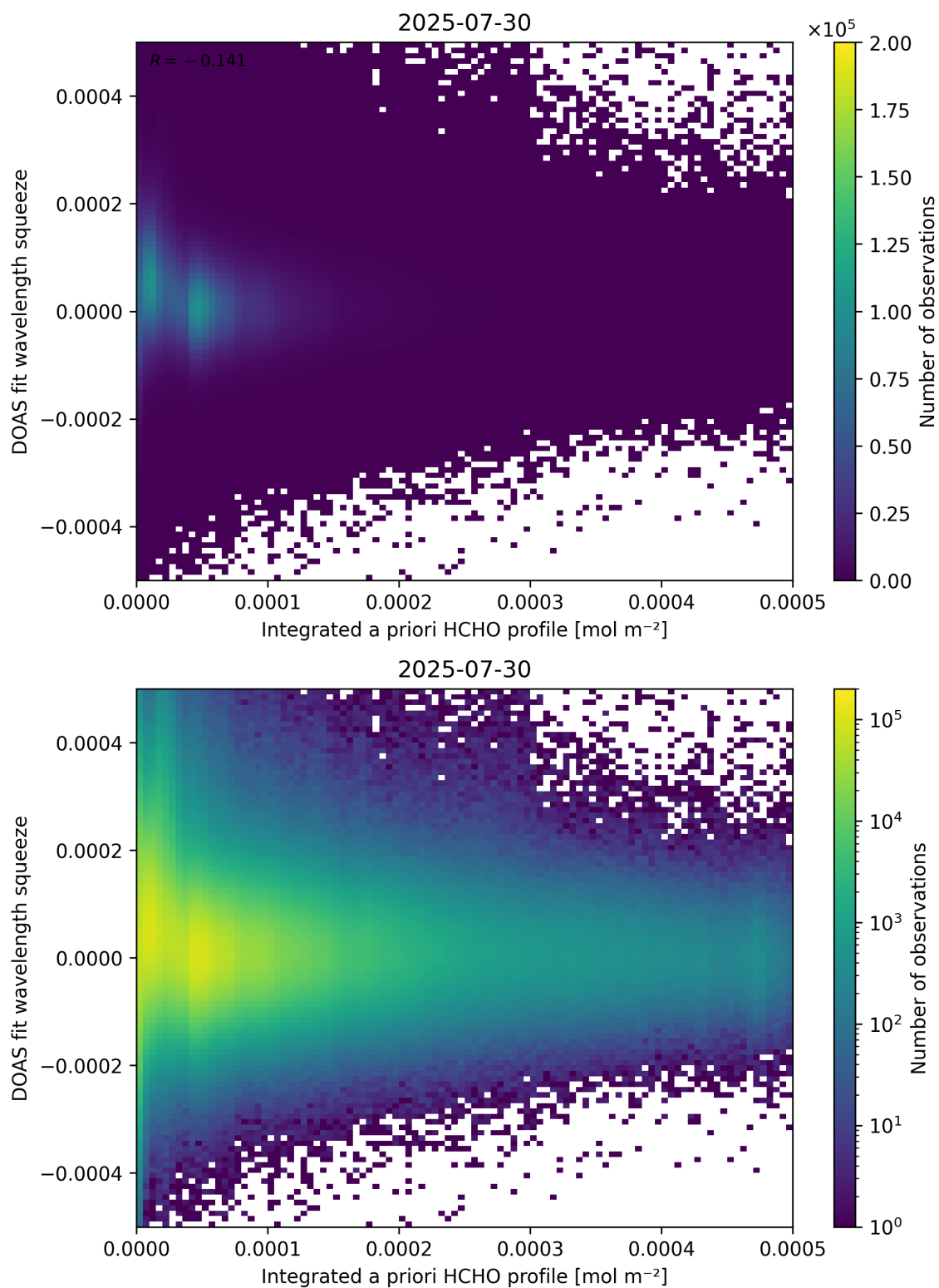
Figure 150: Scatter density plot of “Integrated a priori HCHO profile” against “DOAS fit wavelength squeeze” for 2025-07-29 to 2025-07-31.
