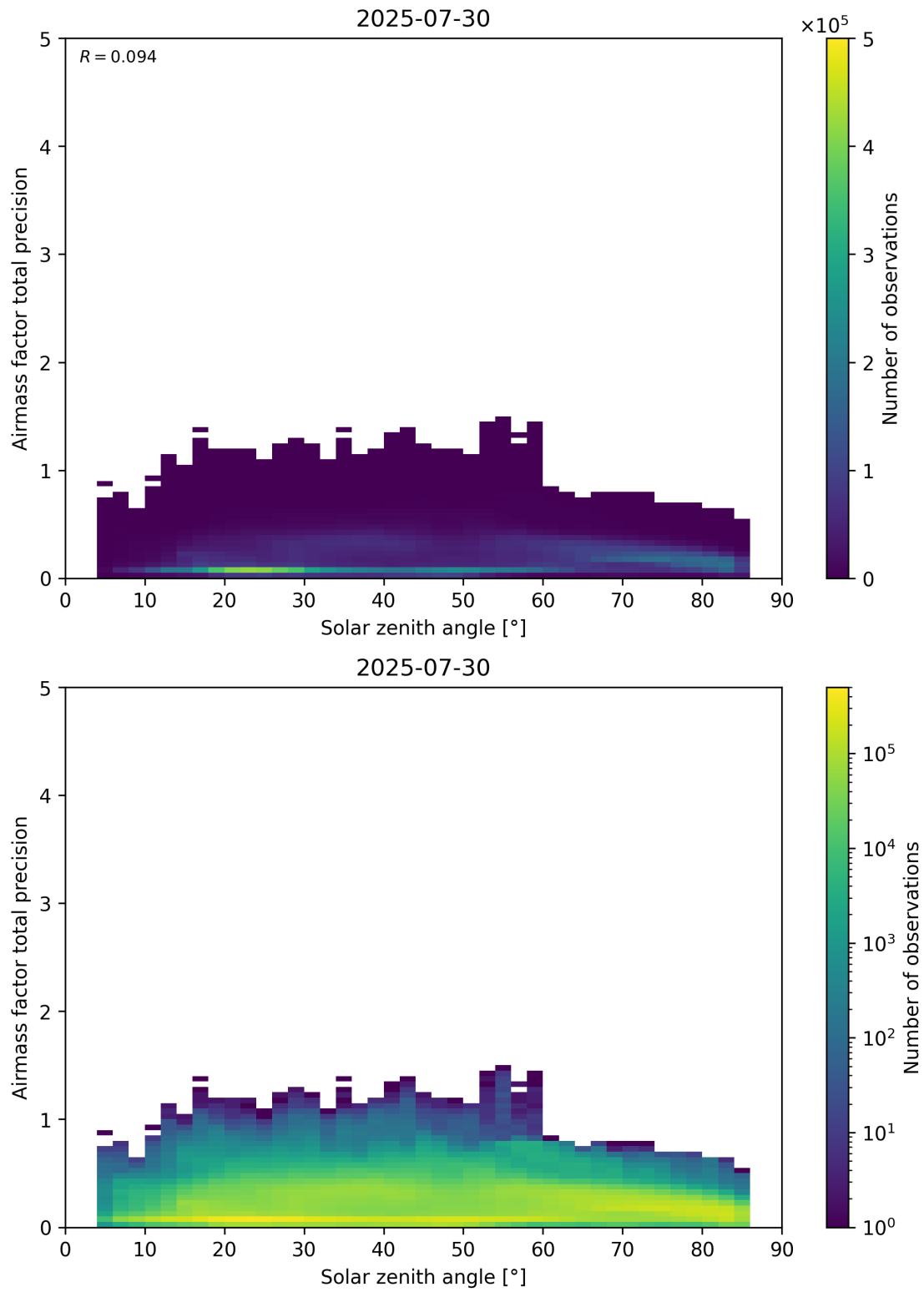
Figure 176: Scatter density plot of “Solar zenith angle” against “Airmass factor total precision” for 2025-07-29 to 2025-07-31.
