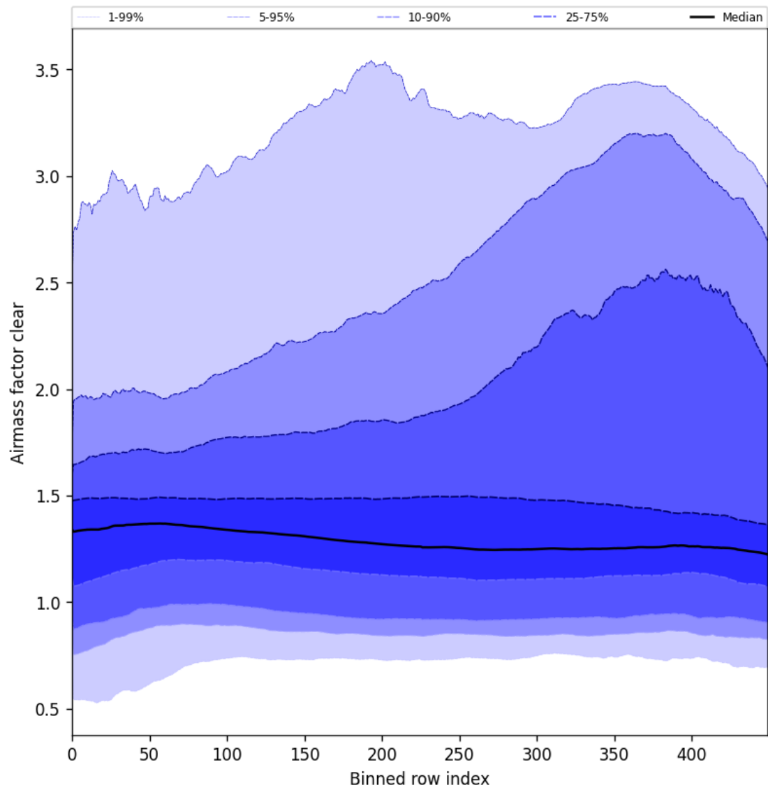
Figure 56: Along track statistics of “Air mass factor clear” for 2025-07-29 to 2025-07-31
