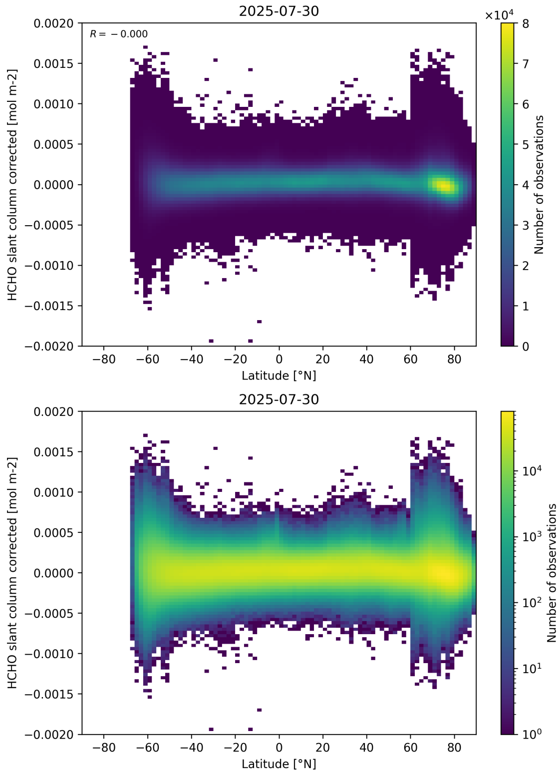
Figure 157: Scatter density plot of “Latitude” against “HCHO slant column corrected” for 2025-07-29 to 2025-07-31.
