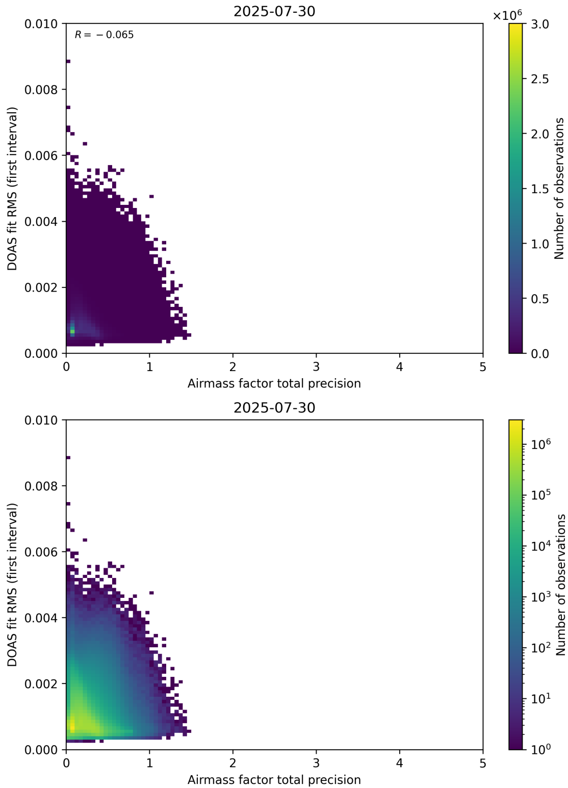
Figure 105: Scatter density plot of “Airmass factor total precision” against “DOAS fit RMS (first interval)” for 2025-07-29 to 2025-07-31.
