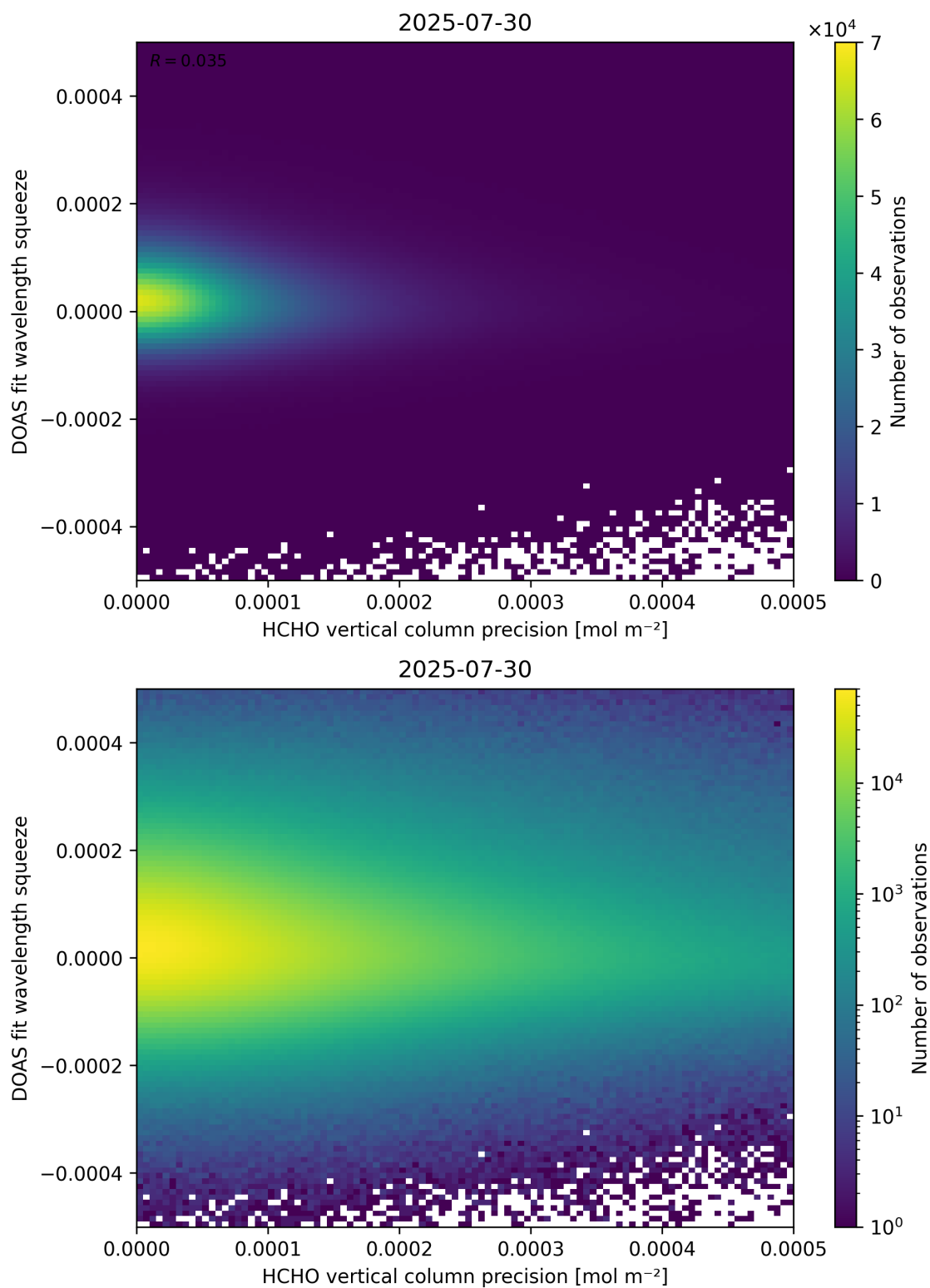
Figure 138: Scatter density plot of “HCHO vertical column precision” against “DOAS fit wavelength squeeze” for 2025-07-29 to 2025-07-31.
