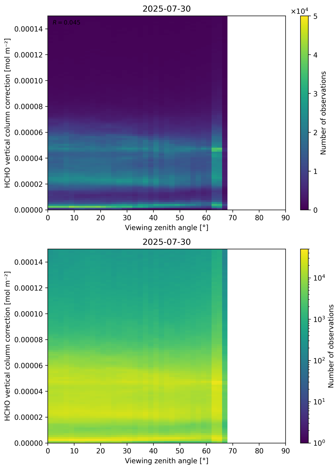
Figure 193: Scatter density plot of “Viewing zenith angle” against “HCHO vertical column correction” for 2025-07-29 to 2025-07-31.
