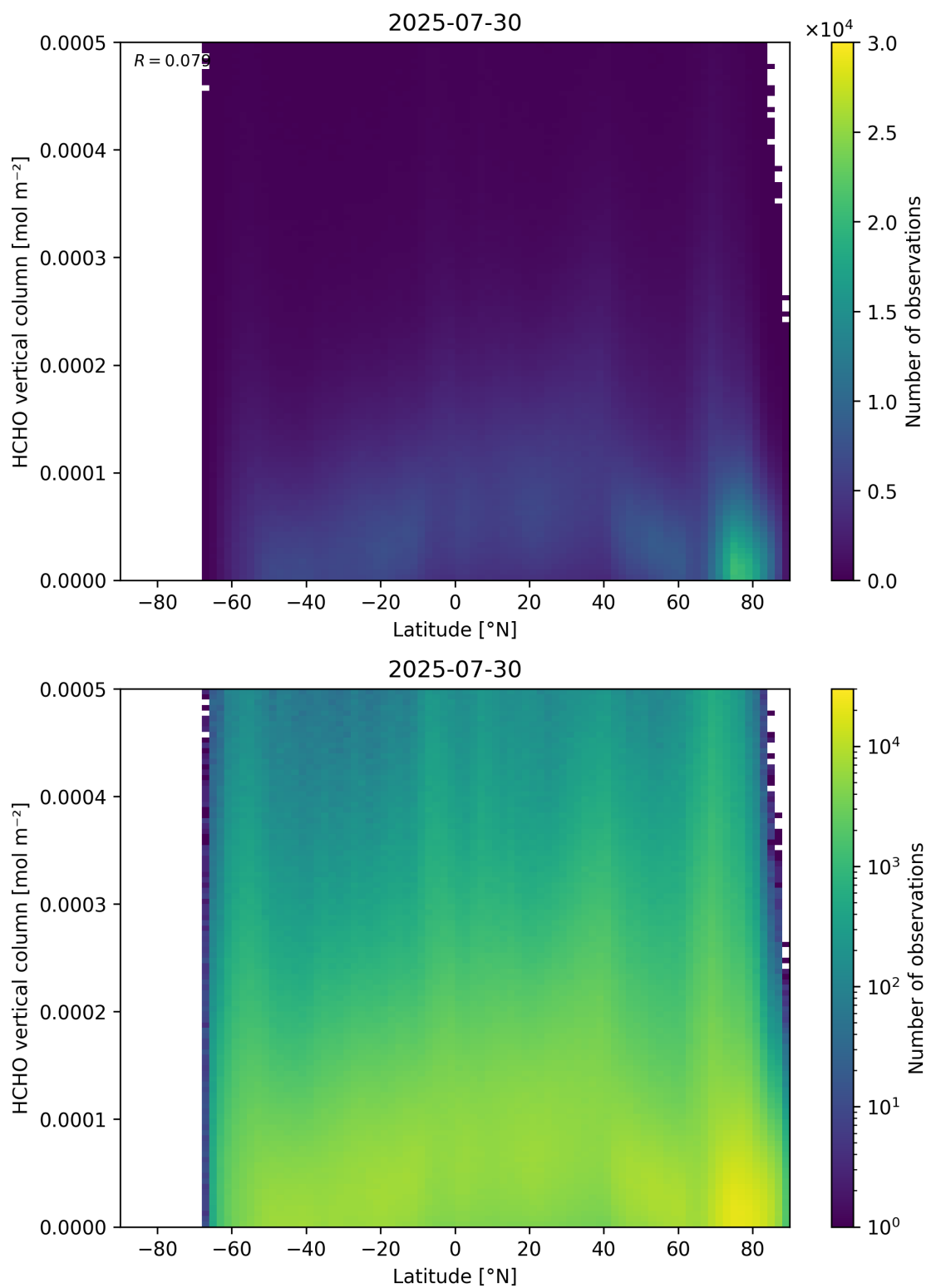
Figure 163: Scatter density plot of “Latitude” against “HCHO vertical column” for 2025-07-29 to 2025-07-31.
