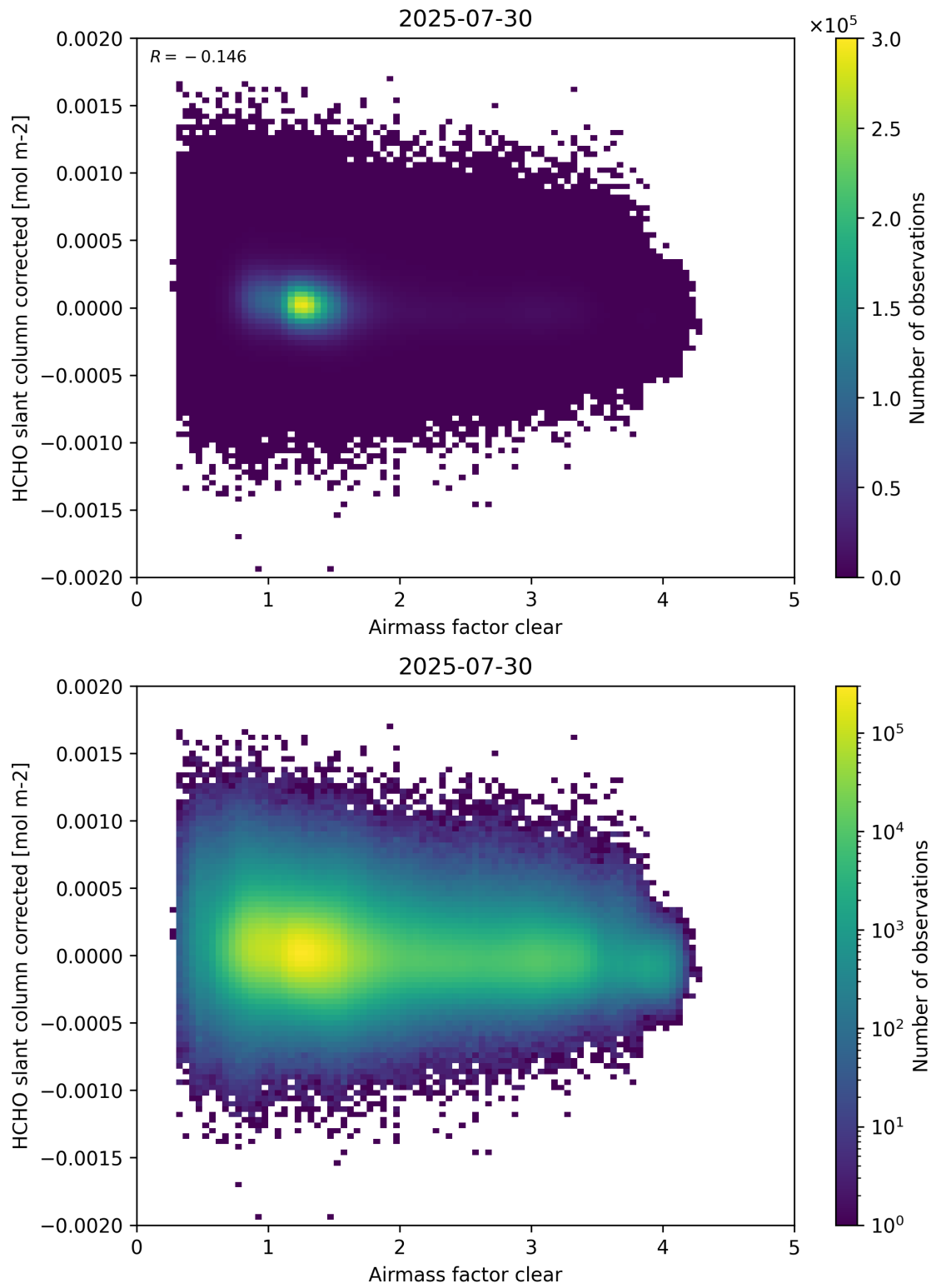
Figure 74: Scatter density plot of “Airmass factor clear” against “HCHO slant column corrected” for 2025-07-29 to 2025-07-31.
