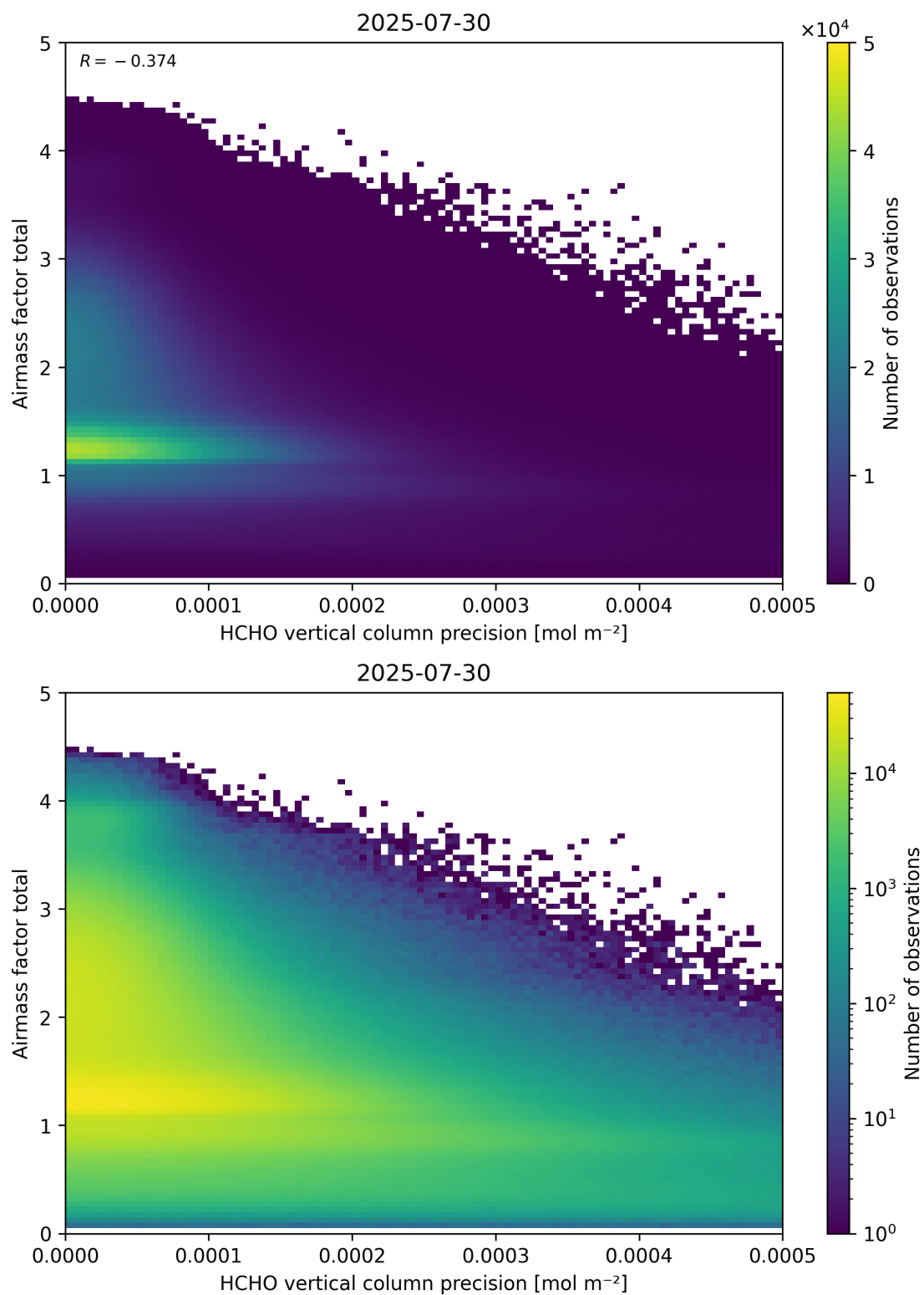
Figure 144: Scatter density plot of “HCHO vertical column precision” against “Airmass factor total” for 2025-07-29 to 2025-07-31.
