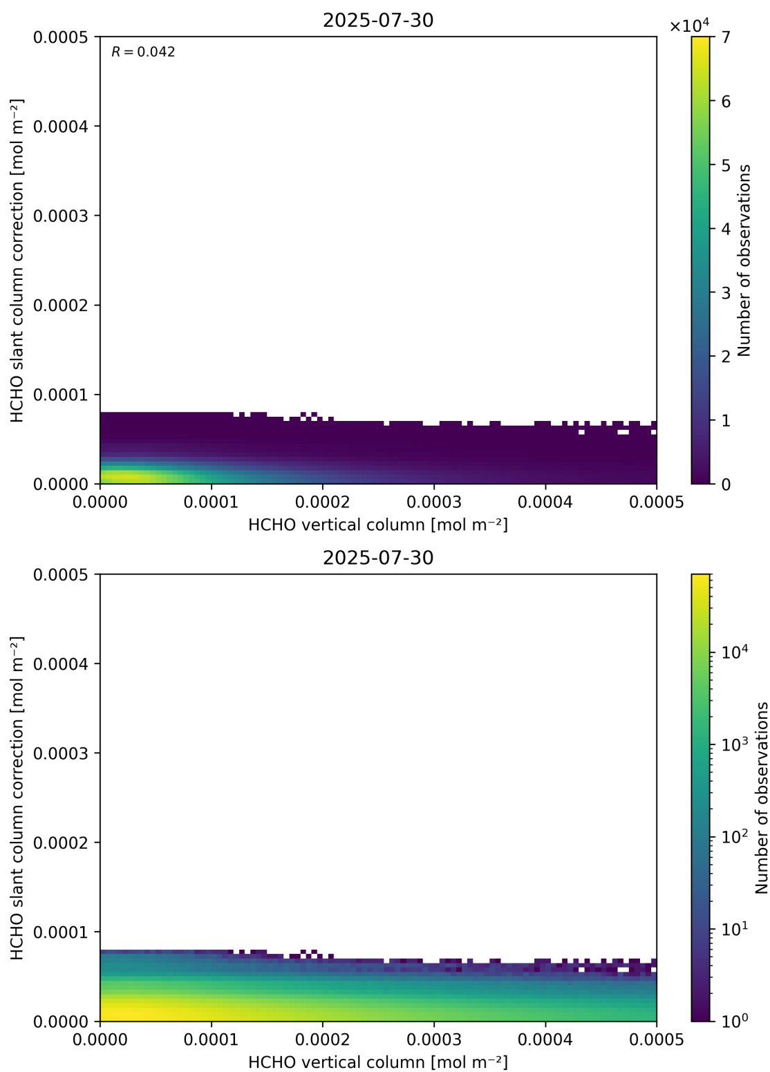
Figure 128: Scatter density plot of “HCHO vertical column” against “HCHO slant column correction” for 2025-07-29 to 2025-07-31.
