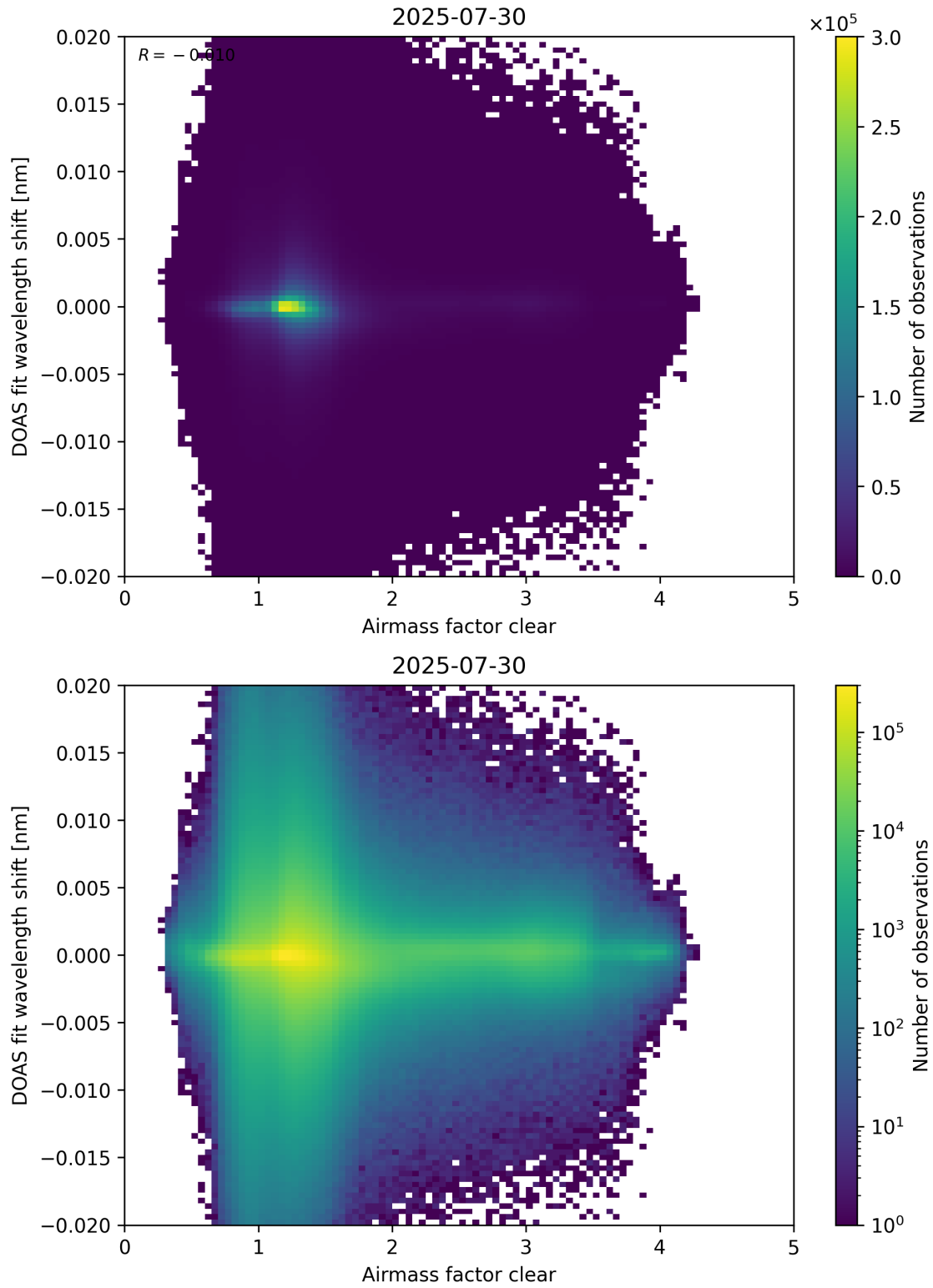
Figure 72: Scatter density plot of “Airmass factor clear” against “DOAS fit wavelength shift” for 2025-07-29 to 2025-07-31.
