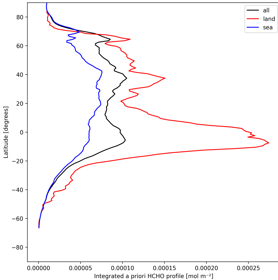
Figure 29: Zonal average of “Integrated a priori HCHO profile” for 2025-07-29 to 2025-07-31.
