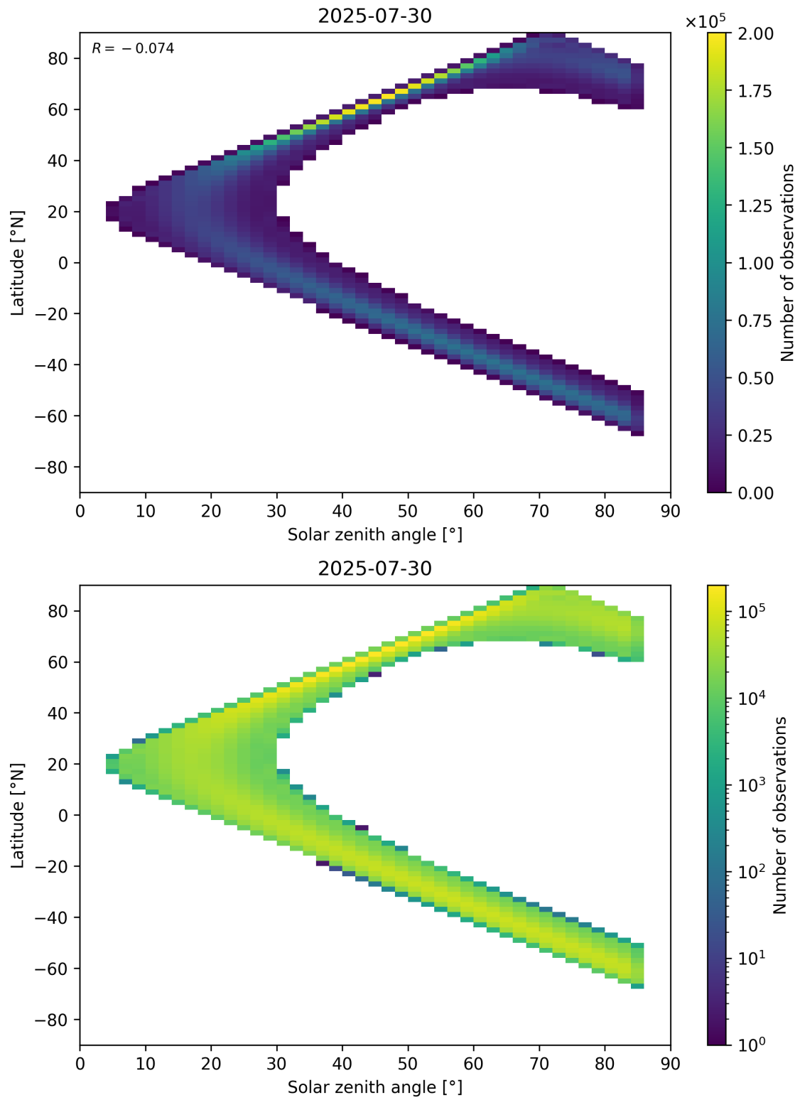
Figure 181: Scatter density plot of “Solar zenith angle” against “Latitude” for 2025-07-29 to 2025-07-31.
