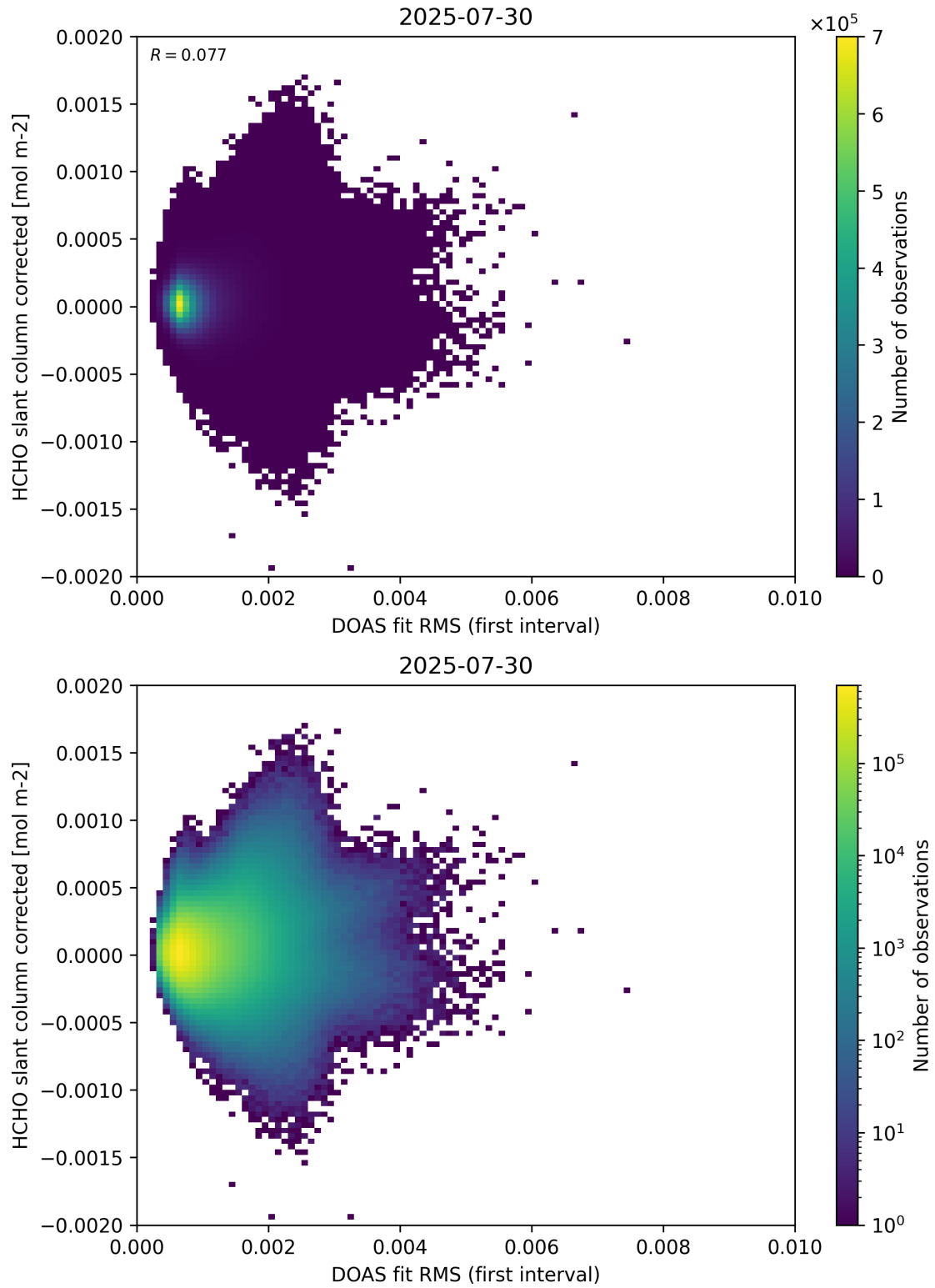
Figure 62: Scatter density plot of “DOAS fit RMS (first interval)” against “HCHO slant column corrected” for 2025-07-29 to 2025-07-31.
