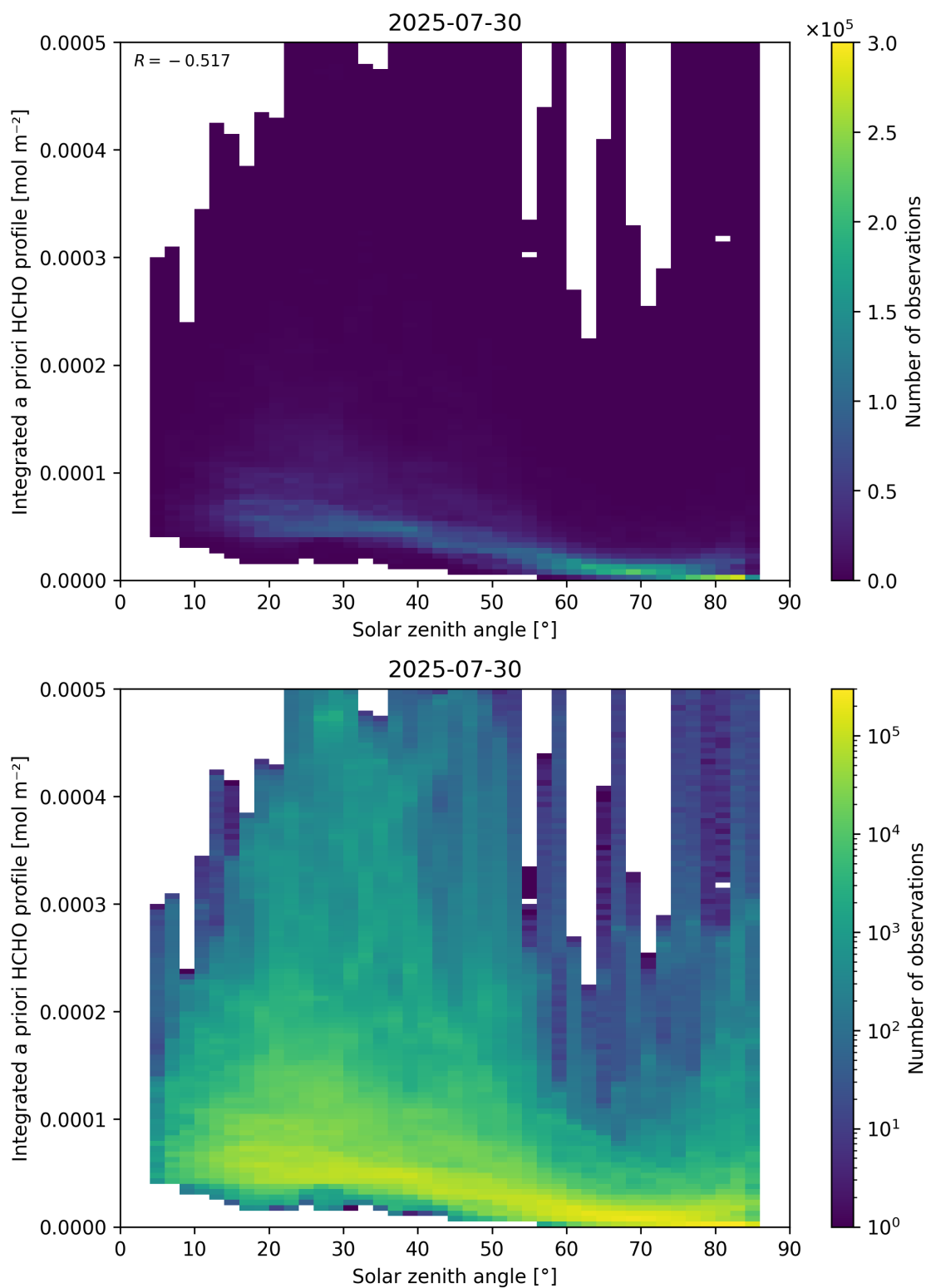
Figure 180: Scatter density plot of “Solar zenith angle” against “Integrated a priori HCHO profile” for 2025-07-29 to 2025-07-31.
