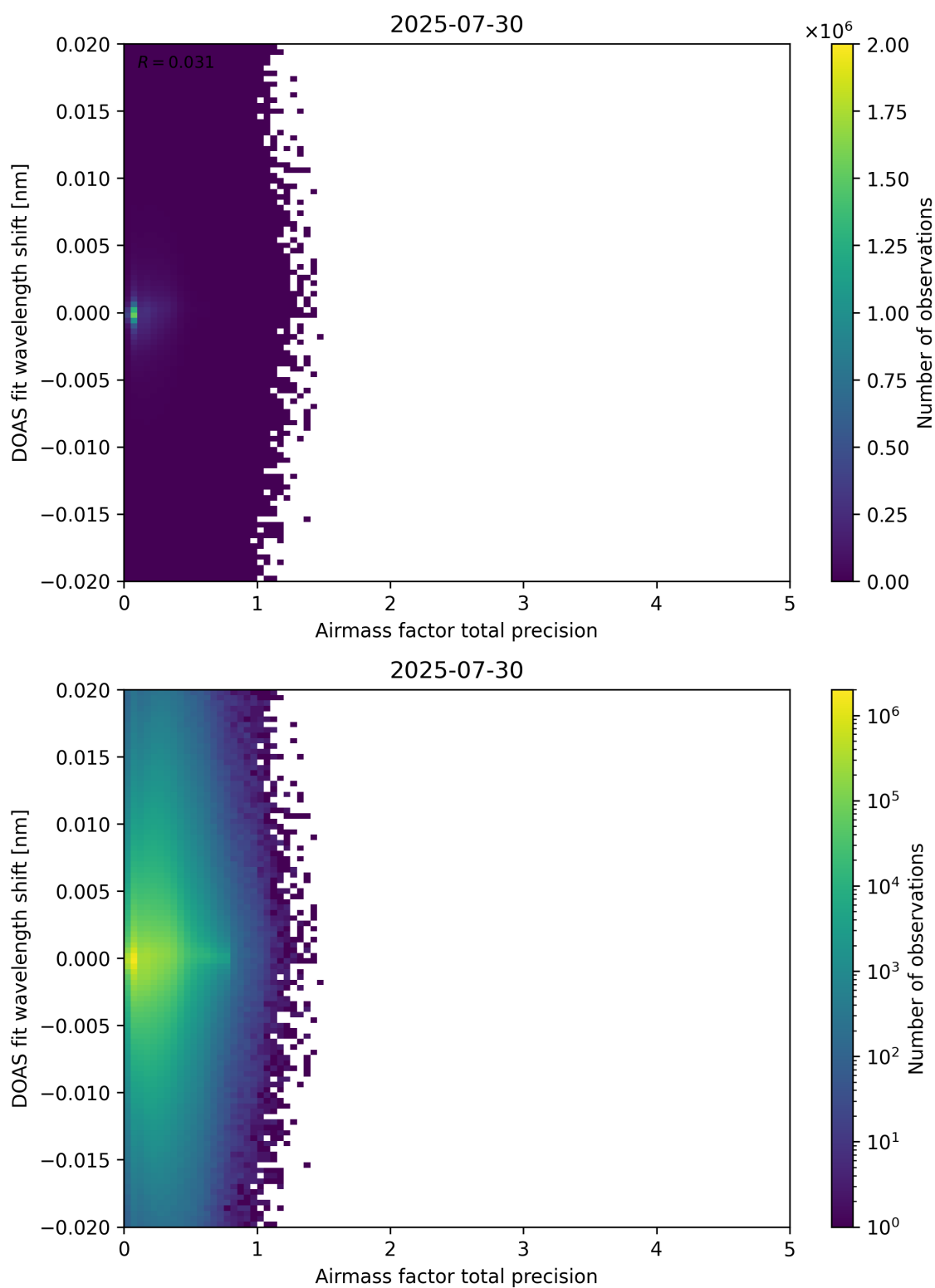
Figure 106: Scatter density plot of “Airmass factor total precision” against “DOAS fit wavelength shift” for 2025-07-29 to 2025-07-31.
