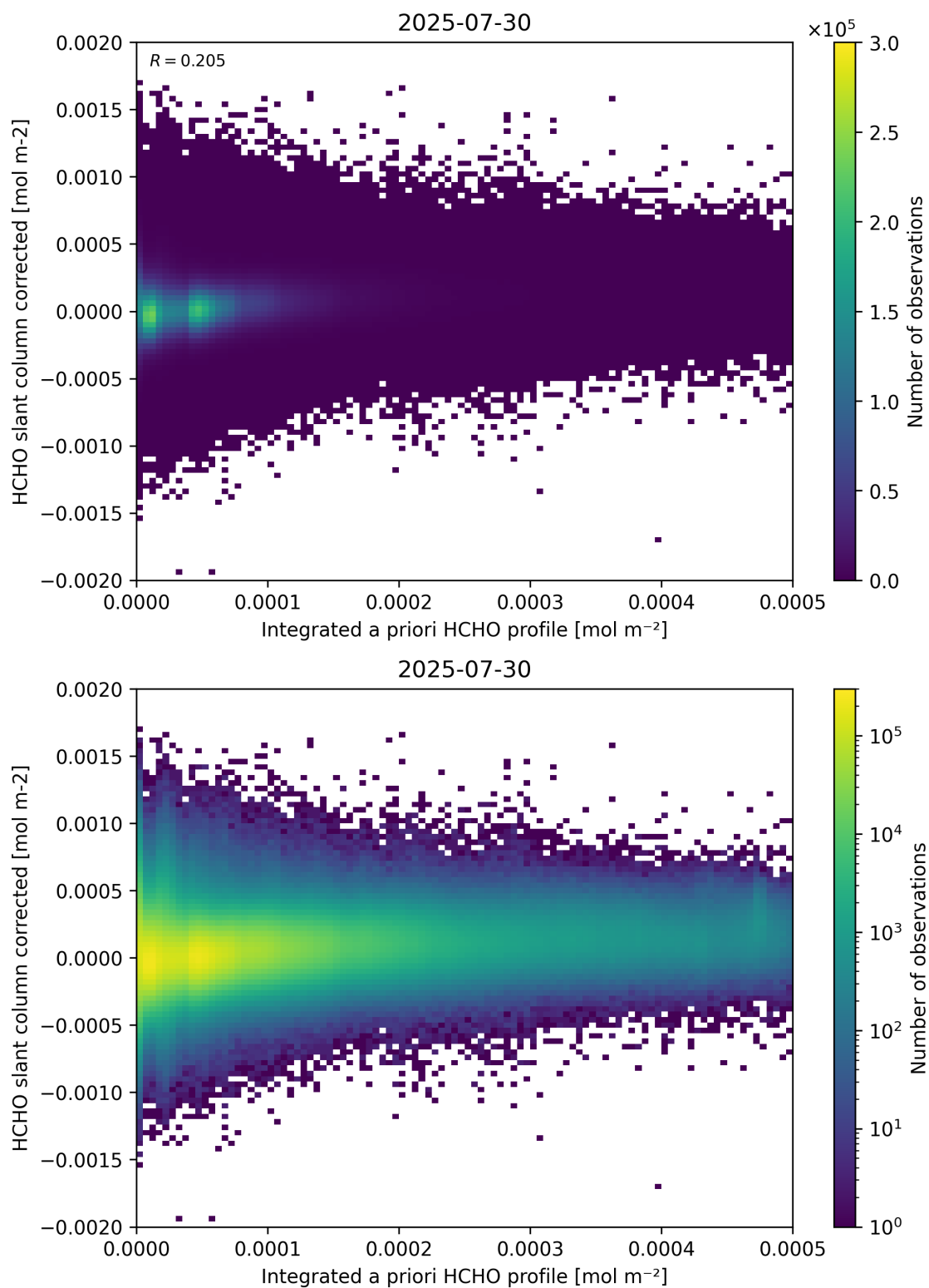
Figure 151: Scatter density plot of “Integrated a priori HCHO profile” against “HCHO slant column corrected” for 2025-07-29 to 2025-07-31.
