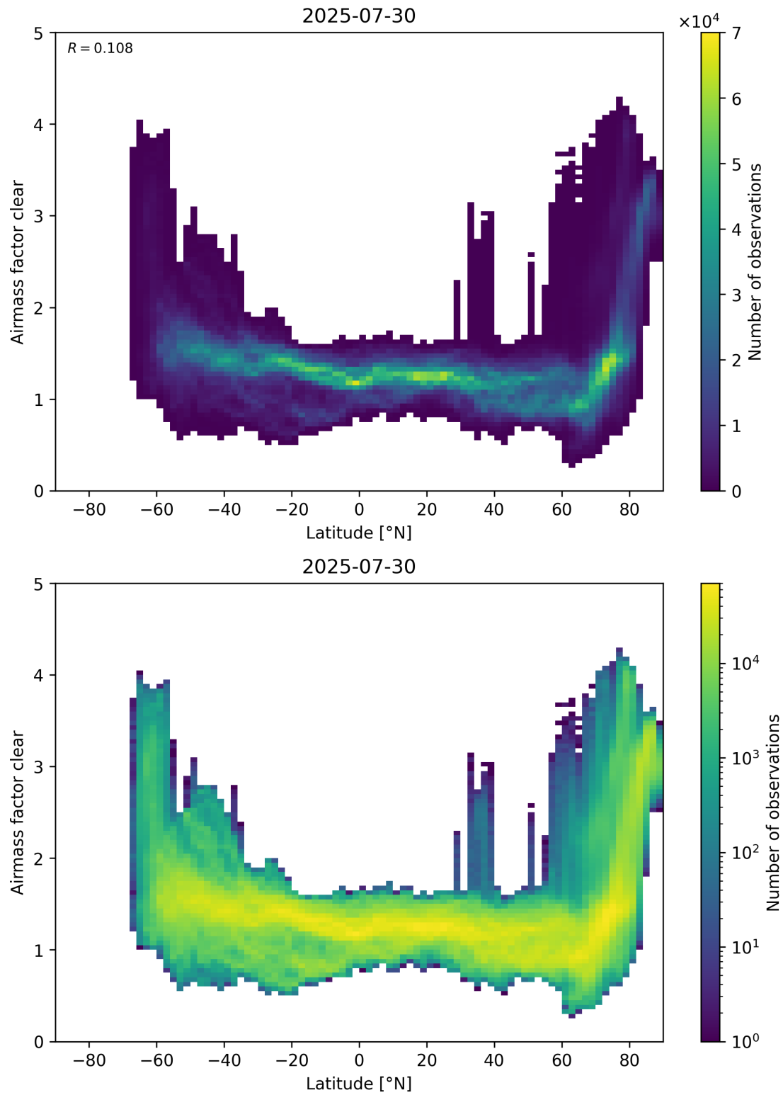
Figure 156: Scatter density plot of “Latitude” against “Airmass factor clear” for 2025-07-29 to 2025-07-31.
