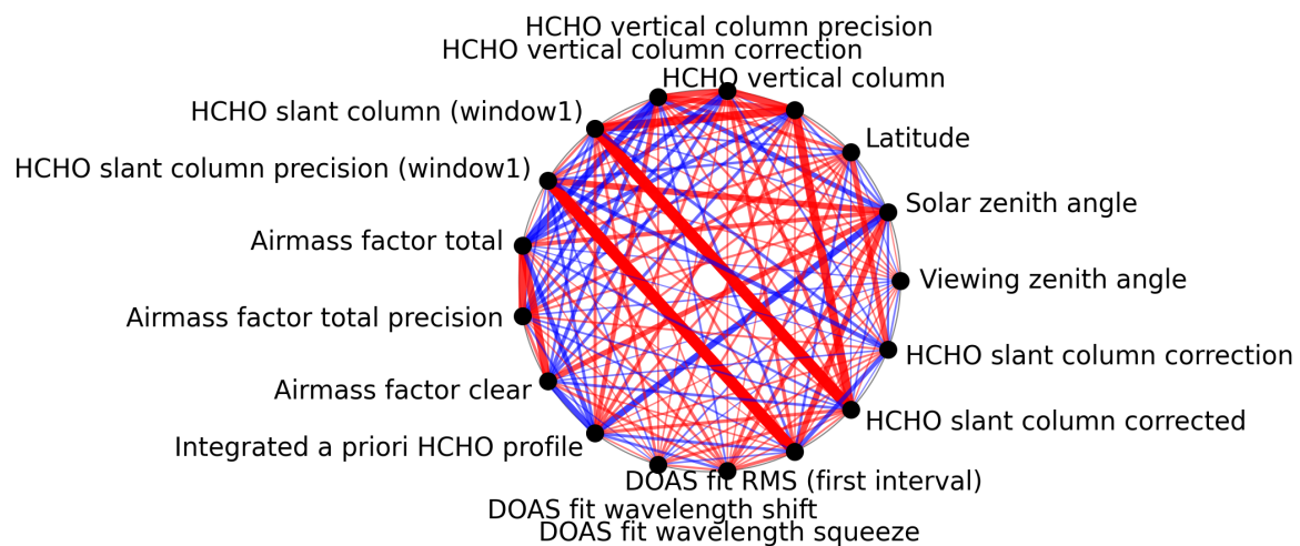
Figure 1: Map of correlation graph for 2025-07-29 to 2025-07-31.
