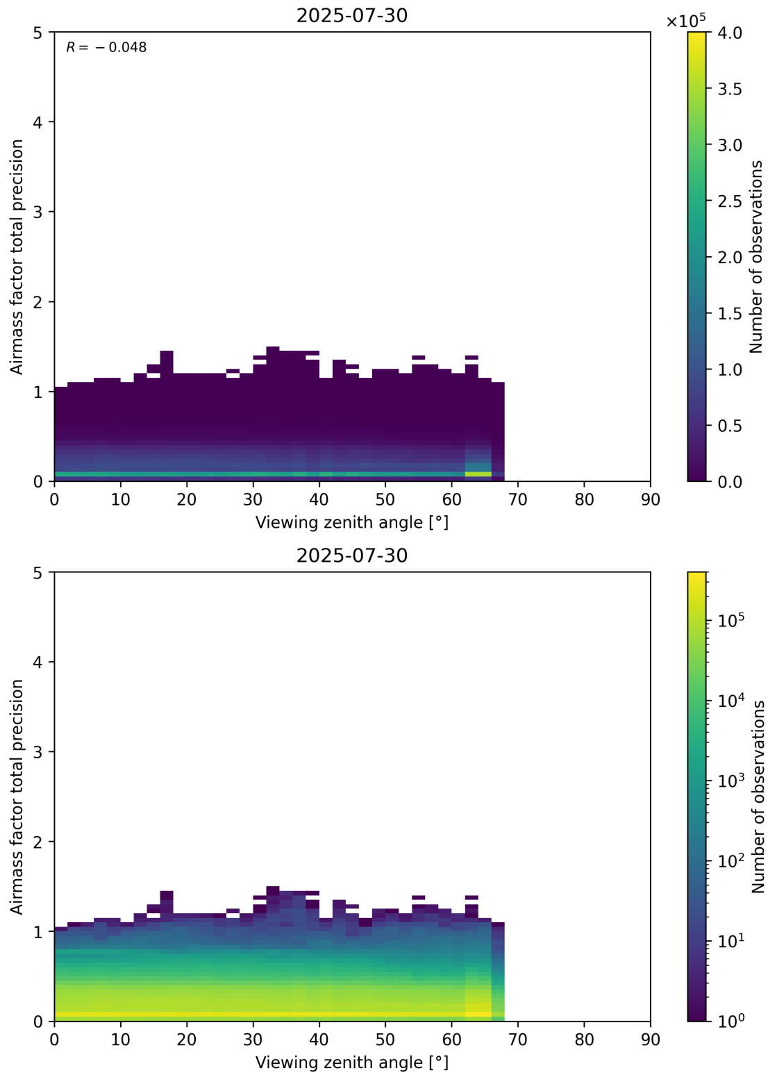
Figure 191: Scatter density plot of “Viewing zenith angle” against “Airmass factor total precision” for 2025-07-29 to 2025-07-31.
