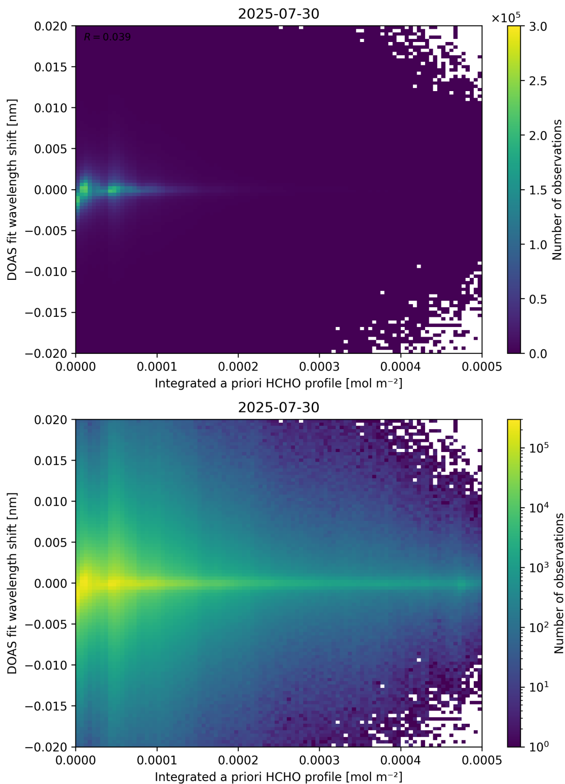
Figure 149: Scatter density plot of “Integrated a priori HCHO profile” against “DOAS fit wavelength shift” for 2025-07-29 to 2025-07-31.
