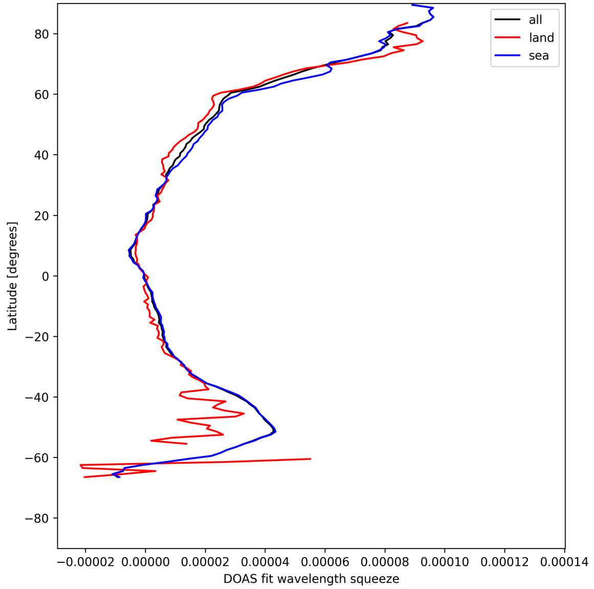
Figure 31: Zonal average of “DOAS fit wavelength squeeze” for 2025-07-29 to 2025-07-31.
