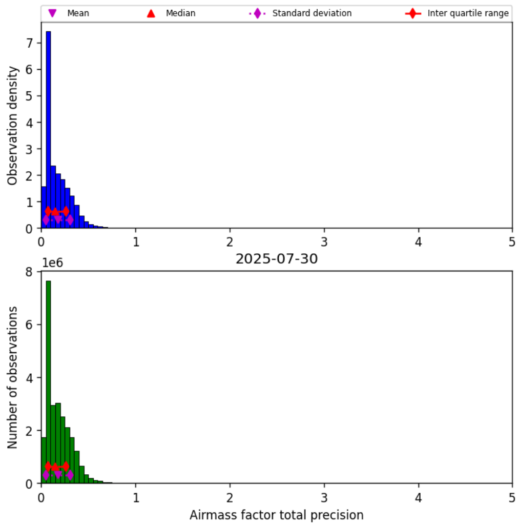
Figure 41: Histogram of “Airmass factor total precision” for 2025-07-29 to 2025-07-31
