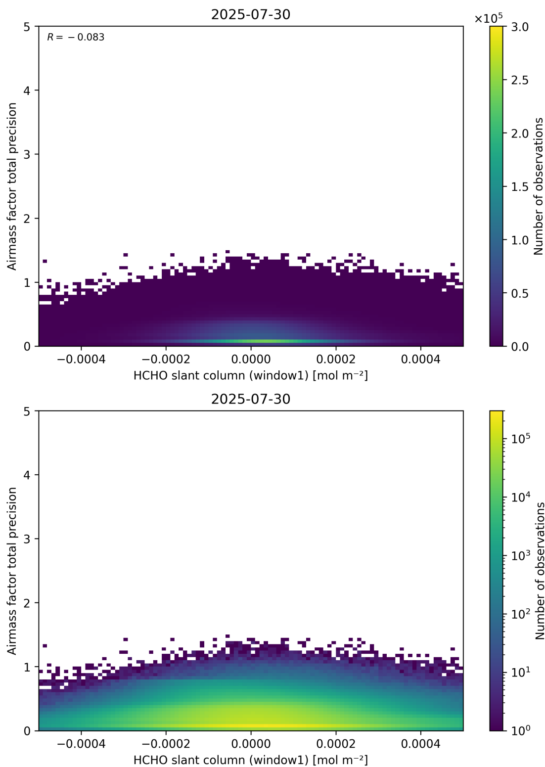
Figure 86: Scatter density plot of “HCHO slant column (window1)” against “Airmass factor total precision” for 2025-07-29 to 2025-07-31.
