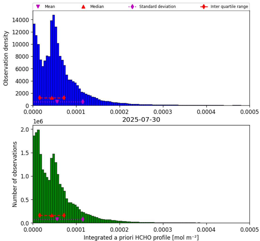
Figure 43: Histogram of “Integrated a priori HCHO profile” for 2025-07-29 to 2025-07-31
