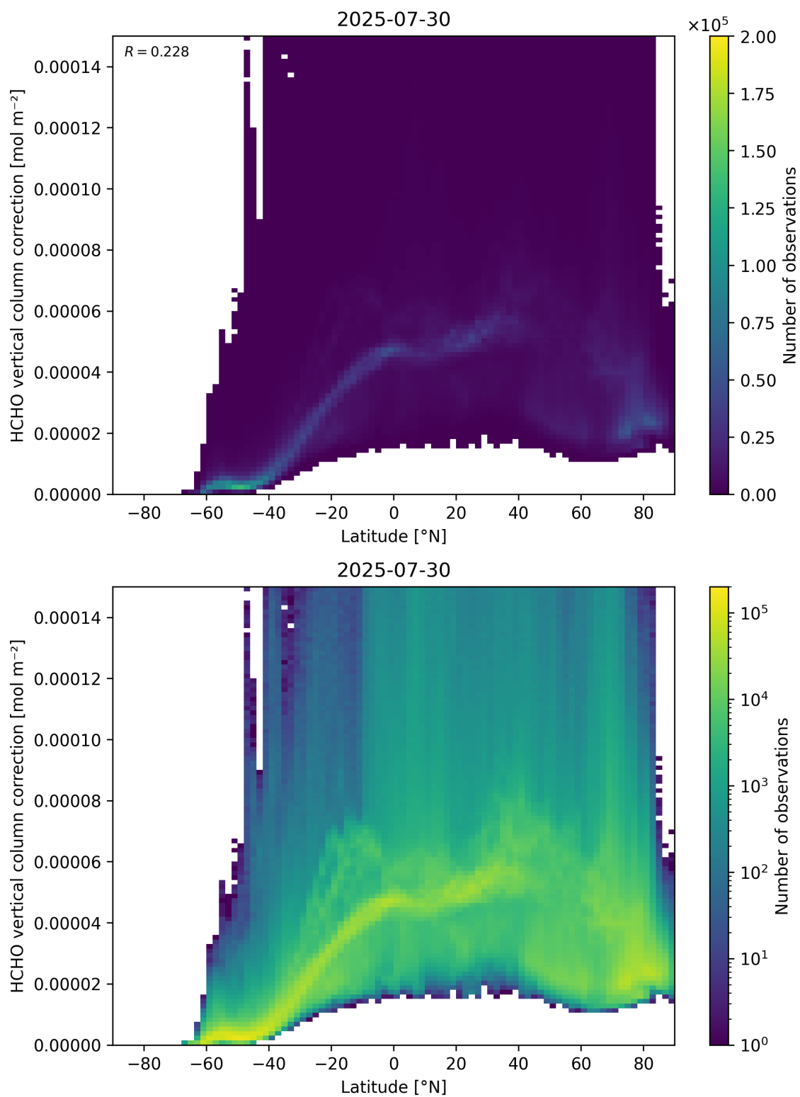
Figure 164: Scatter density plot of “Latitude” against “HCHO vertical column correction” for 2025-07-29 to 2025-07-31.
