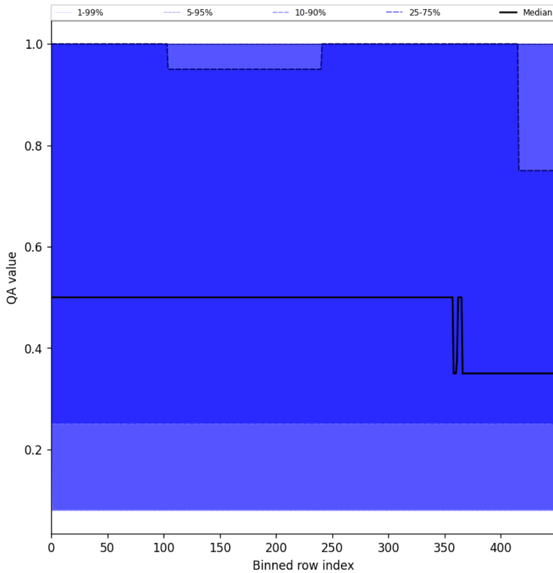
Figure 48: Along track statistics of “QA value” for 2025-07-29 to 2025-07-31
