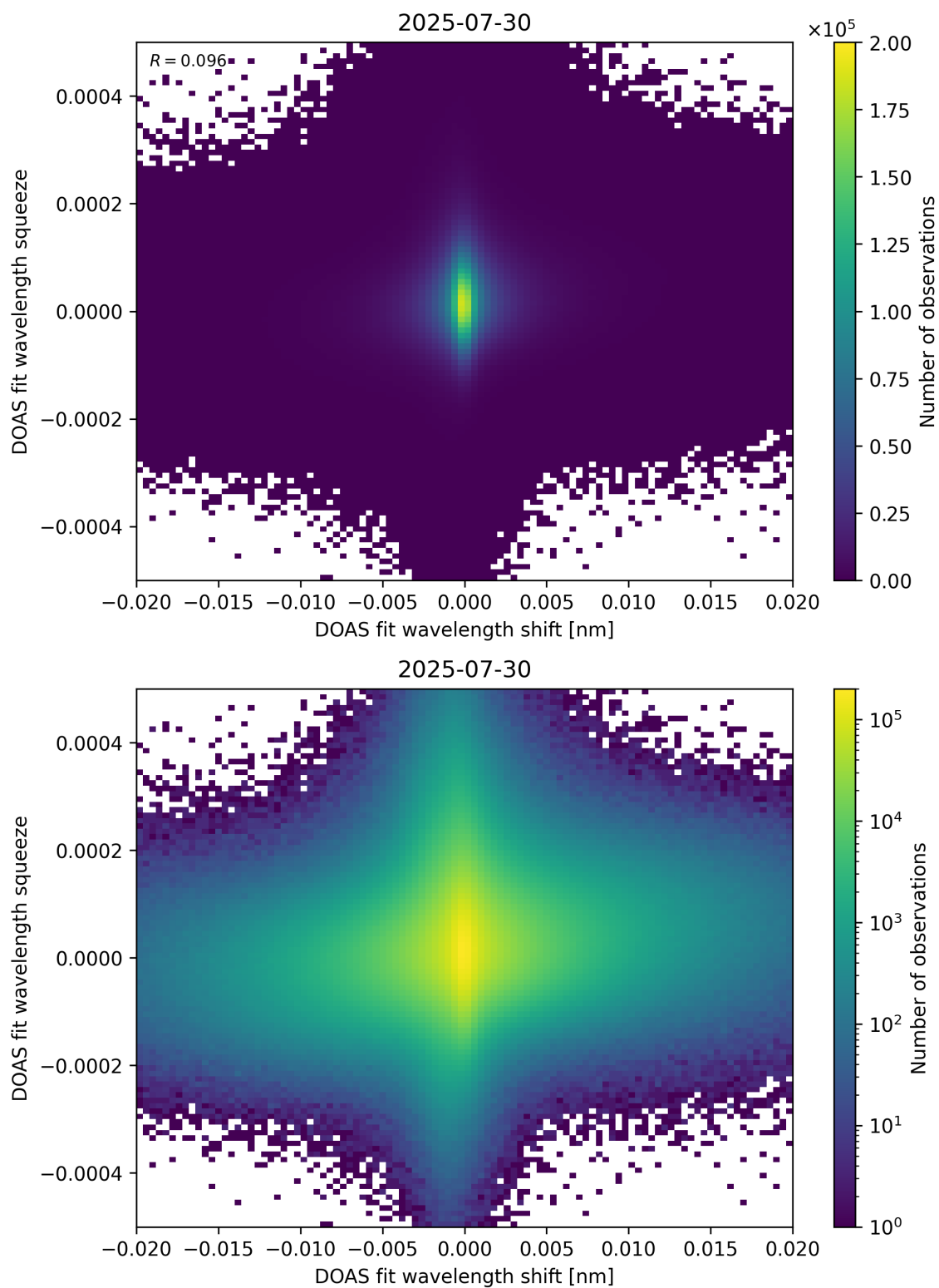
Figure 65: Scatter density plot of “DOAS fit wavelength shift” against “DOAS fit wavelength squeeze” for 2025-07-29 to 2025-07-31.
