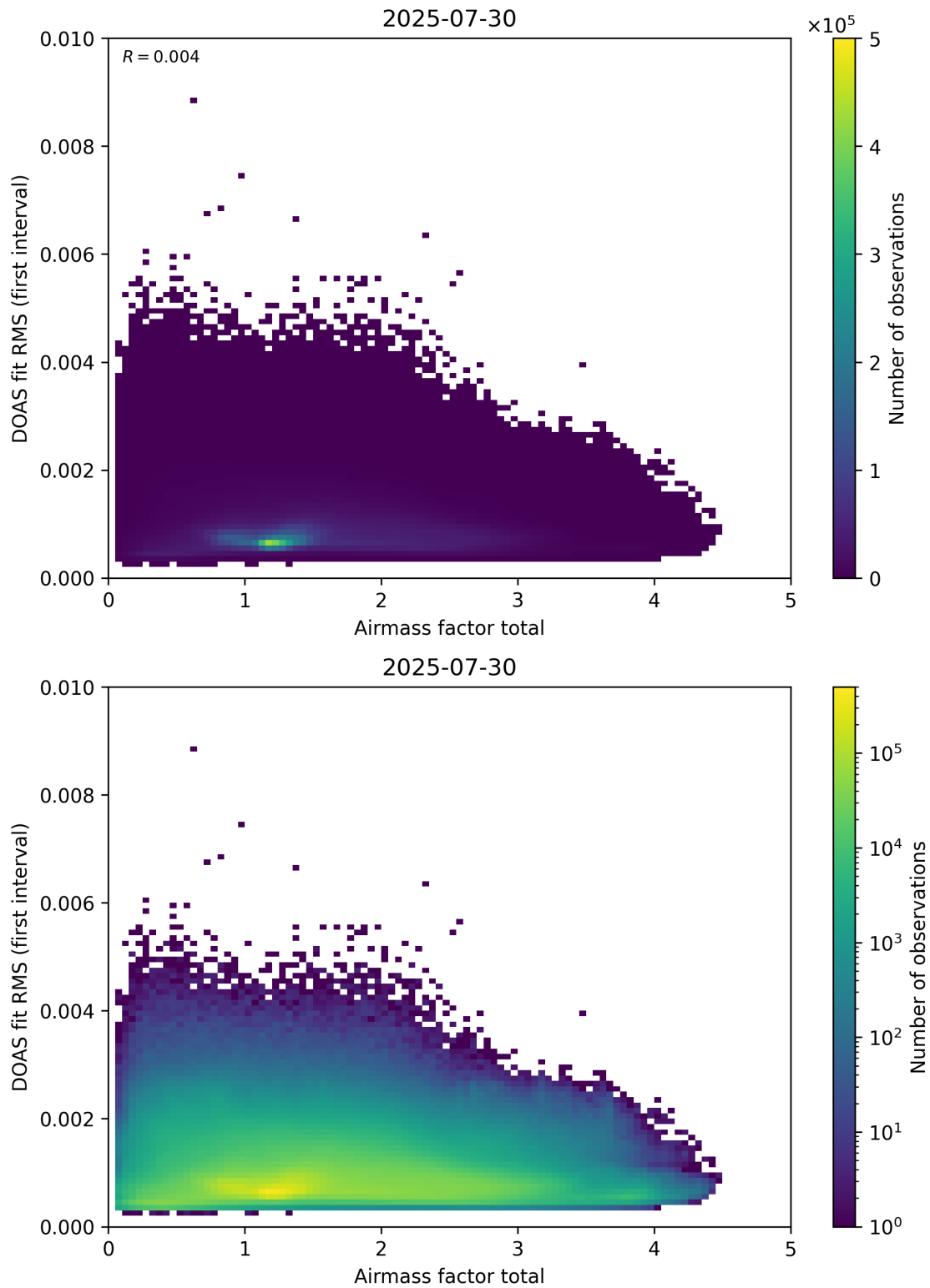
Figure 97: Scatter density plot of “Airmass factor total” against “DOAS fit RMS (first interval)” for 2025-07-29 to 2025-07-31.
