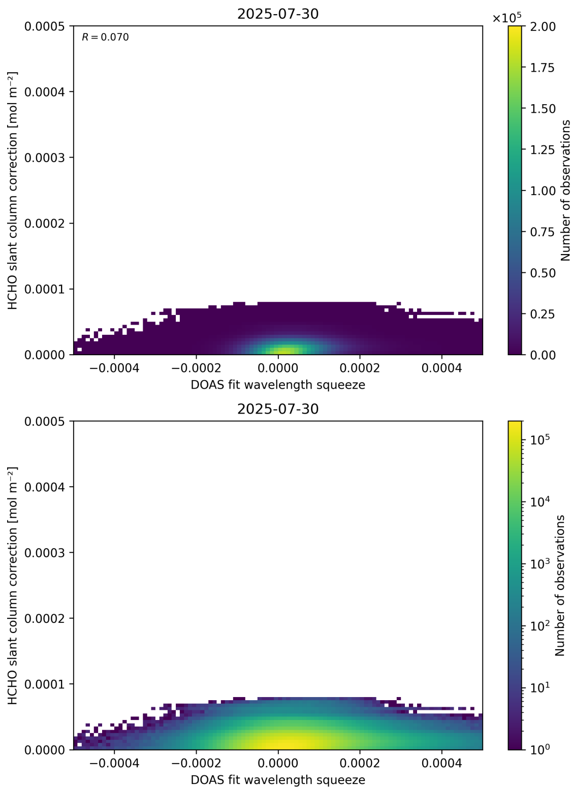
Figure 70: Scatter density plot of “DOAS fit wavelength squeeze” against “HCHO slant column correction” for 2025-07-29 to 2025-07-31.
