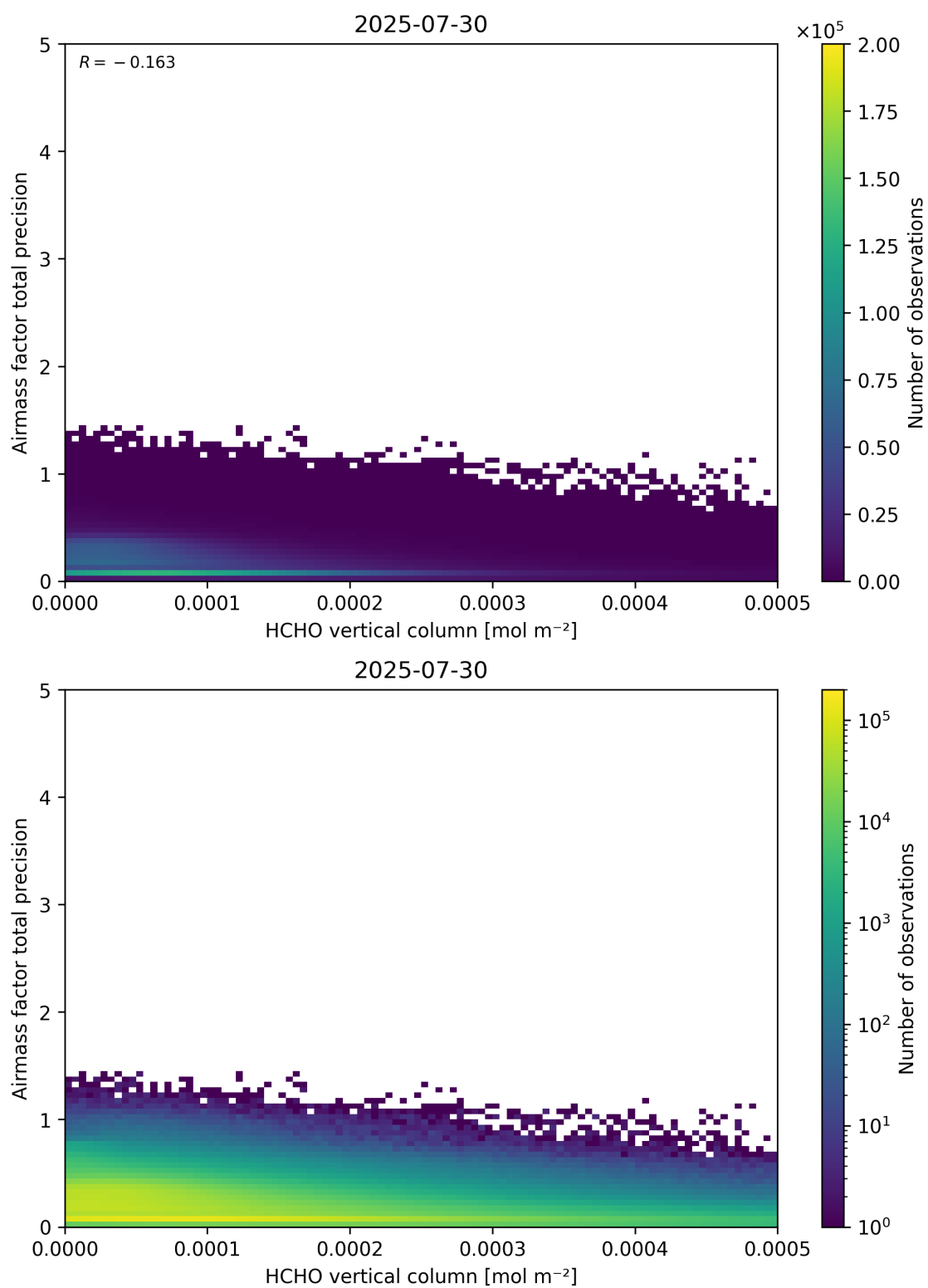
Figure 132: Scatter density plot of “HCHO vertical column” against “Airmass factor total precision” for 2025-07-29 to 2025-07-31.
