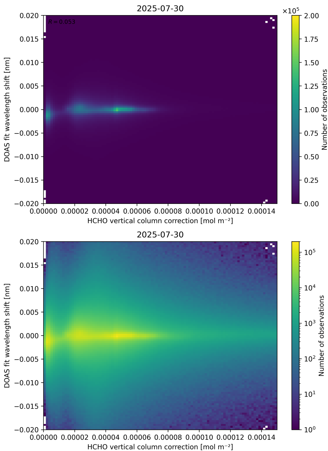
Figure 113: Scatter density plot of “HCHO vertical column correction” against “DOAS fit wavelength shift” for 2025-07-29 to 2025-07-31.
