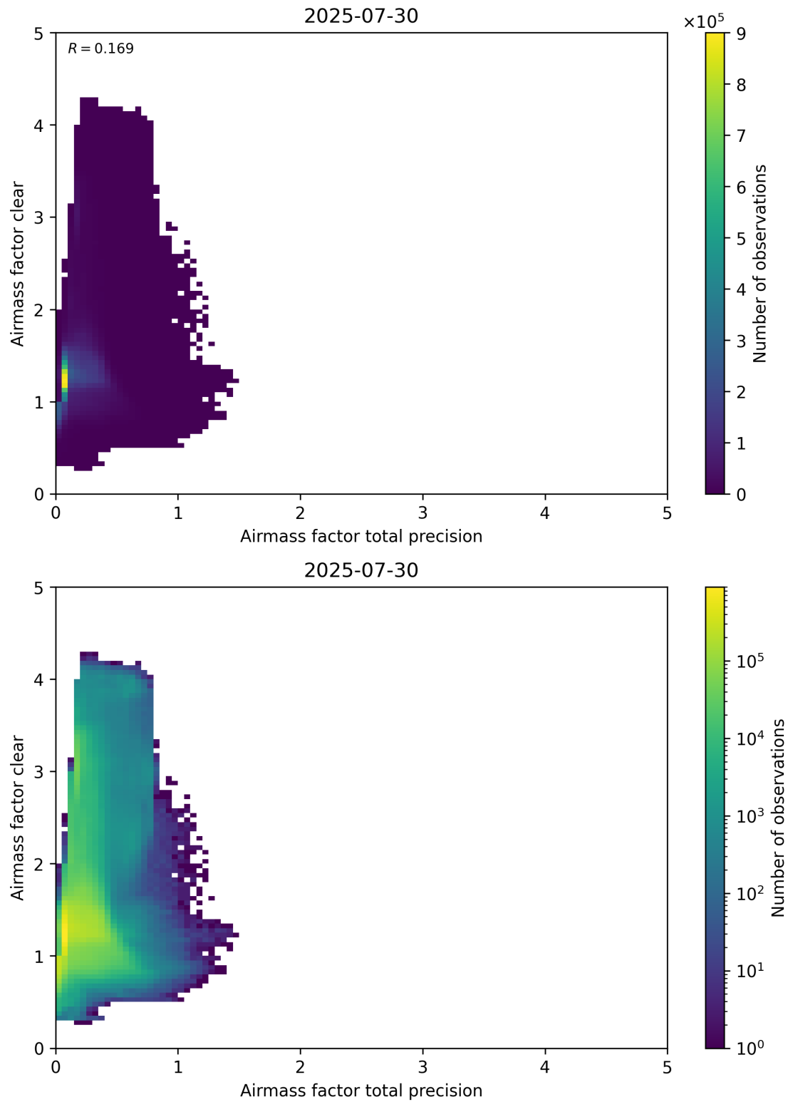
Figure 108: Scatter density plot of “Airmass factor total precision” against “Airmass factor clear” for 2025-07-29 to 2025-07-31.
