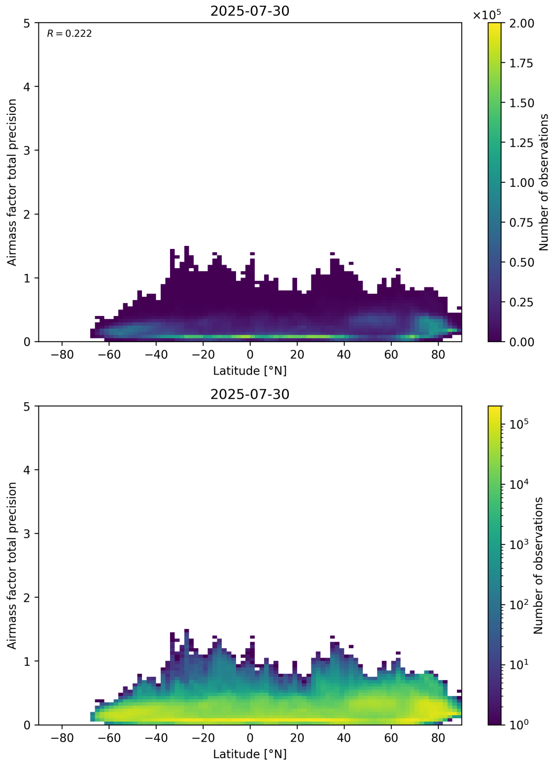
Figure 162: Scatter density plot of “Latitude” against “Airmass factor total precision” for 2025-07-29 to 2025-07-31.
