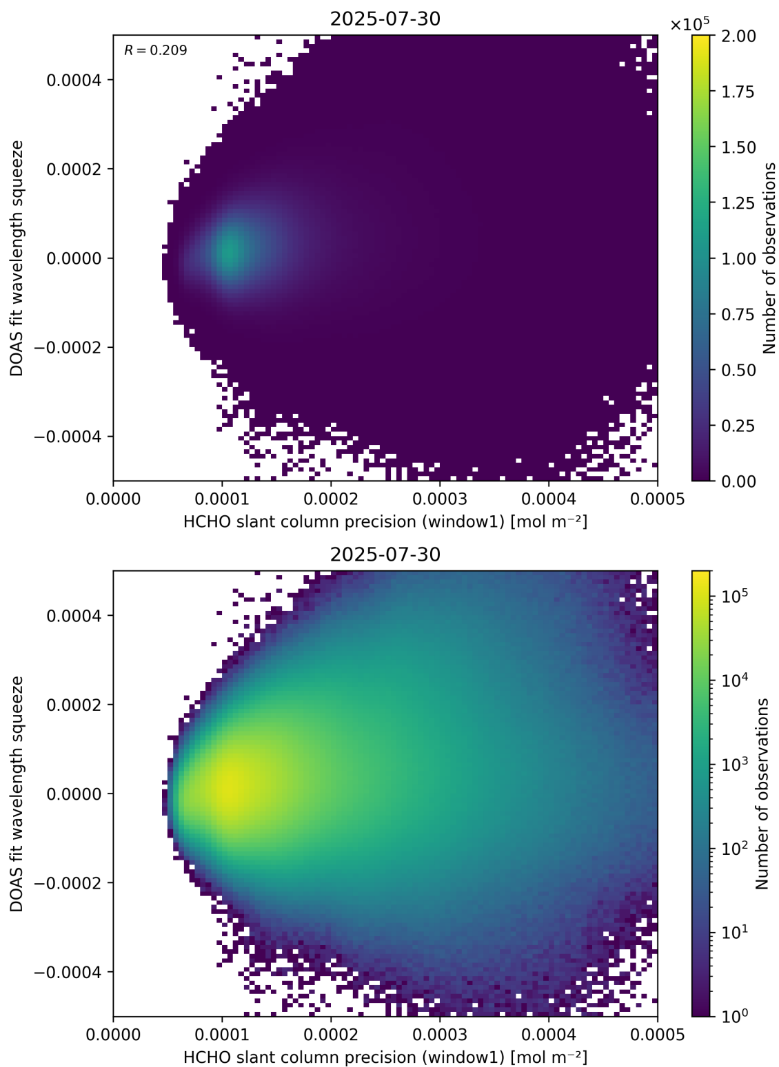
Figure 90: Scatter density plot of “HCHO slant column precision (window1)” against “DOAS fit wavelength squeeze” for 2025-07-29 to 2025-07-31.
