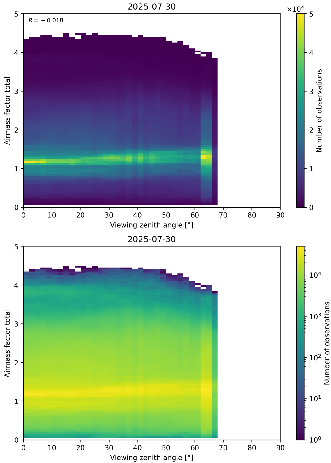
Figure 190: Scatter density plot of “Viewing zenith angle” against “Airmass factor total” for 2025-07-29 to 2025-07-31.
