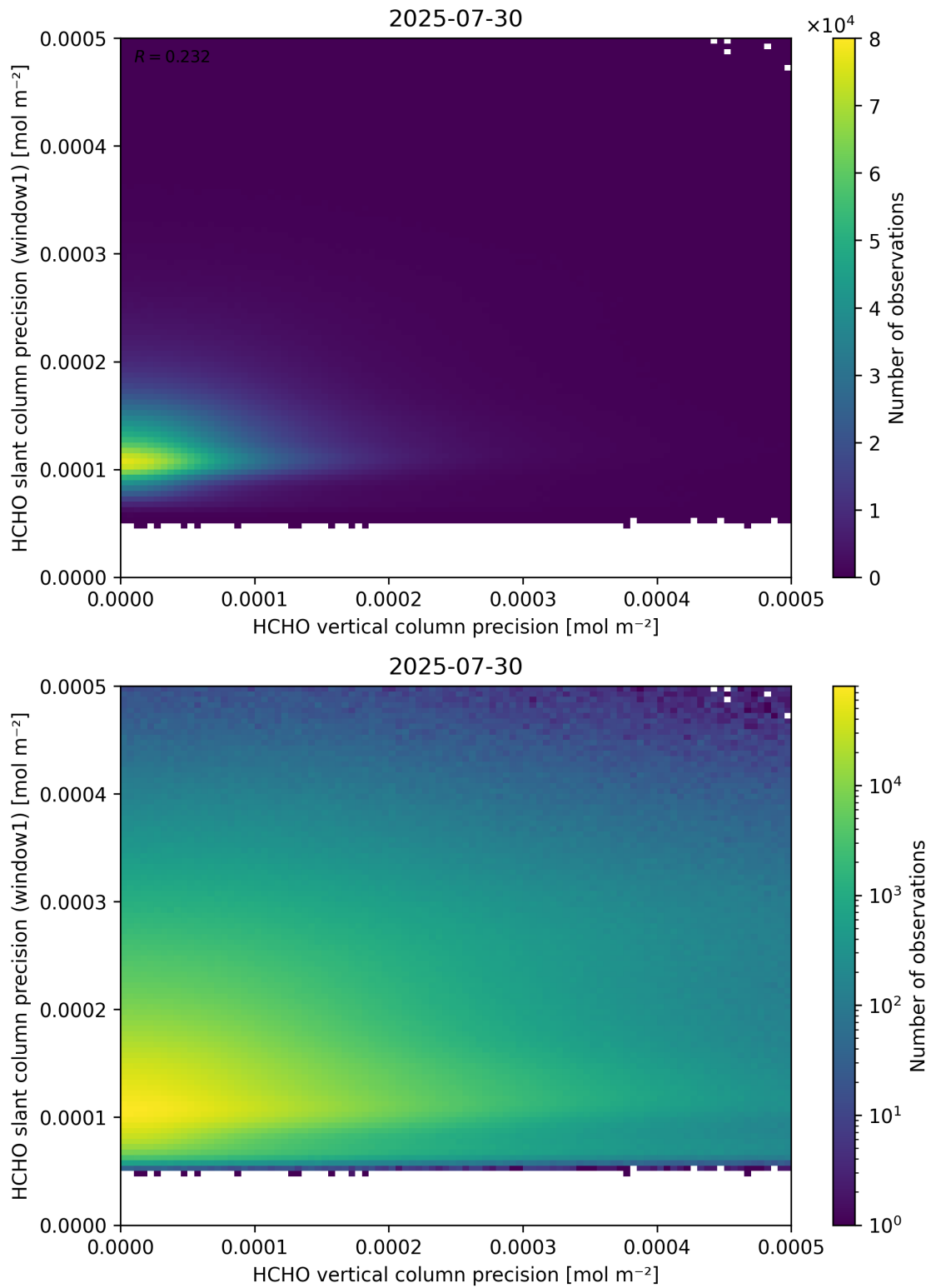
Figure 143: Scatter density plot of “HCHO vertical column precision” against “HCHO slant column precision (window1)” for 2025-07-29 to 2025-07-31.
