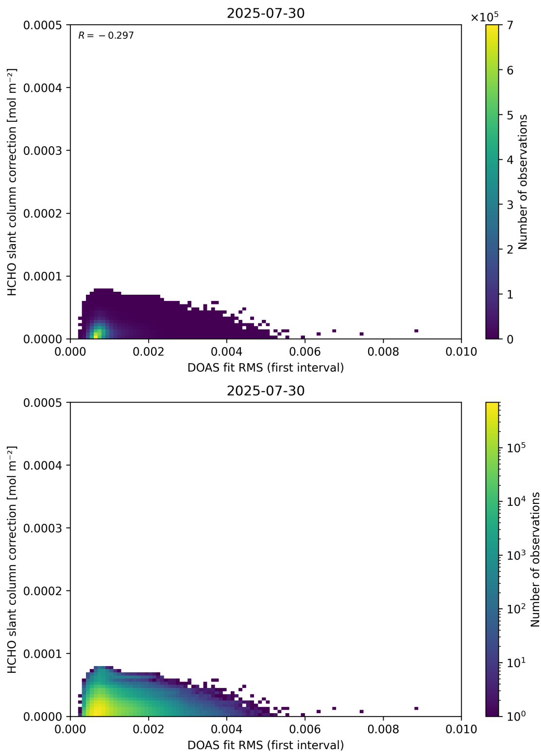
Figure 63: Scatter density plot of “DOAS fit RMS (first interval)” against “HCHO slant column correction” for 2025-07-29 to 2025-07-31.
