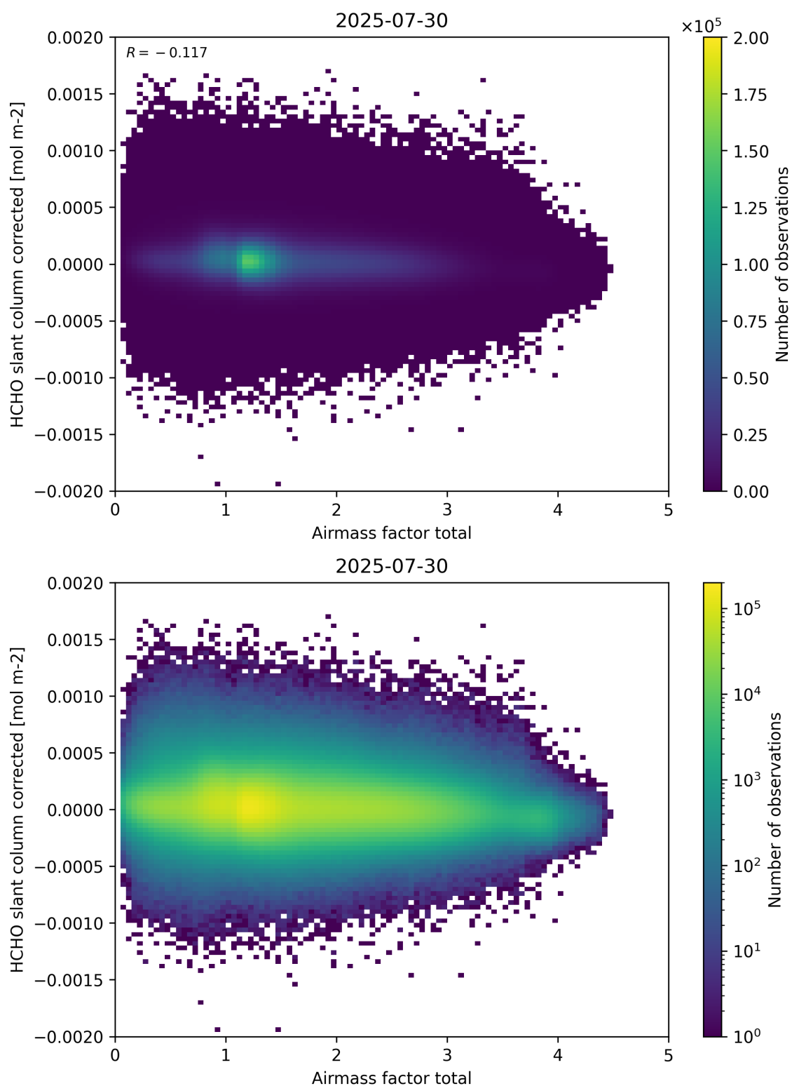
Figure 101: Scatter density plot of “Airmass factor total” against “HCHO slant column corrected” for 2025-07-29 to 2025-07-31.
