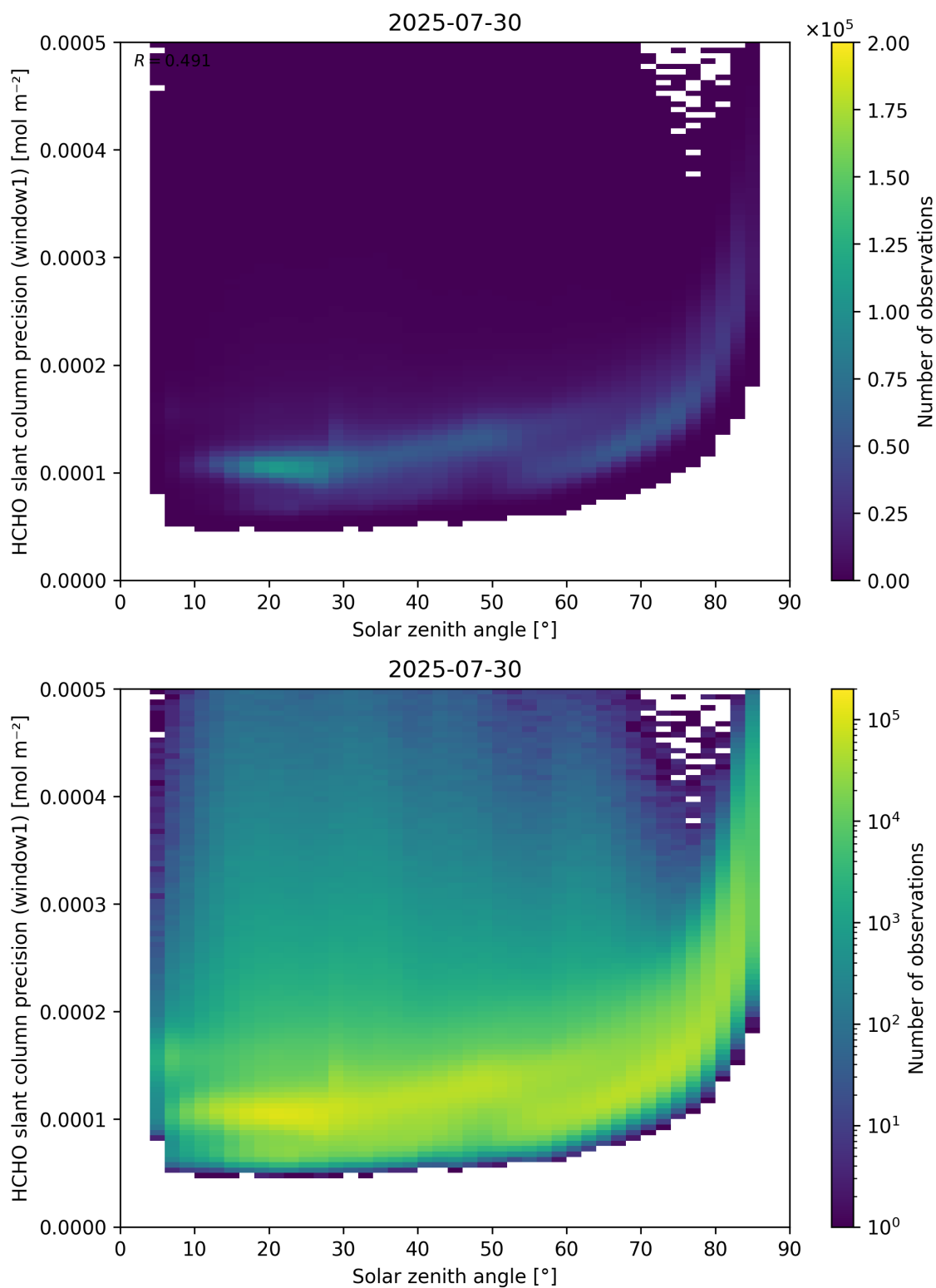
Figure 174: Scatter density plot of “Solar zenith angle” against “HCHO slant column precision (window1)” for 2025-07-29 to 2025-07-31.
