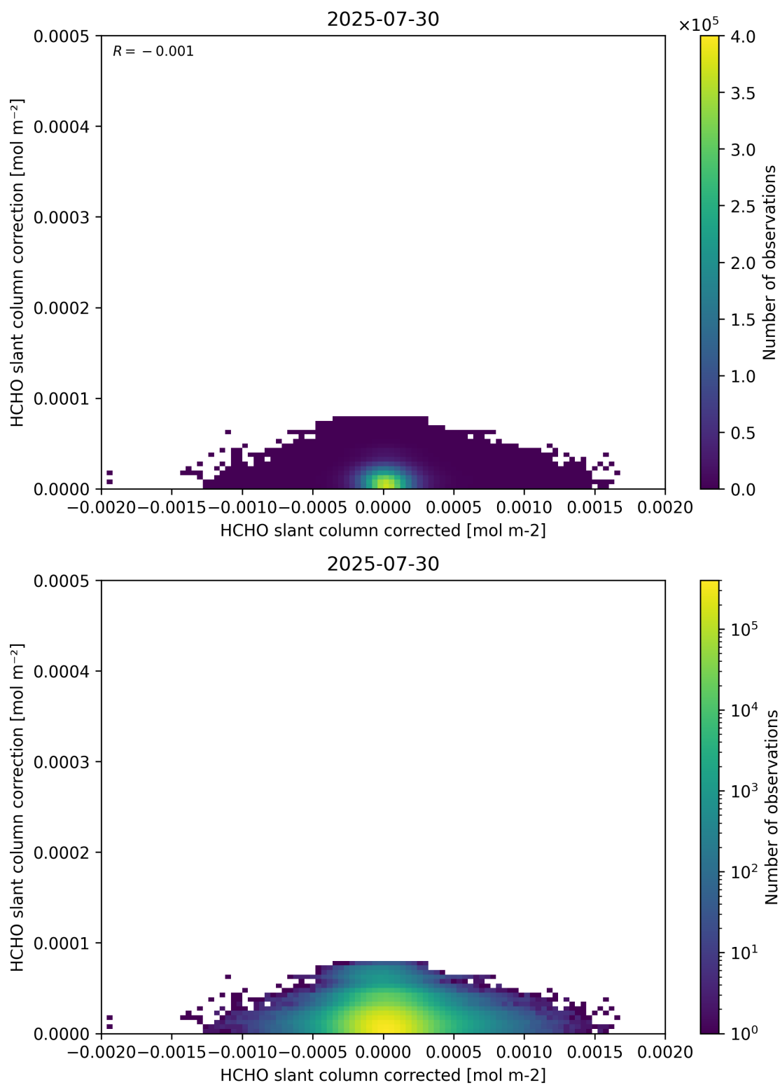
Figure 77: Scatter density plot of “HCHO slant column corrected” against “HCHO slant column correction” for 2025-07-29 to 2025-07-31.
