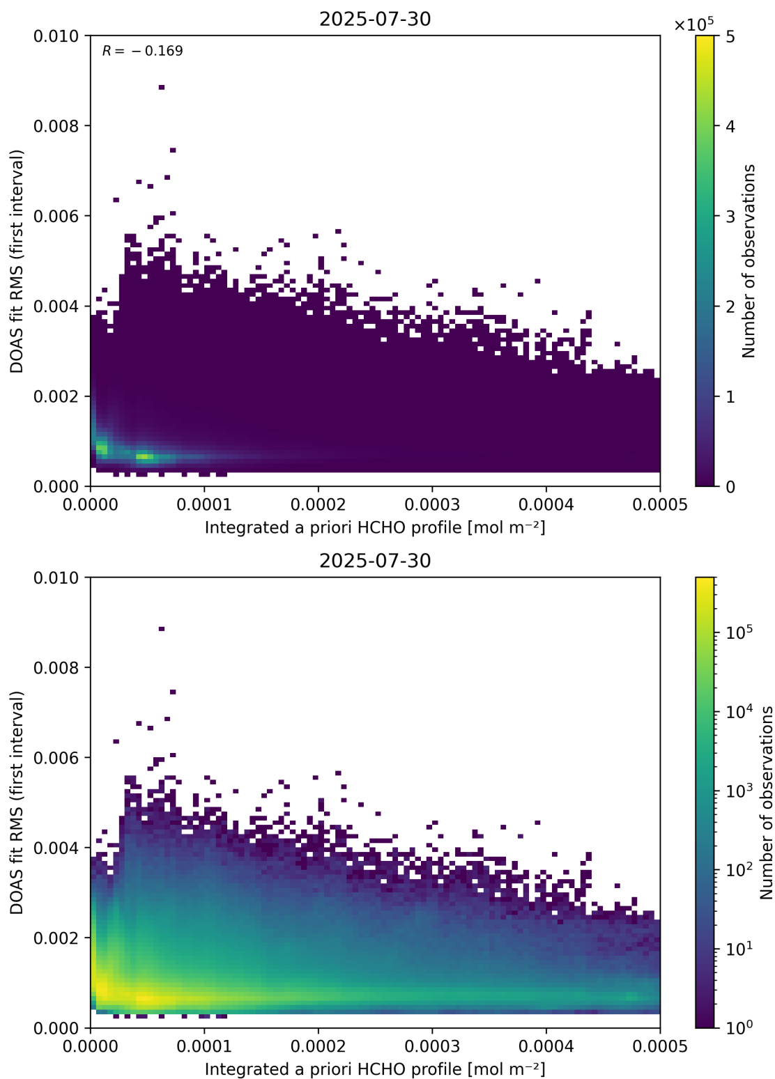
Figure 148: Scatter density plot of “Integrated a priori HCHO profile” against “DOAS fit RMS (first interval)” for 2025-07-29 to 2025-07-31.
