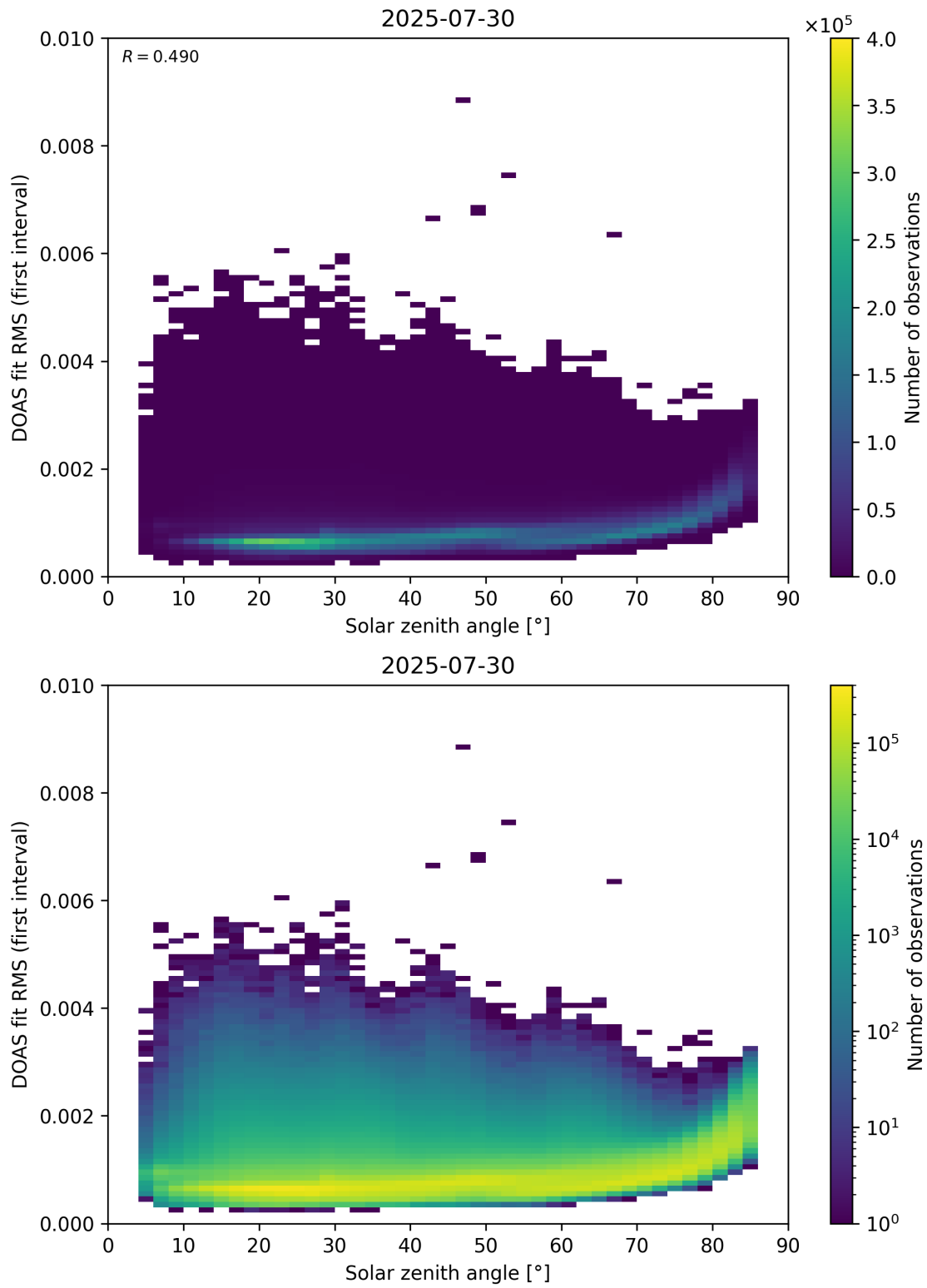
Figure 167: Scatter density plot of “Solar zenith angle” against “DOAS fit RMS (first interval)” for 2025-07-29 to 2025-07-31.
