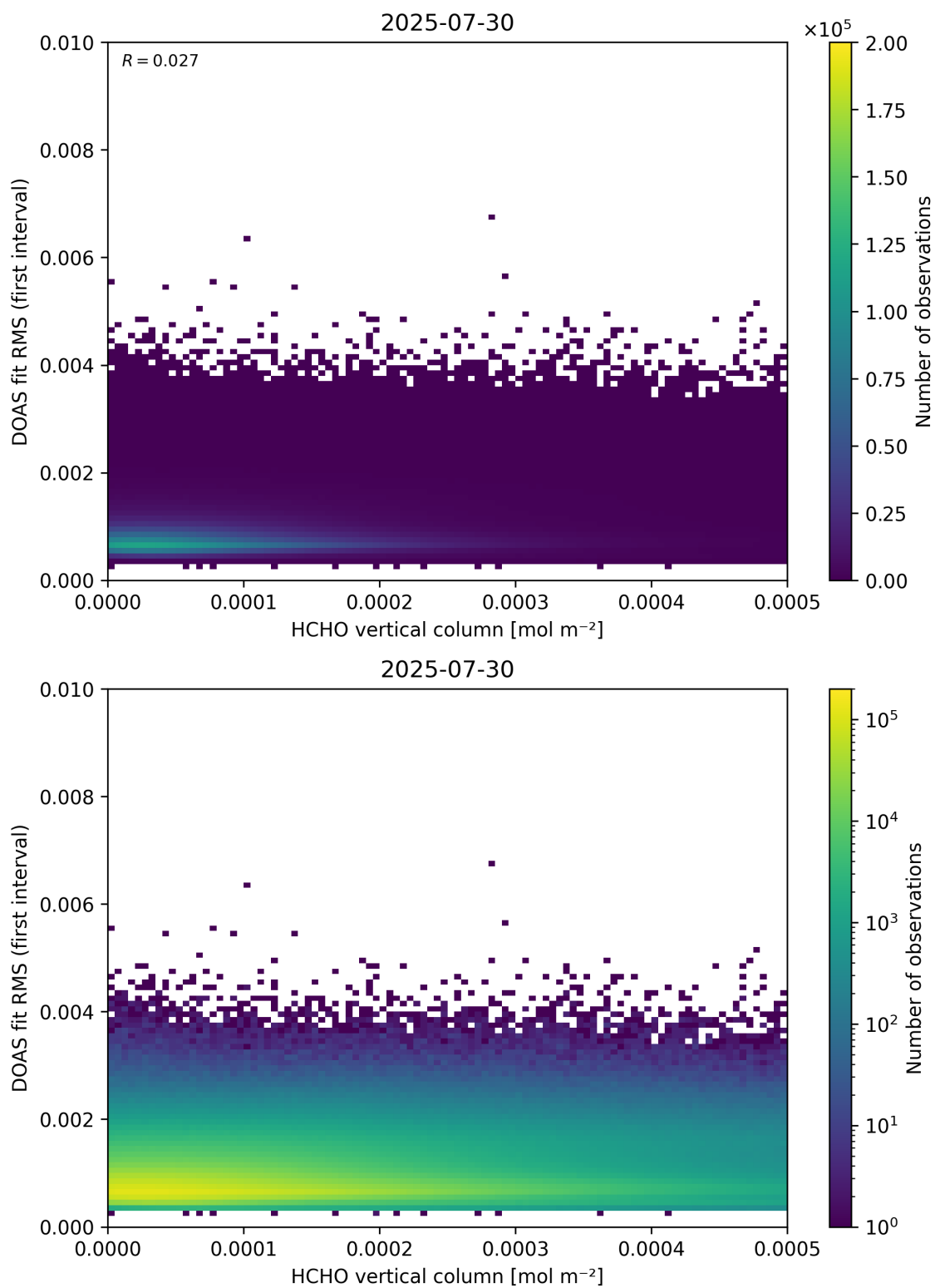
Figure 123: Scatter density plot of “HCHO vertical column” against “DOAS fit RMS (first interval)” for 2025-07-29 to 2025-07-31.
