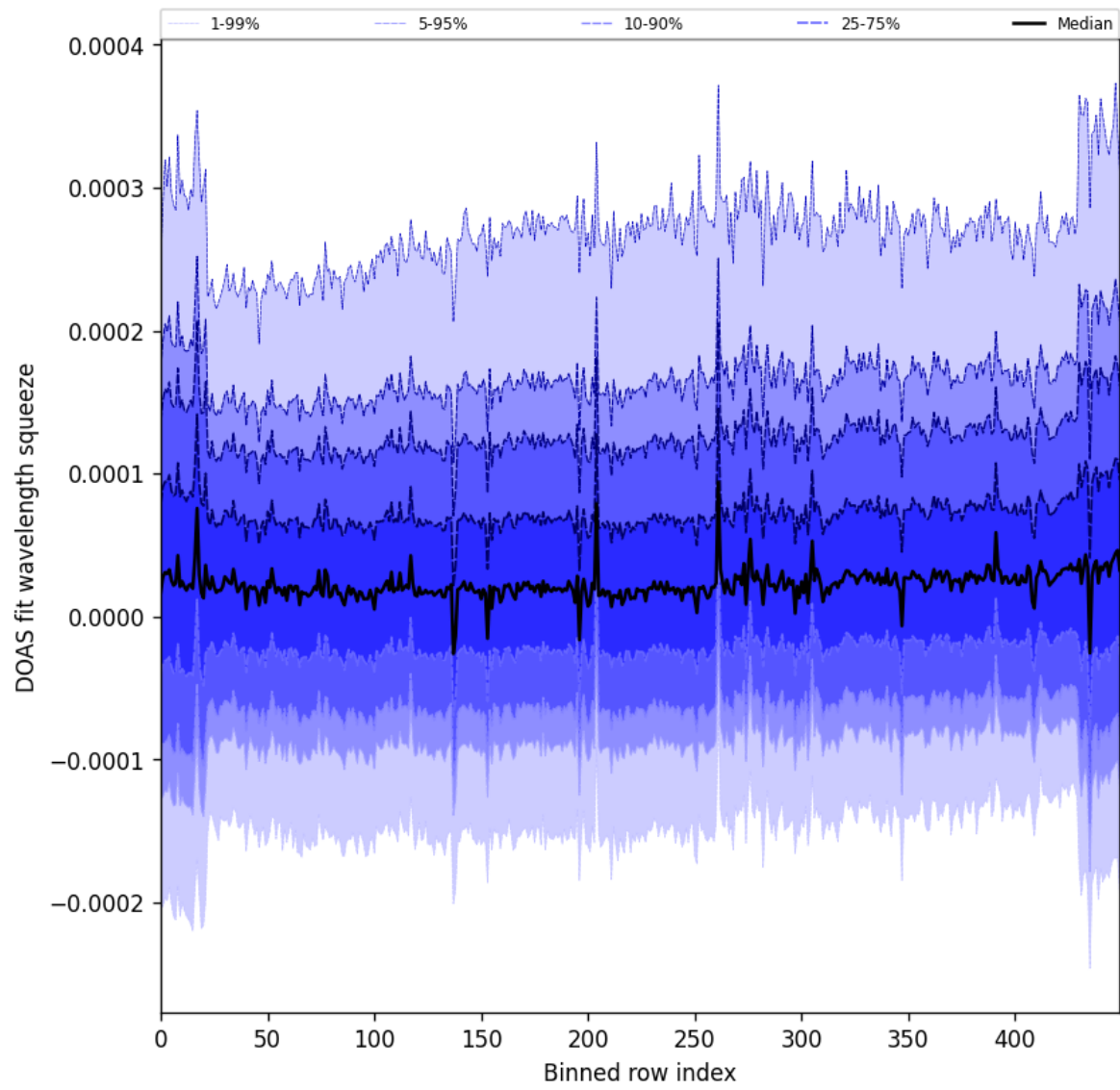
Figure 59: Along track statistics of “DOAS fit wavelength squeeze” for 2025-07-29 to 2025-07-31
