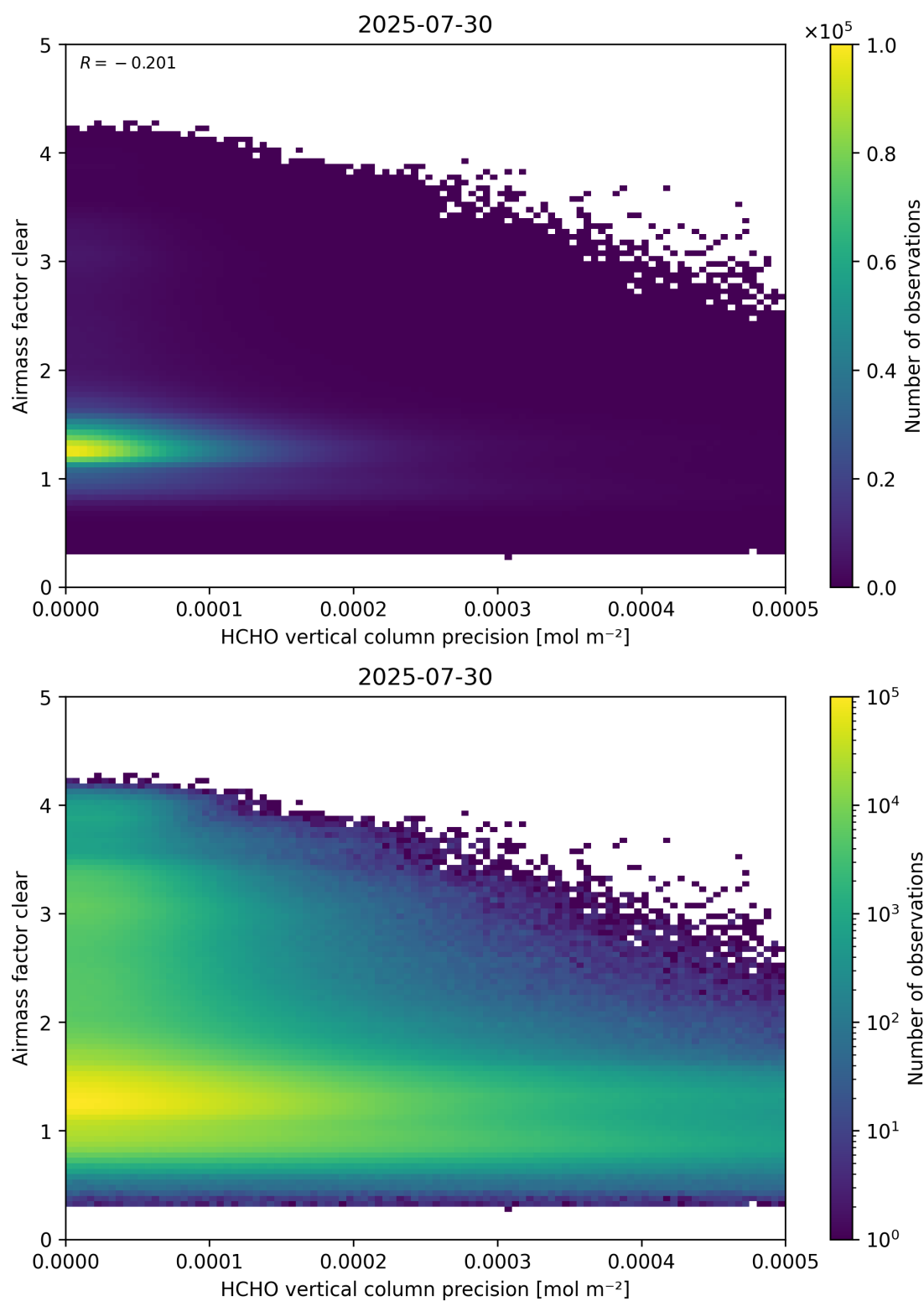
Figure 139: Scatter density plot of “HCHO vertical column precision” against “Airmass factor clear” for 2025-07-29 to 2025-07-31.
