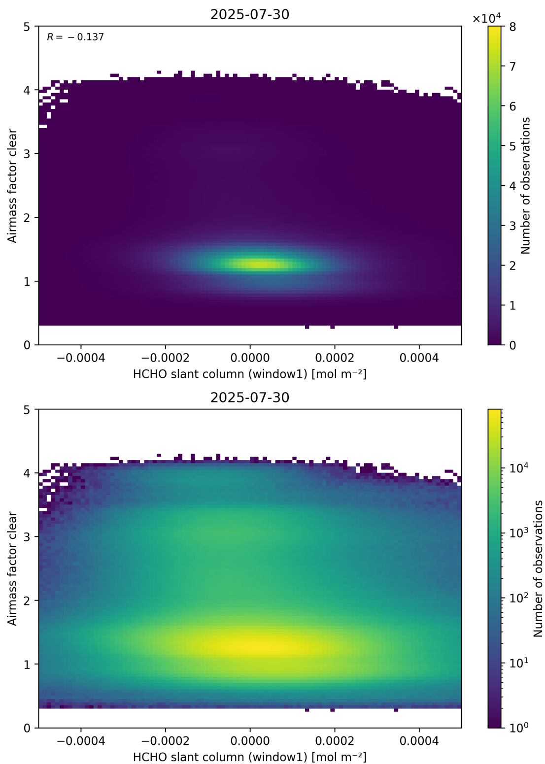
Figure 81: Scatter density plot of “HCHO slant column (window1)” against “Airmass factor clear” for 2025-07-29 to 2025-07-31.
