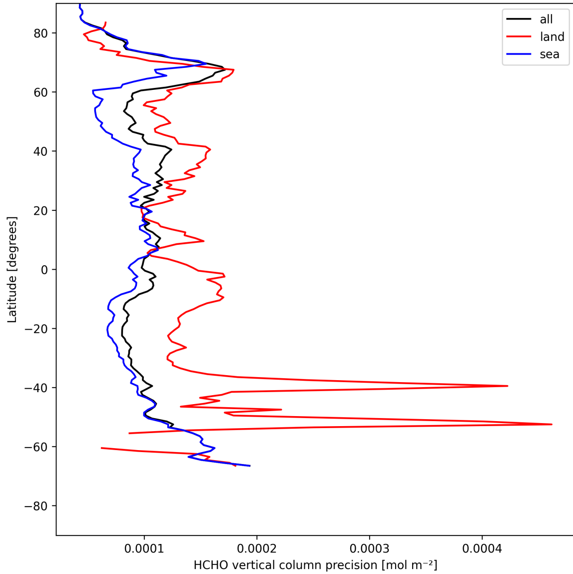
Figure 22: Zonal average of “HCHO vertical column precision” for 2025-07-29 to 2025-07-31.
