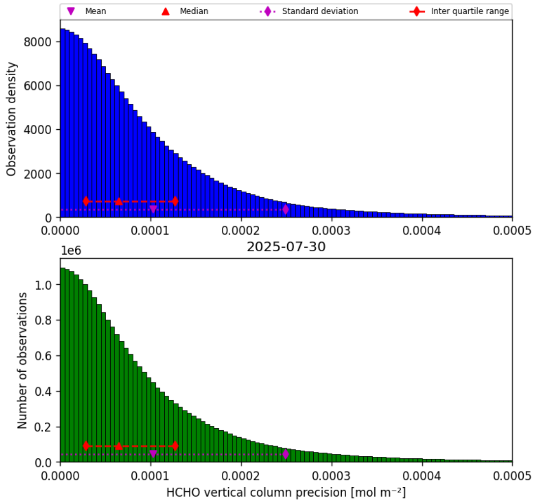
Figure 36: Histogram of “HCHO vertical column precision” for 2025-07-29 to 2025-07-31
