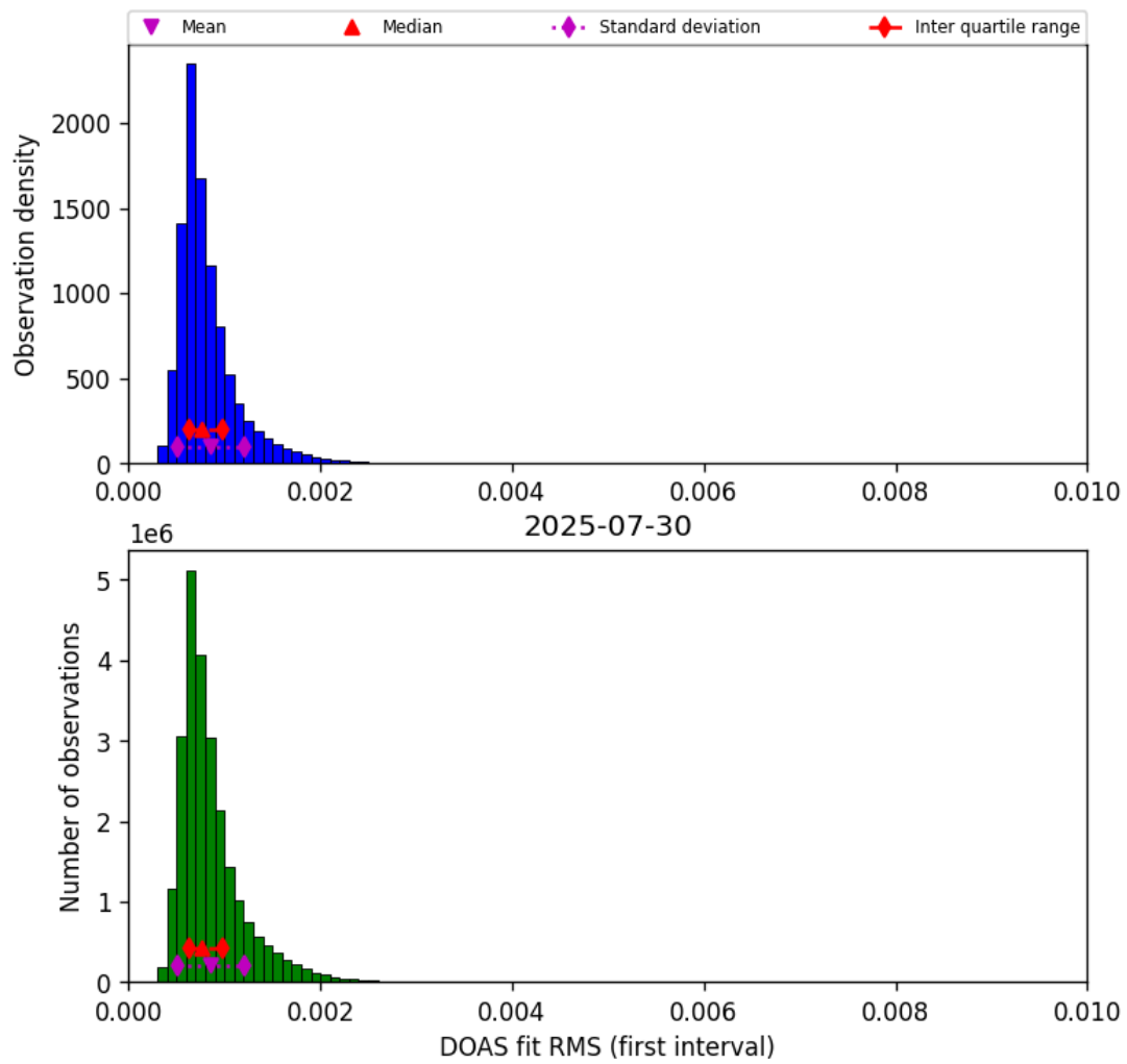
Figure 46: Histogram of “DOAS fit RMS (first interval)” for 2025-07-29 to 2025-07-31
