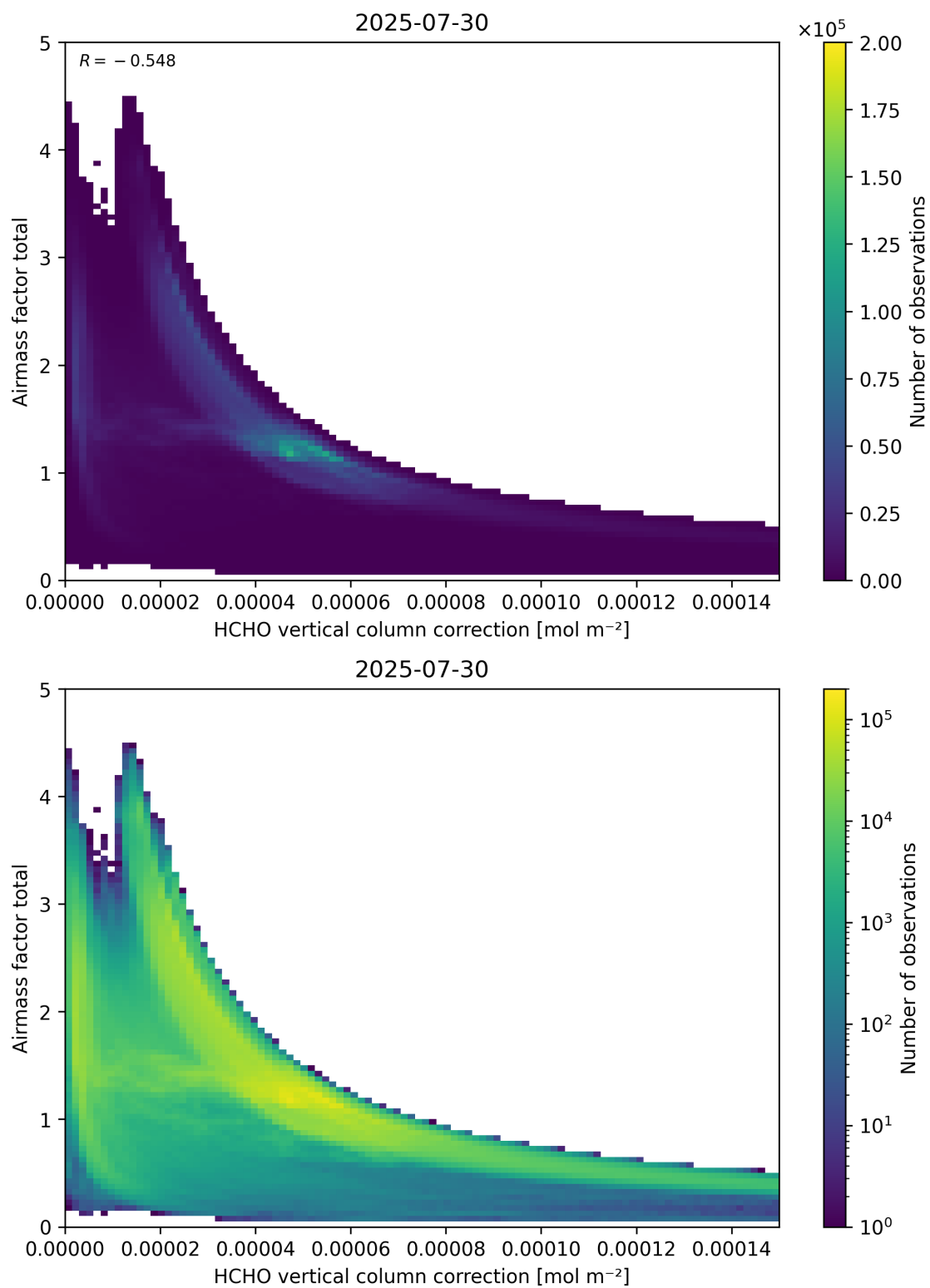
Figure 120: Scatter density plot of “HCHO vertical column correction” against “Airmass factor total” for 2025-07-29 to 2025-07-31.
