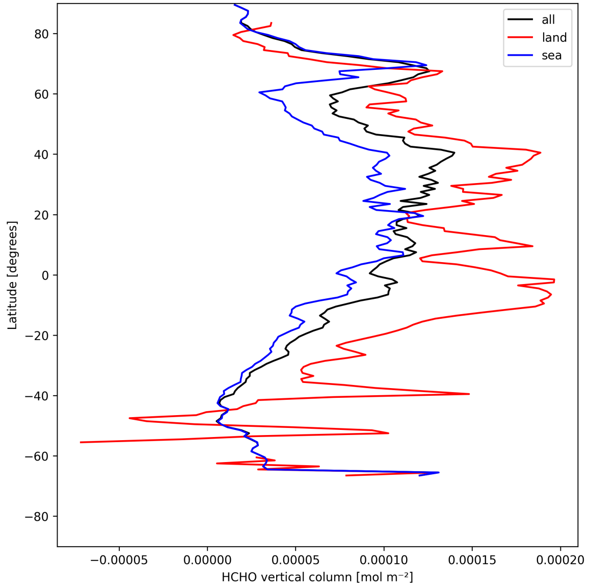
Figure 21: Zonal average of “HCHO vertical column” for 2025-07-29 to 2025-07-31.
