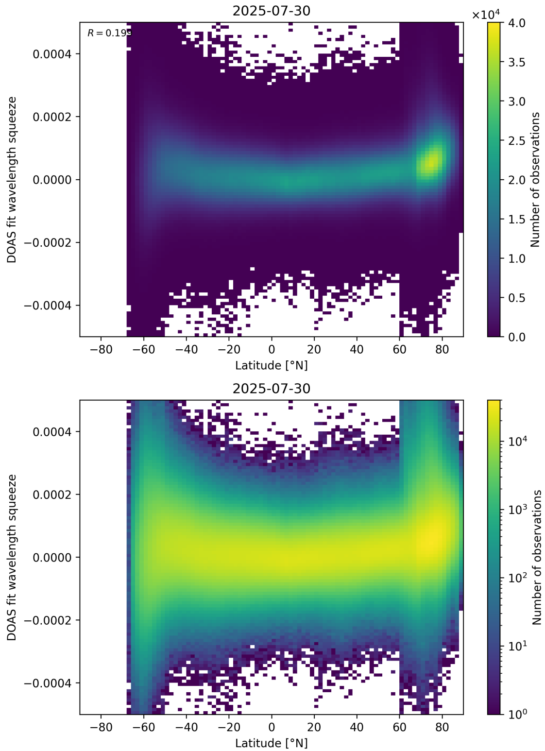
Figure 155: Scatter density plot of “Latitude” against “DOAS fit wavelength squeeze” for 2025-07-29 to 2025-07-31.
