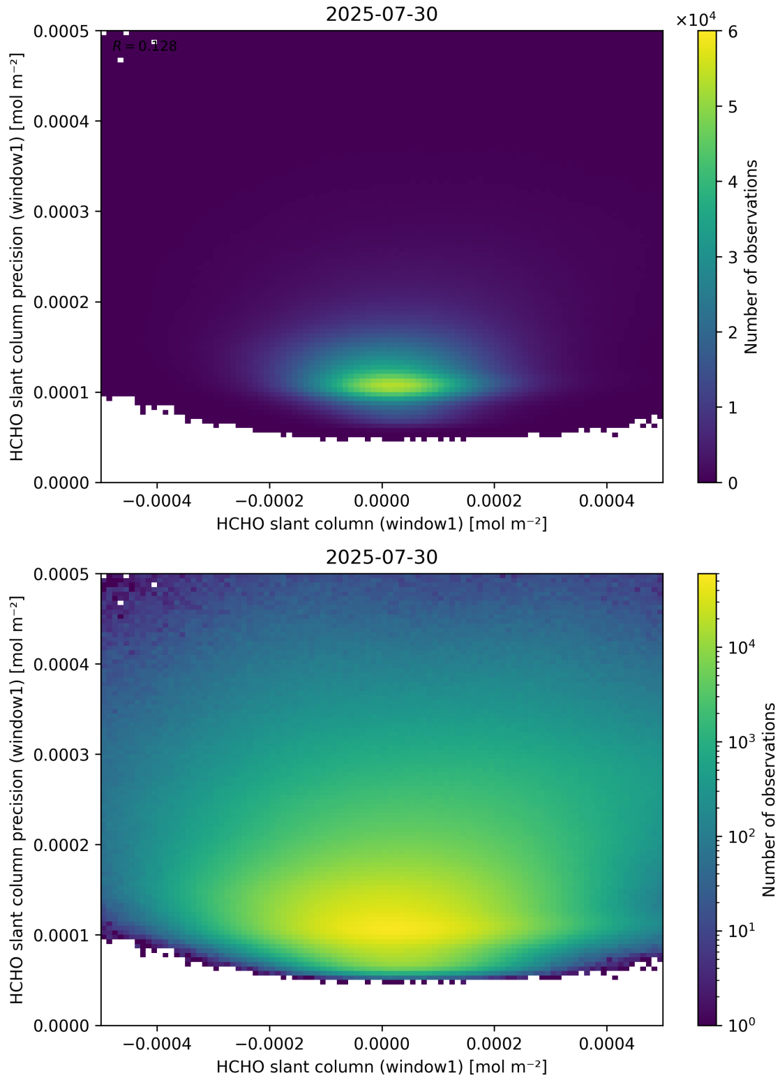
Figure 84: Scatter density plot of “HCHO slant column (window1)” against “HCHO slant column precision (window1)” for 2025-07-29 to 2025-07-31.
