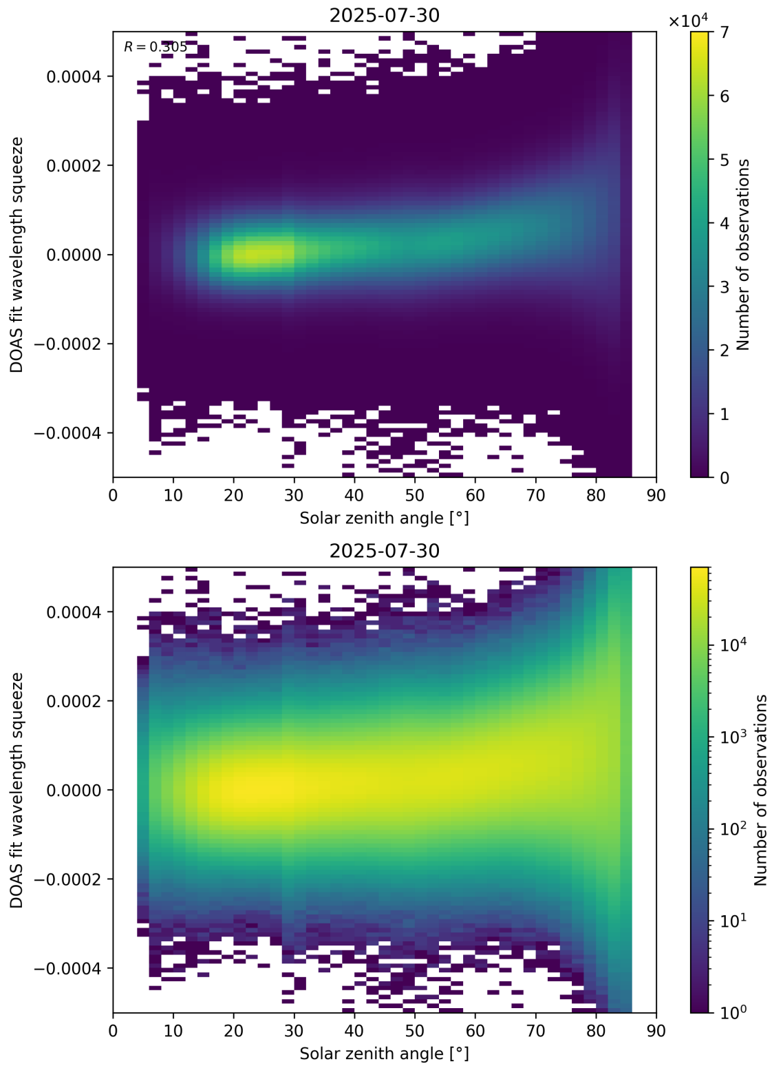
Figure 169: Scatter density plot of “Solar zenith angle” against “DOAS fit wavelength squeeze” for 2025-07-29 to 2025-07-31.
