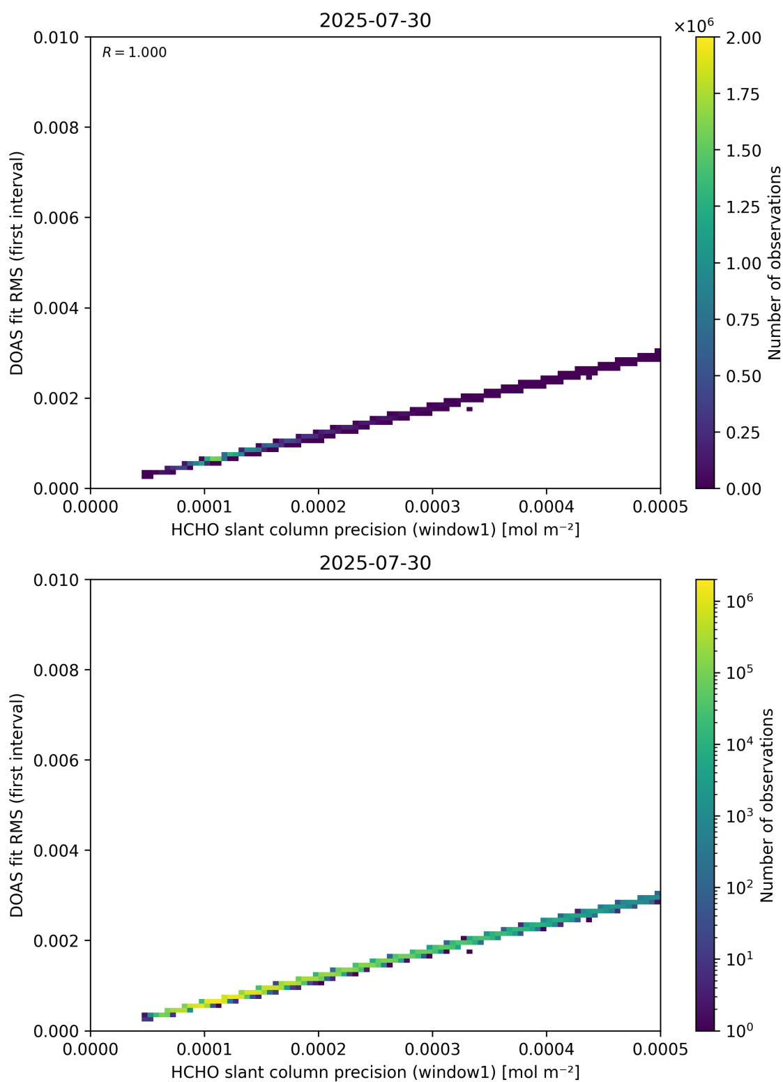
Figure 88: Scatter density plot of “HCHO slant column precision (window1)” against “DOAS fit RMS (first interval)” for 2025-07-29 to 2025-07-31.
