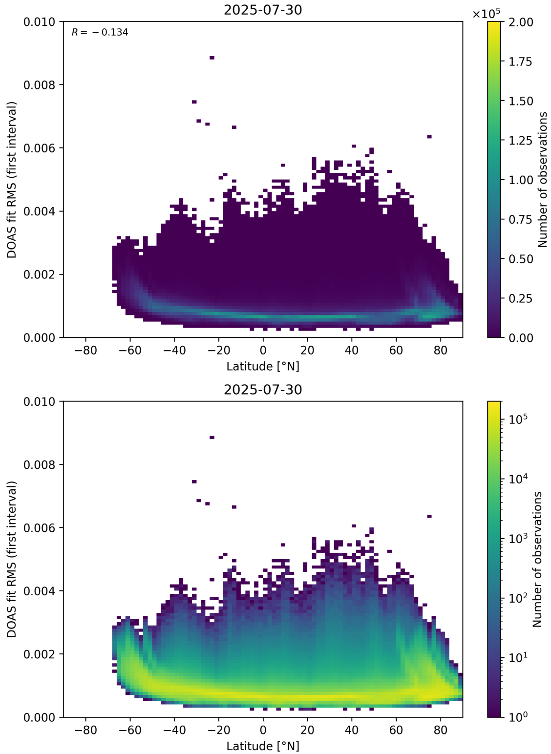
Figure 153: Scatter density plot of “Latitude” against “DOAS fit RMS (first interval)” for 2025-07-29 to 2025-07-31.
