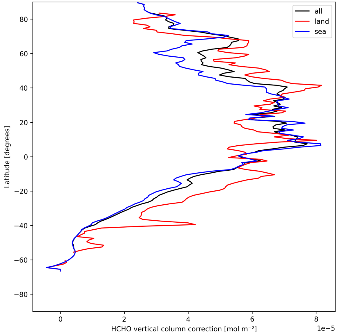
Figure 23: Zonal average of “HCHO vertical column correction” for 2025-07-29 to 2025-07-31.
