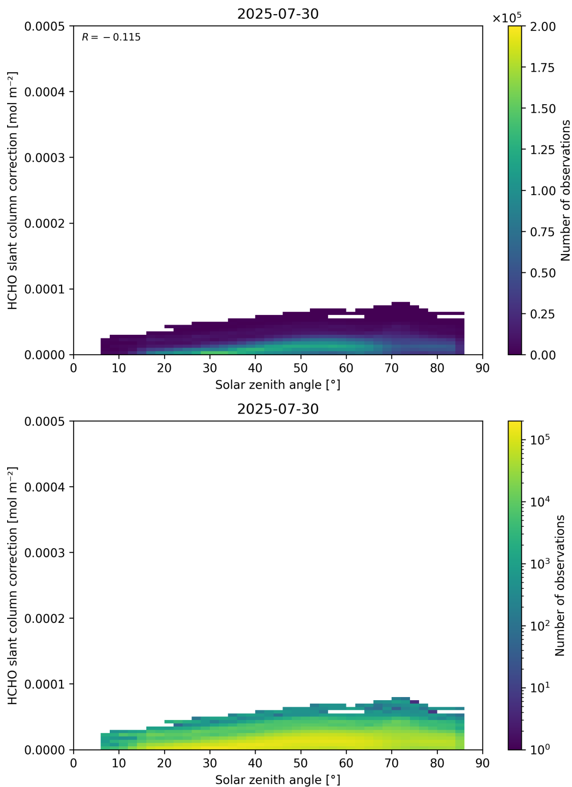
Figure 172: Scatter density plot of “Solar zenith angle” against “HCHO slant column correction” for 2025-07-29 to 2025-07-31.
