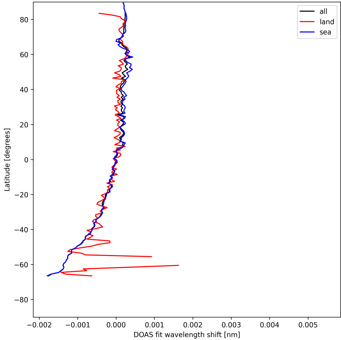
Figure 30: Zonal average of “DOAS fit wavelength shift” for 2025-07-29 to 2025-07-31.
