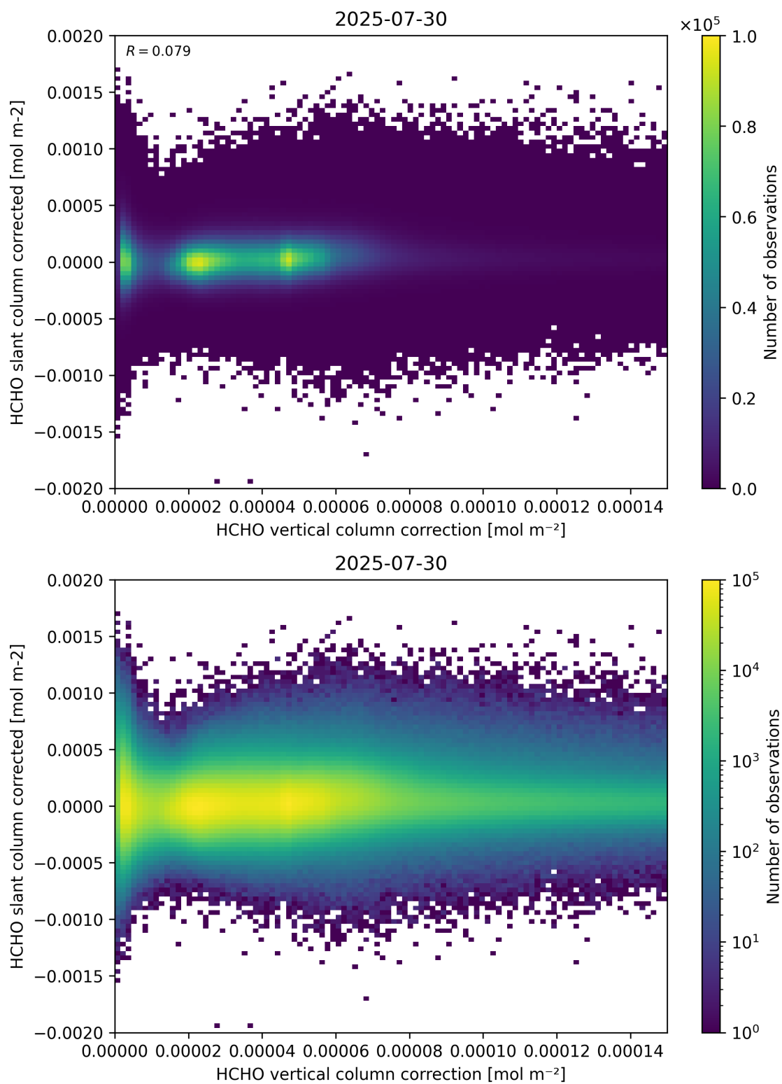
Figure 116: Scatter density plot of “HCHO vertical column correction” against “HCHO slant column corrected” for 2025-07-29 to 2025-07-31.
