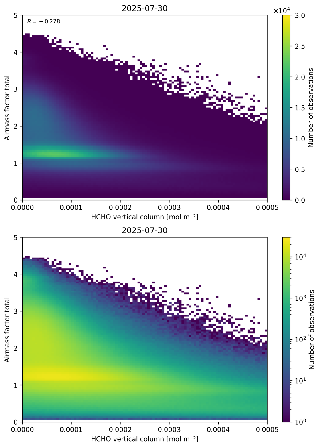
Figure 131: Scatter density plot of “HCHO vertical column” against “Airmass factor total” for 2025-07-29 to 2025-07-31.
