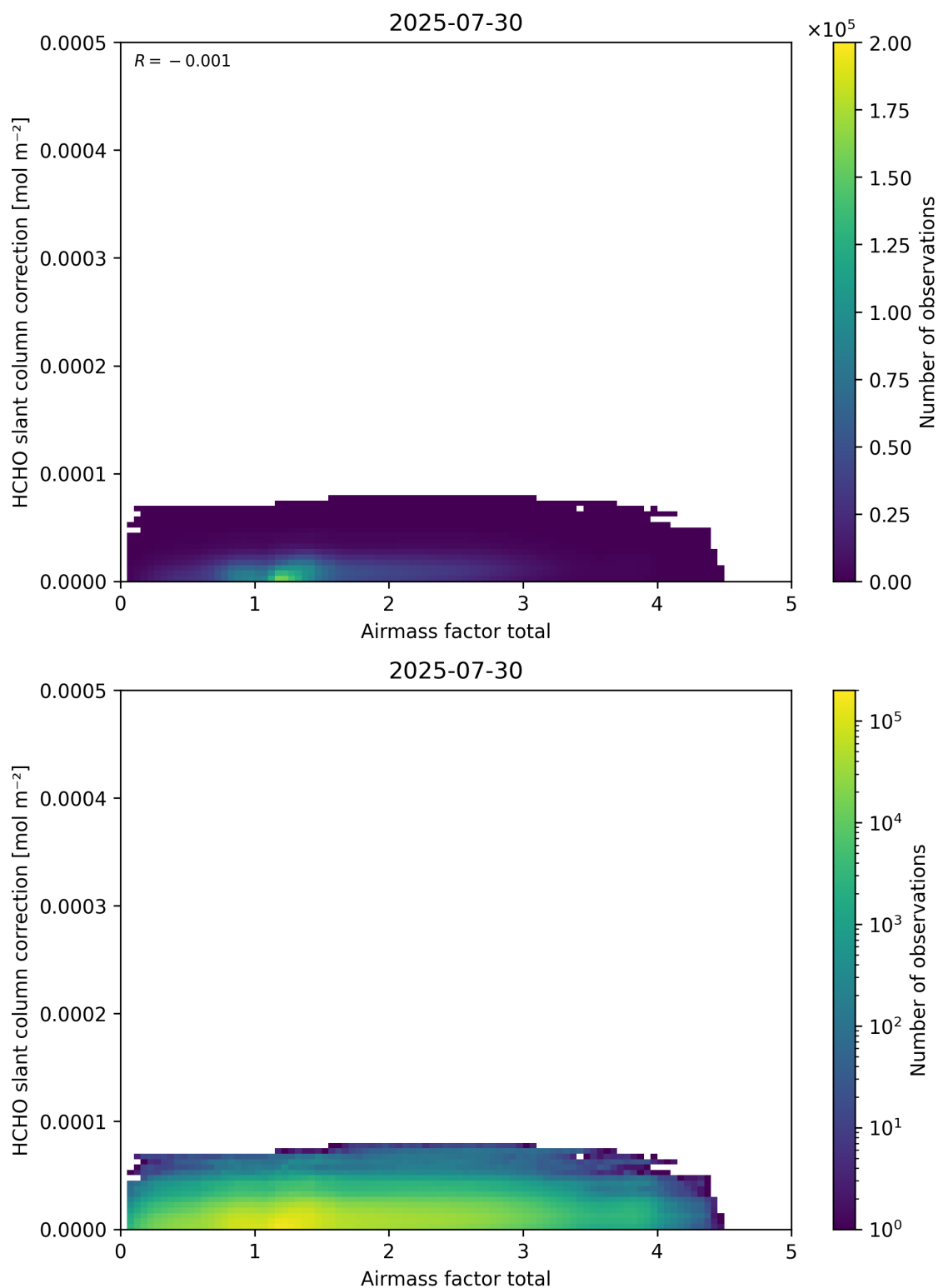
Figure 102: Scatter density plot of “Airmass factor total” against “HCHO slant column correction” for 2025-07-29 to 2025-07-31.
