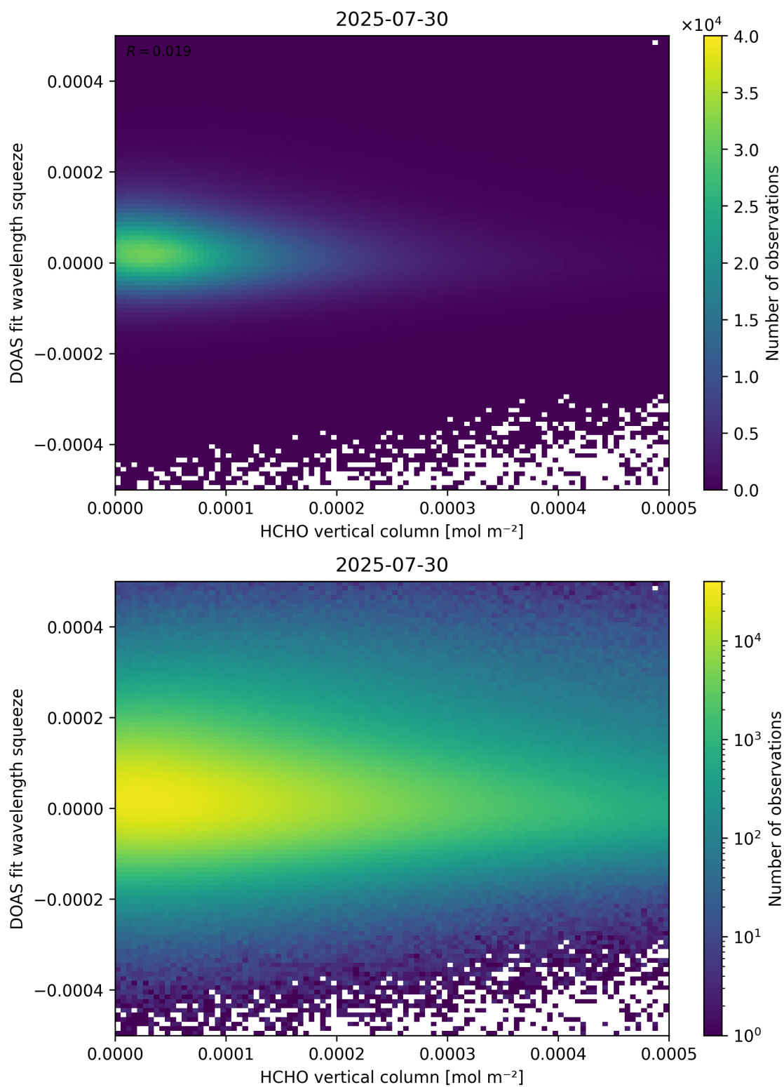
Figure 125: Scatter density plot of “HCHO vertical column” against “DOAS fit wavelength squeeze” for 2025-07-29 to 2025-07-31.
