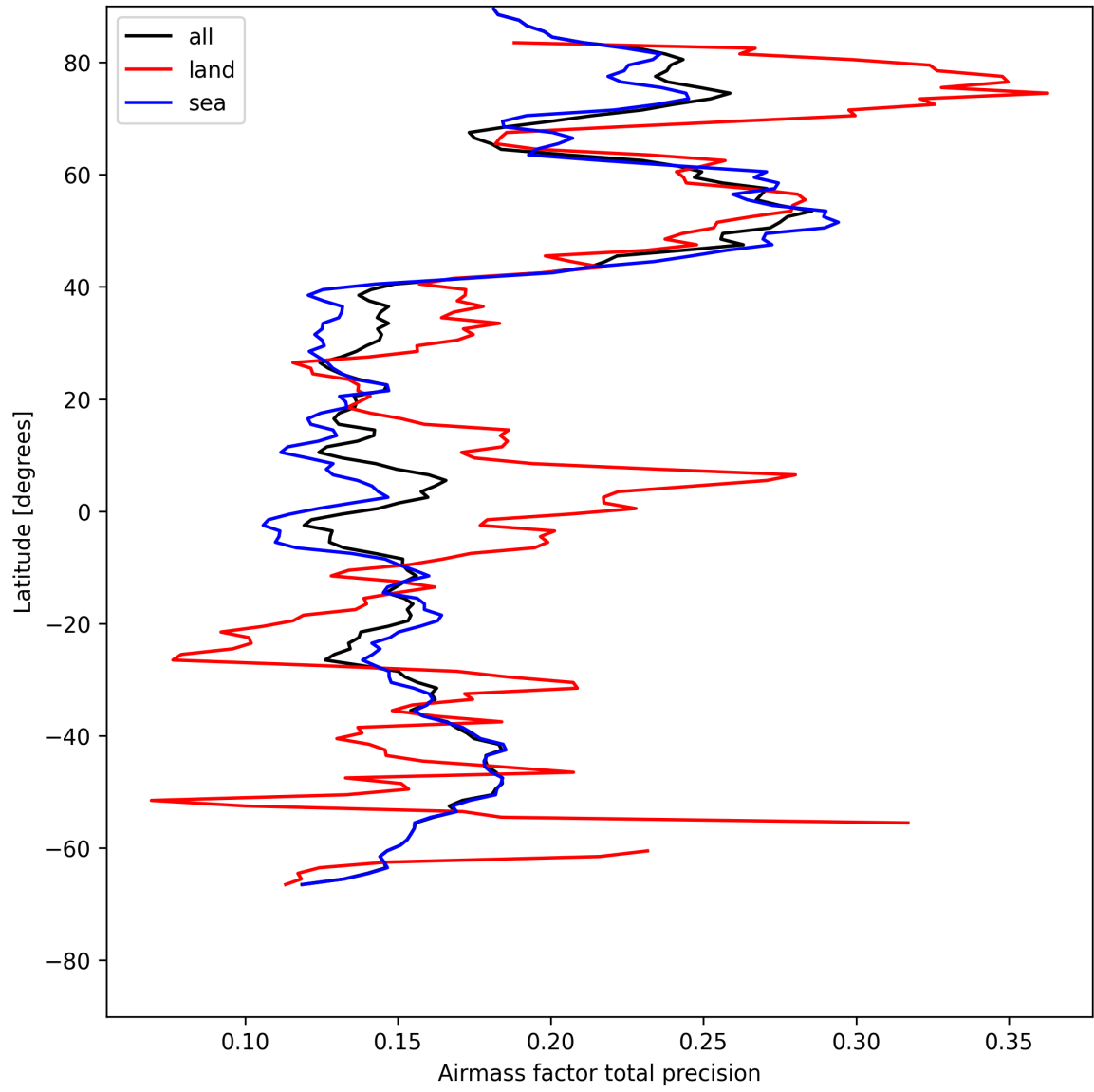
Figure 27: Zonal average of “Airmass factor total precision” for 2025-07-29 to 2025-07-31.
