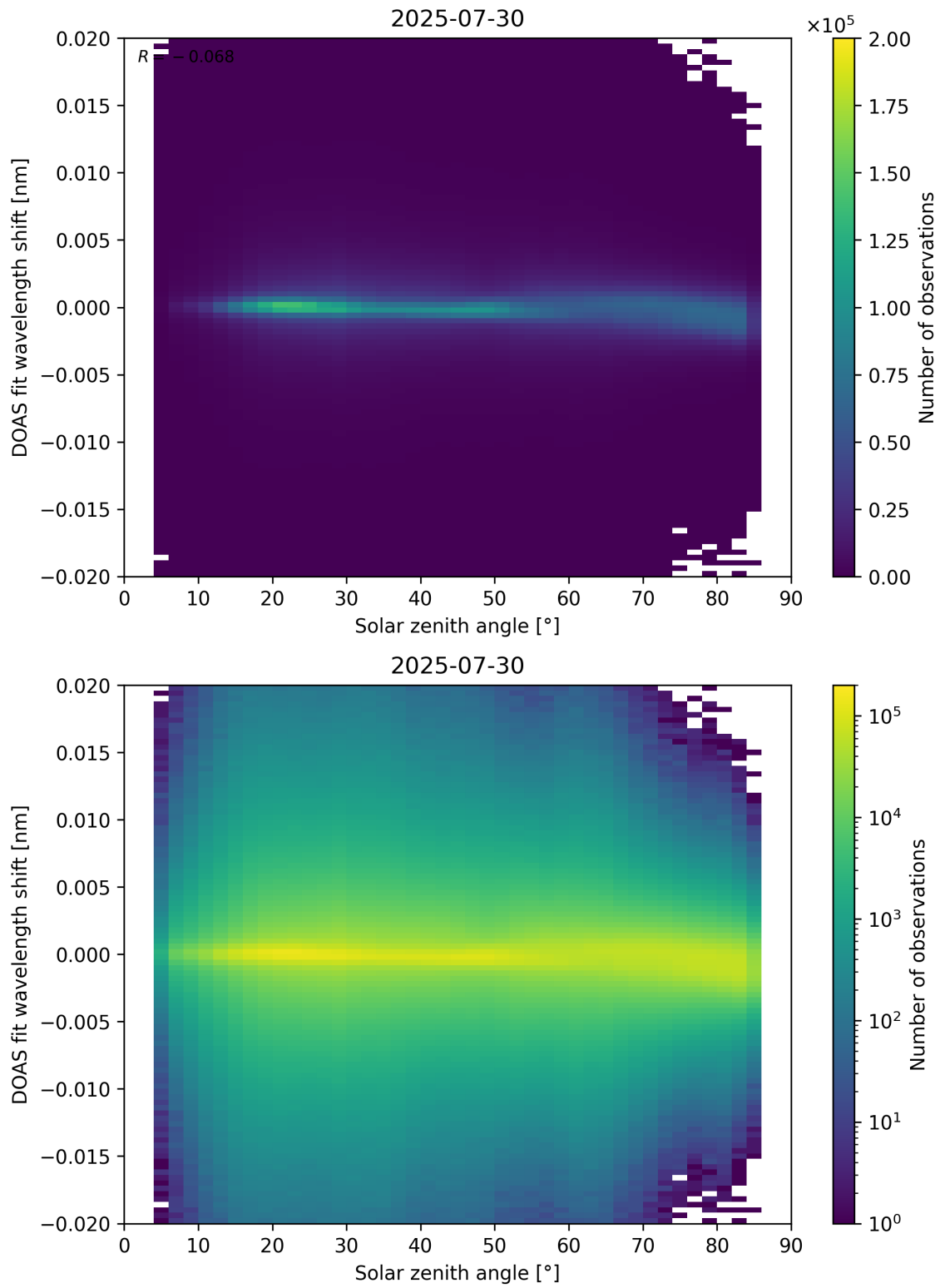
Figure 168: Scatter density plot of “Solar zenith angle” against “DOAS fit wavelength shift” for 2025-07-29 to 2025-07-31.
