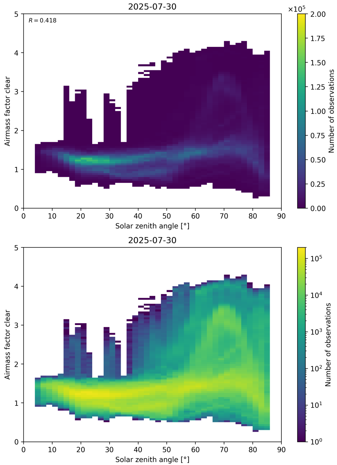
Figure 170: Scatter density plot of “Solar zenith angle” against “Airmass factor clear” for 2025-07-29 to 2025-07-31.
