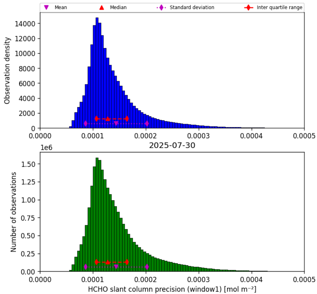
Figure 39: Histogram of “HCHO slant column precision (window1)” for 2025-07-29 to 2025-07-31
