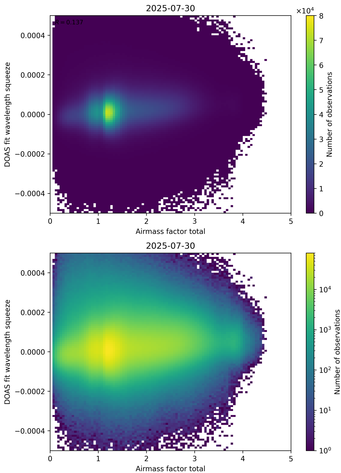
Figure 99: Scatter density plot of “Airmass factor total” against “DOAS fit wavelength squeeze” for 2025-07-29 to 2025-07-31.
