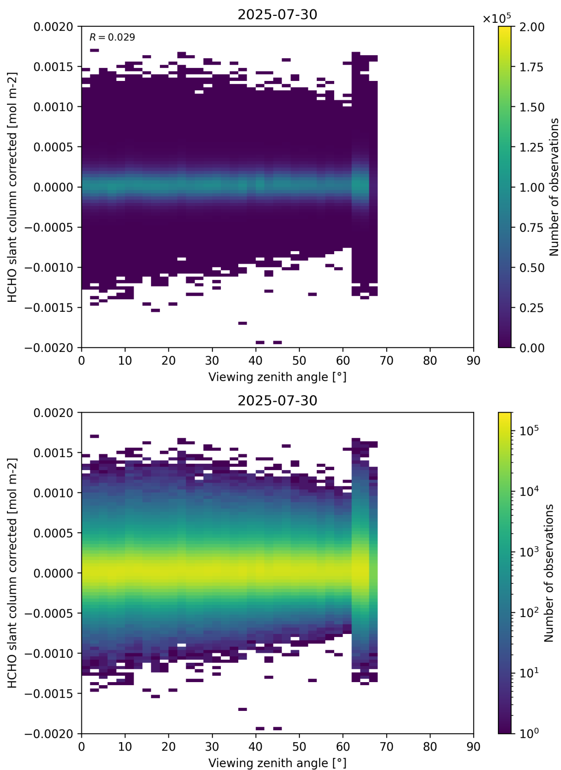
Figure 186: Scatter density plot of “Viewing zenith angle” against “HCHO slant column corrected” for 2025-07-29 to 2025-07-31.
