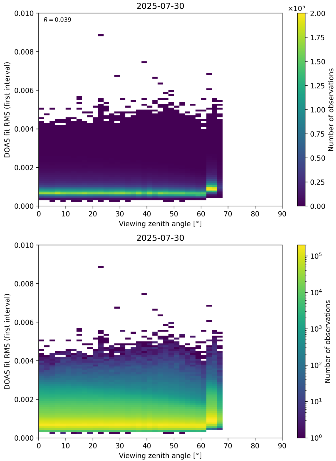
Figure 182: Scatter density plot of “Viewing zenith angle” against “DOAS fit RMS (first interval)” for 2025-07-29 to 2025-07-31.
