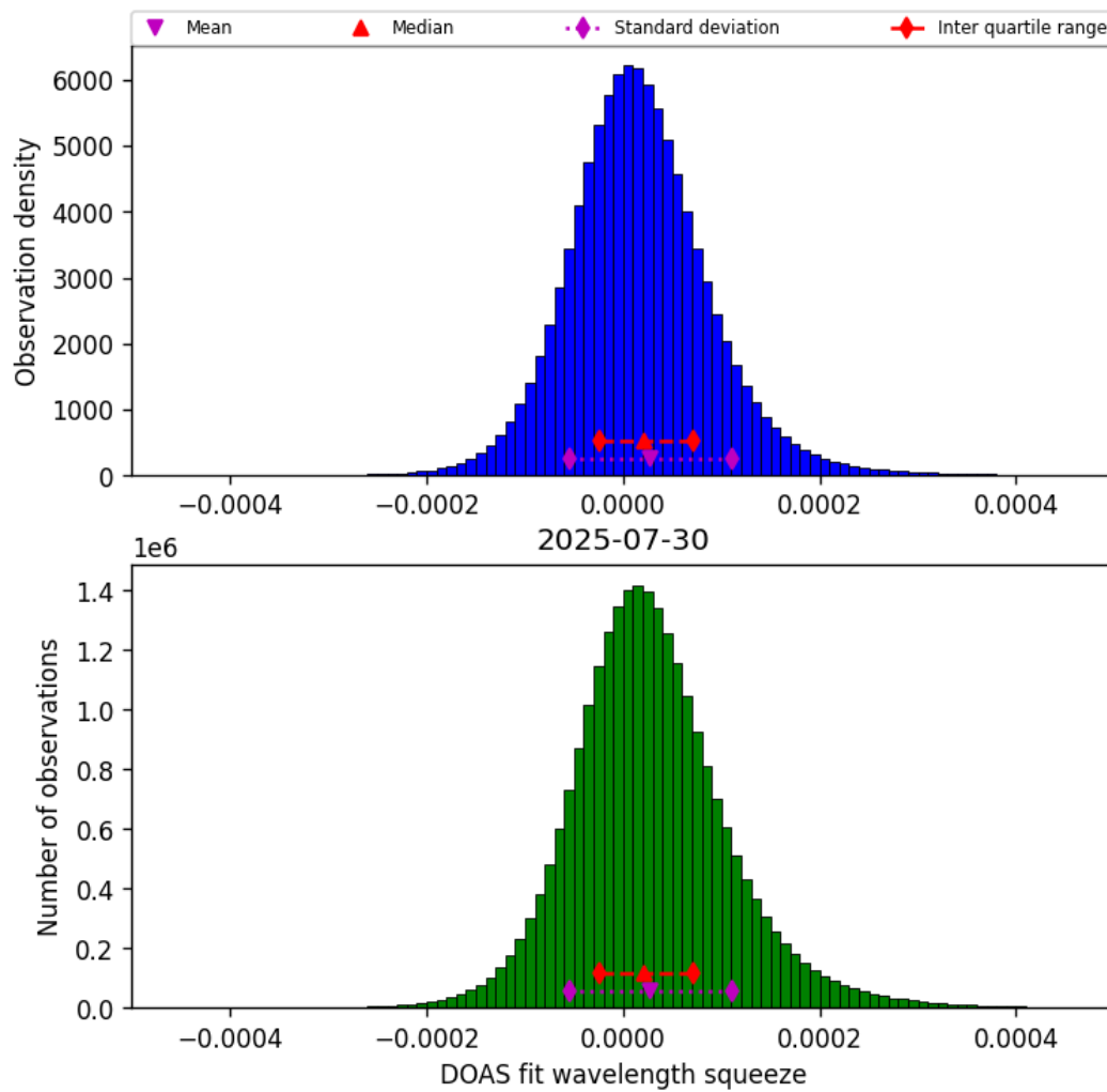
Figure 45: Histogram of “DOAS fit wavelength squeeze” for 2025-07-29 to 2025-07-31
