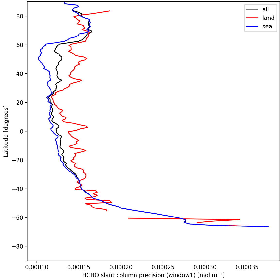
Figure 25: Zonal average of "HCHO slant column precision (window1)" for 2025-07-30 to 2025-08-01.
