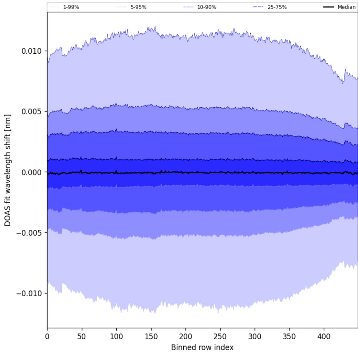
Figure 58: Along track statistics of “DOAS fit wavelength shift” for 2025-07-30 to 2025-08-01
