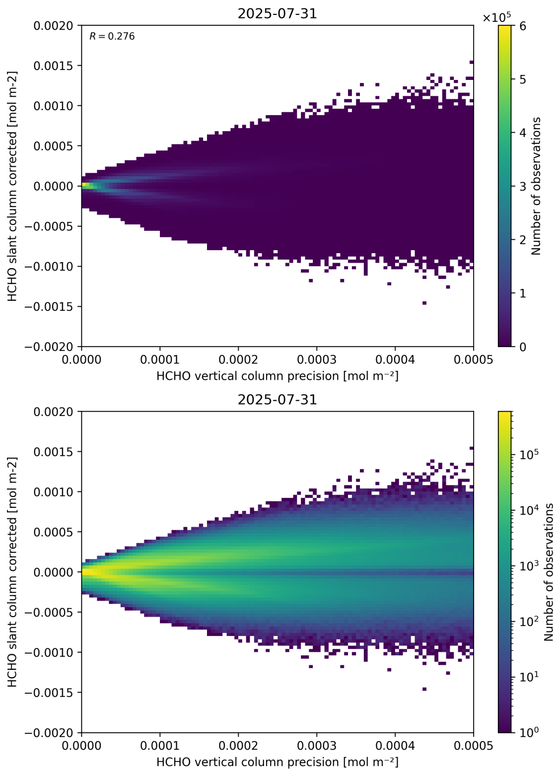
Figure 140: Scatter density plot of “HCHO vertical column precision” against “HCHO slant column corrected” for 2025-07-30 to 2025-08-01.
