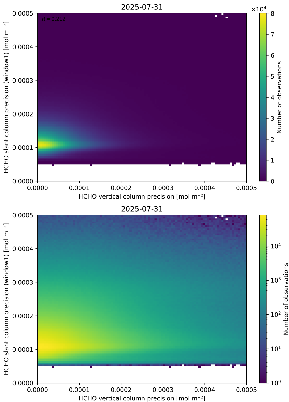
Figure 143: Scatter density plot of “HCHO vertical column precision” against “HCHO slant column precision (window1)” for 2025-07-30 to 2025-08-01.
