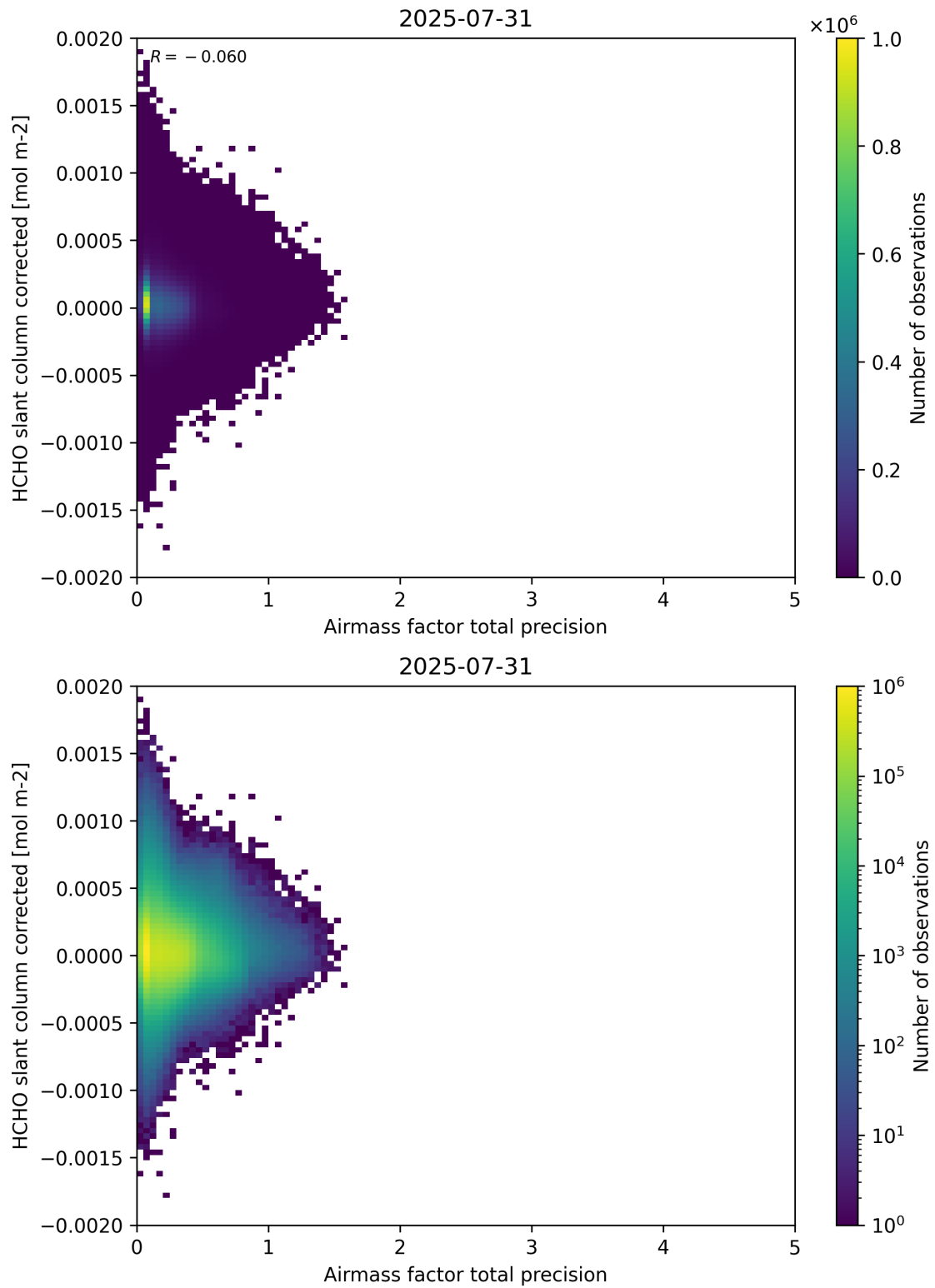
Figure 109: Scatter density plot of “Airmass factor total precision” against “HCHO slant column corrected” for 2025-07-30 to 2025-08-01.
