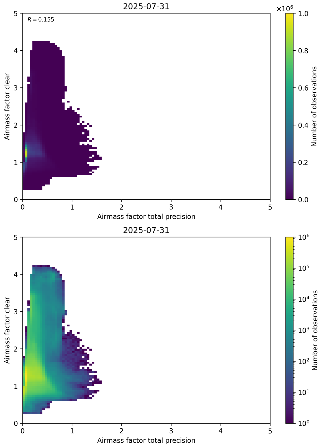
Figure 108: Scatter density plot of “Airmass factor total precision” against “Airmass factor clear” for 2025-07-30 to 2025-08-01.
