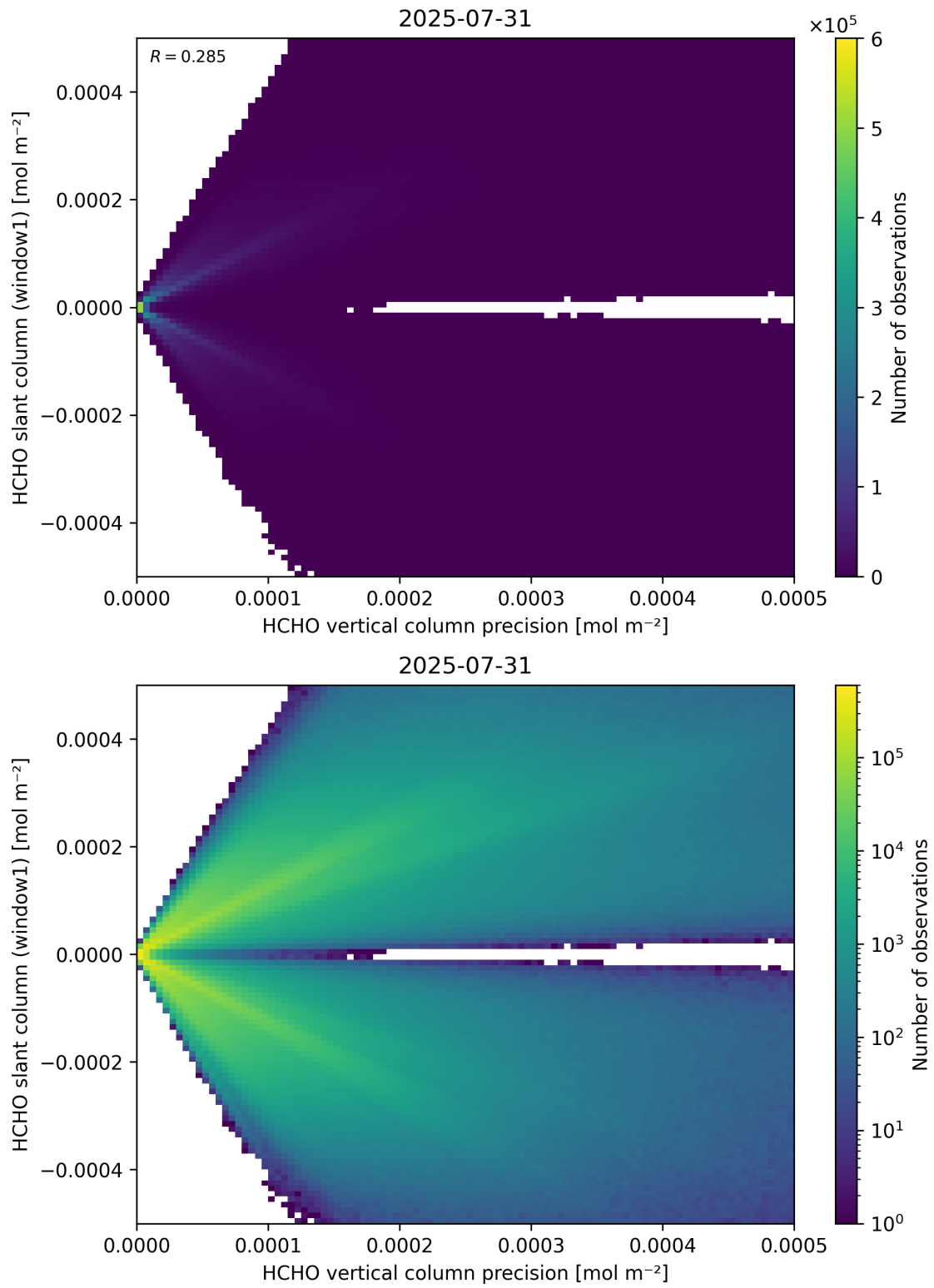
Figure 142: Scatter density plot of “HCHO vertical column precision” against “HCHO slant column (window1)” for 2025-07-30 to 2025-08-01.
