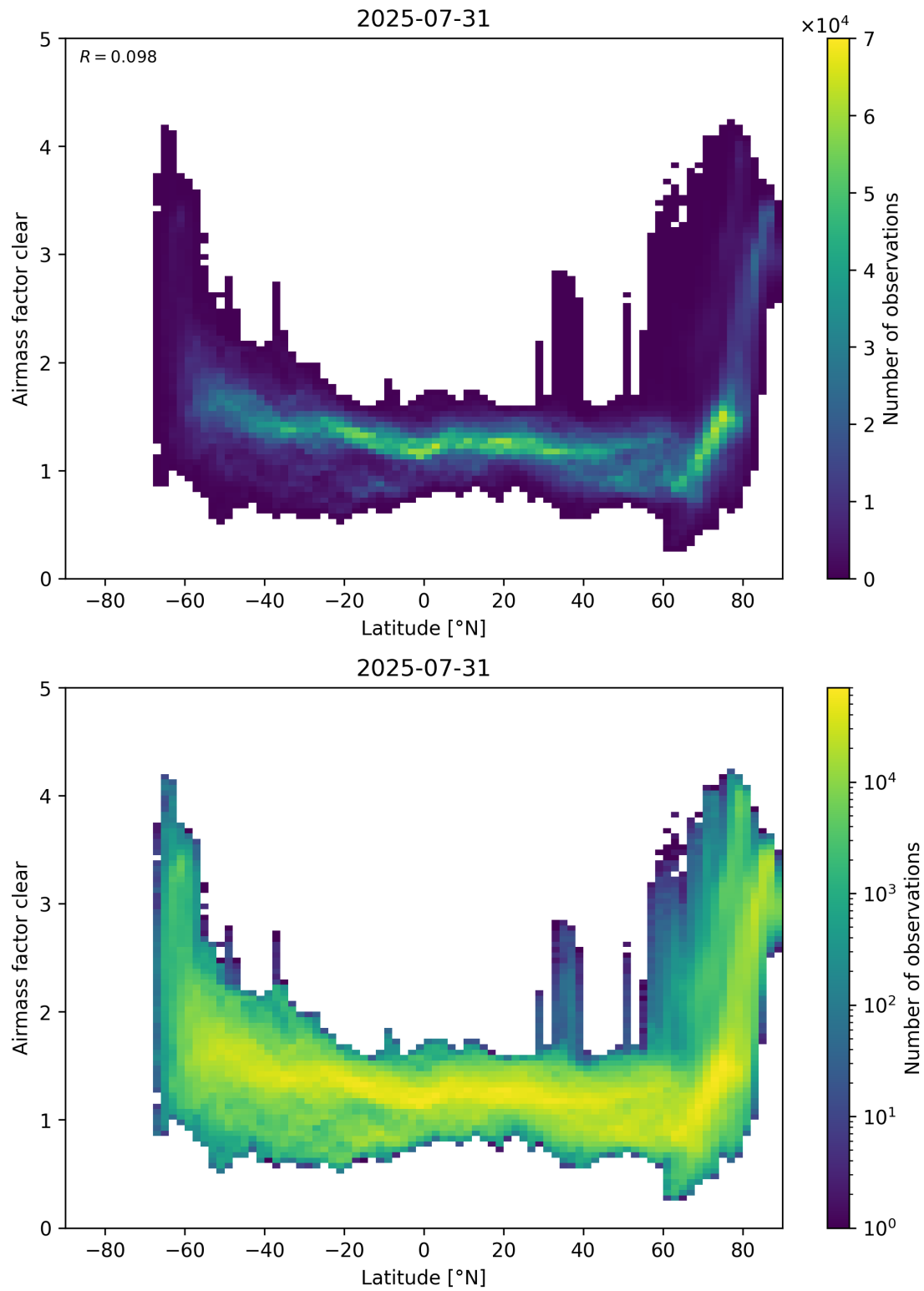
Figure 156: Scatter density plot of “Latitude” against “Airmass factor clear” for 2025-07-30 to 2025-08-01.
