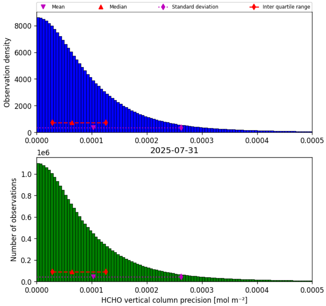
Figure 36: Histogram of “HCHO vertical column precision” for 2025-07-30 to 2025-08-01
