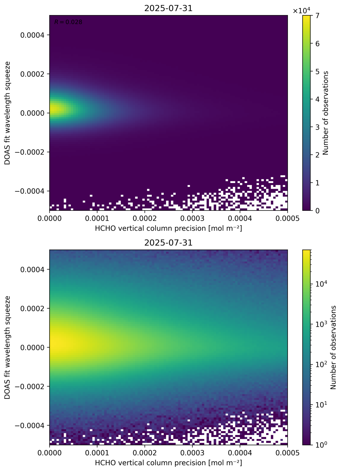
Figure 138: Scatter density plot of “HCHO vertical column precision” against “DOAS fit wavelength squeeze” for 2025-07-30 to 2025-08-01.
