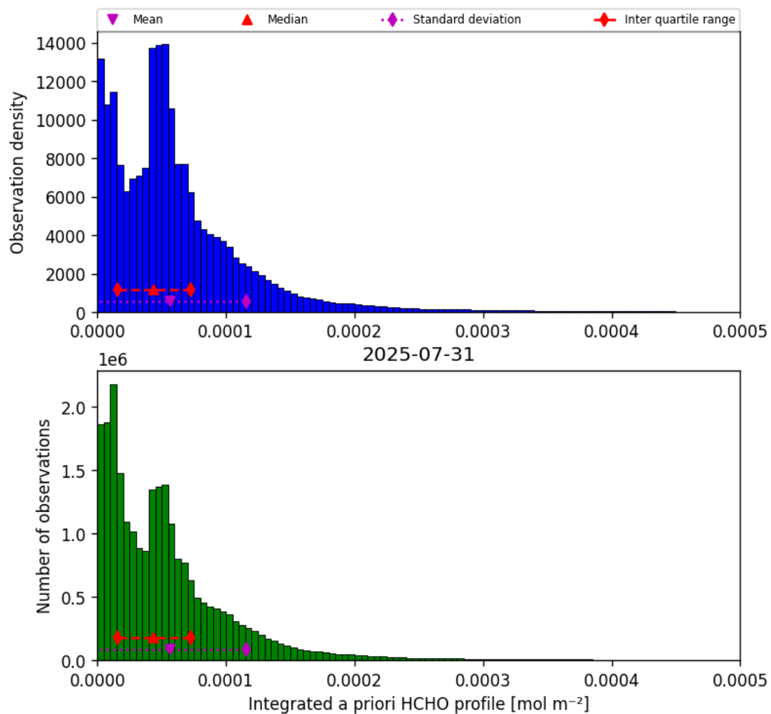
Figure 43: Histogram of “Integrated a priori HCHO profile” for 2025-07-30 to 2025-08-01
