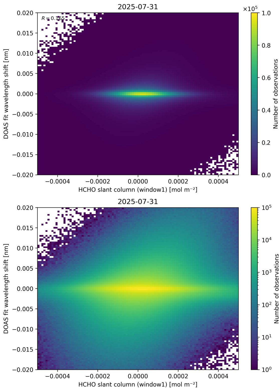
Figure 79: Scatter density plot of “HCHO slant column (window1)” against “DOAS fit wavelength shift” for 2025-07-30 to 2025-08-01.
