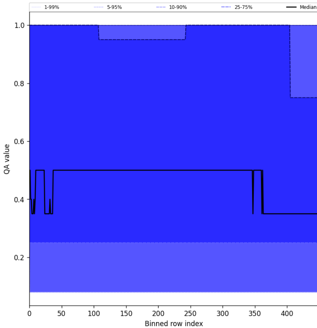
Figure 48: Along track statistics of “QA value” for 2025-07-30 to 2025-08-01
