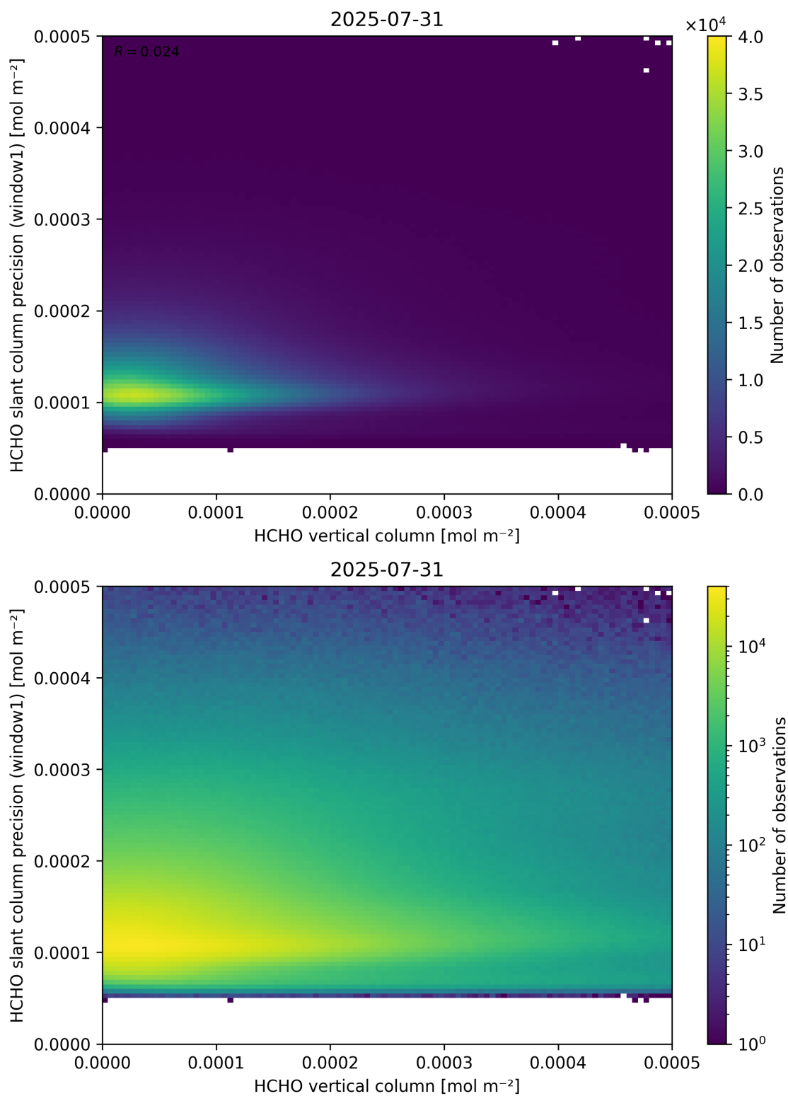
Figure 130: Scatter density plot of “HCHO vertical column” against “HCHO slant column precision (window1)” for 2025-07-30 to 2025-08-01.
