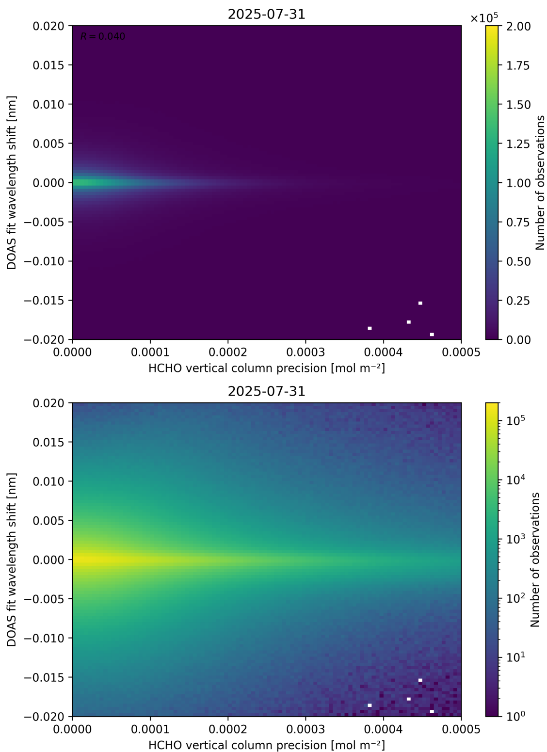
Figure 137: Scatter density plot of “HCHO vertical column precision” against “DOAS fit wavelength shift” for 2025-07-30 to 2025-08-01.
