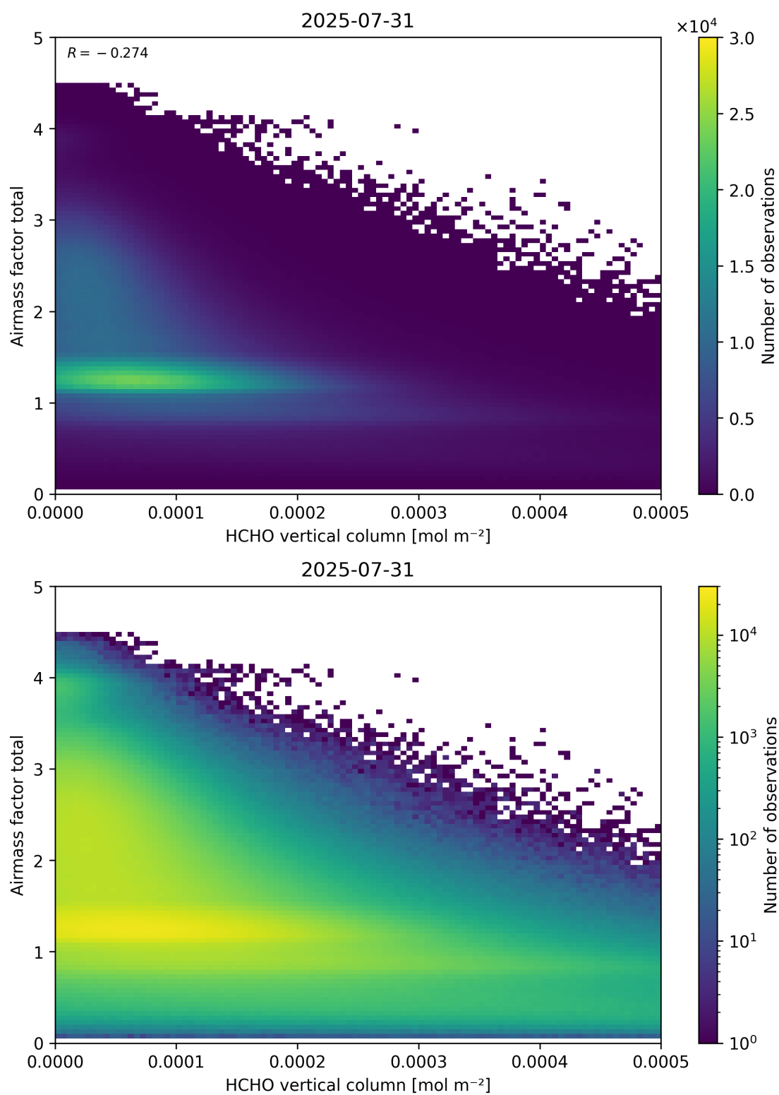
Figure 131: Scatter density plot of “HCHO vertical column” against “Airmass factor total” for 2025-07-30 to 2025-08-01.
