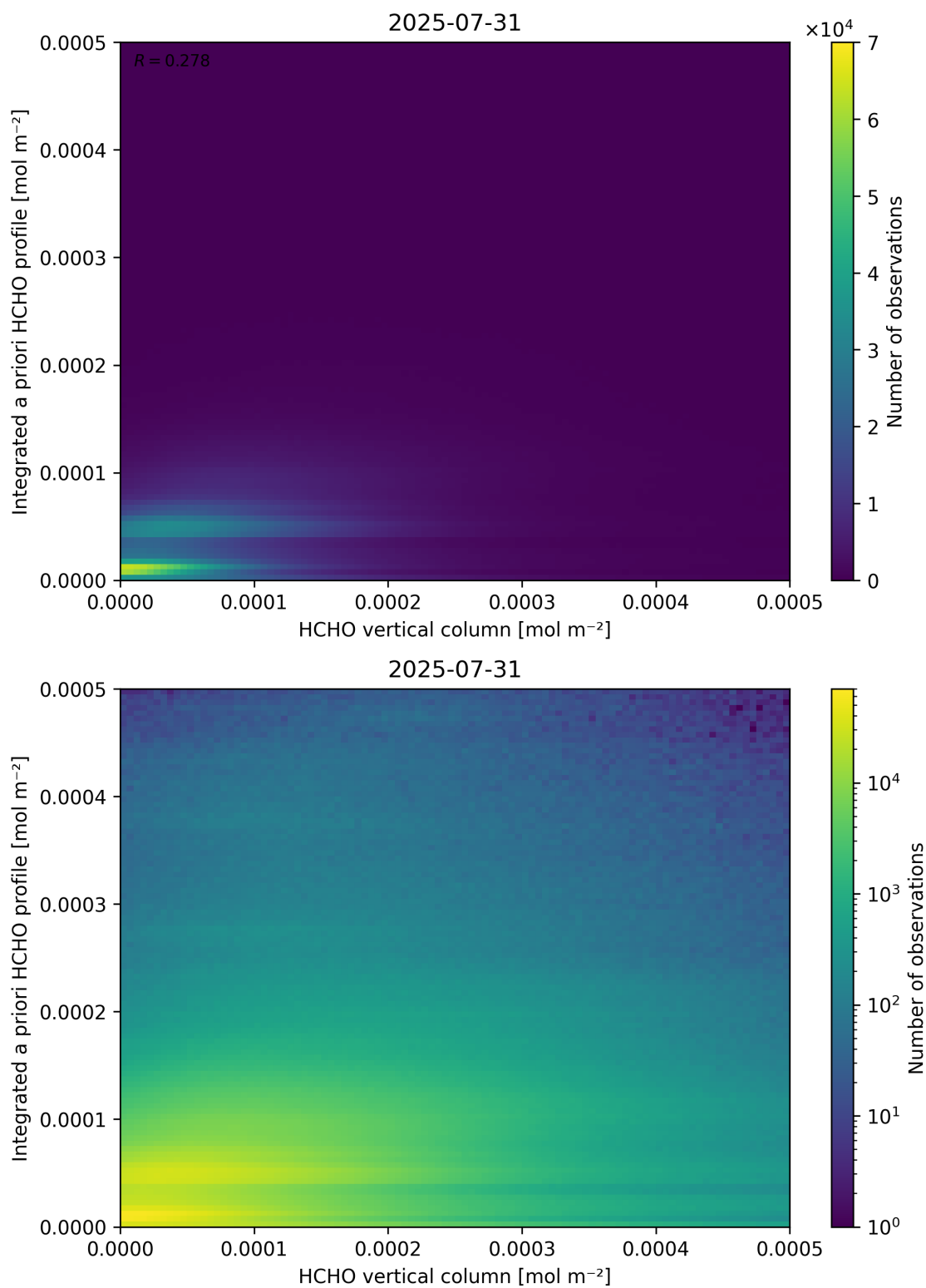
Figure 135: Scatter density plot of “HCHO vertical column” against “Integrated a priori HCHO profile” for 2025-07-30 to 2025-08-01.
