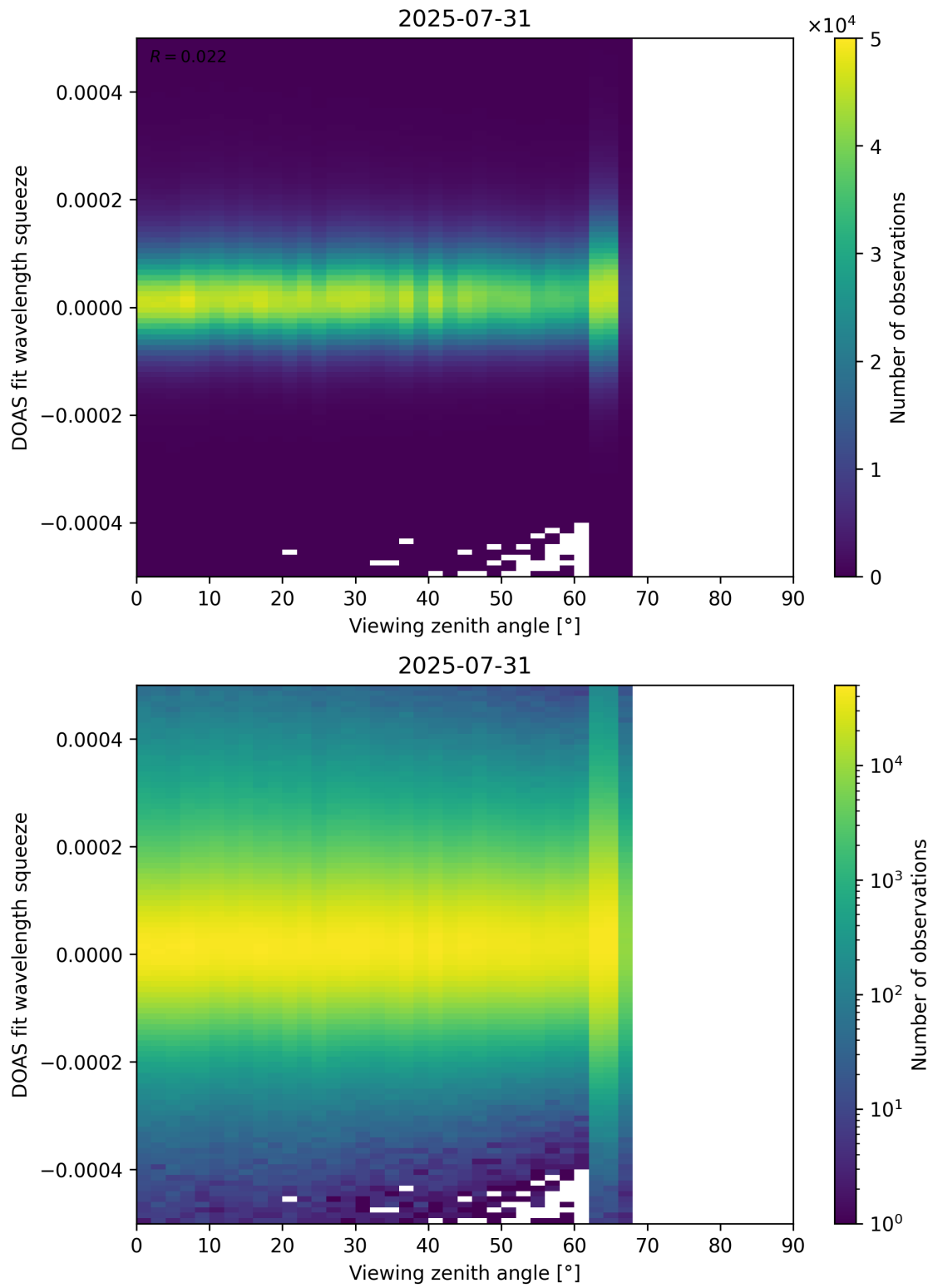
Figure 184: Scatter density plot of “Viewing zenith angle” against “DOAS fit wavelength squeeze” for 2025-07-30 to 2025-08-01.
