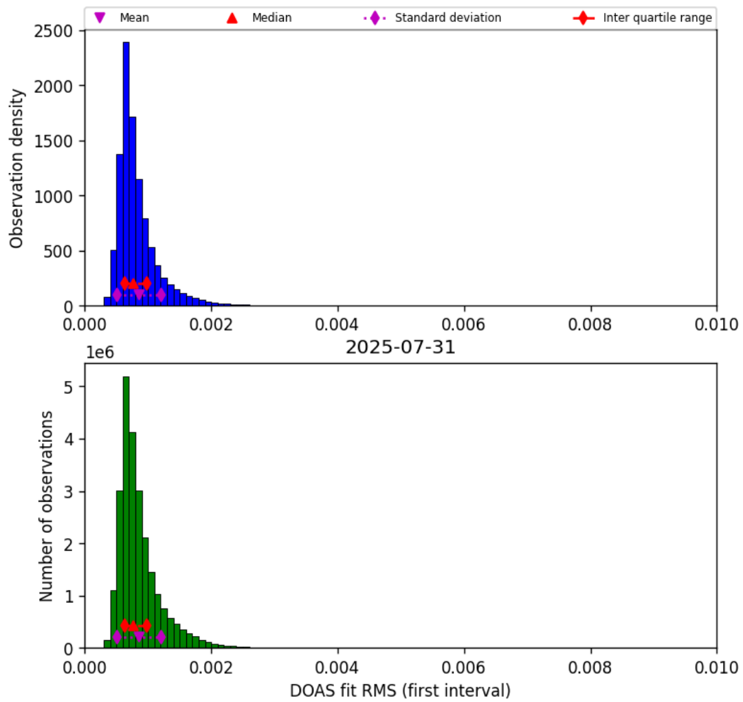
Figure 46: Histogram of “DOAS fit RMS (first interval)” for 2025-07-30 to 2025-08-01
