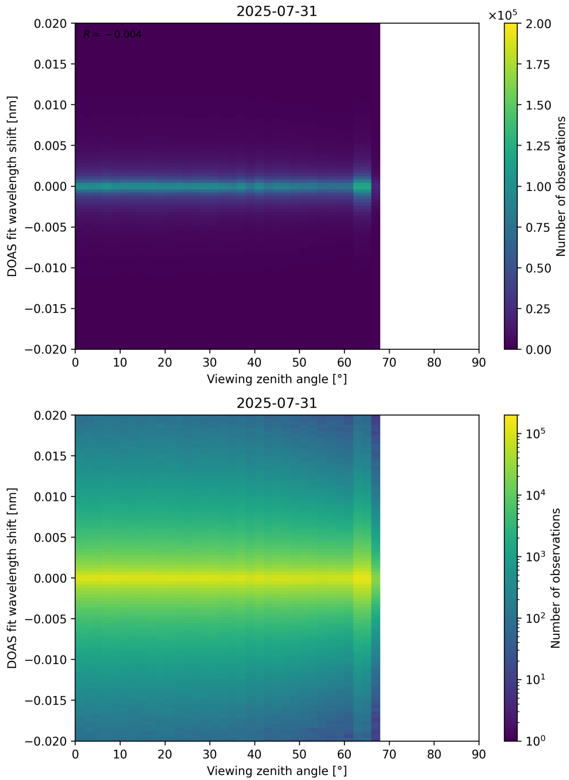
Figure 183: Scatter density plot of “Viewing zenith angle” against “DOAS fit wavelength shift” for 2025-07-30 to 2025-08-01.
