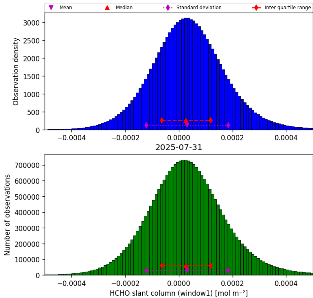
Figure 38: Histogram of “HCHO slant column (window1)” for 2025-07-30 to 2025-08-01
