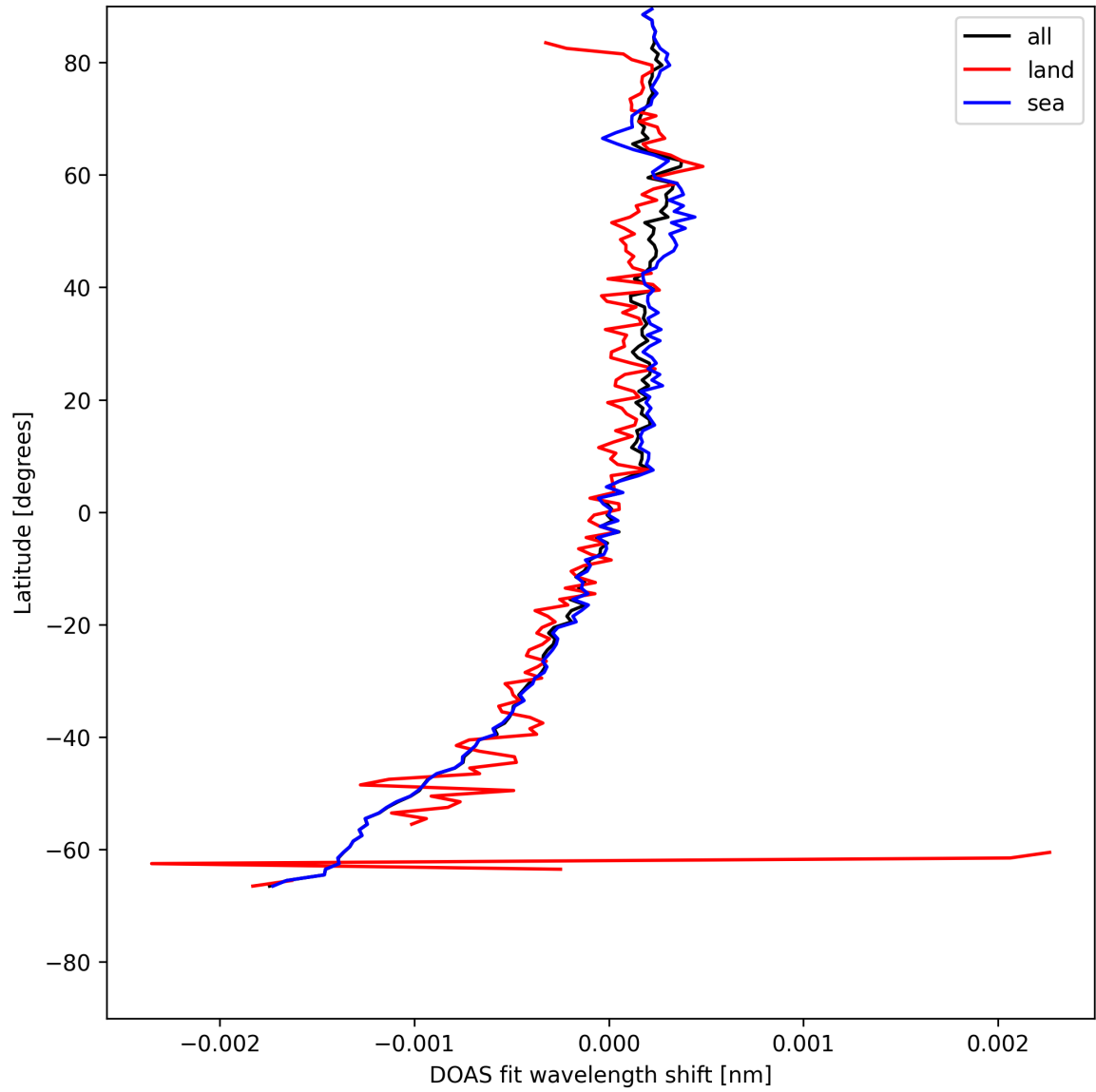
Figure 30: Zonal average of “DOAS fit wavelength shift” for 2025-07-30 to 2025-08-01.
