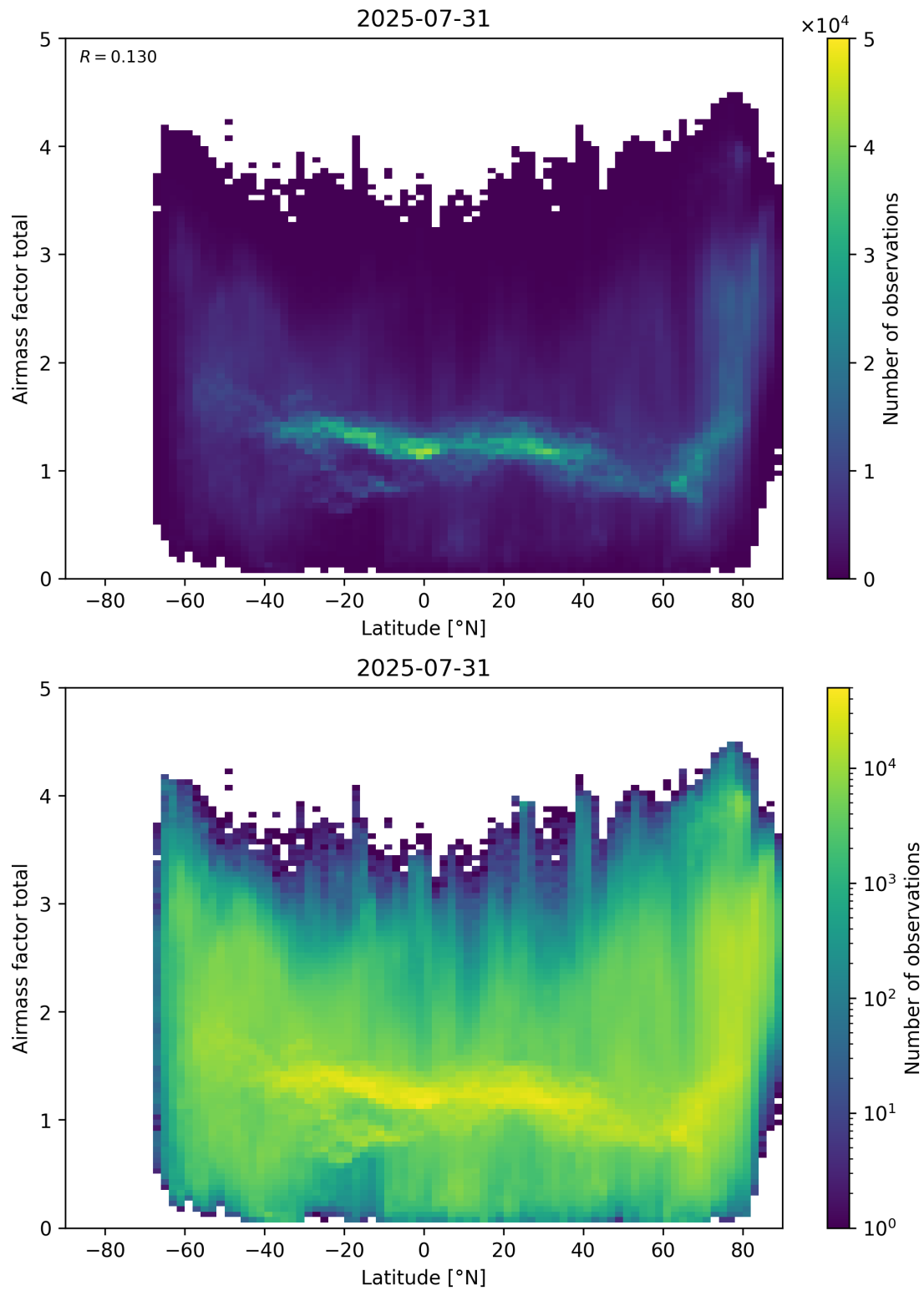
Figure 161: Scatter density plot of “Latitude” against “Airmass factor total” for 2025-07-30 to 2025-08-01.
