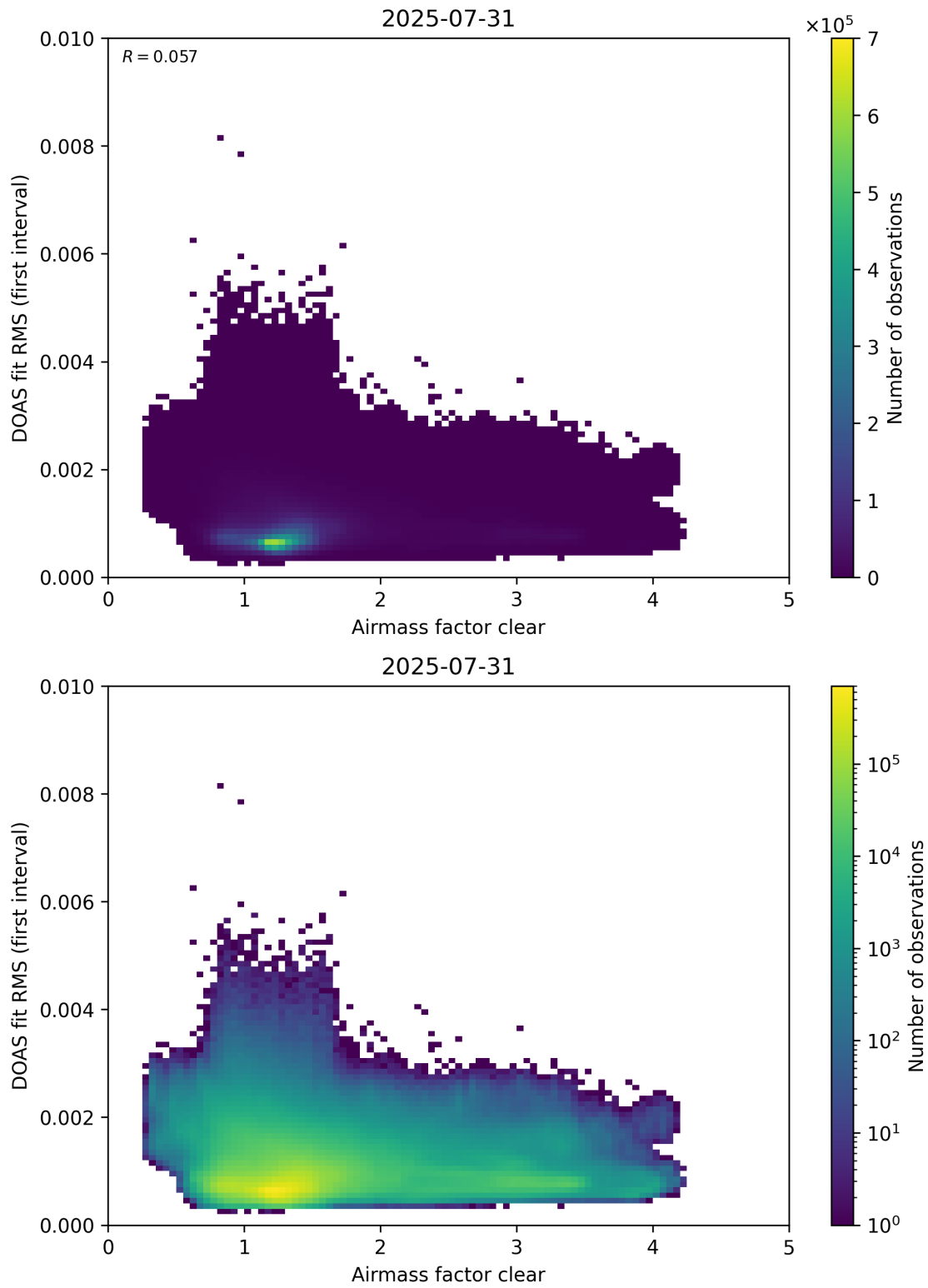
Figure 71: Scatter density plot of “Airmass factor clear” against “DOAS fit RMS (first interval)” for 2025-07-30 to 2025-08-01.
