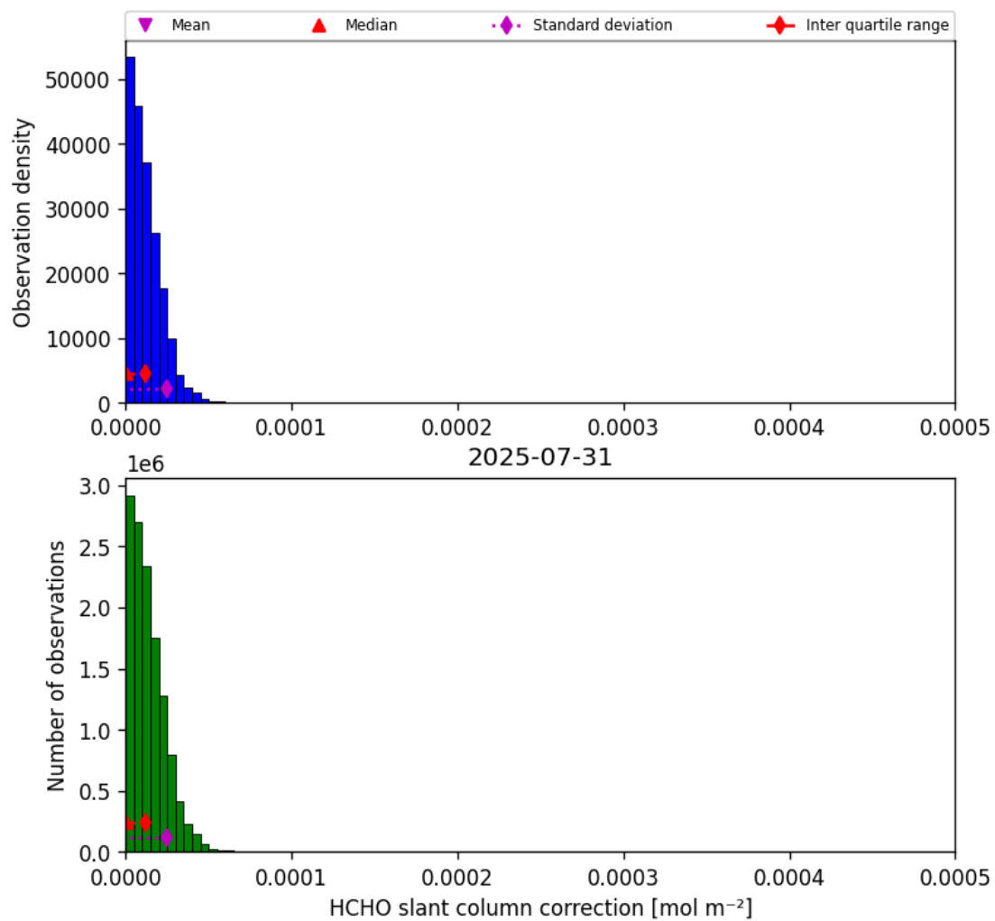
Figure 47: Histogram of “HCHO slant column correction” for 2025-07-30 to 2025-08-01
