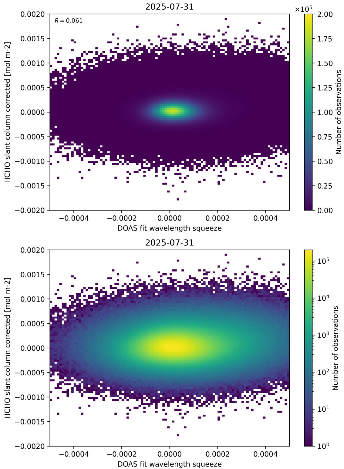
Figure 69: Scatter density plot of “DOAS fit wavelength squeeze” against “HCHO slant column corrected” for 2025-07-30 to 2025-08-01.
