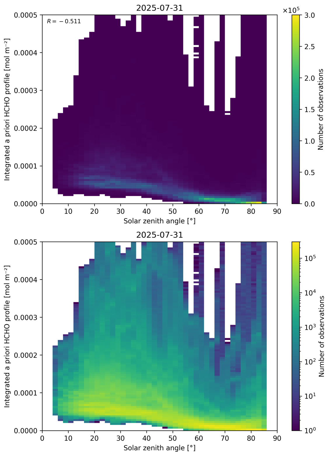
Figure 180: Scatter density plot of “Solar zenith angle” against “Integrated a priori HCHO profile” for 2025-07-30 to 2025-08-01.
