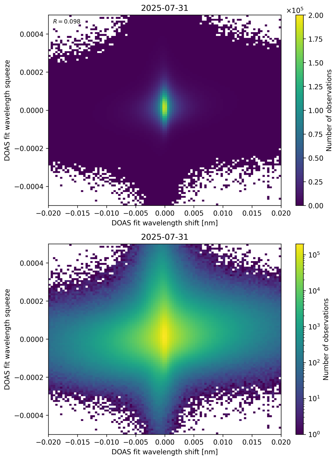
Figure 65: Scatter density plot of “DOAS fit wavelength shift” against “DOAS fit wavelength squeeze” for 2025-07-30 to 2025-08-01.
