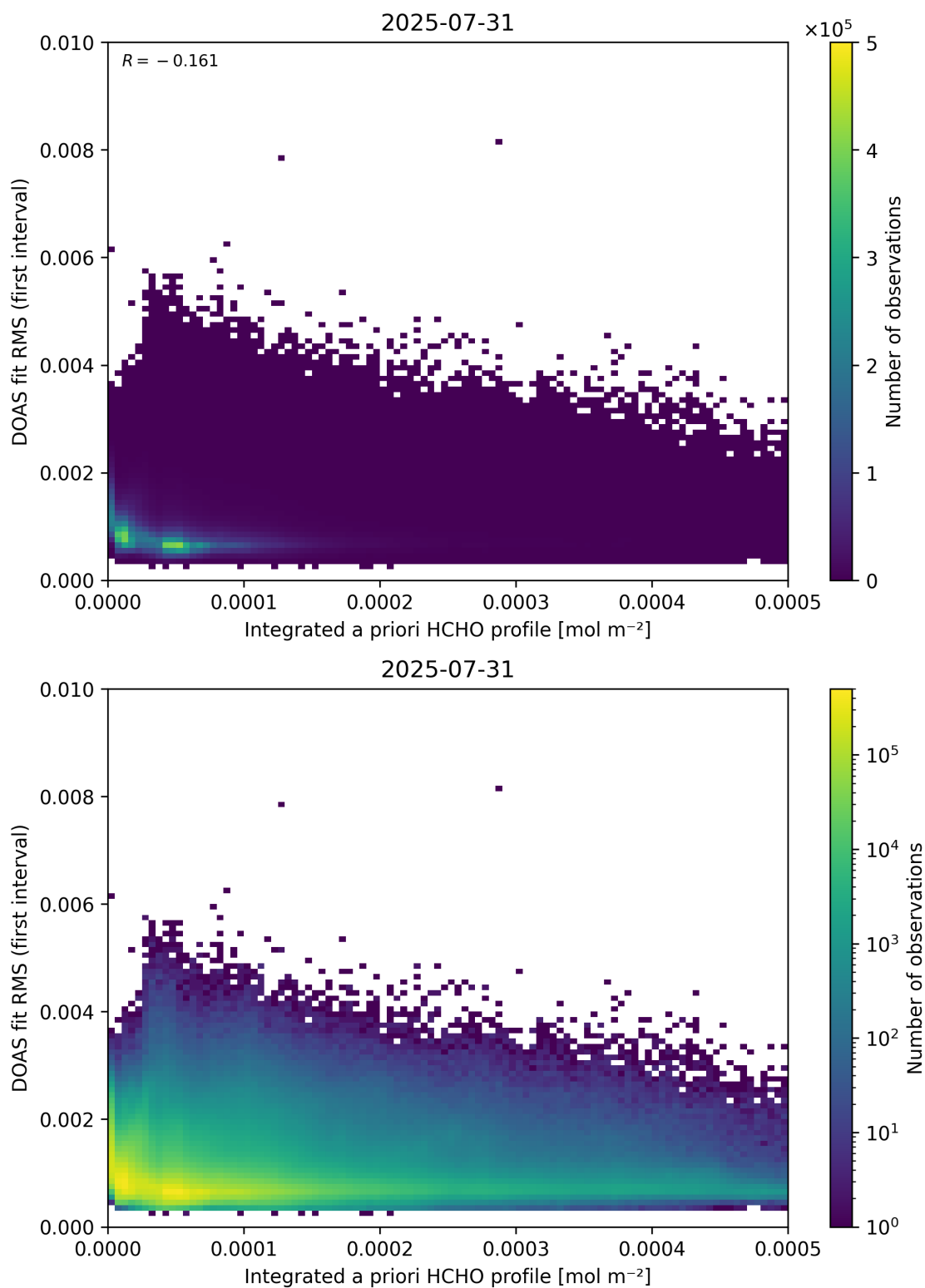
Figure 148: Scatter density plot of “Integrated a priori HCHO profile” against “DOAS fit RMS (first interval)” for 2025-07-30 to 2025-08-01.
