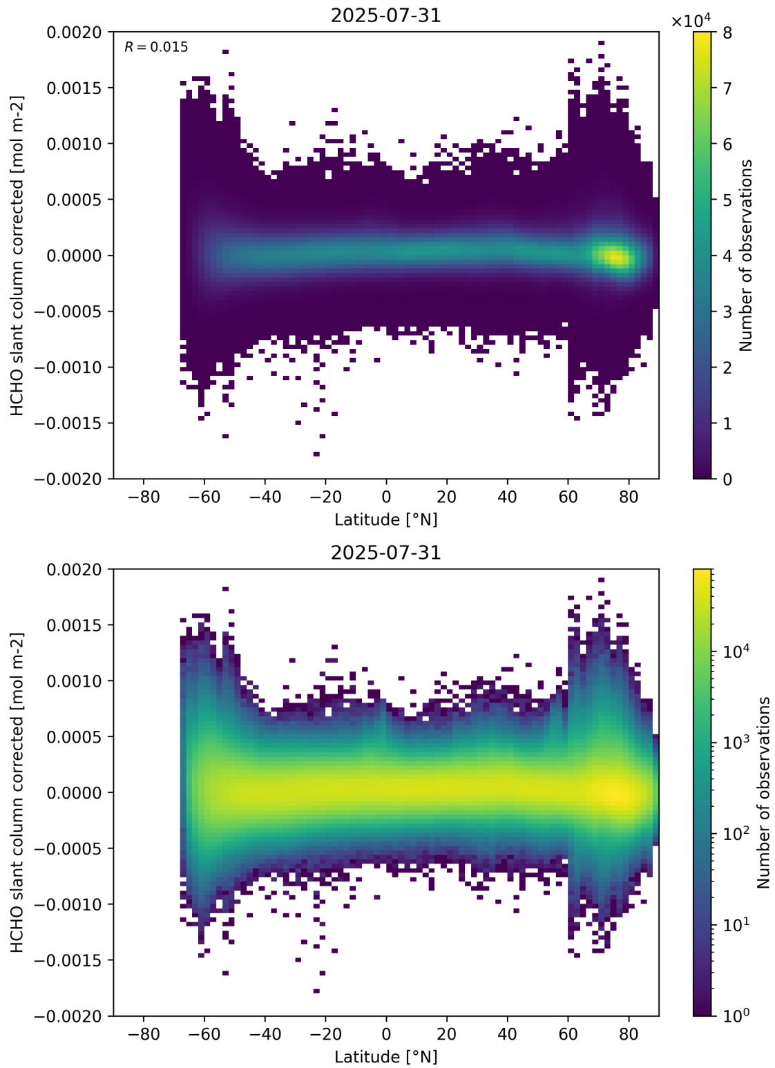
Figure 157: Scatter density plot of “Latitude” against “HCHO slant column corrected” for 2025-07-30 to 2025-08-01.
