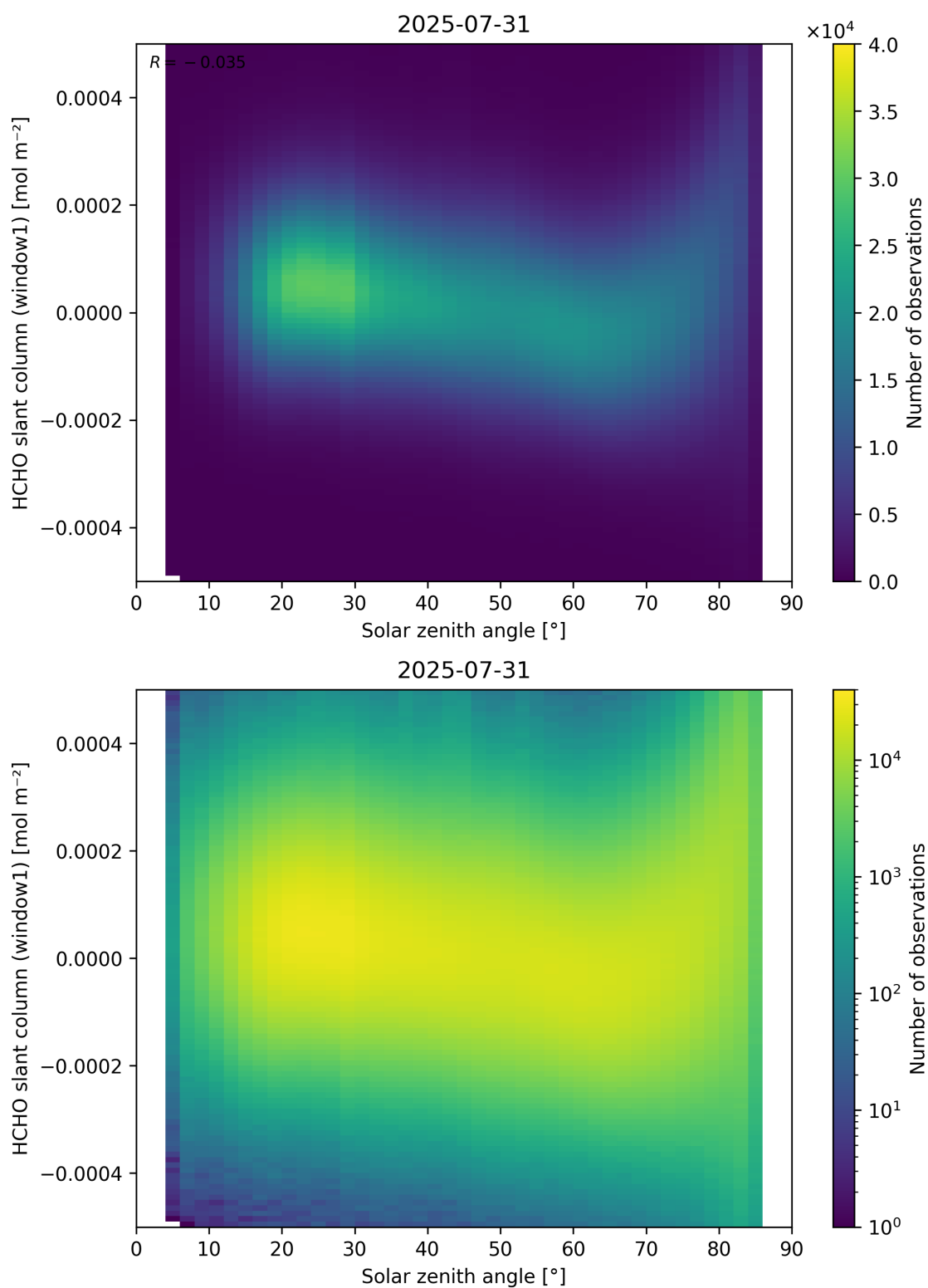
Figure 173: Scatter density plot of “Solar zenith angle” against “HCHO slant column (window1)” for 2025-07-30 to 2025-08-01.
