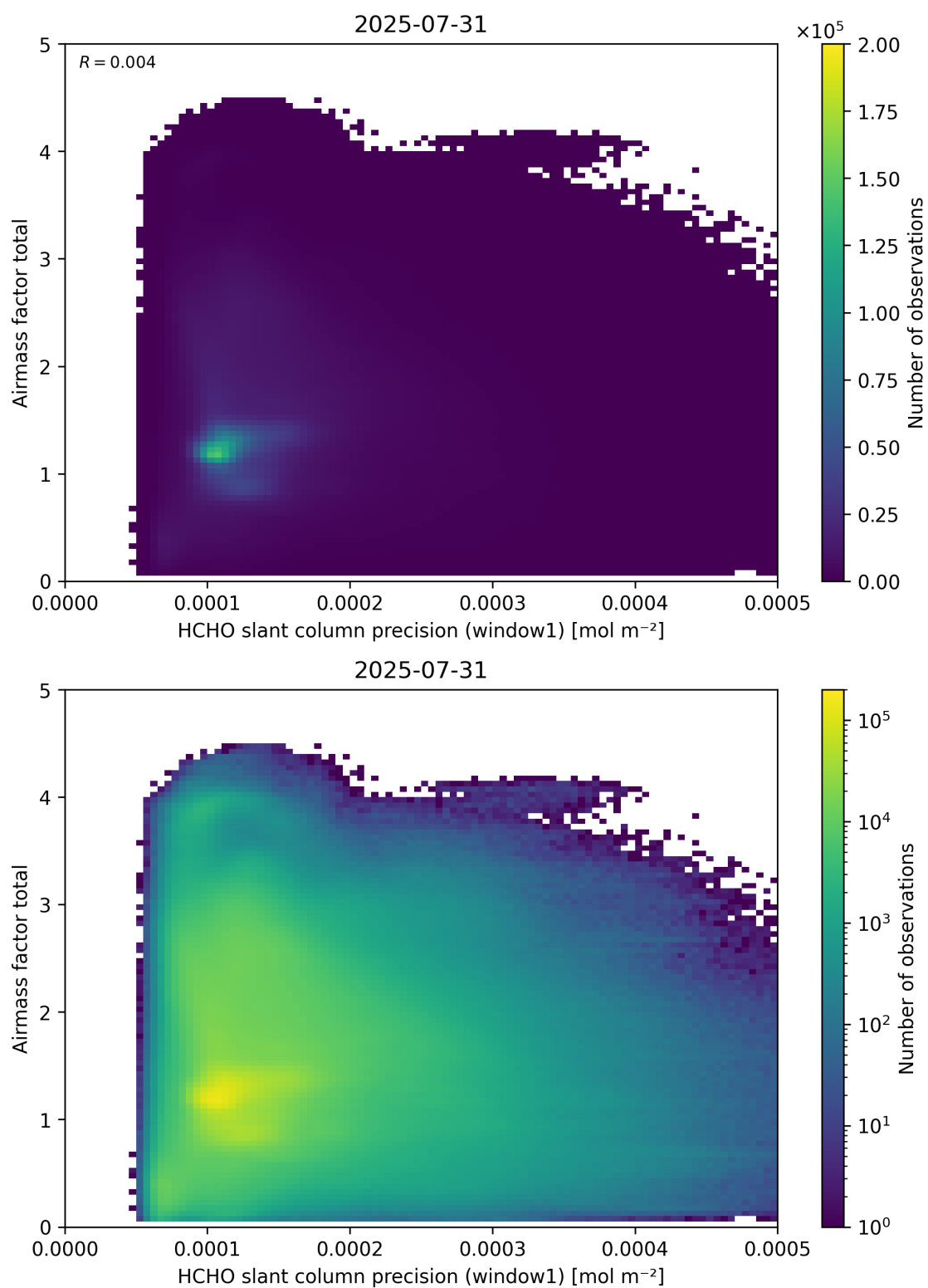
Figure 94: Scatter density plot of “HCHO slant column precision (window1)” against “Airmass factor total” for 2025-07-30 to 2025-08-01.
