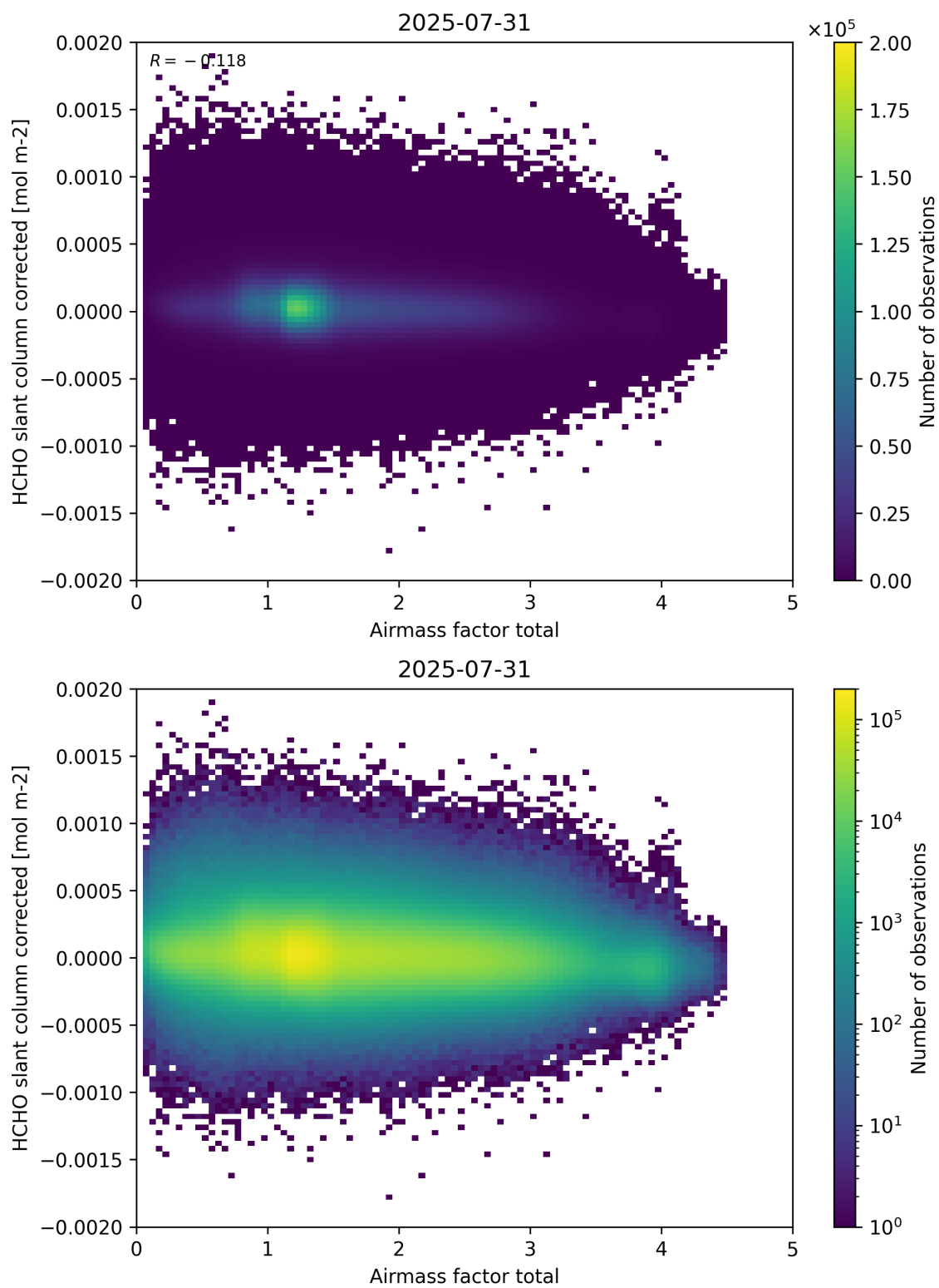
Figure 101: Scatter density plot of “Airmass factor total” against “HCHO slant column corrected” for 2025-07-30 to 2025-08-01.
