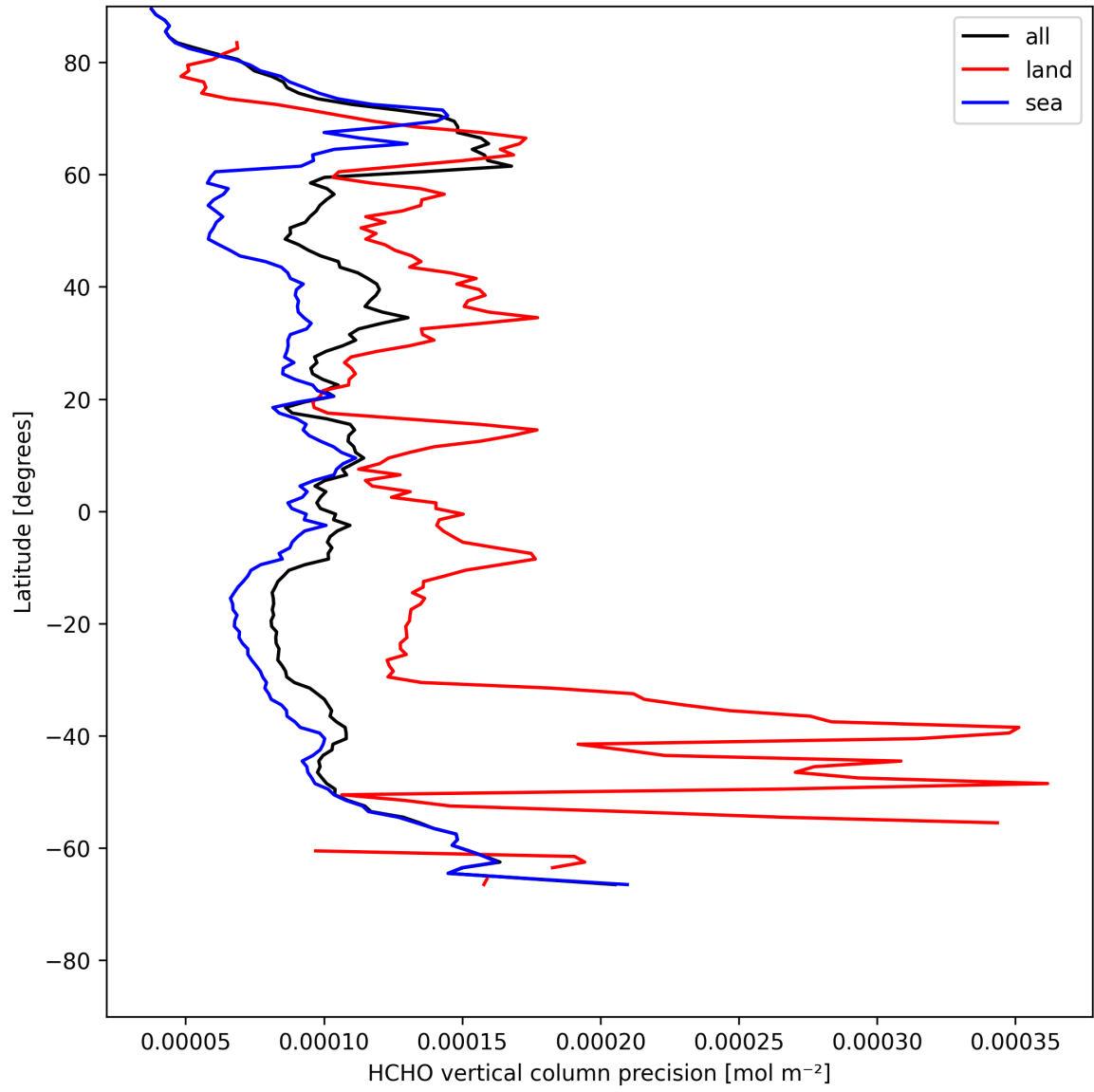
Figure 22: Zonal average of “HCHO vertical column precision” for 2025-07-30 to 2025-08-01.
