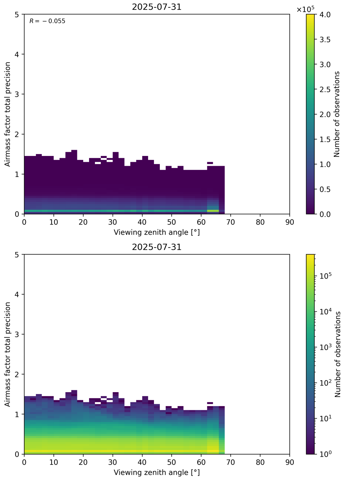
Figure 191: Scatter density plot of “Viewing zenith angle” against “Airmass factor total precision” for 2025-07-30 to 2025-08-01.
