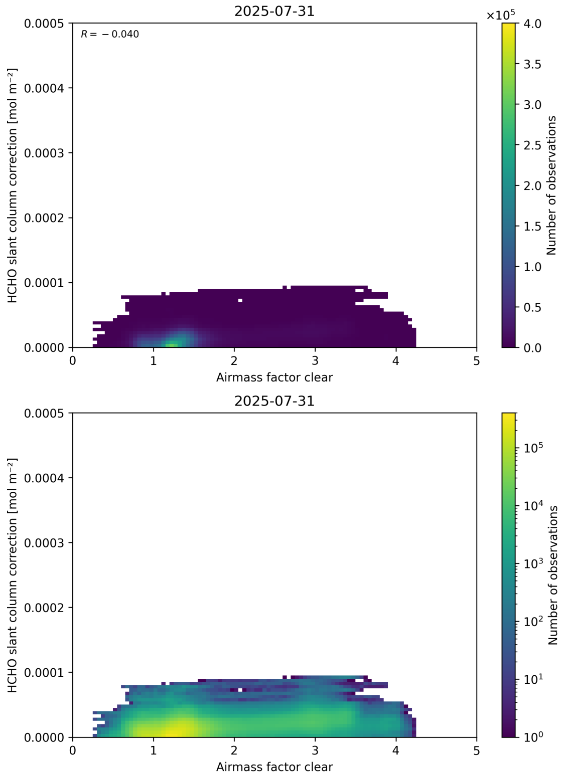
Figure 75: Scatter density plot of “Airmass factor clear” against “HCHO slant column correction” for 2025-07-30 to 2025-08-01.
