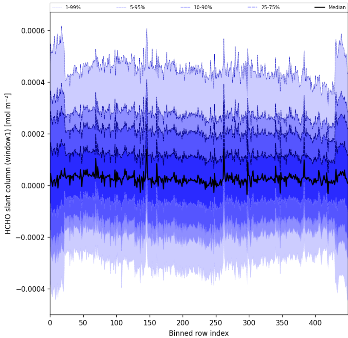
Figure 52: Along track statistics of “HCHO slant column (window1)” for 2025-07-30 to 2025-08-01
