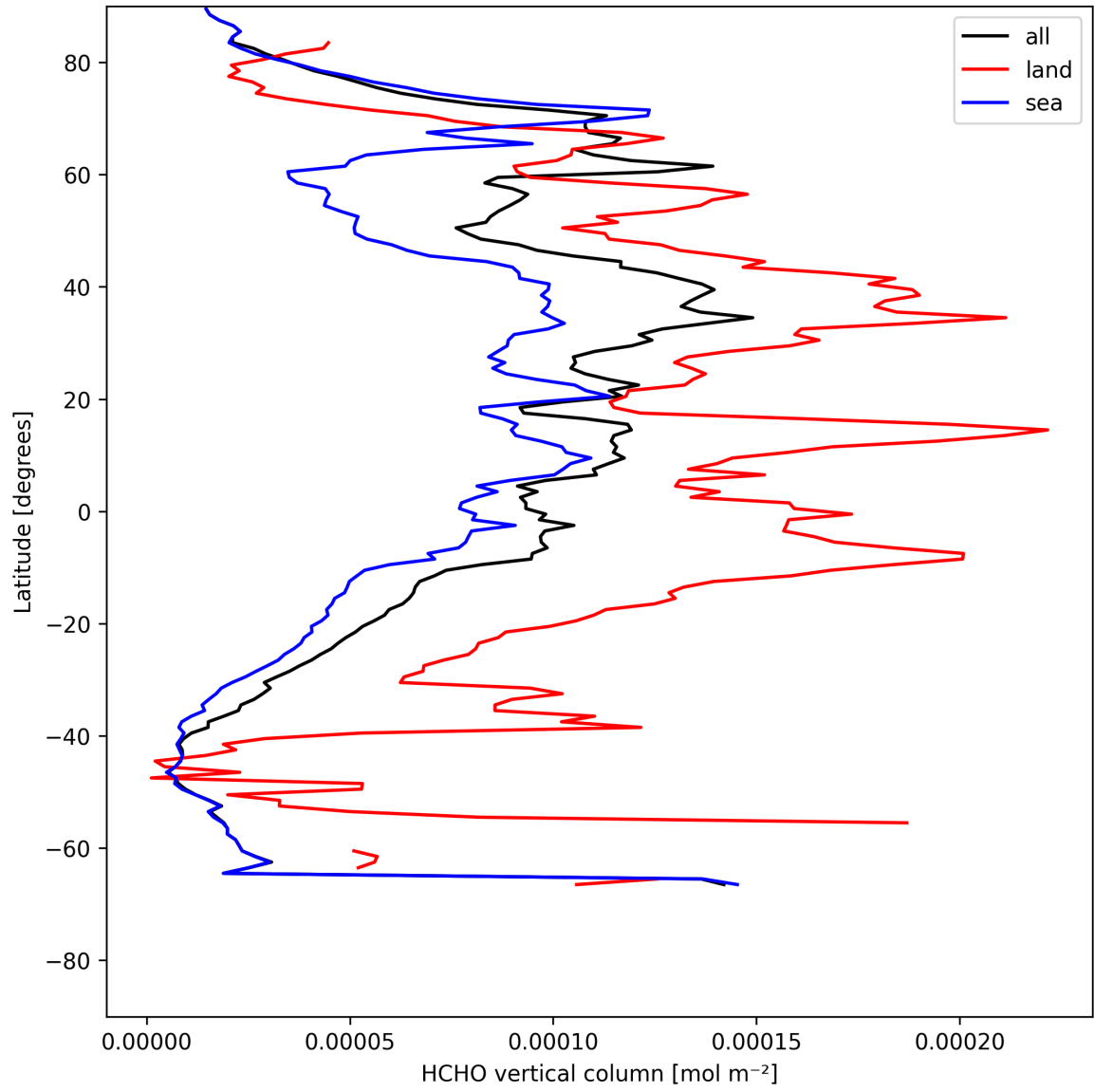
Figure 21: Zonal average of “HCHO vertical column” for 2025-07-30 to 2025-08-01.
