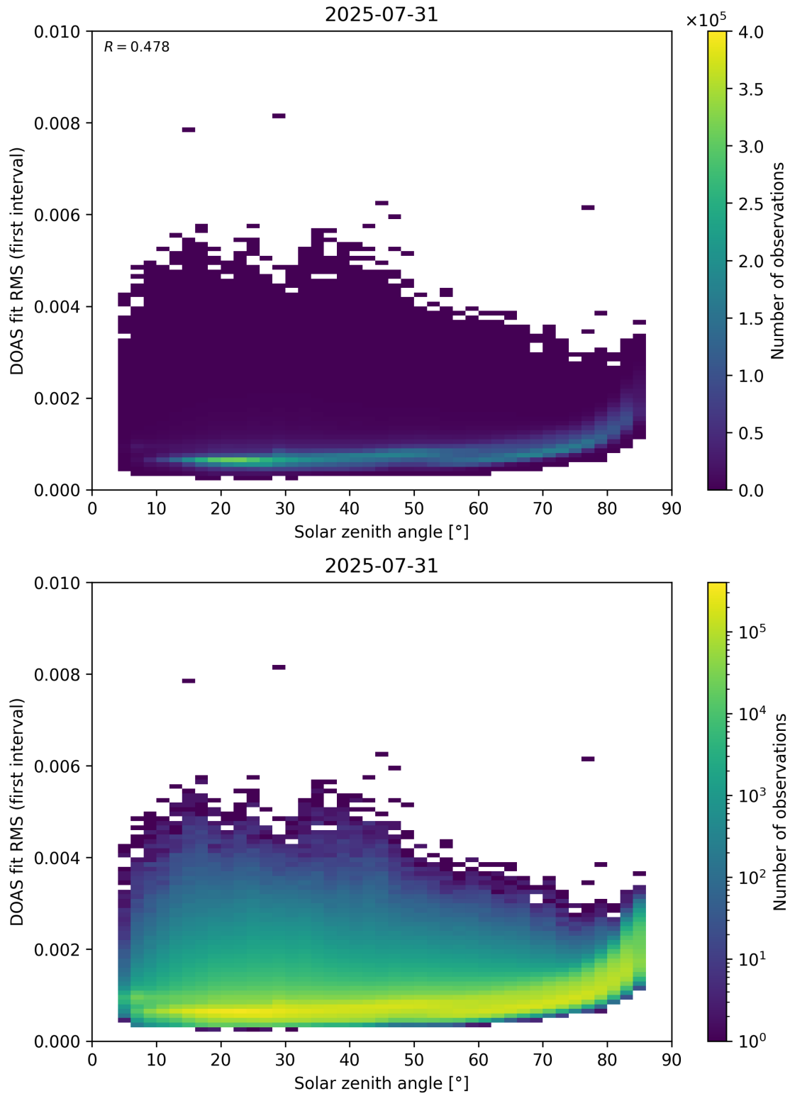
Figure 167: Scatter density plot of “Solar zenith angle” against “DOAS fit RMS (first interval)” for 2025-07-30 to 2025-08-01.
