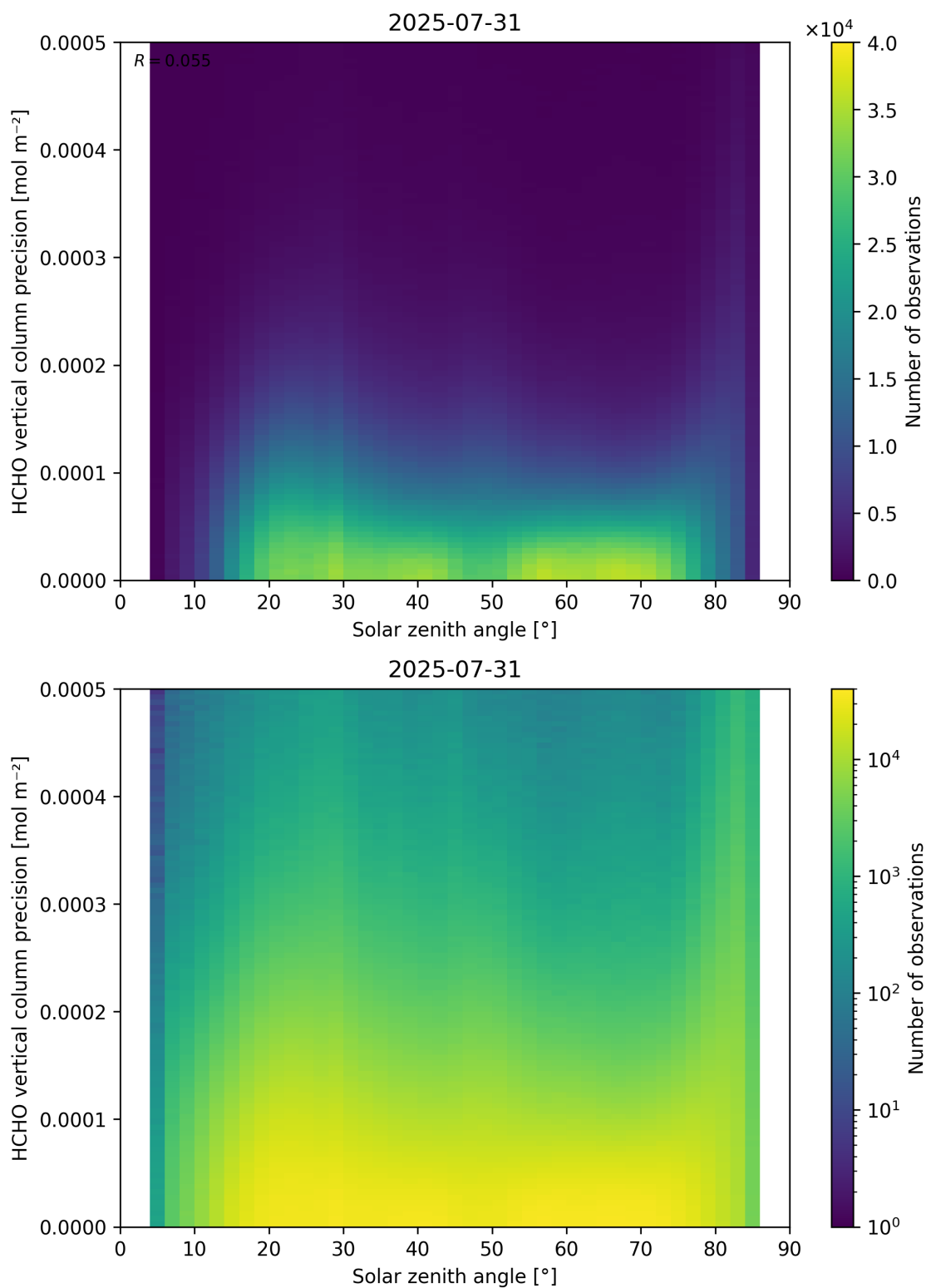
Figure 179: Scatter density plot of “Solar zenith angle” against “HCHO vertical column precision” for 2025-07-30 to 2025-08-01.
