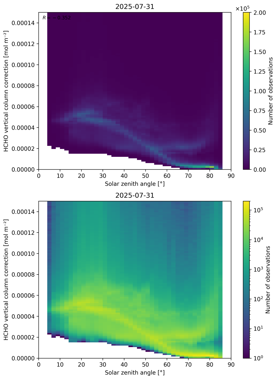
Figure 178: Scatter density plot of “Solar zenith angle” against “HCHO vertical column correction” for 2025-07-30 to 2025-08-01.
