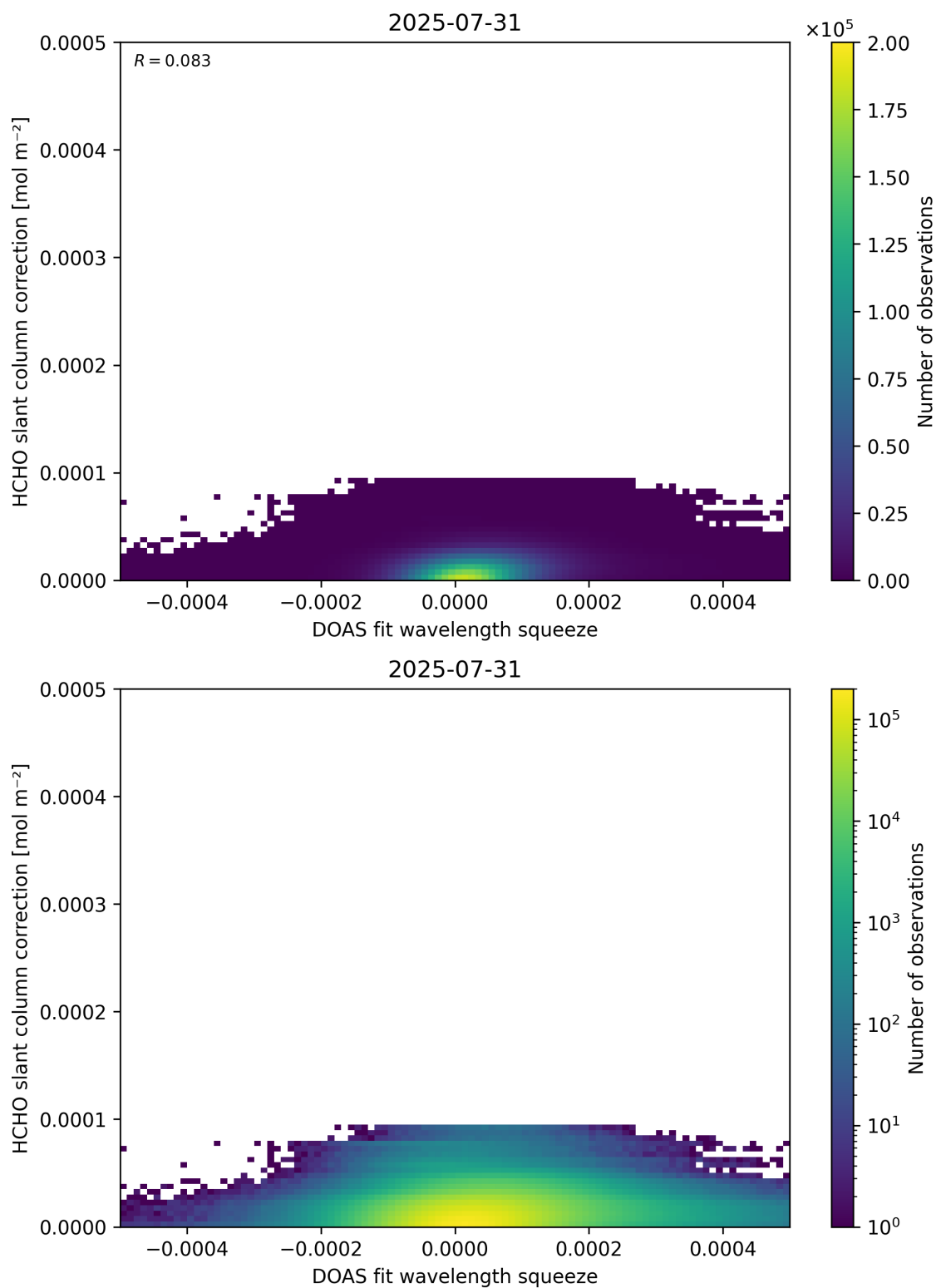
Figure 70: Scatter density plot of “DOAS fit wavelength squeeze” against “HCHO slant column correction” for 2025-07-30 to 2025-08-01.
