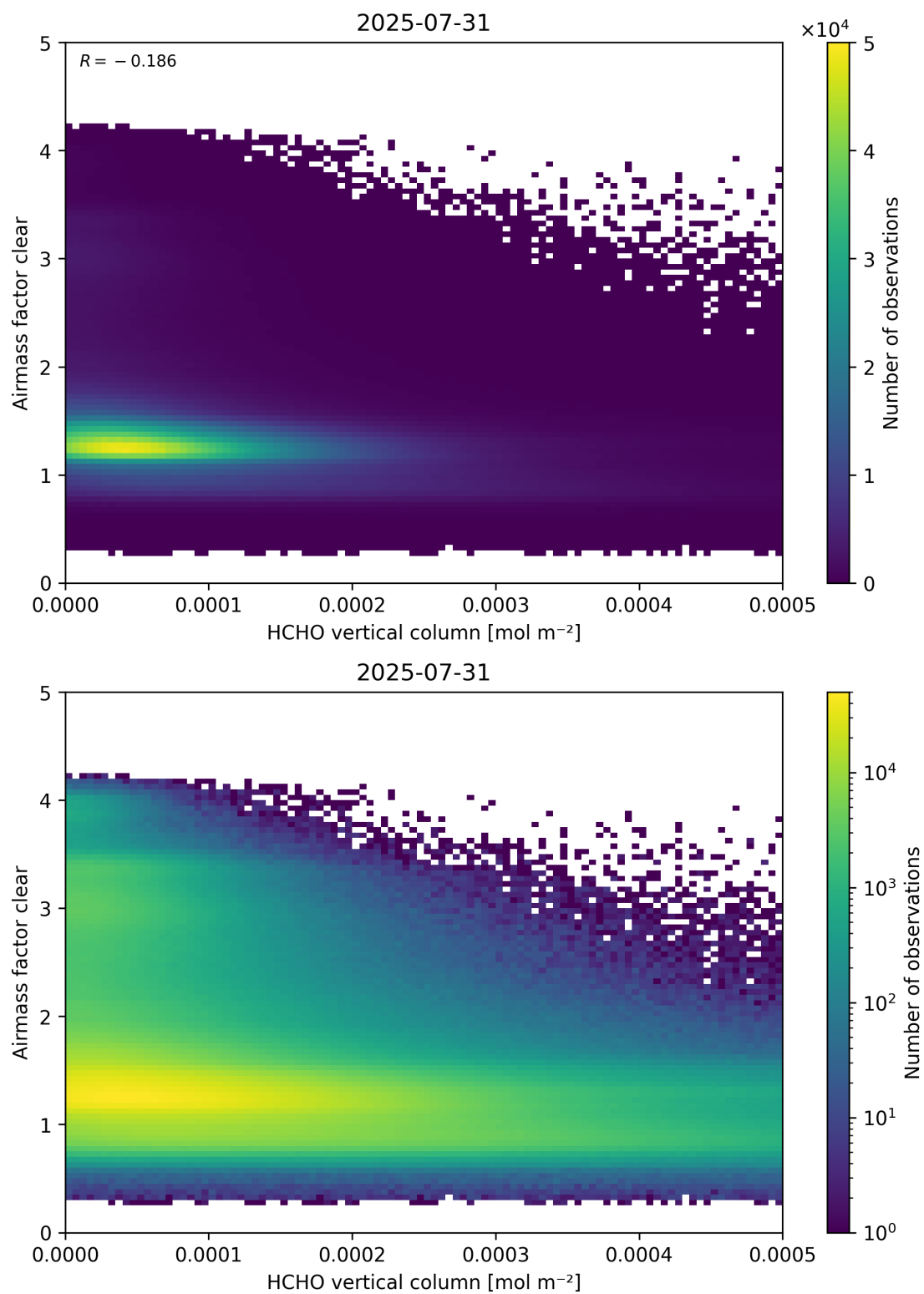
Figure 126: Scatter density plot of “HCHO vertical column” against “Airmass factor clear” for 2025-07-30 to 2025-08-01.
