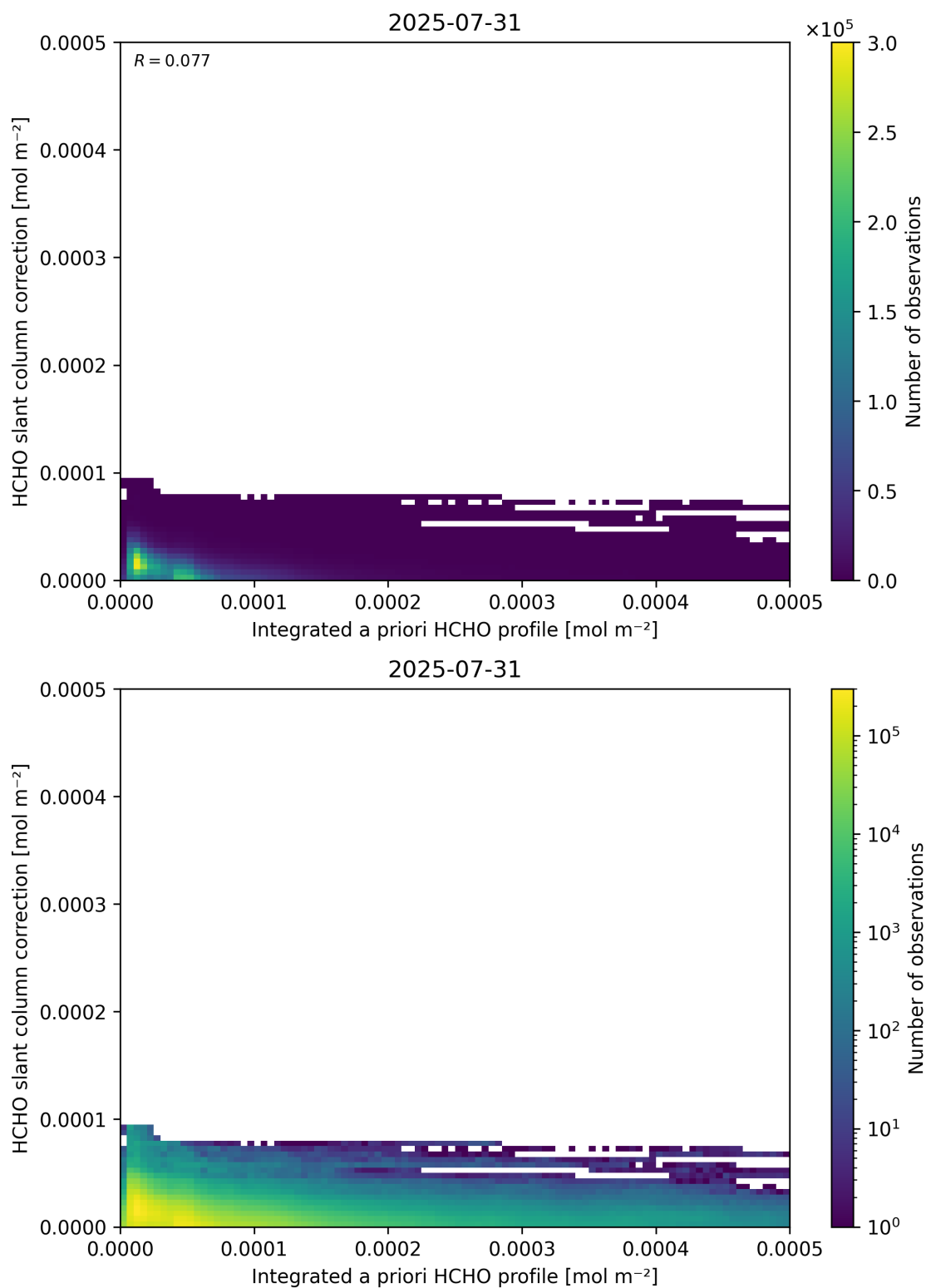
Figure 152: Scatter density plot of “Integrated a priori HCHO profile” against “HCHO slant column correction” for 2025-07-30 to 2025-08-01.
