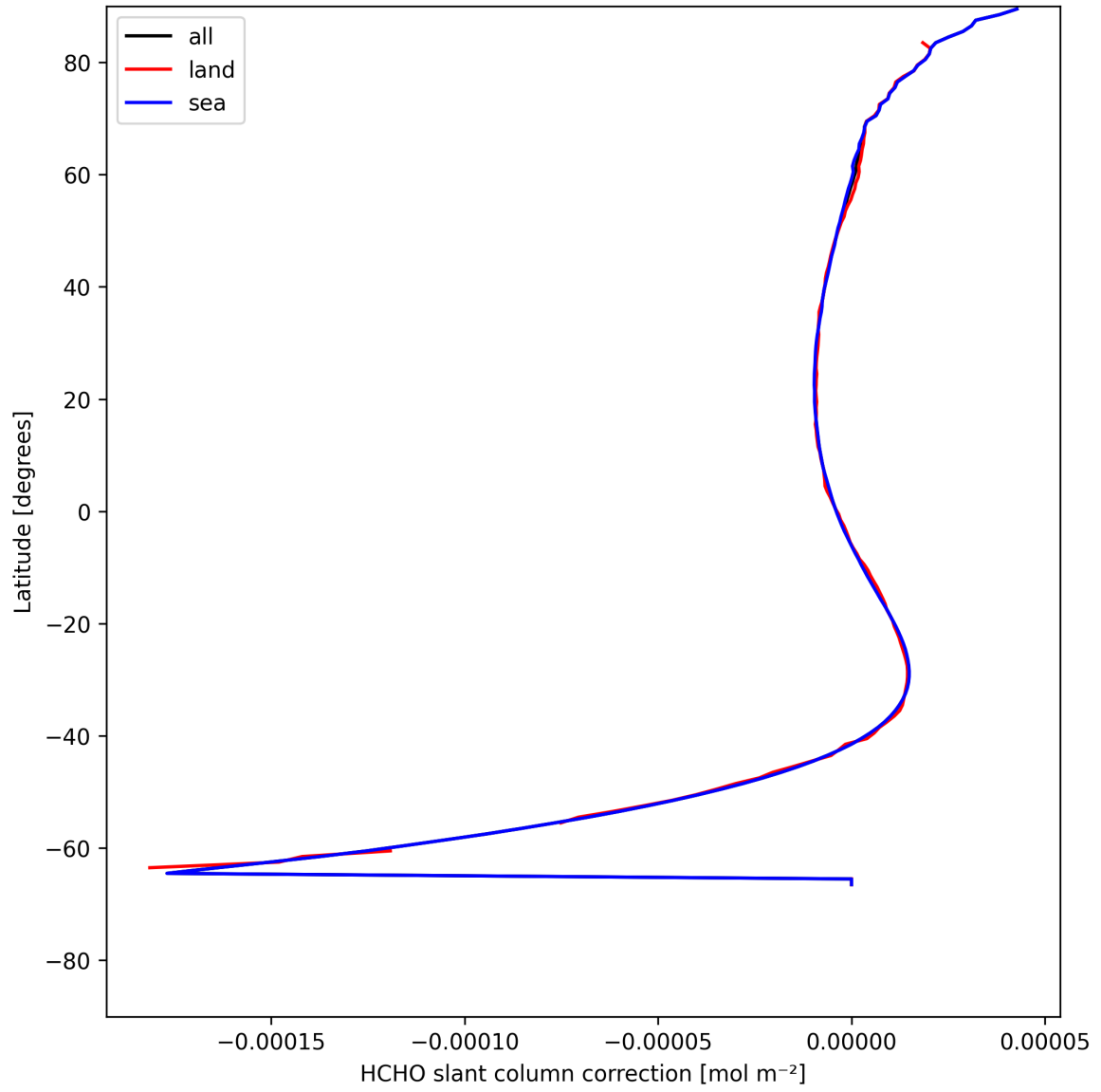
Figure 33: Zonal average of “HCHO slant column correction” for 2025-07-30 to 2025-08-01.
