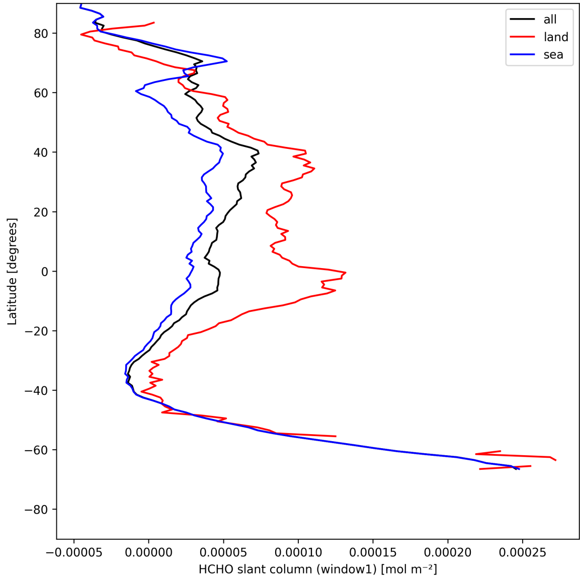
Figure 24: Zonal average of “HCHO slant column (window1)” for 2025-07-30 to 2025-08-01.
