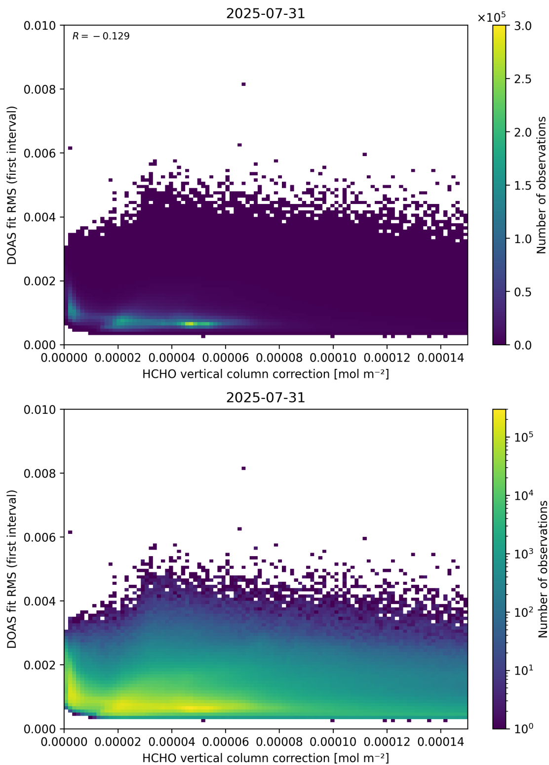
Figure 112: Scatter density plot of “HCHO vertical column correction” against “DOAS fit RMS (first interval)” for 2025-07-30 to 2025-08-01.
