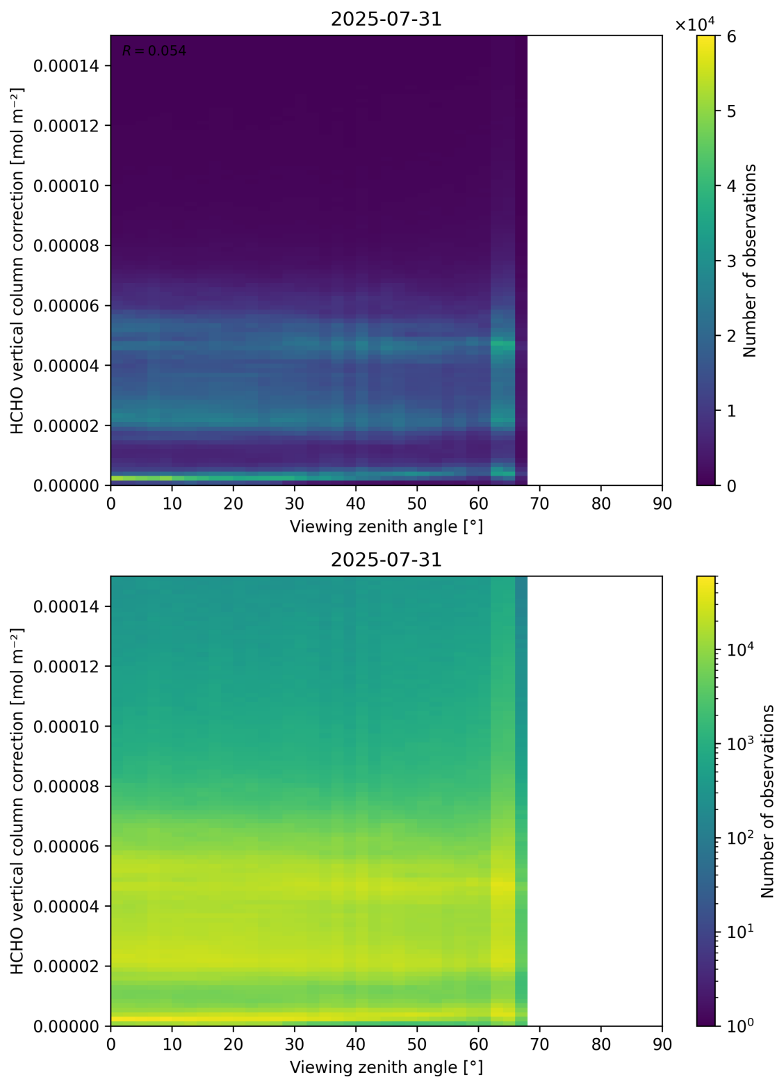
Figure 193: Scatter density plot of “Viewing zenith angle” against “HCHO vertical column correction” for 2025-07-30 to 2025-08-01.
