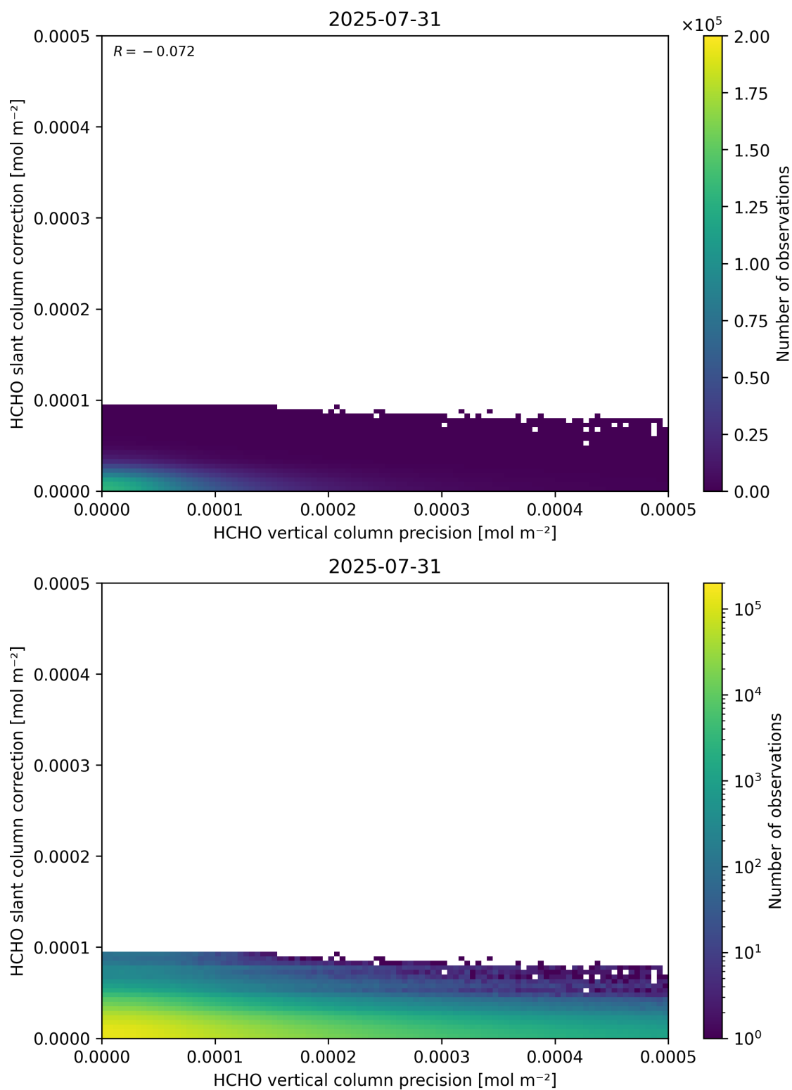
Figure 141: Scatter density plot of “HCHO vertical column precision” against “HCHO slant column correction” for 2025-07-30 to 2025-08-01.
