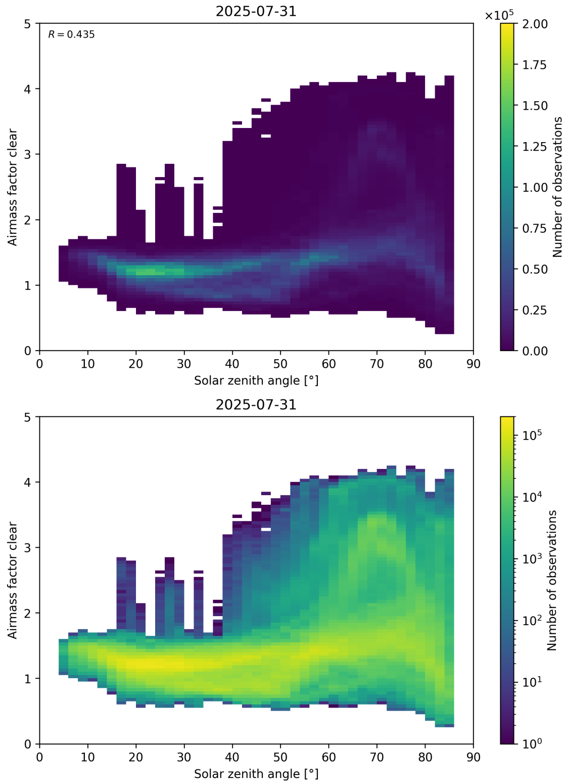
Figure 170: Scatter density plot of “Solar zenith angle” against “Airmass factor clear” for 2025-07-30 to 2025-08-01.
