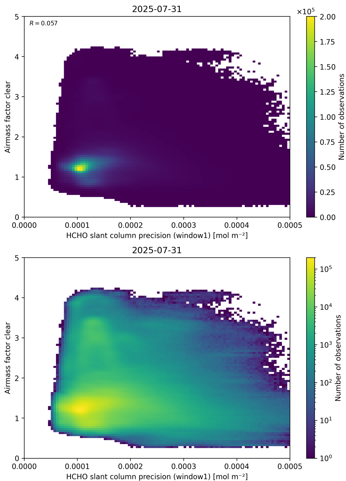
Figure 91: Scatter density plot of “HCHO slant column precision (window1)” against “Airmass factor clear” for 2025-07-30 to 2025-08-01.
