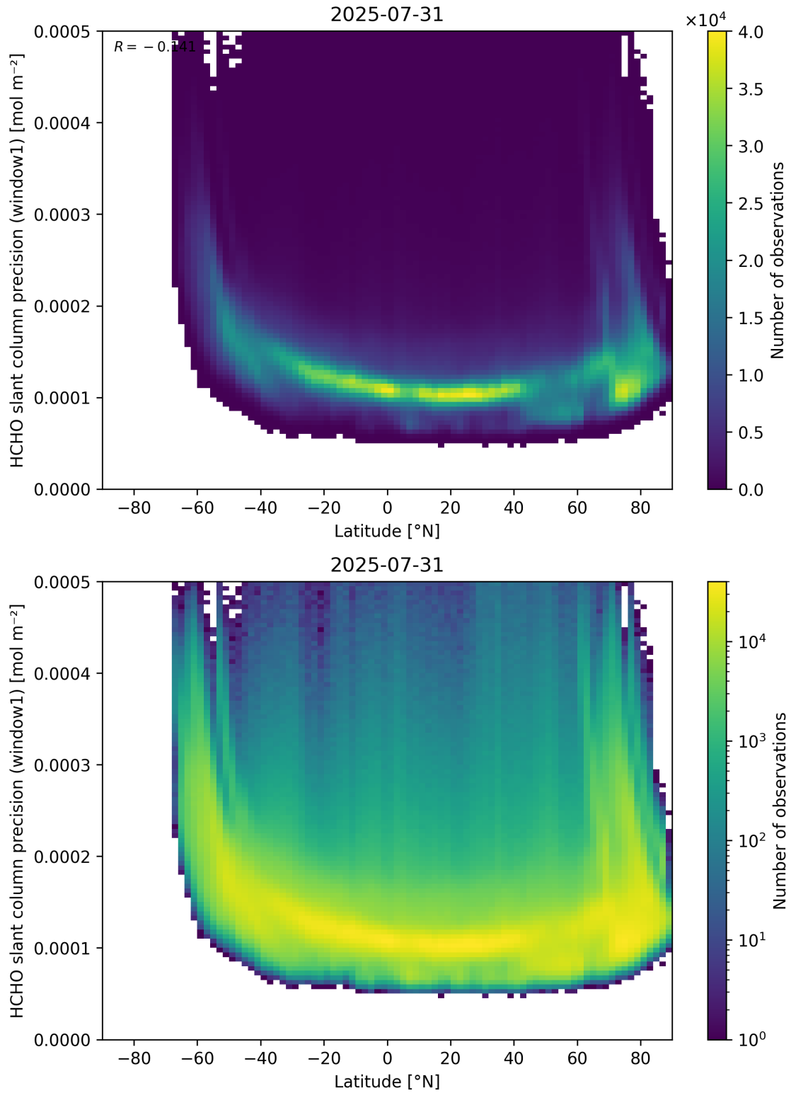
Figure 160: Scatter density plot of “Latitude” against “HCHO slant column precision (window1)” for 2025-07-30 to 2025-08-01.
