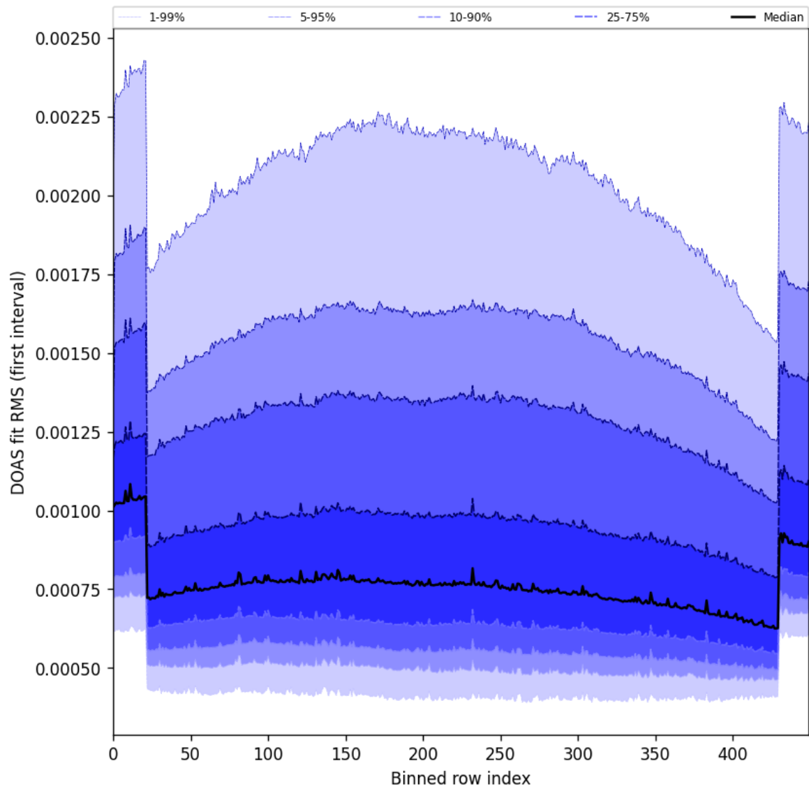
Figure 60: Along track statistics of “DOAS fit RMS (first interval)” for 2025-07-30 to 2025-08-01
