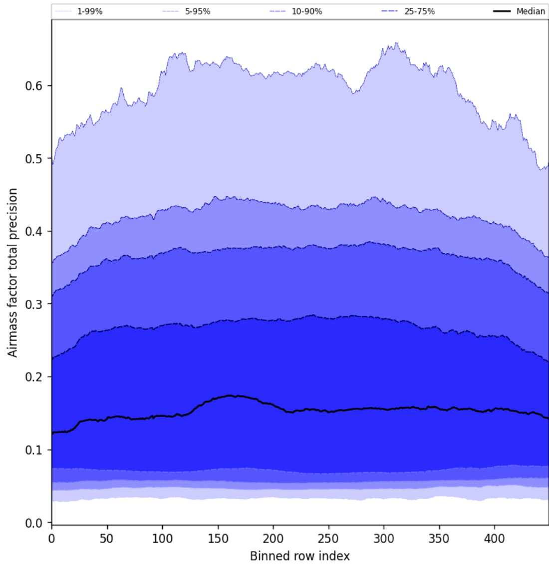
Figure 55: Along track statistics of “Airmass factor total precision” for 2025-07-30 to 2025-08-01
