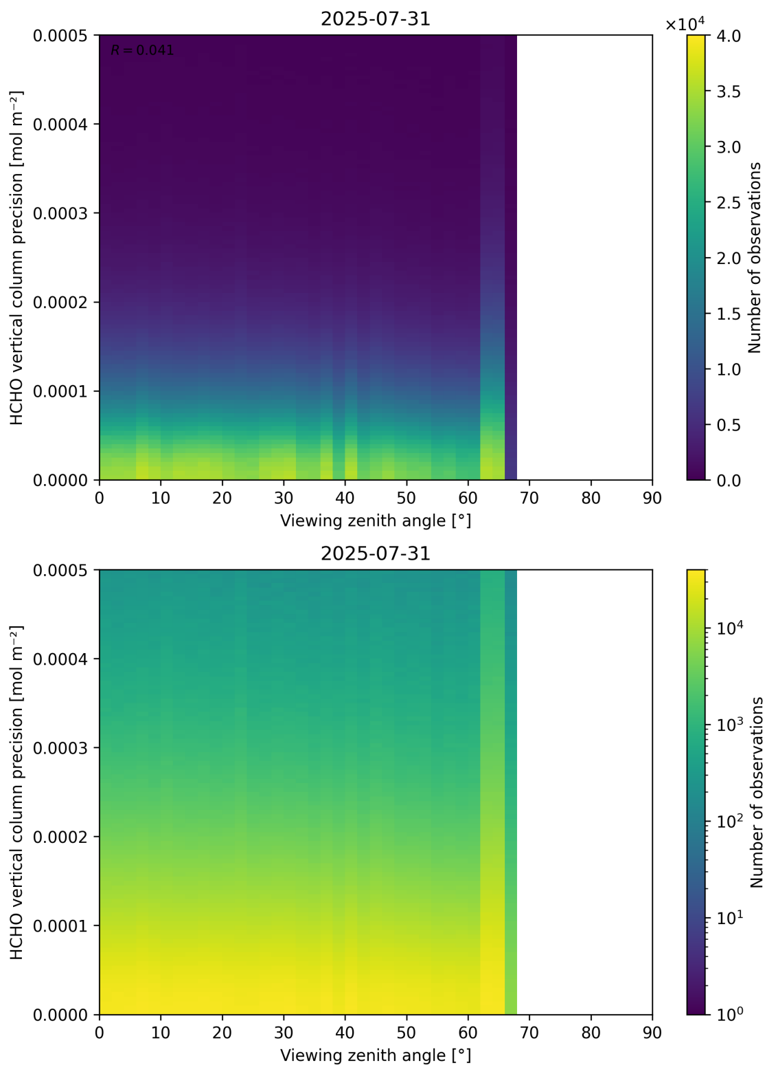
Figure 194: Scatter density plot of “Viewing zenith angle” against “HCHO vertical column precision” for 2025-07-30 to 2025-08-01.
