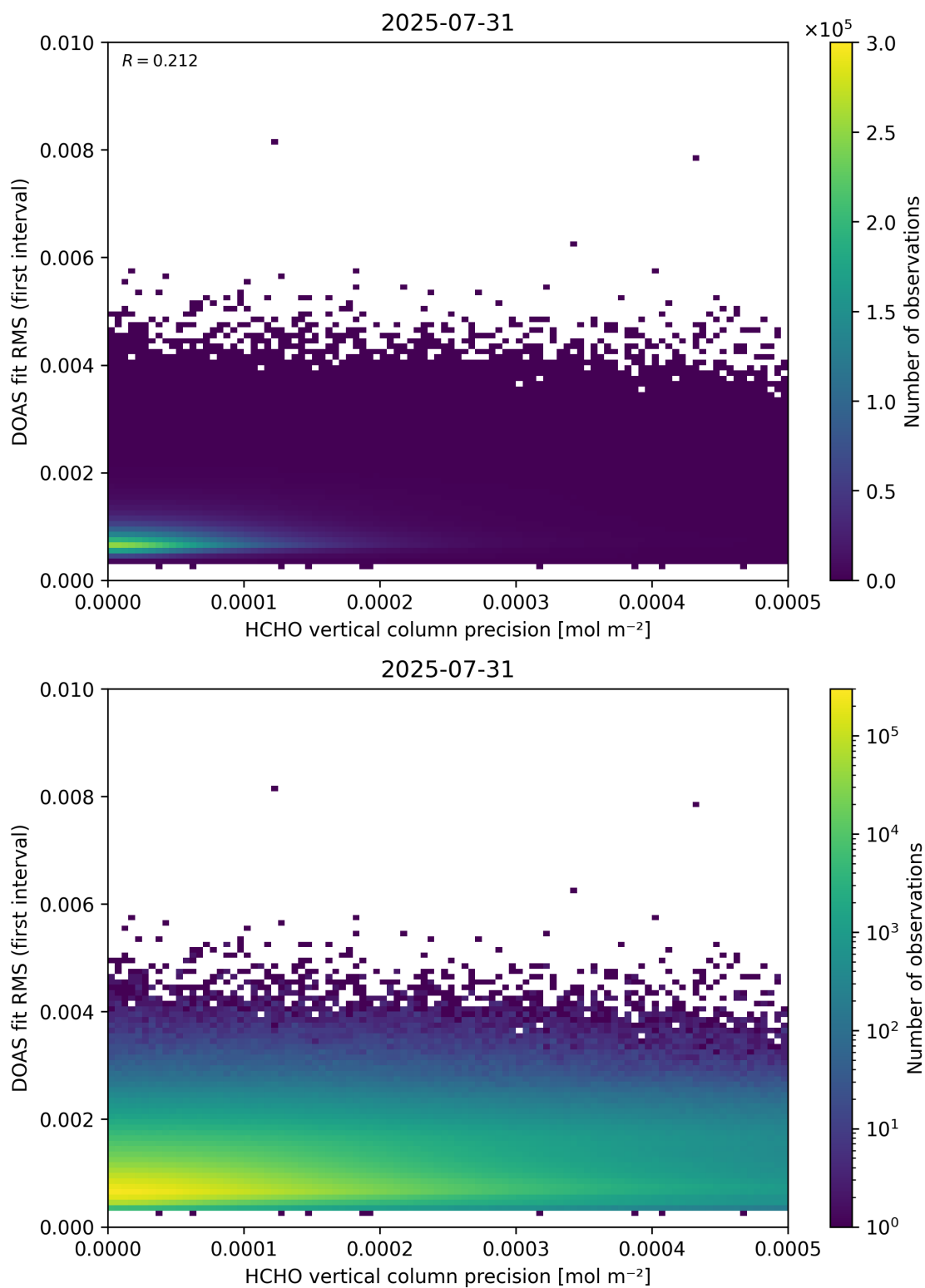
Figure 136: Scatter density plot of “HCHO vertical column precision” against “DOAS fit RMS (first interval)” for 2025-07-30 to 2025-08-01.
