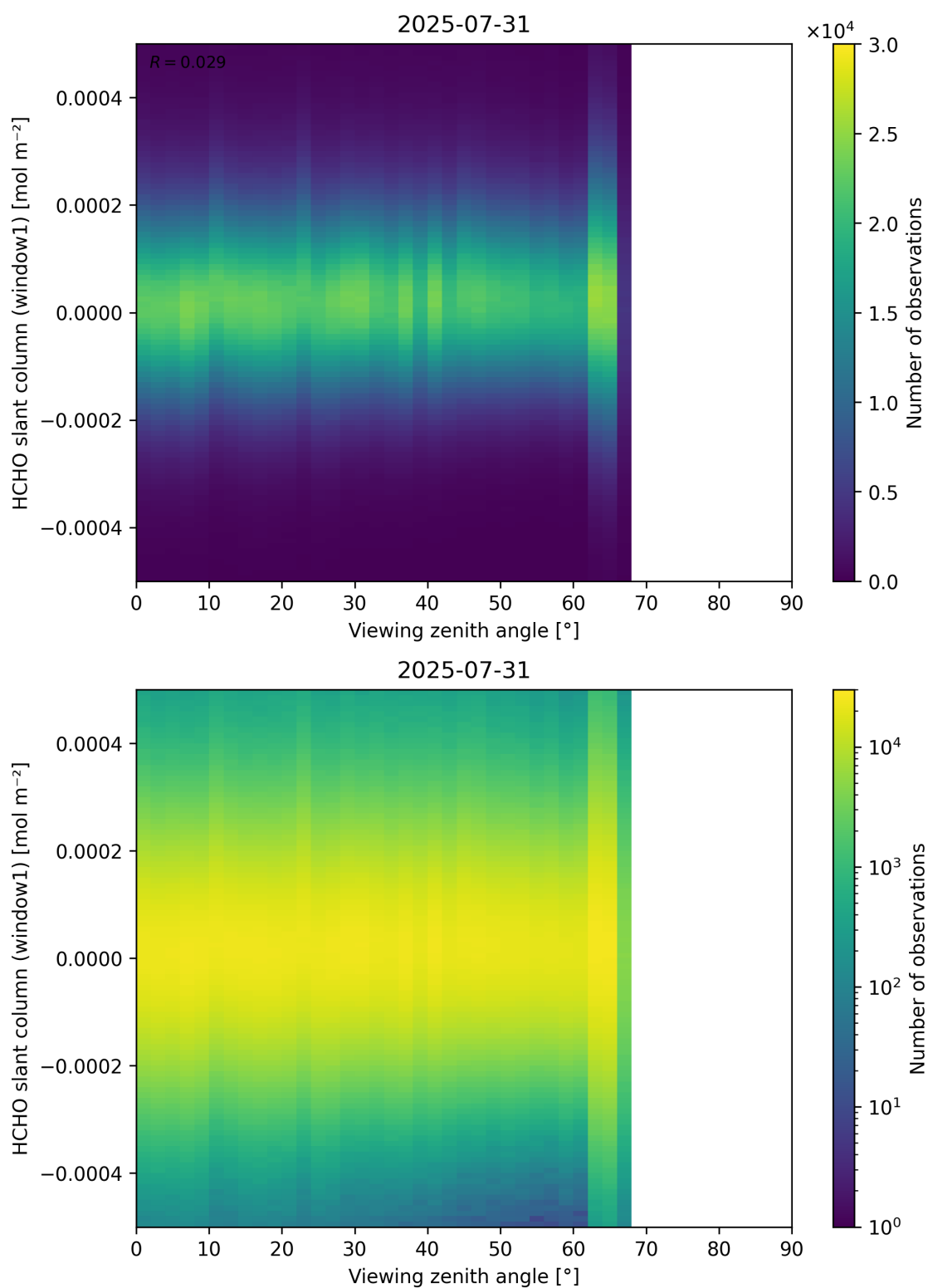
Figure 188: Scatter density plot of “Viewing zenith angle” against “HCHO slant column (window1)” for 2025-07-30 to 2025-08-01.
