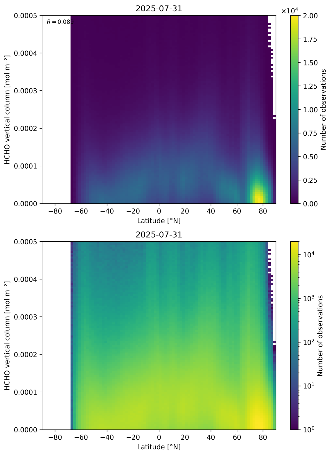
Figure 163: Scatter density plot of “Latitude” against “HCHO vertical column” for 2025-07-30 to 2025-08-01.
