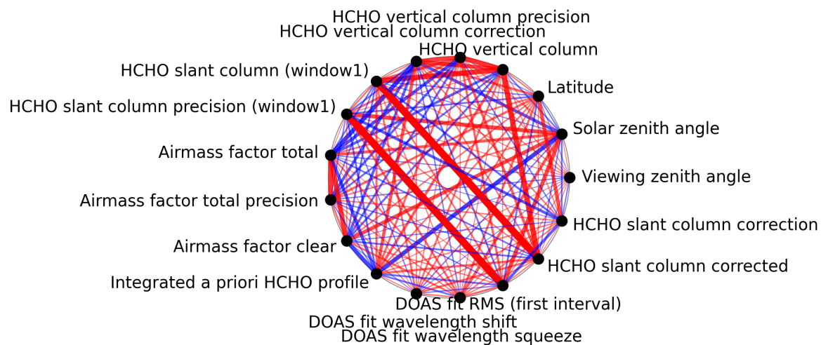
Figure 1: Map of correlation graph for 2025-07-30 to 2025-08-01.
