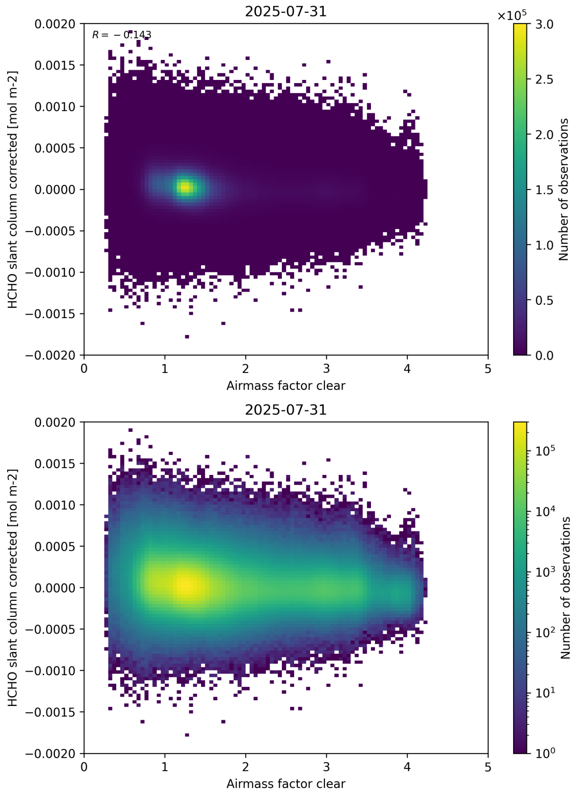
Figure 74: Scatter density plot of “Airmass factor clear” against “HCHO slant column corrected” for 2025-07-30 to 2025-08-01.
