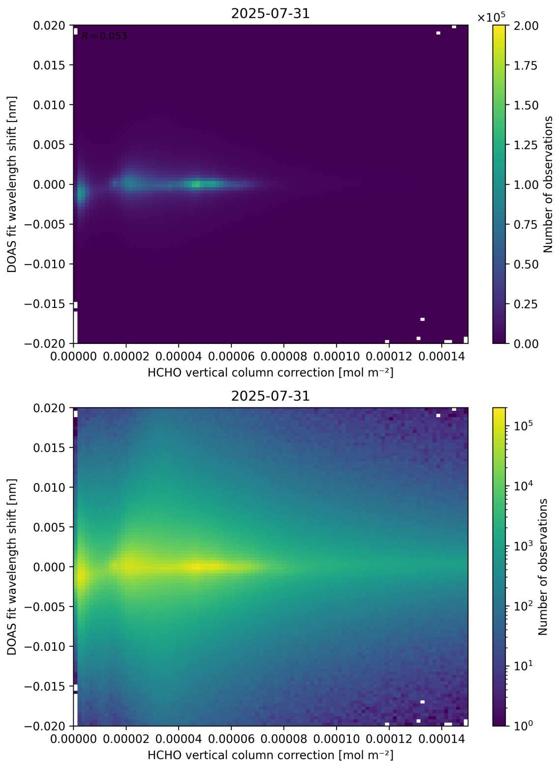
Figure 113: Scatter density plot of “HCHO vertical column correction” against “DOAS fit wavelength shift” for 2025-07-30 to 2025-08-01.
