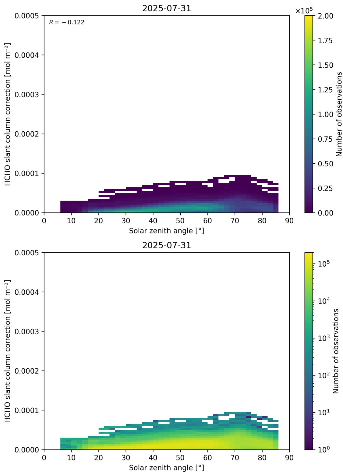
Figure 172: Scatter density plot of “Solar zenith angle” against “HCHO slant column correction” for 2025-07-30 to 2025-08-01.
