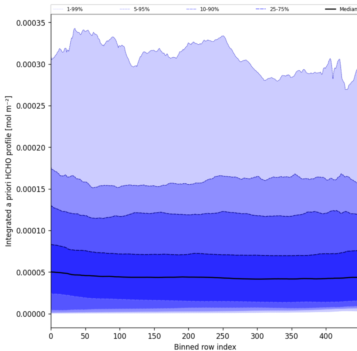
Figure 57: Along track statistics of “Integrated a priori HCHO profile” for 2025-07-30 to 2025-08-01
