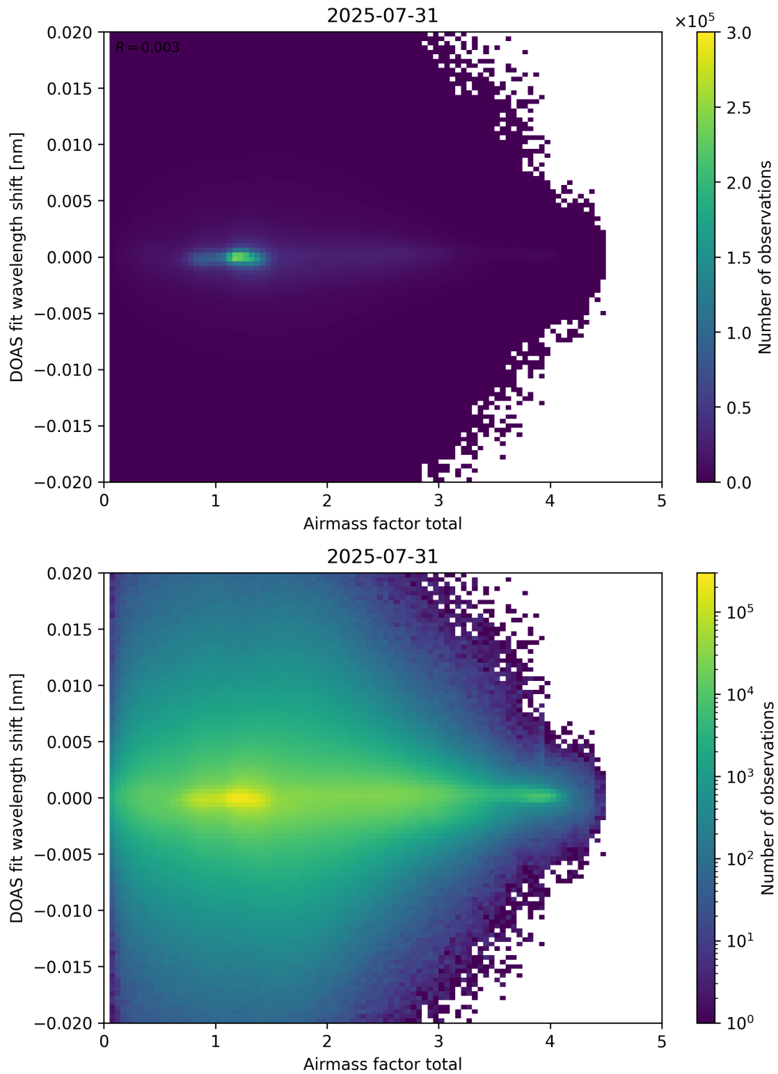
Figure 98: Scatter density plot of “Airmass factor total” against “DOAS fit wavelength shift” for 2025-07-30 to 2025-08-01.
