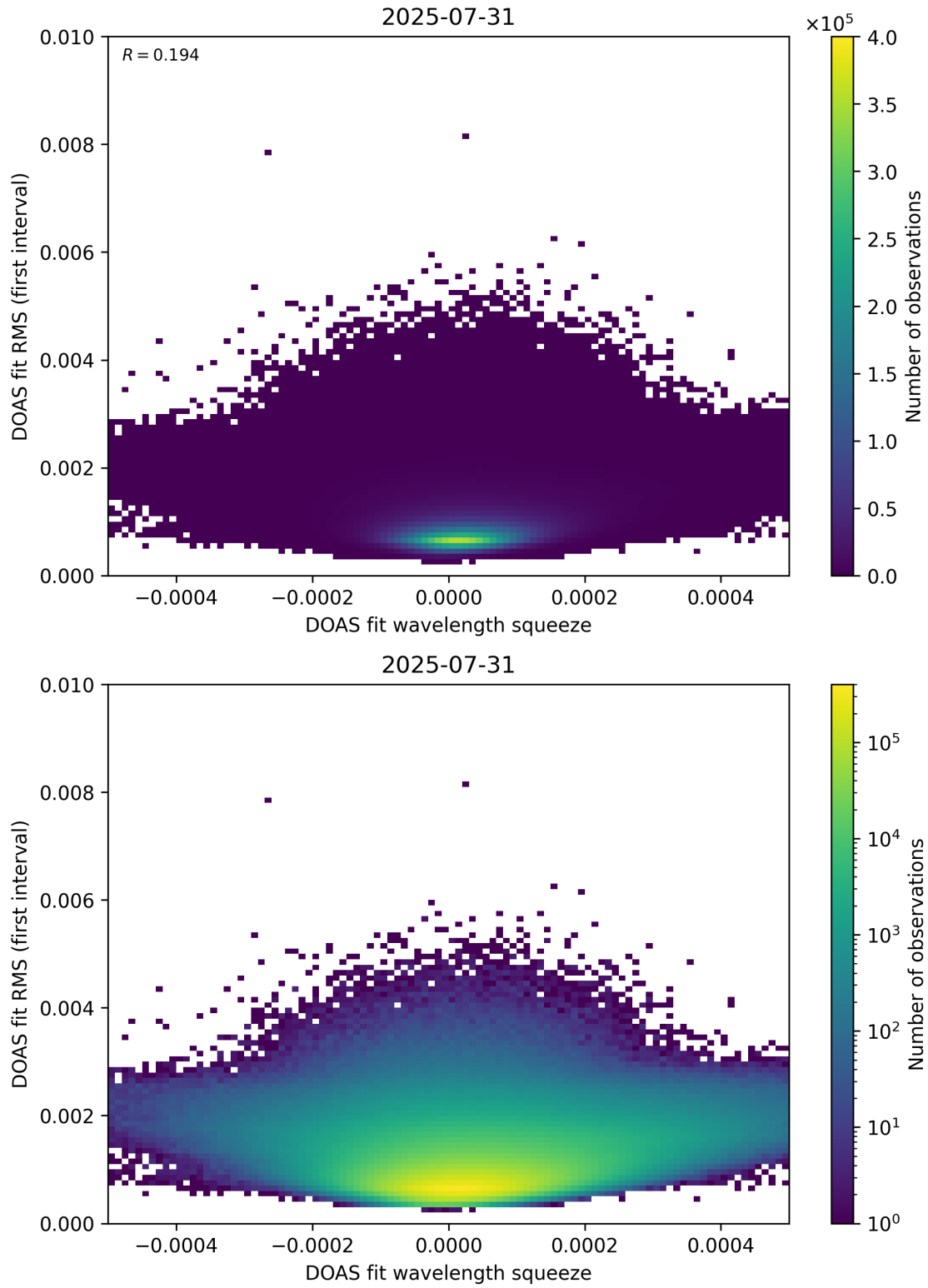
Figure 68: Scatter density plot of “DOAS fit wavelength squeeze” against “DOAS fit RMS (first interval)” for 2025-07-30 to 2025-08-01.
