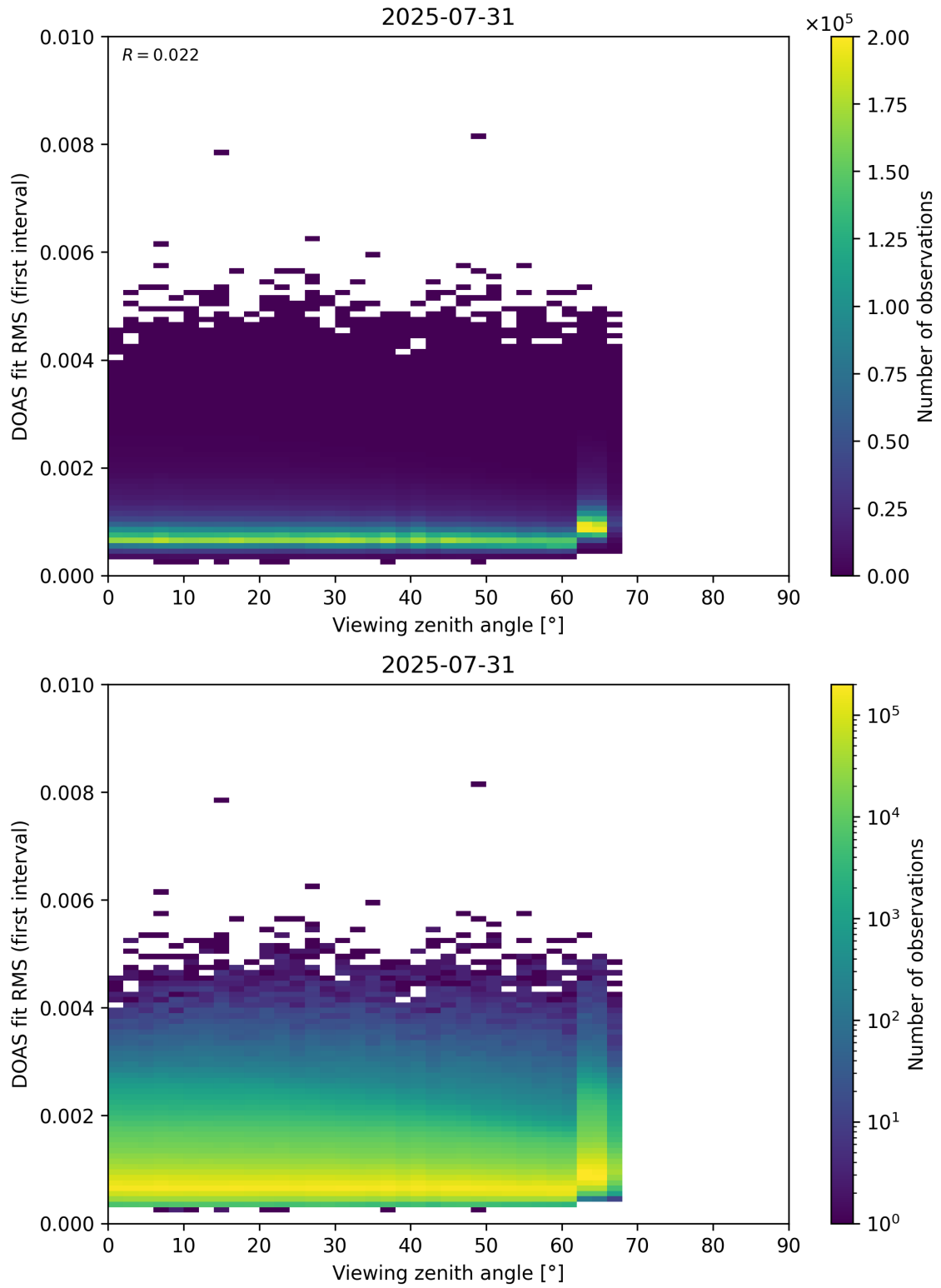
Figure 182: Scatter density plot of “Viewing zenith angle” against “DOAS fit RMS (first interval)” for 2025-07-30 to 2025-08-01.
