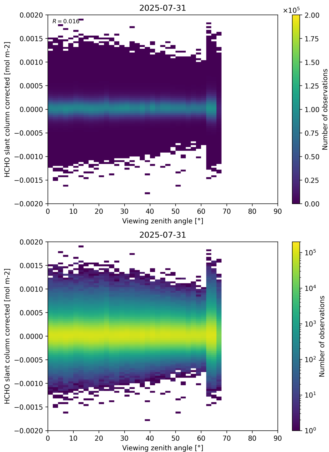
Figure 186: Scatter density plot of “Viewing zenith angle” against “HCHO slant column corrected” for 2025-07-30 to 2025-08-01.
