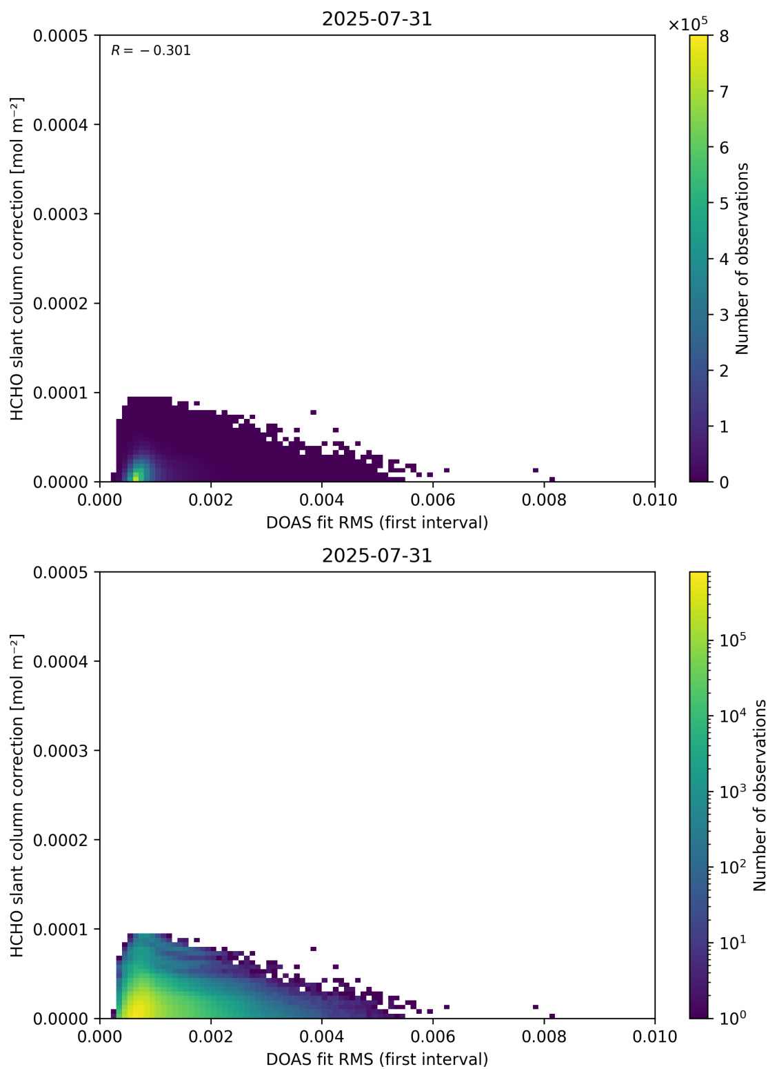
Figure 63: Scatter density plot of “DOAS fit RMS (first interval)” against “HCHO slant column correction” for 2025-07-30 to 2025-08-01.
