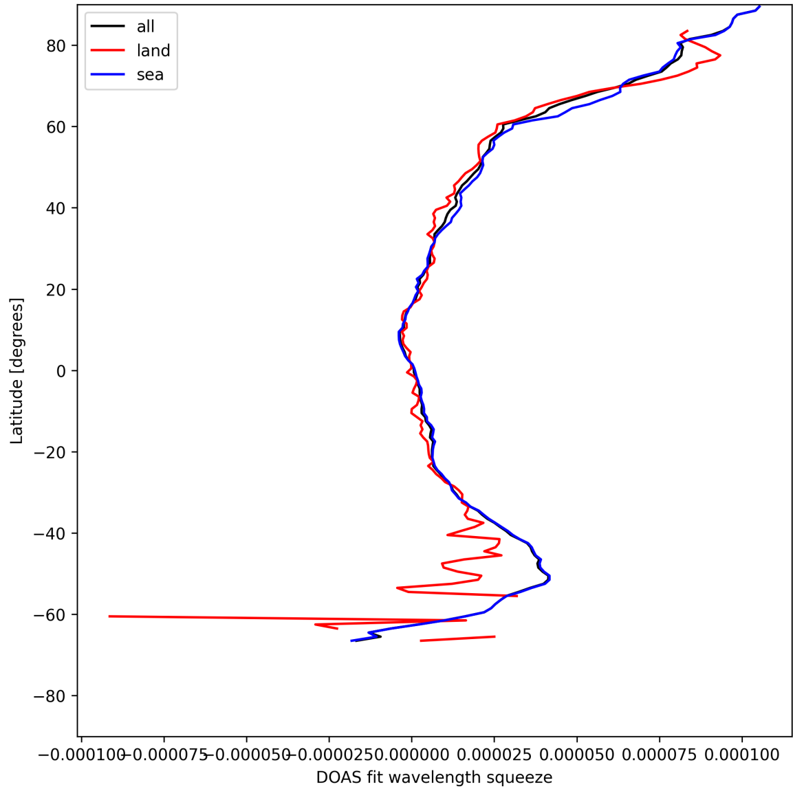
Figure 31: Zonal average of “DOAS fit wavelength squeeze” for 2025-07-30 to 2025-08-01.
