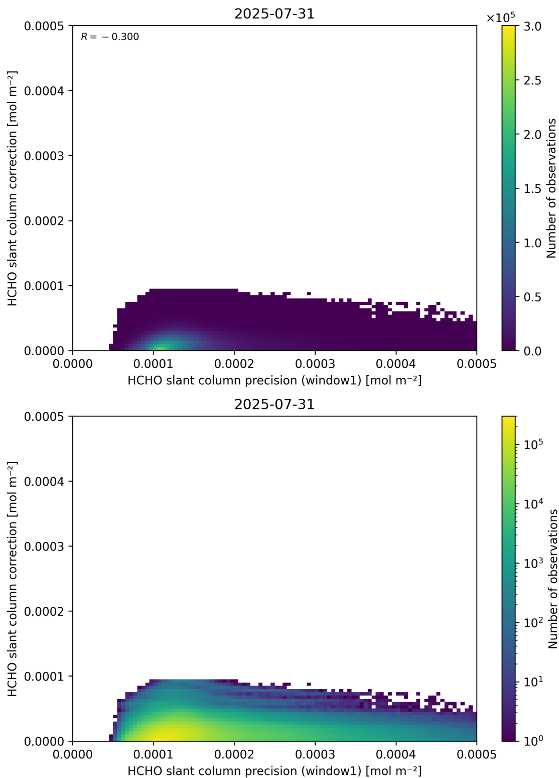
Figure 93: Scatter density plot of “HCHO slant column precision (window1)” against “HCHO slant column correction” for 2025-07-30 to 2025-08-01.
