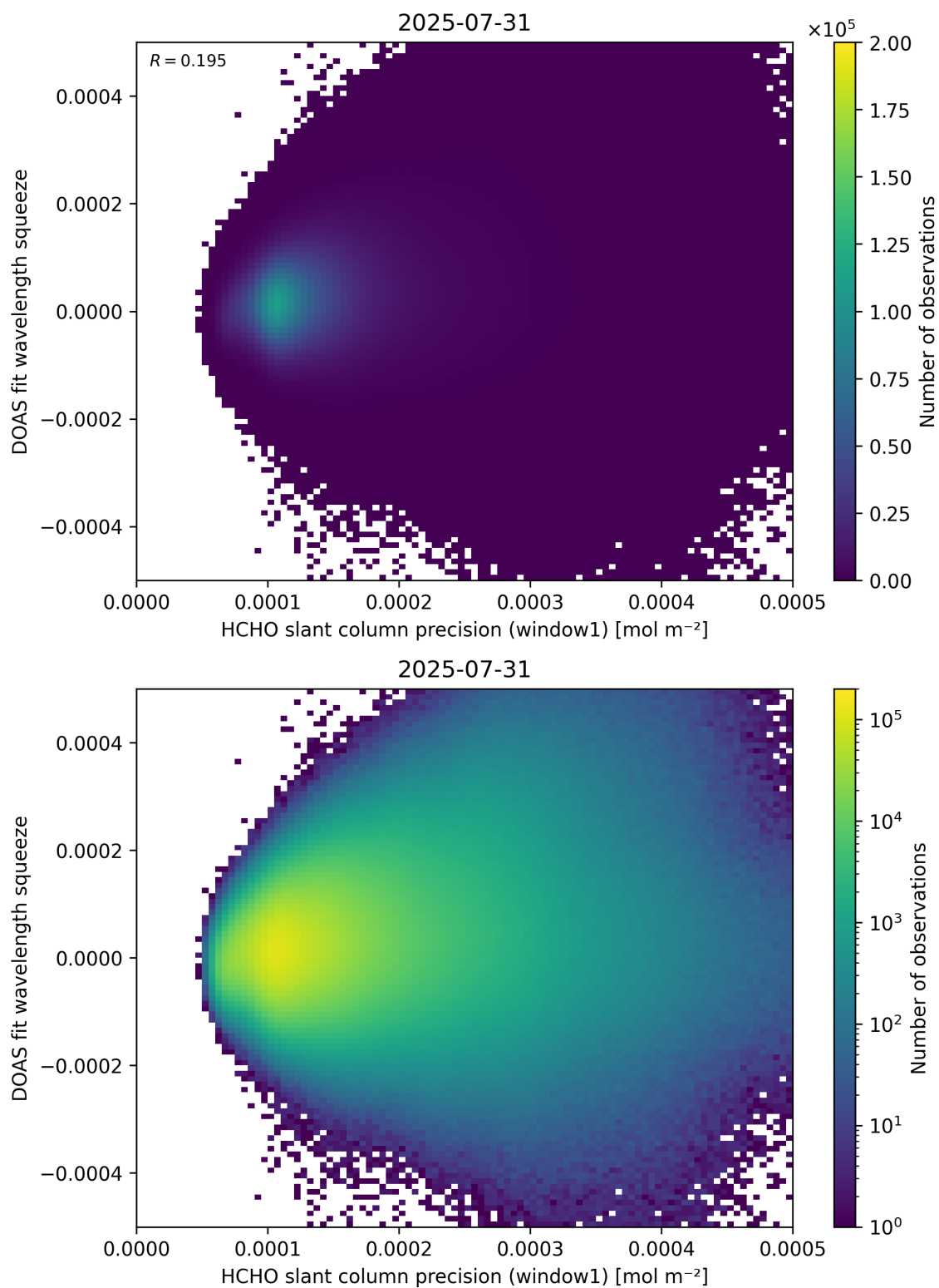
Figure 90: Scatter density plot of “HCHO slant column precision (window1)” against “DOAS fit wavelength squeeze” for 2025-07-30 to 2025-08-01.
