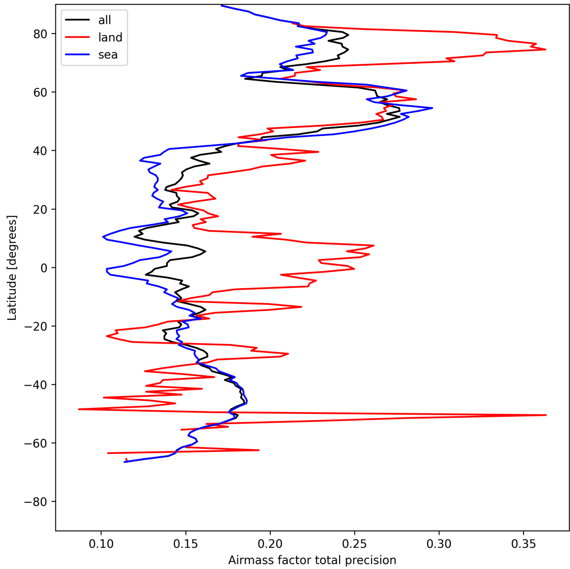
Figure 27: Zonal average of “Airmass factor total precision” for 2025-07-30 to 2025-08-01.
