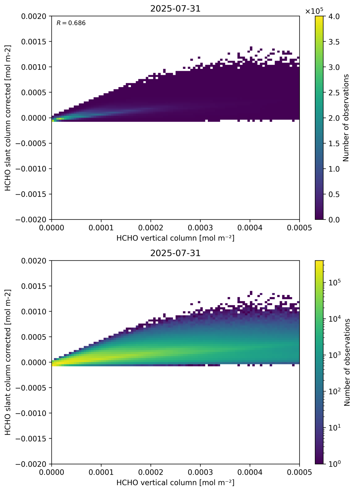
Figure 127: Scatter density plot of “HCHO vertical column” against “HCHO slant column corrected” for 2025-07-30 to 2025-08-01.
