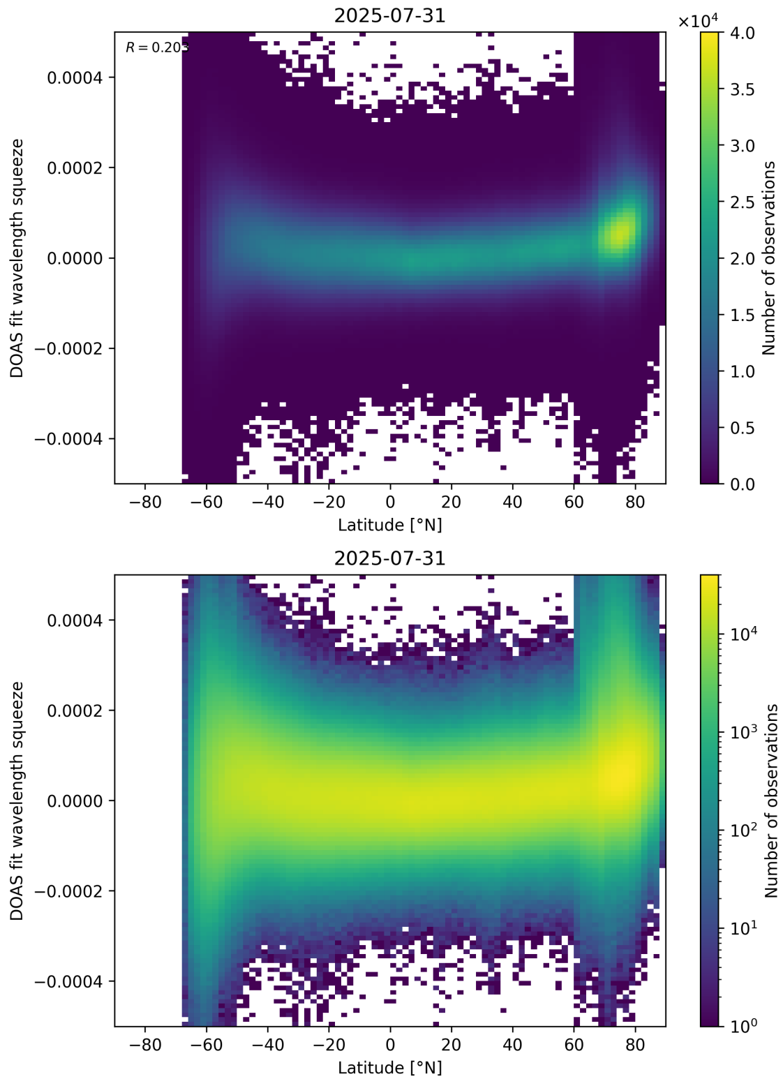
Figure 155: Scatter density plot of “Latitude” against “DOAS fit wavelength squeeze” for 2025-07-30 to 2025-08-01.
