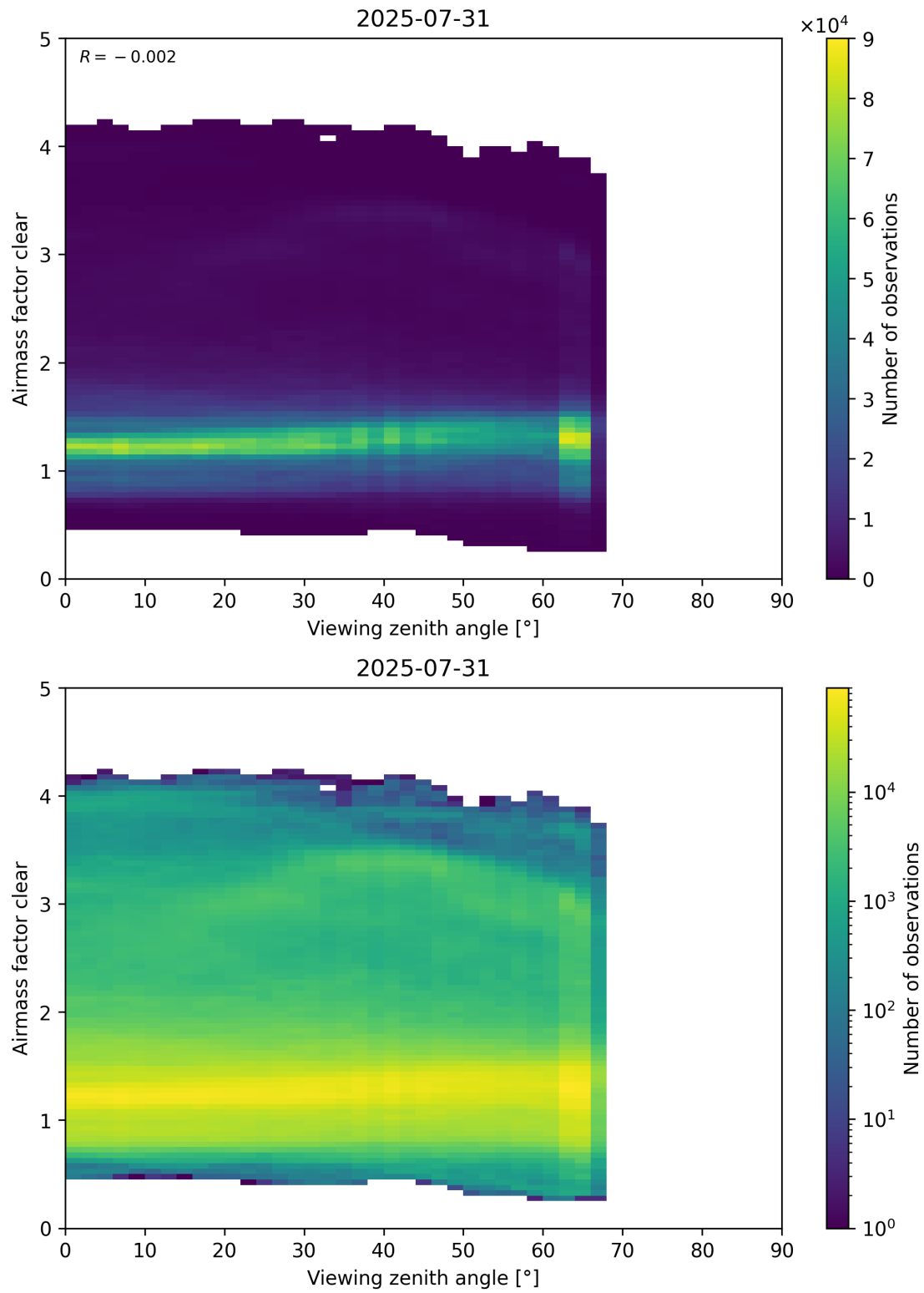
Figure 185: Scatter density plot of “Viewing zenith angle” against “Airmass factor clear” for 2025-07-30 to 2025-08-01.
