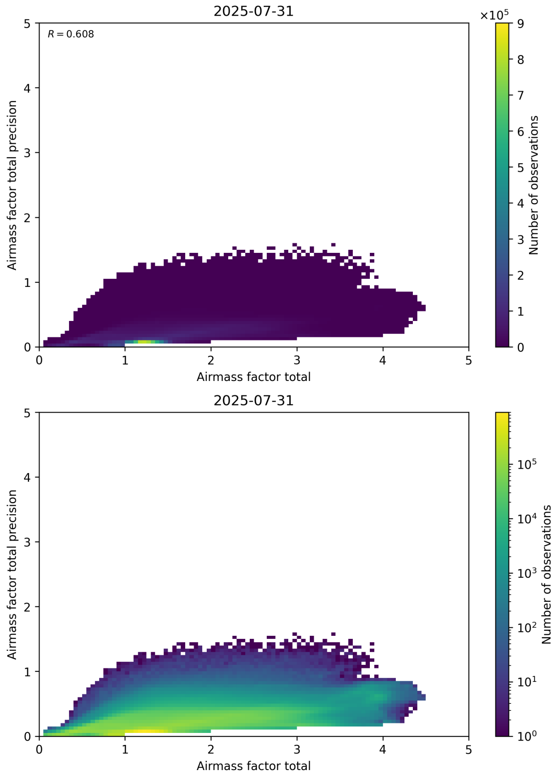
Figure 103: Scatter density plot of “Airmass factor total” against “Airmass factor total precision” for 2025-07-30 to 2025-08-01.
