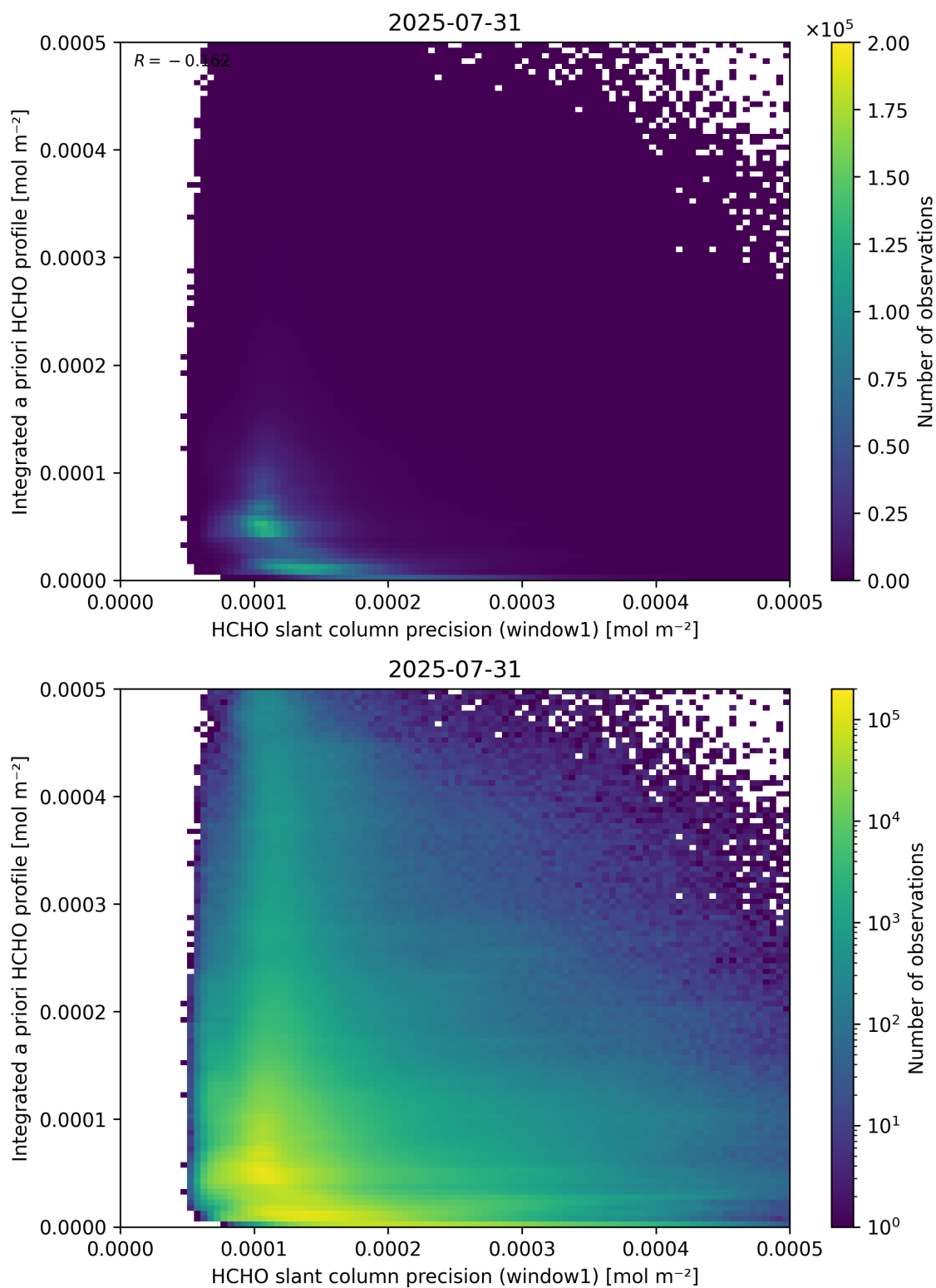
Figure 96: Scatter density plot of “HCHO slant column precision (window1)” against “Integrated a priori HCHO profile” for 2025-07-30 to 2025-08-01.
