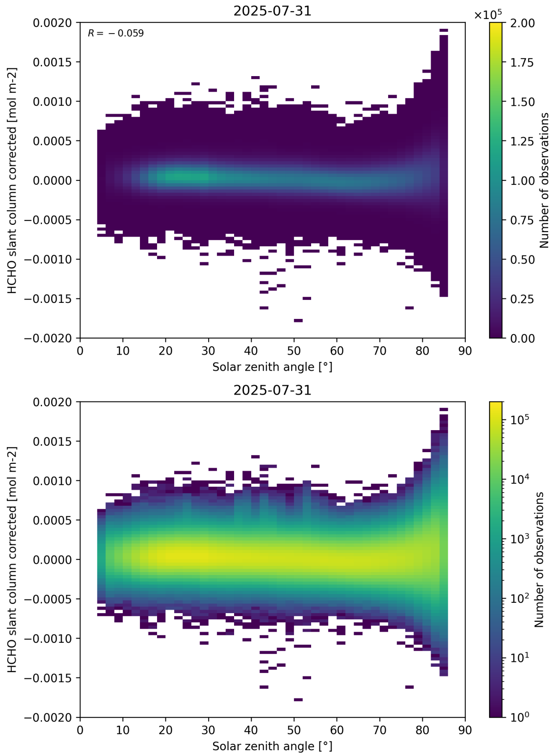
Figure 171: Scatter density plot of “Solar zenith angle” against “HCHO slant column corrected” for 2025-07-30 to 2025-08-01.
