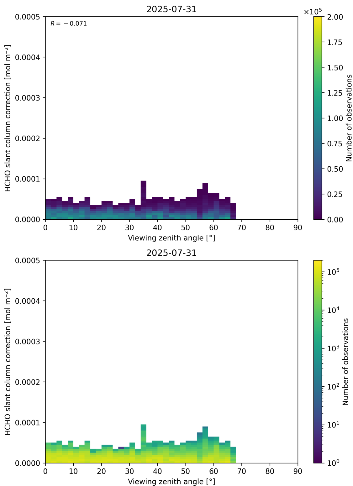
Figure 187: Scatter density plot of “Viewing zenith angle” against “HCHO slant column correction” for 2025-07-30 to 2025-08-01.
