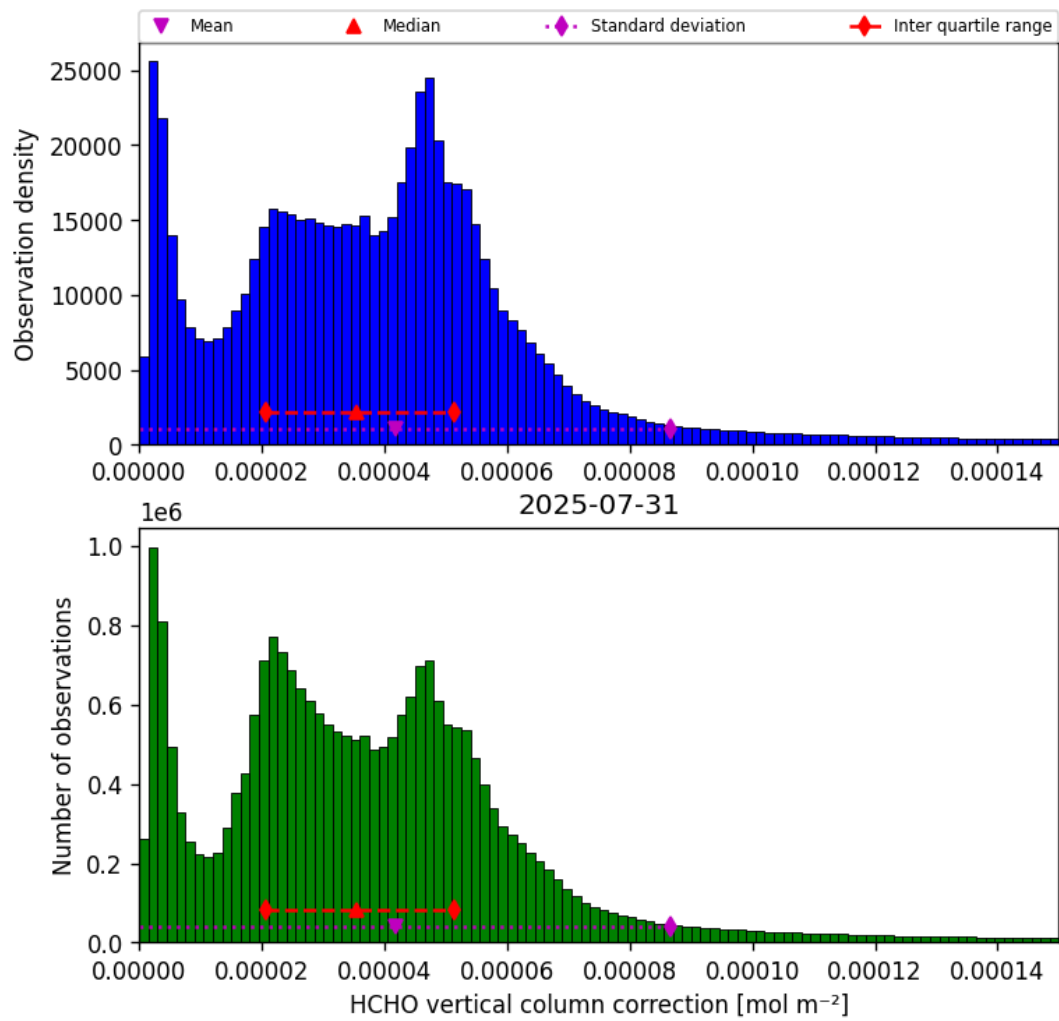
Figure 37: Histogram of “HCHO vertical column correction” for 2025-07-30 to 2025-08-01
