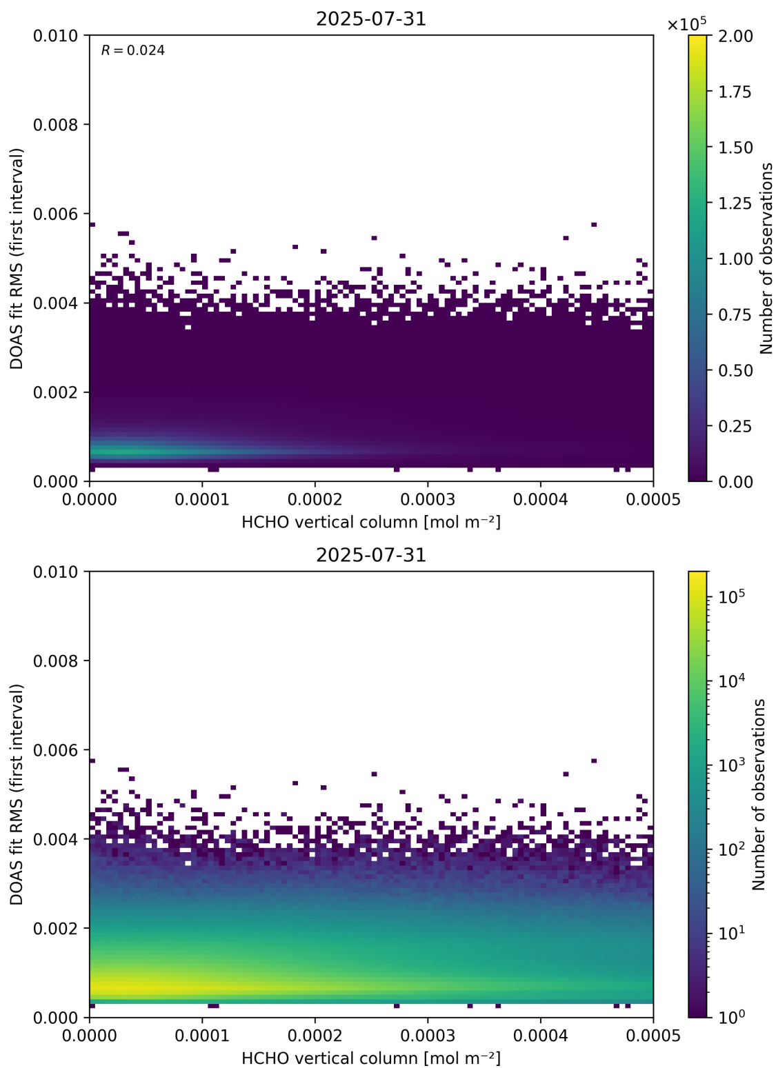
Figure 123: Scatter density plot of “HCHO vertical column” against “DOAS fit RMS (first interval)” for 2025-07-30 to 2025-08-01.
