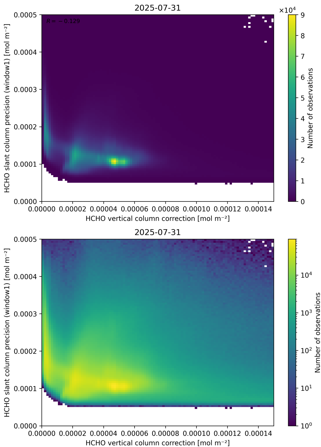
Figure 119: Scatter density plot of “HCHO vertical column correction” against “HCHO slant column precision (window1)” for 2025-07-30 to 2025-08-01.
