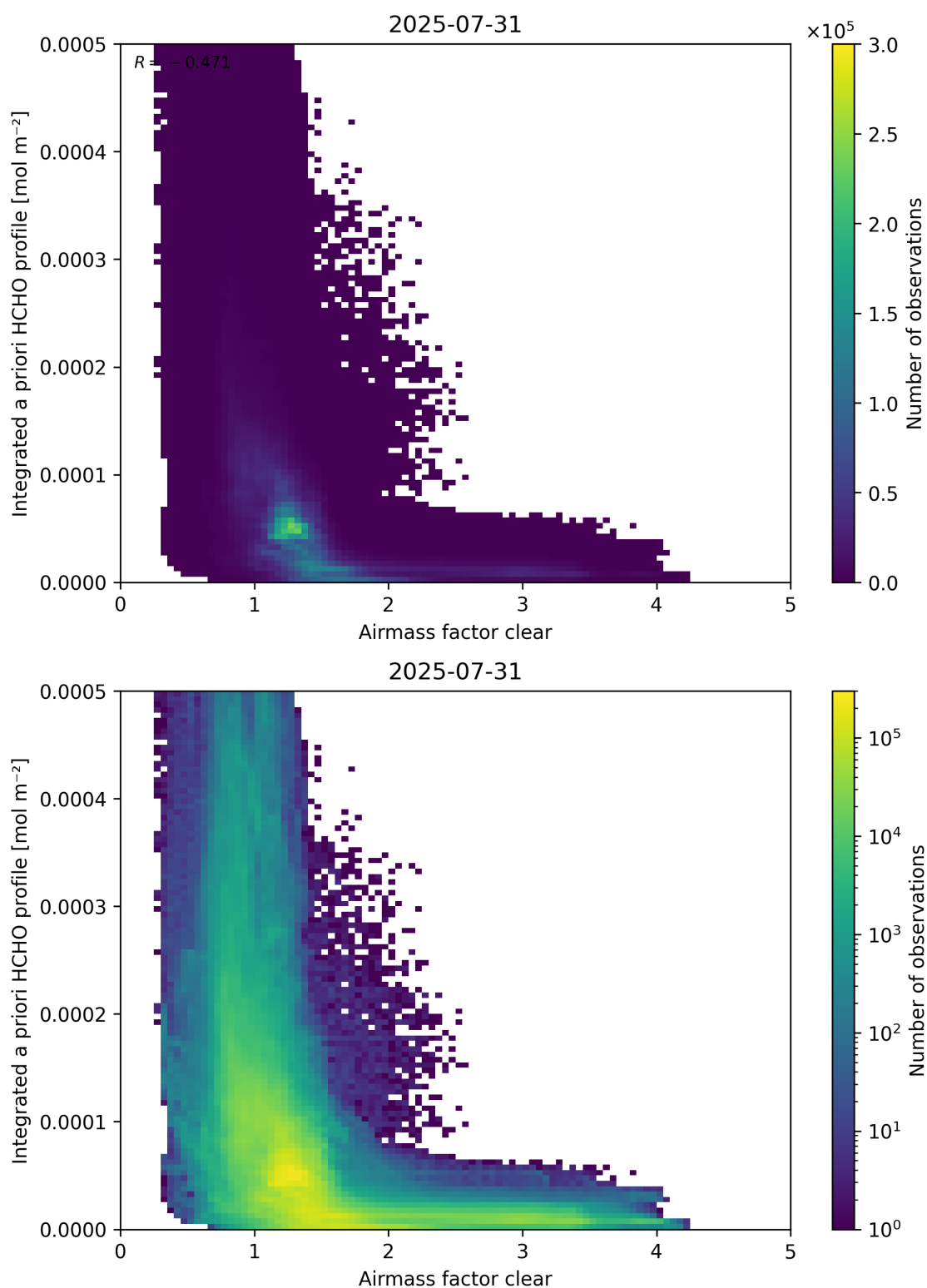
Figure 76: Scatter density plot of “Airmass factor clear” against “Integrated a priori HCHO profile” for 2025-07-30 to 2025-08-01.
