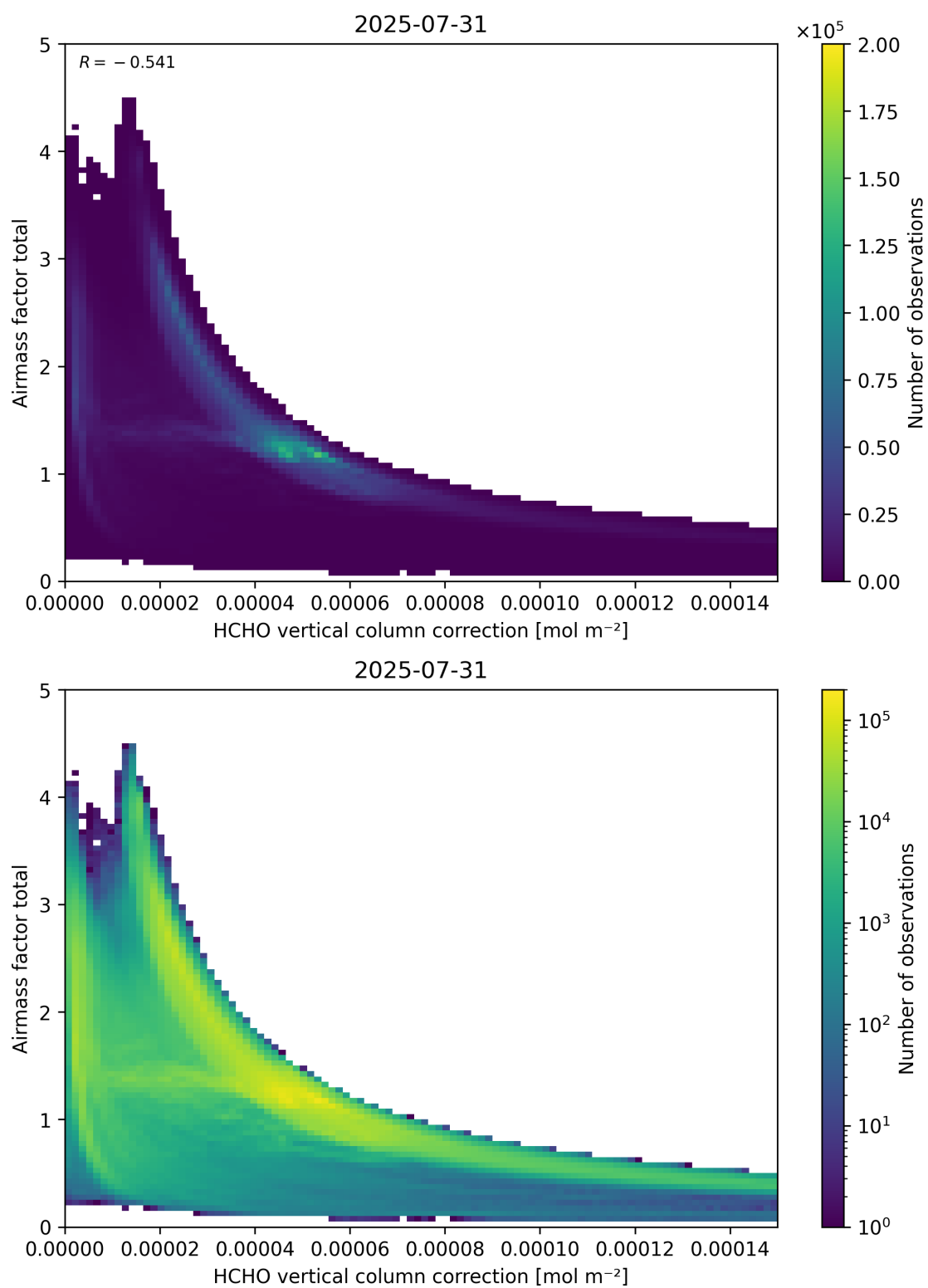
Figure 120: Scatter density plot of “HCHO vertical column correction” against “Airmass factor total” for 2025-07-30 to 2025-08-01.
