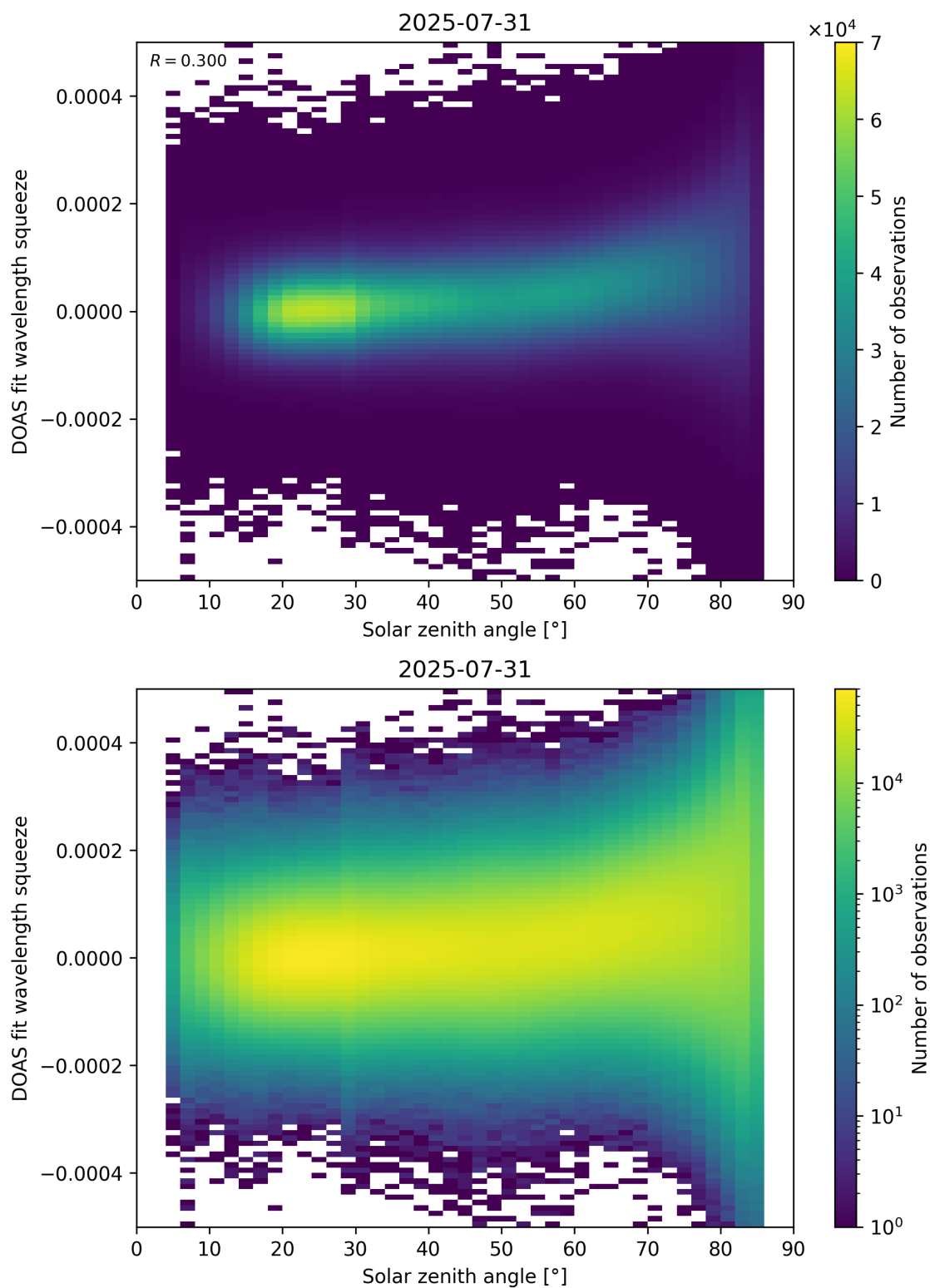
Figure 169: Scatter density plot of “Solar zenith angle” against “DOAS fit wavelength squeeze” for 2025-07-30 to 2025-08-01.
