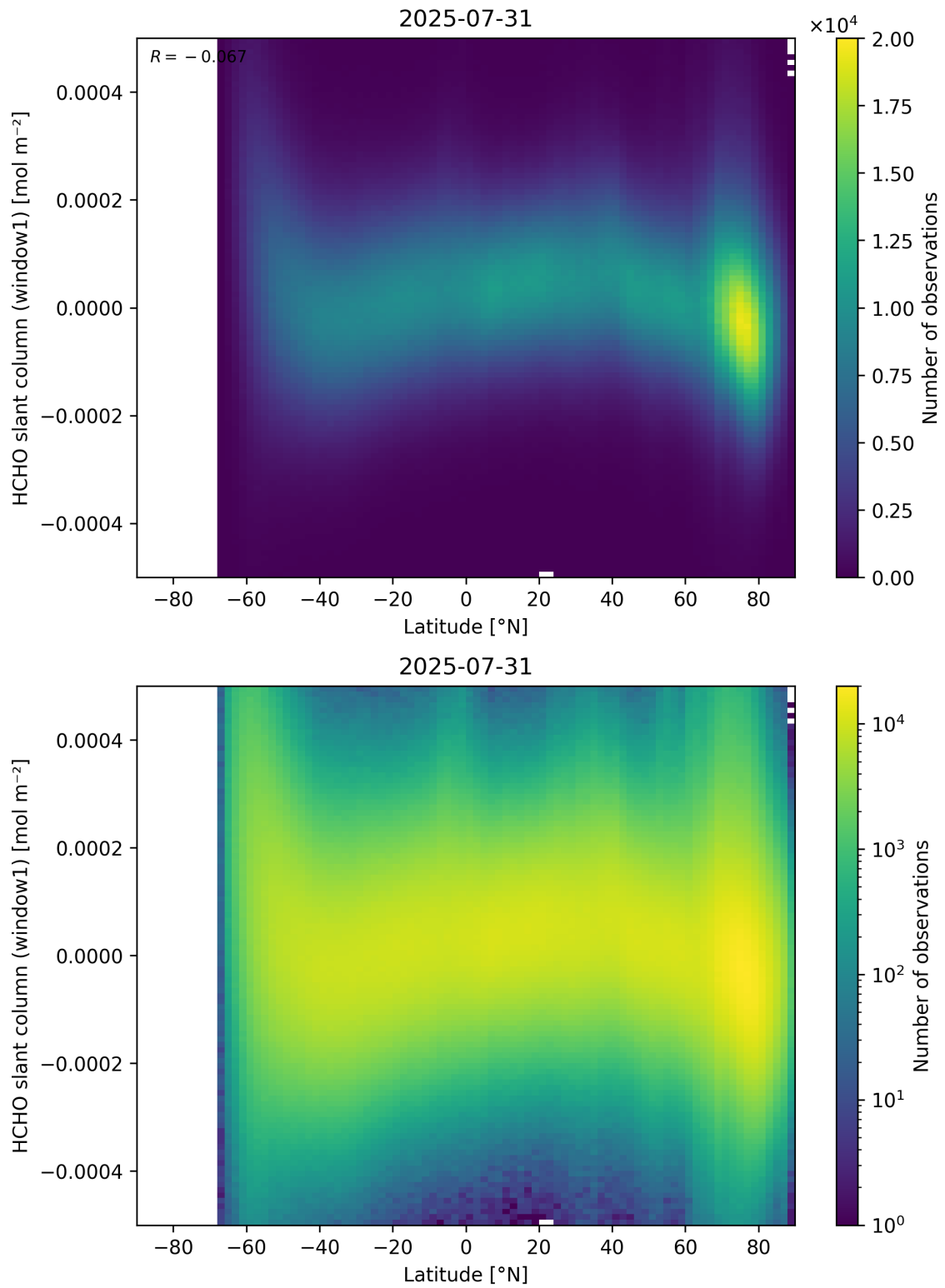
Figure 159: Scatter density plot of “Latitude” against “HCHO slant column (window1)” for 2025-07-30 to 2025-08-01.
