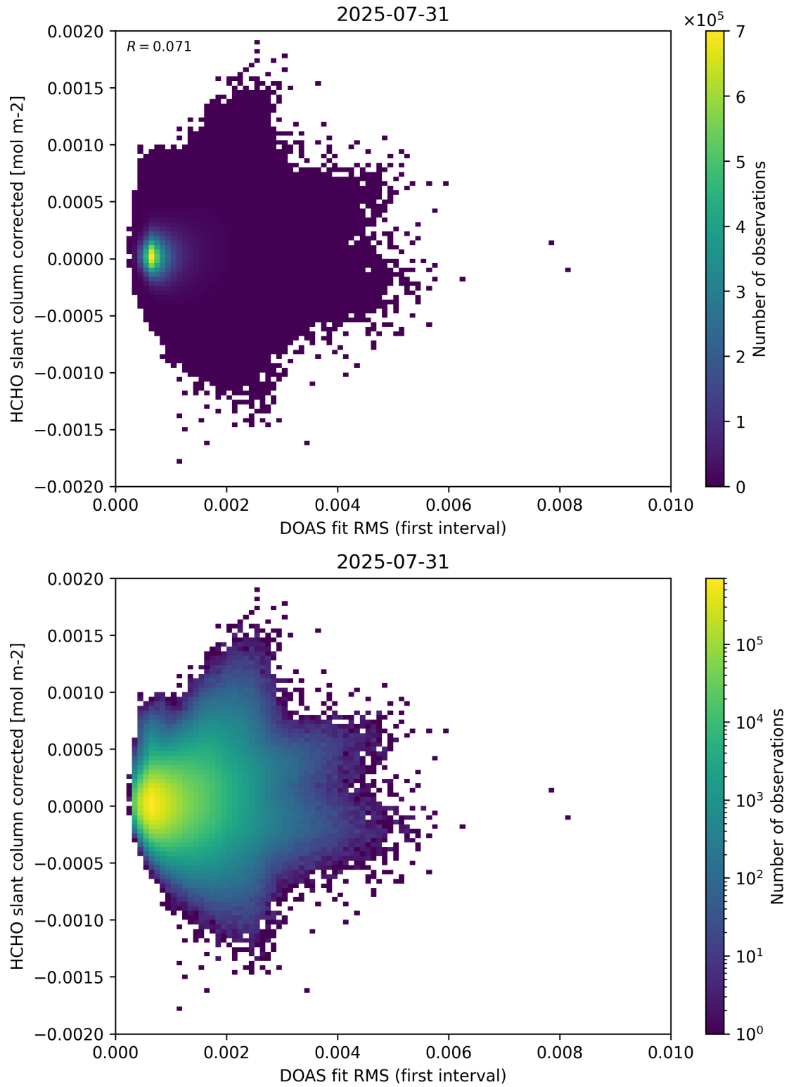
Figure 62: Scatter density plot of “DOAS fit RMS (first interval)” against “HCHO slant column corrected” for 2025-07-30 to 2025-08-01.
