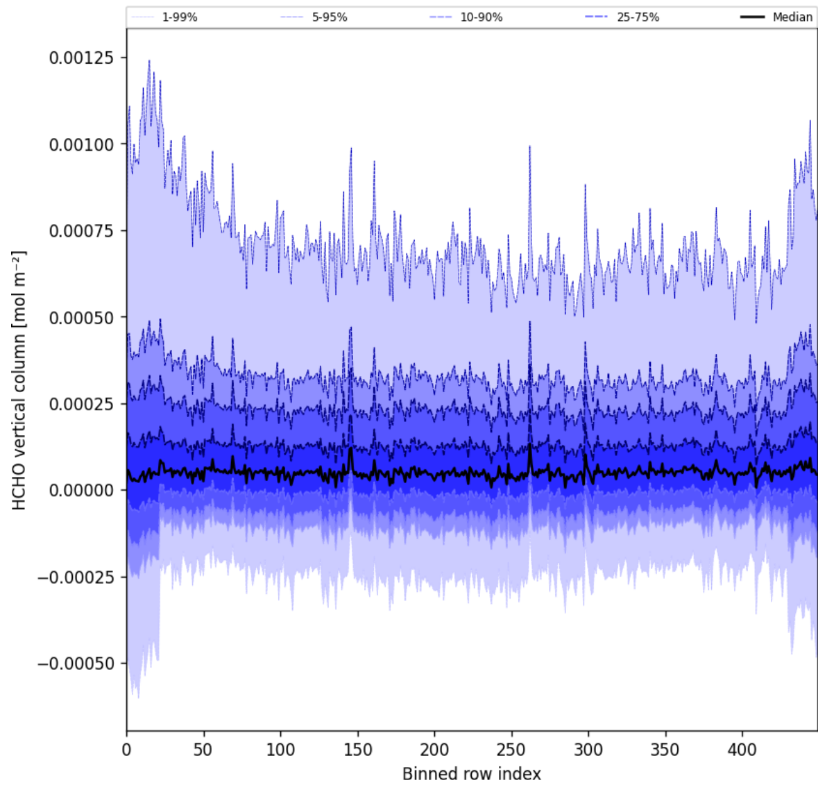
Figure 49: Along track statistics of “HCHO vertical column” for 2025-07-30 to 2025-08-01
