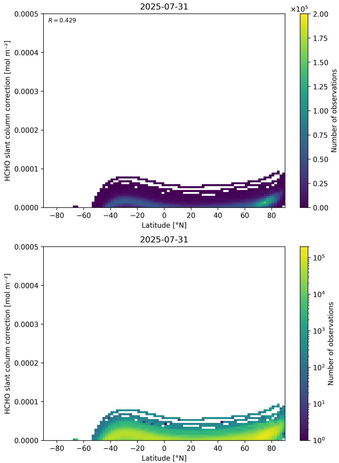
Figure 158: Scatter density plot of “Latitude” against “HCHO slant column correction” for 2025-07-30 to 2025-08-01.
