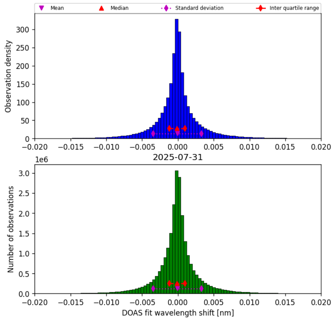
Figure 44: Histogram of “DOAS fit wavelength shift” for 2025-07-30 to 2025-08-01
