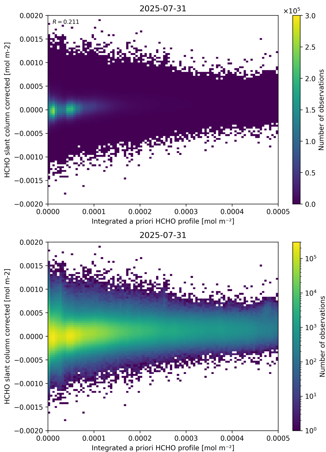
Figure 151: Scatter density plot of “Integrated a priori HCHO profile” against “HCHO slant column corrected” for 2025-07-30 to 2025-08-01.
