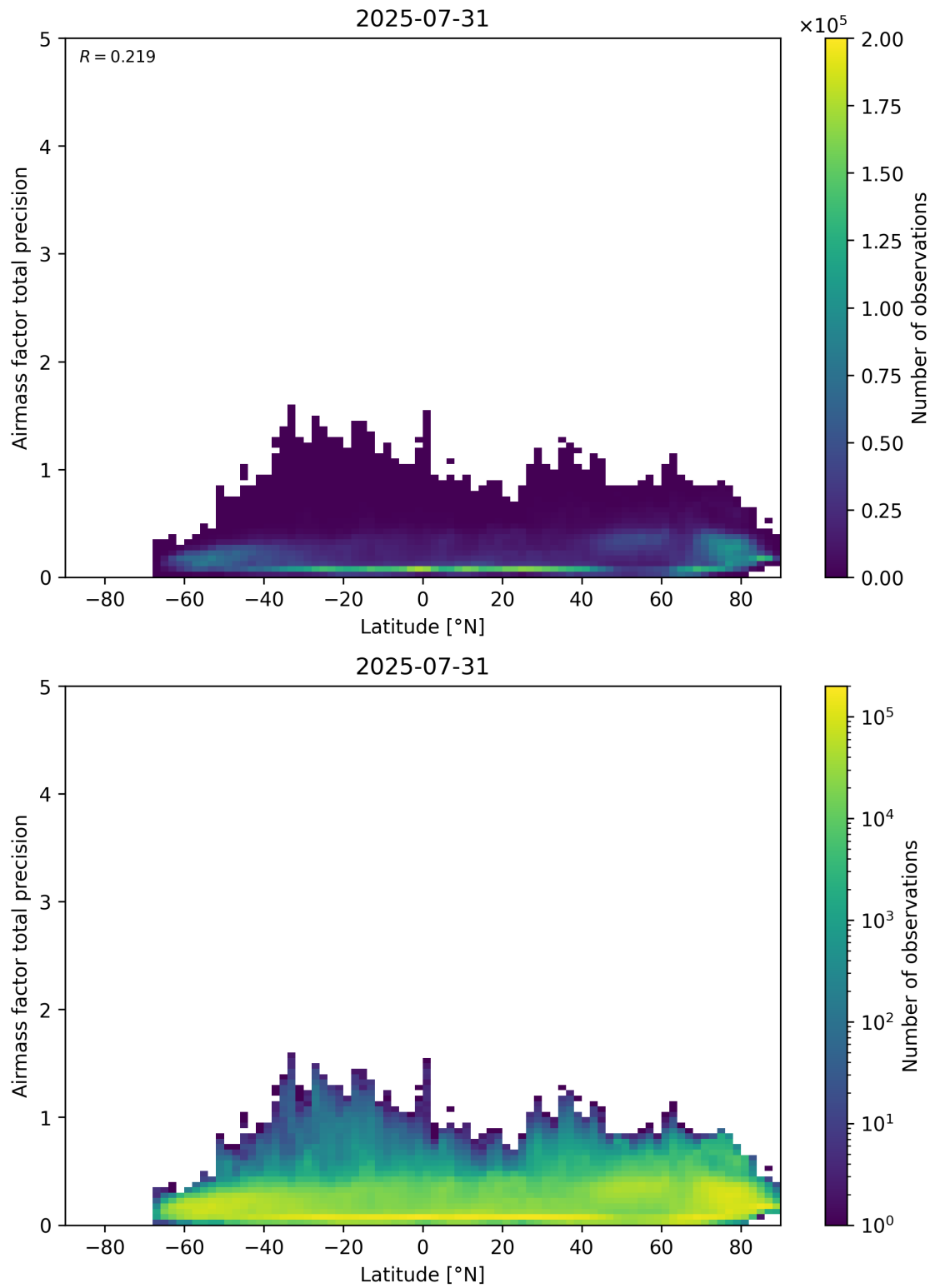
Figure 162: Scatter density plot of “Latitude” against “Airmass factor total precision” for 2025-07-30 to 2025-08-01.
