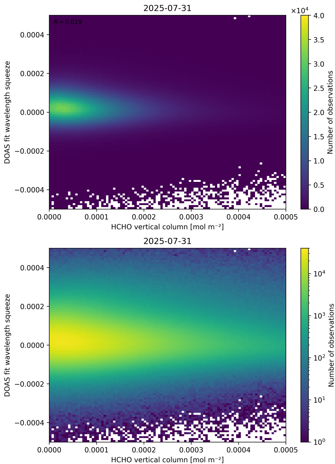
Figure 125: Scatter density plot of “HCHO vertical column” against “DOAS fit wavelength squeeze” for 2025-07-30 to 2025-08-01.
