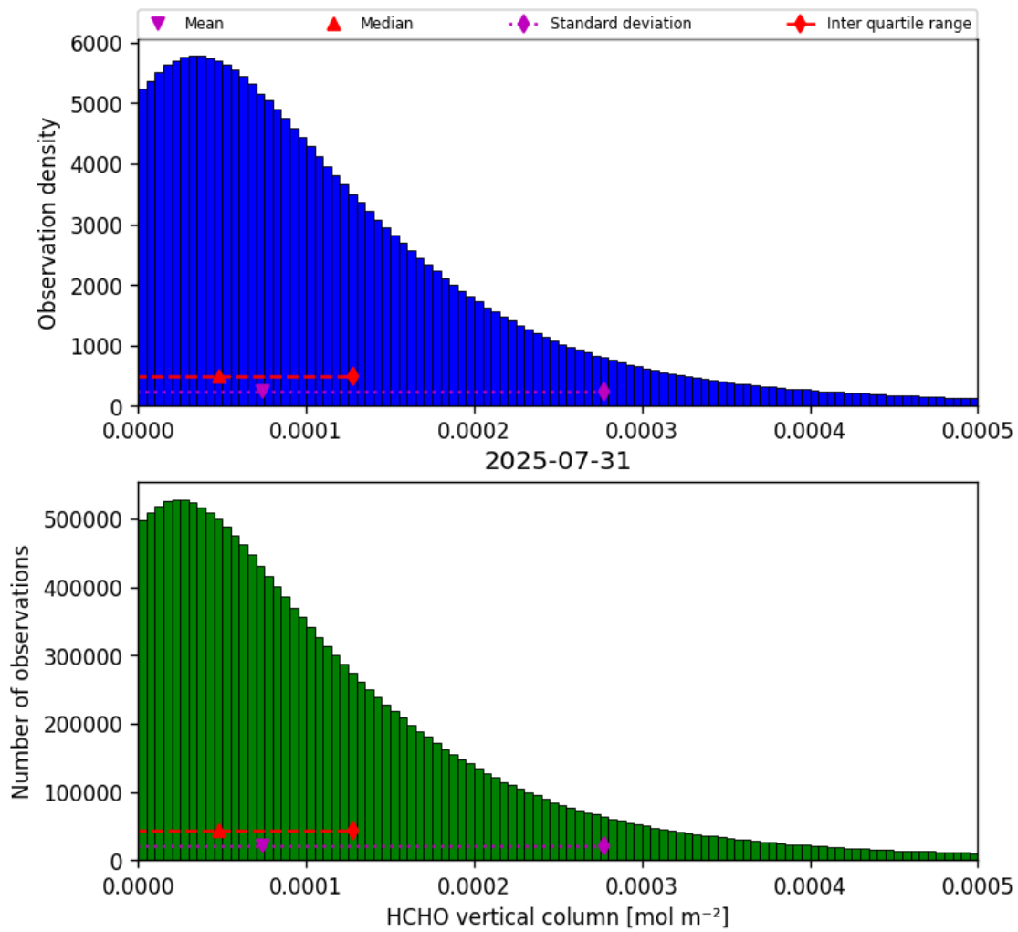
Figure 35: Histogram of “HCHO vertical column” for 2025-07-30 to 2025-08-01
