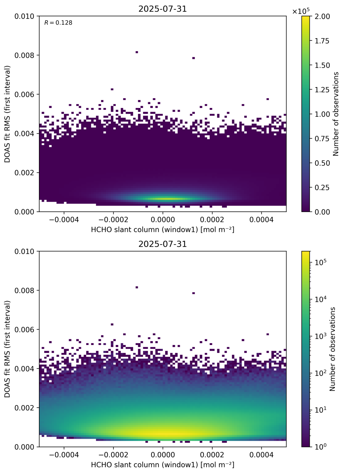
Figure 78: Scatter density plot of “HCHO slant column (window1)” against “DOAS fit RMS (first interval)” for 2025-07-30 to 2025-08-01.
