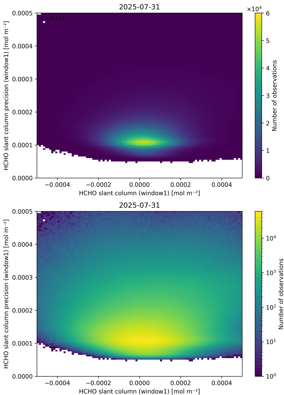
Figure 84: Scatter density plot of “HCHO slant column (window1)” against “HCHO slant column precision (window1)” for 2025-07-30 to 2025-08-01.
