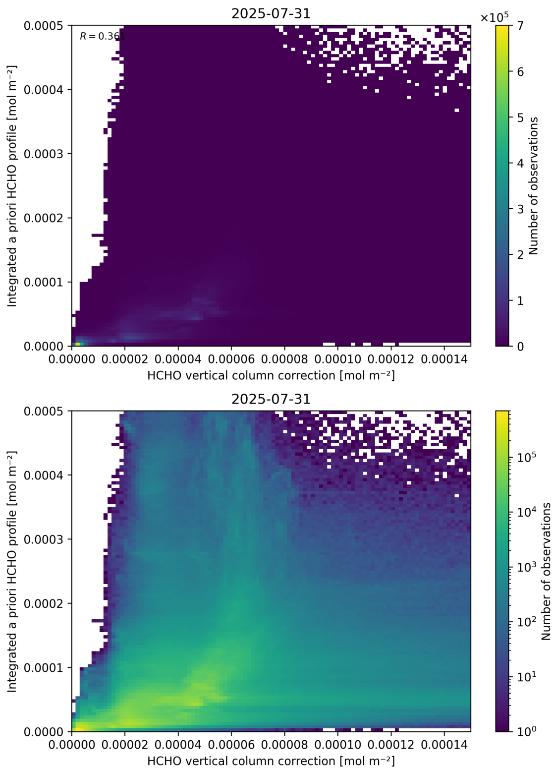
Figure 122: Scatter density plot of “HCHO vertical column correction” against “Integrated a priori HCHO profile” for 2025-07-30 to 2025-08-01.
