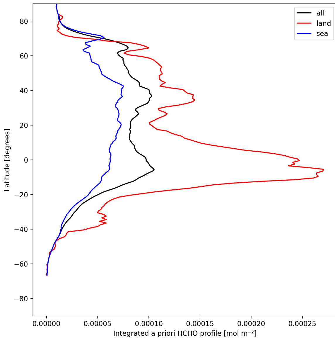
Figure 29: Zonal average of “Integrated a priori HCHO profile” for 2025-07-30 to 2025-08-01.
