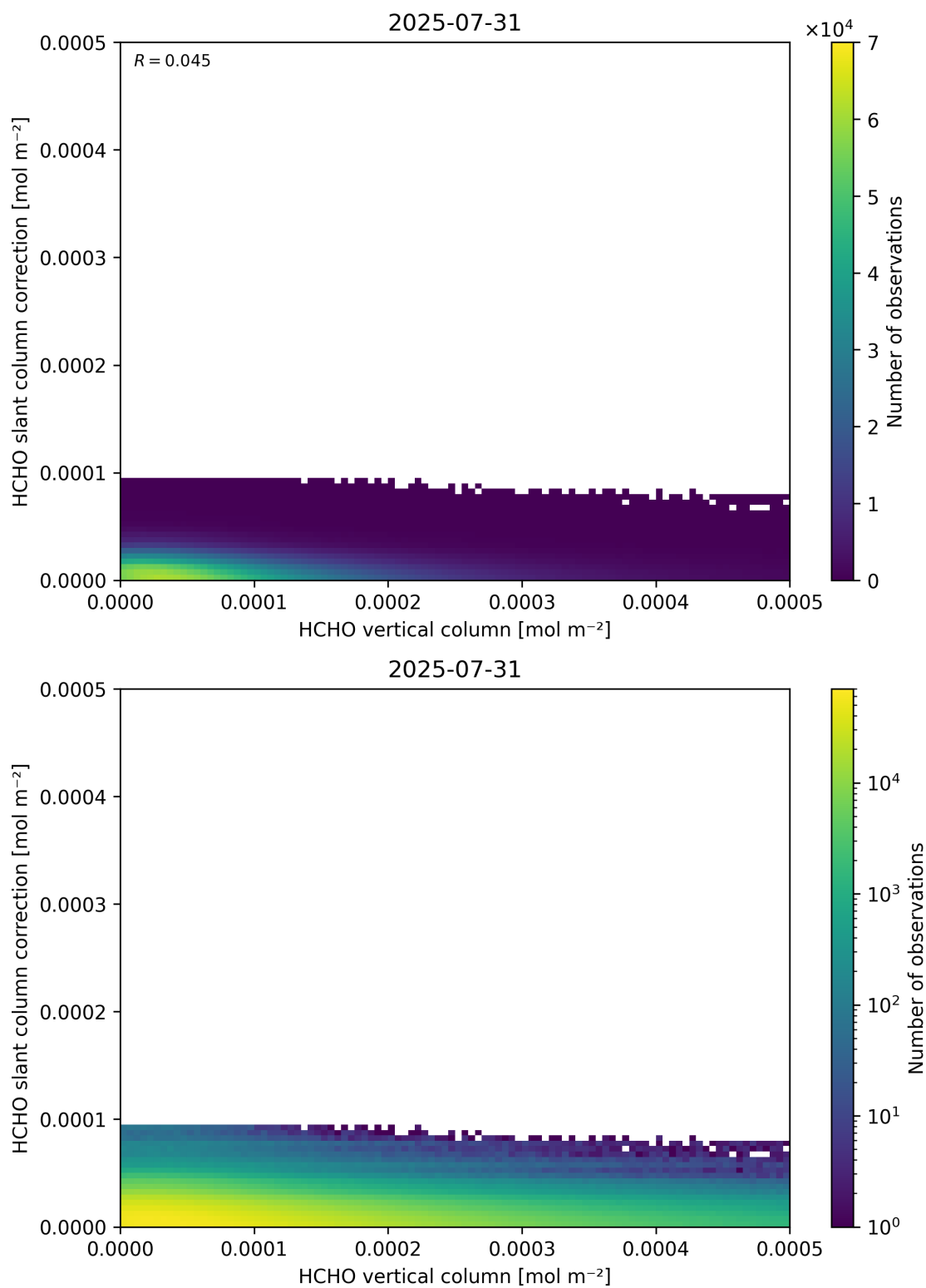
Figure 128: Scatter density plot of “HCHO vertical column” against “HCHO slant column correction” for 2025-07-30 to 2025-08-01.
