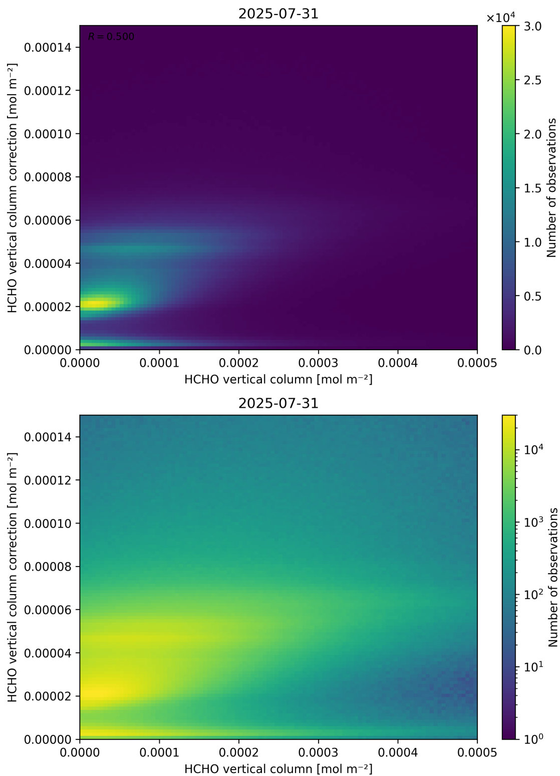
Figure 133: Scatter density plot of “HCHO vertical column” against “HCHO vertical column correction” for 2025-07-30 to 2025-08-01.
