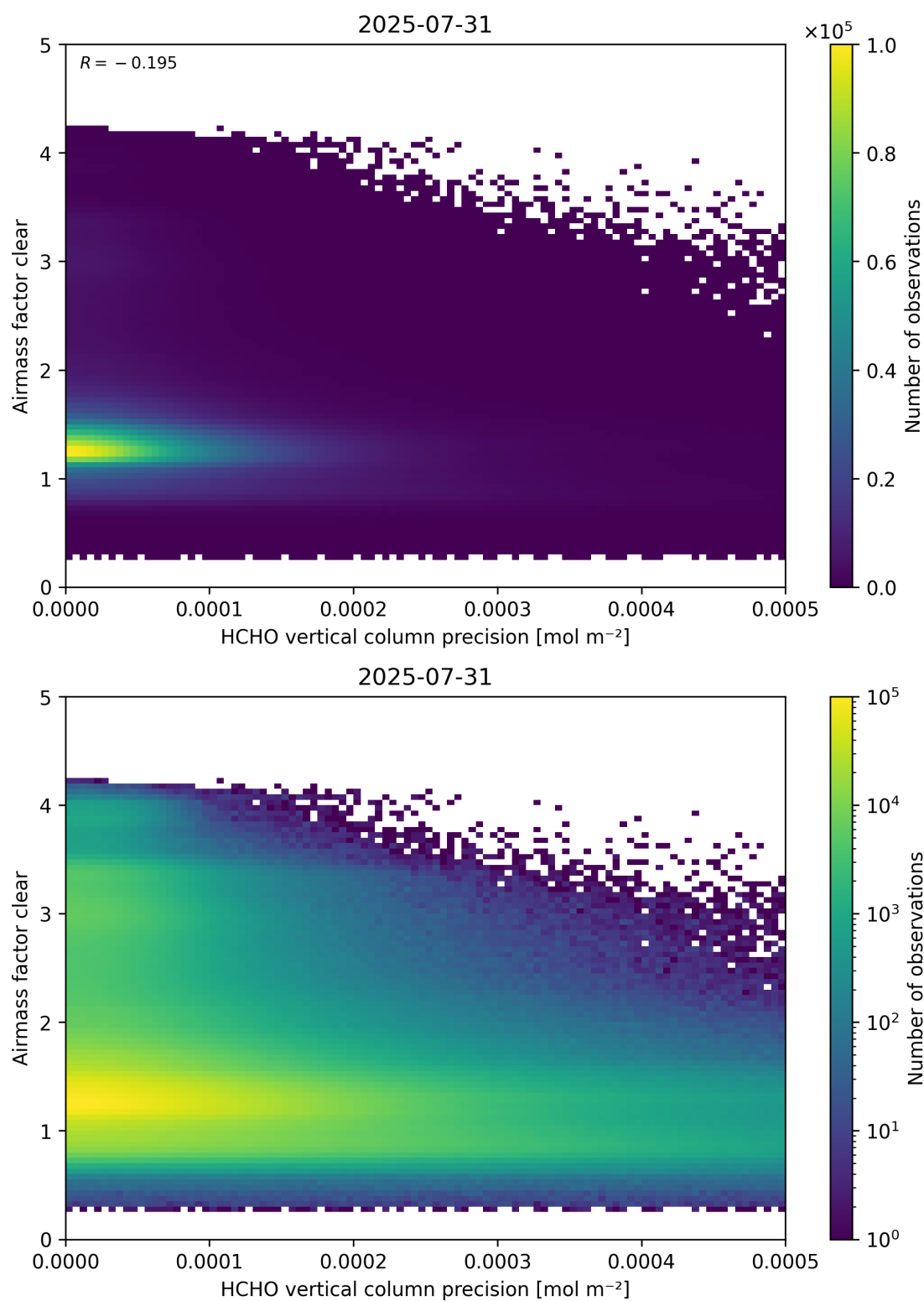
Figure 139: Scatter density plot of “HCHO vertical column precision” against “Airmass factor clear” for 2025-07-30 to 2025-08-01.
