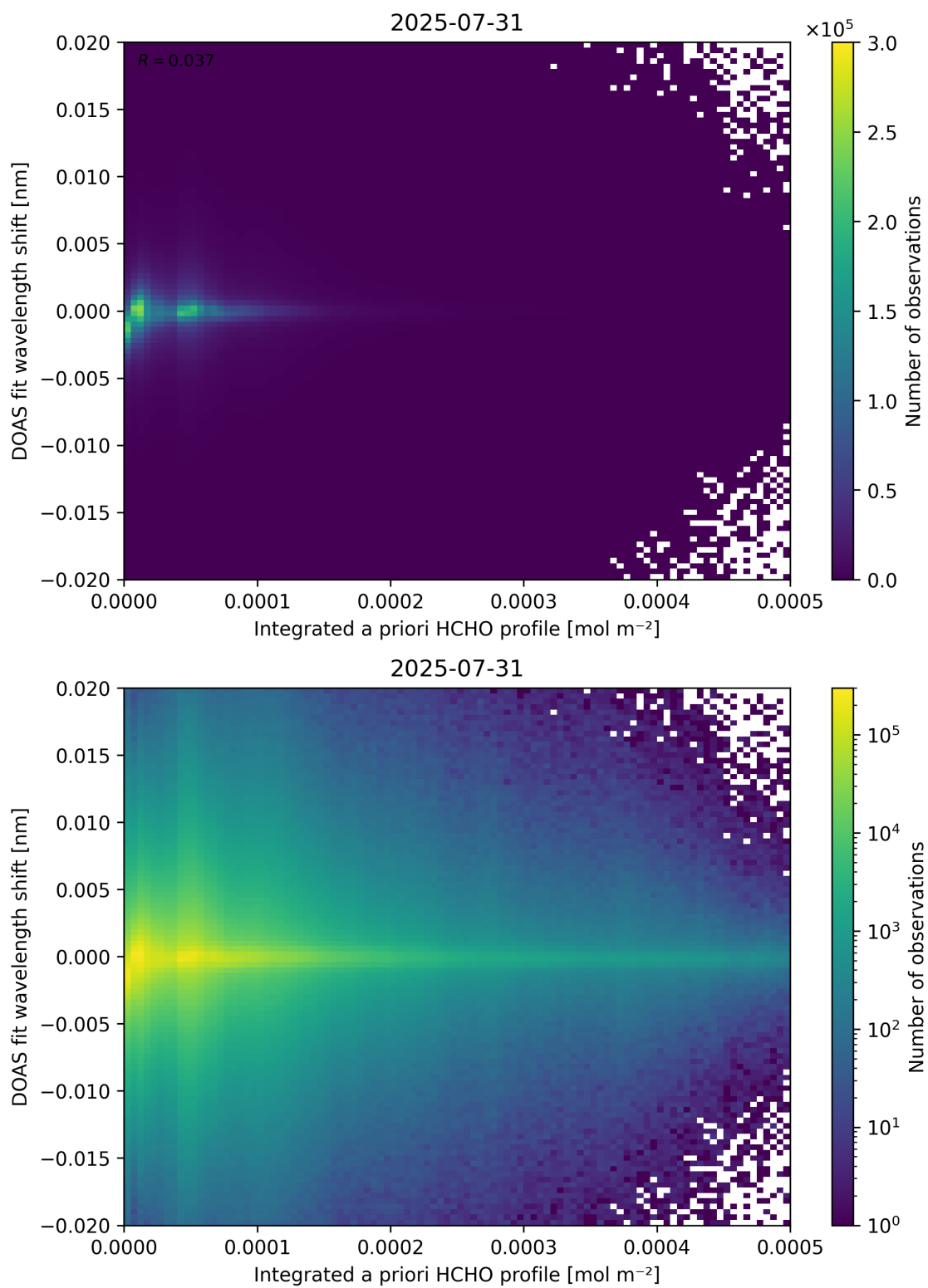
Figure 149: Scatter density plot of “Integrated a priori HCHO profile” against “DOAS fit wavelength shift” for 2025-07-30 to 2025-08-01.
