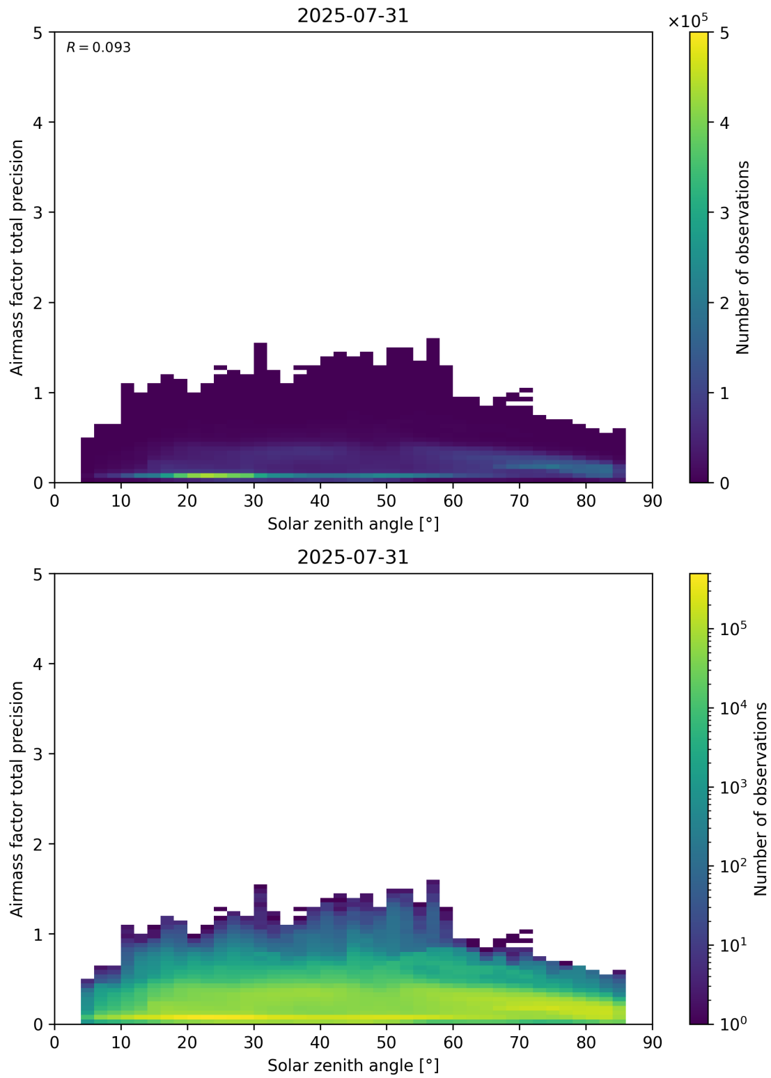
Figure 176: Scatter density plot of “Solar zenith angle” against “Airmass factor total precision” for 2025-07-30 to 2025-08-01.
