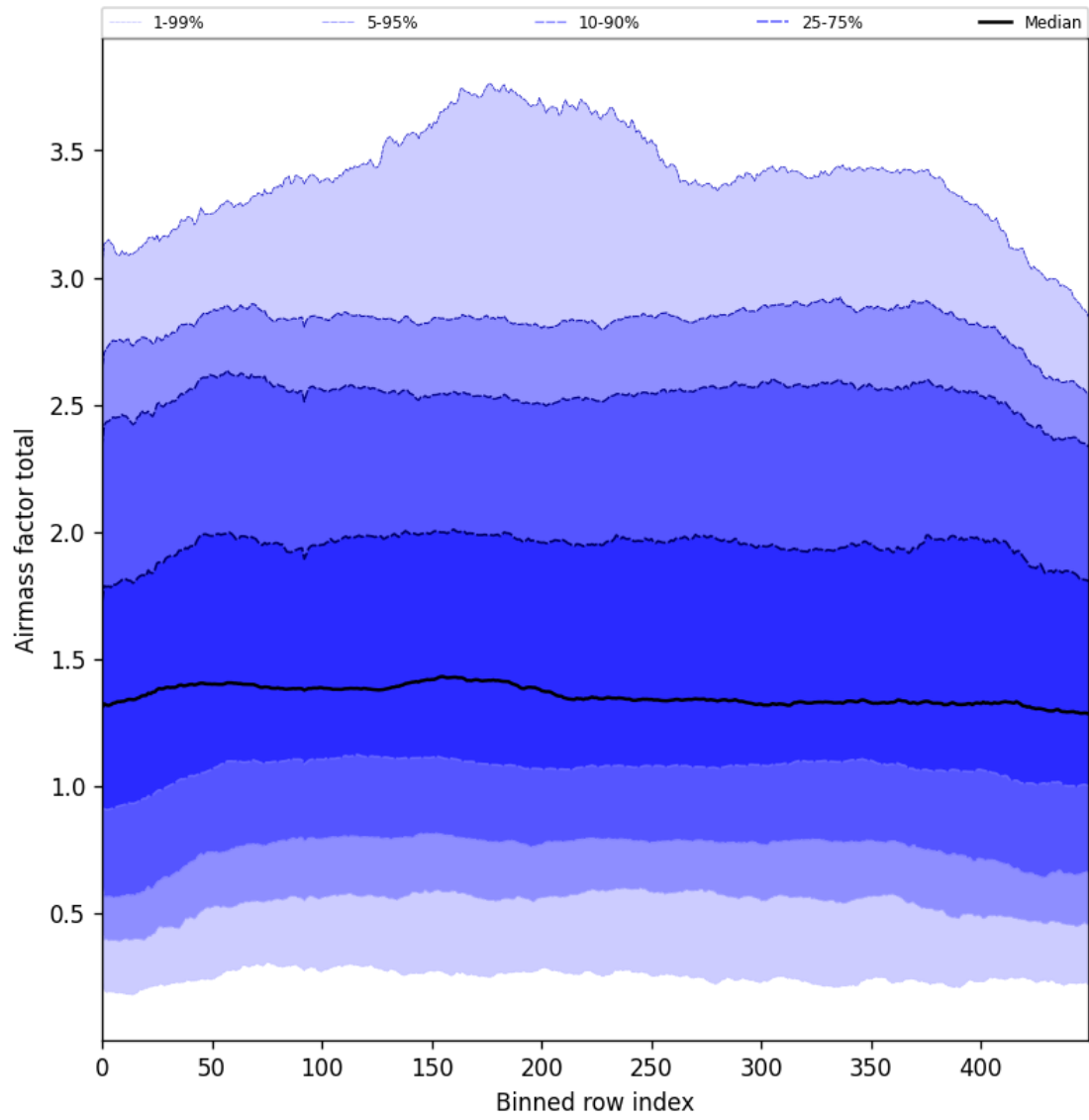
Figure 54: Along track statistics of “Airmass factor total” for 2025-07-30 to 2025-08-01
