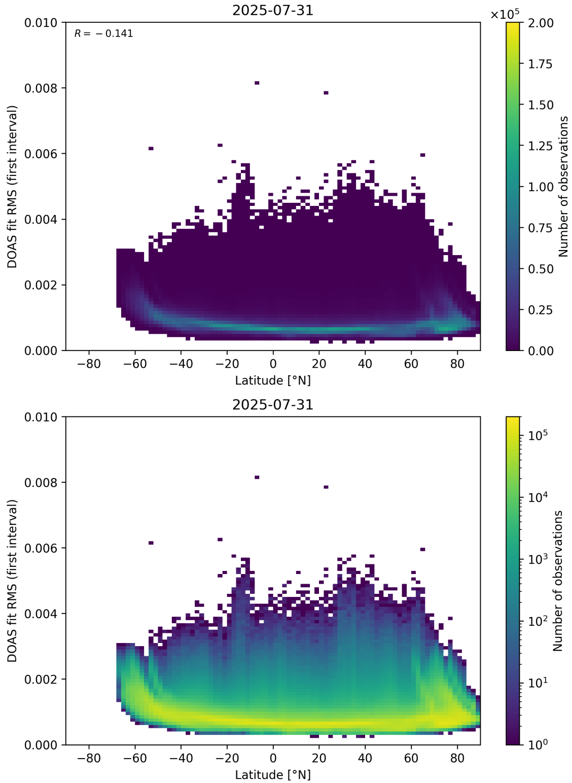
Figure 153: Scatter density plot of “Latitude” against “DOAS fit RMS (first interval)” for 2025-07-30 to 2025-08-01.
