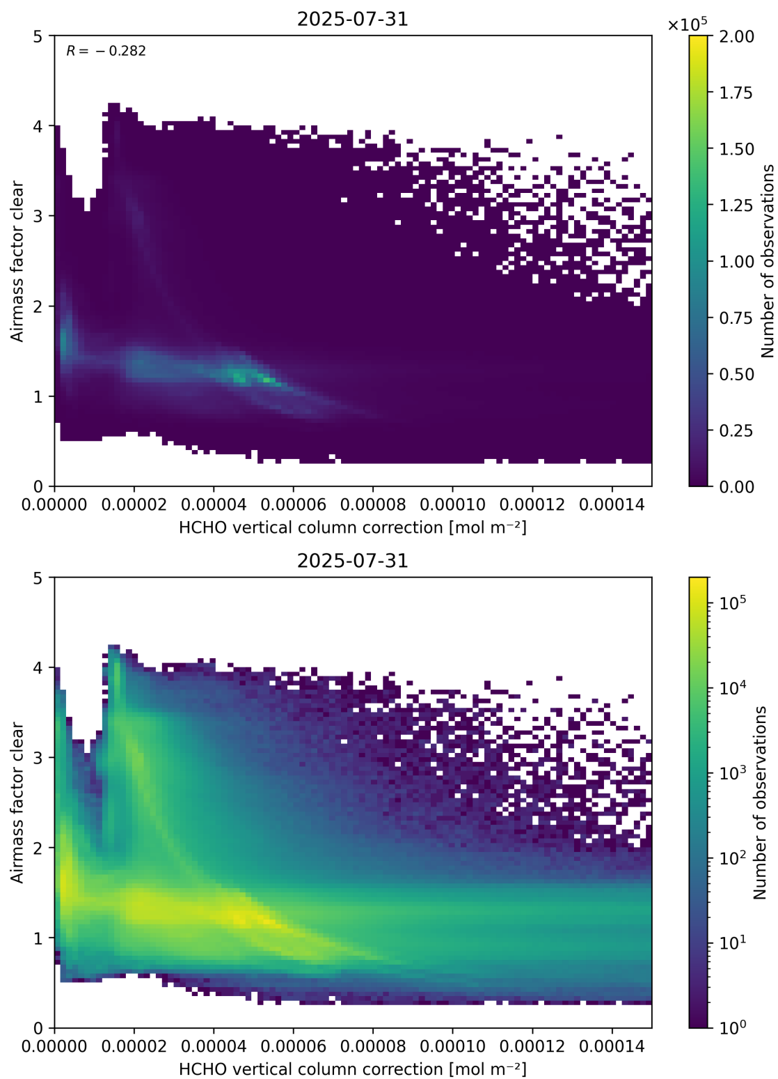
Figure 115: Scatter density plot of “HCHO vertical column correction” against “Airmass factor clear” for 2025-07-30 to 2025-08-01.
