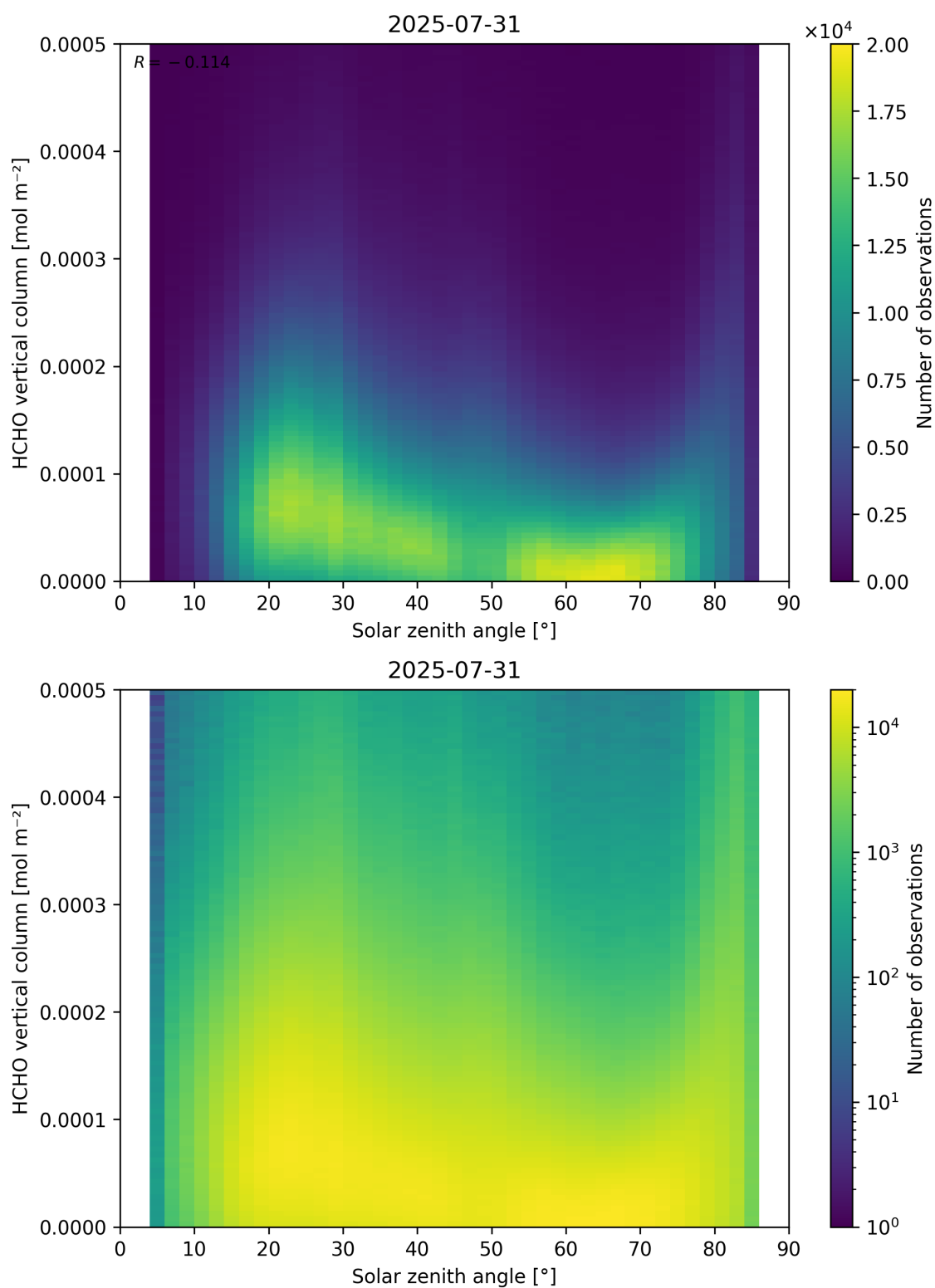
Figure 177: Scatter density plot of “Solar zenith angle” against “HCHO vertical column” for 2025-07-30 to 2025-08-01.
