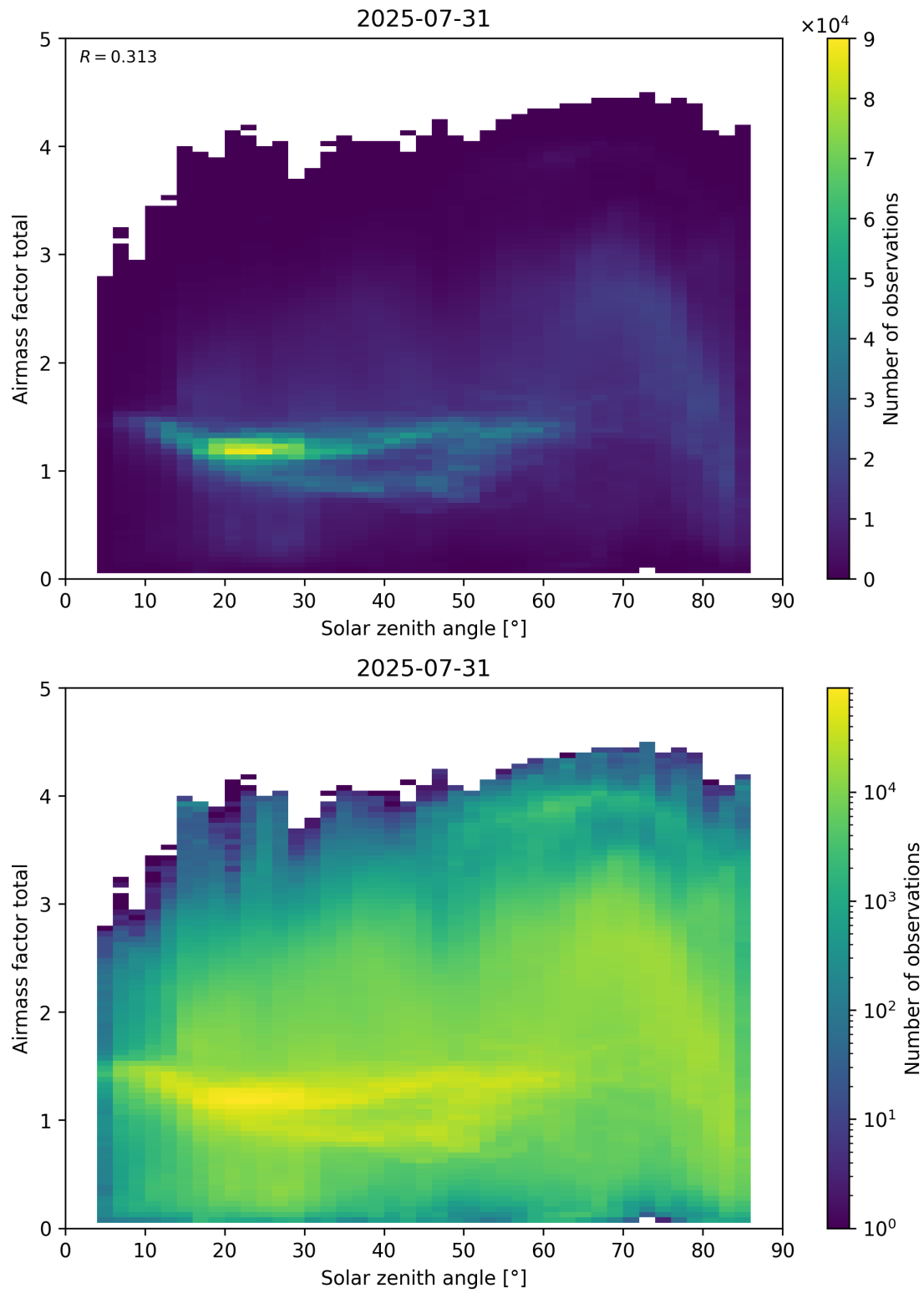
Figure 175: Scatter density plot of “Solar zenith angle” against “Airmass factor total” for 2025-07-30 to 2025-08-01.
