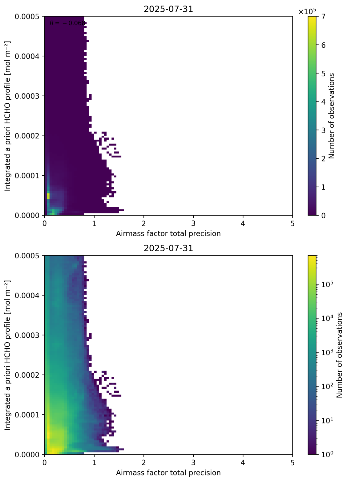
Figure 111: Scatter density plot of “Airmass factor total precision” against “Integrated a priori HCHO profile” for 2025-07-30 to 2025-08-01.
