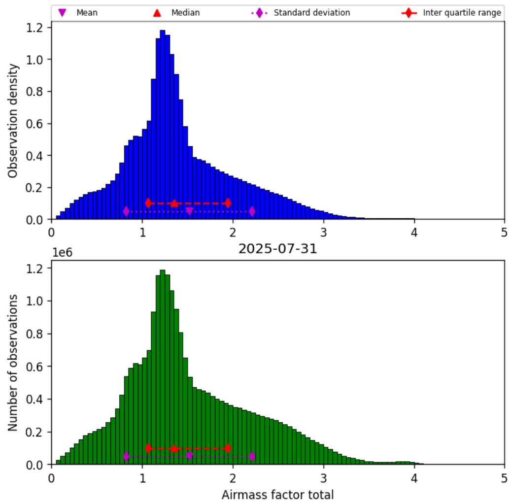
Figure 40: Histogram of “Airmass factor total” for 2025-07-30 to 2025-08-01
