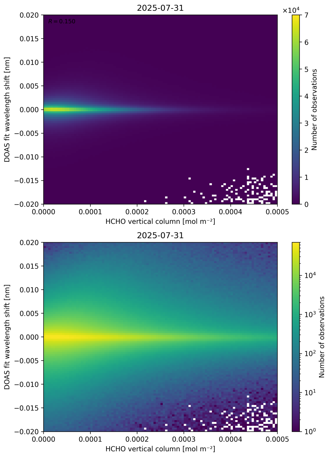
Figure 124: Scatter density plot of “HCHO vertical column” against “DOAS fit wavelength shift” for 2025-07-30 to 2025-08-01.
