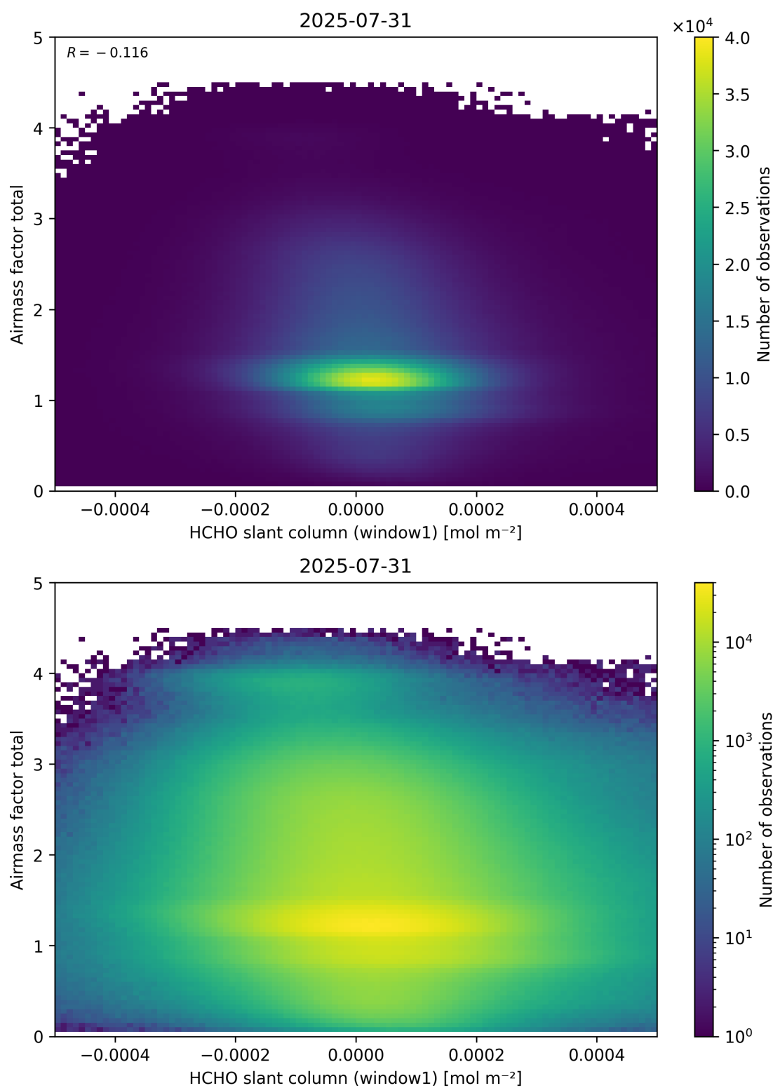
Figure 85: Scatter density plot of “HCHO slant column (window1)” against “Airmass factor total” for 2025-07-30 to 2025-08-01.
