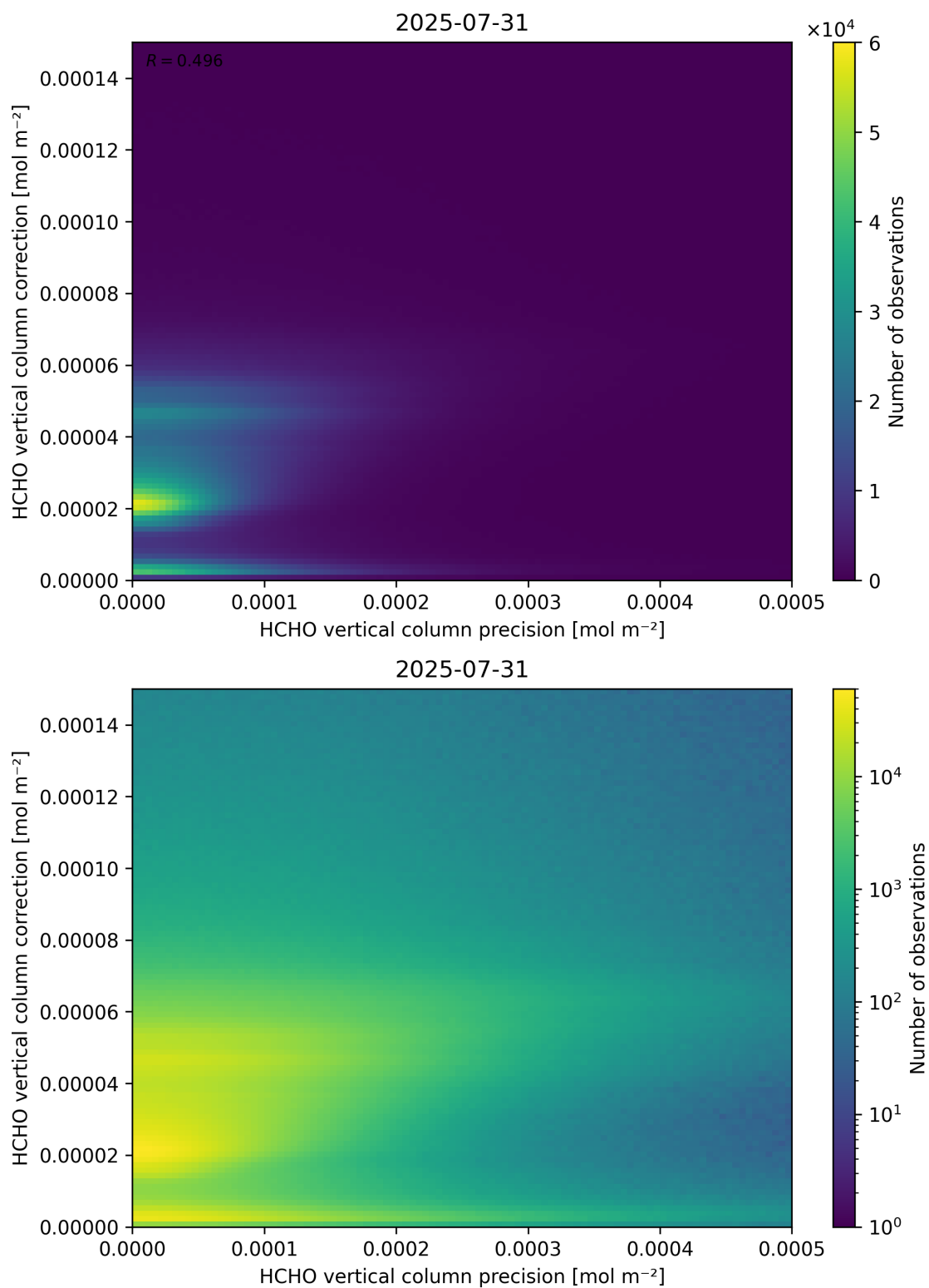
Figure 146: Scatter density plot of “HCHO vertical column precision” against “HCHO vertical column correction” for 2025-07-30 to 2025-08-01.
