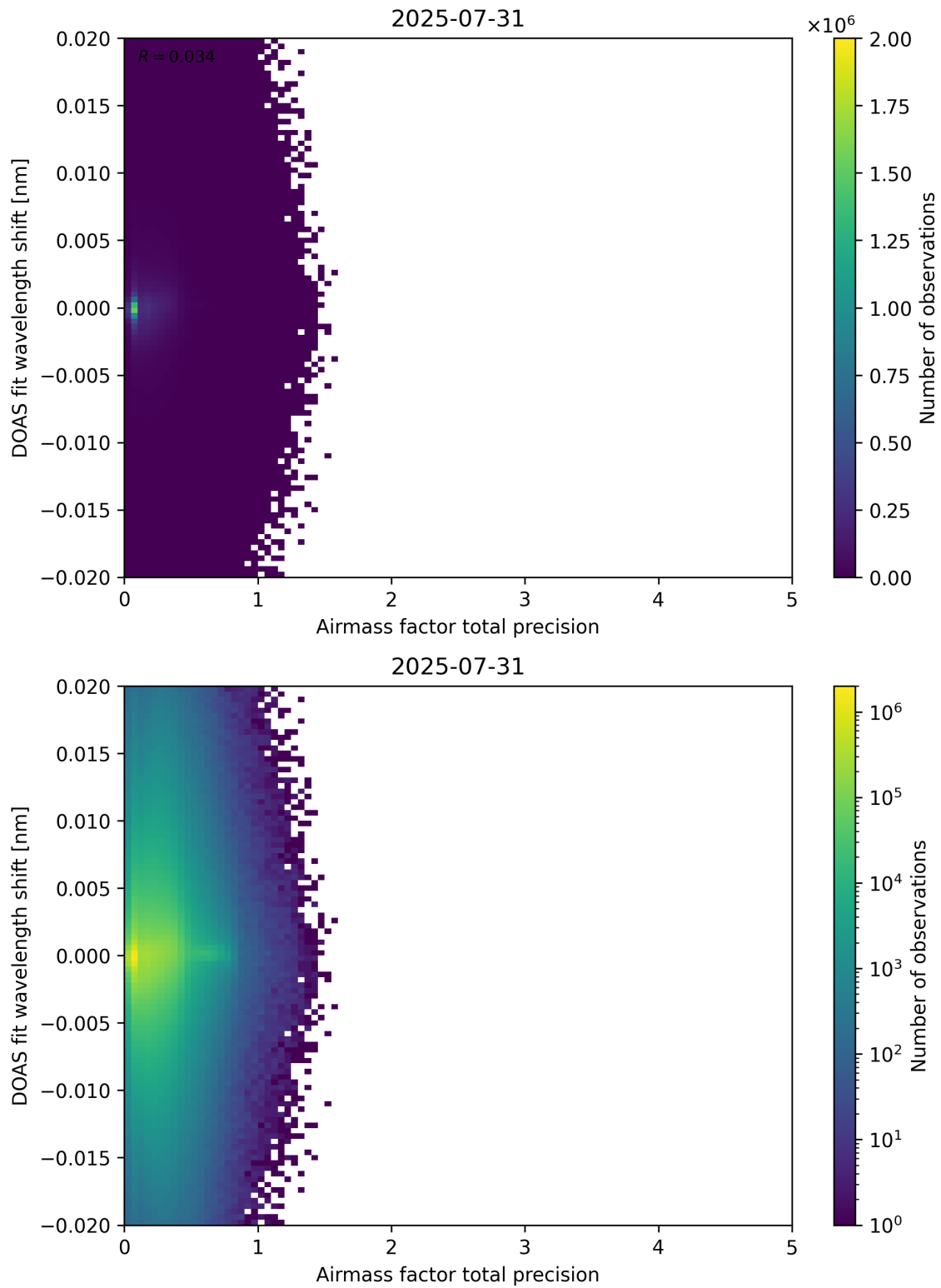
Figure 106: Scatter density plot of “Airmass factor total precision” against “DOAS fit wavelength shift” for 2025-07-30 to 2025-08-01.
