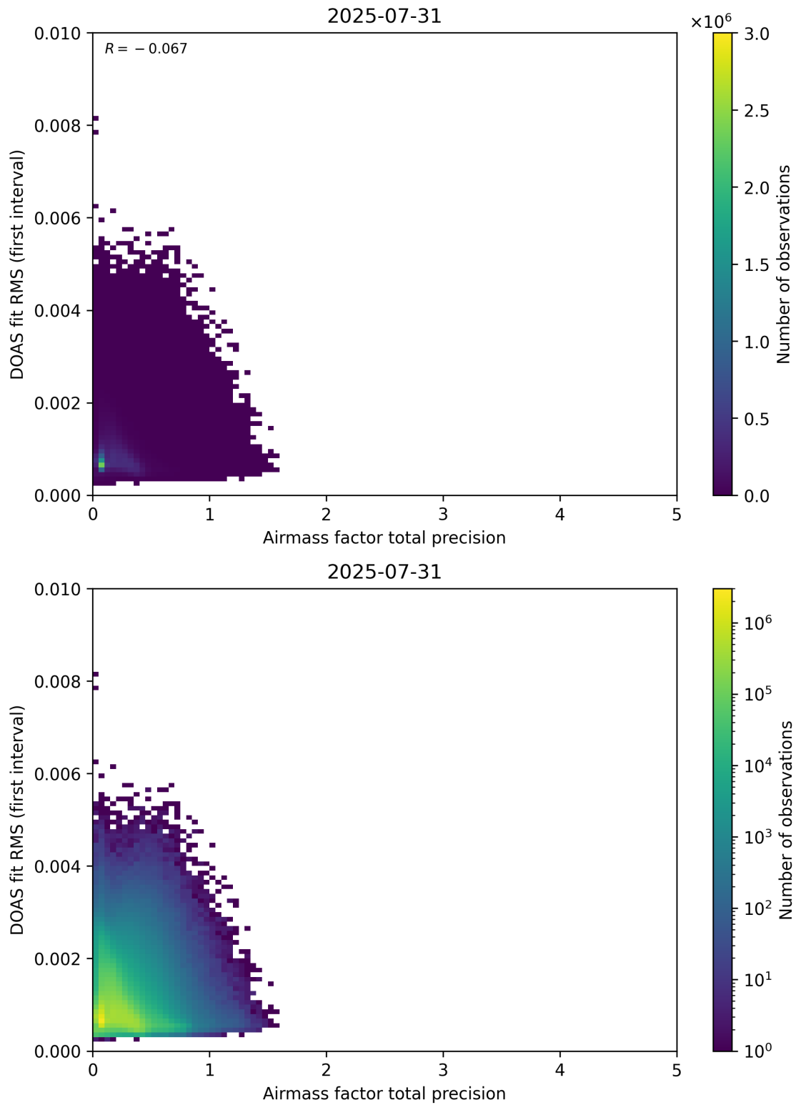
Figure 105: Scatter density plot of “Airmass factor total precision” against “DOAS fit RMS (first interval)” for 2025-07-30 to 2025-08-01.
