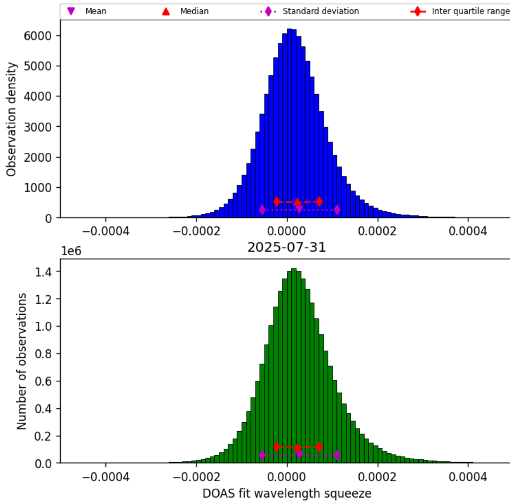
Figure 45: Histogram of “DOAS fit wavelength squeeze” for 2025-07-30 to 2025-08-01
