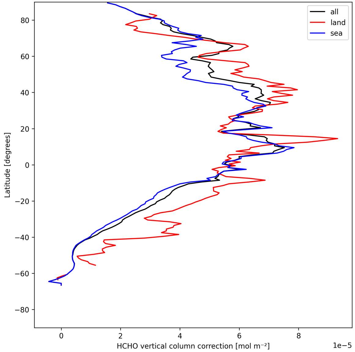
Figure 23: Zonal average of “HCHO vertical column correction” for 2025-07-30 to 2025-08-01.
