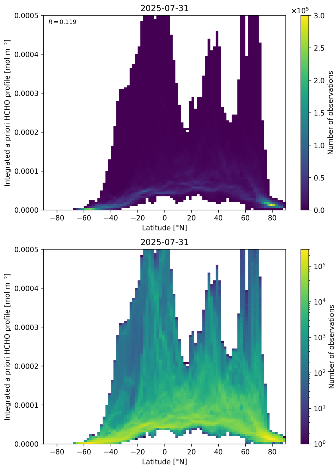
Figure 166: Scatter density plot of “Latitude” against “Integrated a priori HCHO profile” for 2025-07-30 to 2025-08-01.
