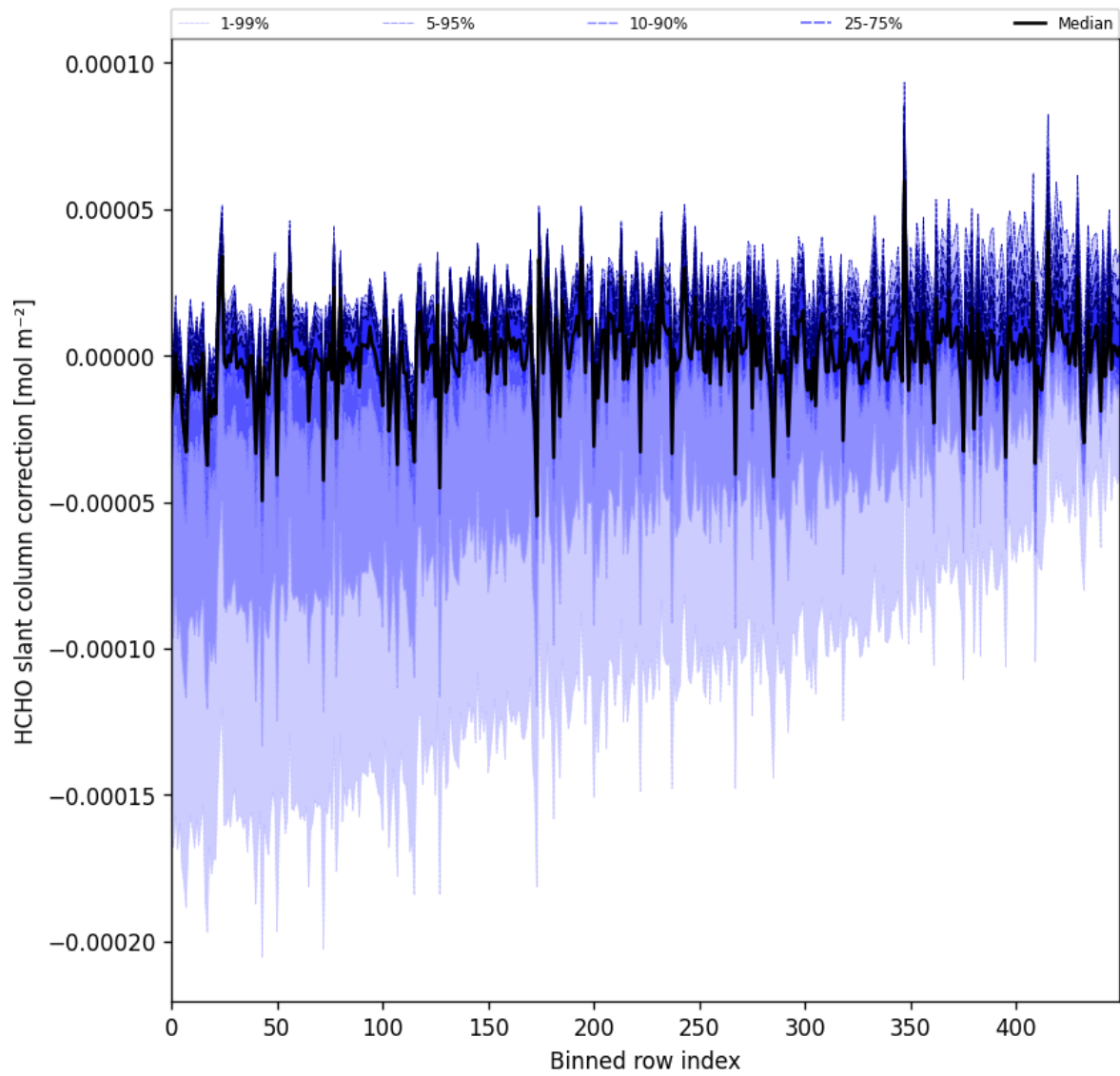
Figure 61: Along track statistics of “HCHO slant column correction” for 2025-07-30 to 2025-08-01
