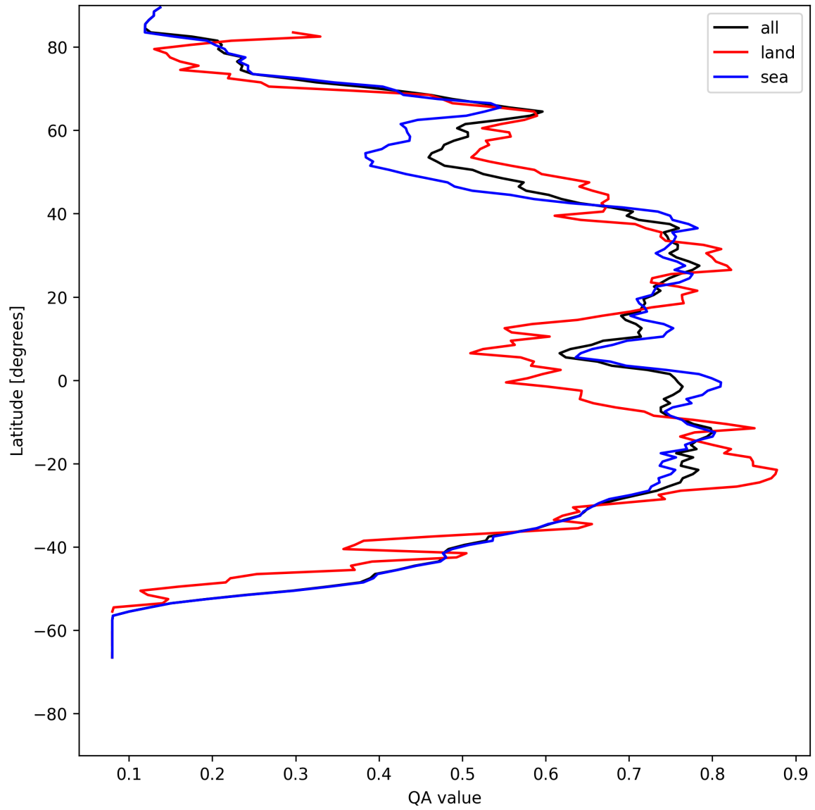
Figure 20: Zonal average of “QA value” for 2025-07-30 to 2025-08-01.
