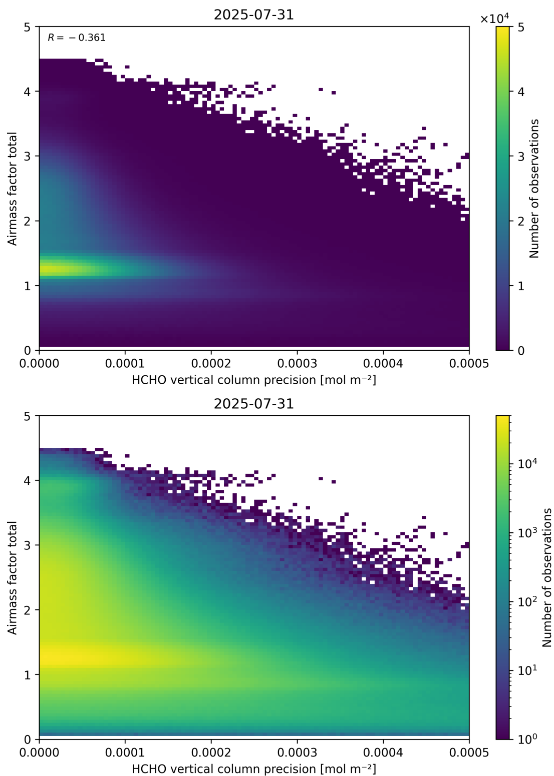
Figure 144: Scatter density plot of “HCHO vertical column precision” against “Airmass factor total” for 2025-07-30 to 2025-08-01.
