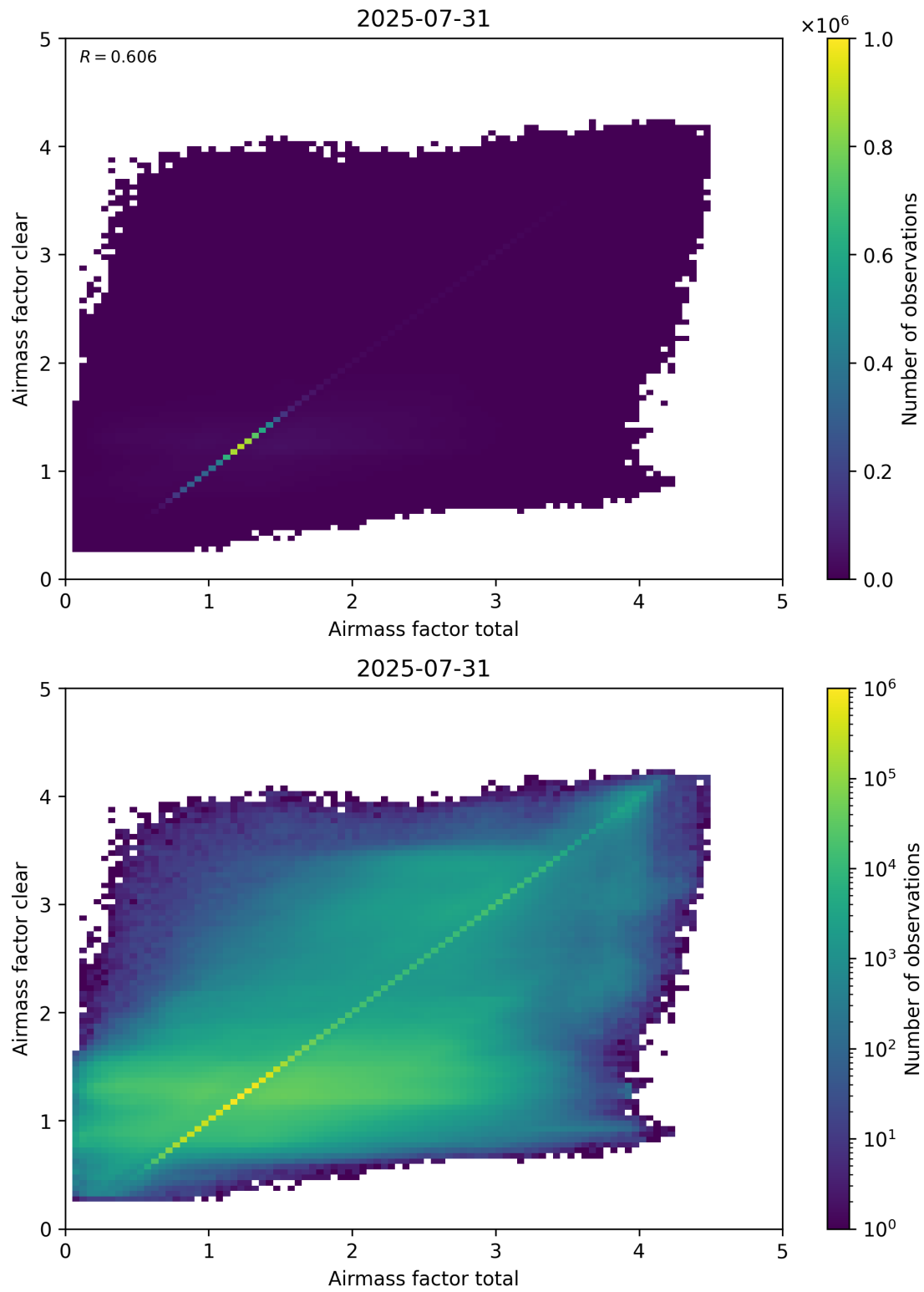
Figure 100: Scatter density plot of “Airmass factor total” against “Airmass factor clear” for 2025-07-30 to 2025-08-01.
