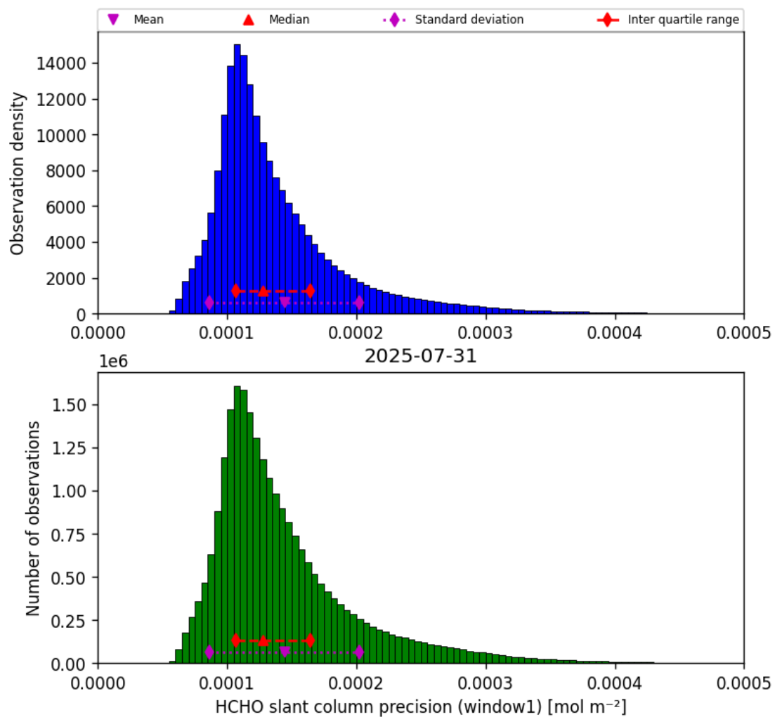
Figure 39: Histogram of “HCHO slant column precision (window1)” for 2025-07-30 to 2025-08-01
