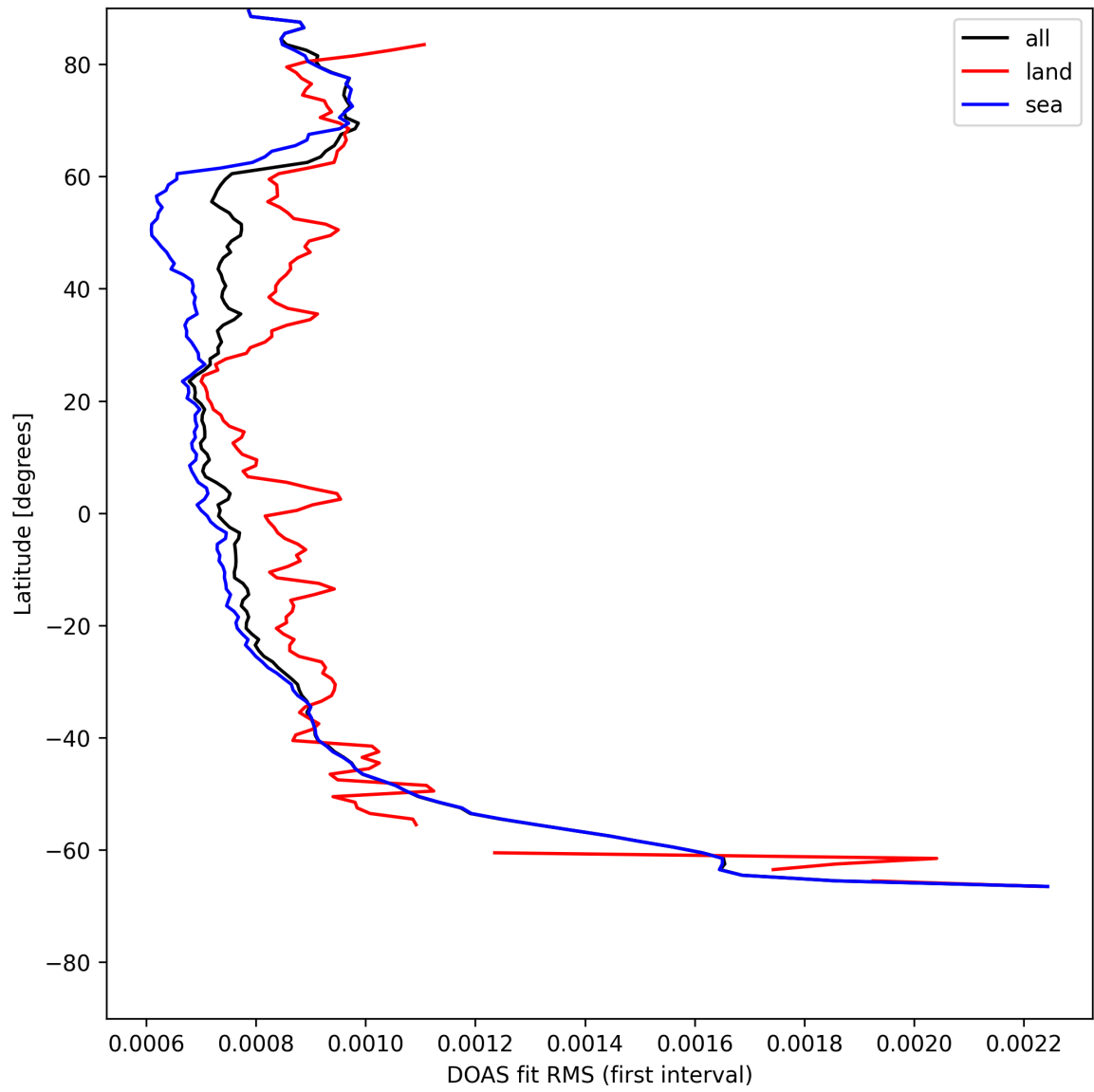
Figure 32: Zonal average of “DOAS fit RMS (first interval)” for 2025-07-30 to 2025-08-01.
