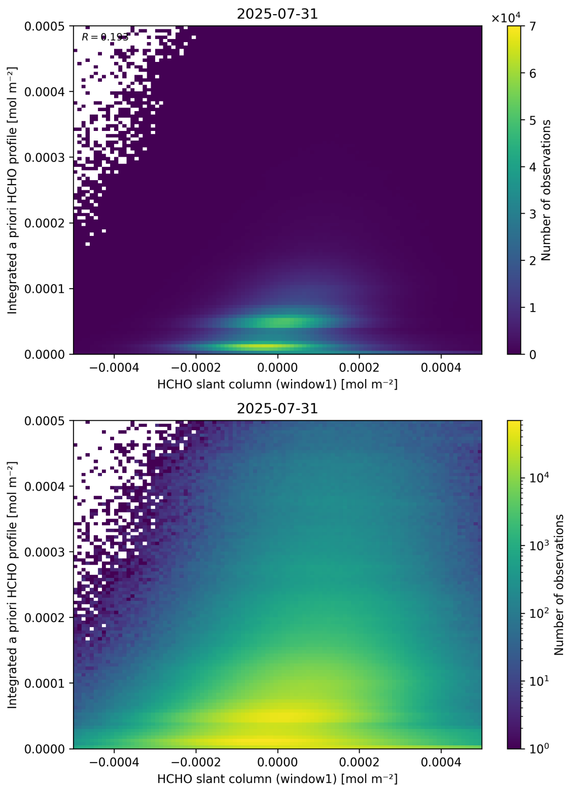
Figure 87: Scatter density plot of “HCHO slant column (window1)” against “Integrated a priori HCHO profile” for 2025-07-30 to 2025-08-01.
