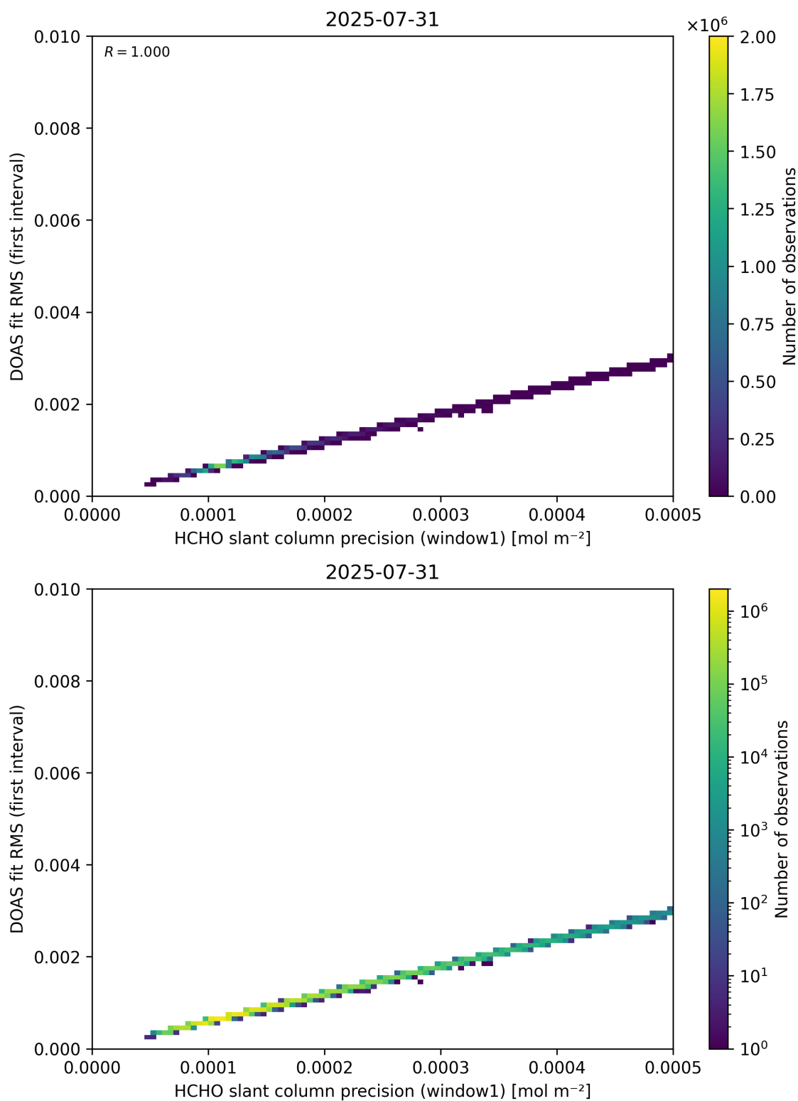
Figure 88: Scatter density plot of “HCHO slant column precision (window1)” against “DOAS fit RMS (first interval)” for 2025-07-30 to 2025-08-01.
