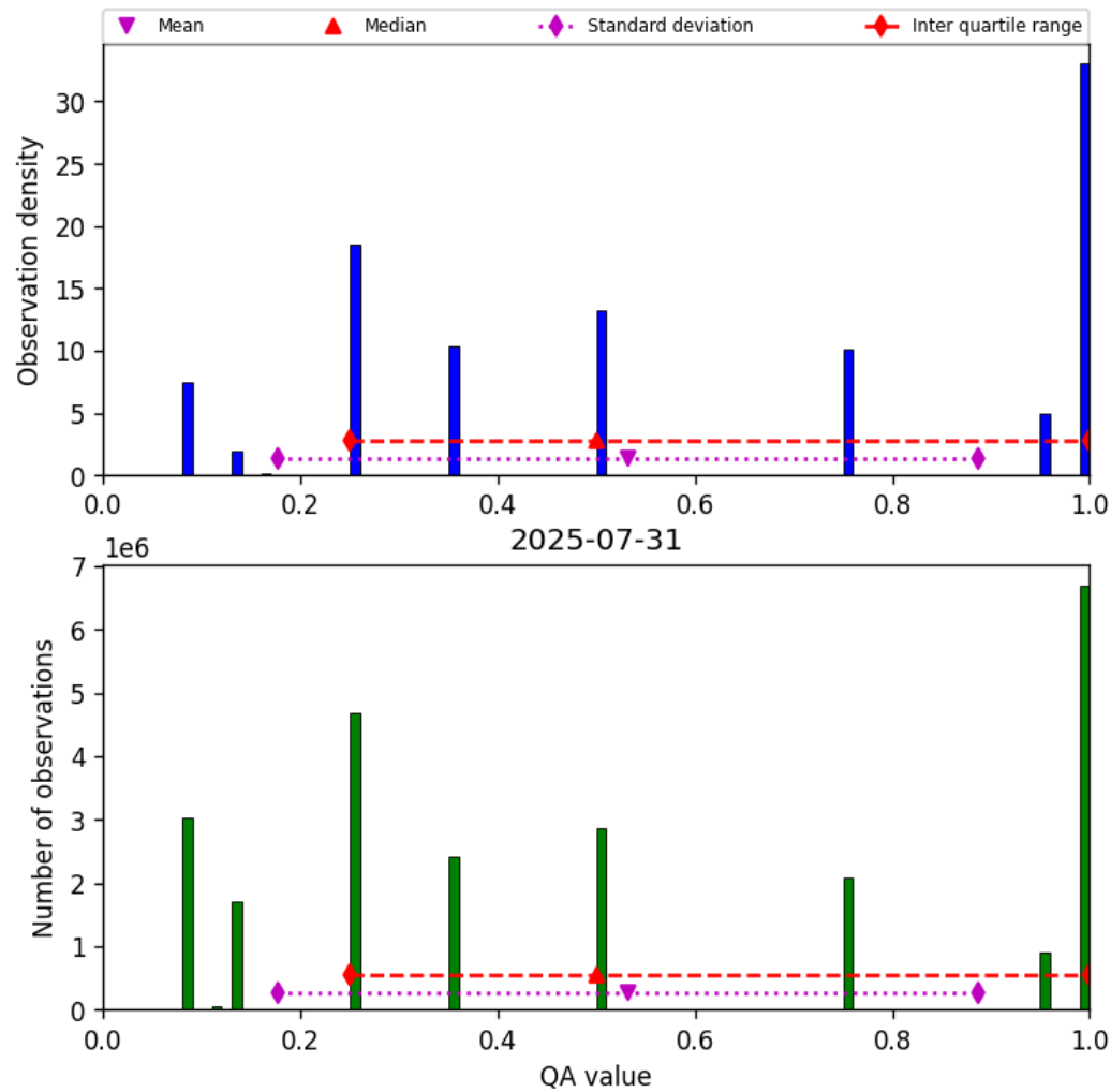
Figure 34: Histogram of “QA value” for 2025-07-30 to 2025-08-01
