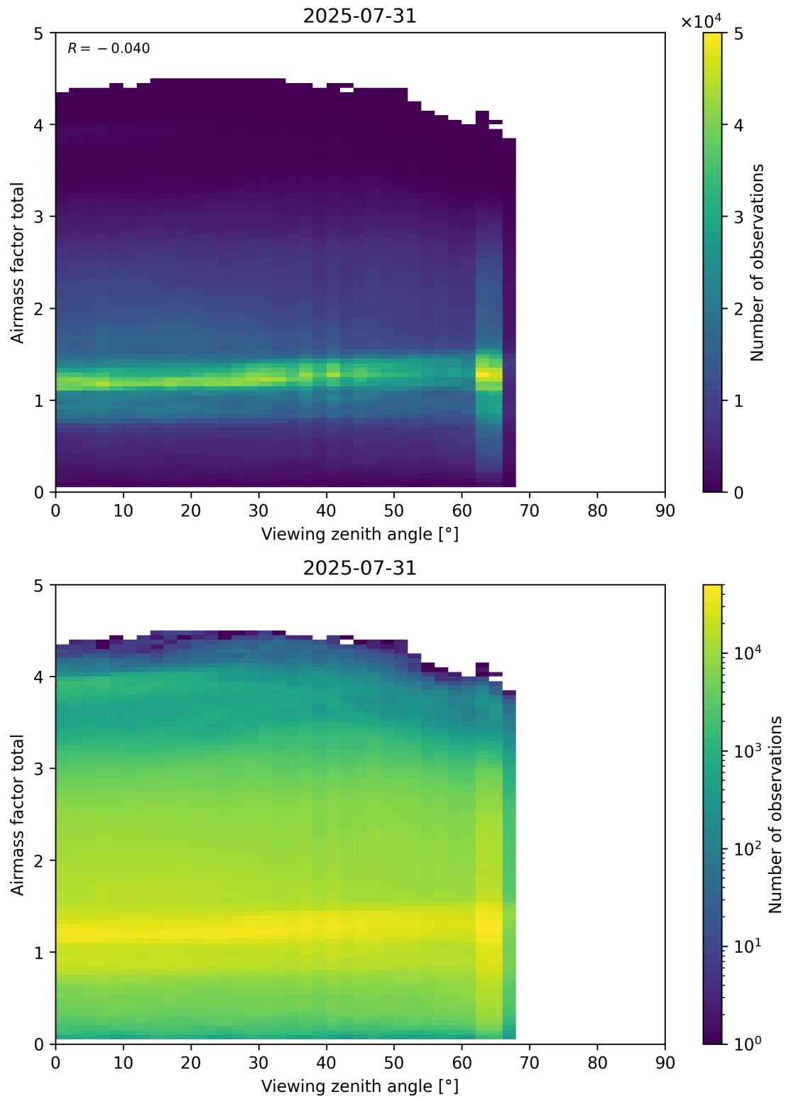
Figure 190: Scatter density plot of “Viewing zenith angle” against “Airmass factor total” for 2025-07-30 to 2025-08-01.
