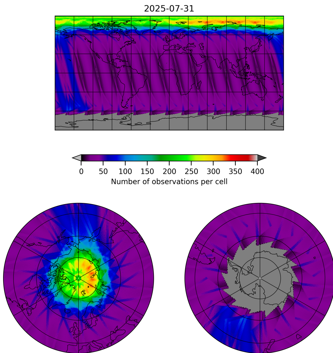
Figure 19: Map of the number of observations for 2025-07-30 to 2025-08-01
