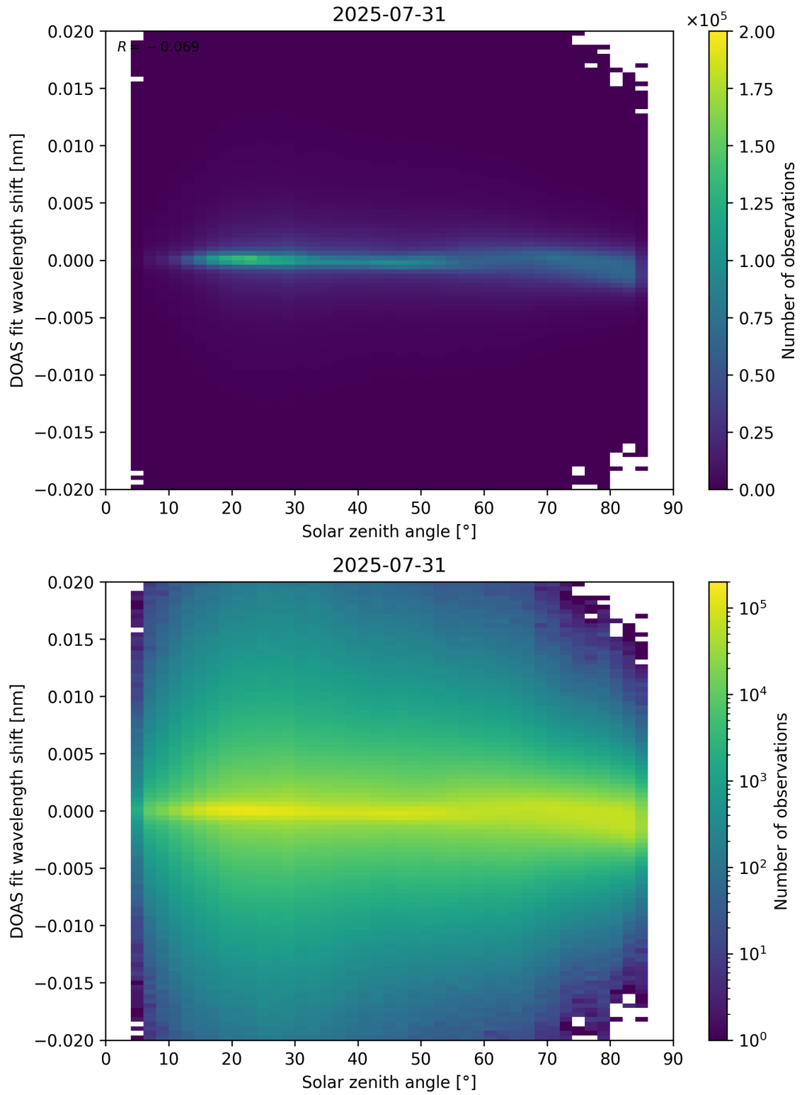
Figure 168: Scatter density plot of “Solar zenith angle” against “DOAS fit wavelength shift” for 2025-07-30 to 2025-08-01.
