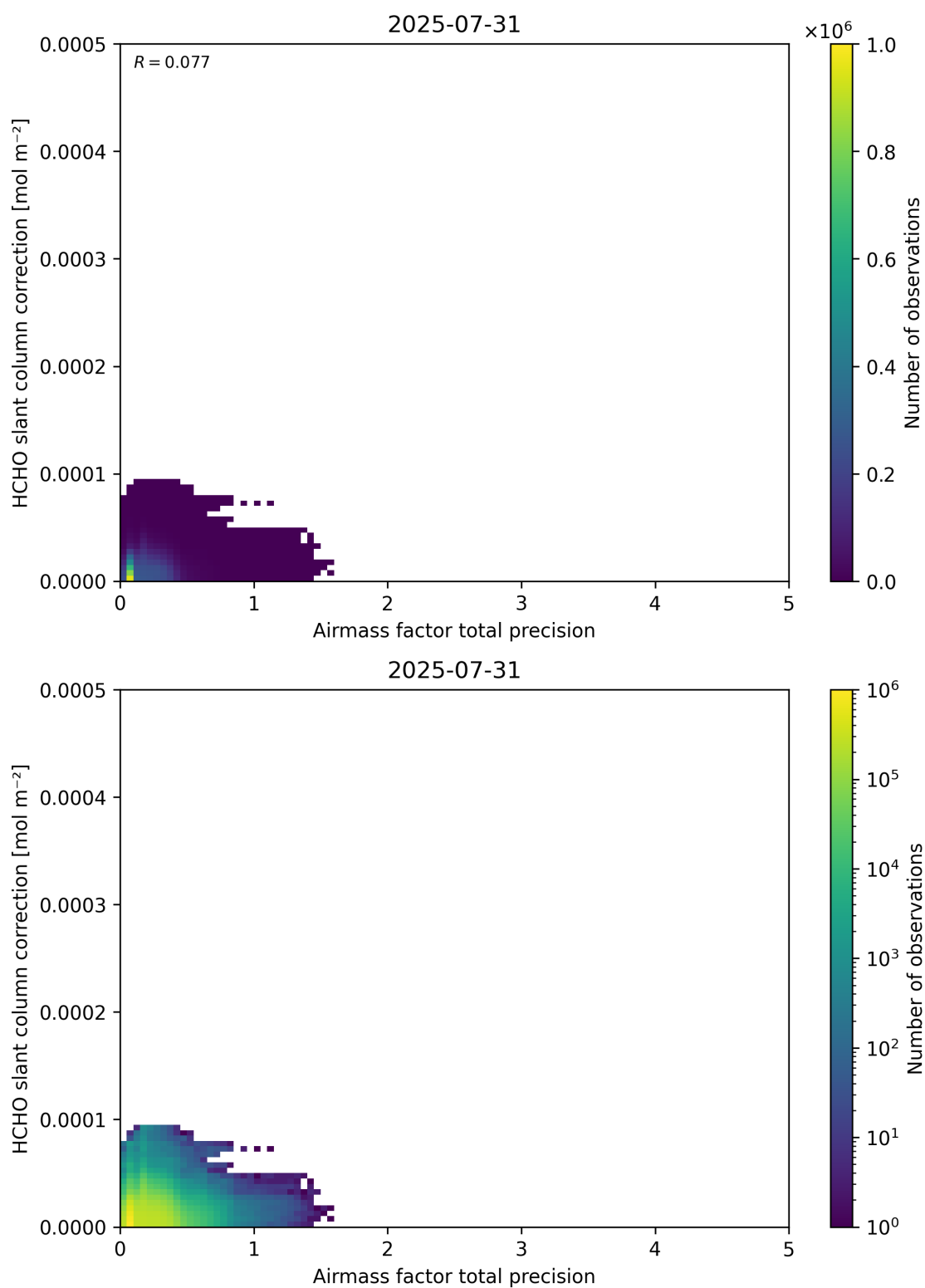
Figure 110: Scatter density plot of “Airmass factor total precision” against “HCHO slant column correction” for 2025-07-30 to 2025-08-01.
