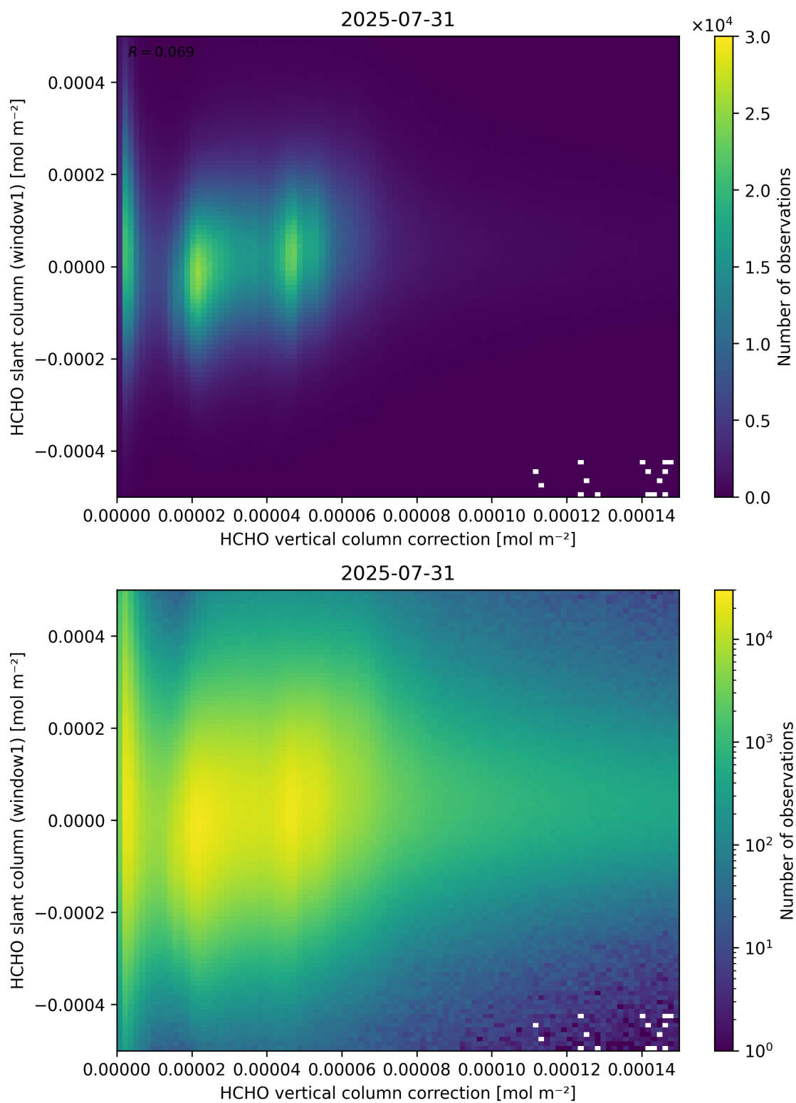
Figure 118: Scatter density plot of “HCHO vertical column correction” against “HCHO slant column (window1)” for 2025-07-30 to 2025-08-01.
