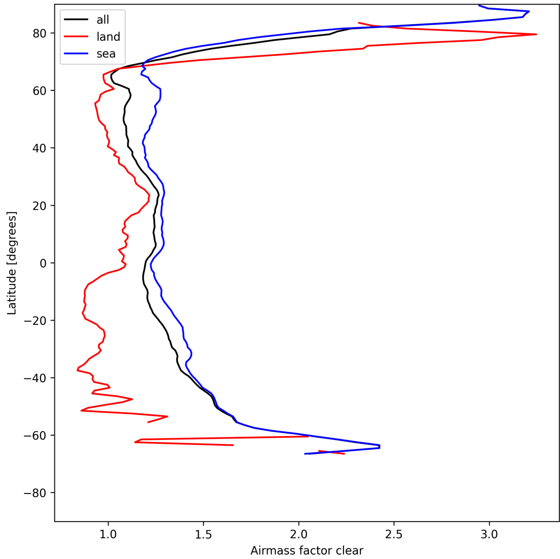
Figure 28: Zonal average of “Airmass factor clear” for 2025-07-30 to 2025-08-01.
