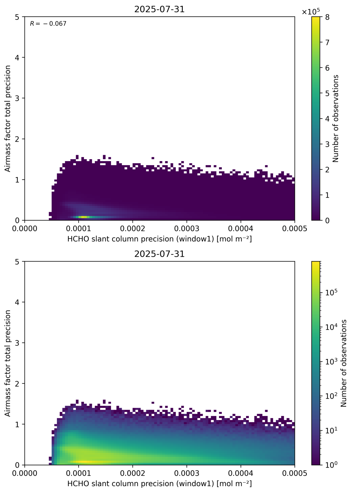
Figure 95: Scatter density plot of “HCHO slant column precision (window1)” against “Airmass factor total precision” for 2025-07-30 to 2025-08-01.
