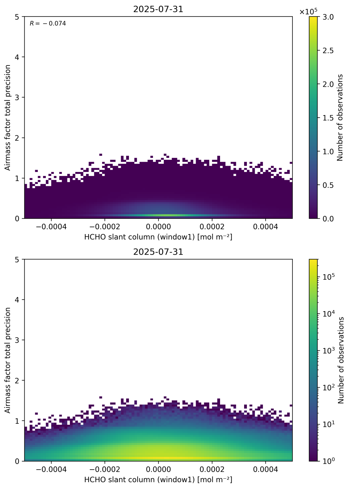
Figure 86: Scatter density plot of “HCHO slant column (window1)” against “Airmass factor total precision” for 2025-07-30 to 2025-08-01.
