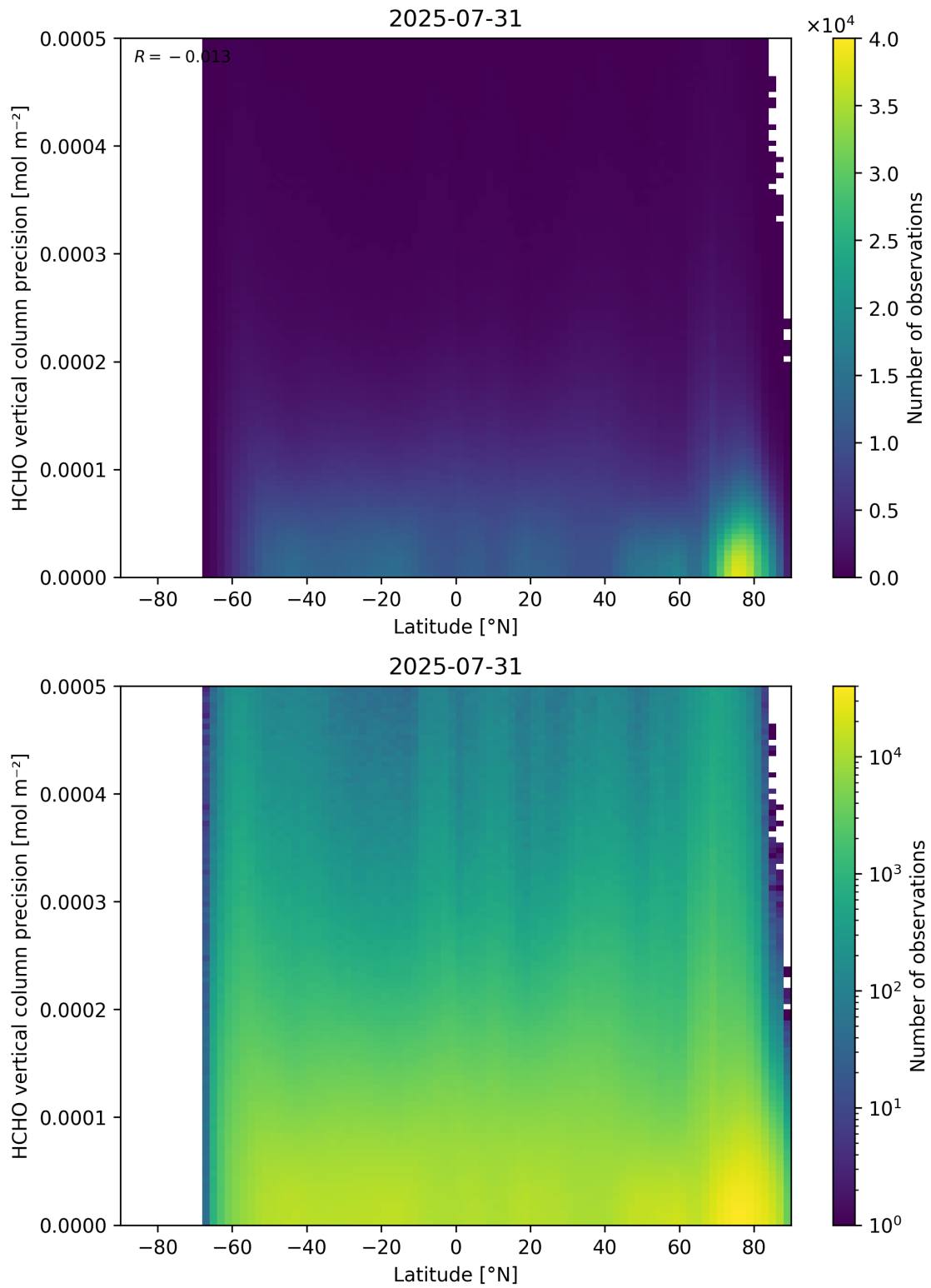
Figure 165: Scatter density plot of “Latitude” against “HCHO vertical column precision” for 2025-07-30 to 2025-08-01.
