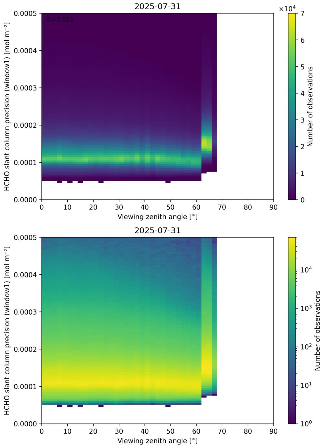
Figure 189: Scatter density plot of “Viewing zenith angle” against “HCHO slant column precision (window1)” for 2025-07-30 to 2025-08-01.
