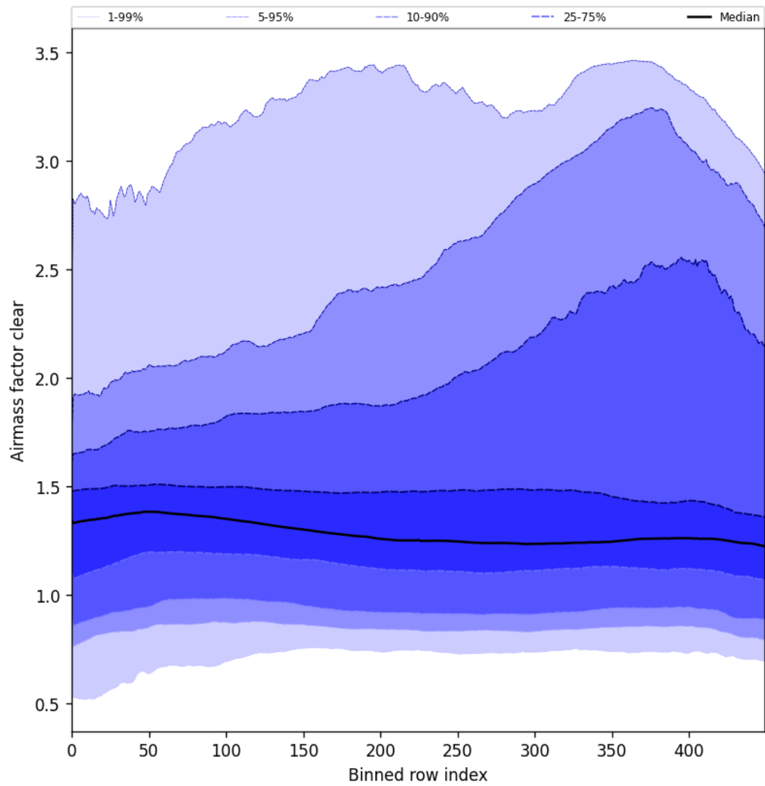
Figure 56: Along track statistics of “Airmass factor clear” for 2025-07-30 to 2025-08-01
