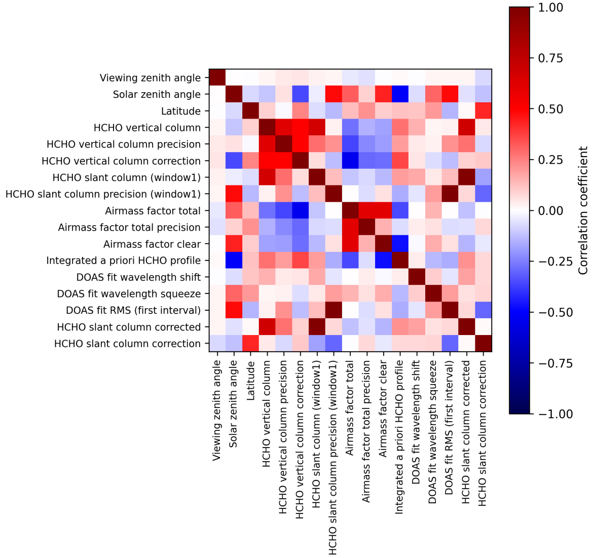
Figure 2: Map of correlation matrix for 2025-07-30 to 2025-08-01.
