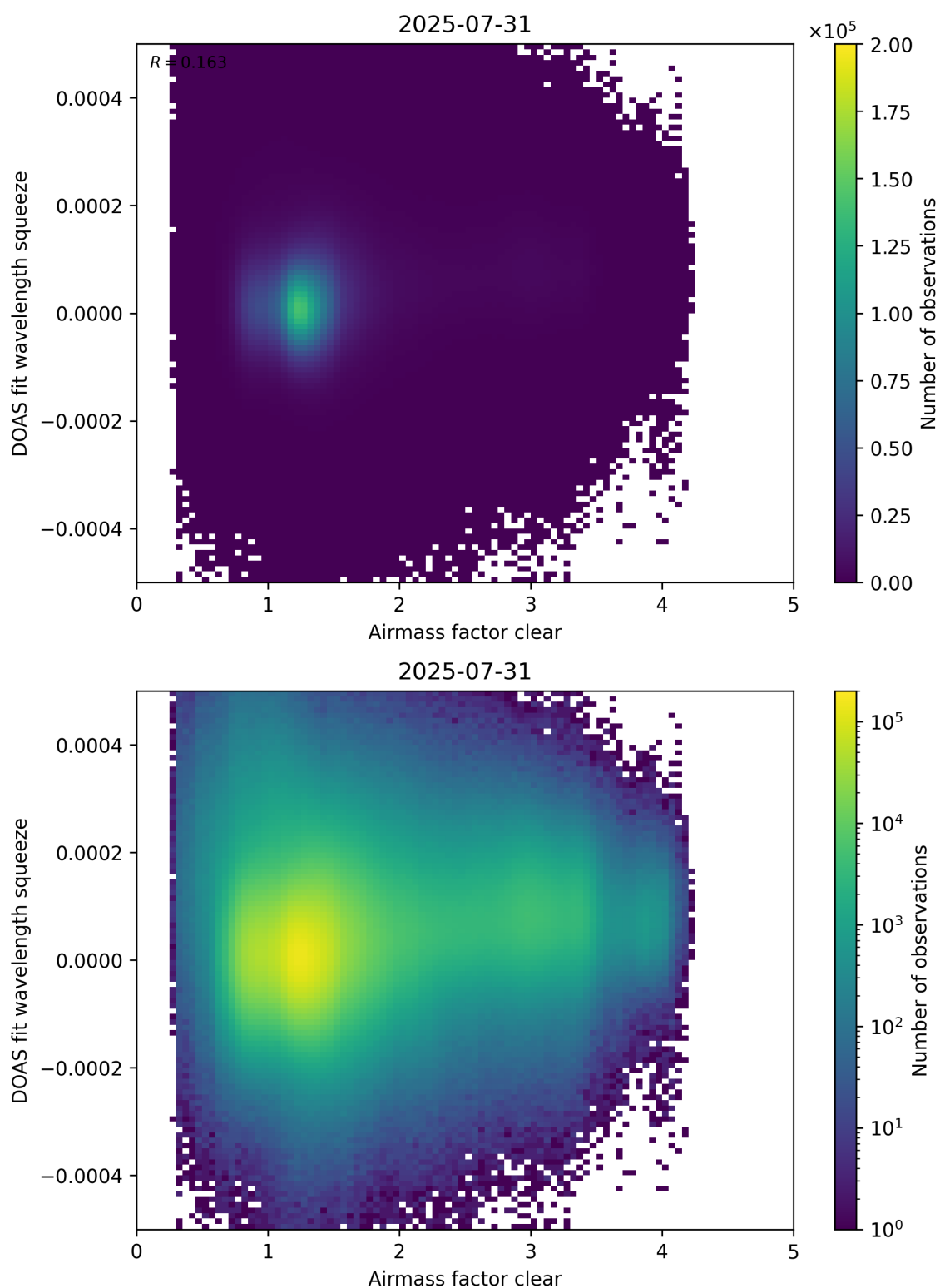
Figure 73: Scatter density plot of “Airmass factor clear” against “DOAS fit wavelength squeeze” for 2025-07-30 to 2025-08-01.
