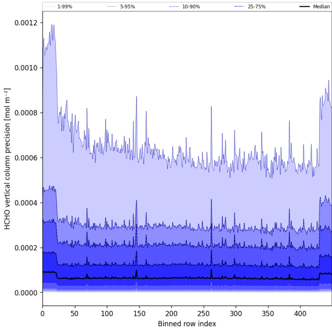
Figure 50: Along track statistics of “HCHO vertical column precision” for 2025-07-30 to 2025-08-01
