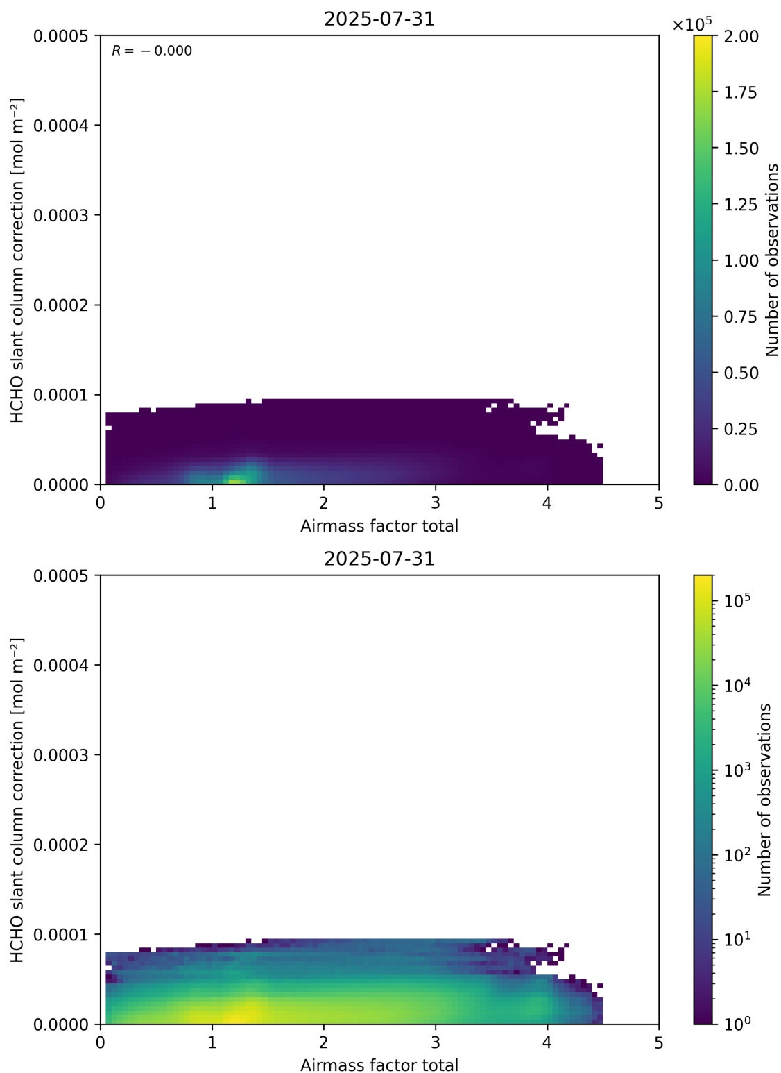
Figure 102: Scatter density plot of “Airmass factor total” against “HCHO slant column correction” for 2025-07-30 to 2025-08-01.
