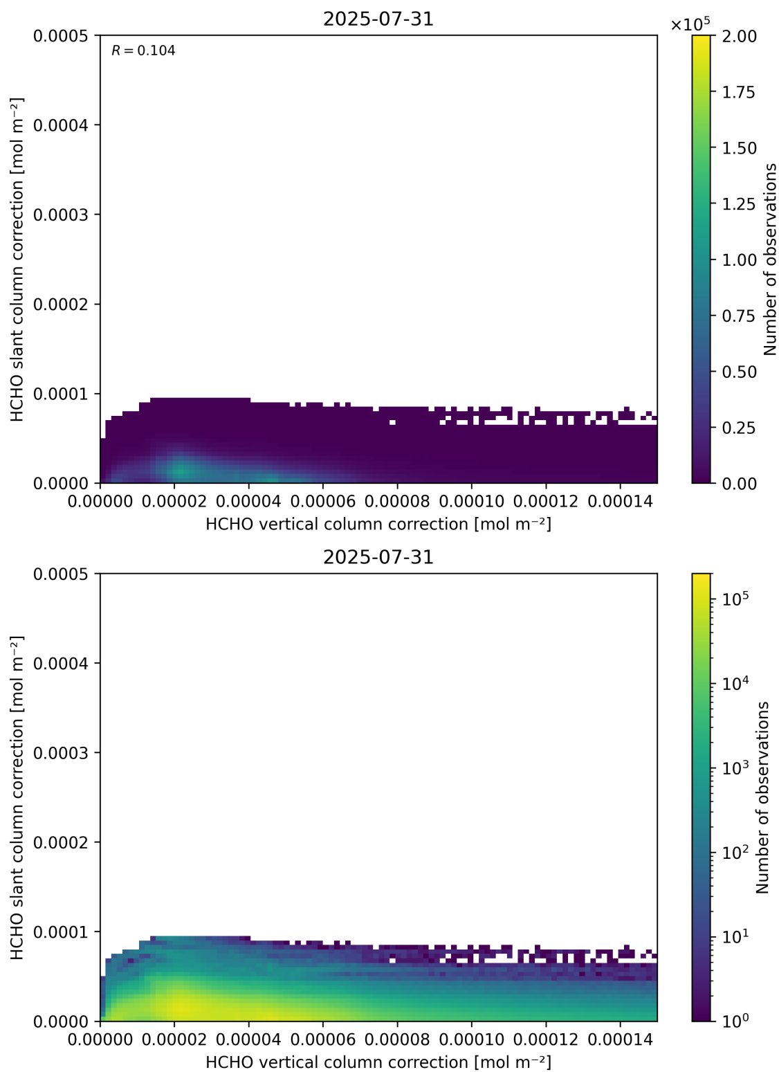
Figure 117: Scatter density plot of “HCHO vertical column correction” against “HCHO slant column correction” for 2025-07-30 to 2025-08-01.
