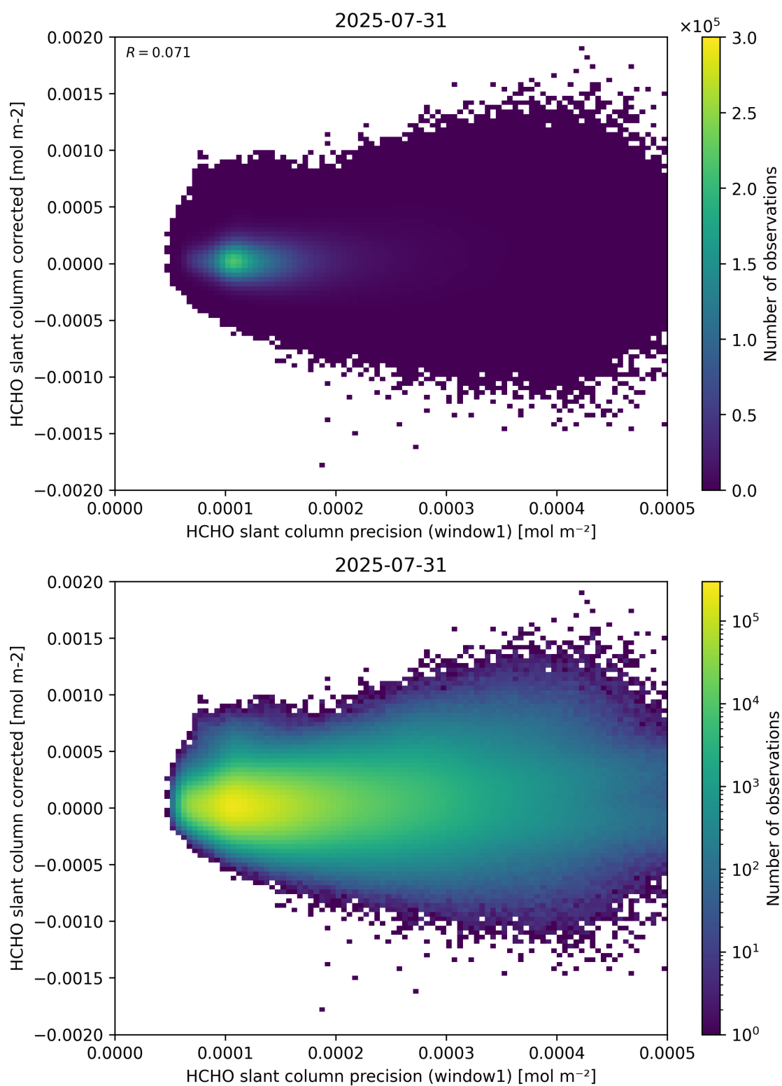
Figure 92: Scatter density plot of “HCHO slant column precision (window1)” against “HCHO slant column corrected” for 2025-07-30 to 2025-08-01.
