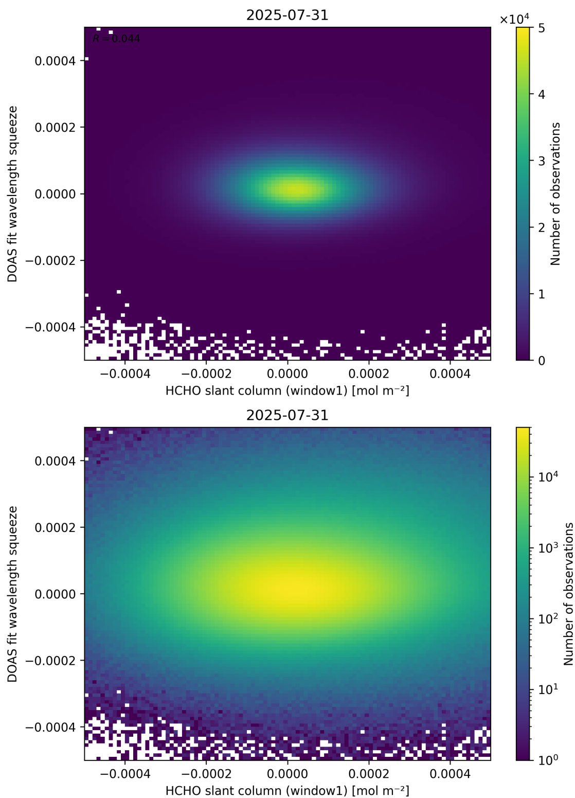
Figure 80: Scatter density plot of “HCHO slant column (window1)” against “DOAS fit wavelength squeeze” for 2025-07-30 to 2025-08-01.
