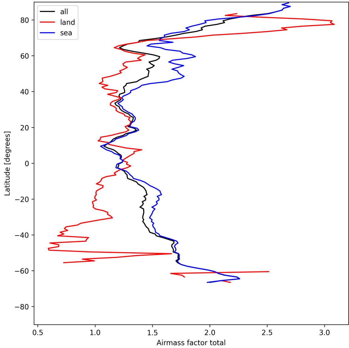
Figure 26: Zonal average of “Airmass factor total” for 2025-07-30 to 2025-08-01.
