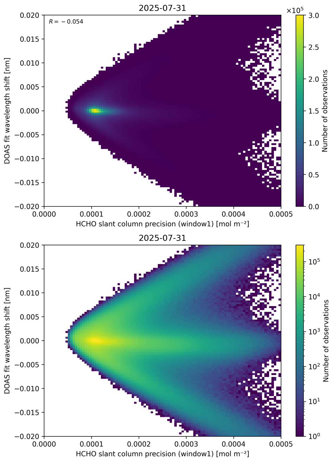
Figure 89: Scatter density plot of “HCHO slant column precision (window1)” against “DOAS fit wavelength shift” for 2025-07-30 to 2025-08-01.
