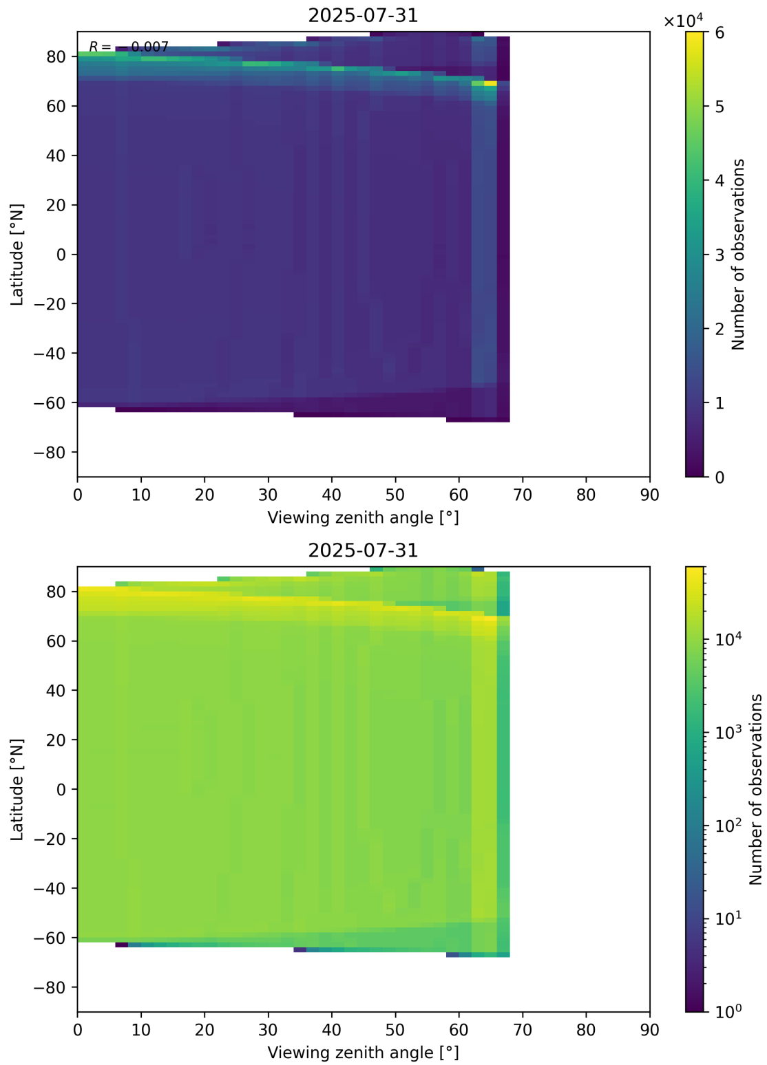
Figure 196: Scatter density plot of “Viewing zenith angle” against “Latitude” for 2025-07-30 to 2025-08-01.
