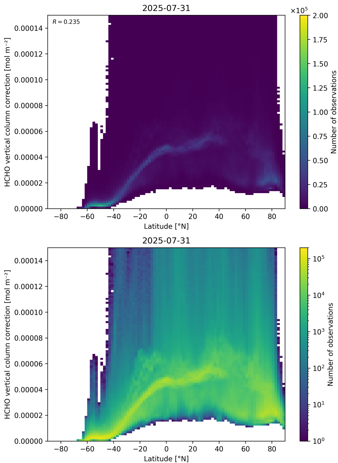
Figure 164: Scatter density plot of “Latitude” against “HCHO vertical column correction” for 2025-07-30 to 2025-08-01.
