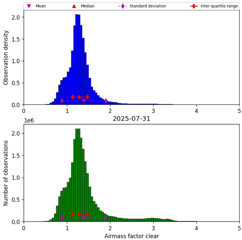
Figure 42: Histogram of “Airmass factor clear” for 2025-07-30 to 2025-08-01
