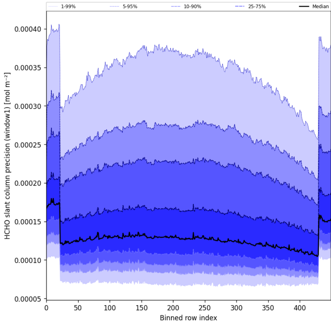
Figure 53: Along track statistics of “HCHO slant column precision (window1)” for 2025-07-30 to 2025-08-01
