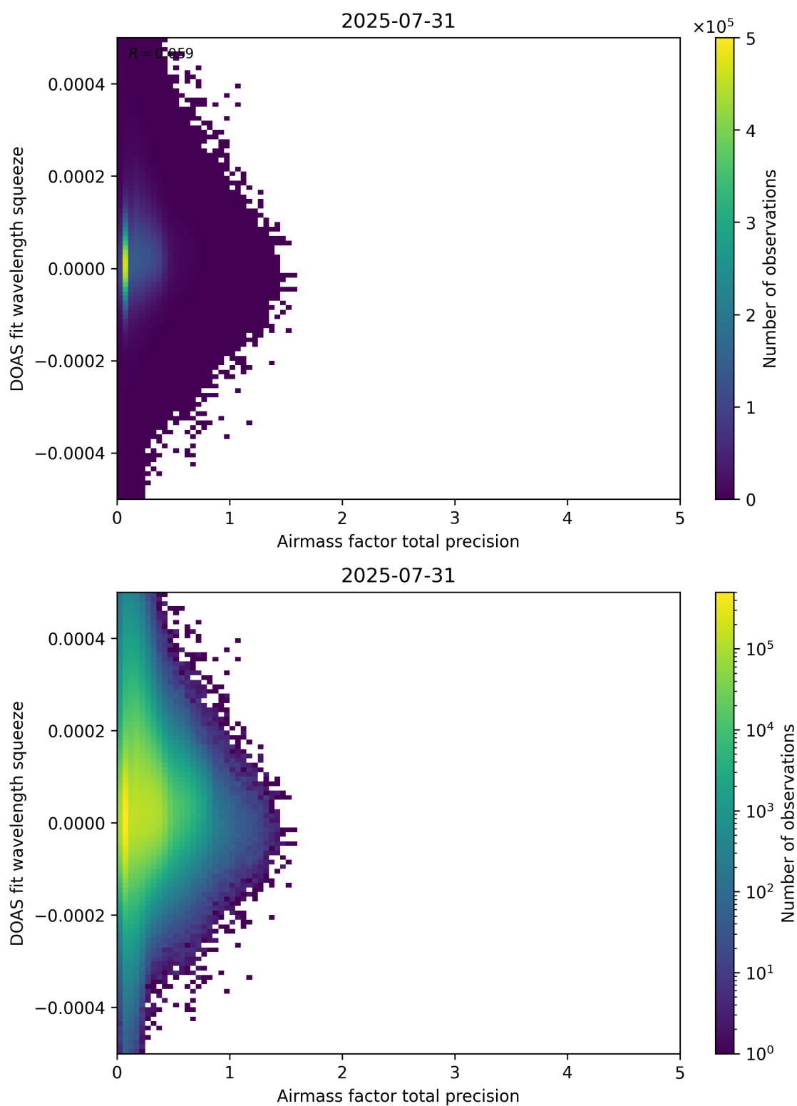
Figure 107: Scatter density plot of “Airmass factor total precision” against “DOAS fit wavelength squeeze” for 2025-07-30 to 2025-08-01.
