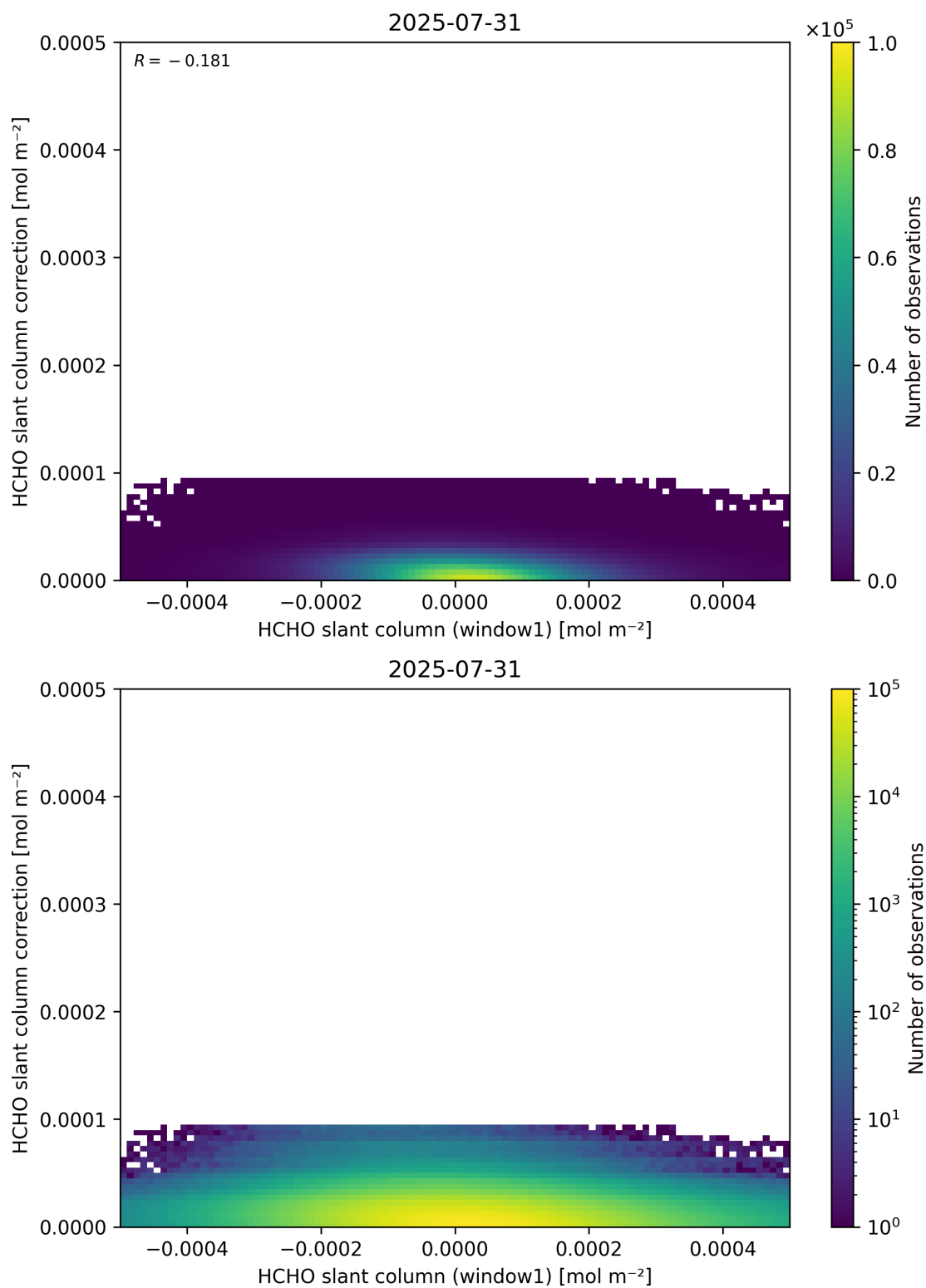
Figure 83: Scatter density plot of “HCHO slant column (window1)” against “HCHO slant column correction” for 2025-07-30 to 2025-08-01.
