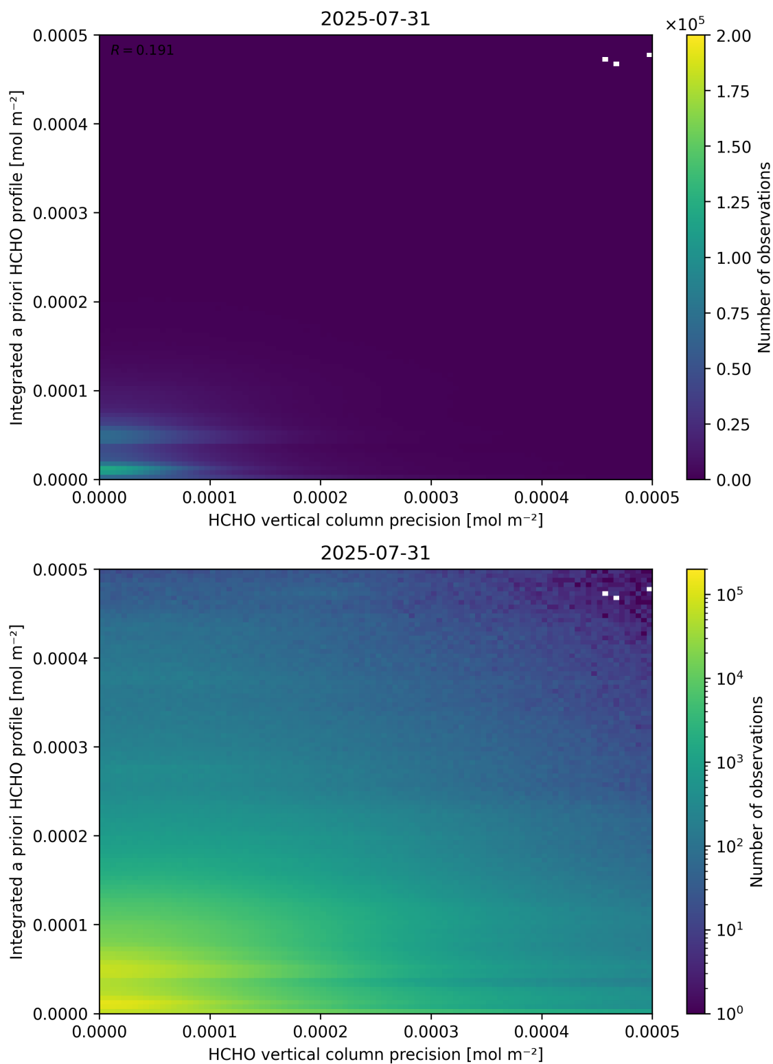
Figure 147: Scatter density plot of “HCHO vertical column precision” against “Integrated a priori HCHO profile” for 2025-07-30 to 2025-08-01.
