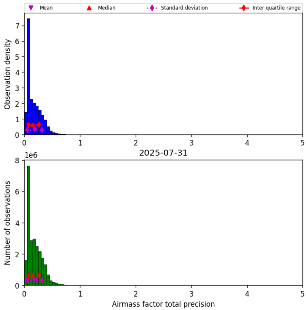
Figure 41: Histogram of “Airmass factor total precision” for 2025-07-30 to 2025-08-01
