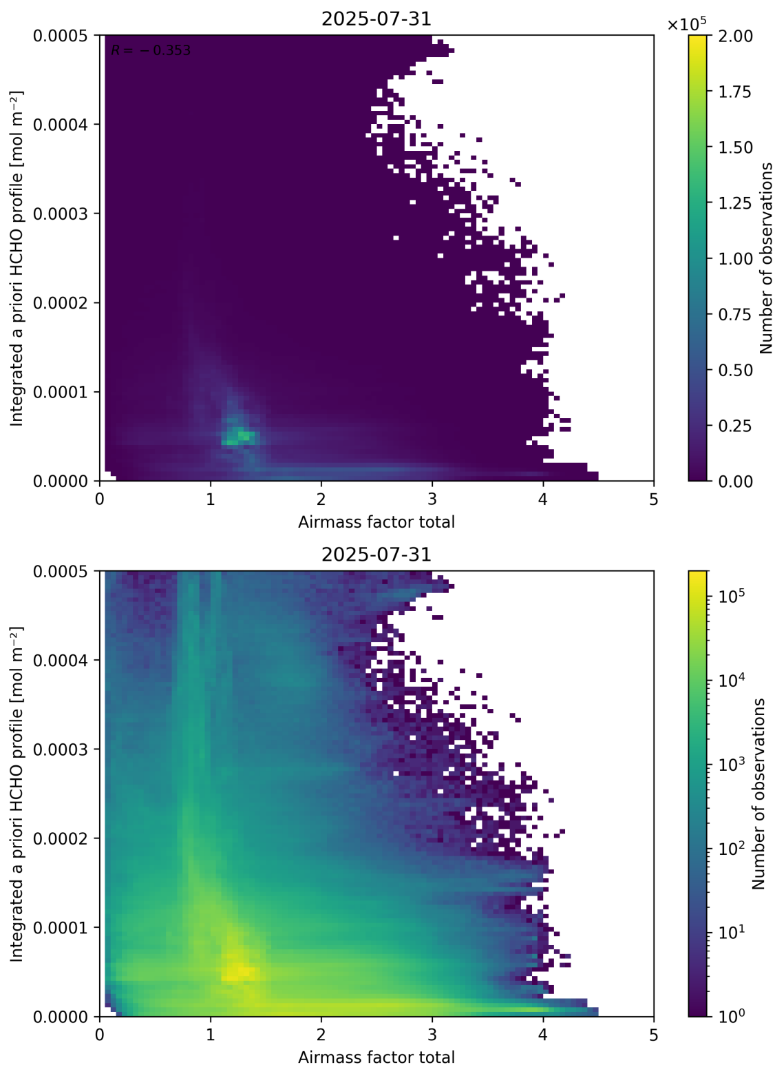
Figure 104: Scatter density plot of “Airmass factor total” against “Integrated a priori HCHO profile” for 2025-07-30 to 2025-08-01.
