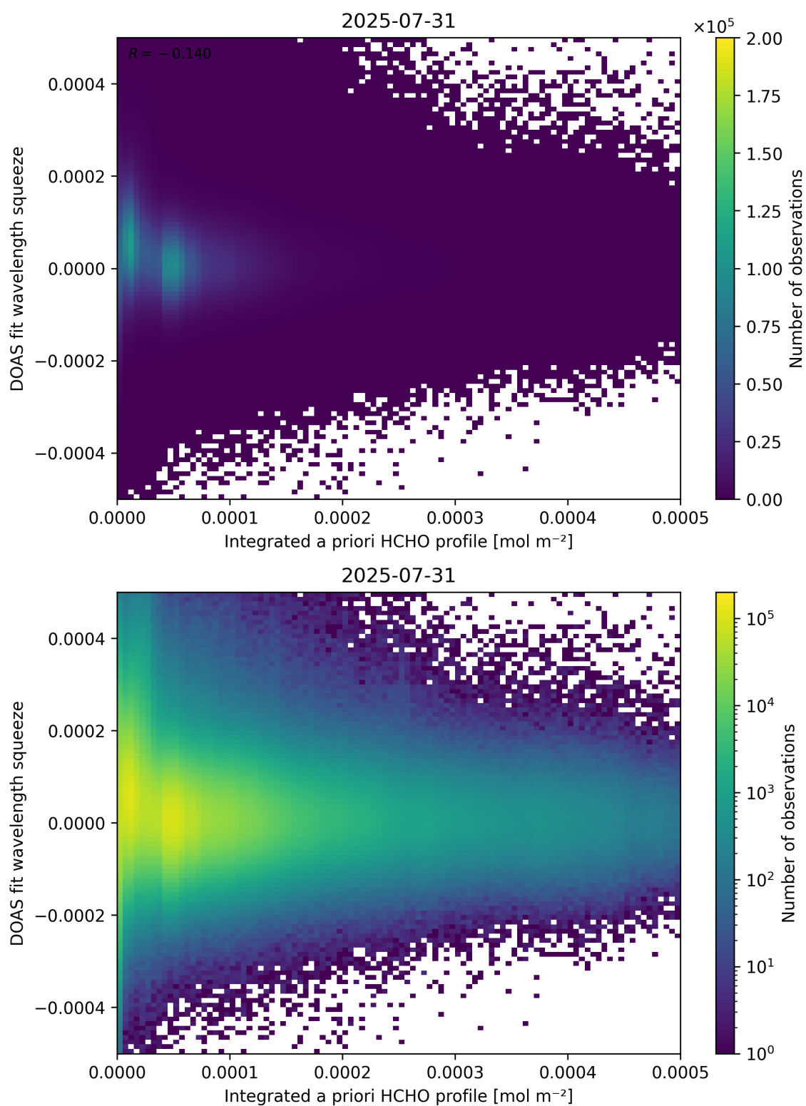
Figure 150: Scatter density plot of “Integrated a priori HCHO profile” against “DOAS fit wavelength squeeze” for 2025-07-30 to 2025-08-01.
