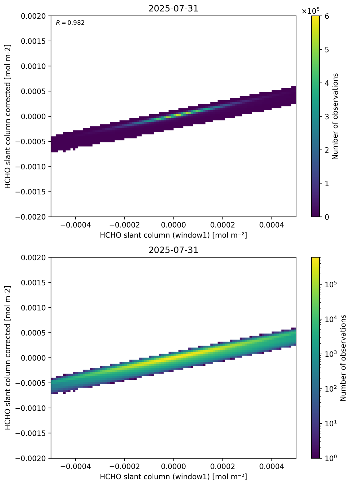
Figure 82: Scatter density plot of “HCHO slant column (window1)” against “HCHO slant column corrected” for 2025-07-30 to 2025-08-01.
