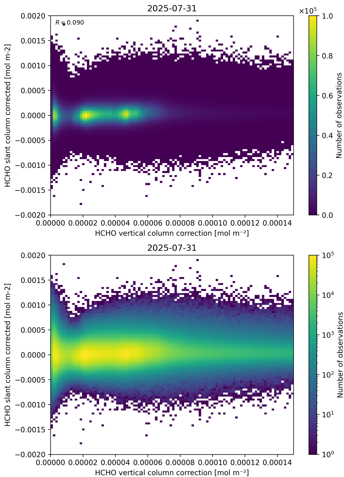
Figure 116: Scatter density plot of “HCHO vertical column correction” against “HCHO slant column corrected” for 2025-07-30 to 2025-08-01.
