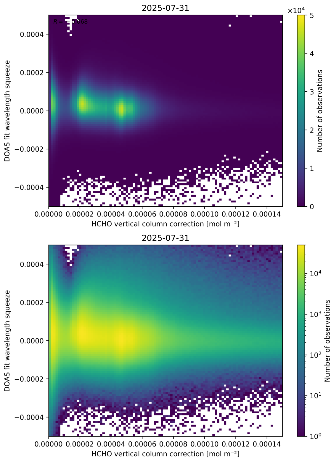
Figure 114: Scatter density plot of “HCHO vertical column correction” against “DOAS fit wavelength squeeze” for 2025-07-30 to 2025-08-01.
