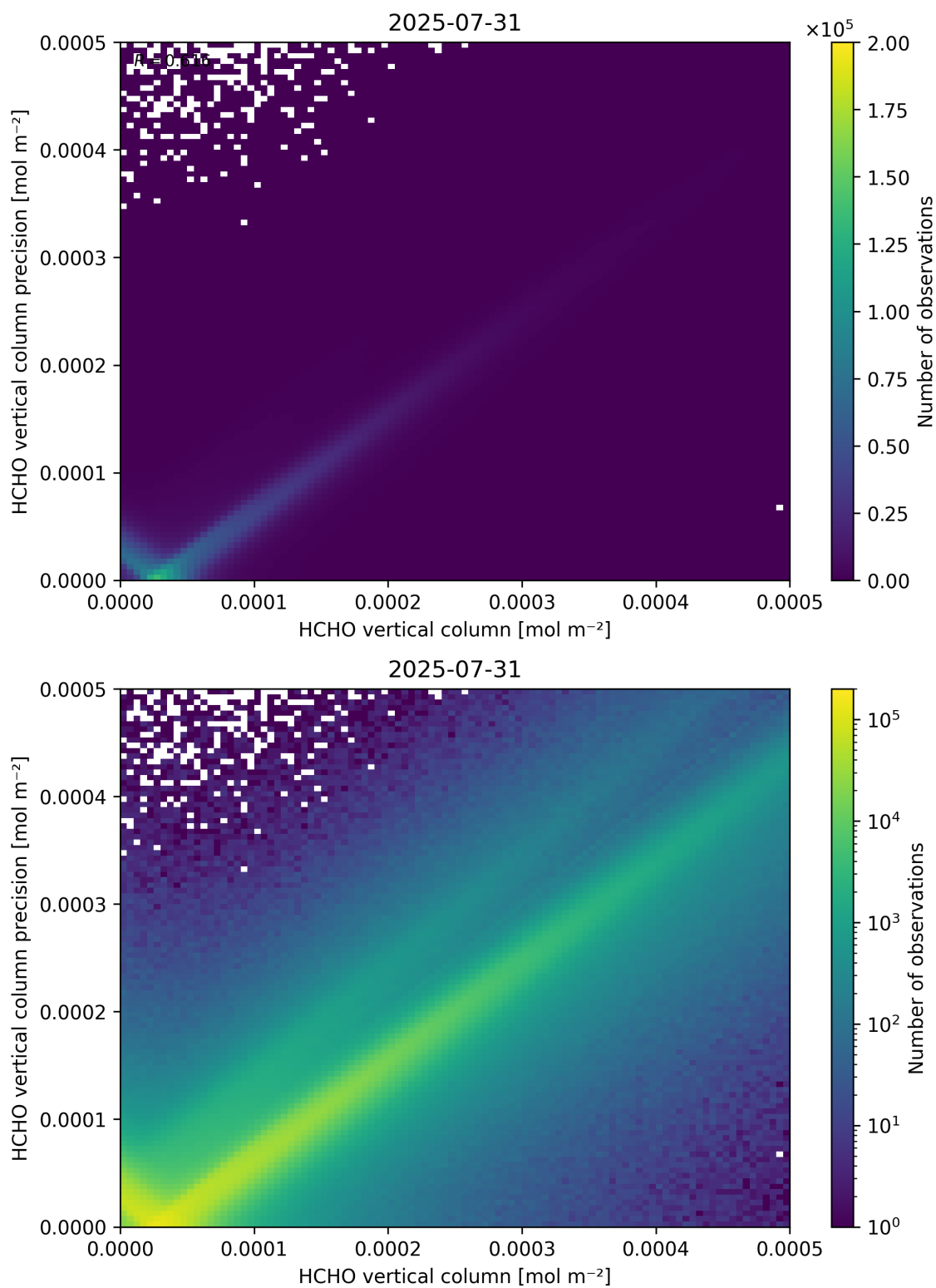
Figure 134: Scatter density plot of “HCHO vertical column” against “HCHO vertical column precision” for 2025-07-30 to 2025-08-01.
