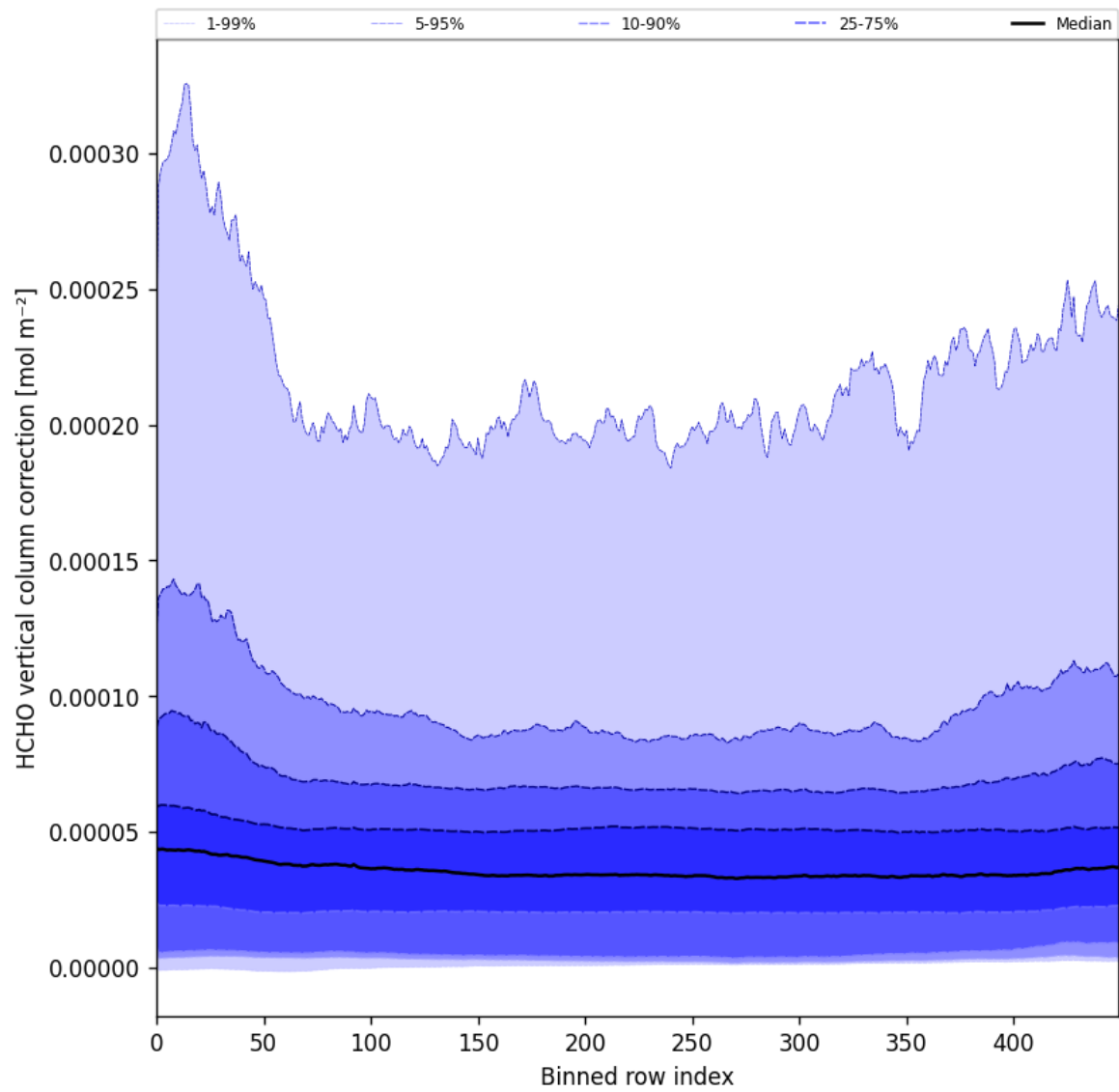
Figure 51: Along track statistics of “HCHO vertical column correction” for 2025-07-30 to 2025-08-01
