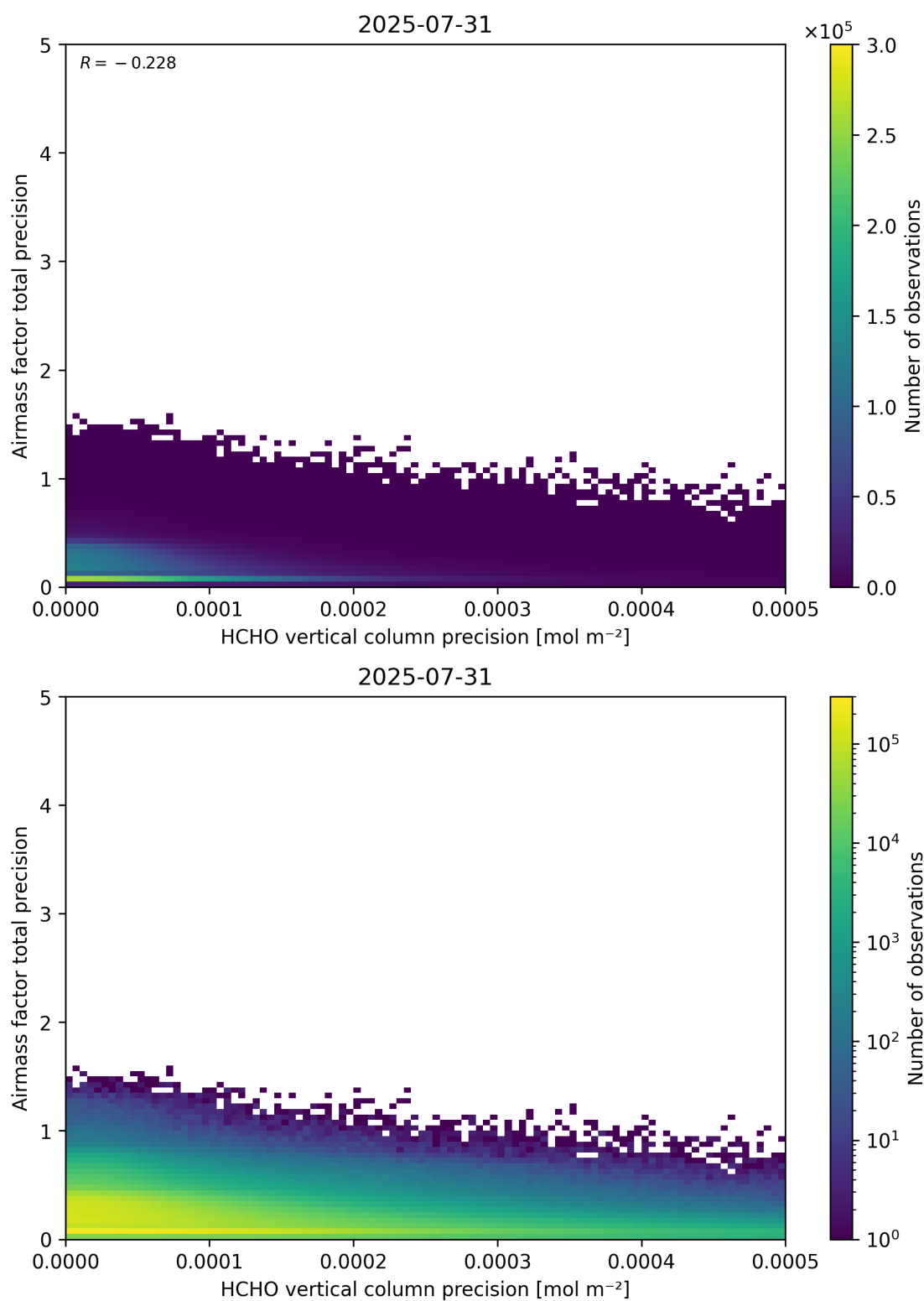
Figure 145: Scatter density plot of “HCHO vertical column precision” against “Airmass factor total precision” for 2025-07-30 to 2025-08-01.
