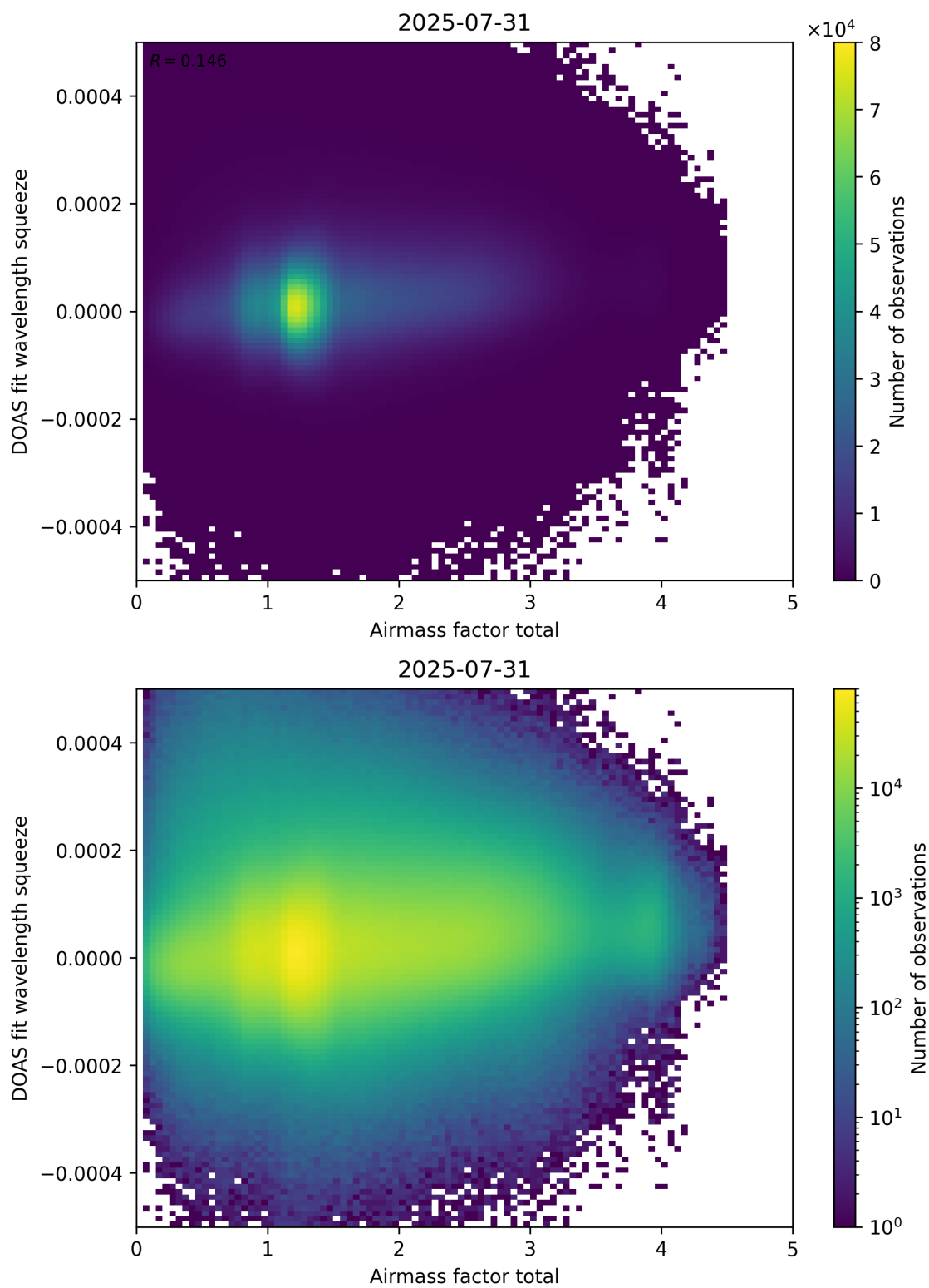
Figure 99: Scatter density plot of “Airmass factor total” against “DOAS fit wavelength squeeze” for 2025-07-30 to 2025-08-01.
