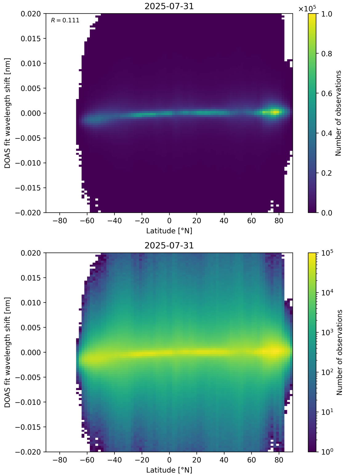
Figure 154: Scatter density plot of “Latitude” against “DOAS fit wavelength shift” for 2025-07-30 to 2025-08-01.
