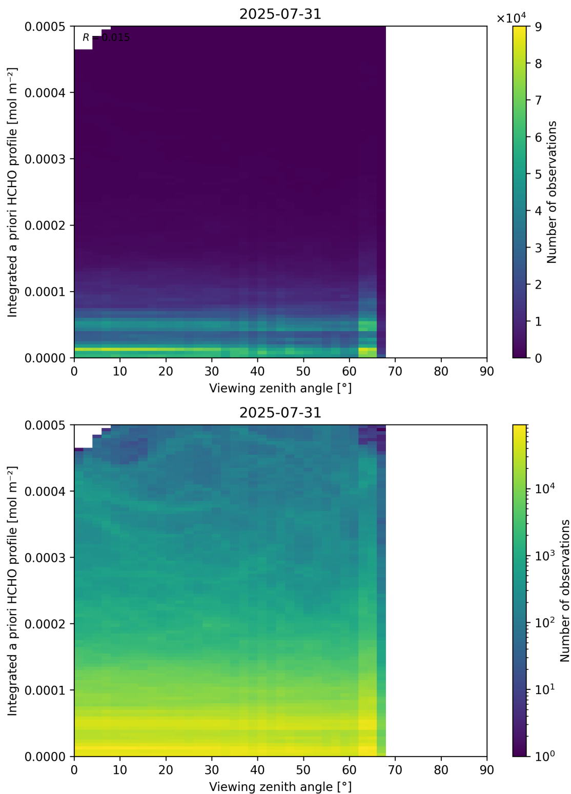
Figure 195: Scatter density plot of “Viewing zenith angle” against “Integrated a priori HCHO profile” for 2025-07-30 to 2025-08-01.
