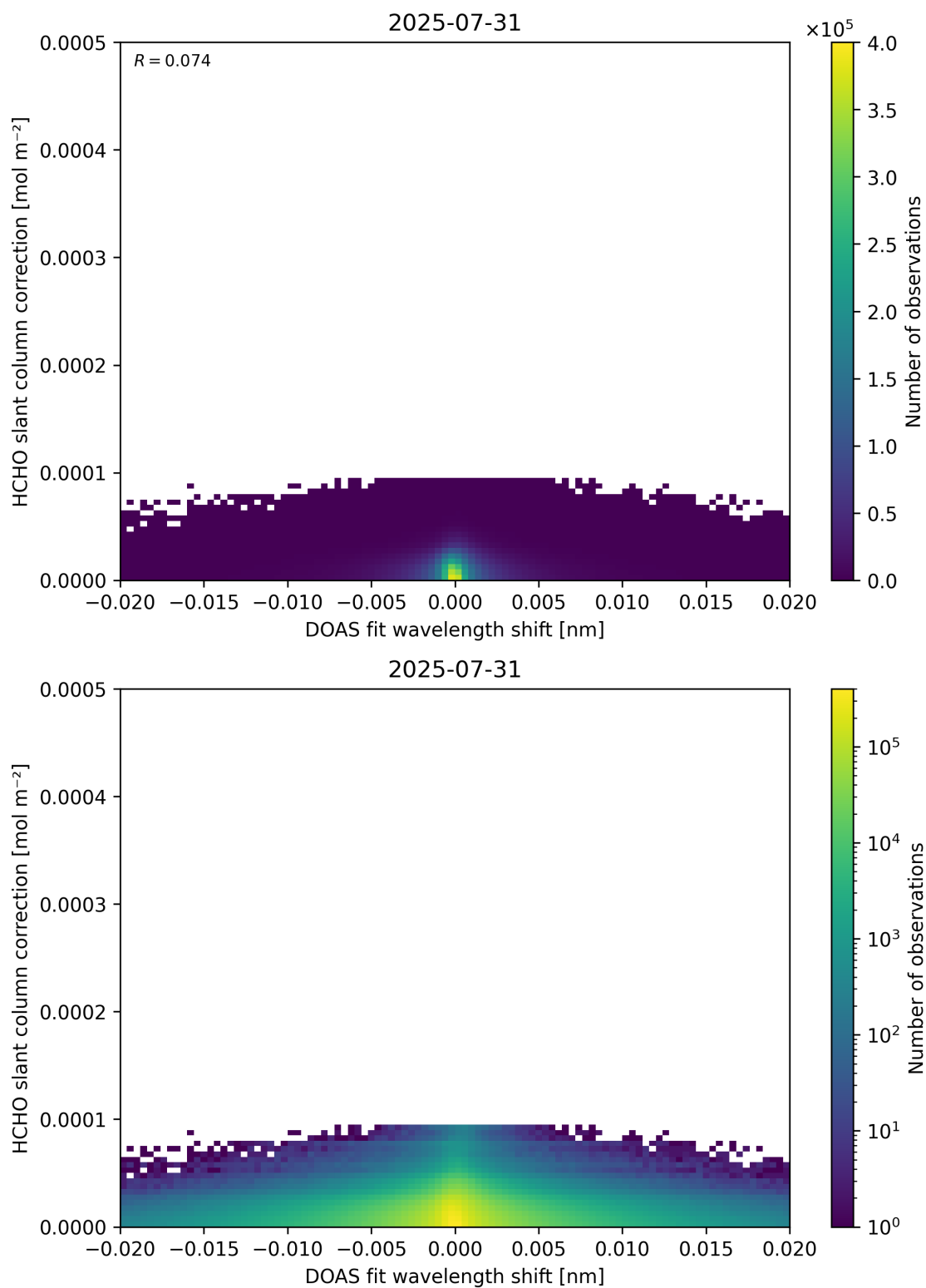
Figure 67: Scatter density plot of “DOAS fit wavelength shift” against “HCHO slant column correction” for 2025-07-30 to 2025-08-01.
