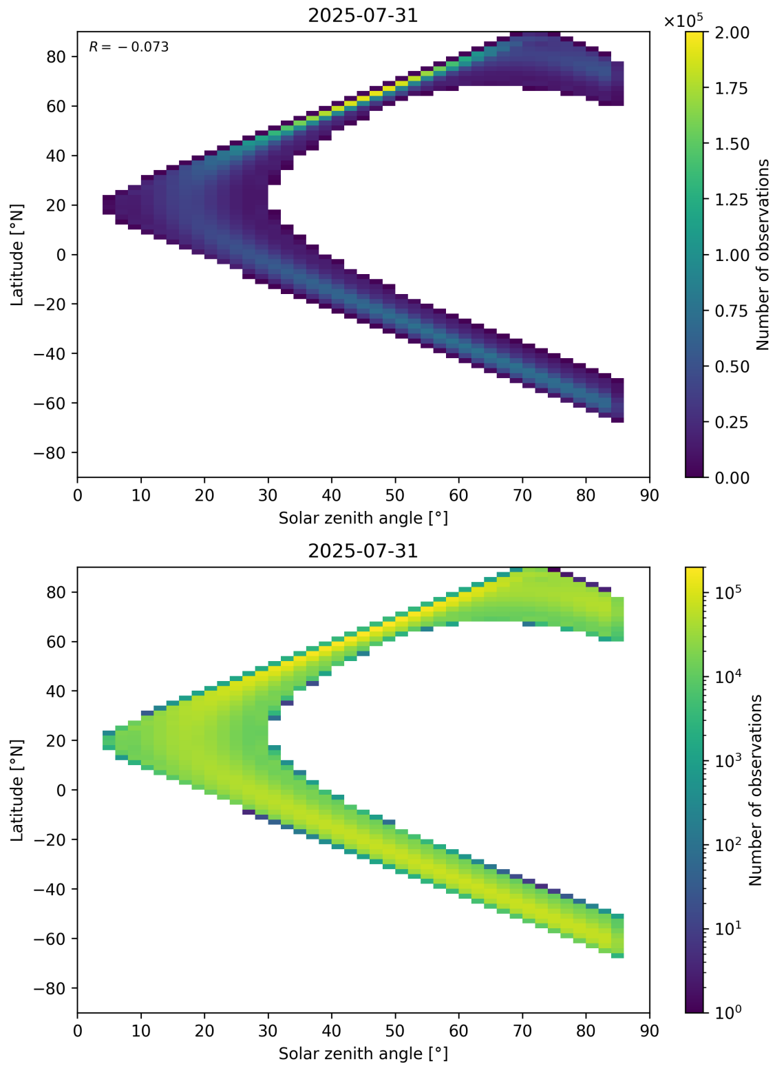
Figure 181: Scatter density plot of “Solar zenith angle” against “Latitude” for 2025-07-30 to 2025-08-01.
