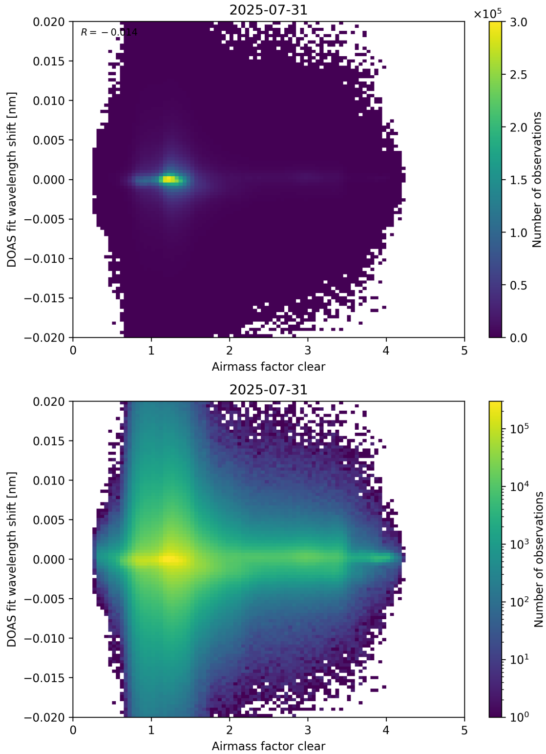
Figure 72: Scatter density plot of “Airmass factor clear” against “DOAS fit wavelength shift” for 2025-07-30 to 2025-08-01.
