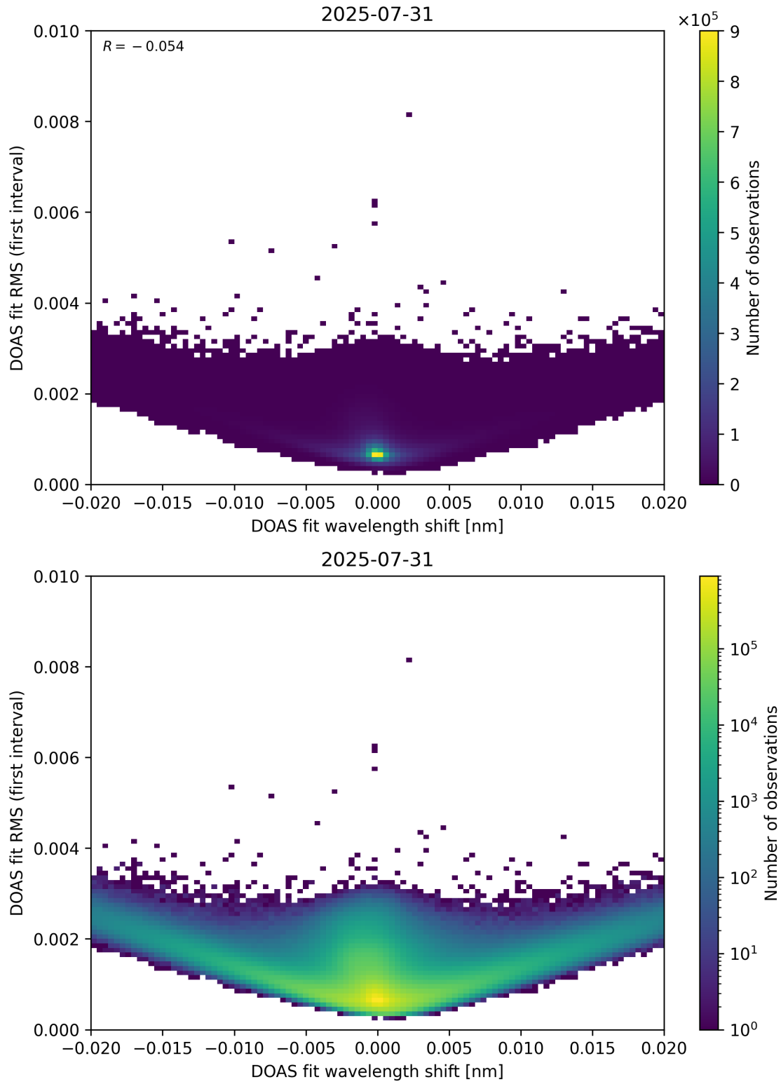
Figure 64: Scatter density plot of “DOAS fit wavelength shift” against “DOAS fit RMS (first interval)” for 2025-07-30 to 2025-08-01.
