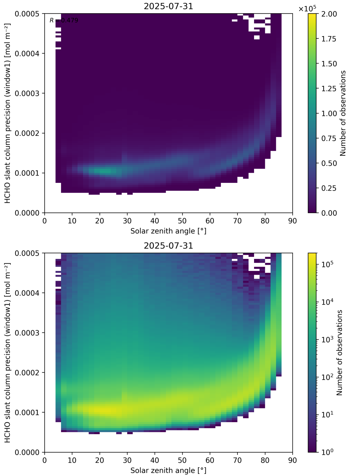
Figure 174: Scatter density plot of “Solar zenith angle” against “HCHO slant column precision (window1)” for 2025-07-30 to 2025-08-01.
