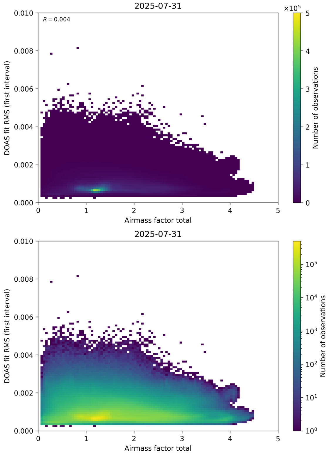
Figure 97: Scatter density plot of “Airmass factor total” against “DOAS fit RMS (first interval)” for 2025-07-30 to 2025-08-01.
