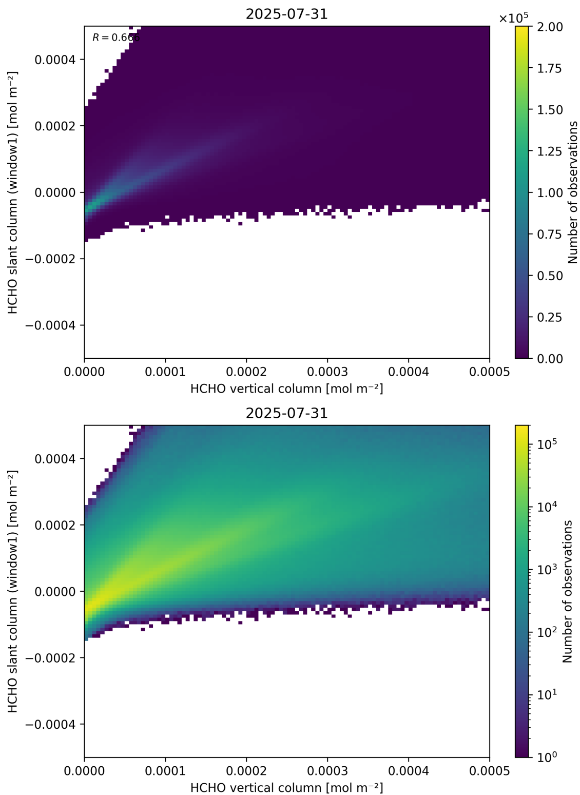
Figure 129: Scatter density plot of “HCHO vertical column” against “HCHO slant column (window1)” for 2025-07-30 to 2025-08-01.
