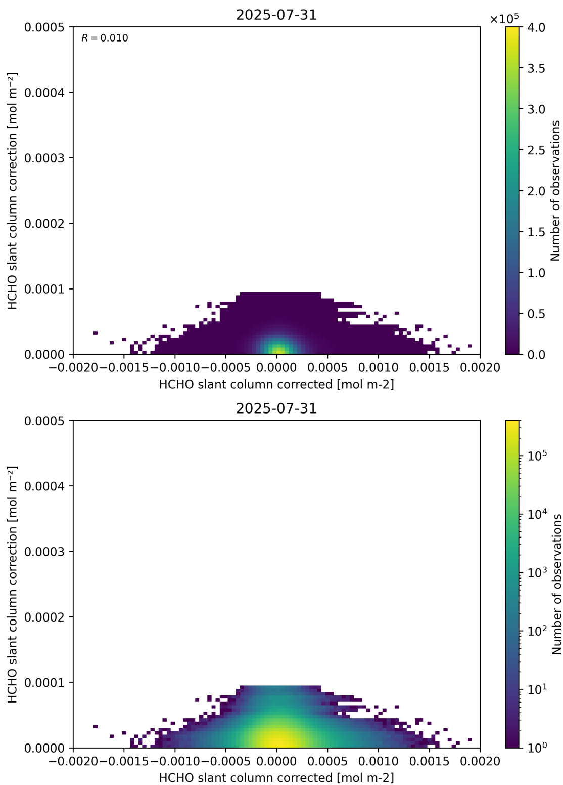
Figure 77: Scatter density plot of “HCHO slant column corrected” against “HCHO slant column correction” for 2025-07-30 to 2025-08-01.
