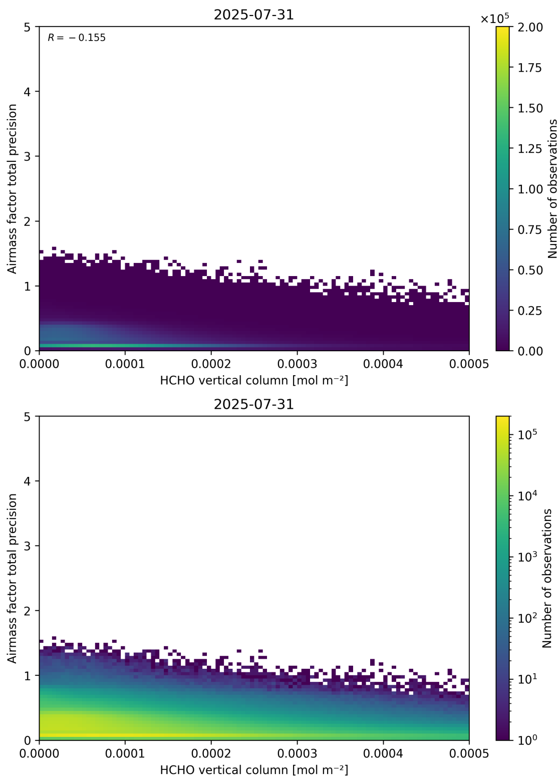
Figure 132: Scatter density plot of “HCHO vertical column” against “Airmass factor total precision” for 2025-07-30 to 2025-08-01.
