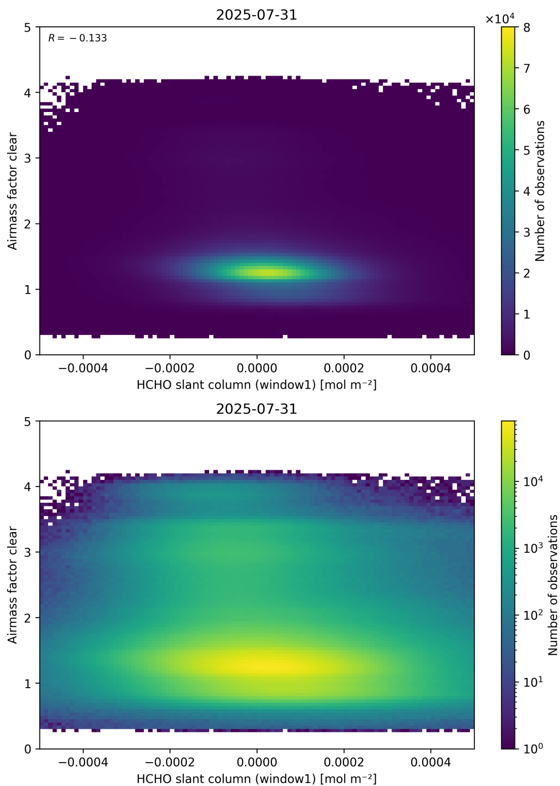
Figure 81: Scatter density plot of “HCHO slant column (window1)” against “Airmass factor clear” for 2025-07-30 to 2025-08-01.
