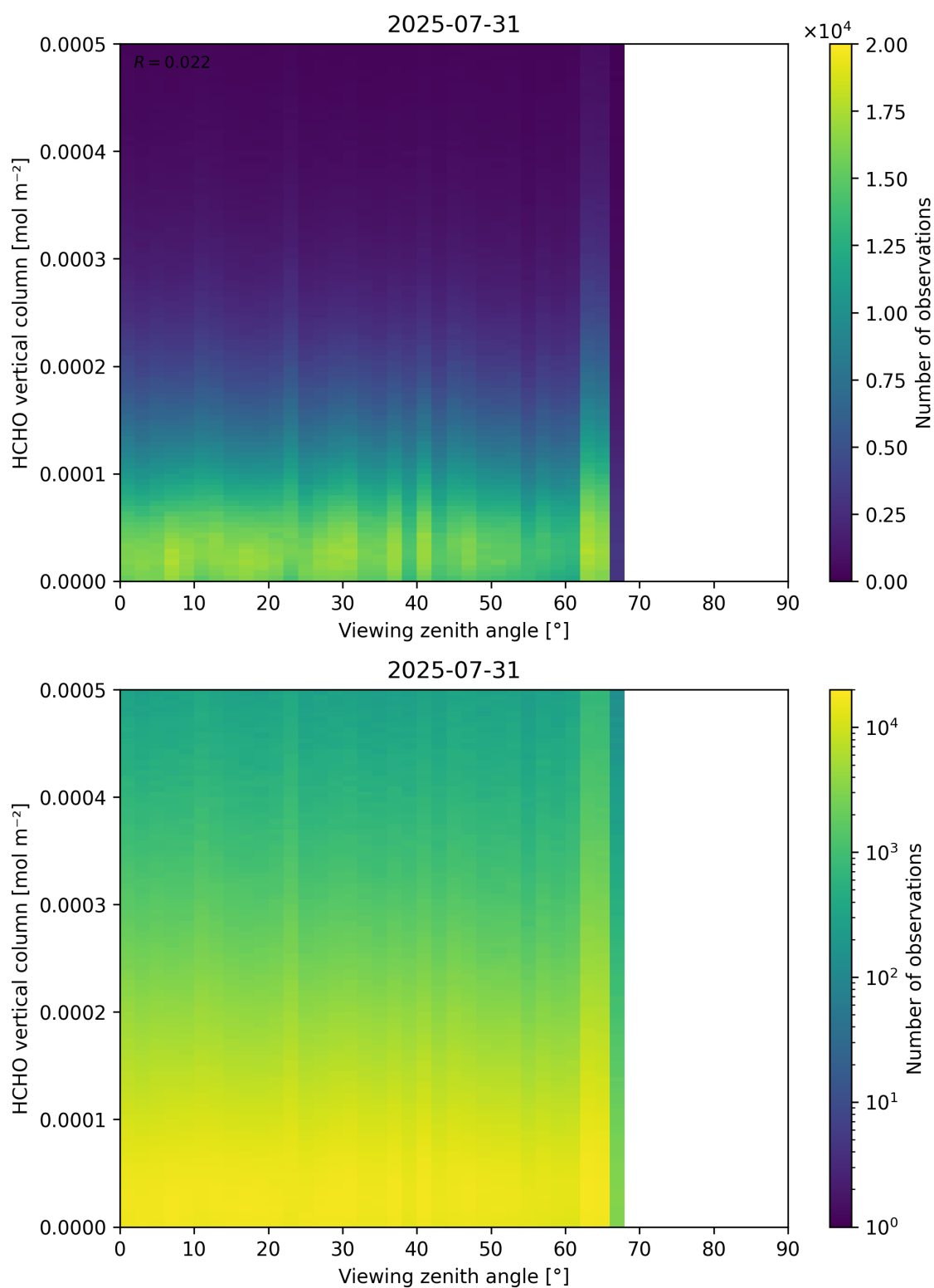
Figure 192: Scatter density plot of “Viewing zenith angle” against “HCHO vertical column” for 2025-07-30 to 2025-08-01.
