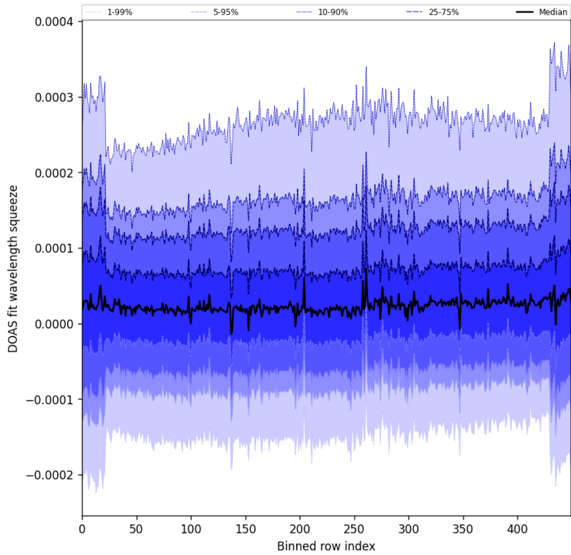
Figure 59: Along track statistics of “DOAS fit wavelength squeeze” for 2025-07-30 to 2025-08-01
