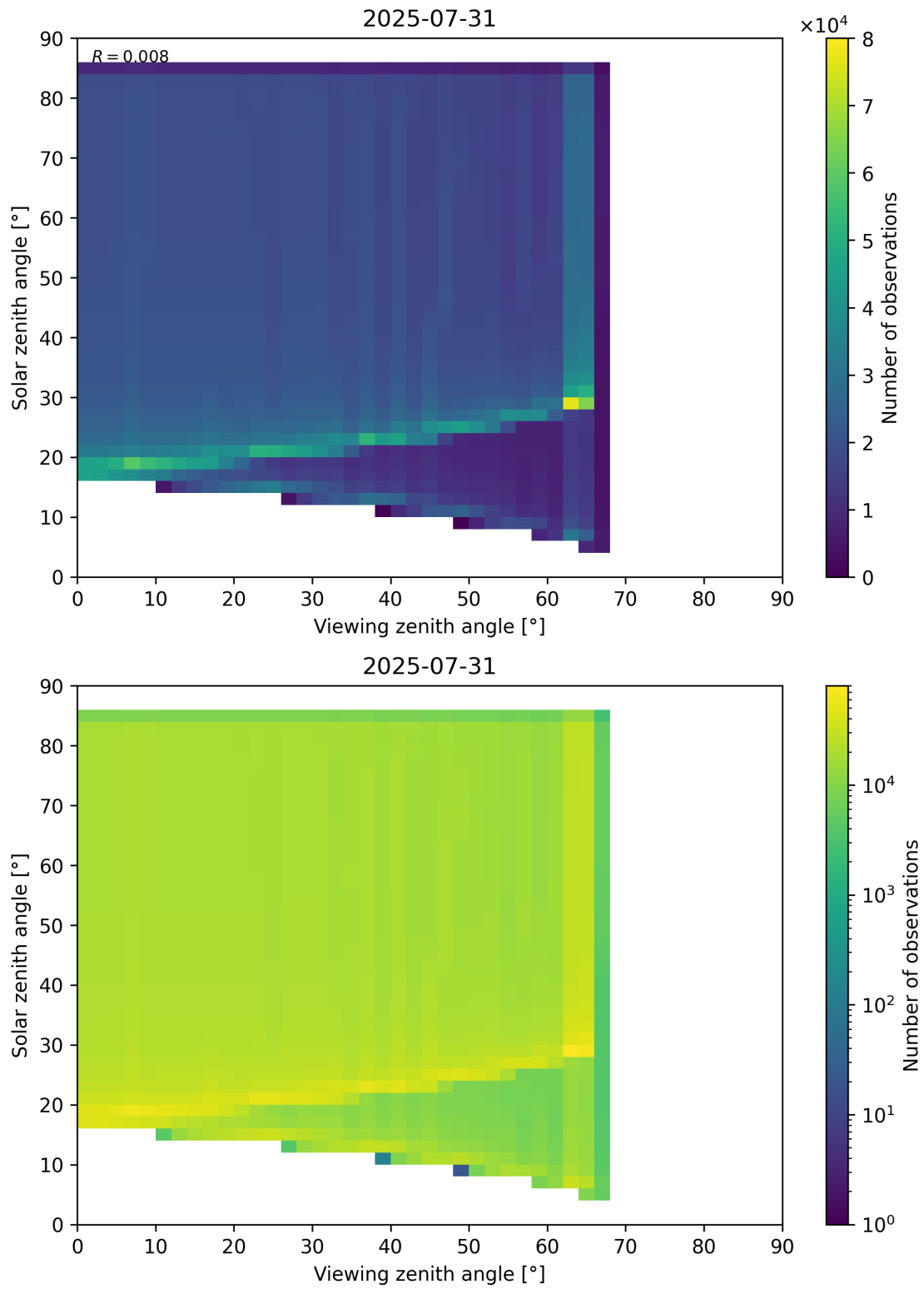
Figure 197: Scatter density plot of “Viewing zenith angle” against “Solar zenith angle” for 2025-07-30 to 2025-08-01.
