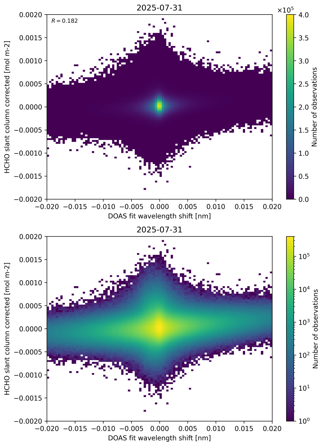
Figure 66: Scatter density plot of “DOAS fit wavelength shift” against “HCHO slant column corrected” for 2025-07-30 to 2025-08-01.
