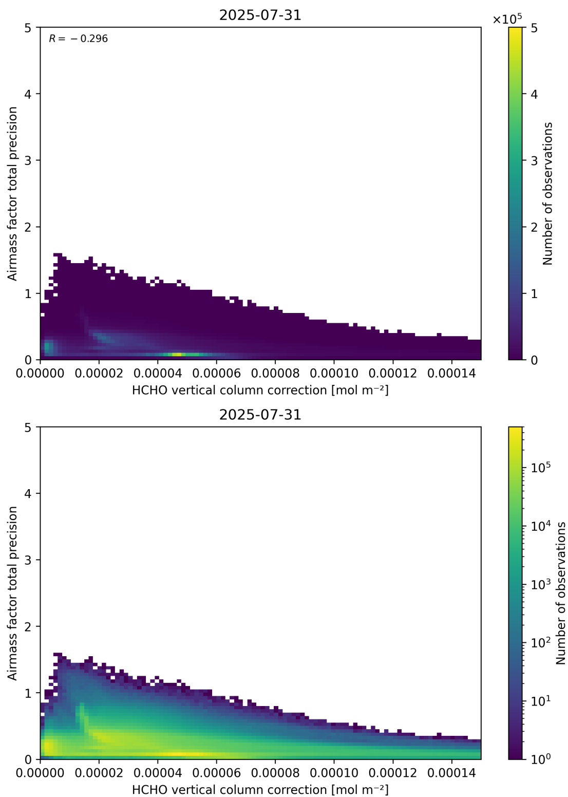
Figure 121: Scatter density plot of “HCHO vertical column correction” against “Airmass factor total precision” for 2025-07-30 to 2025-08-01.
