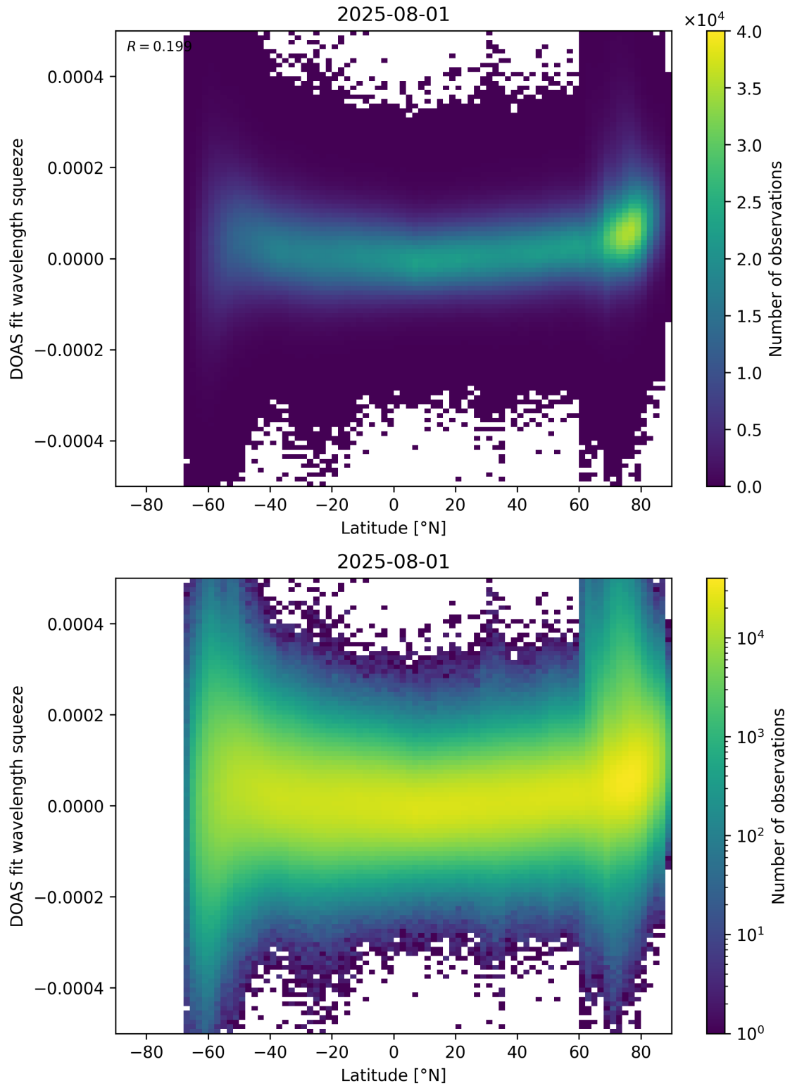
Figure 155: Scatter density plot of “Latitude” against “DOAS fit wavelength squeeze” for 2025-07-31 to 2025-08-02.
