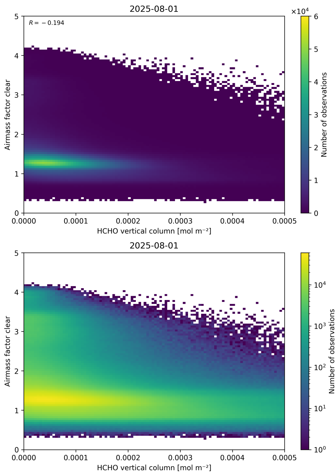
Figure 126: Scatter density plot of “HCHO vertical column” against “Airmass factor clear” for 2025-07-31 to 2025-08-02.
