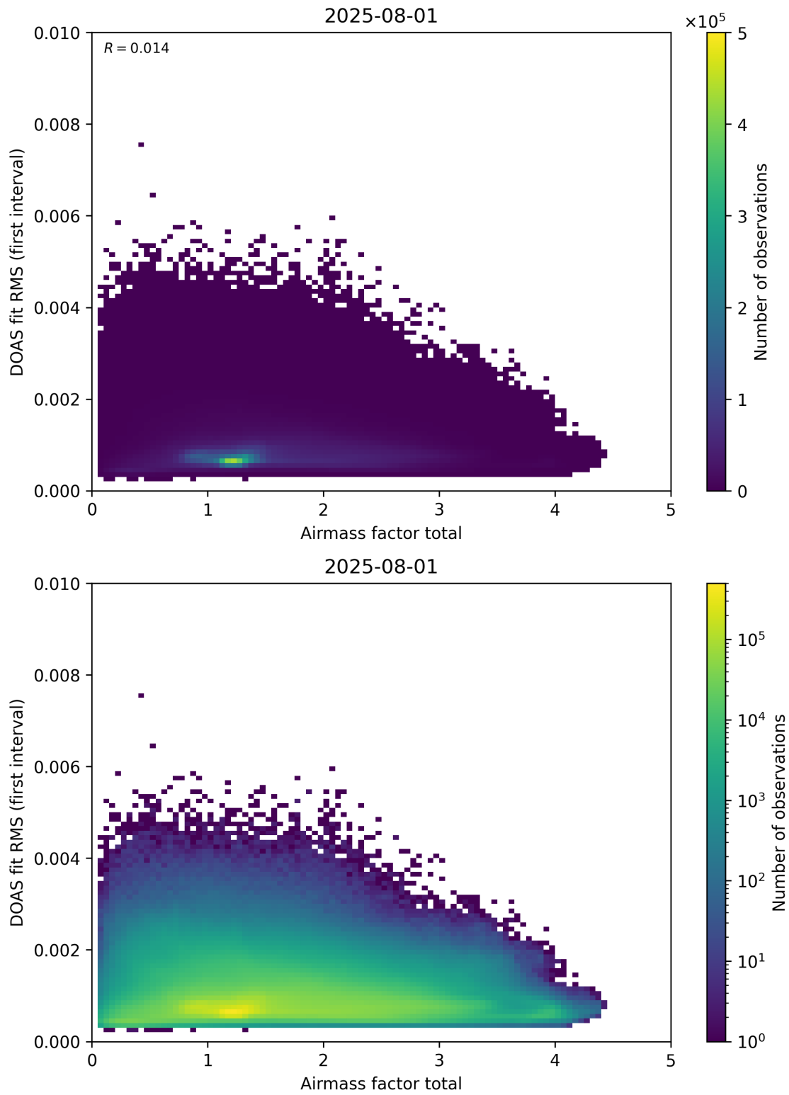
Figure 97: Scatter density plot of “Airmass factor total” against “DOAS fit RMS (first interval)” for 2025-07-31 to 2025-08-02.
