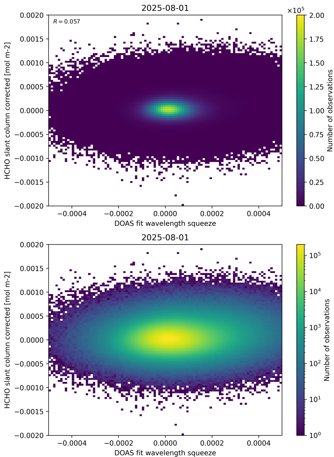
Figure 69: Scatter density plot of “DOAS fit wavelength squeeze” against “HCHO slant column corrected” for 2025-07-31 to 2025-08-02.
