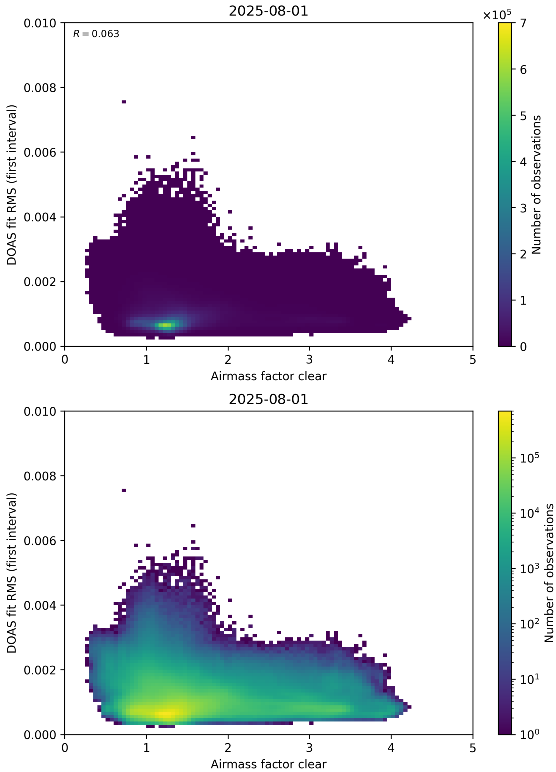
Figure 71: Scatter density plot of “Airmass factor clear” against “DOAS fit RMS (first interval)” for 2025-07-31 to 2025-08-02.
