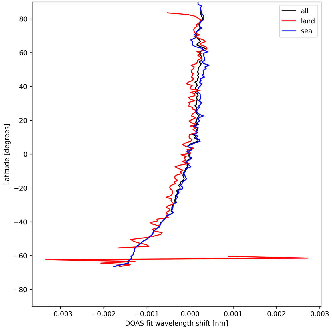
Figure 30: Zonal average of “DOAS fit wavelength shift” for 2025-07-31 to 2025-08-02.
