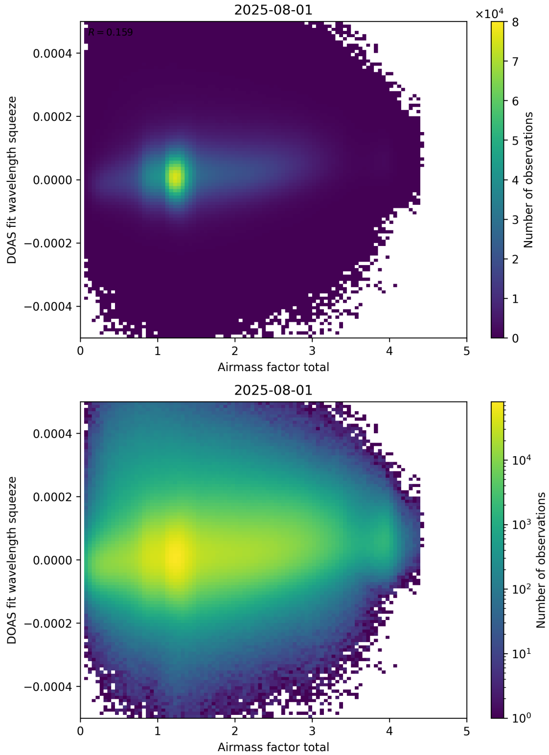
Figure 99: Scatter density plot of “Airmass factor total” against “DOAS fit wavelength squeeze” for 2025-07-31 to 2025-08-02.
