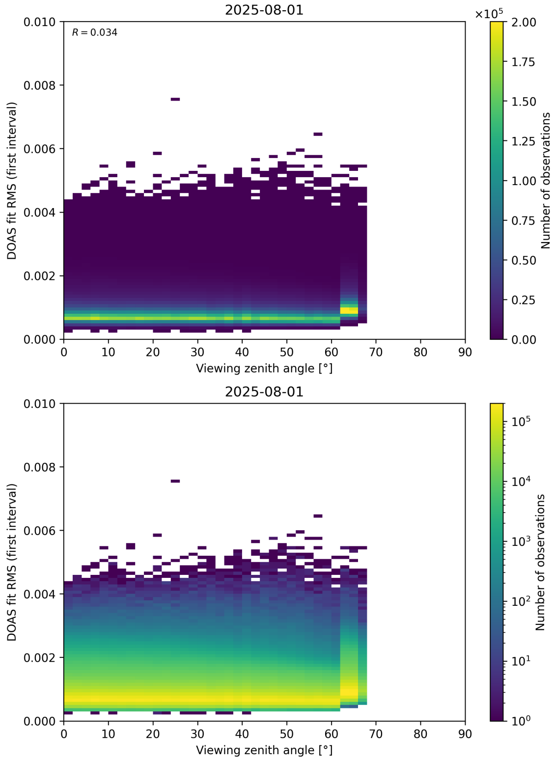
Figure 182: Scatter density plot of “Viewing zenith angle” against “DOAS fit RMS (first interval)” for 2025-07-31 to 2025-08-02.
