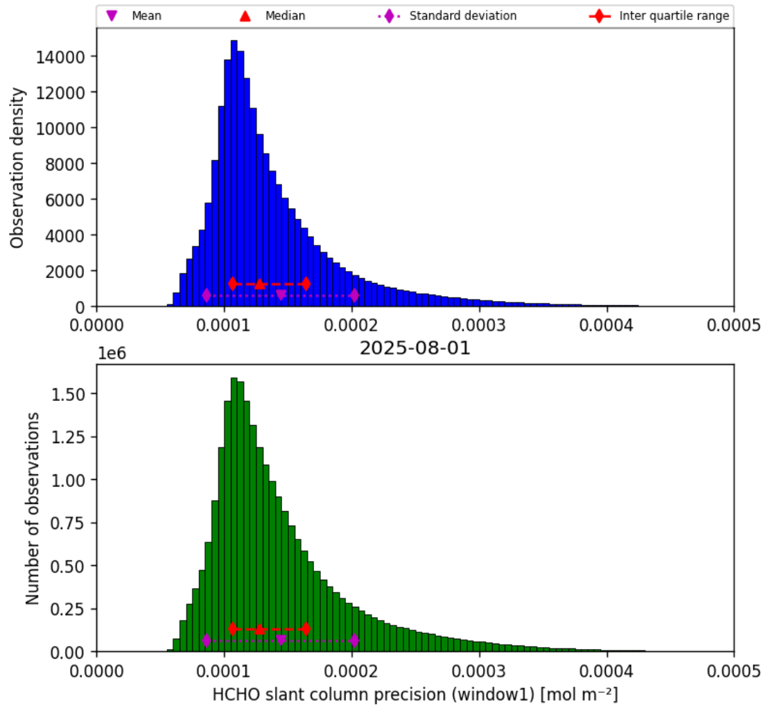
Figure 39: Histogram of “HCHO slant column precision (window1)” for 2025-07-31 to 2025-08-02
