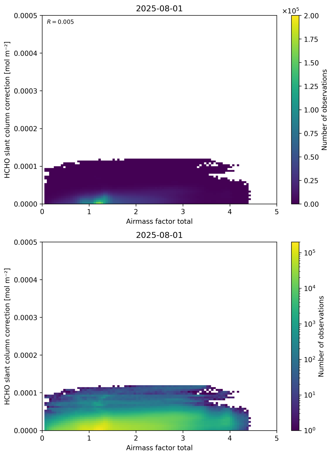
Figure 102: Scatter density plot of “Airmass factor total” against “HCHO slant column correction” for 2025-07-31 to 2025-08-02.
