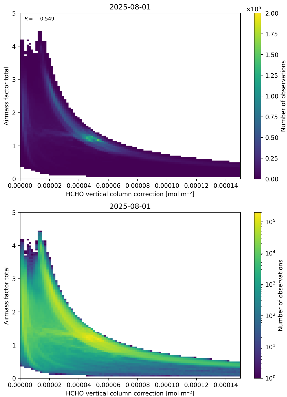
Figure 120: Scatter density plot of “HCHO vertical column correction” against “Airmass factor total” for 2025-07-31 to 2025-08-02.
