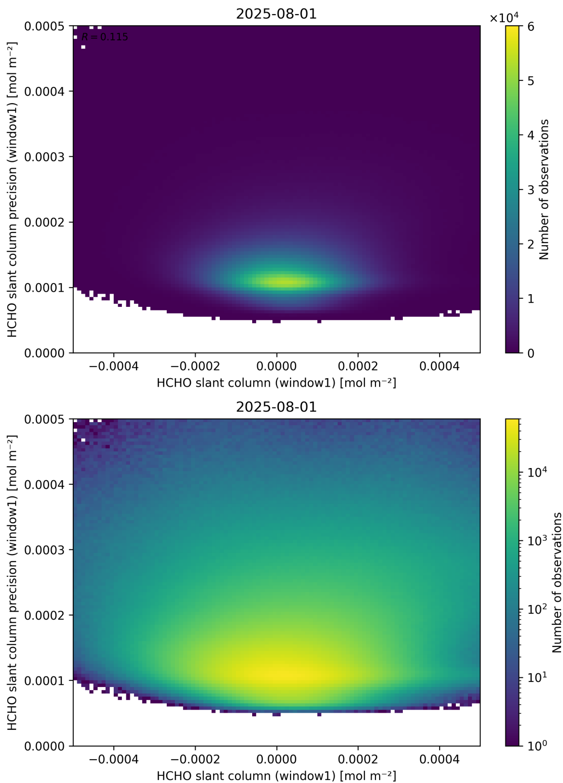
Figure 84: Scatter density plot of “HCHO slant column (window1)” against “HCHO slant column precision (window1)” for 2025-07-31 to 2025-08-02.
