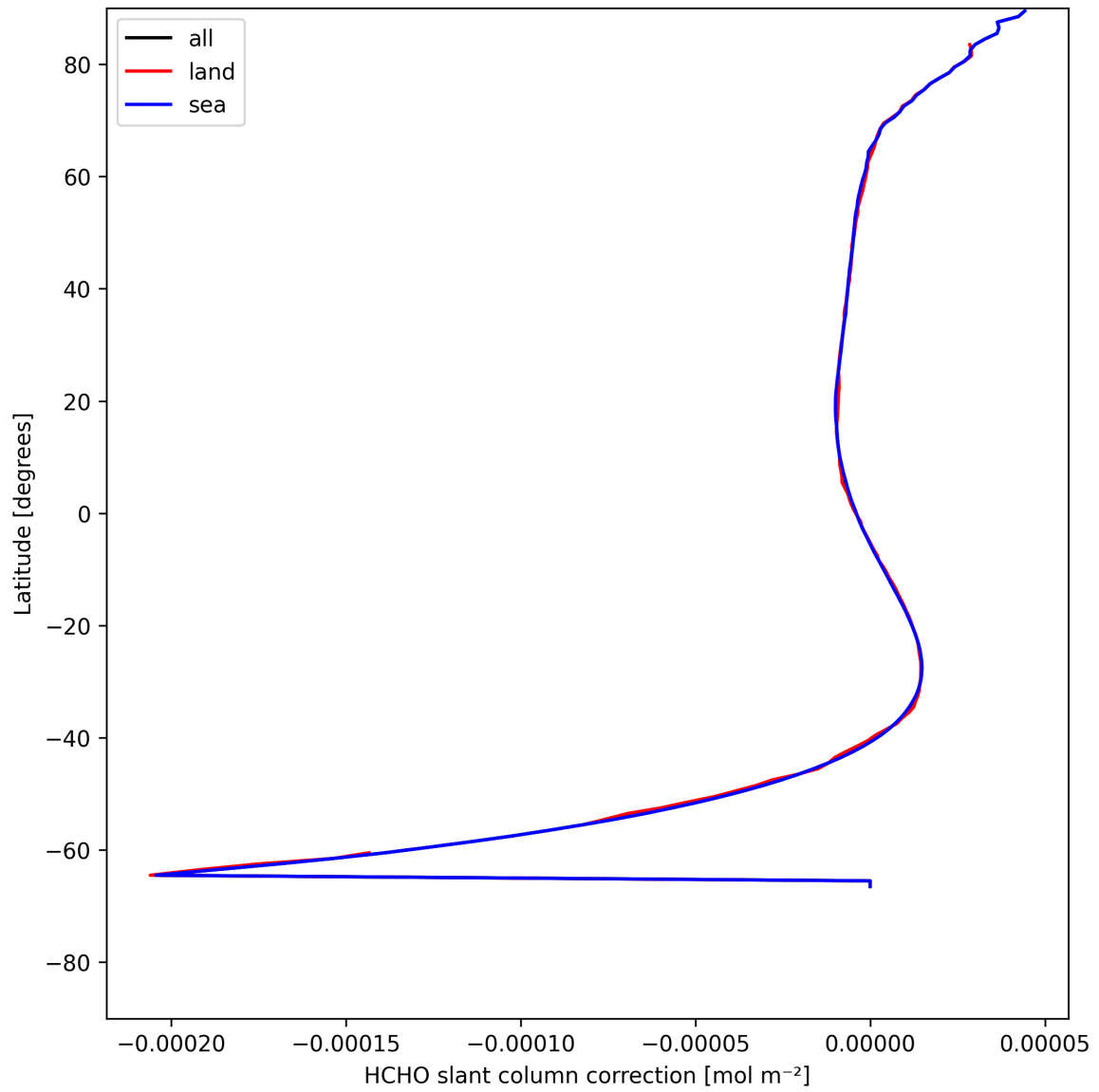
Figure 33: Zonal average of “HCHO slant column correction” for 2025-07-31 to 2025-08-02.
