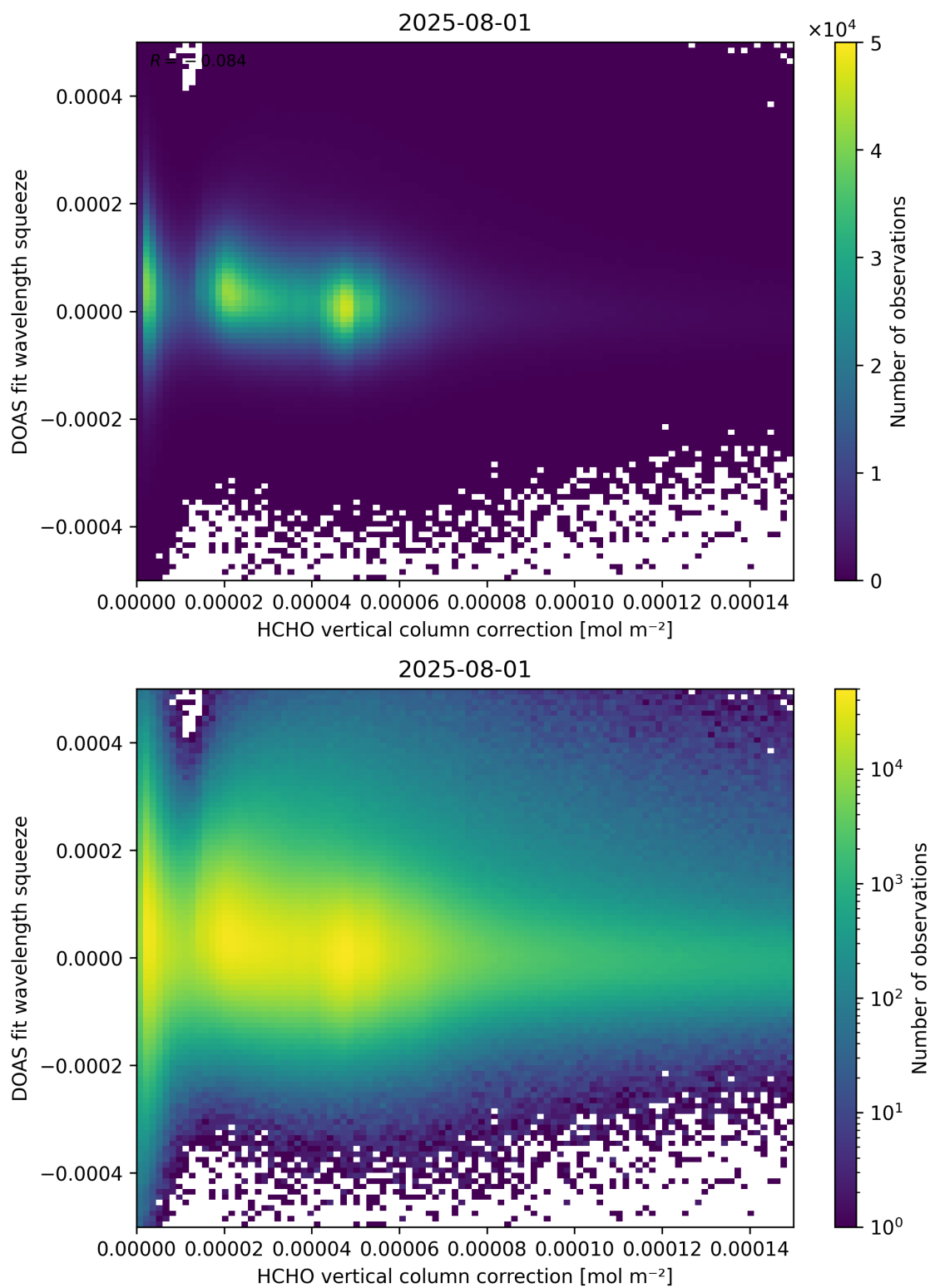
Figure 114: Scatter density plot of “HCHO vertical column correction” against “DOAS fit wavelength squeeze” for 2025-07-31 to 2025-08-02.
