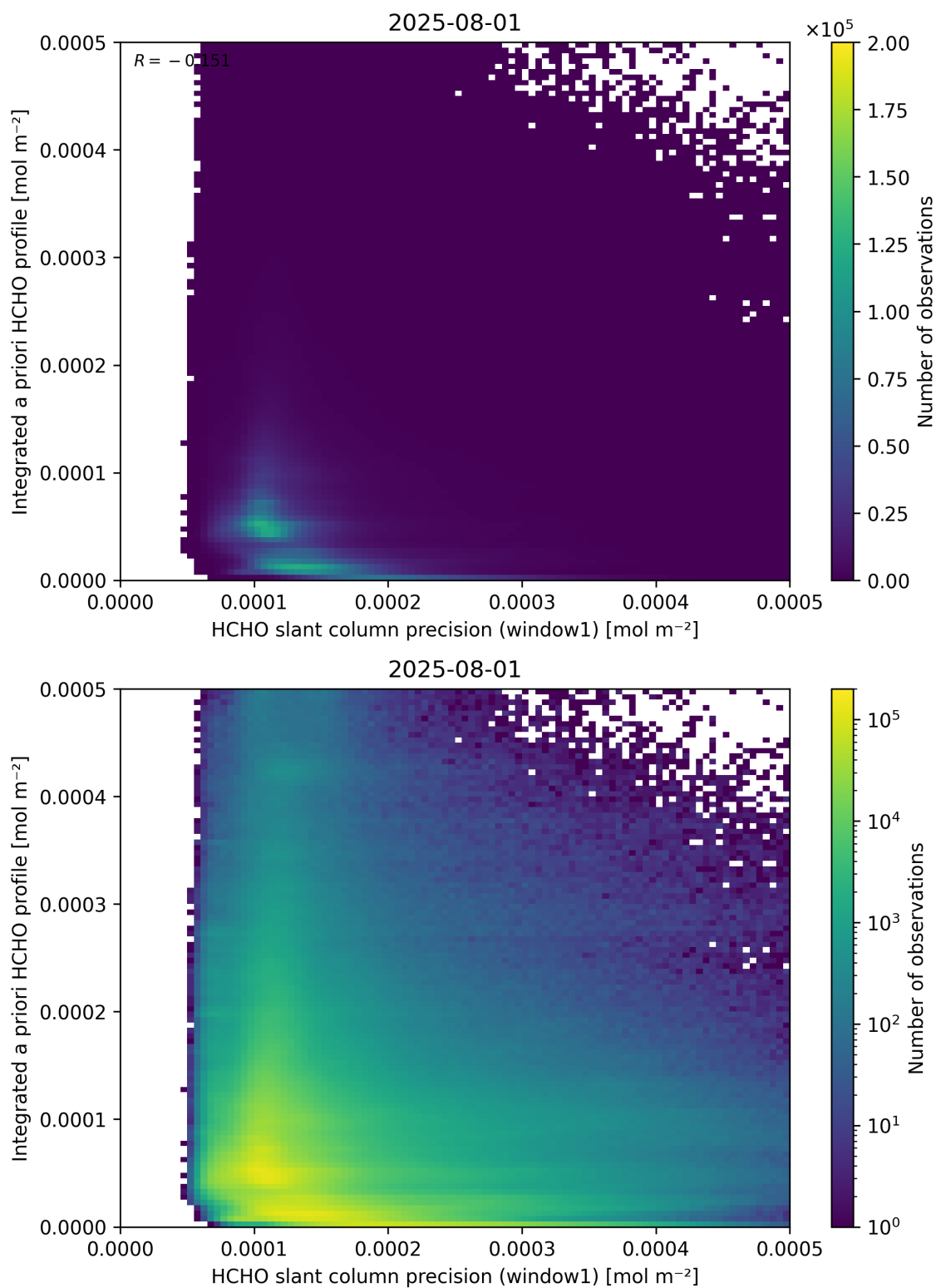
Figure 96: Scatter density plot of “HCHO slant column precision (window1)” against “Integrated a priori HCHO profile” for 2025-07-31 to 2025-08-02.
