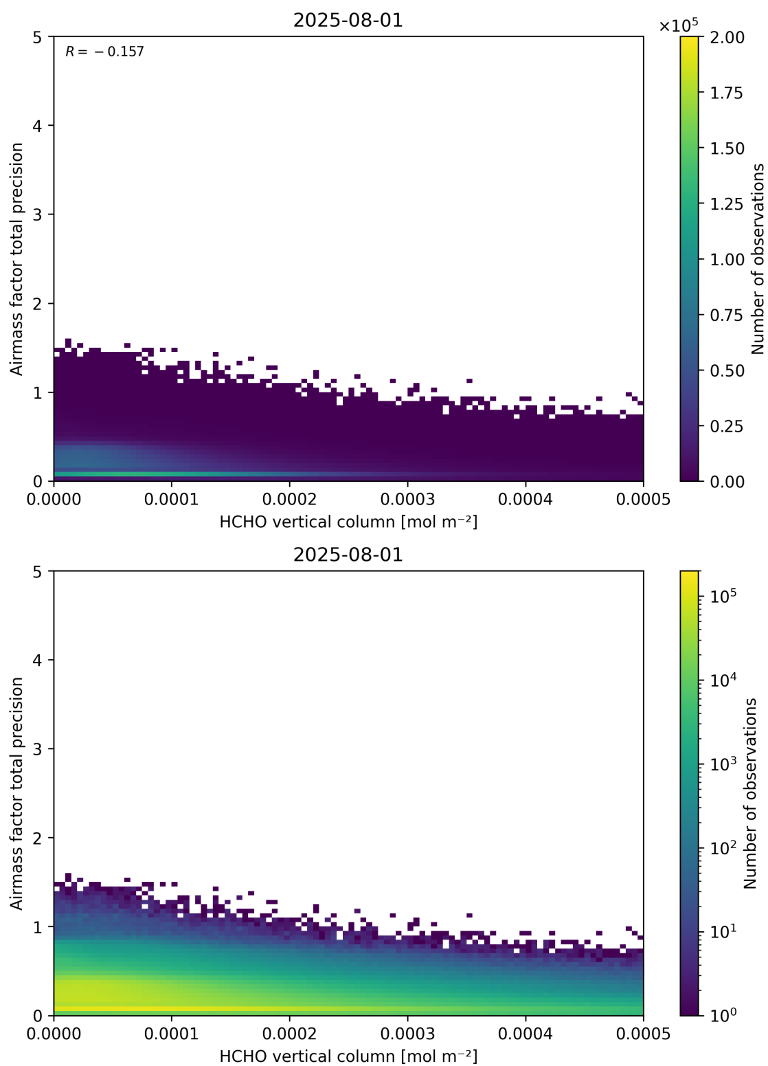
Figure 132: Scatter density plot of “HCHO vertical column” against “Airmass factor total precision” for 2025-07-31 to 2025-08-02.
