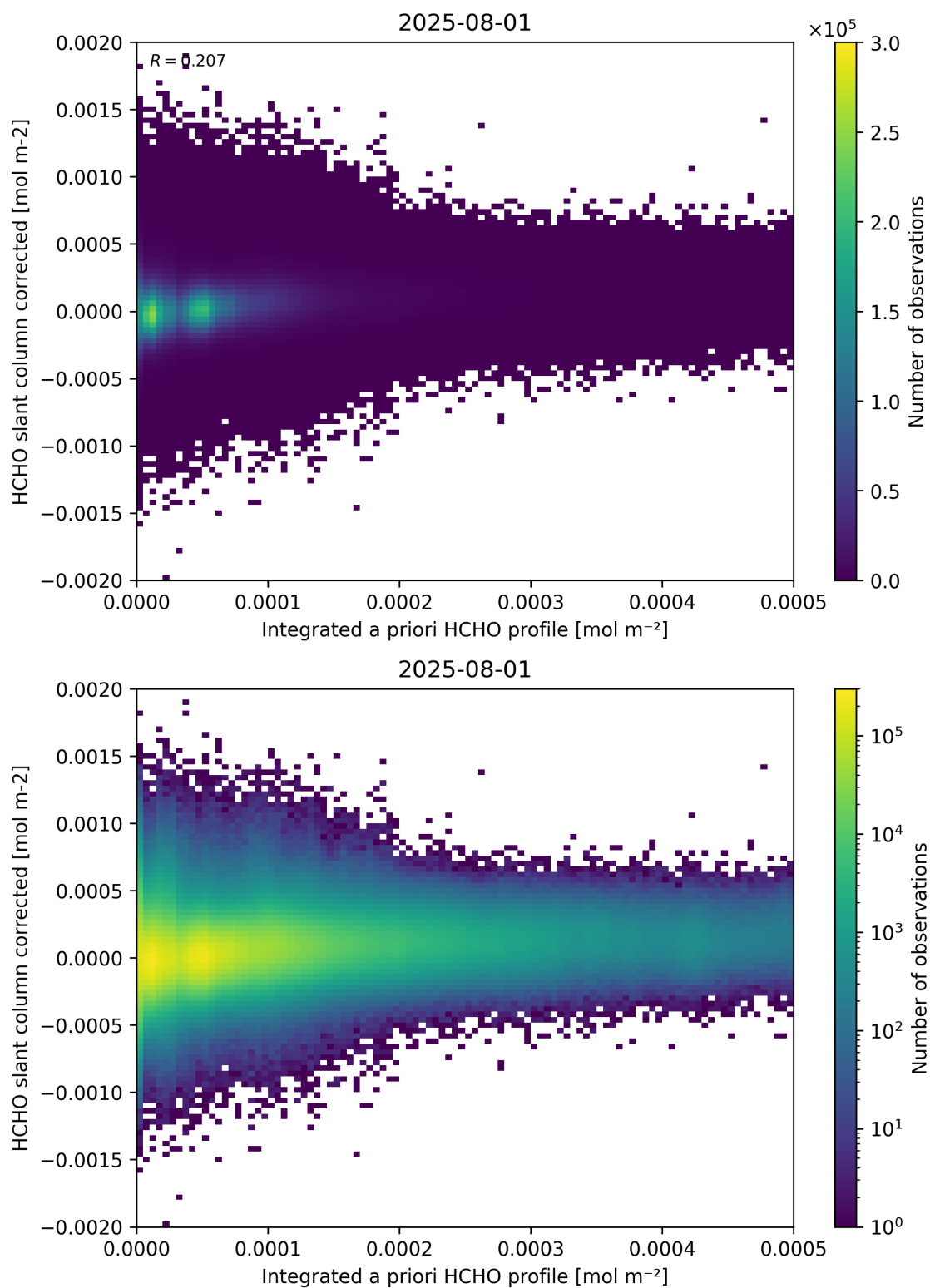
Figure 151: Scatter density plot of “Integrated a priori HCHO profile” against “HCHO slant column corrected” for 2025-07-31 to 2025-08-02.
