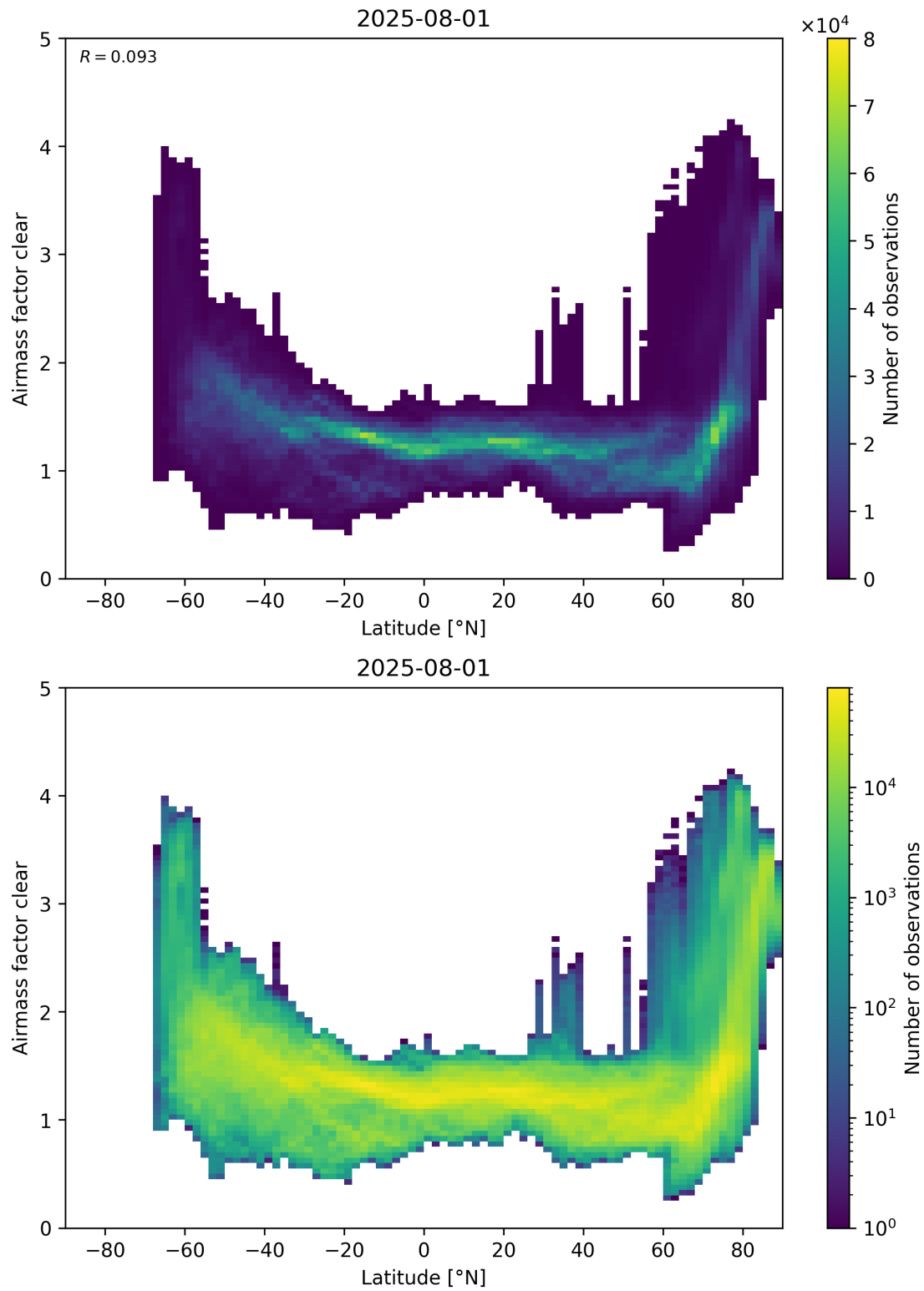
Figure 156: Scatter density plot of “Latitude” against “Airmass factor clear” for 2025-07-31 to 2025-08-02.
