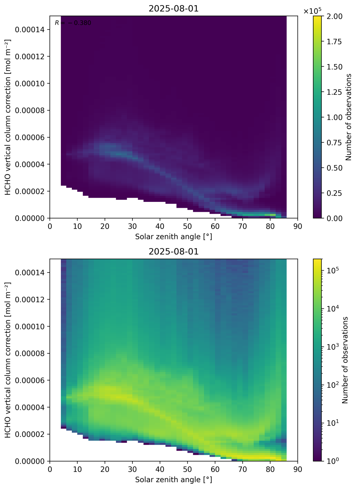
Figure 178: Scatter density plot of “Solar zenith angle” against “HCHO vertical column correction” for 2025-07-31 to 2025-08-02.
