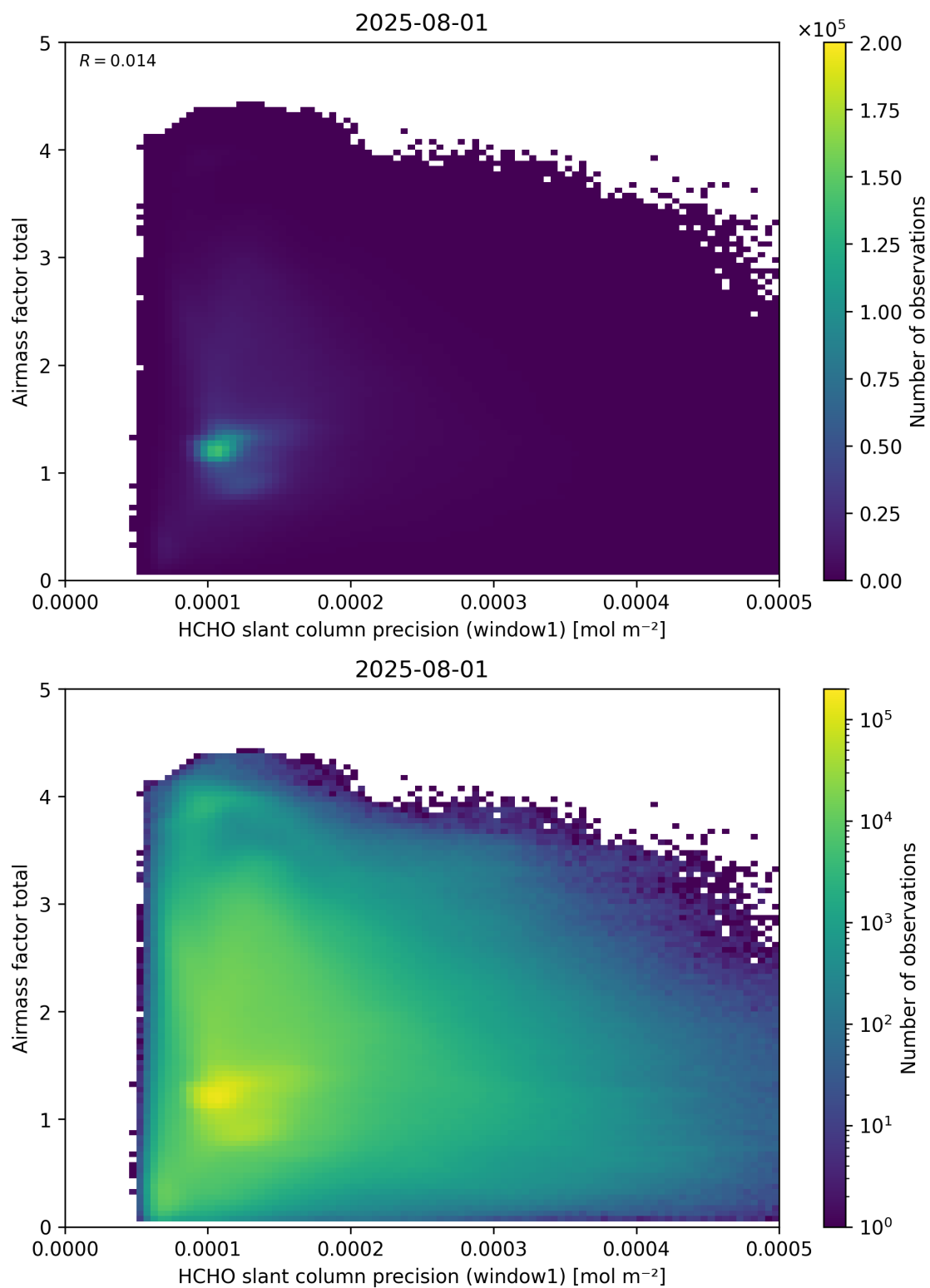
Figure 94: Scatter density plot of “HCHO slant column precision (window1)” against “Airmass factor total” for 2025-07-31 to 2025-08-02.
