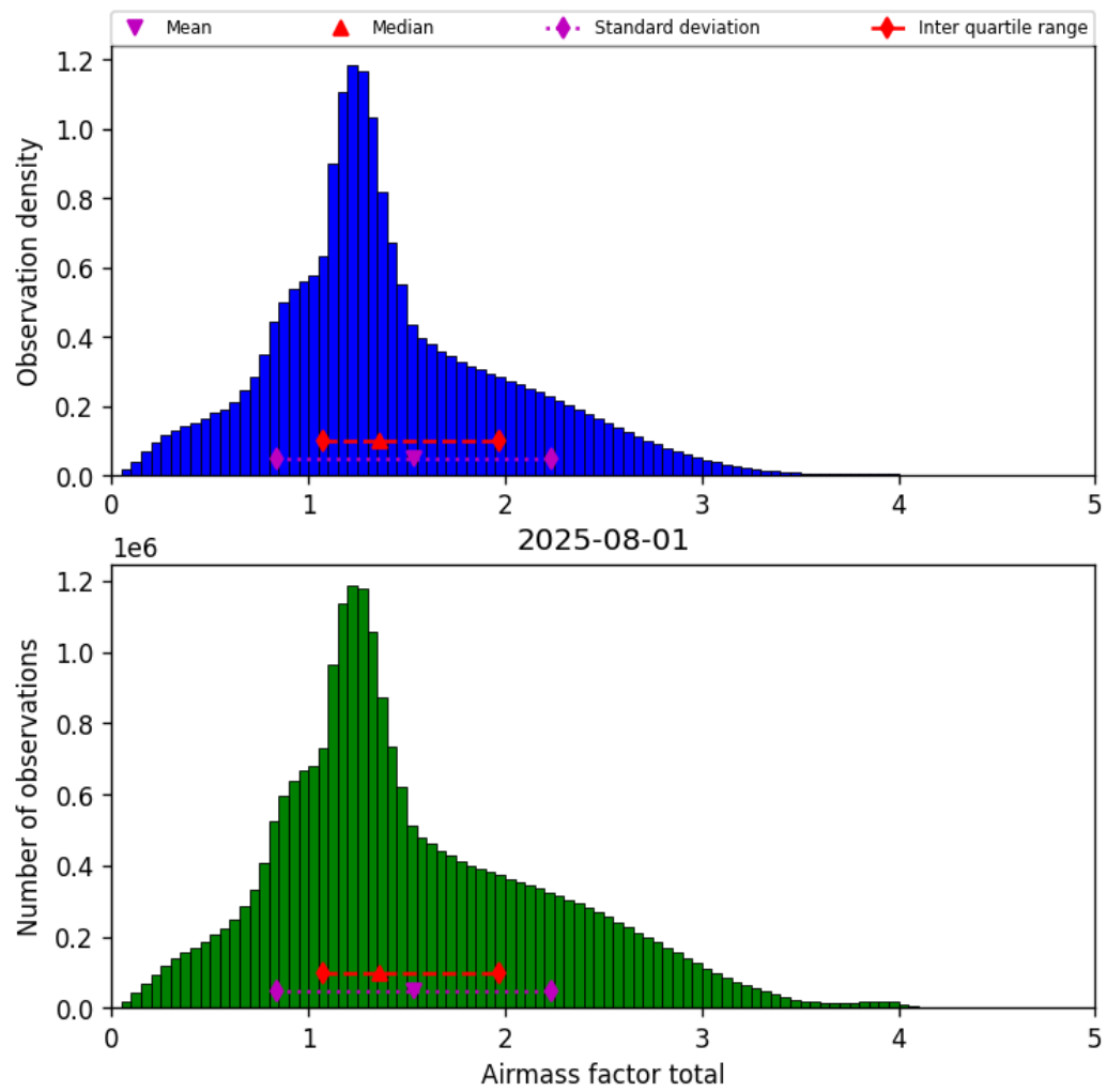
Figure 40: Histogram of “Airmass factor total” for 2025-07-31 to 2025-08-02
