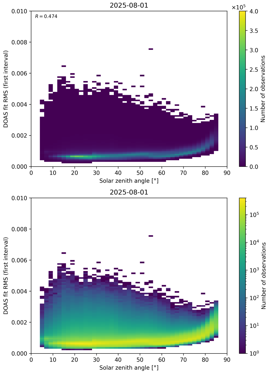
Figure 167: Scatter density plot of “Solar zenith angle” against “DOAS fit RMS (first interval)” for 2025-07-31 to 2025-08-02.
