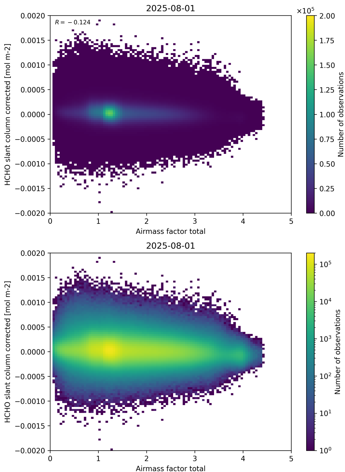
Figure 101: Scatter density plot of “Airmass factor total” against “HCHO slant column corrected” for 2025-07-31 to 2025-08-02.
