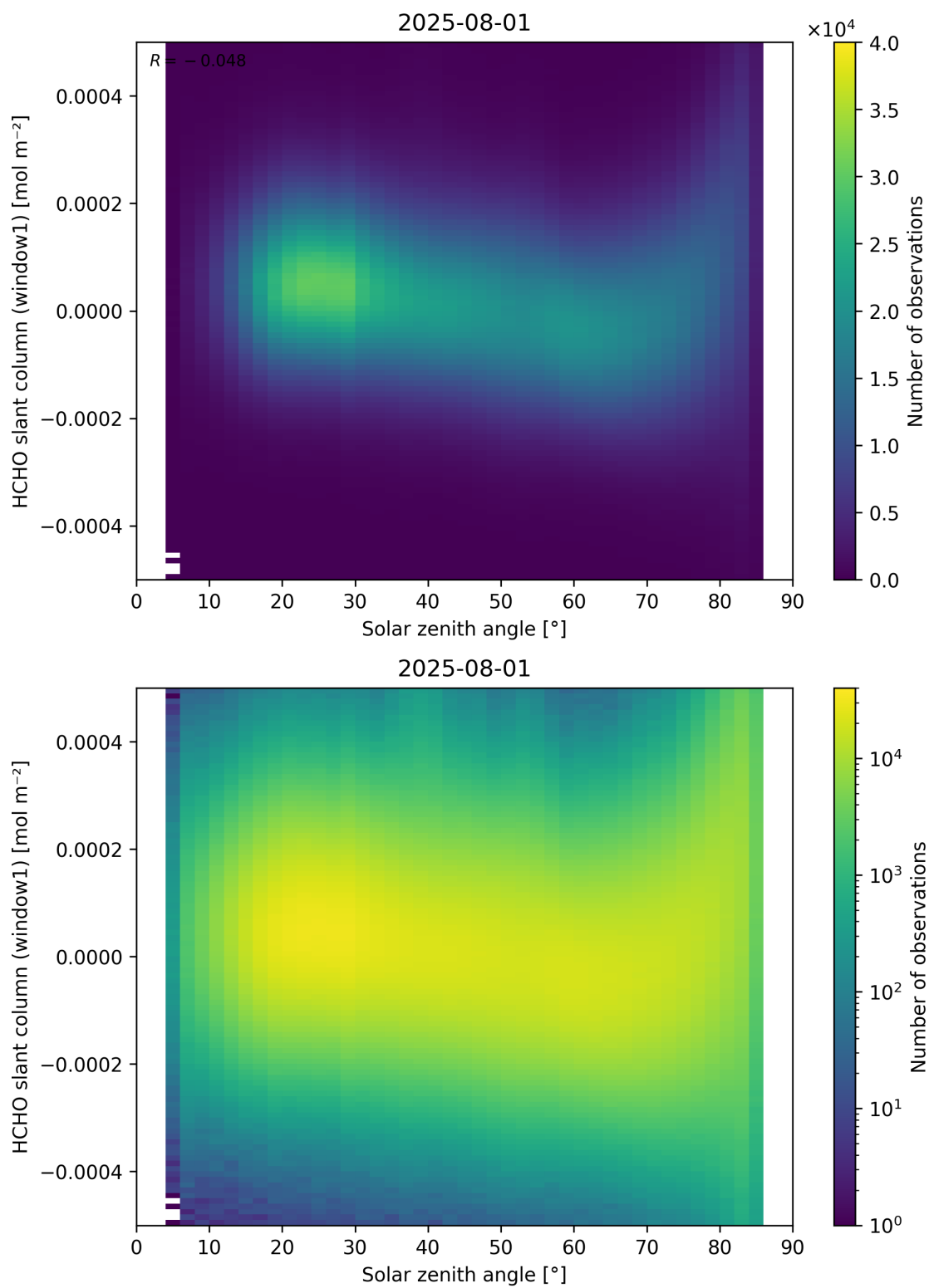
Figure 173: Scatter density plot of “Solar zenith angle” against “HCHO slant column (window1)” for 2025-07-31 to 2025-08-02.
