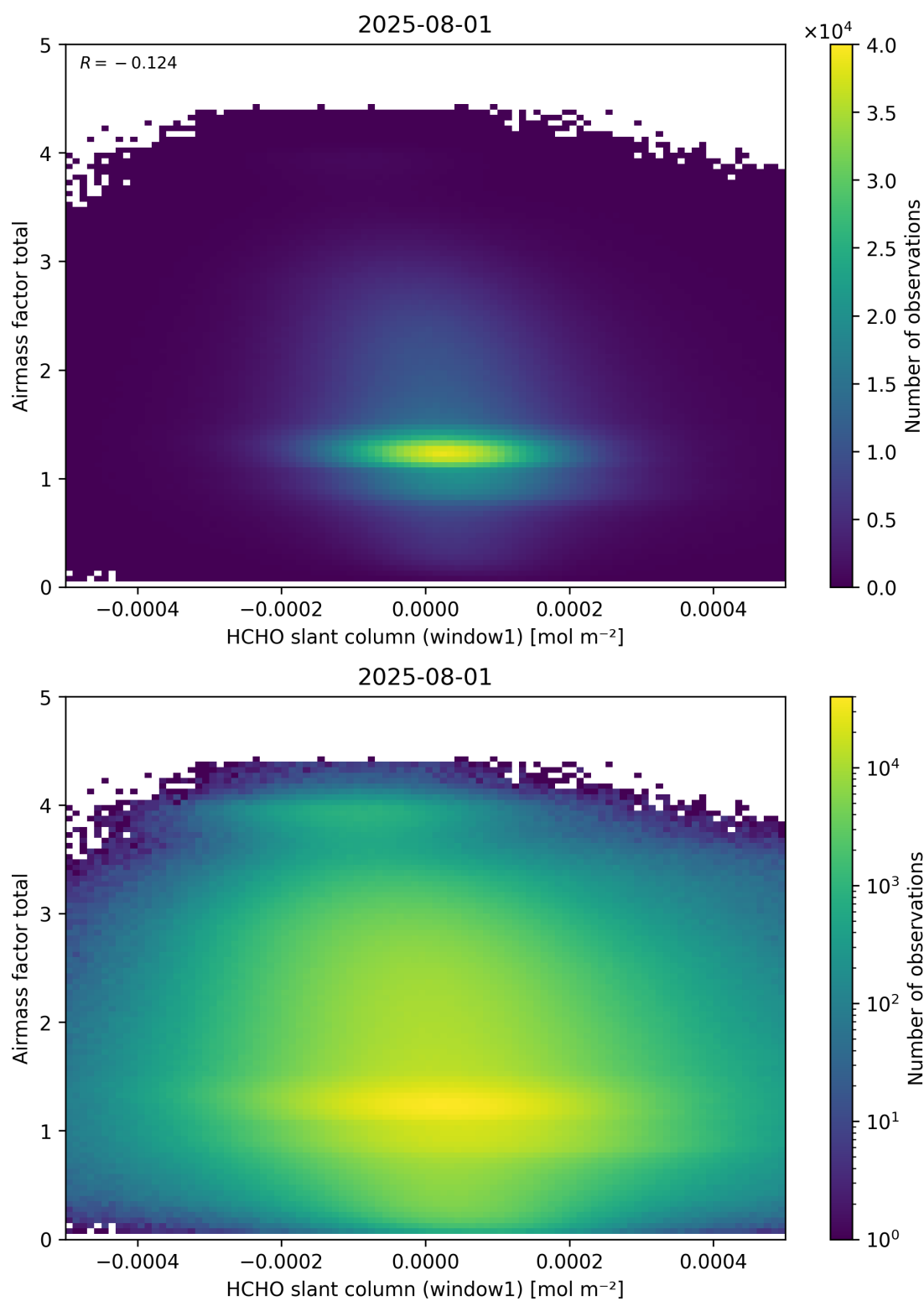
Figure 85: Scatter density plot of “HCHO slant column (window1)” against “Airmass factor total” for 2025-07-31 to 2025-08-02.
