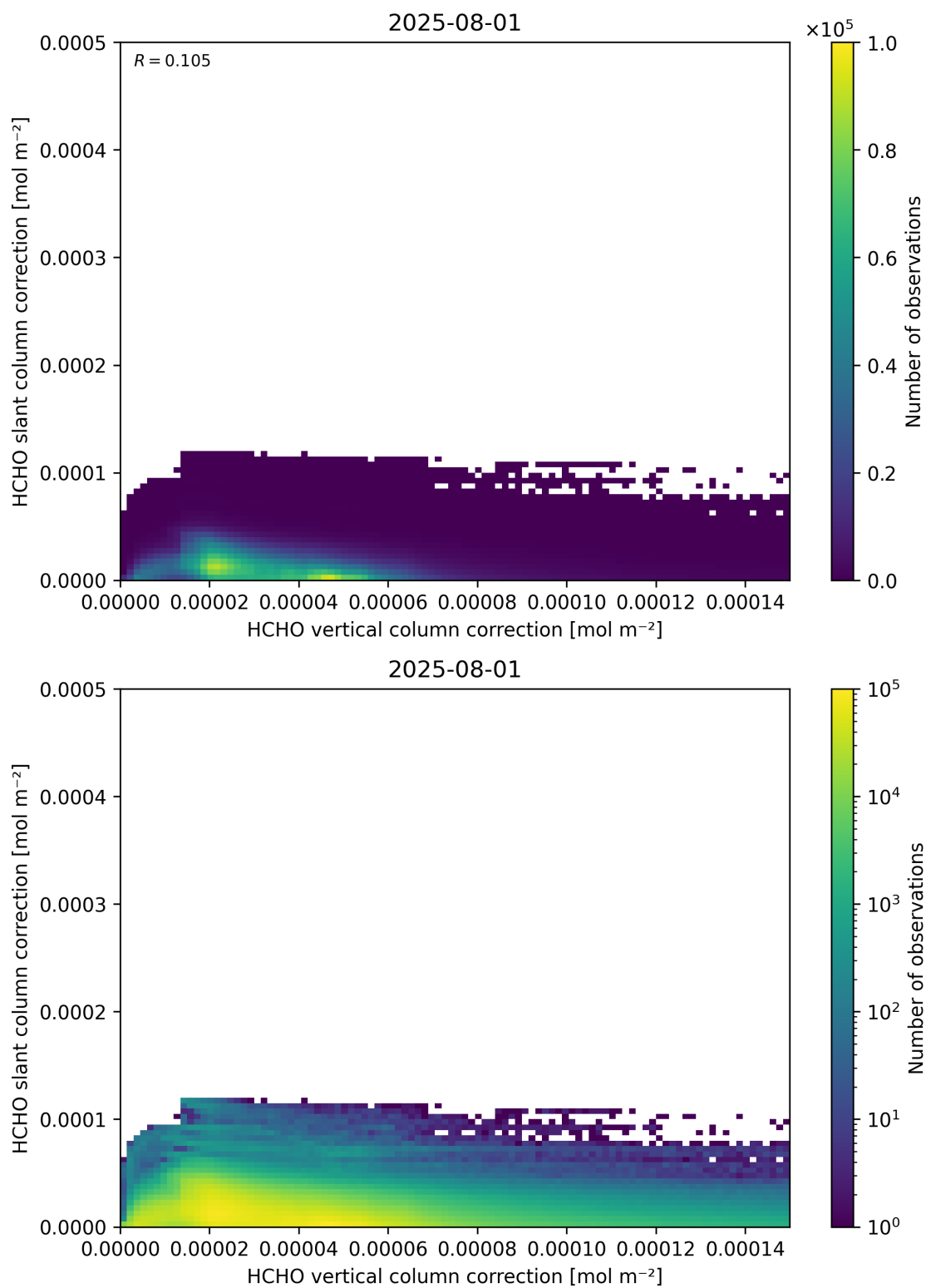
Figure 117: Scatter density plot of “HCHO vertical column correction” against “HCHO slant column correction” for 2025-07-31 to 2025-08-02.
