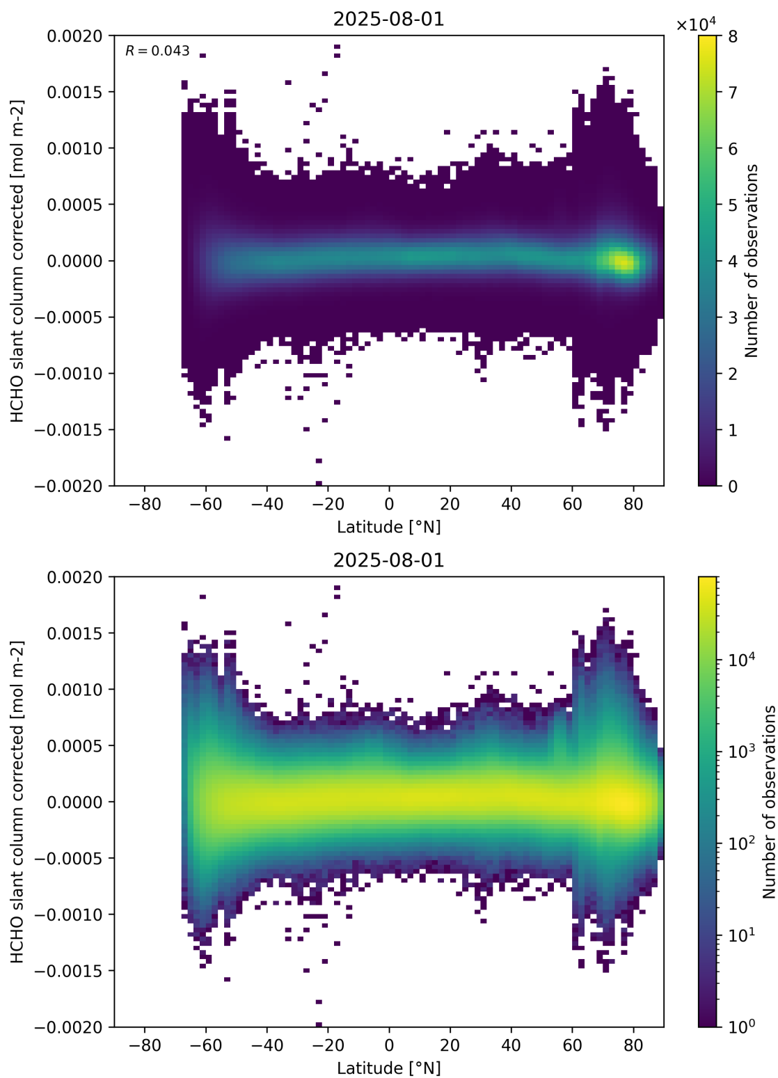
Figure 157: Scatter density plot of “Latitude” against “HCHO slant column corrected” for 2025-07-31 to 2025-08-02.
