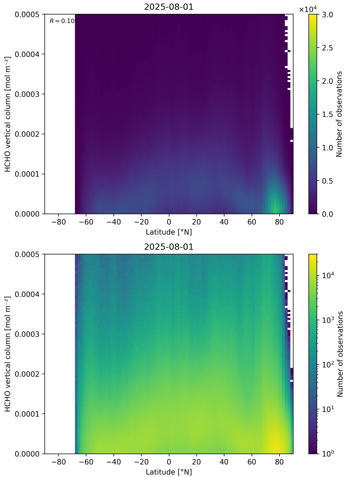
Figure 163: Scatter density plot of “Latitude” against “HCHO vertical column” for 2025-07-31 to 2025-08-02.
