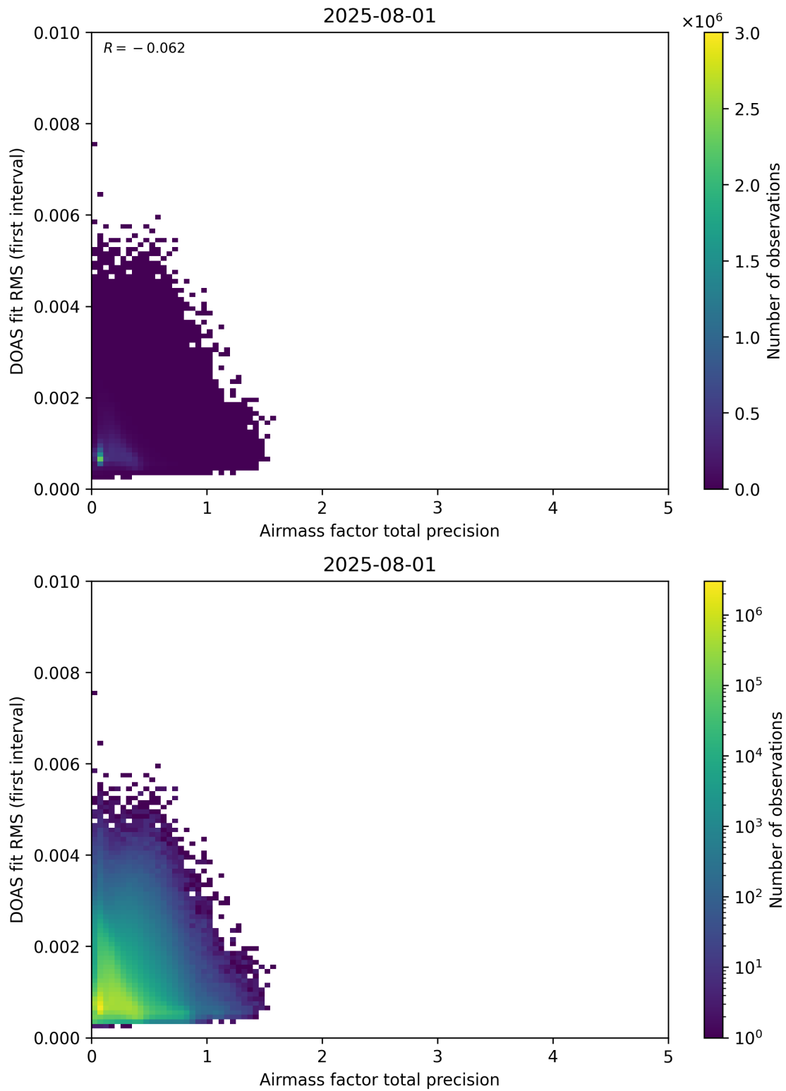
Figure 105: Scatter density plot of “Airmass factor total precision” against “DOAS fit RMS (first interval)” for 2025-07-31 to 2025-08-02.
