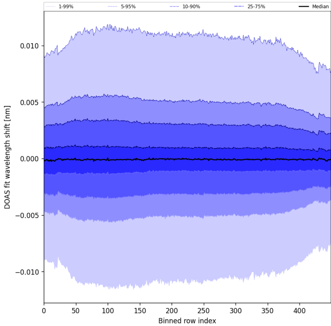
Figure 58: Along track statistics of “DOAS fit wavelength shift” for 2025-07-31 to 2025-08-02
