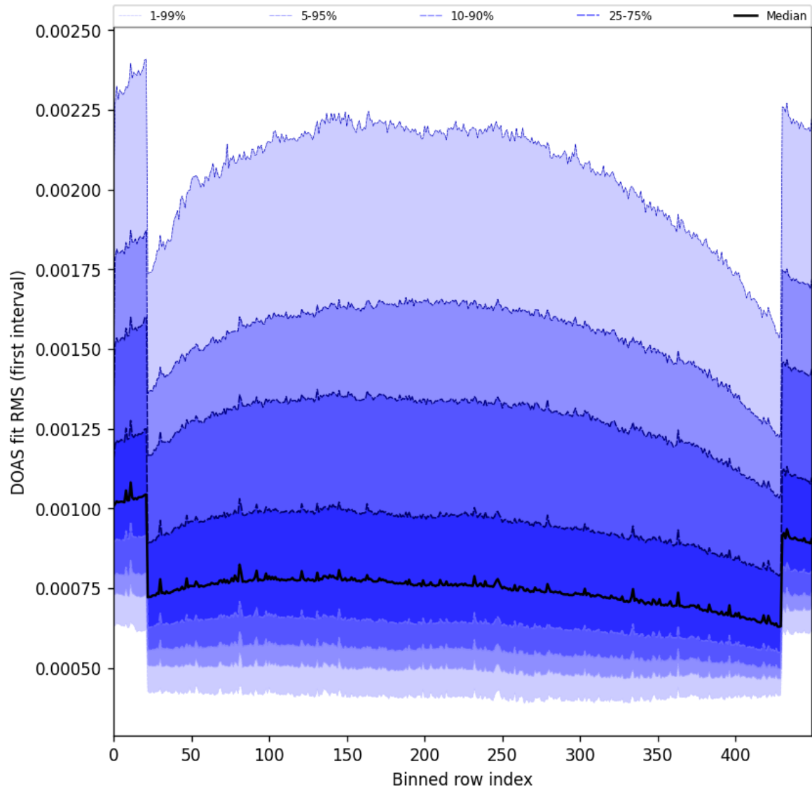
Figure 60: Along track statistics of “DOAS fit RMS (first interval)” for 2025-07-31 to 2025-08-02
