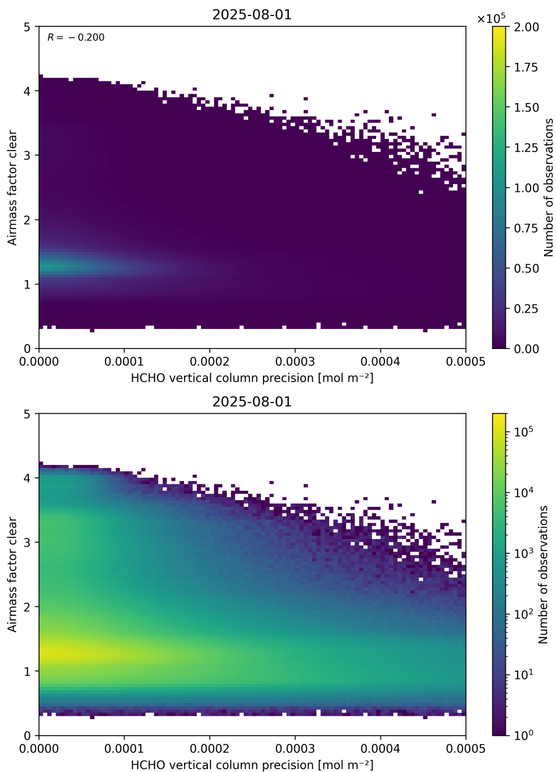
Figure 139: Scatter density plot of “HCHO vertical column precision” against “Airmass factor clear” for 2025-07-31 to 2025-08-02.
