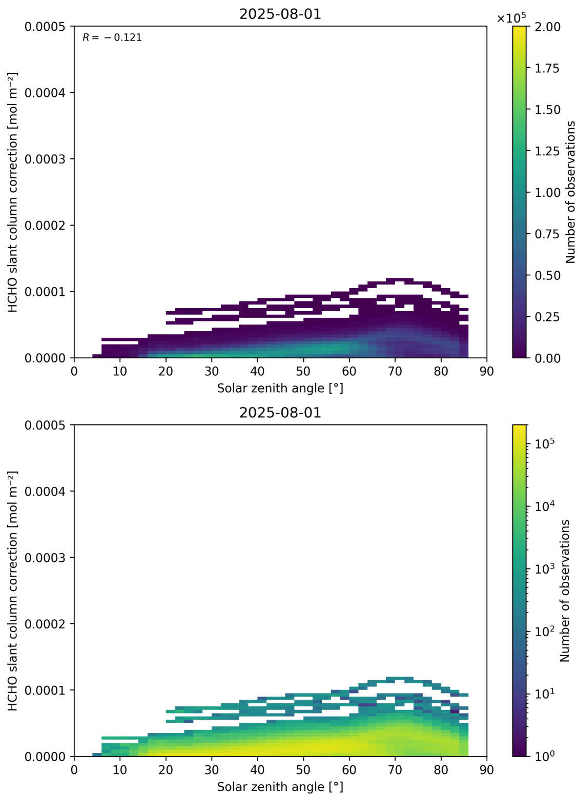
Figure 172: Scatter density plot of “Solar zenith angle” against “HCHO slant column correction” for 2025-07-31 to 2025-08-02.
