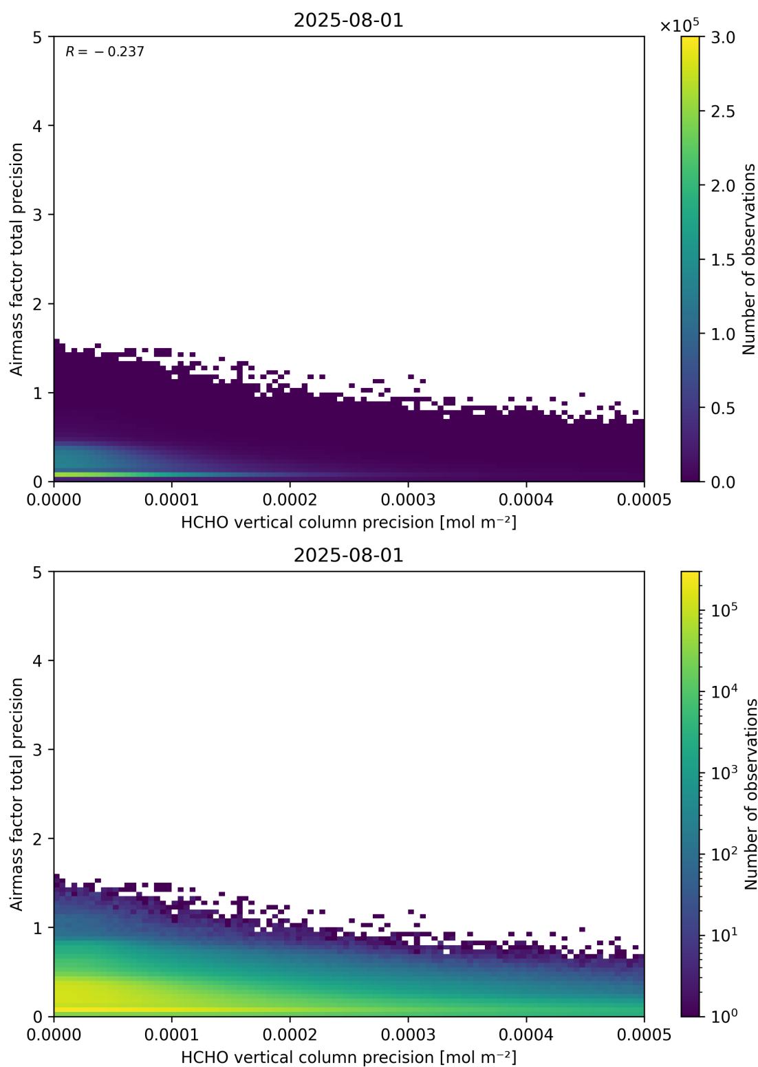
Figure 145: Scatter density plot of “HCHO vertical column precision” against “Airmass factor total precision” for 2025-07-31 to 2025-08-02.
