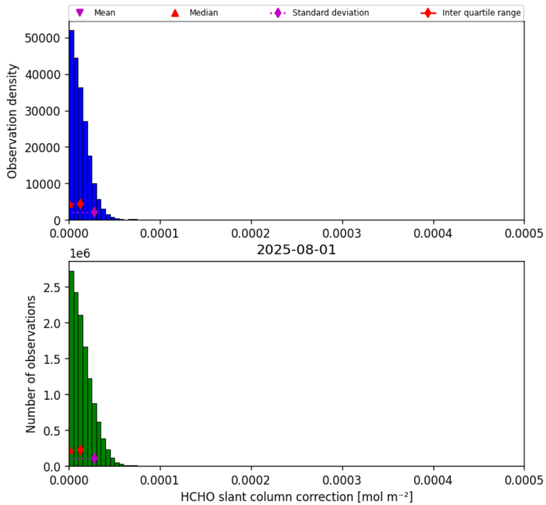
Figure 47: Histogram of “HCHO slant column correction” for 2025-07-31 to 2025-08-02
