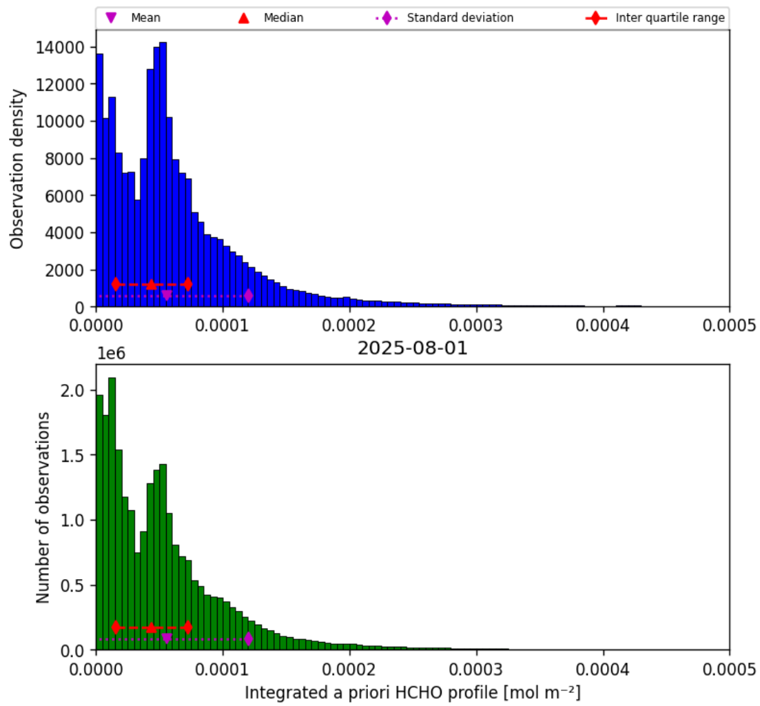
Figure 43: Histogram of “Integrated a priori HCHO profile” for 2025-07-31 to 2025-08-02
