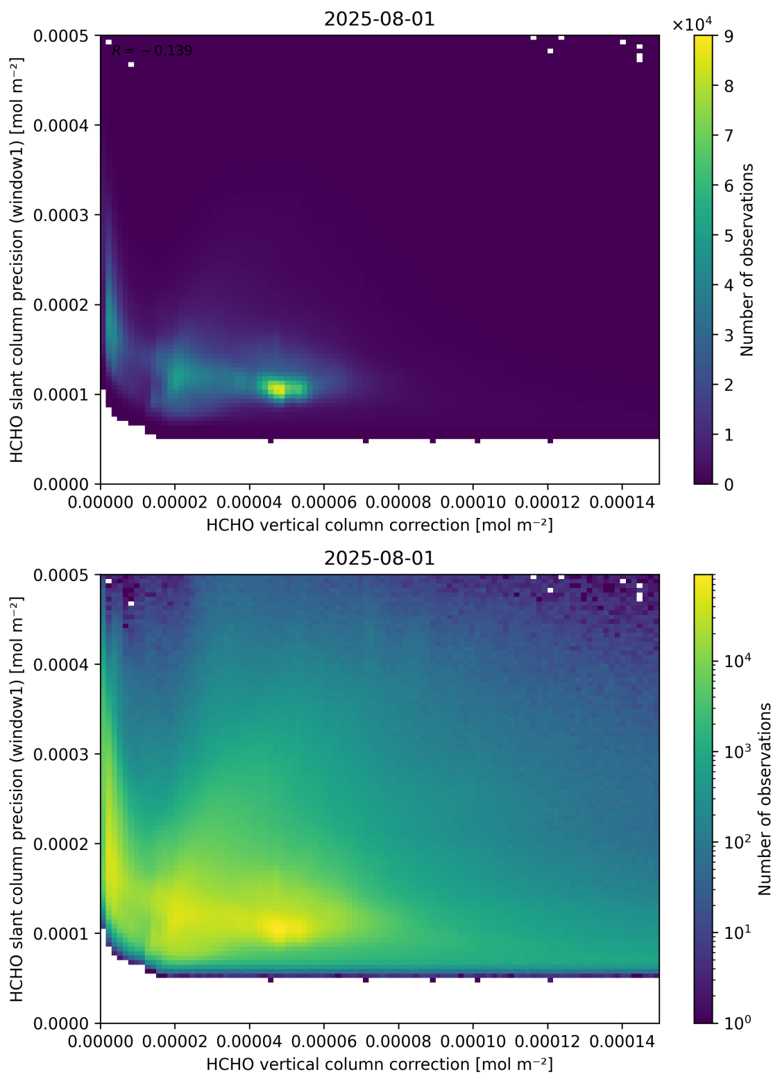
Figure 119: Scatter density plot of “HCHO vertical column correction” against “HCHO slant column precision (window1)” for 2025-07-31 to 2025-08-02.
