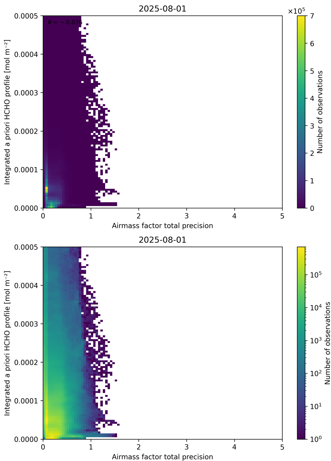
Figure 111: Scatter density plot of “Airmass factor total precision” against “Integrated a priori HCHO profile” for 2025-07-31 to 2025-08-02.
