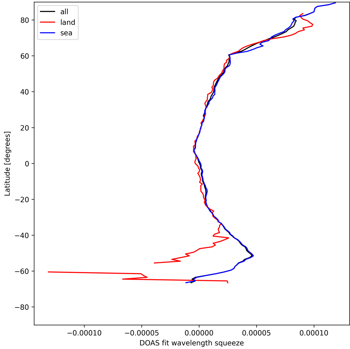
Figure 31: Zonal average of “DOAS fit wavelength squeeze” for 2025-07-31 to 2025-08-02.
