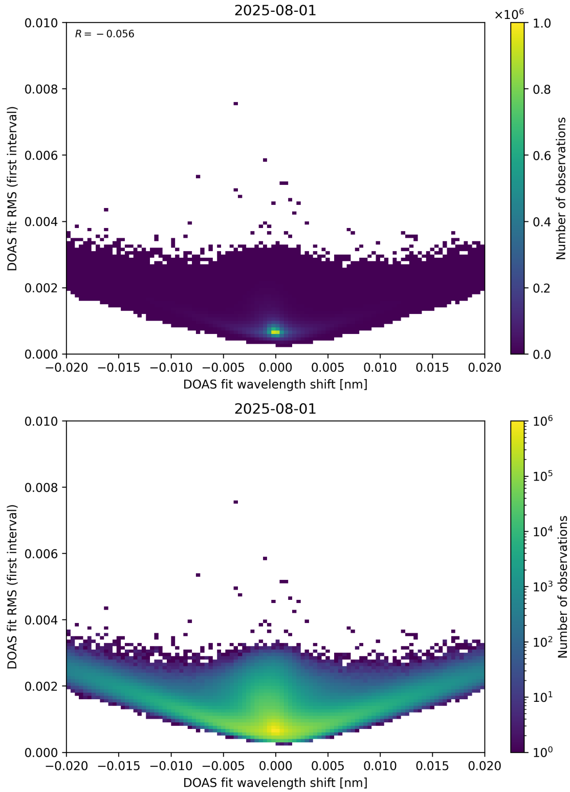
Figure 64: Scatter density plot of “DOAS fit wavelength shift” against “DOAS fit RMS (first interval)” for 2025-07-31 to 2025-08-02.
