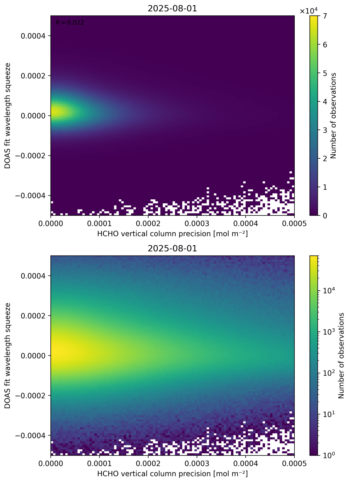
Figure 138: Scatter density plot of “HCHO vertical column precision” against “DOAS fit wavelength squeeze” for 2025-07-31 to 2025-08-02.
