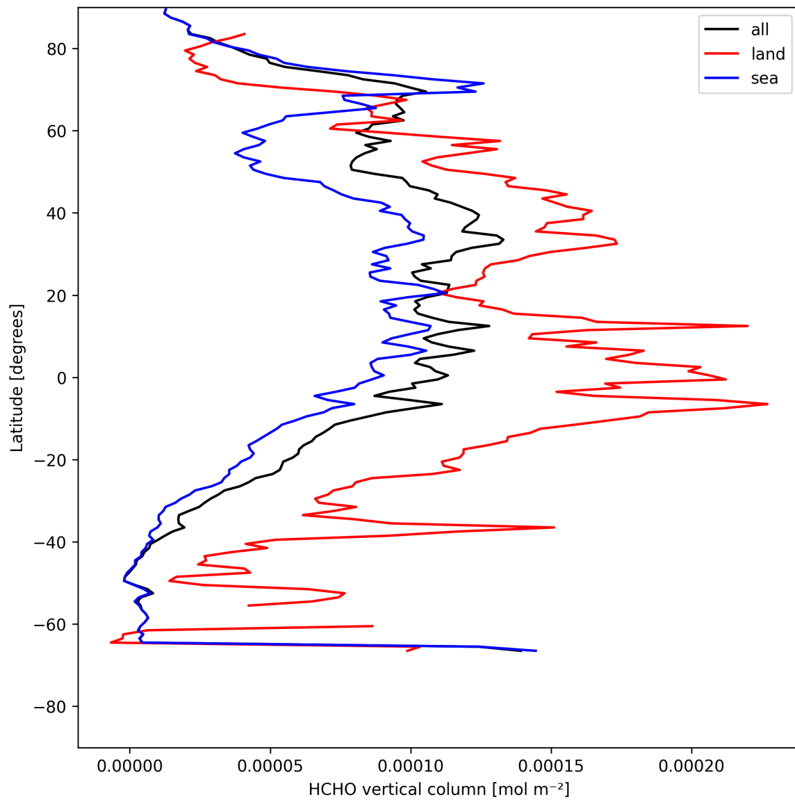
Figure 21: Zonal average of “HCHO vertical column” for 2025-07-31 to 2025-08-02.
