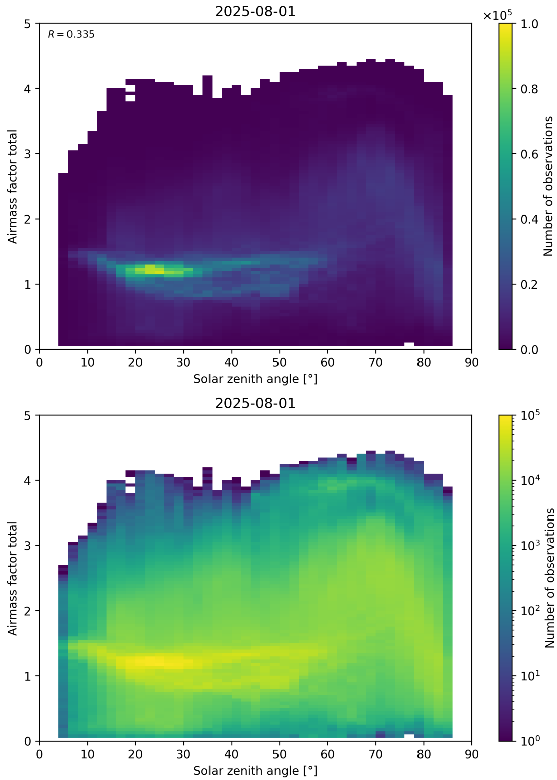
Figure 175: Scatter density plot of “Solar zenith angle” against “Airmass factor total” for 2025-07-31 to 2025-08-02.
