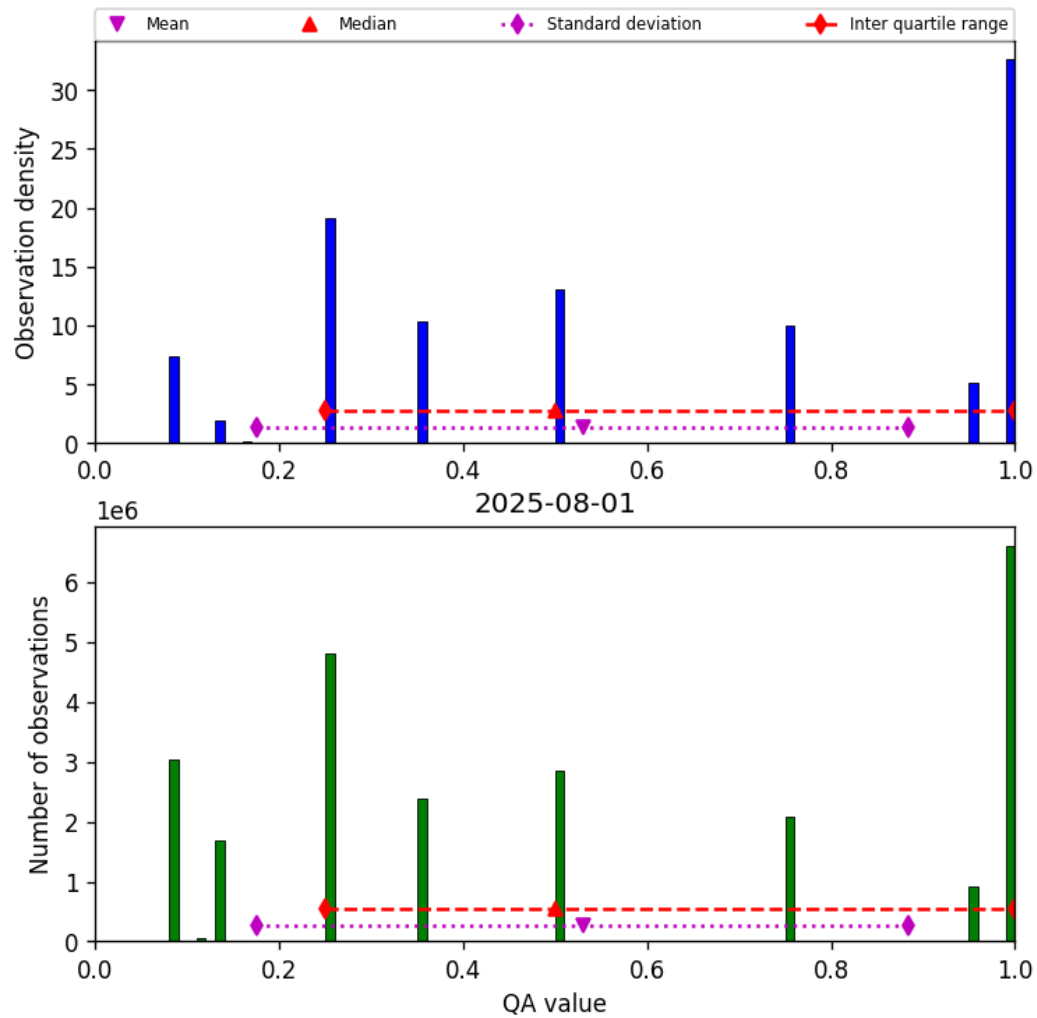
Figure 34: Histogram of “QA value” for 2025-07-31 to 2025-08-02
