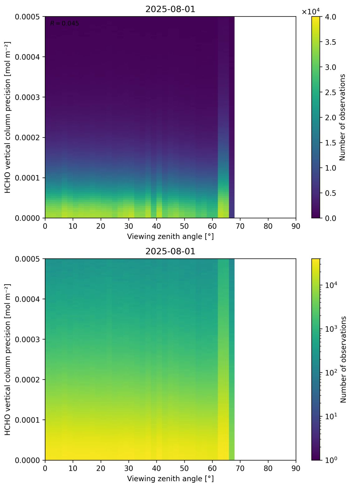
Figure 194: Scatter density plot of “Viewing zenith angle” against “HCHO vertical column precision” for 2025-07-31 to 2025-08-02.
