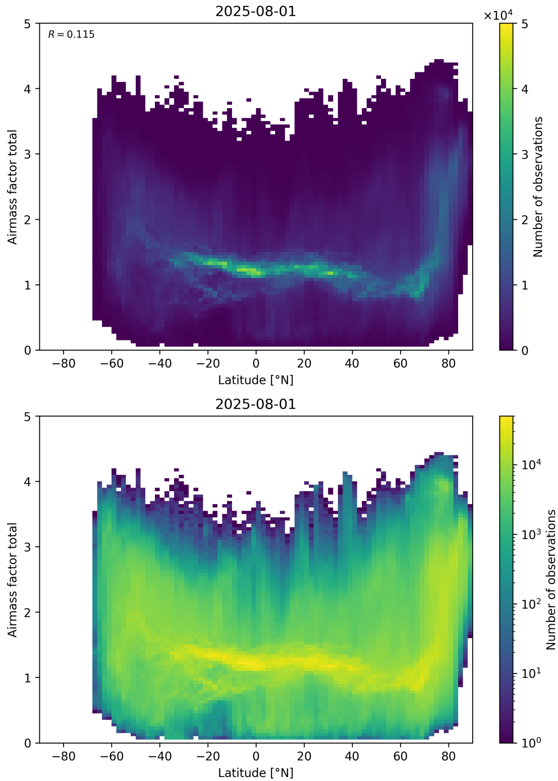
Figure 161: Scatter density plot of “Latitude” against “Airmass factor total” for 2025-07-31 to 2025-08-02.
