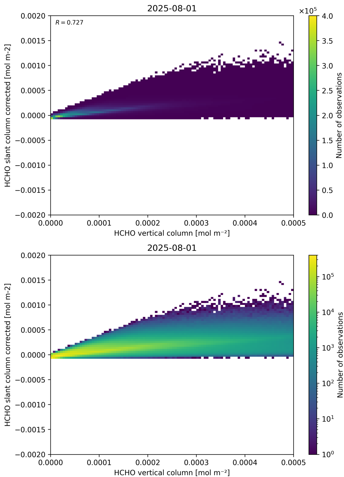
Figure 127: Scatter density plot of “HCHO vertical column” against “HCHO slant column corrected” for 2025-07-31 to 2025-08-02.
