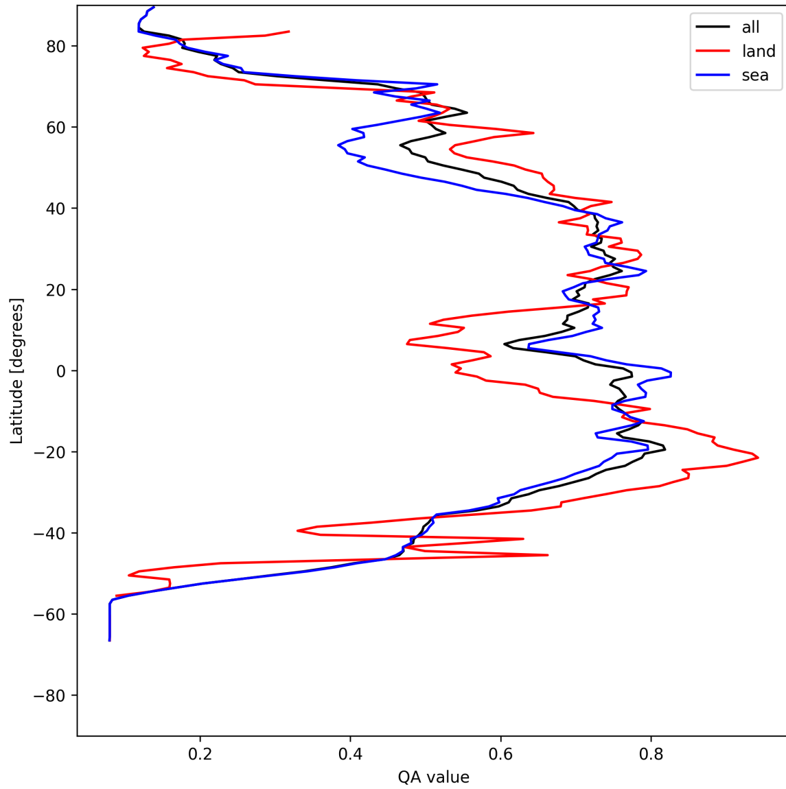
Figure 20: Zonal average of “QA value” for 2025-07-31 to 2025-08-02.
