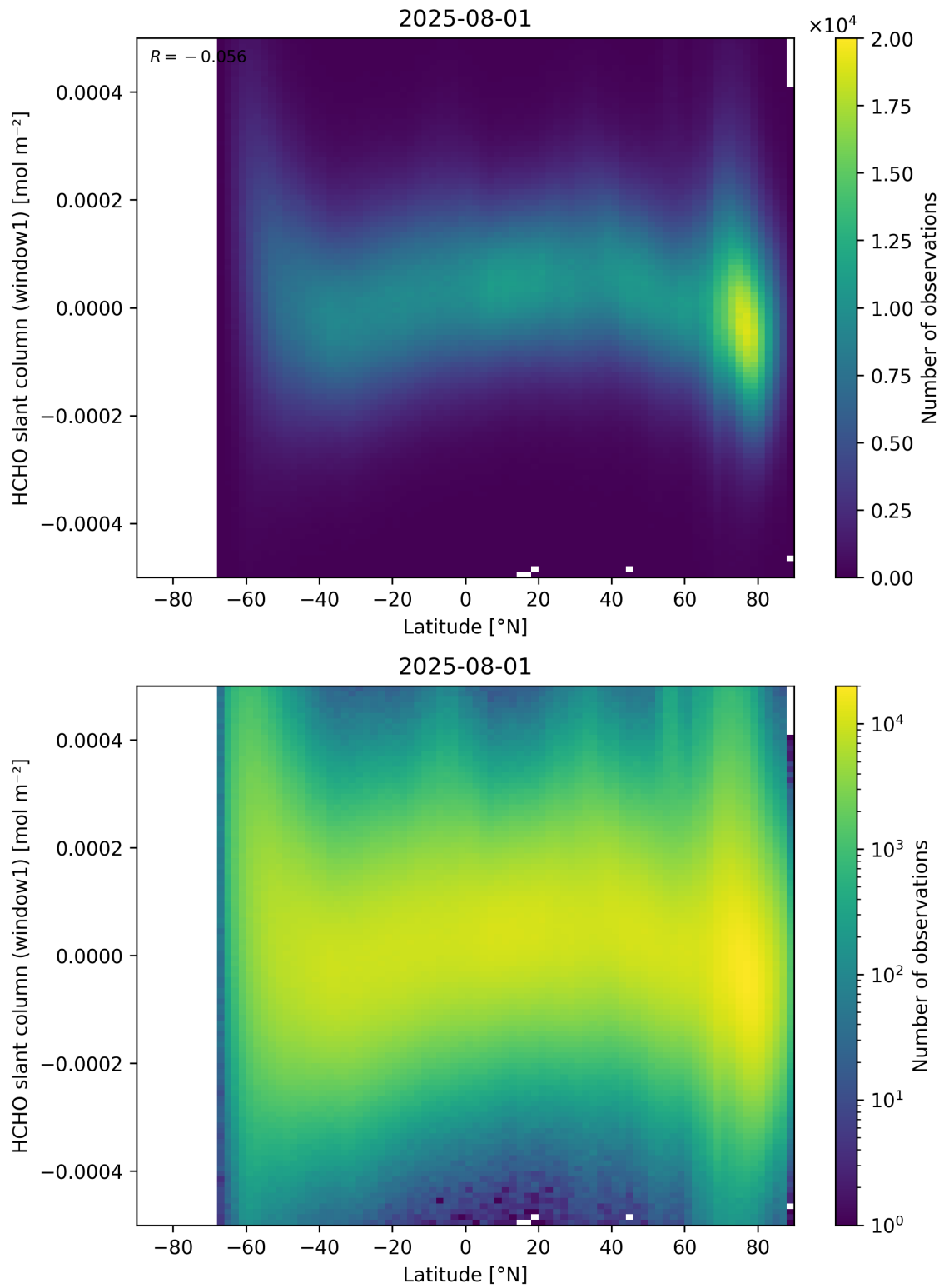
Figure 159: Scatter density plot of “Latitude” against “HCHO slant column (window1)” for 2025-07-31 to 2025-08-02.
