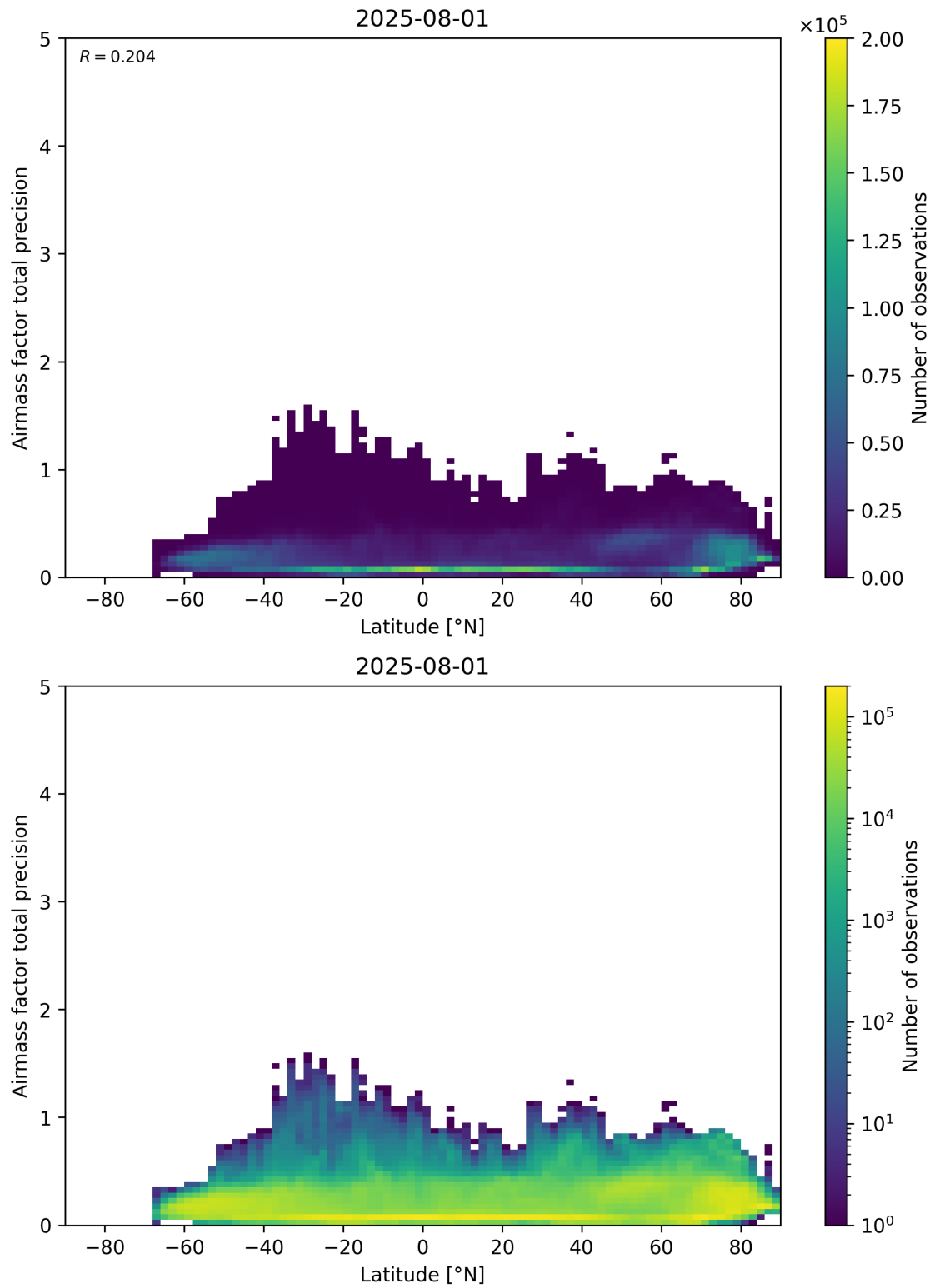
Figure 162: Scatter density plot of “Latitude” against “Airmass factor total precision” for 2025-07-31 to 2025-08-02.
