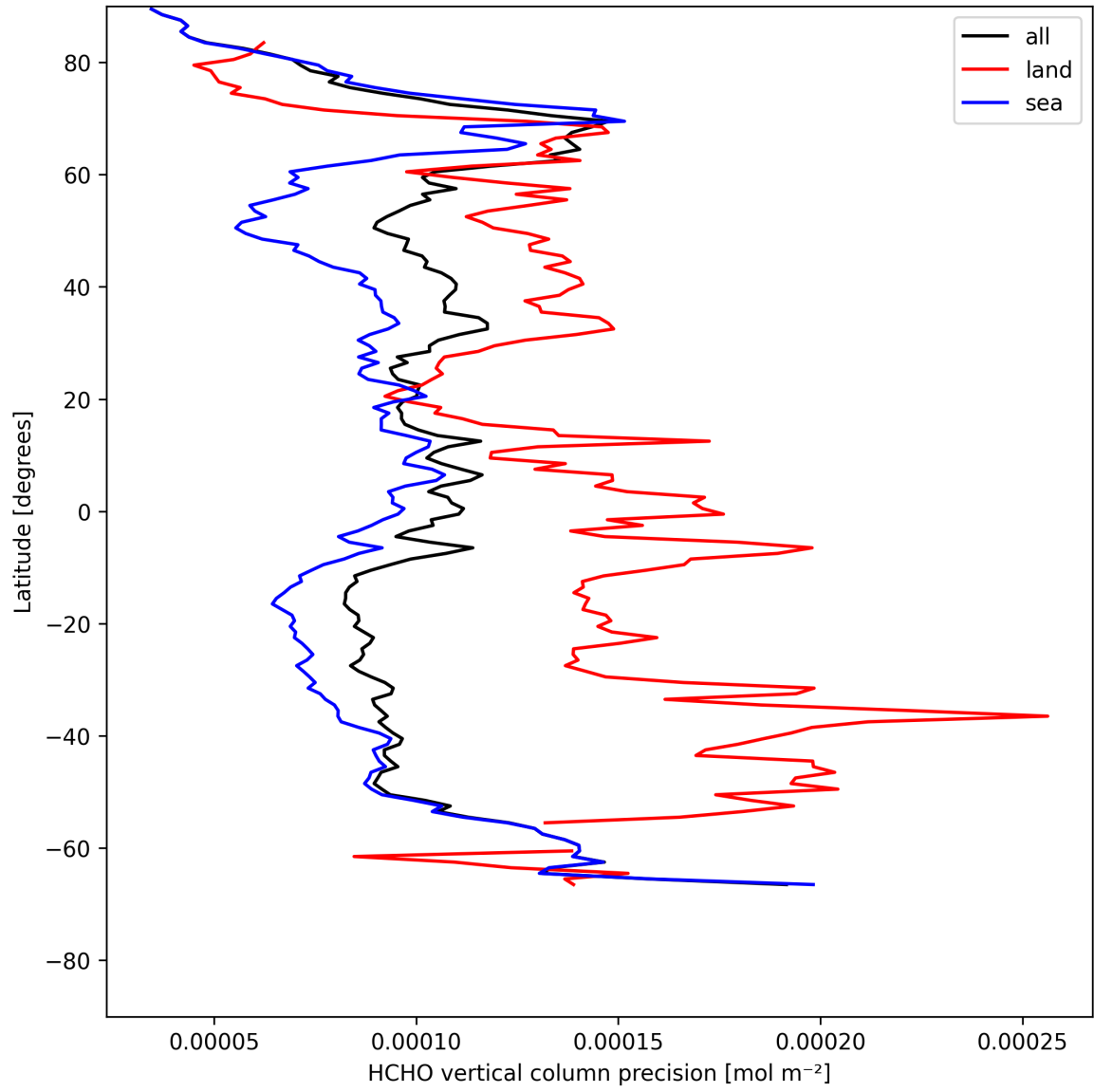
Figure 22: Zonal average of “HCHO vertical column precision” for 2025-07-31 to 2025-08-02.
