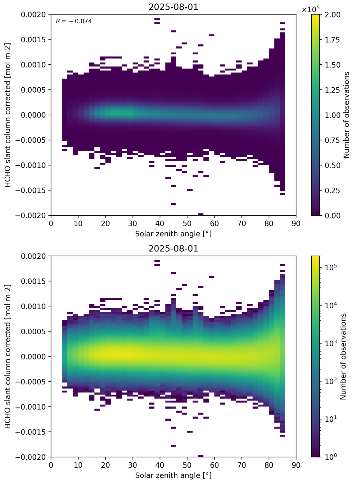
Figure 171: Scatter density plot of “Solar zenith angle” against “HCHO slant column corrected” for 2025-07-31 to 2025-08-02.
