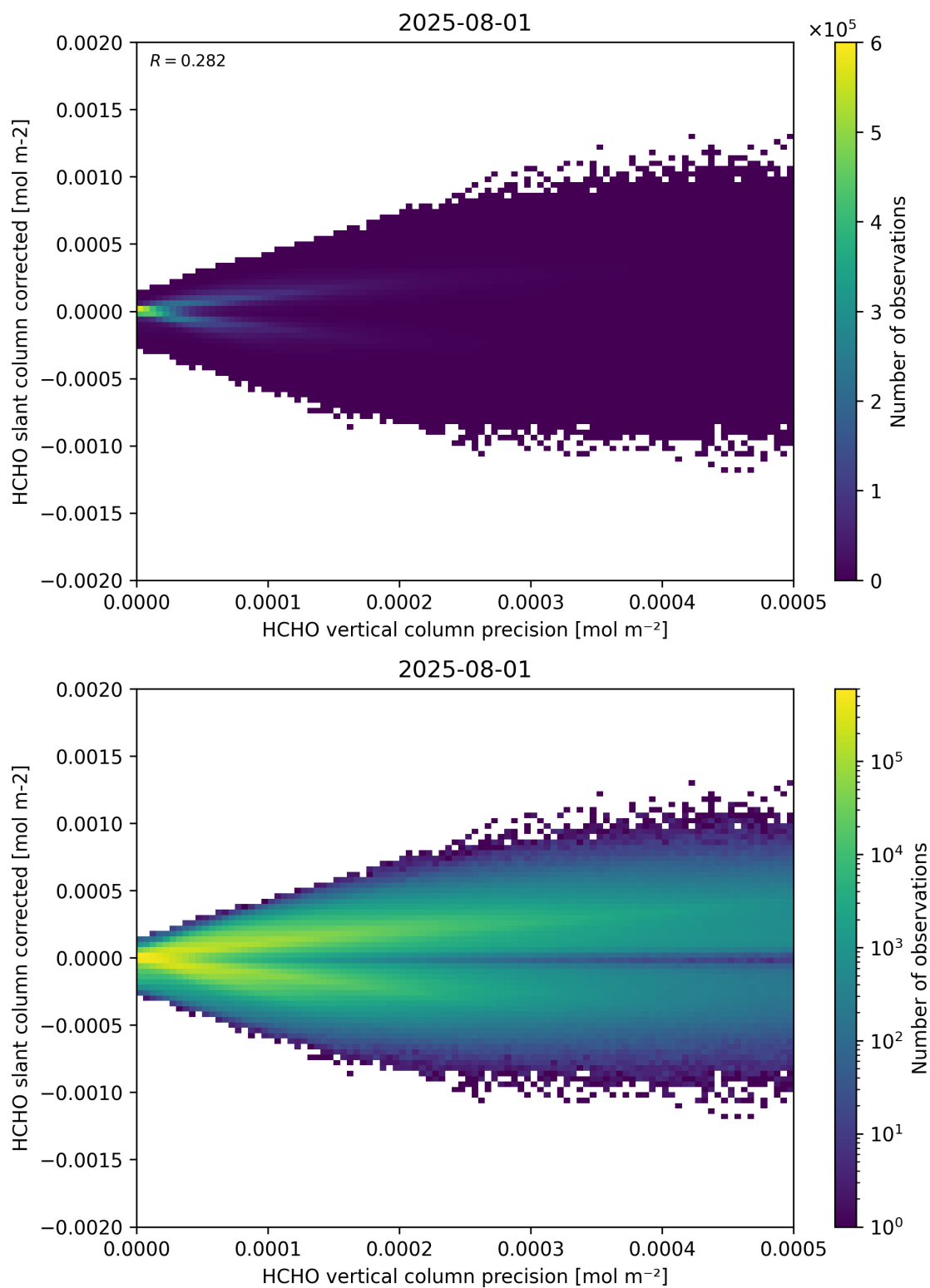
Figure 140: Scatter density plot of “HCHO vertical column precision” against “HCHO slant column corrected” for 2025-07-31 to 2025-08-02.
