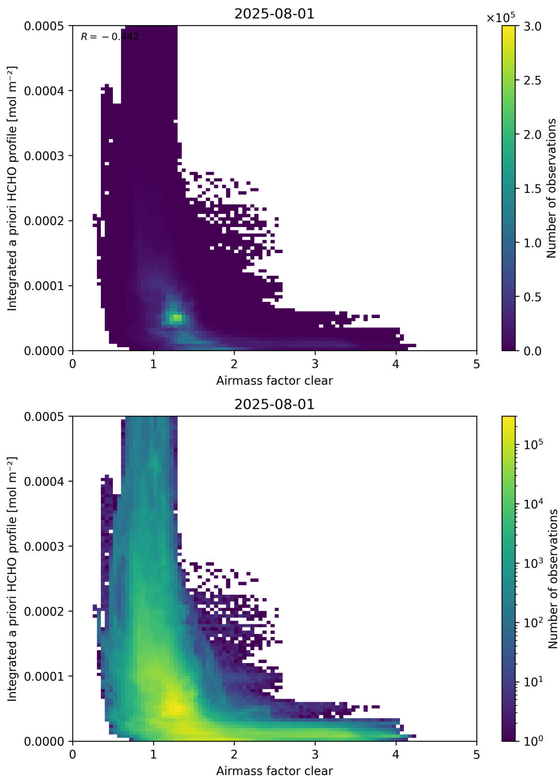
Figure 76: Scatter density plot of “Airmass factor clear” against “Integrated a priori HCHO profile” for 2025-07-31 to 2025-08-02.
