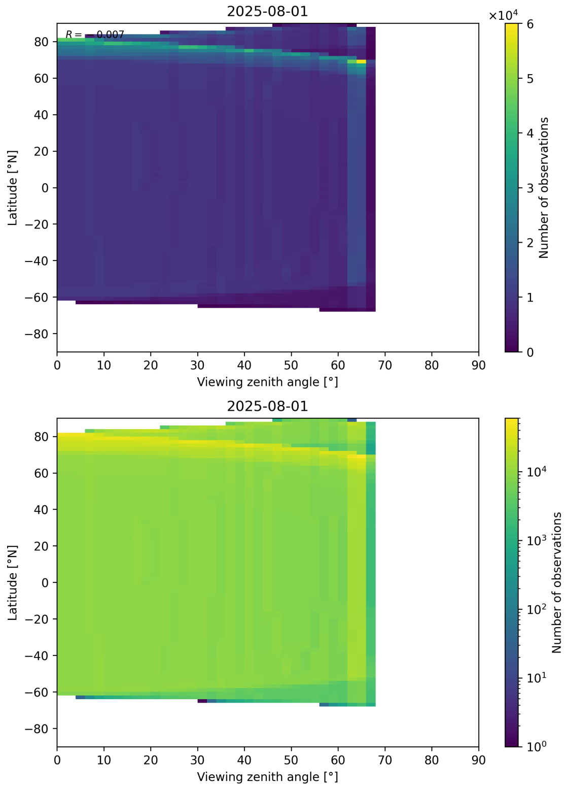
Figure 196: Scatter density plot of “Viewing zenith angle” against “Latitude” for 2025-07-31 to 2025-08-02.
