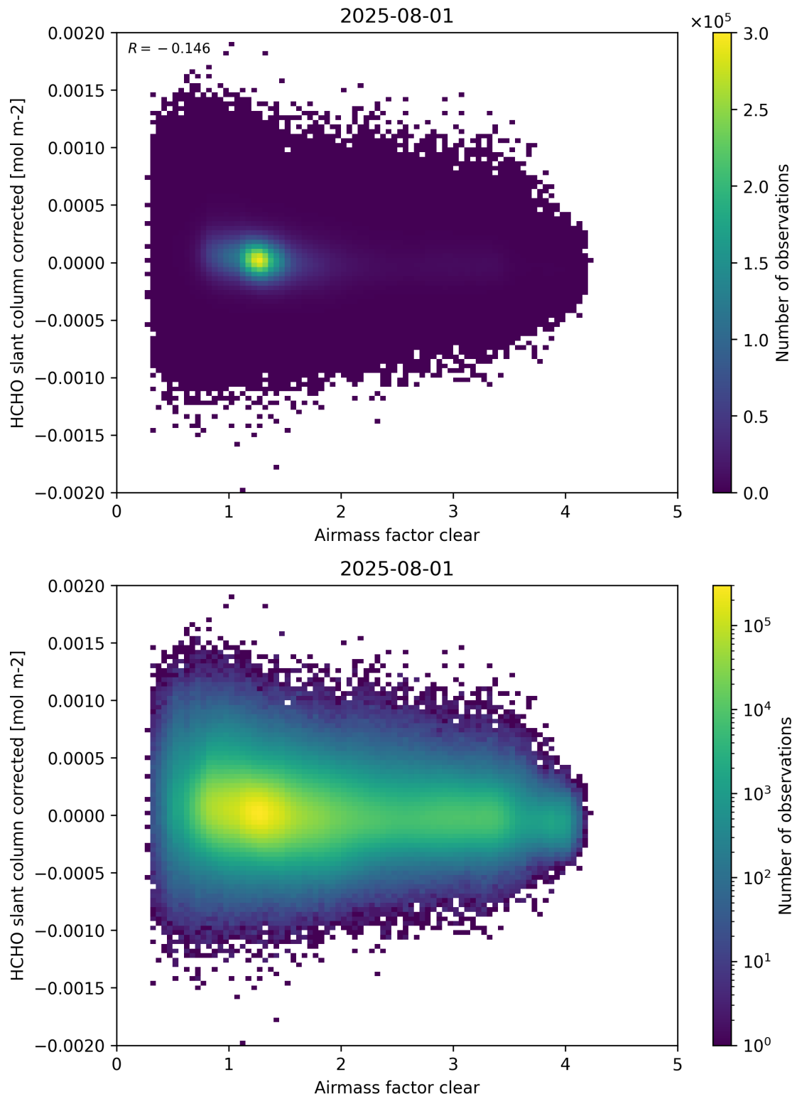
Figure 74: Scatter density plot of “Airmass factor clear” against “HCHO slant column corrected” for 2025-07-31 to 2025-08-02.
