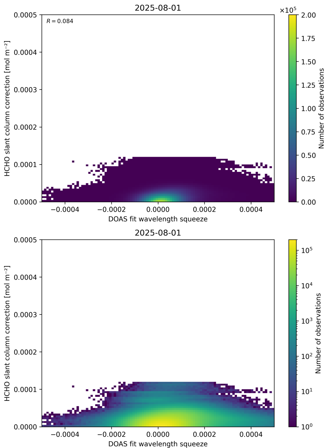
Figure 70: Scatter density plot of “DOAS fit wavelength squeeze” against “HCHO slant column correction” for 2025-07-31 to 2025-08-02.
