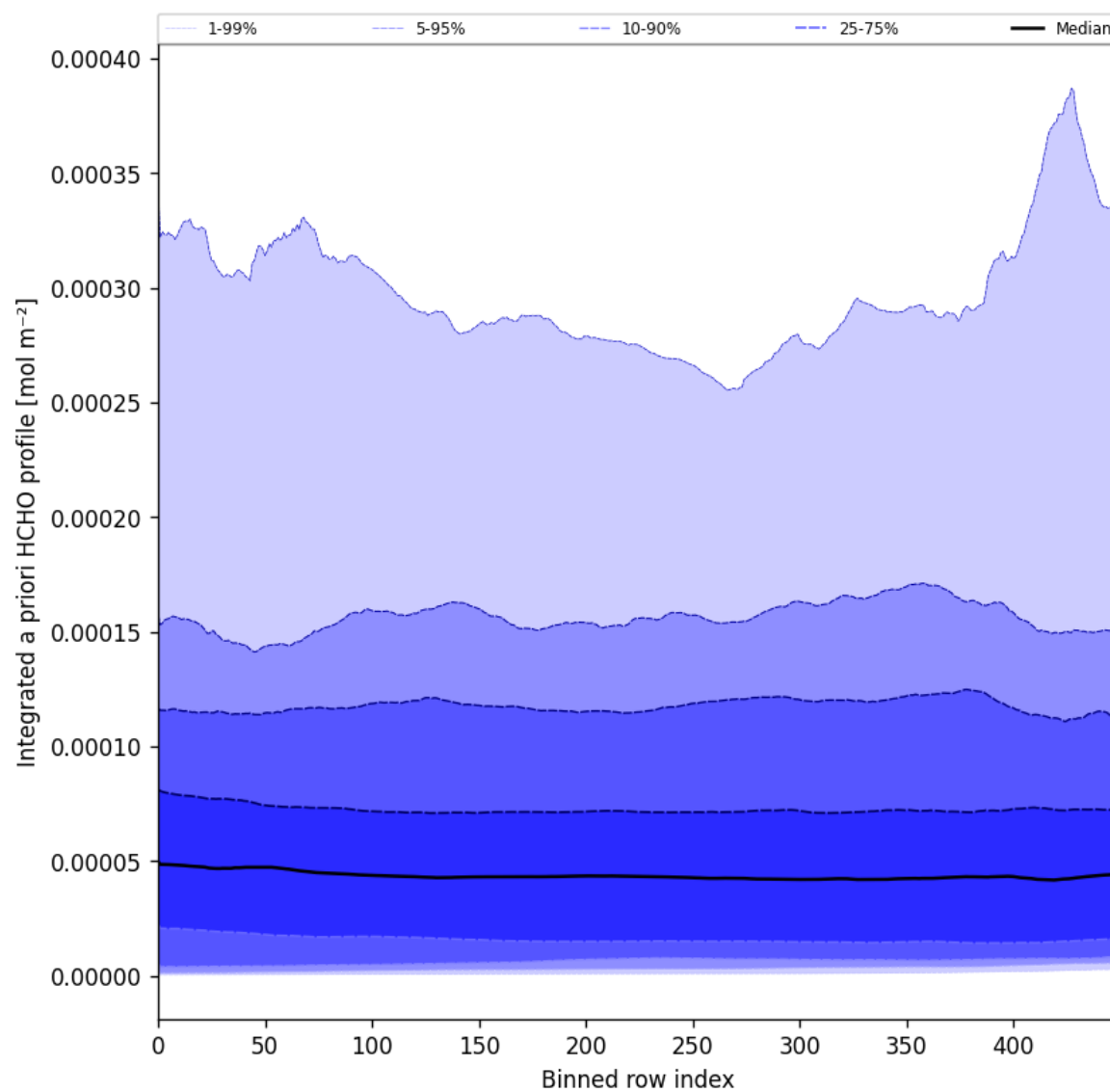
Figure 57: Along track statistics of "Integrated a priori HCHO profile" for 2025-07-31 to 2025-08-02
