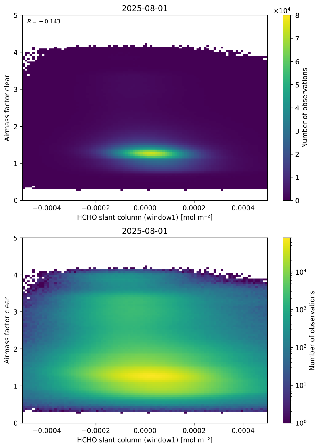
Figure 81: Scatter density plot of “HCHO slant column (window1)” against “Airmass factor clear” for 2025-07-31 to 2025-08-02.
