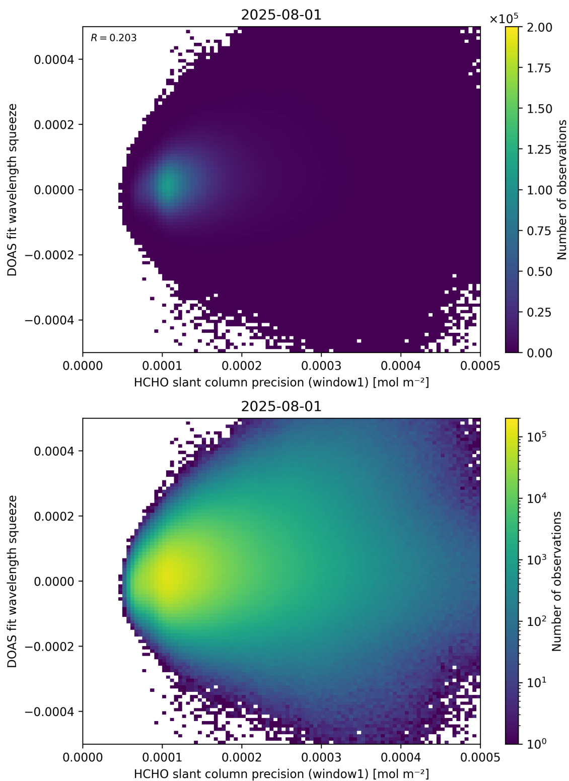
Figure 90: Scatter density plot of “HCHO slant column precision (window1)” against “DOAS fit wavelength squeeze” for 2025-07-31 to 2025-08-02.
