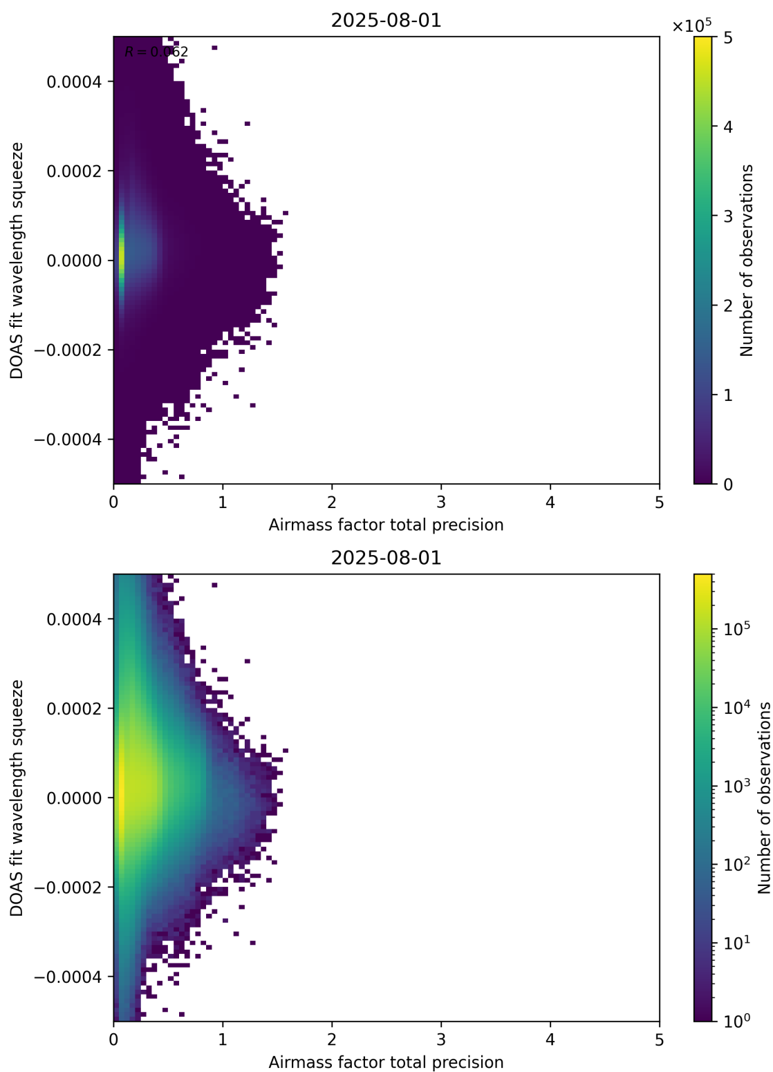
Figure 107: Scatter density plot of “Airmass factor total precision” against “DOAS fit wavelength squeeze” for 2025-07-31 to 2025-08-02.
