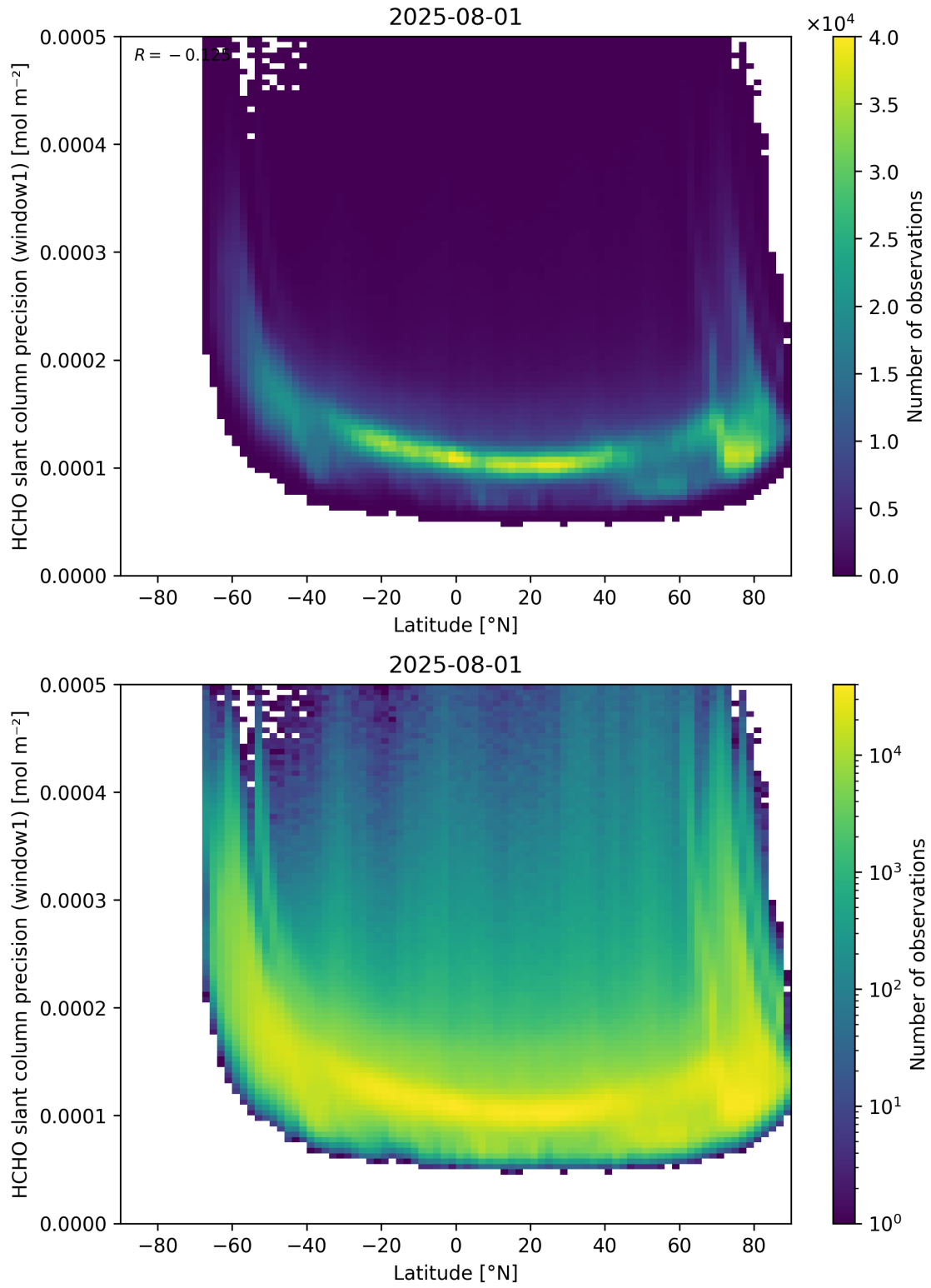
Figure 160: Scatter density plot of “Latitude” against “HCHO slant column precision (window1)” for 2025-07-31 to 2025-08-02.
