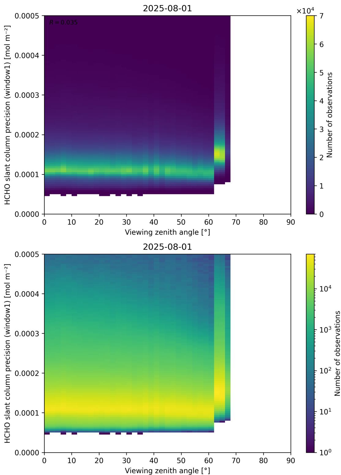
Figure 189: Scatter density plot of “Viewing zenith angle” against “HCHO slant column precision (window1)” for 2025-07-31 to 2025-08-02.
