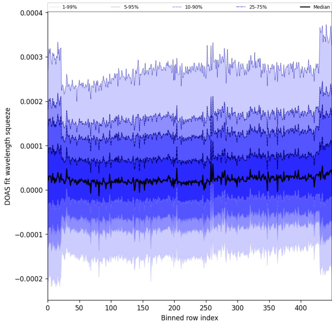
Figure 59: Along track statistics of “DOAS fit wavelength squeeze” for 2025-07-31 to 2025-08-02
