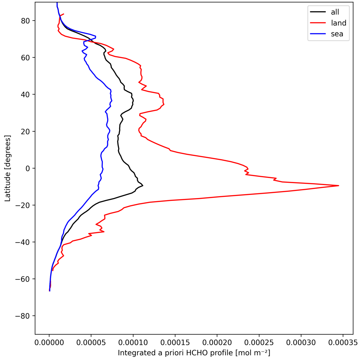
Figure 29: Zonal average of “Integrated a priori HCHO profile” for 2025-07-31 to 2025-08-02.
