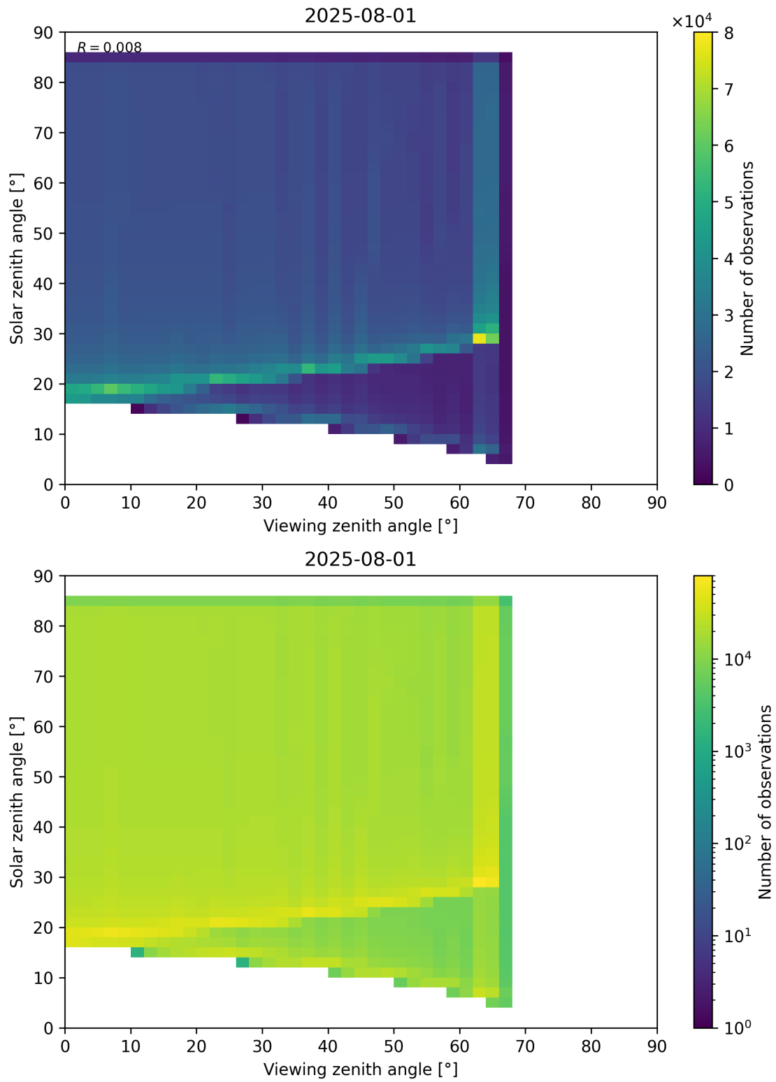
Figure 197: Scatter density plot of “Viewing zenith angle” against “Solar zenith angle” for 2025-07-31 to 2025-08-02.
