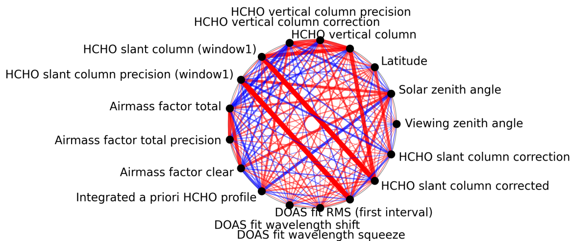
Figure 1: Map of correlation graph for 2025-07-31 to 2025-08-02.
