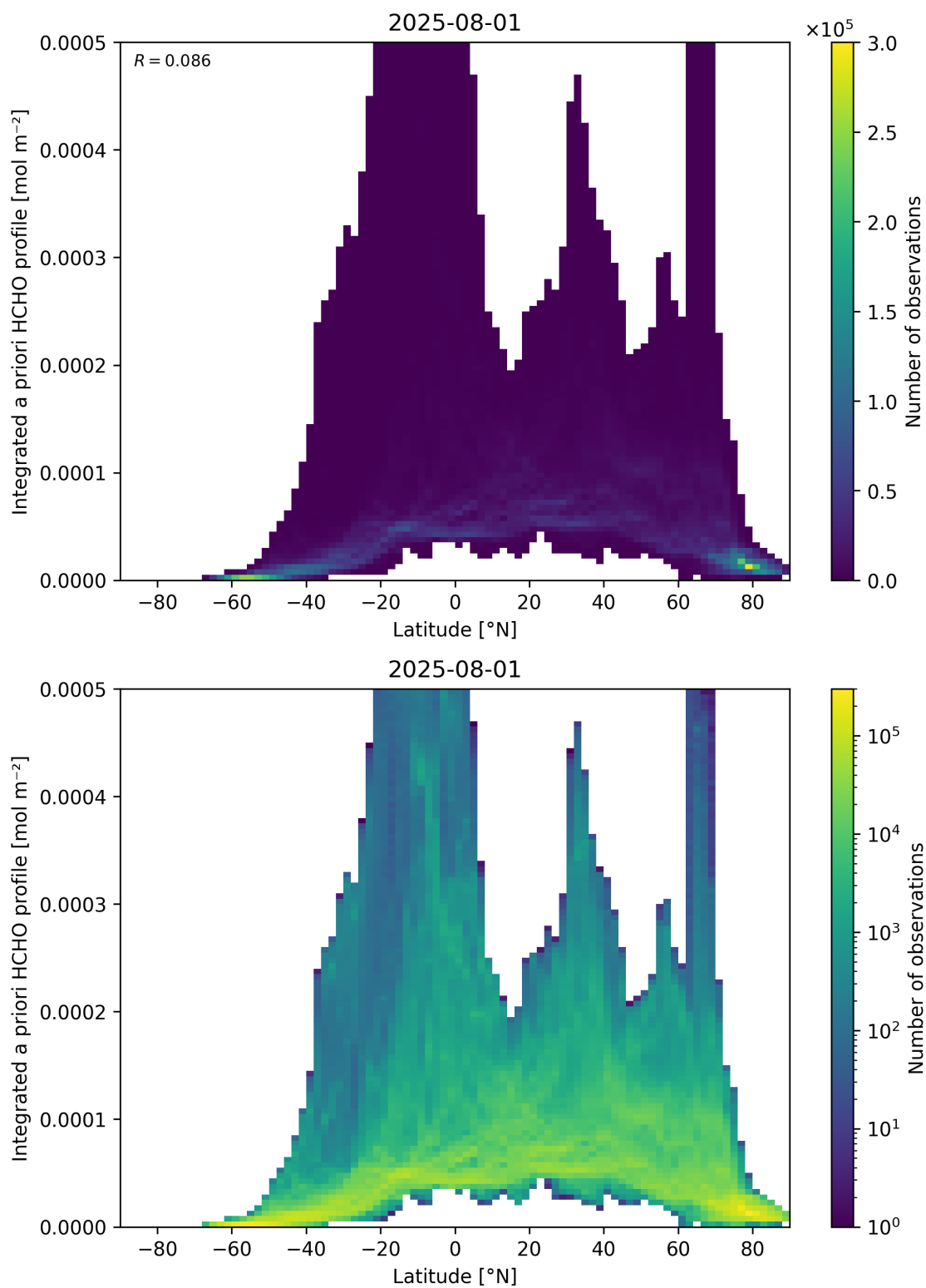
Figure 166: Scatter density plot of “Latitude” against “Integrated a priori HCHO profile” for 2025-07-31 to 2025-08-02.
