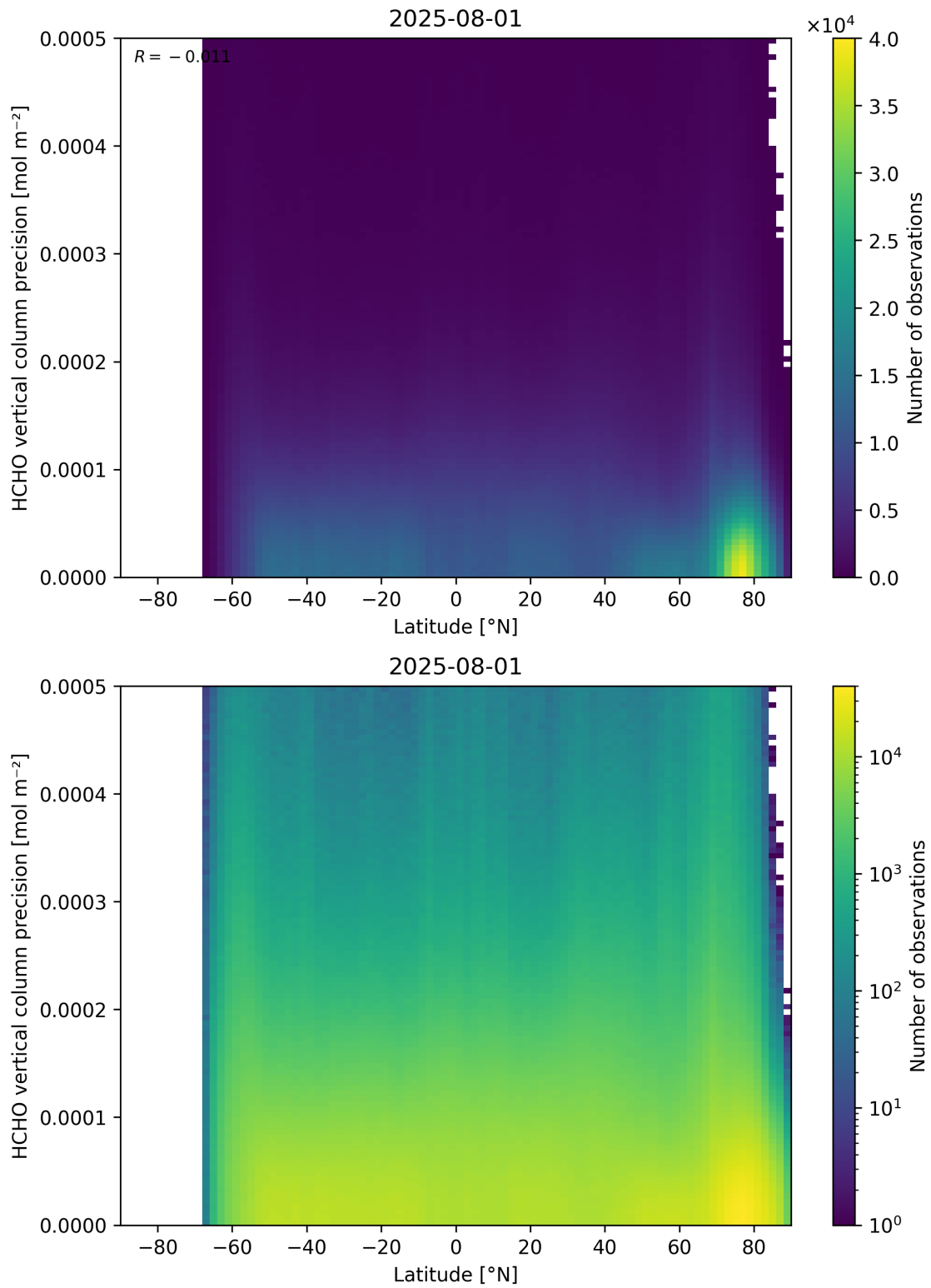
Figure 165: Scatter density plot of “Latitude” against “HCHO vertical column precision” for 2025-07-31 to 2025-08-02.
