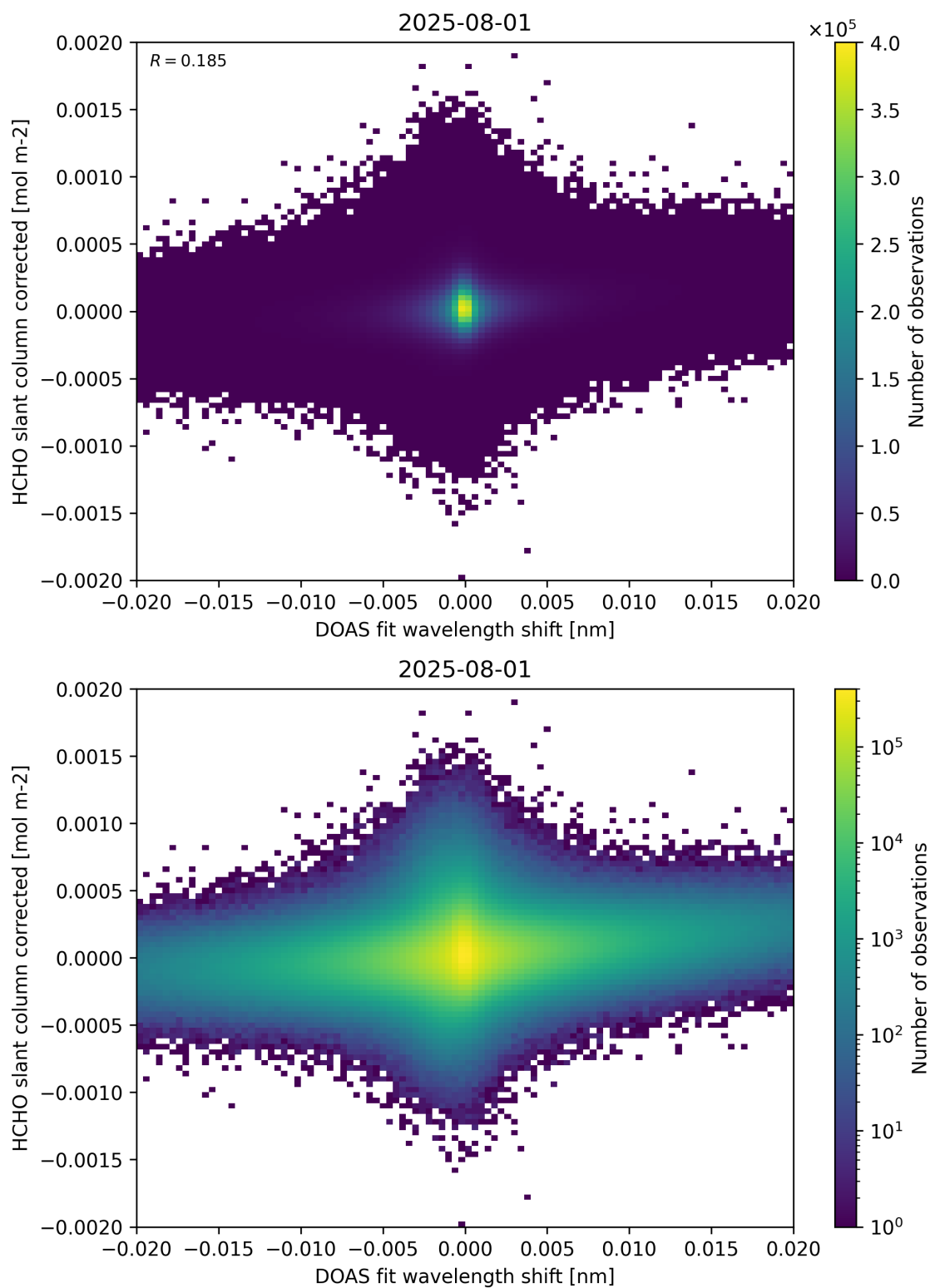
Figure 66: Scatter density plot of “DOAS fit wavelength shift” against “HCHO slant column corrected” for 2025-07-31 to 2025-08-02.
