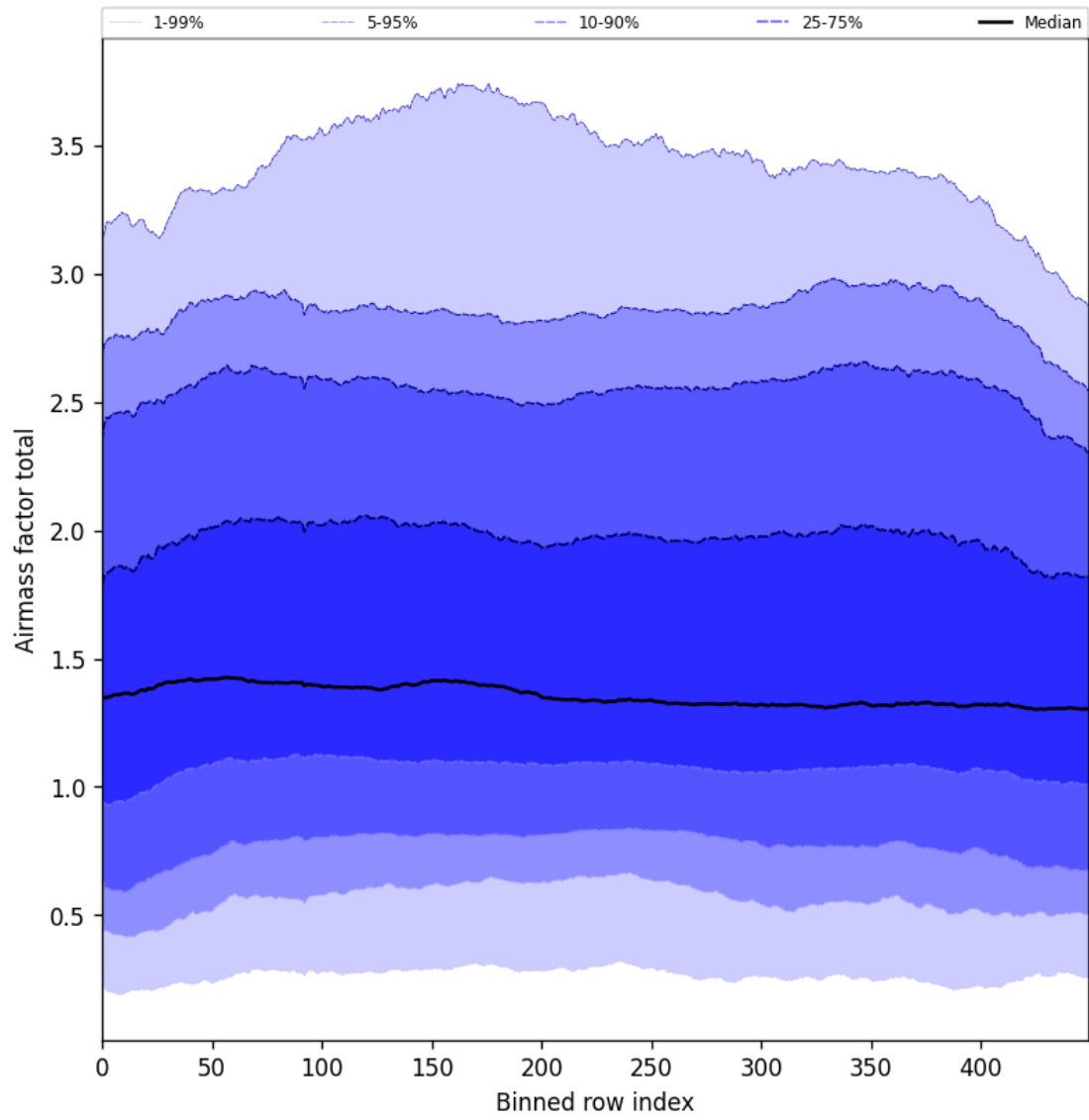
Figure 54: Along track statistics of “Airmass factor total” for 2025-07-31 to 2025-08-02
