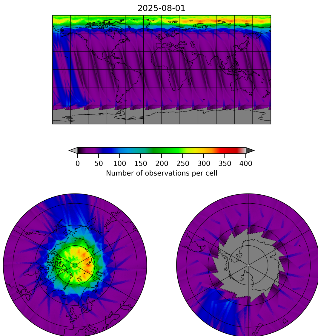
Figure 19: Map of the number of observations for 2025-07-31 to 2025-08-02
