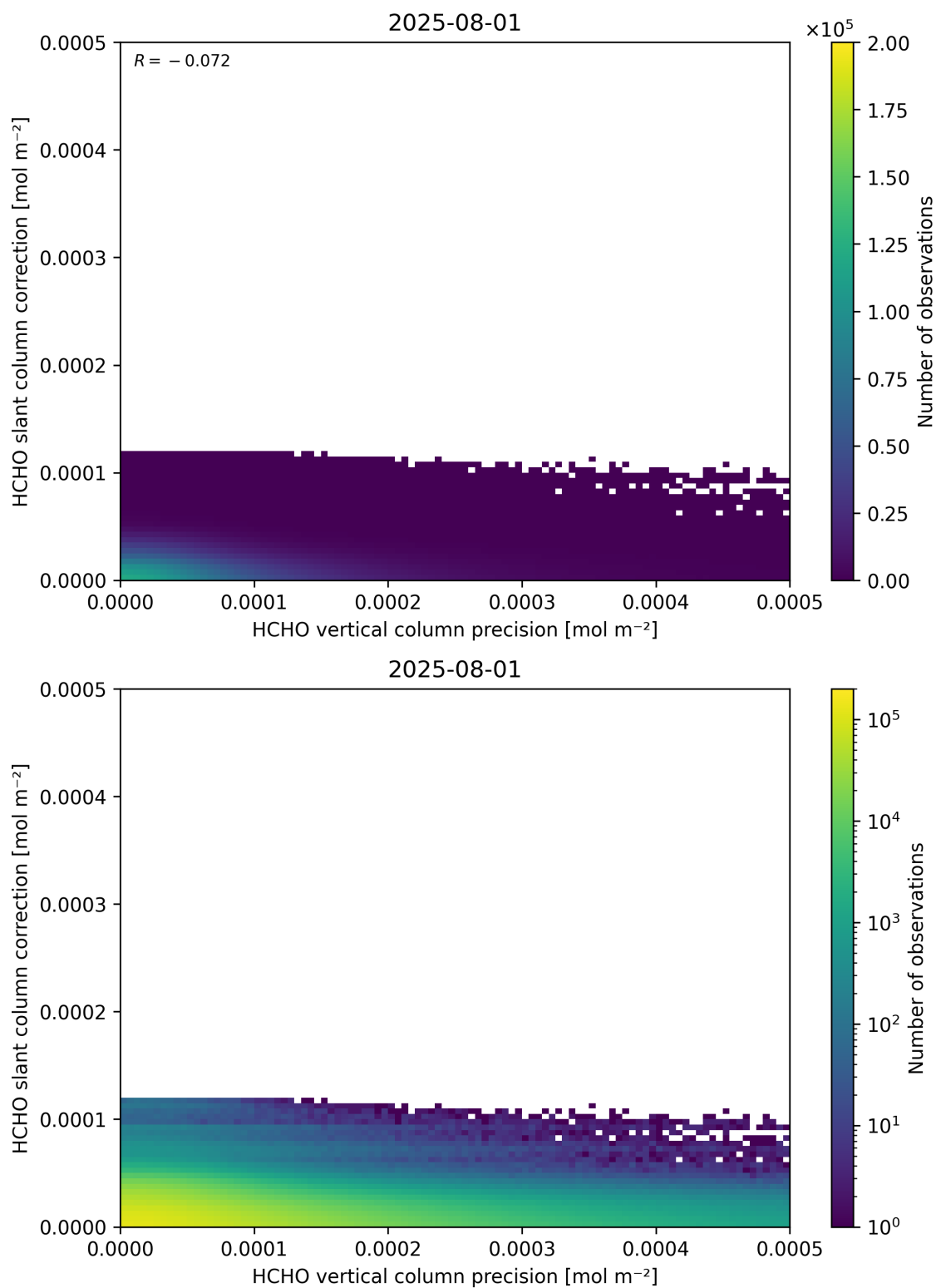
Figure 141: Scatter density plot of “HCHO vertical column precision” against “HCHO slant column correction” for 2025-07-31 to 2025-08-02.
