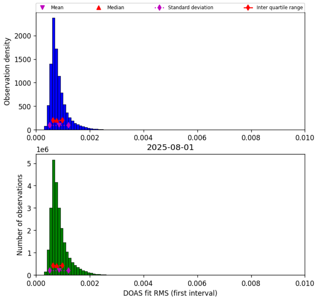
Figure 46: Histogram of “DOAS fit RMS (first interval)” for 2025-07-31 to 2025-08-02
