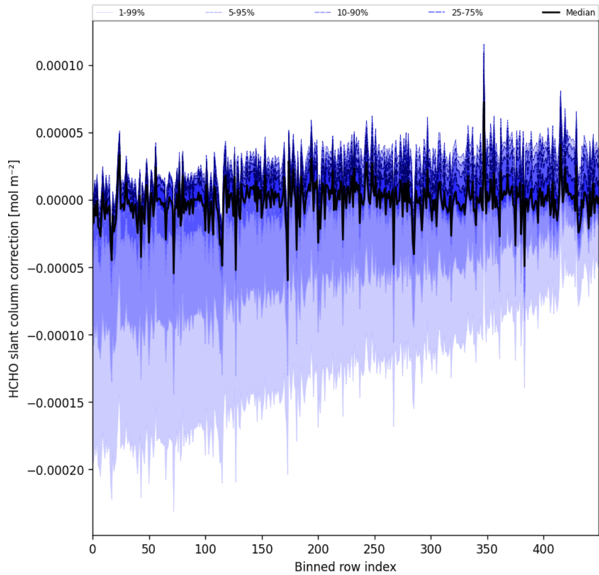
Figure 61: Along track statistics of “HCHO slant column correction” for 2025-07-31 to 2025-08-02
