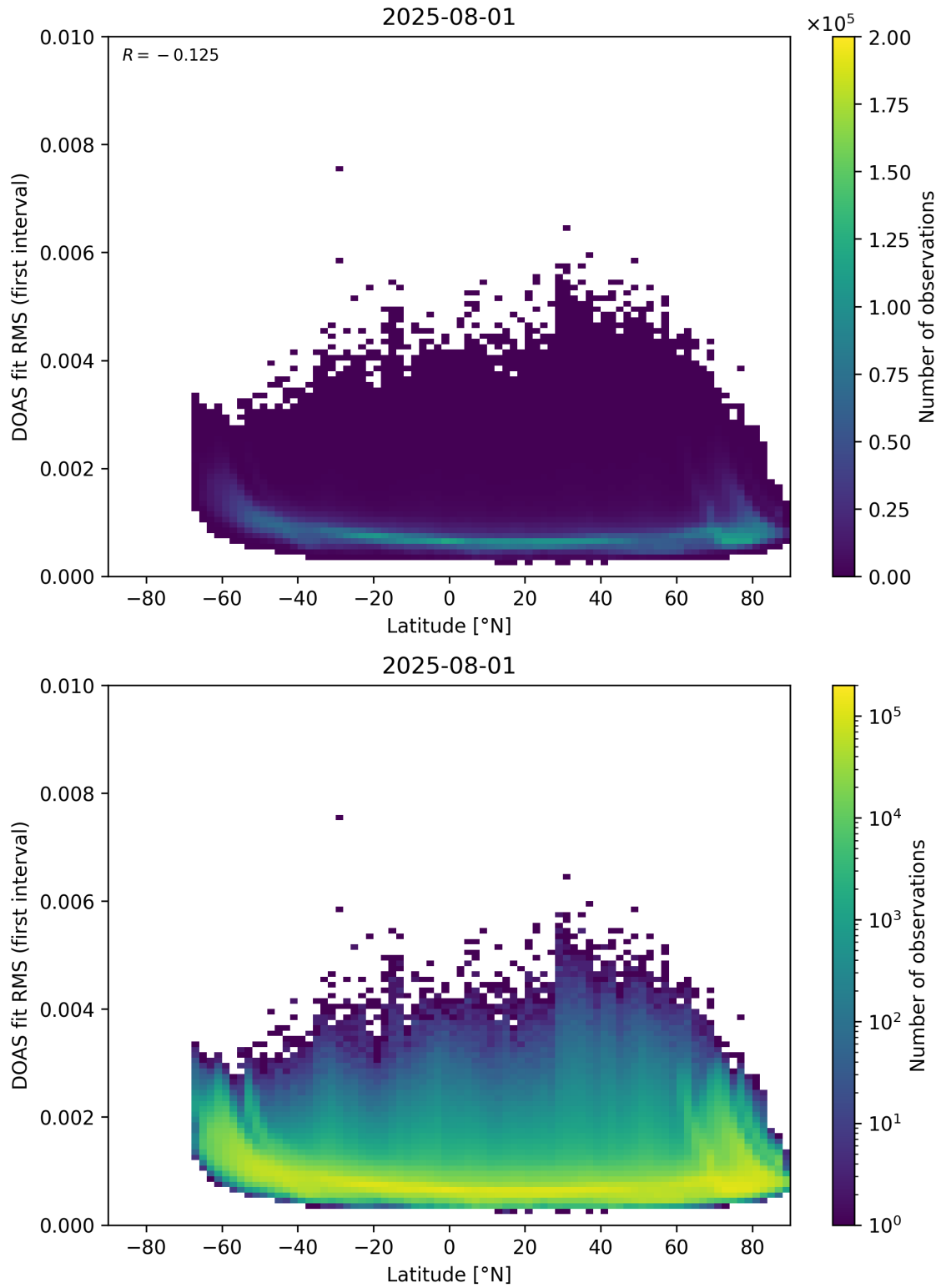
Figure 153: Scatter density plot of “Latitude” against “DOAS fit RMS (first interval)” for 2025-07-31 to 2025-08-02.
