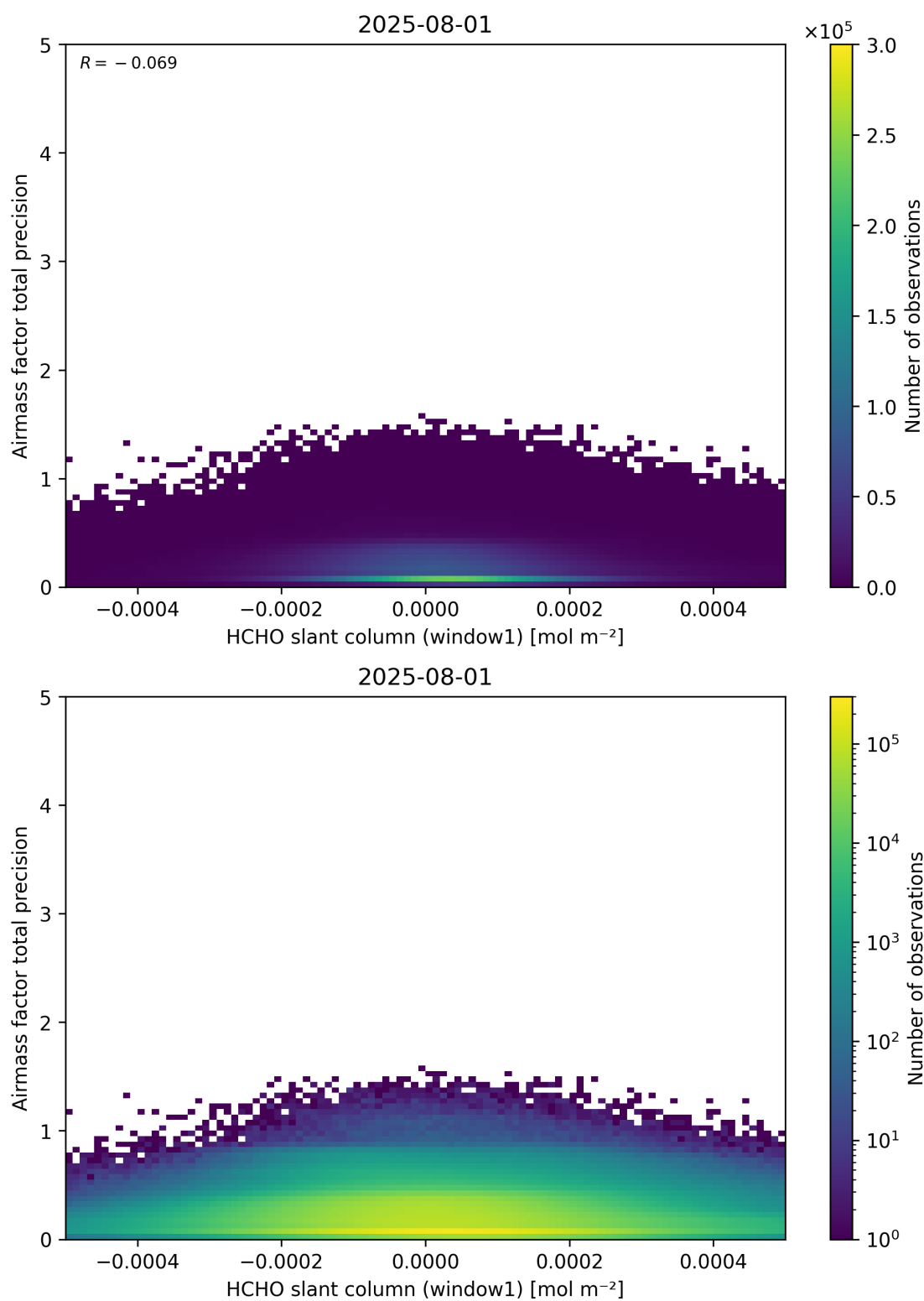
Figure 86: Scatter density plot of “HCHO slant column (window1)” against “Airmass factor total precision” for 2025-07-31 to 2025-08-02.
