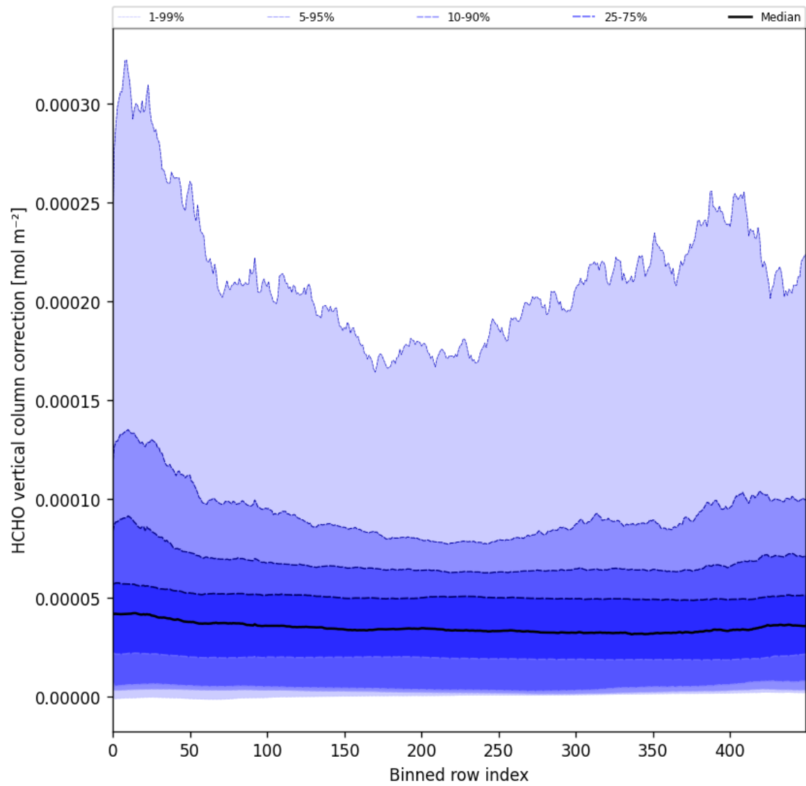
Figure 51: Along track statistics of “HCHO vertical column correction” for 2025-07-31 to 2025-08-02
