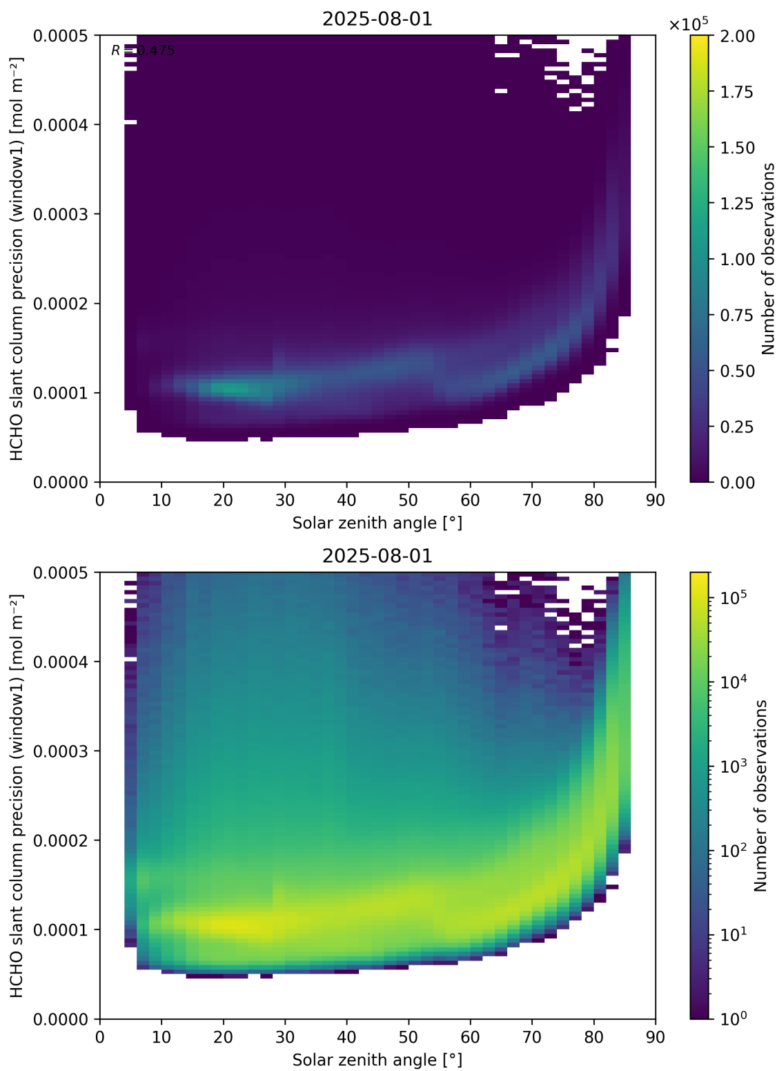
Figure 174: Scatter density plot of “Solar zenith angle” against “HCHO slant column precision (window1)” for 2025-07-31 to 2025-08-02.
