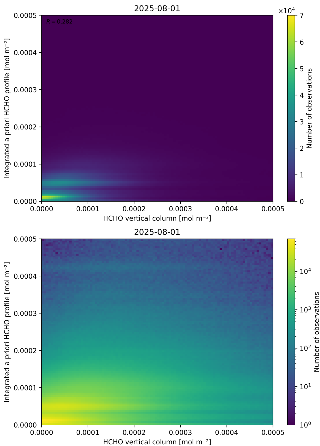
Figure 135: Scatter density plot of “HCHO vertical column” against “Integrated a priori HCHO profile” for 2025-07-31 to 2025-08-02.
