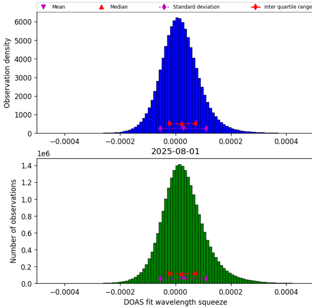
Figure 45: Histogram of “DOAS fit wavelength squeeze” for 2025-07-31 to 2025-08-02
