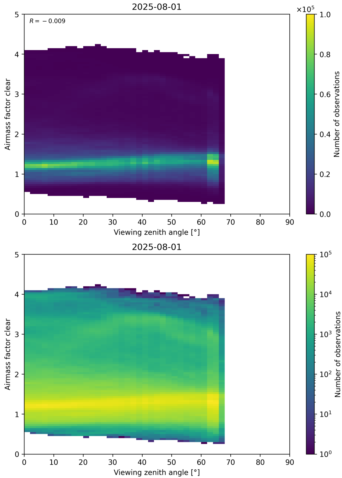
Figure 185: Scatter density plot of “Viewing zenith angle” against “Airmass factor clear” for 2025-07-31 to 2025-08-02.
