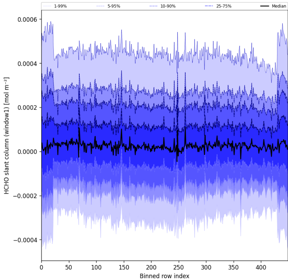
Figure 52: Along track statistics of “HCHO slant column (window1)” for 2025-07-31 to 2025-08-02
