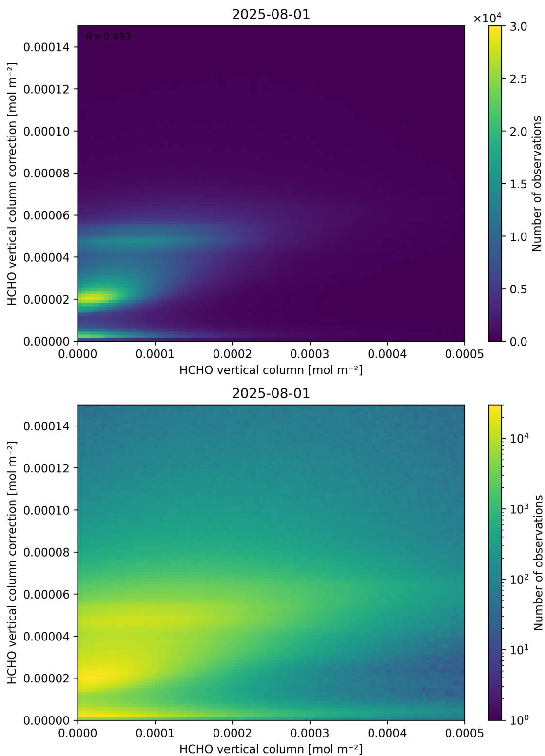
Figure 133: Scatter density plot of “HCHO vertical column” against “HCHO vertical column correction” for 2025-07-31 to 2025-08-02.
