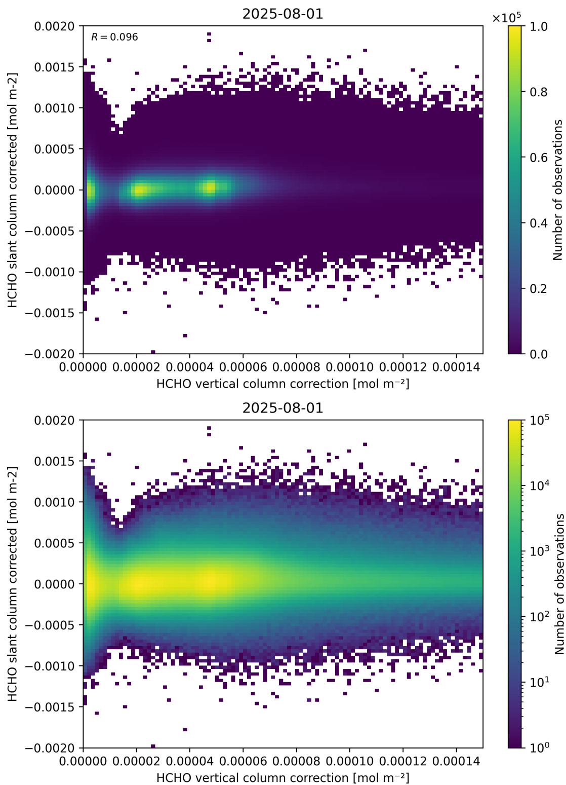
Figure 116: Scatter density plot of “HCHO vertical column correction” against “HCHO slant column corrected” for 2025-07-31 to 2025-08-02.
