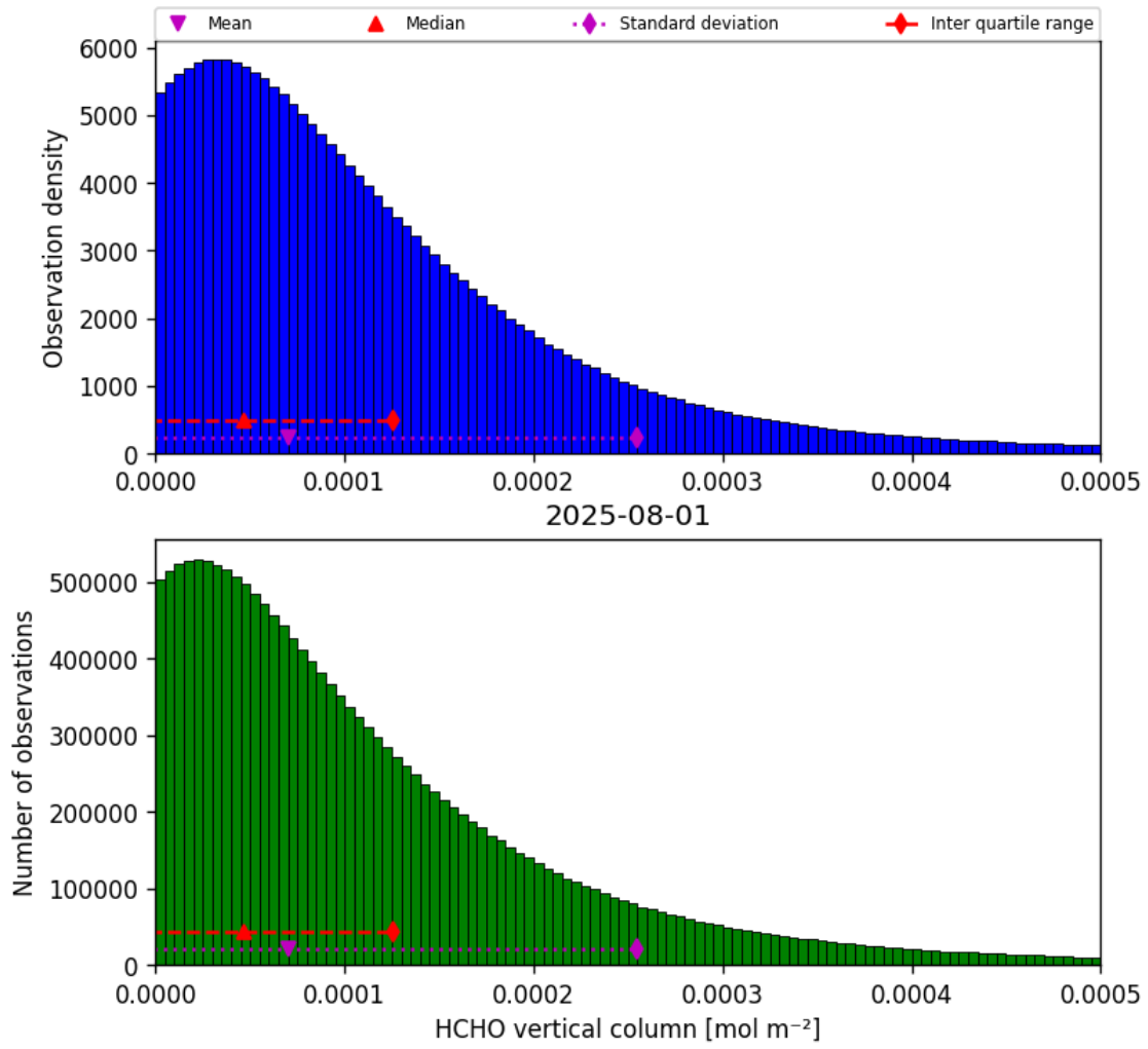
Figure 35: Histogram of “HCHO vertical column” for 2025-07-31 to 2025-08-02
