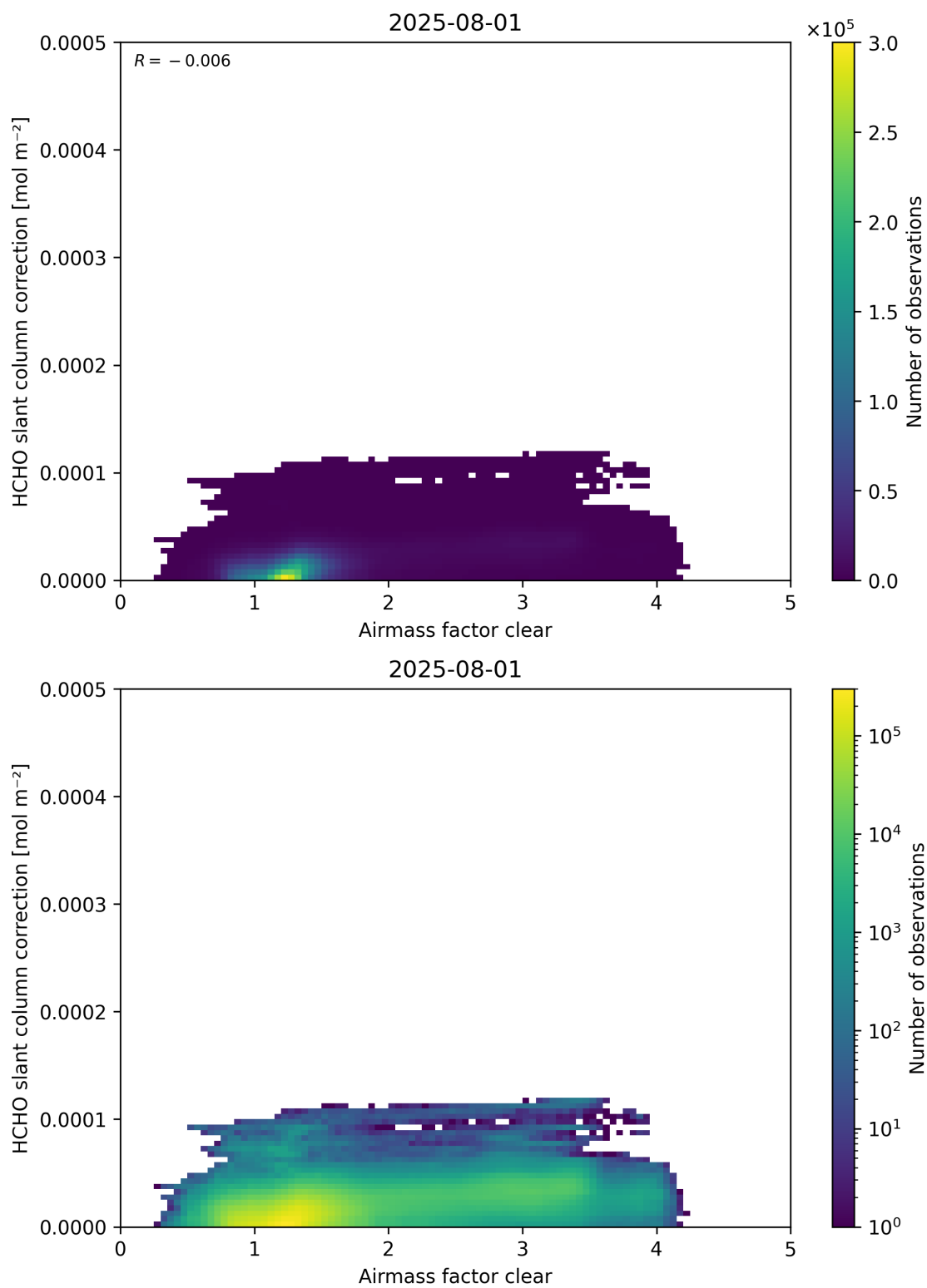
Figure 75: Scatter density plot of “Airmass factor clear” against “HCHO slant column correction” for 2025-07-31 to 2025-08-02.
