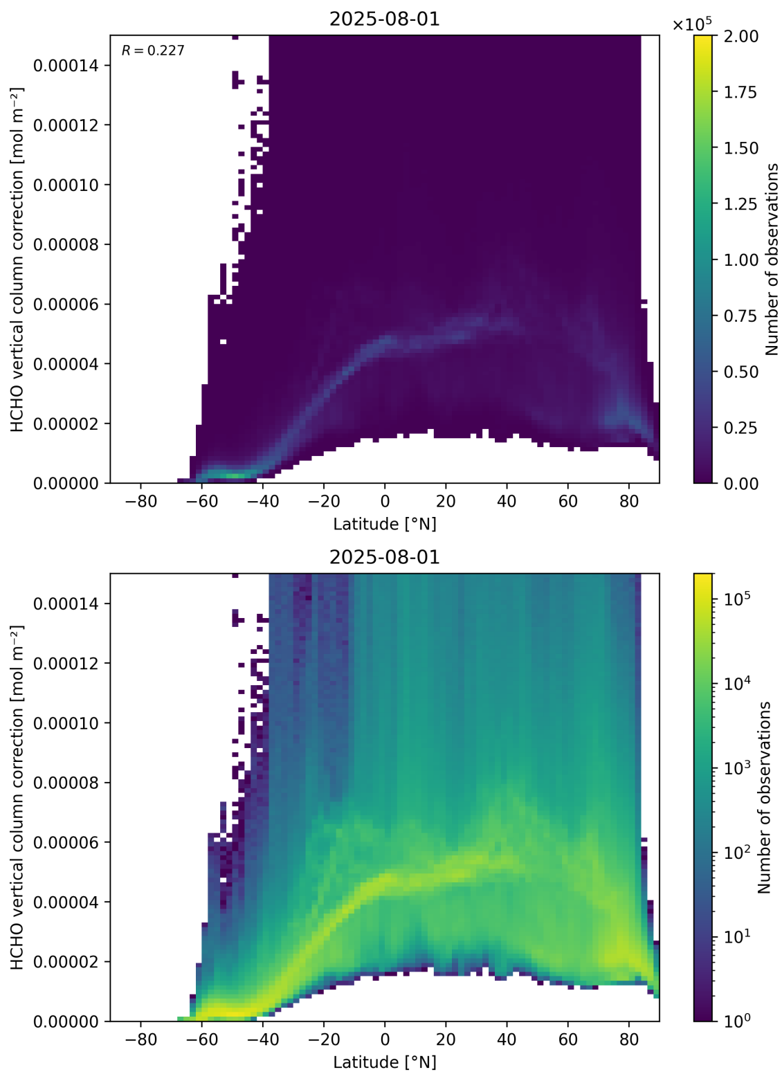
Figure 164: Scatter density plot of “Latitude” against “HCHO vertical column correction” for 2025-07-31 to 2025-08-02.
