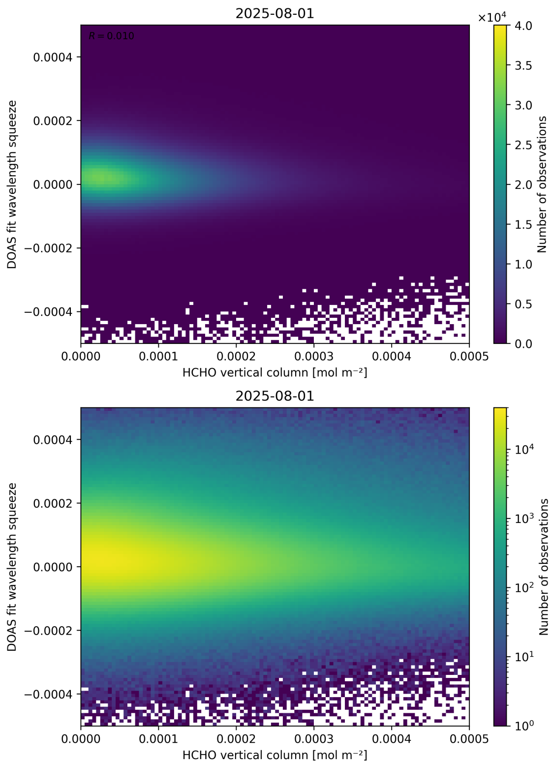
Figure 125: Scatter density plot of “HCHO vertical column” against “DOAS fit wavelength squeeze” for 2025-07-31 to 2025-08-02.
