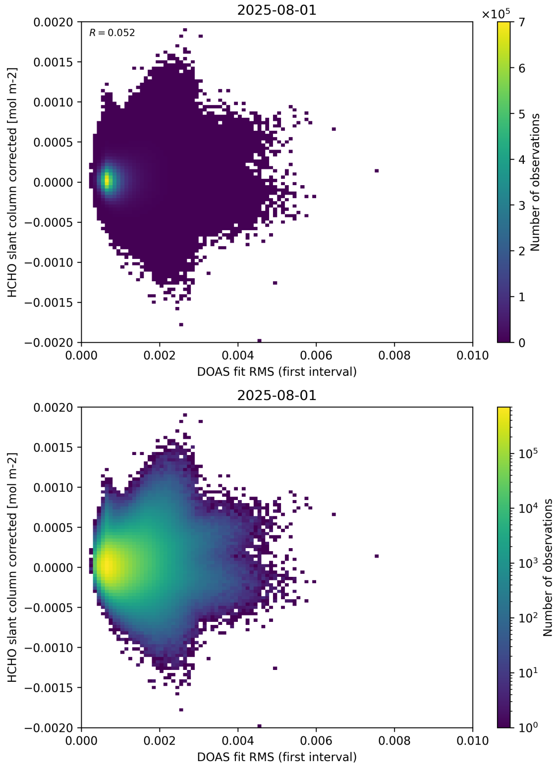
Figure 62: Scatter density plot of “DOAS fit RMS (first interval)” against “HCHO slant column corrected” for 2025-07-31 to 2025-08-02.
