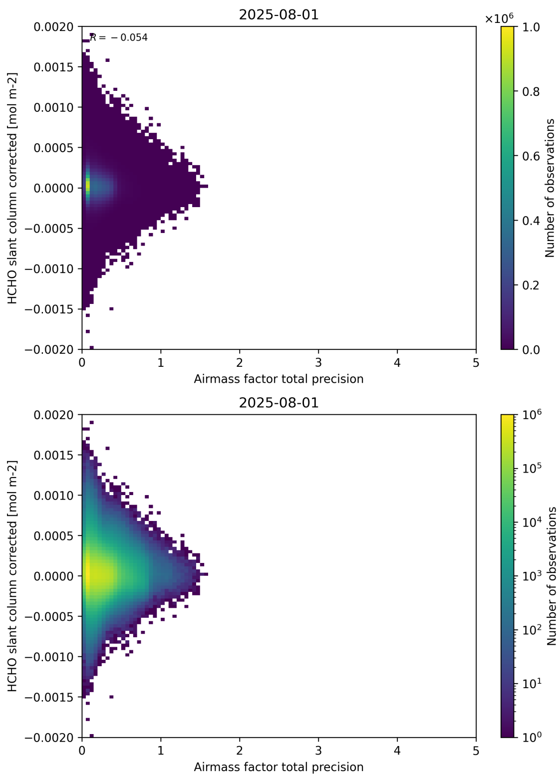
Figure 109: Scatter density plot of “Airmass factor total precision” against “HCHO slant column corrected” for 2025-07-31 to 2025-08-02.
