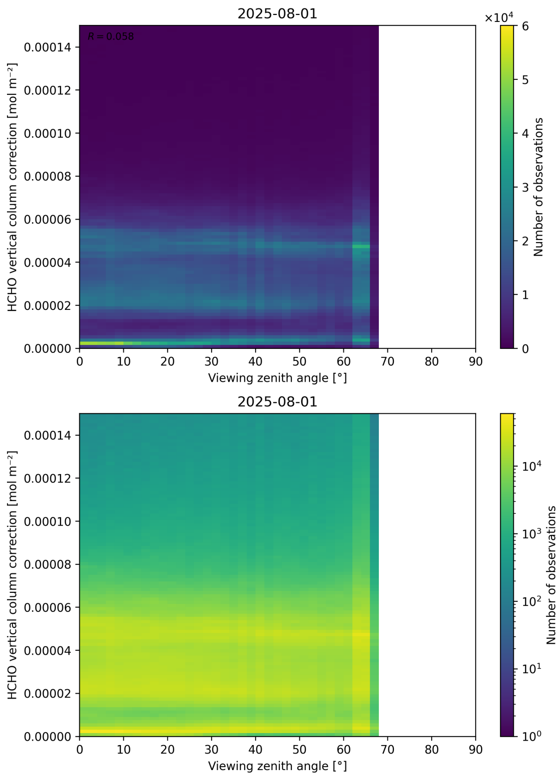
Figure 193: Scatter density plot of “Viewing zenith angle” against “HCHO vertical column correction” for 2025-07-31 to 2025-08-02.
