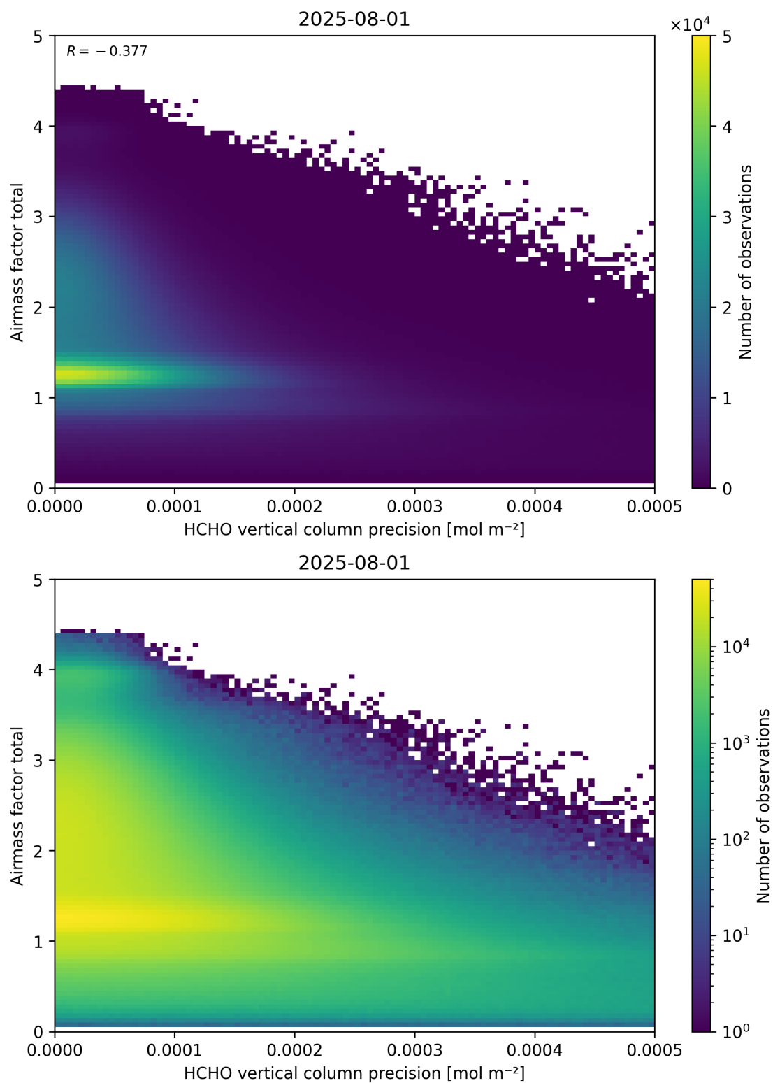
Figure 144: Scatter density plot of “HCHO vertical column precision” against “Airmass factor total” for 2025-07-31 to 2025-08-02.
