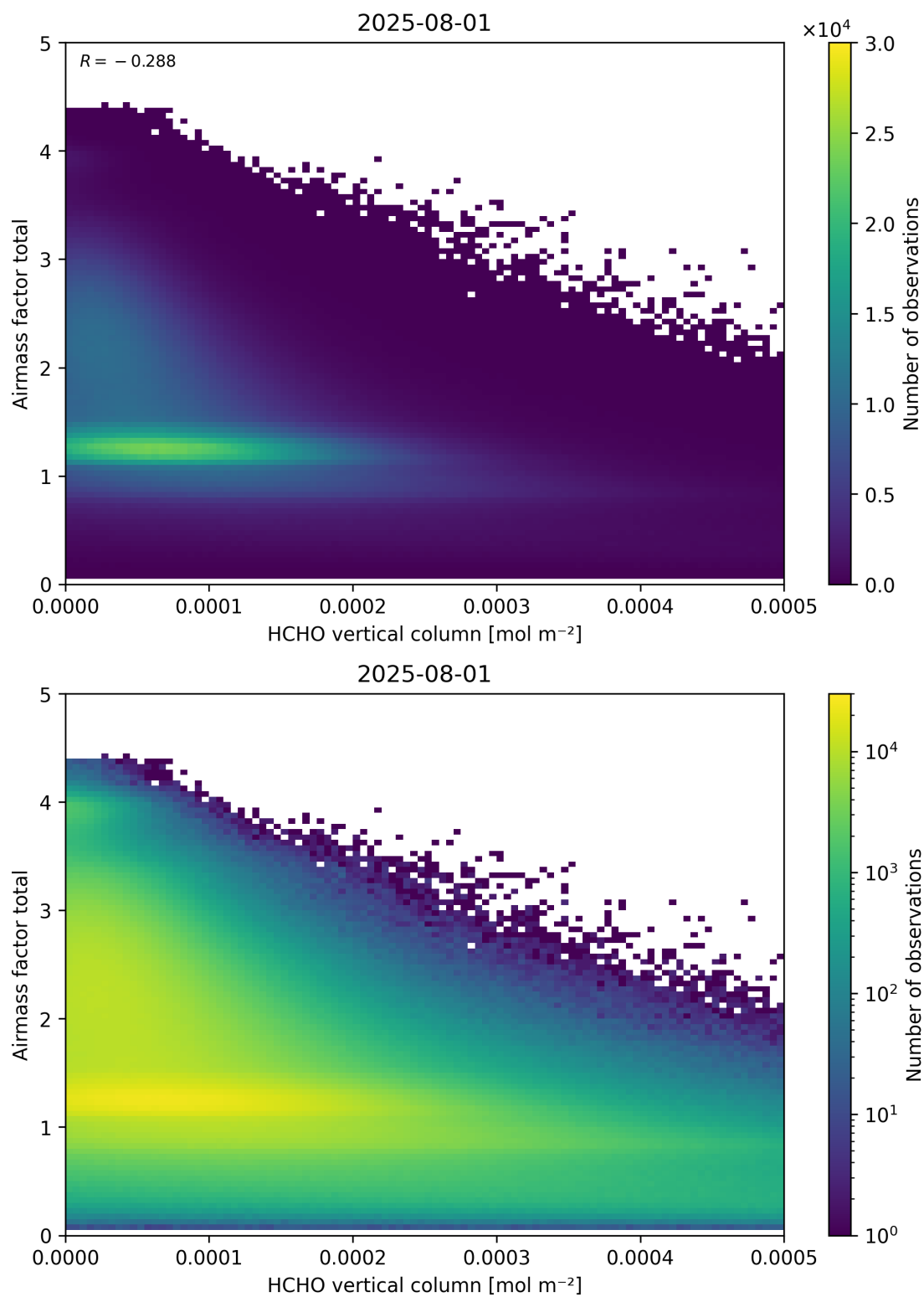
Figure 131: Scatter density plot of “HCHO vertical column” against “Airmass factor total” for 2025-07-31 to 2025-08-02.
