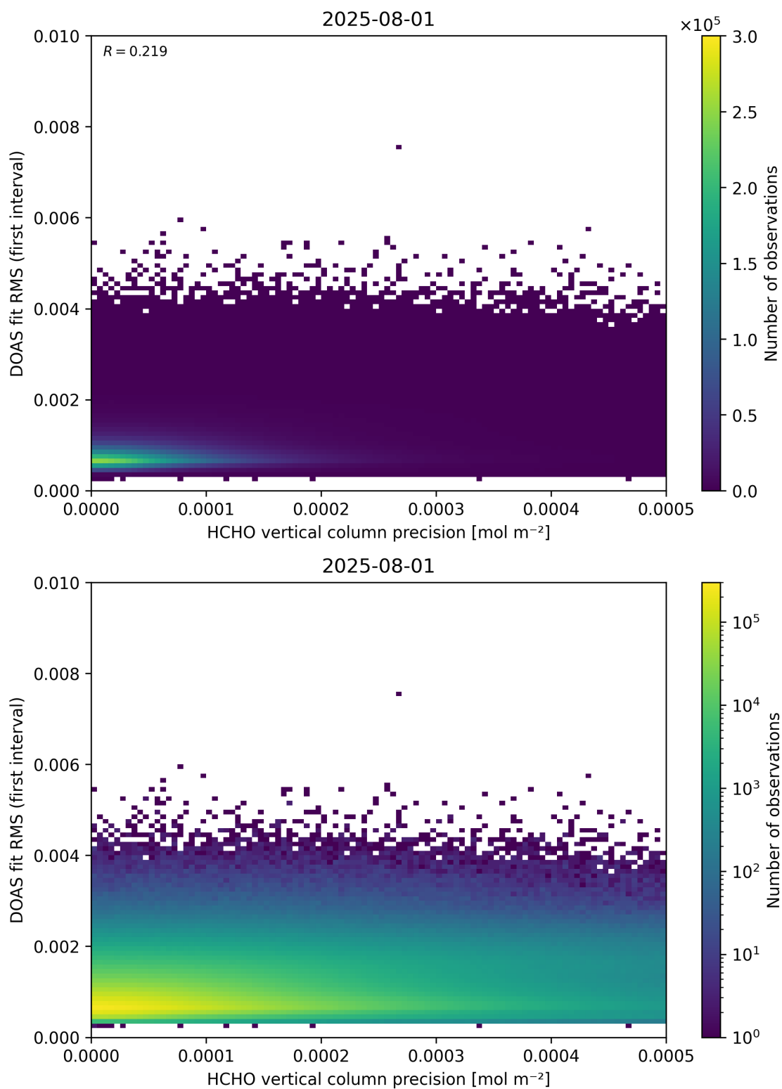
Figure 136: Scatter density plot of “HCHO vertical column precision” against “DOAS fit RMS (first interval)” for 2025-07-31 to 2025-08-02.
