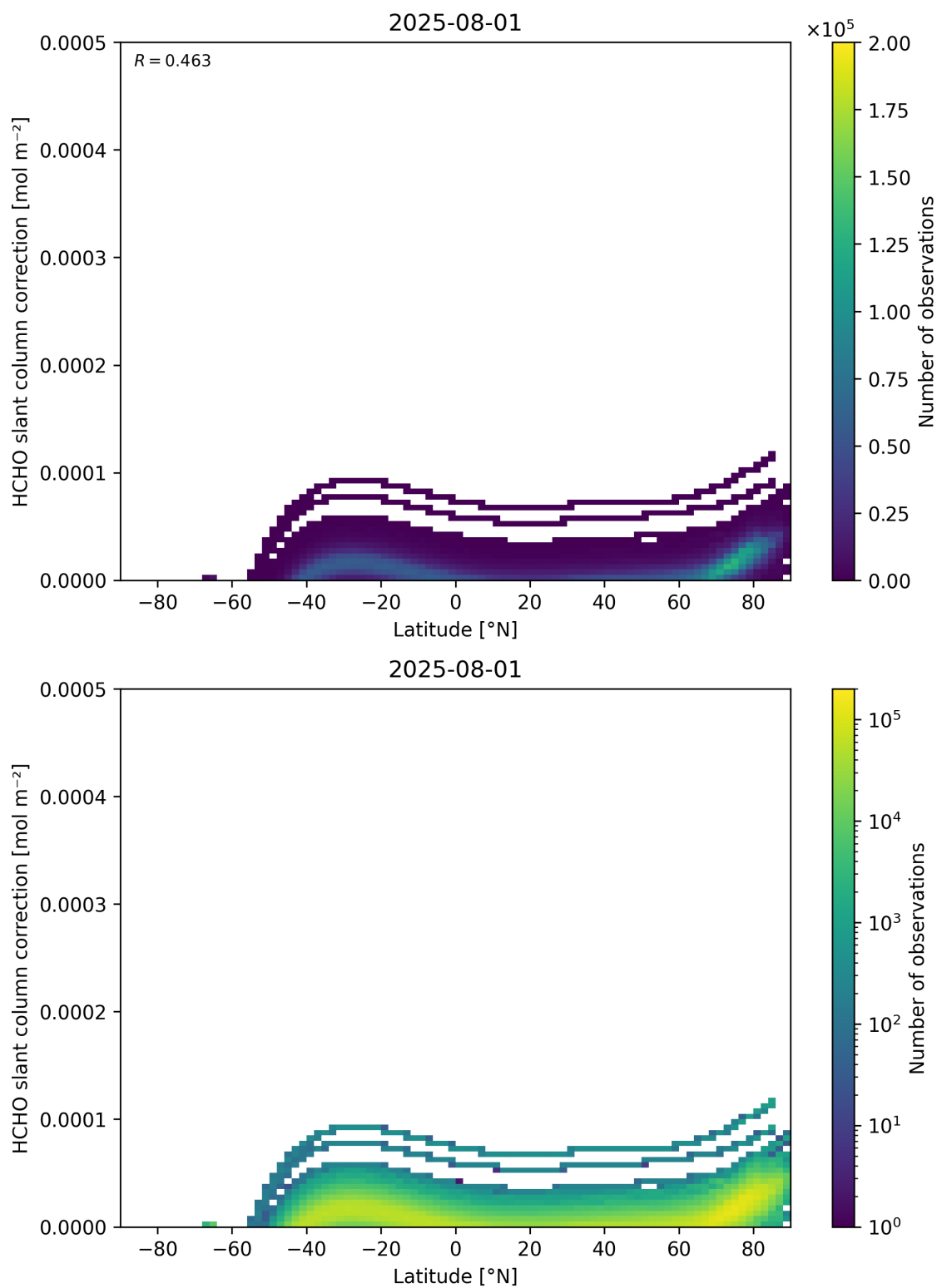
Figure 158: Scatter density plot of “Latitude” against “HCHO slant column correction” for 2025-07-31 to 2025-08-02.
