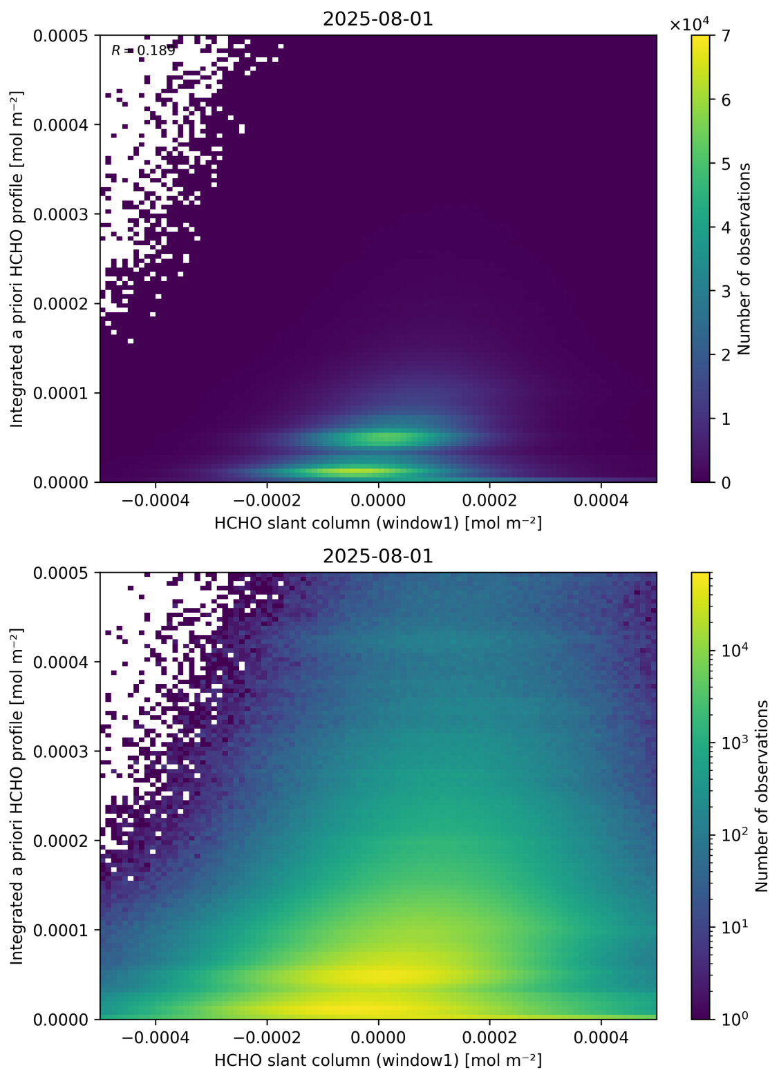
Figure 87: Scatter density plot of “HCHO slant column (window1)” against “Integrated a priori HCHO profile” for 2025-07-31 to 2025-08-02.
