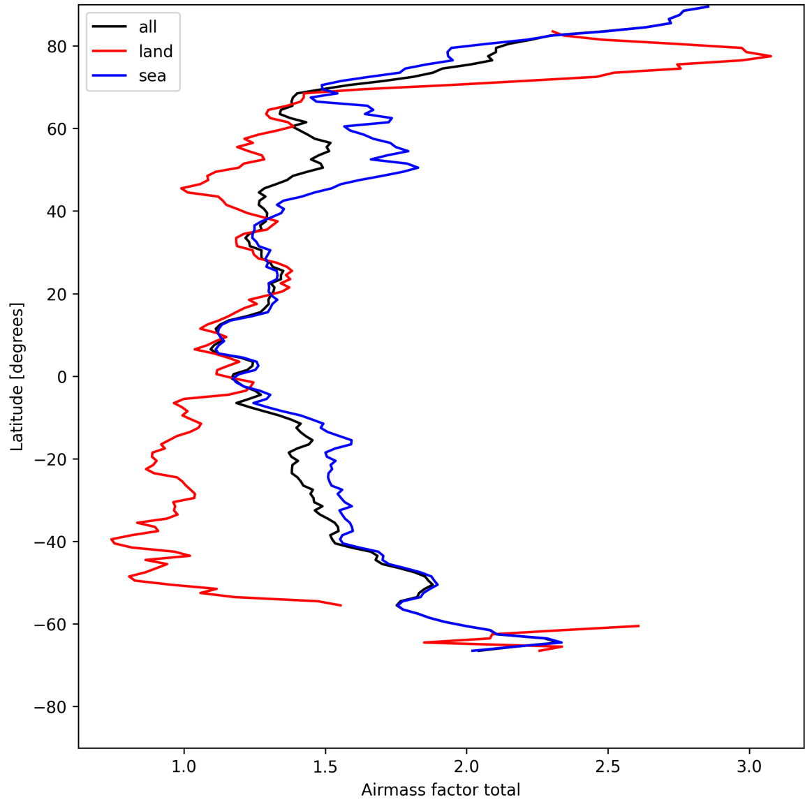
Figure 26: Zonal average of “Airmass factor total” for 2025-07-31 to 2025-08-02.
