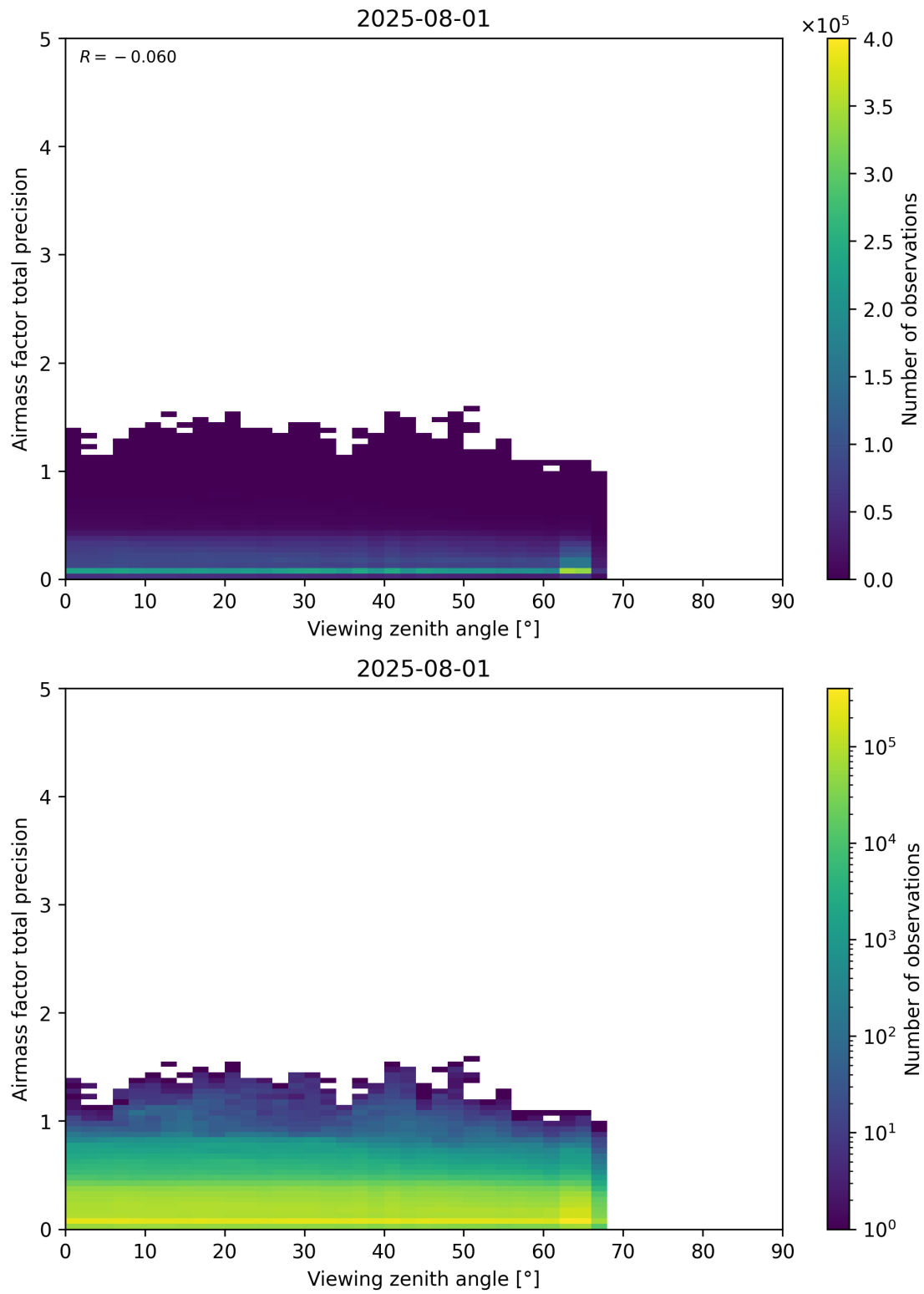
Figure 191: Scatter density plot of “Viewing zenith angle” against “Airmass factor total precision” for 2025-07-31 to 2025-08-02.
