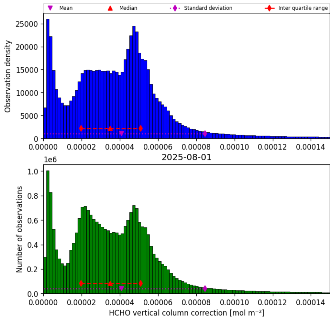
Figure 37: Histogram of “HCHO vertical column correction” for 2025-07-31 to 2025-08-02
