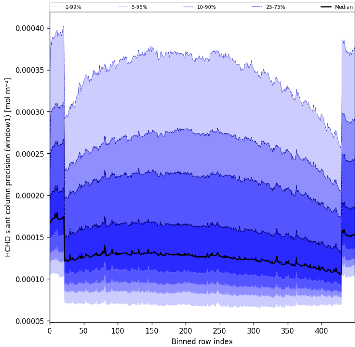
Figure 53: Along track statistics of “HCHO slant column precision (window1)” for 2025-07-31 to 2025-08-02
