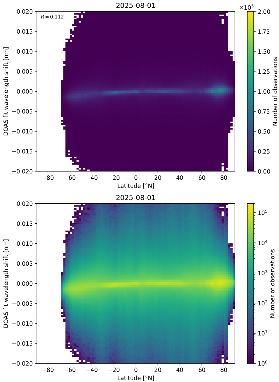
Figure 154: Scatter density plot of “Latitude” against “DOAS fit wavelength shift” for 2025-07-31 to 2025-08-02.
