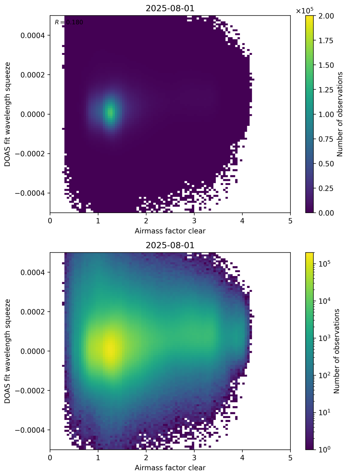
Figure 73: Scatter density plot of “Airmass factor clear” against “DOAS fit wavelength squeeze” for 2025-07-31 to 2025-08-02.
