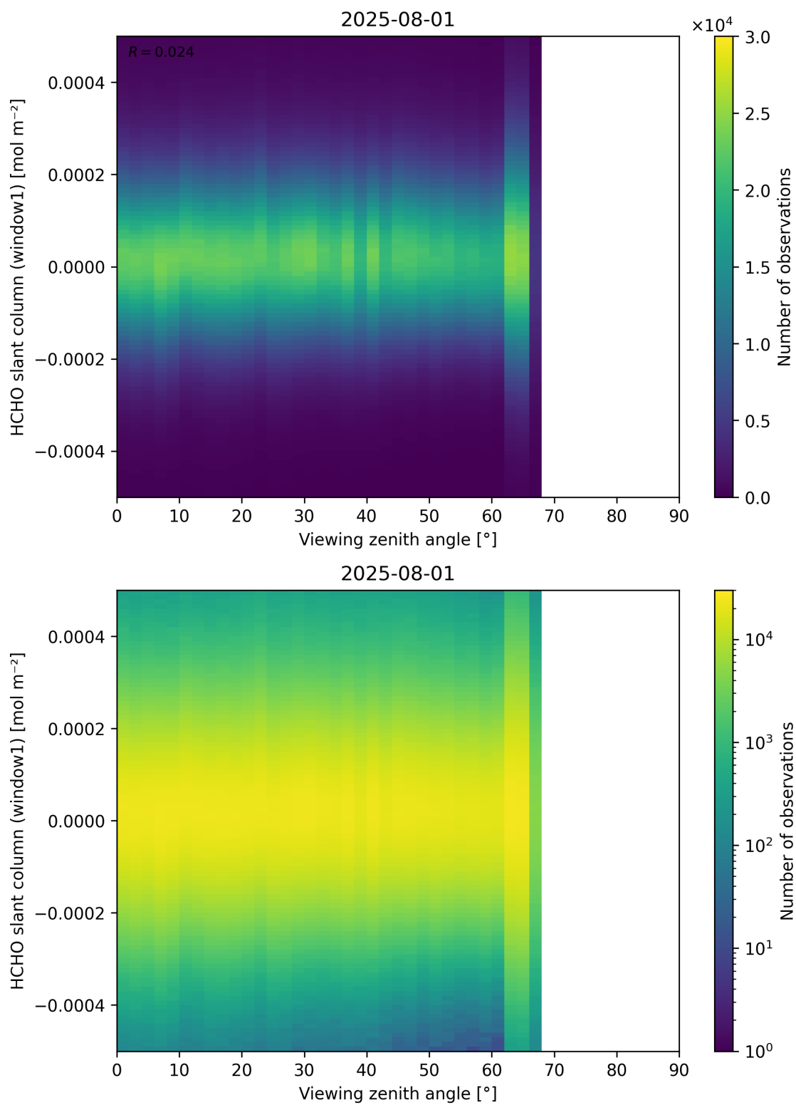
Figure 188: Scatter density plot of “Viewing zenith angle” against “HCHO slant column (window1)” for 2025-07-31 to 2025-08-02.
