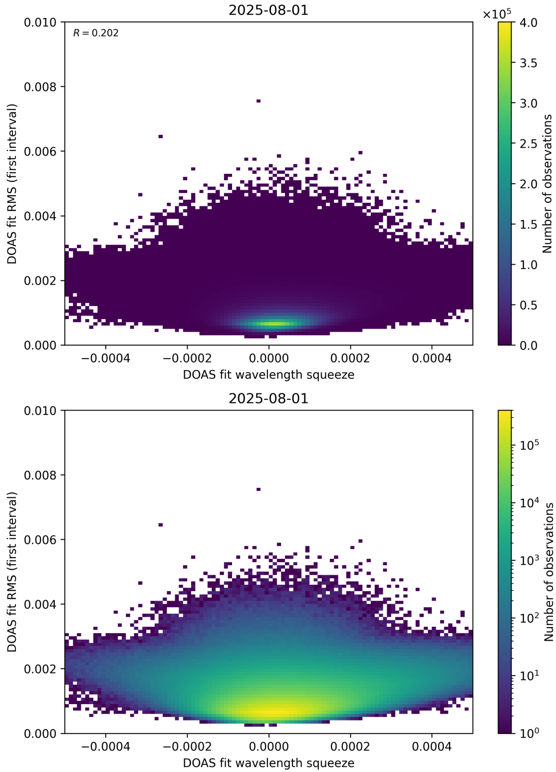
Figure 68: Scatter density plot of “DOAS fit wavelength squeeze” against “DOAS fit RMS (first interval)” for 2025-07-31 to 2025-08-02.
