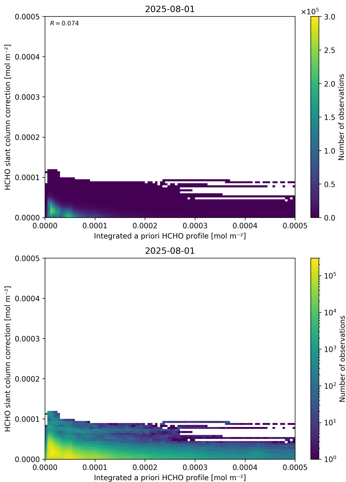
Figure 152: Scatter density plot of “Integrated a priori HCHO profile” against “HCHO slant column correction” for 2025-07-31 to 2025-08-02.
