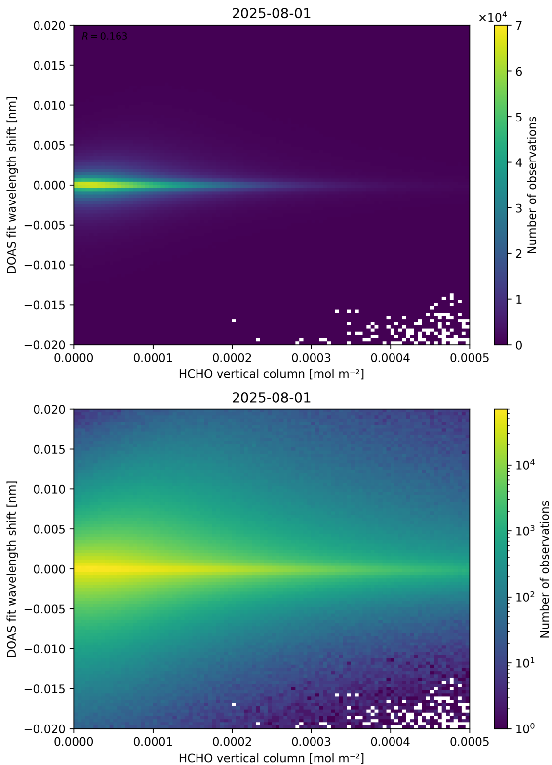
Figure 124: Scatter density plot of “HCHO vertical column” against “DOAS fit wavelength shift” for 2025-07-31 to 2025-08-02.
