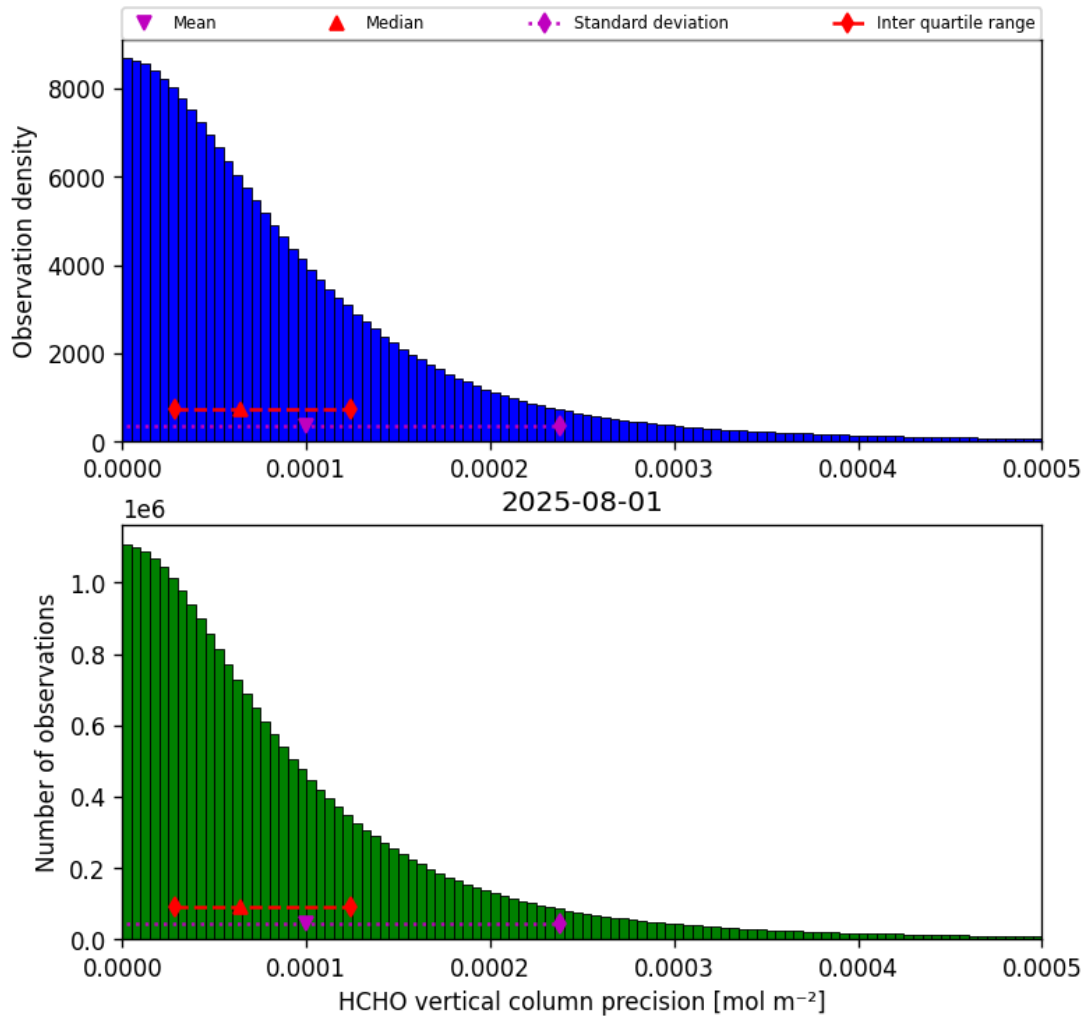
Figure 36: Histogram of “HCHO vertical column precision” for 2025-07-31 to 2025-08-02
