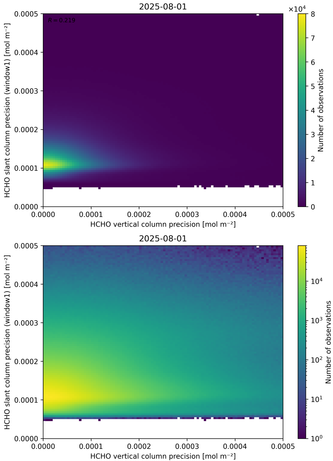
Figure 143: Scatter density plot of “HCHO vertical column precision” against “HCHO slant column precision (window1)” for 2025-07-31 to 2025-08-02.
