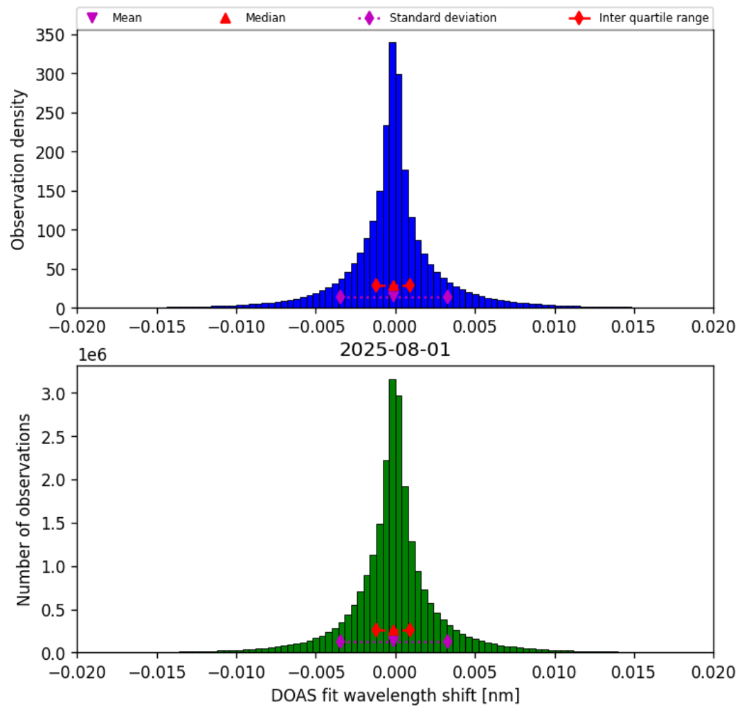
Figure 44: Histogram of “DOAS fit wavelength shift” for 2025-07-31 to 2025-08-02
