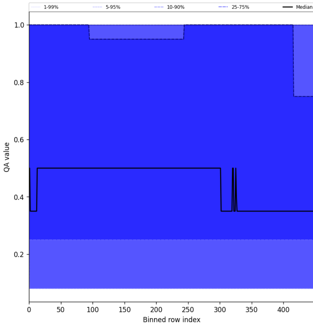
Figure 48: Along track statistics of “QA value” for 2025-07-31 to 2025-08-02
