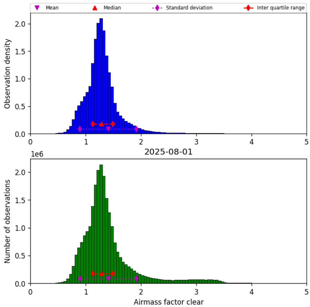
Figure 42: Histogram of “Airmass factor clear” for 2025-07-31 to 2025-08-02
