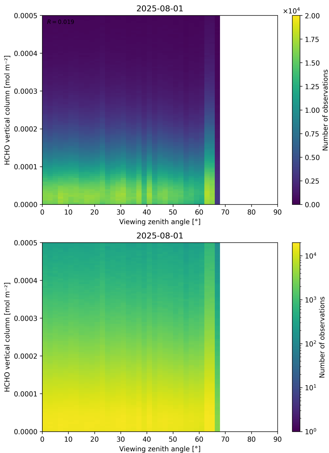
Figure 192: Scatter density plot of “Viewing zenith angle” against “HCHO vertical column” for 2025-07-31 to 2025-08-02.
