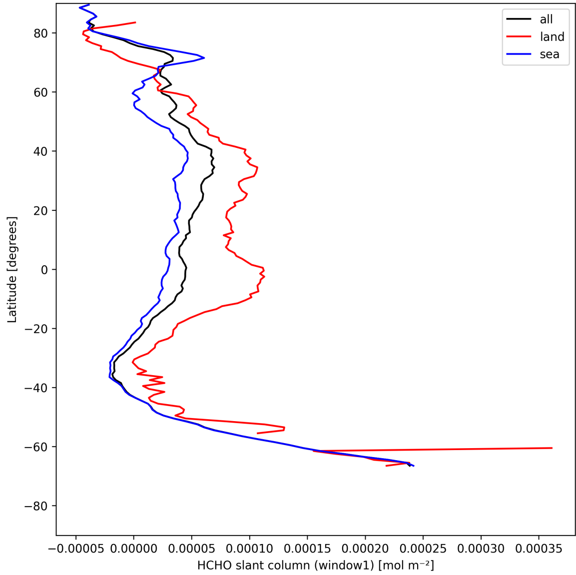
Figure 24: Zonal average of “HCHO slant column (window1)” for 2025-07-31 to 2025-08-02.
