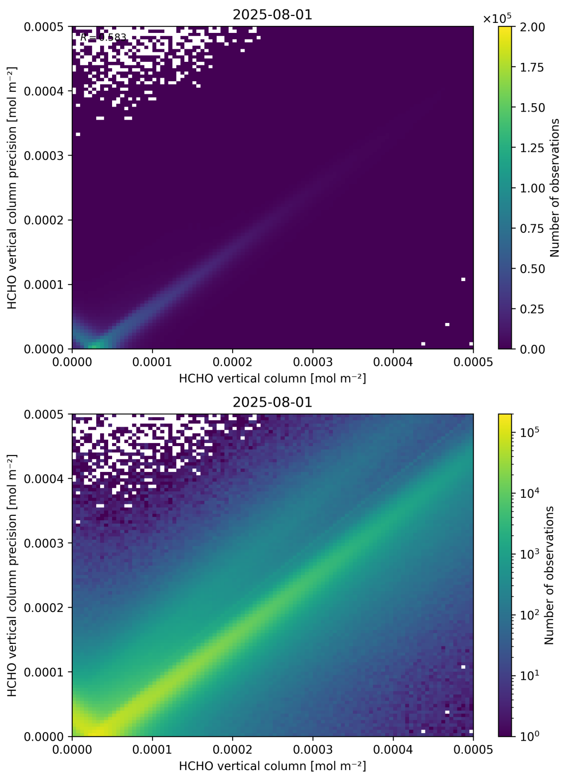
Figure 134: Scatter density plot of “HCHO vertical column” against “HCHO vertical column precision” for 2025-07-31 to 2025-08-02.
