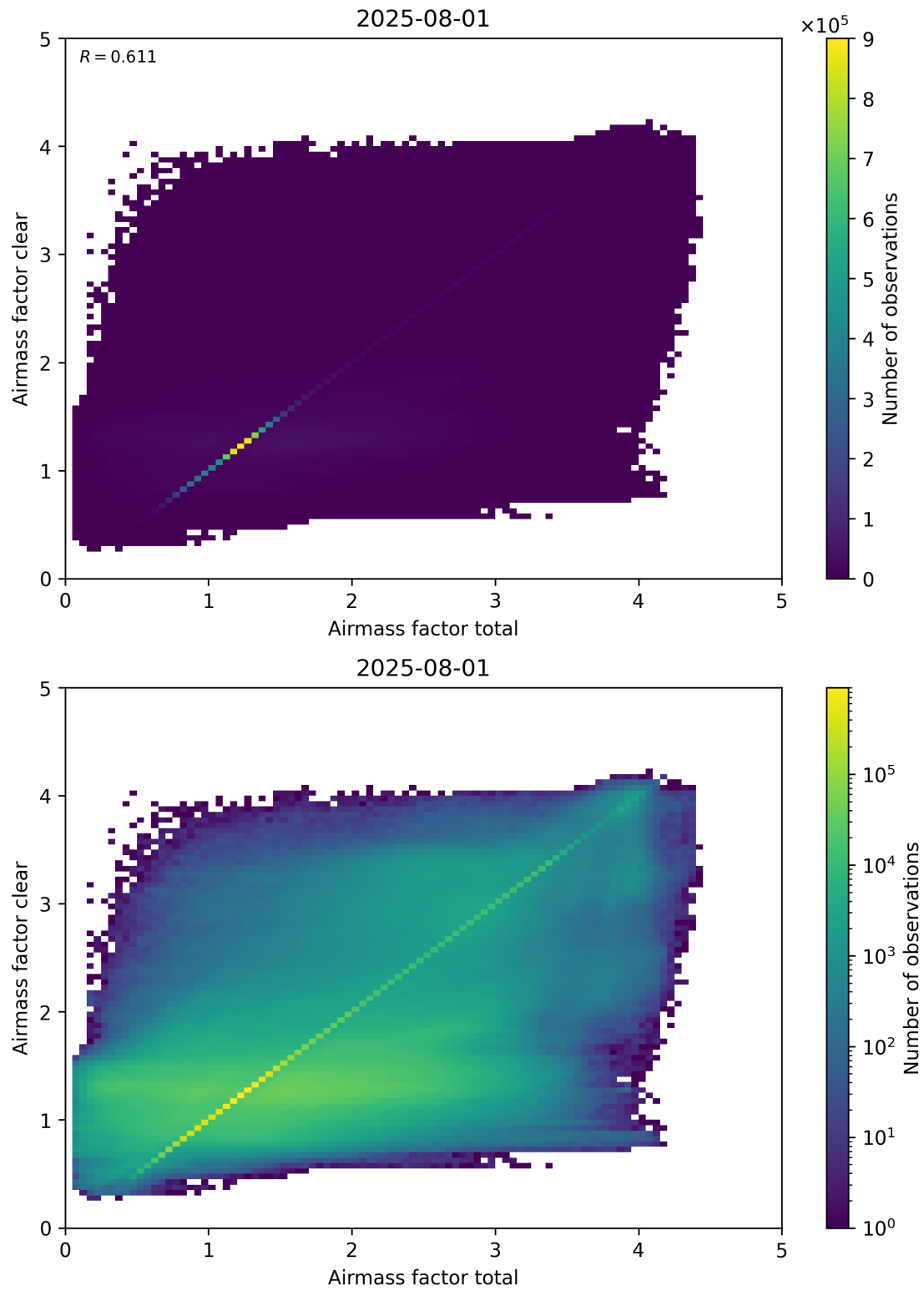
Figure 100: Scatter density plot of “Airmass factor total” against “Airmass factor clear” for 2025-07-31 to 2025-08-02.
