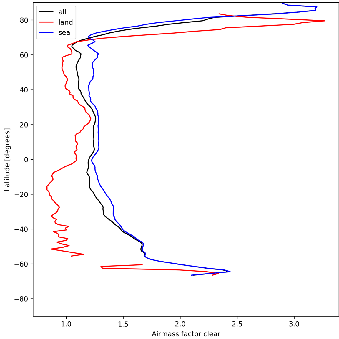
Figure 28: Zonal average of “Airmass factor clear” for 2025-07-31 to 2025-08-02.
