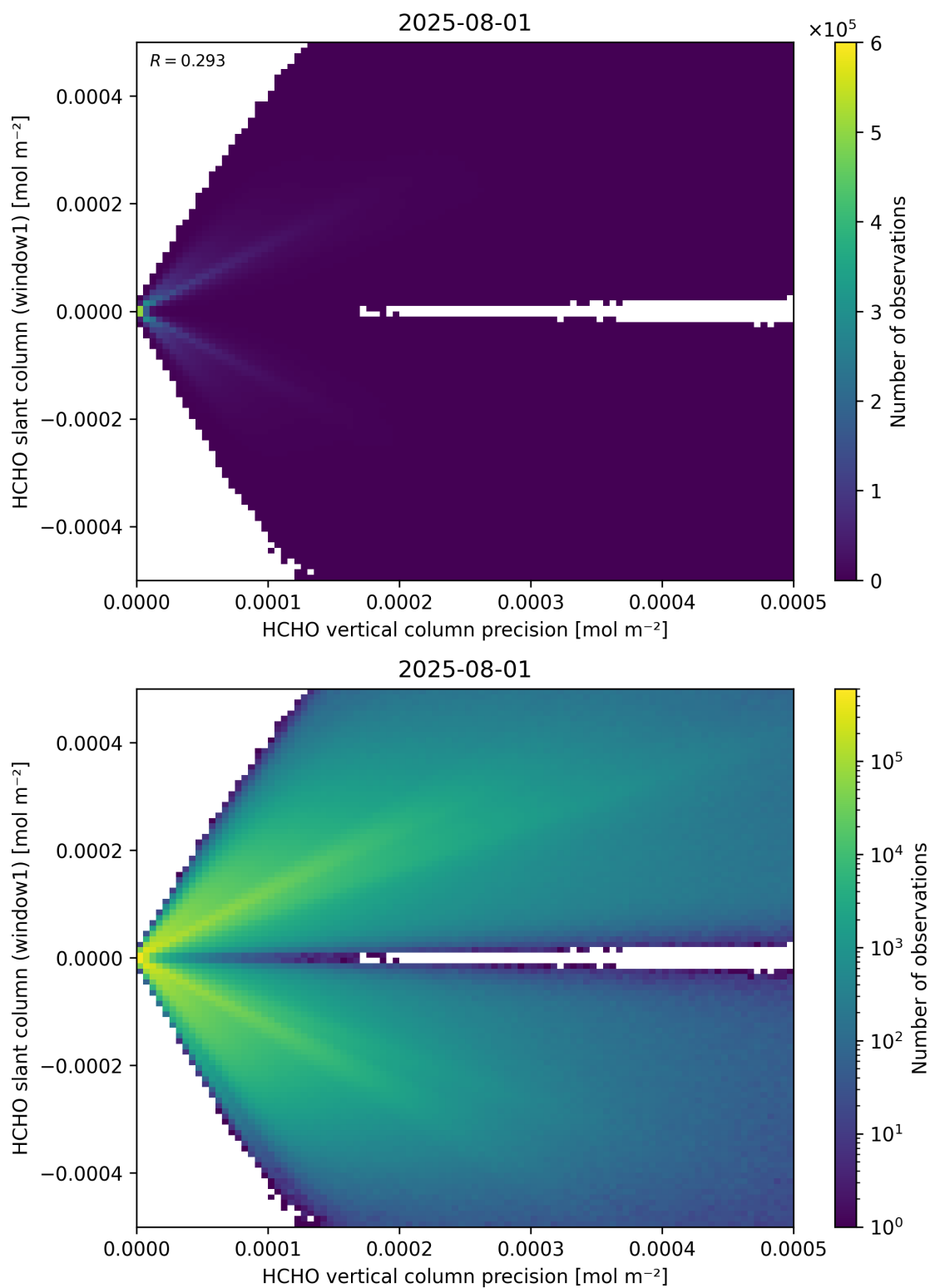
Figure 142: Scatter density plot of “HCHO vertical column precision” against “HCHO slant column (window1)” for 2025-07-31 to 2025-08-02.
