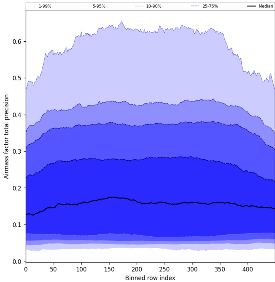
Figure 55: Along track statistics of “Airmass factor total precision” for 2025-07-31 to 2025-08-02
