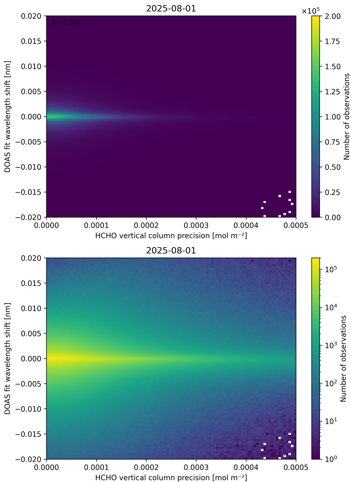
Figure 137: Scatter density plot of “HCHO vertical column precision” against “DOAS fit wavelength shift” for 2025-07-31 to 2025-08-02.
