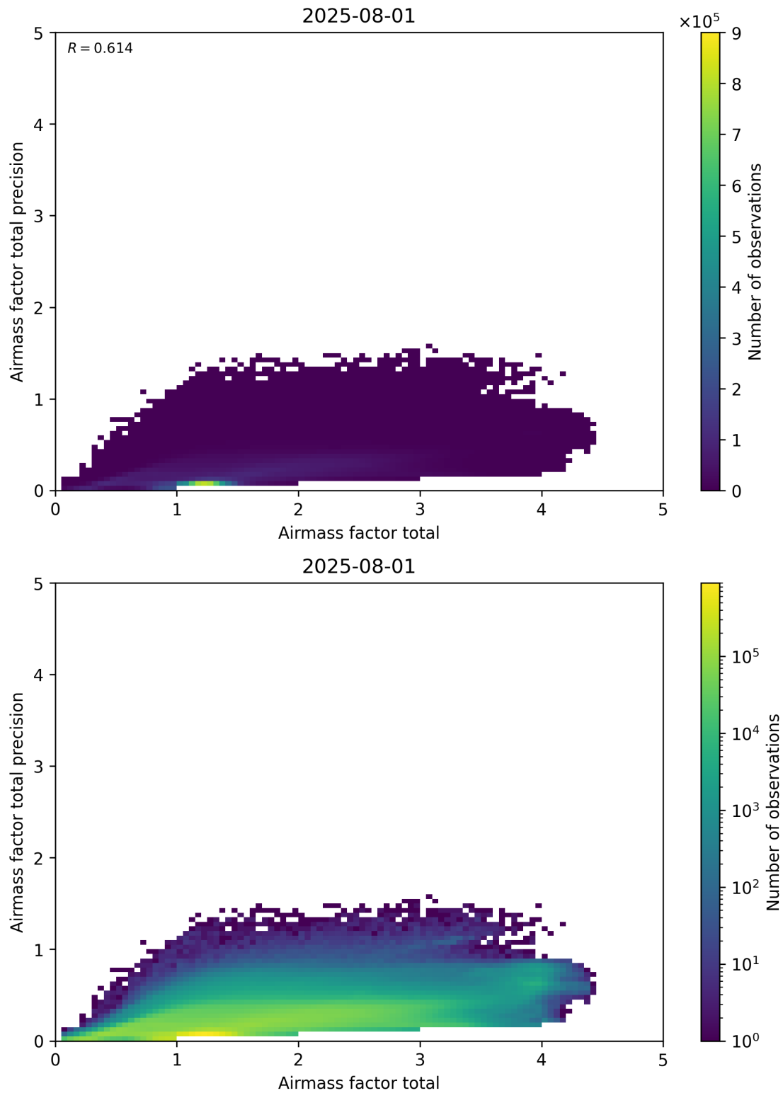
Figure 103: Scatter density plot of “Airmass factor total” against “Airmass factor total precision” for 2025-07-31 to 2025-08-02.
