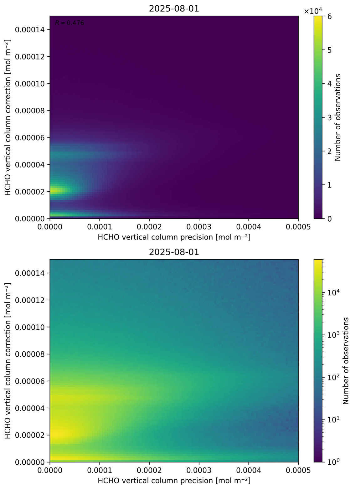
Figure 146: Scatter density plot of “HCHO vertical column precision” against “HCHO vertical column correction” for 2025-07-31 to 2025-08-02.
