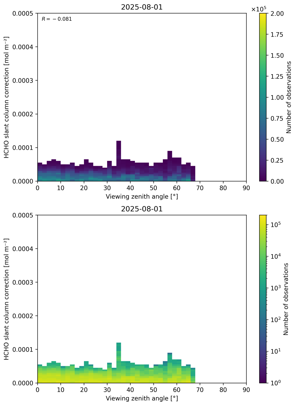
Figure 187: Scatter density plot of “Viewing zenith angle” against “HCHO slant column correction” for 2025-07-31 to 2025-08-02.
