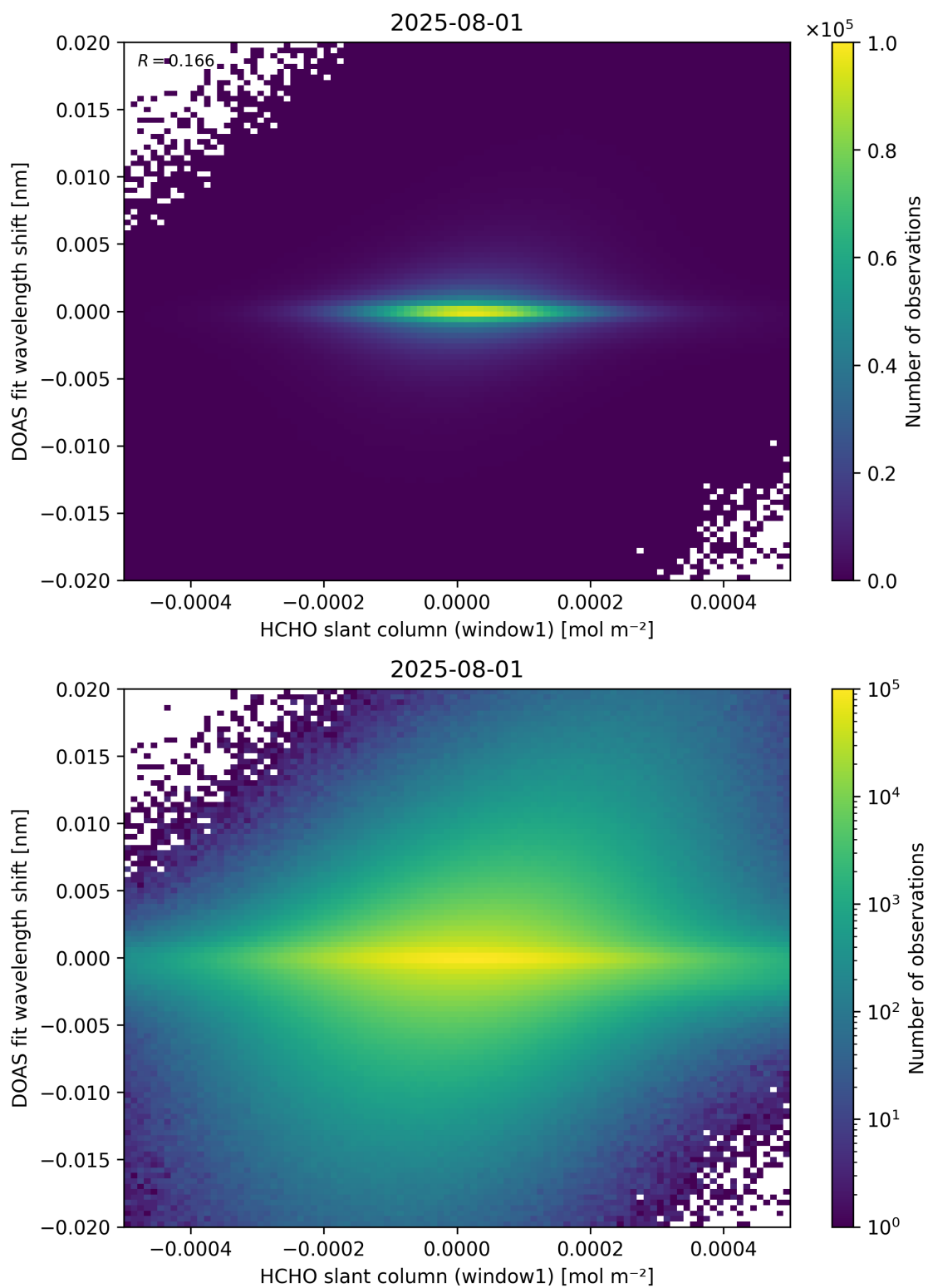
Figure 79: Scatter density plot of “HCHO slant column (window1)” against “DOAS fit wavelength shift” for 2025-07-31 to 2025-08-02.
