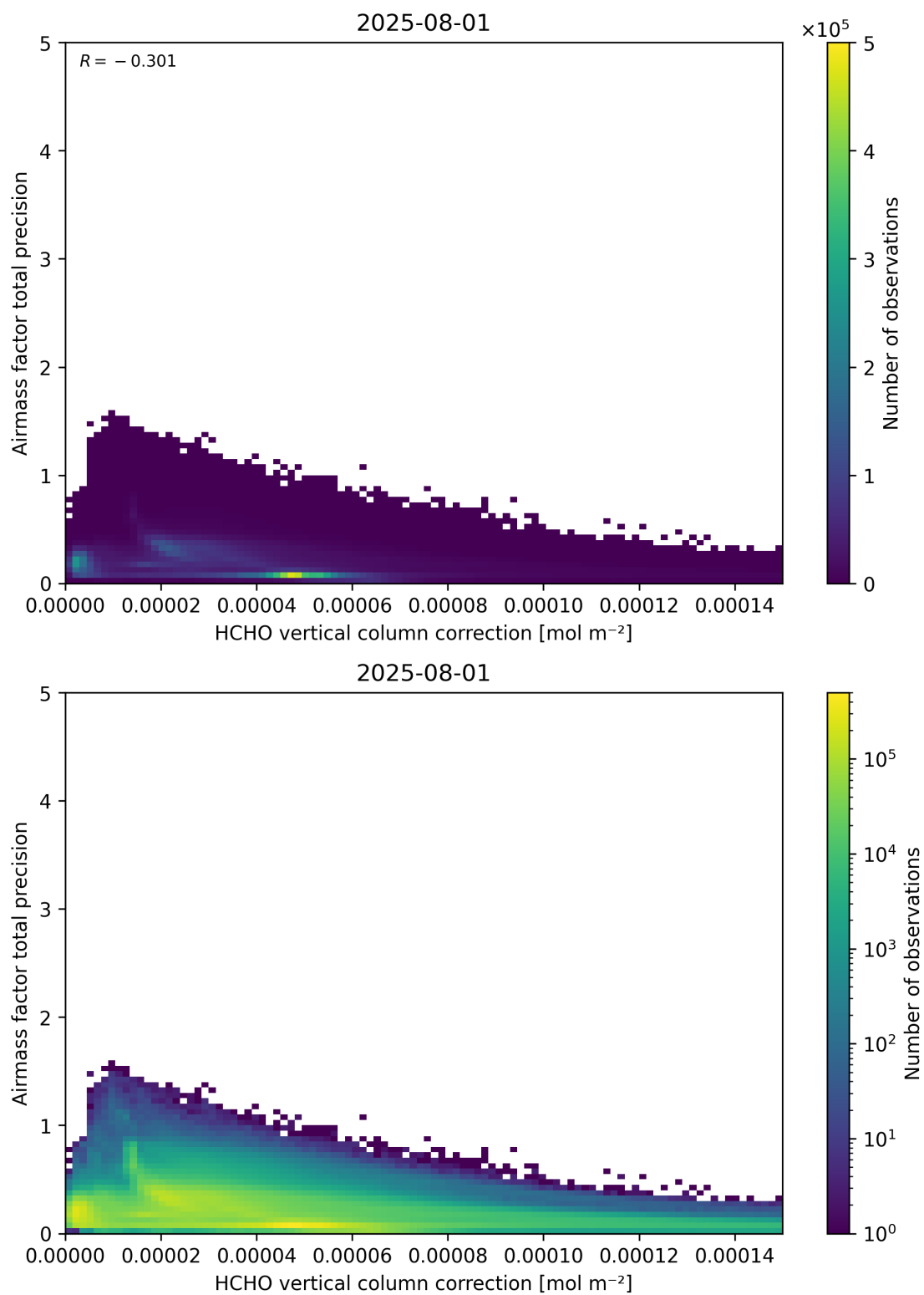
Figure 121: Scatter density plot of “HCHO vertical column correction” against “Airmass factor total precision” for 2025-07-31 to 2025-08-02.
