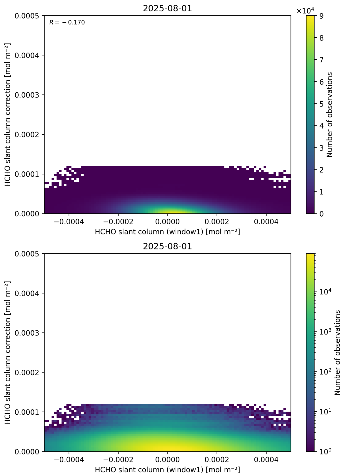
Figure 83: Scatter density plot of “HCHO slant column (window1)” against “HCHO slant column correction” for 2025-07-31 to 2025-08-02.
