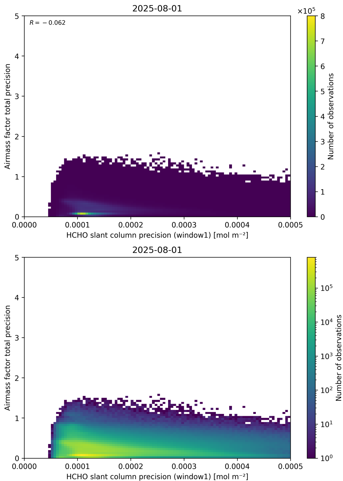
Figure 95: Scatter density plot of “HCHO slant column precision (window1)” against “Airmass factor total precision” for 2025-07-31 to 2025-08-02.
