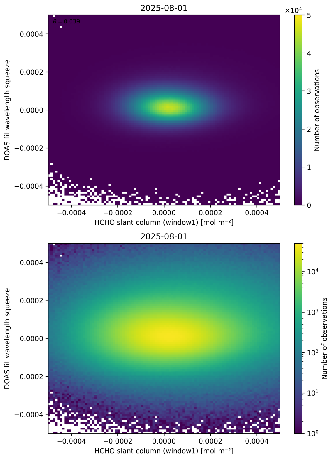
Figure 80: Scatter density plot of “HCHO slant column (window1)” against “DOAS fit wavelength squeeze” for 2025-07-31 to 2025-08-02.
