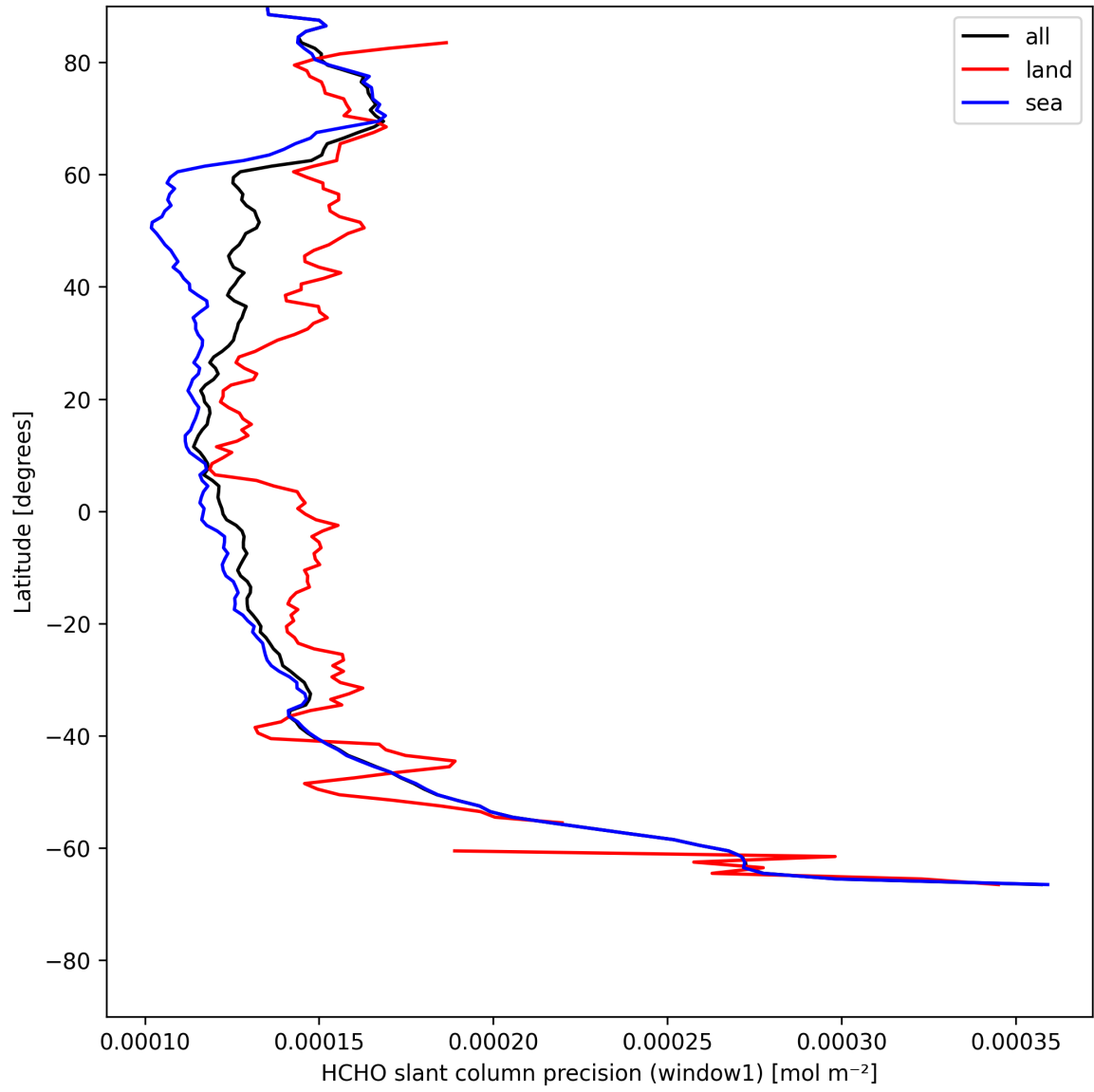
Figure 25: Zonal average of “HCHO slant column precision (window1)” for 2025-07-31 to 2025-08-02.
