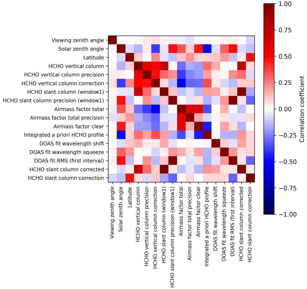
Figure 2: Map of correlation matrix for 2025-07-31 to 2025-08-02.
