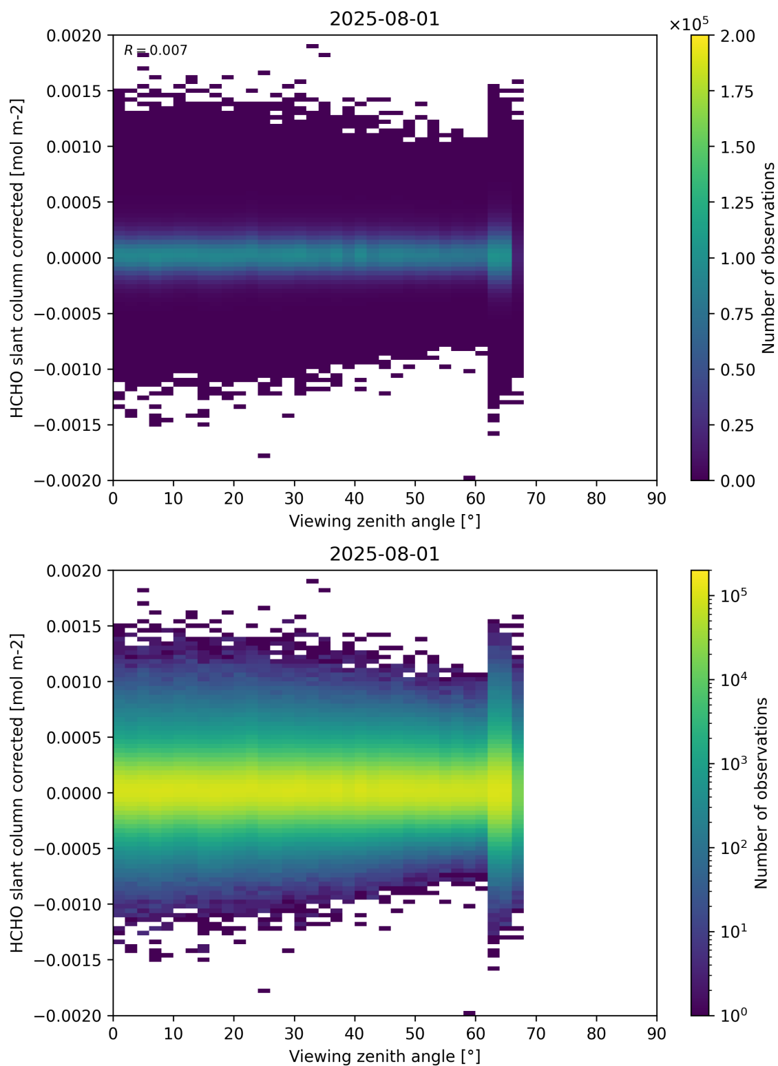
Figure 186: Scatter density plot of “Viewing zenith angle” against “HCHO slant column corrected” for 2025-07-31 to 2025-08-02.
