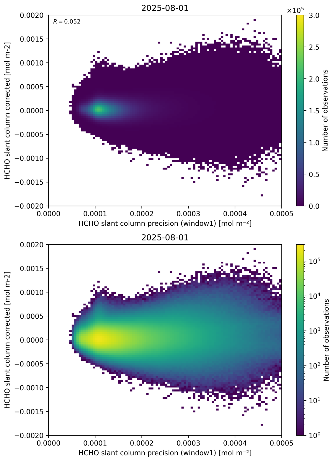
Figure 92: Scatter density plot of “HCHO slant column precision (window1)” against “HCHO slant column corrected” for 2025-07-31 to 2025-08-02.
