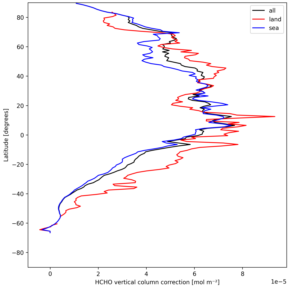
Figure 23: Zonal average of “HCHO vertical column correction” for 2025-07-31 to 2025-08-02.
