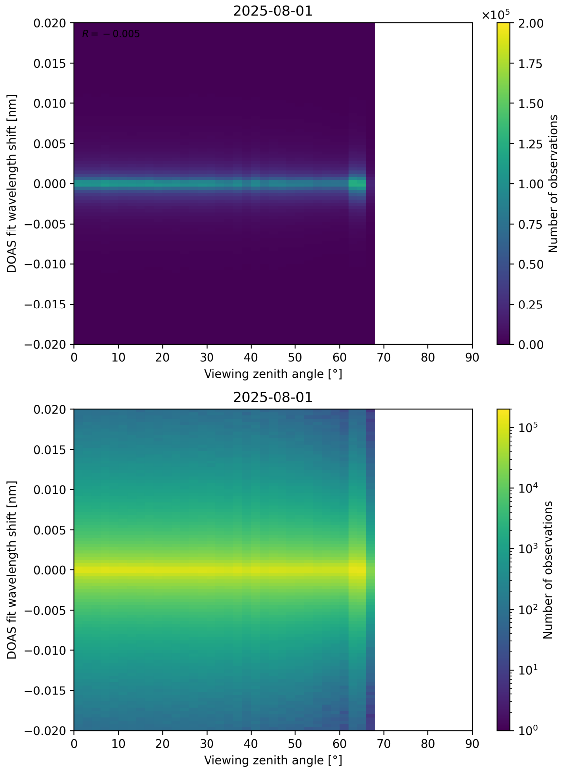
Figure 183: Scatter density plot of “Viewing zenith angle” against “DOAS fit wavelength shift” for 2025-07-31 to 2025-08-02.
