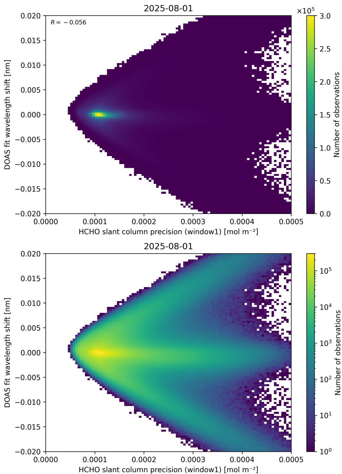
Figure 89: Scatter density plot of “HCHO slant column precision (window1)” against “DOAS fit wavelength shift” for 2025-07-31 to 2025-08-02.
