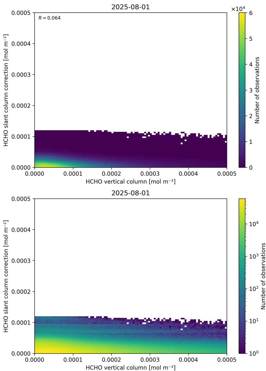
Figure 128: Scatter density plot of “HCHO vertical column” against “HCHO slant column correction” for 2025-07-31 to 2025-08-02.
