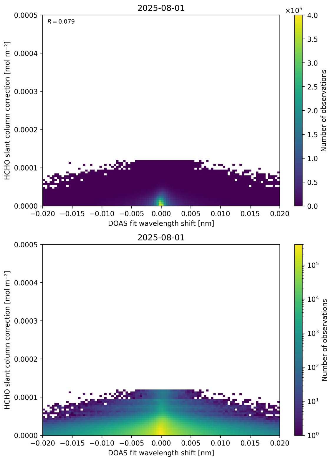
Figure 67: Scatter density plot of “DOAS fit wavelength shift” against “HCHO slant column correction” for 2025-07-31 to 2025-08-02.
