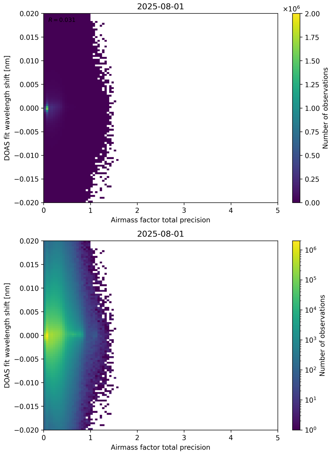
Figure 106: Scatter density plot of “Airmass factor total precision” against “DOAS fit wavelength shift” for 2025-07-31 to 2025-08-02.
