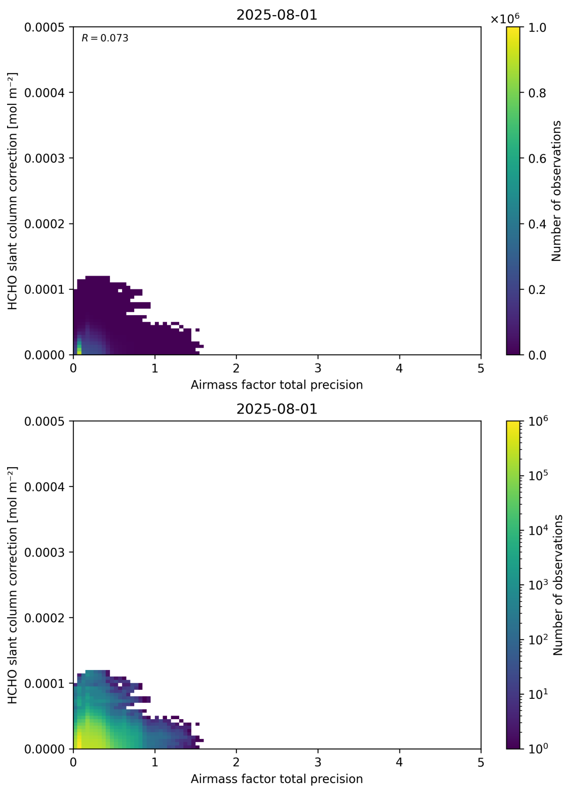
Figure 110: Scatter density plot of “Airmass factor total precision” against “HCHO slant column correction” for 2025-07-31 to 2025-08-02.
