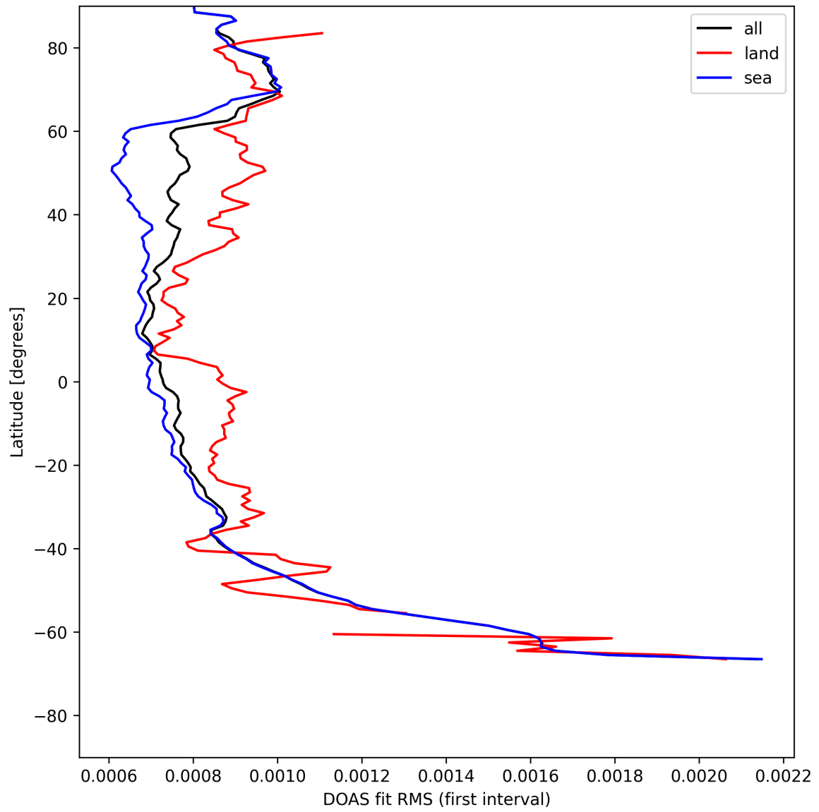
Figure 32: Zonal average of "DOAS fit RMS (first interval)" for 2025-07-31 to 2025-08-02.
