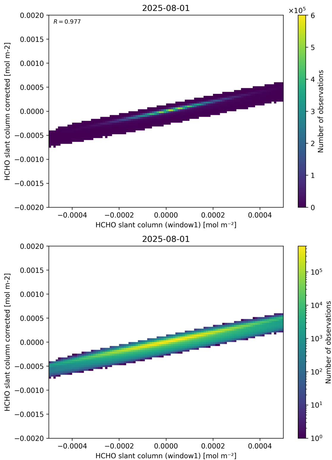
Figure 82: Scatter density plot of “HCHO slant column (window1)” against “HCHO slant column corrected” for 2025-07-31 to 2025-08-02.
