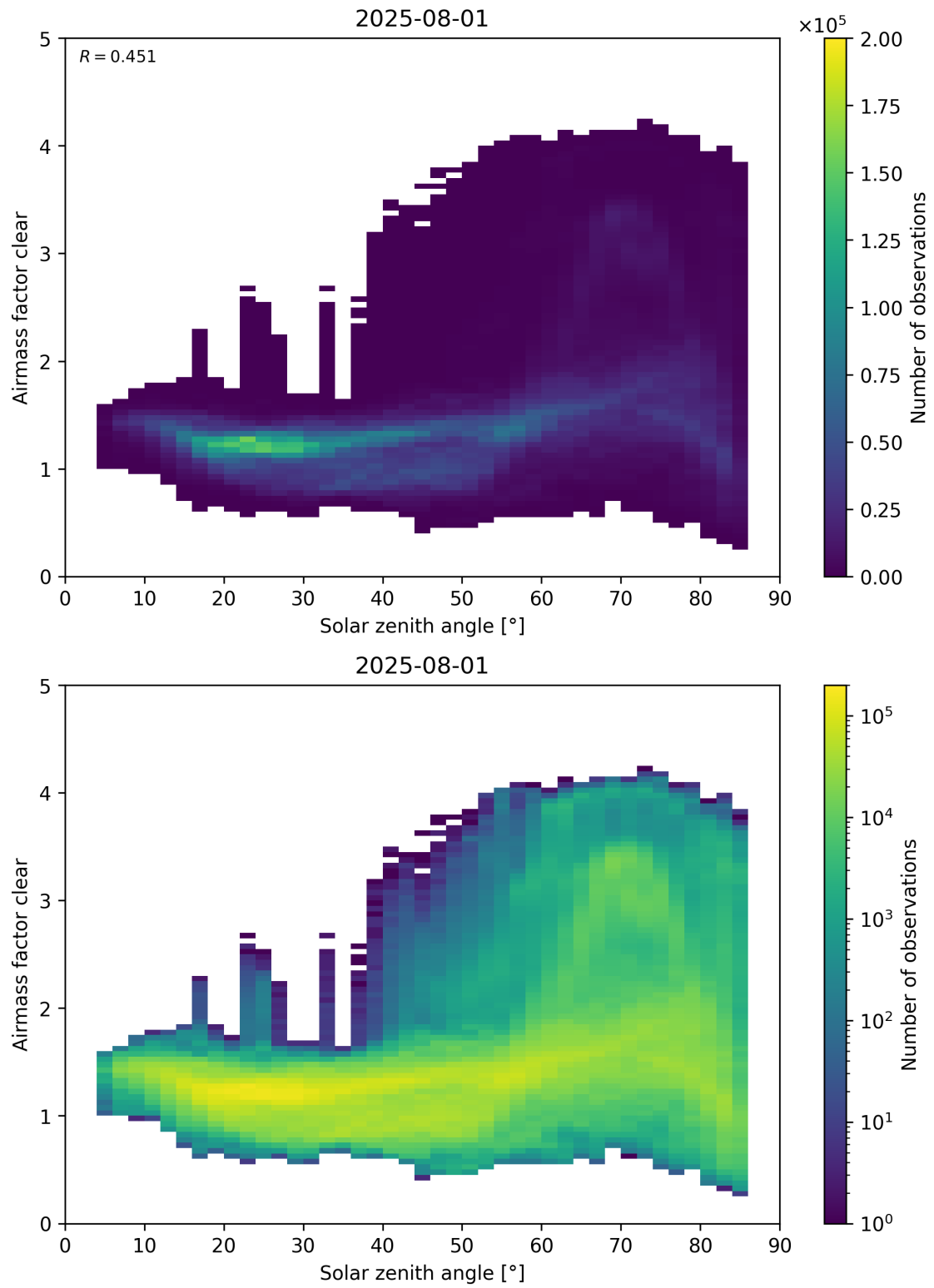
Figure 170: Scatter density plot of “Solar zenith angle” against “Airmass factor clear” for 2025-07-31 to 2025-08-02.
