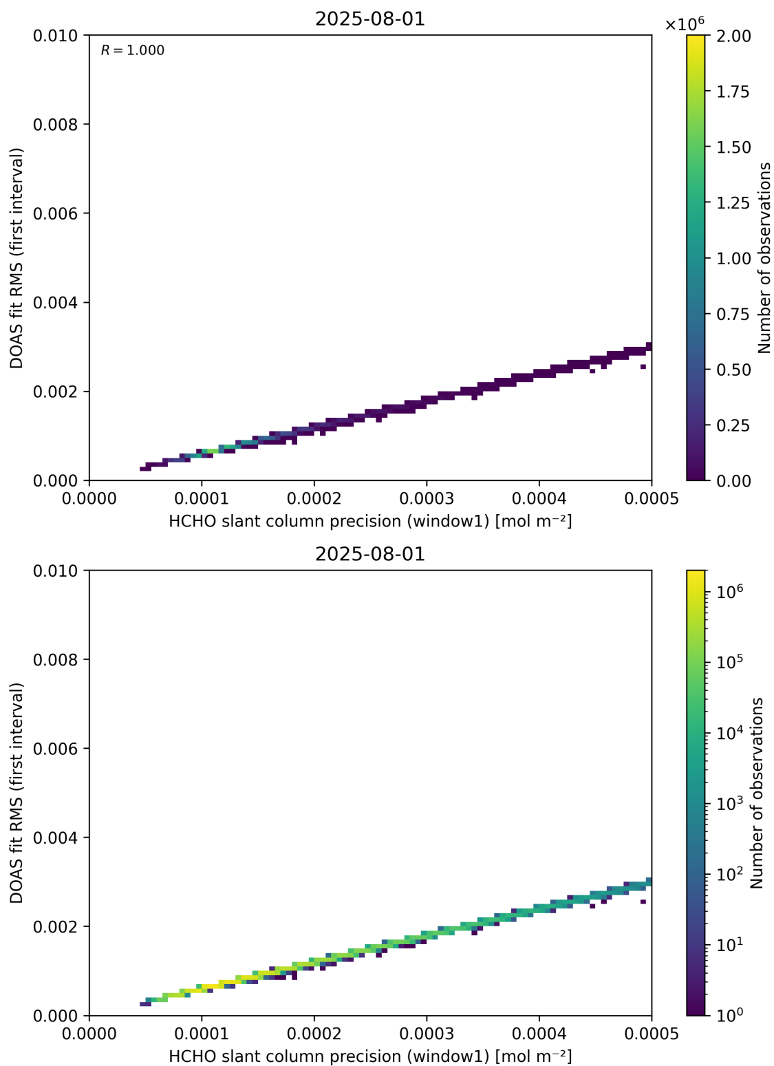
Figure 88: Scatter density plot of “HCHO slant column precision (window1)” against “DOAS fit RMS (first interval)” for 2025-07-31 to 2025-08-02.
