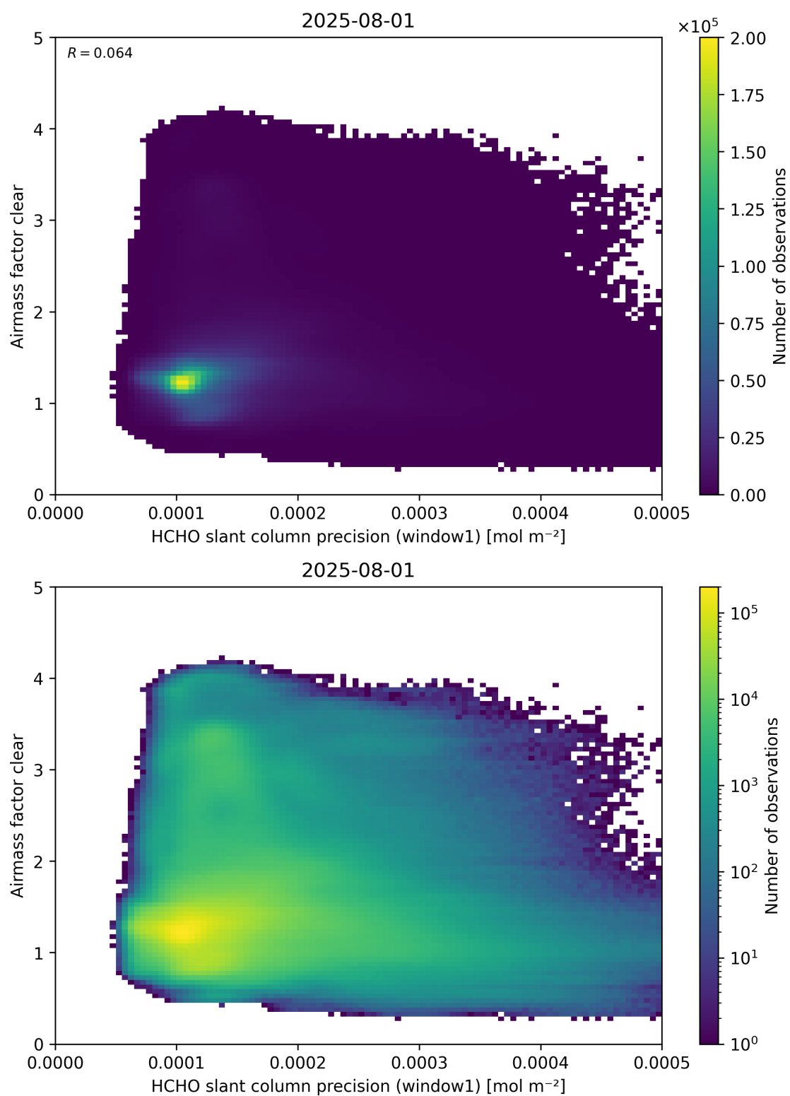
Figure 91: Scatter density plot of “HCHO slant column precision (window1)” against “Airmass factor clear” for 2025-07-31 to 2025-08-02.
