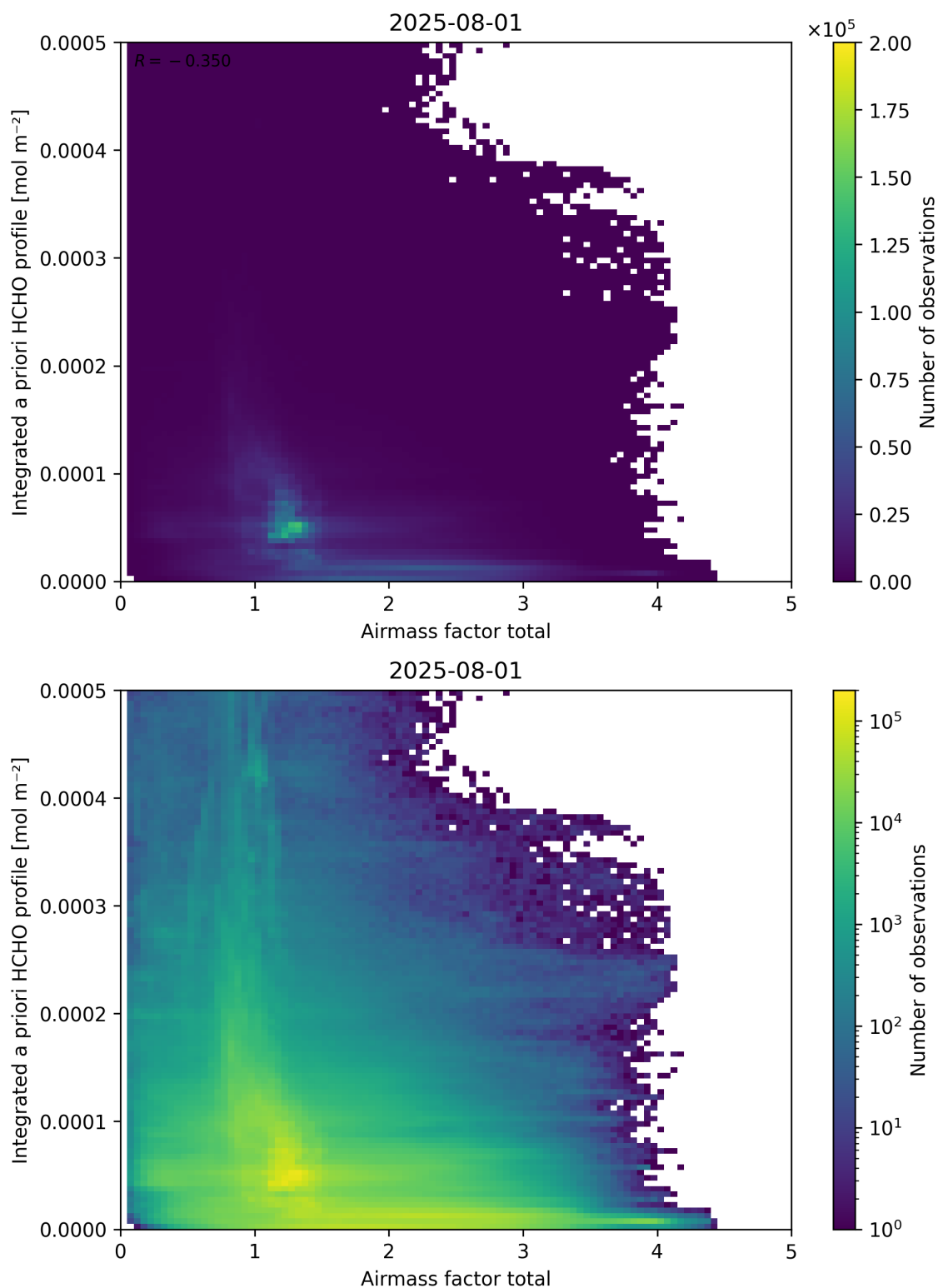
Figure 104: Scatter density plot of “Airmass factor total” against “Integrated a priori HCHO profile” for 2025-07-31 to 2025-08-02.
