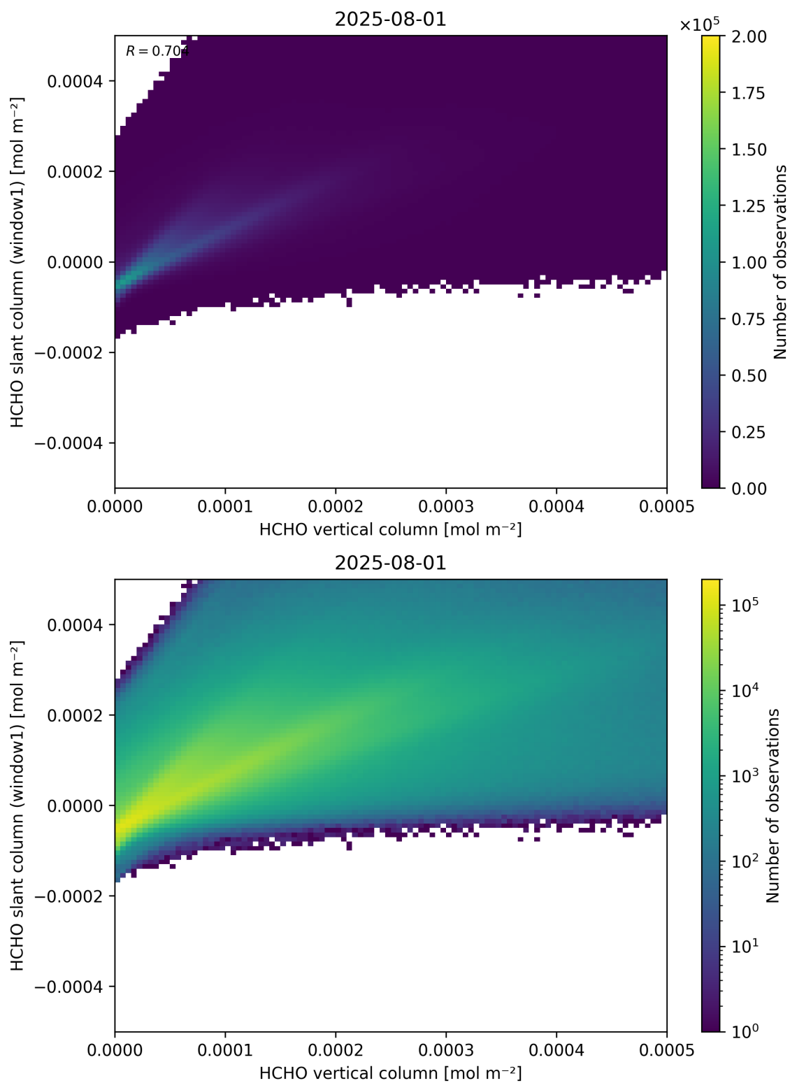
Figure 129: Scatter density plot of “HCHO vertical column” against “HCHO slant column (window1)” for 2025-07-31 to 2025-08-02.
