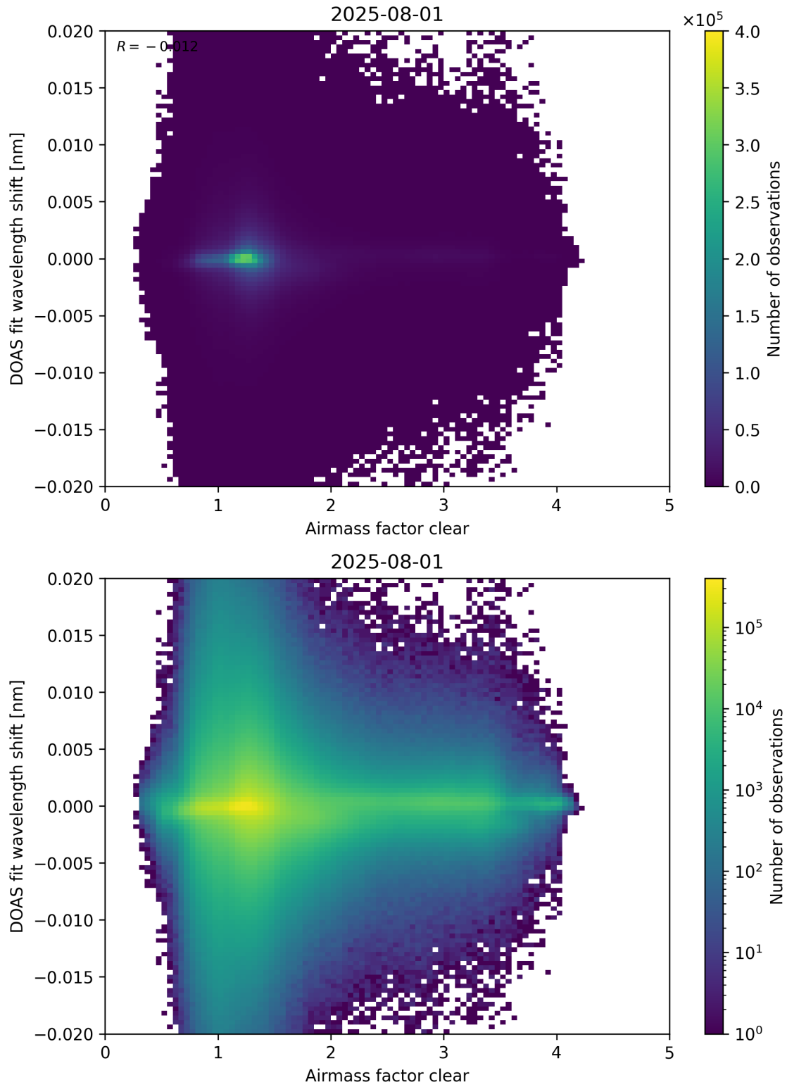
Figure 72: Scatter density plot of “Airmass factor clear” against “DOAS fit wavelength shift” for 2025-07-31 to 2025-08-02.
