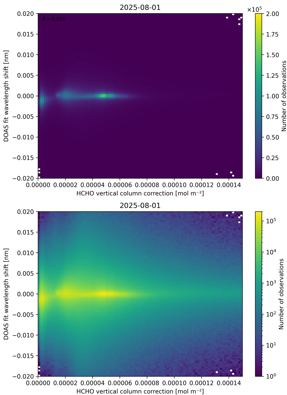
Figure 113: Scatter density plot of “HCHO vertical column correction” against “DOAS fit wavelength shift” for 2025-07-31 to 2025-08-02.
