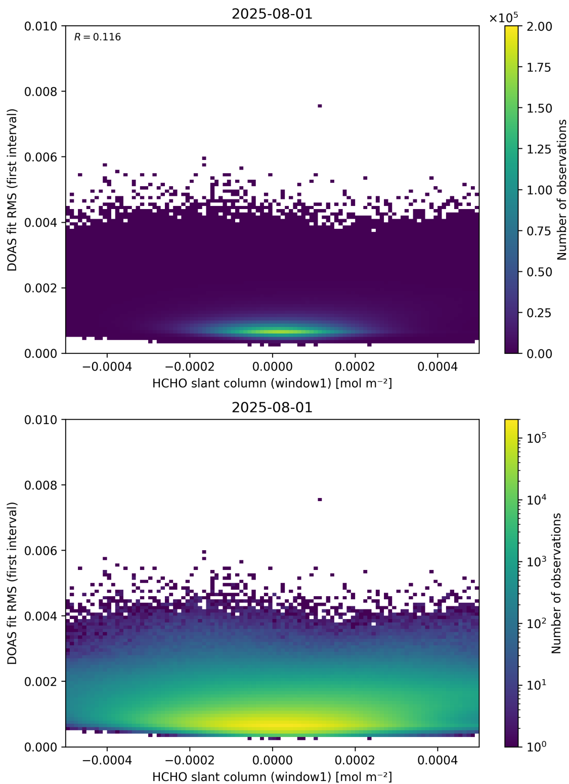
Figure 78: Scatter density plot of “HCHO slant column (window1)” against “DOAS fit RMS (first interval)” for 2025-07-31 to 2025-08-02.
