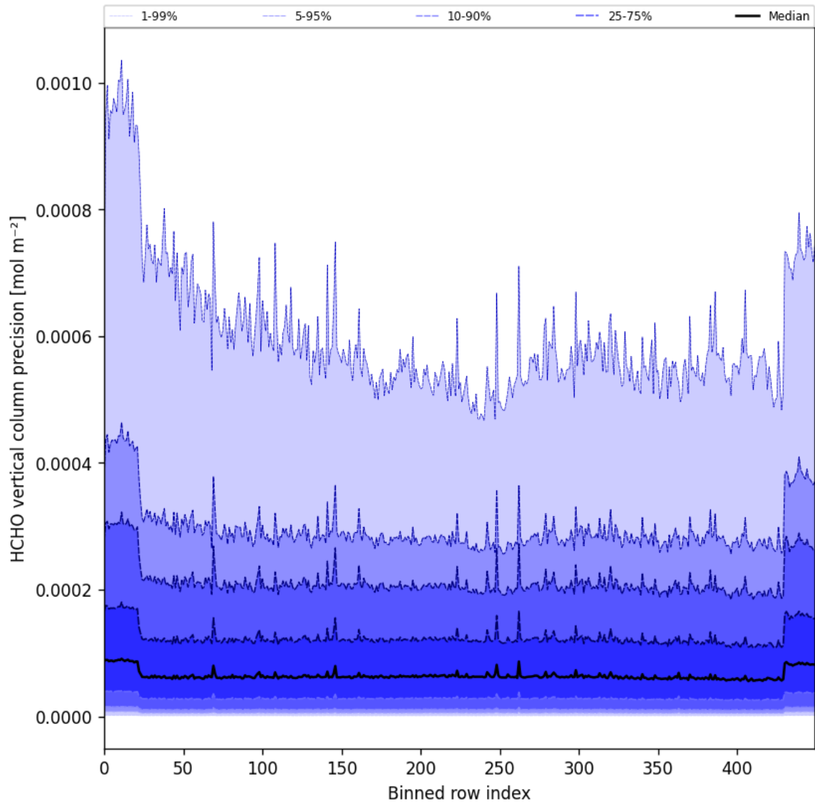
Figure 50: Along track statistics of “HCHO vertical column precision” for 2025-07-31 to 2025-08-02
