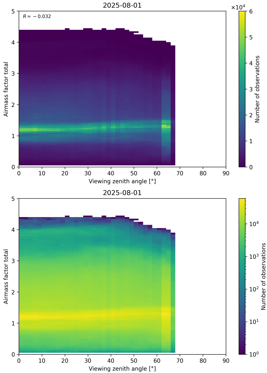
Figure 190: Scatter density plot of “Viewing zenith angle” against “Airmass factor total” for 2025-07-31 to 2025-08-02.
