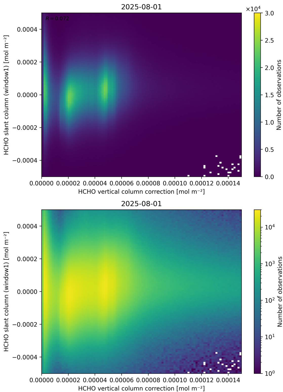
Figure 118: Scatter density plot of “HCHO vertical column correction” against “HCHO slant column (window1)” for 2025-07-31 to 2025-08-02.
