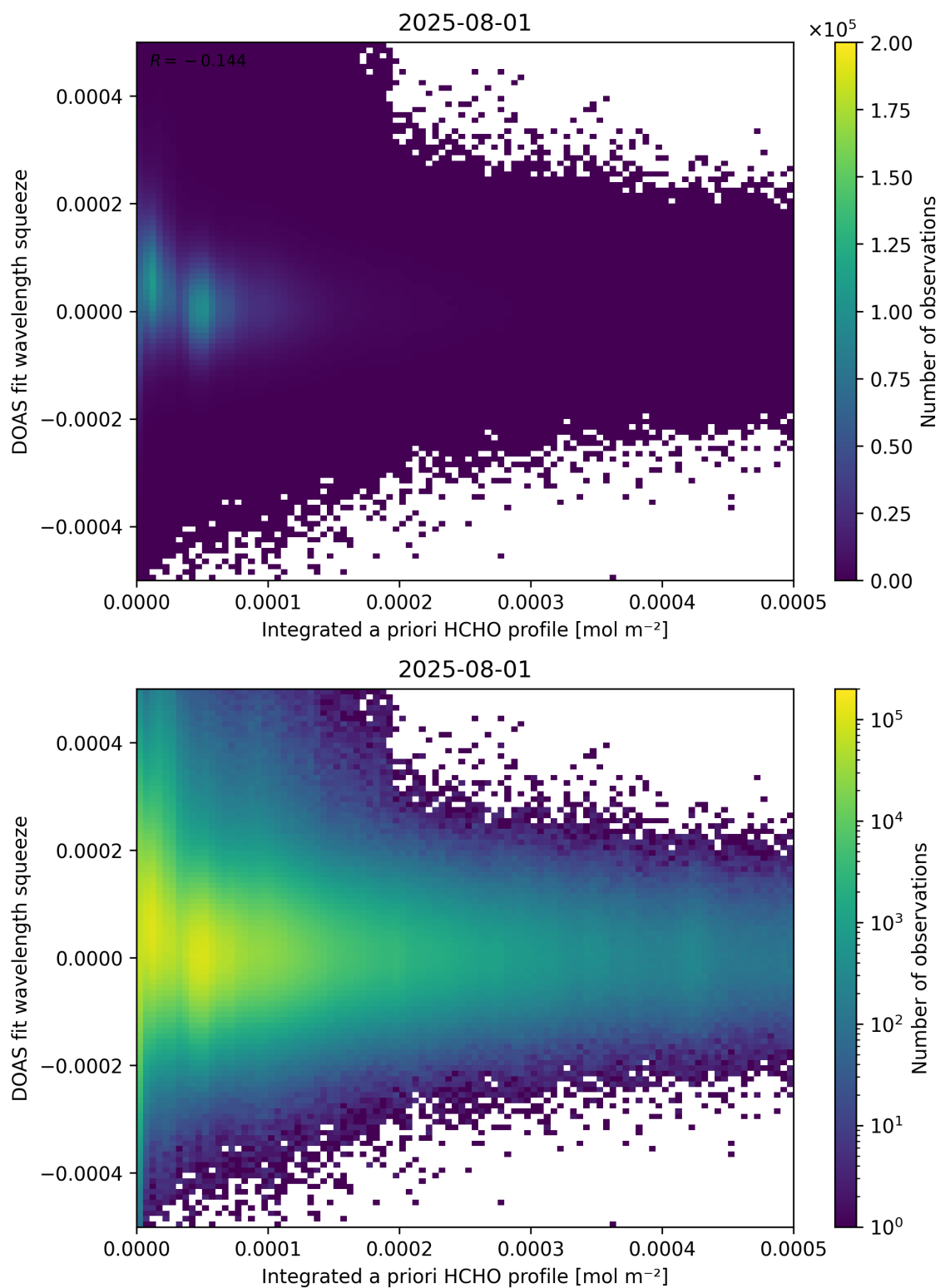
Figure 150: Scatter density plot of “Integrated a priori HCHO profile” against “DOAS fit wavelength squeeze” for 2025-07-31 to 2025-08-02.
