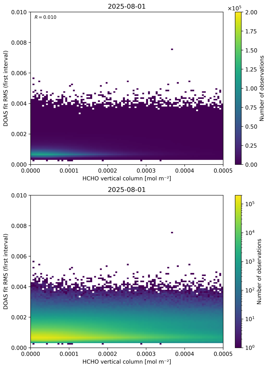
Figure 123: Scatter density plot of “HCHO vertical column” against “DOAS fit RMS (first interval)” for 2025-07-31 to 2025-08-02.
