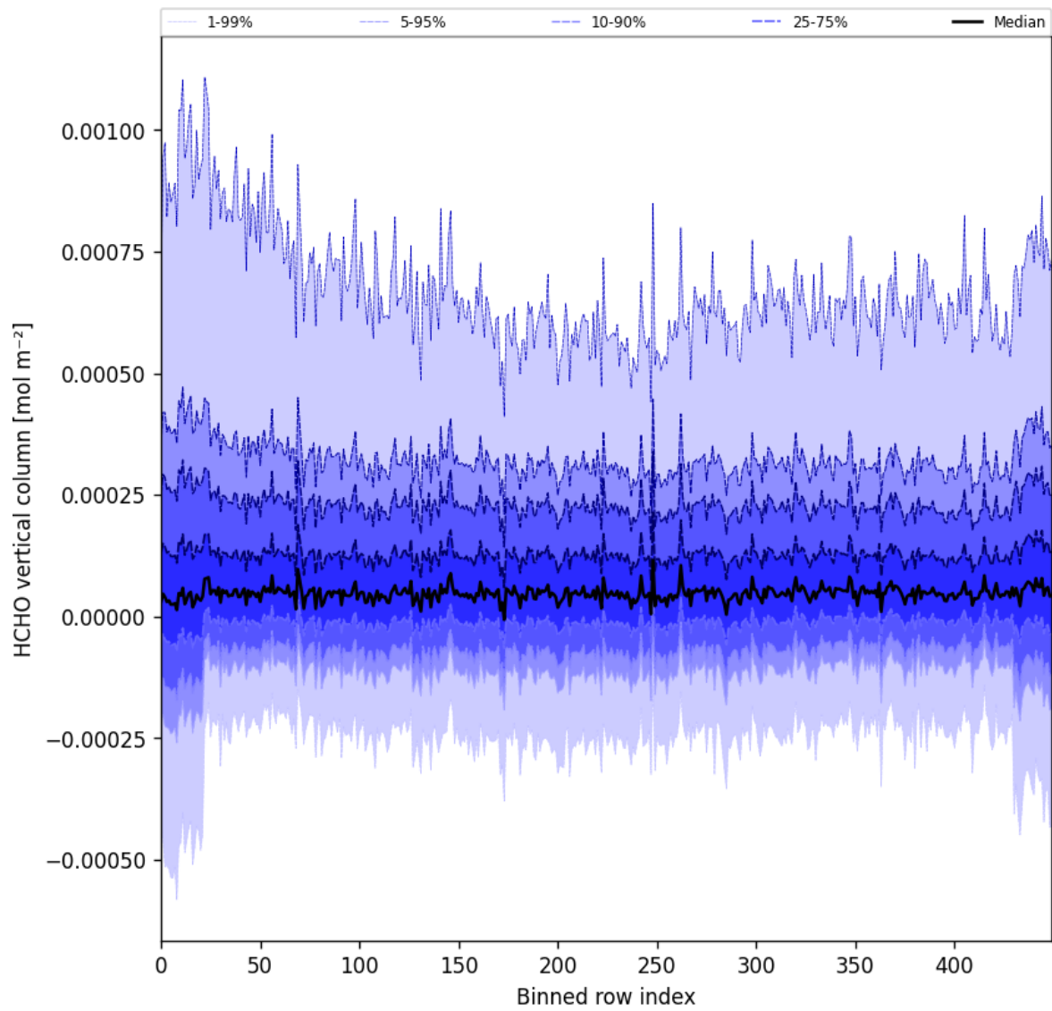
Figure 49: Along track statistics of “HCHO vertical column” for 2025-07-31 to 2025-08-02
