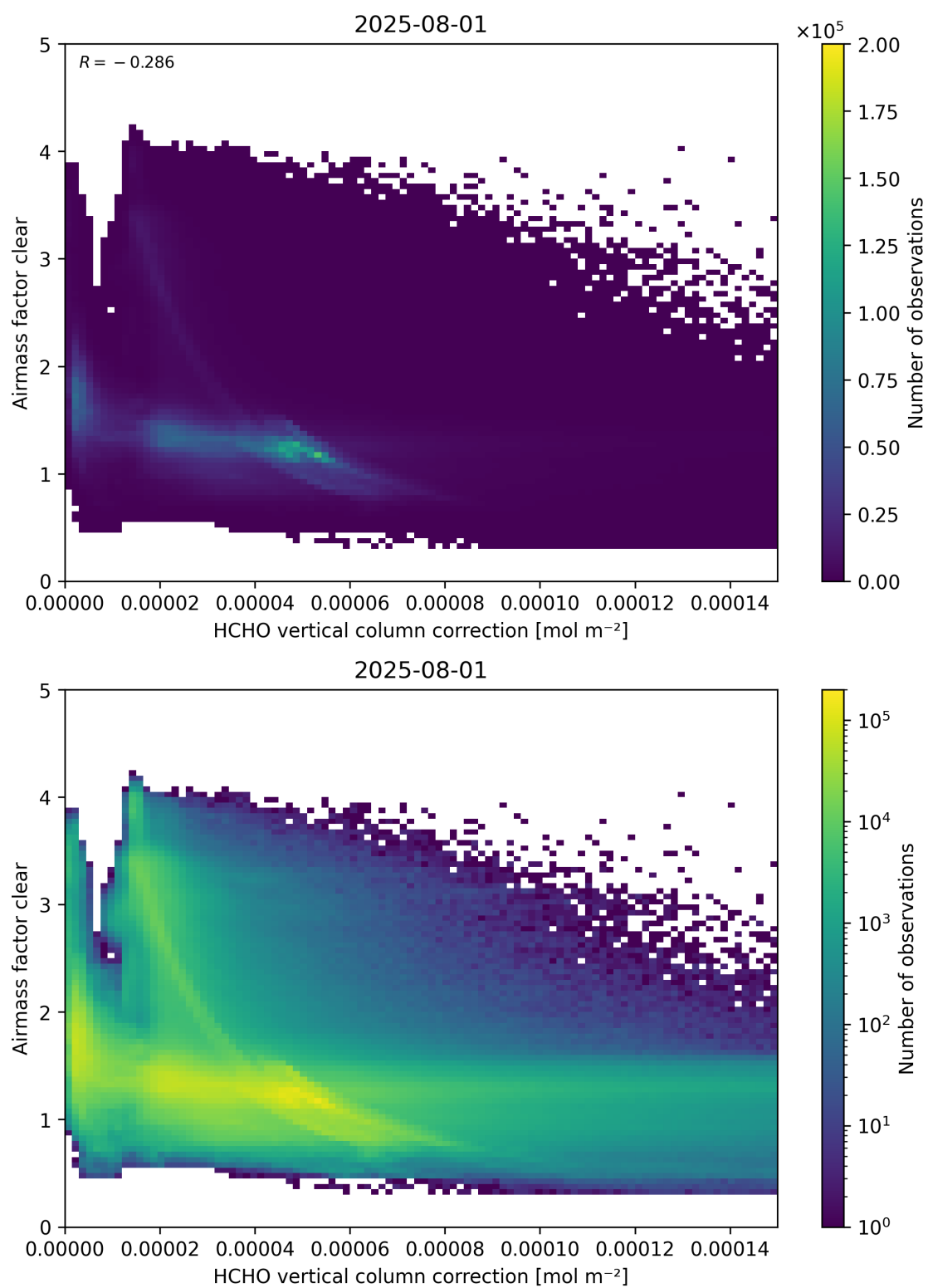
Figure 115: Scatter density plot of “HCHO vertical column correction” against “Airmass factor clear” for 2025-07-31 to 2025-08-02.
