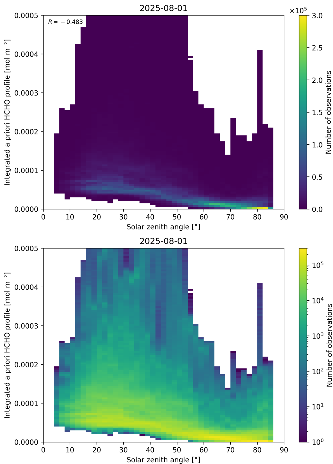
Figure 180: Scatter density plot of “Solar zenith angle” against “Integrated a priori HCHO profile” for 2025-07-31 to 2025-08-02.
