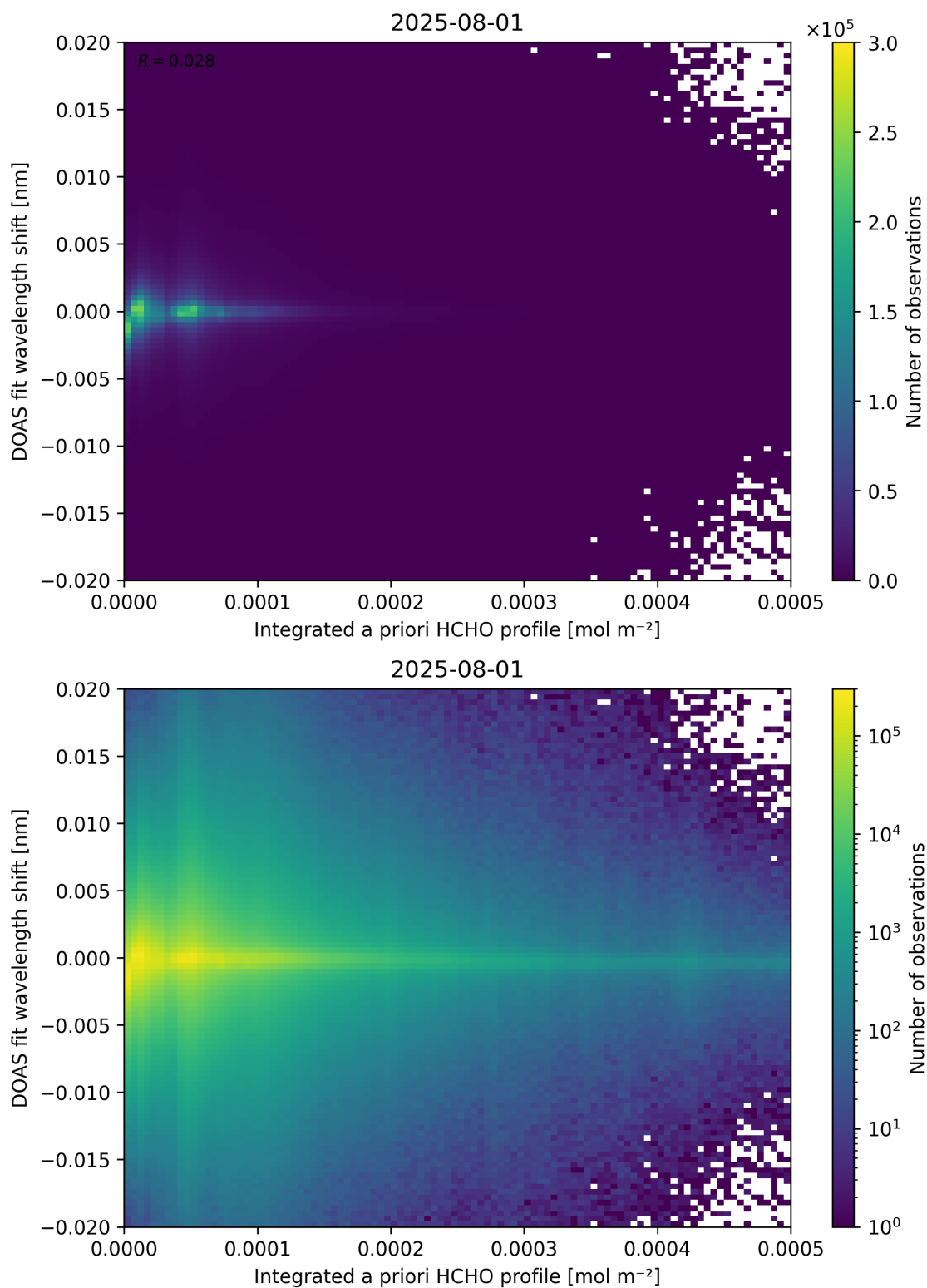
Figure 149: Scatter density plot of “Integrated a priori HCHO profile” against “DOAS fit wavelength shift” for 2025-07-31 to 2025-08-02.
