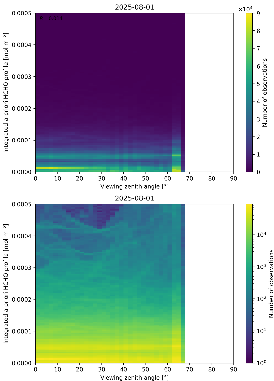
Figure 195: Scatter density plot of “Viewing zenith angle” against “Integrated a priori HCHO profile” for 2025-07-31 to 2025-08-02.
