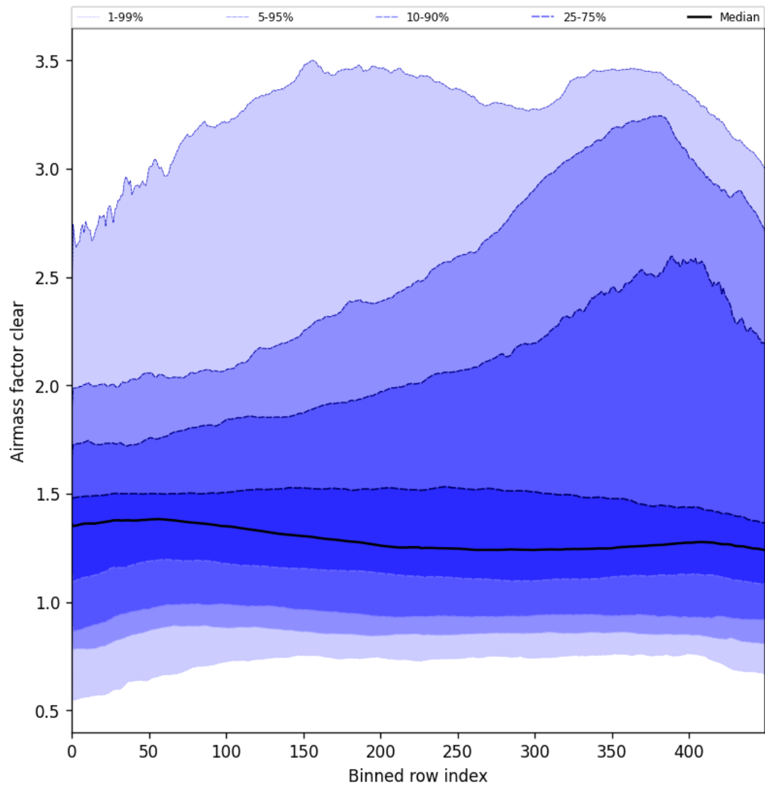
Figure 56: Along track statistics of “Airmass factor clear” for 2025-07-31 to 2025-08-02
