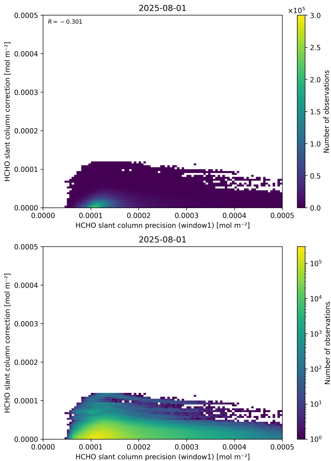
Figure 93: Scatter density plot of “HCHO slant column precision (window1)” against “HCHO slant column correction” for 2025-07-31 to 2025-08-02.
