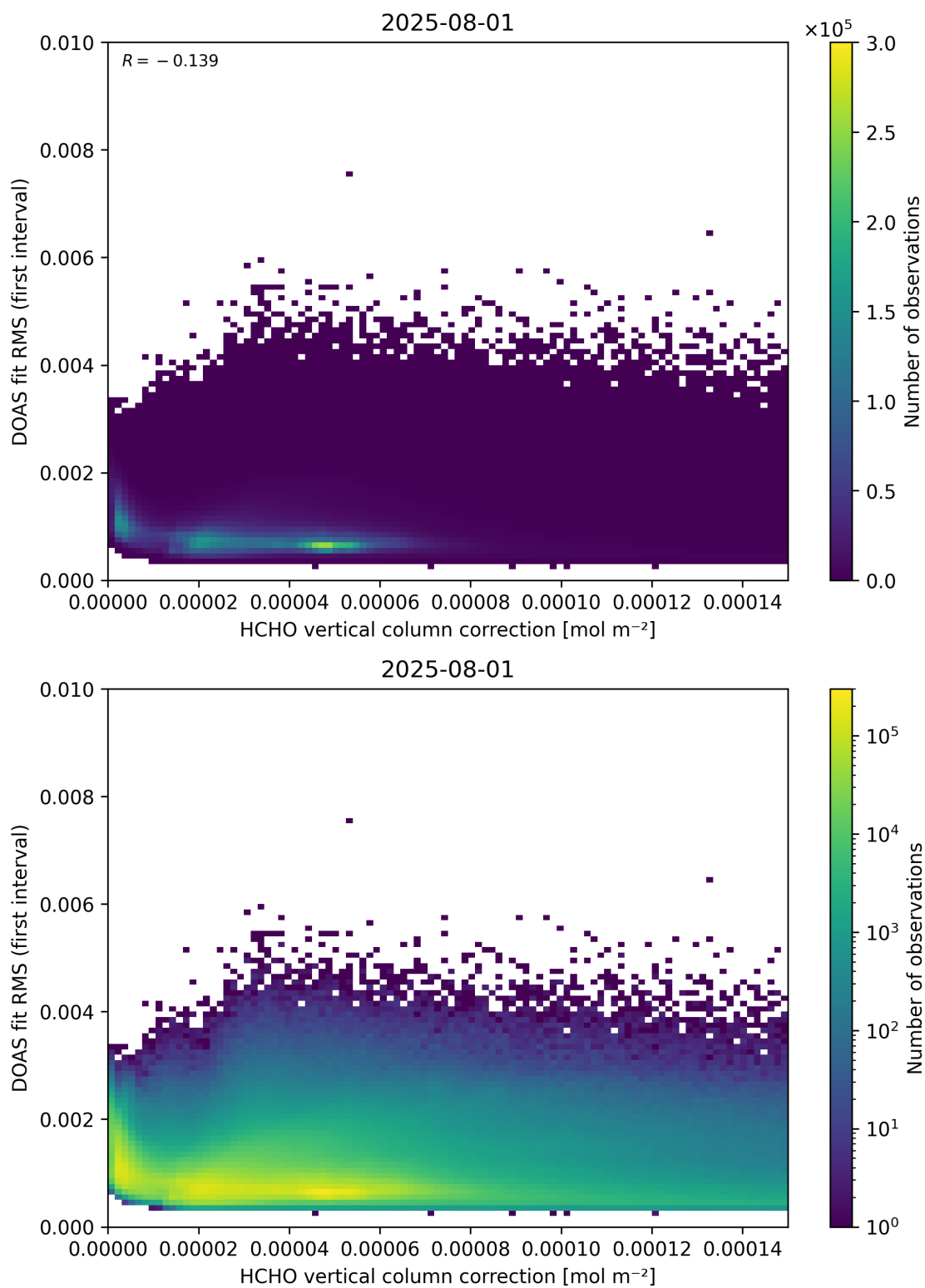
Figure 112: Scatter density plot of “HCHO vertical column correction” against “DOAS fit RMS (first interval)” for 2025-07-31 to 2025-08-02.
