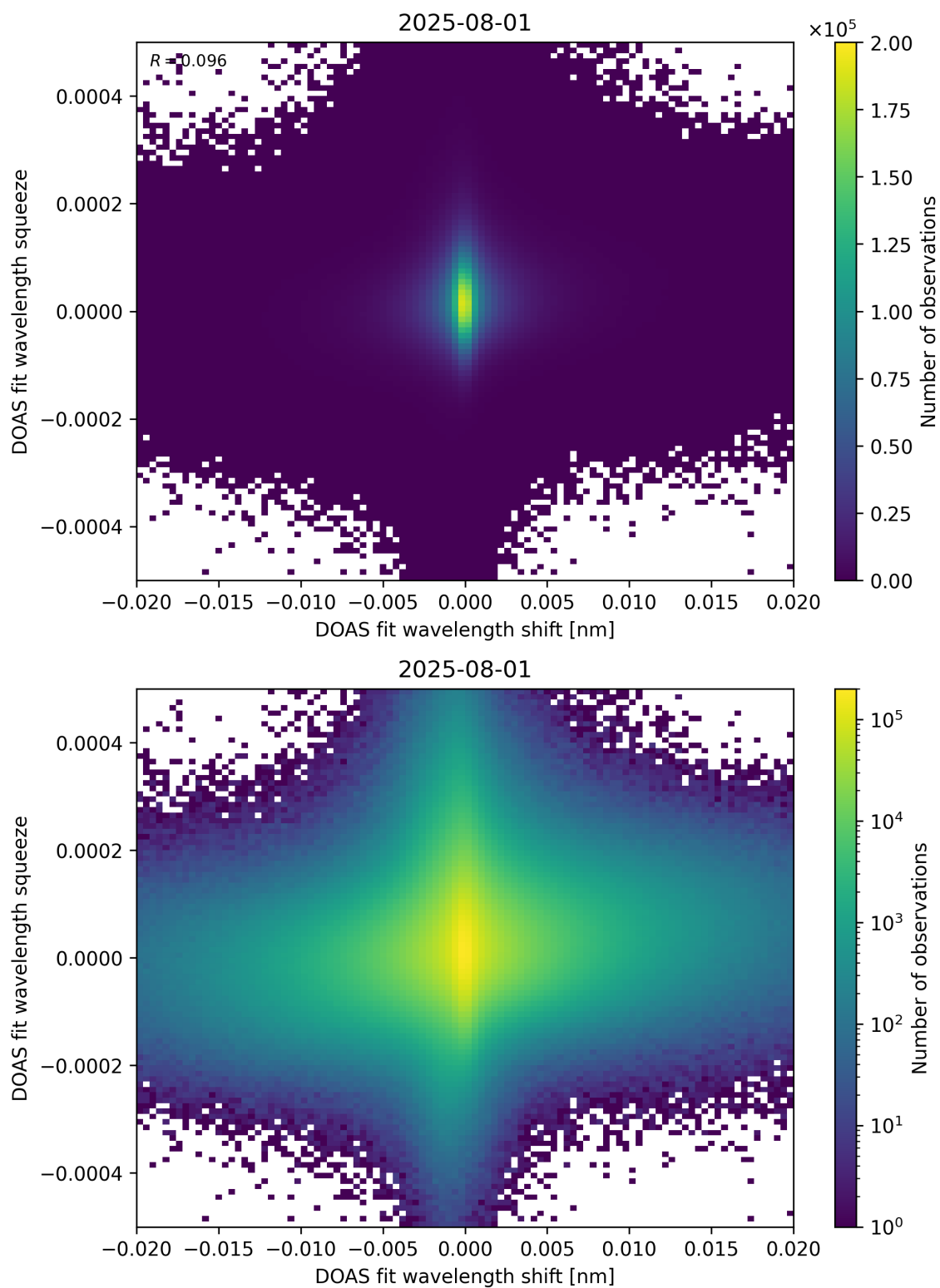
Figure 65: Scatter density plot of “DOAS fit wavelength shift” against “DOAS fit wavelength squeeze” for 2025-07-31 to 2025-08-02.
