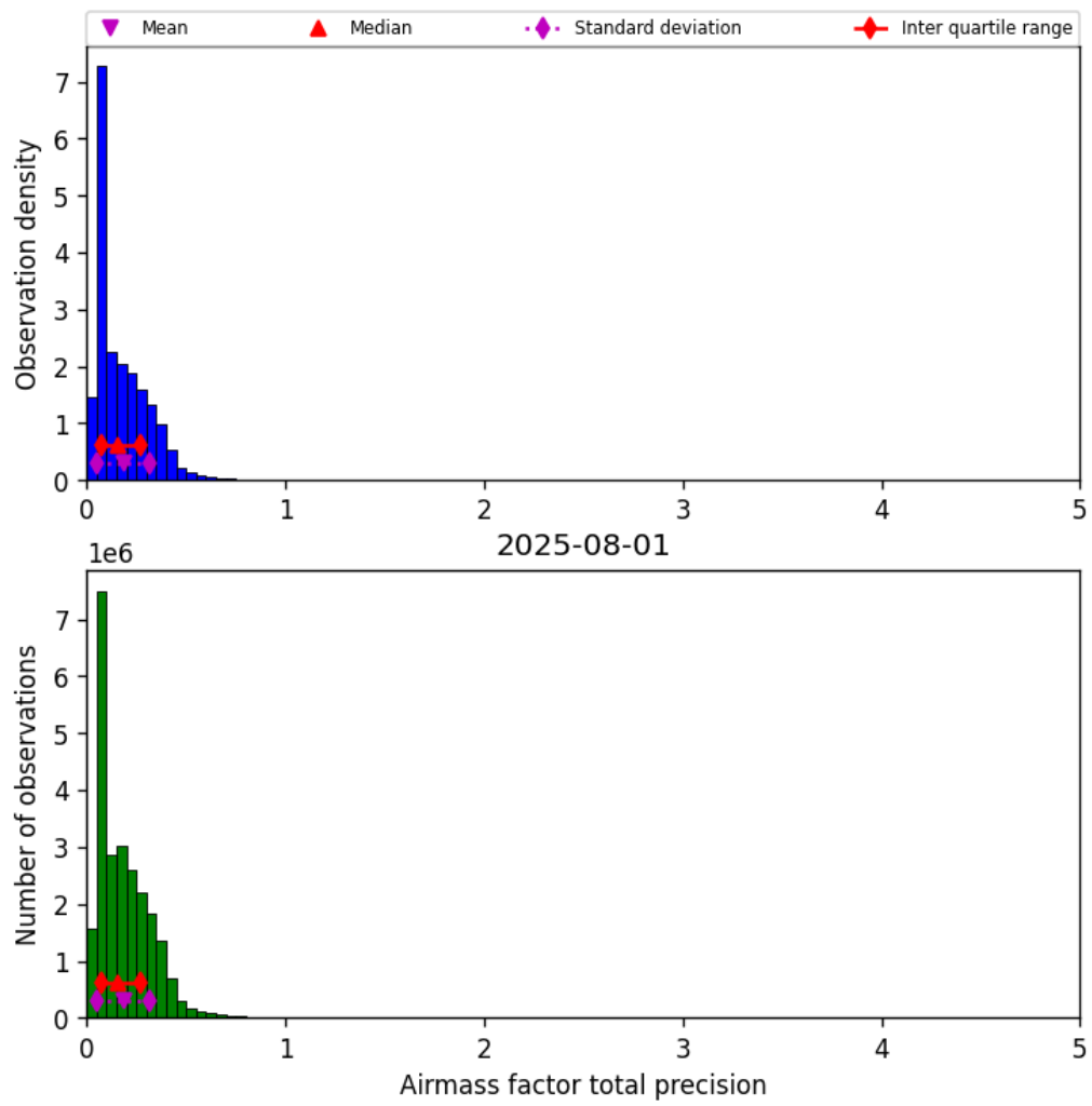
Figure 41: Histogram of “Airmass factor total precision” for 2025-07-31 to 2025-08-02
