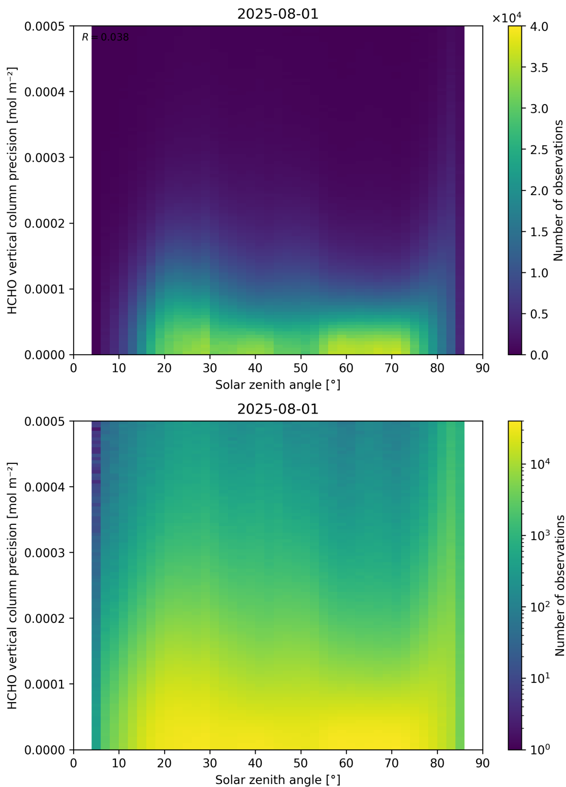
Figure 179: Scatter density plot of “Solar zenith angle” against “HCHO vertical column precision” for 2025-07-31 to 2025-08-02.
