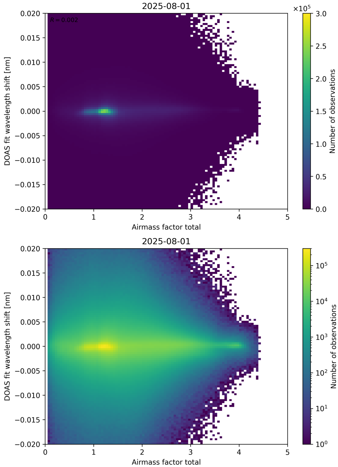
Figure 98: Scatter density plot of “Airmass factor total” against “DOAS fit wavelength shift” for 2025-07-31 to 2025-08-02.
