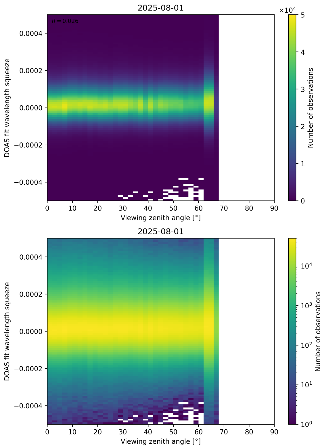
Figure 184: Scatter density plot of “Viewing zenith angle” against “DOAS fit wavelength squeeze” for 2025-07-31 to 2025-08-02.
