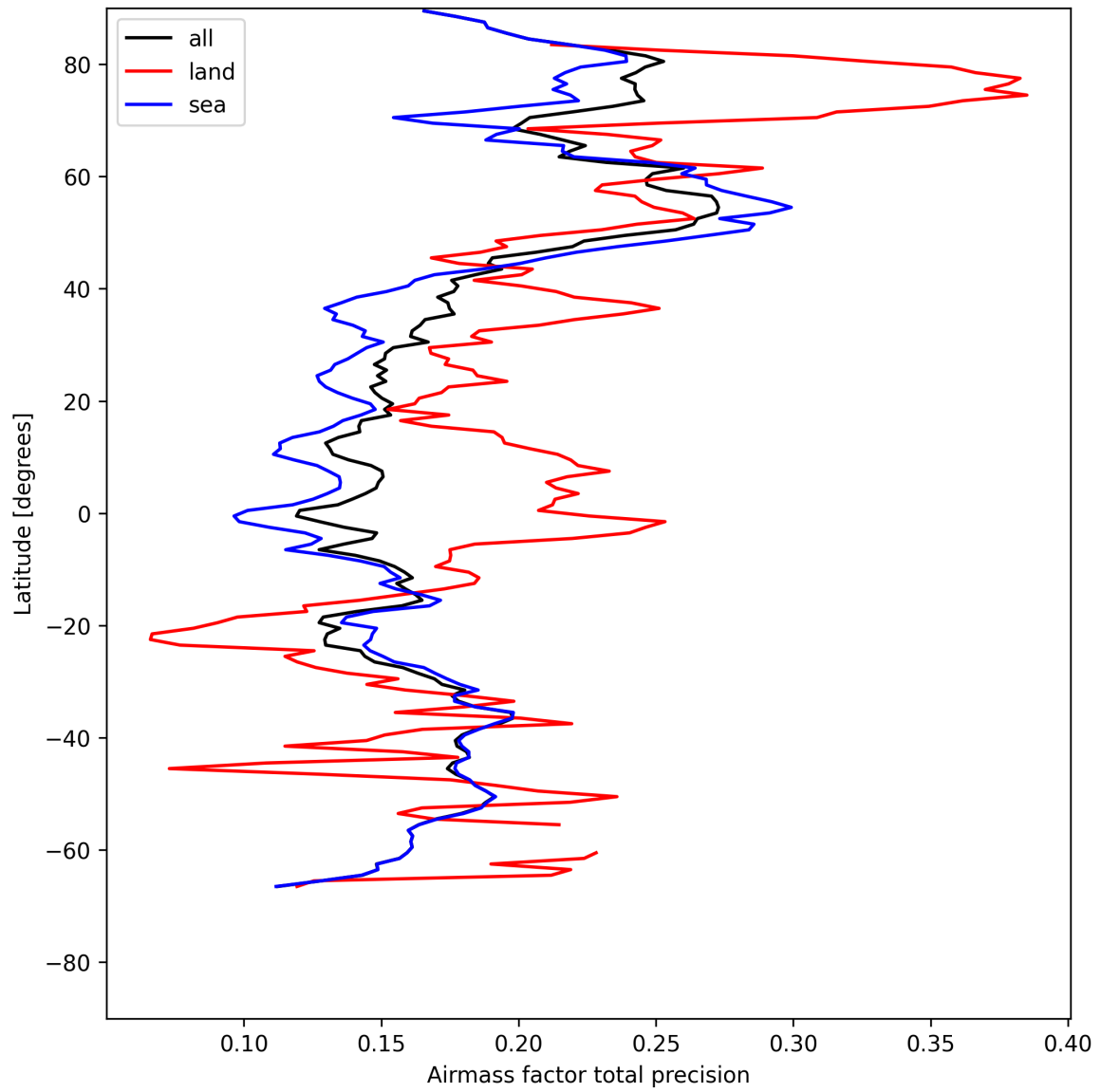
Figure 27: Zonal average of “Airmass factor total precision” for 2025-07-31 to 2025-08-02.
