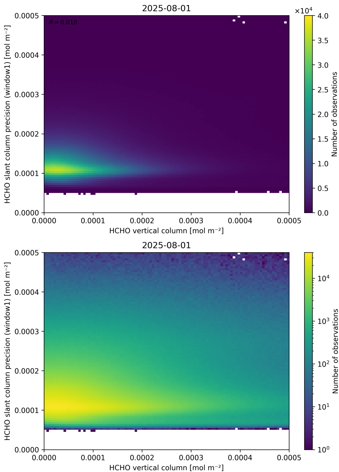
Figure 130: Scatter density plot of “HCHO vertical column” against “HCHO slant column precision (window1)” for 2025-07-31 to 2025-08-02.
