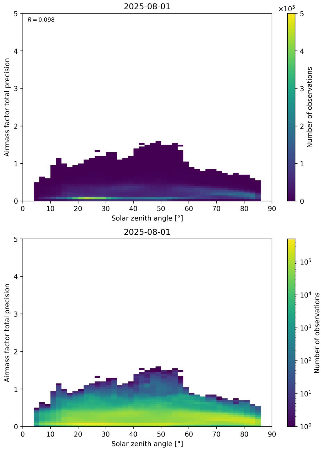
Figure 176: Scatter density plot of “Solar zenith angle” against “Airmass factor total precision” for 2025-07-31 to 2025-08-02.
