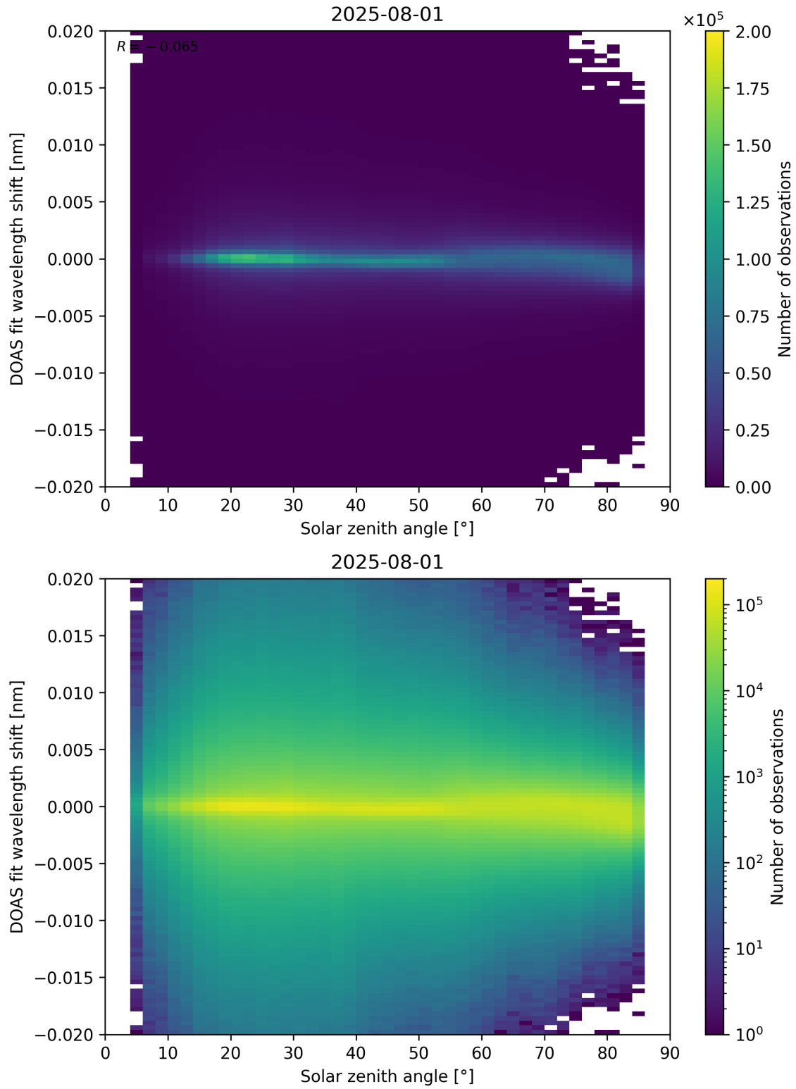
Figure 168: Scatter density plot of “Solar zenith angle” against “DOAS fit wavelength shift” for 2025-07-31 to 2025-08-02.
