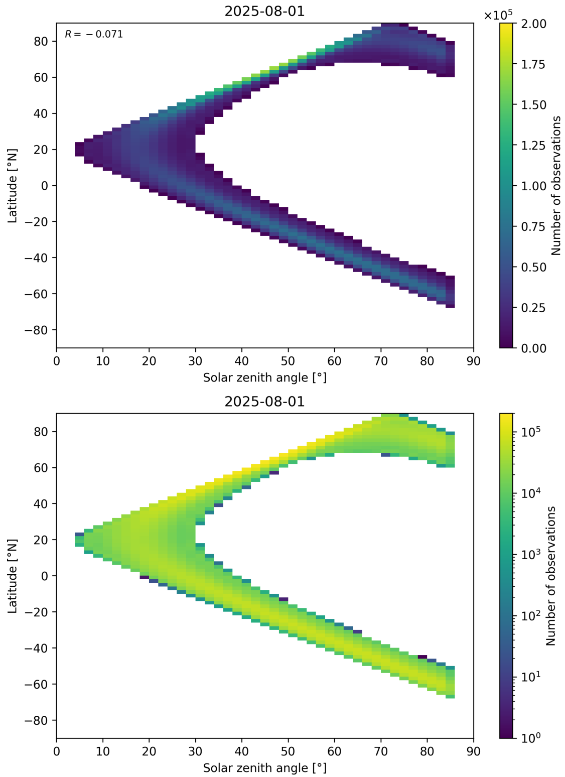
Figure 181: Scatter density plot of “Solar zenith angle” against “Latitude” for 2025-07-31 to 2025-08-02.
