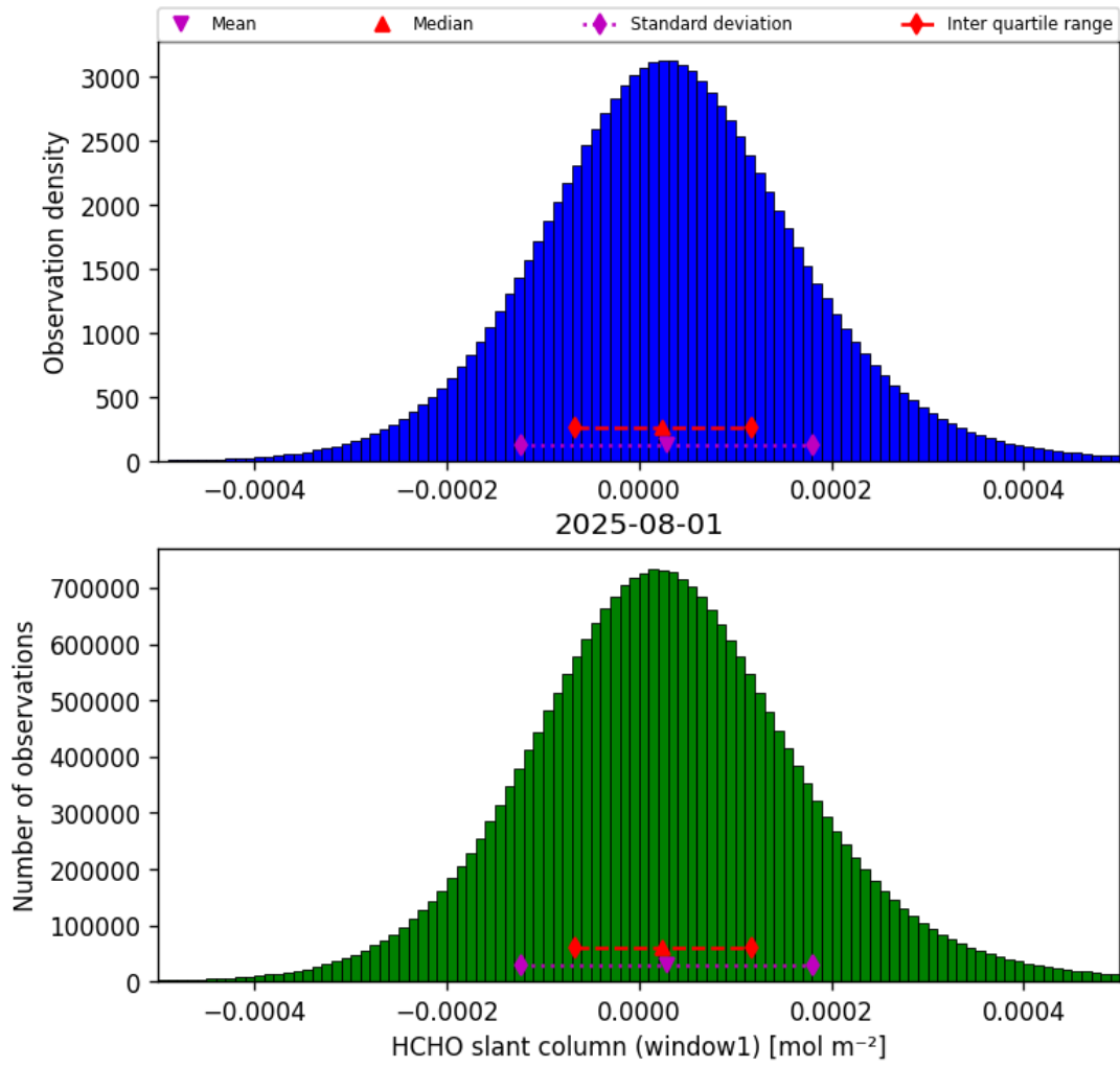
Figure 38: Histogram of “HCHO slant column (window1)” for 2025-07-31 to 2025-08-02
