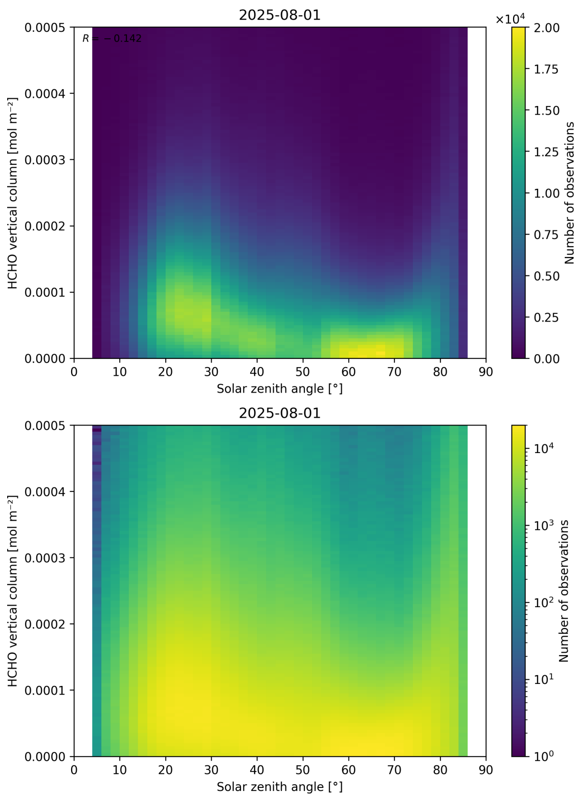
Figure 177: Scatter density plot of “Solar zenith angle” against “HCHO vertical column” for 2025-07-31 to 2025-08-02.
