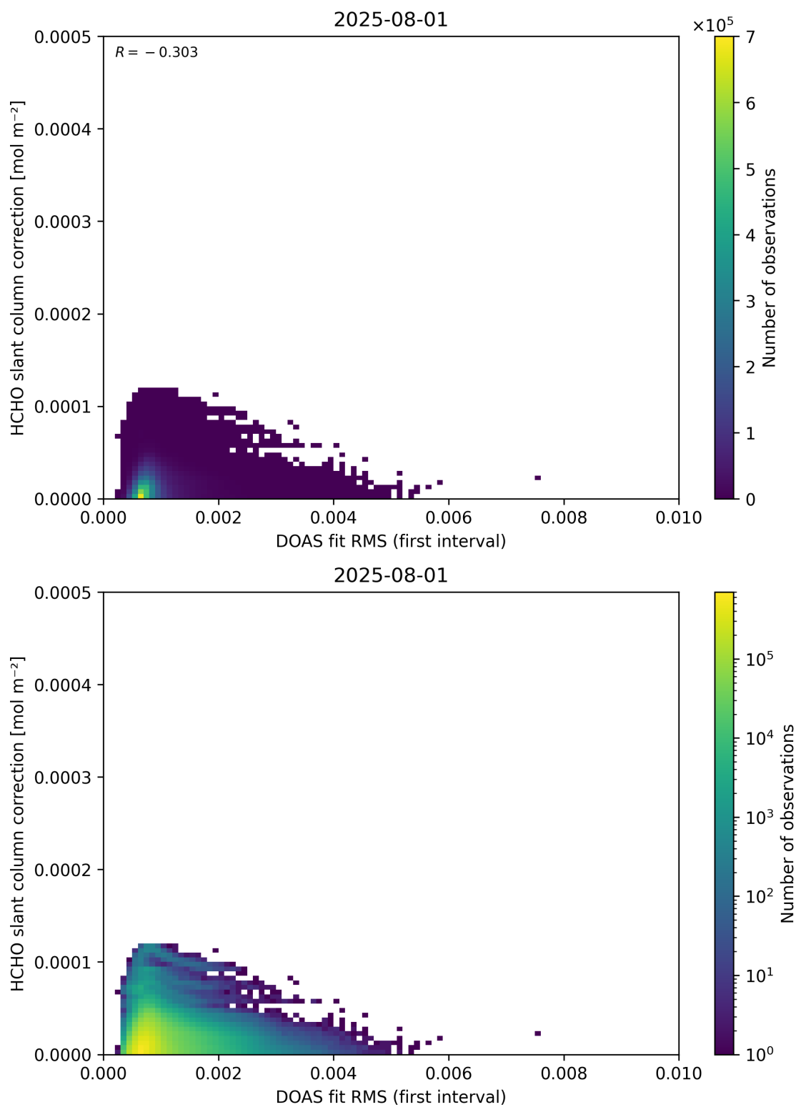
Figure 63: Scatter density plot of “DOAS fit RMS (first interval)” against “HCHO slant column correction” for 2025-07-31 to 2025-08-02.
