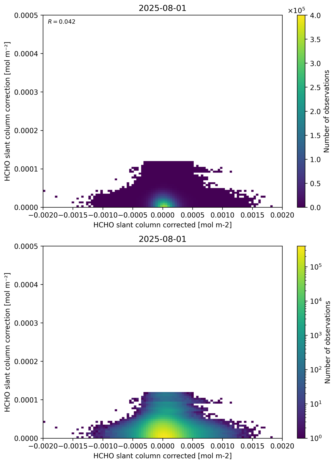
Figure 77: Scatter density plot of “HCHO slant column corrected” against “HCHO slant column correction” for 2025-07-31 to 2025-08-02.
