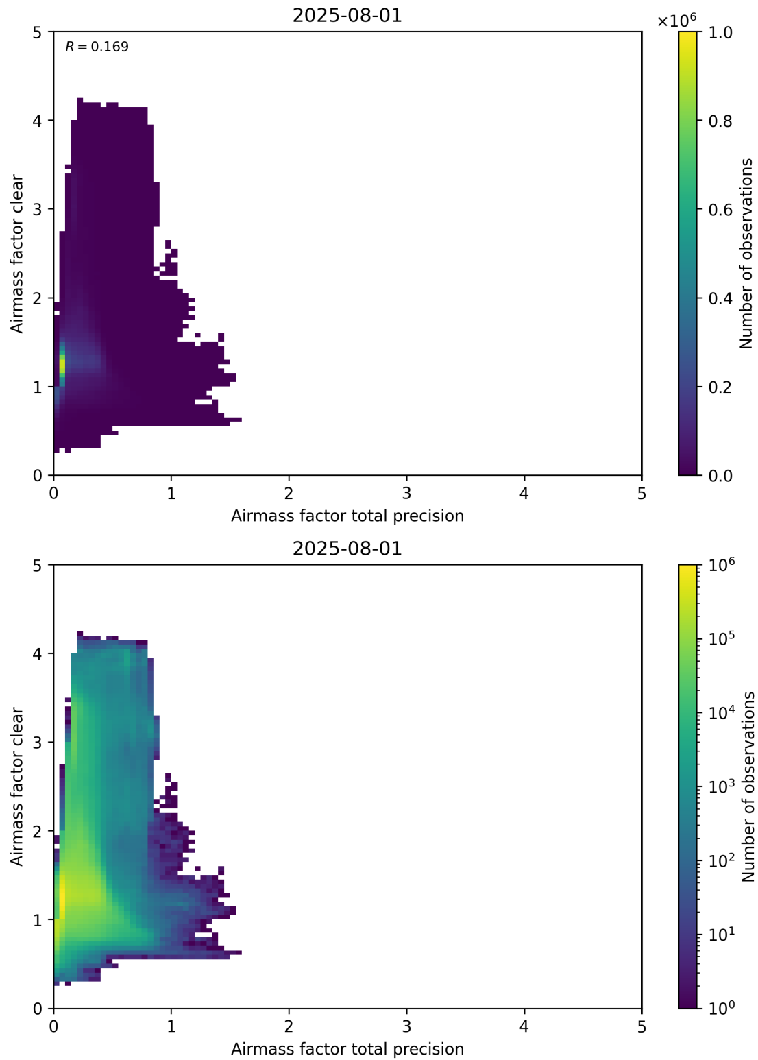
Figure 108: Scatter density plot of “Airmass factor total precision” against “Airmass factor clear” for 2025-07-31 to 2025-08-02.
