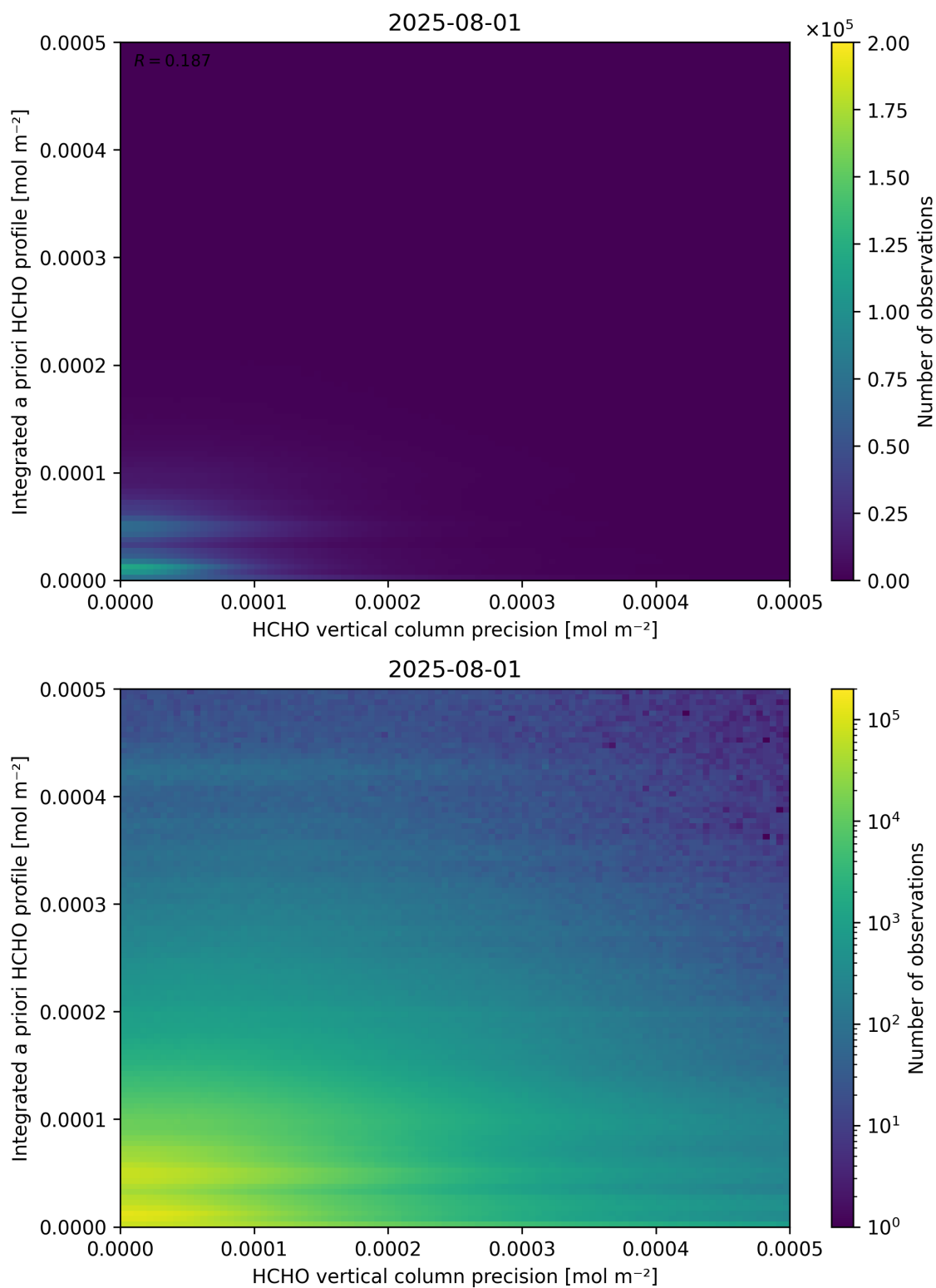
Figure 147: Scatter density plot of “HCHO vertical column precision” against “Integrated a priori HCHO profile” for 2025-07-31 to 2025-08-02.
