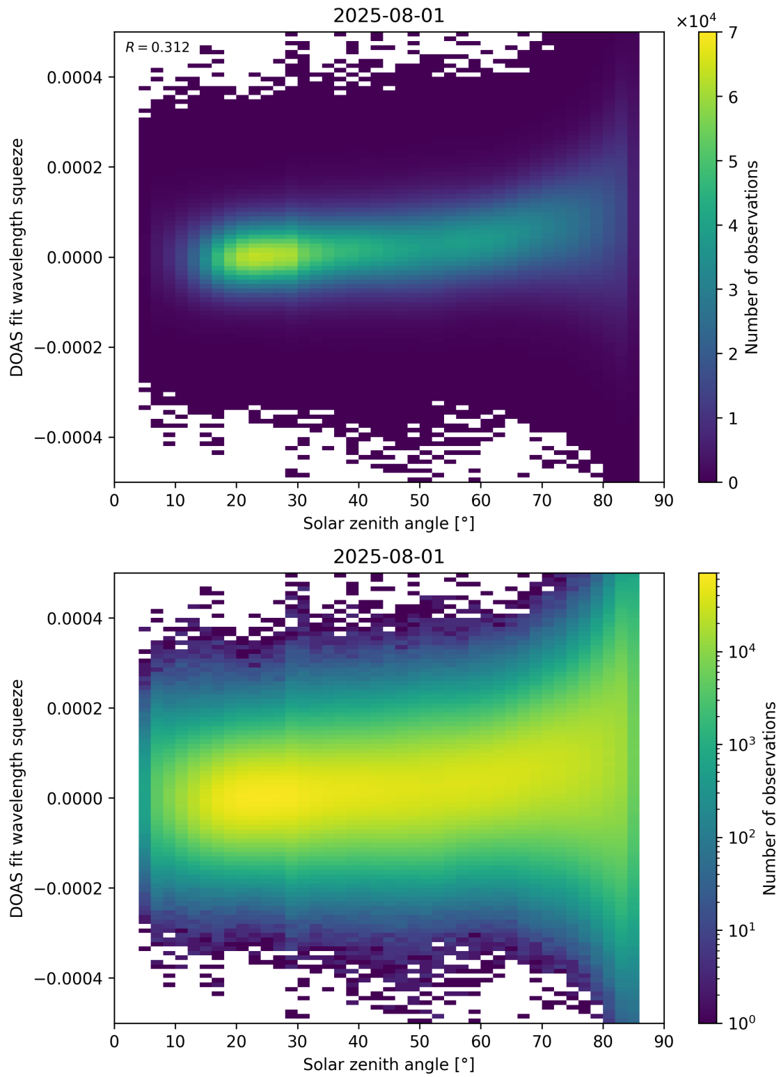
Figure 169: Scatter density plot of “Solar zenith angle” against “DOAS fit wavelength squeeze” for 2025-07-31 to 2025-08-02.
