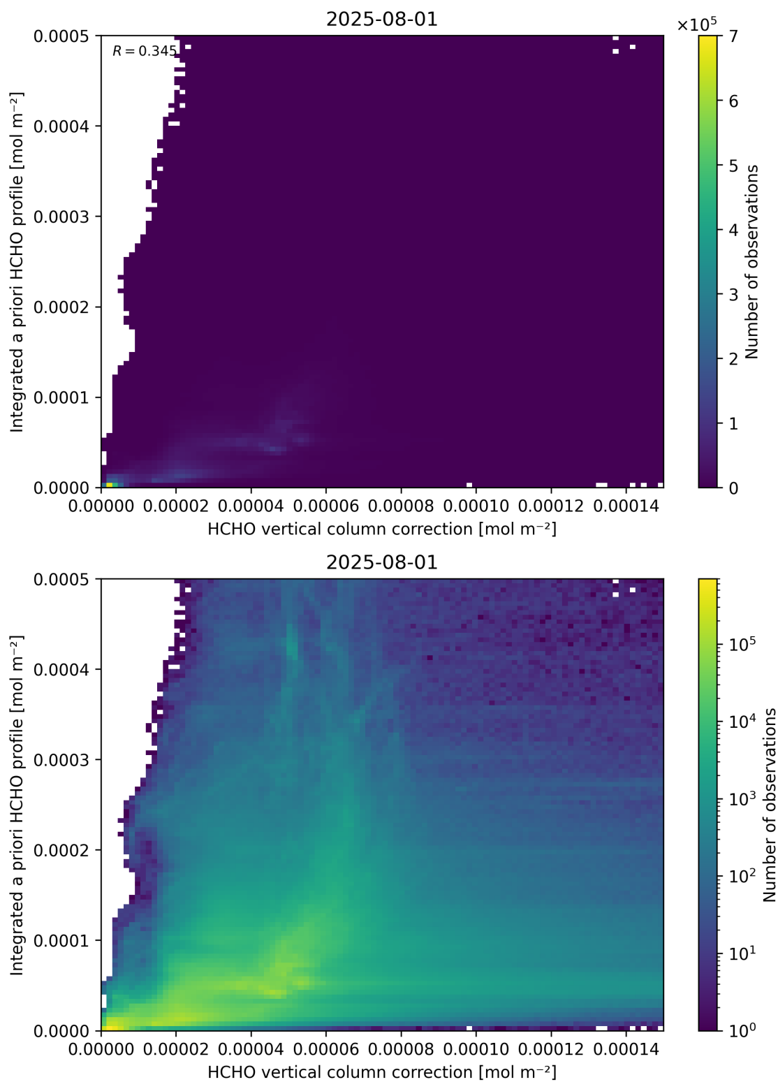
Figure 122: Scatter density plot of “HCHO vertical column correction” against “Integrated a priori HCHO profile” for 2025-07-31 to 2025-08-02.
