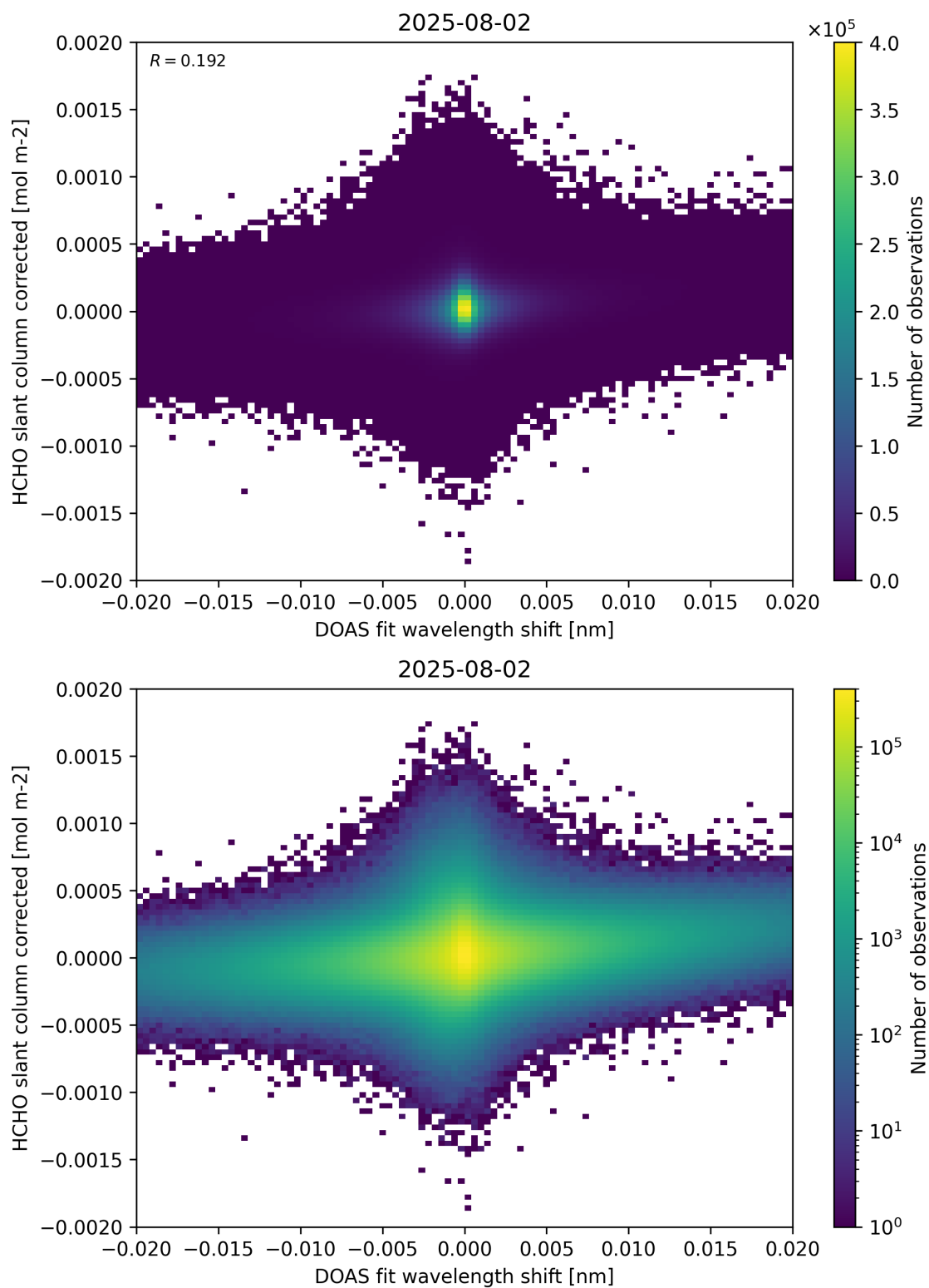
Figure 66: Scatter density plot of “DOAS fit wavelength shift” against “HCHO slant column corrected” for 2025-08-01 to 2025-08-03.
