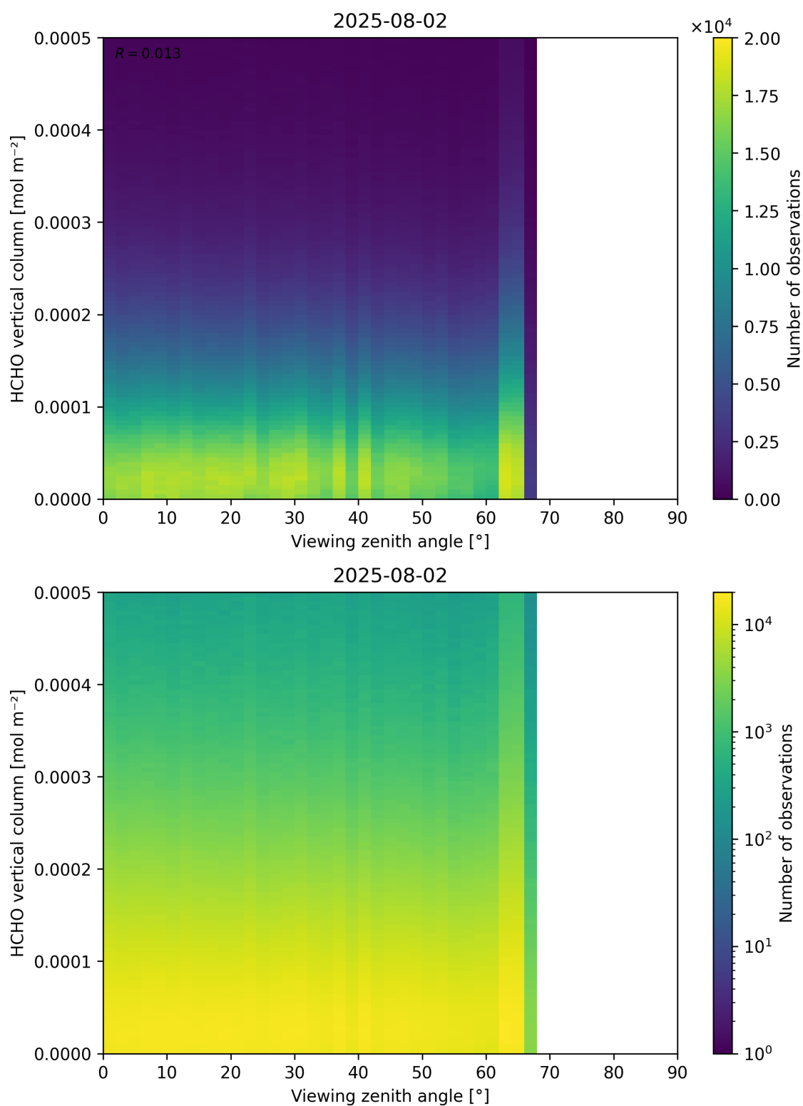
Figure 192: Scatter density plot of “Viewing zenith angle” against “HCHO vertical column” for 2025-08-01 to 2025-08-03.
