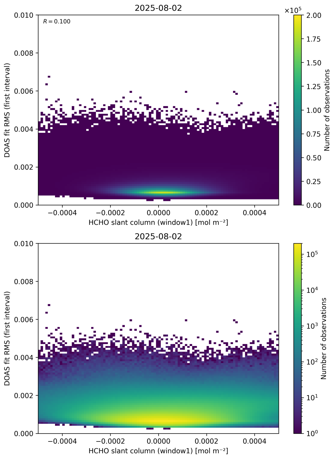
Figure 78: Scatter density plot of “HCHO slant column (window1)” against “DOAS fit RMS (first interval)” for 2025-08-01 to 2025-08-03.
