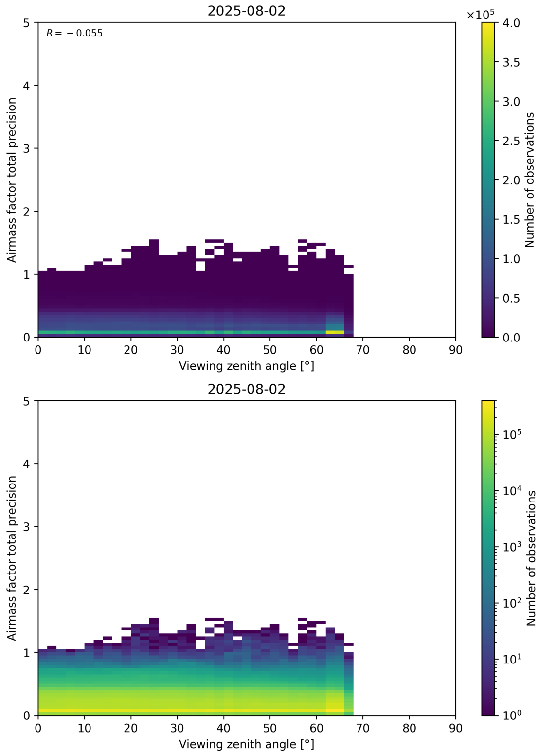
Figure 191: Scatter density plot of “Viewing zenith angle” against “Airmass factor total precision” for 2025-08-01 to 2025-08-03.
