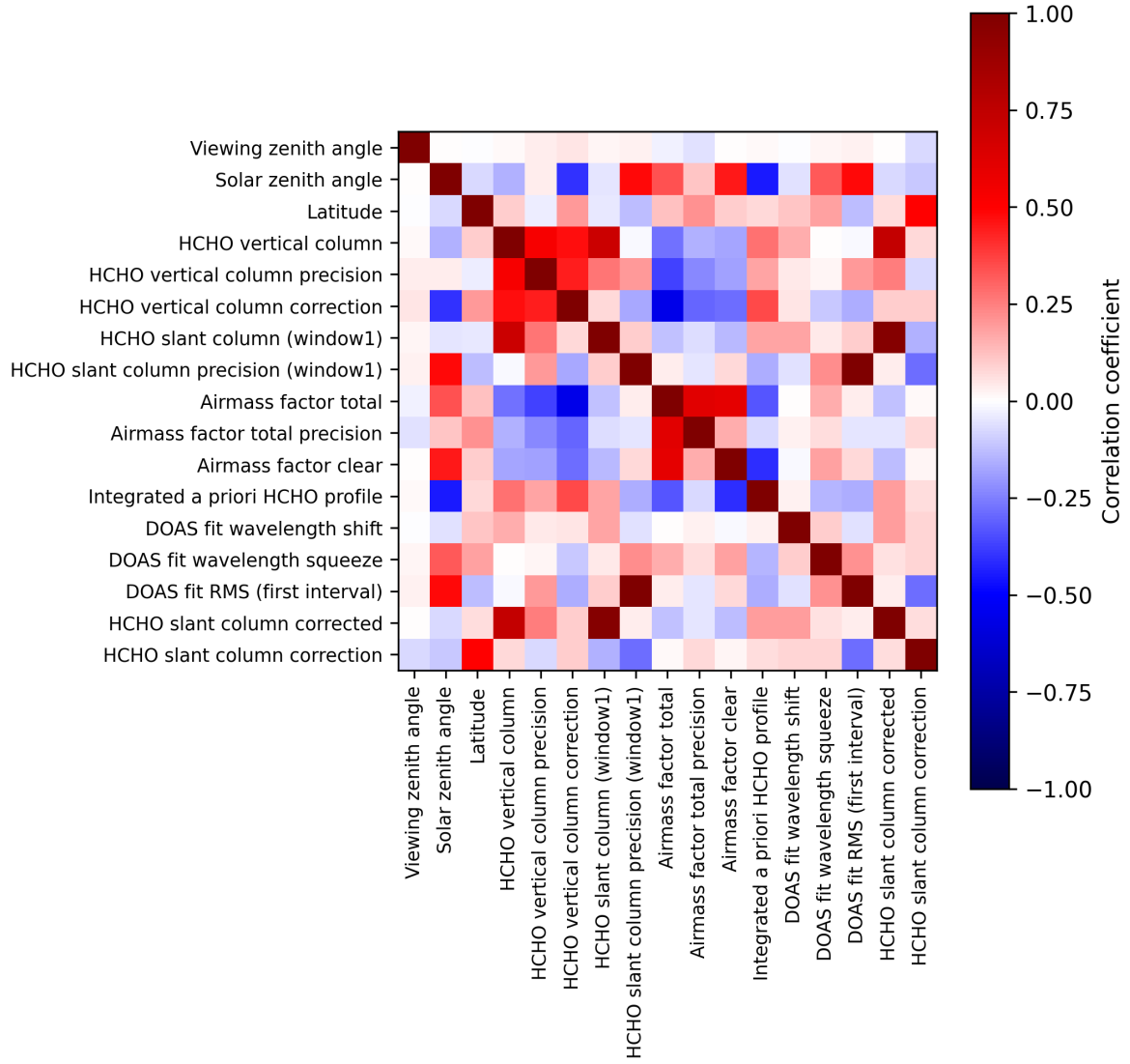
Figure 2: Map of correlation matrix for 2025-08-01 to 2025-08-03.
