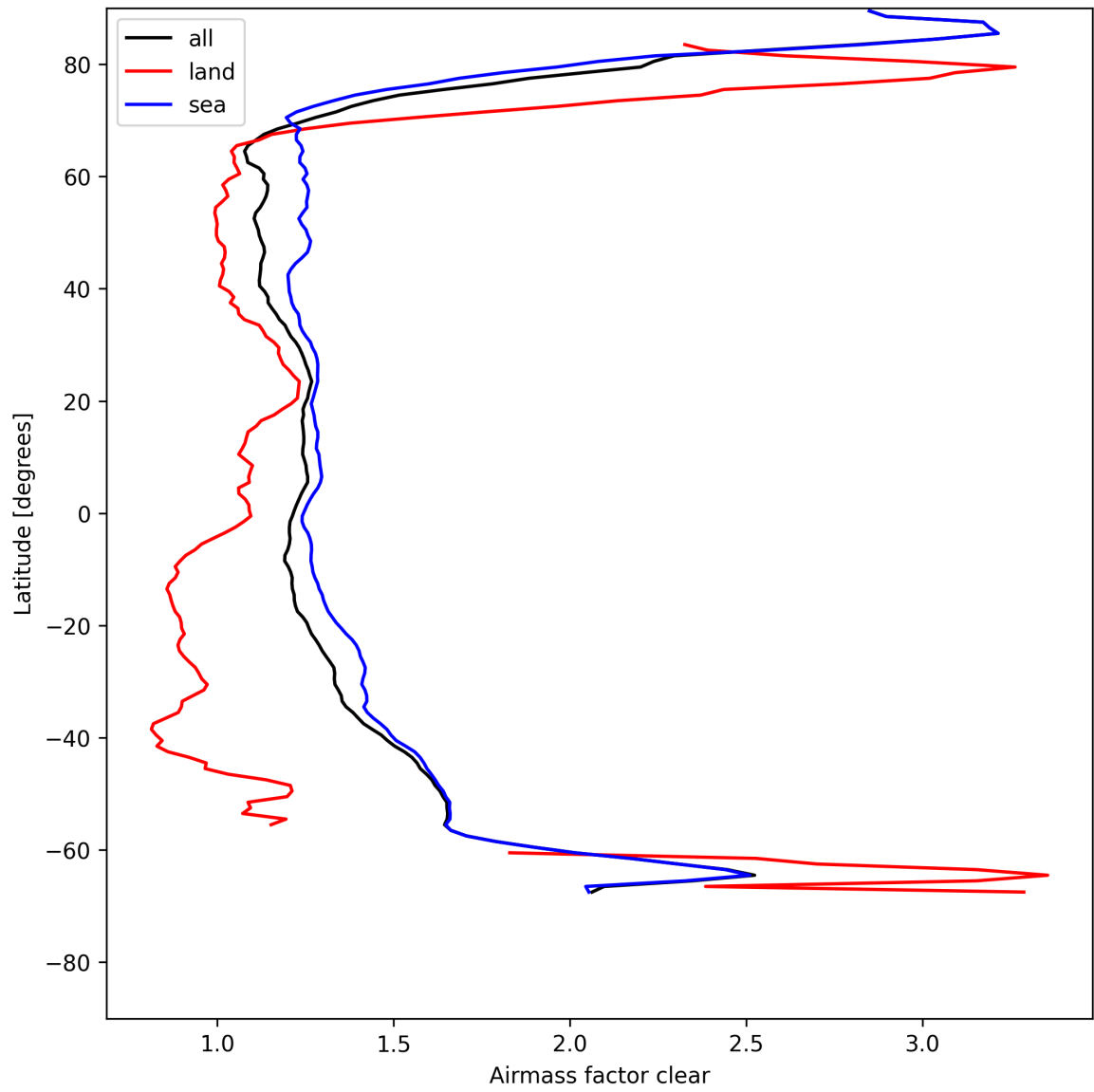
Figure 28: Zonal average of “Airmass factor clear” for 2025-08-01 to 2025-08-03.
