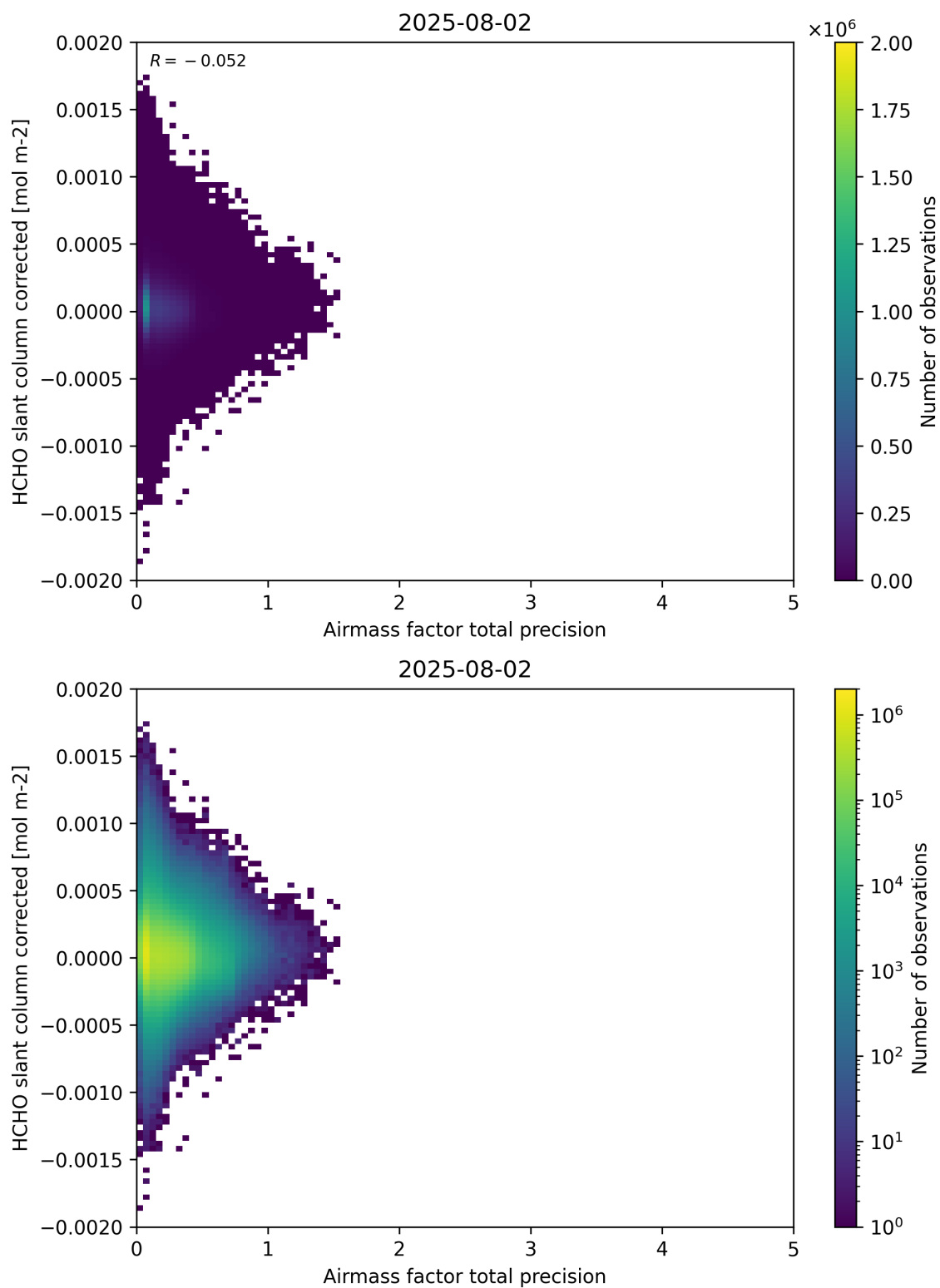
Figure 109: Scatter density plot of “Airmass factor total precision” against “HCHO slant column corrected” for 2025-08-01 to 2025-08-03.
