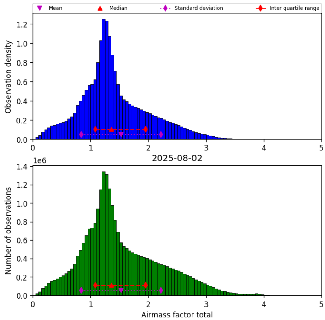
Figure 40: Histogram of “Airmass factor total” for 2025-08-01 to 2025-08-03
