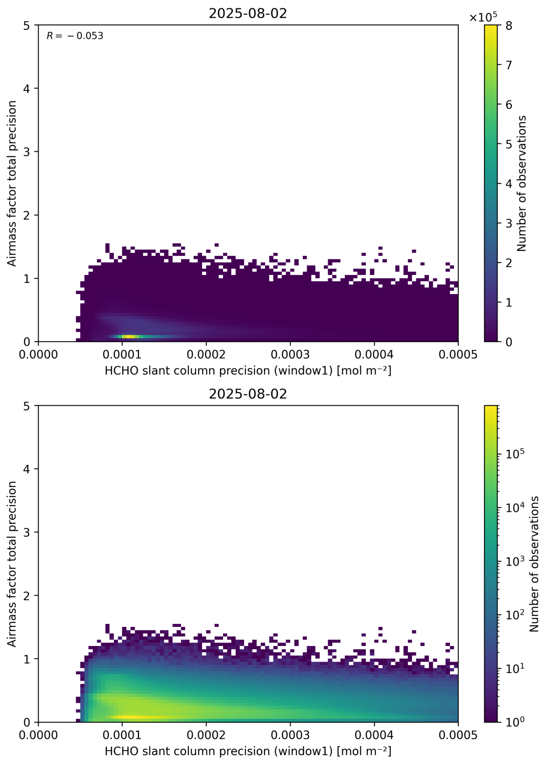
Figure 95: Scatter density plot of “HCHO slant column precision (window1)” against “Airmass factor total precision” for 2025-08-01 to 2025-08-03.
