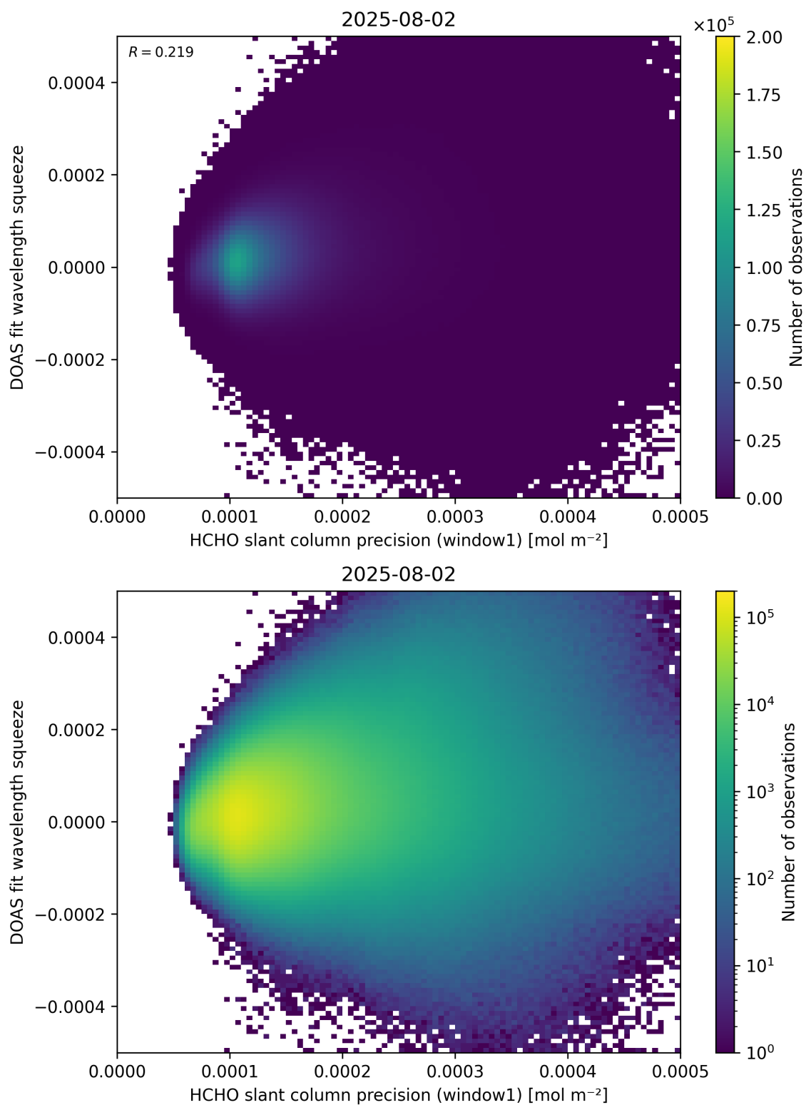
Figure 90: Scatter density plot of “HCHO slant column precision (window1)” against “DOAS fit wavelength squeeze” for 2025-08-01 to 2025-08-03.
