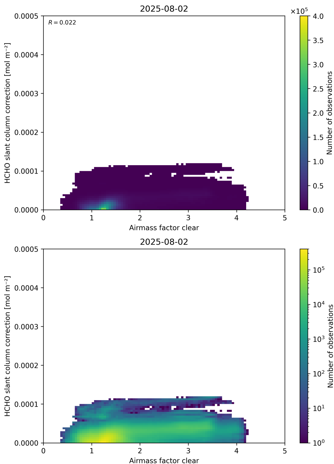
Figure 75: Scatter density plot of “Airmass factor clear” against “HCHO slant column correction” for 2025-08-01 to 2025-08-03.
