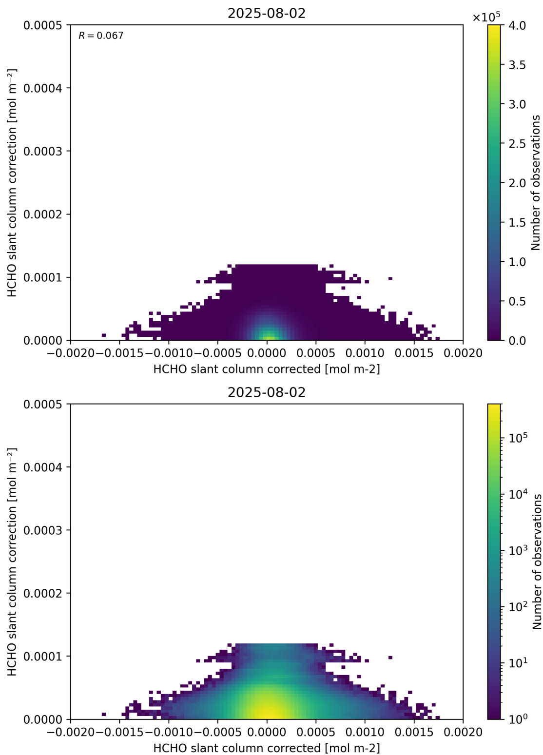
Figure 77: Scatter density plot of “HCHO slant column corrected” against “HCHO slant column correction” for 2025-08-01 to 2025-08-03.
