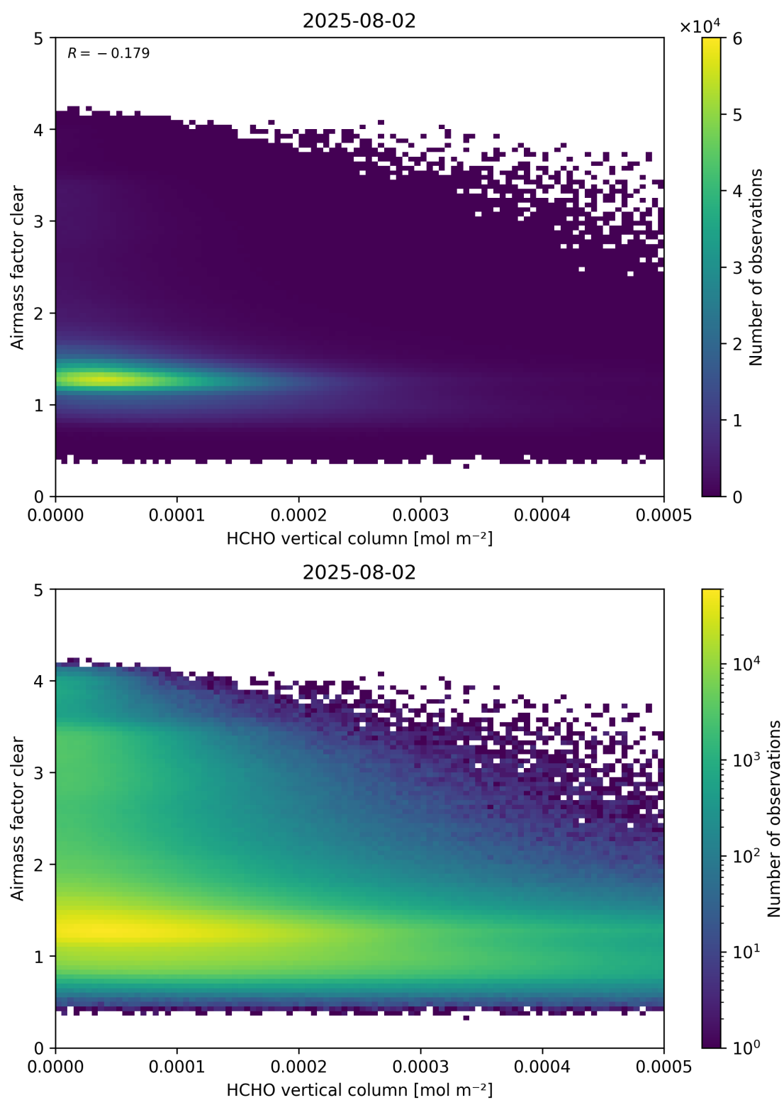
Figure 126: Scatter density plot of “HCHO vertical column” against “Airmass factor clear” for 2025-08-01 to 2025-08-03.
