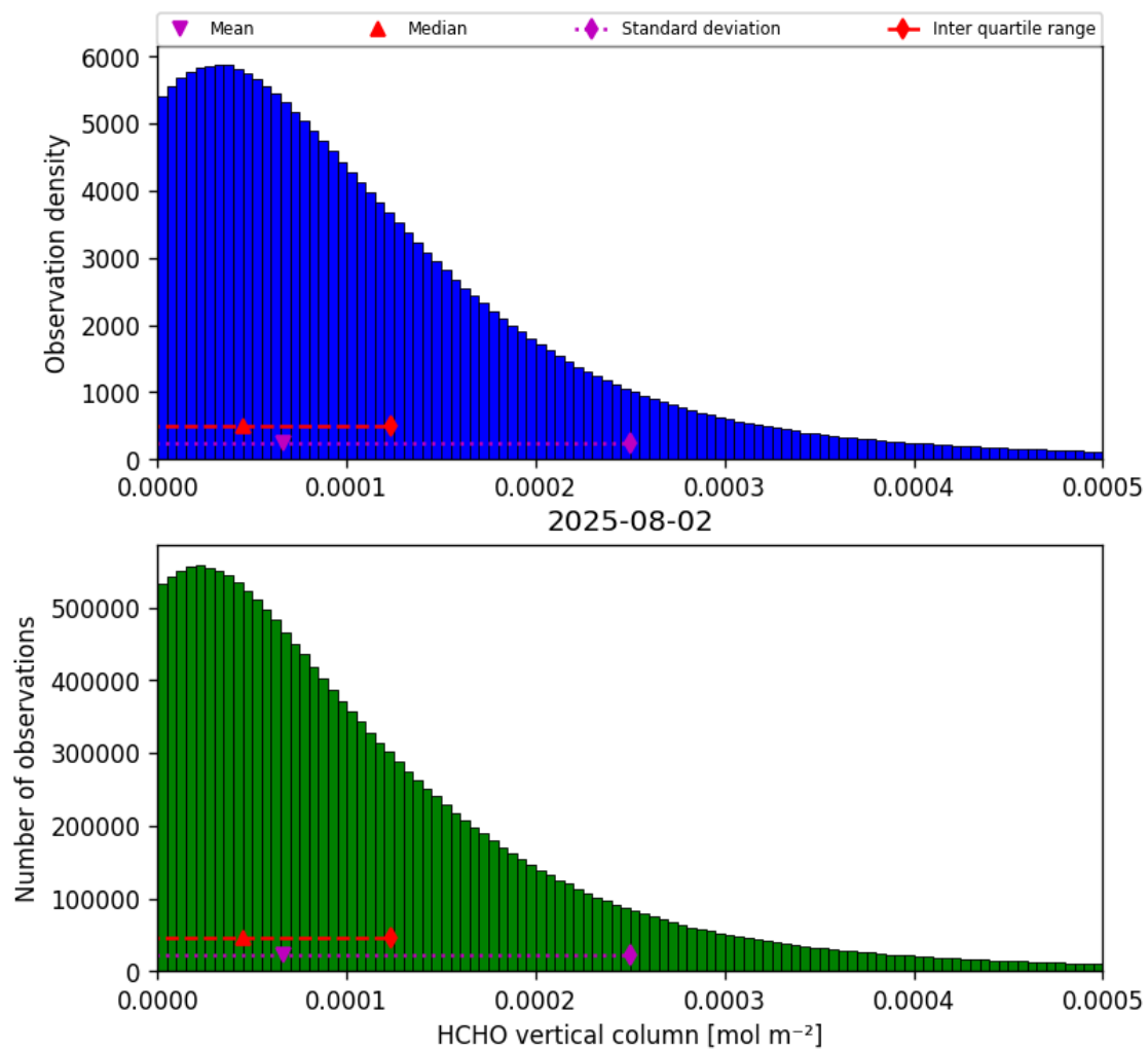
Figure 35: Histogram of “HCHO vertical column” for 2025-08-01 to 2025-08-03
