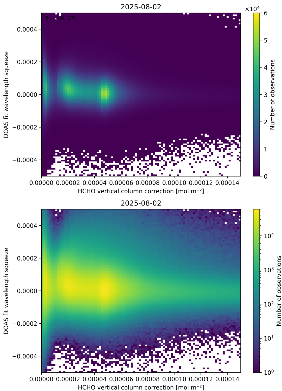
Figure 114: Scatter density plot of “HCHO vertical column correction” against “DOAS fit wavelength squeeze” for 2025-08-01 to 2025-08-03.
