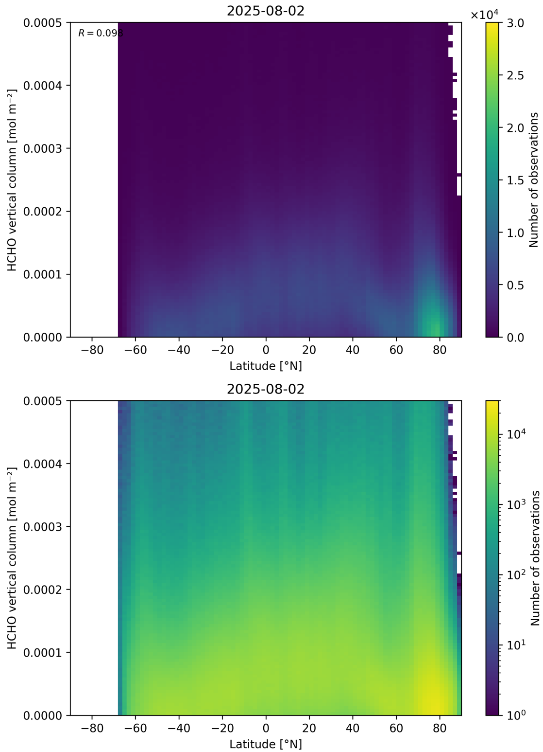
Figure 163: Scatter density plot of “Latitude” against “HCHO vertical column” for 2025-08-01 to 2025-08-03.
