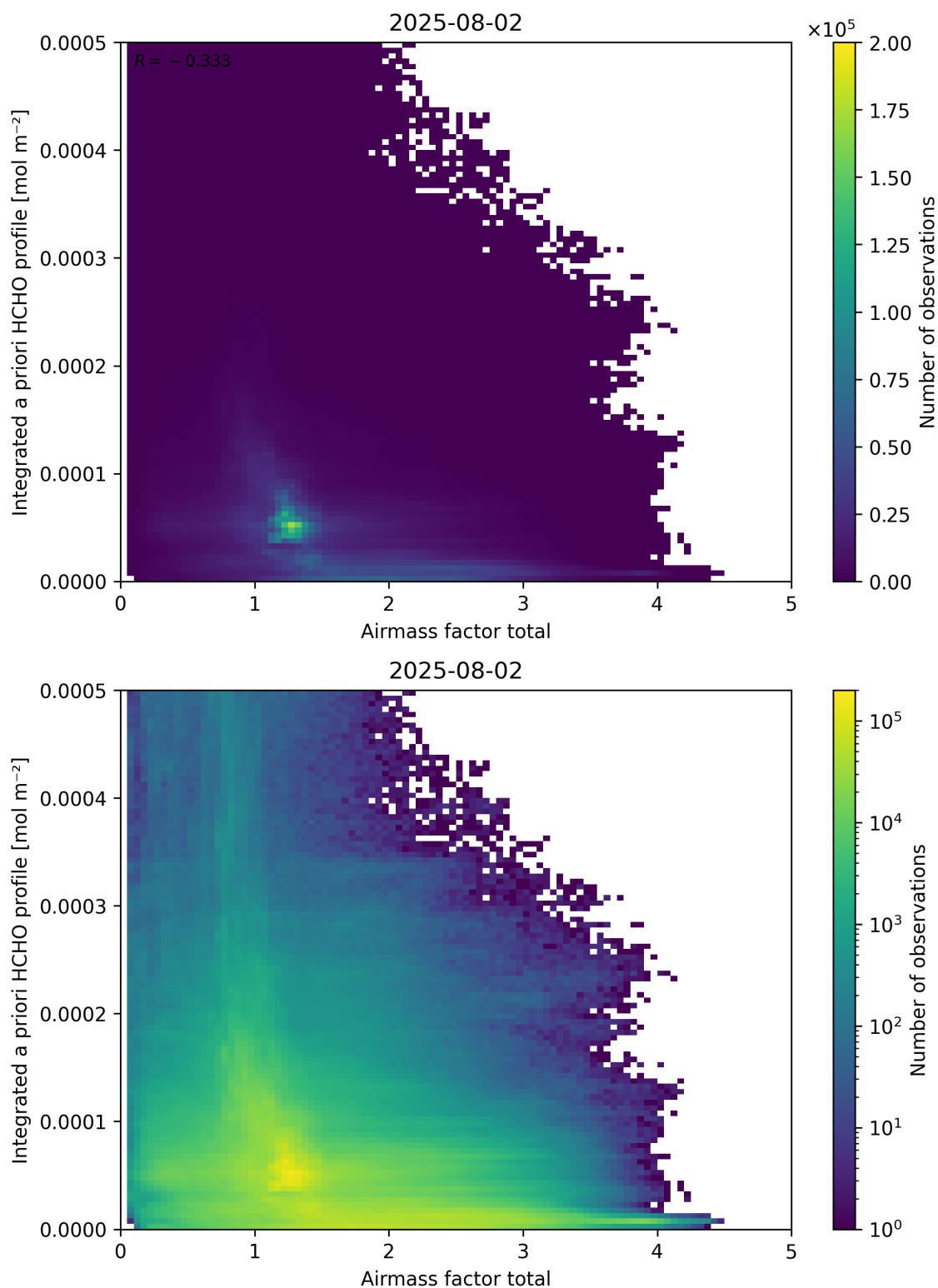
Figure 104: Scatter density plot of “Airmass factor total” against “Integrated a priori HCHO profile” for 2025-08-01 to 2025-08-03.
