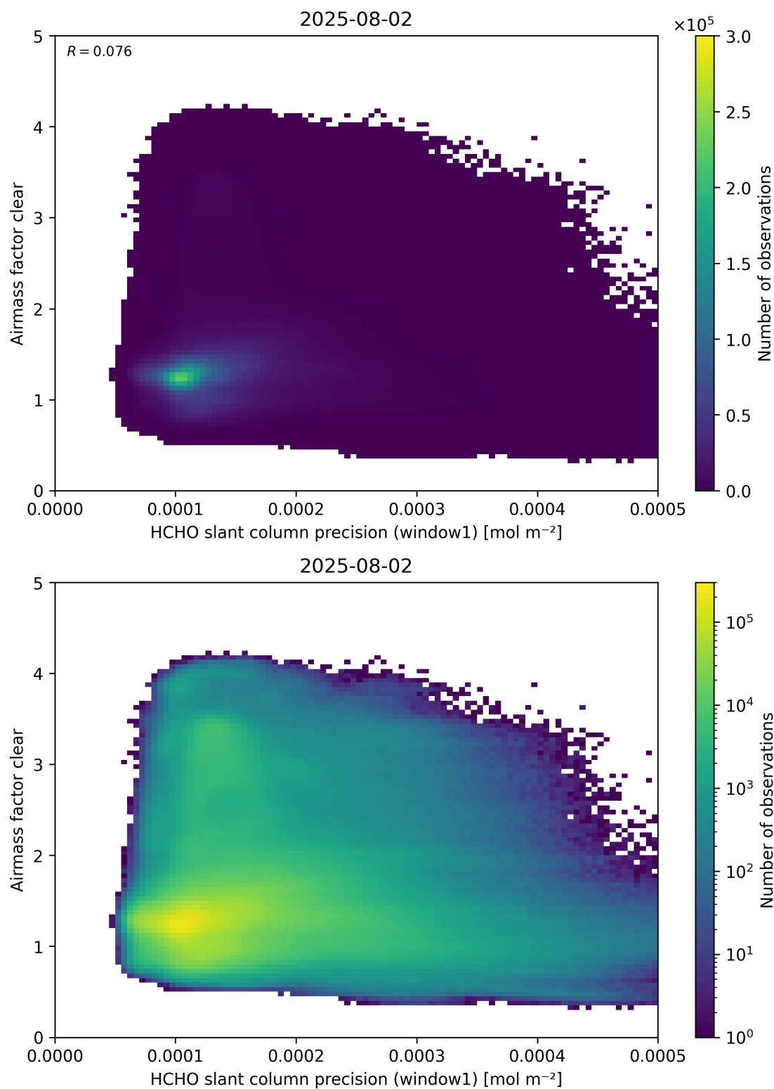
Figure 91: Scatter density plot of “HCHO slant column precision (window1)” against “Airmass factor clear” for 2025-08-01 to 2025-08-03.
