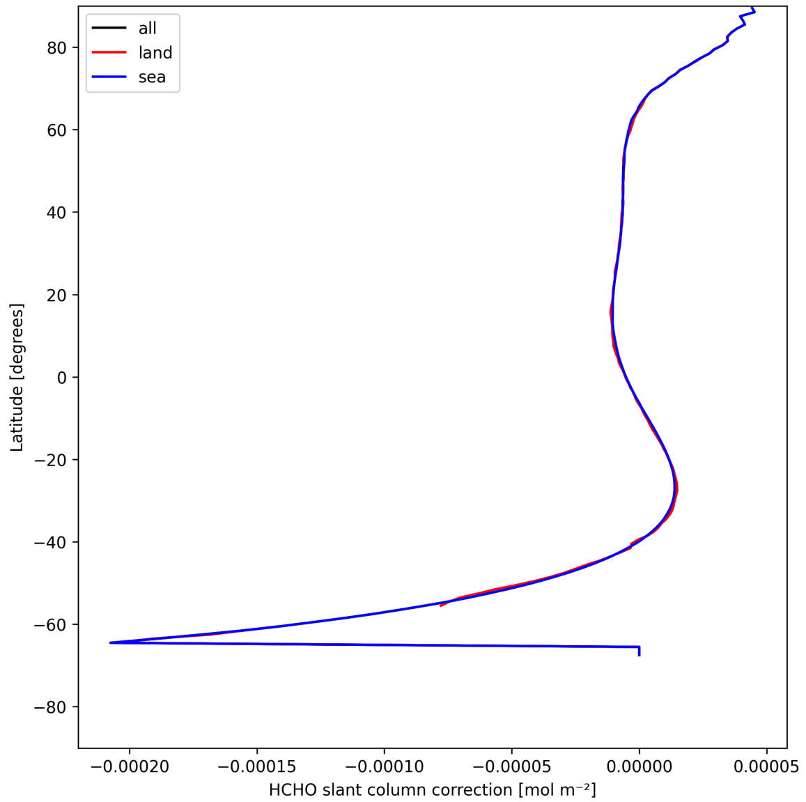
Figure 33: Zonal average of “HCHO slant column correction” for 2025-08-01 to 2025-08-03.
