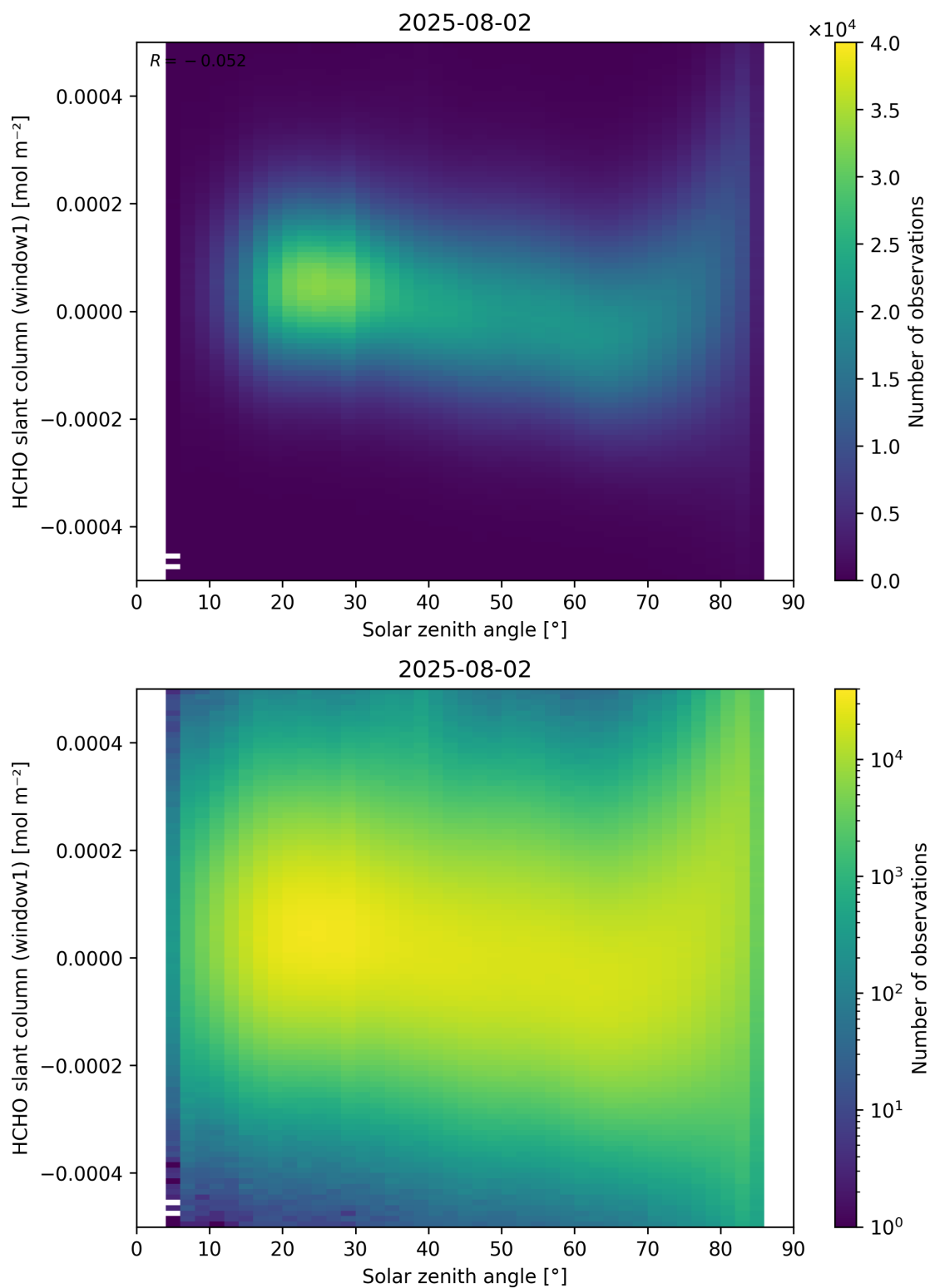
Figure 173: Scatter density plot of “Solar zenith angle” against “HCHO slant column (window1)” for 2025-08-01 to 2025-08-03.
