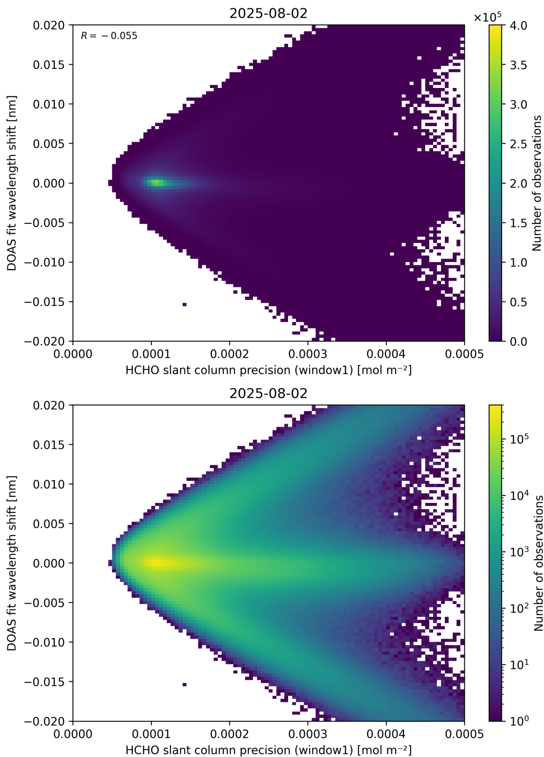
Figure 89: Scatter density plot of “HCHO slant column precision (window1)” against “DOAS fit wavelength shift” for 2025-08-01 to 2025-08-03.
