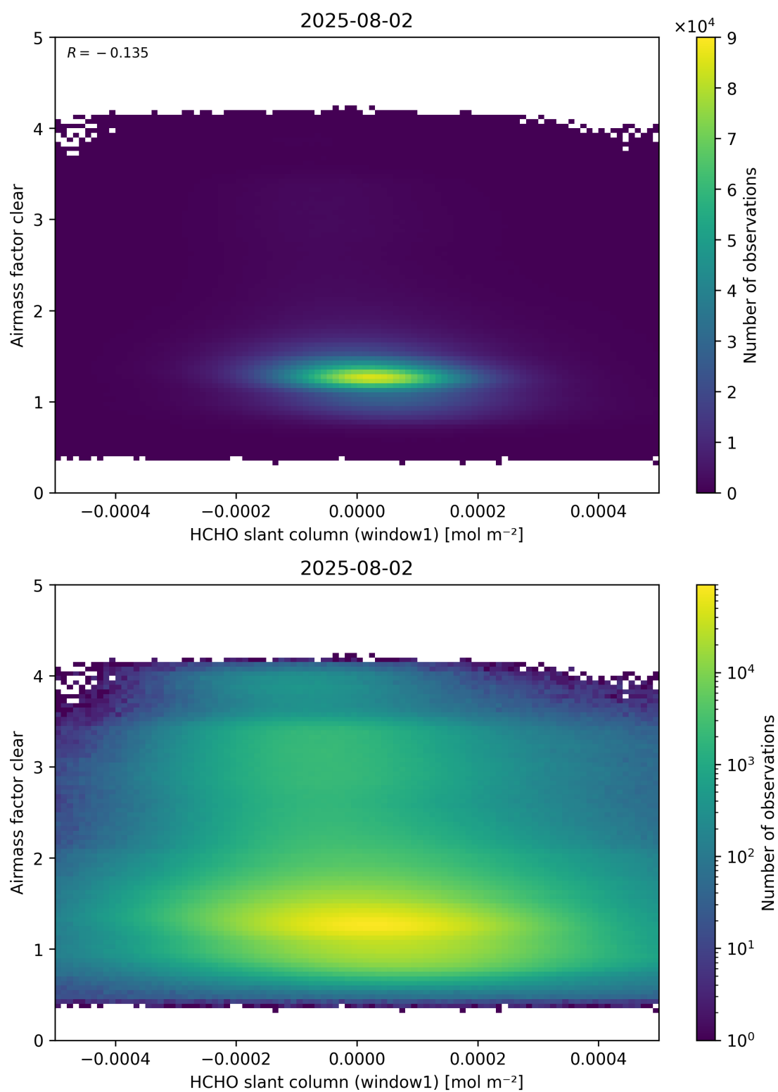
Figure 81: Scatter density plot of “HCHO slant column (window1)” against “Airmass factor clear” for 2025-08-01 to 2025-08-03.
