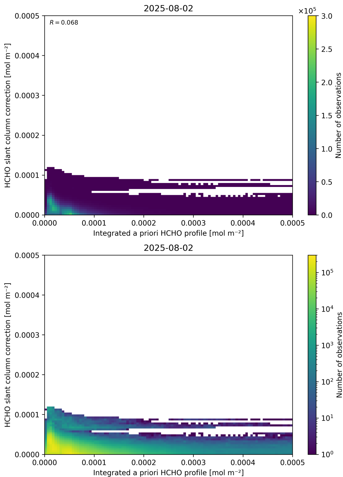
Figure 152: Scatter density plot of “Integrated a priori HCHO profile” against “HCHO slant column correction” for 2025-08-01 to 2025-08-03.
