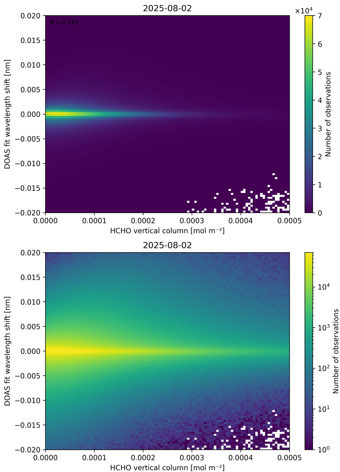
Figure 124: Scatter density plot of “HCHO vertical column” against “DOAS fit wavelength shift” for 2025-08-01 to 2025-08-03.
