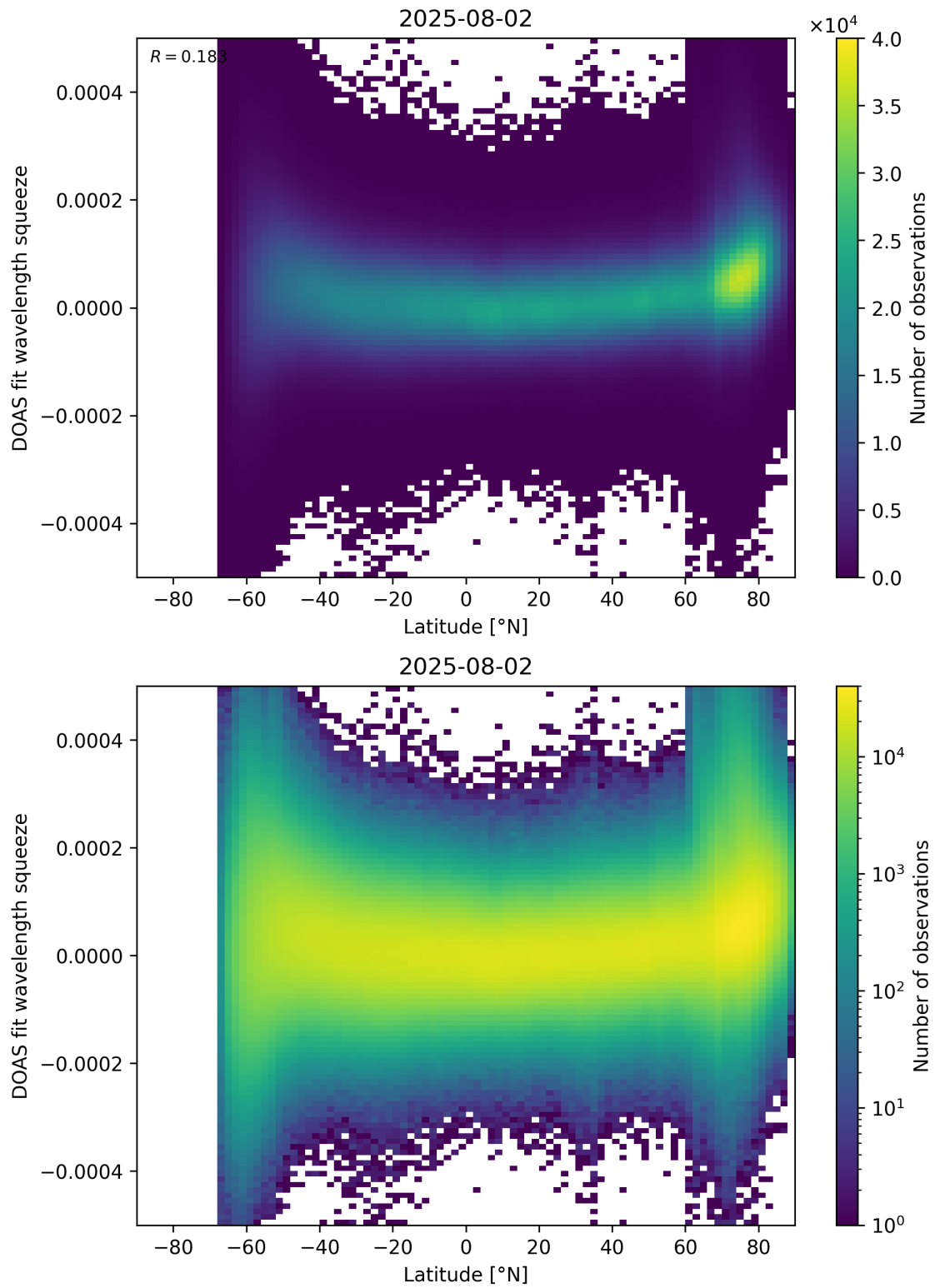
Figure 155: Scatter density plot of “Latitude” against “DOAS fit wavelength squeeze” for 2025-08-01 to 2025-08-03.
