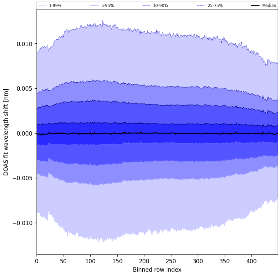
Figure 58: Along track statistics of “DOAS fit wavelength shift” for 2025-08-01 to 2025-08-03
