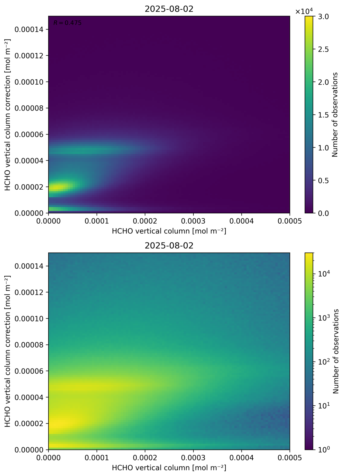
Figure 133: Scatter density plot of “HCHO vertical column” against “HCHO vertical column correction” for 2025-08-01 to 2025-08-03.
