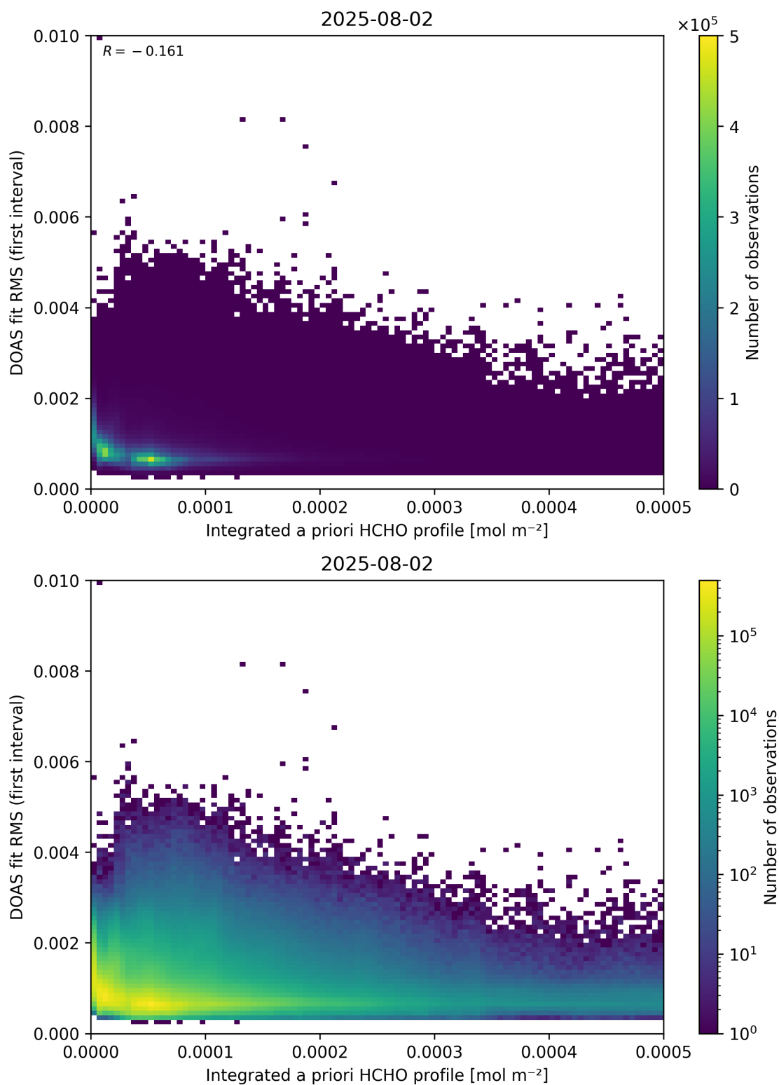
Figure 148: Scatter density plot of “Integrated a priori HCHO profile” against “DOAS fit RMS (first interval)” for 2025-08-01 to 2025-08-03.
