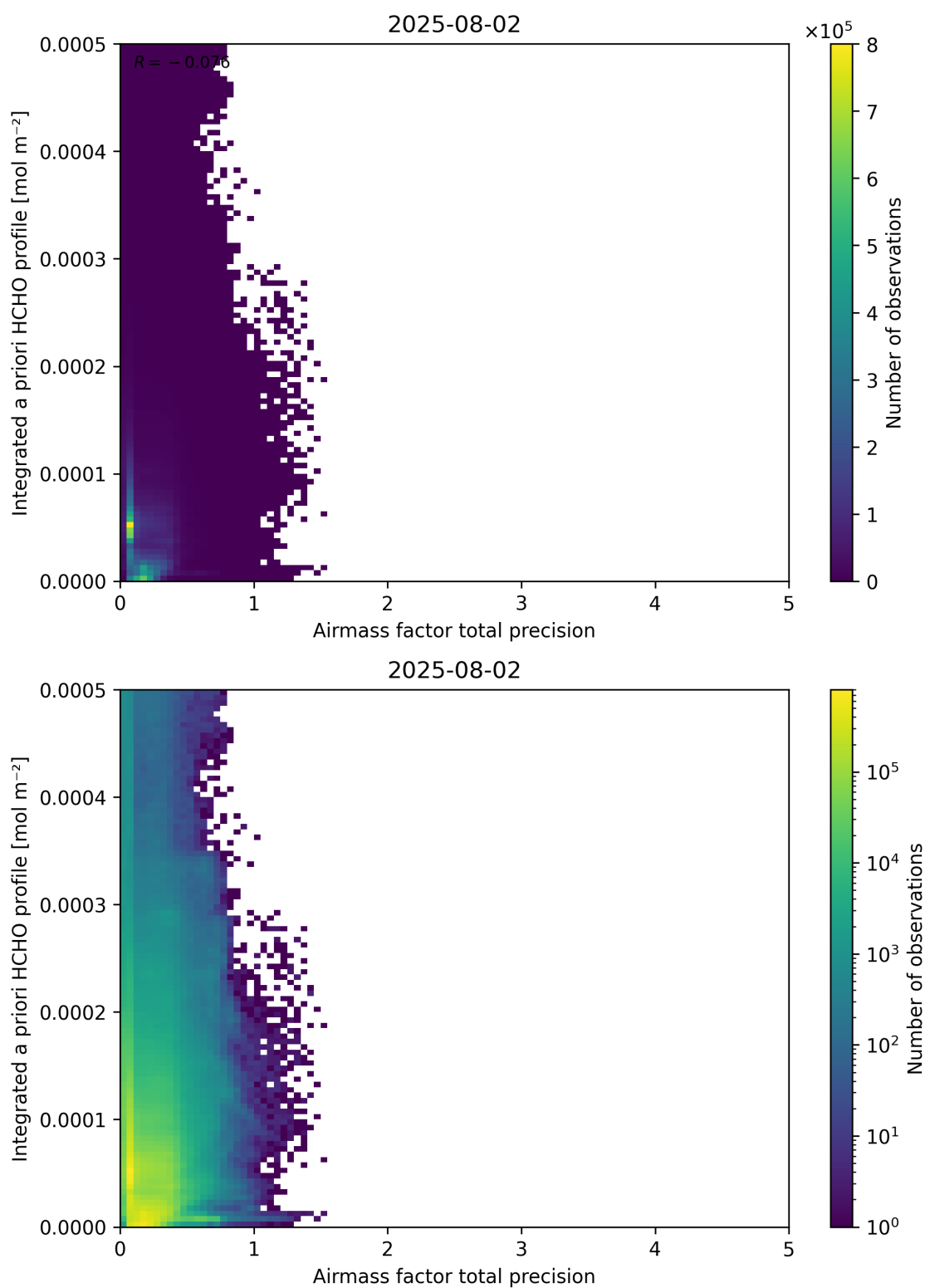
Figure 111: Scatter density plot of “Airmass factor total precision” against “Integrated a priori HCHO profile” for 2025-08-01 to 2025-08-03.
