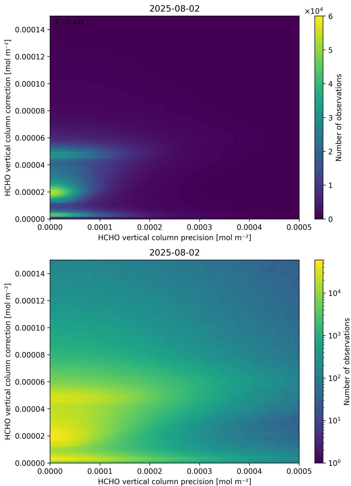
Figure 146: Scatter density plot of “HCHO vertical column precision” against “HCHO vertical column correction” for 2025-08-01 to 2025-08-03.
