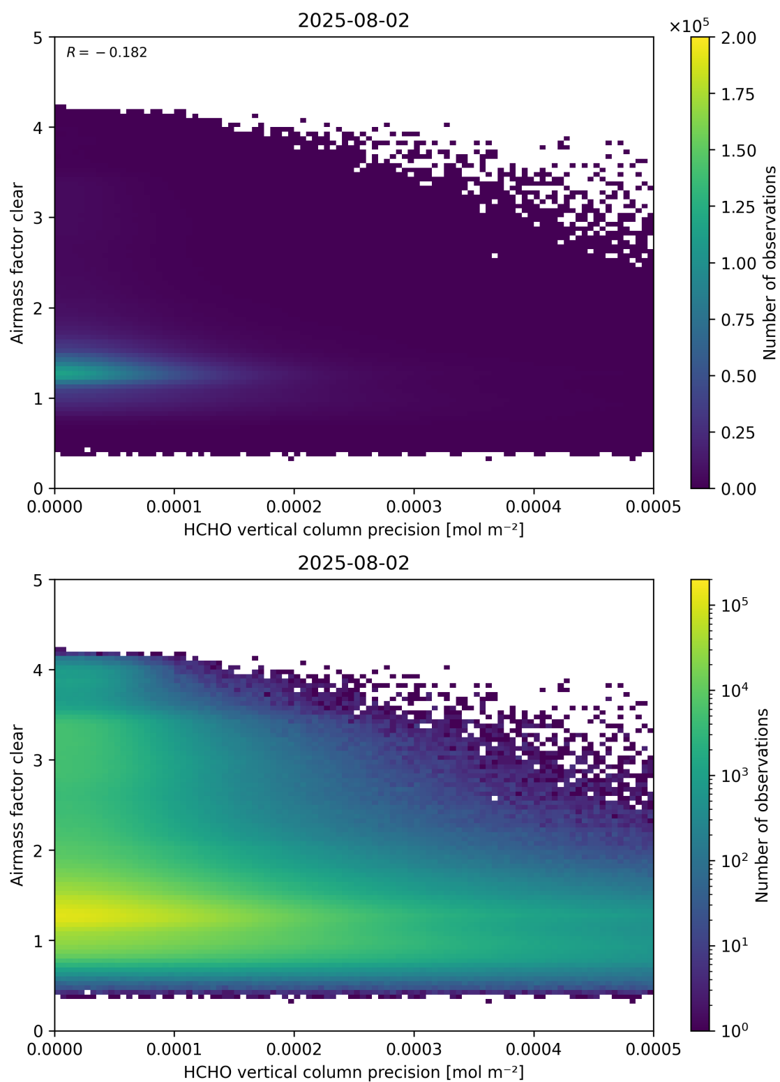
Figure 139: Scatter density plot of “HCHO vertical column precision” against “Airmass factor clear” for 2025-08-01 to 2025-08-03.
