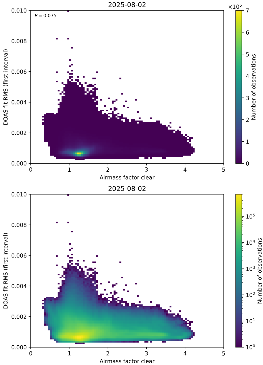
Figure 71: Scatter density plot of “Airmass factor clear” against “DOAS fit RMS (first interval)” for 2025-08-01 to 2025-08-03.
