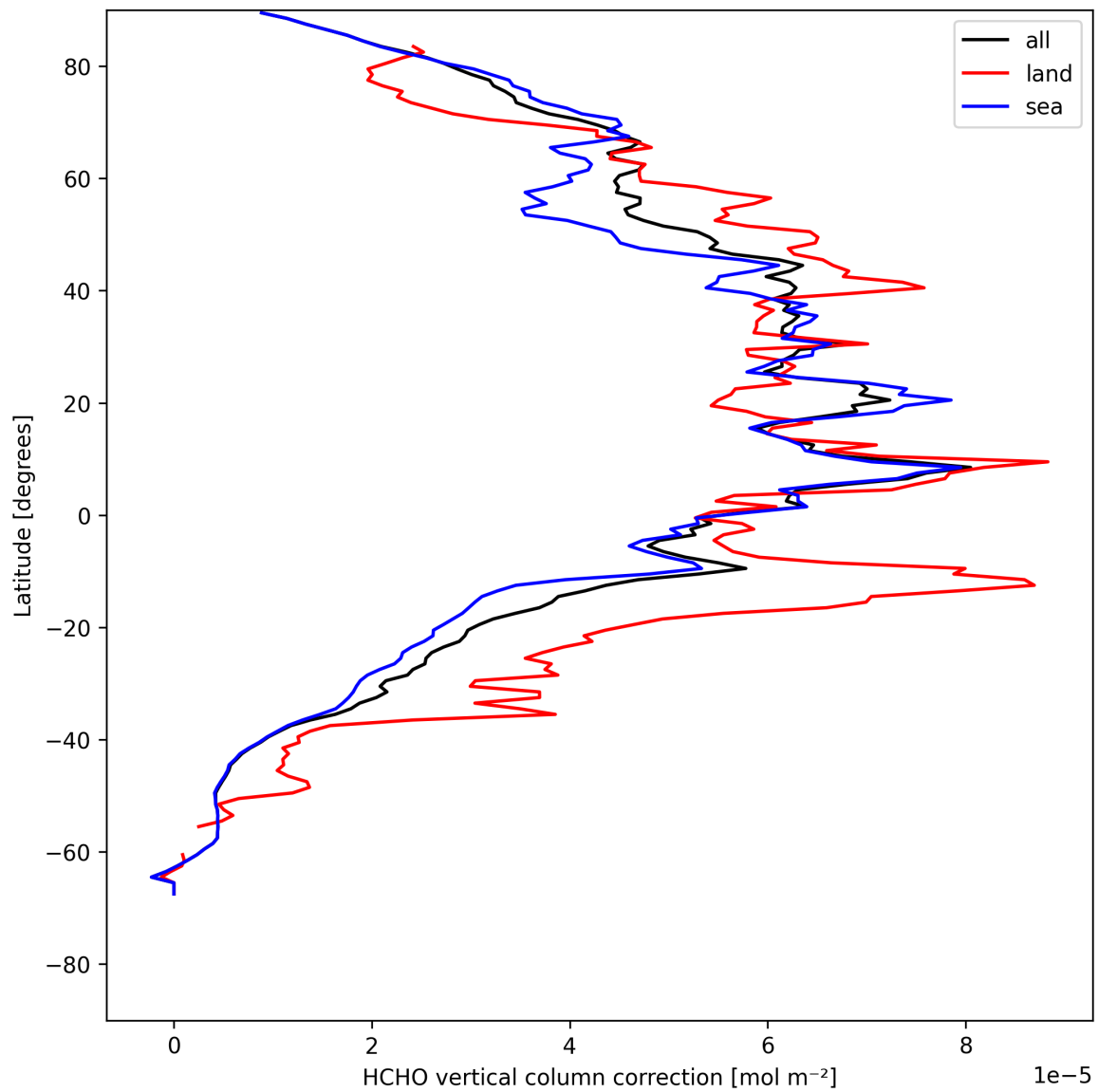
Figure 23: Zonal average of “HCHO vertical column correction” for 2025-08-01 to 2025-08-03.
