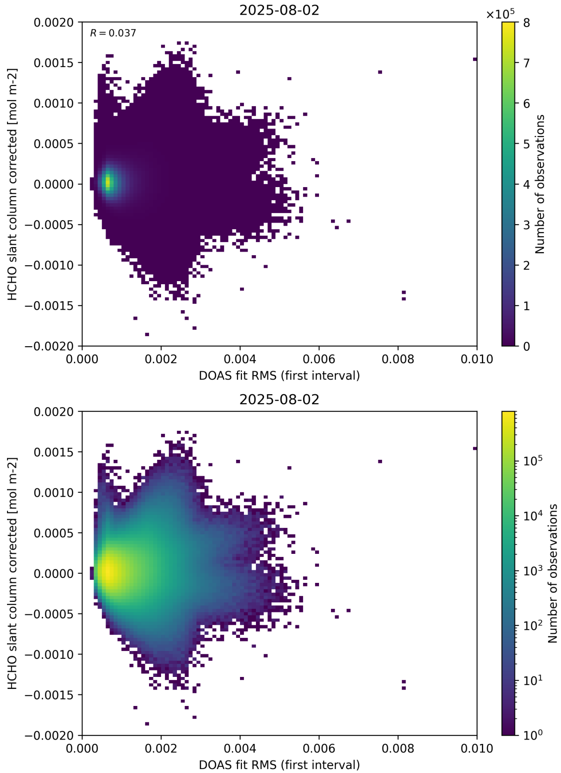
Figure 62: Scatter density plot of “DOAS fit RMS (first interval)” against “HCHO slant column corrected” for 2025-08-01 to 2025-08-03.
