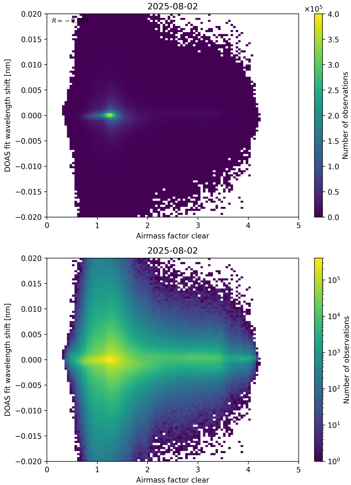
Figure 72: Scatter density plot of “Airmass factor clear” against “DOAS fit wavelength shift” for 2025-08-01 to 2025-08-03.
