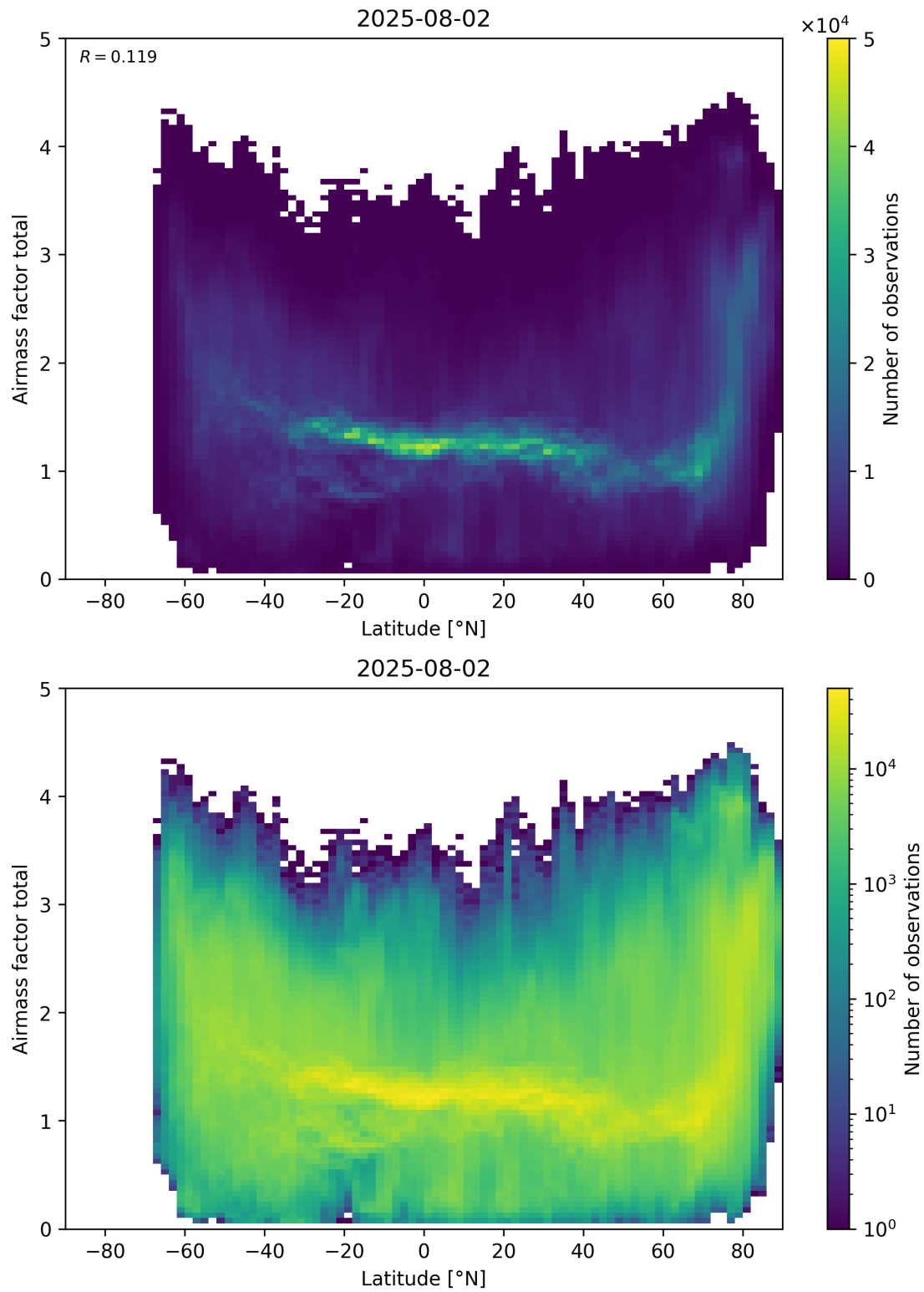
Figure 161: Scatter density plot of “Latitude” against “Airmass factor total” for 2025-08-01 to 2025-08-03.
