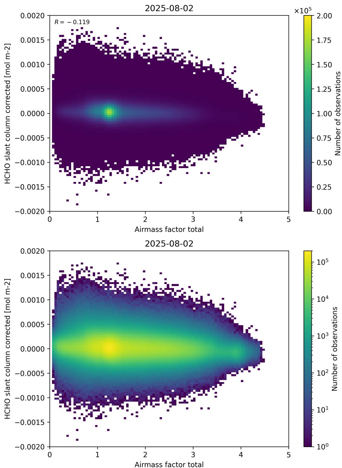
Figure 101: Scatter density plot of “Airmass factor total” against “HCHO slant column corrected” for 2025-08-01 to 2025-08-03.
