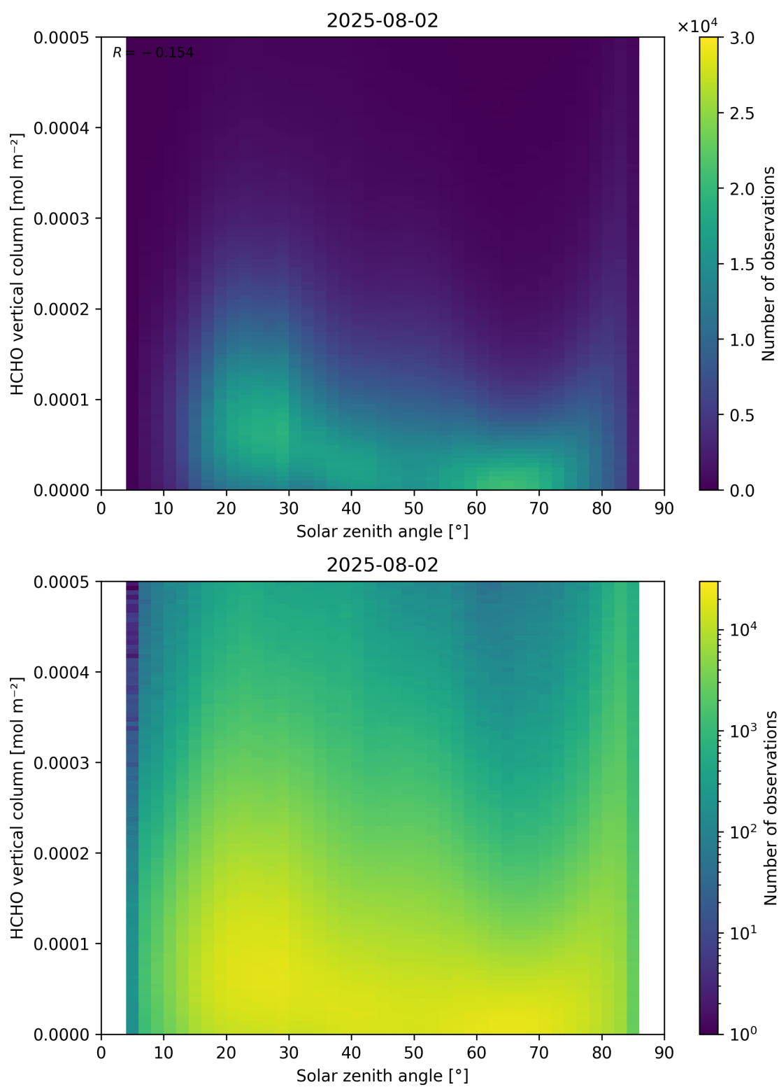
Figure 177: Scatter density plot of “Solar zenith angle” against “HCHO vertical column” for 2025-08-01 to 2025-08-03.
