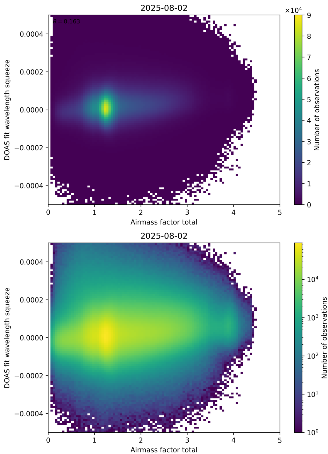
Figure 99: Scatter density plot of “Airmass factor total” against “DOAS fit wavelength squeeze” for 2025-08-01 to 2025-08-03.
