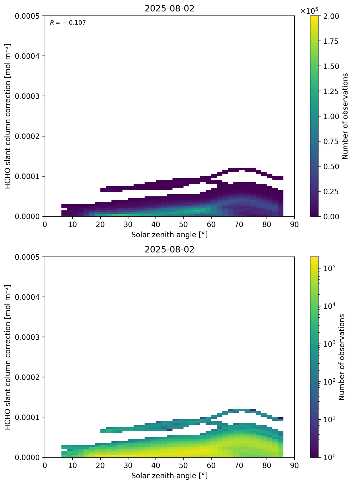
Figure 172: Scatter density plot of “Solar zenith angle” against “HCHO slant column correction” for 2025-08-01 to 2025-08-03.
