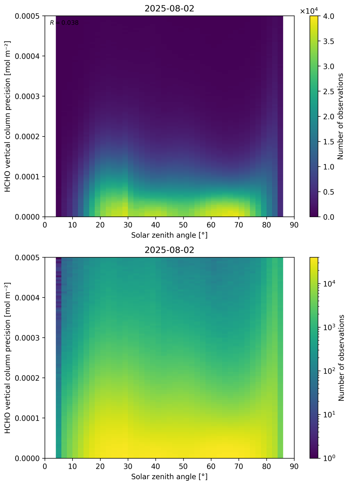
Figure 179: Scatter density plot of “Solar zenith angle” against “HCHO vertical column precision” for 2025-08-01 to 2025-08-03.
