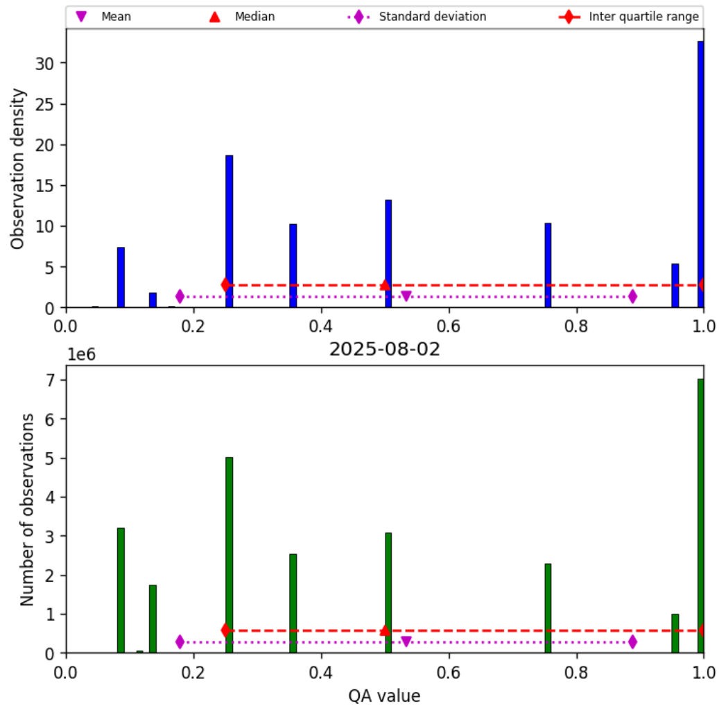
Figure 34: Histogram of “QA value” for 2025-08-01 to 2025-08-03
