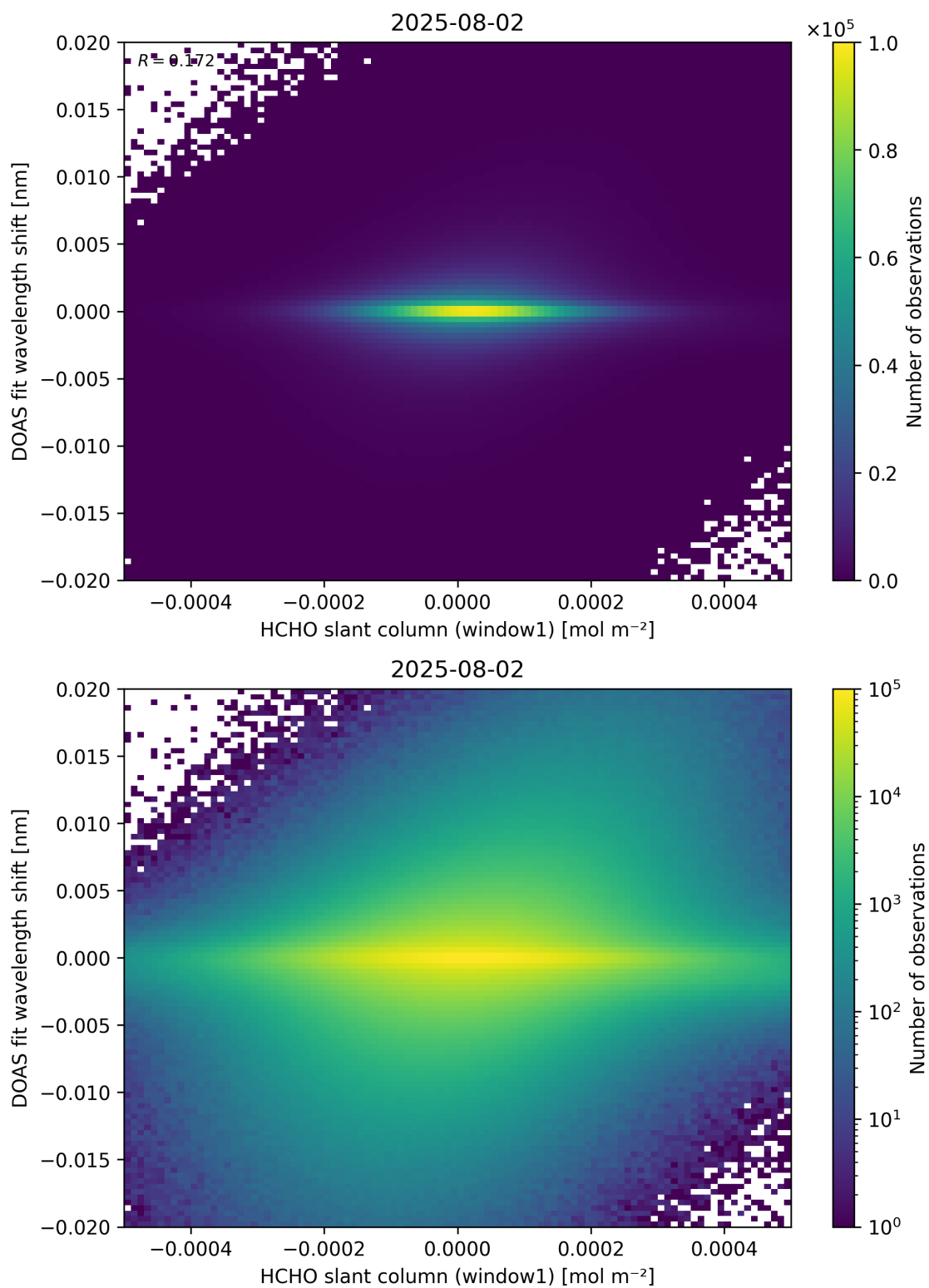
Figure 79: Scatter density plot of “HCHO slant column (window1)” against “DOAS fit wavelength shift” for 2025-08-01 to 2025-08-03.
