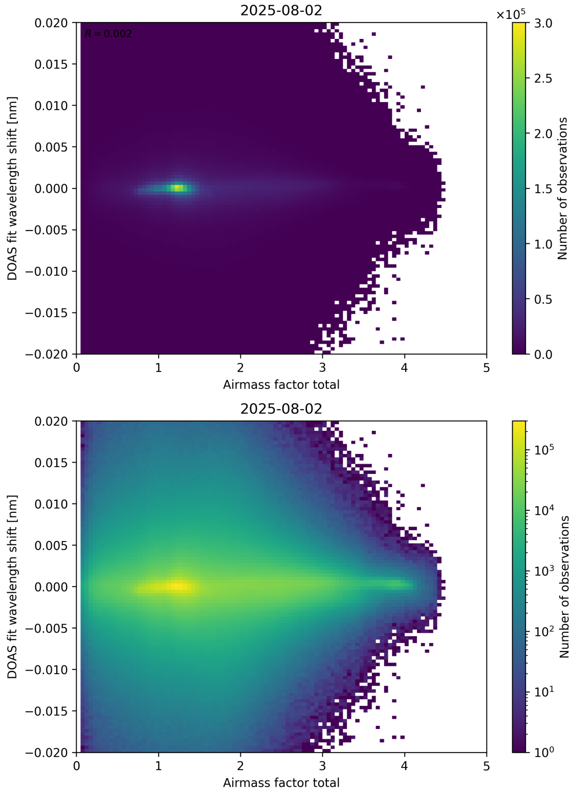
Figure 98: Scatter density plot of “Airmass factor total” against “DOAS fit wavelength shift” for 2025-08-01 to 2025-08-03.
