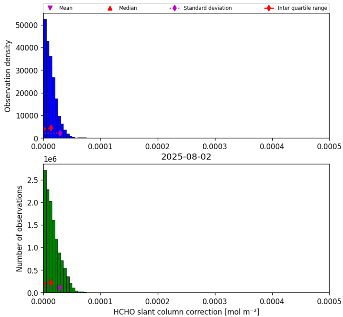
Figure 47: Histogram of “HCHO slant column correction” for 2025-08-01 to 2025-08-03
