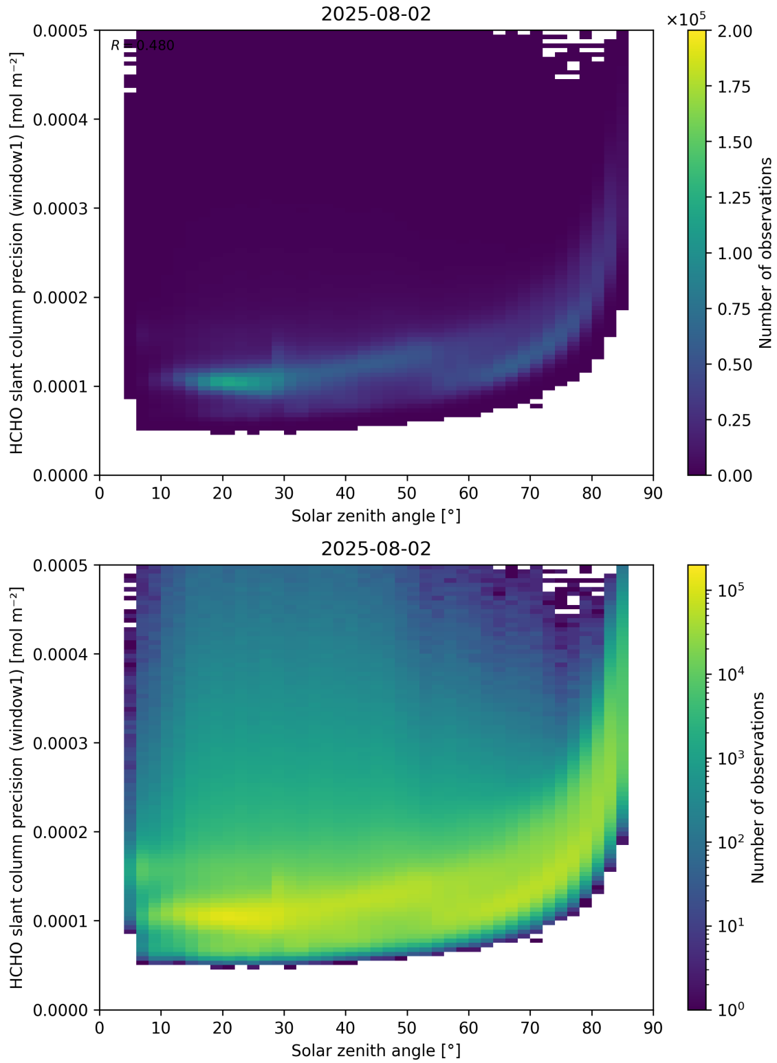
Figure 174: Scatter density plot of “Solar zenith angle” against “HCHO slant column precision (window1)” for 2025-08-01 to 2025-08-03.
