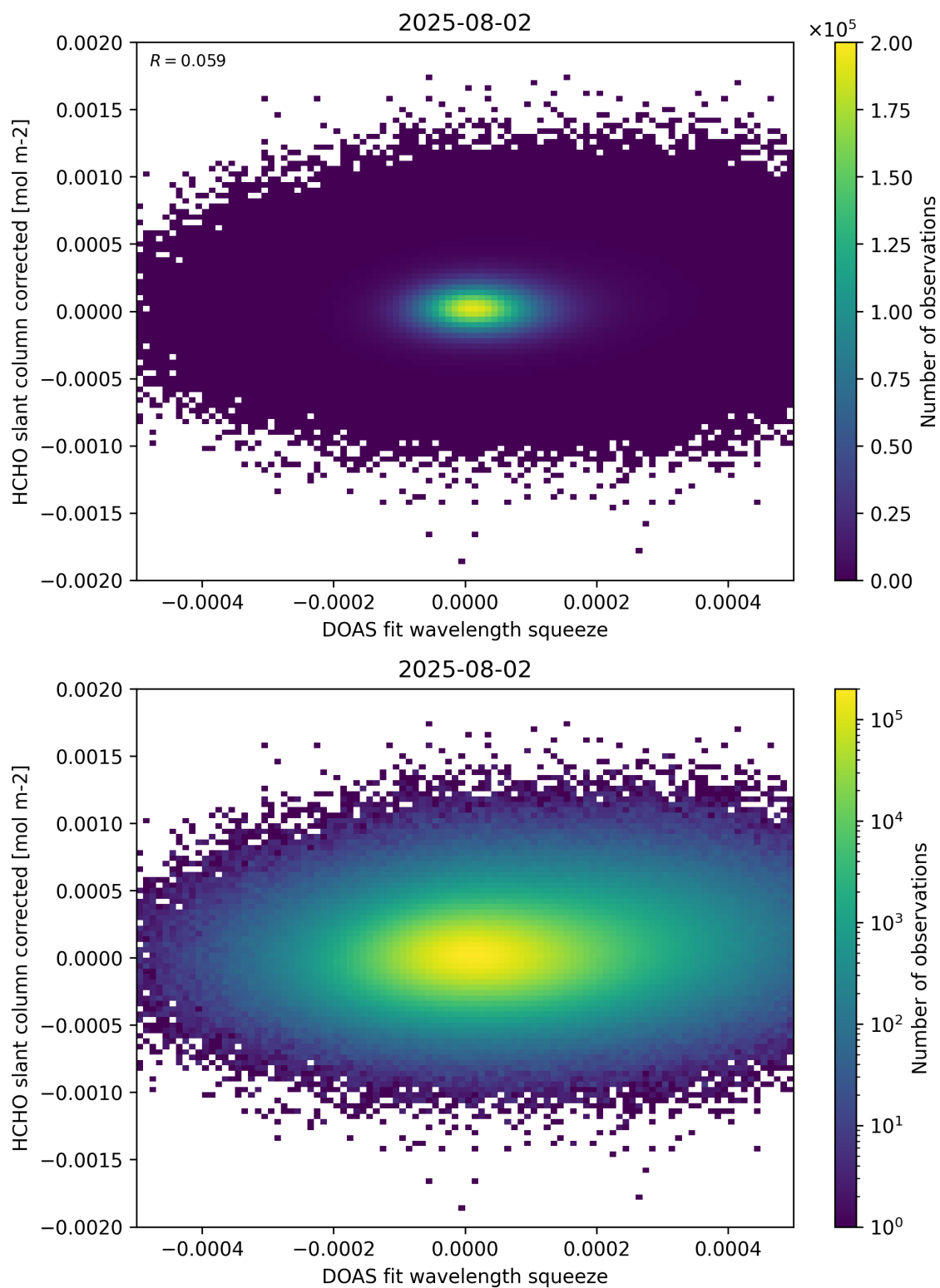
Figure 69: Scatter density plot of “DOAS fit wavelength squeeze” against “HCHO slant column corrected” for 2025-08-01 to 2025-08-03.
