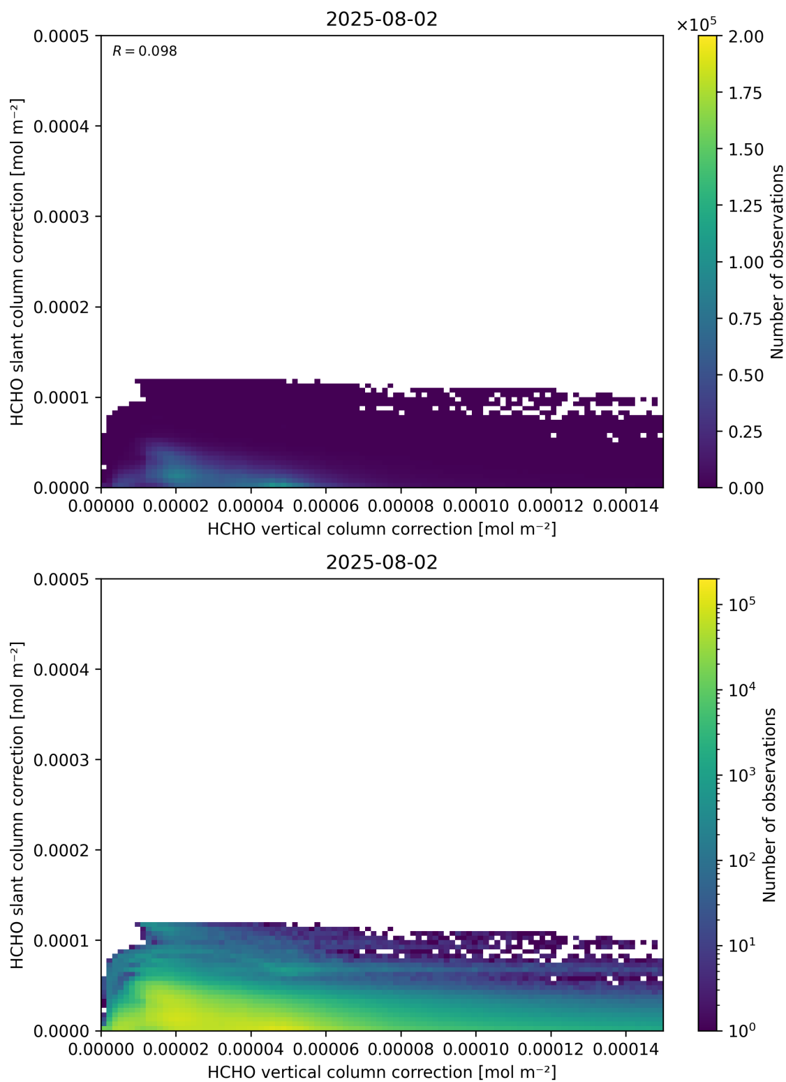
Figure 117: Scatter density plot of “HCHO vertical column correction” against “HCHO slant column correction” for 2025-08-01 to 2025-08-03.
