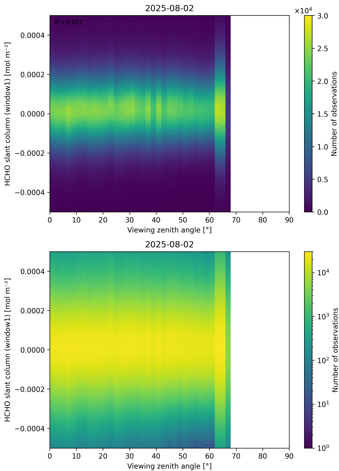
Figure 188: Scatter density plot of “Viewing zenith angle” against “HCHO slant column (window1)” for 2025-08-01 to 2025-08-03.
