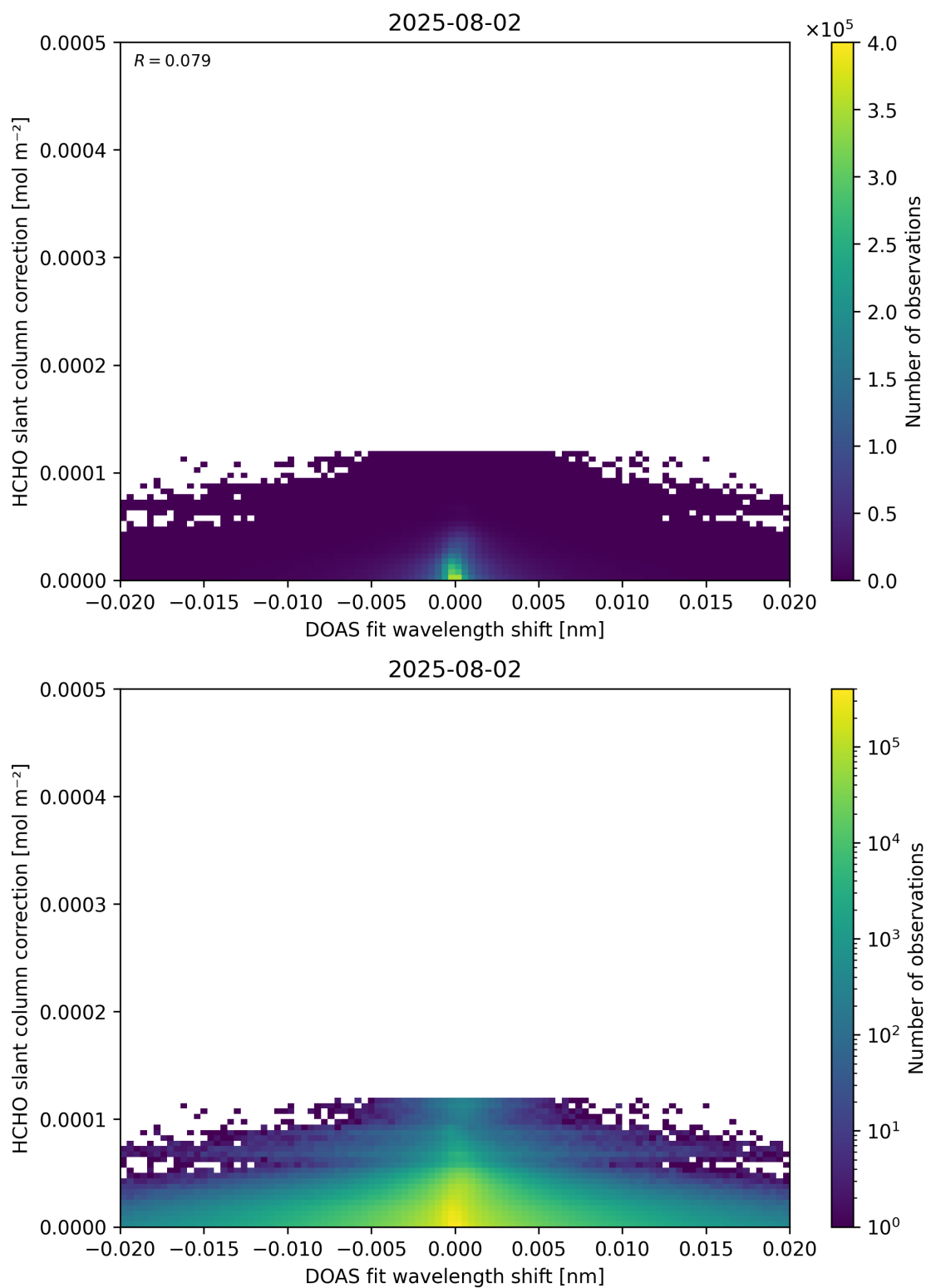
Figure 67: Scatter density plot of “DOAS fit wavelength shift” against “HCHO slant column correction” for 2025-08-01 to 2025-08-03.
