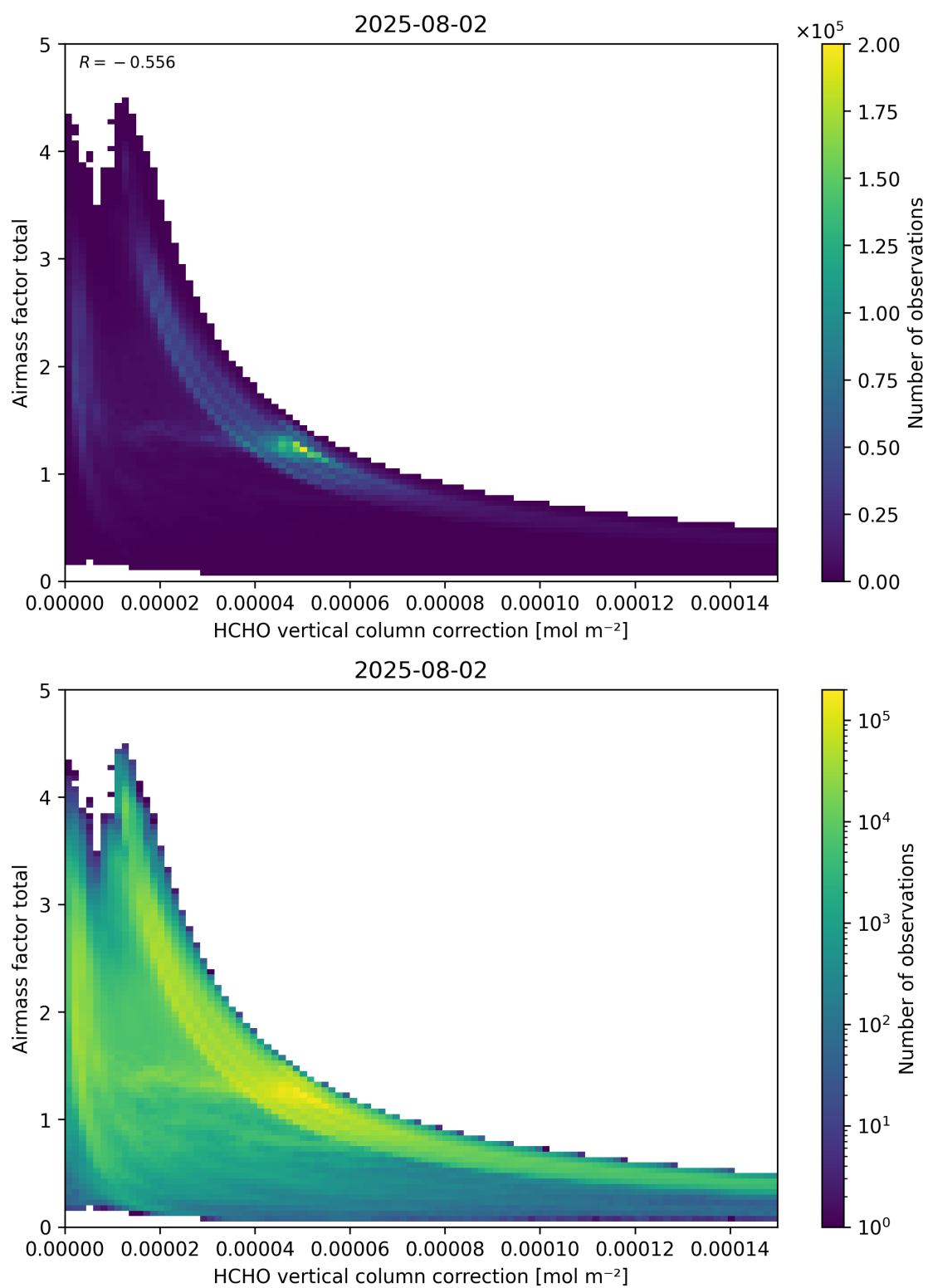
Figure 120: Scatter density plot of “HCHO vertical column correction” against “Airmass factor total” for 2025-08-01 to 2025-08-03.
