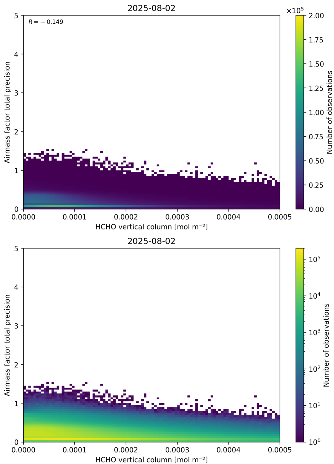
Figure 132: Scatter density plot of “HCHO vertical column” against “Airmass factor total precision” for 2025-08-01 to 2025-08-03.
