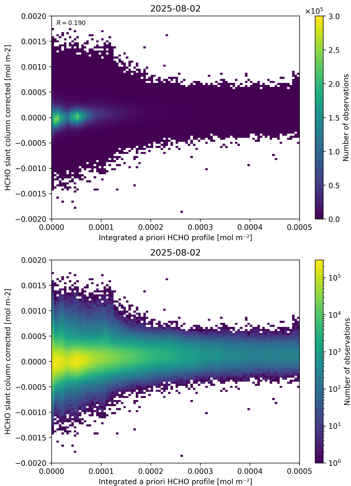
Figure 151: Scatter density plot of “Integrated a priori HCHO profile” against “HCHO slant column corrected” for 2025-08-01 to 2025-08-03.
