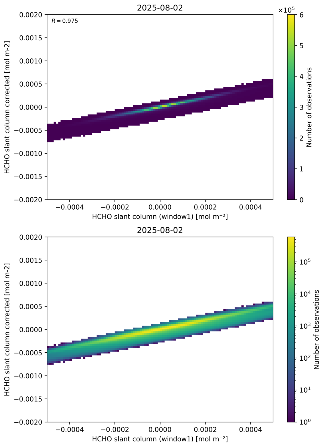
Figure 82: Scatter density plot of “HCHO slant column (window1)” against “HCHO slant column corrected” for 2025-08-01 to 2025-08-03.
