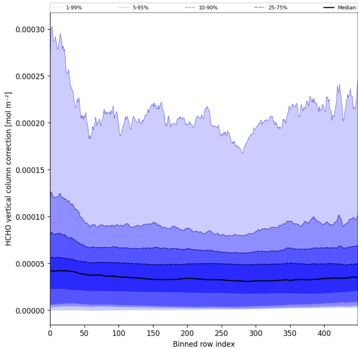
Figure 51: Along track statistics of “HCHO vertical column correction” for 2025-08-01 to 2025-08-03
