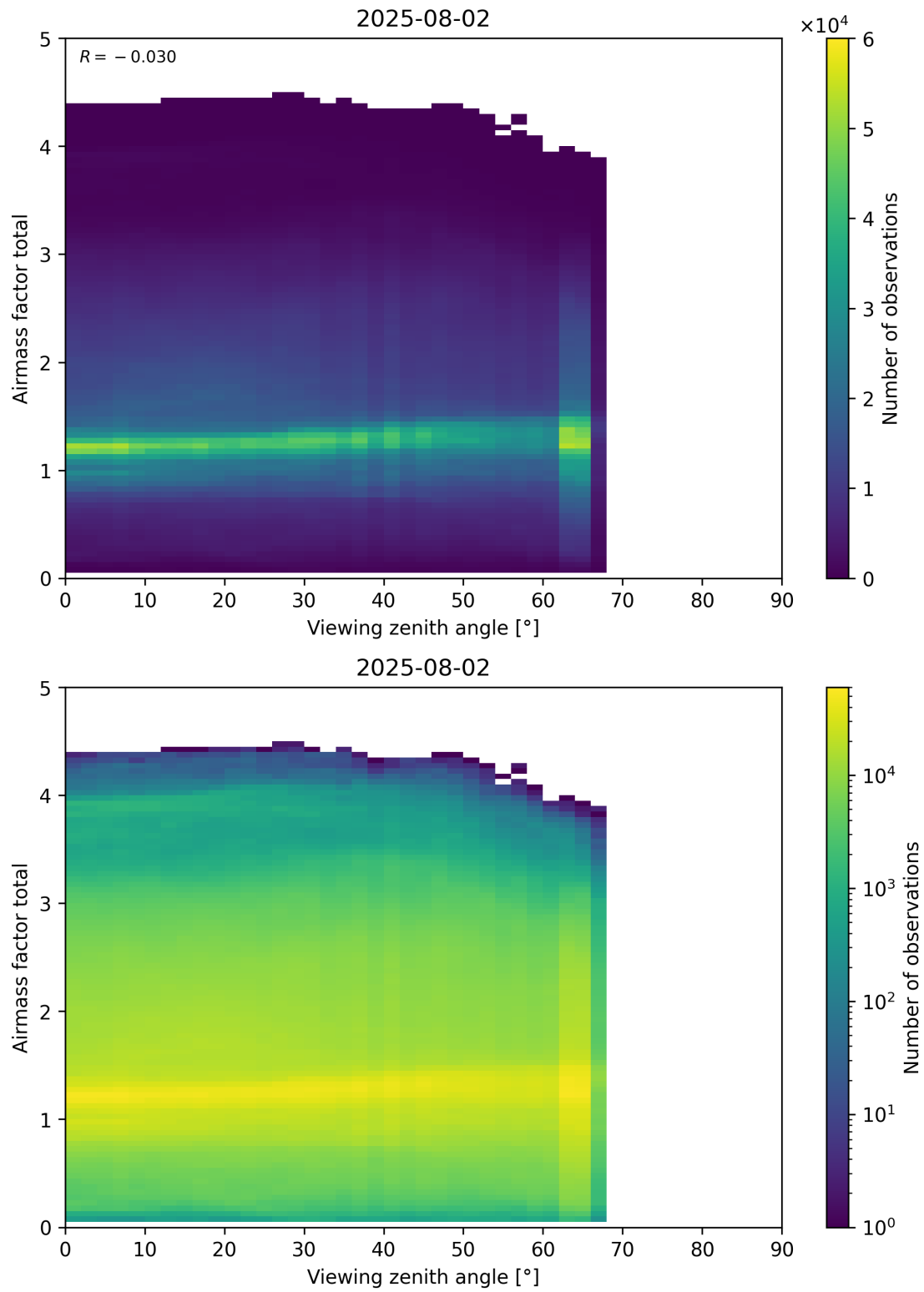
Figure 190: Scatter density plot of “Viewing zenith angle” against “Airmass factor total” for 2025-08-01 to 2025-08-03.
