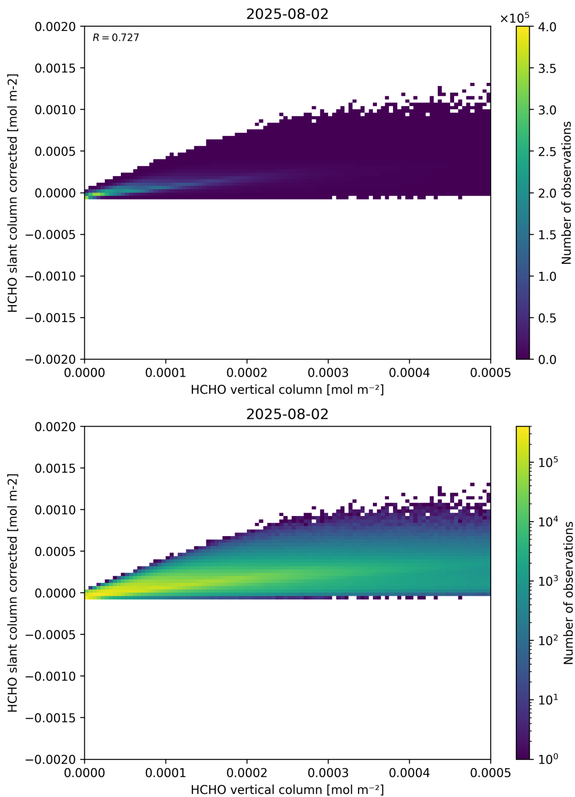
Figure 127: Scatter density plot of “HCHO vertical column” against “HCHO slant column corrected” for 2025-08-01 to 2025-08-03.
