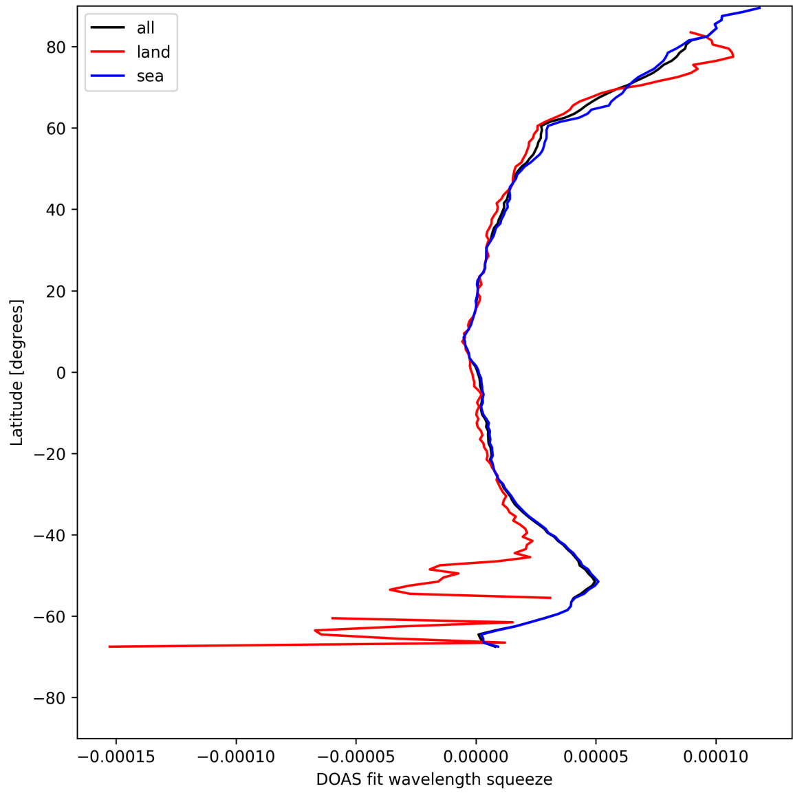
Figure 31: Zonal average of “DOAS fit wavelength squeeze” for 2025-08-01 to 2025-08-03.
