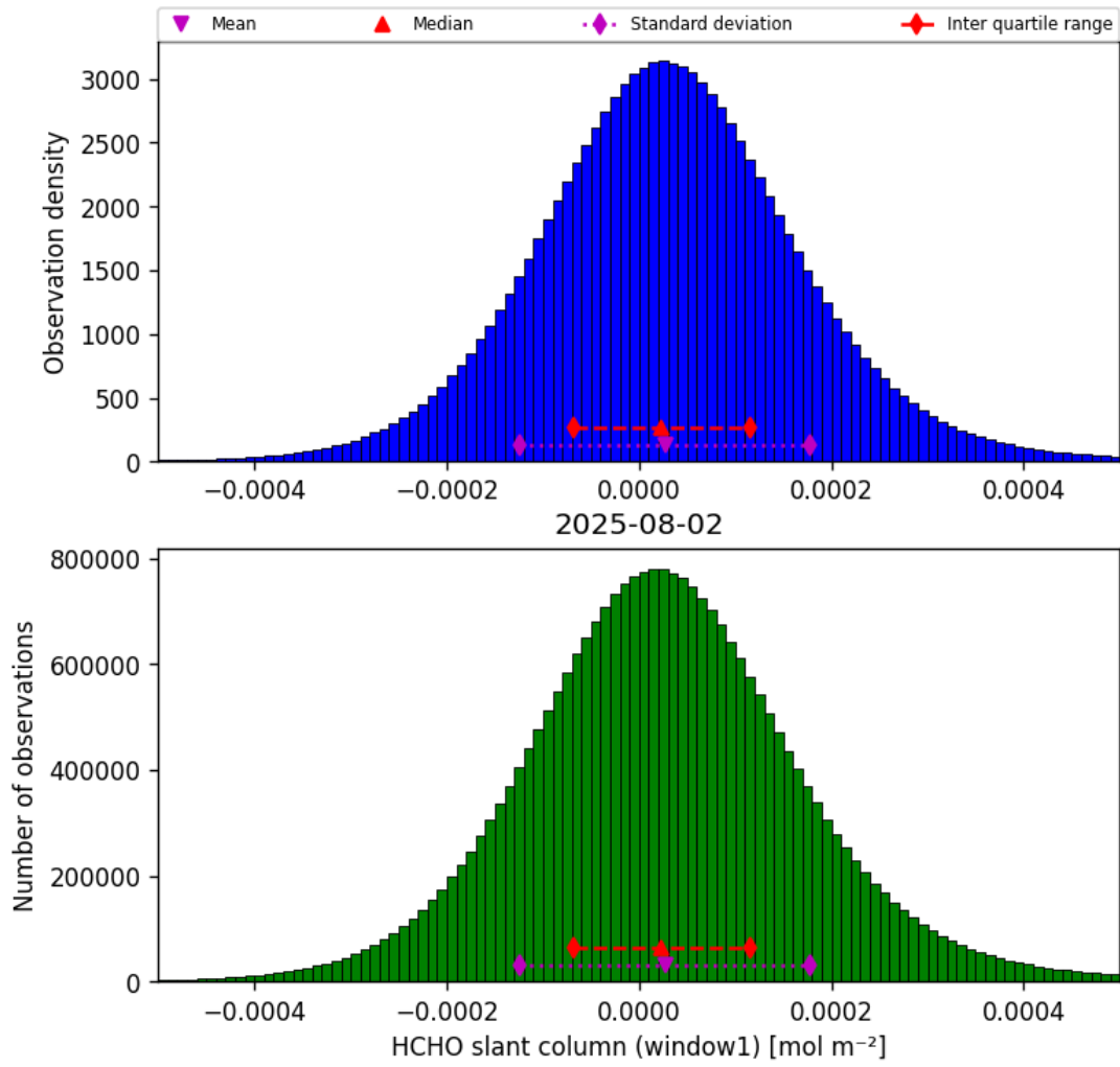
Figure 38: Histogram of “HCHO slant column (window1)” for 2025-08-01 to 2025-08-03
