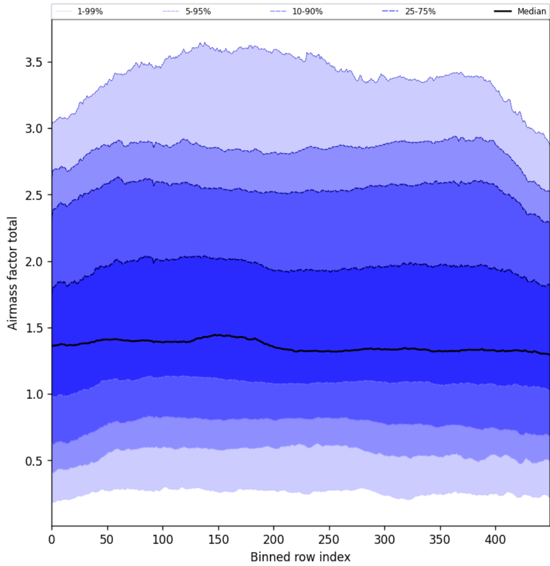
Figure 54: Along track statistics of “Airmass factor total” for 2025-08-01 to 2025-08-03
