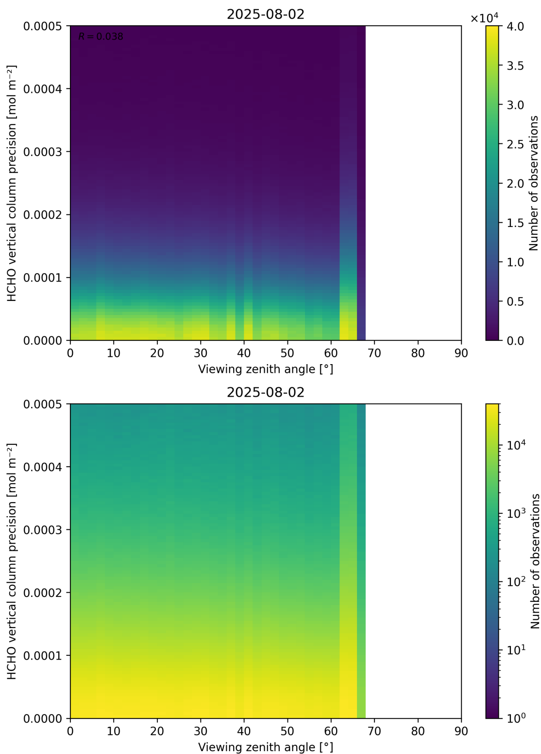
Figure 194: Scatter density plot of “Viewing zenith angle” against “HCHO vertical column precision” for 2025-08-01 to 2025-08-03.
