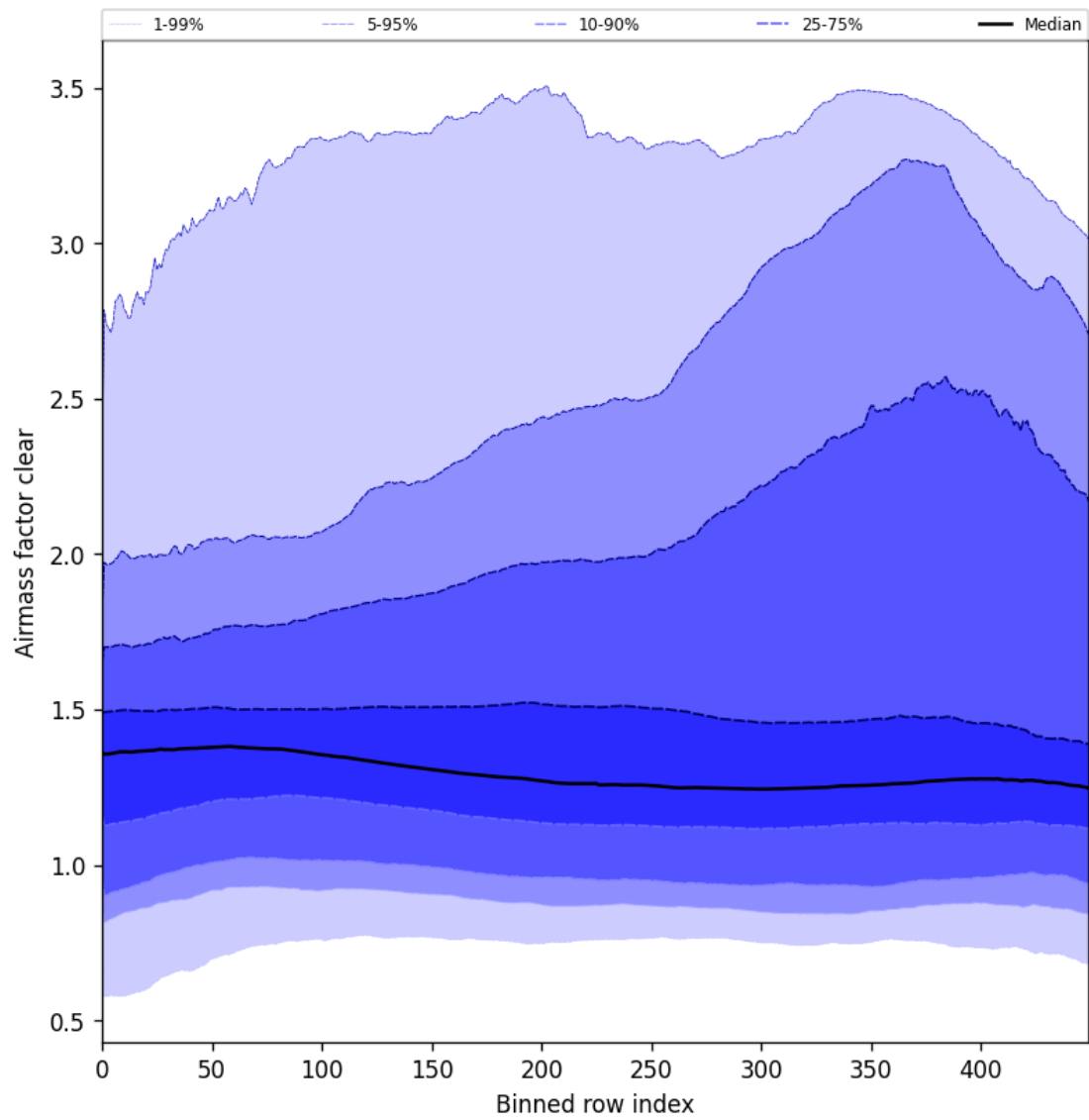
Figure 56: Along track statistics of “Airmass factor clear” for 2025-08-01 to 2025-08-03
