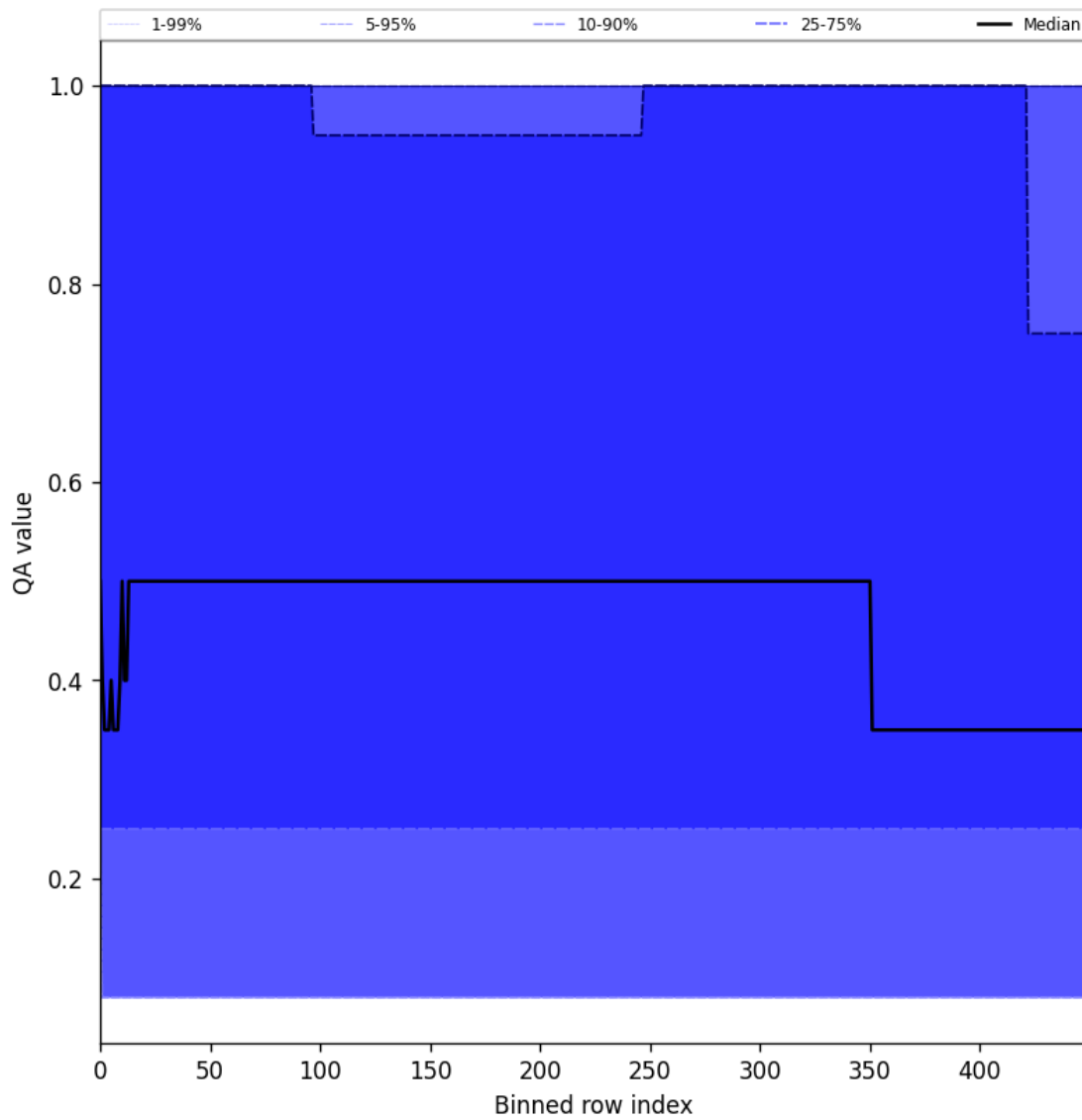
Figure 48: Along track statistics of “QA value” for 2025-08-01 to 2025-08-03
