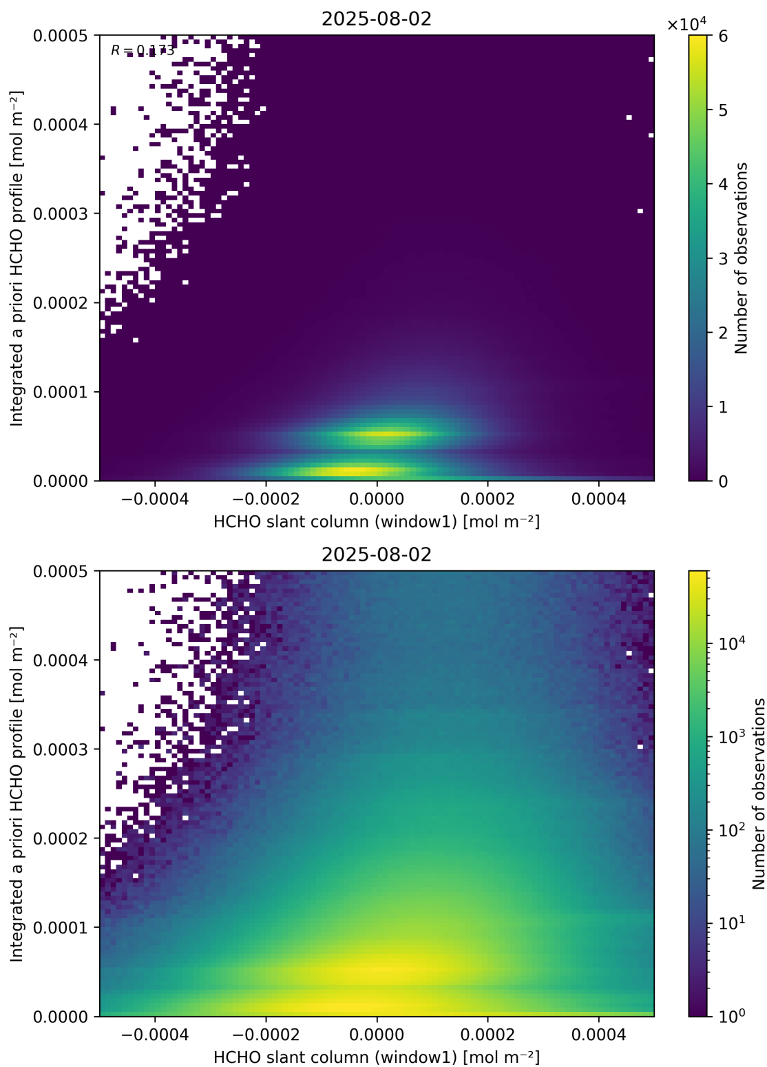
Figure 87: Scatter density plot of “HCHO slant column (window1)” against “Integrated a priori HCHO profile” for 2025-08-01 to 2025-08-03.
