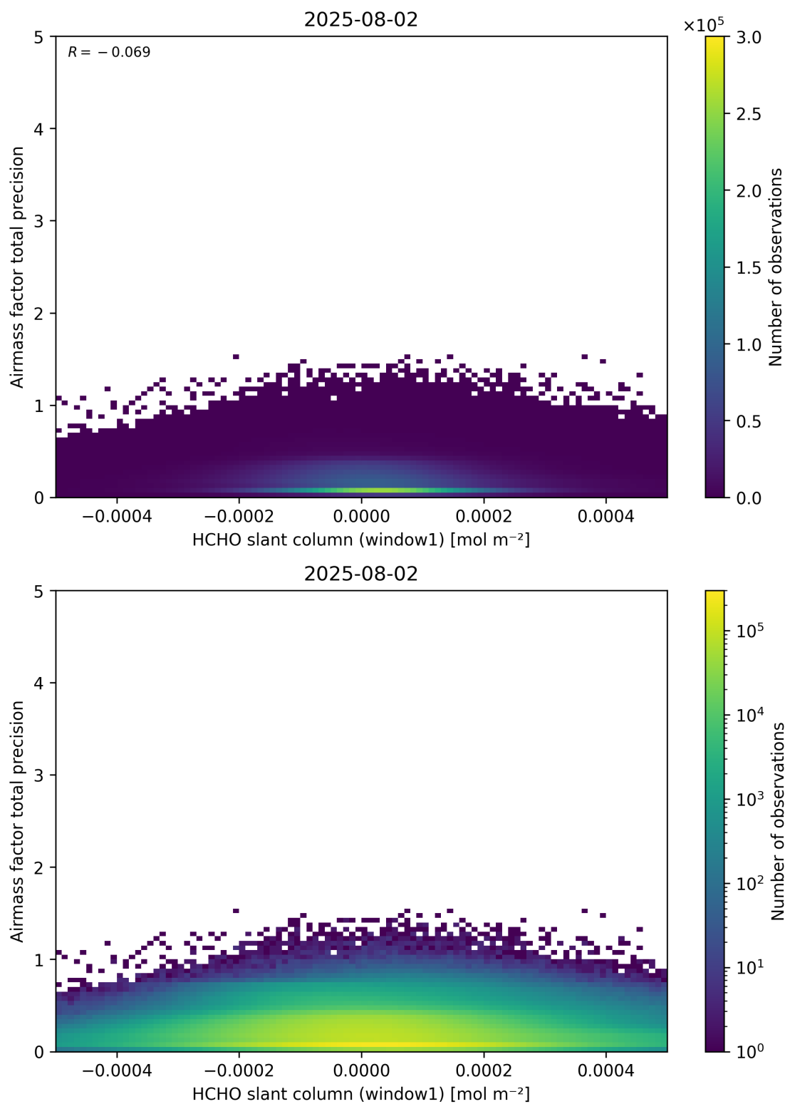
Figure 86: Scatter density plot of “HCHO slant column (window1)” against “Airmass factor total precision” for 2025-08-01 to 2025-08-03.
