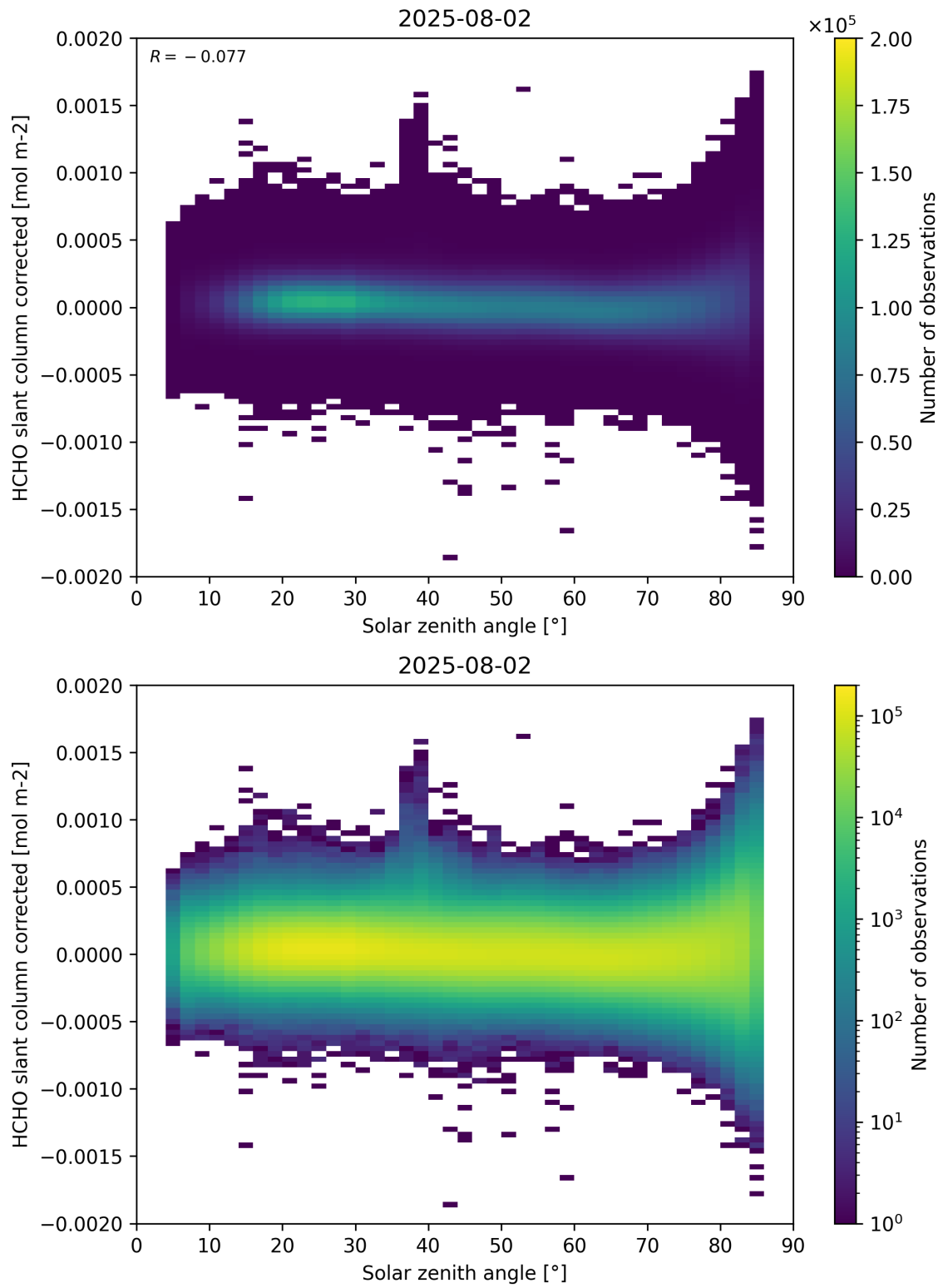
Figure 171: Scatter density plot of “Solar zenith angle” against “HCHO slant column corrected” for 2025-08-01 to 2025-08-03.
