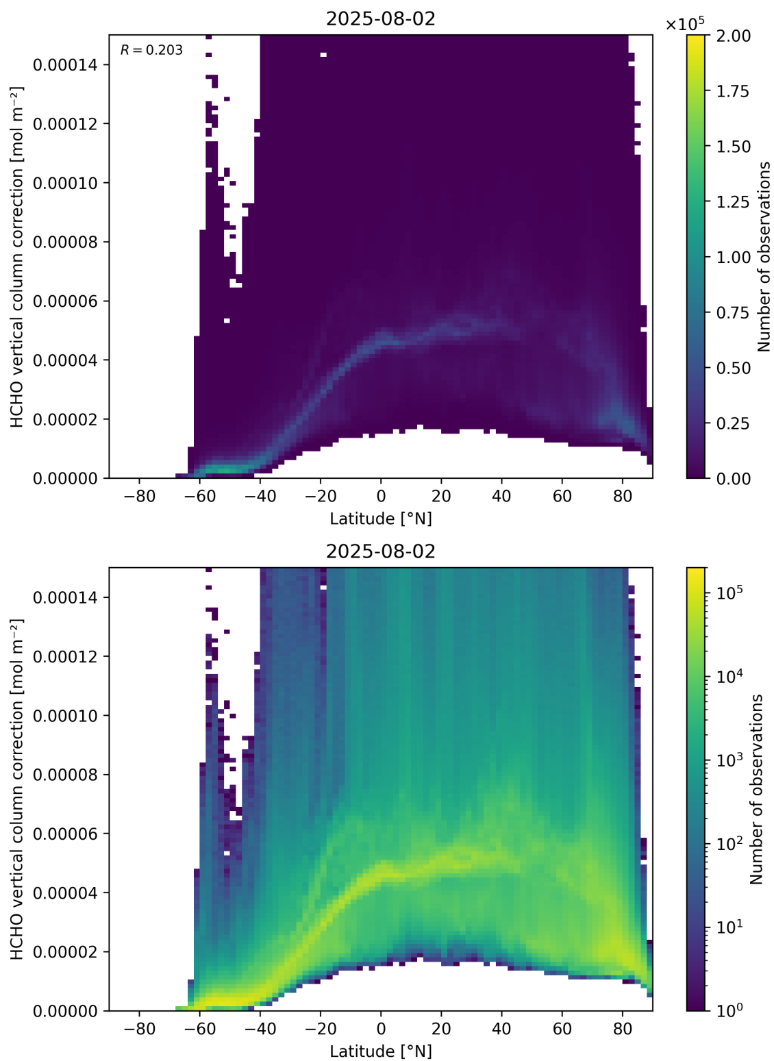
Figure 164: Scatter density plot of “Latitude” against “HCHO vertical column correction” for 2025-08-01 to 2025-08-03.
