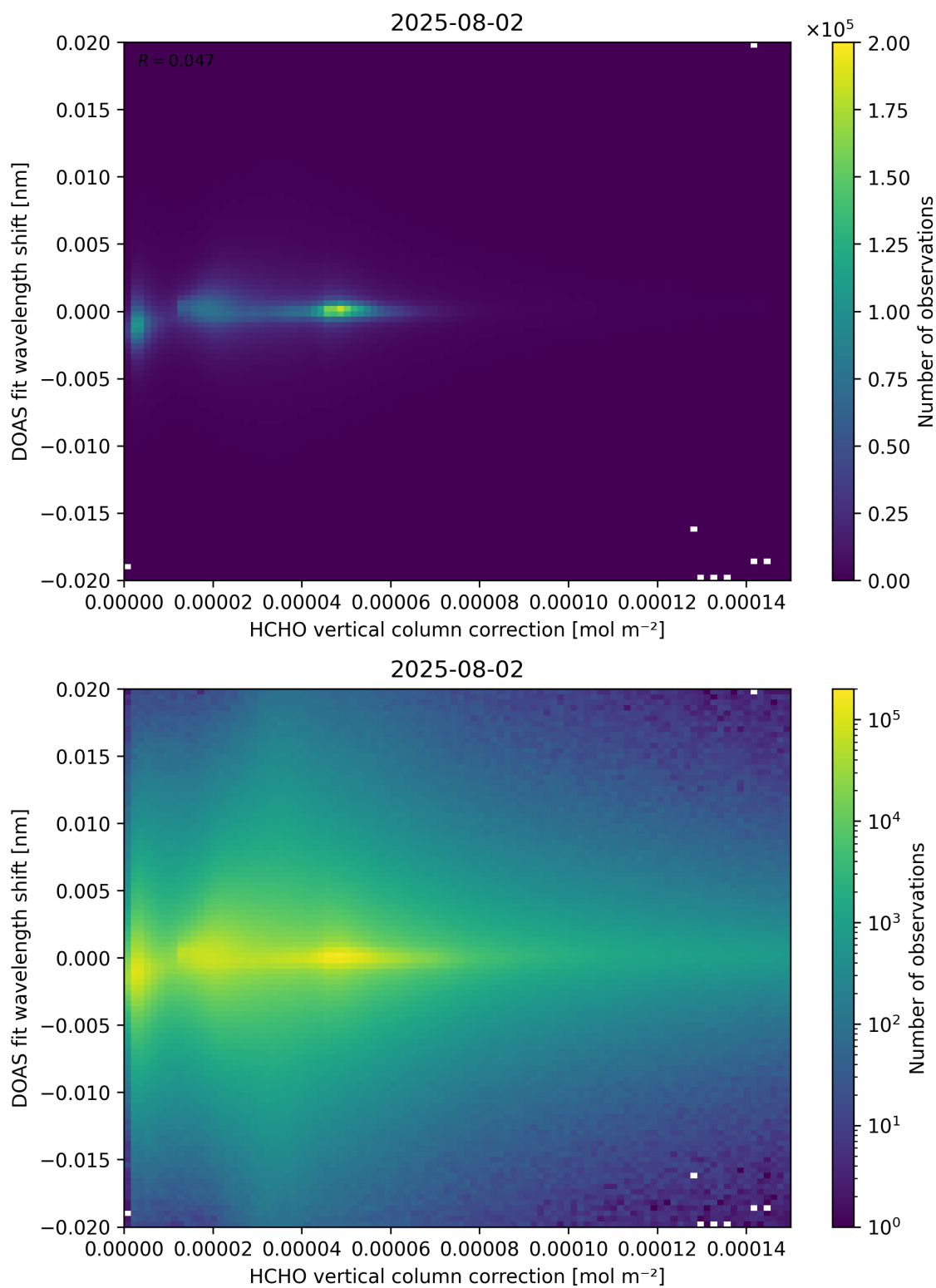
Figure 113: Scatter density plot of “HCHO vertical column correction” against “DOAS fit wavelength shift” for 2025-08-01 to 2025-08-03.
