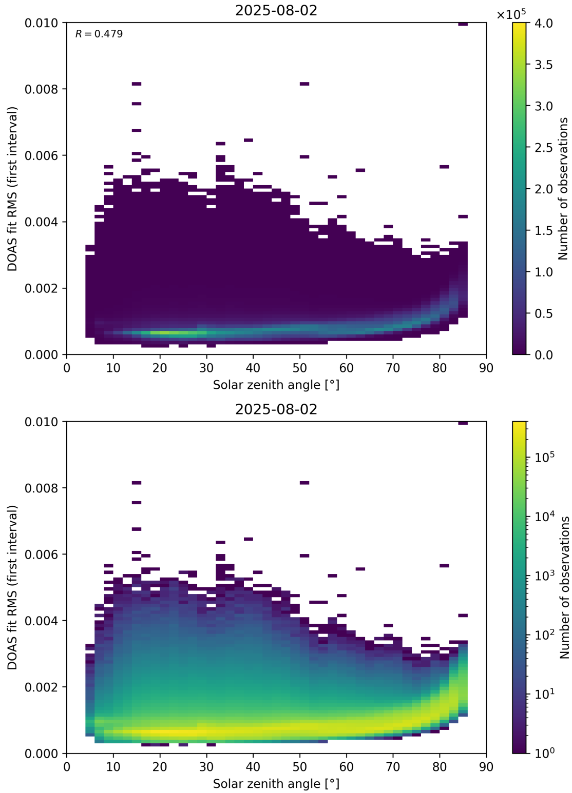
Figure 167: Scatter density plot of “Solar zenith angle” against “DOAS fit RMS (first interval)” for 2025-08-01 to 2025-08-03.
