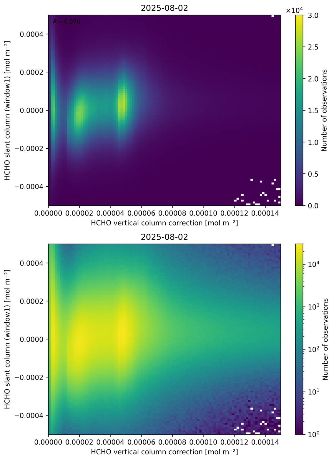
Figure 118: Scatter density plot of “HCHO vertical column correction” against “HCHO slant column (window1)” for 2025-08-01 to 2025-08-03.
