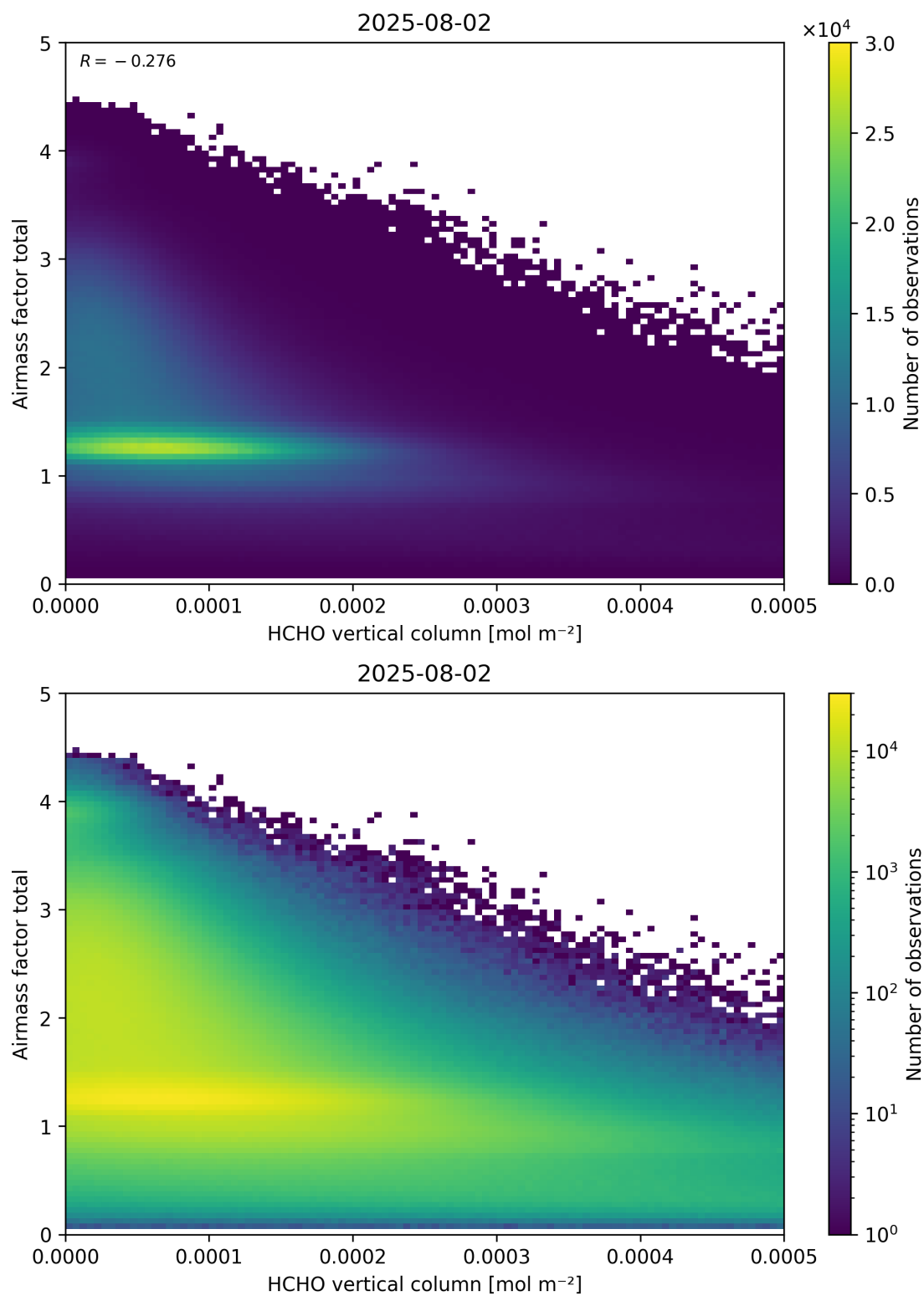
Figure 131: Scatter density plot of “HCHO vertical column” against “Airmass factor total” for 2025-08-01 to 2025-08-03.
