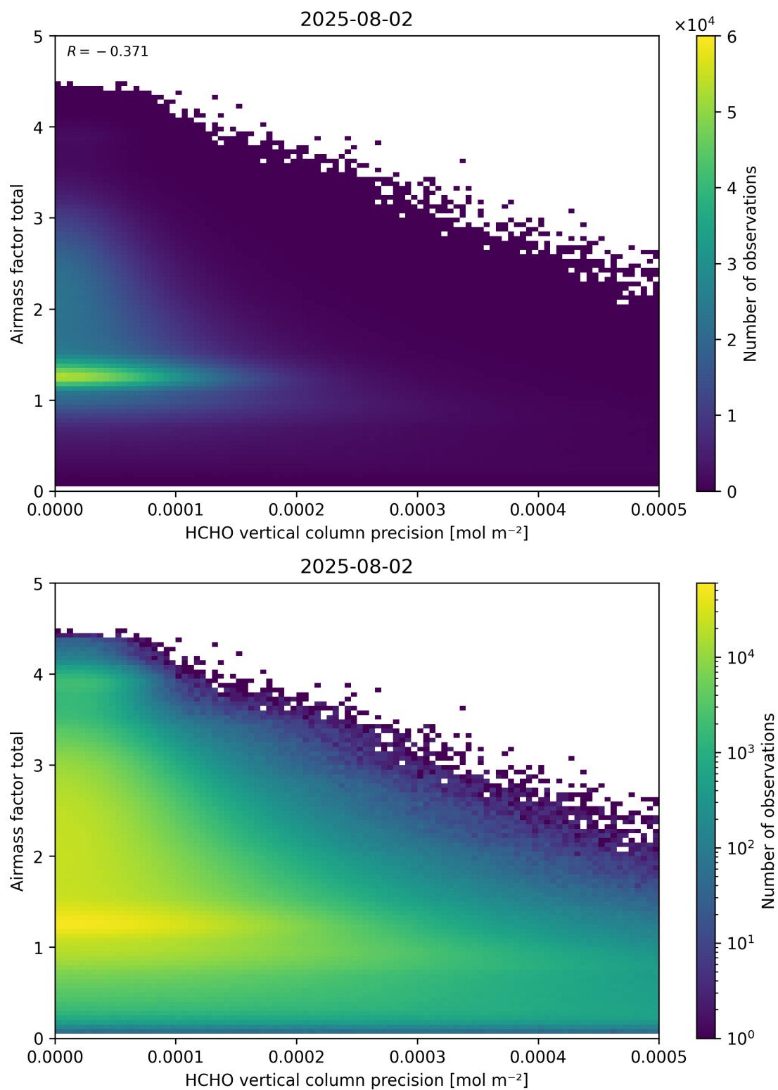
Figure 144: Scatter density plot of “HCHO vertical column precision” against “Airmass factor total” for 2025-08-01 to 2025-08-03.
