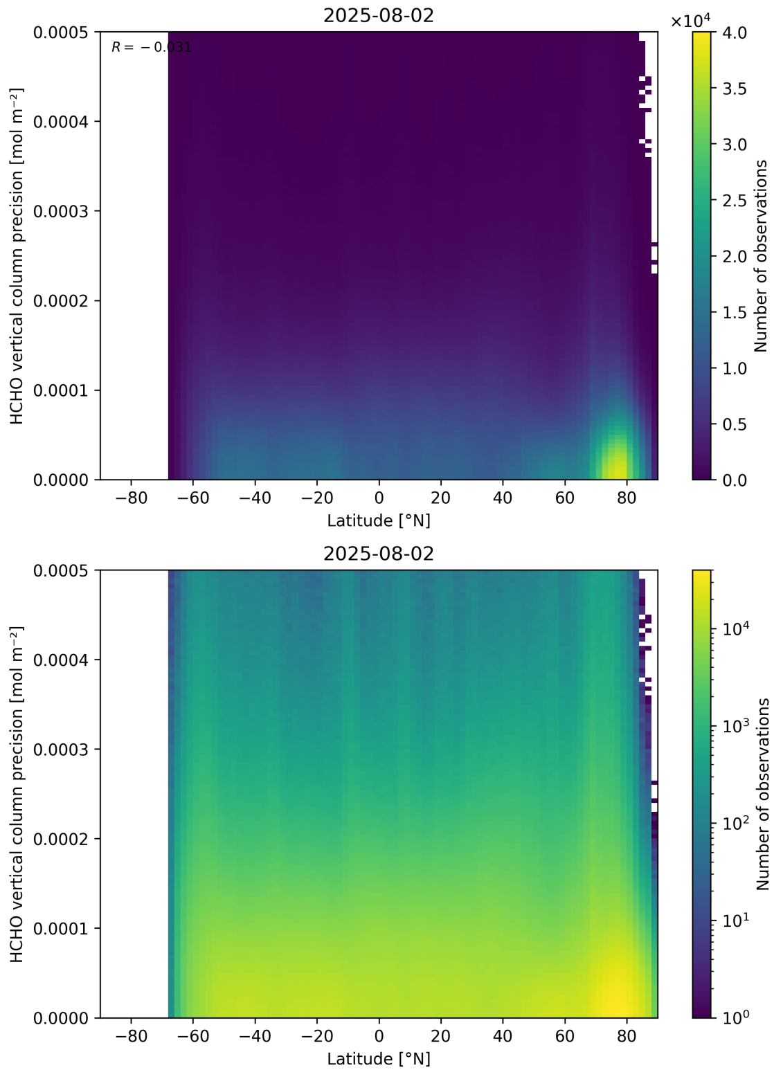
Figure 165: Scatter density plot of “Latitude” against “HCHO vertical column precision” for 2025-08-01 to 2025-08-03.
