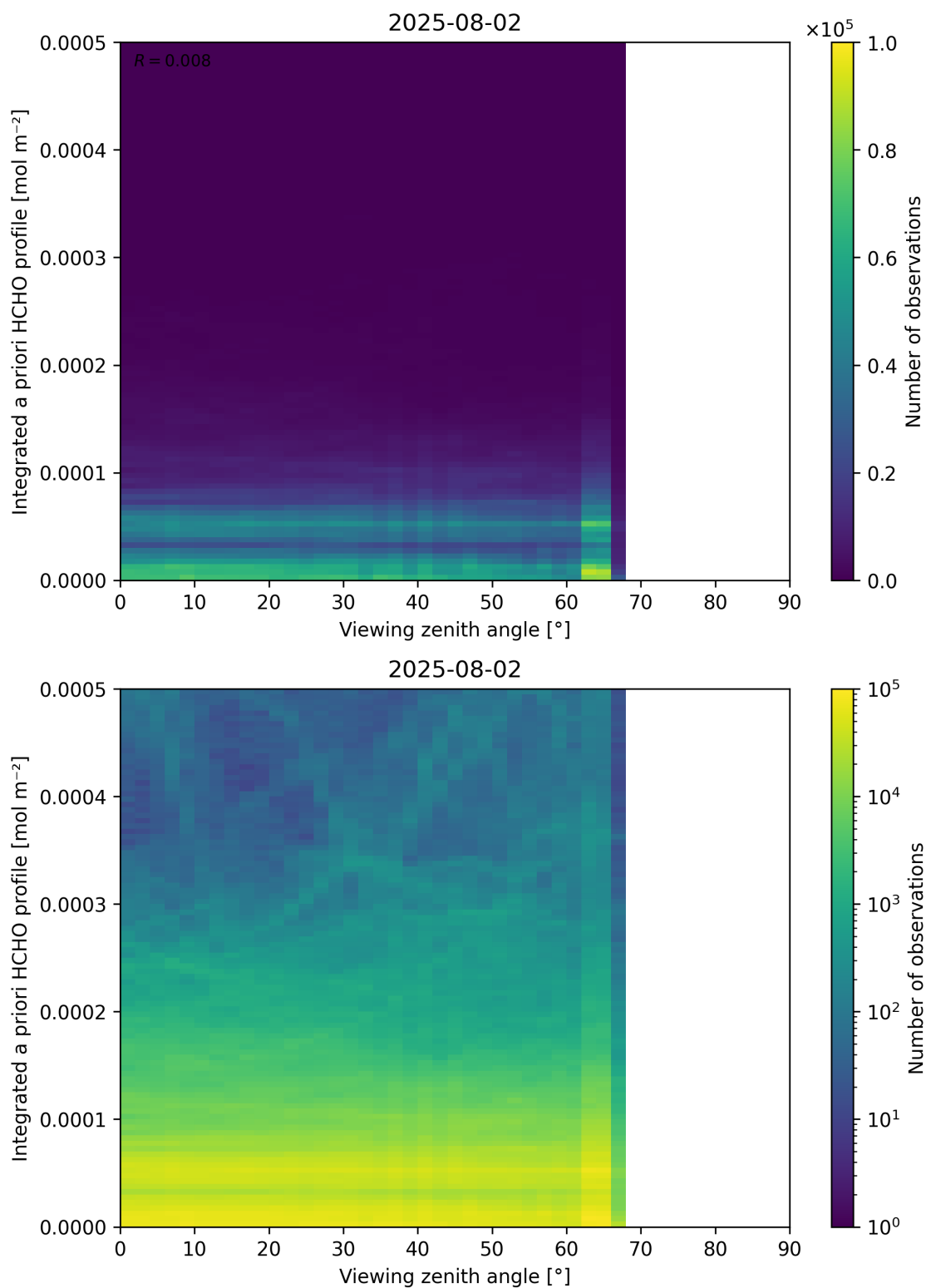
Figure 195: Scatter density plot of “Viewing zenith angle” against “Integrated a priori HCHO profile” for 2025-08-01 to 2025-08-03.
