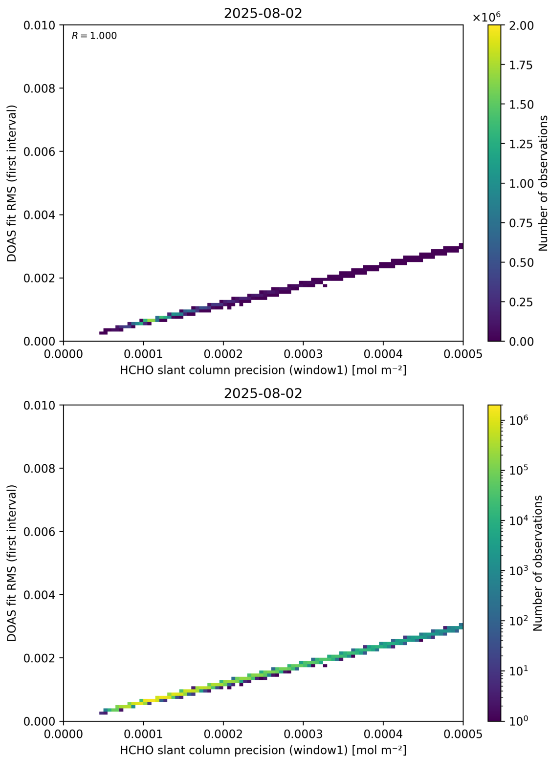
Figure 88: Scatter density plot of “HCHO slant column precision (window1)” against “DOAS fit RMS (first interval)” for 2025-08-01 to 2025-08-03.
