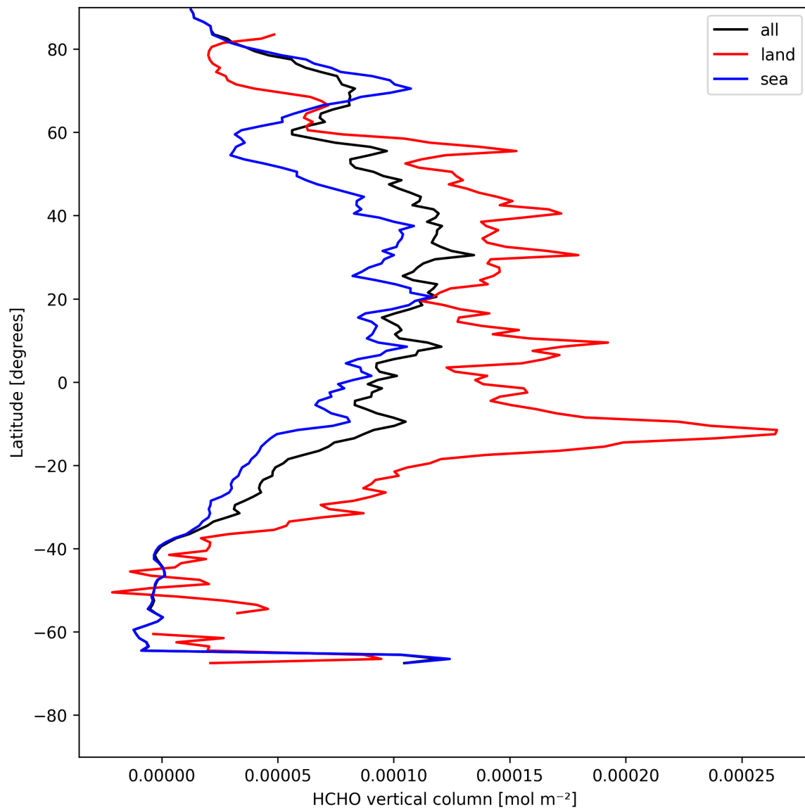
Figure 21: Zonal average of “HCHO vertical column” for 2025-08-01 to 2025-08-03.
