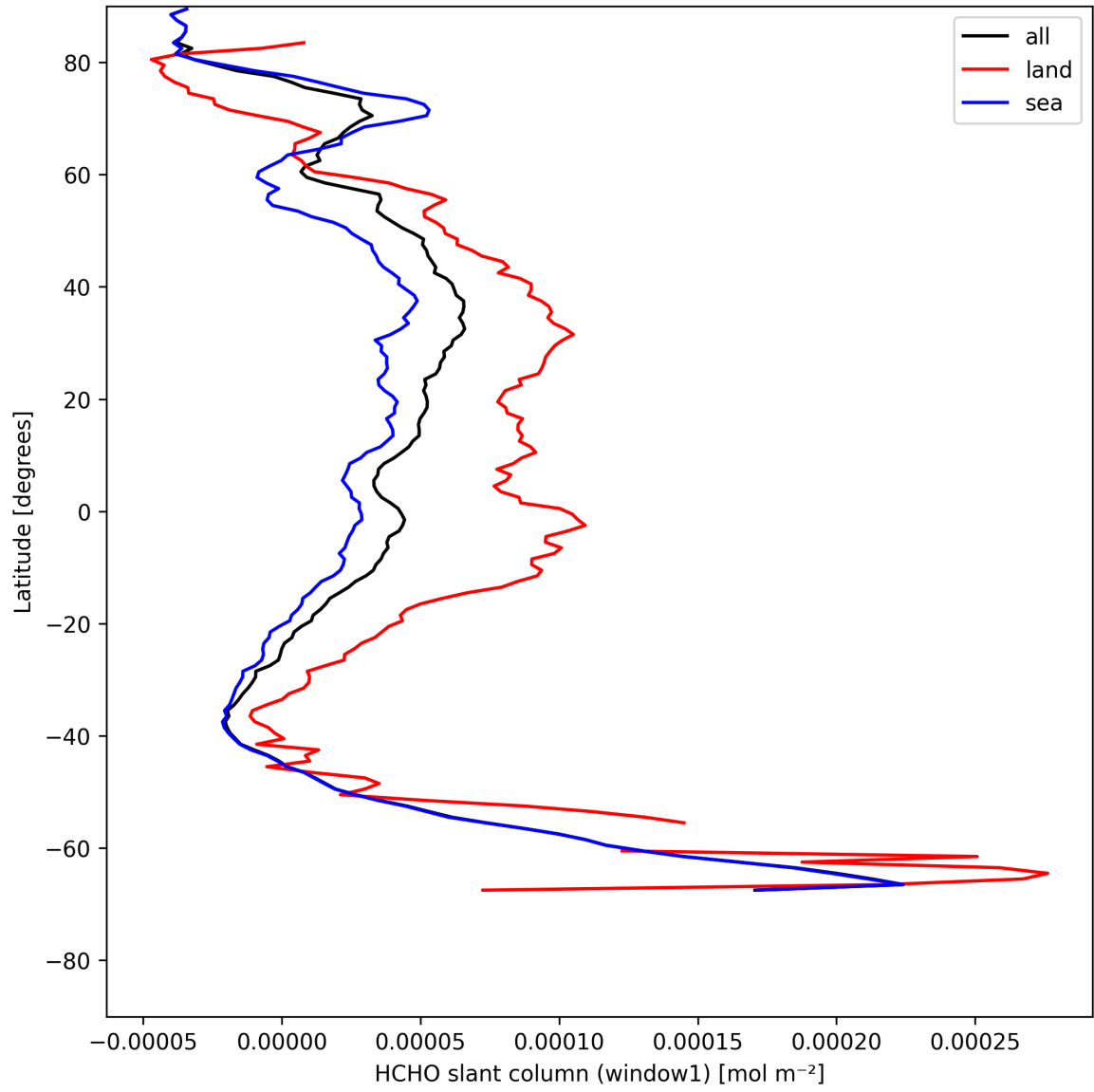
Figure 24: Zonal average of “HCHO slant column (window1)” for 2025-08-01 to 2025-08-03.
