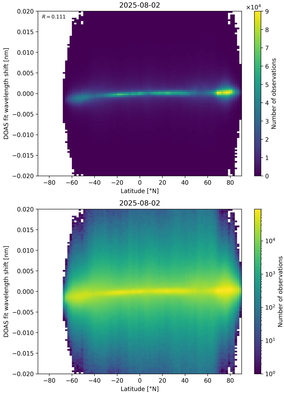
Figure 154: Scatter density plot of “Latitude” against “DOAS fit wavelength shift” for 2025-08-01 to 2025-08-03.
