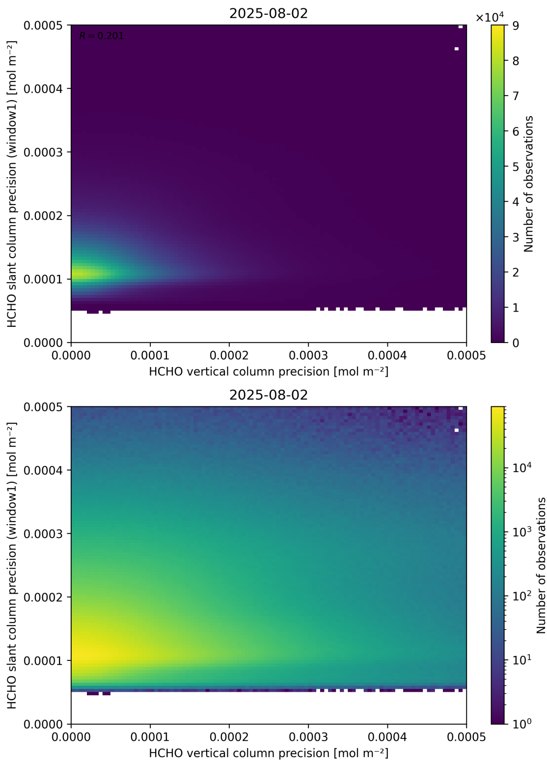
Figure 143: Scatter density plot of “HCHO vertical column precision” against “HCHO slant column precision (window1)” for 2025-08-01 to 2025-08-03.
