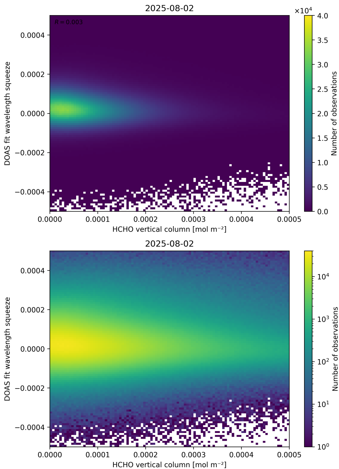
Figure 125: Scatter density plot of “HCHO vertical column” against “DOAS fit wavelength squeeze” for 2025-08-01 to 2025-08-03.
