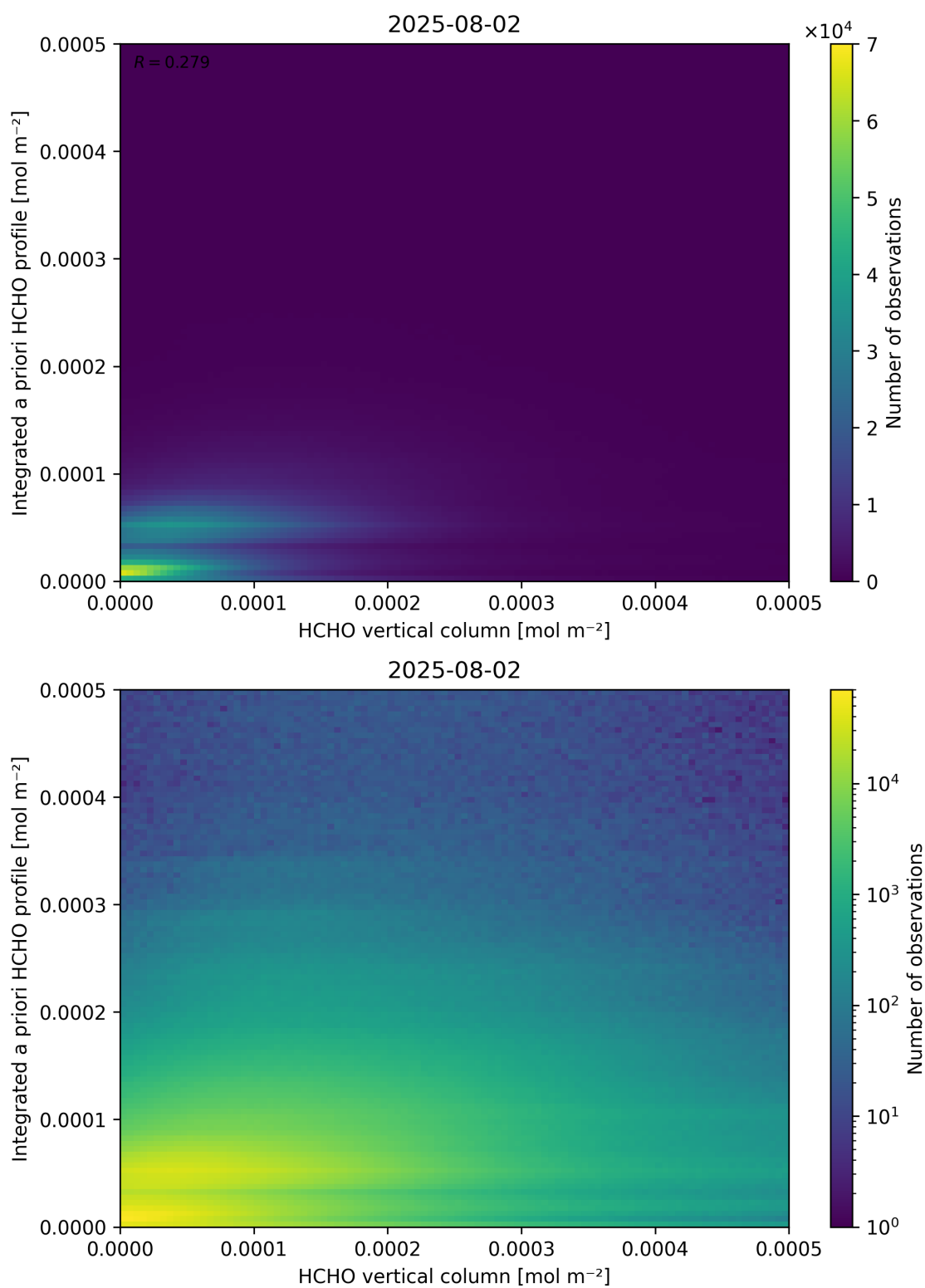
Figure 135: Scatter density plot of “HCHO vertical column” against “Integrated a priori HCHO profile” for 2025-08-01 to 2025-08-03.
