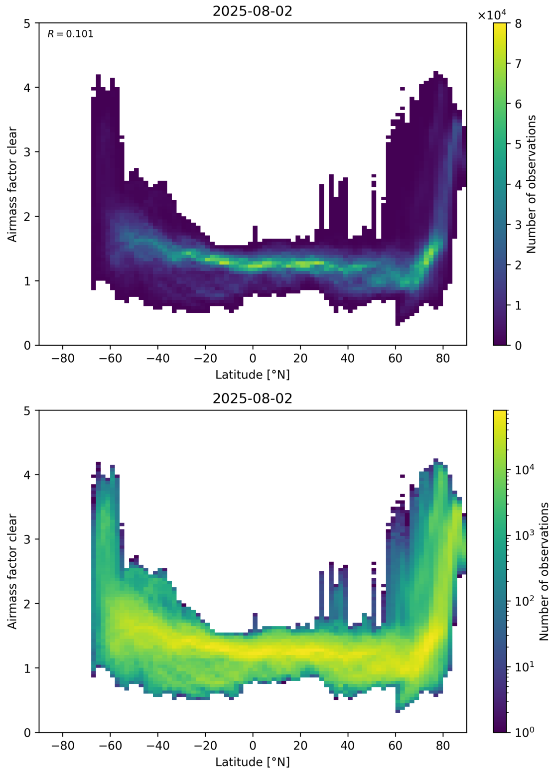
Figure 156: Scatter density plot of “Latitude” against “Airmass factor clear” for 2025-08-01 to 2025-08-03.
