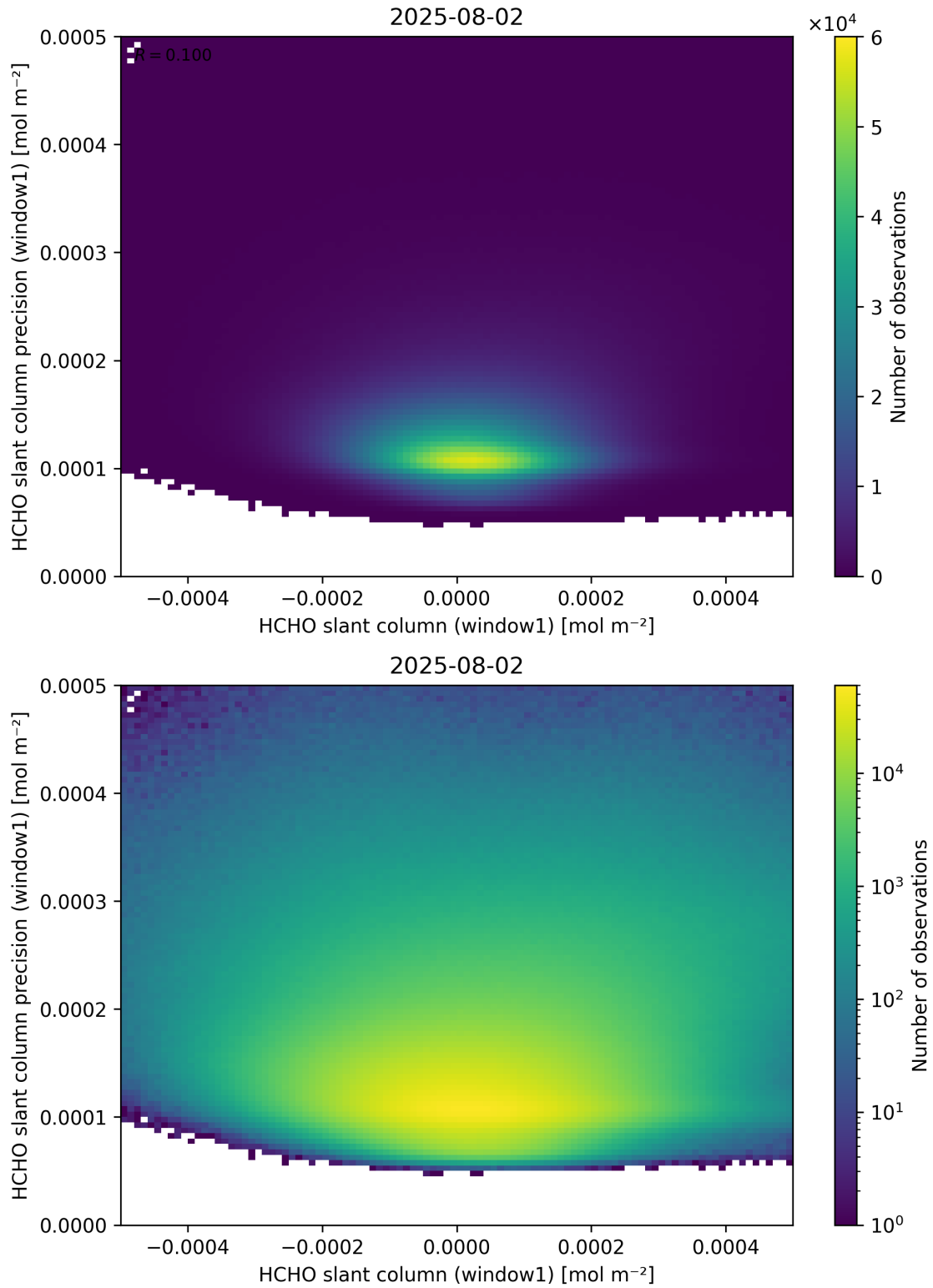
Figure 84: Scatter density plot of “HCHO slant column (window1)” against “HCHO slant column precision (window1)” for 2025-08-01 to 2025-08-03.
