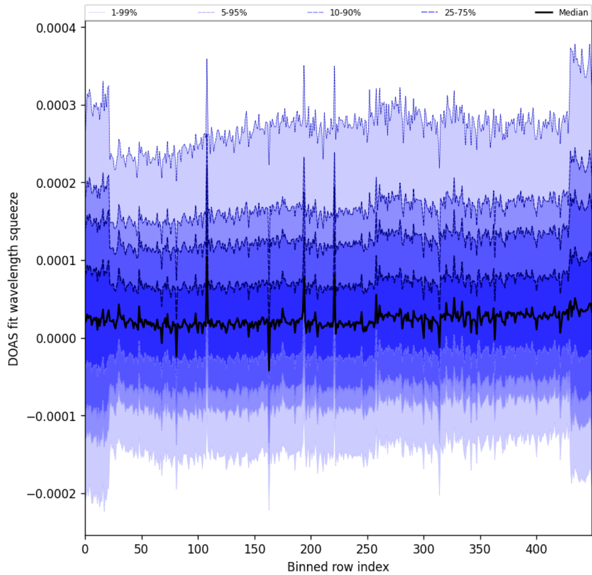
Figure 59: Along track statistics of “DOAS fit wavelength squeeze” for 2025-08-01 to 2025-08-03
