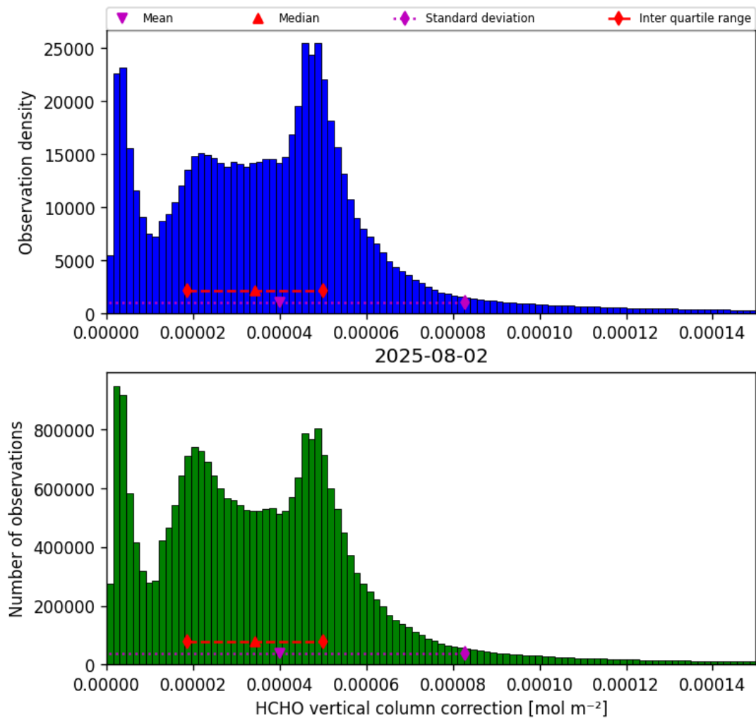
Figure 37: Histogram of “HCHO vertical column correction” for 2025-08-01 to 2025-08-03
