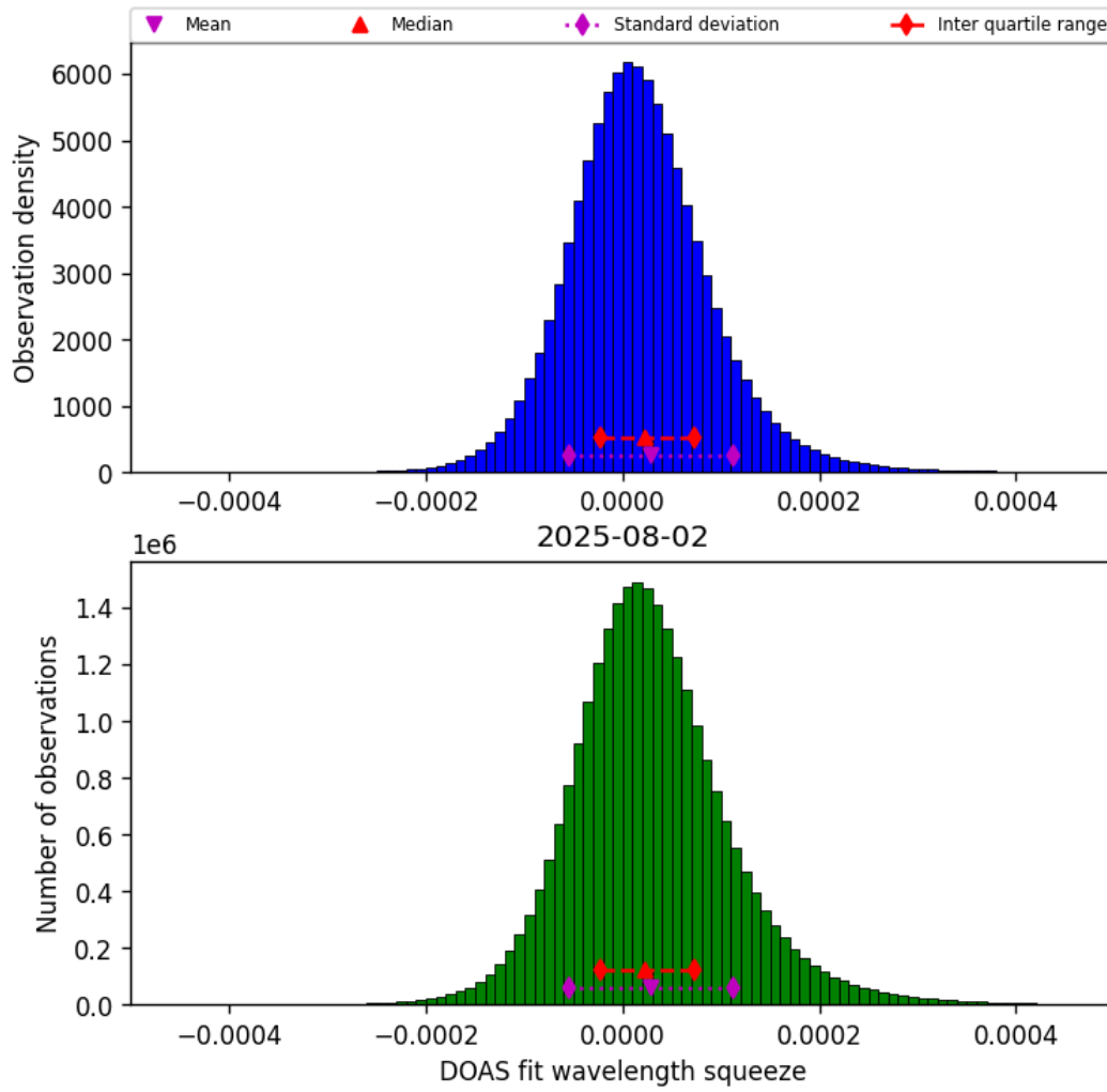
Figure 45: Histogram of “DOAS fit wavelength squeeze” for 2025-08-01 to 2025-08-03
