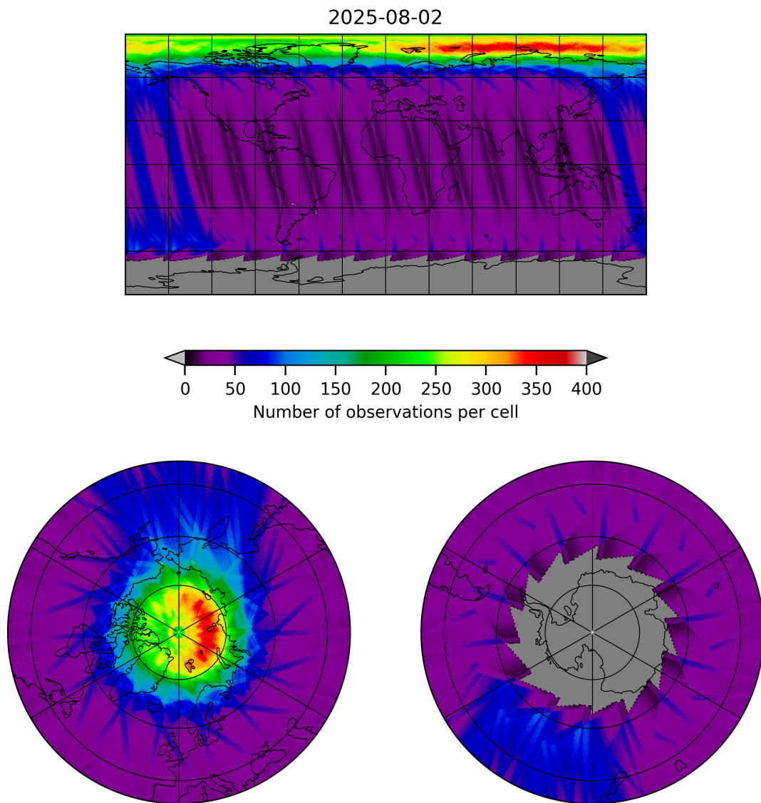
Figure 19: Map of the number of observations for 2025-08-01 to 2025-08-03
