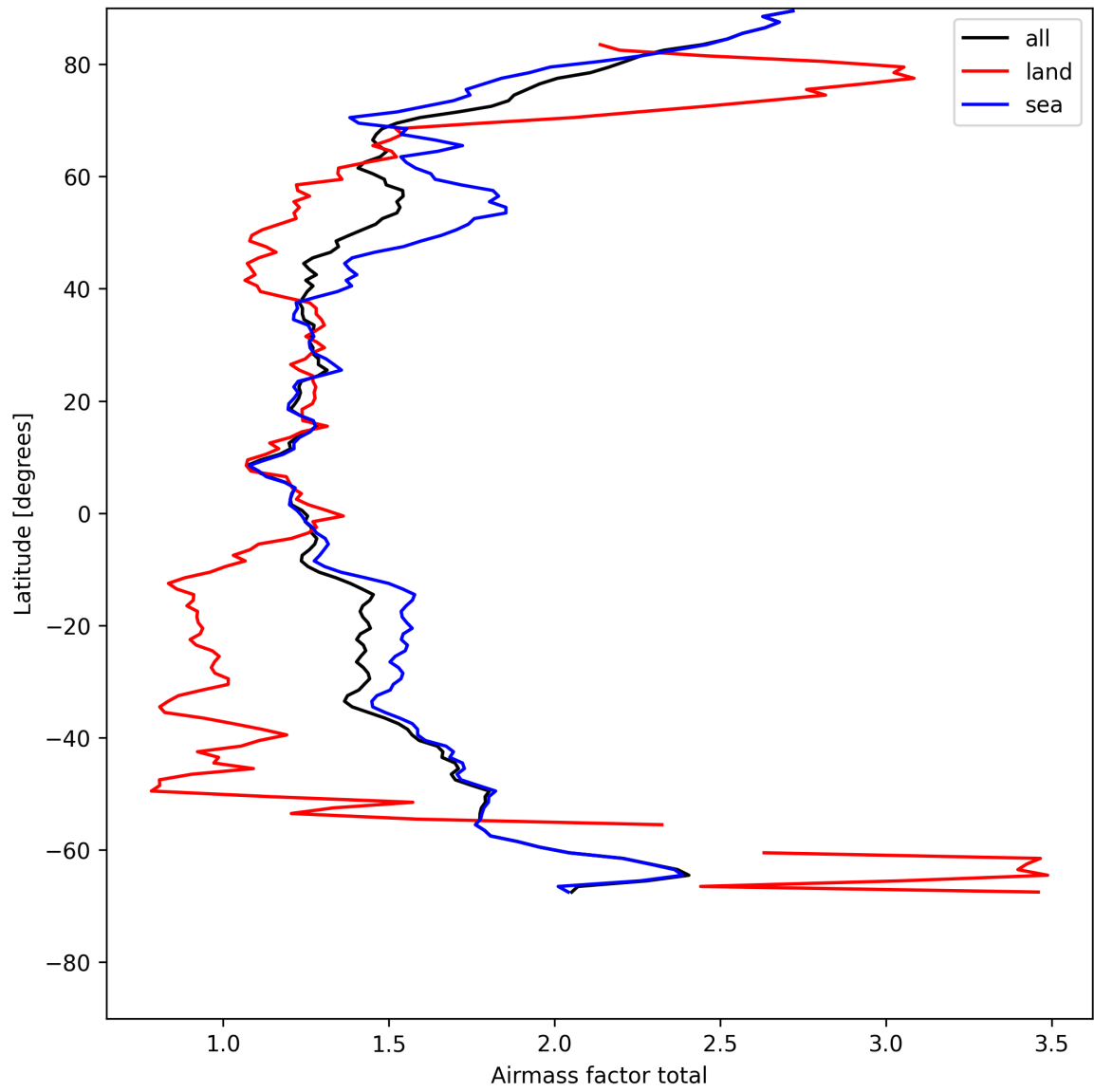
Figure 26: Zonal average of “Airmass factor total” for 2025-08-01 to 2025-08-03.
