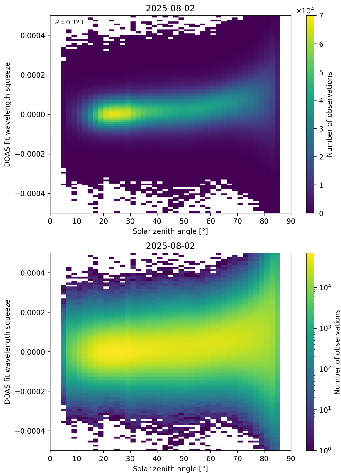
Figure 169: Scatter density plot of “Solar zenith angle” against “DOAS fit wavelength squeeze” for 2025-08-01 to 2025-08-03.
