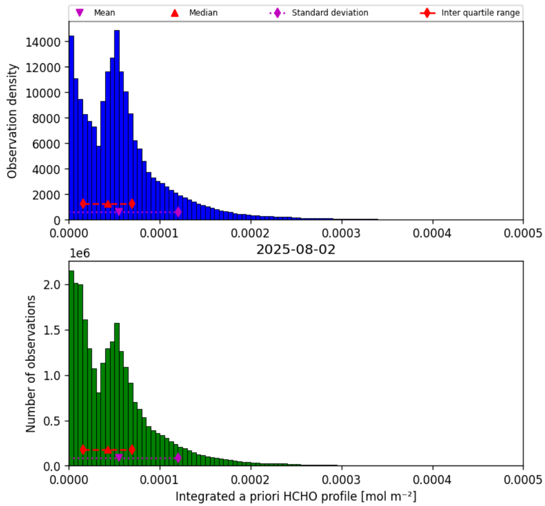
Figure 43: Histogram of “Integrated a priori HCHO profile” for 2025-08-01 to 2025-08-03
