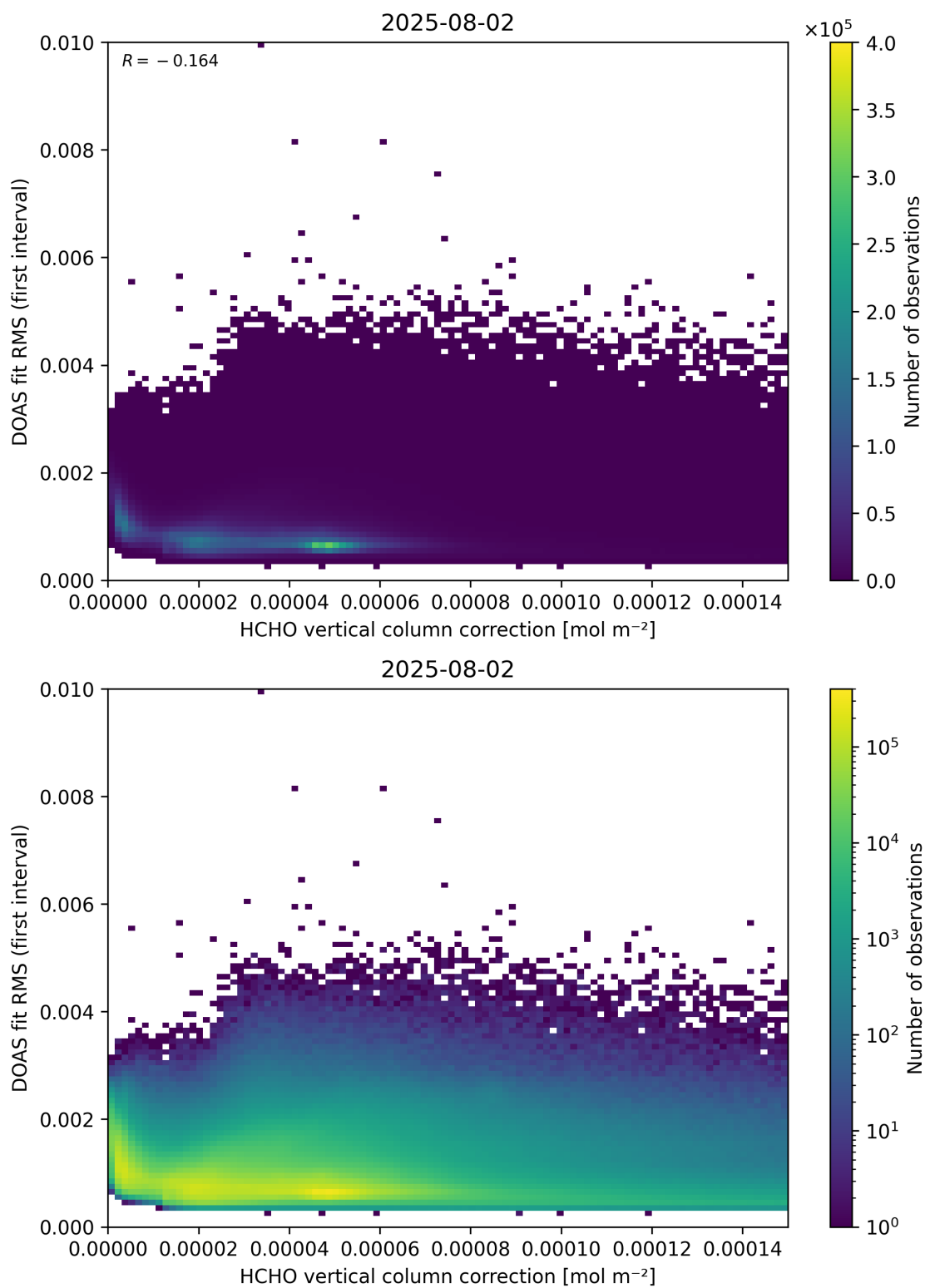
Figure 112: Scatter density plot of “HCHO vertical column correction” against “DOAS fit RMS (first interval)” for 2025-08-01 to 2025-08-03.
