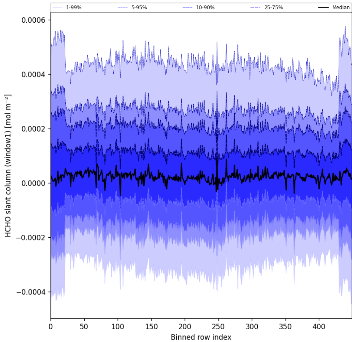
Figure 52: Along track statistics of “HCHO slant column (window1)” for 2025-08-01 to 2025-08-03
