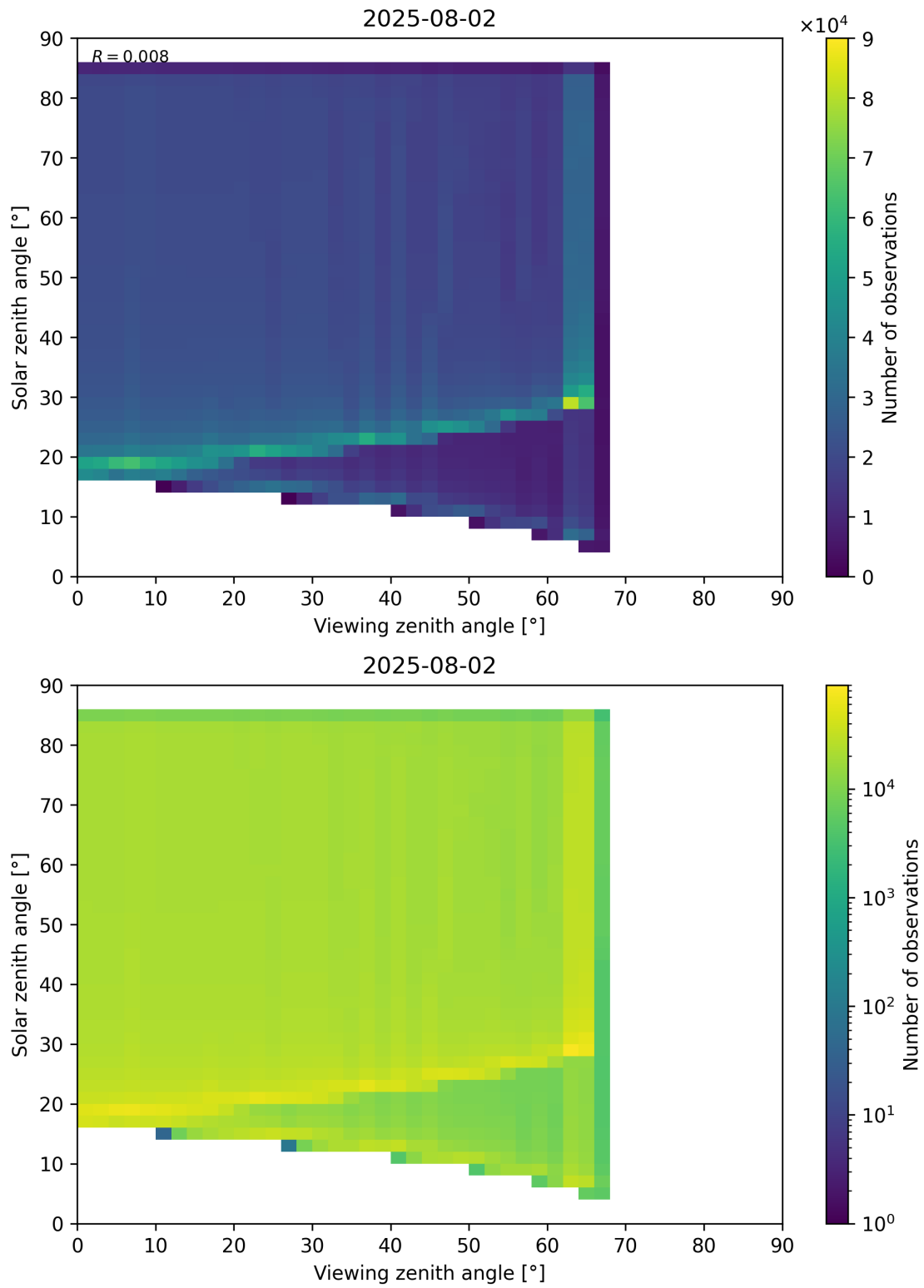
Figure 197: Scatter density plot of “Viewing zenith angle” against “Solar zenith angle” for 2025-08-01 to 2025-08-03.
