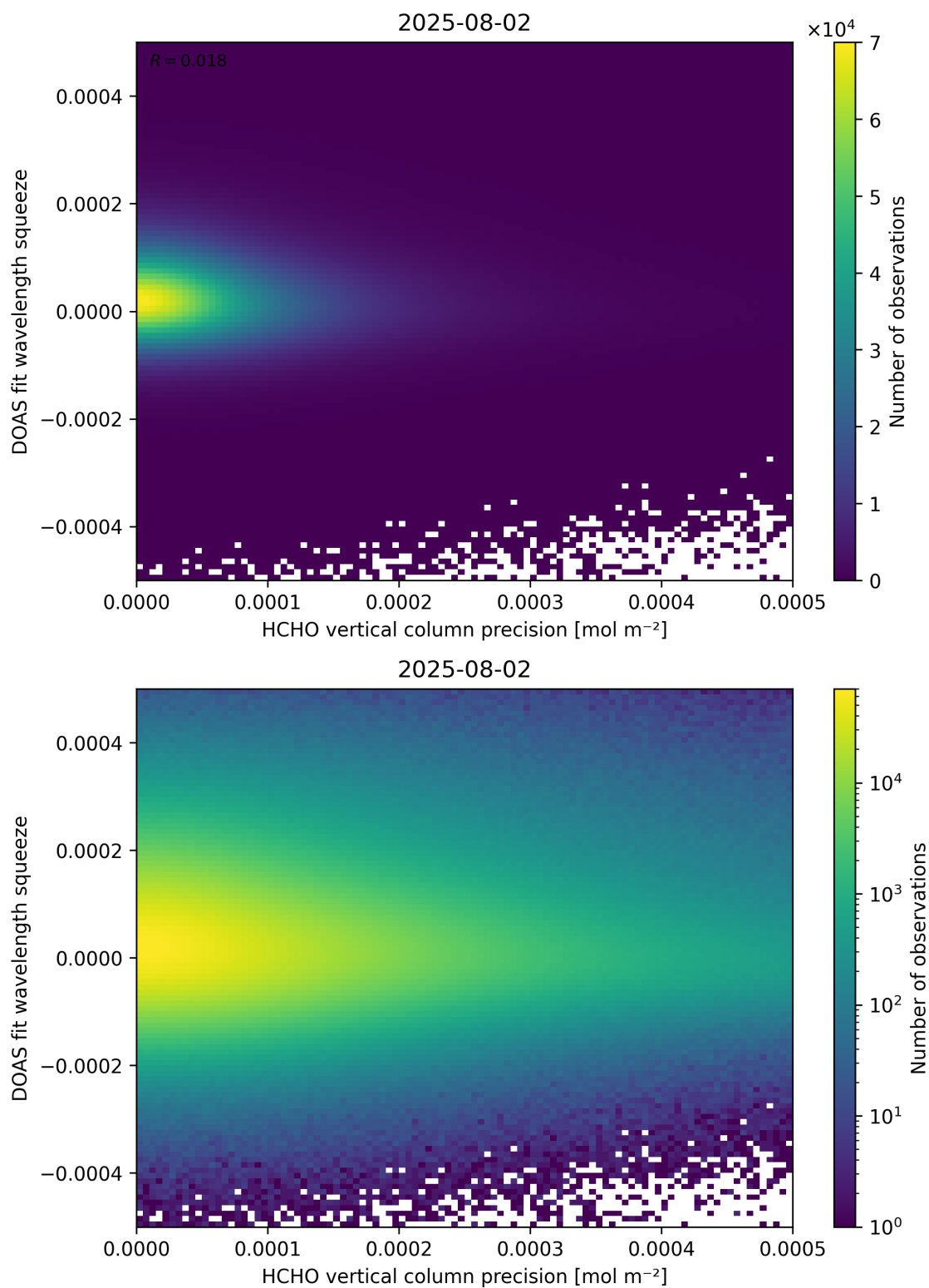
Figure 138: Scatter density plot of “HCHO vertical column precision” against “DOAS fit wavelength squeeze” for 2025-08-01 to 2025-08-03.
