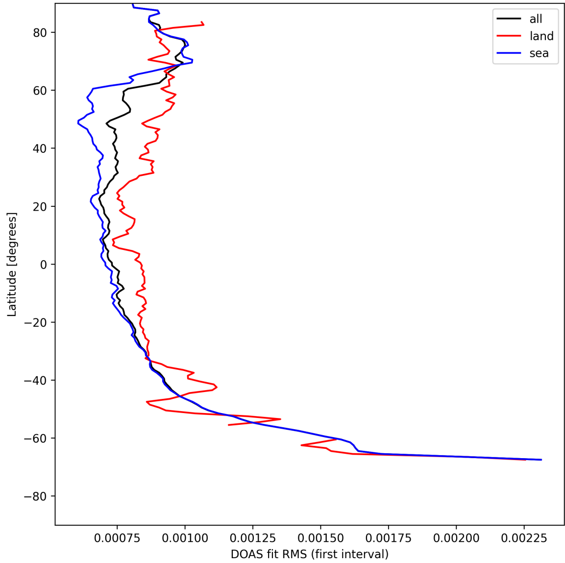
Figure 32: Zonal average of "DOAS fit RMS (first interval)" for 2025-08-01 to 2025-08-03.
