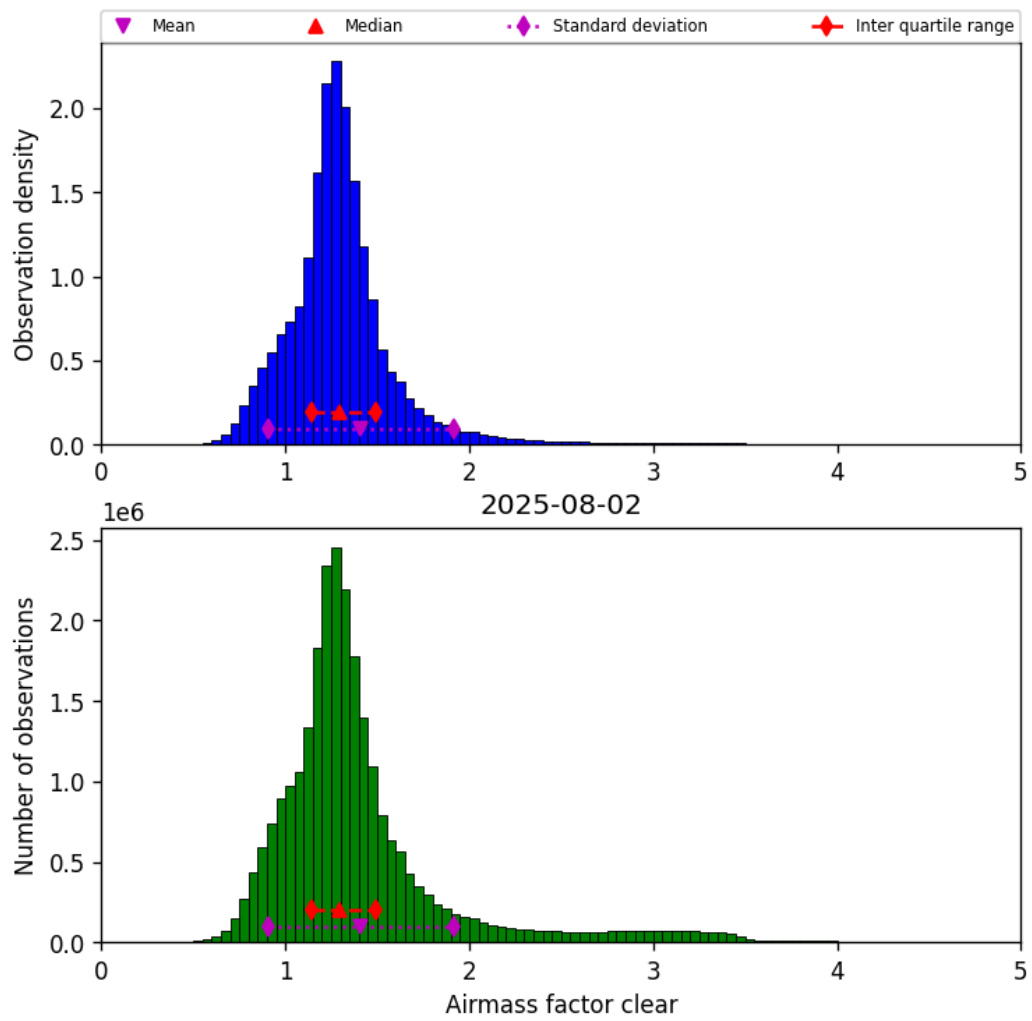
Figure 42: Histogram of “Airmass factor clear” for 2025-08-01 to 2025-08-03
