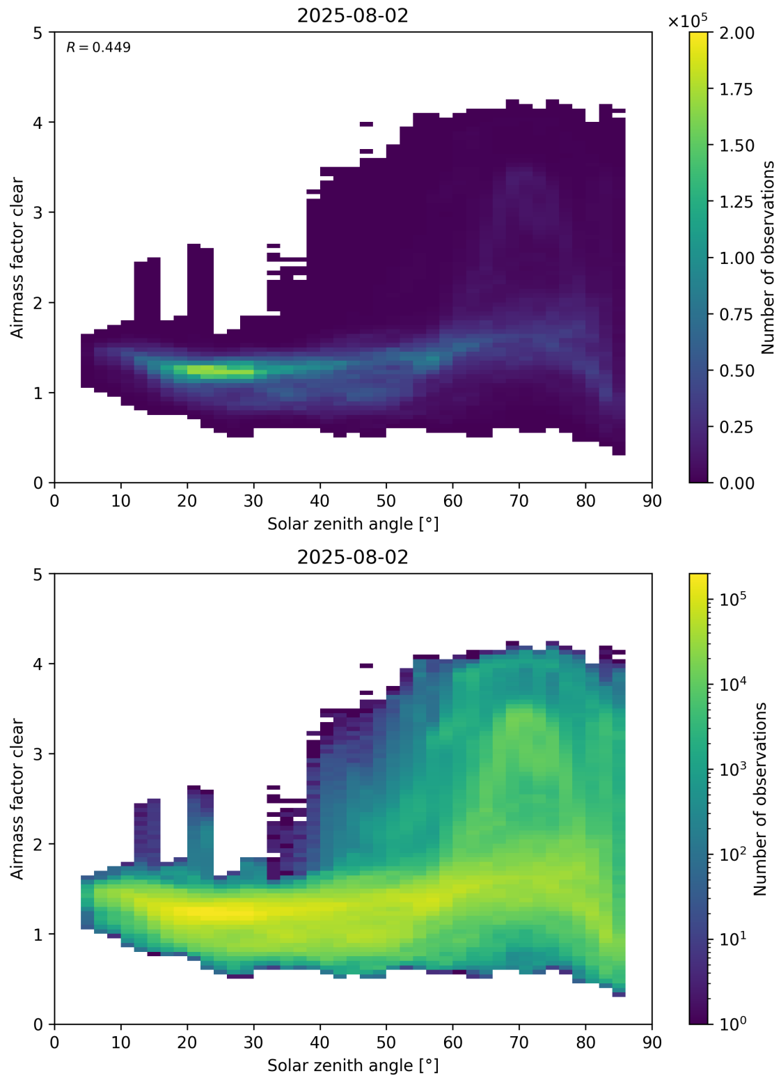
Figure 170: Scatter density plot of “Solar zenith angle” against “Airmass factor clear” for 2025-08-01 to 2025-08-03.
