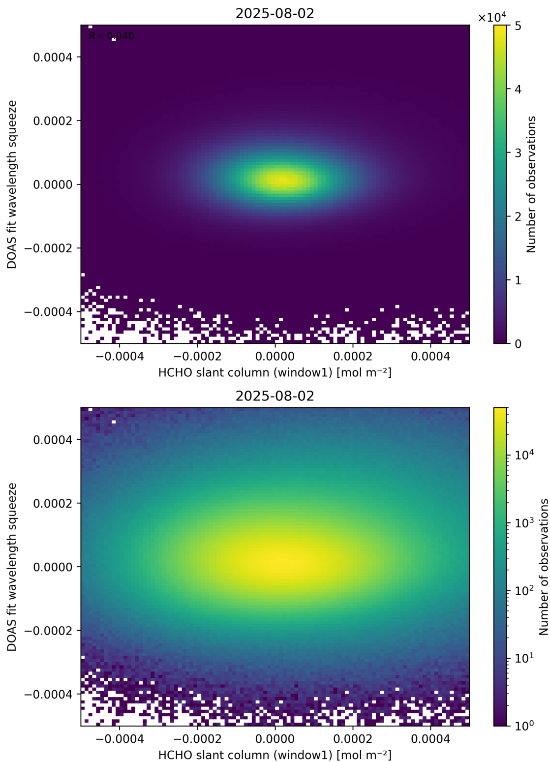
Figure 80: Scatter density plot of “HCHO slant column (window1)” against “DOAS fit wavelength squeeze” for 2025-08-01 to 2025-08-03.
