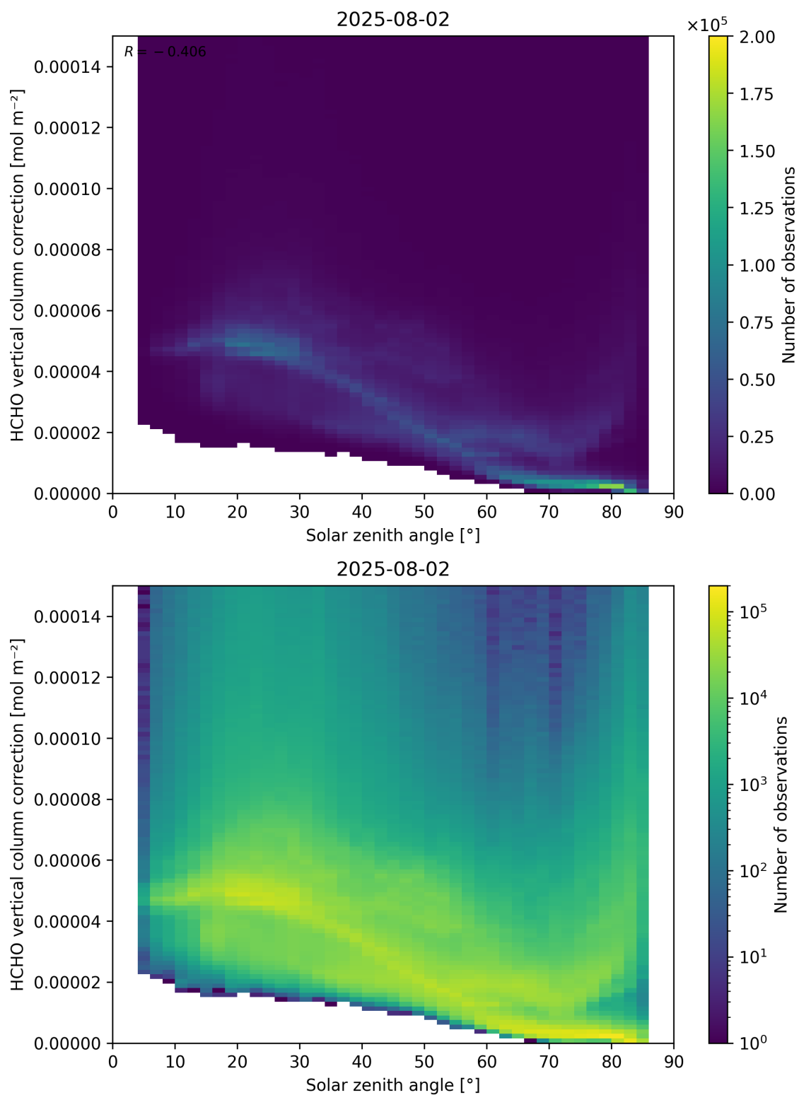
Figure 178: Scatter density plot of “Solar zenith angle” against “HCHO vertical column correction” for 2025-08-01 to 2025-08-03.
