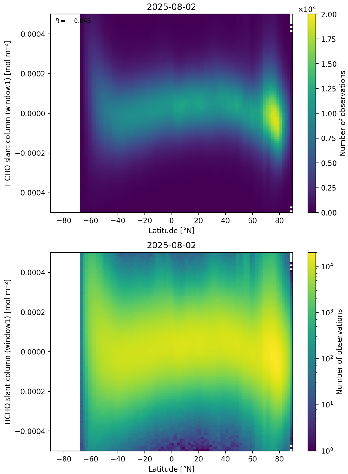
Figure 159: Scatter density plot of “Latitude” against “HCHO slant column (window1)” for 2025-08-01 to 2025-08-03.
