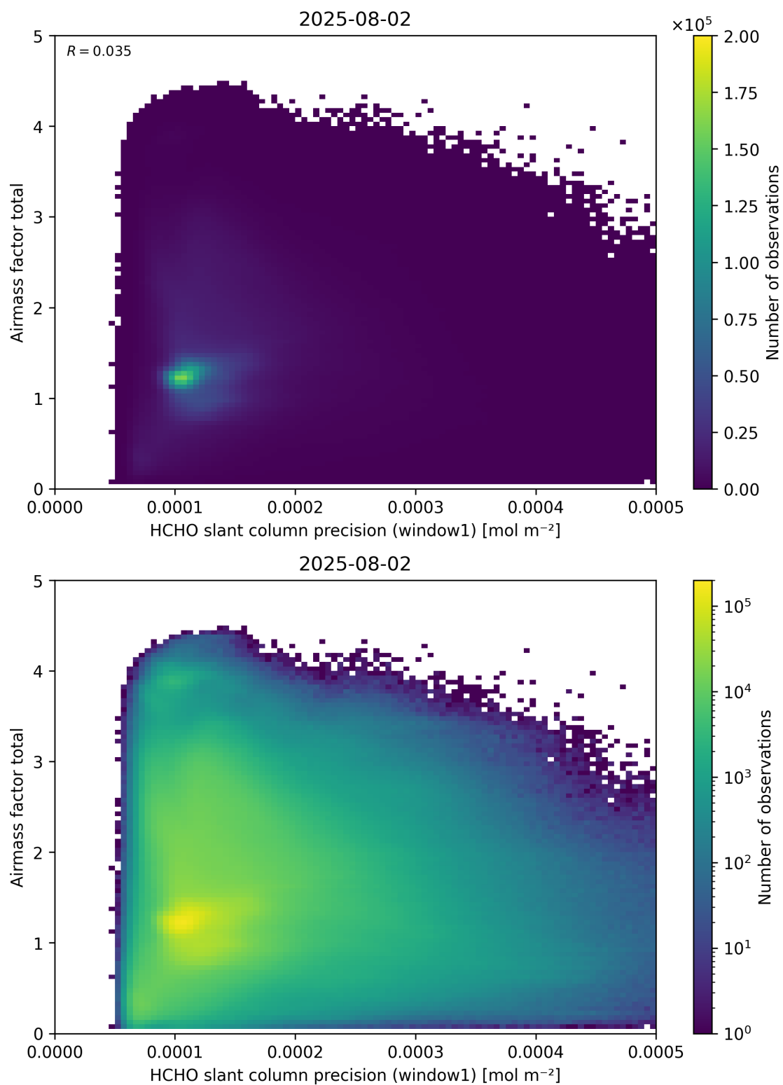
Figure 94: Scatter density plot of “HCHO slant column precision (window1)” against “Airmass factor total” for 2025-08-01 to 2025-08-03.
