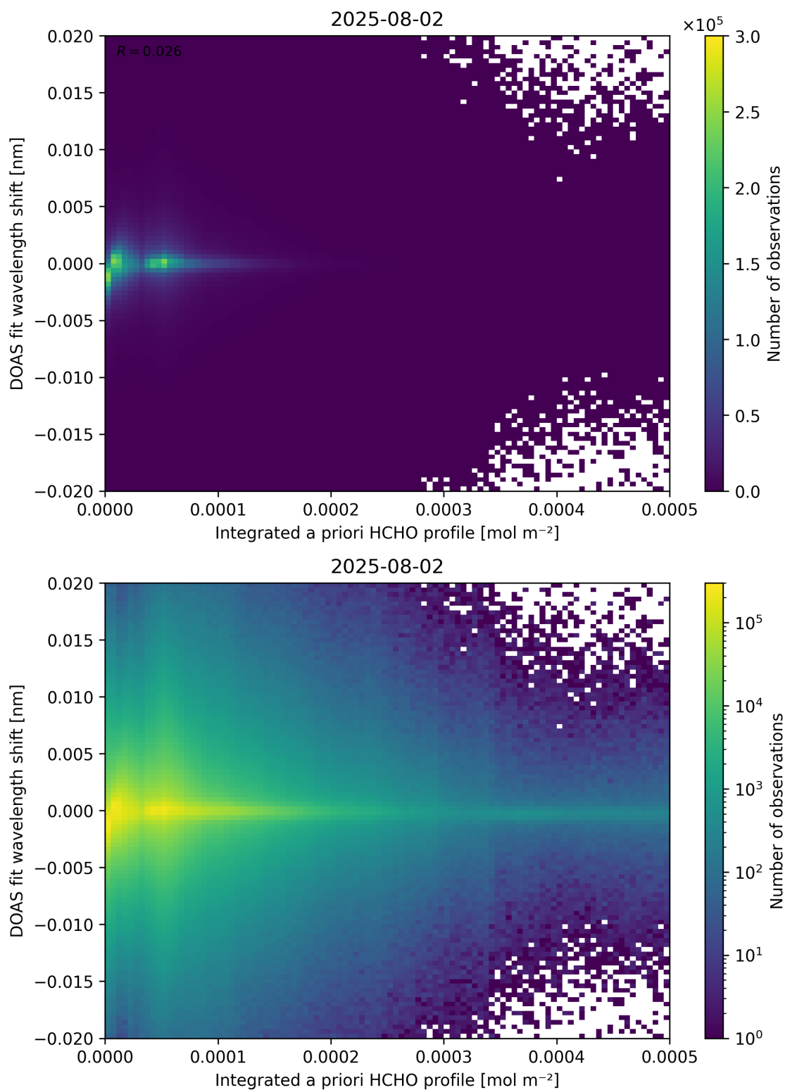
Figure 149: Scatter density plot of “Integrated a priori HCHO profile” against “DOAS fit wavelength shift” for 2025-08-01 to 2025-08-03.
