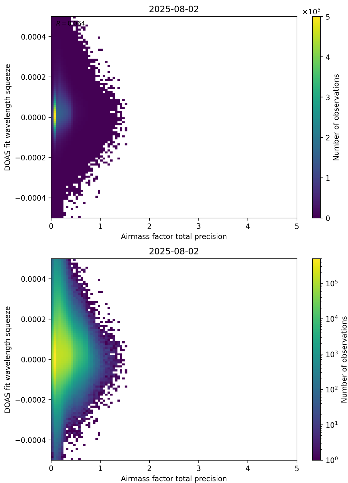
Figure 107: Scatter density plot of “Airmass factor total precision” against “DOAS fit wavelength squeeze” for 2025-08-01 to 2025-08-03.
