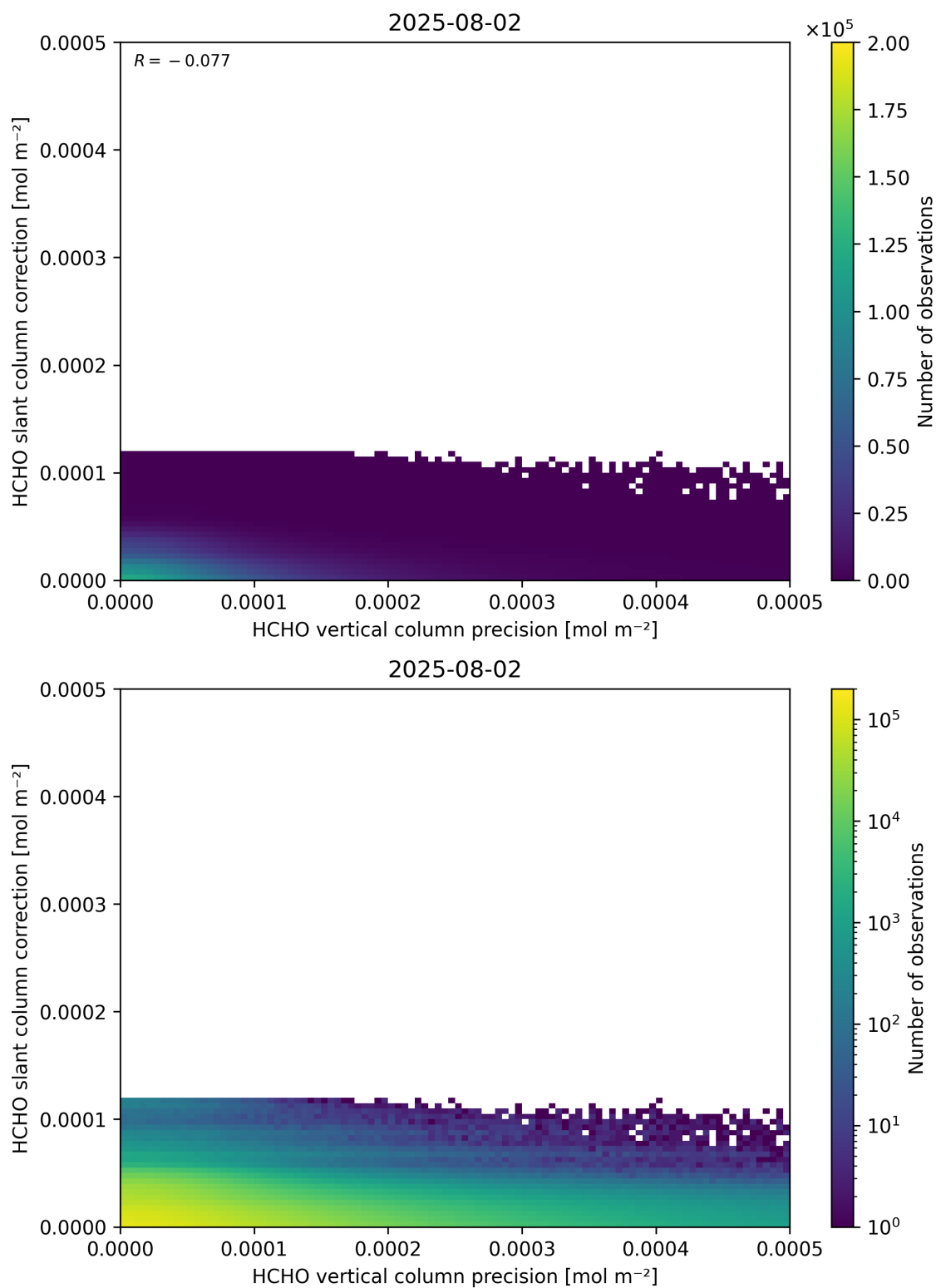
Figure 141: Scatter density plot of “HCHO vertical column precision” against “HCHO slant column correction” for 2025-08-01 to 2025-08-03.
