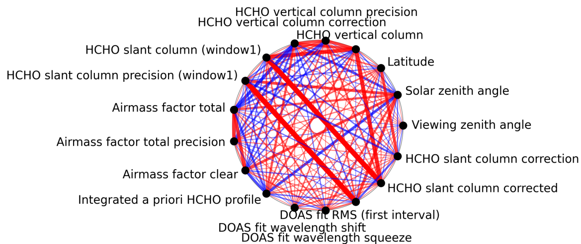
Figure 1: Map of correlation graph for 2025-08-01 to 2025-08-03.
