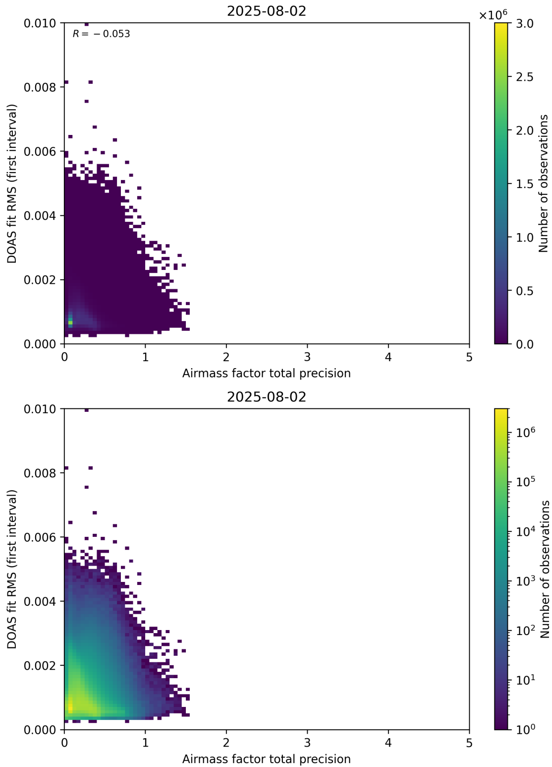
Figure 105: Scatter density plot of “Airmass factor total precision” against “DOAS fit RMS (first interval)” for 2025-08-01 to 2025-08-03.
