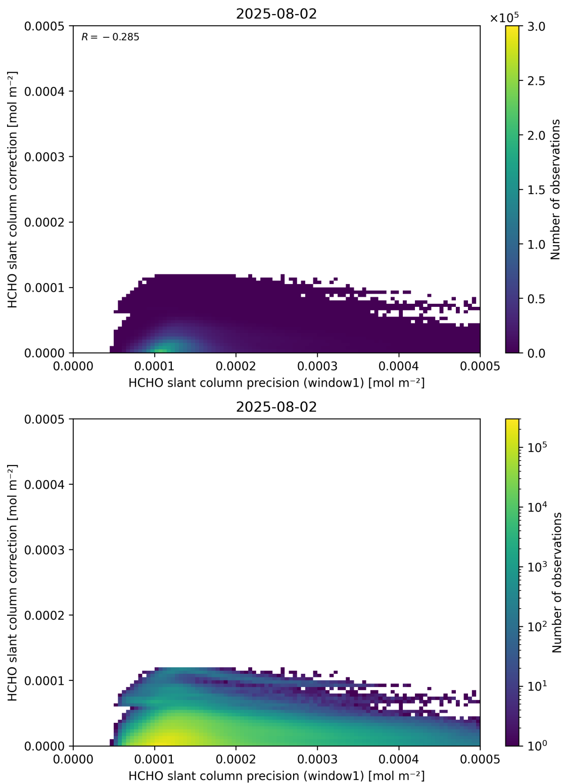
Figure 93: Scatter density plot of “HCHO slant column precision (window1)” against “HCHO slant column correction” for 2025-08-01 to 2025-08-03.
