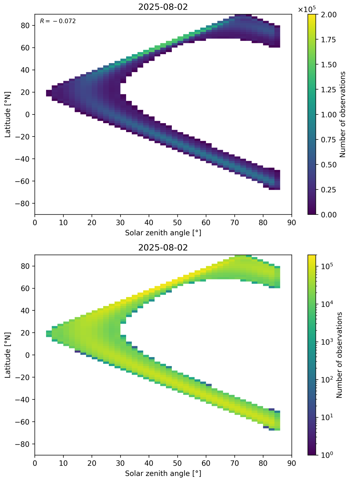
Figure 181: Scatter density plot of “Solar zenith angle” against “Latitude” for 2025-08-01 to 2025-08-03.
