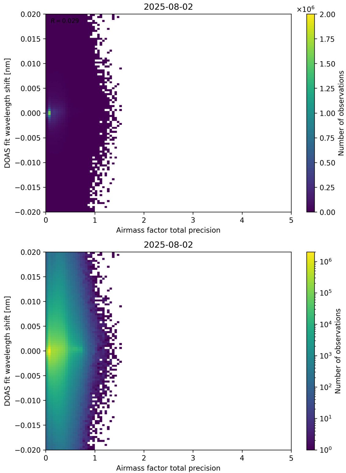
Figure 106: Scatter density plot of “Airmass factor total precision” against “DOAS fit wavelength shift” for 2025-08-01 to 2025-08-03.
