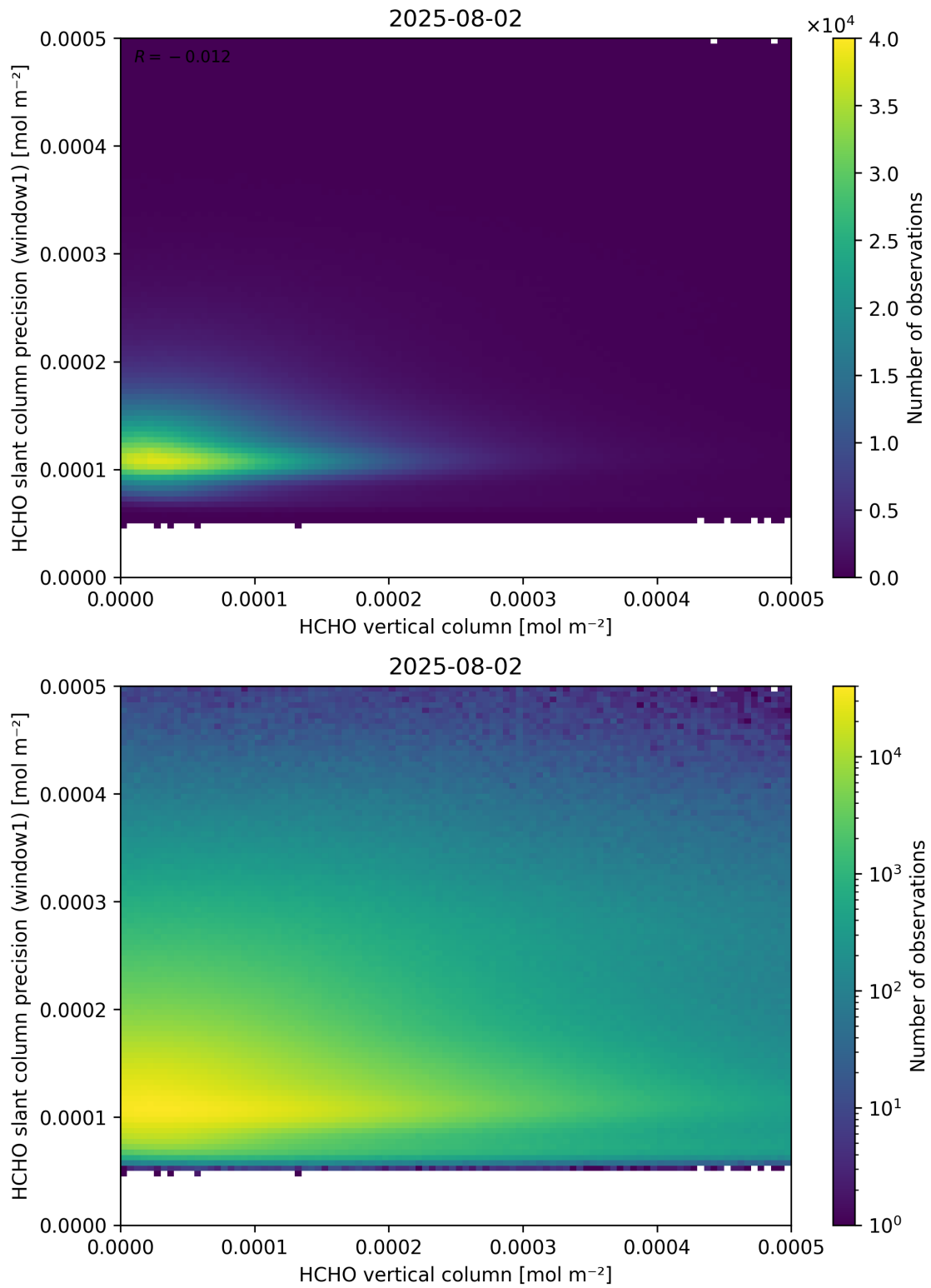
Figure 130: Scatter density plot of “HCHO vertical column” against “HCHO slant column precision (window1)” for 2025-08-01 to 2025-08-03.
