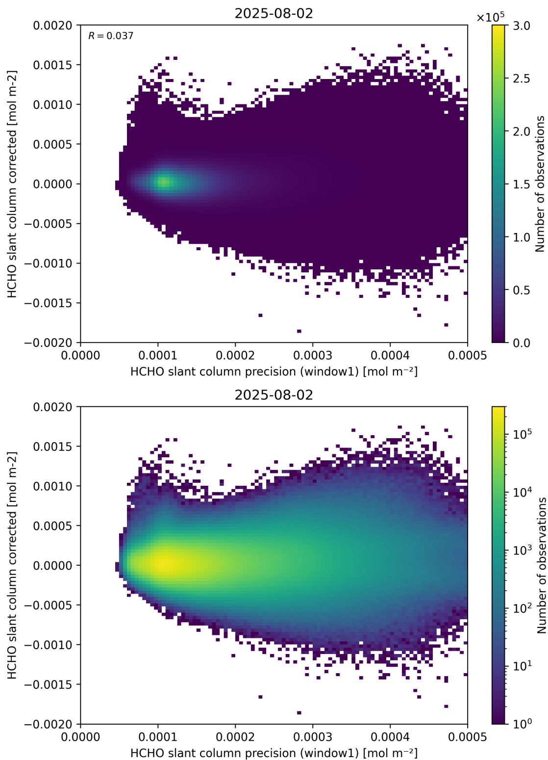
Figure 92: Scatter density plot of “HCHO slant column precision (window1)” against “HCHO slant column corrected” for 2025-08-01 to 2025-08-03.
