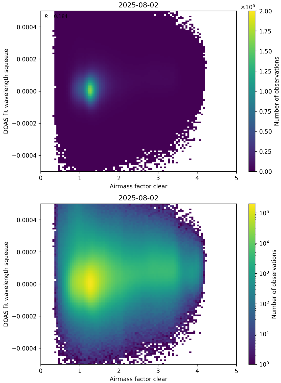
Figure 73: Scatter density plot of “Airmass factor clear” against “DOAS fit wavelength squeeze” for 2025-08-01 to 2025-08-03.
