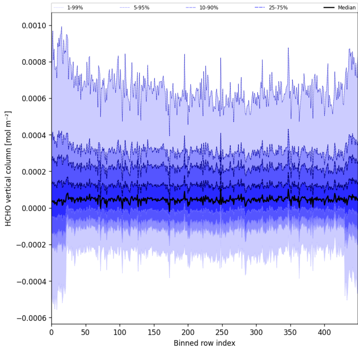
Figure 49: Along track statistics of “HCHO vertical column” for 2025-08-01 to 2025-08-03
