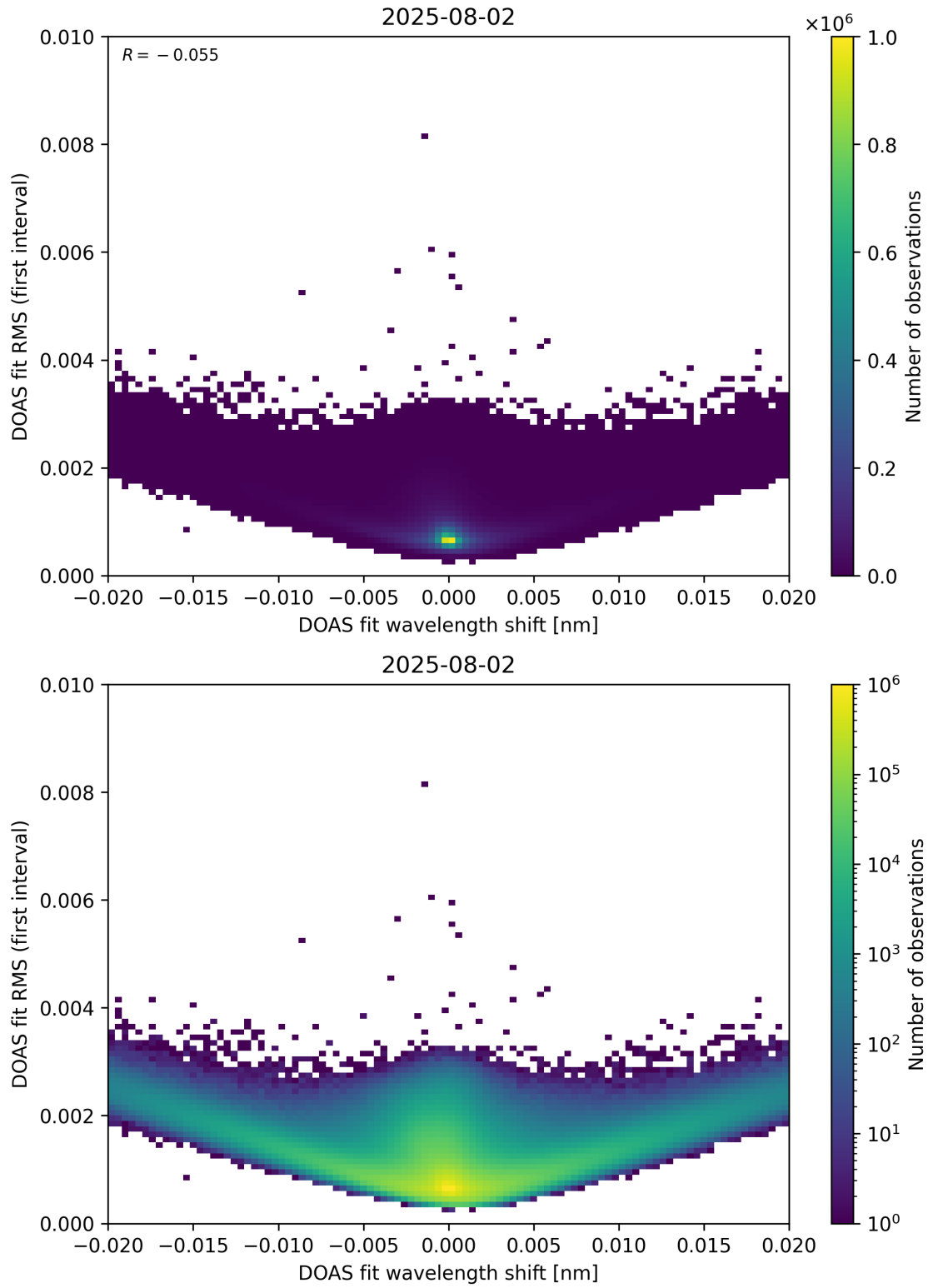
Figure 64: Scatter density plot of “DOAS fit wavelength shift” against “DOAS fit RMS (first interval)” for 2025-08-01 to 2025-08-03.
