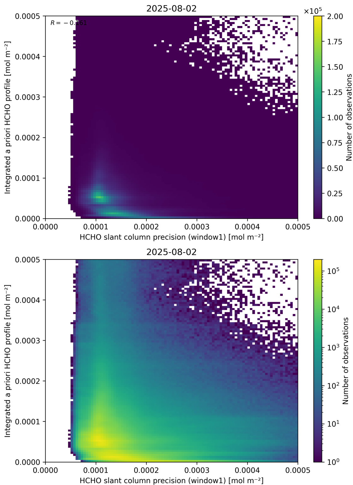
Figure 96: Scatter density plot of “HCHO slant column precision (window1)” against “Integrated a priori HCHO profile” for 2025-08-01 to 2025-08-03.
