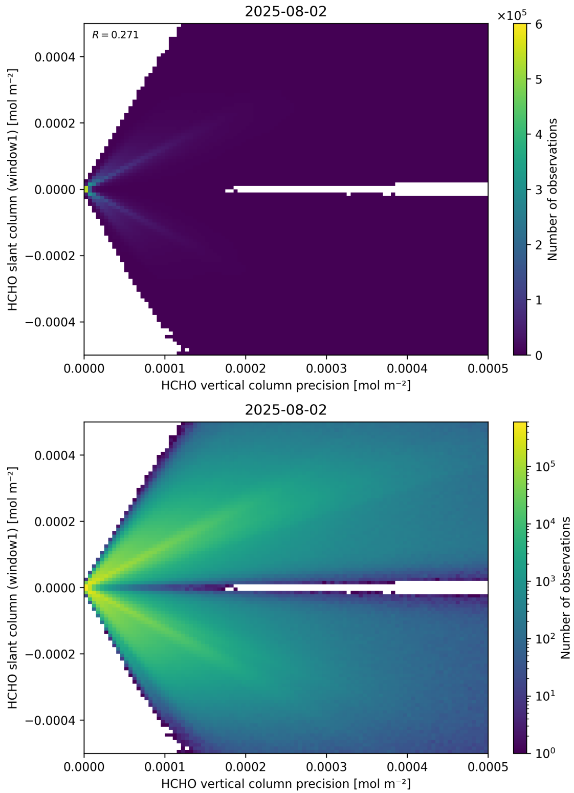
Figure 142: Scatter density plot of “HCHO vertical column precision” against “HCHO slant column (window1)” for 2025-08-01 to 2025-08-03.
