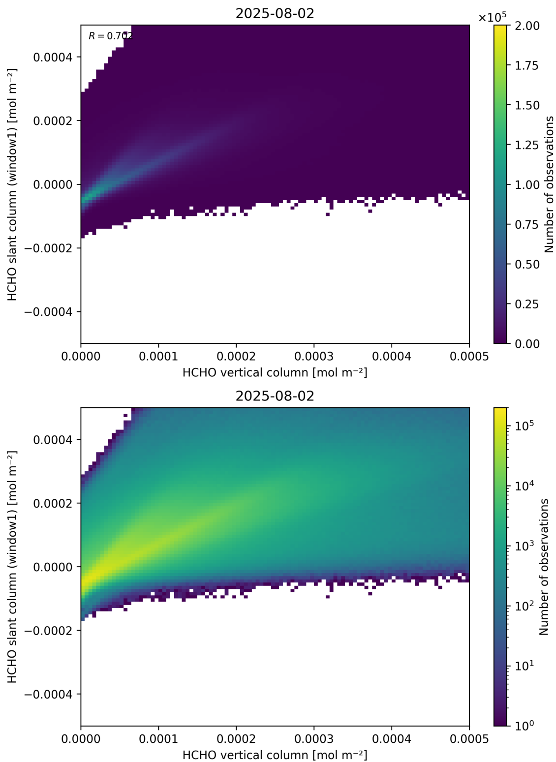
Figure 129: Scatter density plot of “HCHO vertical column” against “HCHO slant column (window1)” for 2025-08-01 to 2025-08-03.
