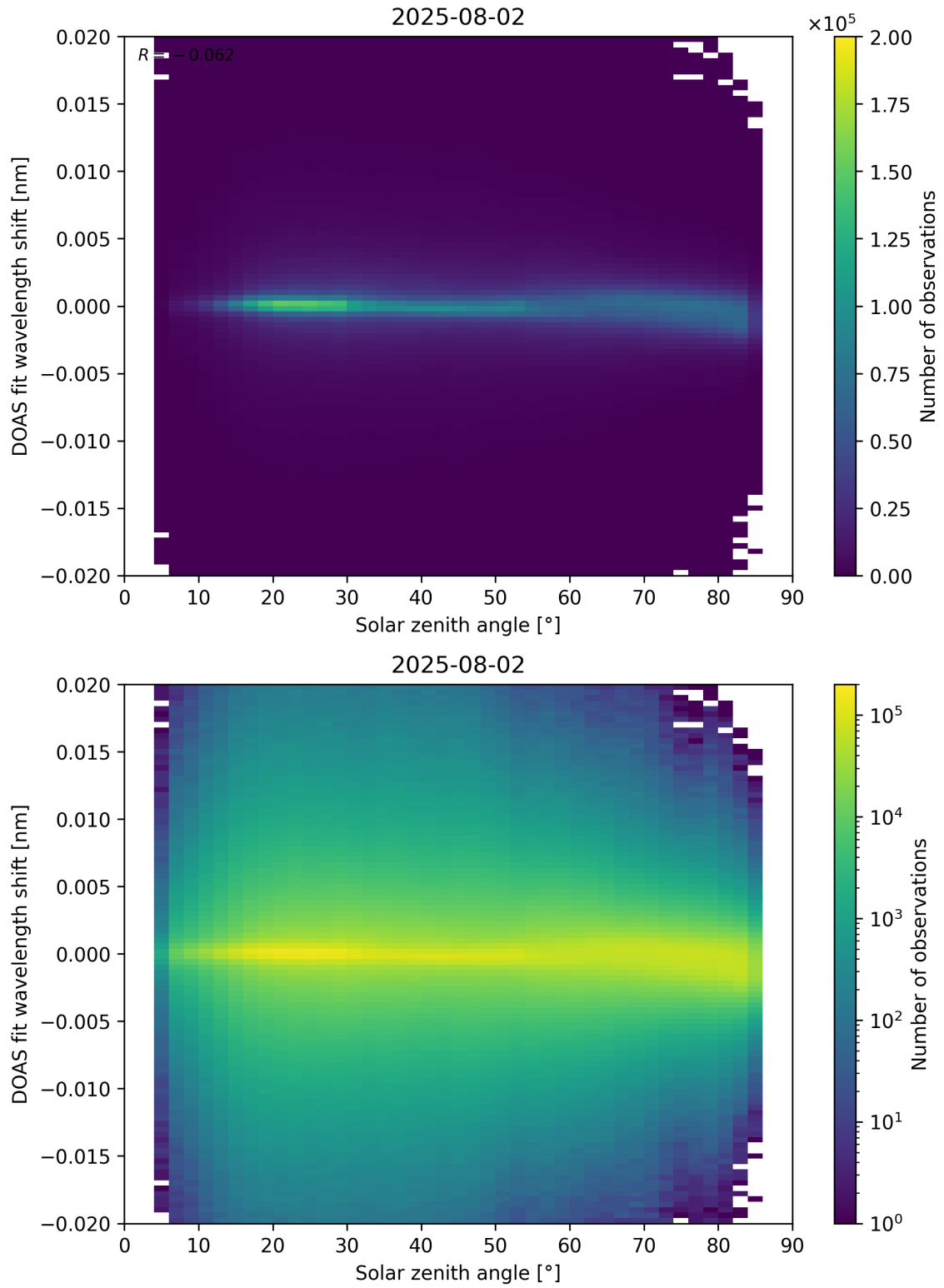
Figure 168: Scatter density plot of “Solar zenith angle” against “DOAS fit wavelength shift” for 2025-08-01 to 2025-08-03.
