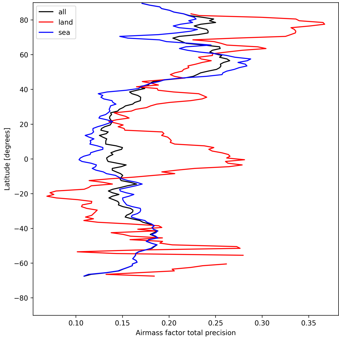
Figure 27: Zonal average of “Airmass factor total precision” for 2025-08-01 to 2025-08-03.
