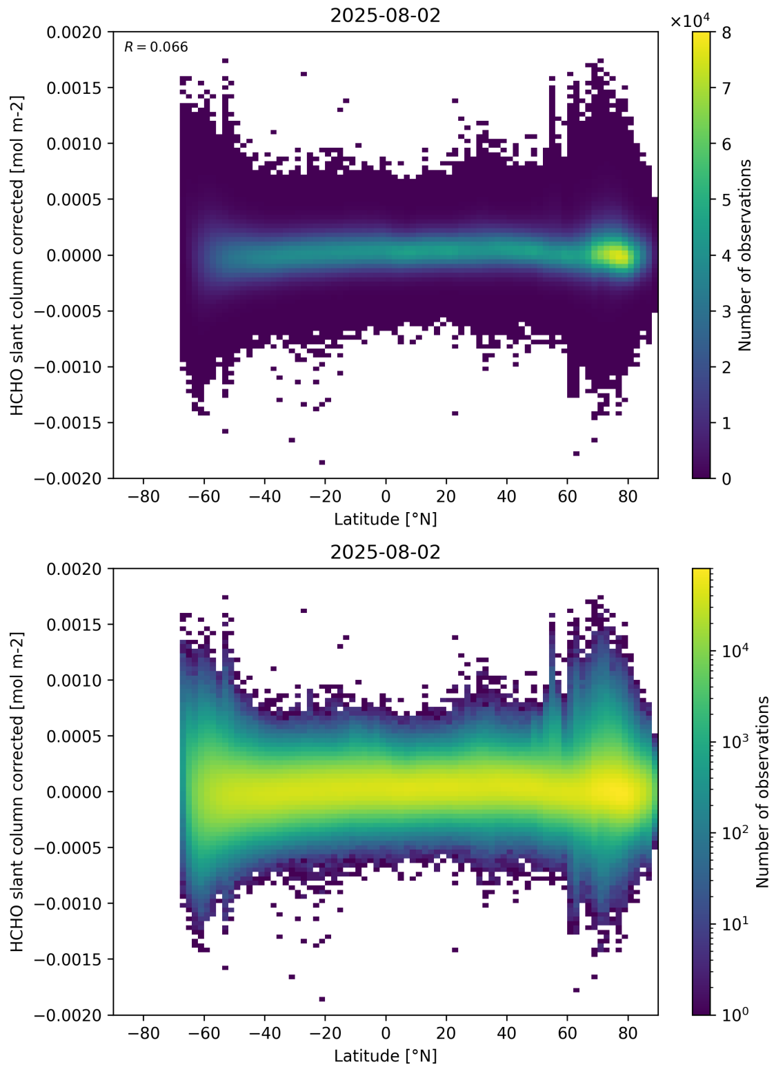
Figure 157: Scatter density plot of “Latitude” against “HCHO slant column corrected” for 2025-08-01 to 2025-08-03.
