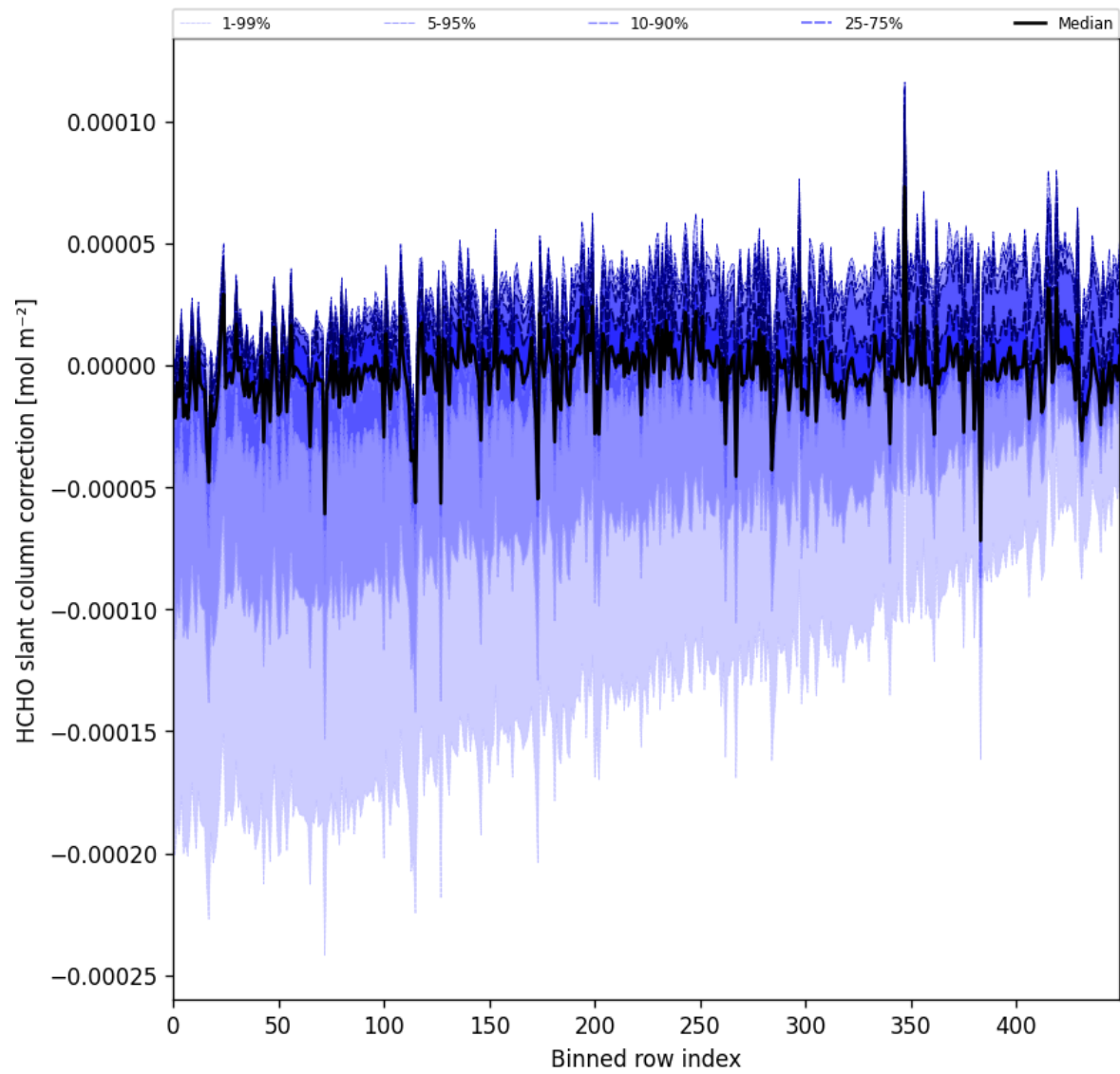
Figure 61: Along track statistics of “HCHO slant column correction” for 2025-08-01 to 2025-08-03
