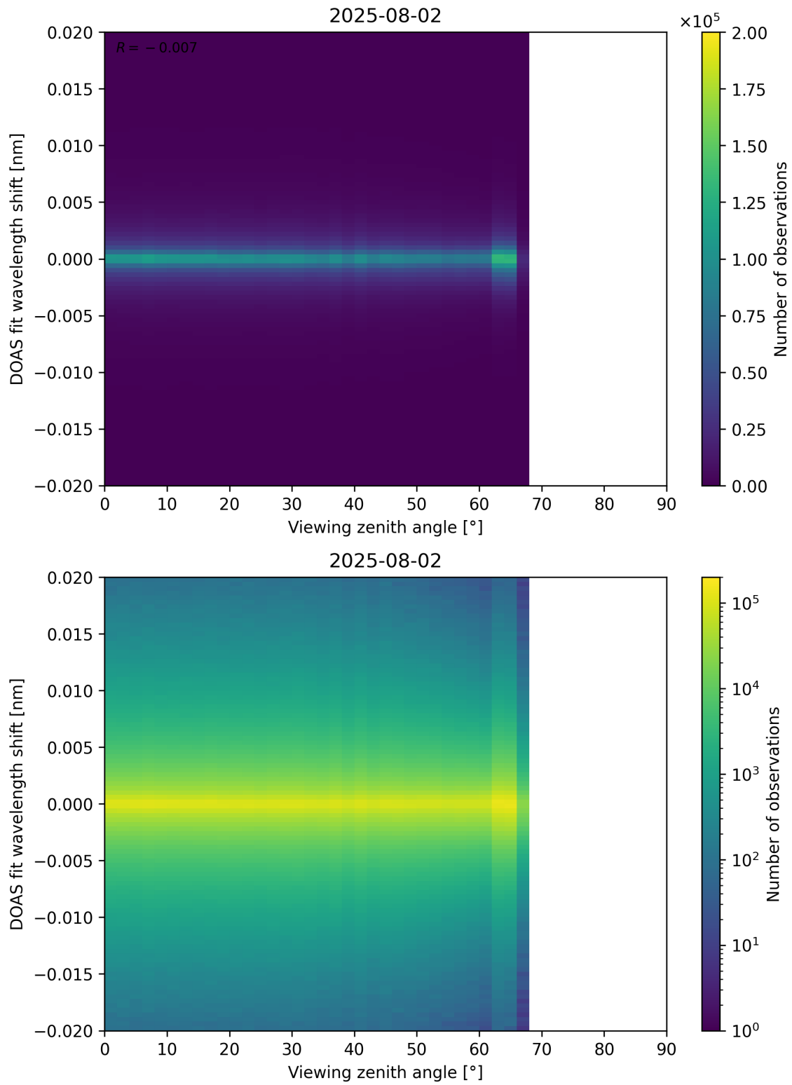
Figure 183: Scatter density plot of “Viewing zenith angle” against “DOAS fit wavelength shift” for 2025-08-01 to 2025-08-03.
