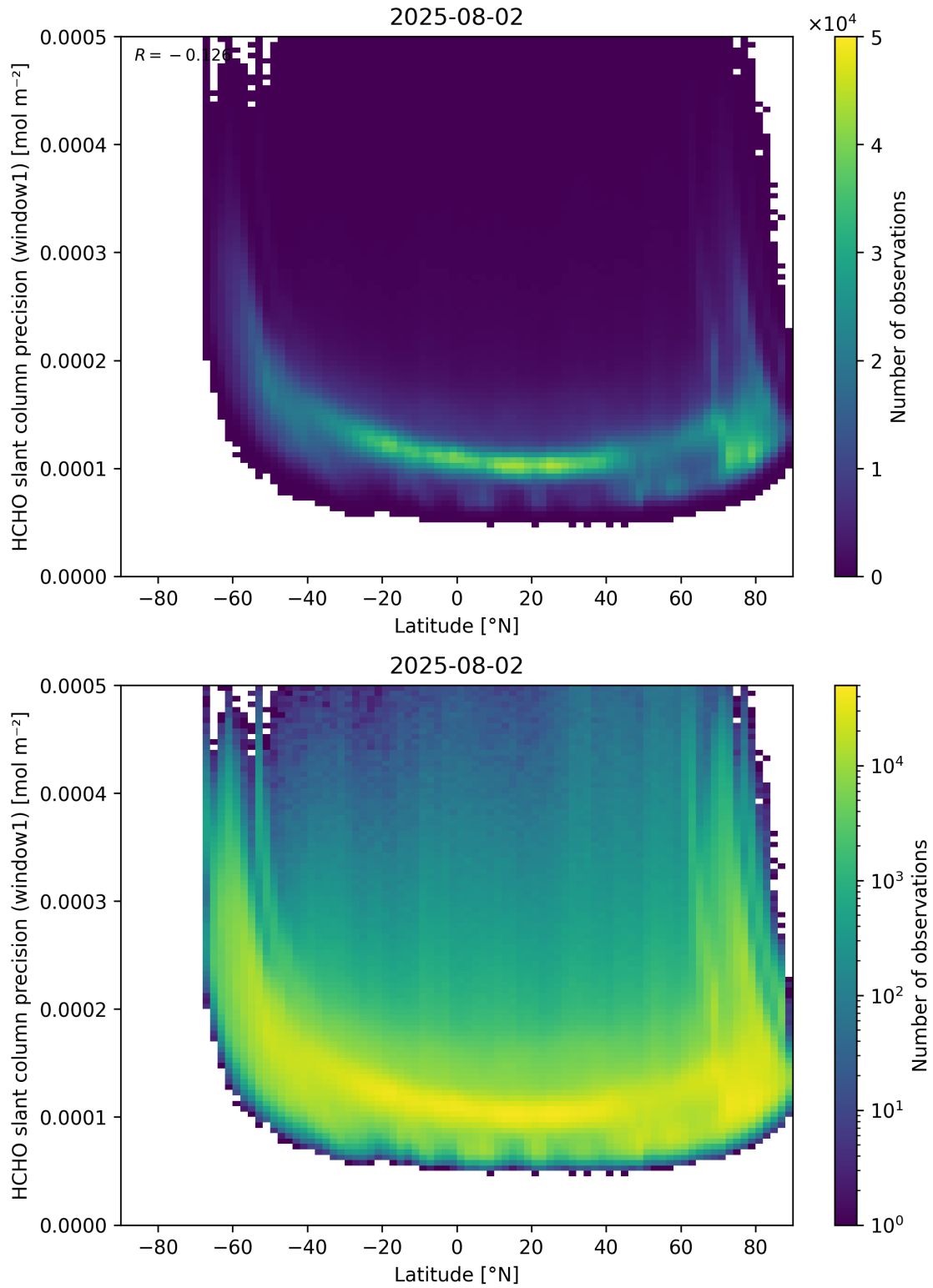
Figure 160: Scatter density plot of “Latitude” against “HCHO slant column precision (window1)” for 2025-08-01 to 2025-08-03.
