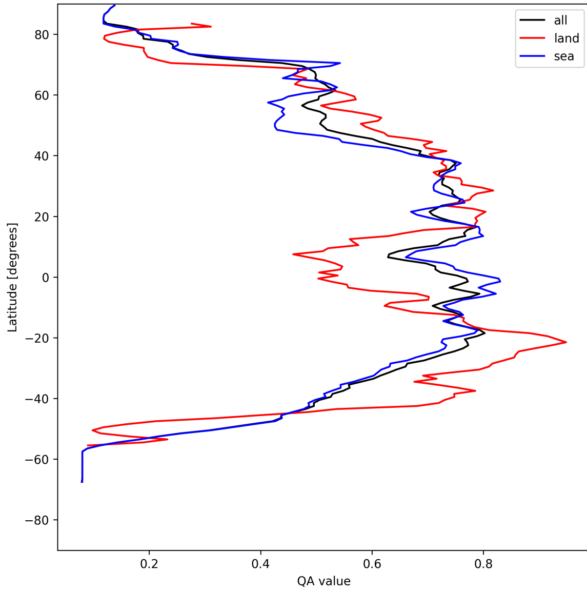
Figure 20: Zonal average of “QA value” for 2025-08-01 to 2025-08-03.
