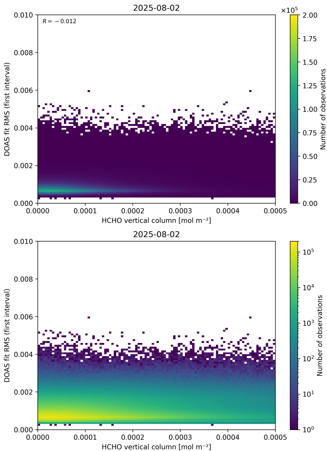
Figure 123: Scatter density plot of “HCHO vertical column” against “DOAS fit RMS (first interval)” for 2025-08-01 to 2025-08-03.
