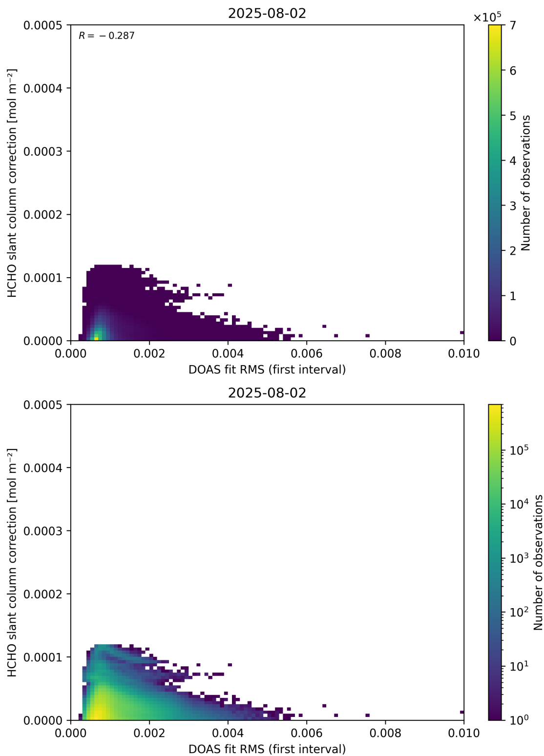
Figure 63: Scatter density plot of “DOAS fit RMS (first interval)” against “HCHO slant column correction” for 2025-08-01 to 2025-08-03.
