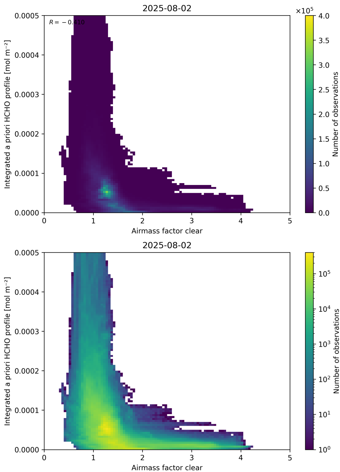
Figure 76: Scatter density plot of “Airmass factor clear” against “Integrated a priori HCHO profile” for 2025-08-01 to 2025-08-03.
