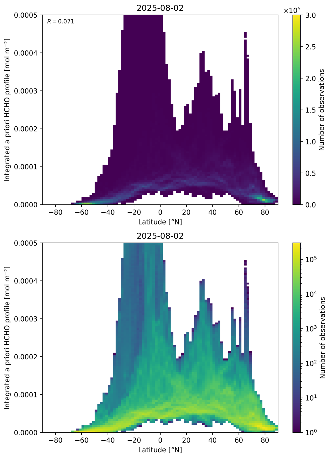
Figure 166: Scatter density plot of “Latitude” against “Integrated a priori HCHO profile” for 2025-08-01 to 2025-08-03.
