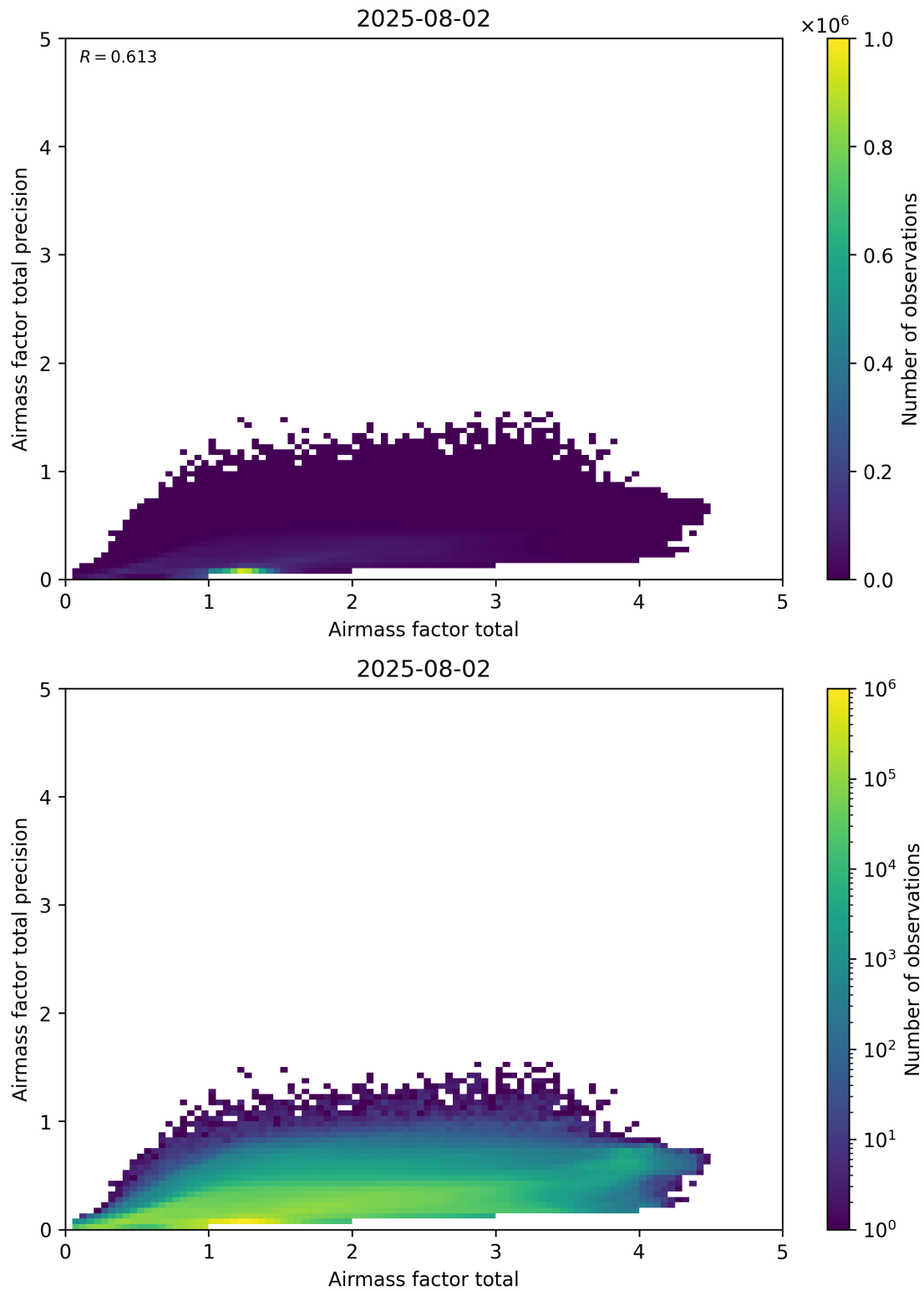
Figure 103: Scatter density plot of “Airmass factor total” against “Airmass factor total precision” for 2025-08-01 to 2025-08-03.
