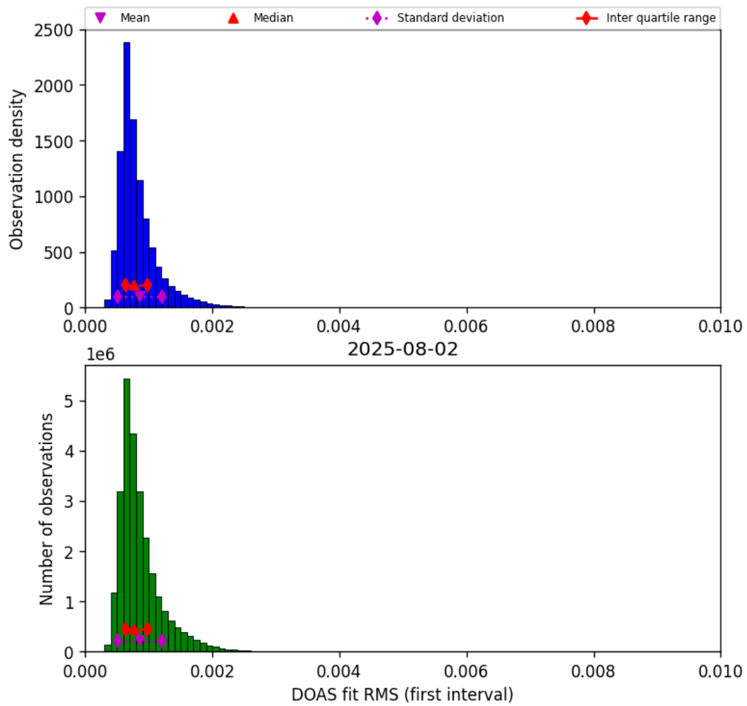
Figure 46: Histogram of “DOAS fit RMS (first interval)” for 2025-08-01 to 2025-08-03
