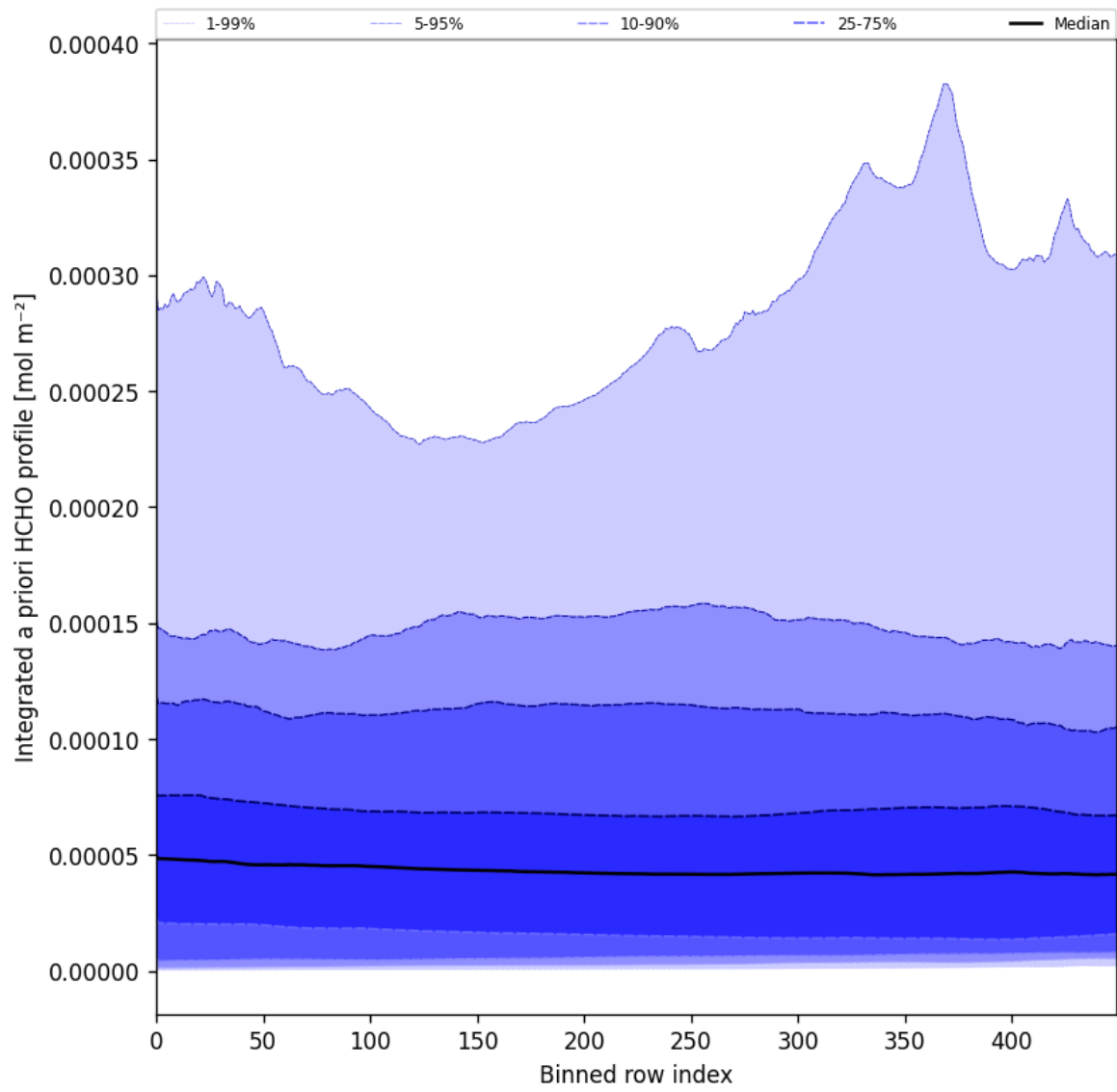
Figure 57: Along track statistics of "Integrated a priori HCHO profile" for 2025-08-01 to 2025-08-03
