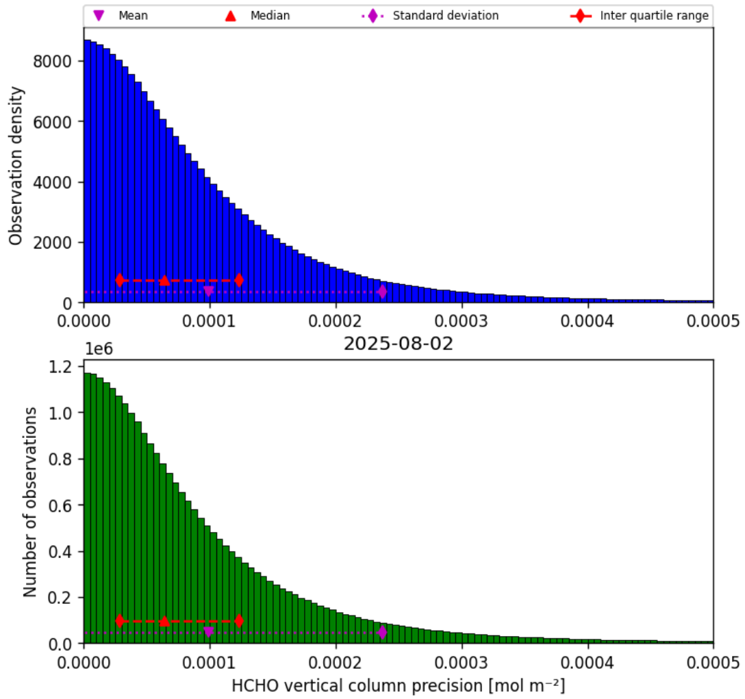
Figure 36: Histogram of “HCHO vertical column precision” for 2025-08-01 to 2025-08-03
