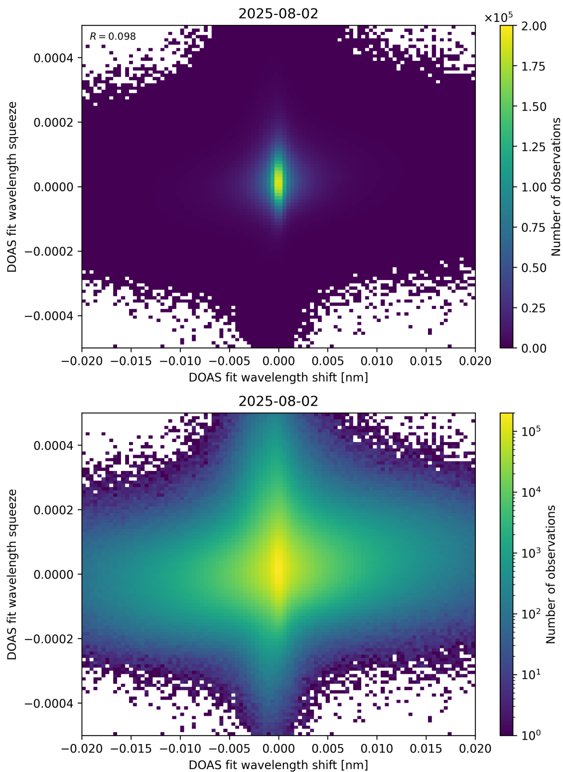
Figure 65: Scatter density plot of “DOAS fit wavelength shift” against “DOAS fit wavelength squeeze” for 2025-08-01 to 2025-08-03.
