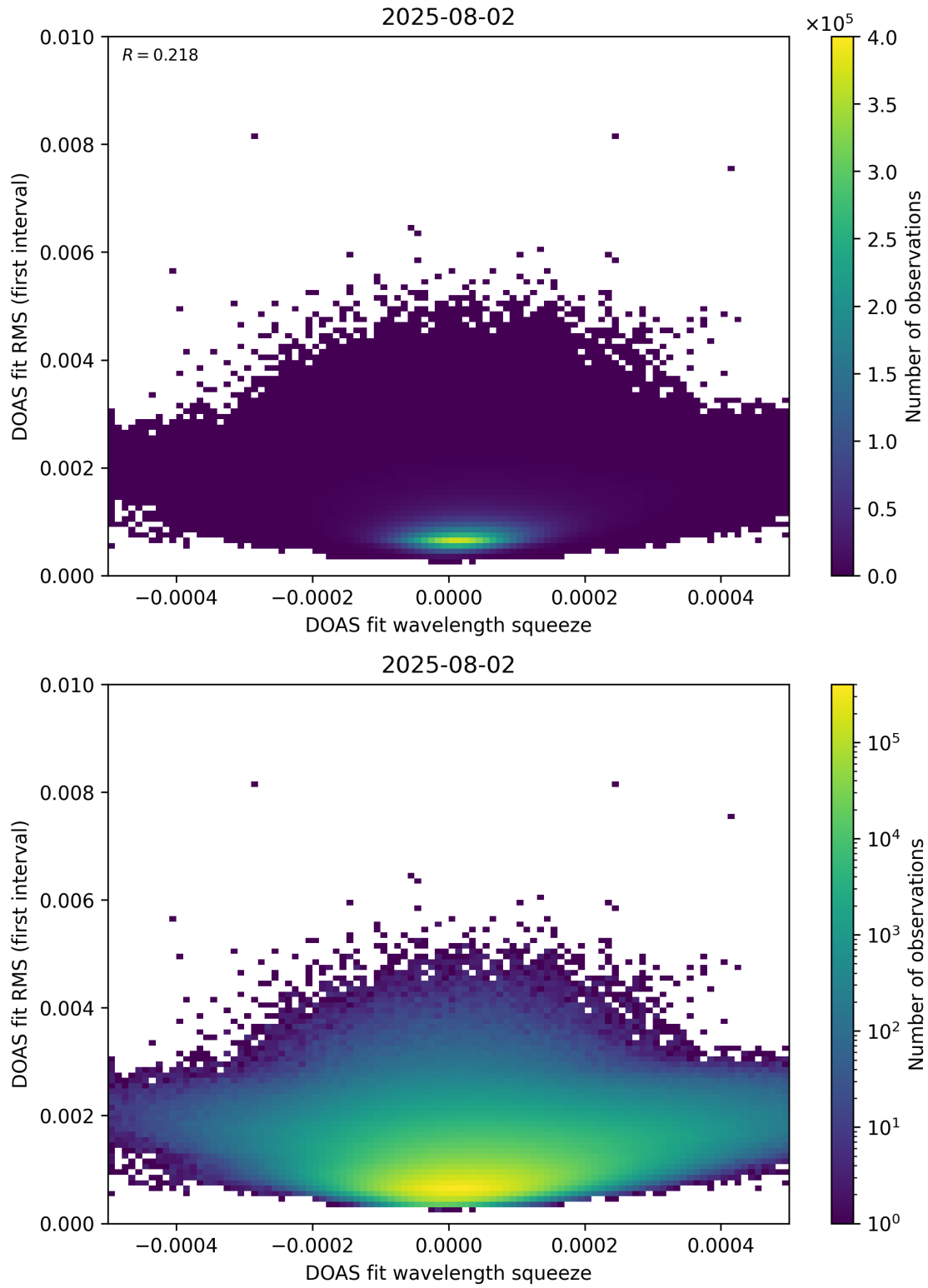
Figure 68: Scatter density plot of “DOAS fit wavelength squeeze” against “DOAS fit RMS (first interval)” for 2025-08-01 to 2025-08-03.
