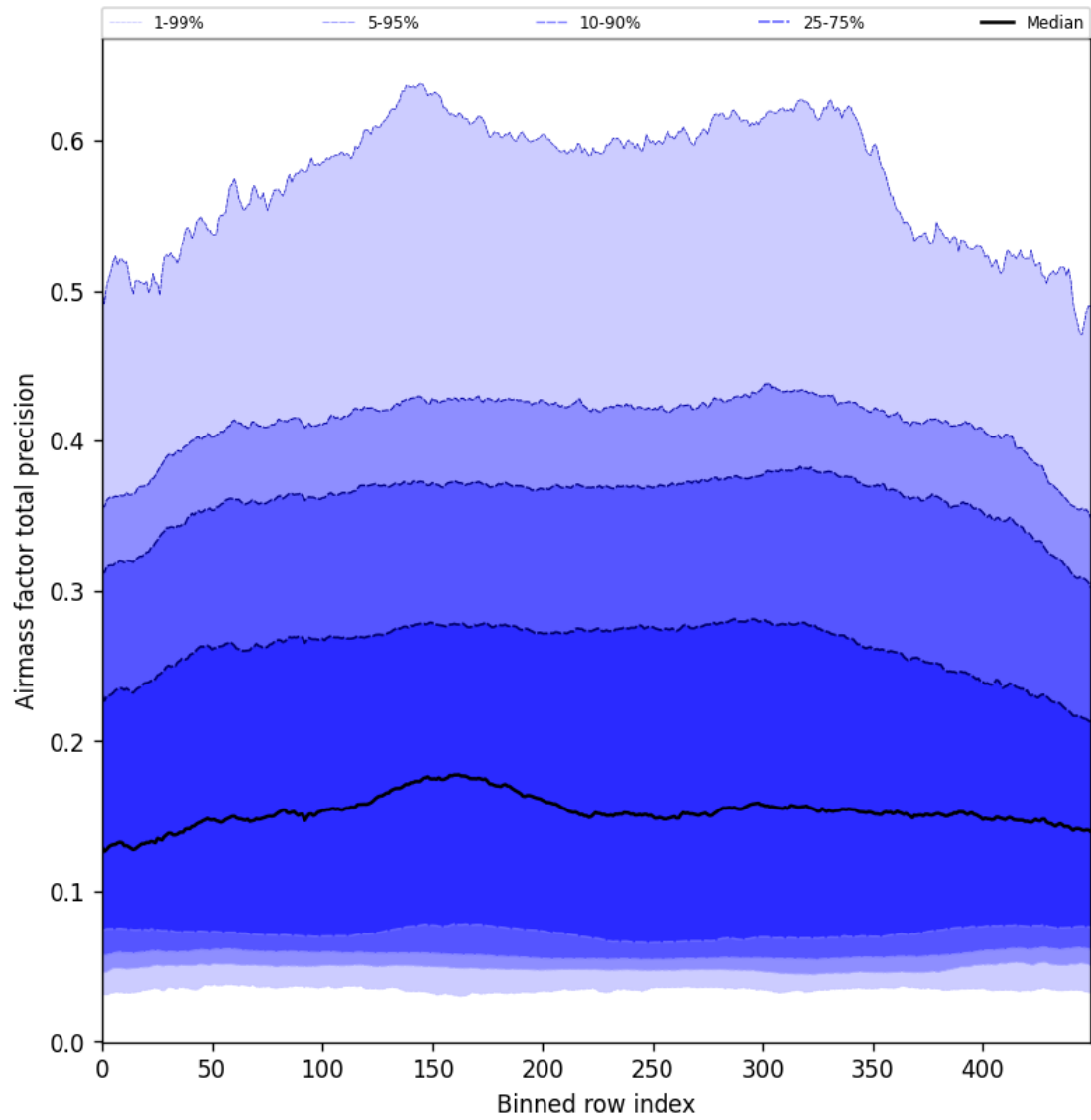
Figure 55: Along track statistics of “Airmass factor total precision” for 2025-08-01 to 2025-08-03
