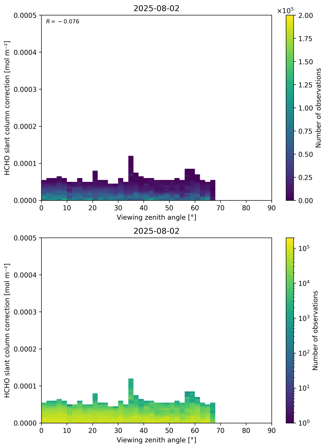
Figure 187: Scatter density plot of “Viewing zenith angle” against “HCHO slant column correction” for 2025-08-01 to 2025-08-03.
