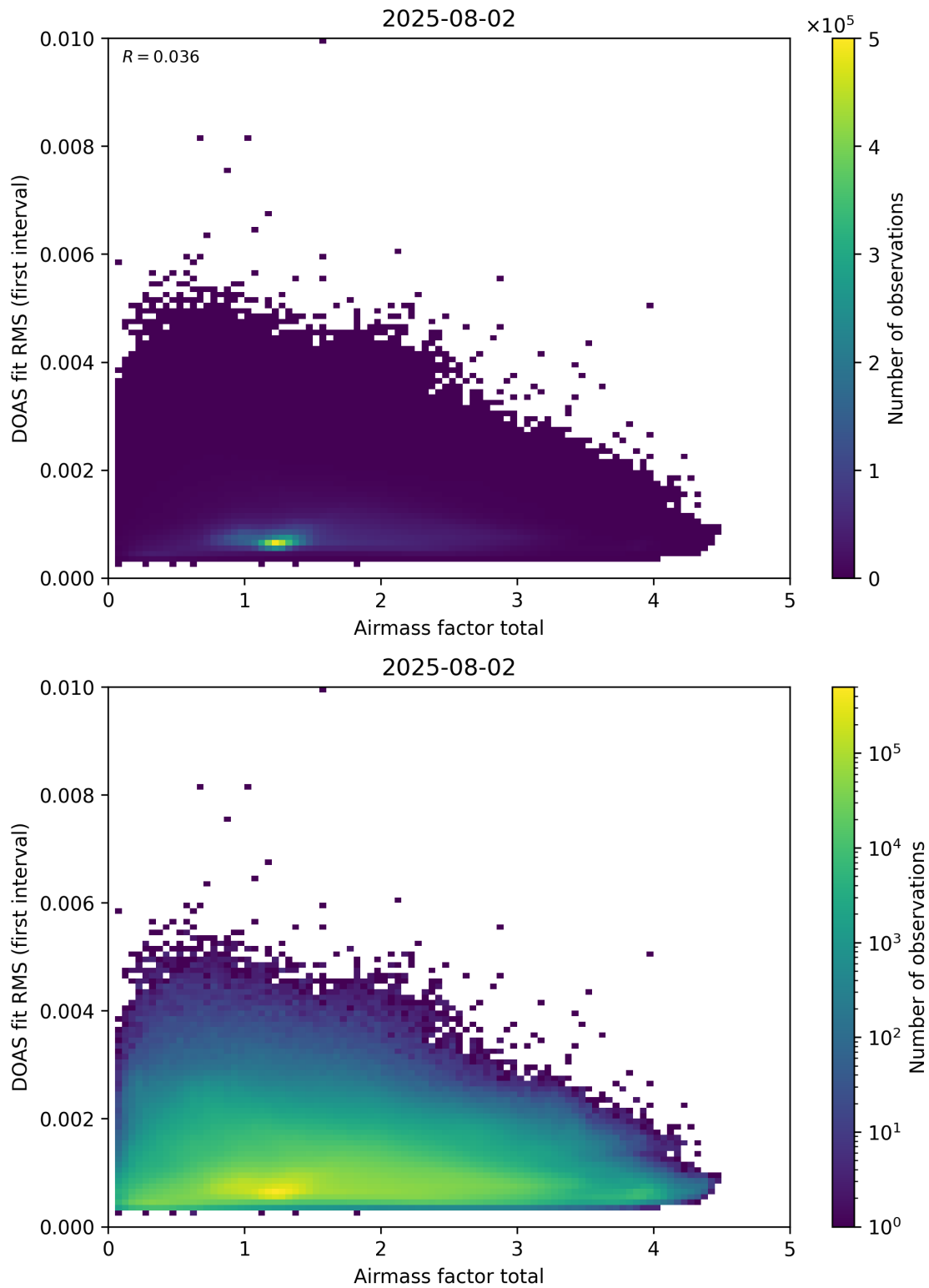
Figure 97: Scatter density plot of “Airmass factor total” against “DOAS fit RMS (first interval)” for 2025-08-01 to 2025-08-03.
