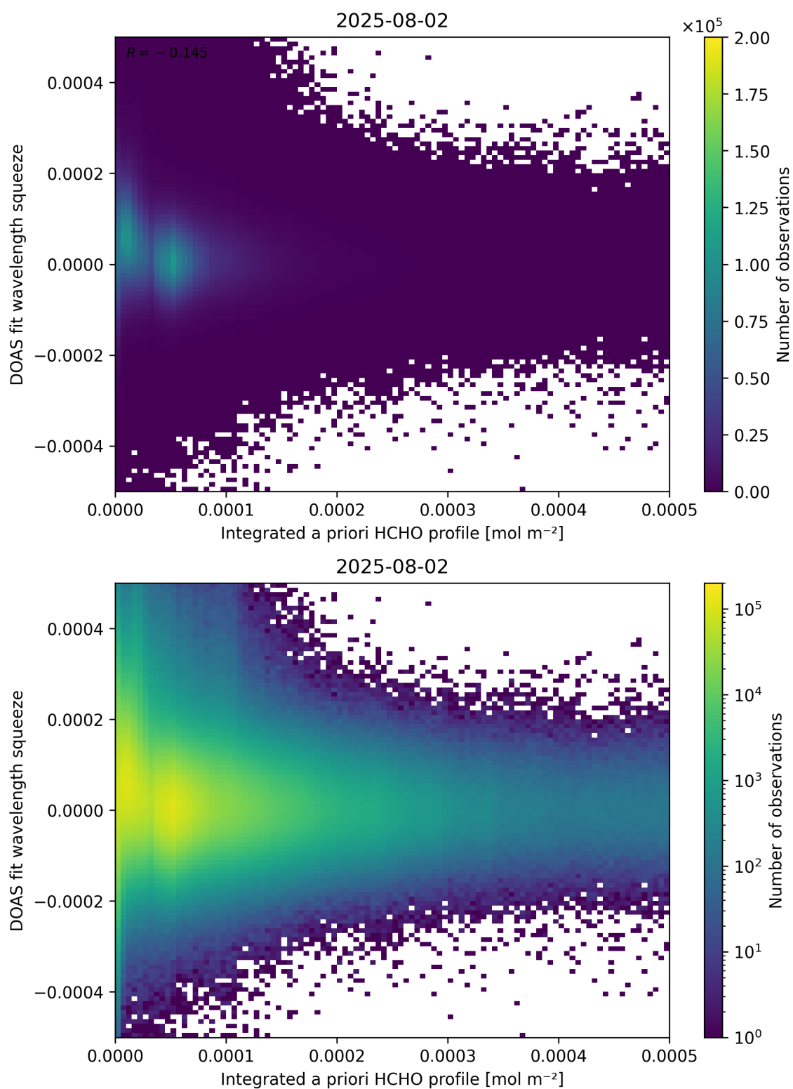
Figure 150: Scatter density plot of “Integrated a priori HCHO profile” against “DOAS fit wavelength squeeze” for 2025-08-01 to 2025-08-03.
