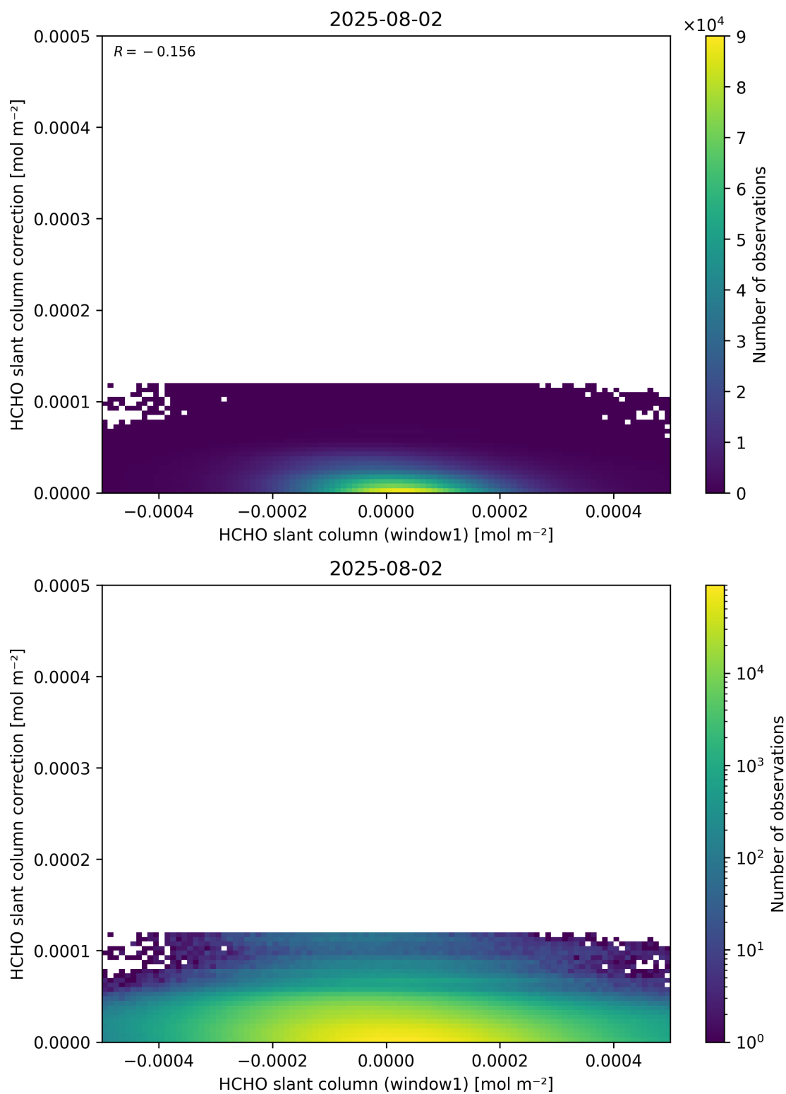
Figure 83: Scatter density plot of “HCHO slant column (window1)” against “HCHO slant column correction” for 2025-08-01 to 2025-08-03.
