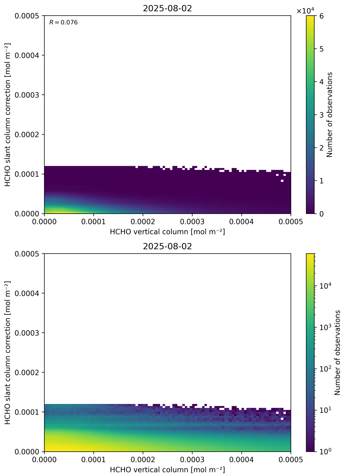
Figure 128: Scatter density plot of “HCHO vertical column” against “HCHO slant column correction” for 2025-08-01 to 2025-08-03.
