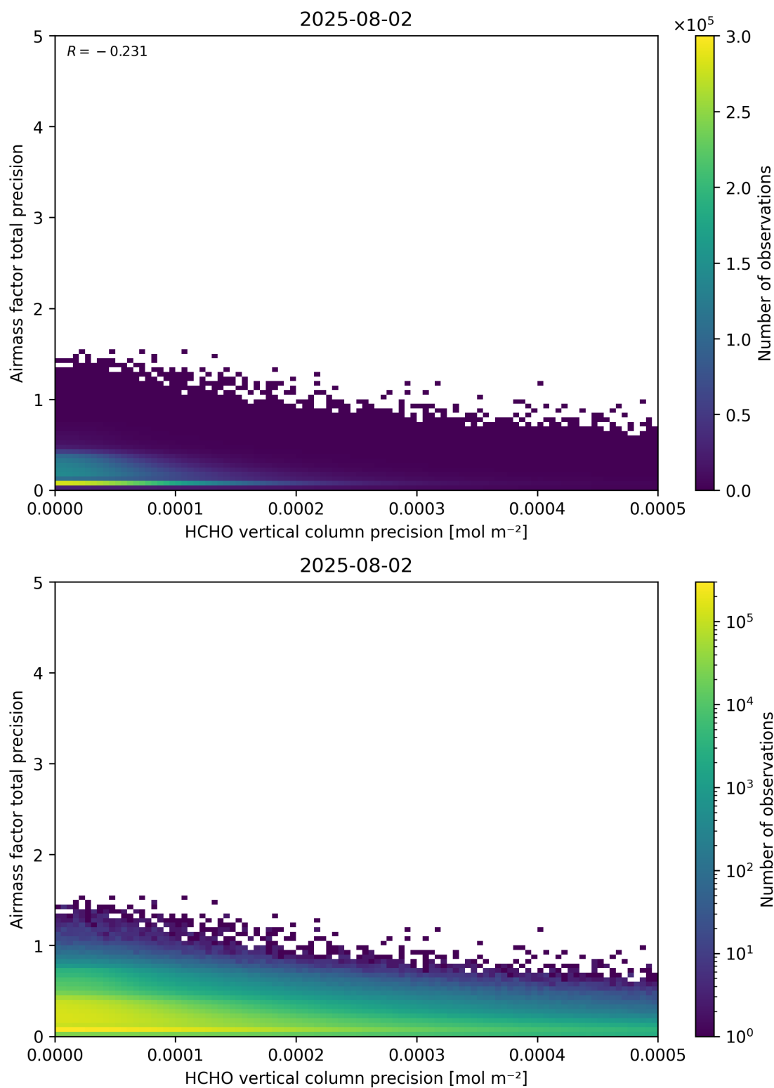
Figure 145: Scatter density plot of “HCHO vertical column precision” against “Airmass factor total precision” for 2025-08-01 to 2025-08-03.
