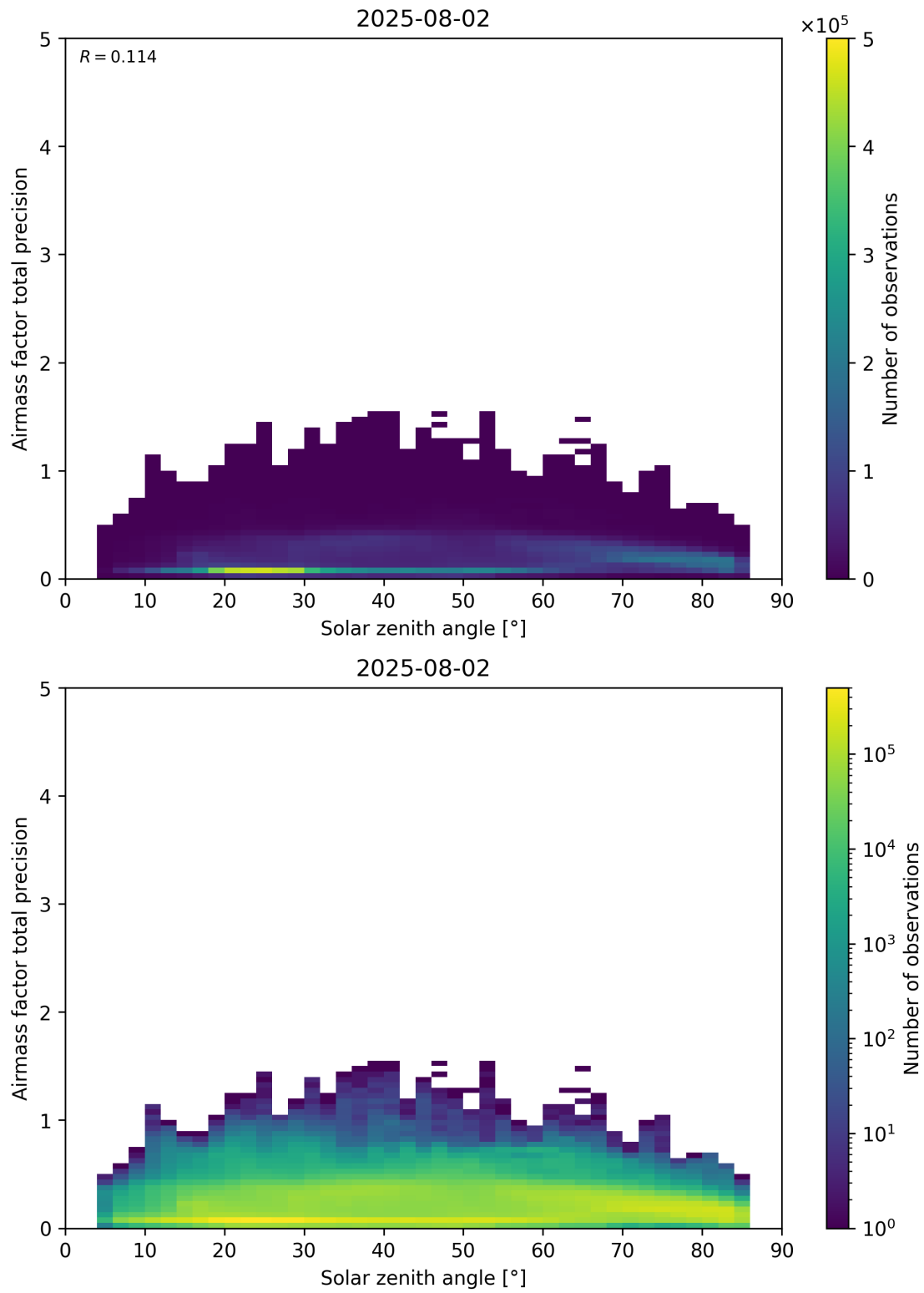
Figure 176: Scatter density plot of “Solar zenith angle” against “Airmass factor total precision” for 2025-08-01 to 2025-08-03.
