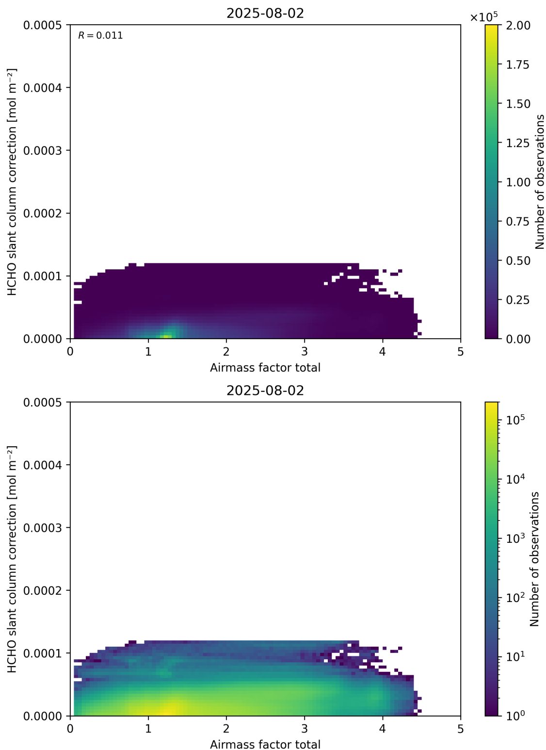
Figure 102: Scatter density plot of “Airmass factor total” against “HCHO slant column correction” for 2025-08-01 to 2025-08-03.
