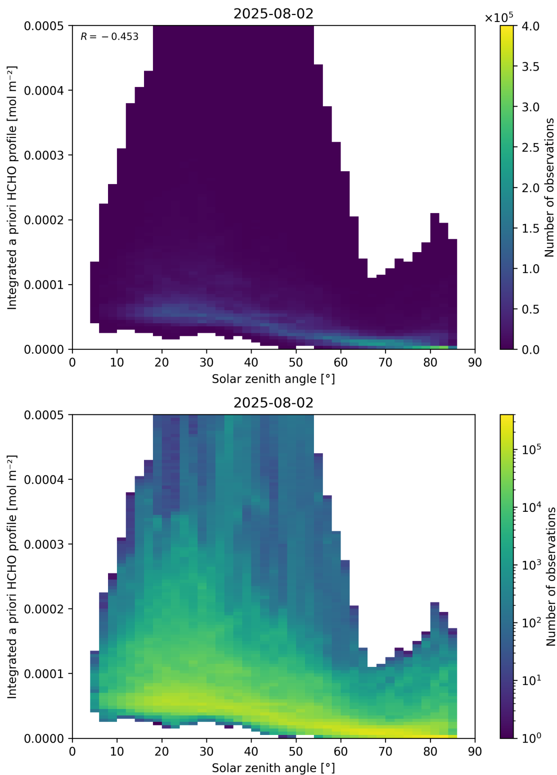
Figure 180: Scatter density plot of “Solar zenith angle” against “Integrated a priori HCHO profile” for 2025-08-01 to 2025-08-03.
