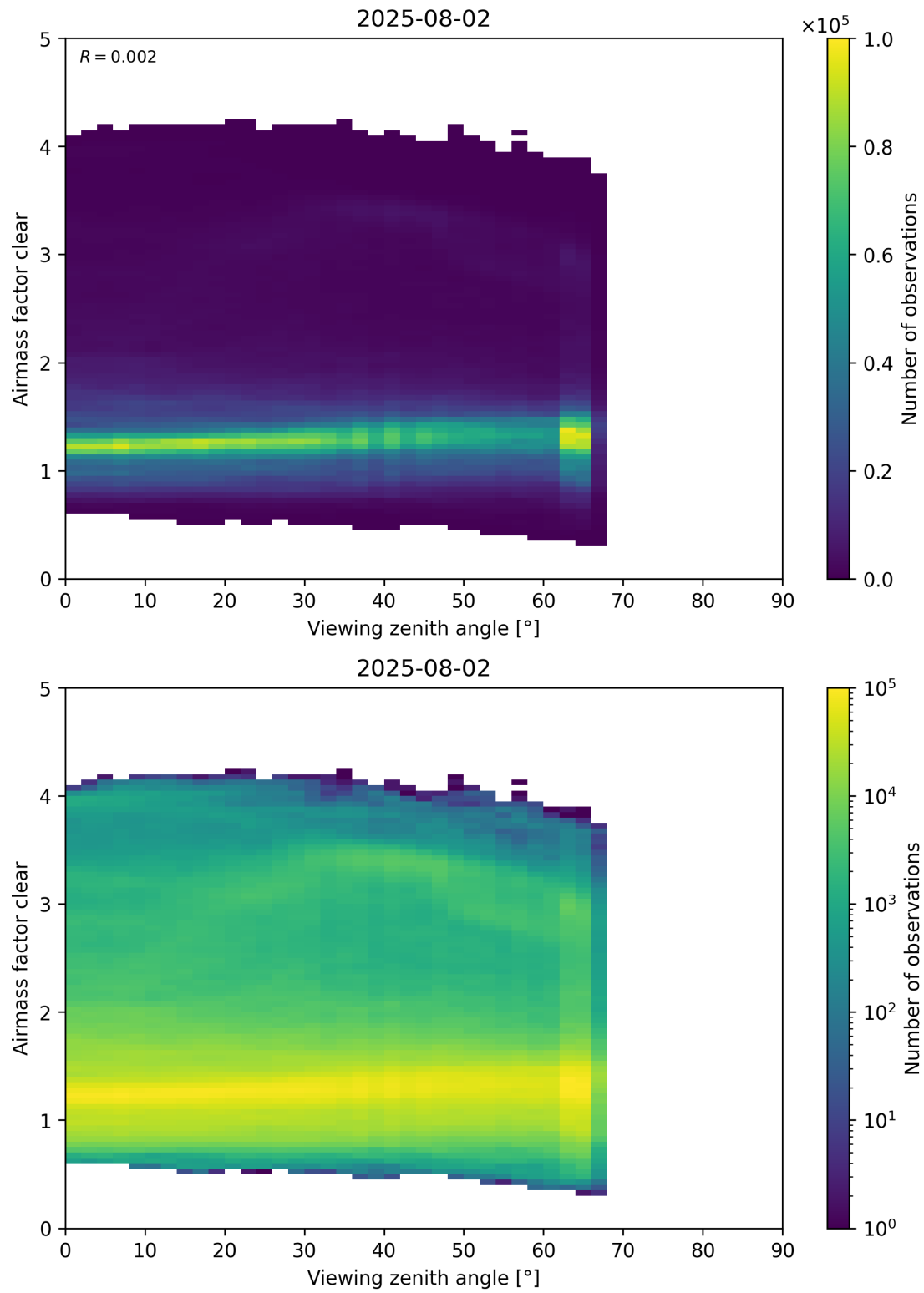
Figure 185: Scatter density plot of “Viewing zenith angle” against “Airmass factor clear” for 2025-08-01 to 2025-08-03.
