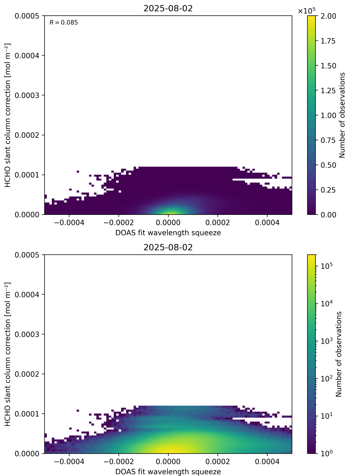
Figure 70: Scatter density plot of “DOAS fit wavelength squeeze” against “HCHO slant column correction” for 2025-08-01 to 2025-08-03.
