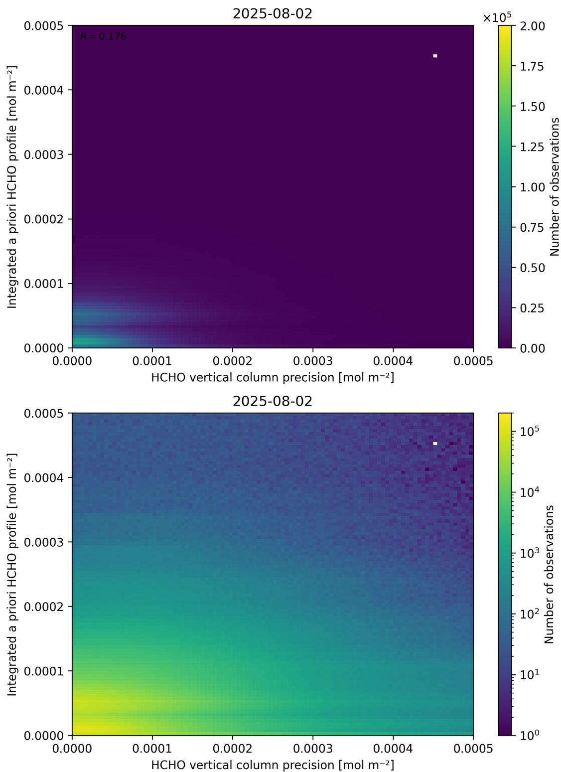
Figure 147: Scatter density plot of “HCHO vertical column precision” against “Integrated a priori HCHO profile” for 2025-08-01 to 2025-08-03.
