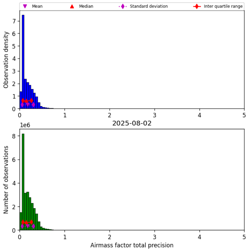
Figure 41: Histogram of “Airmass factor total precision” for 2025-08-01 to 2025-08-03
