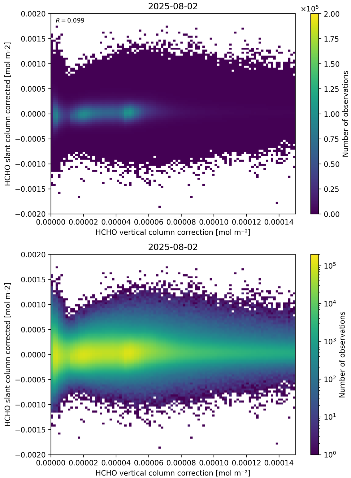
Figure 116: Scatter density plot of “HCHO vertical column correction” against “HCHO slant column corrected” for 2025-08-01 to 2025-08-03.
