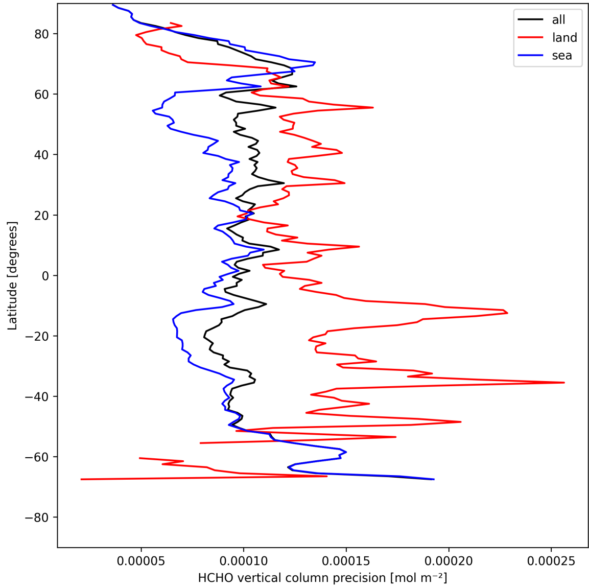
Figure 22: Zonal average of “HCHO vertical column precision” for 2025-08-01 to 2025-08-03.
