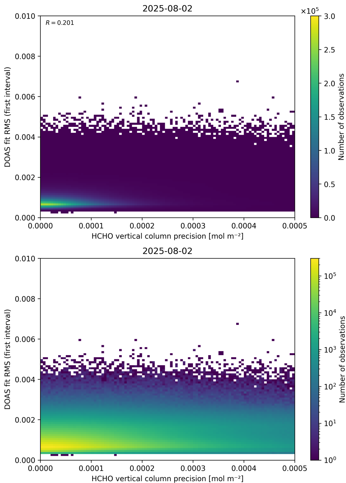
Figure 136: Scatter density plot of “HCHO vertical column precision” against “DOAS fit RMS (first interval)” for 2025-08-01 to 2025-08-03.
