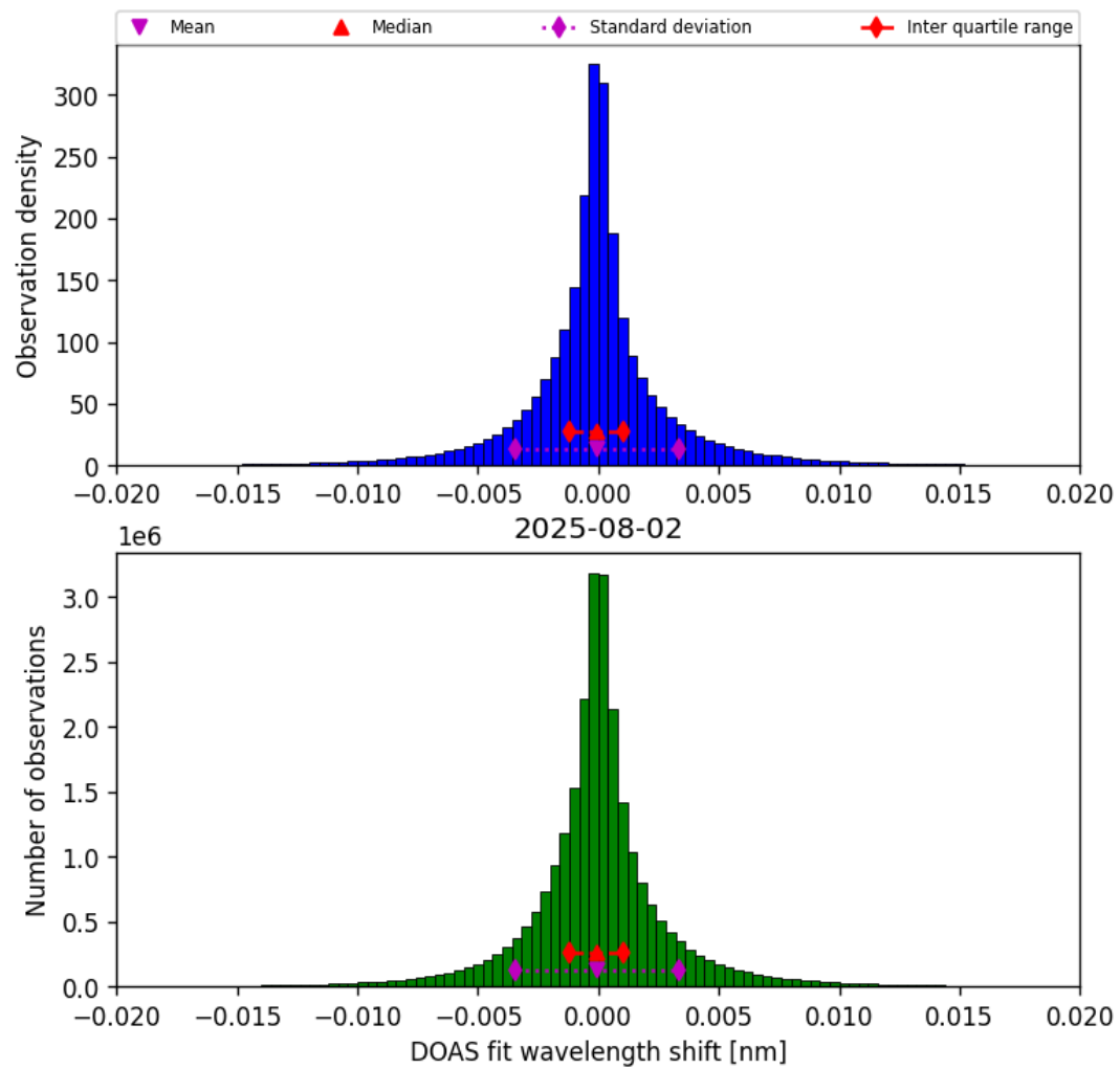
Figure 44: Histogram of “DOAS fit wavelength shift” for 2025-08-01 to 2025-08-03
