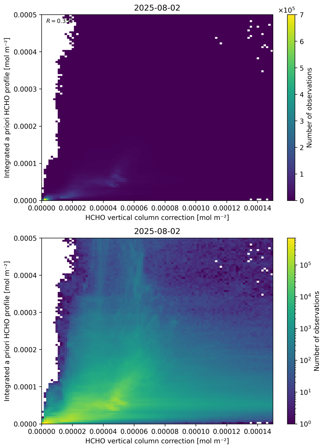
Figure 122: Scatter density plot of “HCHO vertical column correction” against “Integrated a priori HCHO profile” for 2025-08-01 to 2025-08-03.
