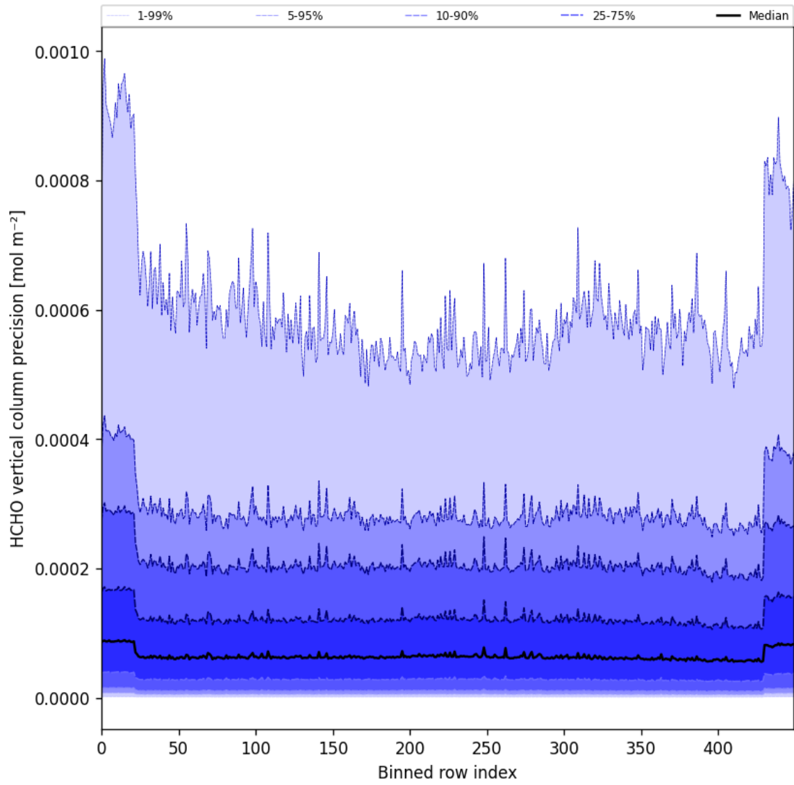
Figure 50: Along track statistics of “HCHO vertical column precision” for 2025-08-01 to 2025-08-03
