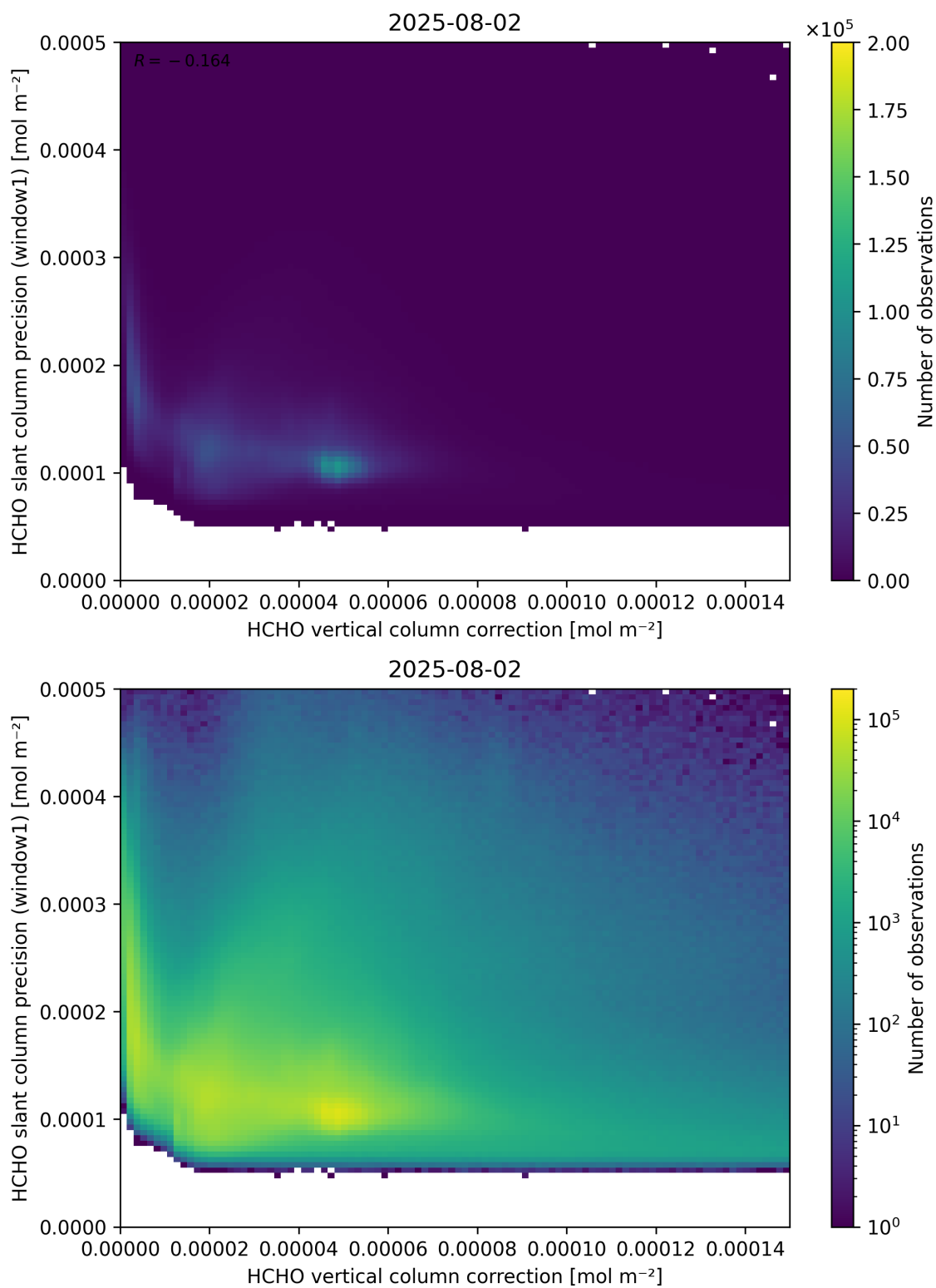
Figure 119: Scatter density plot of “HCHO vertical column correction” against “HCHO slant column precision (window1)” for 2025-08-01 to 2025-08-03.
