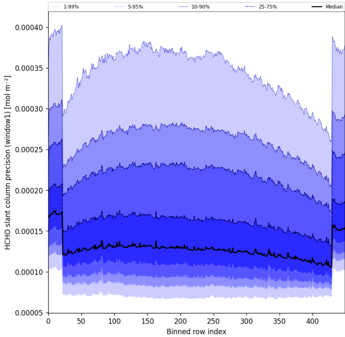
Figure 53: Along track statistics of “HCHO slant column precision (window1)” for 2025-08-01 to 2025-08-03
