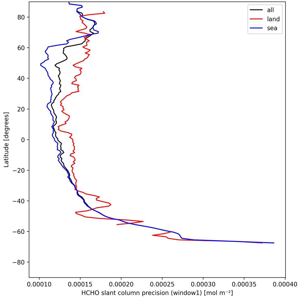
Figure 25: Zonal average of “HCHO slant column precision (window1)” for 2025-08-01 to 2025-08-03.
