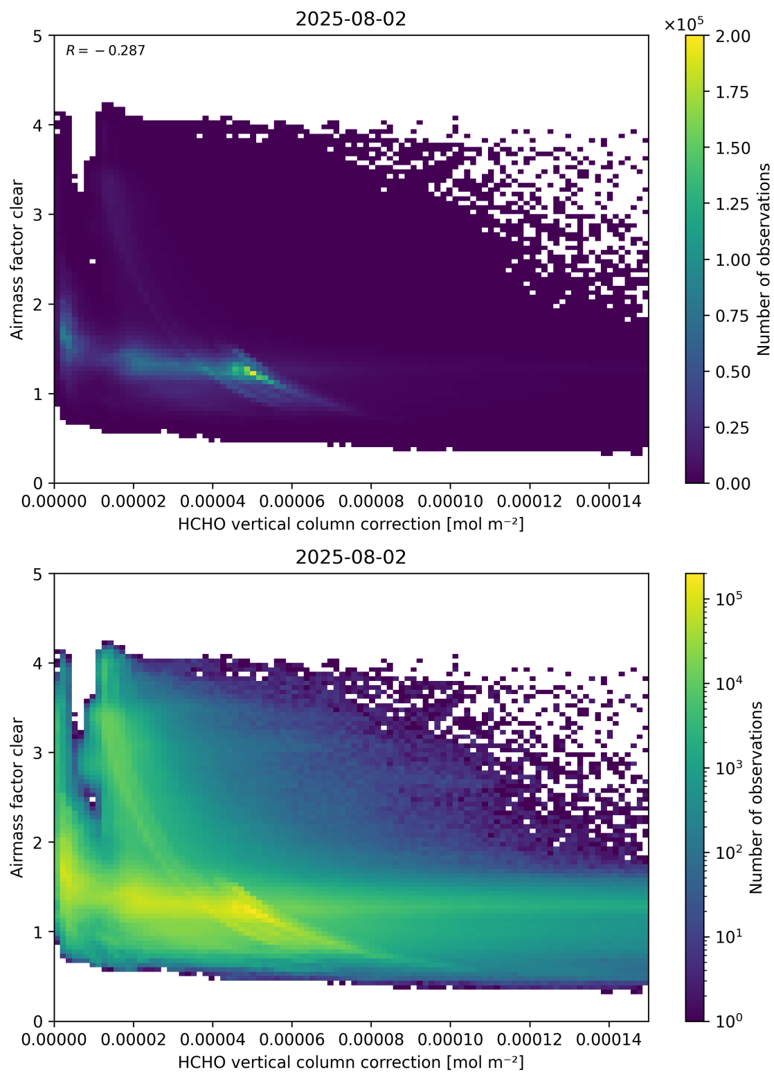
Figure 115: Scatter density plot of “HCHO vertical column correction” against “Airmass factor clear” for 2025-08-01 to 2025-08-03.
