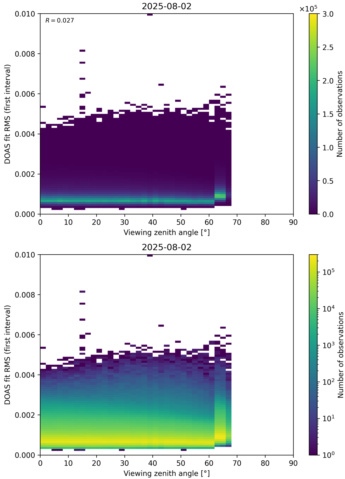
Figure 182: Scatter density plot of “Viewing zenith angle” against “DOAS fit RMS (first interval)” for 2025-08-01 to 2025-08-03.
