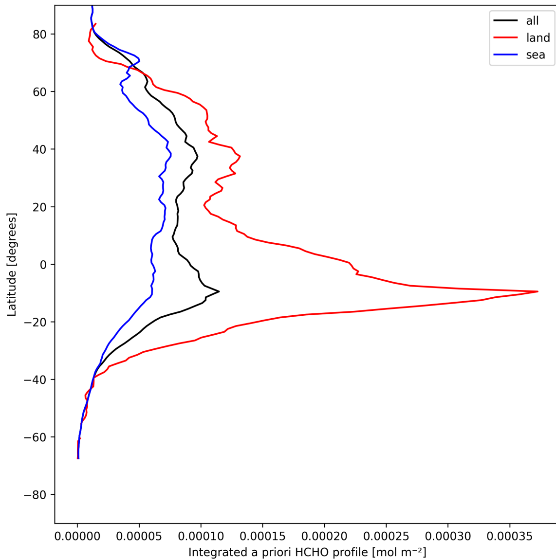
Figure 29: Zonal average of “Integrated a priori HCHO profile” for 2025-08-01 to 2025-08-03.
