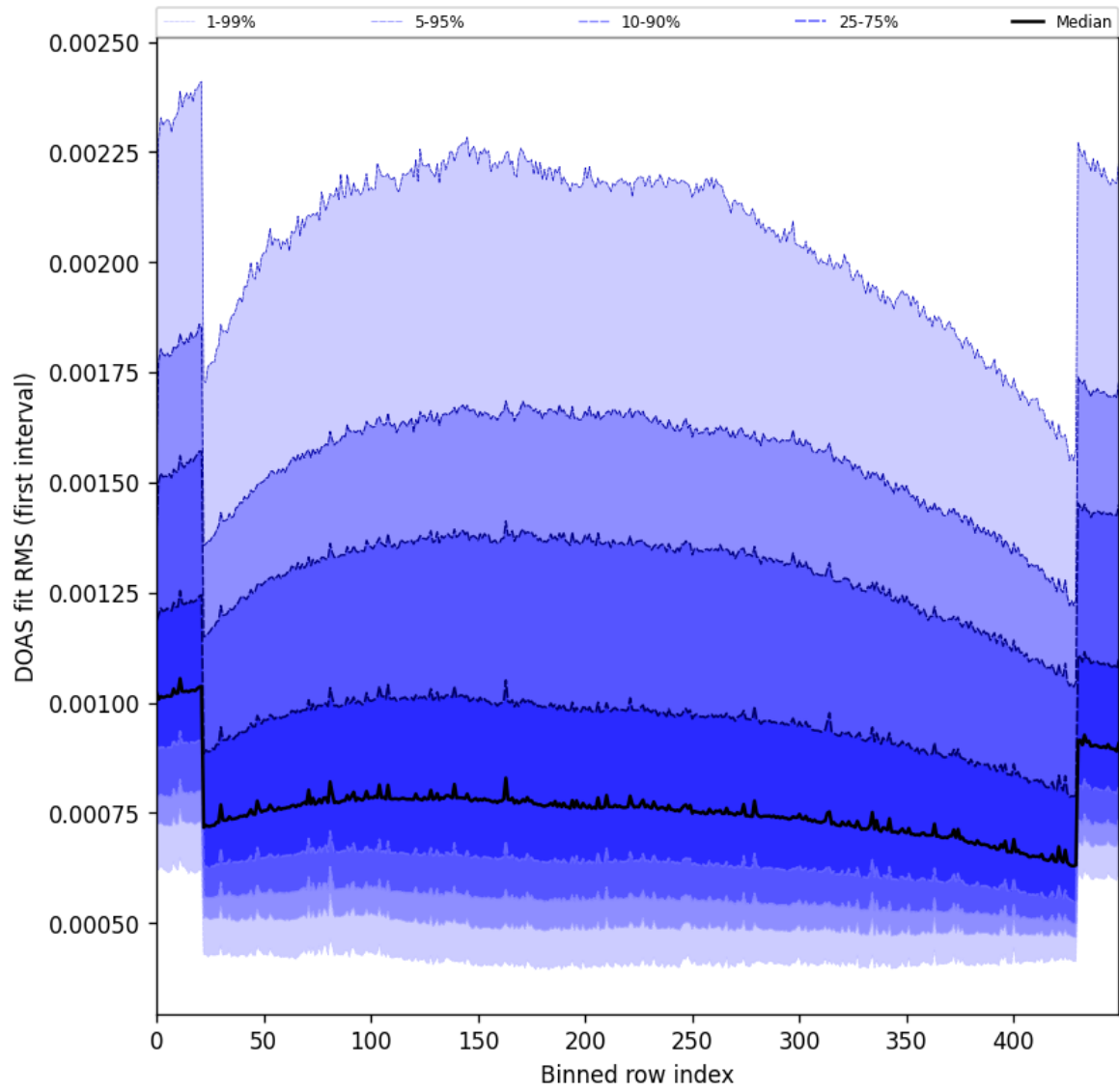
Figure 60: Along track statistics of “DOAS fit RMS (first interval)” for 2025-08-01 to 2025-08-03
