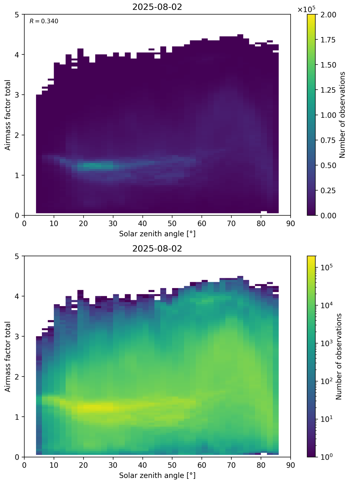
Figure 175: Scatter density plot of “Solar zenith angle” against “Airmass factor total” for 2025-08-01 to 2025-08-03.
