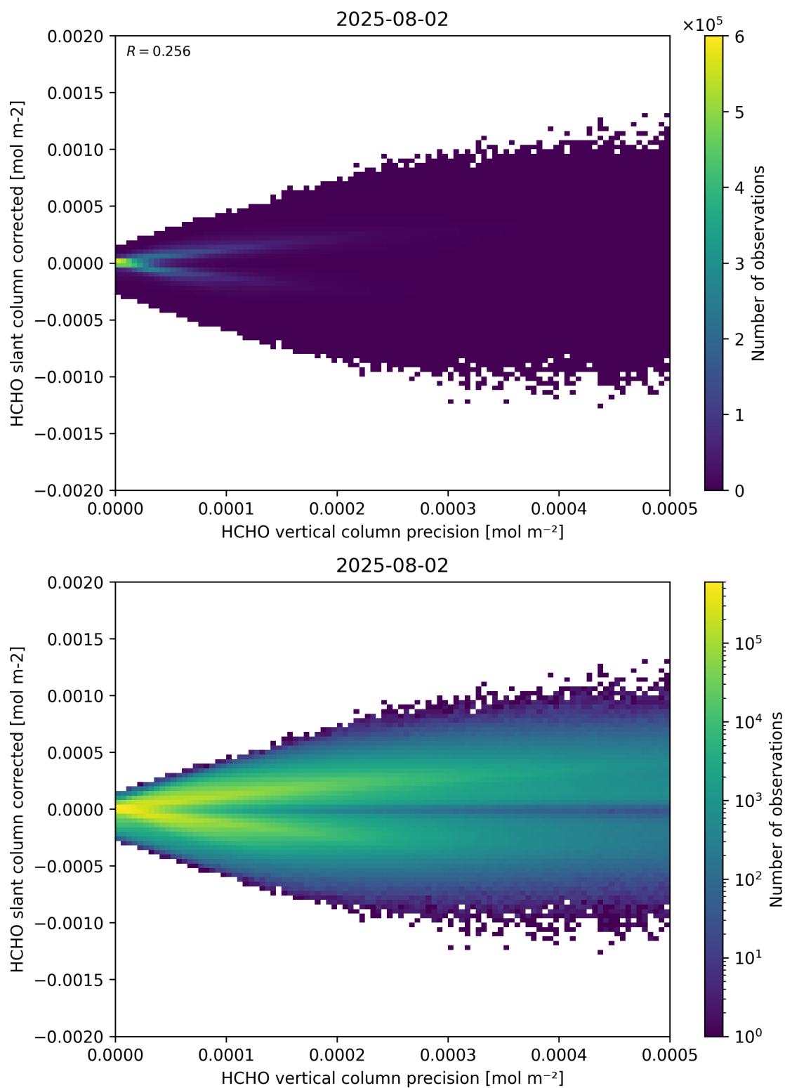
Figure 140: Scatter density plot of “HCHO vertical column precision” against “HCHO slant column corrected” for 2025-08-01 to 2025-08-03.
