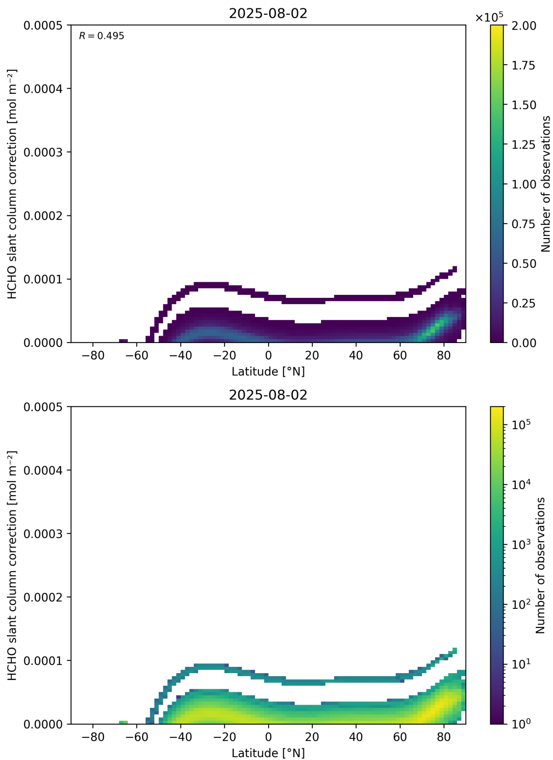
Figure 158: Scatter density plot of “Latitude” against “HCHO slant column correction” for 2025-08-01 to 2025-08-03.
