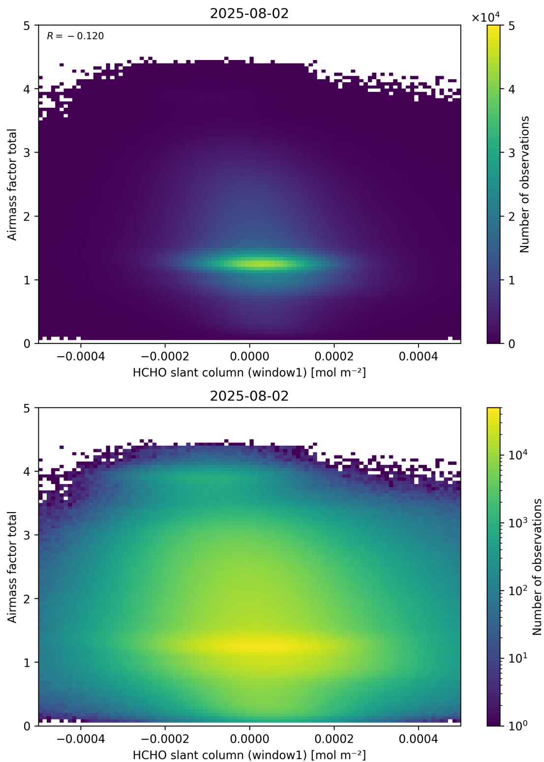
Figure 85: Scatter density plot of “HCHO slant column (window1)” against “Airmass factor total” for 2025-08-01 to 2025-08-03.
