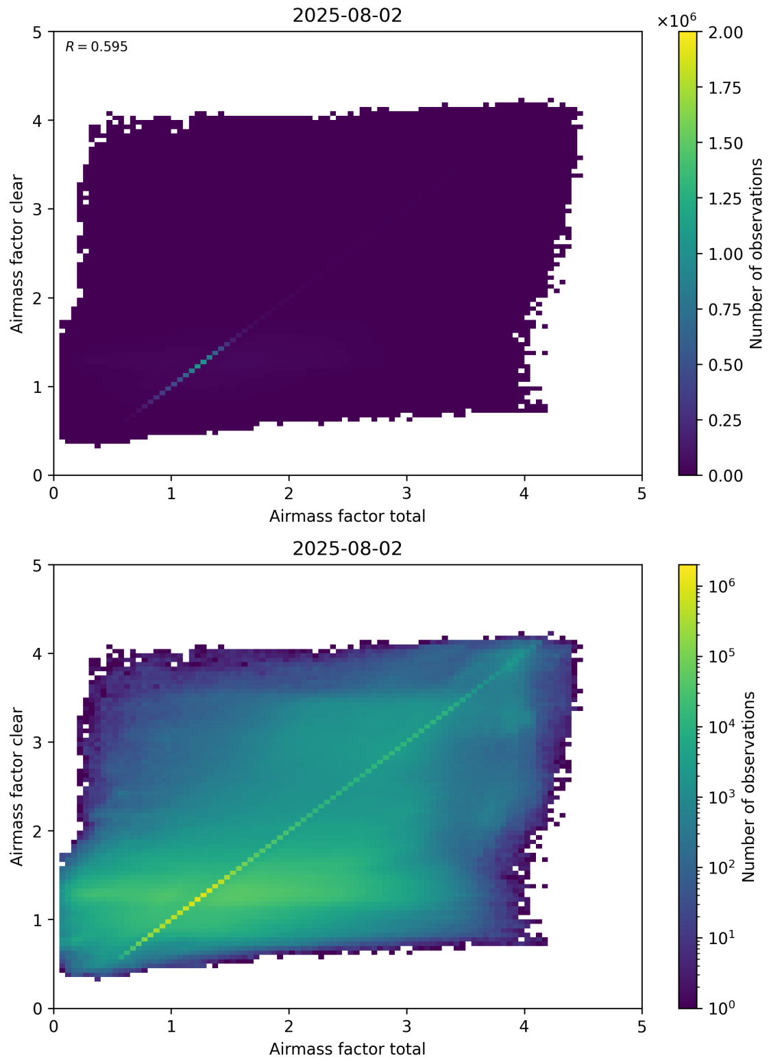
Figure 100: Scatter density plot of “Airmass factor total” against “Airmass factor clear” for 2025-08-01 to 2025-08-03.
