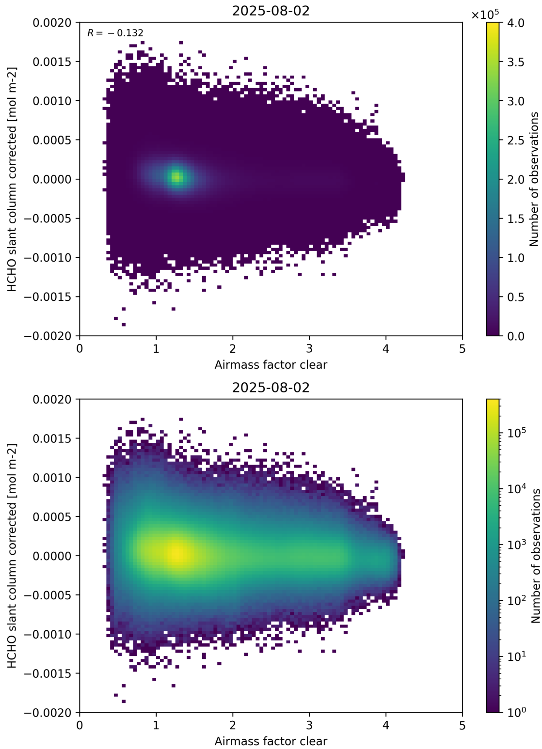
Figure 74: Scatter density plot of “Airmass factor clear” against “HCHO slant column corrected” for 2025-08-01 to 2025-08-03.
