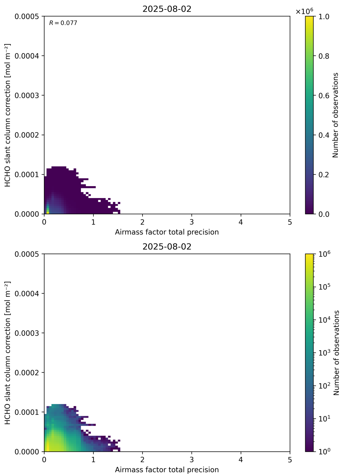
Figure 110: Scatter density plot of “Airmass factor total precision” against “HCHO slant column correction” for 2025-08-01 to 2025-08-03.
