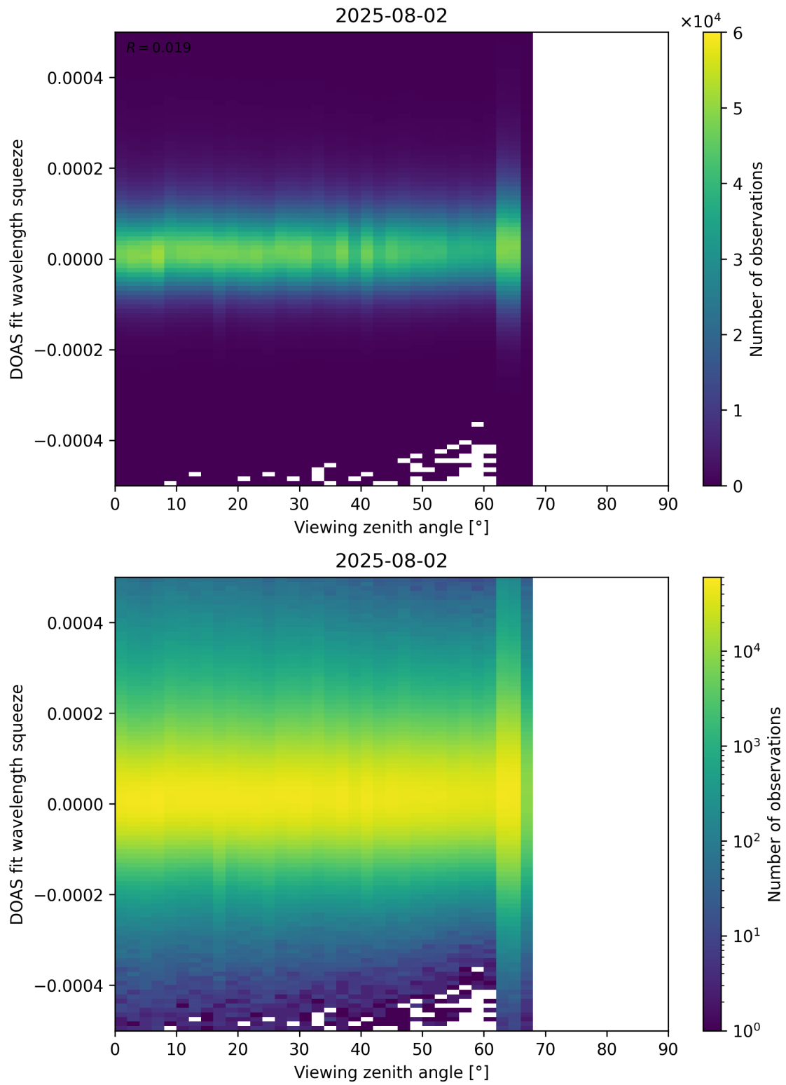
Figure 184: Scatter density plot of “Viewing zenith angle” against “DOAS fit wavelength squeeze” for 2025-08-01 to 2025-08-03.
