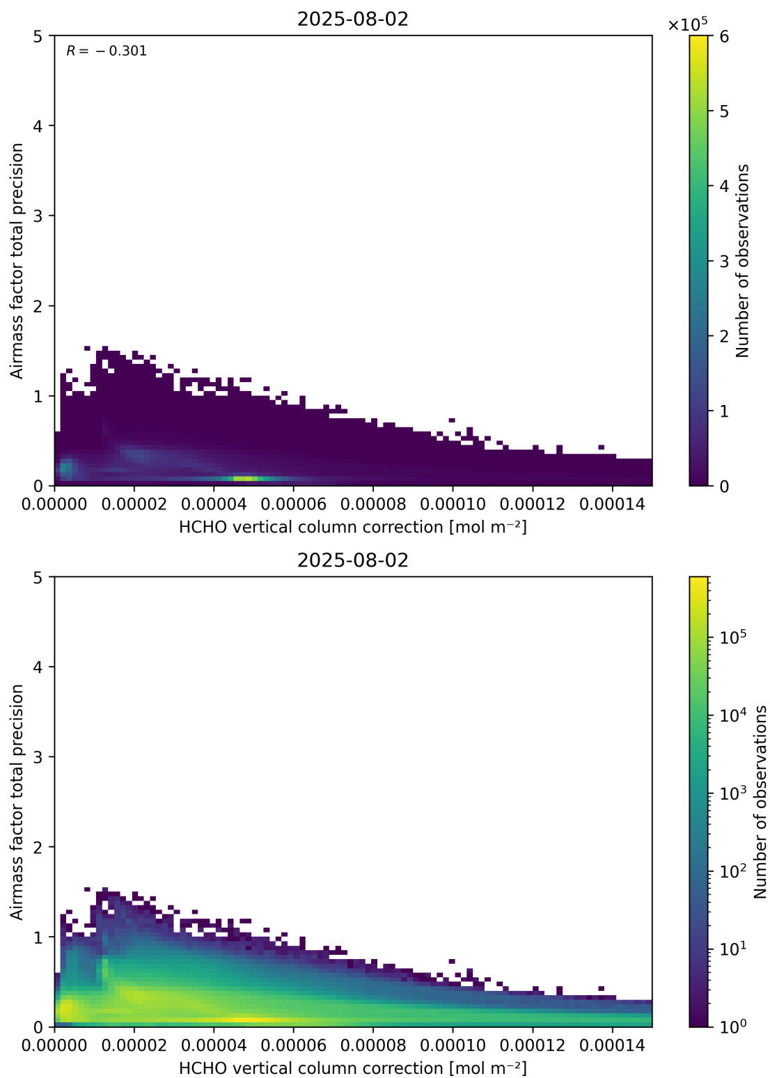
Figure 121: Scatter density plot of “HCHO vertical column correction” against “Airmass factor total precision” for 2025-08-01 to 2025-08-03.
