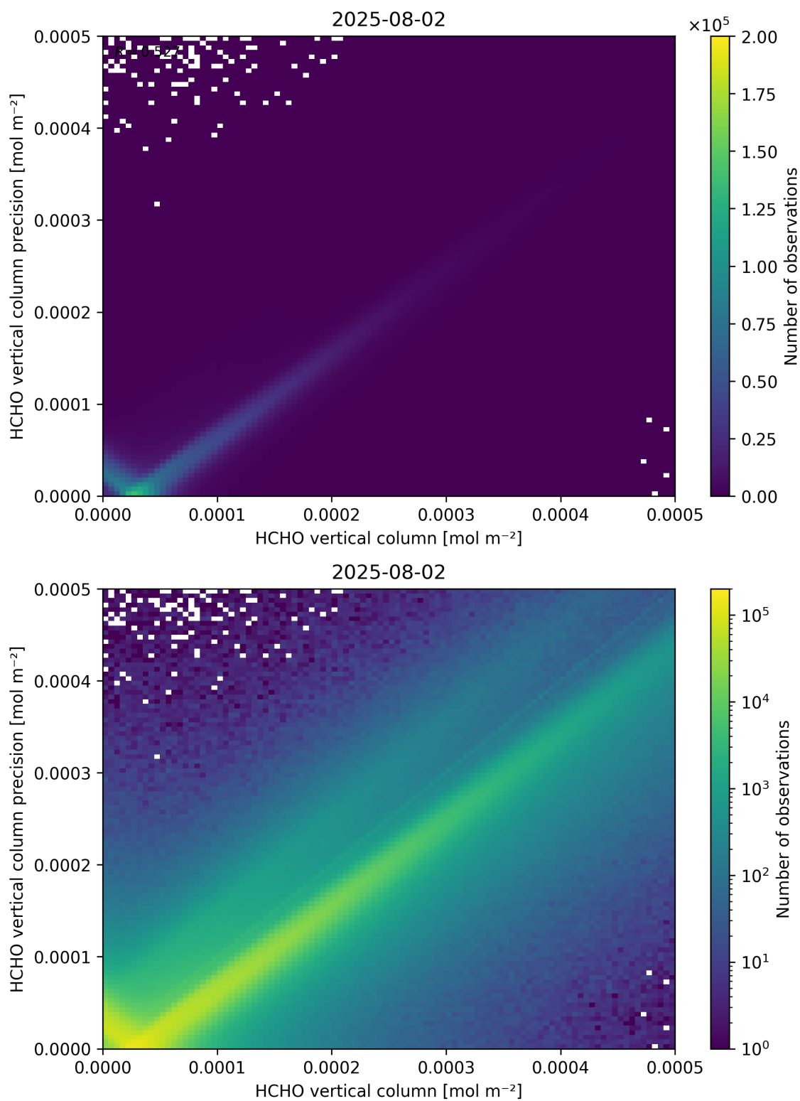
Figure 134: Scatter density plot of “HCHO vertical column” against “HCHO vertical column precision” for 2025-08-01 to 2025-08-03.
