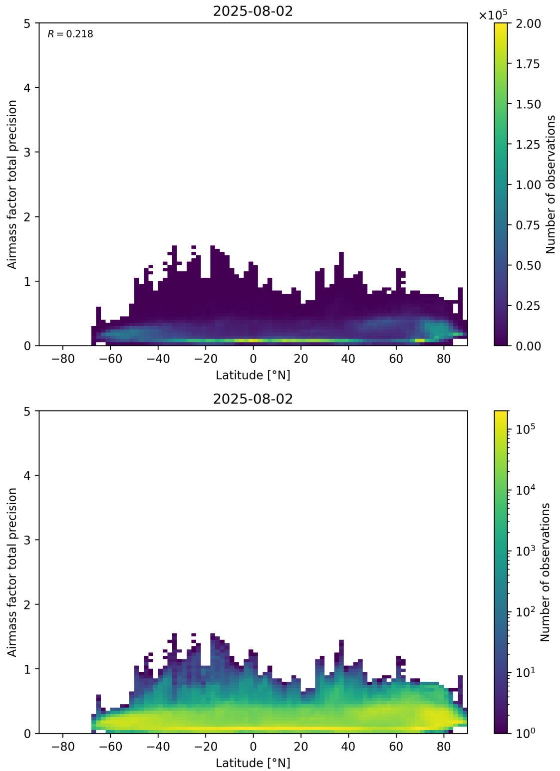
Figure 162: Scatter density plot of “Latitude” against “Airmass factor total precision” for 2025-08-01 to 2025-08-03.
