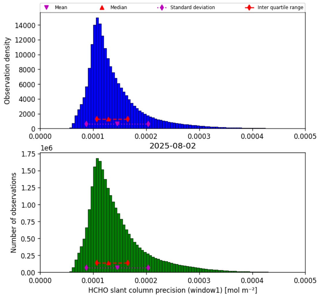
Figure 39: Histogram of “HCHO slant column precision (window1)” for 2025-08-01 to 2025-08-03
