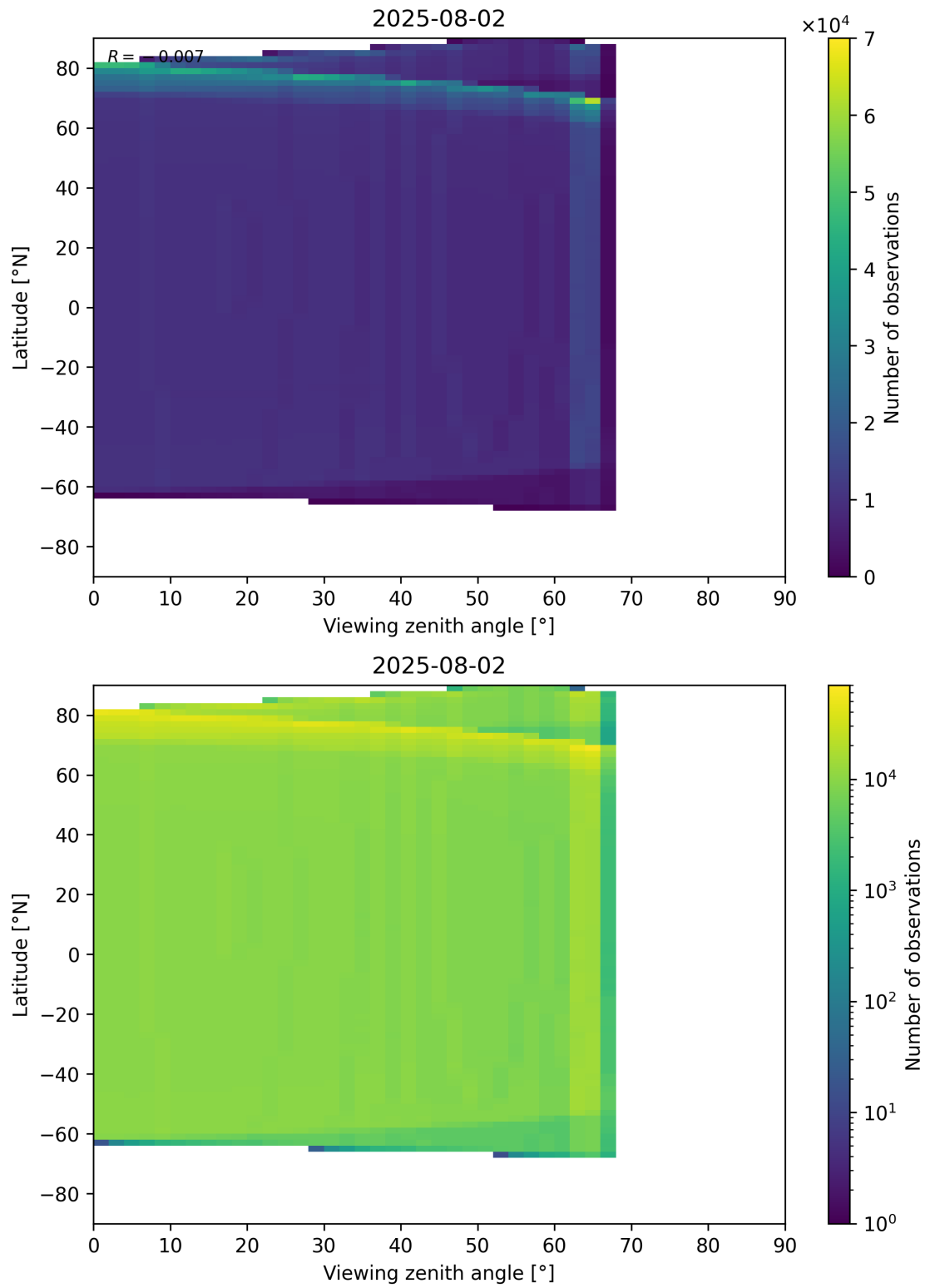
Figure 196: Scatter density plot of “Viewing zenith angle” against “Latitude” for 2025-08-01 to 2025-08-03.
