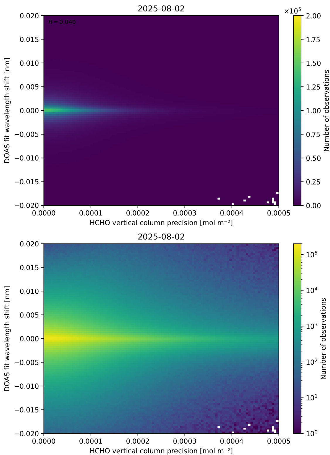
Figure 137: Scatter density plot of “HCHO vertical column precision” against “DOAS fit wavelength shift” for 2025-08-01 to 2025-08-03.
