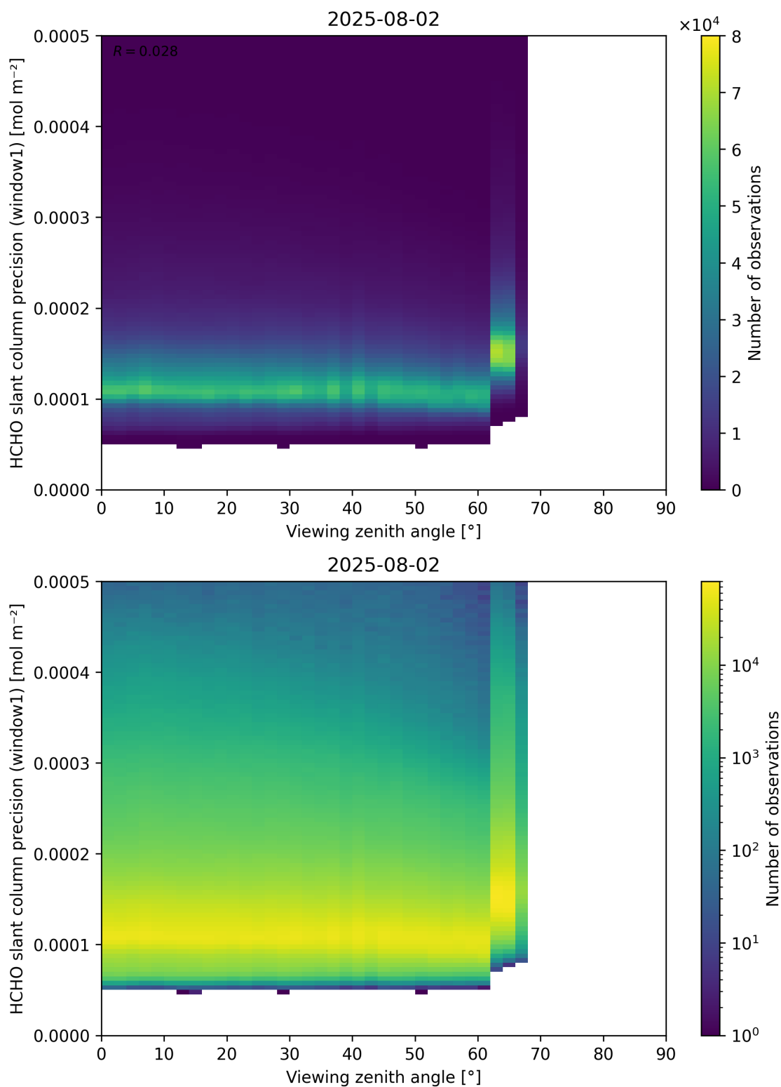
Figure 189: Scatter density plot of “Viewing zenith angle” against “HCHO slant column precision (window1)” for 2025-08-01 to 2025-08-03.
