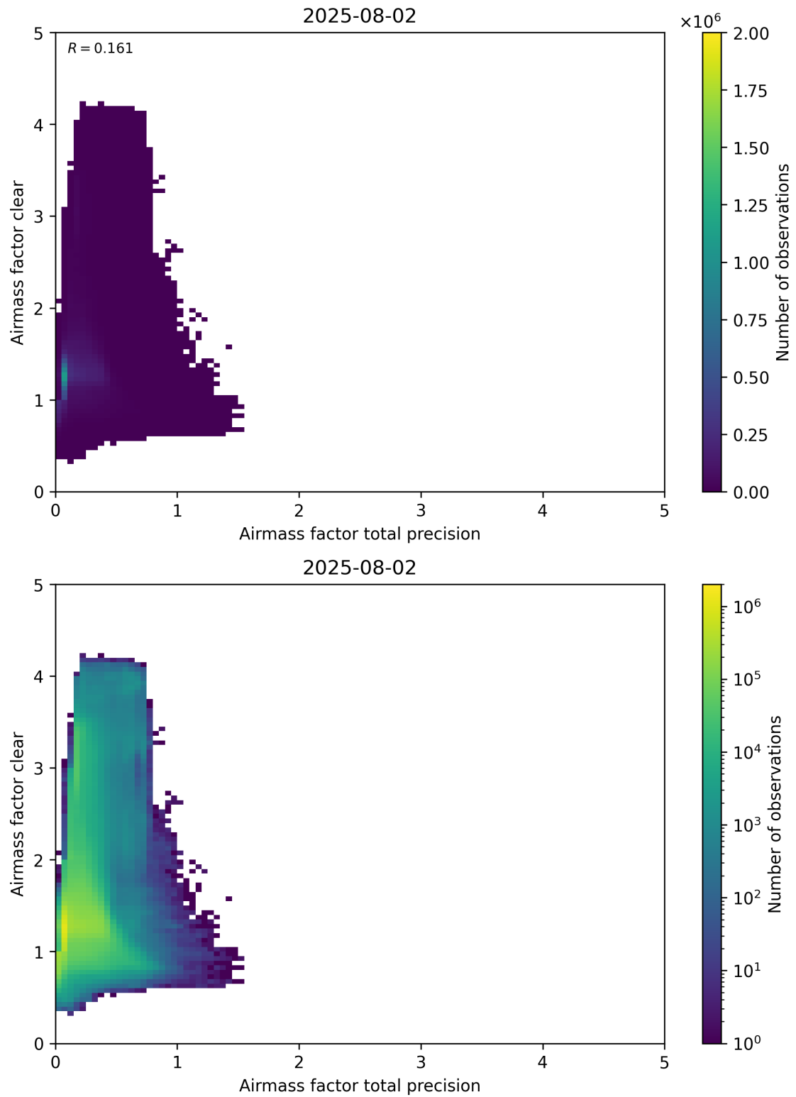
Figure 108: Scatter density plot of “Airmass factor total precision” against “Airmass factor clear” for 2025-08-01 to 2025-08-03.
