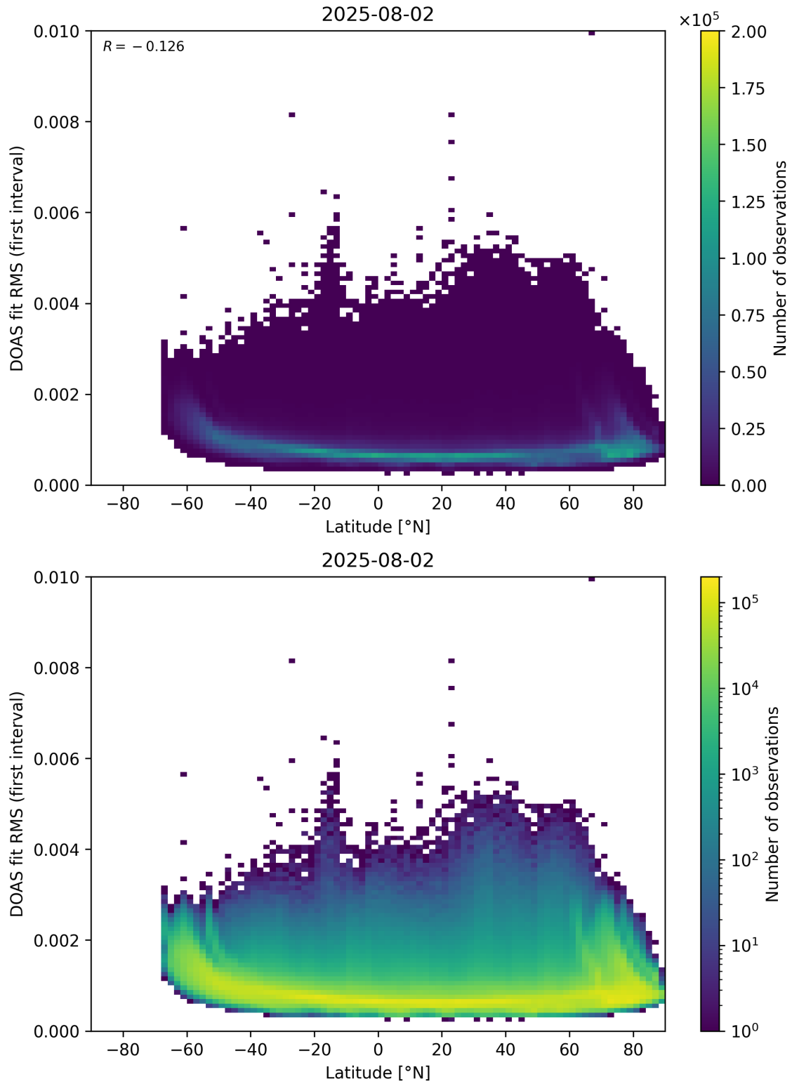
Figure 153: Scatter density plot of “Latitude” against “DOAS fit RMS (first interval)” for 2025-08-01 to 2025-08-03.
