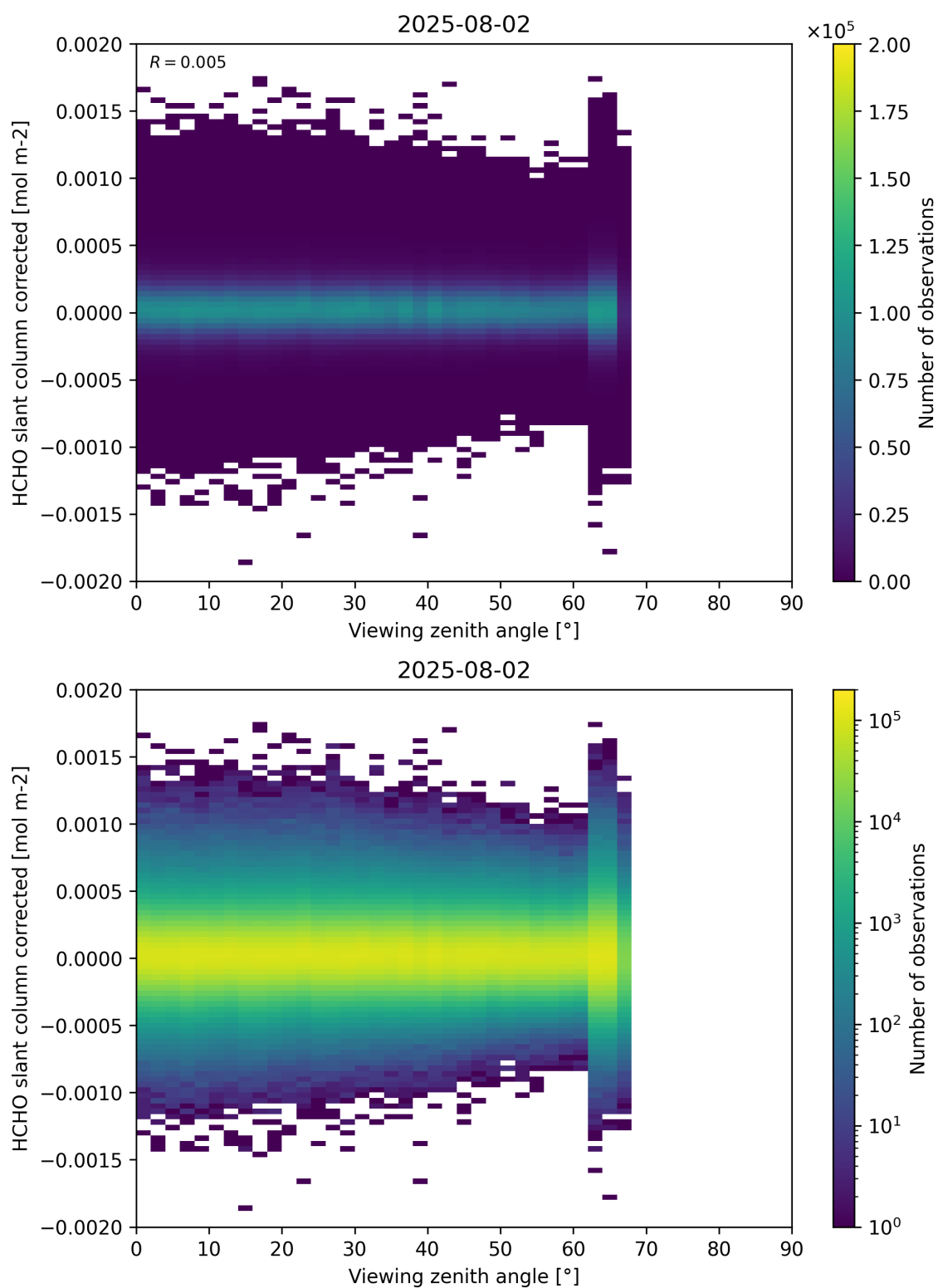
Figure 186: Scatter density plot of “Viewing zenith angle” against “HCHO slant column corrected” for 2025-08-01 to 2025-08-03.
