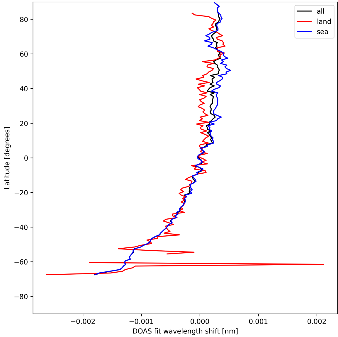
Figure 30: Zonal average of "DOAS fit wavelength shift" for 2025-08-01 to 2025-08-03.
