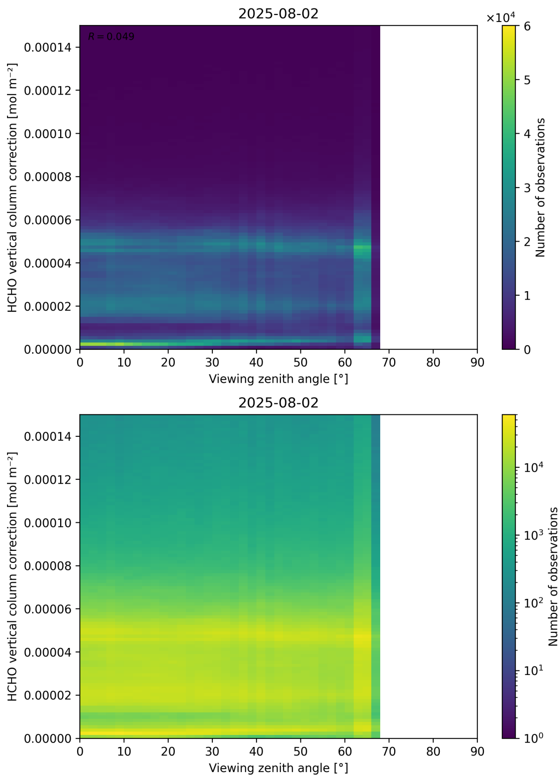
Figure 193: Scatter density plot of “Viewing zenith angle” against “HCHO vertical column correction” for 2025-08-01 to 2025-08-03.
