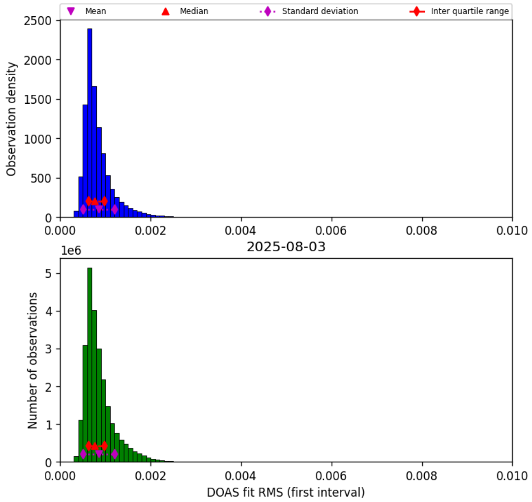
Figure 46: Histogram of “DOAS fit RMS (first interval)” for 2025-08-03 to 2025-08-04
