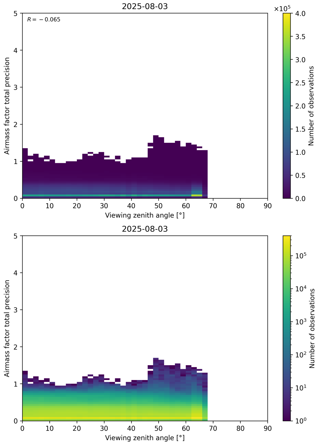
Figure 191: Scatter density plot of “Viewing zenith angle” against “Airmass factor total precision” for 2025-08-03 to 2025-08-04.
