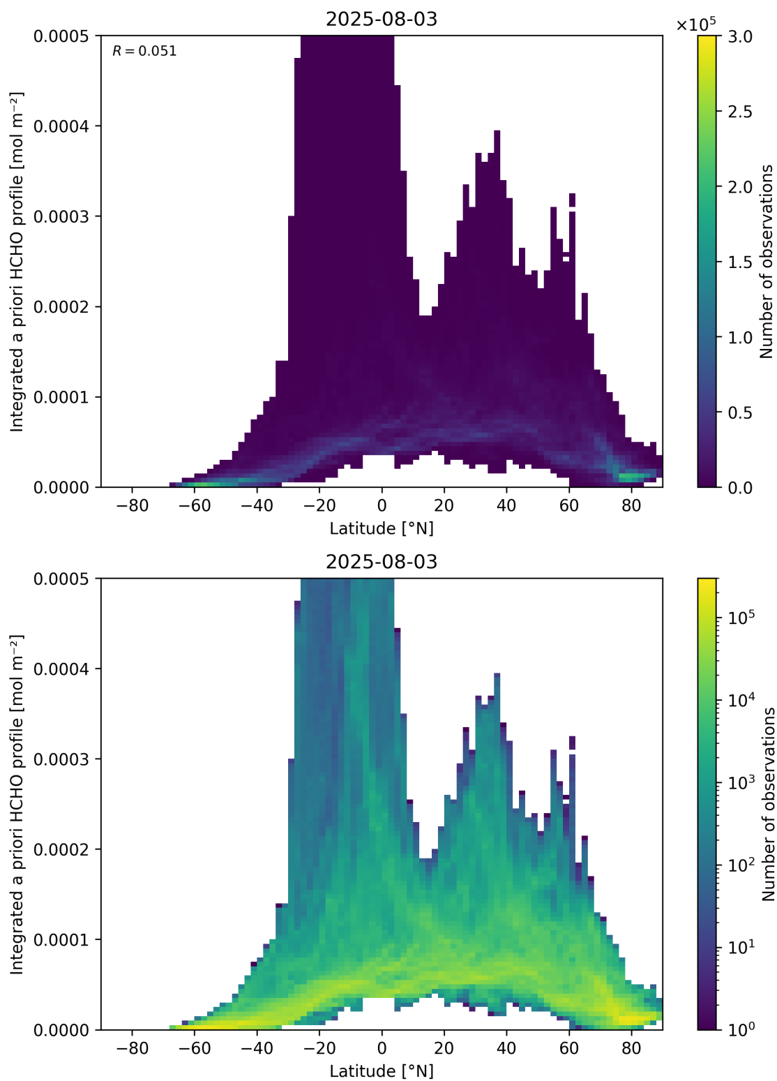
Figure 166: Scatter density plot of “Latitude” against “Integrated a priori HCHO profile” for 2025-08-03 to 2025-08-04.
