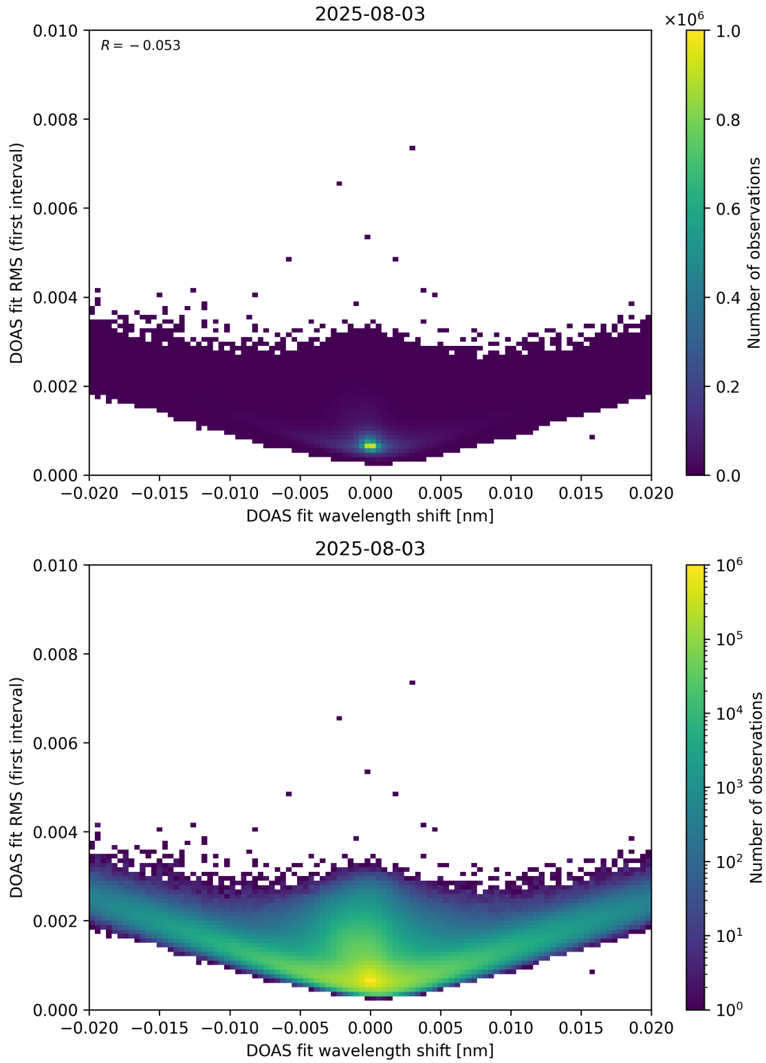
Figure 64: Scatter density plot of “DOAS fit wavelength shift” against “DOAS fit RMS (first interval)” for 2025-08-03 to 2025-08-04.
