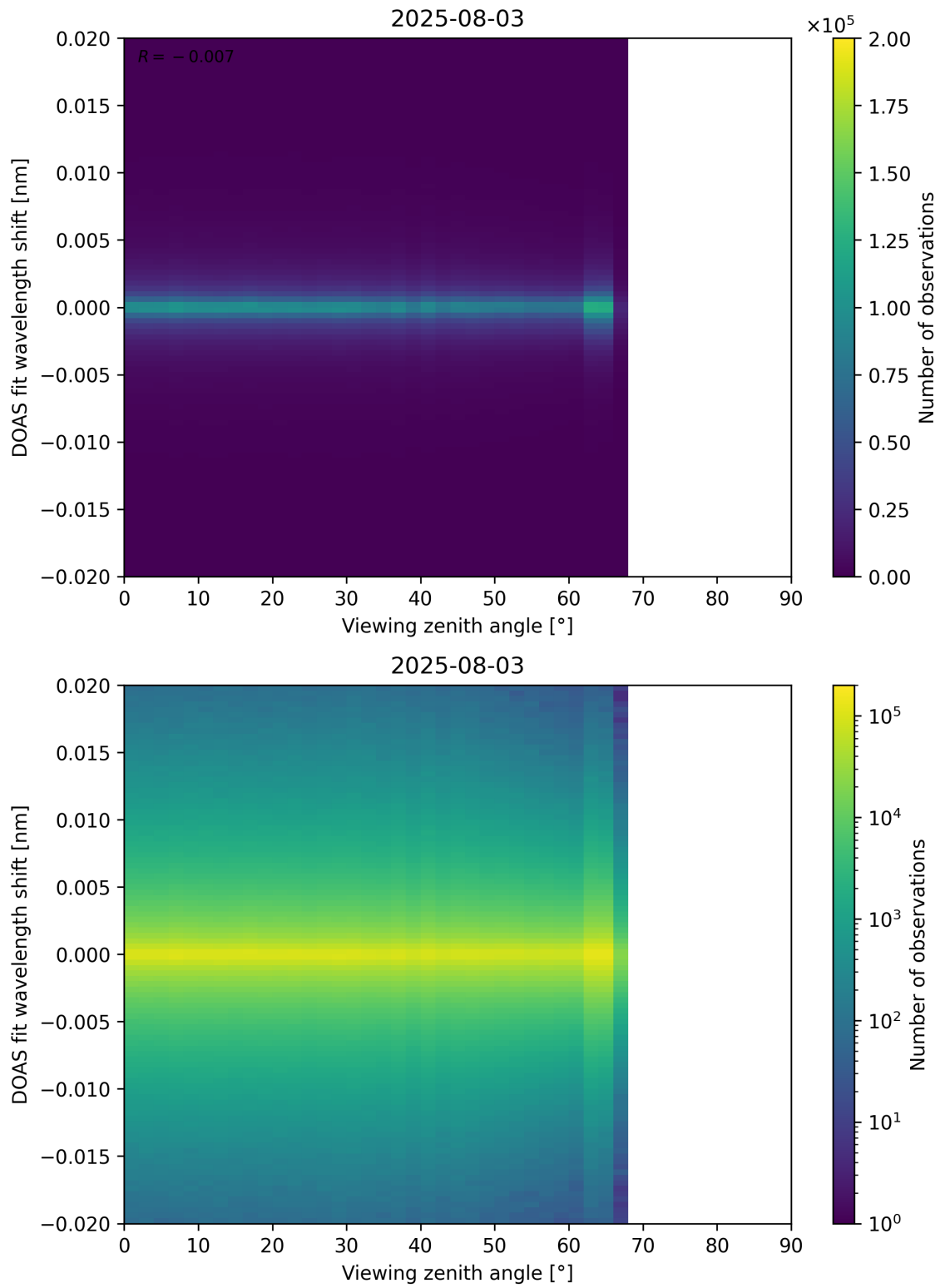
Figure 183: Scatter density plot of “Viewing zenith angle” against “DOAS fit wavelength shift” for 2025-08-03 to 2025-08-04.
