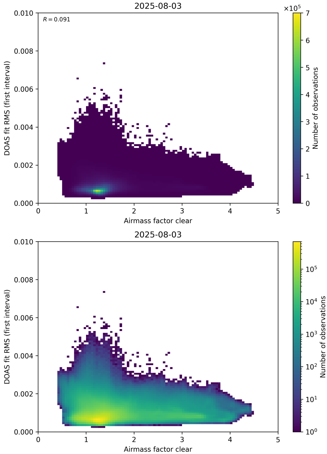
Figure 71: Scatter density plot of “Airmass factor clear” against “DOAS fit RMS (first interval)” for 2025-08-03 to 2025-08-04.
