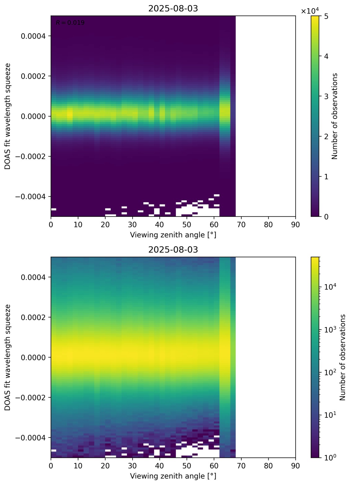
Figure 184: Scatter density plot of “Viewing zenith angle” against “DOAS fit wavelength squeeze” for 2025-08-03 to 2025-08-04.
