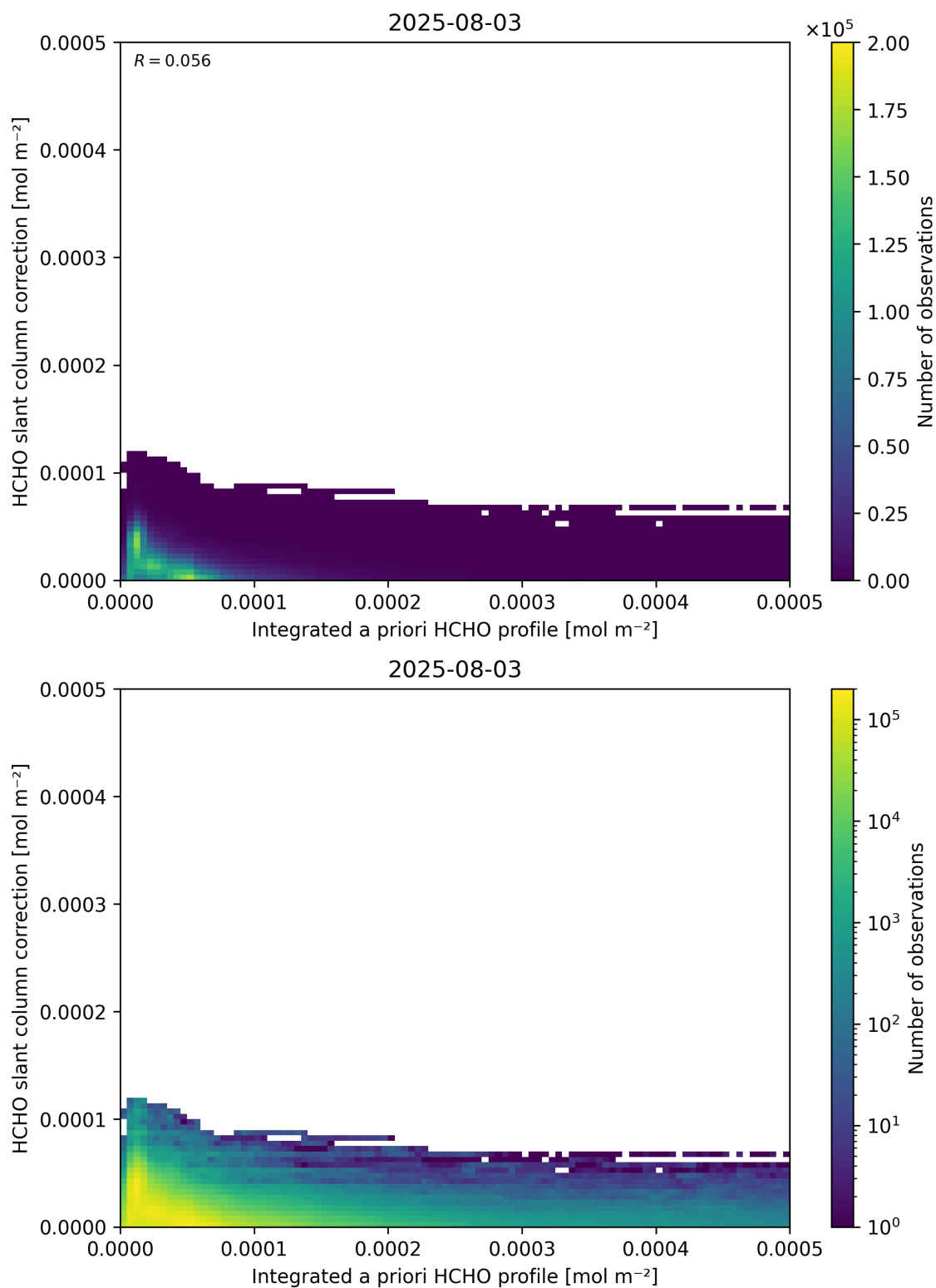
Figure 152: Scatter density plot of “Integrated a priori HCHO profile” against “HCHO slant column correction” for 2025-08-03 to 2025-08-04.
