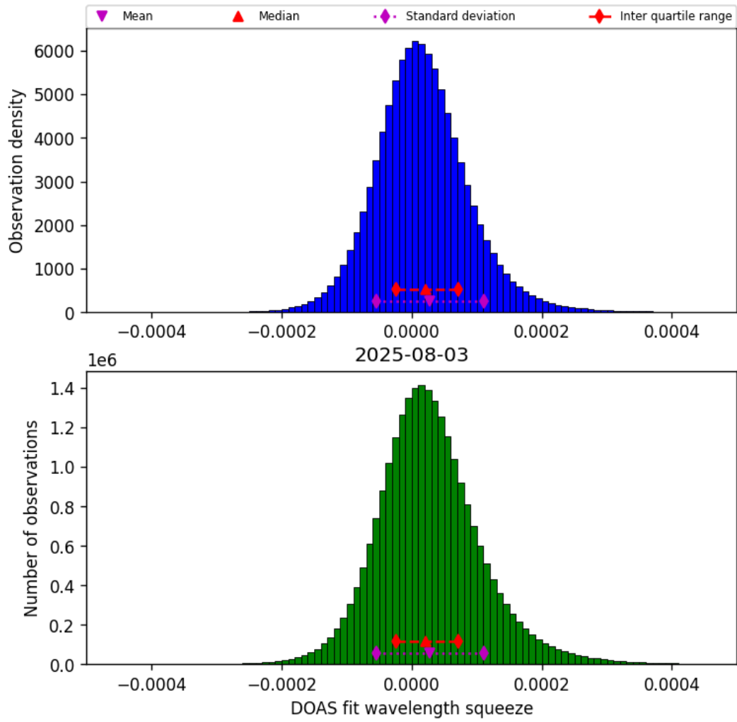
Figure 45: Histogram of “DOAS fit wavelength squeeze” for 2025-08-03 to 2025-08-04
