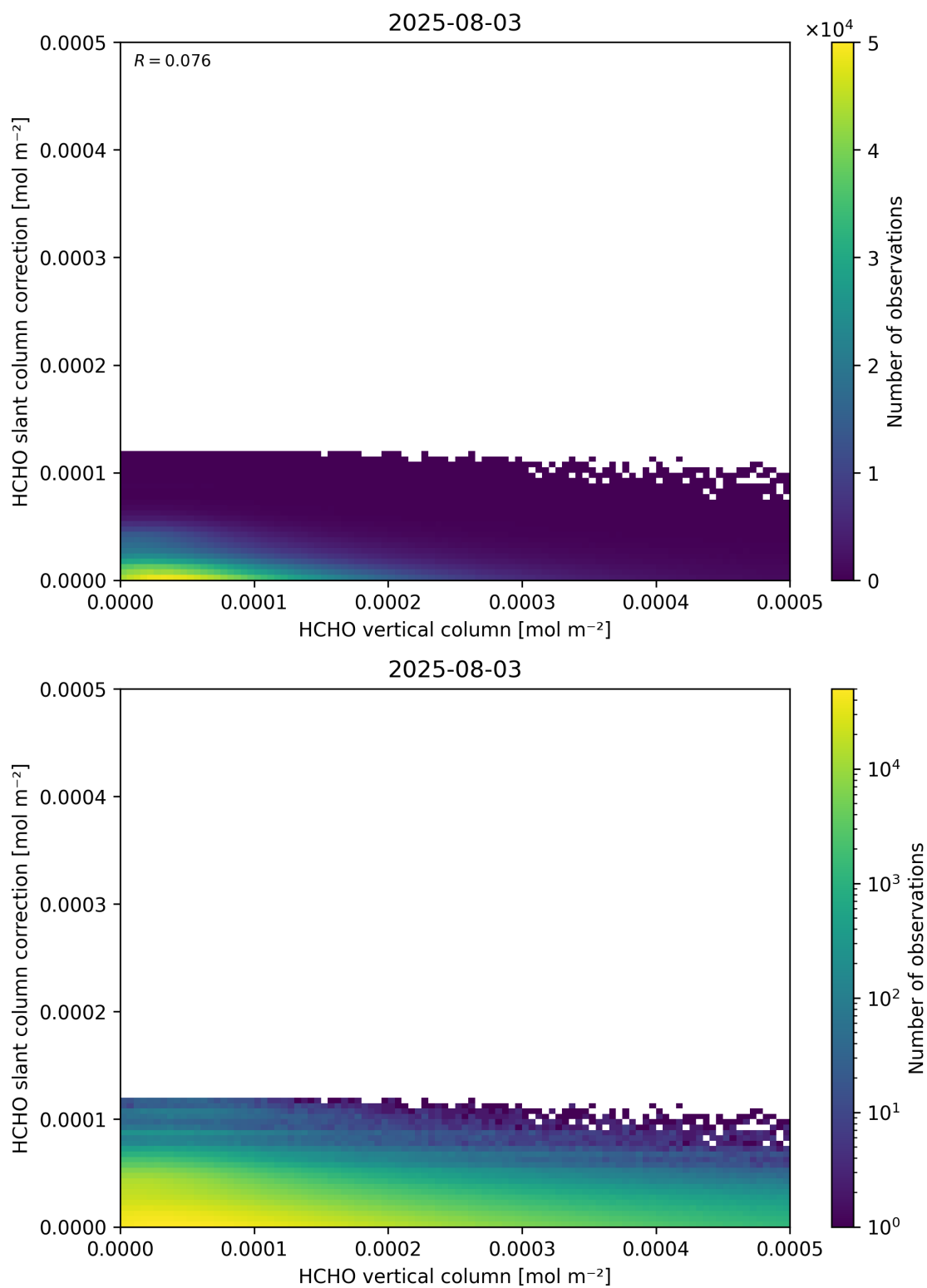
Figure 128: Scatter density plot of “HCHO vertical column” against “HCHO slant column correction” for 2025-08-03 to 2025-08-04.
