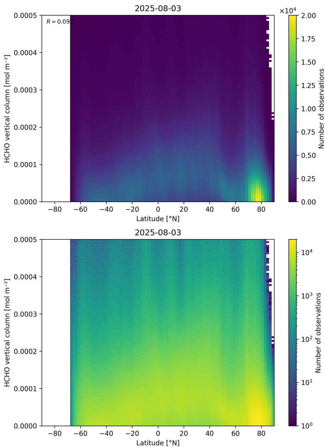
Figure 163: Scatter density plot of “Latitude” against “HCHO vertical column” for 2025-08-03 to 2025-08-04.
