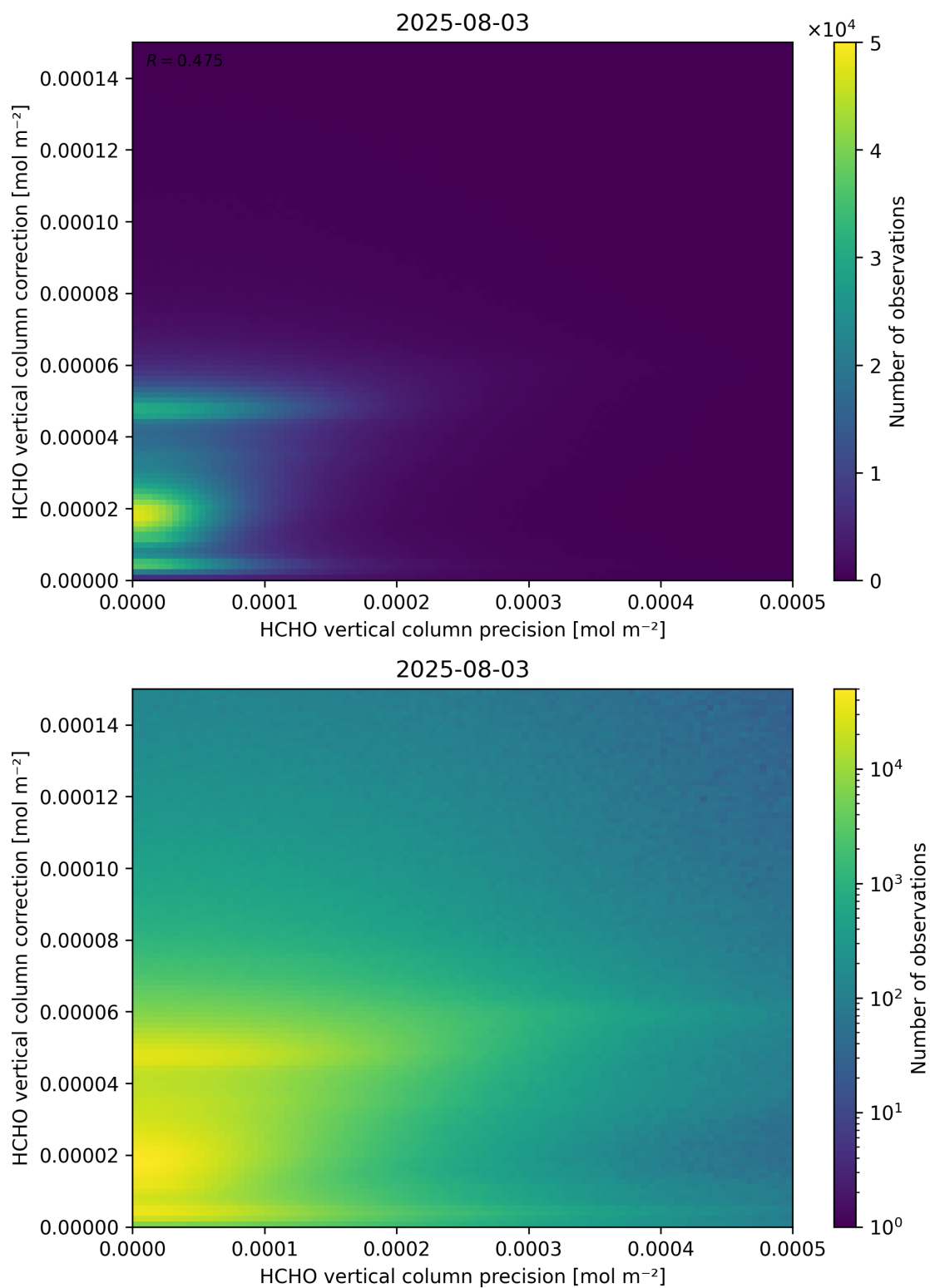
Figure 146: Scatter density plot of “HCHO vertical column precision” against “HCHO vertical column correction” for 2025-08-03 to 2025-08-04.
