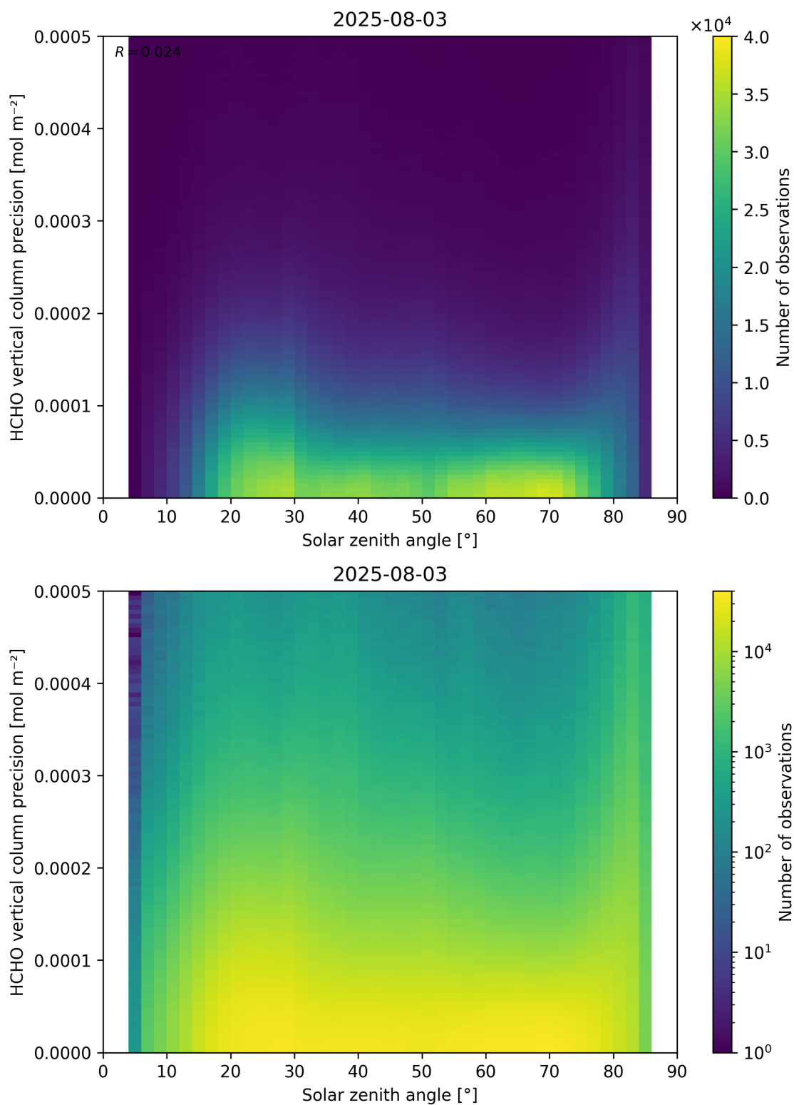
Figure 179: Scatter density plot of “Solar zenith angle” against “HCHO vertical column precision” for 2025-08-03 to 2025-08-04.
