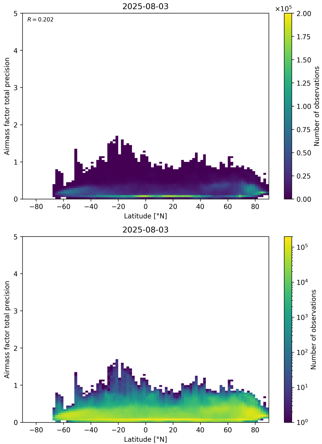
Figure 162: Scatter density plot of “Latitude” against “Airmass factor total precision” for 2025-08-03 to 2025-08-04.
