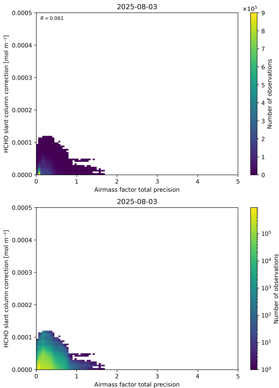
Figure 110: Scatter density plot of “Airmass factor total precision” against “HCHO slant column correction” for 2025-08-03 to 2025-08-04.
