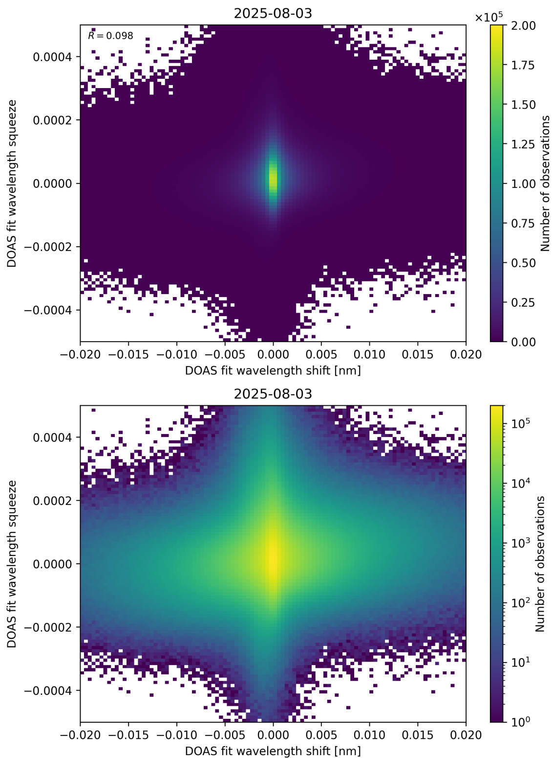
Figure 65: Scatter density plot of “DOAS fit wavelength shift” against “DOAS fit wavelength squeeze” for 2025-08-03 to 2025-08-04.
