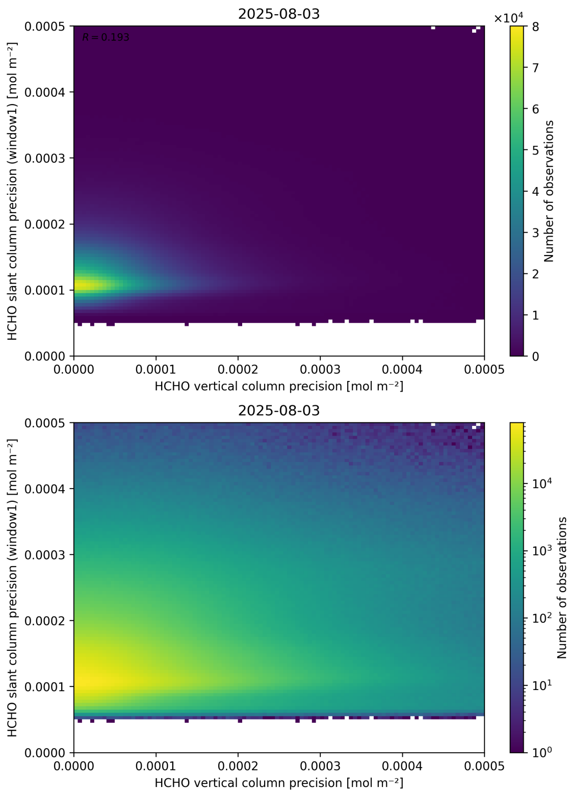
Figure 143: Scatter density plot of “HCHO vertical column precision” against “HCHO slant column precision (window1)” for 2025-08-03 to 2025-08-04.
