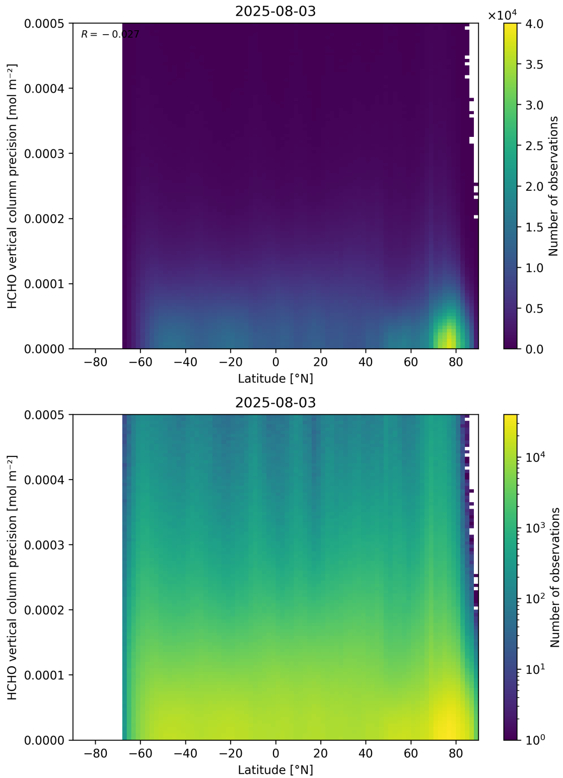
Figure 165: Scatter density plot of “Latitude” against “HCHO vertical column precision” for 2025-08-03 to 2025-08-04.
