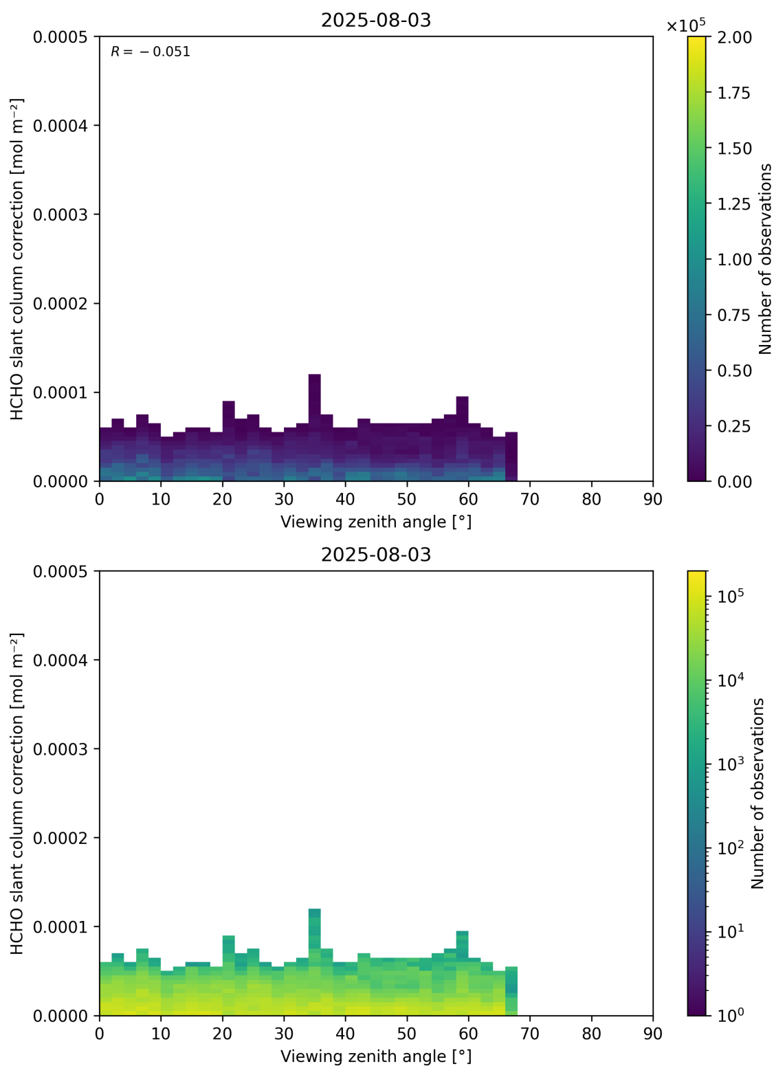
Figure 187: Scatter density plot of “Viewing zenith angle” against “HCHO slant column correction” for 2025-08-03 to 2025-08-04.
