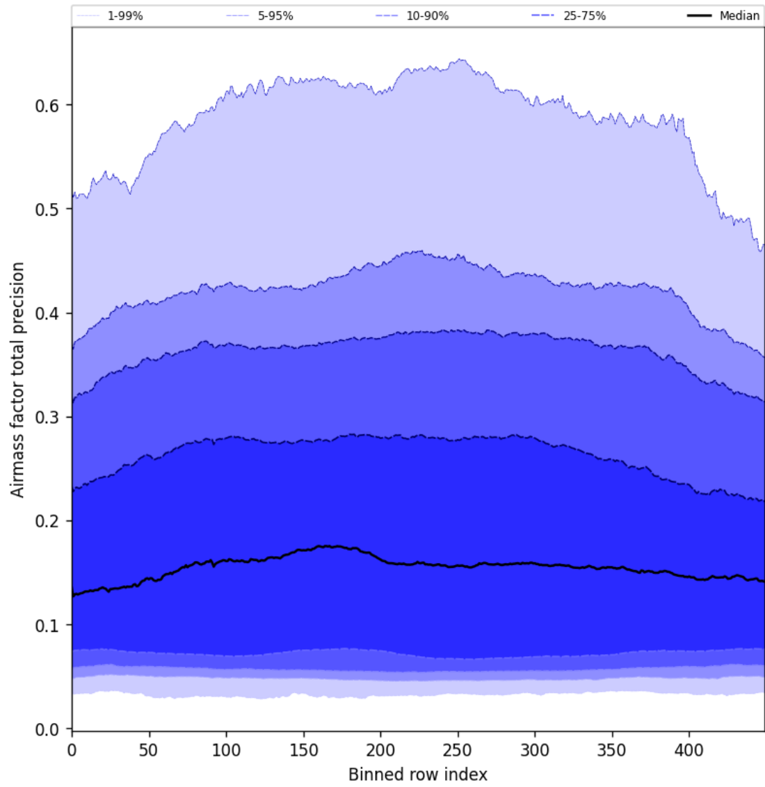
Figure 55: Along track statistics of “Airmass factor total precision” for 2025-08-03 to 2025-08-04
