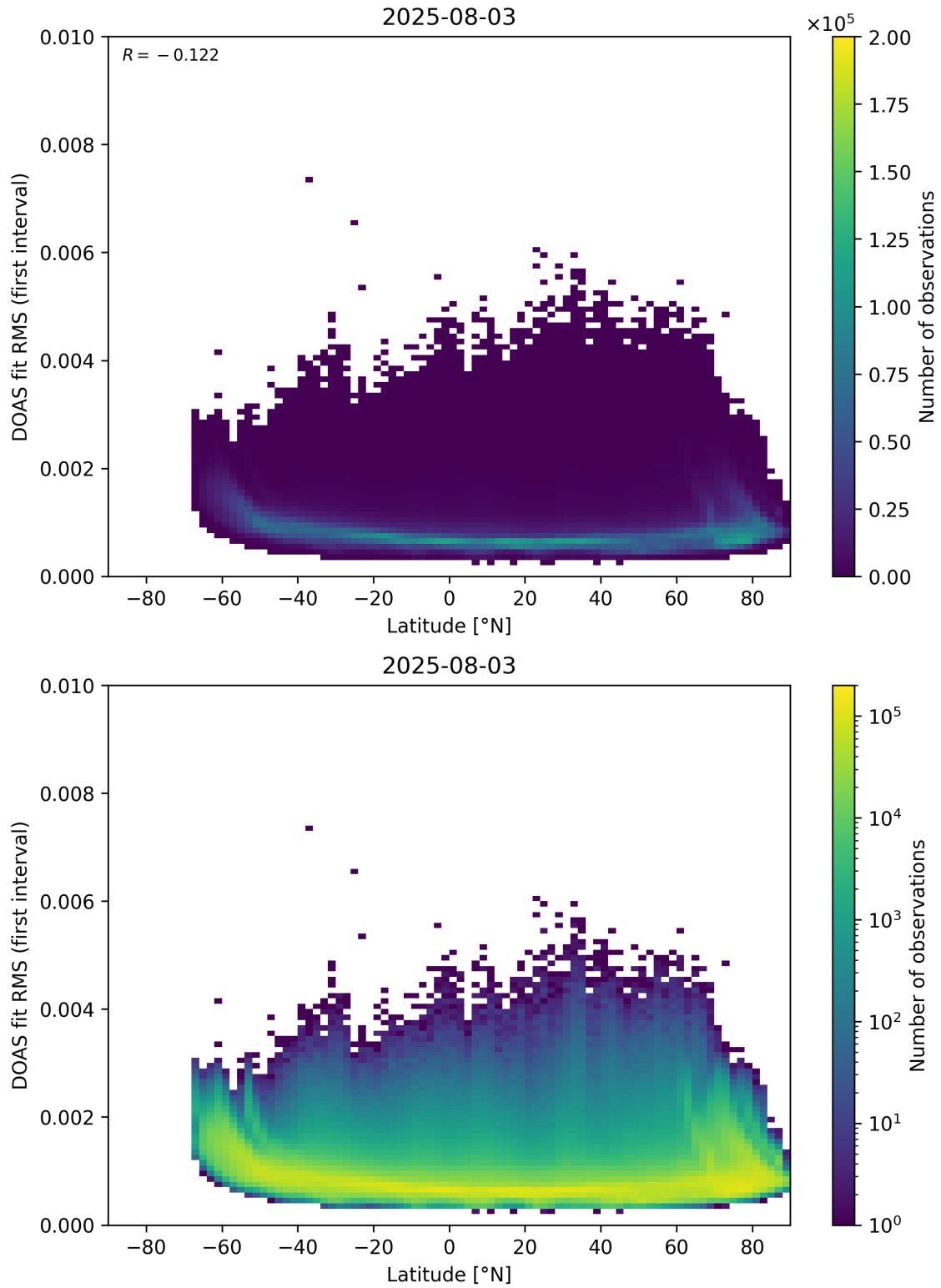
Figure 153: Scatter density plot of “Latitude” against “DOAS fit RMS (first interval)” for 2025-08-03 to 2025-08-04.
