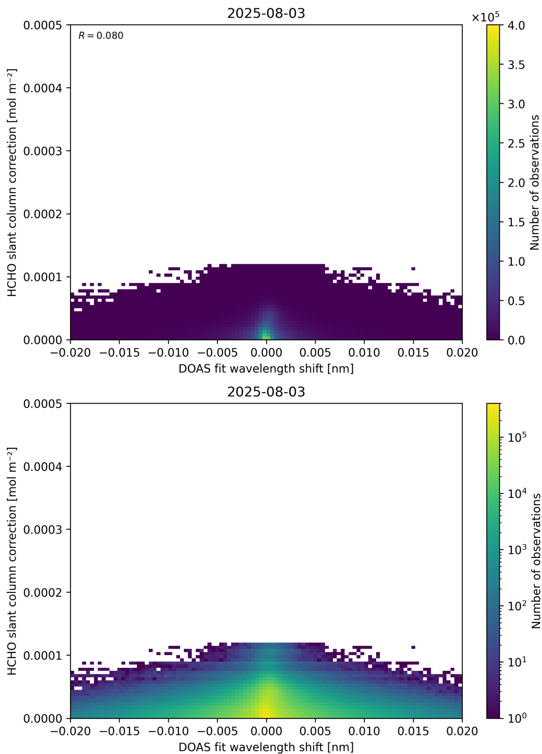
Figure 67: Scatter density plot of “DOAS fit wavelength shift” against “HCHO slant column correction” for 2025-08-03 to 2025-08-04.
