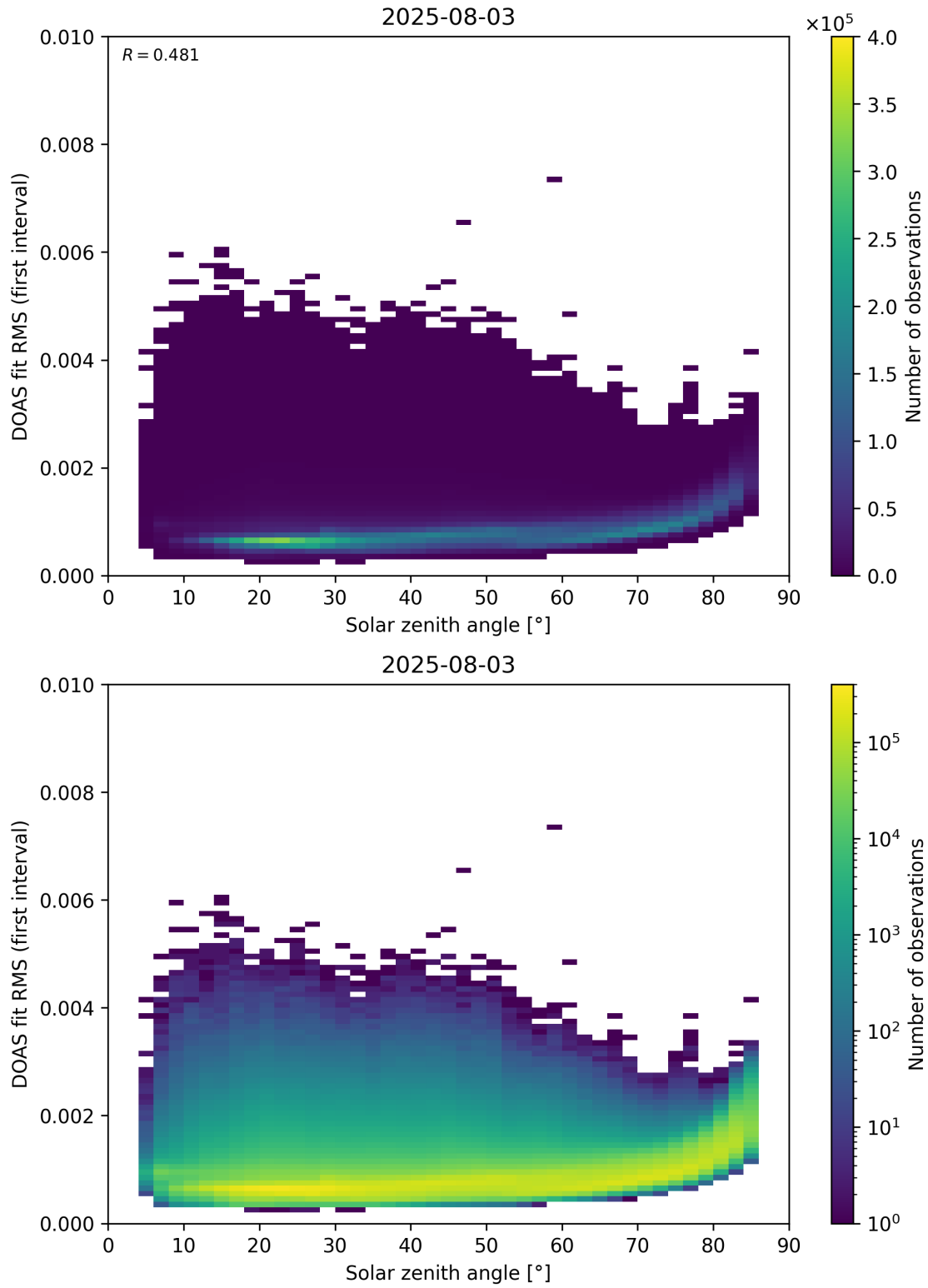
Figure 167: Scatter density plot of “Solar zenith angle” against “DOAS fit RMS (first interval)” for 2025-08-03 to 2025-08-04.
