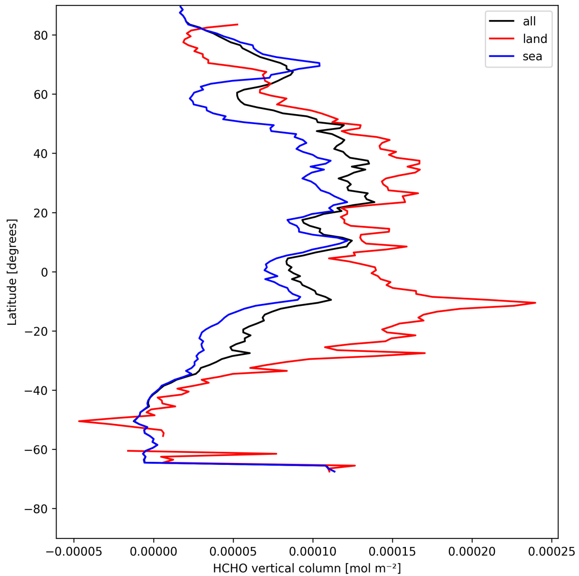
Figure 21: Zonal average of “HCHO vertical column” for 2025-08-03 to 2025-08-04.
