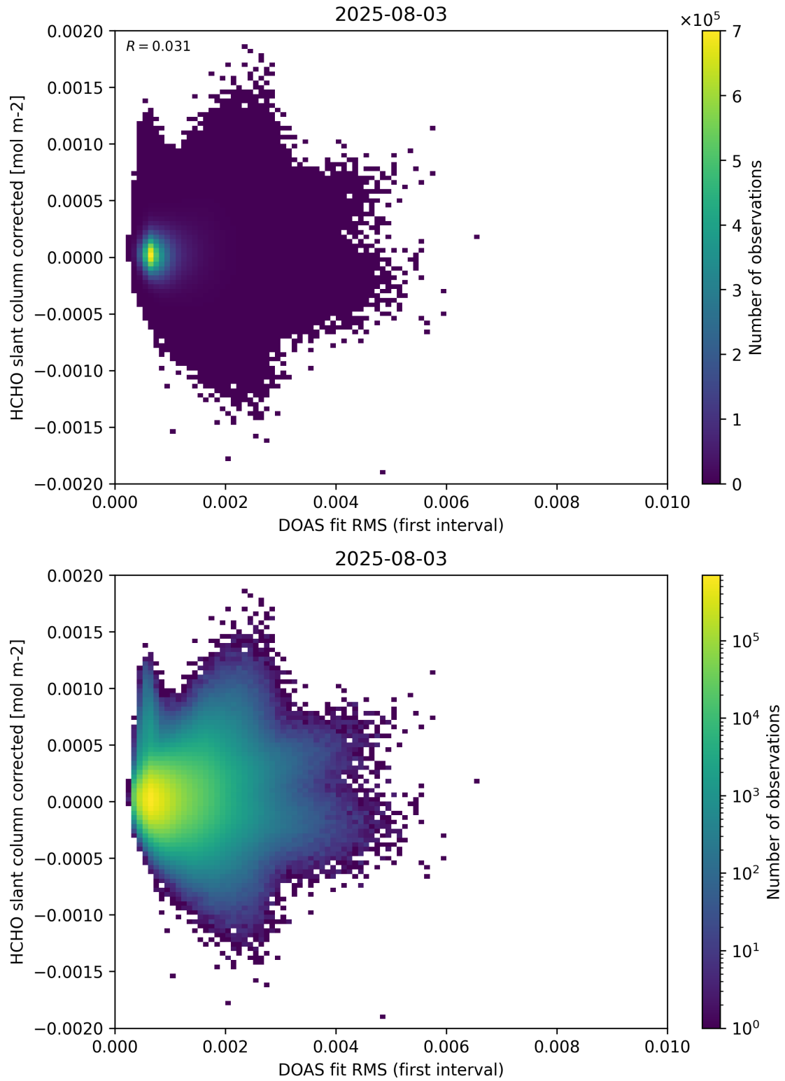
Figure 62: Scatter density plot of “DOAS fit RMS (first interval)” against “HCHO slant column corrected” for 2025-08-03 to 2025-08-04.
