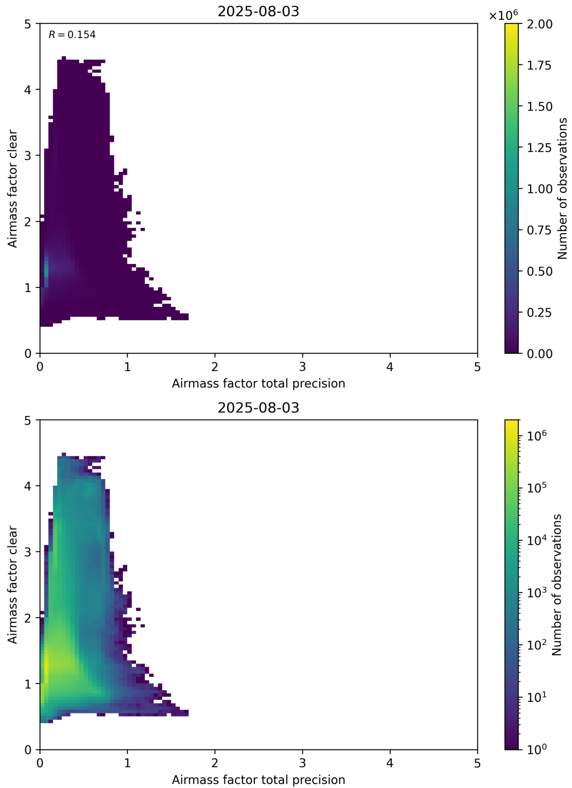
Figure 108: Scatter density plot of “Airmass factor total precision” against “Airmass factor clear” for 2025-08-03 to 2025-08-04.
