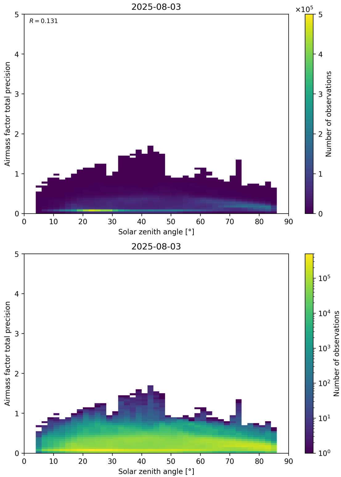
Figure 176: Scatter density plot of “Solar zenith angle” against “Airmass factor total precision” for 2025-08-03 to 2025-08-04.
