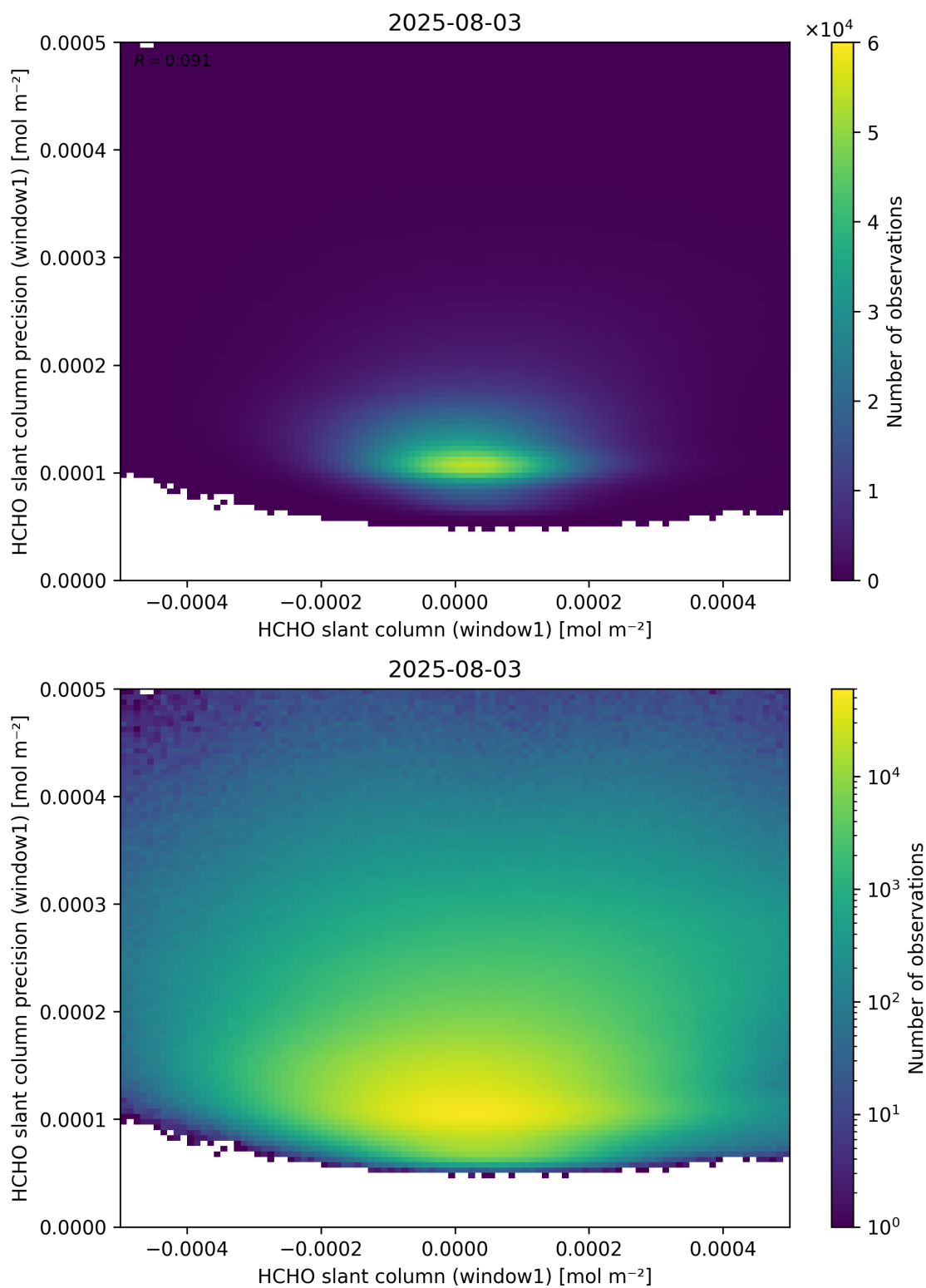
Figure 84: Scatter density plot of “HCHO slant column (window1)” against “HCHO slant column precision (window1)” for 2025-08-03 to 2025-08-04.
