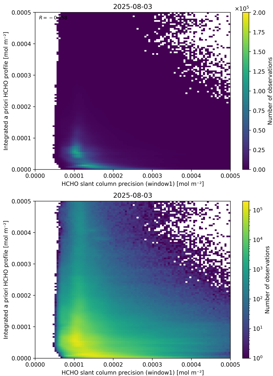
Figure 96: Scatter density plot of “HCHO slant column precision (window1)” against “Integrated a priori HCHO profile” for 2025-08-03 to 2025-08-04.
