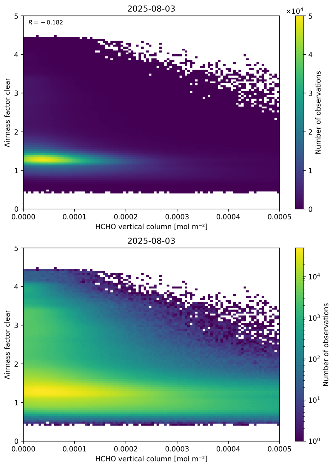
Figure 126: Scatter density plot of “HCHO vertical column” against “Airmass factor clear” for 2025-08-03 to 2025-08-04.
