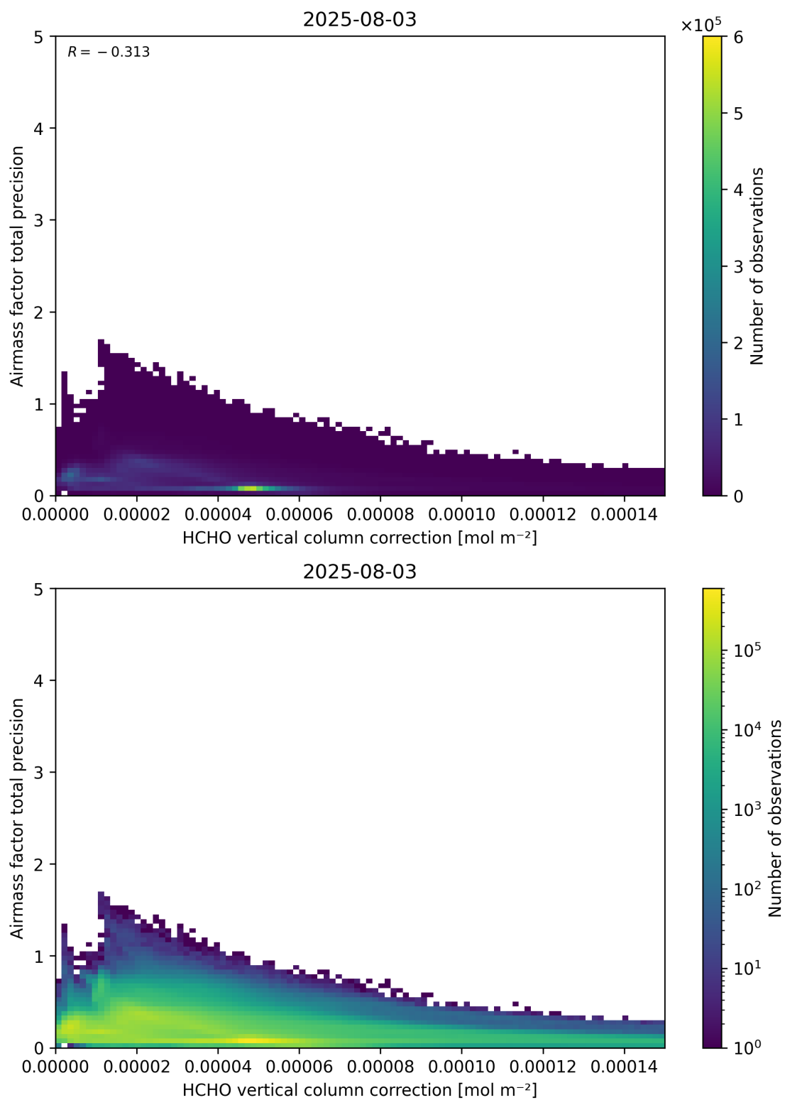
Figure 121: Scatter density plot of “HCHO vertical column correction” against “Airmass factor total precision” for 2025-08-03 to 2025-08-04.
