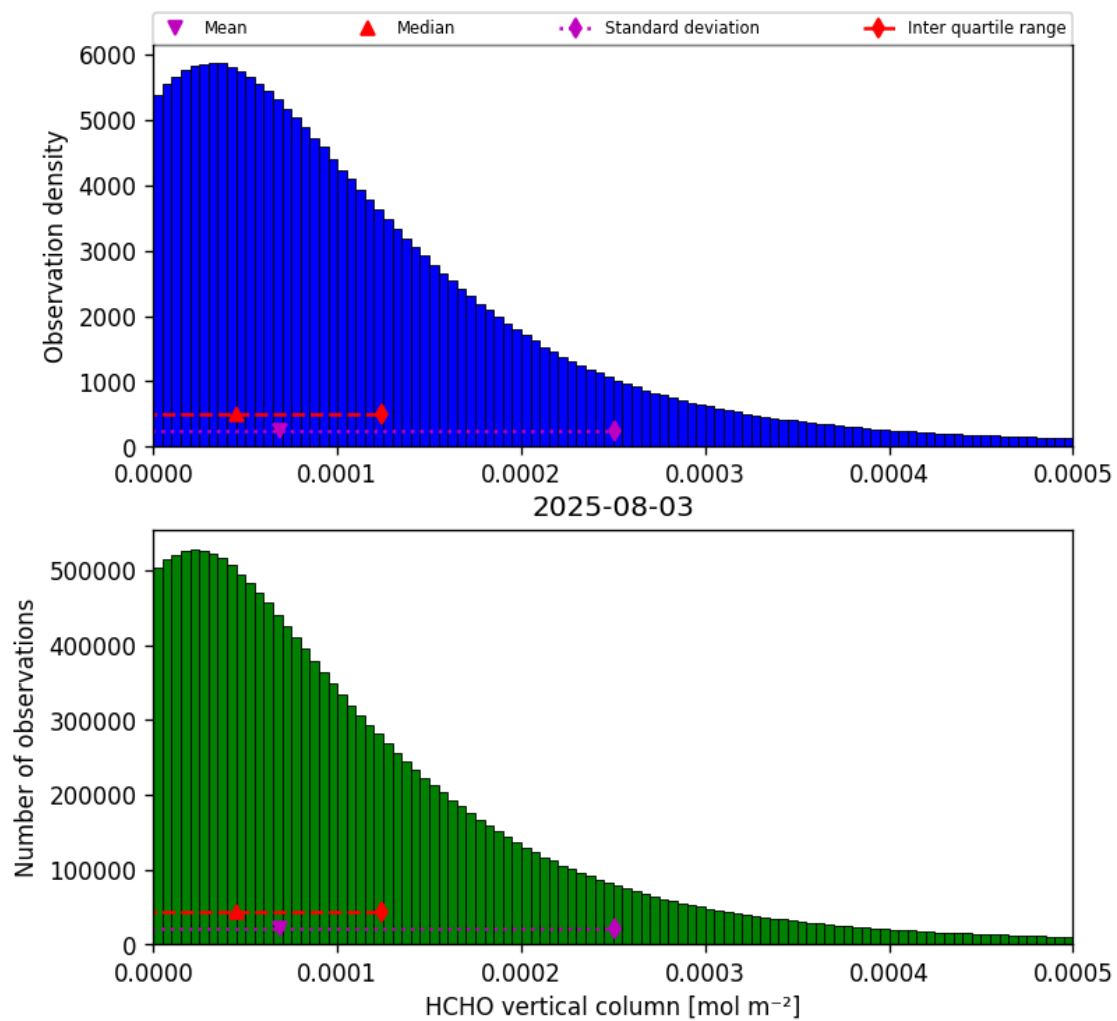
Figure 35: Histogram of “HCHO vertical column” for 2025-08-03 to 2025-08-04
