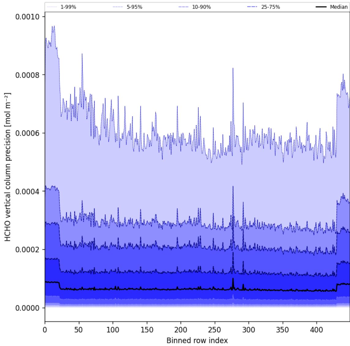
Figure 50: Along track statistics of “HCHO vertical column precision” for 2025-08-03 to 2025-08-04
