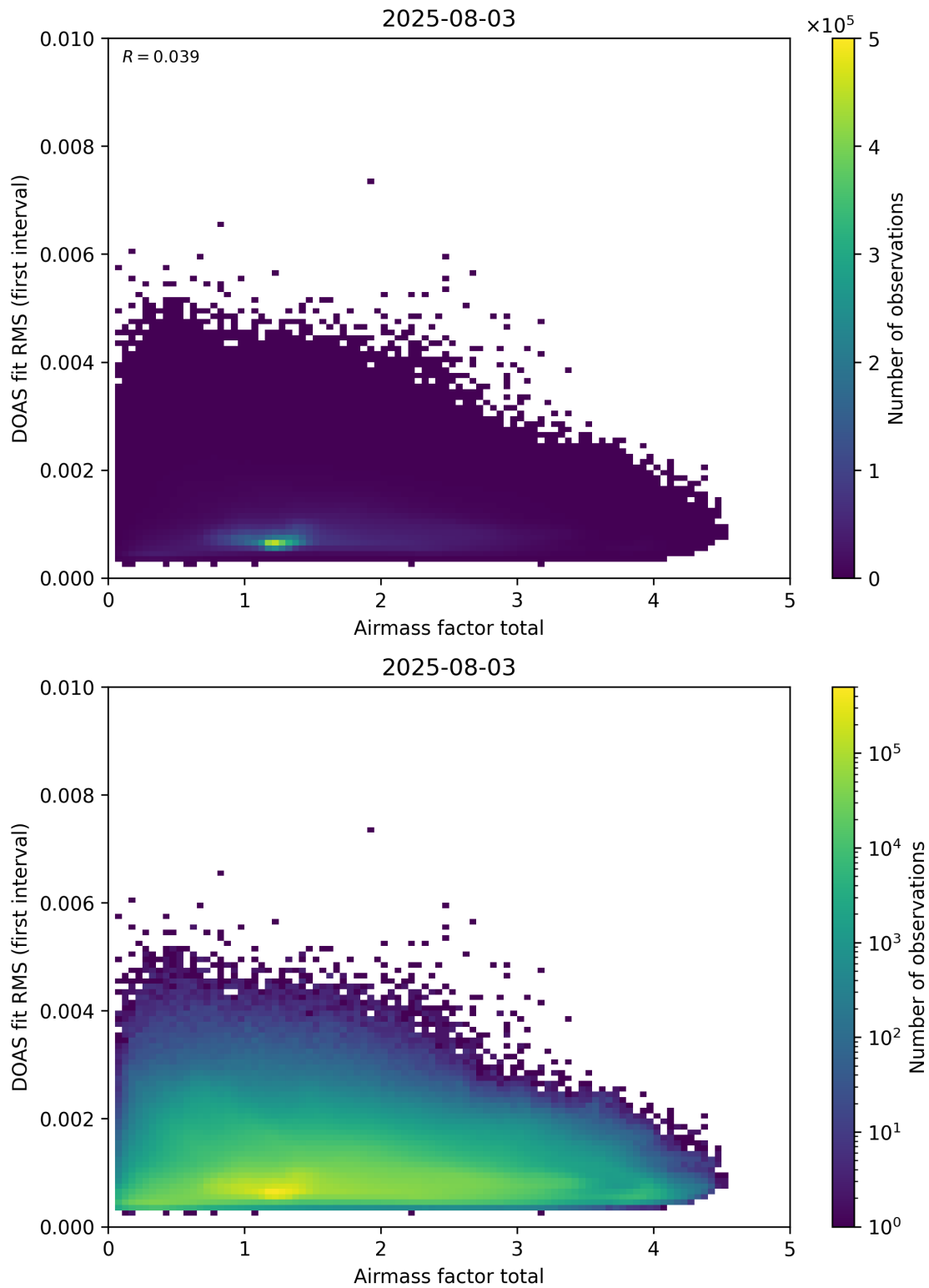
Figure 97: Scatter density plot of “Airmass factor total” against “DOAS fit RMS (first interval)” for 2025-08-03 to 2025-08-04.
