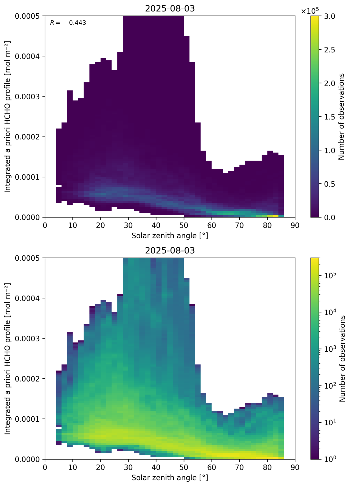
Figure 180: Scatter density plot of “Solar zenith angle” against “Integrated a priori HCHO profile” for 2025-08-03 to 2025-08-04.
