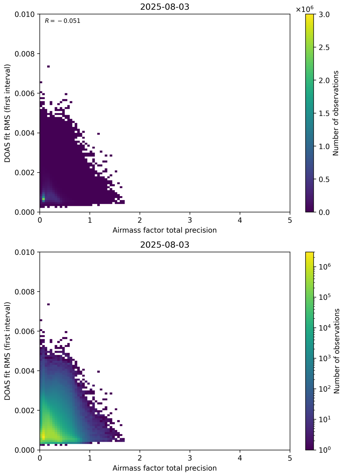
Figure 105: Scatter density plot of “Airmass factor total precision” against “DOAS fit RMS (first interval)” for 2025-08-03 to 2025-08-04.
