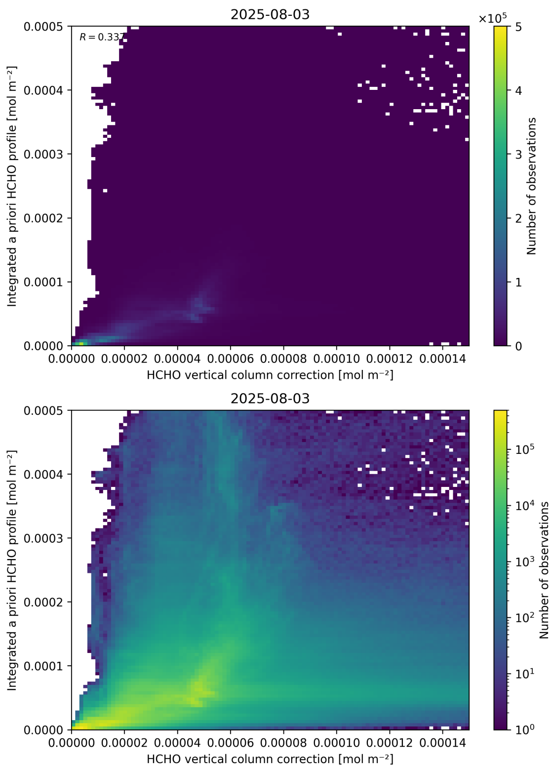
Figure 122: Scatter density plot of “HCHO vertical column correction” against “Integrated a priori HCHO profile” for 2025-08-03 to 2025-08-04.
