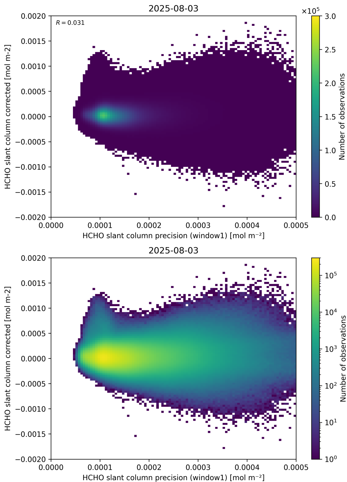
Figure 92: Scatter density plot of “HCHO slant column precision (window1)” against “HCHO slant column corrected” for 2025-08-03 to 2025-08-04.
