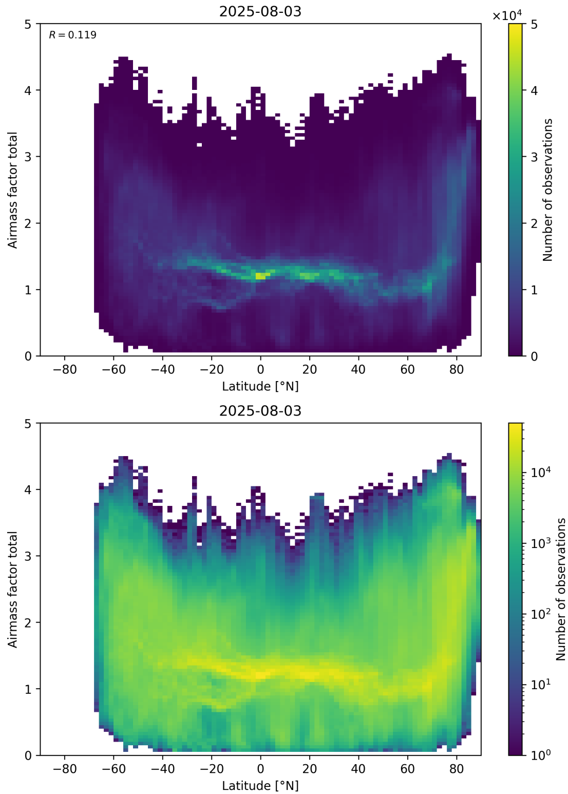
Figure 161: Scatter density plot of “Latitude” against “Airmass factor total” for 2025-08-03 to 2025-08-04.
