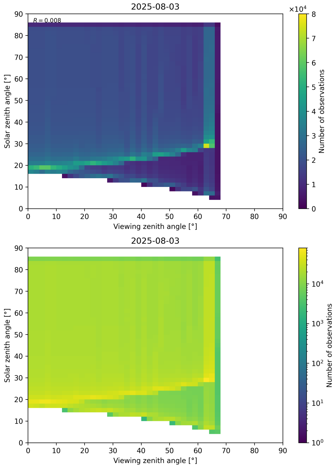
Figure 197: Scatter density plot of “Viewing zenith angle” against “Solar zenith angle” for 2025-08-03 to 2025-08-04.
