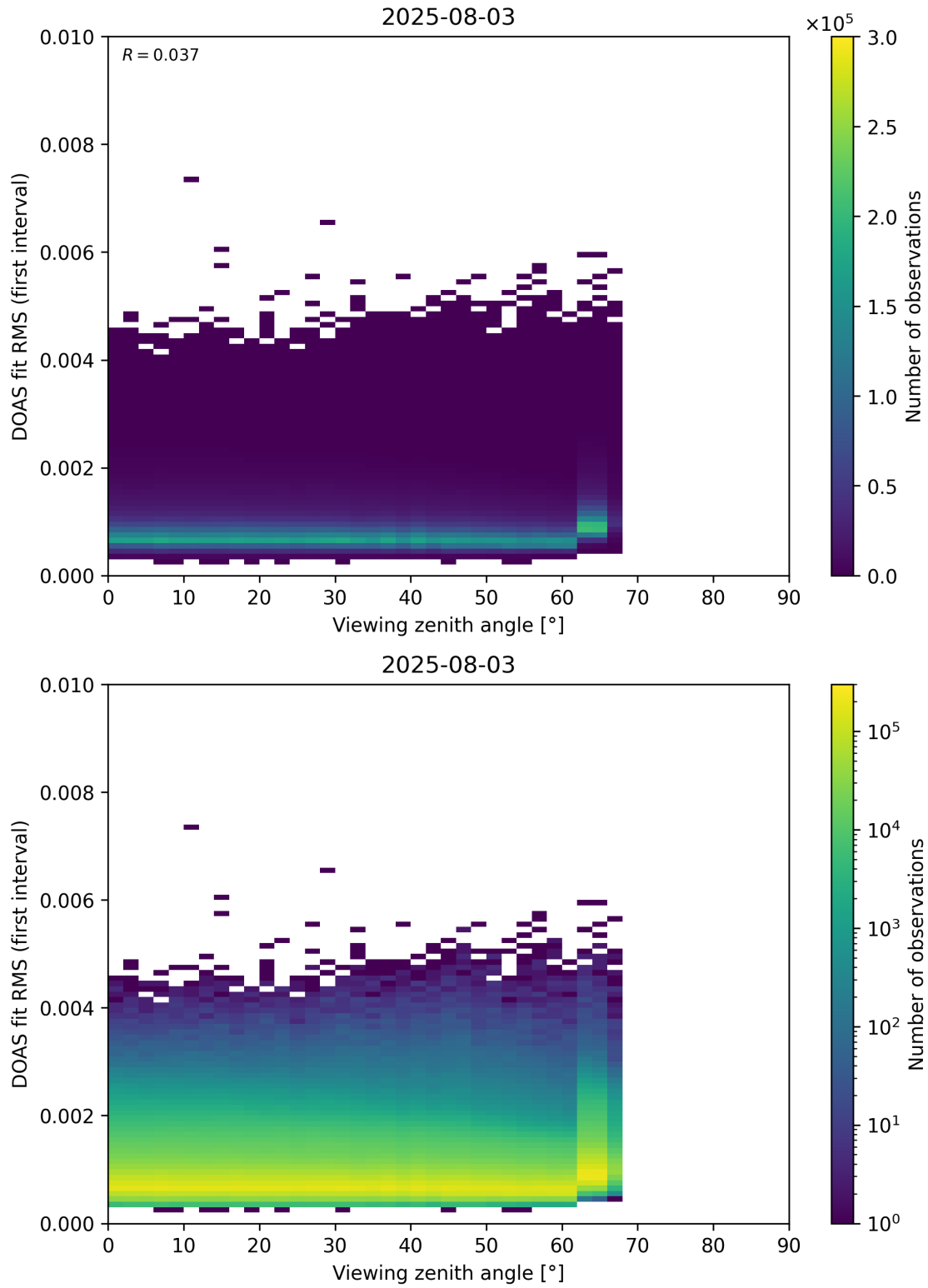
Figure 182: Scatter density plot of “Viewing zenith angle” against “DOAS fit RMS (first interval)” for 2025-08-03 to 2025-08-04.
