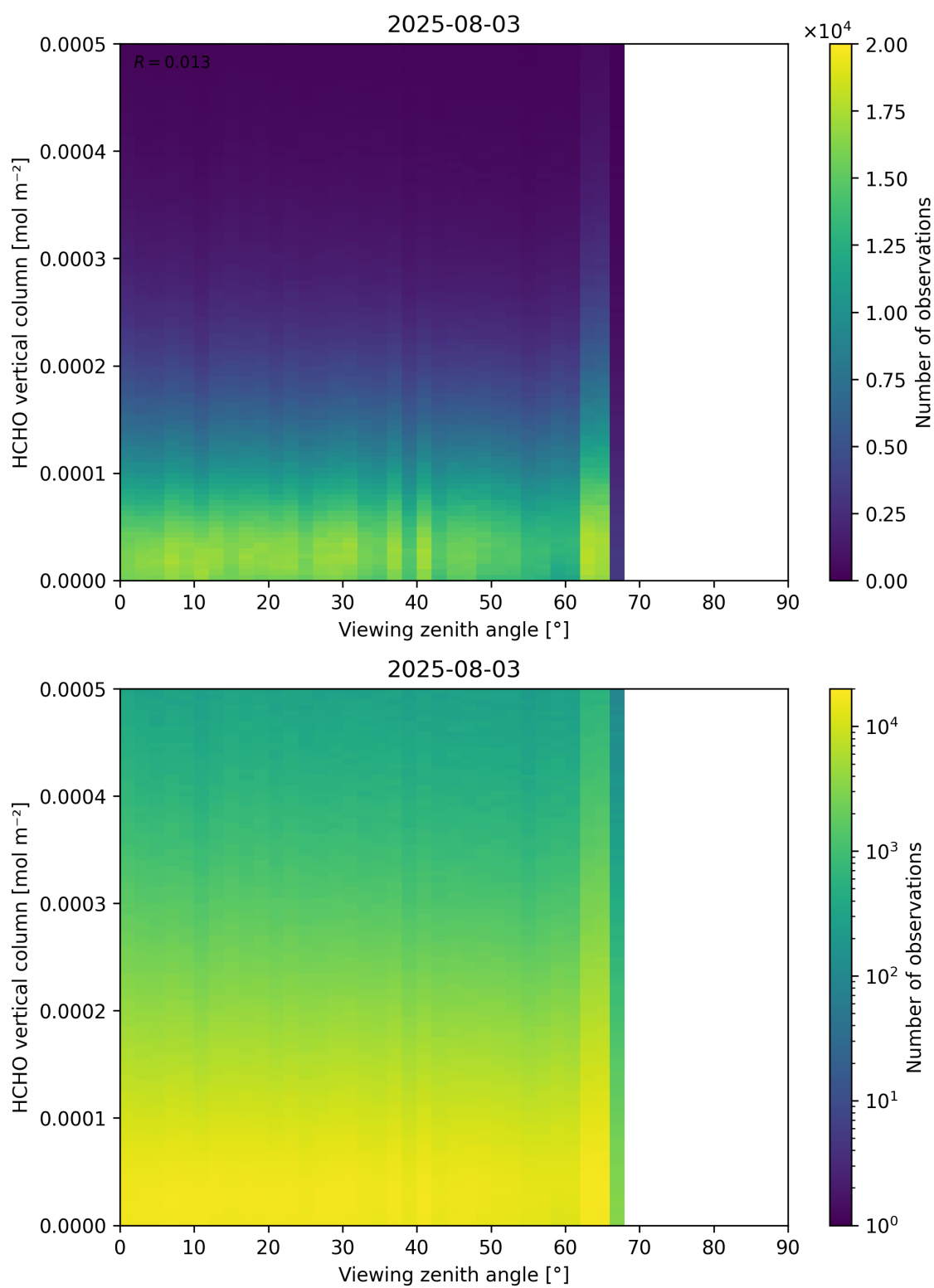
Figure 192: Scatter density plot of “Viewing zenith angle” against “HCHO vertical column” for 2025-08-03 to 2025-08-04.
