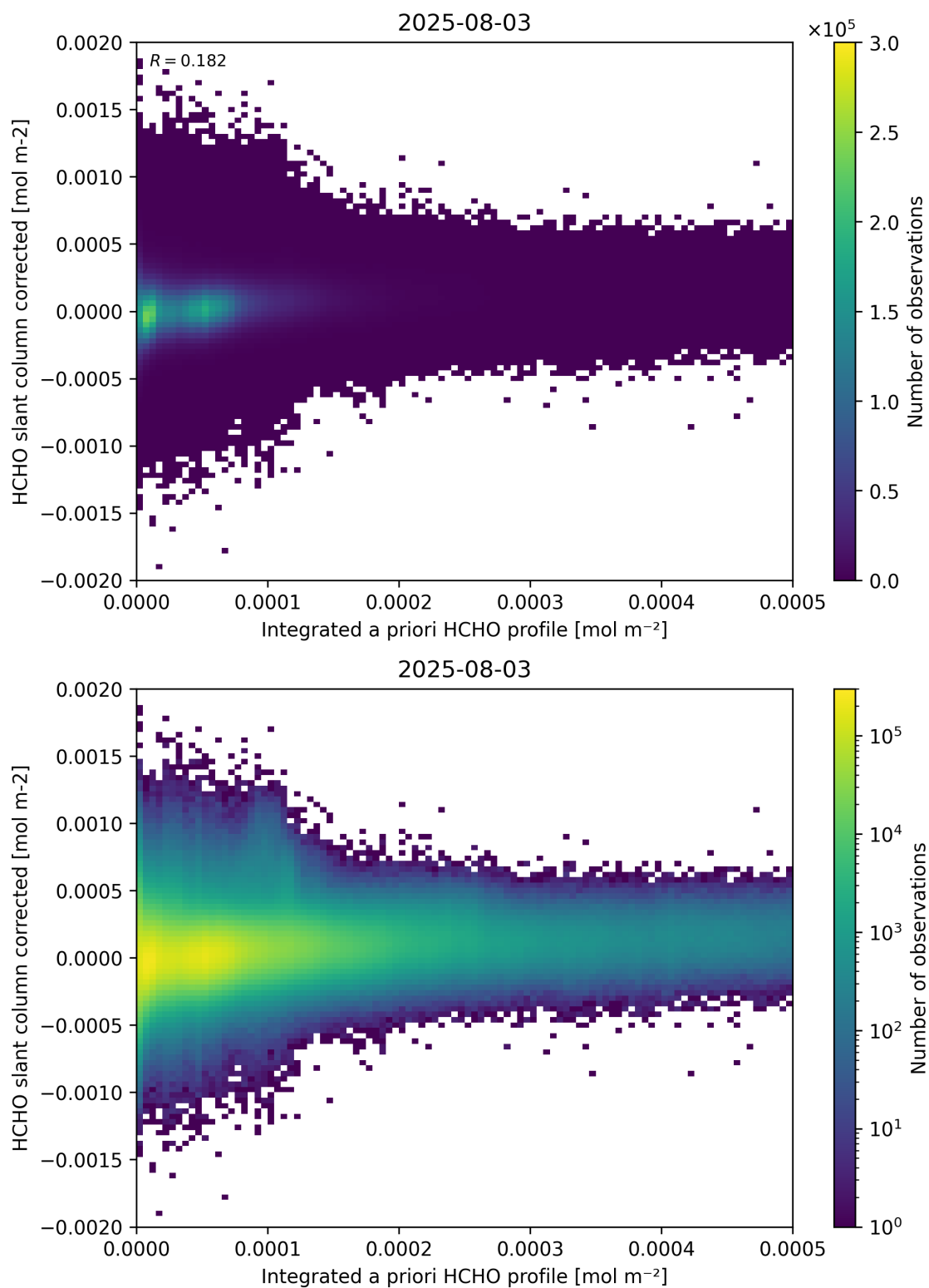
Figure 151: Scatter density plot of “Integrated a priori HCHO profile” against “HCHO slant column corrected” for 2025-08-03 to 2025-08-04.
