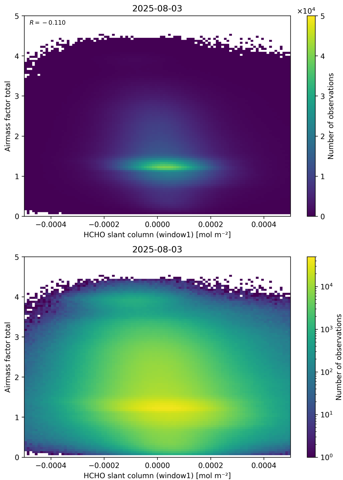
Figure 85: Scatter density plot of “HCHO slant column (window1)” against “Airmass factor total” for 2025-08-03 to 2025-08-04.
