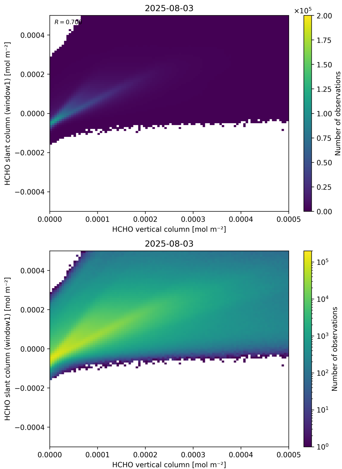
Figure 129: Scatter density plot of “HCHO vertical column” against “HCHO slant column (window1)” for 2025-08-03 to 2025-08-04.
