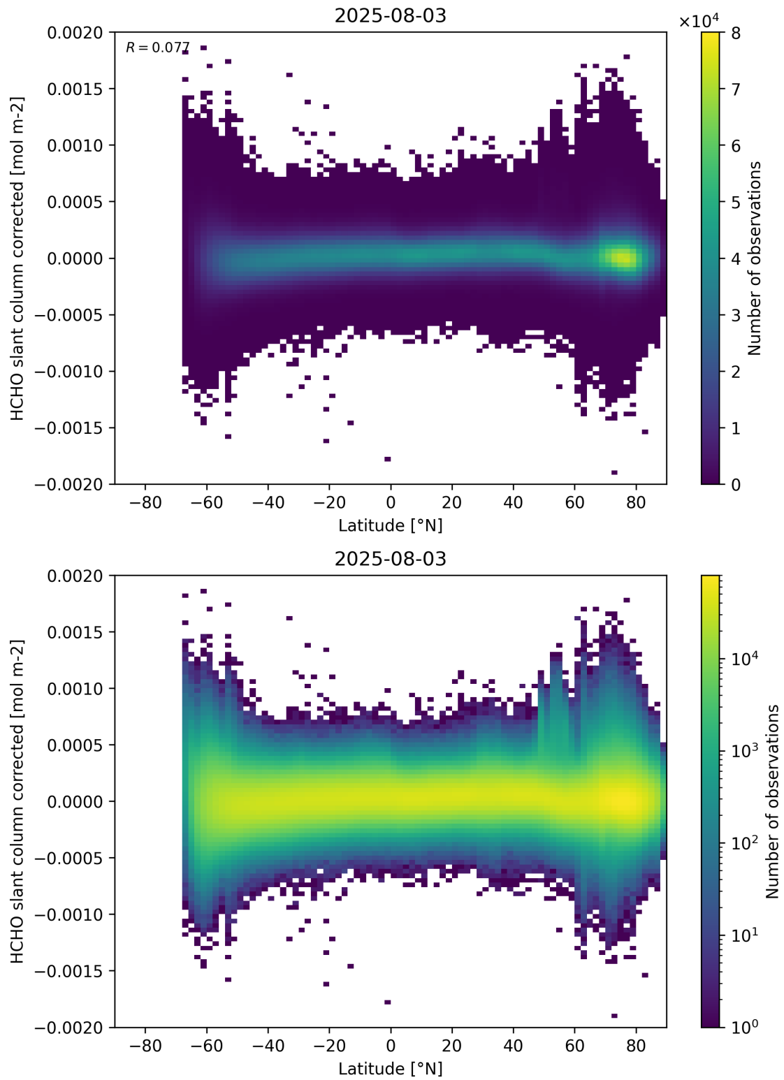
Figure 157: Scatter density plot of “Latitude” against “HCHO slant column corrected” for 2025-08-03 to 2025-08-04.
