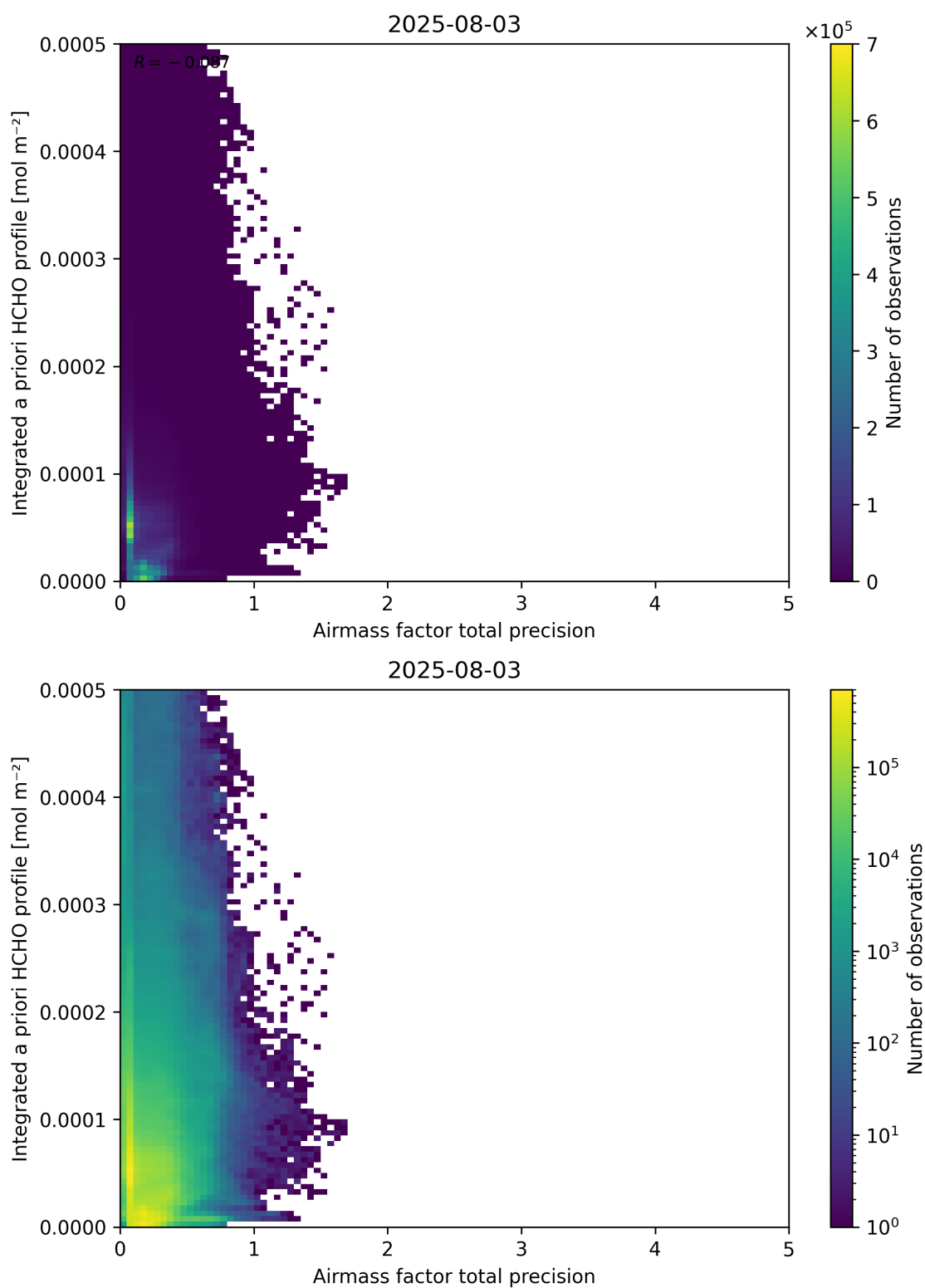
Figure 111: Scatter density plot of “Airmass factor total precision” against “Integrated a priori HCHO profile” for 2025-08-03 to 2025-08-04.
