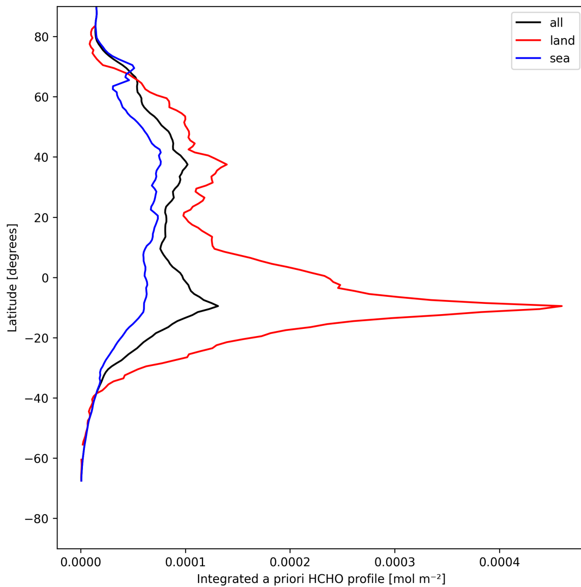
Figure 29: Zonal average of “Integrated a priori HCHO profile” for 2025-08-03 to 2025-08-04.
