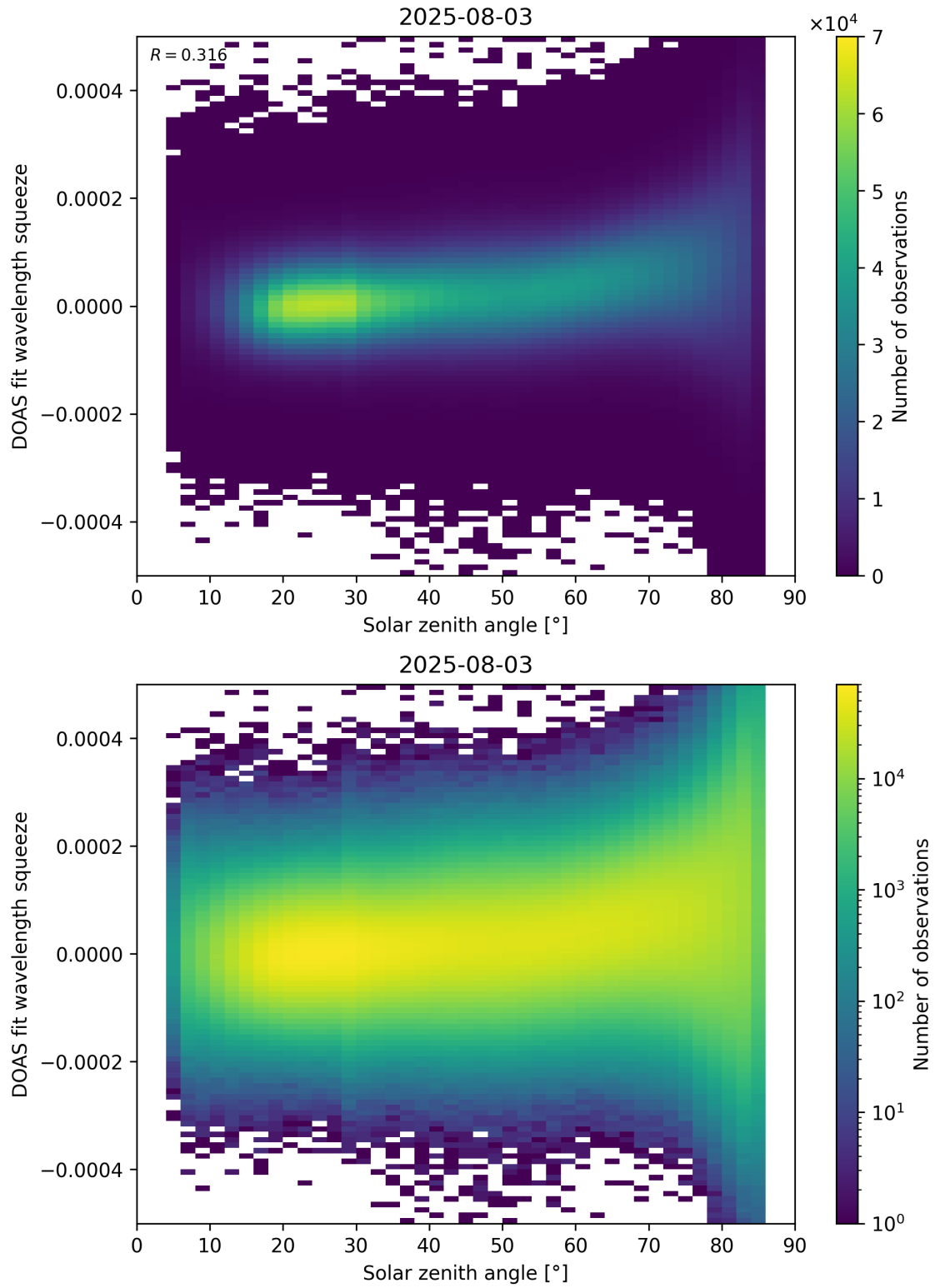
Figure 169: Scatter density plot of “Solar zenith angle” against “DOAS fit wavelength squeeze” for 2025-08-03 to 2025-08-04.
