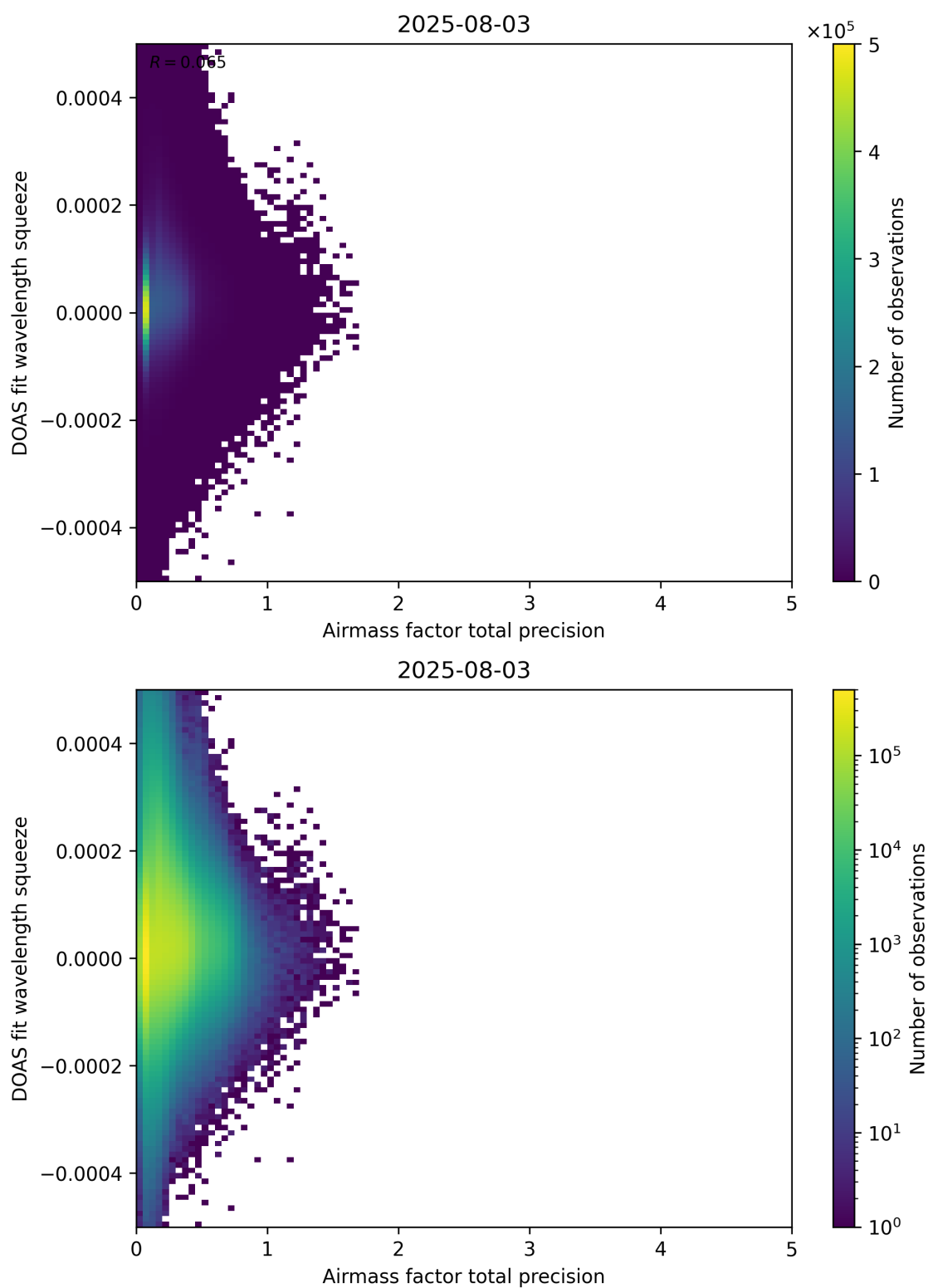
Figure 107: Scatter density plot of “Airmass factor total precision” against “DOAS fit wavelength squeeze” for 2025-08-03 to 2025-08-04.
