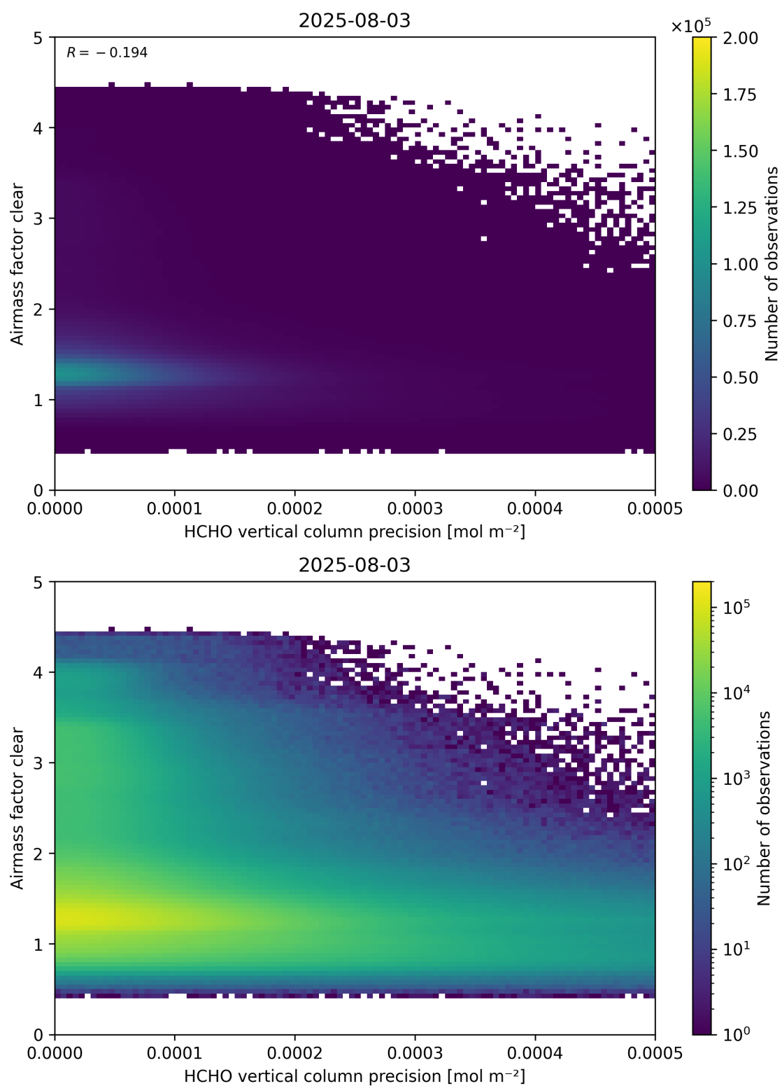
Figure 139: Scatter density plot of “HCHO vertical column precision” against “Airmass factor clear” for 2025-08-03 to 2025-08-04.
