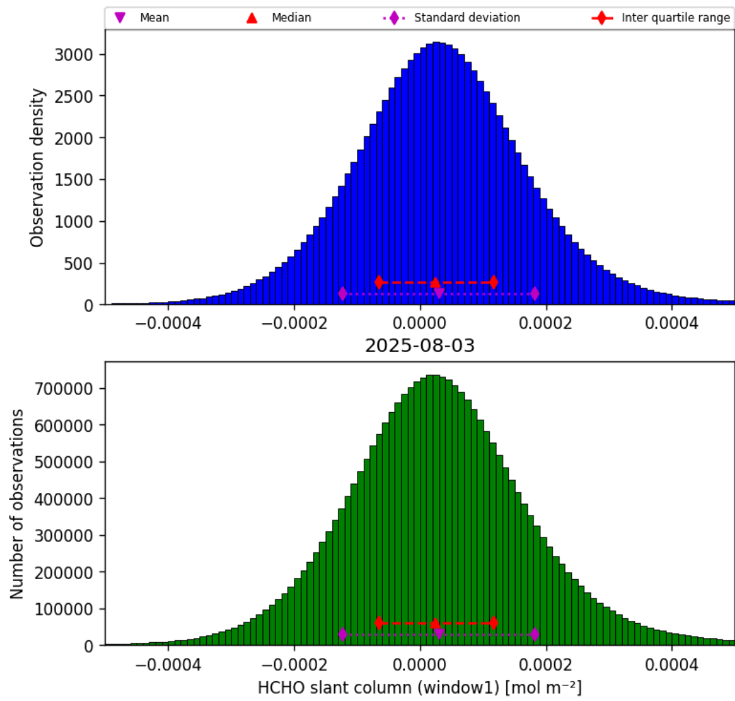
Figure 38: Histogram of “HCHO slant column (window1)” for 2025-08-03 to 2025-08-04
