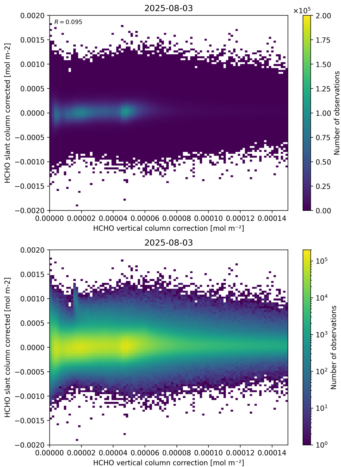
Figure 116: Scatter density plot of “HCHO vertical column correction” against “HCHO slant column corrected” for 2025-08-03 to 2025-08-04.
