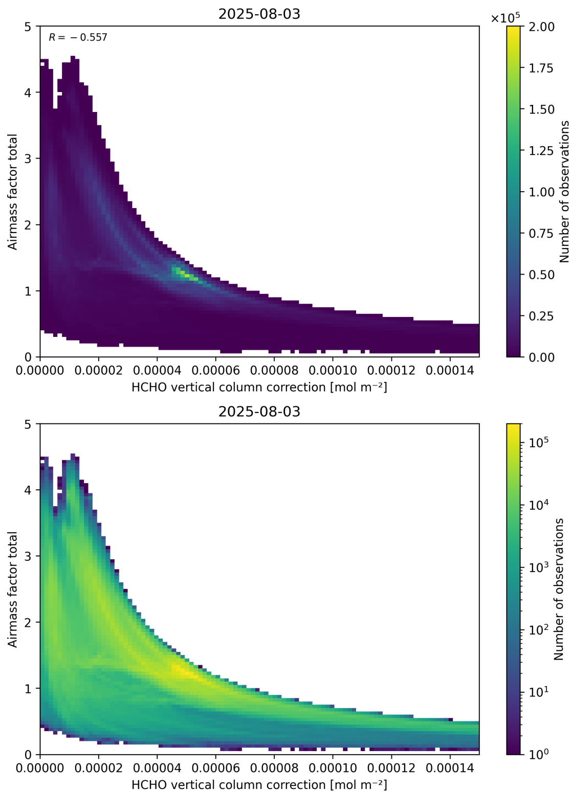
Figure 120: Scatter density plot of “HCHO vertical column correction” against “Airmass factor total” for 2025-08-03 to 2025-08-04.
