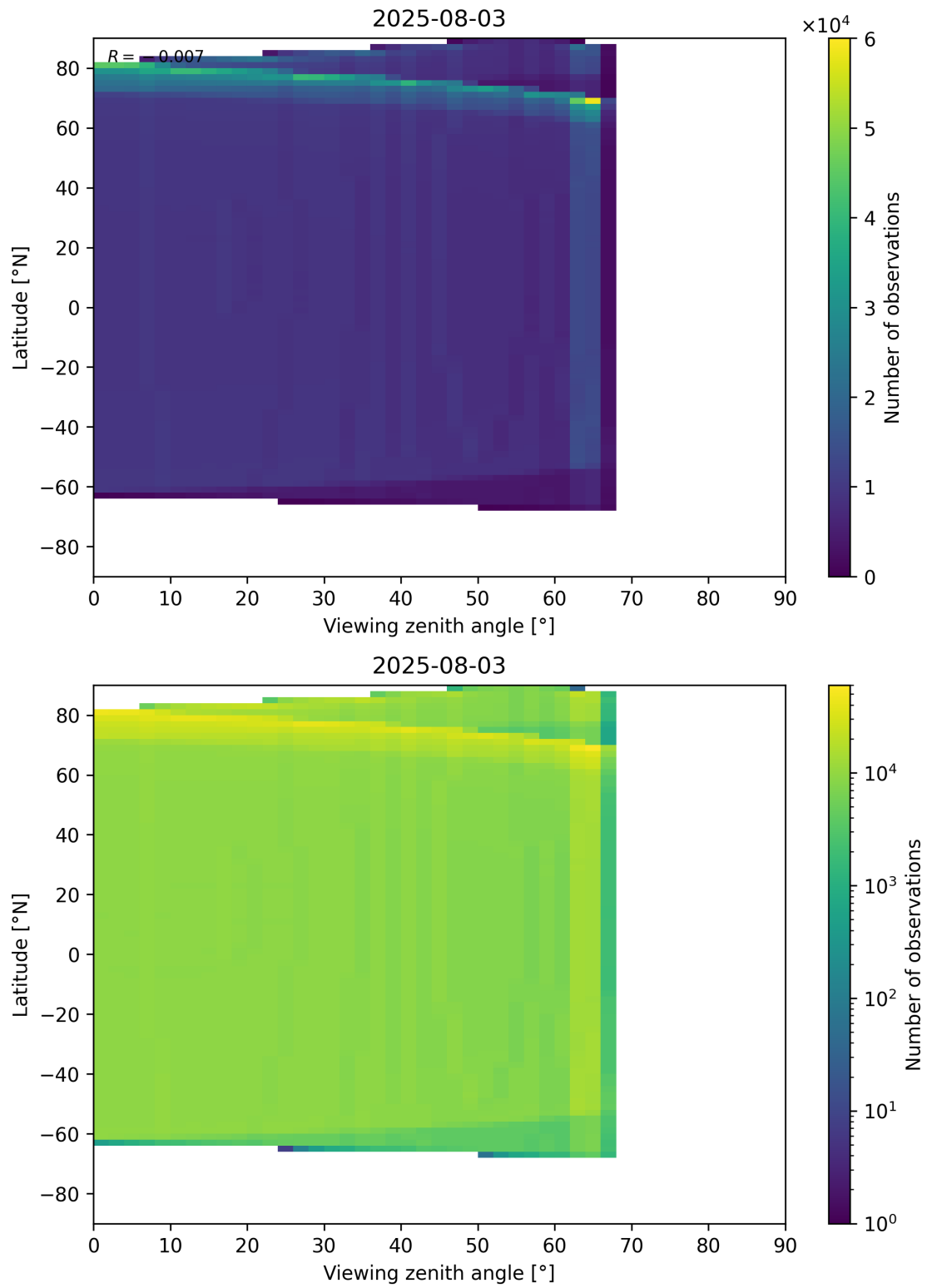
Figure 196: Scatter density plot of “Viewing zenith angle” against “Latitude” for 2025-08-03 to 2025-08-04.
