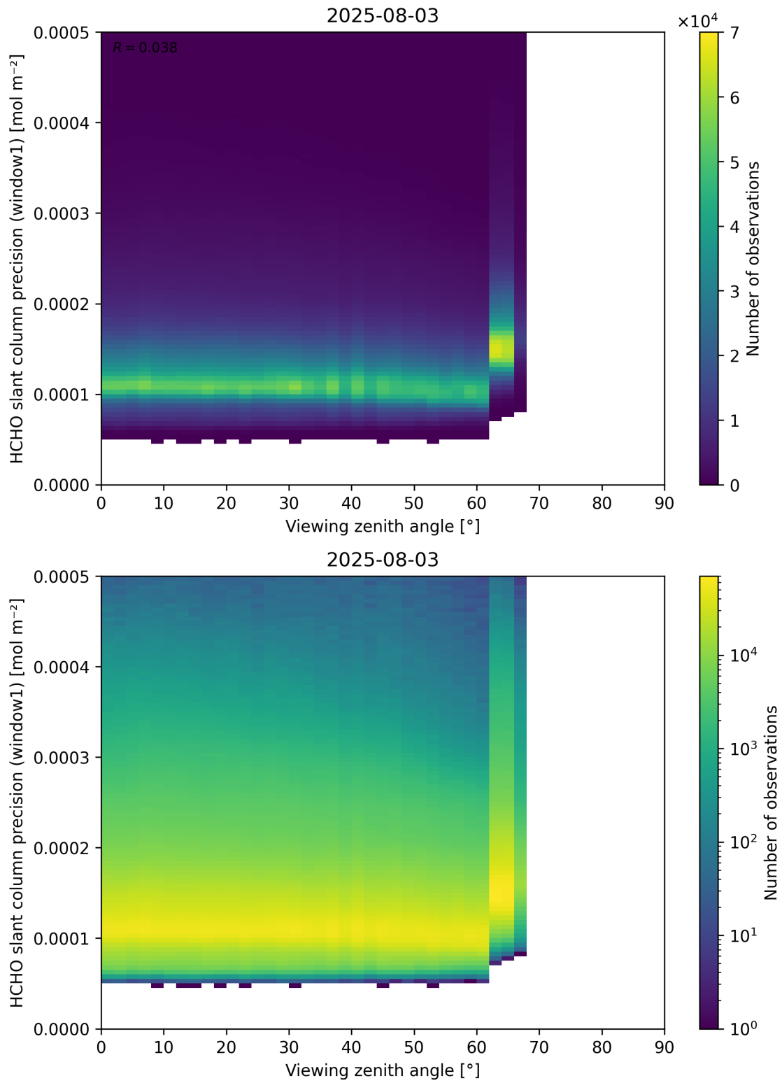
Figure 189: Scatter density plot of “Viewing zenith angle” against “HCHO slant column precision (window1)” for 2025-08-03 to 2025-08-04.
