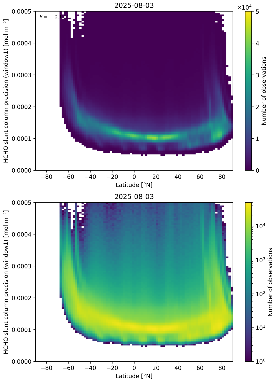
Figure 160: Scatter density plot of “Latitude” against “HCHO slant column precision (window1)” for 2025-08-03 to 2025-08-04.
