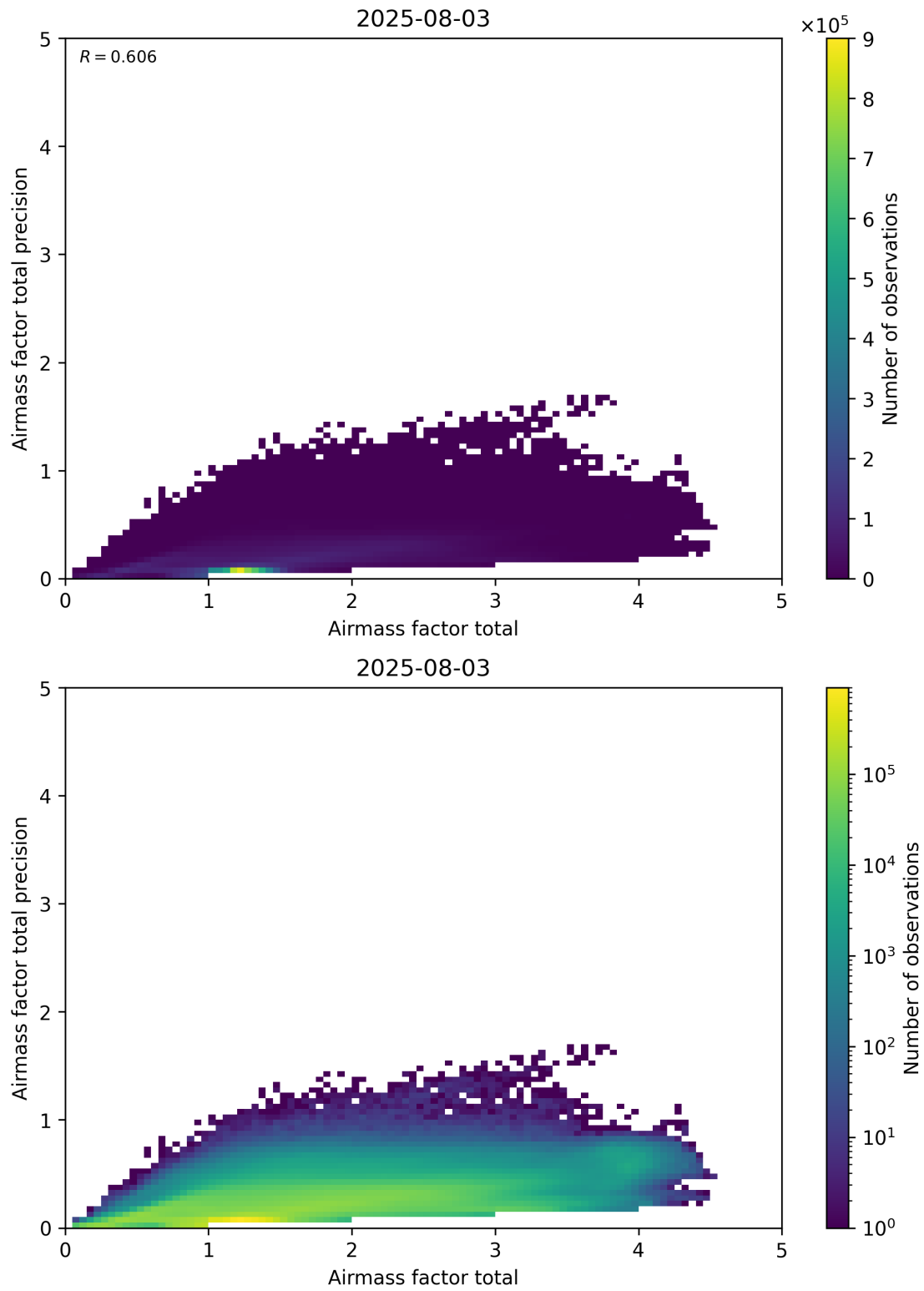
Figure 103: Scatter density plot of “Airmass factor total” against “Airmass factor total precision” for 2025-08-03 to 2025-08-04.
