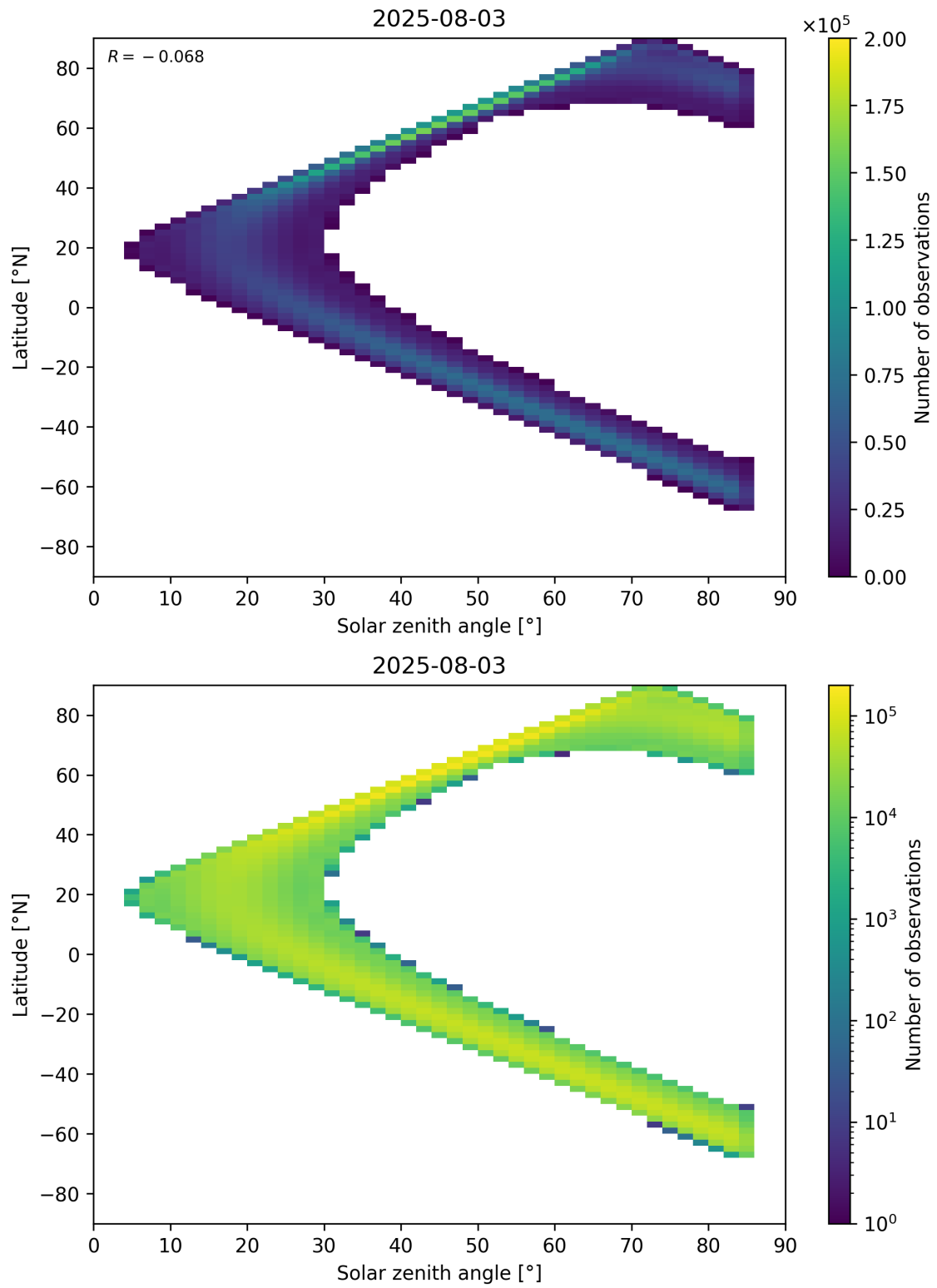
Figure 181: Scatter density plot of “Solar zenith angle” against “Latitude” for 2025-08-03 to 2025-08-04.
