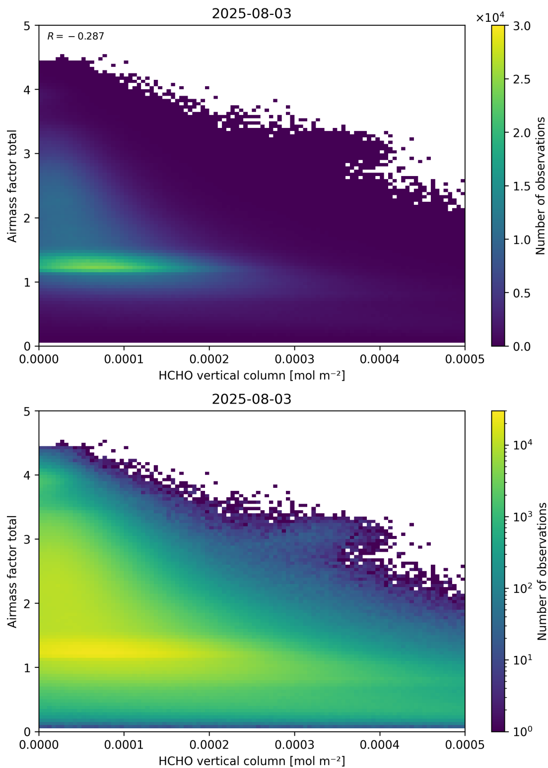
Figure 131: Scatter density plot of “HCHO vertical column” against “Airmass factor total” for 2025-08-03 to 2025-08-04.
