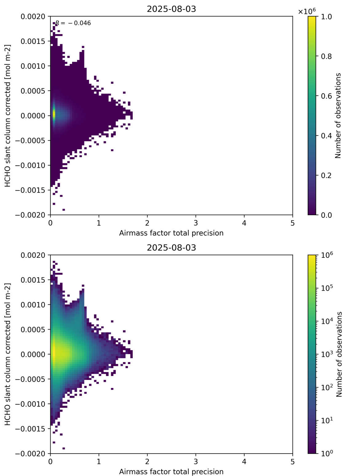
Figure 109: Scatter density plot of “Airmass factor total precision” against “HCHO slant column corrected” for 2025-08-03 to 2025-08-04.
