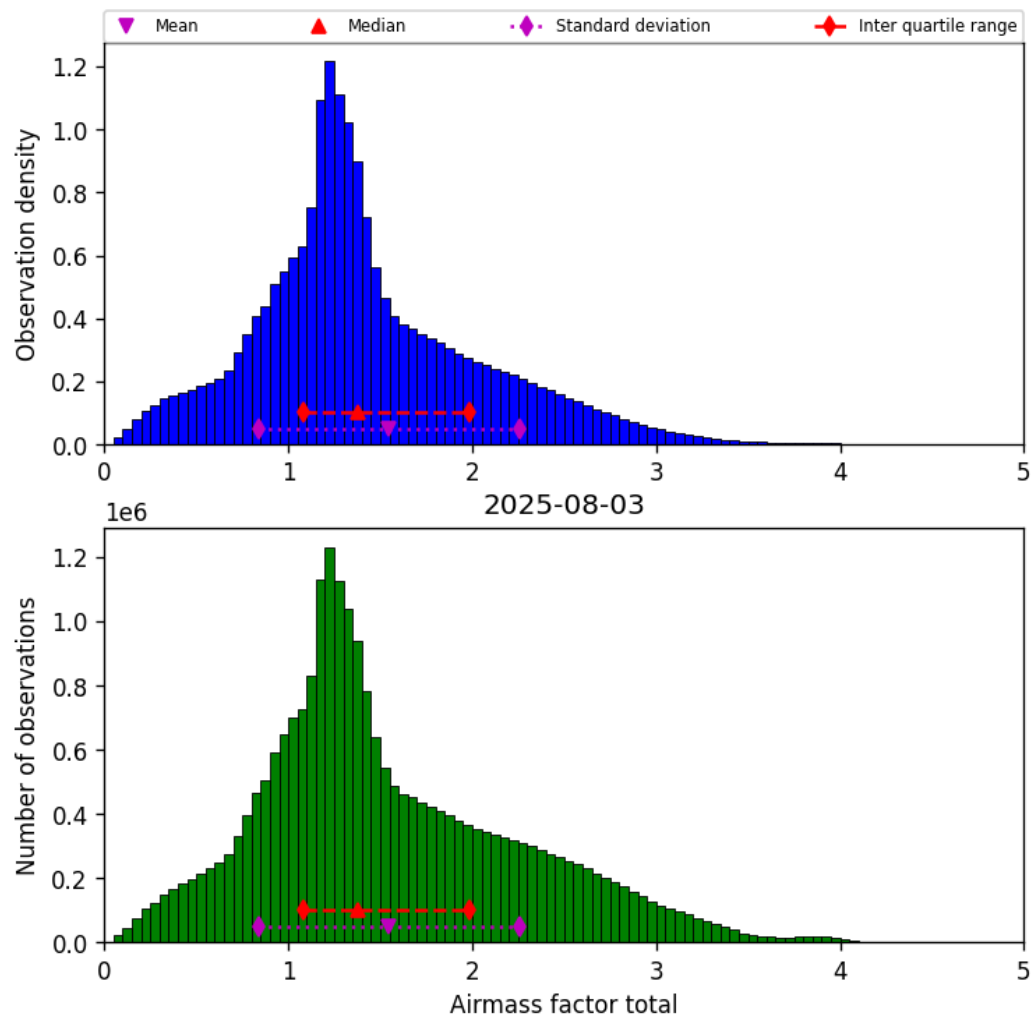
Figure 40: Histogram of “Airmass factor total” for 2025-08-03 to 2025-08-04
