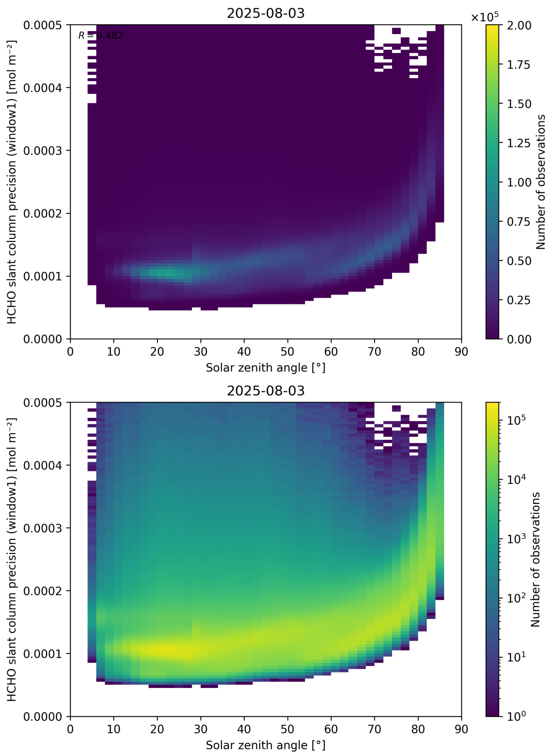
Figure 174: Scatter density plot of “Solar zenith angle” against “HCHO slant column precision (window1)” for 2025-08-03 to 2025-08-04.
