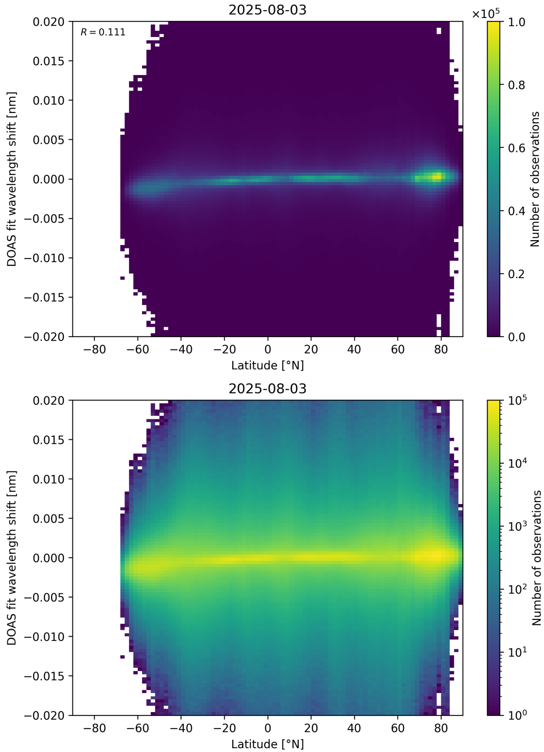
Figure 154: Scatter density plot of “Latitude” against “DOAS fit wavelength shift” for 2025-08-03 to 2025-08-04.
