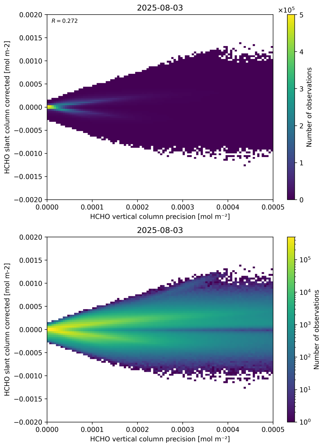
Figure 140: Scatter density plot of “HCHO vertical column precision” against “HCHO slant column corrected” for 2025-08-03 to 2025-08-04.
