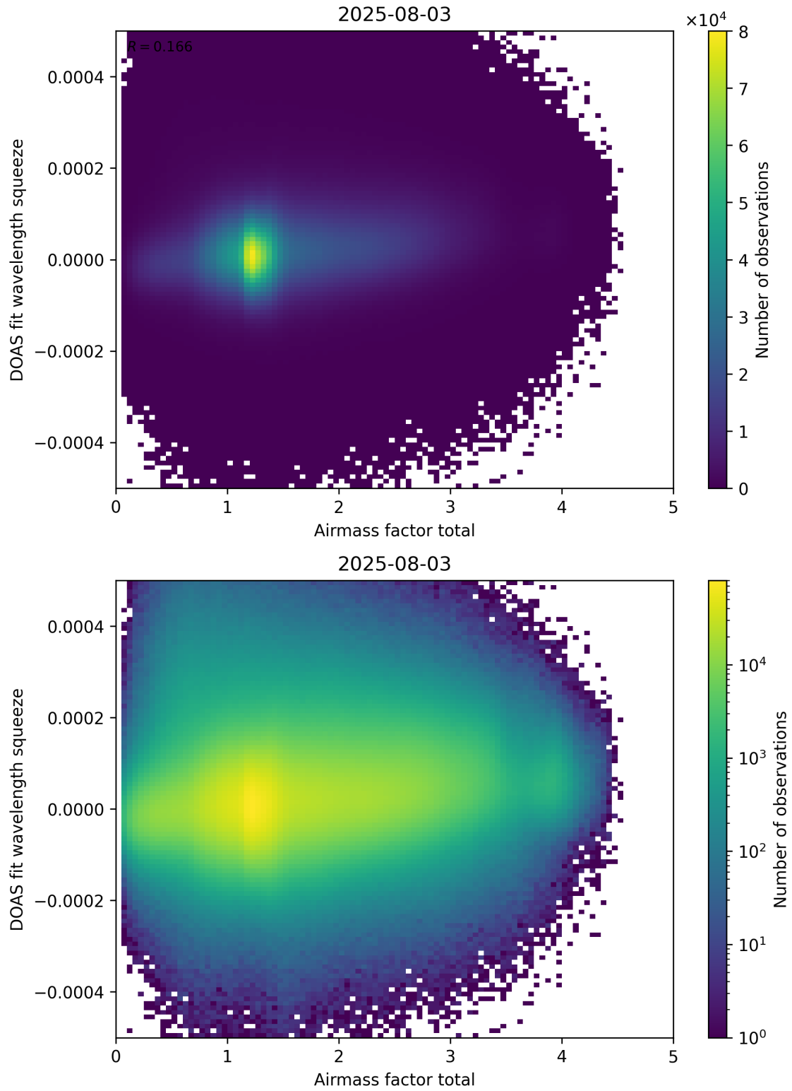
Figure 99: Scatter density plot of “Airmass factor total” against “DOAS fit wavelength squeeze” for 2025-08-03 to 2025-08-04.
