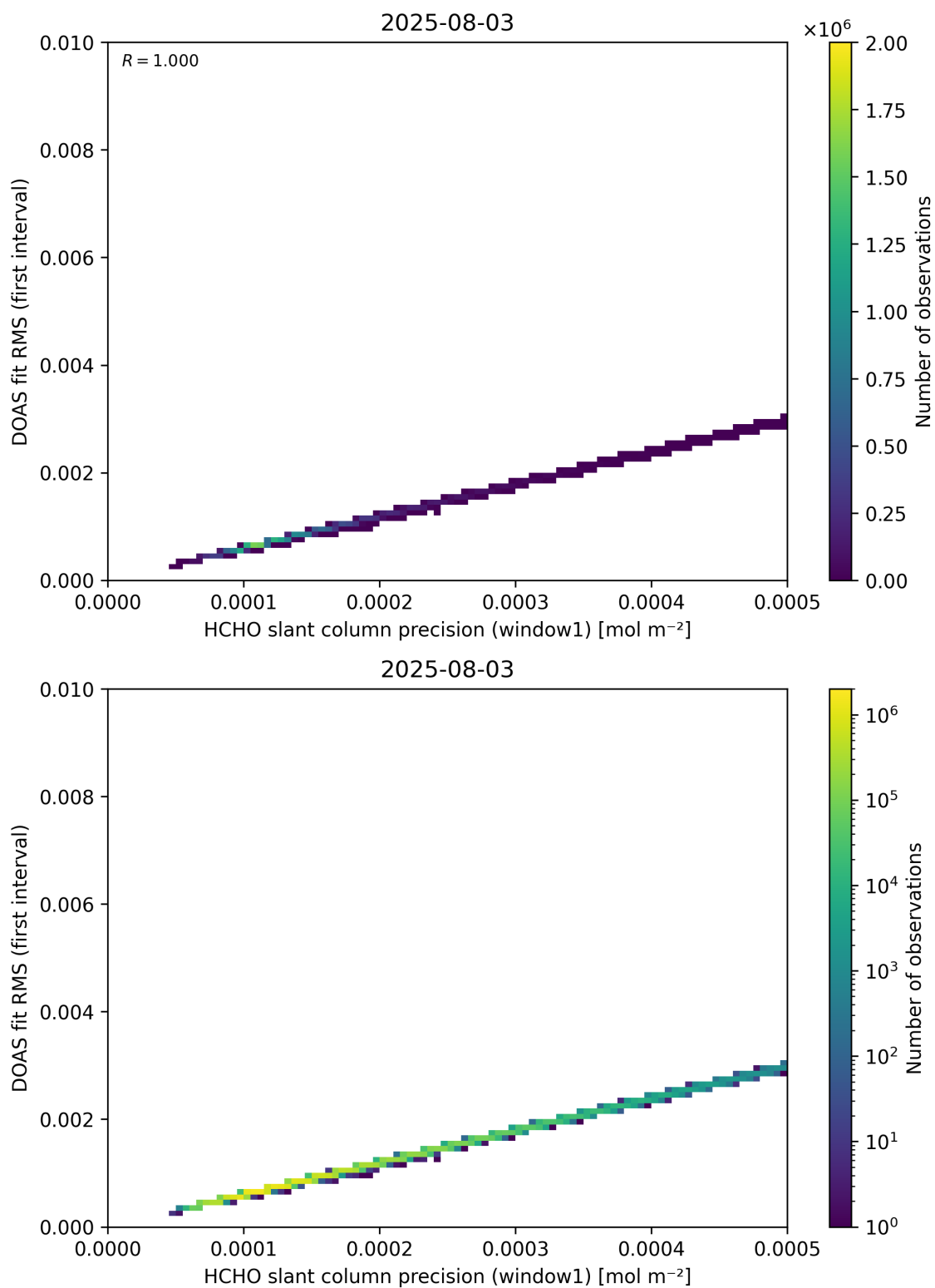
Figure 88: Scatter density plot of “HCHO slant column precision (window1)” against “DOAS fit RMS (first interval)” for 2025-08-03 to 2025-08-04.
