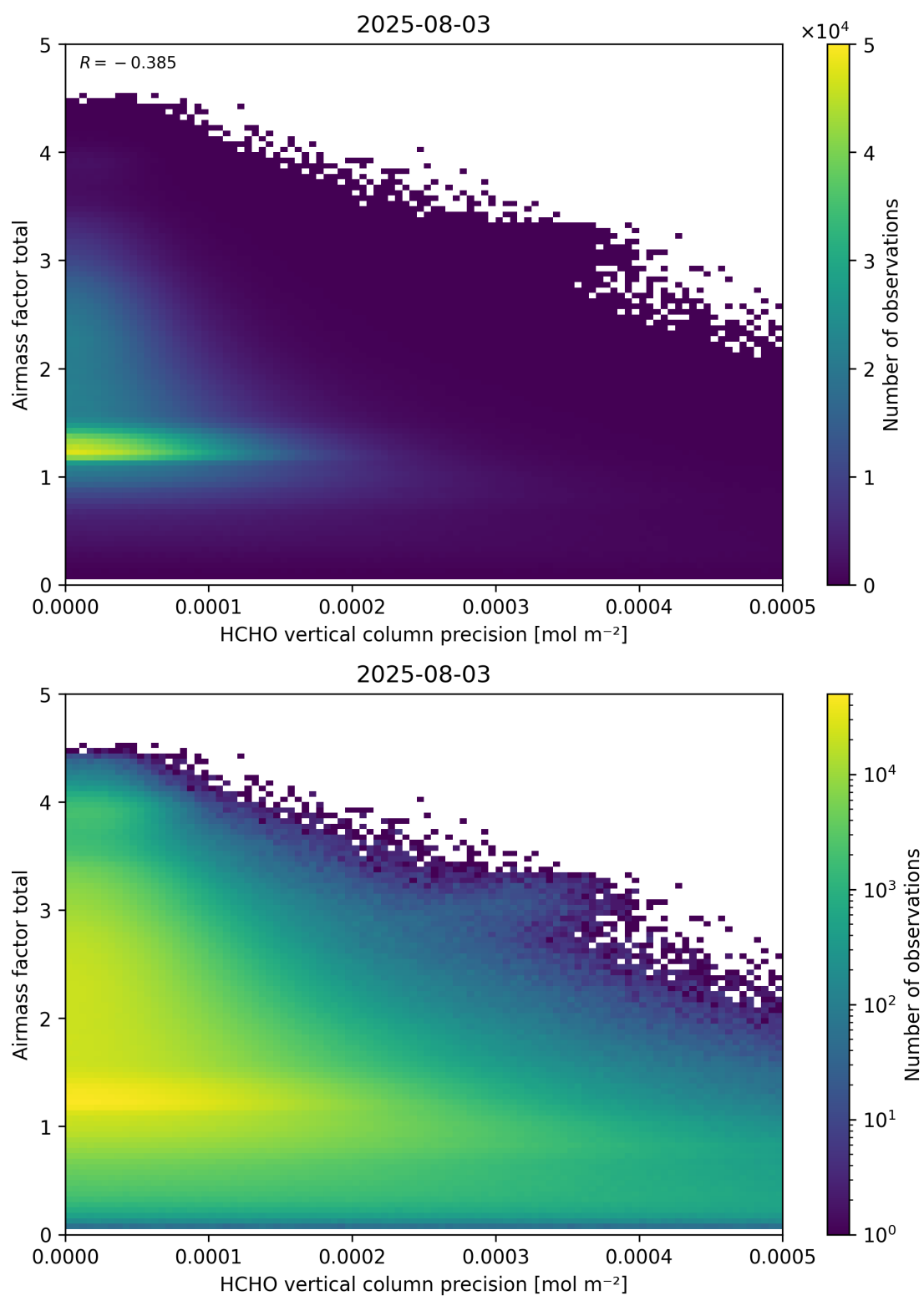
Figure 144: Scatter density plot of “HCHO vertical column precision” against “Airmass factor total” for 2025-08-03 to 2025-08-04.
