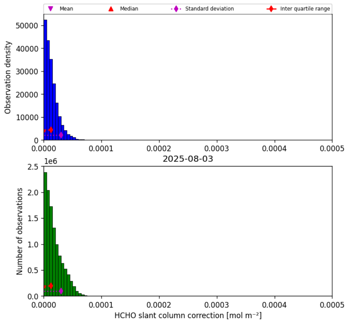
Figure 47: Histogram of “HCHO slant column correction” for 2025-08-03 to 2025-08-04
