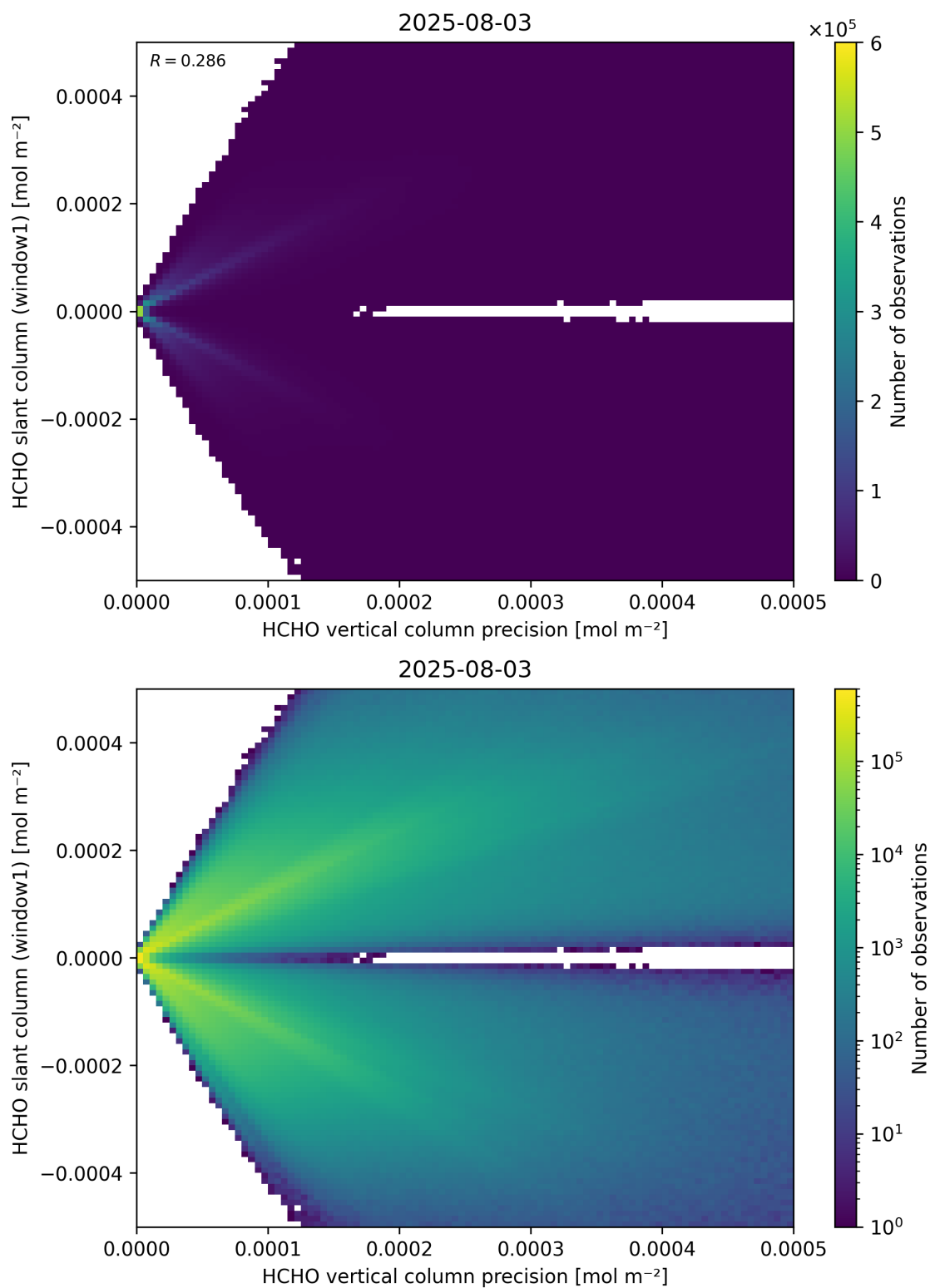
Figure 142: Scatter density plot of “HCHO vertical column precision” against “HCHO slant column (window1)” for 2025-08-03 to 2025-08-04.
