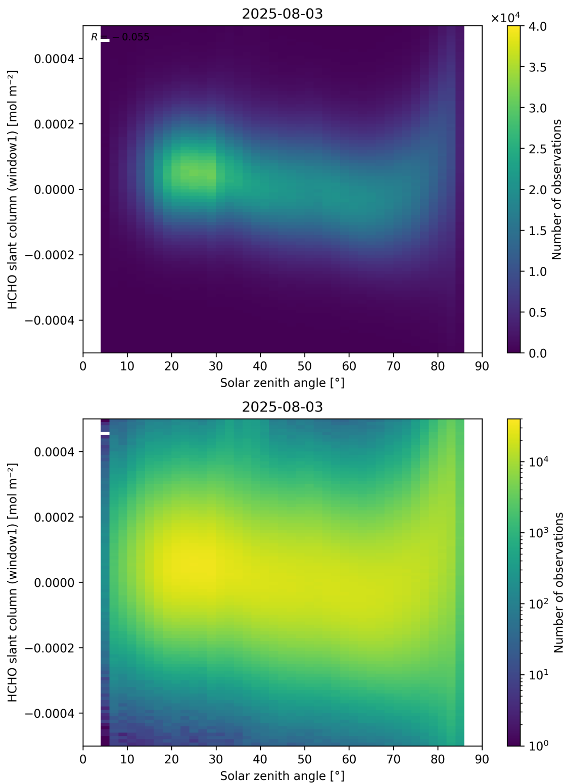
Figure 173: Scatter density plot of “Solar zenith angle” against “HCHO slant column (window1)” for 2025-08-03 to 2025-08-04.
