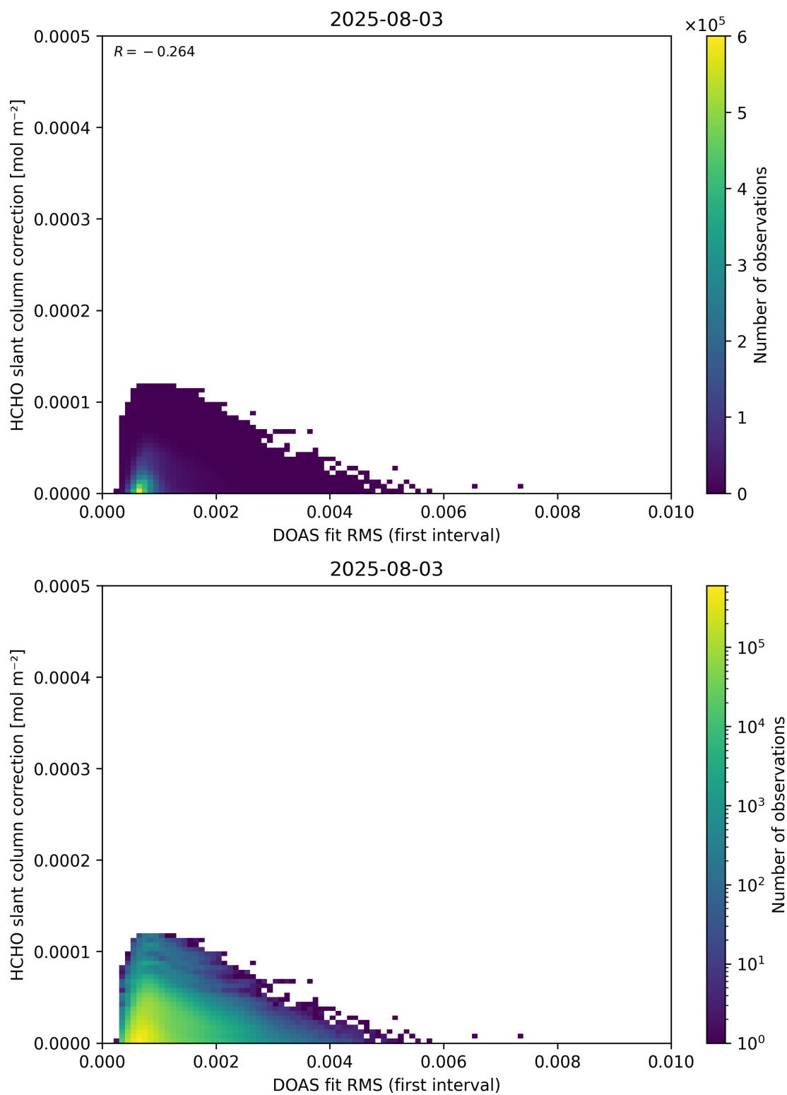
Figure 63: Scatter density plot of “DOAS fit RMS (first interval)” against “HCHO slant column correction” for 2025-08-03 to 2025-08-04.
