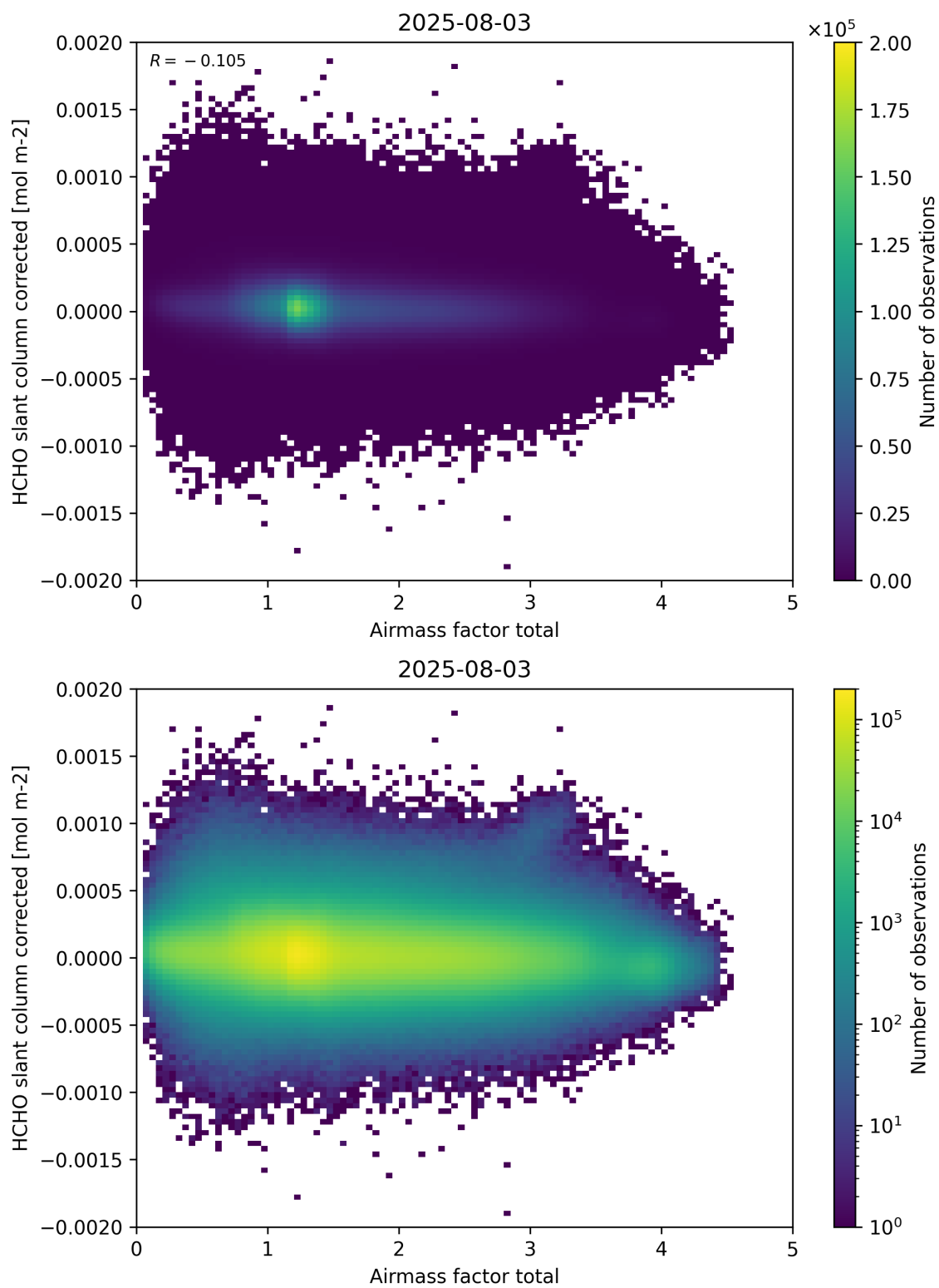
Figure 101: Scatter density plot of “Airmass factor total” against “HCHO slant column corrected” for 2025-08-03 to 2025-08-04.
