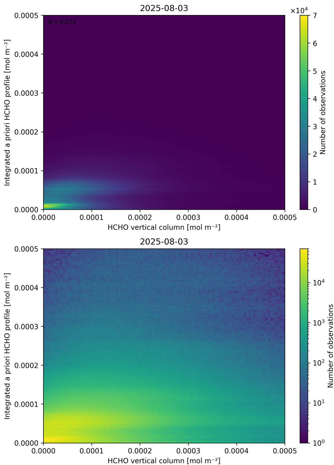
Figure 135: Scatter density plot of “HCHO vertical column” against “Integrated a priori HCHO profile” for 2025-08-03 to 2025-08-04.
