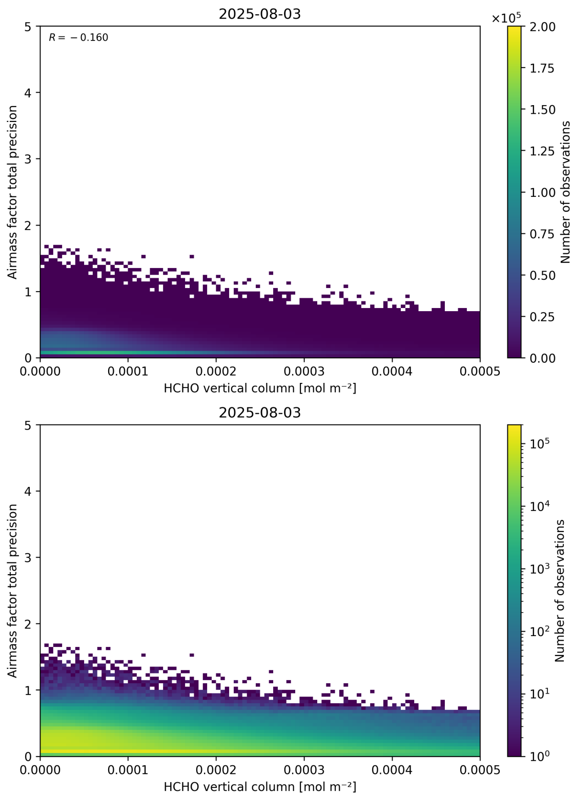
Figure 132: Scatter density plot of “HCHO vertical column” against “Airmass factor total precision” for 2025-08-03 to 2025-08-04.
