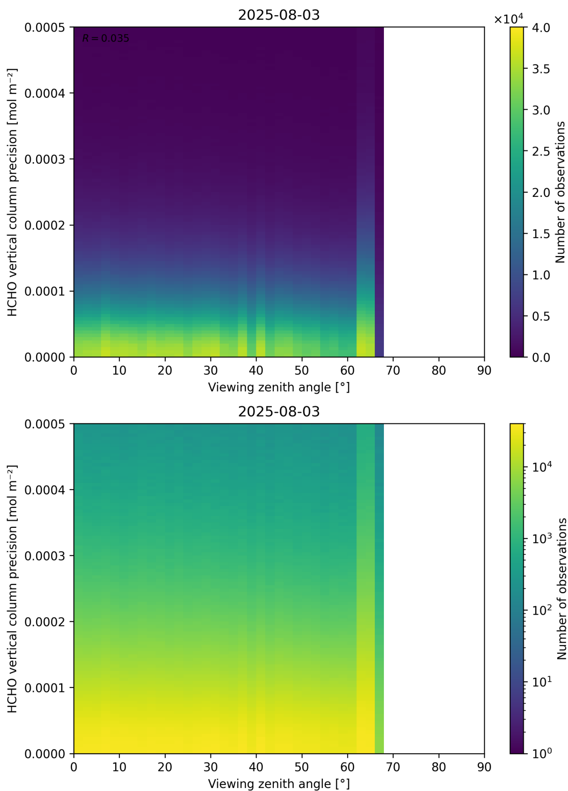
Figure 194: Scatter density plot of “Viewing zenith angle” against “HCHO vertical column precision” for 2025-08-03 to 2025-08-04.
