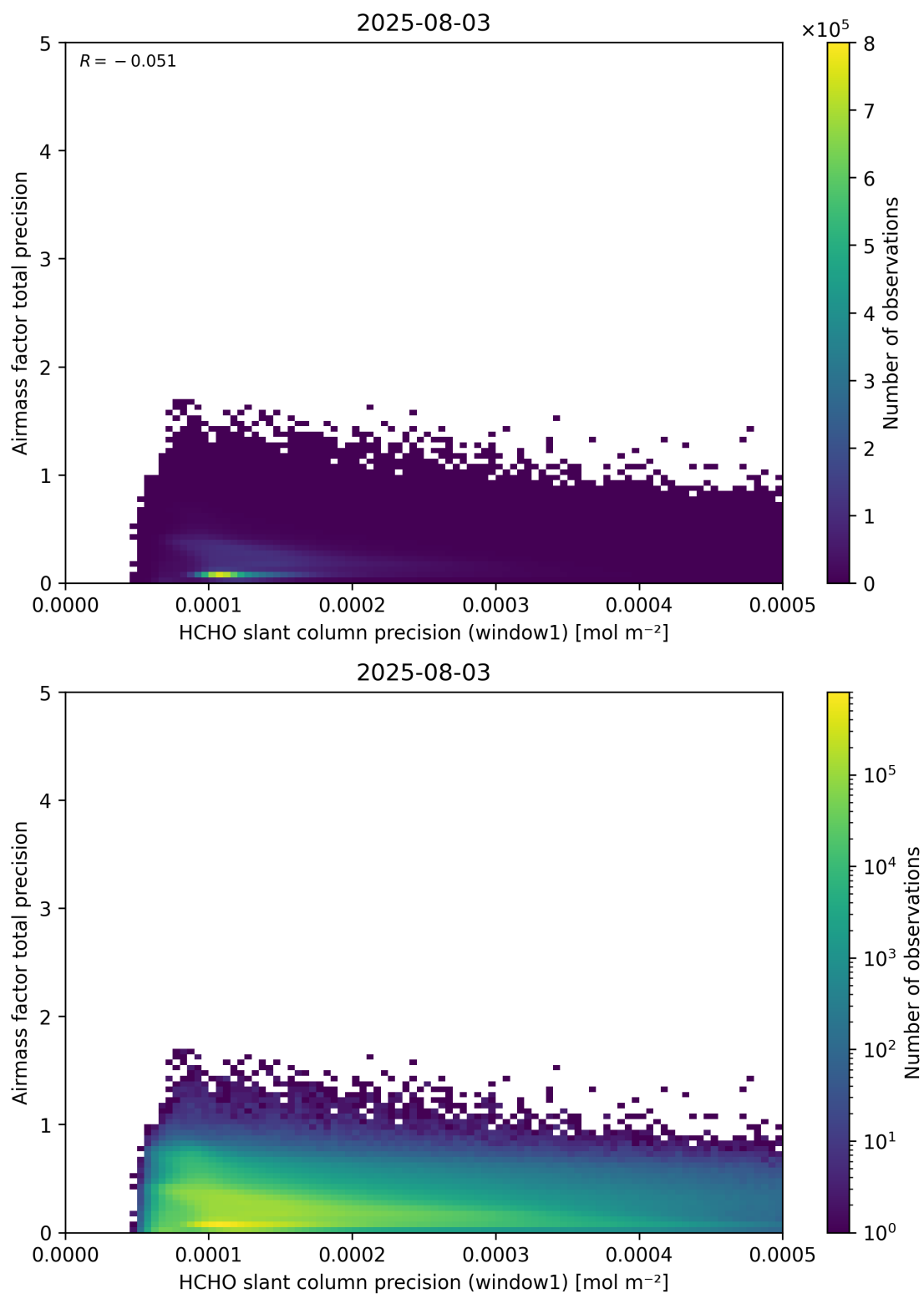
Figure 95: Scatter density plot of “HCHO slant column precision (window1)” against “Airmass factor total precision” for 2025-08-03 to 2025-08-04.
