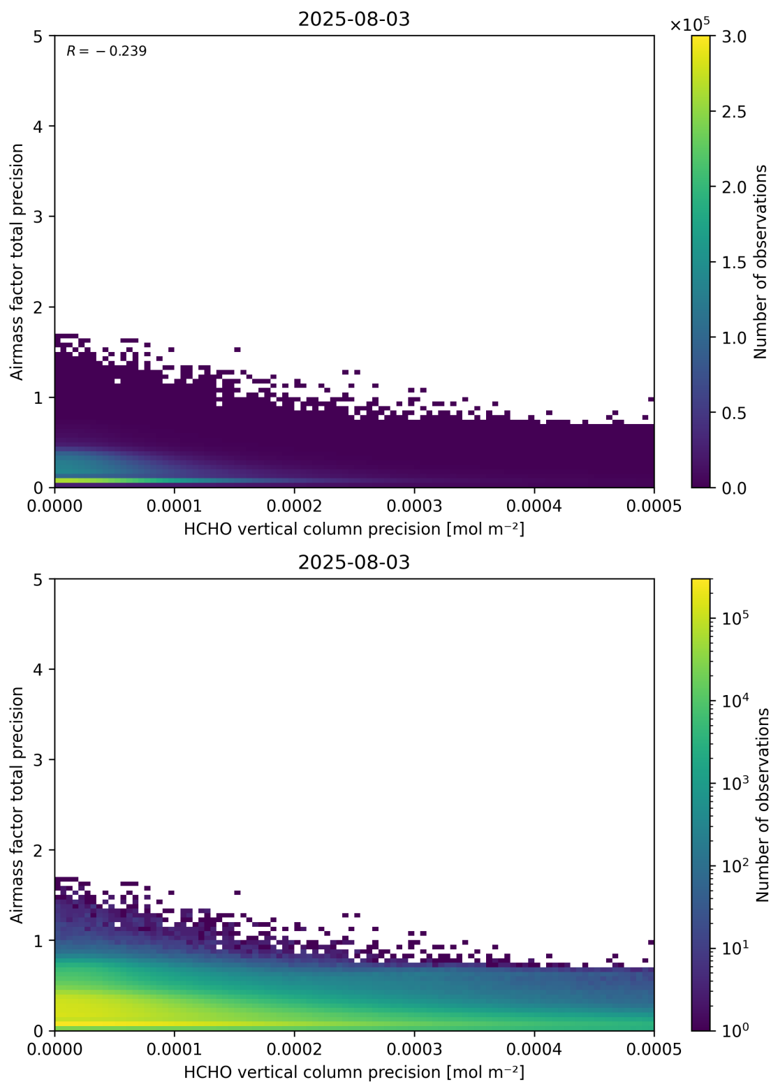
Figure 145: Scatter density plot of “HCHO vertical column precision” against “Airmass factor total precision” for 2025-08-03 to 2025-08-04.
