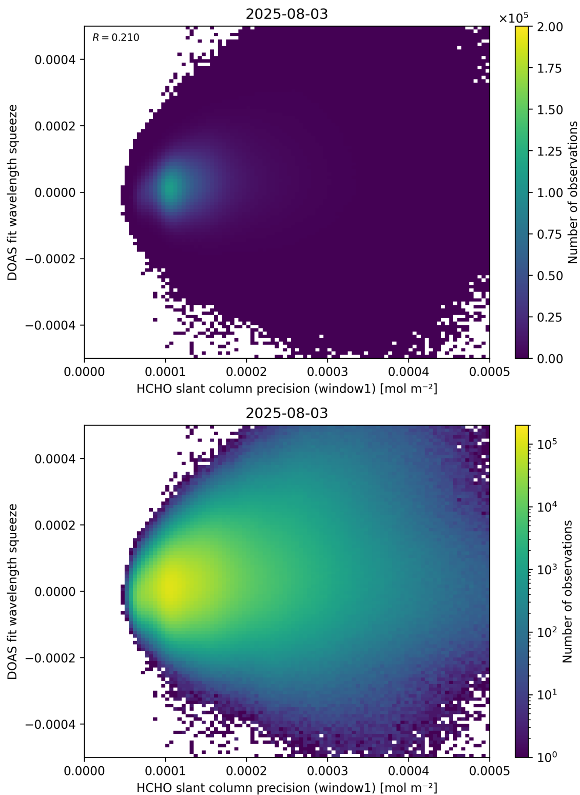
Figure 90: Scatter density plot of “HCHO slant column precision (window1)” against “DOAS fit wavelength squeeze” for 2025-08-03 to 2025-08-04.
