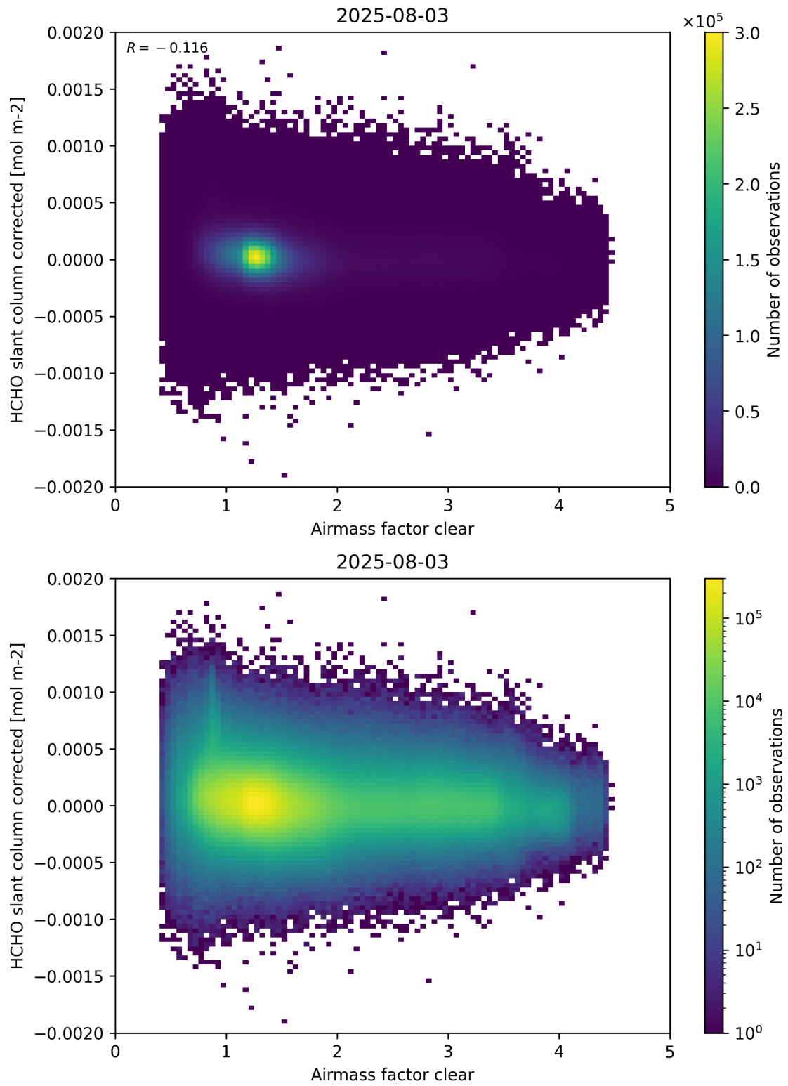
Figure 74: Scatter density plot of “Airmass factor clear” against “HCHO slant column corrected” for 2025-08-03 to 2025-08-04.
