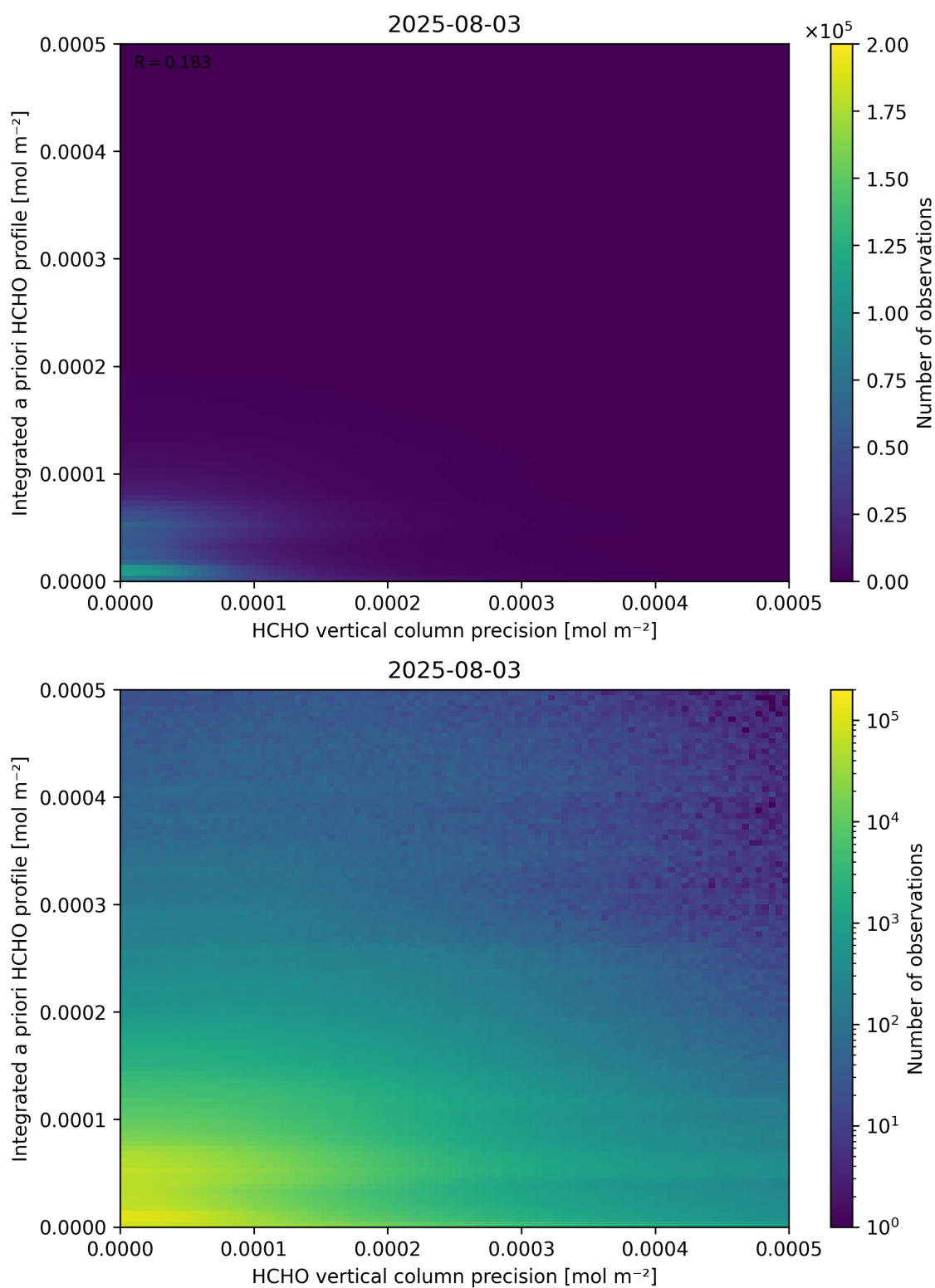
Figure 147: Scatter density plot of “HCHO vertical column precision” against “Integrated a priori HCHO profile” for 2025-08-03 to 2025-08-04.
