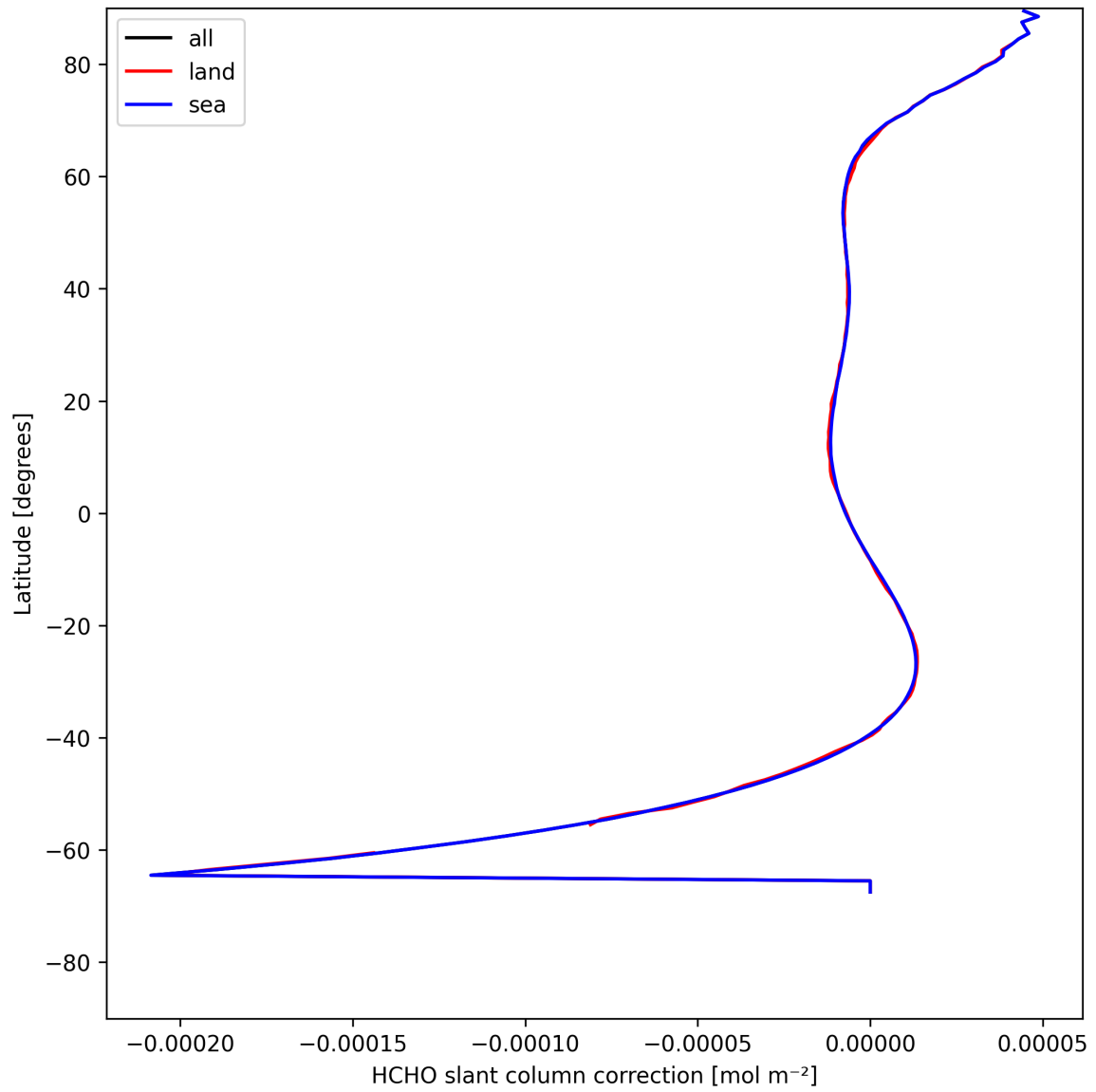
Figure 33: Zonal average of "HCHO slant column correction" for 2025-08-03 to 2025-08-04.
