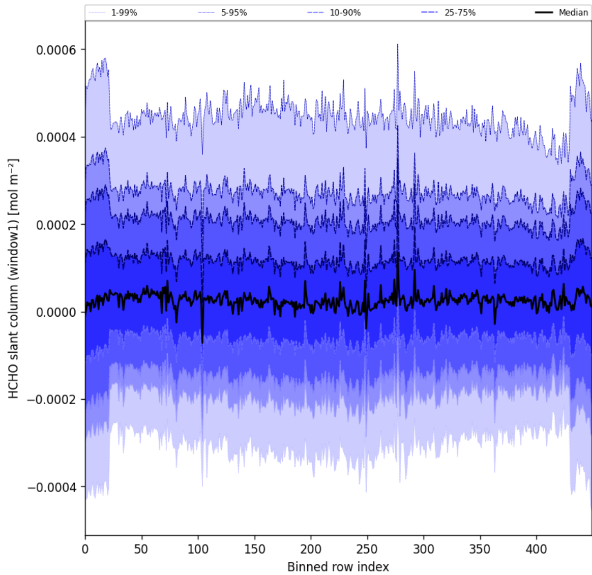
Figure 52: Along track statistics of “HCHO slant column (window1)” for 2025-08-03 to 2025-08-04
