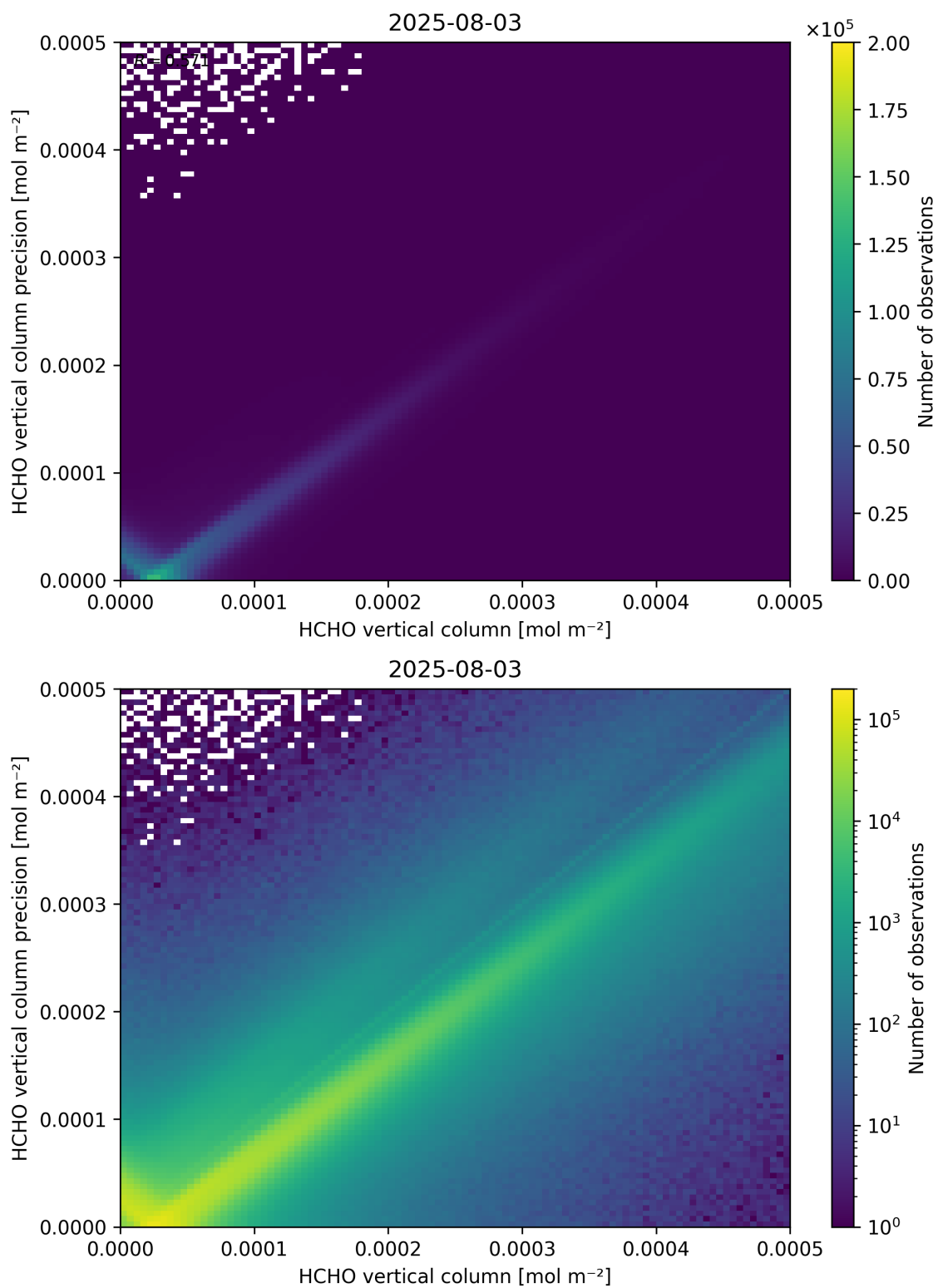
Figure 134: Scatter density plot of “HCHO vertical column” against “HCHO vertical column precision” for 2025-08-03 to 2025-08-04.
