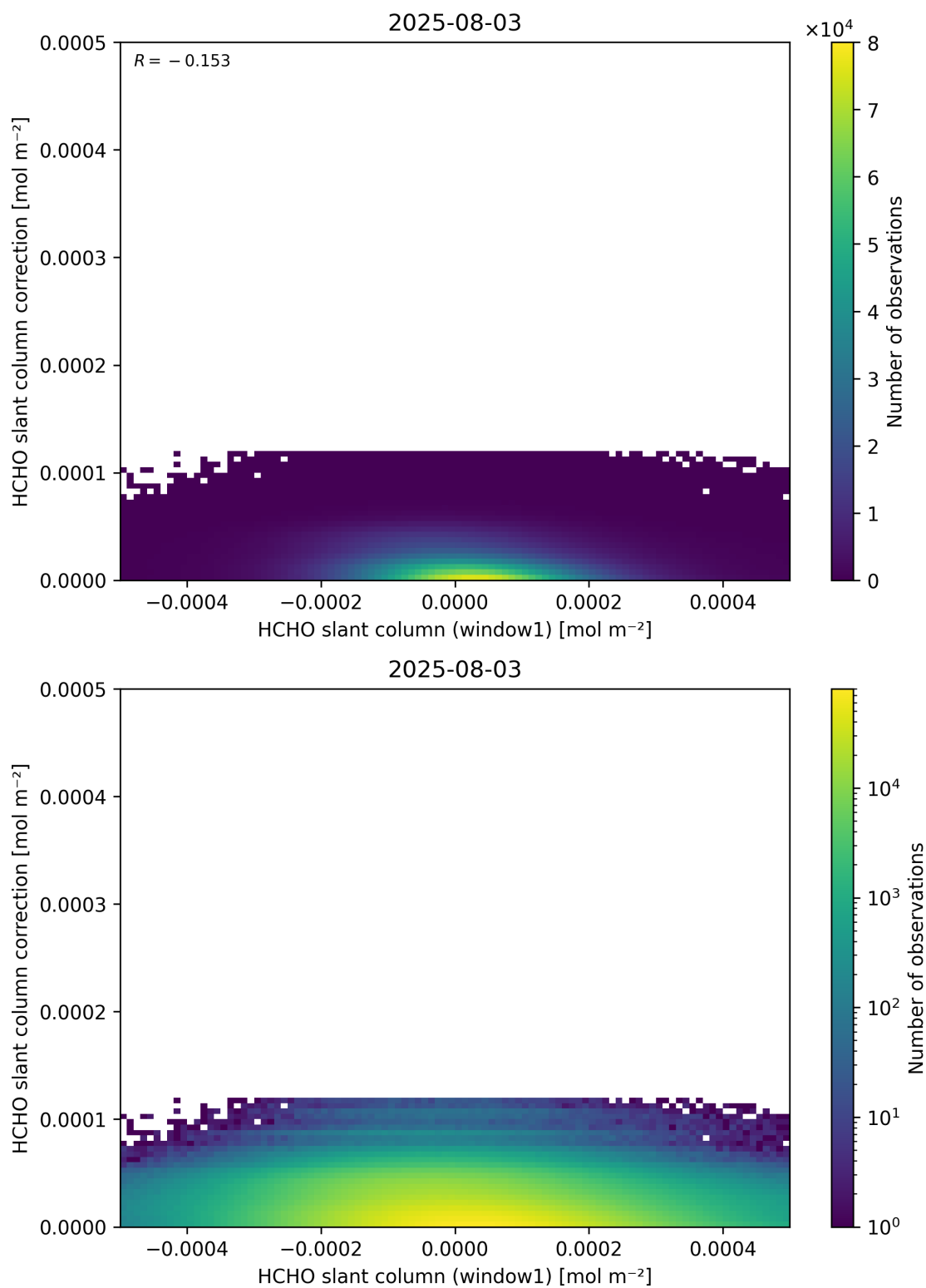
Figure 83: Scatter density plot of “HCHO slant column (window1)” against “HCHO slant column correction” for 2025-08-03 to 2025-08-04.
