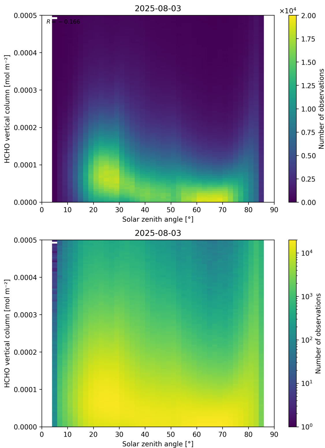
Figure 177: Scatter density plot of “Solar zenith angle” against “HCHO vertical column” for 2025-08-03 to 2025-08-04.
