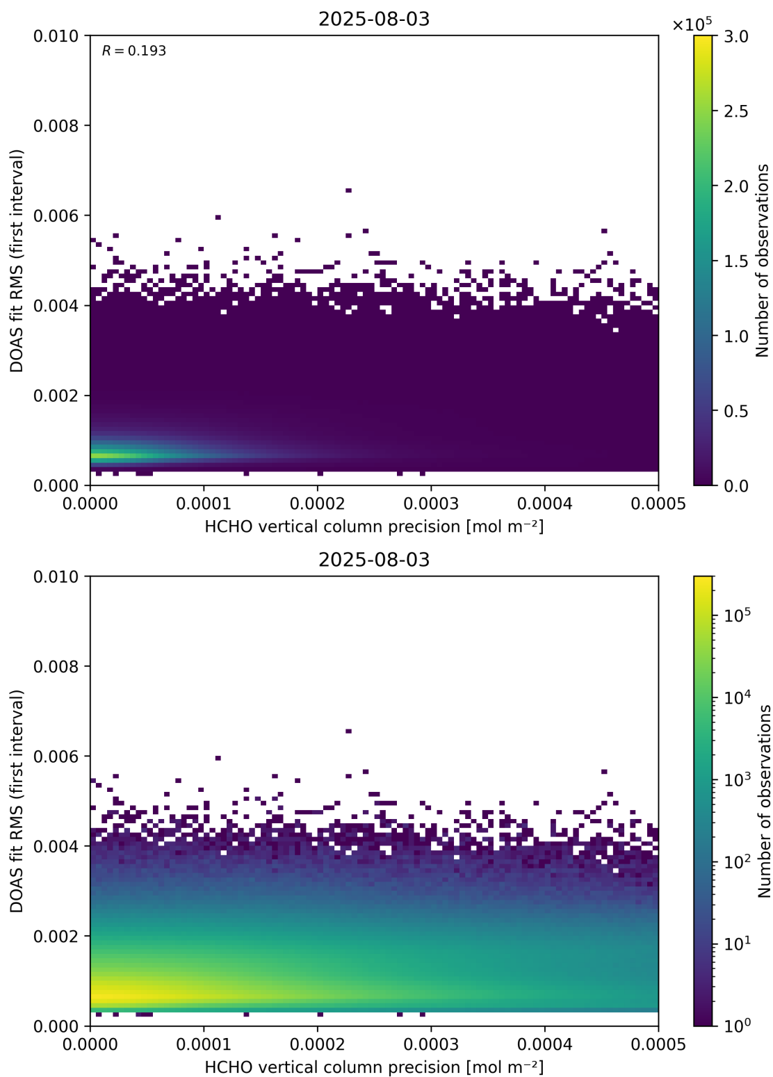
Figure 136: Scatter density plot of “HCHO vertical column precision” against “DOAS fit RMS (first interval)” for 2025-08-03 to 2025-08-04.
