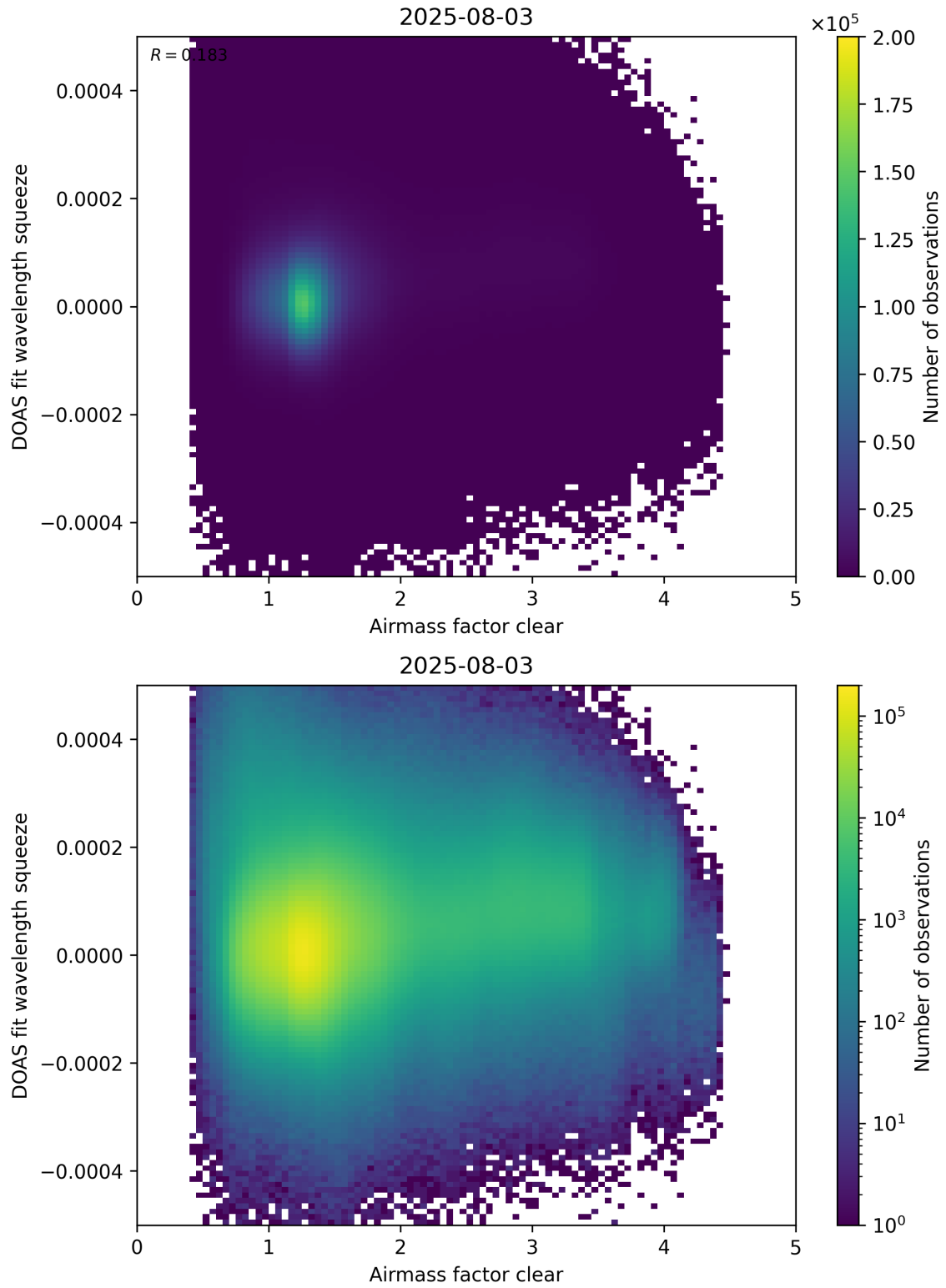
Figure 73: Scatter density plot of “Airmass factor clear” against “DOAS fit wavelength squeeze” for 2025-08-03 to 2025-08-04.
