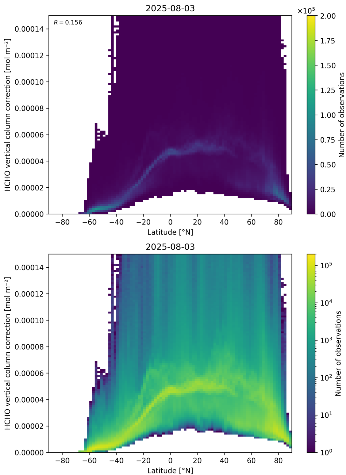
Figure 164: Scatter density plot of “Latitude” against “HCHO vertical column correction” for 2025-08-03 to 2025-08-04.
