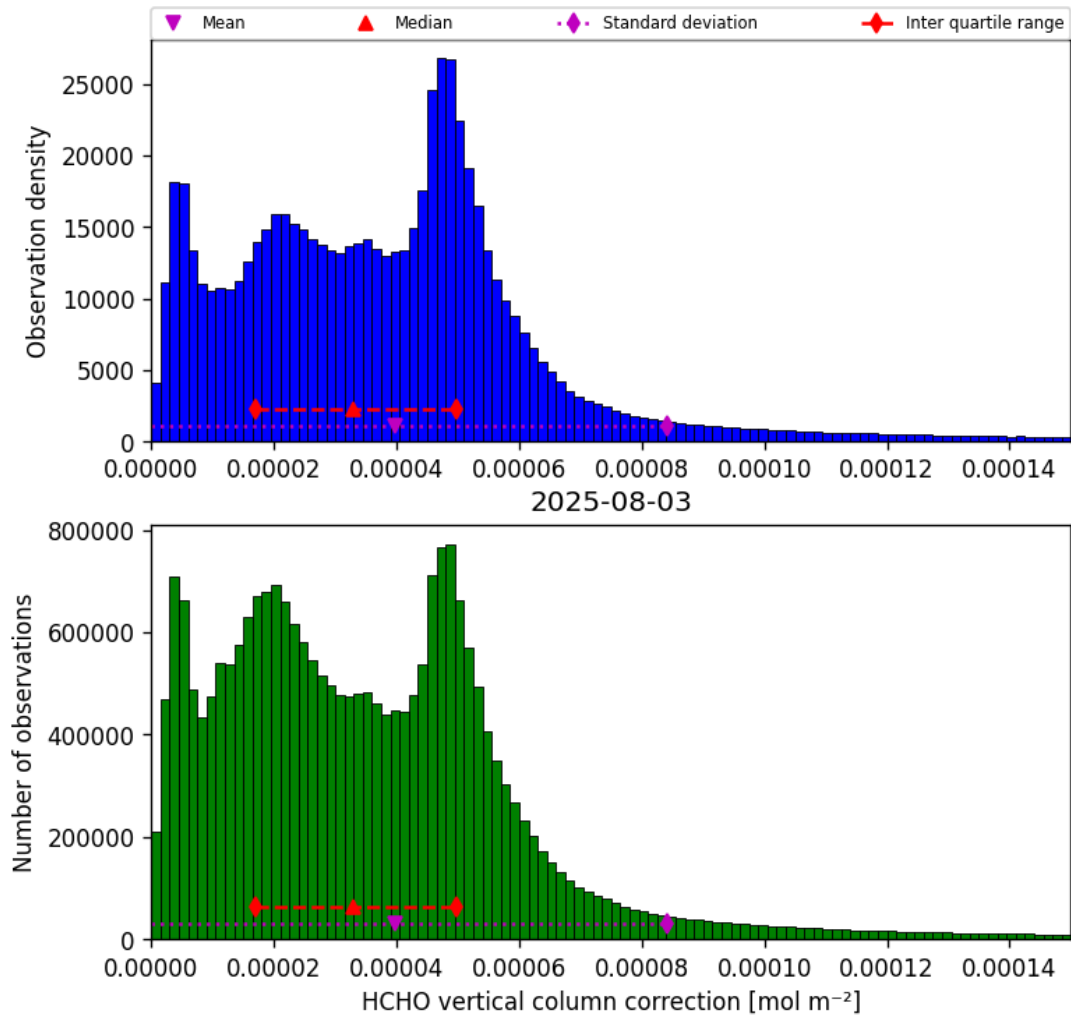
Figure 37: Histogram of “HCHO vertical column correction” for 2025-08-03 to 2025-08-04
