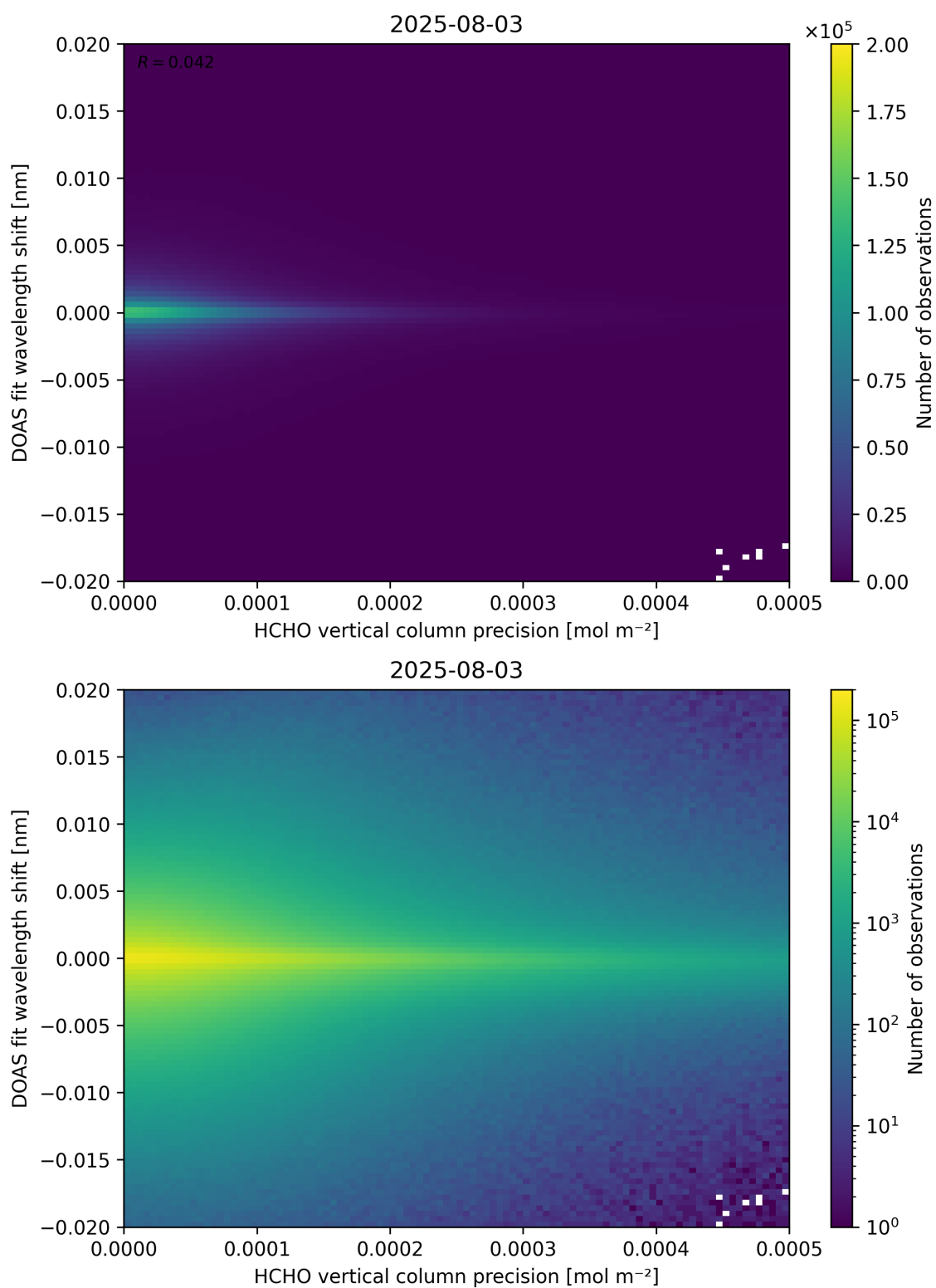
Figure 137: Scatter density plot of “HCHO vertical column precision” against “DOAS fit wavelength shift” for 2025-08-03 to 2025-08-04.
