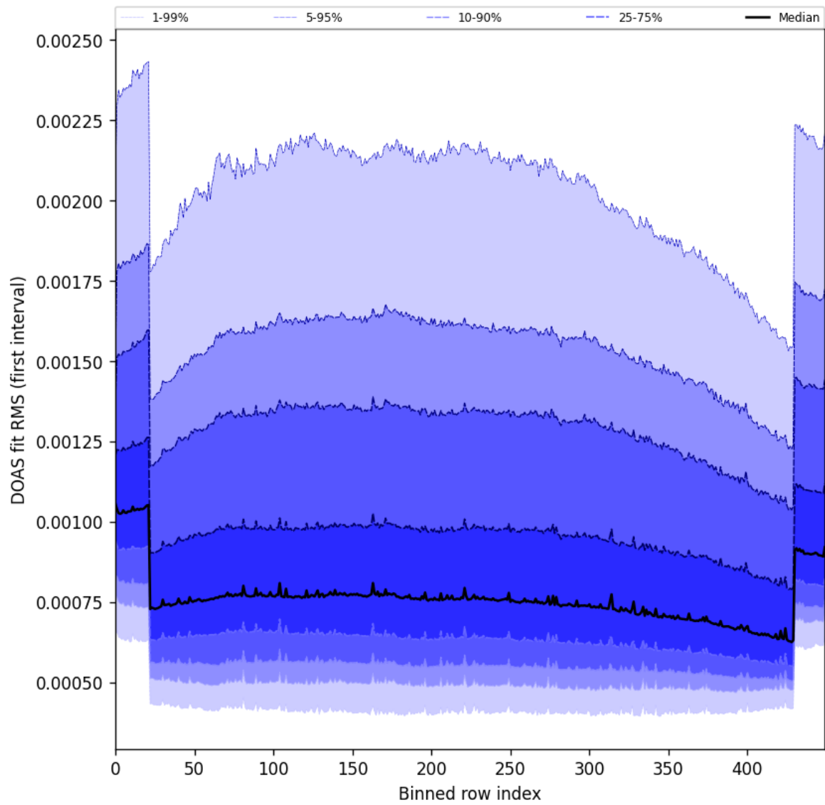
Figure 60: Along track statistics of “DOAS fit RMS (first interval)” for 2025-08-03 to 2025-08-04
