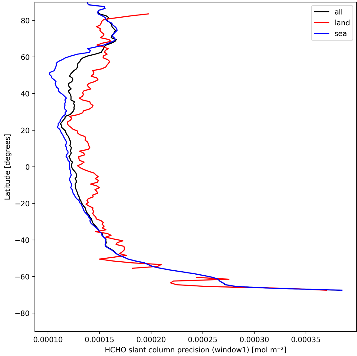
Figure 25: Zonal average of "HCHO slant column precision (window1)" for 2025-08-03 to 2025-08-04.
