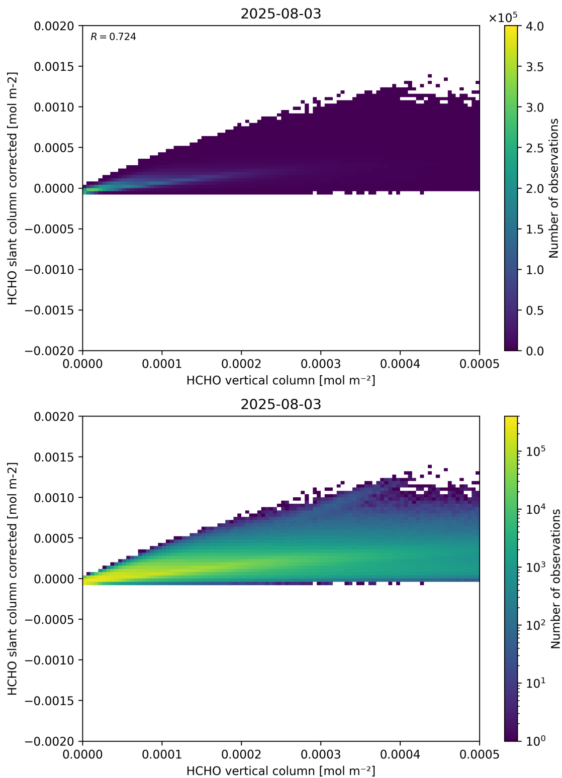
Figure 127: Scatter density plot of “HCHO vertical column” against “HCHO slant column corrected” for 2025-08-03 to 2025-08-04.
