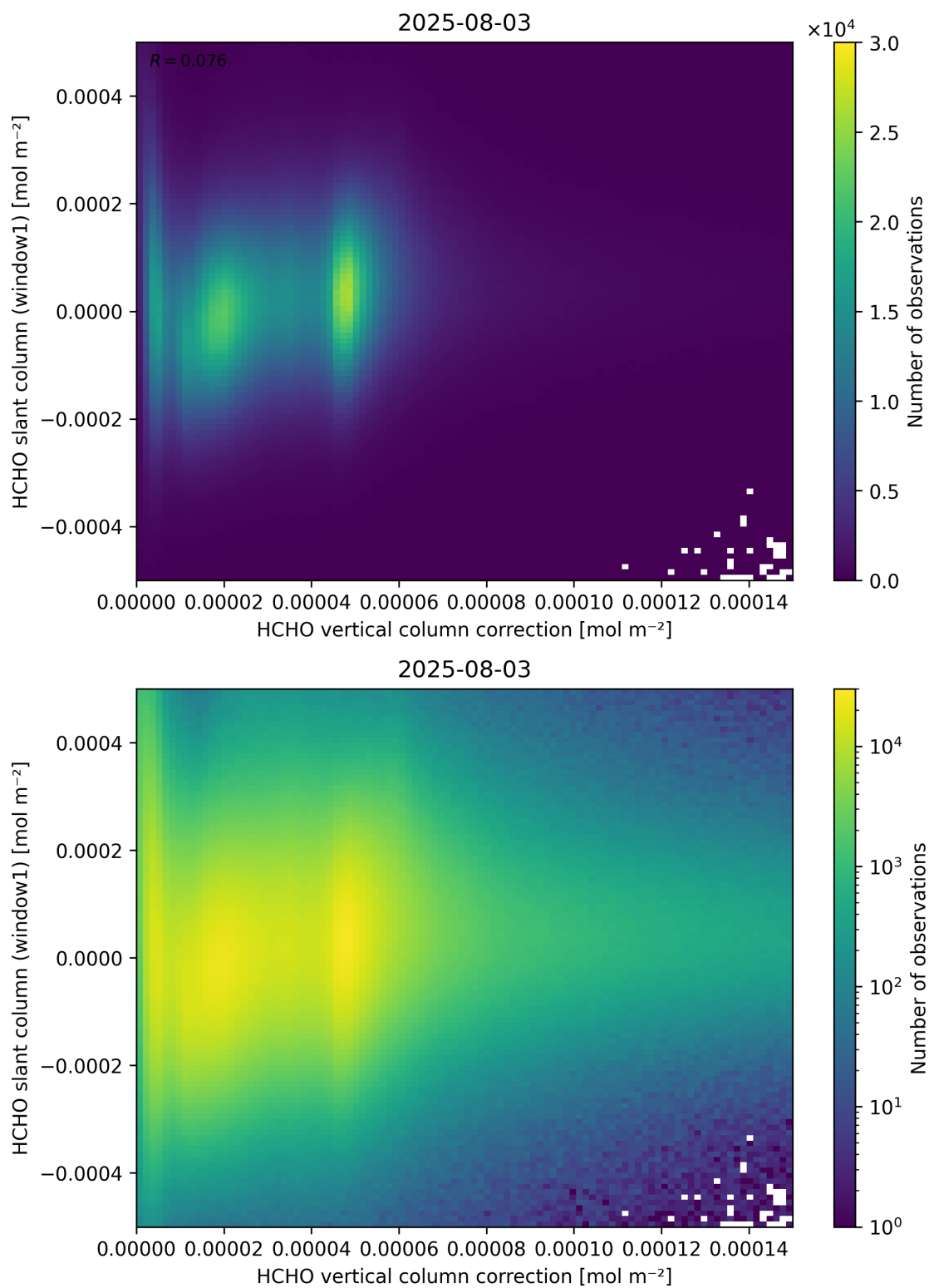
Figure 118: Scatter density plot of “HCHO vertical column correction” against “HCHO slant column (window1)” for 2025-08-03 to 2025-08-04.
