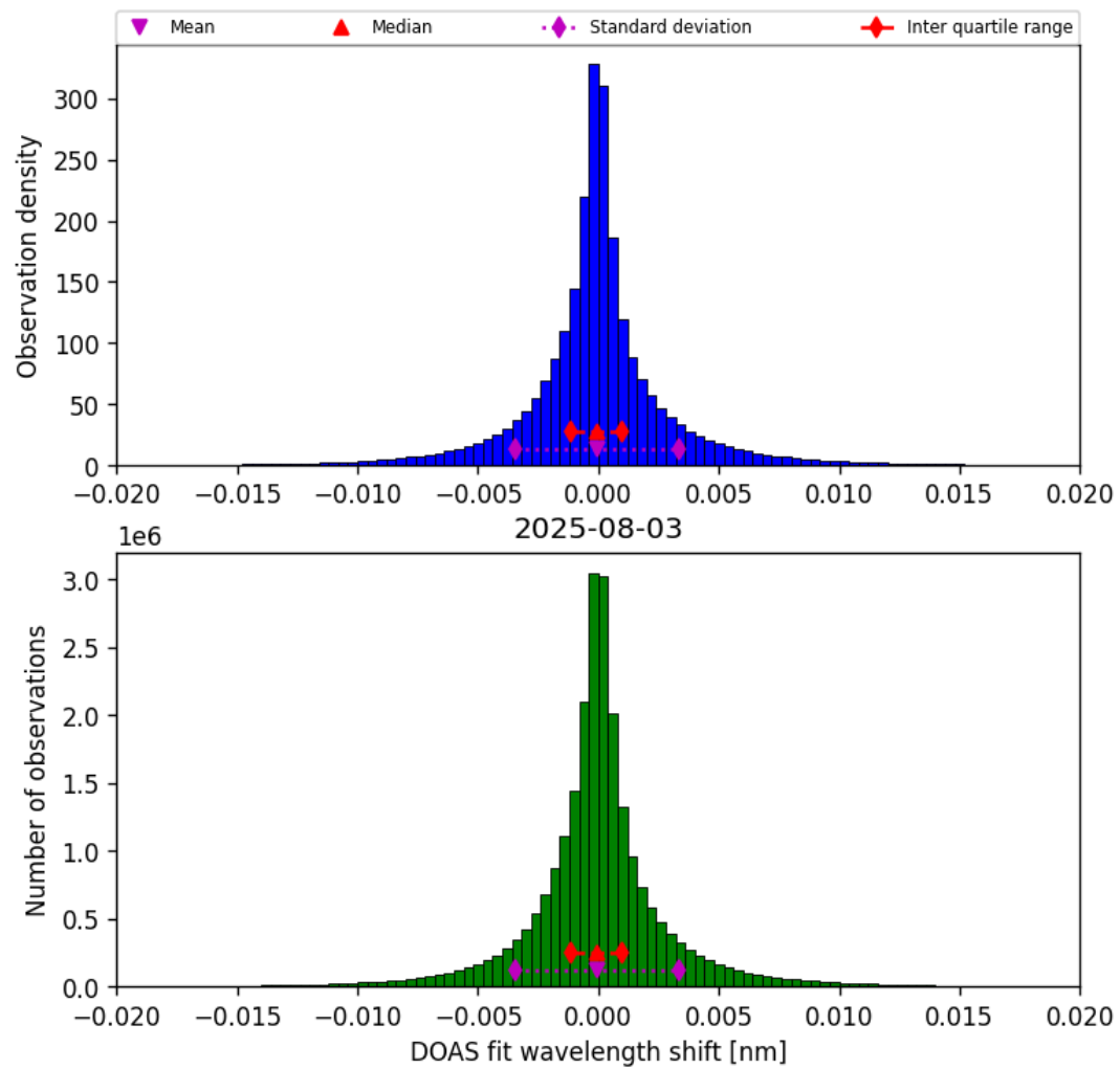
Figure 44: Histogram of “DOAS fit wavelength shift” for 2025-08-03 to 2025-08-04
