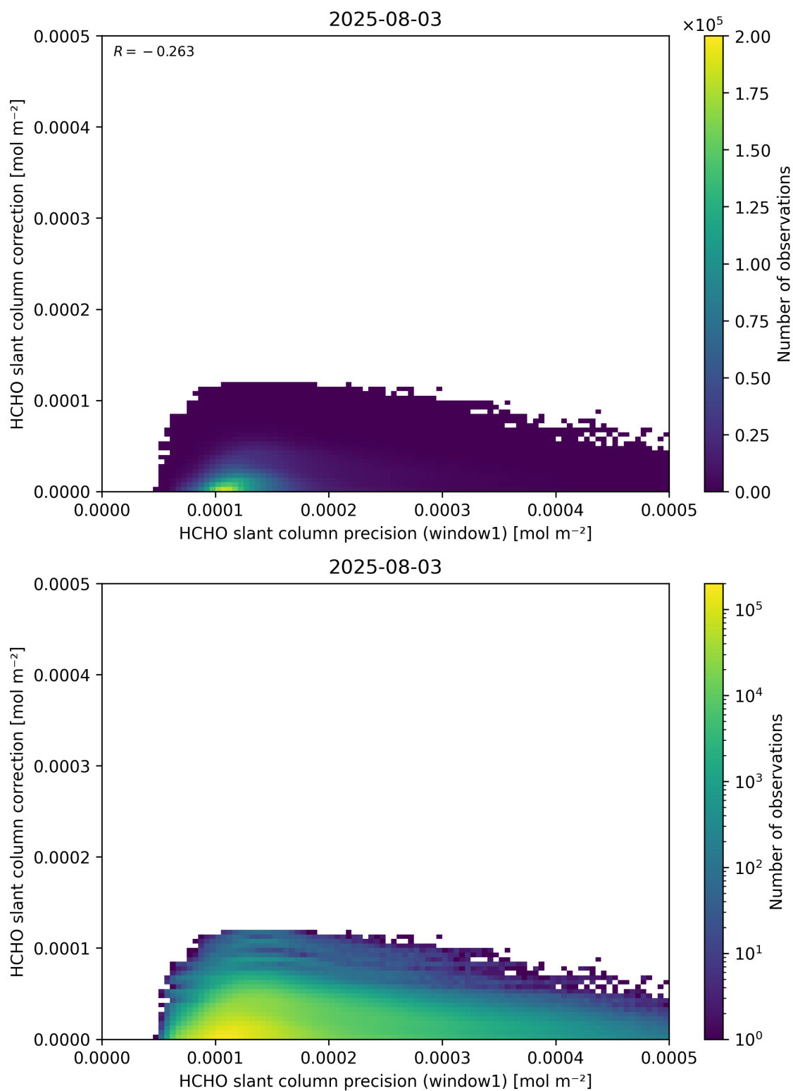
Figure 93: Scatter density plot of “HCHO slant column precision (window1)” against “HCHO slant column correction” for 2025-08-03 to 2025-08-04.
