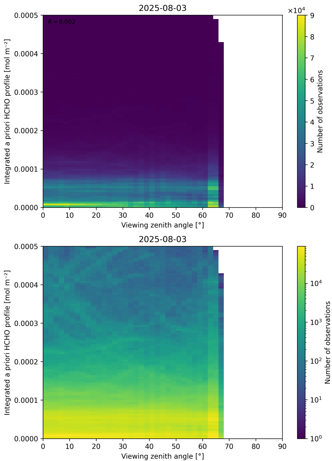
Figure 195: Scatter density plot of “Viewing zenith angle” against “Integrated a priori HCHO profile” for 2025-08-03 to 2025-08-04.
