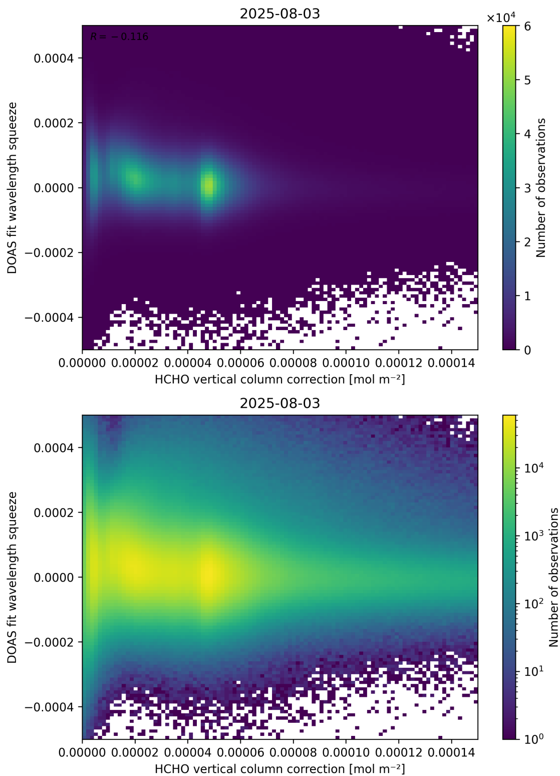
Figure 114: Scatter density plot of “HCHO vertical column correction” against “DOAS fit wavelength squeeze” for 2025-08-03 to 2025-08-04.
