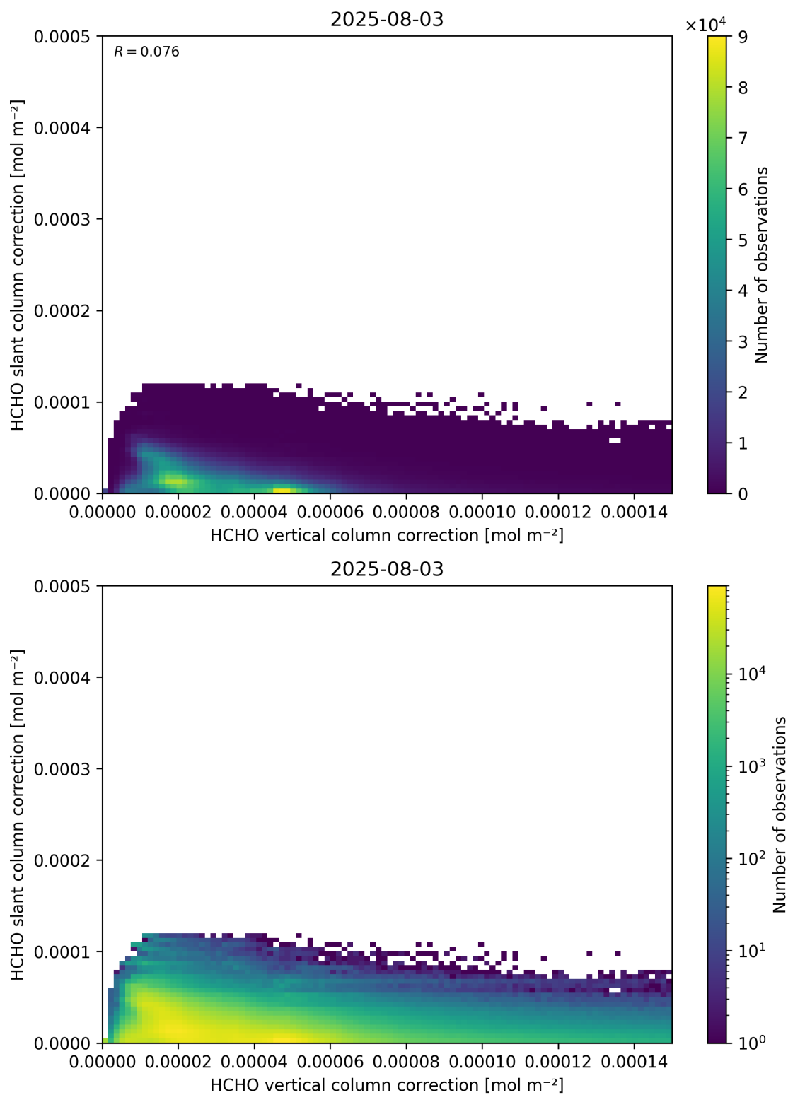
Figure 117: Scatter density plot of “HCHO vertical column correction” against “HCHO slant column correction” for 2025-08-03 to 2025-08-04.
