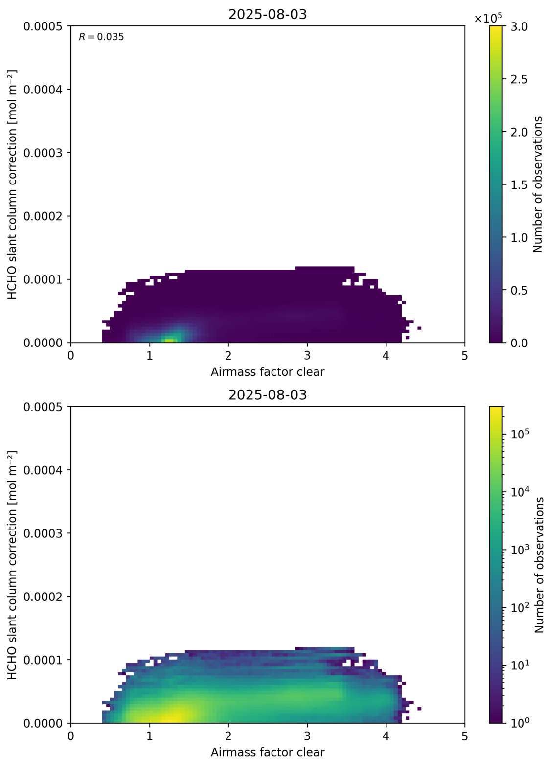
Figure 75: Scatter density plot of “Airmass factor clear” against “HCHO slant column correction” for 2025-08-03 to 2025-08-04.
