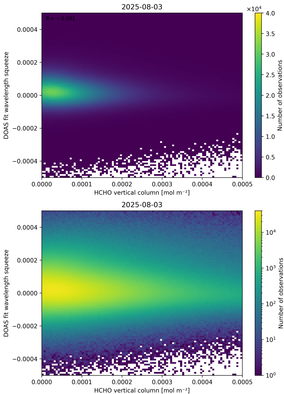
Figure 125: Scatter density plot of “HCHO vertical column” against “DOAS fit wavelength squeeze” for 2025-08-03 to 2025-08-04.
