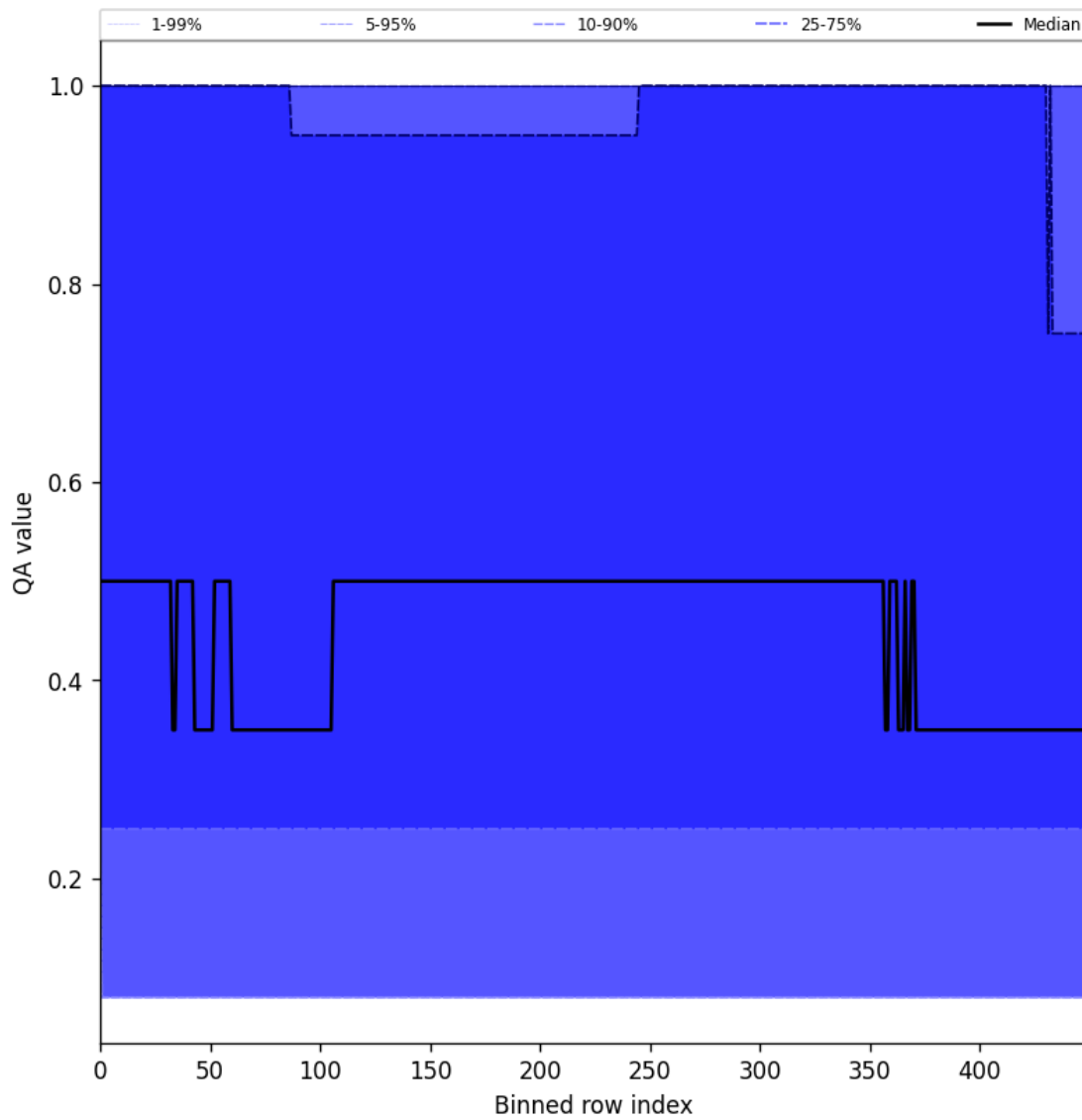
Figure 48: Along track statistics of “QA value” for 2025-08-03 to 2025-08-04
