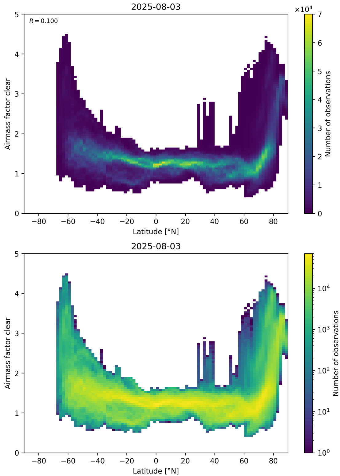
Figure 156: Scatter density plot of “Latitude” against “Airmass factor clear” for 2025-08-03 to 2025-08-04.
