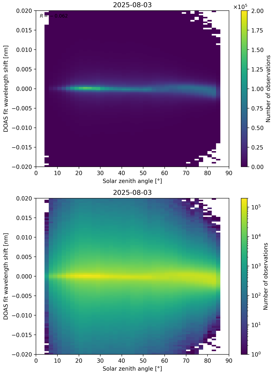
Figure 168: Scatter density plot of “Solar zenith angle” against “DOAS fit wavelength shift” for 2025-08-03 to 2025-08-04.
