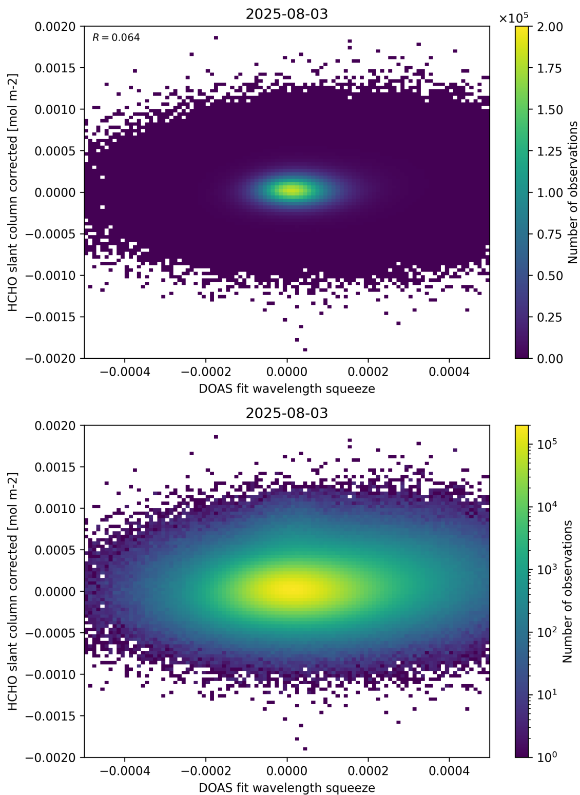
Figure 69: Scatter density plot of “DOAS fit wavelength squeeze” against “HCHO slant column corrected” for 2025-08-03 to 2025-08-04.
