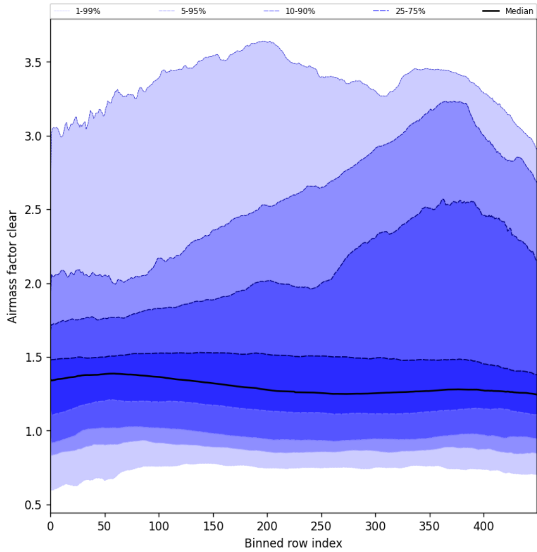
Figure 56: Along track statistics of “Airmass factor clear” for 2025-08-03 to 2025-08-04
