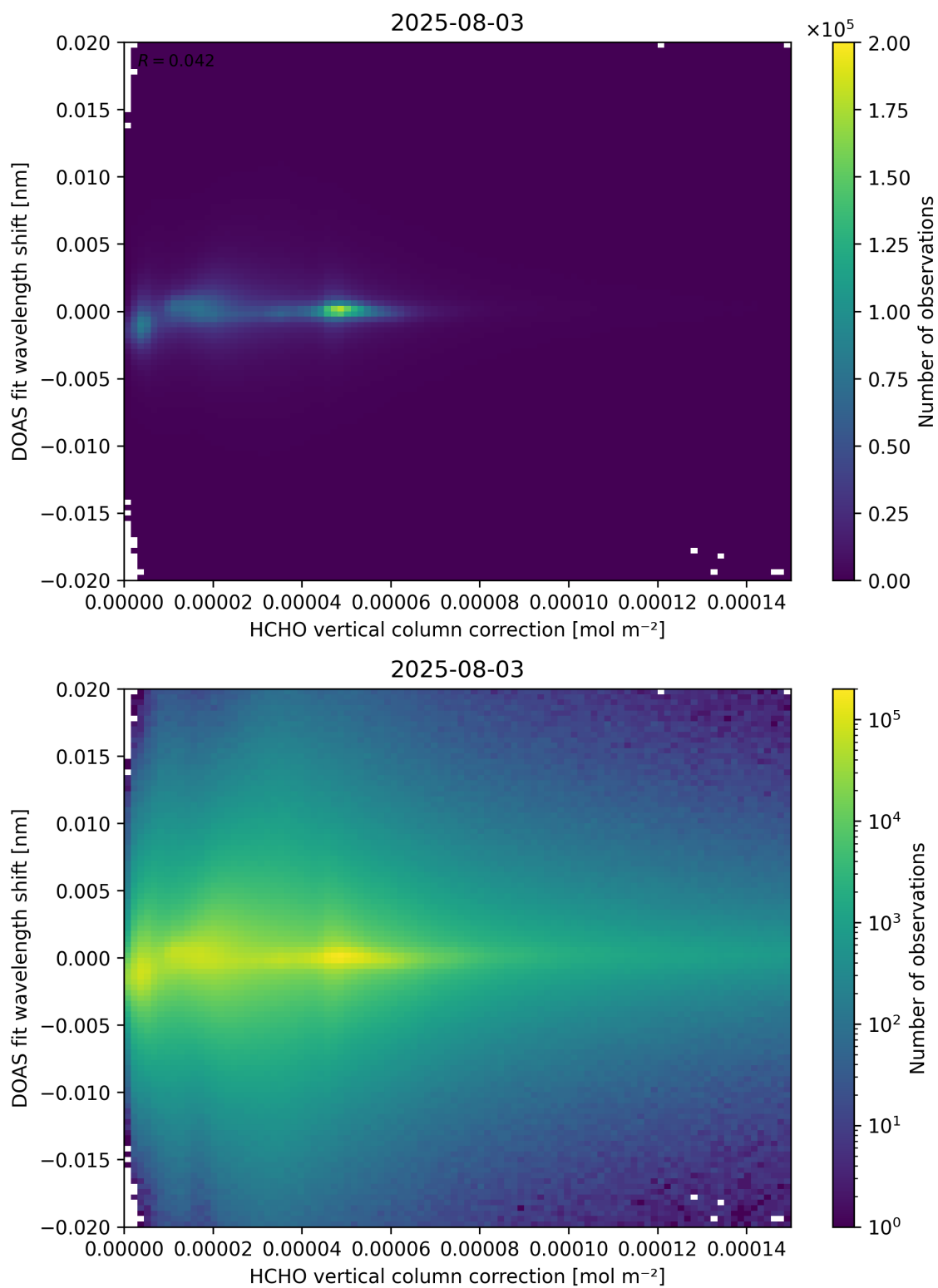
Figure 113: Scatter density plot of “HCHO vertical column correction” against “DOAS fit wavelength shift” for 2025-08-03 to 2025-08-04.
