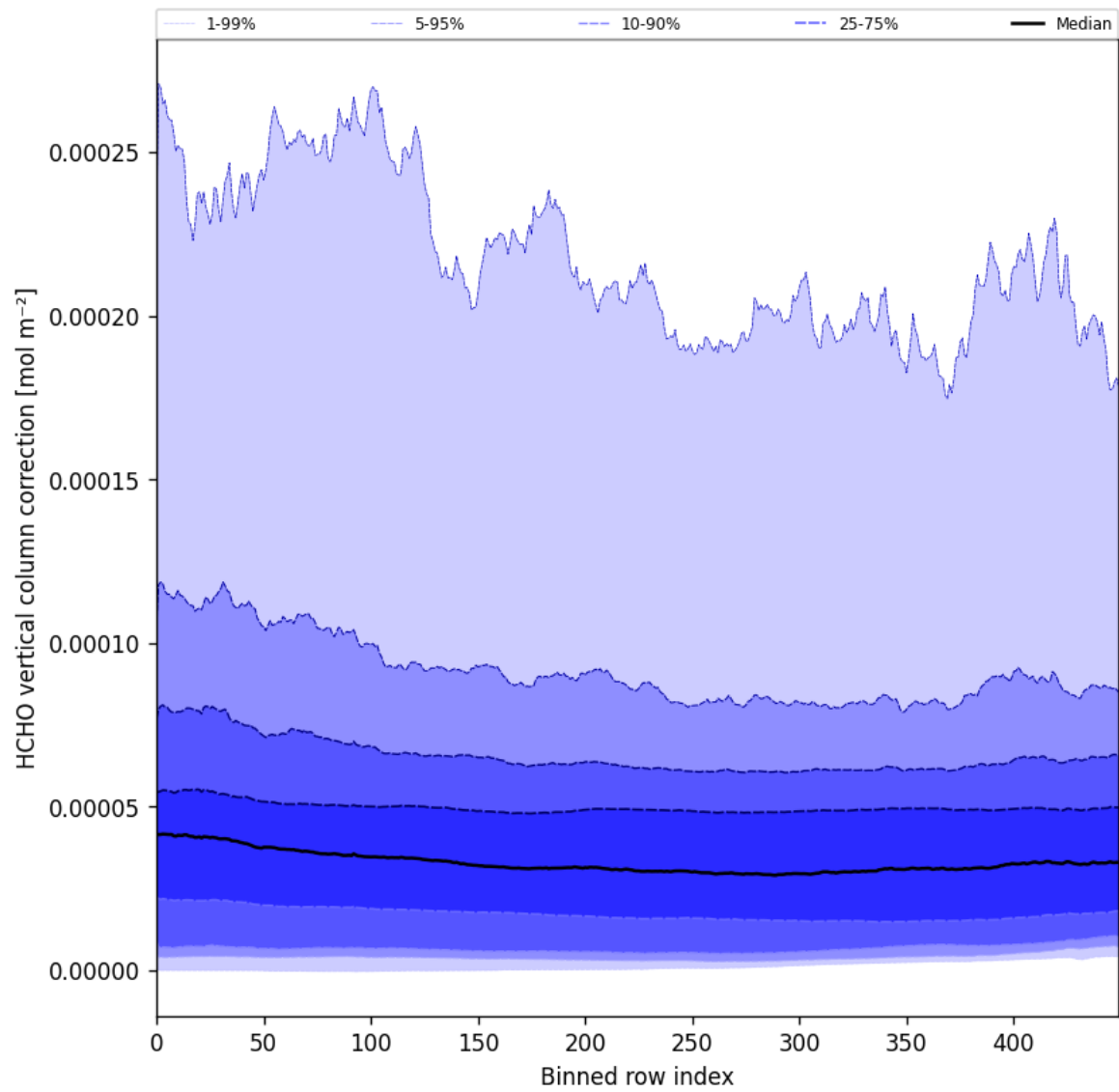
Figure 51: Along track statistics of “HCHO vertical column correction” for 2025-08-03 to 2025-08-04
