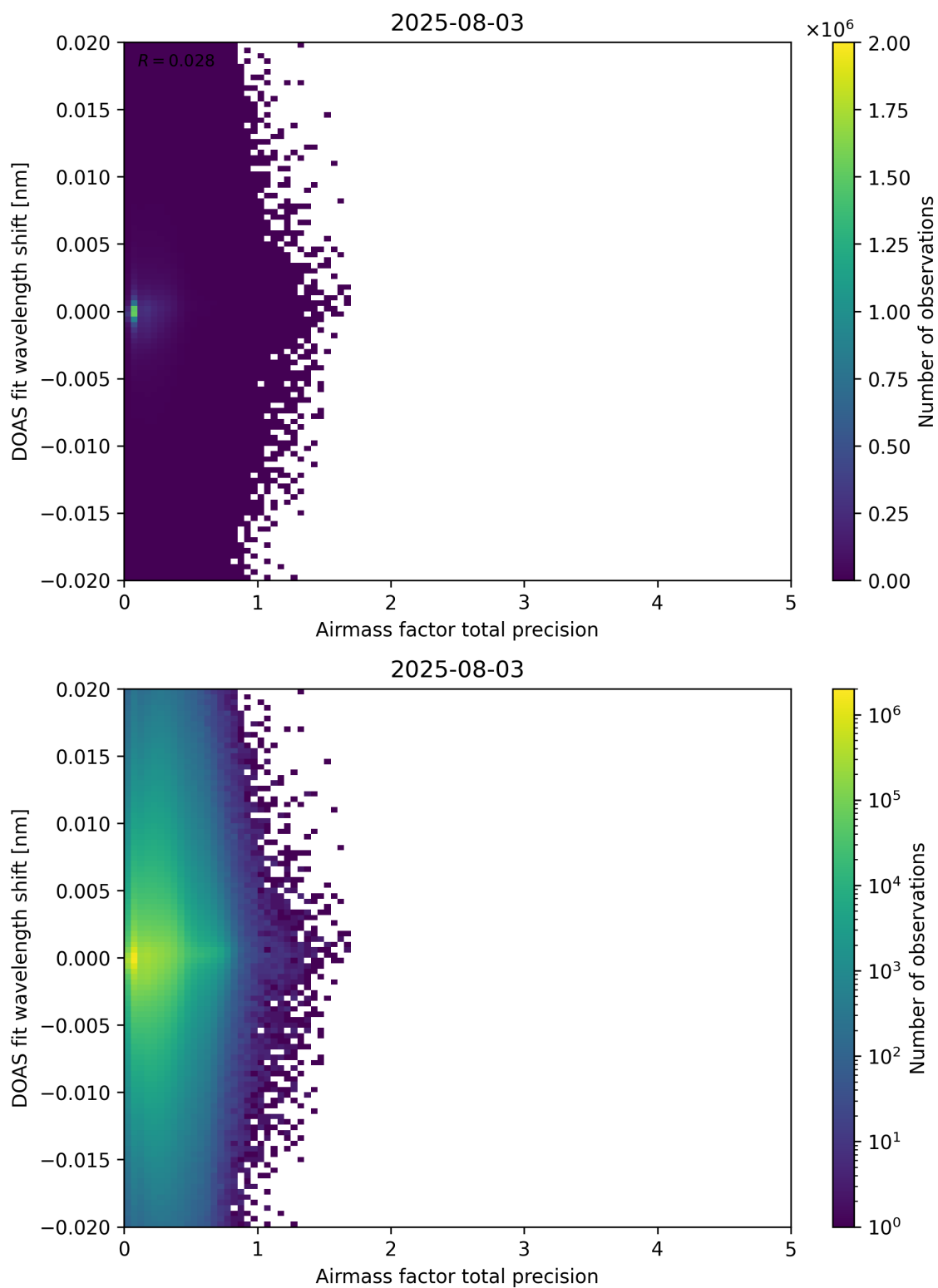
Figure 106: Scatter density plot of “Airmass factor total precision” against “DOAS fit wavelength shift” for 2025-08-03 to 2025-08-04.
