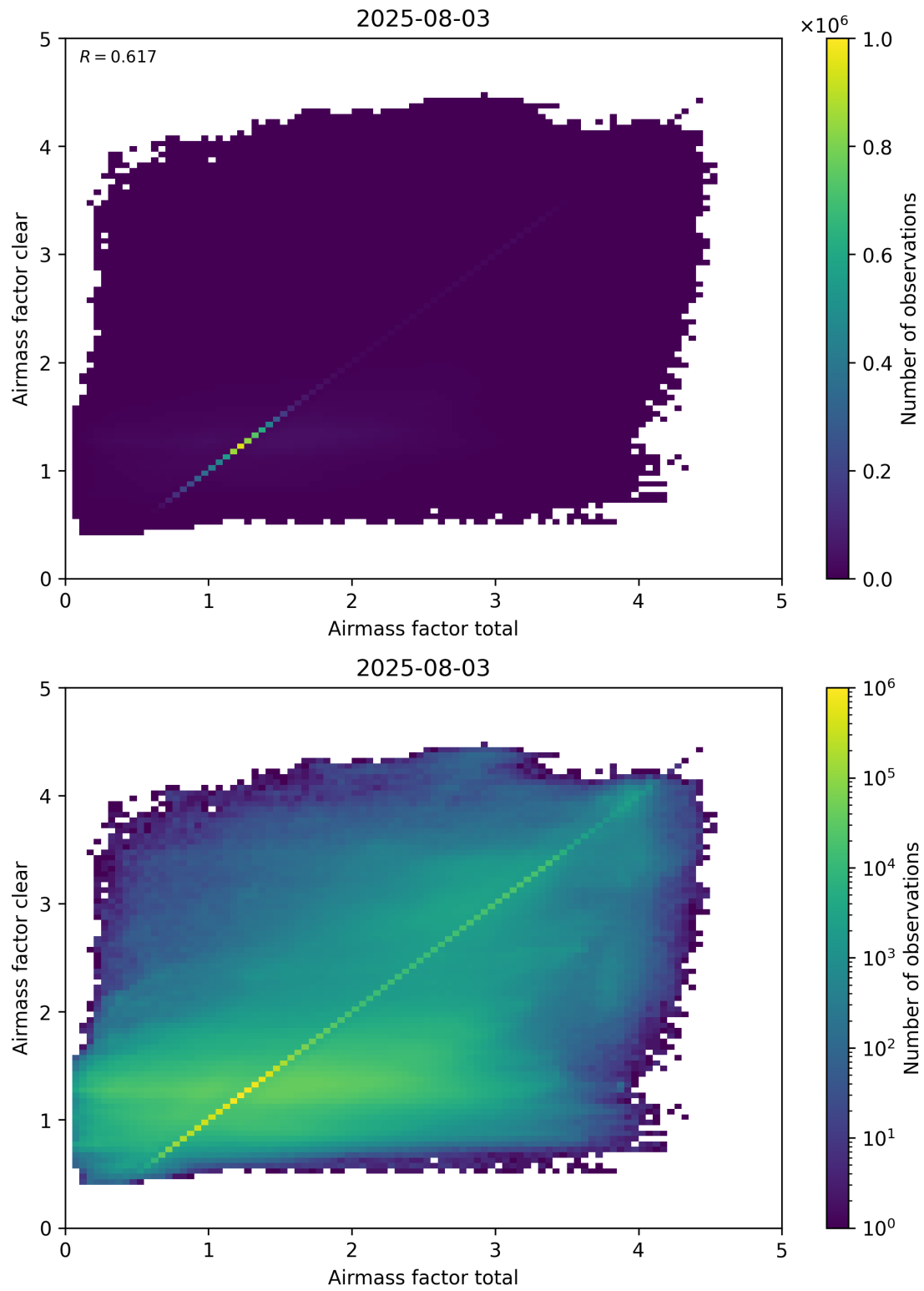
Figure 100: Scatter density plot of “Airmass factor total” against “Airmass factor clear” for 2025-08-03 to 2025-08-04.
