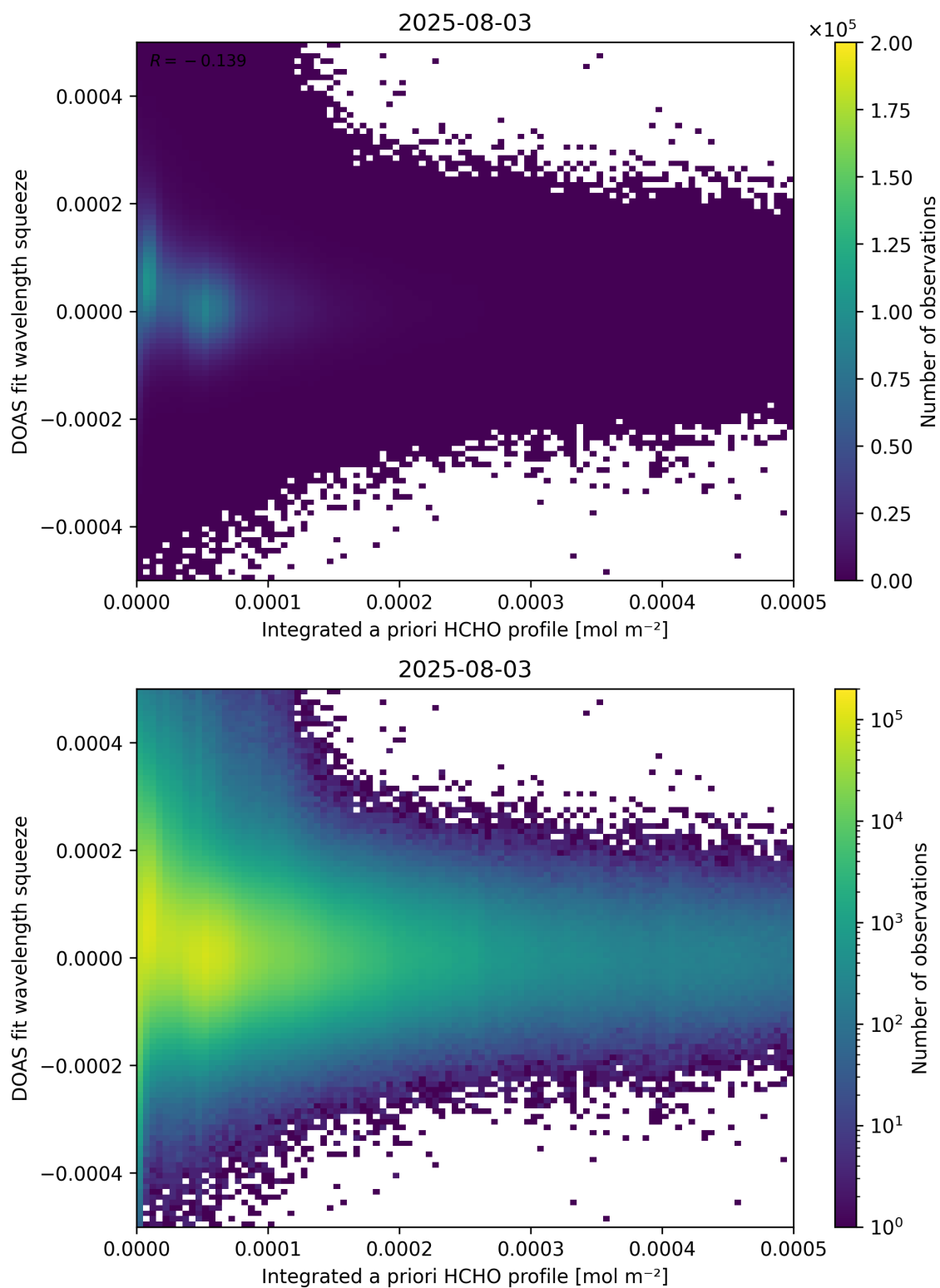
Figure 150: Scatter density plot of “Integrated a priori HCHO profile” against “DOAS fit wavelength squeeze” for 2025-08-03 to 2025-08-04.
