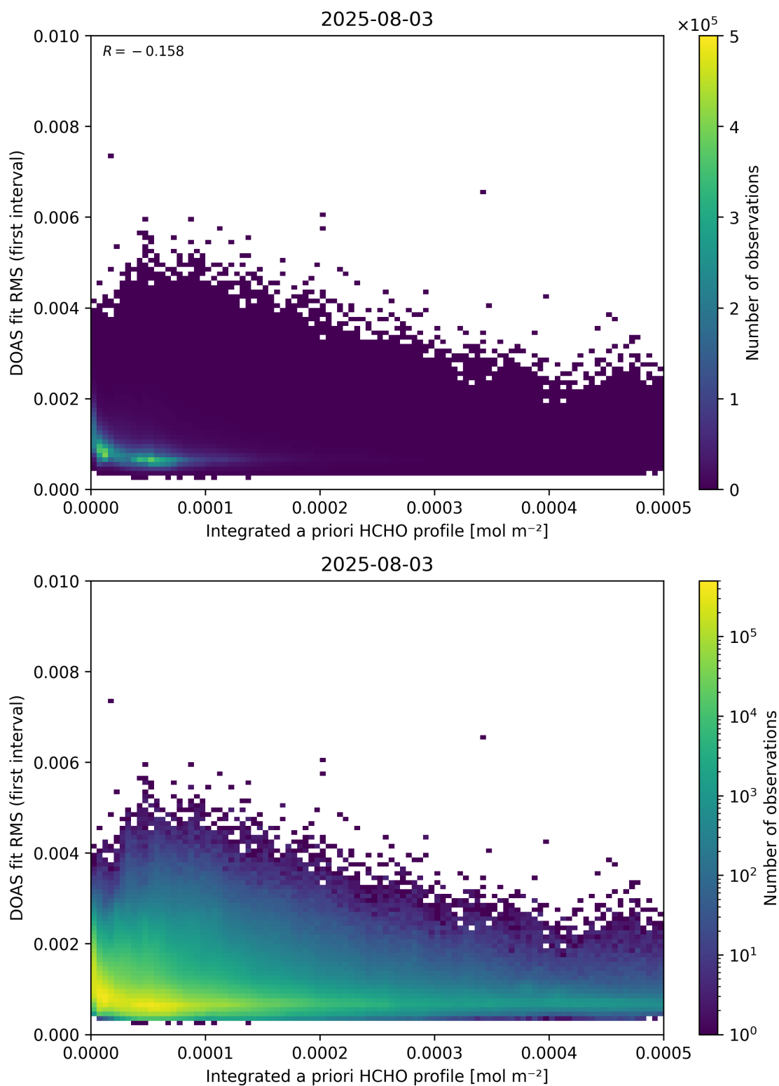
Figure 148: Scatter density plot of “Integrated a priori HCHO profile” against “DOAS fit RMS (first interval)” for 2025-08-03 to 2025-08-04.
