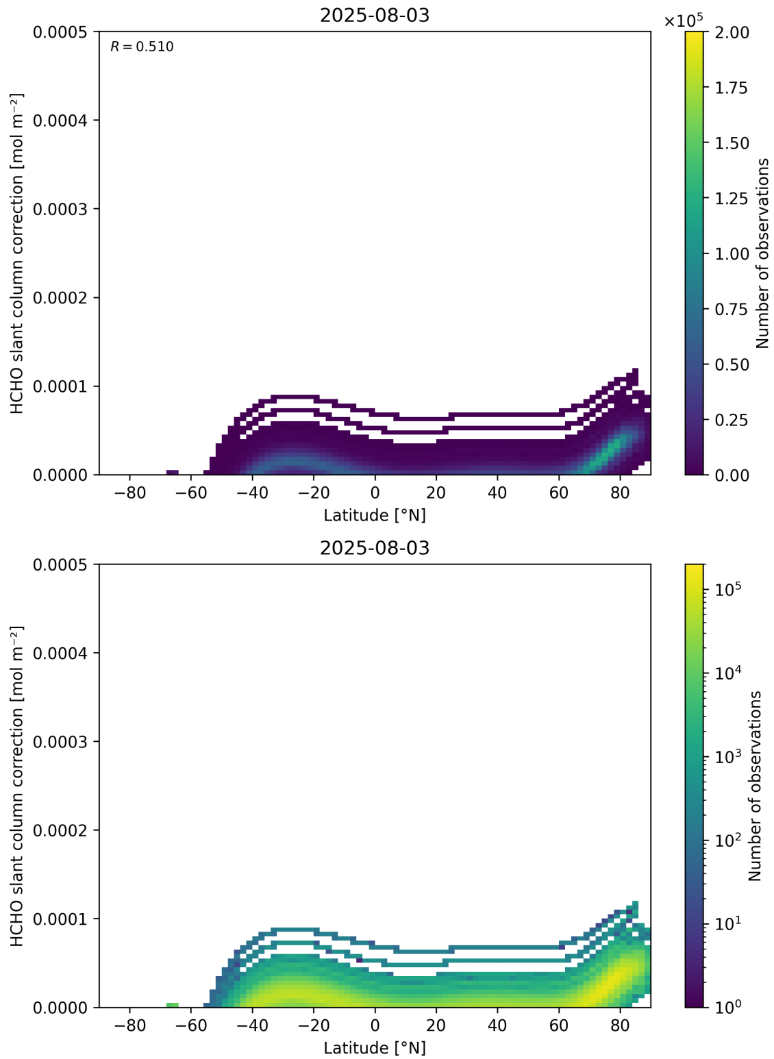
Figure 158: Scatter density plot of “Latitude” against “HCHO slant column correction” for 2025-08-03 to 2025-08-04.
