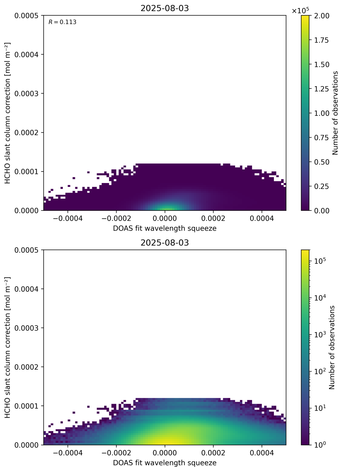
Figure 70: Scatter density plot of “DOAS fit wavelength squeeze” against “HCHO slant column correction” for 2025-08-03 to 2025-08-04.
