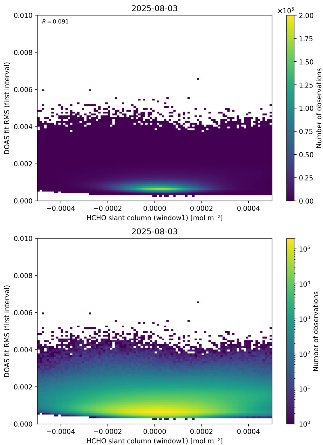
Figure 78: Scatter density plot of “HCHO slant column (window1)” against “DOAS fit RMS (first interval)” for 2025-08-03 to 2025-08-04.
