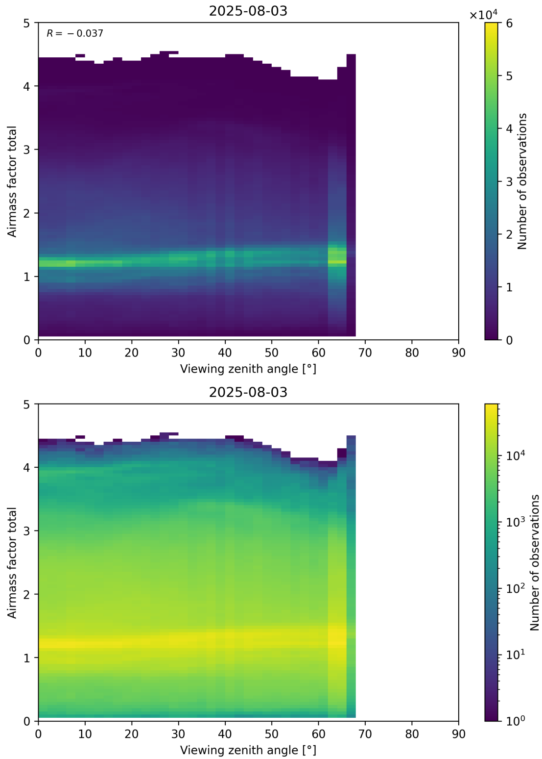
Figure 190: Scatter density plot of “Viewing zenith angle” against “Airmass factor total” for 2025-08-03 to 2025-08-04.
