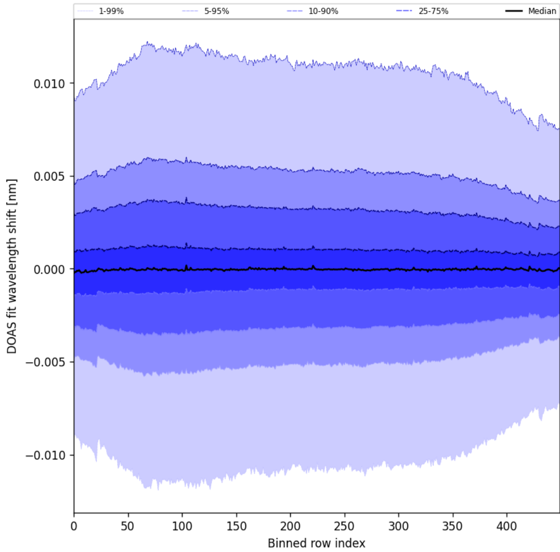
Figure 58: Along track statistics of “DOAS fit wavelength shift” for 2025-08-03 to 2025-08-04
