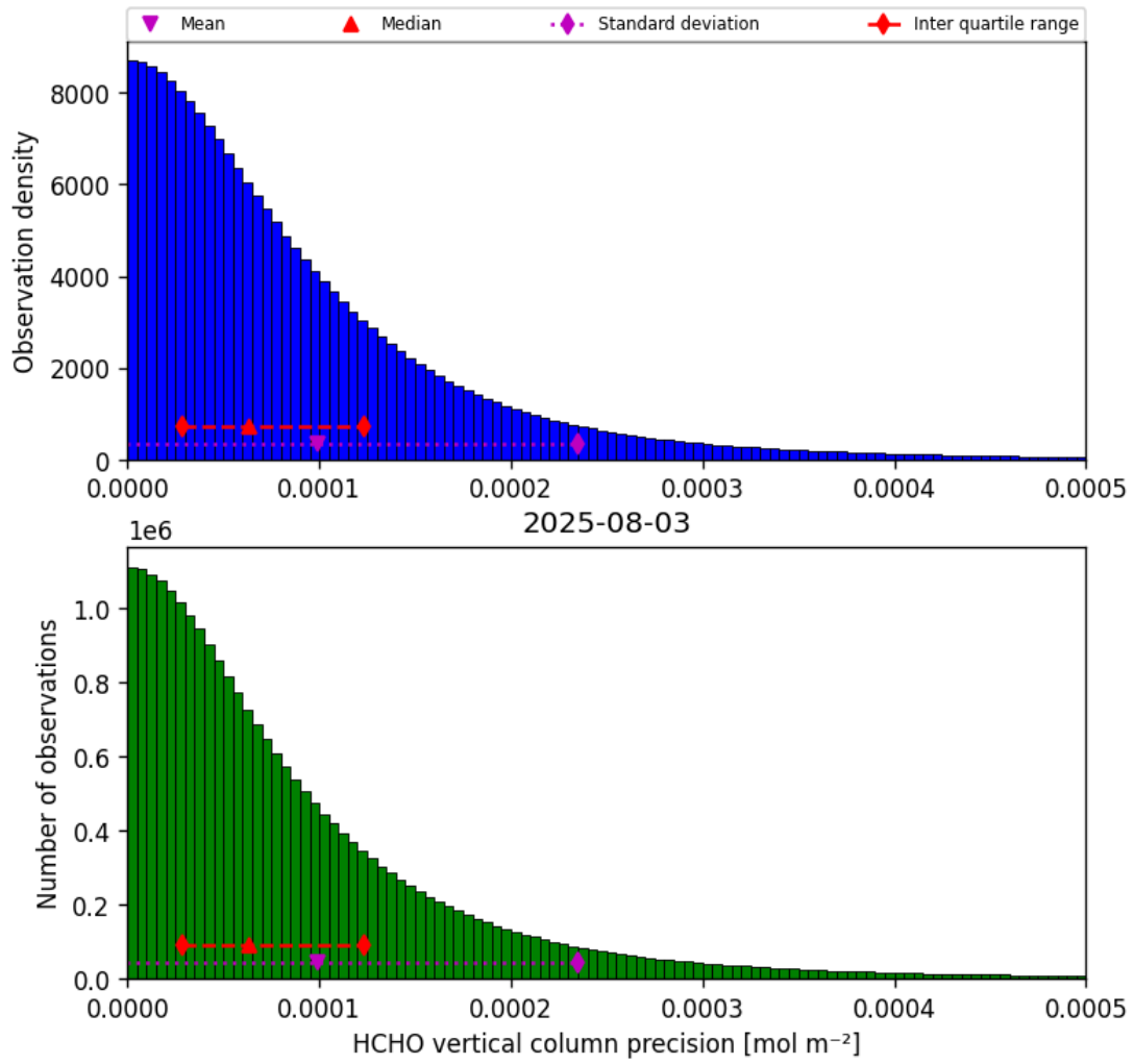
Figure 36: Histogram of “HCHO vertical column precision” for 2025-08-03 to 2025-08-04
