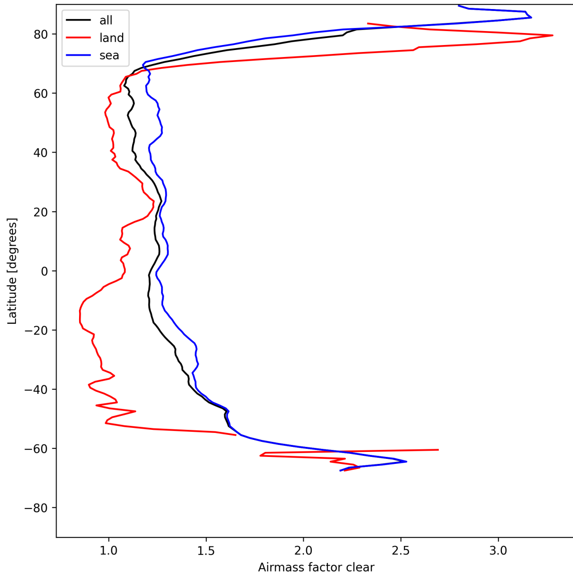
Figure 28: Zonal average of “Airmass factor clear” for 2025-08-03 to 2025-08-04.
