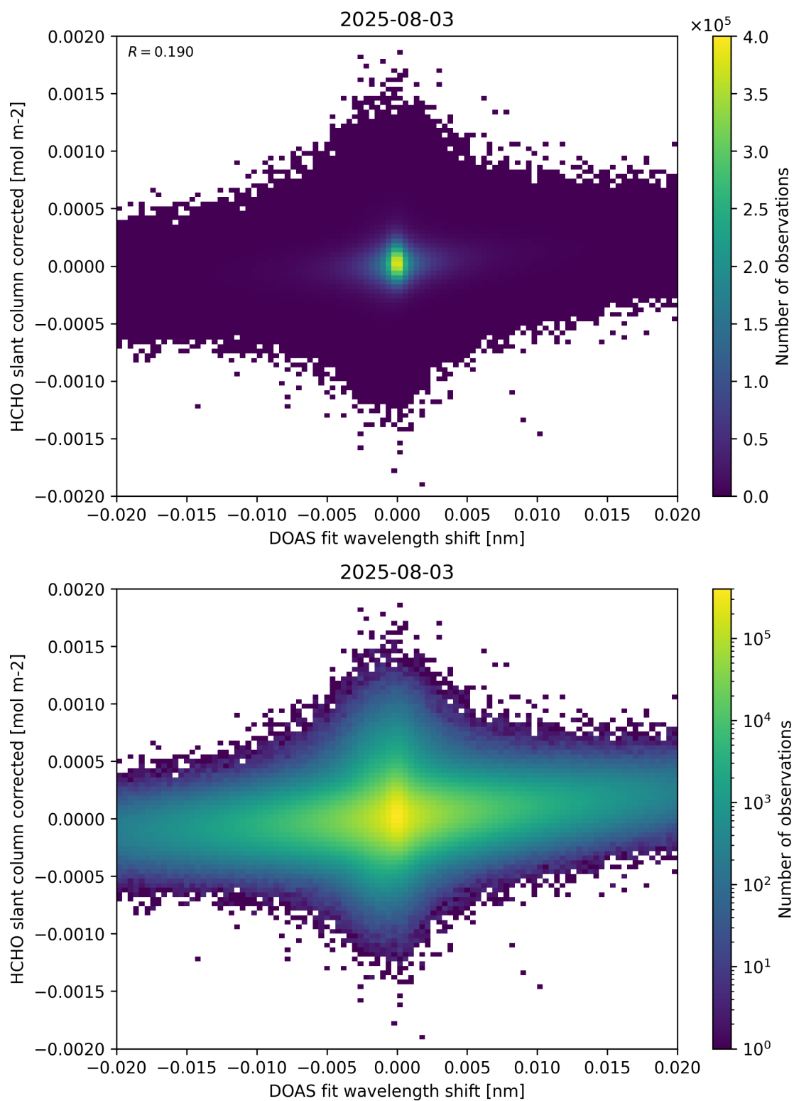
Figure 66: Scatter density plot of “DOAS fit wavelength shift” against “HCHO slant column corrected” for 2025-08-03 to 2025-08-04.
