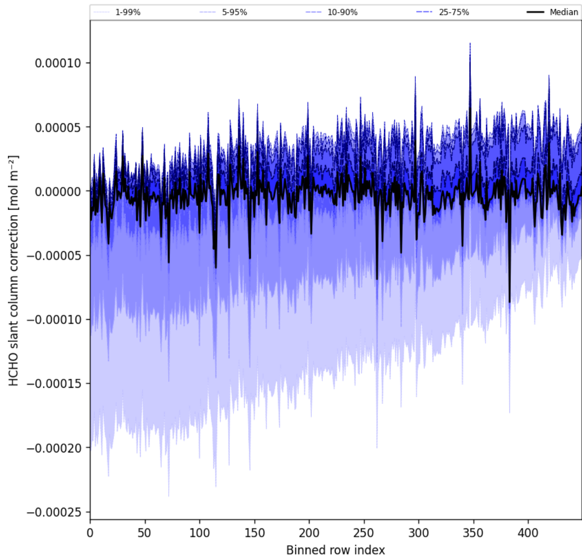
Figure 61: Along track statistics of “HCHO slant column correction” for 2025-08-03 to 2025-08-04
