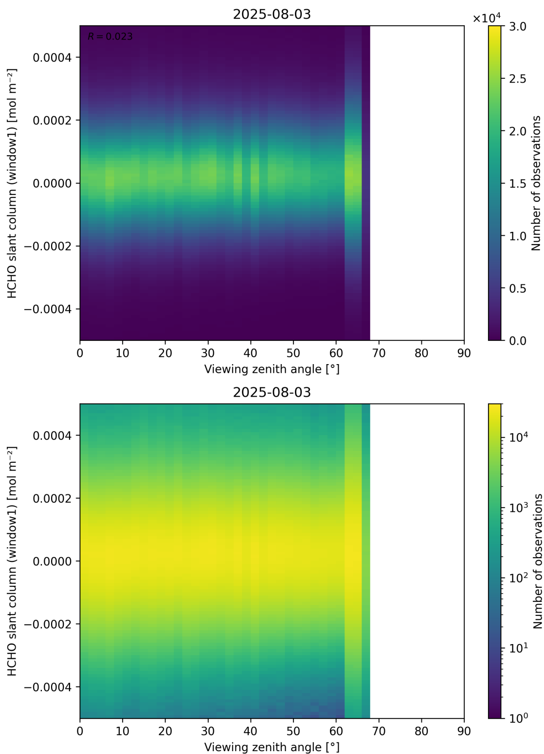
Figure 188: Scatter density plot of “Viewing zenith angle” against “HCHO slant column (window1)” for 2025-08-03 to 2025-08-04.
