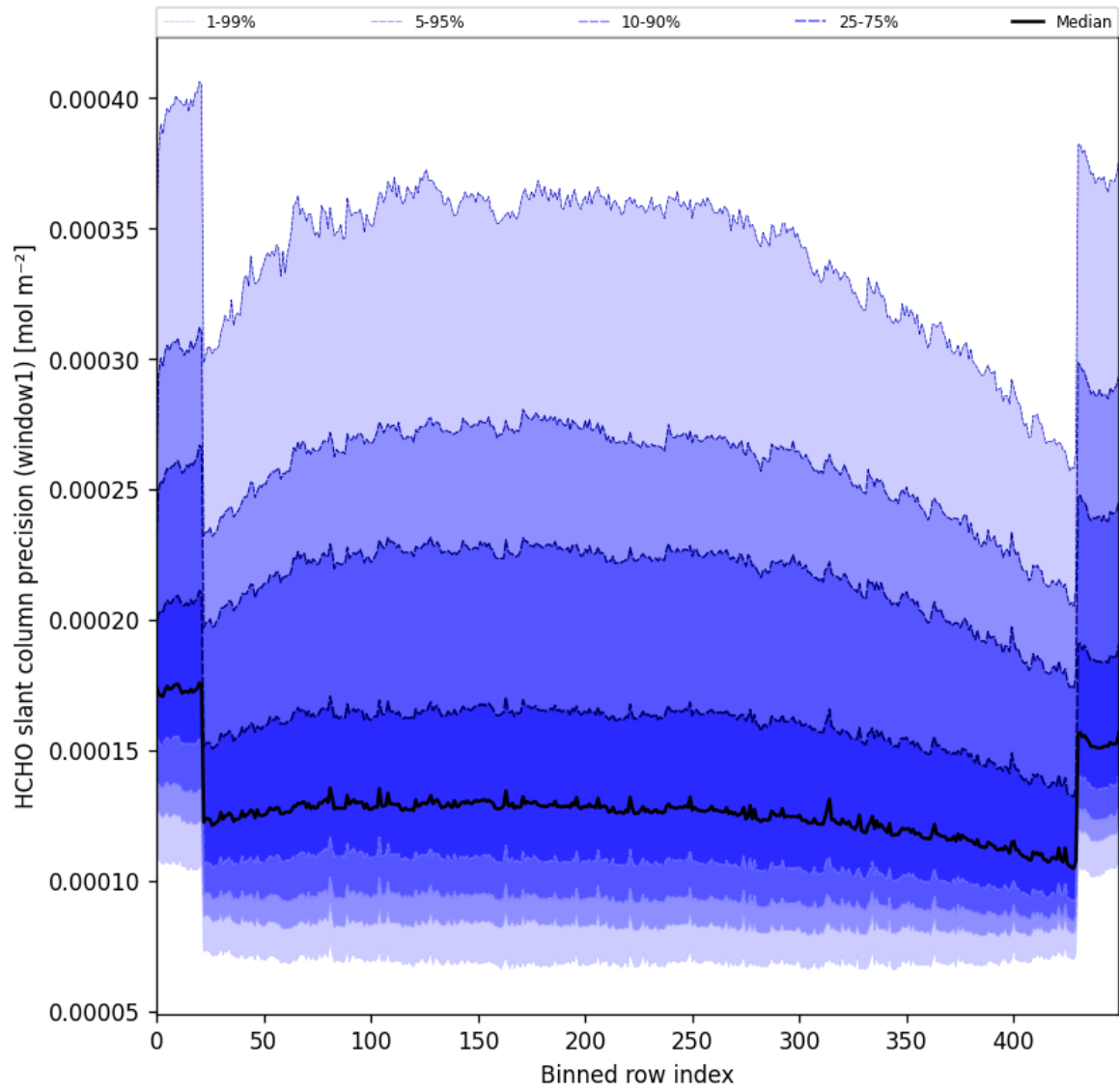
Figure 53: Along track statistics of “HCHO slant column precision (window1)” for 2025-08-03 to 2025-08-04
