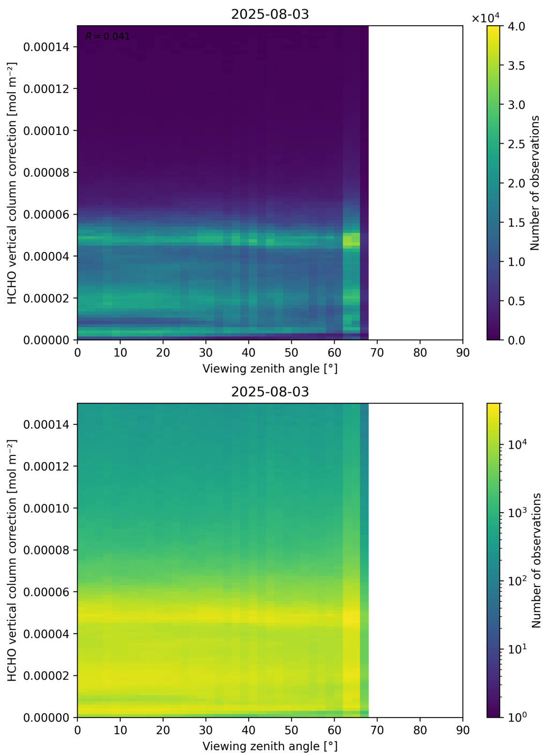
Figure 193: Scatter density plot of “Viewing zenith angle” against “HCHO vertical column correction” for 2025-08-03 to 2025-08-04.
