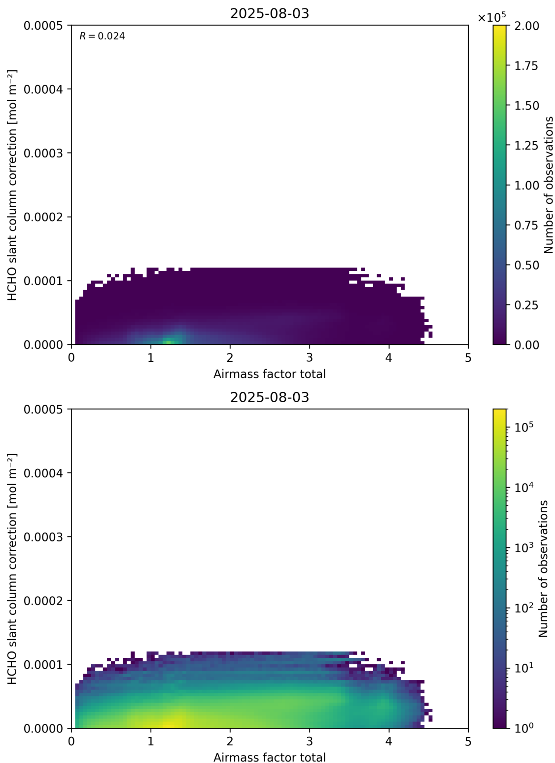
Figure 102: Scatter density plot of “Airmass factor total” against “HCHO slant column correction” for 2025-08-03 to 2025-08-04.
