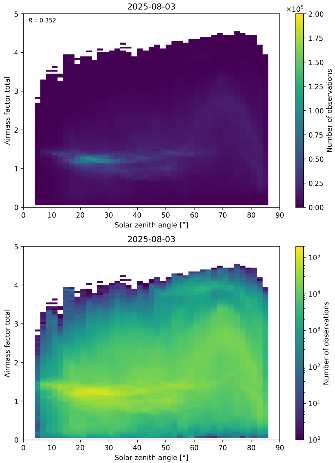
Figure 175: Scatter density plot of “Solar zenith angle” against “Airmass factor total” for 2025-08-03 to 2025-08-04.
