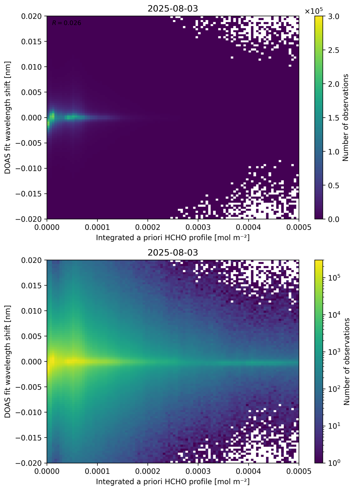
Figure 149: Scatter density plot of “Integrated a priori HCHO profile” against “DOAS fit wavelength shift” for 2025-08-03 to 2025-08-04.
