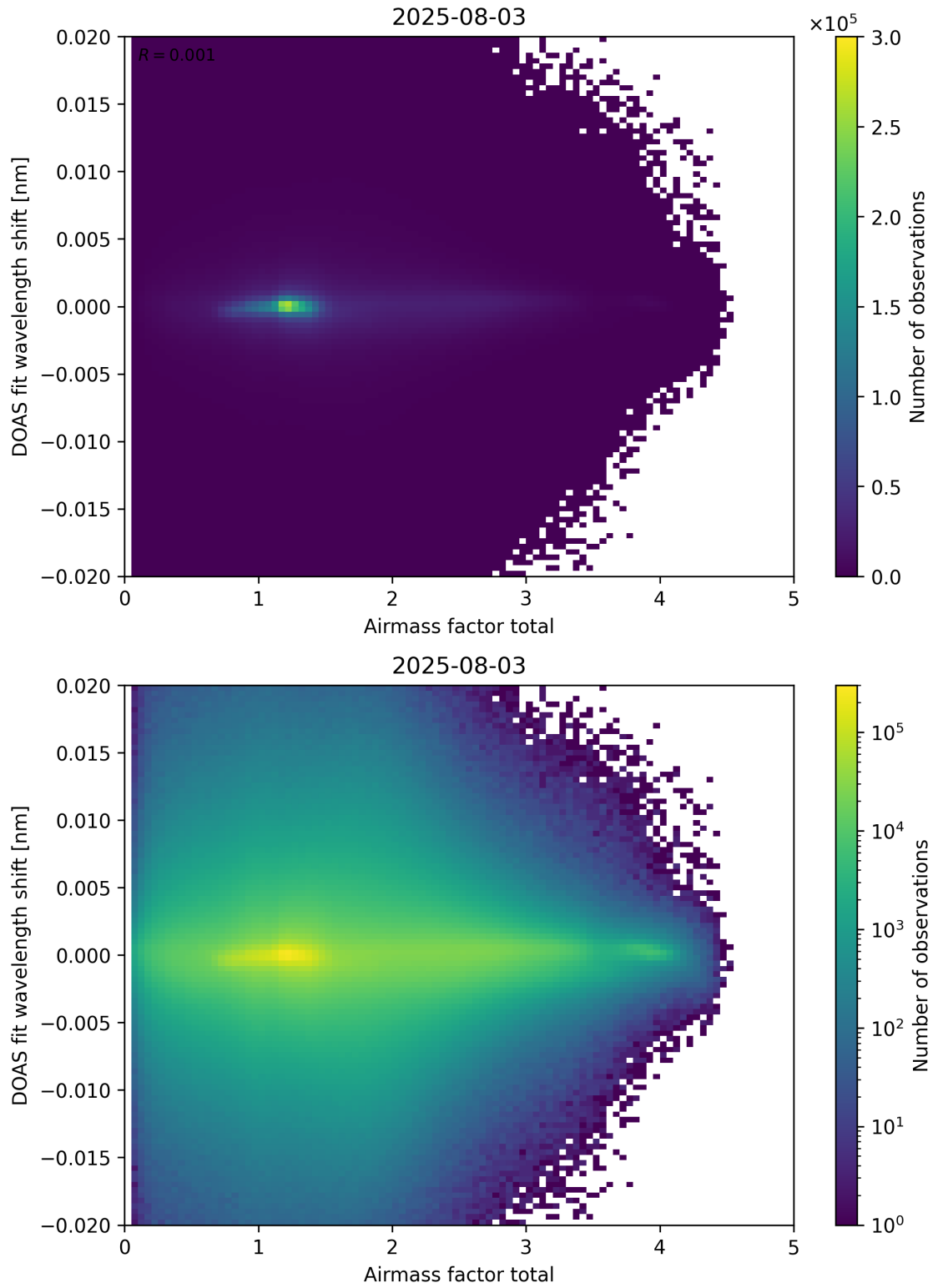
Figure 98: Scatter density plot of “Airmass factor total” against “DOAS fit wavelength shift” for 2025-08-03 to 2025-08-04.
