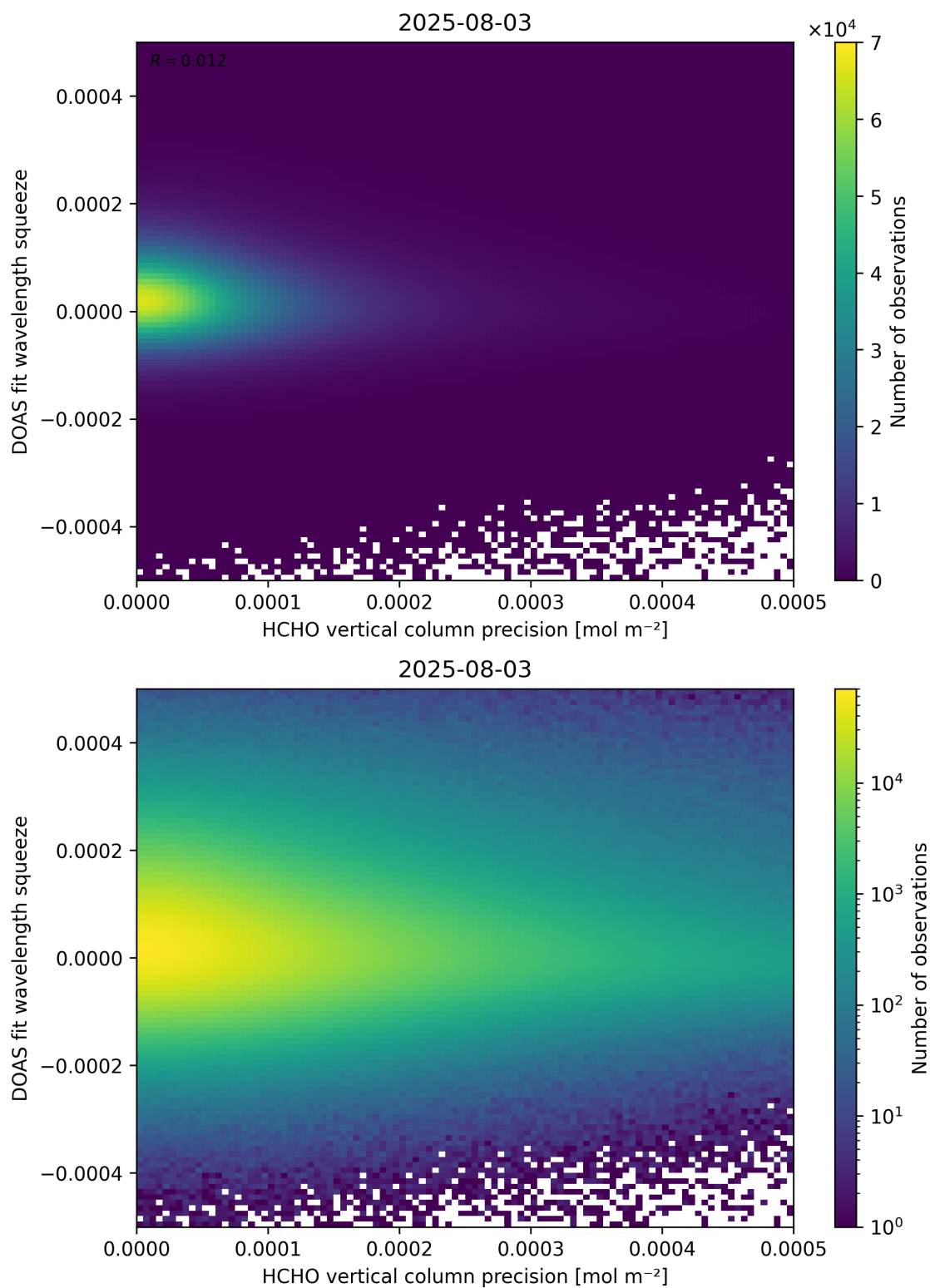
Figure 138: Scatter density plot of “HCHO vertical column precision” against “DOAS fit wavelength squeeze” for 2025-08-03 to 2025-08-04.
