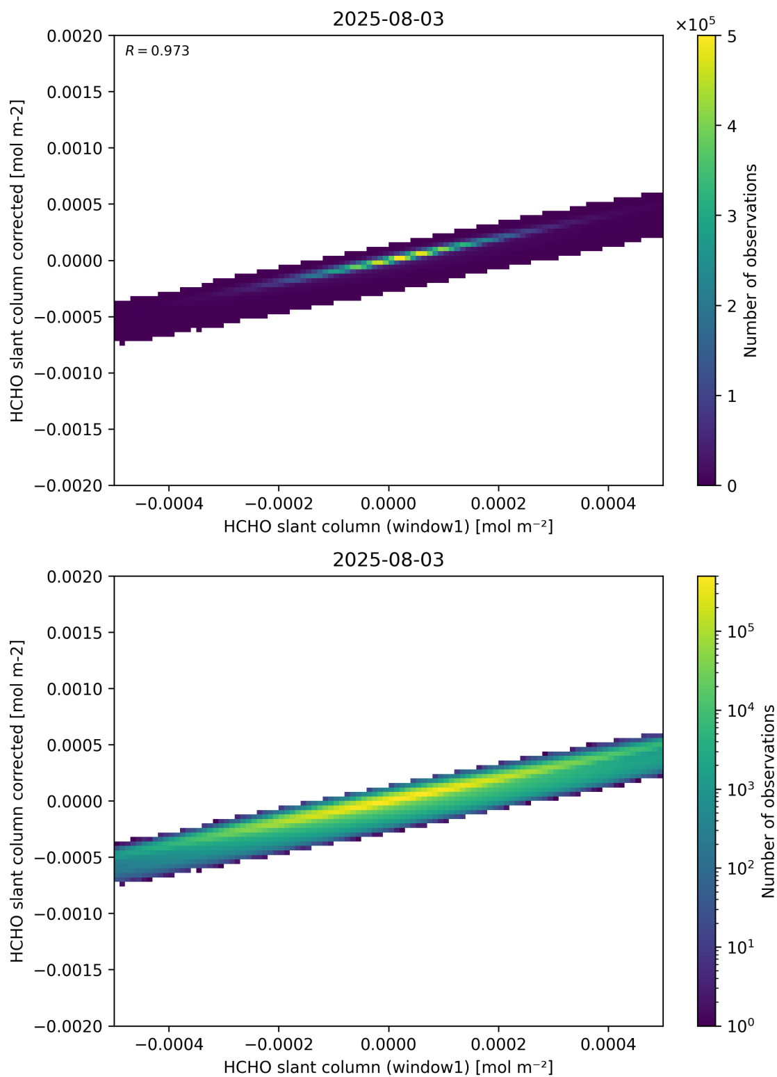
Figure 82: Scatter density plot of “HCHO slant column (window1)” against “HCHO slant column corrected” for 2025-08-03 to 2025-08-04.
