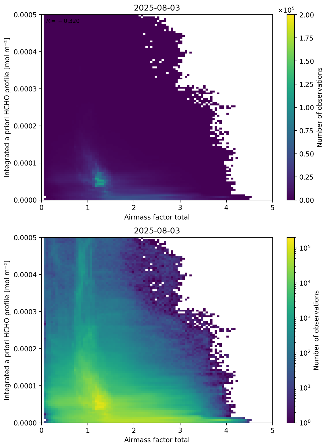
Figure 104: Scatter density plot of “Airmass factor total” against “Integrated a priori HCHO profile” for 2025-08-03 to 2025-08-04.
