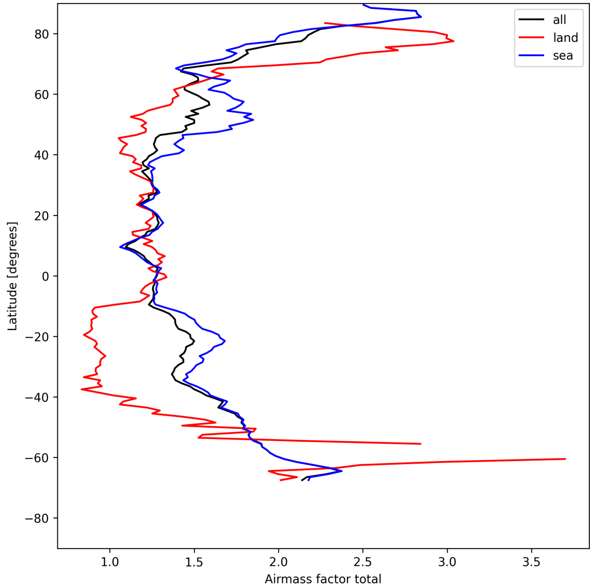
Figure 26: Zonal average of “Airmass factor total” for 2025-08-03 to 2025-08-04.
