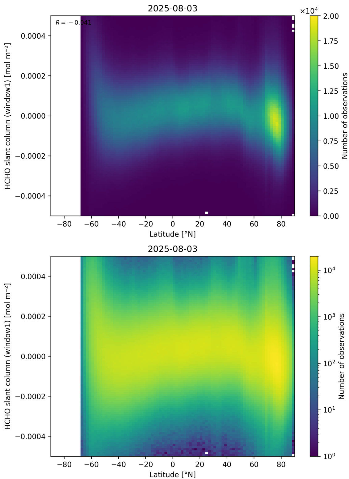
Figure 159: Scatter density plot of “Latitude” against “HCHO slant column (window1)” for 2025-08-03 to 2025-08-04.
