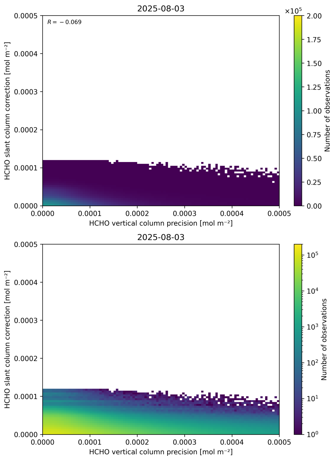
Figure 141: Scatter density plot of “HCHO vertical column precision” against “HCHO slant column correction” for 2025-08-03 to 2025-08-04.
