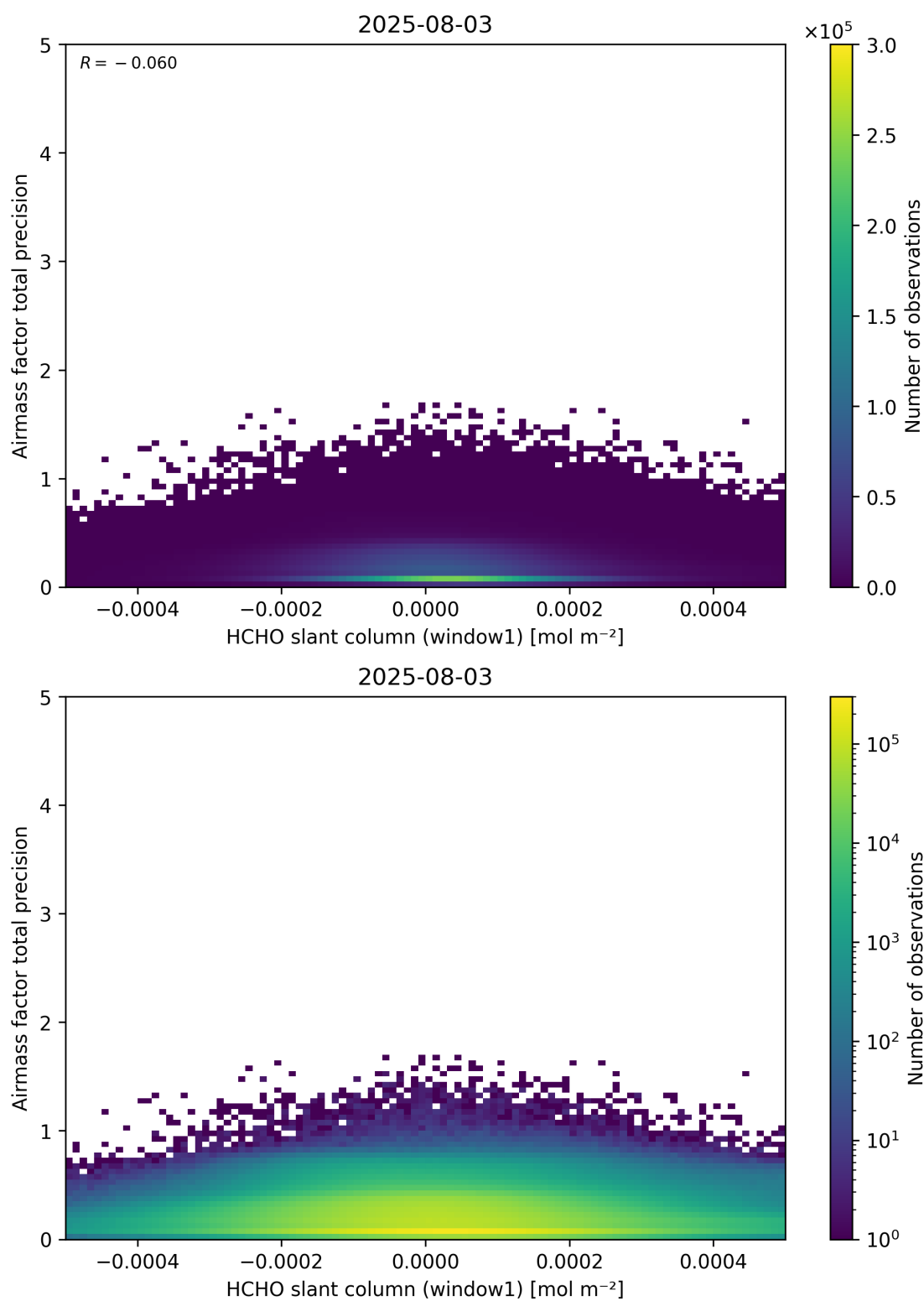
Figure 86: Scatter density plot of “HCHO slant column (window1)” against “Airmass factor total precision” for 2025-08-03 to 2025-08-04.
