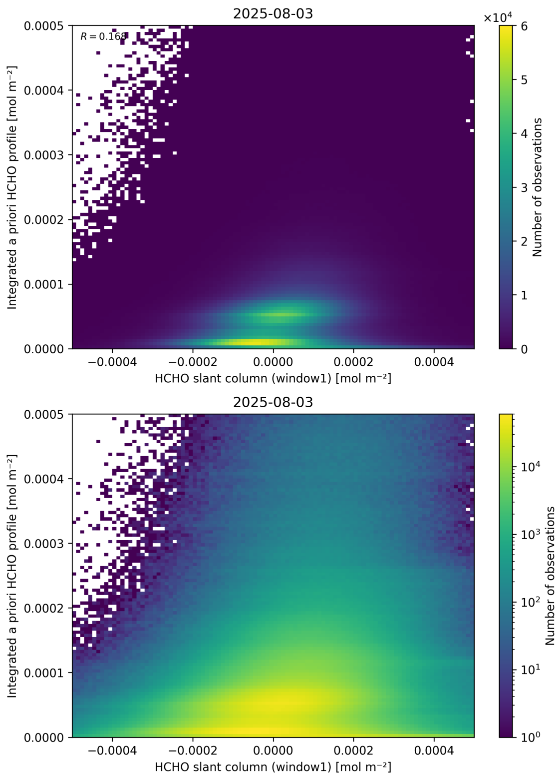
Figure 87: Scatter density plot of “HCHO slant column (window1)” against “Integrated a priori HCHO profile” for 2025-08-03 to 2025-08-04.
