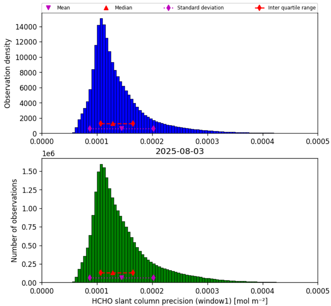
Figure 39: Histogram of “HCHO slant column precision (window1)” for 2025-08-03 to 2025-08-04
