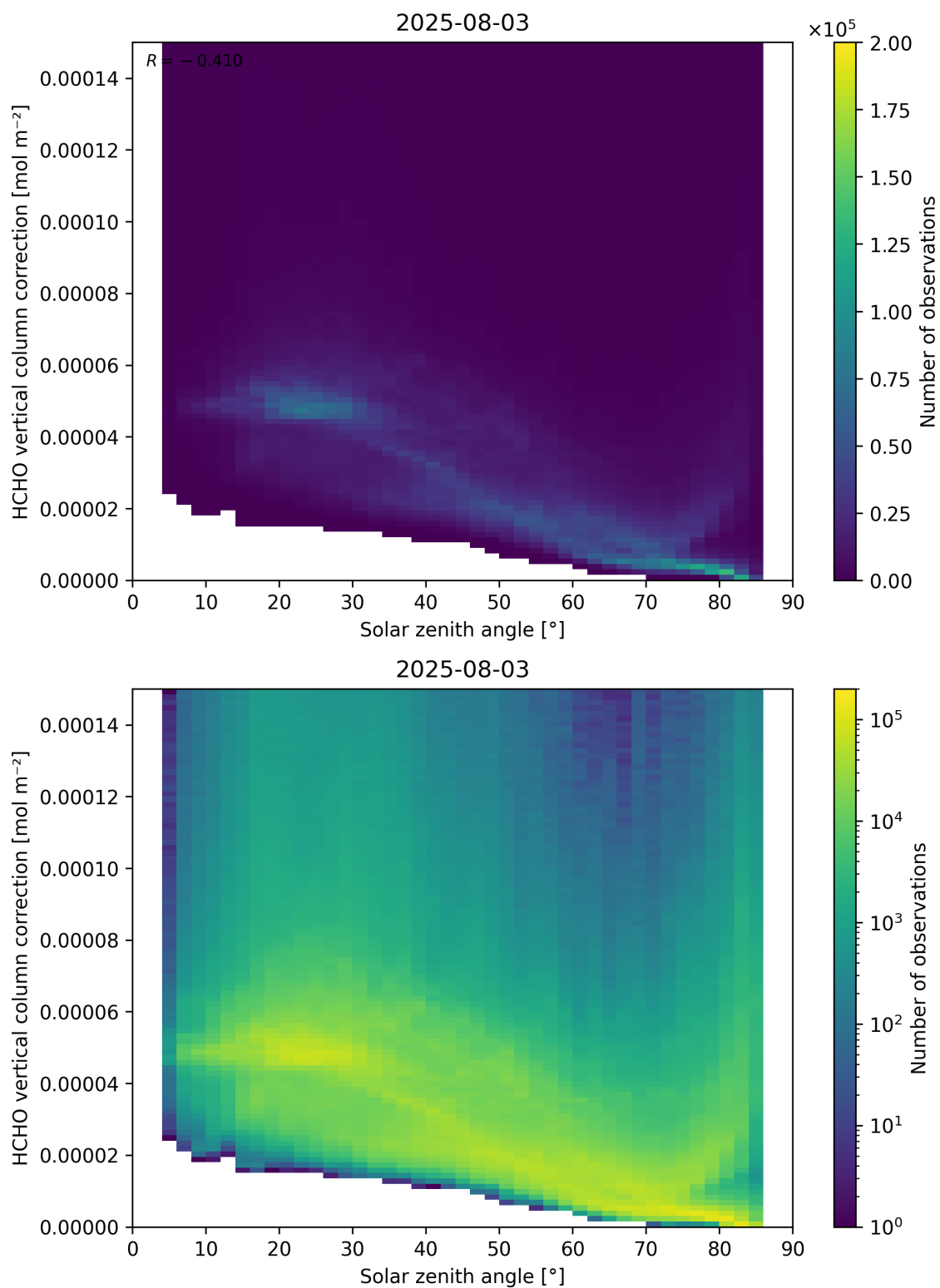
Figure 178: Scatter density plot of “Solar zenith angle” against “HCHO vertical column correction” for 2025-08-03 to 2025-08-04.
