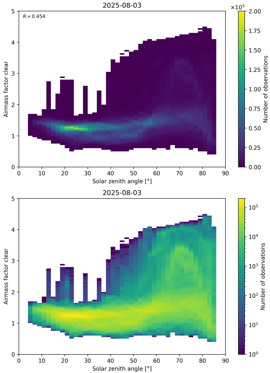
Figure 170: Scatter density plot of “Solar zenith angle” against “Airmass factor clear” for 2025-08-03 to 2025-08-04.
