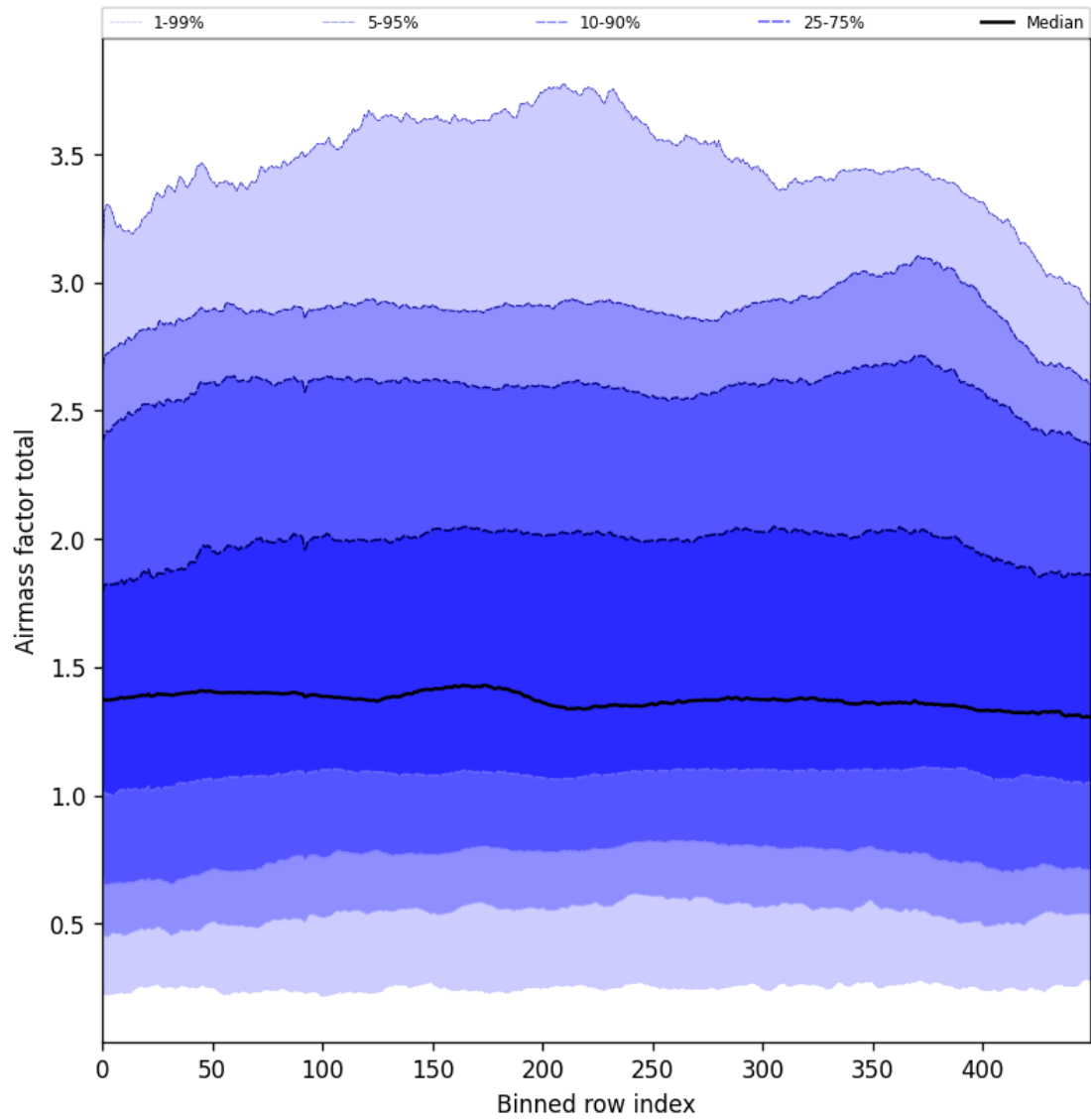
Figure 54: Along track statistics of “Airmass factor total” for 2025-08-03 to 2025-08-04
