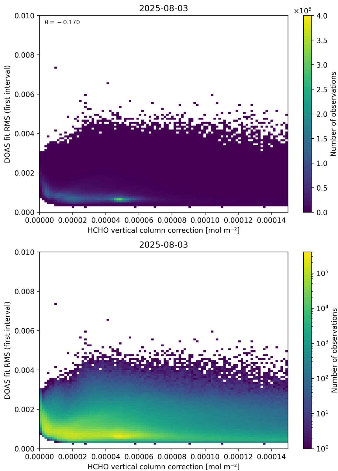
Figure 112: Scatter density plot of “HCHO vertical column correction” against “DOAS fit RMS (first interval)” for 2025-08-03 to 2025-08-04.
