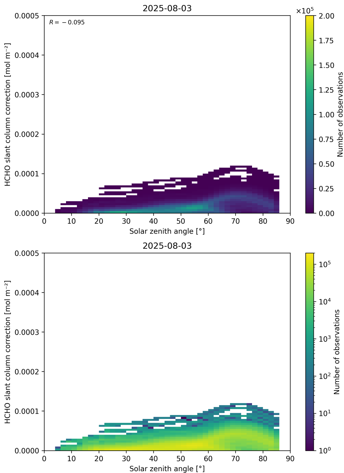
Figure 172: Scatter density plot of “Solar zenith angle” against “HCHO slant column correction” for 2025-08-03 to 2025-08-04.
