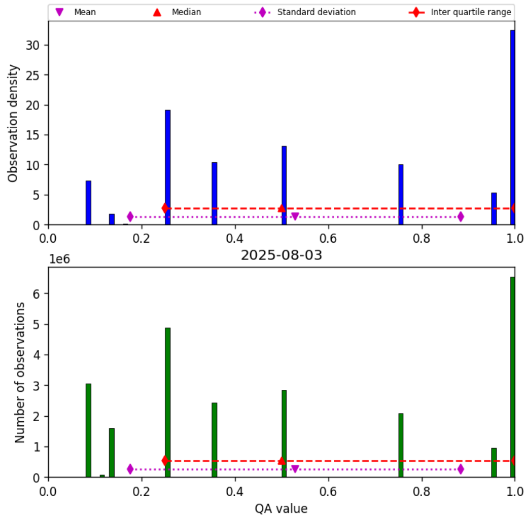
Figure 34: Histogram of “QA value” for 2025-08-03 to 2025-08-04
