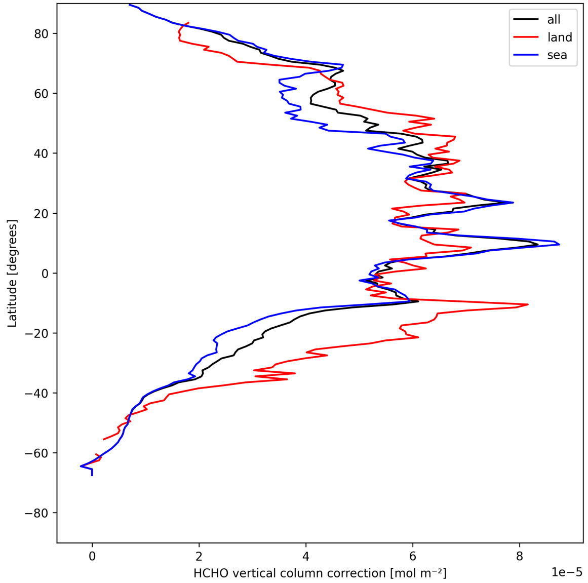
Figure 23: Zonal average of “HCHO vertical column correction” for 2025-08-03 to 2025-08-04.
