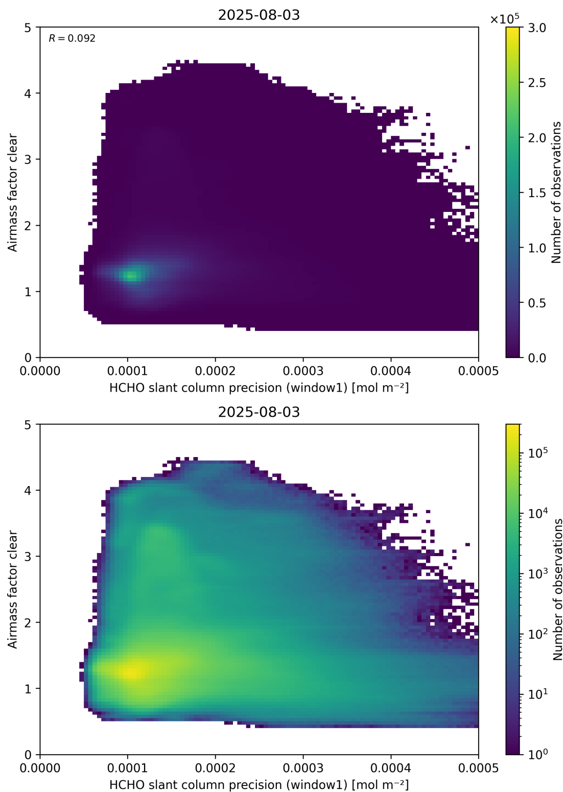
Figure 91: Scatter density plot of “HCHO slant column precision (window1)” against “Airmass factor clear” for 2025-08-03 to 2025-08-04.
