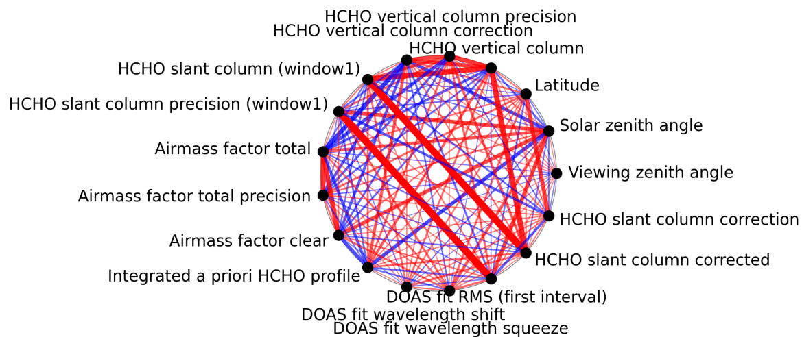
Figure 1: Map of correlation graph for 2025-08-03 to 2025-08-04.
