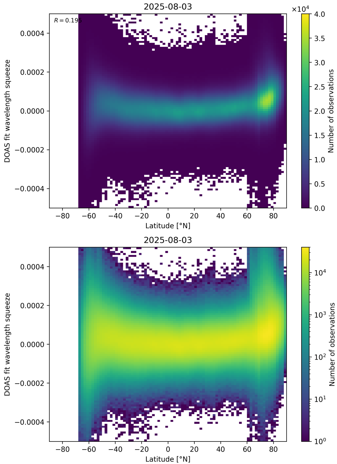
Figure 155: Scatter density plot of “Latitude” against “DOAS fit wavelength squeeze” for 2025-08-03 to 2025-08-04.
