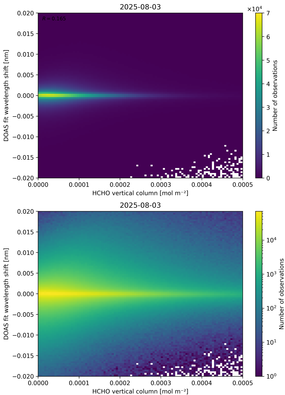
Figure 124: Scatter density plot of “HCHO vertical column” against “DOAS fit wavelength shift” for 2025-08-03 to 2025-08-04.
