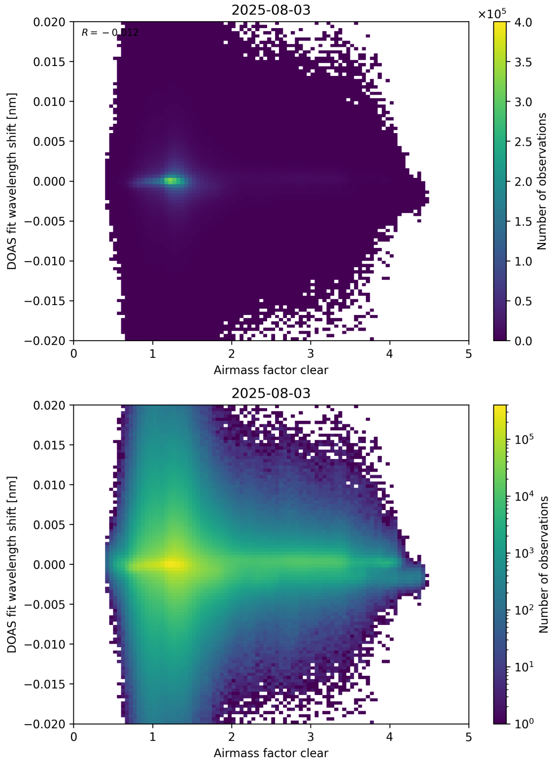
Figure 72: Scatter density plot of “Airmass factor clear” against “DOAS fit wavelength shift” for 2025-08-03 to 2025-08-04.
