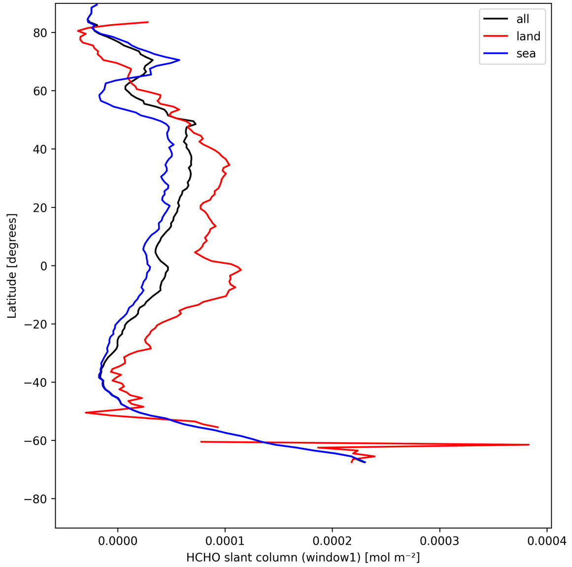
Figure 24: Zonal average of “HCHO slant column (window1)” for 2025-08-03 to 2025-08-04.
