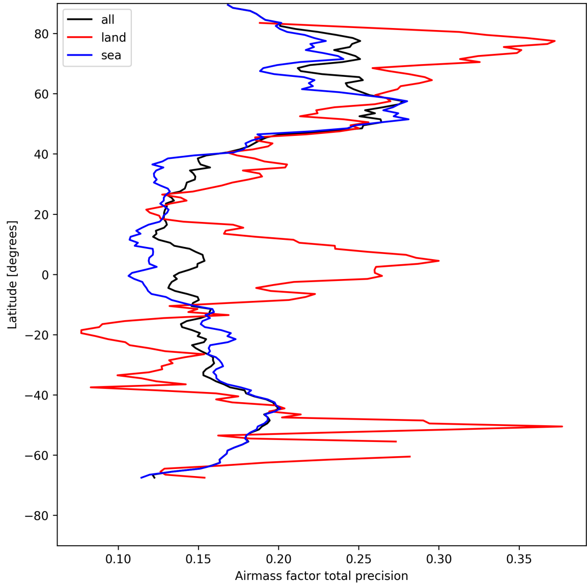
Figure 27: Zonal average of “Airmass factor total precision” for 2025-08-03 to 2025-08-04.
