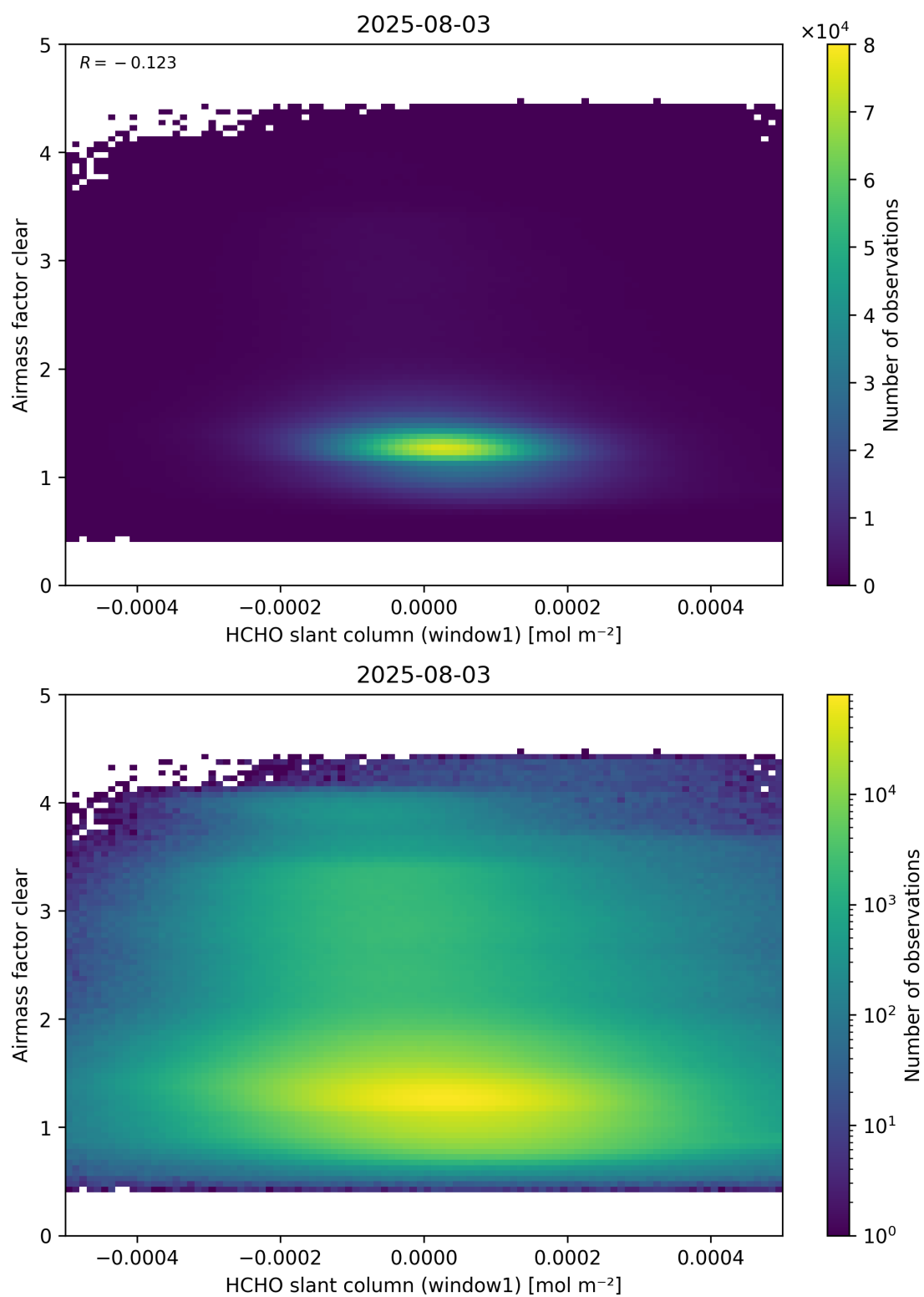
Figure 81: Scatter density plot of “HCHO slant column (window1)” against “Airmass factor clear” for 2025-08-03 to 2025-08-04.
