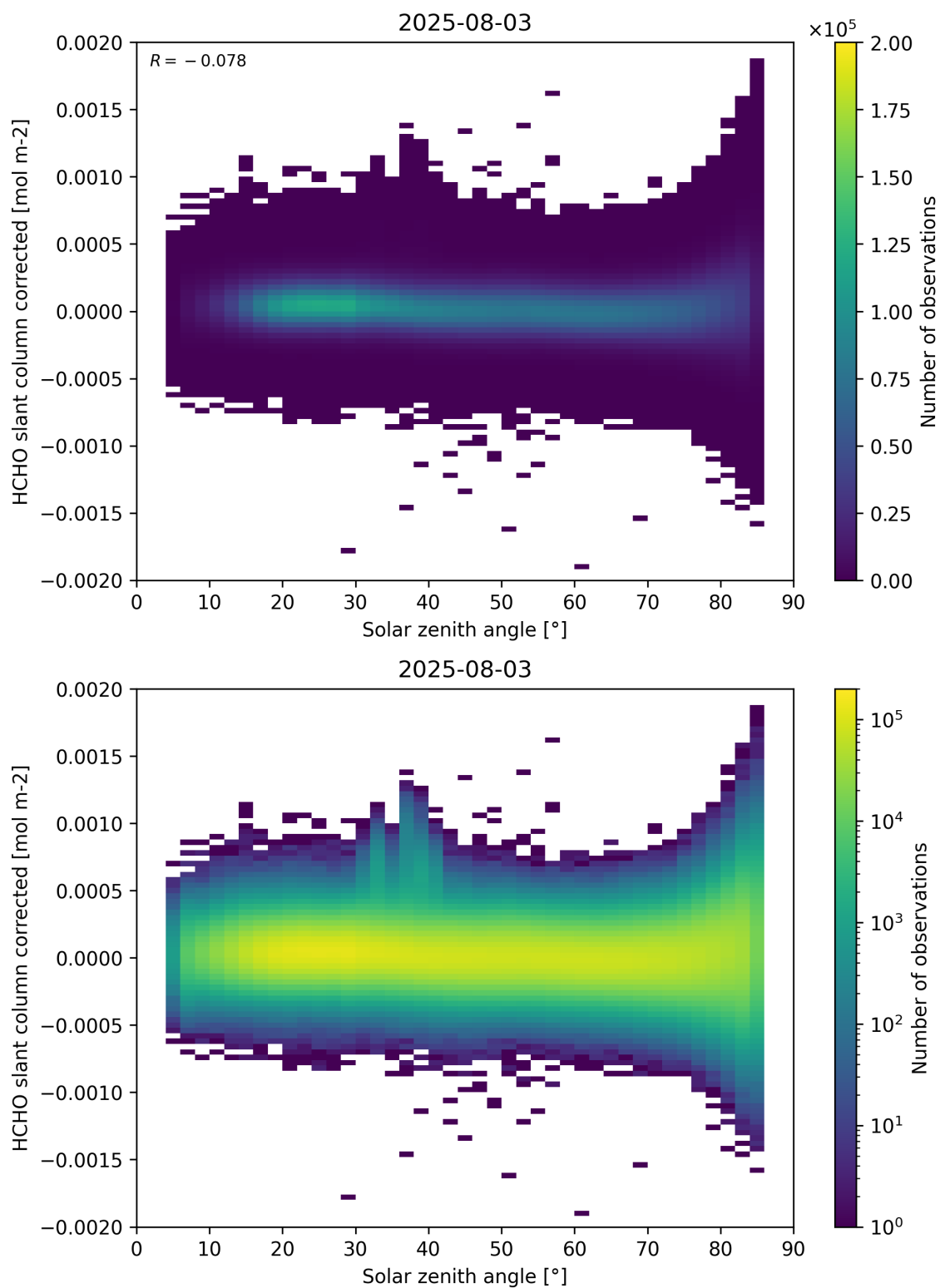
Figure 171: Scatter density plot of “Solar zenith angle” against “HCHO slant column corrected” for 2025-08-03 to 2025-08-04.
