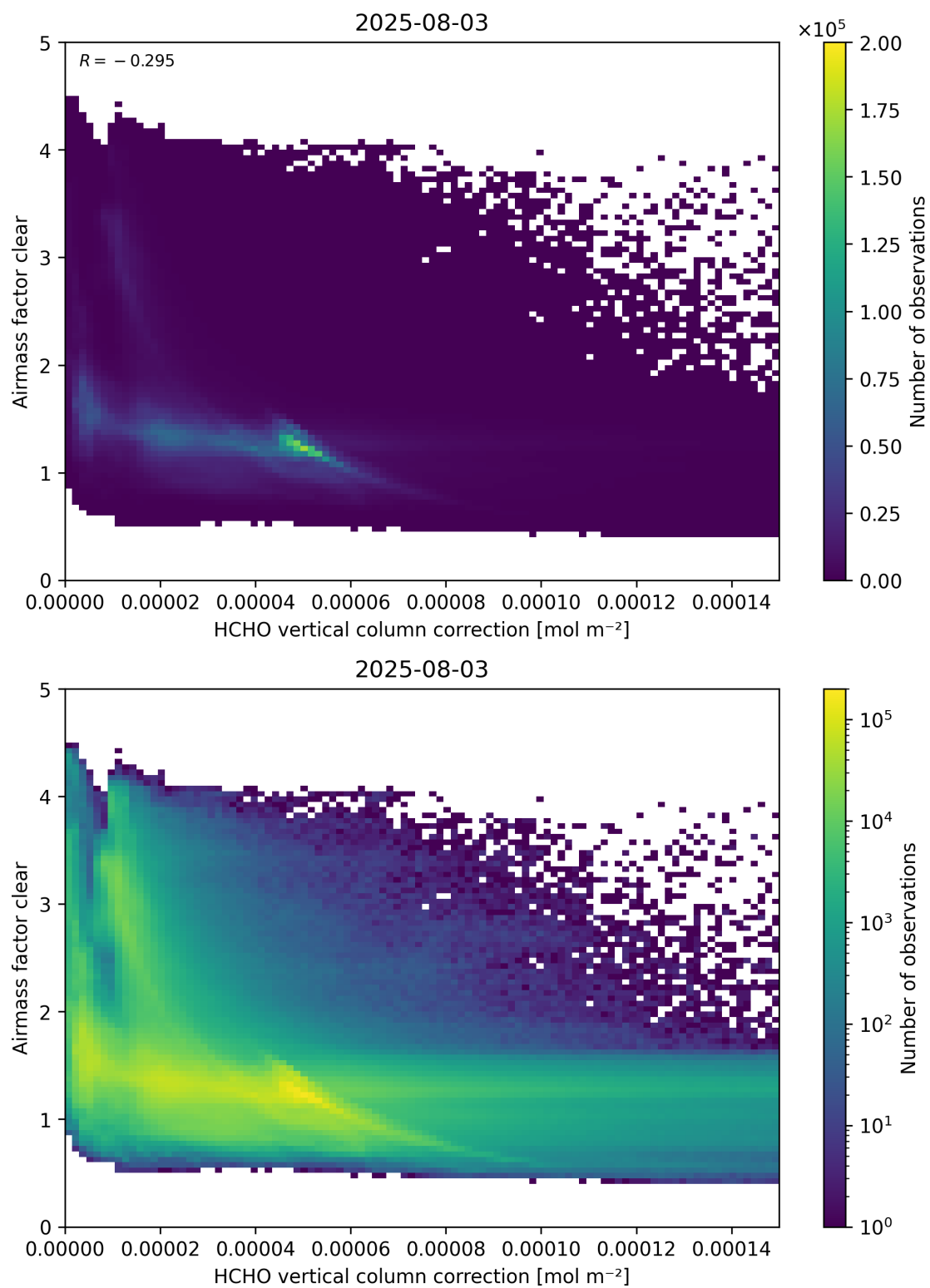
Figure 115: Scatter density plot of “HCHO vertical column correction” against “Airmass factor clear” for 2025-08-03 to 2025-08-04.
