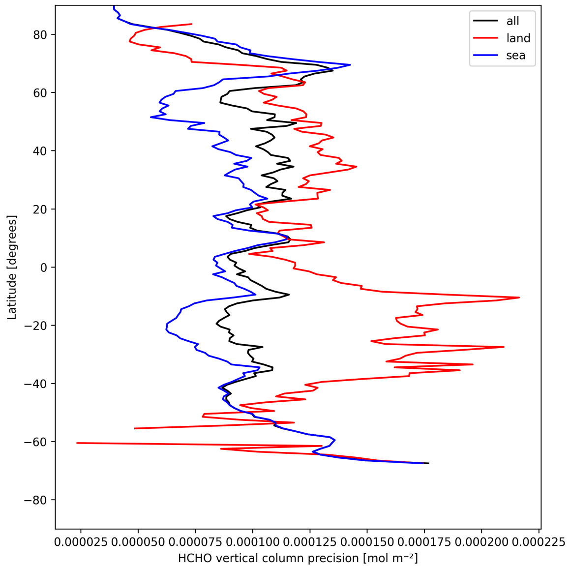
Figure 22: Zonal average of “HCHO vertical column precision” for 2025-08-03 to 2025-08-04.
