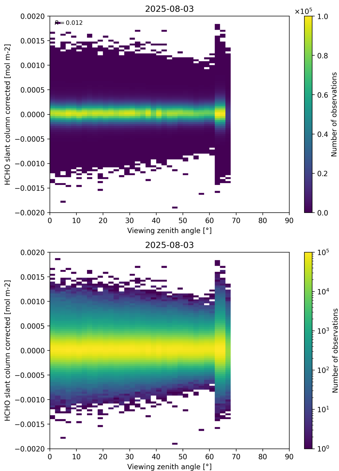
Figure 186: Scatter density plot of “Viewing zenith angle” against “HCHO slant column corrected” for 2025-08-03 to 2025-08-04.
