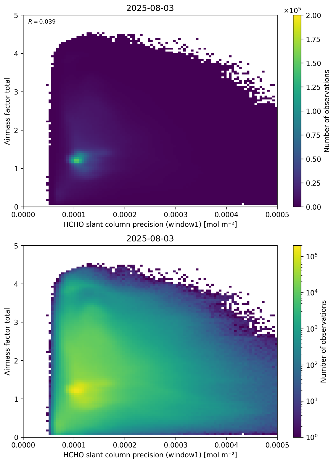
Figure 94: Scatter density plot of “HCHO slant column precision (window1)” against “Airmass factor total” for 2025-08-03 to 2025-08-04.
