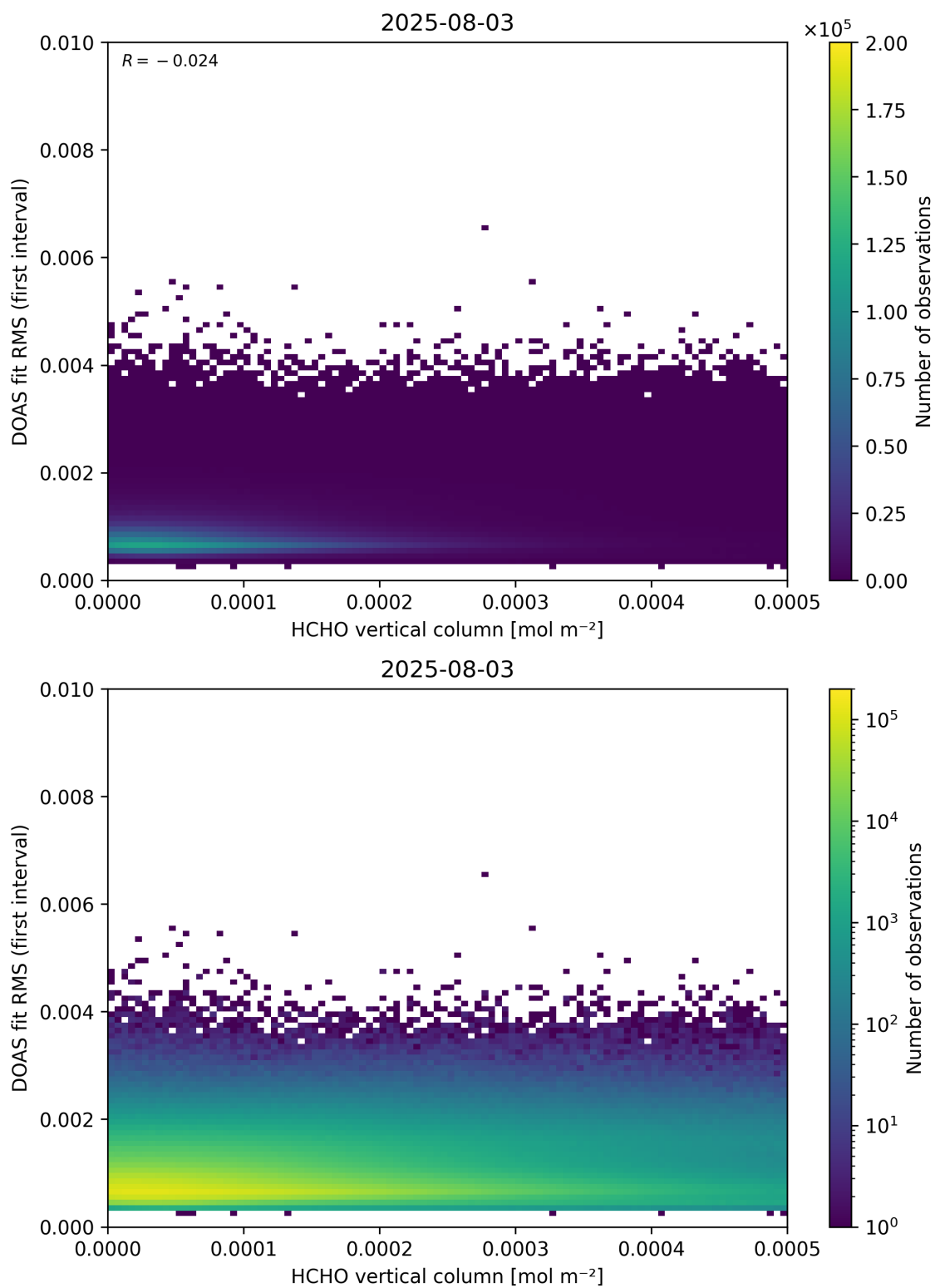
Figure 123: Scatter density plot of “HCHO vertical column” against “DOAS fit RMS (first interval)” for 2025-08-03 to 2025-08-04.
