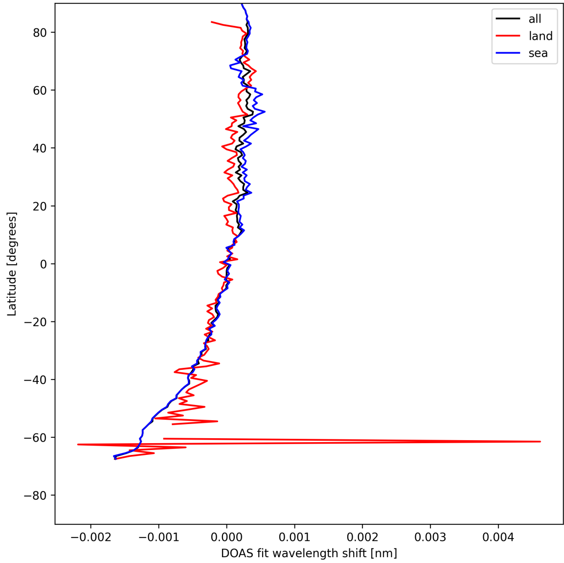
Figure 30: Zonal average of "DOAS fit wavelength shift" for 2025-08-03 to 2025-08-04.
