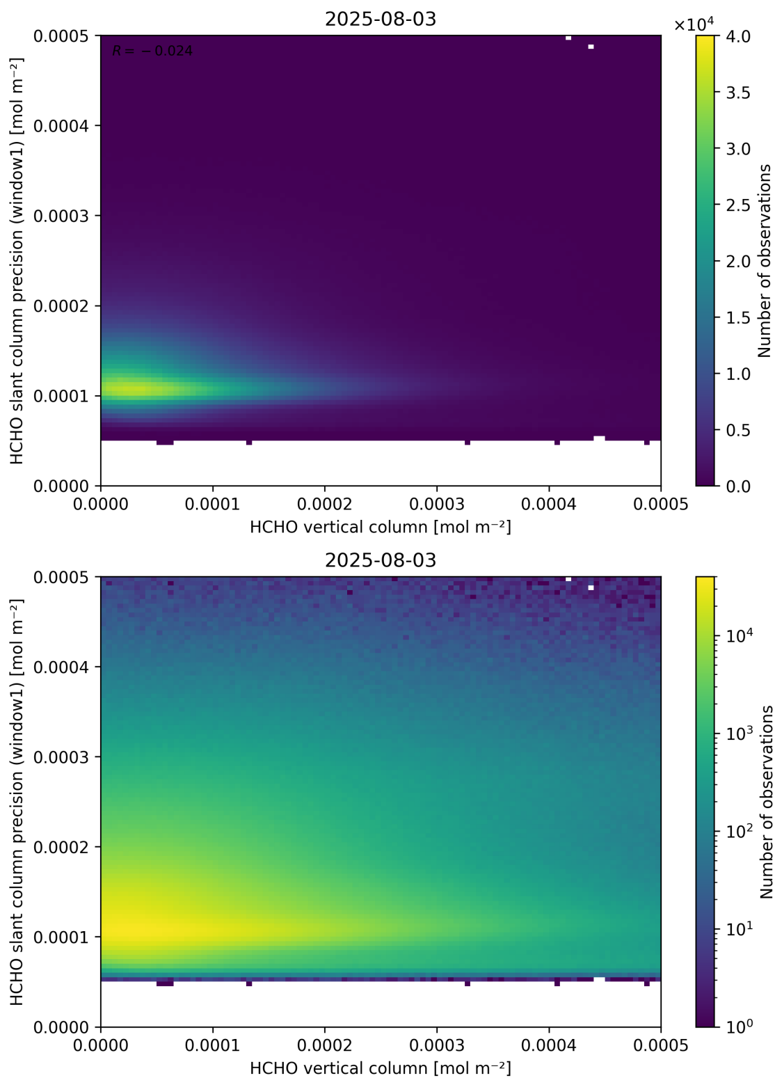
Figure 130: Scatter density plot of “HCHO vertical column” against “HCHO slant column precision (window1)” for 2025-08-03 to 2025-08-04.
