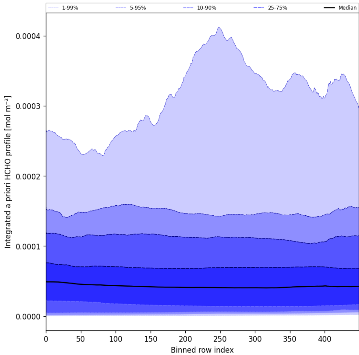
Figure 57: Along track statistics of “Integrated a priori HCHO profile” for 2025-08-03 to 2025-08-04
