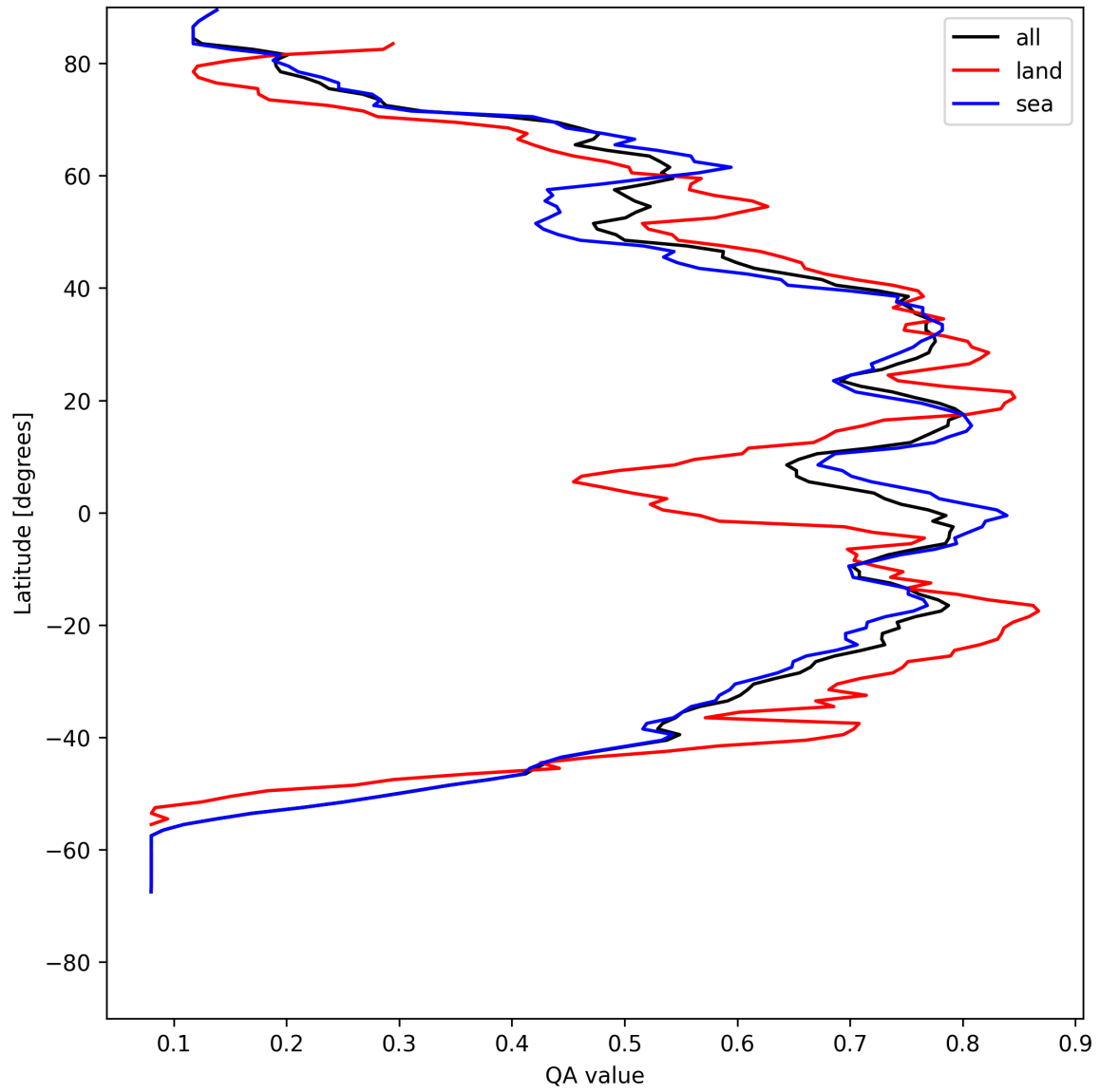
Figure 20: Zonal average of “QA value” for 2025-08-03 to 2025-08-04.
