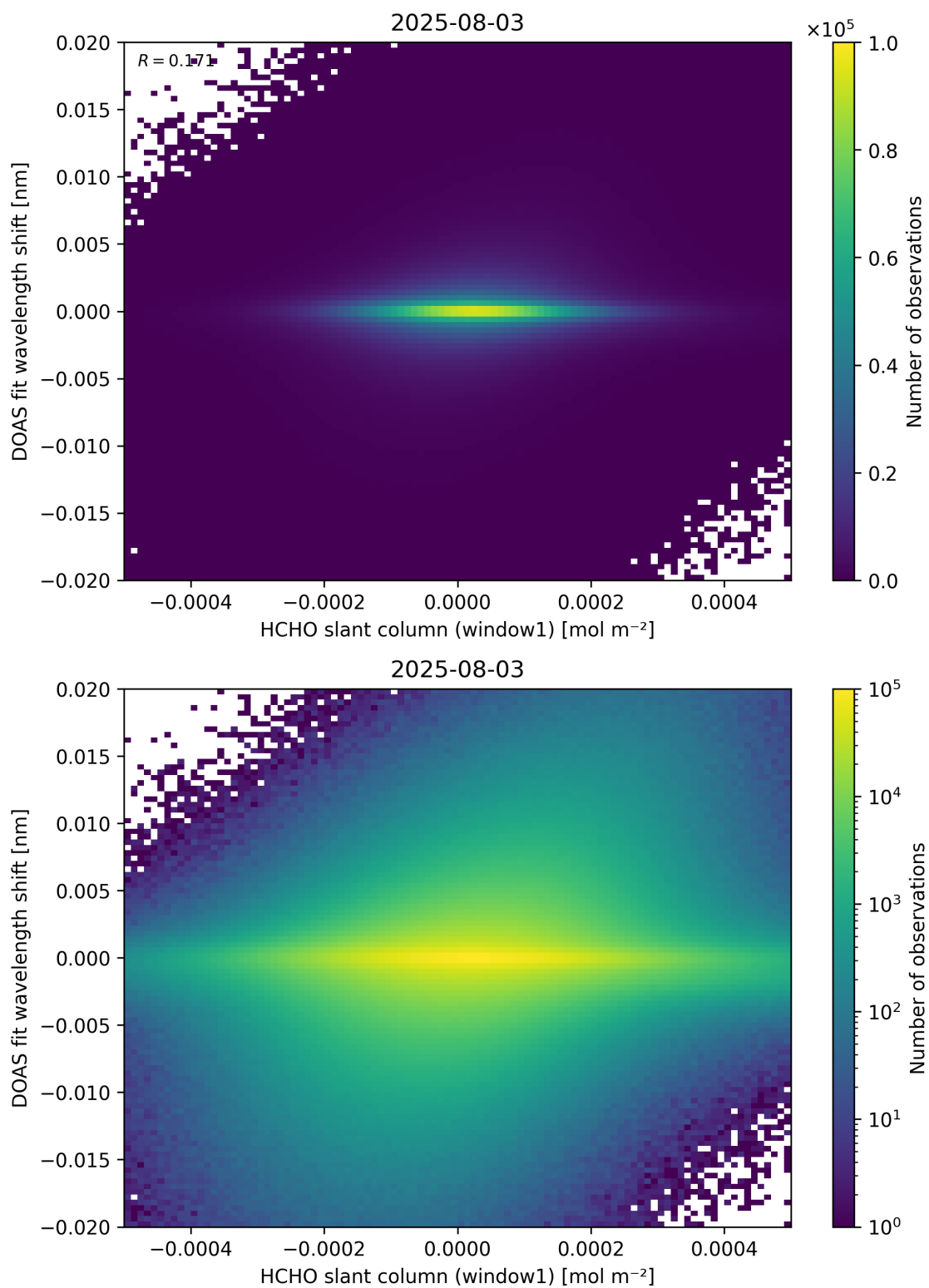
Figure 79: Scatter density plot of “HCHO slant column (window1)” against “DOAS fit wavelength shift” for 2025-08-03 to 2025-08-04.
