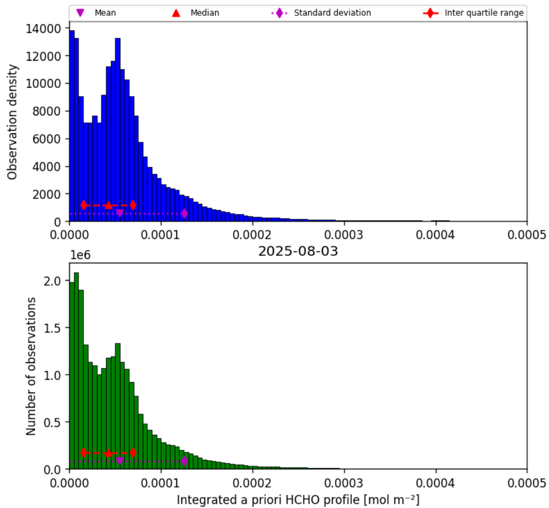
Figure 43: Histogram of “Integrated a priori HCHO profile” for 2025-08-03 to 2025-08-04
