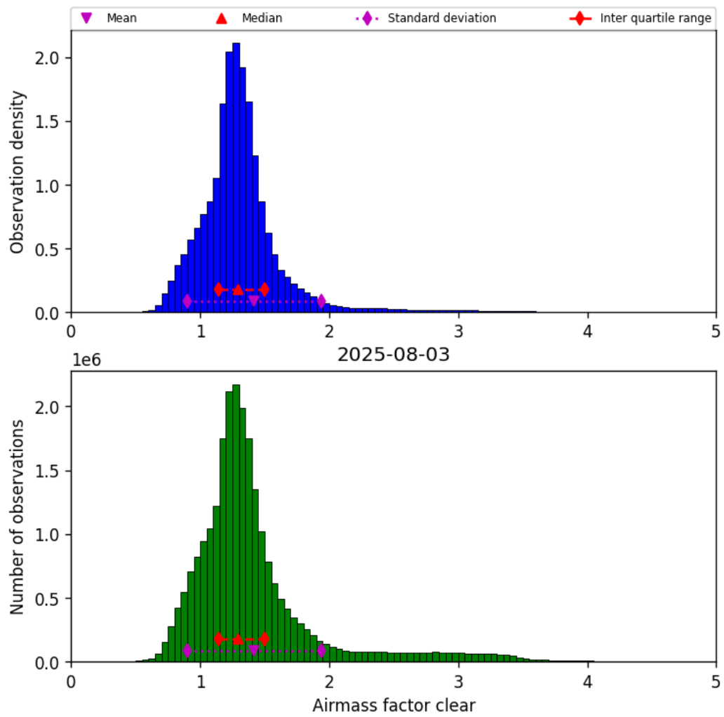
Figure 42: Histogram of “Airmass factor clear” for 2025-08-03 to 2025-08-04
