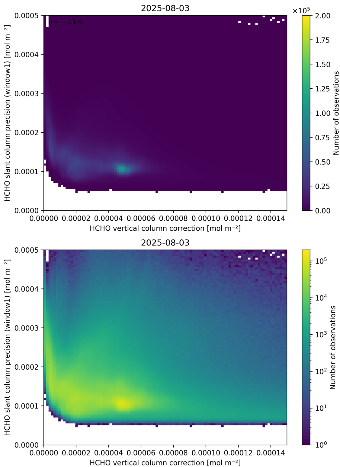
Figure 119: Scatter density plot of “HCHO vertical column correction” against “HCHO slant column precision (window1)” for 2025-08-03 to 2025-08-04.
