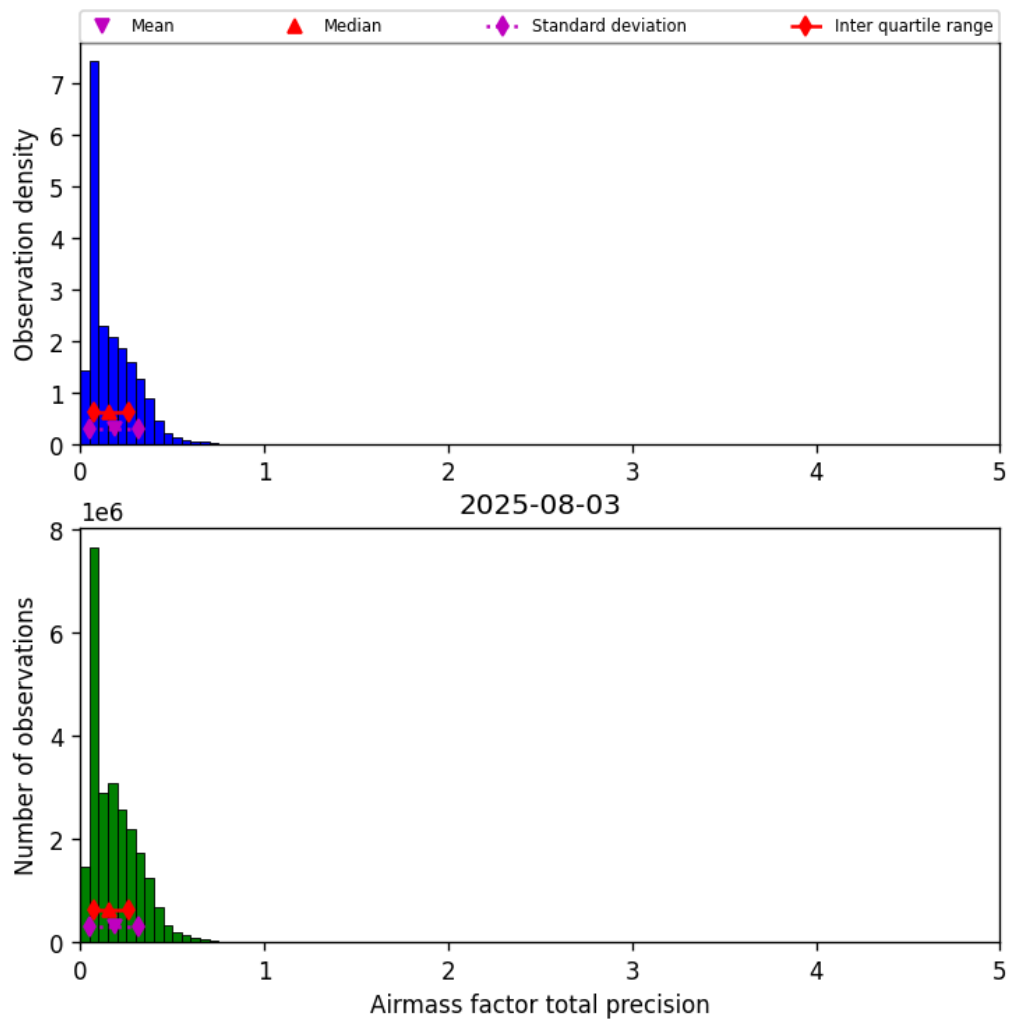
Figure 41: Histogram of “Airmass factor total precision” for 2025-08-03 to 2025-08-04
