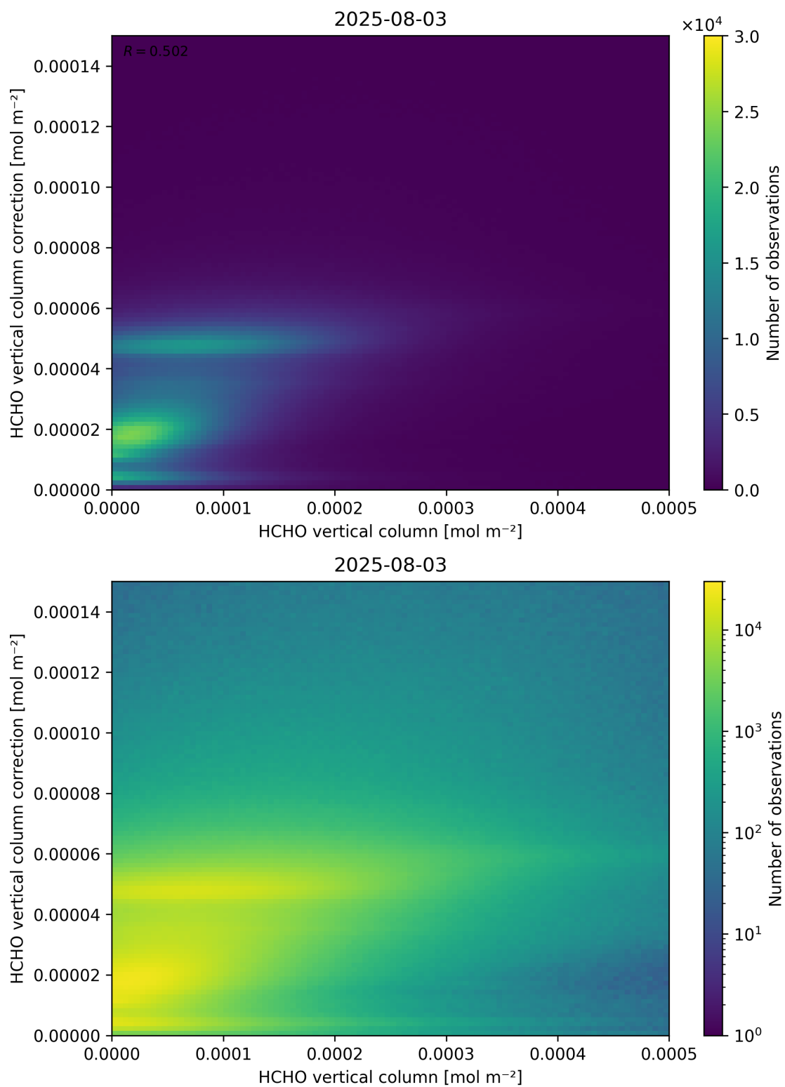
Figure 133: Scatter density plot of “HCHO vertical column” against “HCHO vertical column correction” for 2025-08-03 to 2025-08-04.
