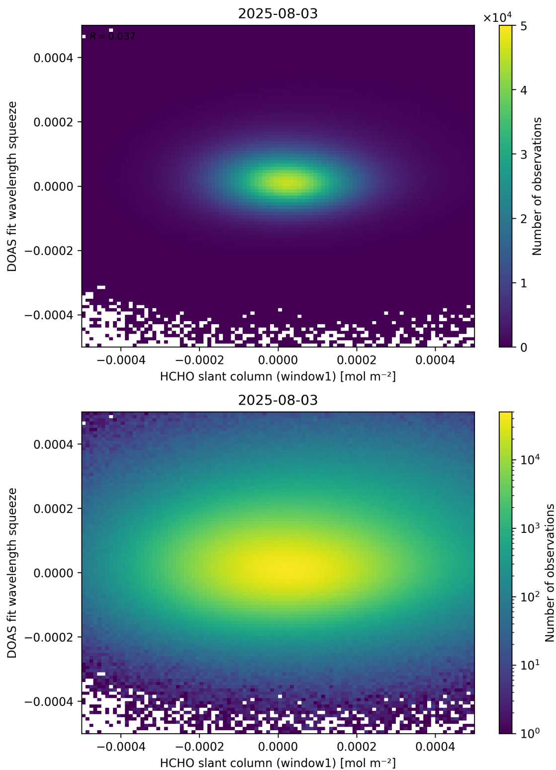
Figure 80: Scatter density plot of “HCHO slant column (window1)” against “DOAS fit wavelength squeeze” for 2025-08-03 to 2025-08-04.
