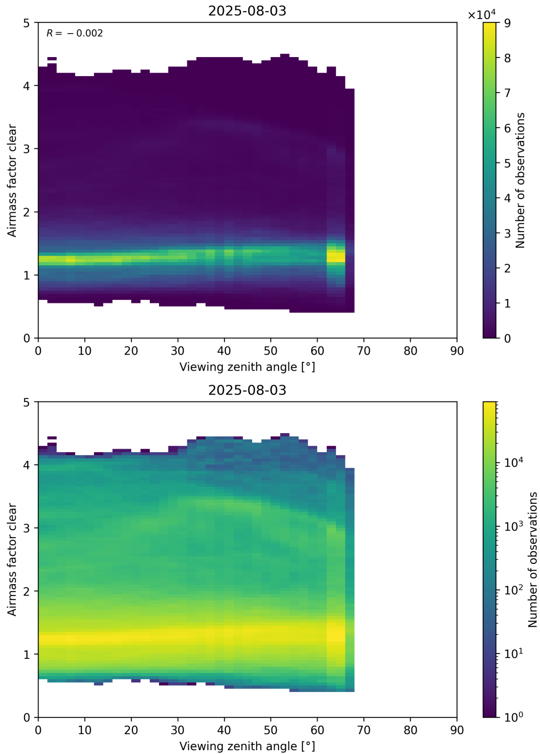
Figure 185: Scatter density plot of “Viewing zenith angle” against “Airmass factor clear” for 2025-08-03 to 2025-08-04.
