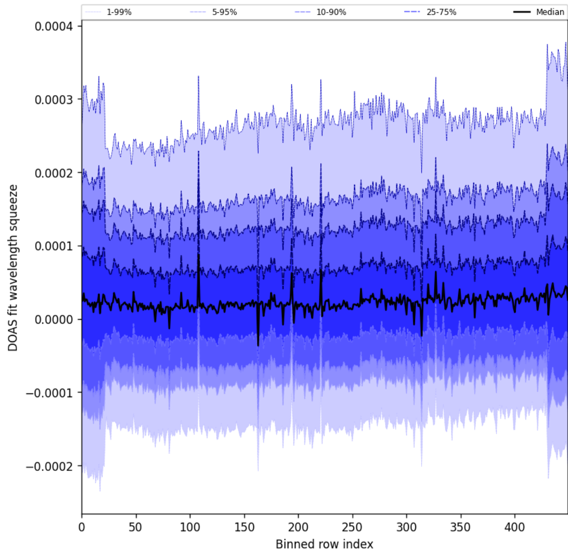
Figure 59: Along track statistics of “DOAS fit wavelength squeeze” for 2025-08-03 to 2025-08-04
