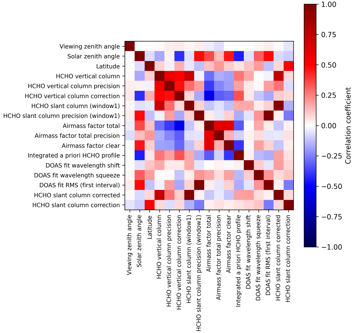
Figure 2: Map of correlation matrix for 2025-08-03 to 2025-08-04.
