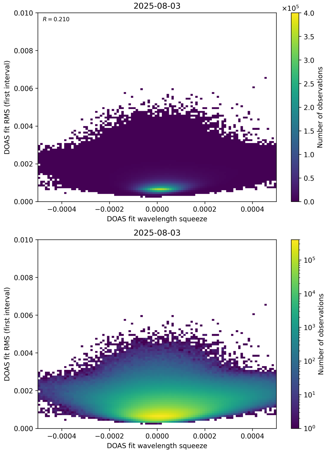
Figure 68: Scatter density plot of “DOAS fit wavelength squeeze” against “DOAS fit RMS (first interval)” for 2025-08-03 to 2025-08-04.
