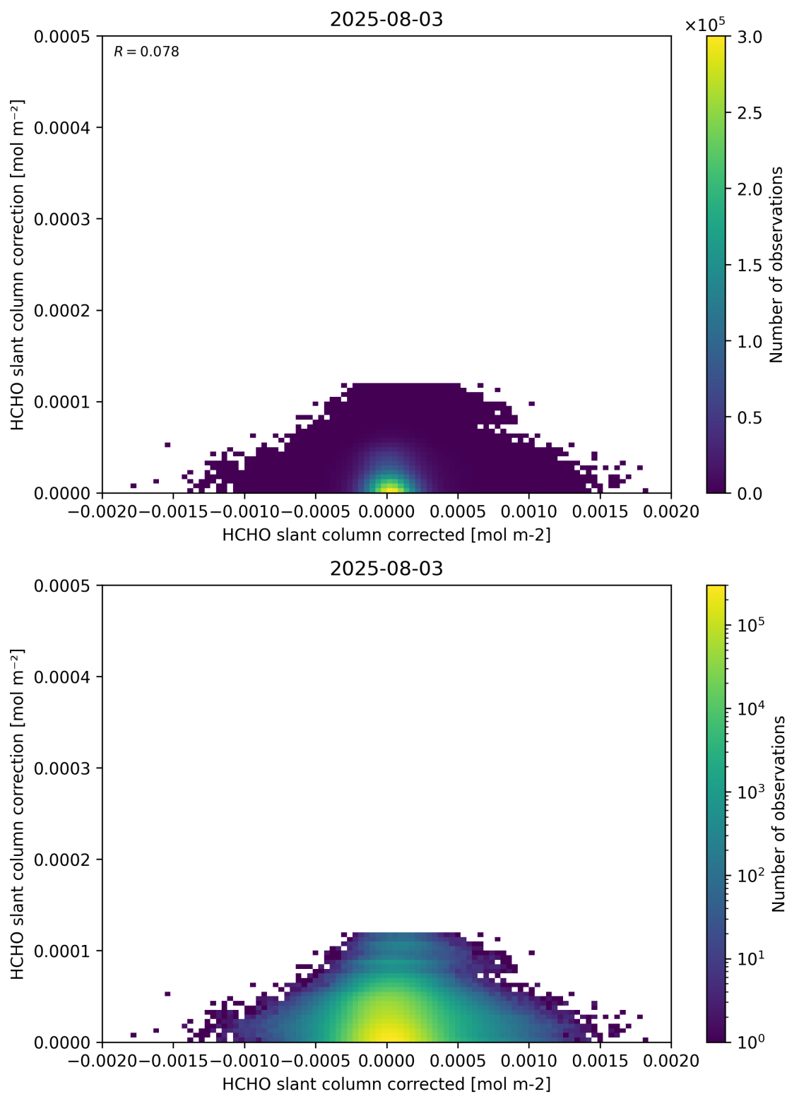
Figure 77: Scatter density plot of “HCHO slant column corrected” against “HCHO slant column correction” for 2025-08-03 to 2025-08-04.
