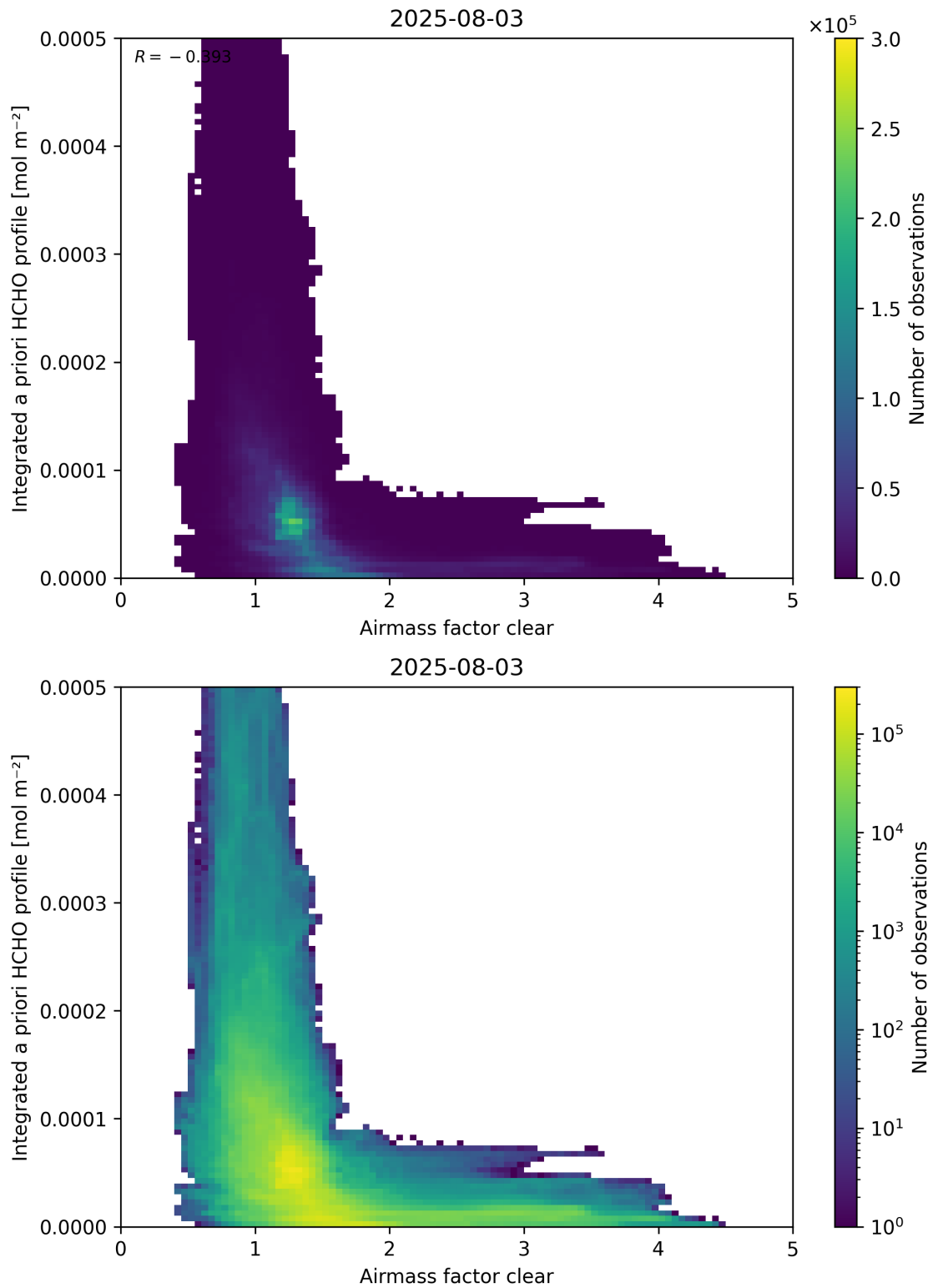
Figure 76: Scatter density plot of “Airmass factor clear” against “Integrated a priori HCHO profile” for 2025-08-03 to 2025-08-04.
