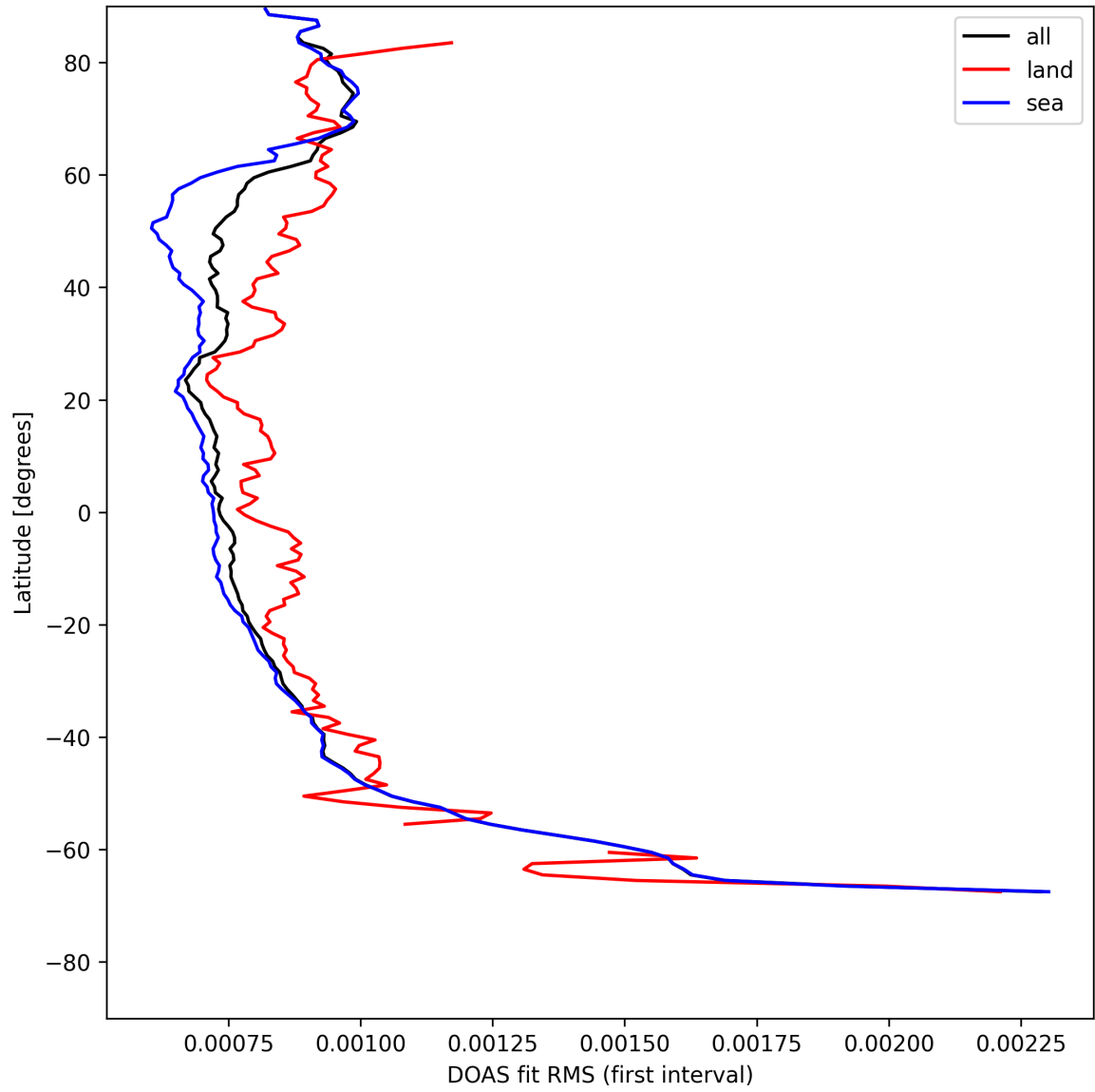
Figure 32: Zonal average of “DOAS fit RMS (first interval)” for 2025-08-03 to 2025-08-04.
