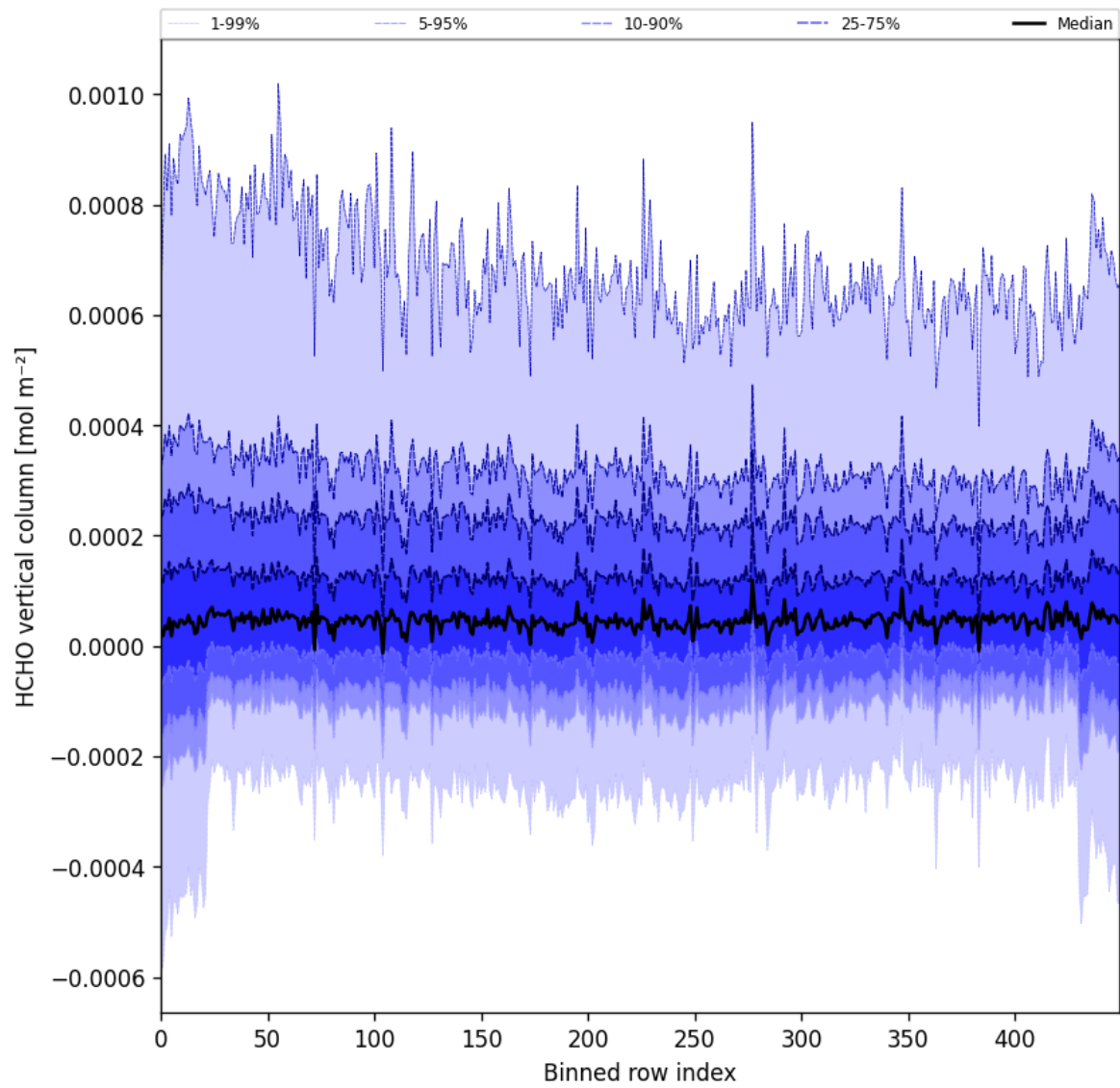
Figure 49: Along track statistics of “HCHO vertical column” for 2025-08-03 to 2025-08-04
