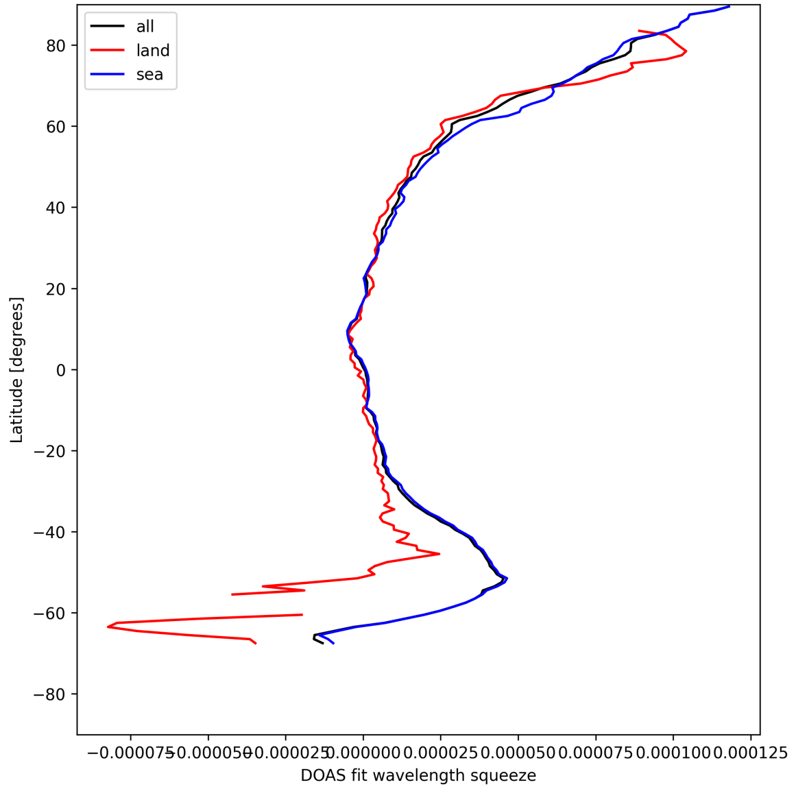
Figure 31: Zonal average of “DOAS fit wavelength squeeze” for 2025-08-03 to 2025-08-04.
