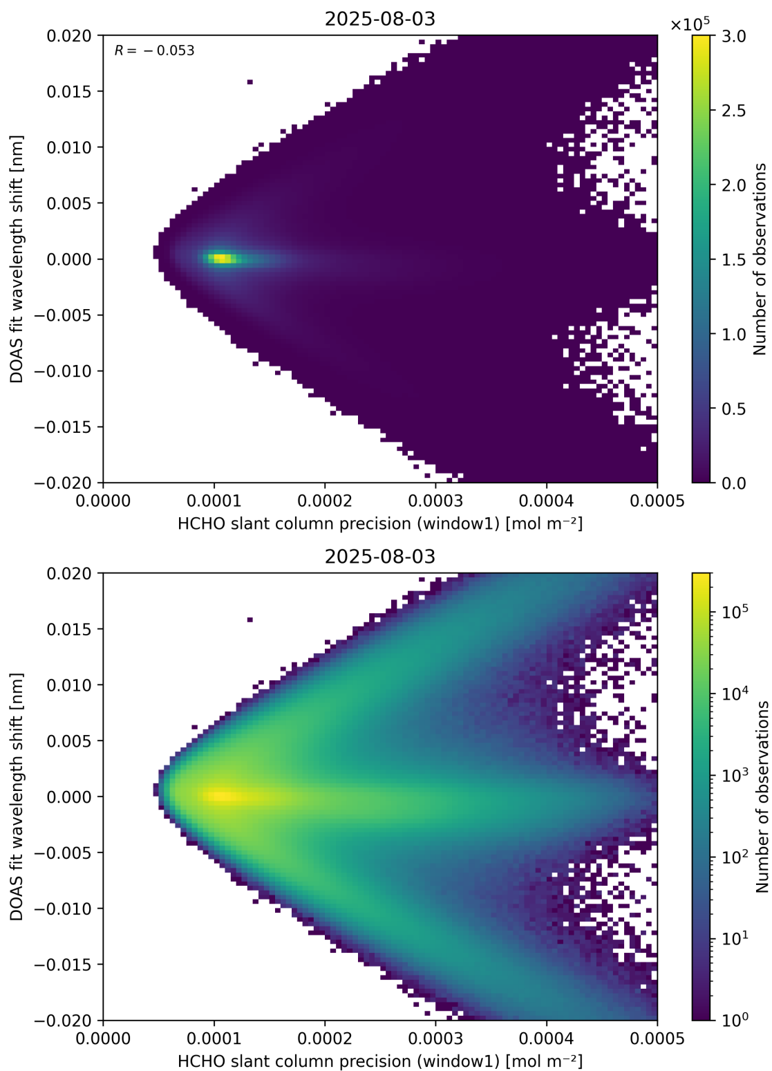
Figure 89: Scatter density plot of “HCHO slant column precision (window1)” against “DOAS fit wavelength shift” for 2025-08-03 to 2025-08-04.
