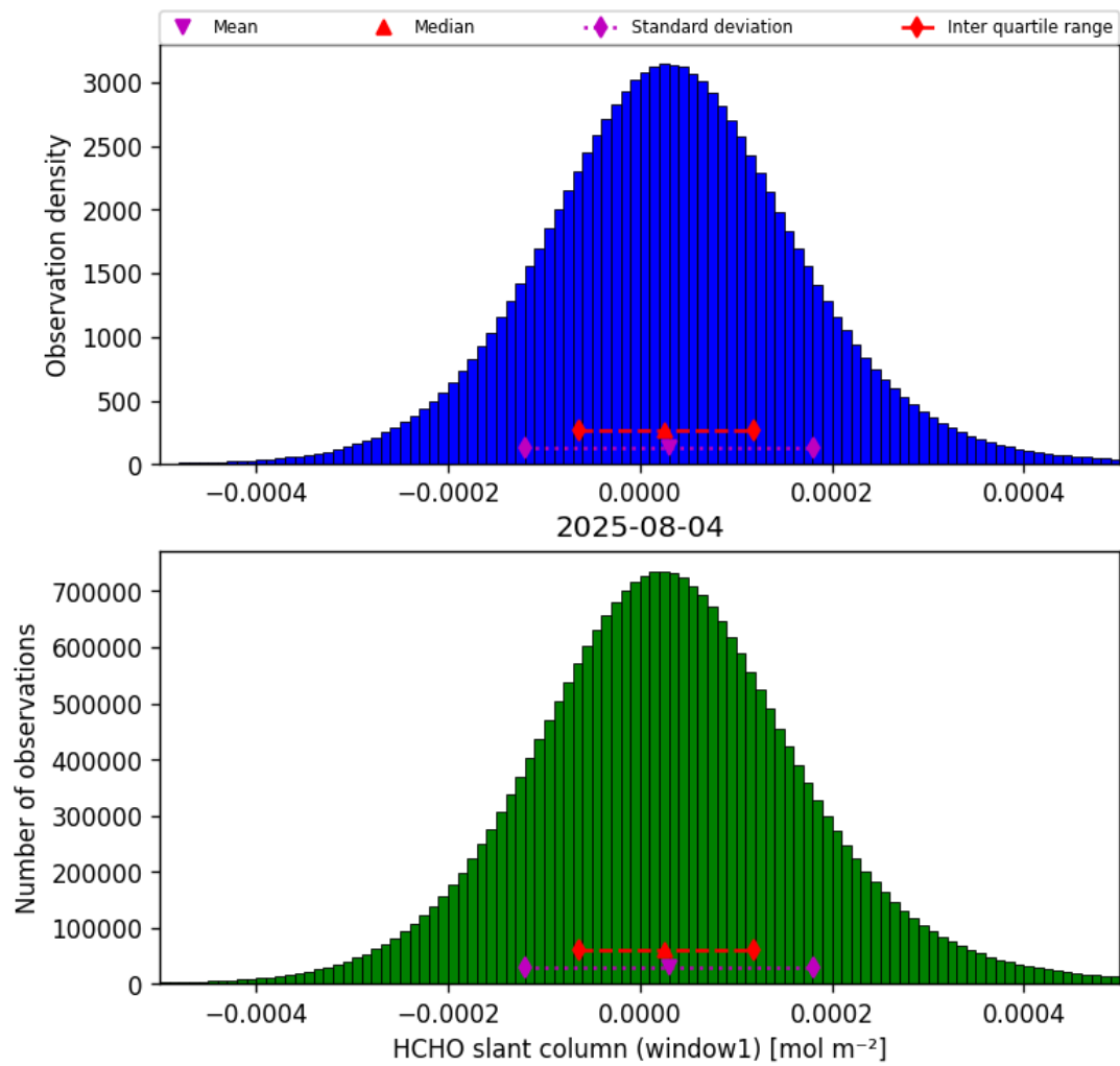
Figure 38: Histogram of “HCHO slant column (window1)” for 2025-08-04 to 2025-08-05
