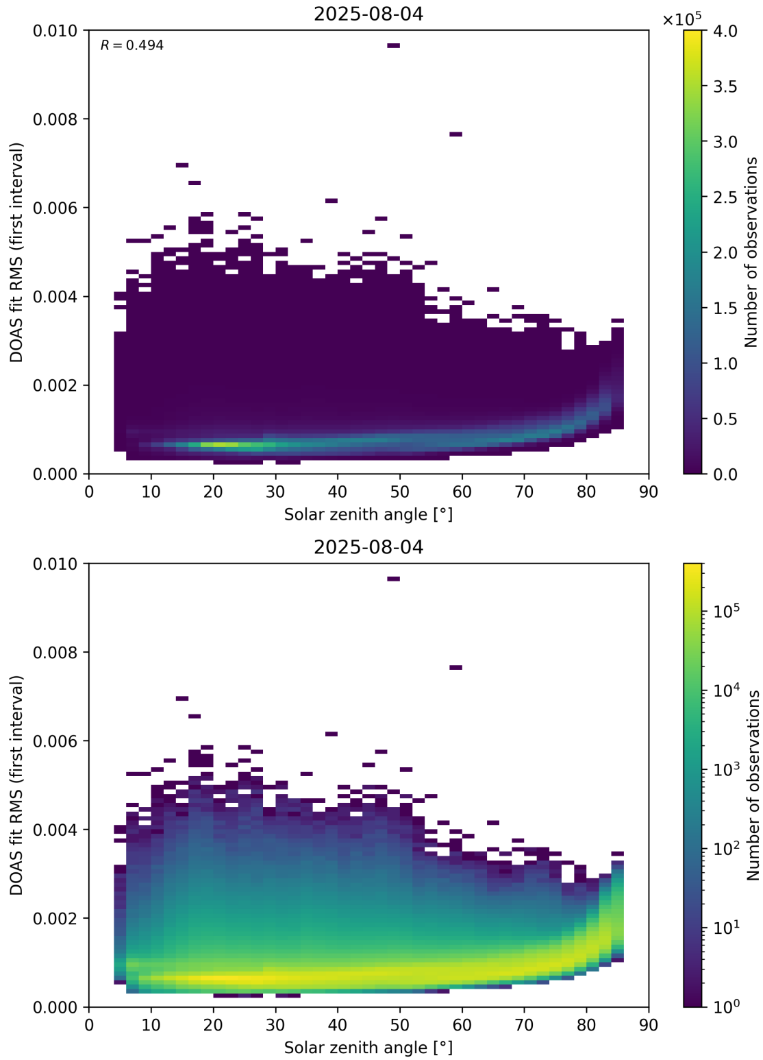
Figure 167: Scatter density plot of “Solar zenith angle” against “DOAS fit RMS (first interval)” for 2025-08-04 to 2025-08-05.
