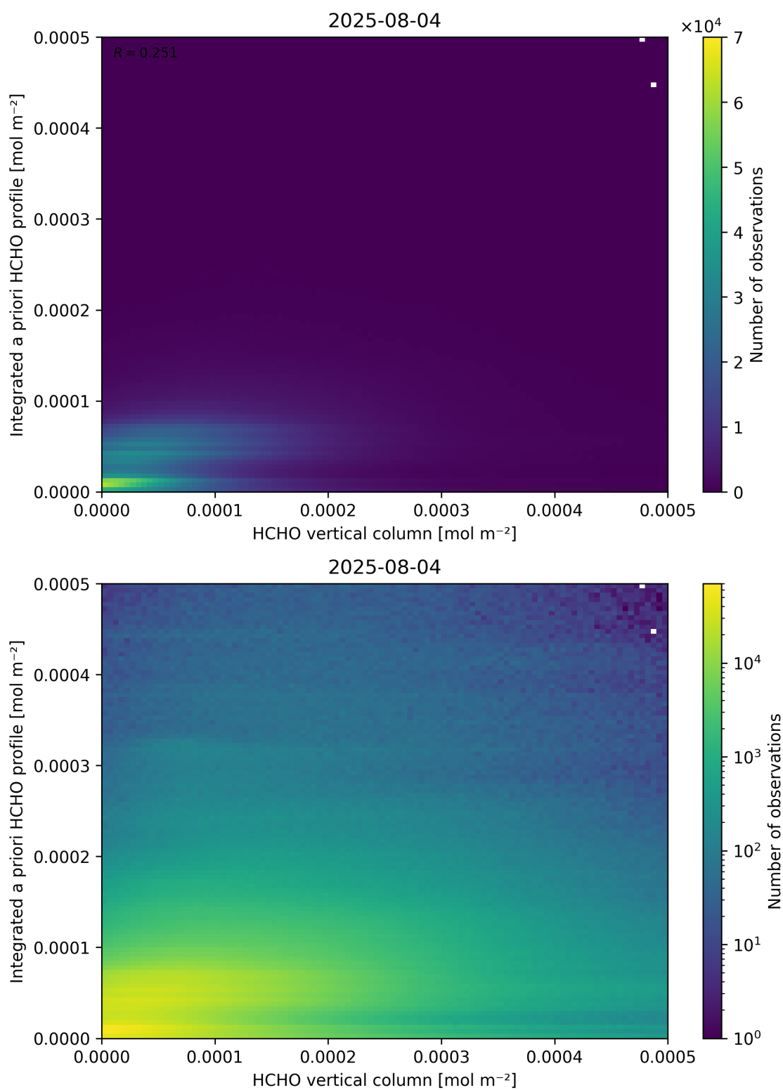
Figure 135: Scatter density plot of “HCHO vertical column” against “Integrated a priori HCHO profile” for 2025-08-04 to 2025-08-05.
