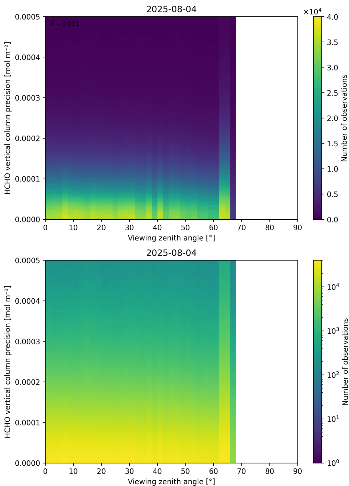
Figure 194: Scatter density plot of “Viewing zenith angle” against “HCHO vertical column precision” for 2025-08-04 to 2025-08-05.
