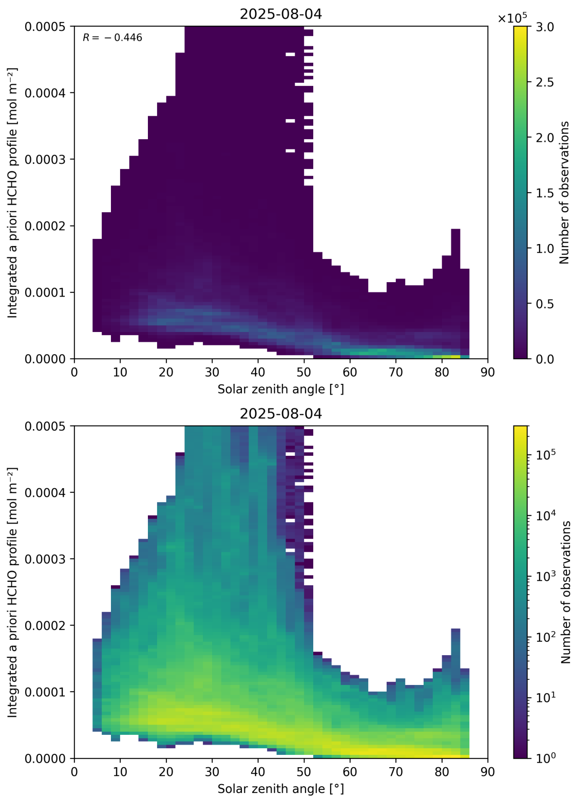
Figure 180: Scatter density plot of “Solar zenith angle” against “Integrated a priori HCHO profile” for 2025-08-04 to 2025-08-05.
