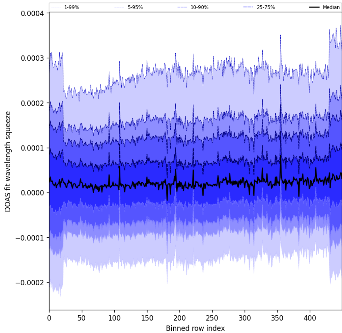
Figure 59: Along track statistics of “DOAS fit wavelength squeeze” for 2025-08-04 to 2025-08-05
