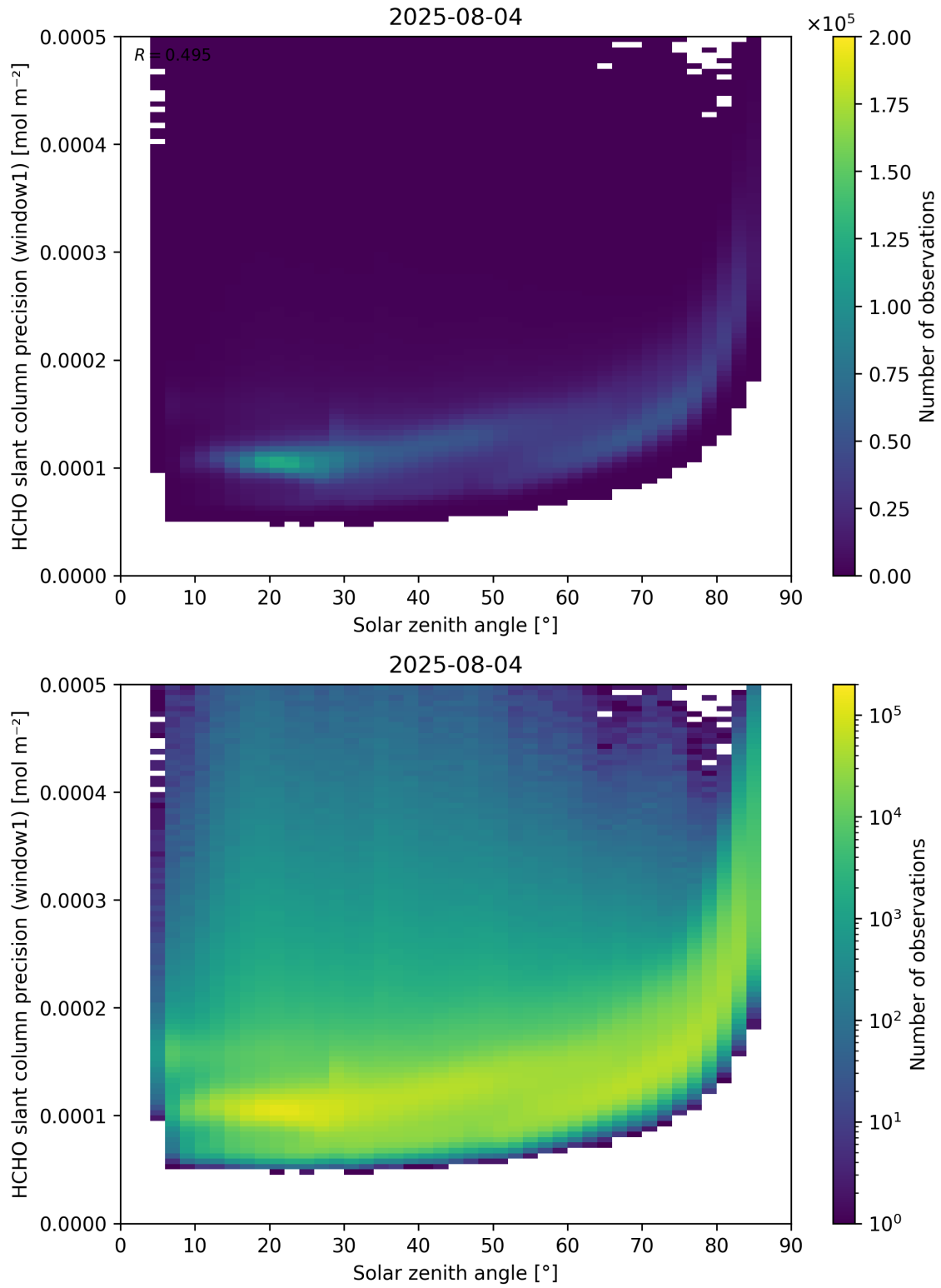
Figure 174: Scatter density plot of “Solar zenith angle” against “HCHO slant column precision (window1)” for 2025-08-04 to 2025-08-05.
