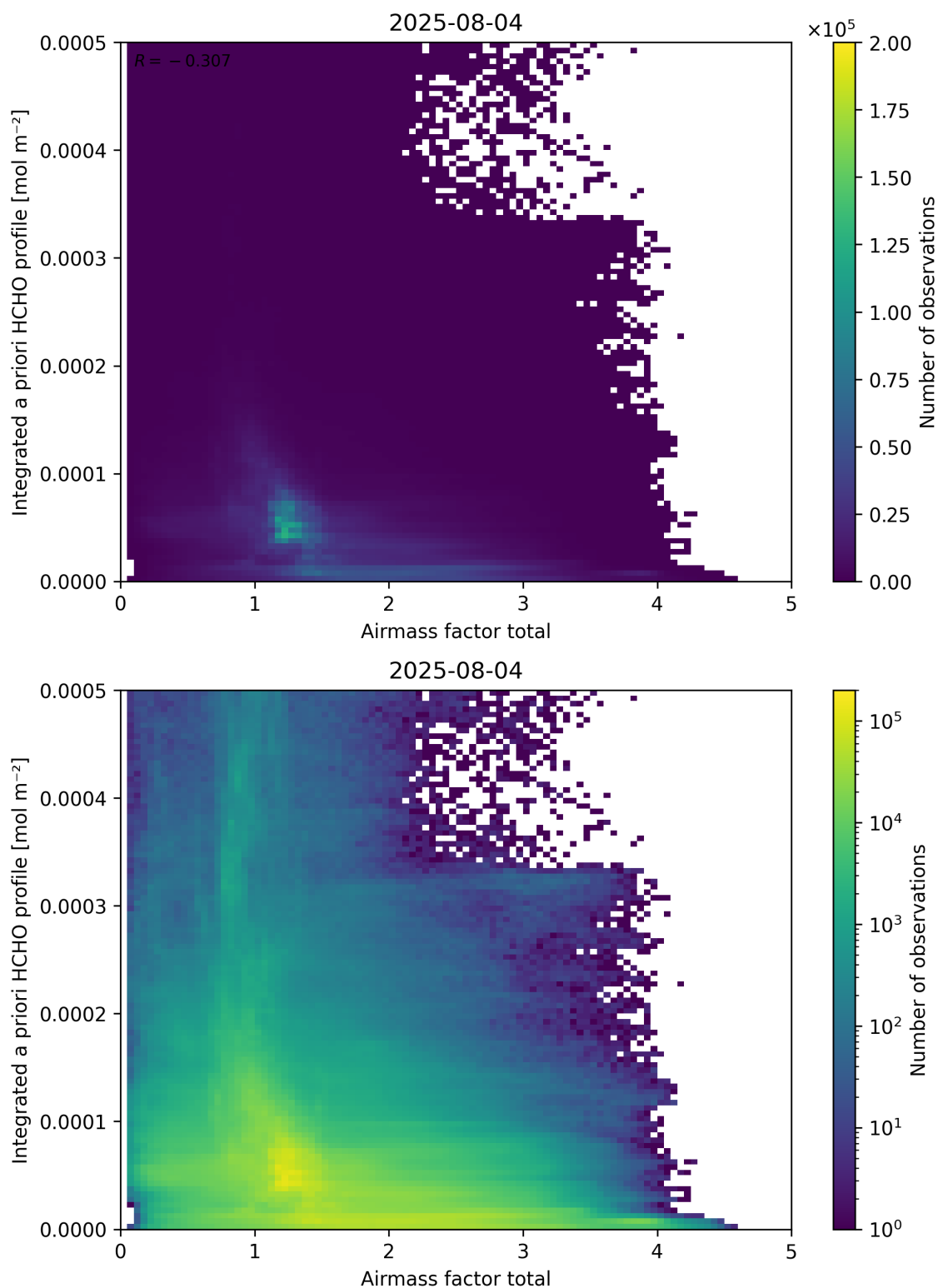
Figure 104: Scatter density plot of “Airmass factor total” against “Integrated a priori HCHO profile” for 2025-08-04 to 2025-08-05.
