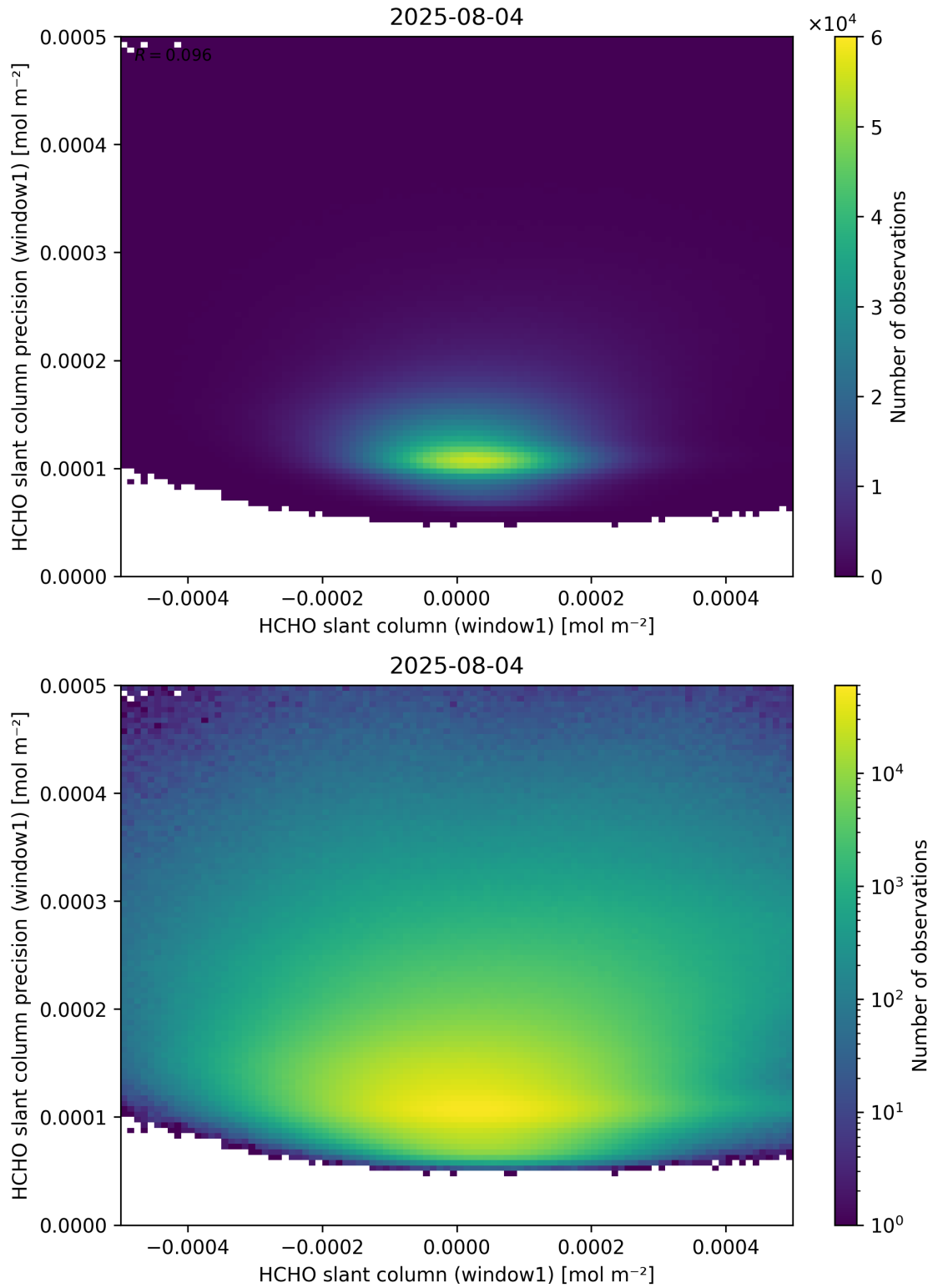
Figure 84: Scatter density plot of “HCHO slant column (window1)” against “HCHO slant column precision (window1)” for 2025-08-04 to 2025-08-05.
