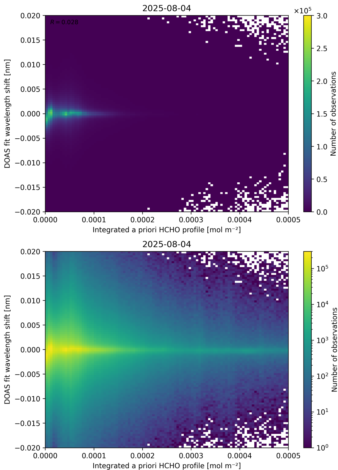
Figure 149: Scatter density plot of “Integrated a priori HCHO profile” against “DOAS fit wavelength shift” for 2025-08-04 to 2025-08-05.
