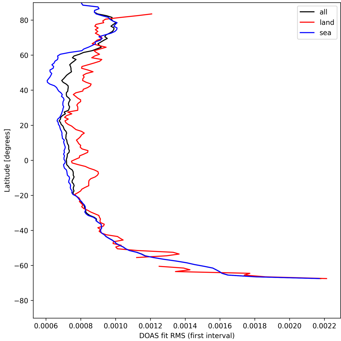
Figure 32: Zonal average of “DOAS fit RMS (first interval)” for 2025-08-04 to 2025-08-05.
