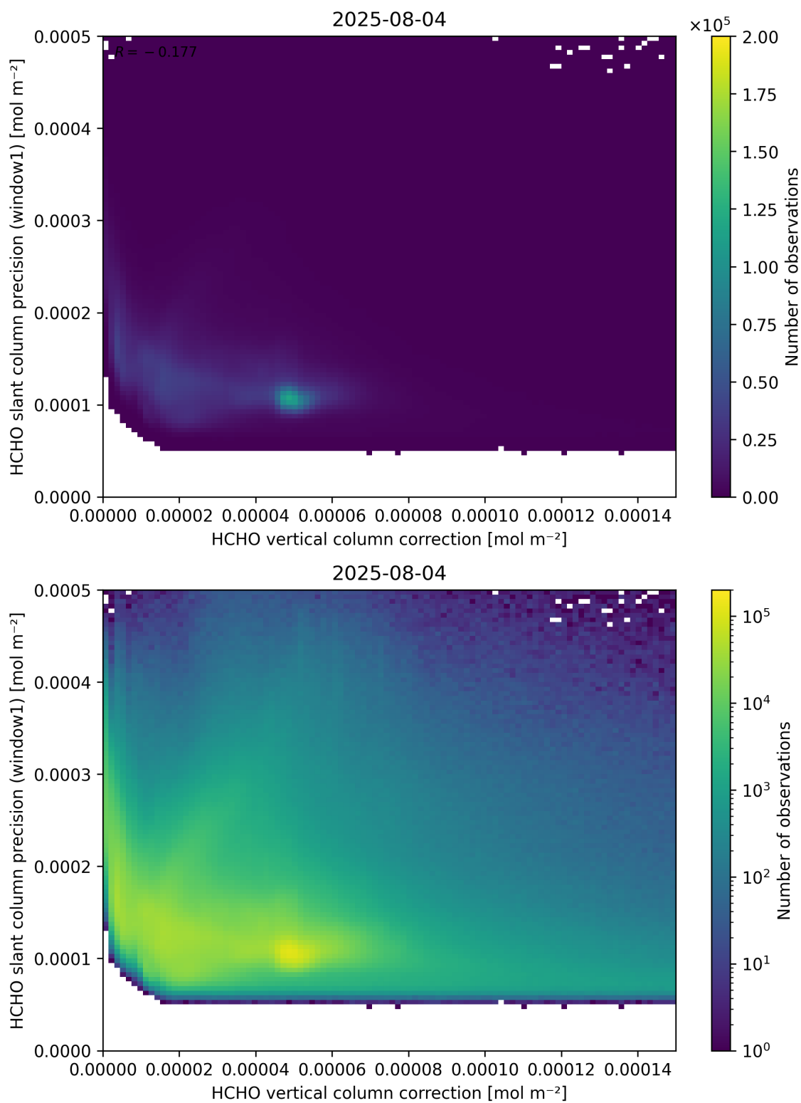
Figure 119: Scatter density plot of “HCHO vertical column correction” against “HCHO slant column precision (window1)” for 2025-08-04 to 2025-08-05.
