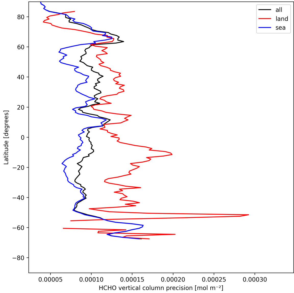
Figure 22: Zonal average of “HCHO vertical column precision” for 2025-08-04 to 2025-08-05.
