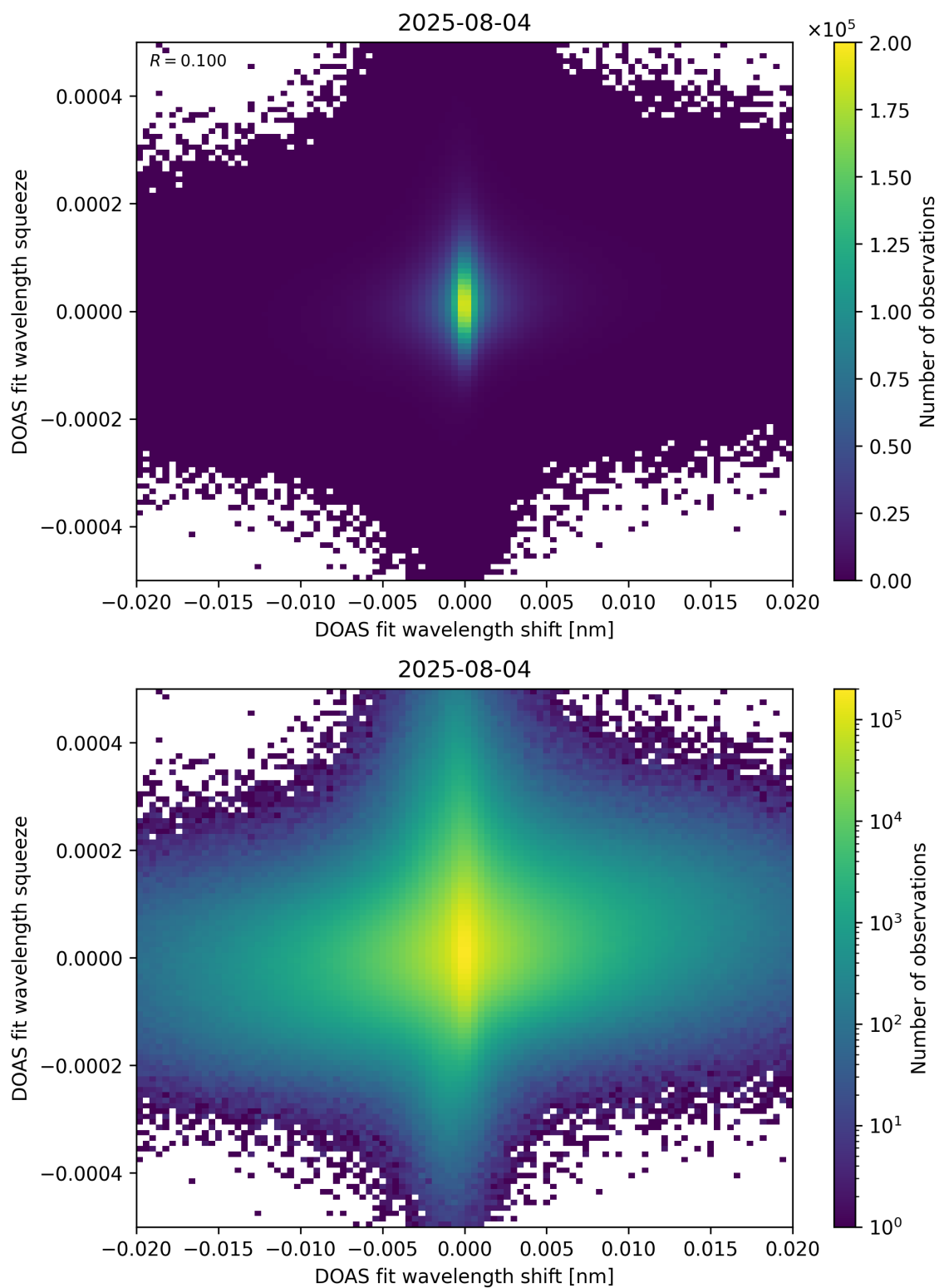
Figure 65: Scatter density plot of “DOAS fit wavelength shift” against “DOAS fit wavelength squeeze” for 2025-08-04 to 2025-08-05.
