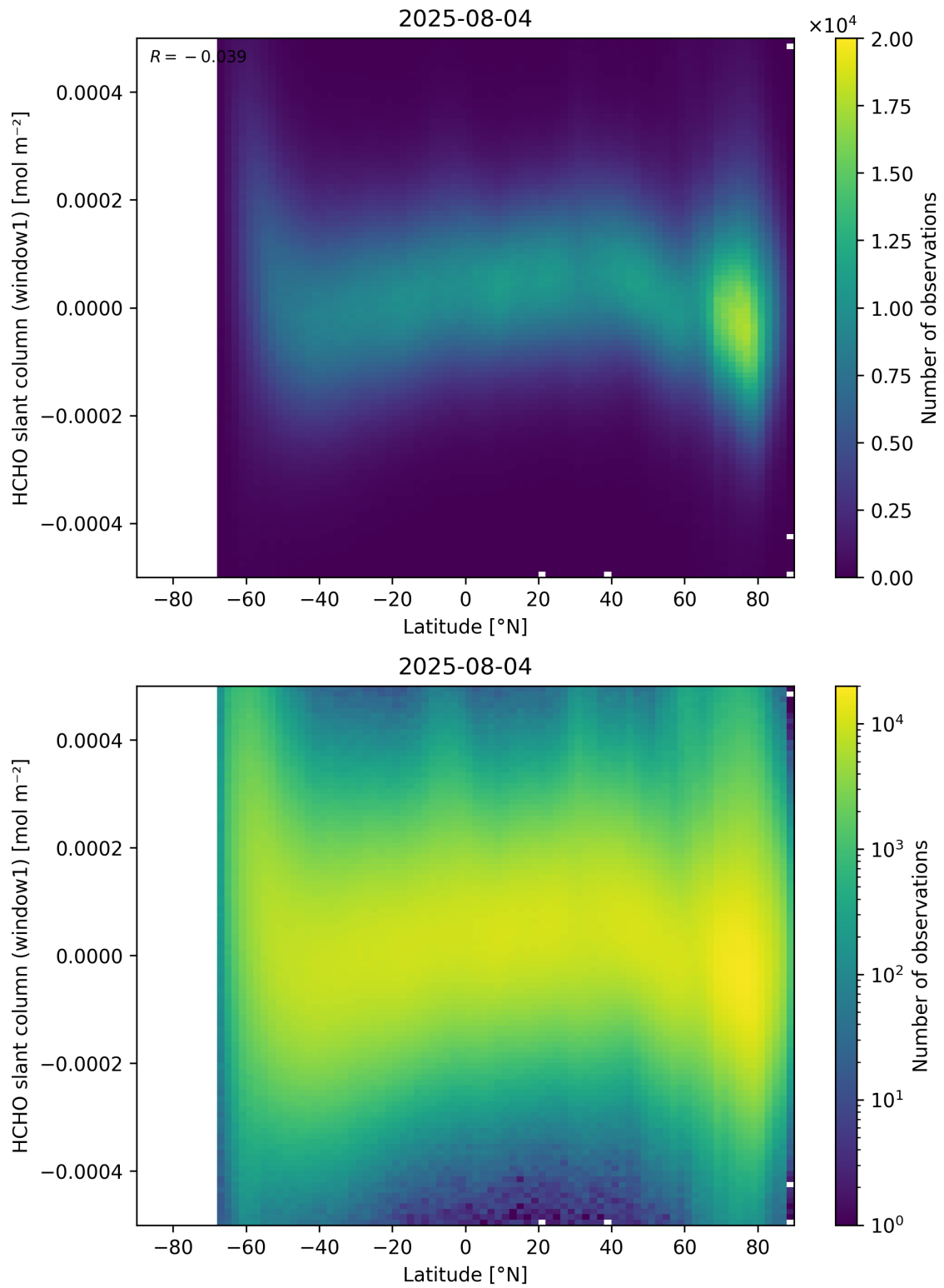
Figure 159: Scatter density plot of “Latitude” against “HCHO slant column (window1)” for 2025-08-04 to 2025-08-05.
