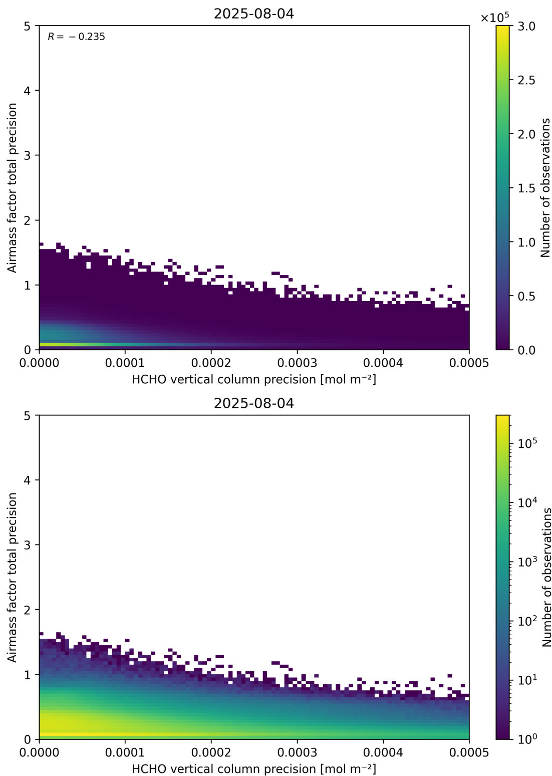
Figure 145: Scatter density plot of “HCHO vertical column precision” against “Airmass factor total precision” for 2025-08-04 to 2025-08-05.
