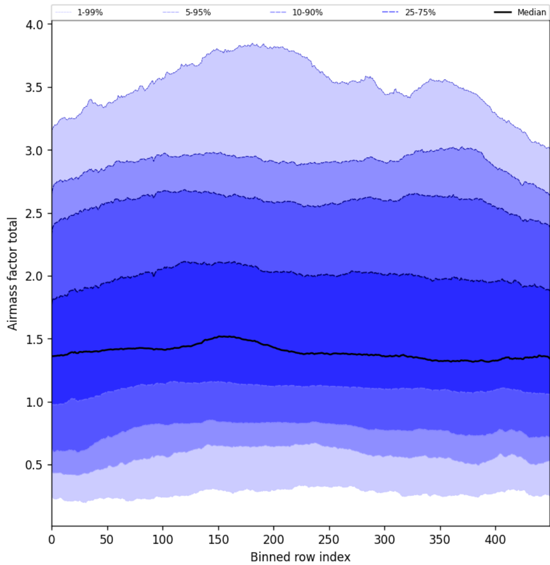
Figure 54: Along track statistics of “Airmass factor total” for 2025-08-04 to 2025-08-05
