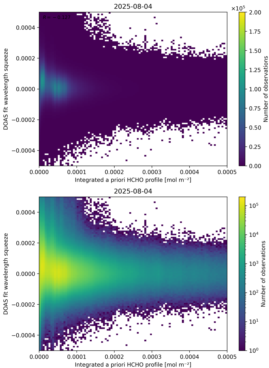
Figure 150: Scatter density plot of “Integrated a priori HCHO profile” against “DOAS fit wavelength squeeze” for 2025-08-04 to 2025-08-05.
