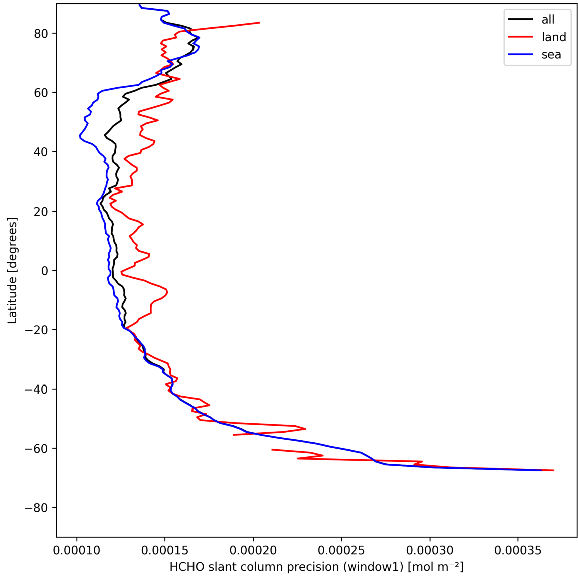
Figure 25: Zonal average of "HCHO slant column precision (window1)" for 2025-08-04 to 2025-08-05.
