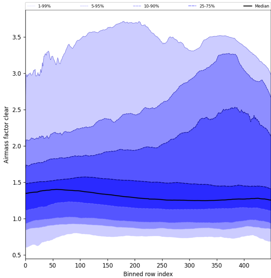
Figure 56: Along track statistics of “Airmass factor clear” for 2025-08-04 to 2025-08-05
