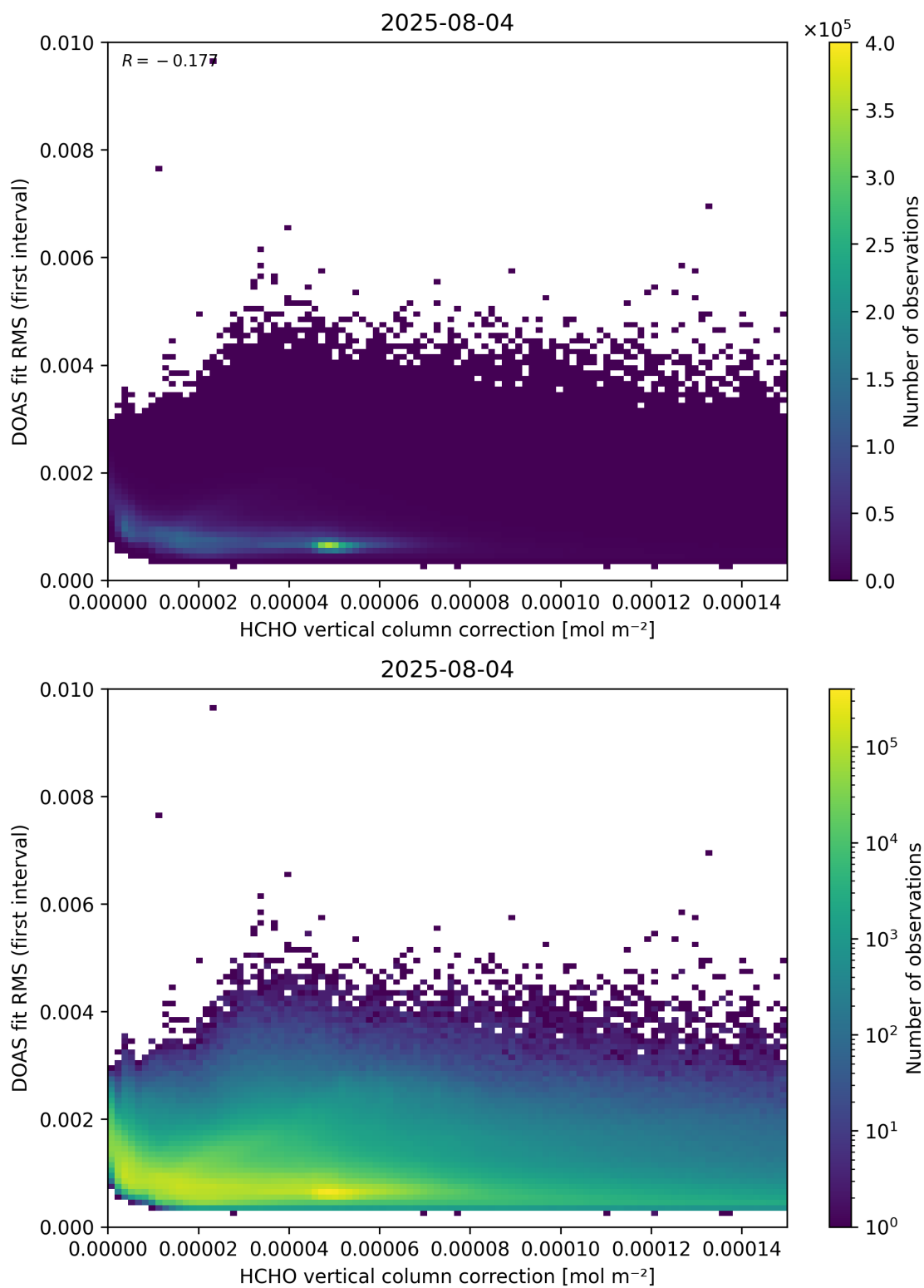
Figure 112: Scatter density plot of “HCHO vertical column correction” against “DOAS fit RMS (first interval)” for 2025-08-04 to 2025-08-05.
