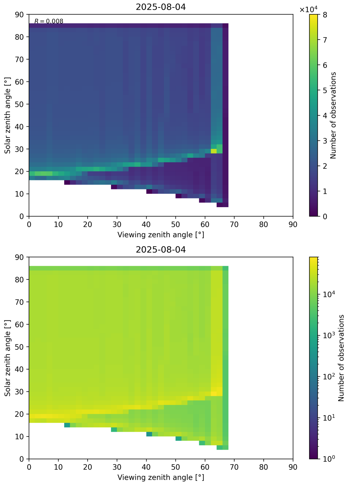
Figure 197: Scatter density plot of “Viewing zenith angle” against “Solar zenith angle” for 2025-08-04 to 2025-08-05.
