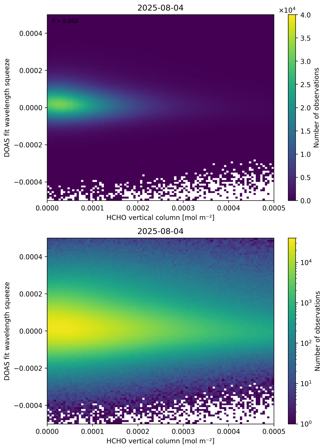
Figure 125: Scatter density plot of “HCHO vertical column” against “DOAS fit wavelength squeeze” for 2025-08-04 to 2025-08-05.
