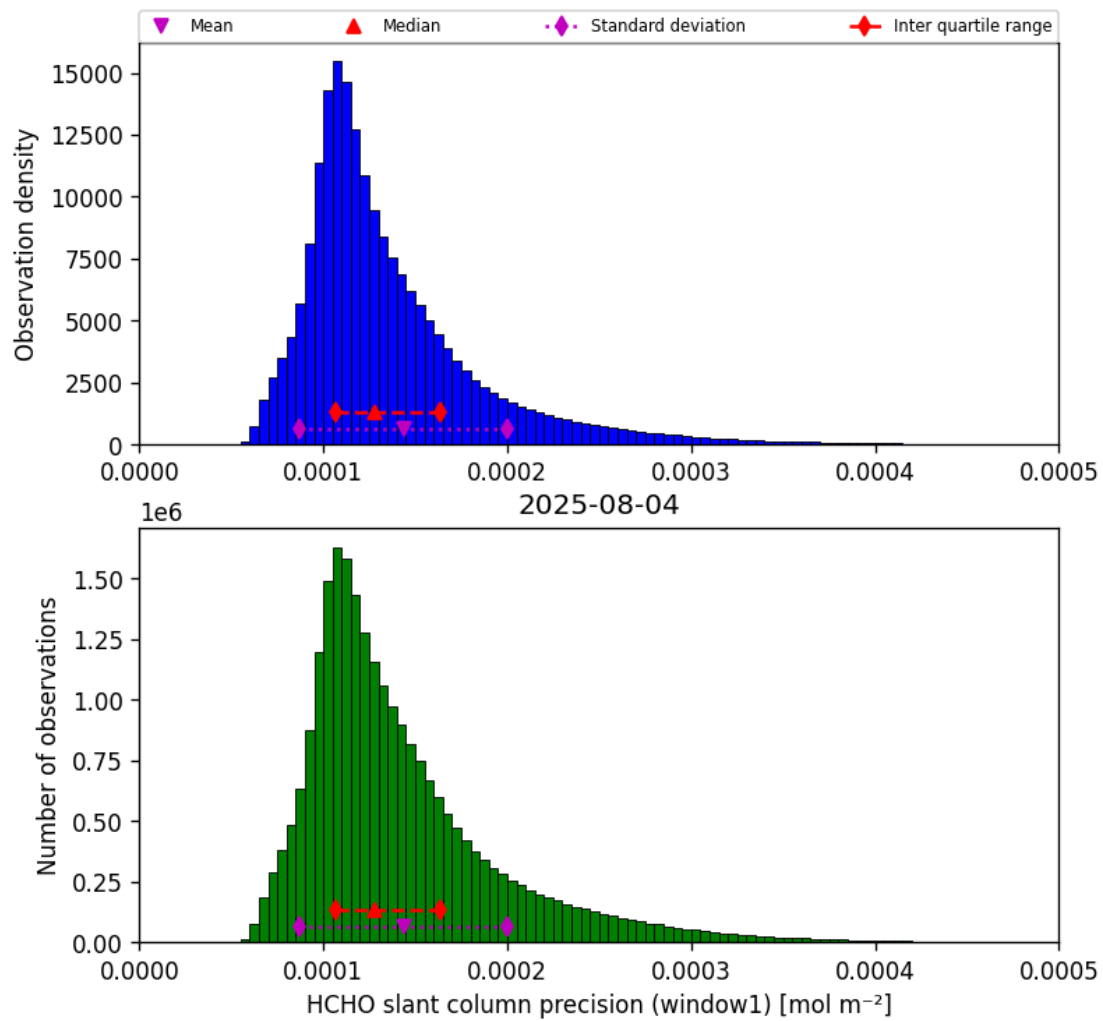
Figure 39: Histogram of “HCHO slant column precision (window1)” for 2025-08-04 to 2025-08-05
