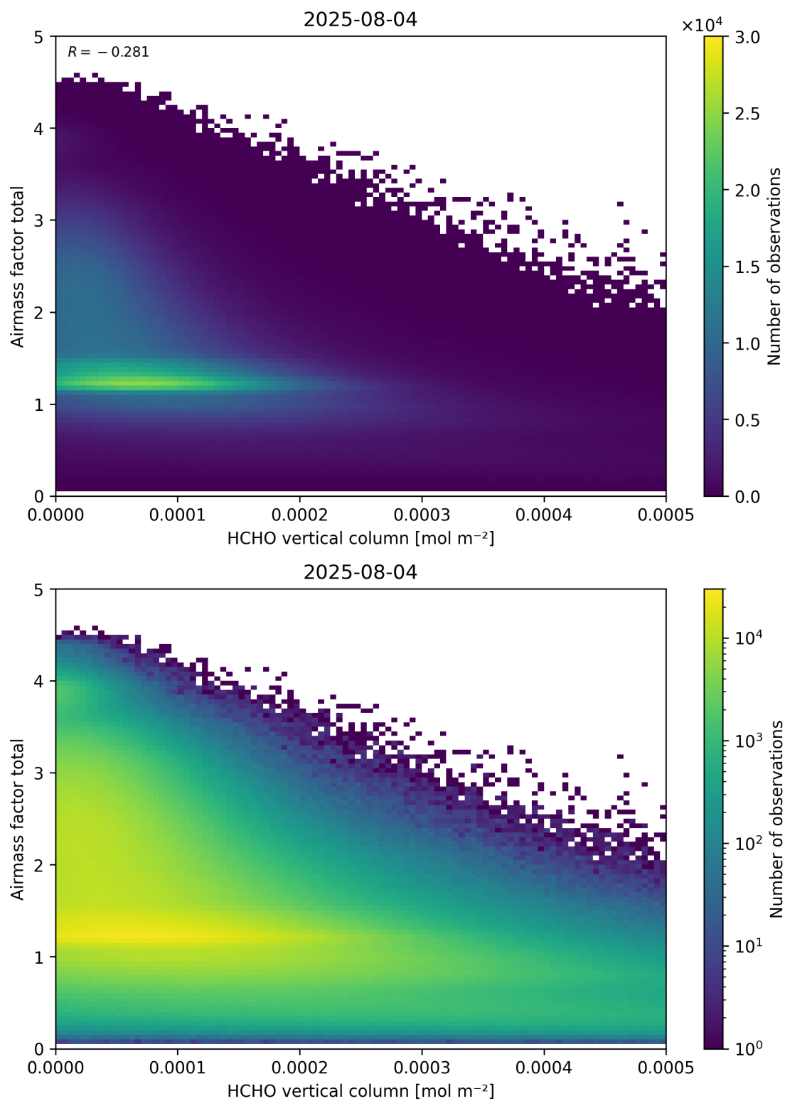
Figure 131: Scatter density plot of “HCHO vertical column” against “Airmass factor total” for 2025-08-04 to 2025-08-05.
