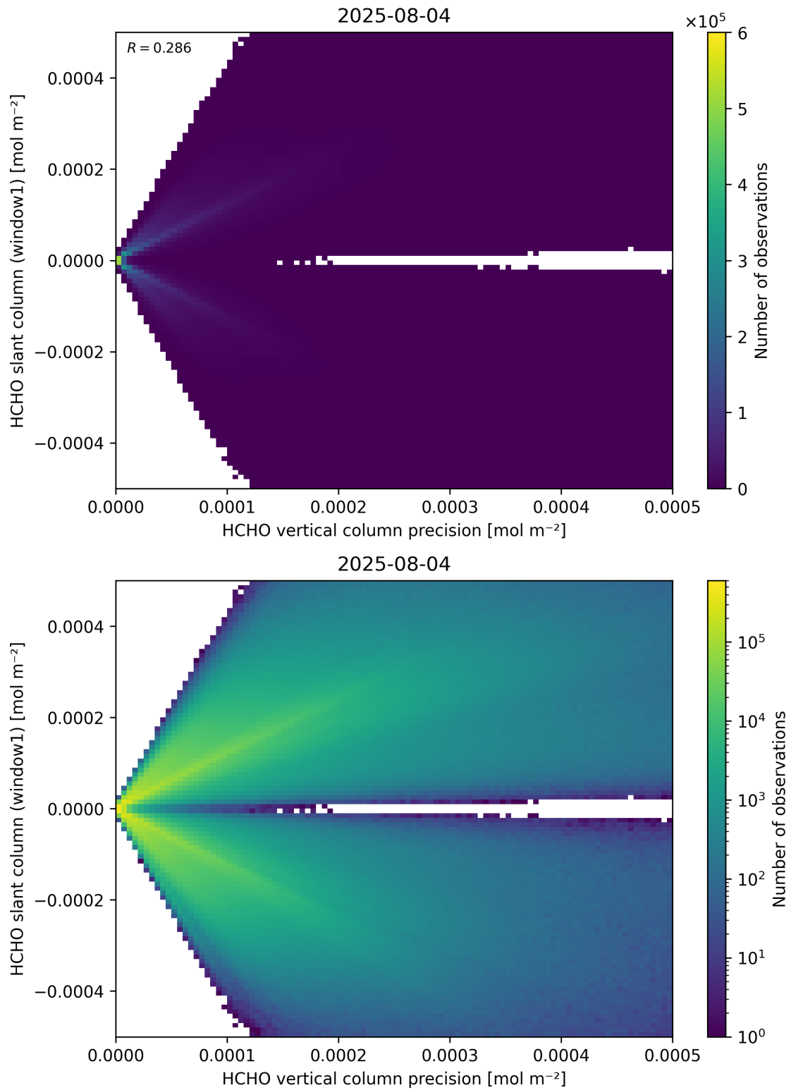
Figure 142: Scatter density plot of “HCHO vertical column precision” against “HCHO slant column (window1)” for 2025-08-04 to 2025-08-05.
