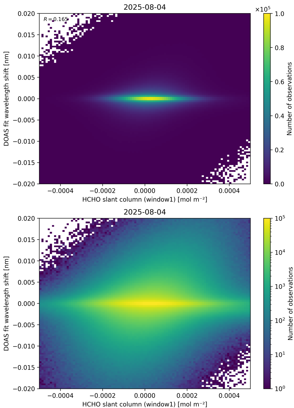
Figure 79: Scatter density plot of “HCHO slant column (window1)” against “DOAS fit wavelength shift” for 2025-08-04 to 2025-08-05.
