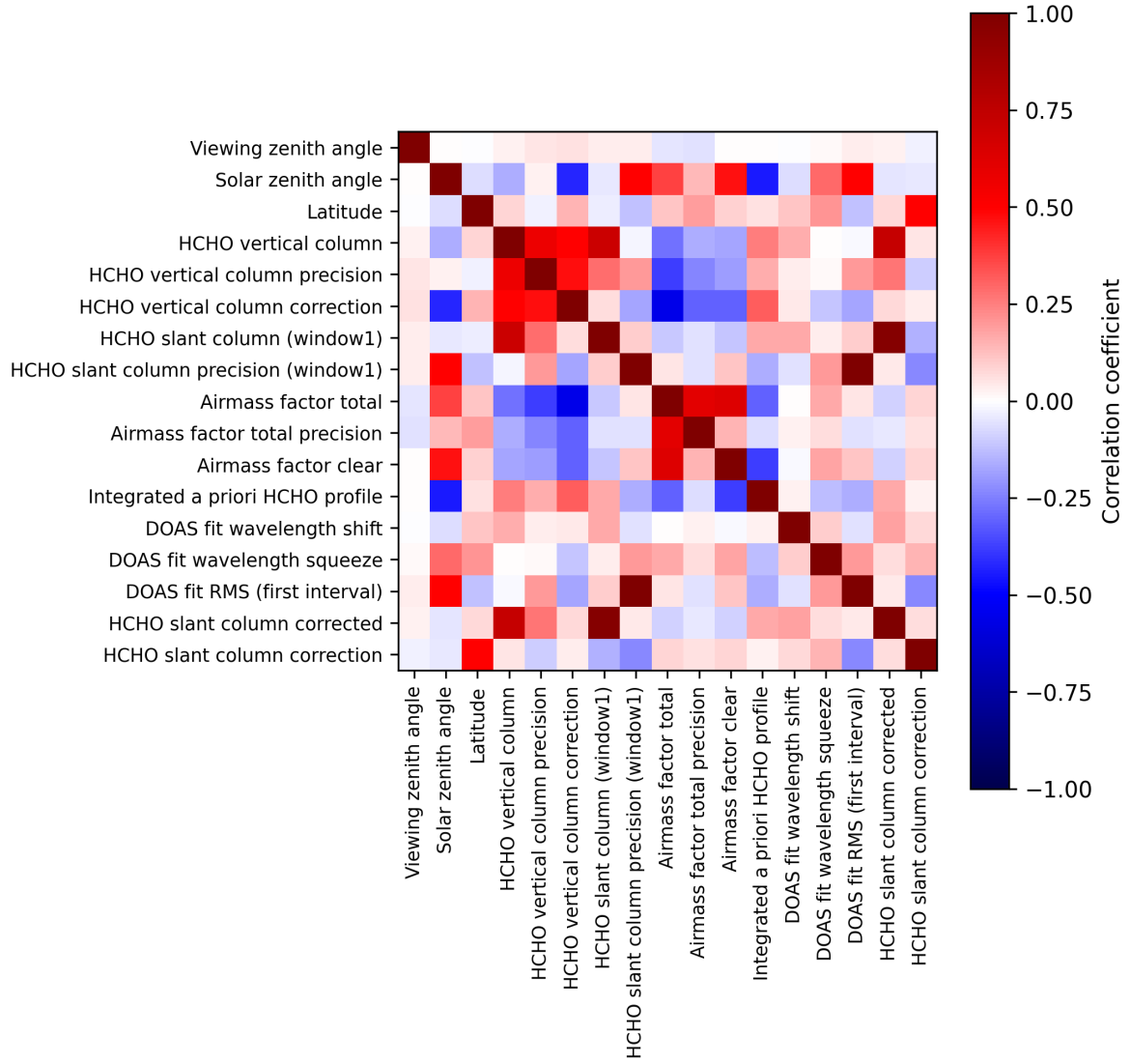
Figure 2: Map of correlation matrix for 2025-08-04 to 2025-08-05.
