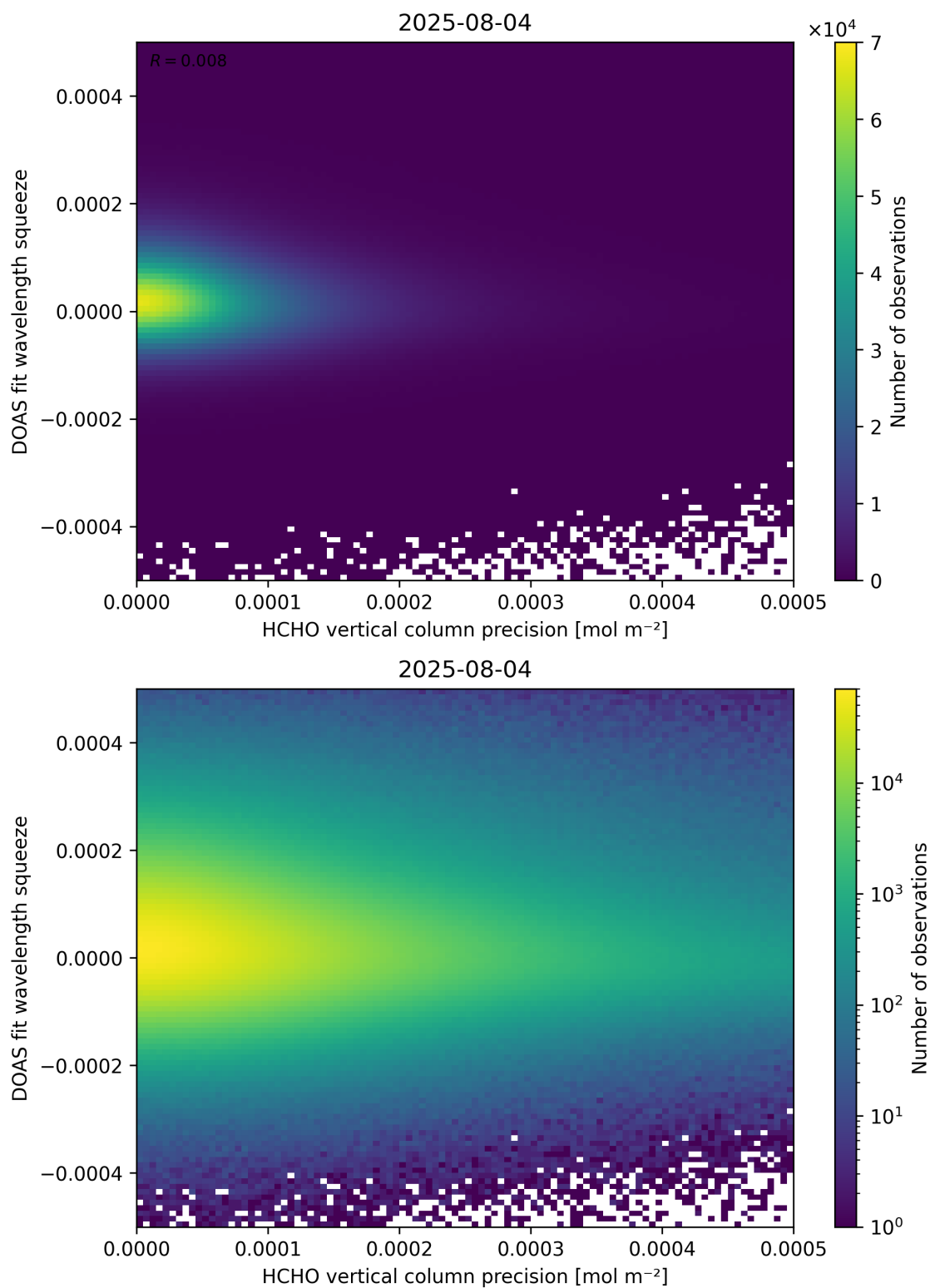
Figure 138: Scatter density plot of “HCHO vertical column precision” against “DOAS fit wavelength squeeze” for 2025-08-04 to 2025-08-05.
