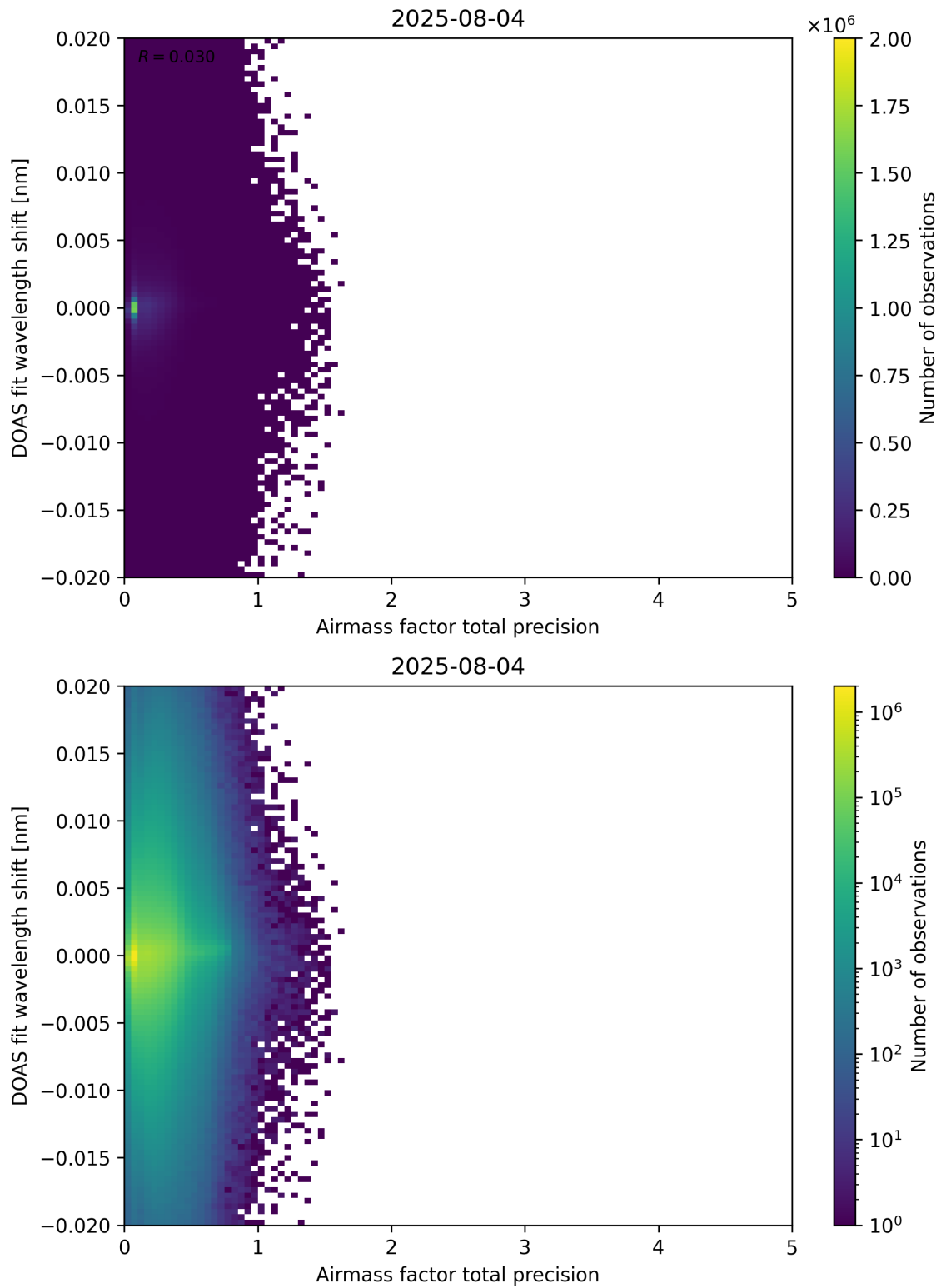
Figure 106: Scatter density plot of “Airmass factor total precision” against “DOAS fit wavelength shift” for 2025-08-04 to 2025-08-05.
