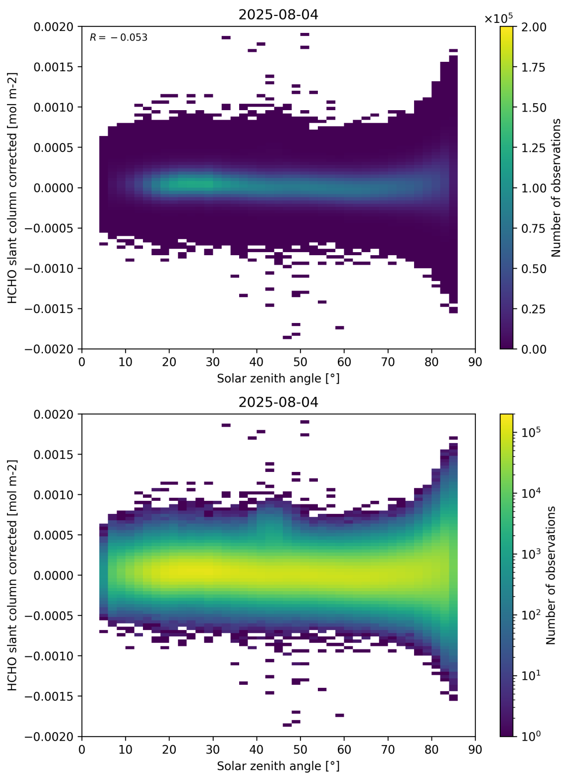
Figure 171: Scatter density plot of “Solar zenith angle” against “HCHO slant column corrected” for 2025-08-04 to 2025-08-05.
