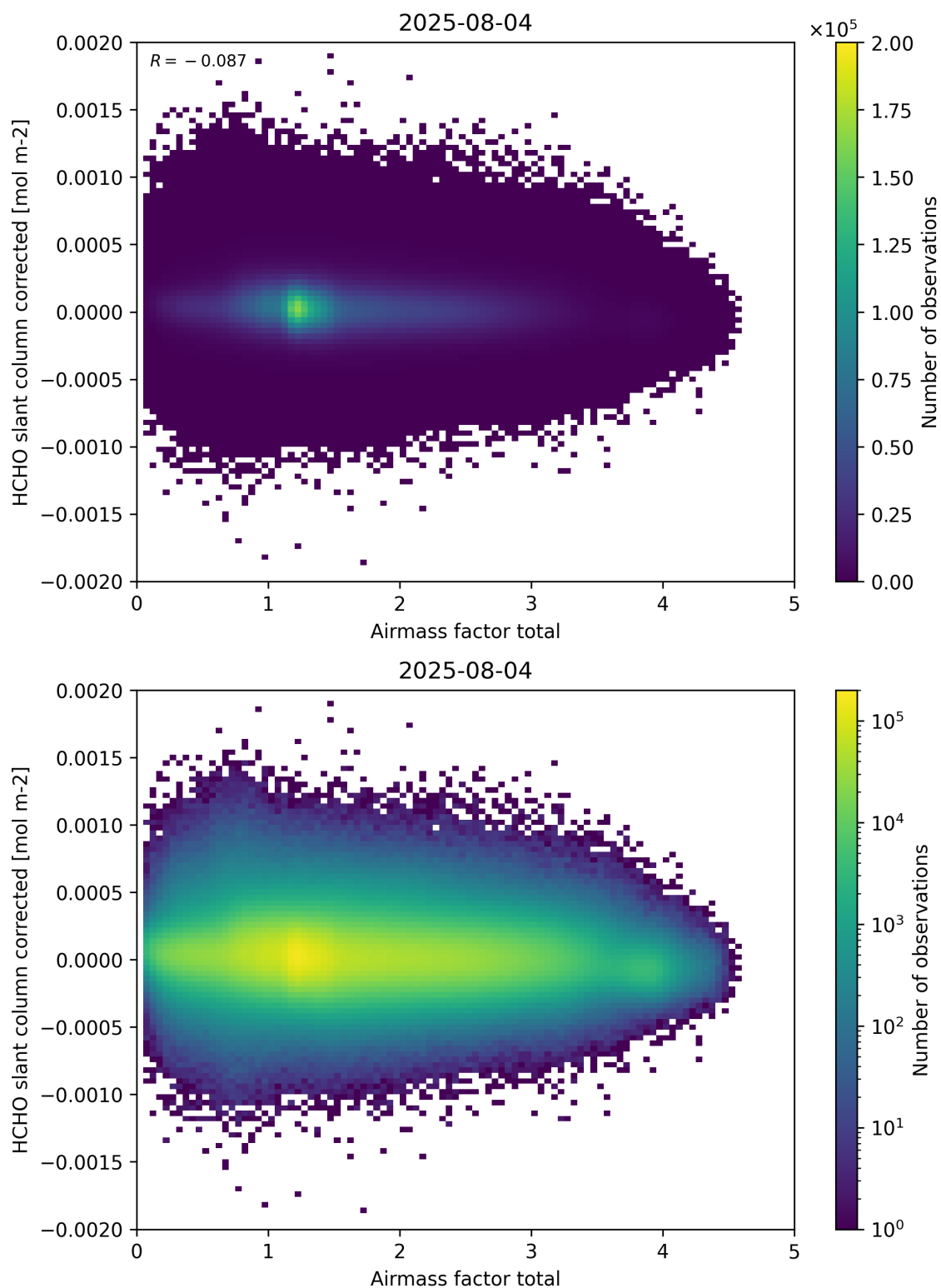
Figure 101: Scatter density plot of “Airmass factor total” against “HCHO slant column corrected” for 2025-08-04 to 2025-08-05.
