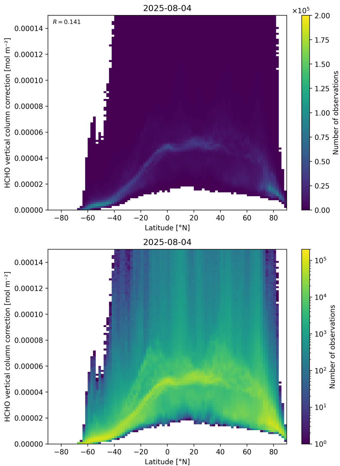
Figure 164: Scatter density plot of “Latitude” against “HCHO vertical column correction” for 2025-08-04 to 2025-08-05.
