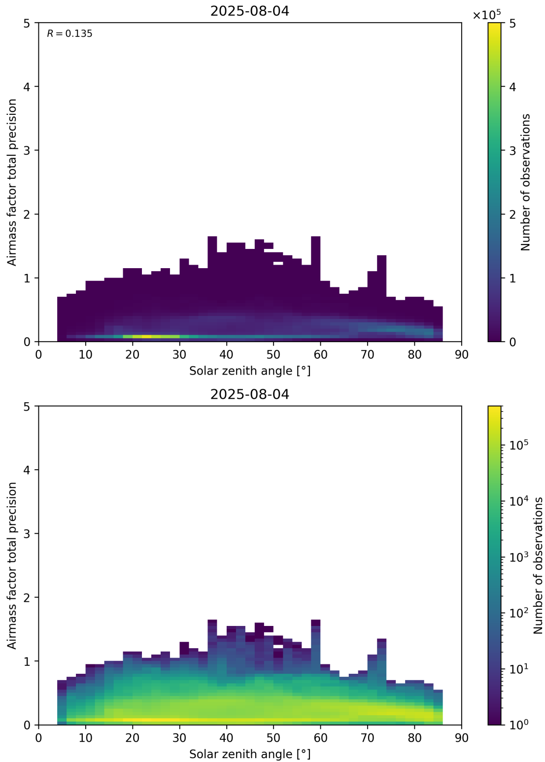
Figure 176: Scatter density plot of “Solar zenith angle” against “Airmass factor total precision” for 2025-08-04 to 2025-08-05.
