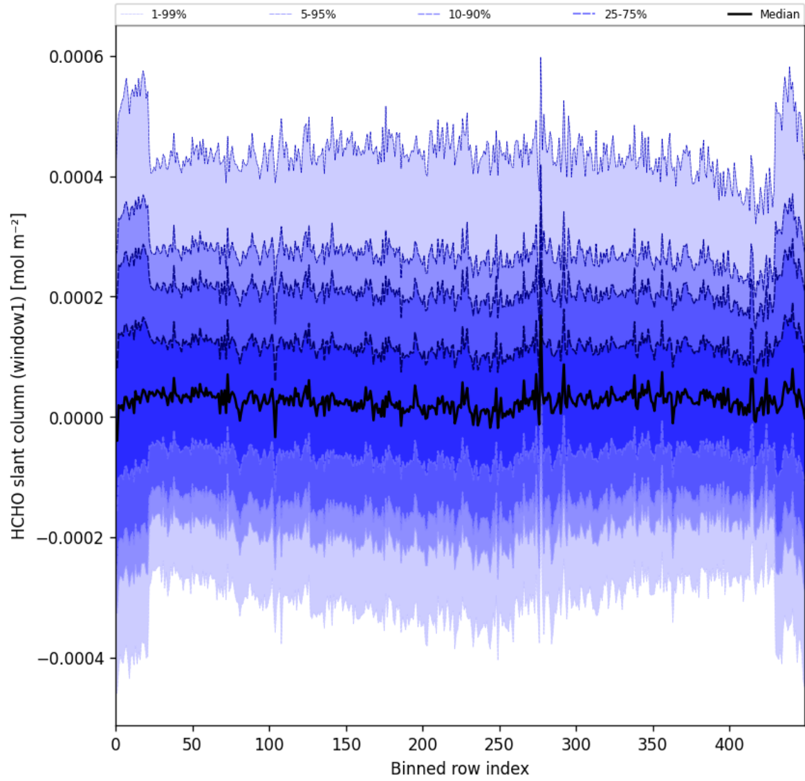
Figure 52: Along track statistics of “HCHO slant column (window1)” for 2025-08-04 to 2025-08-05
