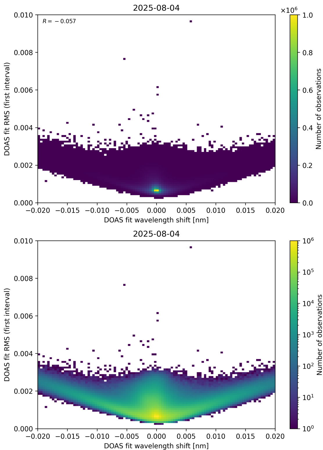
Figure 64: Scatter density plot of “DOAS fit wavelength shift” against “DOAS fit RMS (first interval)” for 2025-08-04 to 2025-08-05.
