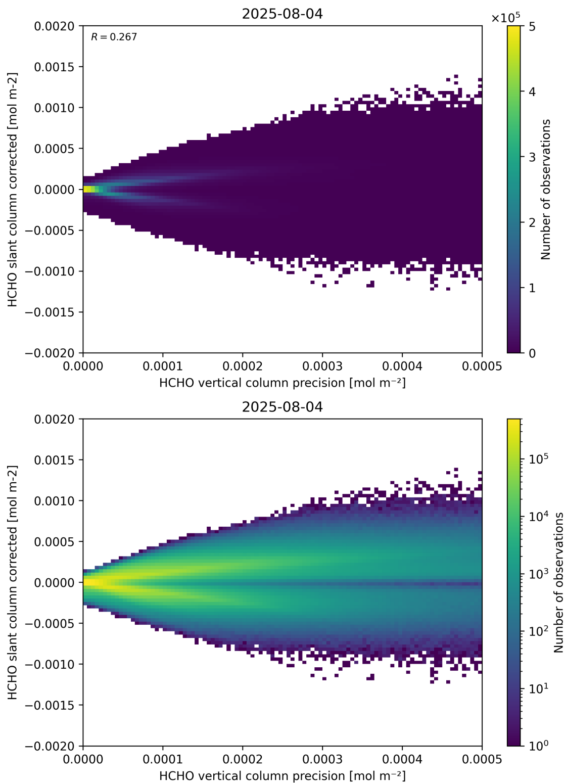
Figure 140: Scatter density plot of “HCHO vertical column precision” against “HCHO slant column corrected” for 2025-08-04 to 2025-08-05.
