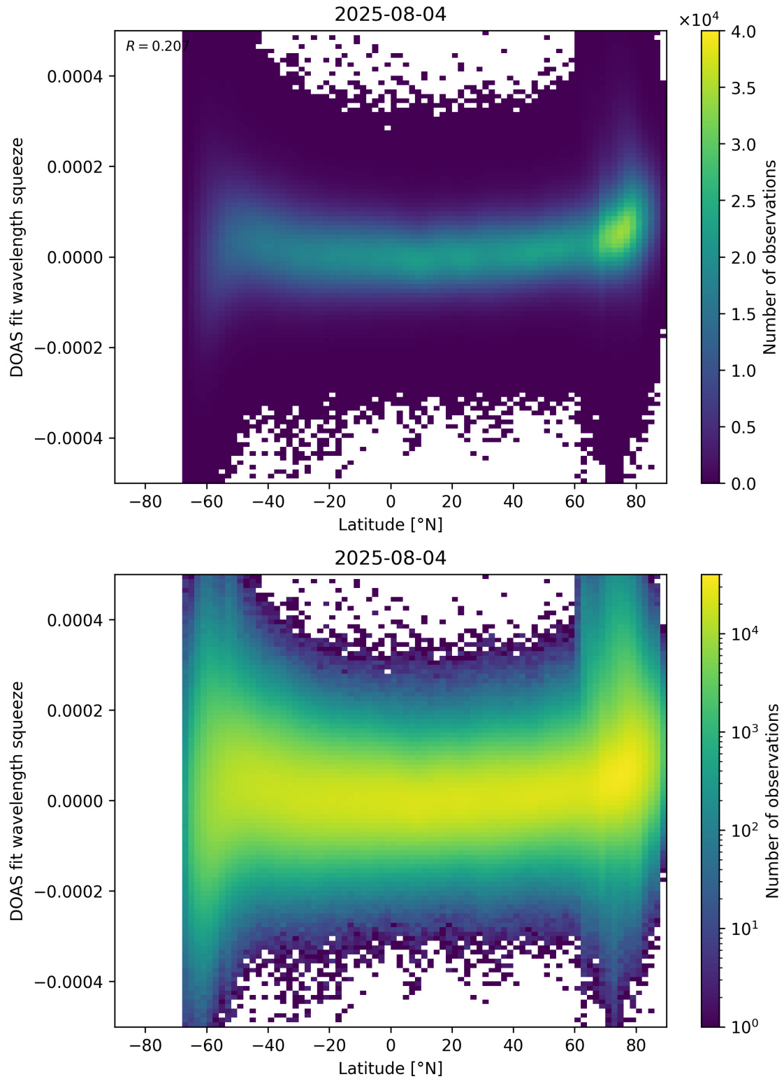
Figure 155: Scatter density plot of “Latitude” against “DOAS fit wavelength squeeze” for 2025-08-04 to 2025-08-05.
