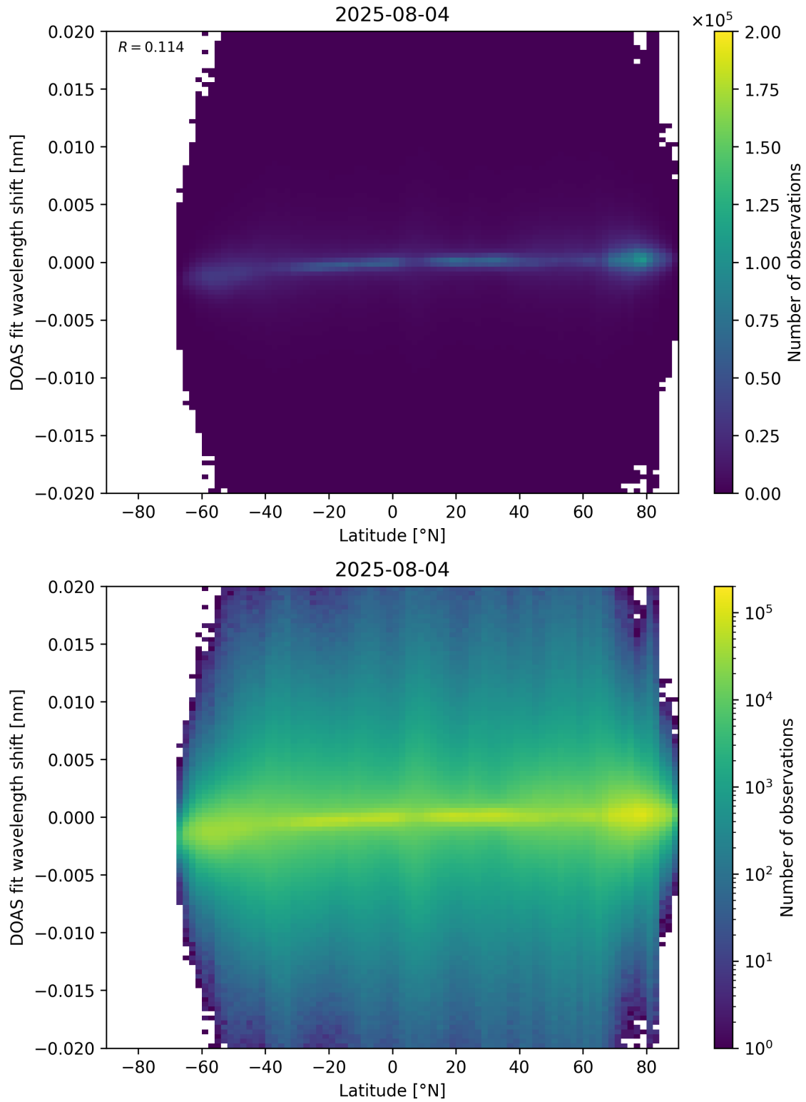
Figure 154: Scatter density plot of “Latitude” against “DOAS fit wavelength shift” for 2025-08-04 to 2025-08-05.
