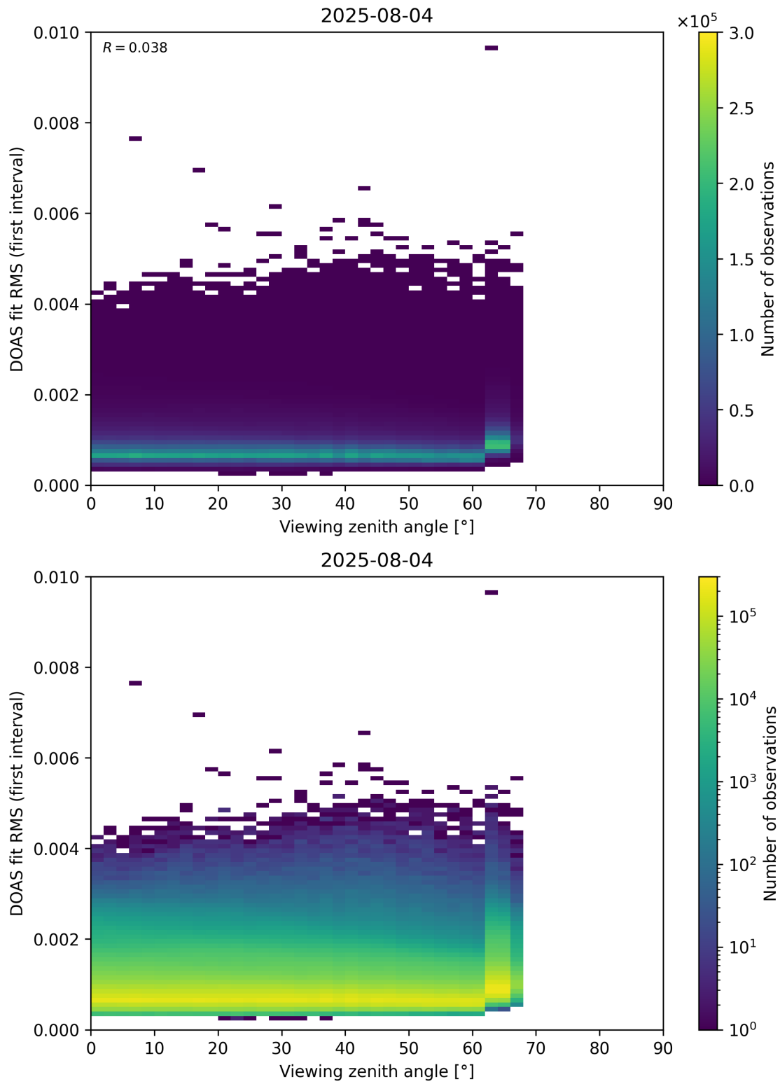
Figure 182: Scatter density plot of “Viewing zenith angle” against “DOAS fit RMS (first interval)” for 2025-08-04 to 2025-08-05.
