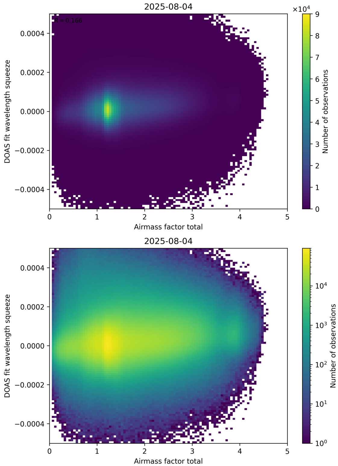
Figure 99: Scatter density plot of “Airmass factor total” against “DOAS fit wavelength squeeze” for 2025-08-04 to 2025-08-05.
