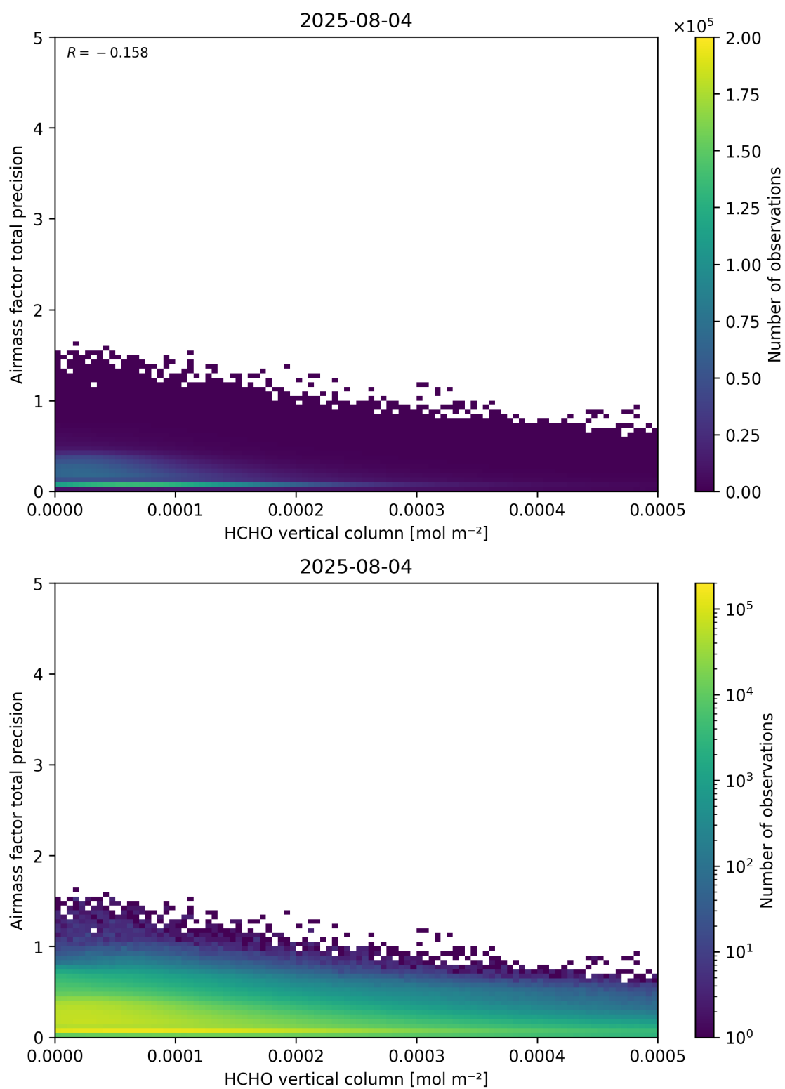
Figure 132: Scatter density plot of “HCHO vertical column” against “Airmass factor total precision” for 2025-08-04 to 2025-08-05.
