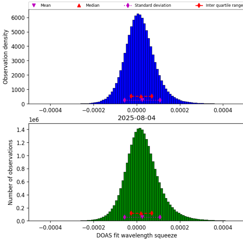
Figure 45: Histogram of “DOAS fit wavelength squeeze” for 2025-08-04 to 2025-08-05
