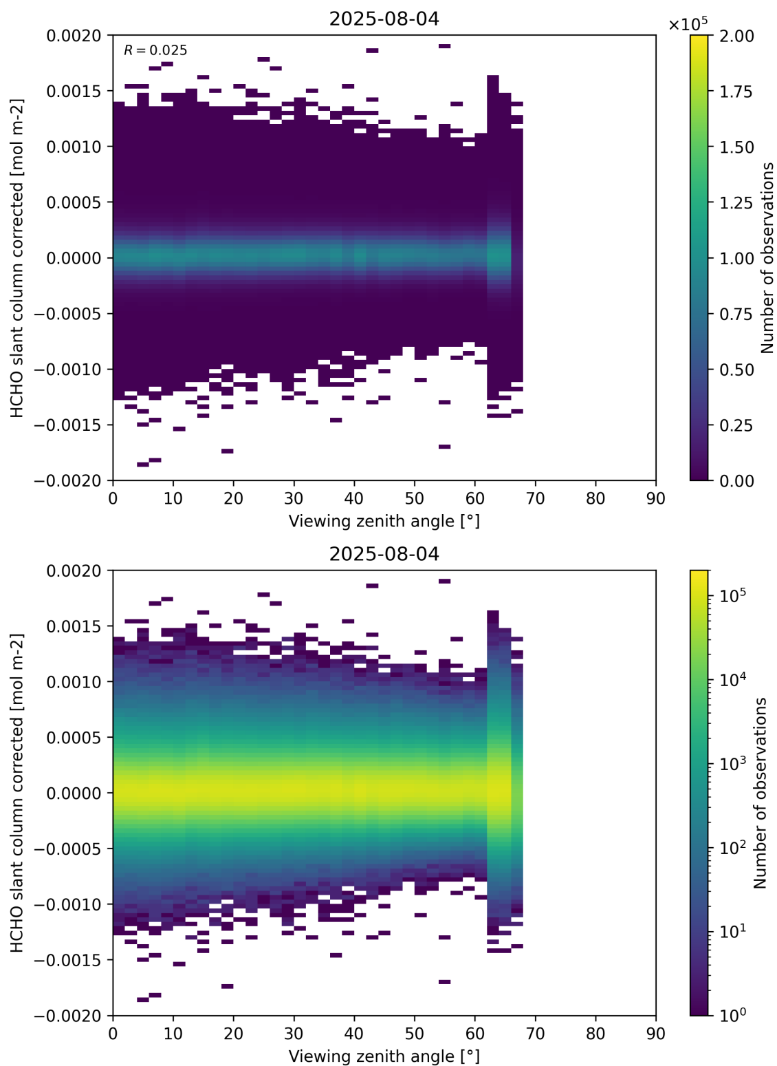
Figure 186: Scatter density plot of “Viewing zenith angle” against “HCHO slant column corrected” for 2025-08-04 to 2025-08-05.
