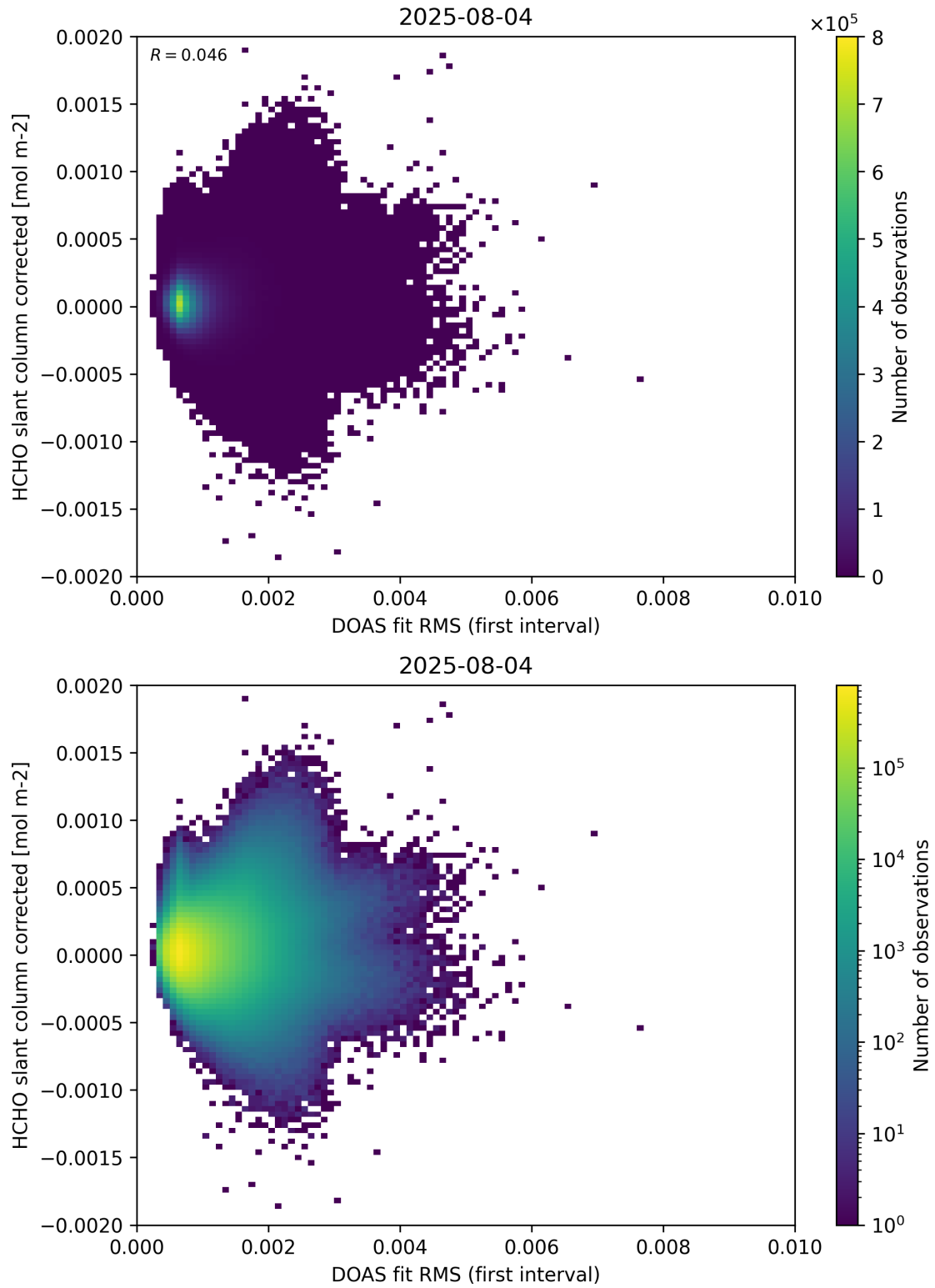
Figure 62: Scatter density plot of “DOAS fit RMS (first interval)” against “HCHO slant column corrected” for 2025-08-04 to 2025-08-05.
