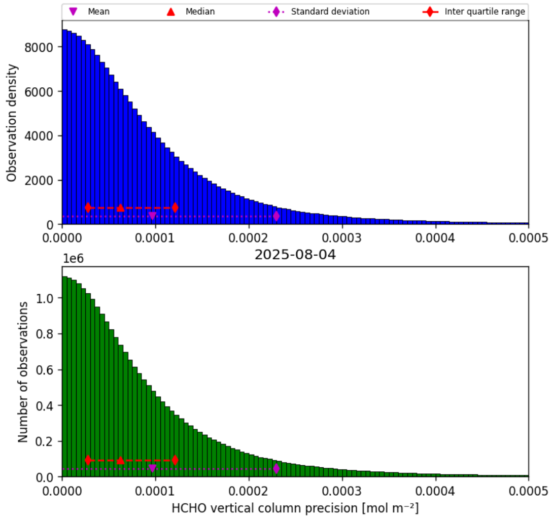
Figure 36: Histogram of “HCHO vertical column precision” for 2025-08-04 to 2025-08-05
