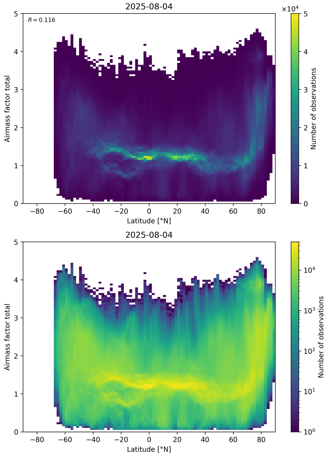
Figure 161: Scatter density plot of “Latitude” against “Airmass factor total” for 2025-08-04 to 2025-08-05.
