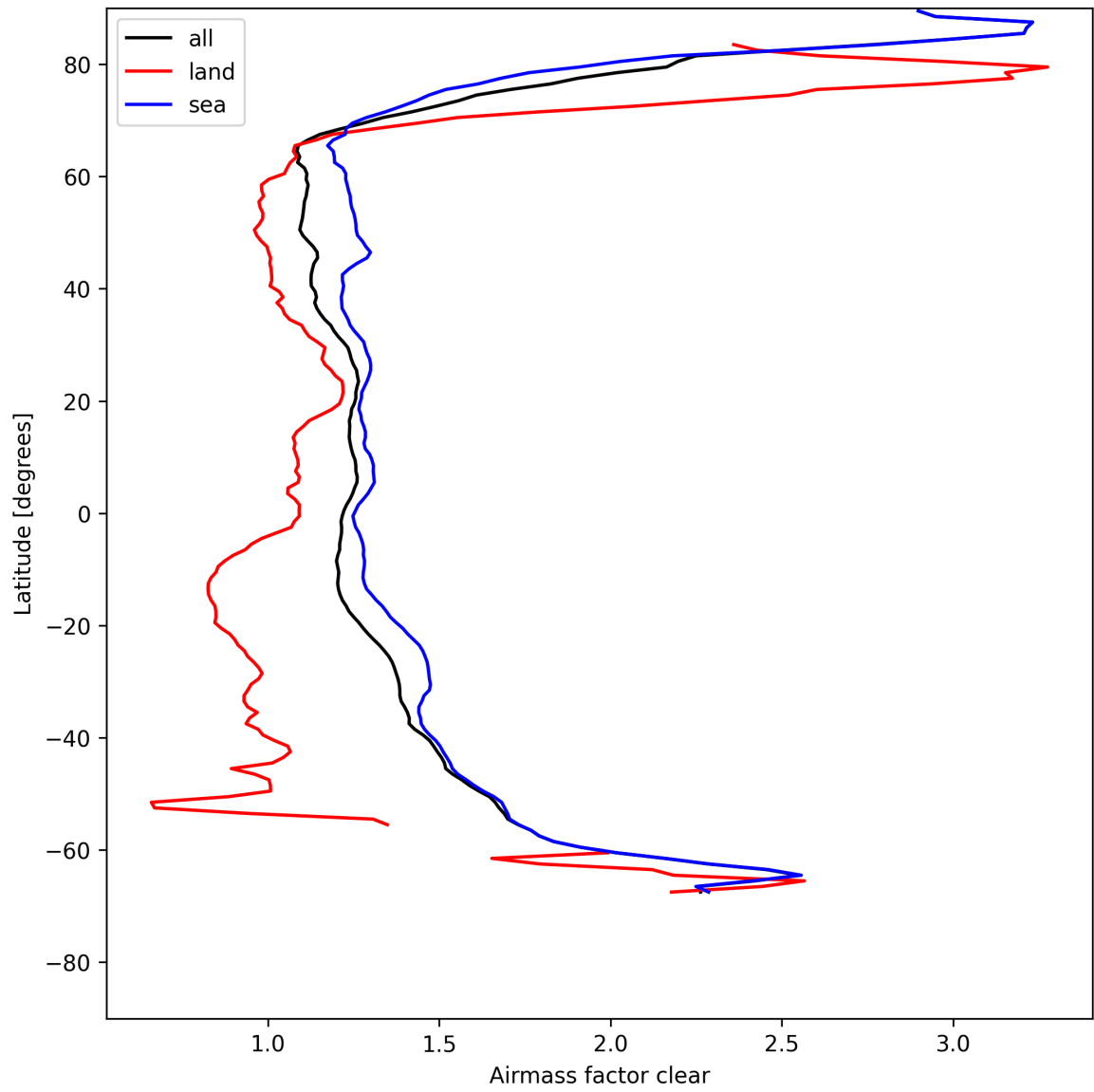
Figure 28: Zonal average of “Airmass factor clear” for 2025-08-04 to 2025-08-05.
