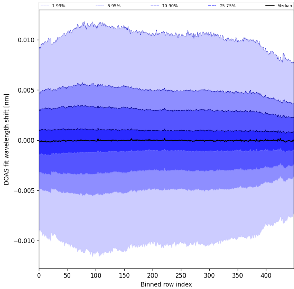
Figure 58: Along track statistics of “DOAS fit wavelength shift” for 2025-08-04 to 2025-08-05
