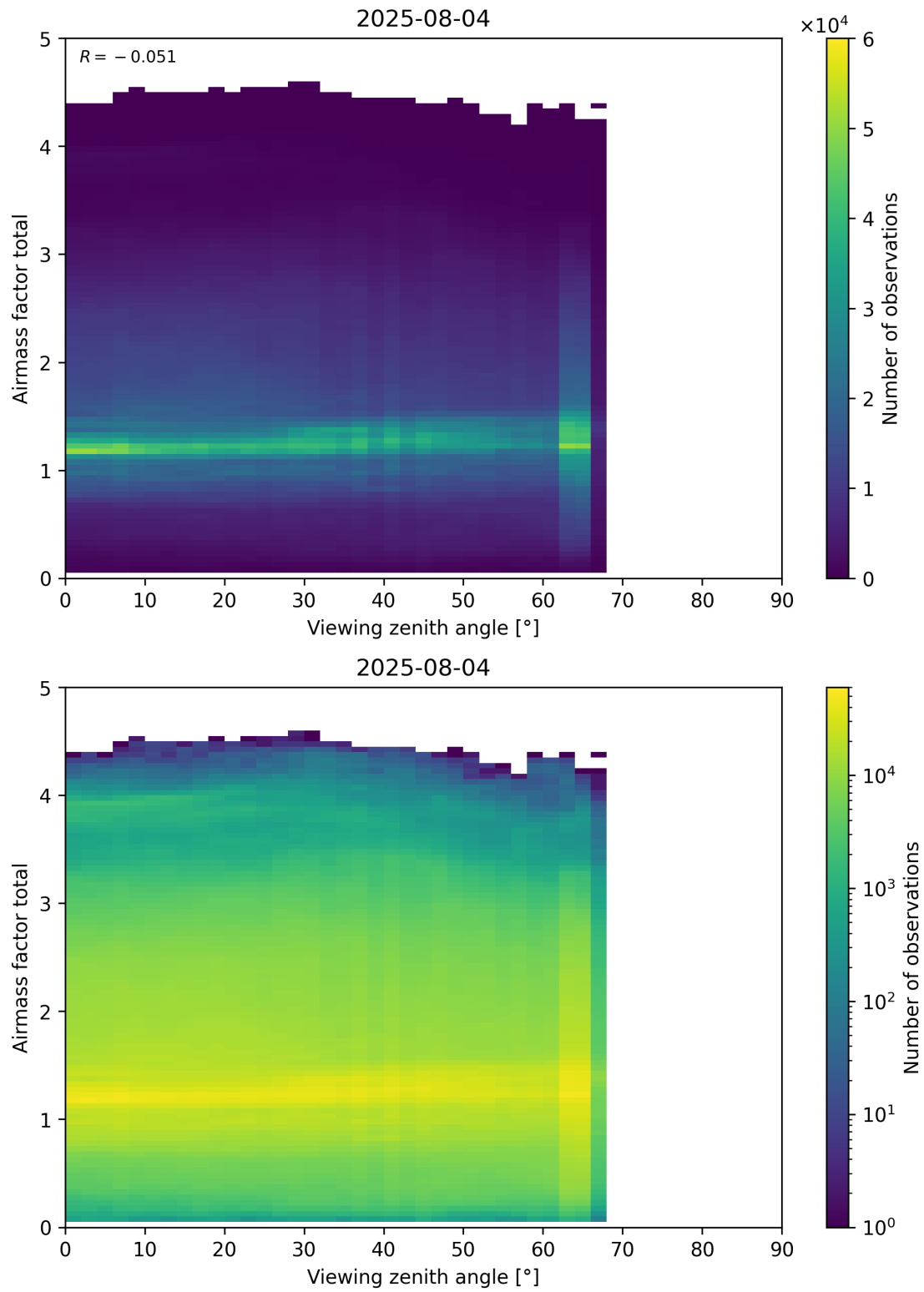
Figure 190: Scatter density plot of “Viewing zenith angle” against “Airmass factor total” for 2025-08-04 to 2025-08-05.
