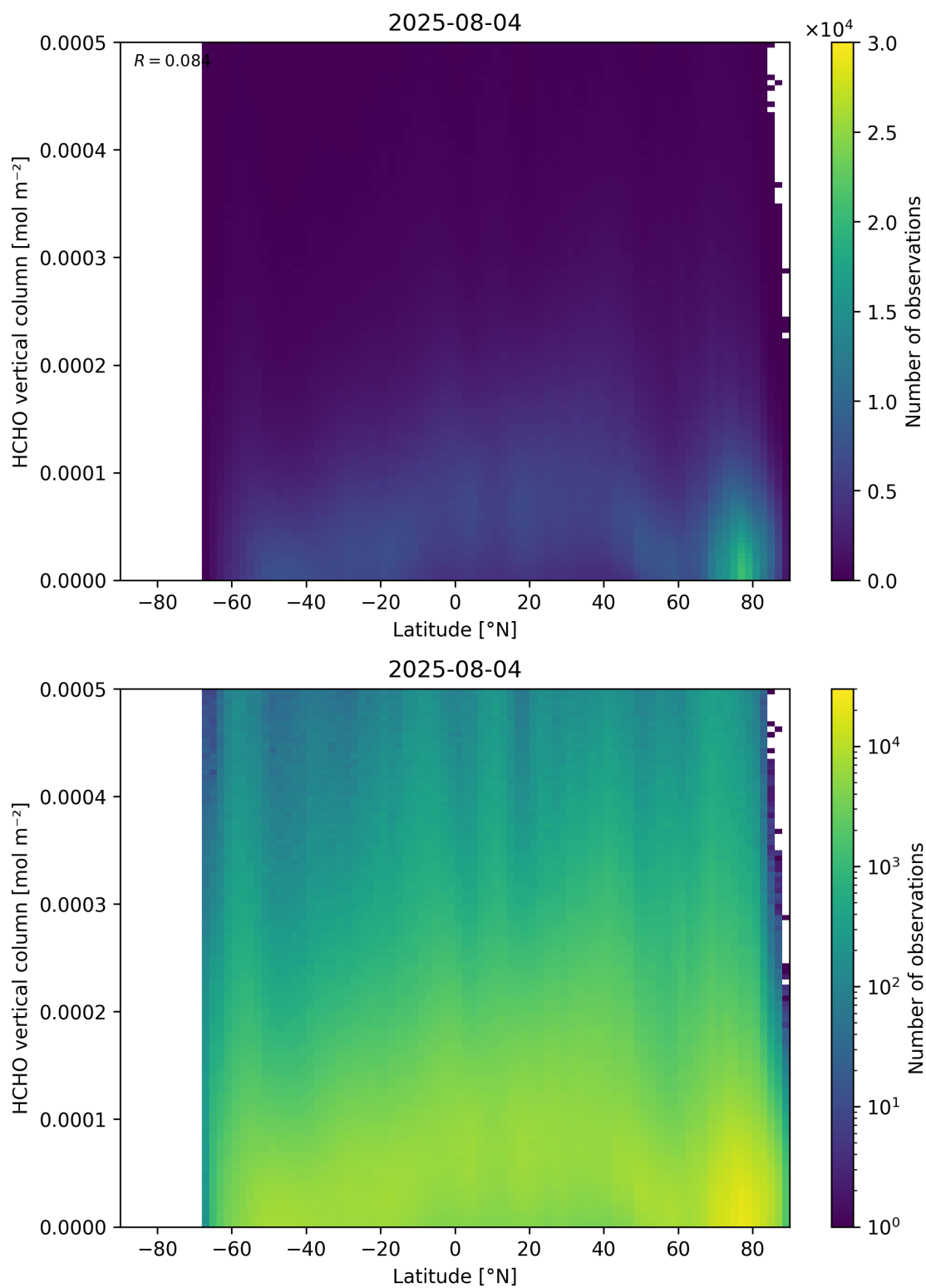
Figure 163: Scatter density plot of “Latitude” against “HCHO vertical column” for 2025-08-04 to 2025-08-05.
