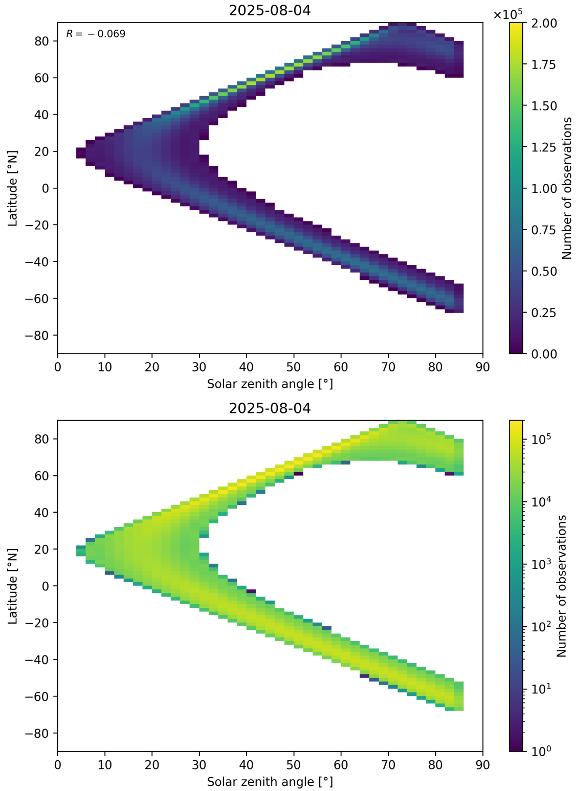
Figure 181: Scatter density plot of “Solar zenith angle” against “Latitude” for 2025-08-04 to 2025-08-05.
