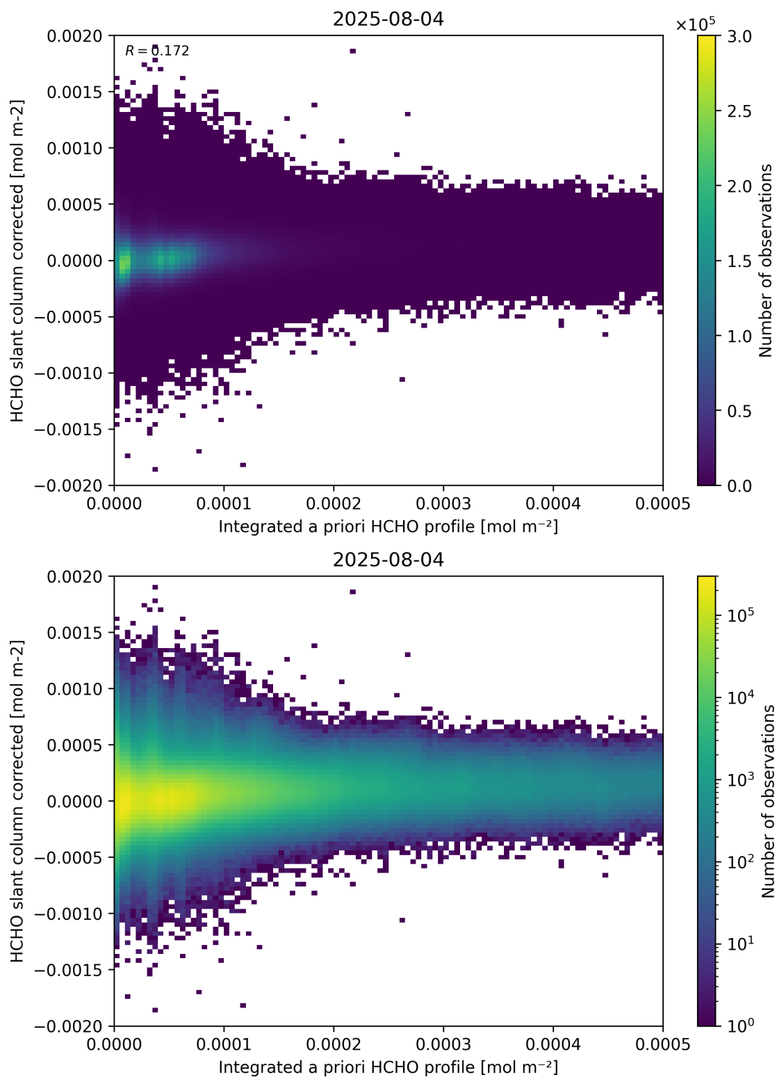
Figure 151: Scatter density plot of “Integrated a priori HCHO profile” against “HCHO slant column corrected” for 2025-08-04 to 2025-08-05.
