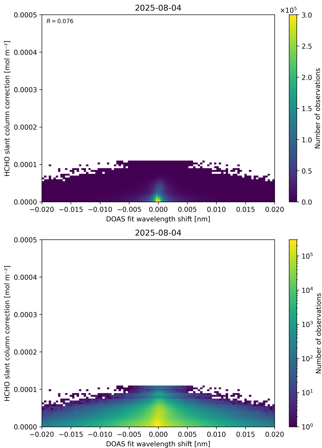
Figure 67: Scatter density plot of “DOAS fit wavelength shift” against “HCHO slant column correction” for 2025-08-04 to 2025-08-05.
