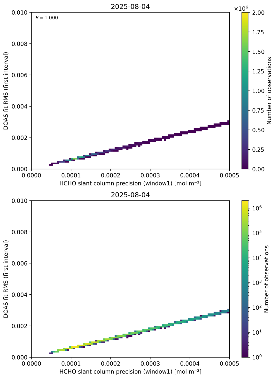
Figure 88: Scatter density plot of “HCHO slant column precision (window1)” against “DOAS fit RMS (first interval)” for 2025-08-04 to 2025-08-05.
