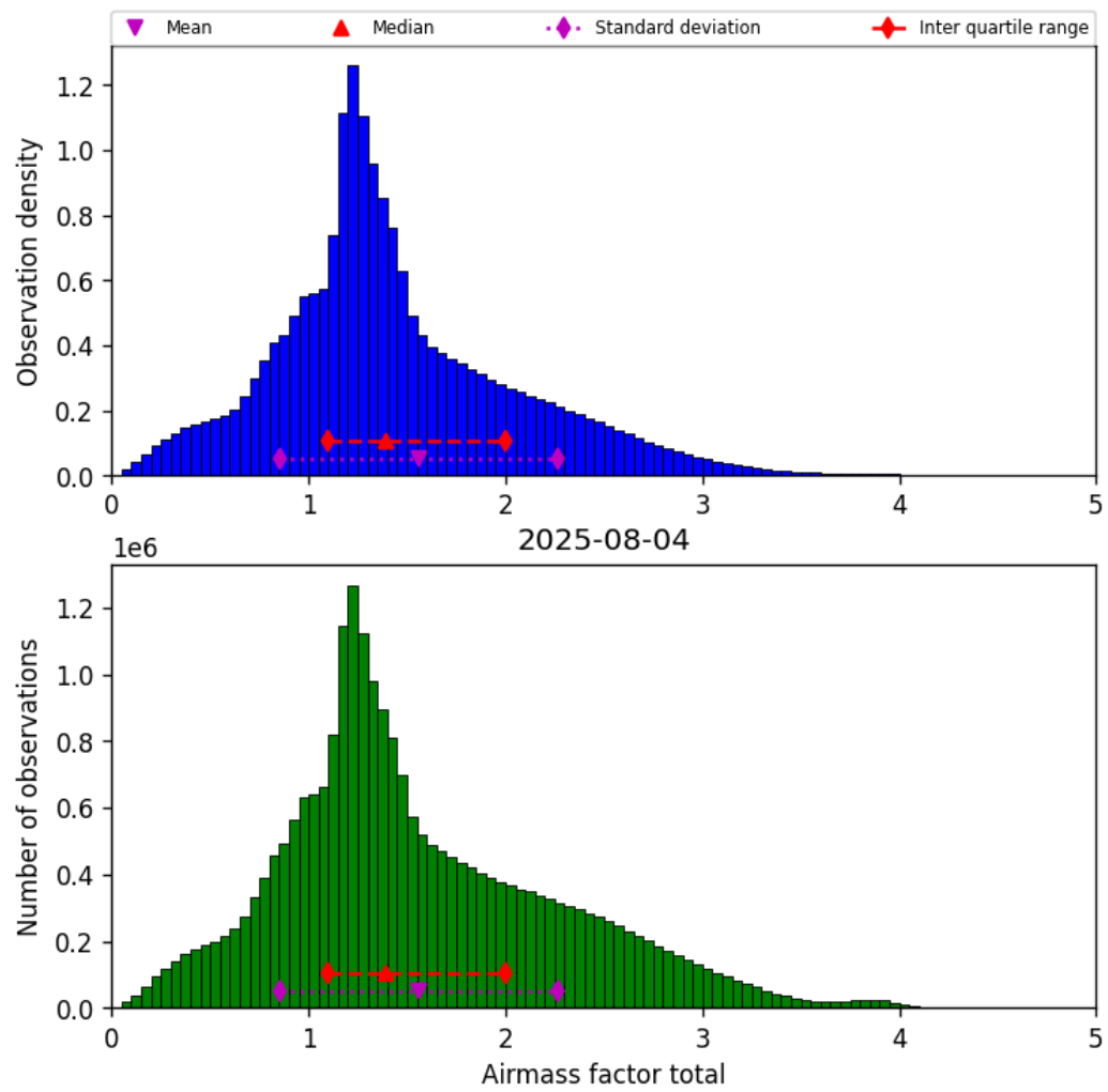
Figure 40: Histogram of “Airmass factor total” for 2025-08-04 to 2025-08-05
