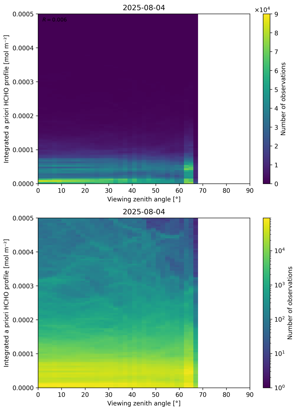
Figure 195: Scatter density plot of “Viewing zenith angle” against “Integrated a priori HCHO profile” for 2025-08-04 to 2025-08-05.
