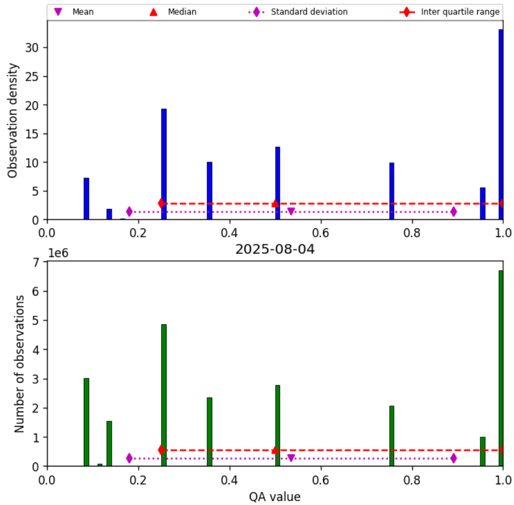
Figure 34: Histogram of “QA value” for 2025-08-04 to 2025-08-05
