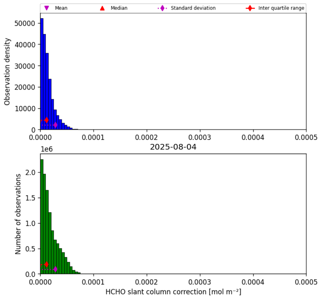
Figure 47: Histogram of “HCHO slant column correction” for 2025-08-04 to 2025-08-05
