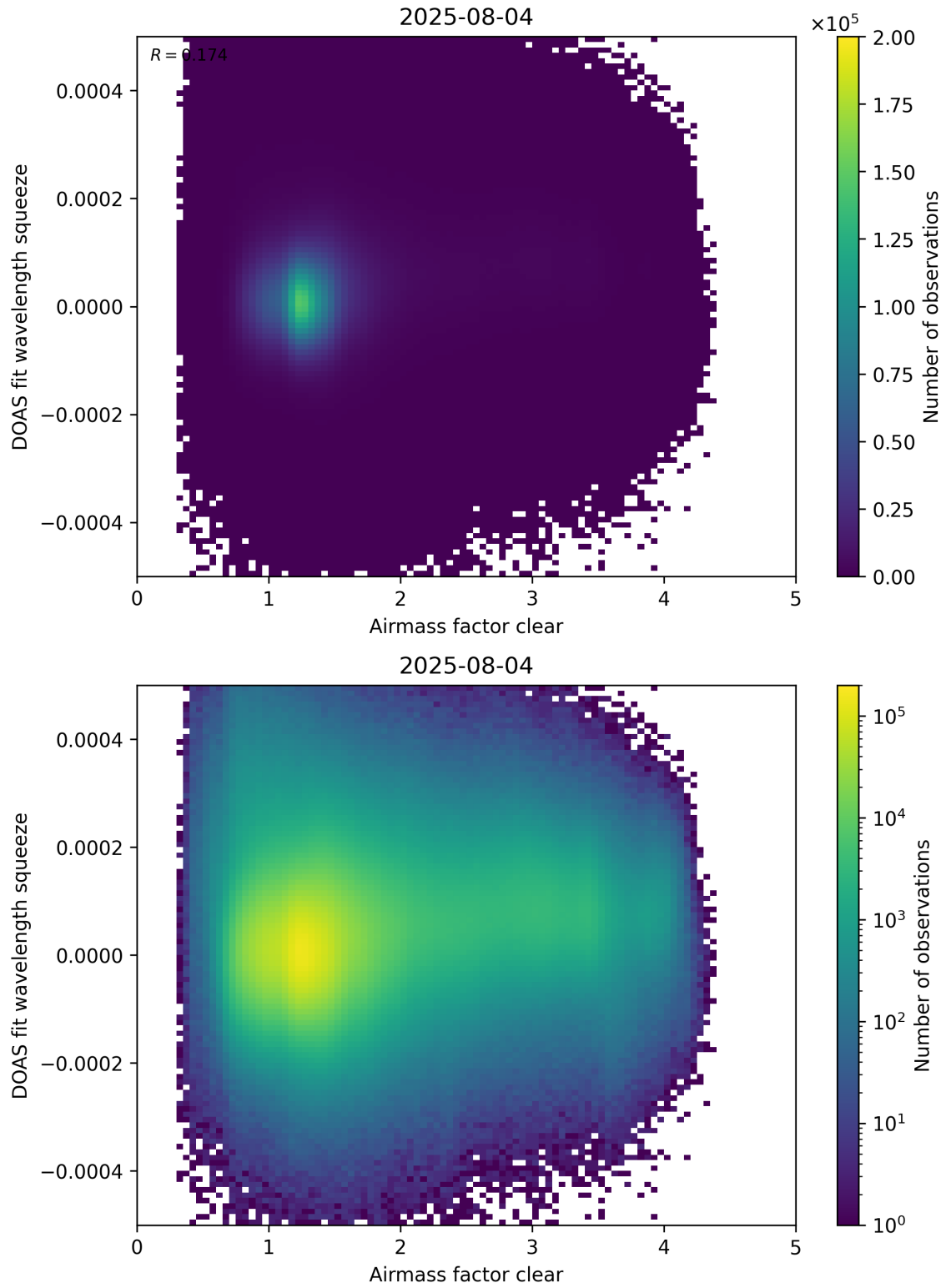
Figure 73: Scatter density plot of “Airmass factor clear” against “DOAS fit wavelength squeeze” for 2025-08-04 to 2025-08-05.
