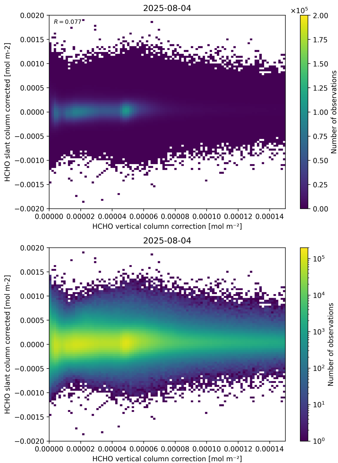
Figure 116: Scatter density plot of “HCHO vertical column correction” against “HCHO slant column corrected” for 2025-08-04 to 2025-08-05.
