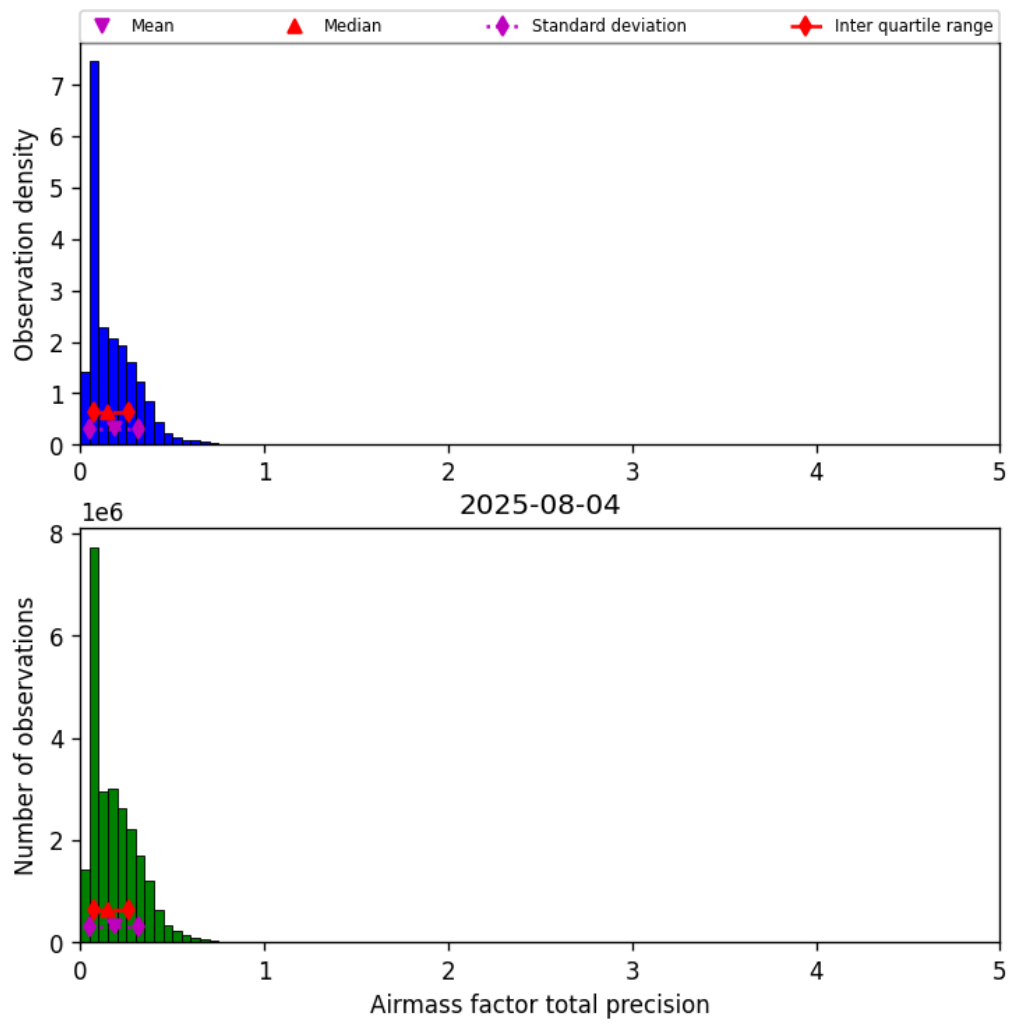
Figure 41: Histogram of “Airmass factor total precision” for 2025-08-04 to 2025-08-05
