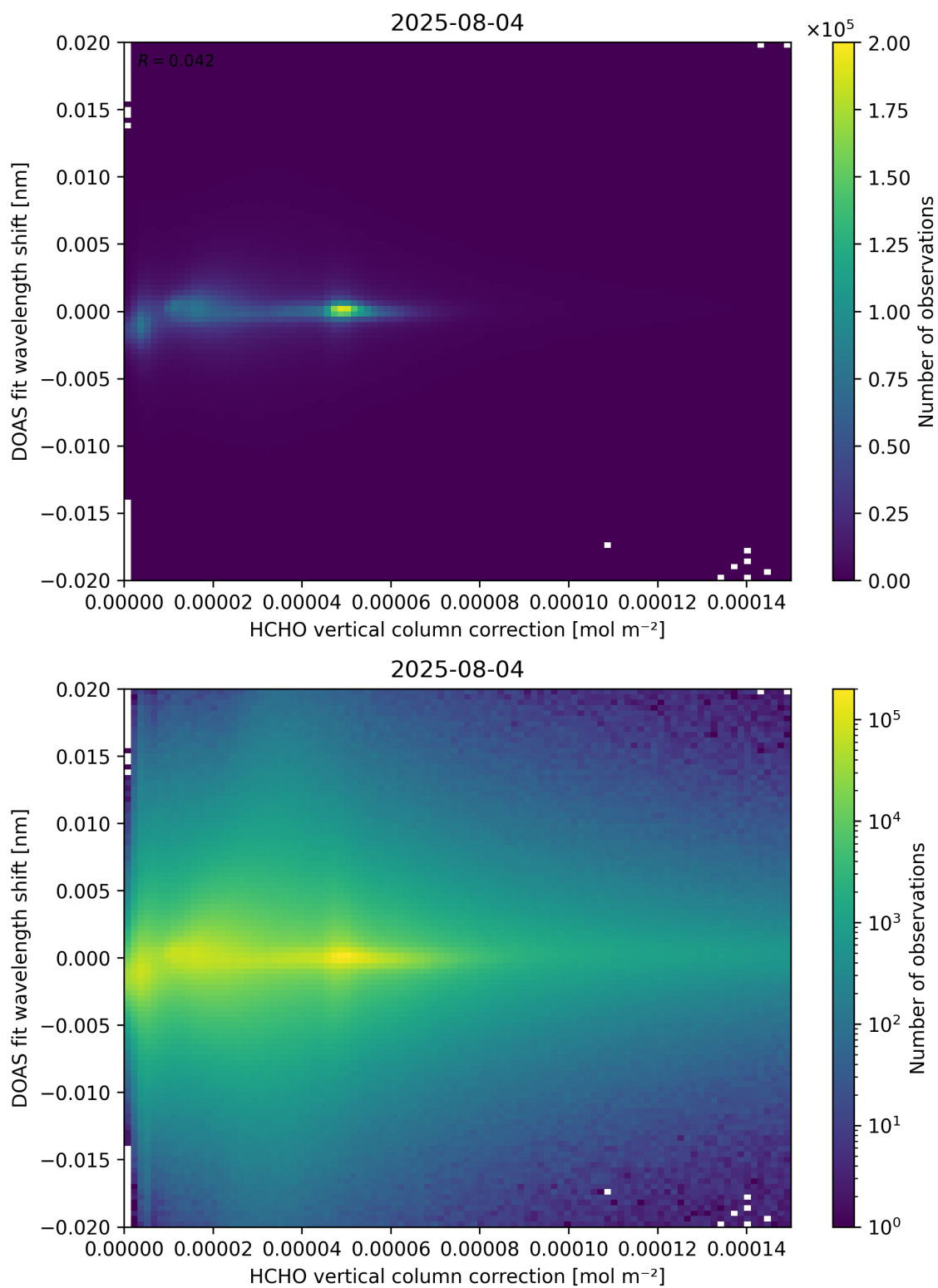
Figure 113: Scatter density plot of “HCHO vertical column correction” against “DOAS fit wavelength shift” for 2025-08-04 to 2025-08-05.
