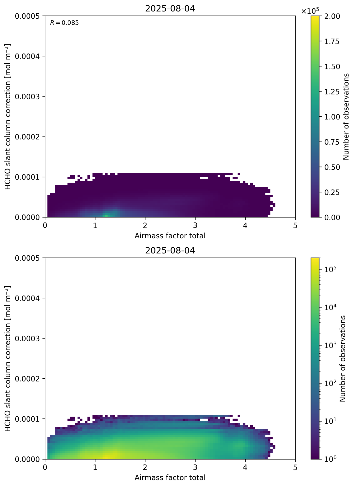
Figure 102: Scatter density plot of “Airmass factor total” against “HCHO slant column correction” for 2025-08-04 to 2025-08-05.
