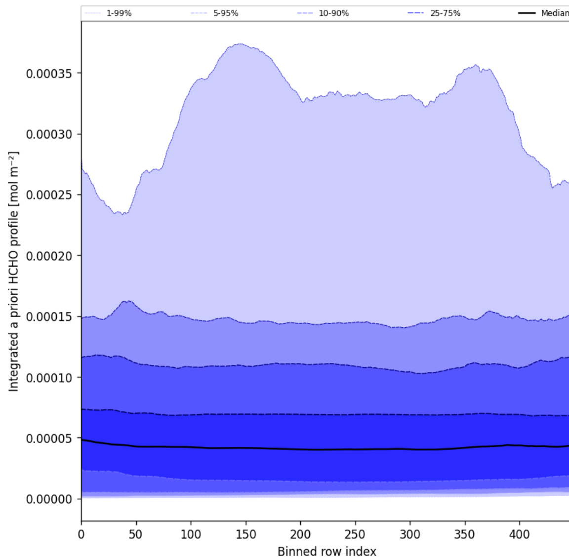
Figure 57: Along track statistics of “Integrated a priori HCHO profile” for 2025-08-04 to 2025-08-05
