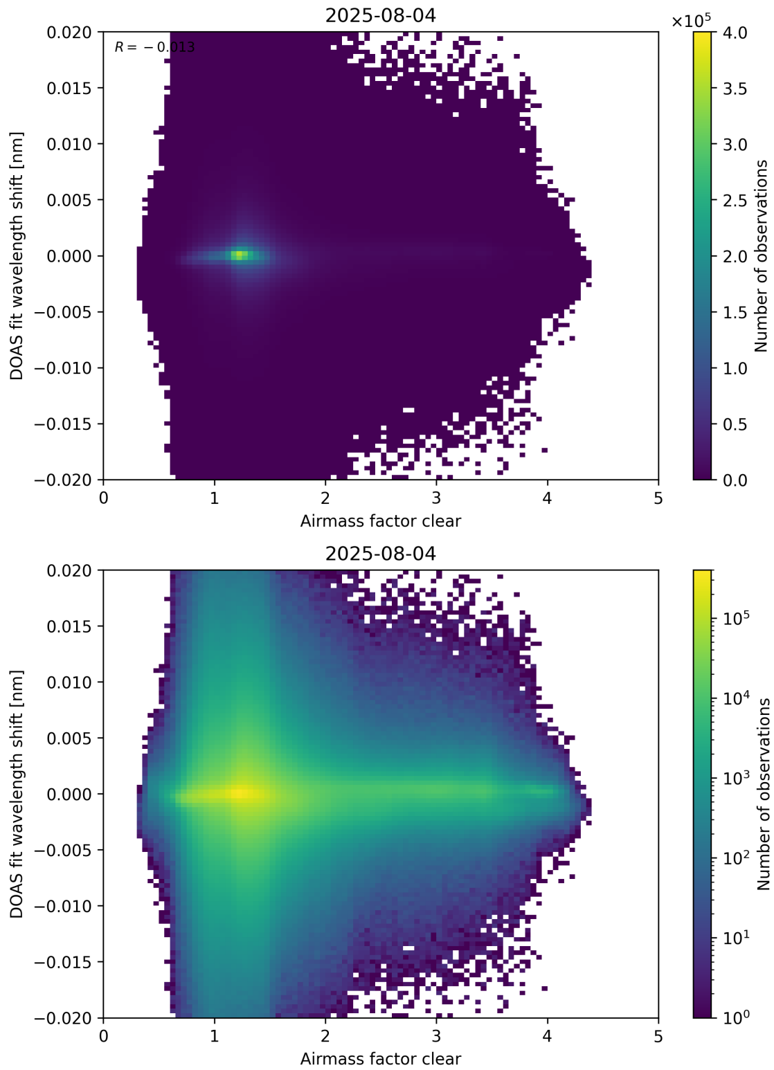
Figure 72: Scatter density plot of “Airmass factor clear” against “DOAS fit wavelength shift” for 2025-08-04 to 2025-08-05.
