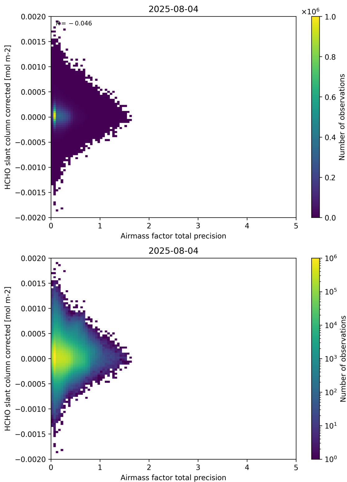
Figure 109: Scatter density plot of “Airmass factor total precision” against “HCHO slant column corrected” for 2025-08-04 to 2025-08-05.
