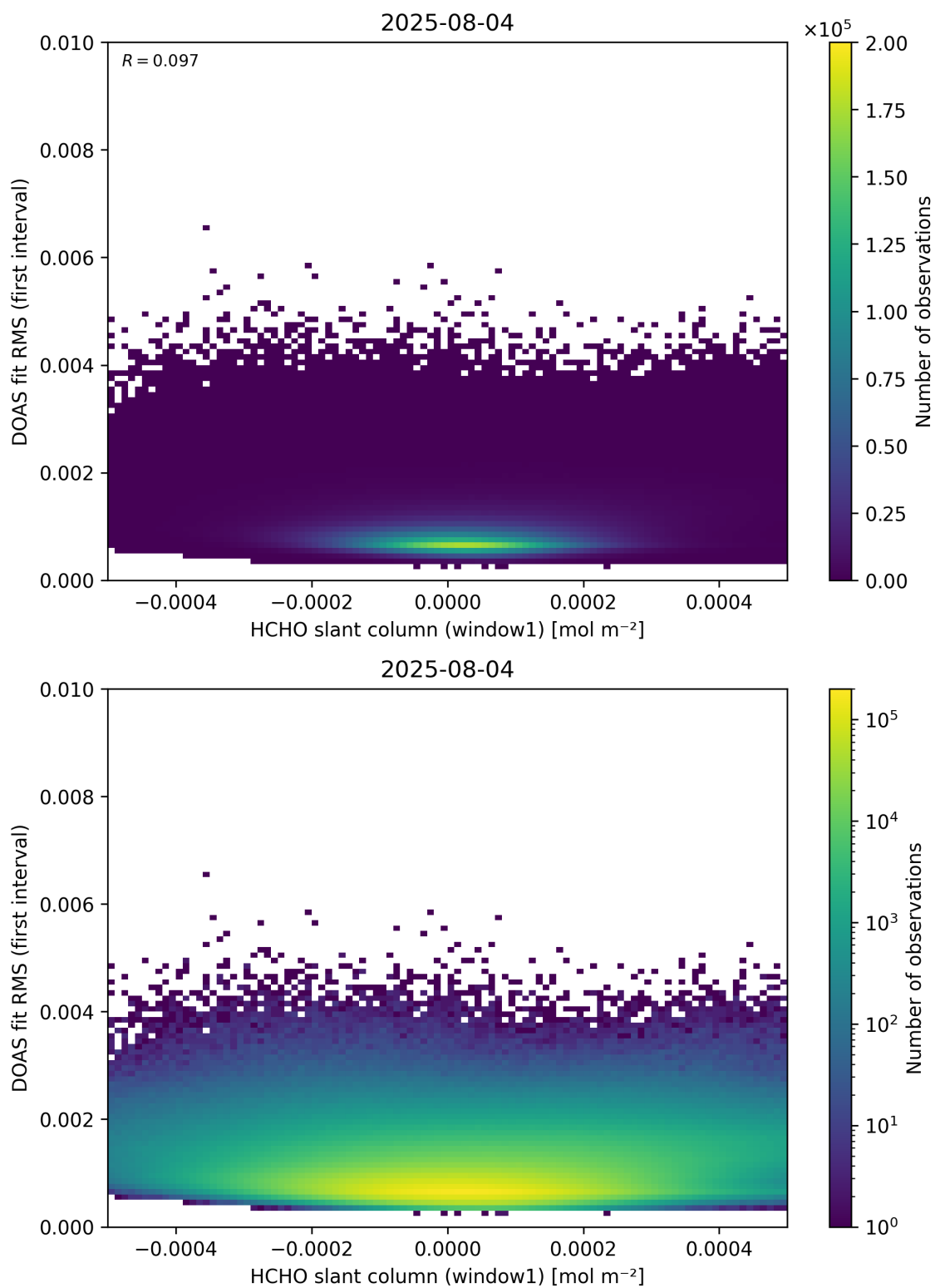
Figure 78: Scatter density plot of “HCHO slant column (window1)” against “DOAS fit RMS (first interval)” for 2025-08-04 to 2025-08-05.
