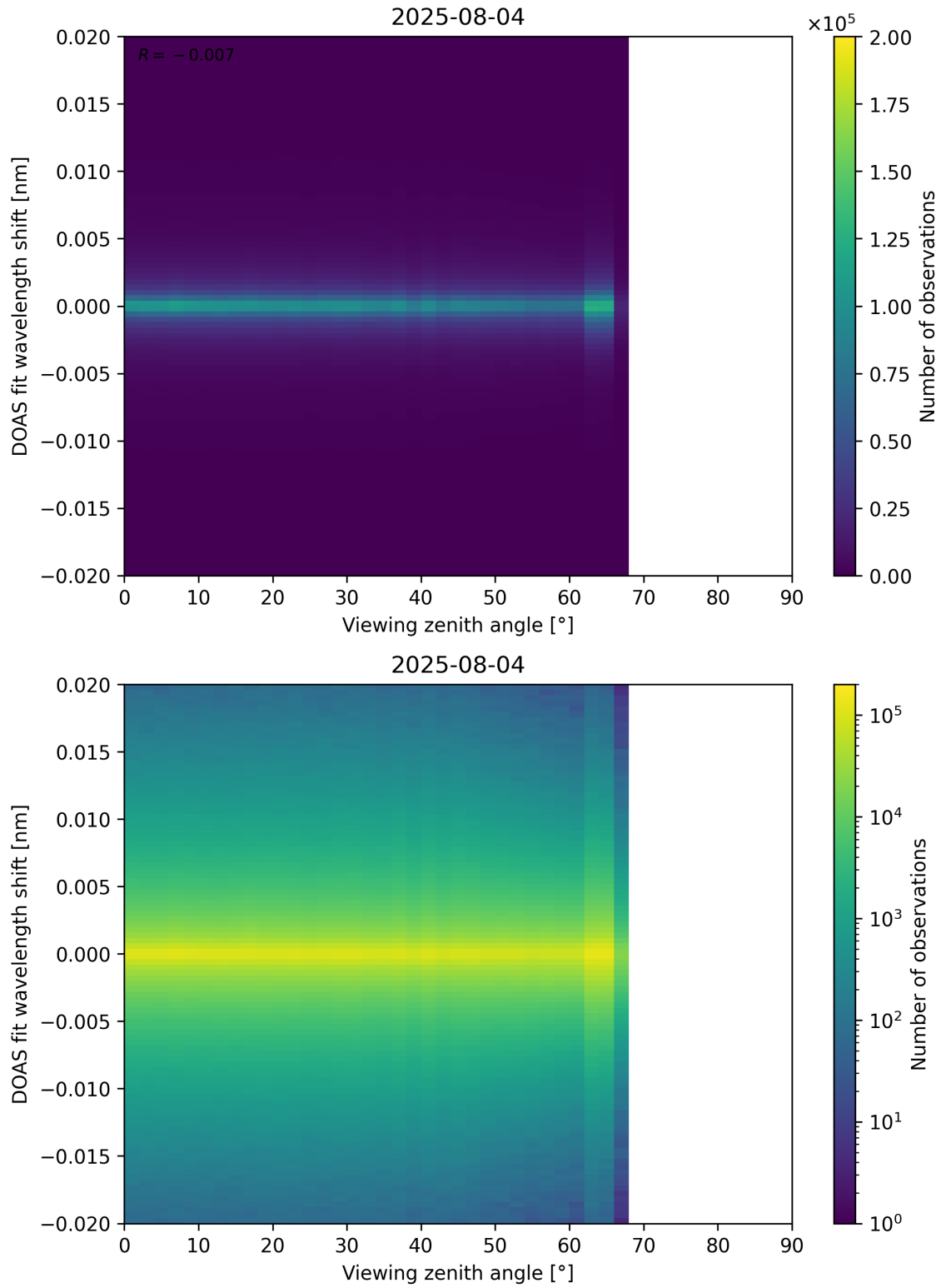
Figure 183: Scatter density plot of “Viewing zenith angle” against “DOAS fit wavelength shift” for 2025-08-04 to 2025-08-05.
