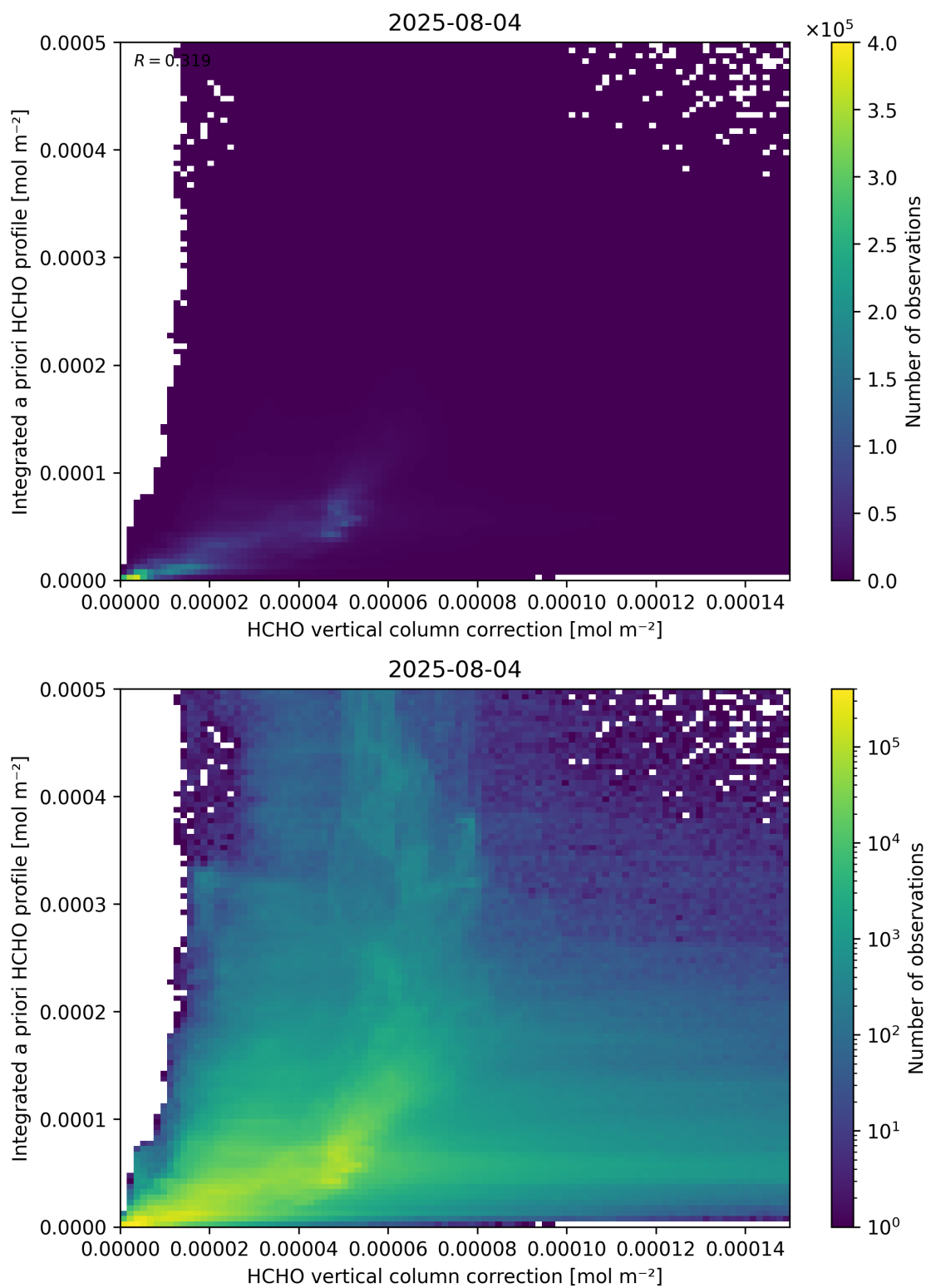
Figure 122: Scatter density plot of “HCHO vertical column correction” against “Integrated a priori HCHO profile” for 2025-08-04 to 2025-08-05.
