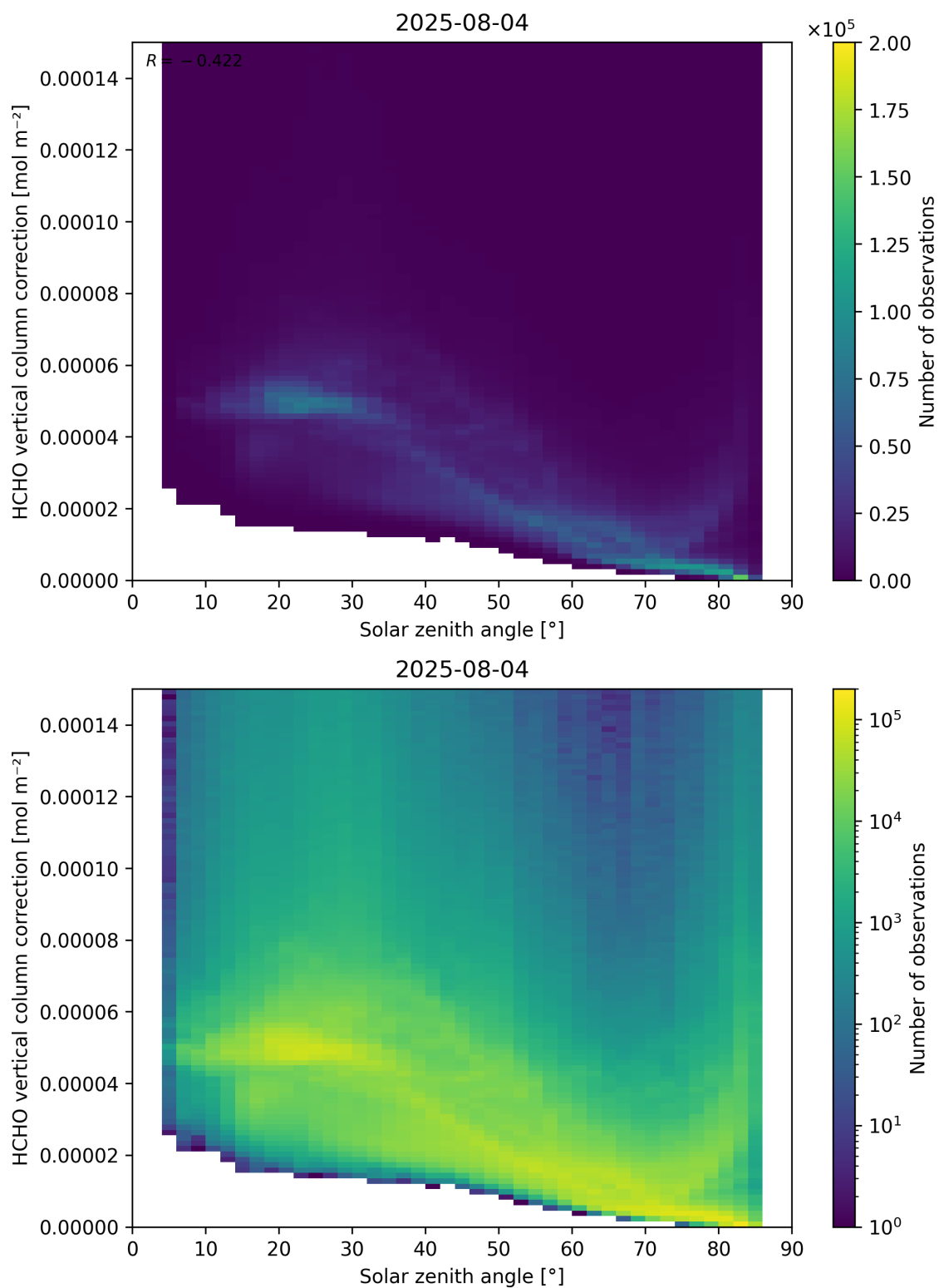
Figure 178: Scatter density plot of “Solar zenith angle” against “HCHO vertical column correction” for 2025-08-04 to 2025-08-05.
