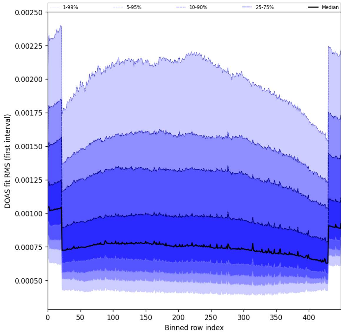
Figure 60: Along track statistics of “DOAS fit RMS (first interval)” for 2025-08-04 to 2025-08-05
