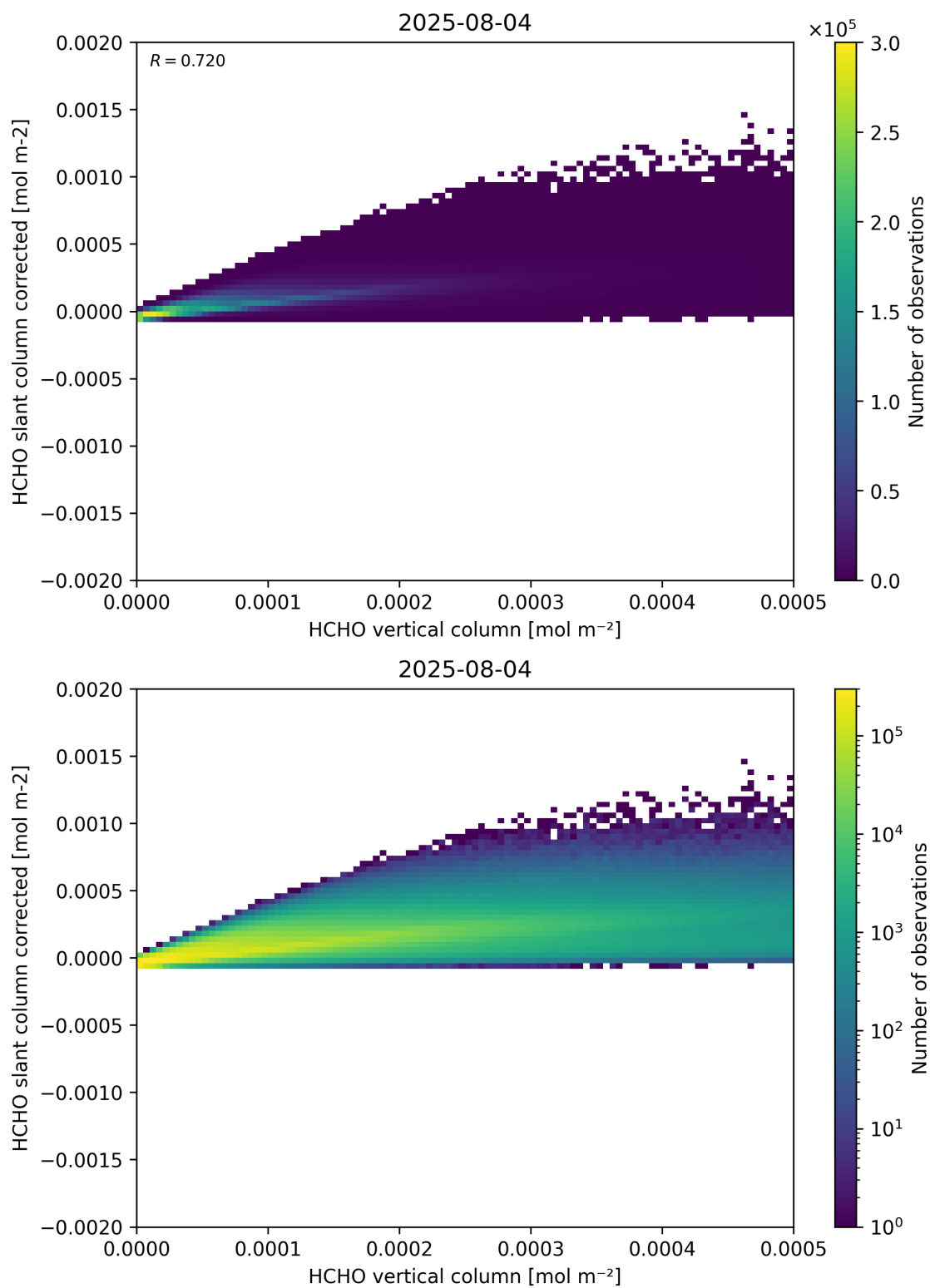
Figure 127: Scatter density plot of “HCHO vertical column” against “HCHO slant column corrected” for 2025-08-04 to 2025-08-05.
