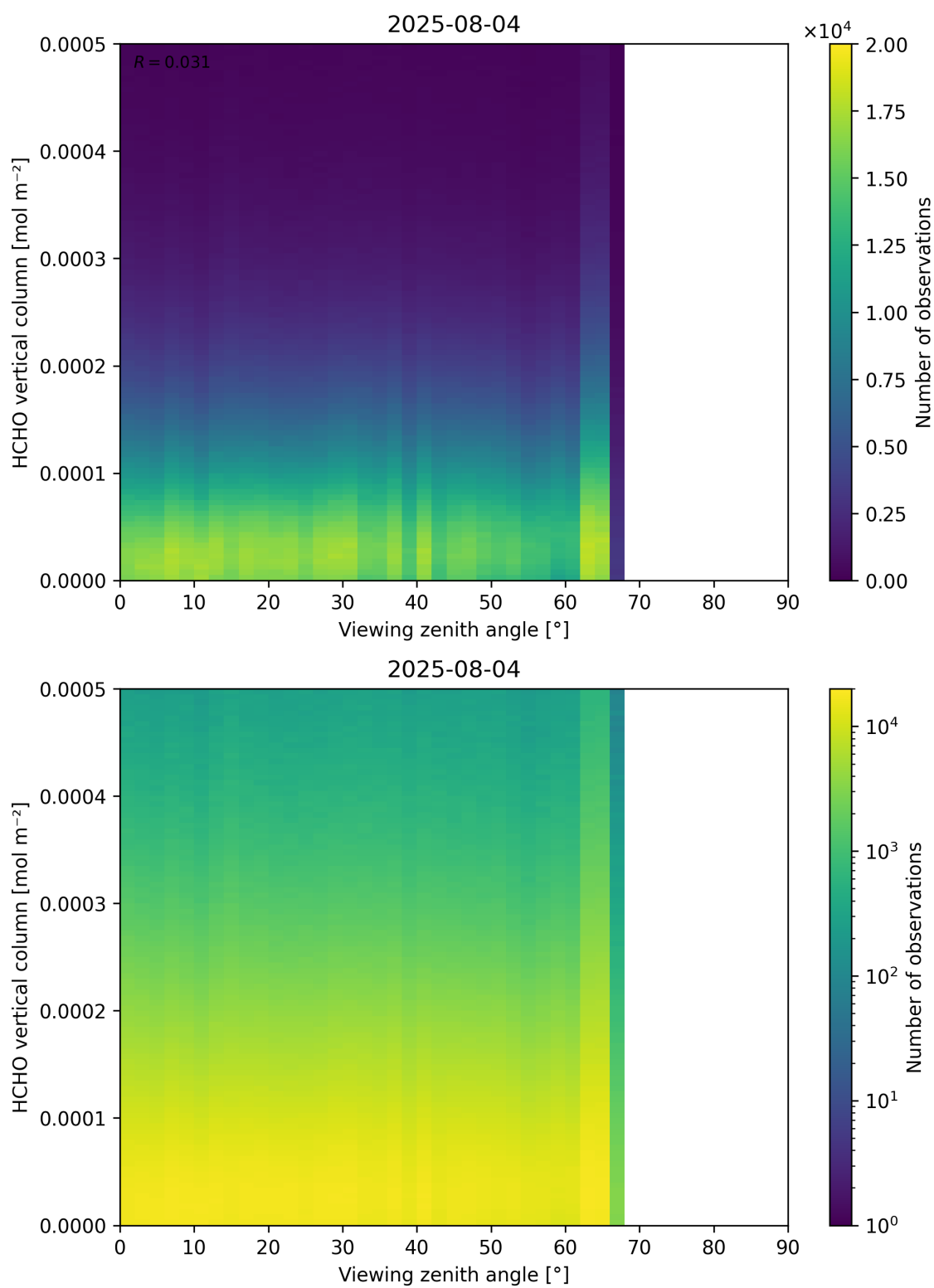
Figure 192: Scatter density plot of “Viewing zenith angle” against “HCHO vertical column” for 2025-08-04 to 2025-08-05.
