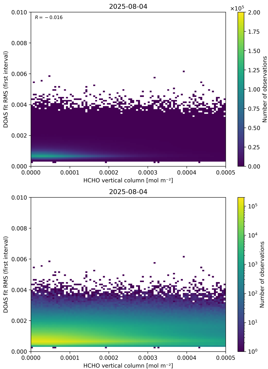
Figure 123: Scatter density plot of “HCHO vertical column” against “DOAS fit RMS (first interval)” for 2025-08-04 to 2025-08-05.
