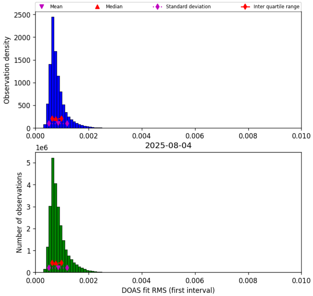
Figure 46: Histogram of “DOAS fit RMS (first interval)” for 2025-08-04 to 2025-08-05
