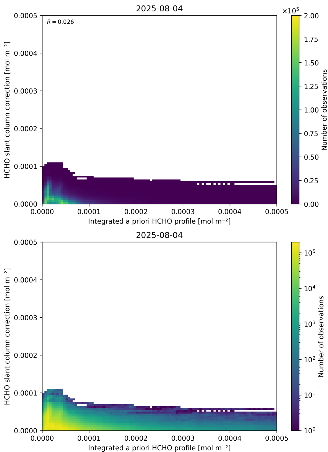
Figure 152: Scatter density plot of “Integrated a priori HCHO profile” against “HCHO slant column correction” for 2025-08-04 to 2025-08-05.
