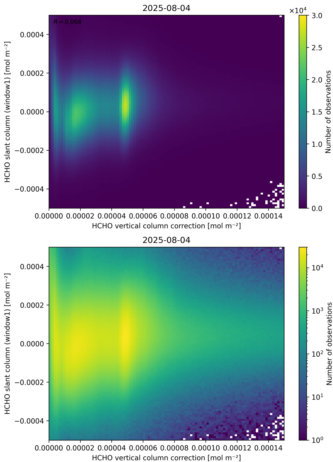
Figure 118: Scatter density plot of “HCHO vertical column correction” against “HCHO slant column (window1)” for 2025-08-04 to 2025-08-05.
