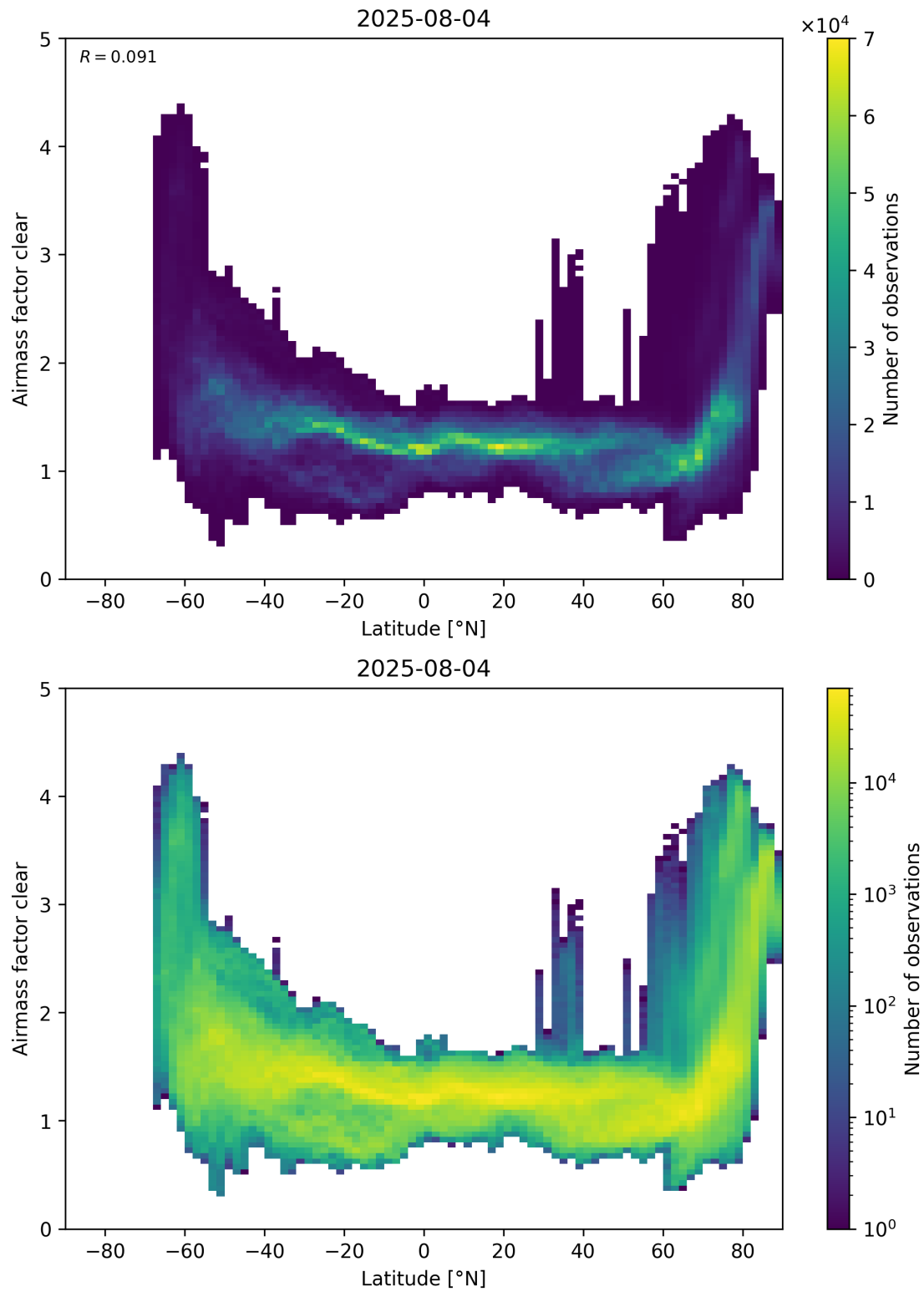
Figure 156: Scatter density plot of “Latitude” against “Airmass factor clear” for 2025-08-04 to 2025-08-05.
