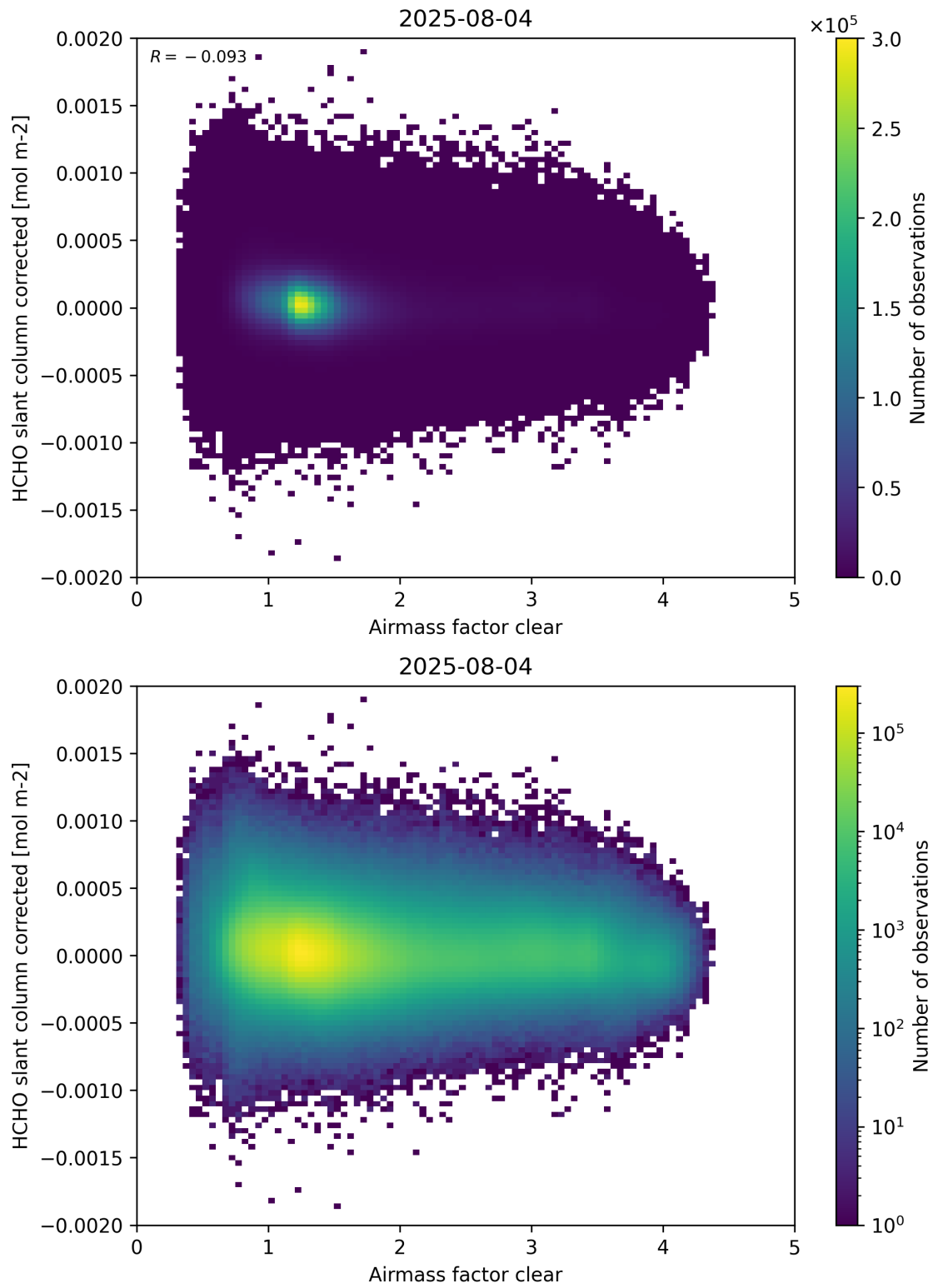
Figure 74: Scatter density plot of “Airmass factor clear” against “HCHO slant column corrected” for 2025-08-04 to 2025-08-05.
