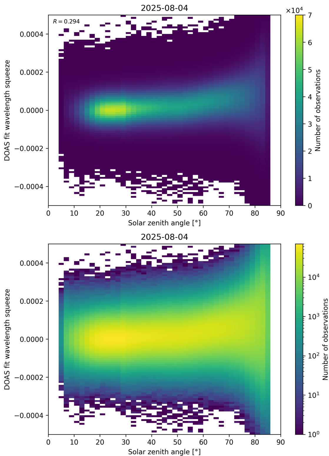
Figure 169: Scatter density plot of “Solar zenith angle” against “DOAS fit wavelength squeeze” for 2025-08-04 to 2025-08-05.
