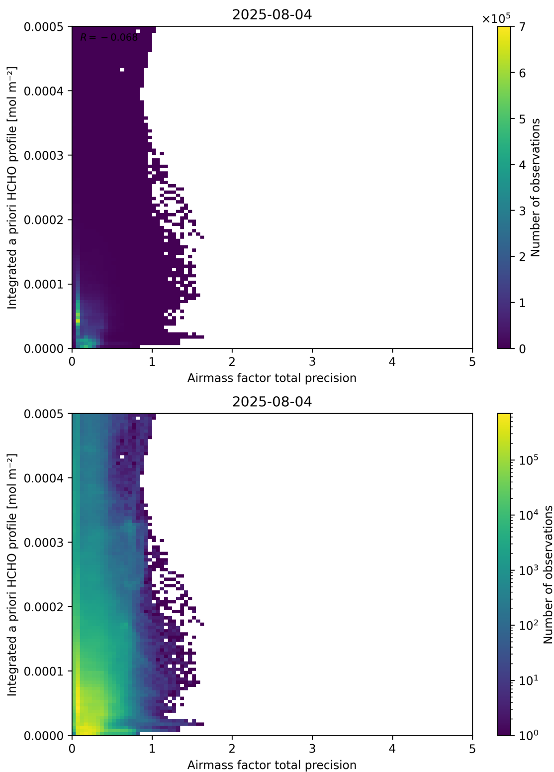
Figure 111: Scatter density plot of “Airmass factor total precision” against “Integrated a priori HCHO profile” for 2025-08-04 to 2025-08-05.
