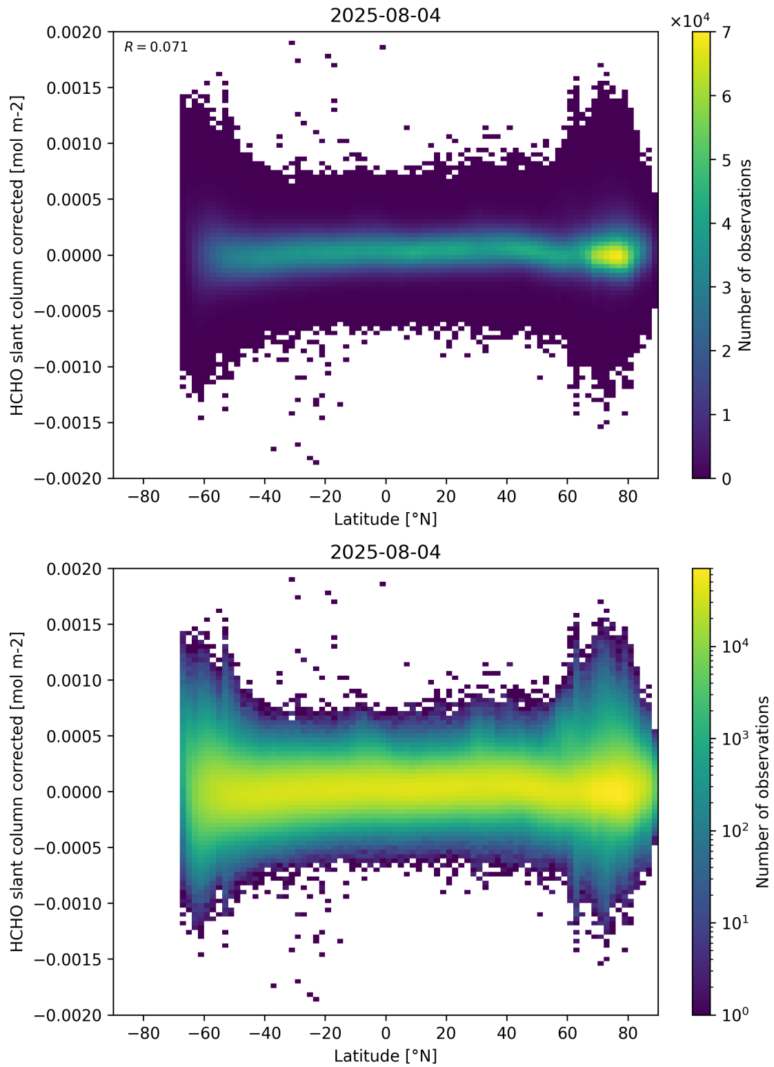
Figure 157: Scatter density plot of “Latitude” against “HCHO slant column corrected” for 2025-08-04 to 2025-08-05.
