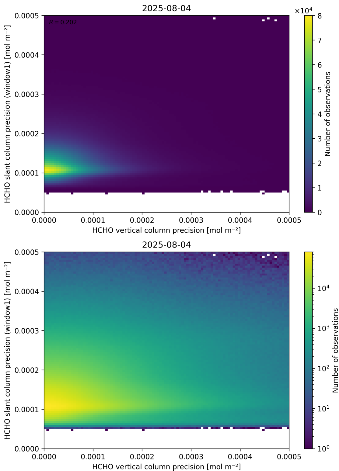
Figure 143: Scatter density plot of “HCHO vertical column precision” against “HCHO slant column precision (window1)” for 2025-08-04 to 2025-08-05.
