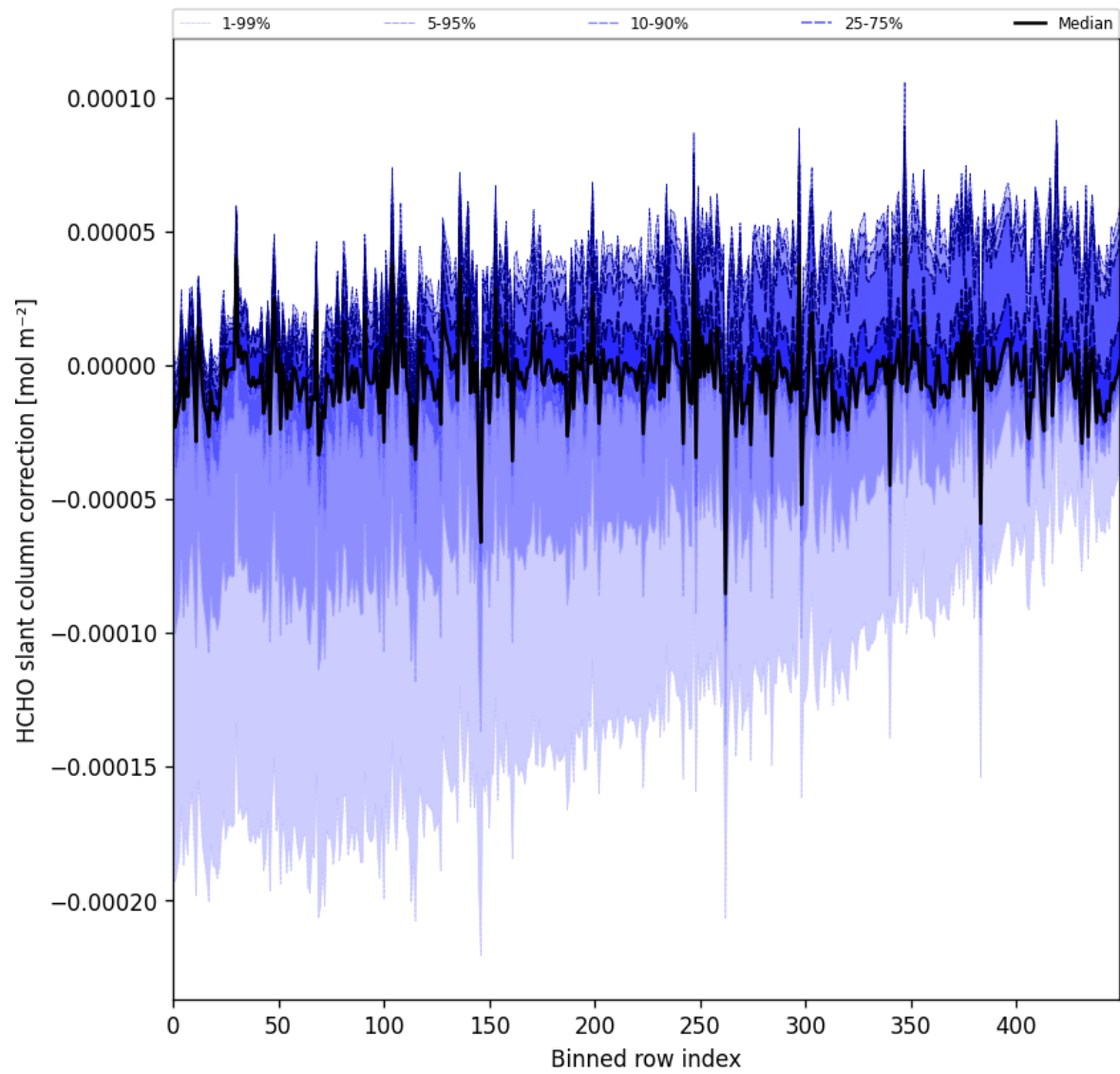
Figure 61: Along track statistics of “HCHO slant column correction” for 2025-08-04 to 2025-08-05
