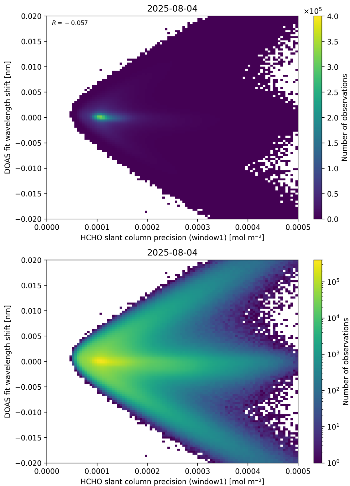
Figure 89: Scatter density plot of “HCHO slant column precision (window1)” against “DOAS fit wavelength shift” for 2025-08-04 to 2025-08-05.
