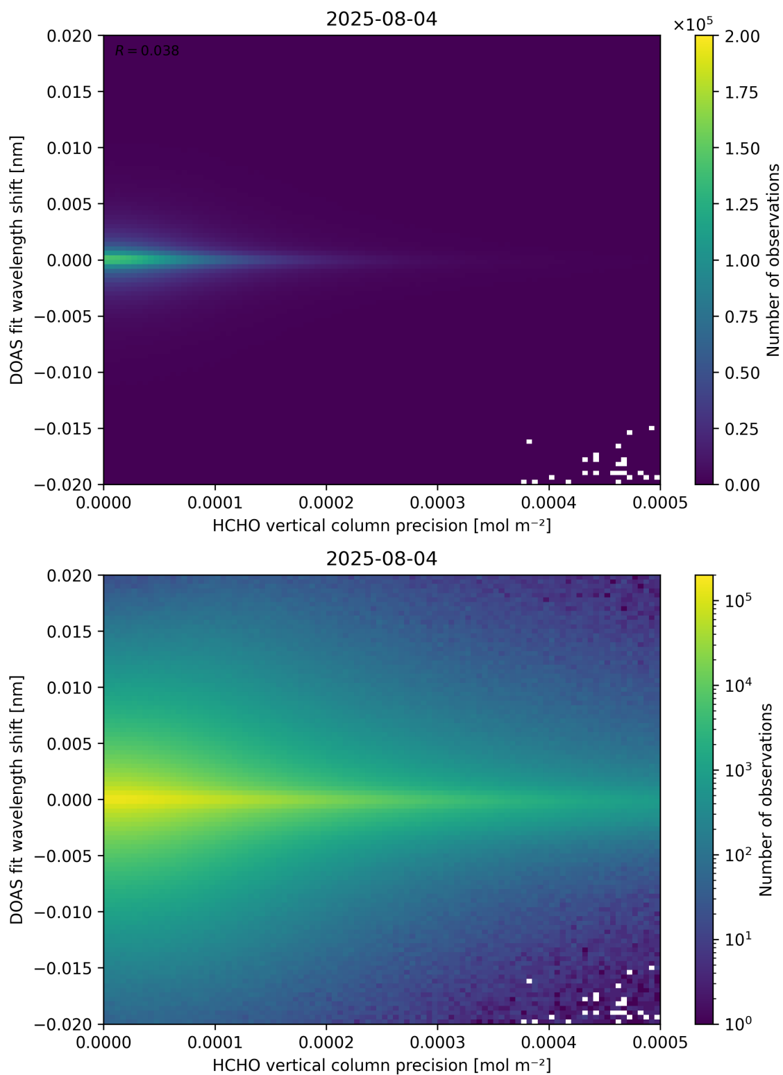
Figure 137: Scatter density plot of “HCHO vertical column precision” against “DOAS fit wavelength shift” for 2025-08-04 to 2025-08-05.
