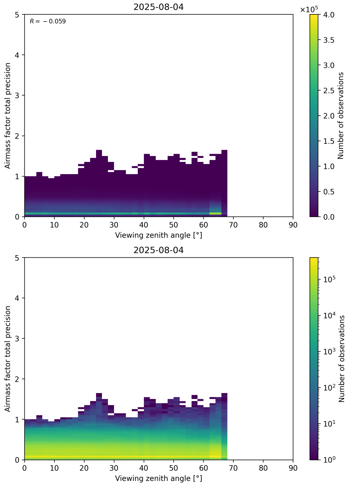
Figure 191: Scatter density plot of “Viewing zenith angle” against “Airmass factor total precision” for 2025-08-04 to 2025-08-05.
