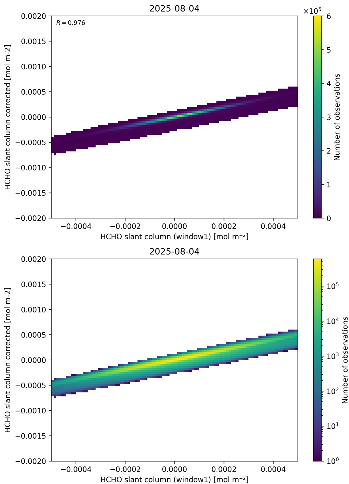
Figure 82: Scatter density plot of “HCHO slant column (window1)” against “HCHO slant column corrected” for 2025-08-04 to 2025-08-05.
