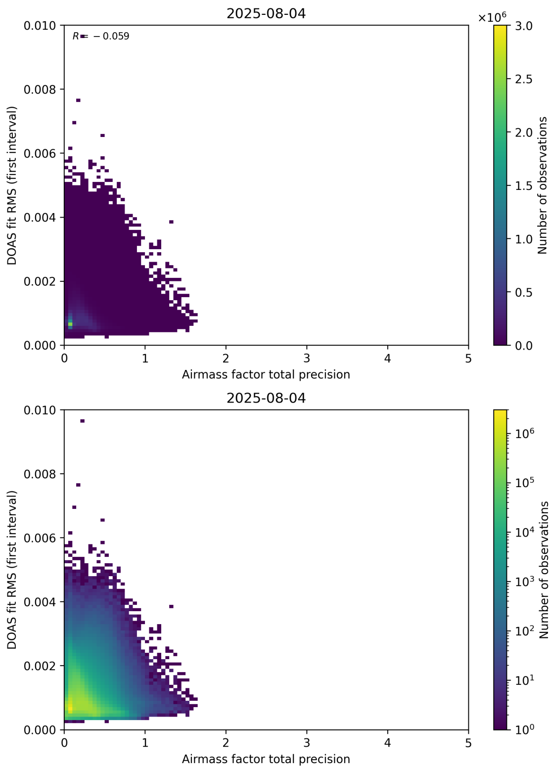
Figure 105: Scatter density plot of “Airmass factor total precision” against “DOAS fit RMS (first interval)” for 2025-08-04 to 2025-08-05.
