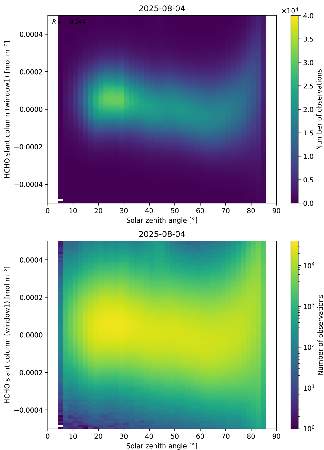
Figure 173: Scatter density plot of “Solar zenith angle” against “HCHO slant column (window1)” for 2025-08-04 to 2025-08-05.
