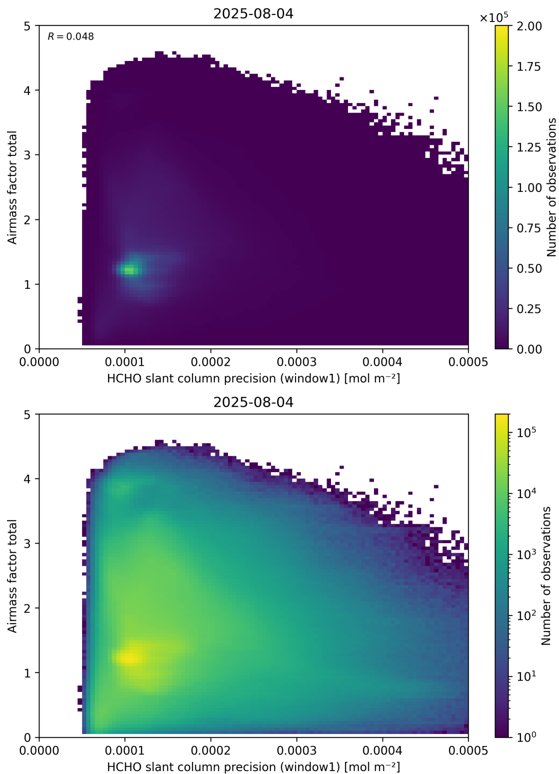
Figure 94: Scatter density plot of “HCHO slant column precision (window1)” against “Airmass factor total” for 2025-08-04 to 2025-08-05.
