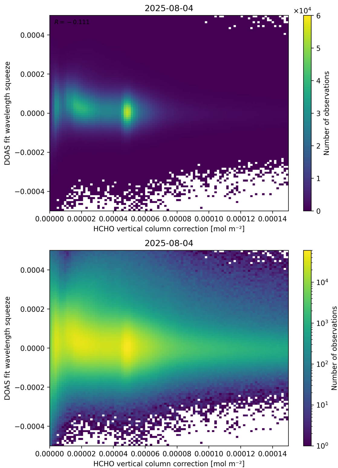
Figure 114: Scatter density plot of “HCHO vertical column correction” against “DOAS fit wavelength squeeze” for 2025-08-04 to 2025-08-05.
