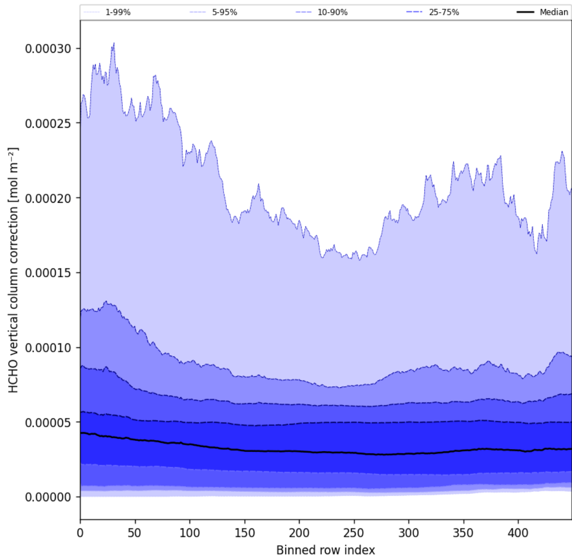
Figure 51: Along track statistics of “HCHO vertical column correction” for 2025-08-04 to 2025-08-05
