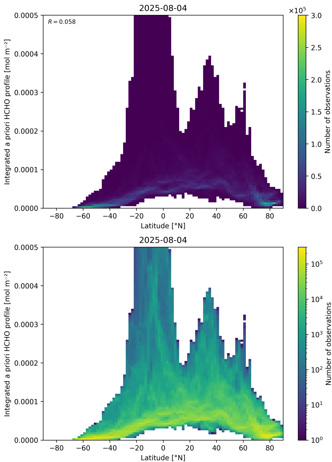
Figure 166: Scatter density plot of “Latitude” against “Integrated a priori HCHO profile” for 2025-08-04 to 2025-08-05.
