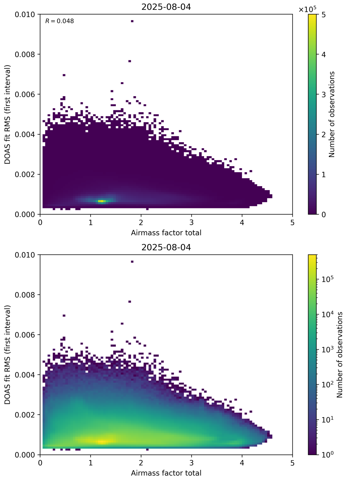
Figure 97: Scatter density plot of “Airmass factor total” against “DOAS fit RMS (first interval)” for 2025-08-04 to 2025-08-05.
