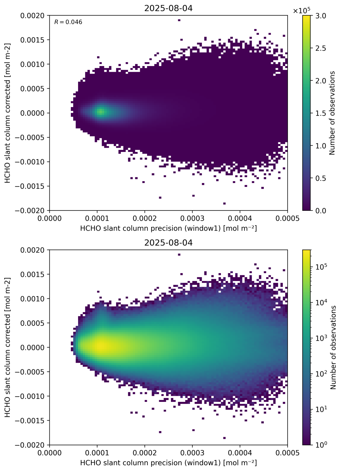
Figure 92: Scatter density plot of “HCHO slant column precision (window1)” against “HCHO slant column corrected” for 2025-08-04 to 2025-08-05.
