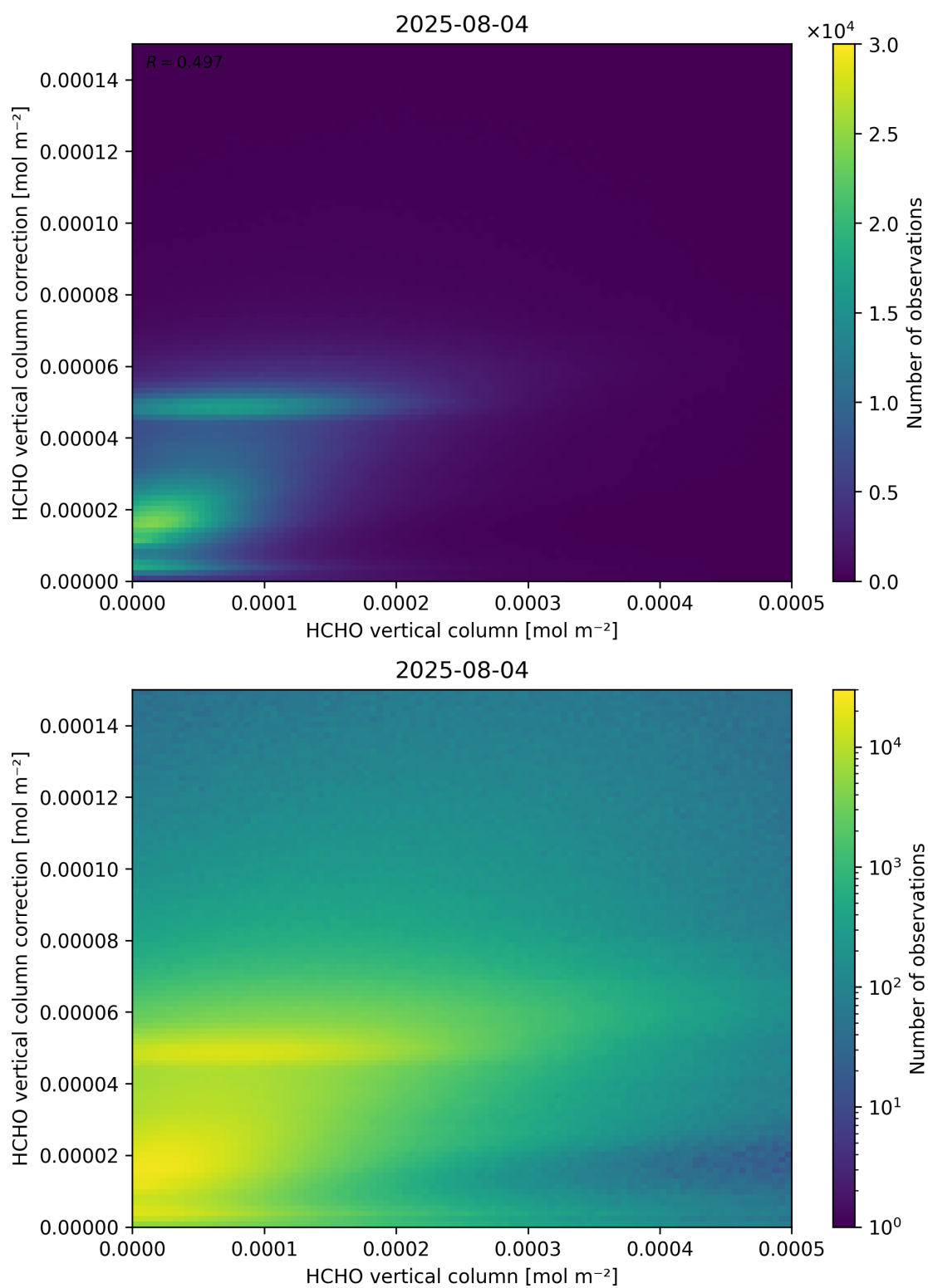
Figure 133: Scatter density plot of “HCHO vertical column” against “HCHO vertical column correction” for 2025-08-04 to 2025-08-05.
