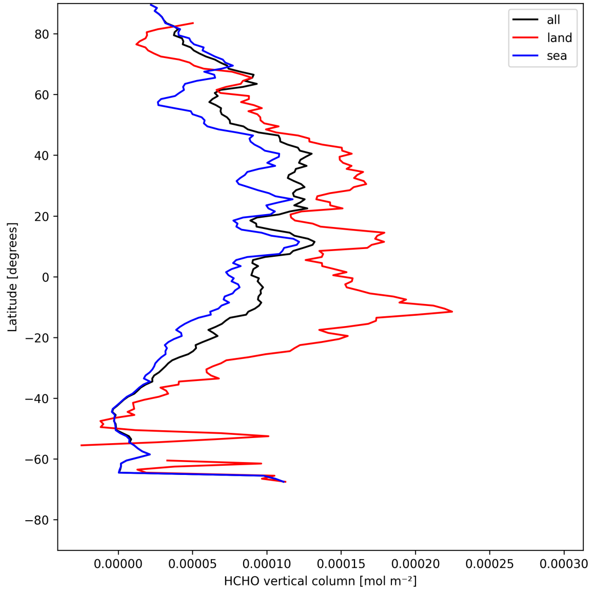
Figure 21: Zonal average of “HCHO vertical column” for 2025-08-04 to 2025-08-05.
