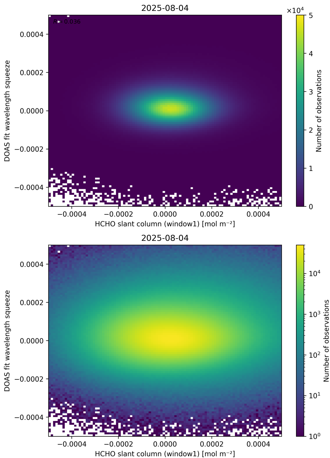
Figure 80: Scatter density plot of “HCHO slant column (window1)” against “DOAS fit wavelength squeeze” for 2025-08-04 to 2025-08-05.
