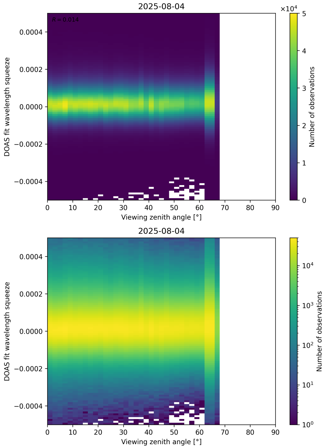
Figure 184: Scatter density plot of “Viewing zenith angle” against “DOAS fit wavelength squeeze” for 2025-08-04 to 2025-08-05.
