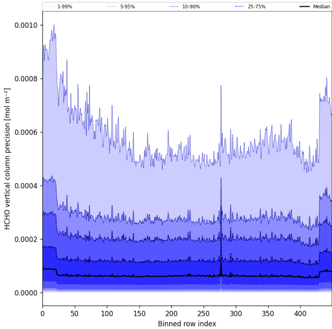
Figure 50: Along track statistics of “HCHO vertical column precision” for 2025-08-04 to 2025-08-05
