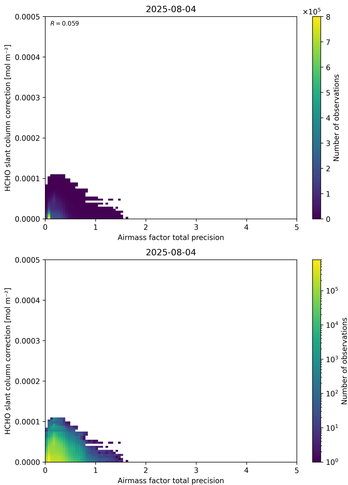
Figure 110: Scatter density plot of “Airmass factor total precision” against “HCHO slant column correction” for 2025-08-04 to 2025-08-05.
