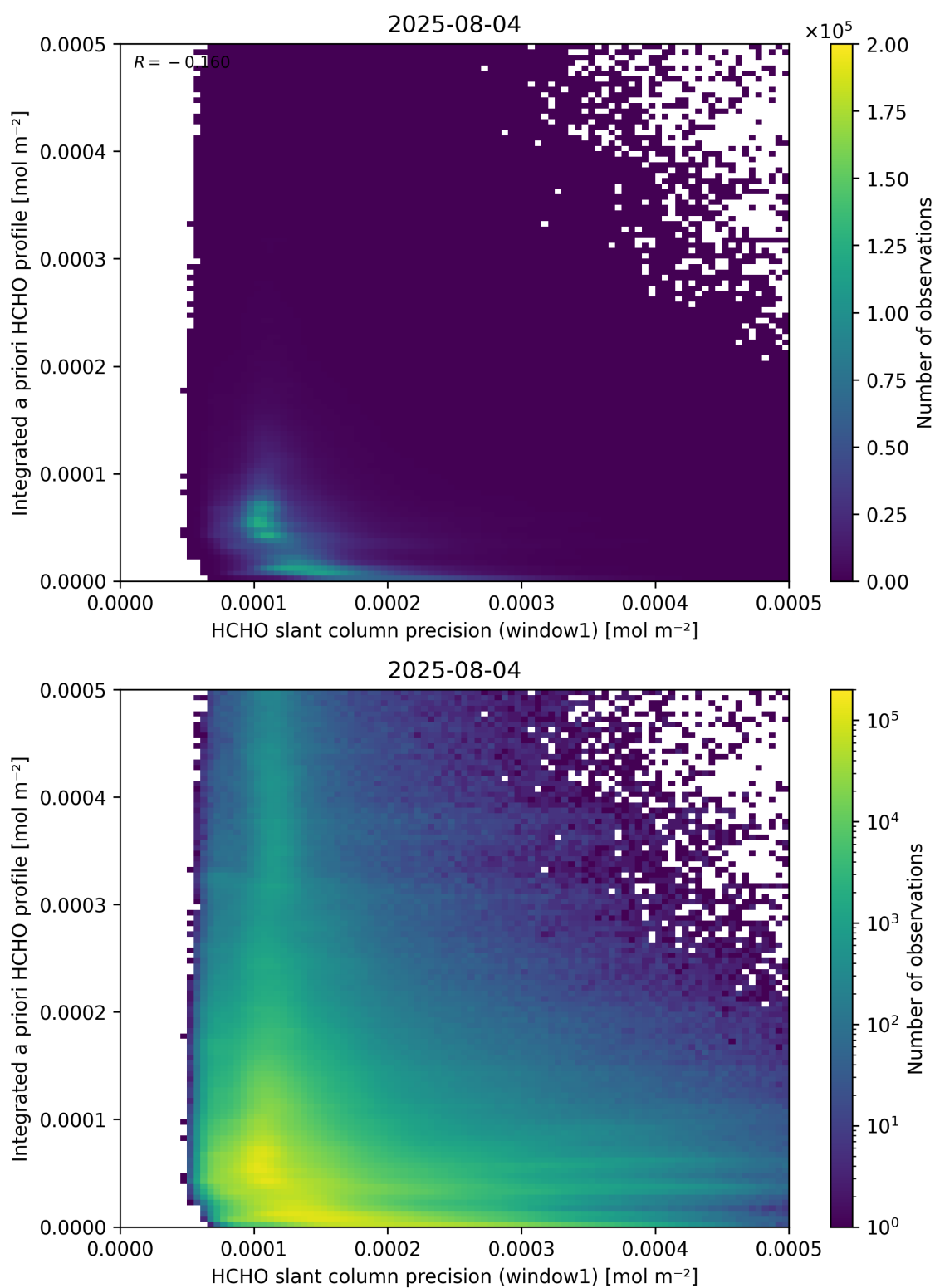
Figure 96: Scatter density plot of “HCHO slant column precision (window1)” against “Integrated a priori HCHO profile” for 2025-08-04 to 2025-08-05.
