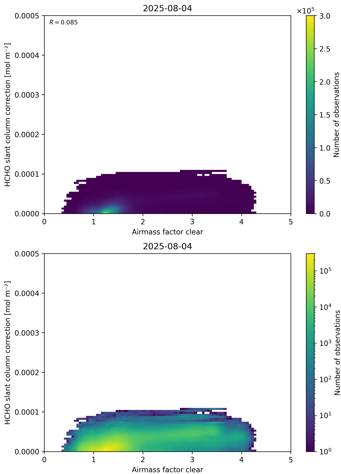
Figure 75: Scatter density plot of “Airmass factor clear” against “HCHO slant column correction” for 2025-08-04 to 2025-08-05.
