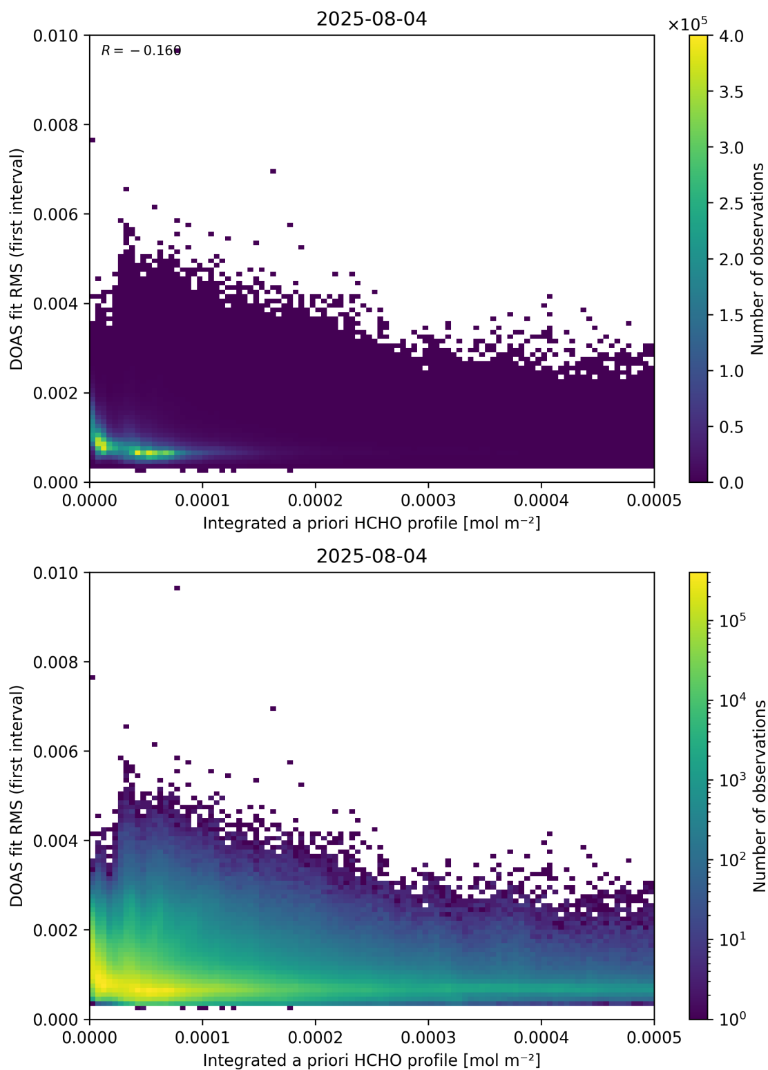
Figure 148: Scatter density plot of “Integrated a priori HCHO profile” against “DOAS fit RMS (first interval)” for 2025-08-04 to 2025-08-05.
