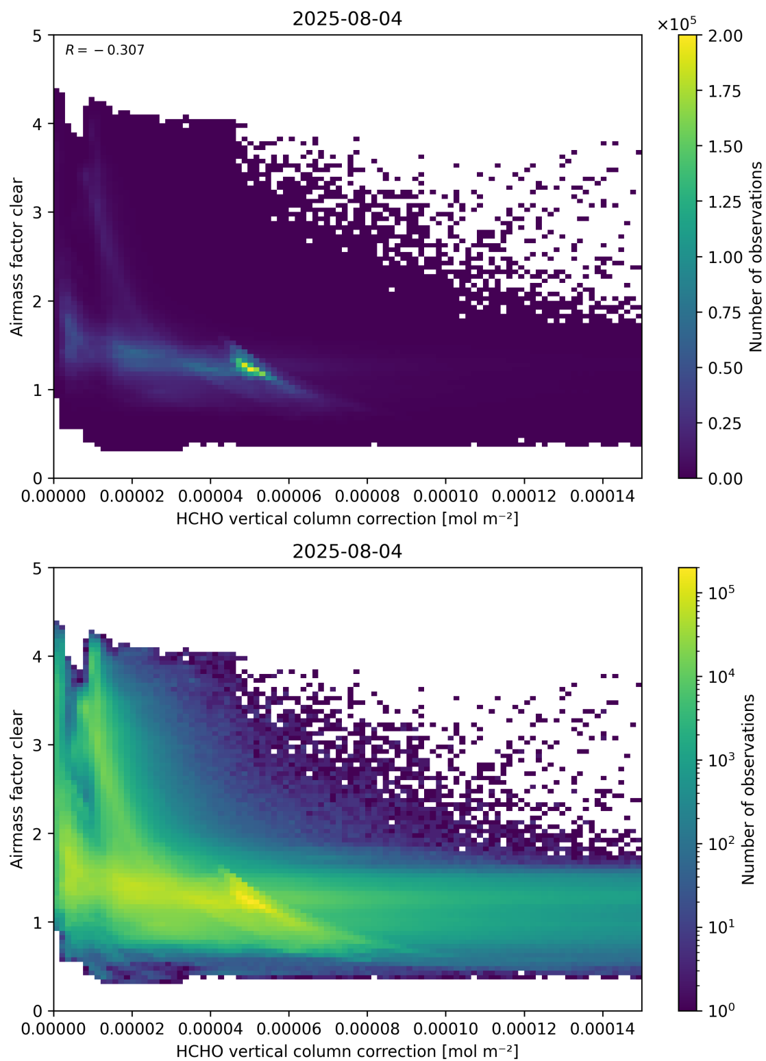
Figure 115: Scatter density plot of “HCHO vertical column correction” against “Airmass factor clear” for 2025-08-04 to 2025-08-05.
