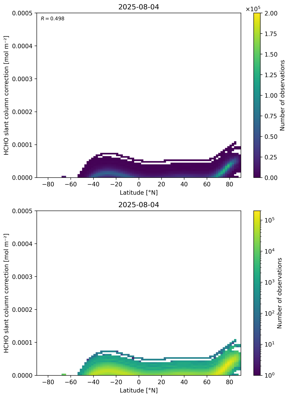
Figure 158: Scatter density plot of “Latitude” against “HCHO slant column correction” for 2025-08-04 to 2025-08-05.
