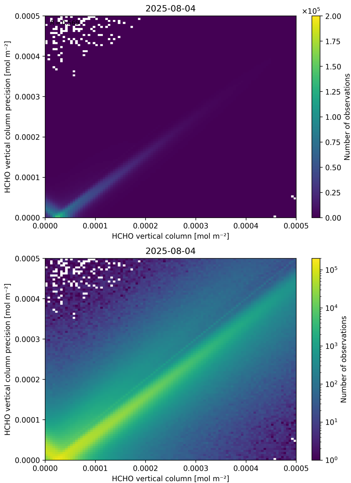
Figure 134: Scatter density plot of “HCHO vertical column” against “HCHO vertical column precision” for 2025-08-04 to 2025-08-05.
