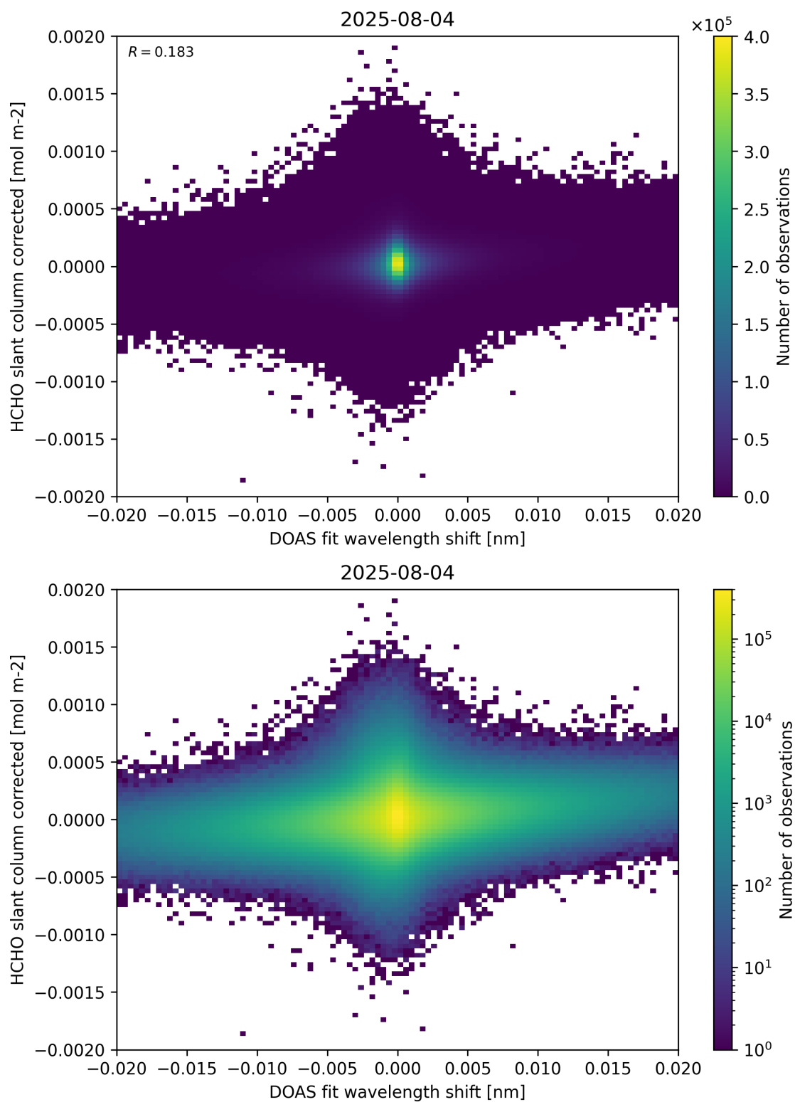
Figure 66: Scatter density plot of “DOAS fit wavelength shift” against “HCHO slant column corrected” for 2025-08-04 to 2025-08-05.
