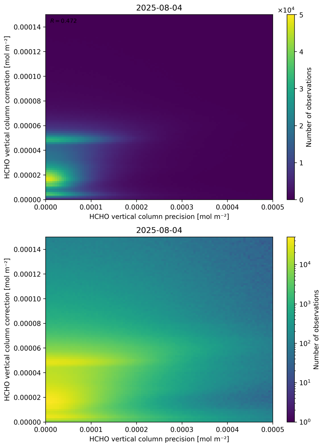
Figure 146: Scatter density plot of “HCHO vertical column precision” against “HCHO vertical column correction” for 2025-08-04 to 2025-08-05.
