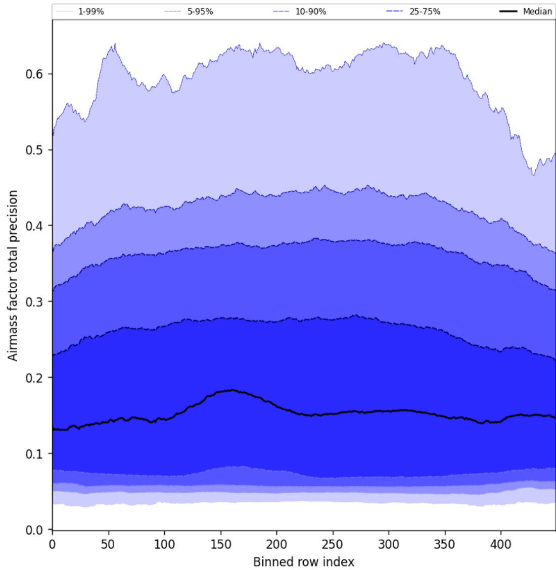
Figure 55: Along track statistics of “Airmass factor total precision” for 2025-08-04 to 2025-08-05
