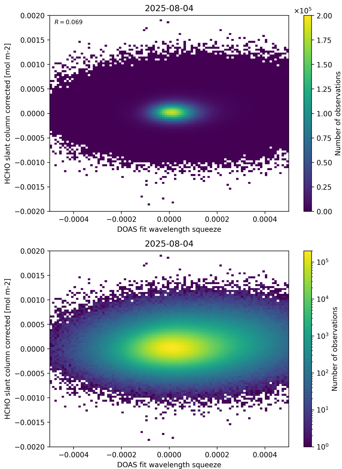
Figure 69: Scatter density plot of “DOAS fit wavelength squeeze” against “HCHO slant column corrected” for 2025-08-04 to 2025-08-05.
