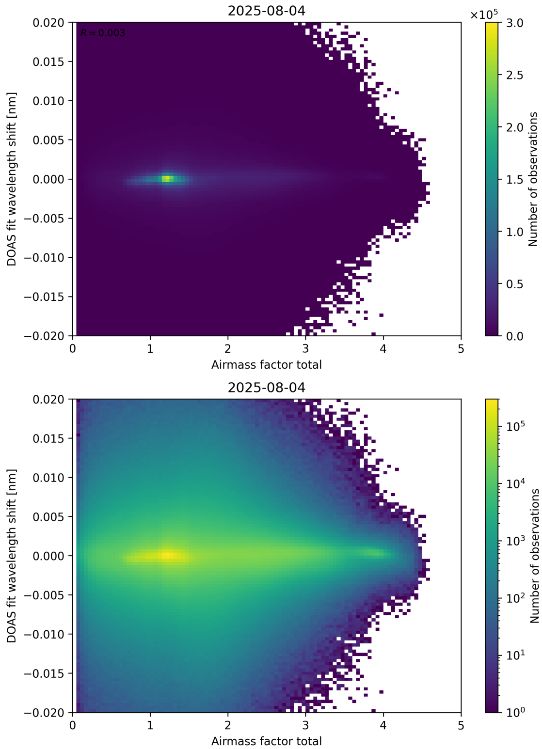
Figure 98: Scatter density plot of “Airmass factor total” against “DOAS fit wavelength shift” for 2025-08-04 to 2025-08-05.
