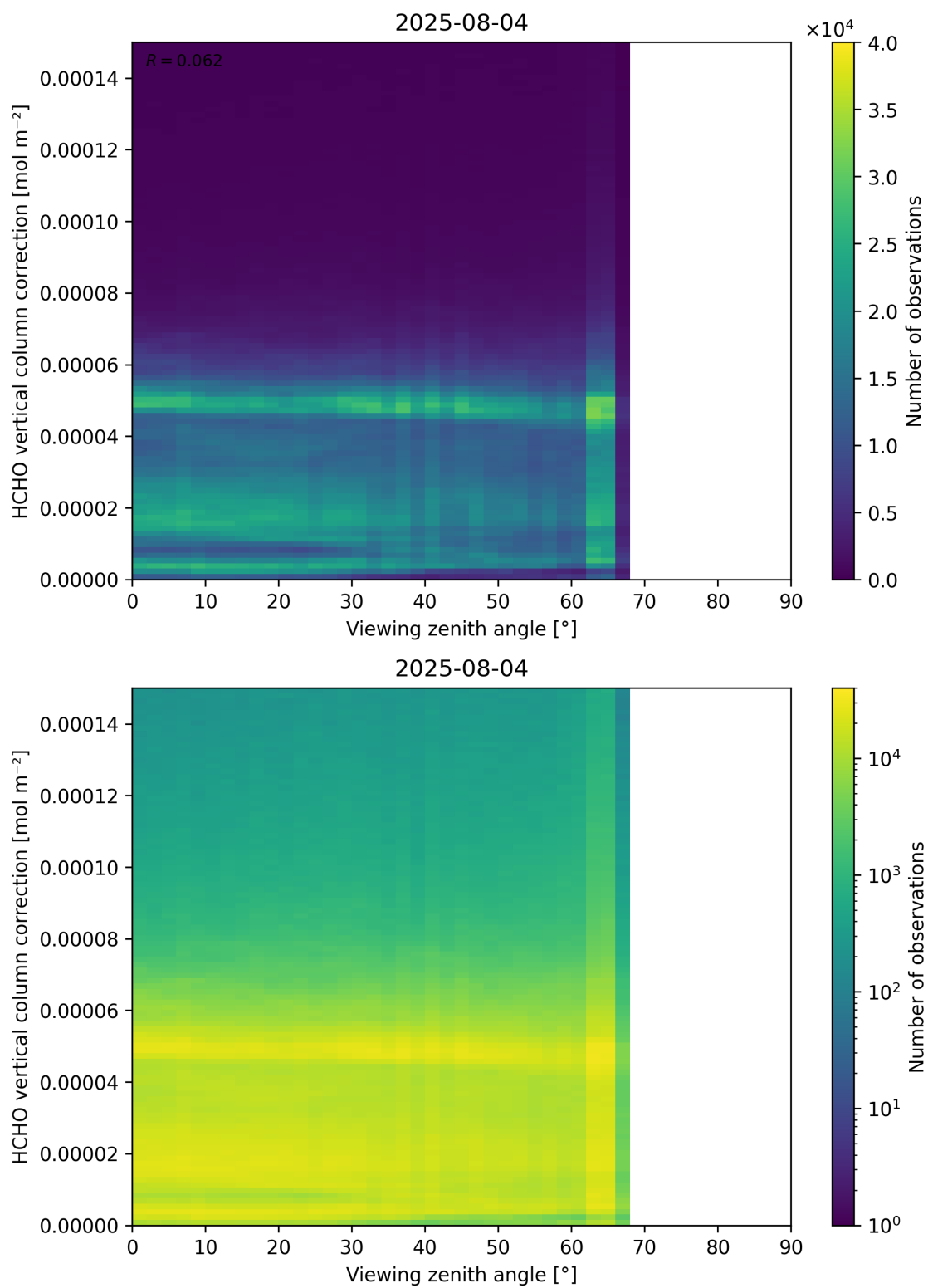
Figure 193: Scatter density plot of “Viewing zenith angle” against “HCHO vertical column correction” for 2025-08-04 to 2025-08-05.
