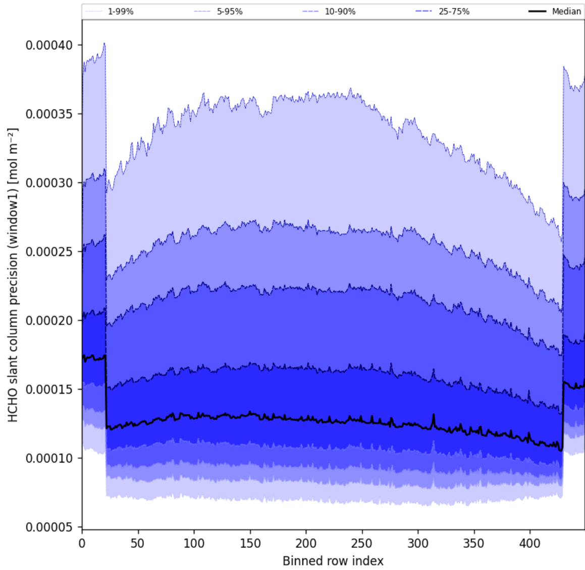
Figure 53: Along track statistics of “HCHO slant column precision (window1)” for 2025-08-04 to 2025-08-05
