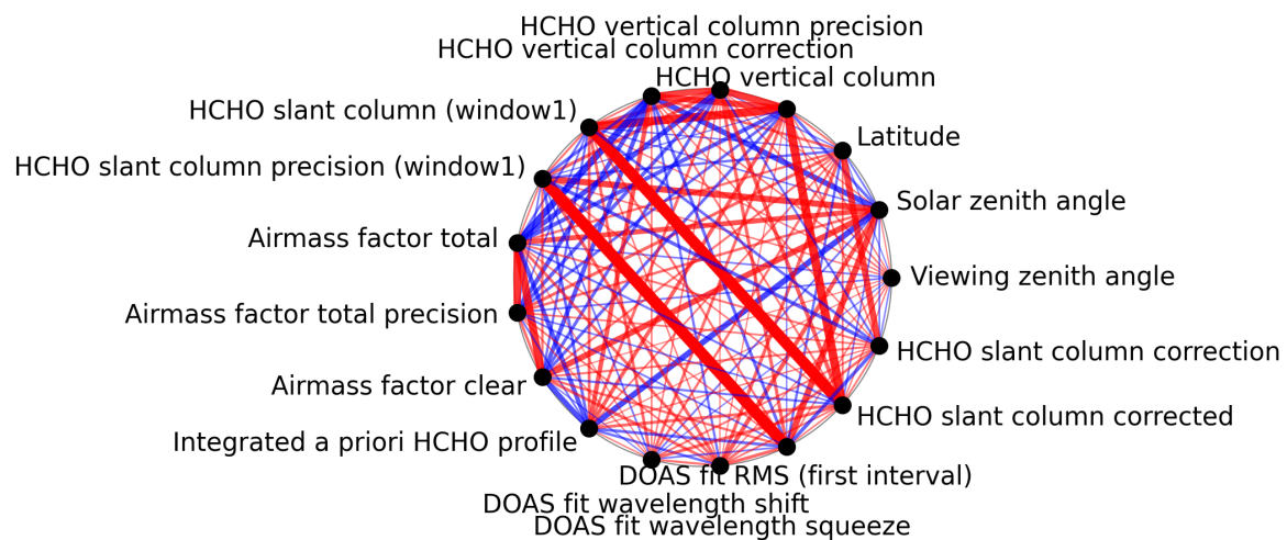
Figure 1: Map of correlation graph for 2025-08-04 to 2025-08-05.
