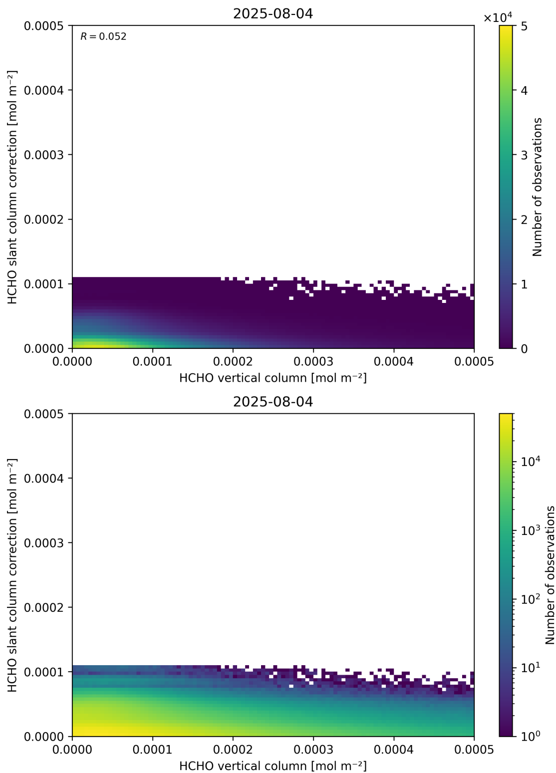
Figure 128: Scatter density plot of “HCHO vertical column” against “HCHO slant column correction” for 2025-08-04 to 2025-08-05.
