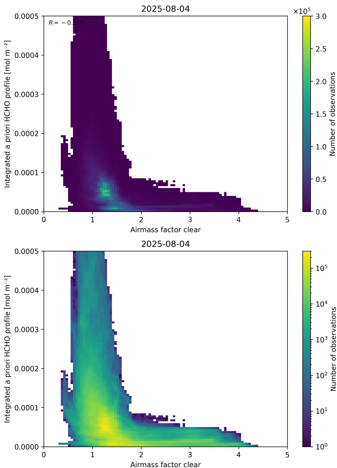
Figure 76: Scatter density plot of “Airmass factor clear” against “Integrated a priori HCHO profile” for 2025-08-04 to 2025-08-05.
