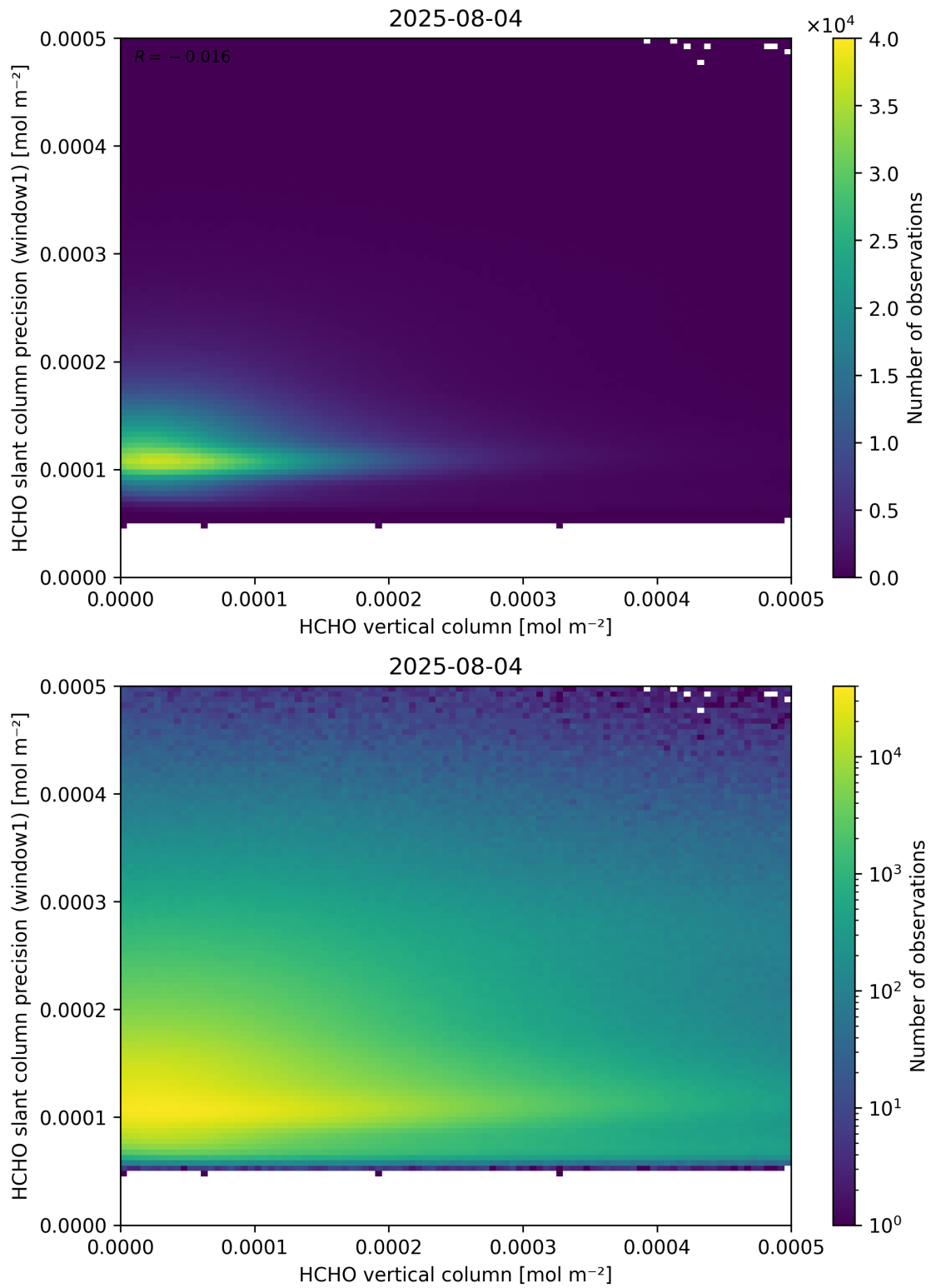
Figure 130: Scatter density plot of “HCHO vertical column” against “HCHO slant column precision (window1)” for 2025-08-04 to 2025-08-05.
