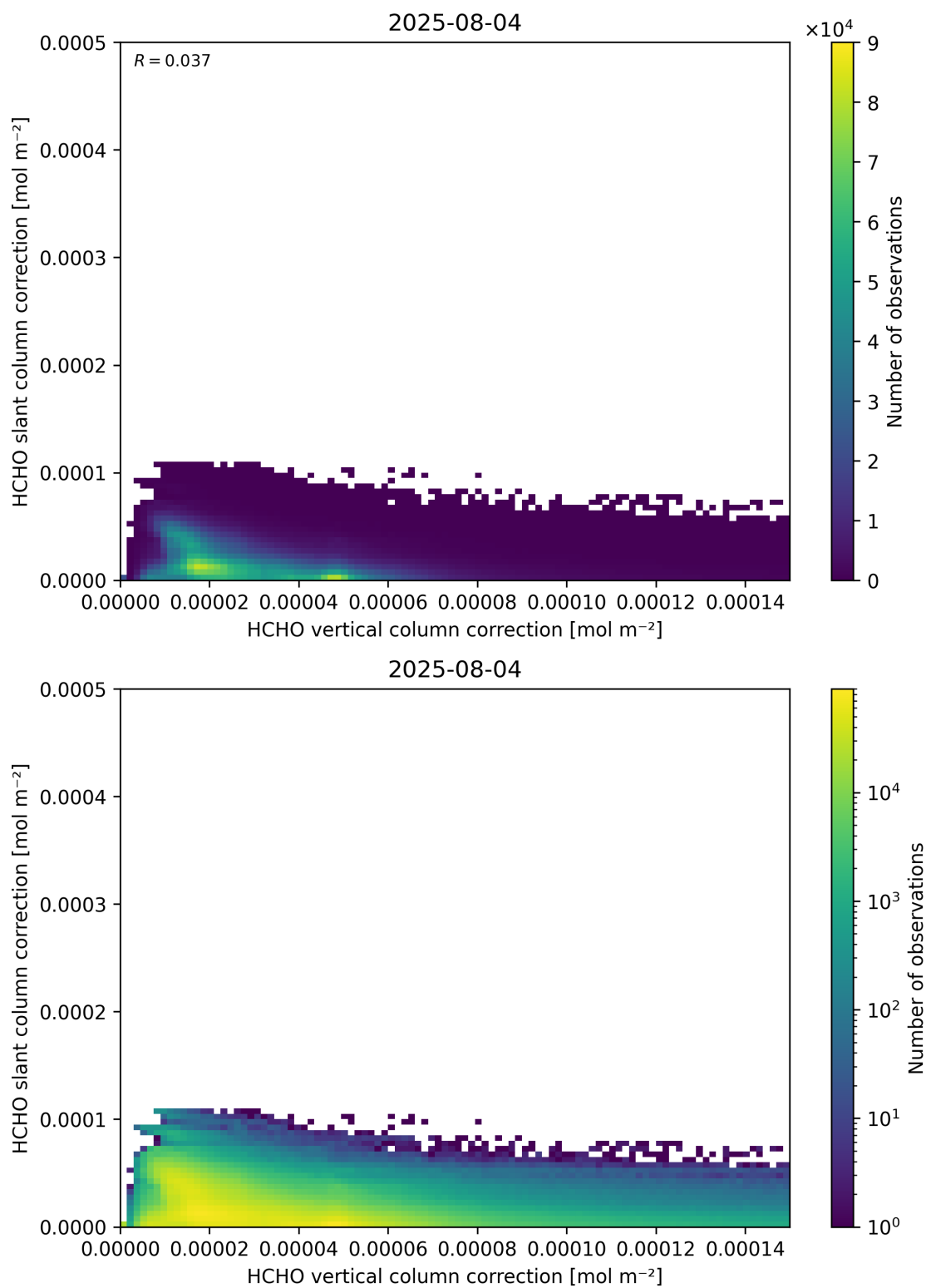
Figure 117: Scatter density plot of “HCHO vertical column correction” against “HCHO slant column correction” for 2025-08-04 to 2025-08-05.
