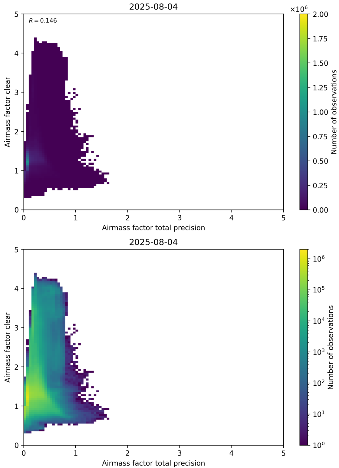
Figure 108: Scatter density plot of “Airmass factor total precision” against “Airmass factor clear” for 2025-08-04 to 2025-08-05.
