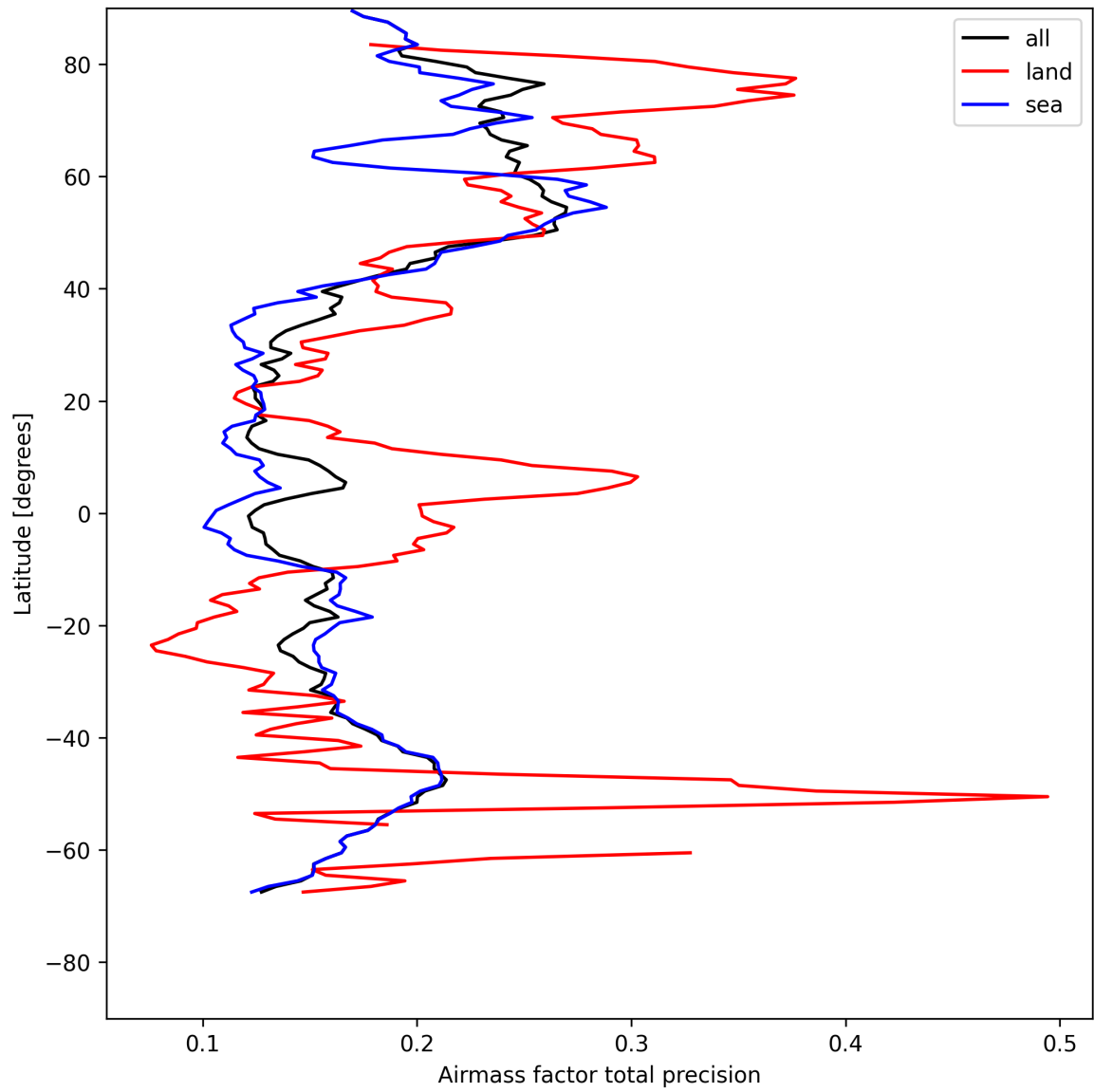
Figure 27: Zonal average of “Airmass factor total precision” for 2025-08-04 to 2025-08-05.
