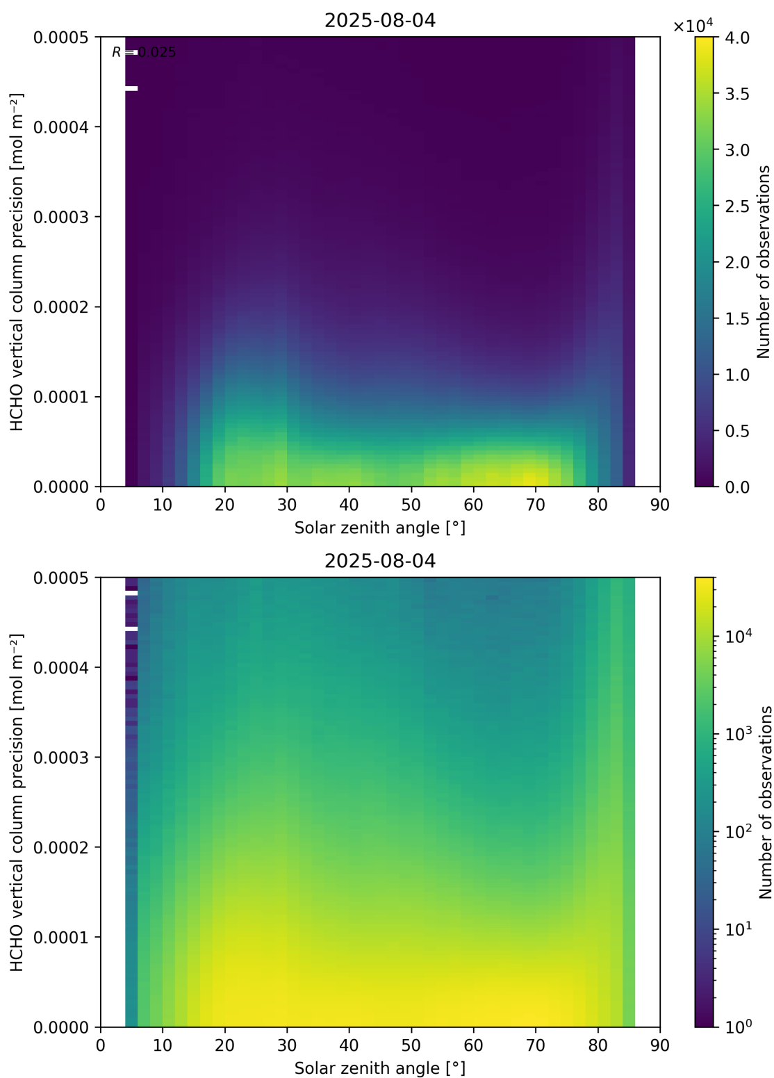
Figure 179: Scatter density plot of “Solar zenith angle” against “HCHO vertical column precision” for 2025-08-04 to 2025-08-05.
