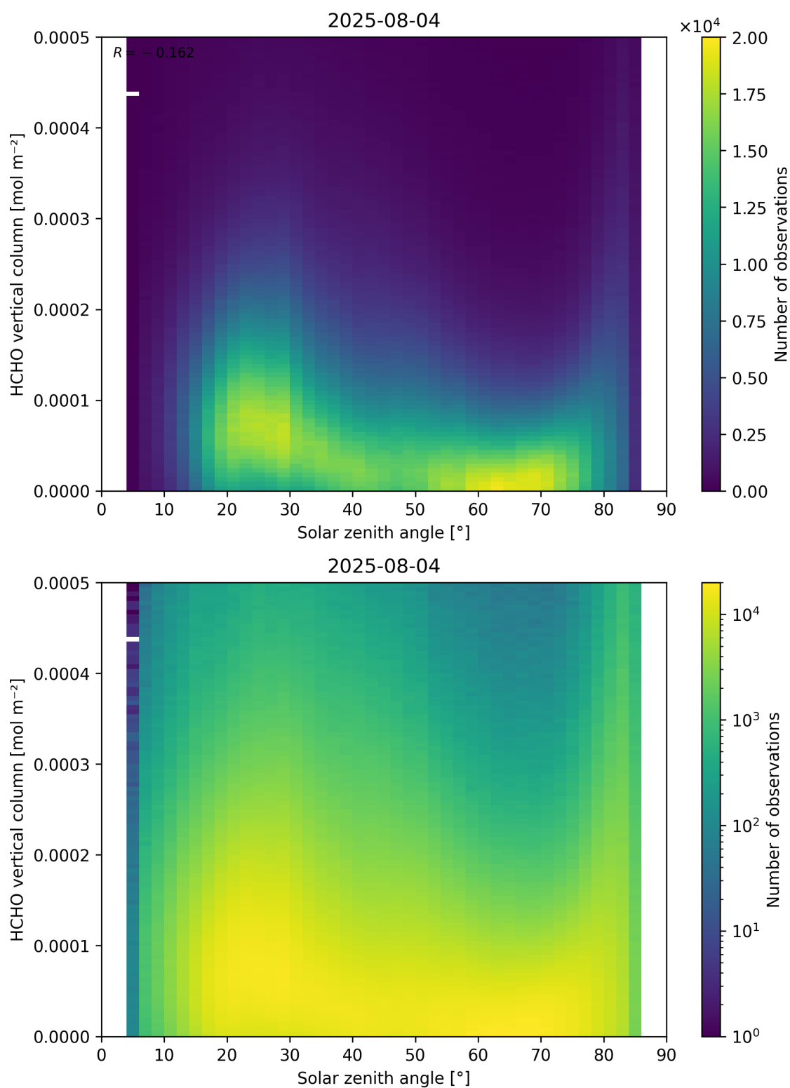
Figure 177: Scatter density plot of “Solar zenith angle” against “HCHO vertical column” for 2025-08-04 to 2025-08-05.
