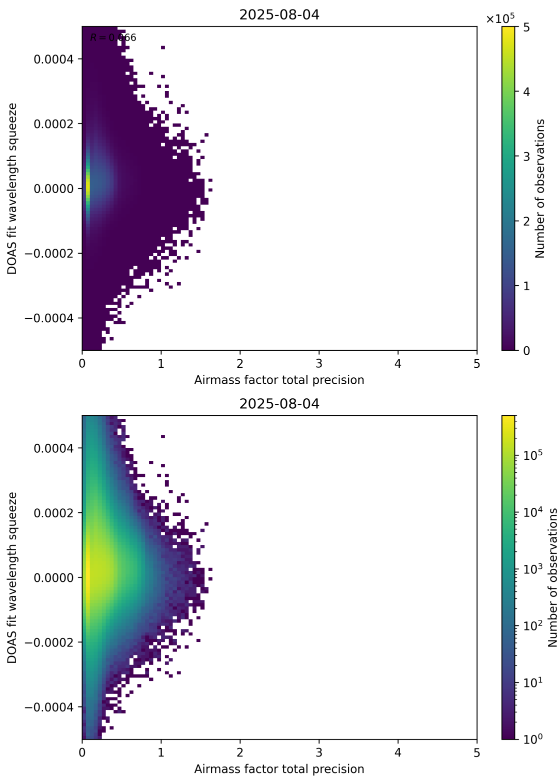
Figure 107: Scatter density plot of “Airmass factor total precision” against “DOAS fit wavelength squeeze” for 2025-08-04 to 2025-08-05.
