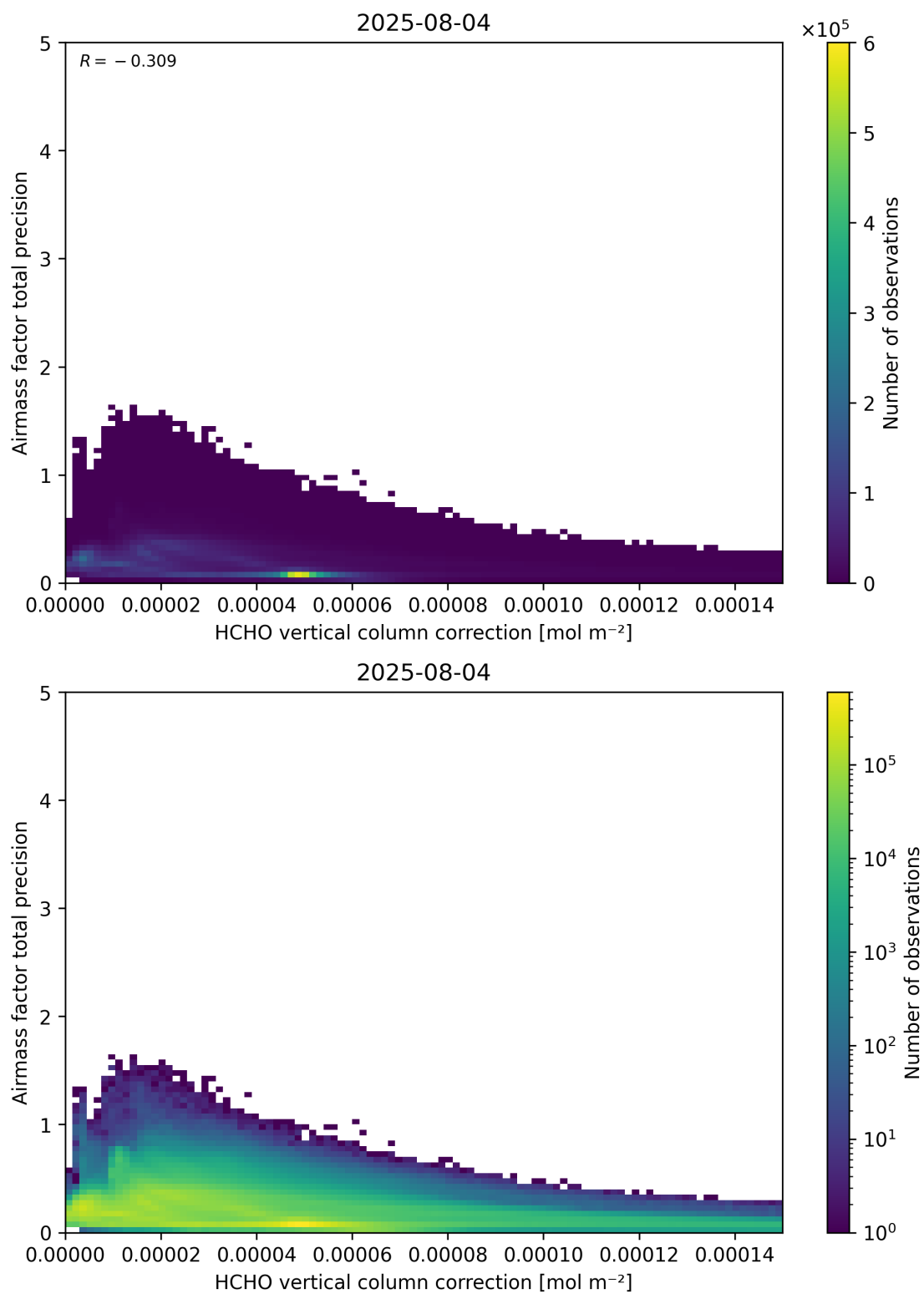
Figure 121: Scatter density plot of “HCHO vertical column correction” against “Airmass factor total precision” for 2025-08-04 to 2025-08-05.
