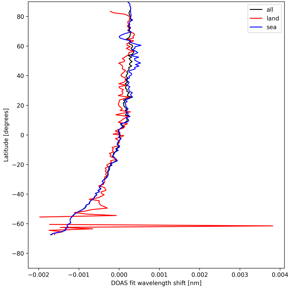
Figure 30: Zonal average of "DOAS fit wavelength shift" for 2025-08-04 to 2025-08-05.
