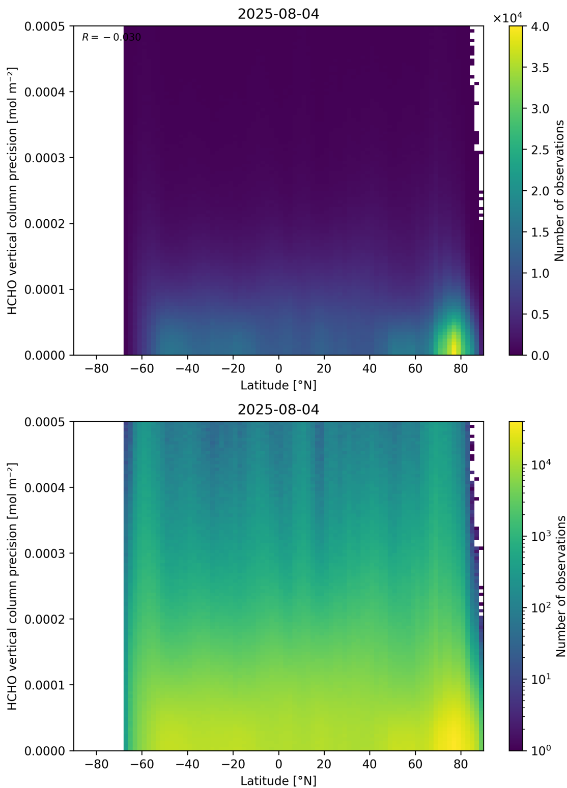
Figure 165: Scatter density plot of “Latitude” against “HCHO vertical column precision” for 2025-08-04 to 2025-08-05.
