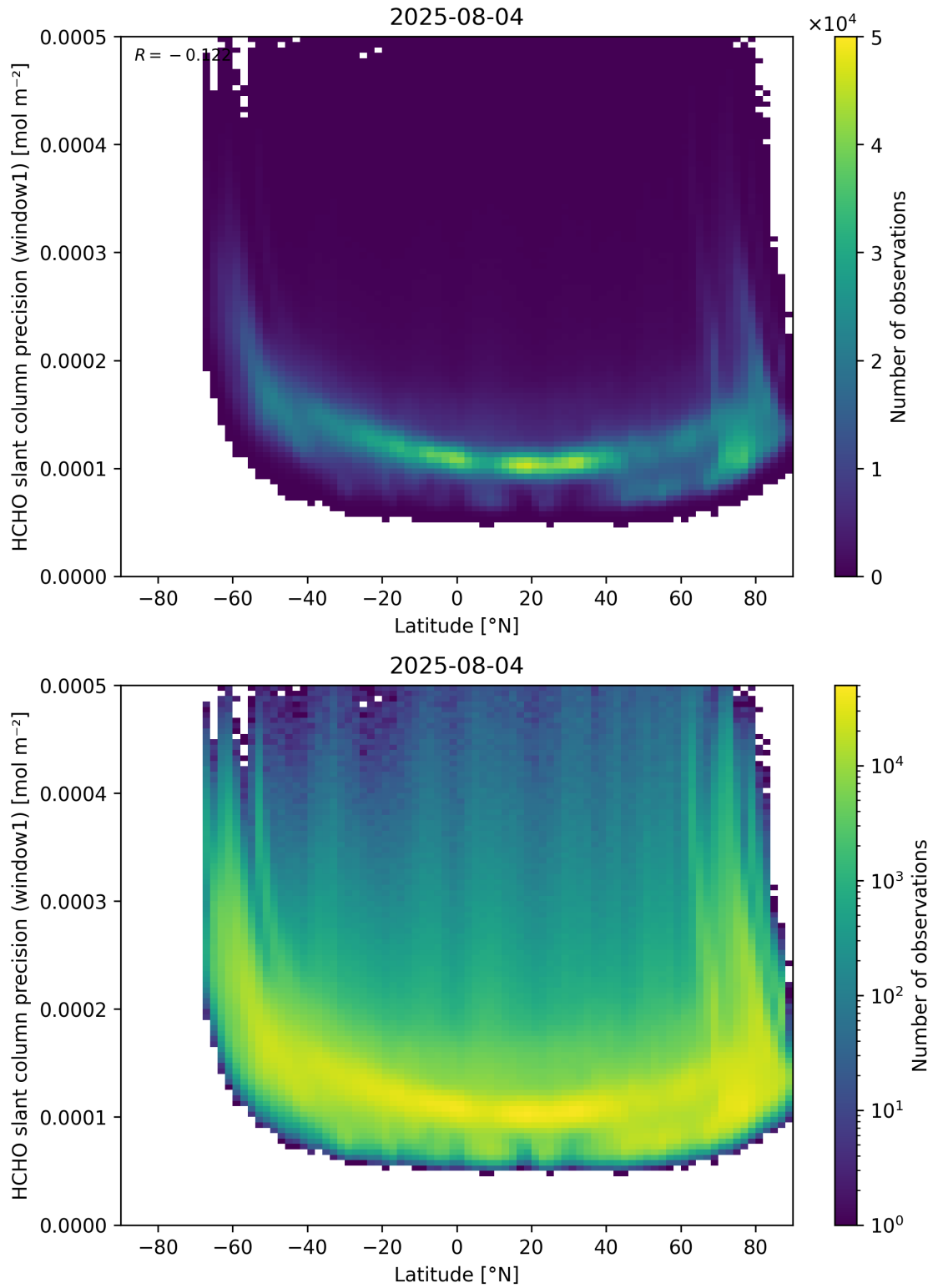
Figure 160: Scatter density plot of “Latitude” against “HCHO slant column precision (window1)” for 2025-08-04 to 2025-08-05.
