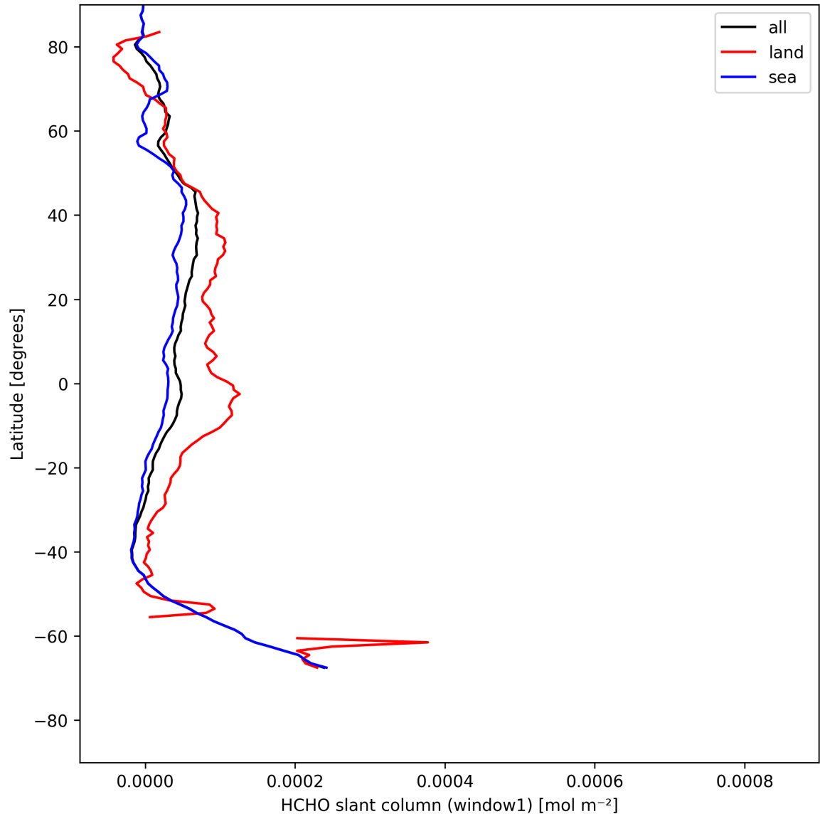
Figure 24: Zonal average of “HCHO slant column (window1)” for 2025-08-04 to 2025-08-05.
