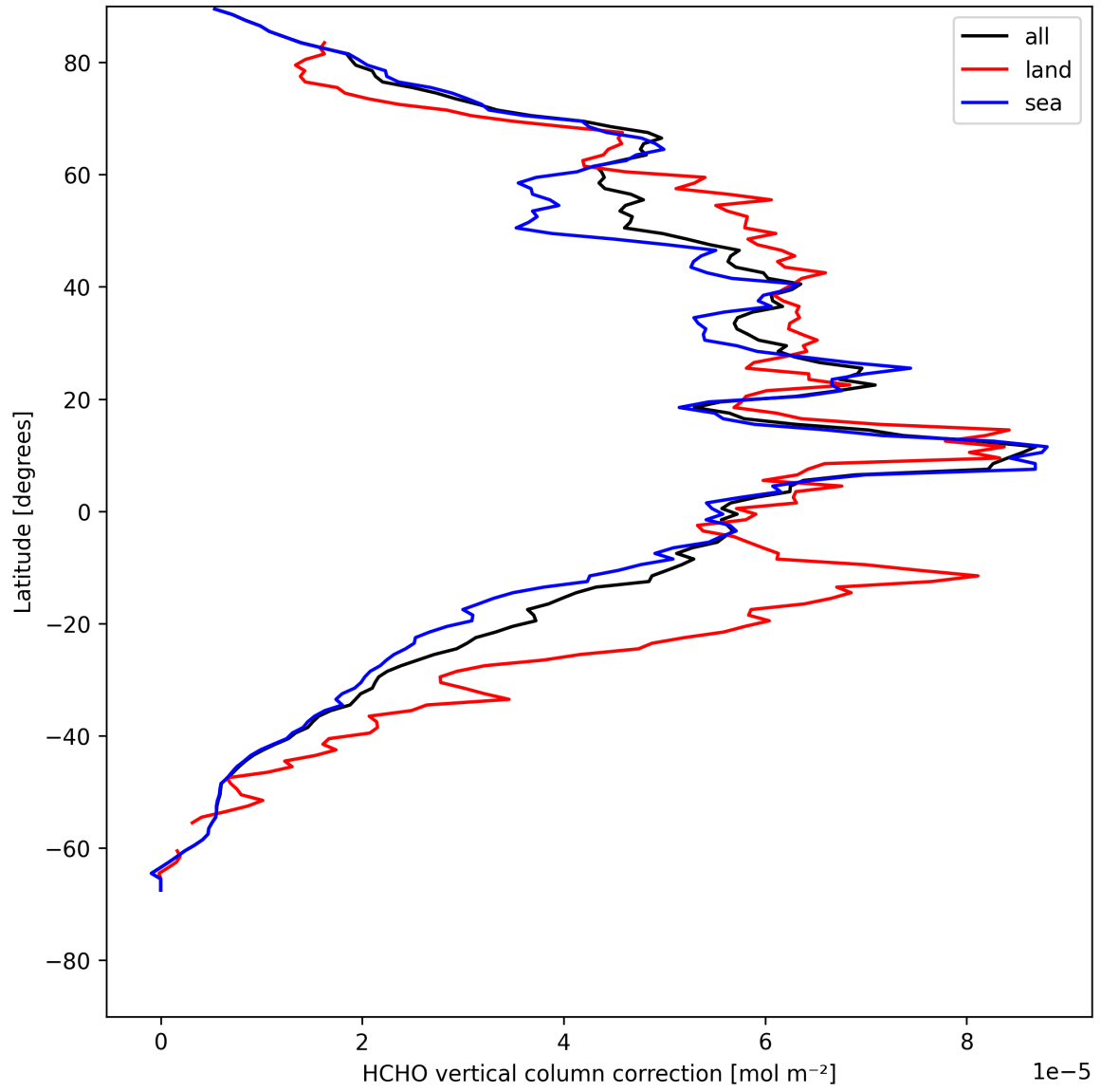
Figure 23: Zonal average of “HCHO vertical column correction” for 2025-08-04 to 2025-08-05.
