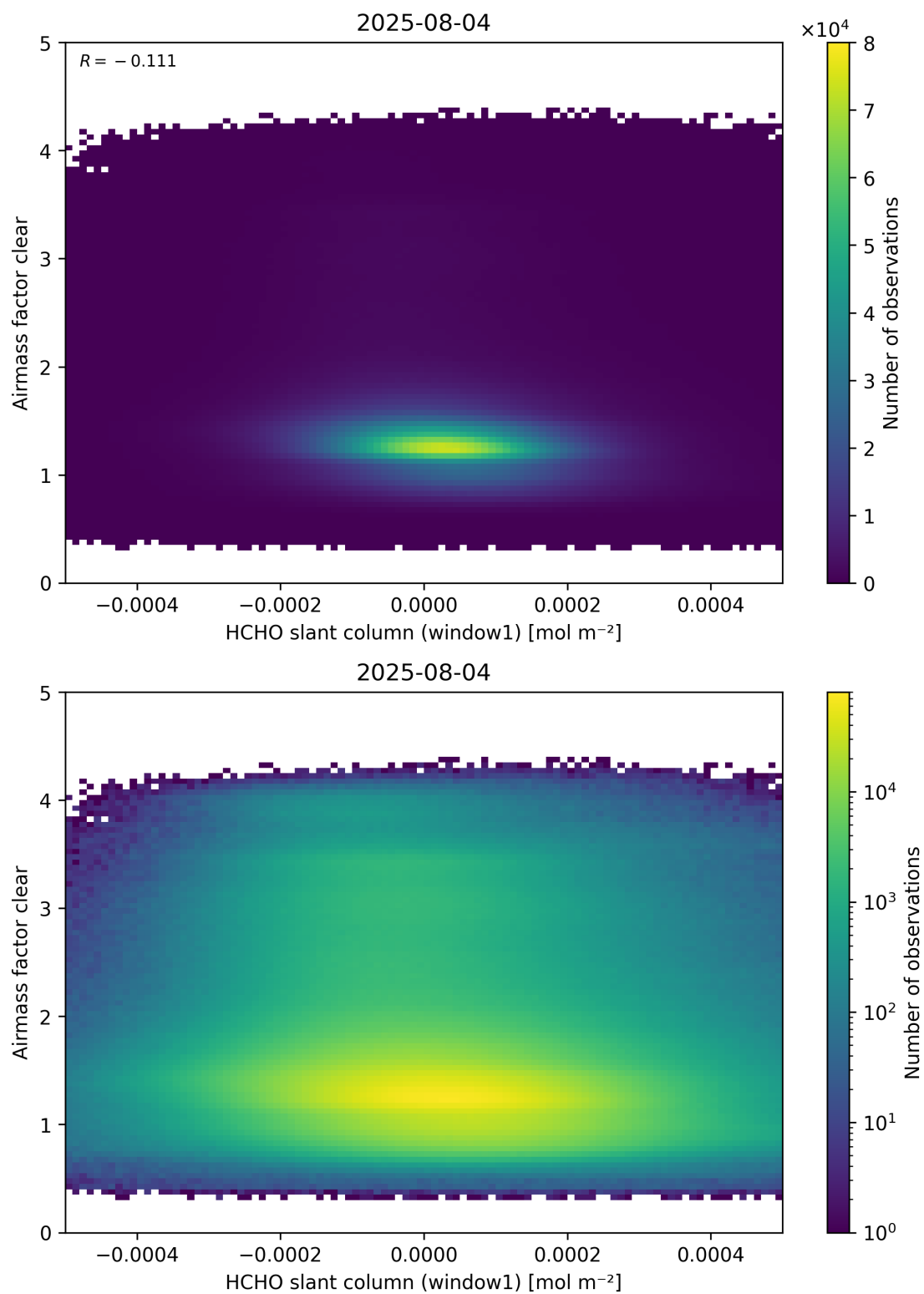
Figure 81: Scatter density plot of “HCHO slant column (window1)” against “Airmass factor clear” for 2025-08-04 to 2025-08-05.
