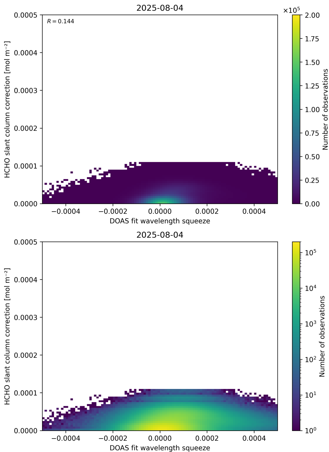
Figure 70: Scatter density plot of “DOAS fit wavelength squeeze” against “HCHO slant column correction” for 2025-08-04 to 2025-08-05.
