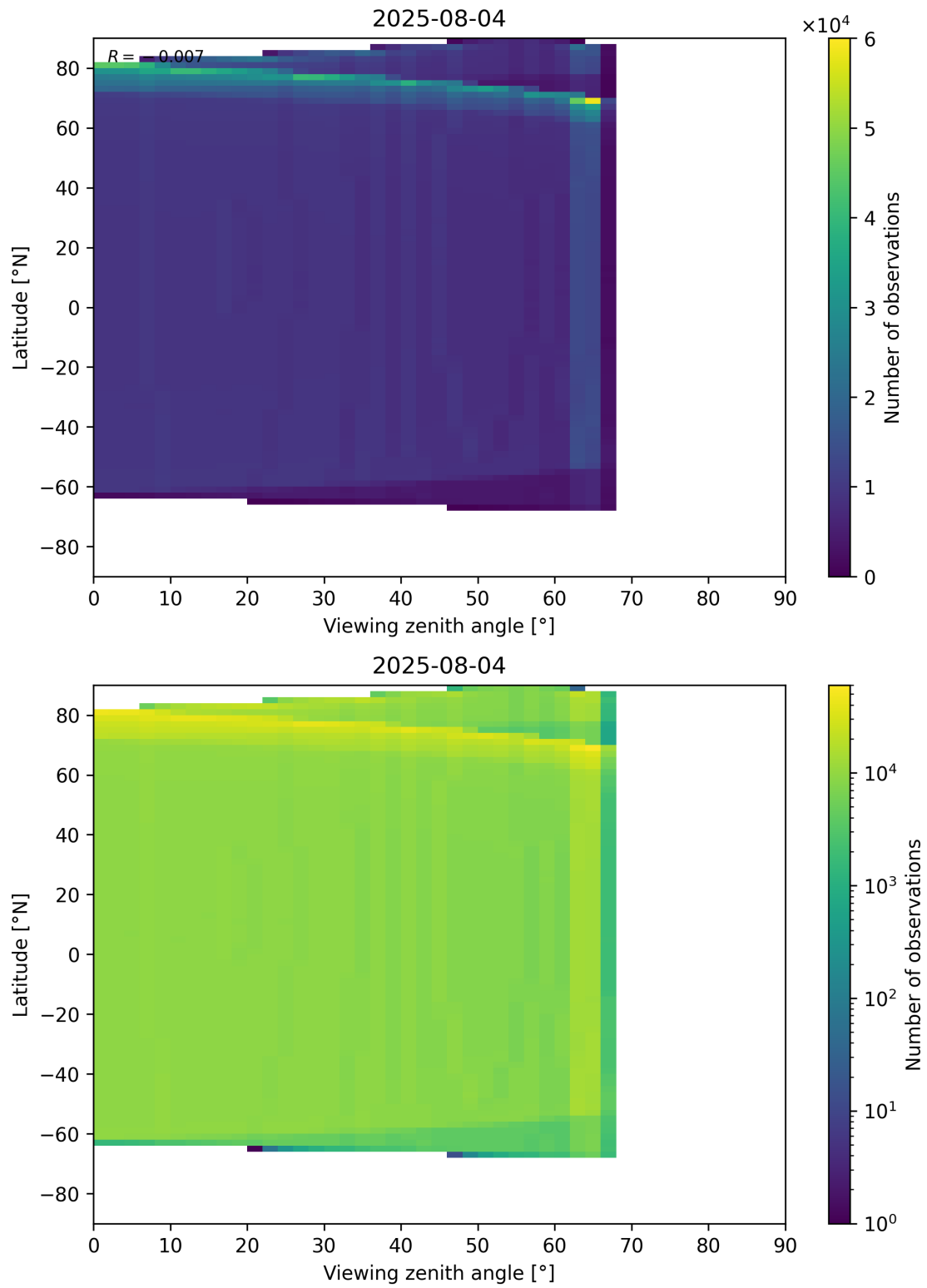
Figure 196: Scatter density plot of “Viewing zenith angle” against “Latitude” for 2025-08-04 to 2025-08-05.
