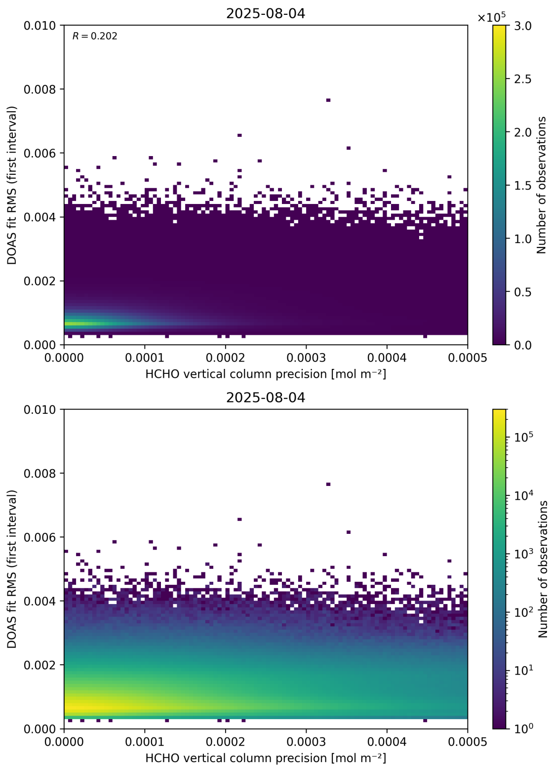
Figure 136: Scatter density plot of “HCHO vertical column precision” against “DOAS fit RMS (first interval)” for 2025-08-04 to 2025-08-05.
