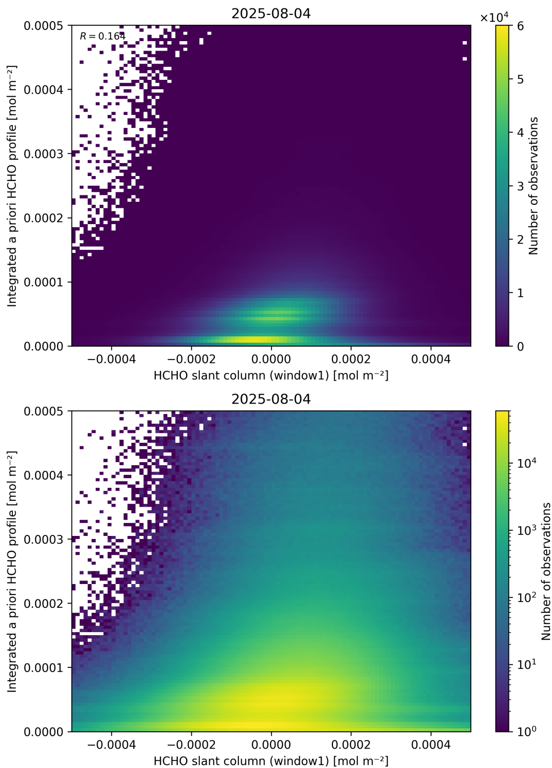
Figure 87: Scatter density plot of “HCHO slant column (window1)” against “Integrated a priori HCHO profile” for 2025-08-04 to 2025-08-05.
