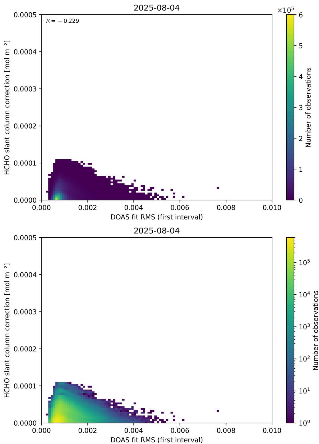
Figure 63: Scatter density plot of “DOAS fit RMS (first interval)” against “HCHO slant column correction” for 2025-08-04 to 2025-08-05.
