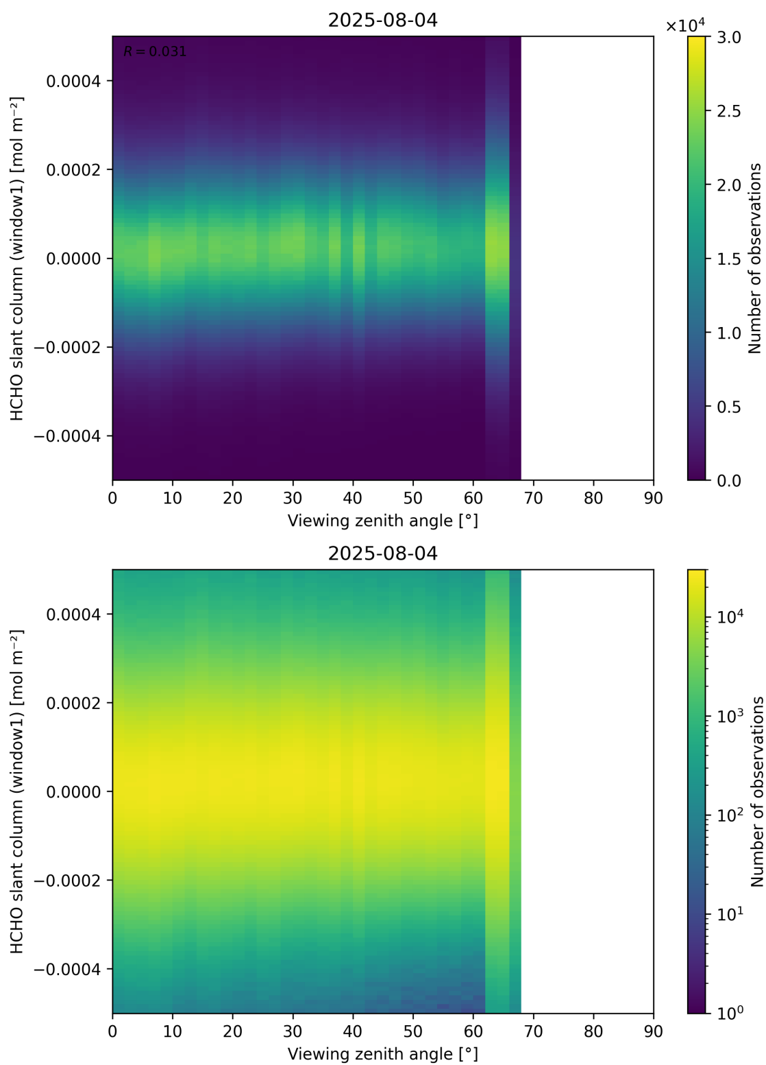
Figure 188: Scatter density plot of “Viewing zenith angle” against “HCHO slant column (window1)” for 2025-08-04 to 2025-08-05.
