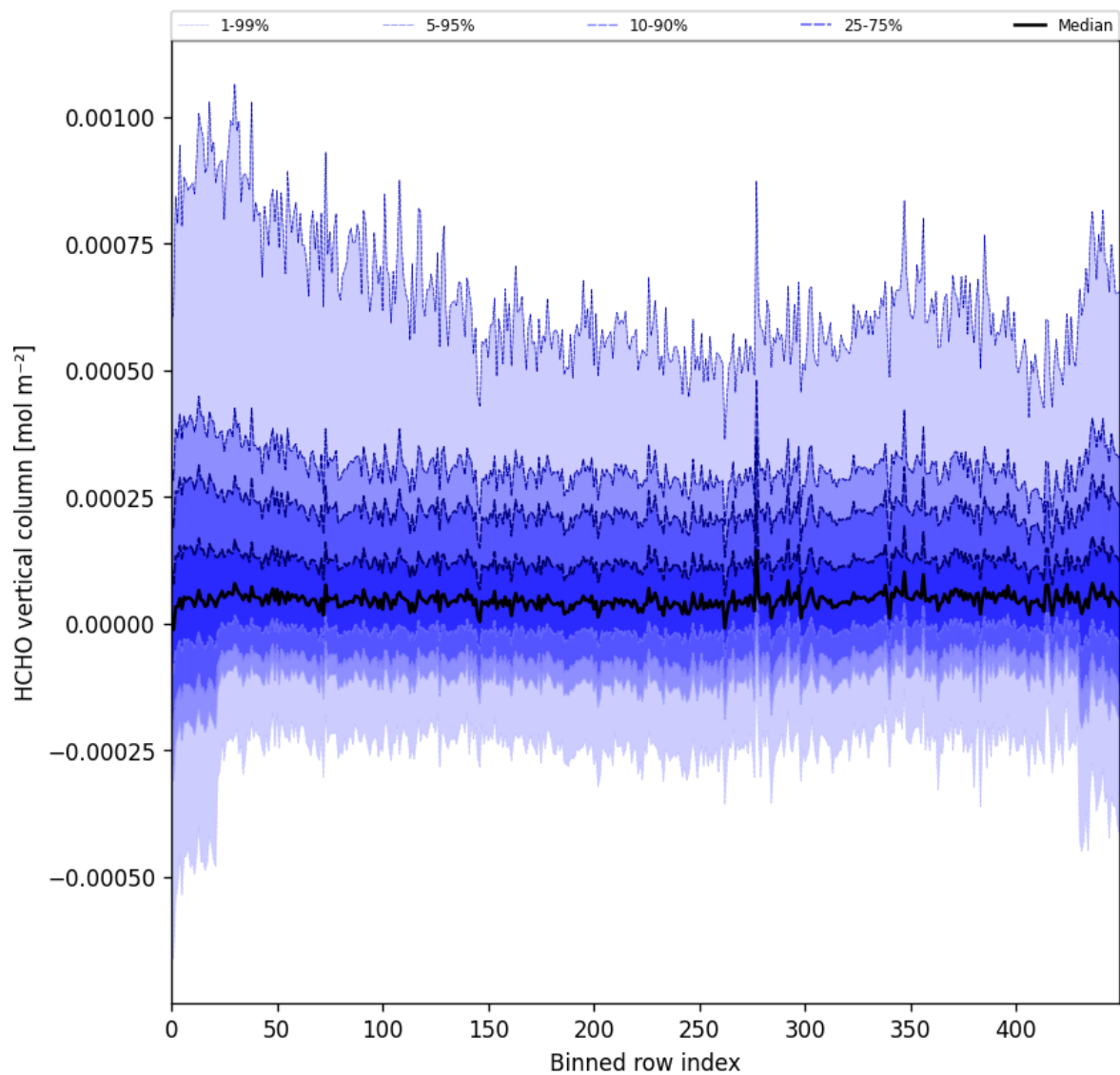
Figure 49: Along track statistics of “HCHO vertical column” for 2025-08-04 to 2025-08-05
