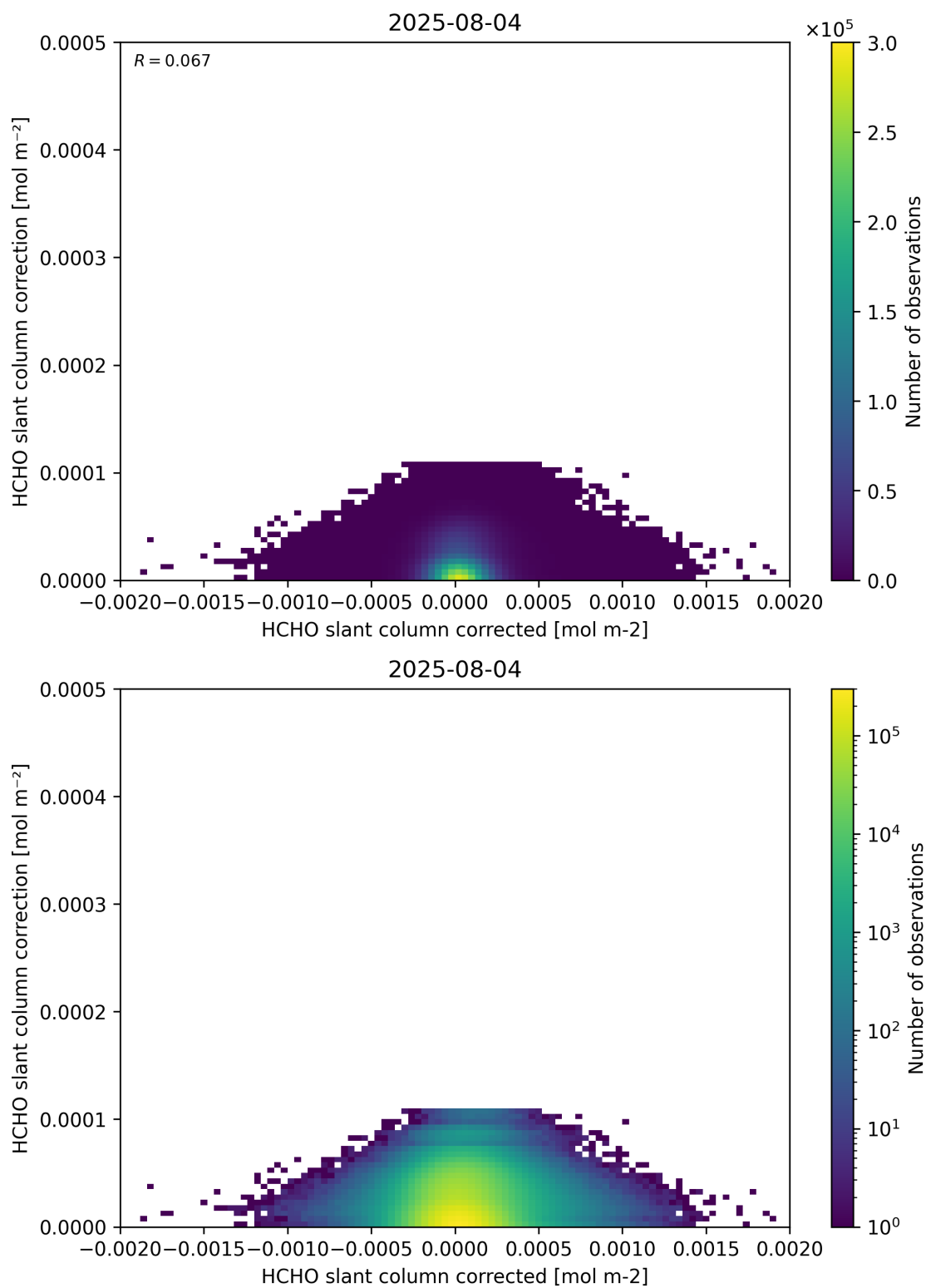
Figure 77: Scatter density plot of “HCHO slant column corrected” against “HCHO slant column correction” for 2025-08-04 to 2025-08-05.
