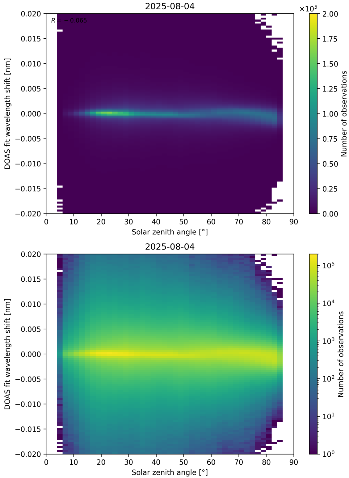
Figure 168: Scatter density plot of “Solar zenith angle” against “DOAS fit wavelength shift” for 2025-08-04 to 2025-08-05.
