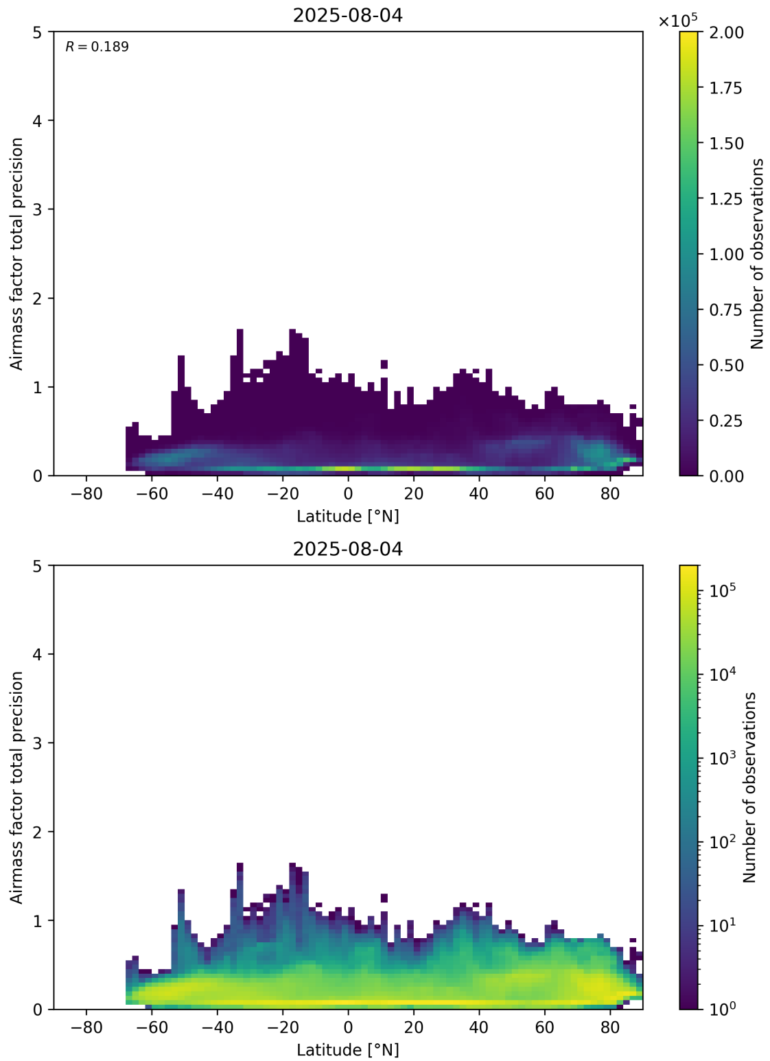
Figure 162: Scatter density plot of “Latitude” against “Airmass factor total precision” for 2025-08-04 to 2025-08-05.
