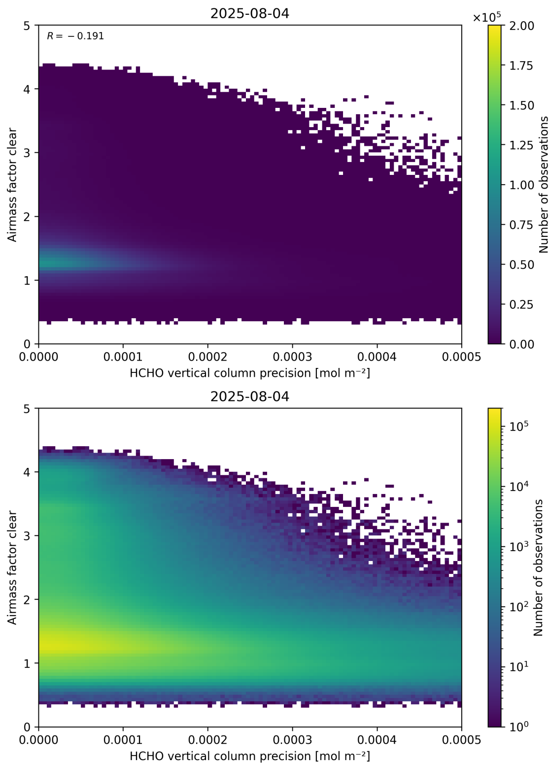
Figure 139: Scatter density plot of “HCHO vertical column precision” against “Airmass factor clear” for 2025-08-04 to 2025-08-05.
