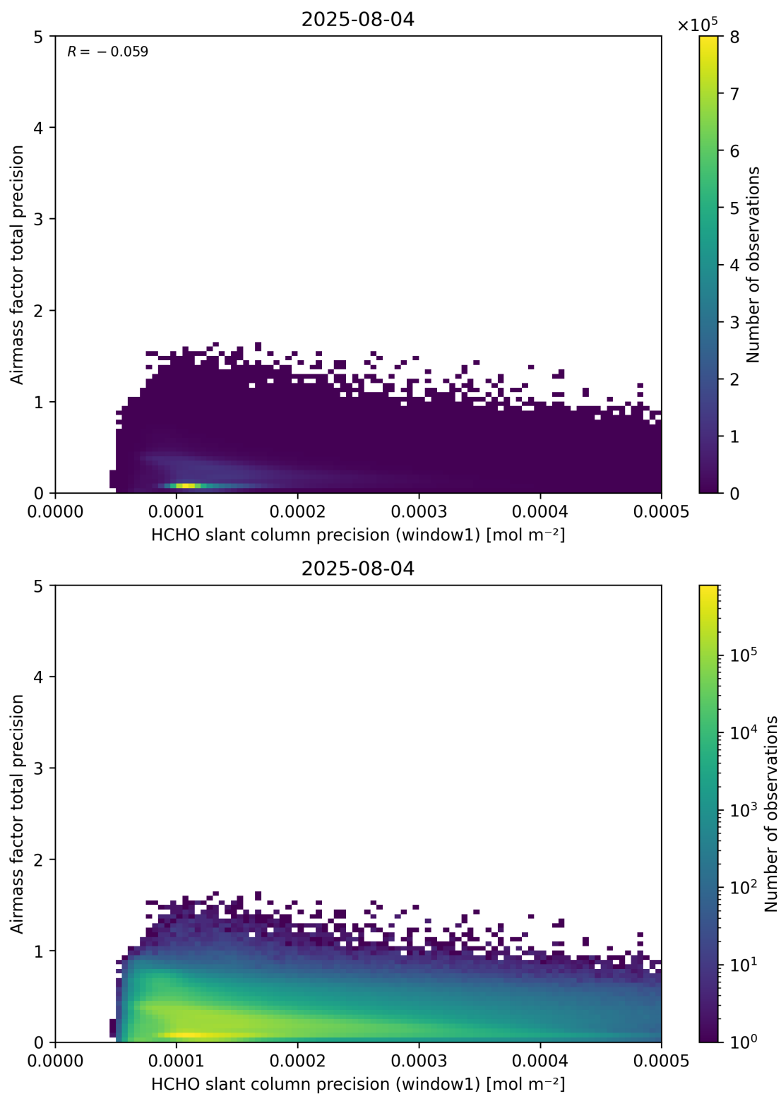
Figure 95: Scatter density plot of “HCHO slant column precision (window1)” against “Airmass factor total precision” for 2025-08-04 to 2025-08-05.
