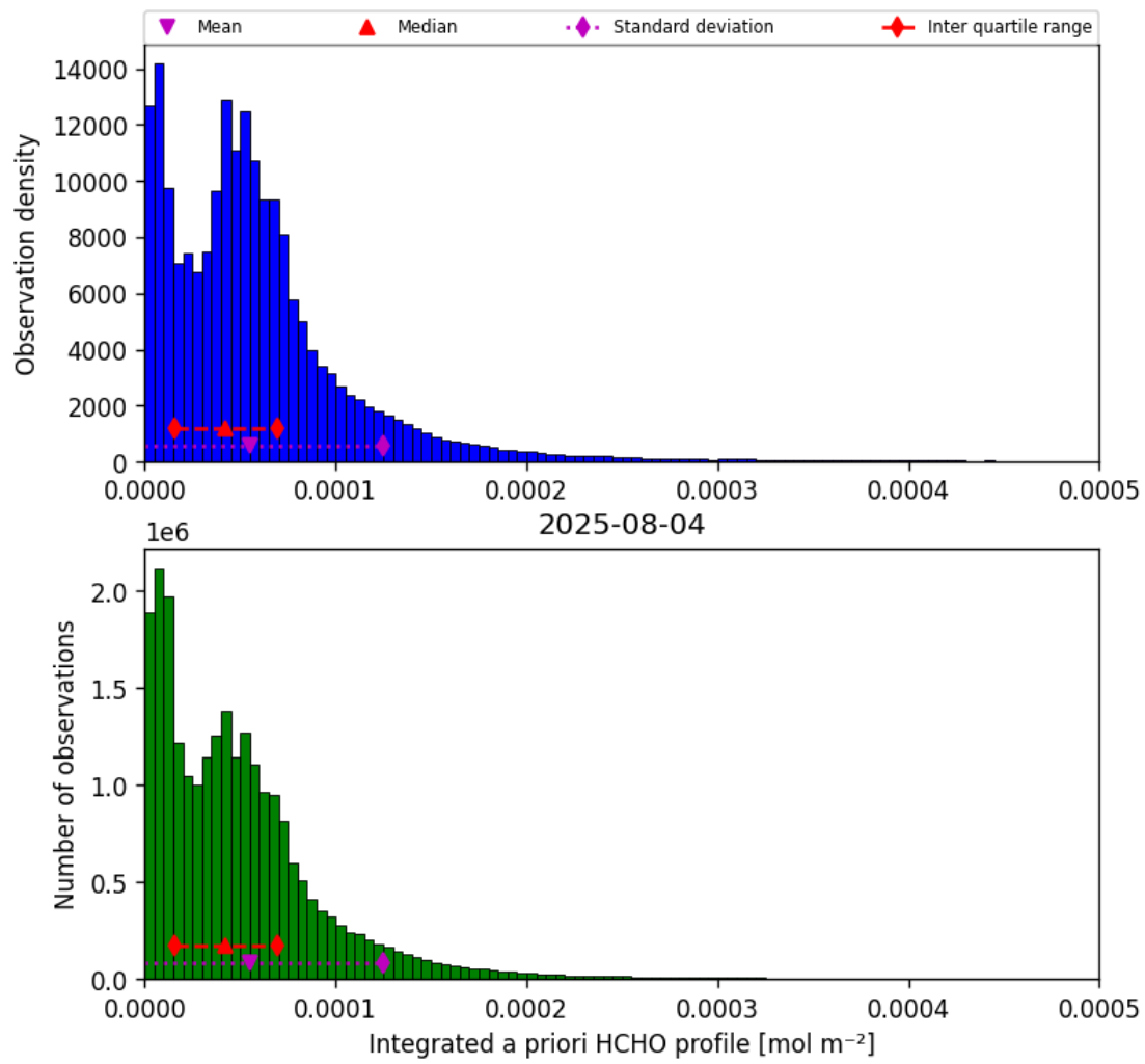
Figure 43: Histogram of “Integrated a priori HCHO profile” for 2025-08-04 to 2025-08-05
