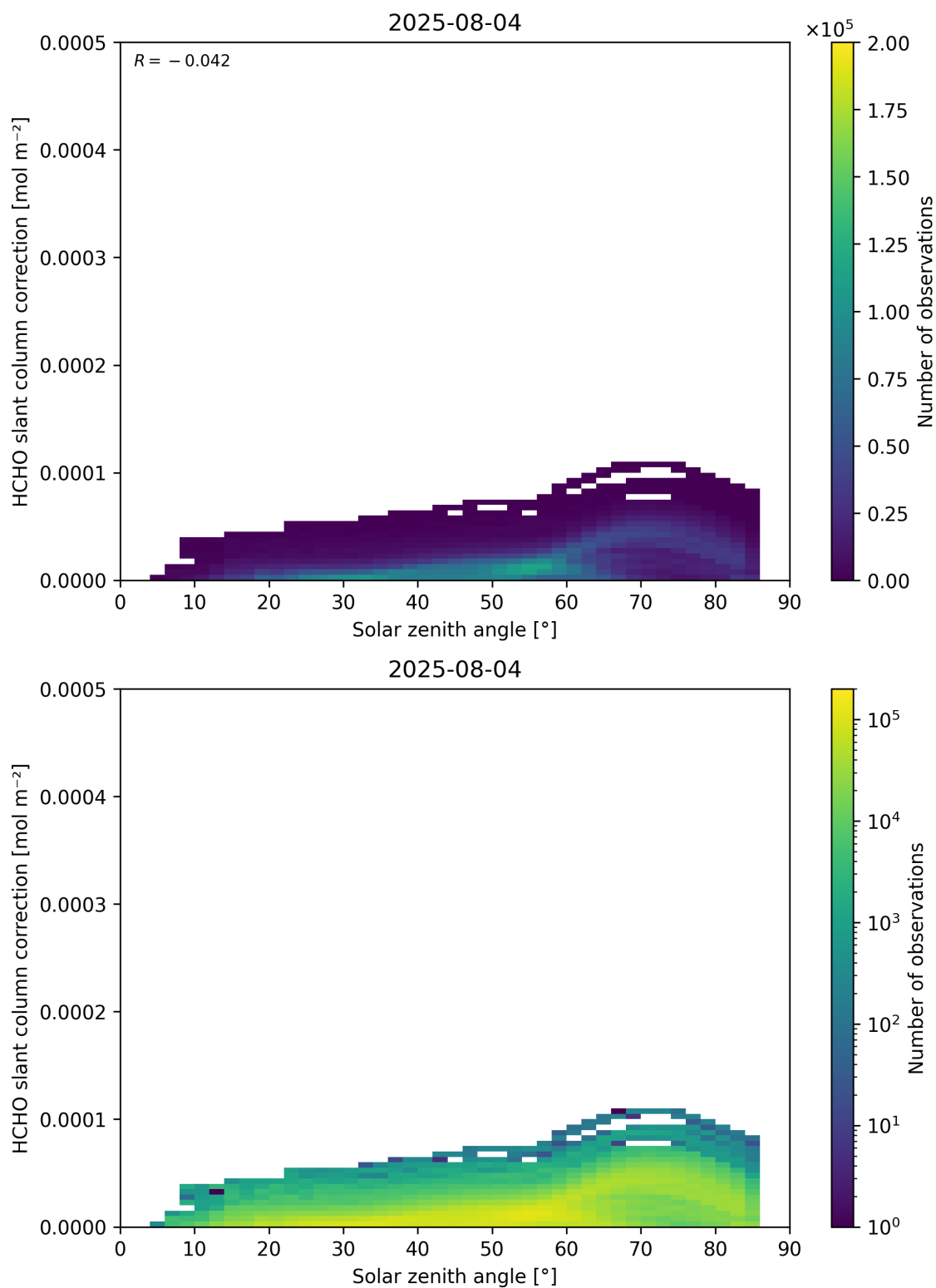
Figure 172: Scatter density plot of “Solar zenith angle” against “HCHO slant column correction” for 2025-08-04 to 2025-08-05.
