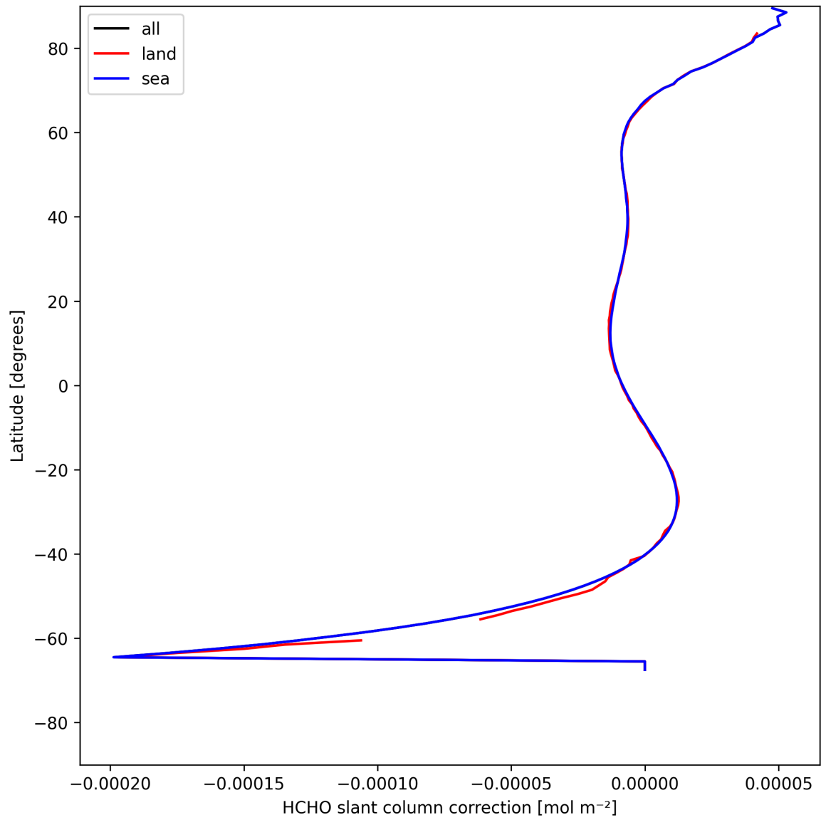
Figure 33: Zonal average of “HCHO slant column correction” for 2025-08-04 to 2025-08-05.
