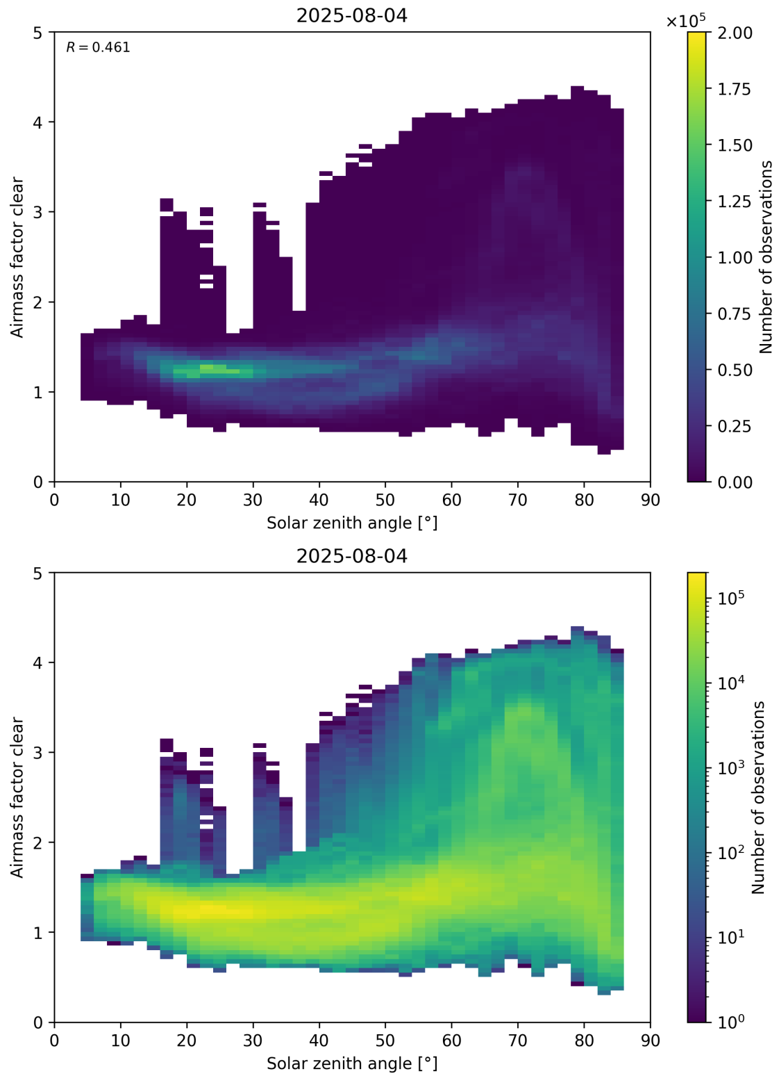
Figure 170: Scatter density plot of “Solar zenith angle” against “Airmass factor clear” for 2025-08-04 to 2025-08-05.
