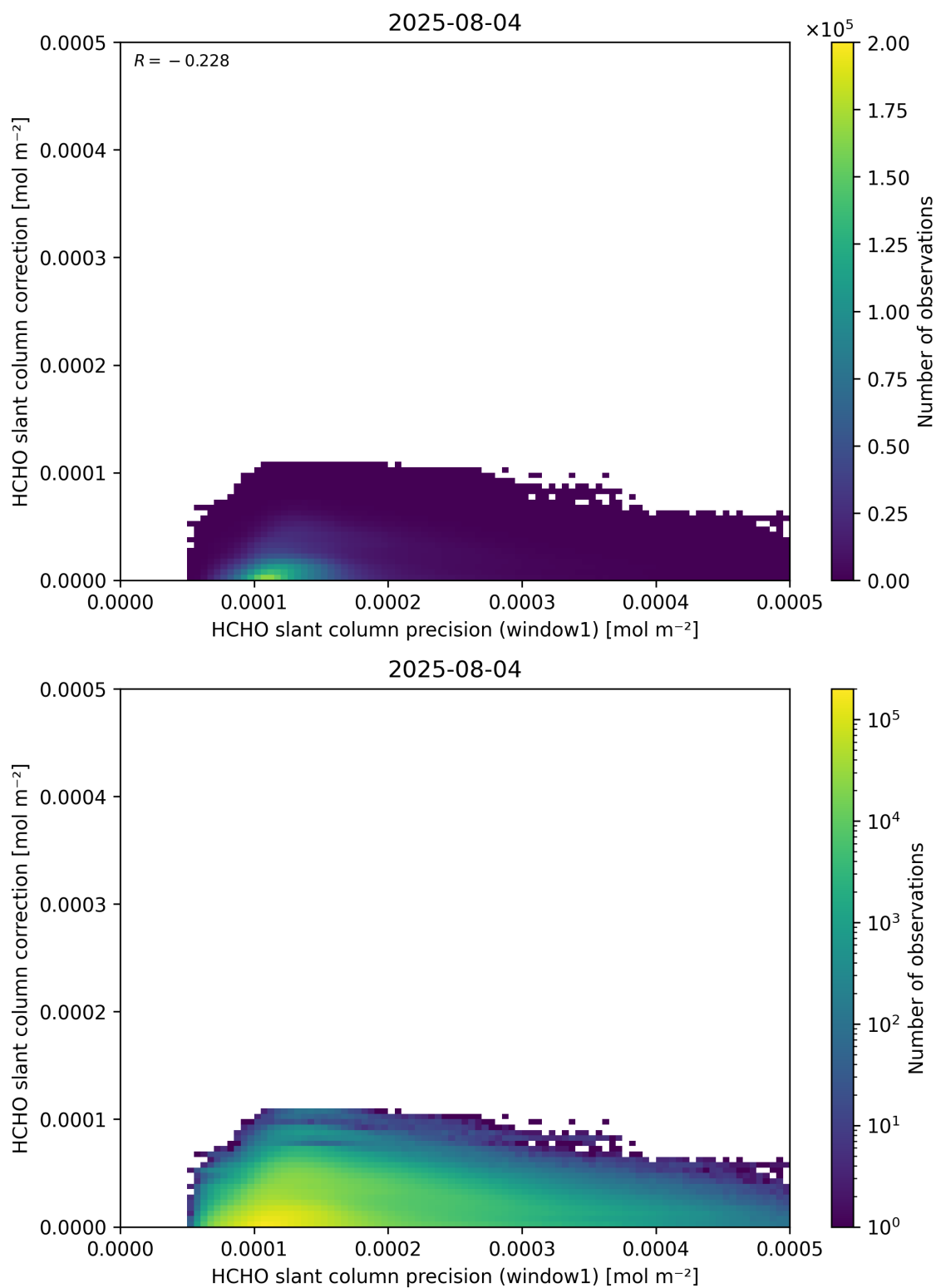
Figure 93: Scatter density plot of “HCHO slant column precision (window1)” against “HCHO slant column correction” for 2025-08-04 to 2025-08-05.
