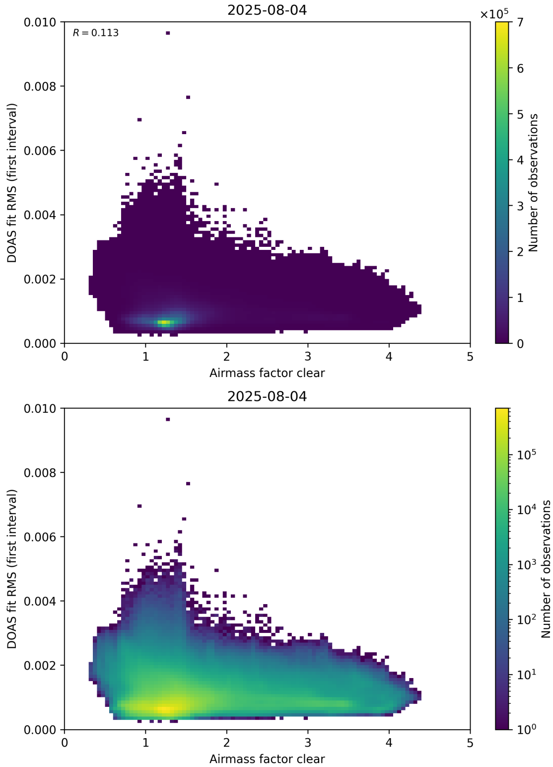
Figure 71: Scatter density plot of “Airmass factor clear” against “DOAS fit RMS (first interval)” for 2025-08-04 to 2025-08-05.
