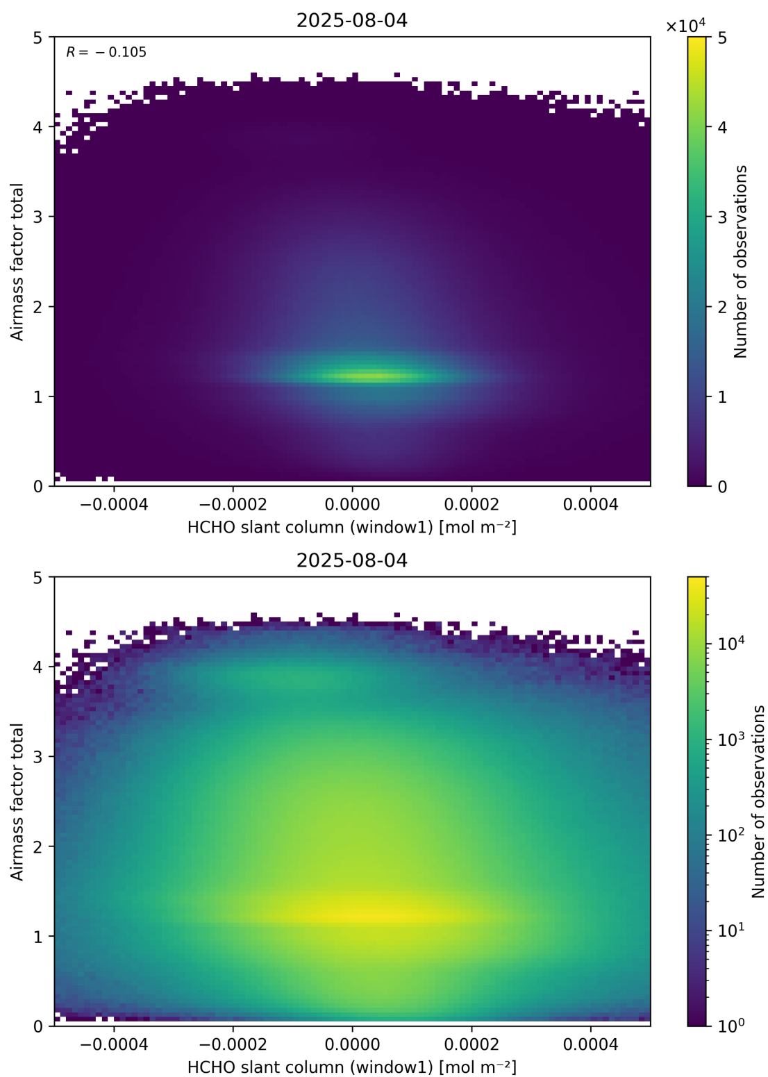
Figure 85: Scatter density plot of “HCHO slant column (window1)” against “Airmass factor total” for 2025-08-04 to 2025-08-05.
