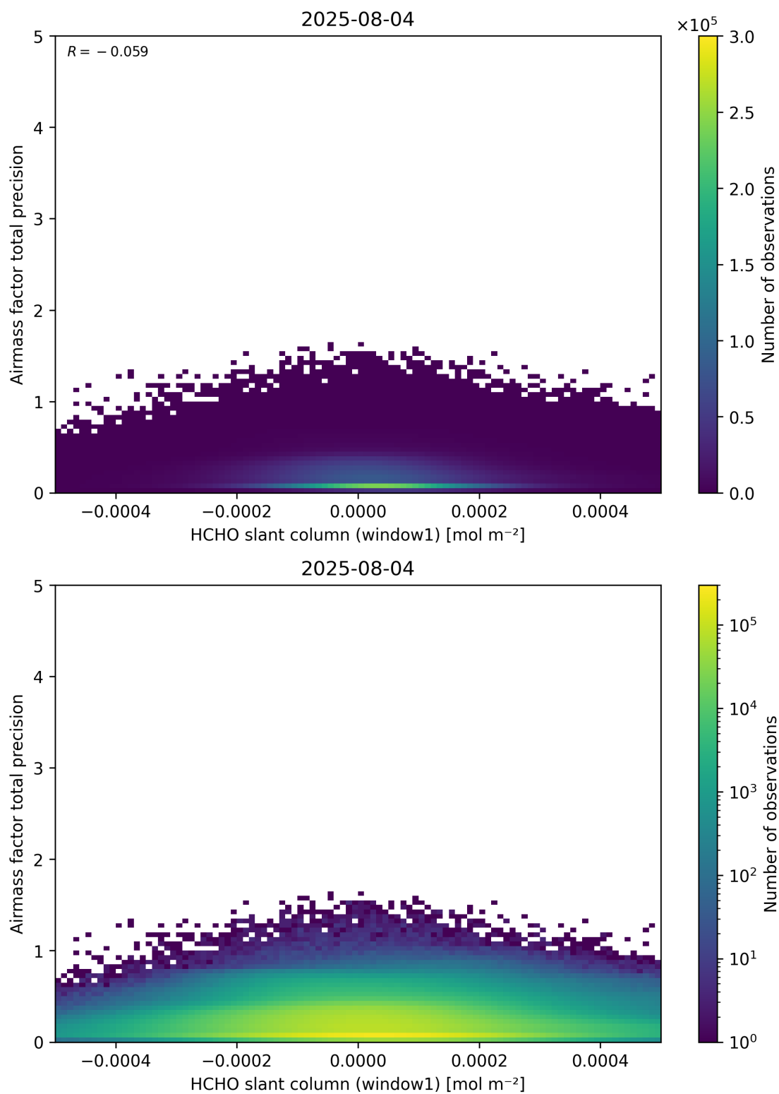
Figure 86: Scatter density plot of “HCHO slant column (window1)” against “Airmass factor total precision” for 2025-08-04 to 2025-08-05.
