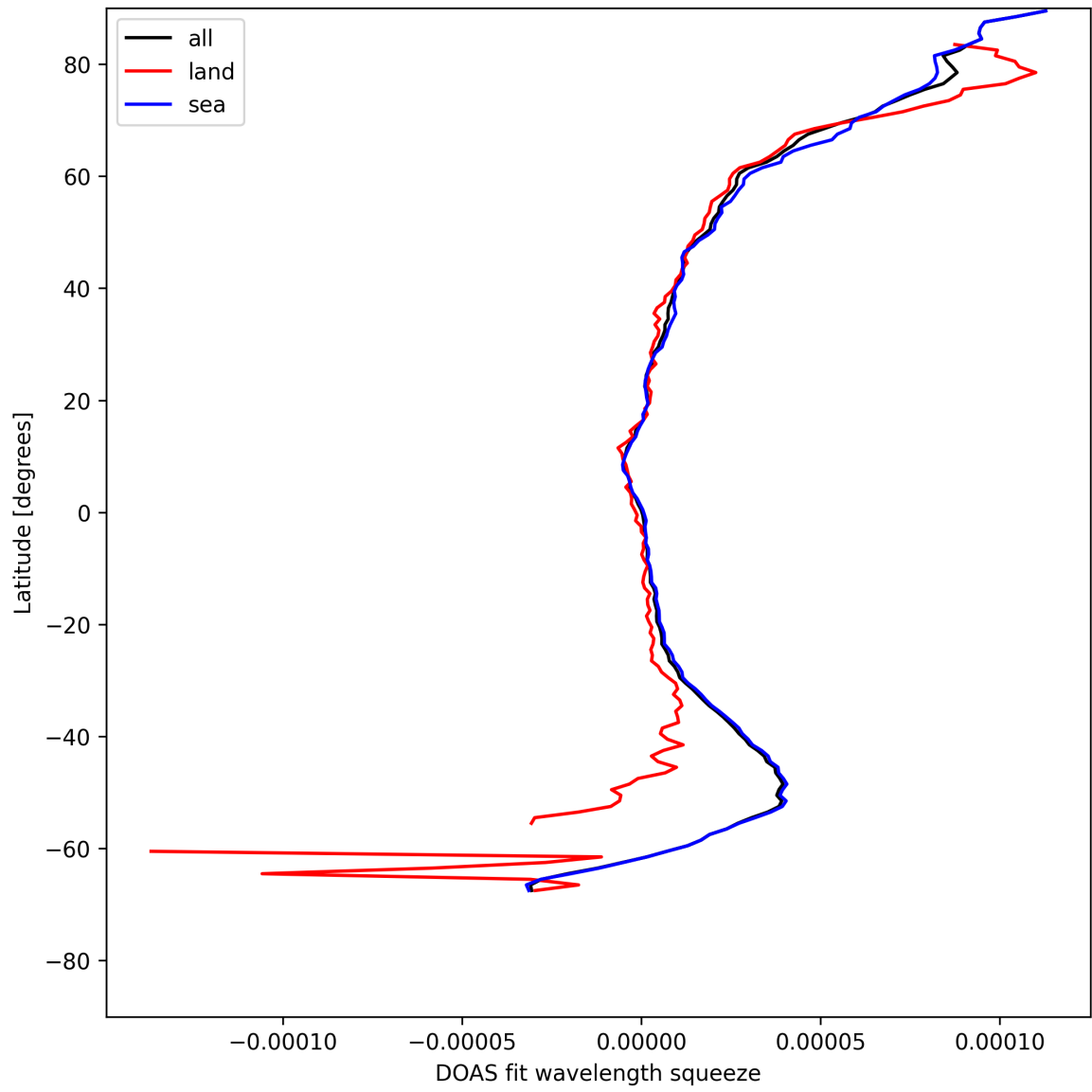
Figure 31: Zonal average of “DOAS fit wavelength squeeze” for 2025-08-04 to 2025-08-05.
