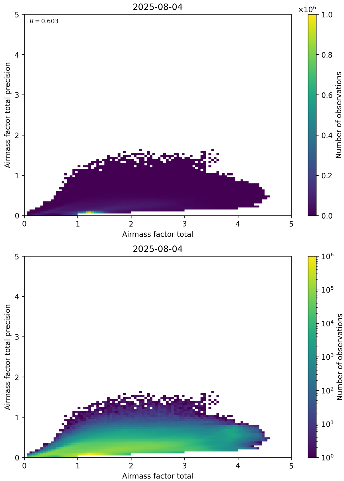
Figure 103: Scatter density plot of “Airmass factor total” against “Airmass factor total precision” for 2025-08-04 to 2025-08-05.
