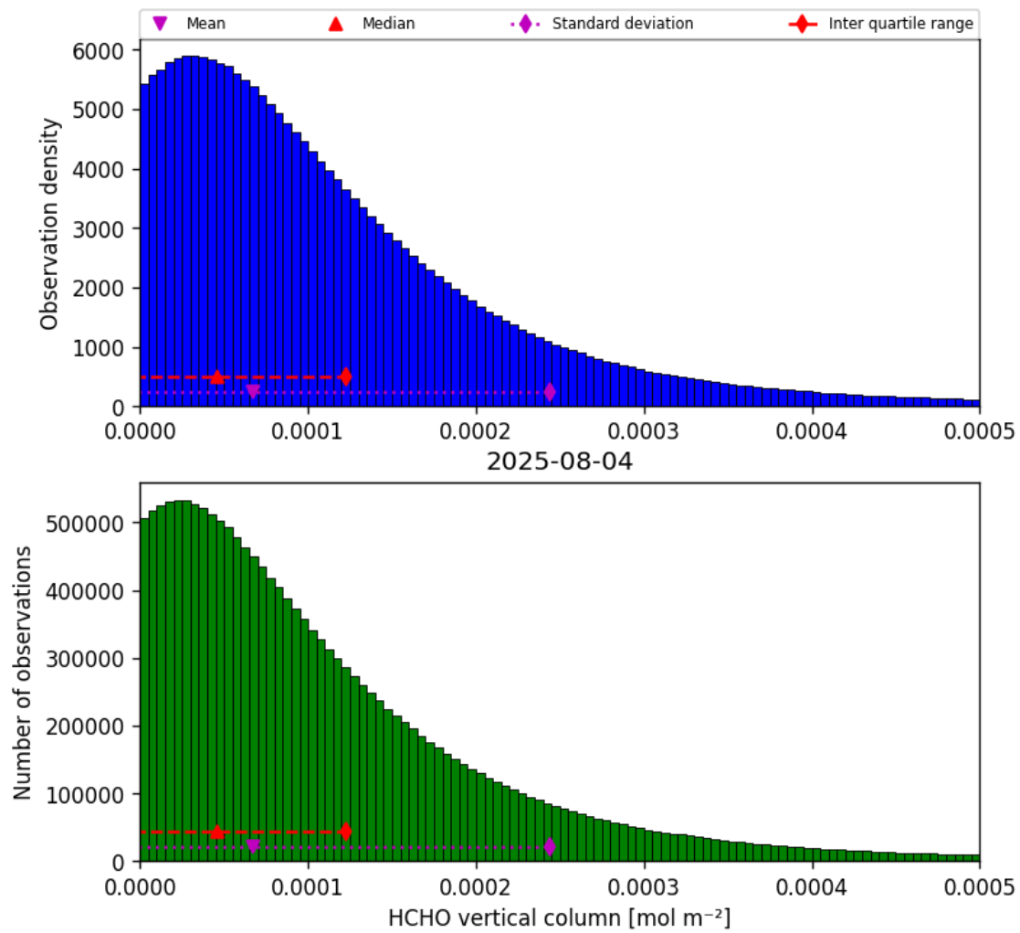
Figure 35: Histogram of “HCHO vertical column” for 2025-08-04 to 2025-08-05
