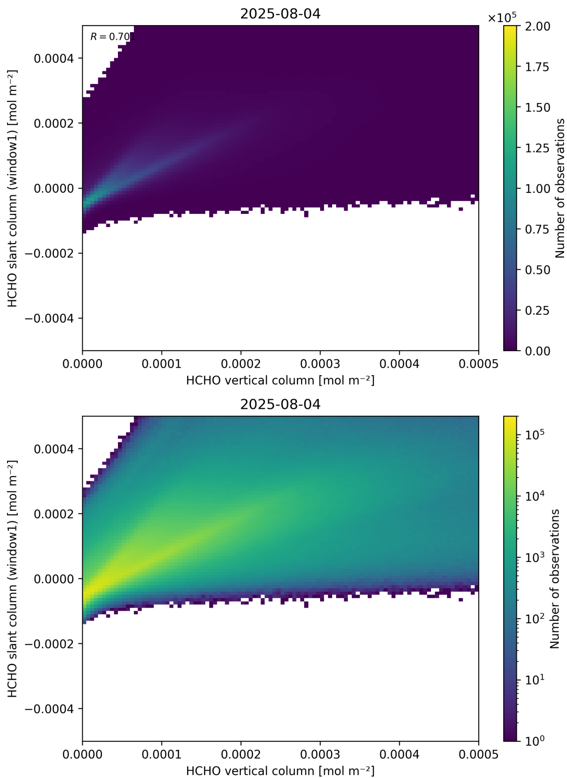
Figure 129: Scatter density plot of “HCHO vertical column” against “HCHO slant column (window1)” for 2025-08-04 to 2025-08-05.
