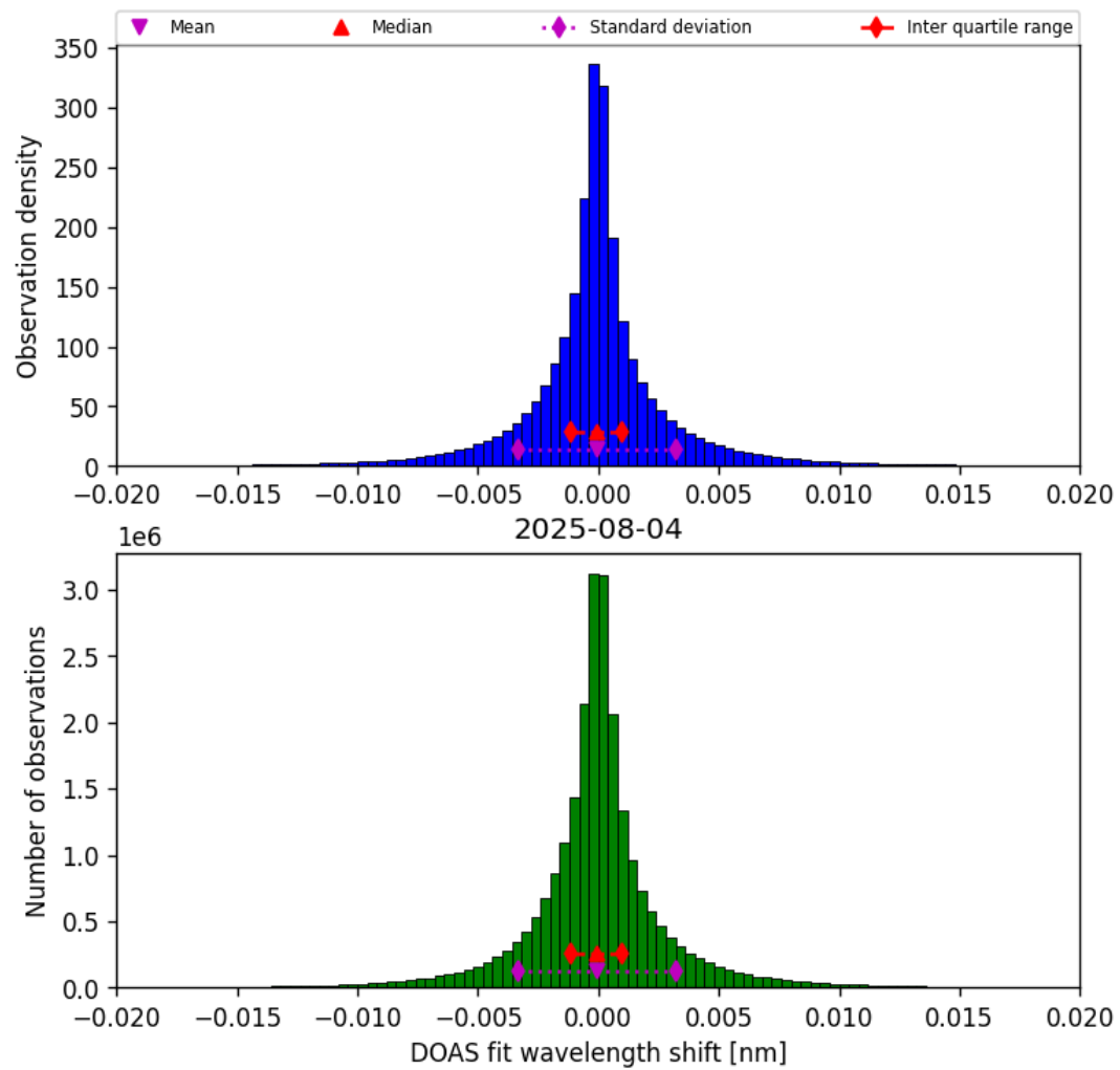
Figure 44: Histogram of “DOAS fit wavelength shift” for 2025-08-04 to 2025-08-05
