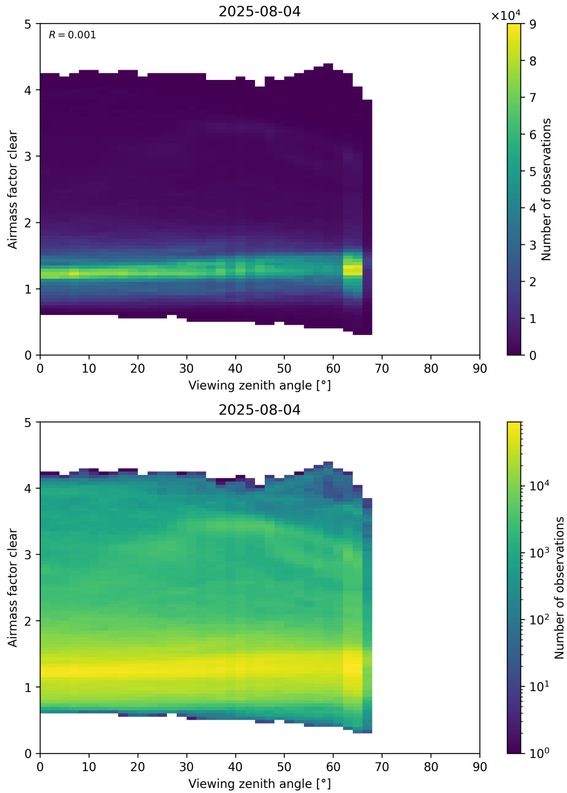
Figure 185: Scatter density plot of “Viewing zenith angle” against “Airmass factor clear” for 2025-08-04 to 2025-08-05.
