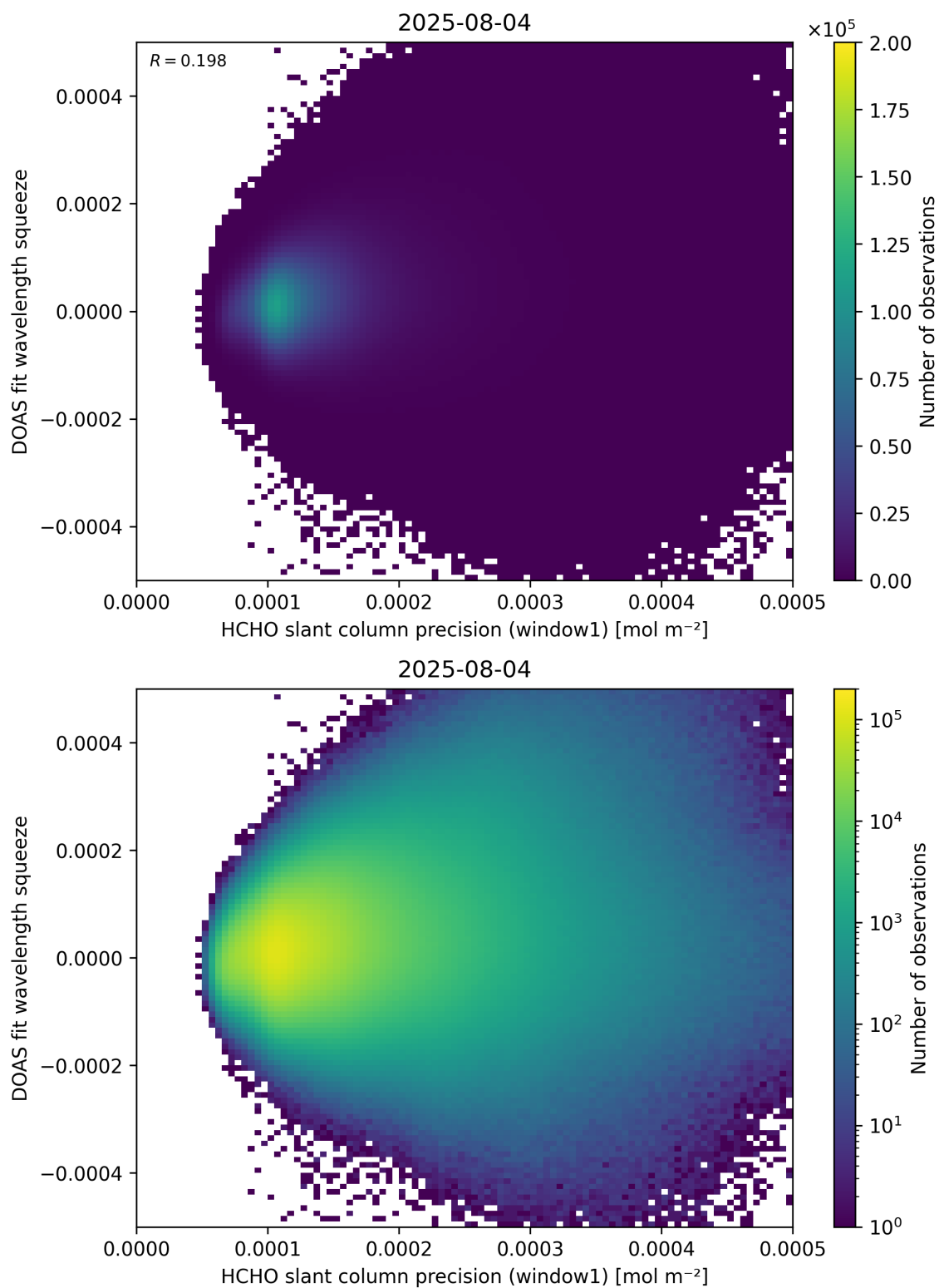
Figure 90: Scatter density plot of “HCHO slant column precision (window1)” against “DOAS fit wavelength squeeze” for 2025-08-04 to 2025-08-05.
