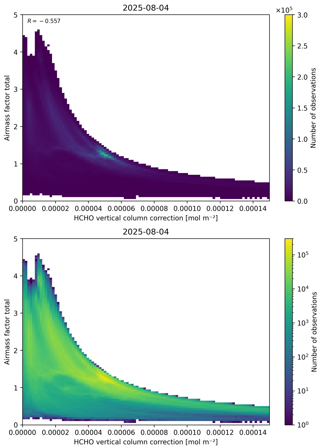
Figure 120: Scatter density plot of “HCHO vertical column correction” against “Airmass factor total” for 2025-08-04 to 2025-08-05.
