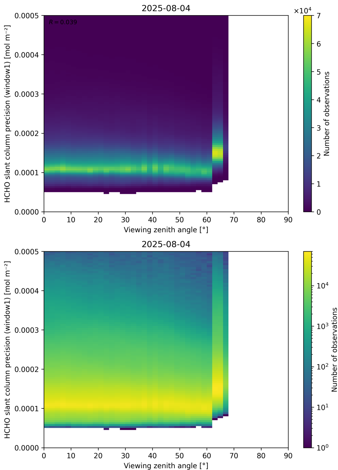
Figure 189: Scatter density plot of “Viewing zenith angle” against “HCHO slant column precision (window1)” for 2025-08-04 to 2025-08-05.
