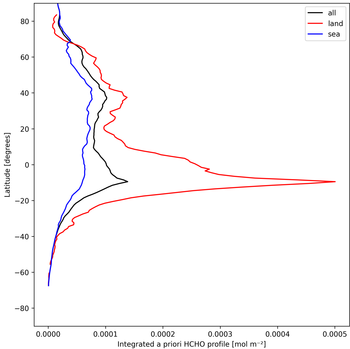
Figure 29: Zonal average of “Integrated a priori HCHO profile” for 2025-08-04 to 2025-08-05.
