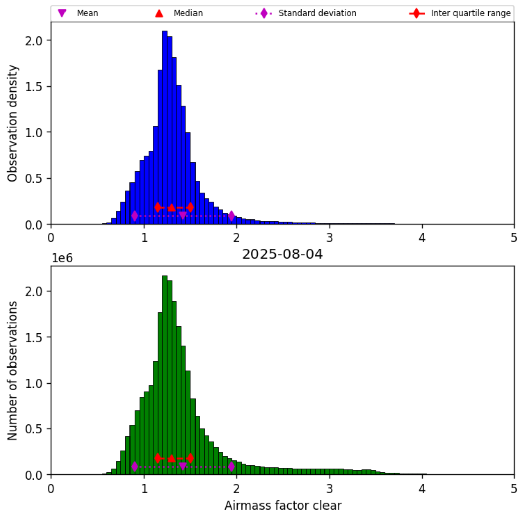
Figure 42: Histogram of “Airmass factor clear” for 2025-08-04 to 2025-08-05
