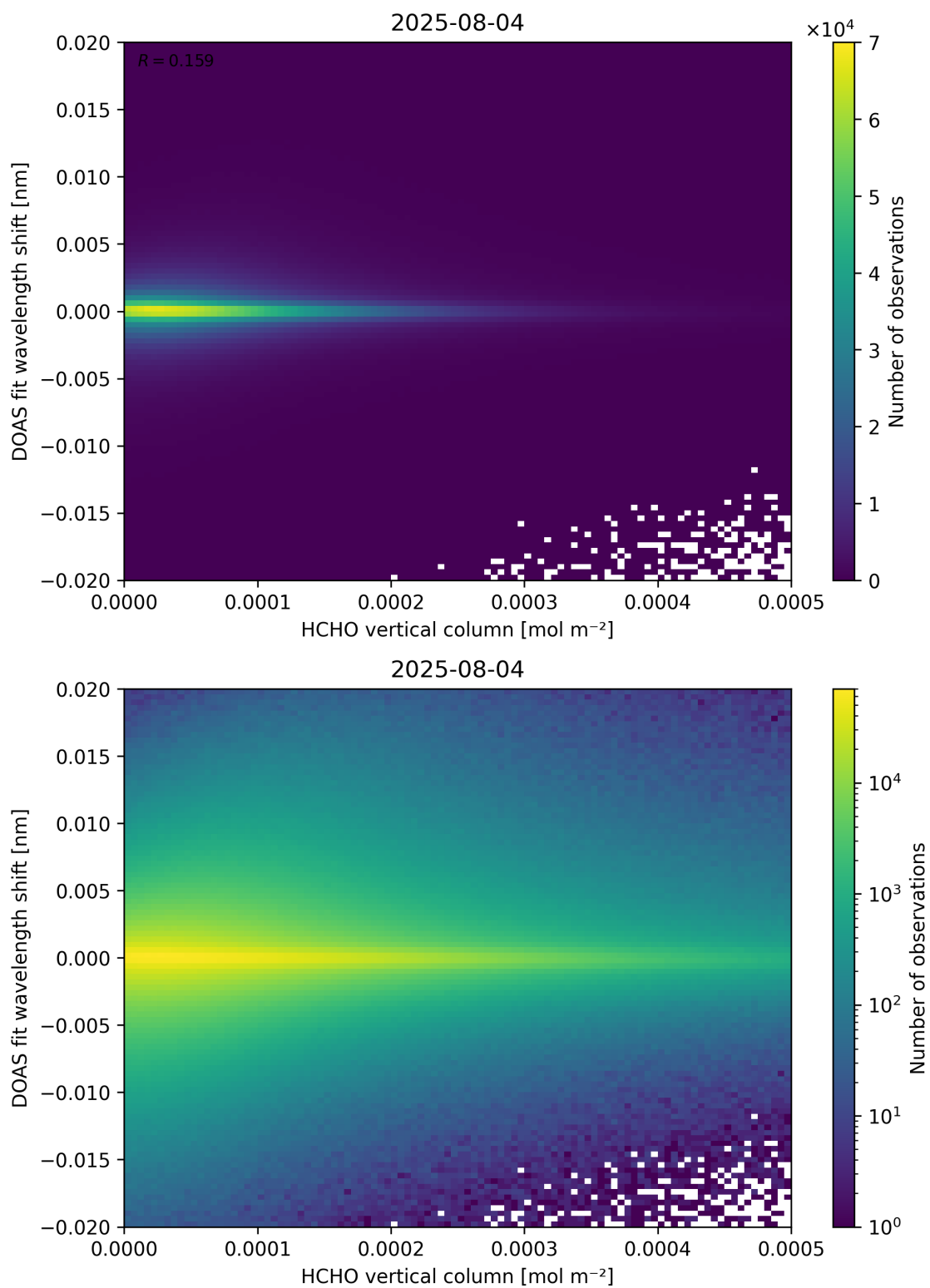
Figure 124: Scatter density plot of “HCHO vertical column” against “DOAS fit wavelength shift” for 2025-08-04 to 2025-08-05.
