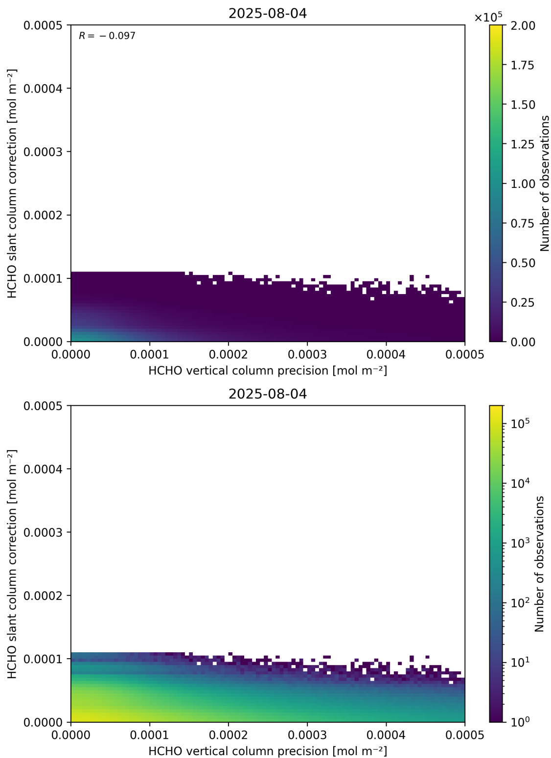
Figure 141: Scatter density plot of “HCHO vertical column precision” against “HCHO slant column correction” for 2025-08-04 to 2025-08-05.
