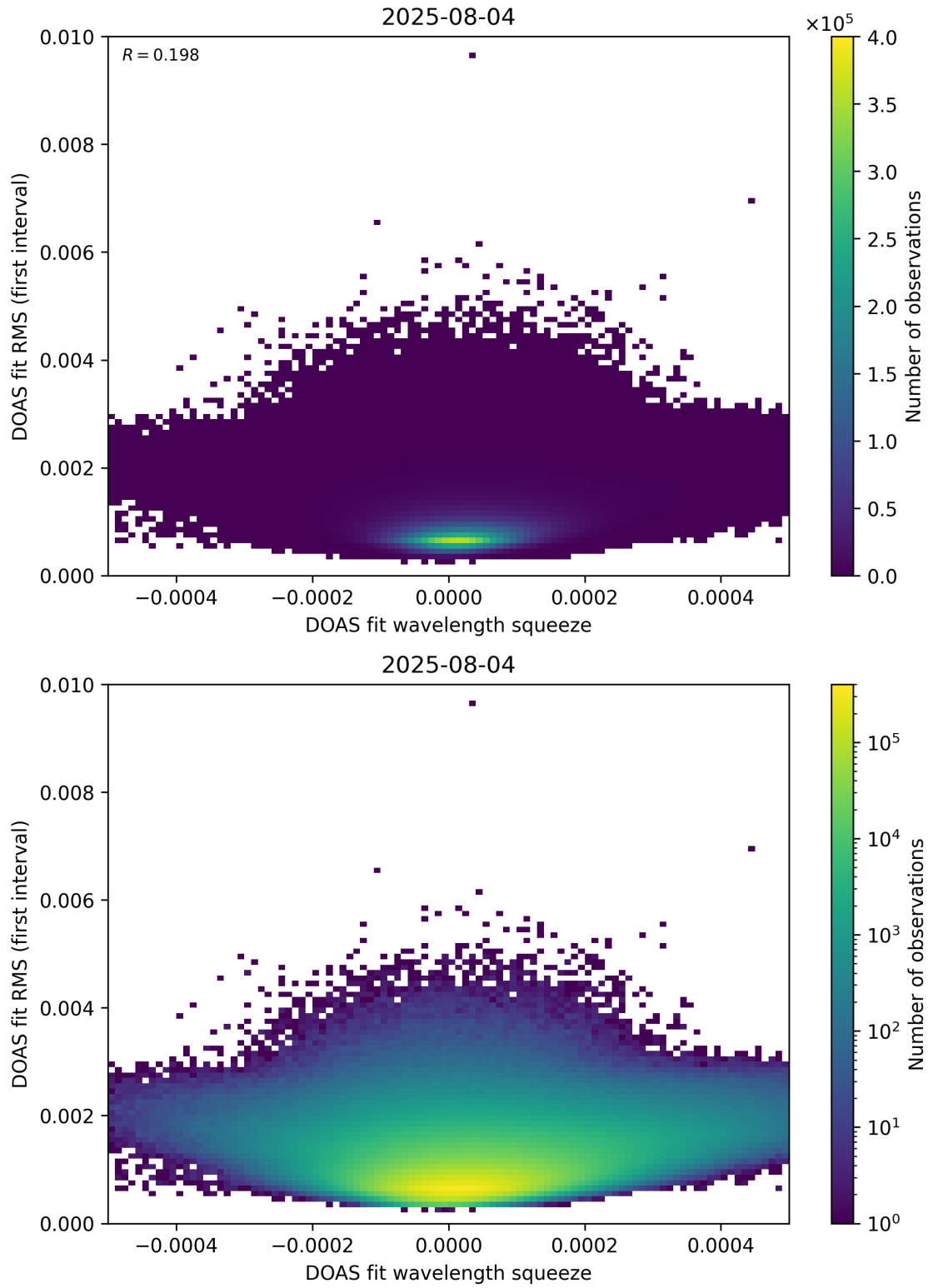
Figure 68: Scatter density plot of “DOAS fit wavelength squeeze” against “DOAS fit RMS (first interval)” for 2025-08-04 to 2025-08-05.
