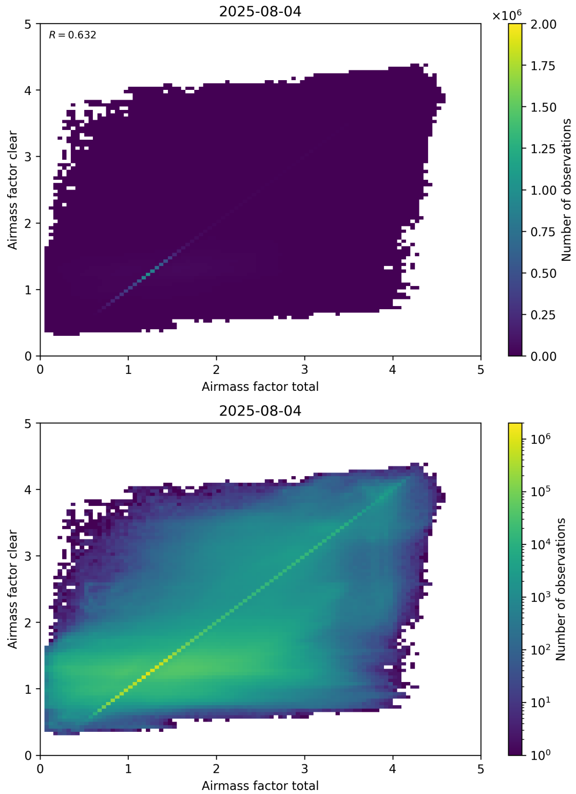
Figure 100: Scatter density plot of “Airmass factor total” against “Airmass factor clear” for 2025-08-04 to 2025-08-05.
