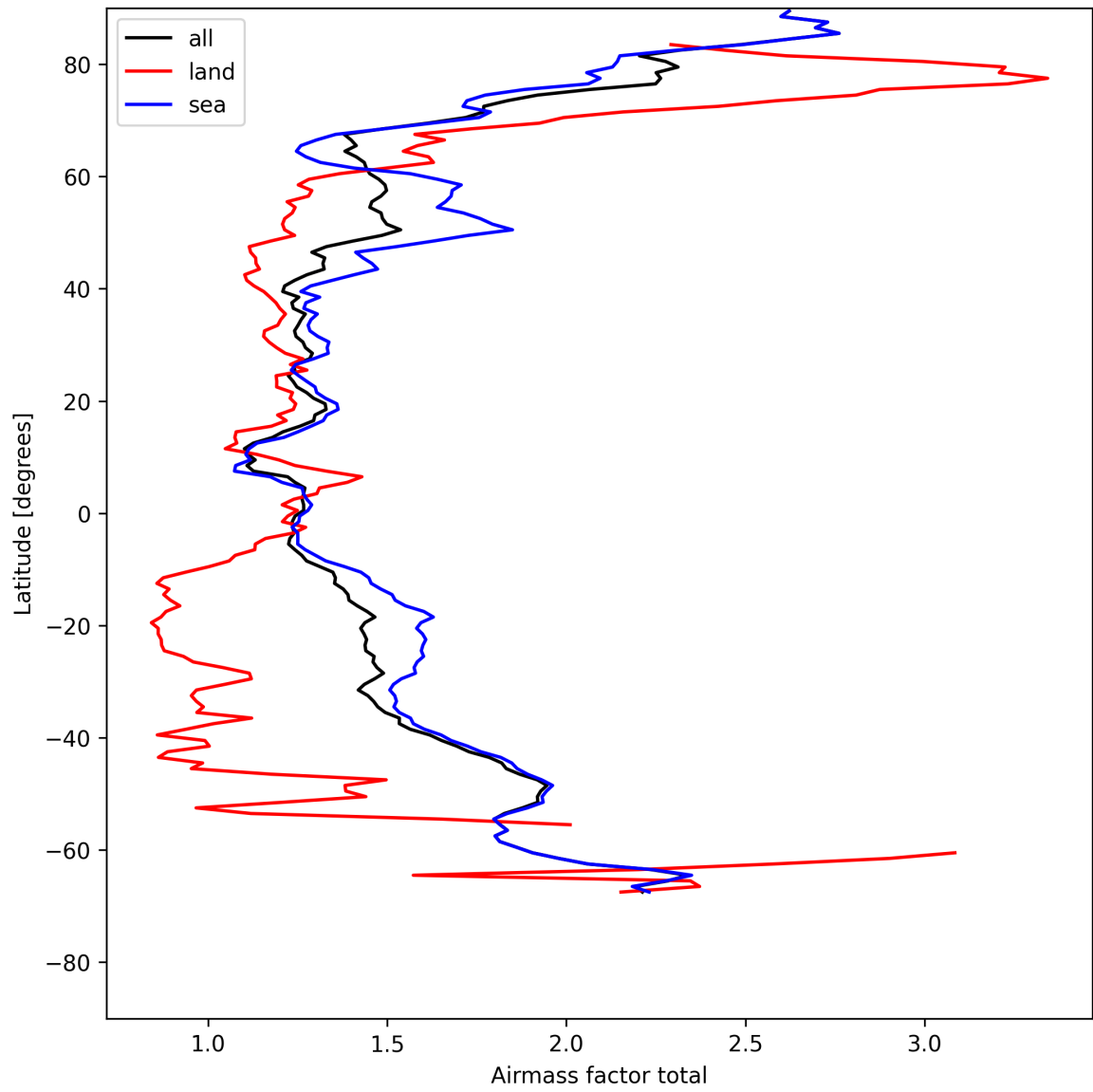
Figure 26: Zonal average of “Airmass factor total” for 2025-08-04 to 2025-08-05.
