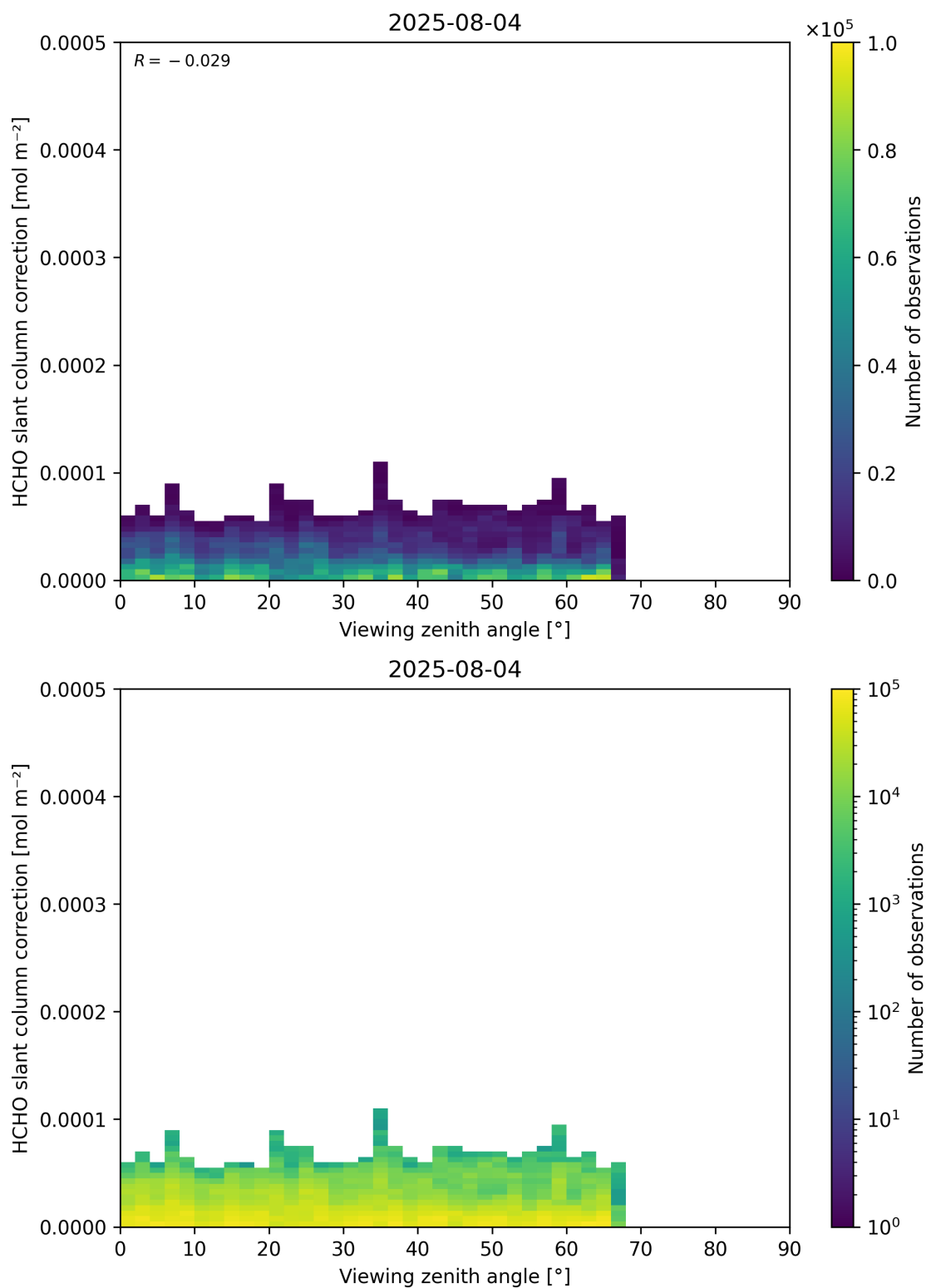
Figure 187: Scatter density plot of “Viewing zenith angle” against “HCHO slant column correction” for 2025-08-04 to 2025-08-05.
