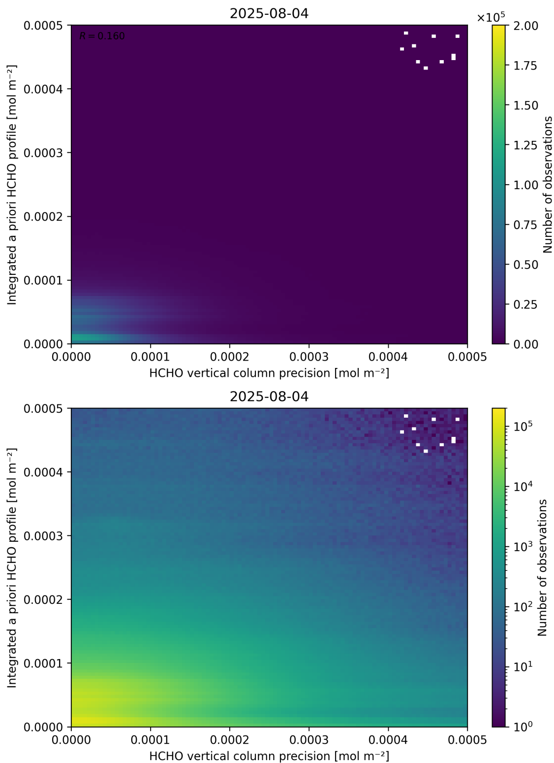
Figure 147: Scatter density plot of “HCHO vertical column precision” against “Integrated a priori HCHO profile” for 2025-08-04 to 2025-08-05.
