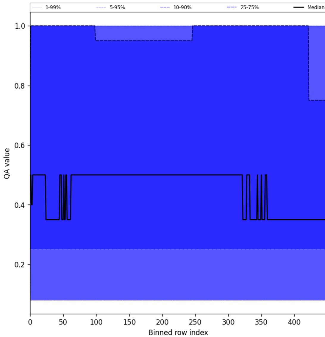
Figure 48: Along track statistics of “QA value” for 2025-08-04 to 2025-08-05
