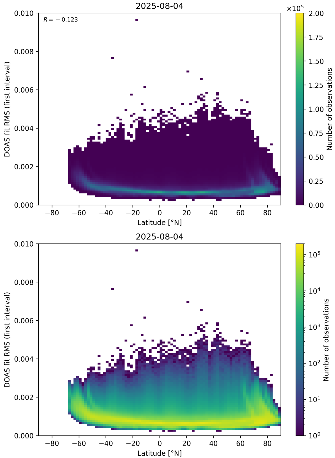
Figure 153: Scatter density plot of “Latitude” against “DOAS fit RMS (first interval)” for 2025-08-04 to 2025-08-05.
