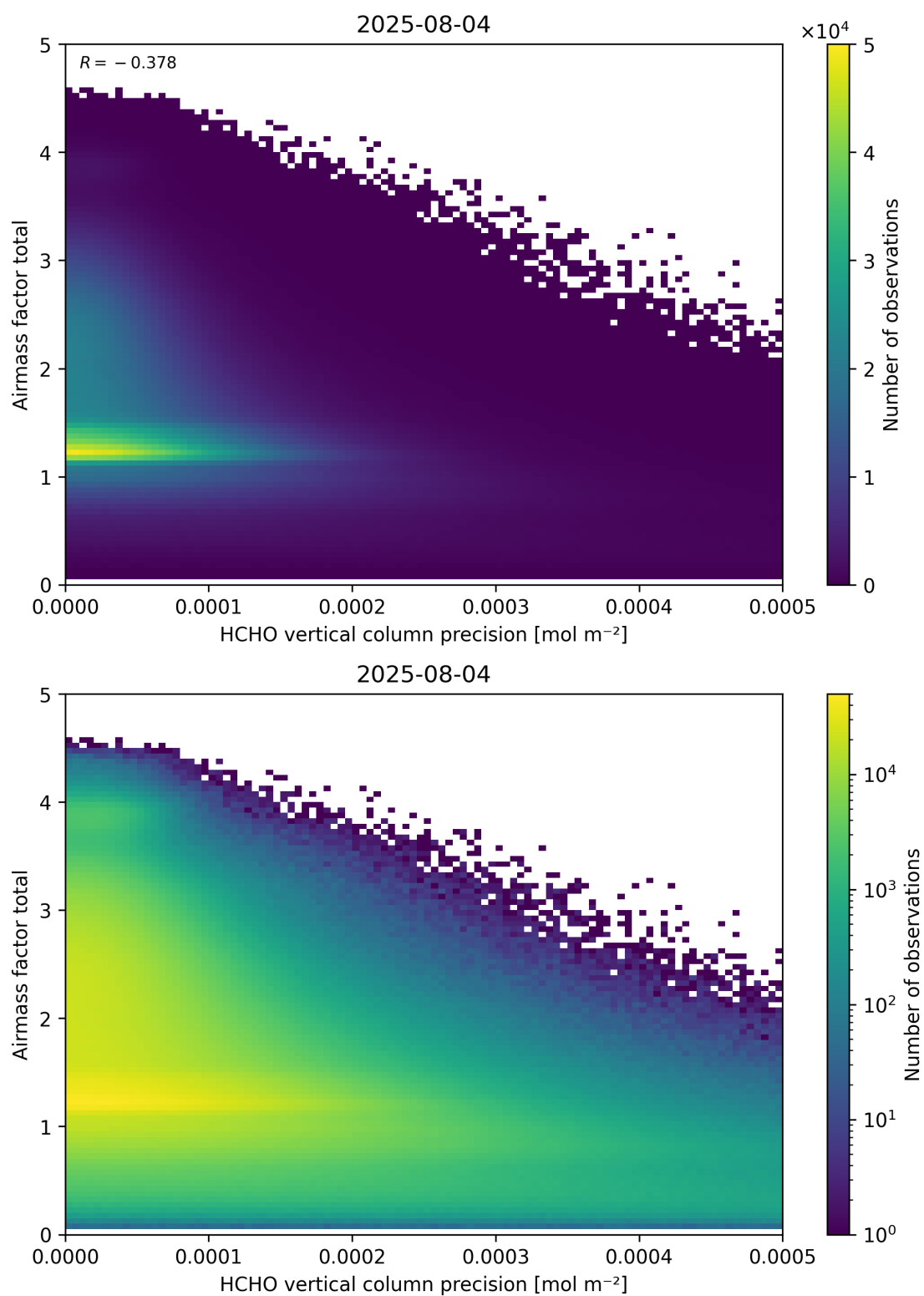
Figure 144: Scatter density plot of “HCHO vertical column precision” against “Airmass factor total” for 2025-08-04 to 2025-08-05.
