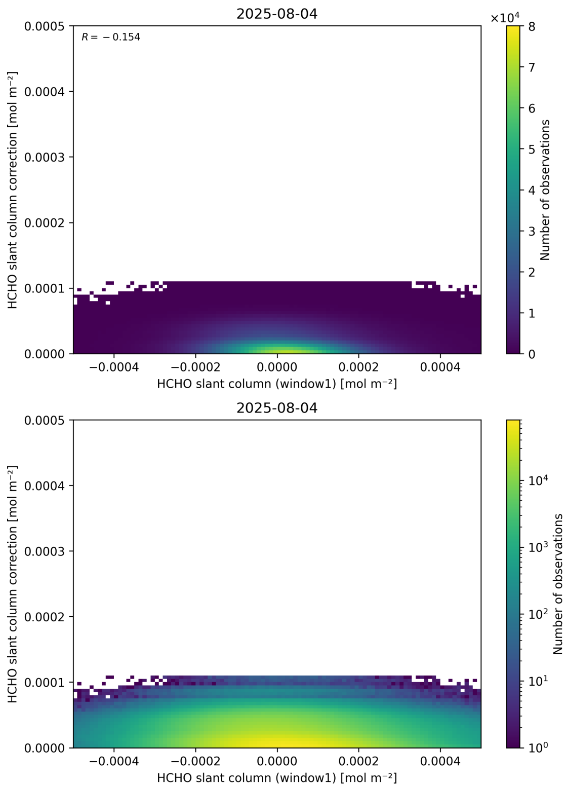
Figure 83: Scatter density plot of “HCHO slant column (window1)” against “HCHO slant column correction” for 2025-08-04 to 2025-08-05.
