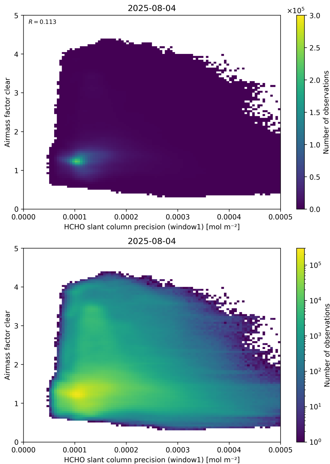
Figure 91: Scatter density plot of “HCHO slant column precision (window1)” against “Airmass factor clear” for 2025-08-04 to 2025-08-05.
