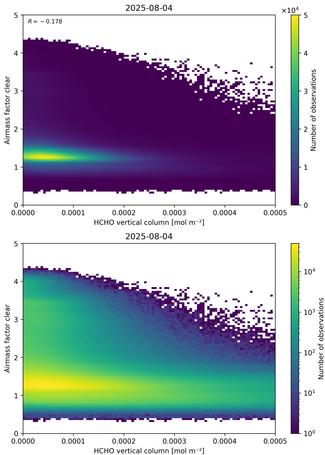
Figure 126: Scatter density plot of “HCHO vertical column” against “Airmass factor clear” for 2025-08-04 to 2025-08-05.
