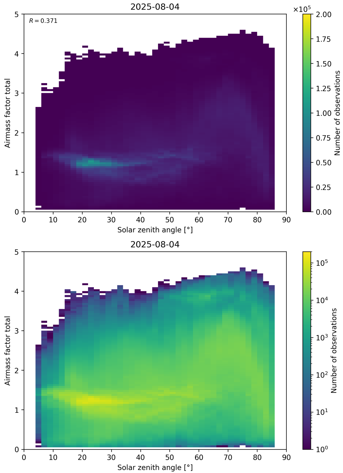
Figure 175: Scatter density plot of “Solar zenith angle” against “Airmass factor total” for 2025-08-04 to 2025-08-05.
