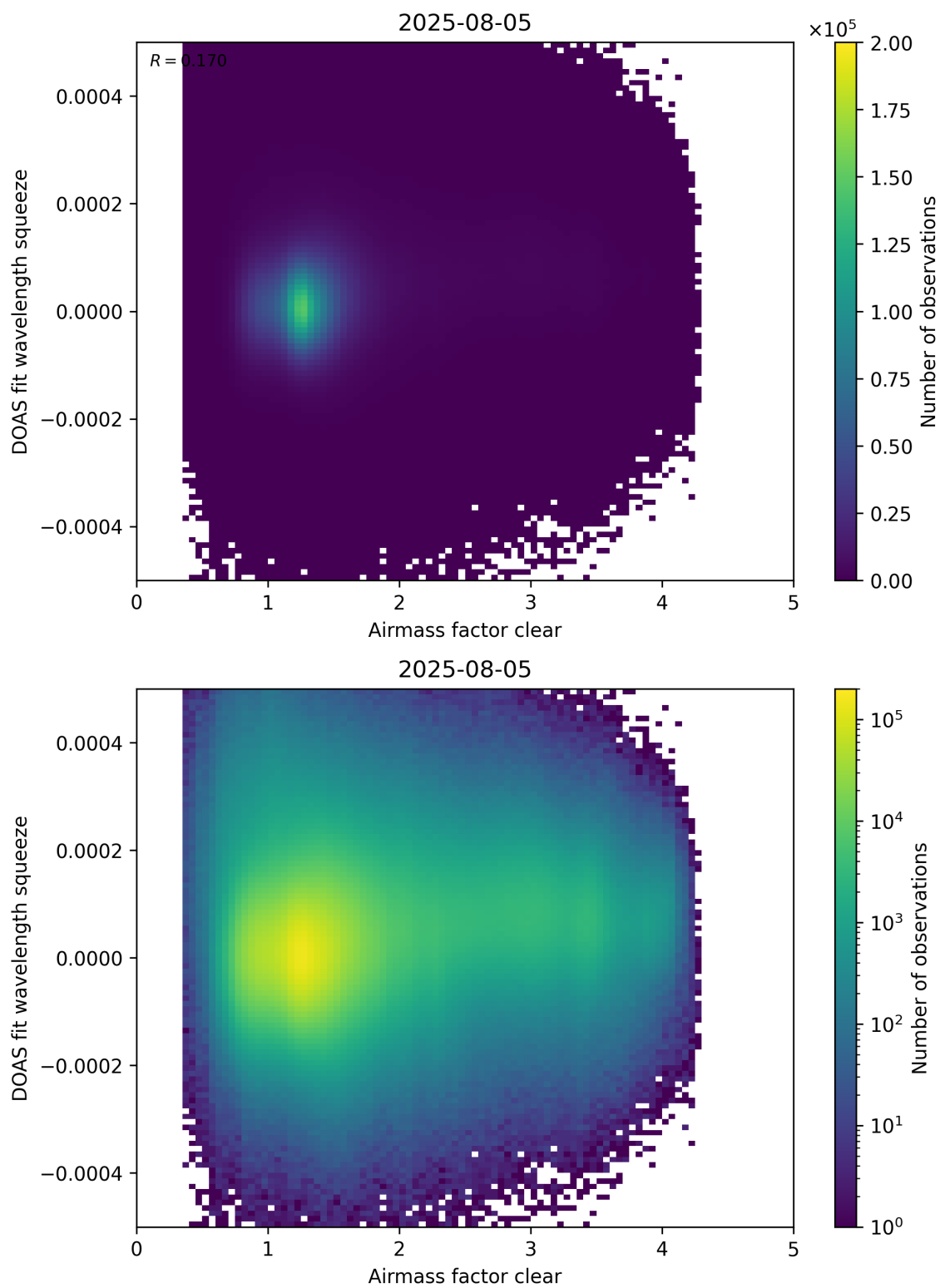
Figure 73: Scatter density plot of “Airmass factor clear” against “DOAS fit wavelength squeeze” for 2025-08-04 to 2025-08-06.
