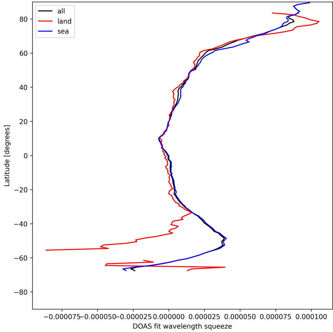
Figure 31: Zonal average of “DOAS fit wavelength squeeze” for 2025-08-04 to 2025-08-06.
