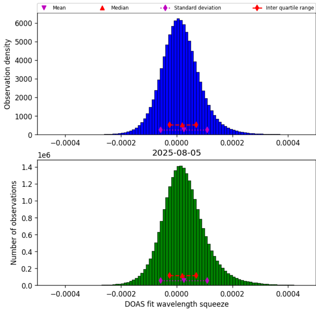
Figure 45: Histogram of “DOAS fit wavelength squeeze” for 2025-08-04 to 2025-08-06
