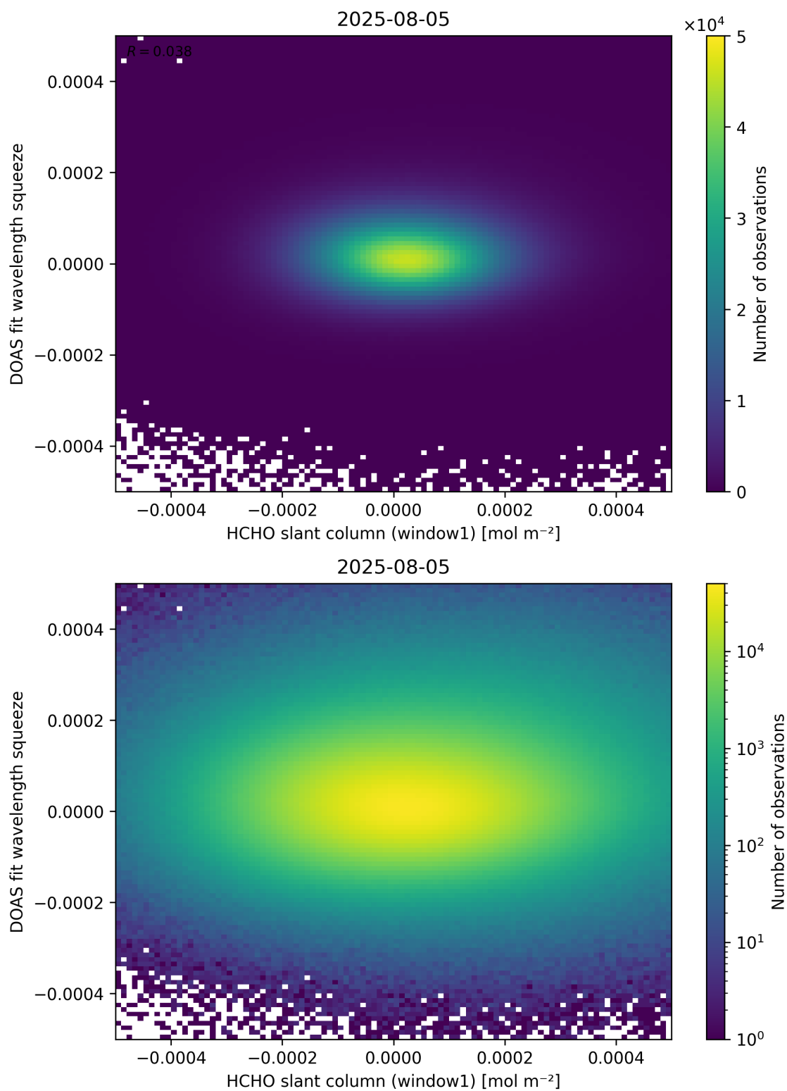
Figure 80: Scatter density plot of “HCHO slant column (window1)” against “DOAS fit wavelength squeeze” for 2025-08-04 to 2025-08-06.
