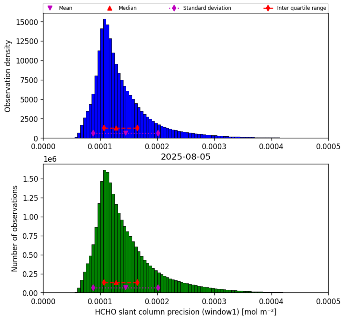
Figure 39: Histogram of “HCHO slant column precision (window1)” for 2025-08-04 to 2025-08-06
