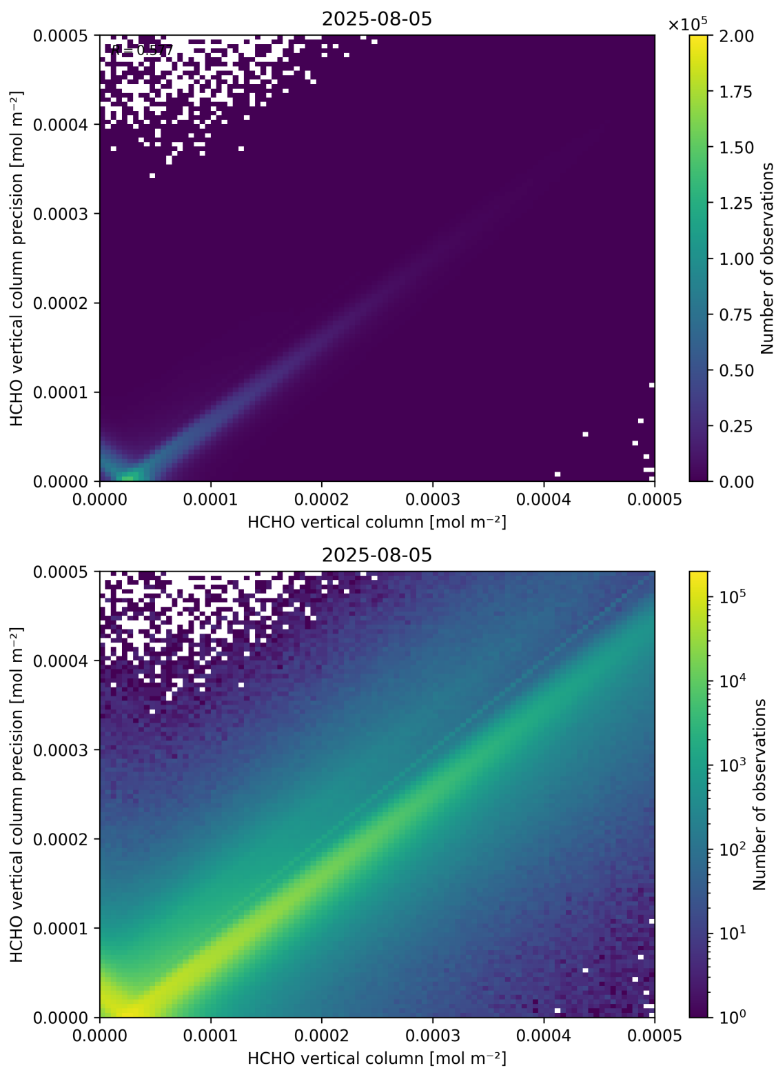
Figure 134: Scatter density plot of “HCHO vertical column” against “HCHO vertical column precision” for 2025-08-04 to 2025-08-06.
