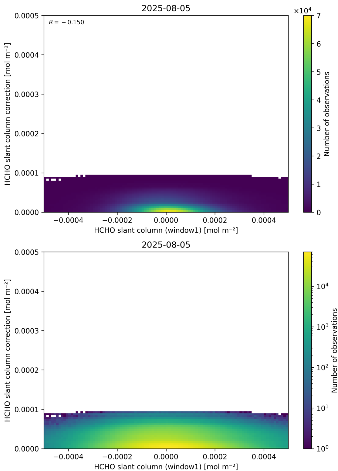
Figure 83: Scatter density plot of “HCHO slant column (window1)” against “HCHO slant column correction” for 2025-08-04 to 2025-08-06.
