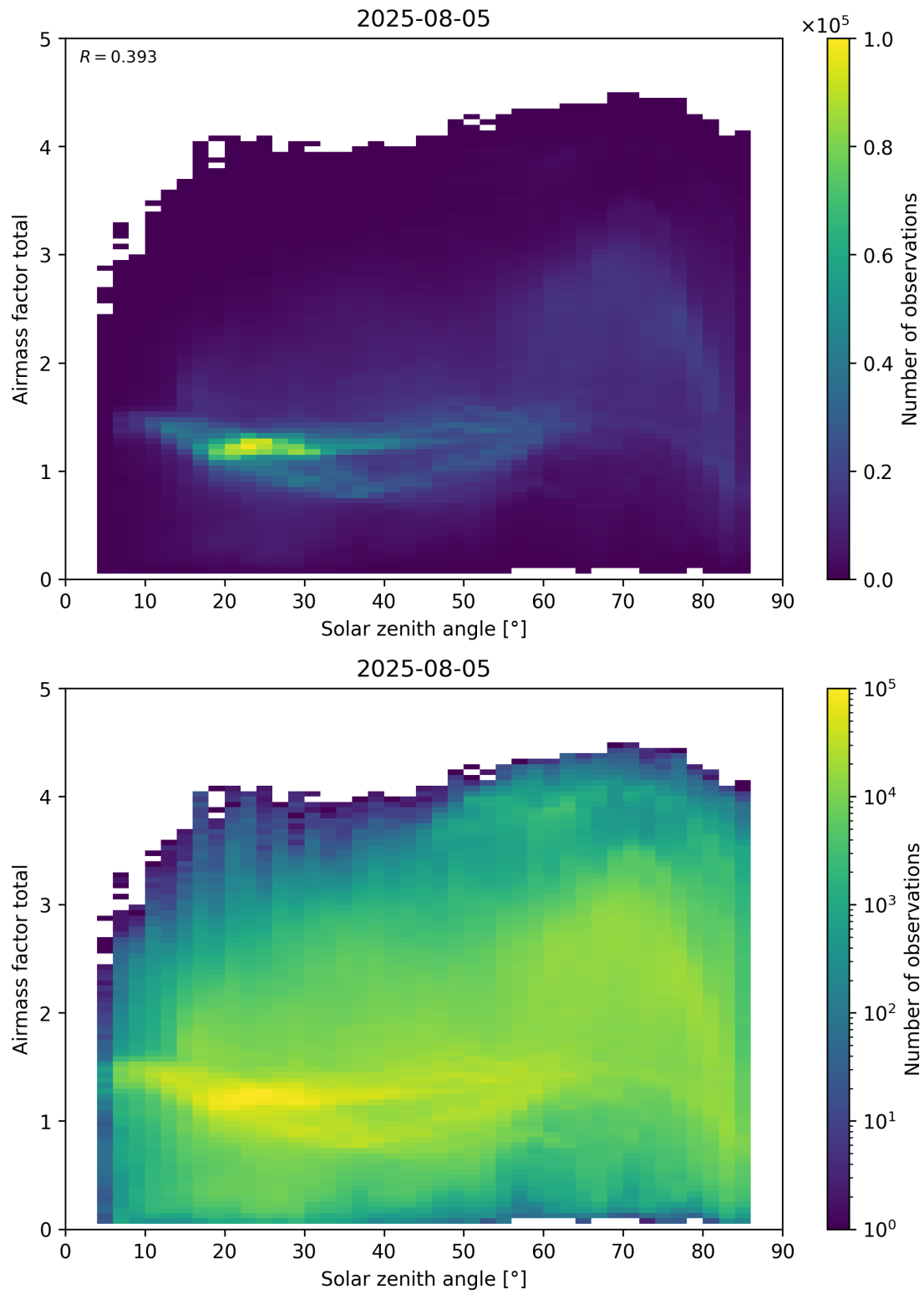
Figure 175: Scatter density plot of “Solar zenith angle” against “Airmass factor total” for 2025-08-04 to 2025-08-06.
