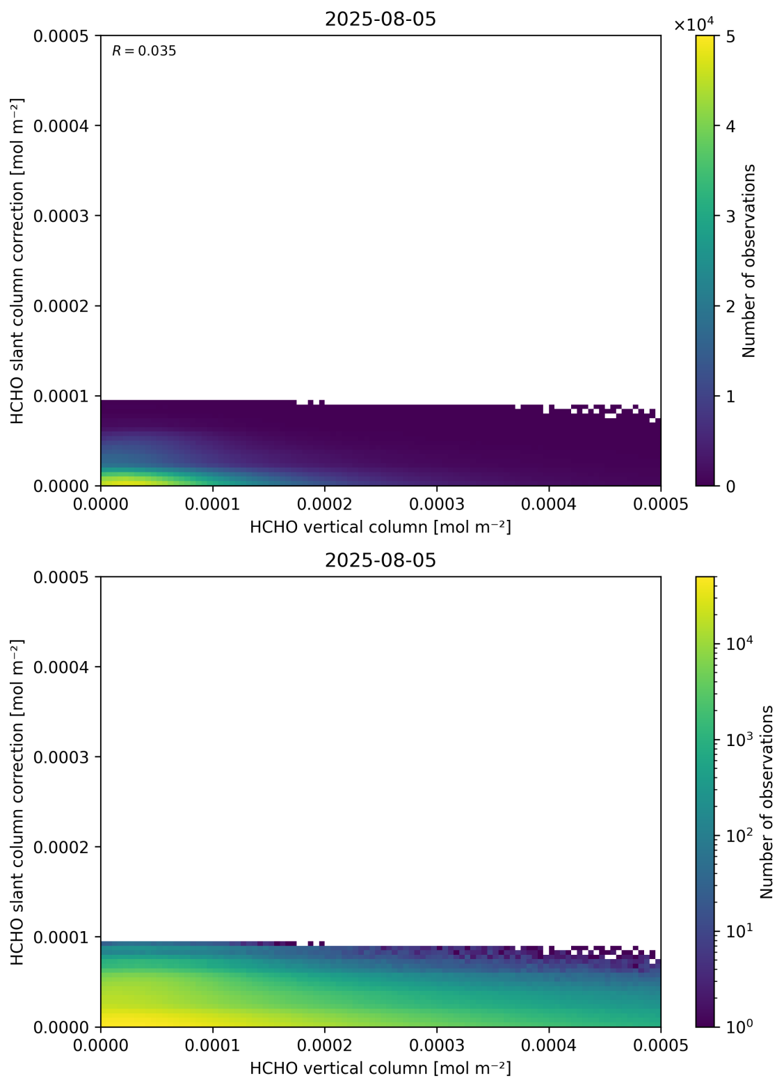
Figure 128: Scatter density plot of “HCHO vertical column” against “HCHO slant column correction” for 2025-08-04 to 2025-08-06.
