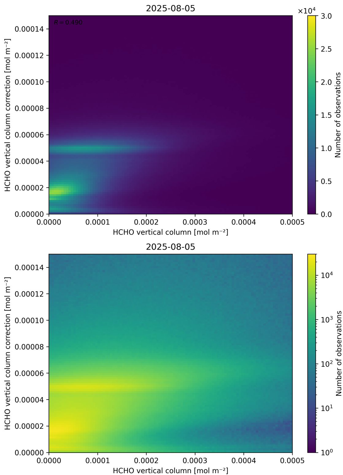
Figure 133: Scatter density plot of “HCHO vertical column” against “HCHO vertical column correction” for 2025-08-04 to 2025-08-06.
