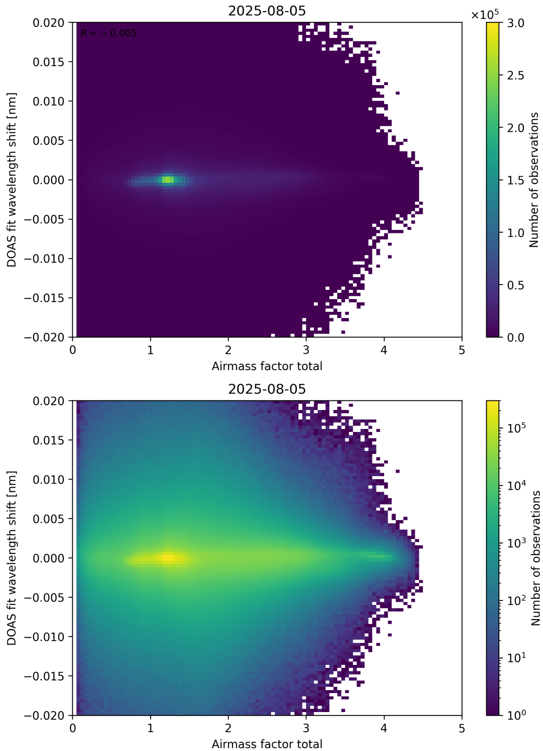
Figure 98: Scatter density plot of “Airmass factor total” against “DOAS fit wavelength shift” for 2025-08-04 to 2025-08-06.
