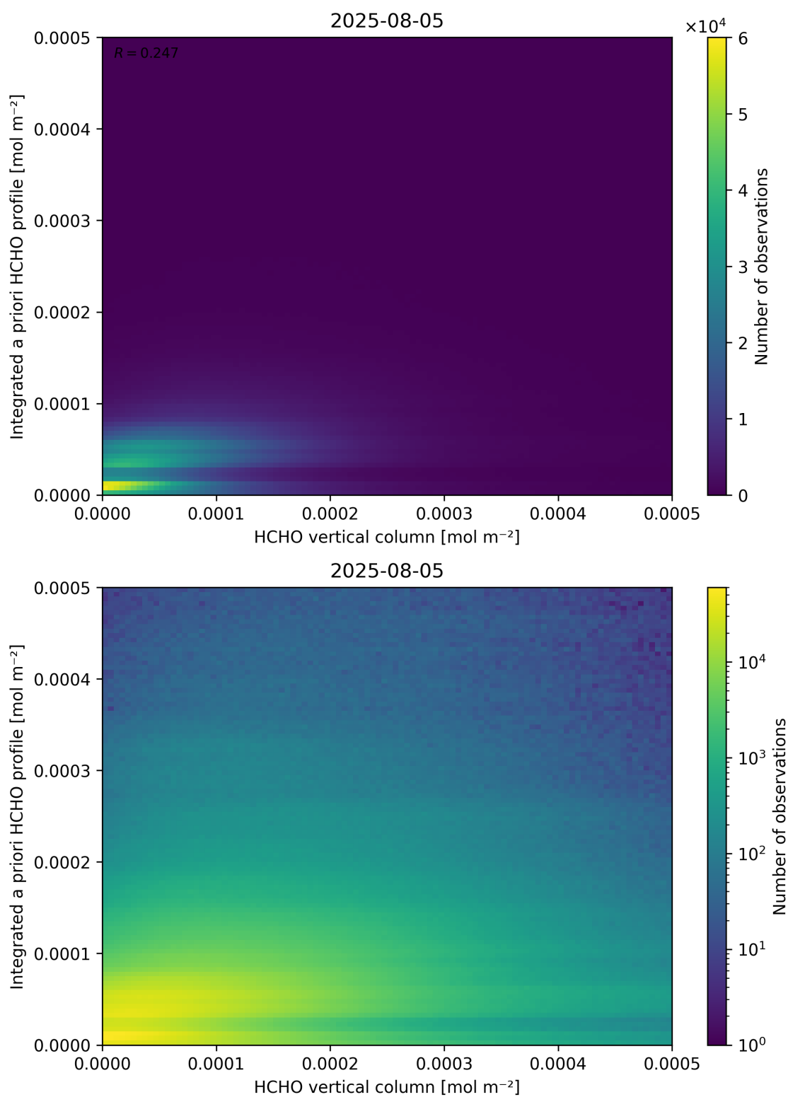
Figure 135: Scatter density plot of “HCHO vertical column” against “Integrated a priori HCHO profile” for 2025-08-04 to 2025-08-06.
