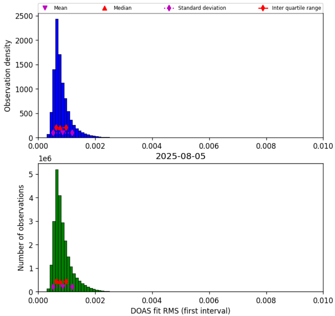
Figure 46: Histogram of “DOAS fit RMS (first interval)” for 2025-08-04 to 2025-08-06
