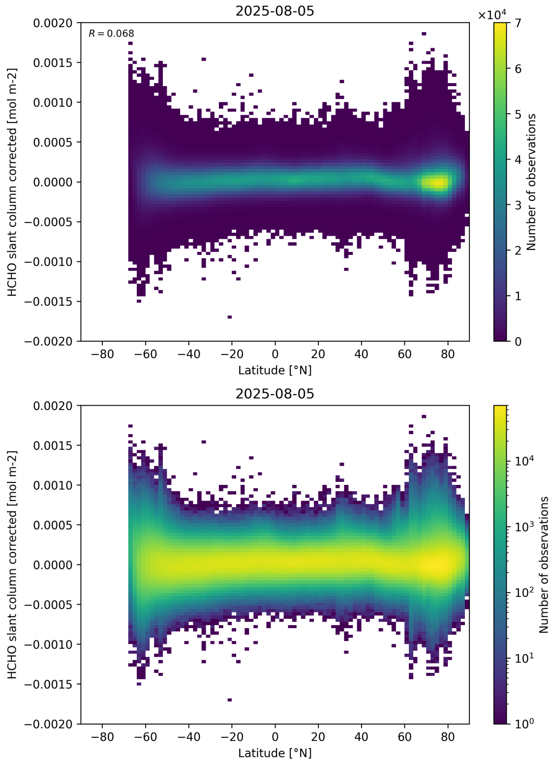
Figure 157: Scatter density plot of “Latitude” against “HCHO slant column corrected” for 2025-08-04 to 2025-08-06.
