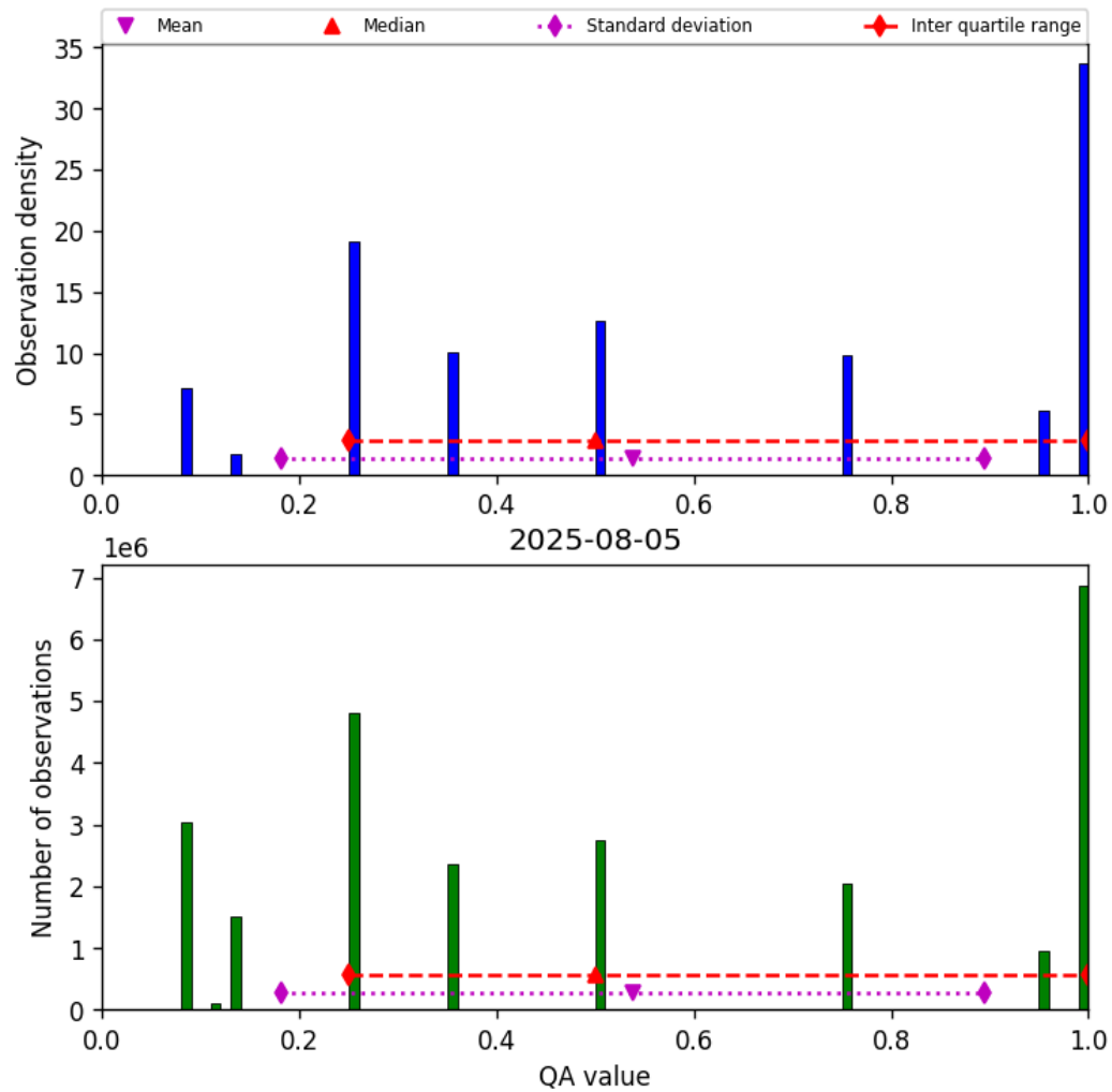
Figure 34: Histogram of “QA value” for 2025-08-04 to 2025-08-06
