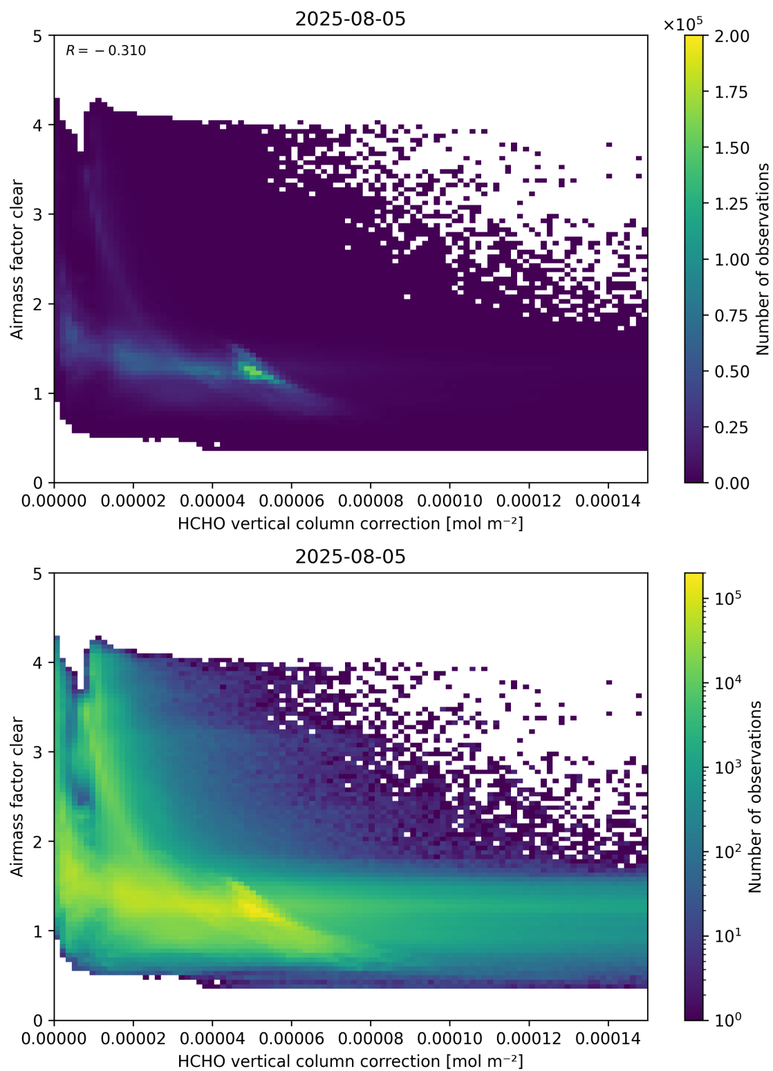
Figure 115: Scatter density plot of “HCHO vertical column correction” against “Airmass factor clear” for 2025-08-04 to 2025-08-06.
