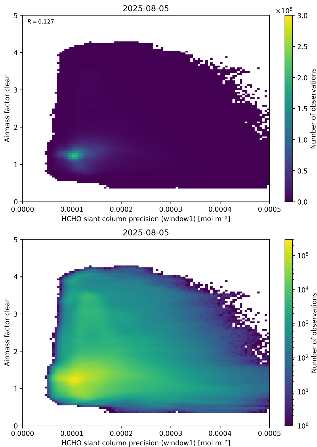
Figure 91: Scatter density plot of “HCHO slant column precision (window1)” against “Airmass factor clear” for 2025-08-04 to 2025-08-06.
