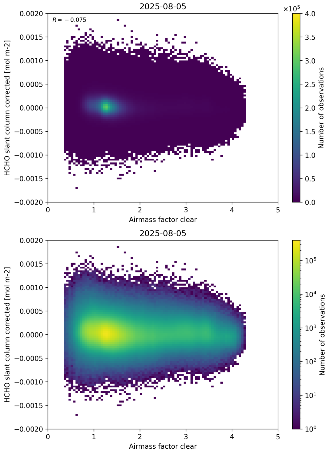
Figure 74: Scatter density plot of “Airmass factor clear” against “HCHO slant column corrected” for 2025-08-04 to 2025-08-06.
