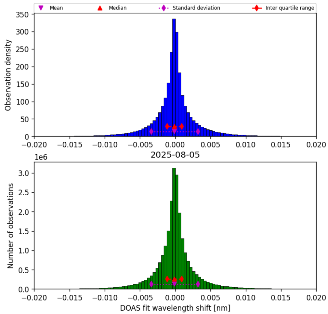
Figure 44: Histogram of “DOAS fit wavelength shift” for 2025-08-04 to 2025-08-06
