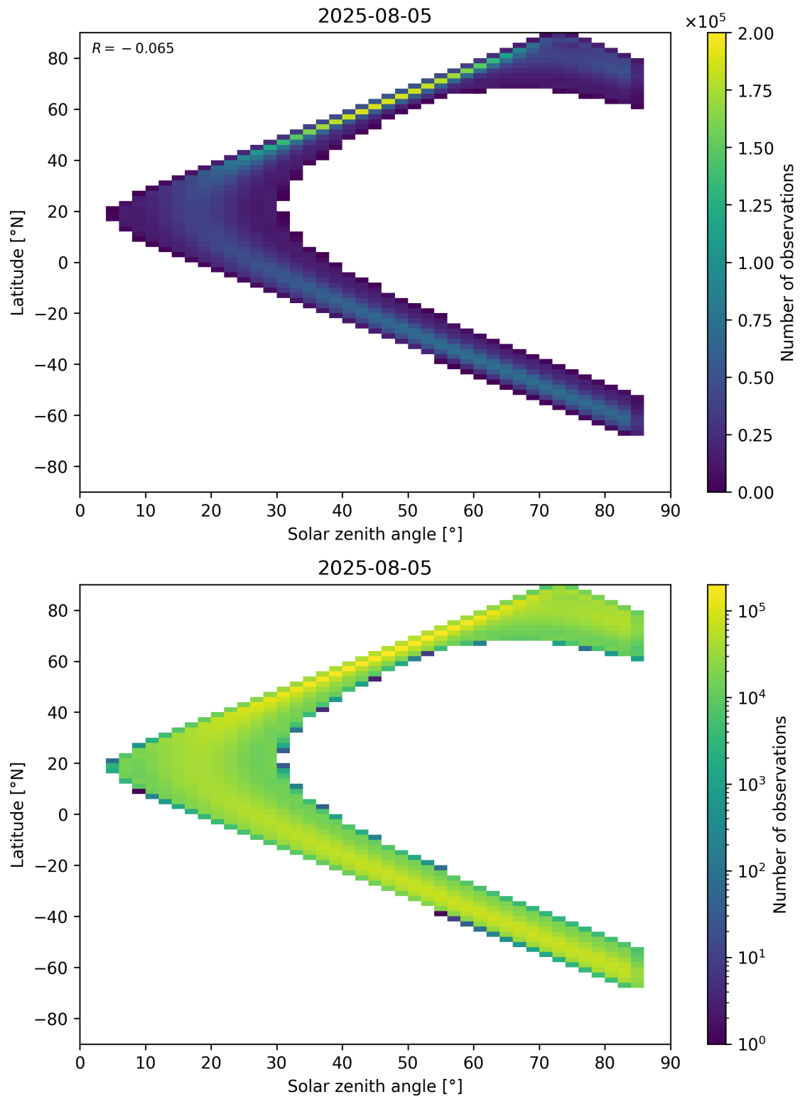
Figure 181: Scatter density plot of “Solar zenith angle” against “Latitude” for 2025-08-04 to 2025-08-06.
