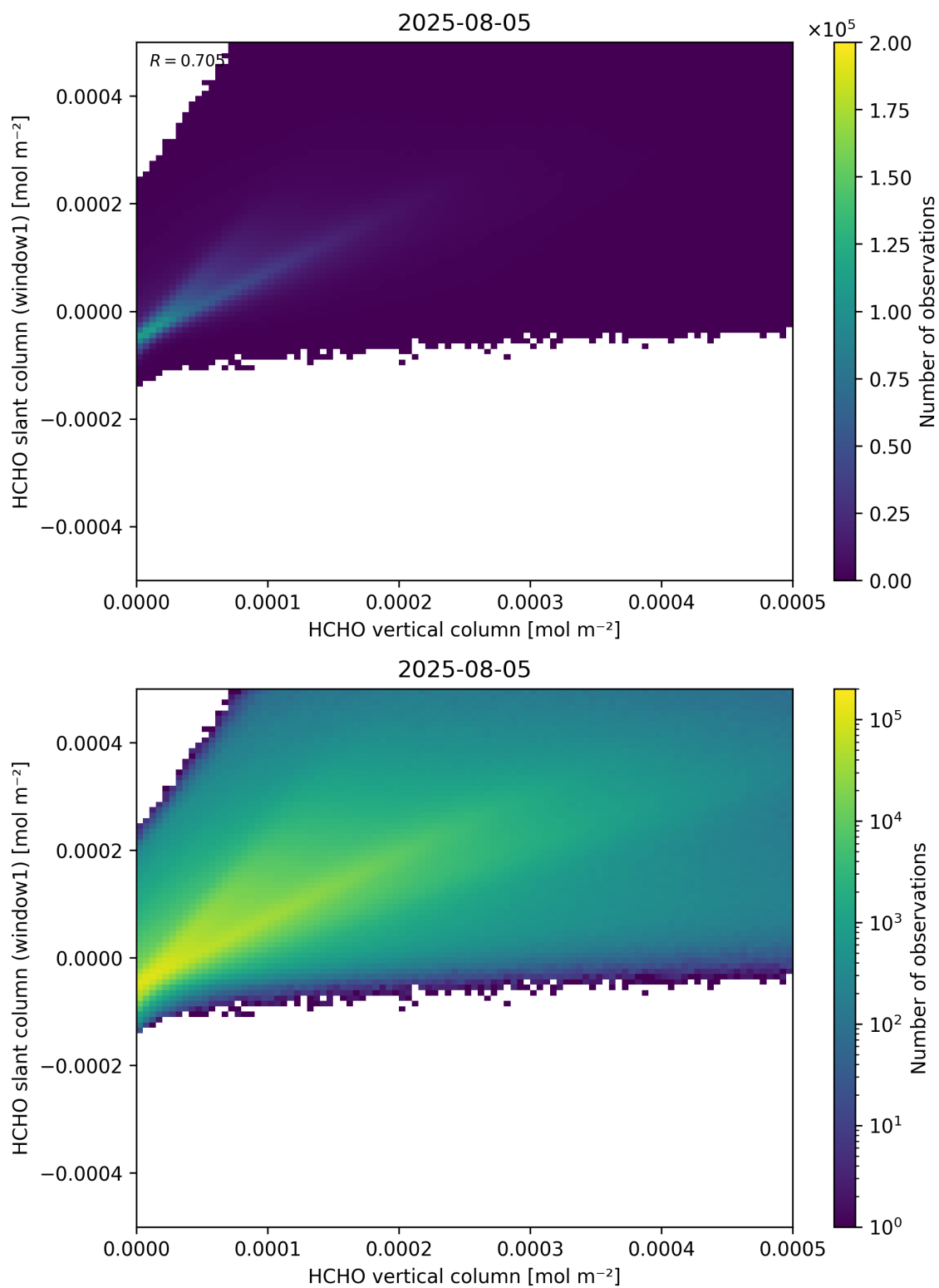
Figure 129: Scatter density plot of “HCHO vertical column” against “HCHO slant column (window1)” for 2025-08-04 to 2025-08-06.
