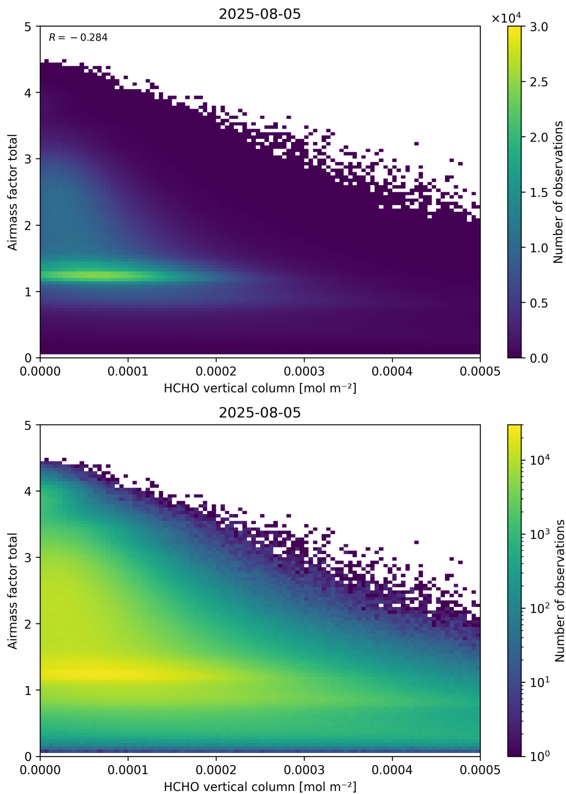
Figure 131: Scatter density plot of “HCHO vertical column” against “Airmass factor total” for 2025-08-04 to 2025-08-06.
