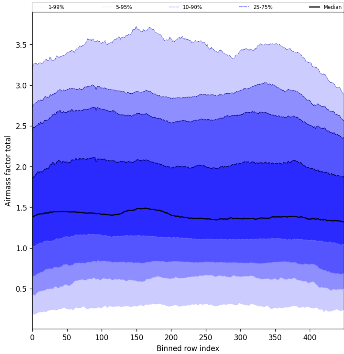
Figure 54: Along track statistics of “Airmass factor total” for 2025-08-04 to 2025-08-06
