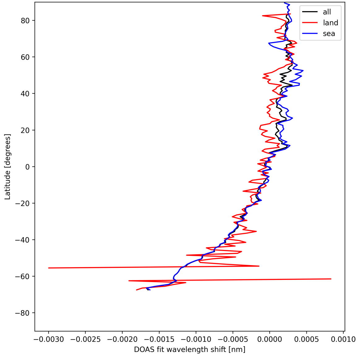
Figure 30: Zonal average of “DOAS fit wavelength shift” for 2025-08-04 to 2025-08-06.
