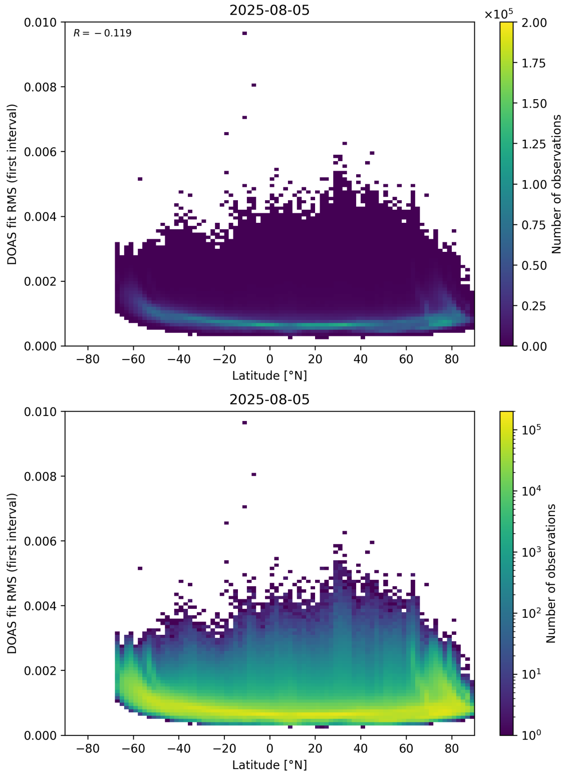
Figure 153: Scatter density plot of “Latitude” against “DOAS fit RMS (first interval)” for 2025-08-04 to 2025-08-06.
