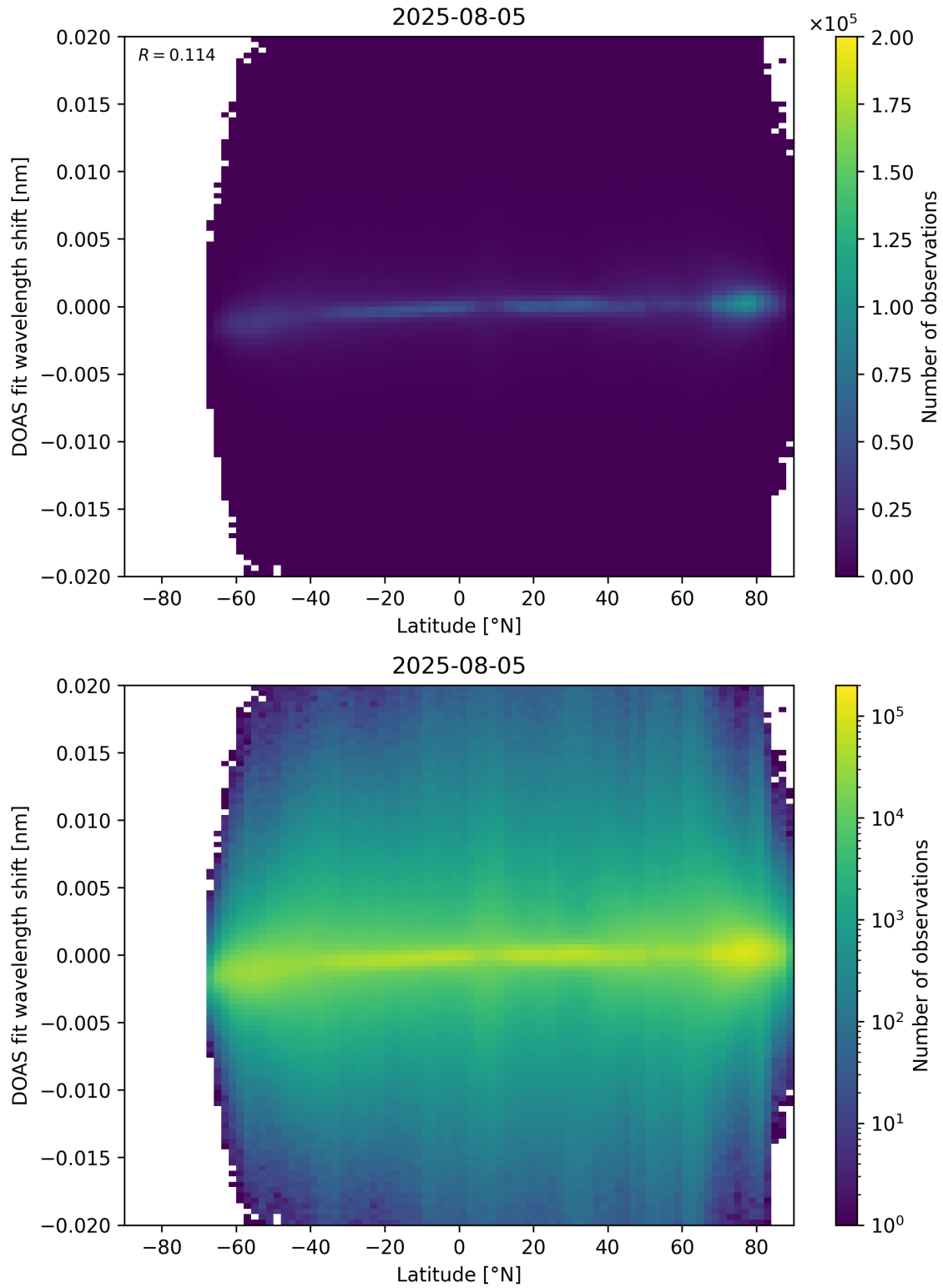
Figure 154: Scatter density plot of “Latitude” against “DOAS fit wavelength shift” for 2025-08-04 to 2025-08-06.
