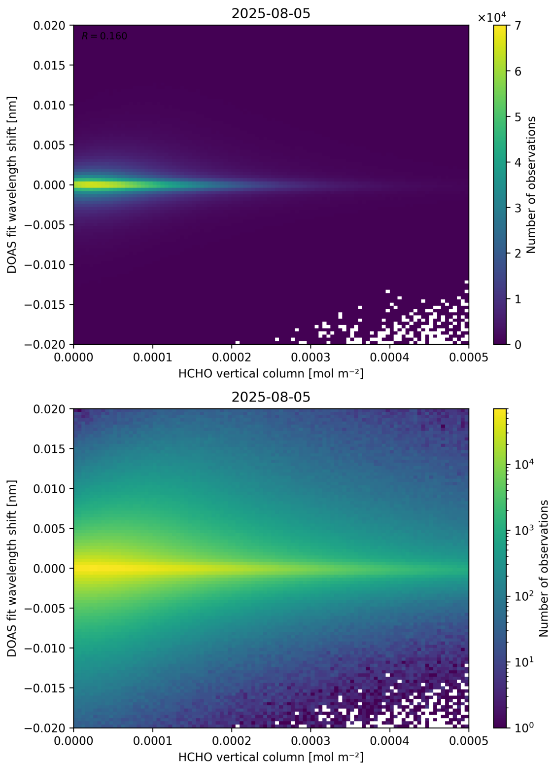
Figure 124: Scatter density plot of “HCHO vertical column” against “DOAS fit wavelength shift” for 2025-08-04 to 2025-08-06.
