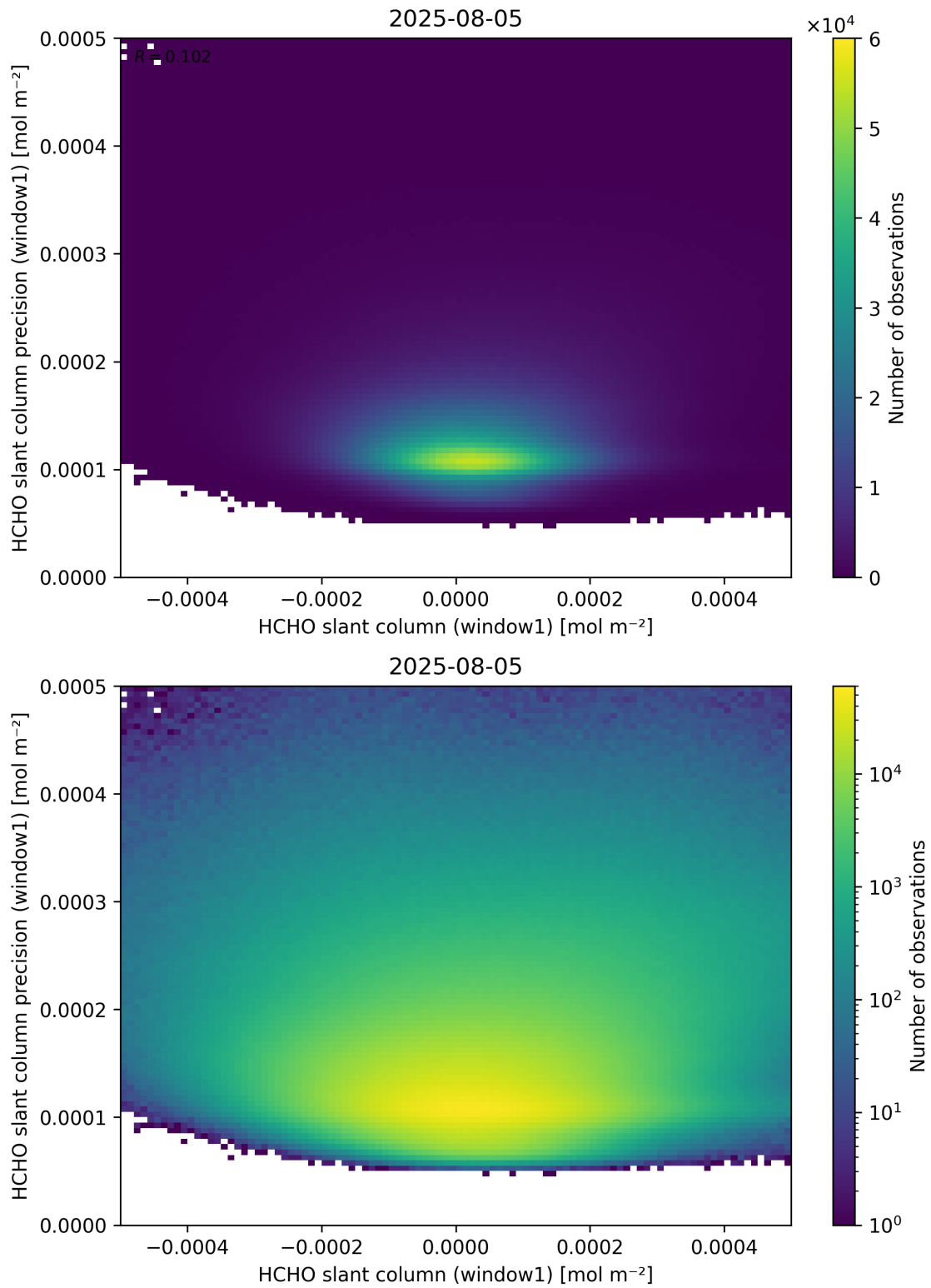
Figure 84: Scatter density plot of “HCHO slant column (window1)” against “HCHO slant column precision (window1)” for 2025-08-04 to 2025-08-06.
