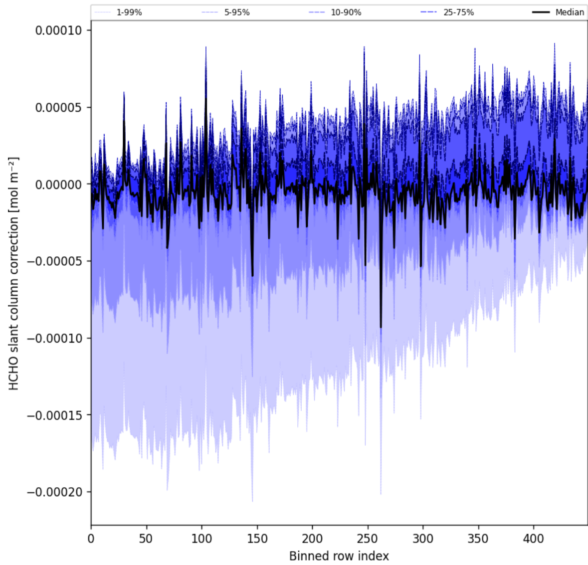
Figure 61: Along track statistics of “HCHO slant column correction” for 2025-08-04 to 2025-08-06
