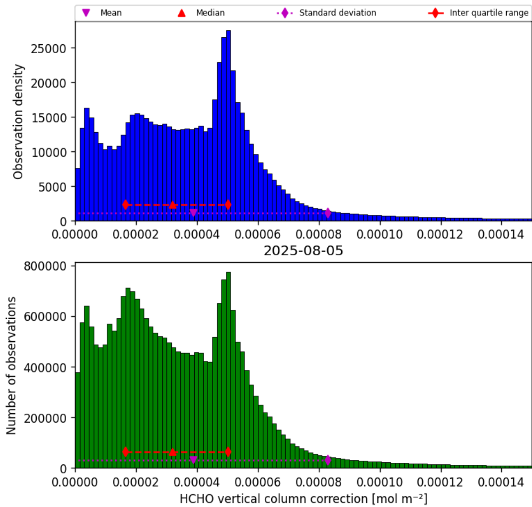
Figure 37: Histogram of “HCHO vertical column correction” for 2025-08-04 to 2025-08-06
