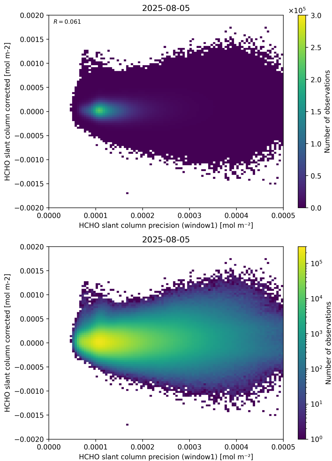
Figure 92: Scatter density plot of “HCHO slant column precision (window1)” against “HCHO slant column corrected” for 2025-08-04 to 2025-08-06.
