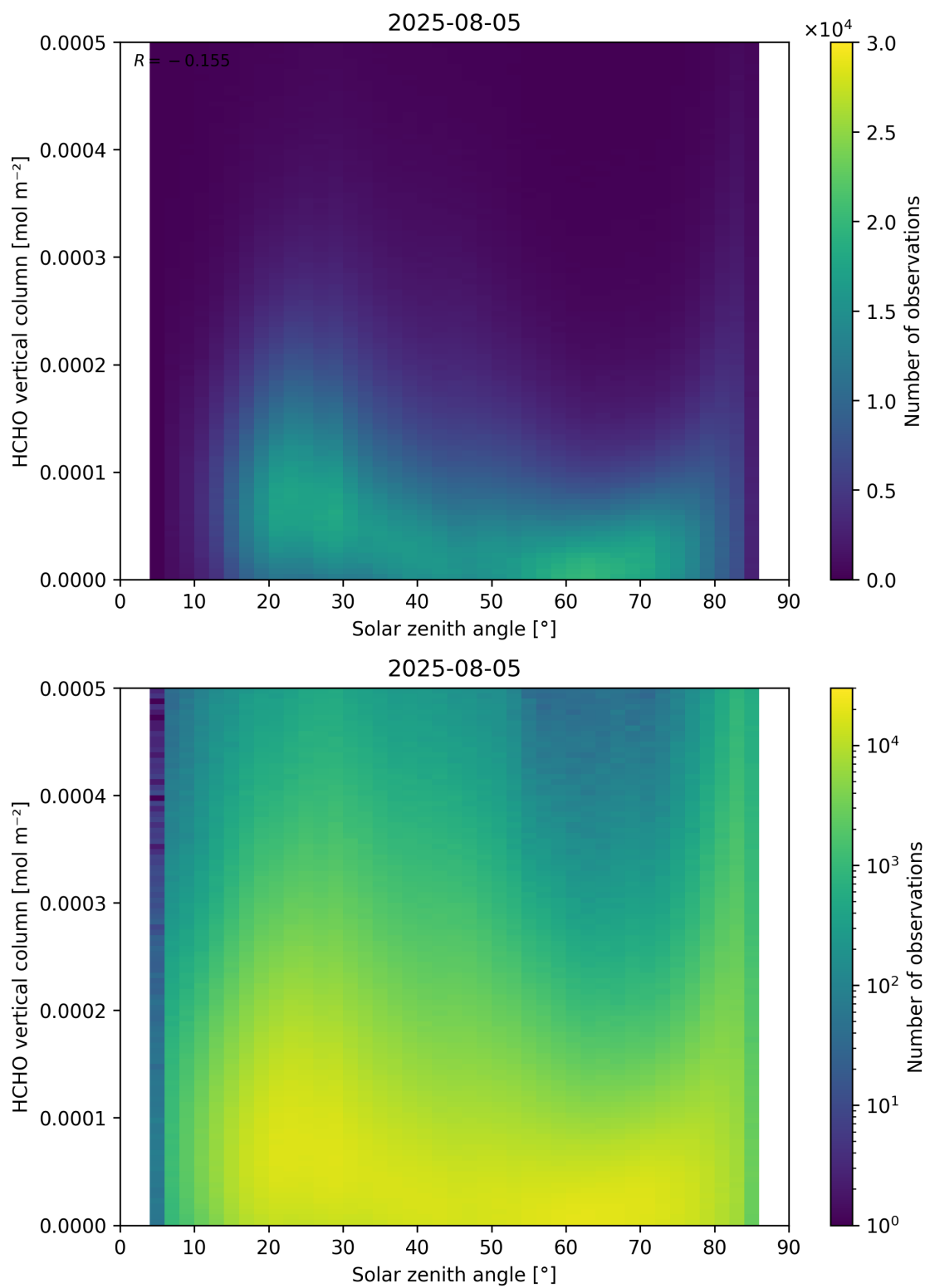
Figure 177: Scatter density plot of “Solar zenith angle” against “HCHO vertical column” for 2025-08-04 to 2025-08-06.
