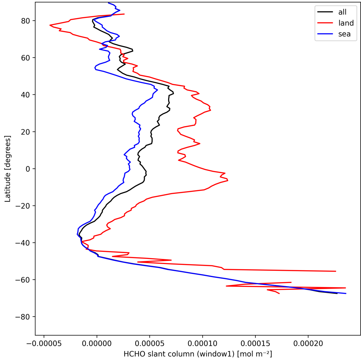
Figure 24: Zonal average of “HCHO slant column (window1)” for 2025-08-04 to 2025-08-06.
