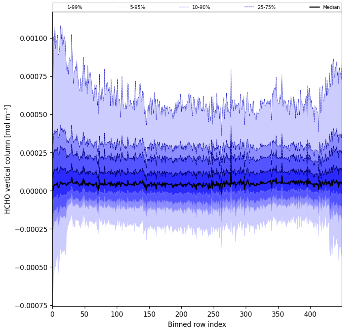
Figure 49: Along track statistics of “HCHO vertical column” for 2025-08-04 to 2025-08-06
