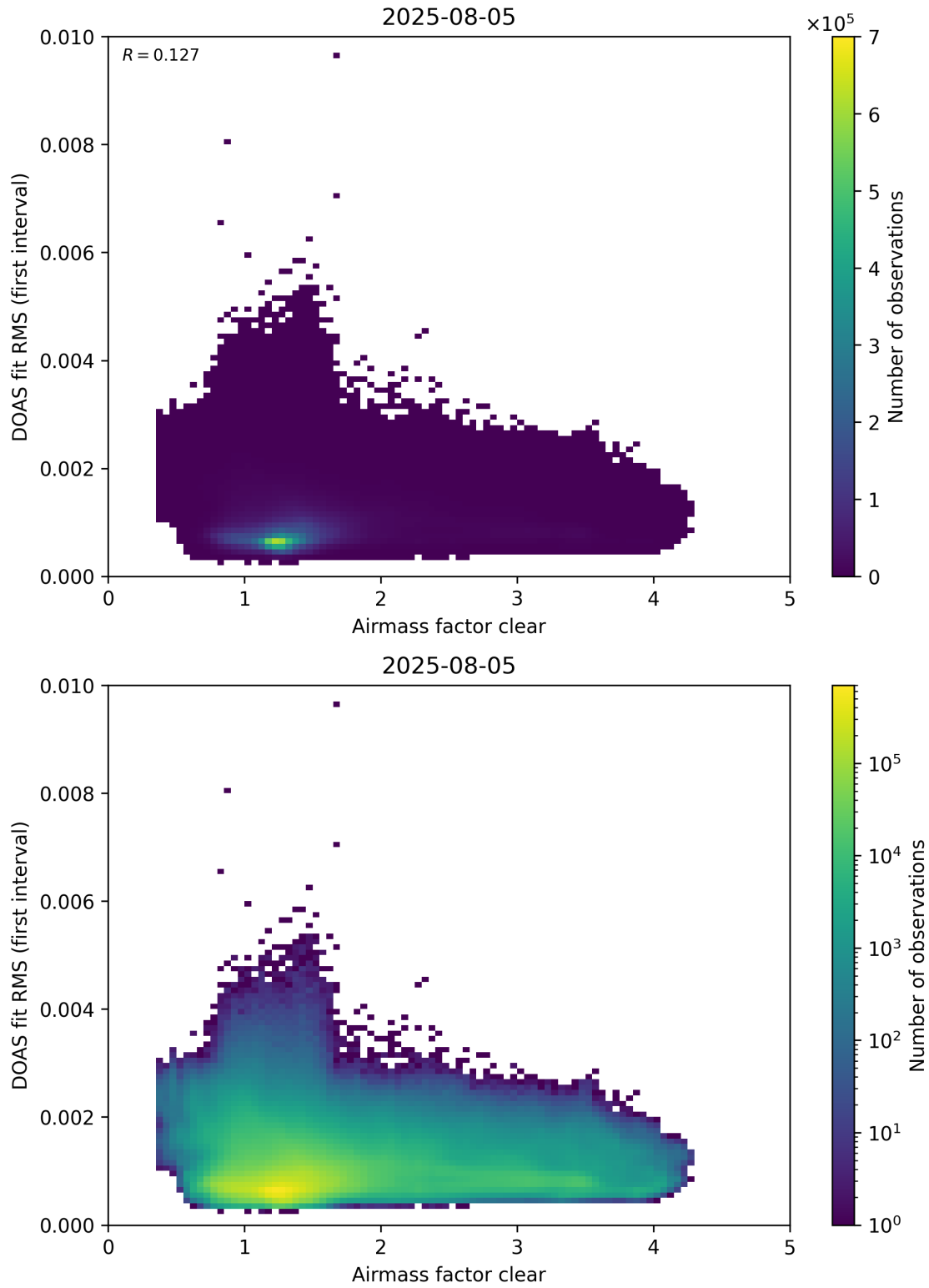
Figure 71: Scatter density plot of “Airmass factor clear” against “DOAS fit RMS (first interval)” for 2025-08-04 to 2025-08-06.
