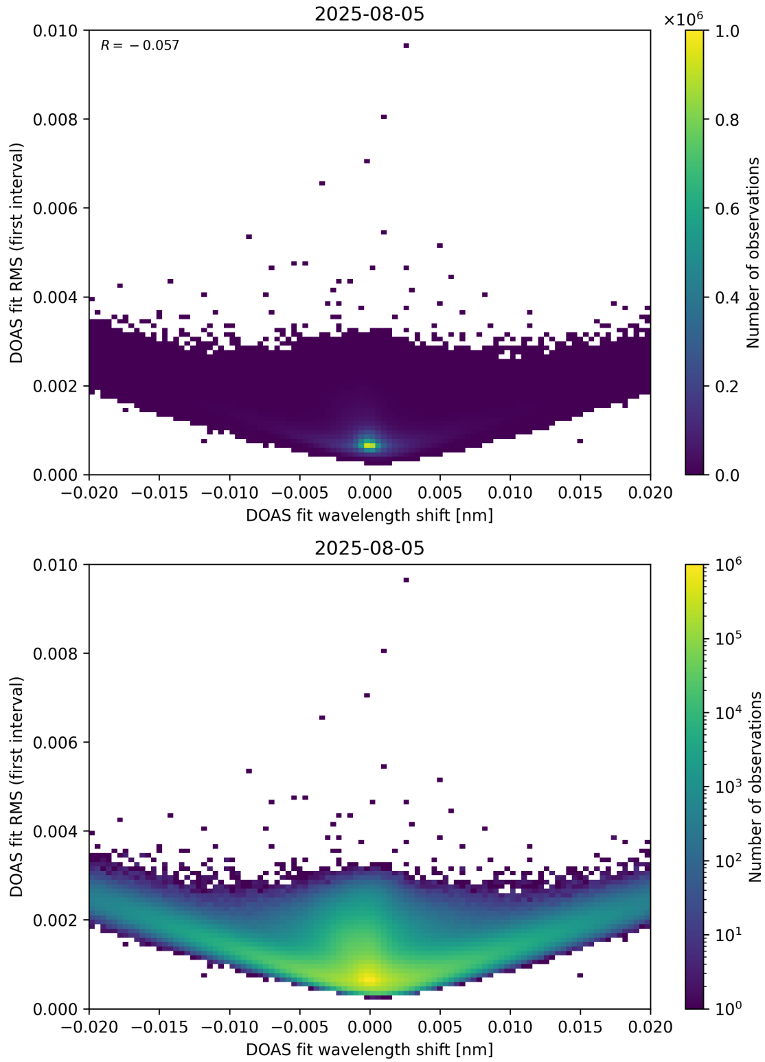
Figure 64: Scatter density plot of “DOAS fit wavelength shift” against “DOAS fit RMS (first interval)” for 2025-08-04 to 2025-08-06.
