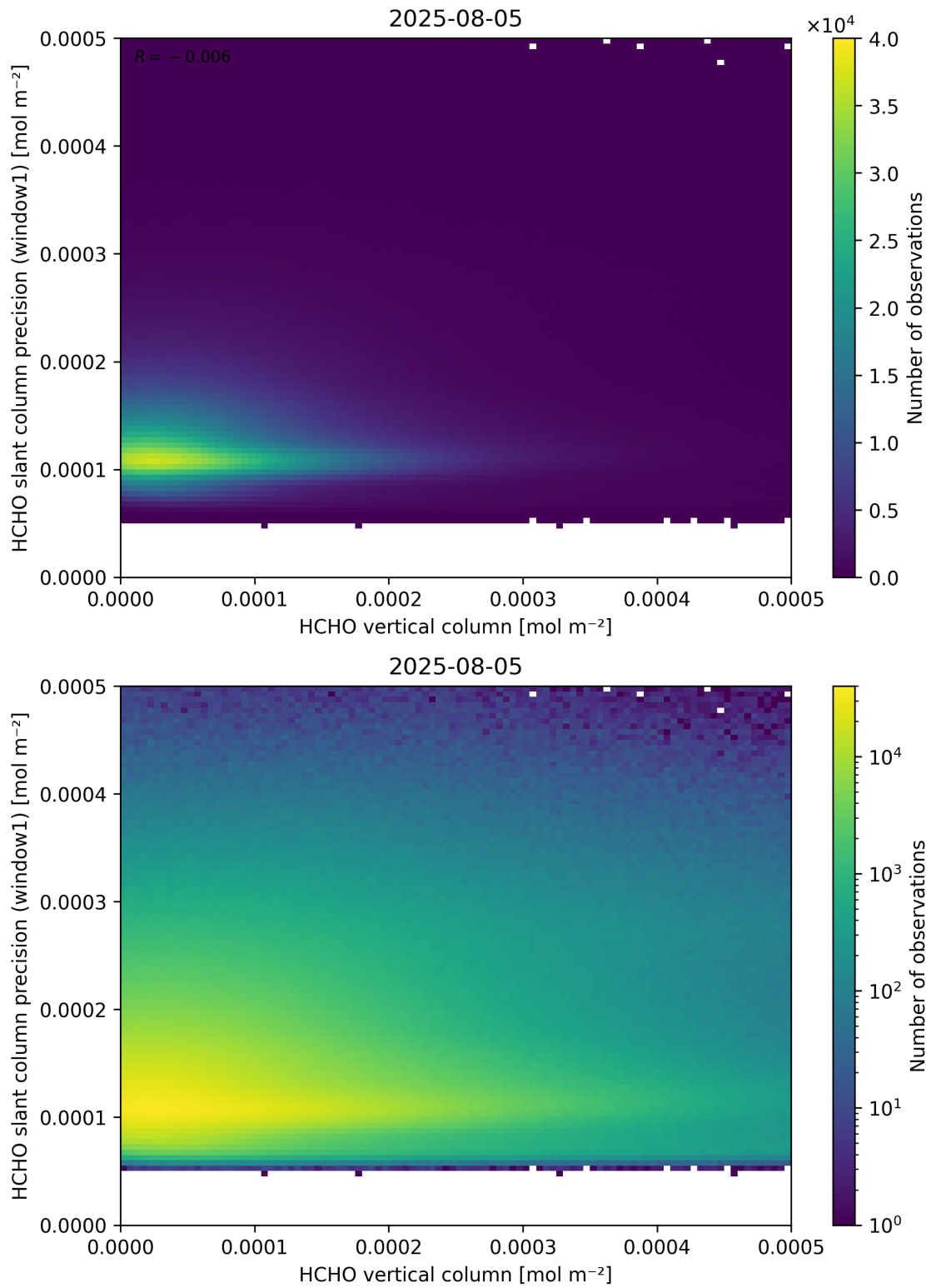
Figure 130: Scatter density plot of “HCHO vertical column” against “HCHO slant column precision (window1)” for 2025-08-04 to 2025-08-06.
