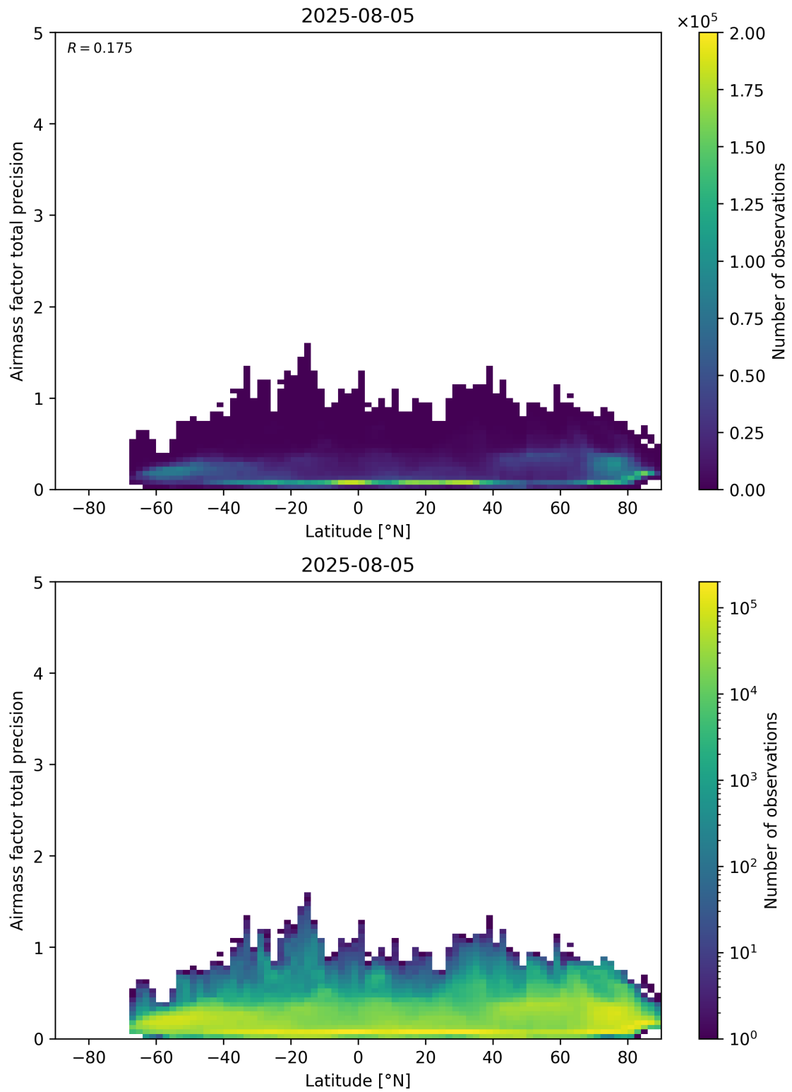
Figure 162: Scatter density plot of “Latitude” against “Airmass factor total precision” for 2025-08-04 to 2025-08-06.
