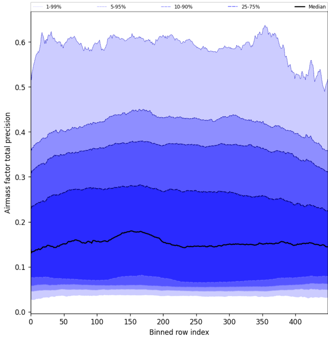
Figure 55: Along track statistics of “Airmass factor total precision” for 2025-08-04 to 2025-08-06
