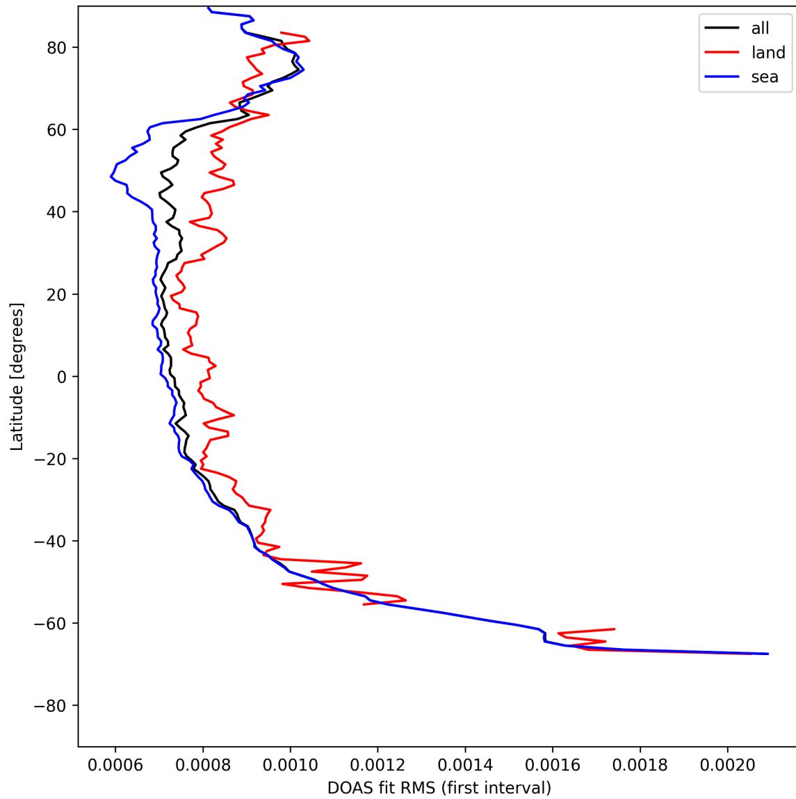
Figure 32: Zonal average of "DOAS fit RMS (first interval)" for 2025-08-04 to 2025-08-06.
