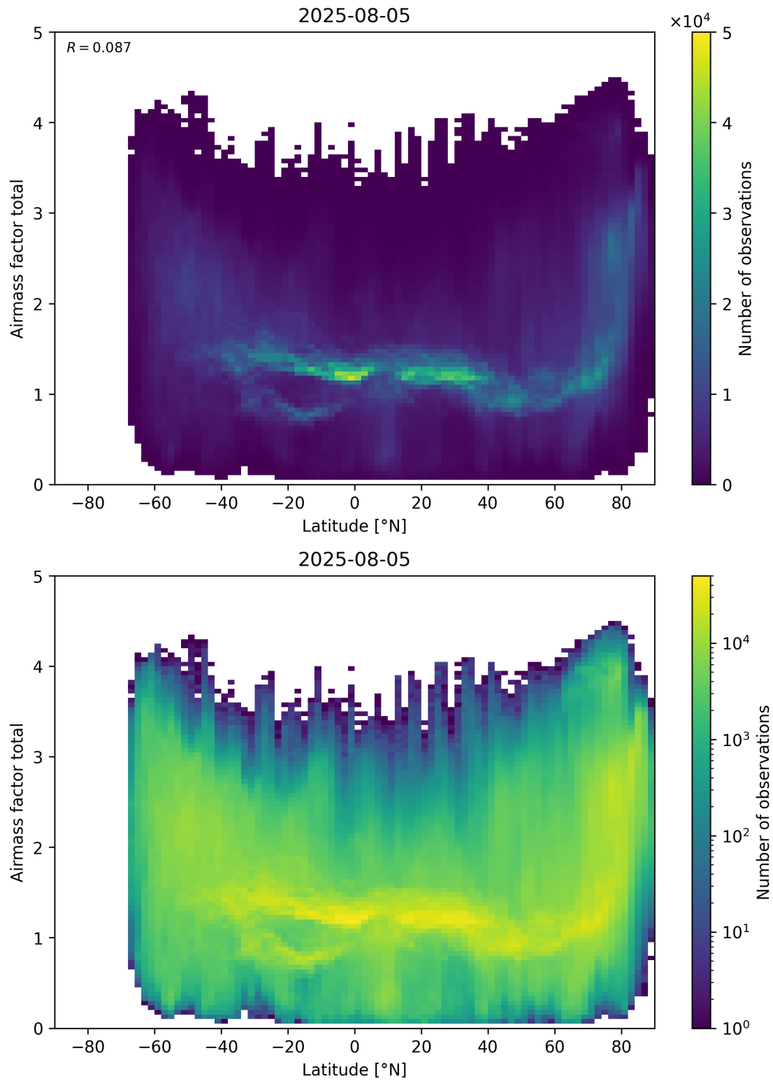
Figure 161: Scatter density plot of “Latitude” against “Airmass factor total” for 2025-08-04 to 2025-08-06.
