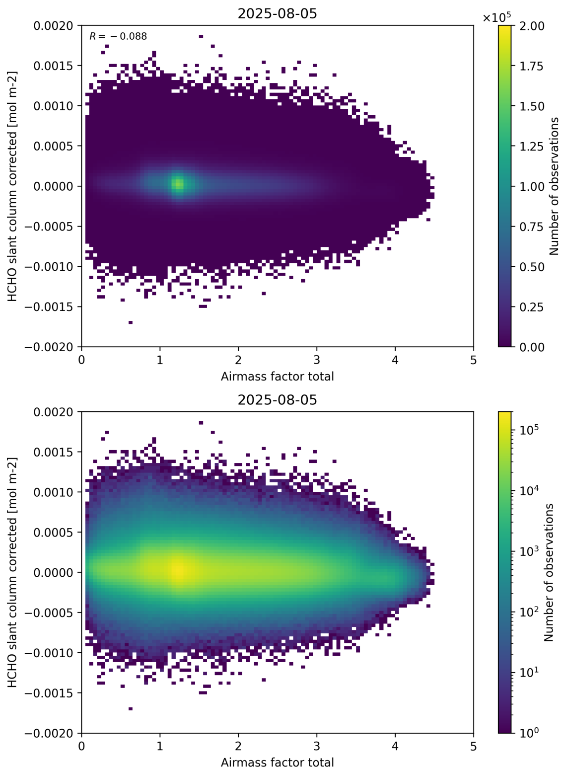
Figure 101: Scatter density plot of “Airmass factor total” against “HCHO slant column corrected” for 2025-08-04 to 2025-08-06.
