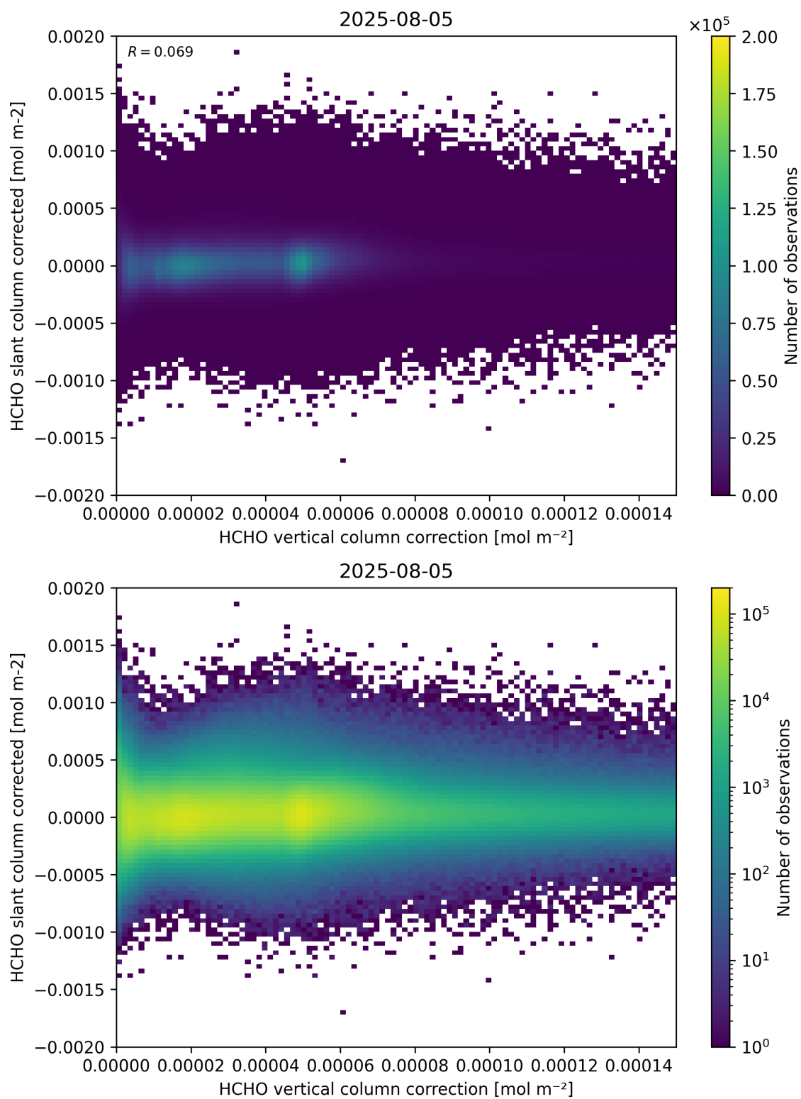
Figure 116: Scatter density plot of “HCHO vertical column correction” against “HCHO slant column corrected” for 2025-08-04 to 2025-08-06.
