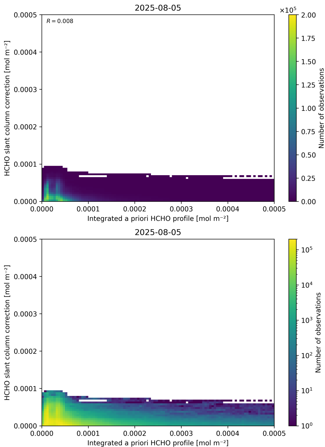
Figure 152: Scatter density plot of “Integrated a priori HCHO profile” against “HCHO slant column correction” for 2025-08-04 to 2025-08-06.
