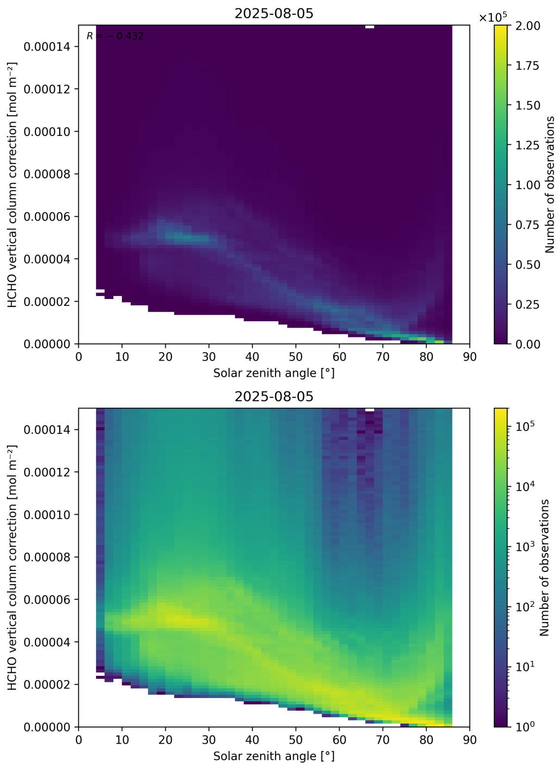
Figure 178: Scatter density plot of “Solar zenith angle” against “HCHO vertical column correction” for 2025-08-04 to 2025-08-06.
