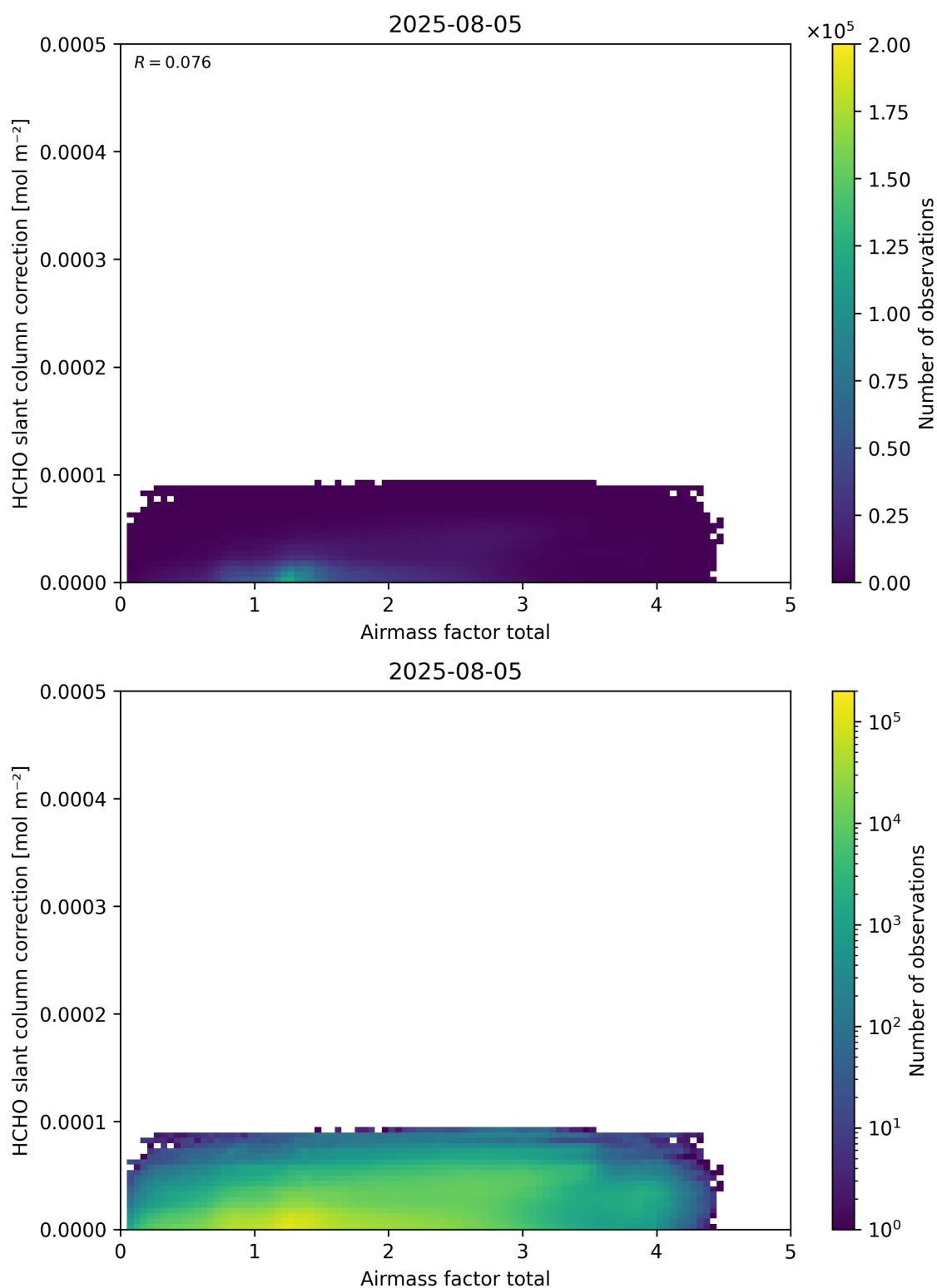
Figure 102: Scatter density plot of “Airmass factor total” against “HCHO slant column correction” for 2025-08-04 to 2025-08-06.
