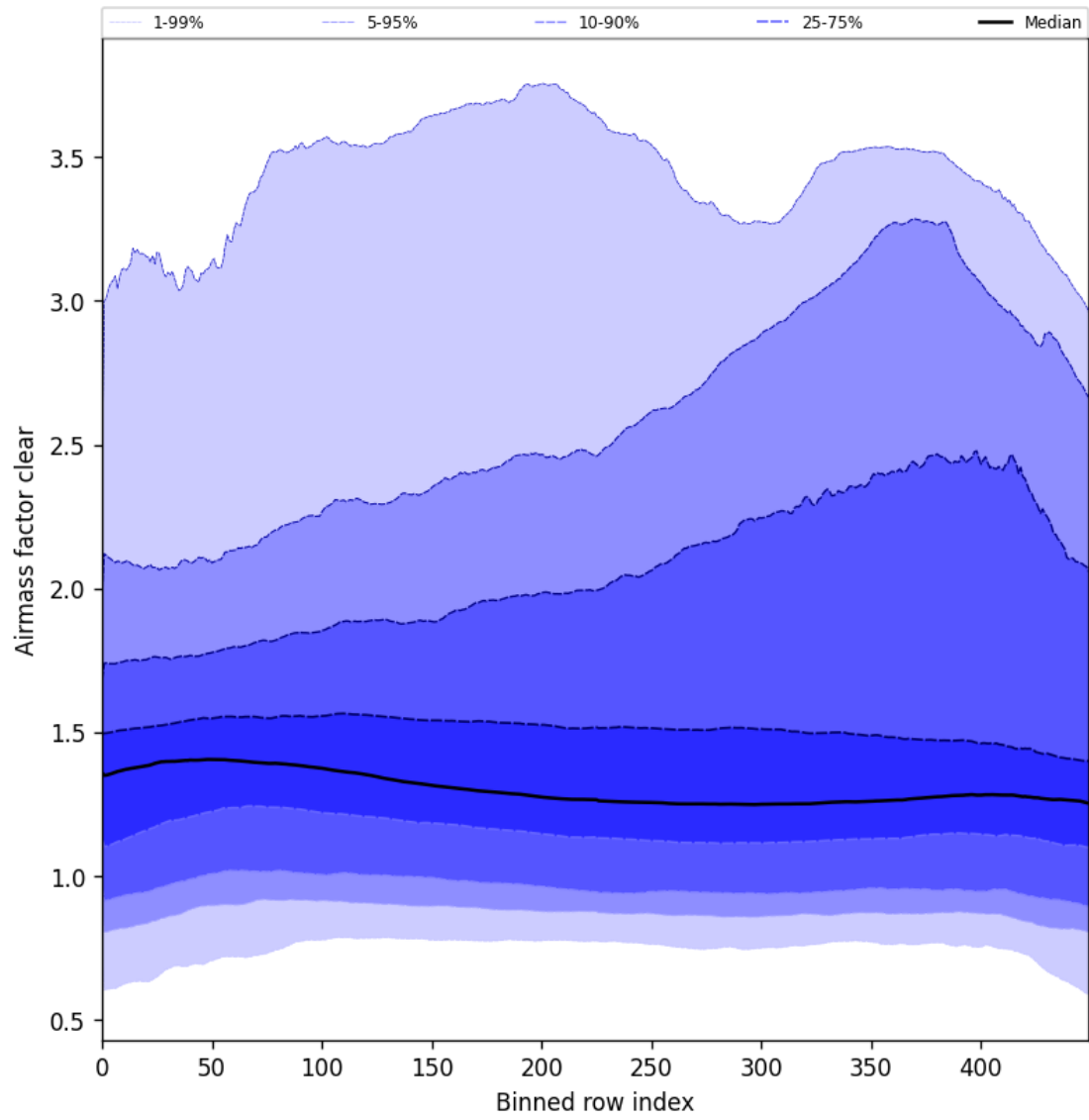
Figure 56: Along track statistics of “Airmass factor clear” for 2025-08-04 to 2025-08-06
