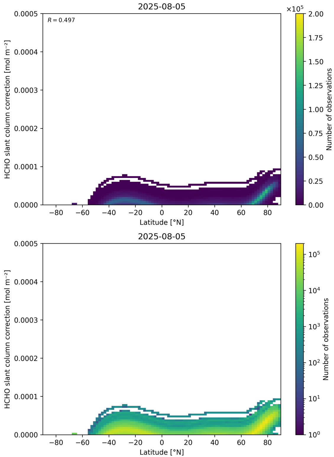
Figure 158: Scatter density plot of “Latitude” against “HCHO slant column correction” for 2025-08-04 to 2025-08-06.
