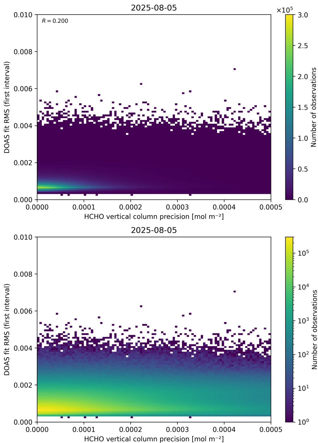
Figure 136: Scatter density plot of “HCHO vertical column precision” against “DOAS fit RMS (first interval)” for 2025-08-04 to 2025-08-06.
