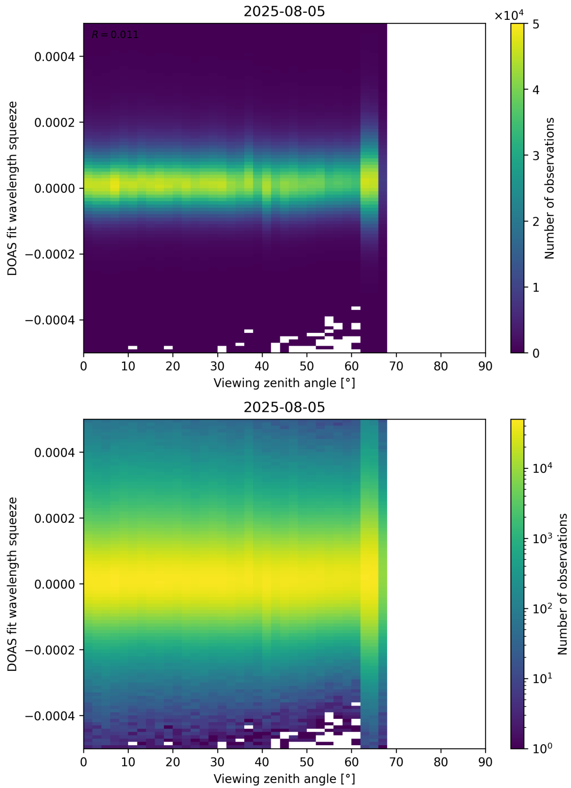
Figure 184: Scatter density plot of “Viewing zenith angle” against “DOAS fit wavelength squeeze” for 2025-08-04 to 2025-08-06.
