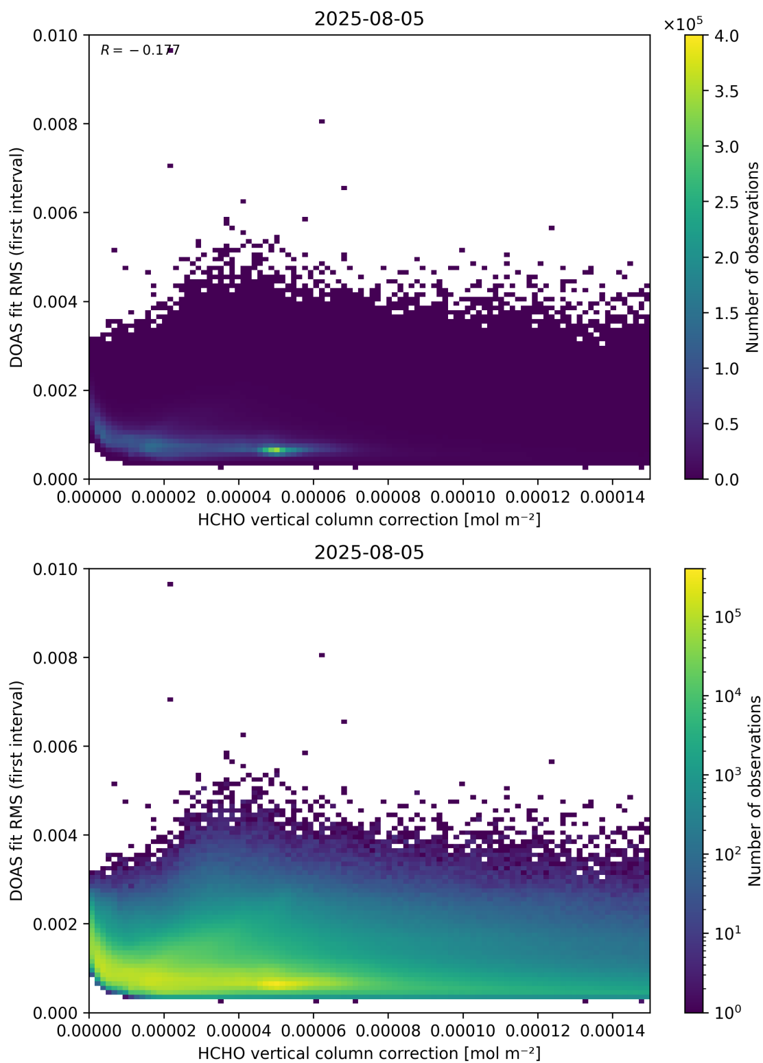
Figure 112: Scatter density plot of “HCHO vertical column correction” against “DOAS fit RMS (first interval)” for 2025-08-04 to 2025-08-06.
