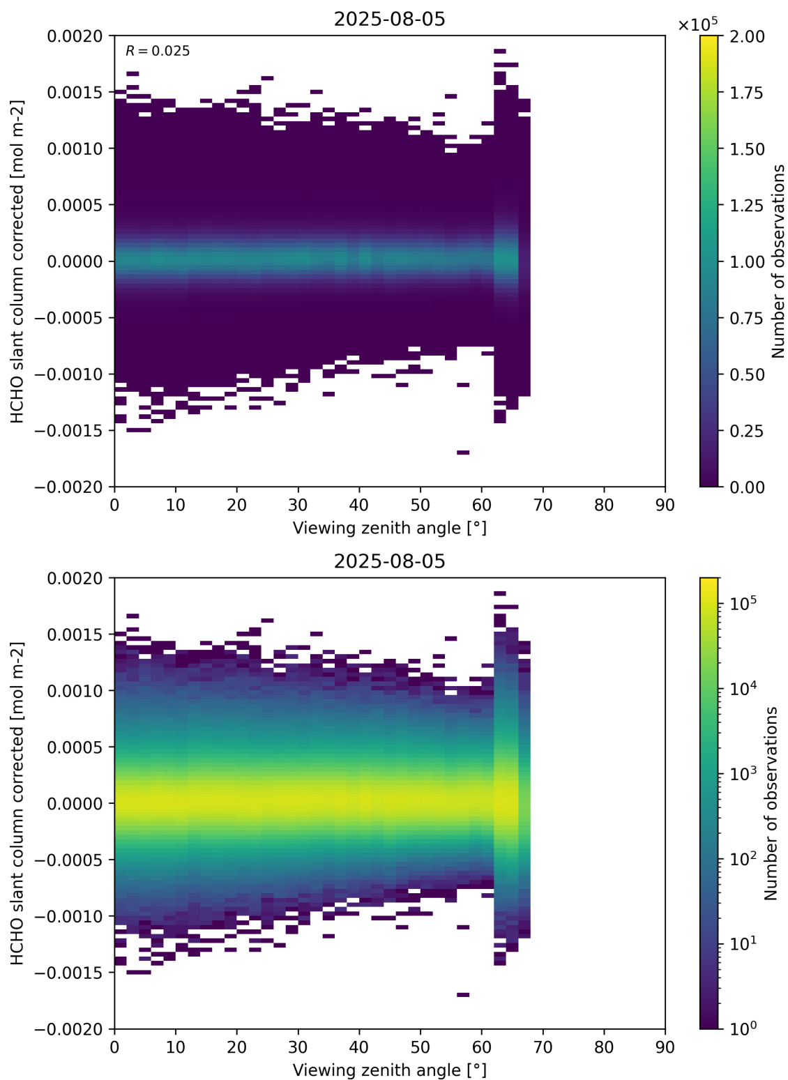
Figure 186: Scatter density plot of “Viewing zenith angle” against “HCHO slant column corrected” for 2025-08-04 to 2025-08-06.
