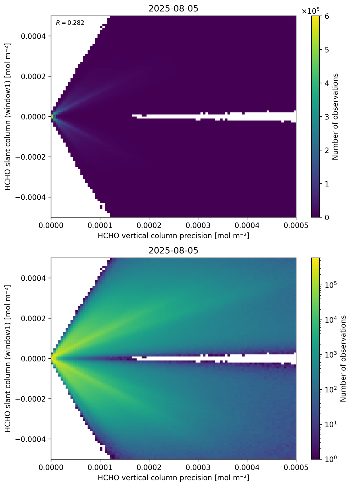
Figure 142: Scatter density plot of “HCHO vertical column precision” against “HCHO slant column (window1)” for 2025-08-04 to 2025-08-06.
