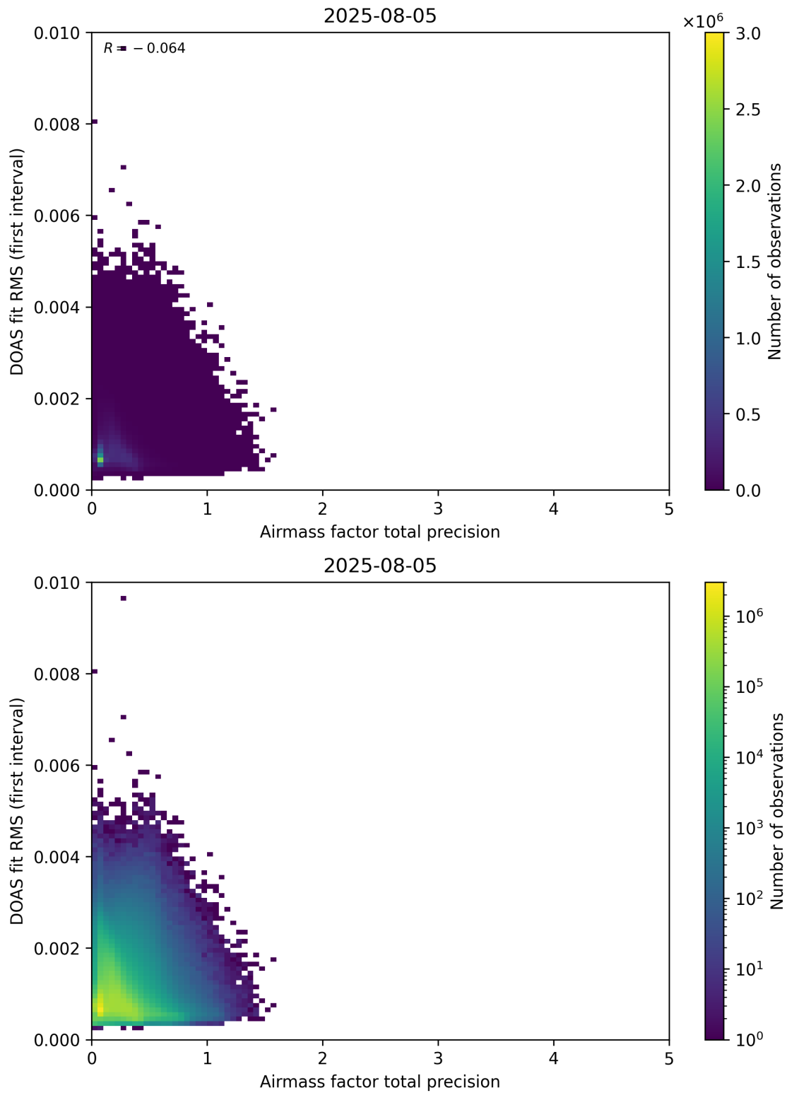
Figure 105: Scatter density plot of “Airmass factor total precision” against “DOAS fit RMS (first interval)” for 2025-08-04 to 2025-08-06.
