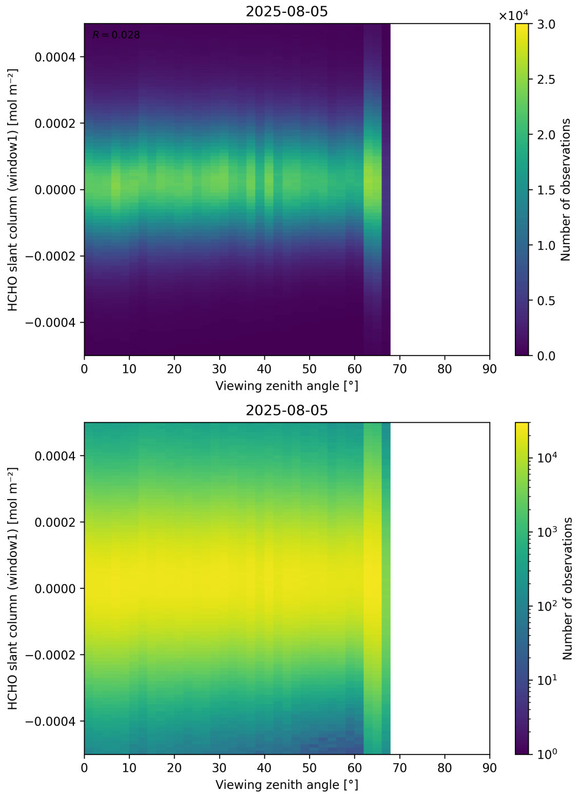
Figure 188: Scatter density plot of “Viewing zenith angle” against “HCHO slant column (window1)” for 2025-08-04 to 2025-08-06.
