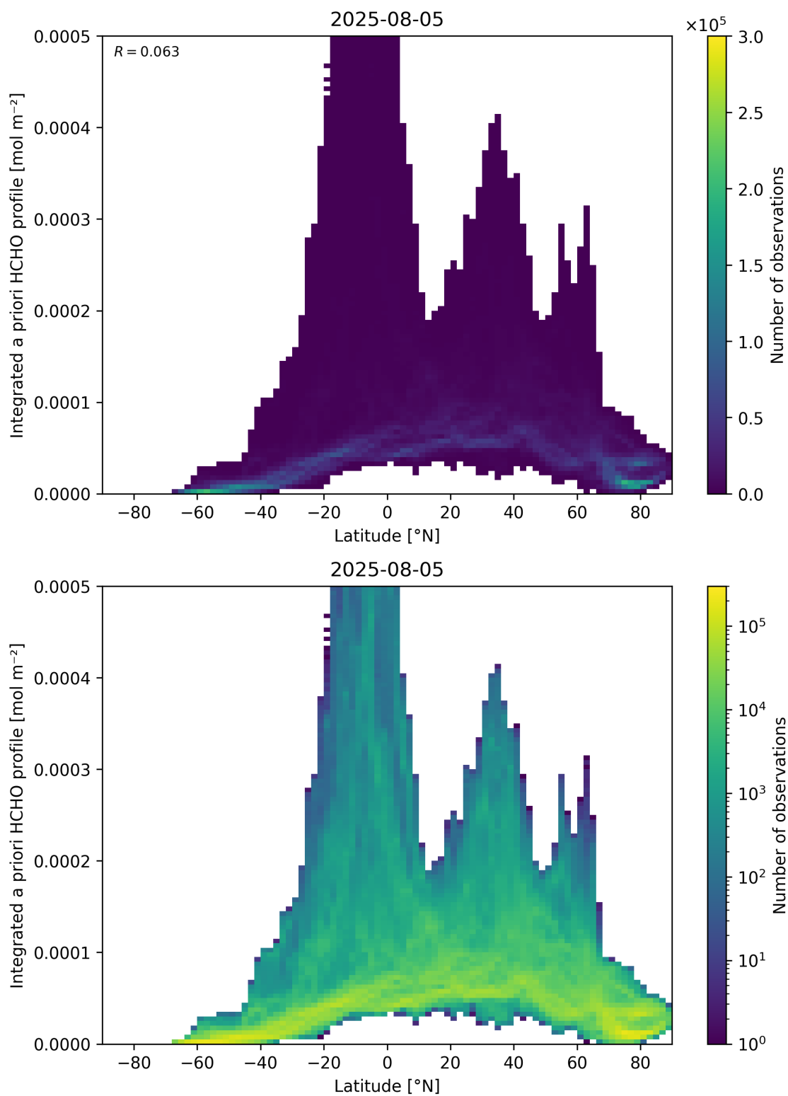
Figure 166: Scatter density plot of “Latitude” against “Integrated a priori HCHO profile” for 2025-08-04 to 2025-08-06.
