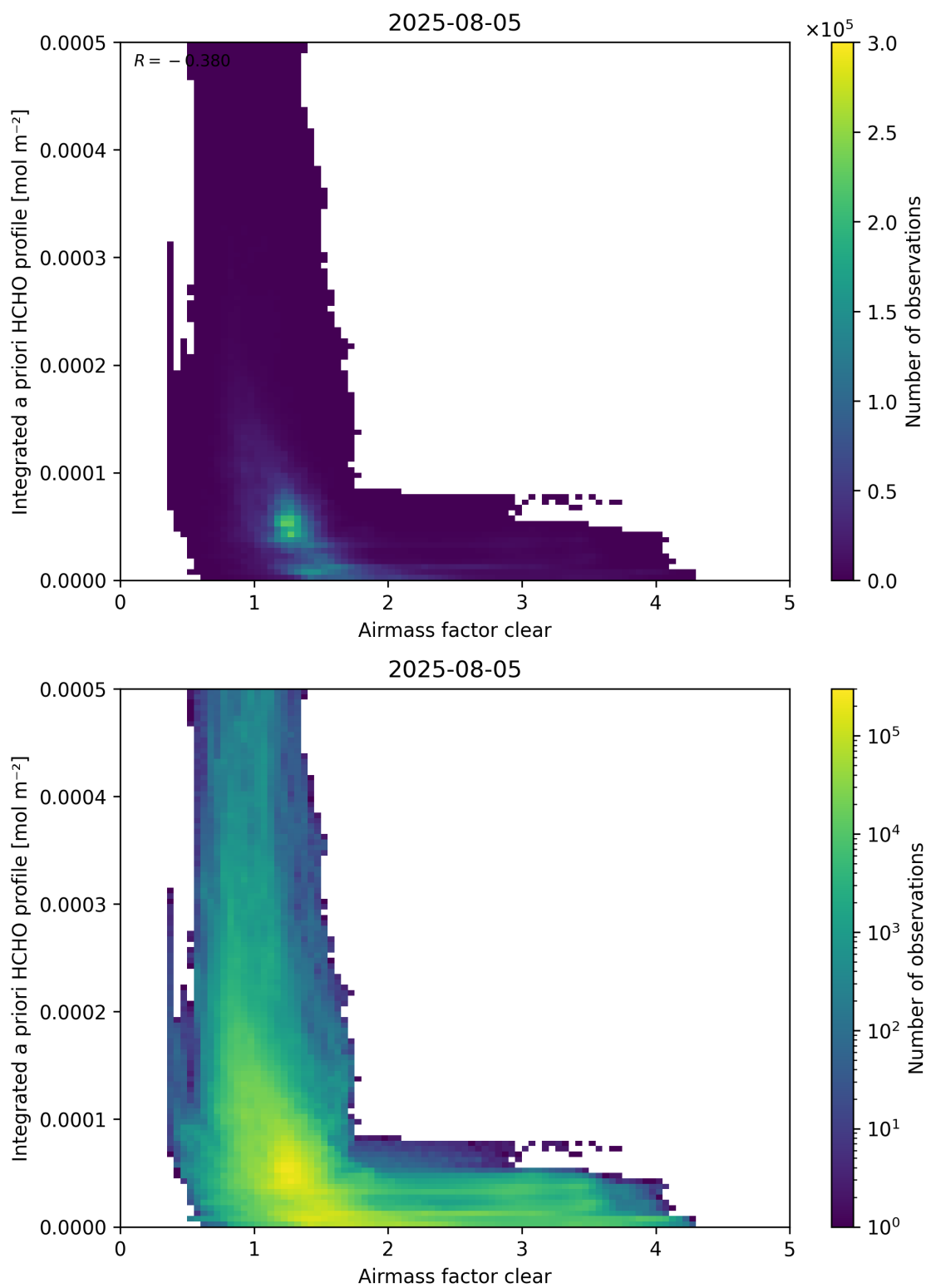
Figure 76: Scatter density plot of “Airmass factor clear” against “Integrated a priori HCHO profile” for 2025-08-04 to 2025-08-06.
