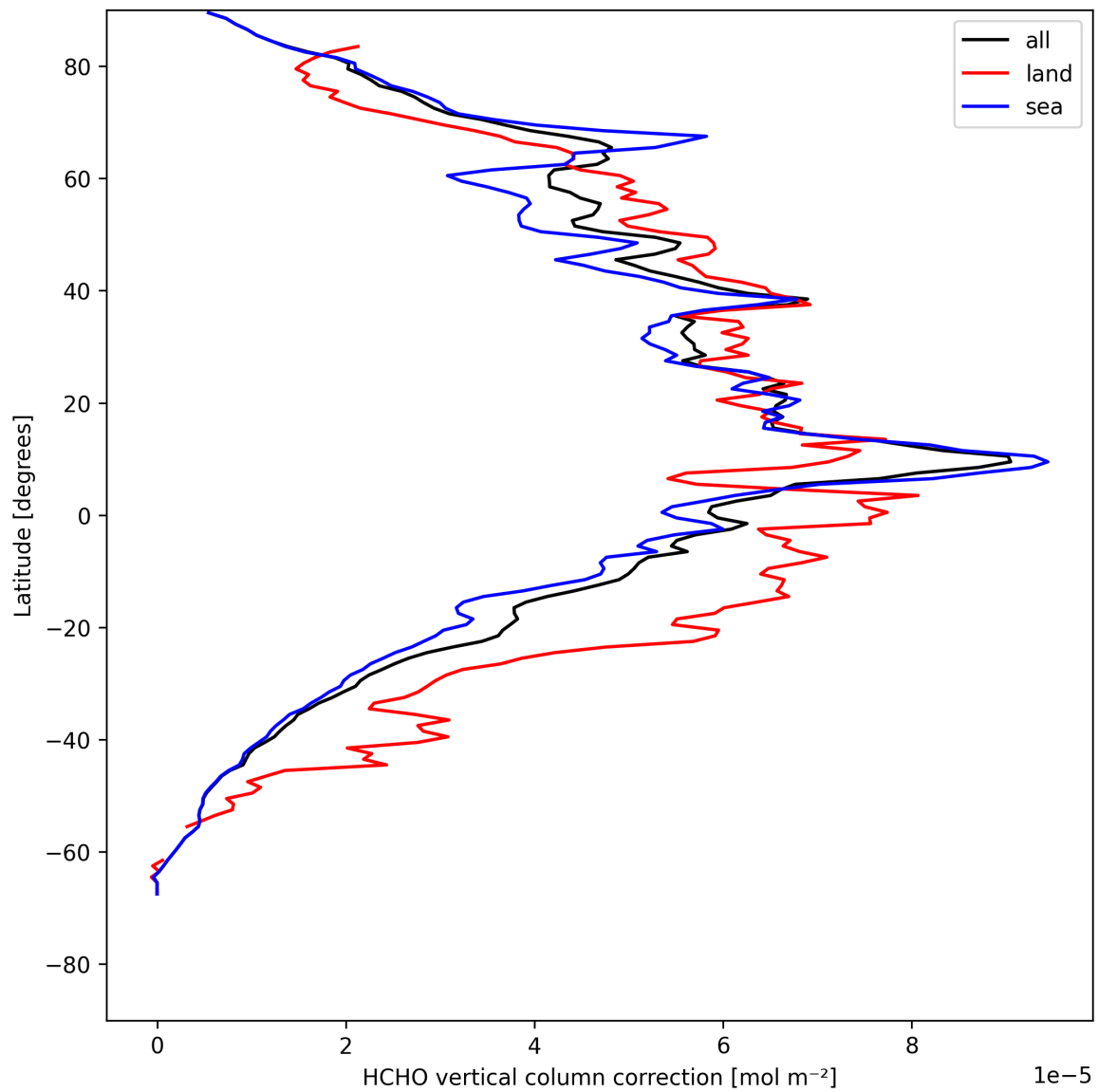
Figure 23: Zonal average of “HCHO vertical column correction” for 2025-08-04 to 2025-08-06.
