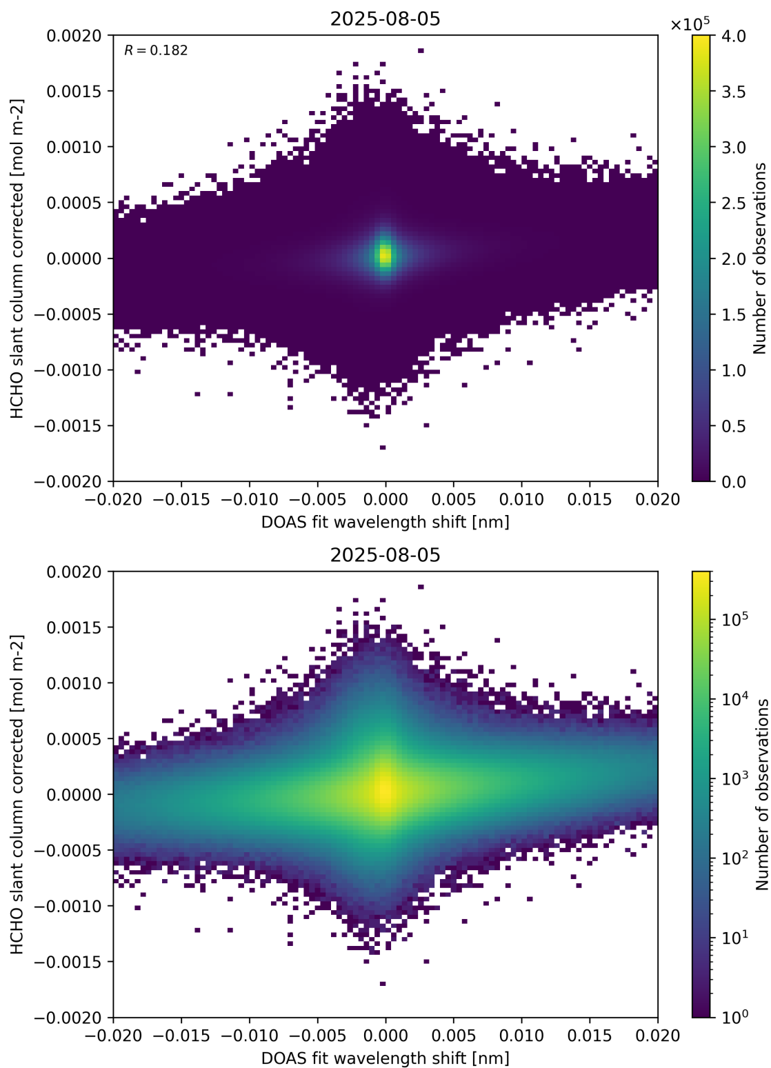
Figure 66: Scatter density plot of “DOAS fit wavelength shift” against “HCHO slant column corrected” for 2025-08-04 to 2025-08-06.
