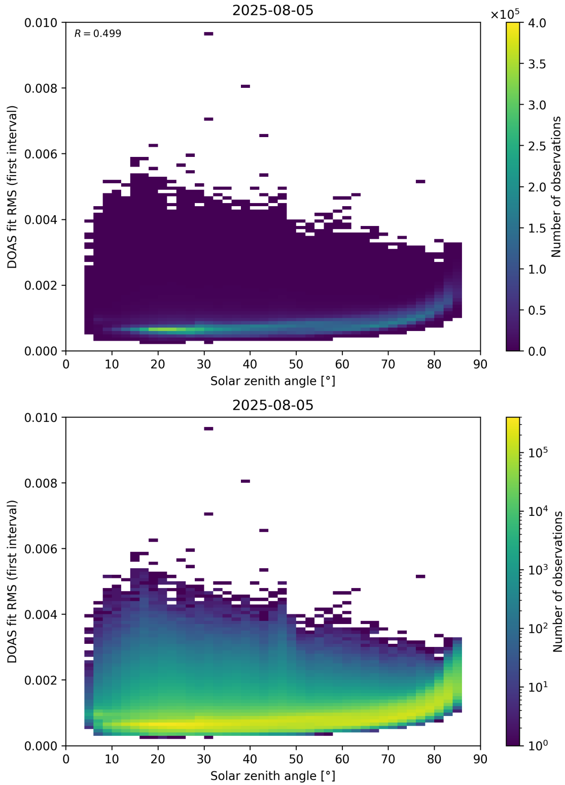
Figure 167: Scatter density plot of “Solar zenith angle” against “DOAS fit RMS (first interval)” for 2025-08-04 to 2025-08-06.
