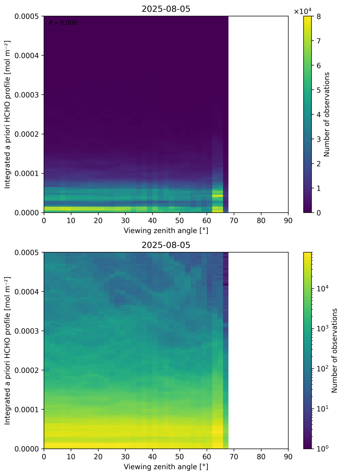
Figure 195: Scatter density plot of “Viewing zenith angle” against “Integrated a priori HCHO profile” for 2025-08-04 to 2025-08-06.
