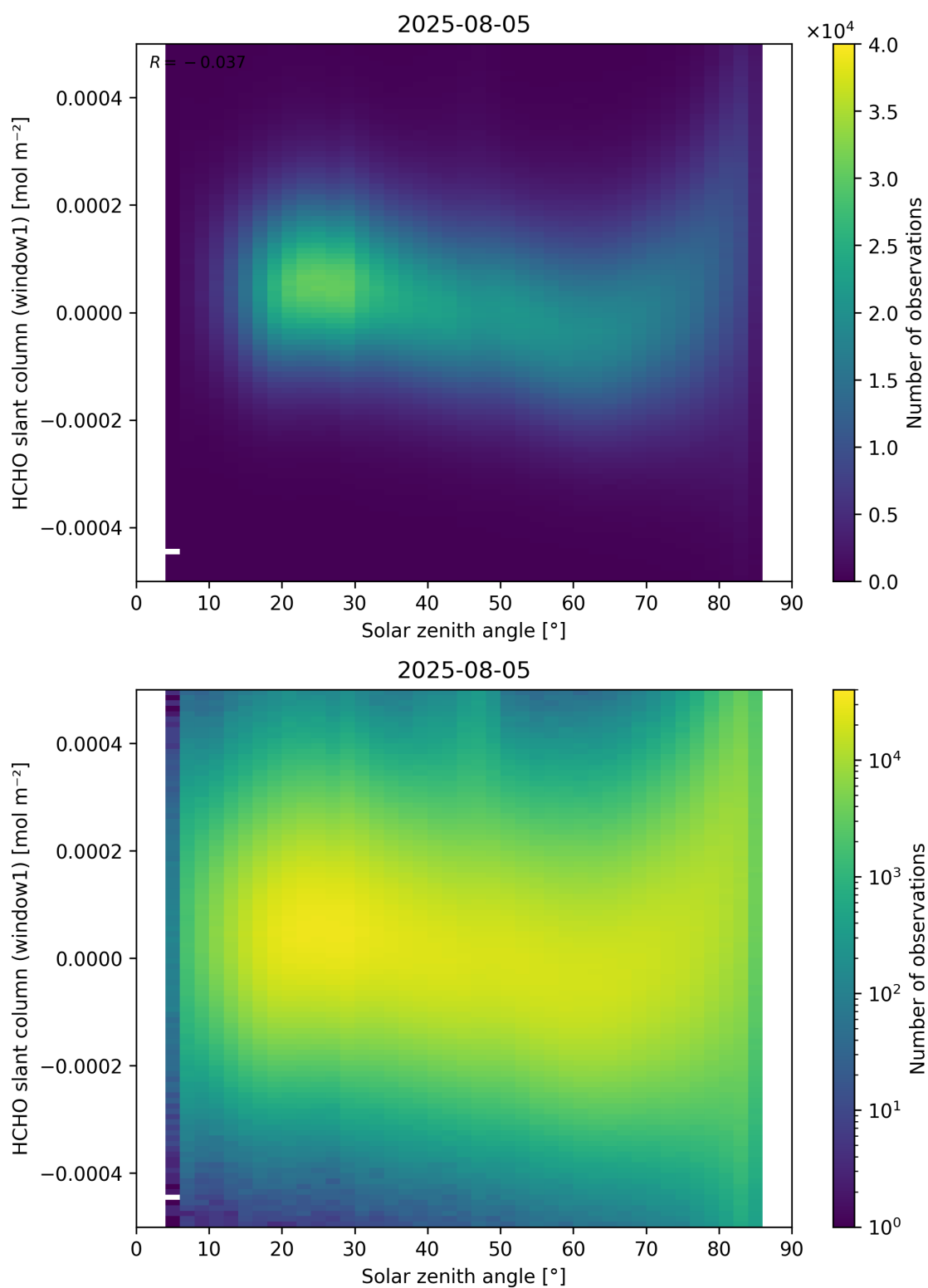
Figure 173: Scatter density plot of “Solar zenith angle” against “HCHO slant column (window1)” for 2025-08-04 to 2025-08-06.
