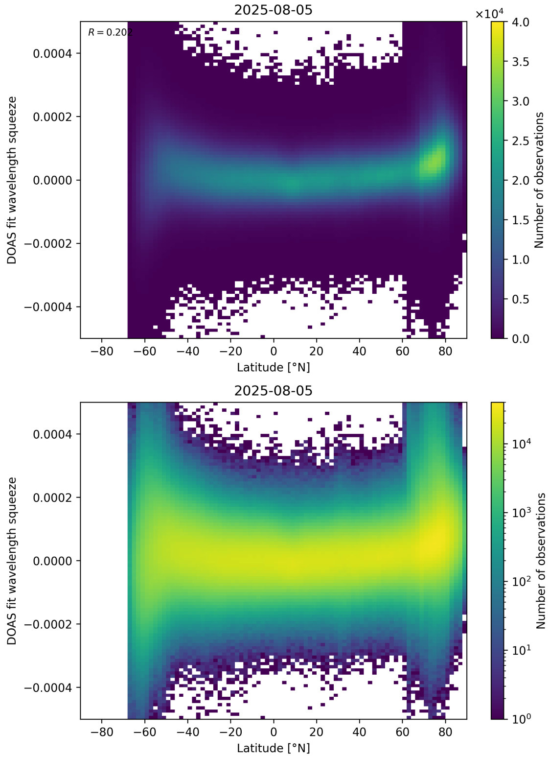
Figure 155: Scatter density plot of “Latitude” against “DOAS fit wavelength squeeze” for 2025-08-04 to 2025-08-06.
