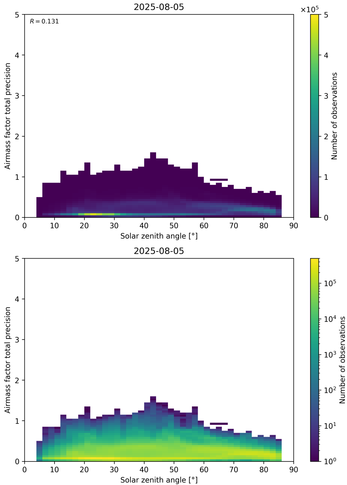
Figure 176: Scatter density plot of “Solar zenith angle” against “Airmass factor total precision” for 2025-08-04 to 2025-08-06.
