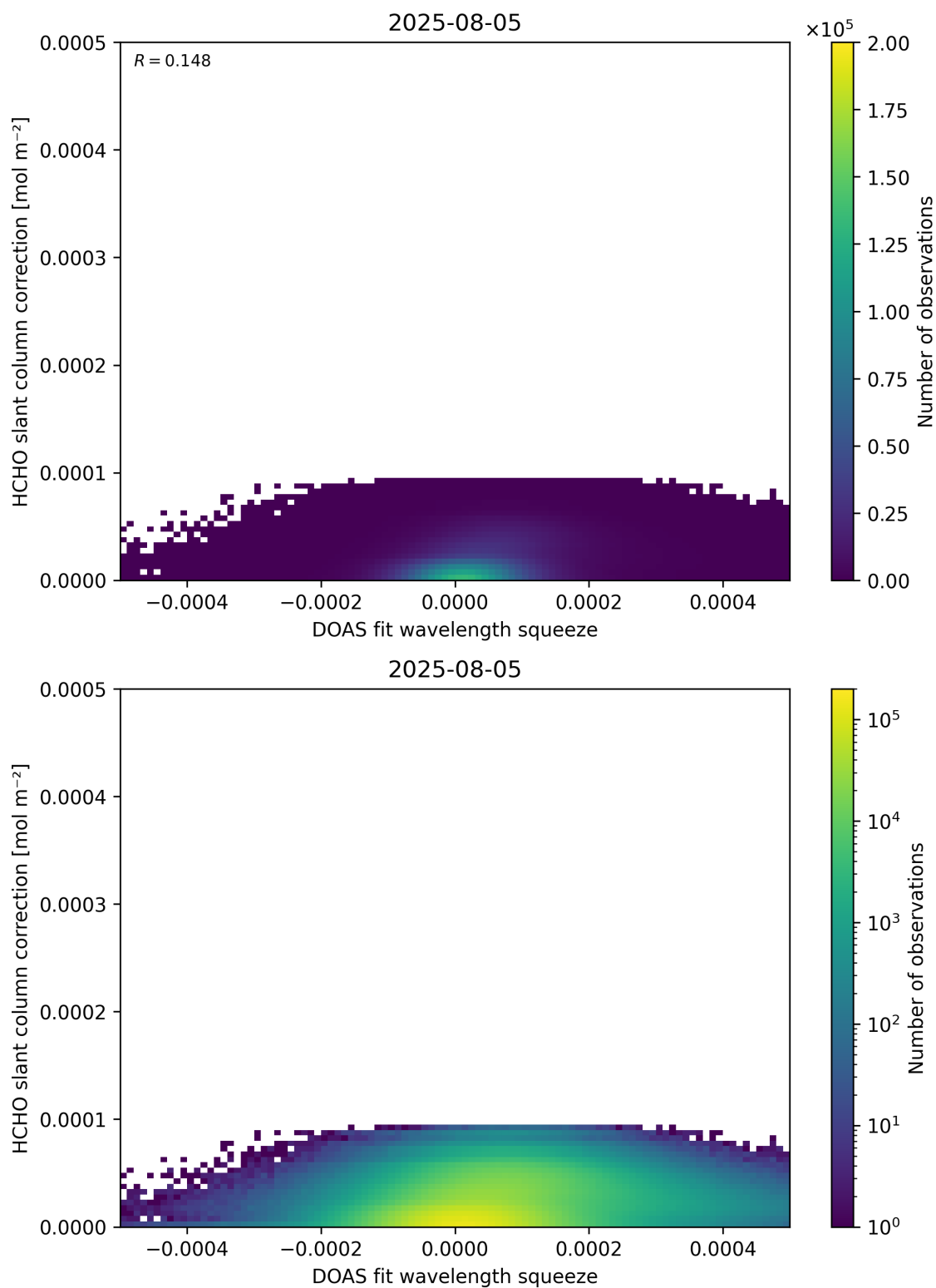
Figure 70: Scatter density plot of “DOAS fit wavelength squeeze” against “HCHO slant column correction” for 2025-08-04 to 2025-08-06.
