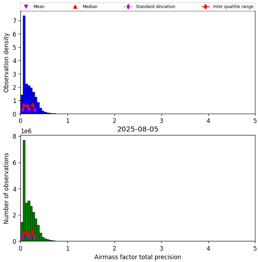
Figure 41: Histogram of “Airmass factor total precision” for 2025-08-04 to 2025-08-06
