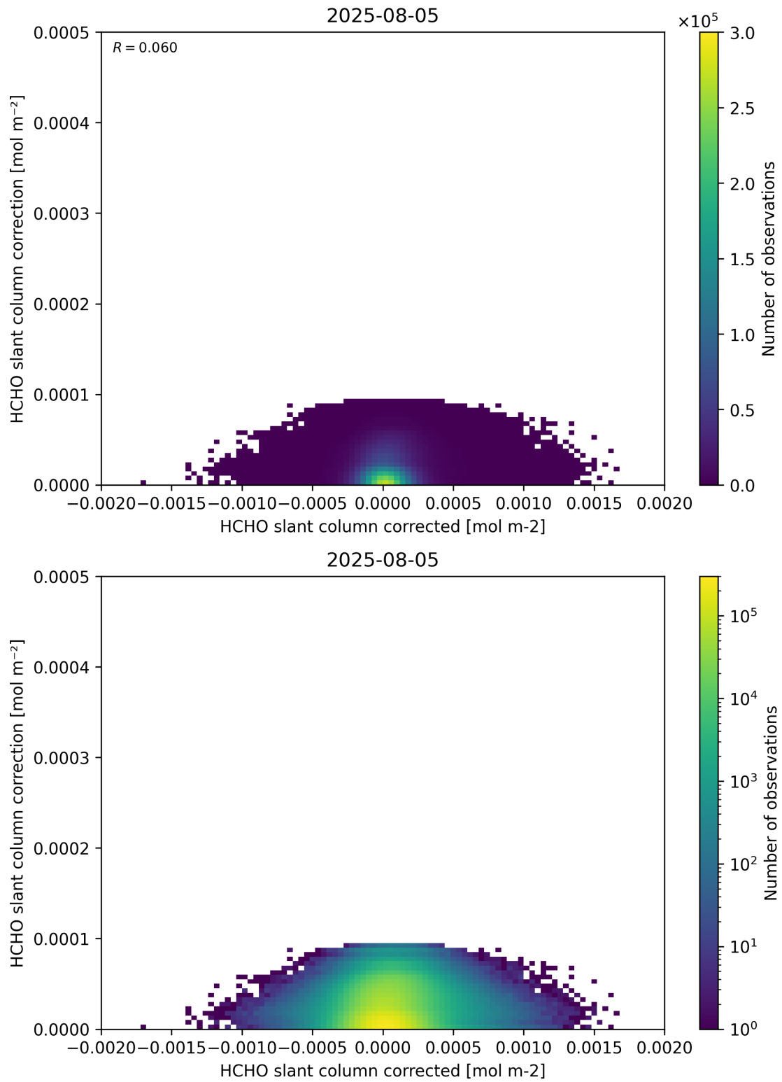
Figure 77: Scatter density plot of “HCHO slant column corrected” against “HCHO slant column correction” for 2025-08-04 to 2025-08-06.
