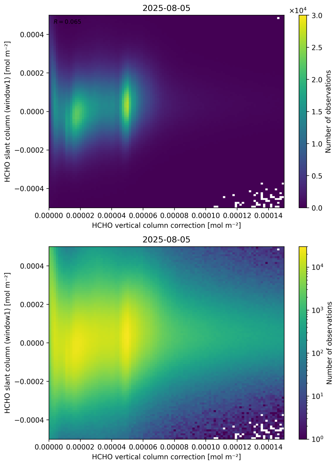
Figure 118: Scatter density plot of “HCHO vertical column correction” against “HCHO slant column (window1)” for 2025-08-04 to 2025-08-06.
