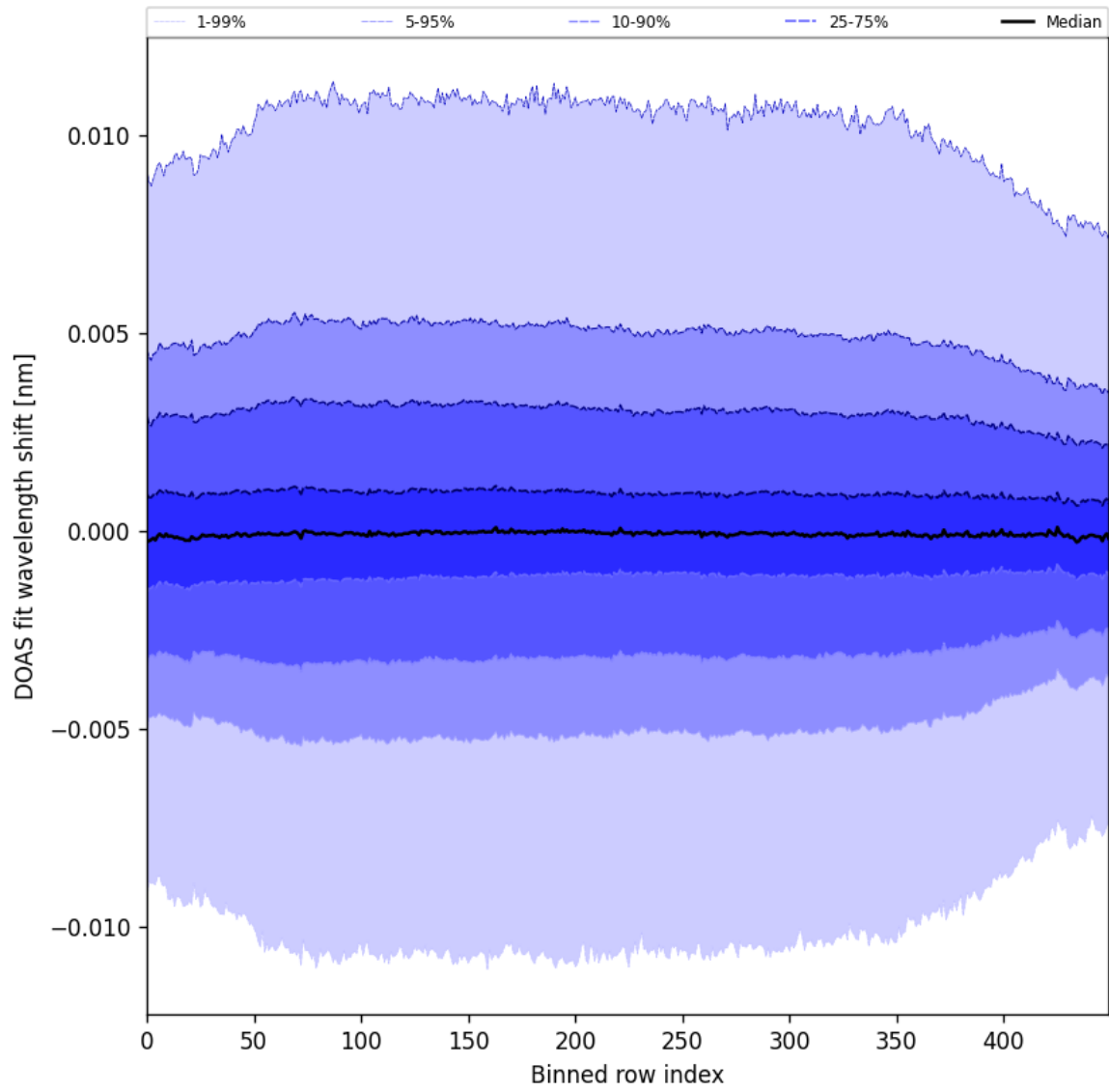
Figure 58: Along track statistics of “DOAS fit wavelength shift” for 2025-08-04 to 2025-08-06
