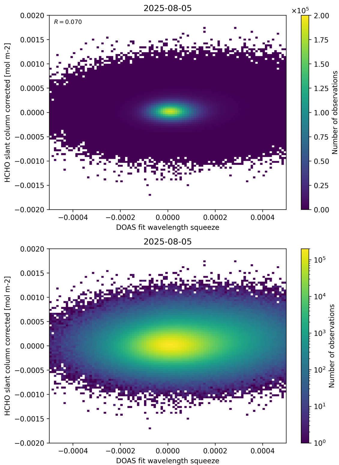
Figure 69: Scatter density plot of “DOAS fit wavelength squeeze” against “HCHO slant column corrected” for 2025-08-04 to 2025-08-06.
