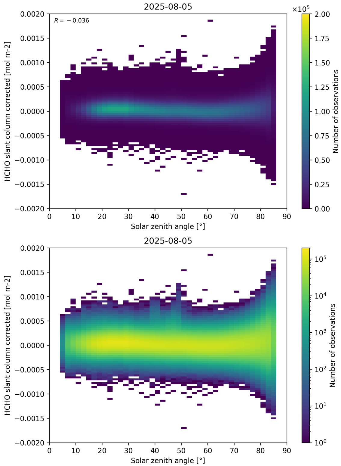
Figure 171: Scatter density plot of “Solar zenith angle” against “HCHO slant column corrected” for 2025-08-04 to 2025-08-06.
