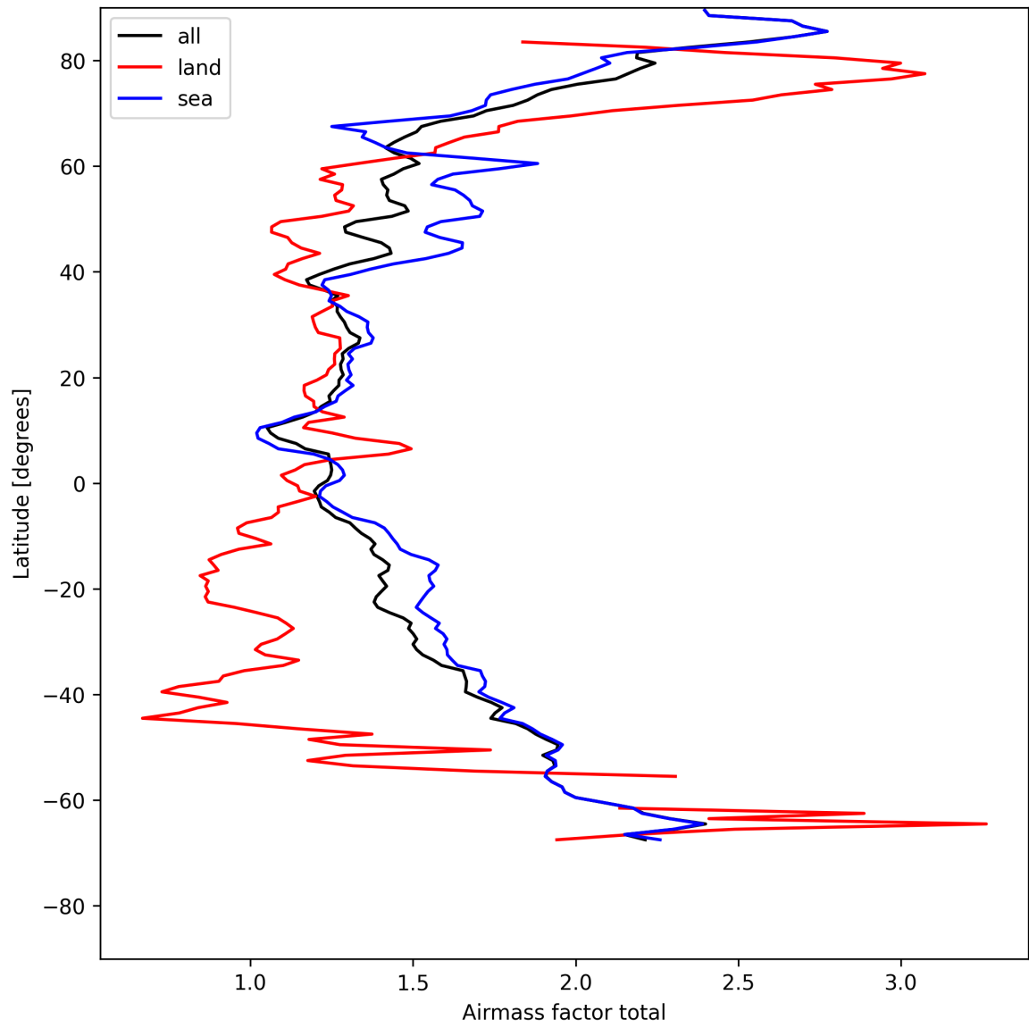
Figure 26: Zonal average of “Airmass factor total” for 2025-08-04 to 2025-08-06.
