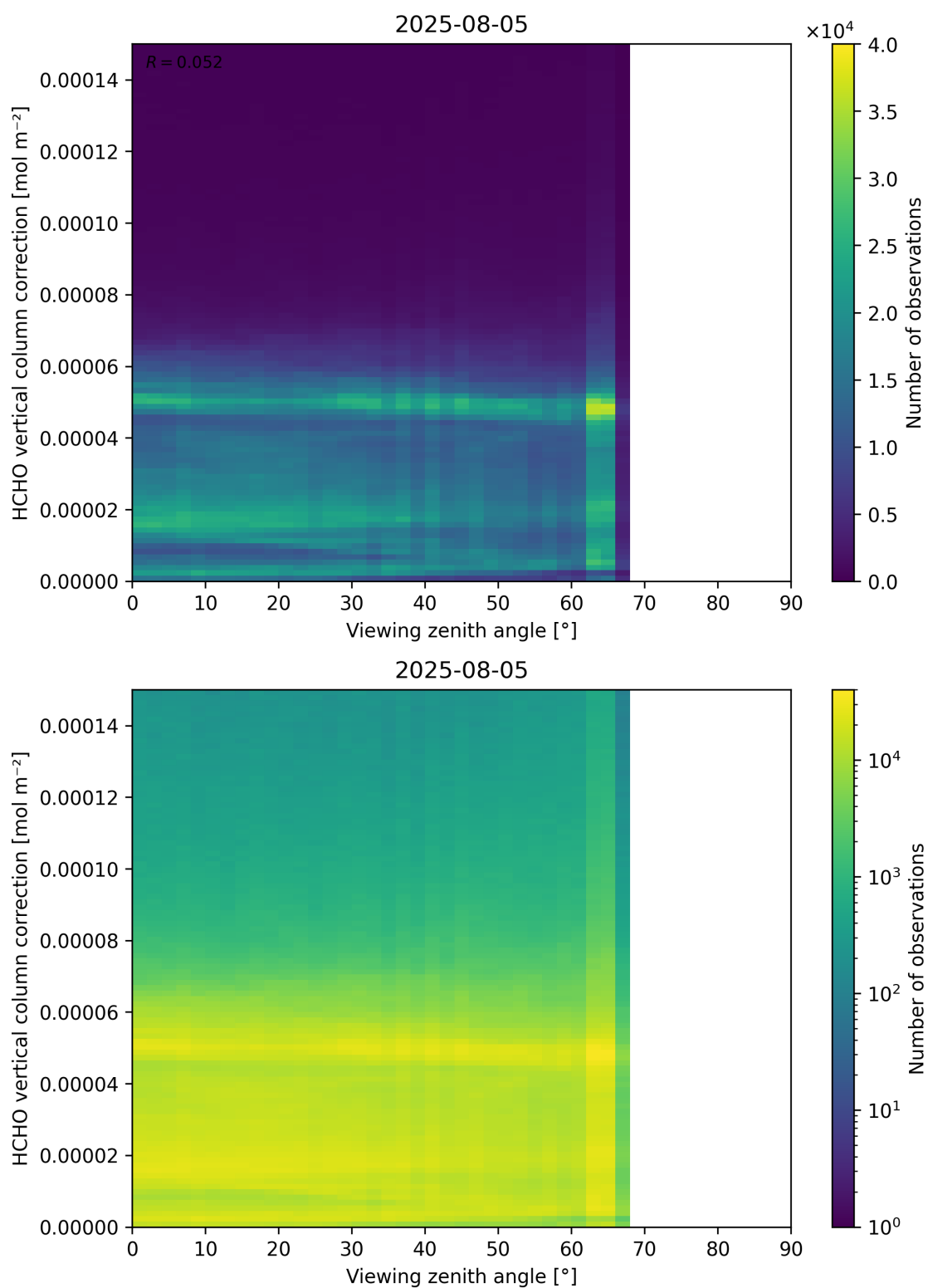
Figure 193: Scatter density plot of “Viewing zenith angle” against “HCHO vertical column correction” for 2025-08-04 to 2025-08-06.
