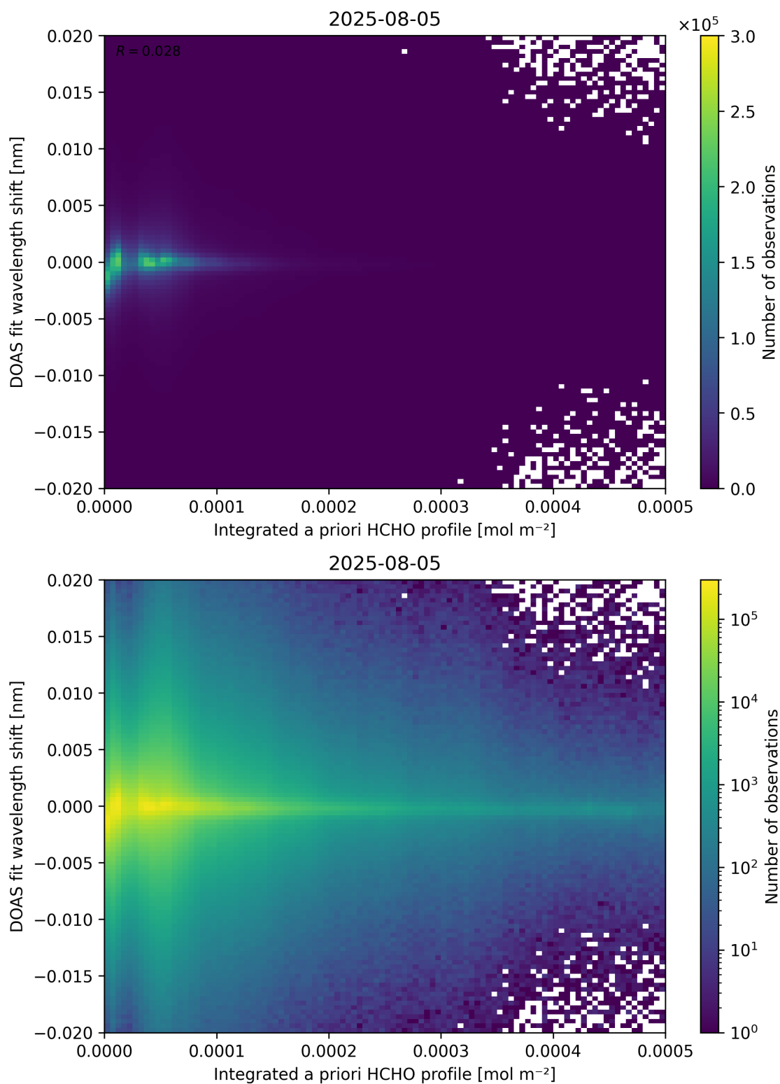
Figure 149: Scatter density plot of “Integrated a priori HCHO profile” against “DOAS fit wavelength shift” for 2025-08-04 to 2025-08-06.
