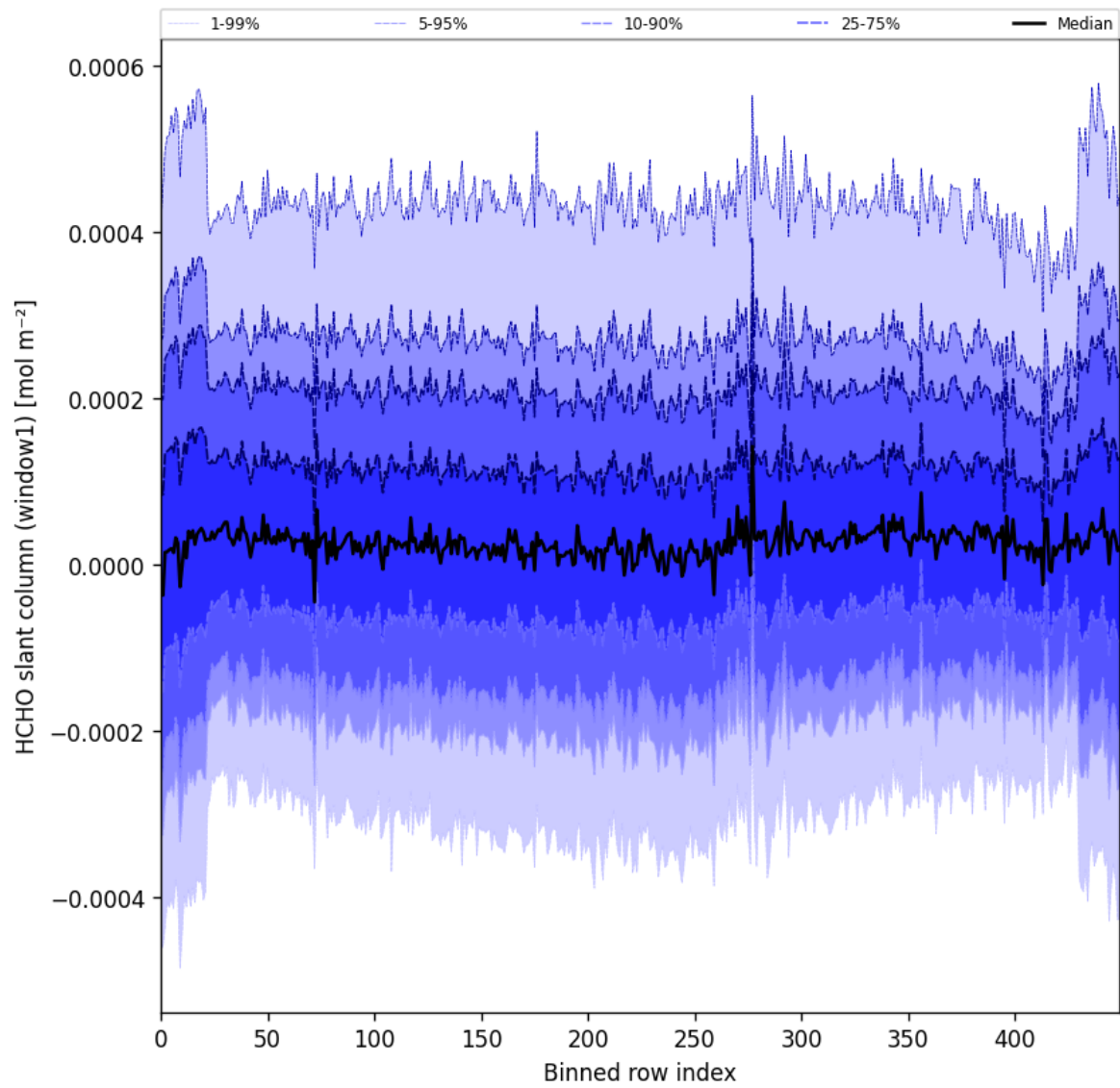
Figure 52: Along track statistics of “HCHO slant column (window1)” for 2025-08-04 to 2025-08-06
