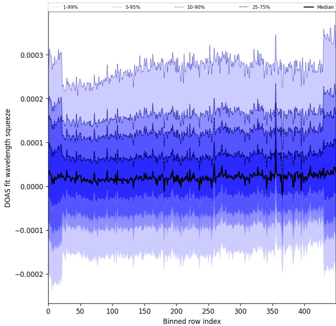
Figure 59: Along track statistics of “DOAS fit wavelength squeeze” for 2025-08-04 to 2025-08-06
