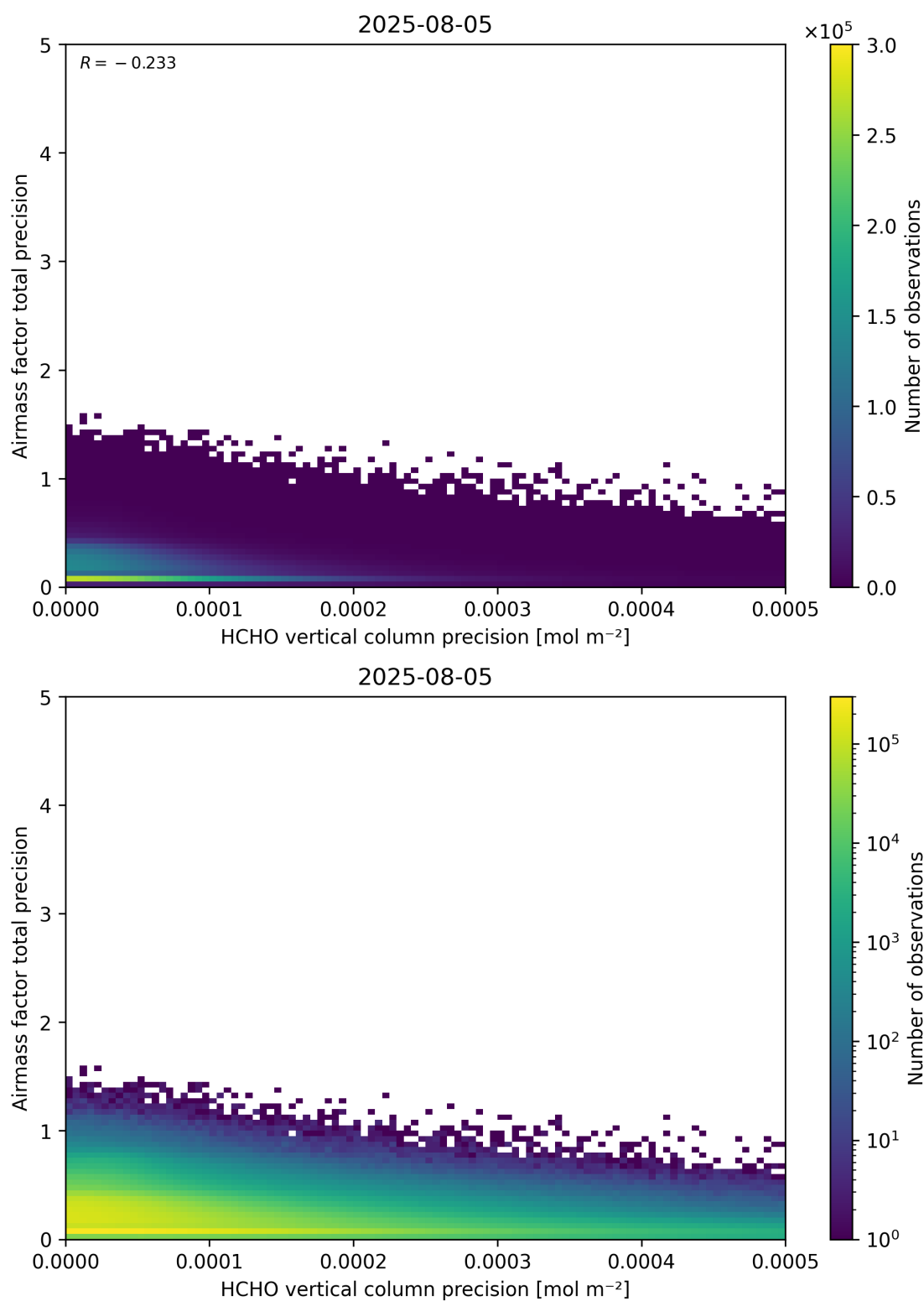
Figure 145: Scatter density plot of “HCHO vertical column precision” against “Airmass factor total precision” for 2025-08-04 to 2025-08-06.
