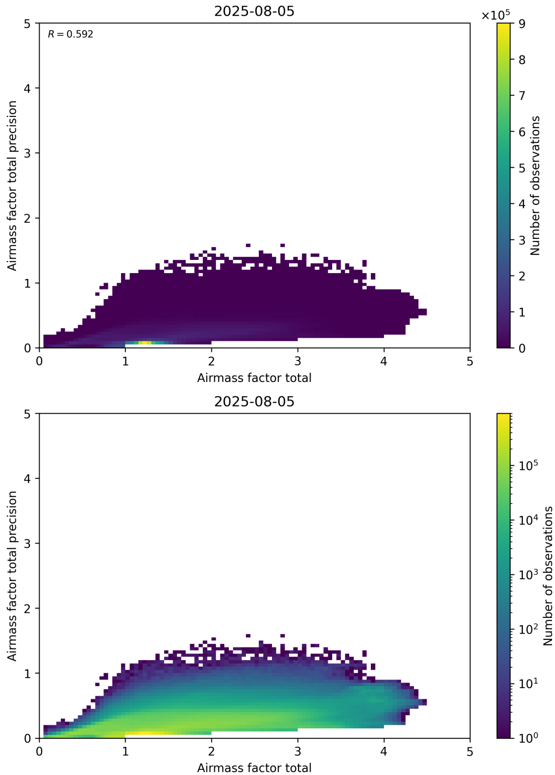
Figure 103: Scatter density plot of “Airmass factor total” against “Airmass factor total precision” for 2025-08-04 to 2025-08-06.
