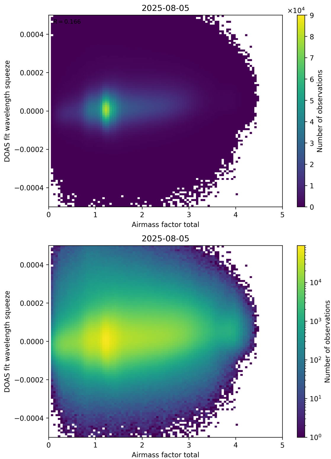
Figure 99: Scatter density plot of “Airmass factor total” against “DOAS fit wavelength squeeze” for 2025-08-04 to 2025-08-06.
