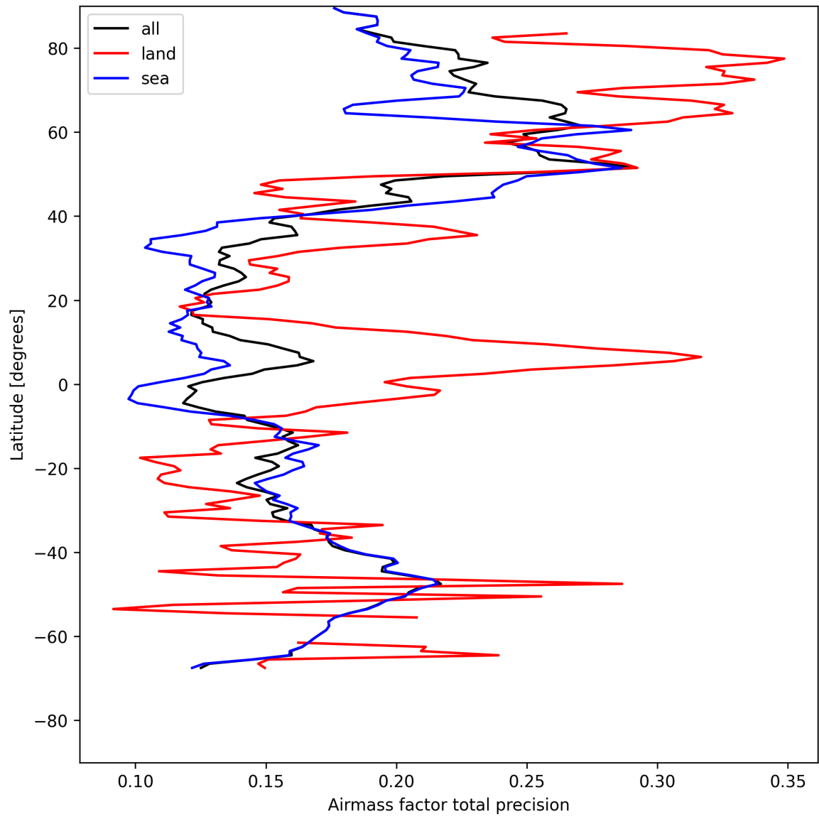
Figure 27: Zonal average of “Airmass factor total precision” for 2025-08-04 to 2025-08-06.
