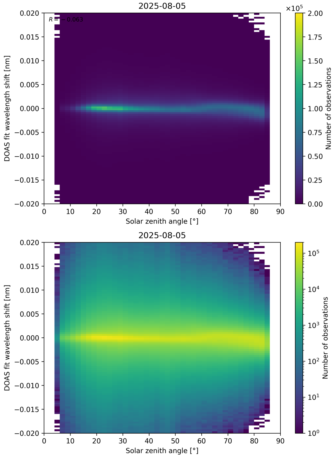
Figure 168: Scatter density plot of “Solar zenith angle” against “DOAS fit wavelength shift” for 2025-08-04 to 2025-08-06.
