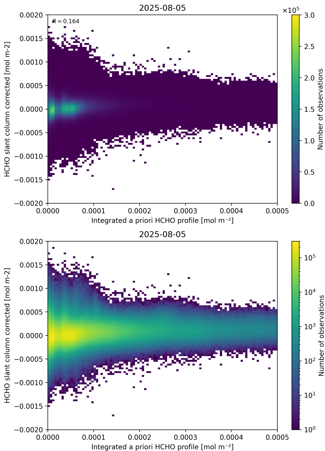
Figure 151: Scatter density plot of “Integrated a priori HCHO profile” against “HCHO slant column corrected” for 2025-08-04 to 2025-08-06.
