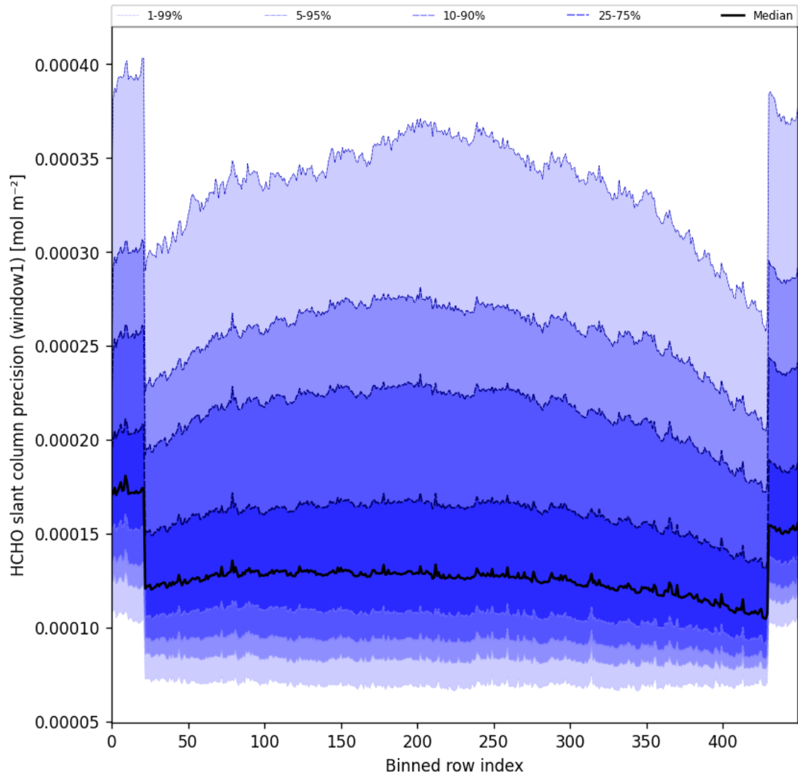
Figure 53: Along track statistics of “HCHO slant column precision (window1)” for 2025-08-04 to 2025-08-06
