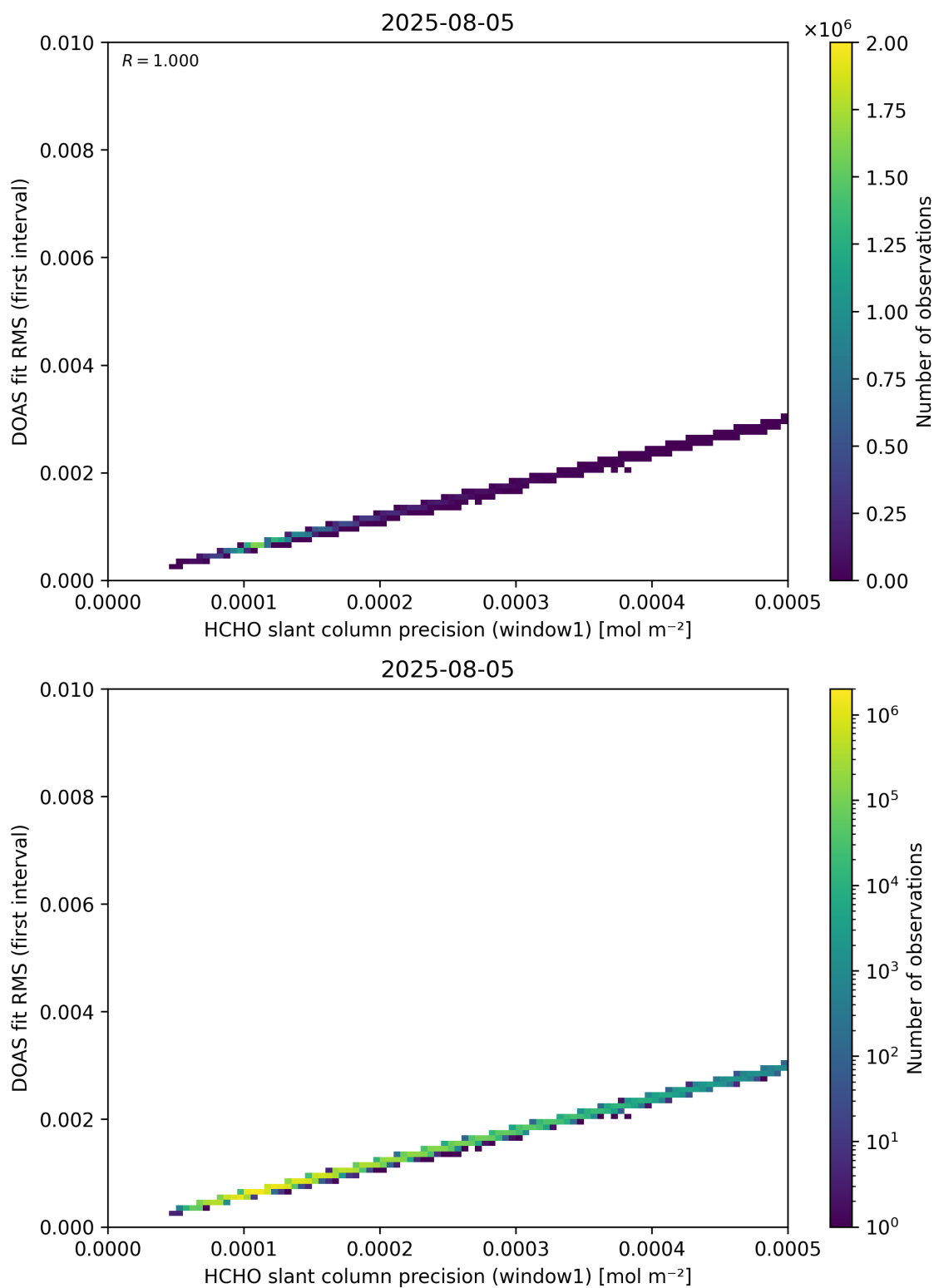
Figure 88: Scatter density plot of “HCHO slant column precision (window1)” against “DOAS fit RMS (first interval)” for 2025-08-04 to 2025-08-06.
