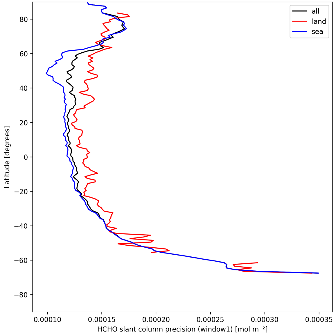
Figure 25: Zonal average of “HCHO slant column precision (window1)” for 2025-08-04 to 2025-08-06.
