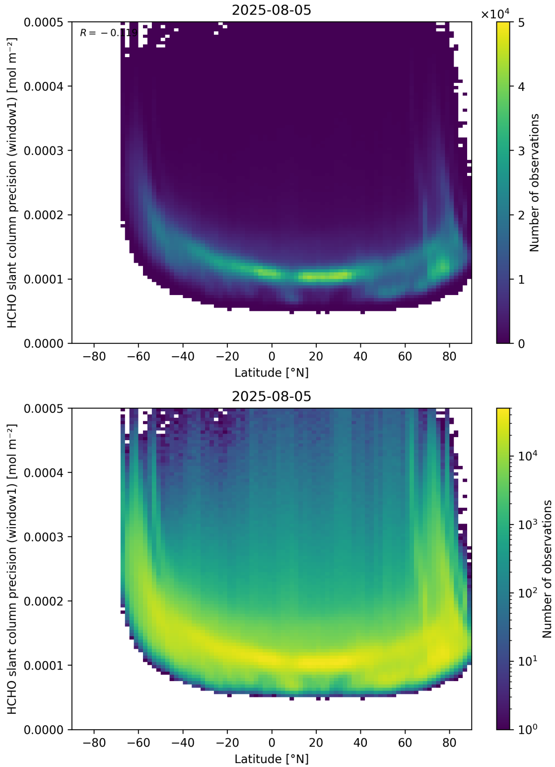
Figure 160: Scatter density plot of “Latitude” against “HCHO slant column precision (window1)” for 2025-08-04 to 2025-08-06.
