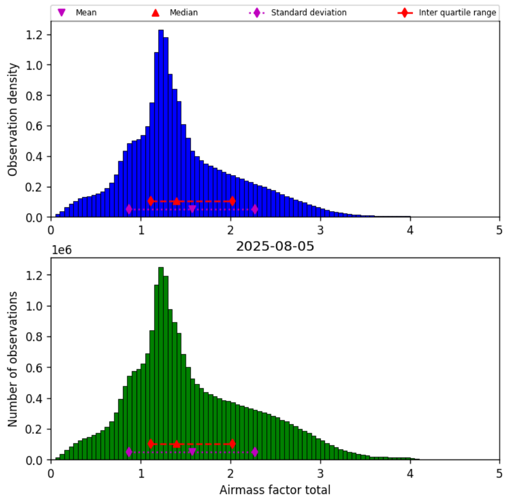
Figure 40: Histogram of “Airmass factor total” for 2025-08-04 to 2025-08-06
