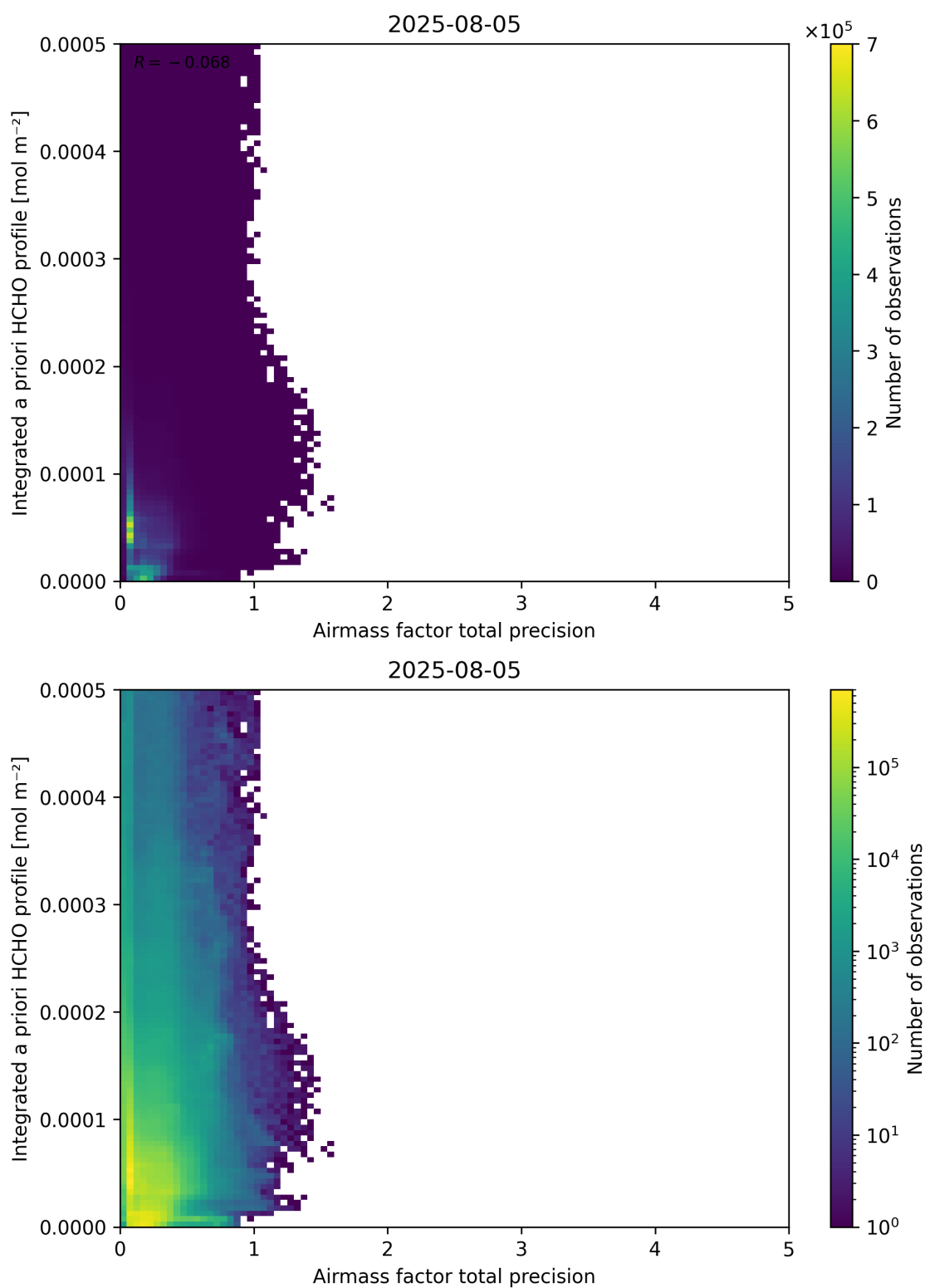
Figure 111: Scatter density plot of “Airmass factor total precision” against “Integrated a priori HCHO profile” for 2025-08-04 to 2025-08-06.
