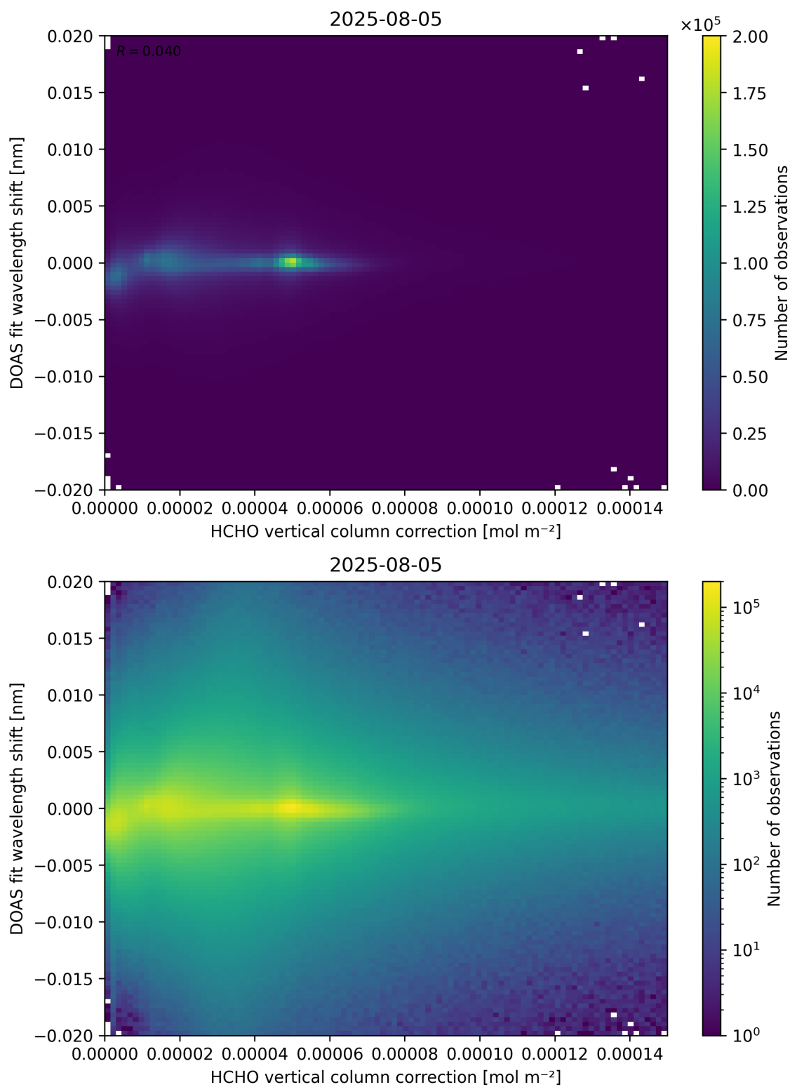
Figure 113: Scatter density plot of “HCHO vertical column correction” against “DOAS fit wavelength shift” for 2025-08-04 to 2025-08-06.
