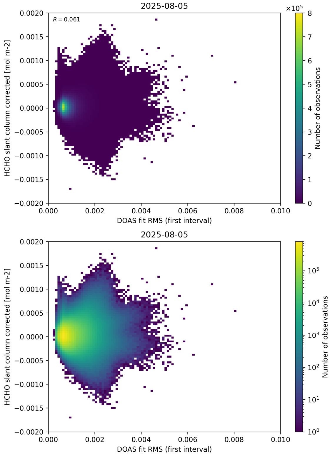
Figure 62: Scatter density plot of “DOAS fit RMS (first interval)” against “HCHO slant column corrected” for 2025-08-04 to 2025-08-06.
