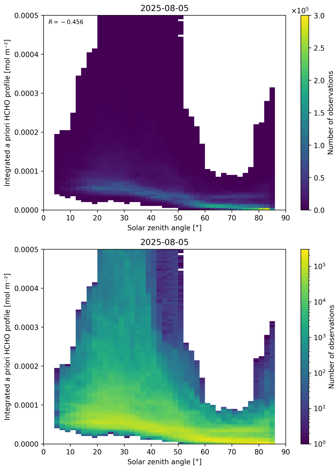
Figure 180: Scatter density plot of “Solar zenith angle” against “Integrated a priori HCHO profile” for 2025-08-04 to 2025-08-06.
