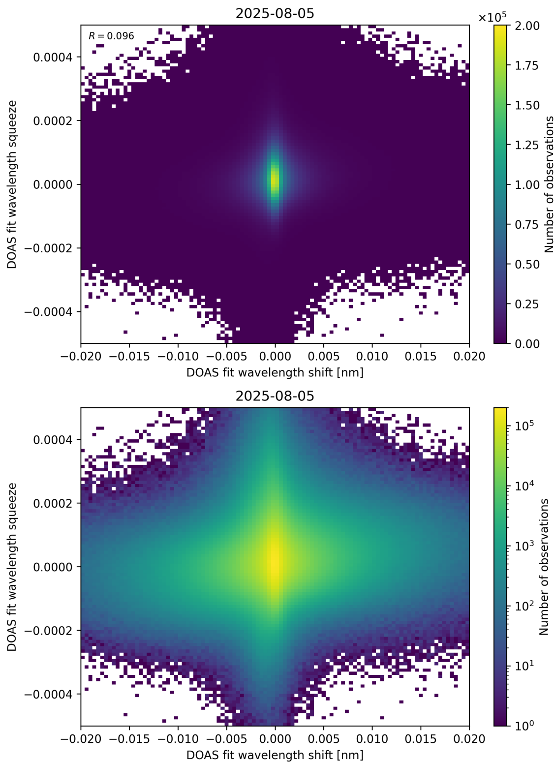
Figure 65: Scatter density plot of “DOAS fit wavelength shift” against “DOAS fit wavelength squeeze” for 2025-08-04 to 2025-08-06.
