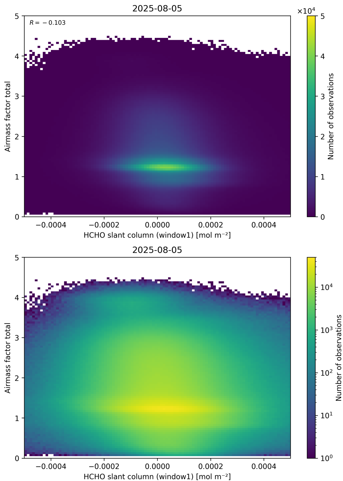
Figure 85: Scatter density plot of “HCHO slant column (window1)” against “Airmass factor total” for 2025-08-04 to 2025-08-06.
