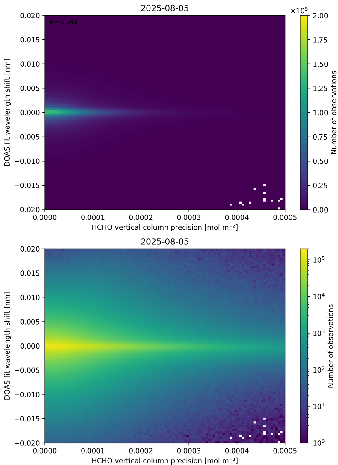
Figure 137: Scatter density plot of “HCHO vertical column precision” against “DOAS fit wavelength shift” for 2025-08-04 to 2025-08-06.
