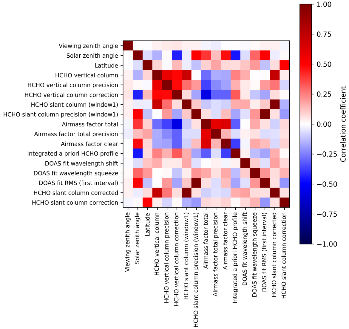
Figure 2: Map of correlation matrix for 2025-08-04 to 2025-08-06.
