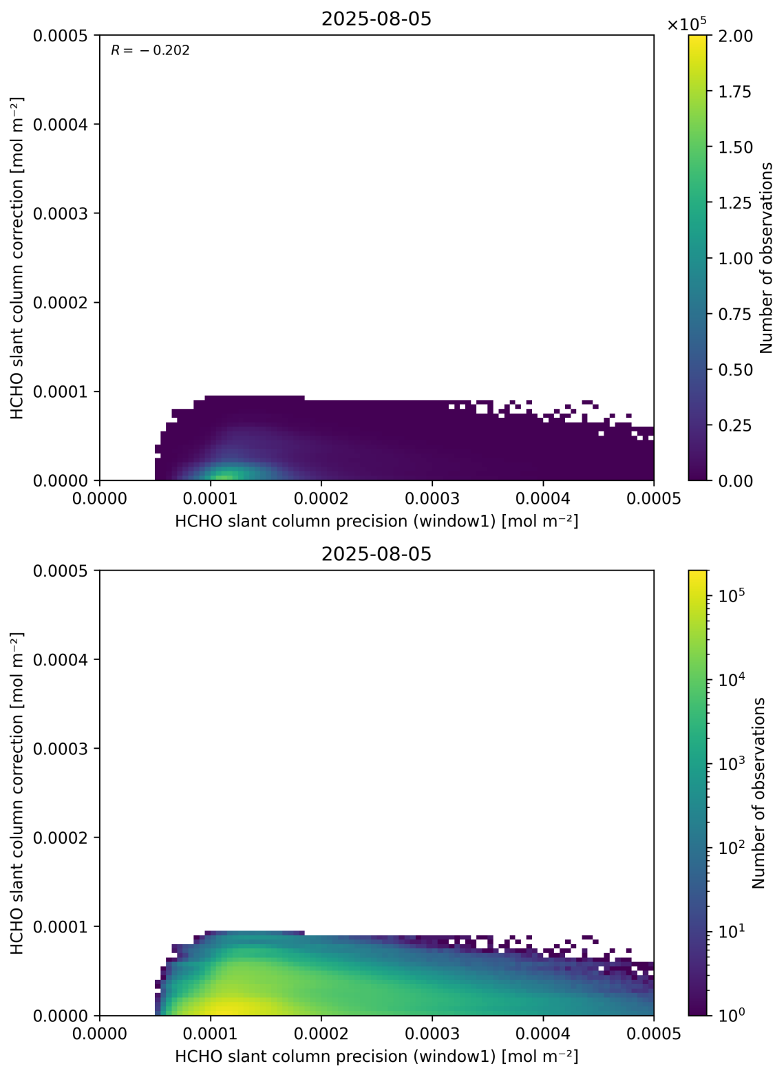
Figure 93: Scatter density plot of “HCHO slant column precision (window1)” against “HCHO slant column correction” for 2025-08-04 to 2025-08-06.
