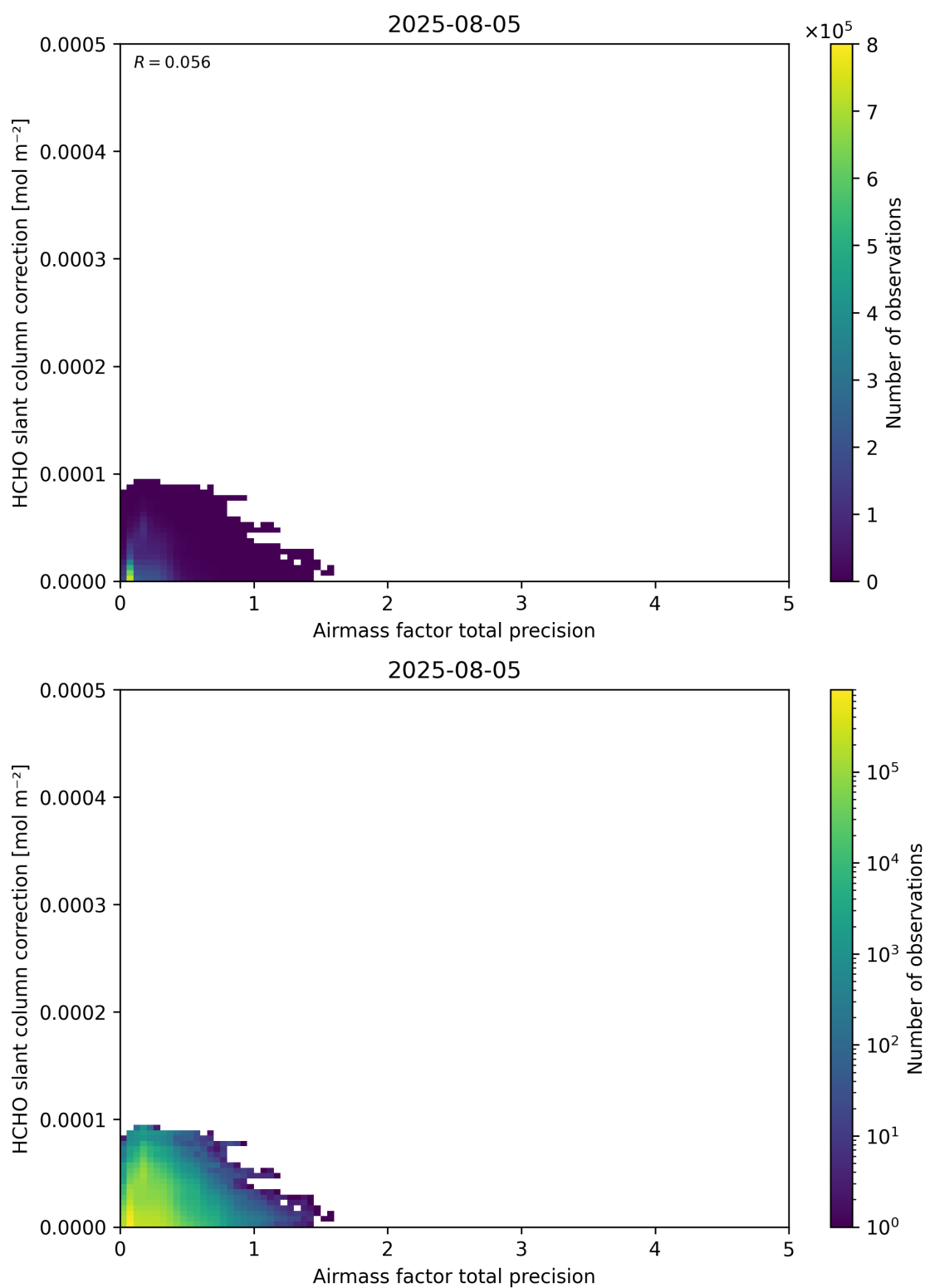
Figure 110: Scatter density plot of “Airmass factor total precision” against “HCHO slant column correction” for 2025-08-04 to 2025-08-06.
