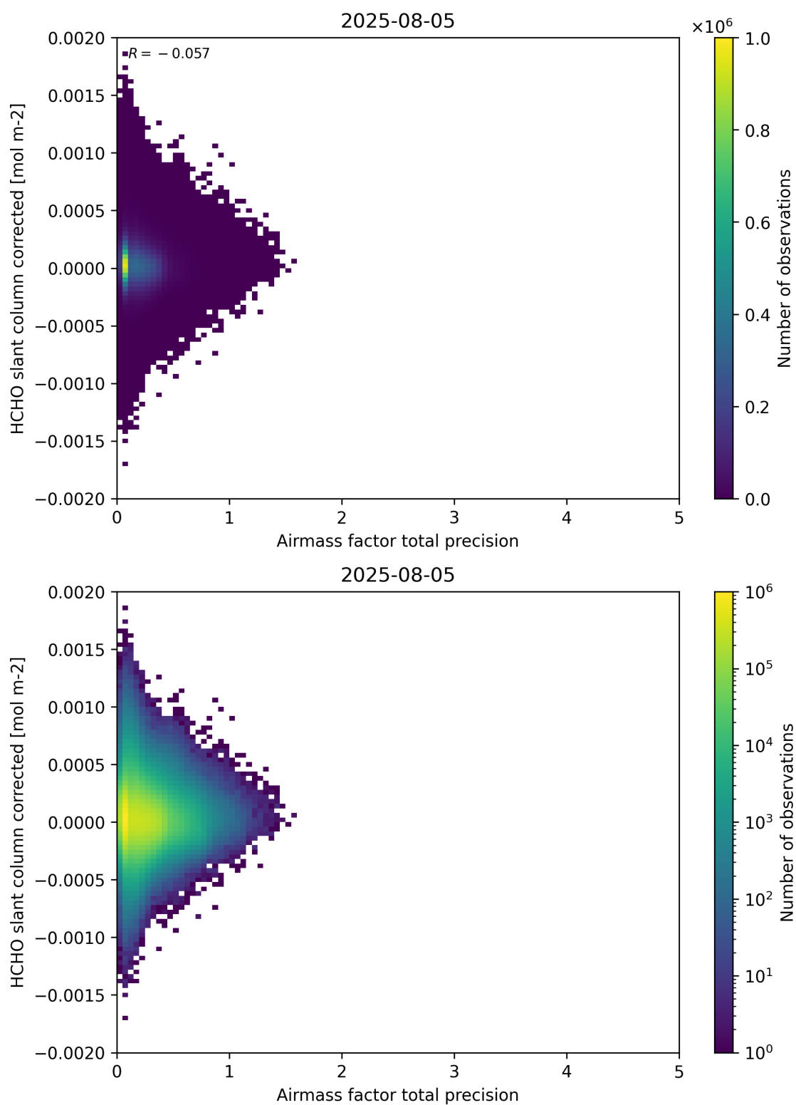
Figure 109: Scatter density plot of “Airmass factor total precision” against “HCHO slant column corrected” for 2025-08-04 to 2025-08-06.
