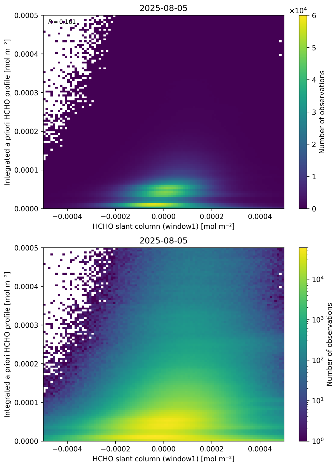
Figure 87: Scatter density plot of “HCHO slant column (window1)” against “Integrated a priori HCHO profile” for 2025-08-04 to 2025-08-06.
