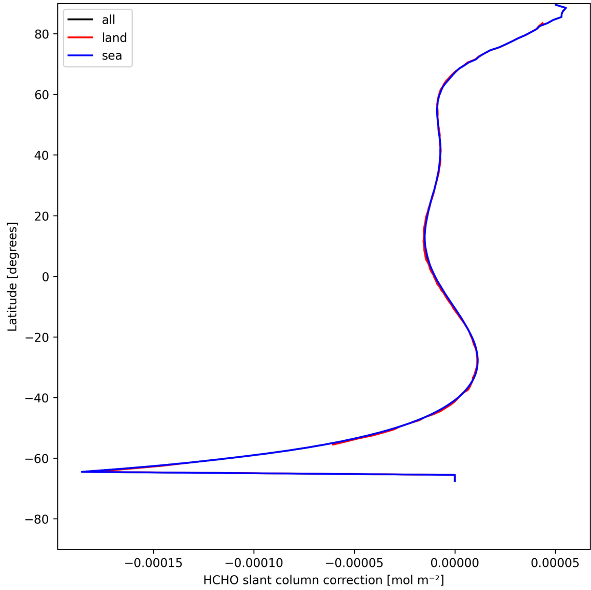
Figure 33: Zonal average of "HCHO slant column correction" for 2025-08-04 to 2025-08-06.
