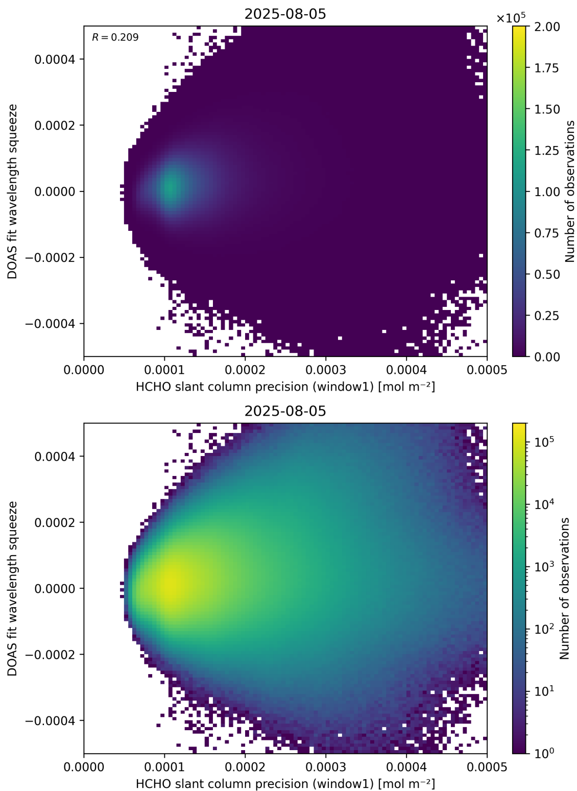
Figure 90: Scatter density plot of “HCHO slant column precision (window1)” against “DOAS fit wavelength squeeze” for 2025-08-04 to 2025-08-06.
