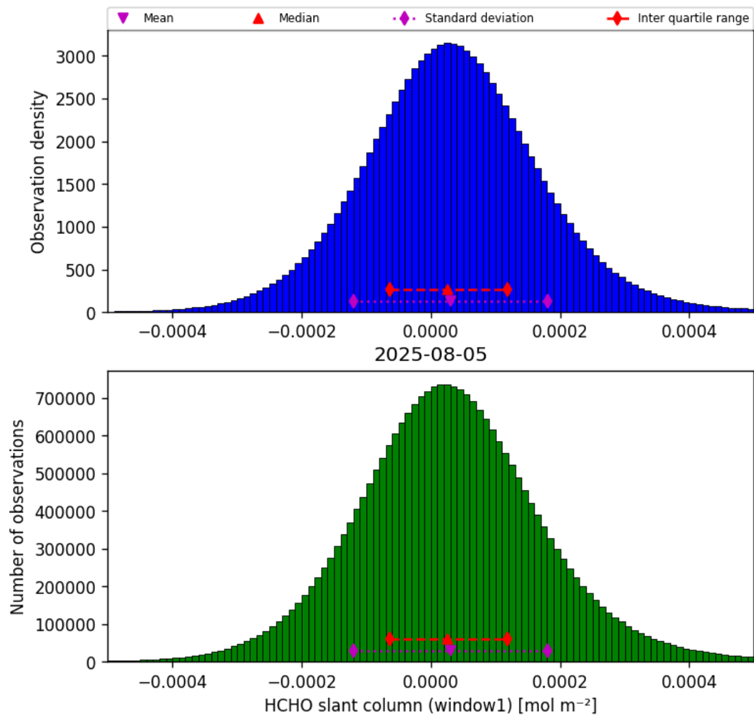
Figure 38: Histogram of “HCHO slant column (window1)” for 2025-08-04 to 2025-08-06
