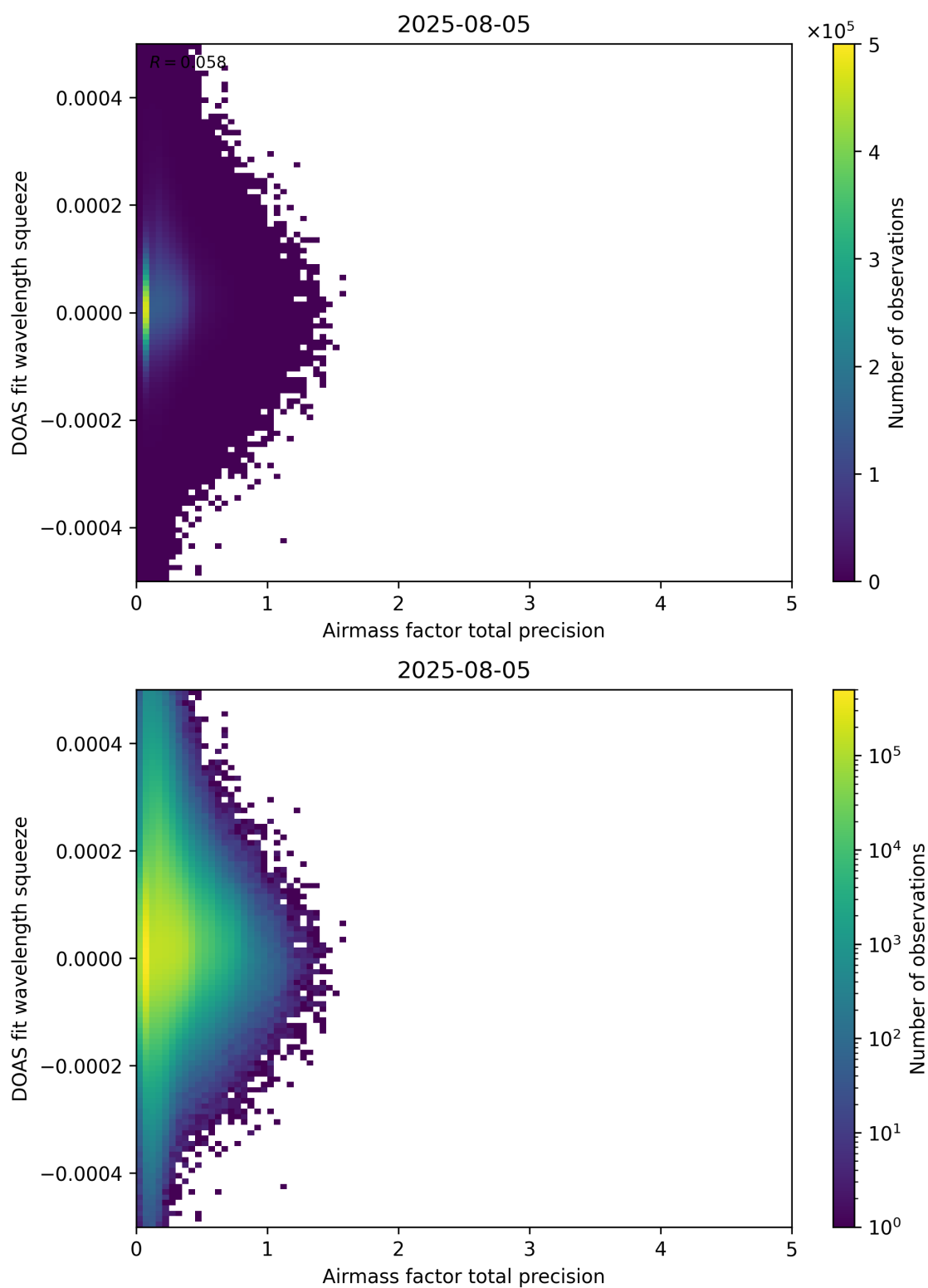
Figure 107: Scatter density plot of “Airmass factor total precision” against “DOAS fit wavelength squeeze” for 2025-08-04 to 2025-08-06.
