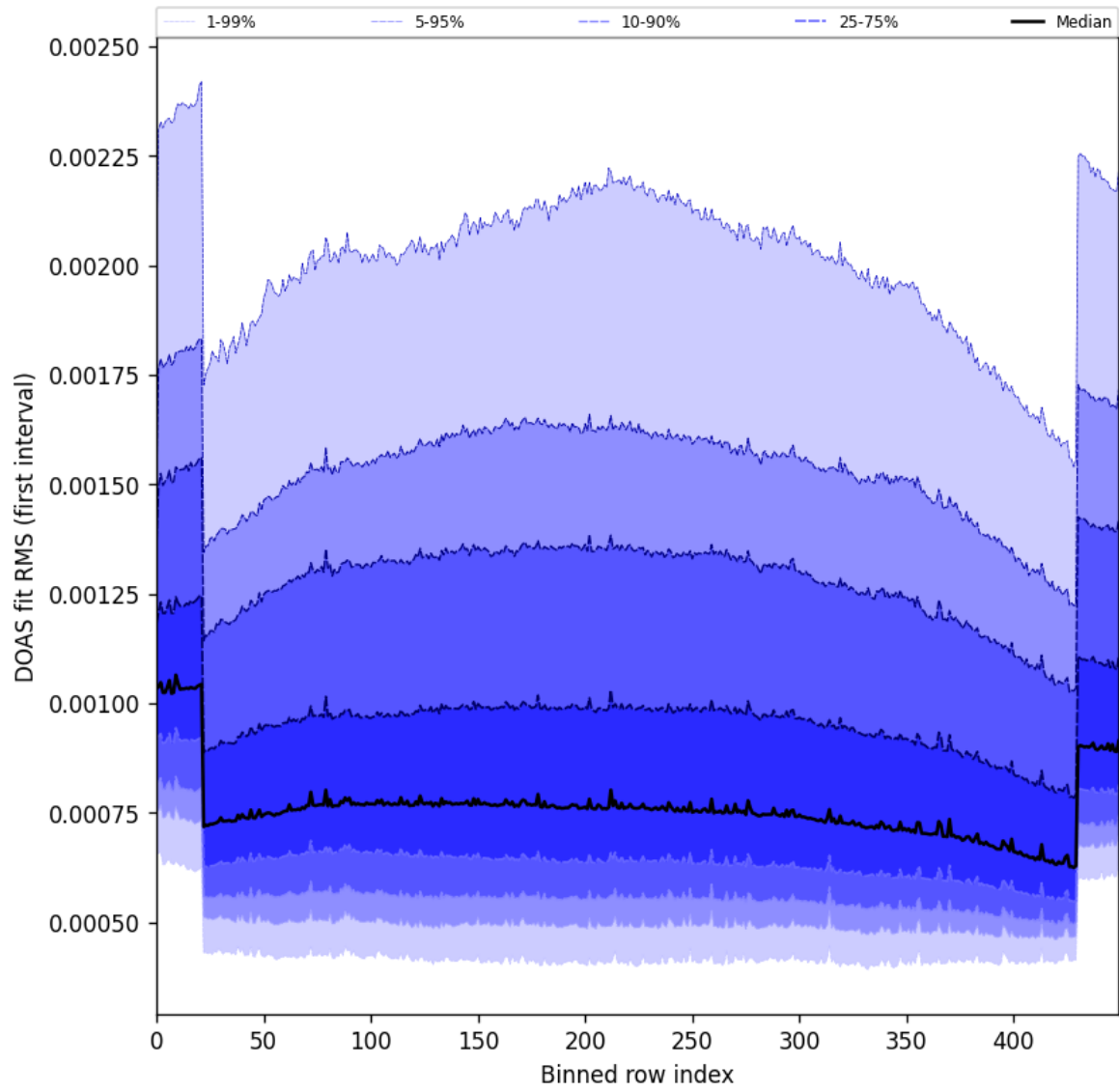
Figure 60: Along track statistics of “DOAS fit RMS (first interval)” for 2025-08-04 to 2025-08-06
