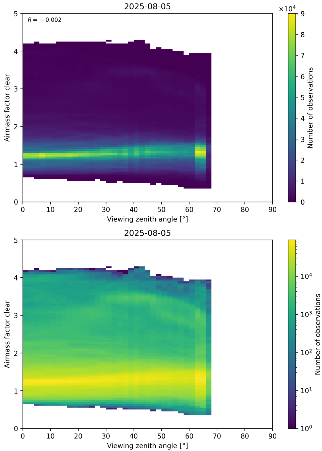
Figure 185: Scatter density plot of “Viewing zenith angle” against “Airmass factor clear” for 2025-08-04 to 2025-08-06.
