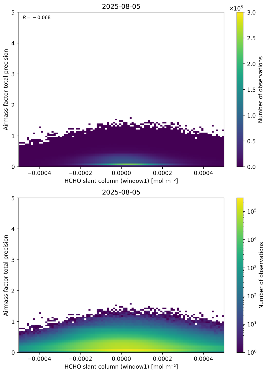
Figure 86: Scatter density plot of “HCHO slant column (window1)” against “Airmass factor total precision” for 2025-08-04 to 2025-08-06.
