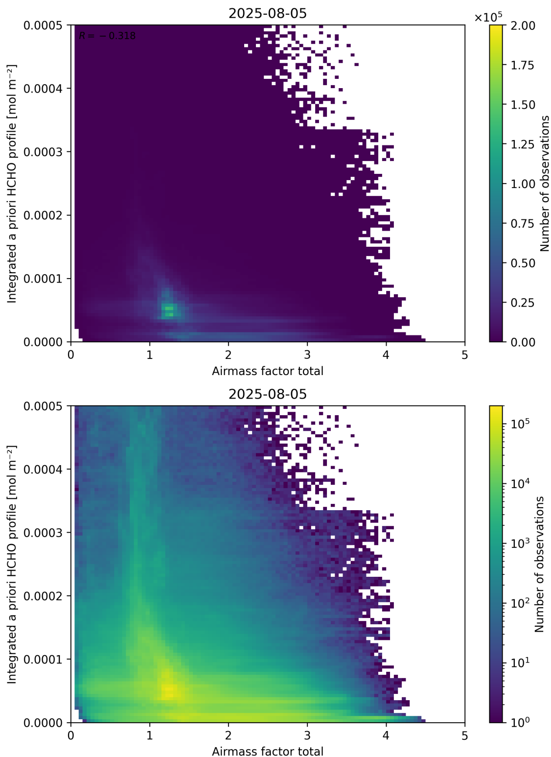
Figure 104: Scatter density plot of “Airmass factor total” against “Integrated a priori HCHO profile” for 2025-08-04 to 2025-08-06.
