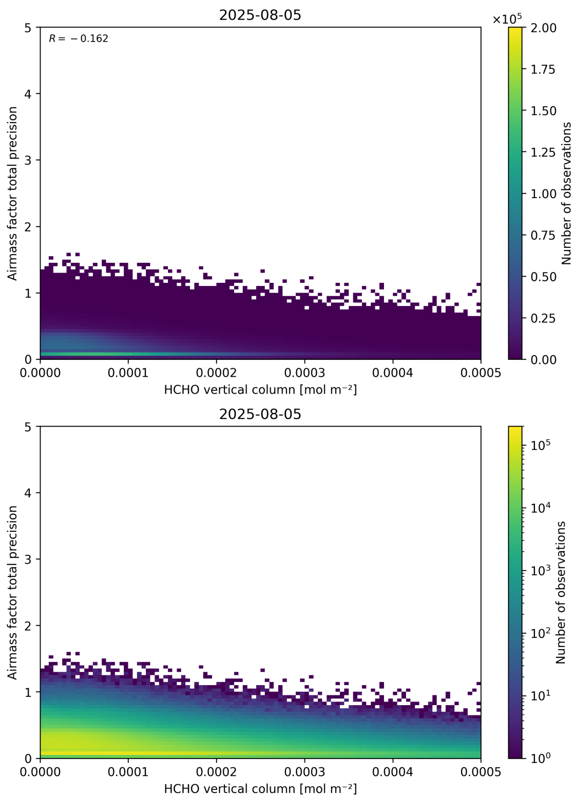
Figure 132: Scatter density plot of “HCHO vertical column” against “Airmass factor total precision” for 2025-08-04 to 2025-08-06.
