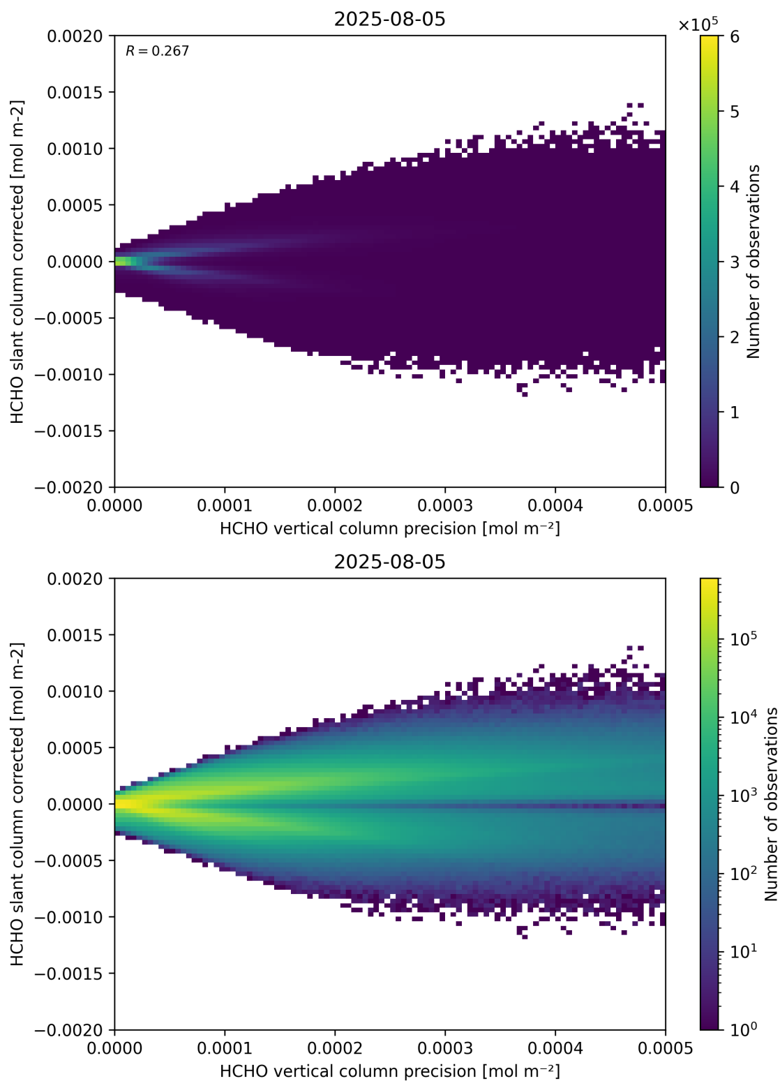
Figure 140: Scatter density plot of “HCHO vertical column precision” against “HCHO slant column corrected” for 2025-08-04 to 2025-08-06.
