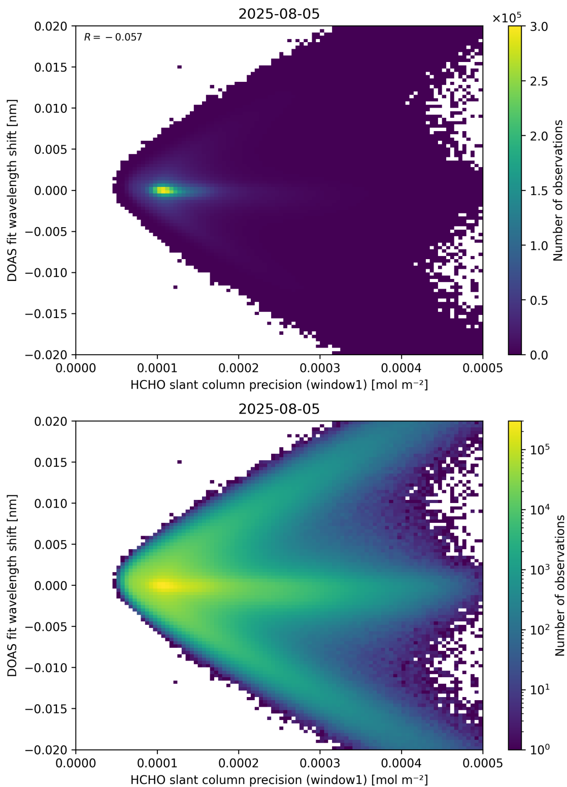
Figure 89: Scatter density plot of “HCHO slant column precision (window1)” against “DOAS fit wavelength shift” for 2025-08-04 to 2025-08-06.
