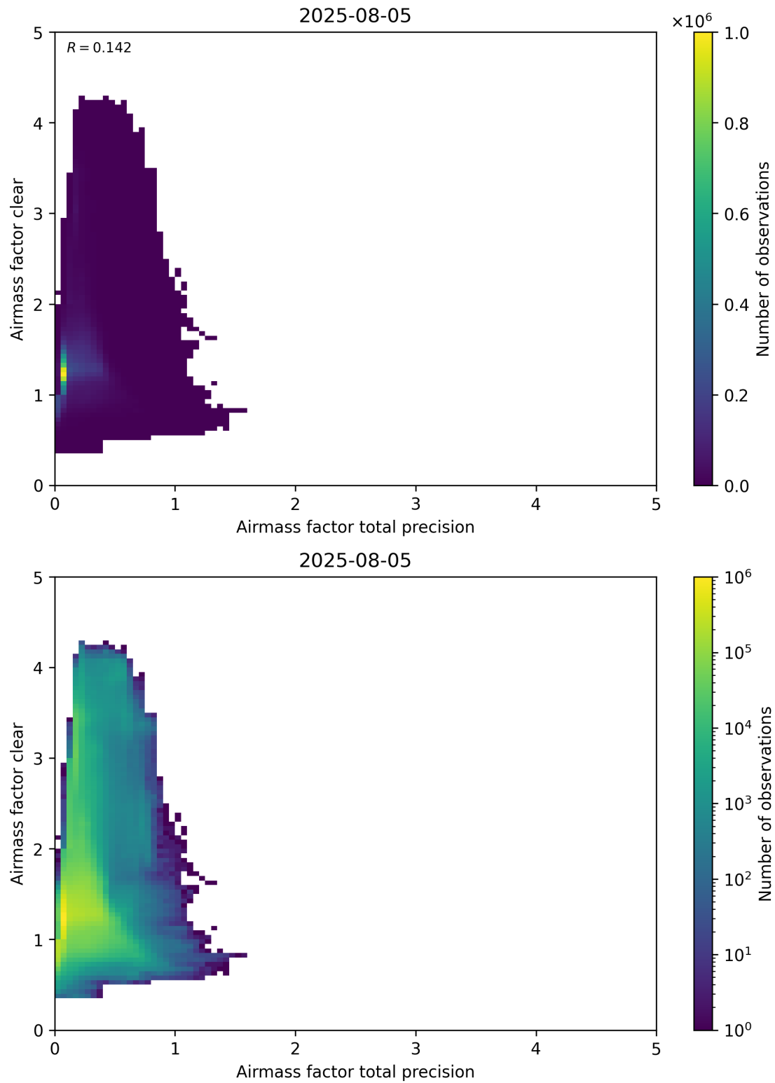
Figure 108: Scatter density plot of “Airmass factor total precision” against “Airmass factor clear” for 2025-08-04 to 2025-08-06.
