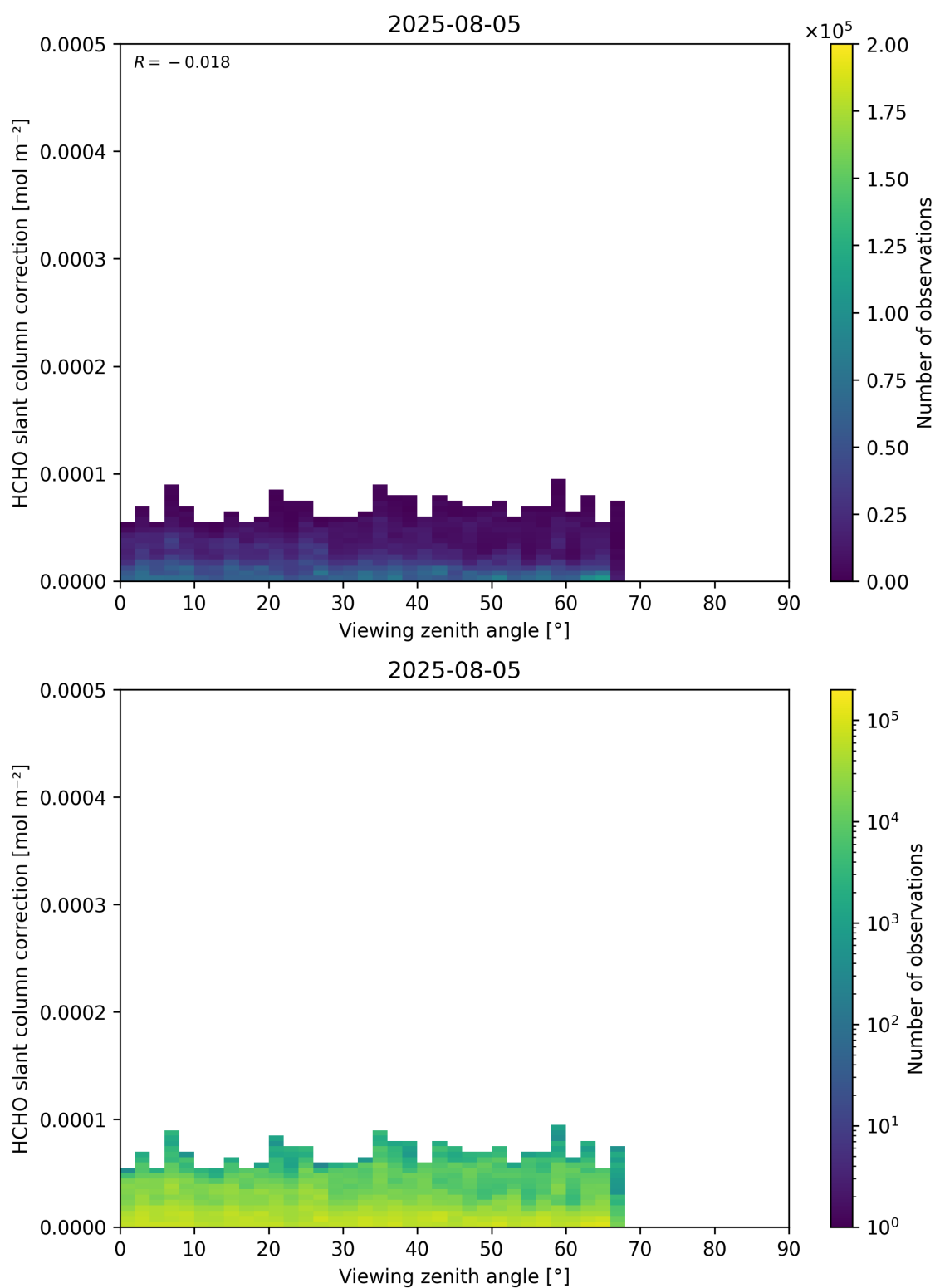
Figure 187: Scatter density plot of “Viewing zenith angle” against “HCHO slant column correction” for 2025-08-04 to 2025-08-06.
