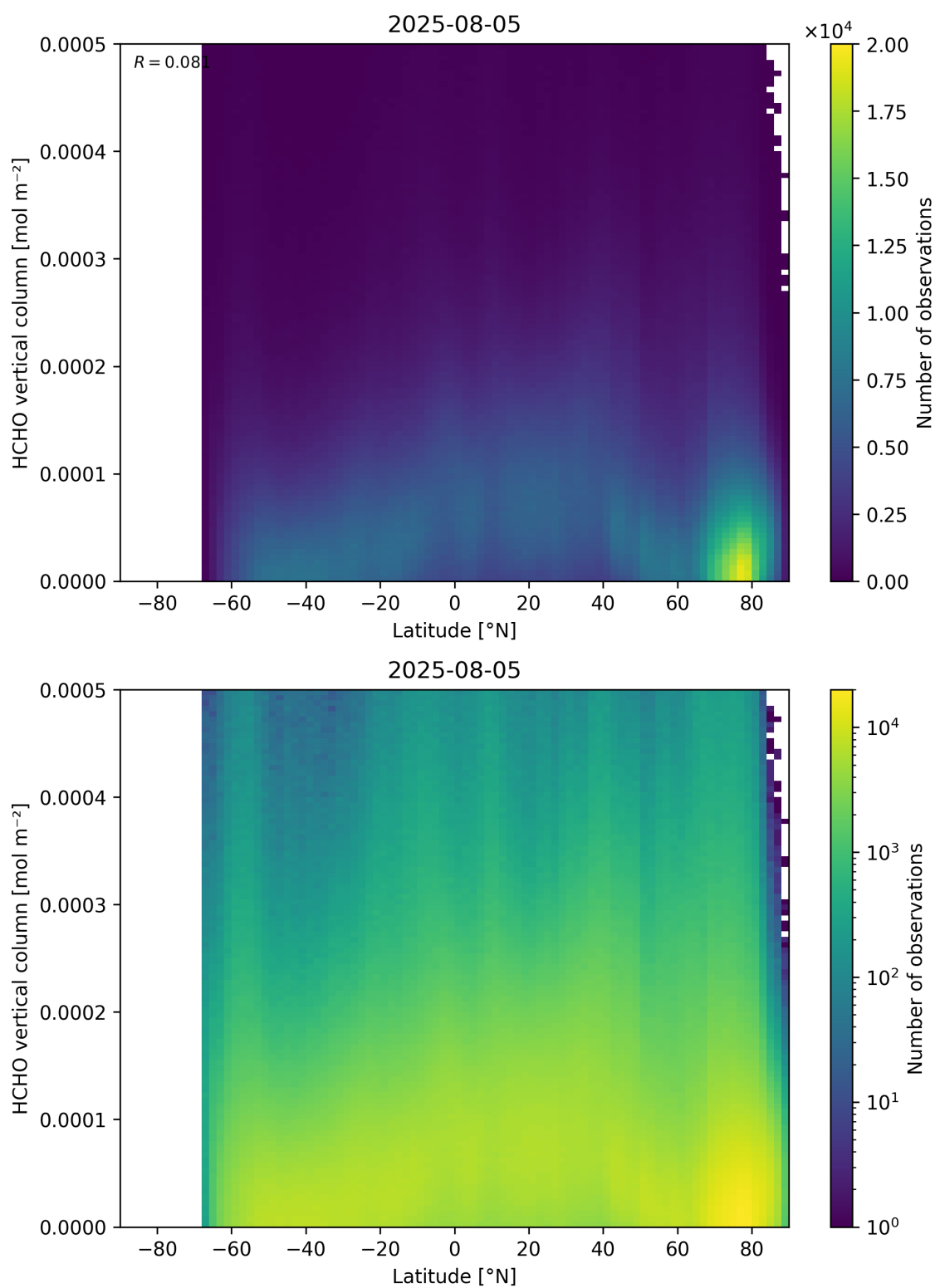
Figure 163: Scatter density plot of “Latitude” against “HCHO vertical column” for 2025-08-04 to 2025-08-06.
