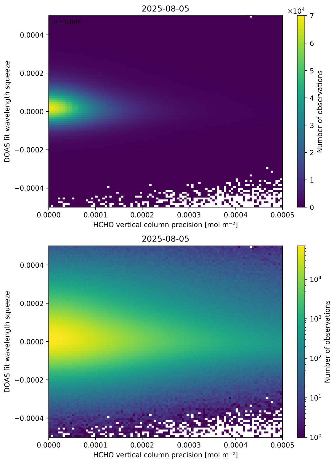
Figure 138: Scatter density plot of “HCHO vertical column precision” against “DOAS fit wavelength squeeze” for 2025-08-04 to 2025-08-06.
