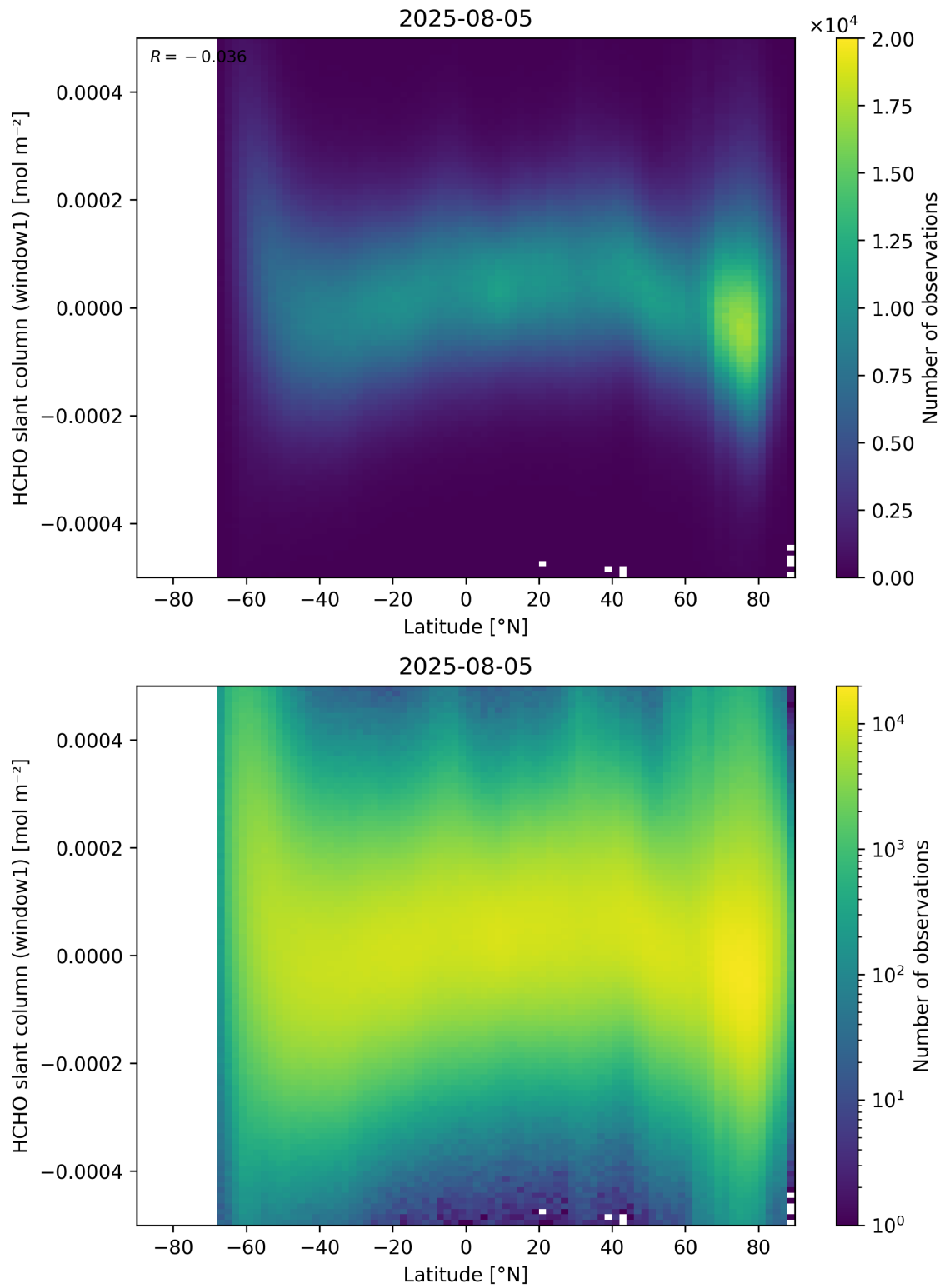
Figure 159: Scatter density plot of “Latitude” against “HCHO slant column (window1)” for 2025-08-04 to 2025-08-06.
