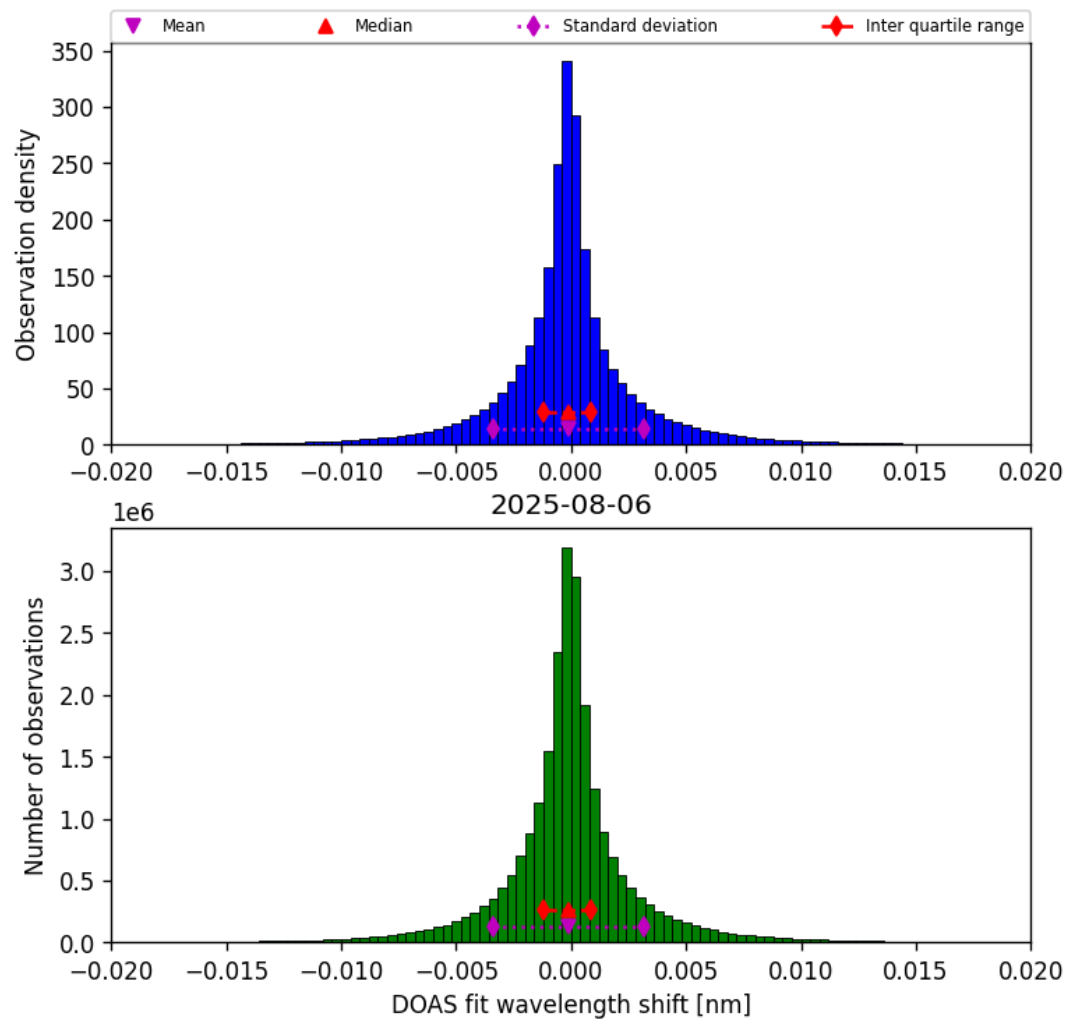
Figure 44: Histogram of “DOAS fit wavelength shift” for 2025-08-05 to 2025-08-07
