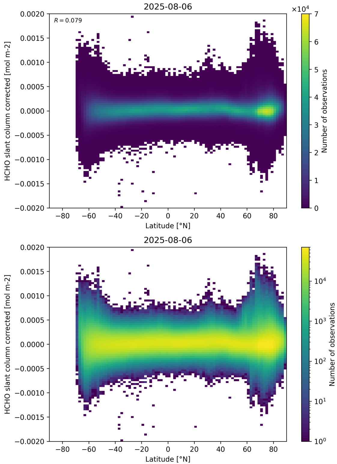
Figure 157: Scatter density plot of “Latitude” against “HCHO slant column corrected” for 2025-08-05 to 2025-08-07.
