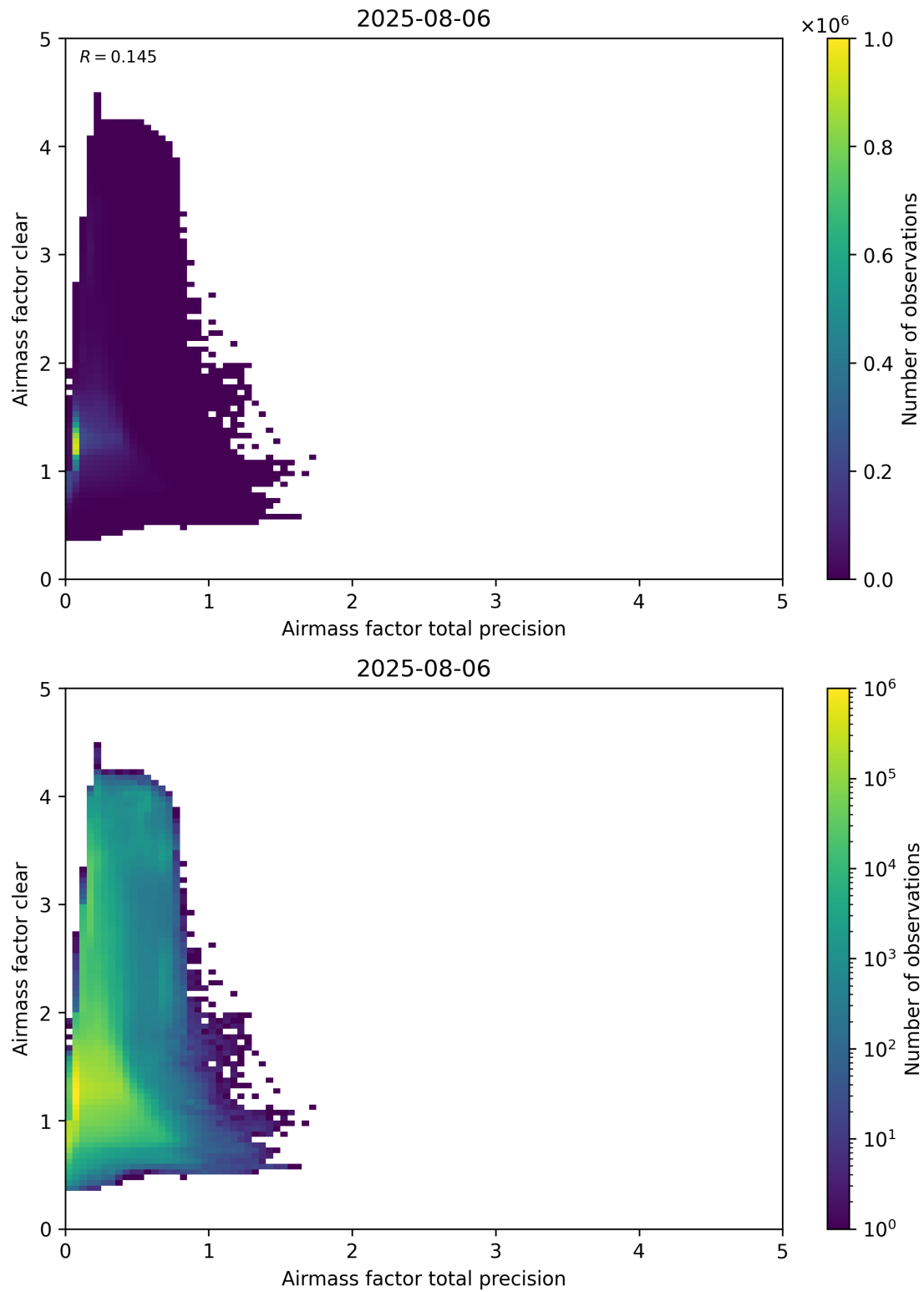
Figure 108: Scatter density plot of “Airmass factor total precision” against “Airmass factor clear” for 2025-08-05 to 2025-08-07.
