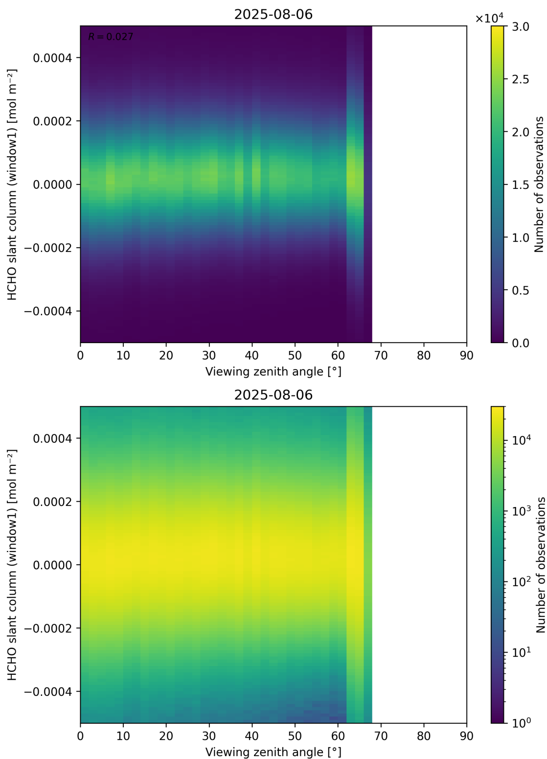
Figure 188: Scatter density plot of “Viewing zenith angle” against “HCHO slant column (window1)” for 2025-08-05 to 2025-08-07.
