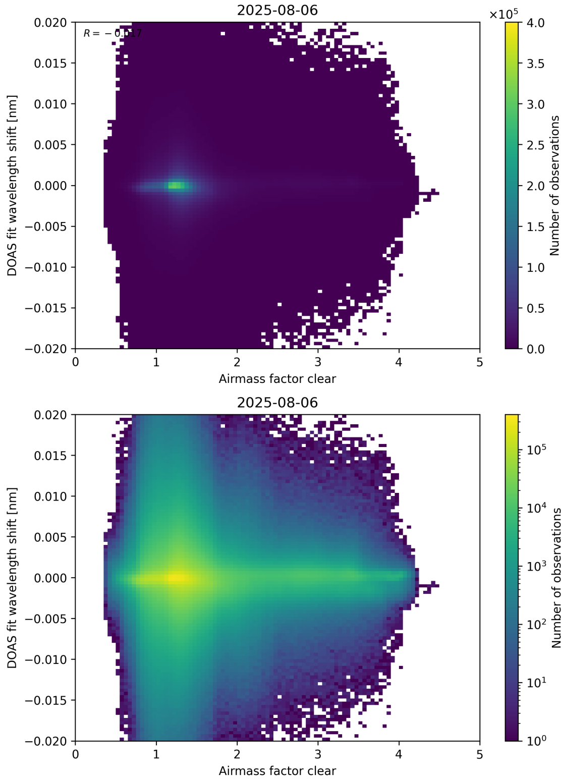
Figure 72: Scatter density plot of “Airmass factor clear” against “DOAS fit wavelength shift” for 2025-08-05 to 2025-08-07.
