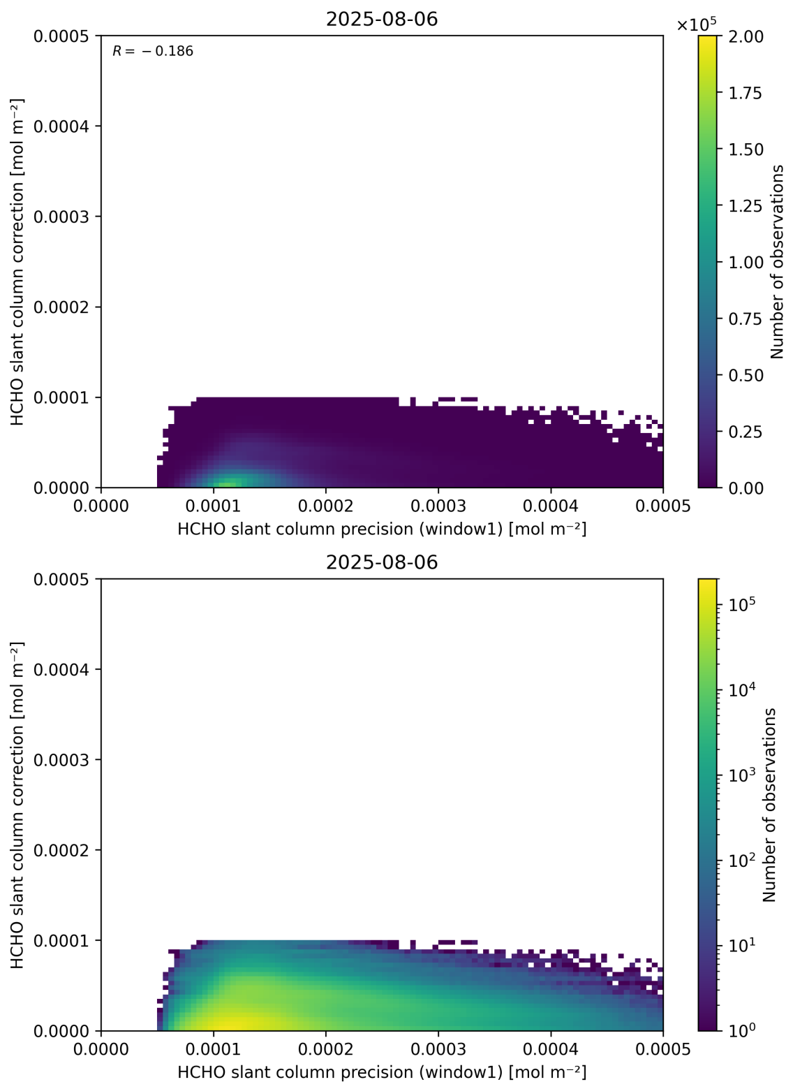
Figure 93: Scatter density plot of “HCHO slant column precision (window1)” against “HCHO slant column correction” for 2025-08-05 to 2025-08-07.
