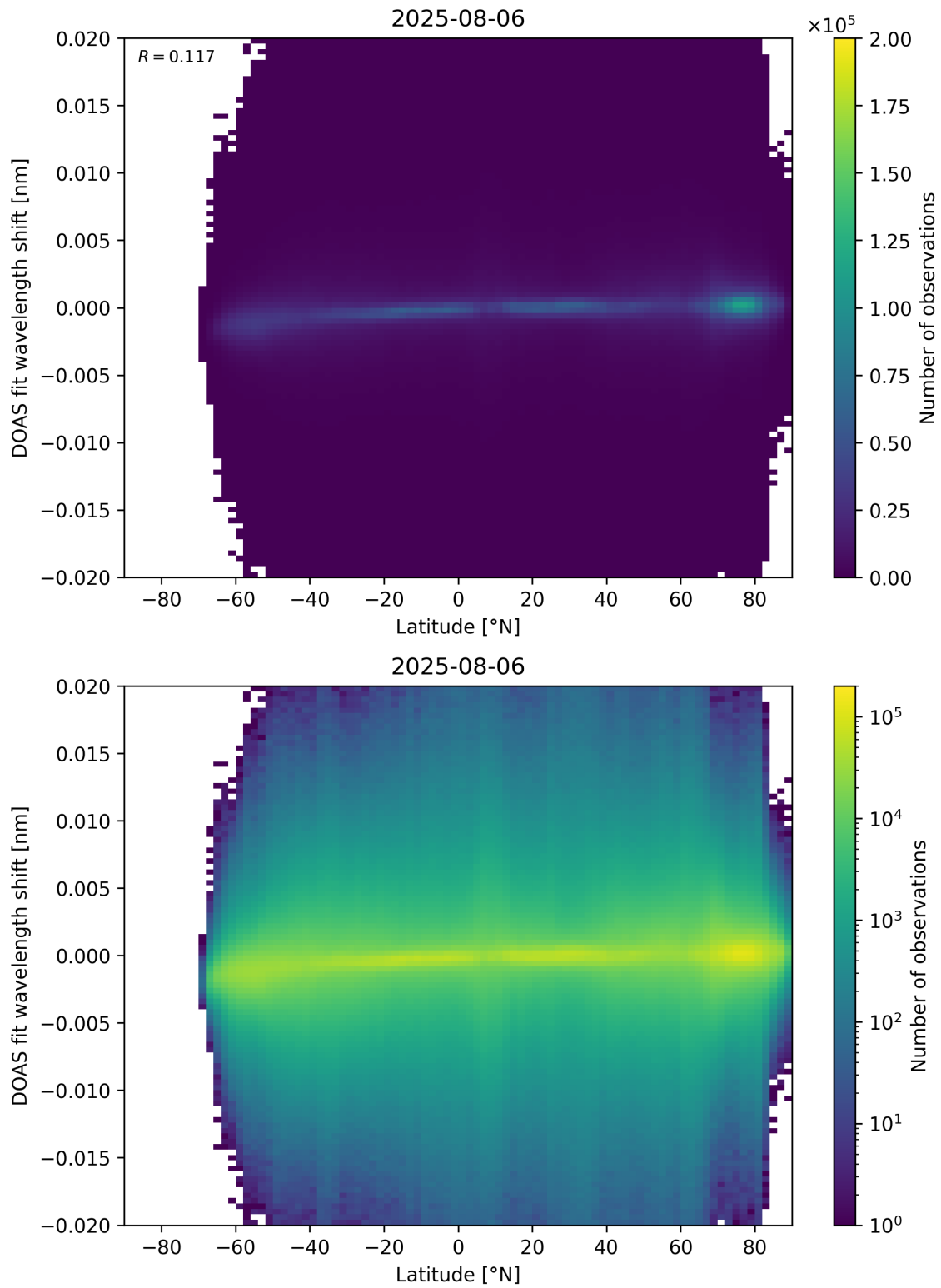
Figure 154: Scatter density plot of “Latitude” against “DOAS fit wavelength shift” for 2025-08-05 to 2025-08-07.
