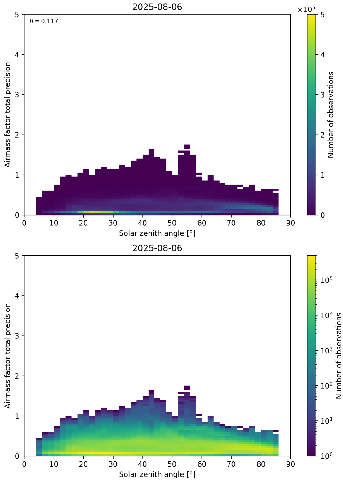
Figure 176: Scatter density plot of “Solar zenith angle” against “Airmass factor total precision” for 2025-08-05 to 2025-08-07.
