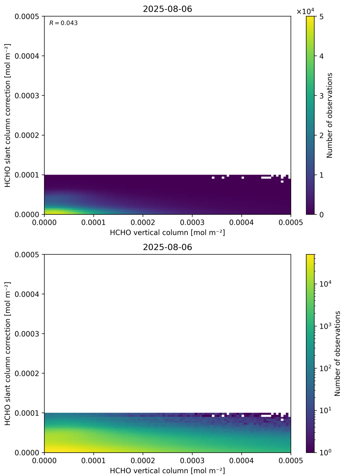
Figure 128: Scatter density plot of “HCHO vertical column” against “HCHO slant column correction” for 2025-08-05 to 2025-08-07.
