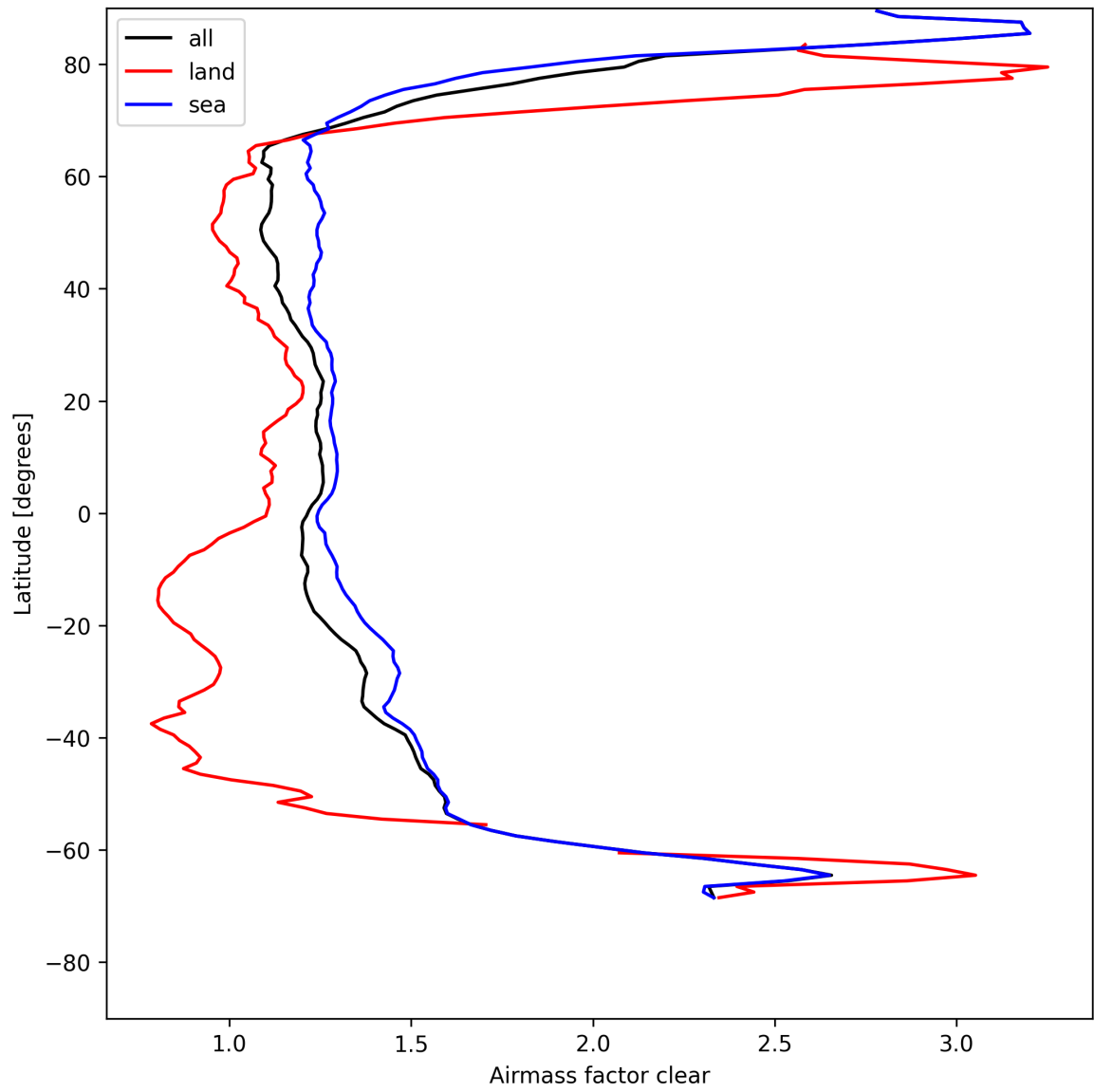
Figure 28: Zonal average of “Airmass factor clear” for 2025-08-05 to 2025-08-07.
