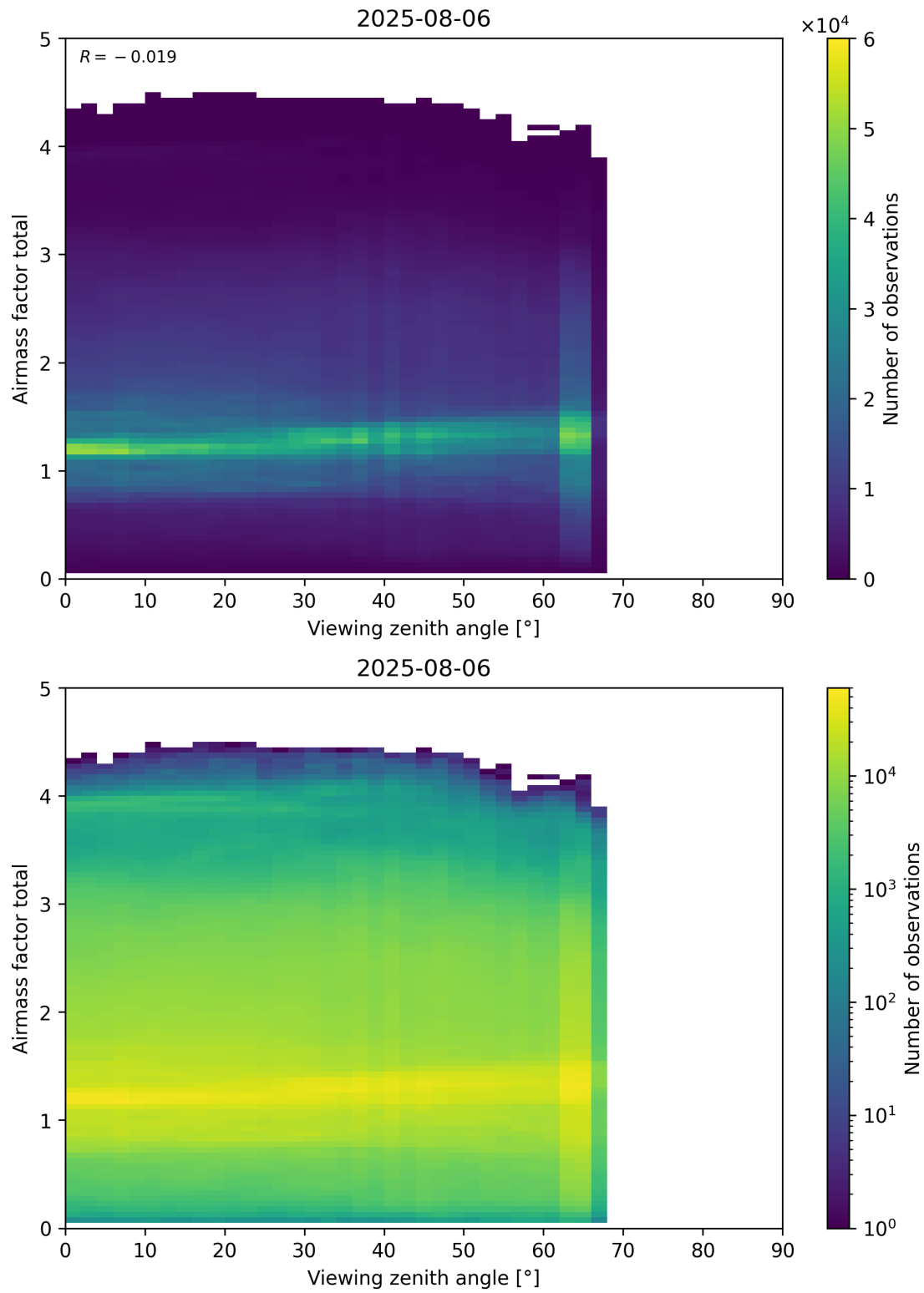
Figure 190: Scatter density plot of “Viewing zenith angle” against “Airmass factor total” for 2025-08-05 to 2025-08-07.
