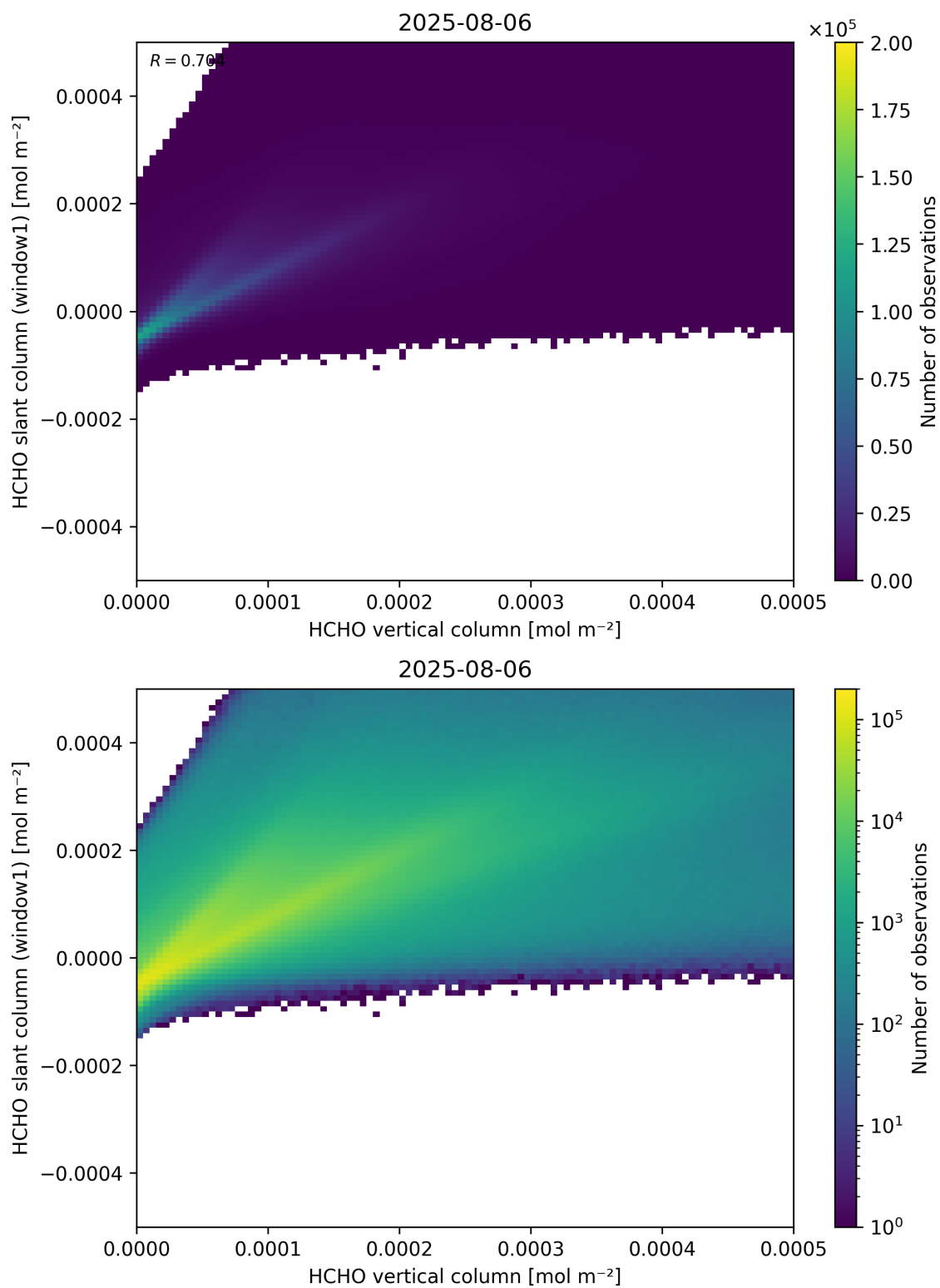
Figure 129: Scatter density plot of “HCHO vertical column” against “HCHO slant column (window1)” for 2025-08-05 to 2025-08-07.
