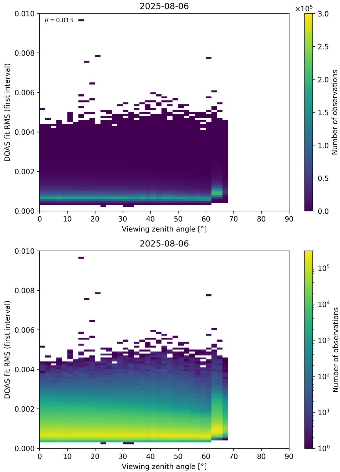
Figure 182: Scatter density plot of “Viewing zenith angle” against “DOAS fit RMS (first interval)” for 2025-08-05 to 2025-08-07.
