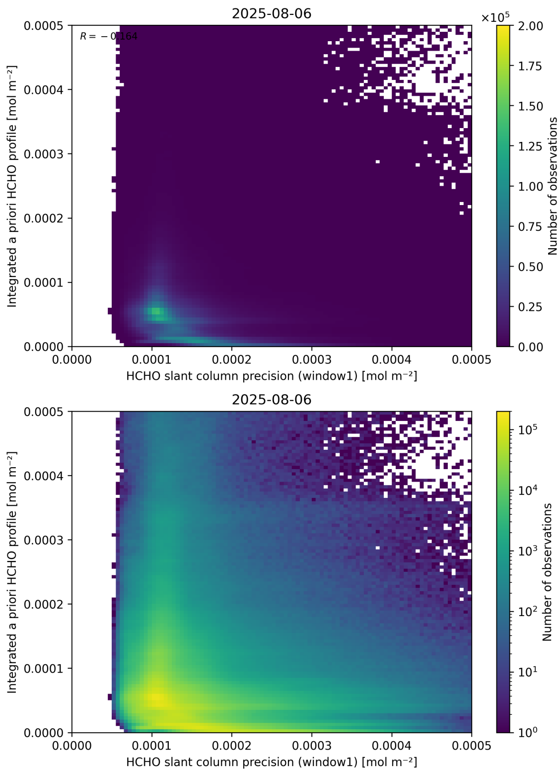
Figure 96: Scatter density plot of “HCHO slant column precision (window1)” against “Integrated a priori HCHO profile” for 2025-08-05 to 2025-08-07.
