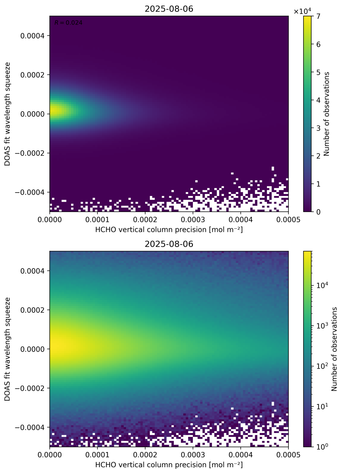
Figure 138: Scatter density plot of “HCHO vertical column precision” against “DOAS fit wavelength squeeze” for 2025-08-05 to 2025-08-07.
