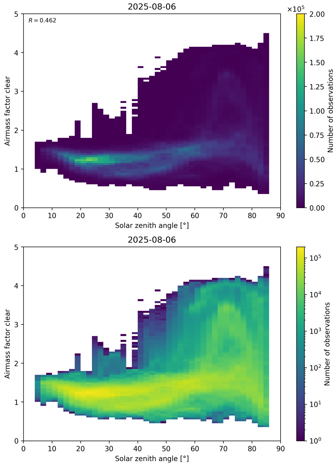
Figure 170: Scatter density plot of “Solar zenith angle” against “Airmass factor clear” for 2025-08-05 to 2025-08-07.
