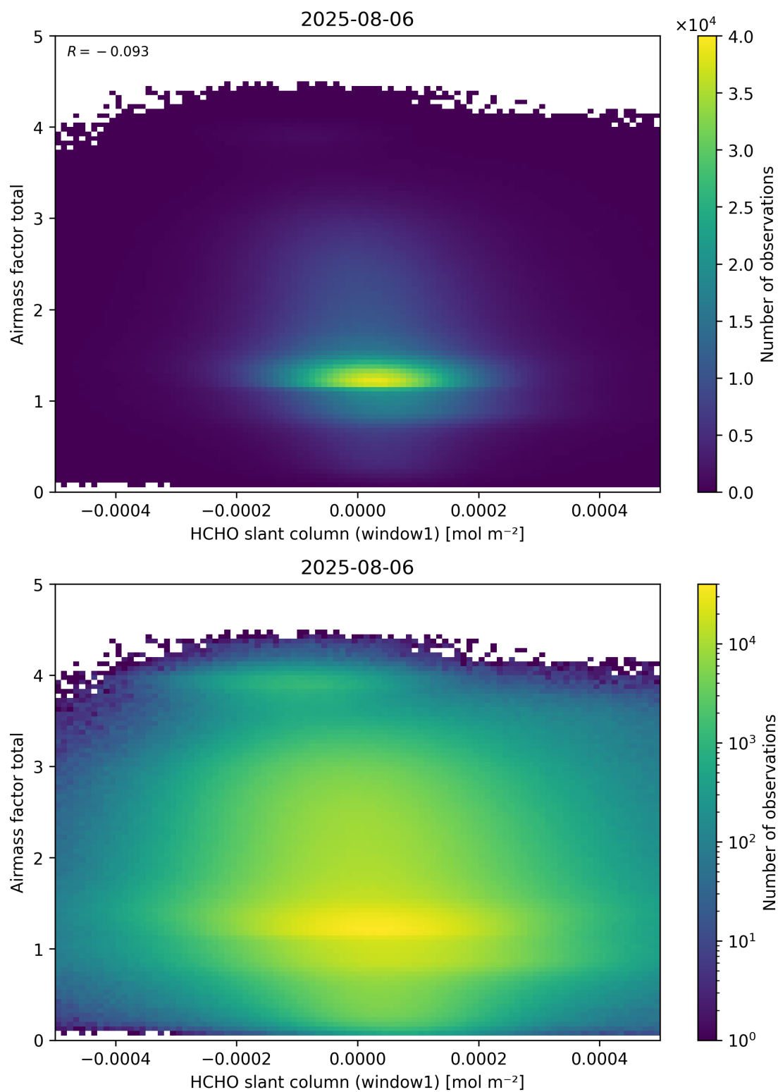
Figure 85: Scatter density plot of “HCHO slant column (window1)” against “Airmass factor total” for 2025-08-05 to 2025-08-07.
