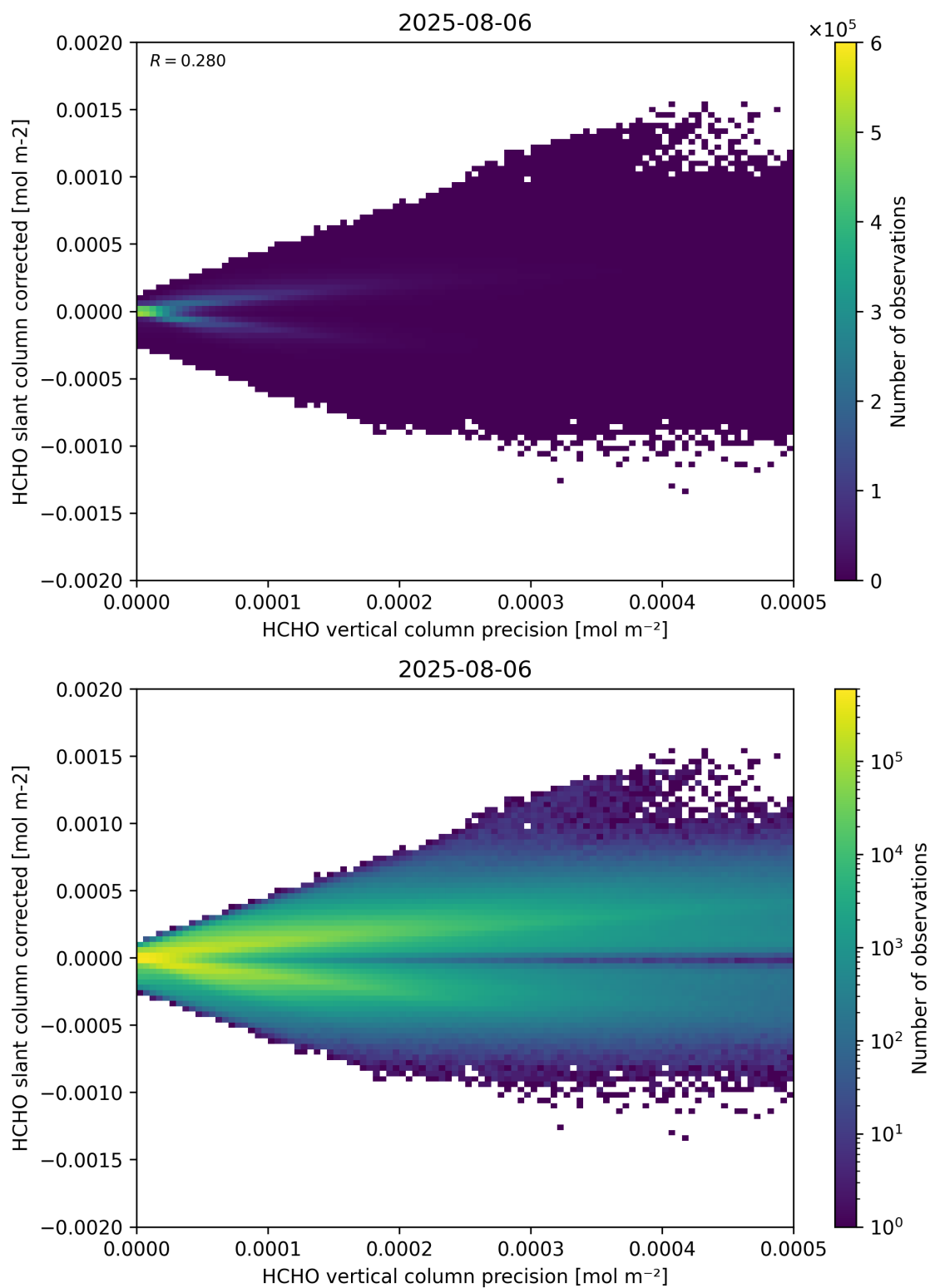
Figure 140: Scatter density plot of “HCHO vertical column precision” against “HCHO slant column corrected” for 2025-08-05 to 2025-08-07.
