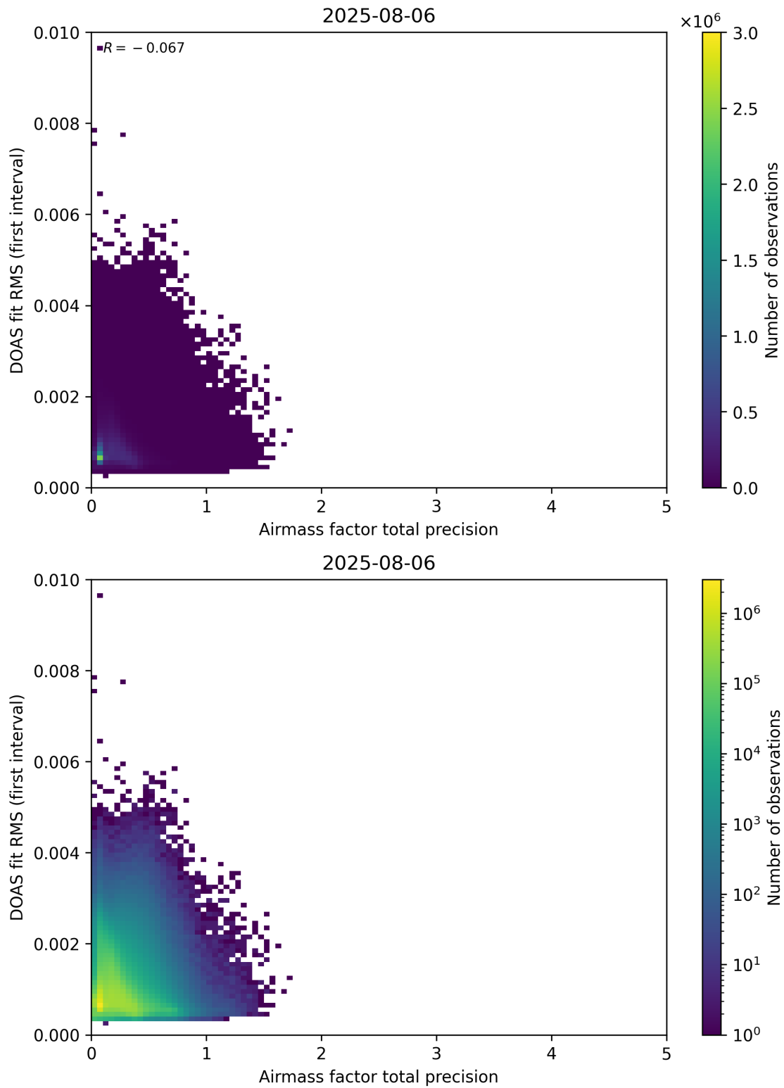
Figure 105: Scatter density plot of “Airmass factor total precision” against “DOAS fit RMS (first interval)” for 2025-08-05 to 2025-08-07.
