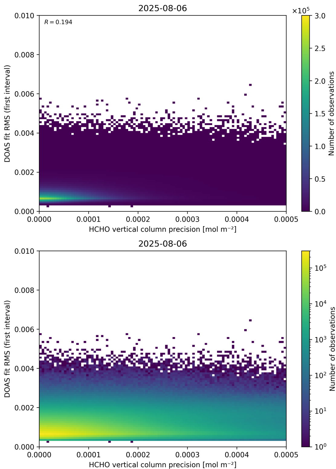
Figure 136: Scatter density plot of “HCHO vertical column precision” against “DOAS fit RMS (first interval)” for 2025-08-05 to 2025-08-07.
