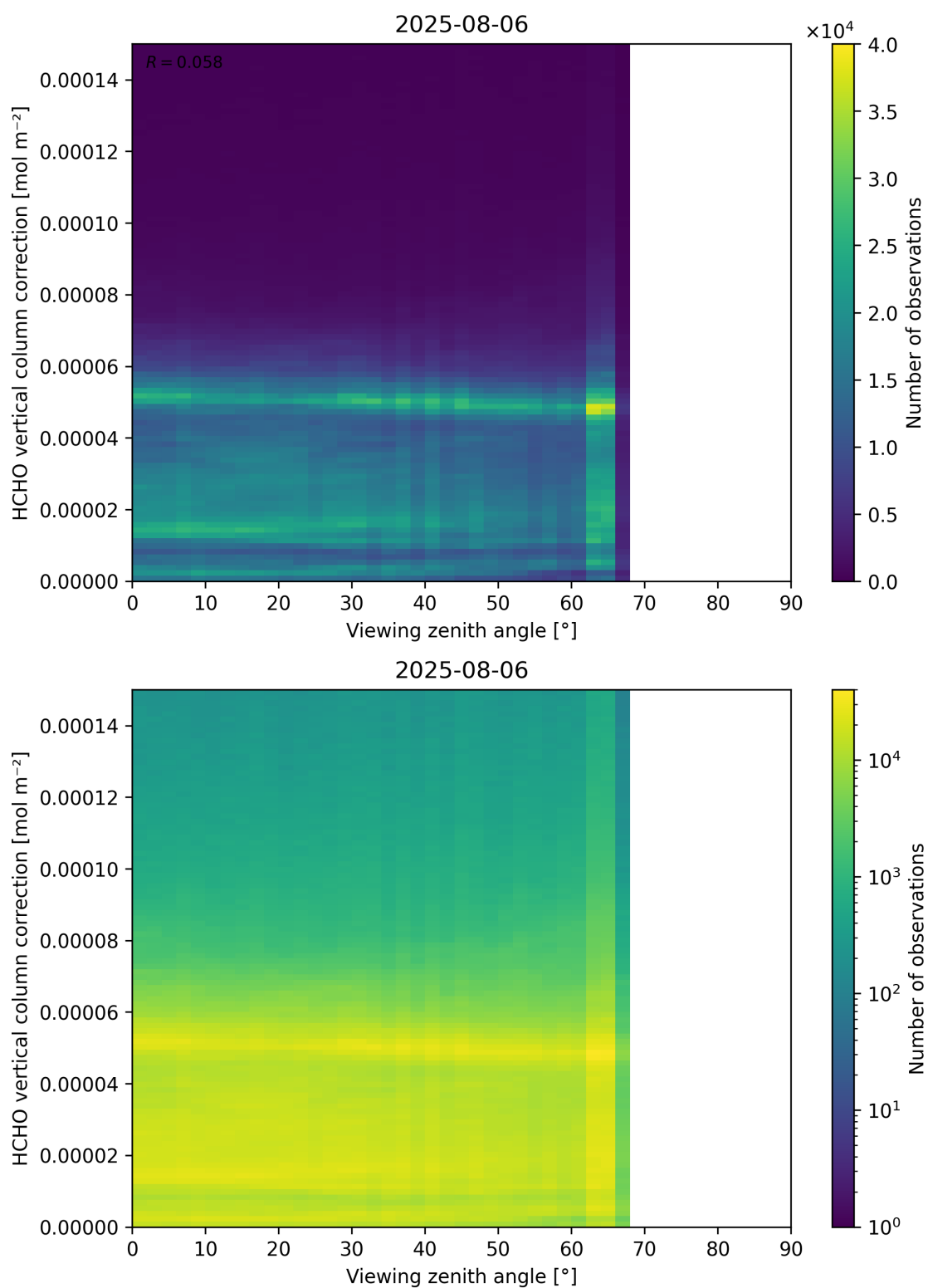
Figure 193: Scatter density plot of “Viewing zenith angle” against “HCHO vertical column correction” for 2025-08-05 to 2025-08-07.
