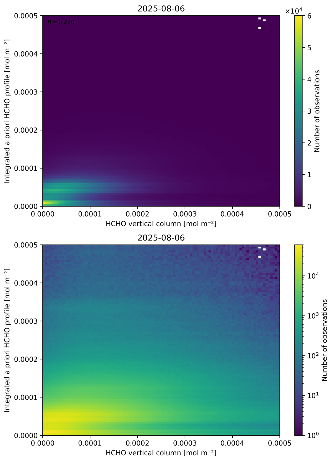
Figure 135: Scatter density plot of “HCHO vertical column” against “Integrated a priori HCHO profile” for 2025-08-05 to 2025-08-07.
