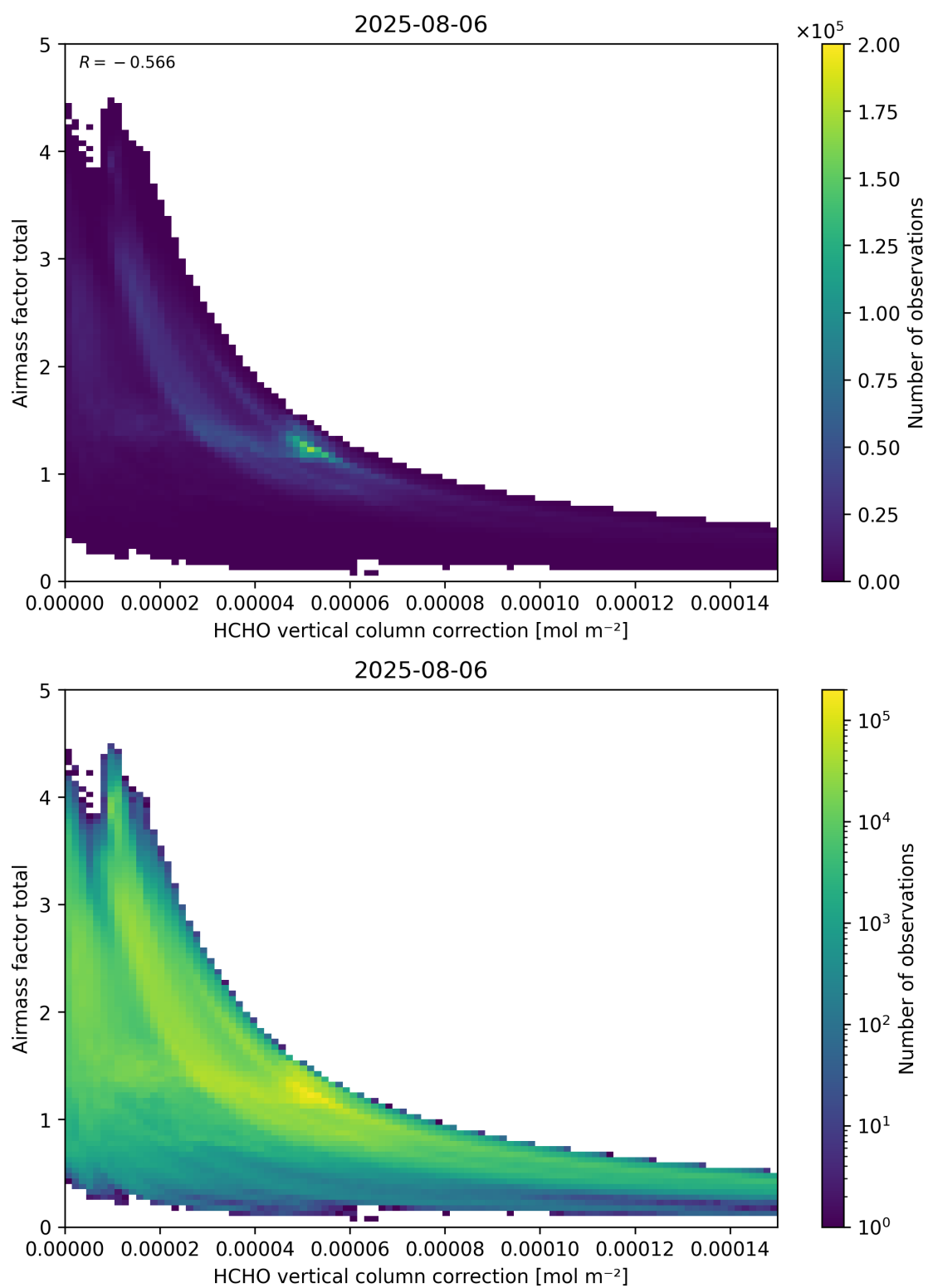
Figure 120: Scatter density plot of “HCHO vertical column correction” against “Airmass factor total” for 2025-08-05 to 2025-08-07.
