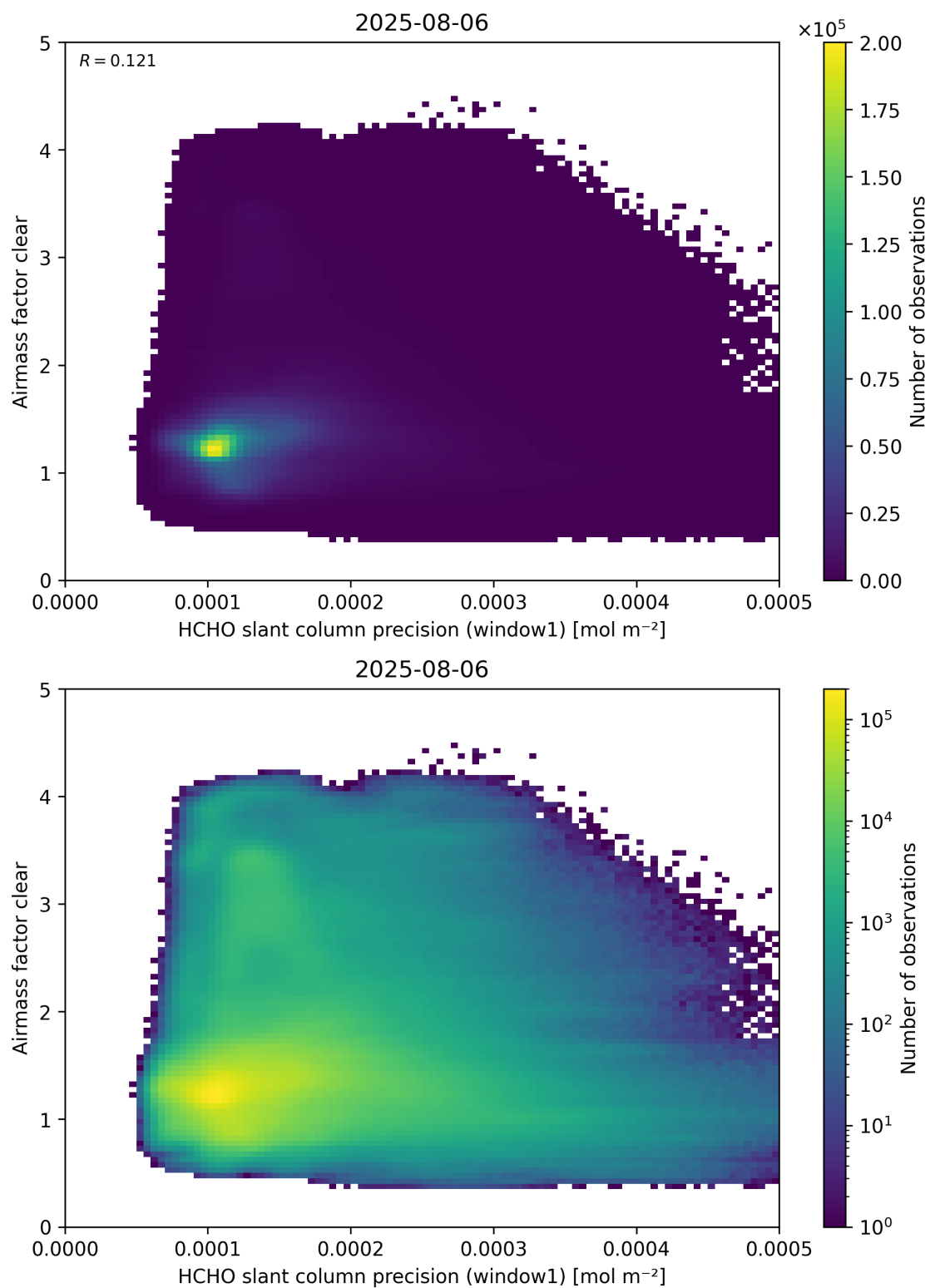
Figure 91: Scatter density plot of “HCHO slant column precision (window1)” against “Airmass factor clear” for 2025-08-05 to 2025-08-07.
