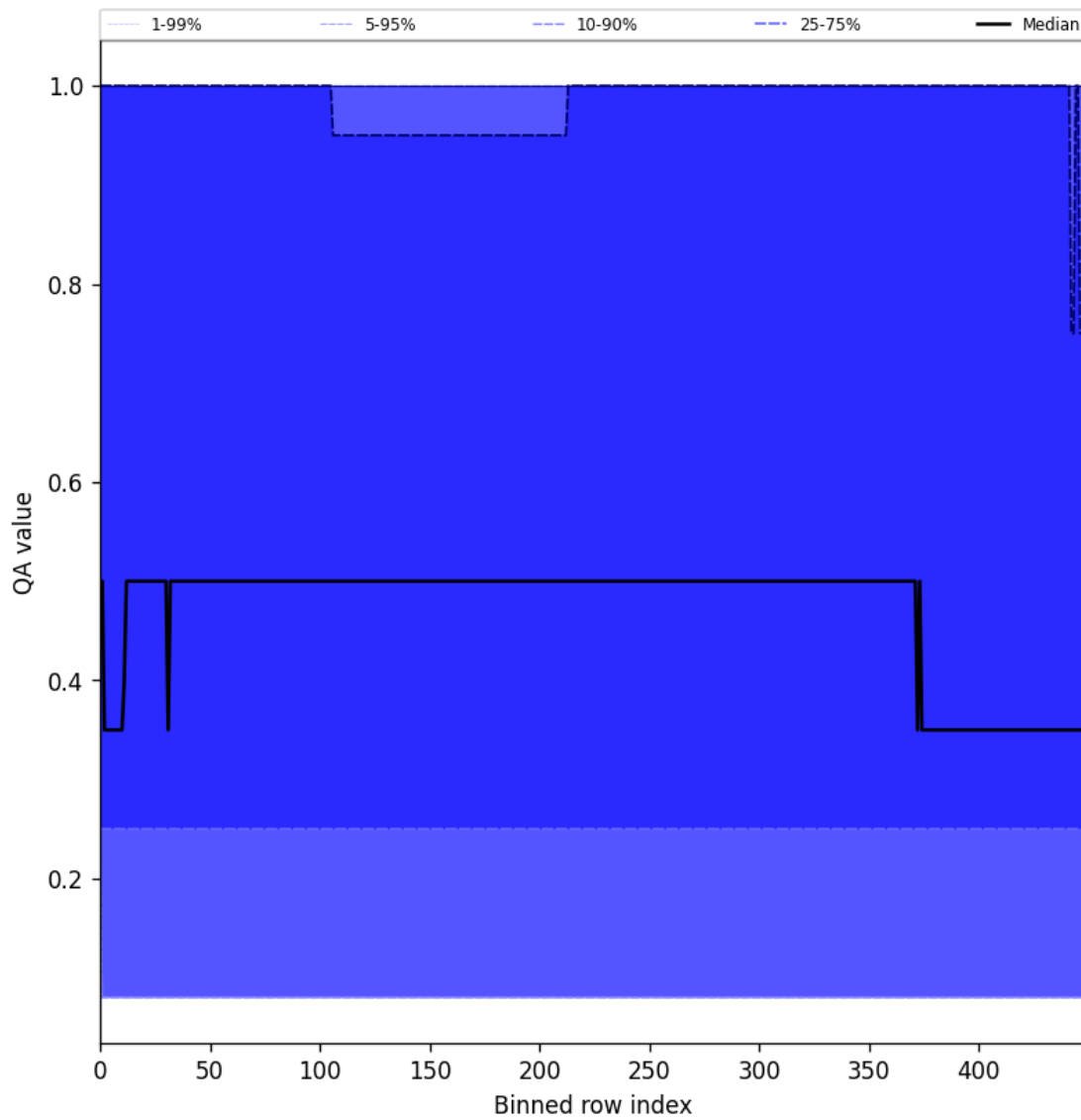
Figure 48: Along track statistics of “QA value” for 2025-08-05 to 2025-08-07
