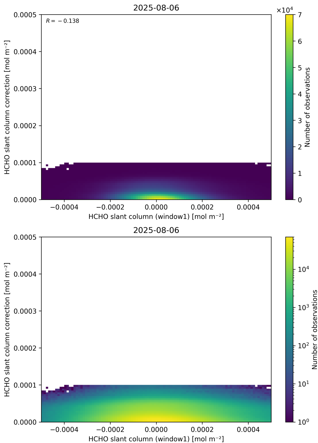
Figure 83: Scatter density plot of “HCHO slant column (window1)” against “HCHO slant column correction” for 2025-08-05 to 2025-08-07.
