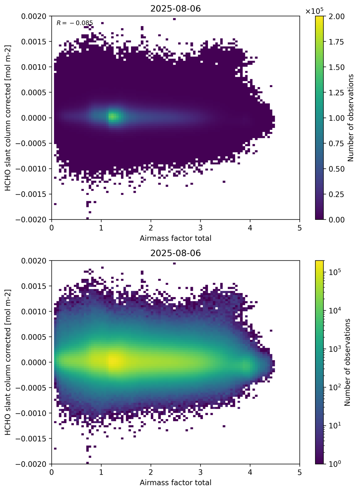
Figure 101: Scatter density plot of “Airmass factor total” against “HCHO slant column corrected” for 2025-08-05 to 2025-08-07.
