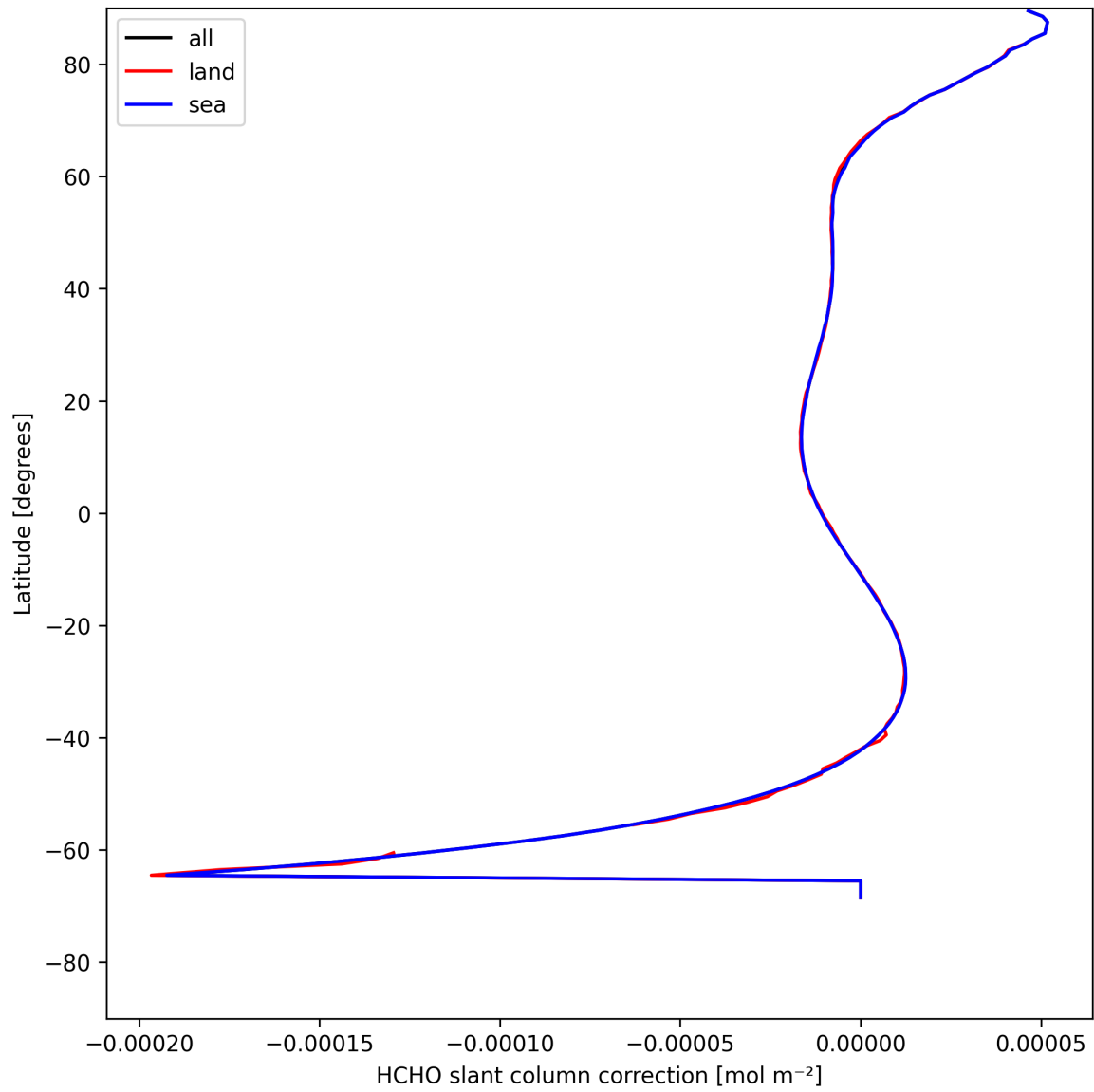
Figure 33: Zonal average of “HCHO slant column correction” for 2025-08-05 to 2025-08-07.
