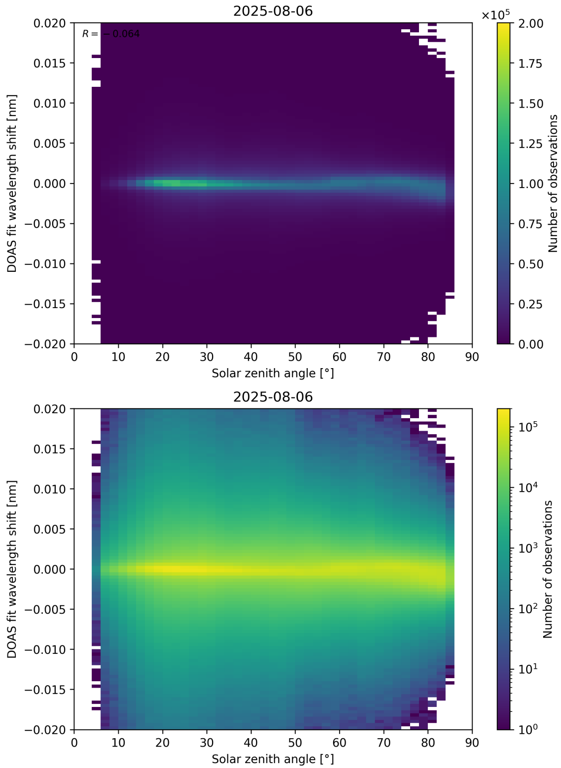
Figure 168: Scatter density plot of “Solar zenith angle” against “DOAS fit wavelength shift” for 2025-08-05 to 2025-08-07.
