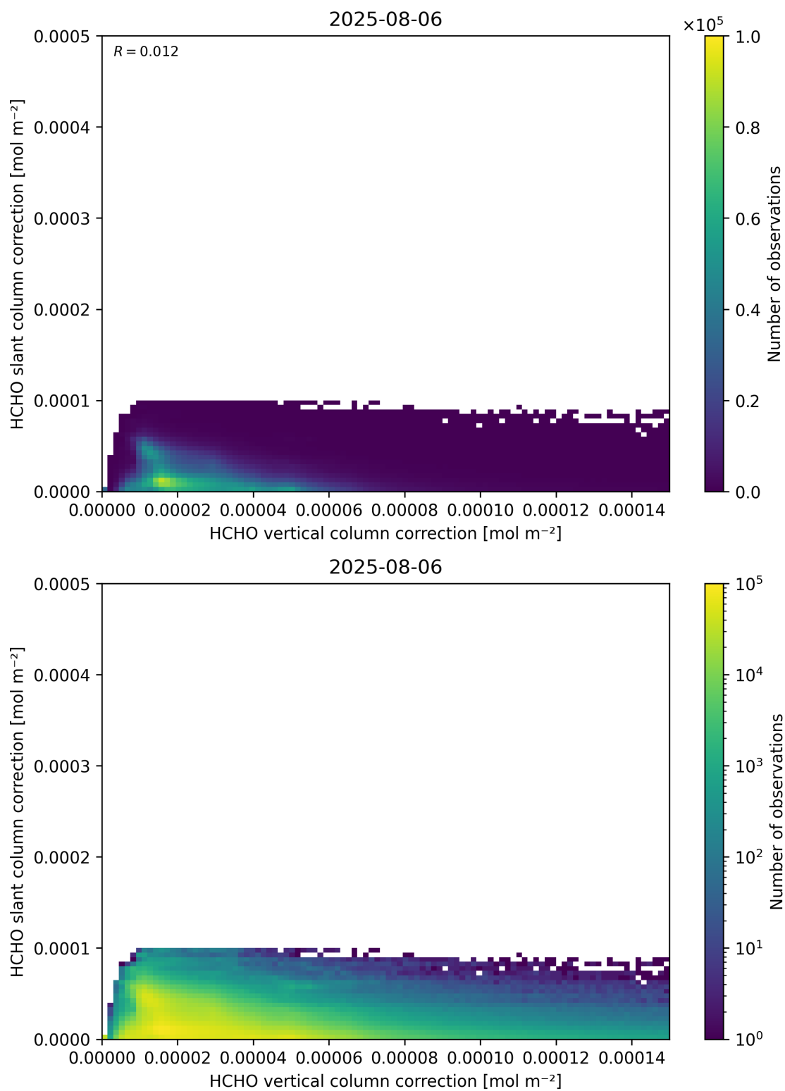
Figure 117: Scatter density plot of “HCHO vertical column correction” against “HCHO slant column correction” for 2025-08-05 to 2025-08-07.
