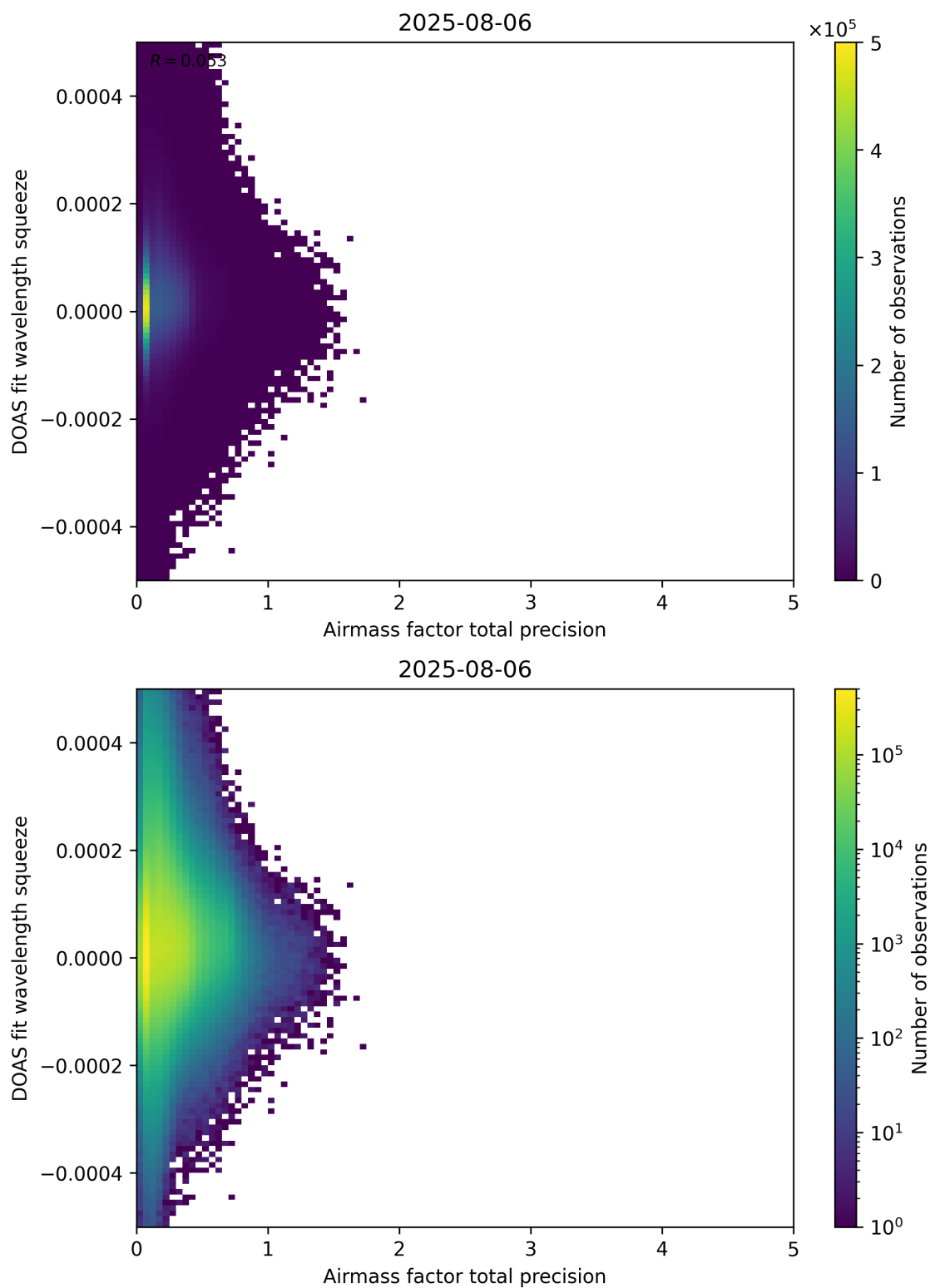
Figure 107: Scatter density plot of “Airmass factor total precision” against “DOAS fit wavelength squeeze” for 2025-08-05 to 2025-08-07.
