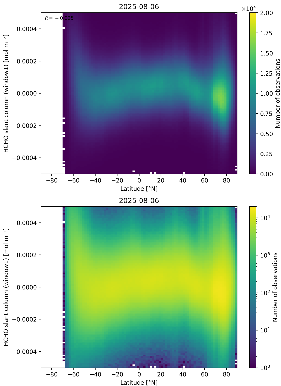
Figure 159: Scatter density plot of “Latitude” against “HCHO slant column (window1)” for 2025-08-05 to 2025-08-07.
