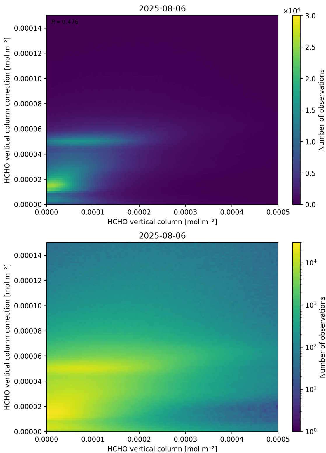
Figure 133: Scatter density plot of “HCHO vertical column” against “HCHO vertical column correction” for 2025-08-05 to 2025-08-07.
