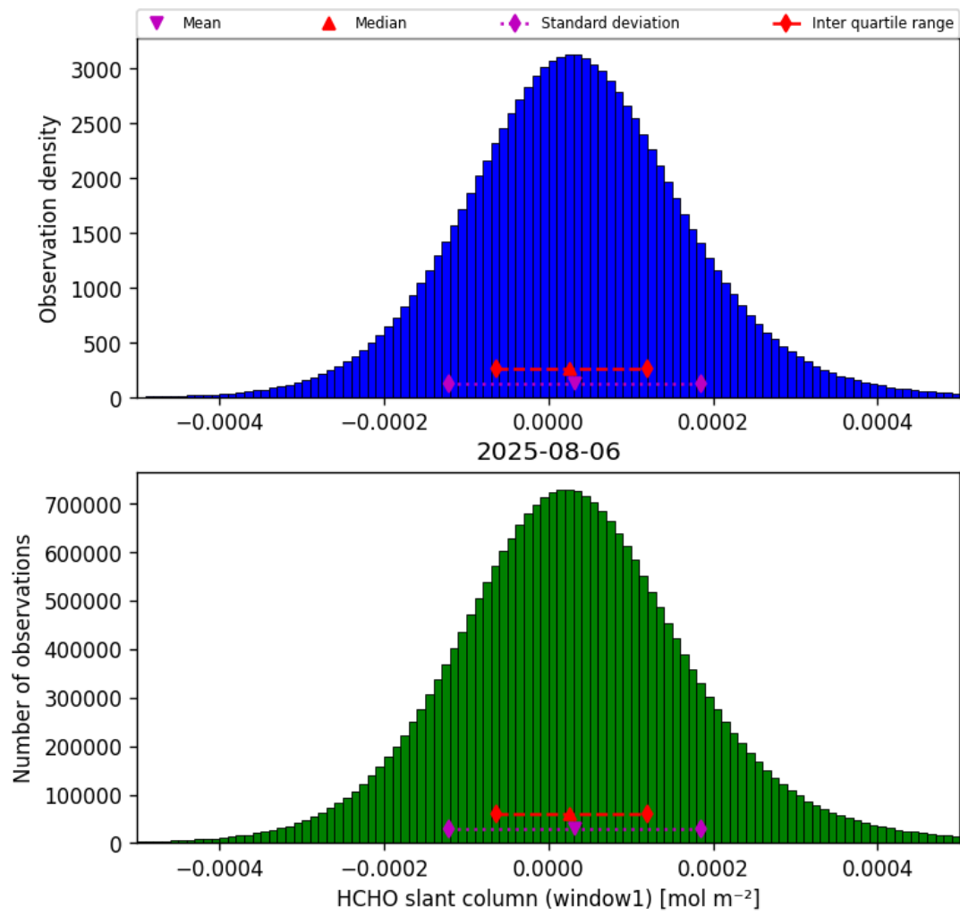
Figure 38: Histogram of “HCHO slant column (window1)” for 2025-08-05 to 2025-08-07
