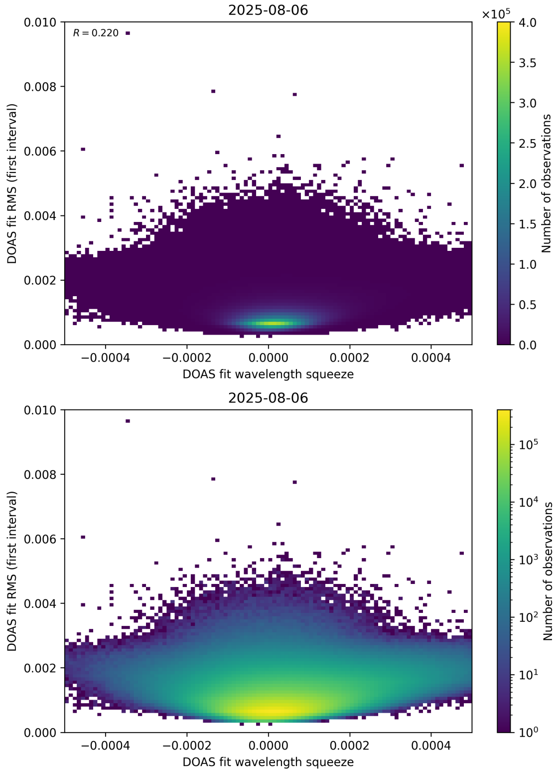
Figure 68: Scatter density plot of “DOAS fit wavelength squeeze” against “DOAS fit RMS (first interval)” for 2025-08-05 to 2025-08-07.
