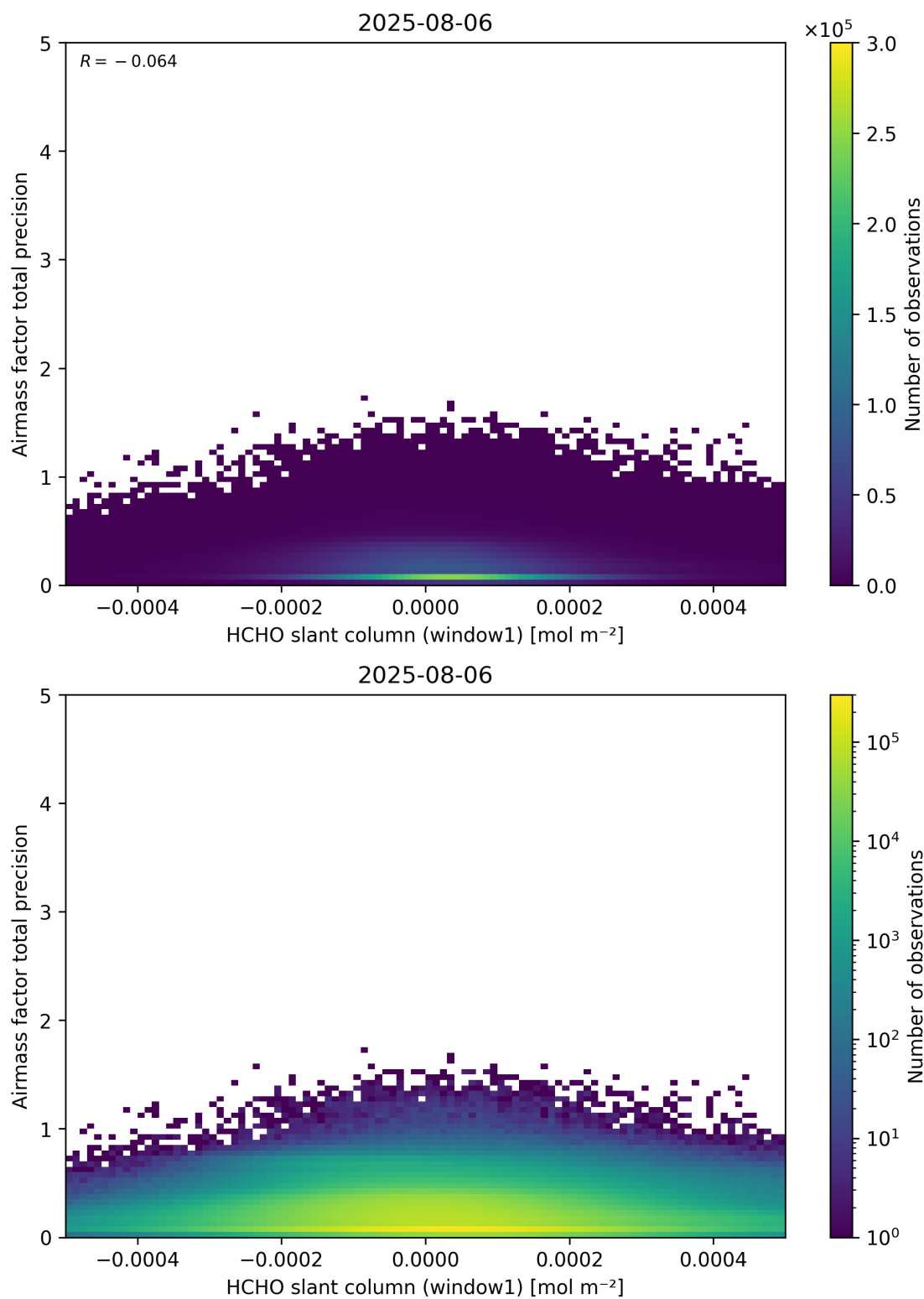
Figure 86: Scatter density plot of “HCHO slant column (window1)” against “Airmass factor total precision” for 2025-08-05 to 2025-08-07.
