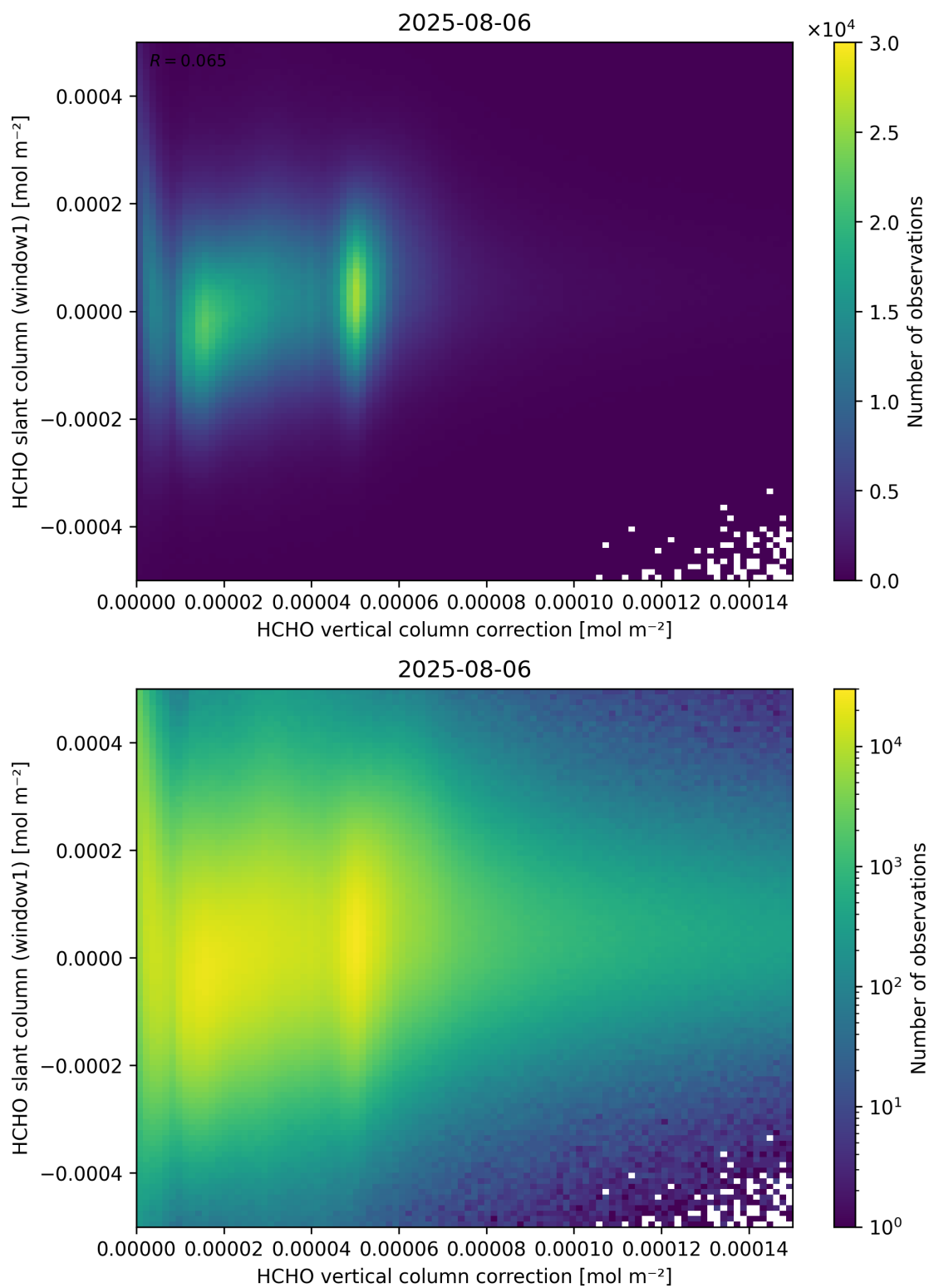
Figure 118: Scatter density plot of “HCHO vertical column correction” against “HCHO slant column (window1)” for 2025-08-05 to 2025-08-07.
