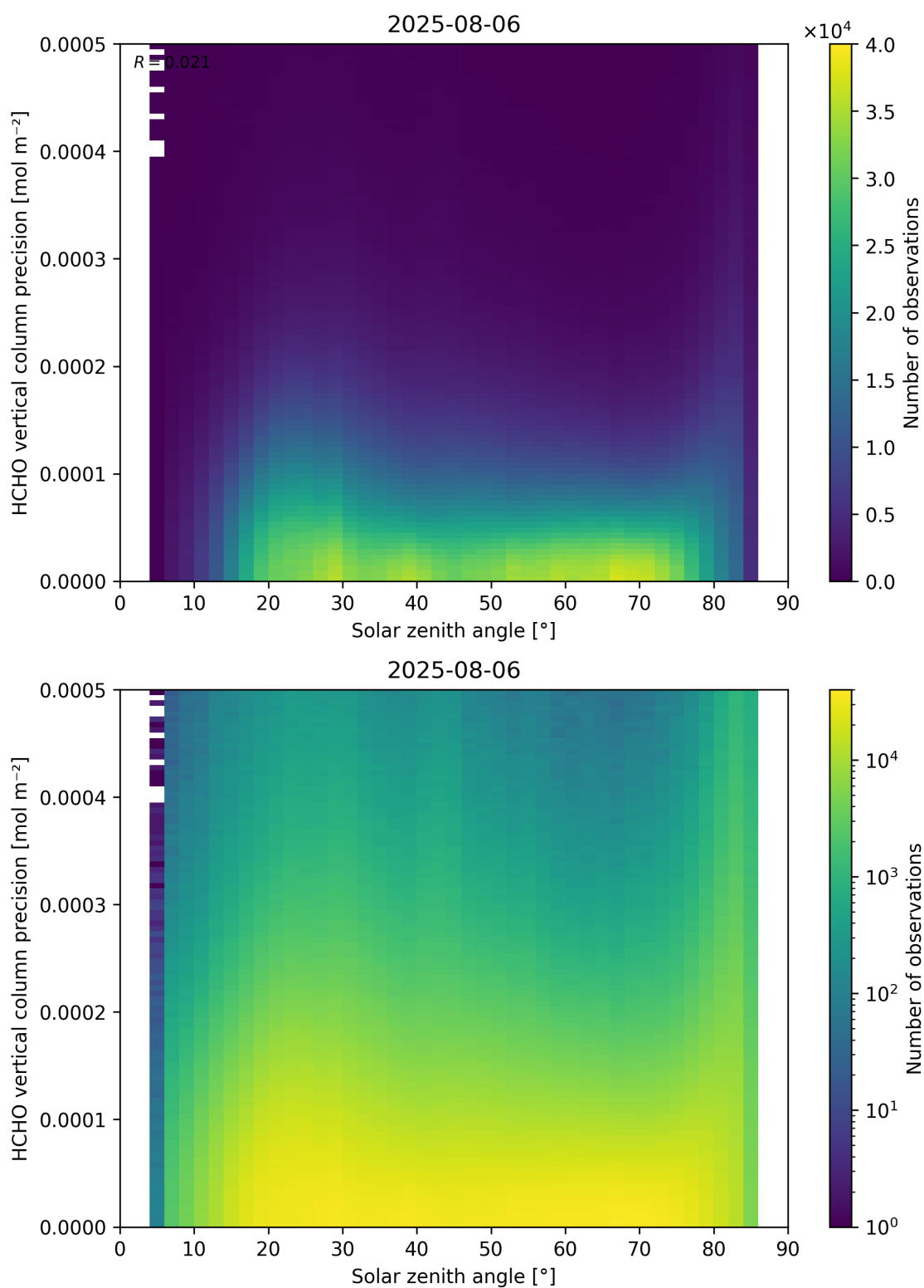
Figure 179: Scatter density plot of “Solar zenith angle” against “HCHO vertical column precision” for 2025-08-05 to 2025-08-07.
