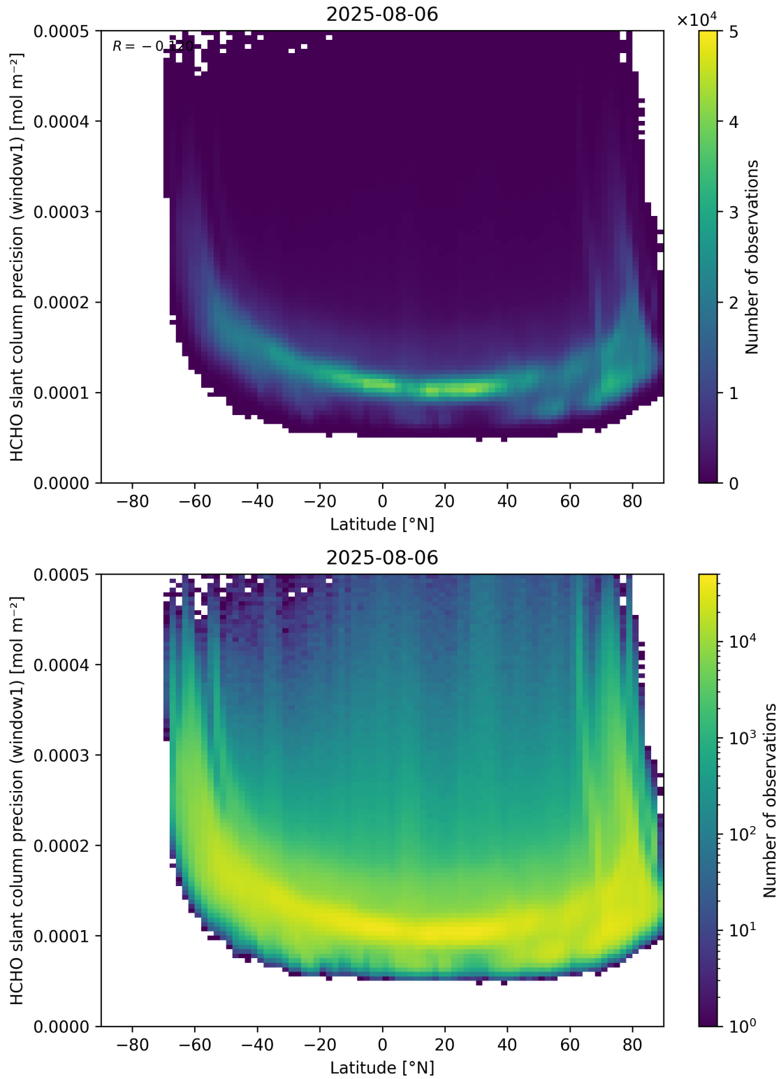
Figure 160: Scatter density plot of “Latitude” against “HCHO slant column precision (window1)” for 2025-08-05 to 2025-08-07.
