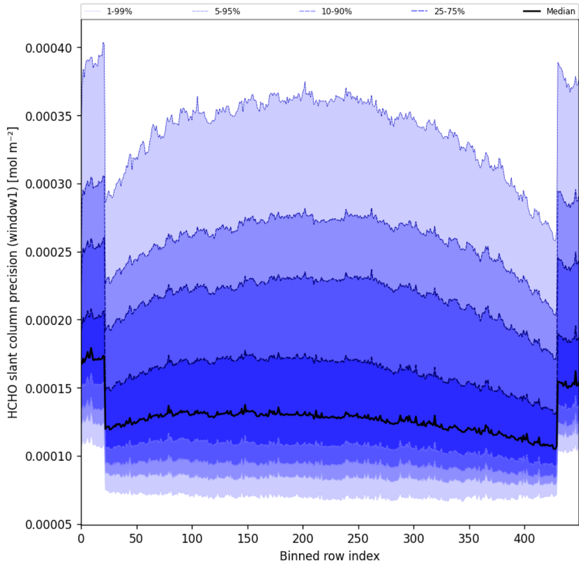
Figure 53: Along track statistics of “HCHO slant column precision (window1)” for 2025-08-05 to 2025-08-07
