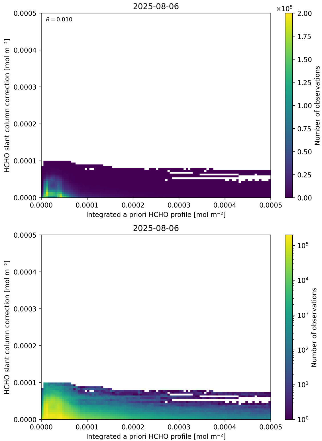
Figure 152: Scatter density plot of “Integrated a priori HCHO profile” against “HCHO slant column correction” for 2025-08-05 to 2025-08-07.
