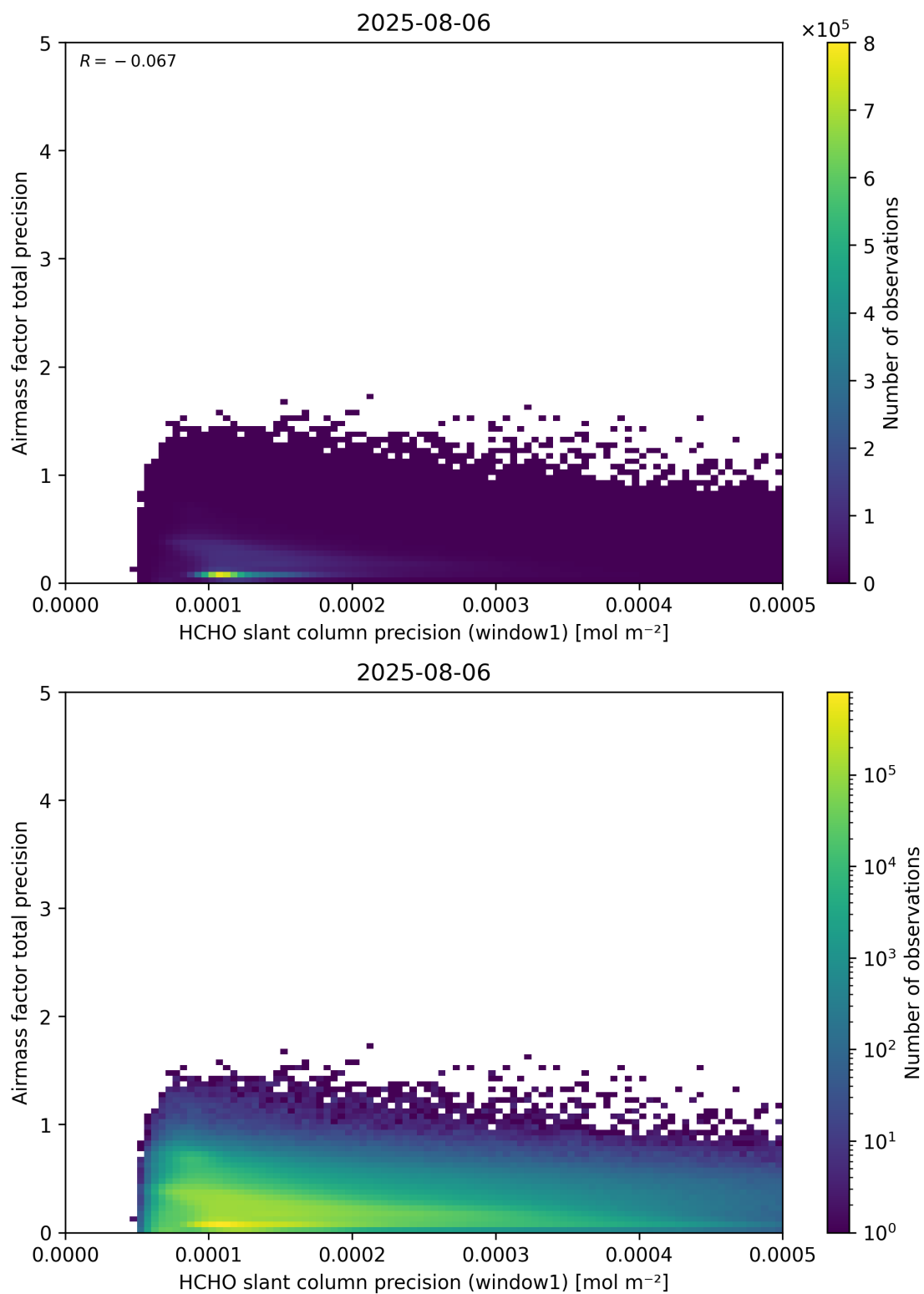
Figure 95: Scatter density plot of “HCHO slant column precision (window1)” against “Airmass factor total precision” for 2025-08-05 to 2025-08-07.
