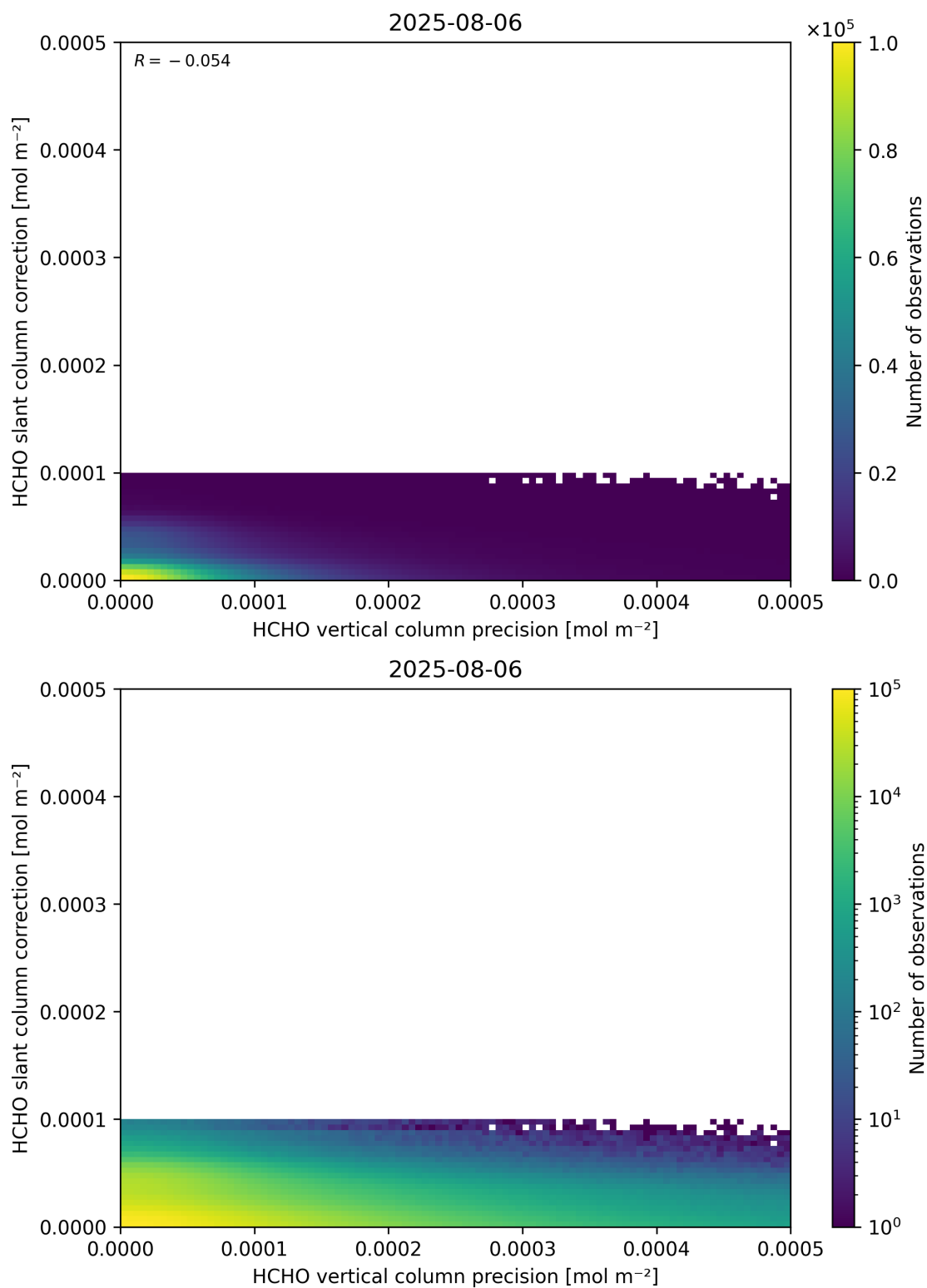
Figure 141: Scatter density plot of “HCHO vertical column precision” against “HCHO slant column correction” for 2025-08-05 to 2025-08-07.
