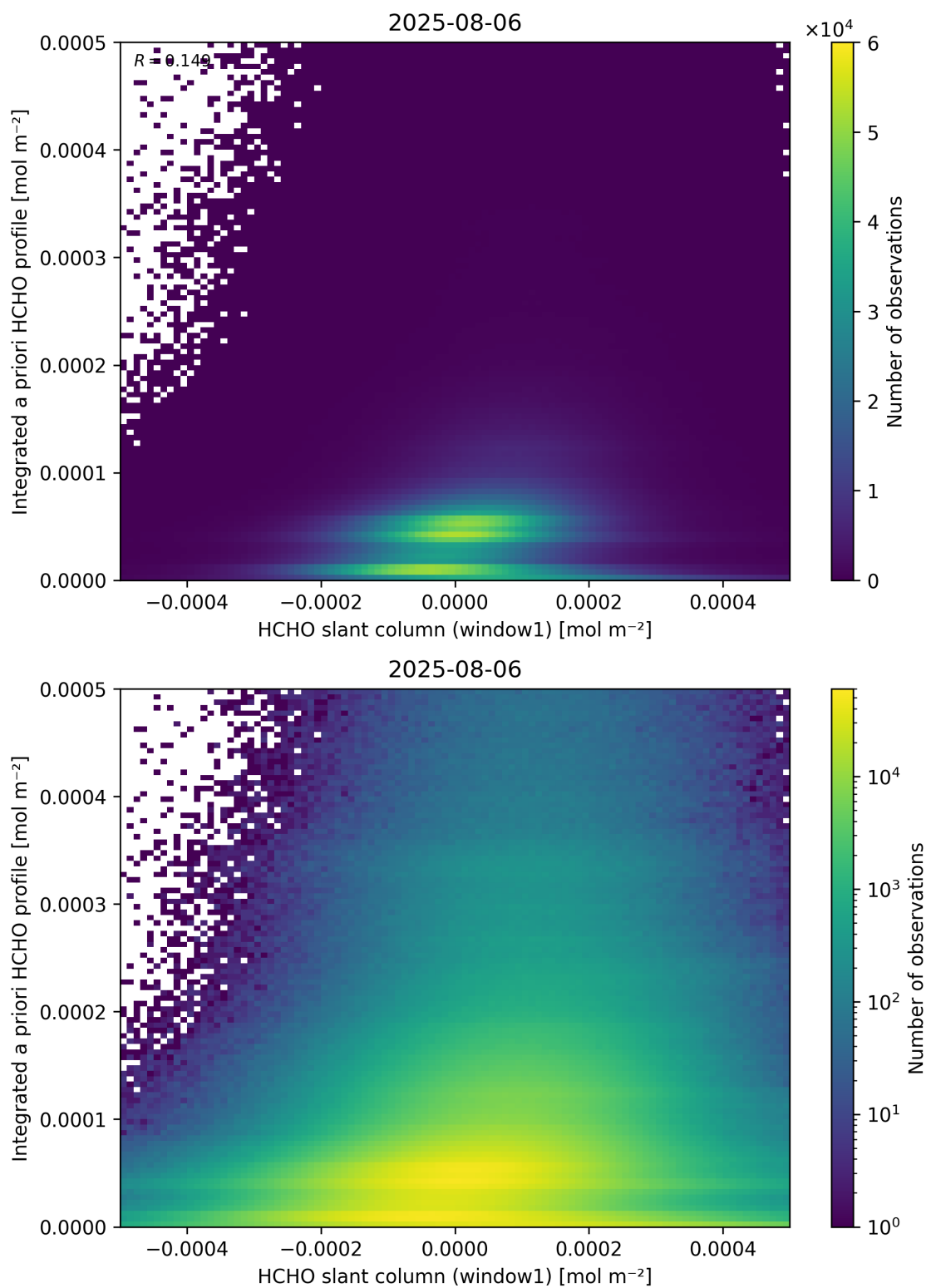
Figure 87: Scatter density plot of “HCHO slant column (window1)” against “Integrated a priori HCHO profile” for 2025-08-05 to 2025-08-07.
