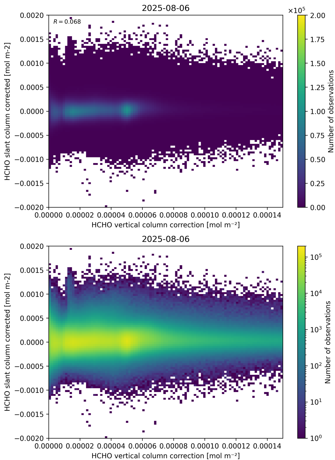
Figure 116: Scatter density plot of “HCHO vertical column correction” against “HCHO slant column corrected” for 2025-08-05 to 2025-08-07.
