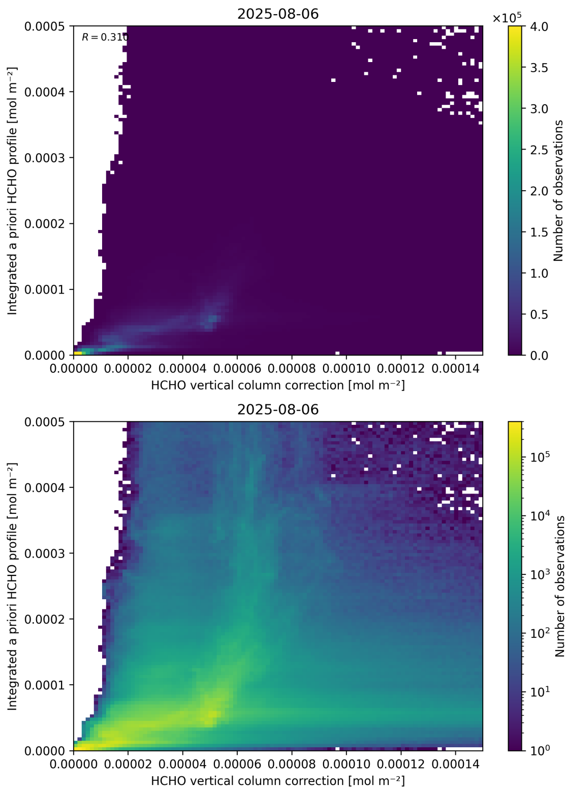
Figure 122: Scatter density plot of “HCHO vertical column correction” against “Integrated a priori HCHO profile” for 2025-08-05 to 2025-08-07.
