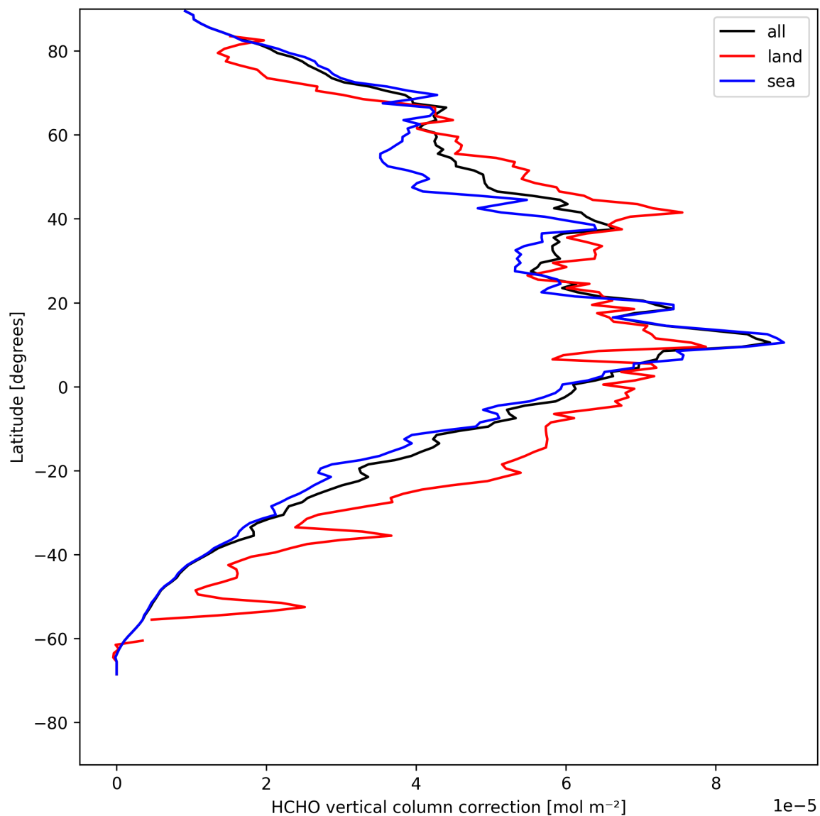
Figure 23: Zonal average of “HCHO vertical column correction” for 2025-08-05 to 2025-08-07.
