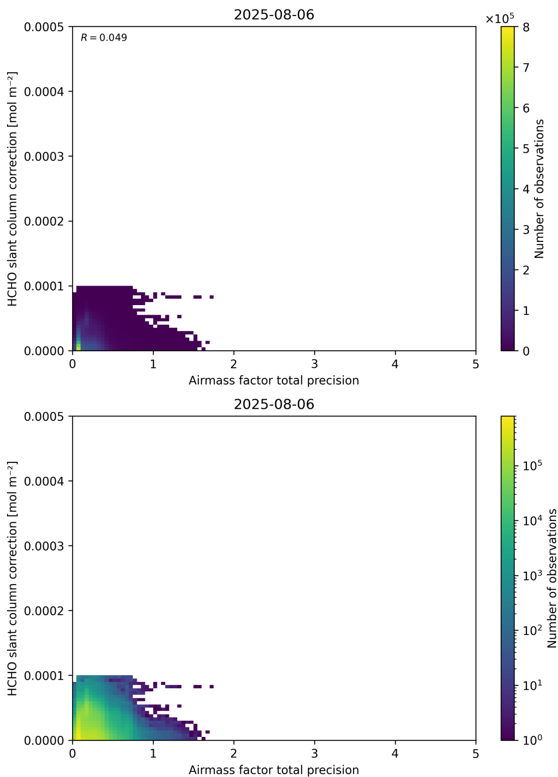
Figure 110: Scatter density plot of “Airmass factor total precision” against “HCHO slant column correction” for 2025-08-05 to 2025-08-07.
