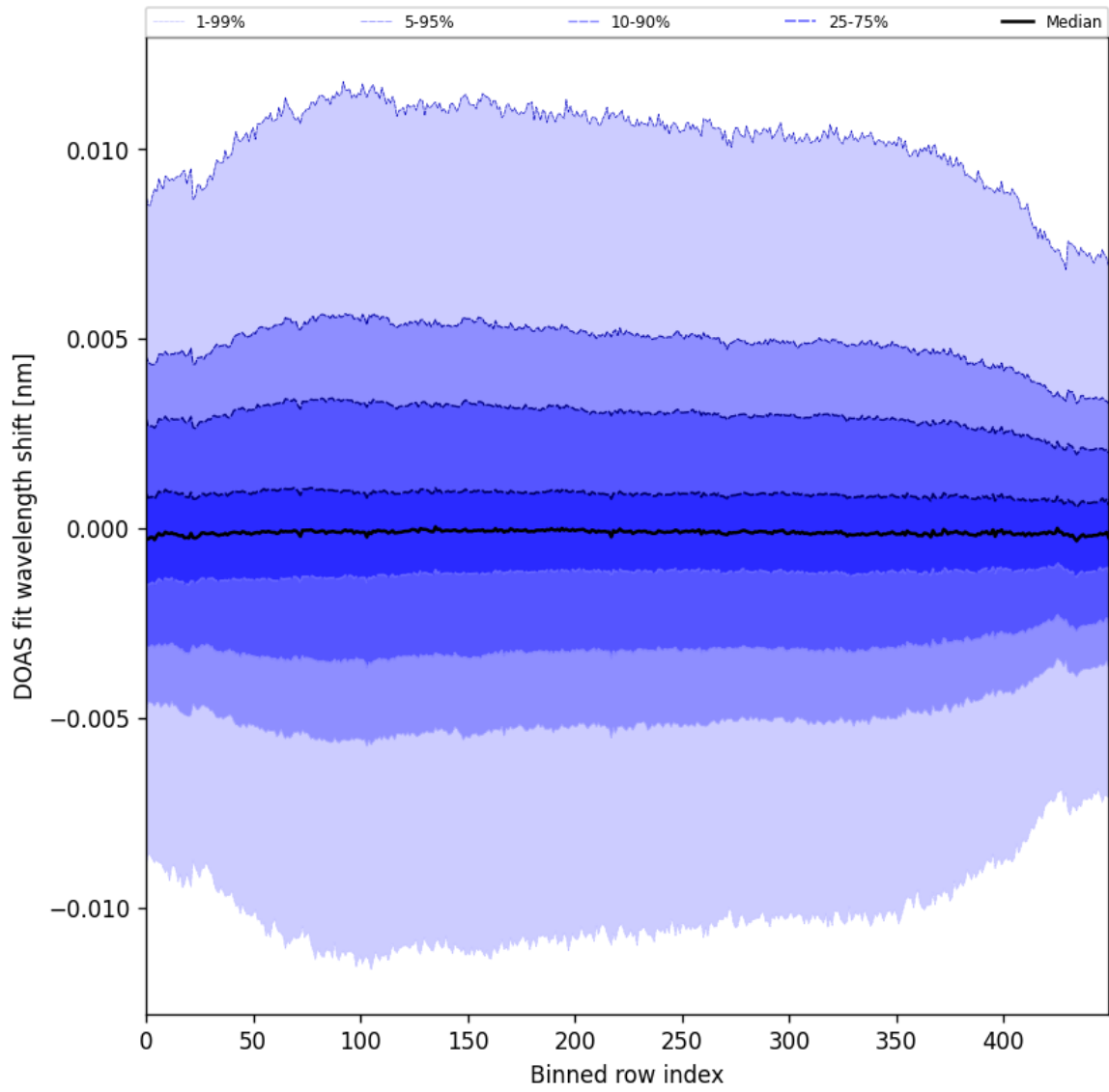
Figure 58: Along track statistics of “DOAS fit wavelength shift” for 2025-08-05 to 2025-08-07
