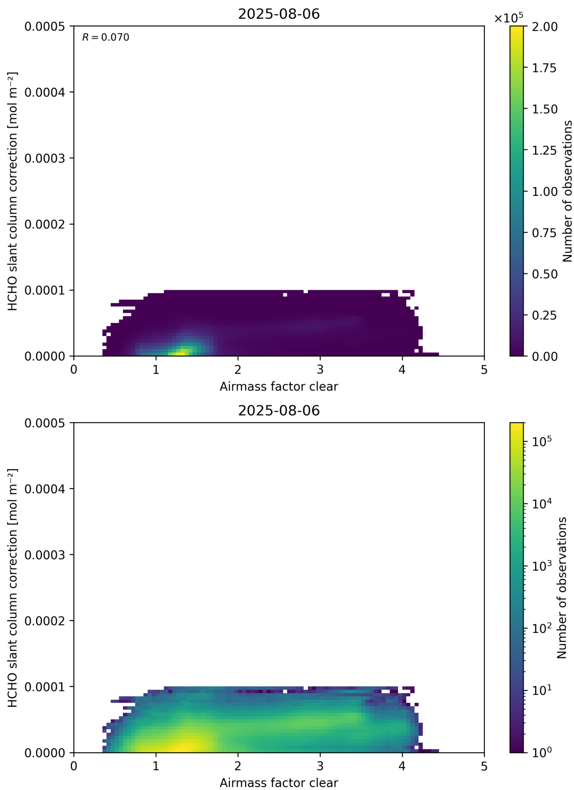
Figure 75: Scatter density plot of “Airmass factor clear” against “HCHO slant column correction” for 2025-08-05 to 2025-08-07.
