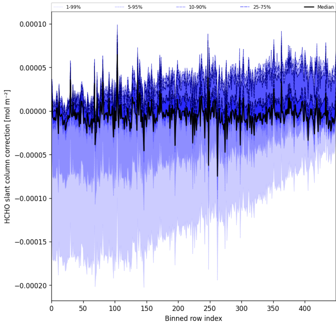
Figure 61: Along track statistics of “HCHO slant column correction” for 2025-08-05 to 2025-08-07
