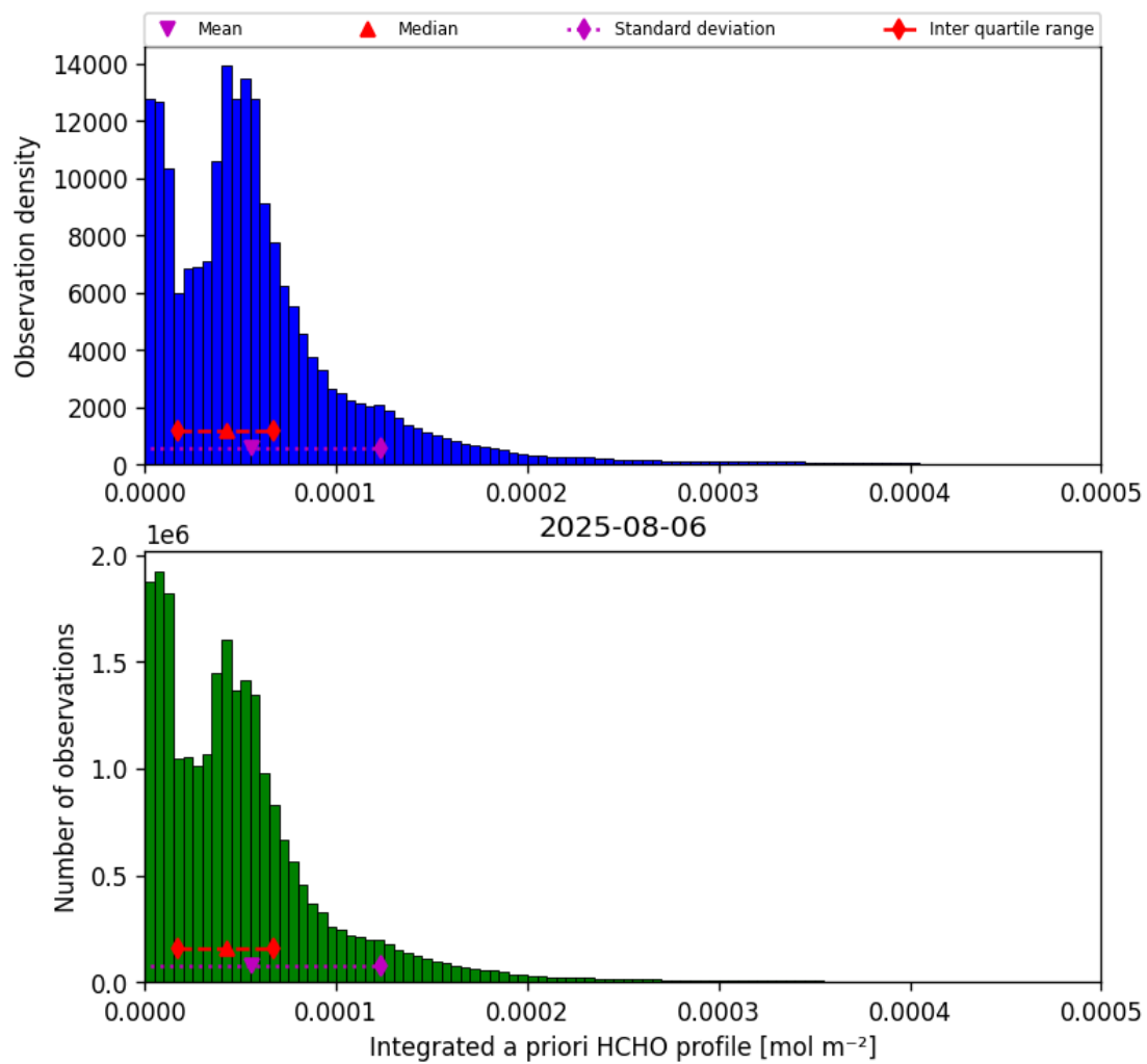
Figure 43: Histogram of “Integrated a priori HCHO profile” for 2025-08-05 to 2025-08-07
