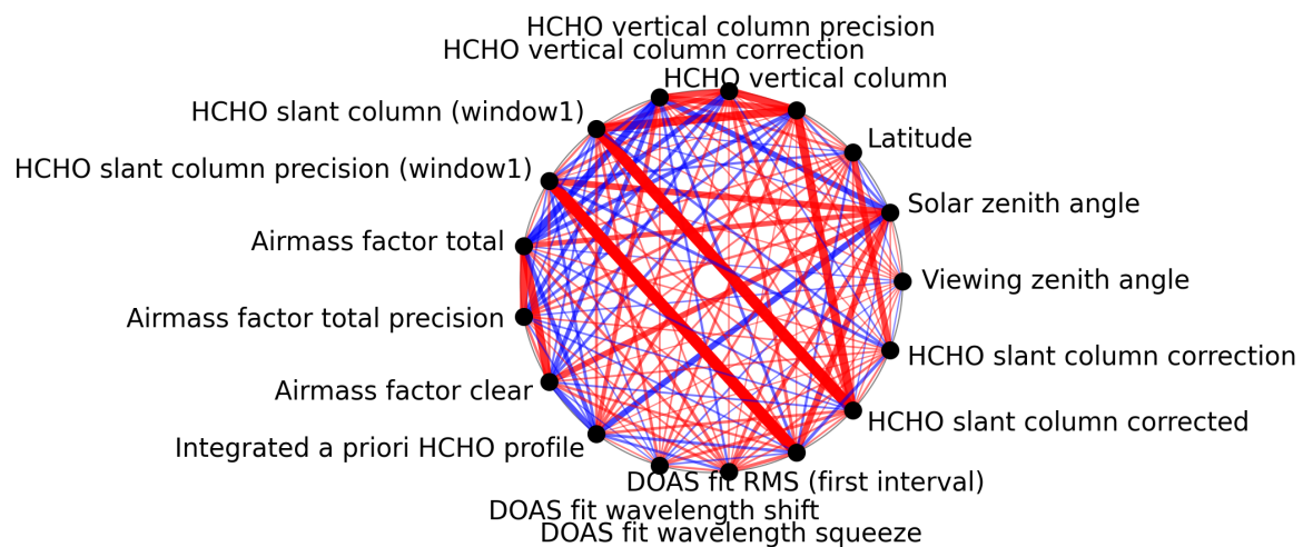
Figure 1: Map of correlation graph for 2025-08-05 to 2025-08-07.
