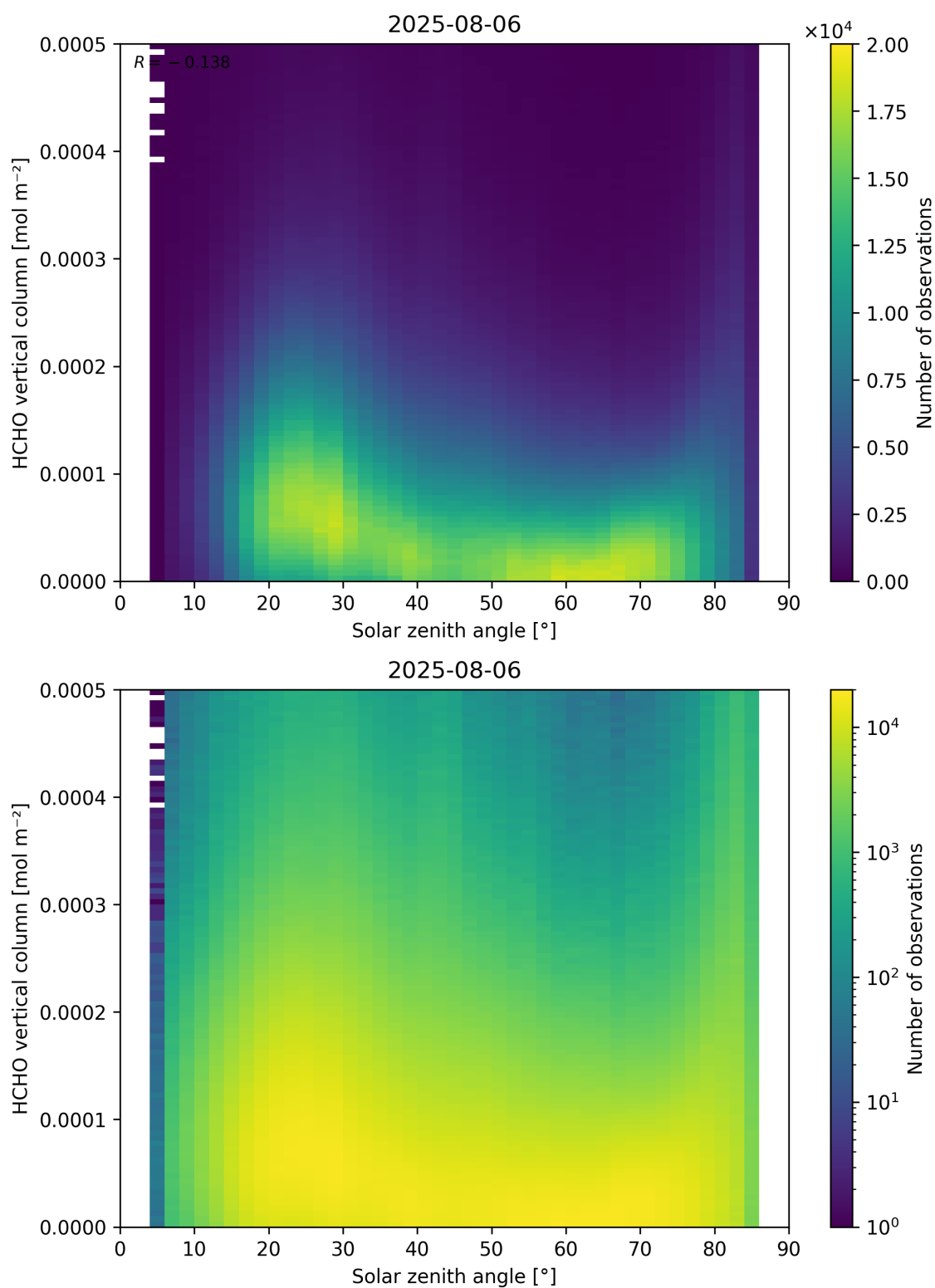
Figure 177: Scatter density plot of “Solar zenith angle” against “HCHO vertical column” for 2025-08-05 to 2025-08-07.
