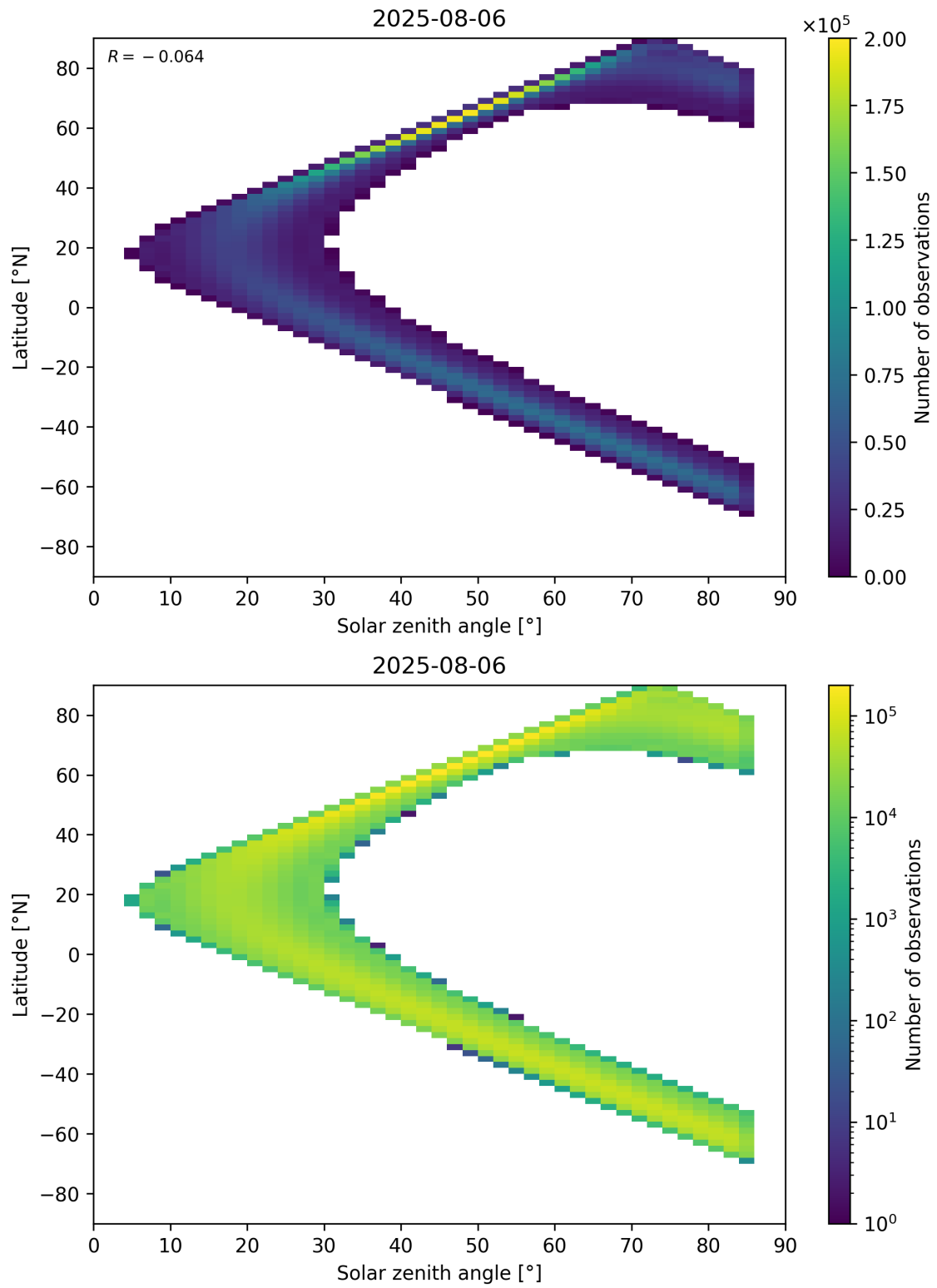
Figure 181: Scatter density plot of “Solar zenith angle” against “Latitude” for 2025-08-05 to 2025-08-07.
