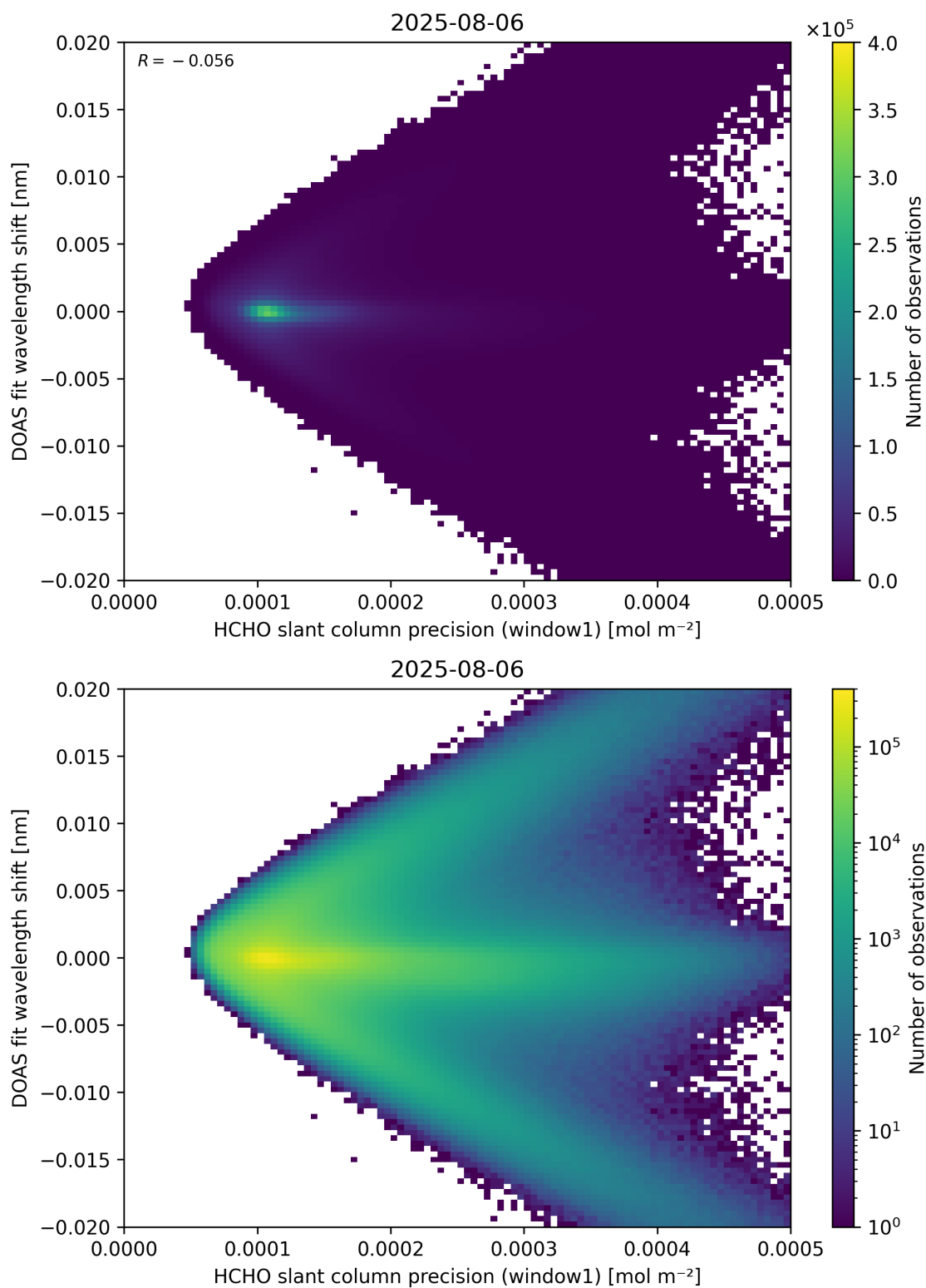
Figure 89: Scatter density plot of “HCHO slant column precision (window1)” against “DOAS fit wavelength shift” for 2025-08-05 to 2025-08-07.
