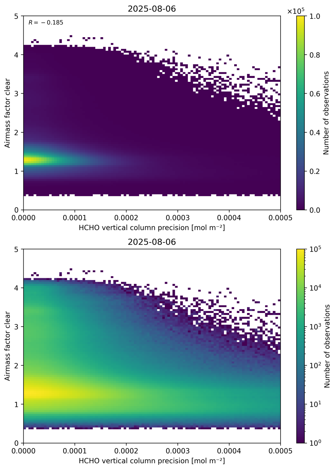
Figure 139: Scatter density plot of “HCHO vertical column precision” against “Airmass factor clear” for 2025-08-05 to 2025-08-07.
