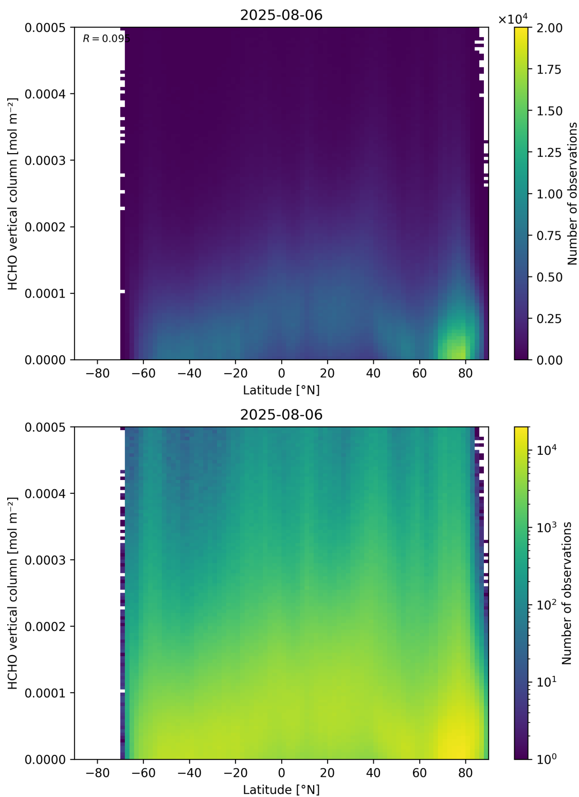
Figure 163: Scatter density plot of “Latitude” against “HCHO vertical column” for 2025-08-05 to 2025-08-07.
