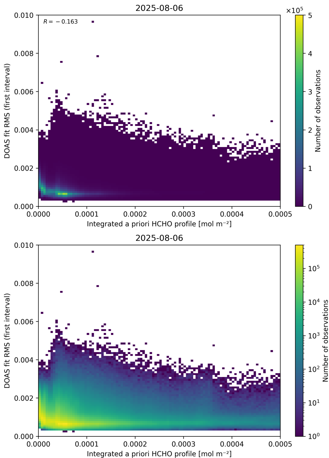
Figure 148: Scatter density plot of “Integrated a priori HCHO profile” against “DOAS fit RMS (first interval)” for 2025-08-05 to 2025-08-07.
