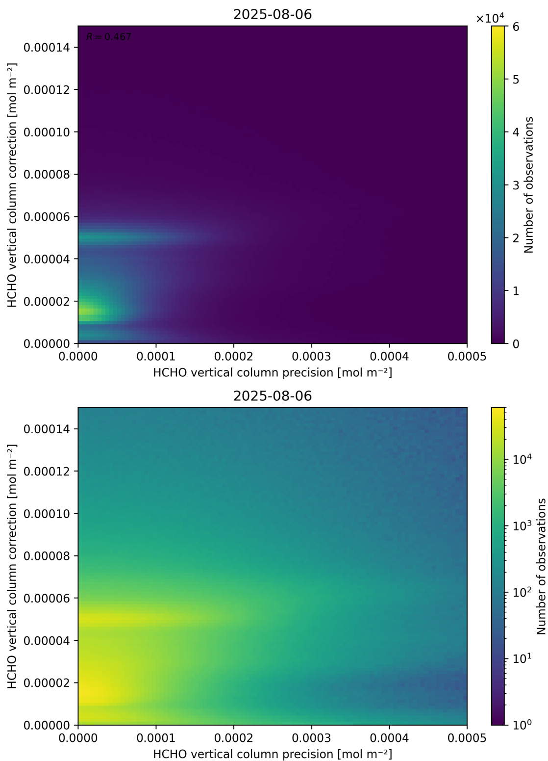
Figure 146: Scatter density plot of “HCHO vertical column precision” against “HCHO vertical column correction” for 2025-08-05 to 2025-08-07.
