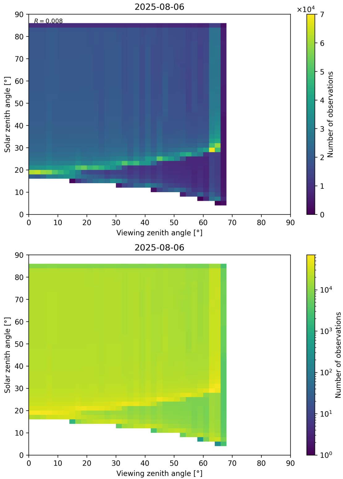
Figure 197: Scatter density plot of “Viewing zenith angle” against “Solar zenith angle” for 2025-08-05 to 2025-08-07.
