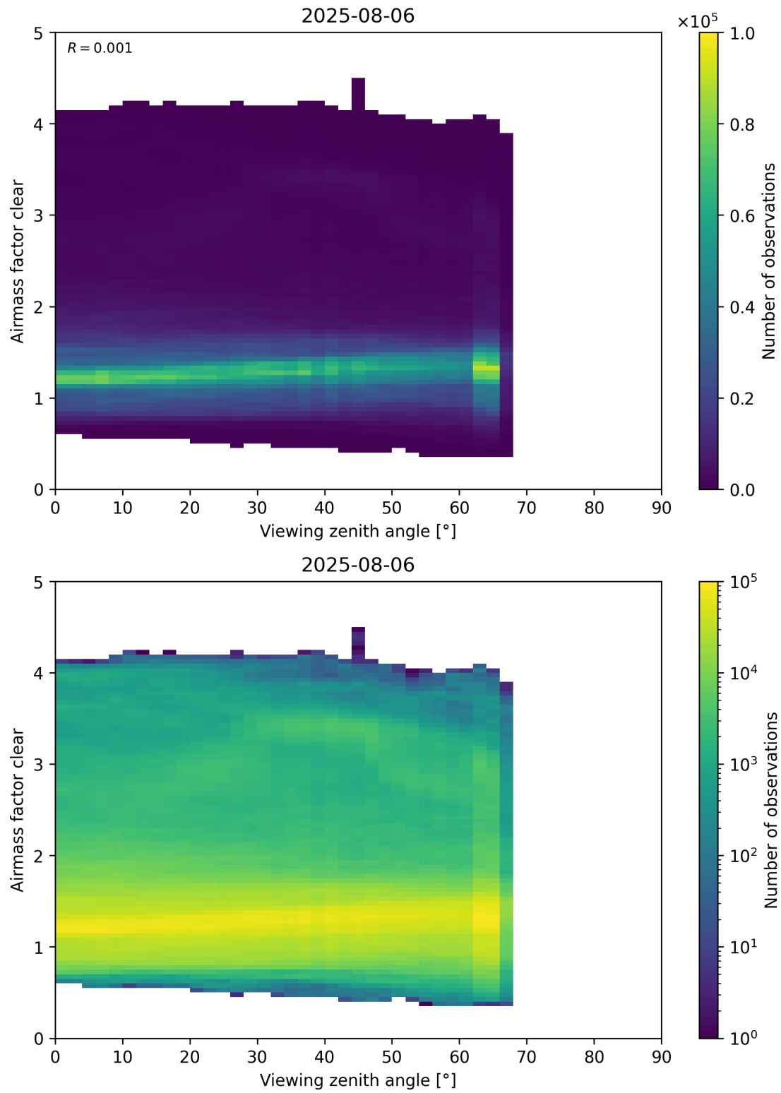
Figure 185: Scatter density plot of “Viewing zenith angle” against “Airmass factor clear” for 2025-08-05 to 2025-08-07.
