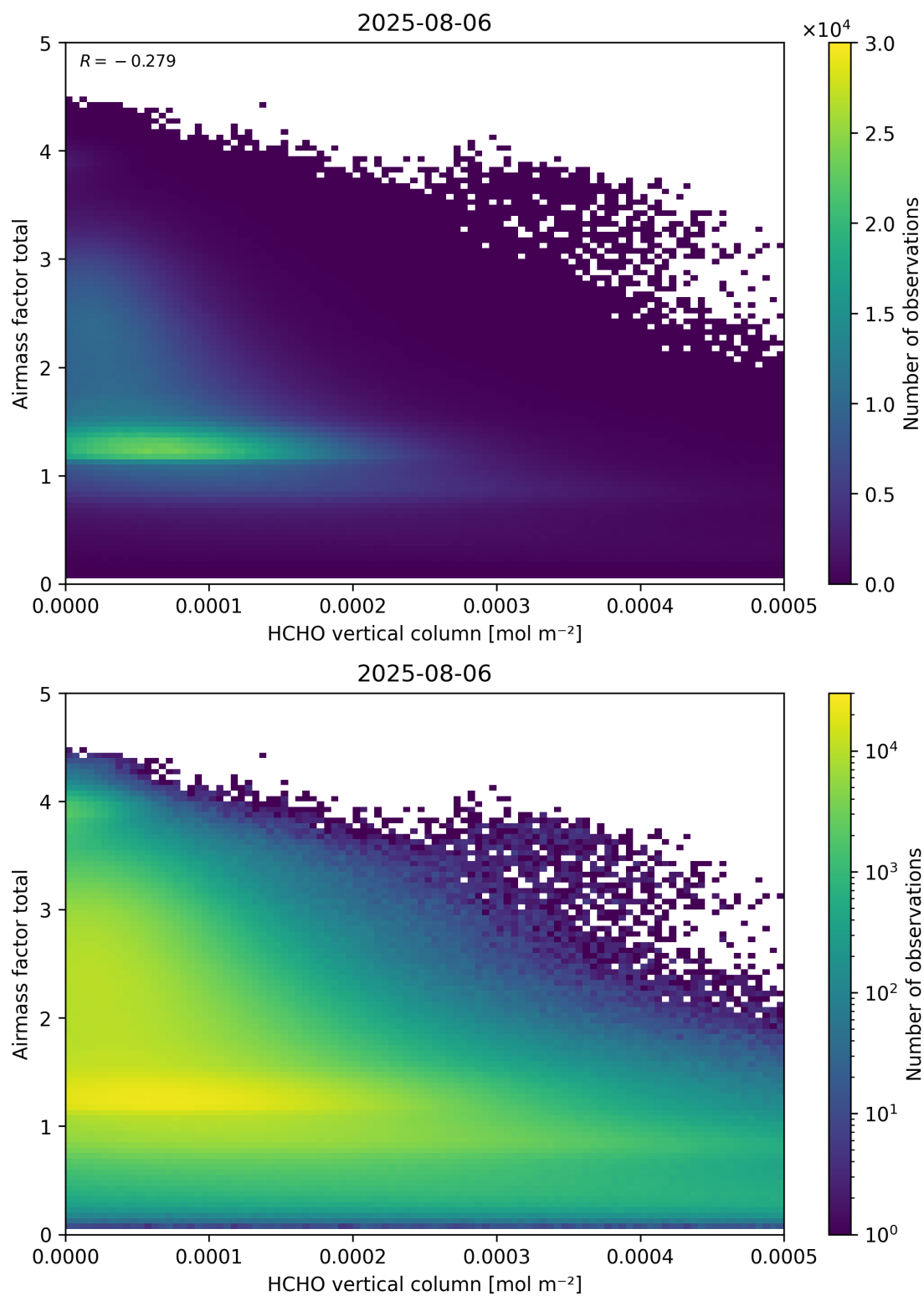
Figure 131: Scatter density plot of “HCHO vertical column” against “Airmass factor total” for 2025-08-05 to 2025-08-07.
