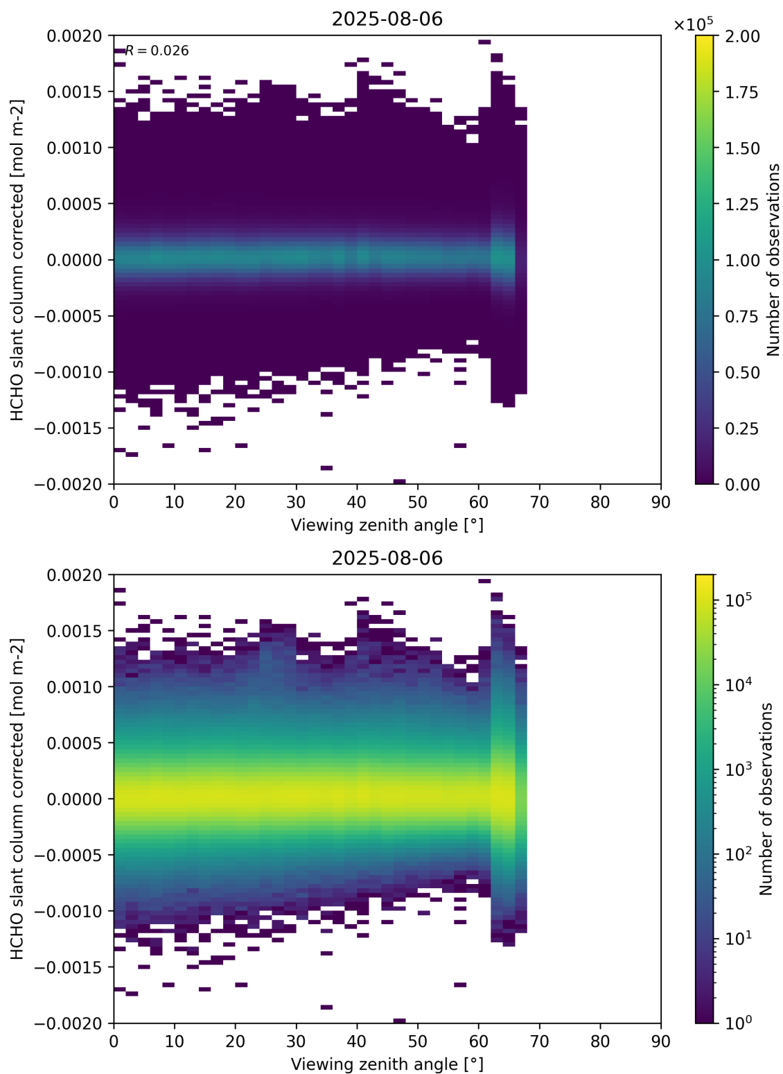
Figure 186: Scatter density plot of “Viewing zenith angle” against “HCHO slant column corrected” for 2025-08-05 to 2025-08-07.
