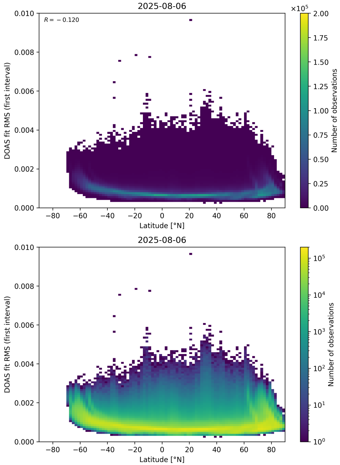
Figure 153: Scatter density plot of “Latitude” against “DOAS fit RMS (first interval)” for 2025-08-05 to 2025-08-07.
