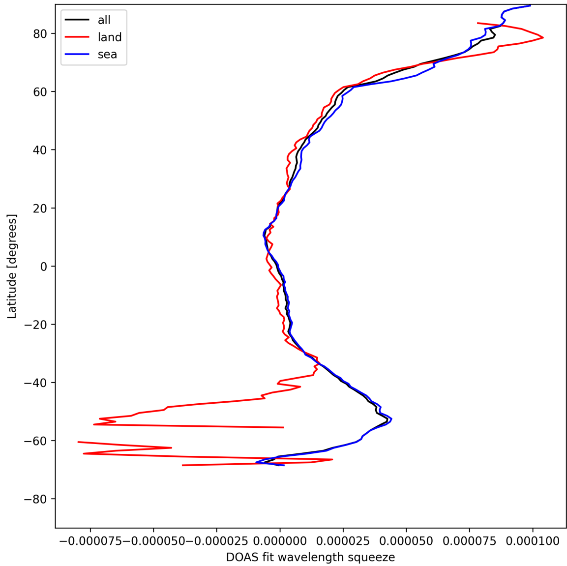
Figure 31: Zonal average of “DOAS fit wavelength squeeze” for 2025-08-05 to 2025-08-07.
