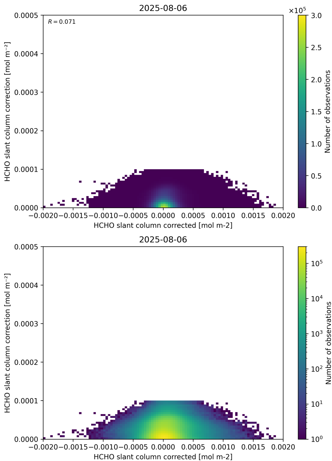
Figure 77: Scatter density plot of “HCHO slant column corrected” against “HCHO slant column correction” for 2025-08-05 to 2025-08-07.
