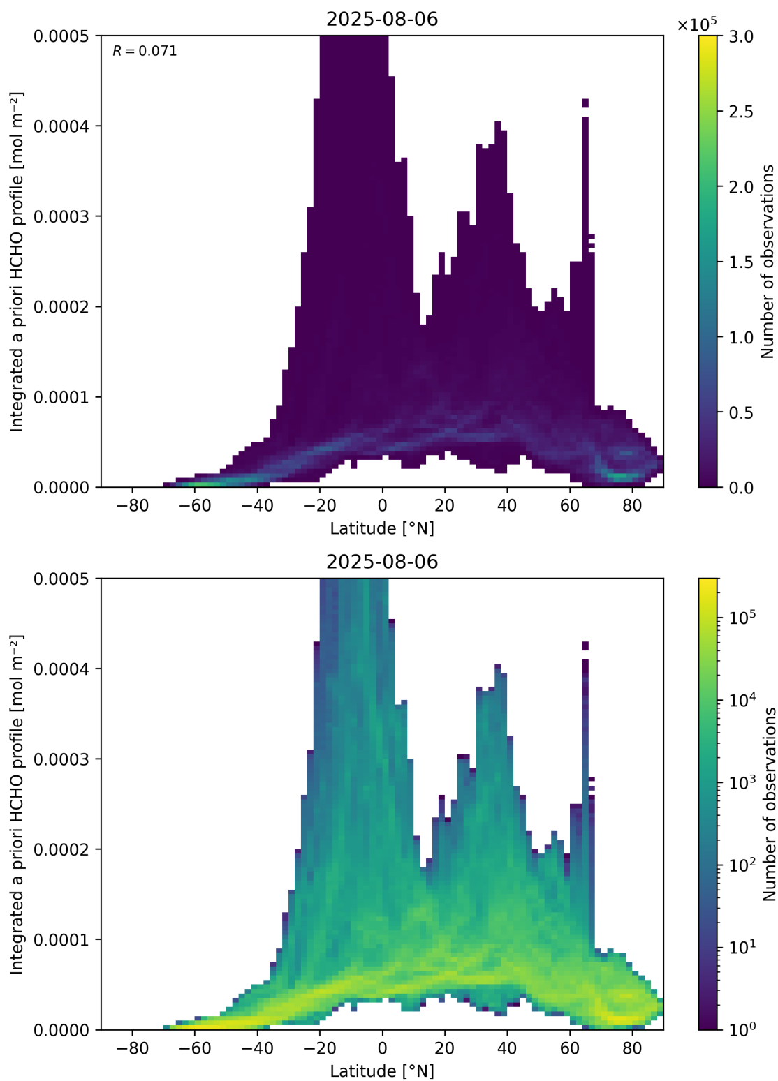
Figure 166: Scatter density plot of “Latitude” against “Integrated a priori HCHO profile” for 2025-08-05 to 2025-08-07.
