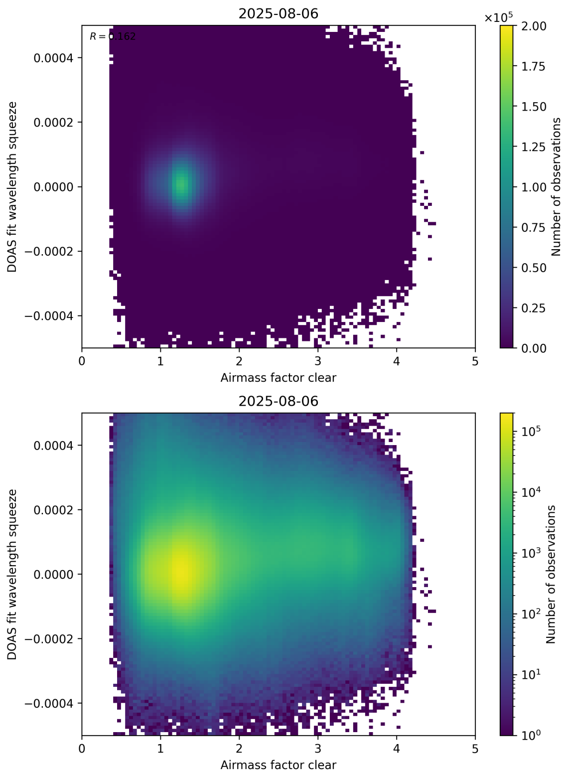
Figure 73: Scatter density plot of “Airmass factor clear” against “DOAS fit wavelength squeeze” for 2025-08-05 to 2025-08-07.
