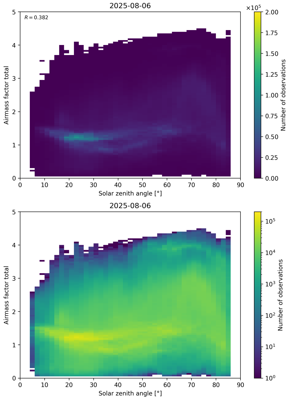
Figure 175: Scatter density plot of “Solar zenith angle” against “Airmass factor total” for 2025-08-05 to 2025-08-07.
