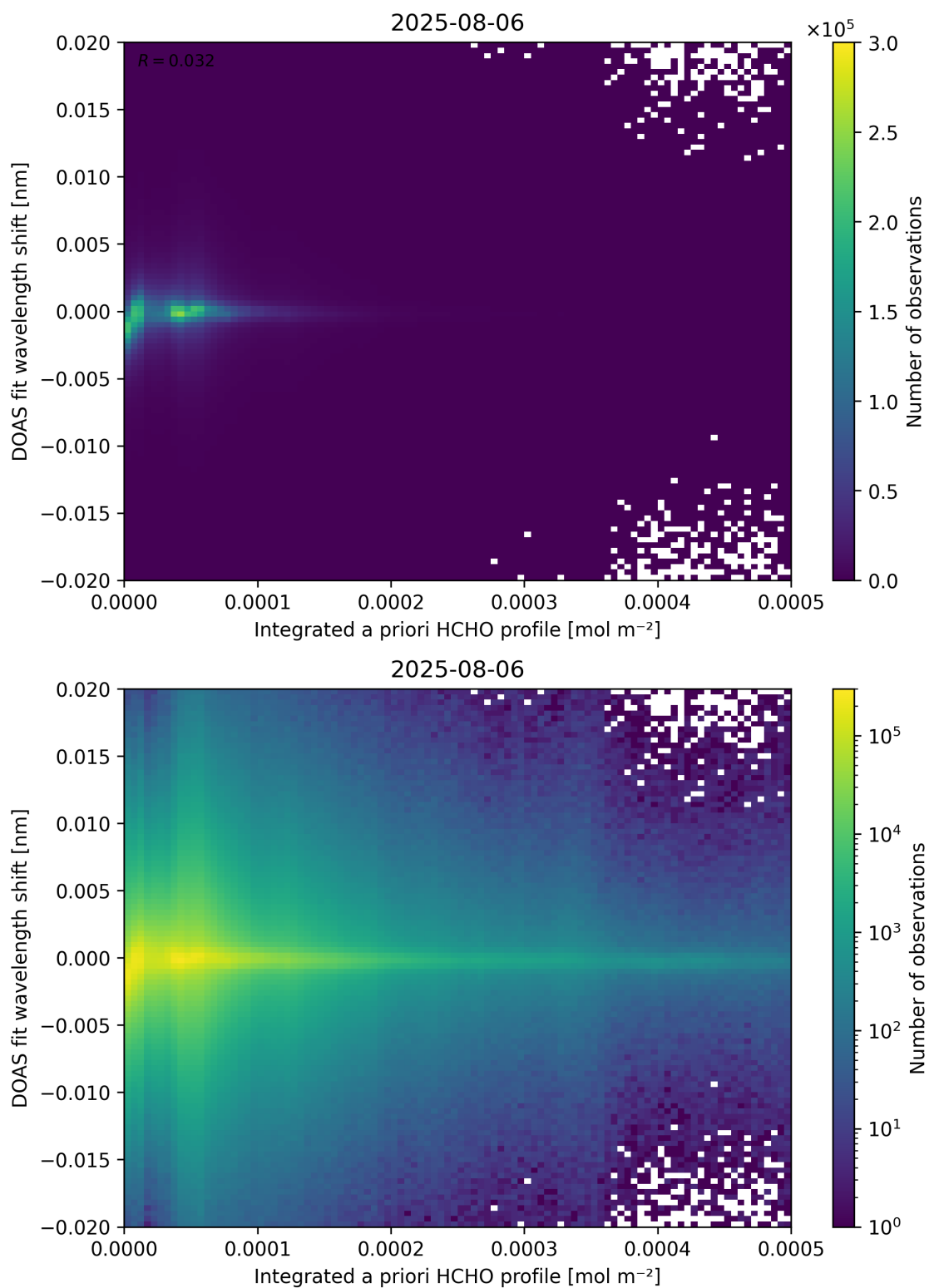
Figure 149: Scatter density plot of “Integrated a priori HCHO profile” against “DOAS fit wavelength shift” for 2025-08-05 to 2025-08-07.
