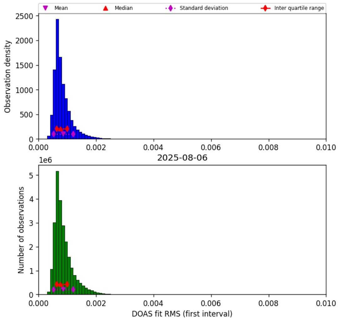
Figure 46: Histogram of “DOAS fit RMS (first interval)” for 2025-08-05 to 2025-08-07
