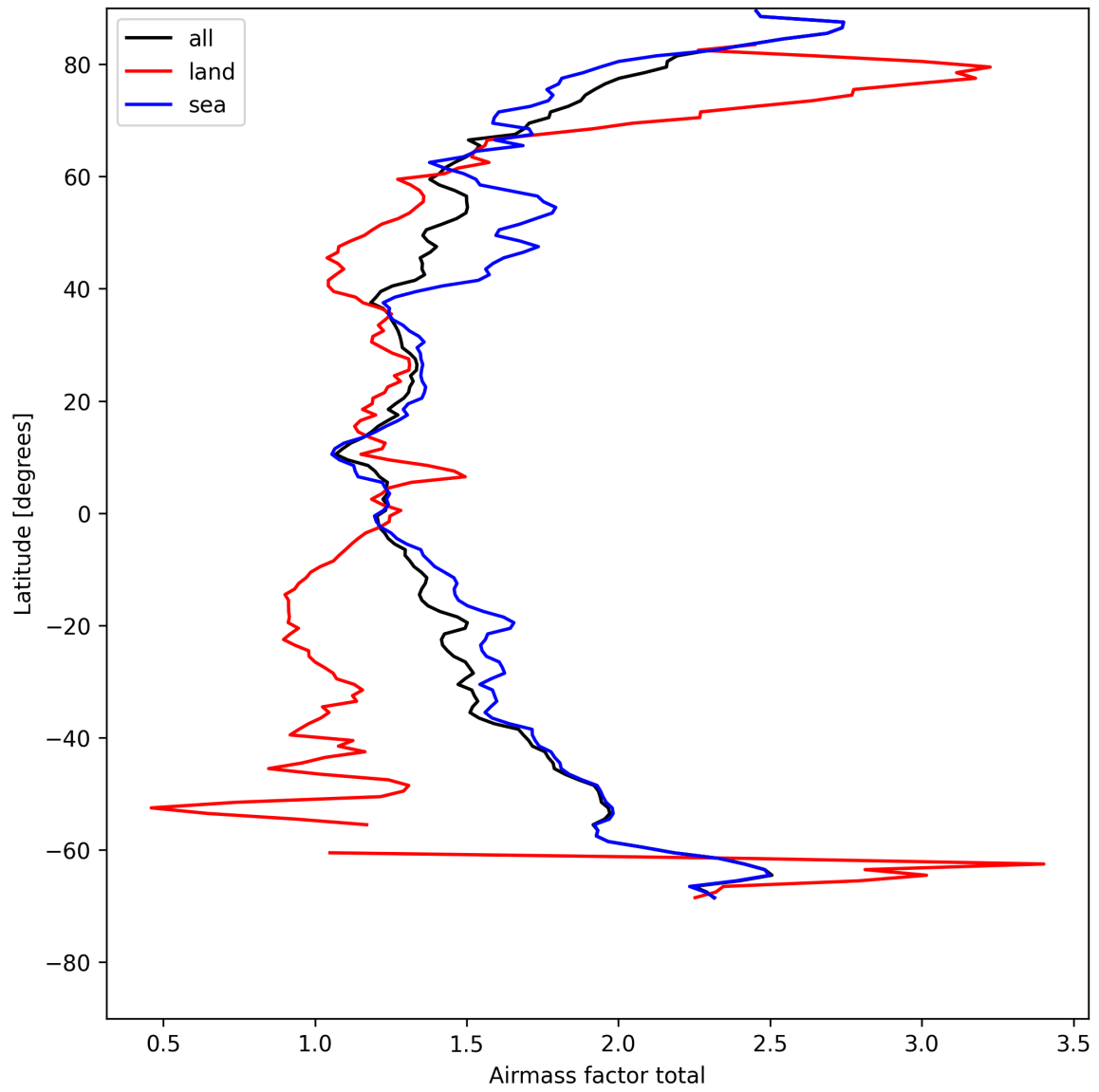
Figure 26: Zonal average of “Airmass factor total” for 2025-08-05 to 2025-08-07.
