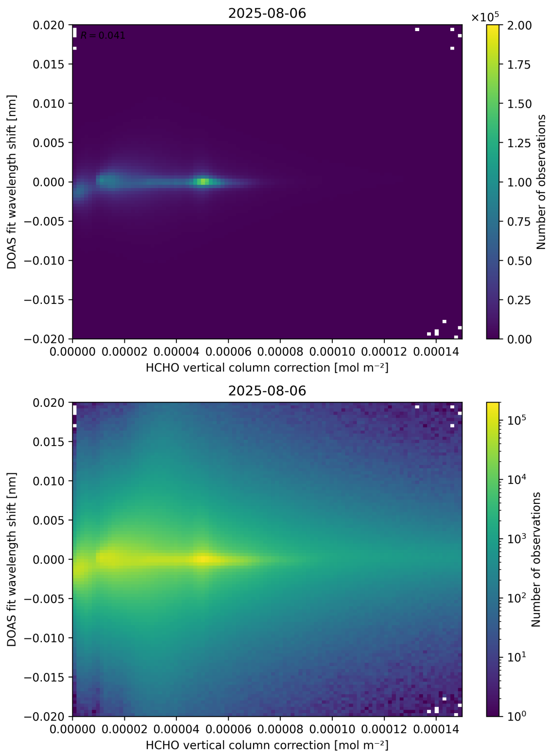
Figure 113: Scatter density plot of “HCHO vertical column correction” against “DOAS fit wavelength shift” for 2025-08-05 to 2025-08-07.
