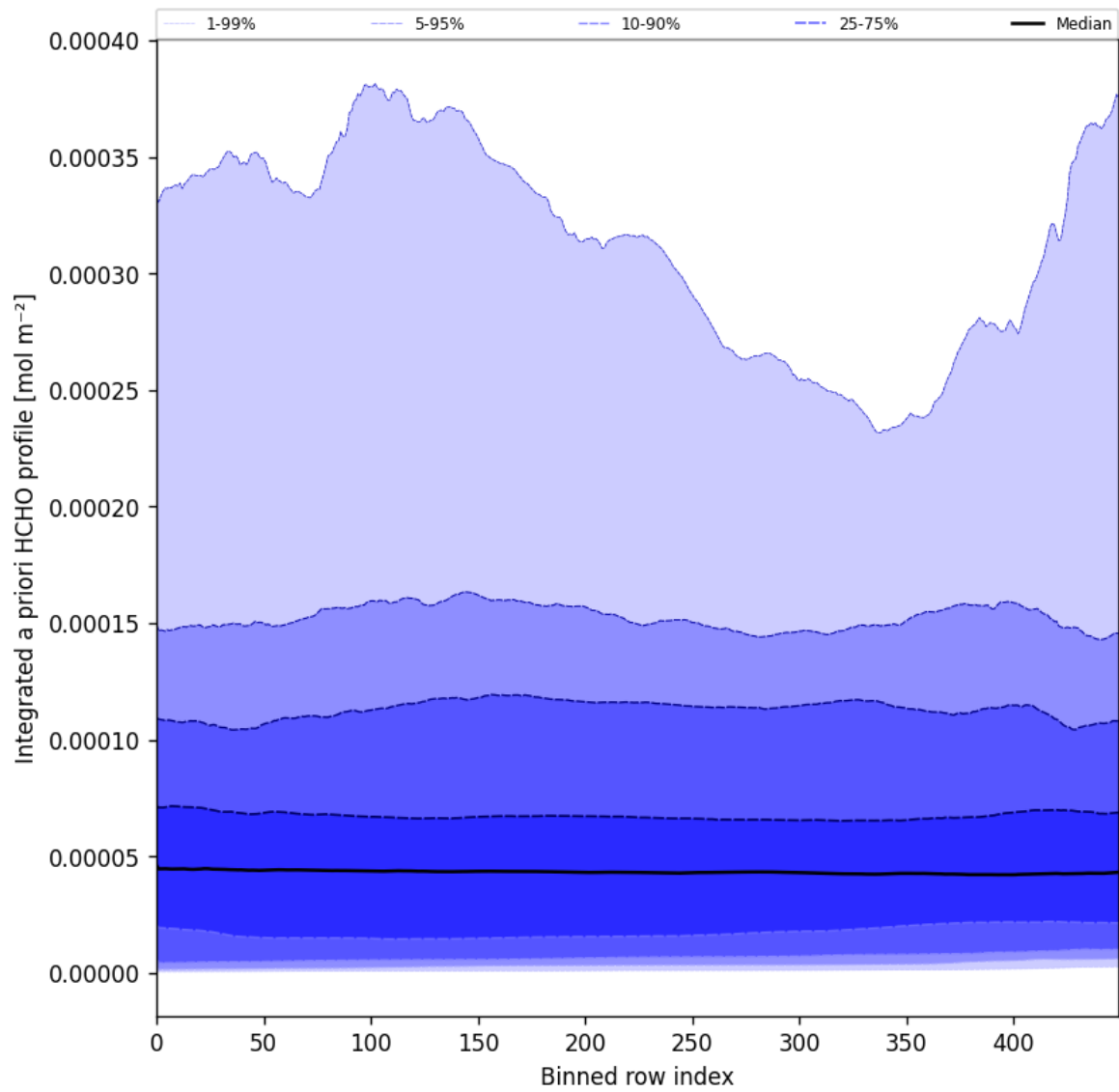
Figure 57: Along track statistics of “Integrated a priori HCHO profile” for 2025-08-05 to 2025-08-07
