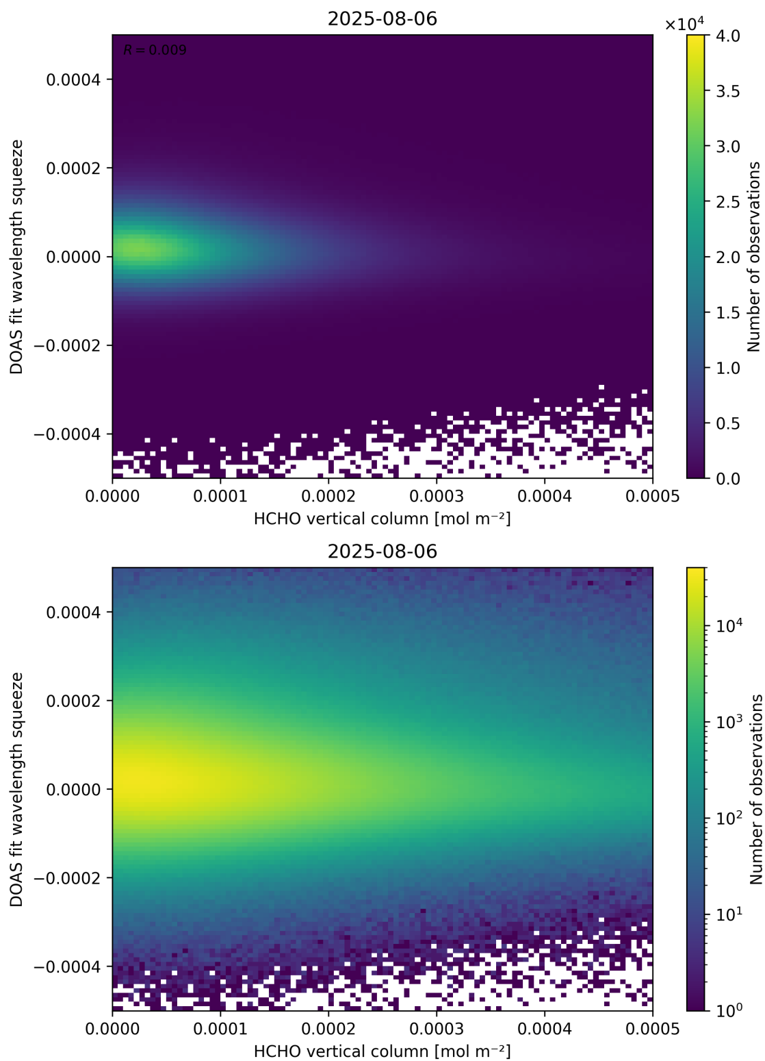
Figure 125: Scatter density plot of “HCHO vertical column” against “DOAS fit wavelength squeeze” for 2025-08-05 to 2025-08-07.
