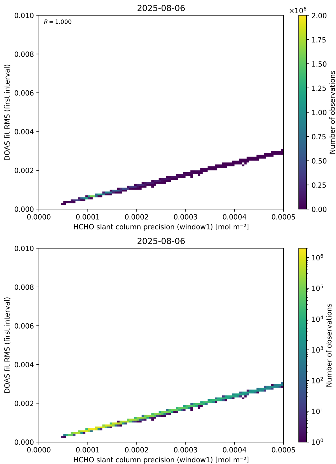
Figure 88: Scatter density plot of “HCHO slant column precision (window1)” against “DOAS fit RMS (first interval)” for 2025-08-05 to 2025-08-07.
