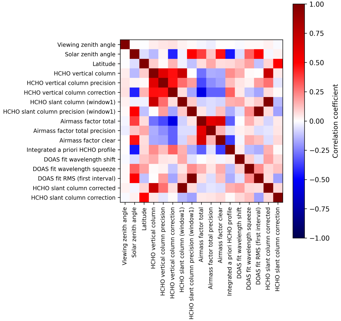
Figure 2: Map of correlation matrix for 2025-08-05 to 2025-08-07.
