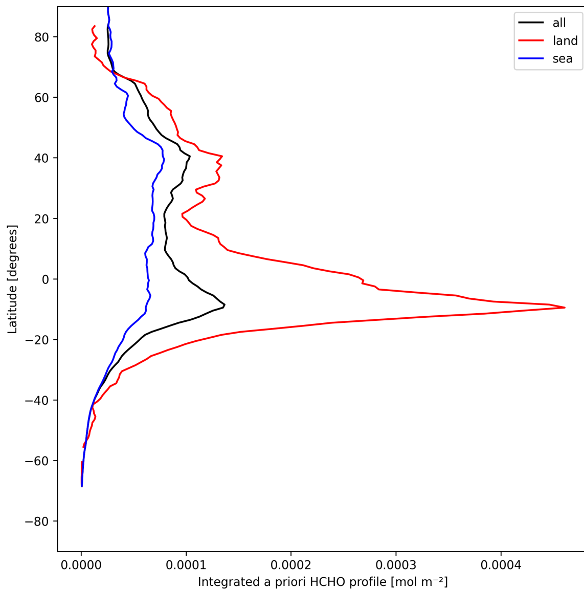
Figure 29: Zonal average of “Integrated a priori HCHO profile” for 2025-08-05 to 2025-08-07.
