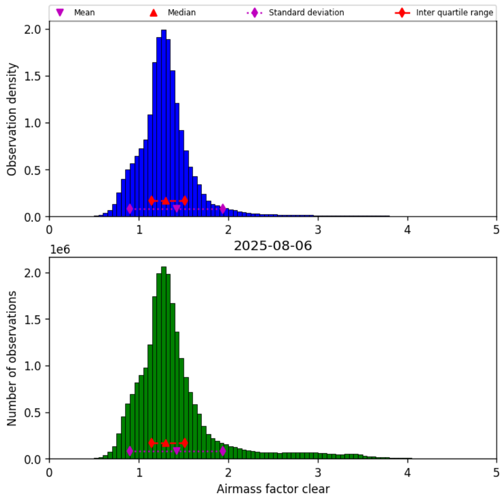
Figure 42: Histogram of “Airmass factor clear” for 2025-08-05 to 2025-08-07
