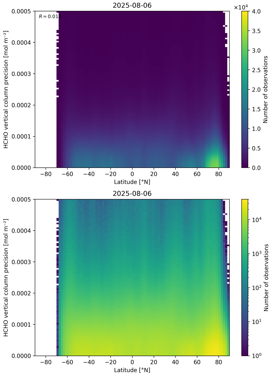
Figure 165: Scatter density plot of “Latitude” against “HCHO vertical column precision” for 2025-08-05 to 2025-08-07.
