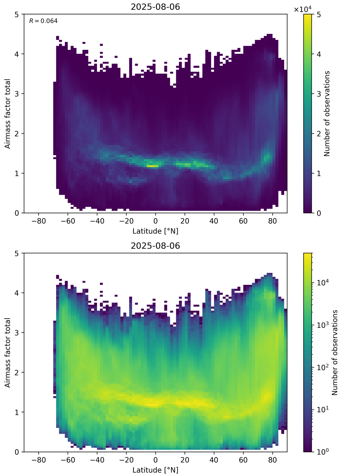
Figure 161: Scatter density plot of “Latitude” against “Airmass factor total” for 2025-08-05 to 2025-08-07.
