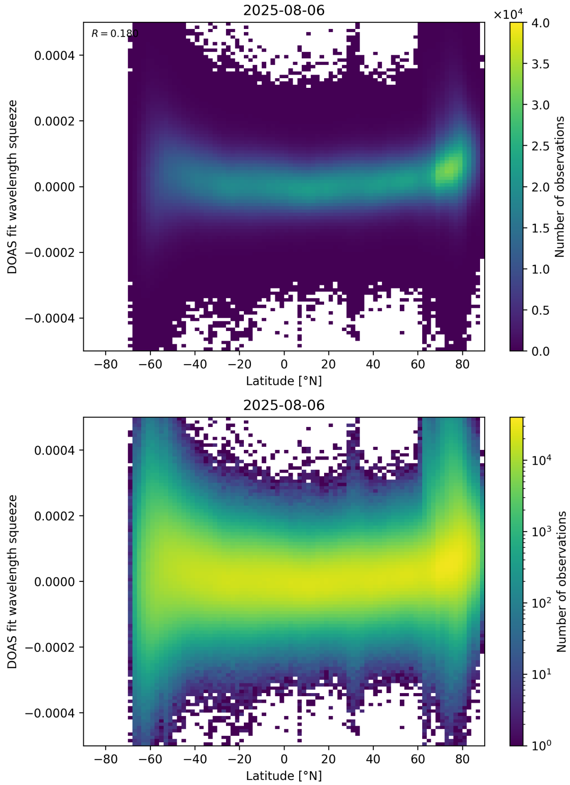
Figure 155: Scatter density plot of “Latitude” against “DOAS fit wavelength squeeze” for 2025-08-05 to 2025-08-07.
