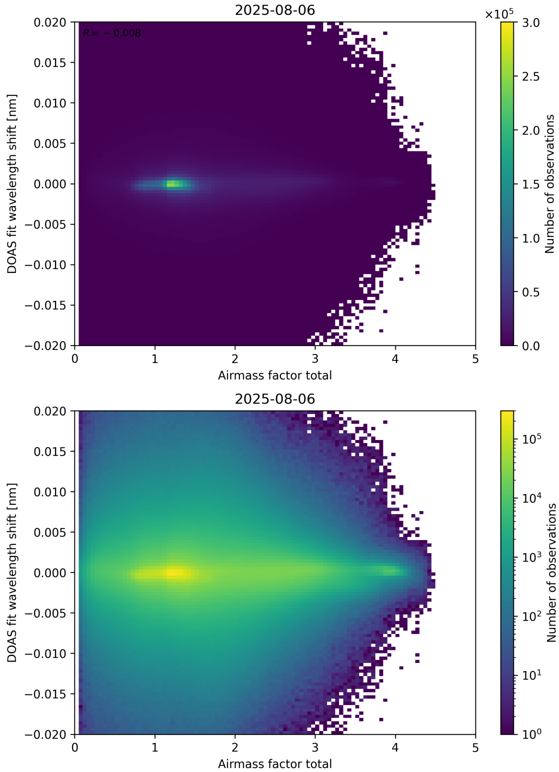
Figure 98: Scatter density plot of “Airmass factor total” against “DOAS fit wavelength shift” for 2025-08-05 to 2025-08-07.
