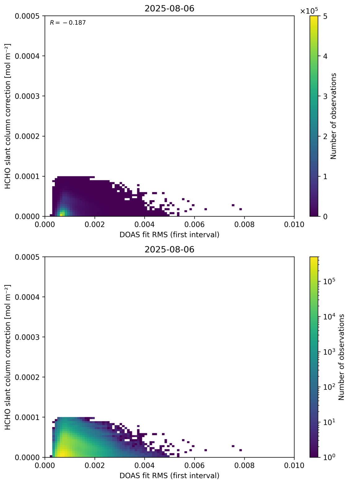
Figure 63: Scatter density plot of “DOAS fit RMS (first interval)” against “HCHO slant column correction” for 2025-08-05 to 2025-08-07.
