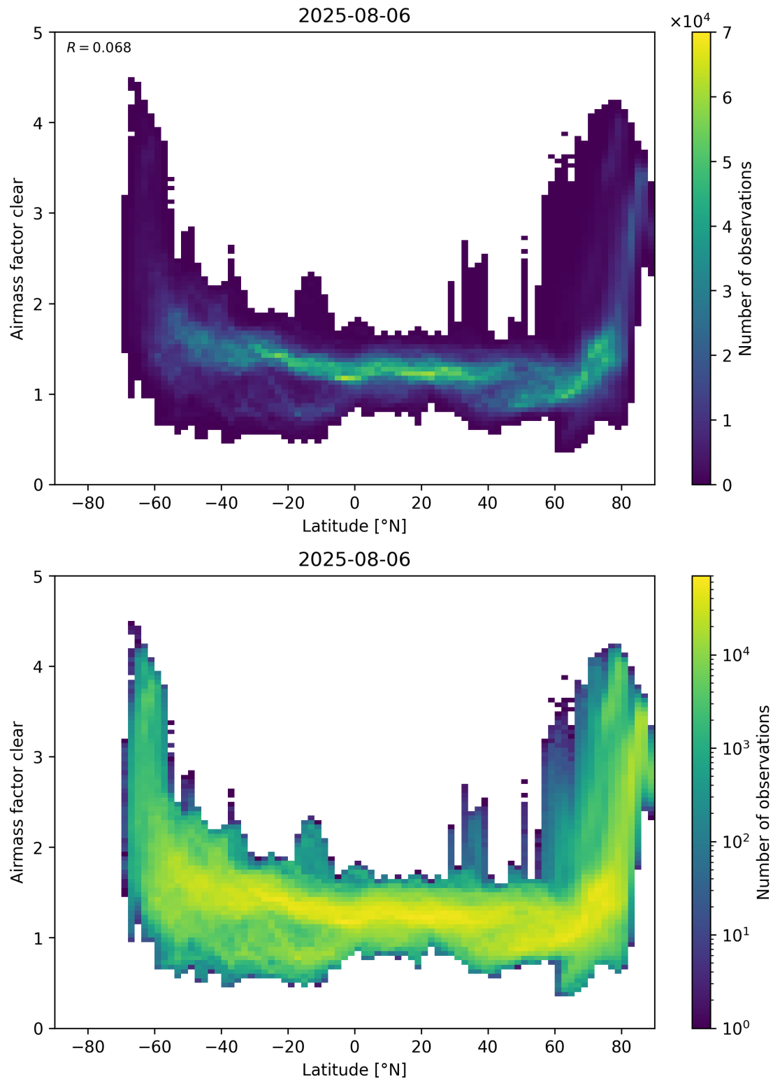
Figure 156: Scatter density plot of “Latitude” against “Airmass factor clear” for 2025-08-05 to 2025-08-07.
