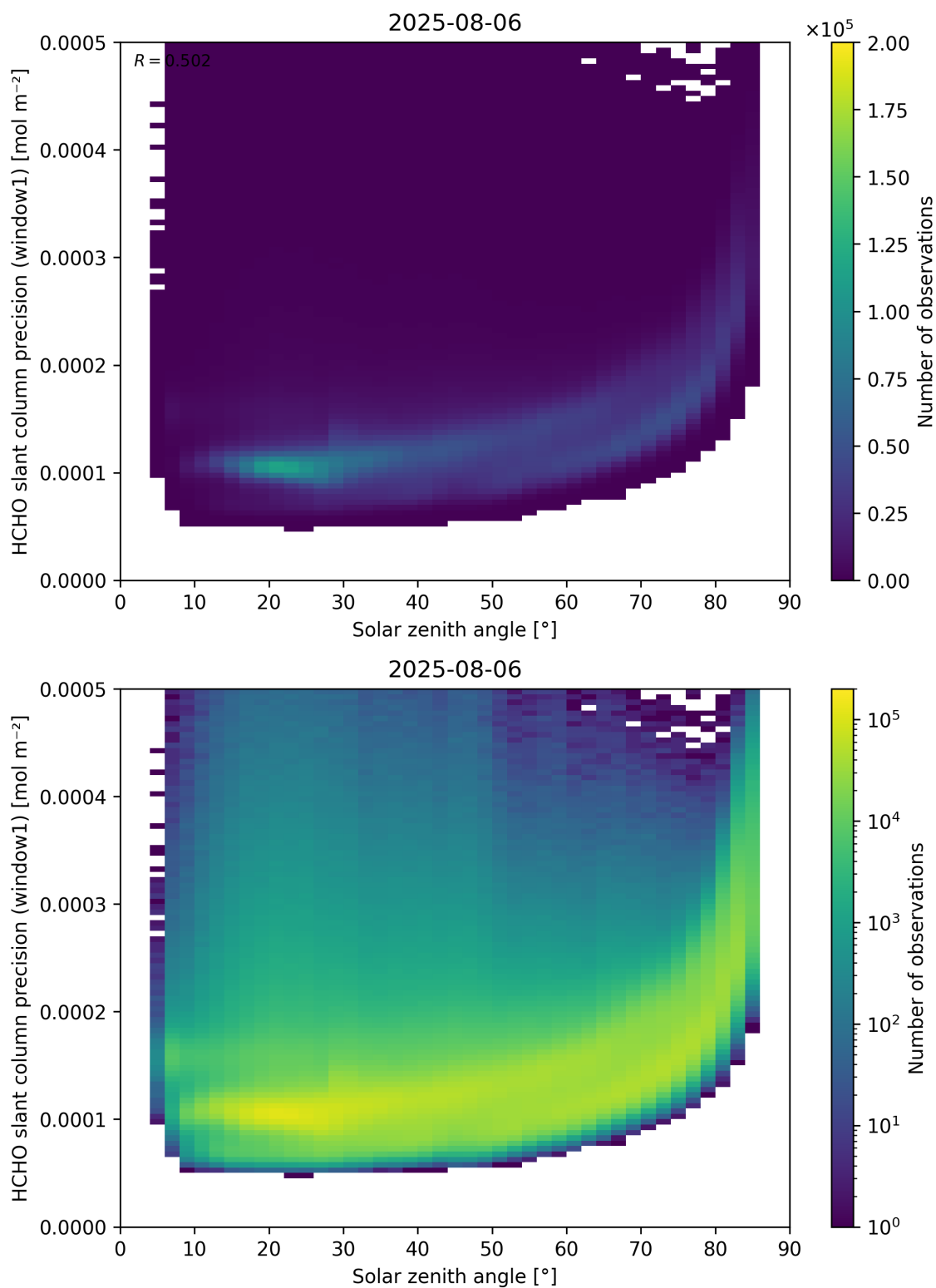
Figure 174: Scatter density plot of “Solar zenith angle” against “HCHO slant column precision (window1)” for 2025-08-05 to 2025-08-07.
