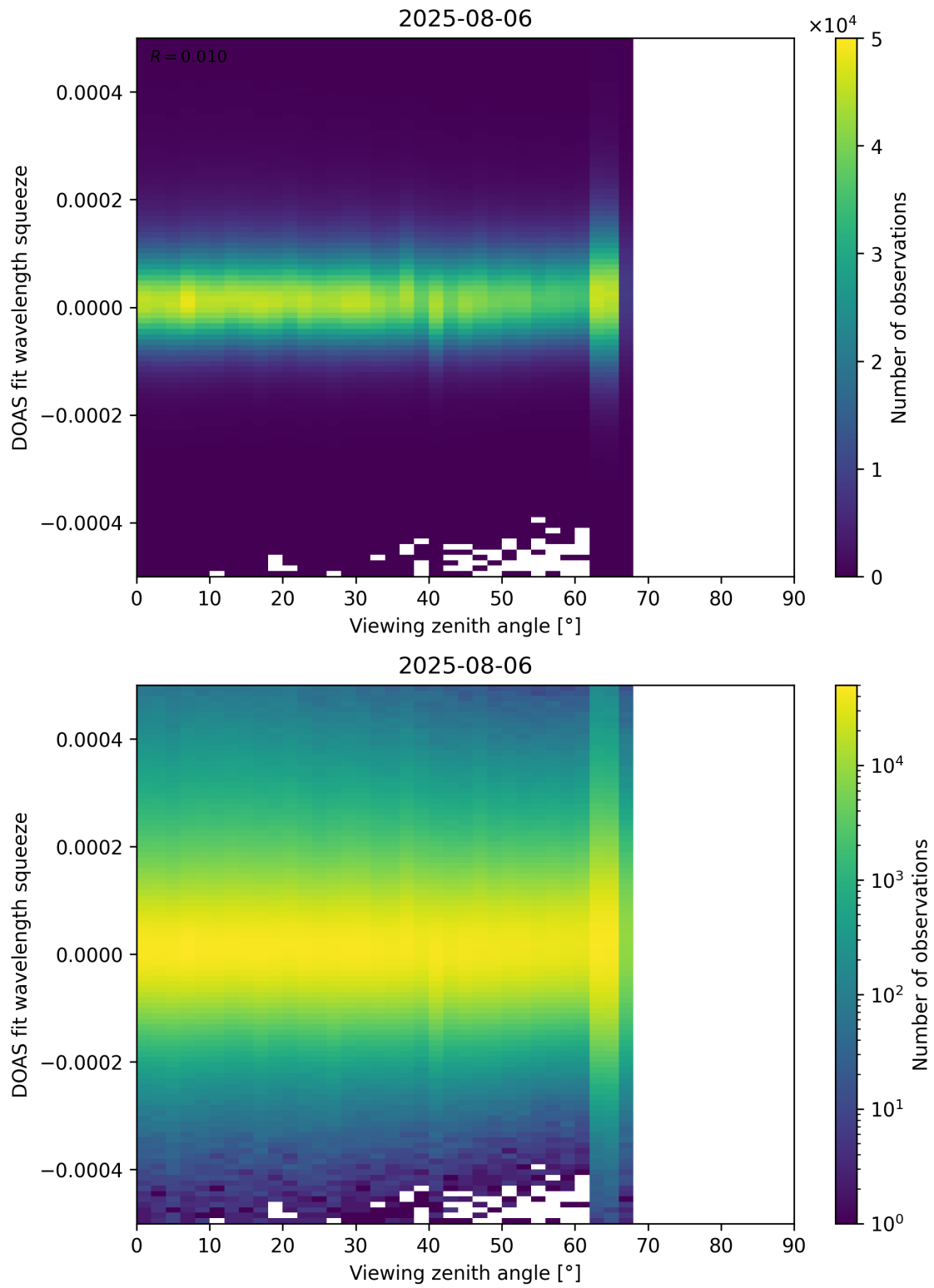
Figure 184: Scatter density plot of “Viewing zenith angle” against “DOAS fit wavelength squeeze” for 2025-08-05 to 2025-08-07.
