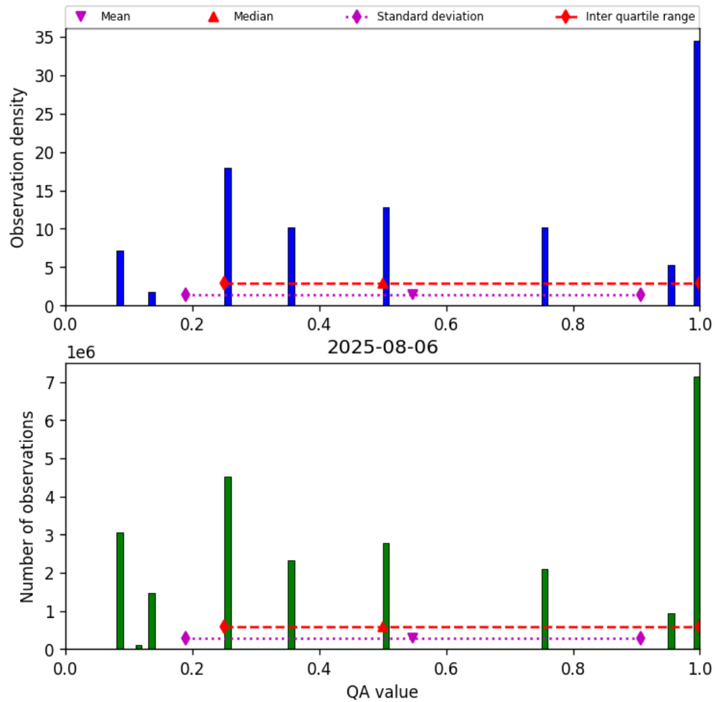
Figure 34: Histogram of “QA value” for 2025-08-05 to 2025-08-07
