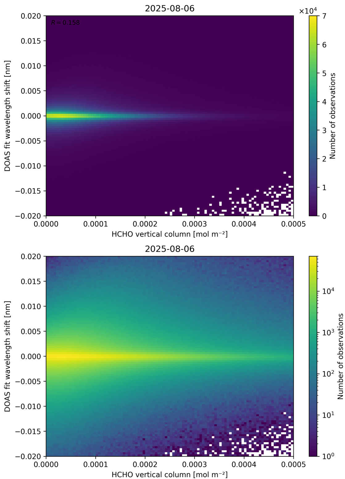
Figure 124: Scatter density plot of “HCHO vertical column” against “DOAS fit wavelength shift” for 2025-08-05 to 2025-08-07.
