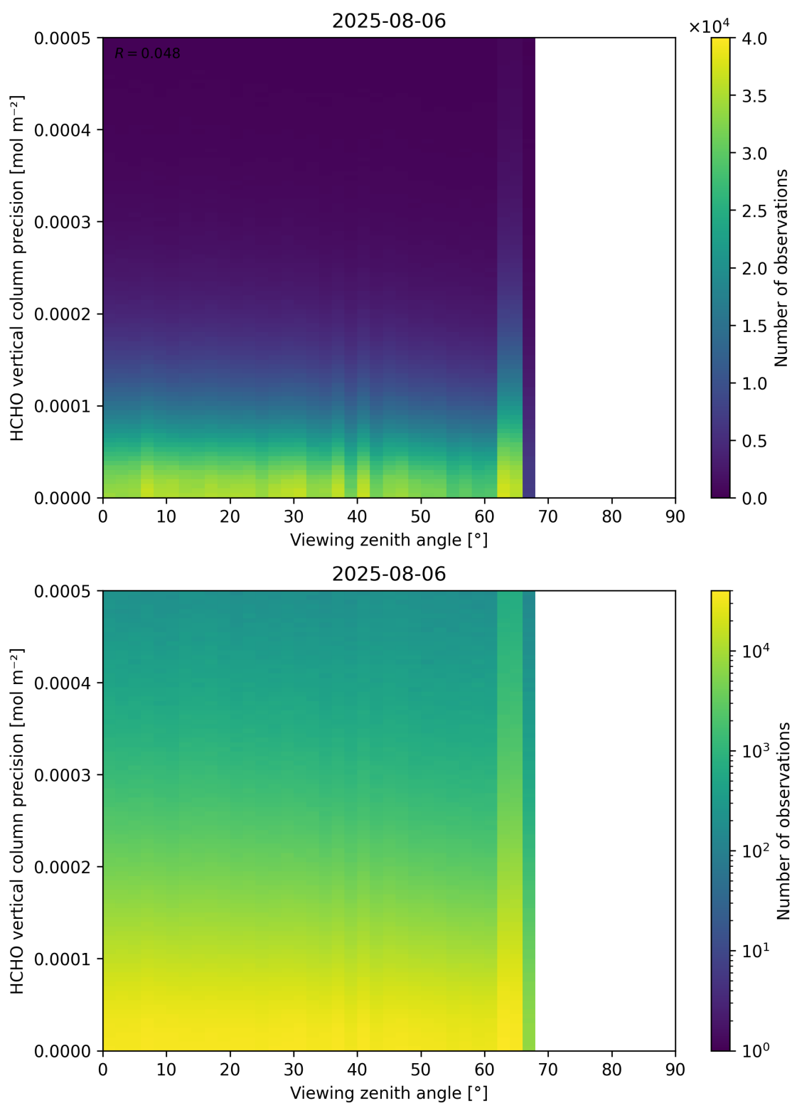
Figure 194: Scatter density plot of “Viewing zenith angle” against “HCHO vertical column precision” for 2025-08-05 to 2025-08-07.
