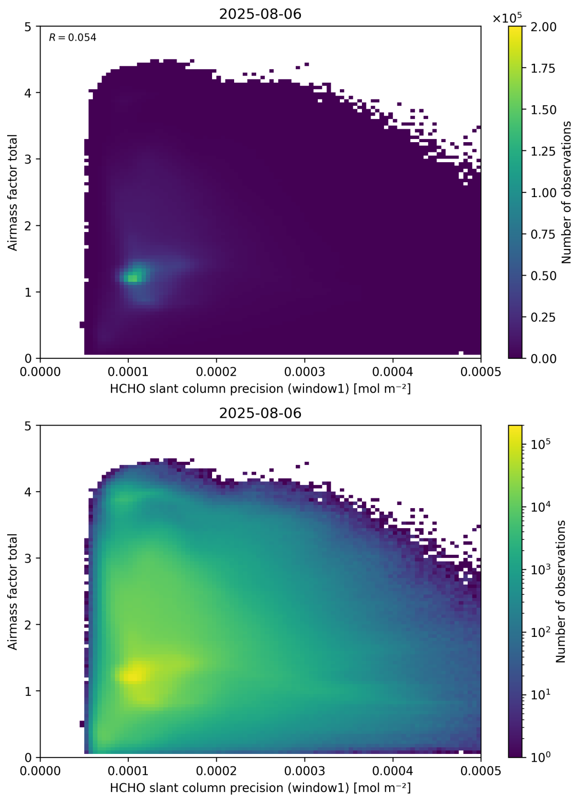
Figure 94: Scatter density plot of “HCHO slant column precision (window1)” against “Airmass factor total” for 2025-08-05 to 2025-08-07.
