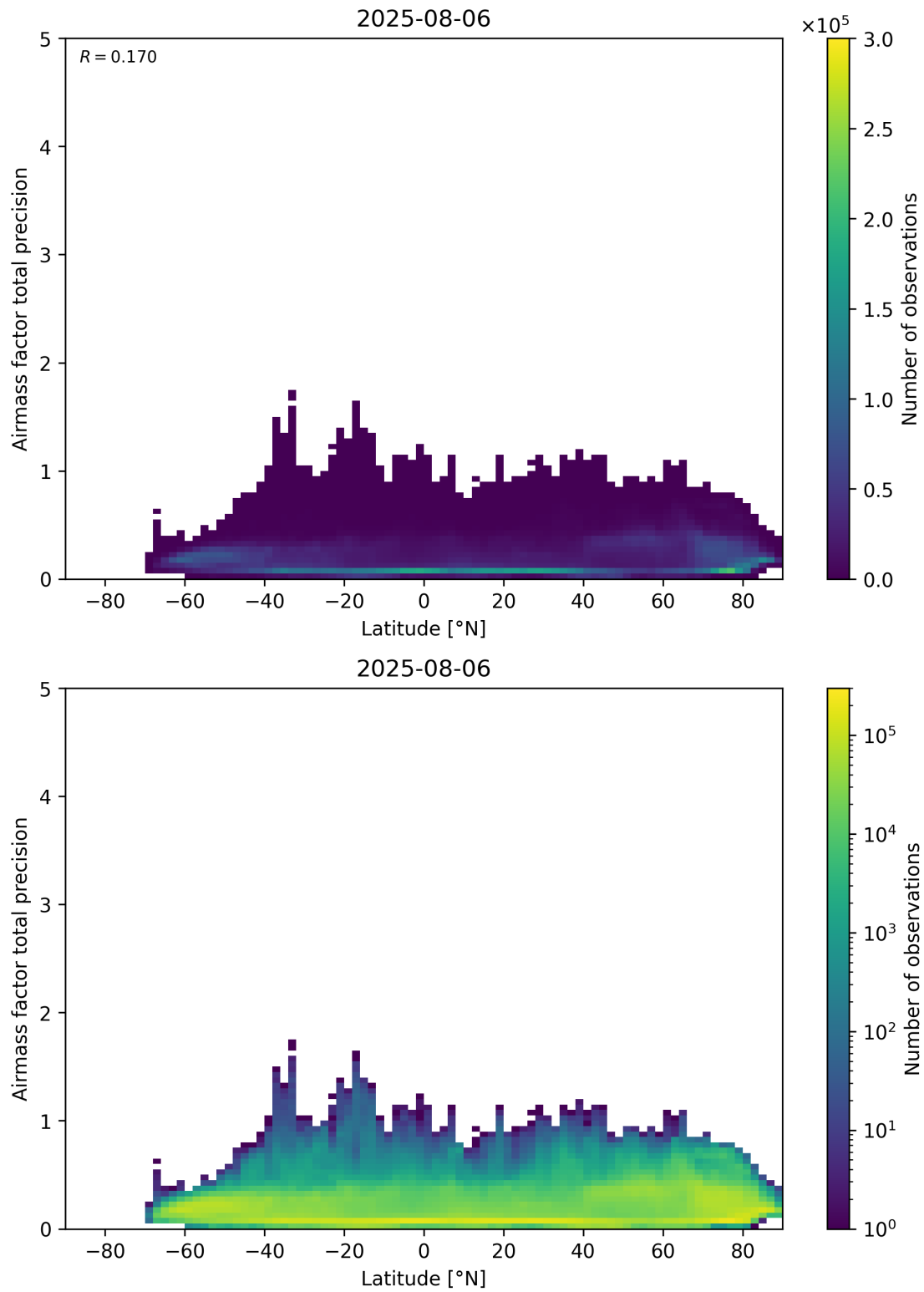
Figure 162: Scatter density plot of “Latitude” against “Airmass factor total precision” for 2025-08-05 to 2025-08-07.
