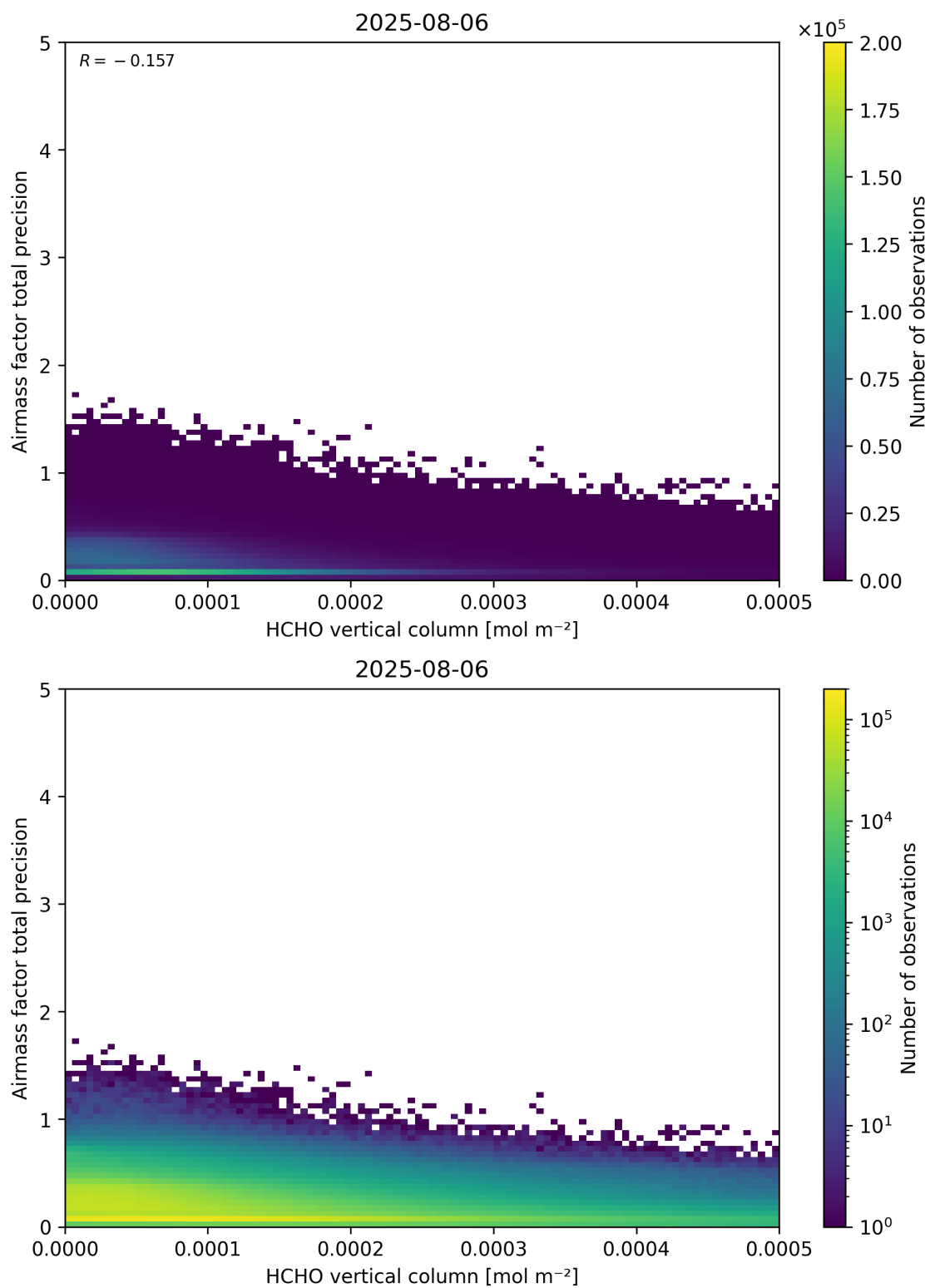
Figure 132: Scatter density plot of “HCHO vertical column” against “Airmass factor total precision” for 2025-08-05 to 2025-08-07.
