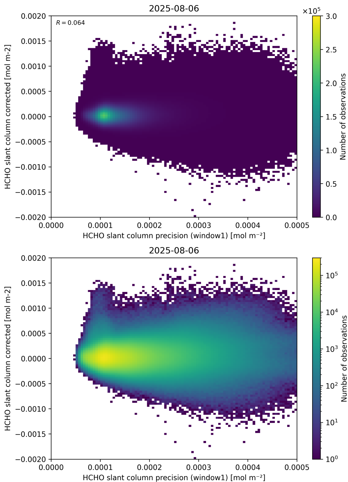
Figure 92: Scatter density plot of “HCHO slant column precision (window1)” against “HCHO slant column corrected” for 2025-08-05 to 2025-08-07.
