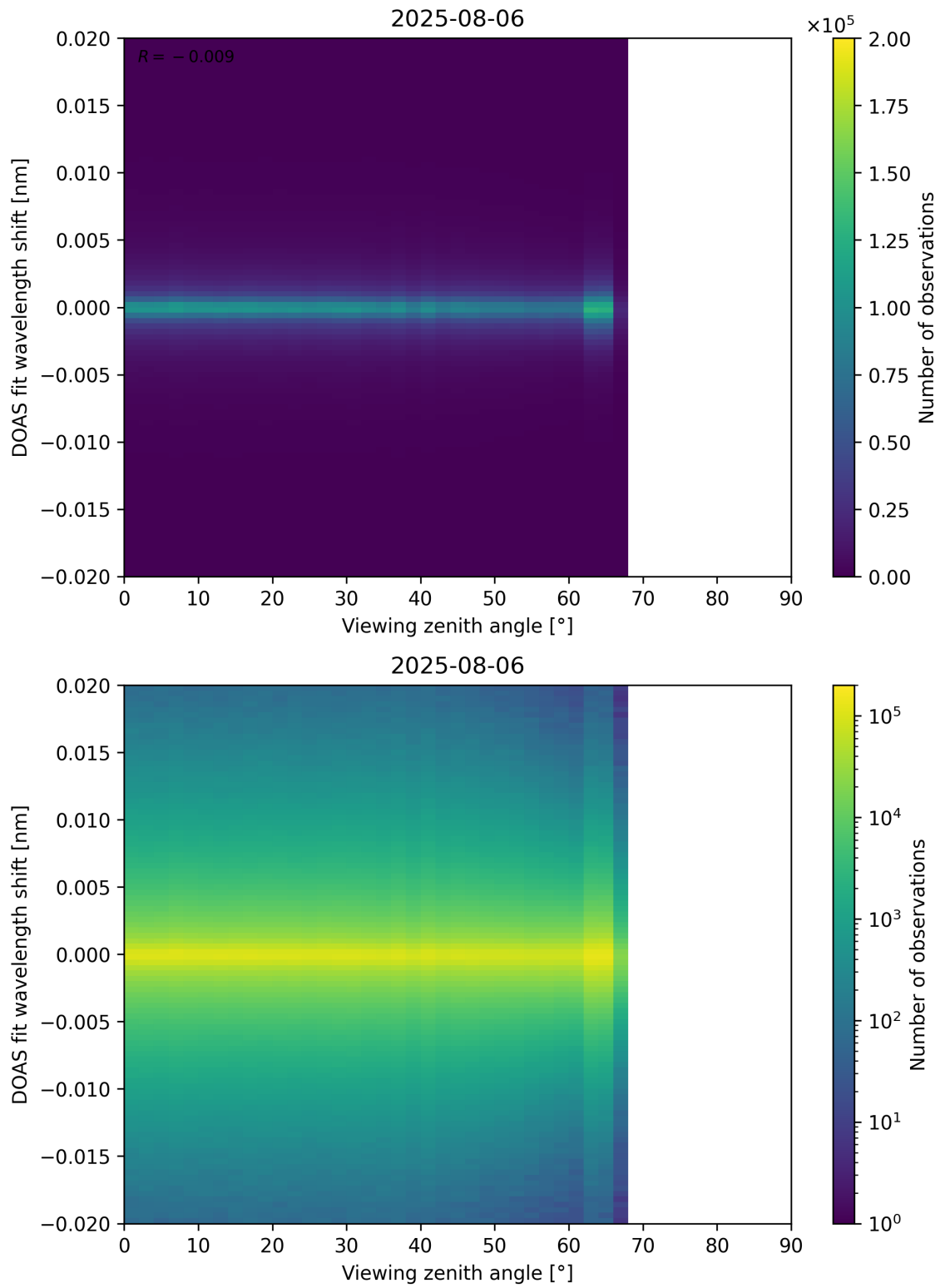
Figure 183: Scatter density plot of “Viewing zenith angle” against “DOAS fit wavelength shift” for 2025-08-05 to 2025-08-07.
