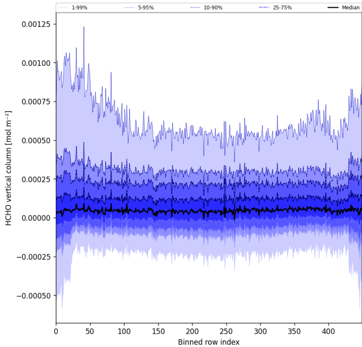
Figure 49: Along track statistics of “HCHO vertical column” for 2025-08-05 to 2025-08-07
