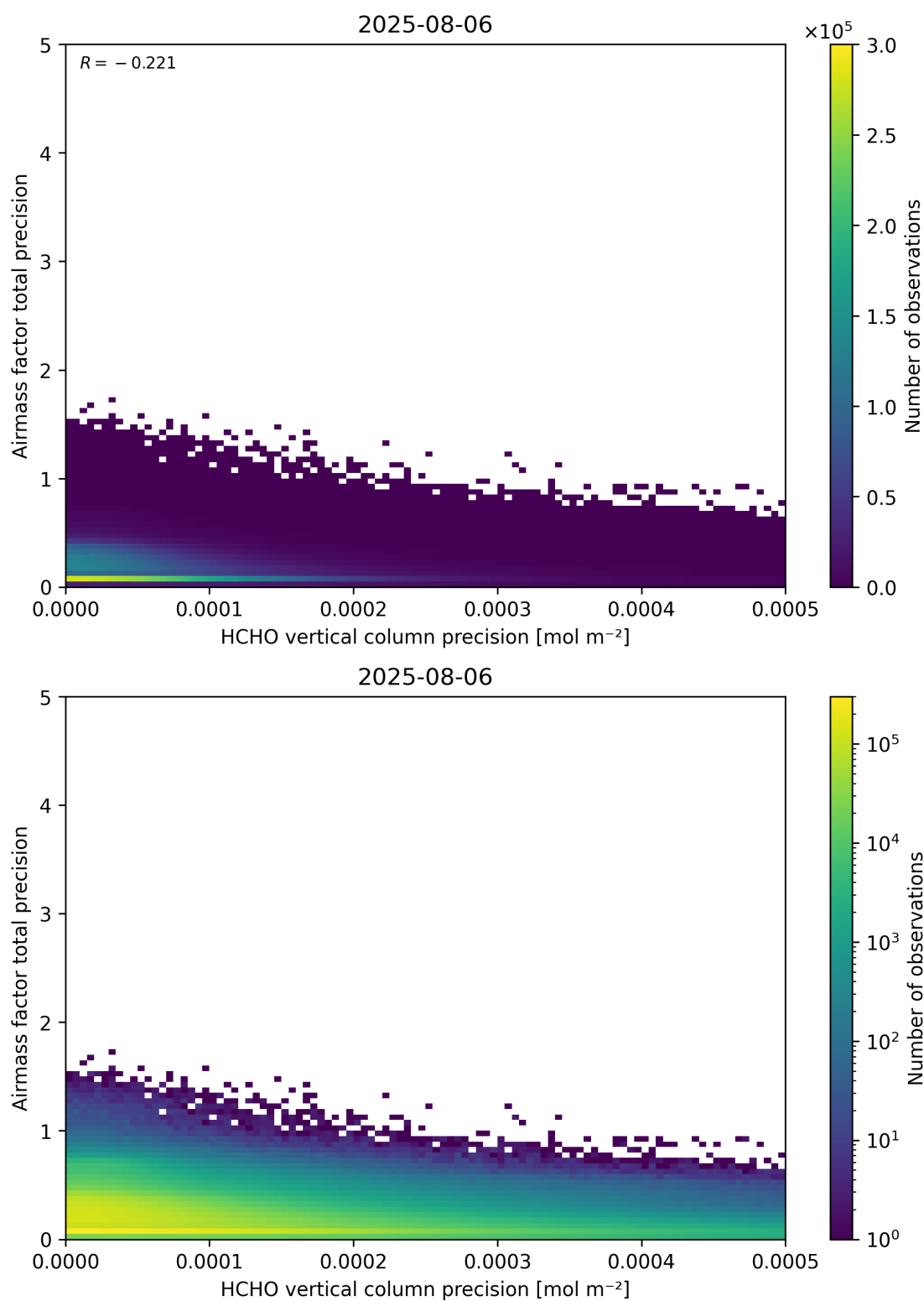
Figure 145: Scatter density plot of “HCHO vertical column precision” against “Airmass factor total precision” for 2025-08-05 to 2025-08-07.
