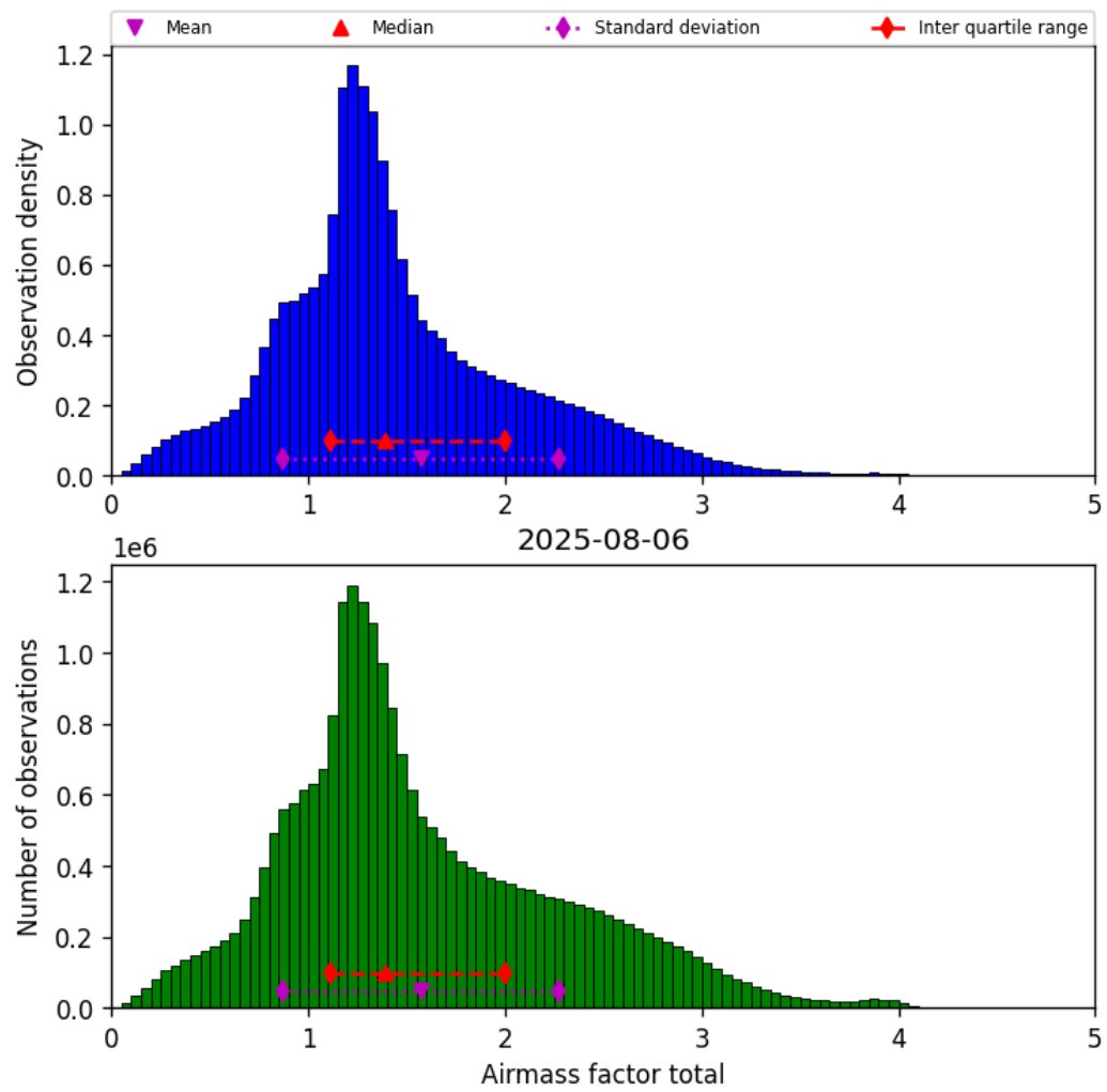
Figure 40: Histogram of “Airmass factor total” for 2025-08-05 to 2025-08-07
