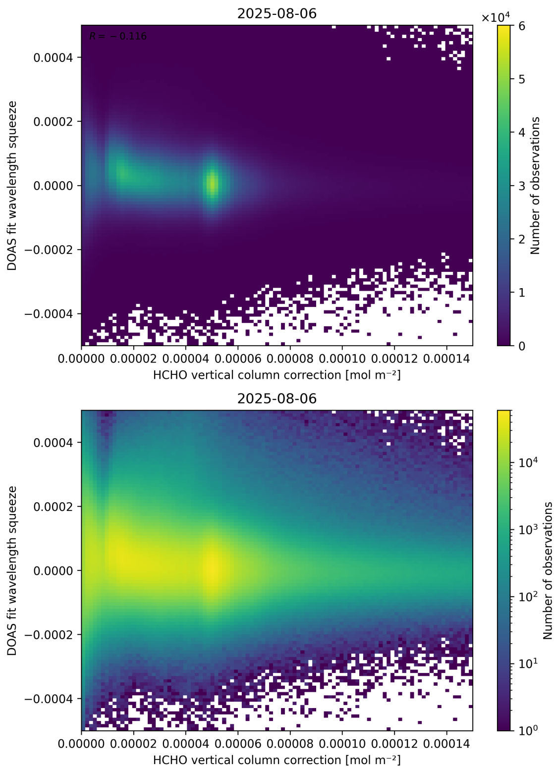
Figure 114: Scatter density plot of “HCHO vertical column correction” against “DOAS fit wavelength squeeze” for 2025-08-05 to 2025-08-07.
