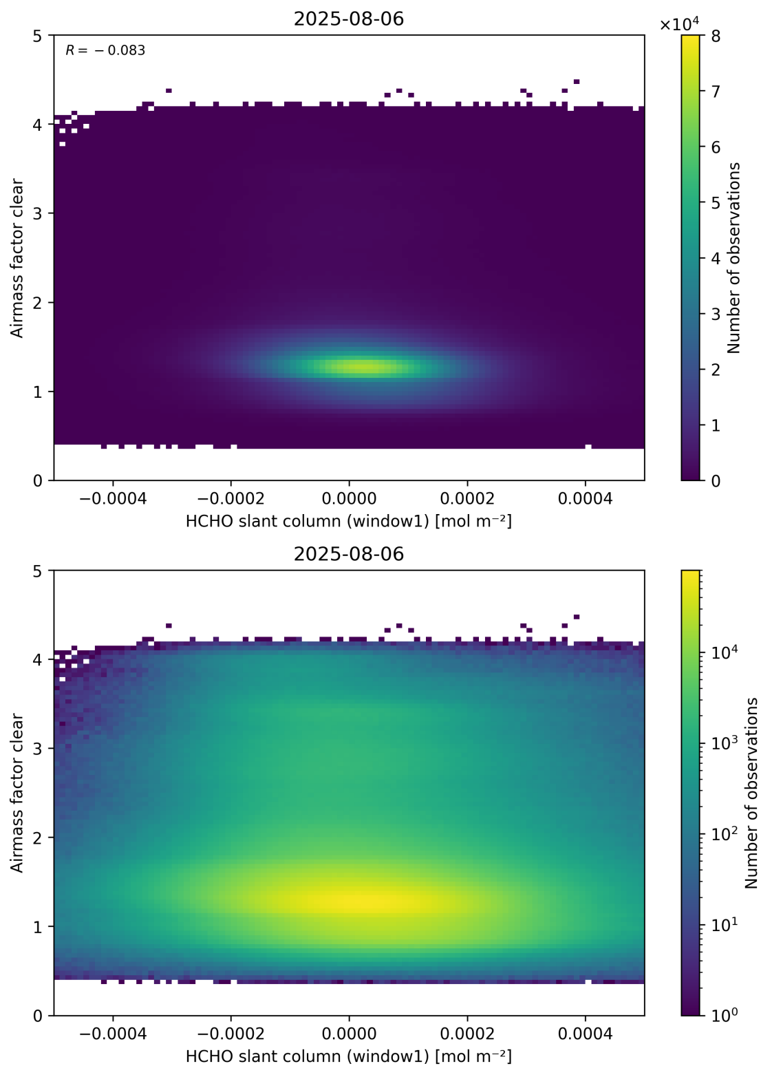
Figure 81: Scatter density plot of “HCHO slant column (window1)” against “Airmass factor clear” for 2025-08-05 to 2025-08-07.
