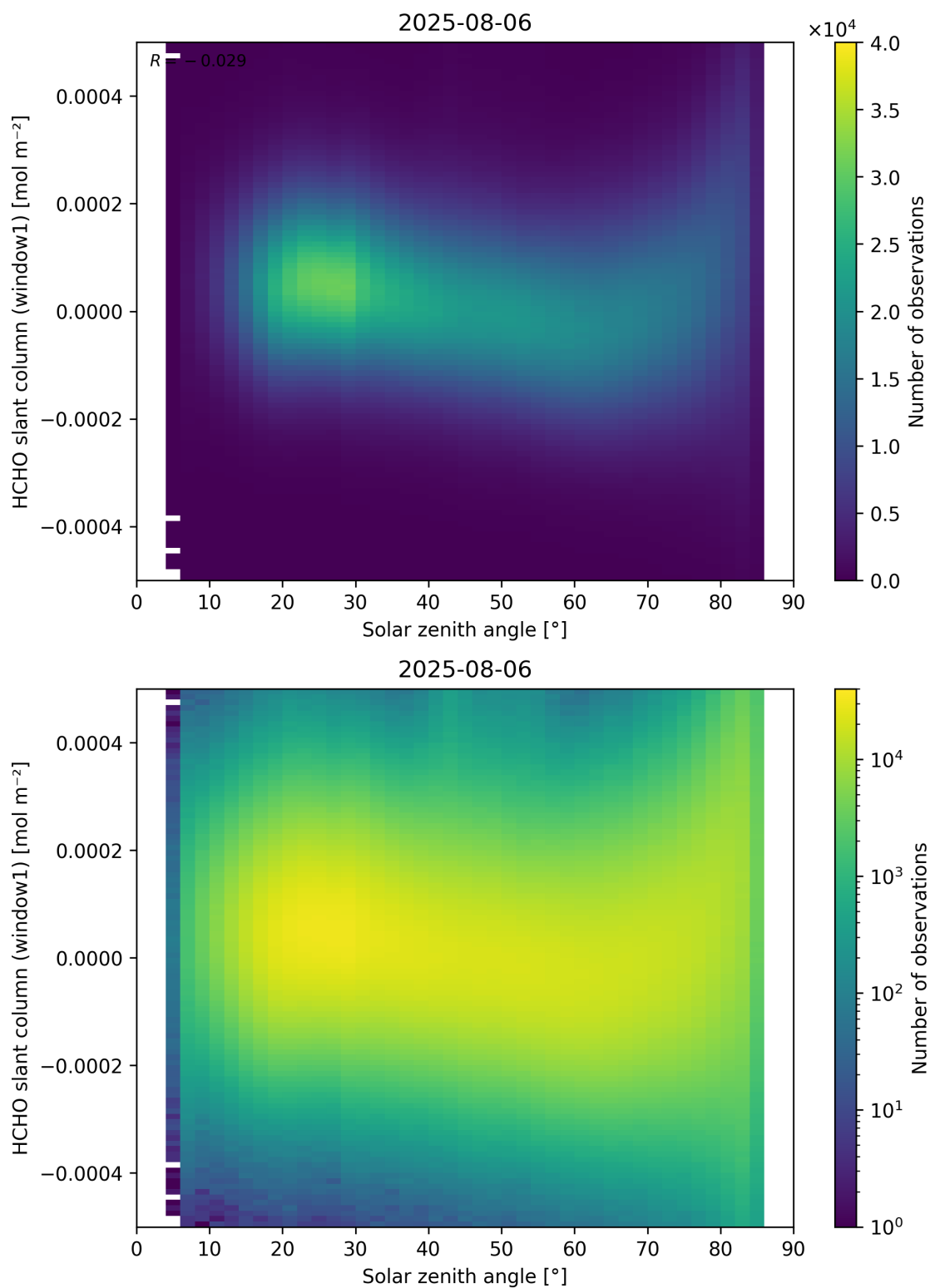
Figure 173: Scatter density plot of “Solar zenith angle” against “HCHO slant column (window1)” for 2025-08-05 to 2025-08-07.
