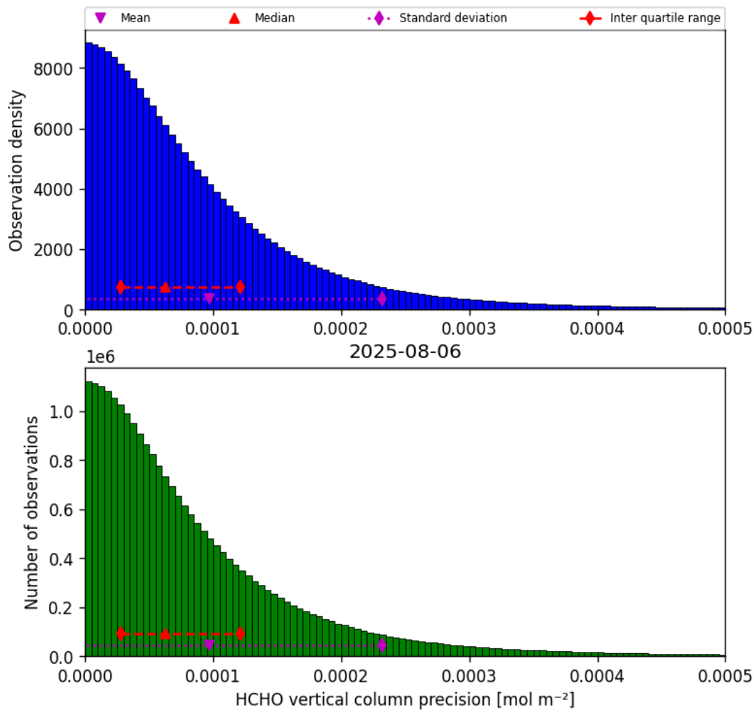
Figure 36: Histogram of “HCHO vertical column precision” for 2025-08-05 to 2025-08-07
