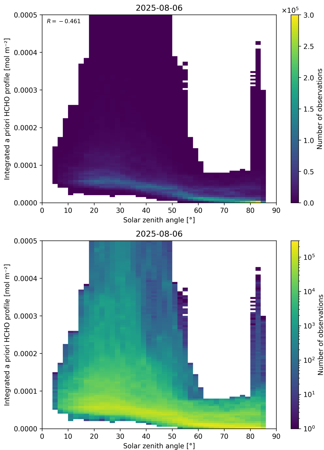
Figure 180: Scatter density plot of “Solar zenith angle” against “Integrated a priori HCHO profile” for 2025-08-05 to 2025-08-07.
