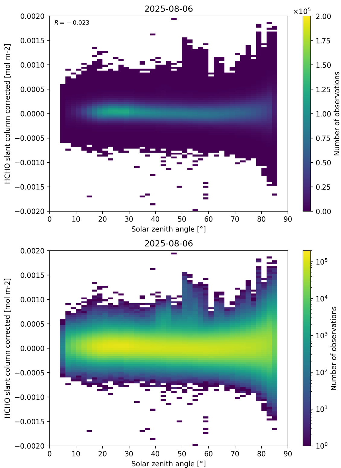
Figure 171: Scatter density plot of “Solar zenith angle” against “HCHO slant column corrected” for 2025-08-05 to 2025-08-07.
