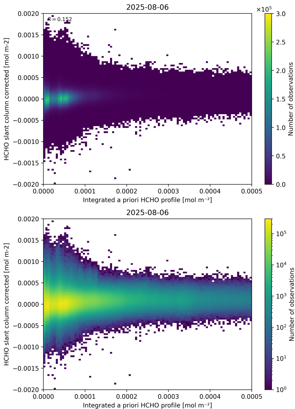
Figure 151: Scatter density plot of “Integrated a priori HCHO profile” against “HCHO slant column corrected” for 2025-08-05 to 2025-08-07.
