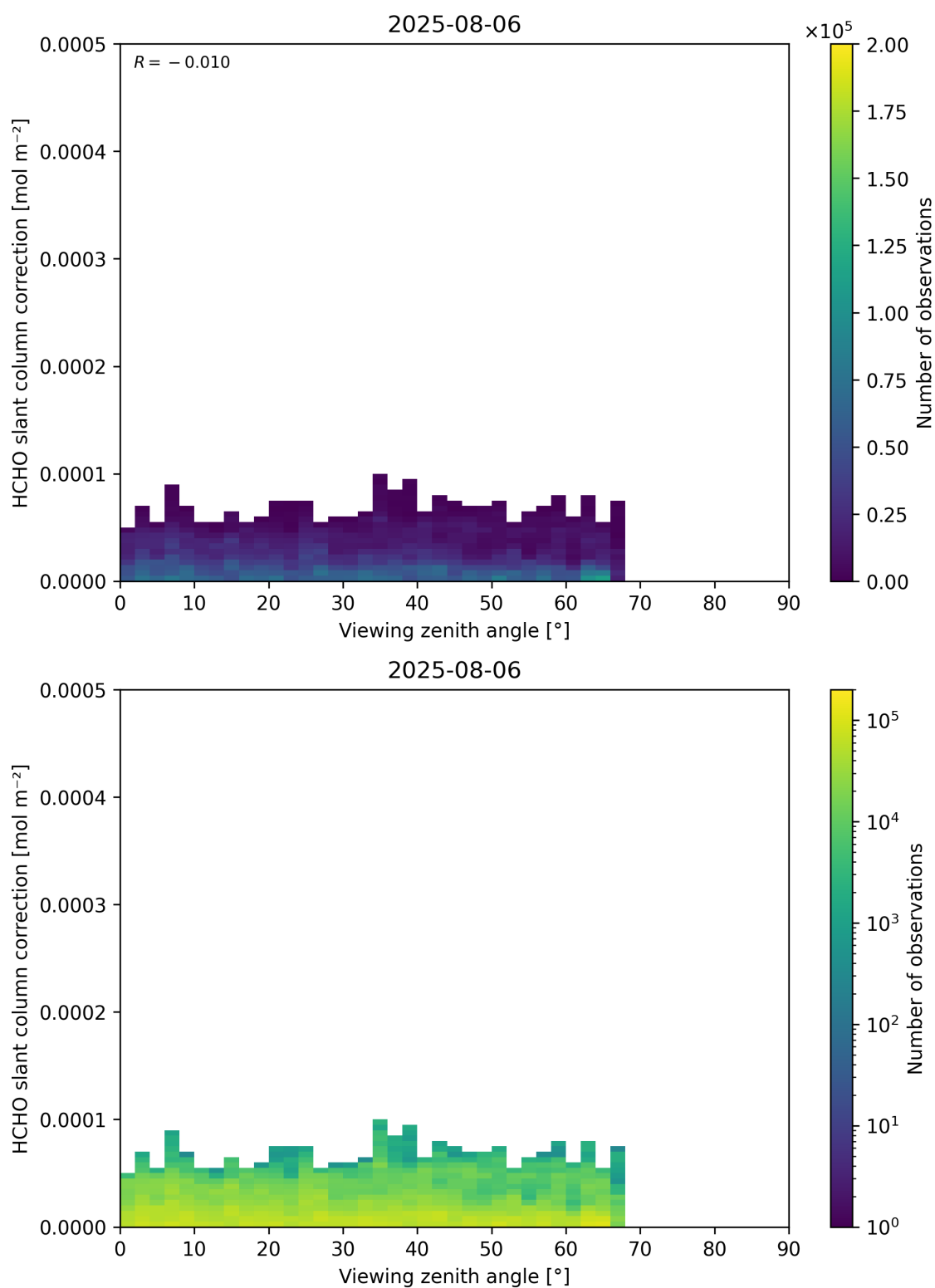
Figure 187: Scatter density plot of “Viewing zenith angle” against “HCHO slant column correction” for 2025-08-05 to 2025-08-07.
