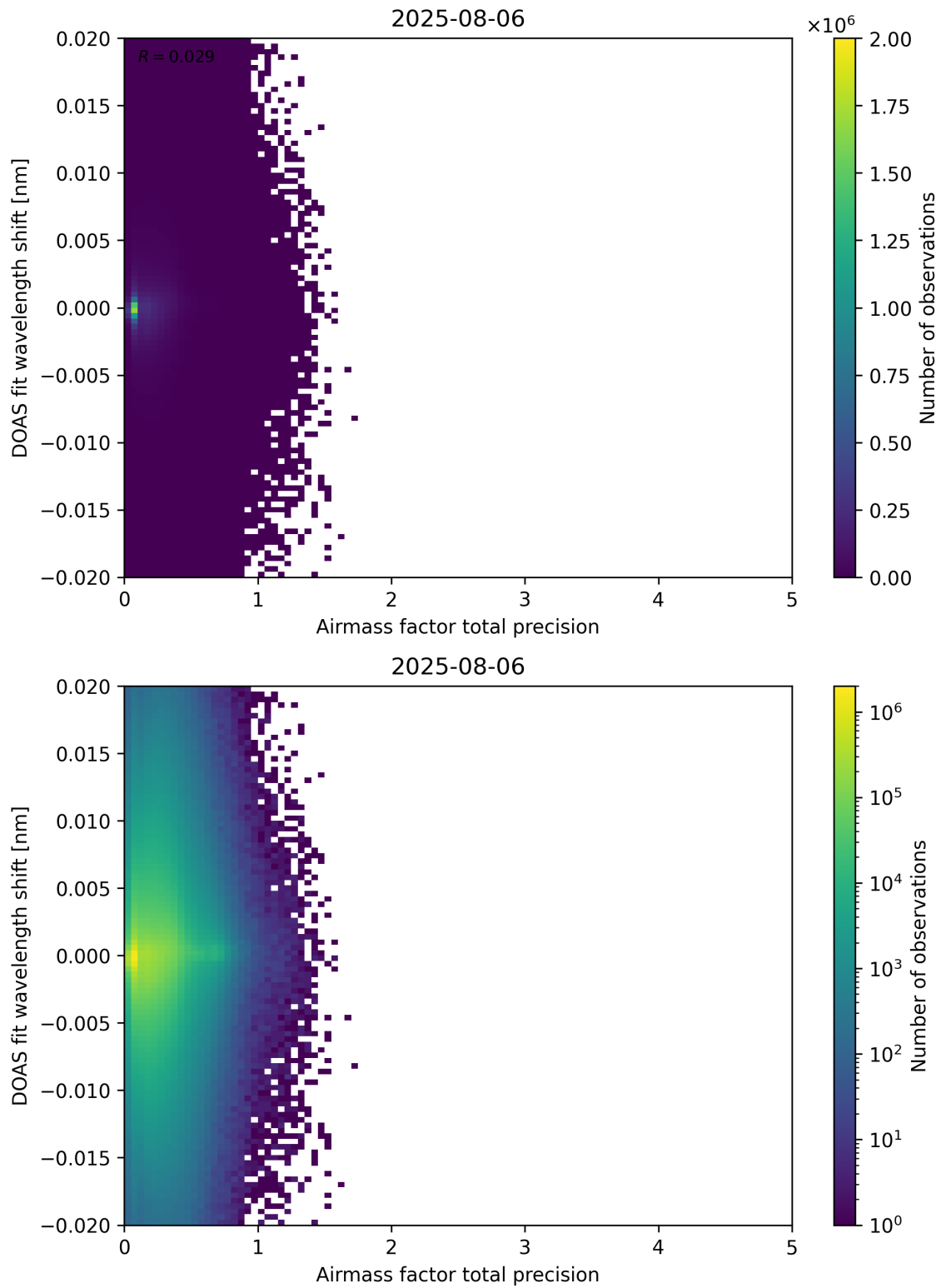
Figure 106: Scatter density plot of “Airmass factor total precision” against “DOAS fit wavelength shift” for 2025-08-05 to 2025-08-07.
