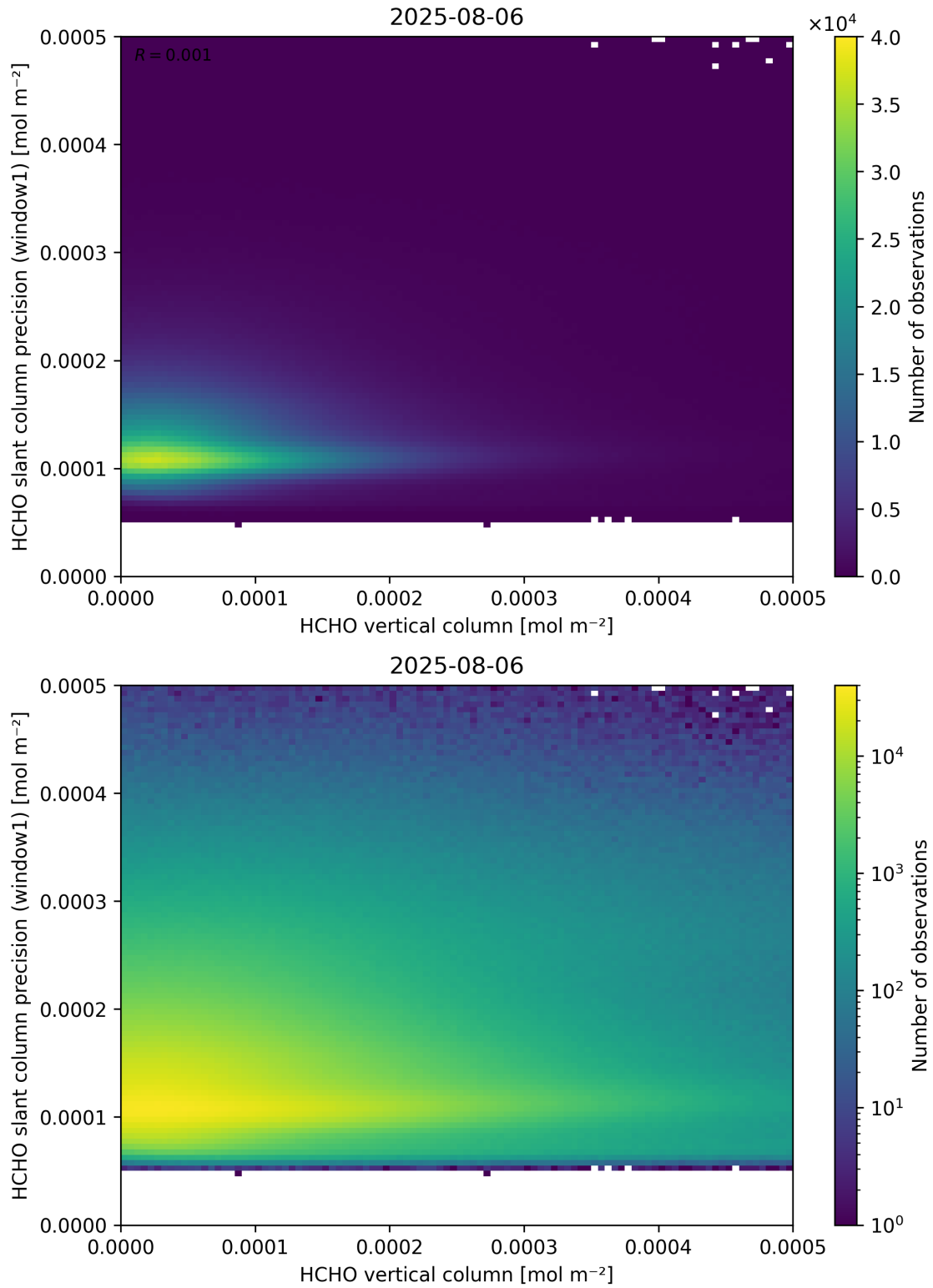
Figure 130: Scatter density plot of “HCHO vertical column” against “HCHO slant column precision (window1)” for 2025-08-05 to 2025-08-07.
