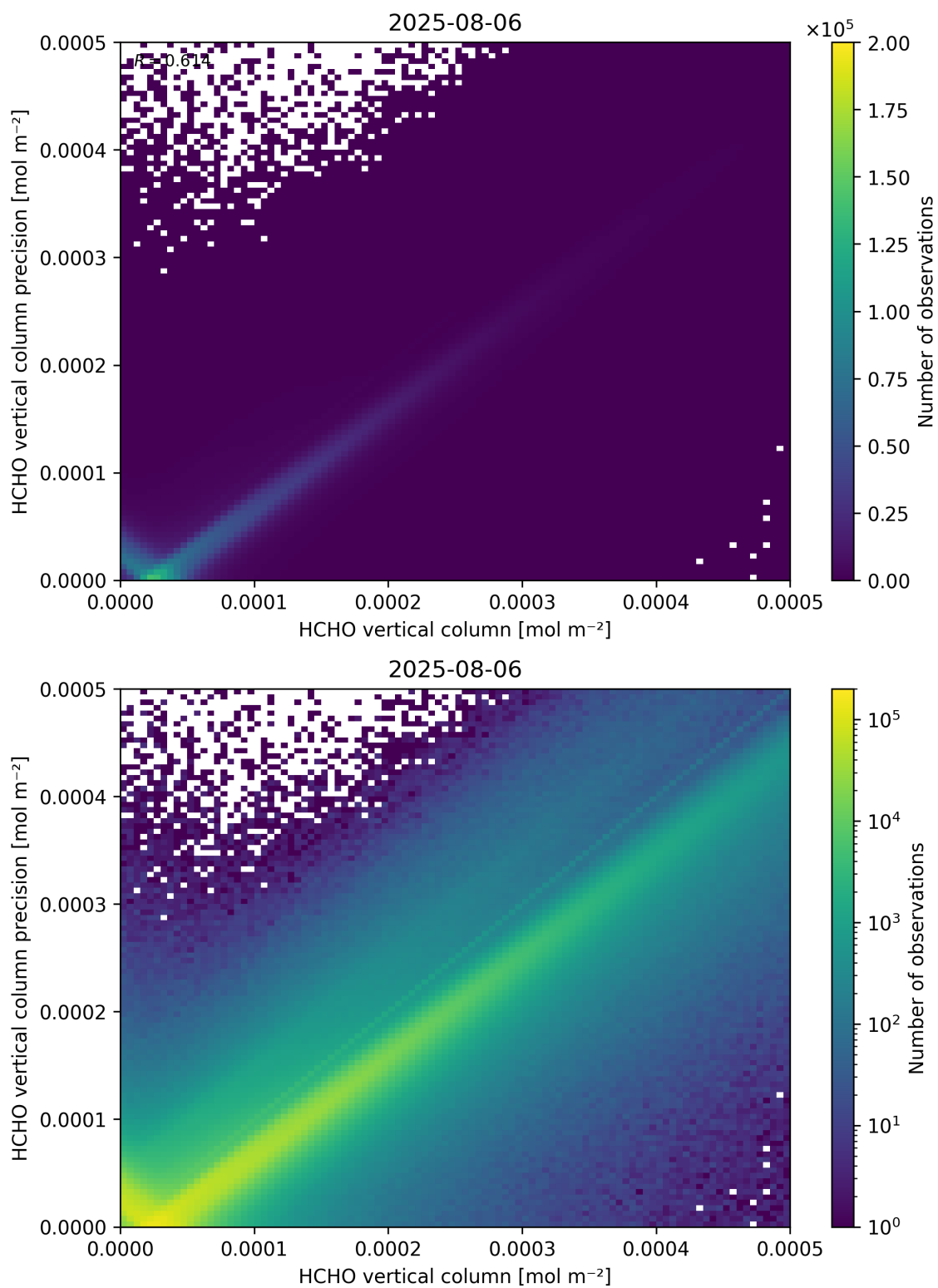
Figure 134: Scatter density plot of “HCHO vertical column” against “HCHO vertical column precision” for 2025-08-05 to 2025-08-07.
