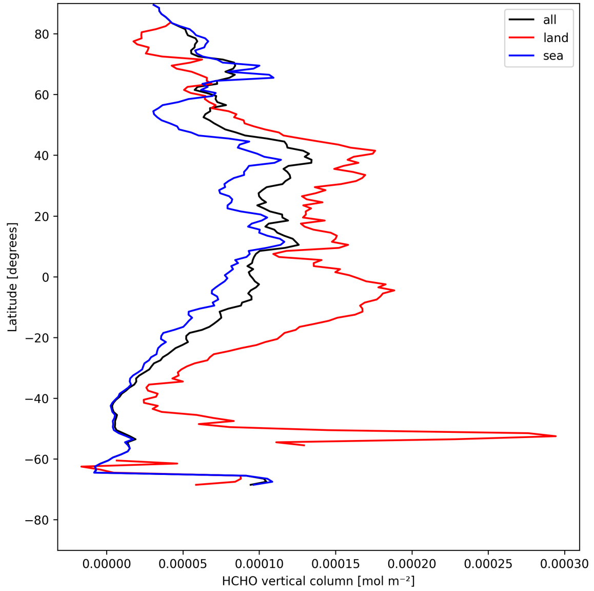
Figure 21: Zonal average of “HCHO vertical column” for 2025-08-05 to 2025-08-07.
