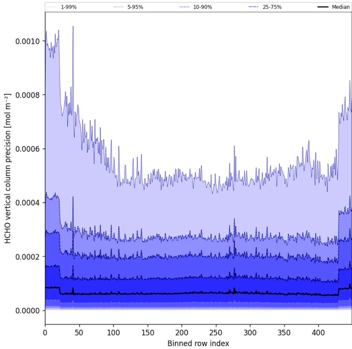
Figure 50: Along track statistics of “HCHO vertical column precision” for 2025-08-05 to 2025-08-07
