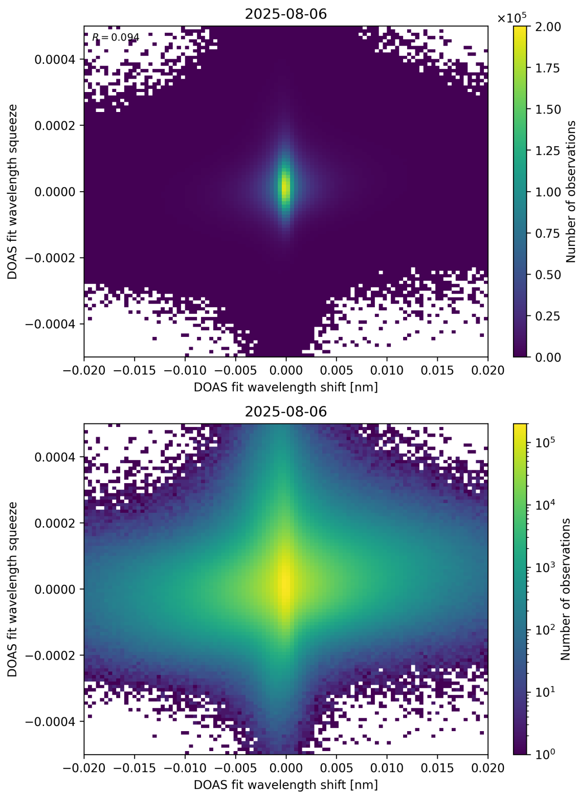
Figure 65: Scatter density plot of “DOAS fit wavelength shift” against “DOAS fit wavelength squeeze” for 2025-08-05 to 2025-08-07.
