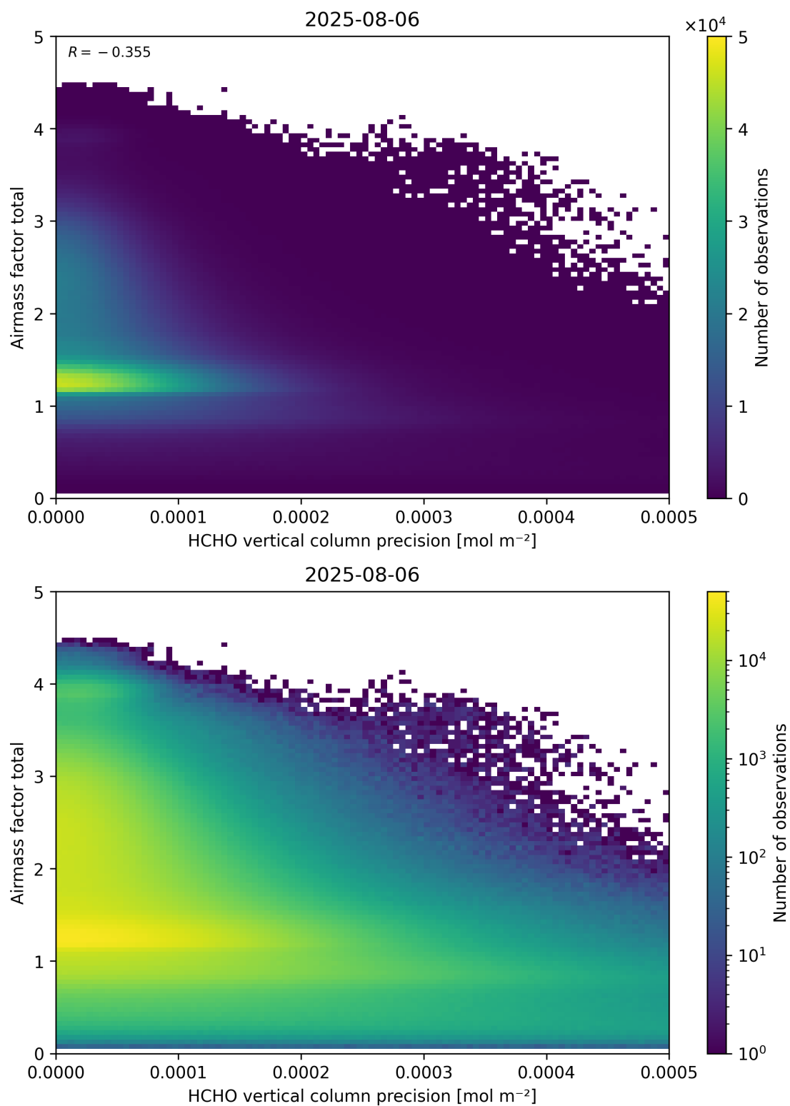
Figure 144: Scatter density plot of “HCHO vertical column precision” against “Airmass factor total” for 2025-08-05 to 2025-08-07.
