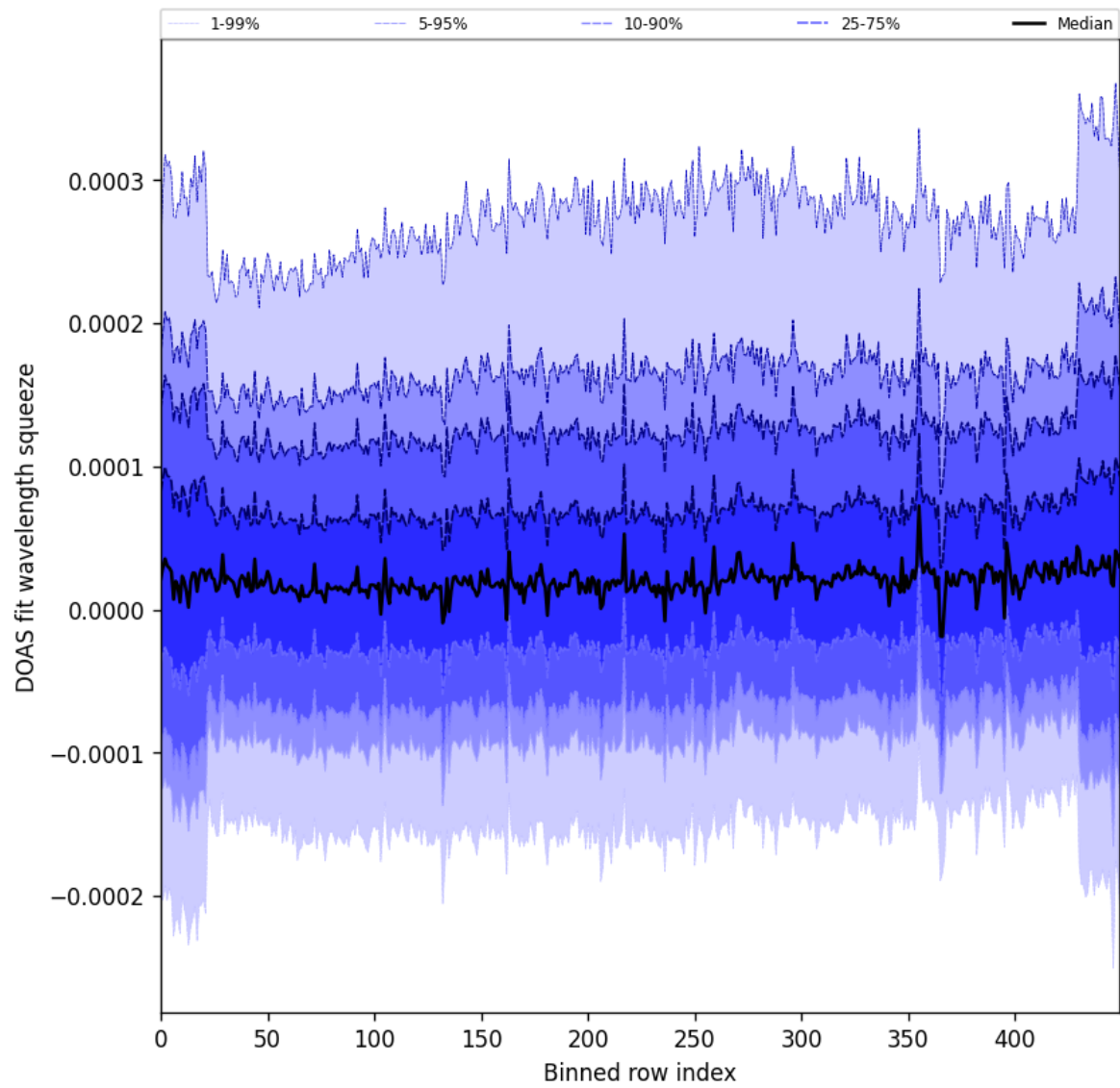
Figure 59: Along track statistics of “DOAS fit wavelength squeeze” for 2025-08-05 to 2025-08-07
