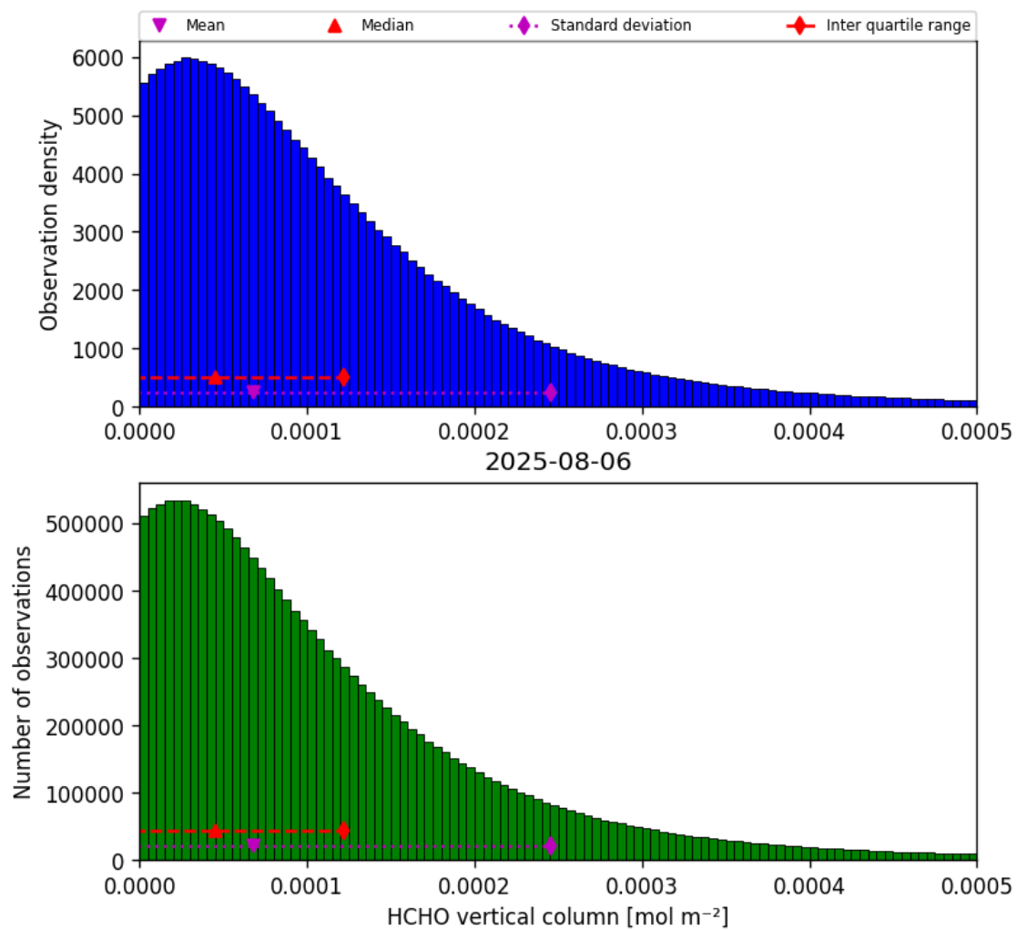
Figure 35: Histogram of “HCHO vertical column” for 2025-08-05 to 2025-08-07
