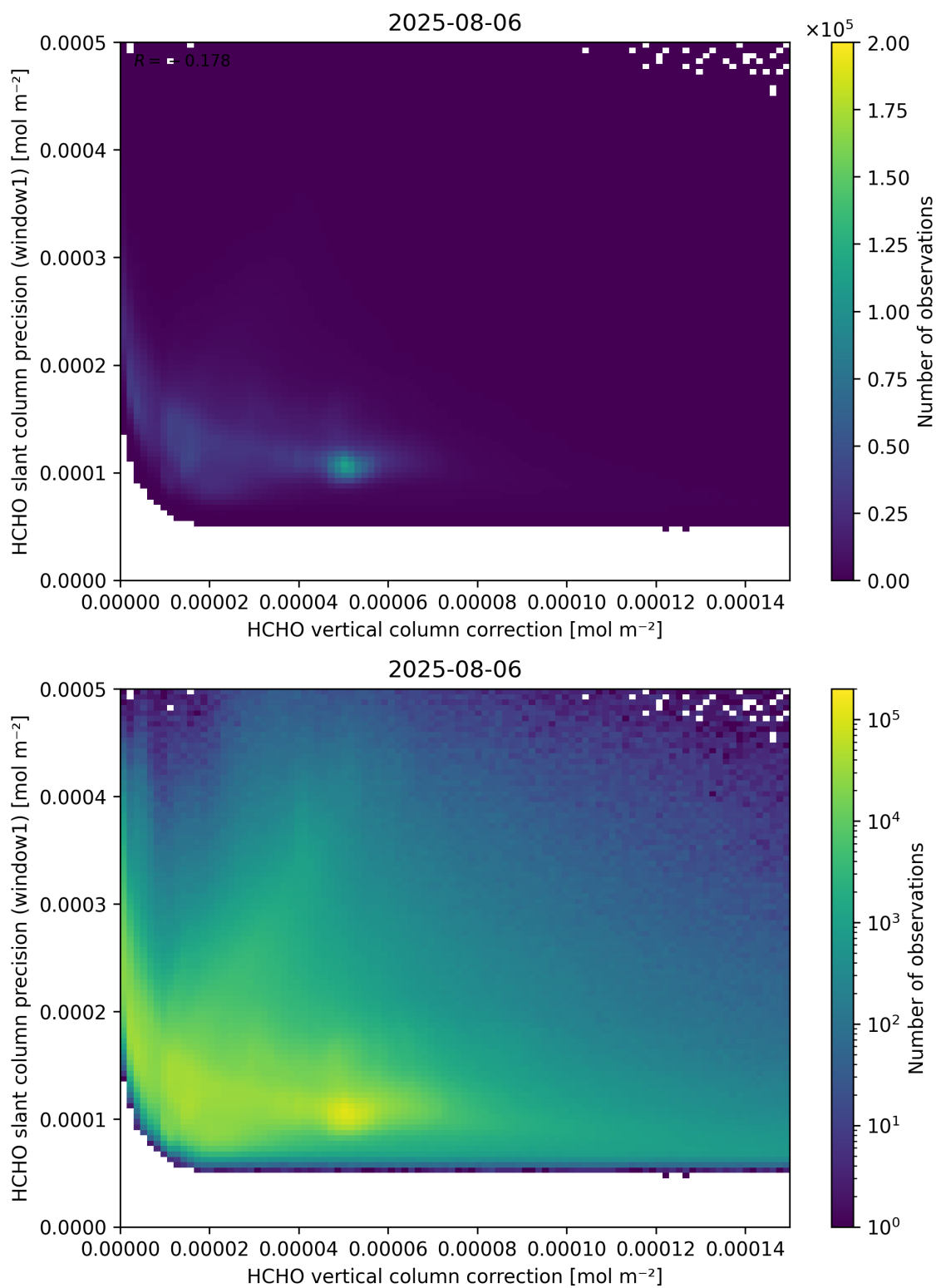
Figure 119: Scatter density plot of “HCHO vertical column correction” against “HCHO slant column precision (window1)” for 2025-08-05 to 2025-08-07.
