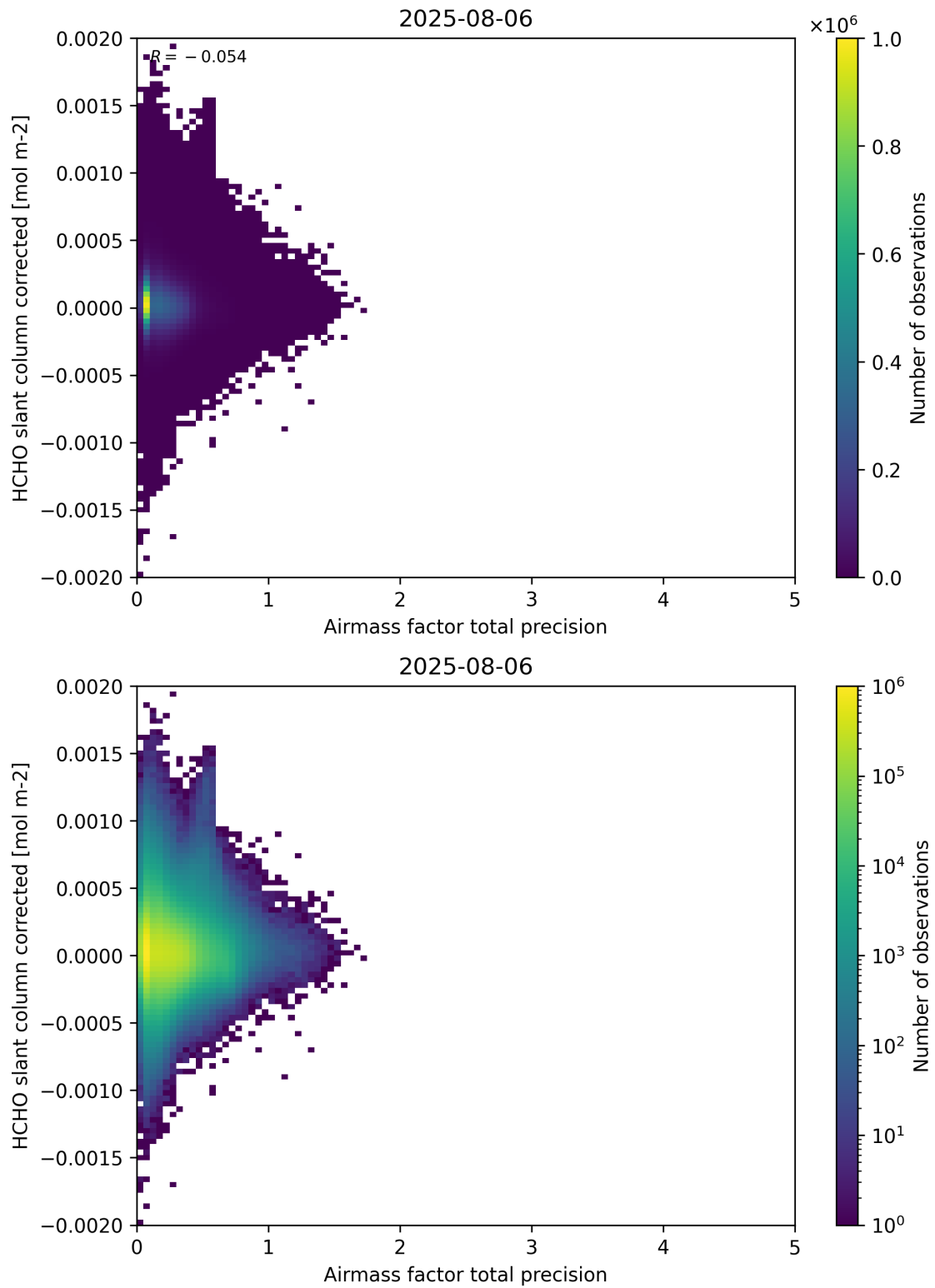
Figure 109: Scatter density plot of “Airmass factor total precision” against “HCHO slant column corrected” for 2025-08-05 to 2025-08-07.
