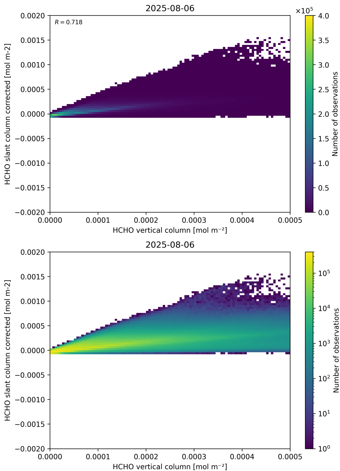
Figure 127: Scatter density plot of “HCHO vertical column” against “HCHO slant column corrected” for 2025-08-05 to 2025-08-07.
