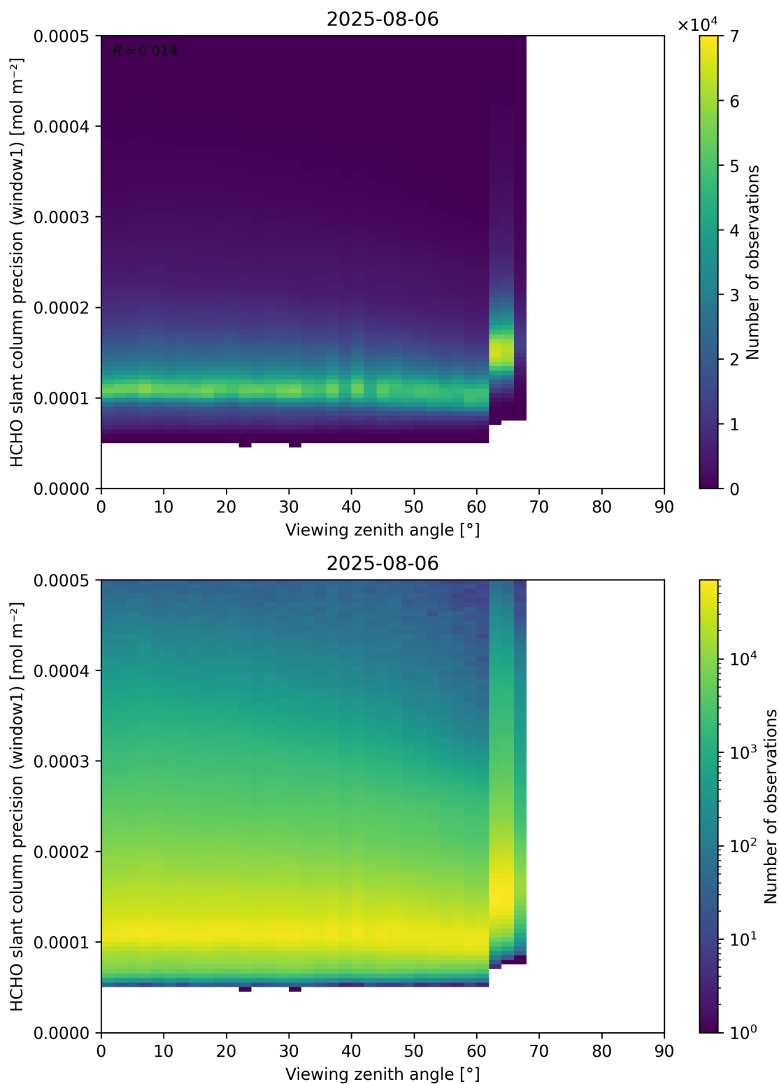
Figure 189: Scatter density plot of “Viewing zenith angle” against “HCHO slant column precision (window1)” for 2025-08-05 to 2025-08-07.
