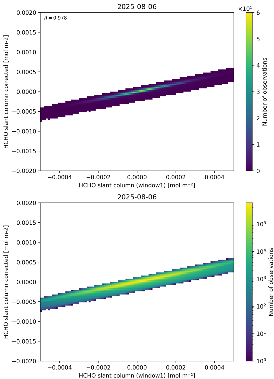
Figure 82: Scatter density plot of “HCHO slant column (window1)” against “HCHO slant column corrected” for 2025-08-05 to 2025-08-07.
