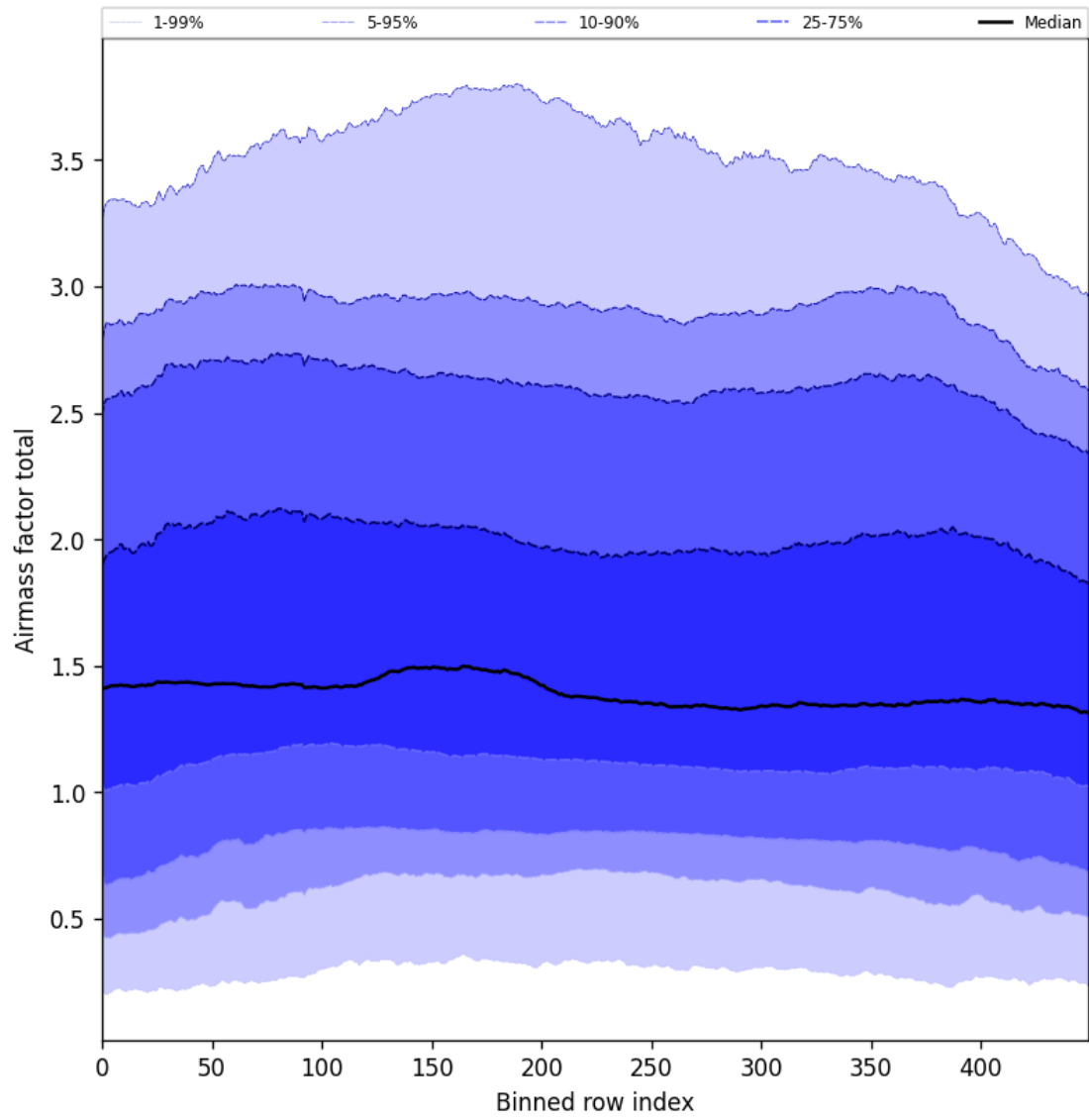
Figure 54: Along track statistics of “Airmass factor total” for 2025-08-05 to 2025-08-07
