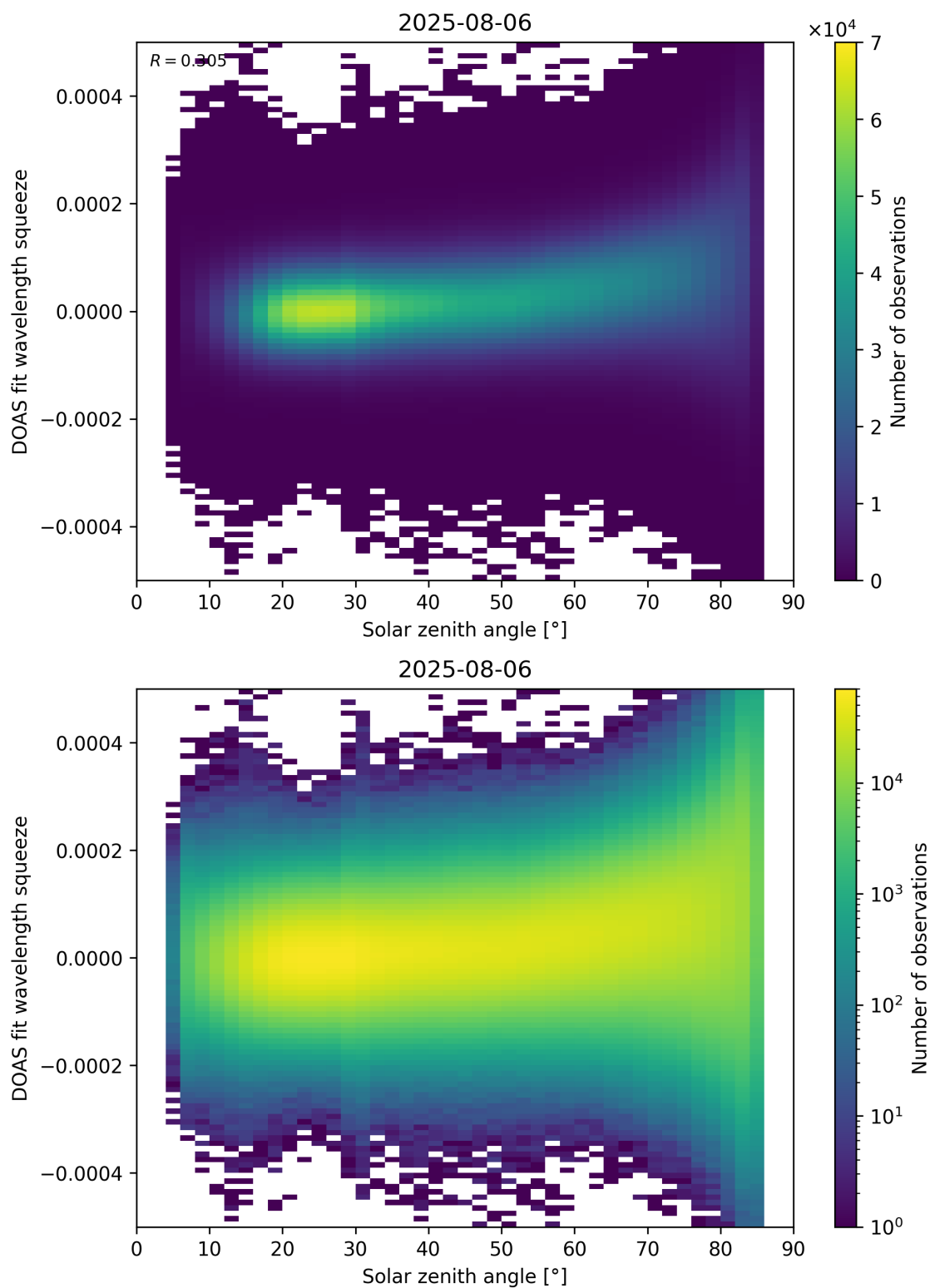
Figure 169: Scatter density plot of “Solar zenith angle” against “DOAS fit wavelength squeeze” for 2025-08-05 to 2025-08-07.
