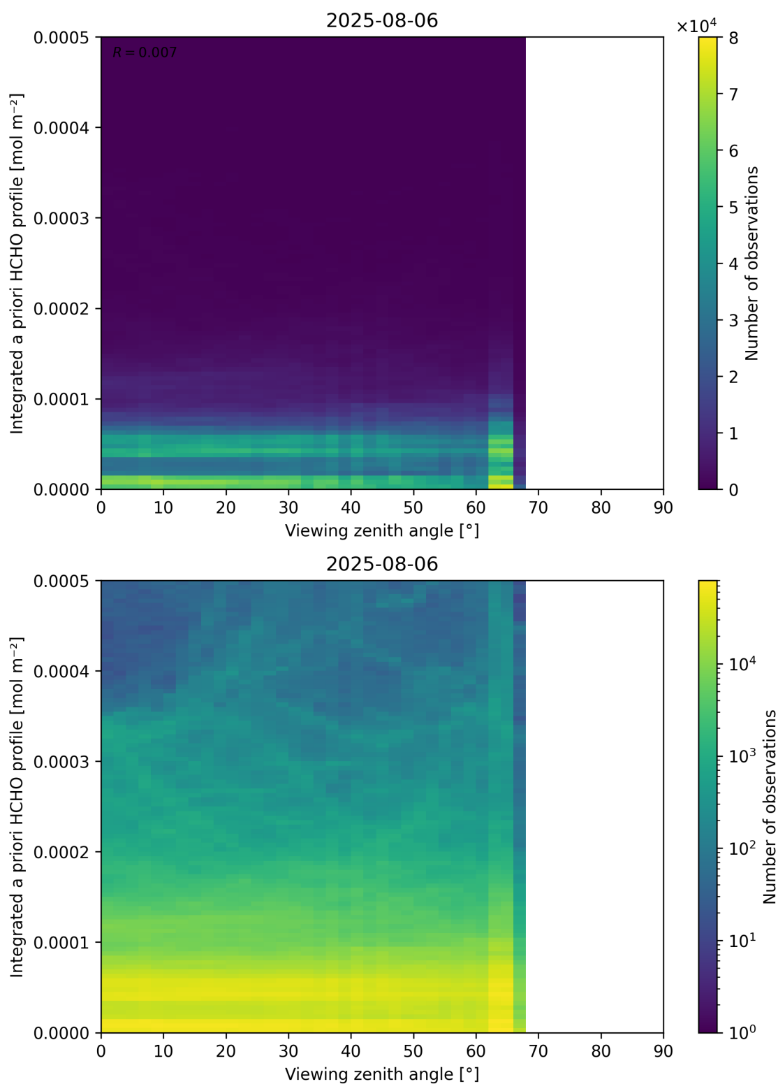
Figure 195: Scatter density plot of “Viewing zenith angle” against “Integrated a priori HCHO profile” for 2025-08-05 to 2025-08-07.
