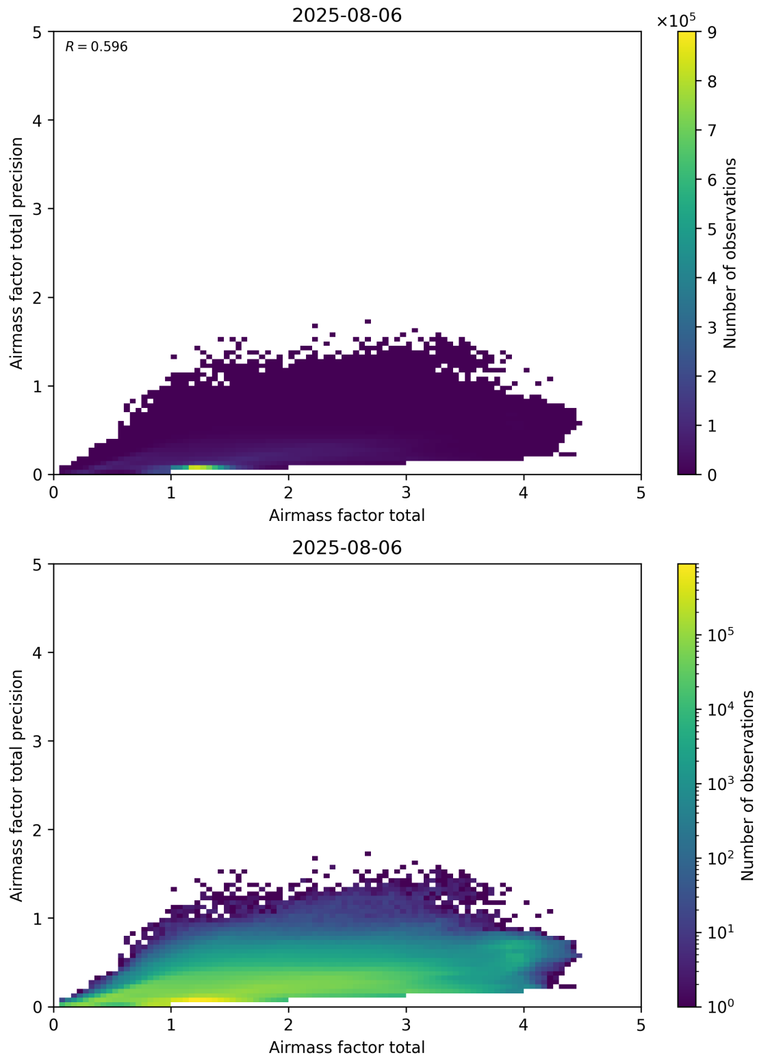
Figure 103: Scatter density plot of “Airmass factor total” against “Airmass factor total precision” for 2025-08-05 to 2025-08-07.
