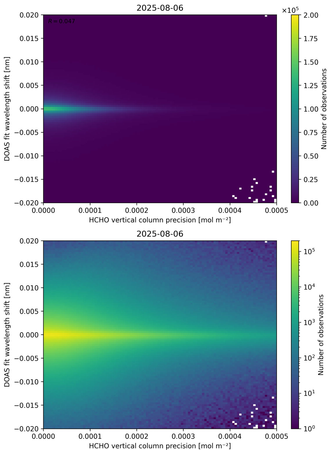
Figure 137: Scatter density plot of “HCHO vertical column precision” against “DOAS fit wavelength shift” for 2025-08-05 to 2025-08-07.
