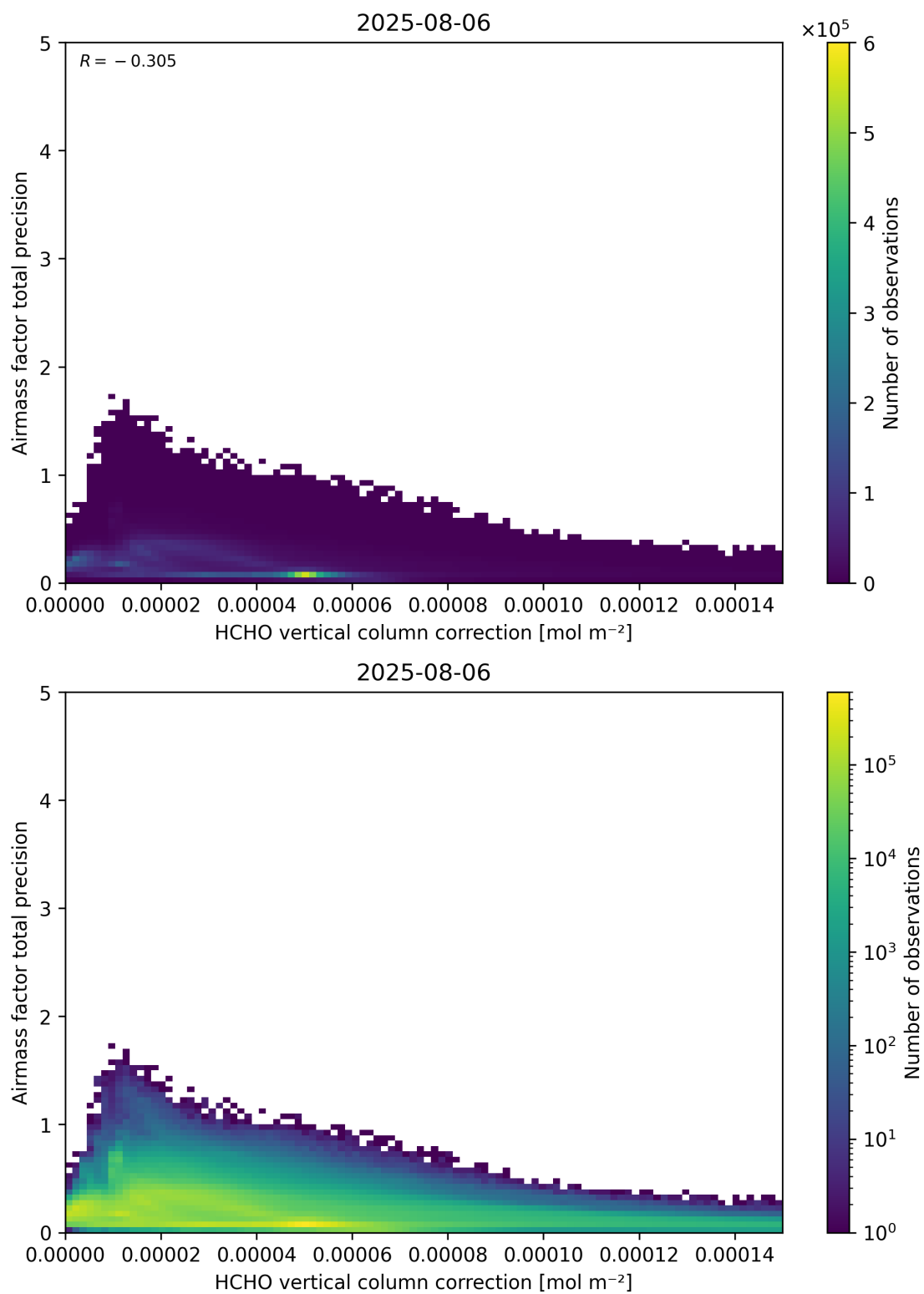
Figure 121: Scatter density plot of “HCHO vertical column correction” against “Airmass factor total precision” for 2025-08-05 to 2025-08-07.
