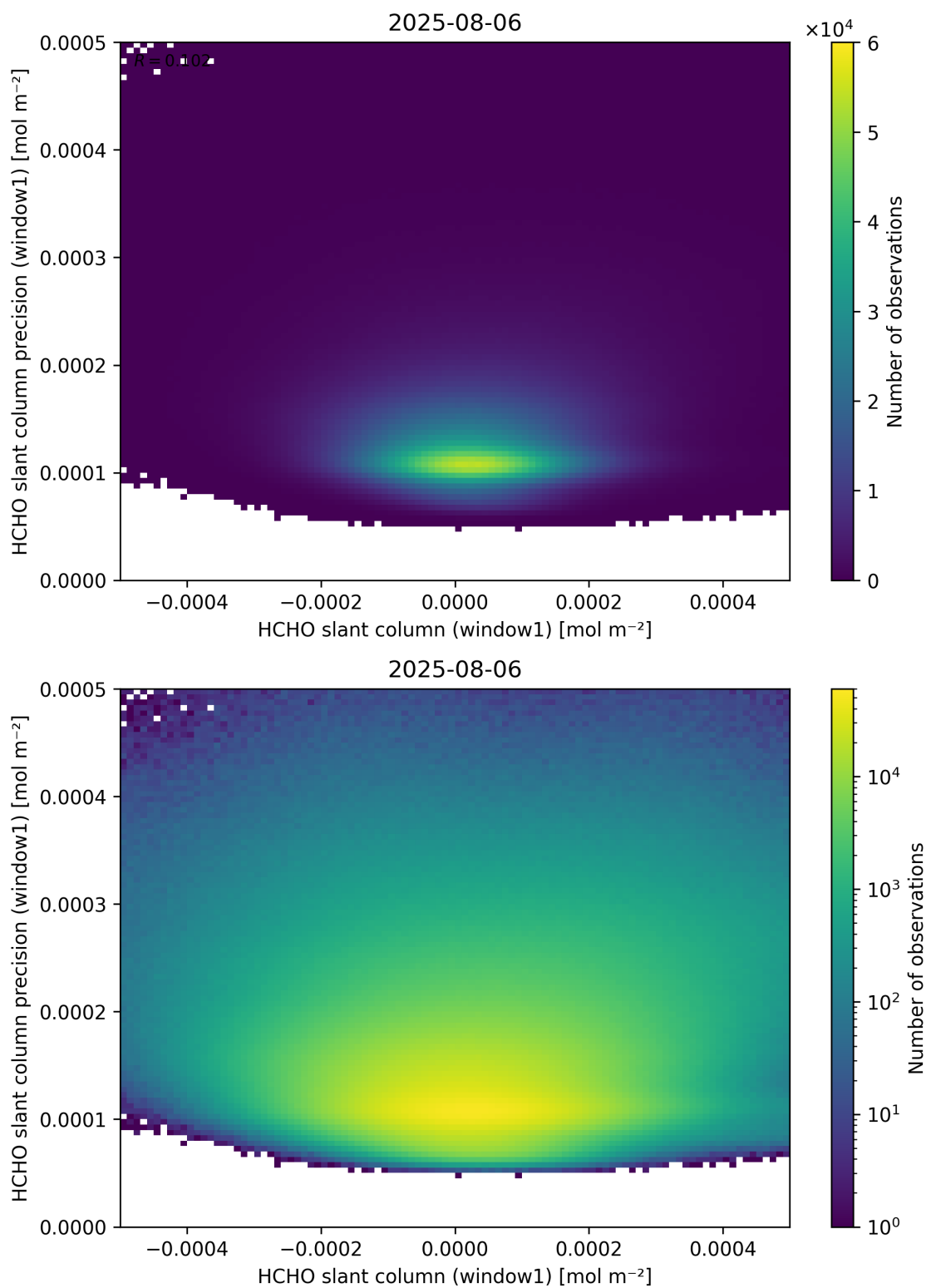
Figure 84: Scatter density plot of “HCHO slant column (window1)” against “HCHO slant column precision (window1)” for 2025-08-05 to 2025-08-07.
