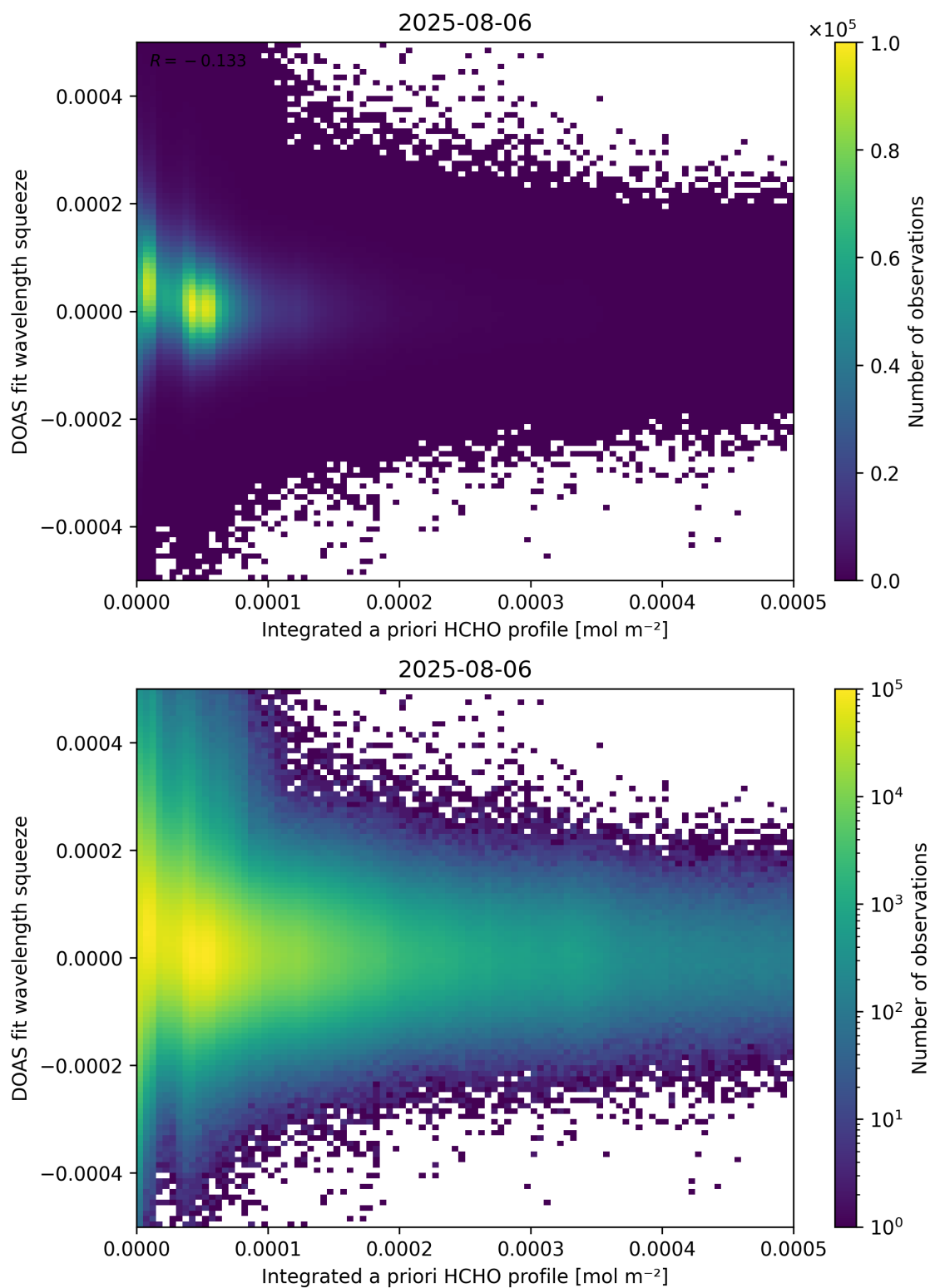
Figure 150: Scatter density plot of “Integrated a priori HCHO profile” against “DOAS fit wavelength squeeze” for 2025-08-05 to 2025-08-07.
