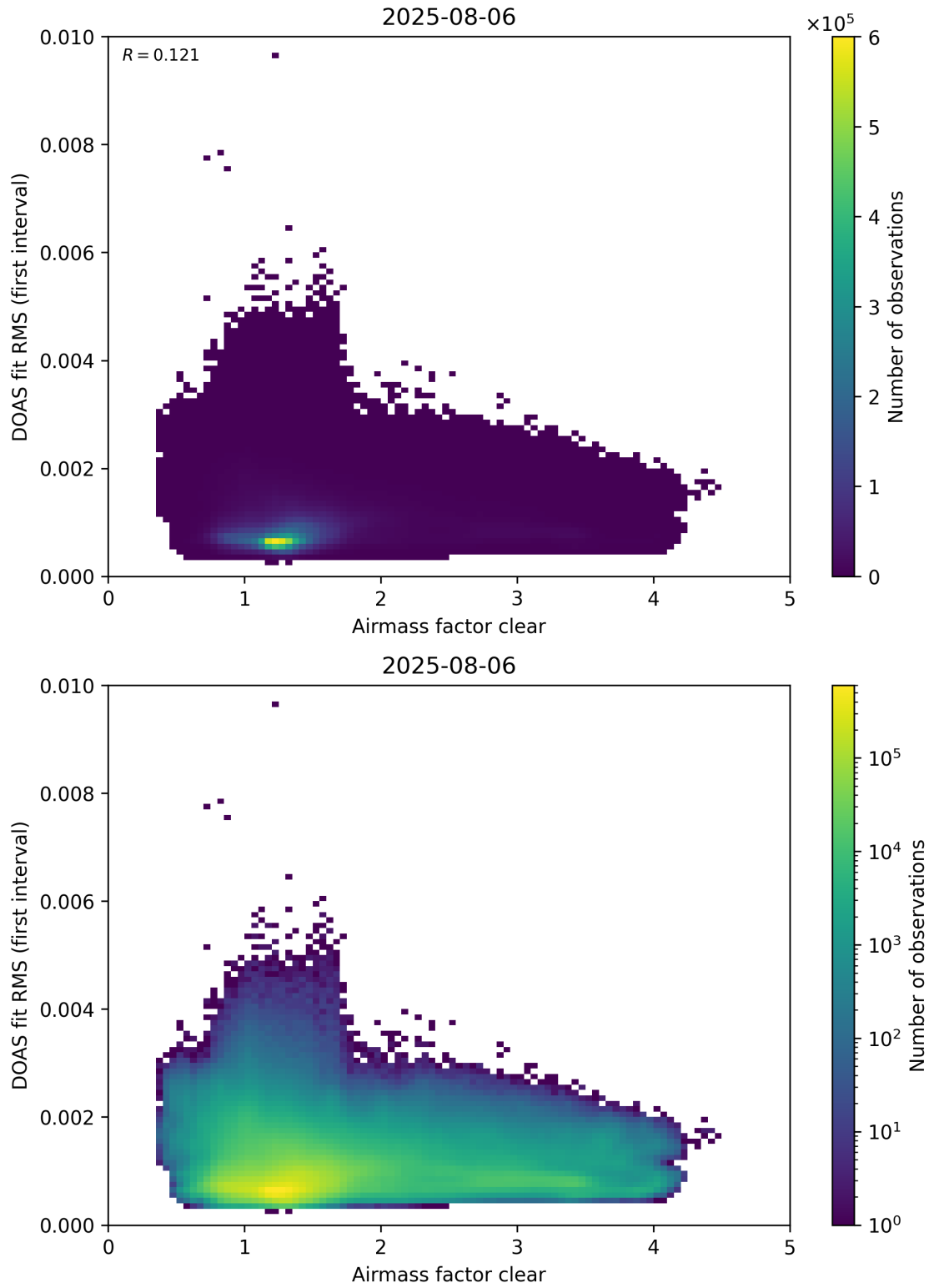
Figure 71: Scatter density plot of “Airmass factor clear” against “DOAS fit RMS (first interval)” for 2025-08-05 to 2025-08-07.
