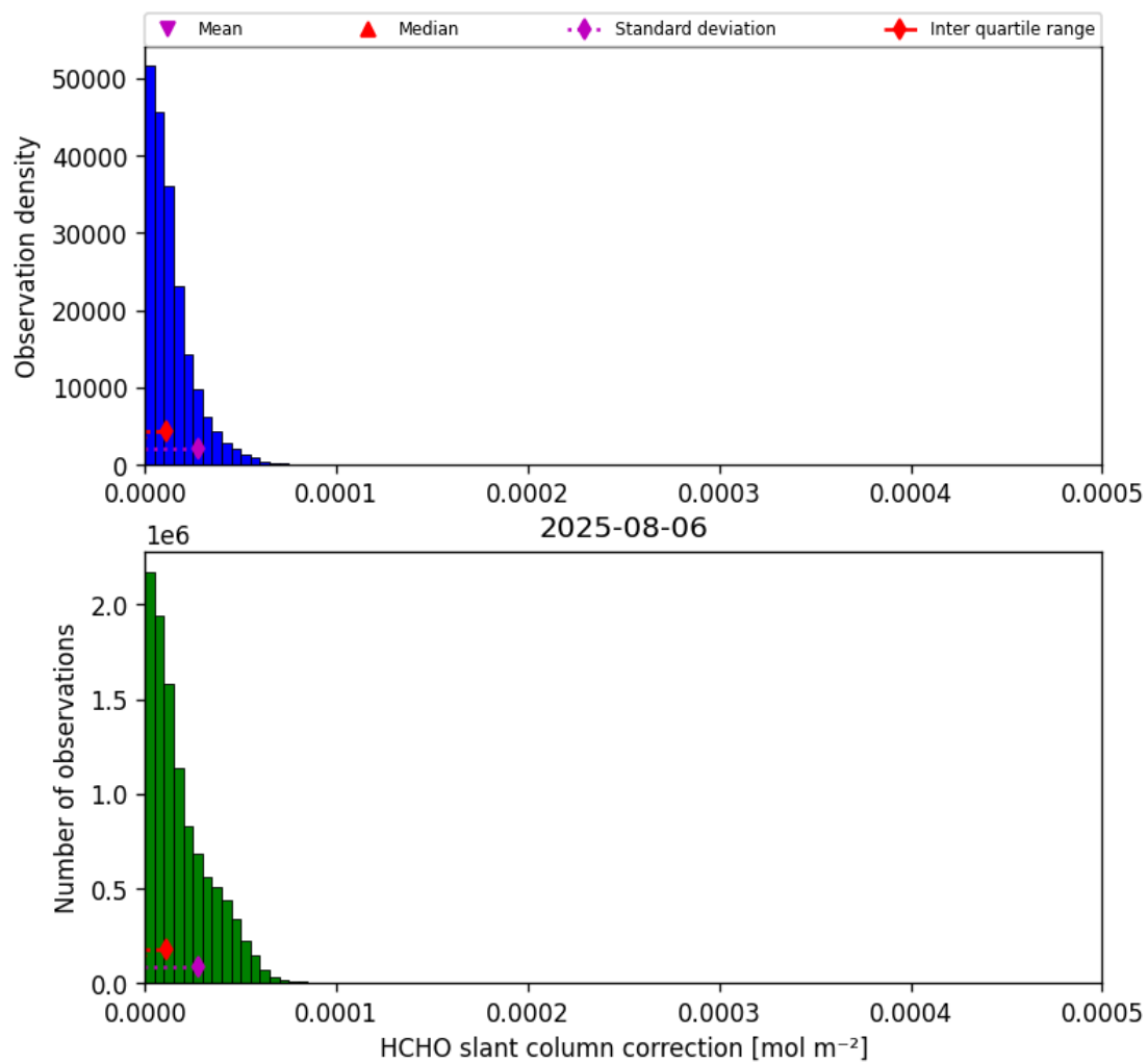
Figure 47: Histogram of “HCHO slant column correction” for 2025-08-05 to 2025-08-07
