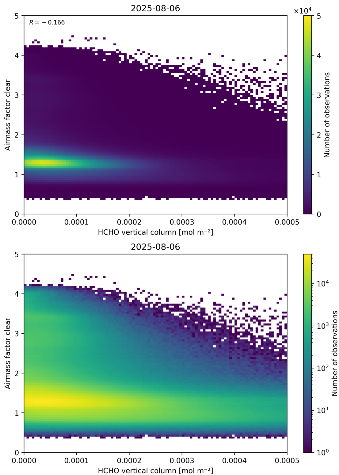
Figure 126: Scatter density plot of “HCHO vertical column” against “Airmass factor clear” for 2025-08-05 to 2025-08-07.
