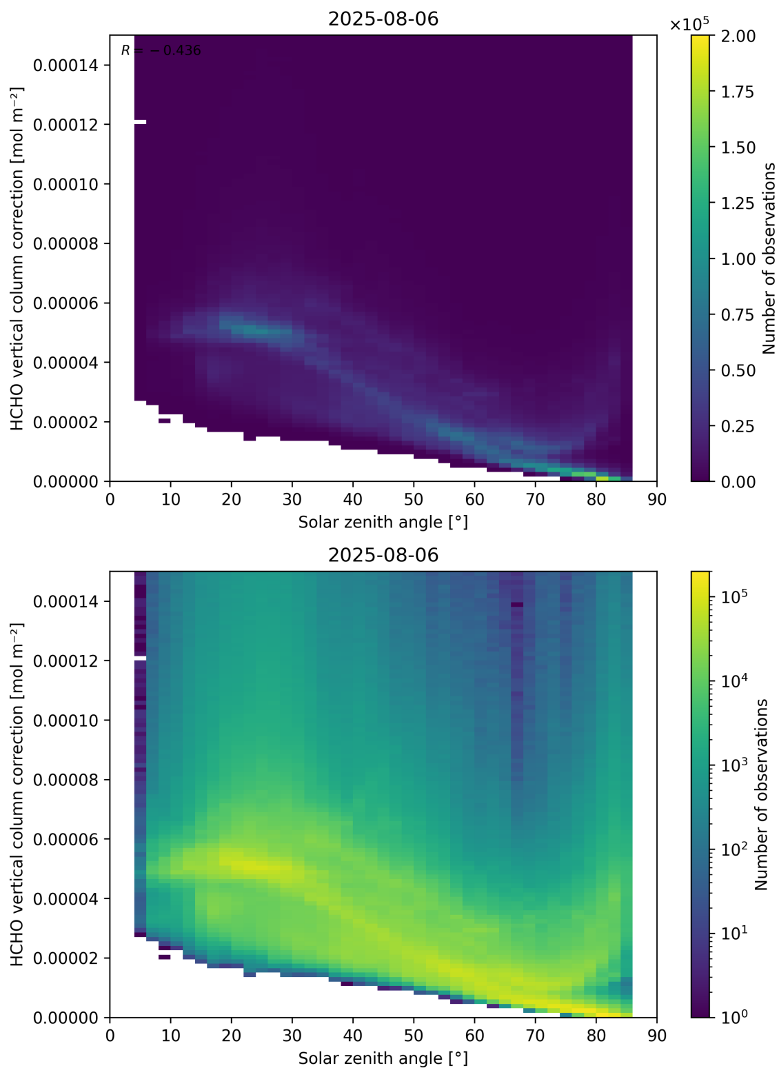
Figure 178: Scatter density plot of “Solar zenith angle” against “HCHO vertical column correction” for 2025-08-05 to 2025-08-07.
