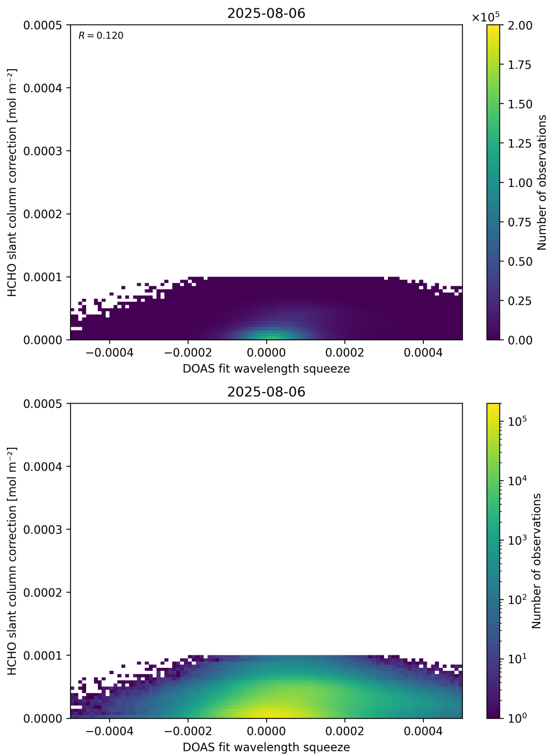
Figure 70: Scatter density plot of “DOAS fit wavelength squeeze” against “HCHO slant column correction” for 2025-08-05 to 2025-08-07.
