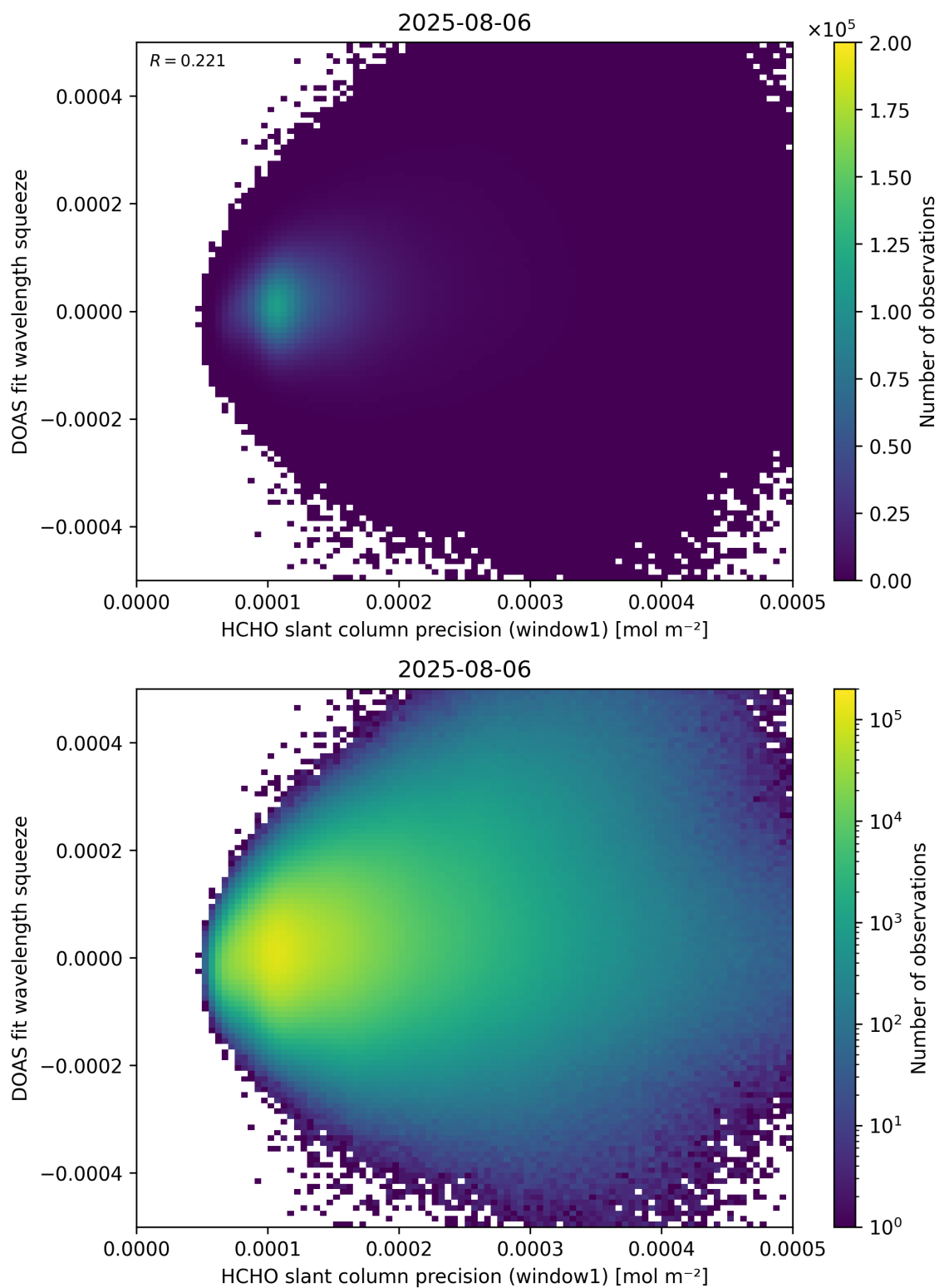
Figure 90: Scatter density plot of “HCHO slant column precision (window1)” against “DOAS fit wavelength squeeze” for 2025-08-05 to 2025-08-07.
