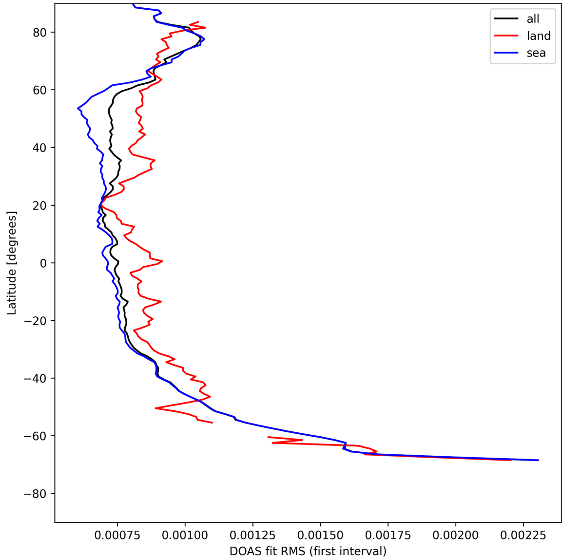
Figure 32: Zonal average of "DOAS fit RMS (first interval)" for 2025-08-05 to 2025-08-07.
