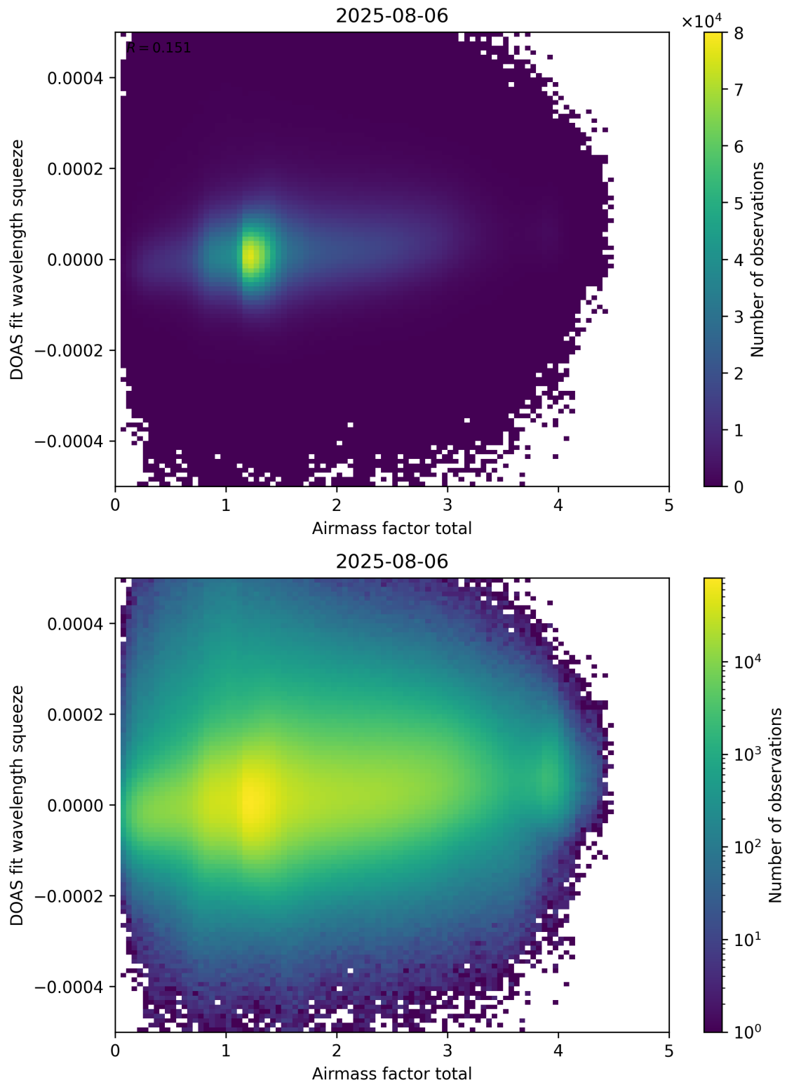
Figure 99: Scatter density plot of “Airmass factor total” against “DOAS fit wavelength squeeze” for 2025-08-05 to 2025-08-07.
