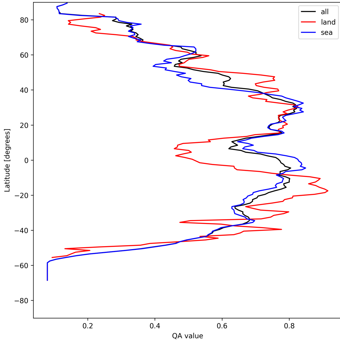
Figure 20: Zonal average of “QA value” for 2025-08-05 to 2025-08-07.
