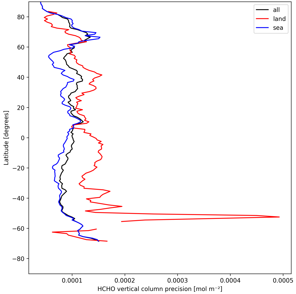
Figure 22: Zonal average of “HCHO vertical column precision” for 2025-08-05 to 2025-08-07.
