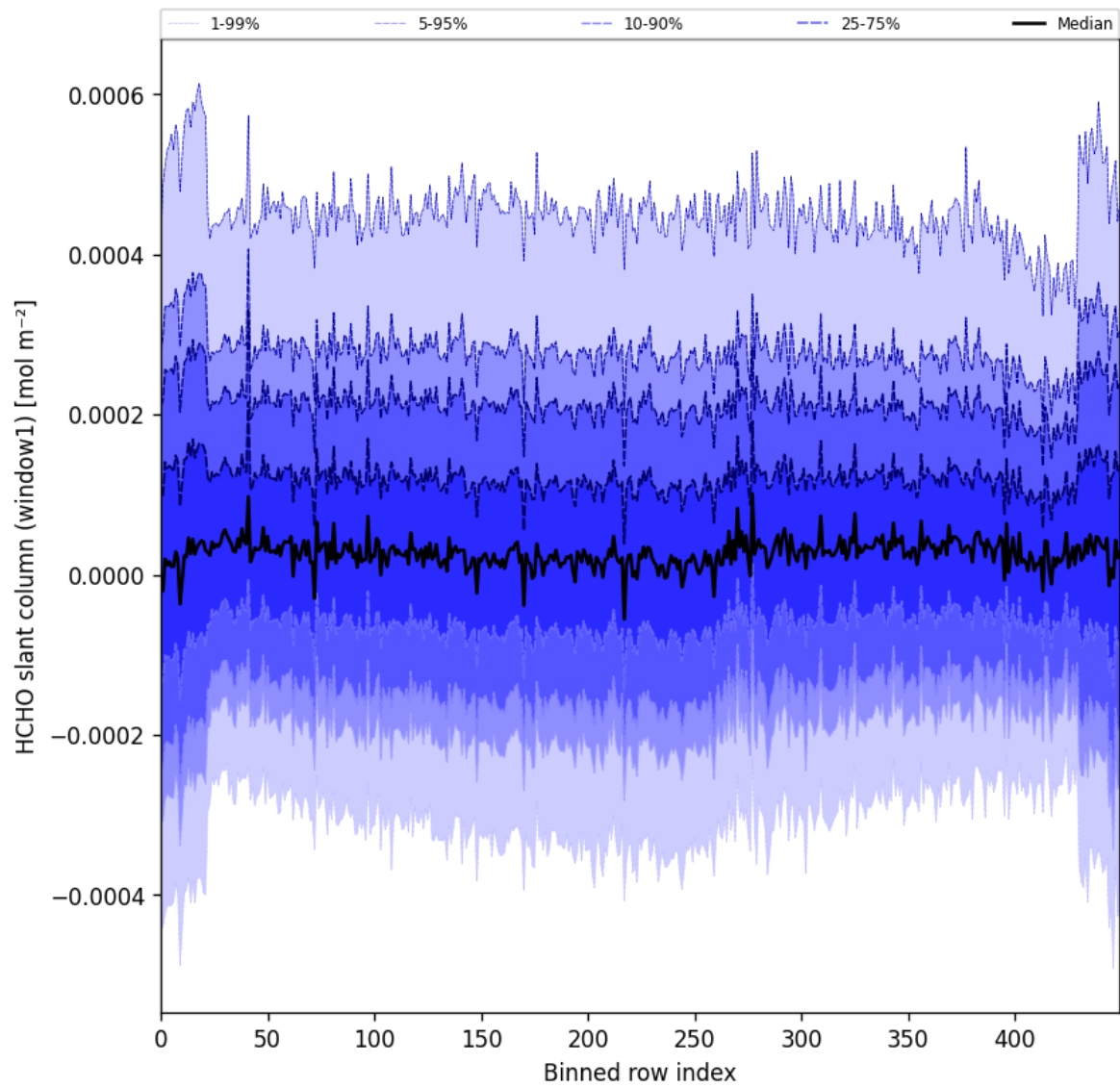
Figure 52: Along track statistics of “HCHO slant column (window1)” for 2025-08-05 to 2025-08-07
