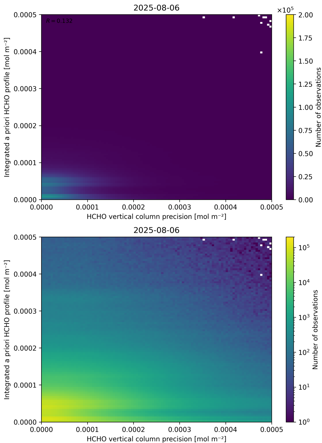
Figure 147: Scatter density plot of “HCHO vertical column precision” against “Integrated a priori HCHO profile” for 2025-08-05 to 2025-08-07.
