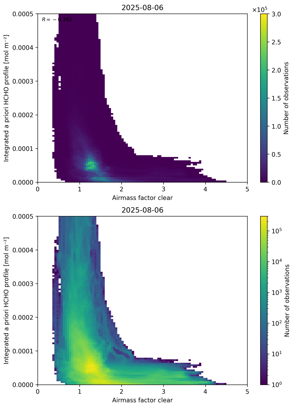
Figure 76: Scatter density plot of “Airmass factor clear” against “Integrated a priori HCHO profile” for 2025-08-05 to 2025-08-07.
