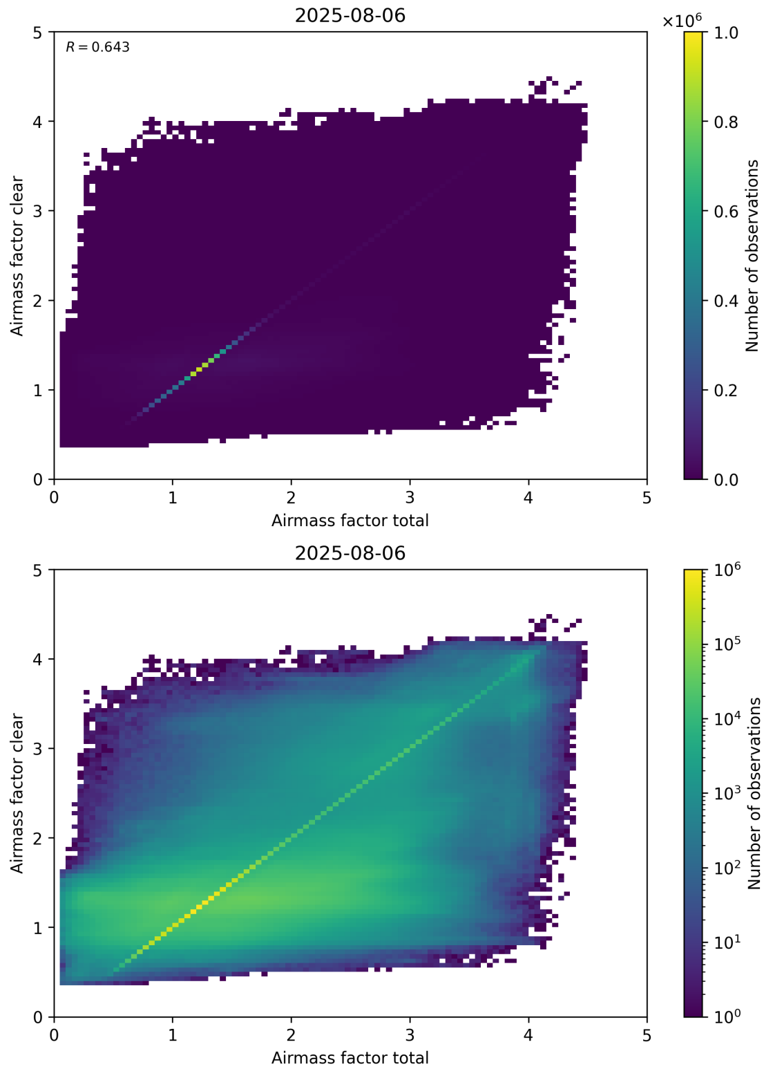
Figure 100: Scatter density plot of “Airmass factor total” against “Airmass factor clear” for 2025-08-05 to 2025-08-07.
