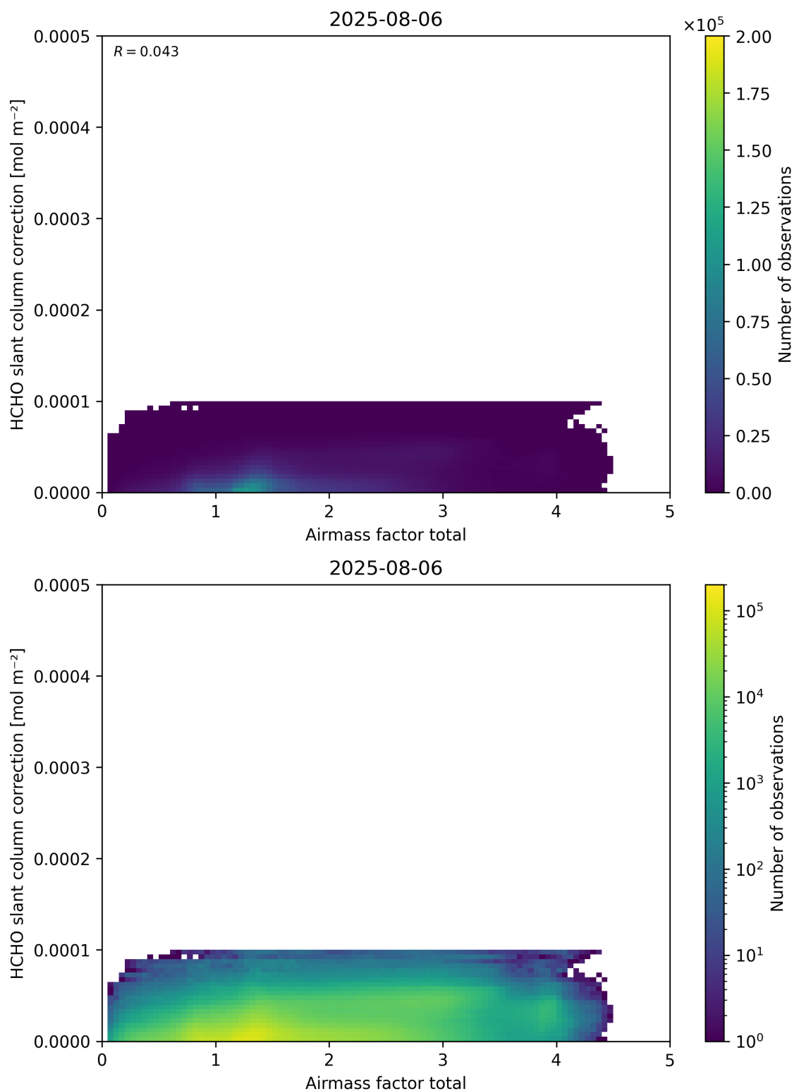
Figure 102: Scatter density plot of “Airmass factor total” against “HCHO slant column correction” for 2025-08-05 to 2025-08-07.
