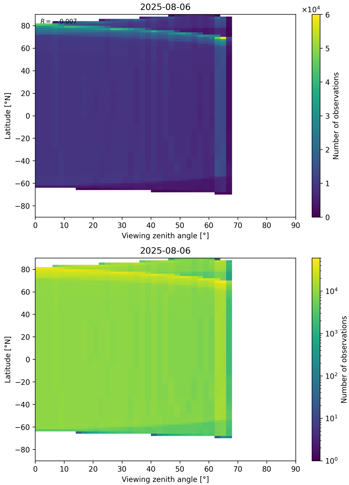
Figure 196: Scatter density plot of “Viewing zenith angle” against “Latitude” for 2025-08-05 to 2025-08-07.
