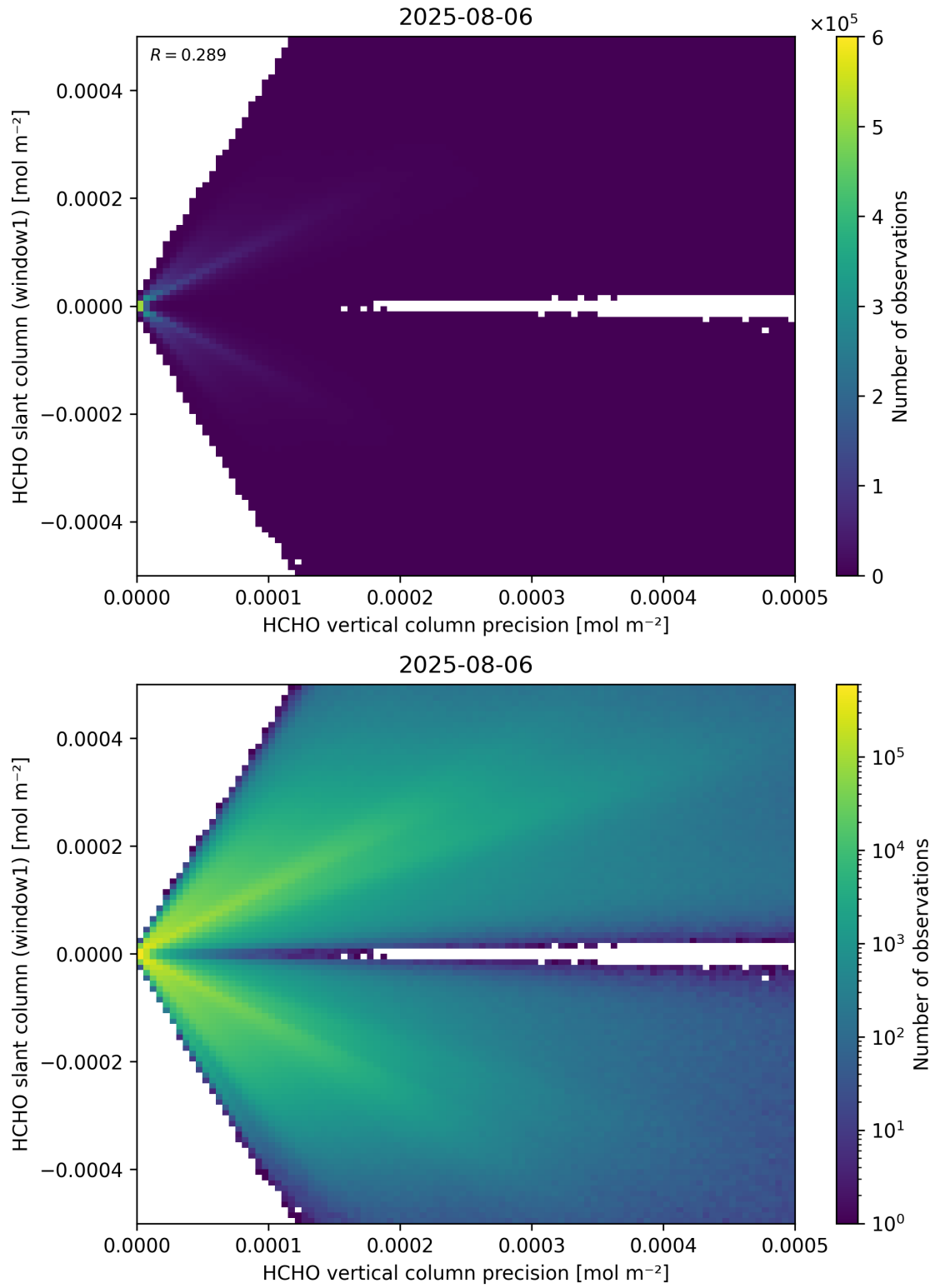
Figure 142: Scatter density plot of “HCHO vertical column precision” against “HCHO slant column (window1)” for 2025-08-05 to 2025-08-07.
