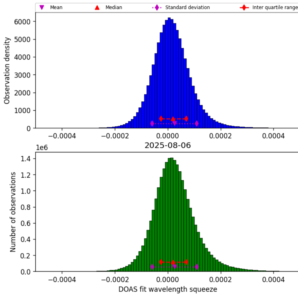
Figure 45: Histogram of “DOAS fit wavelength squeeze” for 2025-08-05 to 2025-08-07
