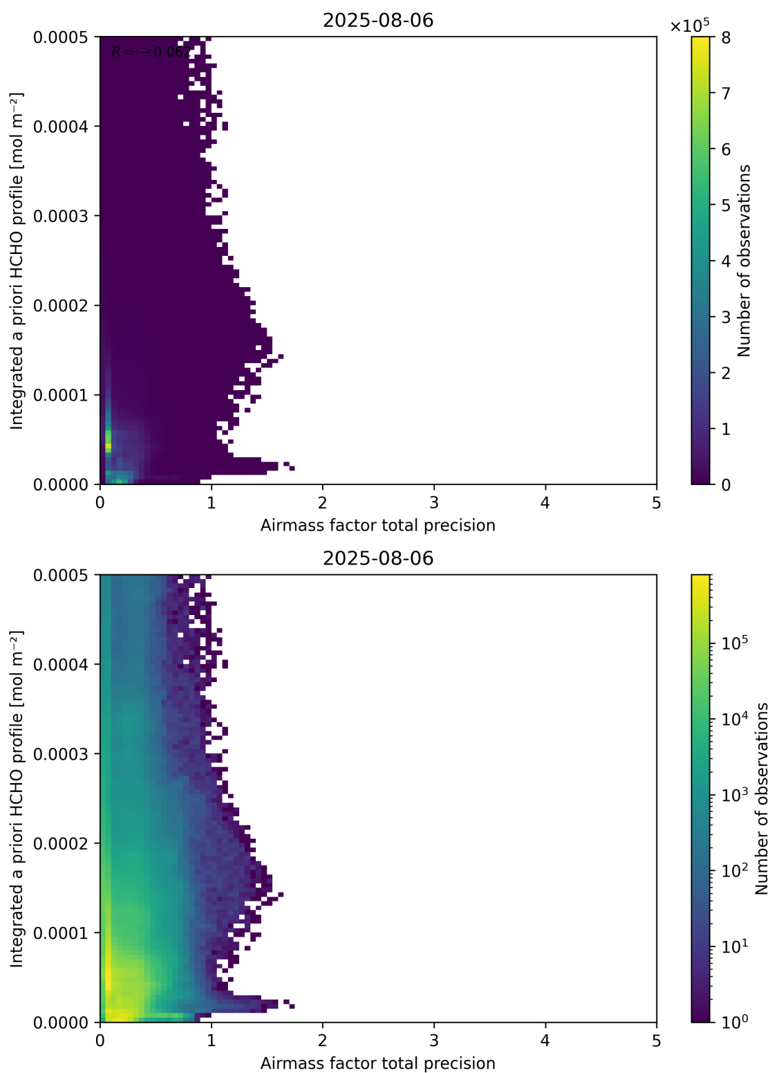
Figure 111: Scatter density plot of “Airmass factor total precision” against “Integrated a priori HCHO profile” for 2025-08-05 to 2025-08-07.
