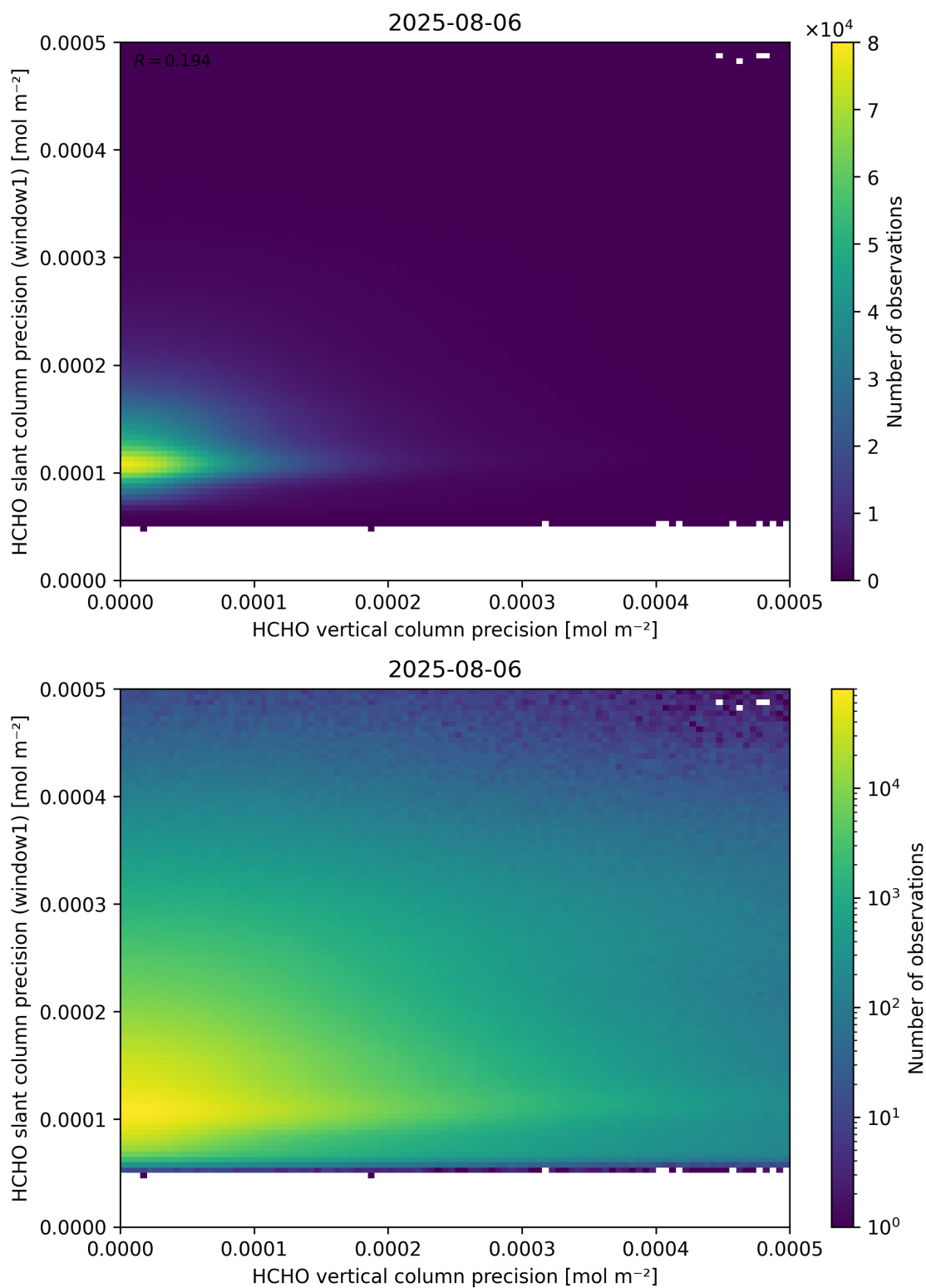
Figure 143: Scatter density plot of “HCHO vertical column precision” against “HCHO slant column precision (window1)” for 2025-08-05 to 2025-08-07.
