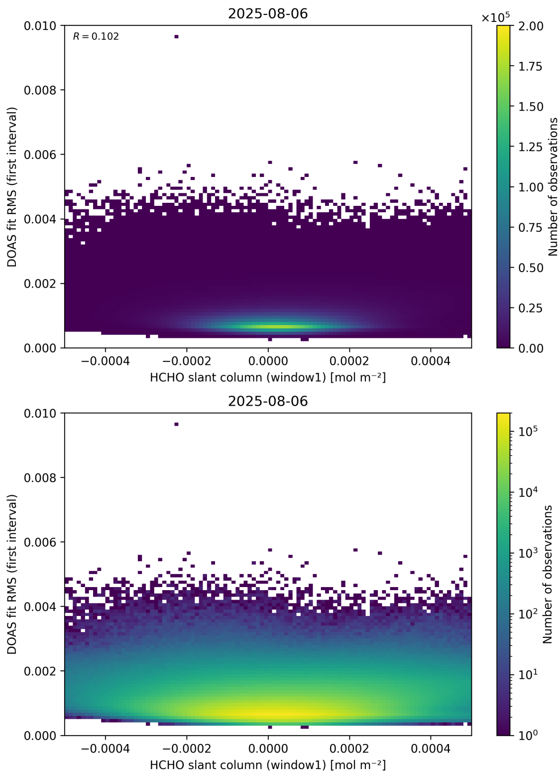
Figure 78: Scatter density plot of “HCHO slant column (window1)” against “DOAS fit RMS (first interval)” for 2025-08-05 to 2025-08-07.
