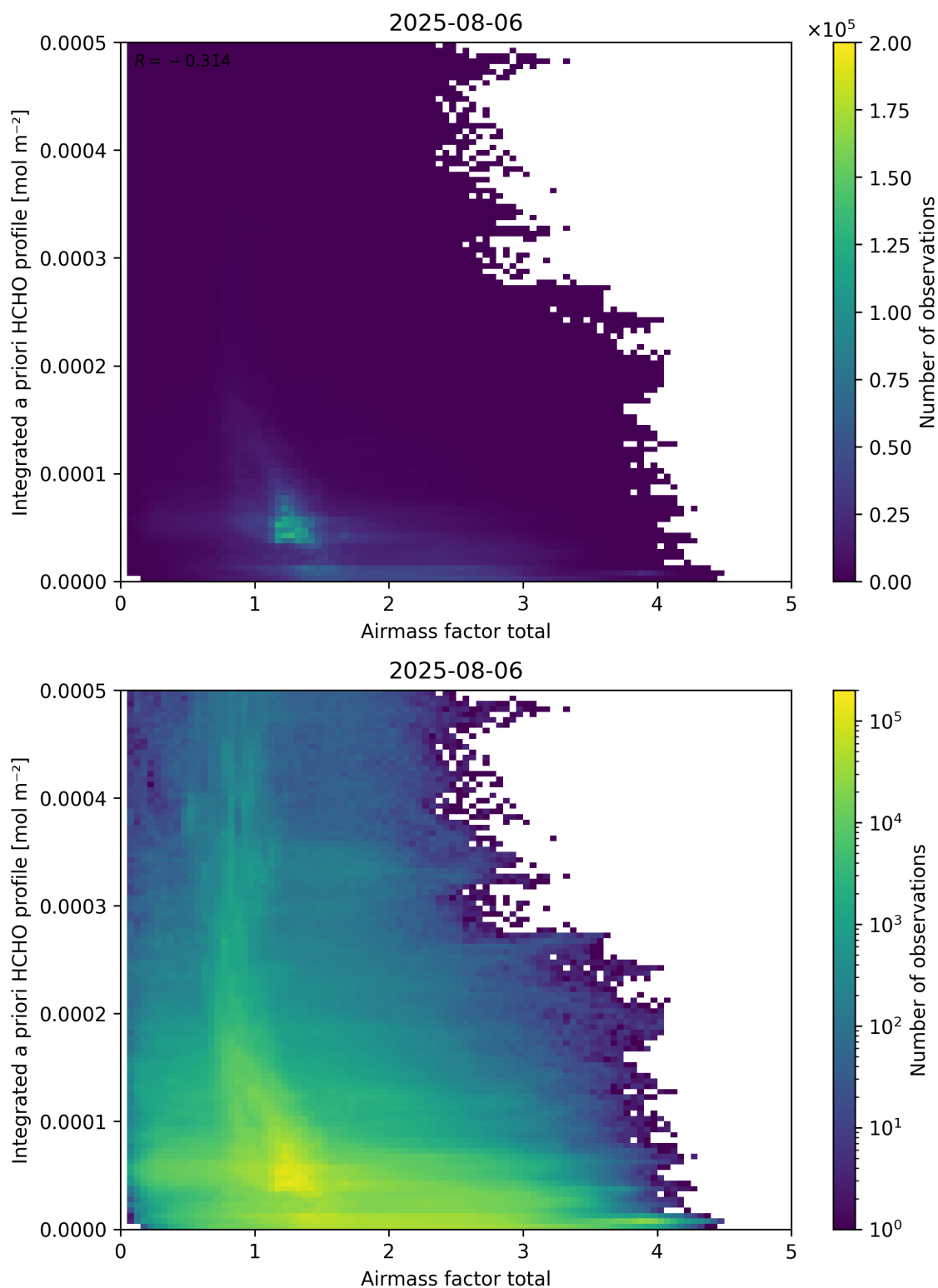
Figure 104: Scatter density plot of “Airmass factor total” against “Integrated a priori HCHO profile” for 2025-08-05 to 2025-08-07.
