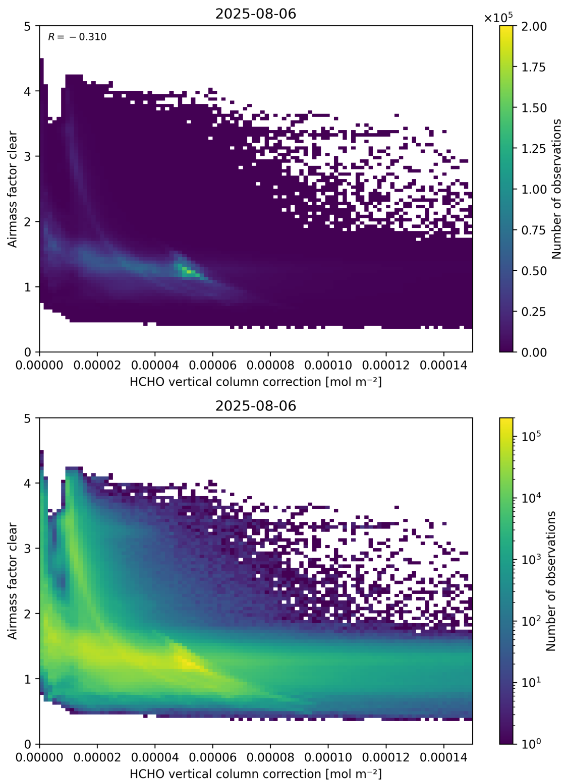
Figure 115: Scatter density plot of “HCHO vertical column correction” against “Airmass factor clear” for 2025-08-05 to 2025-08-07.
