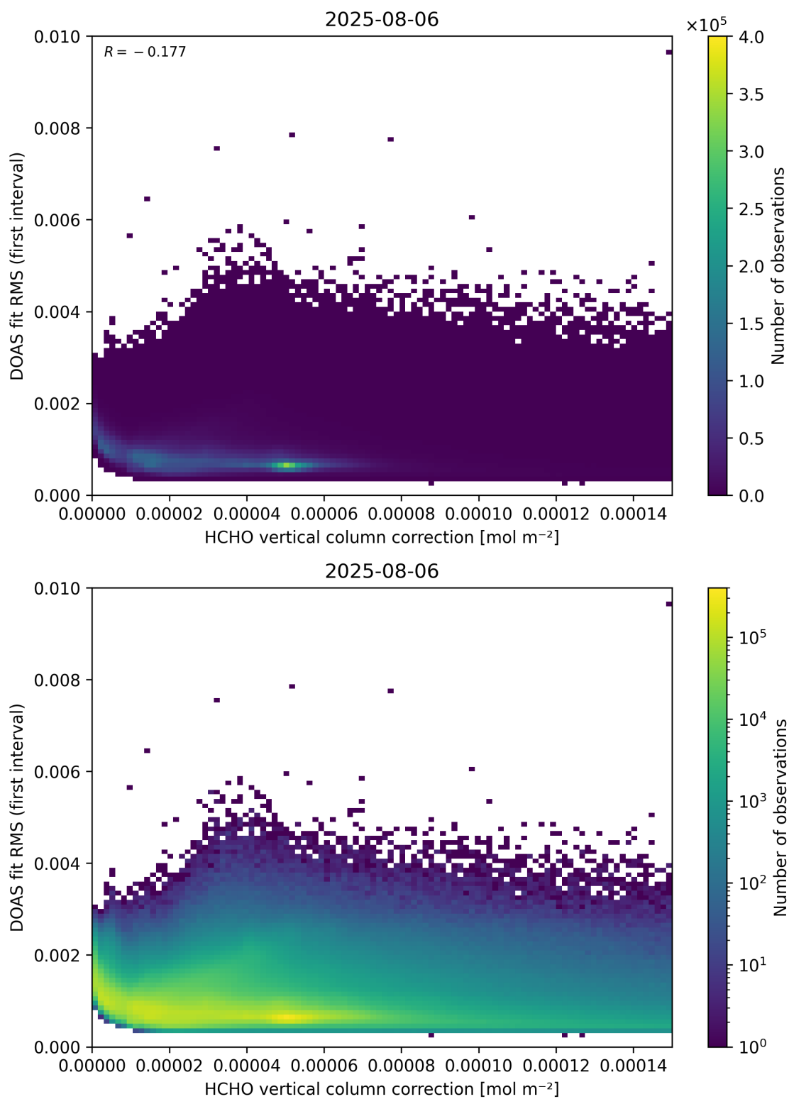
Figure 112: Scatter density plot of “HCHO vertical column correction” against “DOAS fit RMS (first interval)” for 2025-08-05 to 2025-08-07.
