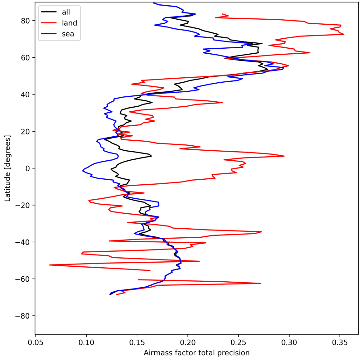
Figure 27: Zonal average of “Airmass factor total precision” for 2025-08-05 to 2025-08-07.
