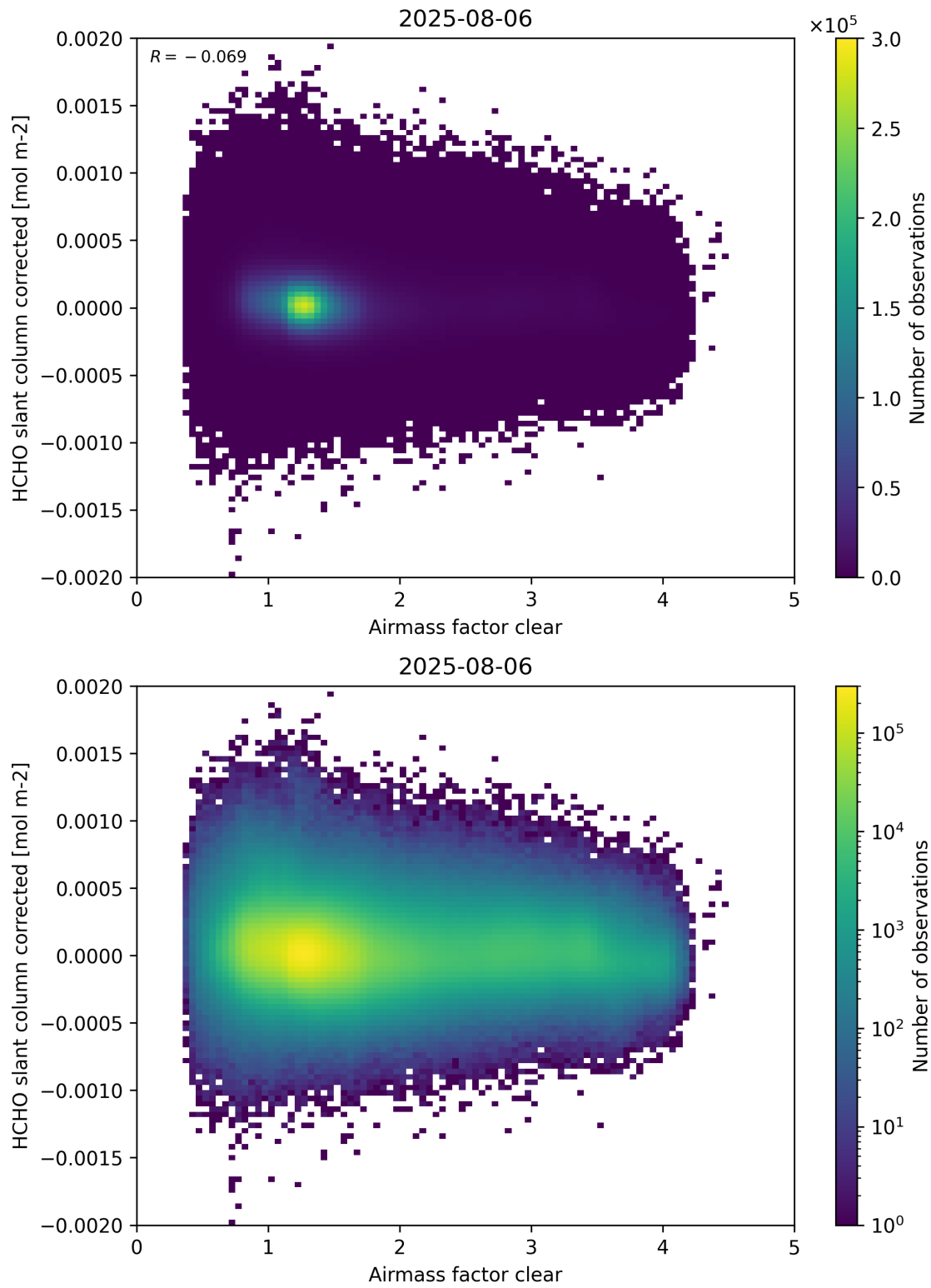
Figure 74: Scatter density plot of “Airmass factor clear” against “HCHO slant column corrected” for 2025-08-05 to 2025-08-07.
