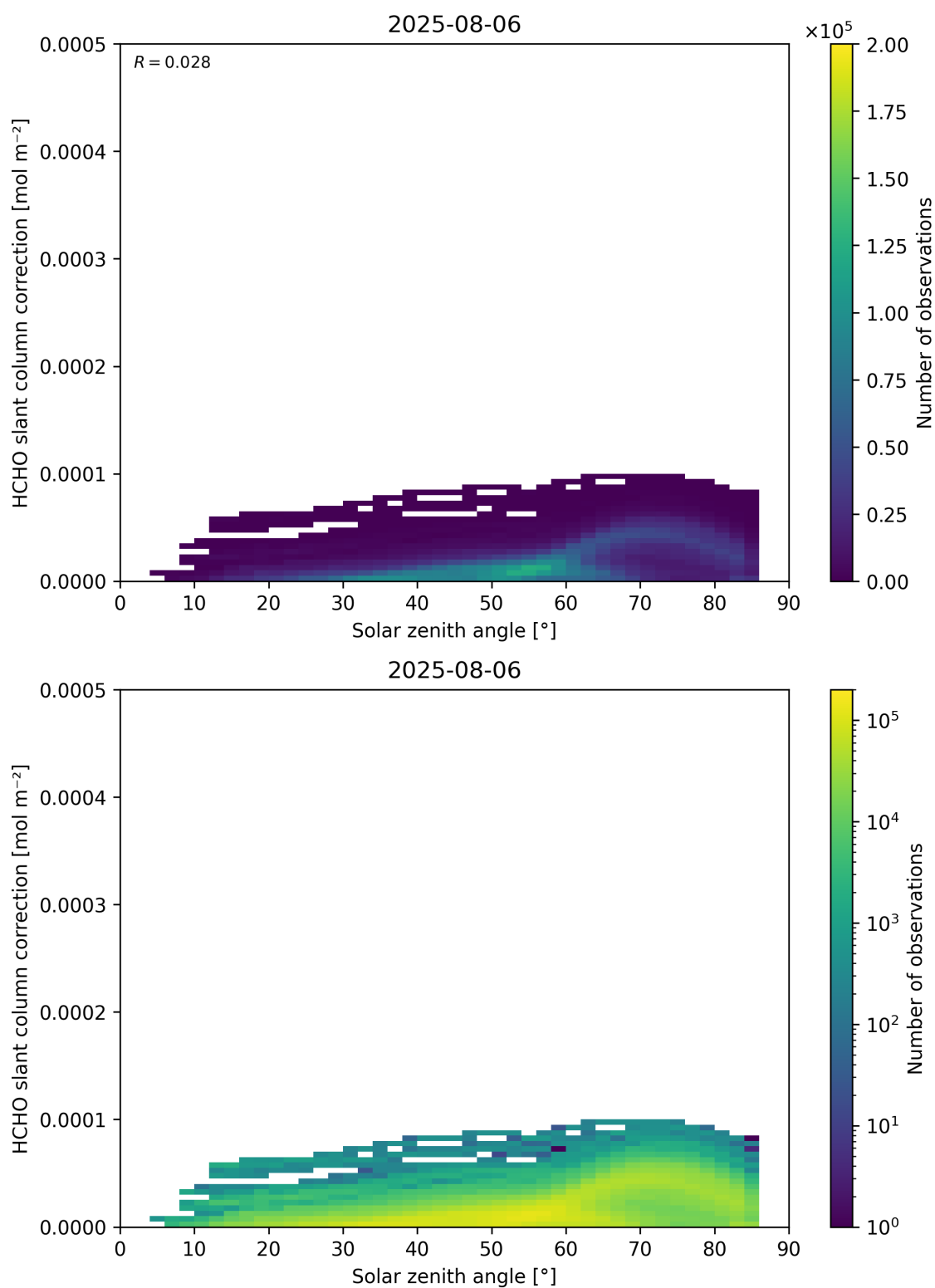
Figure 172: Scatter density plot of “Solar zenith angle” against “HCHO slant column correction” for 2025-08-05 to 2025-08-07.
