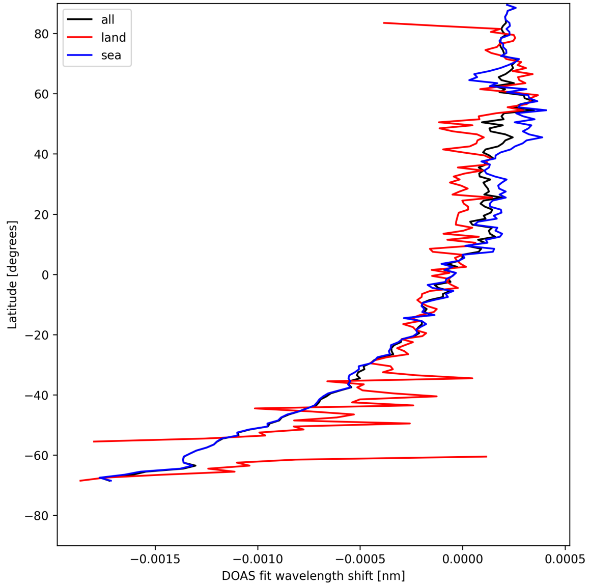
Figure 30: Zonal average of “DOAS fit wavelength shift” for 2025-08-05 to 2025-08-07.
