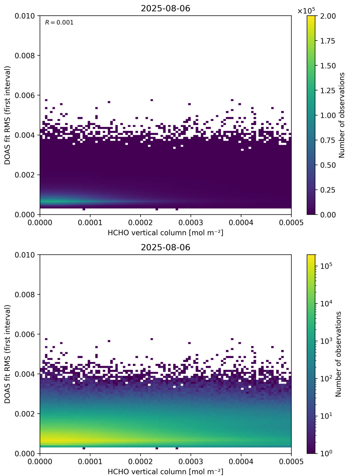
Figure 123: Scatter density plot of “HCHO vertical column” against “DOAS fit RMS (first interval)” for 2025-08-05 to 2025-08-07.
