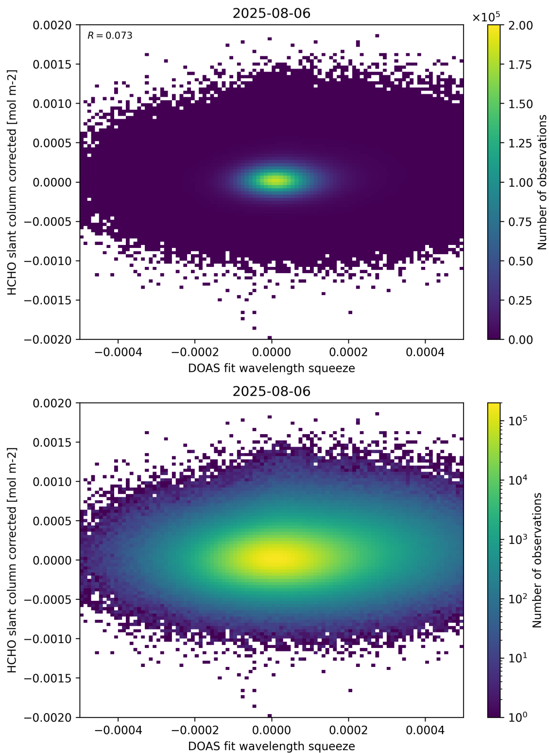
Figure 69: Scatter density plot of “DOAS fit wavelength squeeze” against “HCHO slant column corrected” for 2025-08-05 to 2025-08-07.
