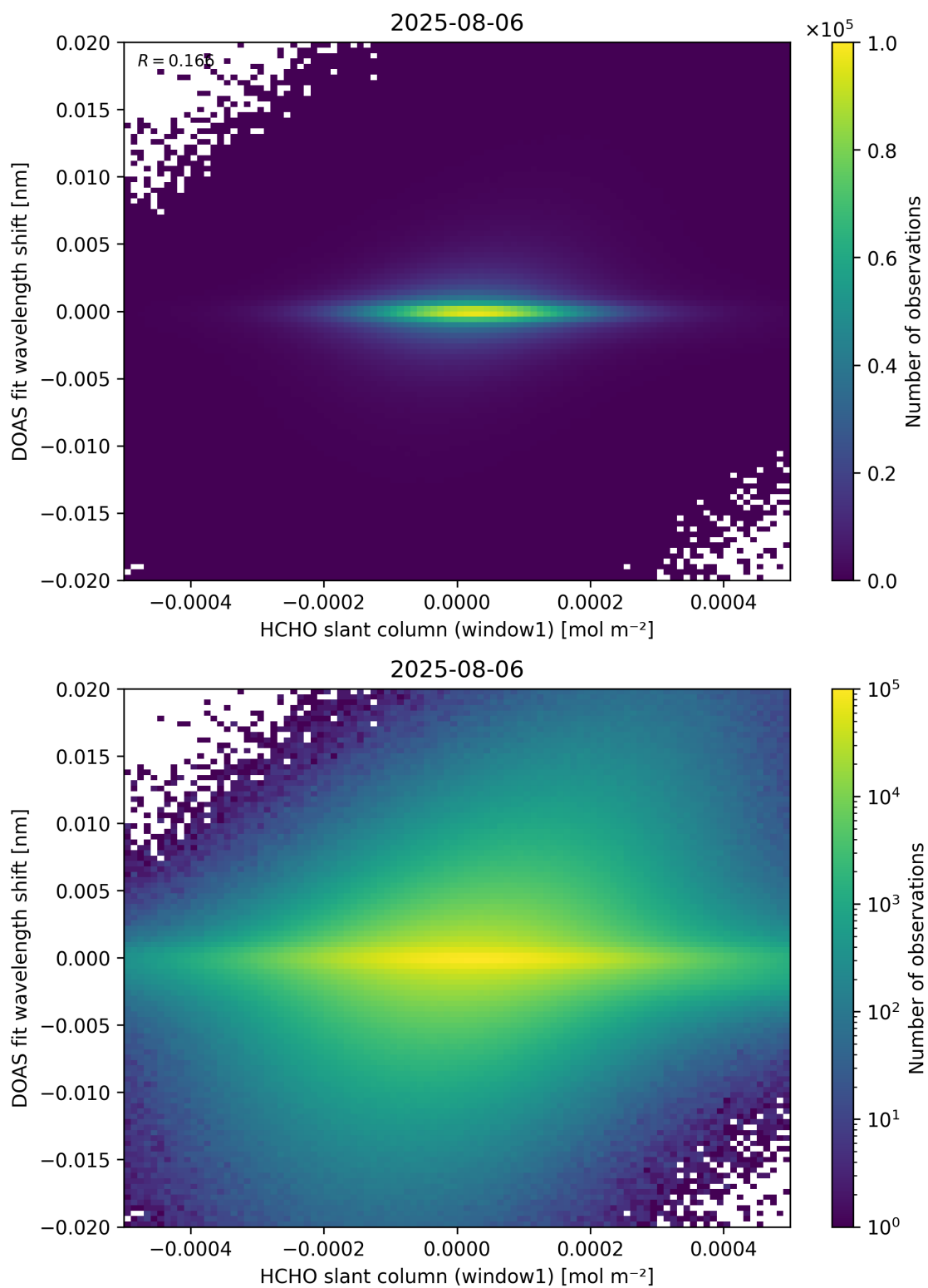
Figure 79: Scatter density plot of “HCHO slant column (window1)” against “DOAS fit wavelength shift” for 2025-08-05 to 2025-08-07.
