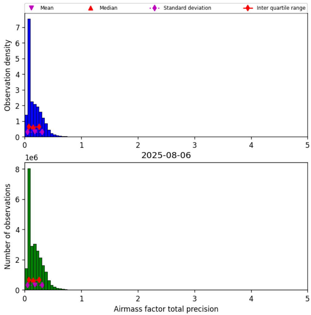
Figure 41: Histogram of “Airmass factor total precision” for 2025-08-05 to 2025-08-07
