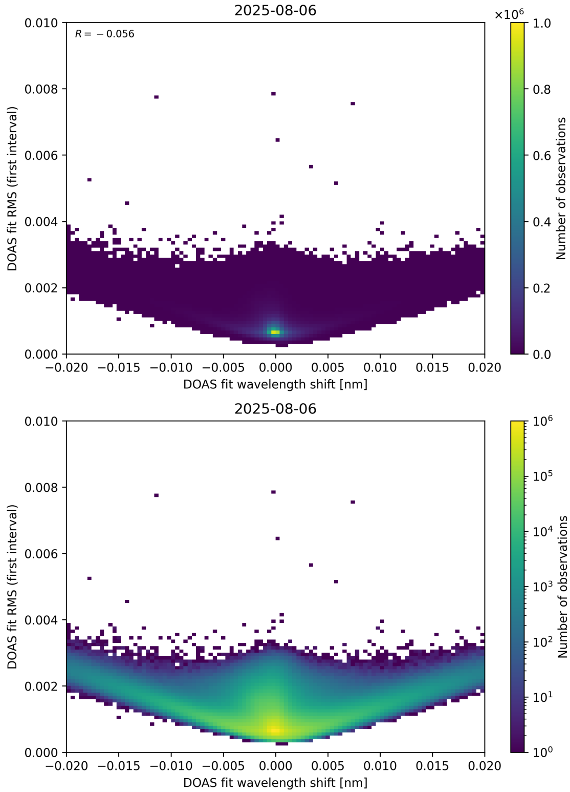
Figure 64: Scatter density plot of “DOAS fit wavelength shift” against “DOAS fit RMS (first interval)” for 2025-08-05 to 2025-08-07.
