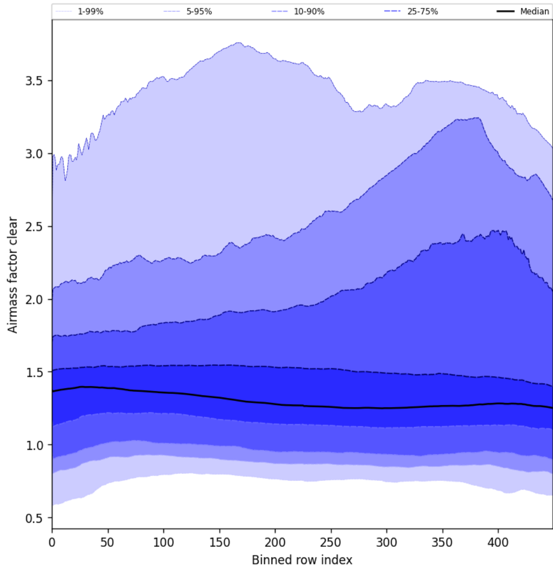
Figure 56: Along track statistics of “Airmass factor clear” for 2025-08-05 to 2025-08-07
