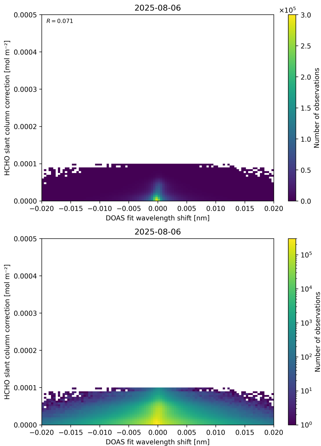
Figure 67: Scatter density plot of “DOAS fit wavelength shift” against “HCHO slant column correction” for 2025-08-05 to 2025-08-07.
