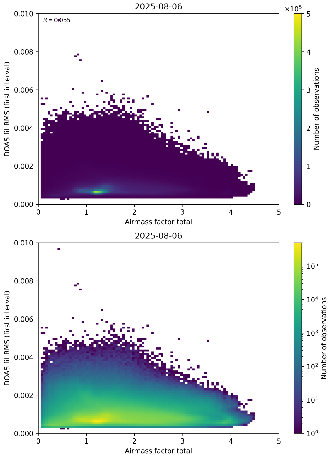
Figure 97: Scatter density plot of “Airmass factor total” against “DOAS fit RMS (first interval)” for 2025-08-05 to 2025-08-07.
