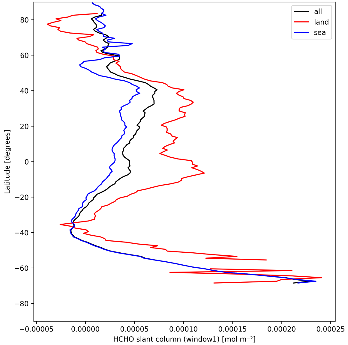
Figure 24: Zonal average of “HCHO slant column (window1)” for 2025-08-05 to 2025-08-07.
