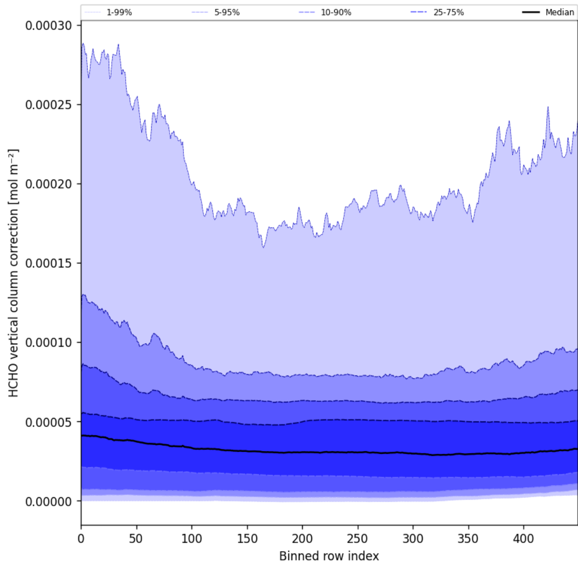
Figure 51: Along track statistics of “HCHO vertical column correction” for 2025-08-05 to 2025-08-07
