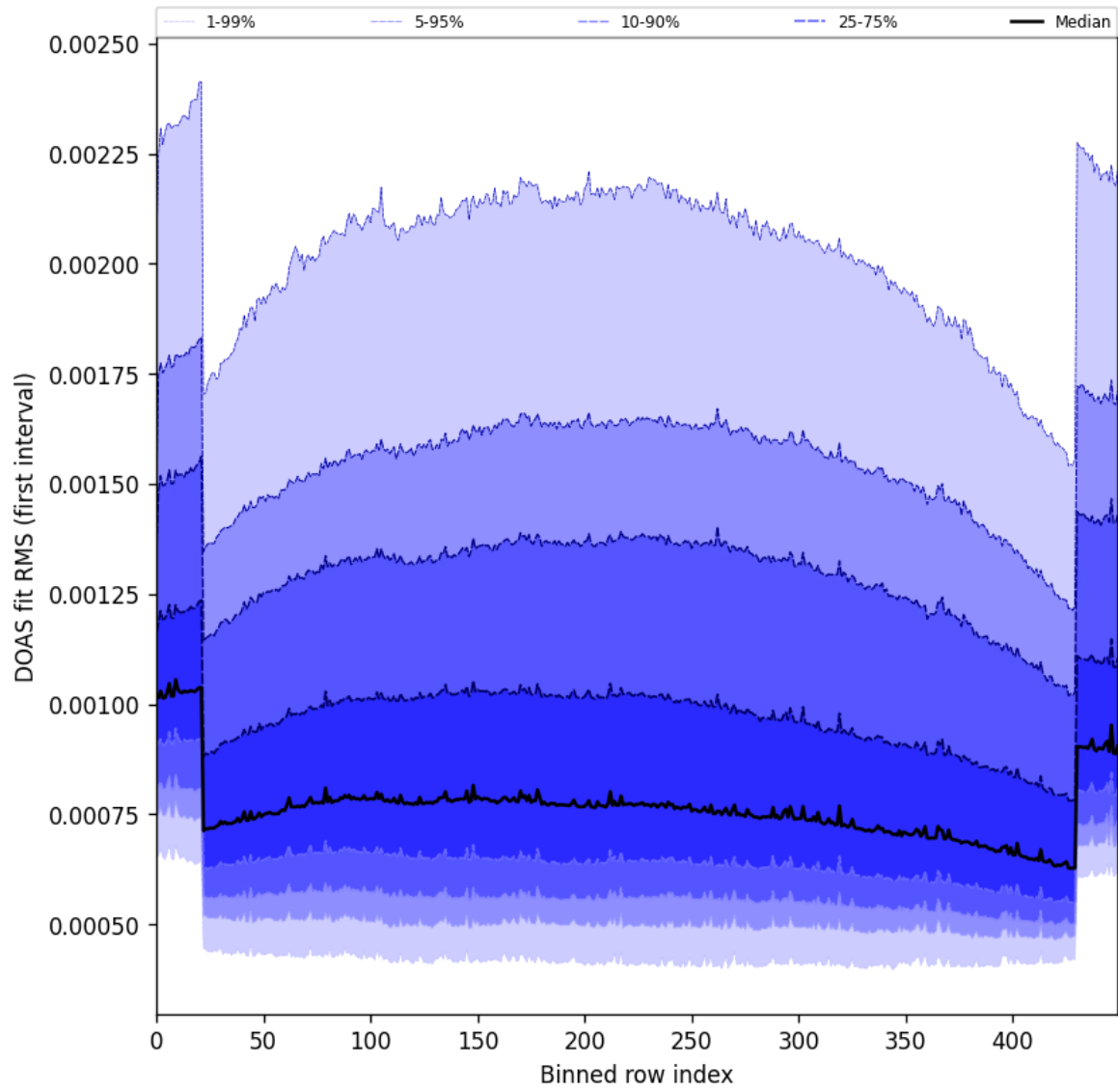
Figure 60: Along track statistics of “DOAS fit RMS (first interval)” for 2025-08-05 to 2025-08-07
