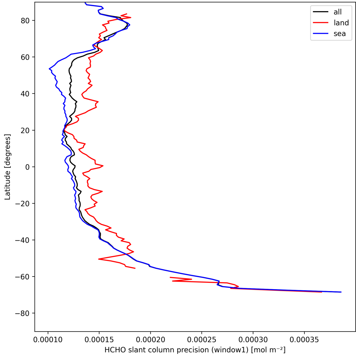
Figure 25: Zonal average of “HCHO slant column precision (window1)” for 2025-08-05 to 2025-08-07.
