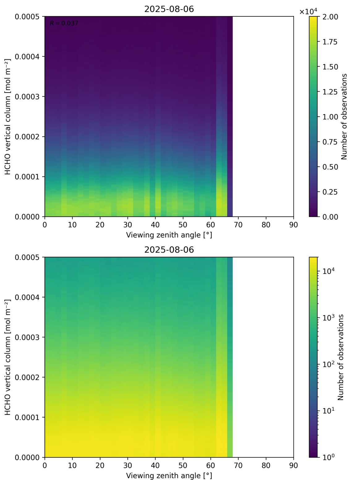
Figure 192: Scatter density plot of “Viewing zenith angle” against “HCHO vertical column” for 2025-08-05 to 2025-08-07.
