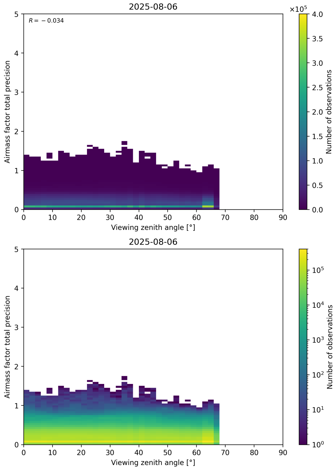
Figure 191: Scatter density plot of “Viewing zenith angle” against “Airmass factor total precision” for 2025-08-05 to 2025-08-07.
