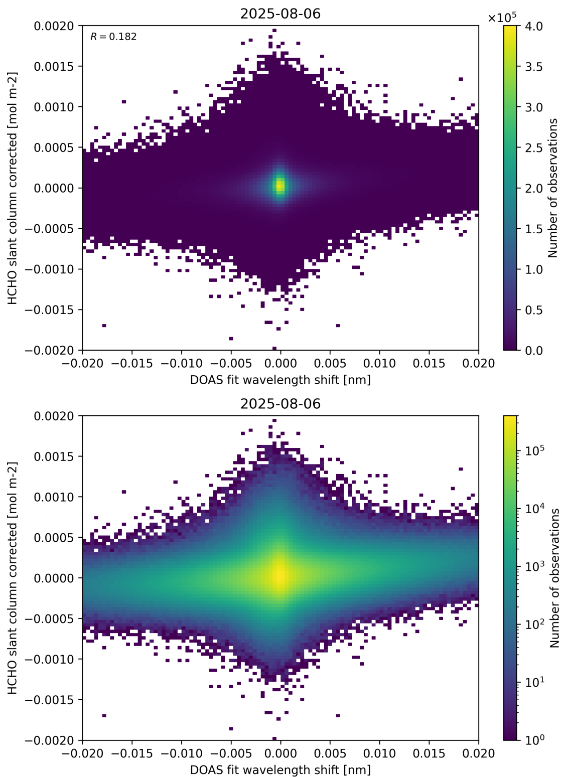
Figure 66: Scatter density plot of “DOAS fit wavelength shift” against “HCHO slant column corrected” for 2025-08-05 to 2025-08-07.
