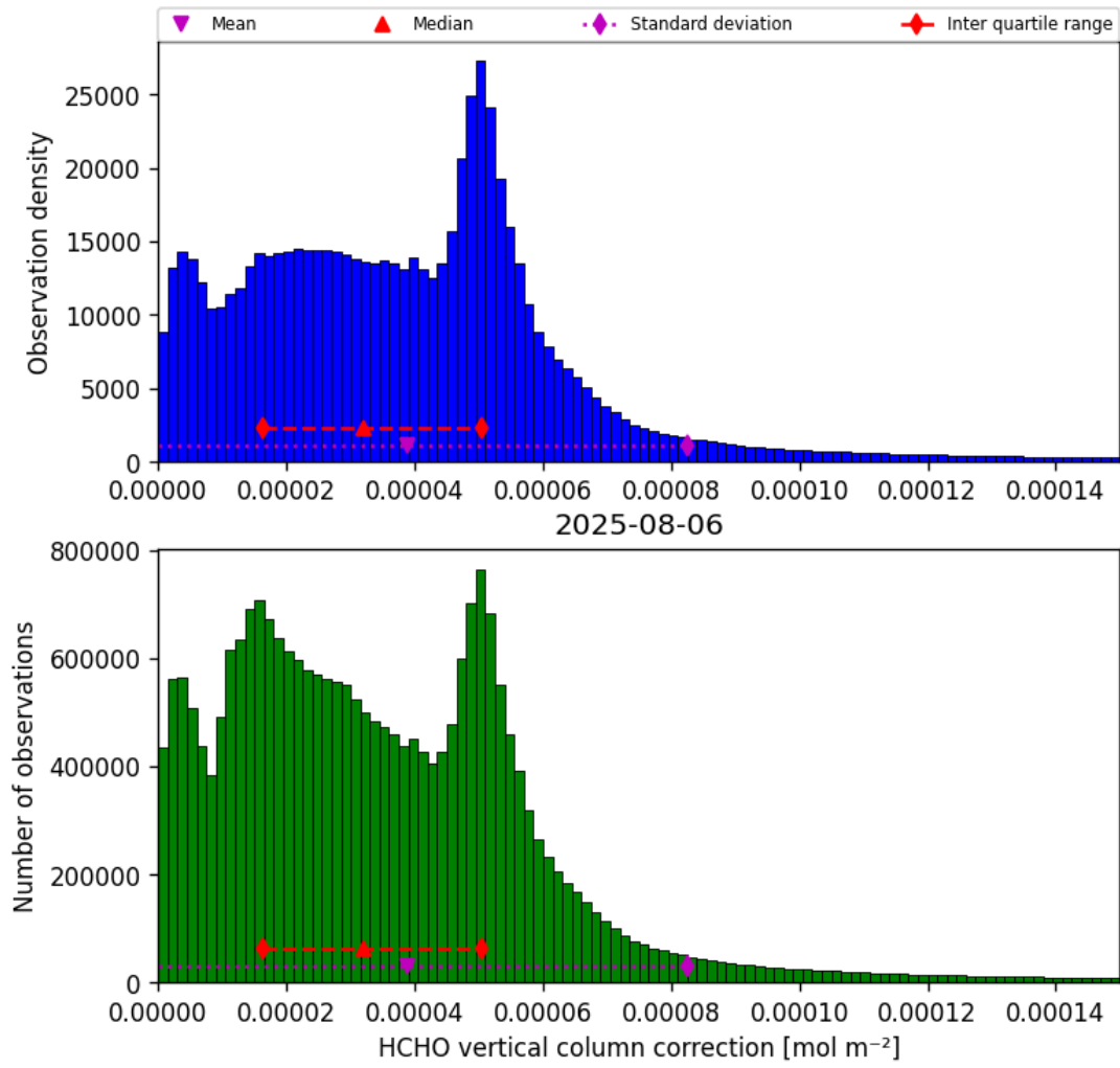
Figure 37: Histogram of “HCHO vertical column correction” for 2025-08-05 to 2025-08-07
