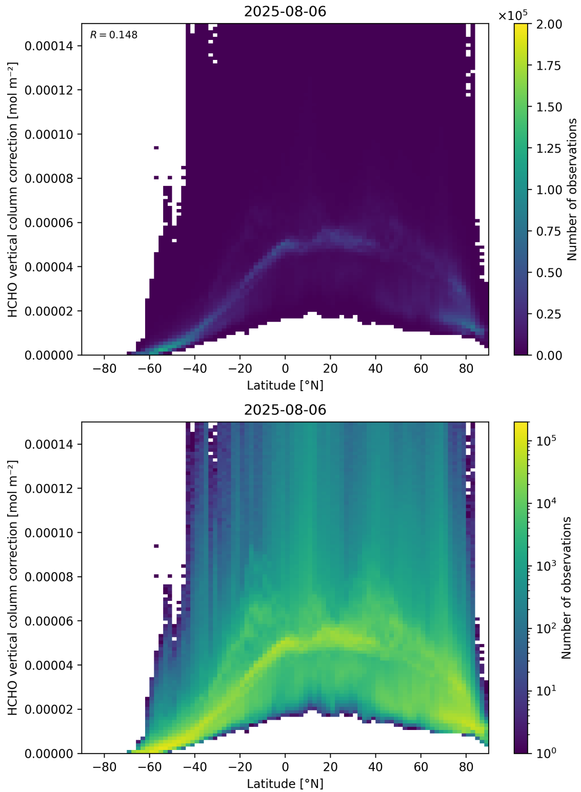
Figure 164: Scatter density plot of “Latitude” against “HCHO vertical column correction” for 2025-08-05 to 2025-08-07.
