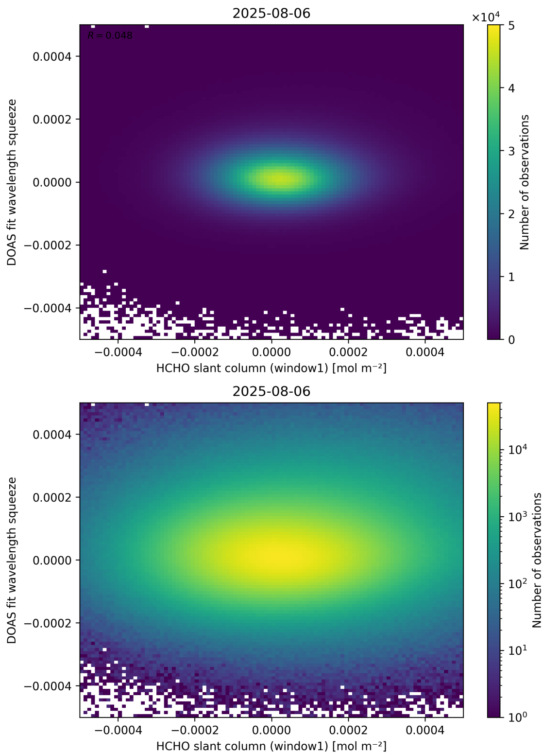
Figure 80: Scatter density plot of “HCHO slant column (window1)” against “DOAS fit wavelength squeeze” for 2025-08-05 to 2025-08-07.
