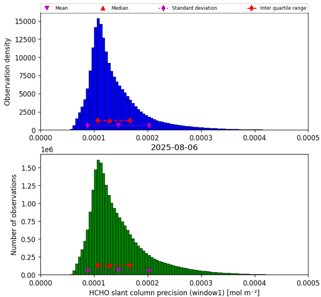
Figure 39: Histogram of “HCHO slant column precision (window1)” for 2025-08-05 to 2025-08-07
