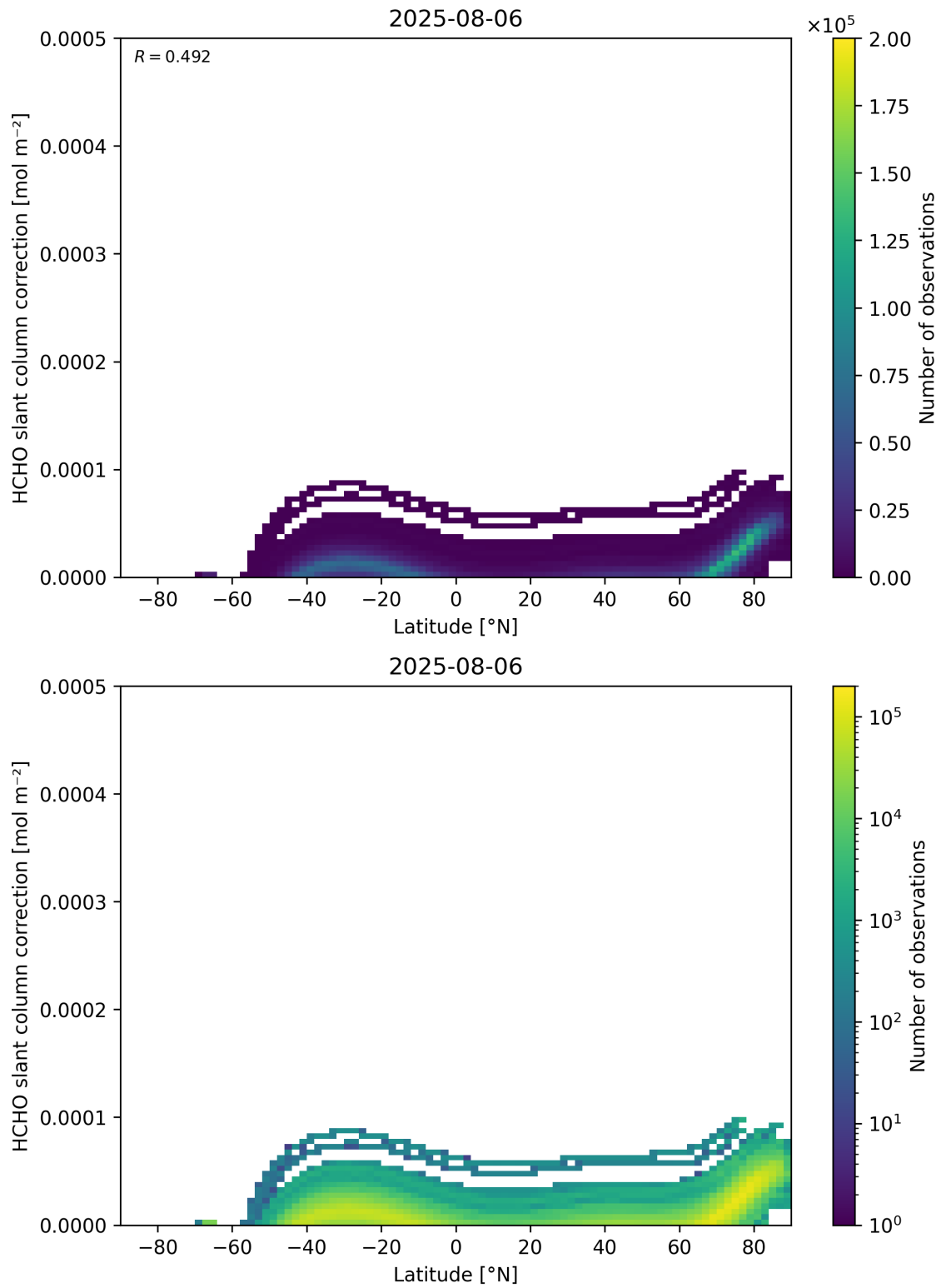
Figure 158: Scatter density plot of “Latitude” against “HCHO slant column correction” for 2025-08-05 to 2025-08-07.
