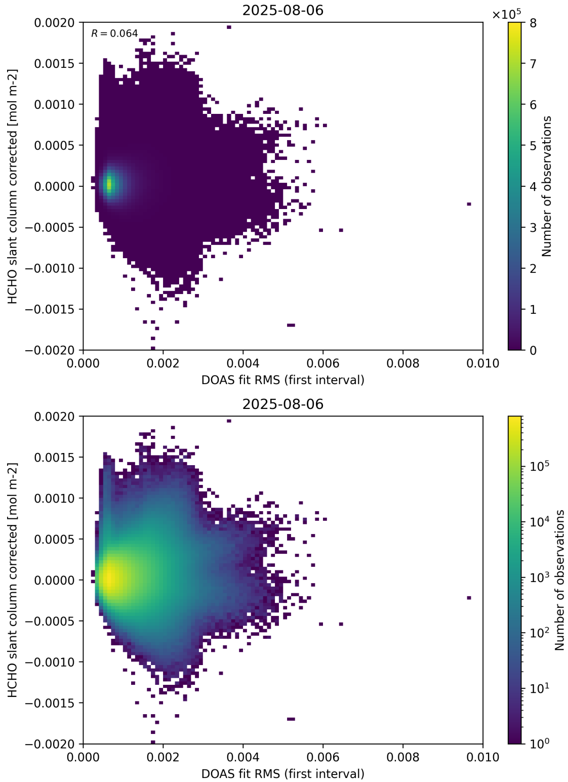
Figure 62: Scatter density plot of “DOAS fit RMS (first interval)” against “HCHO slant column corrected” for 2025-08-05 to 2025-08-07.
