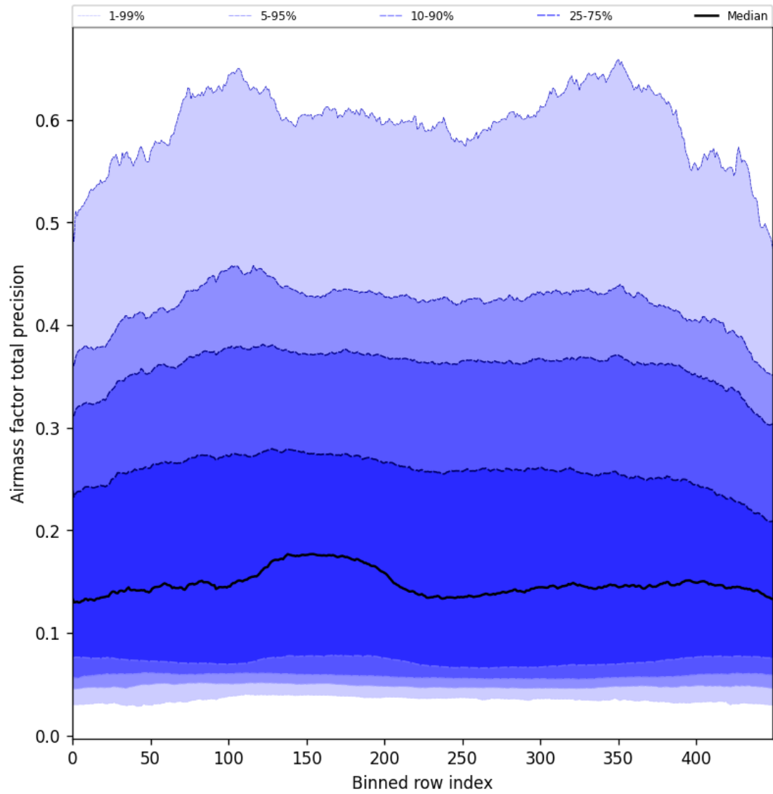
Figure 55: Along track statistics of “Airmass factor total precision” for 2025-08-05 to 2025-08-07
