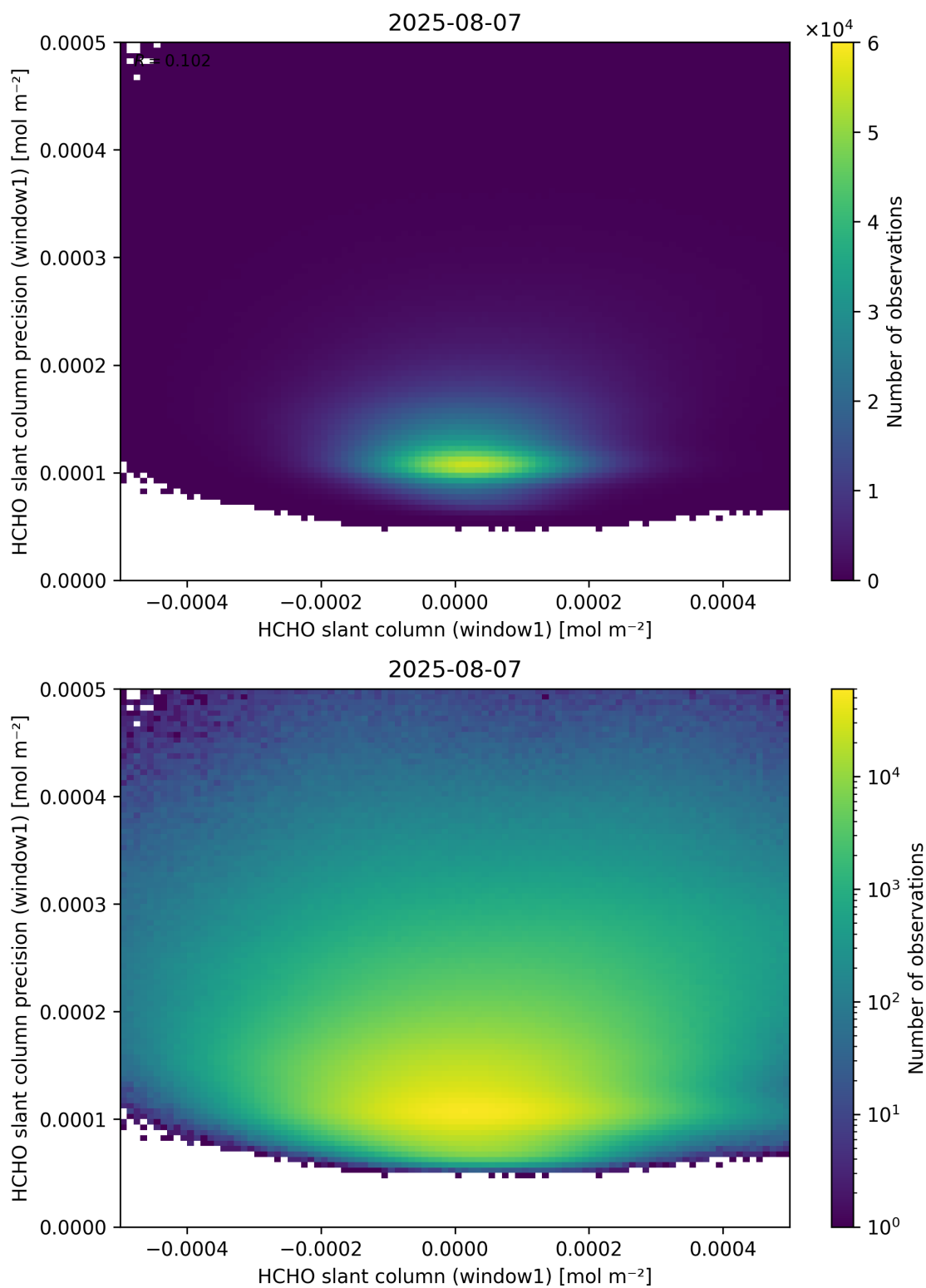
Figure 84: Scatter density plot of “HCHO slant column (window1)” against “HCHO slant column precision (window1)” for 2025-08-06 to 2025-08-08.
