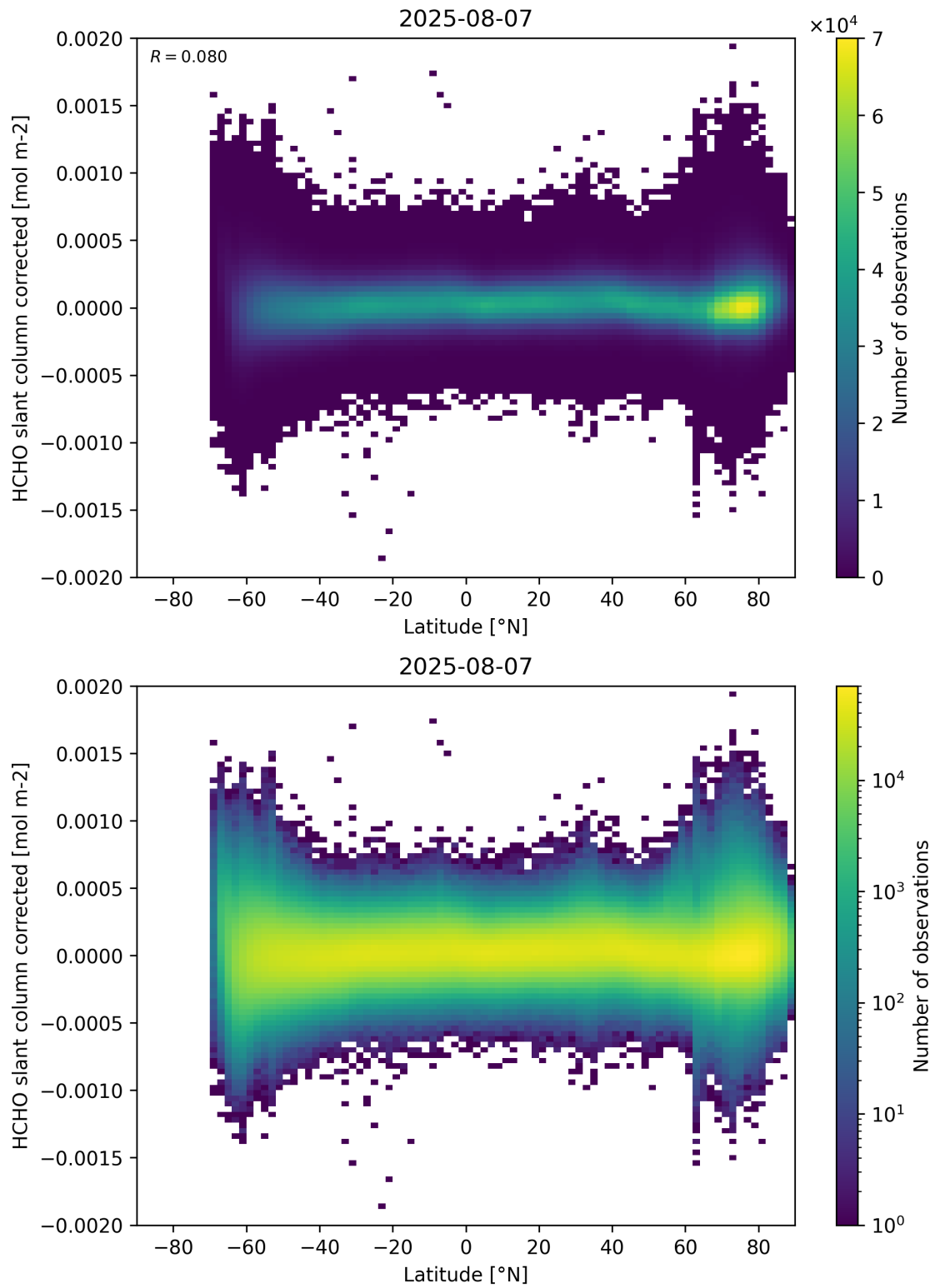
Figure 157: Scatter density plot of “Latitude” against “HCHO slant column corrected” for 2025-08-06 to 2025-08-08.
