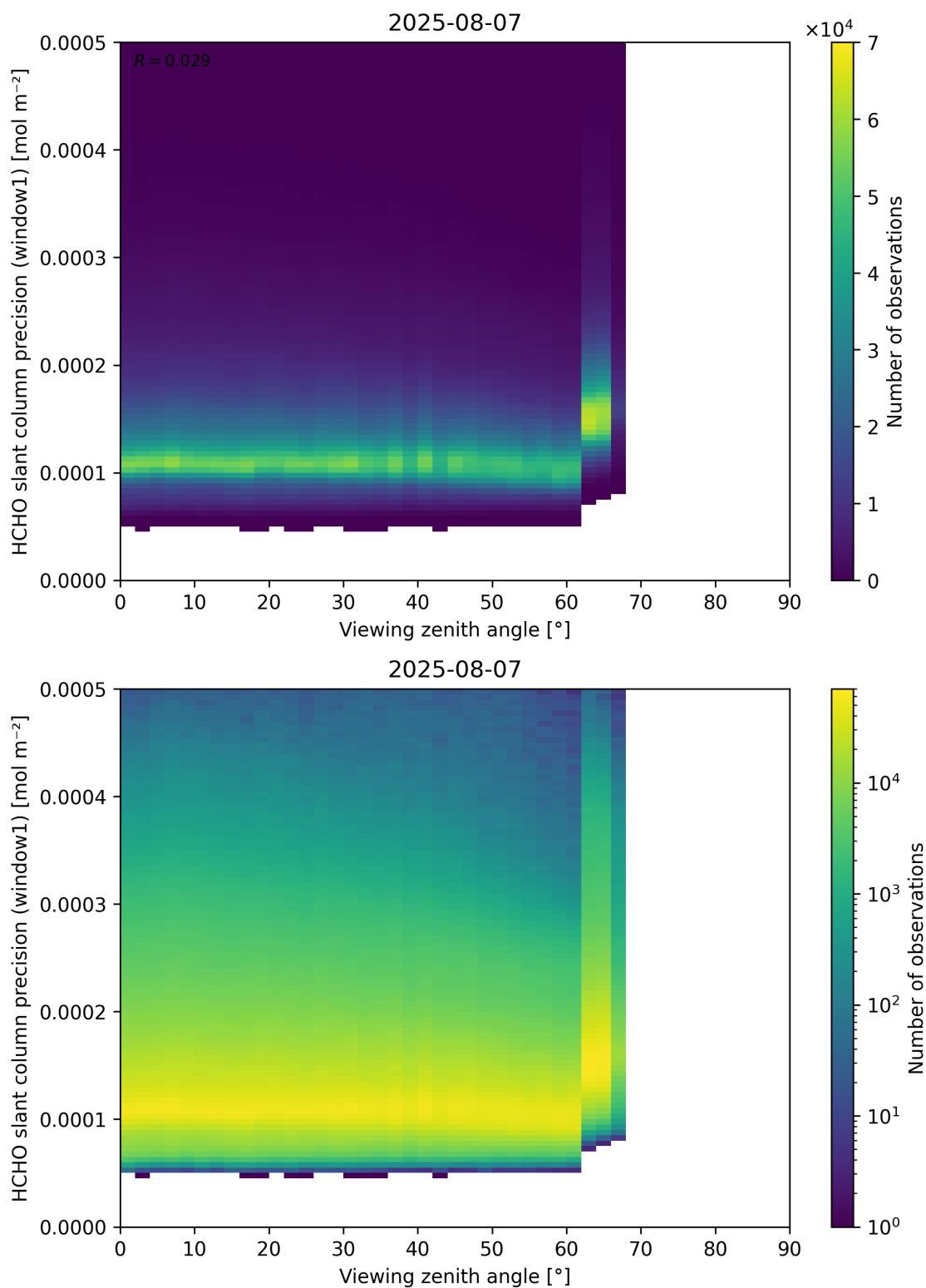
Figure 189: Scatter density plot of “Viewing zenith angle” against “HCHO slant column precision (window1)” for 2025-08-06 to 2025-08-08.
