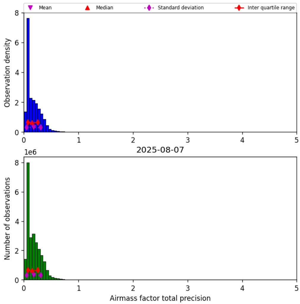
Figure 41: Histogram of “Airmass factor total precision” for 2025-08-06 to 2025-08-08
