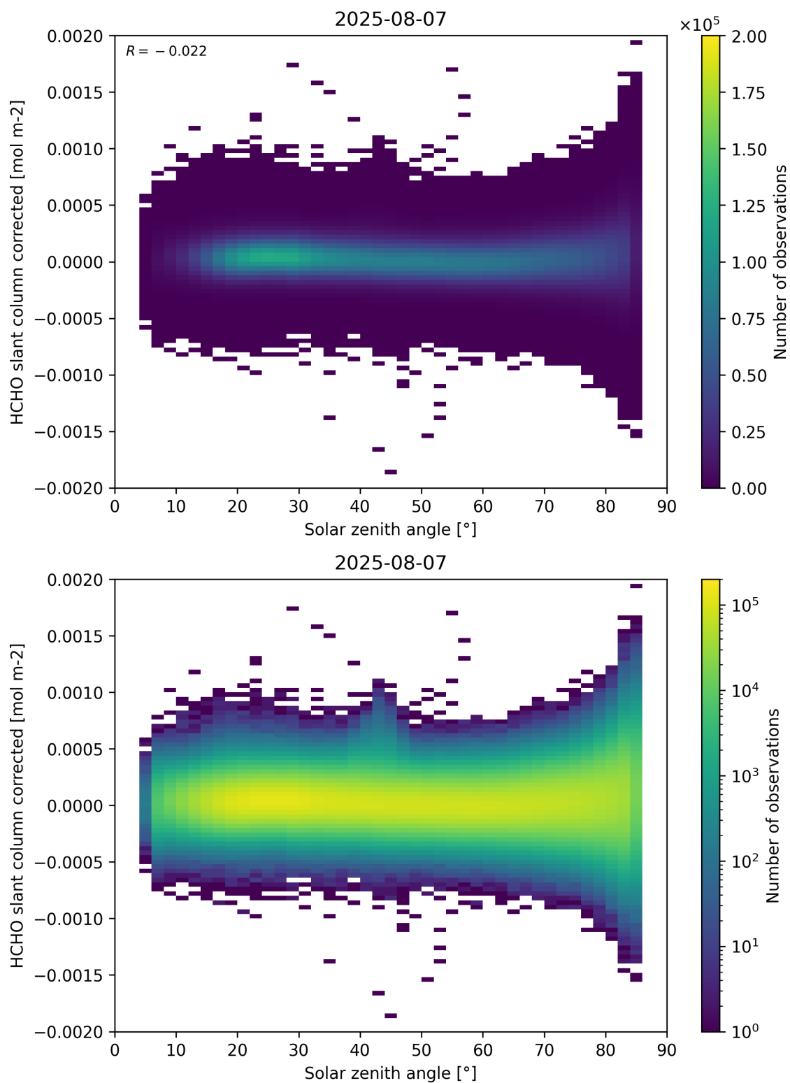
Figure 171: Scatter density plot of “Solar zenith angle” against “HCHO slant column corrected” for 2025-08-06 to 2025-08-08.
