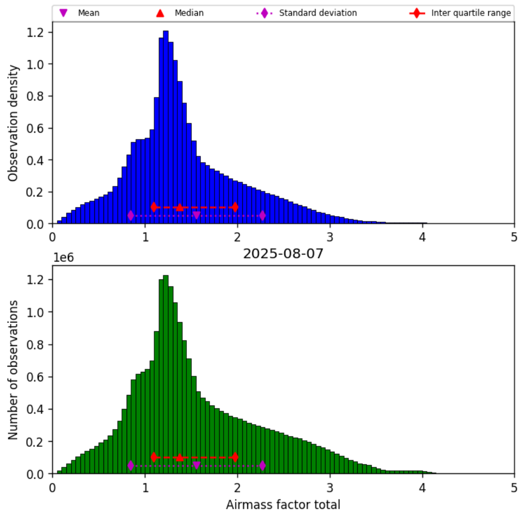
Figure 40: Histogram of “Airmass factor total” for 2025-08-06 to 2025-08-08
