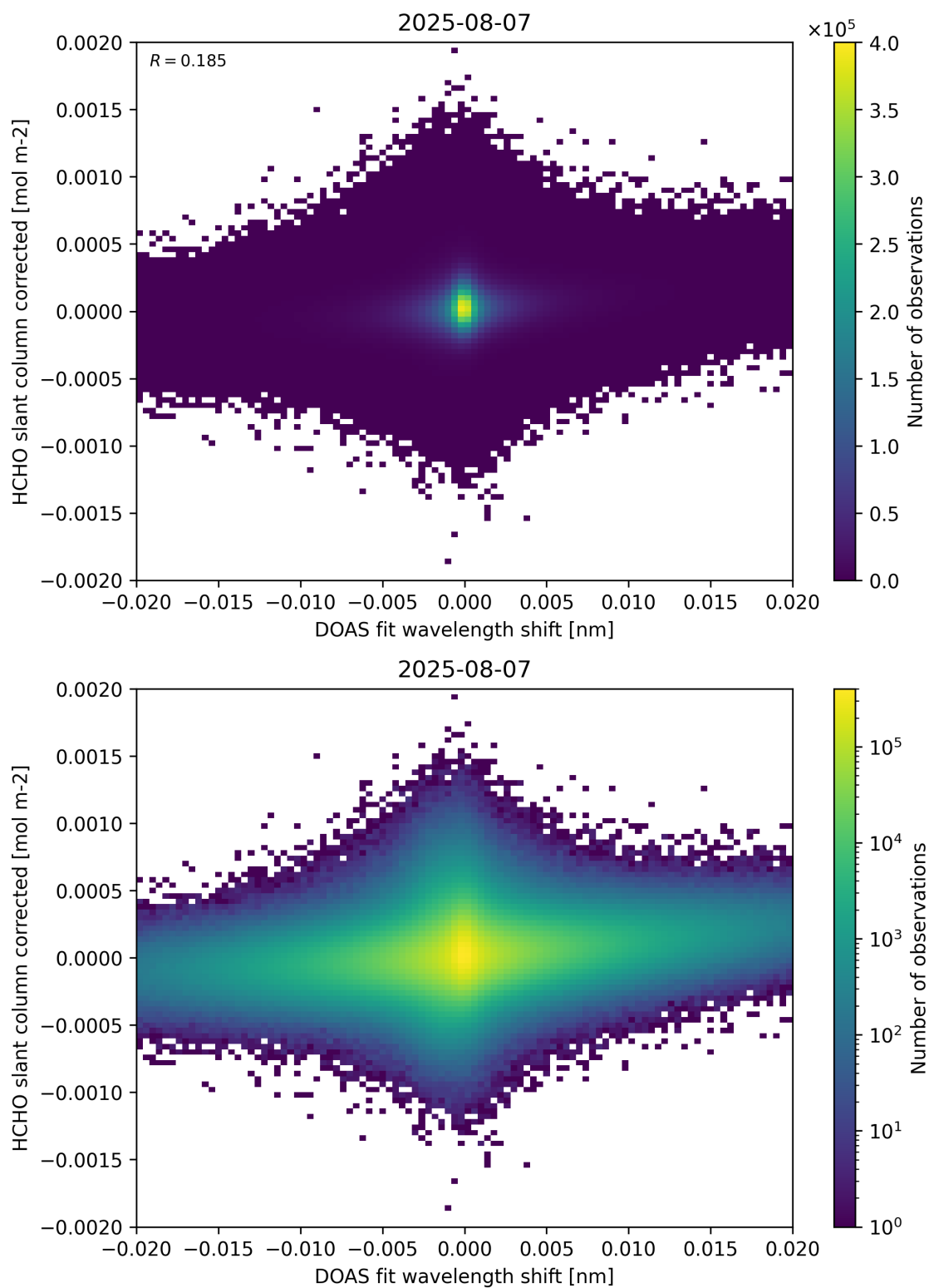
Figure 66: Scatter density plot of “DOAS fit wavelength shift” against “HCHO slant column corrected” for 2025-08-06 to 2025-08-08.
