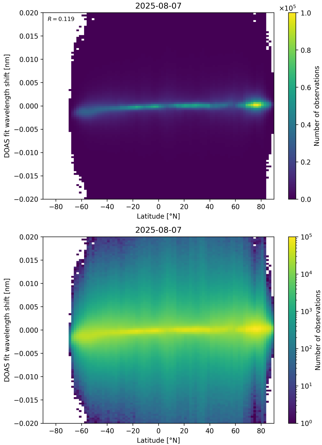
Figure 154: Scatter density plot of “Latitude” against “DOAS fit wavelength shift” for 2025-08-06 to 2025-08-08.
