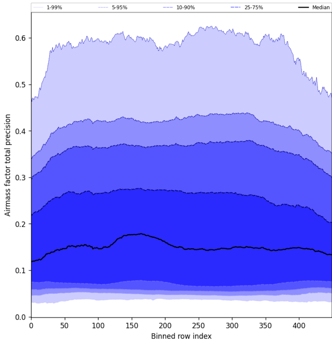
Figure 55: Along track statistics of “Airmass factor total precision” for 2025-08-06 to 2025-08-08
