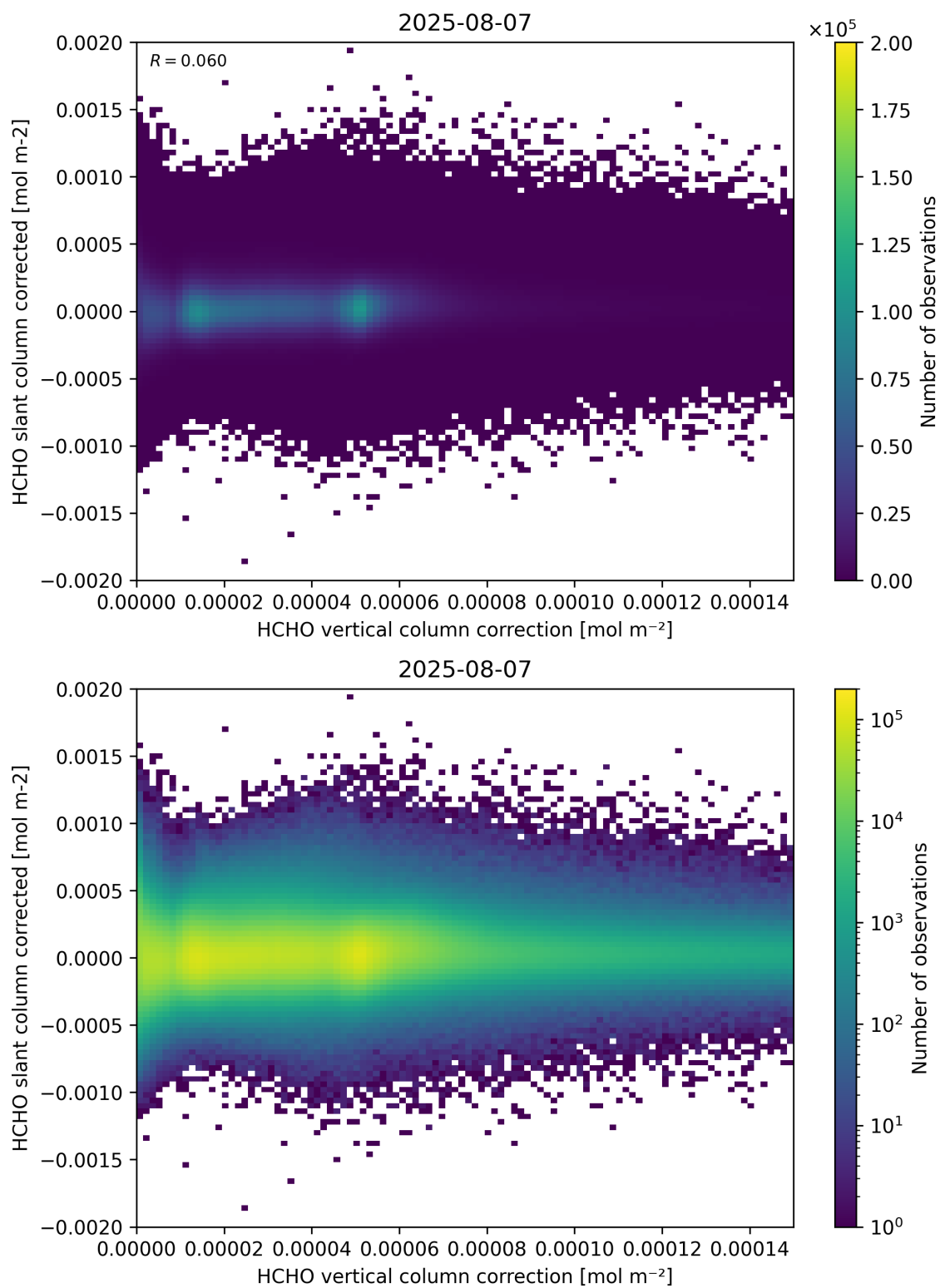
Figure 116: Scatter density plot of “HCHO vertical column correction” against “HCHO slant column corrected” for 2025-08-06 to 2025-08-08.
