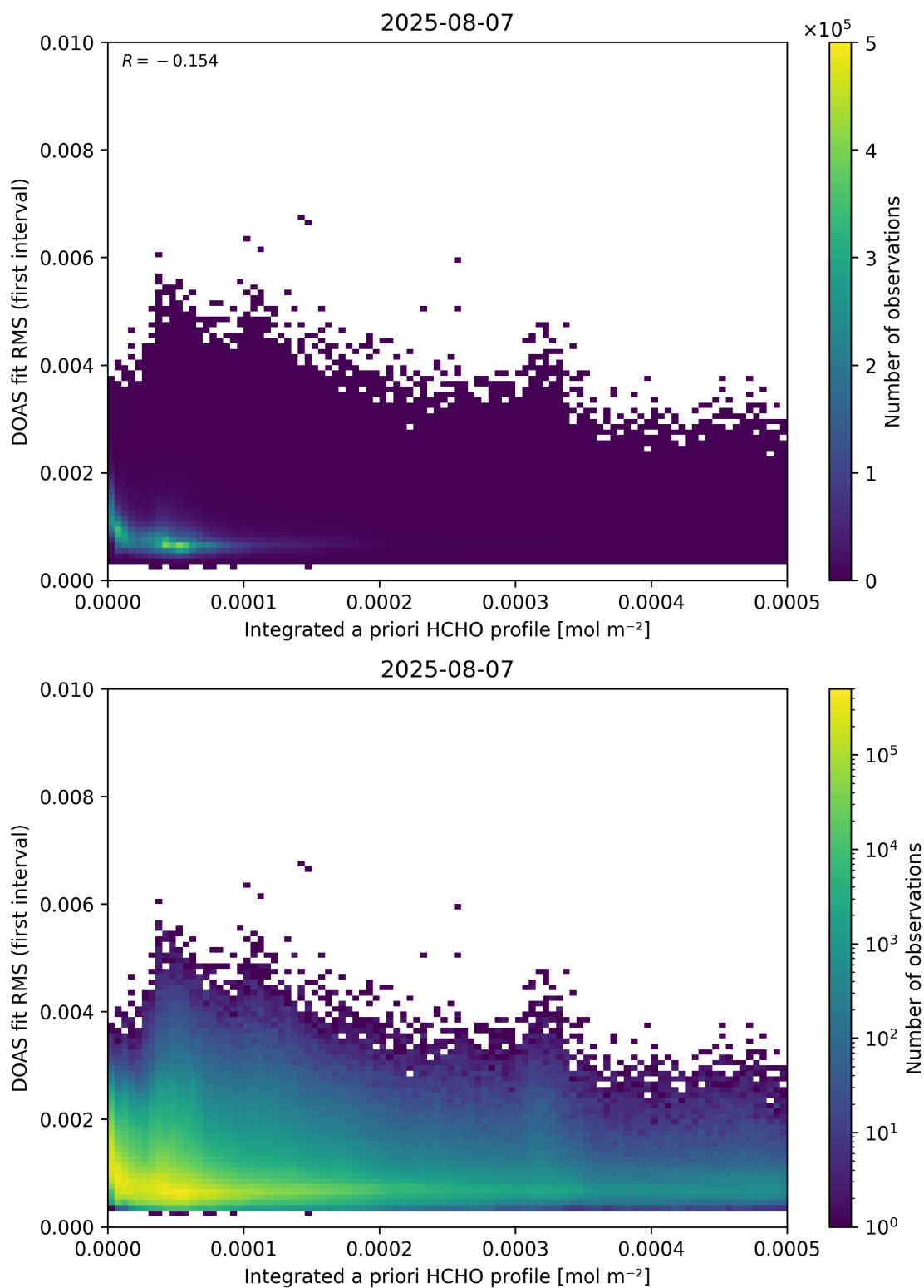
Figure 148: Scatter density plot of “Integrated a priori HCHO profile” against “DOAS fit RMS (first interval)” for 2025-08-06 to 2025-08-08.
