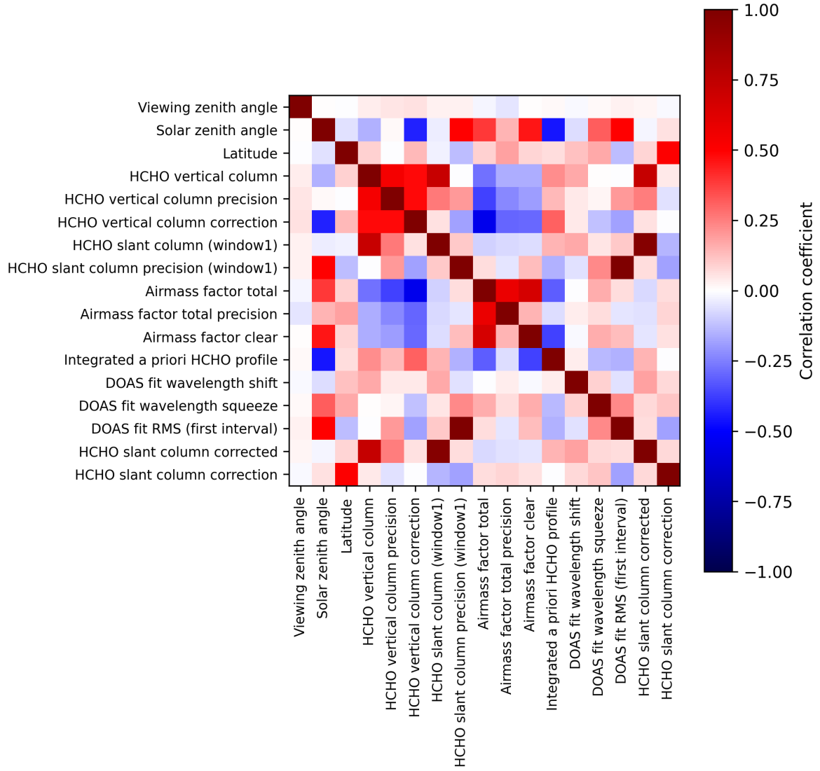
Figure 2: Map of correlation matrix for 2025-08-06 to 2025-08-08.
