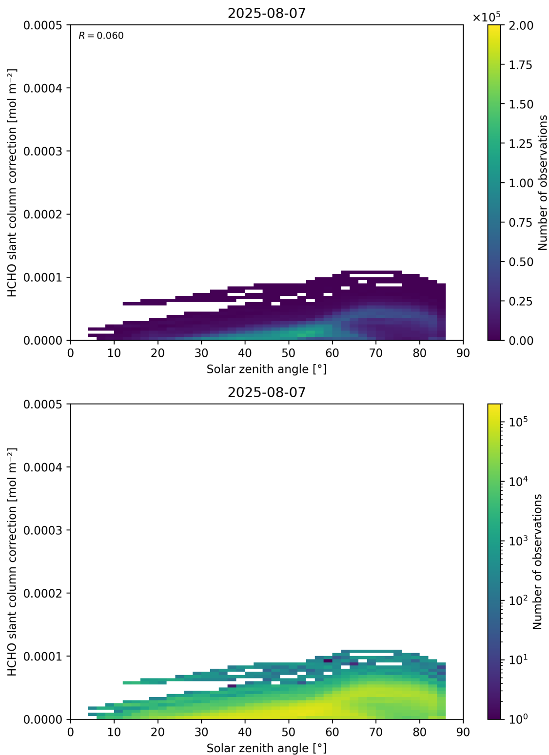
Figure 172: Scatter density plot of “Solar zenith angle” against “HCHO slant column correction” for 2025-08-06 to 2025-08-08.
