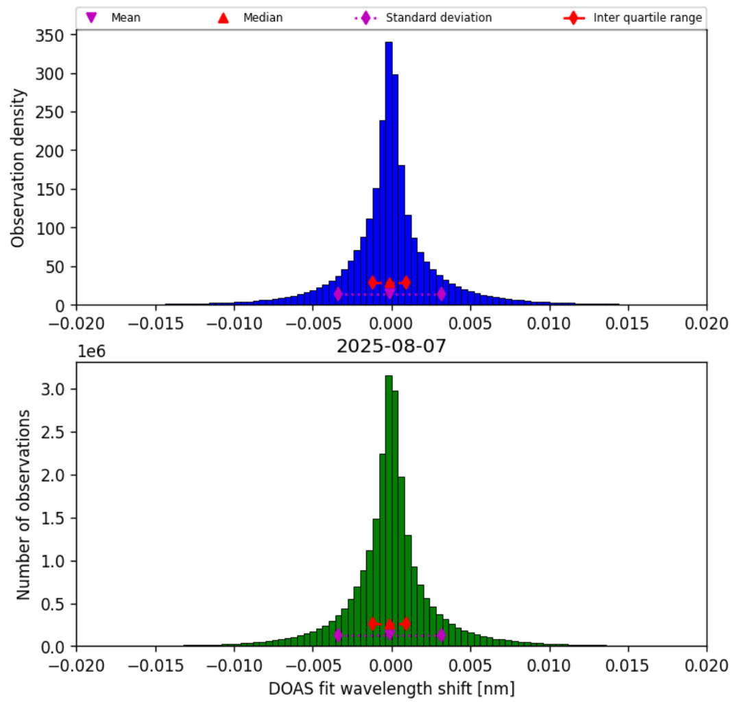
Figure 44: Histogram of “DOAS fit wavelength shift” for 2025-08-06 to 2025-08-08
