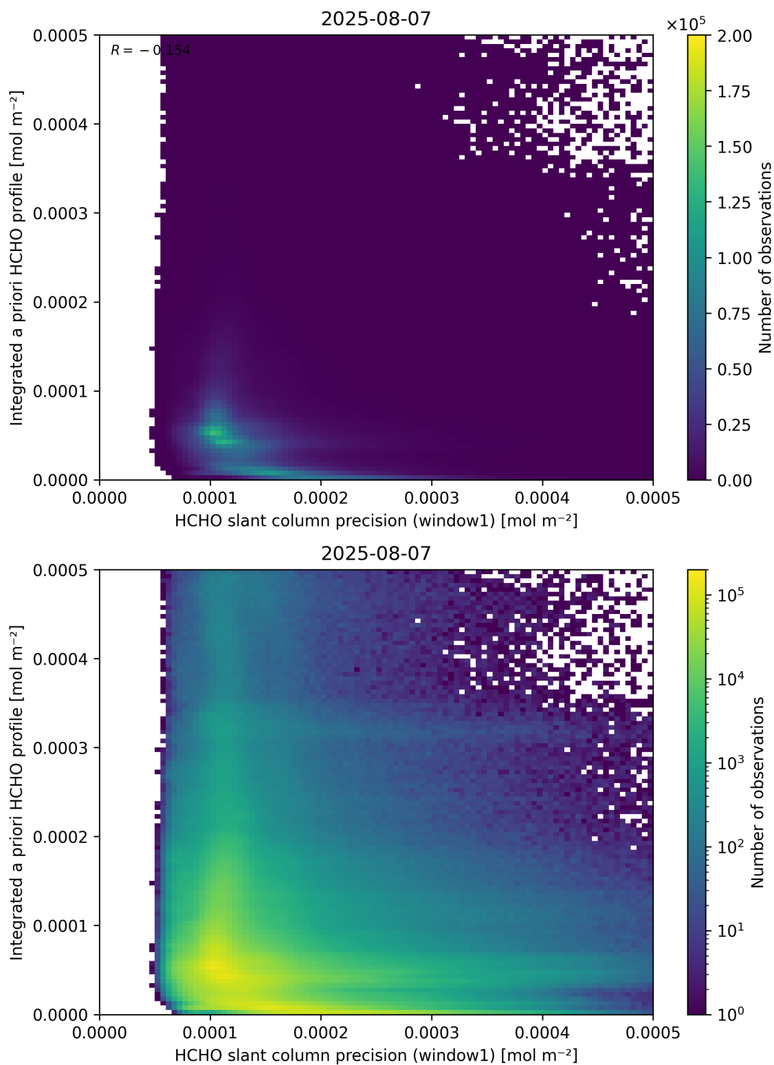
Figure 96: Scatter density plot of “HCHO slant column precision (window1)” against “Integrated a priori HCHO profile” for 2025-08-06 to 2025-08-08.
