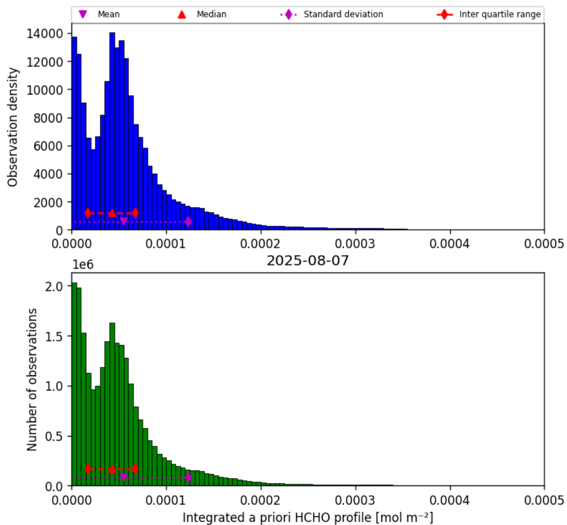
Figure 43: Histogram of “Integrated a priori HCHO profile” for 2025-08-06 to 2025-08-08
