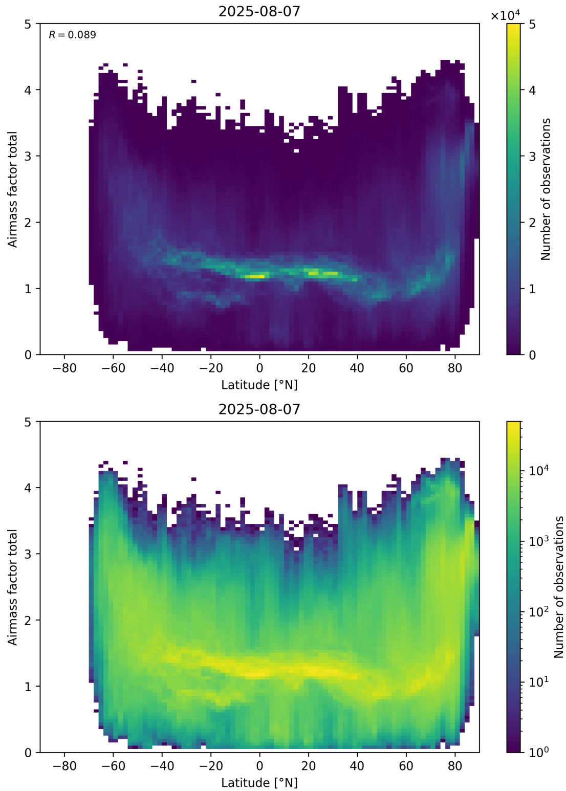
Figure 161: Scatter density plot of “Latitude” against “Airmass factor total” for 2025-08-06 to 2025-08-08.
