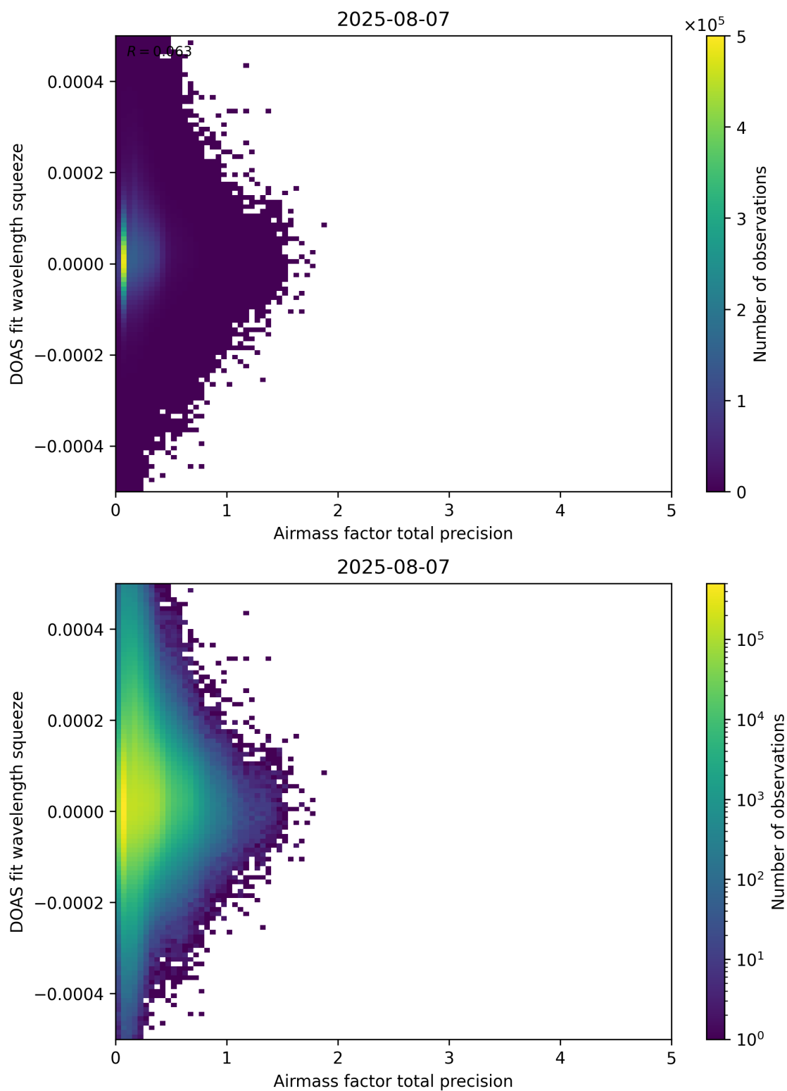
Figure 107: Scatter density plot of “Airmass factor total precision” against “DOAS fit wavelength squeeze” for 2025-08-06 to 2025-08-08.
