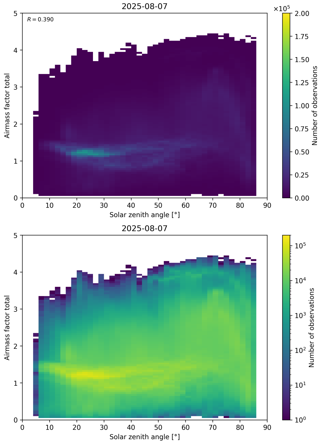
Figure 175: Scatter density plot of “Solar zenith angle” against “Airmass factor total” for 2025-08-06 to 2025-08-08.
