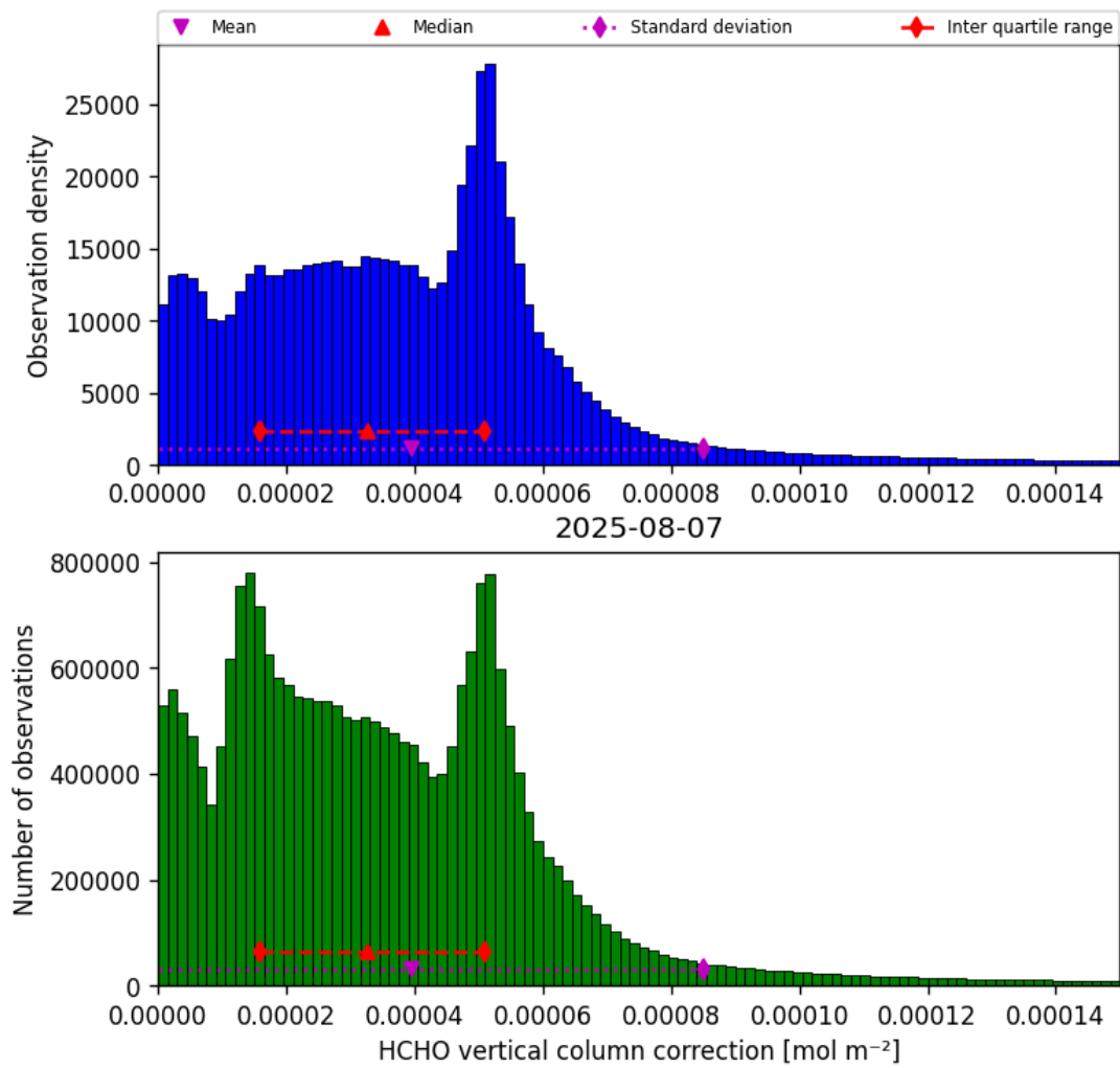
Figure 37: Histogram of “HCHO vertical column correction” for 2025-08-06 to 2025-08-08
