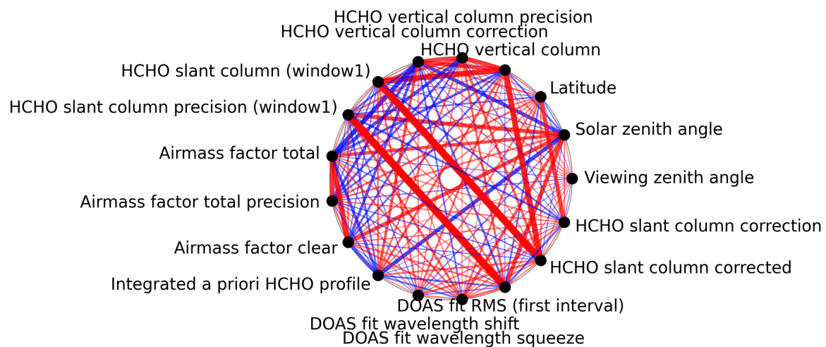
Figure 1: Map of correlation graph for 2025-08-06 to 2025-08-08.
