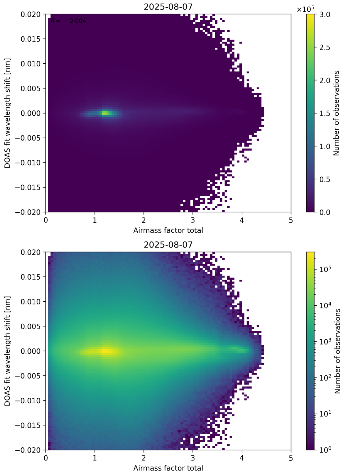
Figure 98: Scatter density plot of “Airmass factor total” against “DOAS fit wavelength shift” for 2025-08-06 to 2025-08-08.
