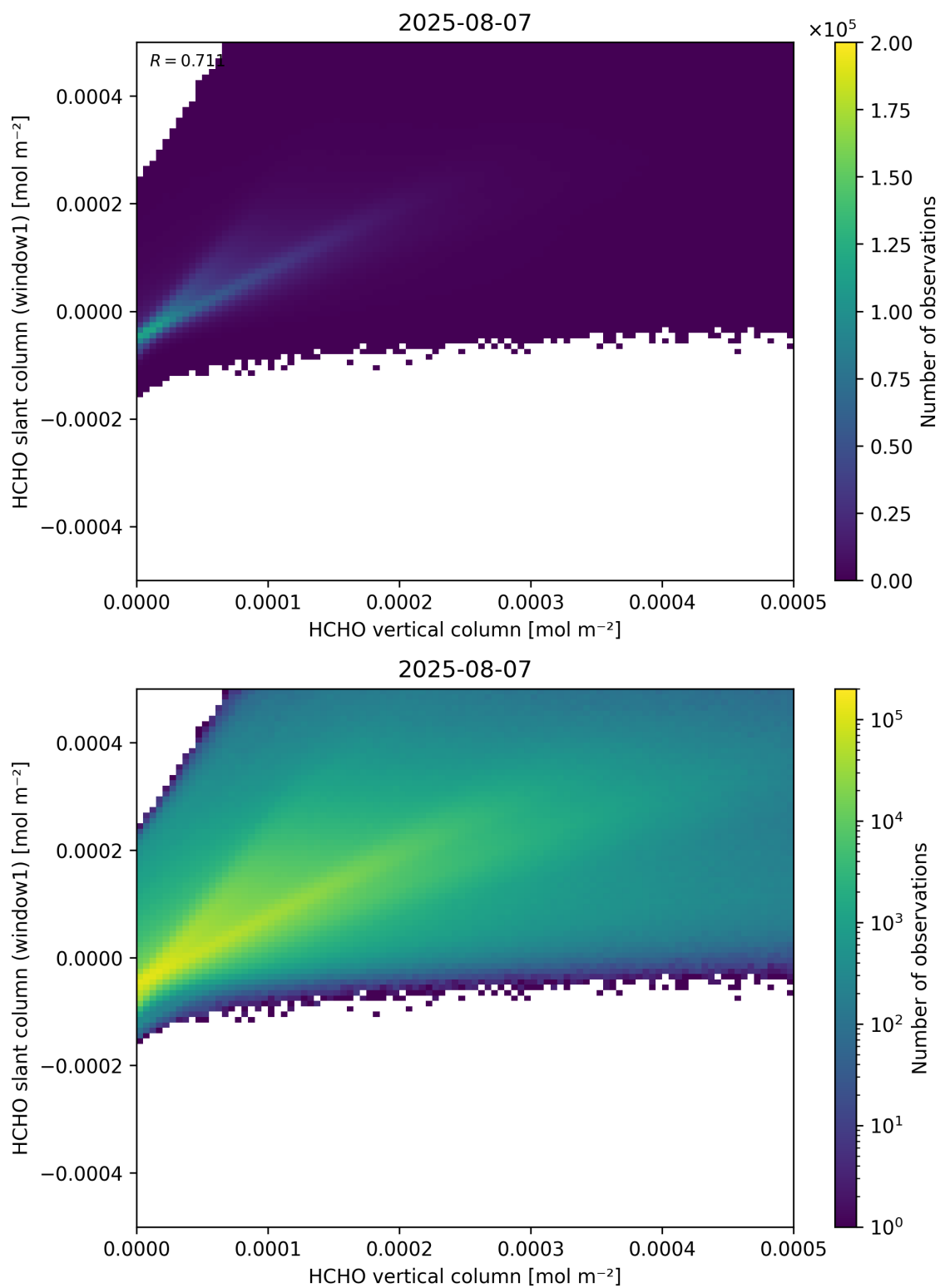
Figure 129: Scatter density plot of “HCHO vertical column” against “HCHO slant column (window1)” for 2025-08-06 to 2025-08-08.
