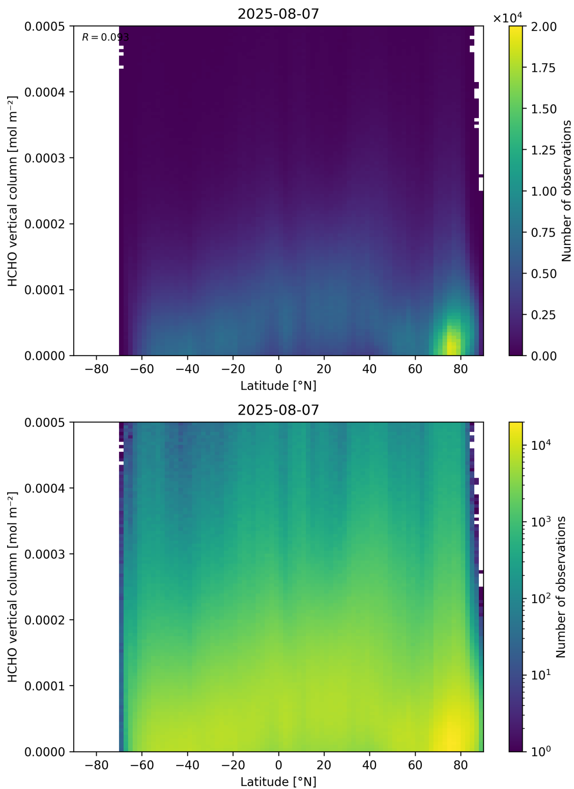
Figure 163: Scatter density plot of “Latitude” against “HCHO vertical column” for 2025-08-06 to 2025-08-08.
