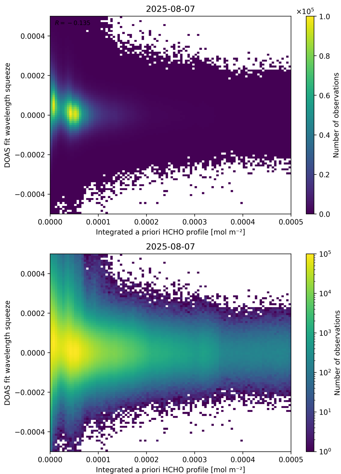
Figure 150: Scatter density plot of “Integrated a priori HCHO profile” against “DOAS fit wavelength squeeze” for 2025-08-06 to 2025-08-08.
