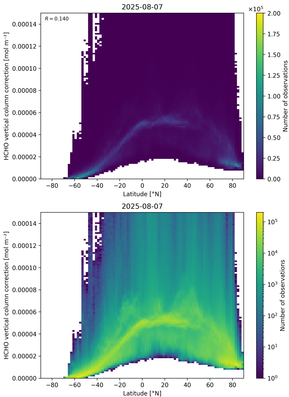
Figure 164: Scatter density plot of “Latitude” against “HCHO vertical column correction” for 2025-08-06 to 2025-08-08.
