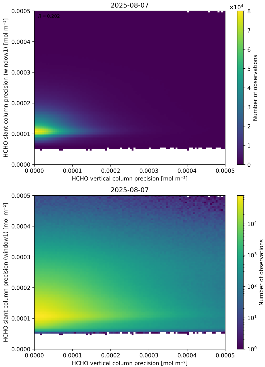
Figure 143: Scatter density plot of “HCHO vertical column precision” against “HCHO slant column precision (window1)” for 2025-08-06 to 2025-08-08.
