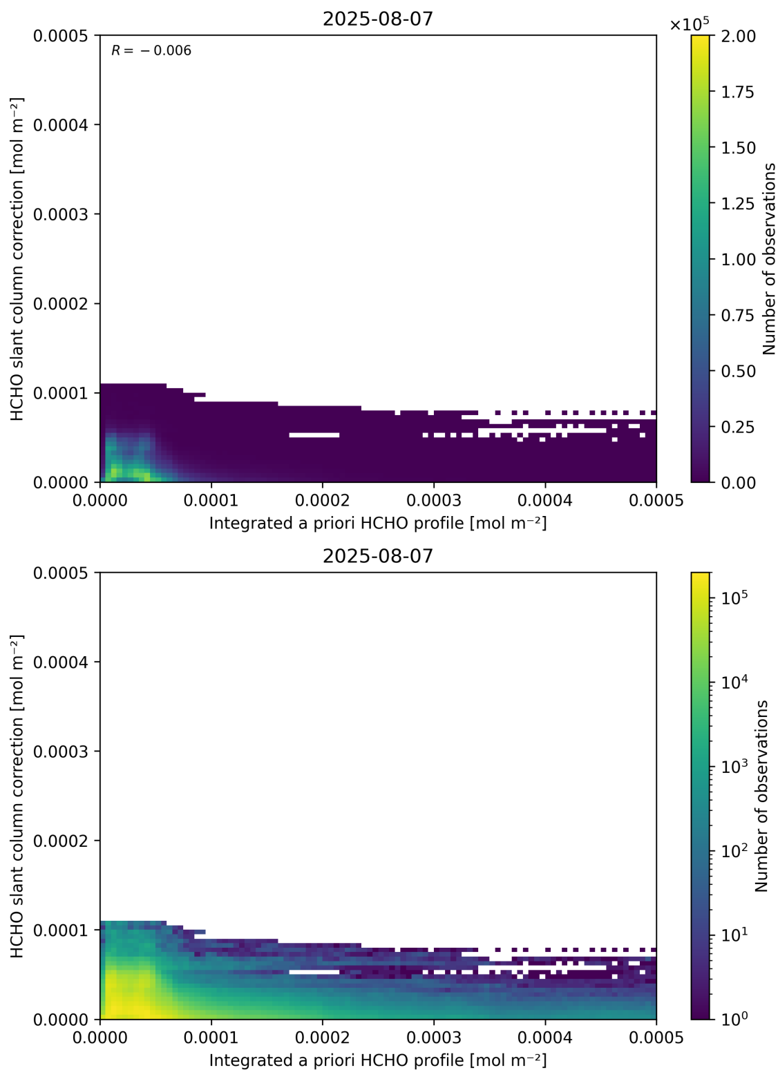
Figure 152: Scatter density plot of “Integrated a priori HCHO profile” against “HCHO slant column correction” for 2025-08-06 to 2025-08-08.
