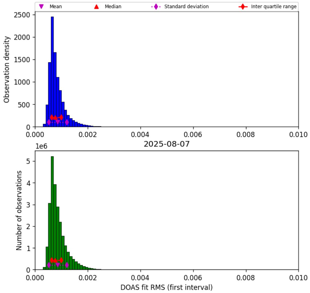
Figure 46: Histogram of “DOAS fit RMS (first interval)” for 2025-08-06 to 2025-08-08
