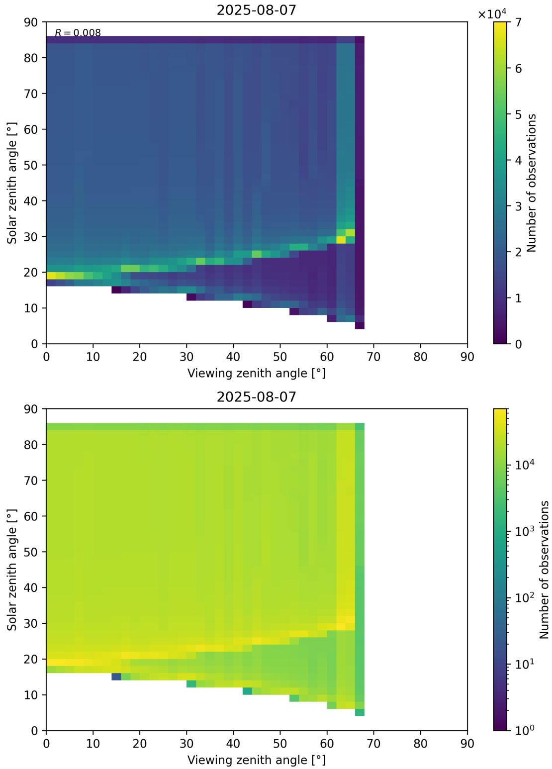
Figure 197: Scatter density plot of “Viewing zenith angle” against “Solar zenith angle” for 2025-08-06 to 2025-08-08.
