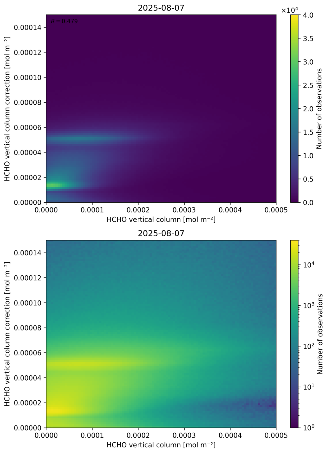
Figure 133: Scatter density plot of “HCHO vertical column” against “HCHO vertical column correction” for 2025-08-06 to 2025-08-08.
