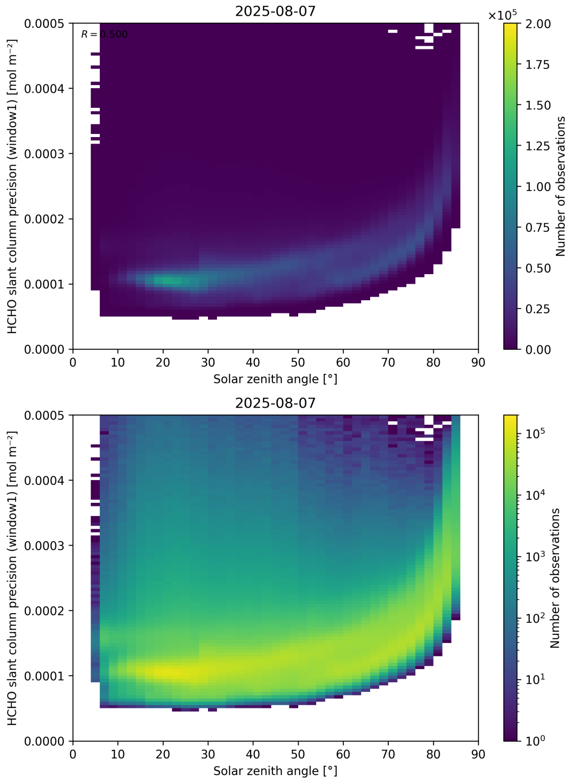
Figure 174: Scatter density plot of “Solar zenith angle” against “HCHO slant column precision (window1)” for 2025-08-06 to 2025-08-08.
