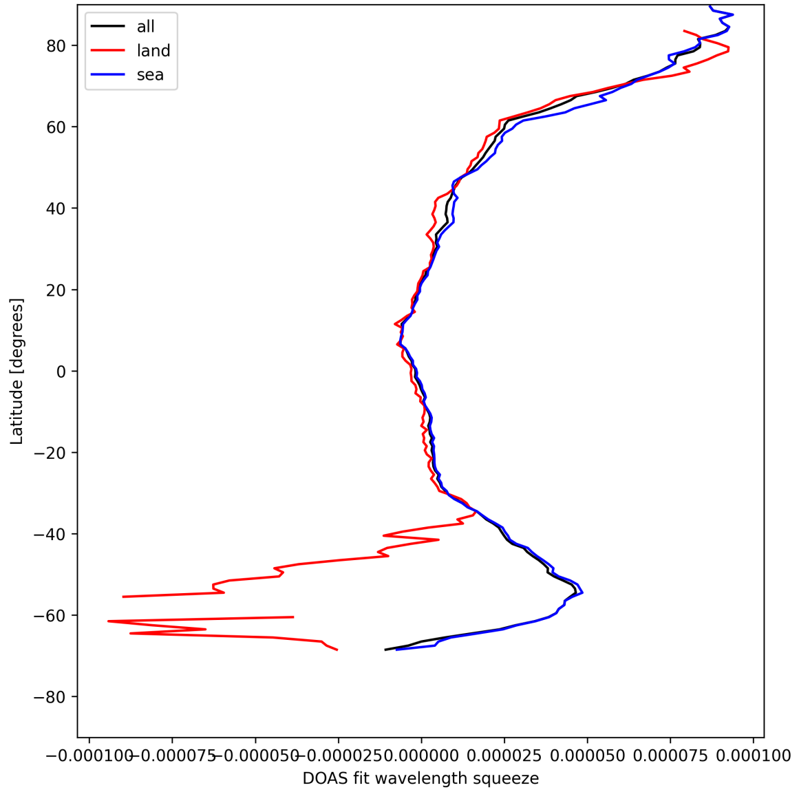
Figure 31: Zonal average of “DOAS fit wavelength squeeze” for 2025-08-06 to 2025-08-08.
