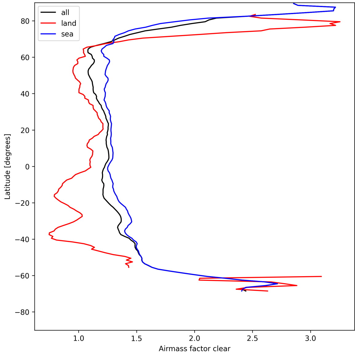
Figure 28: Zonal average of “Airmass factor clear” for 2025-08-06 to 2025-08-08.
