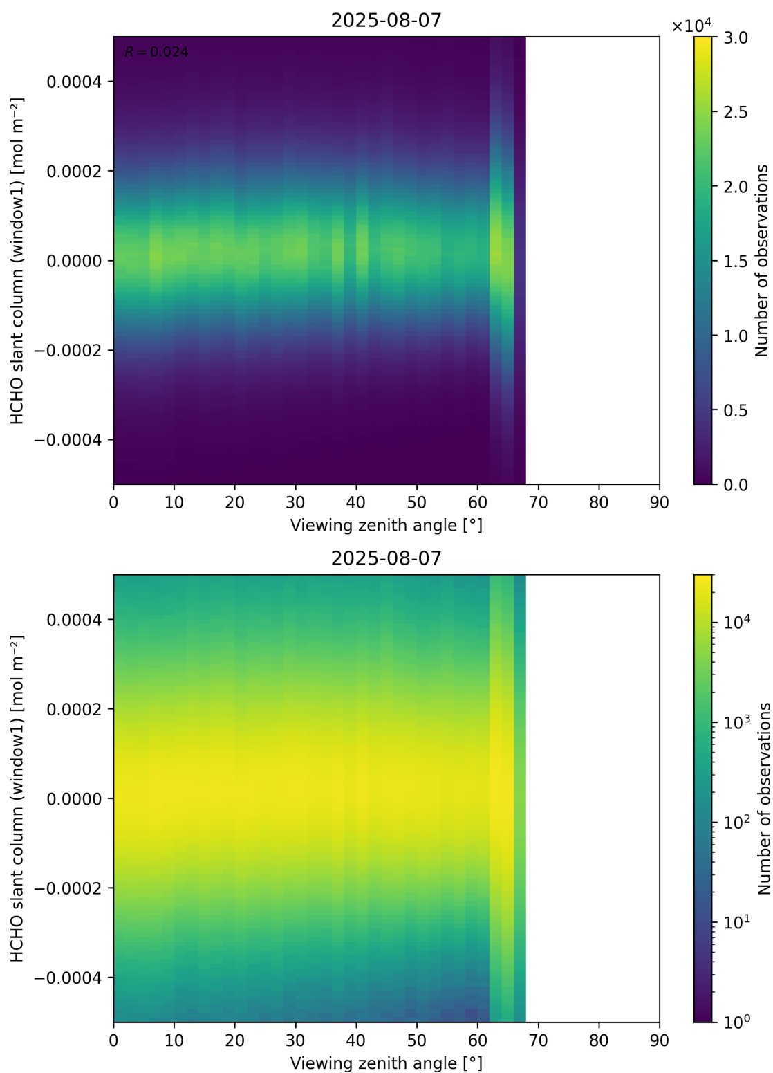
Figure 188: Scatter density plot of “Viewing zenith angle” against “HCHO slant column (window1)” for 2025-08-06 to 2025-08-08.
