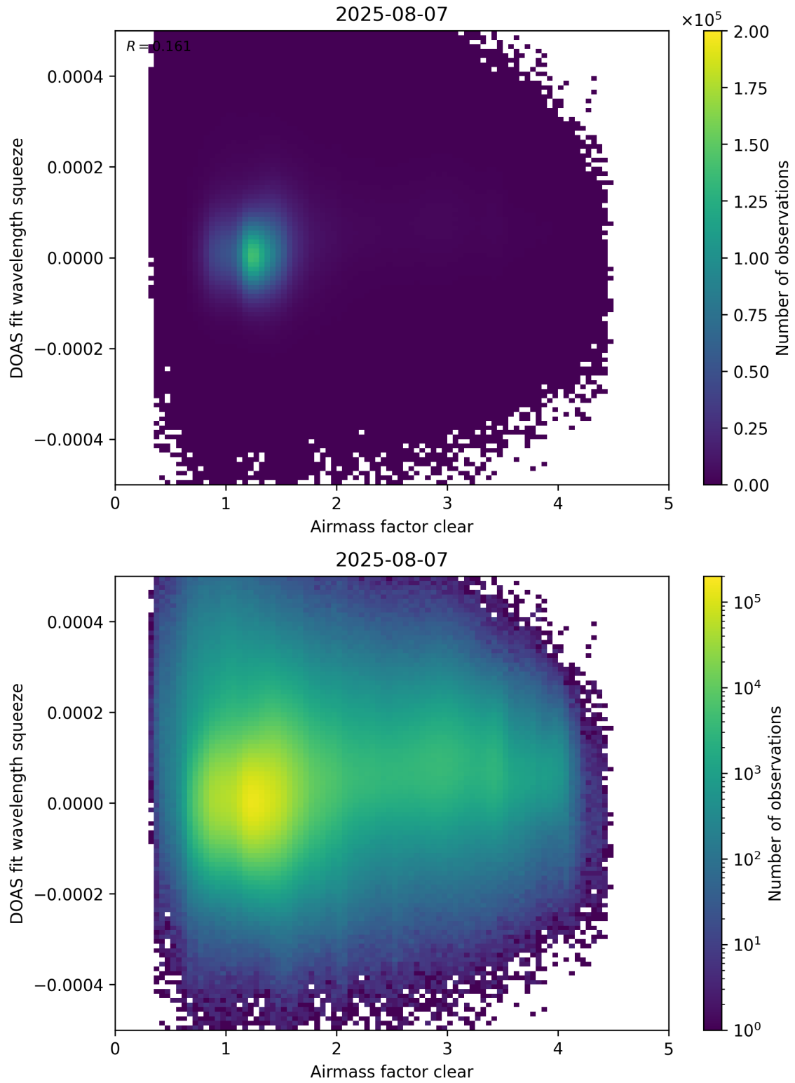
Figure 73: Scatter density plot of “Airmass factor clear” against “DOAS fit wavelength squeeze” for 2025-08-06 to 2025-08-08.
