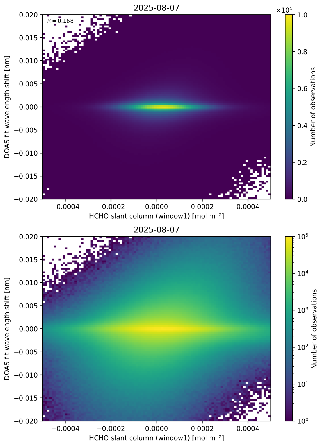
Figure 79: Scatter density plot of “HCHO slant column (window1)” against “DOAS fit wavelength shift” for 2025-08-06 to 2025-08-08.
