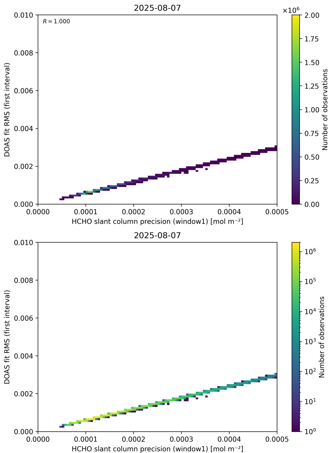
Figure 88: Scatter density plot of “HCHO slant column precision (window1)” against “DOAS fit RMS (first interval)” for 2025-08-06 to 2025-08-08.
