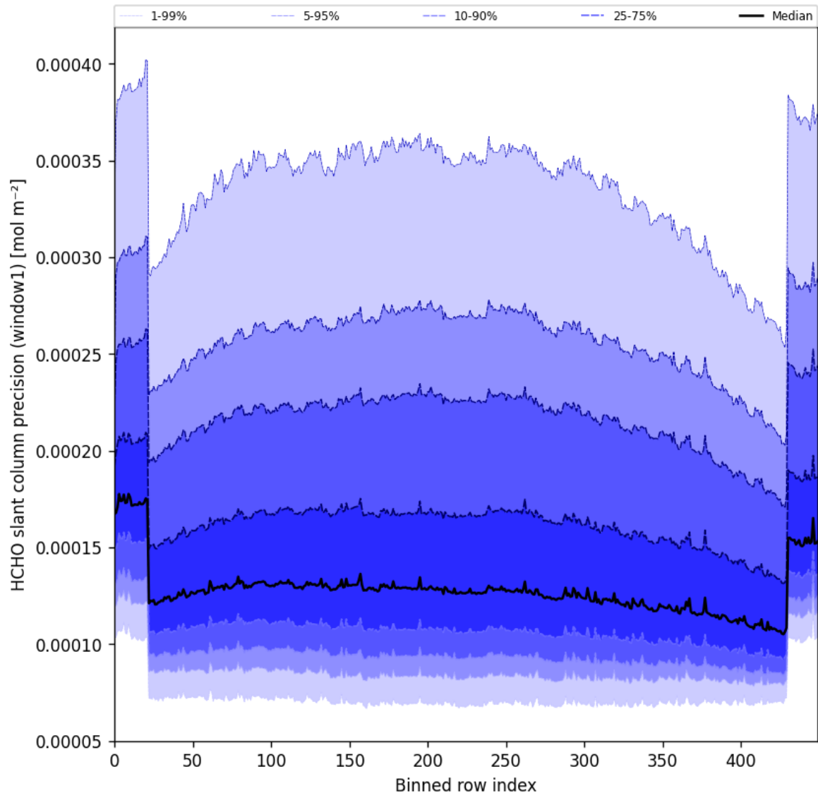
Figure 53: Along track statistics of “HCHO slant column precision (window1)” for 2025-08-06 to 2025-08-08
