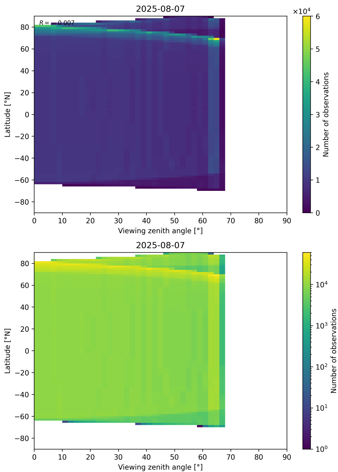
Figure 196: Scatter density plot of “Viewing zenith angle” against “Latitude” for 2025-08-06 to 2025-08-08.
