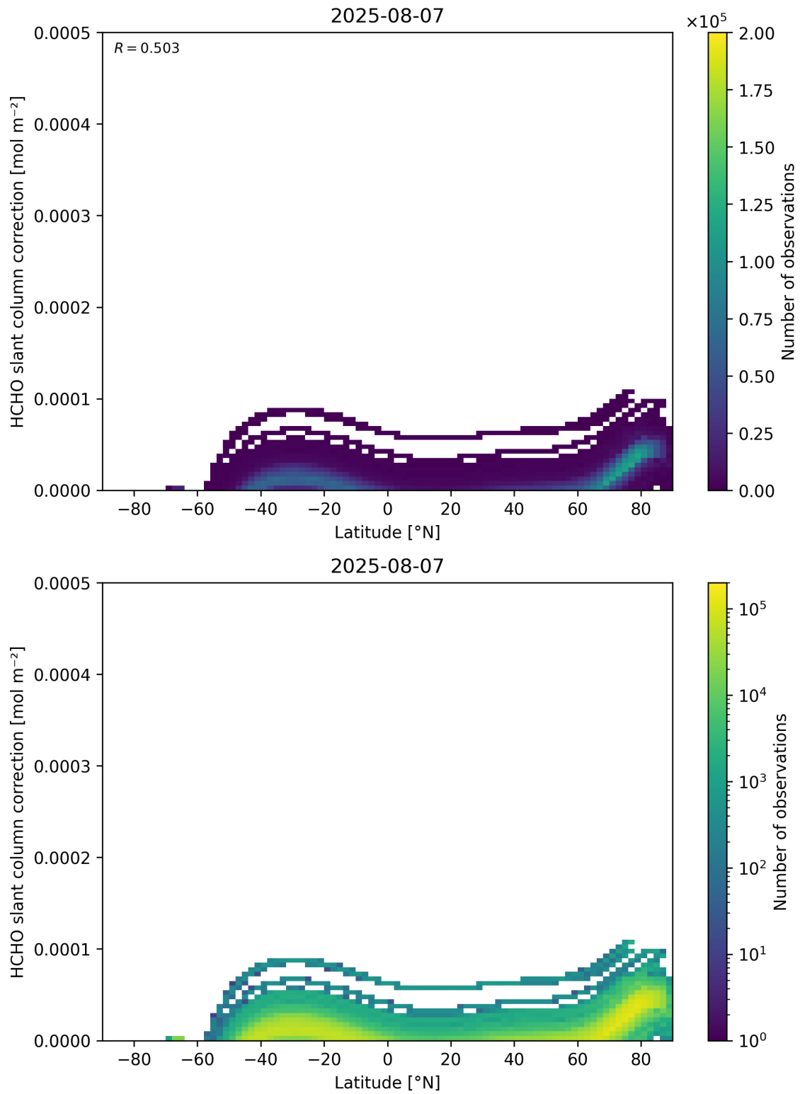
Figure 158: Scatter density plot of “Latitude” against “HCHO slant column correction” for 2025-08-06 to 2025-08-08.
