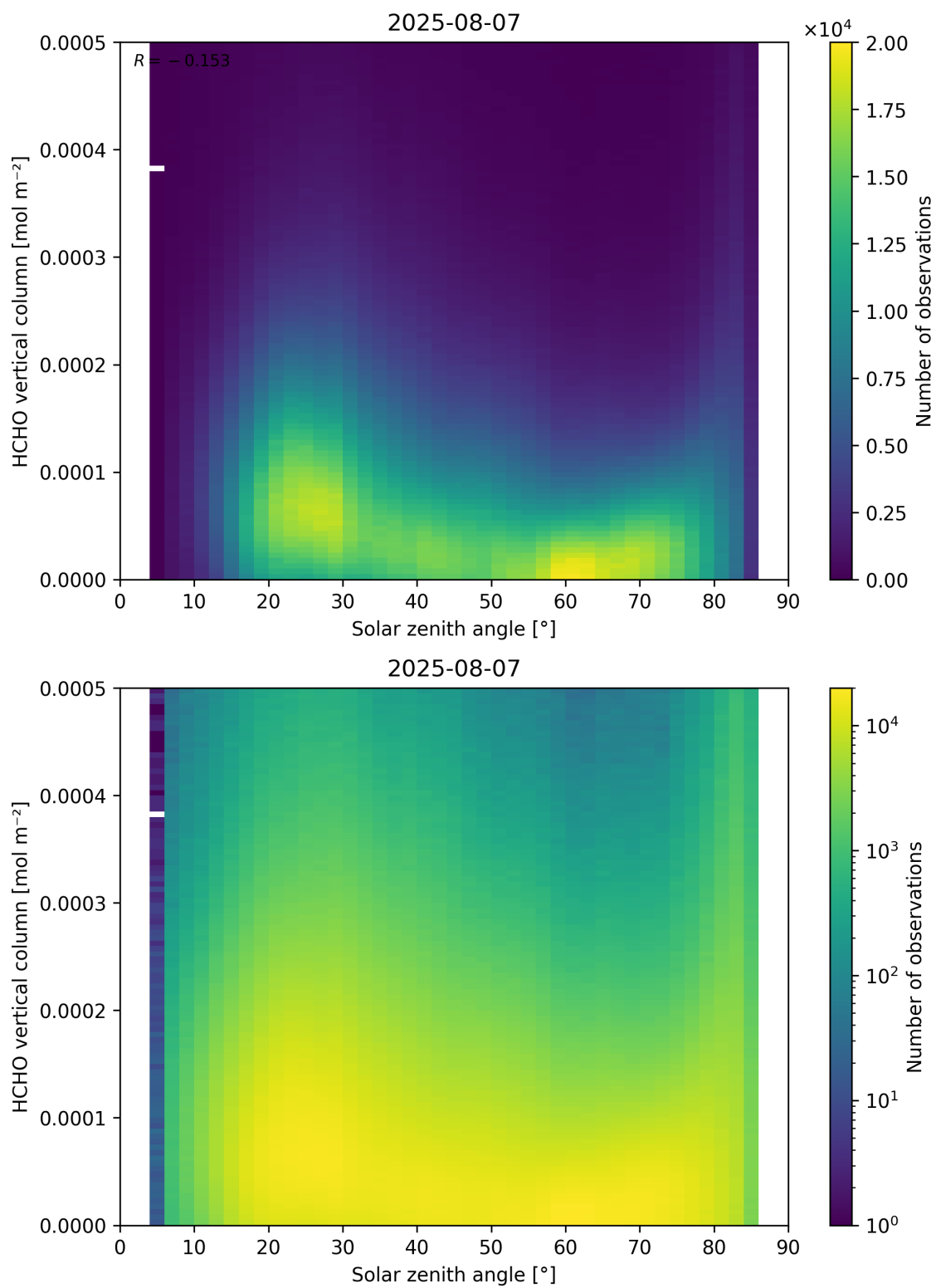
Figure 177: Scatter density plot of “Solar zenith angle” against “HCHO vertical column” for 2025-08-06 to 2025-08-08.
