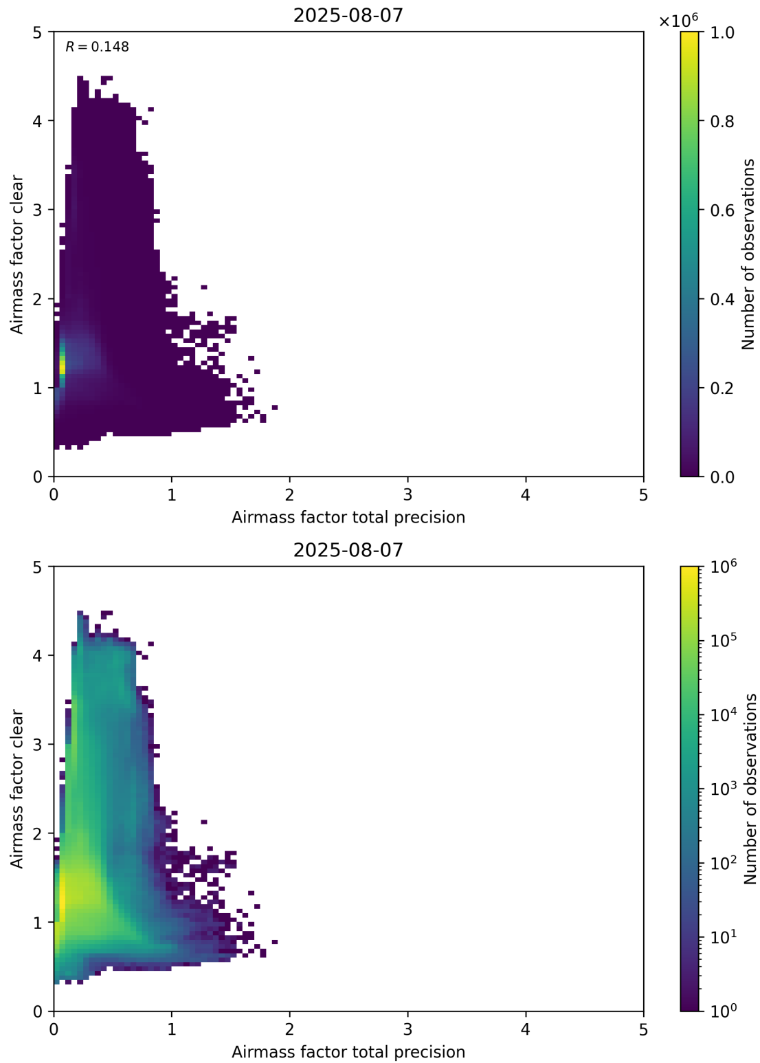
Figure 108: Scatter density plot of “Airmass factor total precision” against “Airmass factor clear” for 2025-08-06 to 2025-08-08.
