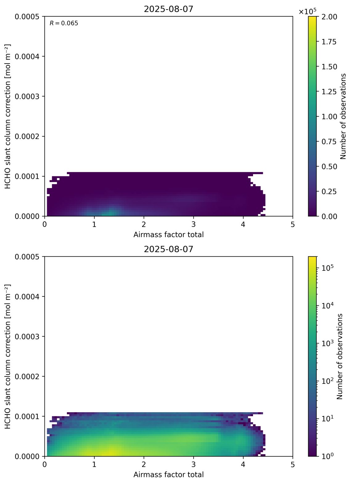
Figure 102: Scatter density plot of “Airmass factor total” against “HCHO slant column correction” for 2025-08-06 to 2025-08-08.
