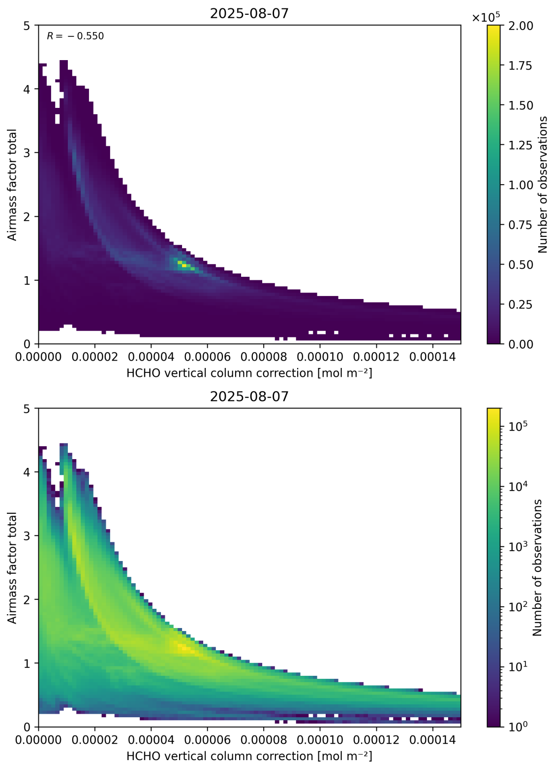
Figure 120: Scatter density plot of “HCHO vertical column correction” against “Airmass factor total” for 2025-08-06 to 2025-08-08.
