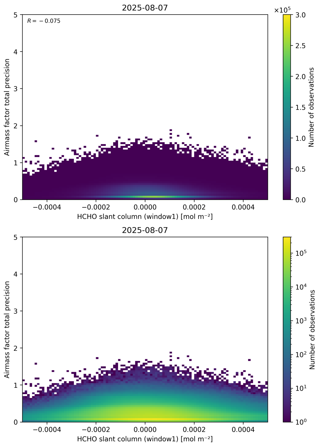
Figure 86: Scatter density plot of “HCHO slant column (window1)” against “Airmass factor total precision” for 2025-08-06 to 2025-08-08.
