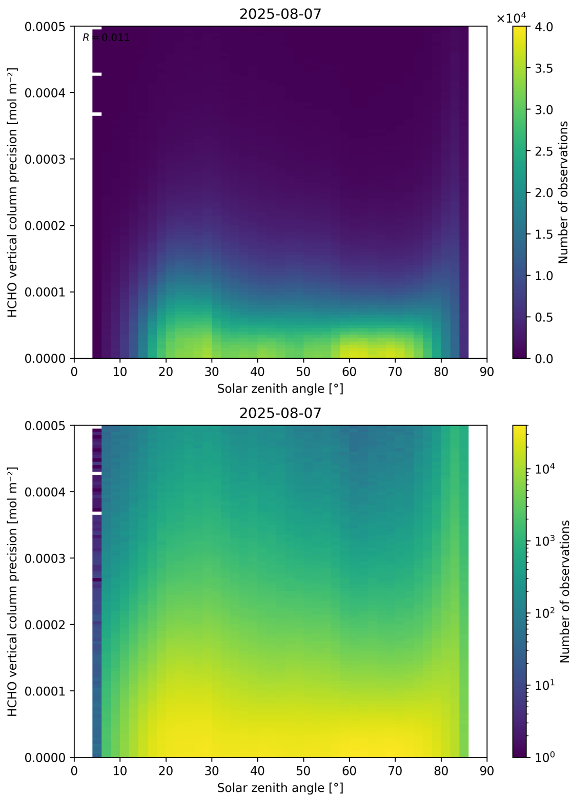
Figure 179: Scatter density plot of “Solar zenith angle” against “HCHO vertical column precision” for 2025-08-06 to 2025-08-08.
