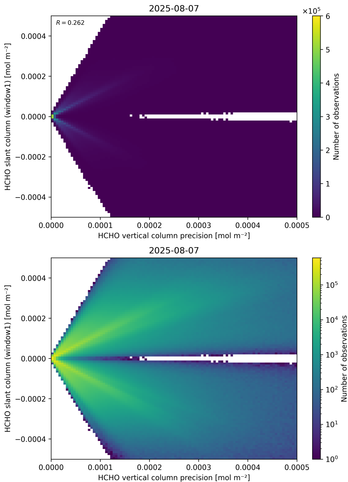
Figure 142: Scatter density plot of “HCHO vertical column precision” against “HCHO slant column (window1)” for 2025-08-06 to 2025-08-08.
