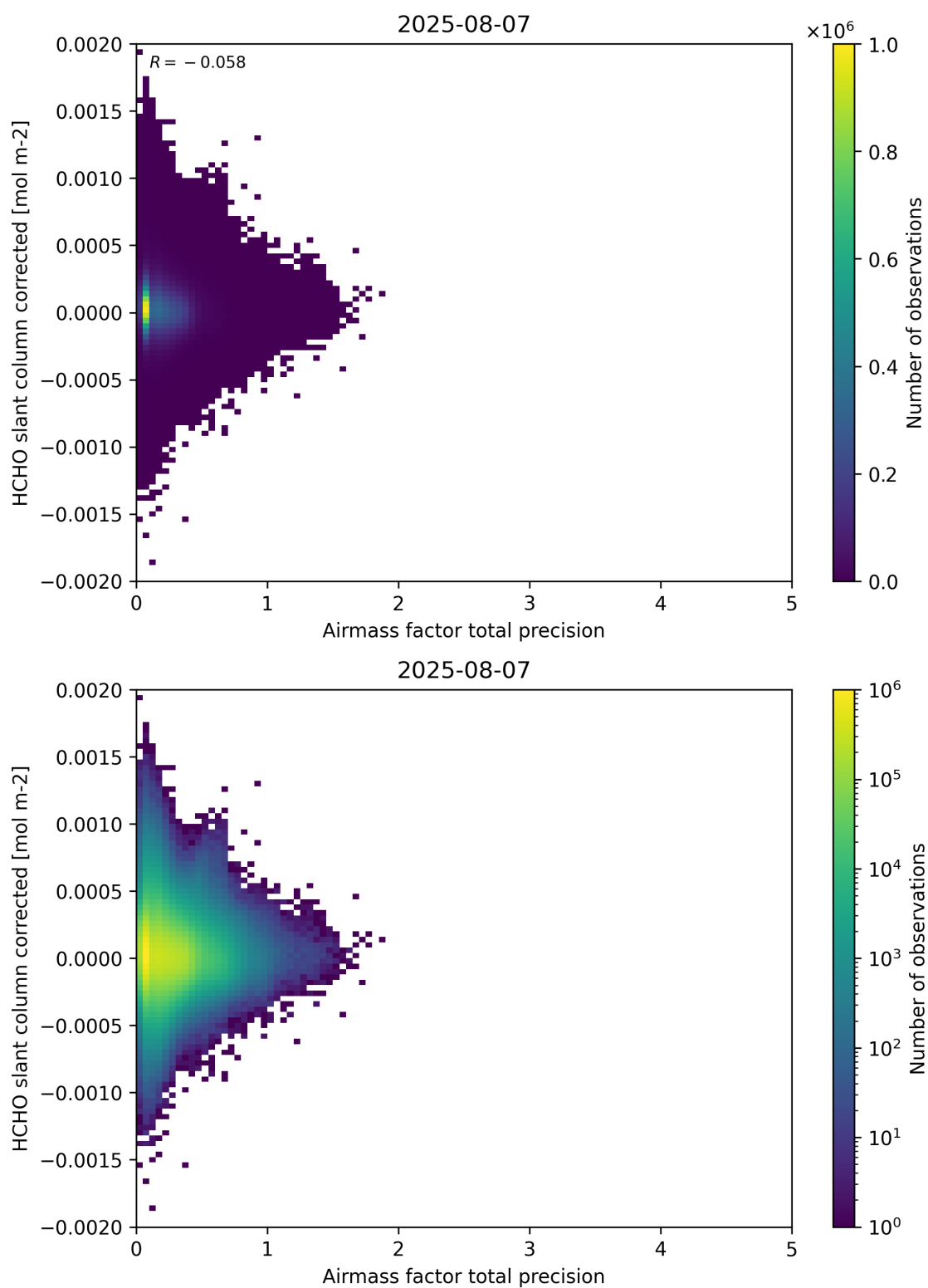
Figure 109: Scatter density plot of “Airmass factor total precision” against “HCHO slant column corrected” for 2025-08-06 to 2025-08-08.
