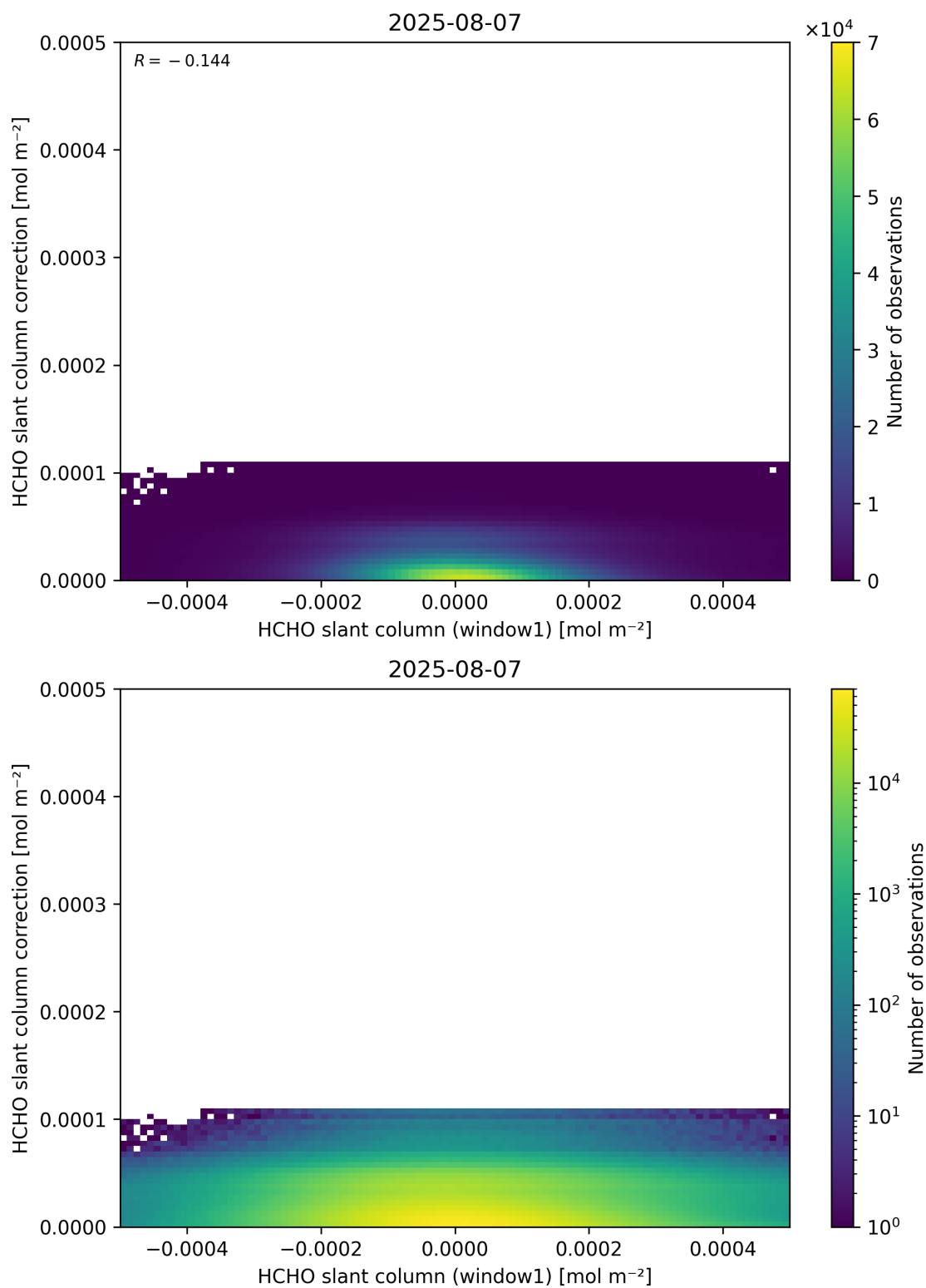
Figure 83: Scatter density plot of “HCHO slant column (window1)” against “HCHO slant column correction” for 2025-08-06 to 2025-08-08.
