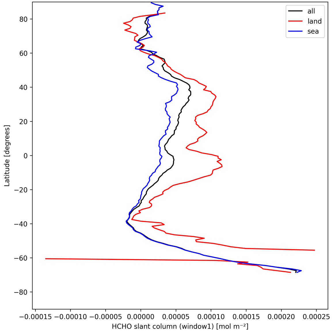
Figure 24: Zonal average of “HCHO slant column (window1)” for 2025-08-06 to 2025-08-08.
