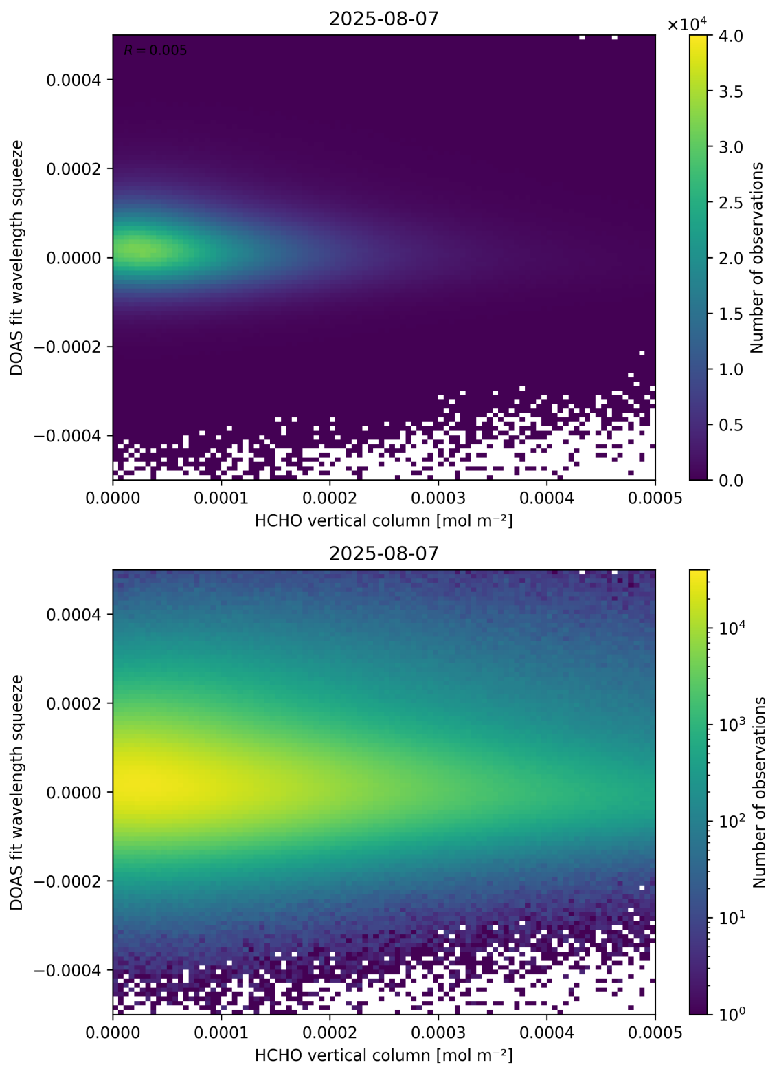
Figure 125: Scatter density plot of “HCHO vertical column” against “DOAS fit wavelength squeeze” for 2025-08-06 to 2025-08-08.
