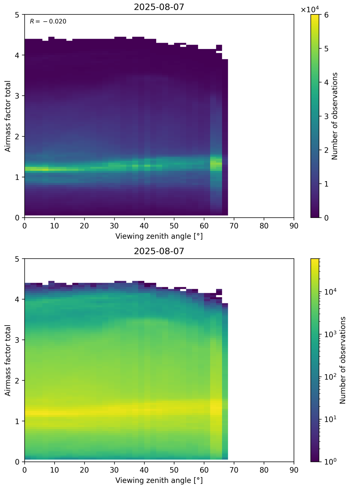
Figure 190: Scatter density plot of “Viewing zenith angle” against “Airmass factor total” for 2025-08-06 to 2025-08-08.
