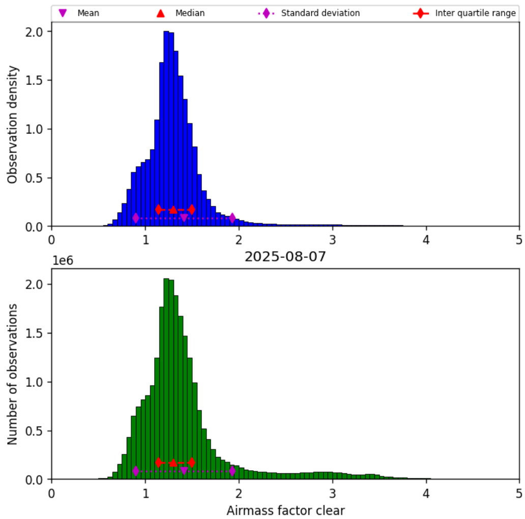
Figure 42: Histogram of “Airmass factor clear” for 2025-08-06 to 2025-08-08
