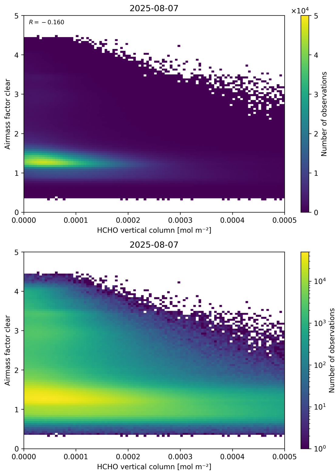
Figure 126: Scatter density plot of “HCHO vertical column” against “Airmass factor clear” for 2025-08-06 to 2025-08-08.
