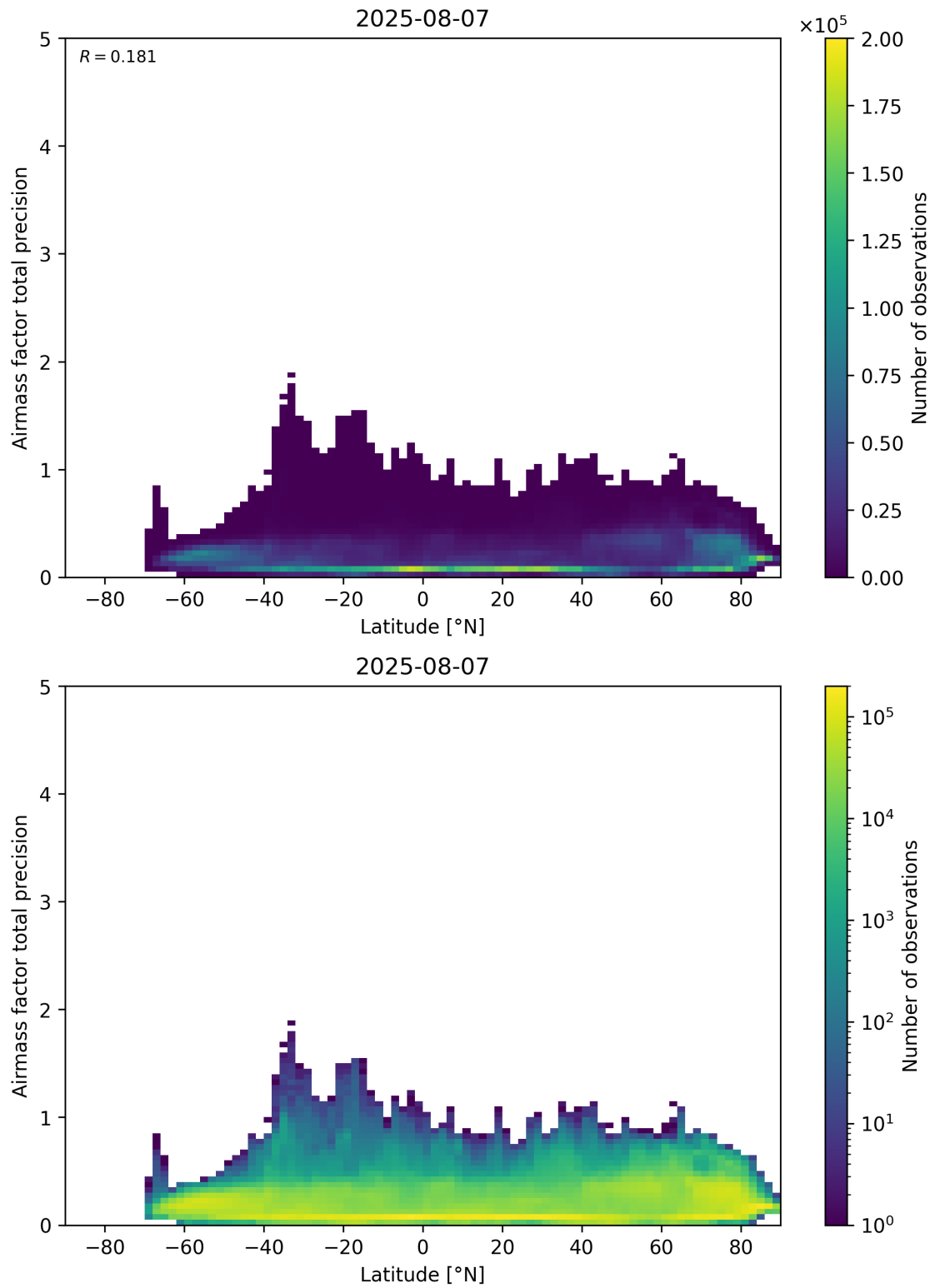
Figure 162: Scatter density plot of “Latitude” against “Airmass factor total precision” for 2025-08-06 to 2025-08-08.
