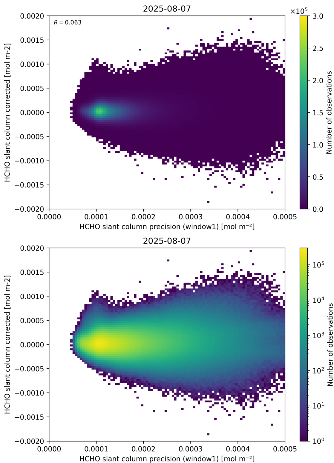
Figure 92: Scatter density plot of “HCHO slant column precision (window1)” against “HCHO slant column corrected” for 2025-08-06 to 2025-08-08.
