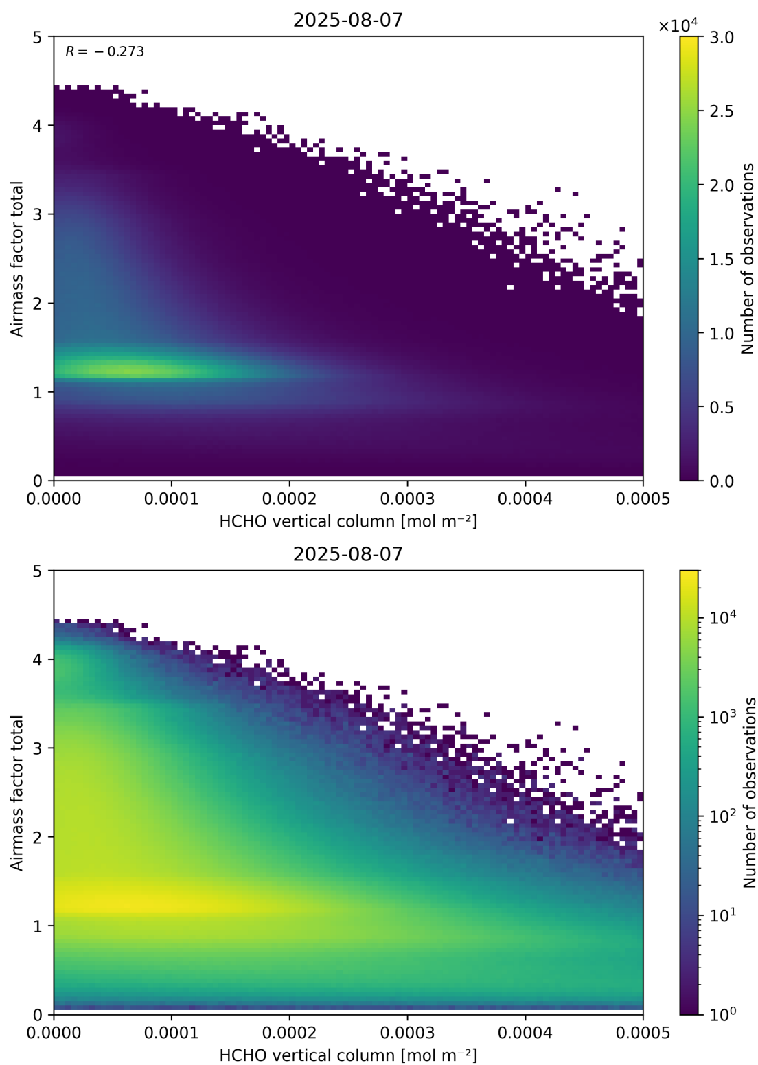
Figure 131: Scatter density plot of “HCHO vertical column” against “Airmass factor total” for 2025-08-06 to 2025-08-08.
