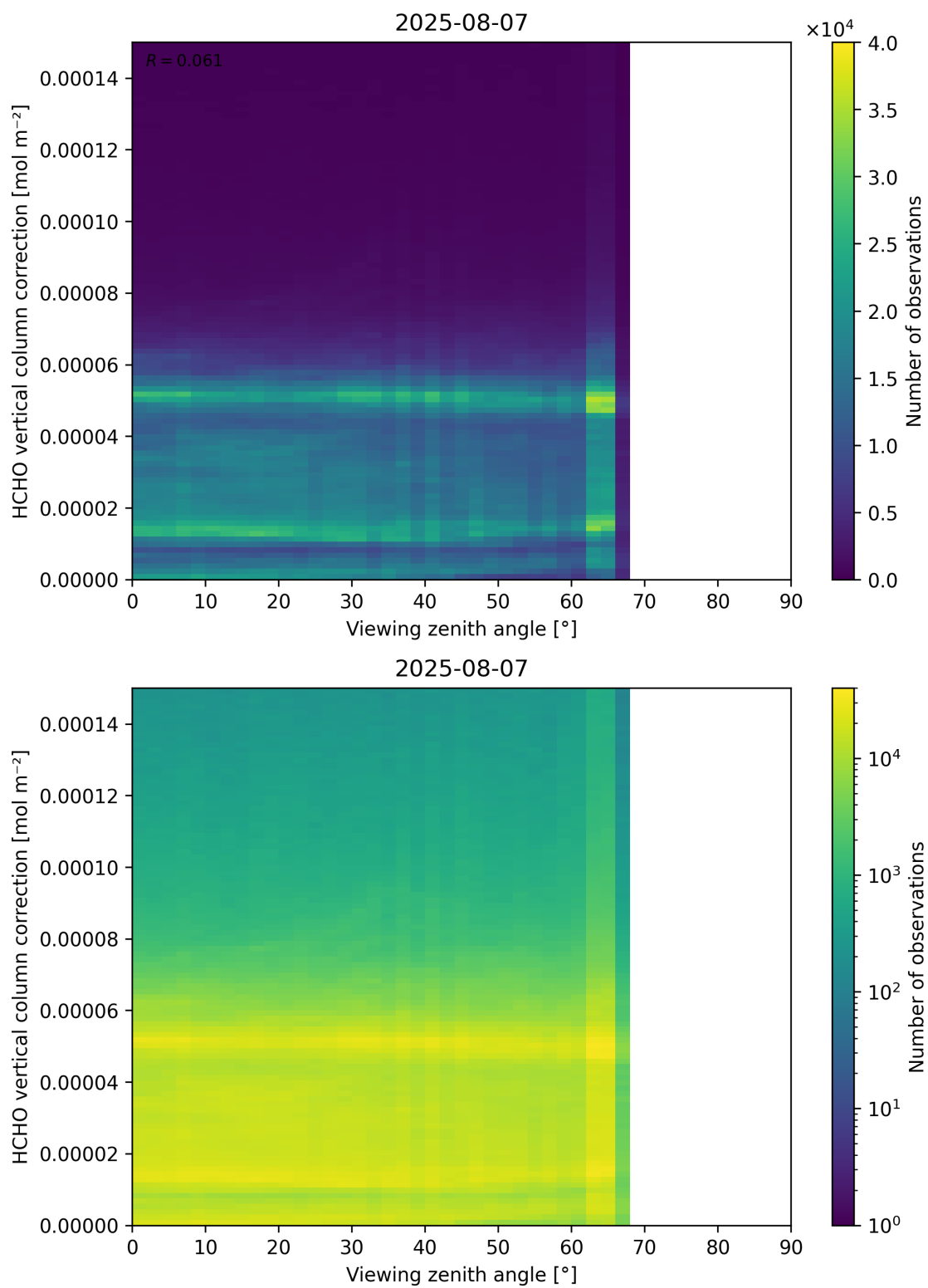
Figure 193: Scatter density plot of “Viewing zenith angle” against “HCHO vertical column correction” for 2025-08-06 to 2025-08-08.
