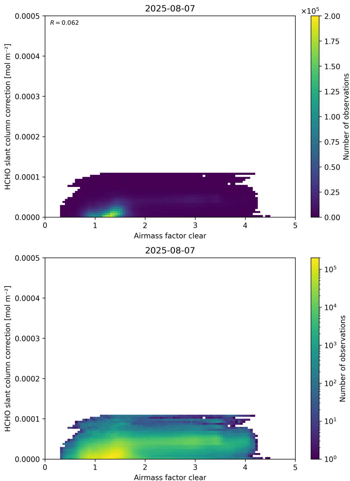
Figure 75: Scatter density plot of “Airmass factor clear” against “HCHO slant column correction” for 2025-08-06 to 2025-08-08.
