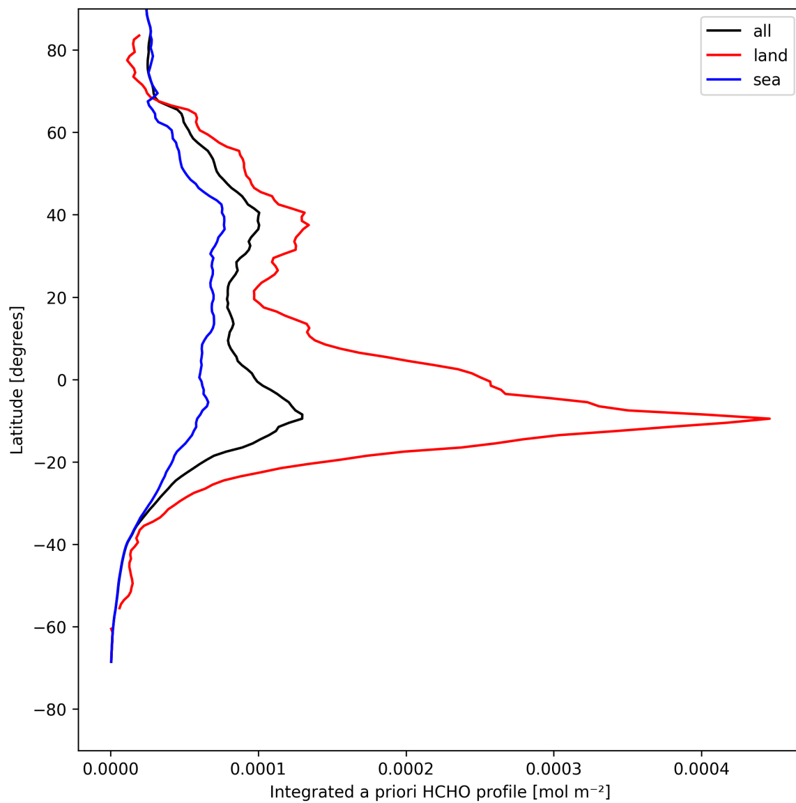
Figure 29: Zonal average of “Integrated a priori HCHO profile” for 2025-08-06 to 2025-08-08.
