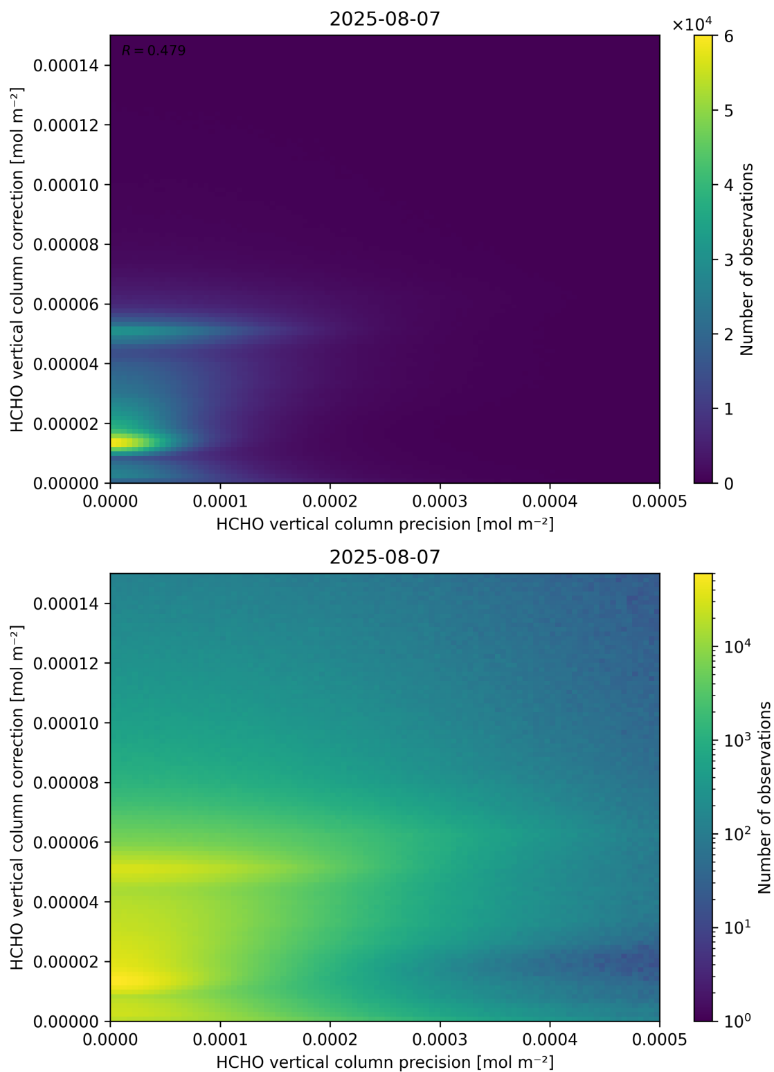
Figure 146: Scatter density plot of “HCHO vertical column precision” against “HCHO vertical column correction” for 2025-08-06 to 2025-08-08.
