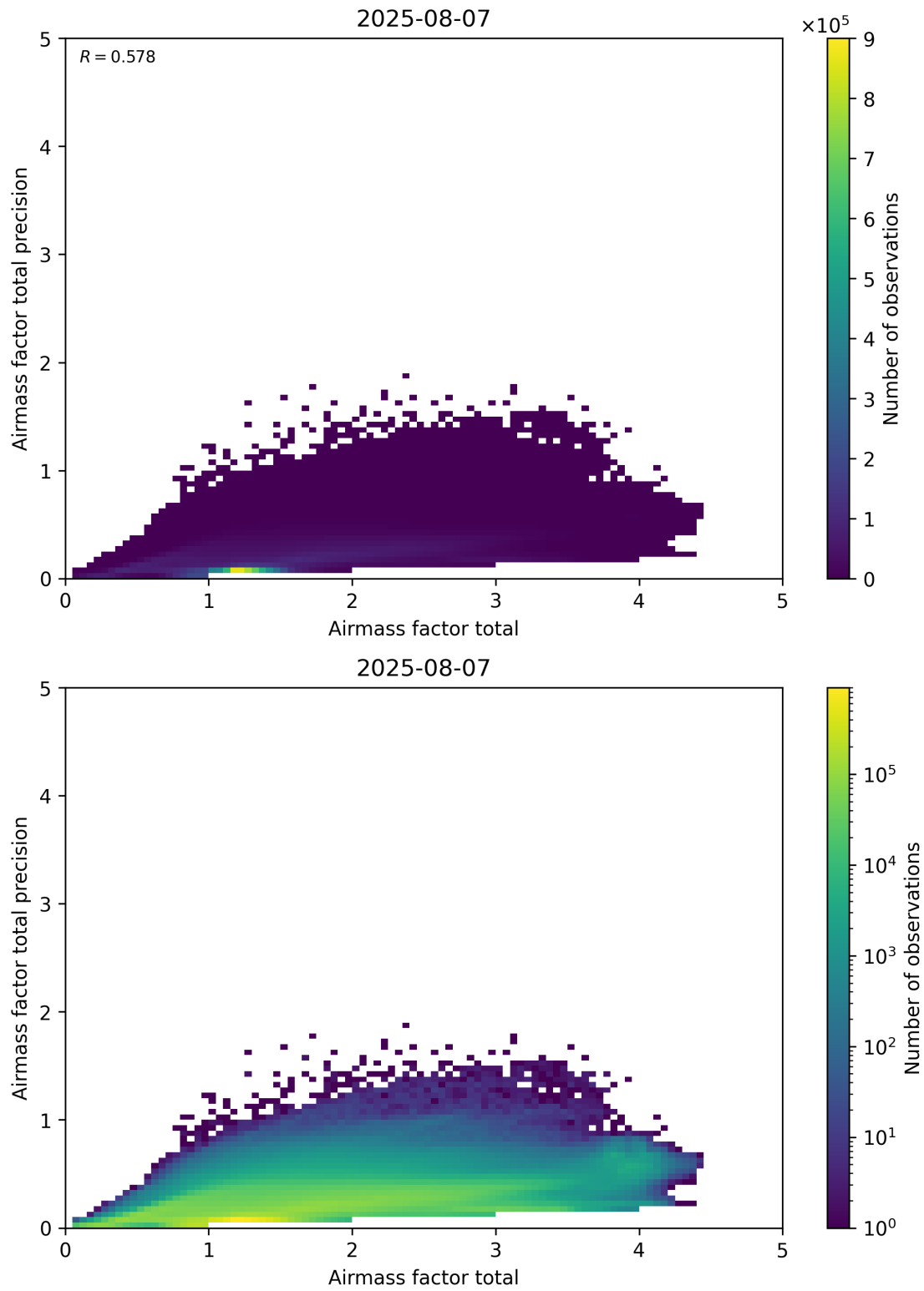
Figure 103: Scatter density plot of “Airmass factor total” against “Airmass factor total precision” for 2025-08-06 to 2025-08-08.
