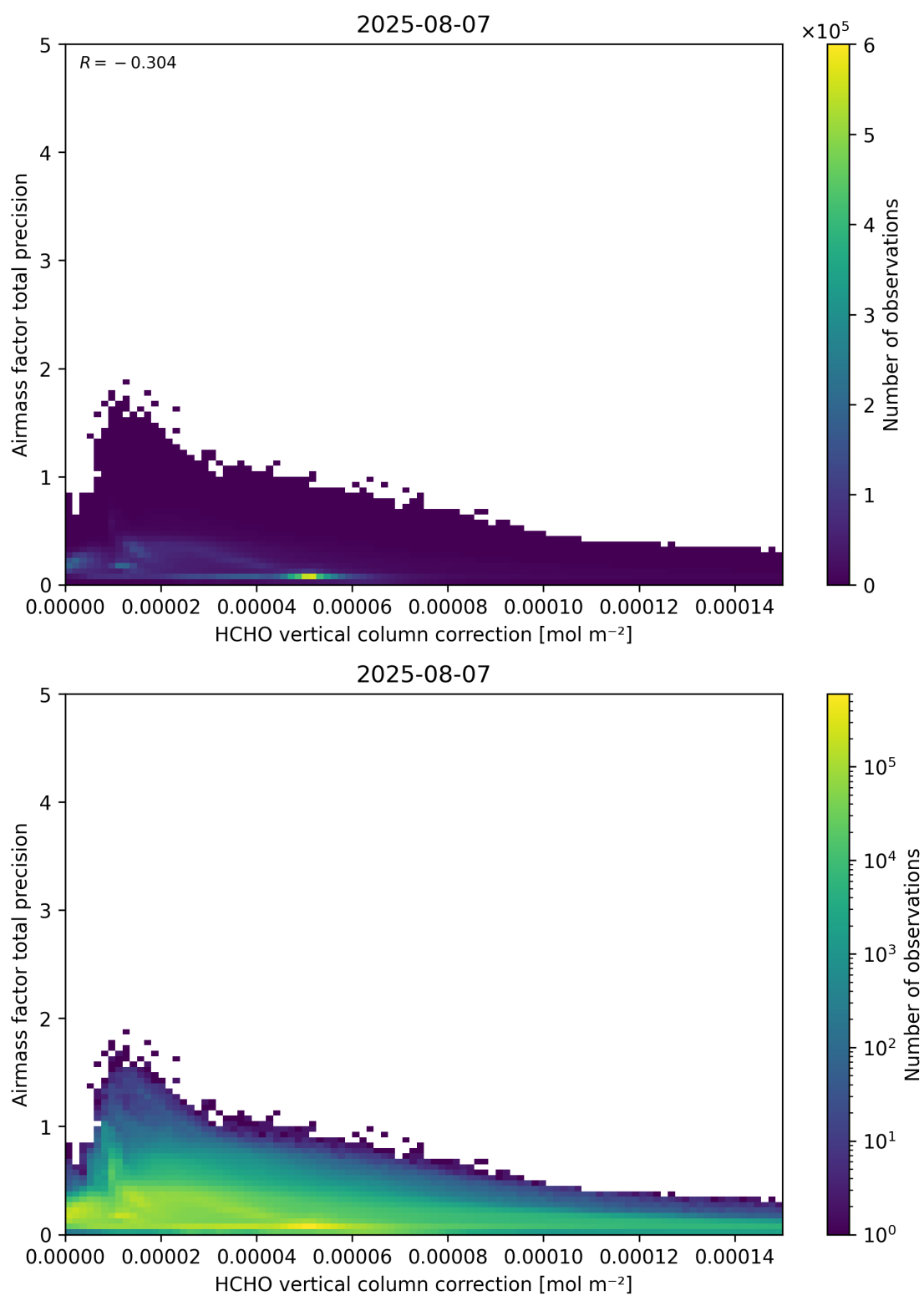
Figure 121: Scatter density plot of “HCHO vertical column correction” against “Airmass factor total precision” for 2025-08-06 to 2025-08-08.
