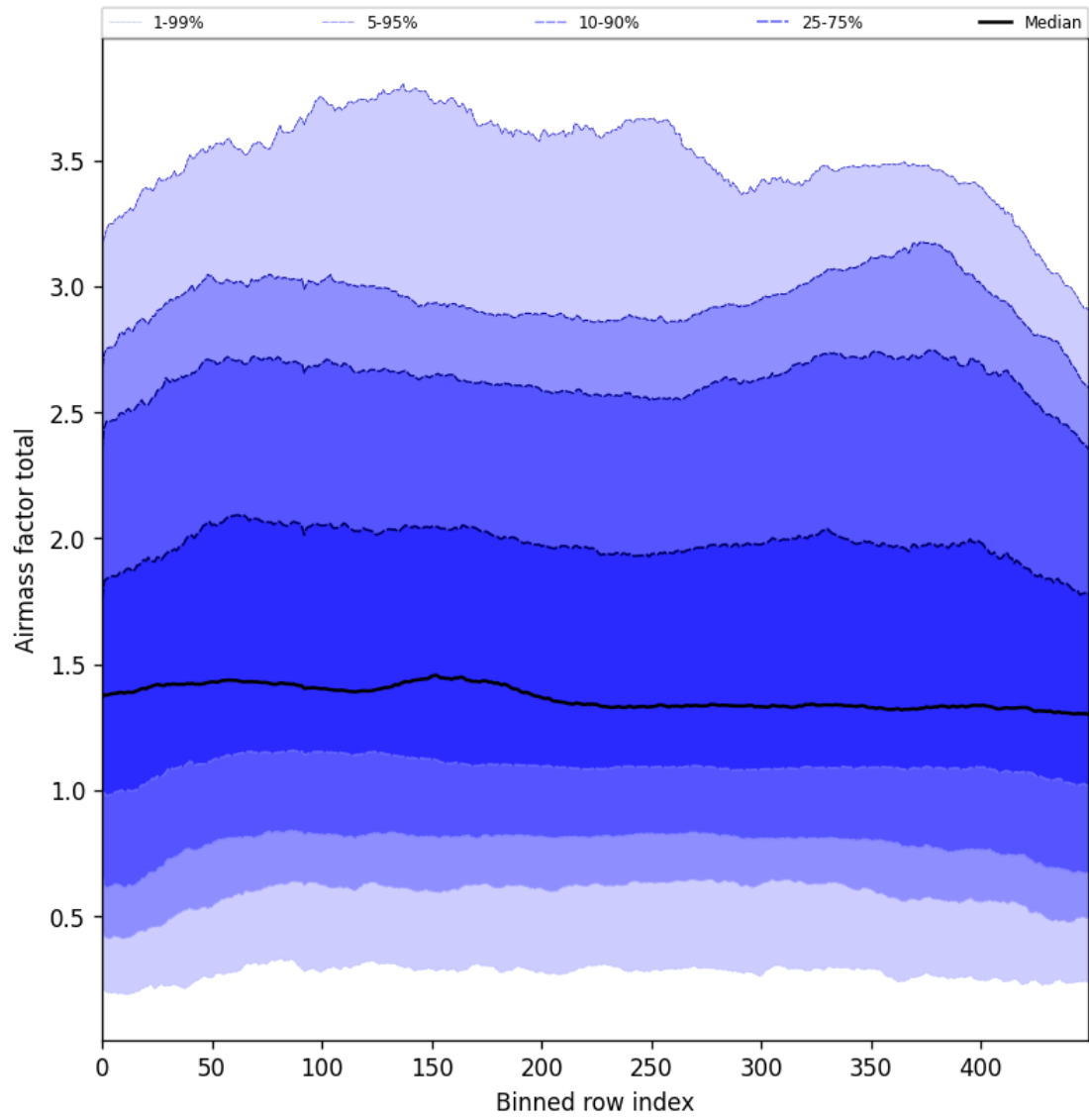
Figure 54: Along track statistics of “Airmass factor total” for 2025-08-06 to 2025-08-08
