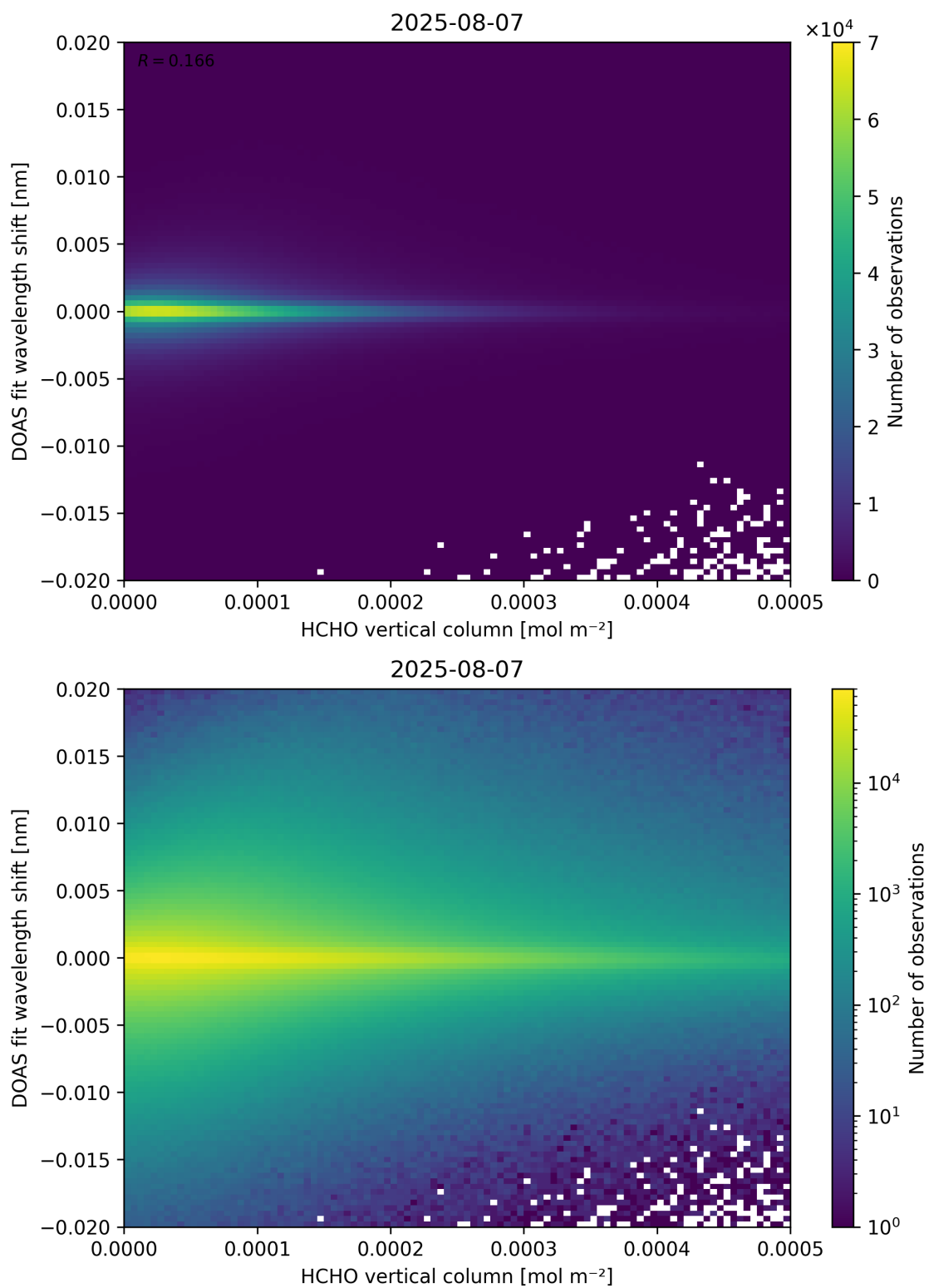
Figure 124: Scatter density plot of “HCHO vertical column” against “DOAS fit wavelength shift” for 2025-08-06 to 2025-08-08.
