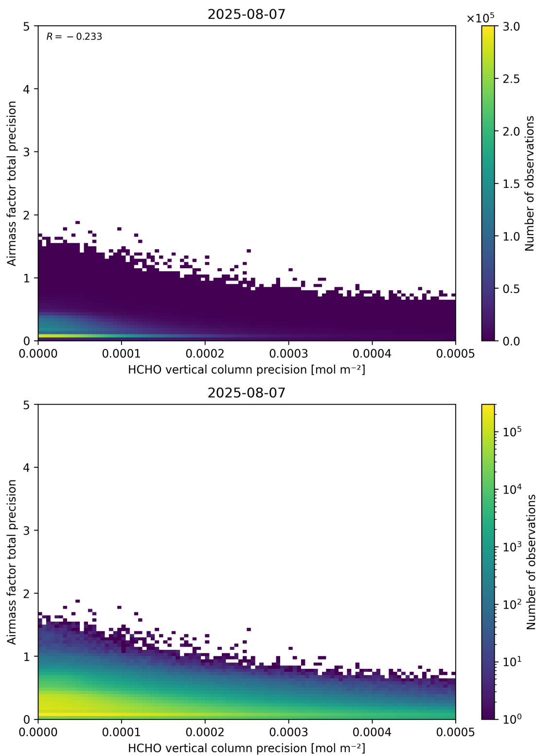
Figure 145: Scatter density plot of “HCHO vertical column precision” against “Airmass factor total precision” for 2025-08-06 to 2025-08-08.
