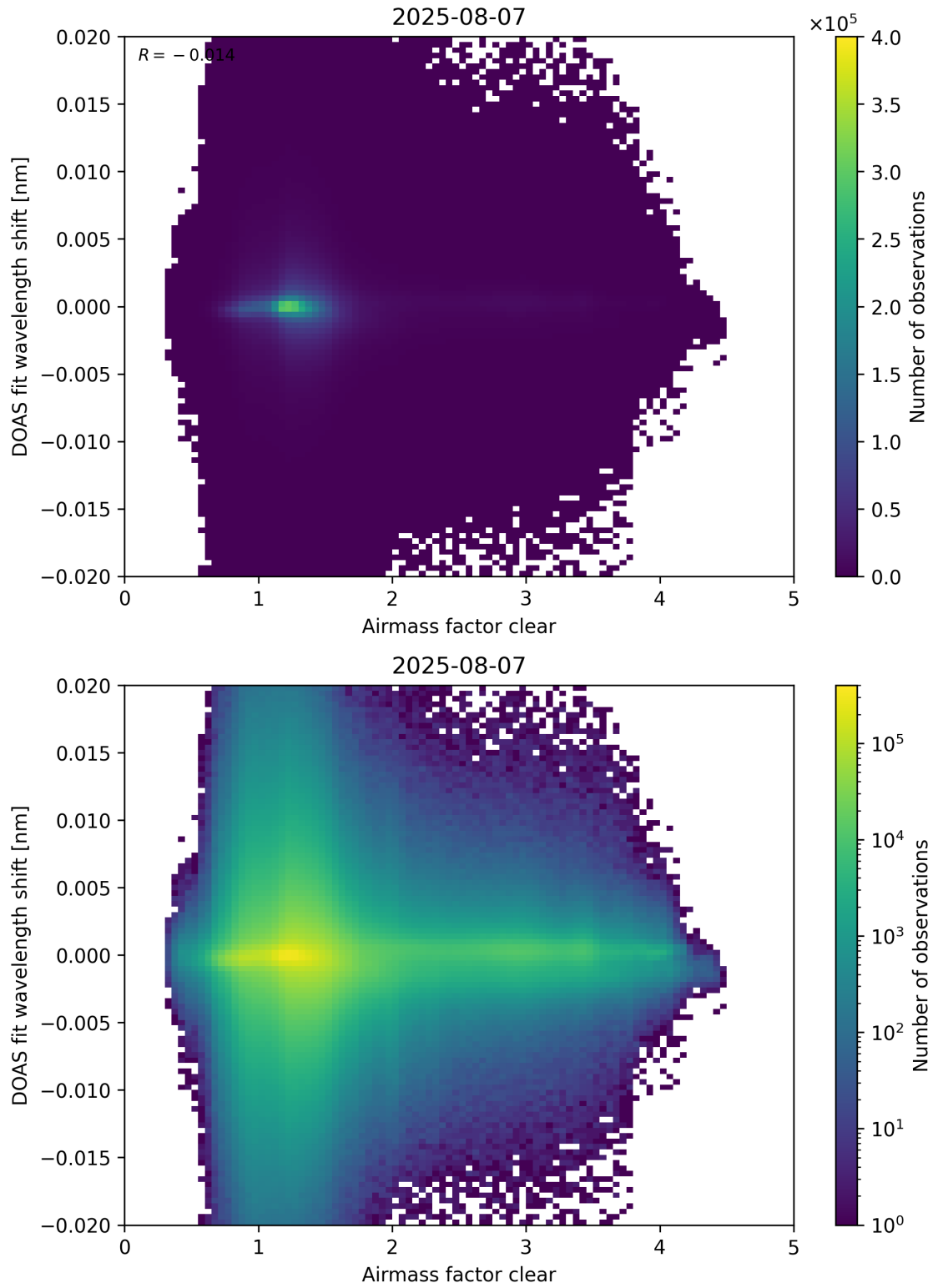
Figure 72: Scatter density plot of “Airmass factor clear” against “DOAS fit wavelength shift” for 2025-08-06 to 2025-08-08.
