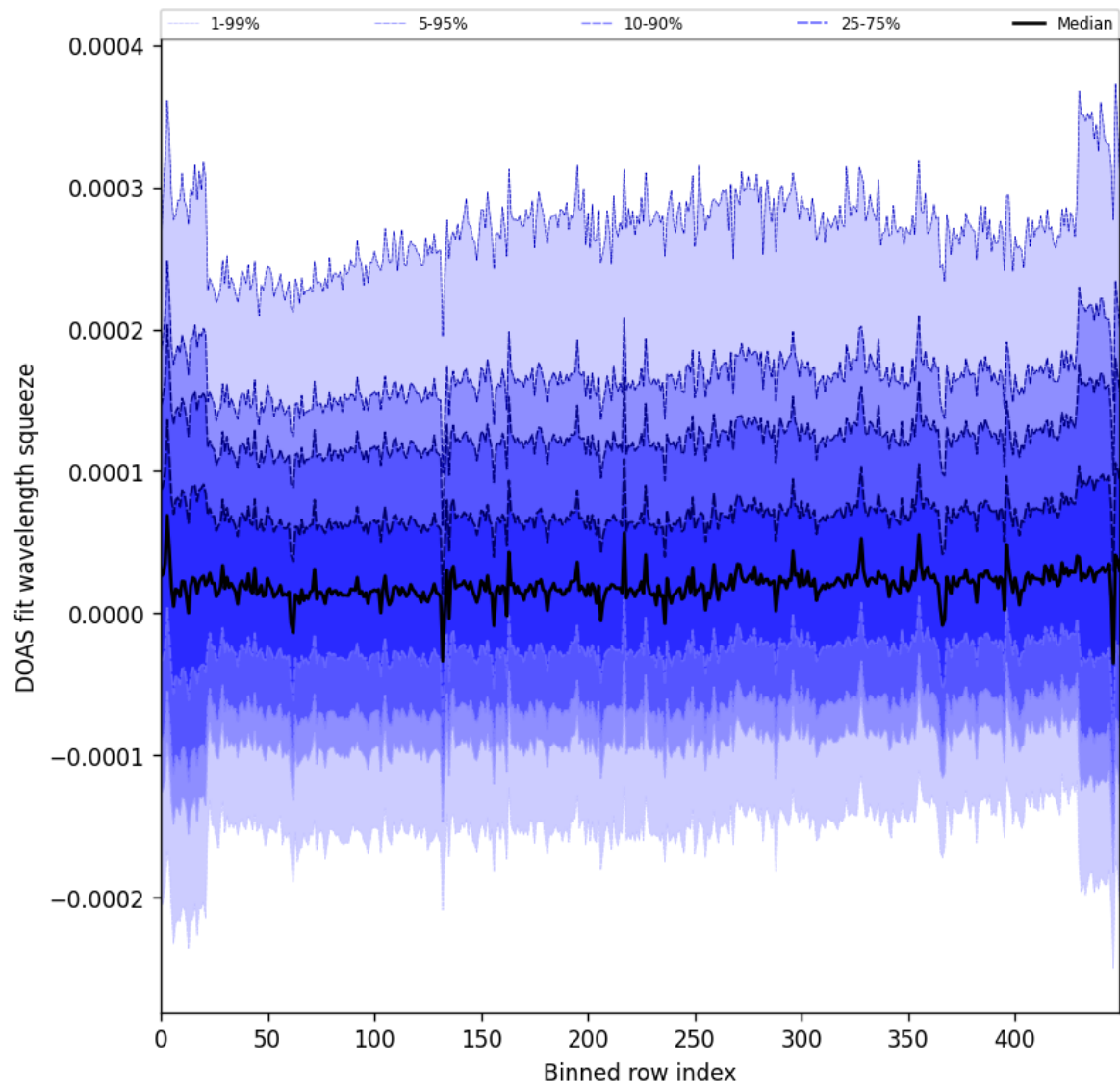
Figure 59: Along track statistics of “DOAS fit wavelength squeeze” for 2025-08-06 to 2025-08-08
