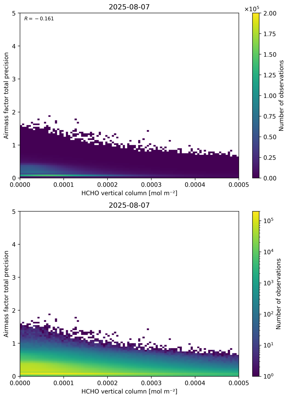
Figure 132: Scatter density plot of “HCHO vertical column” against “Airmass factor total precision” for 2025-08-06 to 2025-08-08.
