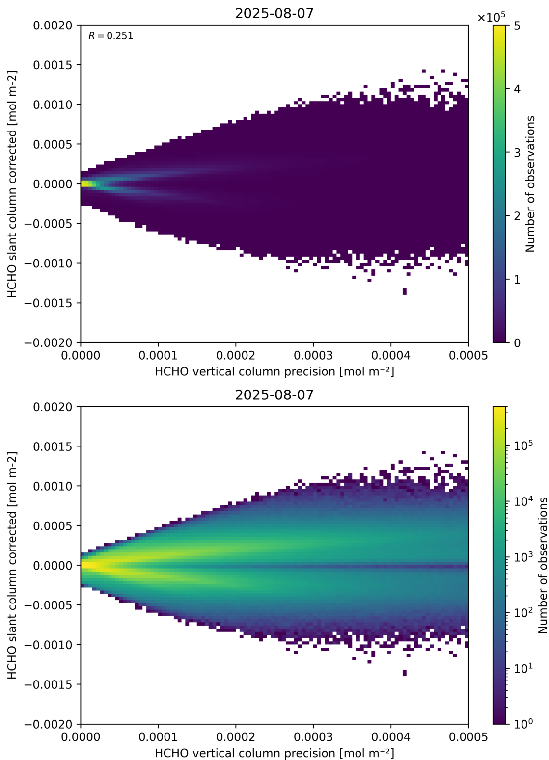
Figure 140: Scatter density plot of “HCHO vertical column precision” against “HCHO slant column corrected” for 2025-08-06 to 2025-08-08.
