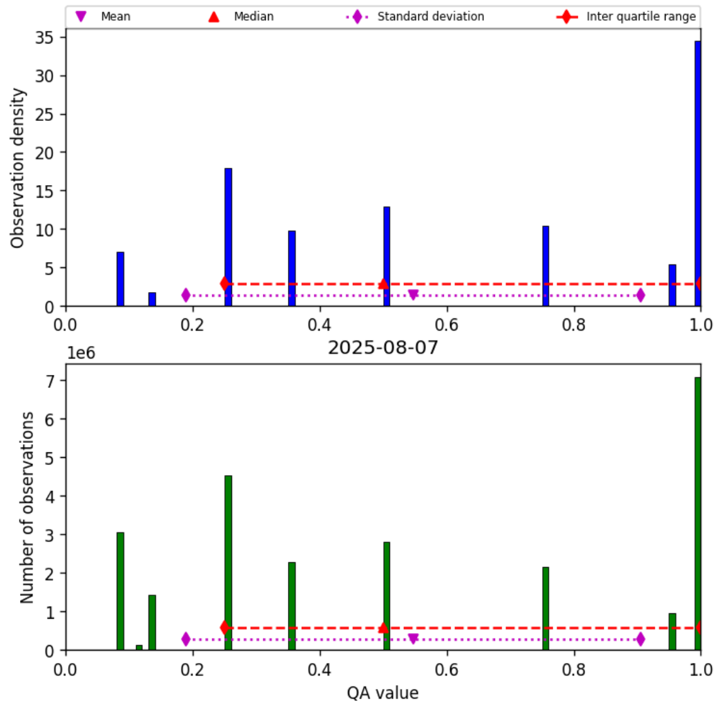
Figure 34: Histogram of “QA value” for 2025-08-06 to 2025-08-08
