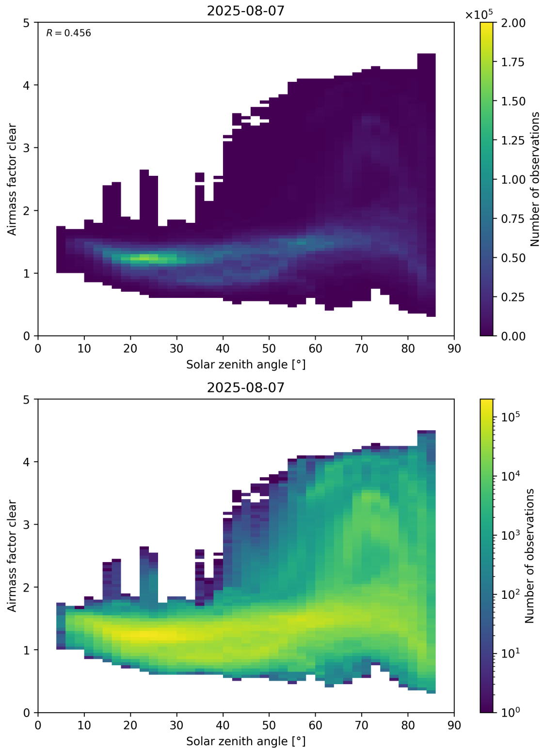
Figure 170: Scatter density plot of “Solar zenith angle” against “Airmass factor clear” for 2025-08-06 to 2025-08-08.
