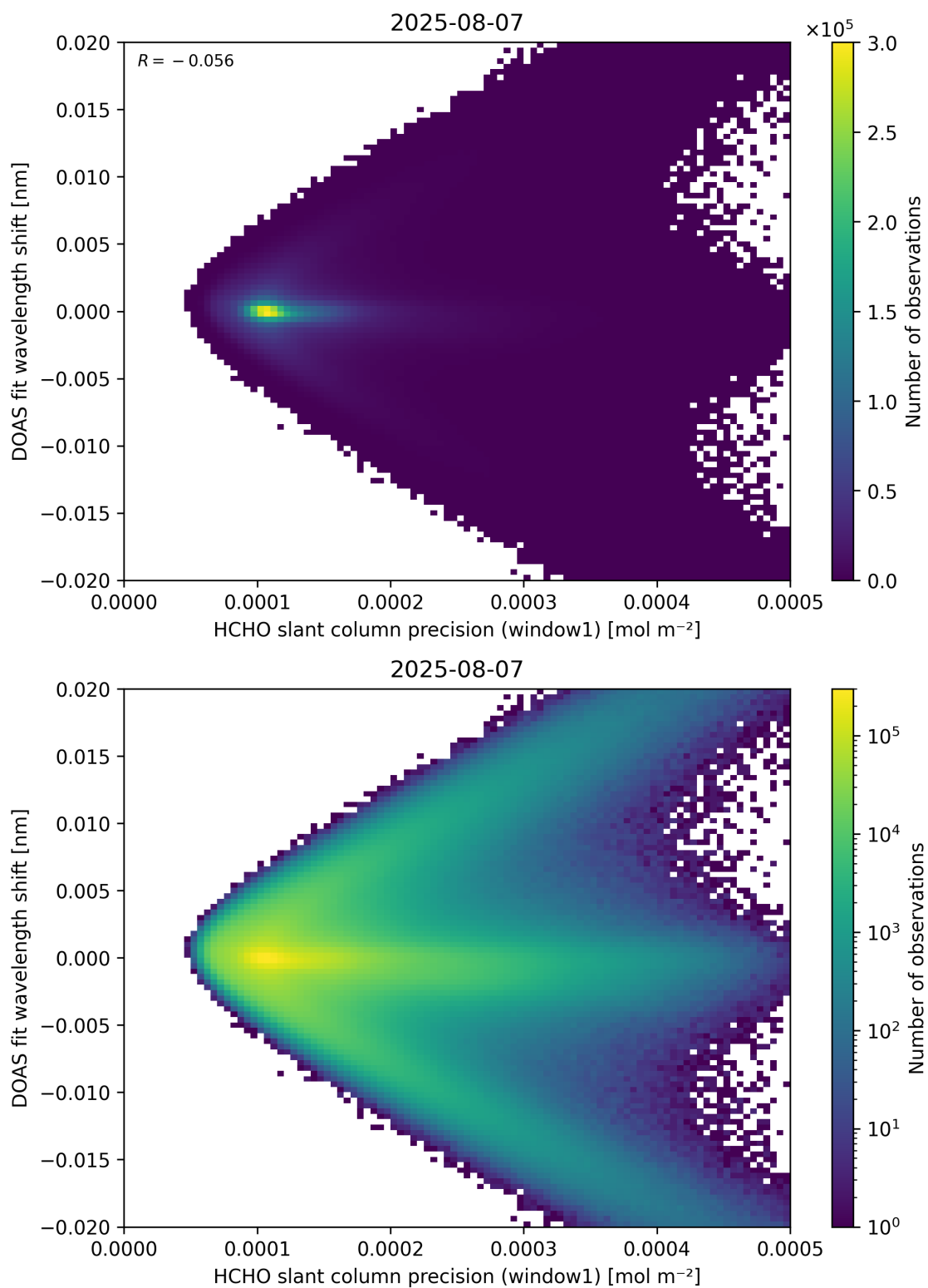
Figure 89: Scatter density plot of “HCHO slant column precision (window1)” against “DOAS fit wavelength shift” for 2025-08-06 to 2025-08-08.
