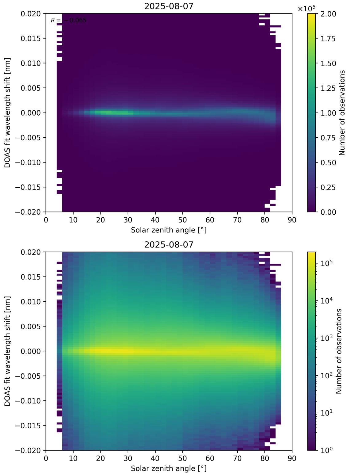
Figure 168: Scatter density plot of “Solar zenith angle” against “DOAS fit wavelength shift” for 2025-08-06 to 2025-08-08.
