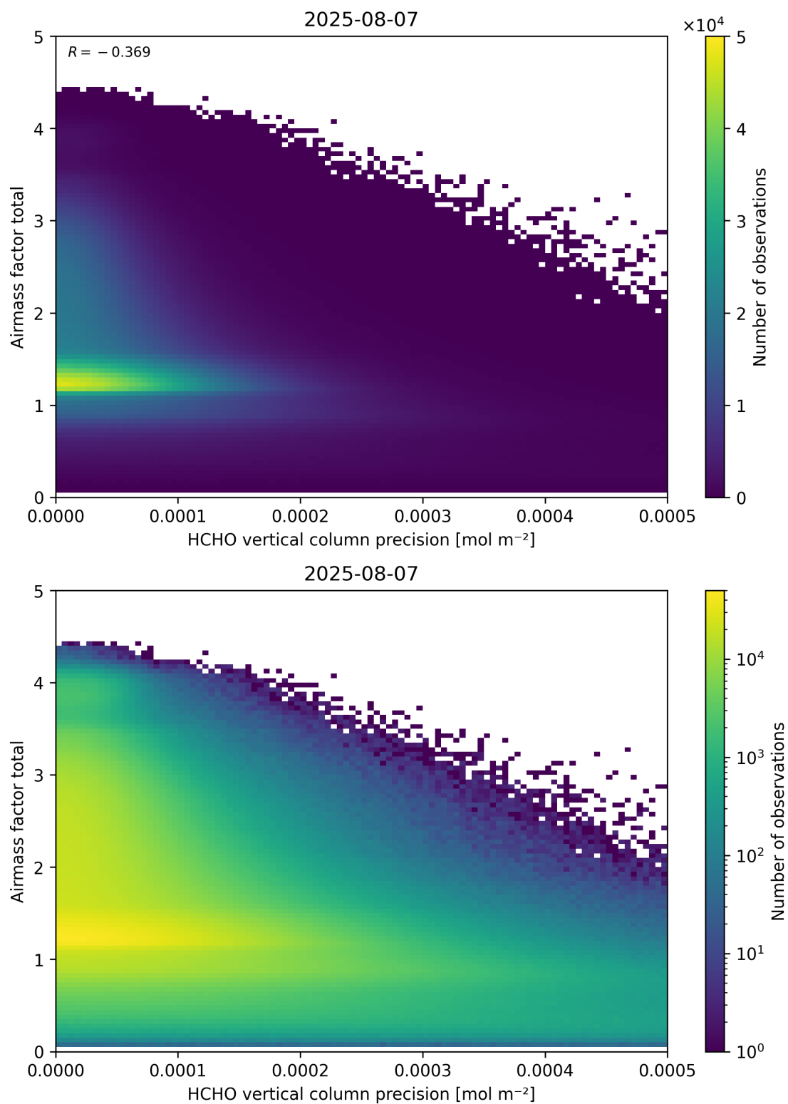
Figure 144: Scatter density plot of “HCHO vertical column precision” against “Airmass factor total” for 2025-08-06 to 2025-08-08.
