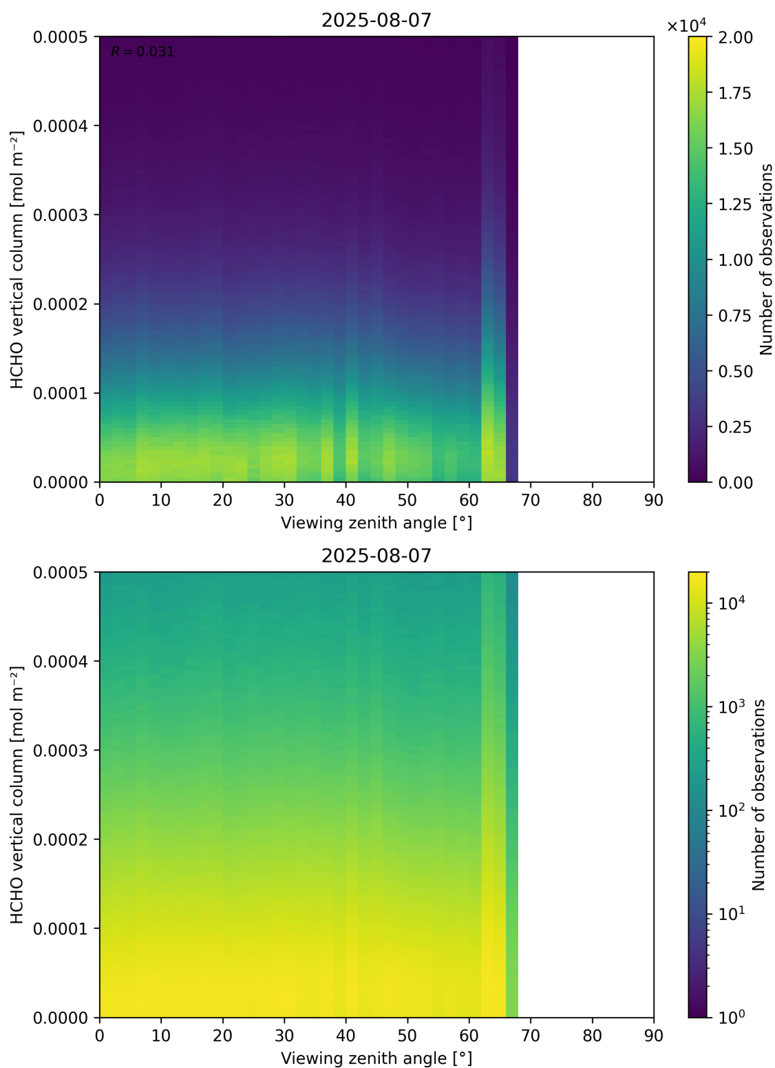
Figure 192: Scatter density plot of “Viewing zenith angle” against “HCHO vertical column” for 2025-08-06 to 2025-08-08.
