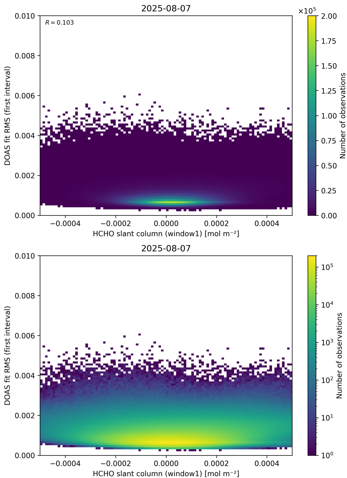
Figure 78: Scatter density plot of “HCHO slant column (window1)” against “DOAS fit RMS (first interval)” for 2025-08-06 to 2025-08-08.
