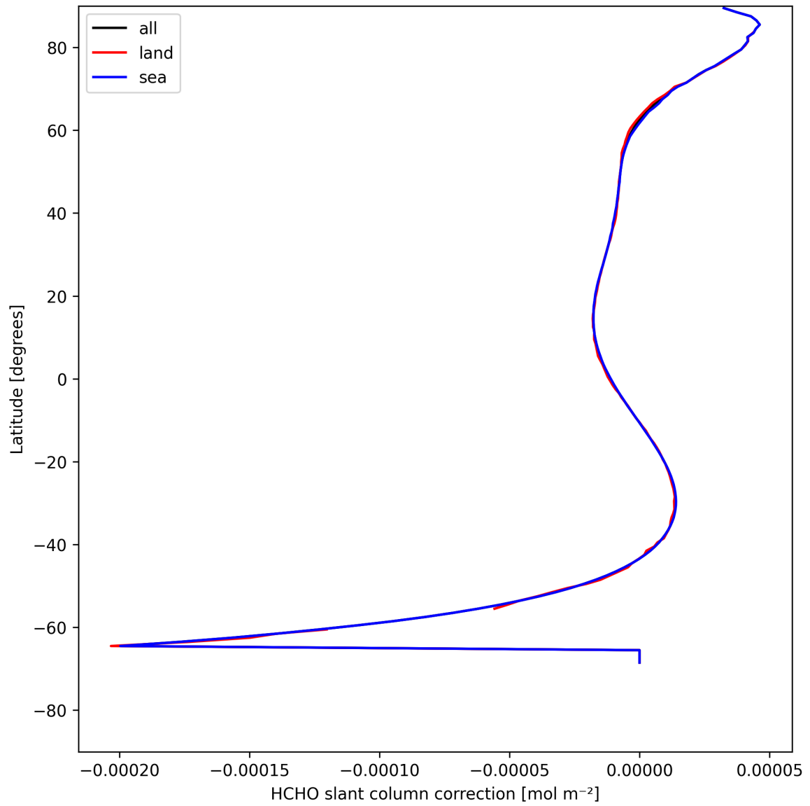
Figure 33: Zonal average of “HCHO slant column correction” for 2025-08-06 to 2025-08-08.
