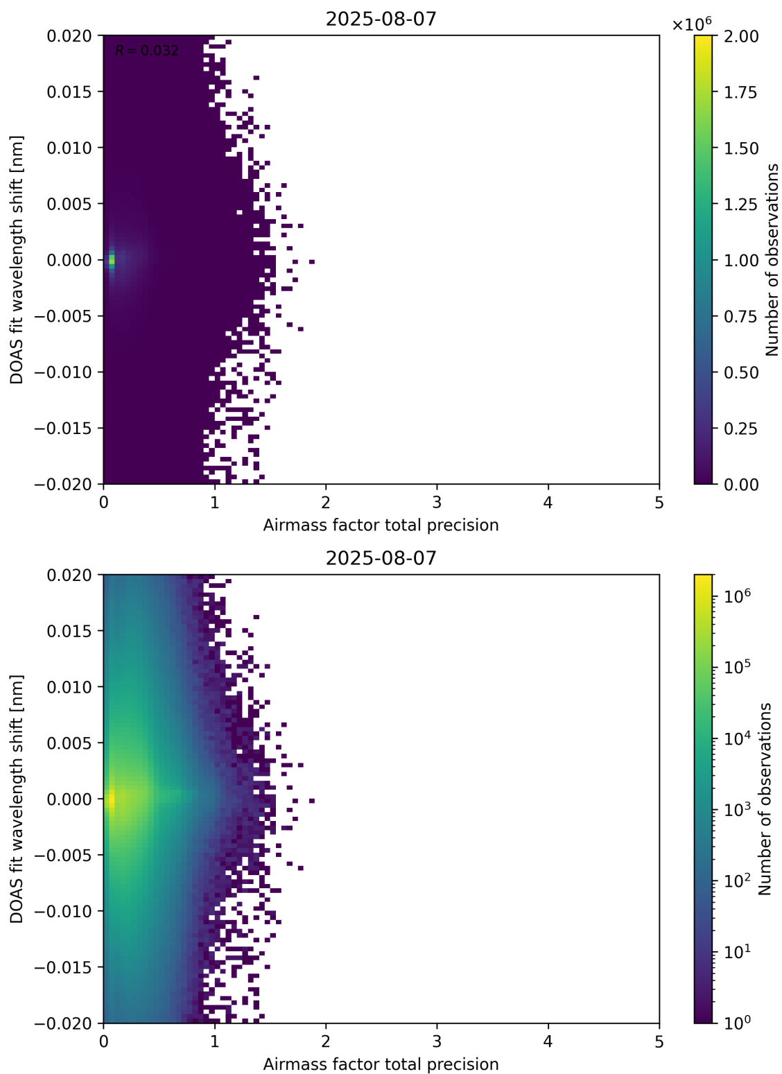
Figure 106: Scatter density plot of “Airmass factor total precision” against “DOAS fit wavelength shift” for 2025-08-06 to 2025-08-08.
