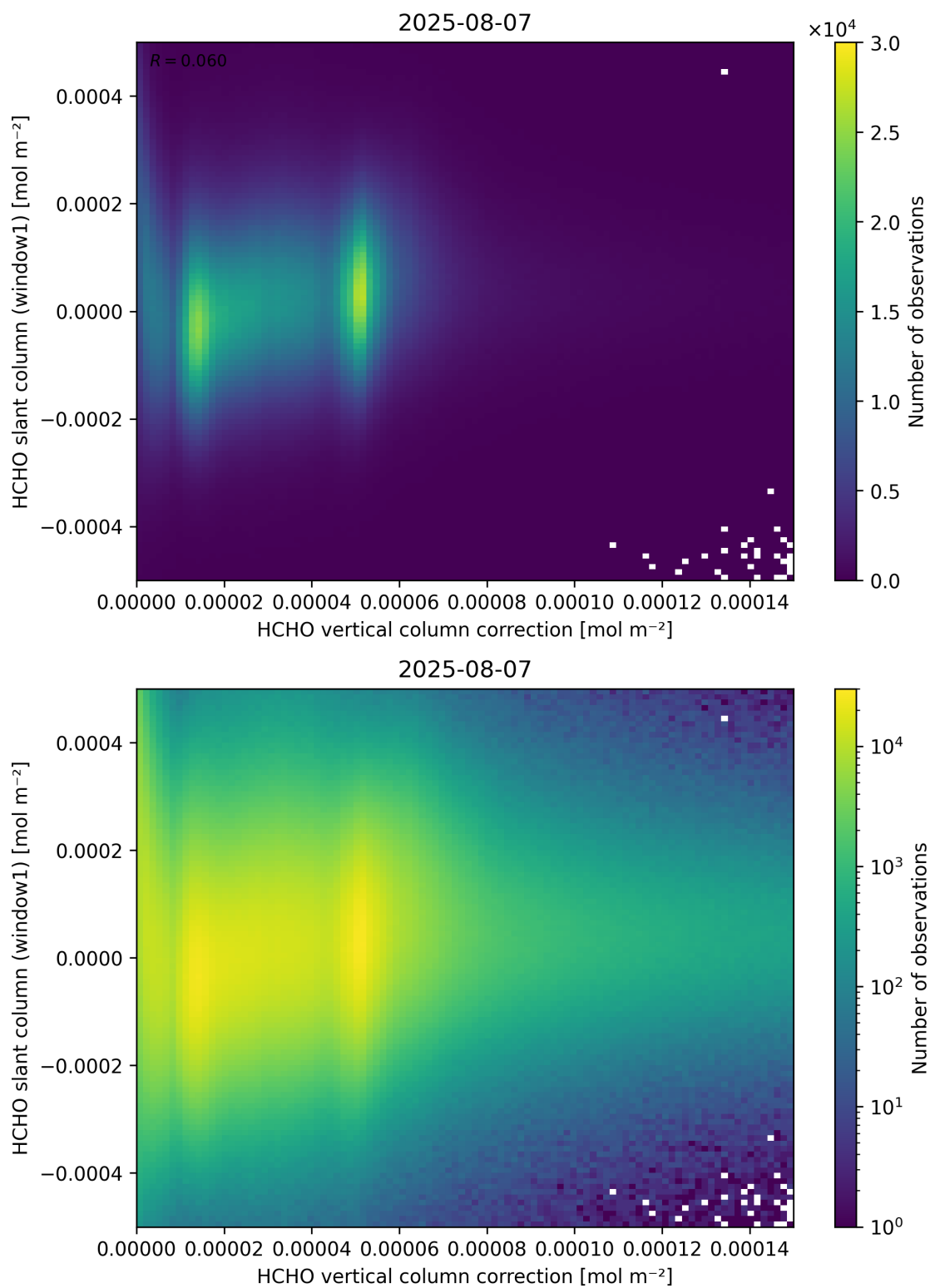
Figure 118: Scatter density plot of “HCHO vertical column correction” against “HCHO slant column (window1)” for 2025-08-06 to 2025-08-08.
