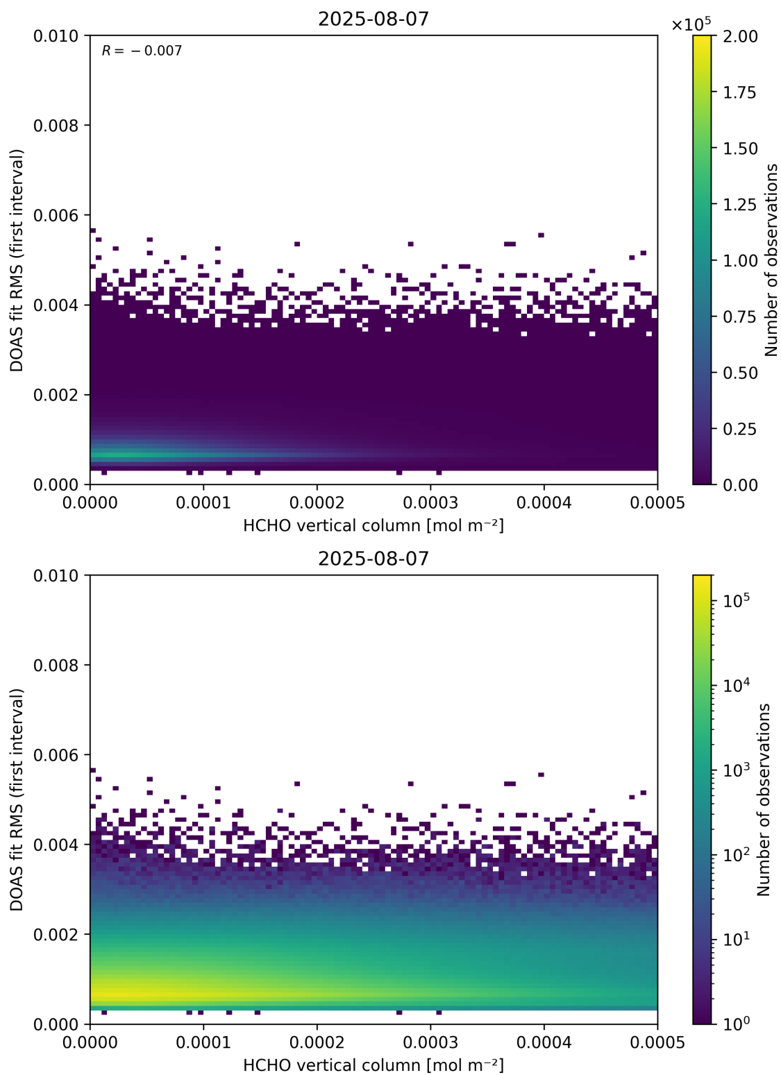
Figure 123: Scatter density plot of “HCHO vertical column” against “DOAS fit RMS (first interval)” for 2025-08-06 to 2025-08-08.
