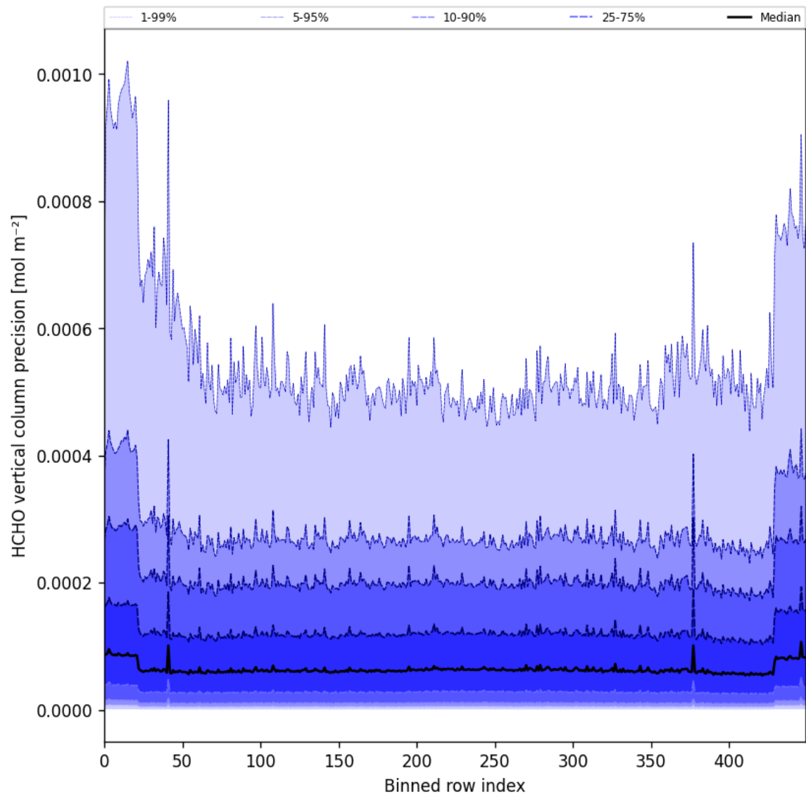
Figure 50: Along track statistics of “HCHO vertical column precision” for 2025-08-06 to 2025-08-08
