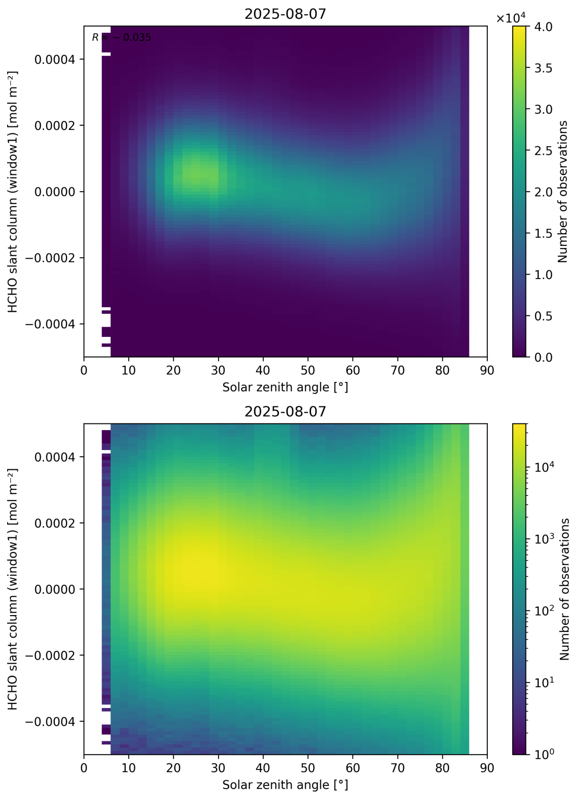
Figure 173: Scatter density plot of “Solar zenith angle” against “HCHO slant column (window1)” for 2025-08-06 to 2025-08-08.
