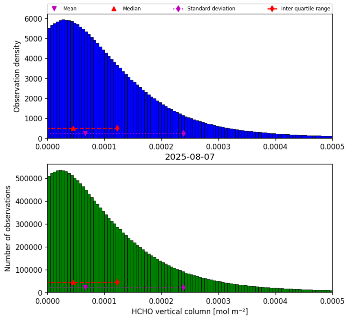
Figure 35: Histogram of “HCHO vertical column” for 2025-08-06 to 2025-08-08
