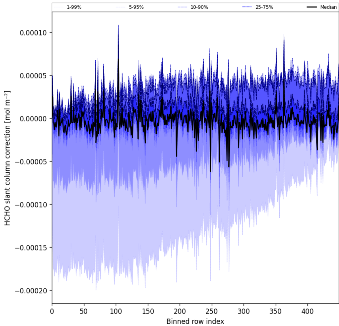
Figure 61: Along track statistics of “HCHO slant column correction” for 2025-08-06 to 2025-08-08
