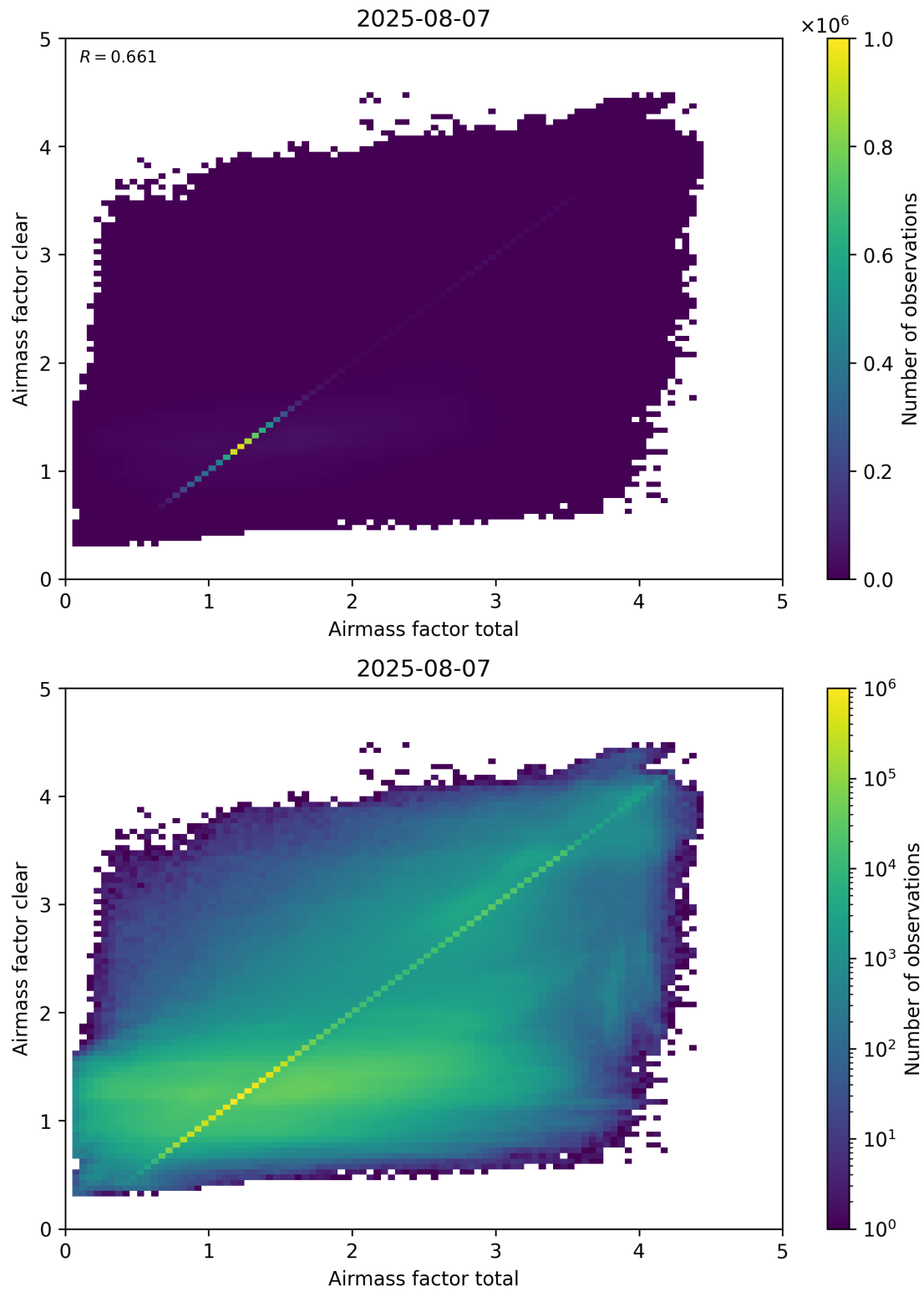
Figure 100: Scatter density plot of “Airmass factor total” against “Airmass factor clear” for 2025-08-06 to 2025-08-08.
