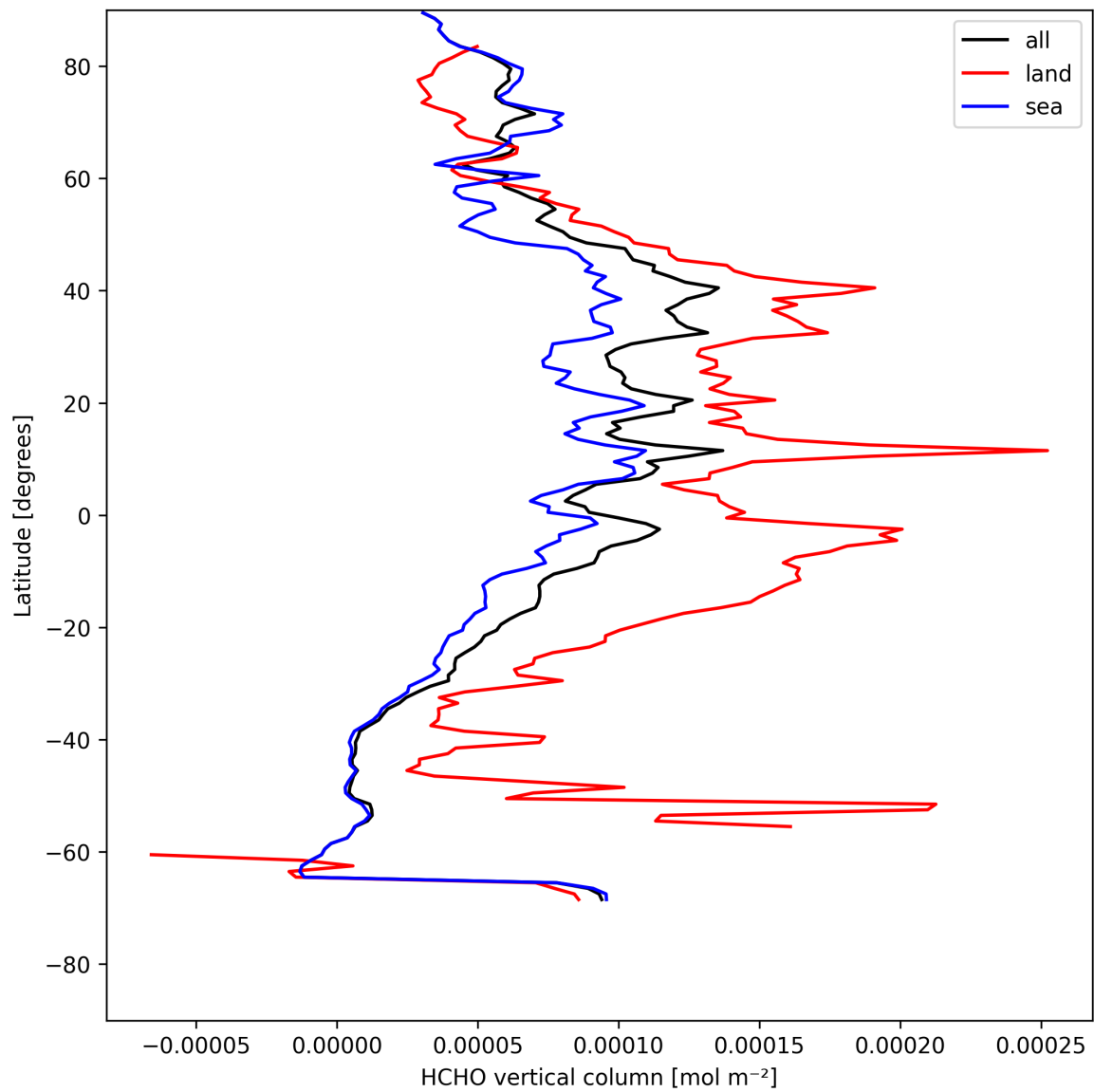
Figure 21: Zonal average of “HCHO vertical column” for 2025-08-06 to 2025-08-08.
