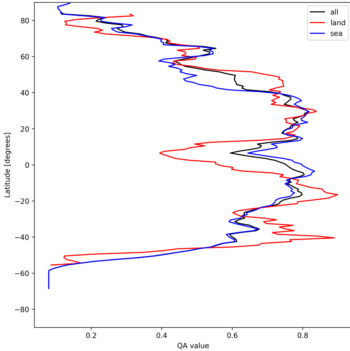
Figure 20: Zonal average of “QA value” for 2025-08-06 to 2025-08-08.
