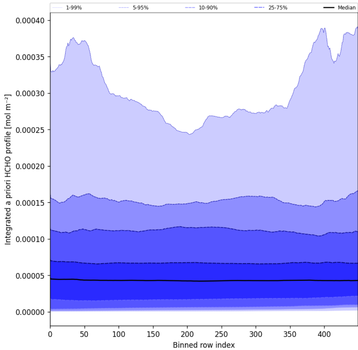
Figure 57: Along track statistics of “Integrated a priori HCHO profile” for 2025-08-06 to 2025-08-08
