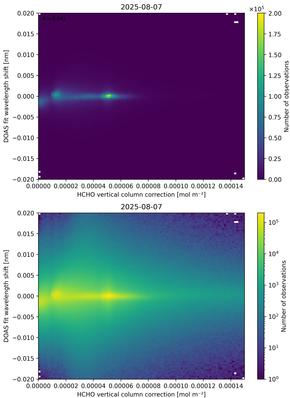
Figure 113: Scatter density plot of “HCHO vertical column correction” against “DOAS fit wavelength shift” for 2025-08-06 to 2025-08-08.
