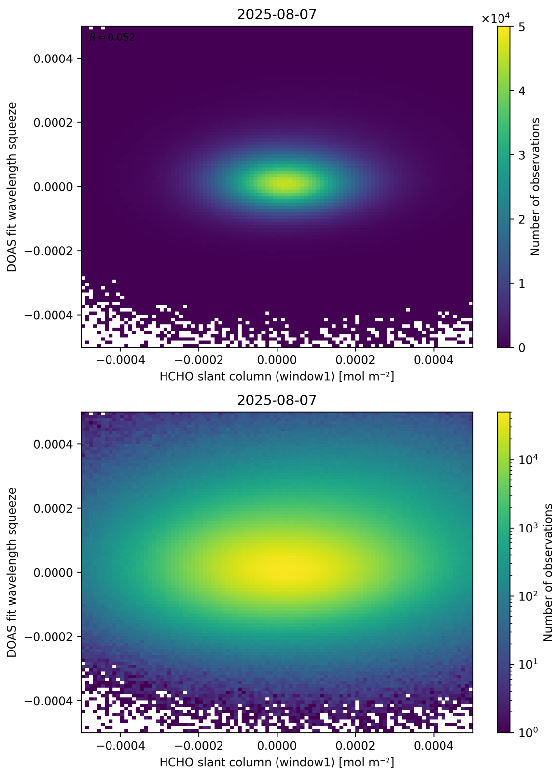
Figure 80: Scatter density plot of “HCHO slant column (window1)” against “DOAS fit wavelength squeeze” for 2025-08-06 to 2025-08-08.
