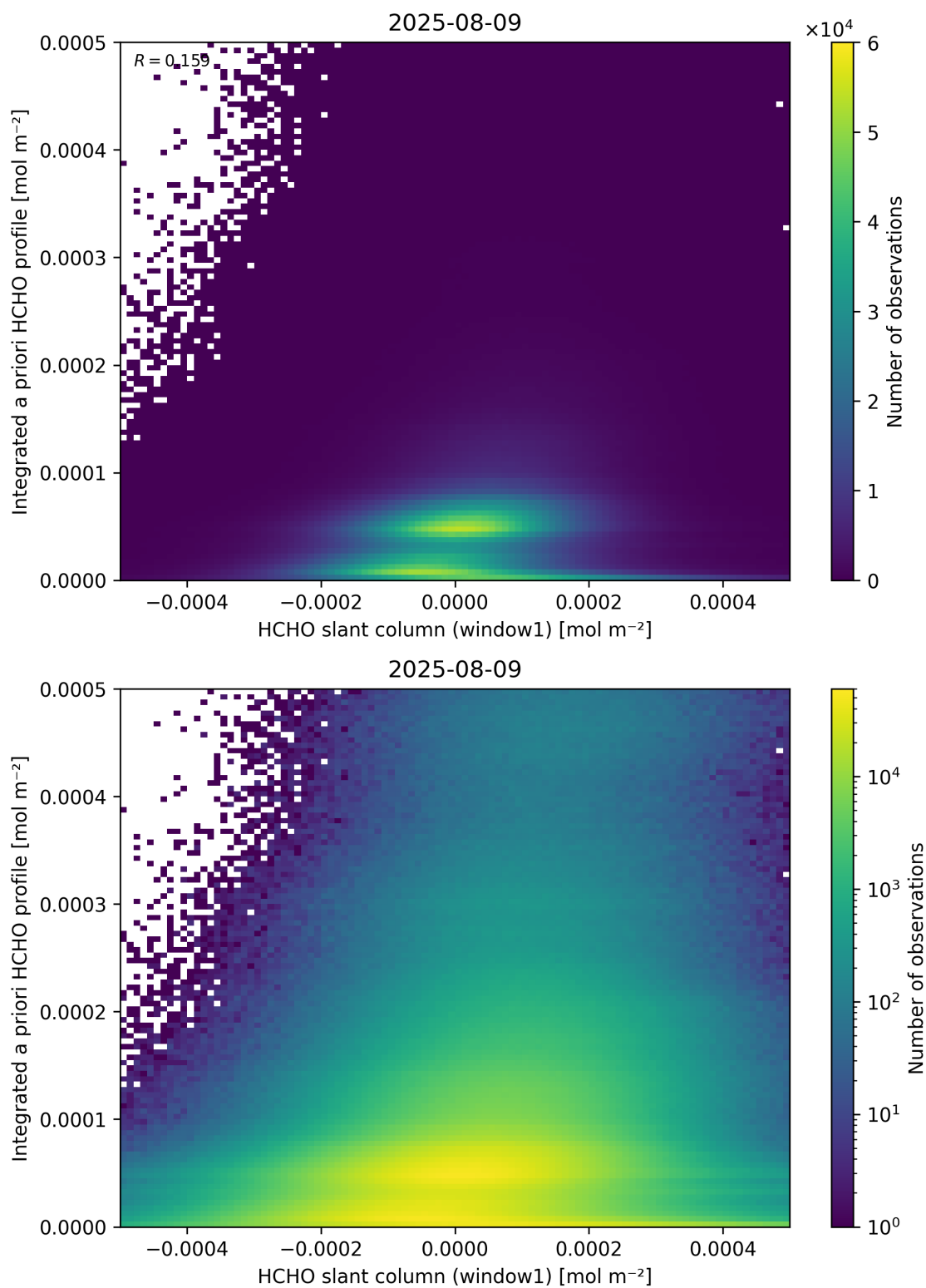
Figure 87: Scatter density plot of “HCHO slant column (window1)” against “Integrated a priori HCHO profile” for 2025-08-09 to 2025-08-10.
