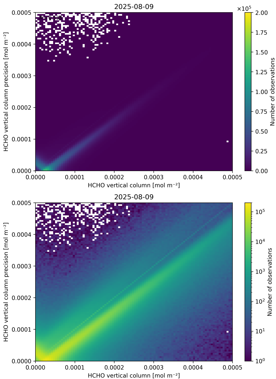
Figure 134: Scatter density plot of “HCHO vertical column” against “HCHO vertical column precision” for 2025-08-09 to 2025-08-10.
