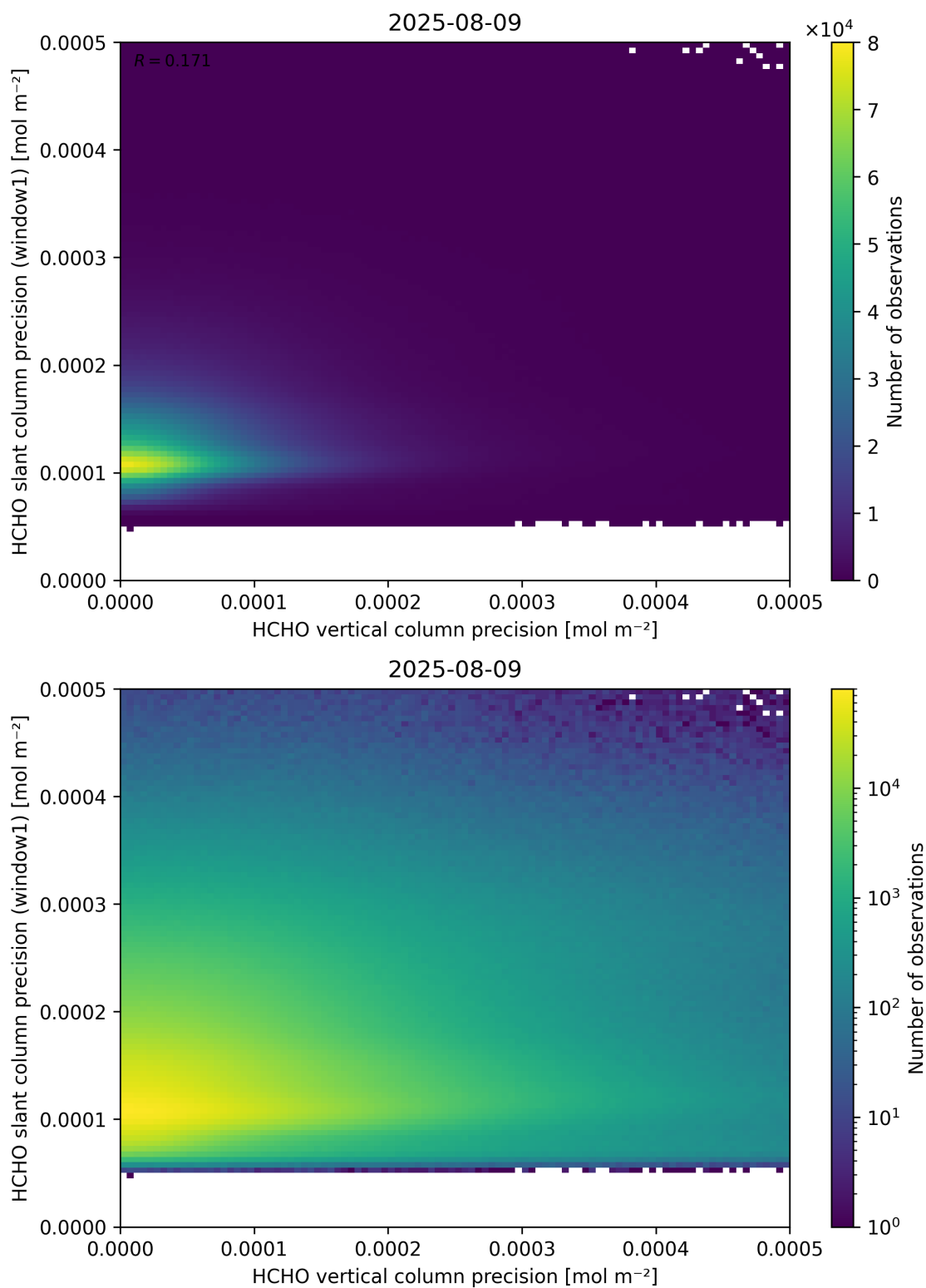
Figure 143: Scatter density plot of “HCHO vertical column precision” against “HCHO slant column precision (window1)” for 2025-08-09 to 2025-08-10.
