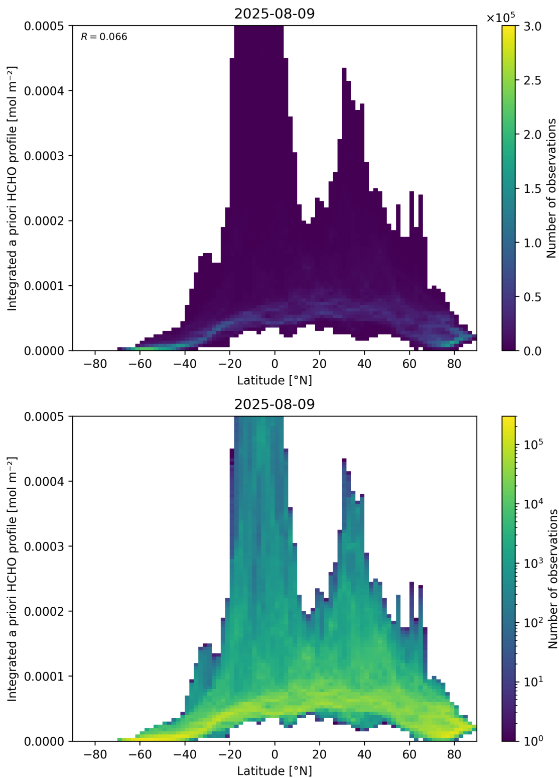
Figure 166: Scatter density plot of “Latitude” against “Integrated a priori HCHO profile” for 2025-08-09 to 2025-08-10.
