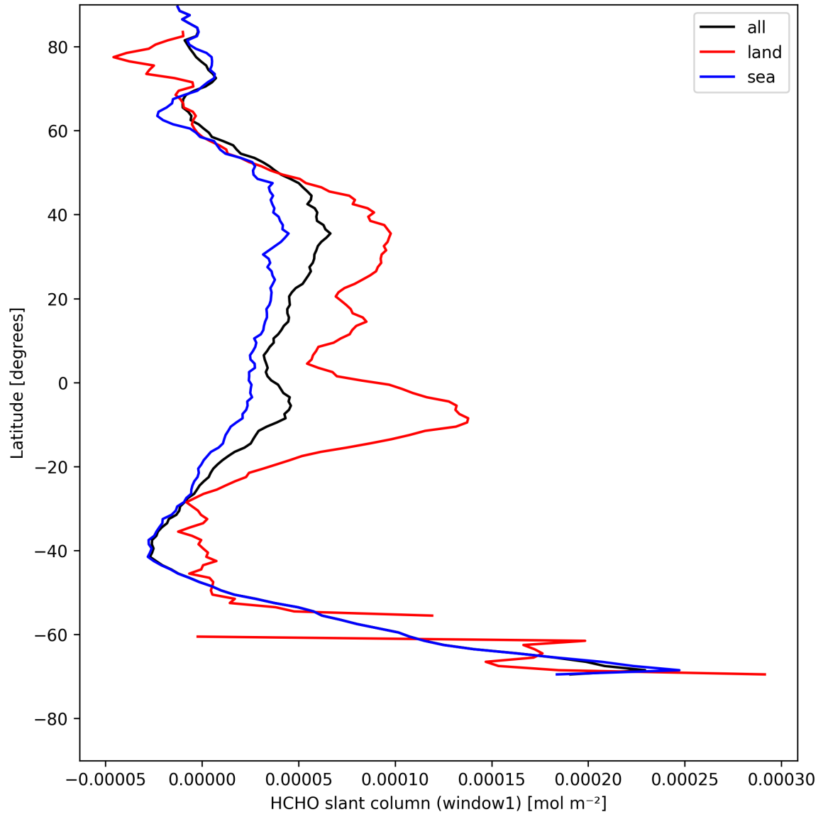
Figure 24: Zonal average of “HCHO slant column (window1)” for 2025-08-09 to 2025-08-10.
