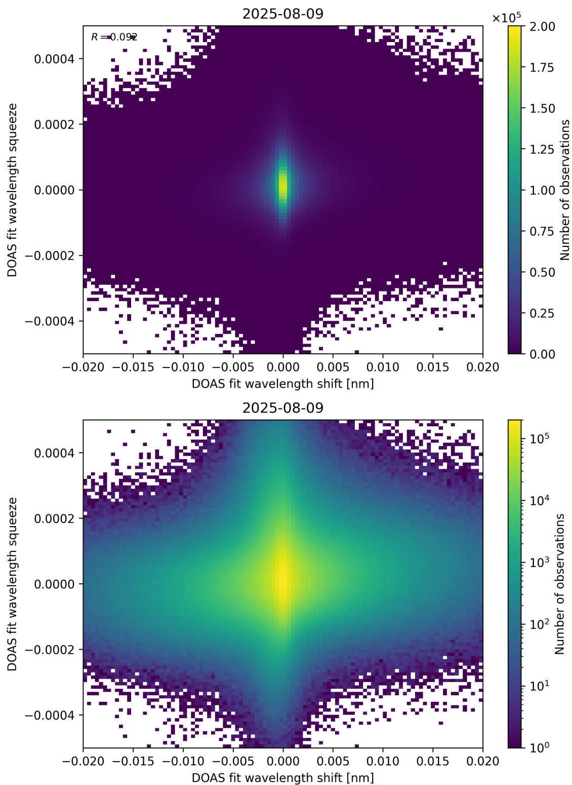
Figure 65: Scatter density plot of “DOAS fit wavelength shift” against “DOAS fit wavelength squeeze” for 2025-08-09 to 2025-08-10.
