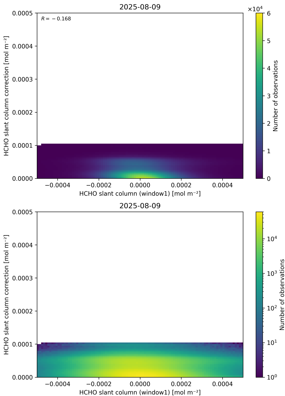
Figure 83: Scatter density plot of “HCHO slant column (window1)” against “HCHO slant column correction” for 2025-08-09 to 2025-08-10.
