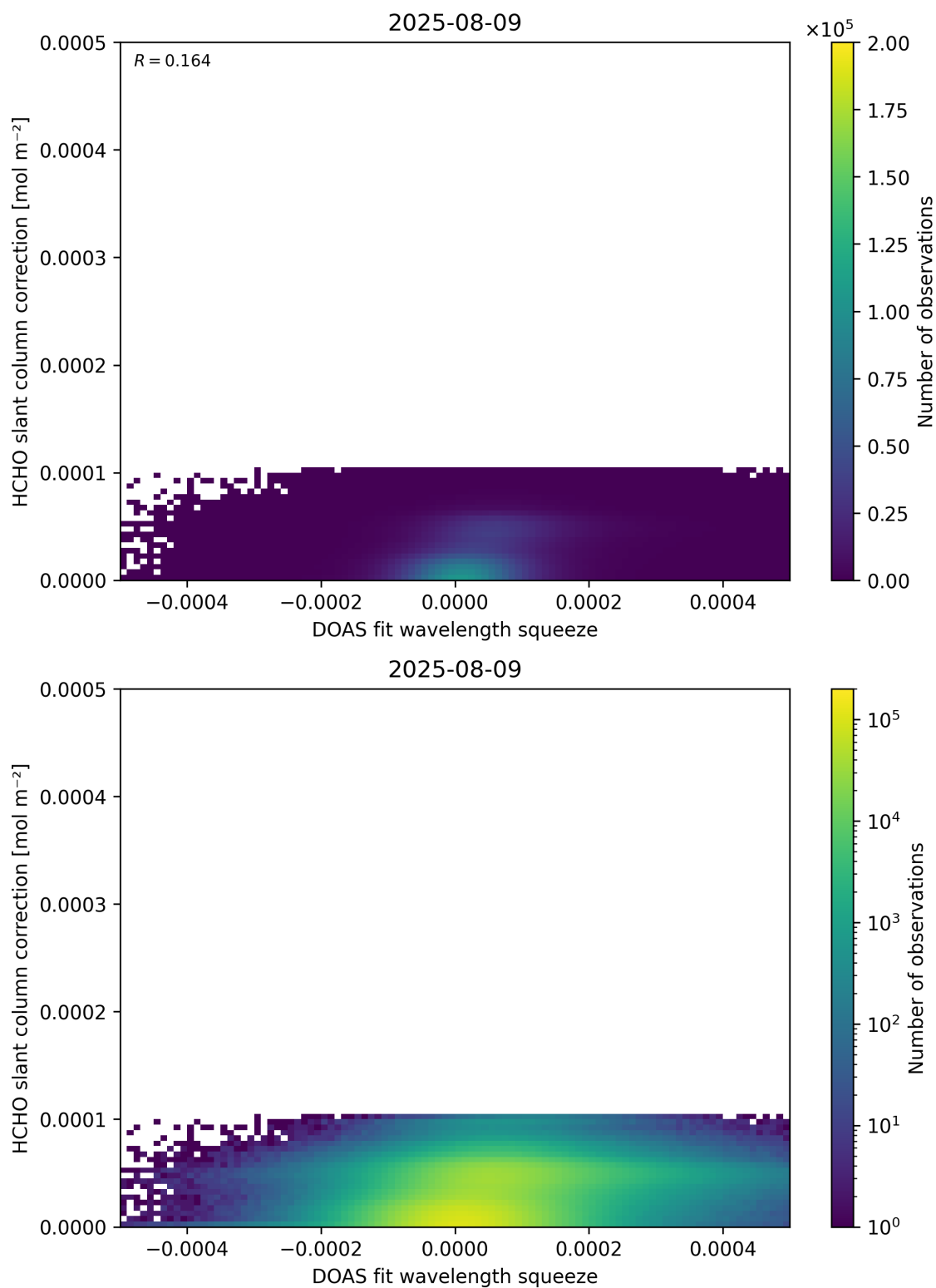
Figure 70: Scatter density plot of “DOAS fit wavelength squeeze” against “HCHO slant column correction” for 2025-08-09 to 2025-08-10.
