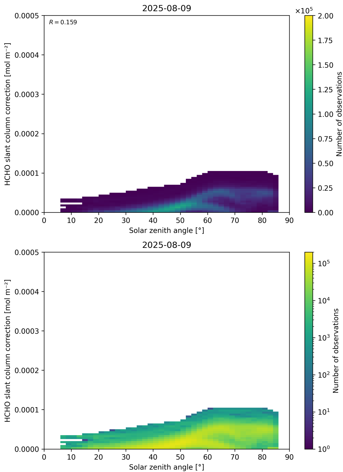
Figure 172: Scatter density plot of “Solar zenith angle” against “HCHO slant column correction” for 2025-08-09 to 2025-08-10.
