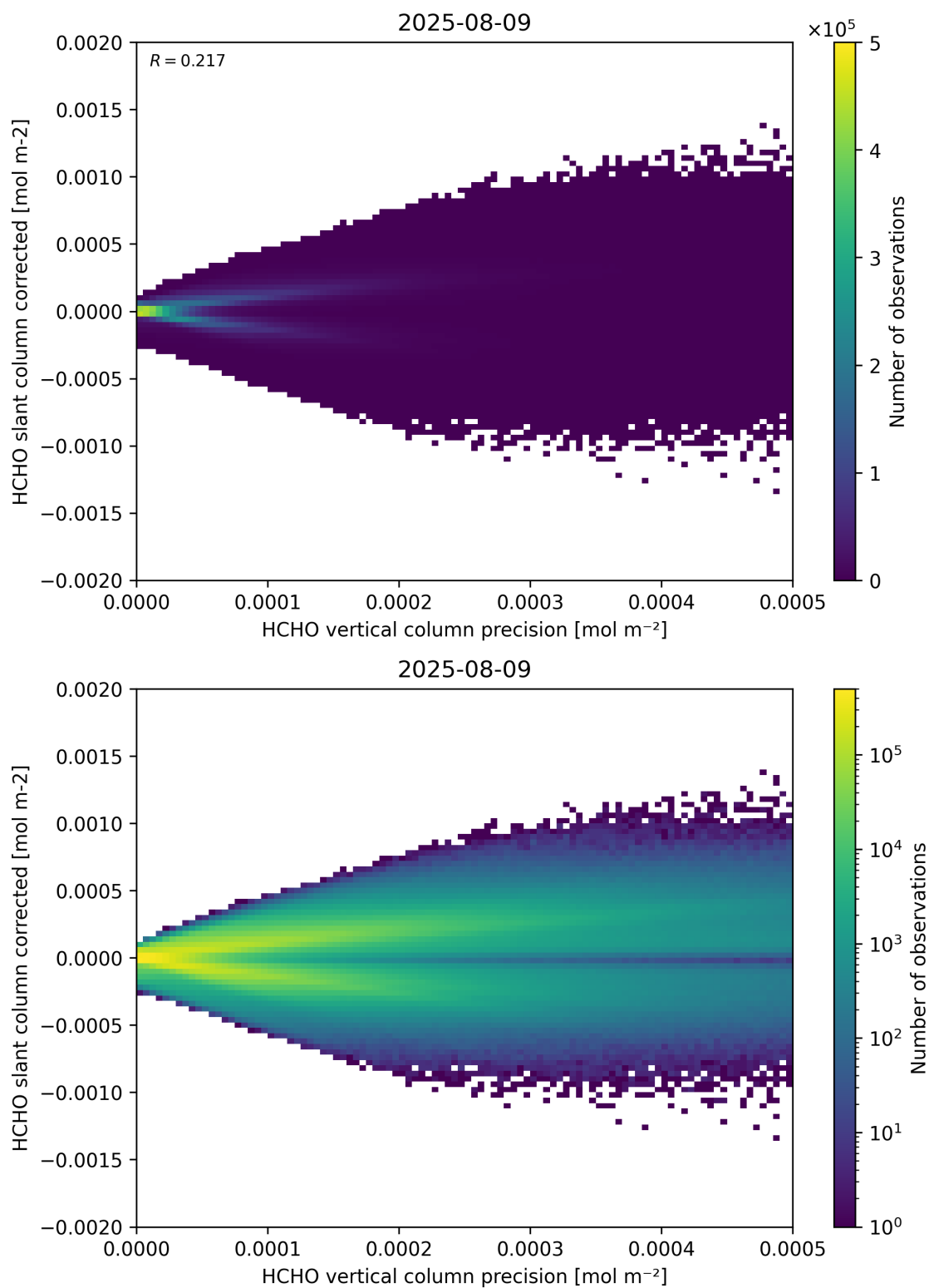
Figure 140: Scatter density plot of “HCHO vertical column precision” against “HCHO slant column corrected” for 2025-08-09 to 2025-08-10.
