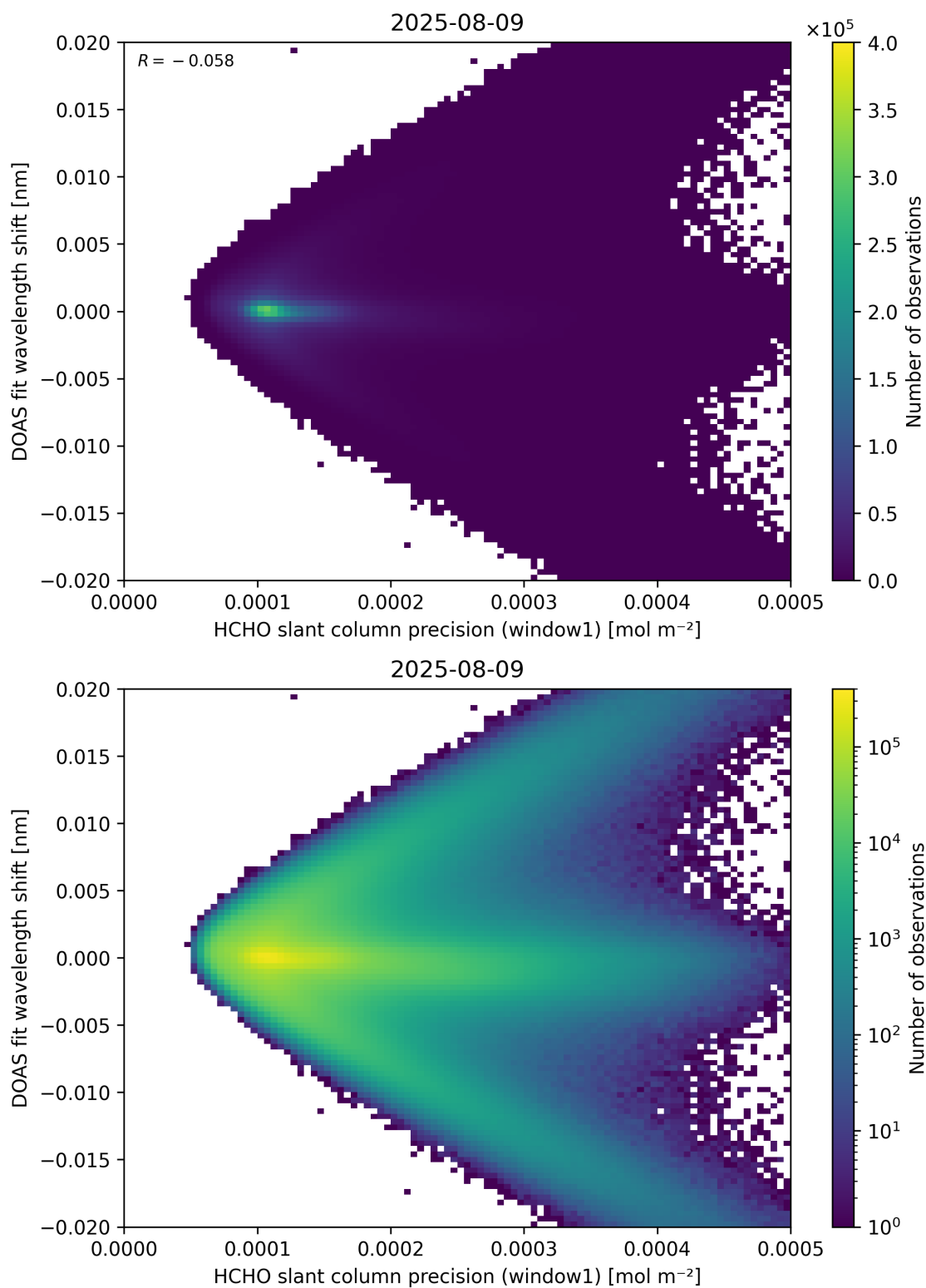
Figure 89: Scatter density plot of “HCHO slant column precision (window1)” against “DOAS fit wavelength shift” for 2025-08-09 to 2025-08-10.
