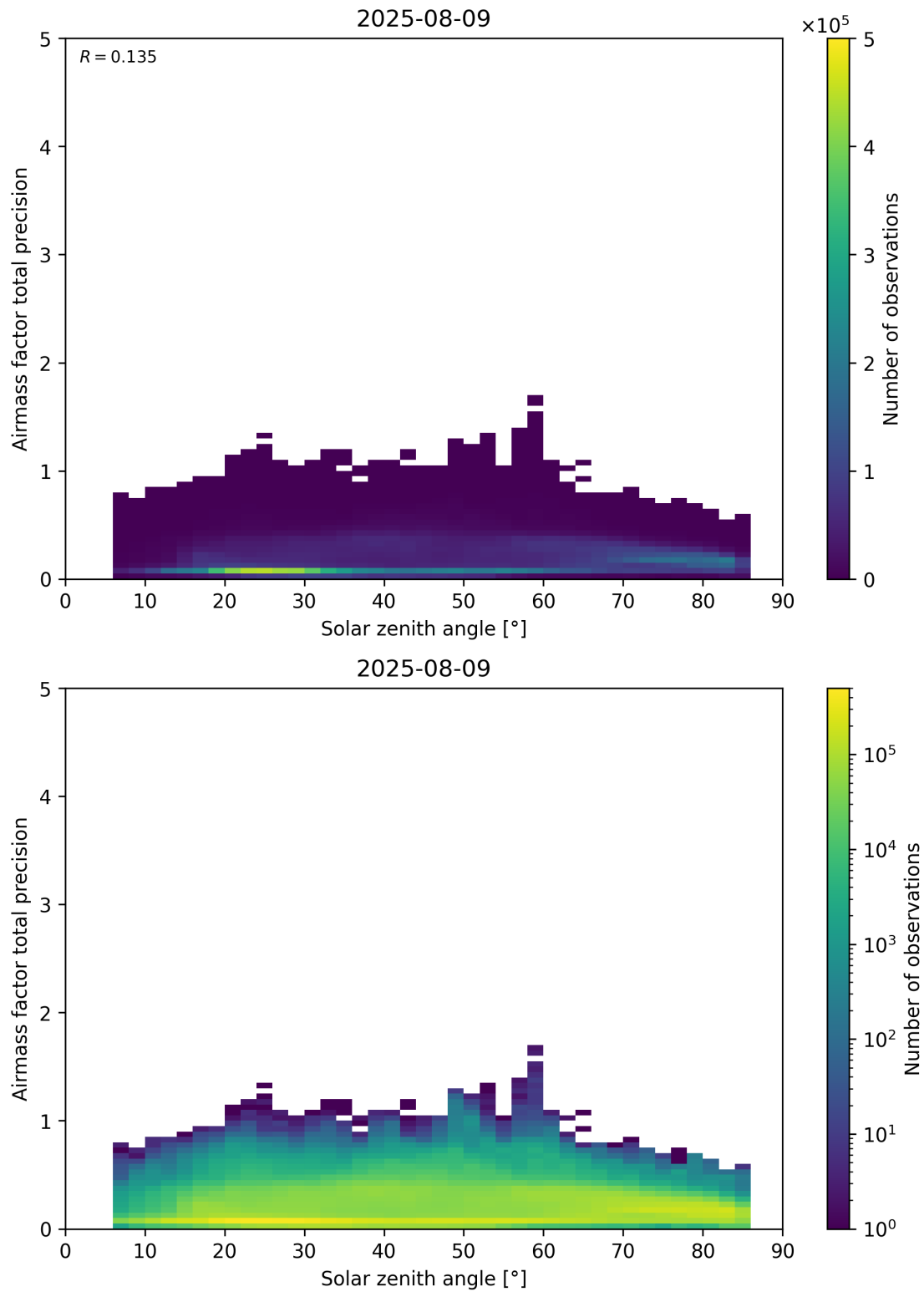
Figure 176: Scatter density plot of “Solar zenith angle” against “Airmass factor total precision” for 2025-08-09 to 2025-08-10.
