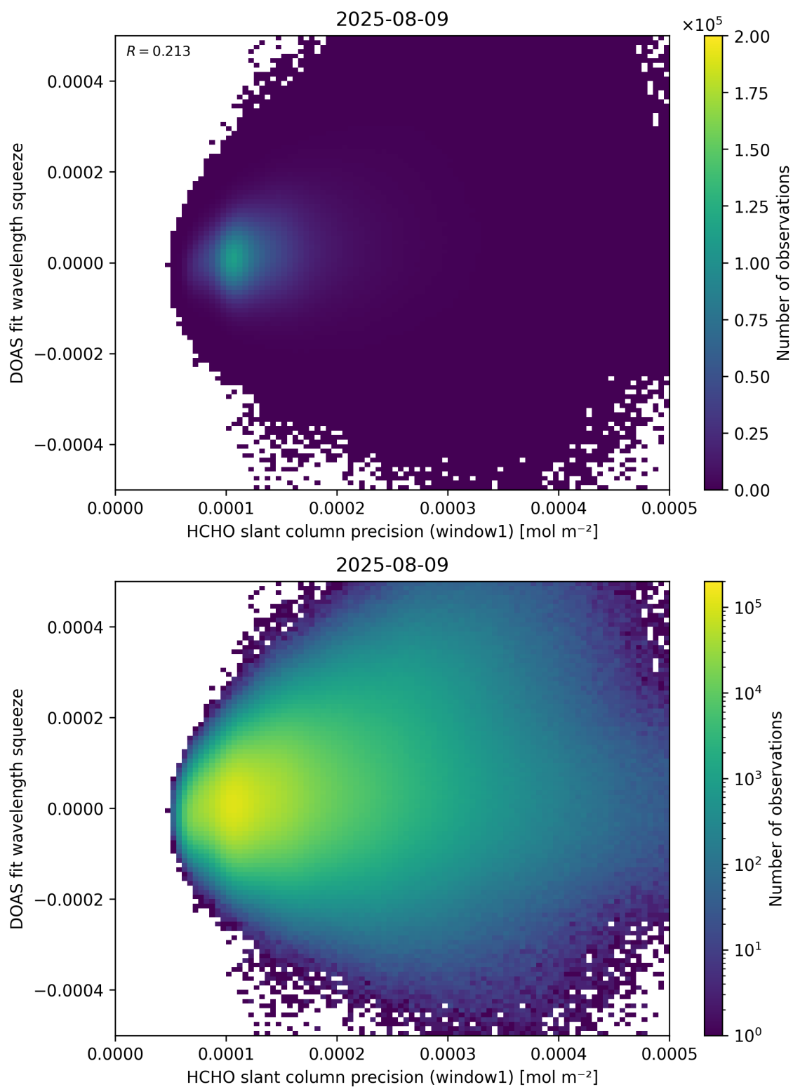
Figure 90: Scatter density plot of “HCHO slant column precision (window1)” against “DOAS fit wavelength squeeze” for 2025-08-09 to 2025-08-10.
