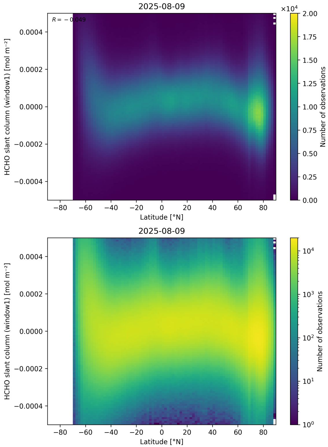
Figure 159: Scatter density plot of “Latitude” against “HCHO slant column (window1)” for 2025-08-09 to 2025-08-10.
