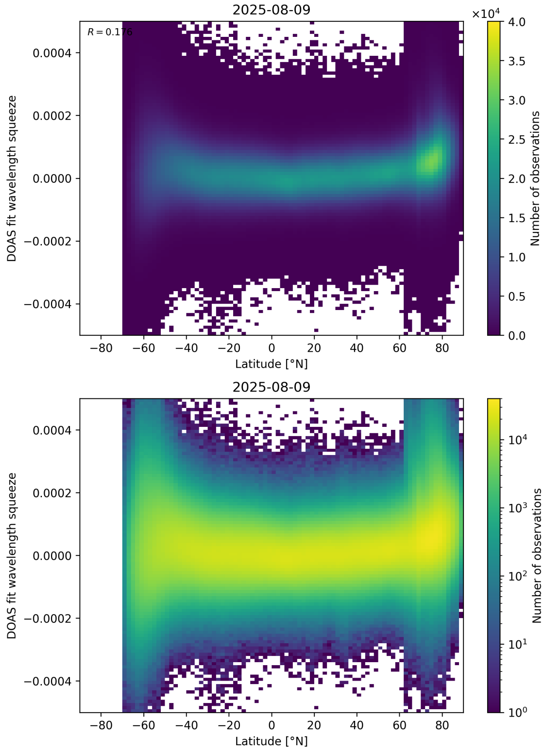
Figure 155: Scatter density plot of “Latitude” against “DOAS fit wavelength squeeze” for 2025-08-09 to 2025-08-10.
