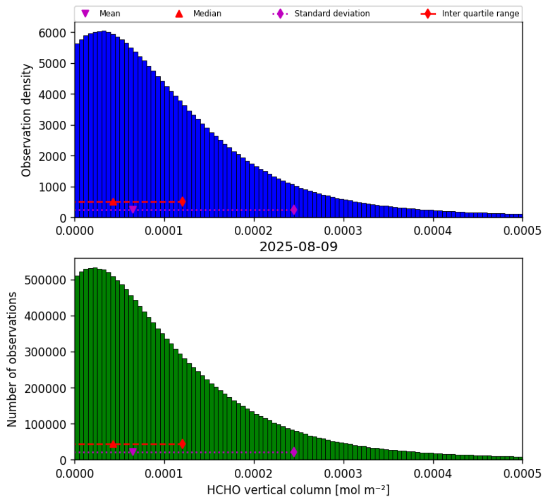
Figure 35: Histogram of “HCHO vertical column” for 2025-08-09 to 2025-08-10
