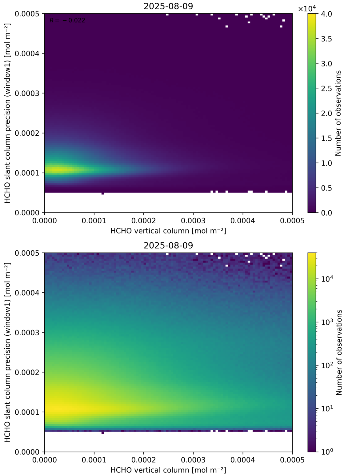
Figure 130: Scatter density plot of “HCHO vertical column” against “HCHO slant column precision (window1)” for 2025-08-09 to 2025-08-10.
