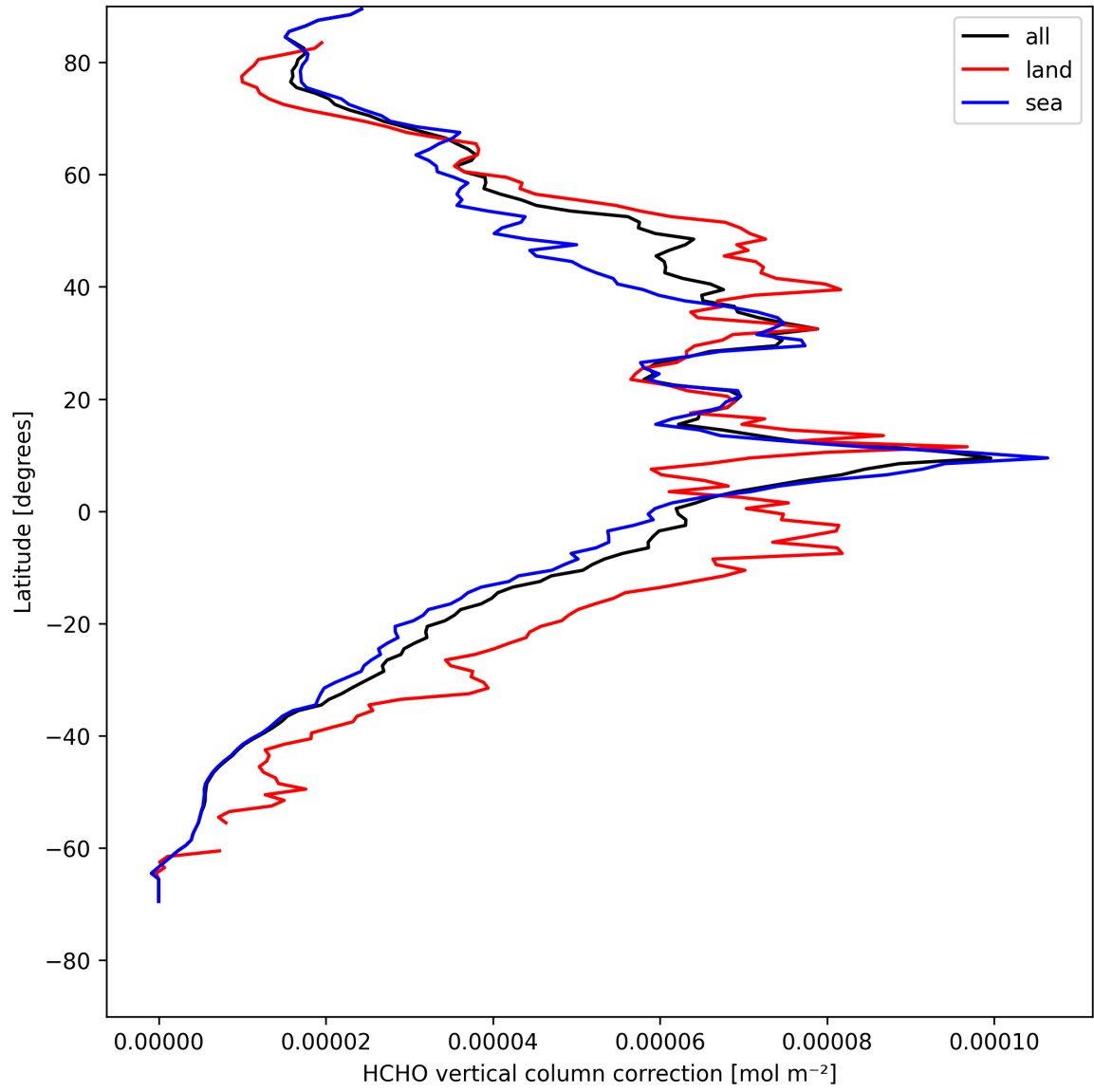
Figure 23: Zonal average of “HCHO vertical column correction” for 2025-08-09 to 2025-08-10.
