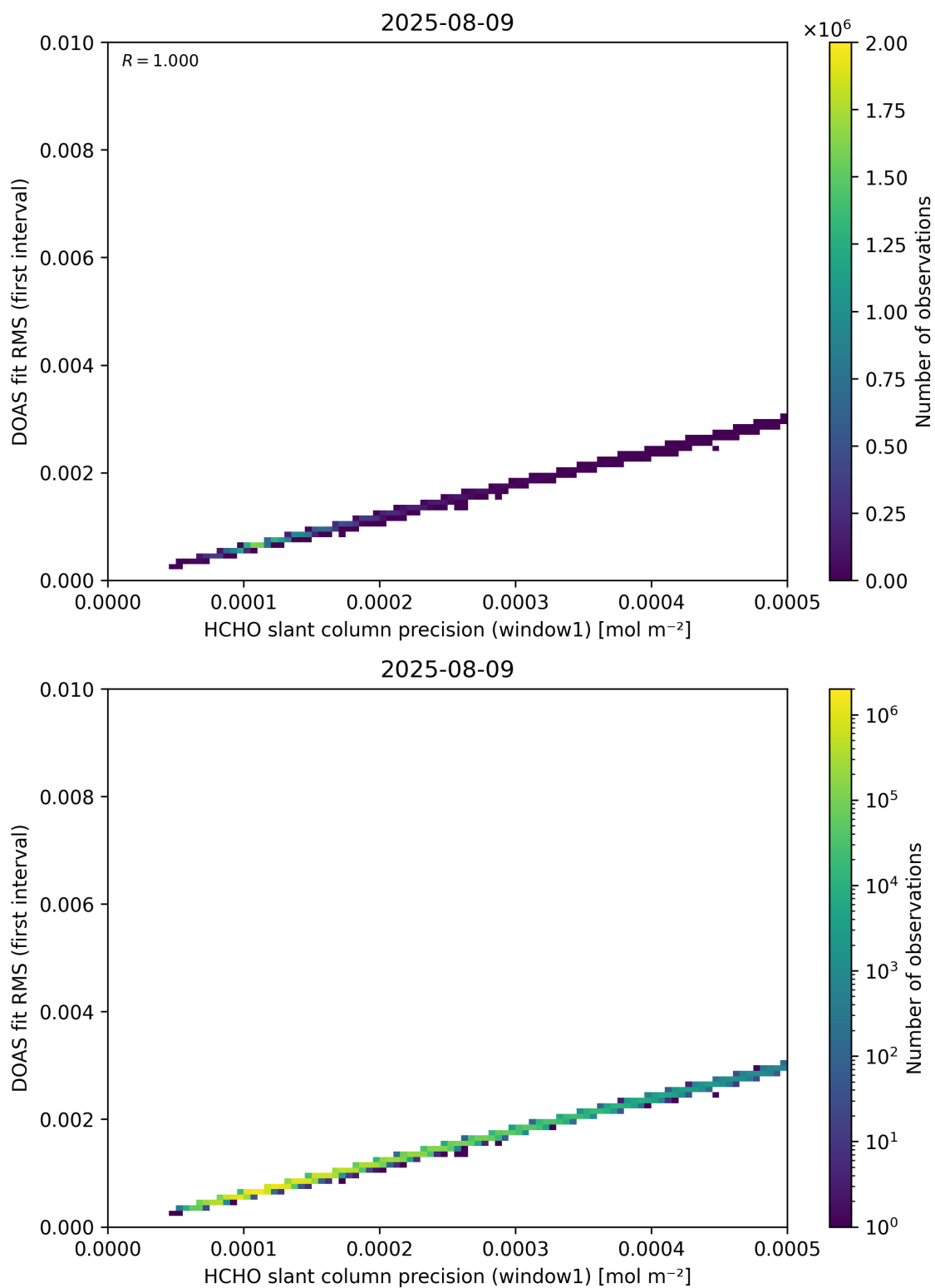
Figure 88: Scatter density plot of “HCHO slant column precision (window1)” against “DOAS fit RMS (first interval)” for 2025-08-09 to 2025-08-10.
