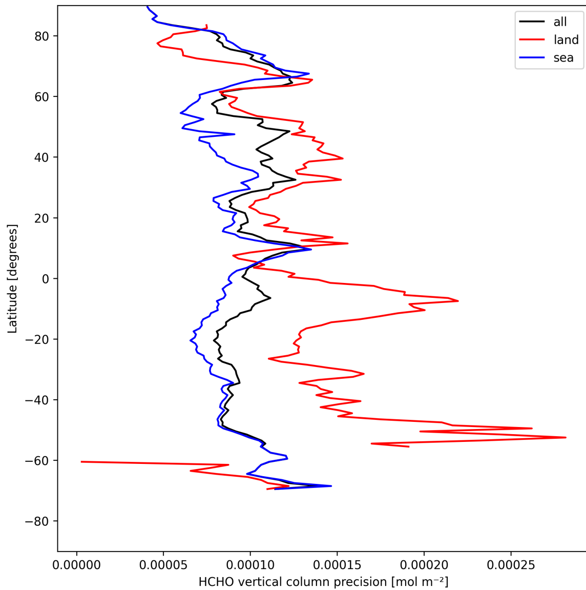
Figure 22: Zonal average of “HCHO vertical column precision” for 2025-08-09 to 2025-08-10.
