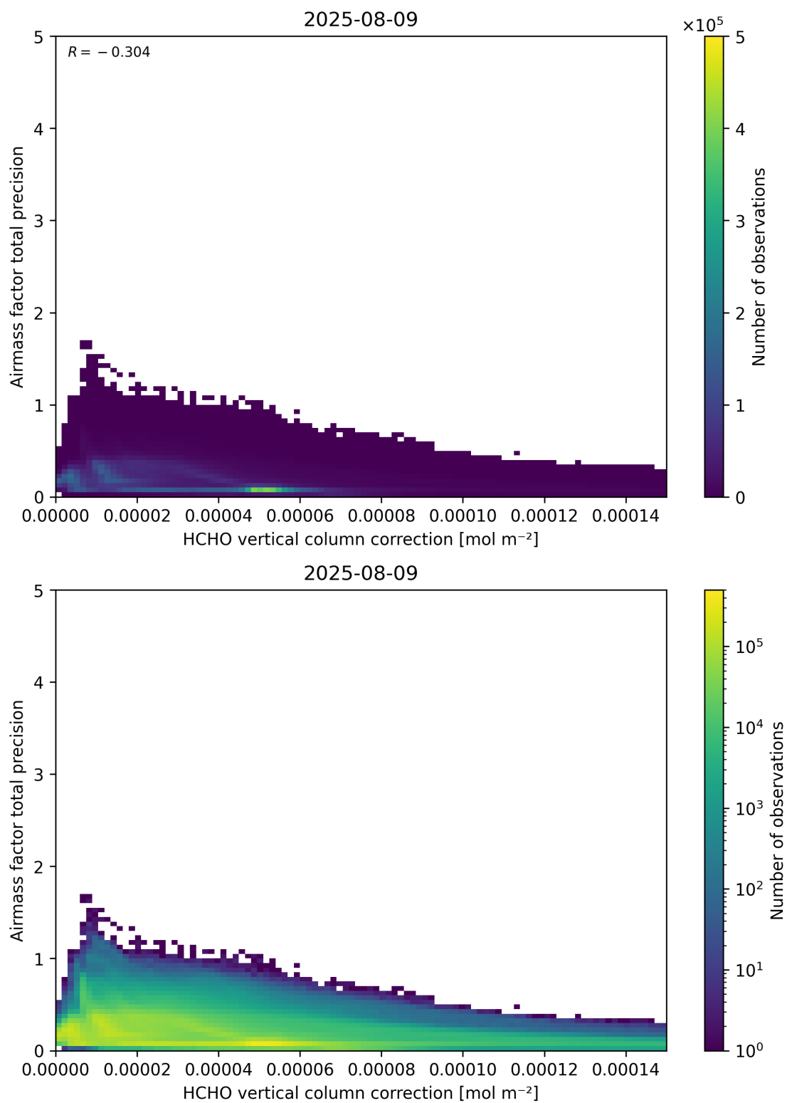
Figure 121: Scatter density plot of “HCHO vertical column correction” against “Airmass factor total precision” for 2025-08-09 to 2025-08-10.
