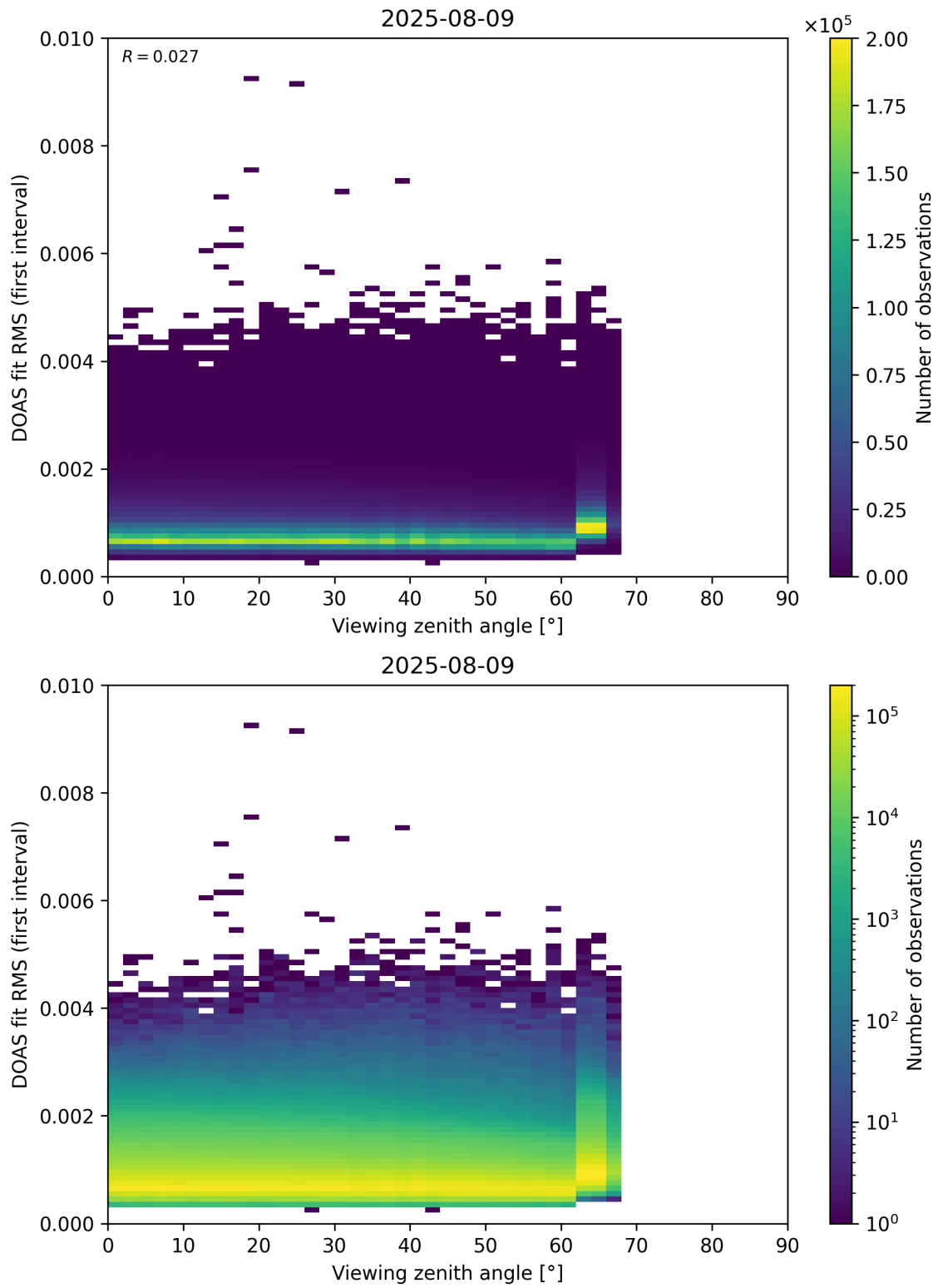
Figure 182: Scatter density plot of “Viewing zenith angle” against “DOAS fit RMS (first interval)” for 2025-08-09 to 2025-08-10.
