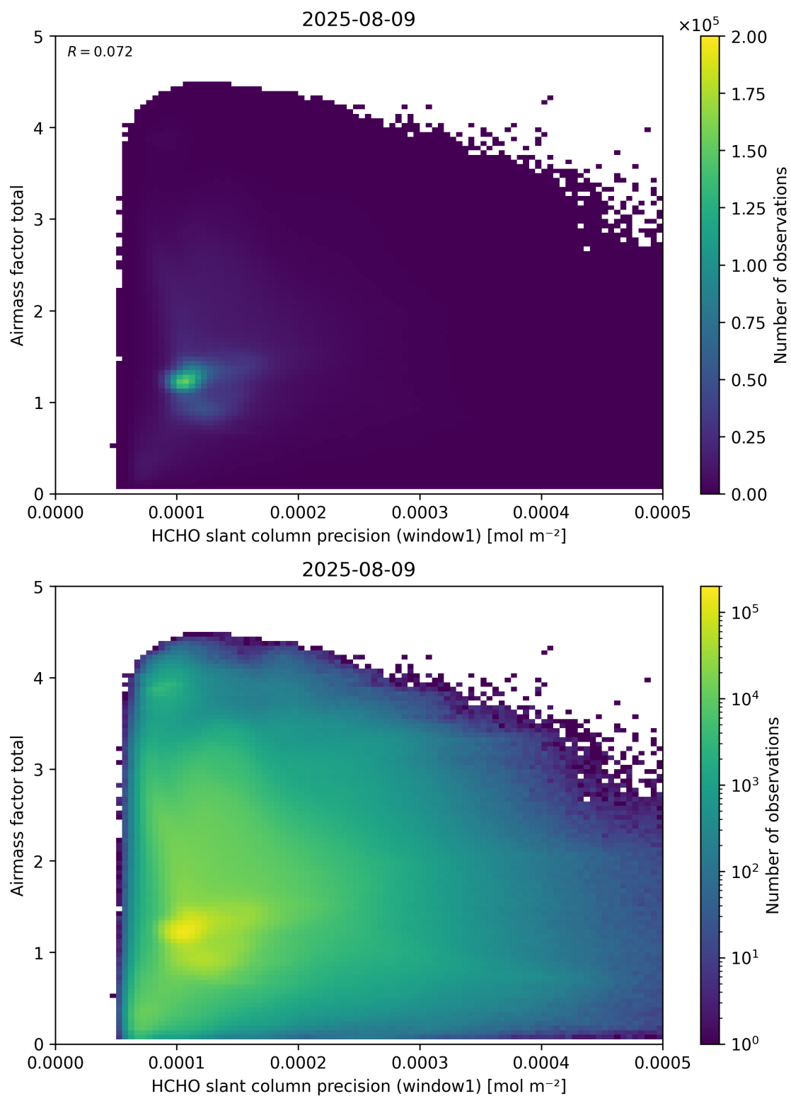
Figure 94: Scatter density plot of “HCHO slant column precision (window1)” against “Airmass factor total” for 2025-08-09 to 2025-08-10.
