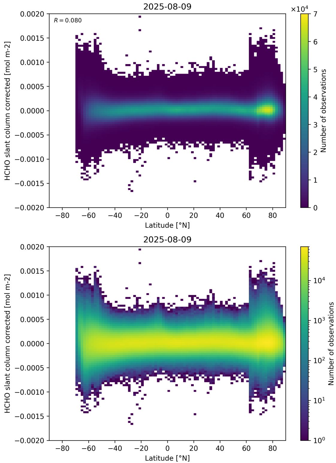
Figure 157: Scatter density plot of “Latitude” against “HCHO slant column corrected” for 2025-08-09 to 2025-08-10.
