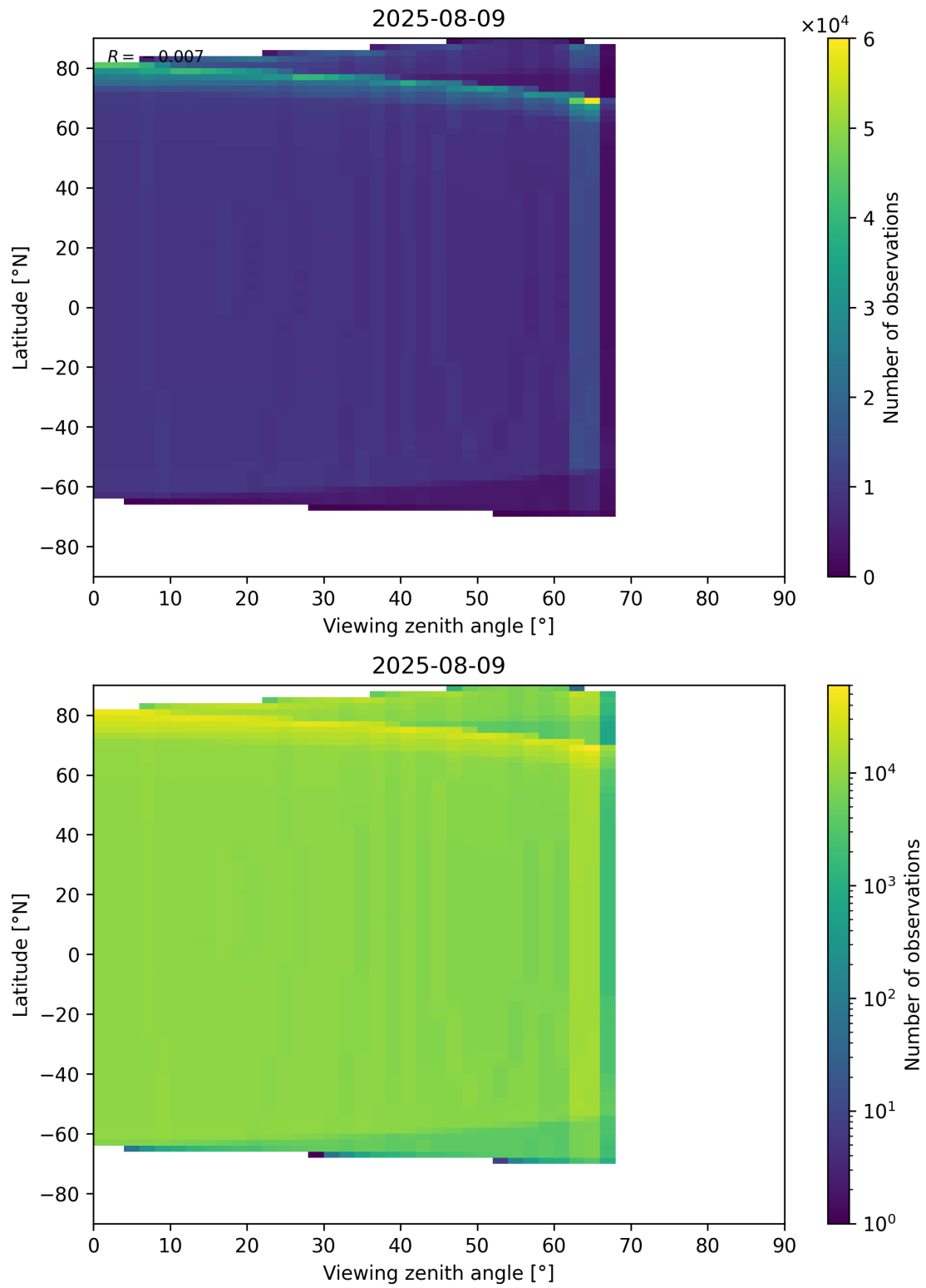
Figure 196: Scatter density plot of “Viewing zenith angle” against “Latitude” for 2025-08-09 to 2025-08-10.
