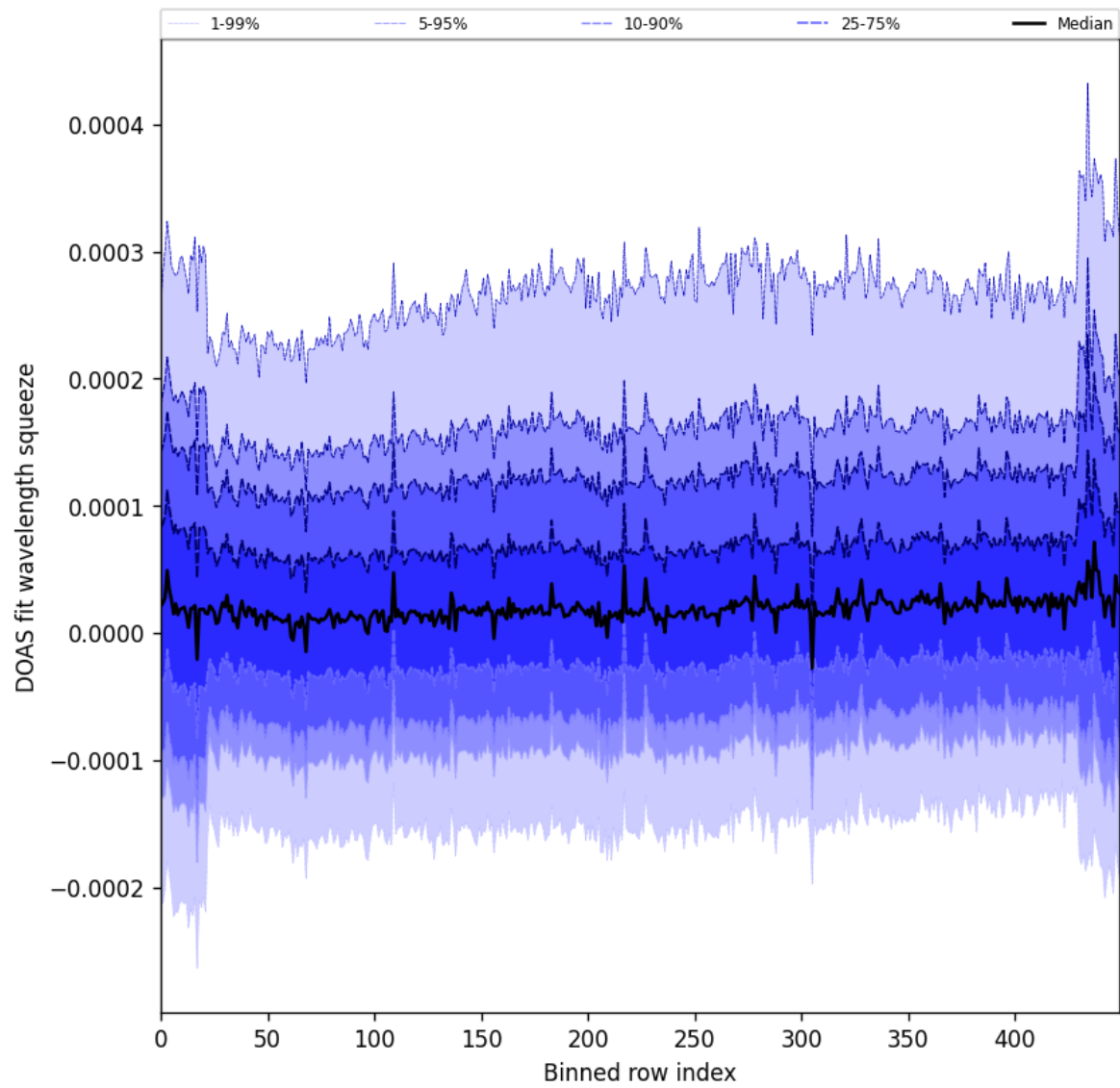
Figure 59: Along track statistics of “DOAS fit wavelength squeeze” for 2025-08-09 to 2025-08-10
