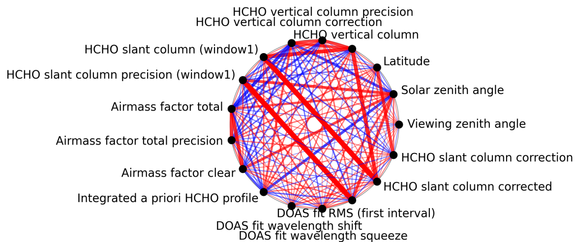
Figure 1: Map of correlation graph for 2025-08-09 to 2025-08-10.
