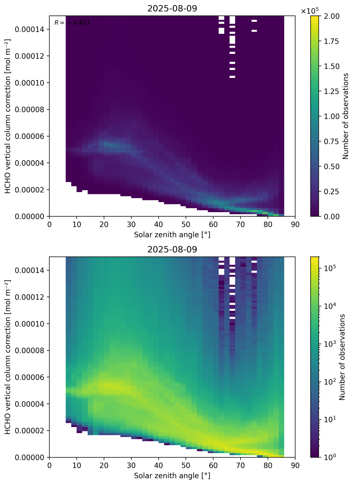
Figure 178: Scatter density plot of “Solar zenith angle” against “HCHO vertical column correction” for 2025-08-09 to 2025-08-10.
