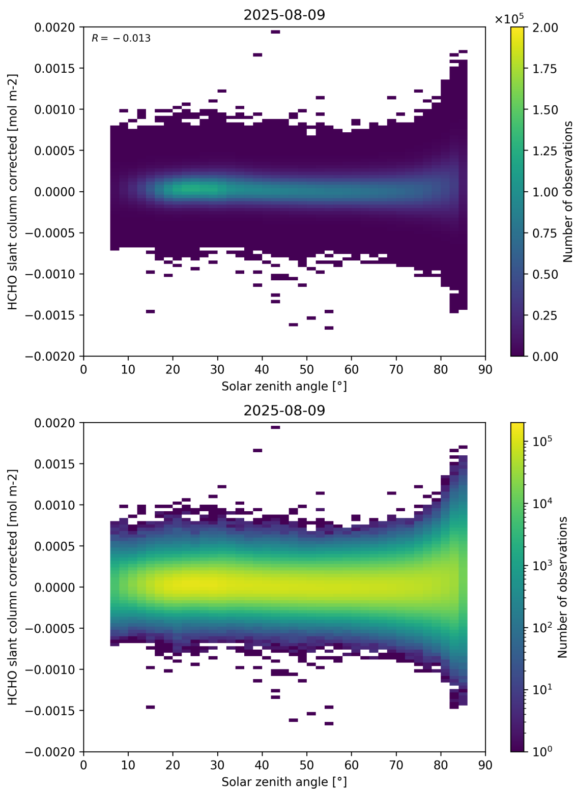
Figure 171: Scatter density plot of “Solar zenith angle” against “HCHO slant column corrected” for 2025-08-09 to 2025-08-10.
