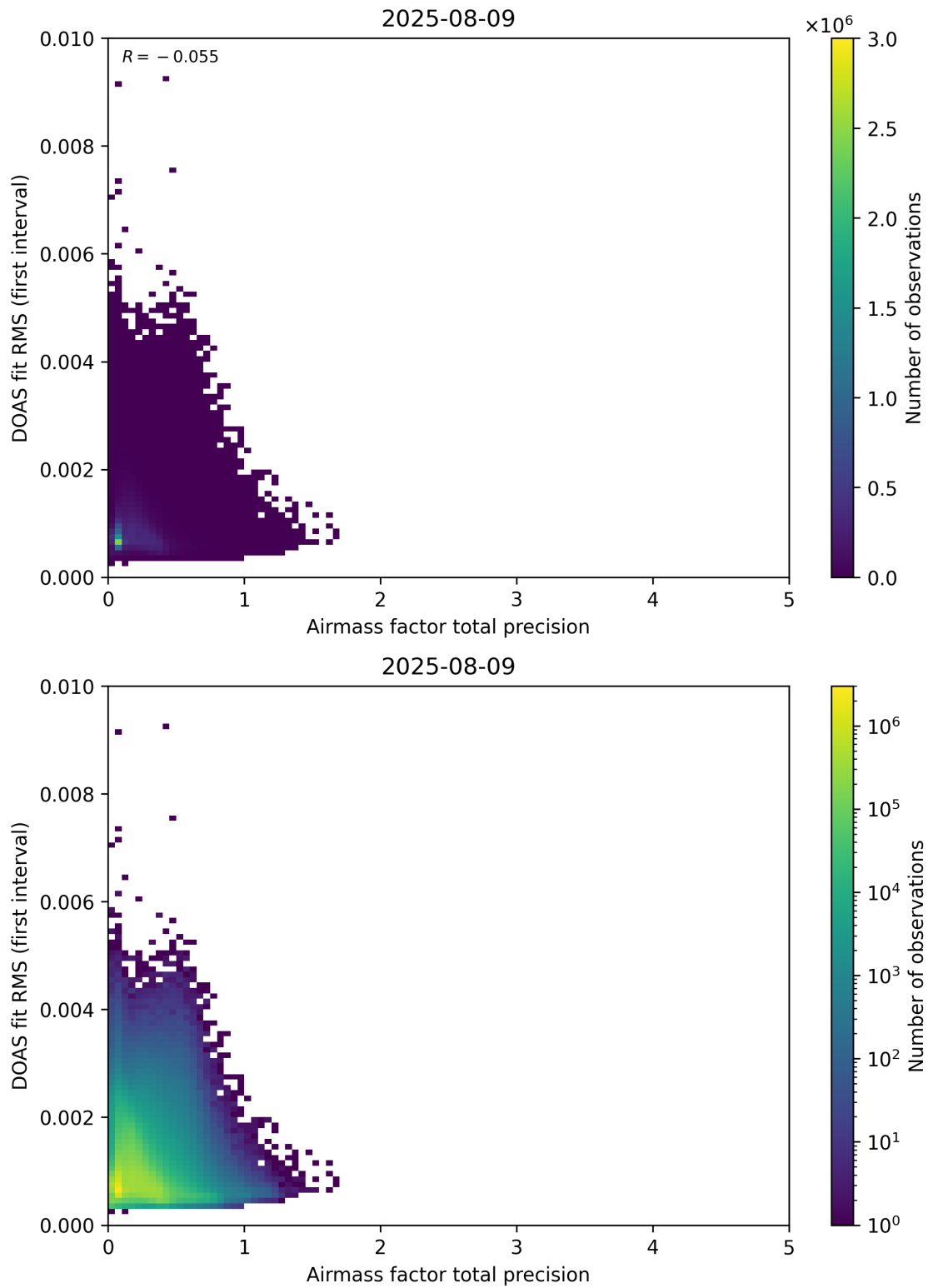
Figure 105: Scatter density plot of “Airmass factor total precision” against “DOAS fit RMS (first interval)” for 2025-08-09 to 2025-08-10.
