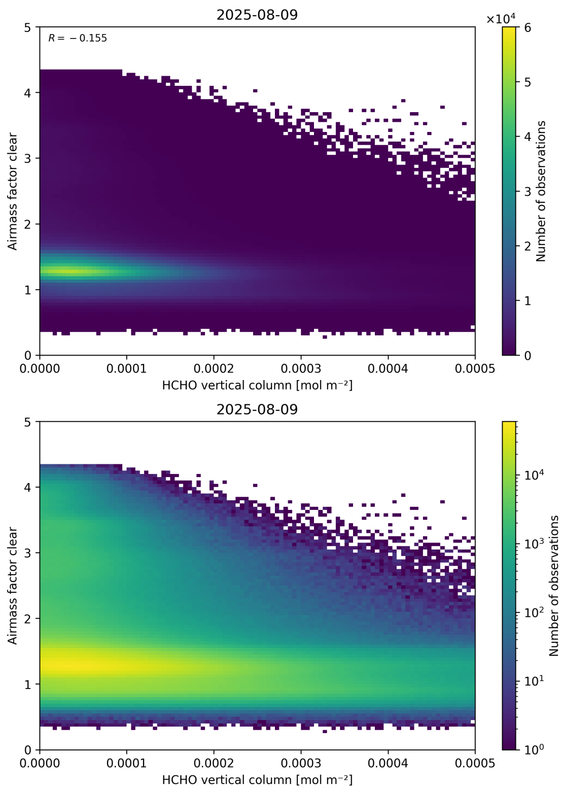
Figure 126: Scatter density plot of “HCHO vertical column” against “Airmass factor clear” for 2025-08-09 to 2025-08-10.
