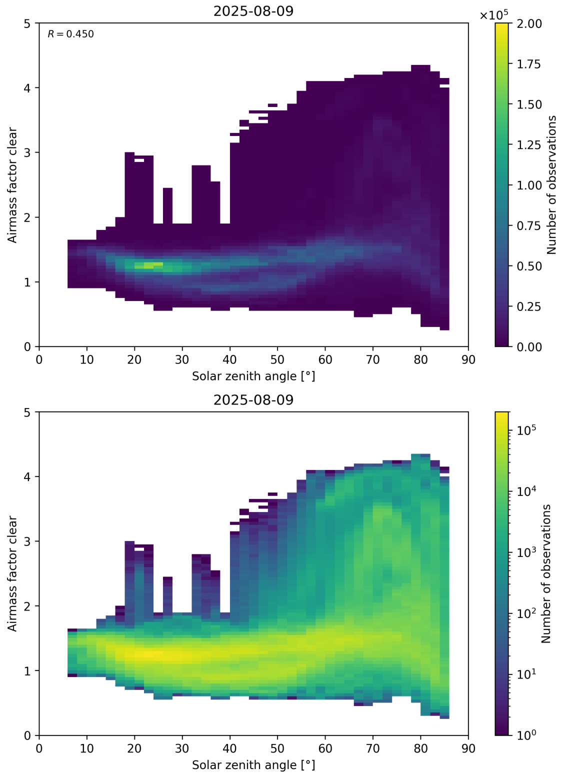
Figure 170: Scatter density plot of “Solar zenith angle” against “Airmass factor clear” for 2025-08-09 to 2025-08-10.
