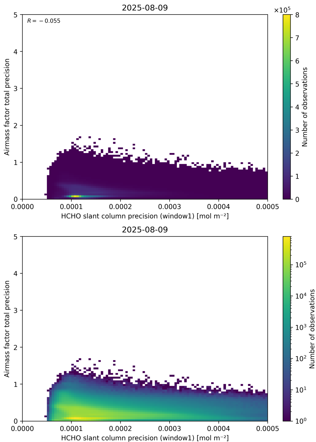
Figure 95: Scatter density plot of “HCHO slant column precision (window1)” against “Airmass factor total precision” for 2025-08-09 to 2025-08-10.
