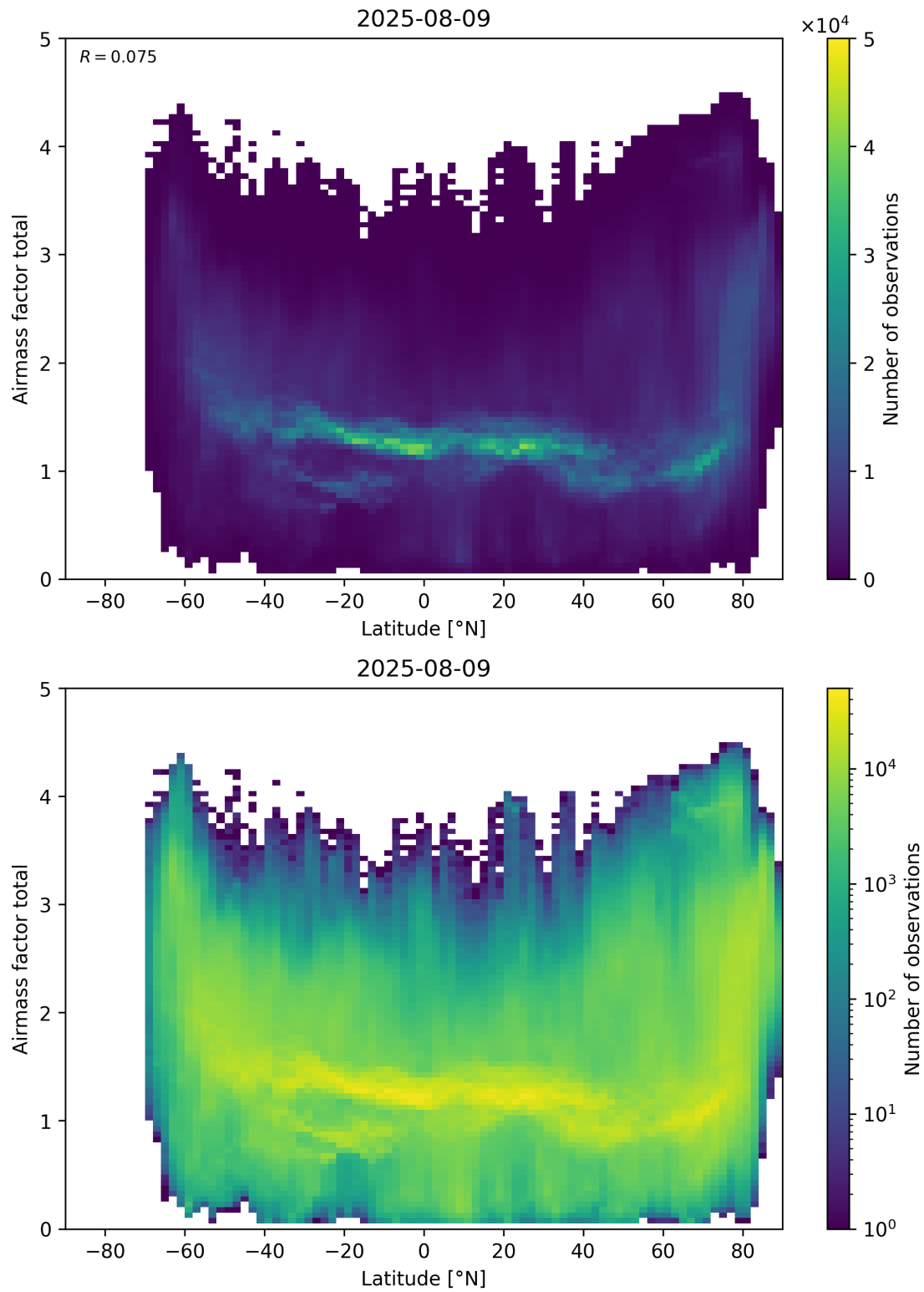
Figure 161: Scatter density plot of “Latitude” against “Airmass factor total” for 2025-08-09 to 2025-08-10.
