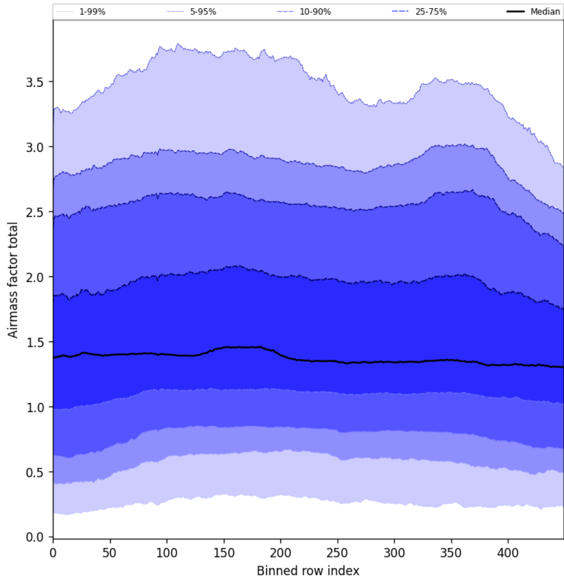
Figure 54: Along track statistics of “Airmass factor total” for 2025-08-09 to 2025-08-10
