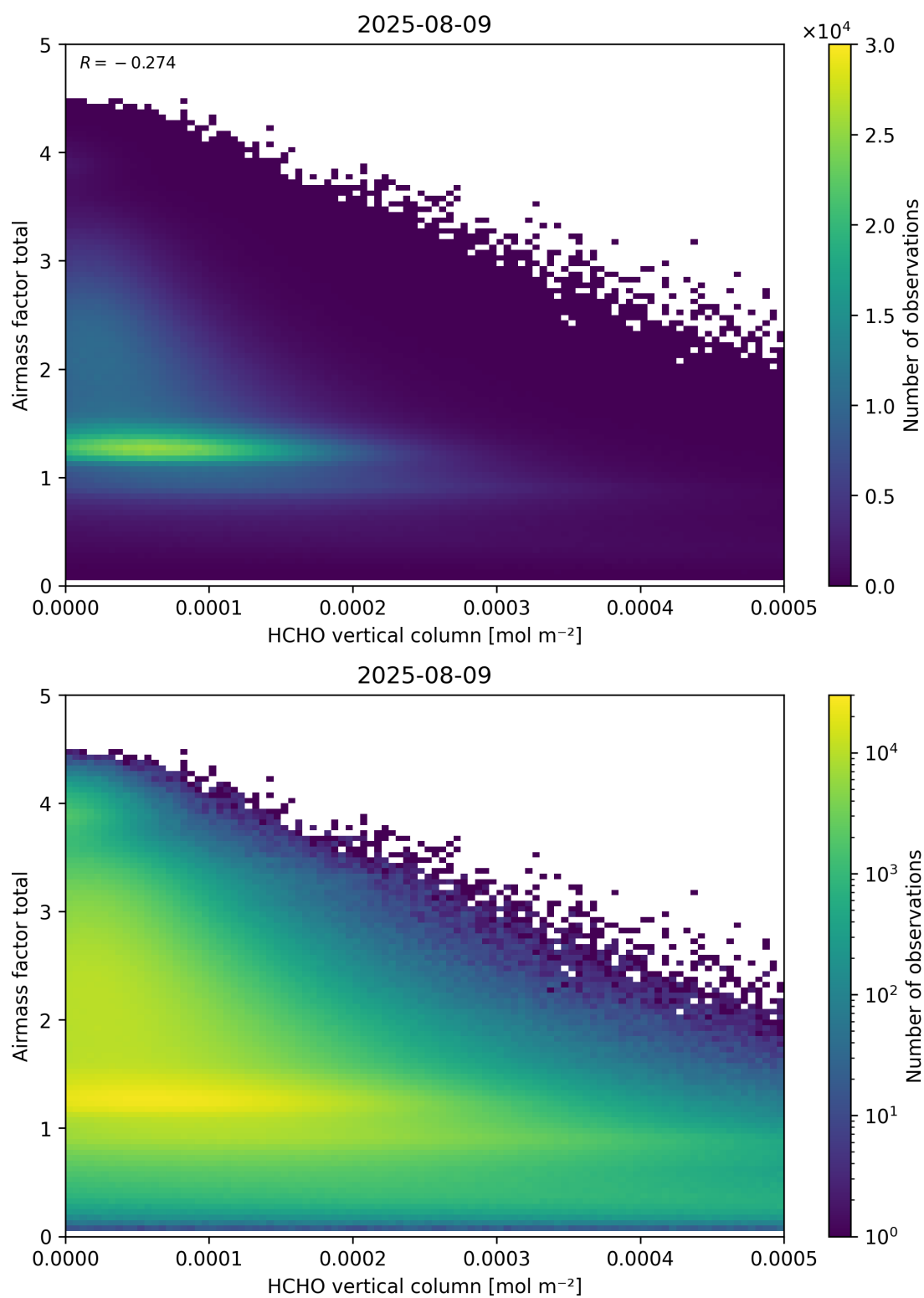
Figure 131: Scatter density plot of “HCHO vertical column” against “Airmass factor total” for 2025-08-09 to 2025-08-10.
