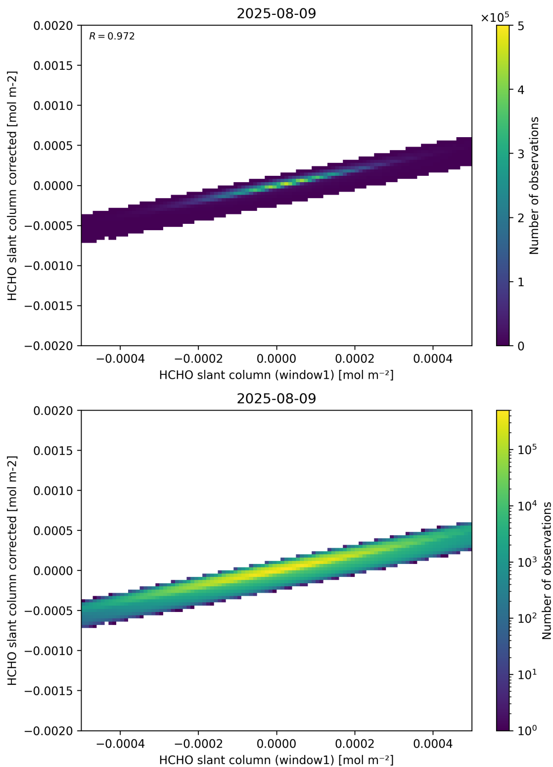
Figure 82: Scatter density plot of “HCHO slant column (window1)” against “HCHO slant column corrected” for 2025-08-09 to 2025-08-10.
