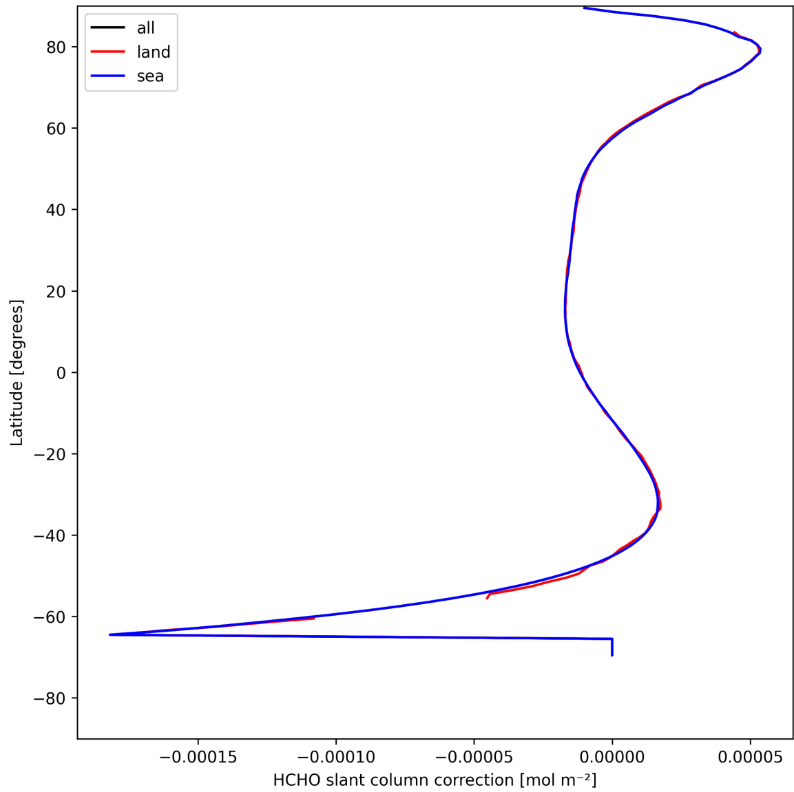
Figure 33: Zonal average of “HCHO slant column correction” for 2025-08-09 to 2025-08-10.
