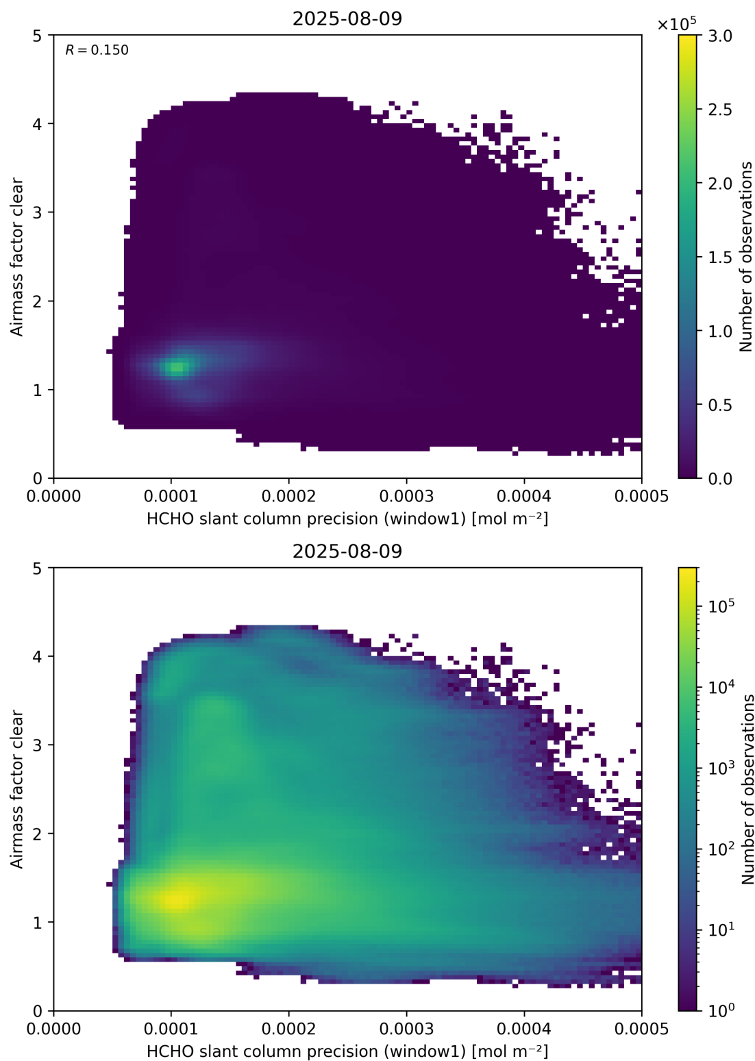
Figure 91: Scatter density plot of “HCHO slant column precision (window1)” against “Airmass factor clear” for 2025-08-09 to 2025-08-10.
