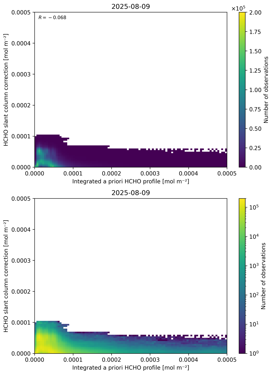
Figure 152: Scatter density plot of “Integrated a priori HCHO profile” against “HCHO slant column correction” for 2025-08-09 to 2025-08-10.
