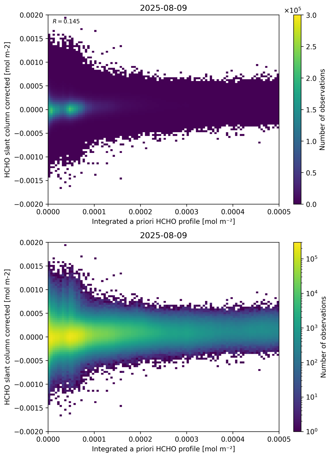
Figure 151: Scatter density plot of “Integrated a priori HCHO profile” against “HCHO slant column corrected” for 2025-08-09 to 2025-08-10.
