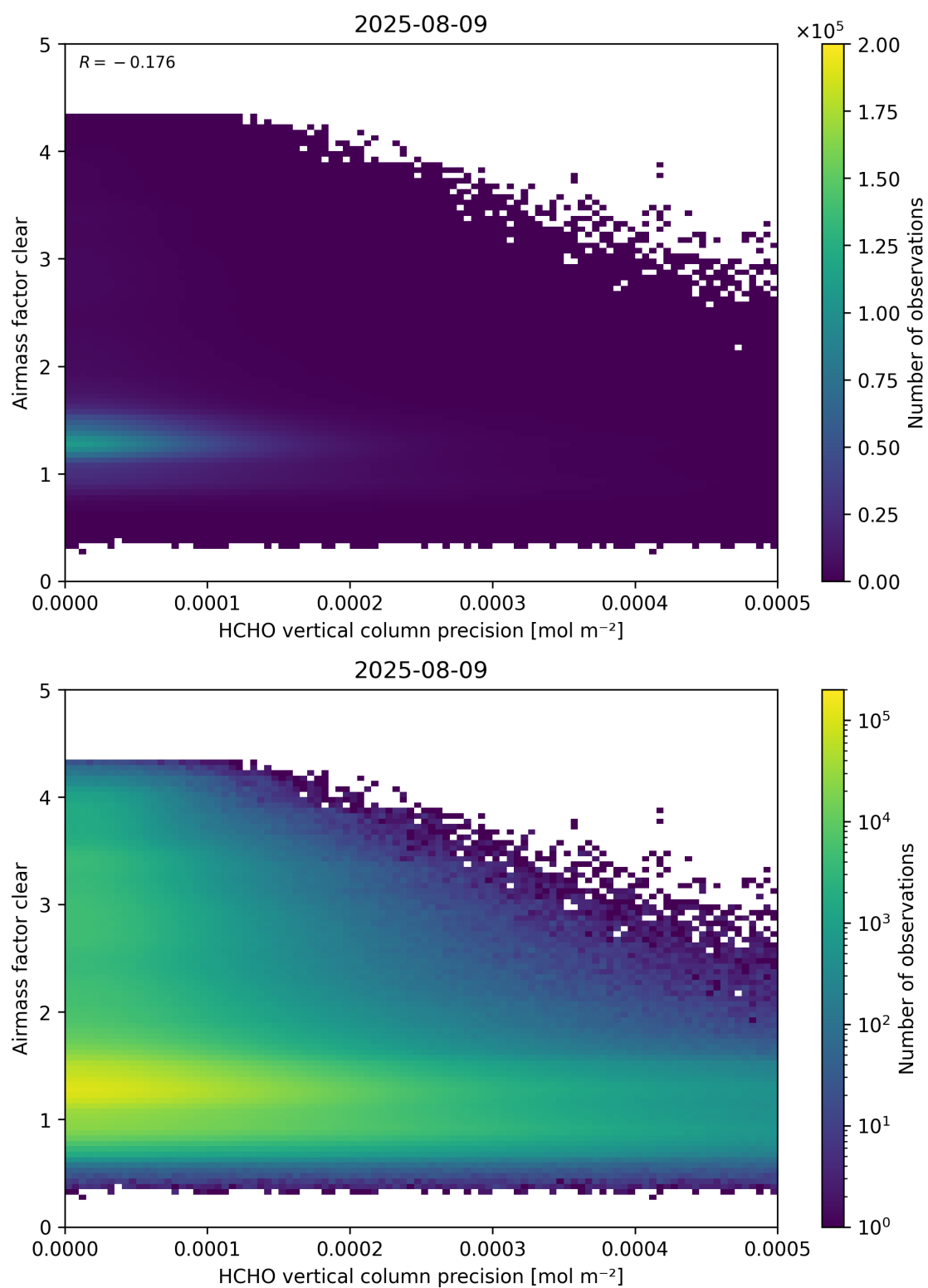
Figure 139: Scatter density plot of “HCHO vertical column precision” against “Airmass factor clear” for 2025-08-09 to 2025-08-10.
