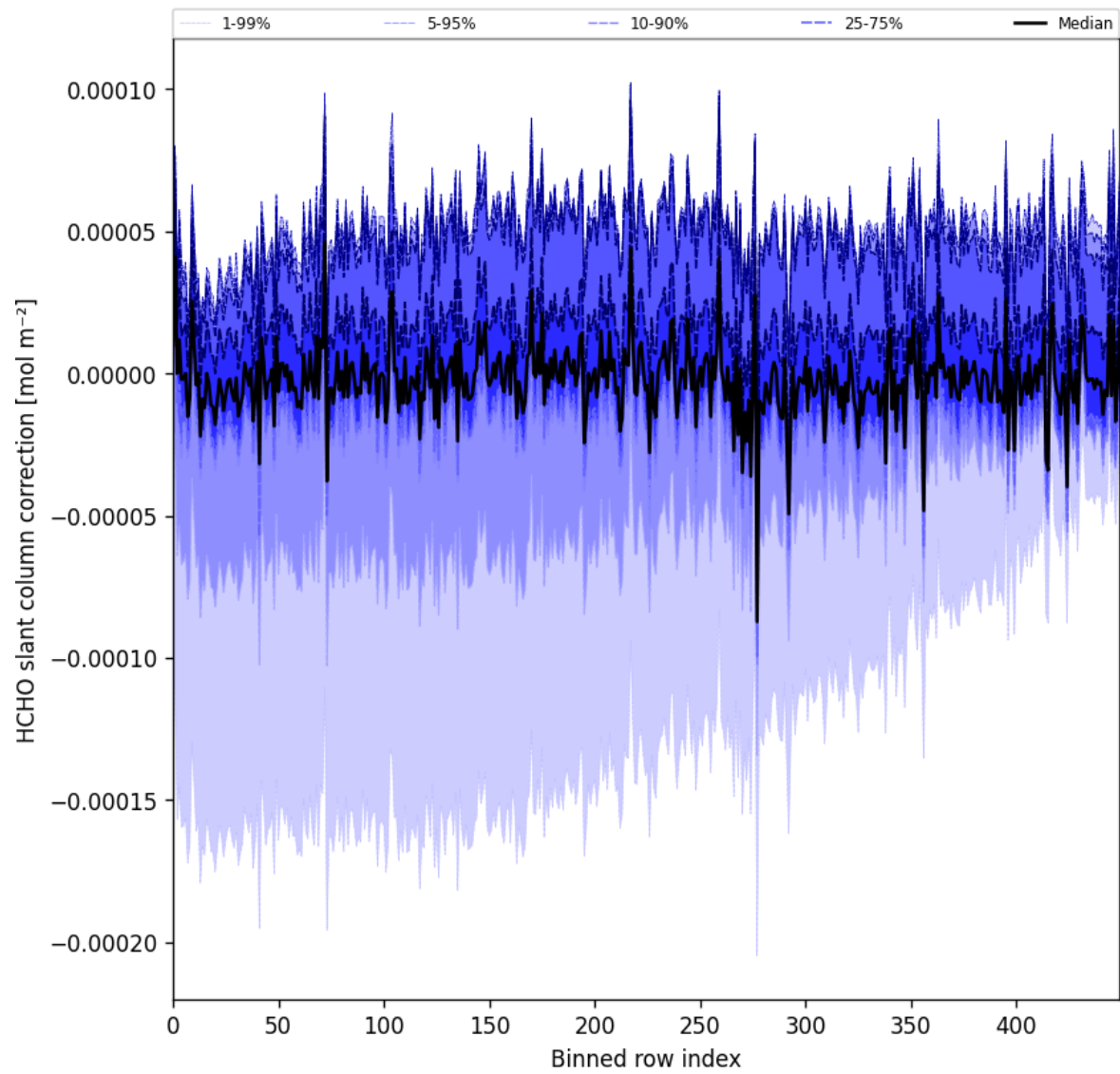
Figure 61: Along track statistics of “HCHO slant column correction” for 2025-08-09 to 2025-08-10
