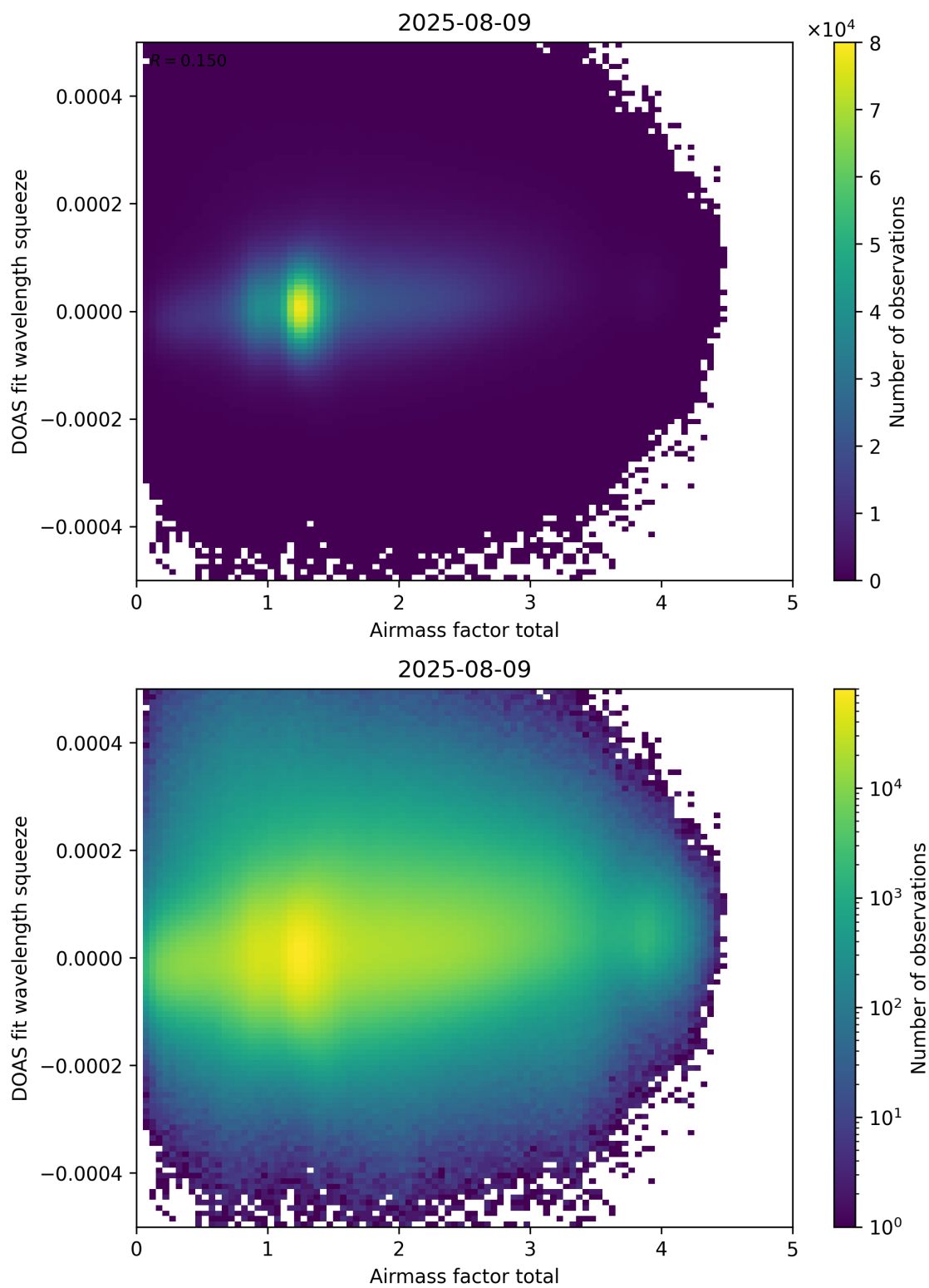
Figure 99: Scatter density plot of “Airmass factor total” against “DOAS fit wavelength squeeze” for 2025-08-09 to 2025-08-10.
