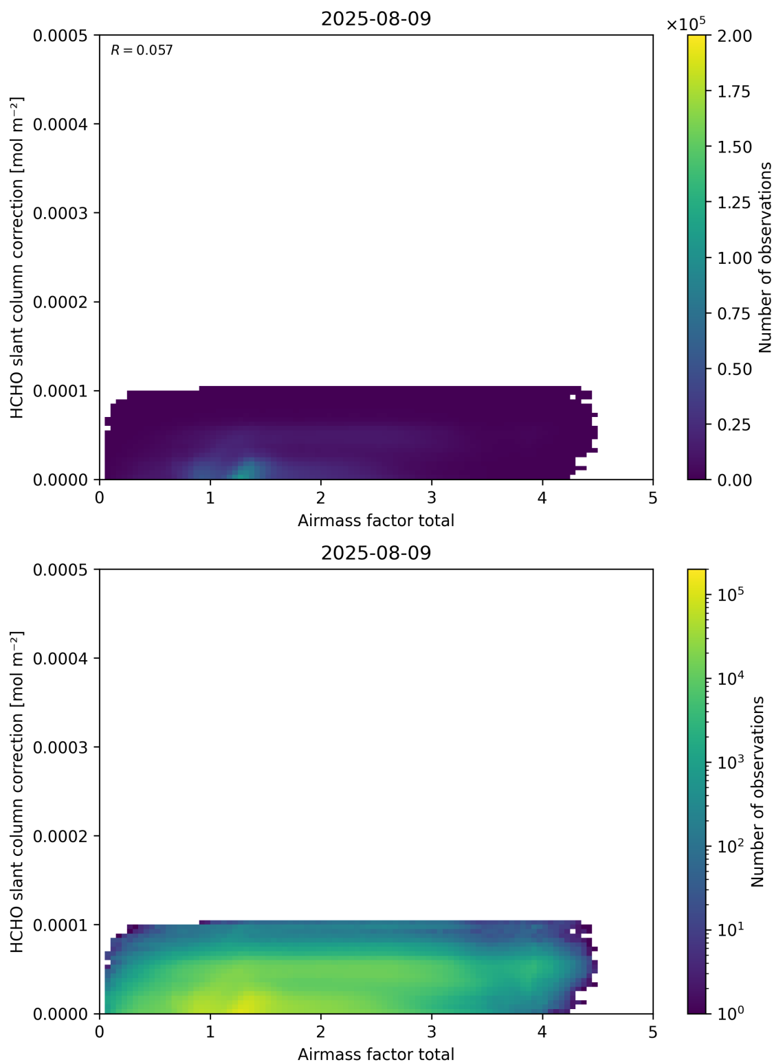
Figure 102: Scatter density plot of “Airmass factor total” against “HCHO slant column correction” for 2025-08-09 to 2025-08-10.
