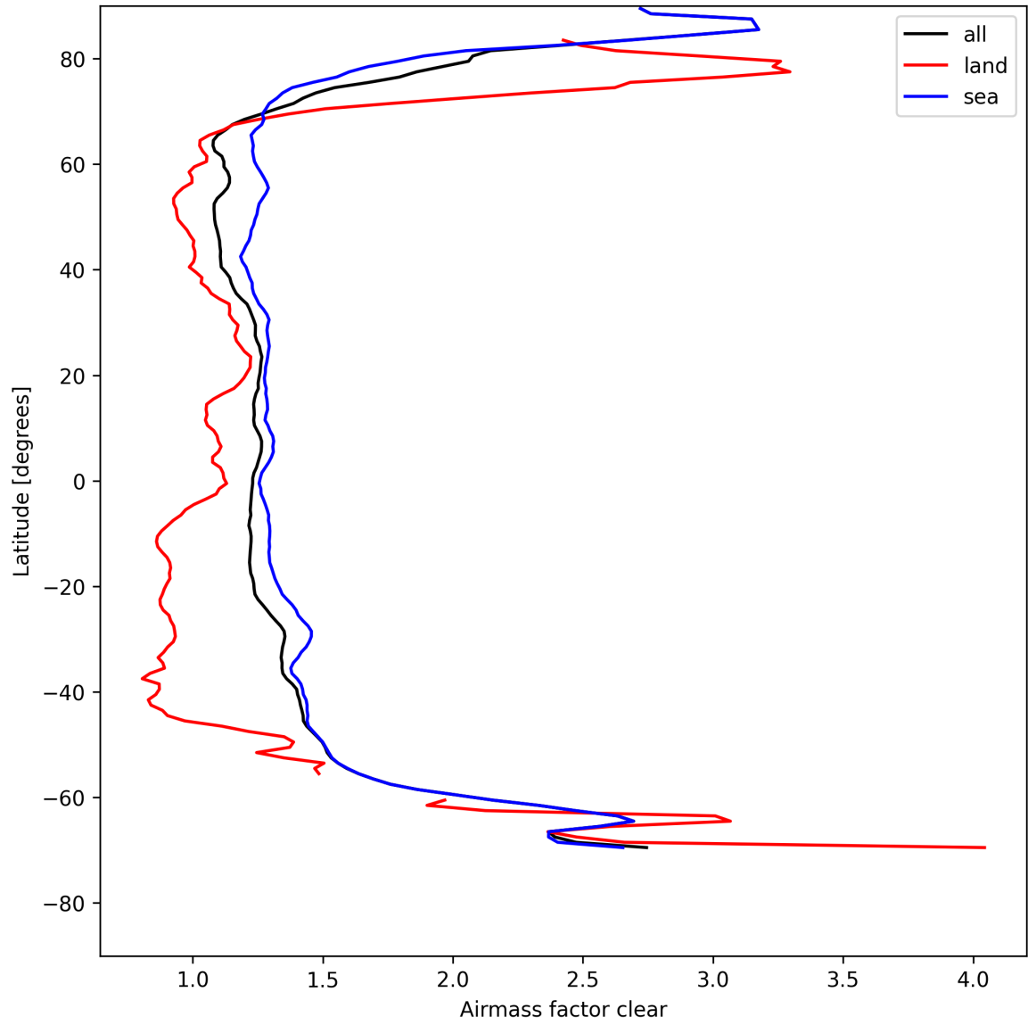
Figure 28: Zonal average of “Airmass factor clear” for 2025-08-09 to 2025-08-10.
