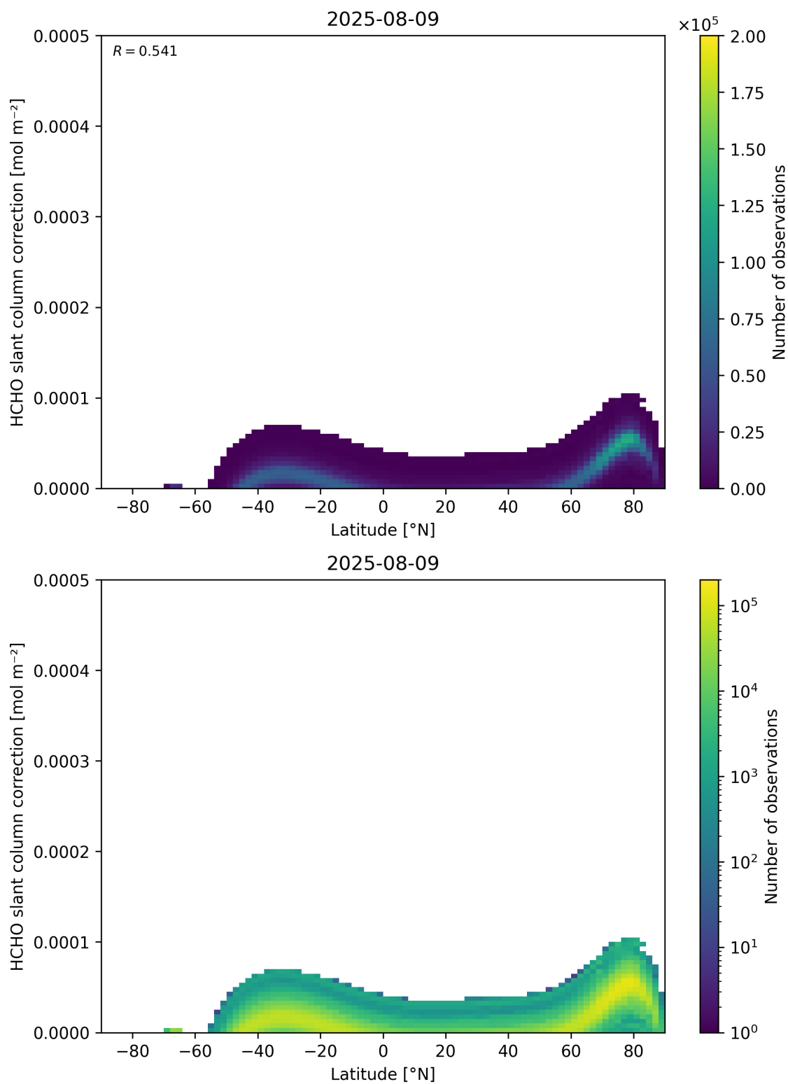
Figure 158: Scatter density plot of “Latitude” against “HCHO slant column correction” for 2025-08-09 to 2025-08-10.
