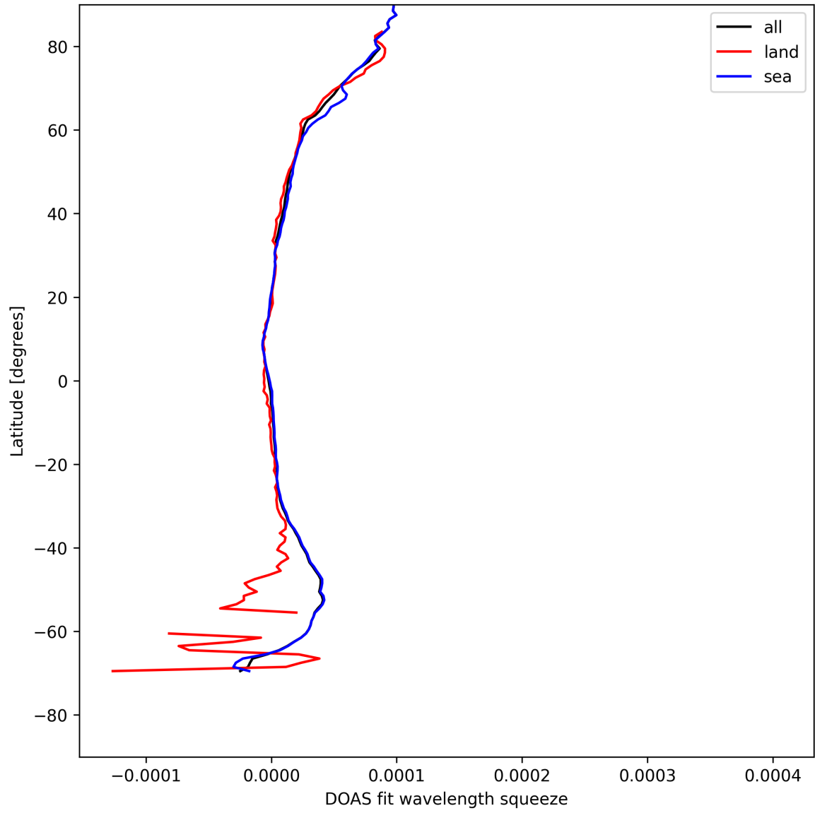
Figure 31: Zonal average of “DOAS fit wavelength squeeze” for 2025-08-09 to 2025-08-10.
