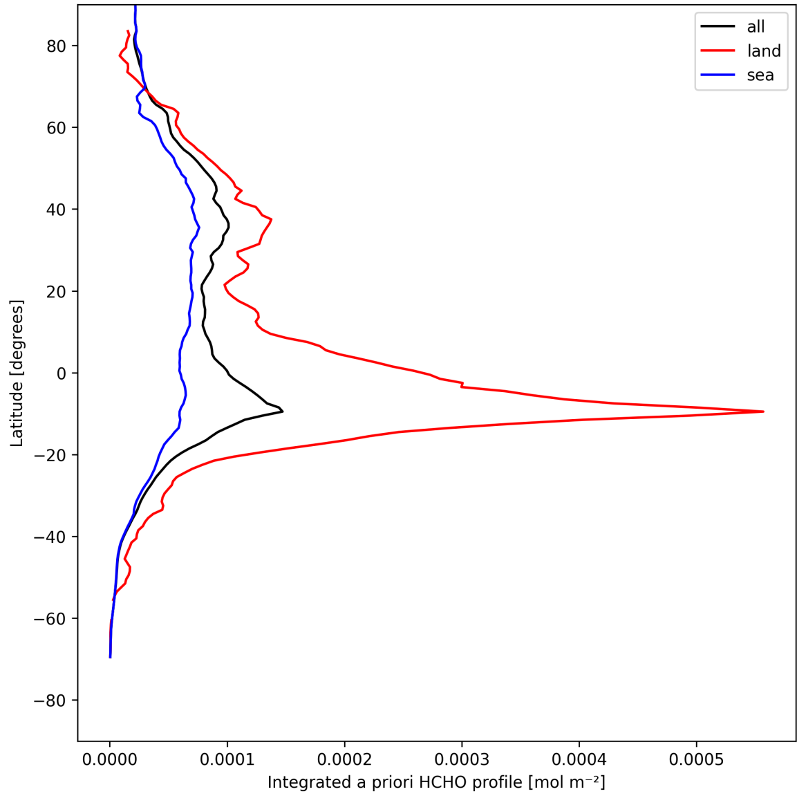
Figure 29: Zonal average of “Integrated a priori HCHO profile” for 2025-08-09 to 2025-08-10.
