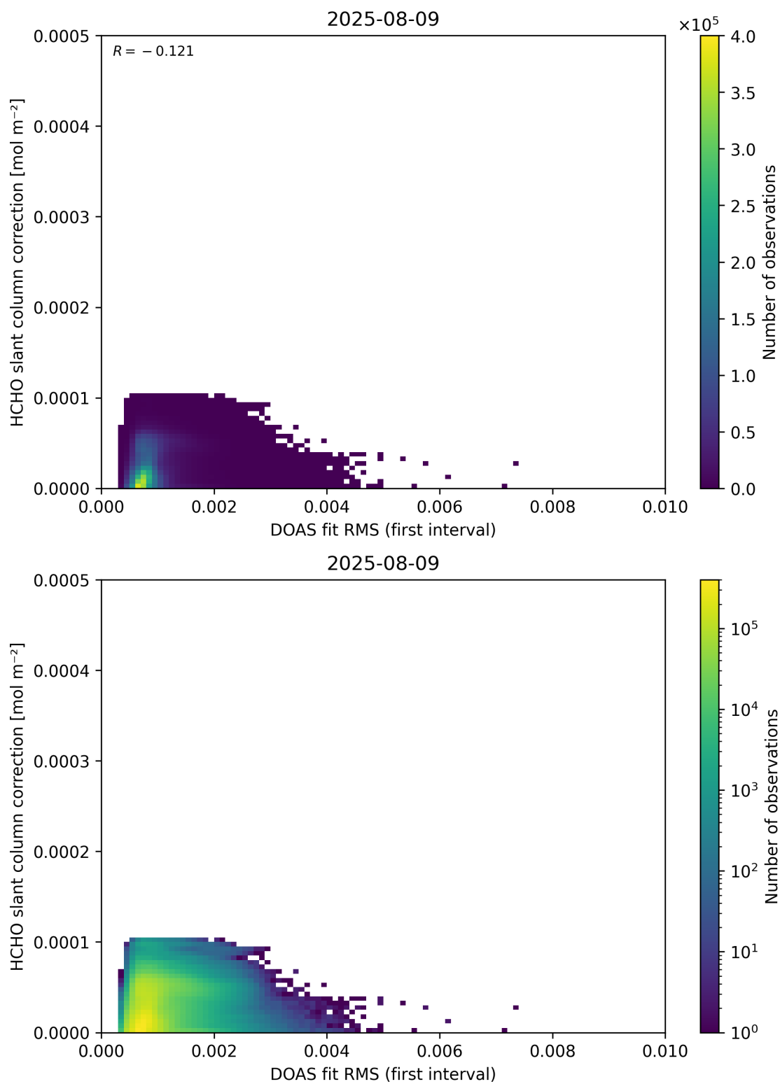
Figure 63: Scatter density plot of “DOAS fit RMS (first interval)” against “HCHO slant column correction” for 2025-08-09 to 2025-08-10.
