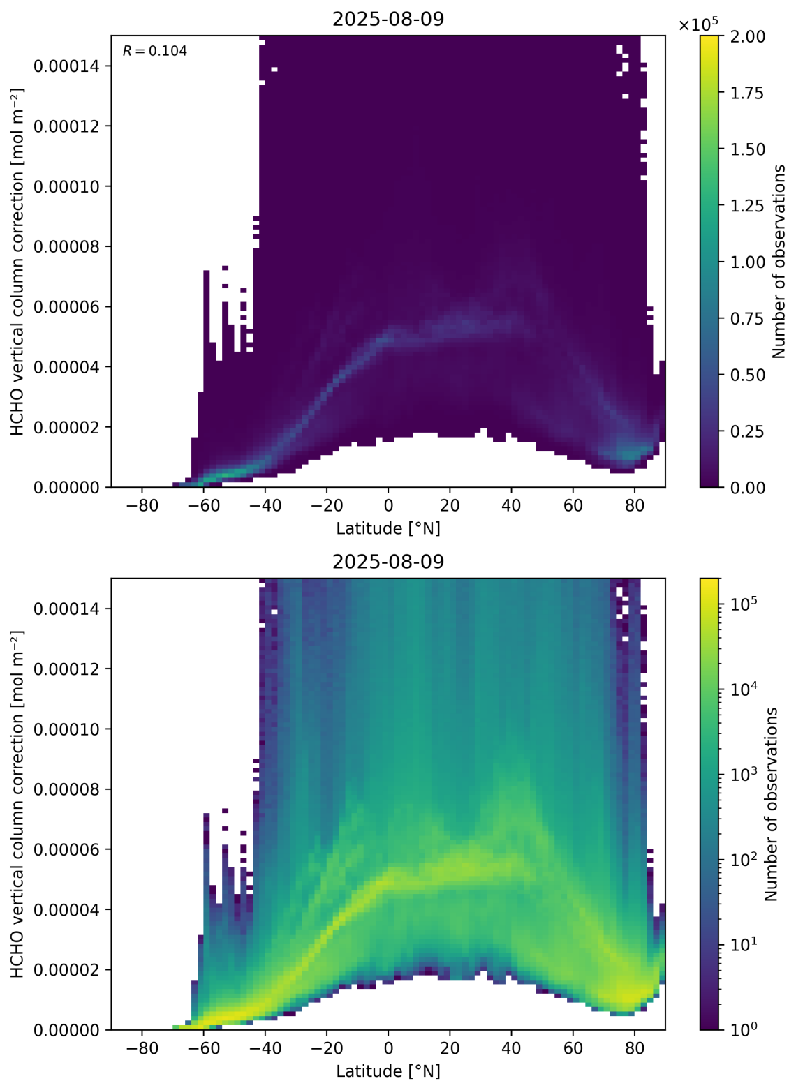
Figure 164: Scatter density plot of “Latitude” against “HCHO vertical column correction” for 2025-08-09 to 2025-08-10.
