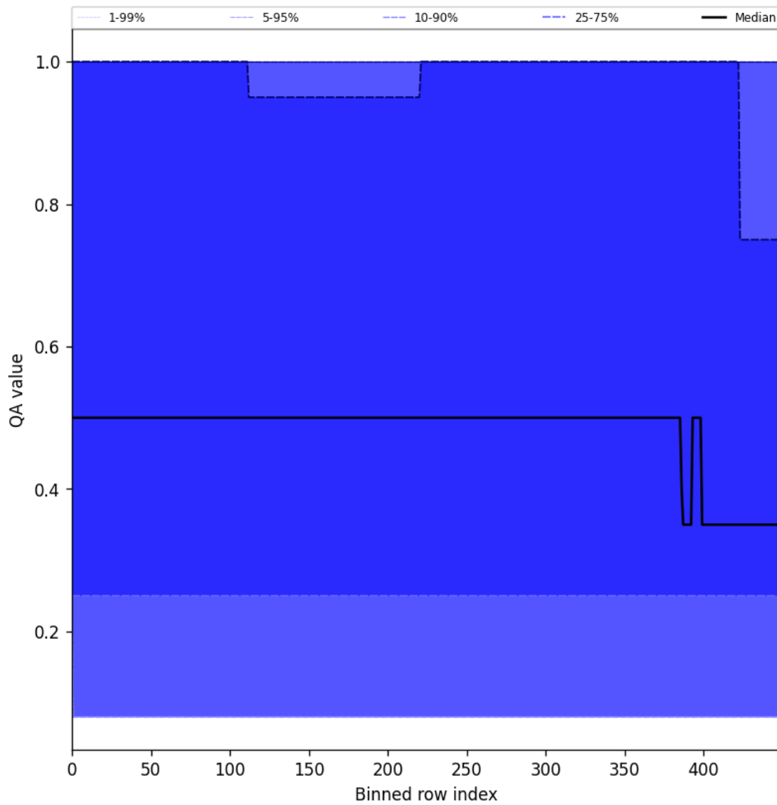
Figure 48: Along track statistics of “QA value” for 2025-08-09 to 2025-08-10
