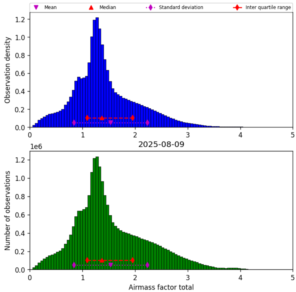
Figure 40: Histogram of “Airmass factor total” for 2025-08-09 to 2025-08-10
