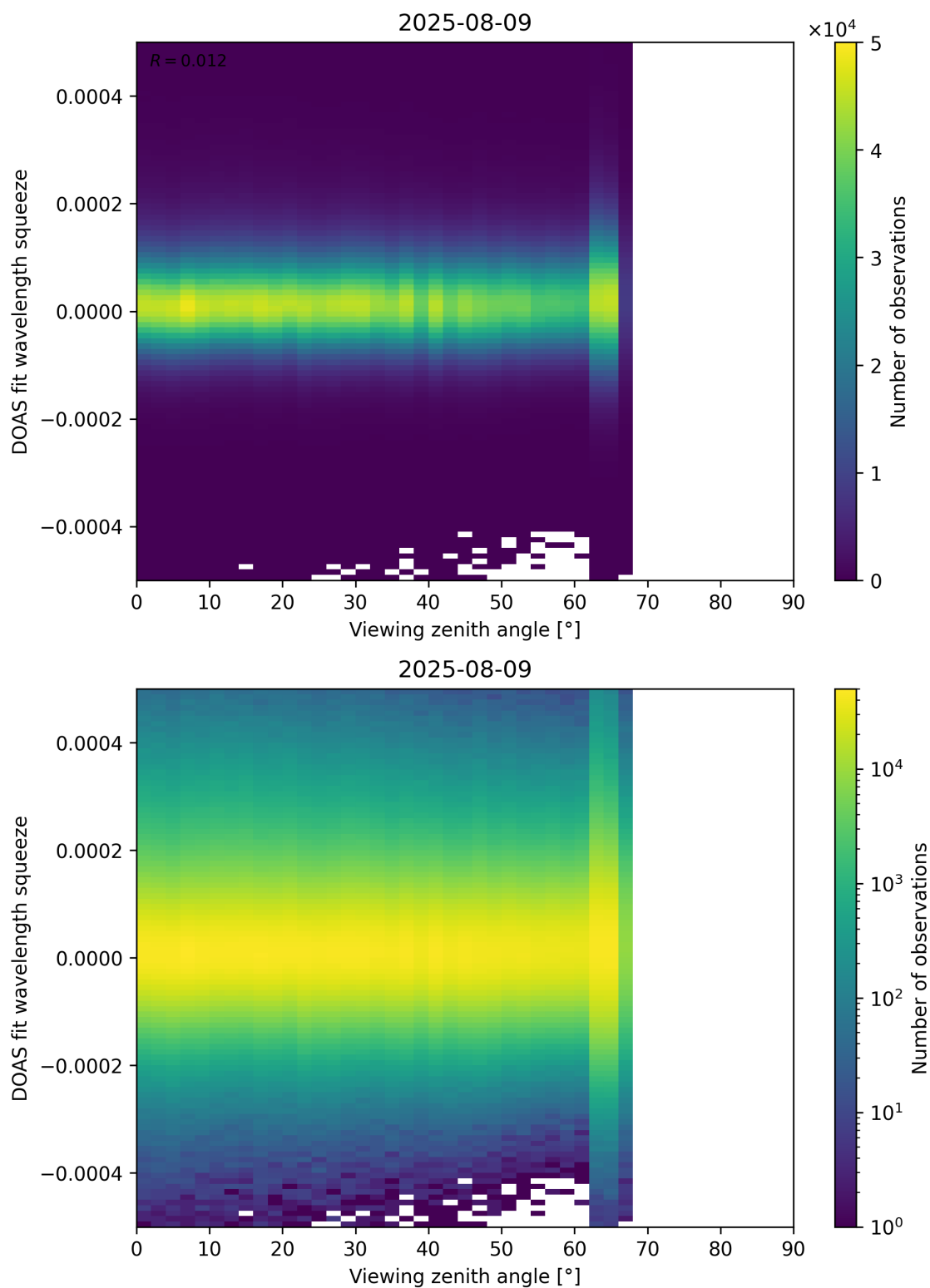
Figure 184: Scatter density plot of “Viewing zenith angle” against “DOAS fit wavelength squeeze” for 2025-08-09 to 2025-08-10.
