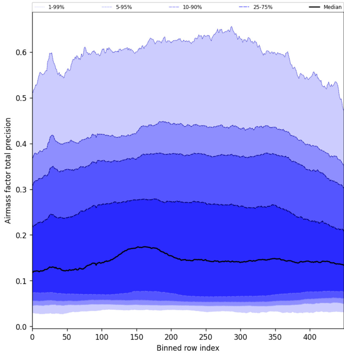
Figure 55: Along track statistics of “Airmass factor total precision” for 2025-08-09 to 2025-08-10
