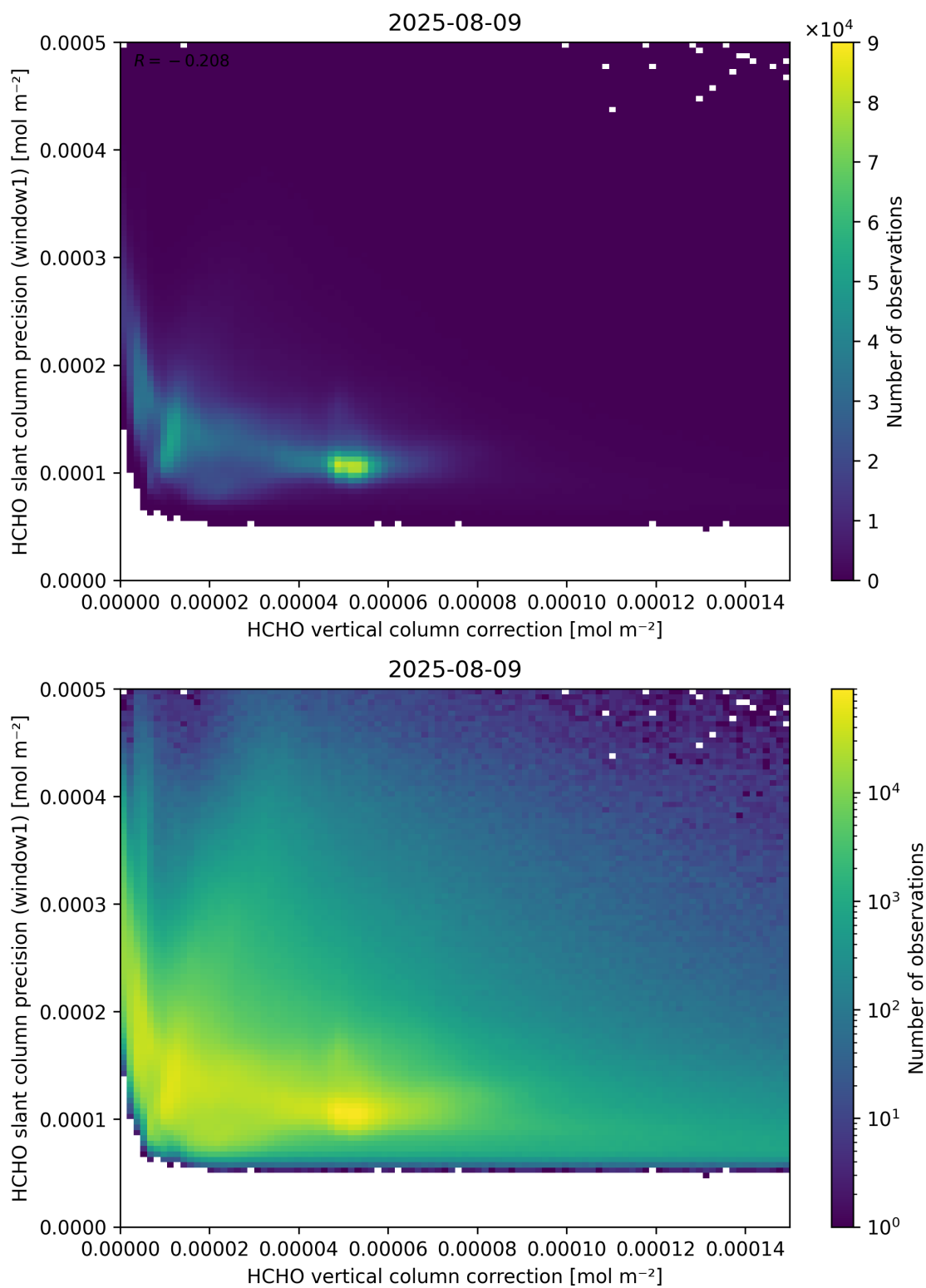
Figure 119: Scatter density plot of “HCHO vertical column correction” against “HCHO slant column precision (window1)” for 2025-08-09 to 2025-08-10.
