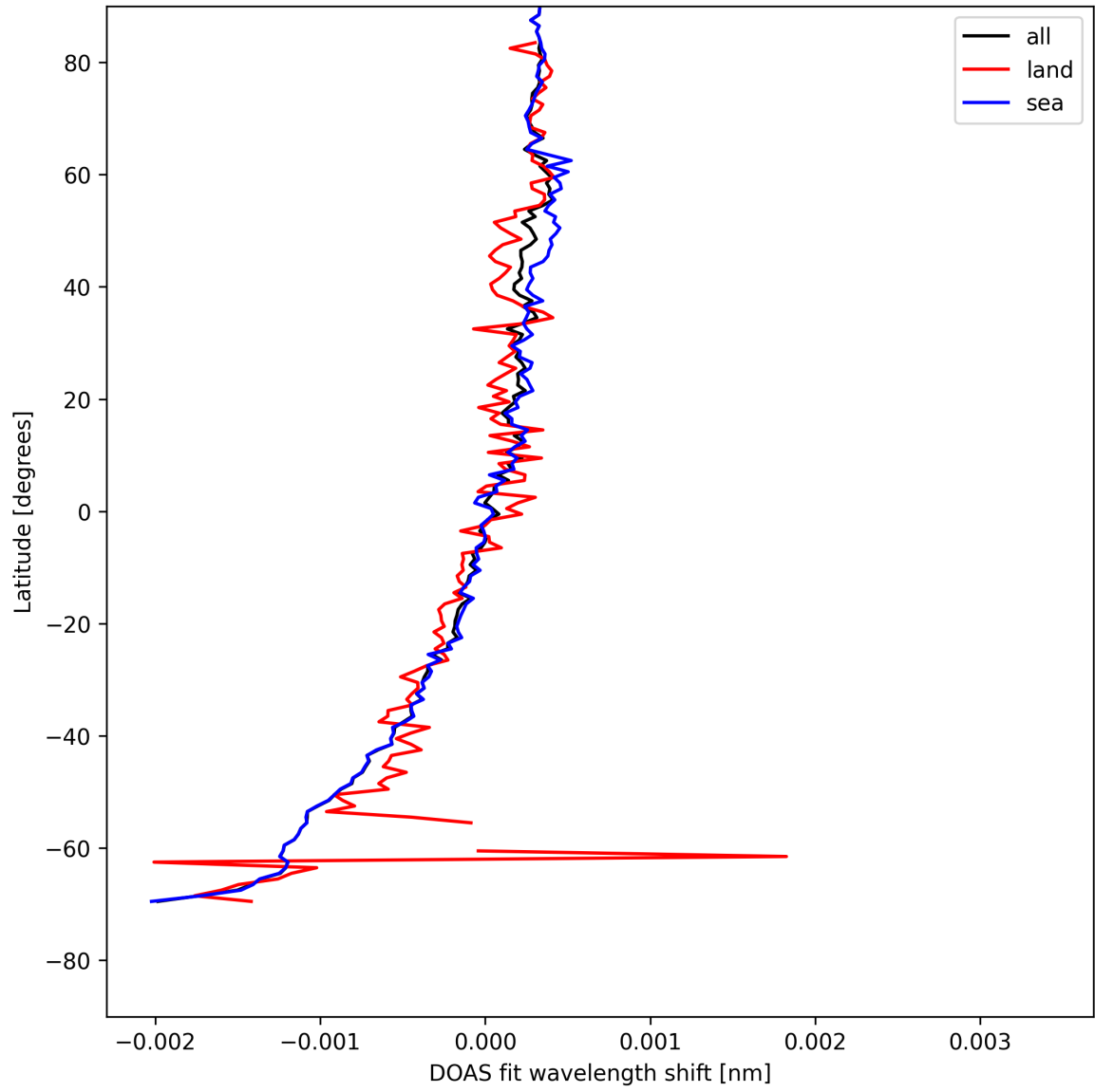
Figure 30: Zonal average of "DOAS fit wavelength shift" for 2025-08-09 to 2025-08-10.
