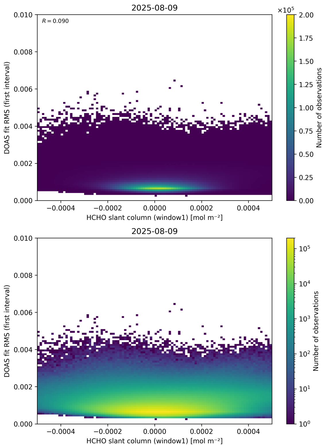
Figure 78: Scatter density plot of “HCHO slant column (window1)” against “DOAS fit RMS (first interval)” for 2025-08-09 to 2025-08-10.
