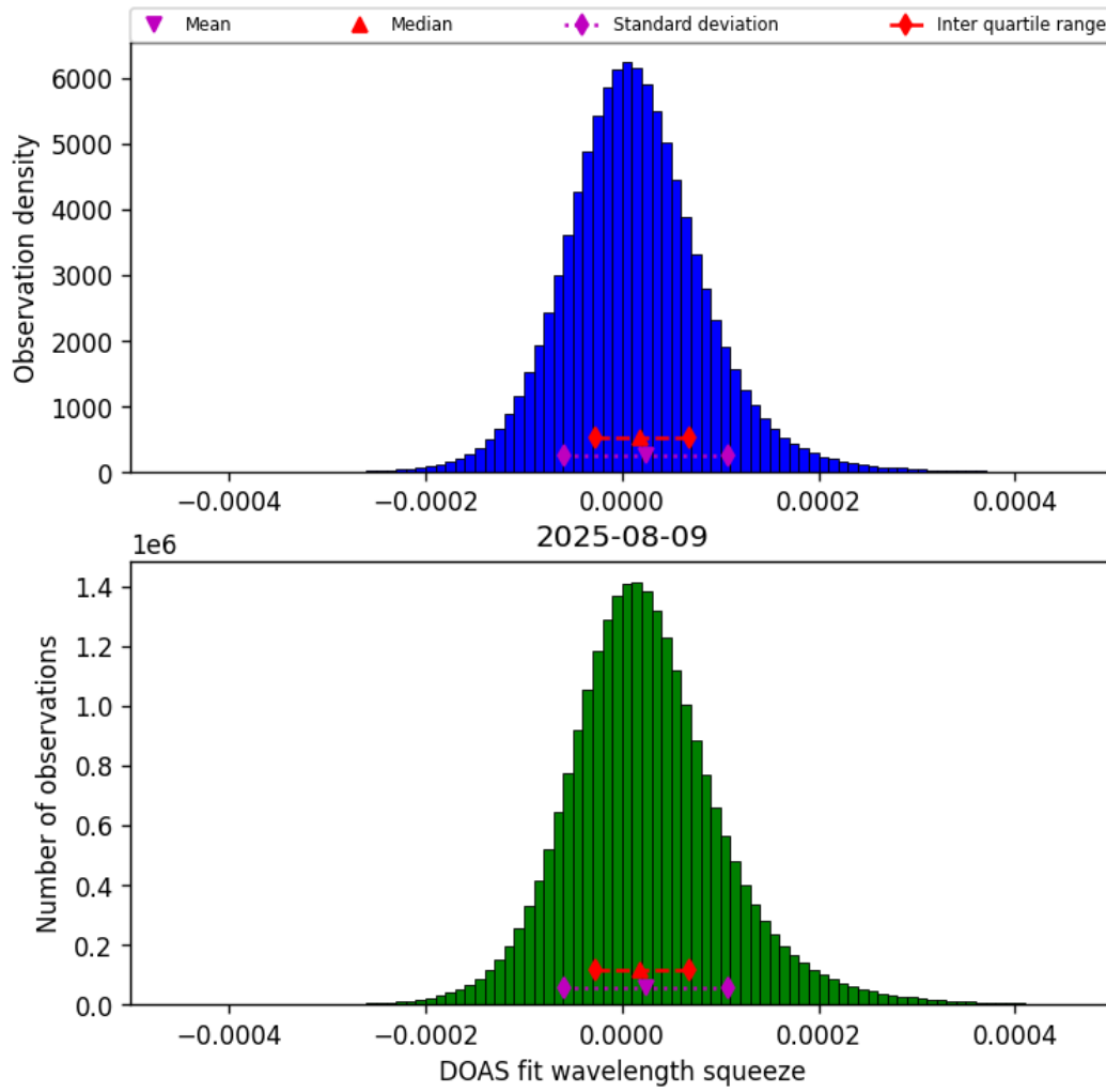
Figure 45: Histogram of “DOAS fit wavelength squeeze” for 2025-08-09 to 2025-08-10
