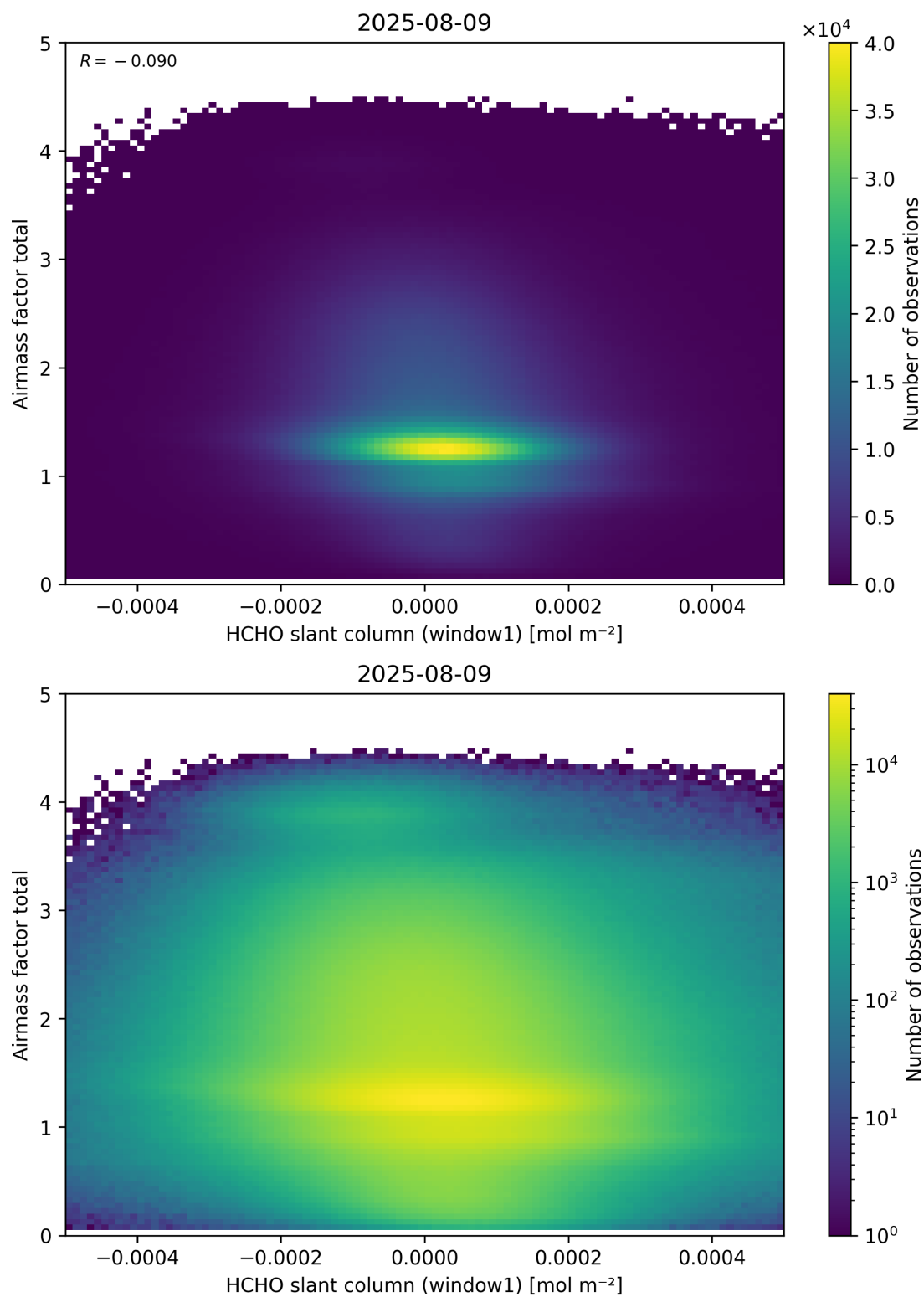
Figure 85: Scatter density plot of “HCHO slant column (window1)” against “Airmass factor total” for 2025-08-09 to 2025-08-10.
