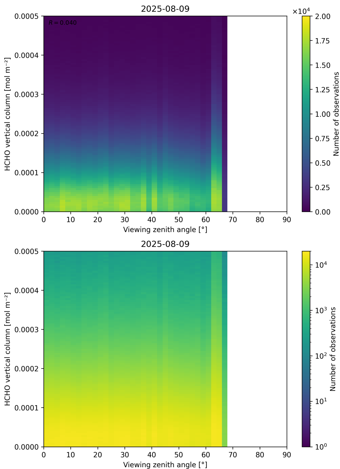
Figure 192: Scatter density plot of “Viewing zenith angle” against “HCHO vertical column” for 2025-08-09 to 2025-08-10.
