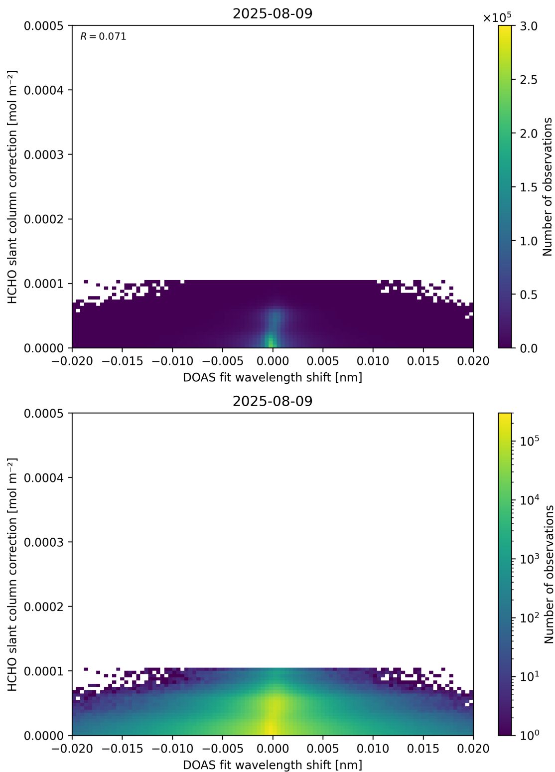
Figure 67: Scatter density plot of “DOAS fit wavelength shift” against “HCHO slant column correction” for 2025-08-09 to 2025-08-10.
