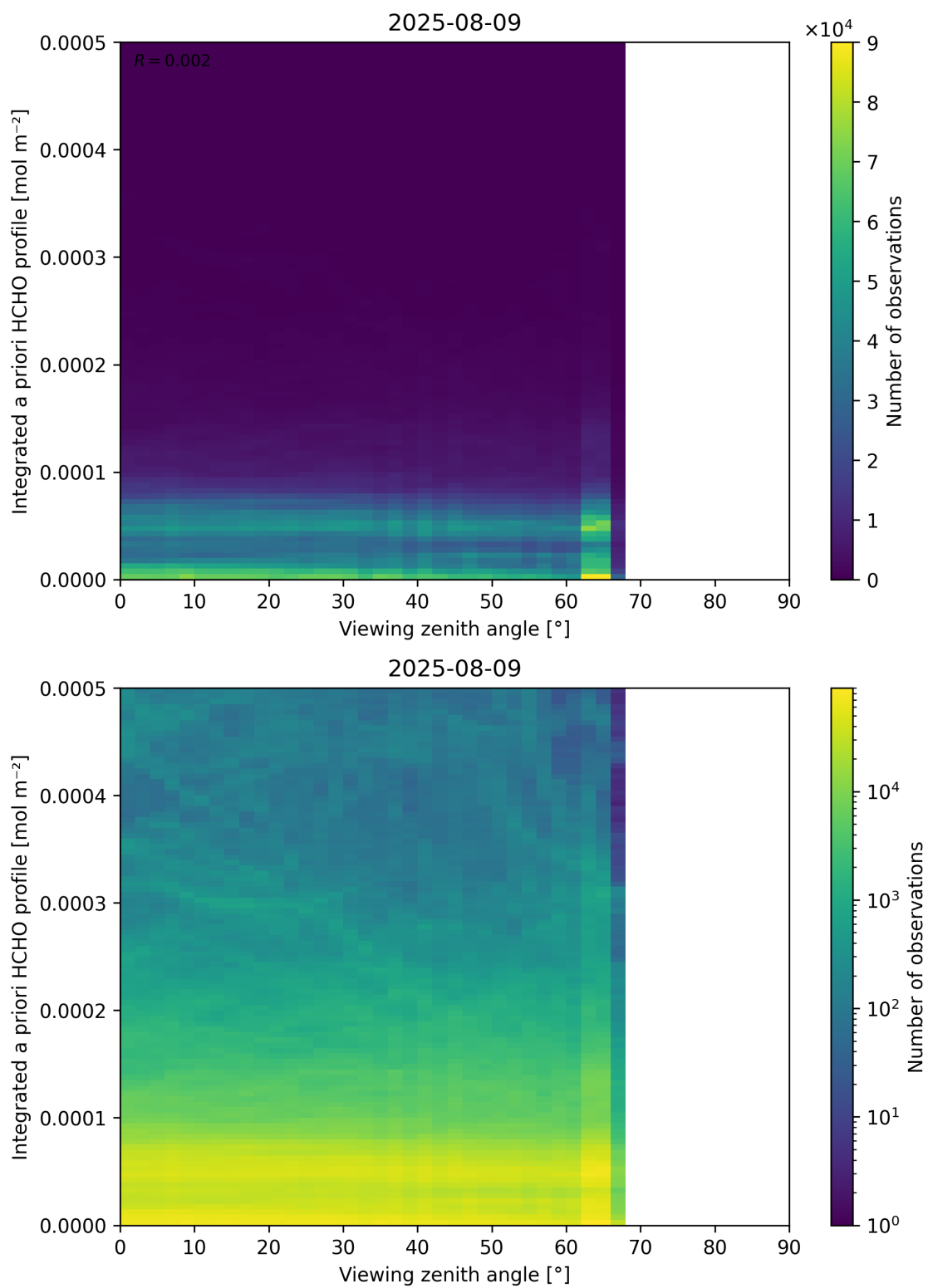
Figure 195: Scatter density plot of “Viewing zenith angle” against “Integrated a priori HCHO profile” for 2025-08-09 to 2025-08-10.
