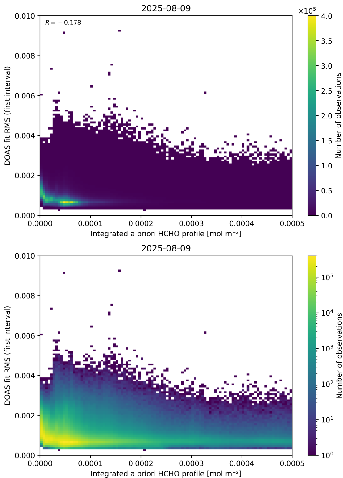
Figure 148: Scatter density plot of “Integrated a priori HCHO profile” against “DOAS fit RMS (first interval)” for 2025-08-09 to 2025-08-10.
