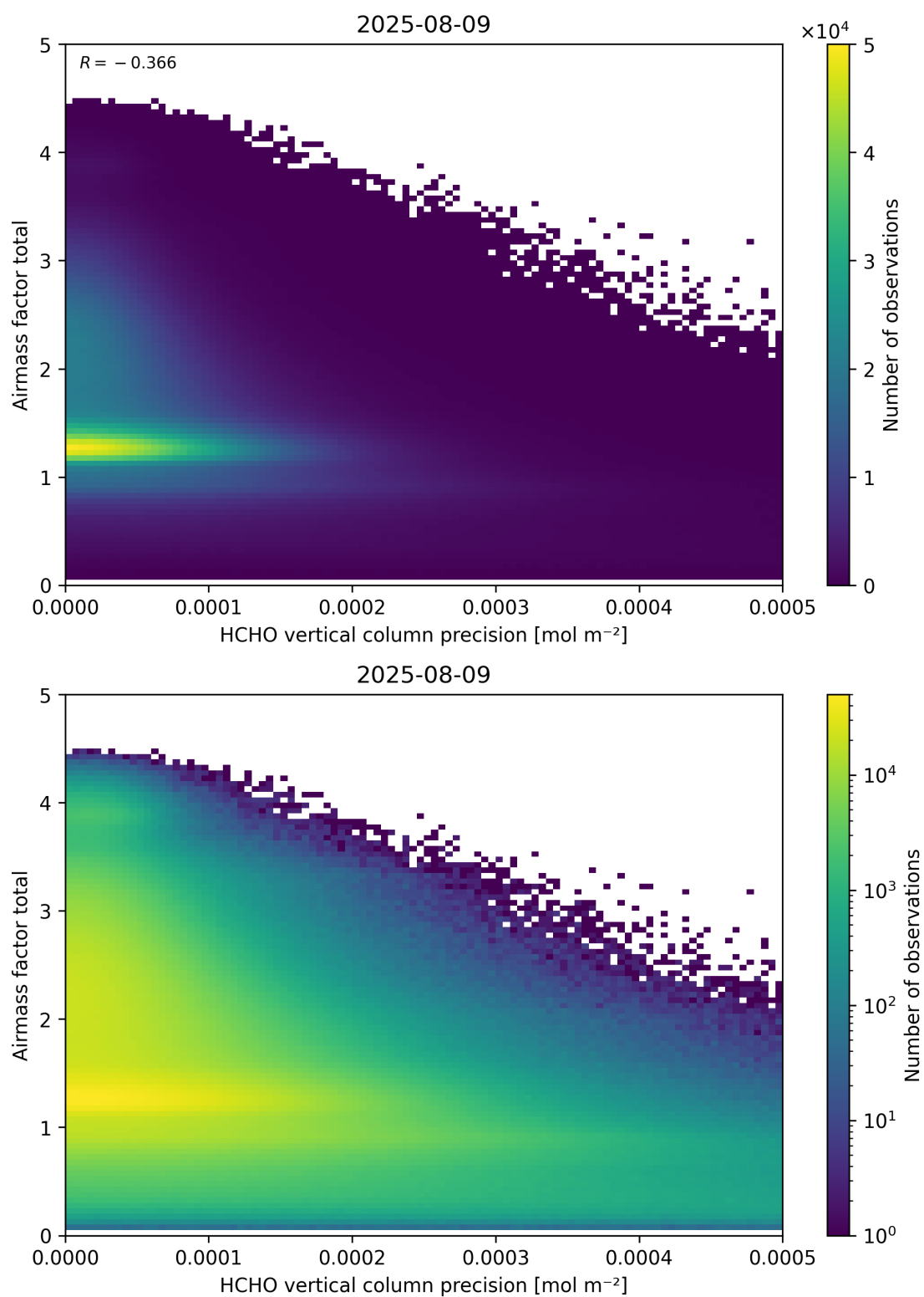
Figure 144: Scatter density plot of “HCHO vertical column precision” against “Airmass factor total” for 2025-08-09 to 2025-08-10.
