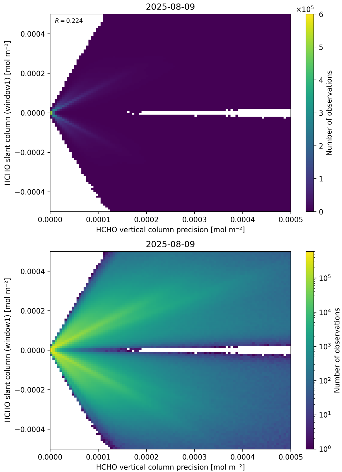
Figure 142: Scatter density plot of “HCHO vertical column precision” against “HCHO slant column (window1)” for 2025-08-09 to 2025-08-10.
