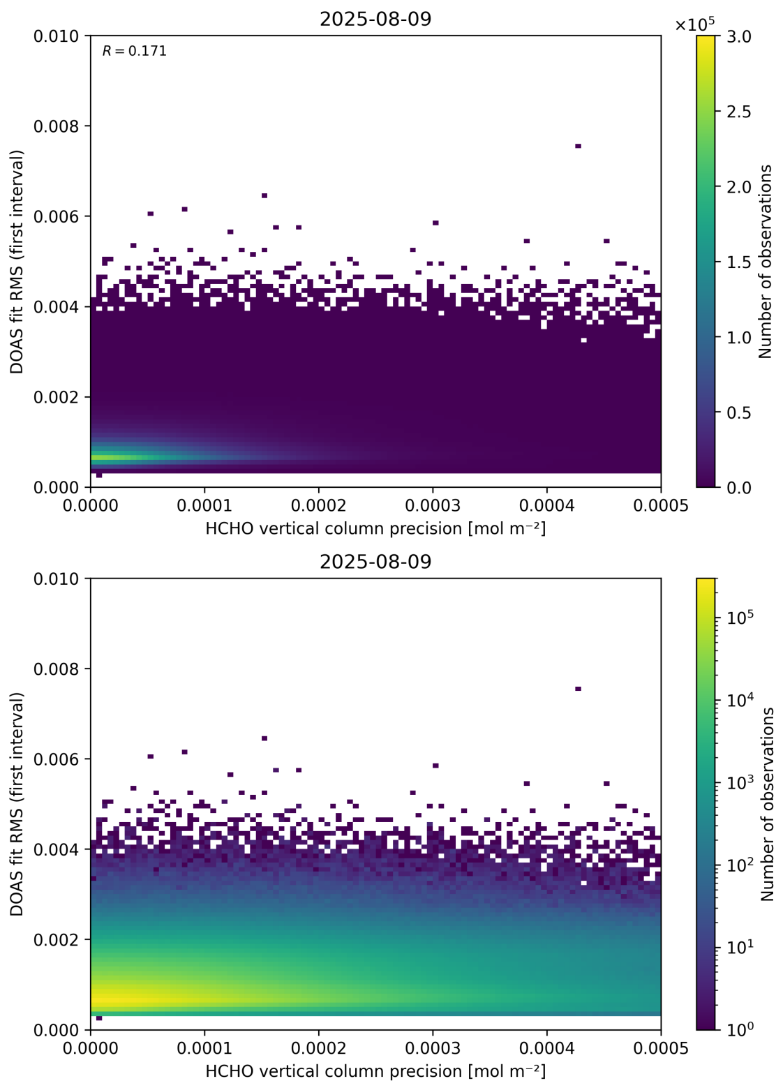
Figure 136: Scatter density plot of “HCHO vertical column precision” against “DOAS fit RMS (first interval)” for 2025-08-09 to 2025-08-10.
