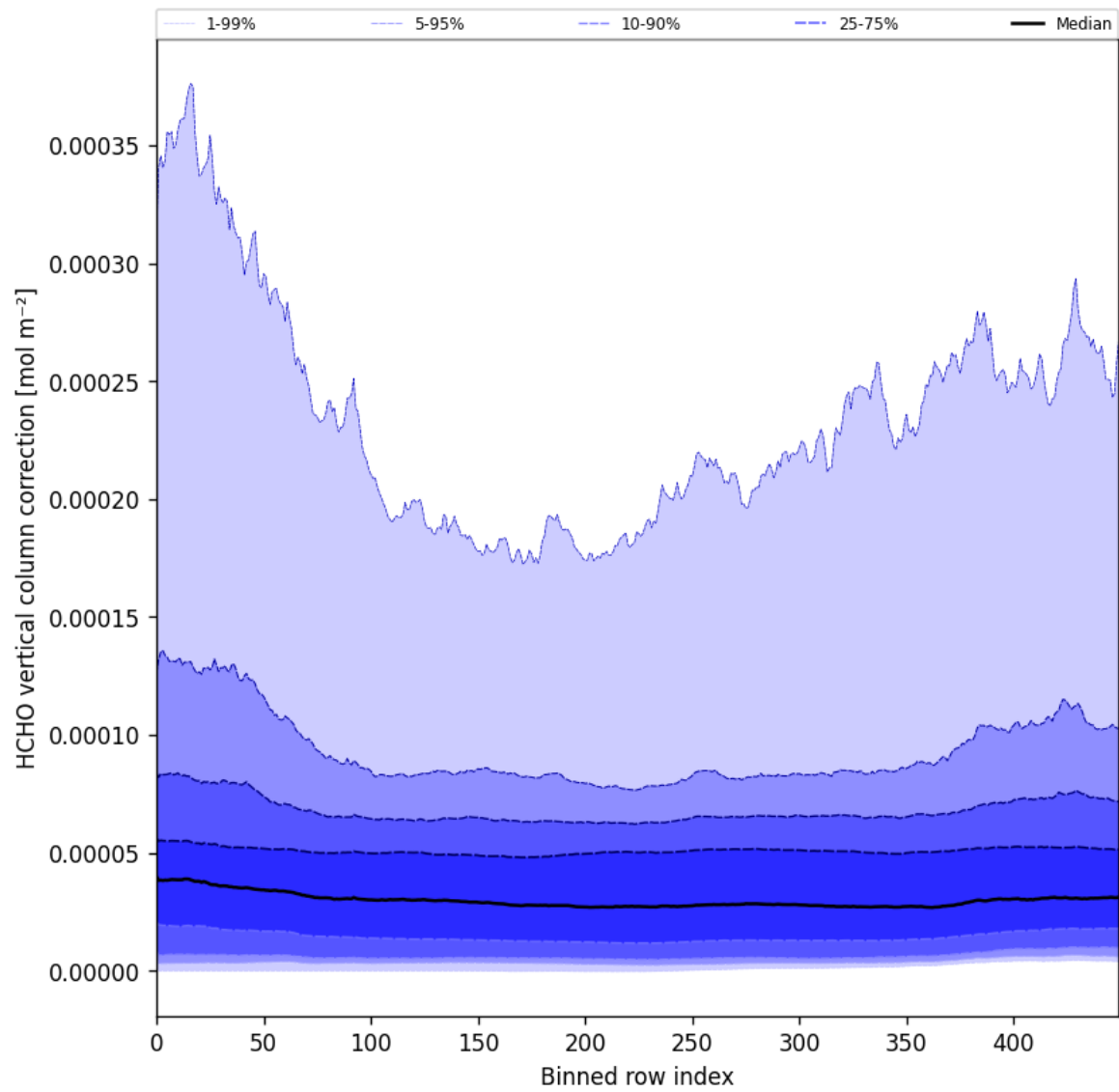
Figure 51: Along track statistics of “HCHO vertical column correction” for 2025-08-09 to 2025-08-10
