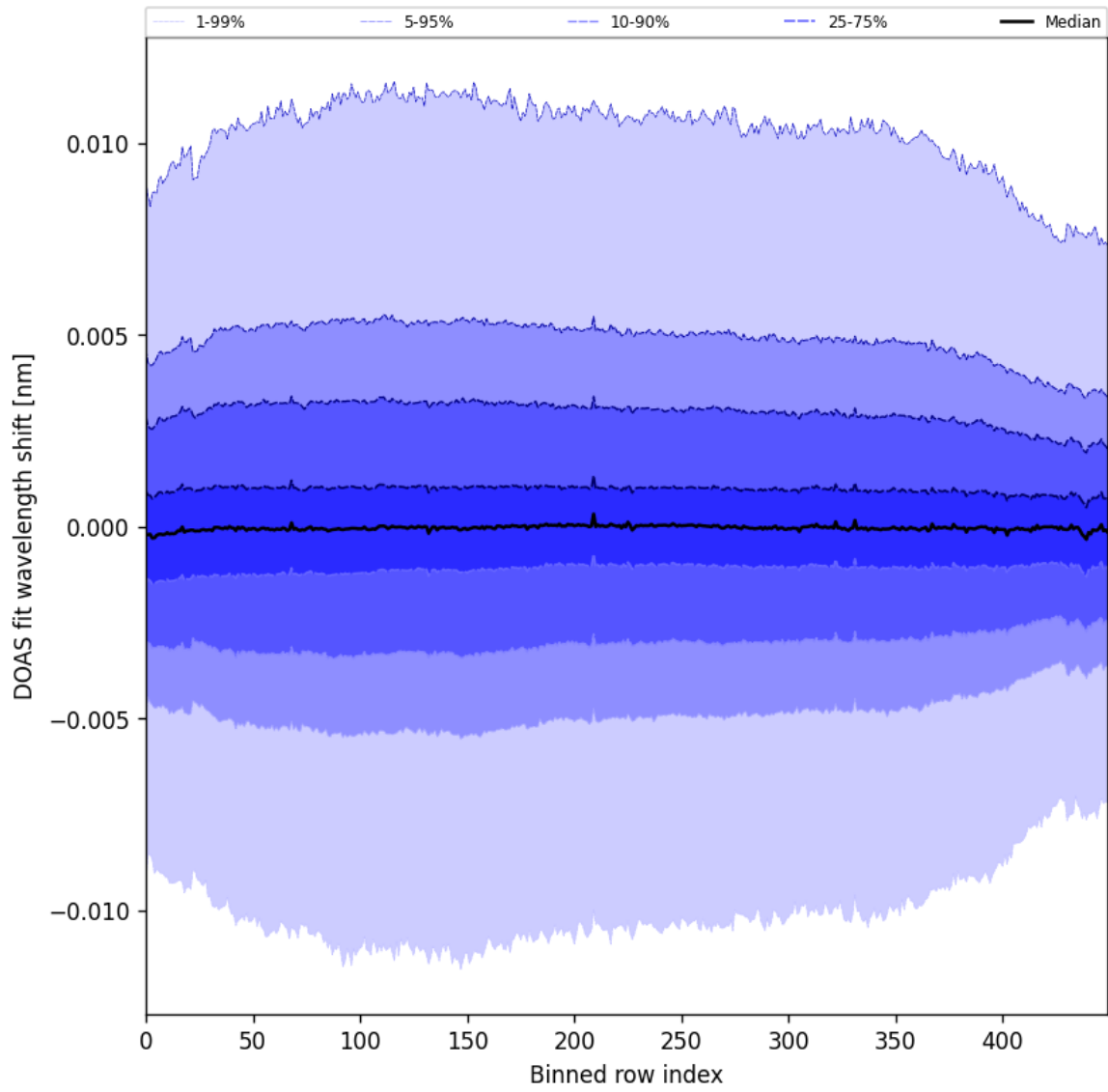
Figure 58: Along track statistics of “DOAS fit wavelength shift” for 2025-08-09 to 2025-08-10
