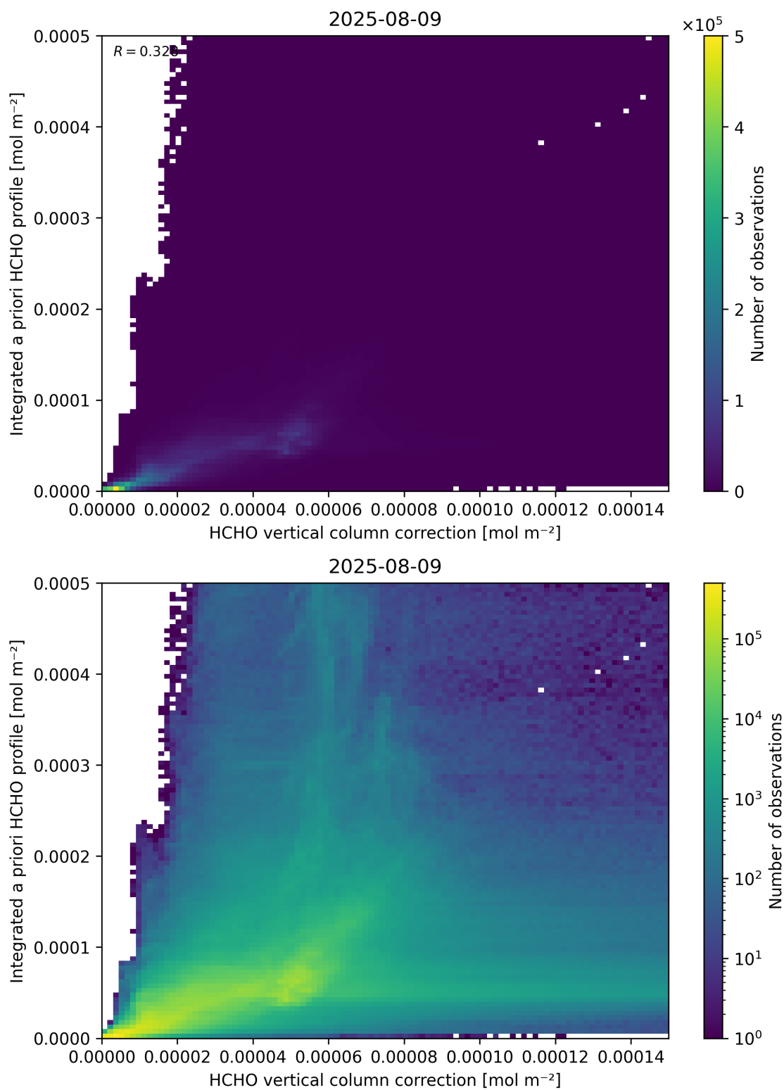
Figure 122: Scatter density plot of “HCHO vertical column correction” against “Integrated a priori HCHO profile” for 2025-08-09 to 2025-08-10.
