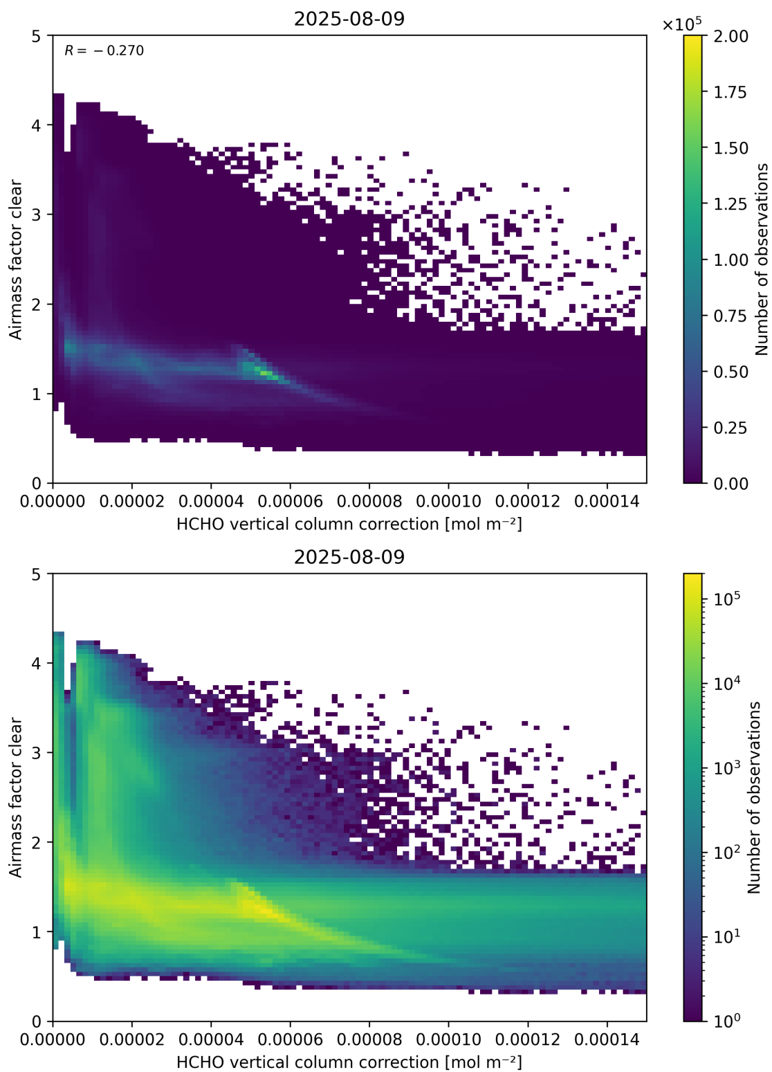
Figure 115: Scatter density plot of “HCHO vertical column correction” against “Airmass factor clear” for 2025-08-09 to 2025-08-10.
