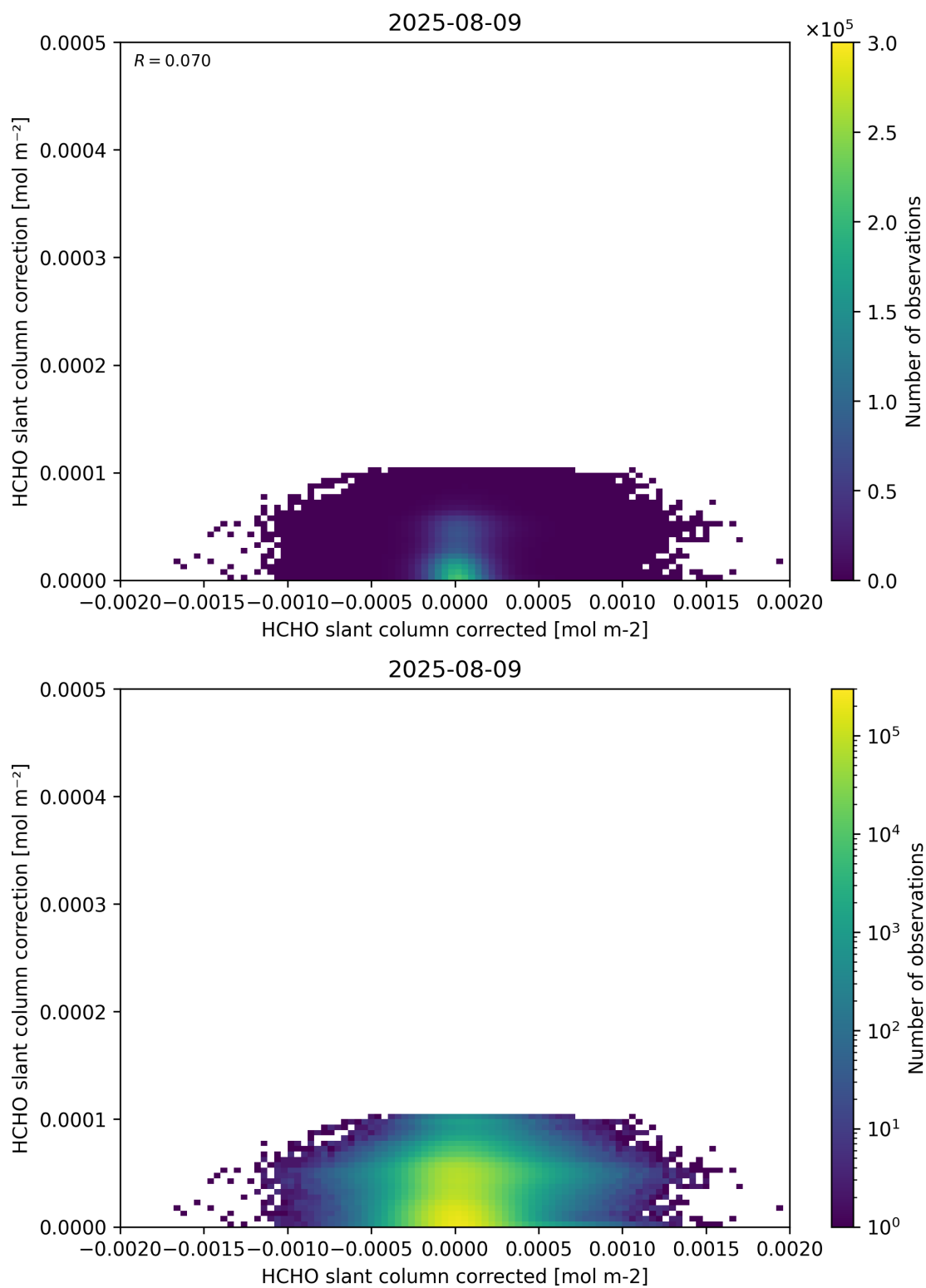
Figure 77: Scatter density plot of “HCHO slant column corrected” against “HCHO slant column correction” for 2025-08-09 to 2025-08-10.
