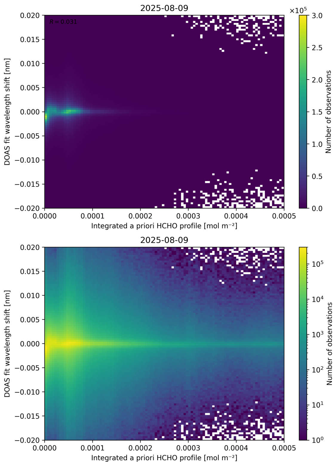
Figure 149: Scatter density plot of “Integrated a priori HCHO profile” against “DOAS fit wavelength shift” for 2025-08-09 to 2025-08-10.
