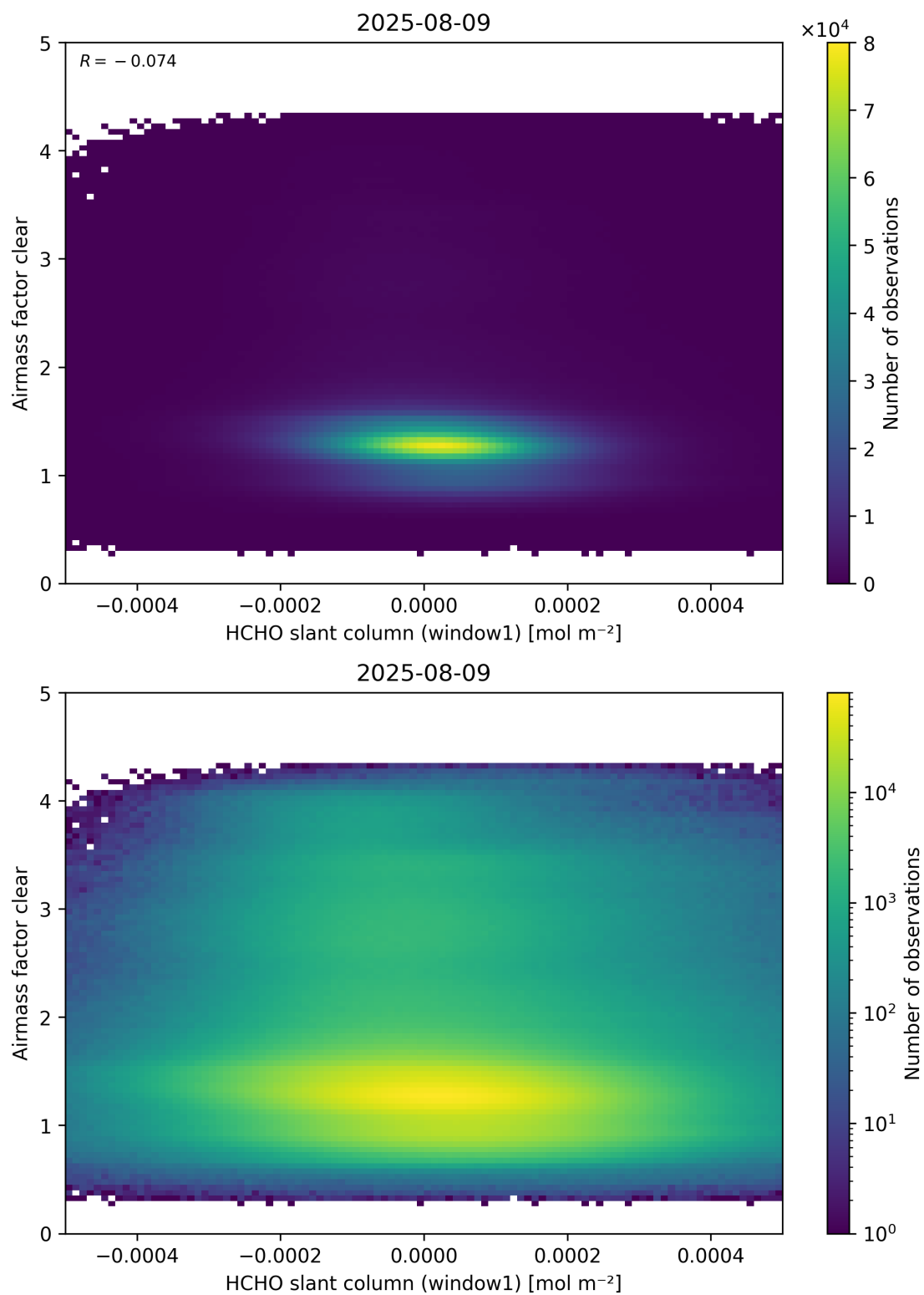
Figure 81: Scatter density plot of “HCHO slant column (window1)” against “Airmass factor clear” for 2025-08-09 to 2025-08-10.
