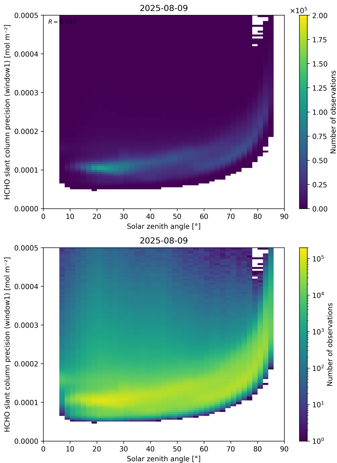
Figure 174: Scatter density plot of “Solar zenith angle” against “HCHO slant column precision (window1)” for 2025-08-09 to 2025-08-10.
