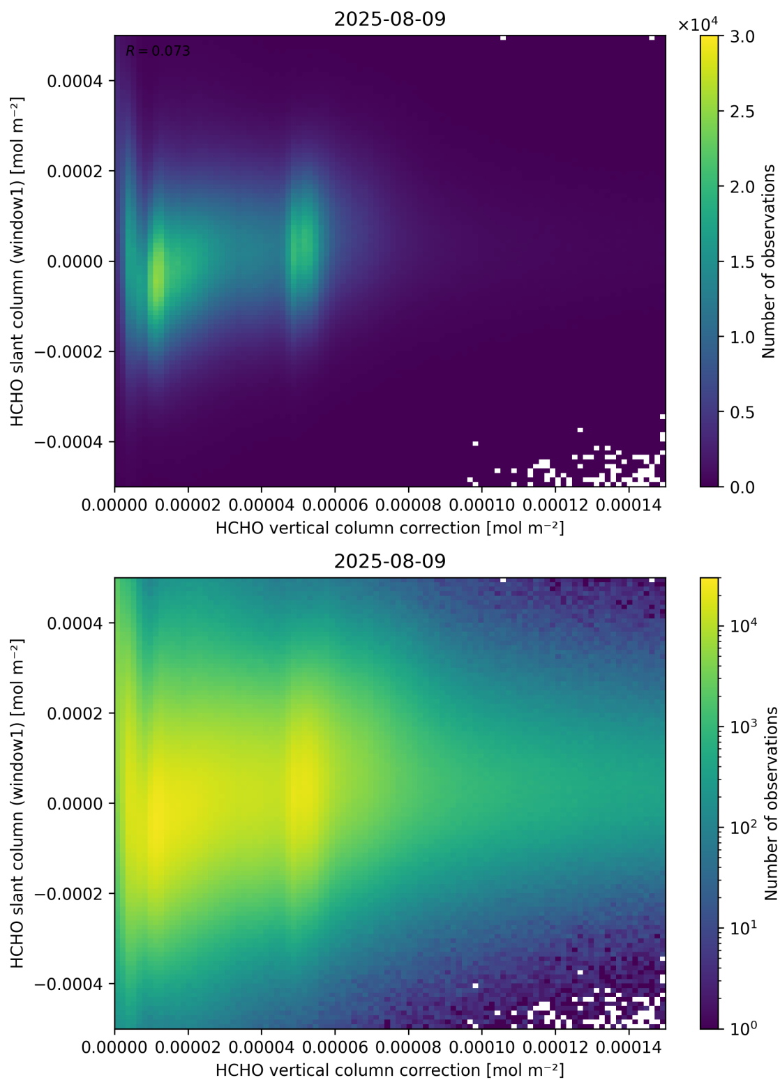
Figure 118: Scatter density plot of “HCHO vertical column correction” against “HCHO slant column (window1)” for 2025-08-09 to 2025-08-10.
