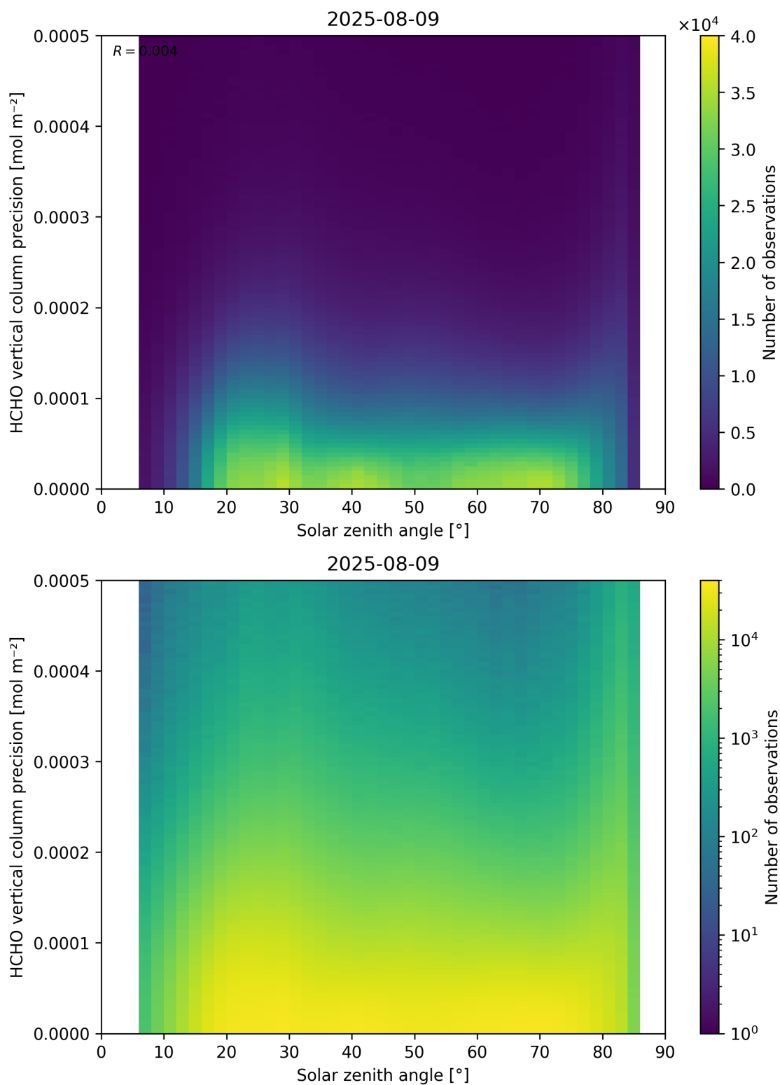
Figure 179: Scatter density plot of “Solar zenith angle” against “HCHO vertical column precision” for 2025-08-09 to 2025-08-10.
