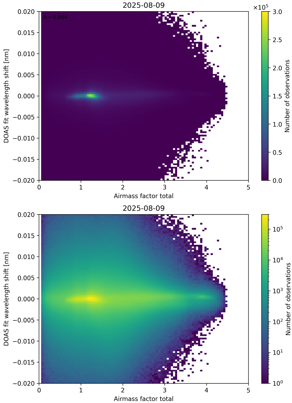
Figure 98: Scatter density plot of “Airmass factor total” against “DOAS fit wavelength shift” for 2025-08-09 to 2025-08-10.
