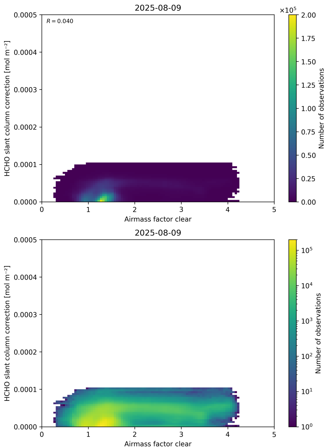
Figure 75: Scatter density plot of “Airmass factor clear” against “HCHO slant column correction” for 2025-08-09 to 2025-08-10.
