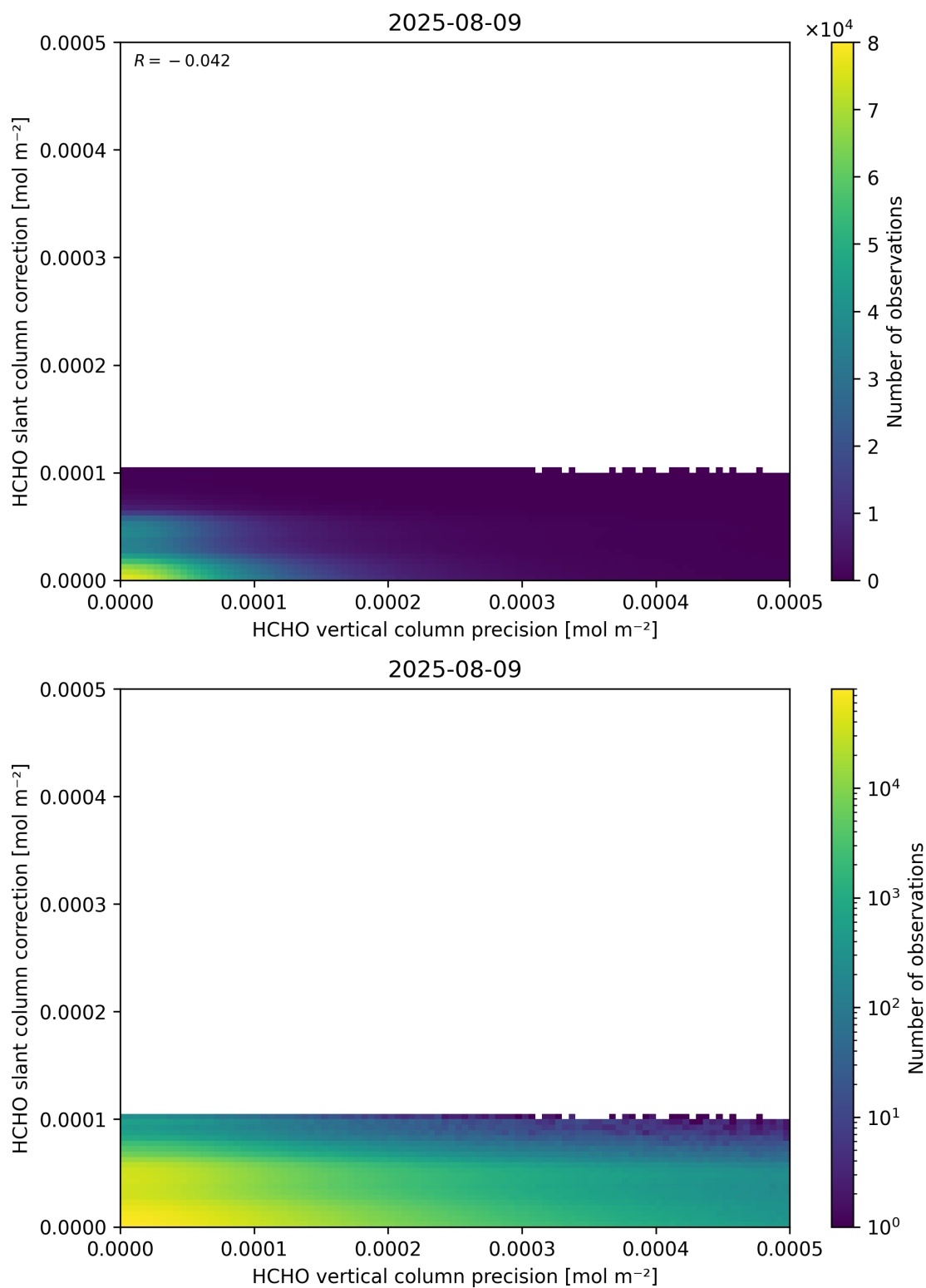
Figure 141: Scatter density plot of “HCHO vertical column precision” against “HCHO slant column correction” for 2025-08-09 to 2025-08-10.
