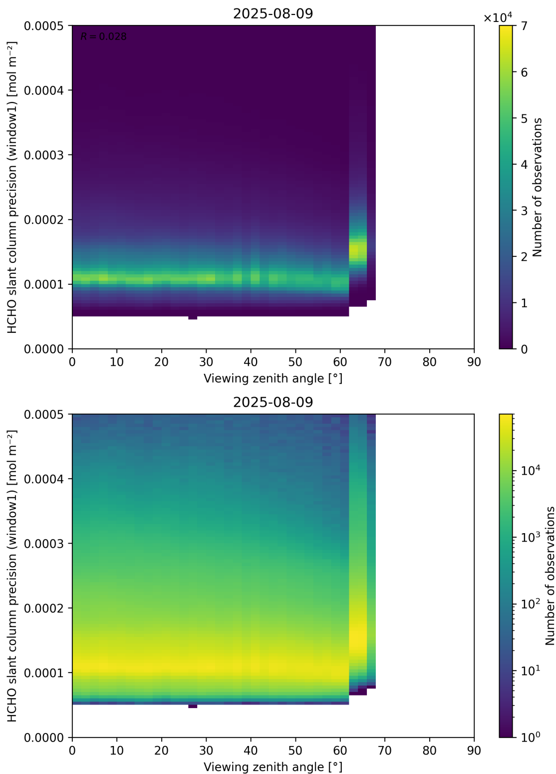
Figure 189: Scatter density plot of “Viewing zenith angle” against “HCHO slant column precision (window1)” for 2025-08-09 to 2025-08-10.
