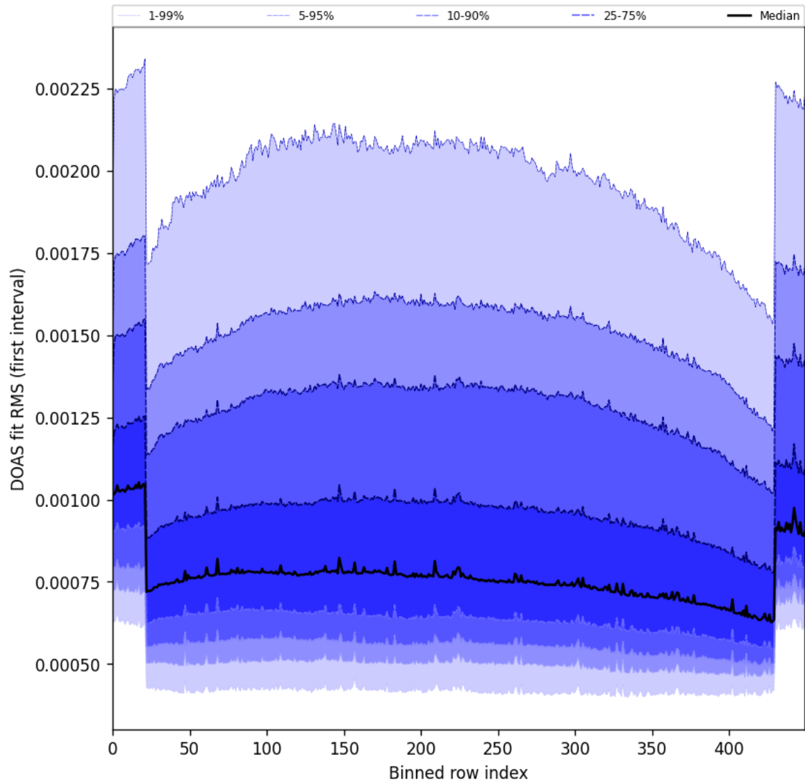
Figure 60: Along track statistics of “DOAS fit RMS (first interval)” for 2025-08-09 to 2025-08-10
