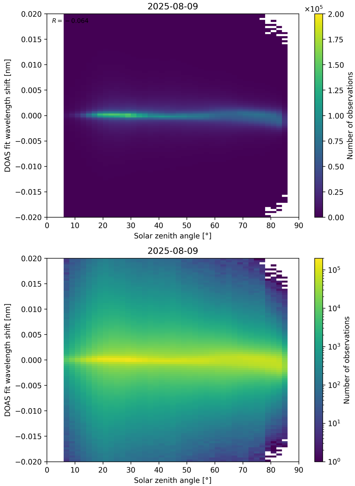
Figure 168: Scatter density plot of “Solar zenith angle” against “DOAS fit wavelength shift” for 2025-08-09 to 2025-08-10.
