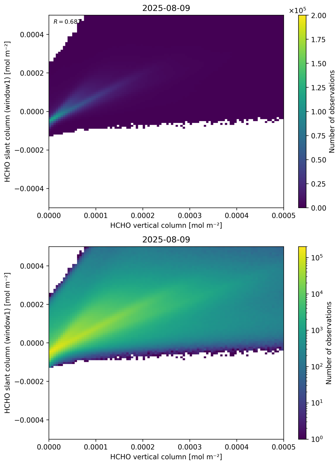
Figure 129: Scatter density plot of “HCHO vertical column” against “HCHO slant column (window1)” for 2025-08-09 to 2025-08-10.
