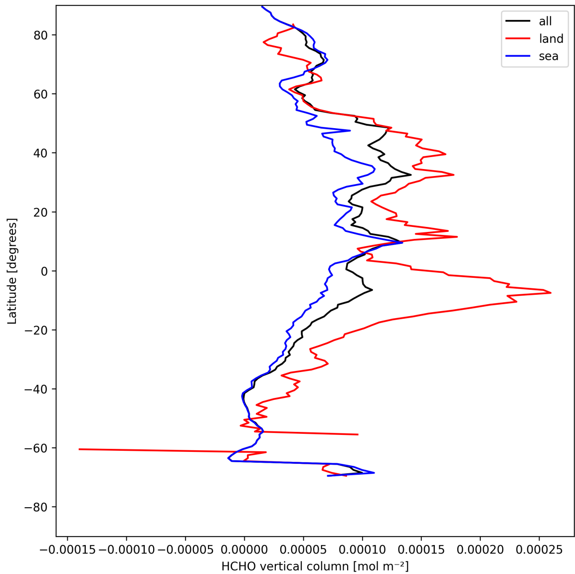
Figure 21: Zonal average of “HCHO vertical column” for 2025-08-09 to 2025-08-10.
