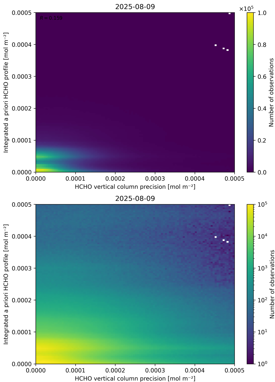
Figure 147: Scatter density plot of “HCHO vertical column precision” against “Integrated a priori HCHO profile” for 2025-08-09 to 2025-08-10.
