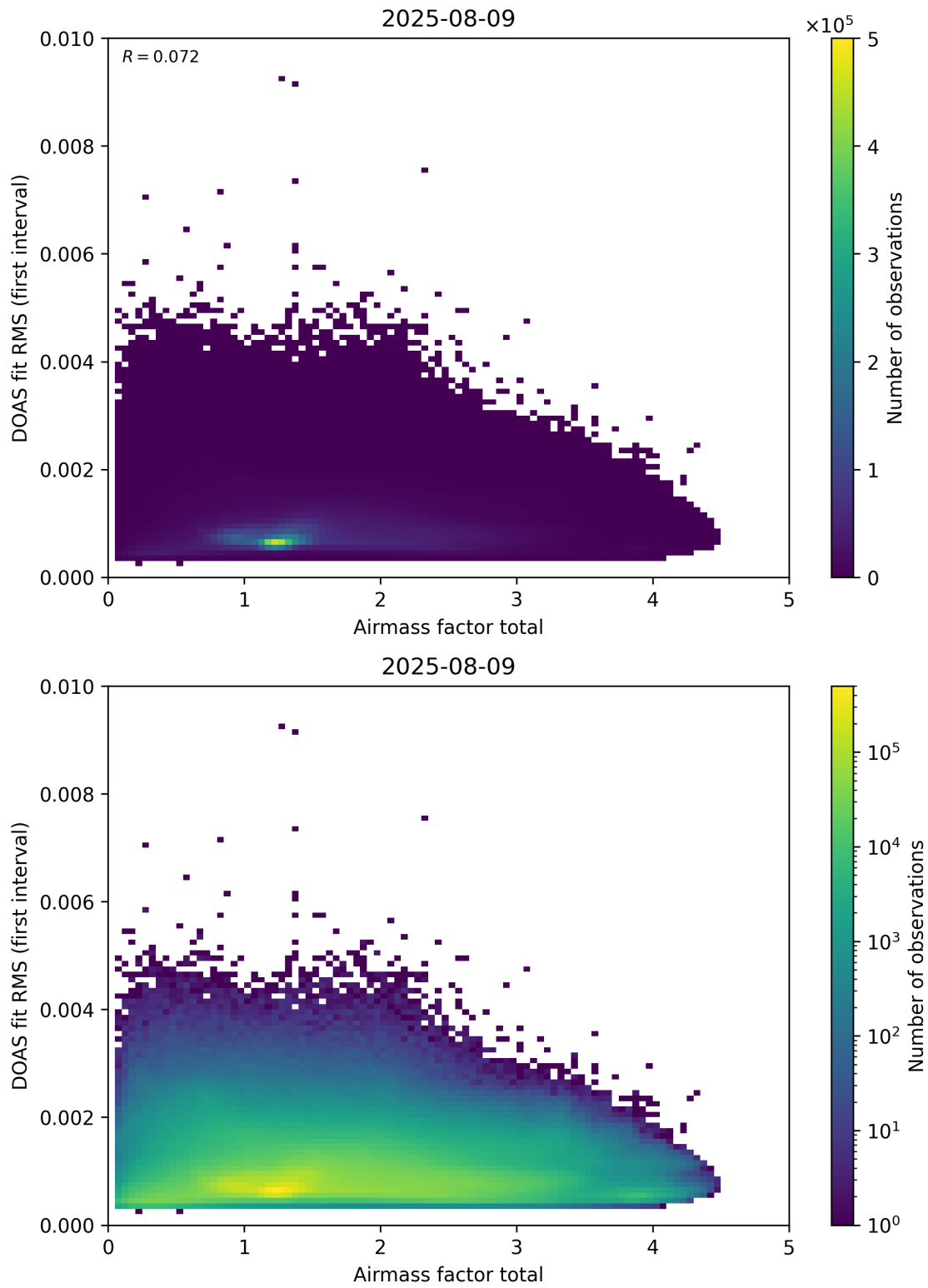
Figure 97: Scatter density plot of “Airmass factor total” against “DOAS fit RMS (first interval)” for 2025-08-09 to 2025-08-10.
