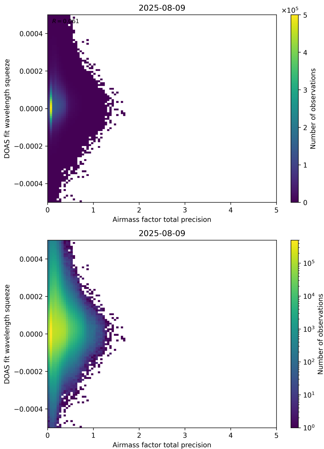
Figure 107: Scatter density plot of “Airmass factor total precision” against “DOAS fit wavelength squeeze” for 2025-08-09 to 2025-08-10.
