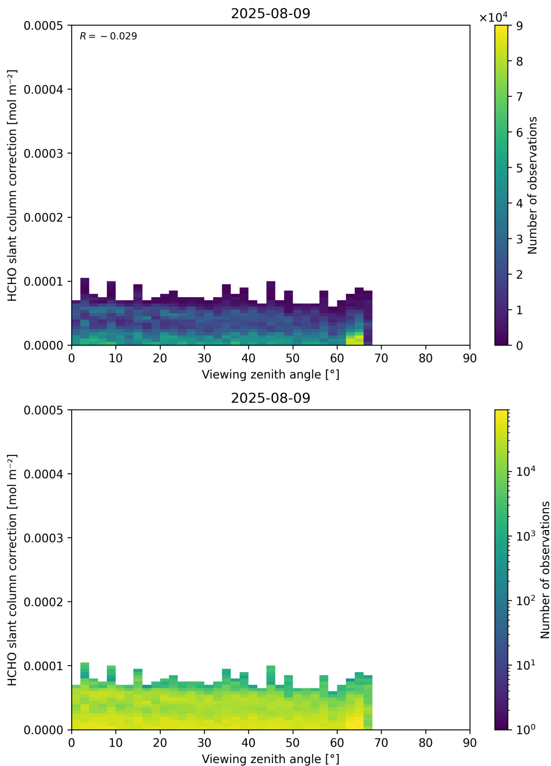
Figure 187: Scatter density plot of “Viewing zenith angle” against “HCHO slant column correction” for 2025-08-09 to 2025-08-10.
