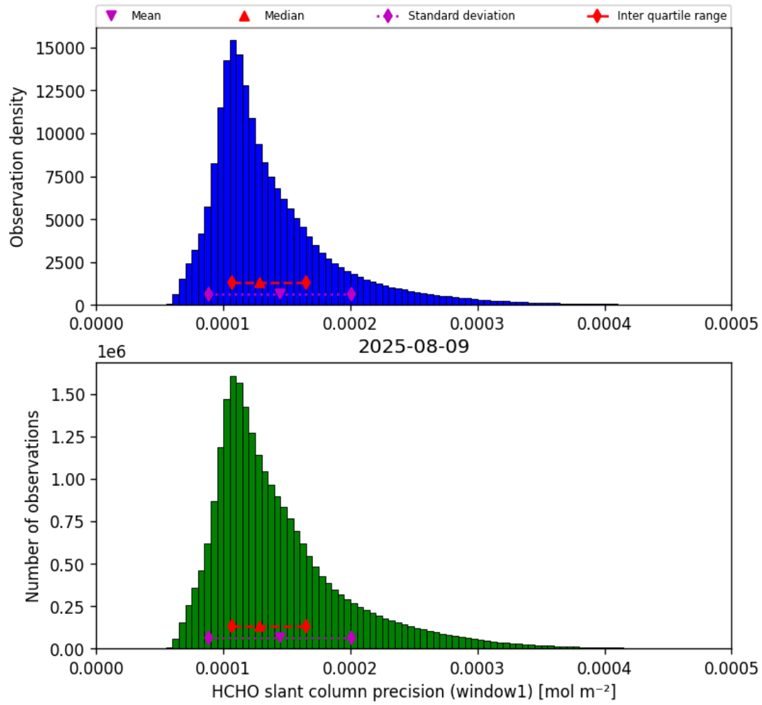
Figure 39: Histogram of “HCHO slant column precision (window1)” for 2025-08-09 to 2025-08-10
