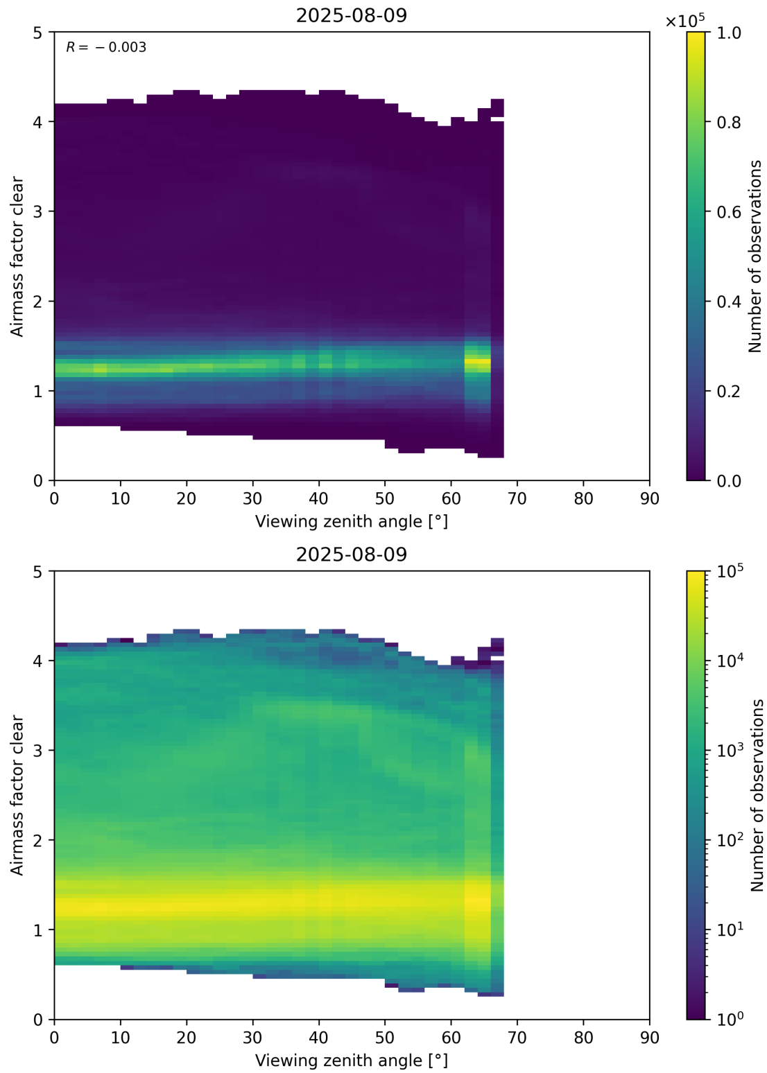
Figure 185: Scatter density plot of “Viewing zenith angle” against “Airmass factor clear” for 2025-08-09 to 2025-08-10.
