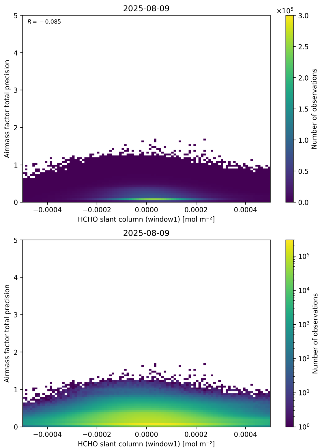
Figure 86: Scatter density plot of “HCHO slant column (window1)” against “Airmass factor total precision” for 2025-08-09 to 2025-08-10.
