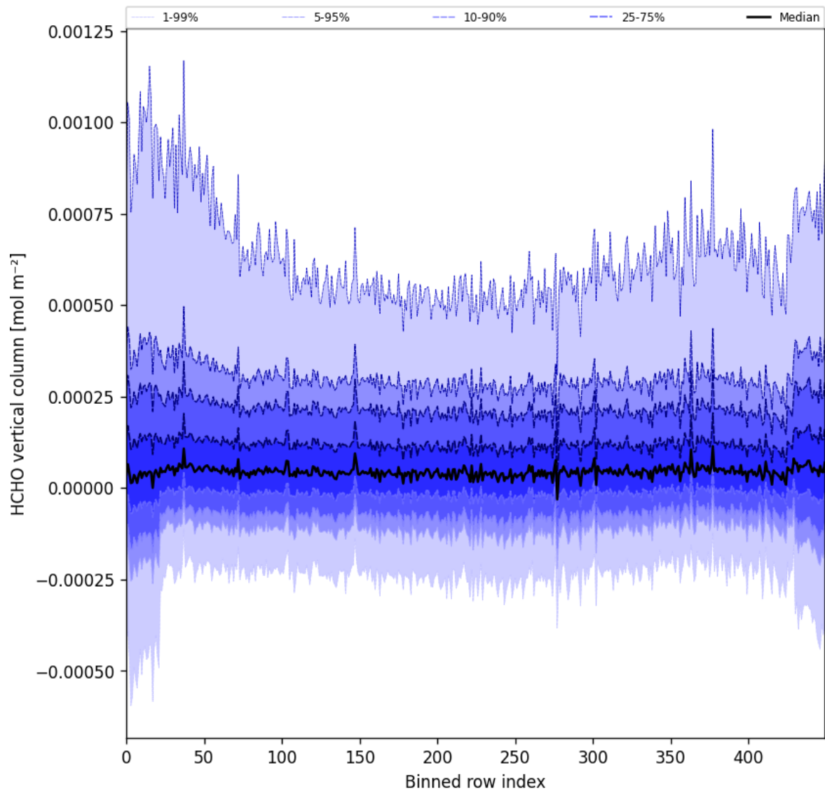
Figure 49: Along track statistics of “HCHO vertical column” for 2025-08-09 to 2025-08-10
