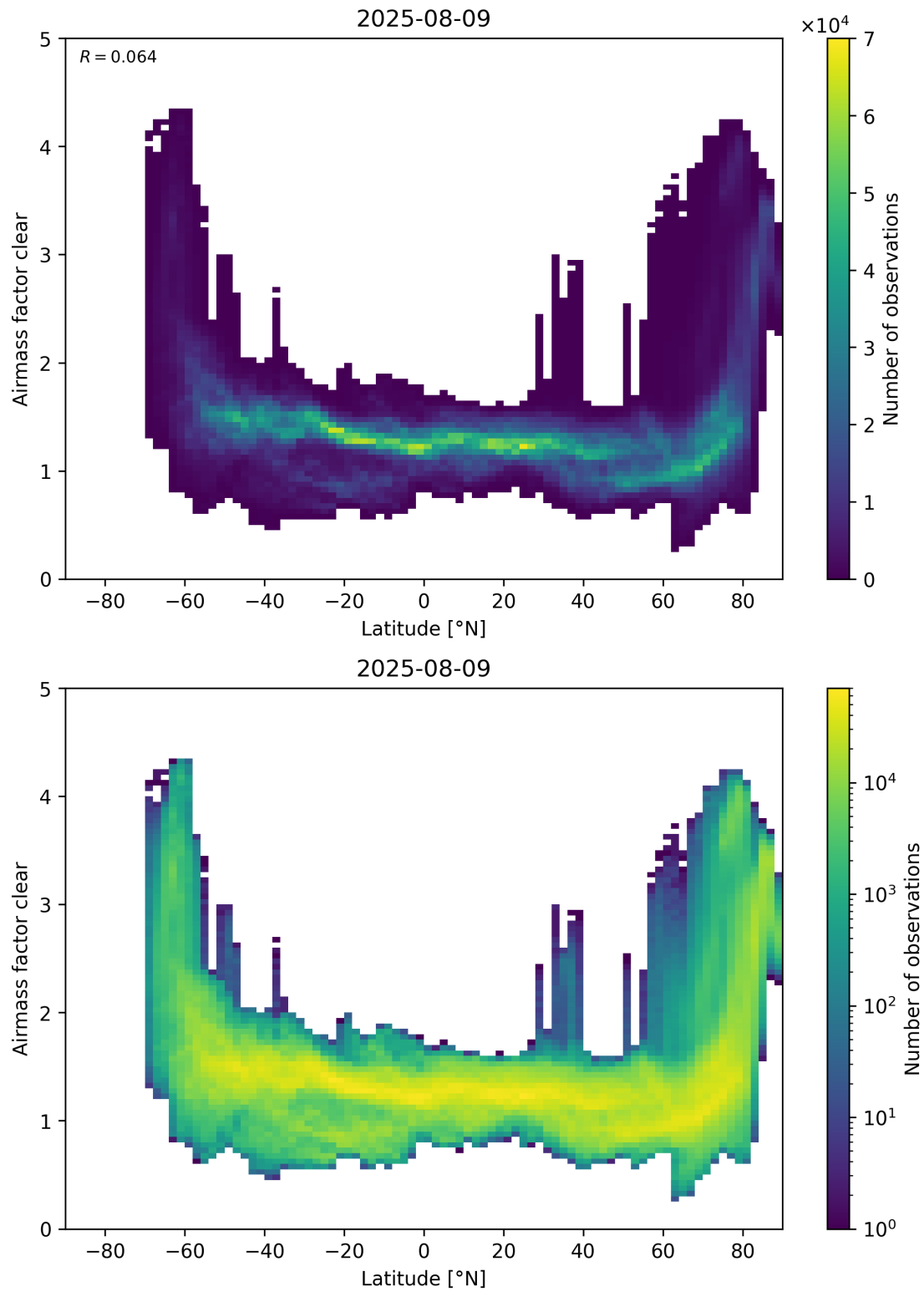
Figure 156: Scatter density plot of “Latitude” against “Airmass factor clear” for 2025-08-09 to 2025-08-10.
