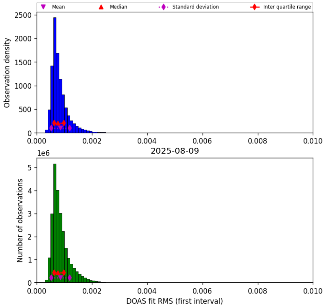
Figure 46: Histogram of “DOAS fit RMS (first interval)” for 2025-08-09 to 2025-08-10
