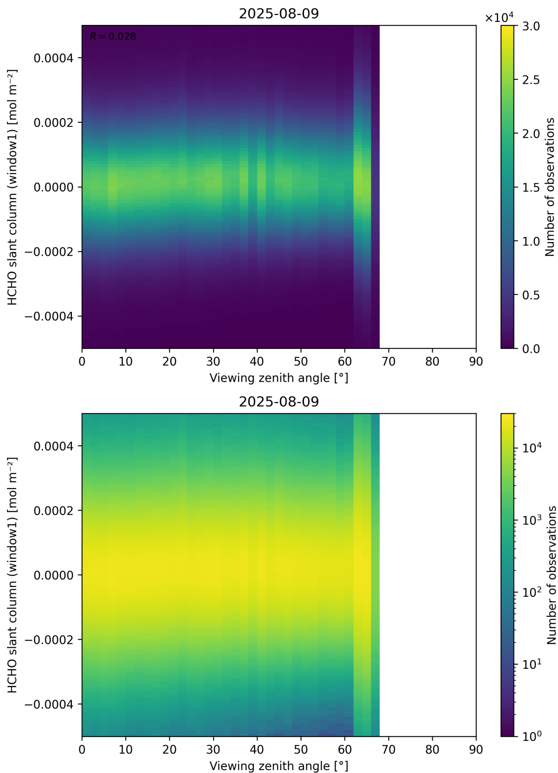
Figure 188: Scatter density plot of “Viewing zenith angle” against “HCHO slant column (window1)” for 2025-08-09 to 2025-08-10.
