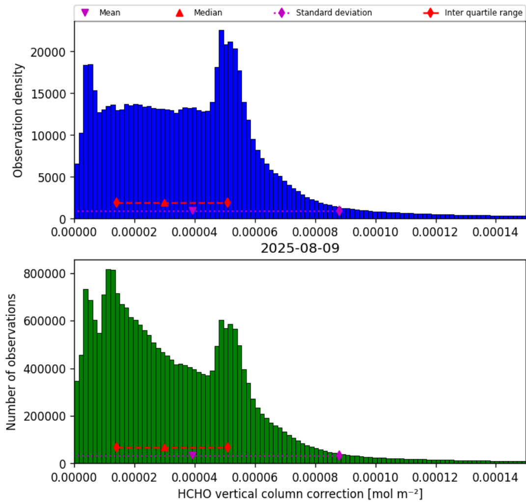
Figure 37: Histogram of “HCHO vertical column correction” for 2025-08-09 to 2025-08-10
