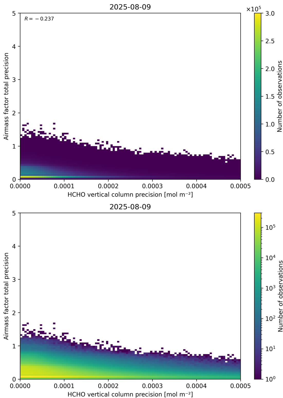
Figure 145: Scatter density plot of “HCHO vertical column precision” against “Airmass factor total precision” for 2025-08-09 to 2025-08-10.
