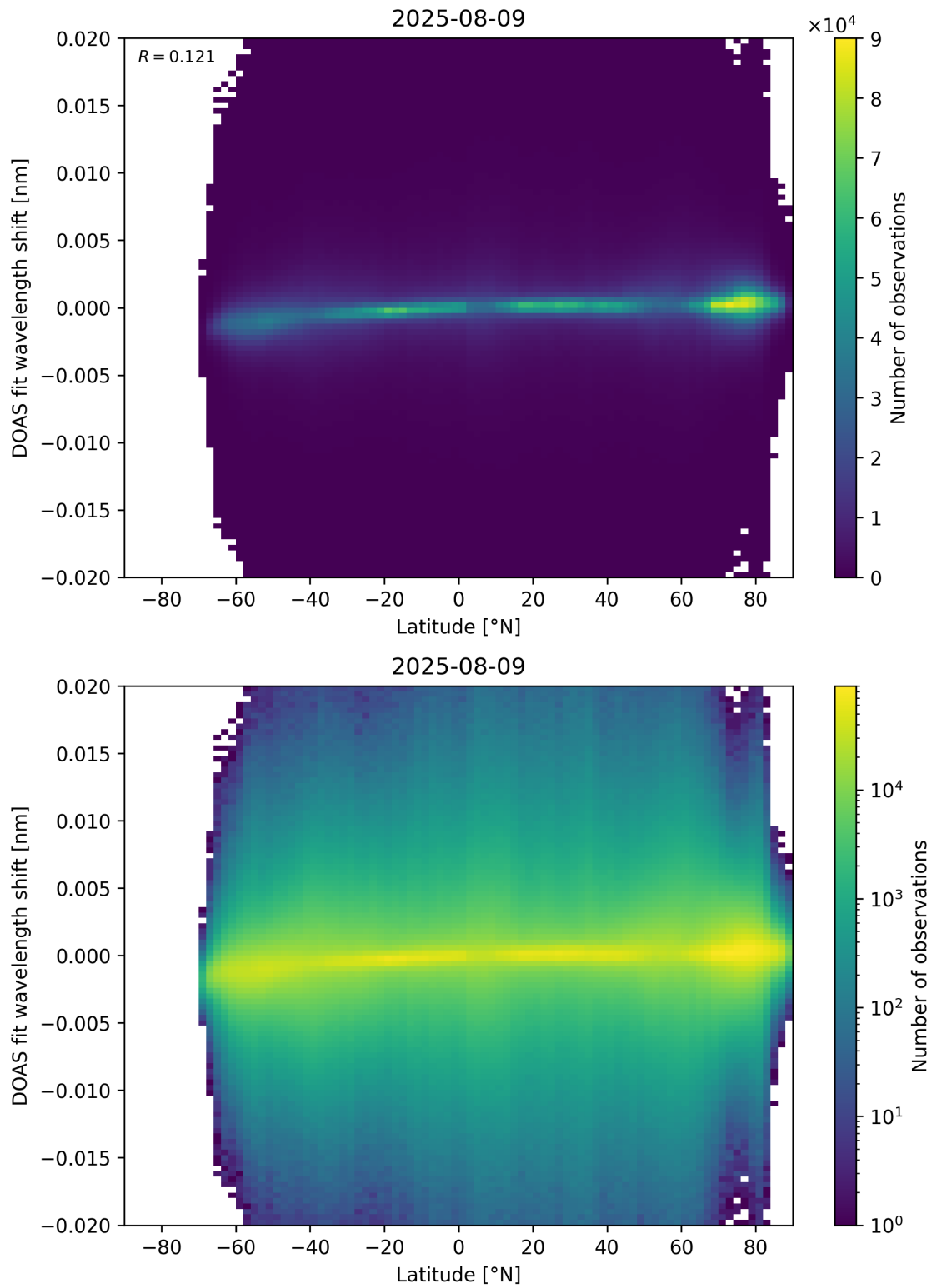
Figure 154: Scatter density plot of “Latitude” against “DOAS fit wavelength shift” for 2025-08-09 to 2025-08-10.
