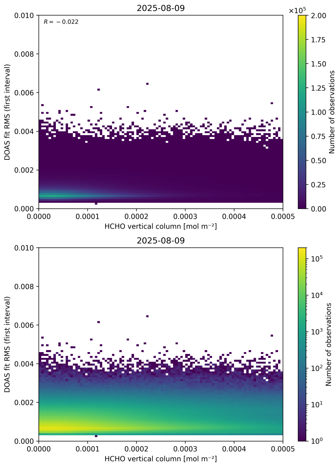
Figure 123: Scatter density plot of “HCHO vertical column” against “DOAS fit RMS (first interval)” for 2025-08-09 to 2025-08-10.
