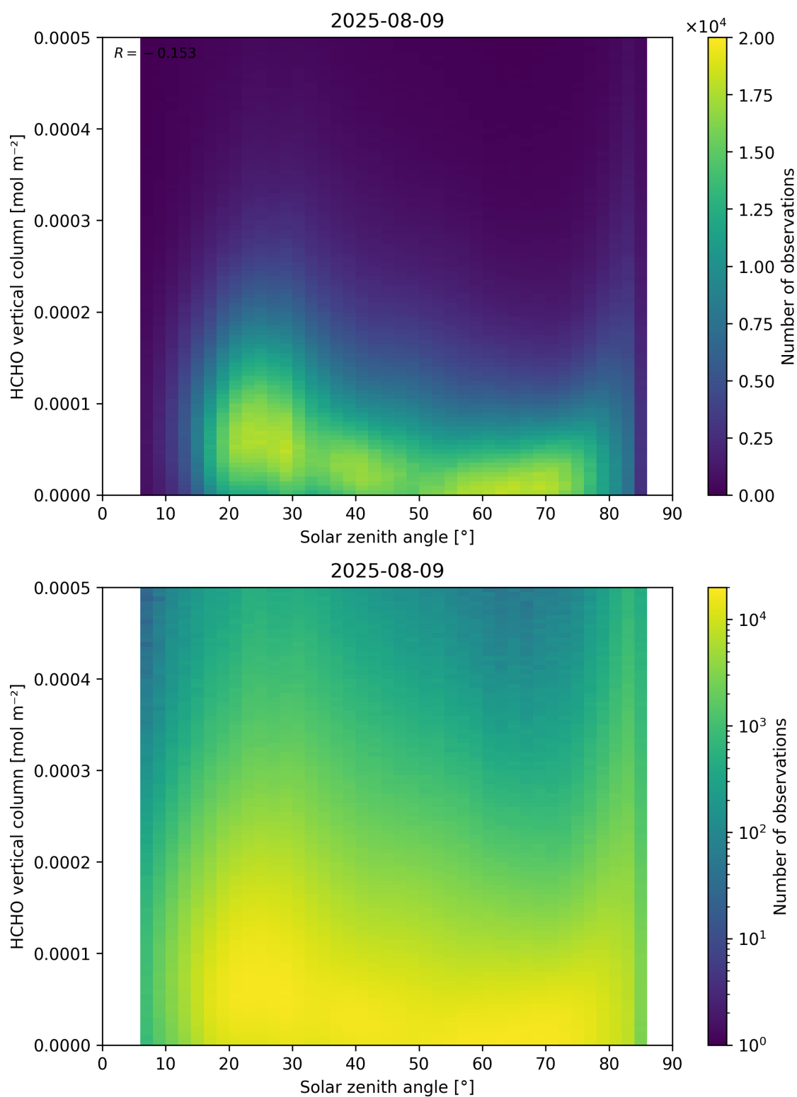
Figure 177: Scatter density plot of “Solar zenith angle” against “HCHO vertical column” for 2025-08-09 to 2025-08-10.
