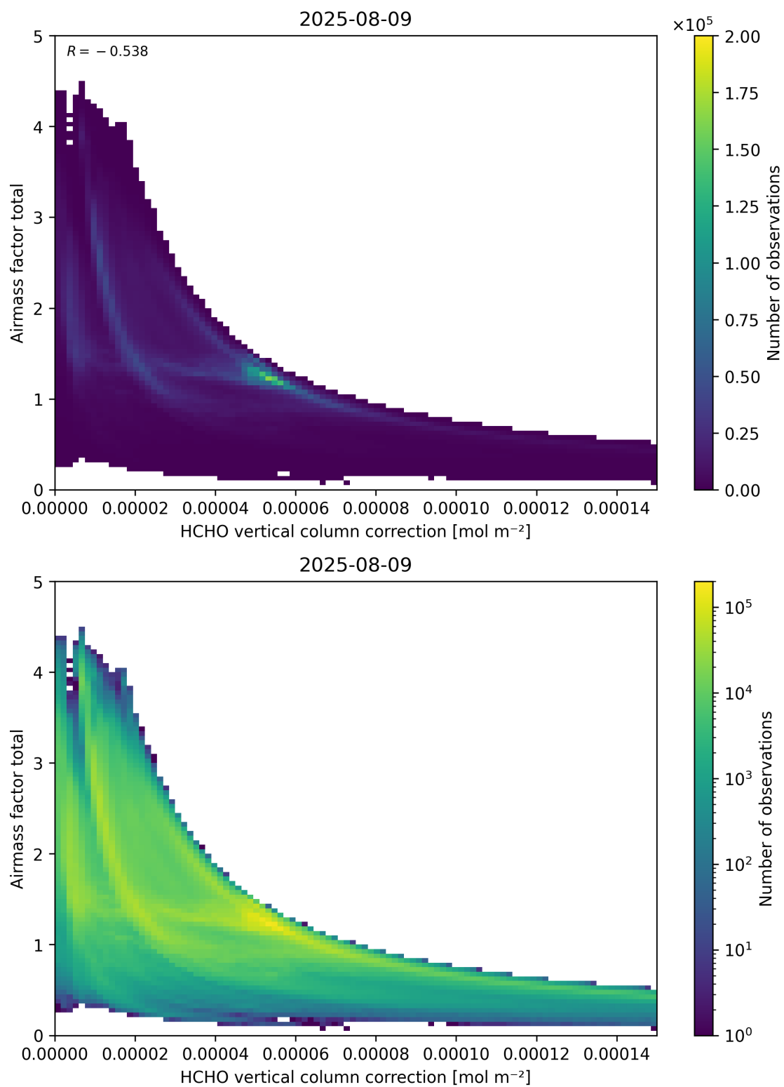
Figure 120: Scatter density plot of “HCHO vertical column correction” against “Airmass factor total” for 2025-08-09 to 2025-08-10.
