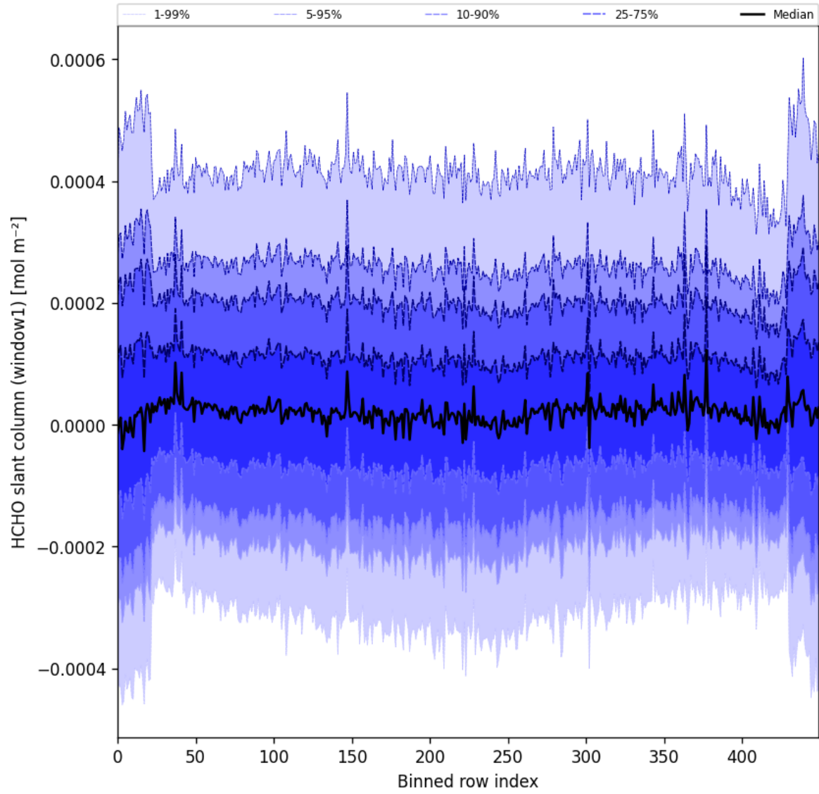
Figure 52: Along track statistics of “HCHO slant column (window1)” for 2025-08-09 to 2025-08-10
