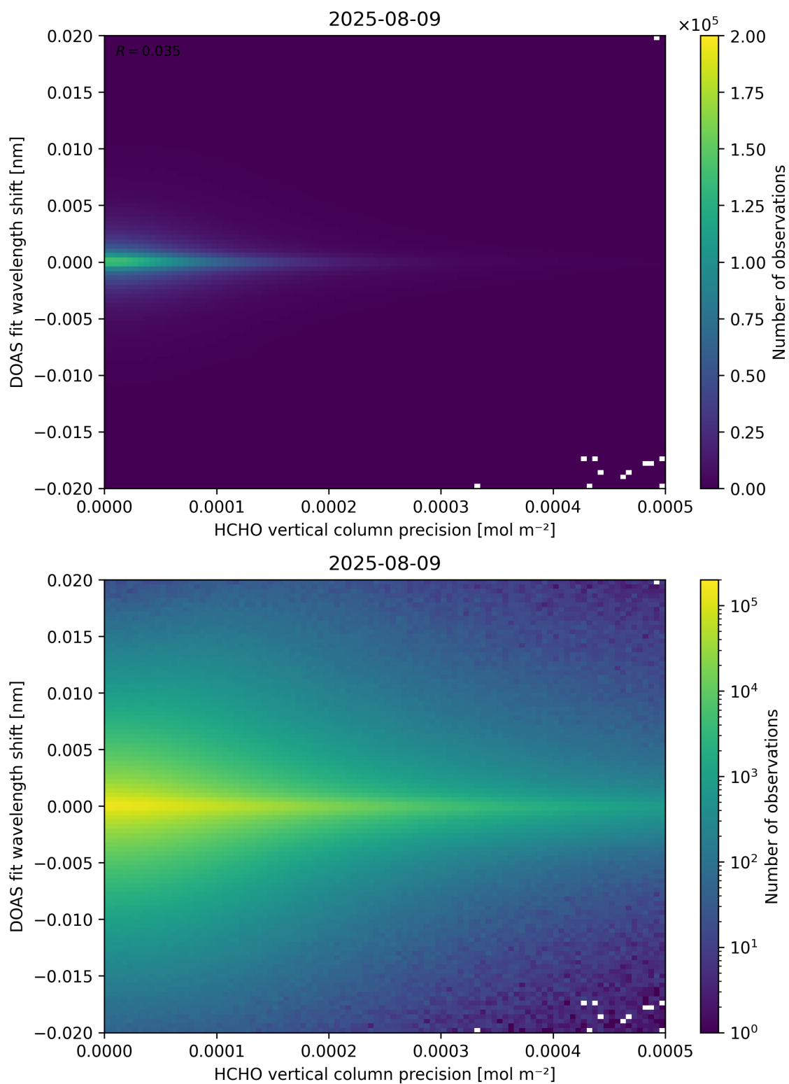
Figure 137: Scatter density plot of “HCHO vertical column precision” against “DOAS fit wavelength shift” for 2025-08-09 to 2025-08-10.
