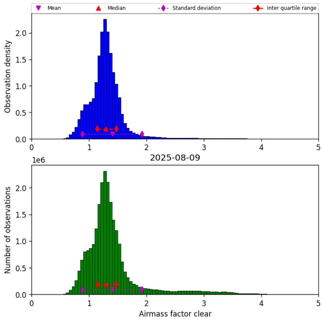
Figure 42: Histogram of “Airmass factor clear” for 2025-08-09 to 2025-08-10
