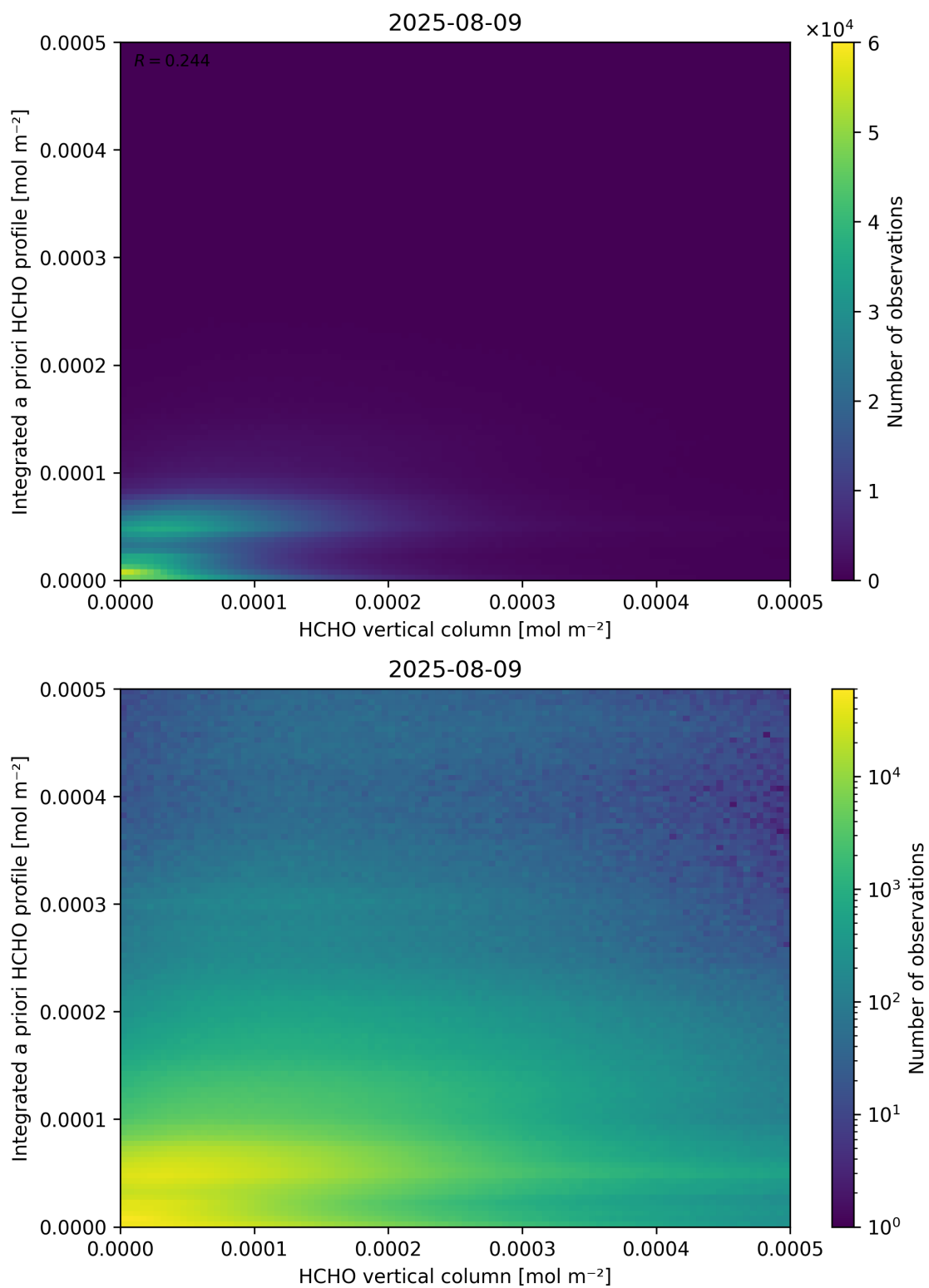
Figure 135: Scatter density plot of “HCHO vertical column” against “Integrated a priori HCHO profile” for 2025-08-09 to 2025-08-10.
