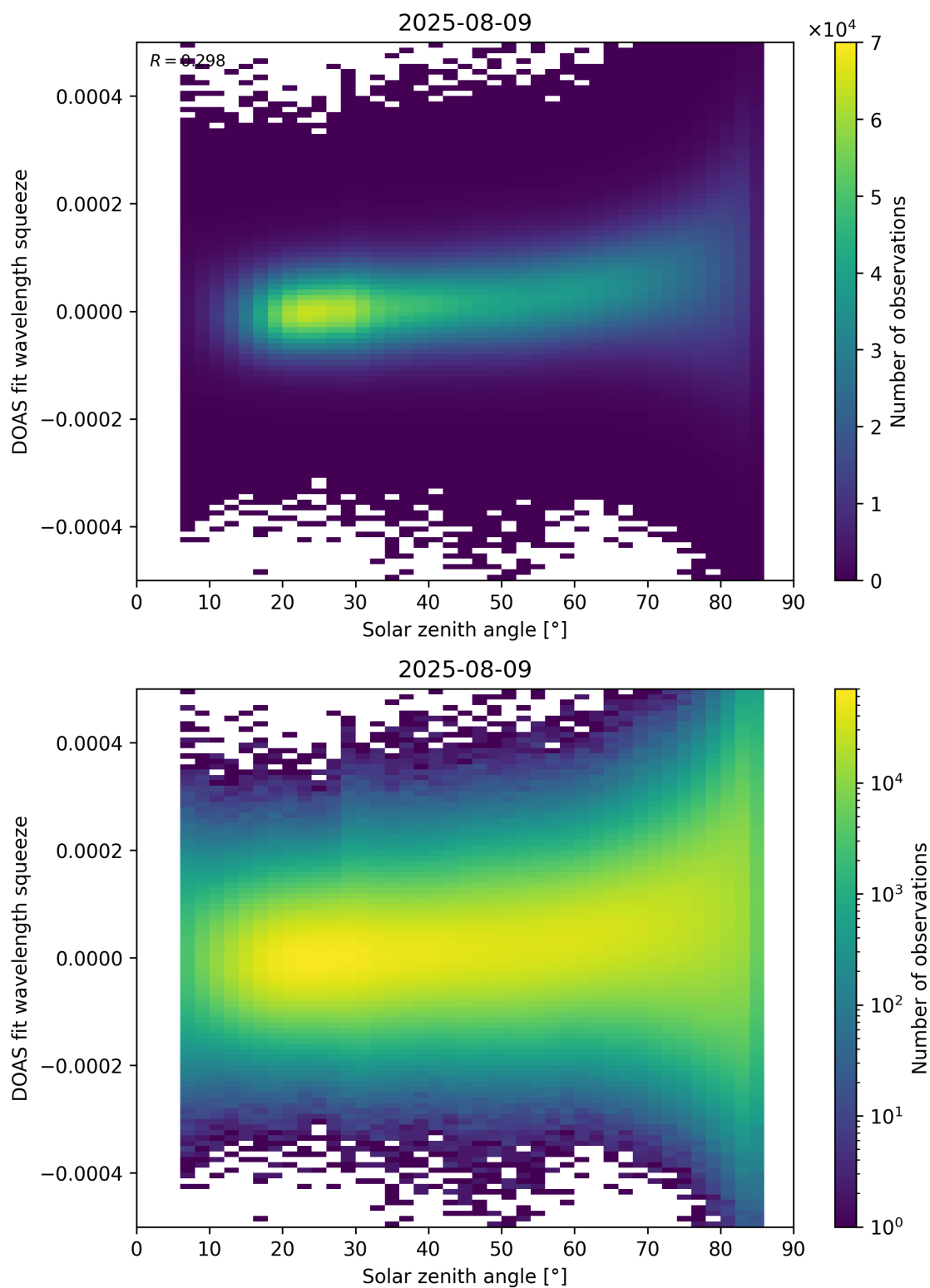
Figure 169: Scatter density plot of “Solar zenith angle” against “DOAS fit wavelength squeeze” for 2025-08-09 to 2025-08-10.
