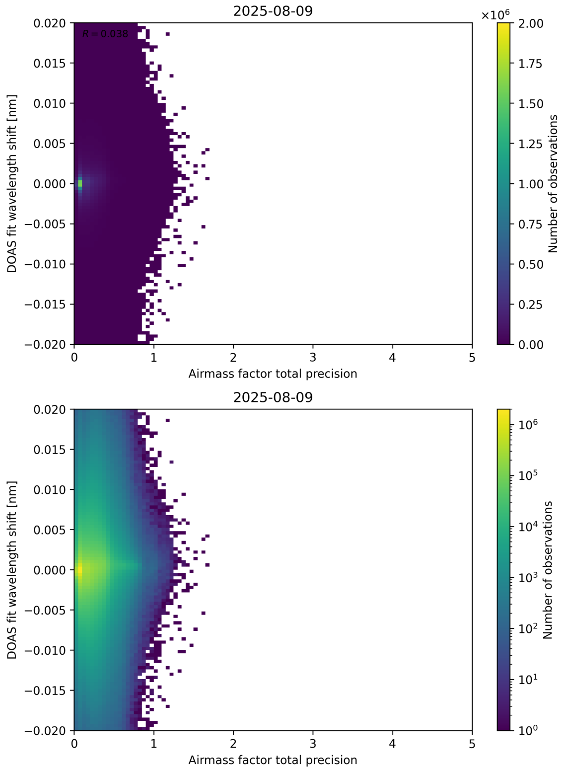
Figure 106: Scatter density plot of “Airmass factor total precision” against “DOAS fit wavelength shift” for 2025-08-09 to 2025-08-10.
