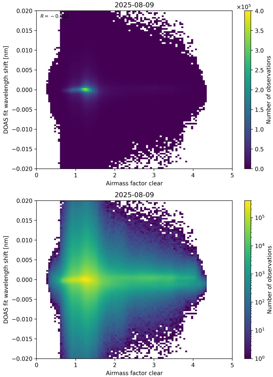
Figure 72: Scatter density plot of “Airmass factor clear” against “DOAS fit wavelength shift” for 2025-08-09 to 2025-08-10.
