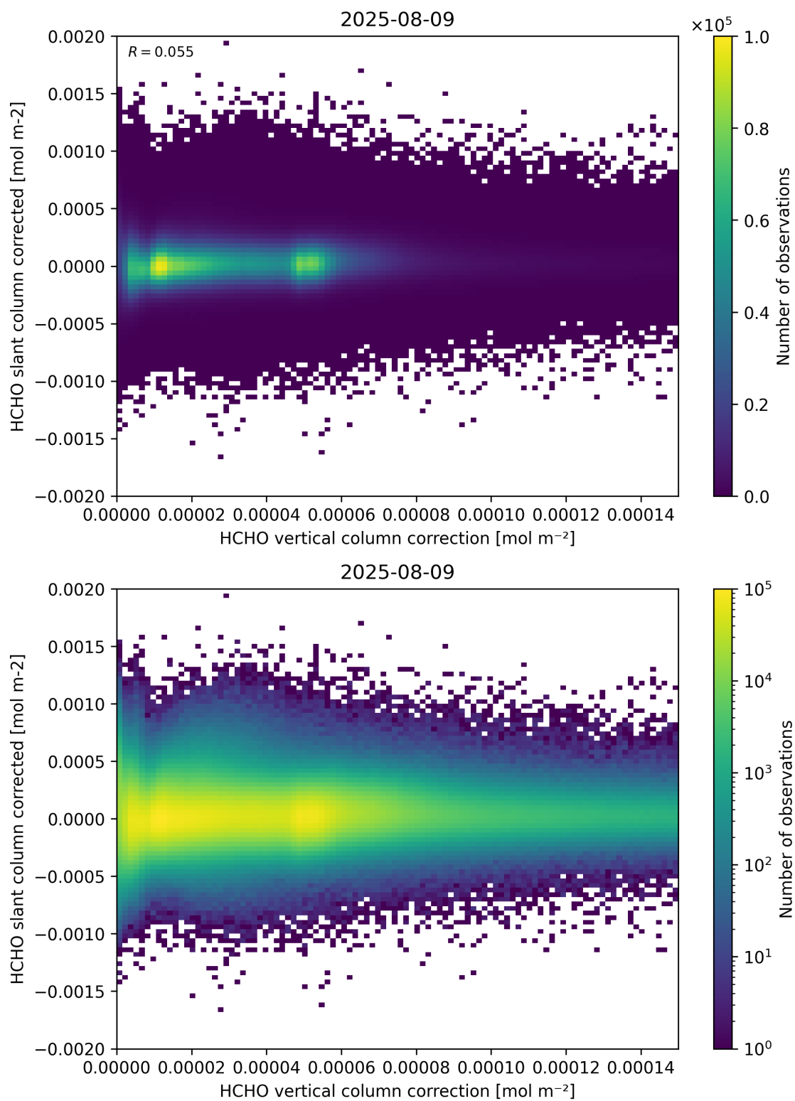
Figure 116: Scatter density plot of “HCHO vertical column correction” against “HCHO slant column corrected” for 2025-08-09 to 2025-08-10.
