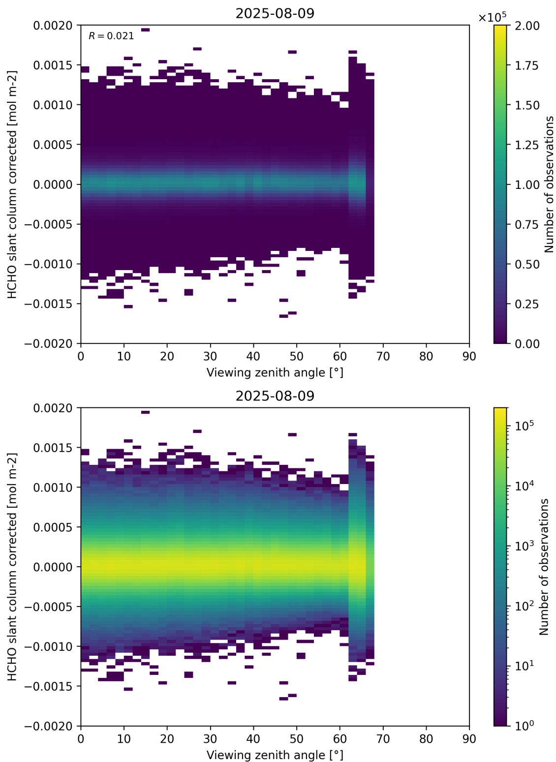
Figure 186: Scatter density plot of “Viewing zenith angle” against “HCHO slant column corrected” for 2025-08-09 to 2025-08-10.
