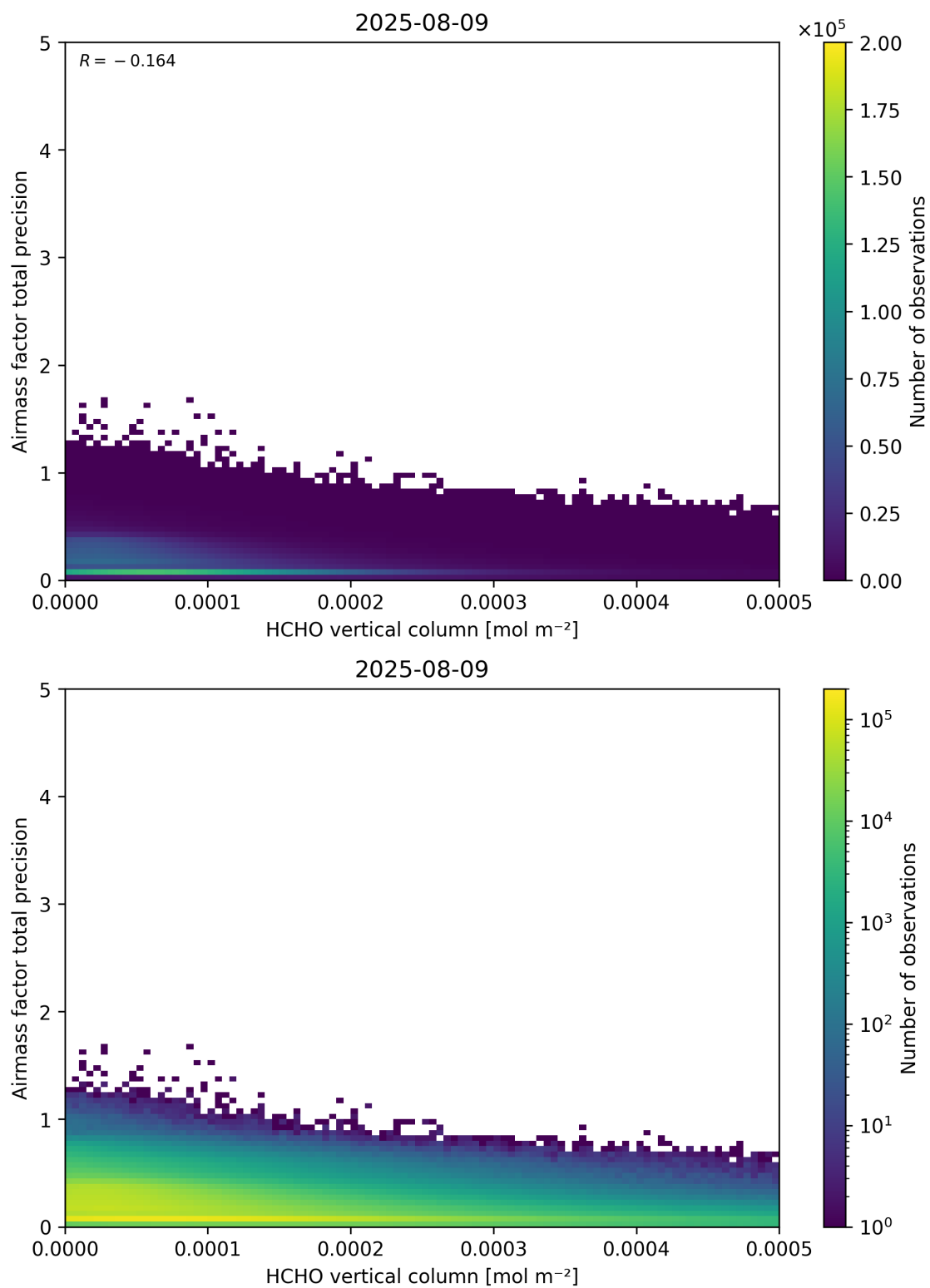
Figure 132: Scatter density plot of “HCHO vertical column” against “Airmass factor total precision” for 2025-08-09 to 2025-08-10.
