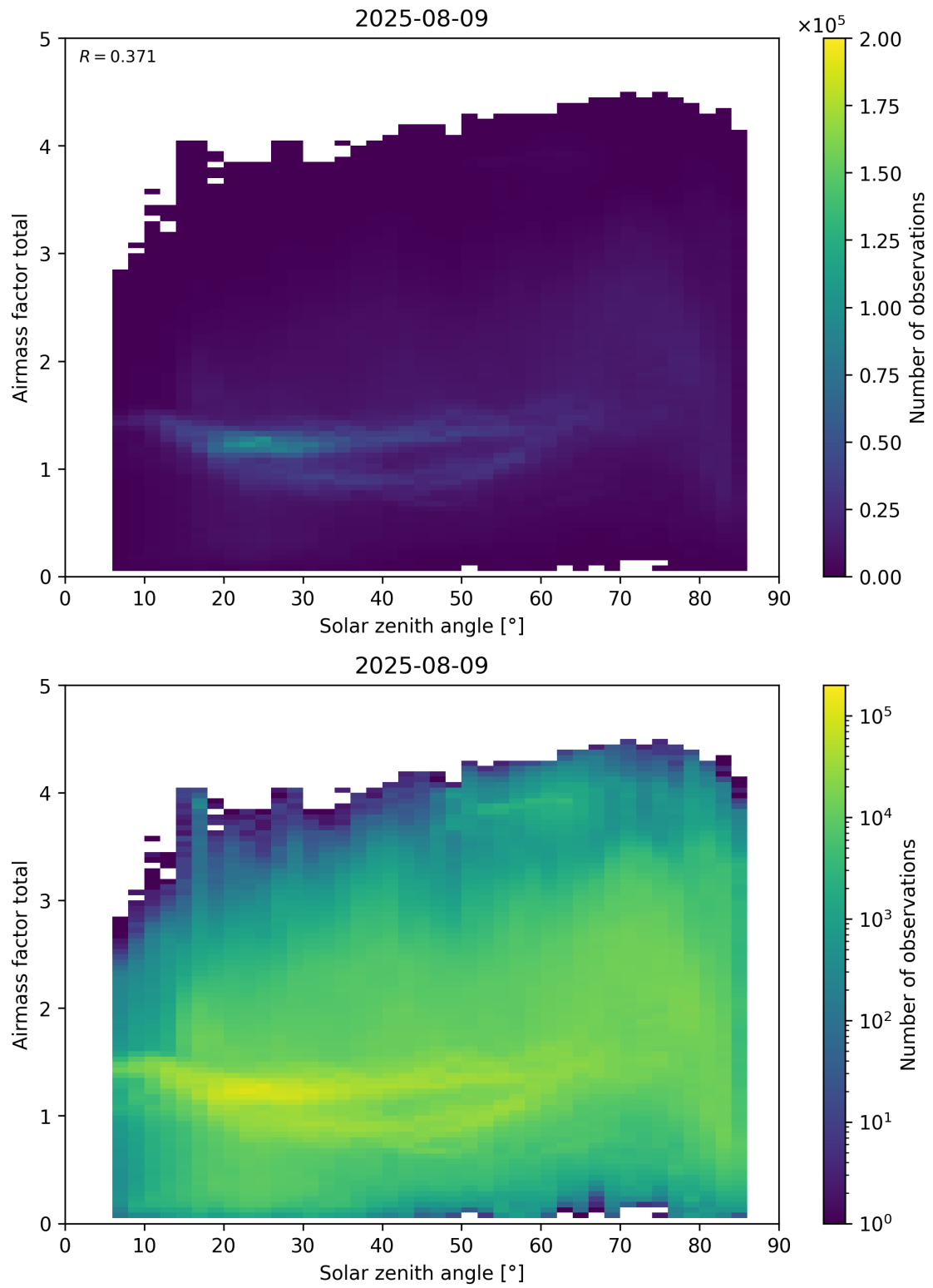
Figure 175: Scatter density plot of “Solar zenith angle” against “Airmass factor total” for 2025-08-09 to 2025-08-10.
