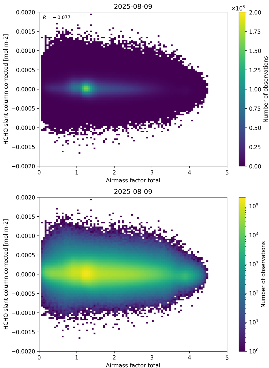
Figure 101: Scatter density plot of “Airmass factor total” against “HCHO slant column corrected” for 2025-08-09 to 2025-08-10.
