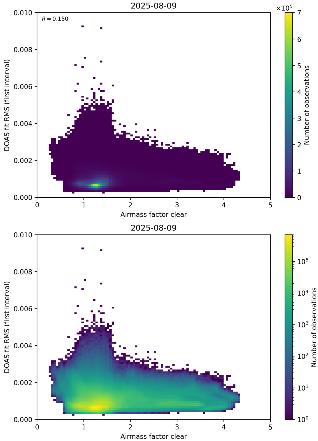
Figure 71: Scatter density plot of “Airmass factor clear” against “DOAS fit RMS (first interval)” for 2025-08-09 to 2025-08-10.
