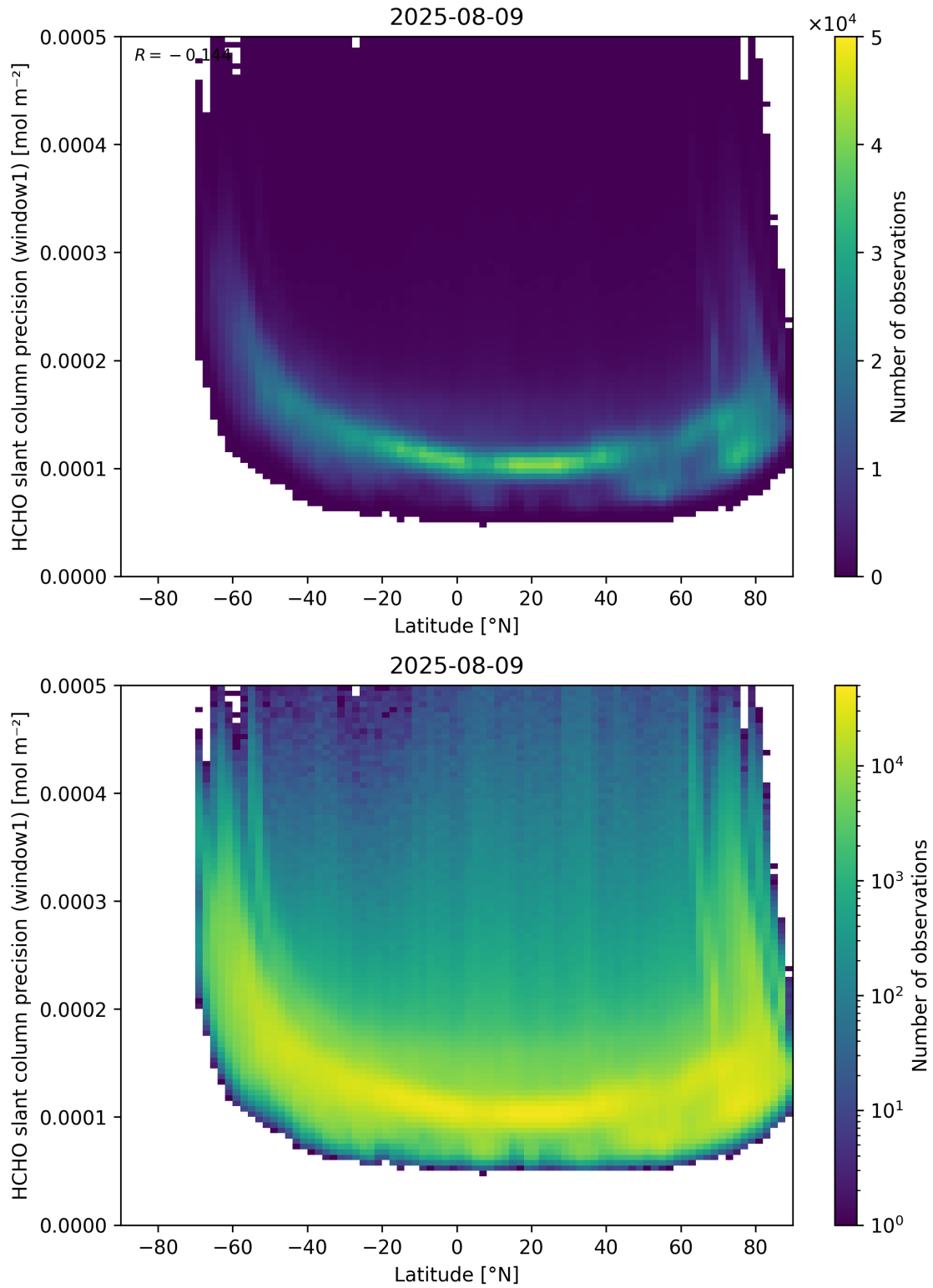
Figure 160: Scatter density plot of “Latitude” against “HCHO slant column precision (window1)” for 2025-08-09 to 2025-08-10.
