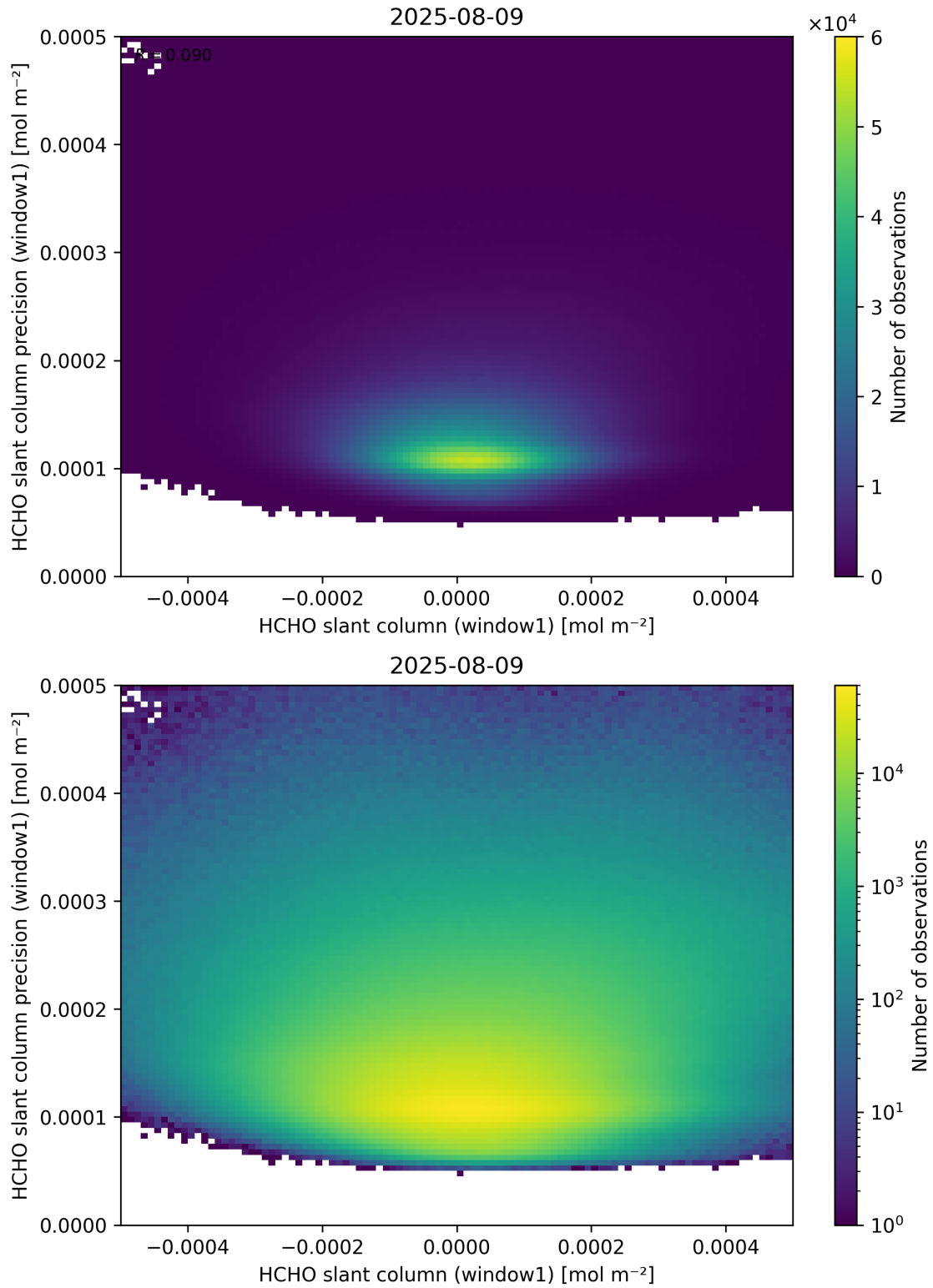
Figure 84: Scatter density plot of “HCHO slant column (window1)” against “HCHO slant column precision (window1)” for 2025-08-09 to 2025-08-10.
