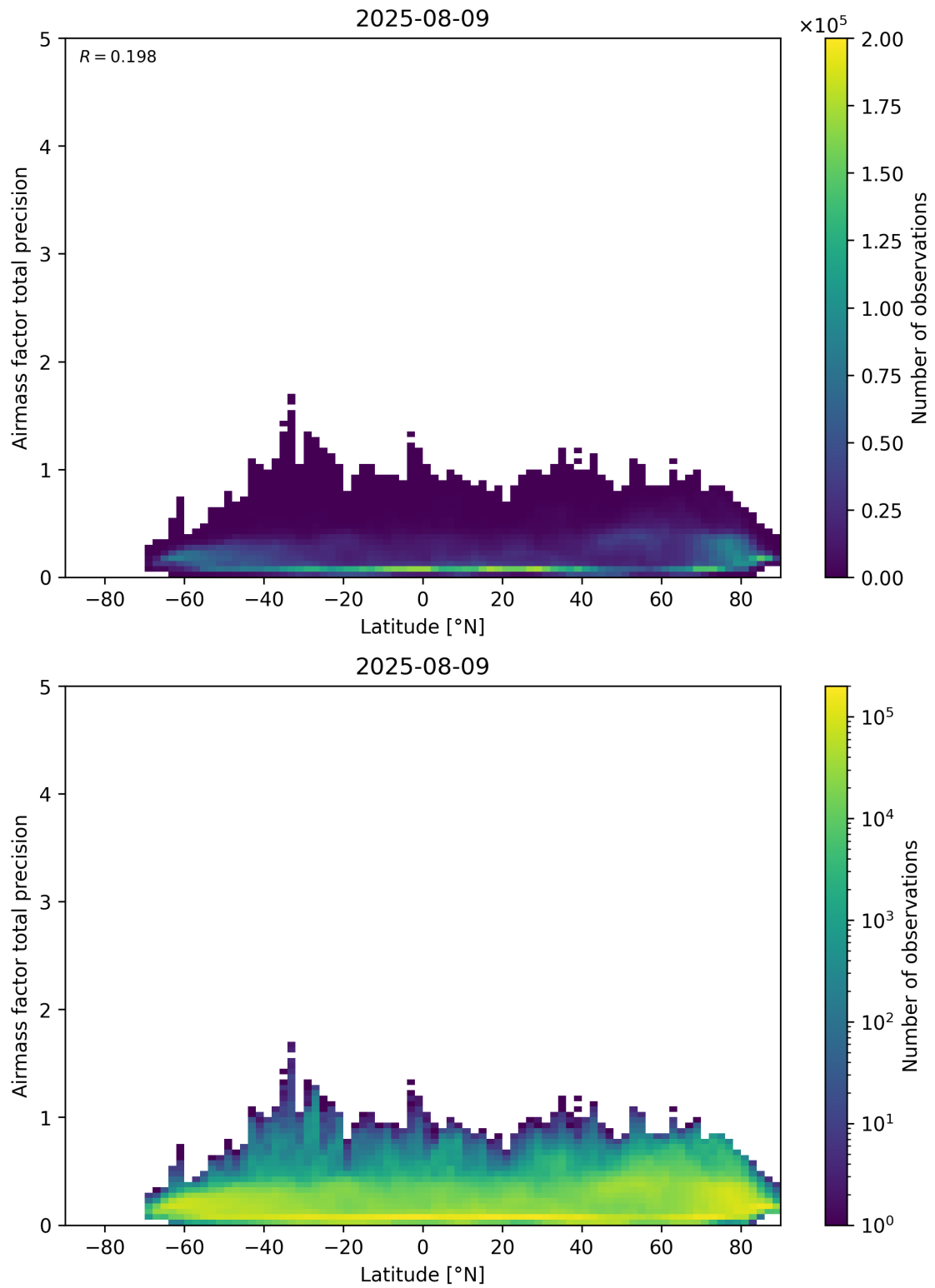
Figure 162: Scatter density plot of “Latitude” against “Airmass factor total precision” for 2025-08-09 to 2025-08-10.
