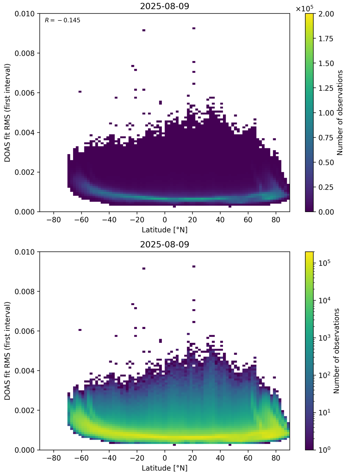
Figure 153: Scatter density plot of “Latitude” against “DOAS fit RMS (first interval)” for 2025-08-09 to 2025-08-10.
