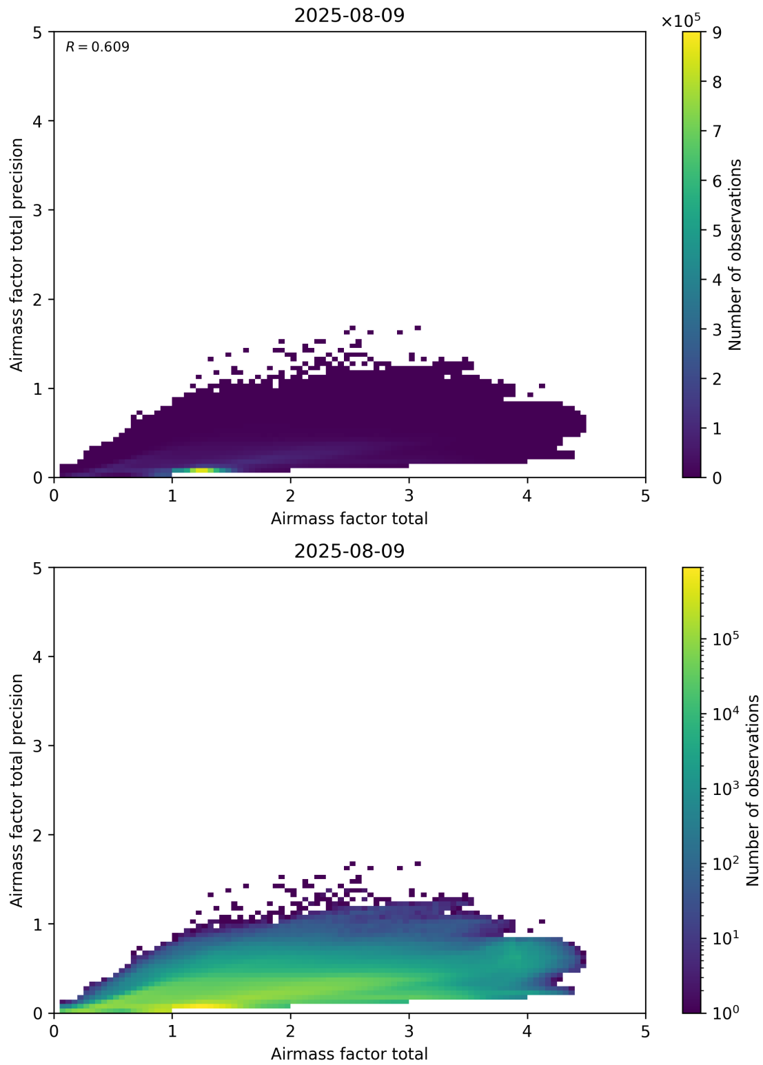
Figure 103: Scatter density plot of “Airmass factor total” against “Airmass factor total precision” for 2025-08-09 to 2025-08-10.
