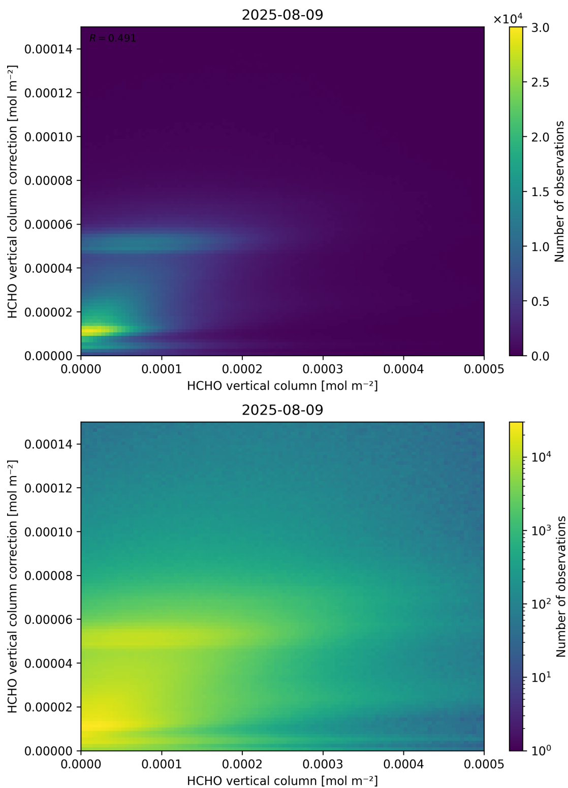
Figure 133: Scatter density plot of “HCHO vertical column” against “HCHO vertical column correction” for 2025-08-09 to 2025-08-10.
