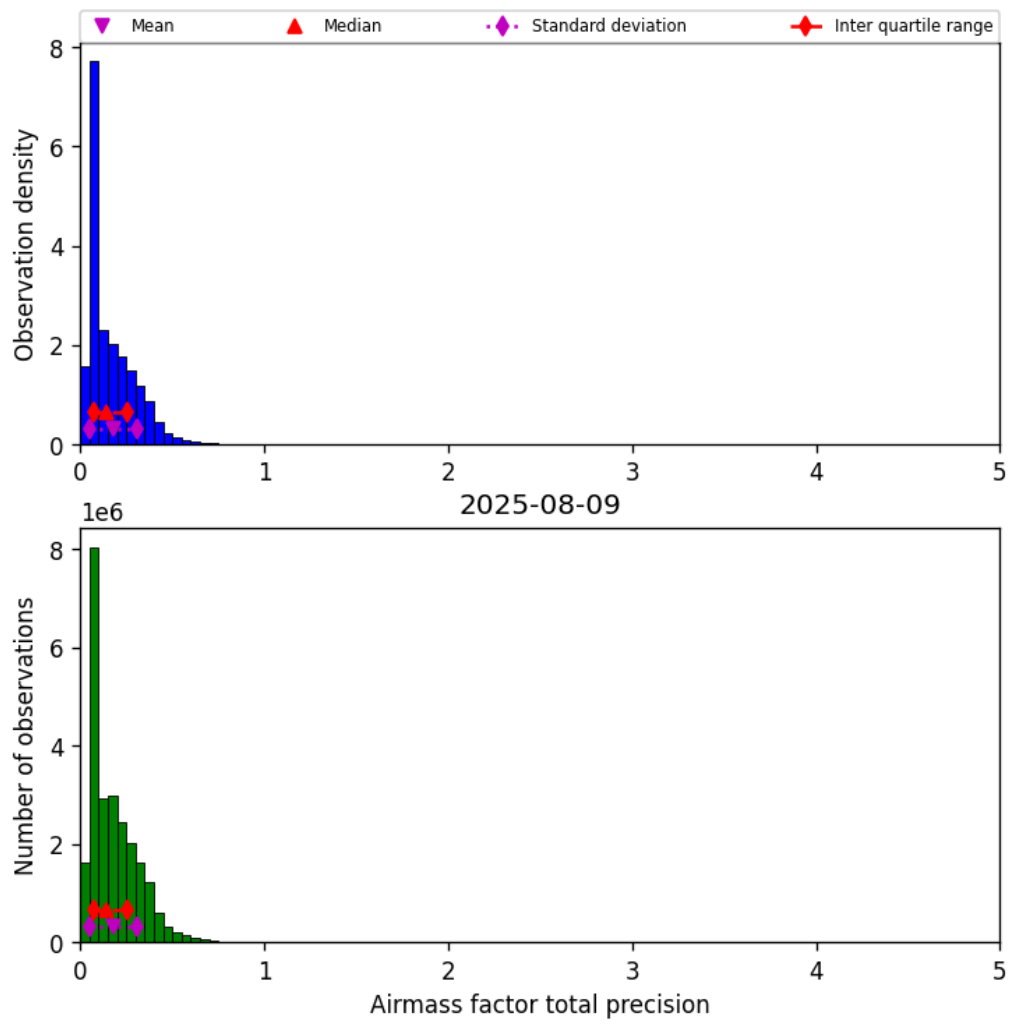
Figure 41: Histogram of “Airmass factor total precision” for 2025-08-09 to 2025-08-10
