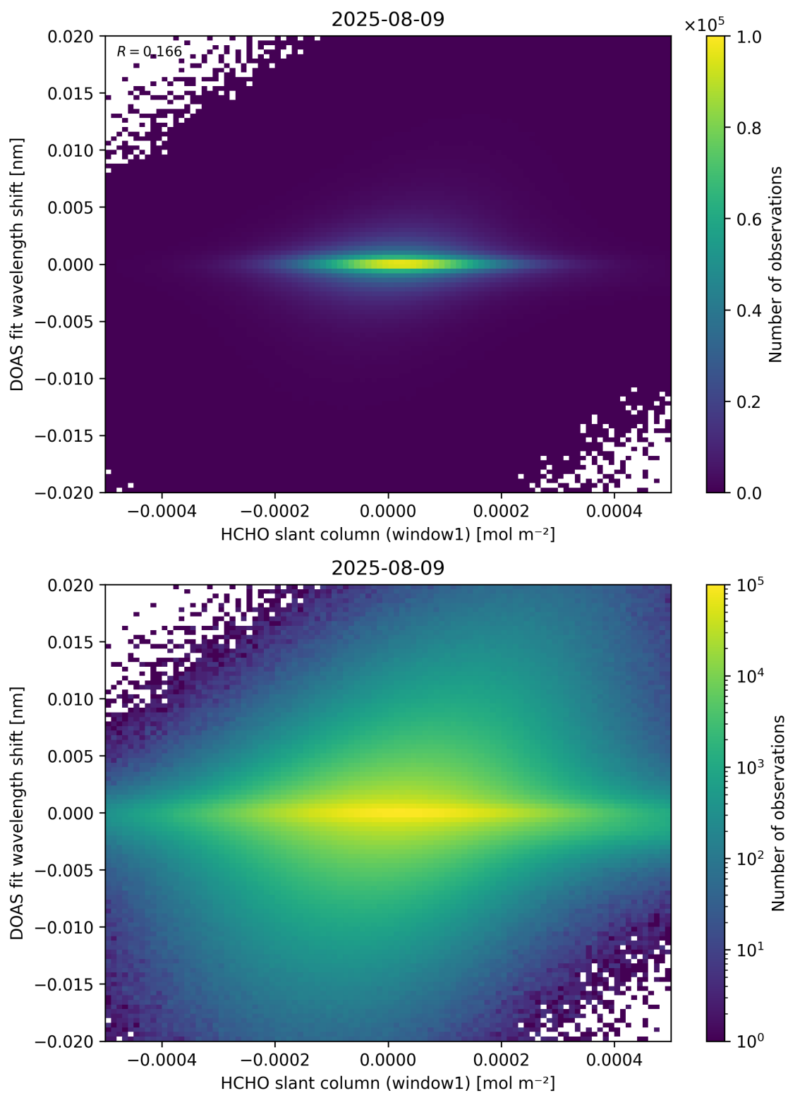
Figure 79: Scatter density plot of “HCHO slant column (window1)” against “DOAS fit wavelength shift” for 2025-08-09 to 2025-08-10.
