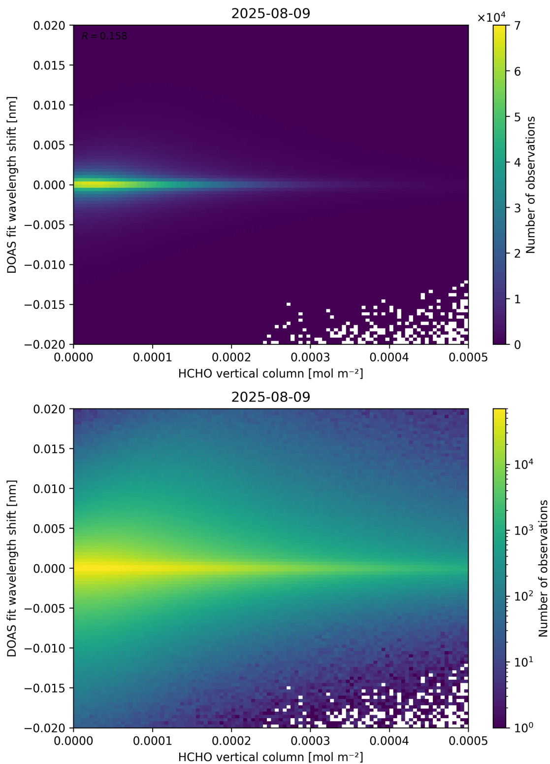
Figure 124: Scatter density plot of “HCHO vertical column” against “DOAS fit wavelength shift” for 2025-08-09 to 2025-08-10.
