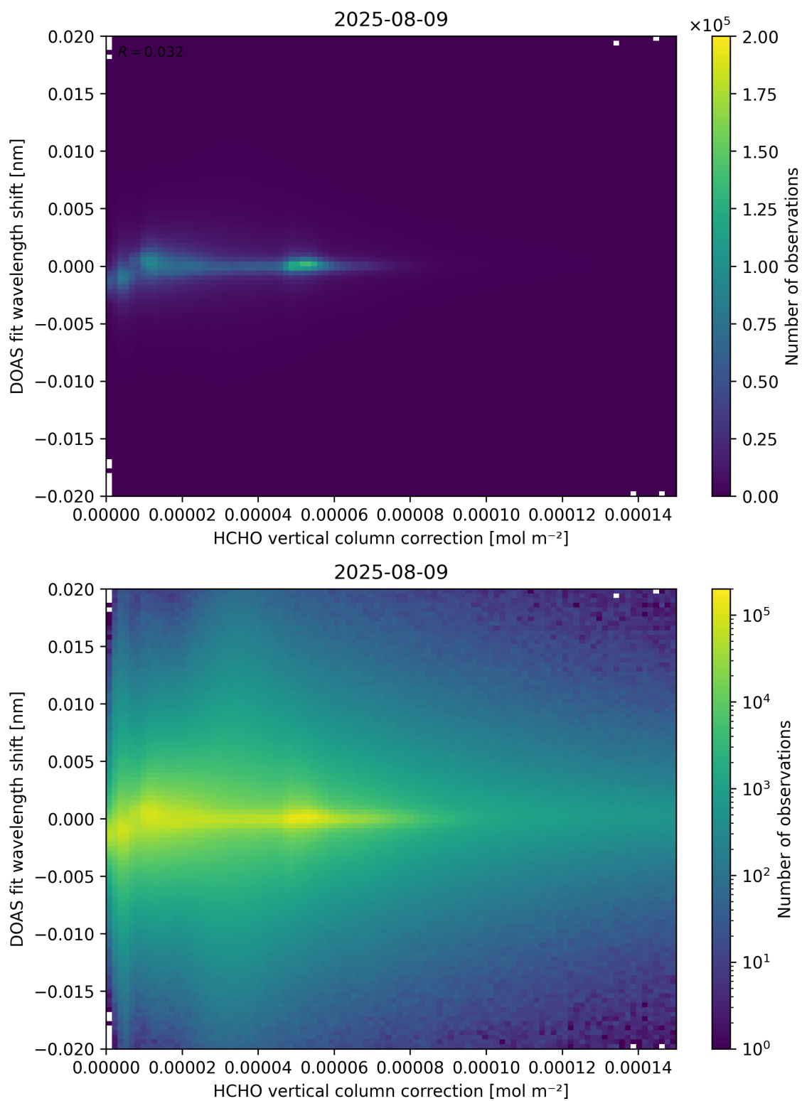
Figure 113: Scatter density plot of “HCHO vertical column correction” against “DOAS fit wavelength shift” for 2025-08-09 to 2025-08-10.
