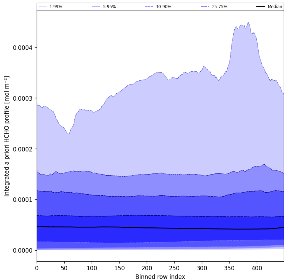
Figure 57: Along track statistics of “Integrated a priori HCHO profile” for 2025-08-09 to 2025-08-10
