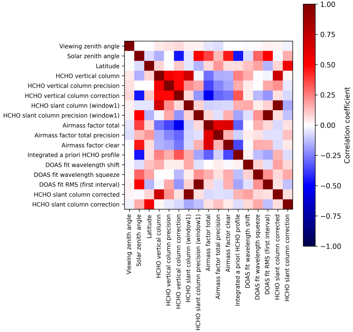
Figure 2: Map of correlation matrix for 2025-08-09 to 2025-08-10.
