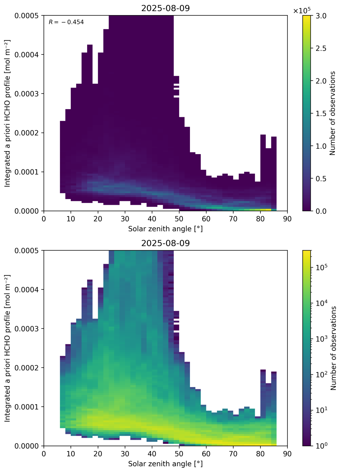
Figure 180: Scatter density plot of “Solar zenith angle” against “Integrated a priori HCHO profile” for 2025-08-09 to 2025-08-10.
