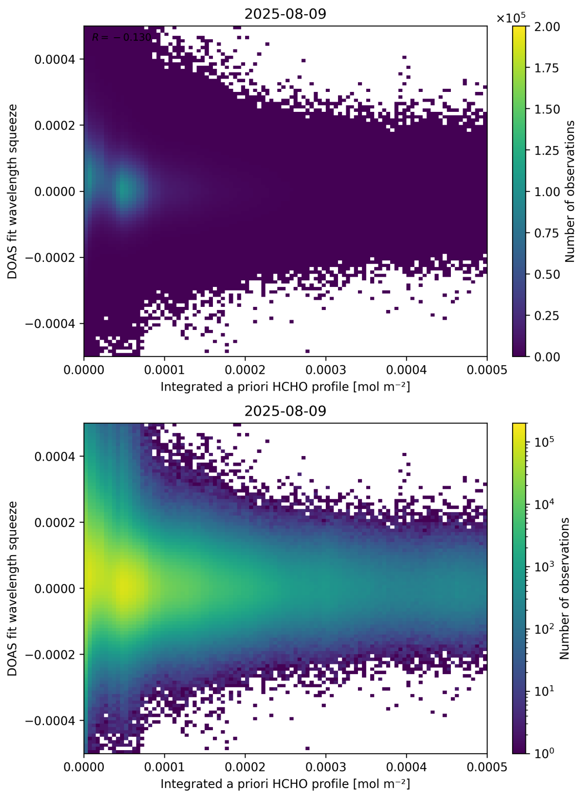
Figure 150: Scatter density plot of “Integrated a priori HCHO profile” against “DOAS fit wavelength squeeze” for 2025-08-09 to 2025-08-10.
