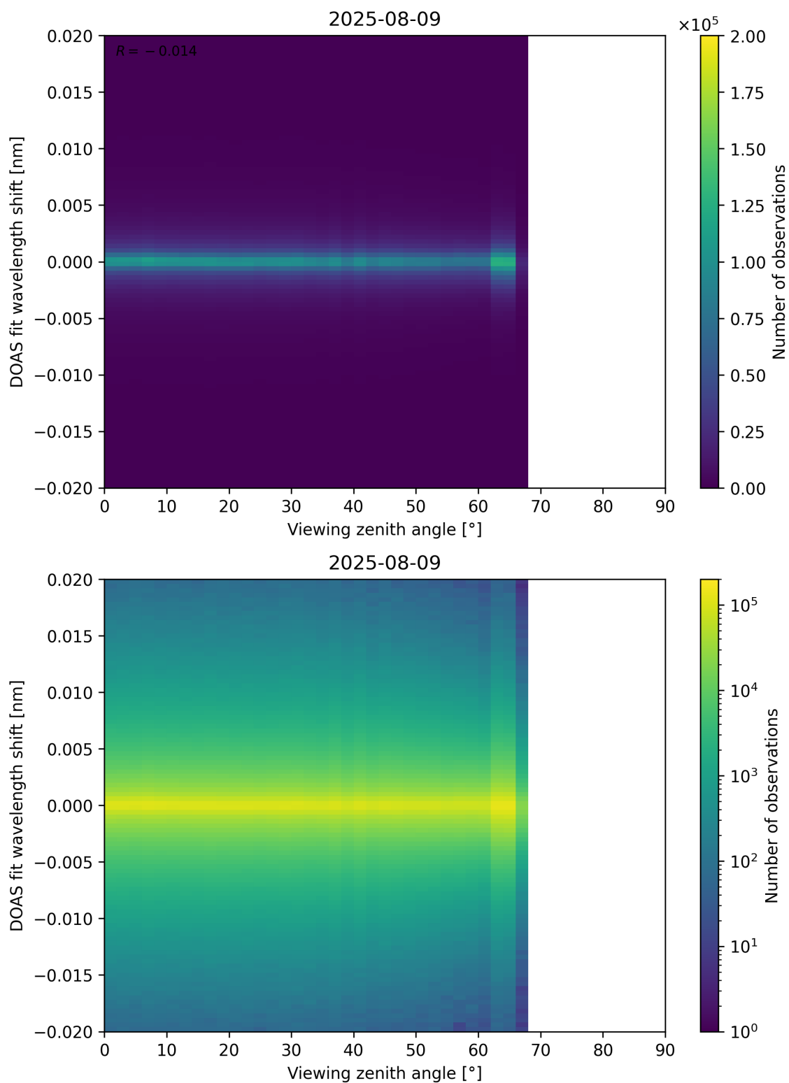
Figure 183: Scatter density plot of “Viewing zenith angle” against “DOAS fit wavelength shift” for 2025-08-09 to 2025-08-10.
