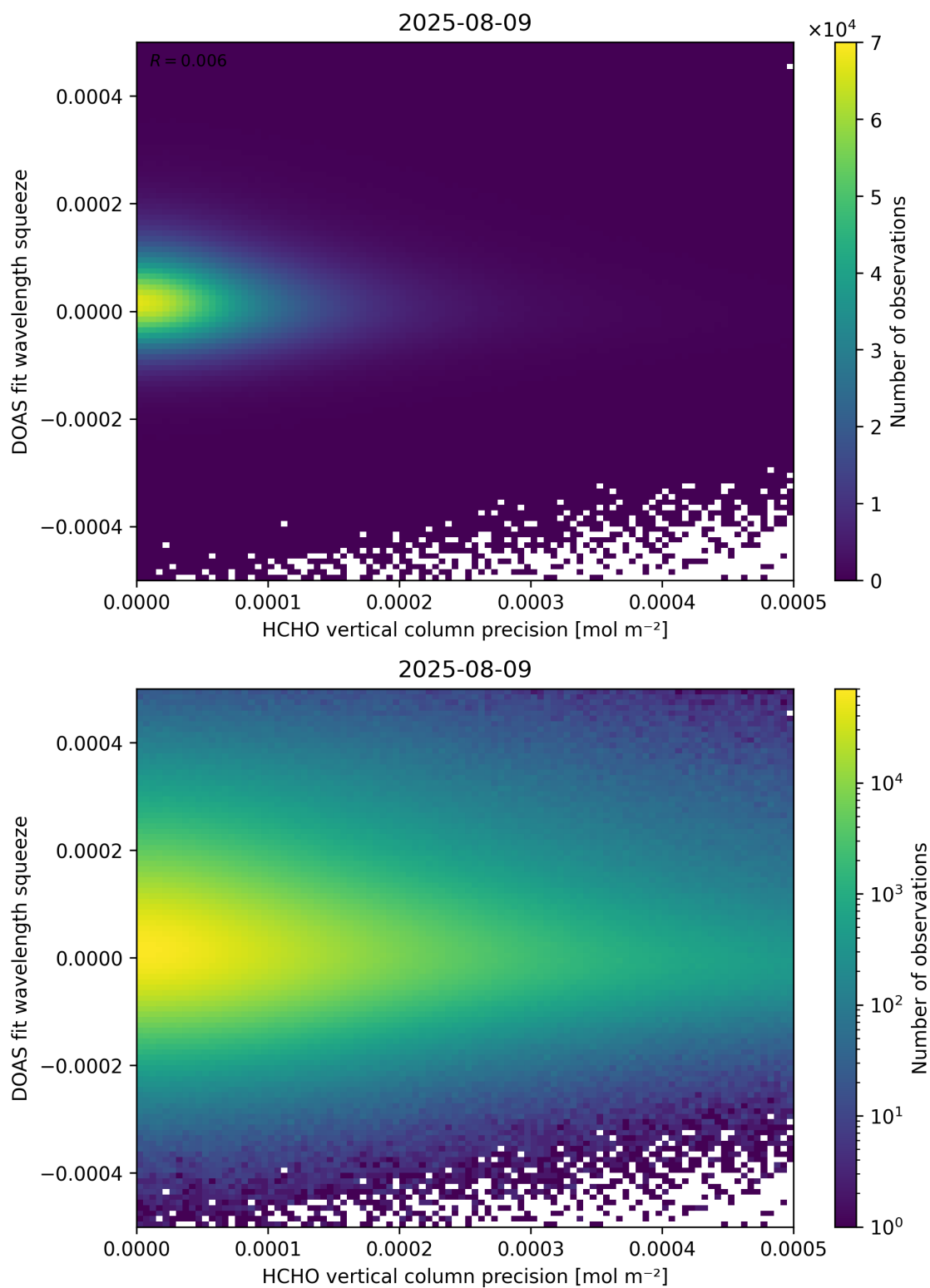
Figure 138: Scatter density plot of “HCHO vertical column precision” against “DOAS fit wavelength squeeze” for 2025-08-09 to 2025-08-10.
