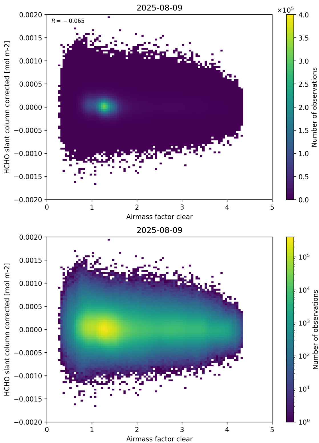
Figure 74: Scatter density plot of “Airmass factor clear” against “HCHO slant column corrected” for 2025-08-09 to 2025-08-10.
