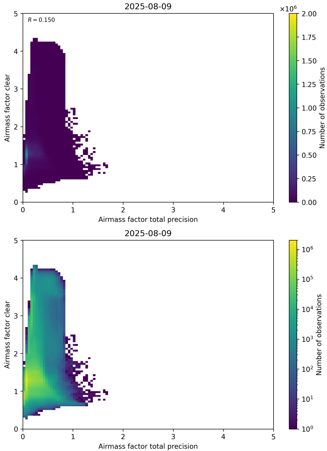
Figure 108: Scatter density plot of “Airmass factor total precision” against “Airmass factor clear” for 2025-08-09 to 2025-08-10.
