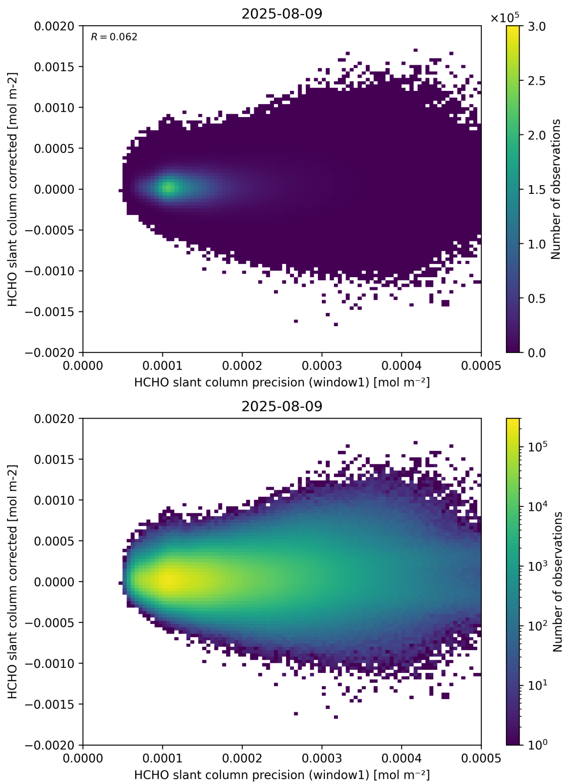
Figure 92: Scatter density plot of “HCHO slant column precision (window1)” against “HCHO slant column corrected” for 2025-08-09 to 2025-08-10.
