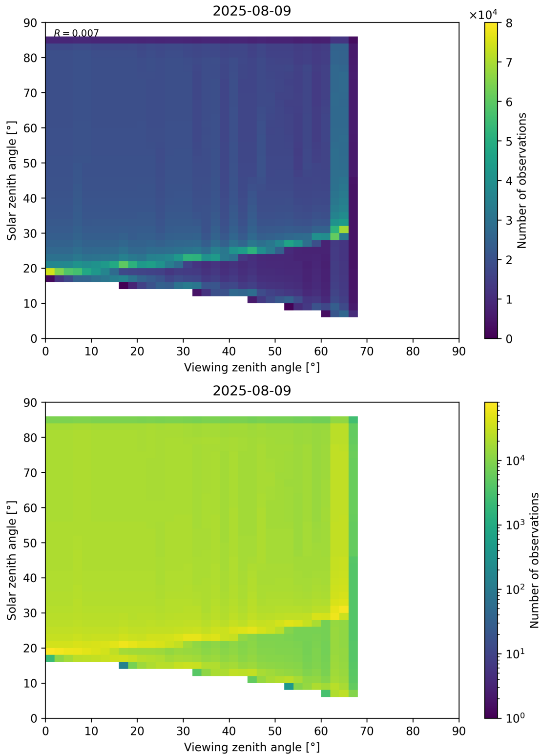
Figure 197: Scatter density plot of “Viewing zenith angle” against “Solar zenith angle” for 2025-08-09 to 2025-08-10.
