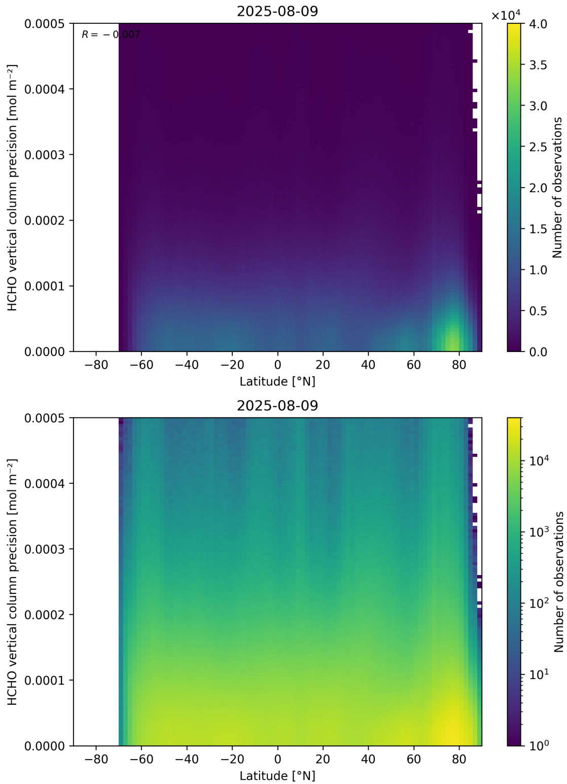
Figure 165: Scatter density plot of “Latitude” against “HCHO vertical column precision” for 2025-08-09 to 2025-08-10.
