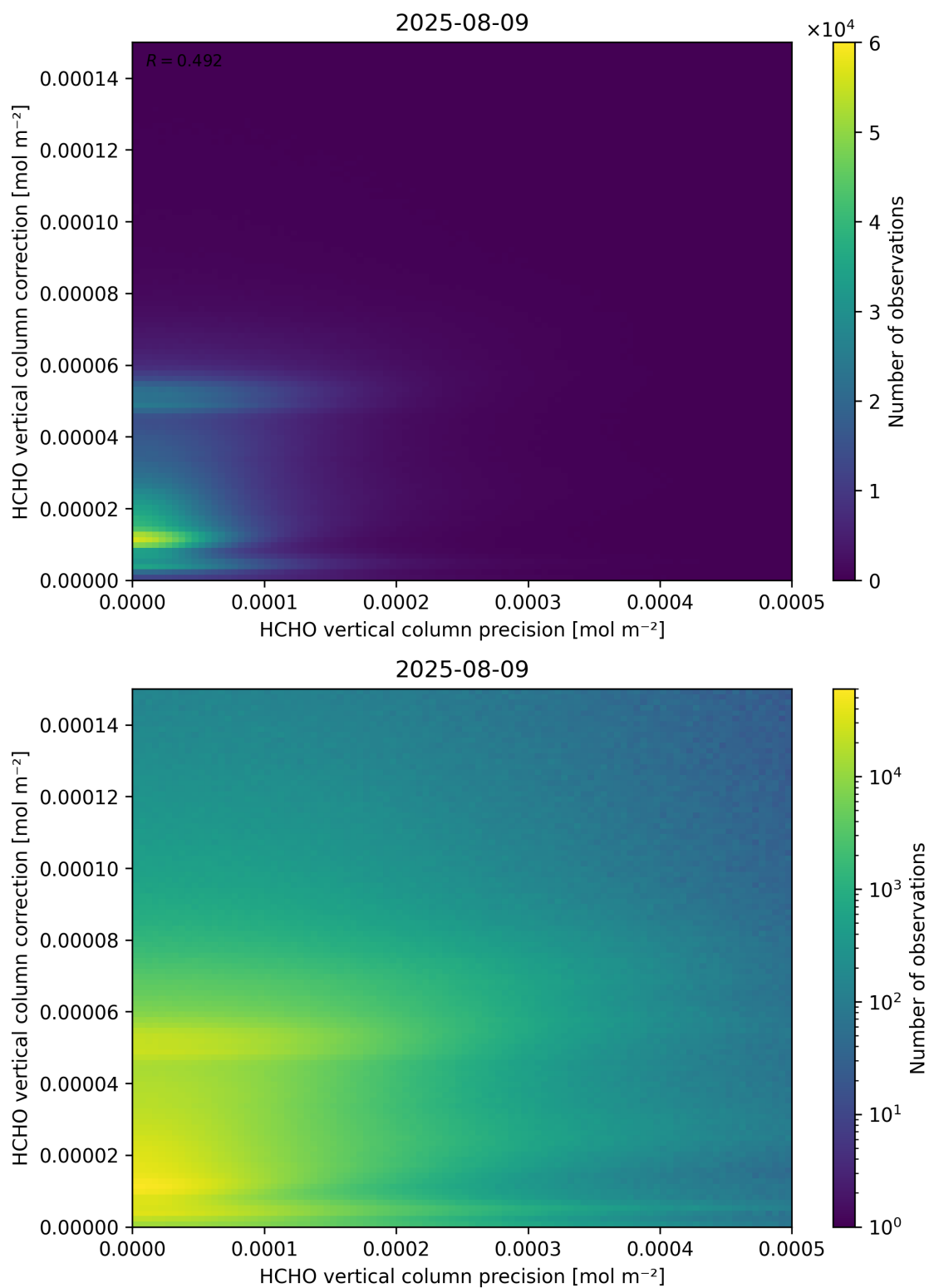
Figure 146: Scatter density plot of “HCHO vertical column precision” against “HCHO vertical column correction” for 2025-08-09 to 2025-08-10.
