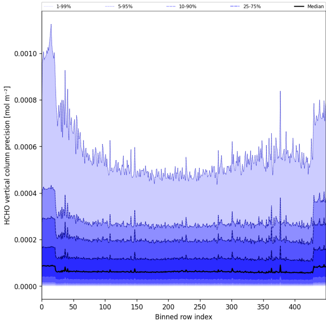
Figure 50: Along track statistics of “HCHO vertical column precision” for 2025-08-09 to 2025-08-10
