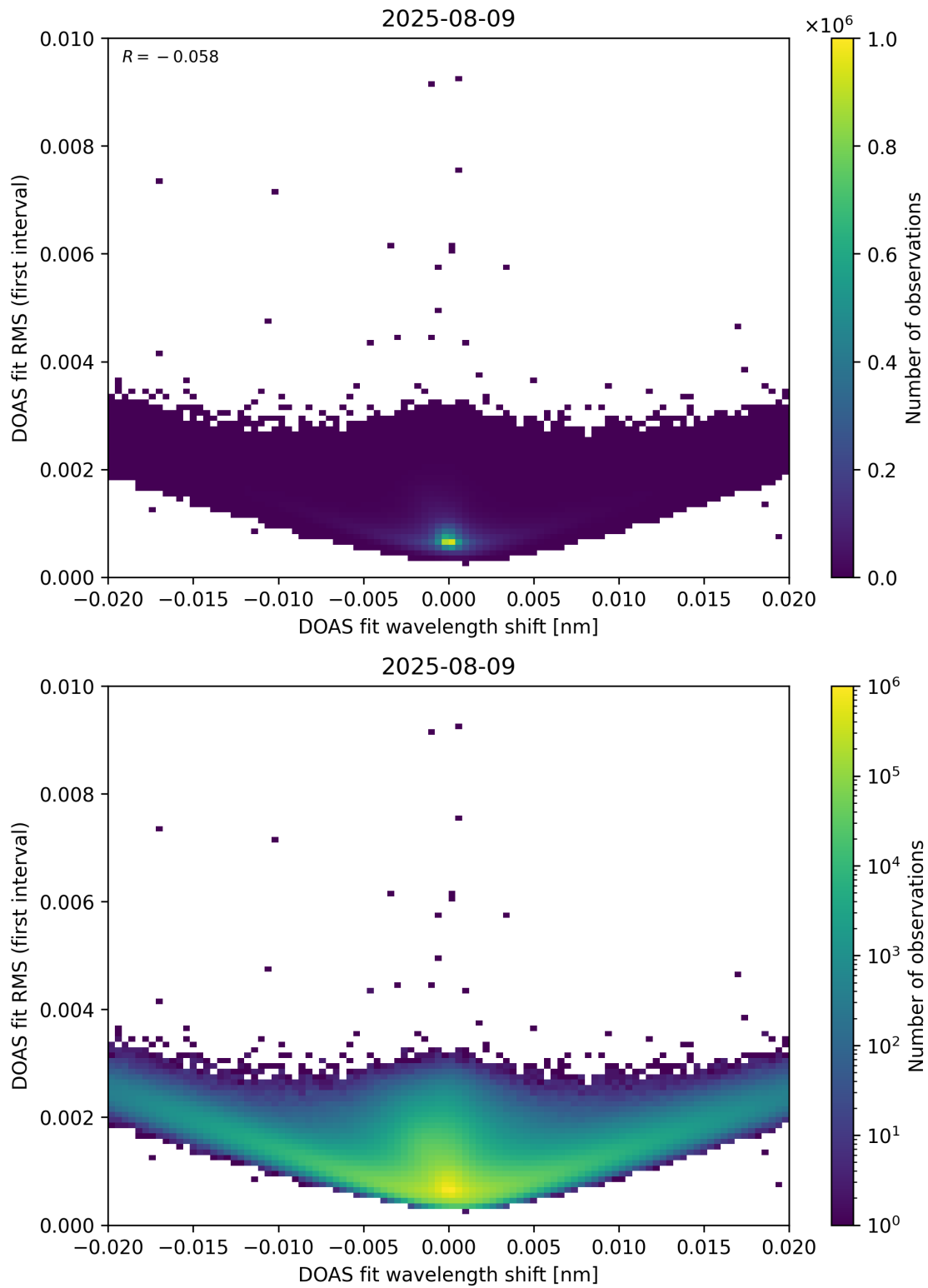
Figure 64: Scatter density plot of “DOAS fit wavelength shift” against “DOAS fit RMS (first interval)” for 2025-08-09 to 2025-08-10.
