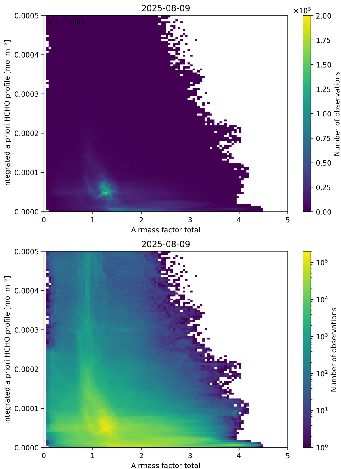
Figure 104: Scatter density plot of “Airmass factor total” against “Integrated a priori HCHO profile” for 2025-08-09 to 2025-08-10.
