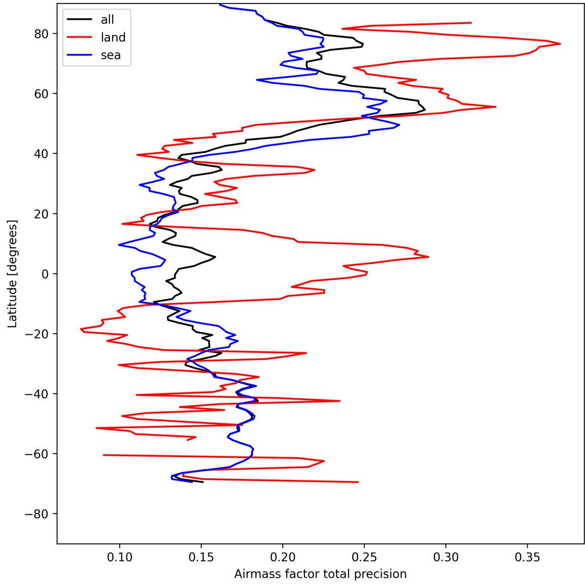
Figure 27: Zonal average of “Airmass factor total precision” for 2025-08-09 to 2025-08-10.
