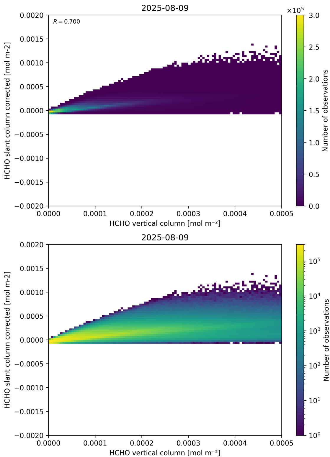
Figure 127: Scatter density plot of “HCHO vertical column” against “HCHO slant column corrected” for 2025-08-09 to 2025-08-10.
