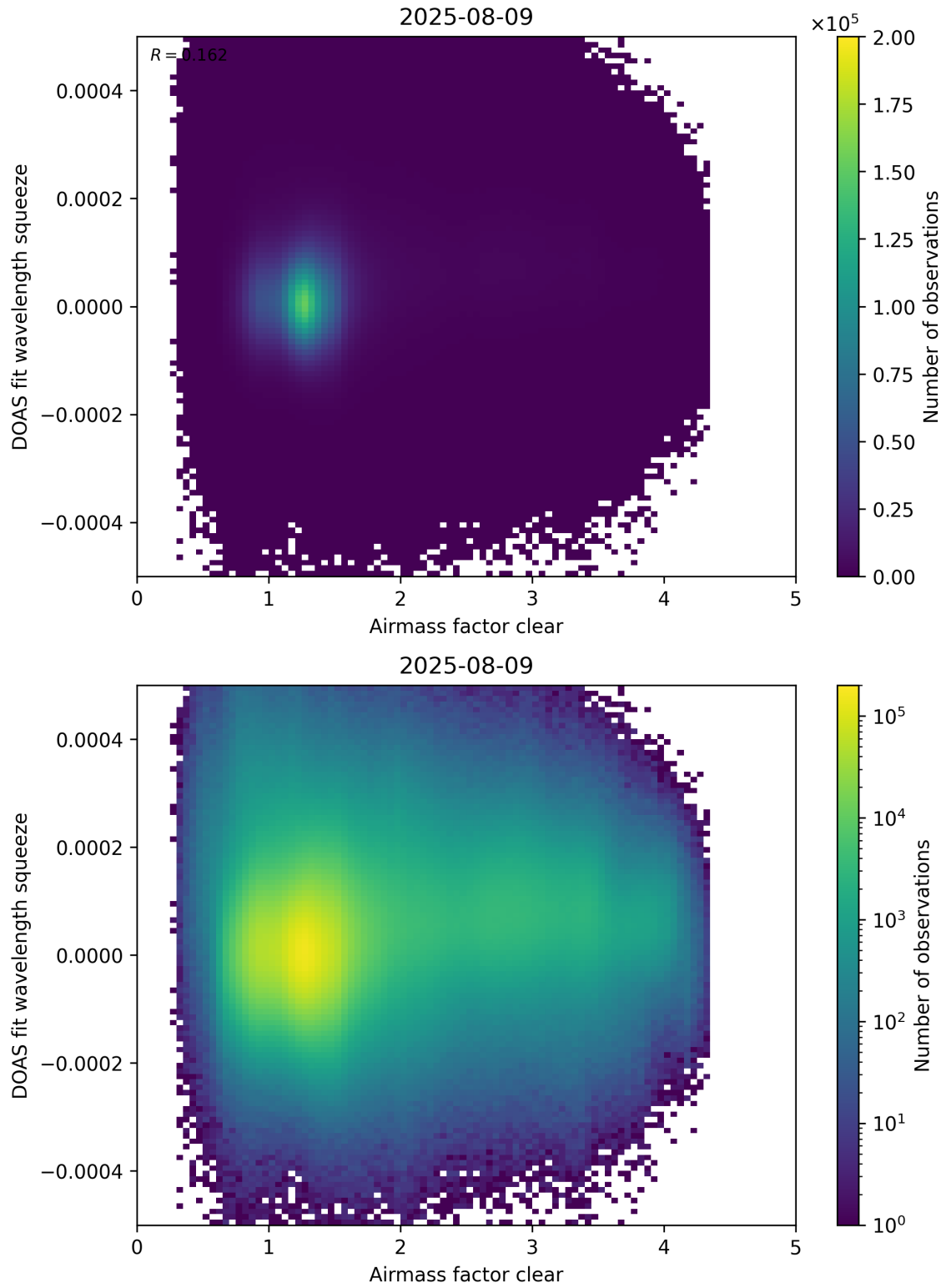
Figure 73: Scatter density plot of “Airmass factor clear” against “DOAS fit wavelength squeeze” for 2025-08-09 to 2025-08-10.
