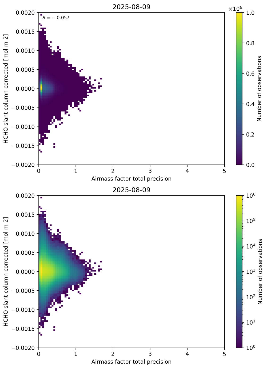
Figure 109: Scatter density plot of “Airmass factor total precision” against “HCHO slant column corrected” for 2025-08-09 to 2025-08-10.
