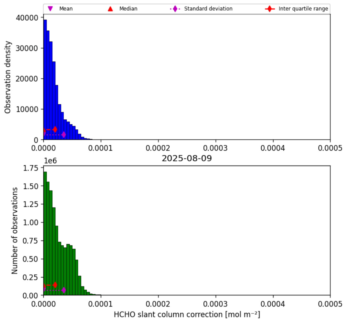
Figure 47: Histogram of “HCHO slant column correction” for 2025-08-09 to 2025-08-10
