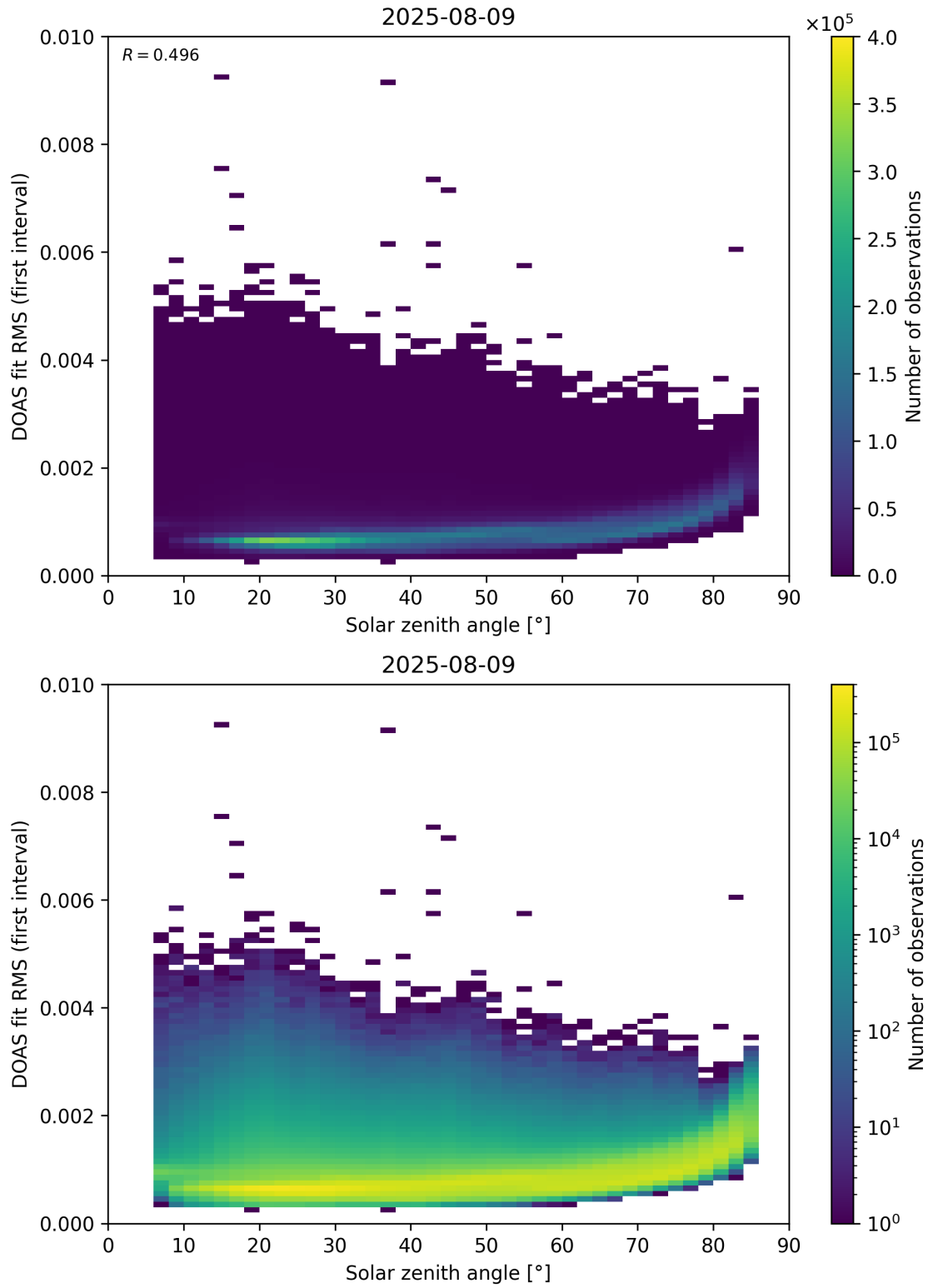
Figure 167: Scatter density plot of “Solar zenith angle” against “DOAS fit RMS (first interval)” for 2025-08-09 to 2025-08-10.
