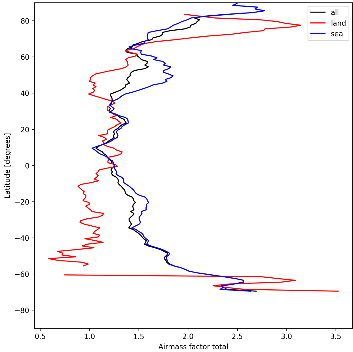
Figure 26: Zonal average of “Airmass factor total” for 2025-08-09 to 2025-08-10.
