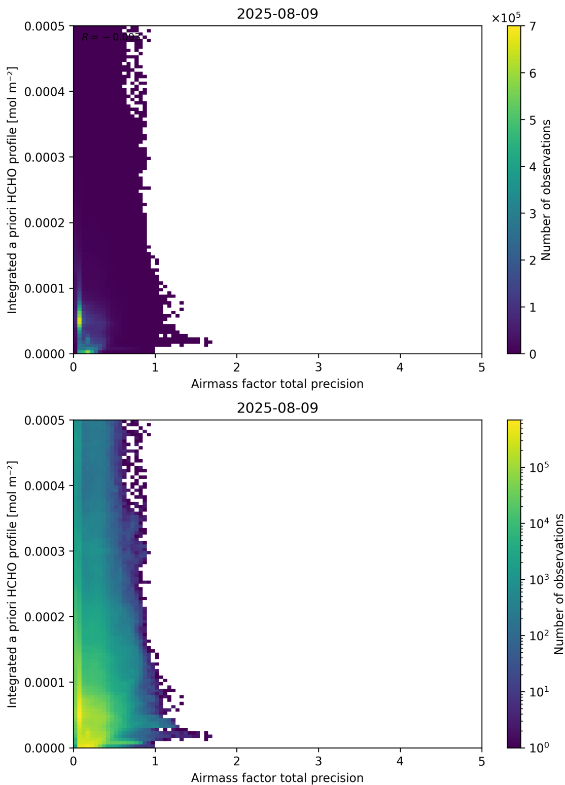
Figure 111: Scatter density plot of “Airmass factor total precision” against “Integrated a priori HCHO profile” for 2025-08-09 to 2025-08-10.
