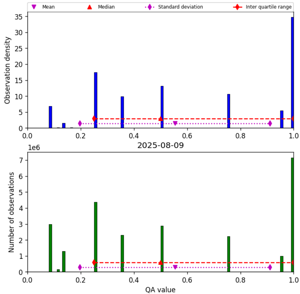
Figure 34: Histogram of “QA value” for 2025-08-09 to 2025-08-10
