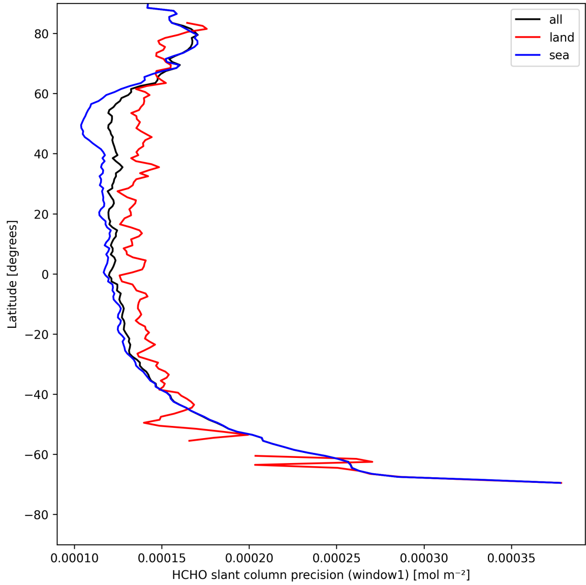
Figure 25: Zonal average of “HCHO slant column precision (window1)” for 2025-08-09 to 2025-08-10.
