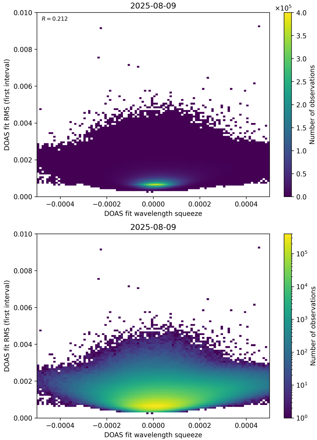
Figure 68: Scatter density plot of “DOAS fit wavelength squeeze” against “DOAS fit RMS (first interval)” for 2025-08-09 to 2025-08-10.
