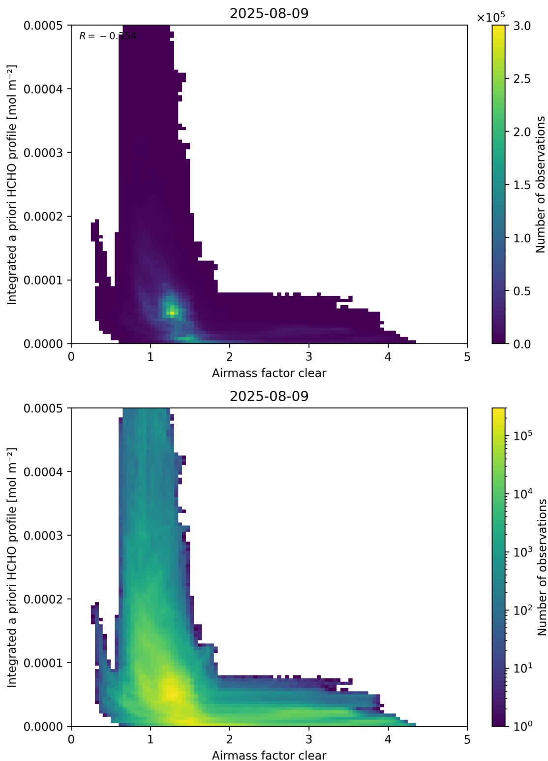
Figure 76: Scatter density plot of “Airmass factor clear” against “Integrated a priori HCHO profile” for 2025-08-09 to 2025-08-10.
