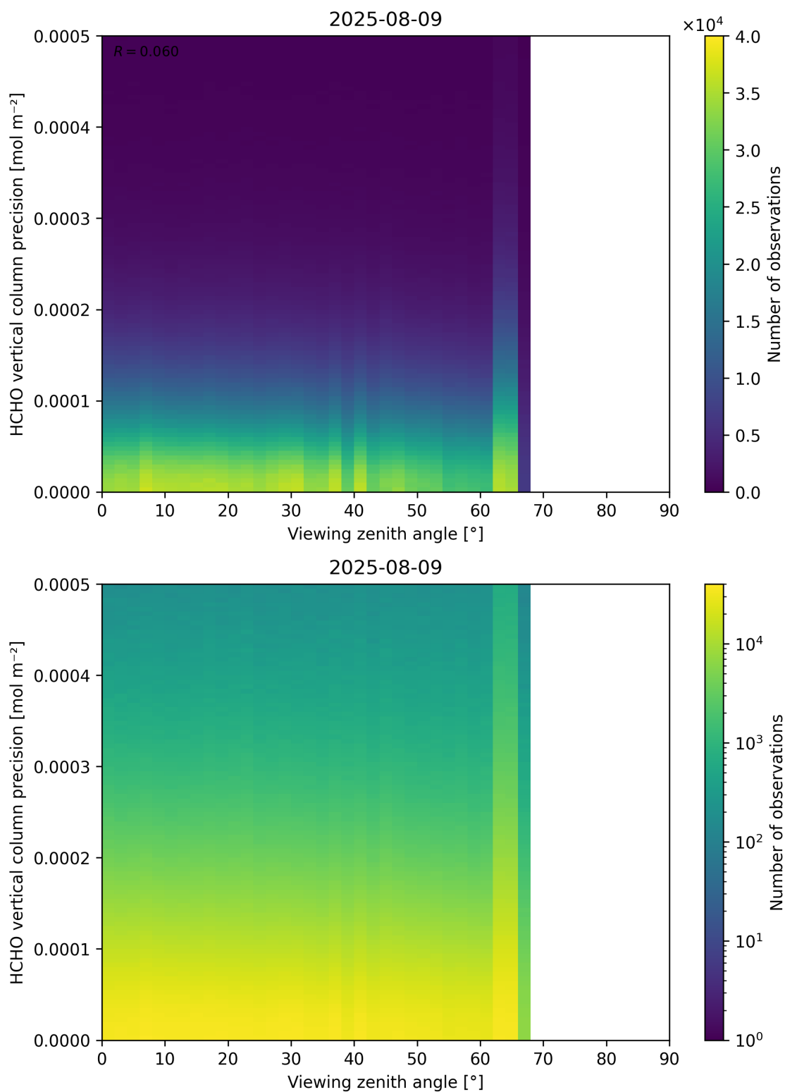
Figure 194: Scatter density plot of “Viewing zenith angle” against “HCHO vertical column precision” for 2025-08-09 to 2025-08-10.
