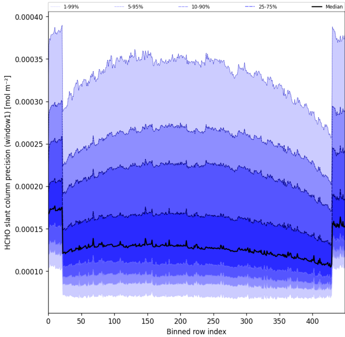
Figure 53: Along track statistics of “HCHO slant column precision (window1)” for 2025-08-09 to 2025-08-10
