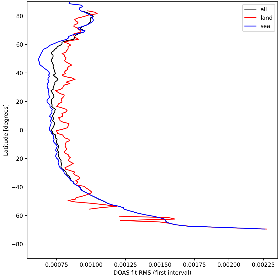
Figure 32: Zonal average of "DOAS fit RMS (first interval)" for 2025-08-09 to 2025-08-10.
