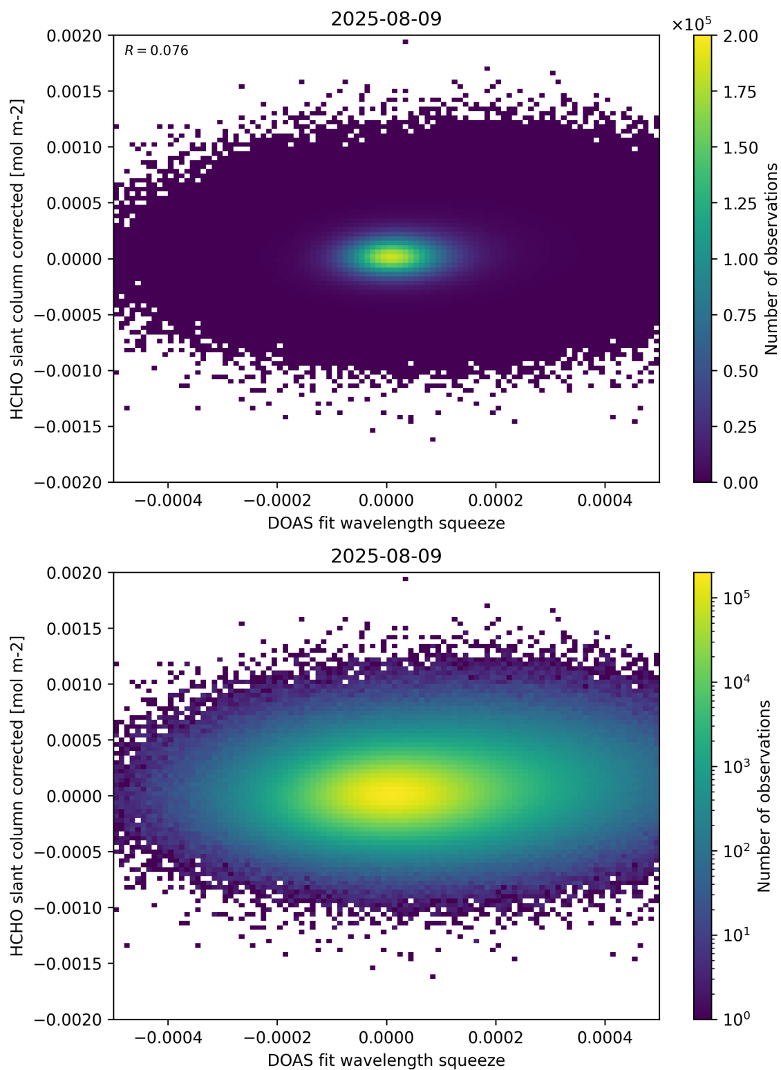
Figure 69: Scatter density plot of “DOAS fit wavelength squeeze” against “HCHO slant column corrected” for 2025-08-09 to 2025-08-10.
