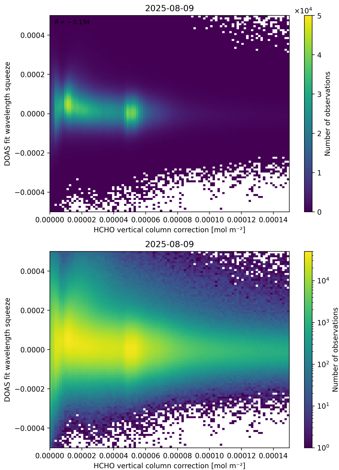
Figure 114: Scatter density plot of “HCHO vertical column correction” against “DOAS fit wavelength squeeze” for 2025-08-09 to 2025-08-10.
