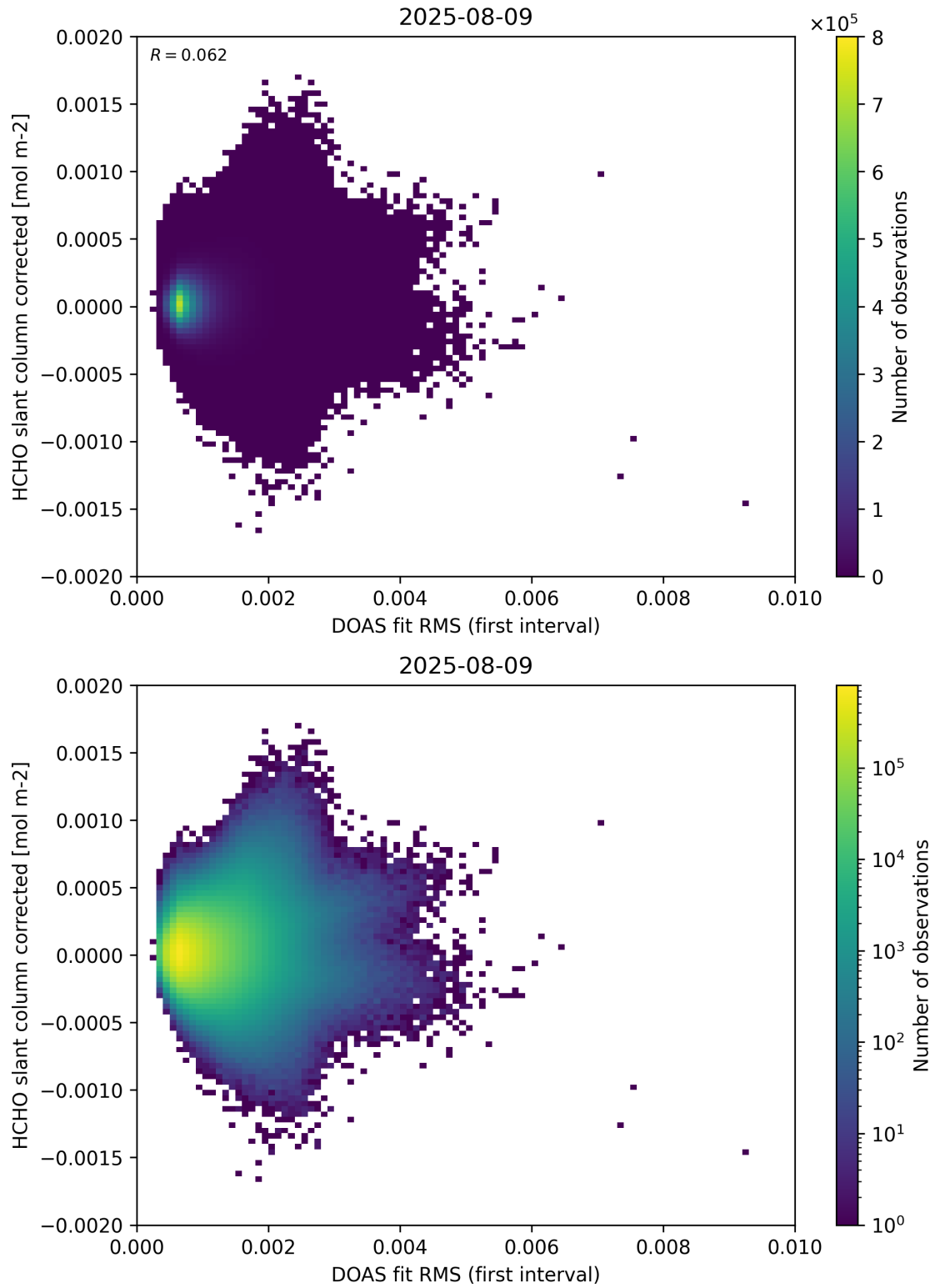
Figure 62: Scatter density plot of “DOAS fit RMS (first interval)” against “HCHO slant column corrected” for 2025-08-09 to 2025-08-10.
