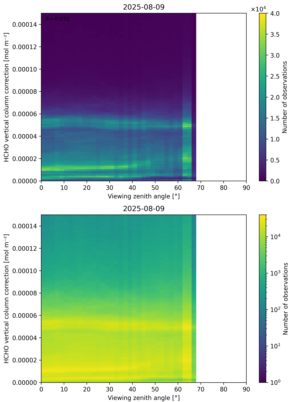
Figure 193: Scatter density plot of “Viewing zenith angle” against “HCHO vertical column correction” for 2025-08-09 to 2025-08-10.
