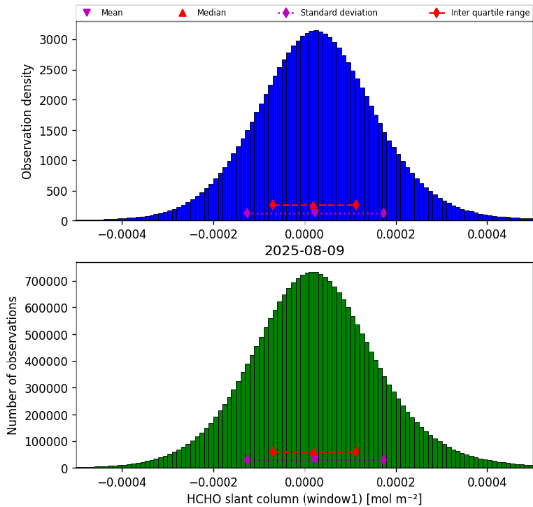
Figure 38: Histogram of “HCHO slant column (window1)” for 2025-08-09 to 2025-08-10
