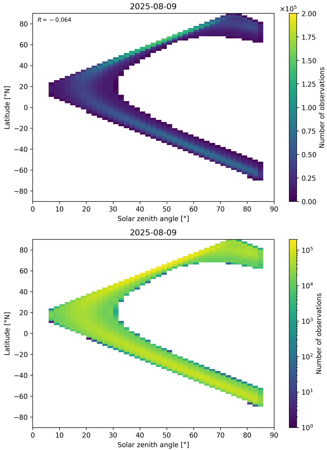
Figure 181: Scatter density plot of “Solar zenith angle” against “Latitude” for 2025-08-09 to 2025-08-10.
