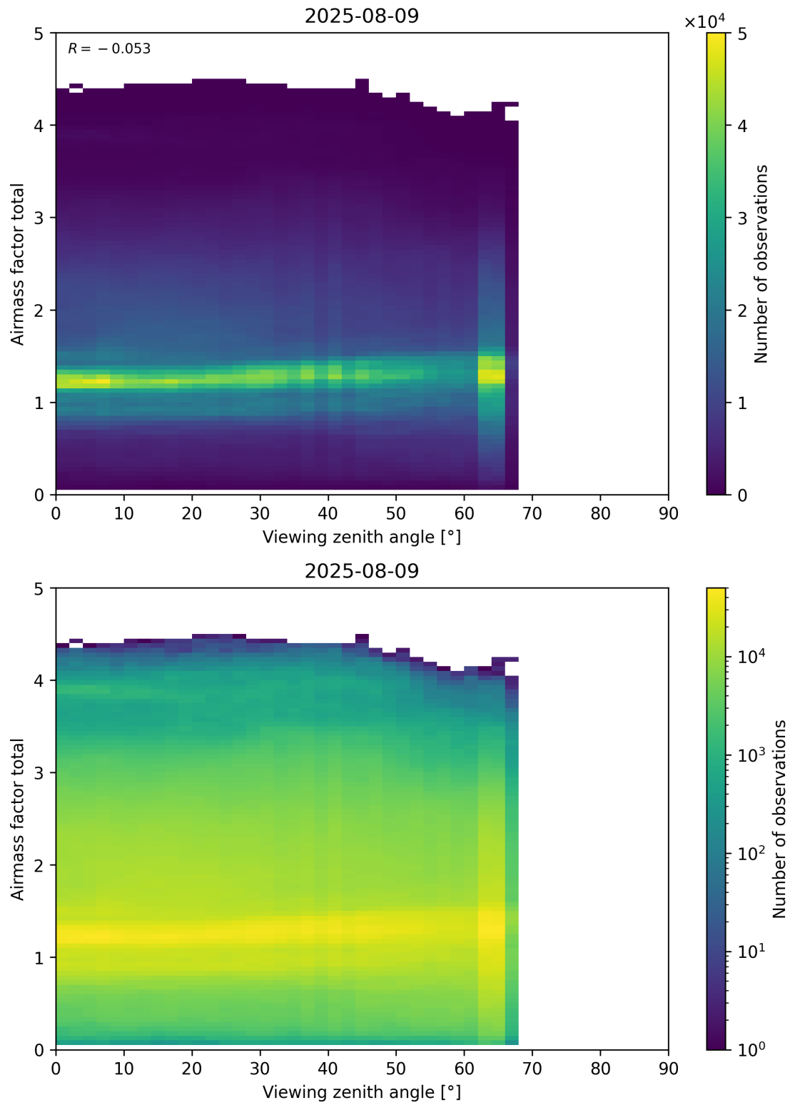
Figure 190: Scatter density plot of “Viewing zenith angle” against “Airmass factor total” for 2025-08-09 to 2025-08-10.
