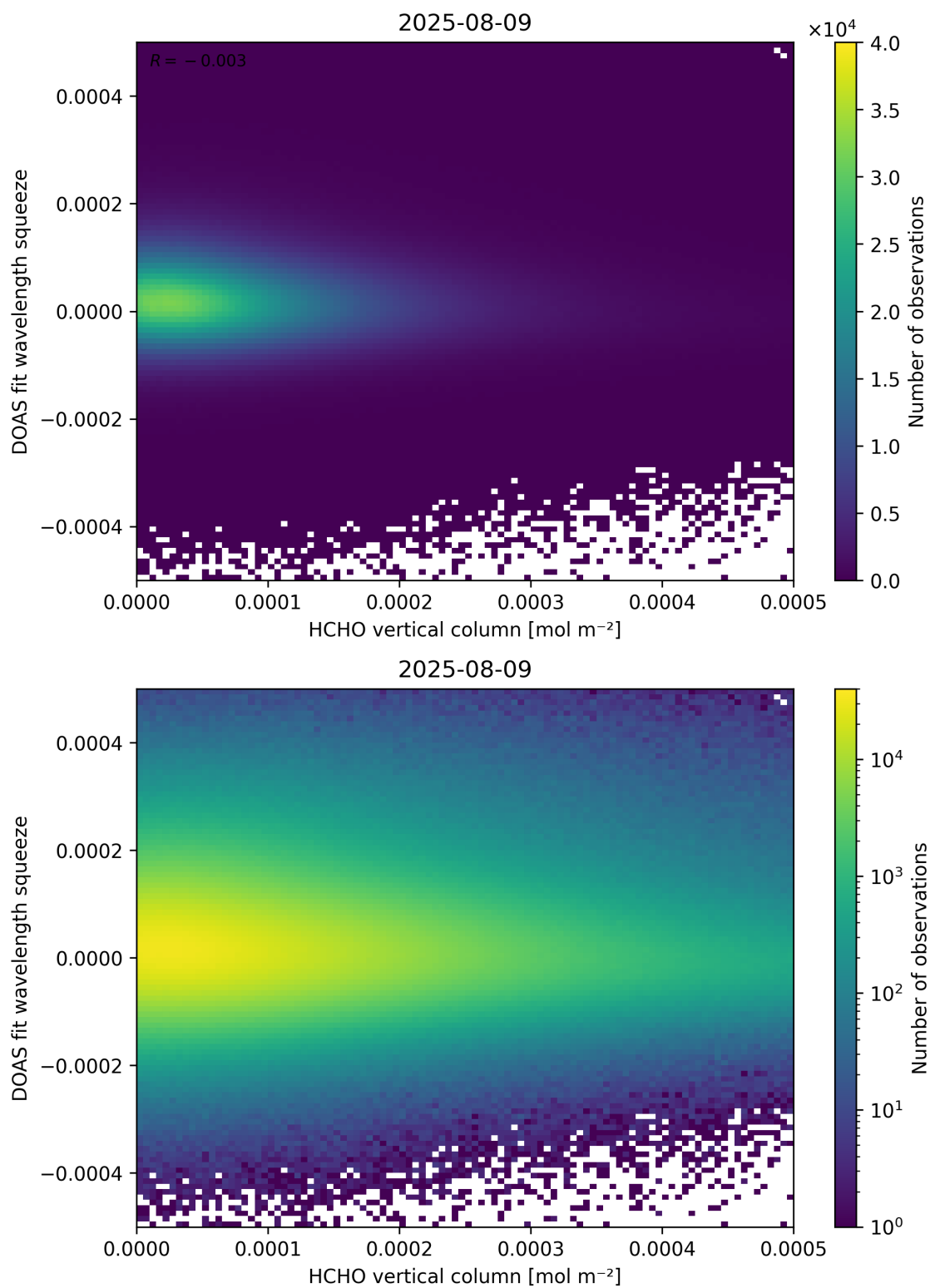
Figure 125: Scatter density plot of “HCHO vertical column” against “DOAS fit wavelength squeeze” for 2025-08-09 to 2025-08-10.
