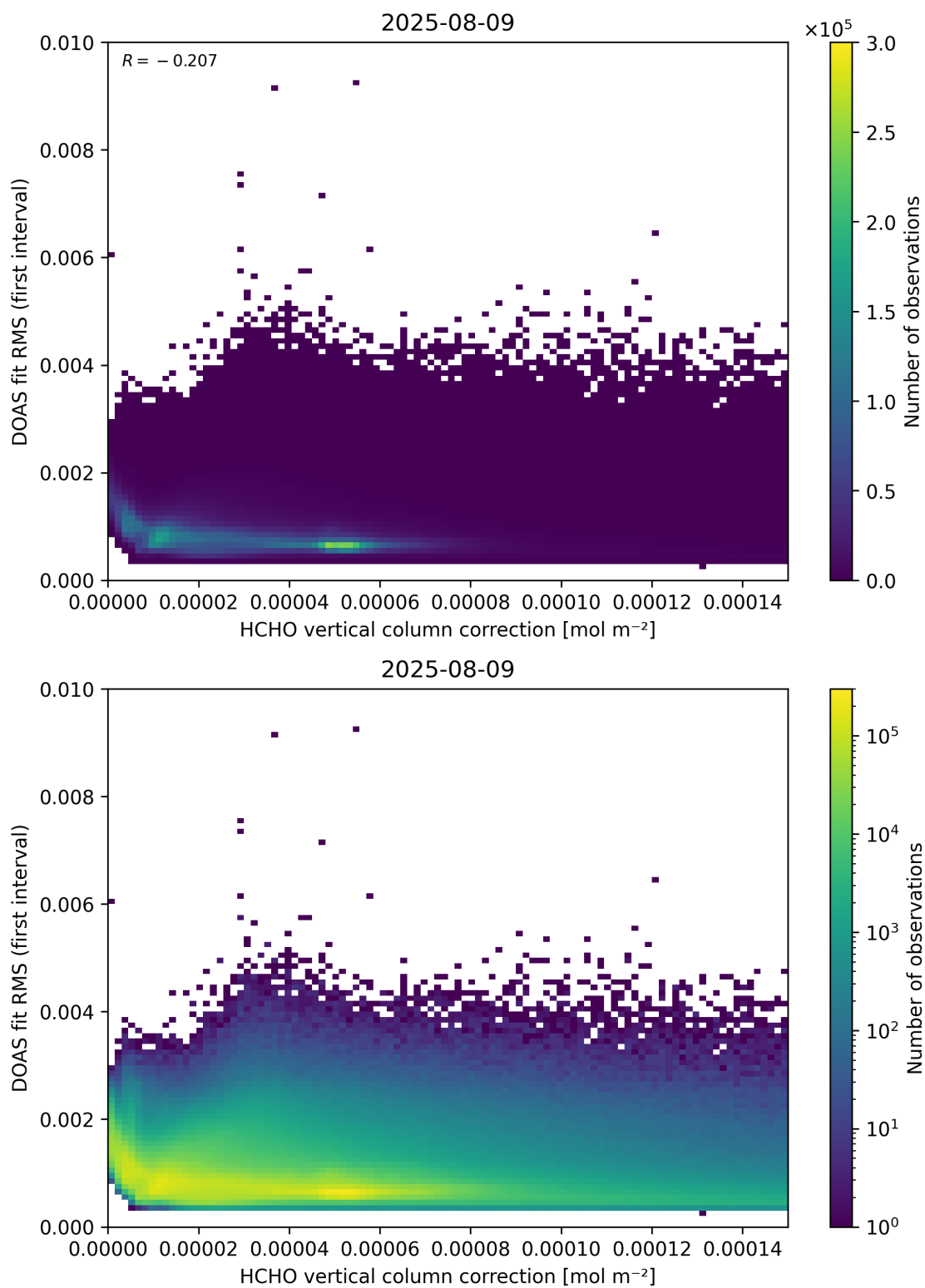
Figure 112: Scatter density plot of “HCHO vertical column correction” against “DOAS fit RMS (first interval)” for 2025-08-09 to 2025-08-10.
