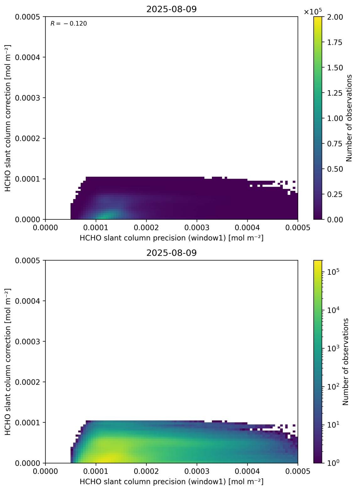
Figure 93: Scatter density plot of “HCHO slant column precision (window1)” against “HCHO slant column correction” for 2025-08-09 to 2025-08-10.
