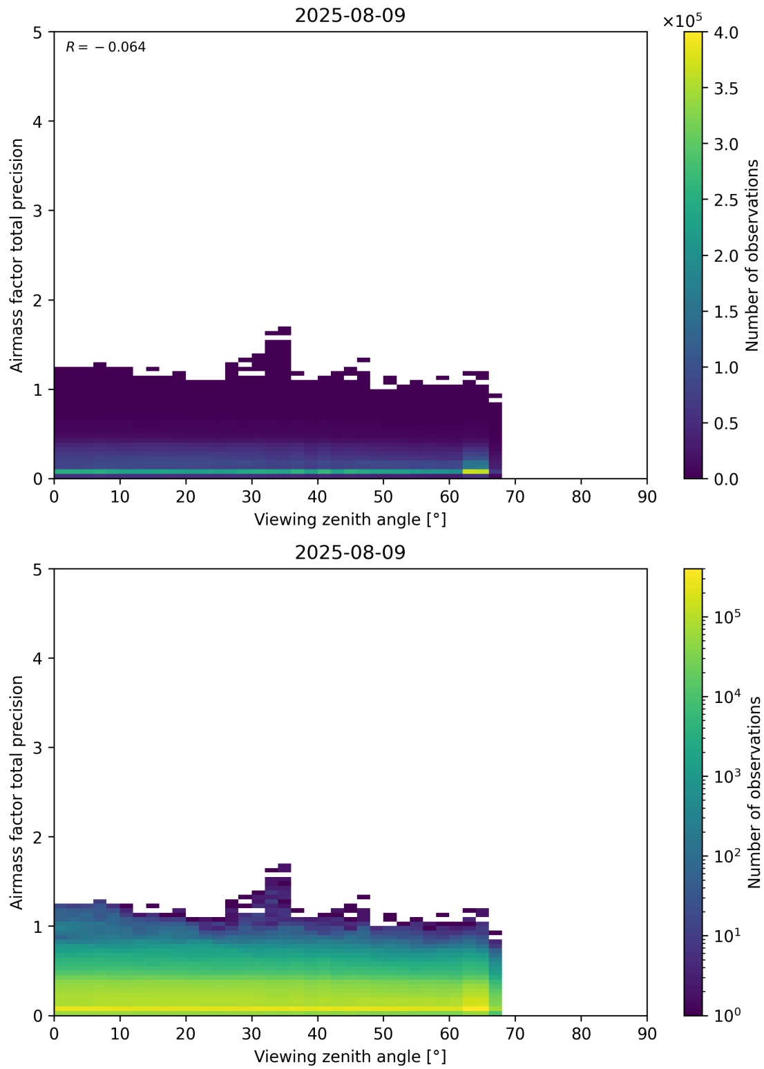
Figure 191: Scatter density plot of “Viewing zenith angle” against “Airmass factor total precision” for 2025-08-09 to 2025-08-10.
