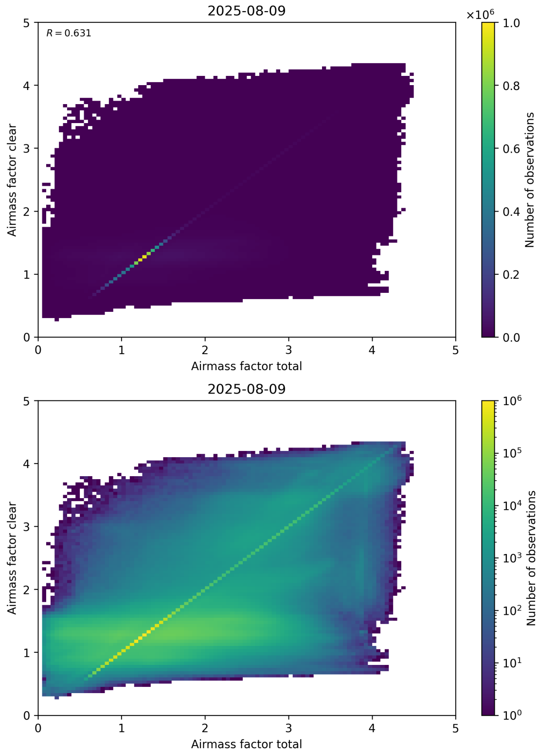
Figure 100: Scatter density plot of “Airmass factor total” against “Airmass factor clear” for 2025-08-09 to 2025-08-10.
