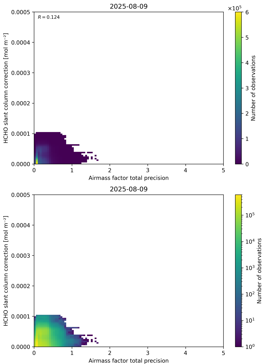
Figure 110: Scatter density plot of “Airmass factor total precision” against “HCHO slant column correction” for 2025-08-09 to 2025-08-10.
