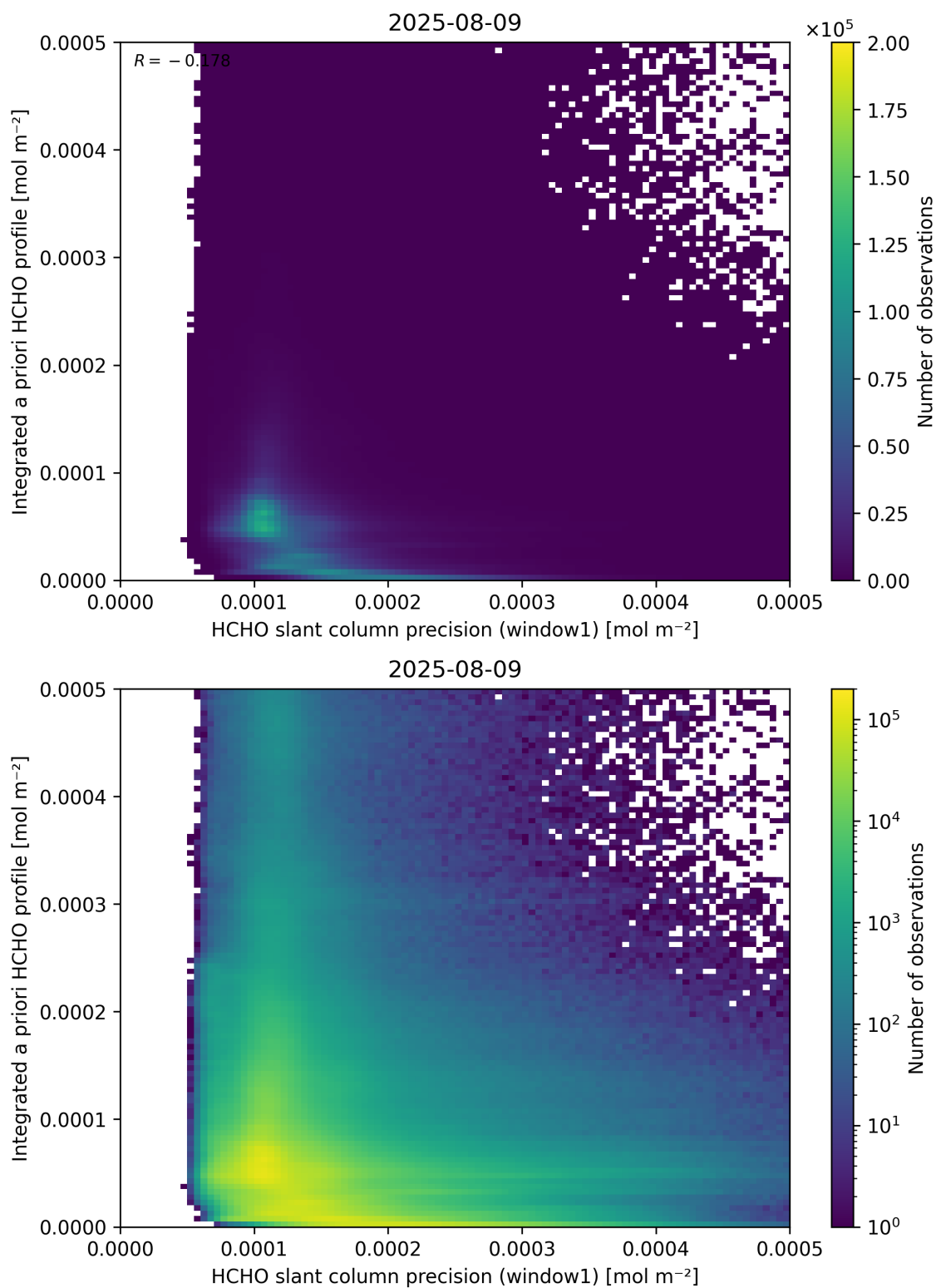
Figure 96: Scatter density plot of “HCHO slant column precision (window1)” against “Integrated a priori HCHO profile” for 2025-08-09 to 2025-08-10.
