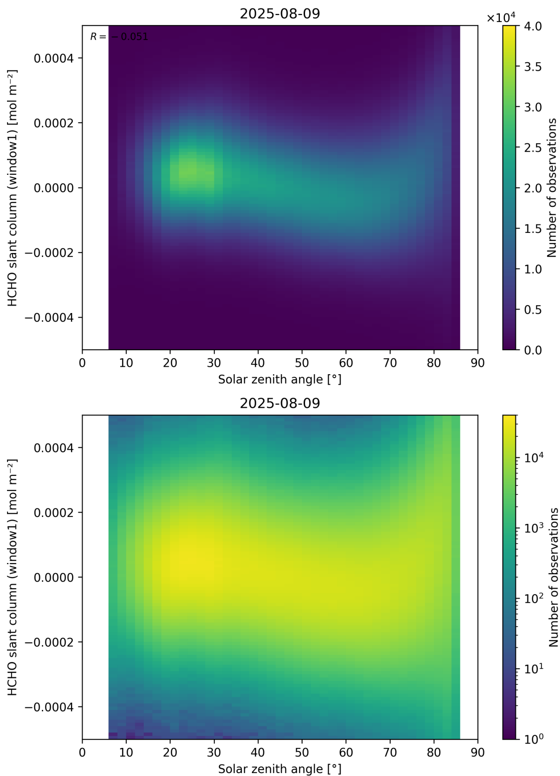
Figure 173: Scatter density plot of “Solar zenith angle” against “HCHO slant column (window1)” for 2025-08-09 to 2025-08-10.
