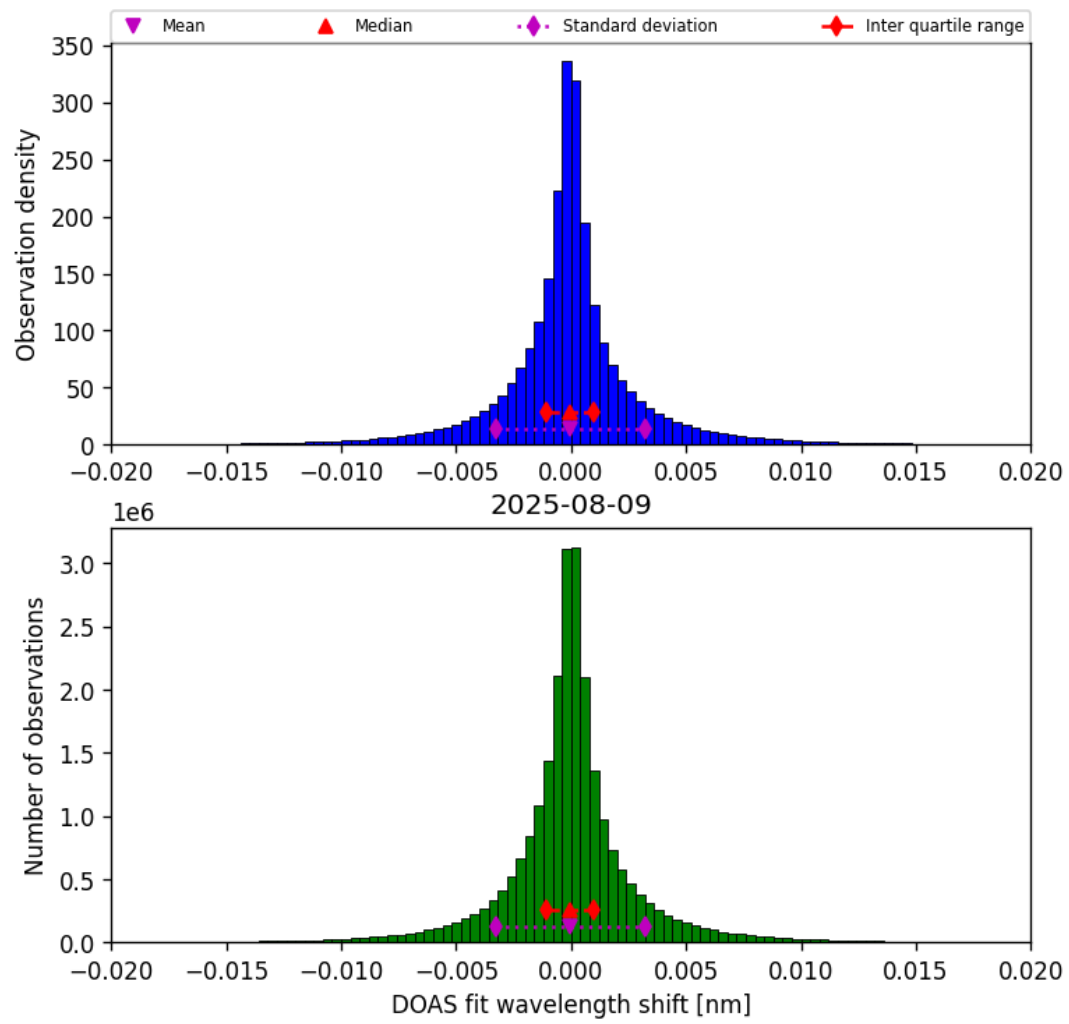
Figure 44: Histogram of “DOAS fit wavelength shift” for 2025-08-09 to 2025-08-10
