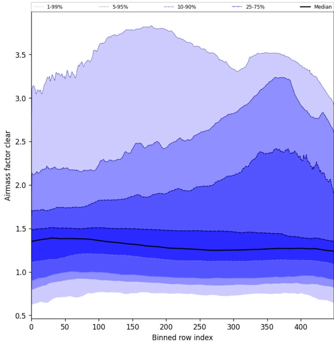
Figure 56: Along track statistics of “Airmass factor clear” for 2025-08-09 to 2025-08-10
