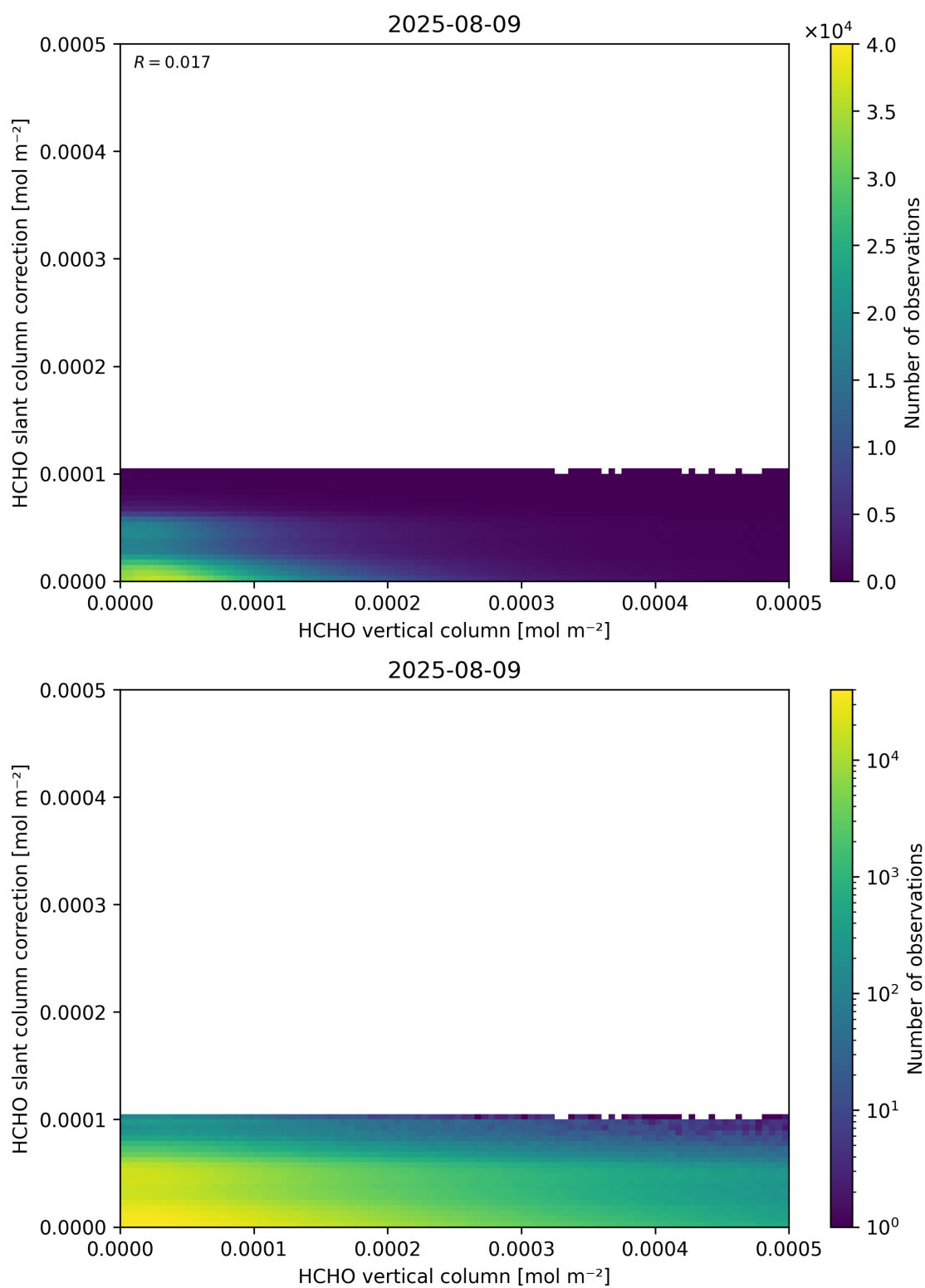
Figure 128: Scatter density plot of “HCHO vertical column” against “HCHO slant column correction” for 2025-08-09 to 2025-08-10.
