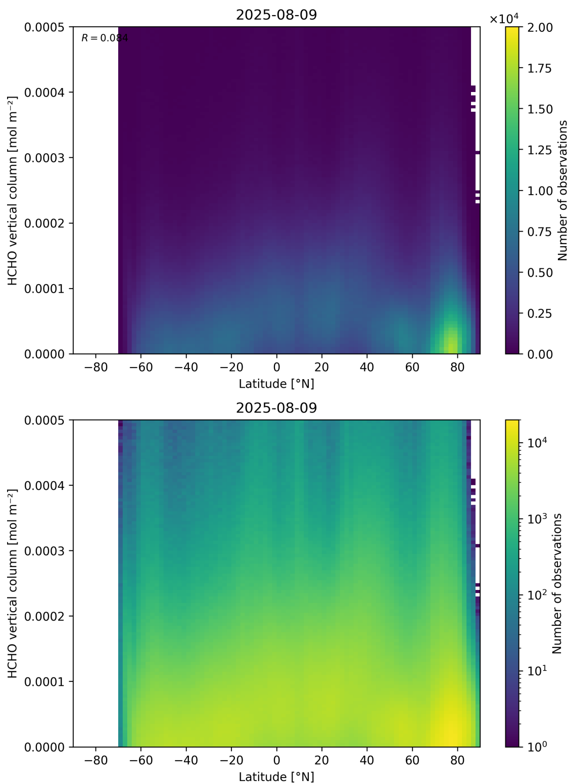
Figure 163: Scatter density plot of “Latitude” against “HCHO vertical column” for 2025-08-09 to 2025-08-10.
