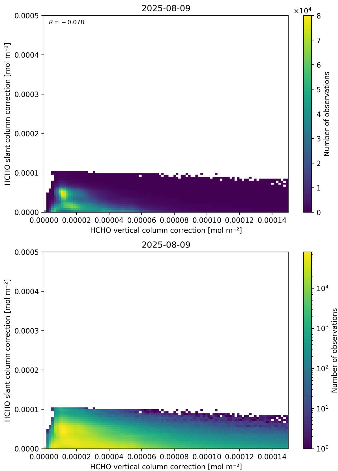
Figure 117: Scatter density plot of “HCHO vertical column correction” against “HCHO slant column correction” for 2025-08-09 to 2025-08-10.
