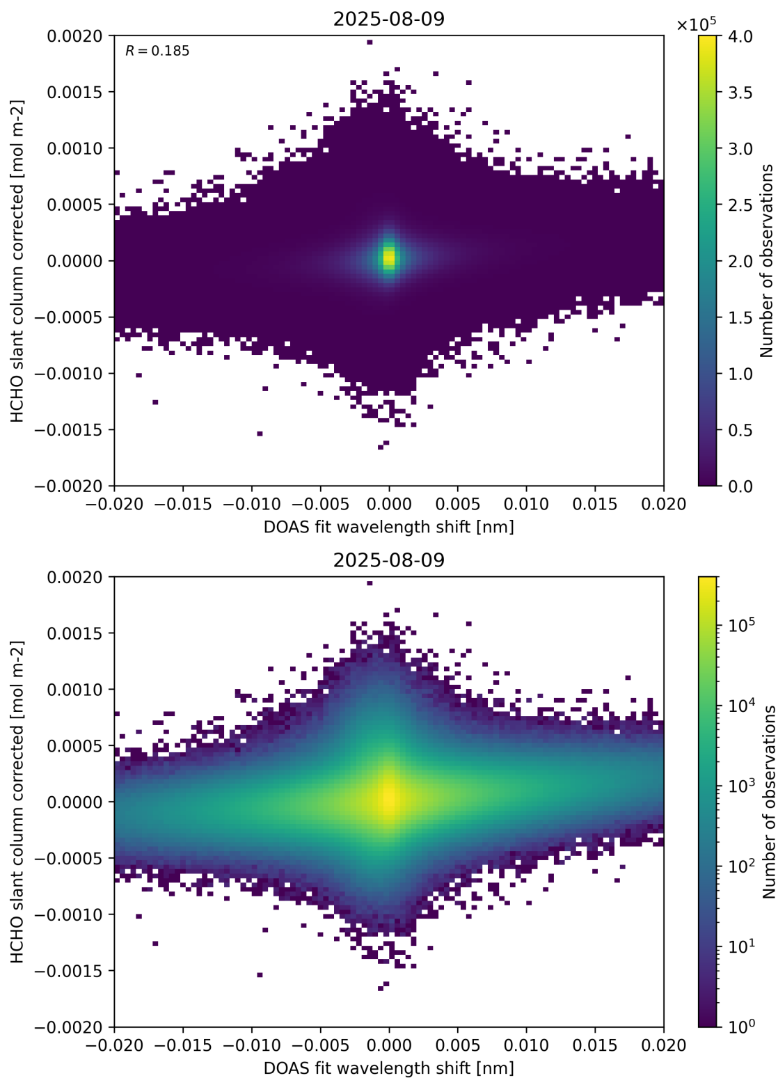
Figure 66: Scatter density plot of “DOAS fit wavelength shift” against “HCHO slant column corrected” for 2025-08-09 to 2025-08-10.
