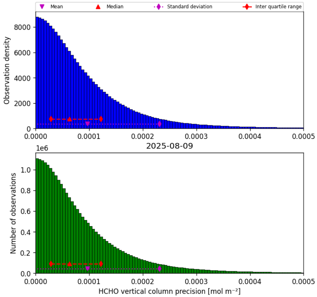
Figure 36: Histogram of “HCHO vertical column precision” for 2025-08-09 to 2025-08-10
