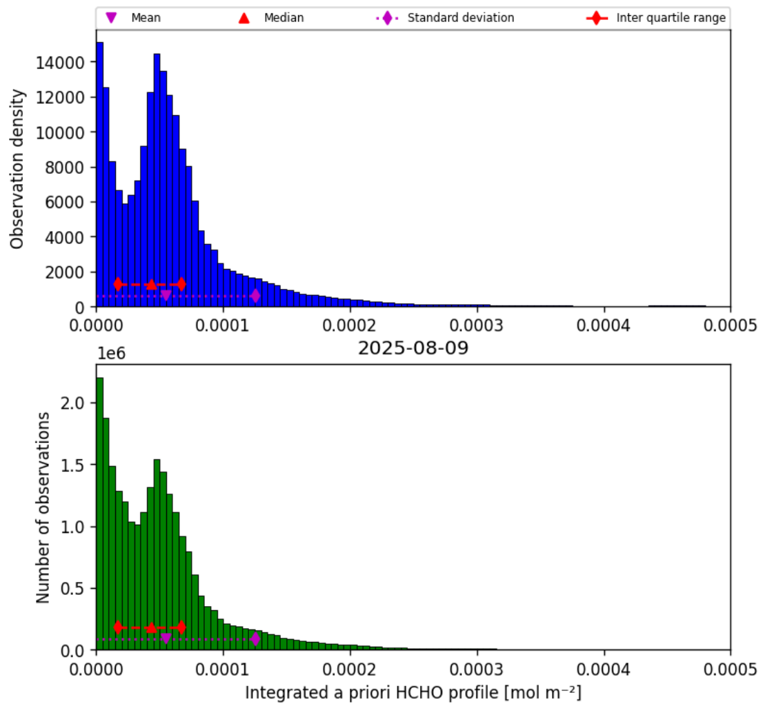
Figure 43: Histogram of “Integrated a priori HCHO profile” for 2025-08-09 to 2025-08-10
