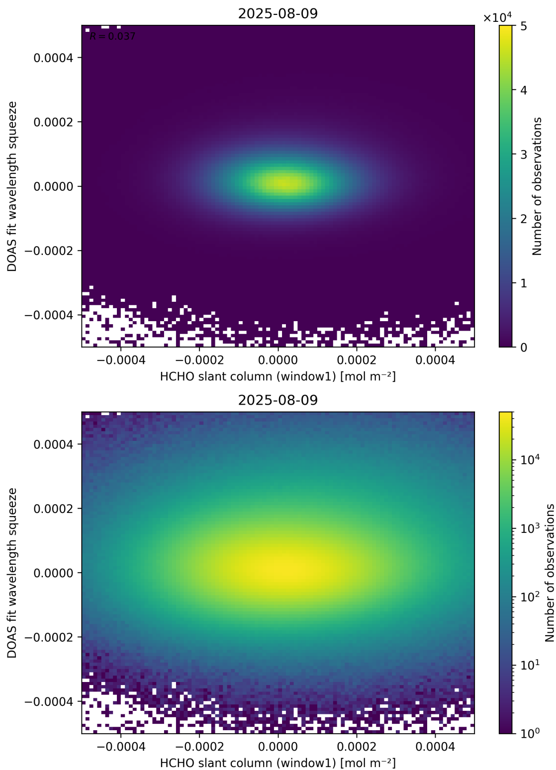
Figure 80: Scatter density plot of “HCHO slant column (window1)” against “DOAS fit wavelength squeeze” for 2025-08-09 to 2025-08-10.
