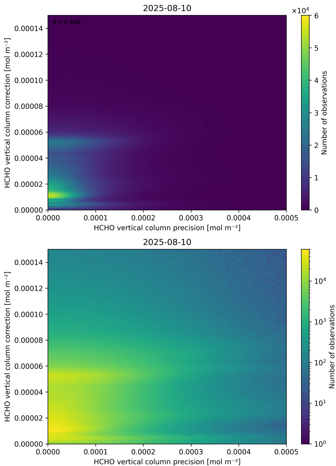
Figure 146: Scatter density plot of “HCHO vertical column precision” against “HCHO vertical column correction” for 2025-08-09 to 2025-08-11.
