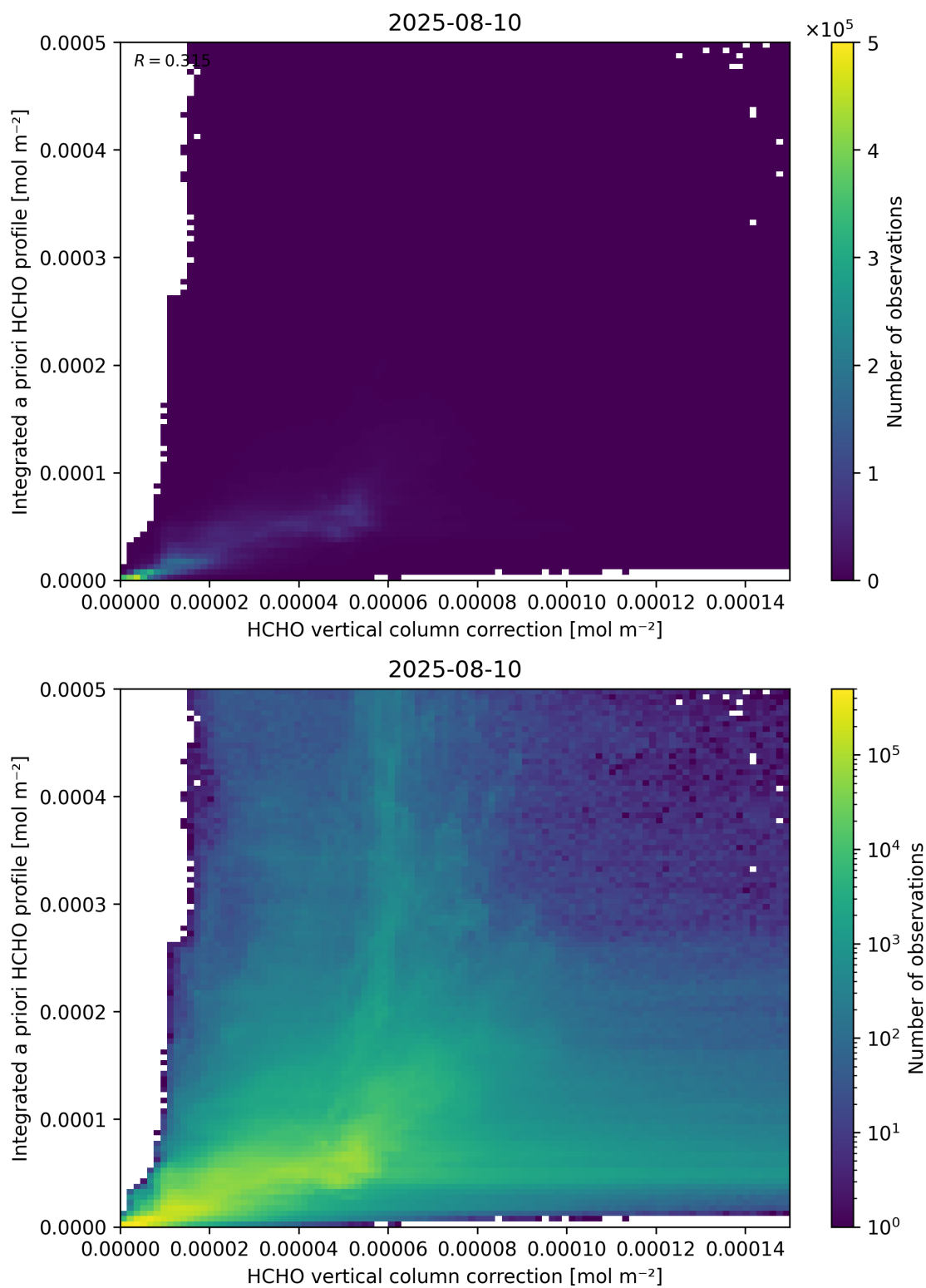
Figure 122: Scatter density plot of “HCHO vertical column correction” against “Integrated a priori HCHO profile” for 2025-08-09 to 2025-08-11.
