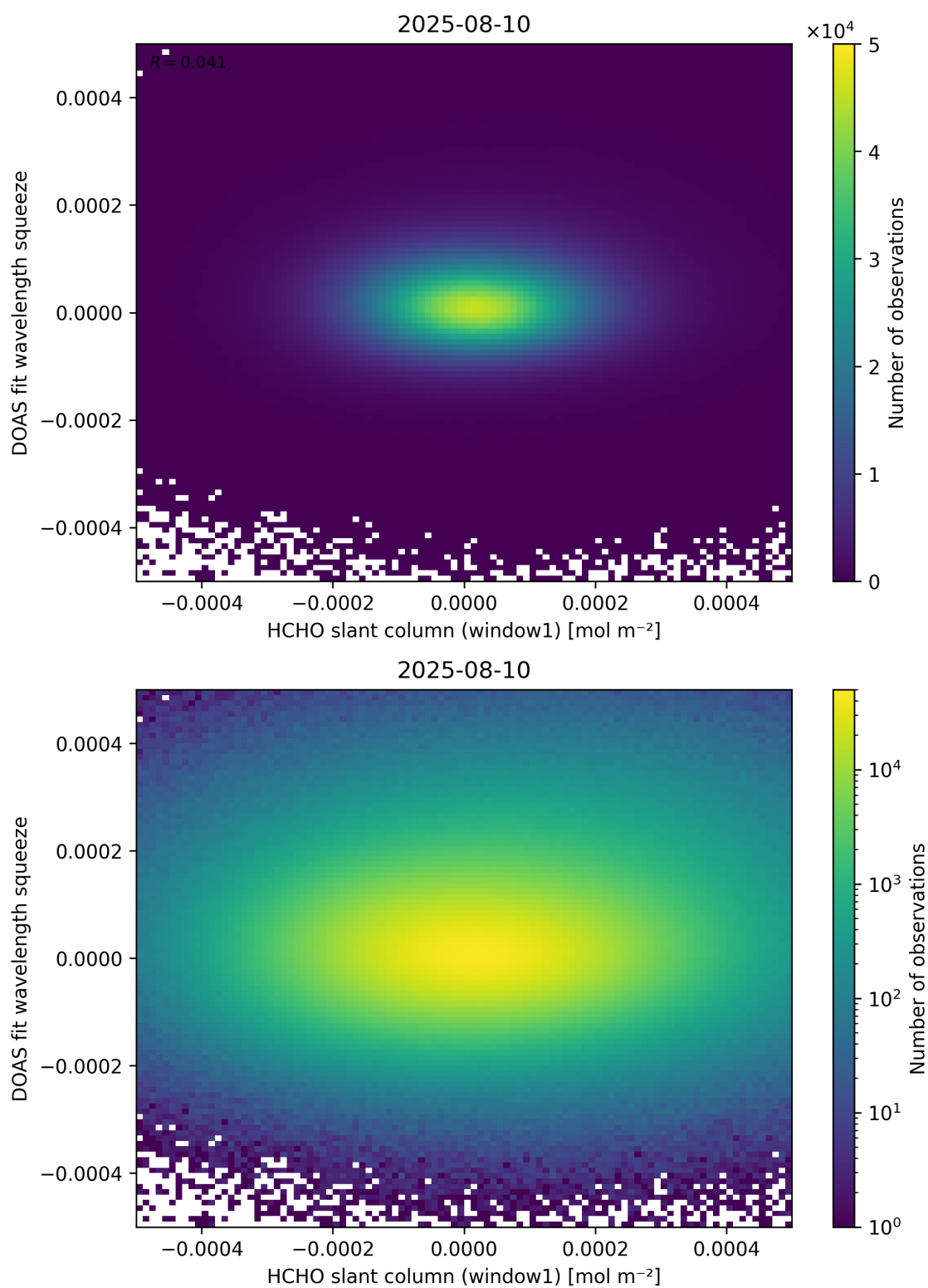
Figure 80: Scatter density plot of “HCHO slant column (window1)” against “DOAS fit wavelength squeeze” for 2025-08-09 to 2025-08-11.
