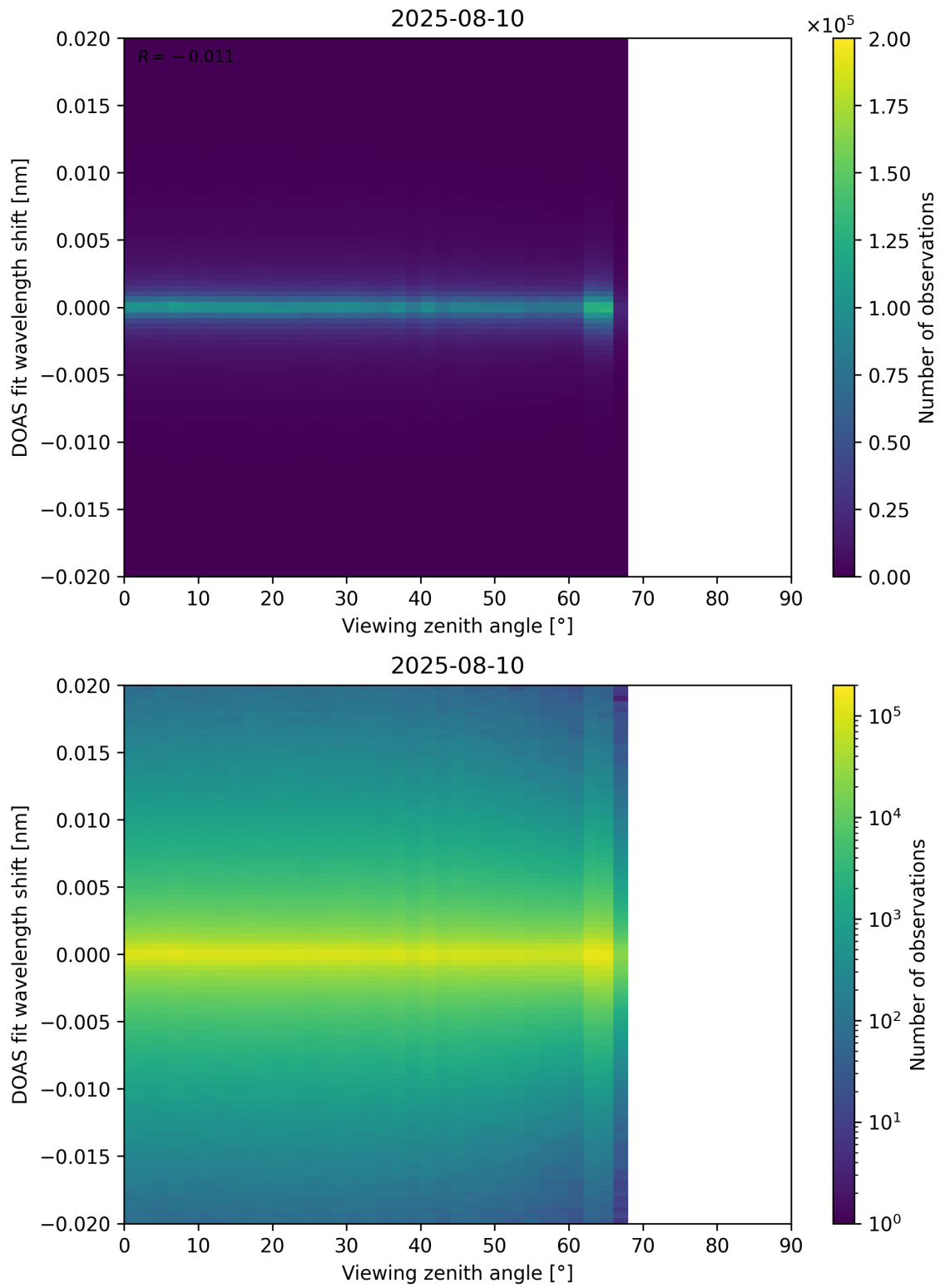
Figure 183: Scatter density plot of “Viewing zenith angle” against “DOAS fit wavelength shift” for 2025-08-09 to 2025-08-11.
