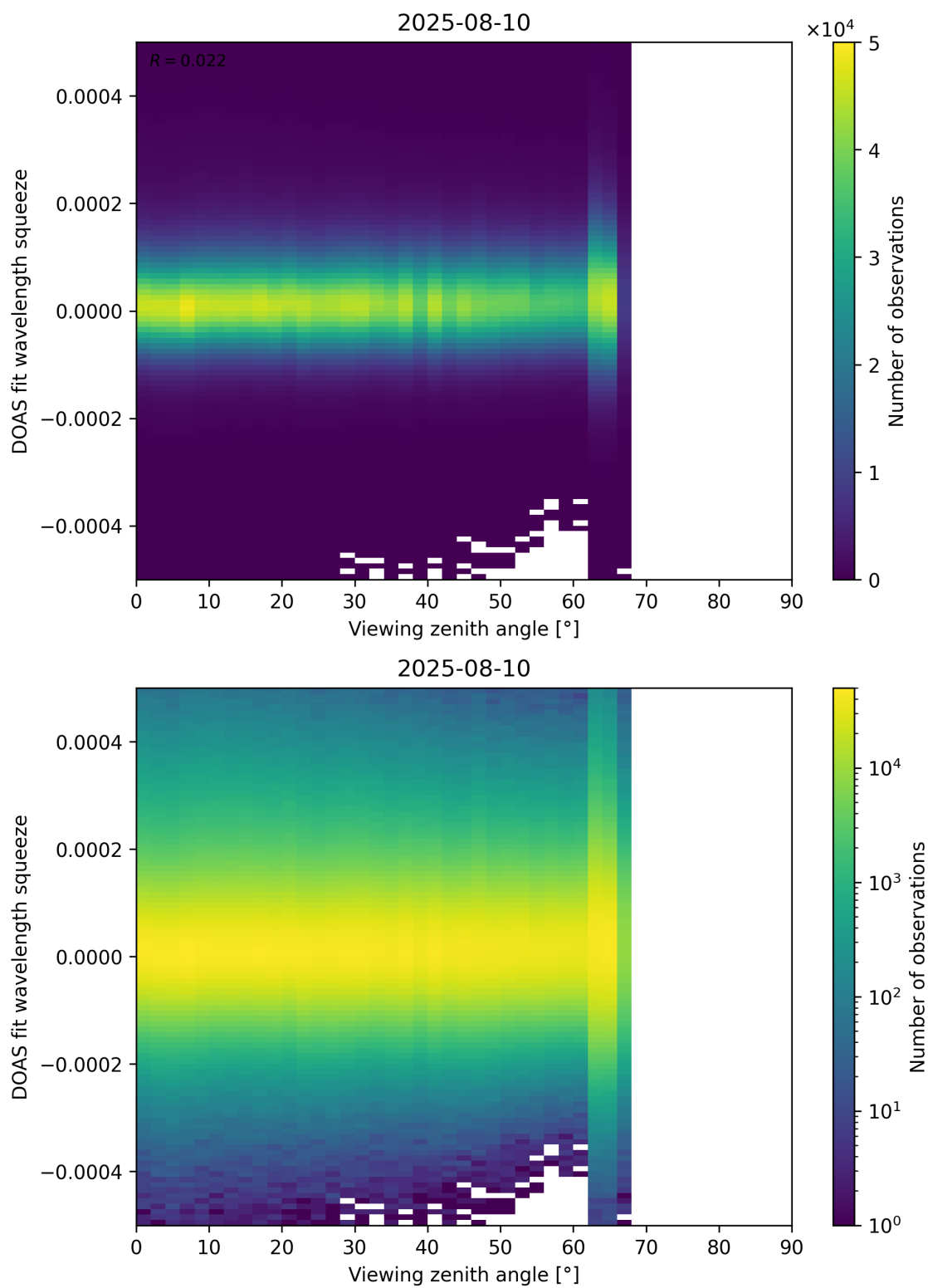
Figure 184: Scatter density plot of “Viewing zenith angle” against “DOAS fit wavelength squeeze” for 2025-08-09 to 2025-08-11.
