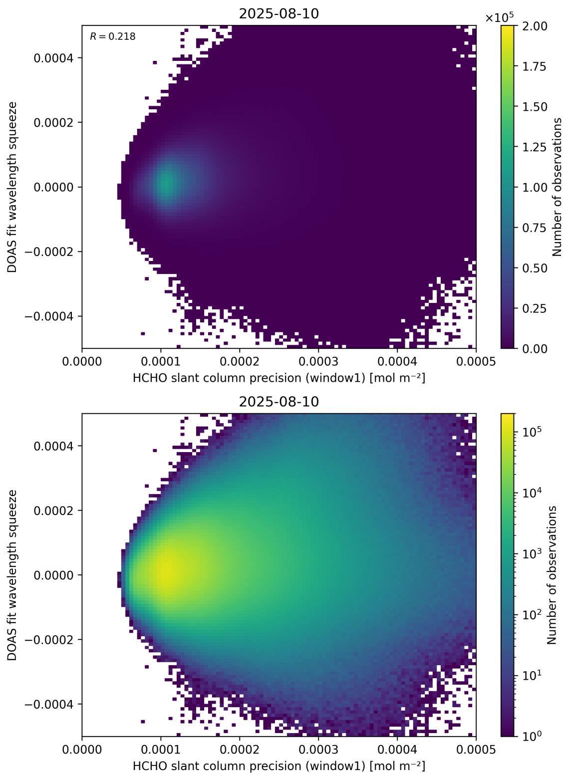
Figure 90: Scatter density plot of “HCHO slant column precision (window1)” against “DOAS fit wavelength squeeze” for 2025-08-09 to 2025-08-11.
