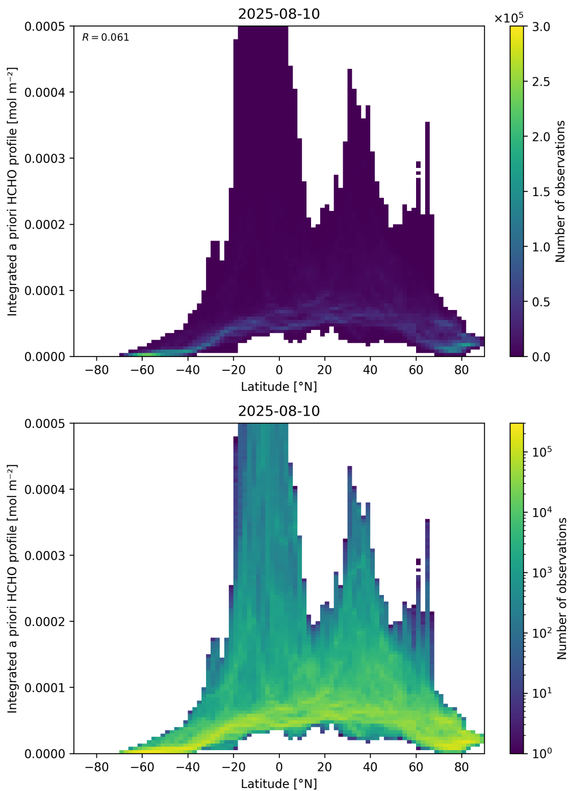
Figure 166: Scatter density plot of “Latitude” against “Integrated a priori HCHO profile” for 2025-08-09 to 2025-08-11.
