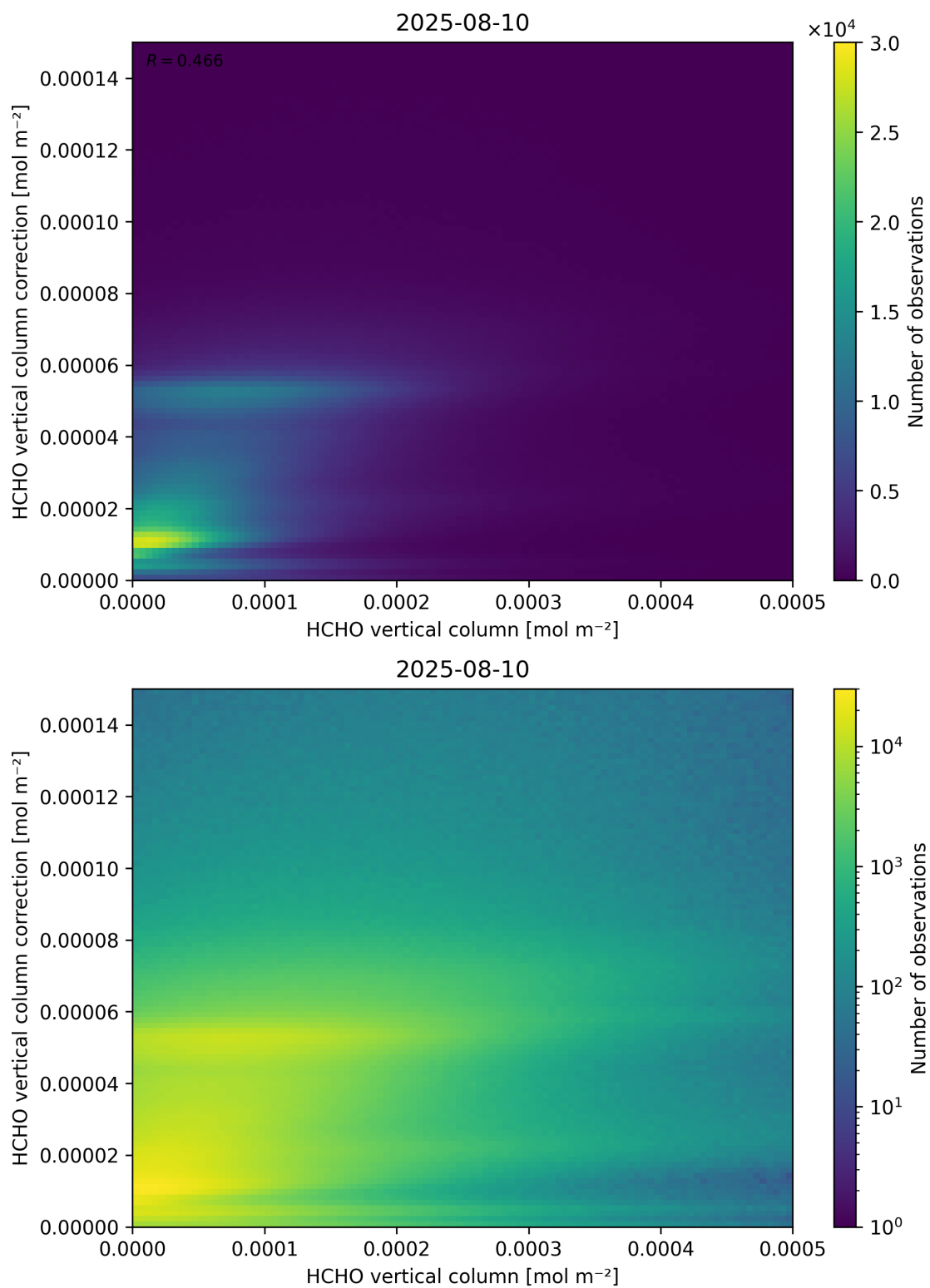
Figure 133: Scatter density plot of “HCHO vertical column” against “HCHO vertical column correction” for 2025-08-09 to 2025-08-11.
