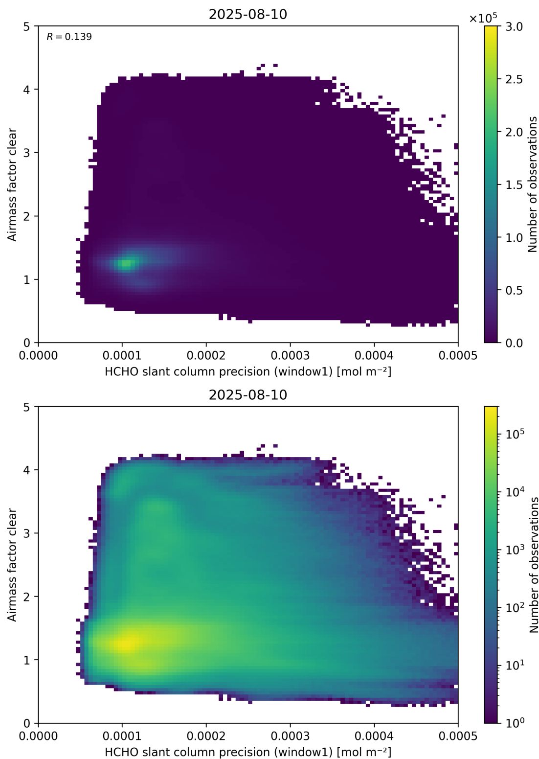
Figure 91: Scatter density plot of “HCHO slant column precision (window1)” against “Airmass factor clear” for 2025-08-09 to 2025-08-11.
