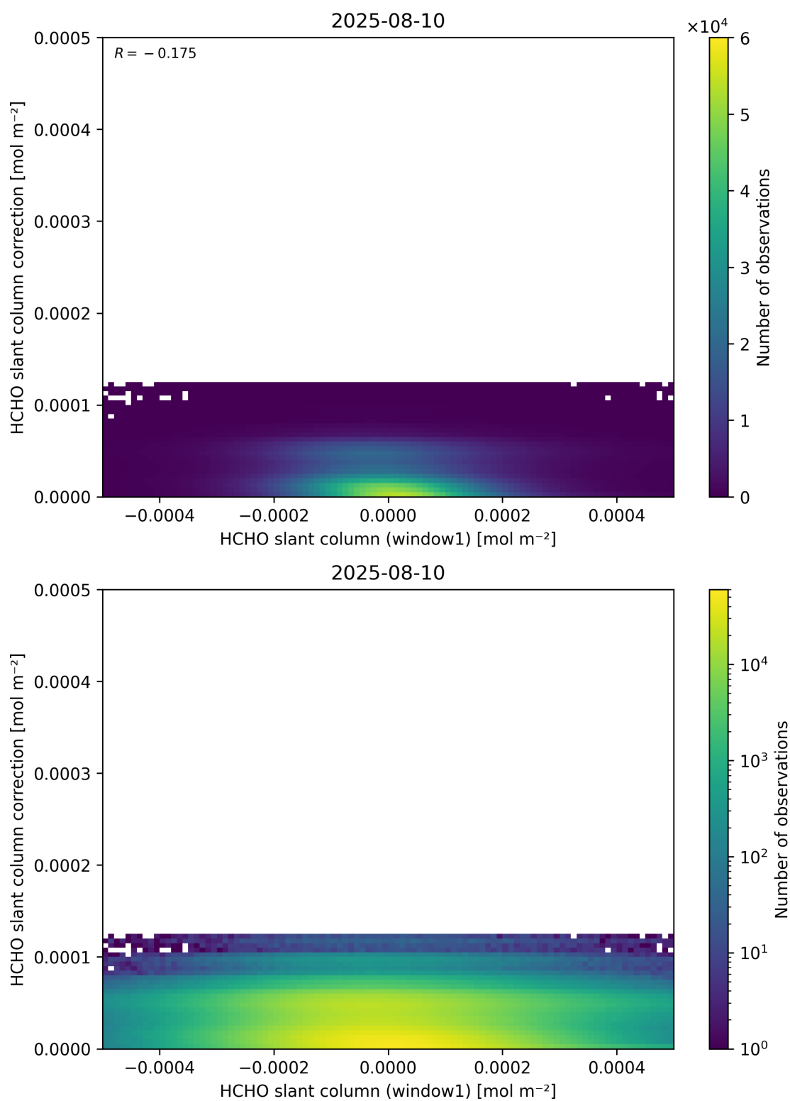
Figure 83: Scatter density plot of “HCHO slant column (window1)” against “HCHO slant column correction” for 2025-08-09 to 2025-08-11.
