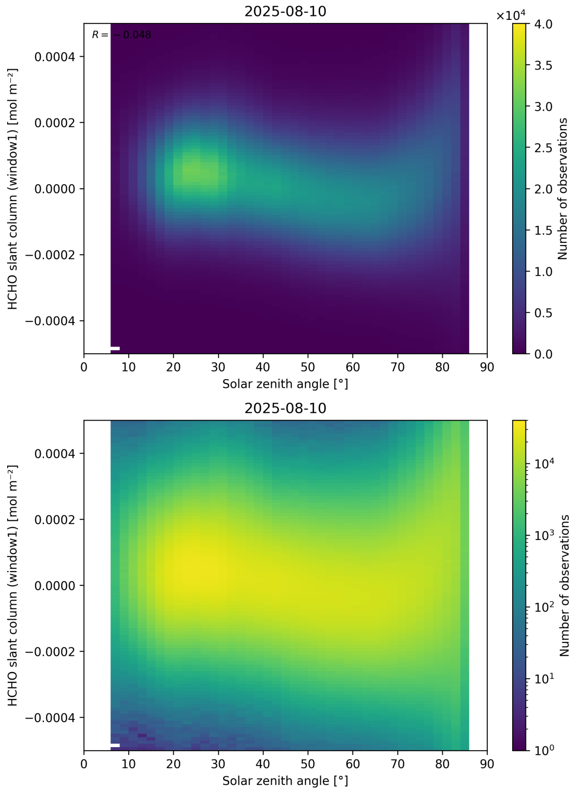
Figure 173: Scatter density plot of “Solar zenith angle” against “HCHO slant column (window1)” for 2025-08-09 to 2025-08-11.
