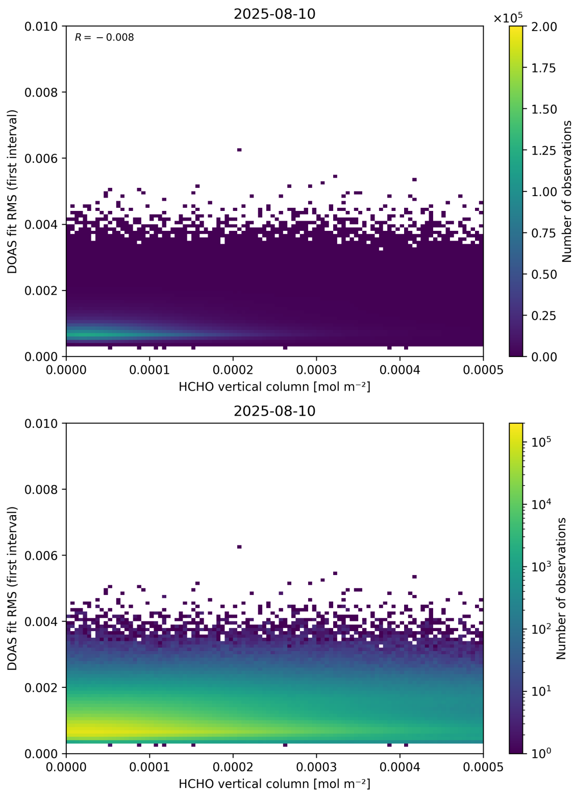
Figure 123: Scatter density plot of “HCHO vertical column” against “DOAS fit RMS (first interval)” for 2025-08-09 to 2025-08-11.
