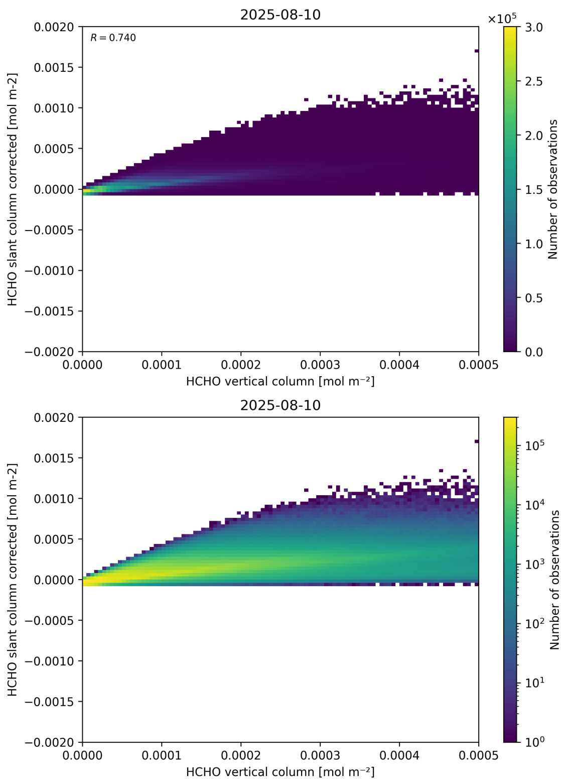
Figure 127: Scatter density plot of “HCHO vertical column” against “HCHO slant column corrected” for 2025-08-09 to 2025-08-11.
