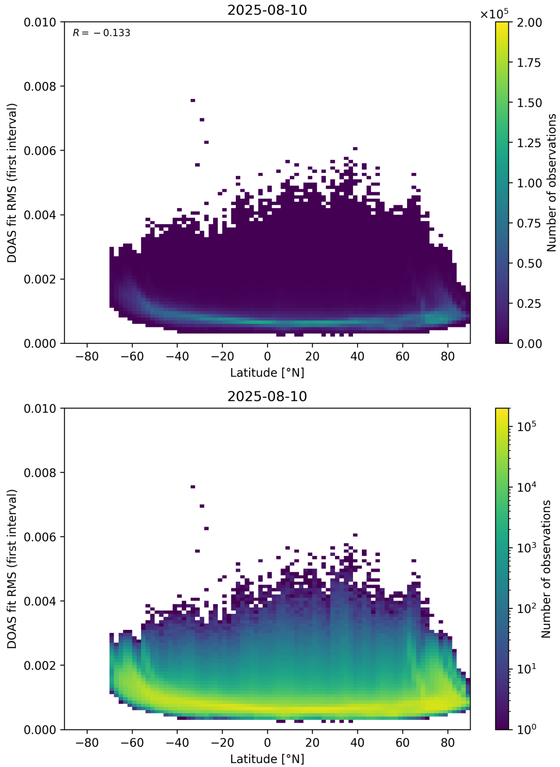
Figure 153: Scatter density plot of “Latitude” against “DOAS fit RMS (first interval)” for 2025-08-09 to 2025-08-11.
