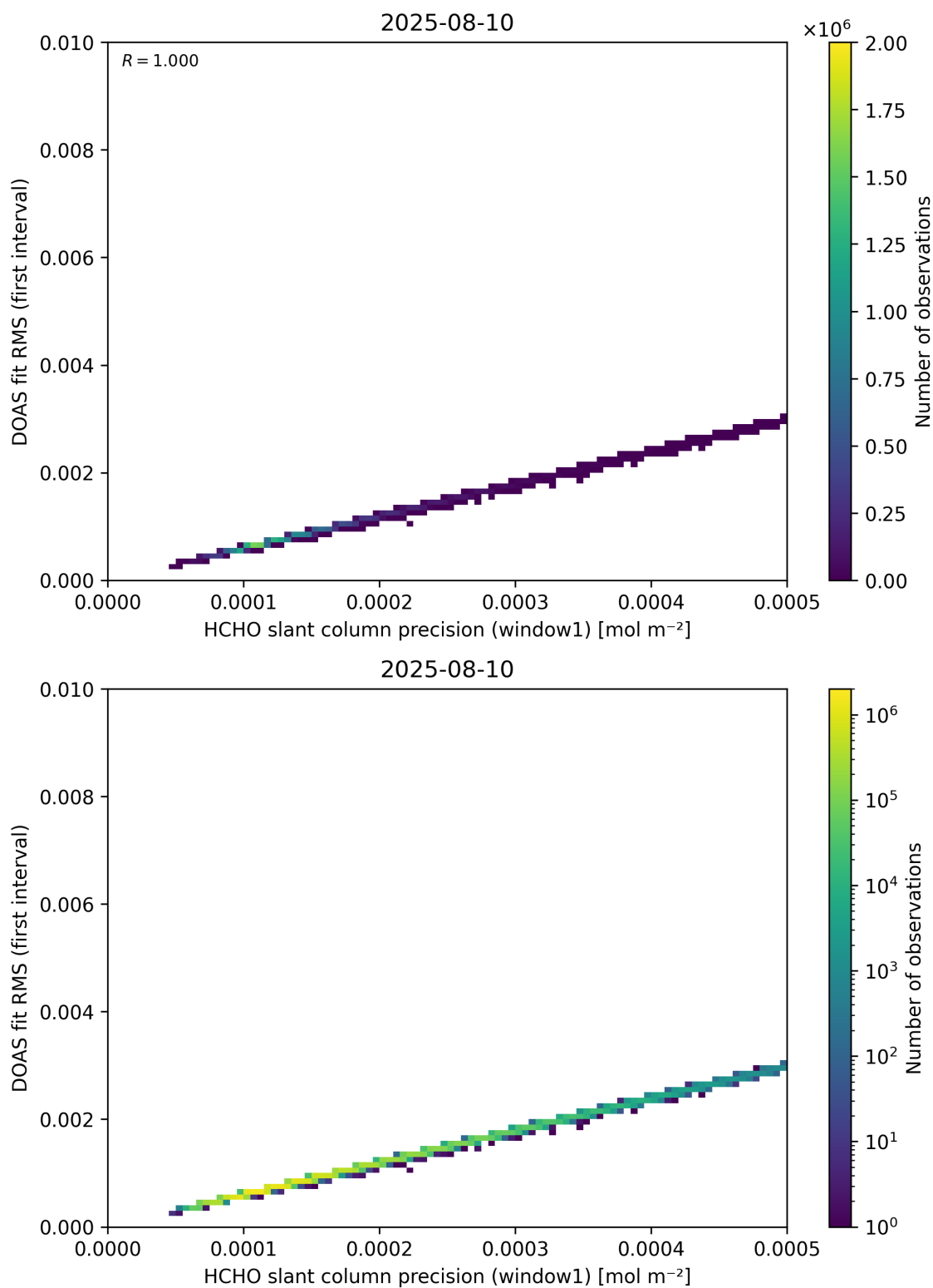
Figure 88: Scatter density plot of “HCHO slant column precision (window1)” against “DOAS fit RMS (first interval)” for 2025-08-09 to 2025-08-11.
