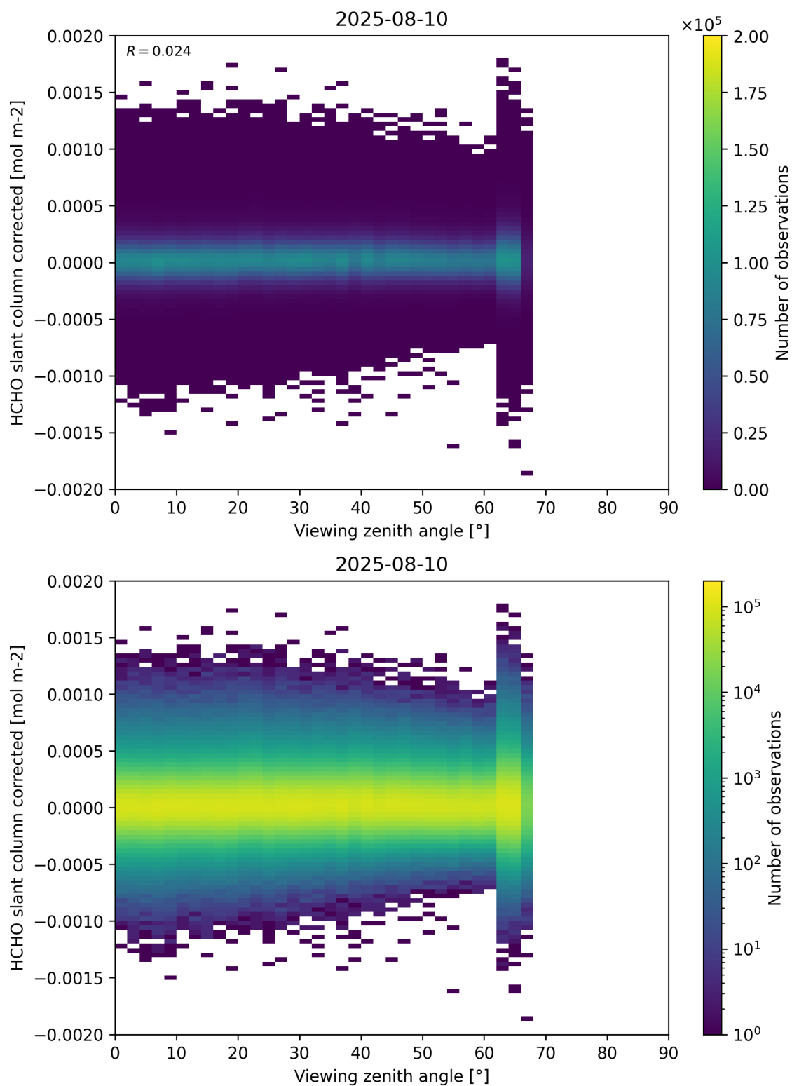
Figure 186: Scatter density plot of “Viewing zenith angle” against “HCHO slant column corrected” for 2025-08-09 to 2025-08-11.
