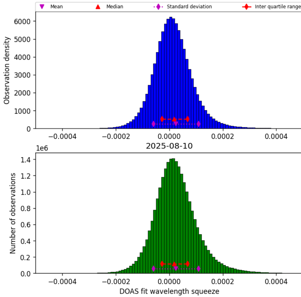
Figure 45: Histogram of “DOAS fit wavelength squeeze” for 2025-08-09 to 2025-08-11
