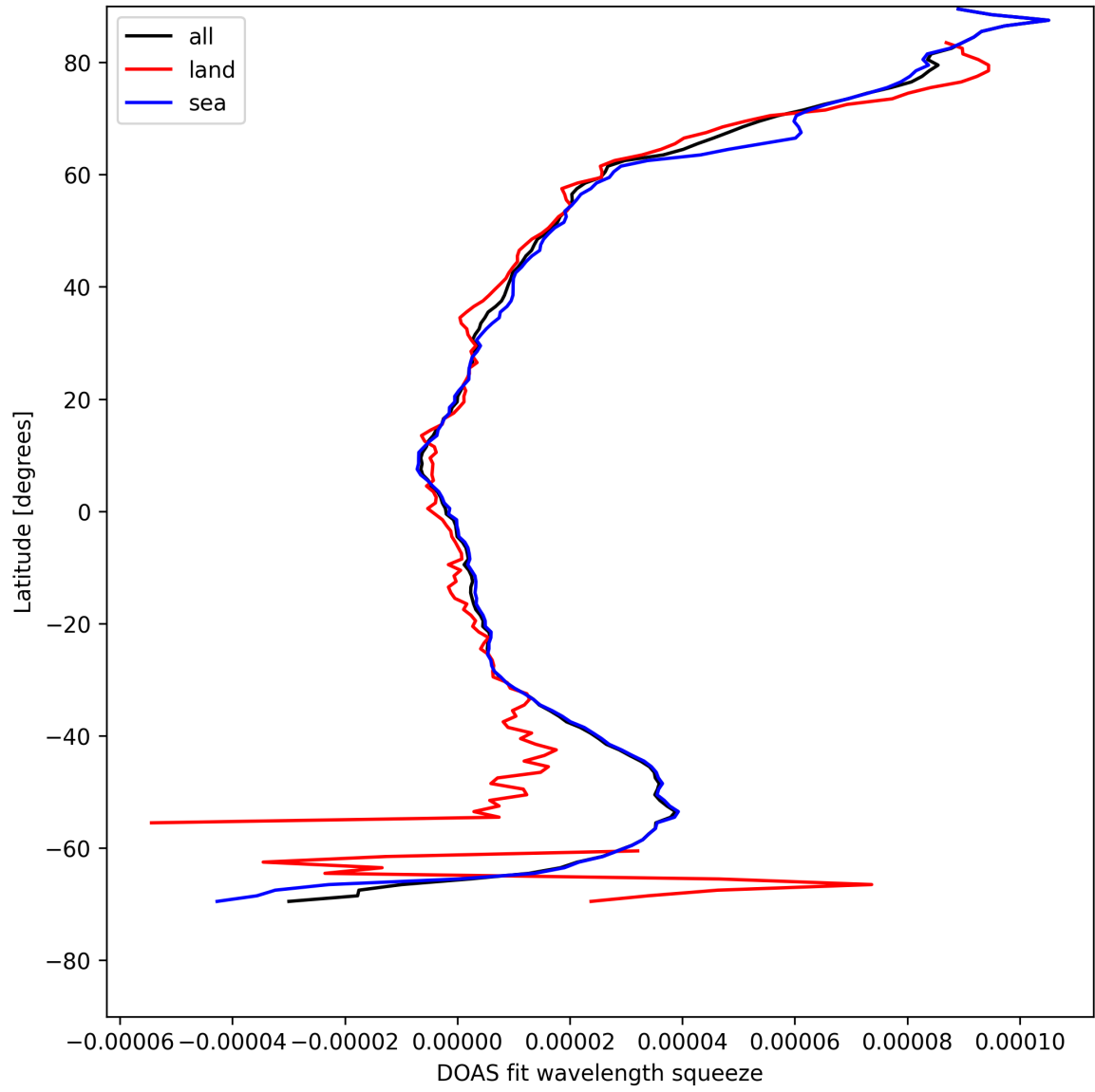
Figure 31: Zonal average of “DOAS fit wavelength squeeze” for 2025-08-09 to 2025-08-11.
