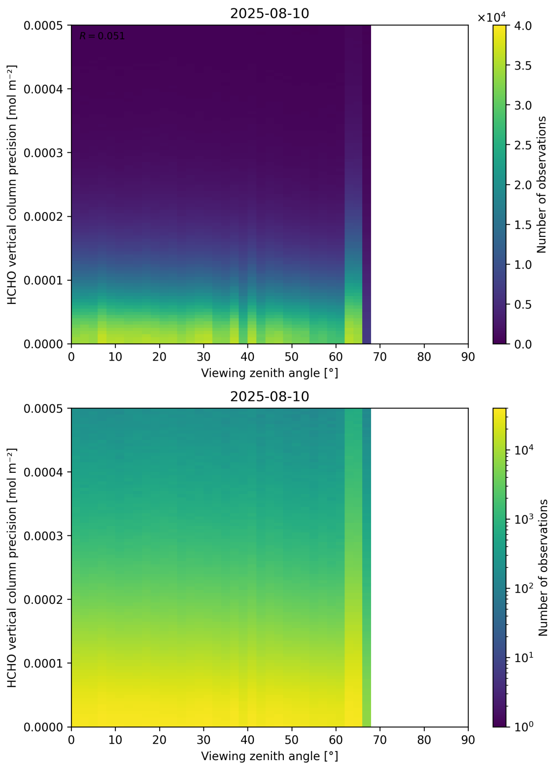
Figure 194: Scatter density plot of “Viewing zenith angle” against “HCHO vertical column precision” for 2025-08-09 to 2025-08-11.
