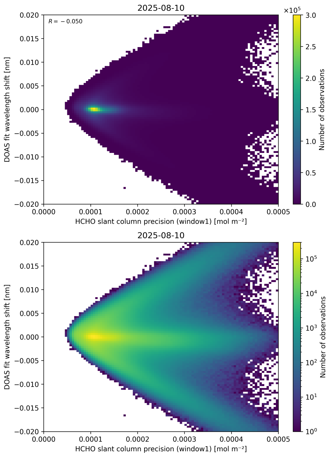
Figure 89: Scatter density plot of “HCHO slant column precision (window1)” against “DOAS fit wavelength shift” for 2025-08-09 to 2025-08-11.
