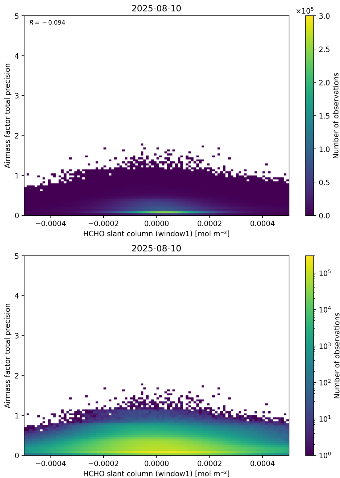
Figure 86: Scatter density plot of “HCHO slant column (window1)” against “Airmass factor total precision” for 2025-08-09 to 2025-08-11.
