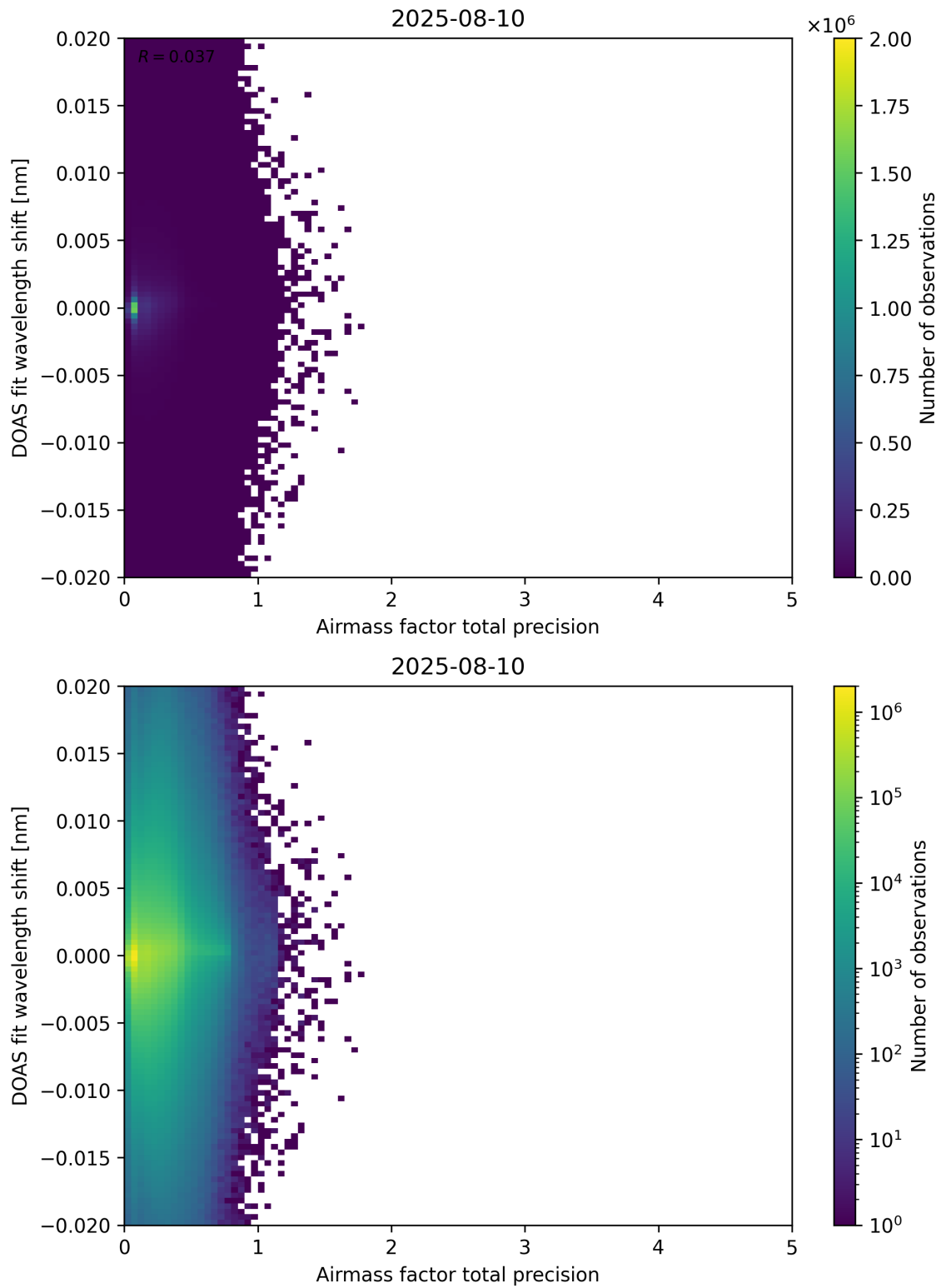
Figure 106: Scatter density plot of “Airmass factor total precision” against “DOAS fit wavelength shift” for 2025-08-09 to 2025-08-11.
