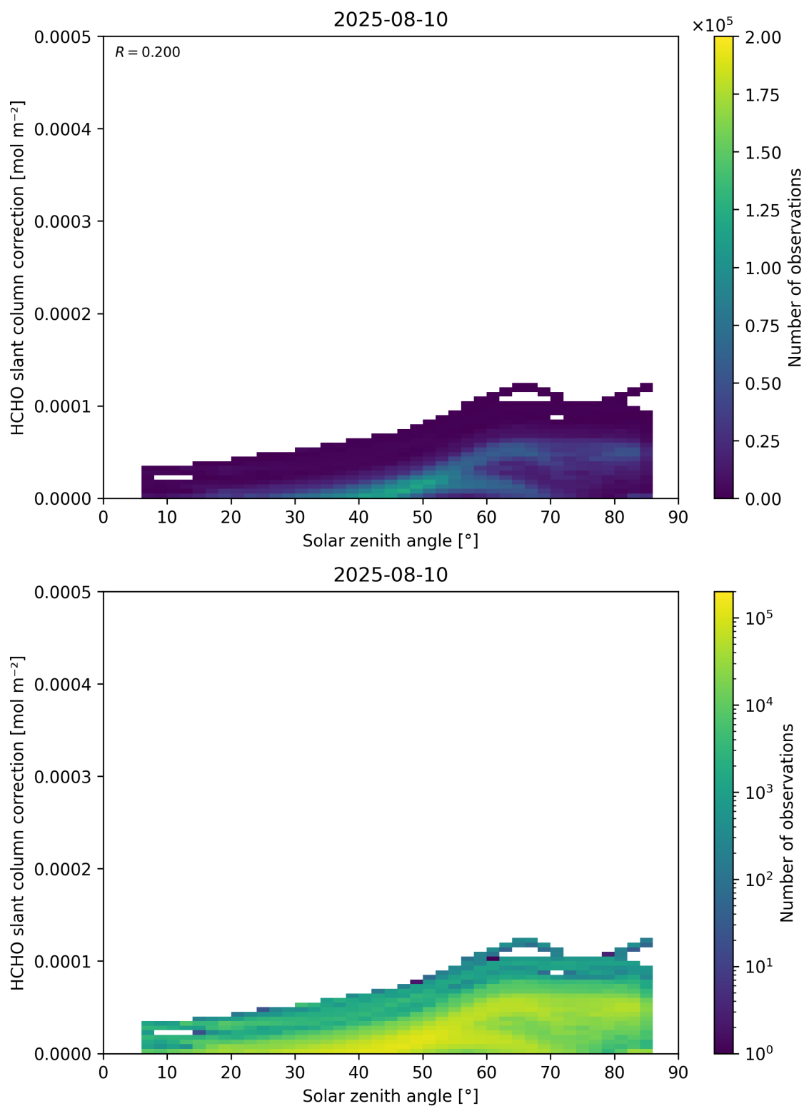
Figure 172: Scatter density plot of “Solar zenith angle” against “HCHO slant column correction” for 2025-08-09 to 2025-08-11.
