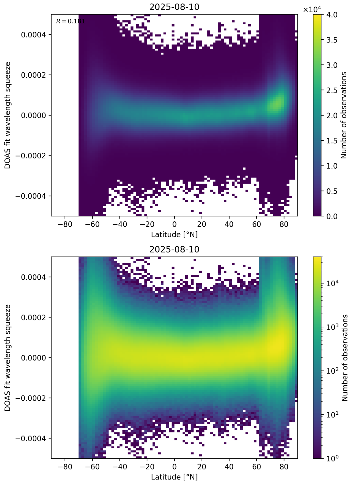
Figure 155: Scatter density plot of “Latitude” against “DOAS fit wavelength squeeze” for 2025-08-09 to 2025-08-11.
