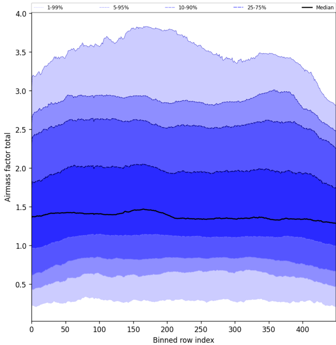
Figure 54: Along track statistics of “Airmass factor total” for 2025-08-09 to 2025-08-11
