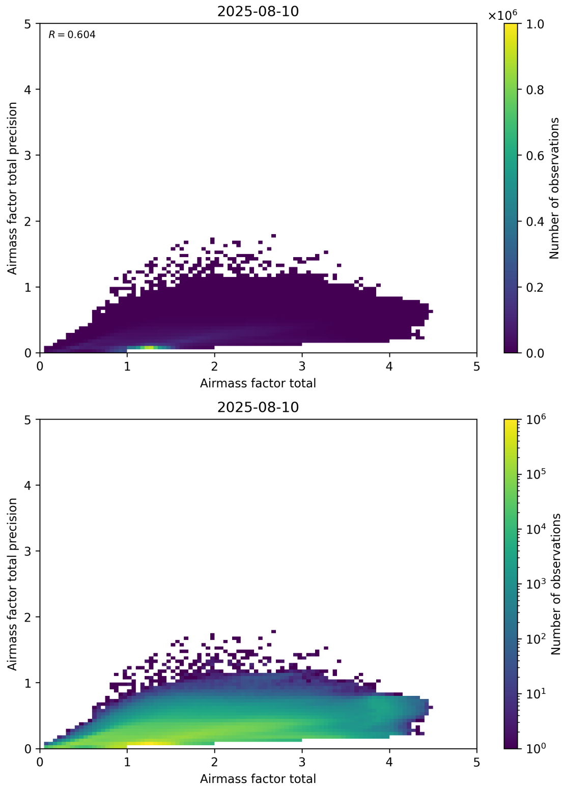
Figure 103: Scatter density plot of “Airmass factor total” against “Airmass factor total precision” for 2025-08-09 to 2025-08-11.
