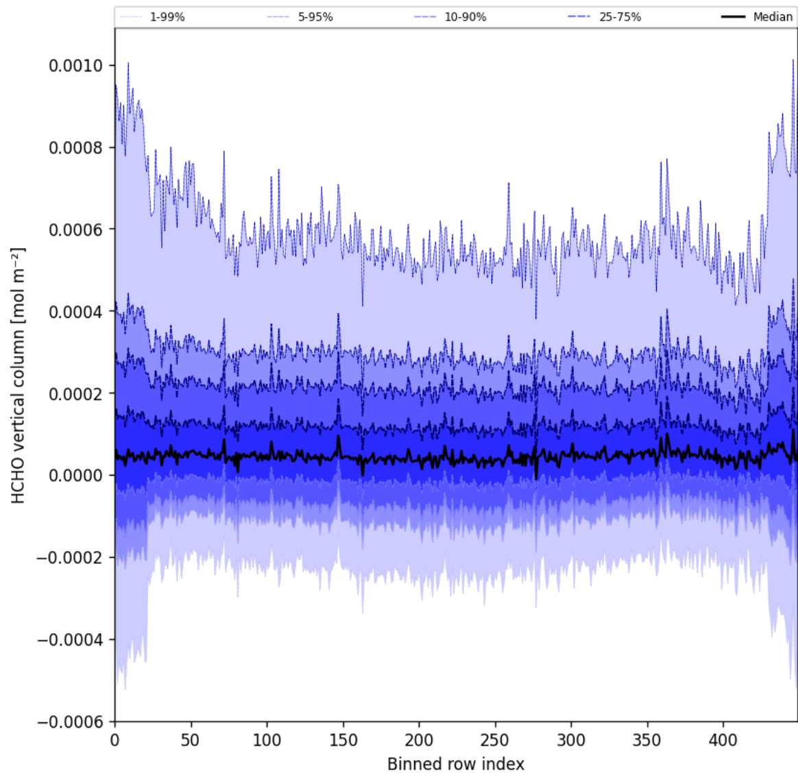
Figure 49: Along track statistics of “HCHO vertical column” for 2025-08-09 to 2025-08-11
