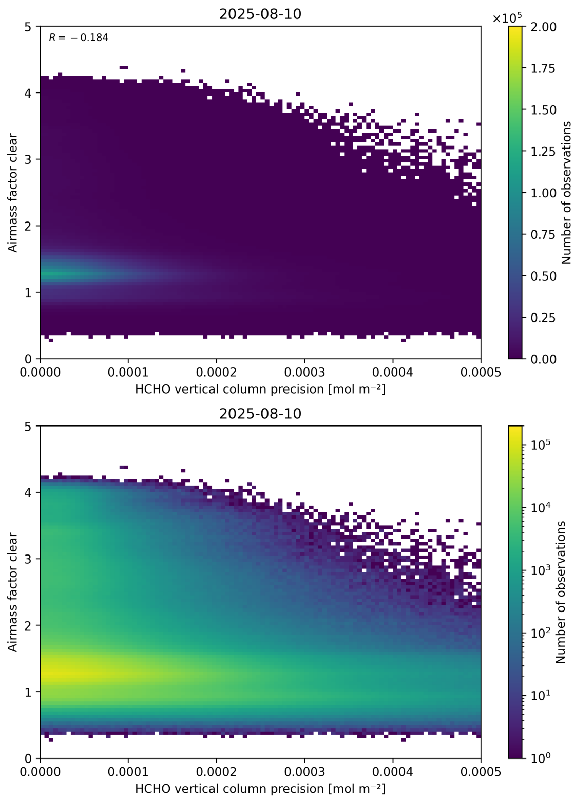
Figure 139: Scatter density plot of “HCHO vertical column precision” against “Airmass factor clear” for 2025-08-09 to 2025-08-11.
