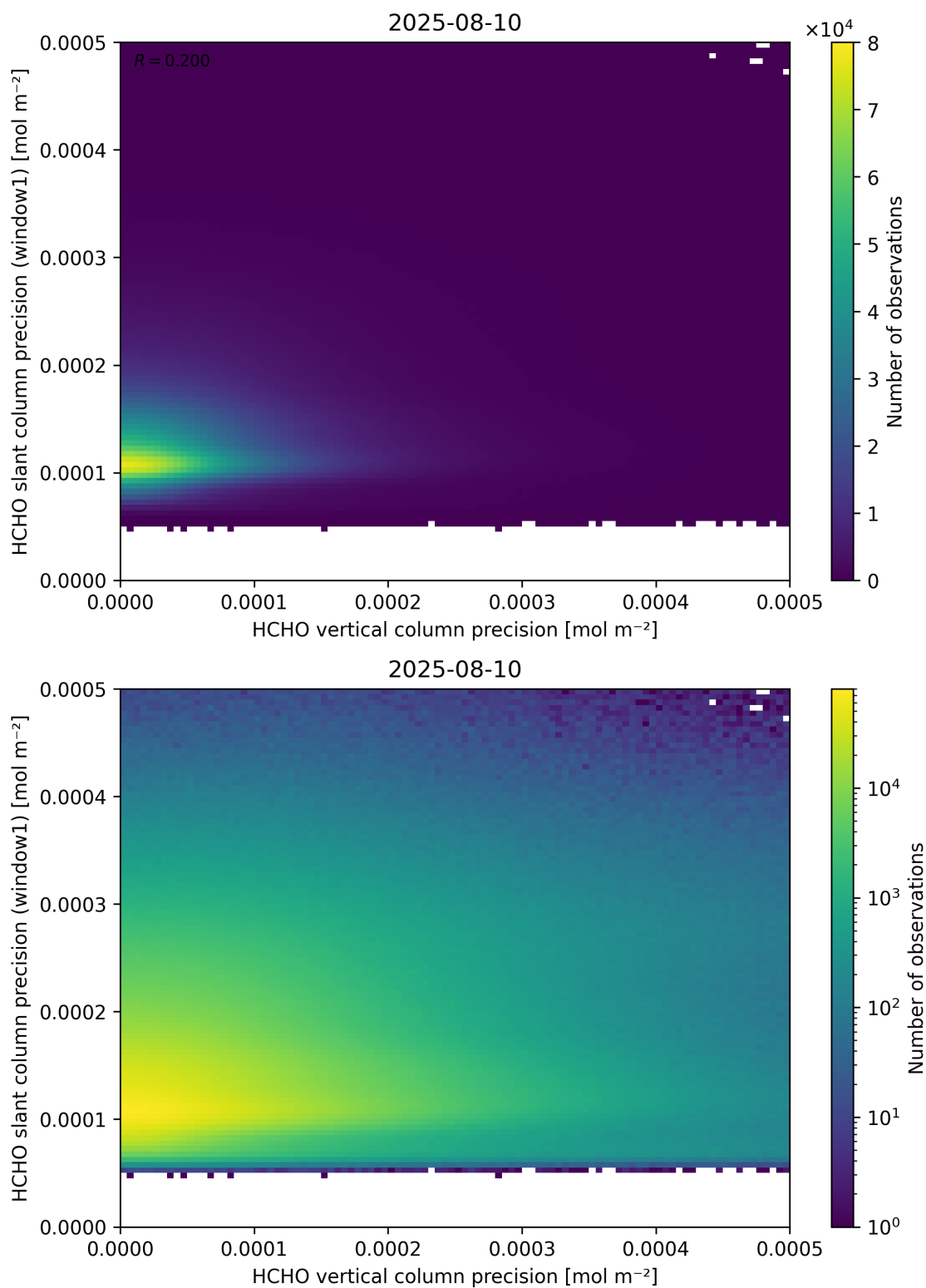
Figure 143: Scatter density plot of “HCHO vertical column precision” against “HCHO slant column precision (window1)” for 2025-08-09 to 2025-08-11.
