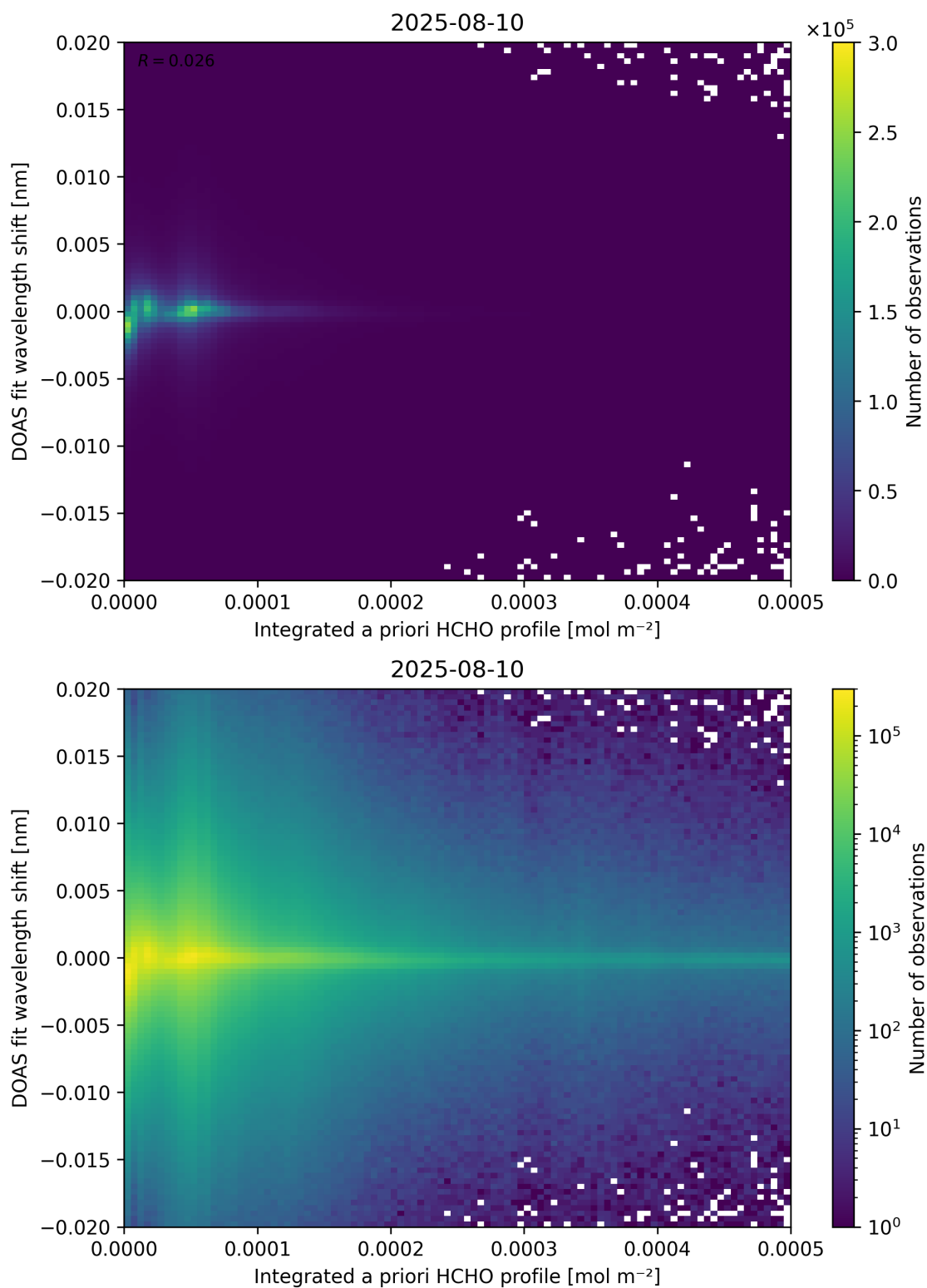
Figure 149: Scatter density plot of “Integrated a priori HCHO profile” against “DOAS fit wavelength shift” for 2025-08-09 to 2025-08-11.
