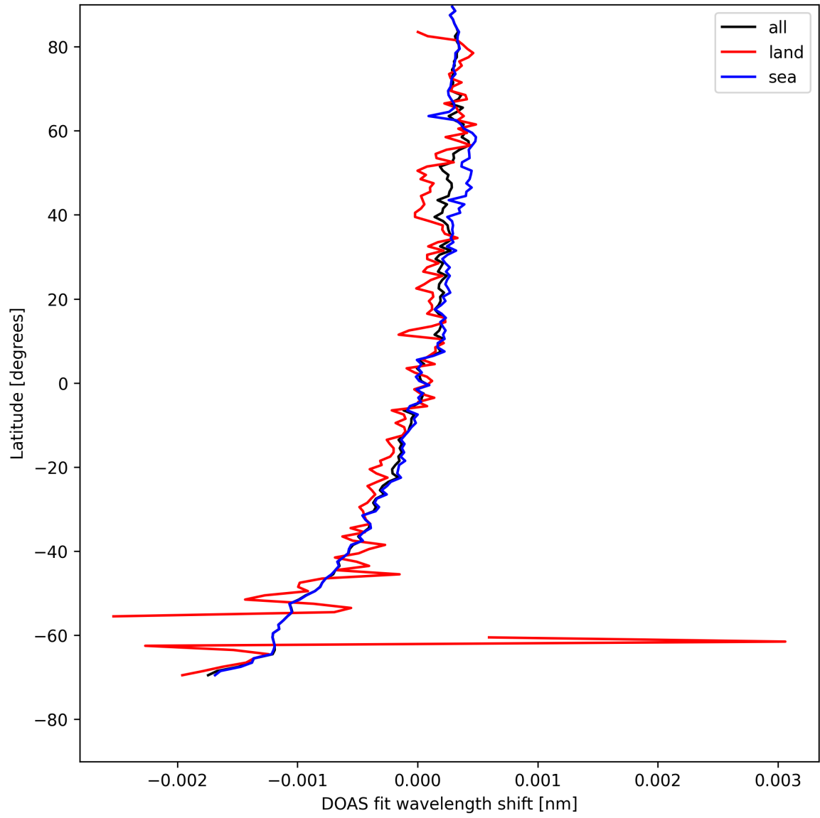
Figure 30: Zonal average of “DOAS fit wavelength shift” for 2025-08-09 to 2025-08-11.
