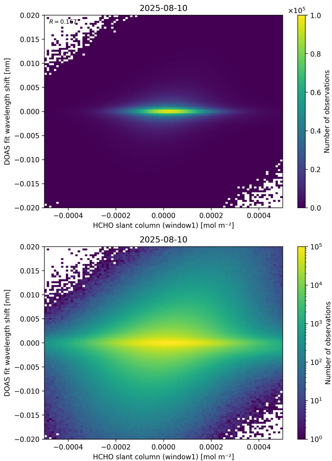
Figure 79: Scatter density plot of “HCHO slant column (window1)” against “DOAS fit wavelength shift” for 2025-08-09 to 2025-08-11.
