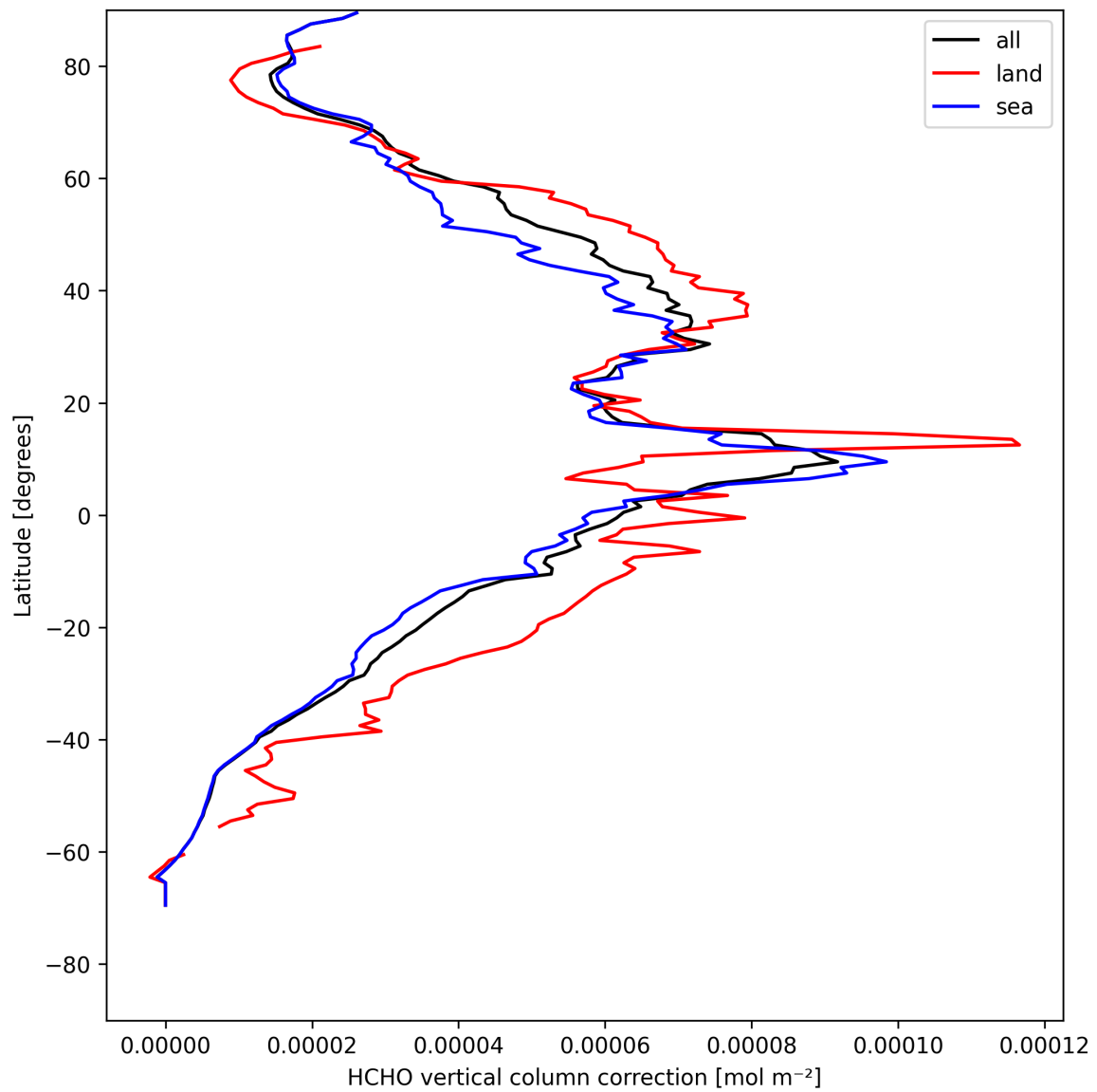
Figure 23: Zonal average of “HCHO vertical column correction” for 2025-08-09 to 2025-08-11.
