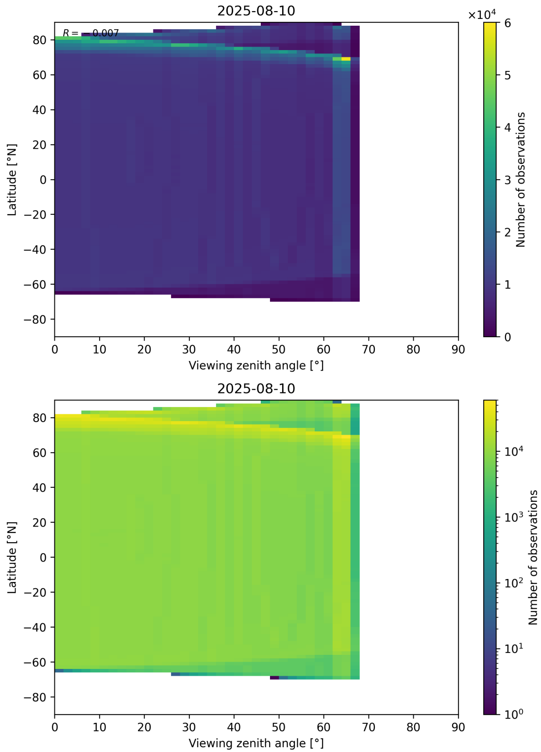
Figure 196: Scatter density plot of “Viewing zenith angle” against “Latitude” for 2025-08-09 to 2025-08-11.
