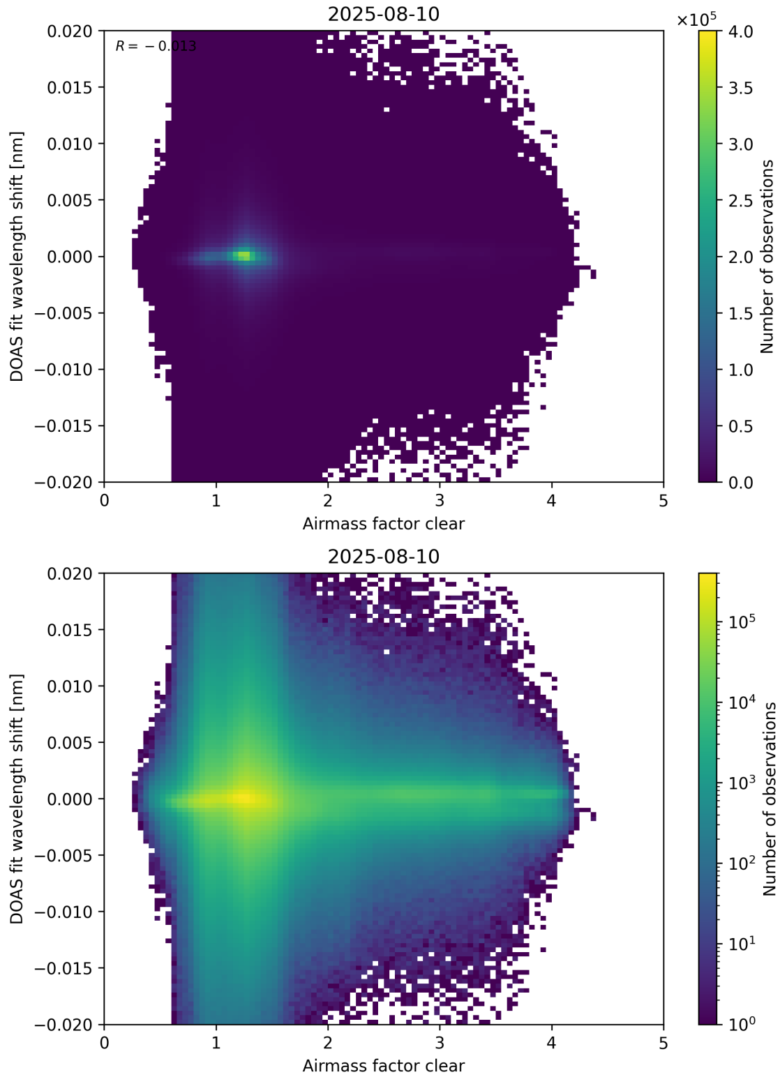
Figure 72: Scatter density plot of “Airmass factor clear” against “DOAS fit wavelength shift” for 2025-08-09 to 2025-08-11.
