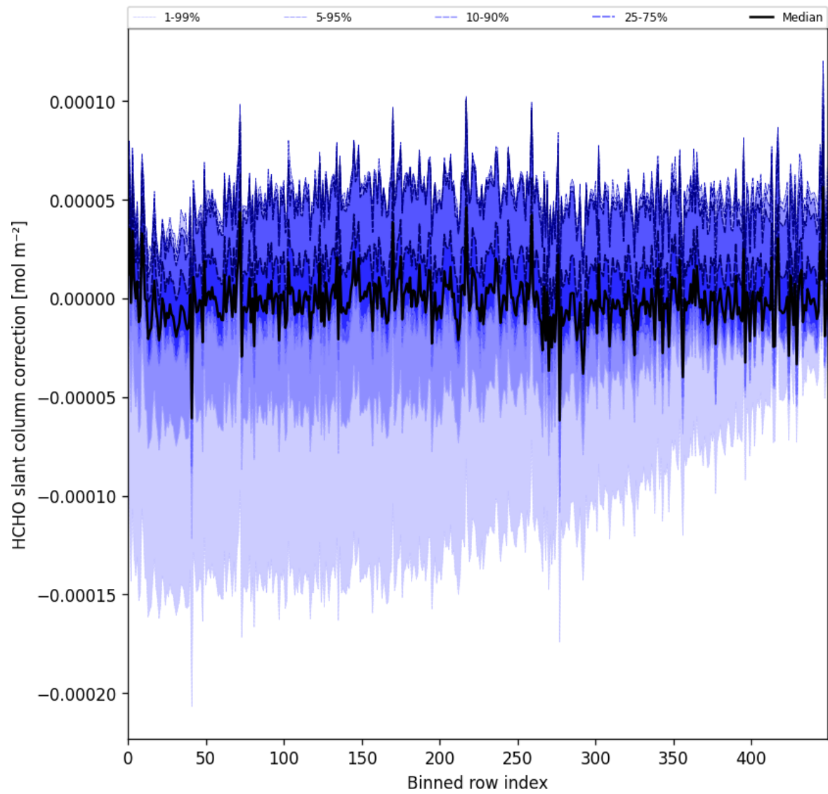
Figure 61: Along track statistics of “HCHO slant column correction” for 2025-08-09 to 2025-08-11
