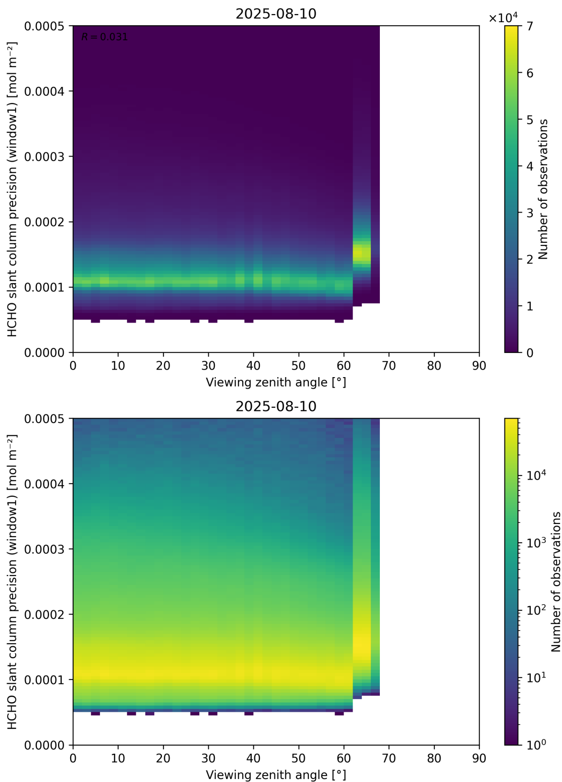
Figure 189: Scatter density plot of “Viewing zenith angle” against “HCHO slant column precision (window1)” for 2025-08-09 to 2025-08-11.
