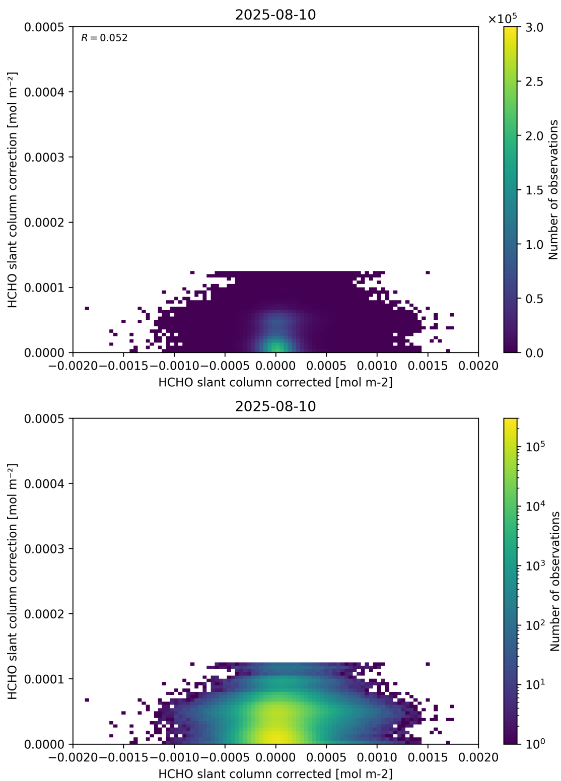
Figure 77: Scatter density plot of “HCHO slant column corrected” against “HCHO slant column correction” for 2025-08-09 to 2025-08-11.
