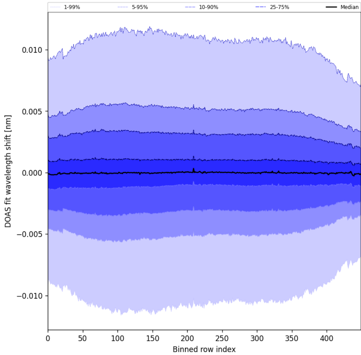
Figure 58: Along track statistics of “DOAS fit wavelength shift” for 2025-08-09 to 2025-08-11
