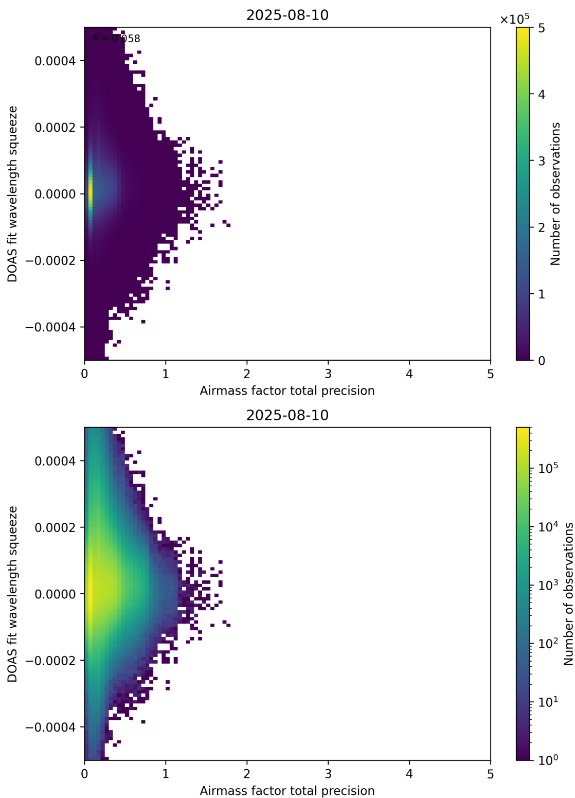
Figure 107: Scatter density plot of “Airmass factor total precision” against “DOAS fit wavelength squeeze” for 2025-08-09 to 2025-08-11.
