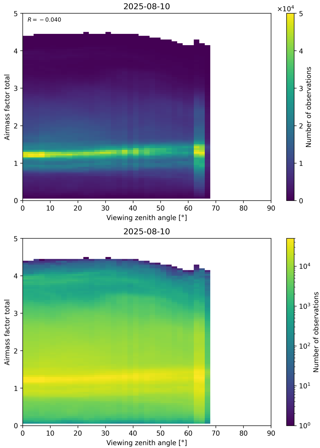
Figure 190: Scatter density plot of “Viewing zenith angle” against “Airmass factor total” for 2025-08-09 to 2025-08-11.
