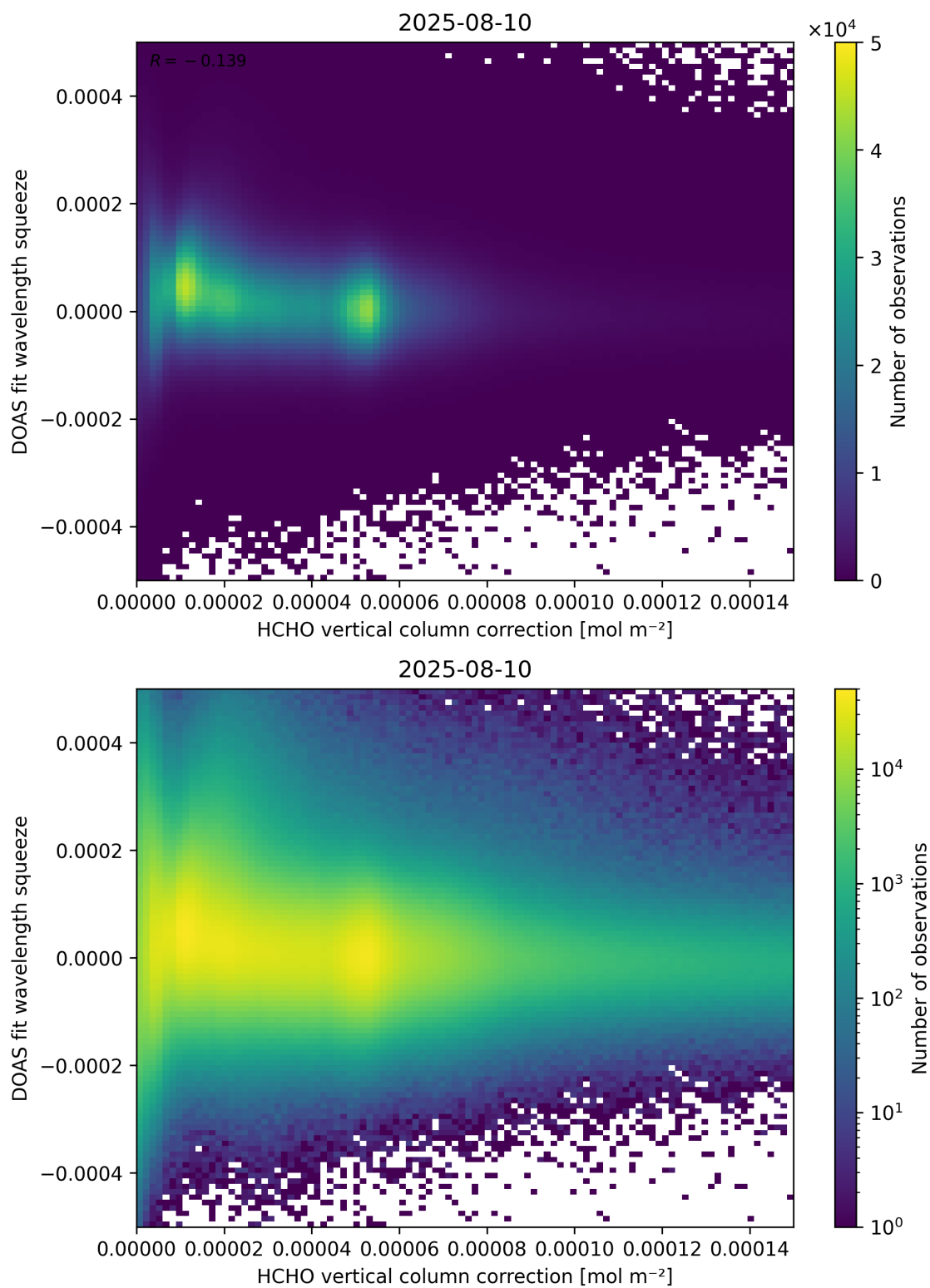
Figure 114: Scatter density plot of “HCHO vertical column correction” against “DOAS fit wavelength squeeze” for 2025-08-09 to 2025-08-11.
