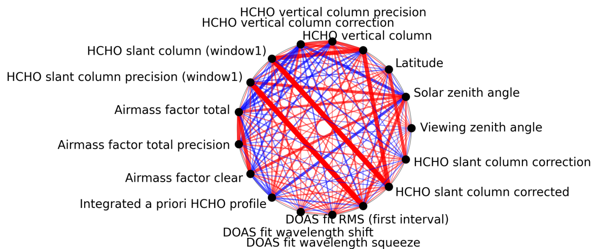
Figure 1: Map of correlation graph for 2025-08-09 to 2025-08-11.
