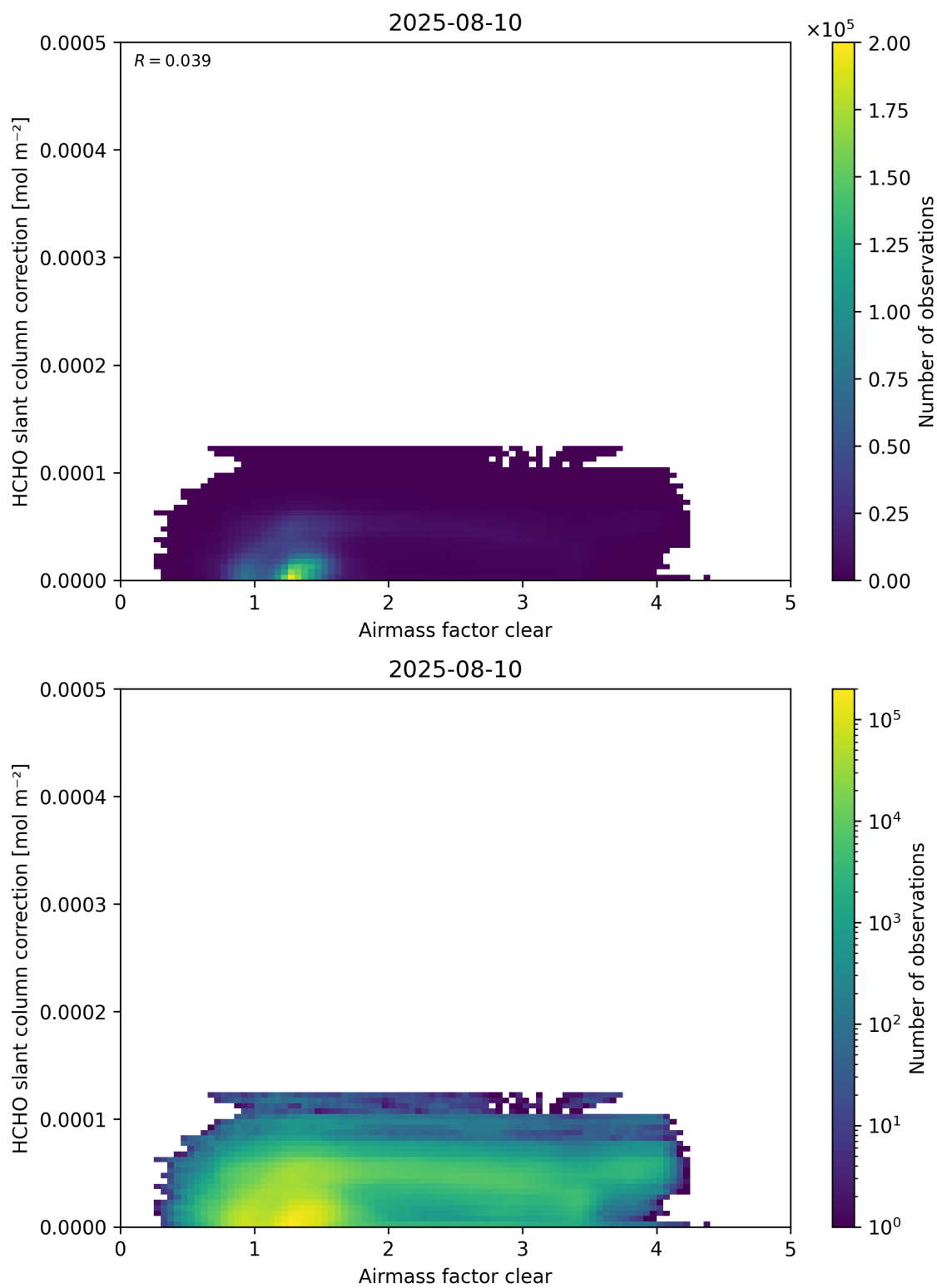
Figure 75: Scatter density plot of “Airmass factor clear” against “HCHO slant column correction” for 2025-08-09 to 2025-08-11.
