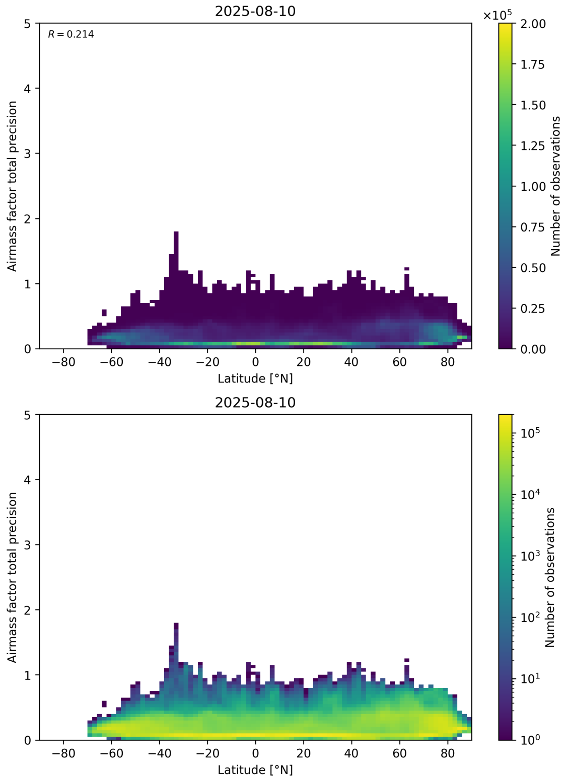
Figure 162: Scatter density plot of “Latitude” against “Airmass factor total precision” for 2025-08-09 to 2025-08-11.
