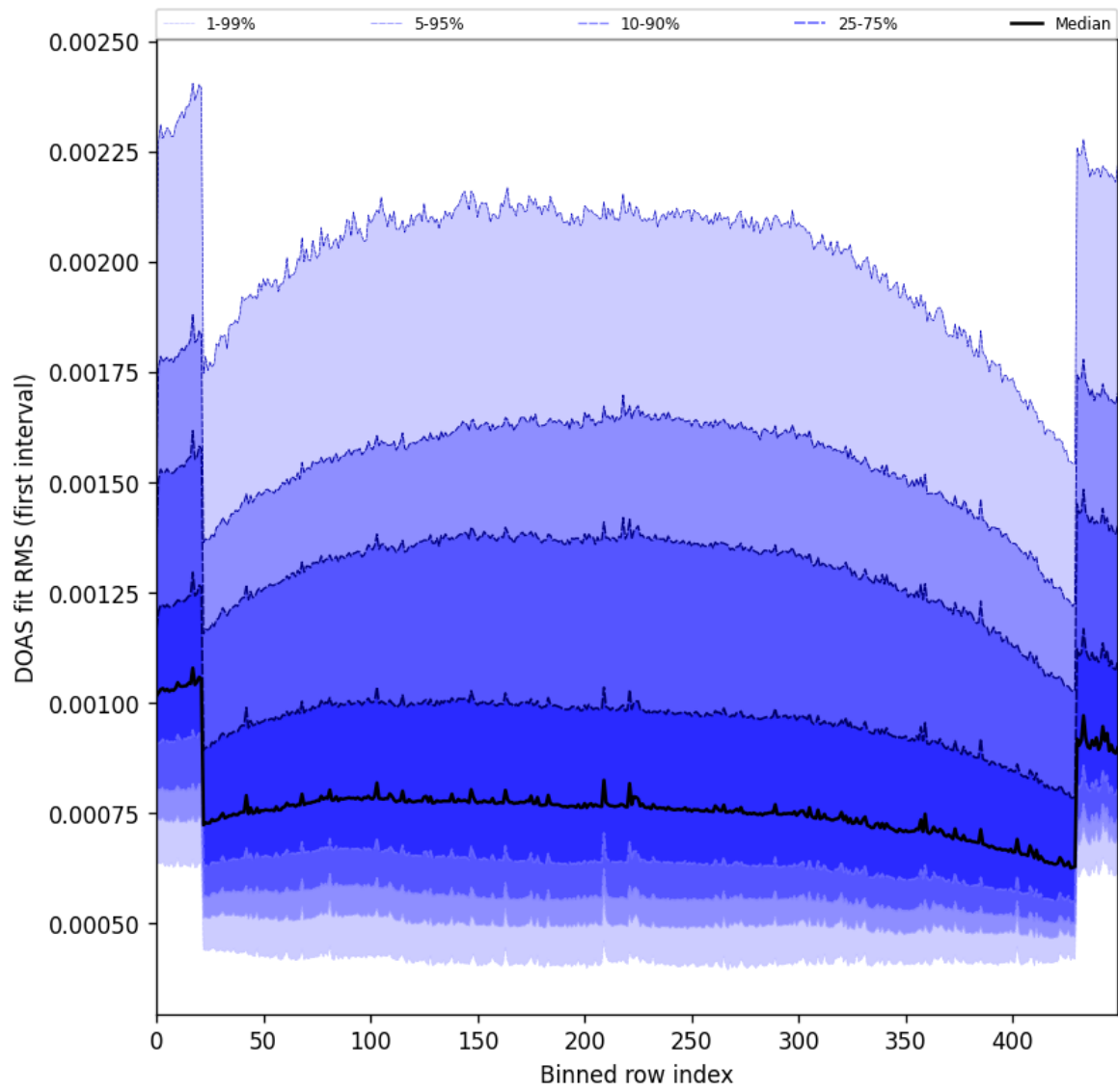
Figure 60: Along track statistics of “DOAS fit RMS (first interval)” for 2025-08-09 to 2025-08-11
