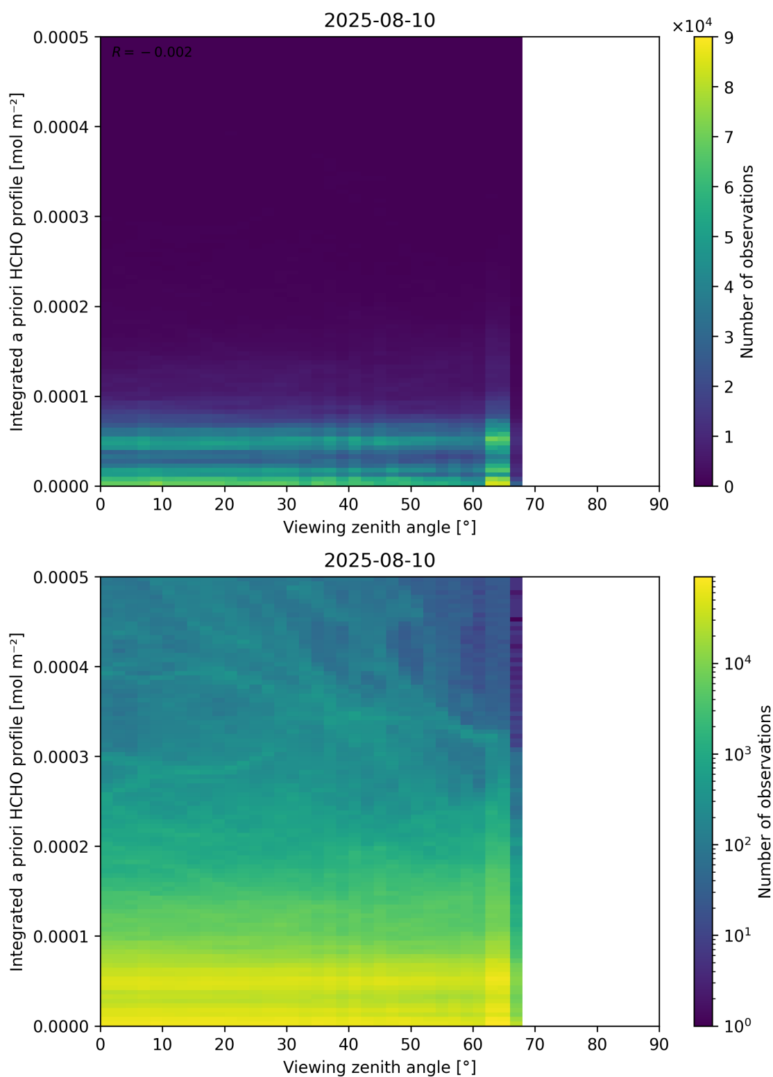
Figure 195: Scatter density plot of “Viewing zenith angle” against “Integrated a priori HCHO profile” for 2025-08-09 to 2025-08-11.
