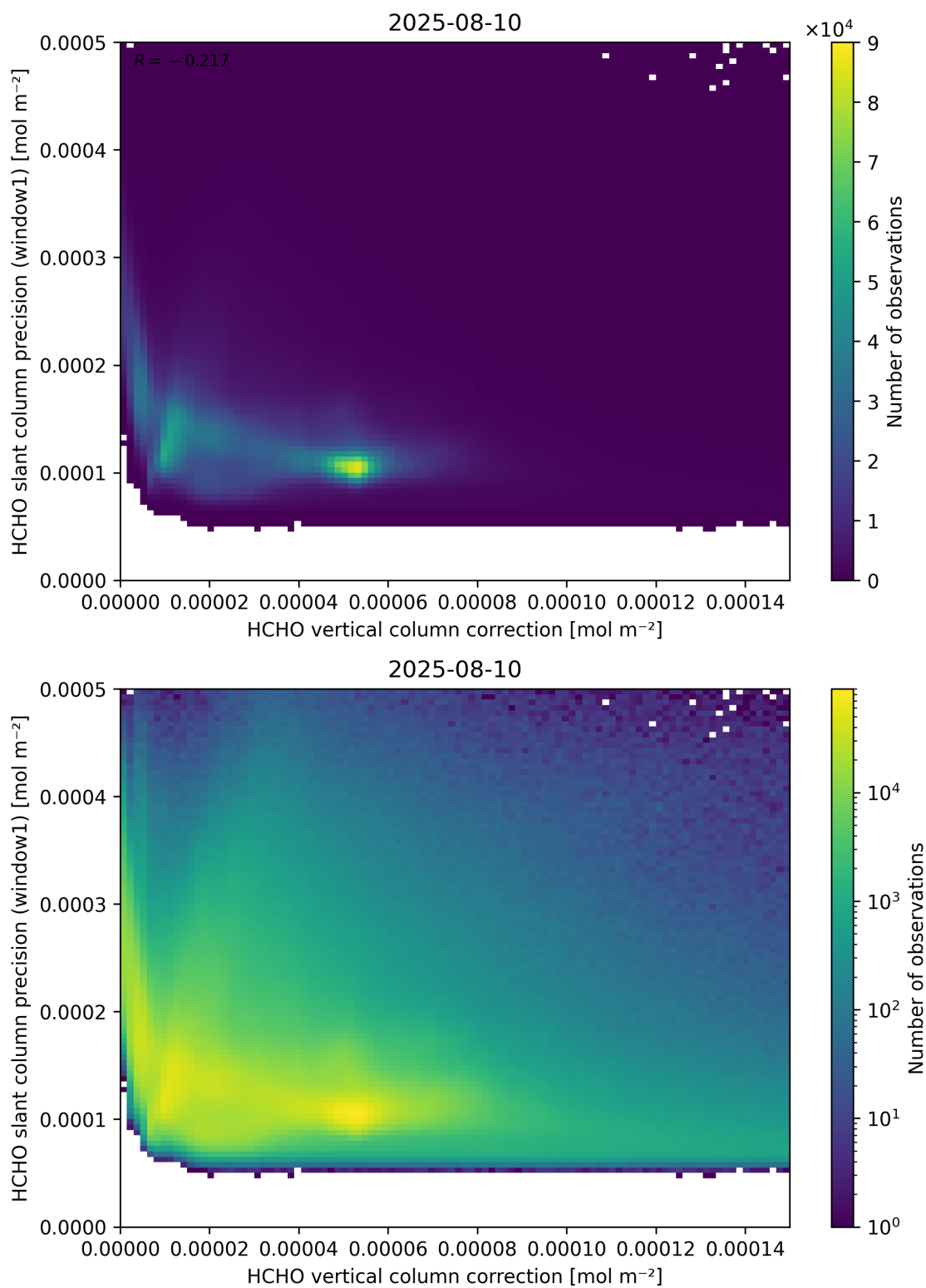
Figure 119: Scatter density plot of “HCHO vertical column correction” against “HCHO slant column precision (window1)” for 2025-08-09 to 2025-08-11.
