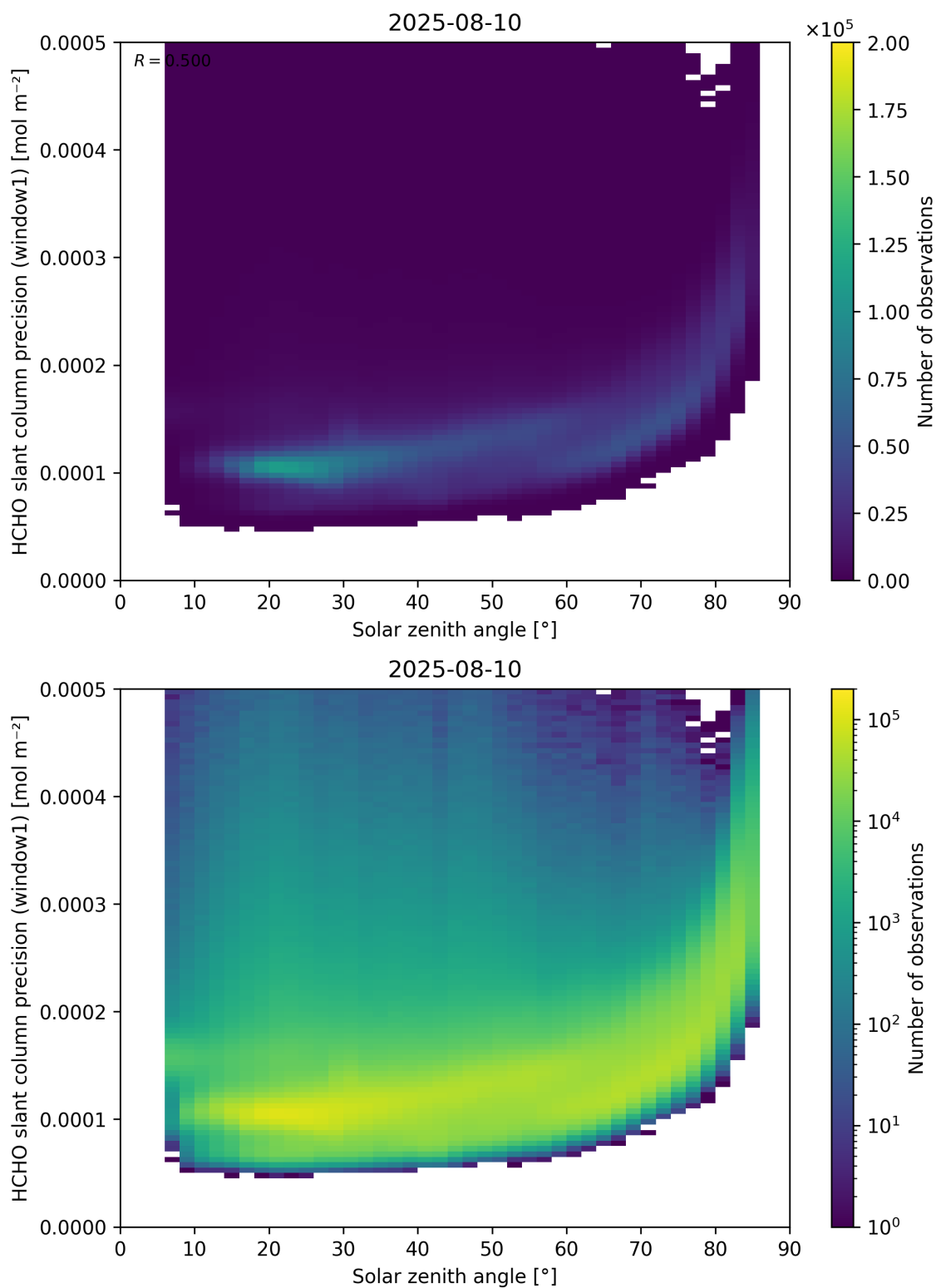
Figure 174: Scatter density plot of “Solar zenith angle” against “HCHO slant column precision (window1)” for 2025-08-09 to 2025-08-11.
