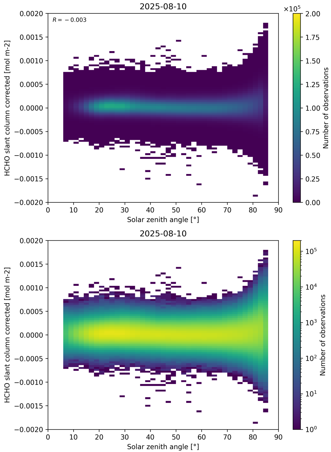
Figure 171: Scatter density plot of “Solar zenith angle” against “HCHO slant column corrected” for 2025-08-09 to 2025-08-11.
