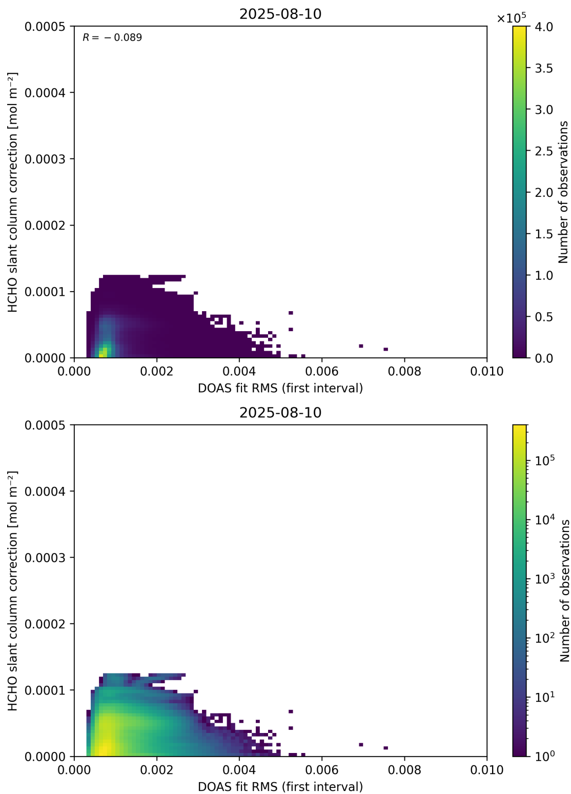
Figure 63: Scatter density plot of “DOAS fit RMS (first interval)” against “HCHO slant column correction” for 2025-08-09 to 2025-08-11.
