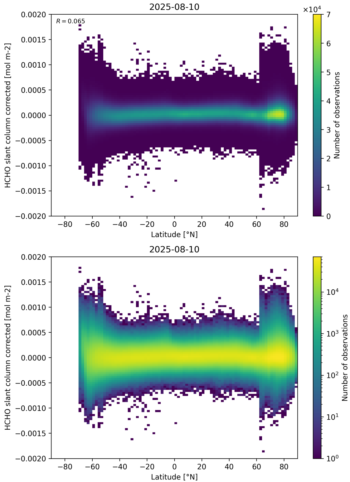
Figure 157: Scatter density plot of “Latitude” against “HCHO slant column corrected” for 2025-08-09 to 2025-08-11.
