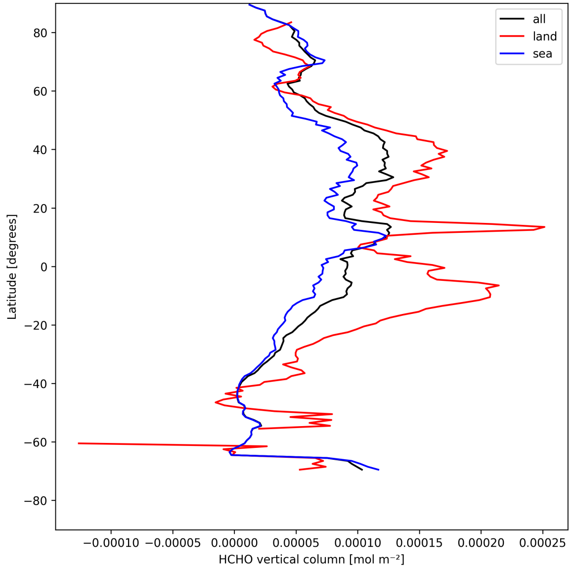
Figure 21: Zonal average of “HCHO vertical column” for 2025-08-09 to 2025-08-11.
