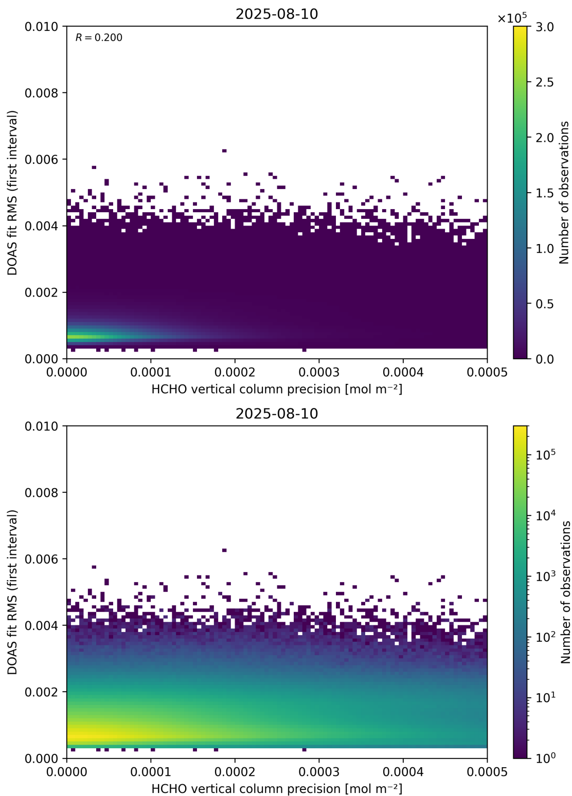
Figure 136: Scatter density plot of “HCHO vertical column precision” against “DOAS fit RMS (first interval)” for 2025-08-09 to 2025-08-11.
