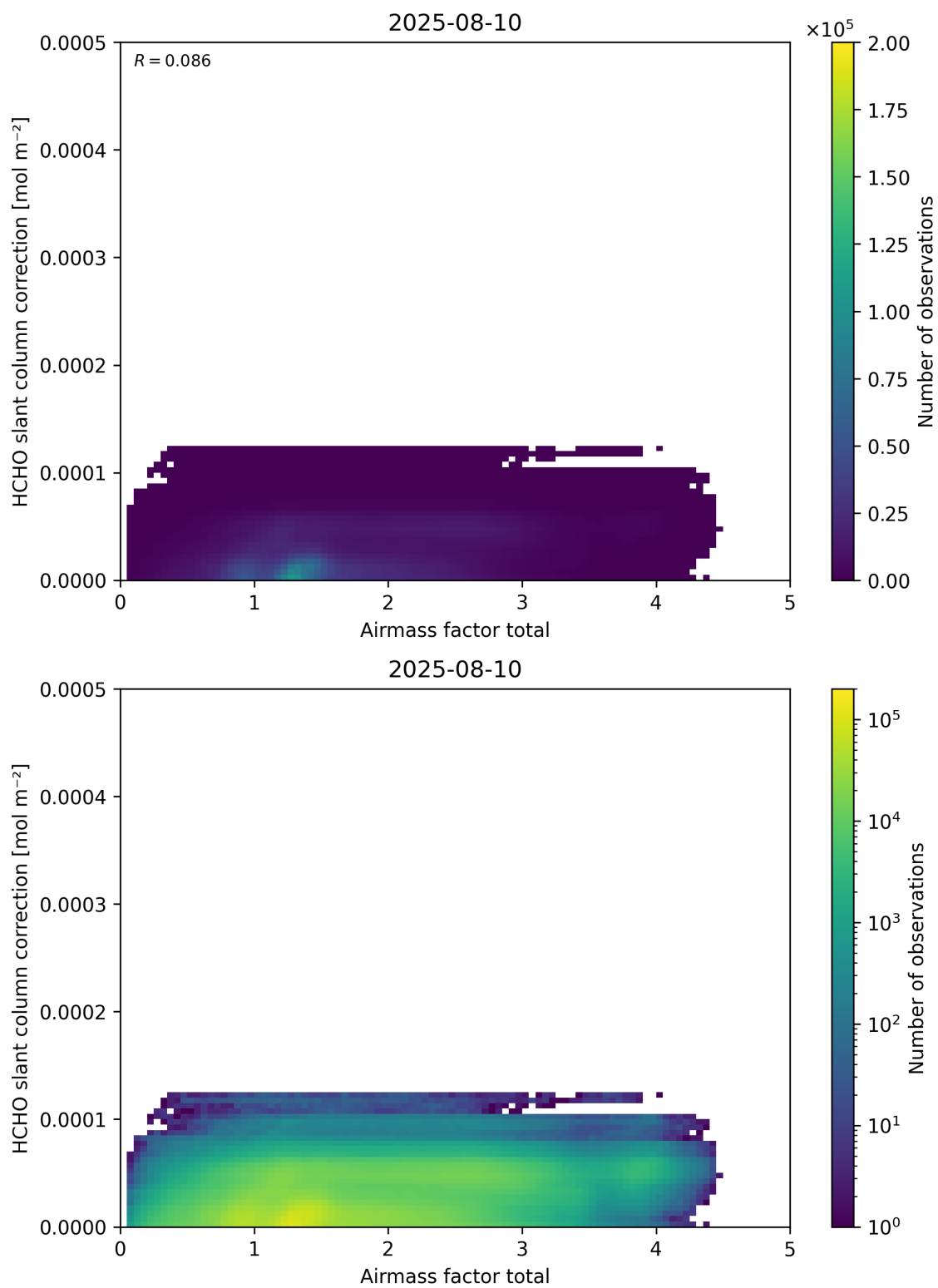
Figure 102: Scatter density plot of “Airmass factor total” against “HCHO slant column correction” for 2025-08-09 to 2025-08-11.
