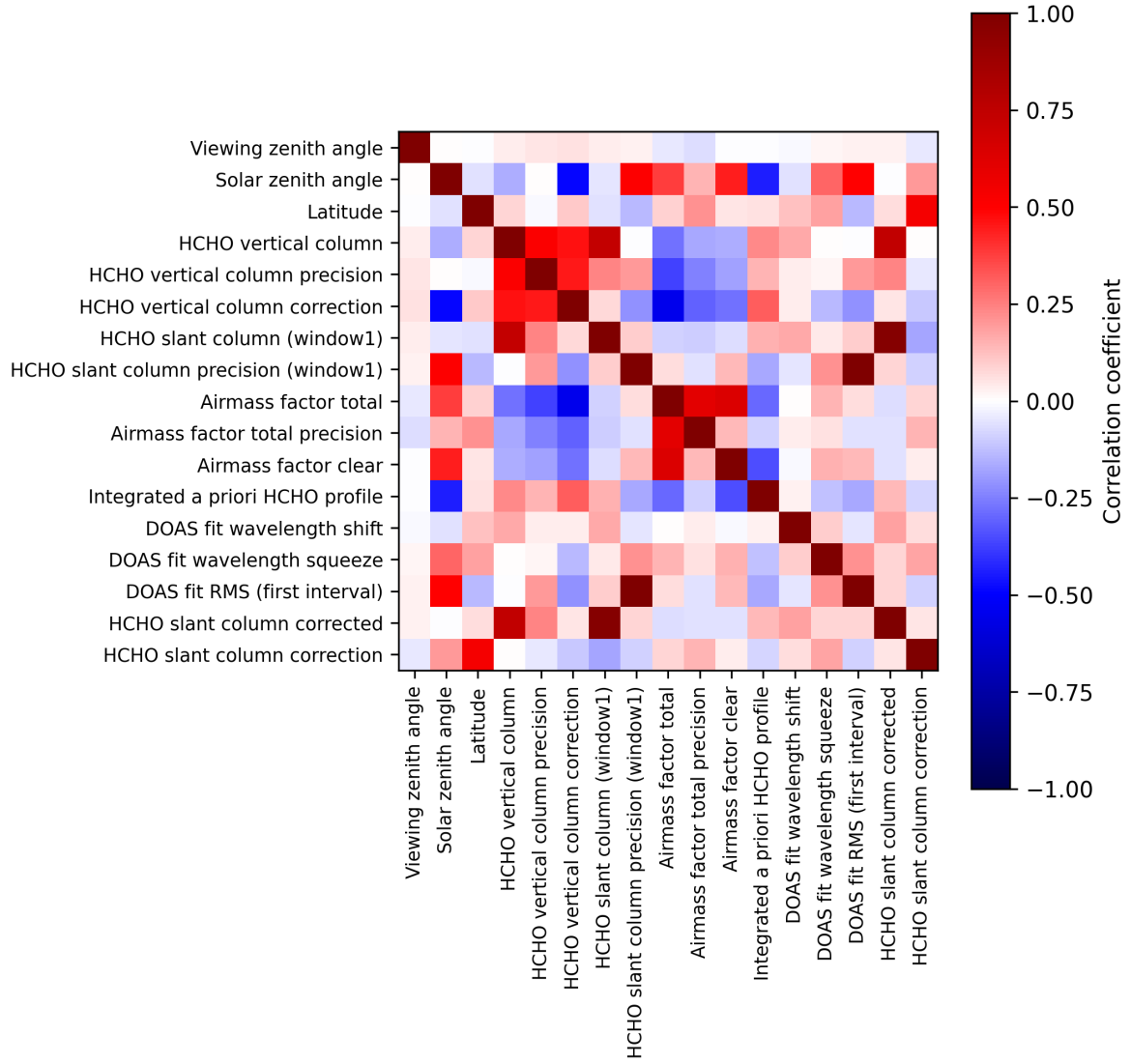
Figure 2: Map of correlation matrix for 2025-08-09 to 2025-08-11.
