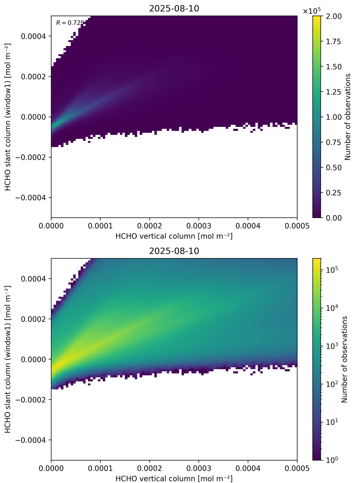
Figure 129: Scatter density plot of “HCHO vertical column” against “HCHO slant column (window1)” for 2025-08-09 to 2025-08-11.
