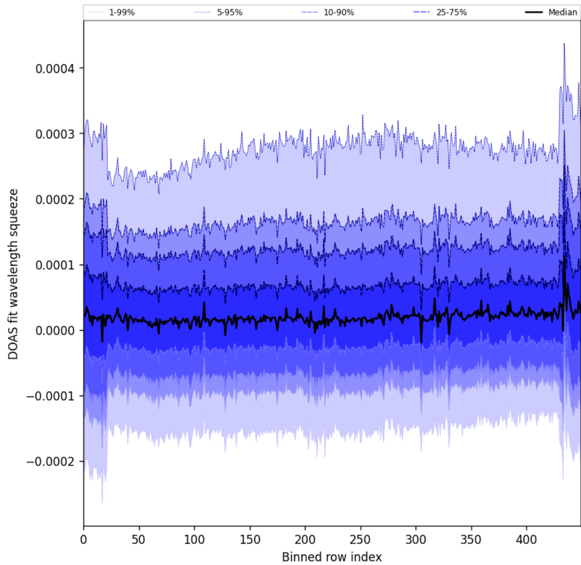
Figure 59: Along track statistics of “DOAS fit wavelength squeeze” for 2025-08-09 to 2025-08-11
