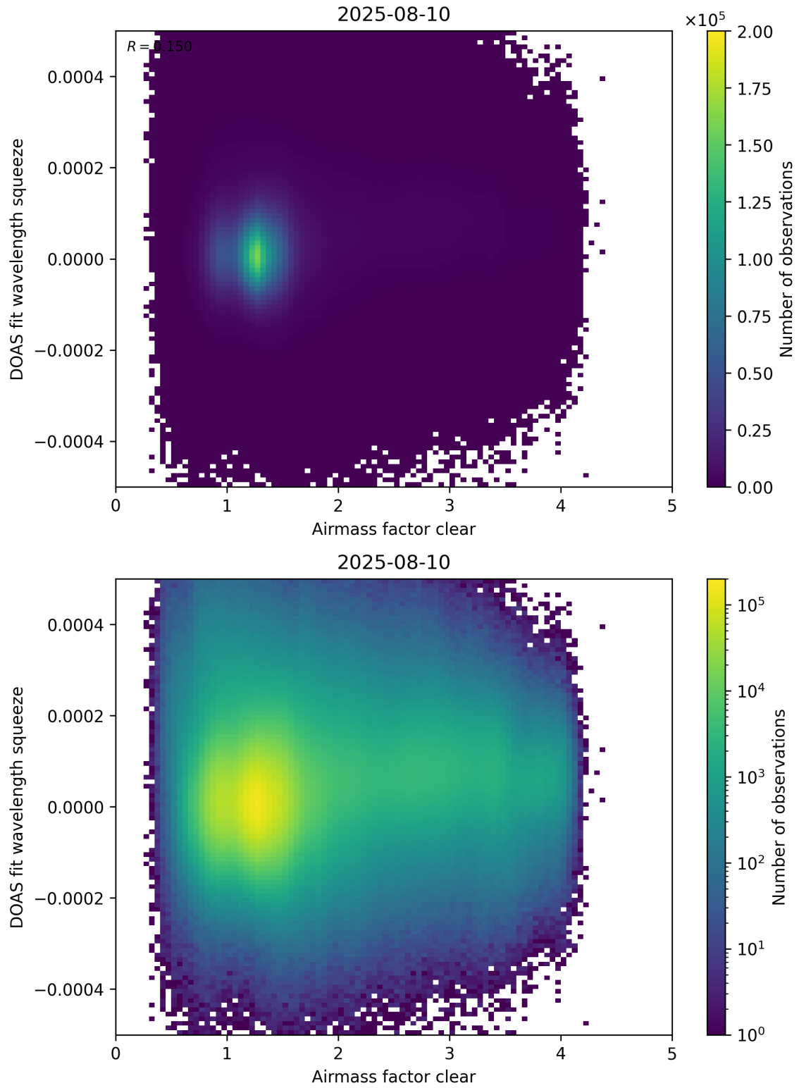
Figure 73: Scatter density plot of “Airmass factor clear” against “DOAS fit wavelength squeeze” for 2025-08-09 to 2025-08-11.
