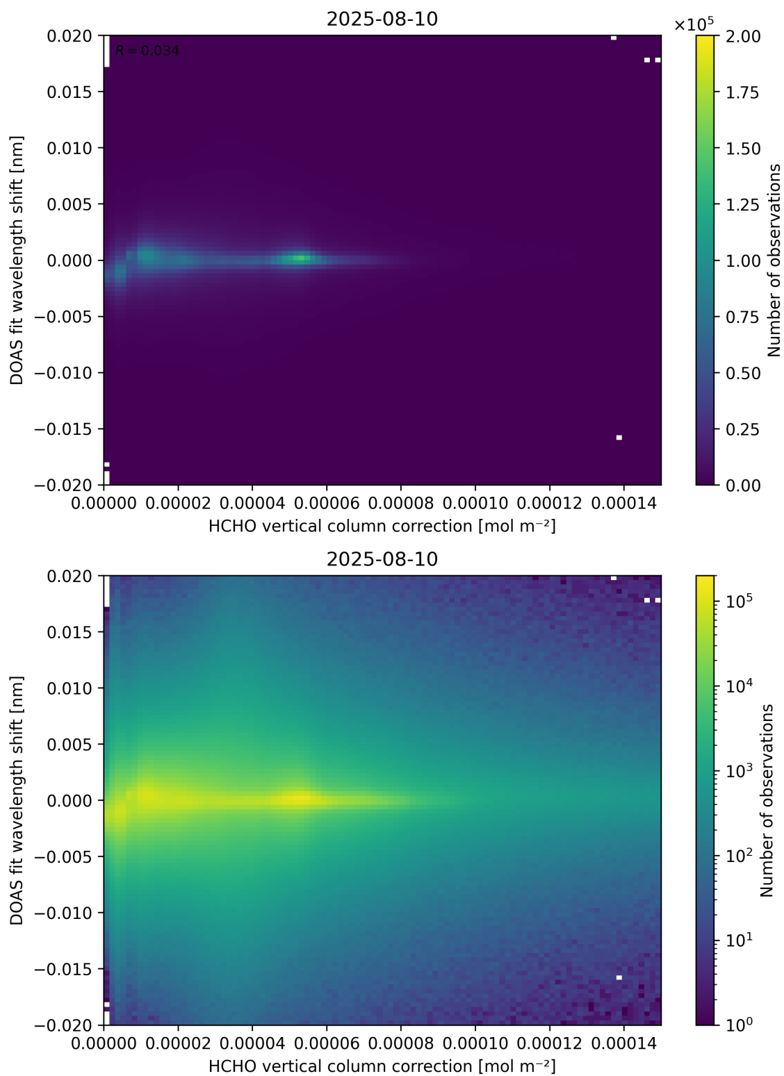
Figure 113: Scatter density plot of “HCHO vertical column correction” against “DOAS fit wavelength shift” for 2025-08-09 to 2025-08-11.
