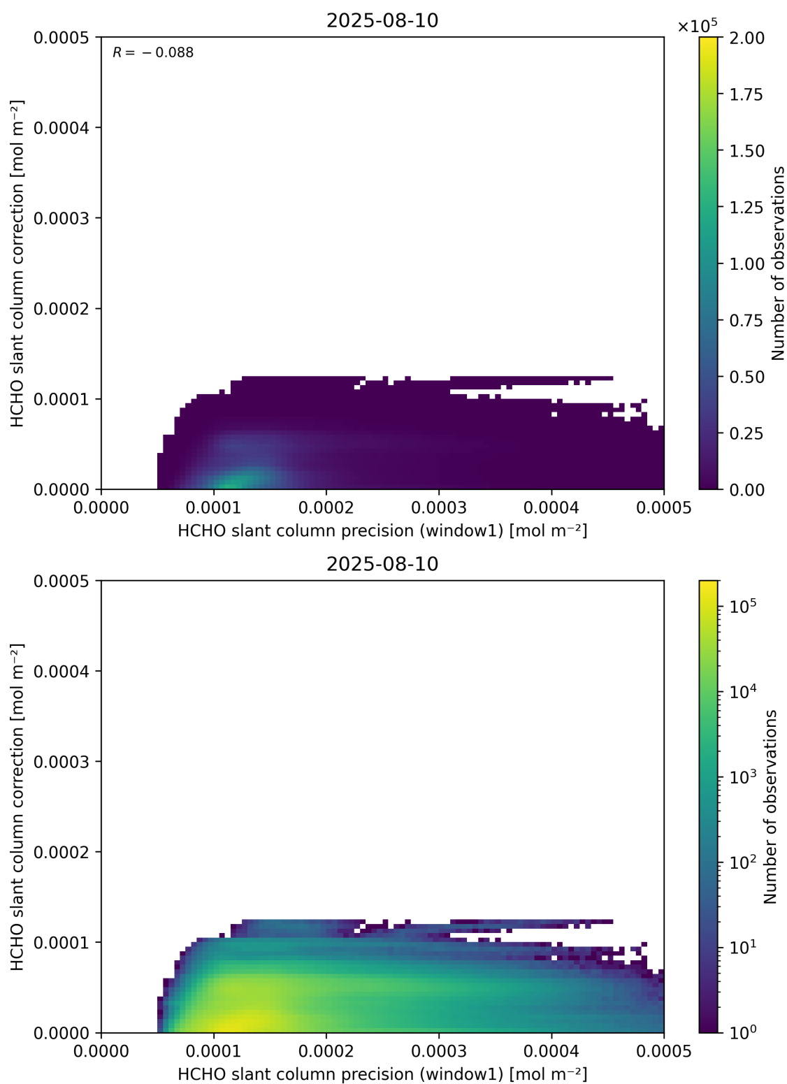
Figure 93: Scatter density plot of “HCHO slant column precision (window1)” against “HCHO slant column correction” for 2025-08-09 to 2025-08-11.
