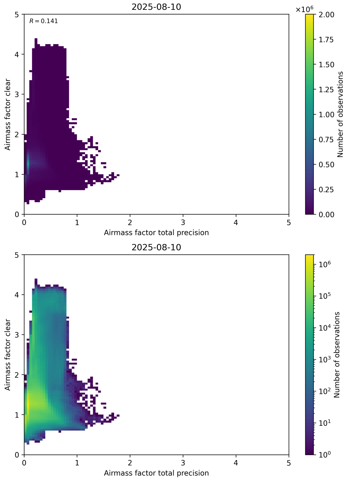
Figure 108: Scatter density plot of “Airmass factor total precision” against “Airmass factor clear” for 2025-08-09 to 2025-08-11.
