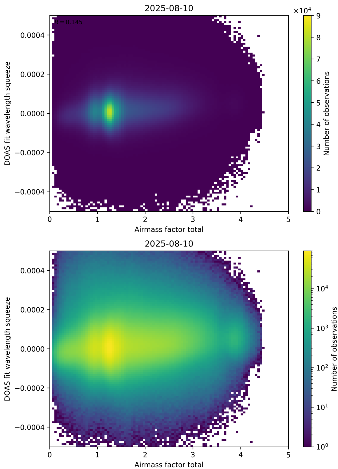
Figure 99: Scatter density plot of “Airmass factor total” against “DOAS fit wavelength squeeze” for 2025-08-09 to 2025-08-11.
