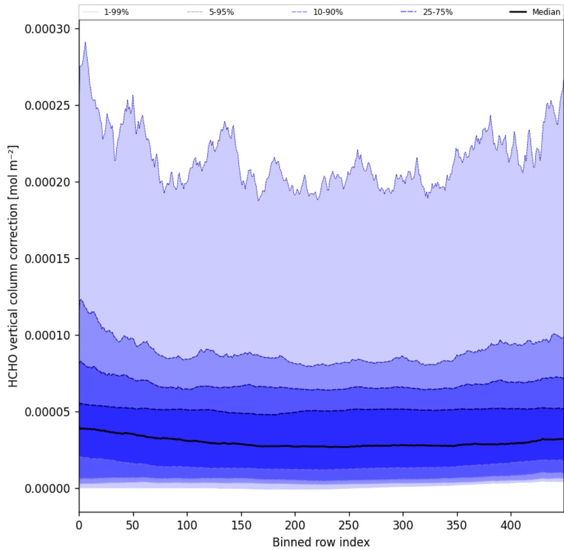
Figure 51: Along track statistics of “HCHO vertical column correction” for 2025-08-09 to 2025-08-11
