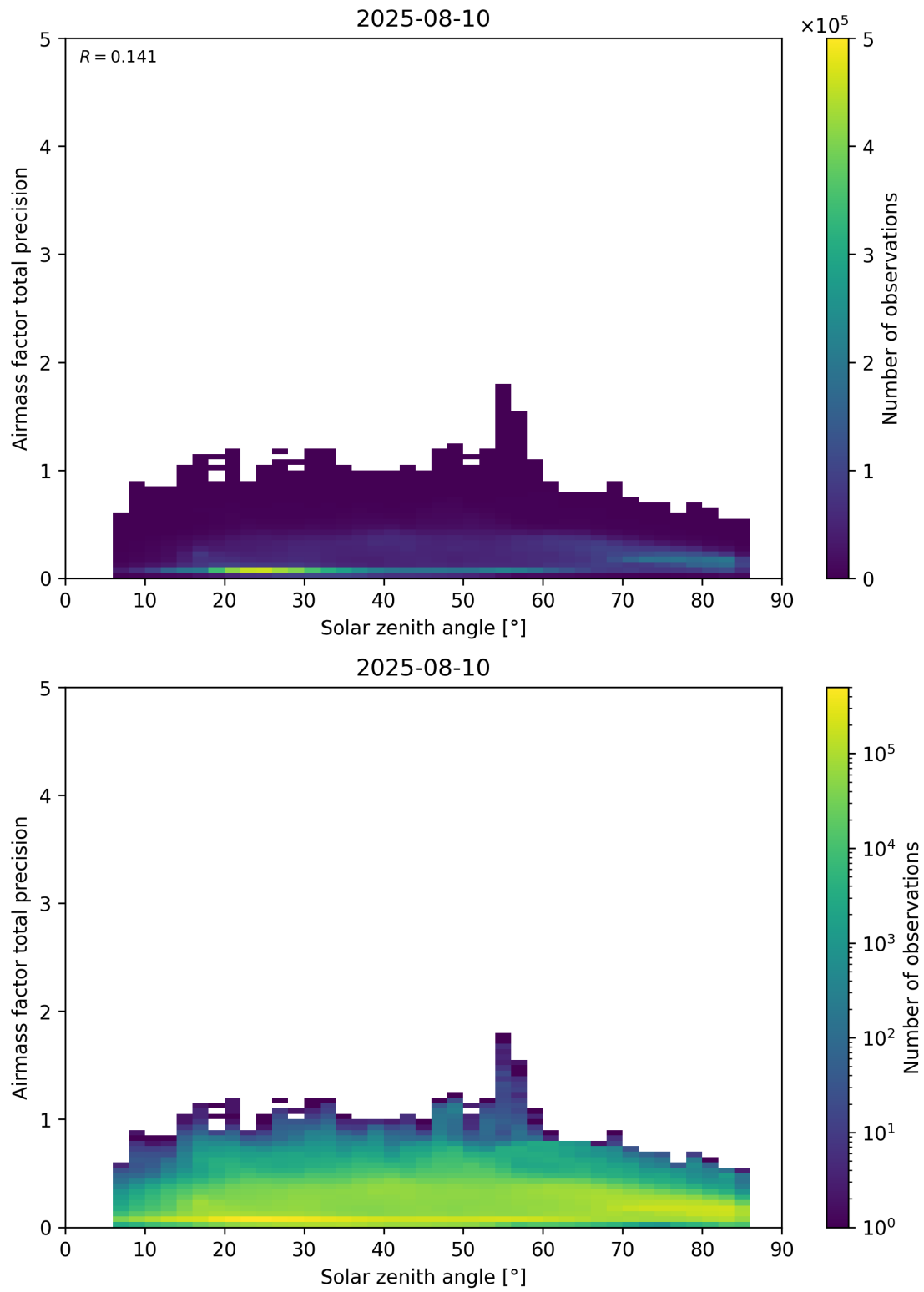
Figure 176: Scatter density plot of “Solar zenith angle” against “Airmass factor total precision” for 2025-08-09 to 2025-08-11.
