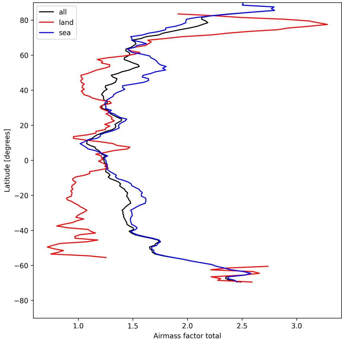
Figure 26: Zonal average of “Airmass factor total” for 2025-08-09 to 2025-08-11.
