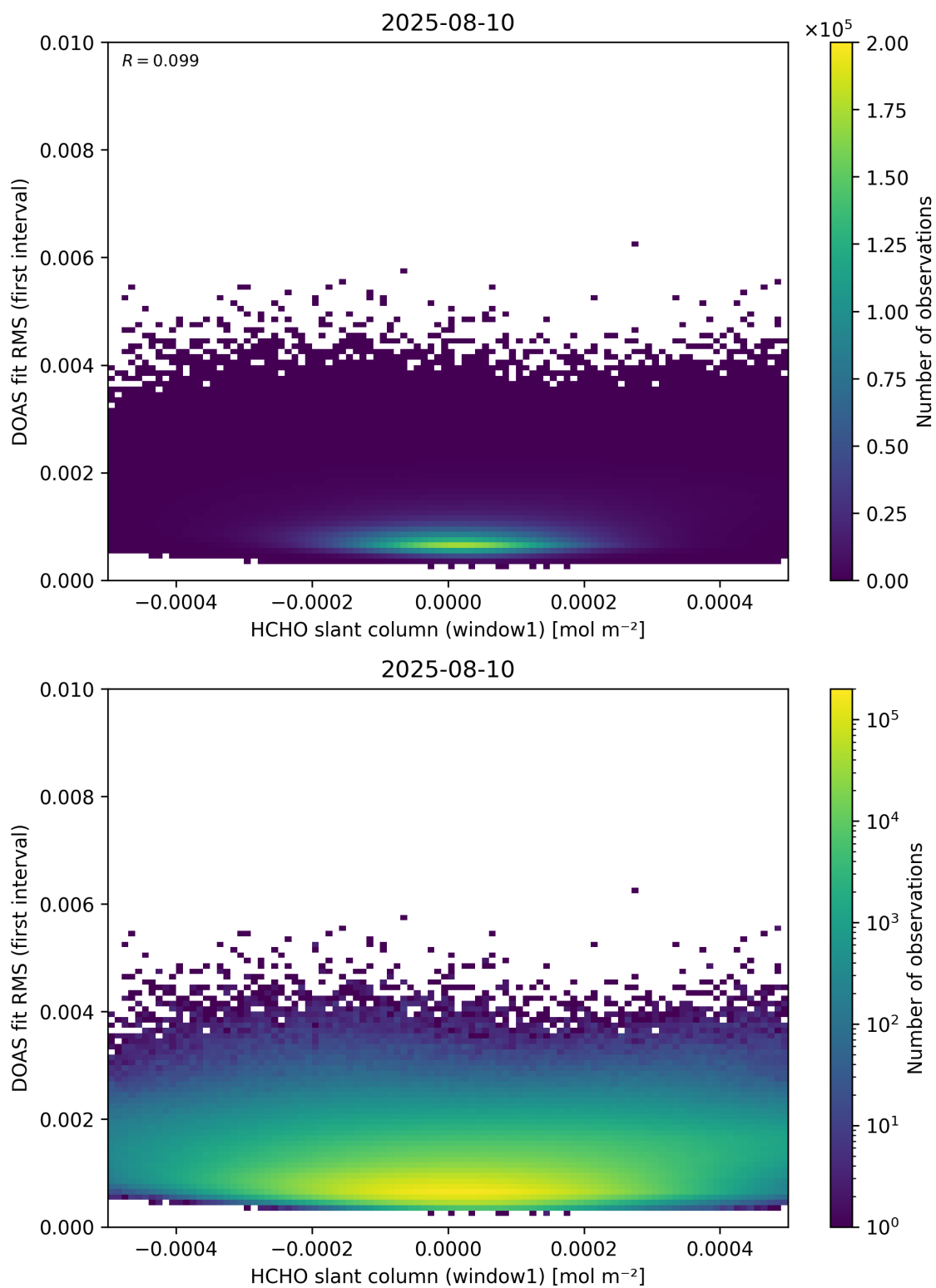
Figure 78: Scatter density plot of “HCHO slant column (window1)” against “DOAS fit RMS (first interval)” for 2025-08-09 to 2025-08-11.
