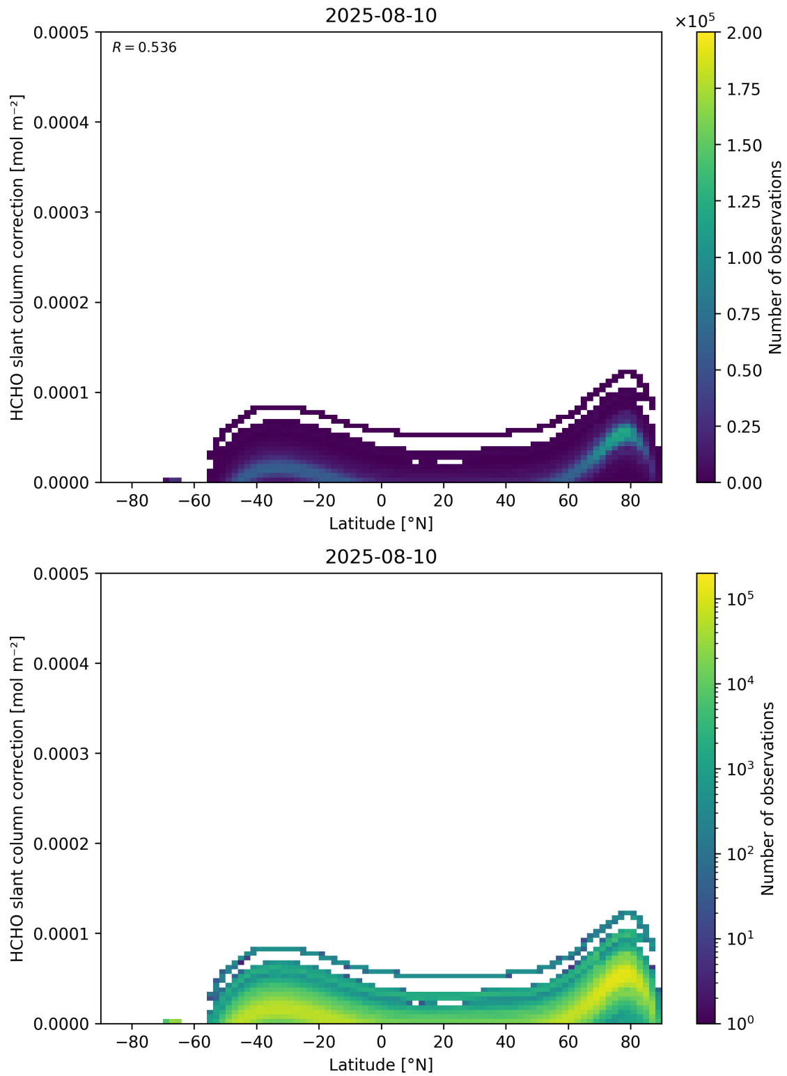
Figure 158: Scatter density plot of “Latitude” against “HCHO slant column correction” for 2025-08-09 to 2025-08-11.
