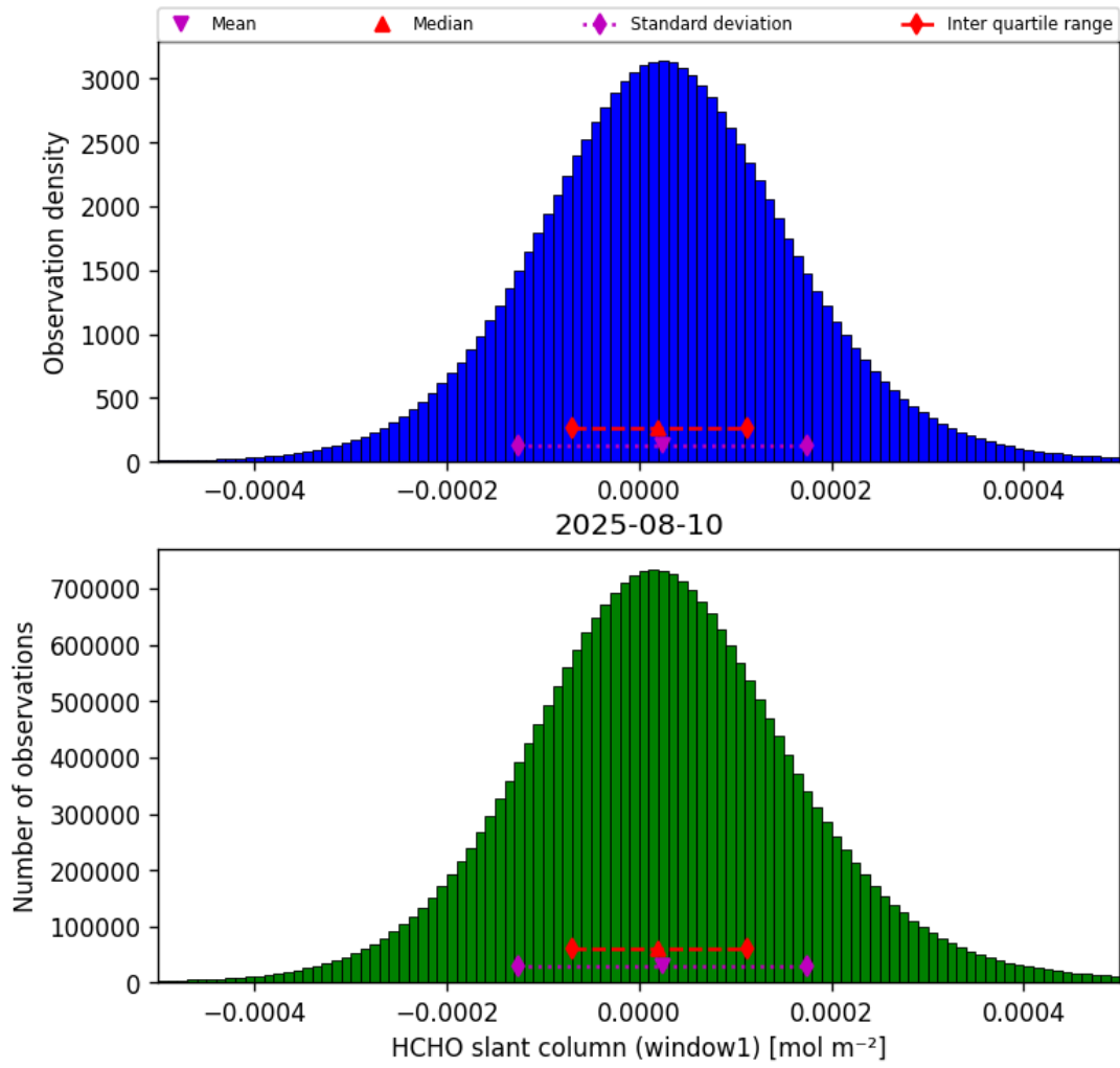
Figure 38: Histogram of “HCHO slant column (window1)” for 2025-08-09 to 2025-08-11
