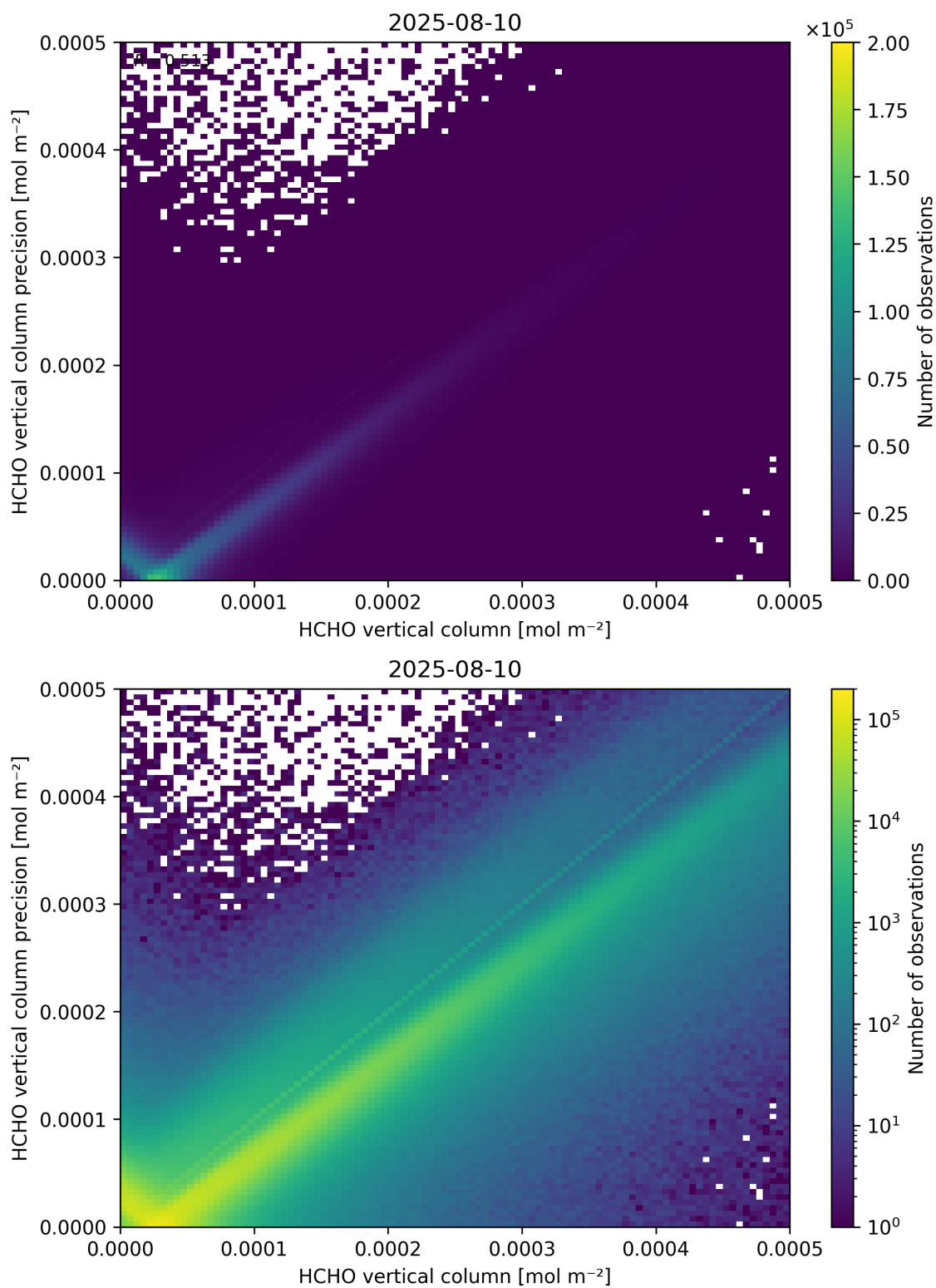
Figure 134: Scatter density plot of “HCHO vertical column” against “HCHO vertical column precision” for 2025-08-09 to 2025-08-11.
