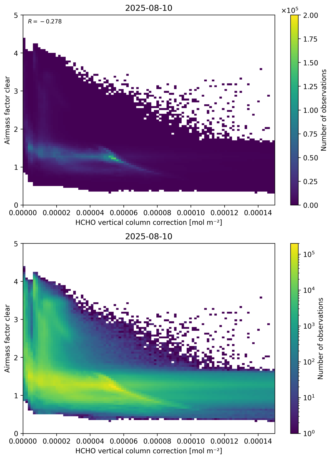
Figure 115: Scatter density plot of “HCHO vertical column correction” against “Airmass factor clear” for 2025-08-09 to 2025-08-11.
