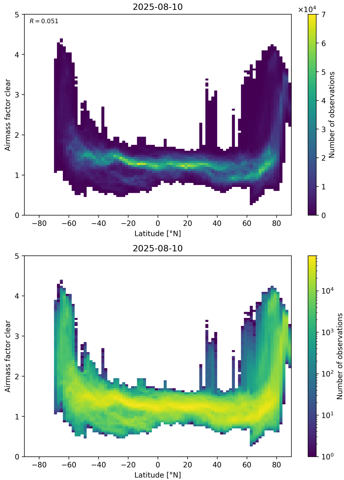
Figure 156: Scatter density plot of “Latitude” against “Airmass factor clear” for 2025-08-09 to 2025-08-11.
