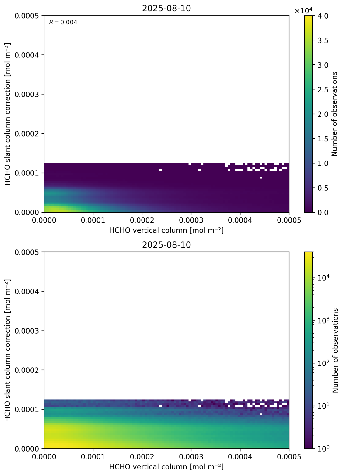
Figure 128: Scatter density plot of “HCHO vertical column” against “HCHO slant column correction” for 2025-08-09 to 2025-08-11.
