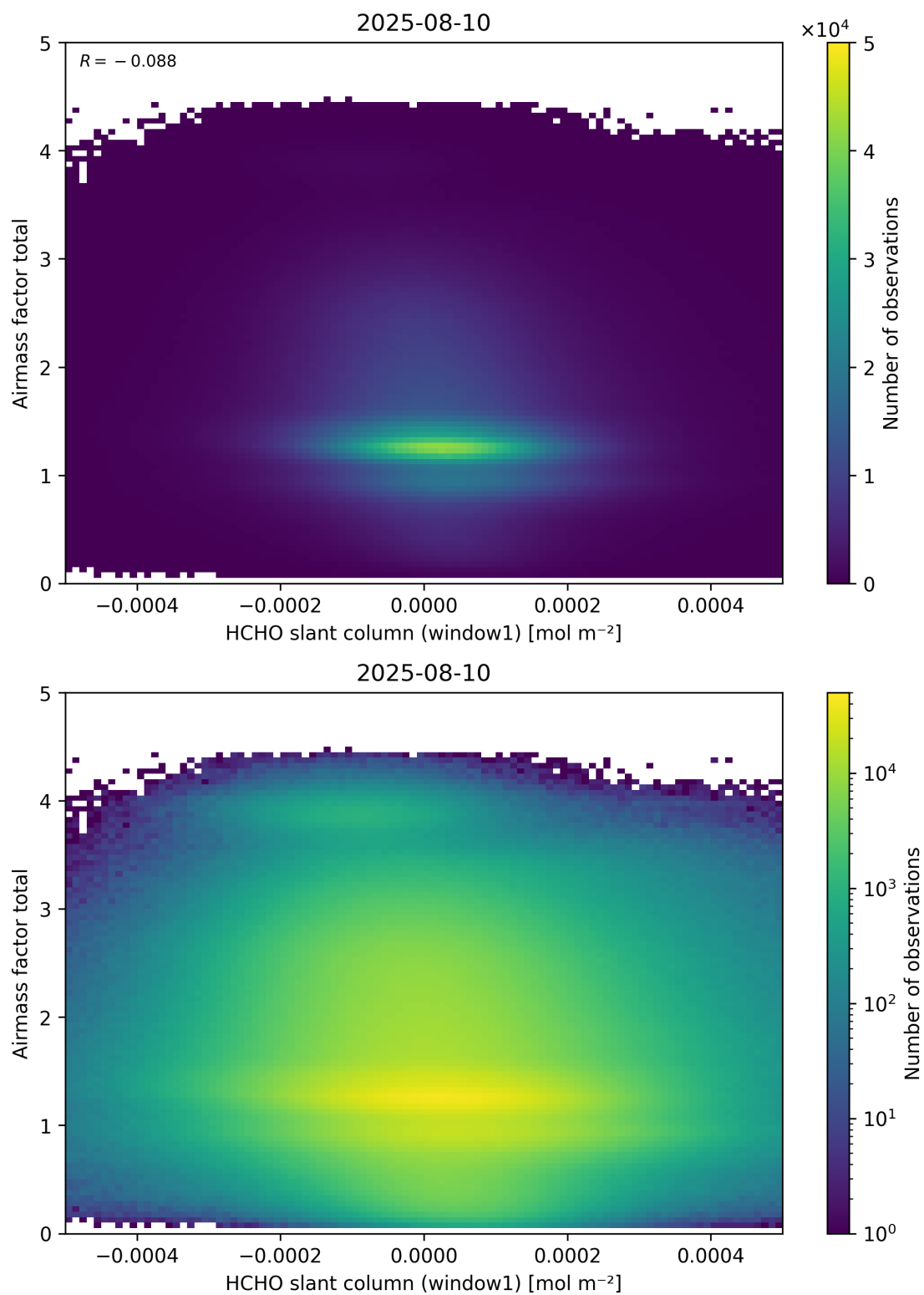
Figure 85: Scatter density plot of “HCHO slant column (window1)” against “Airmass factor total” for 2025-08-09 to 2025-08-11.
