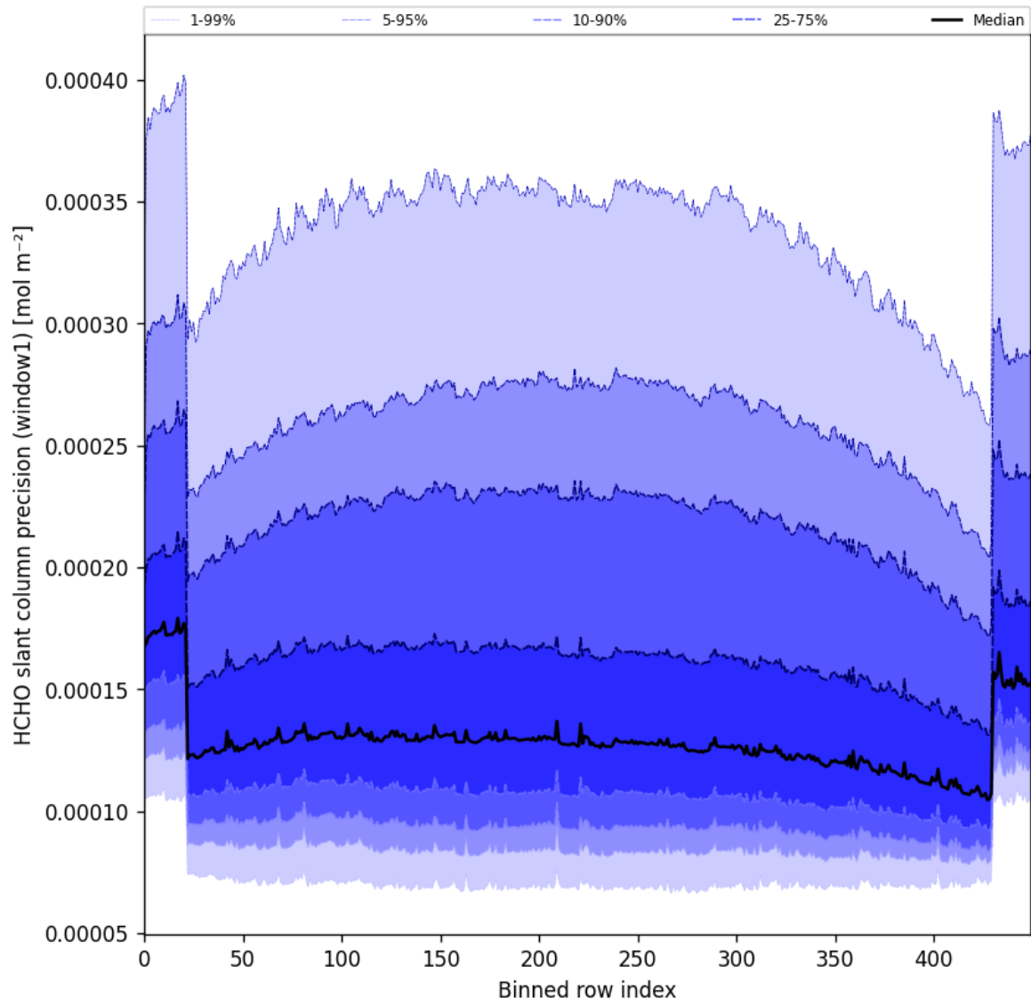
Figure 53: Along track statistics of “HCHO slant column precision (window1)” for 2025-08-09 to 2025-08-11
