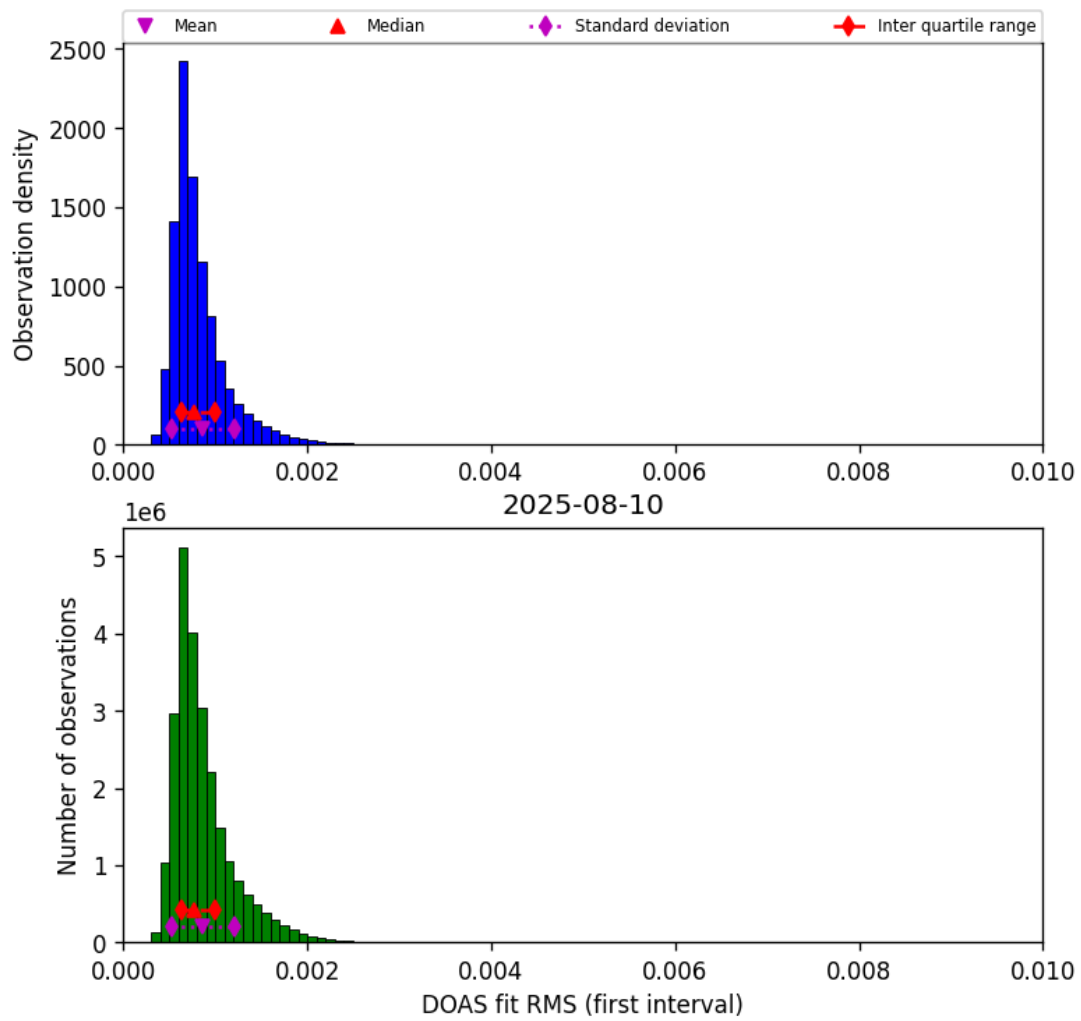
Figure 46: Histogram of “DOAS fit RMS (first interval)” for 2025-08-09 to 2025-08-11
