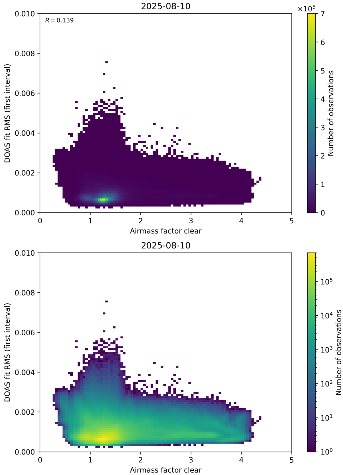
Figure 71: Scatter density plot of “Airmass factor clear” against “DOAS fit RMS (first interval)” for 2025-08-09 to 2025-08-11.
