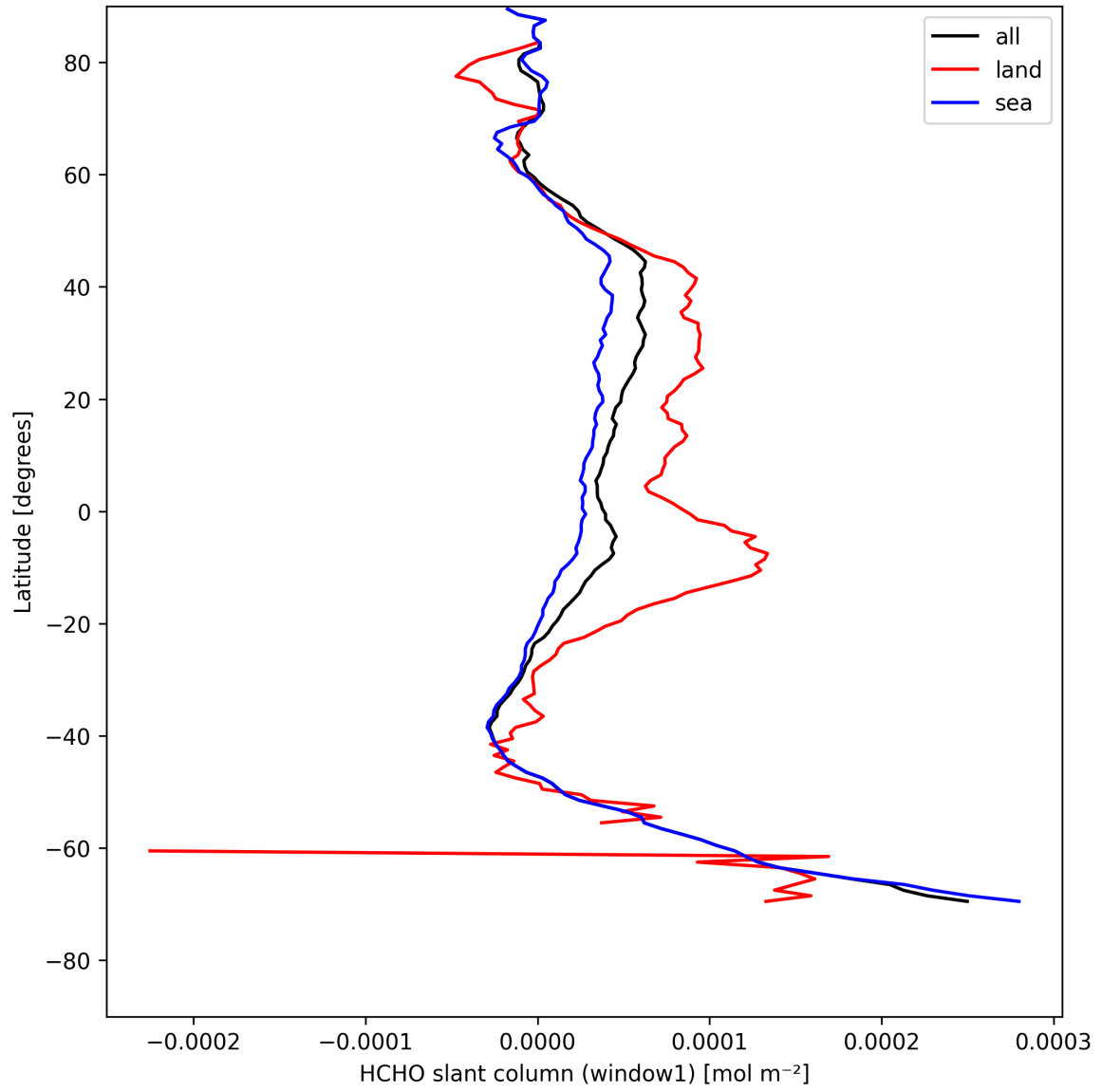
Figure 24: Zonal average of “HCHO slant column (window1)” for 2025-08-09 to 2025-08-11.
