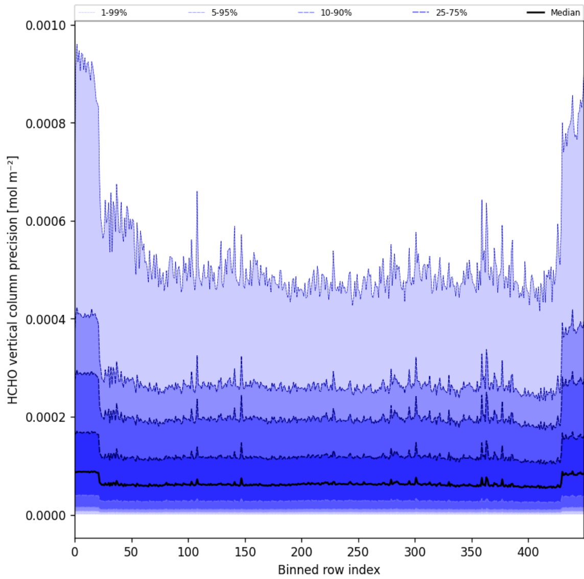
Figure 50: Along track statistics of “HCHO vertical column precision” for 2025-08-09 to 2025-08-11
