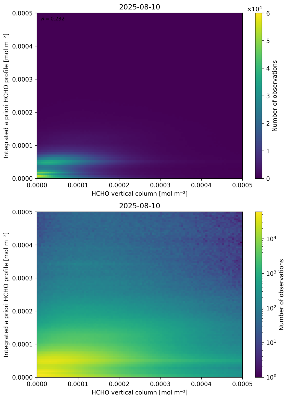
Figure 135: Scatter density plot of “HCHO vertical column” against “Integrated a priori HCHO profile” for 2025-08-09 to 2025-08-11.
