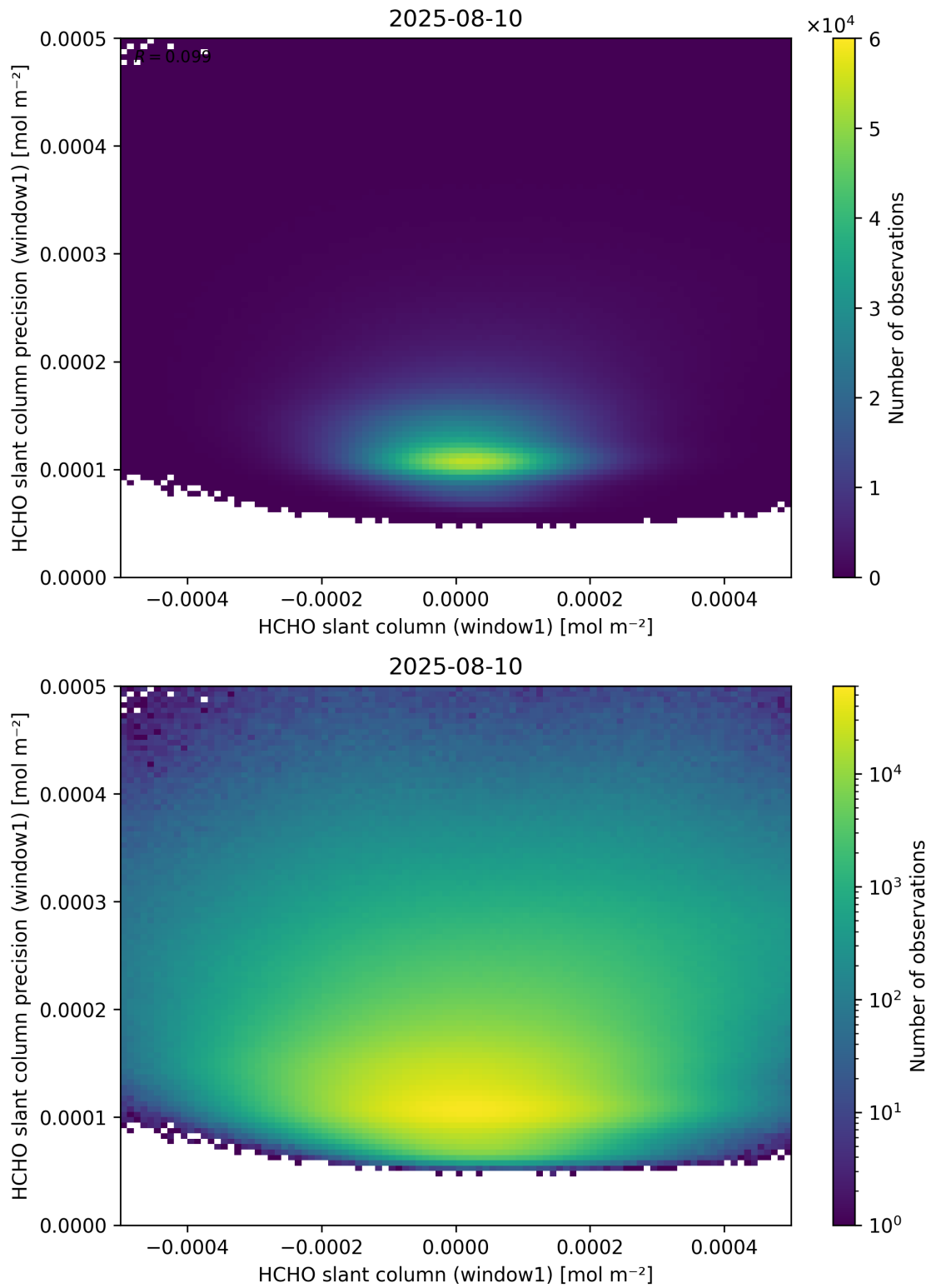
Figure 84: Scatter density plot of “HCHO slant column (window1)” against “HCHO slant column precision (window1)” for 2025-08-09 to 2025-08-11.
