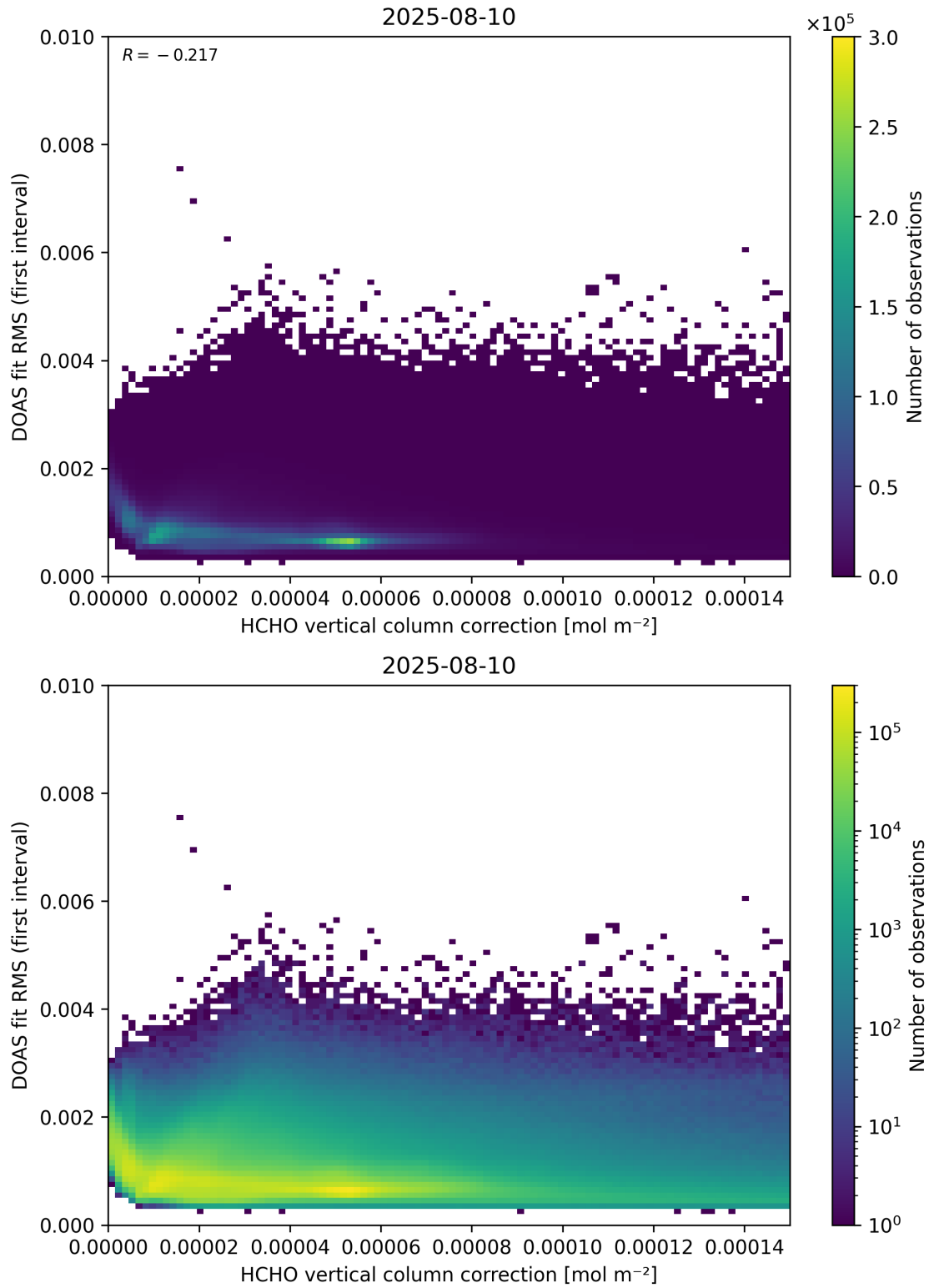
Figure 112: Scatter density plot of “HCHO vertical column correction” against “DOAS fit RMS (first interval)” for 2025-08-09 to 2025-08-11.
