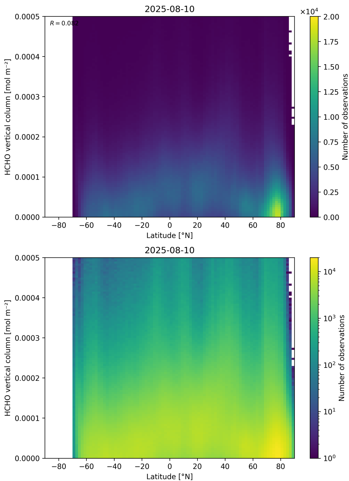
Figure 163: Scatter density plot of “Latitude” against “HCHO vertical column” for 2025-08-09 to 2025-08-11.
