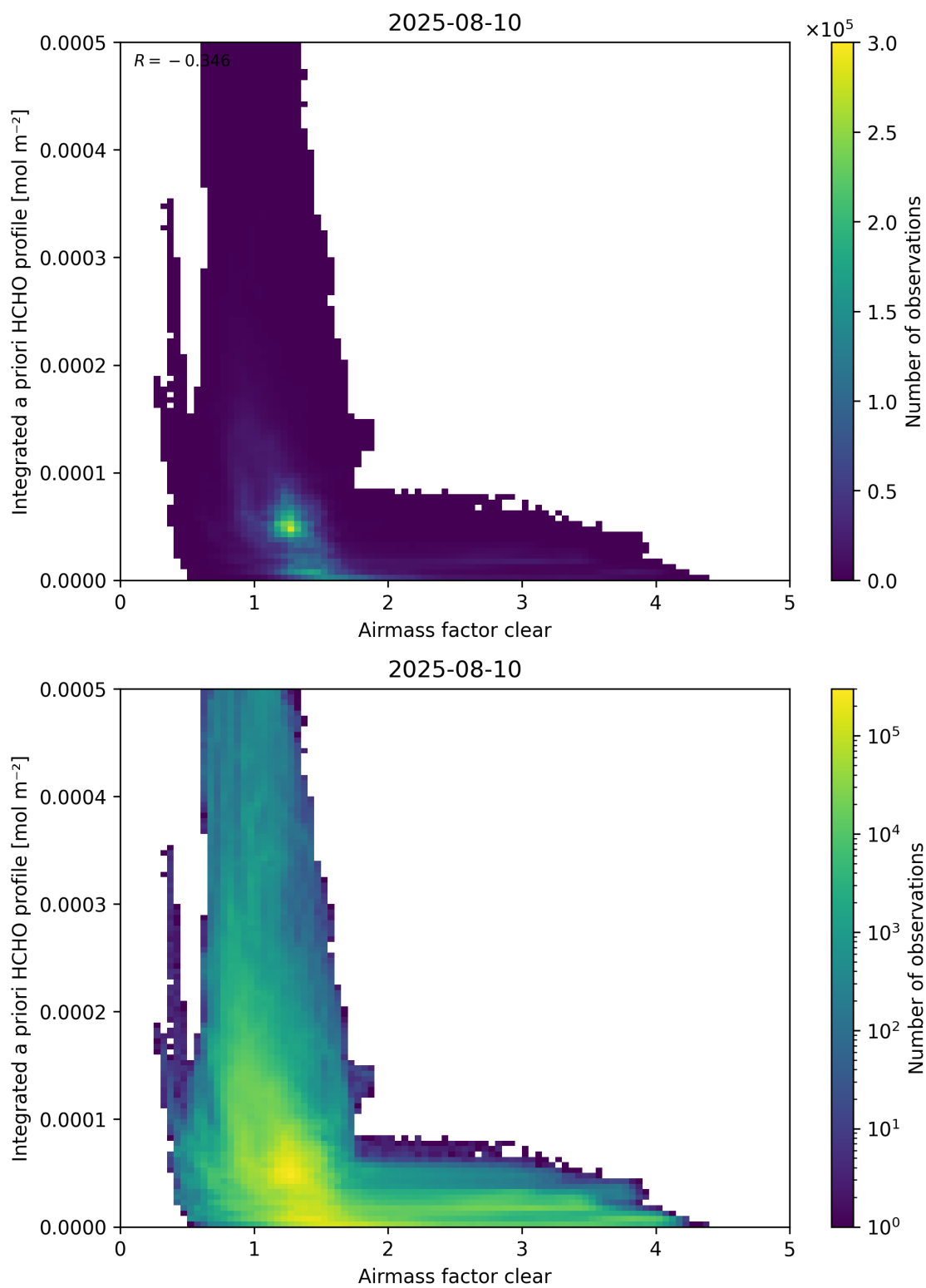
Figure 76: Scatter density plot of “Airmass factor clear” against “Integrated a priori HCHO profile” for 2025-08-09 to 2025-08-11.
