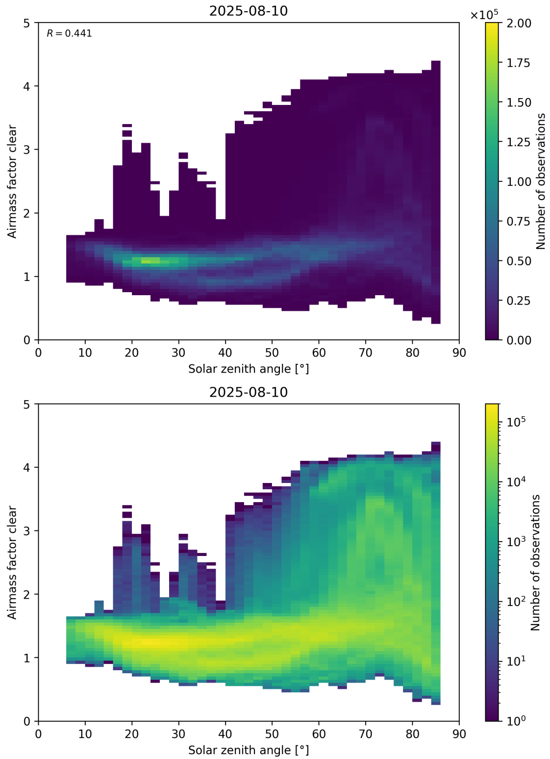
Figure 170: Scatter density plot of “Solar zenith angle” against “Airmass factor clear” for 2025-08-09 to 2025-08-11.
