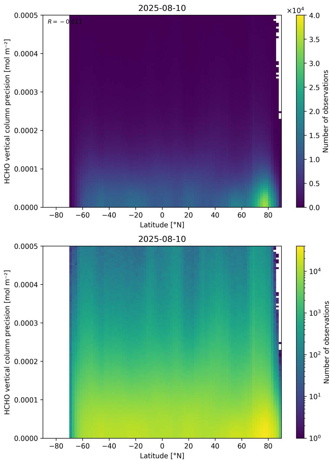
Figure 165: Scatter density plot of “Latitude” against “HCHO vertical column precision” for 2025-08-09 to 2025-08-11.
