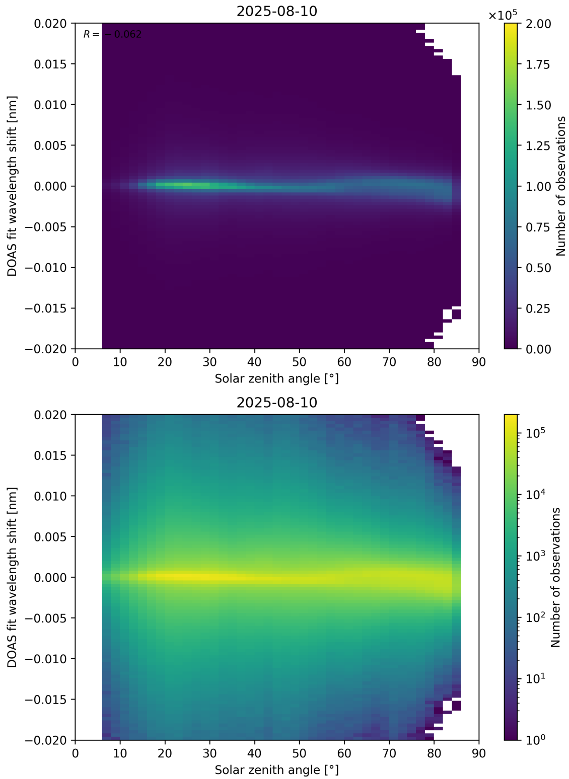
Figure 168: Scatter density plot of “Solar zenith angle” against “DOAS fit wavelength shift” for 2025-08-09 to 2025-08-11.
