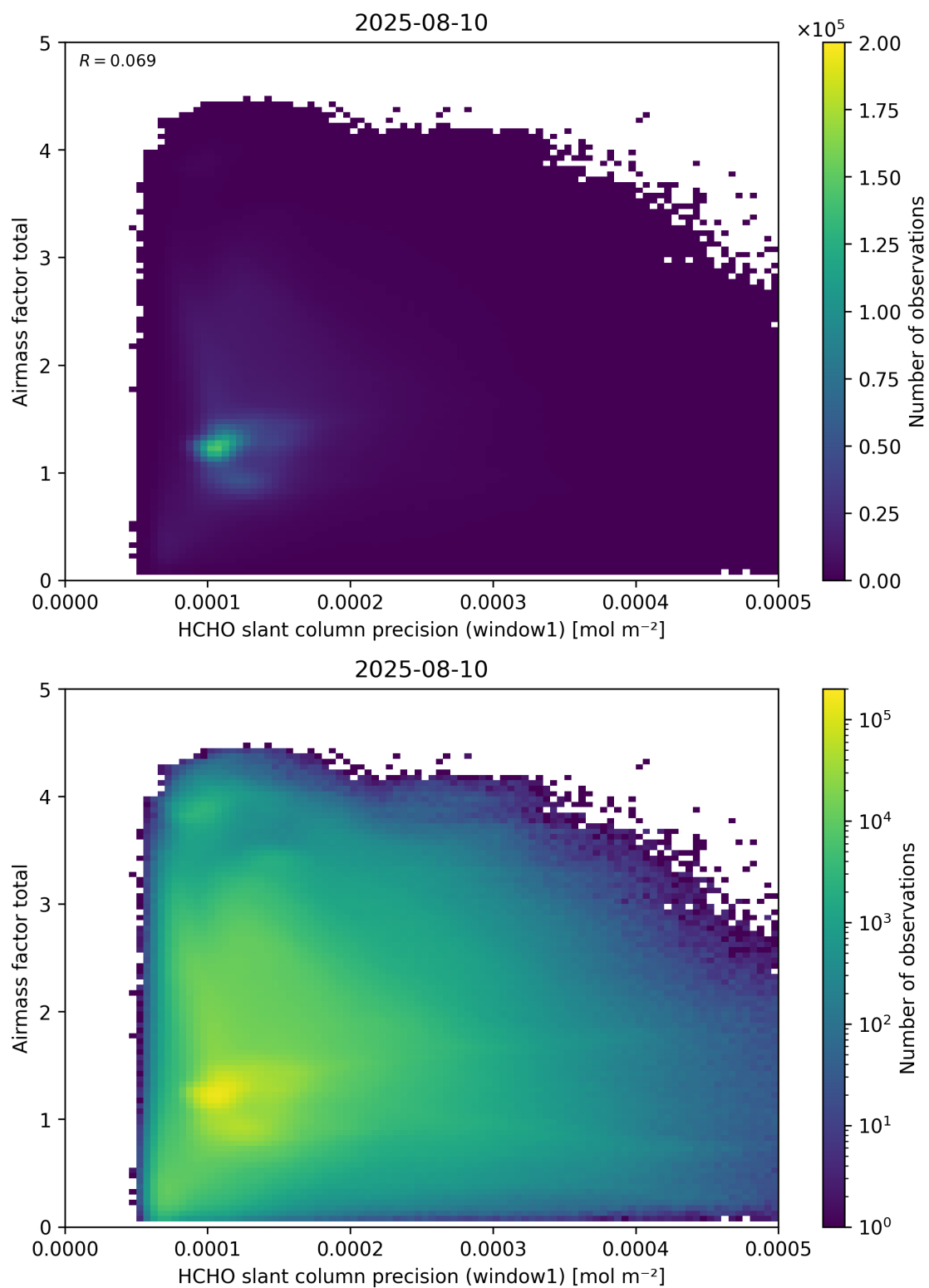
Figure 94: Scatter density plot of “HCHO slant column precision (window1)” against “Airmass factor total” for 2025-08-09 to 2025-08-11.
