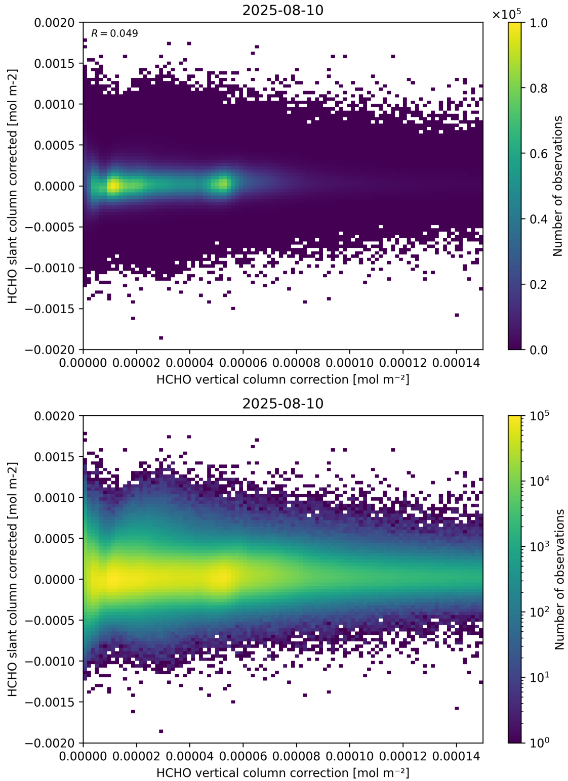
Figure 116: Scatter density plot of “HCHO vertical column correction” against “HCHO slant column corrected” for 2025-08-09 to 2025-08-11.
