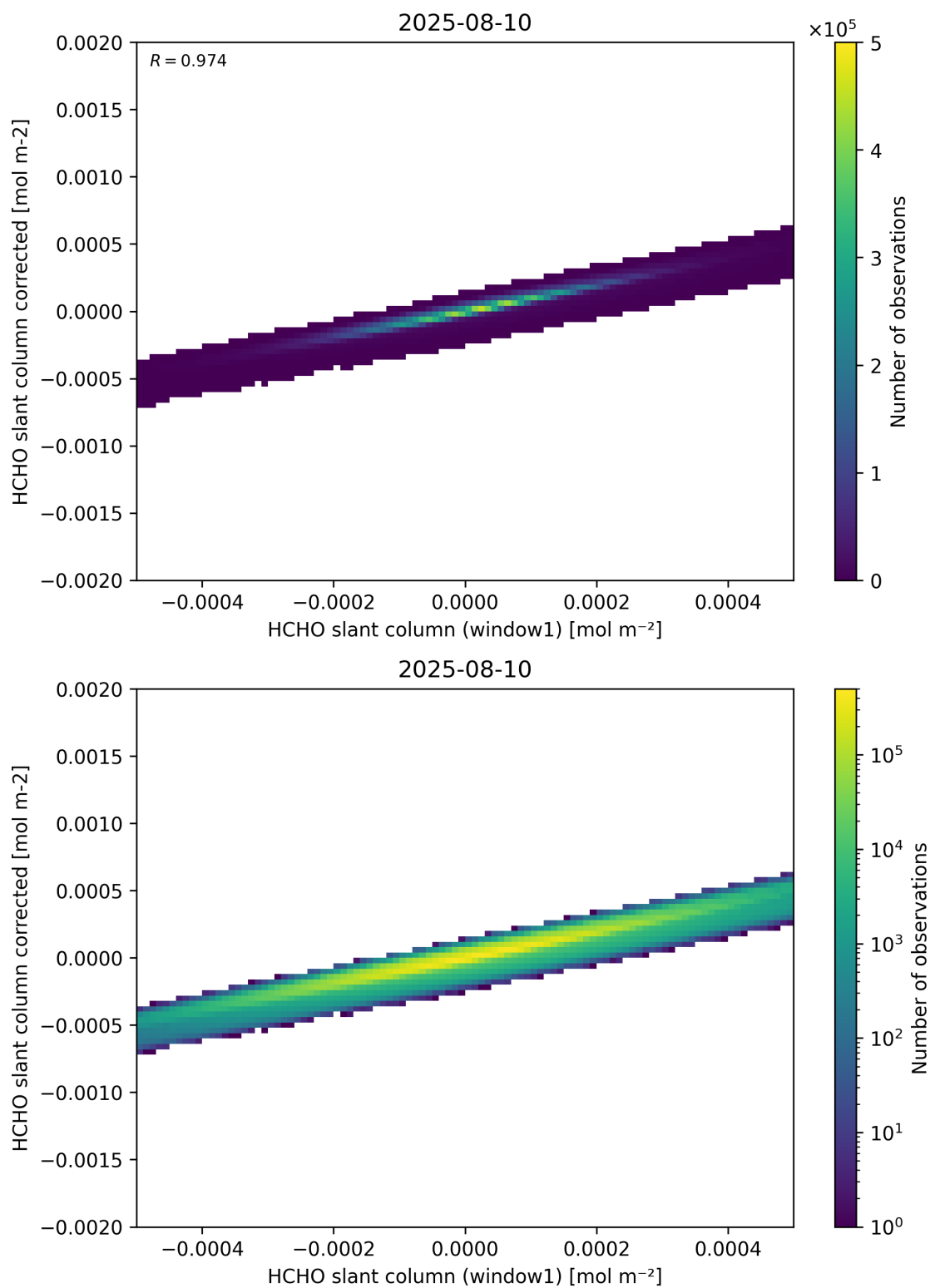
Figure 82: Scatter density plot of “HCHO slant column (window1)” against “HCHO slant column corrected” for 2025-08-09 to 2025-08-11.
