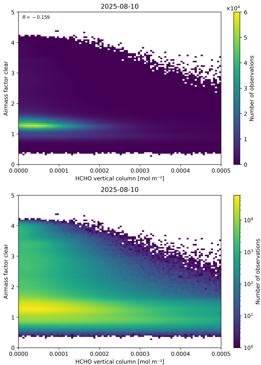
Figure 126: Scatter density plot of “HCHO vertical column” against “Airmass factor clear” for 2025-08-09 to 2025-08-11.
