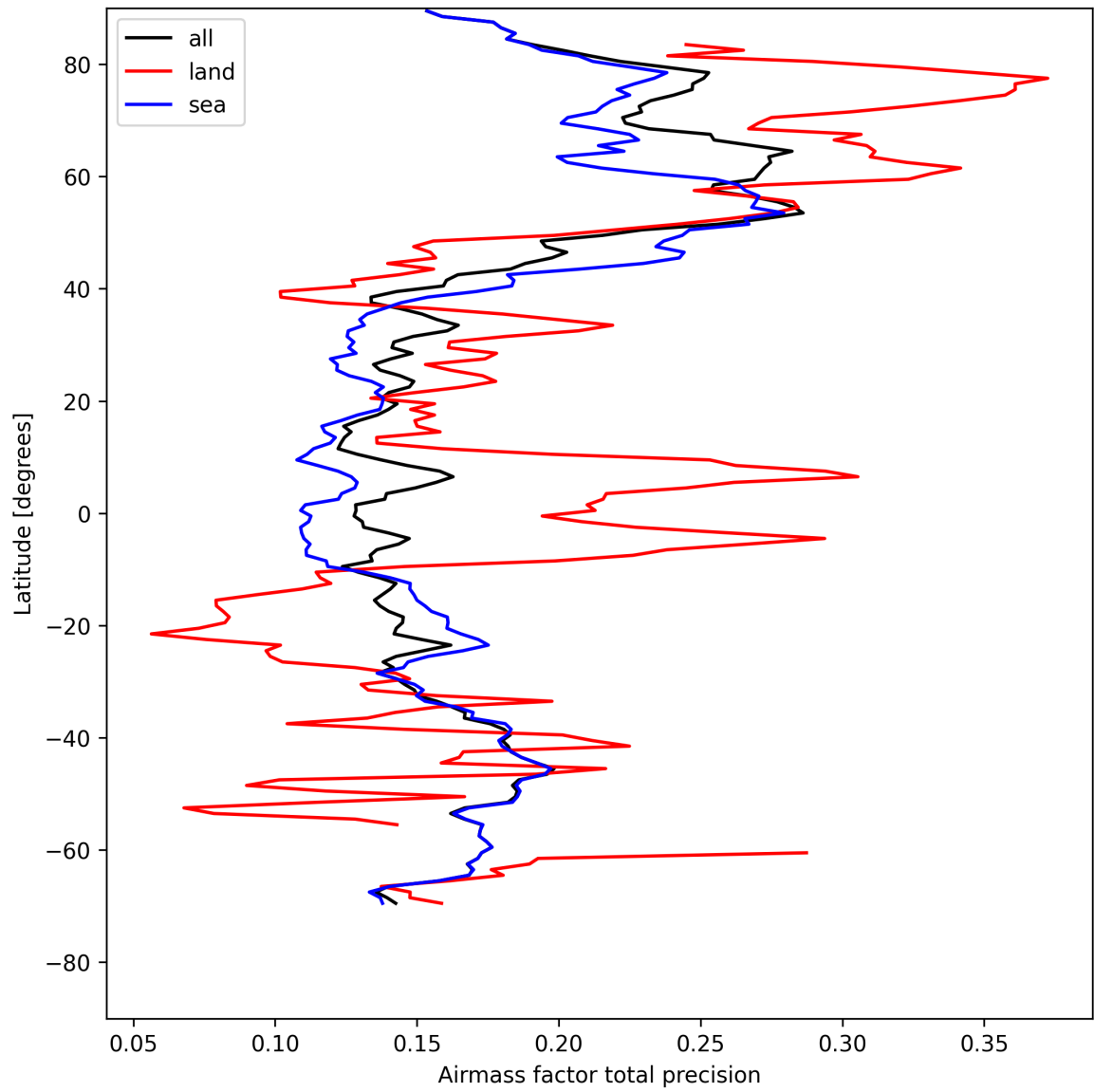
Figure 27: Zonal average of “Airmass factor total precision” for 2025-08-09 to 2025-08-11.
