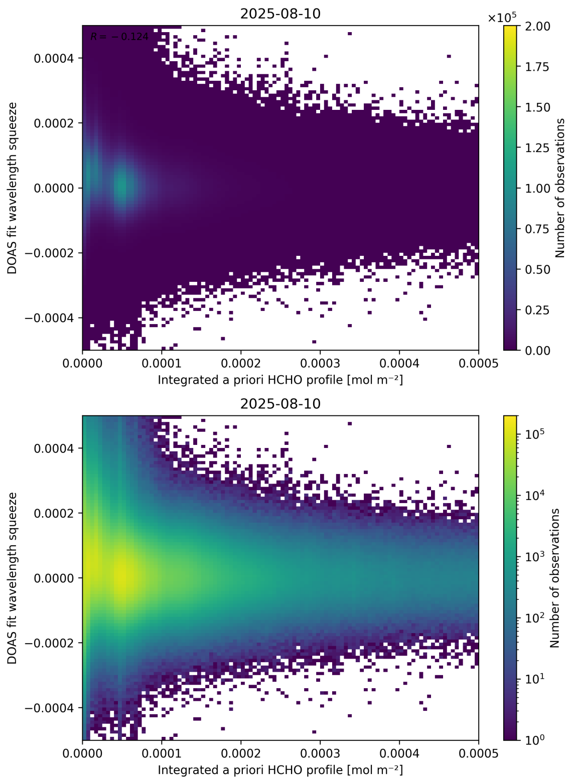
Figure 150: Scatter density plot of “Integrated a priori HCHO profile” against “DOAS fit wavelength squeeze” for 2025-08-09 to 2025-08-11.
