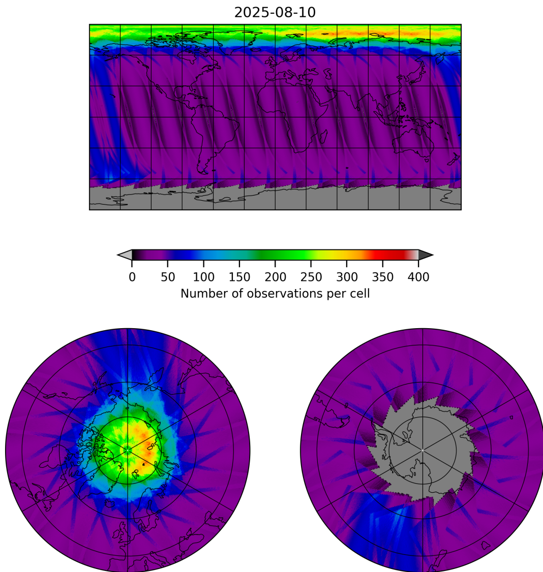
Figure 19: Map of the number of observations for 2025-08-09 to 2025-08-11
