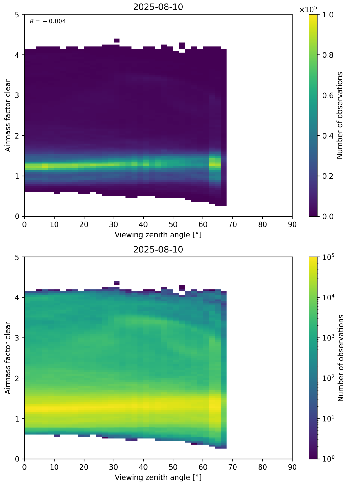
Figure 185: Scatter density plot of “Viewing zenith angle” against “Airmass factor clear” for 2025-08-09 to 2025-08-11.
