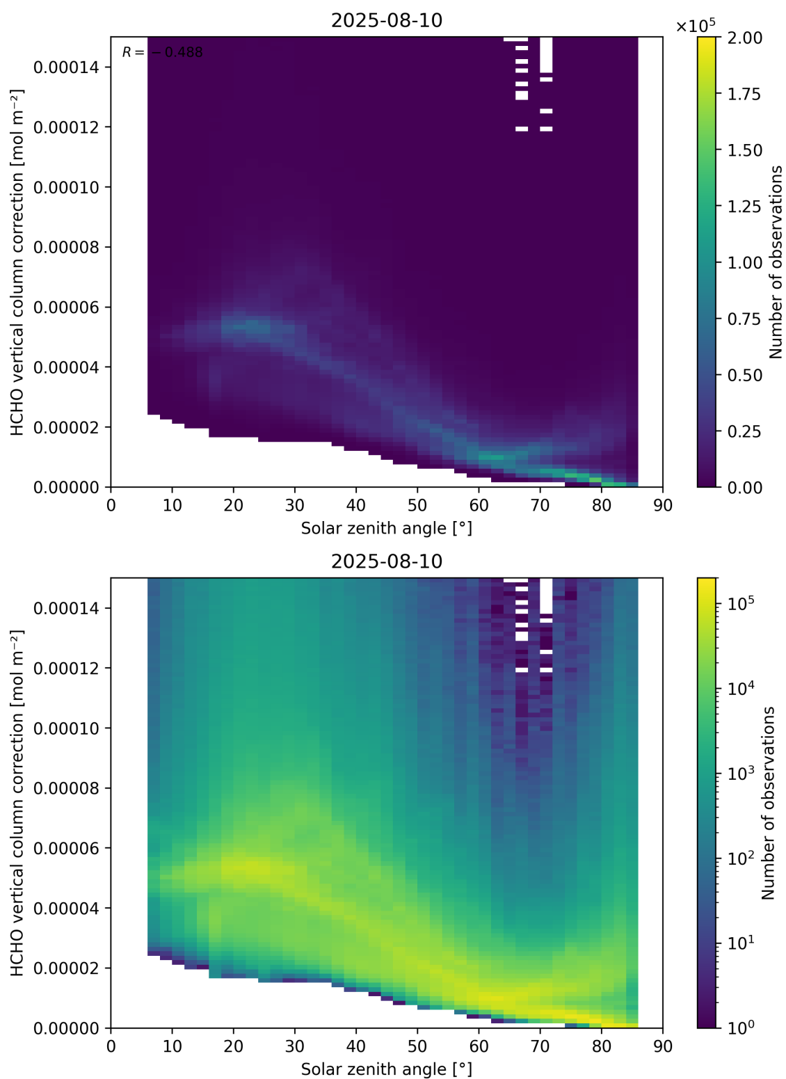
Figure 178: Scatter density plot of “Solar zenith angle” against “HCHO vertical column correction” for 2025-08-09 to 2025-08-11.
