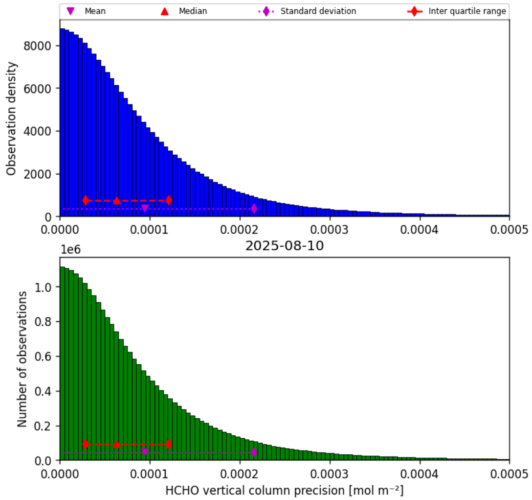
Figure 36: Histogram of “HCHO vertical column precision” for 2025-08-09 to 2025-08-11
