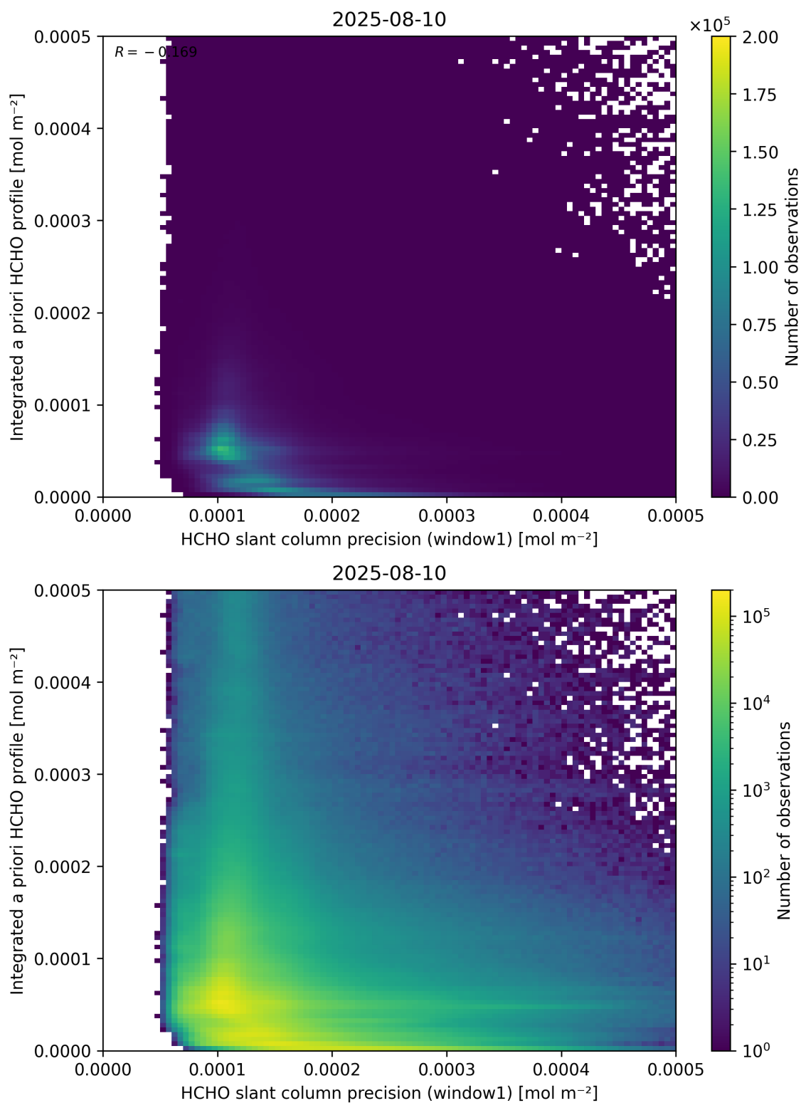
Figure 96: Scatter density plot of “HCHO slant column precision (window1)” against “Integrated a priori HCHO profile” for 2025-08-09 to 2025-08-11.
