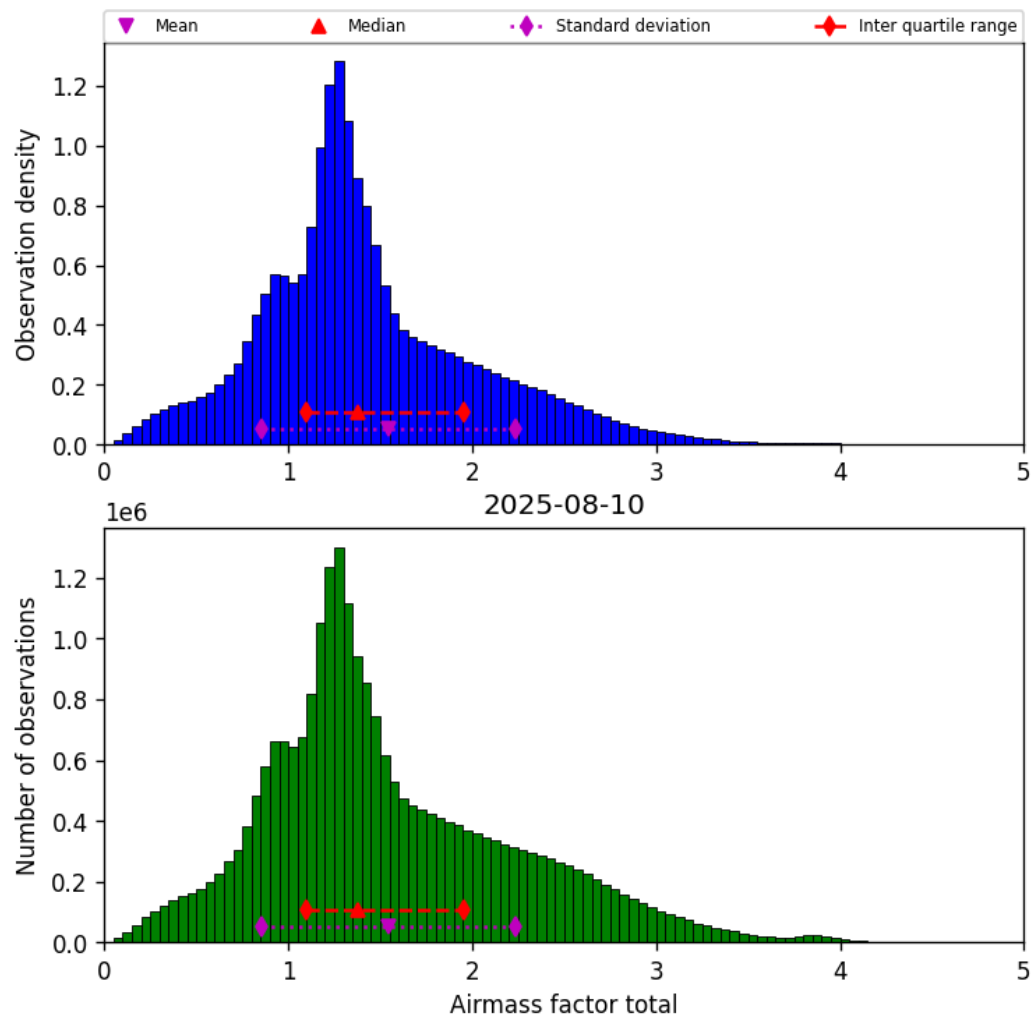
Figure 40: Histogram of “Airmass factor total” for 2025-08-09 to 2025-08-11
