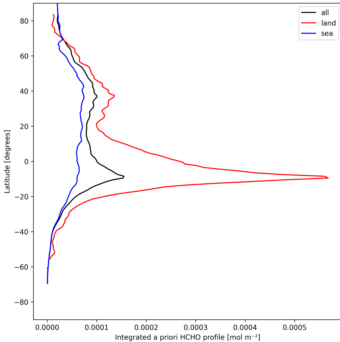
Figure 29: Zonal average of “Integrated a priori HCHO profile” for 2025-08-09 to 2025-08-11.
