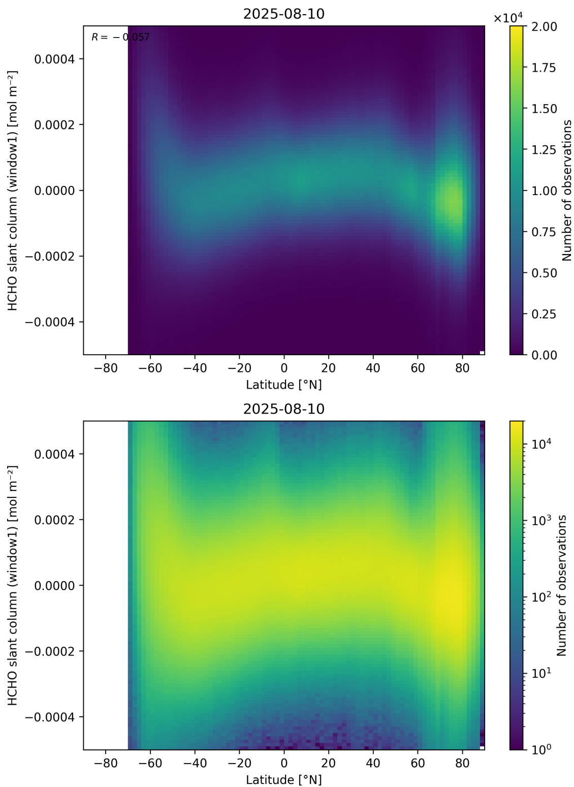
Figure 159: Scatter density plot of “Latitude” against “HCHO slant column (window1)” for 2025-08-09 to 2025-08-11.
