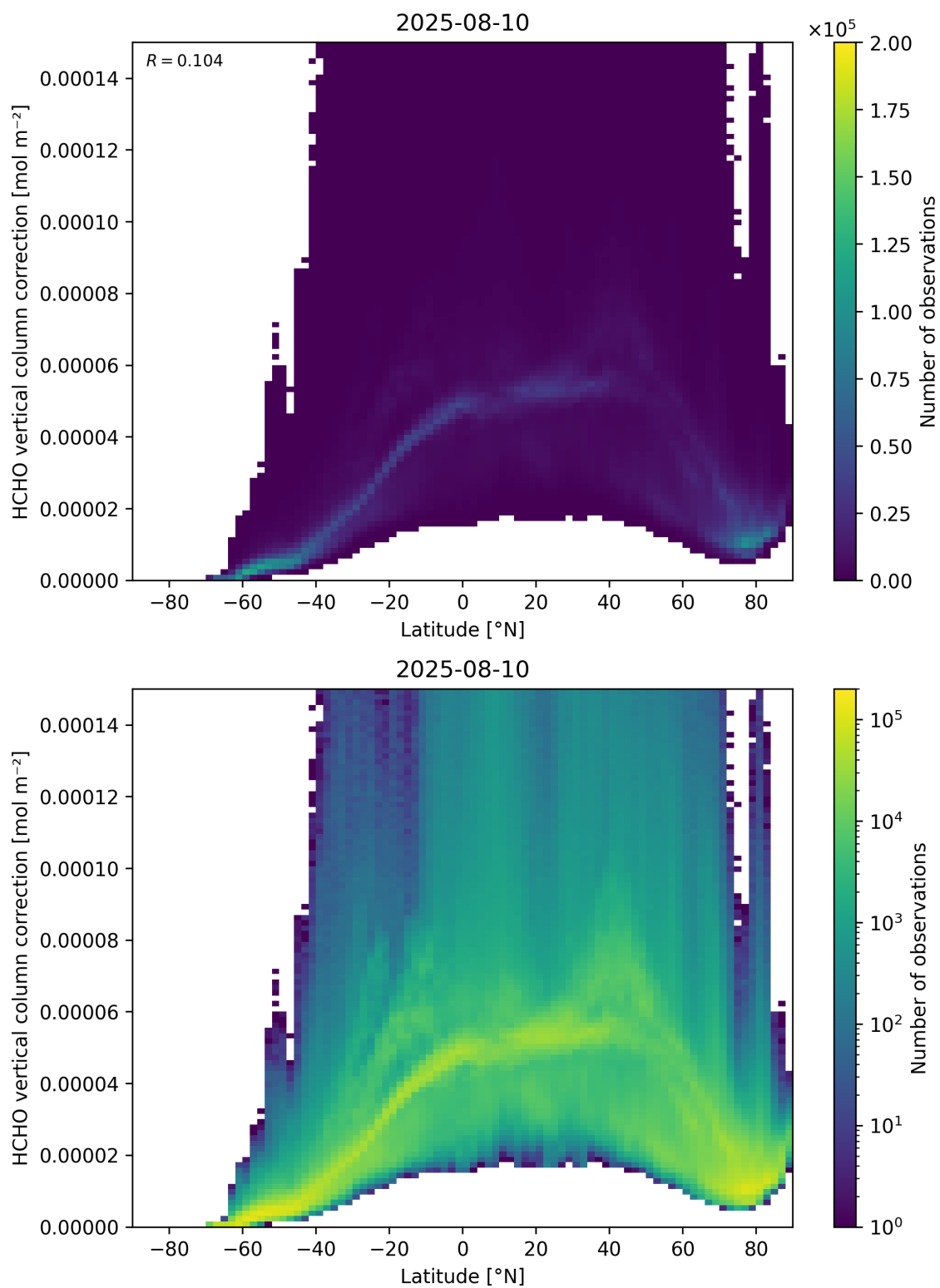
Figure 164: Scatter density plot of “Latitude” against “HCHO vertical column correction” for 2025-08-09 to 2025-08-11.
