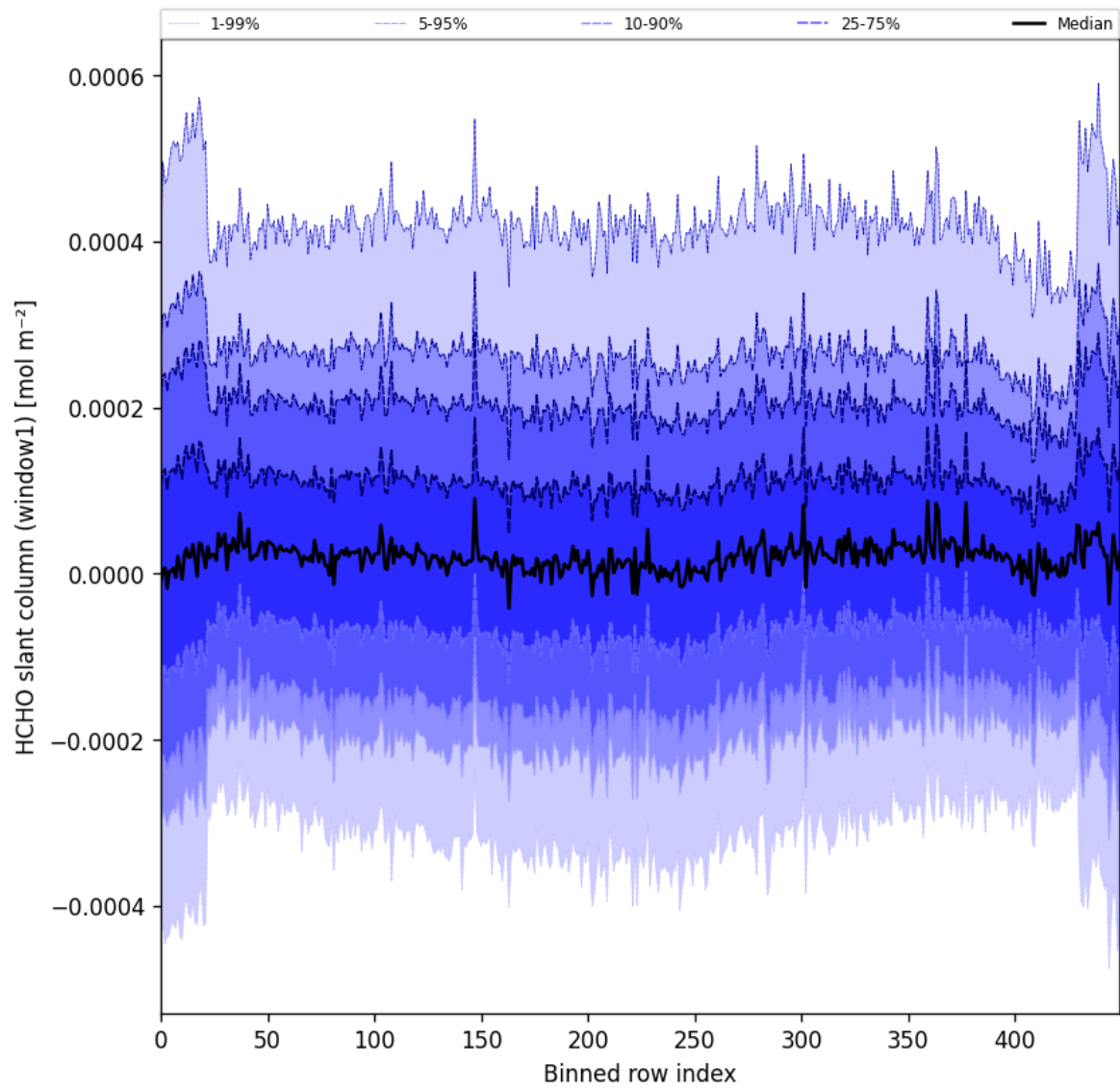
Figure 52: Along track statistics of “HCHO slant column (window1)” for 2025-08-09 to 2025-08-11
