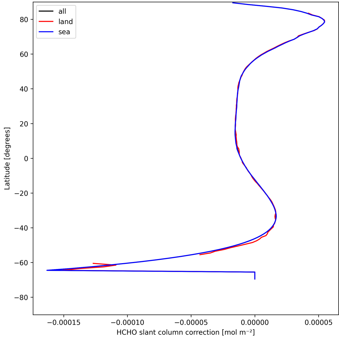
Figure 33: Zonal average of “HCHO slant column correction” for 2025-08-09 to 2025-08-11.
