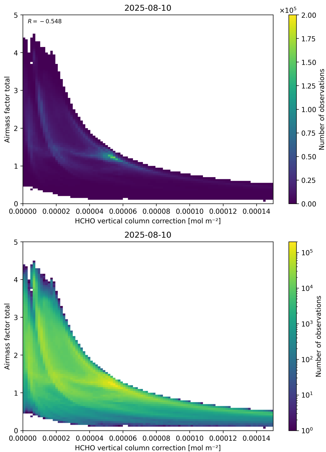
Figure 120: Scatter density plot of “HCHO vertical column correction” against “Airmass factor total” for 2025-08-09 to 2025-08-11.
