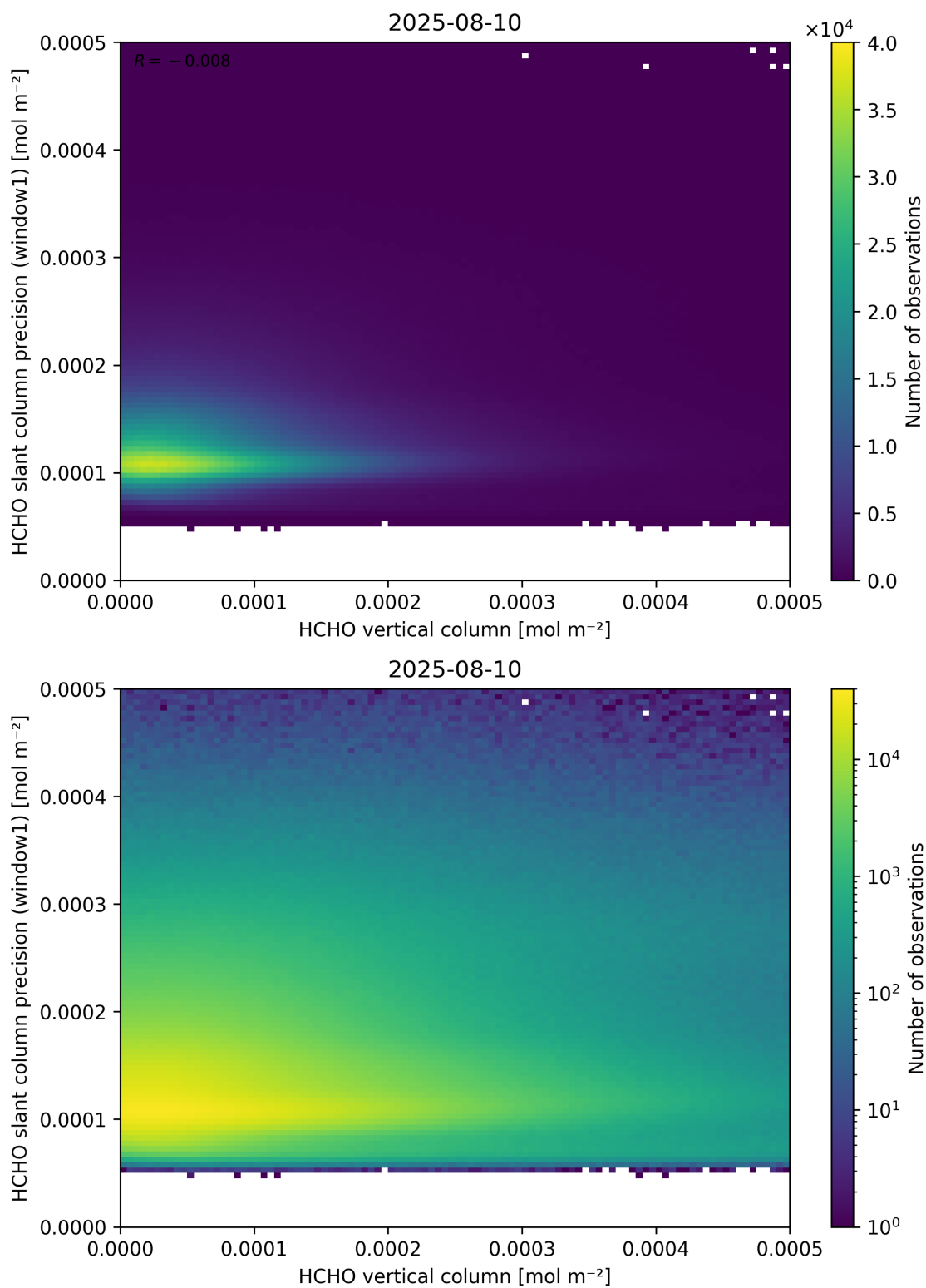
Figure 130: Scatter density plot of “HCHO vertical column” against “HCHO slant column precision (window1)” for 2025-08-09 to 2025-08-11.
