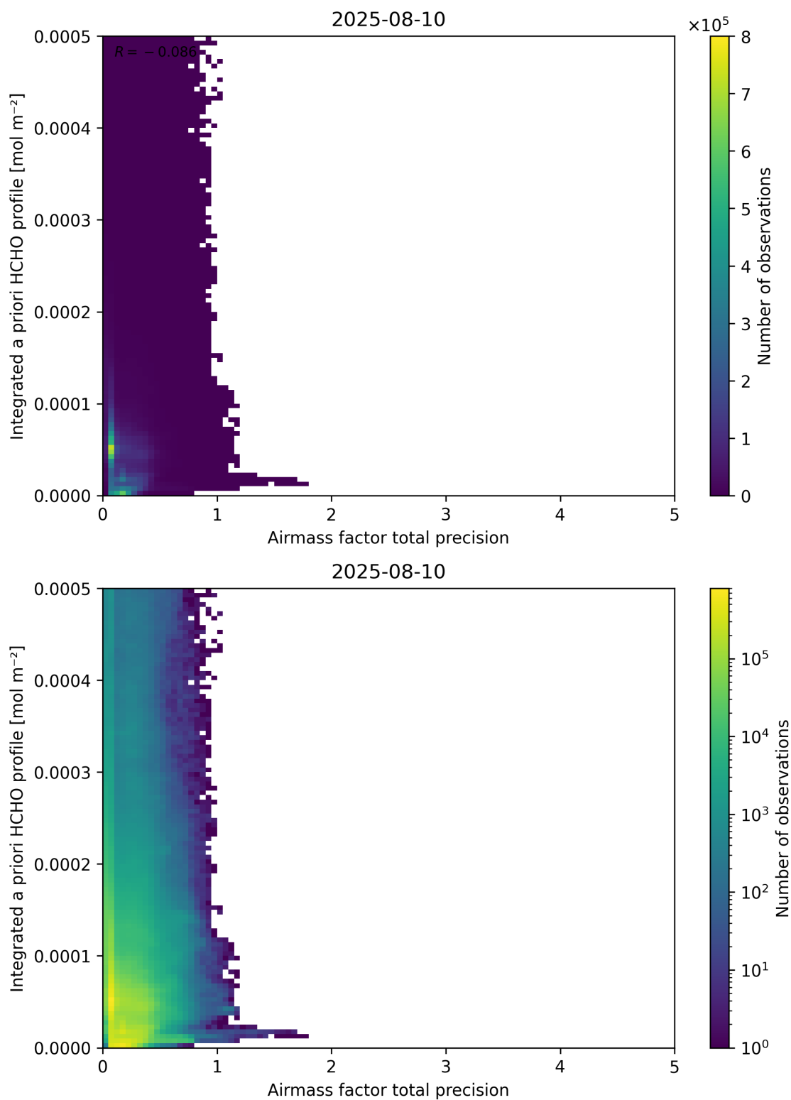
Figure 111: Scatter density plot of “Airmass factor total precision” against “Integrated a priori HCHO profile” for 2025-08-09 to 2025-08-11.
