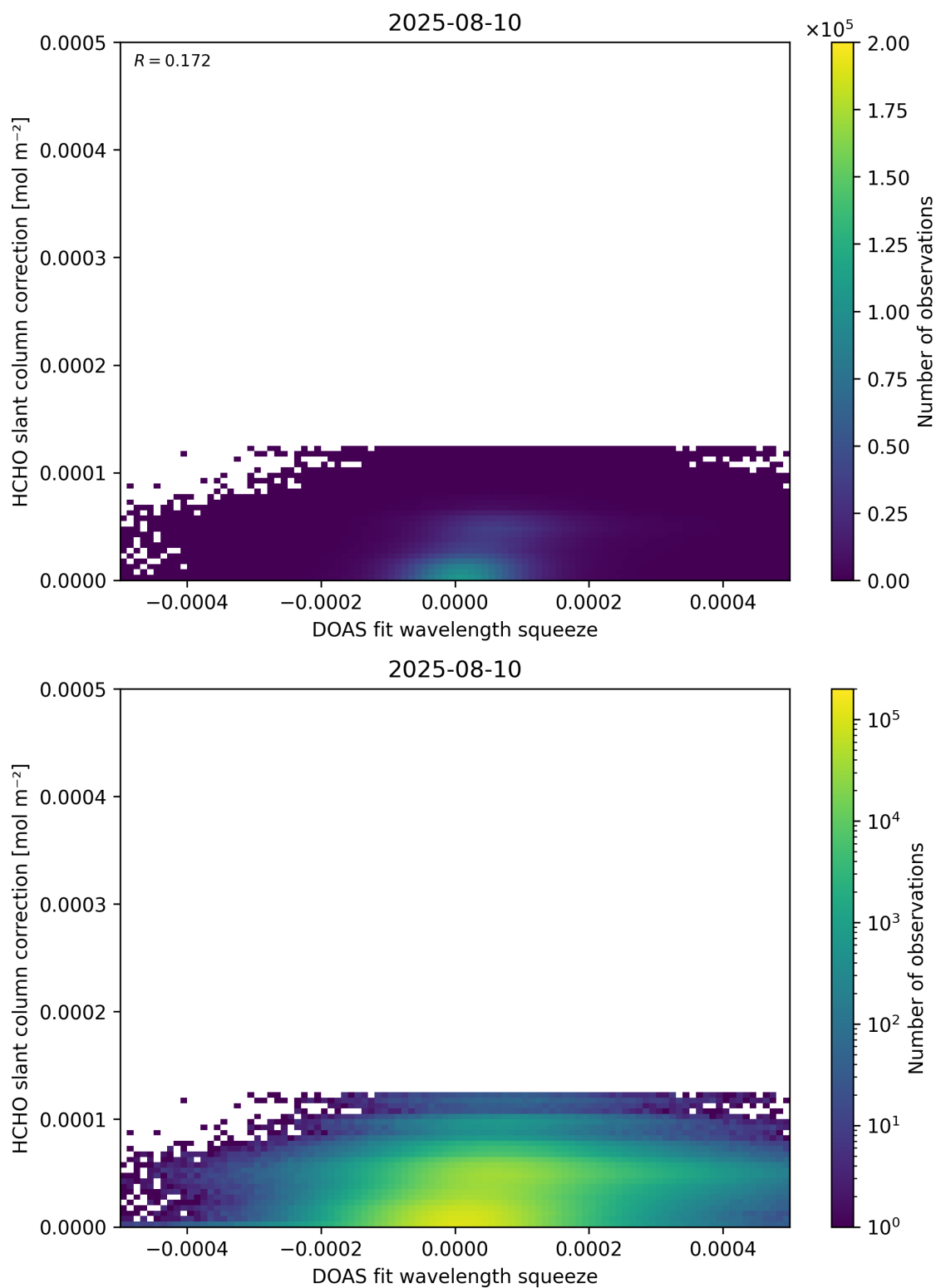
Figure 70: Scatter density plot of “DOAS fit wavelength squeeze” against “HCHO slant column correction” for 2025-08-09 to 2025-08-11.
