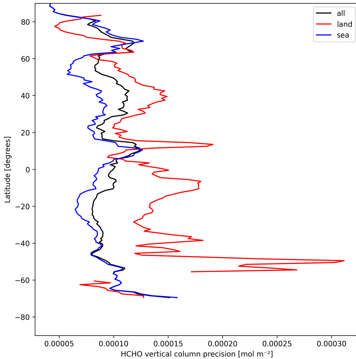
Figure 22: Zonal average of “HCHO vertical column precision” for 2025-08-09 to 2025-08-11.
