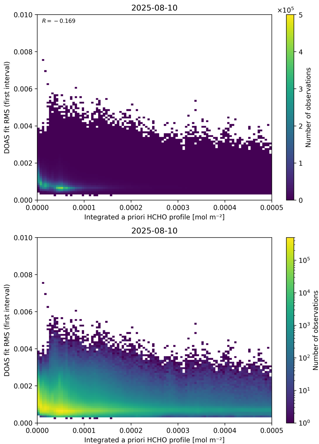
Figure 148: Scatter density plot of “Integrated a priori HCHO profile” against “DOAS fit RMS (first interval)” for 2025-08-09 to 2025-08-11.
