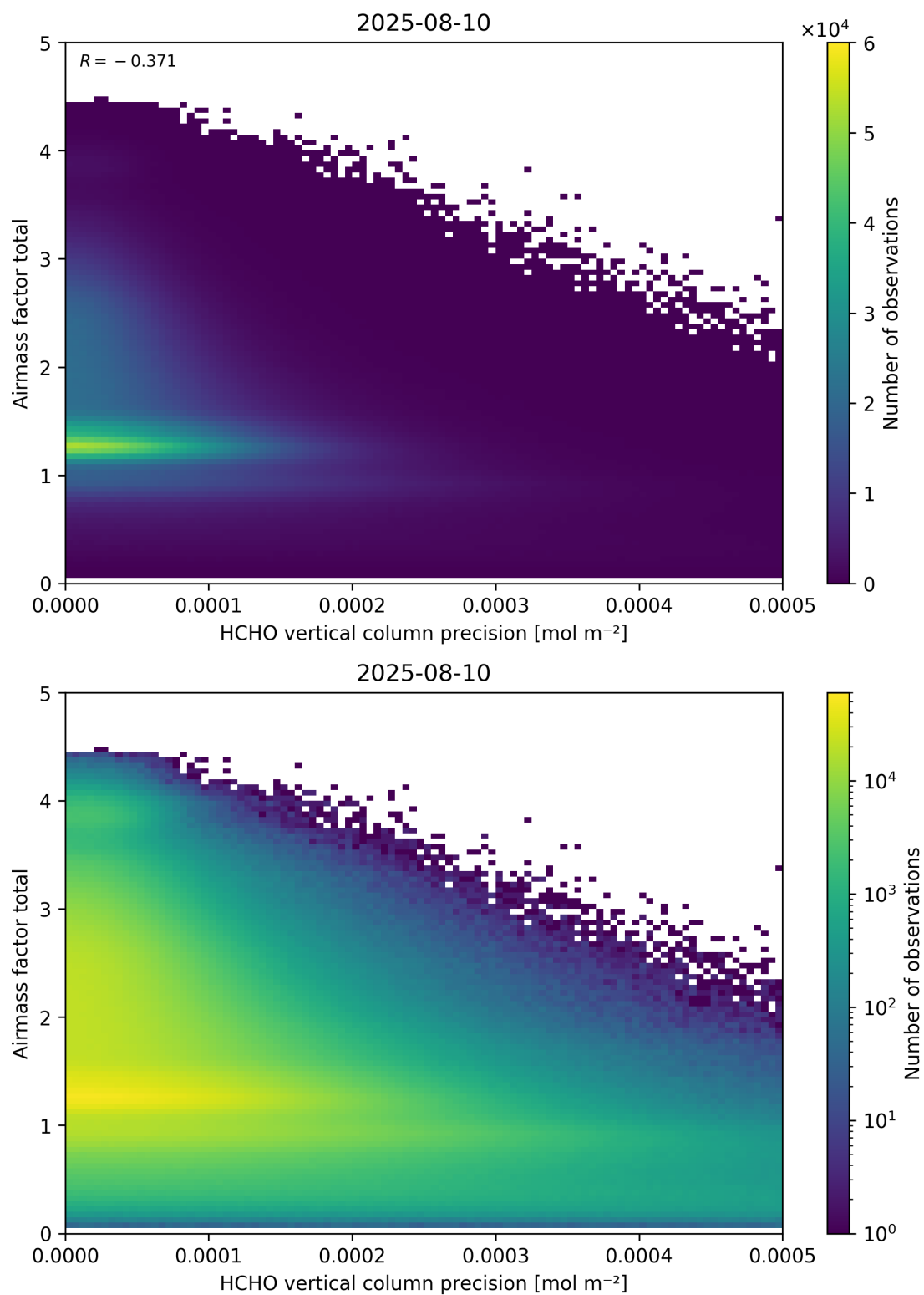
Figure 144: Scatter density plot of “HCHO vertical column precision” against “Airmass factor total” for 2025-08-09 to 2025-08-11.
