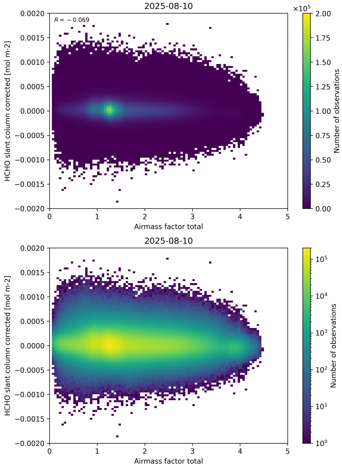
Figure 101: Scatter density plot of “Airmass factor total” against “HCHO slant column corrected” for 2025-08-09 to 2025-08-11.
