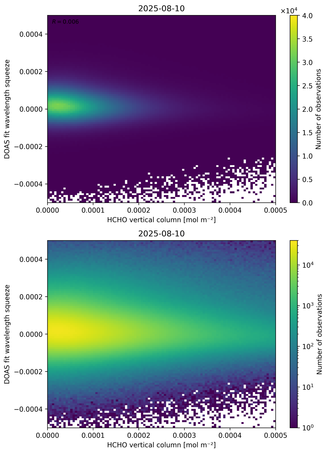
Figure 125: Scatter density plot of “HCHO vertical column” against “DOAS fit wavelength squeeze” for 2025-08-09 to 2025-08-11.
