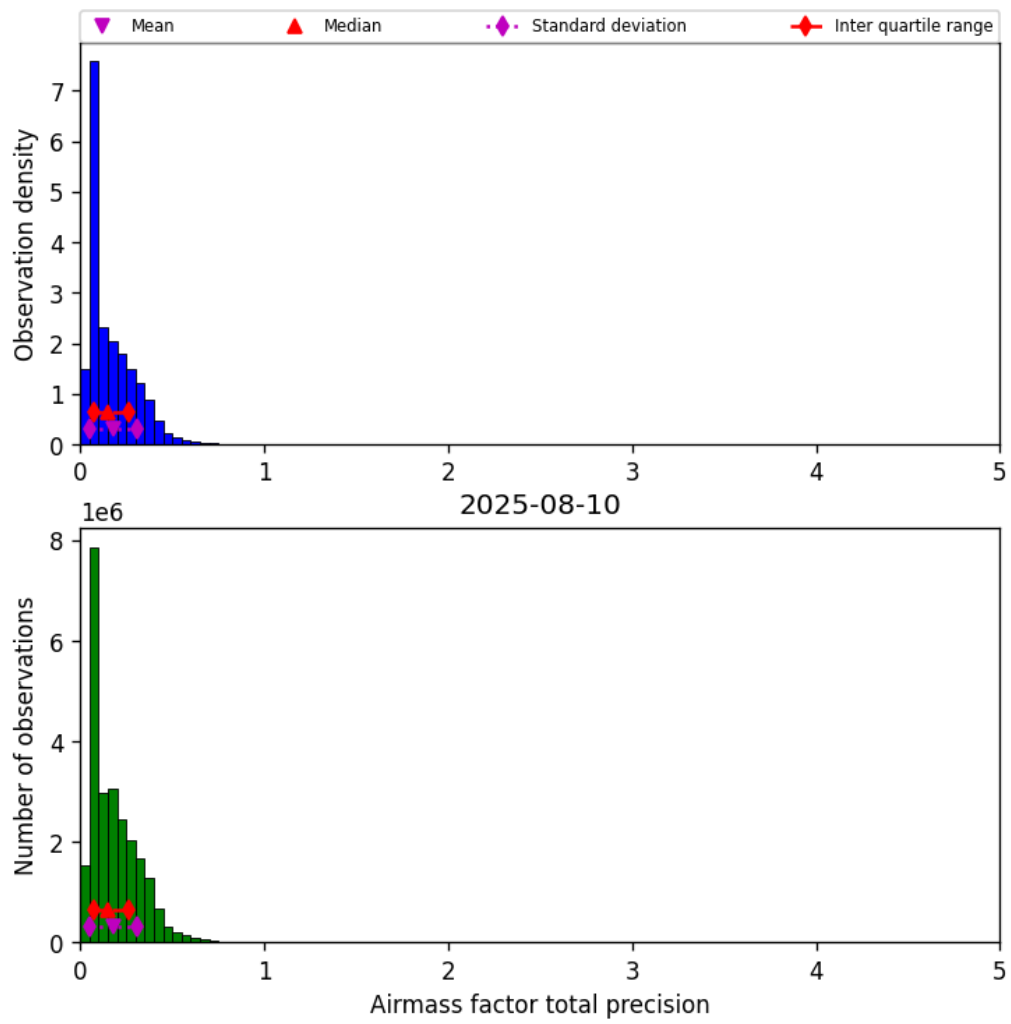
Figure 41: Histogram of “Airmass factor total precision” for 2025-08-09 to 2025-08-11
