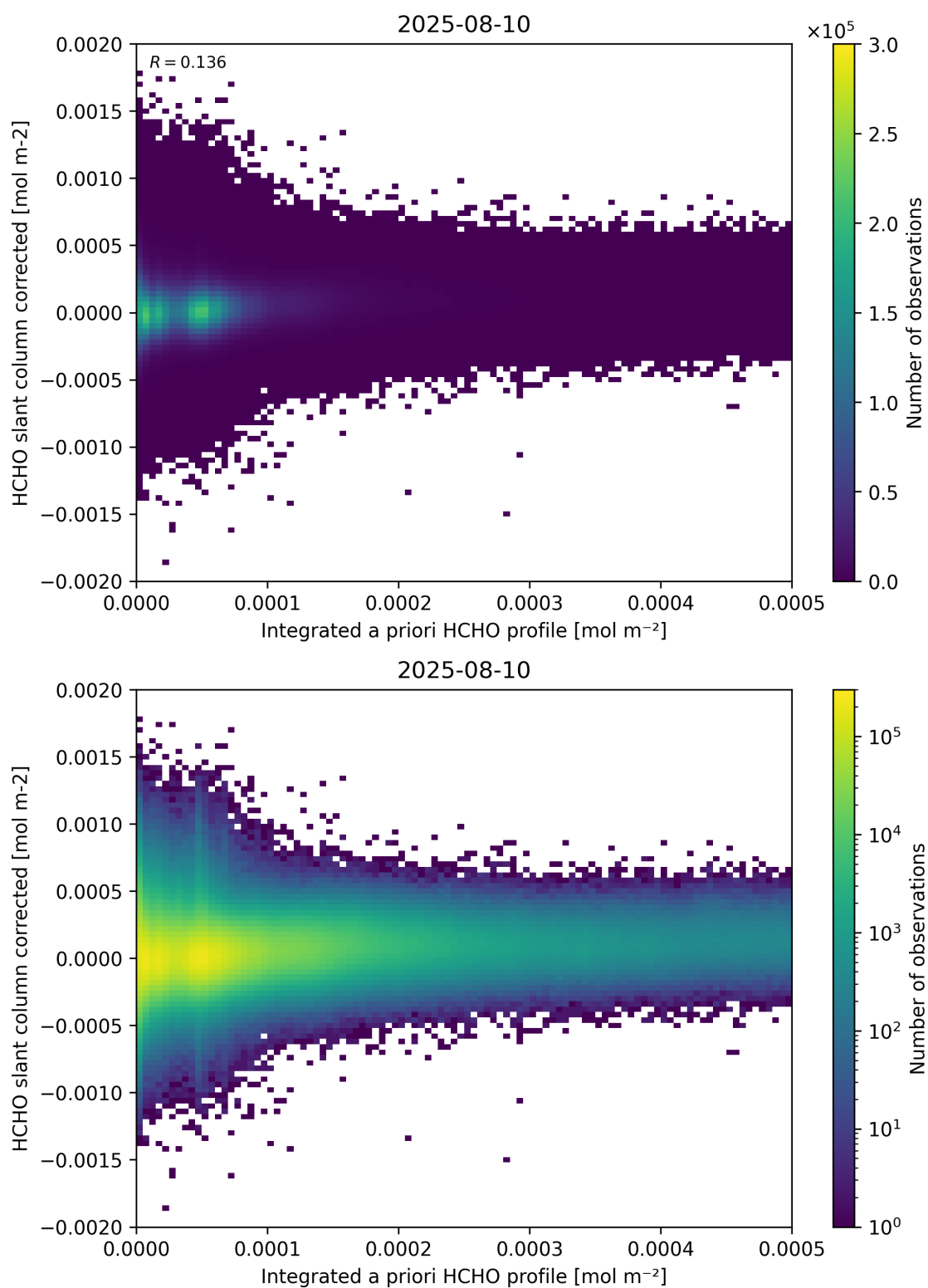
Figure 151: Scatter density plot of “Integrated a priori HCHO profile” against “HCHO slant column corrected” for 2025-08-09 to 2025-08-11.
