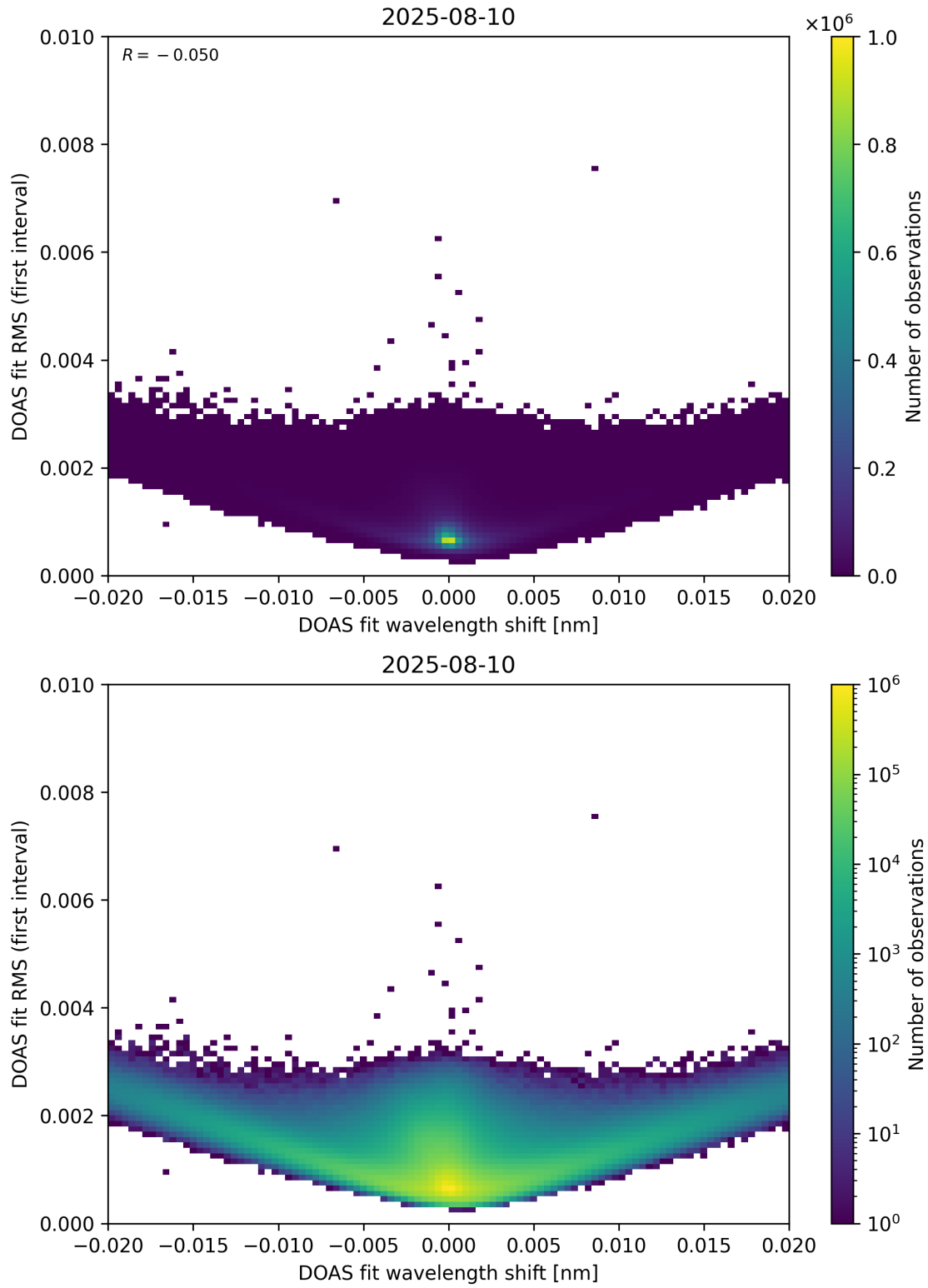
Figure 64: Scatter density plot of “DOAS fit wavelength shift” against “DOAS fit RMS (first interval)” for 2025-08-09 to 2025-08-11.
