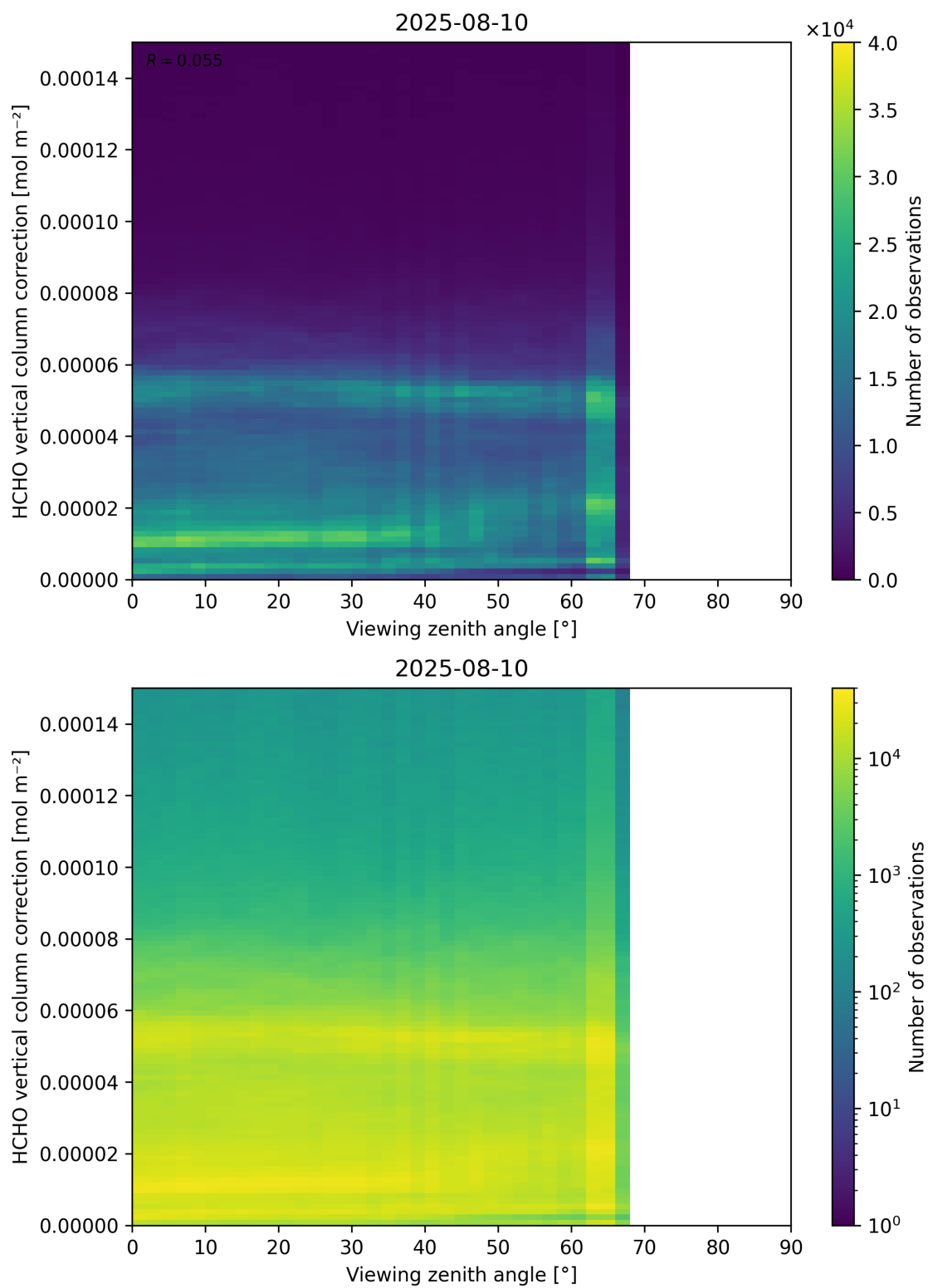
Figure 193: Scatter density plot of “Viewing zenith angle” against “HCHO vertical column correction” for 2025-08-09 to 2025-08-11.
