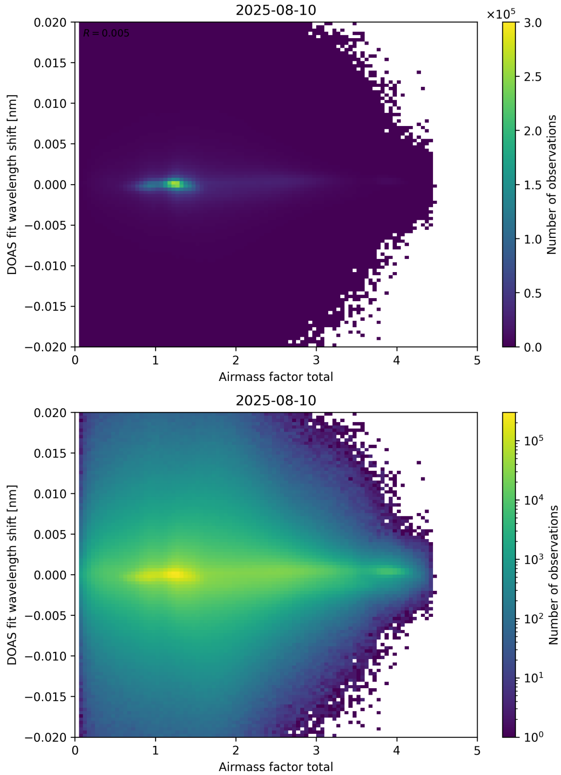
Figure 98: Scatter density plot of “Airmass factor total” against “DOAS fit wavelength shift” for 2025-08-09 to 2025-08-11.
