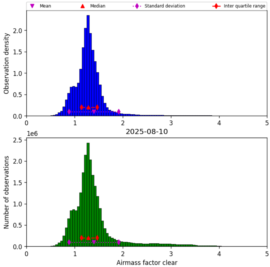
Figure 42: Histogram of “Airmass factor clear” for 2025-08-09 to 2025-08-11
