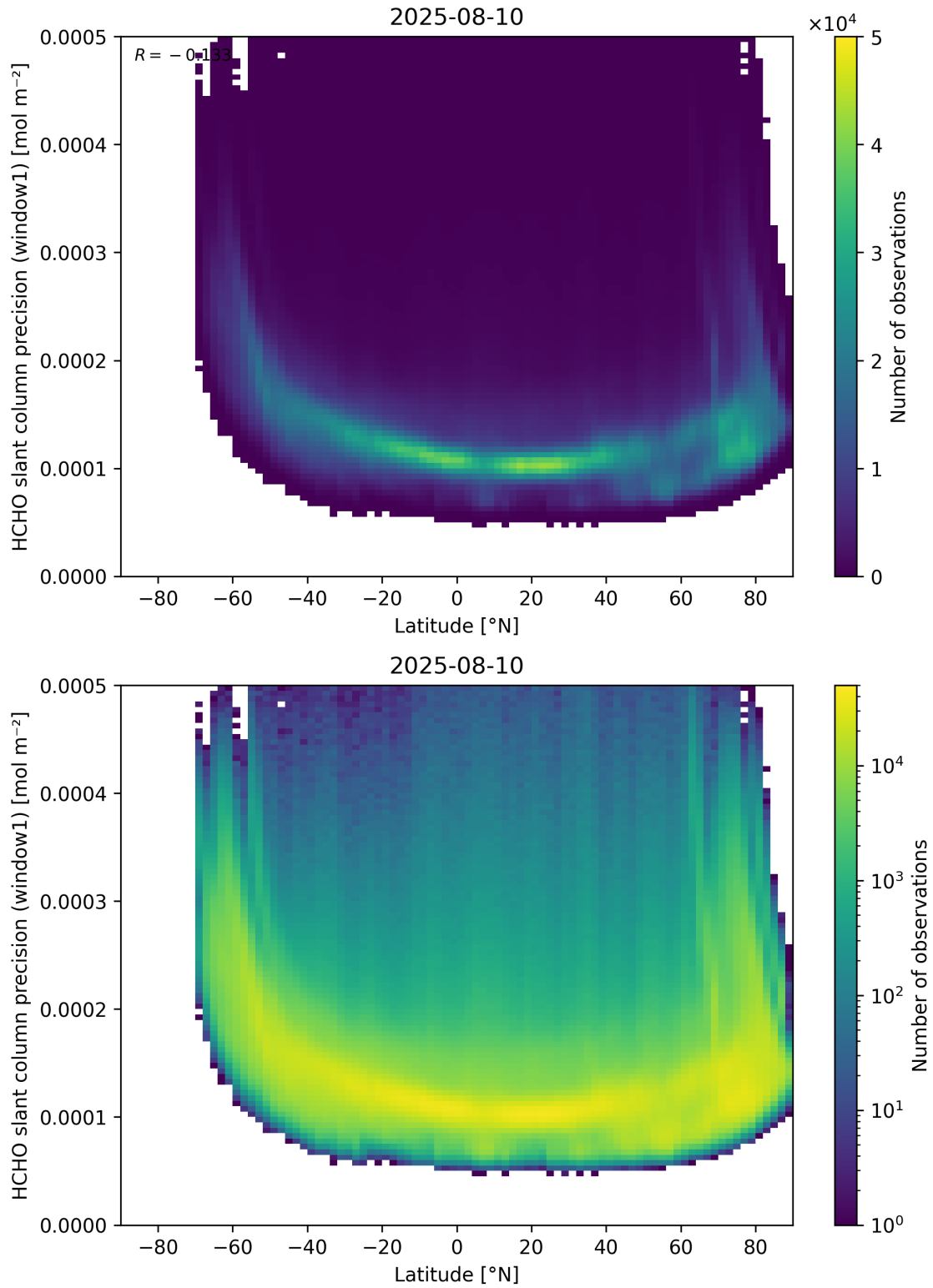
Figure 160: Scatter density plot of “Latitude” against “HCHO slant column precision (window1)” for 2025-08-09 to 2025-08-11.
