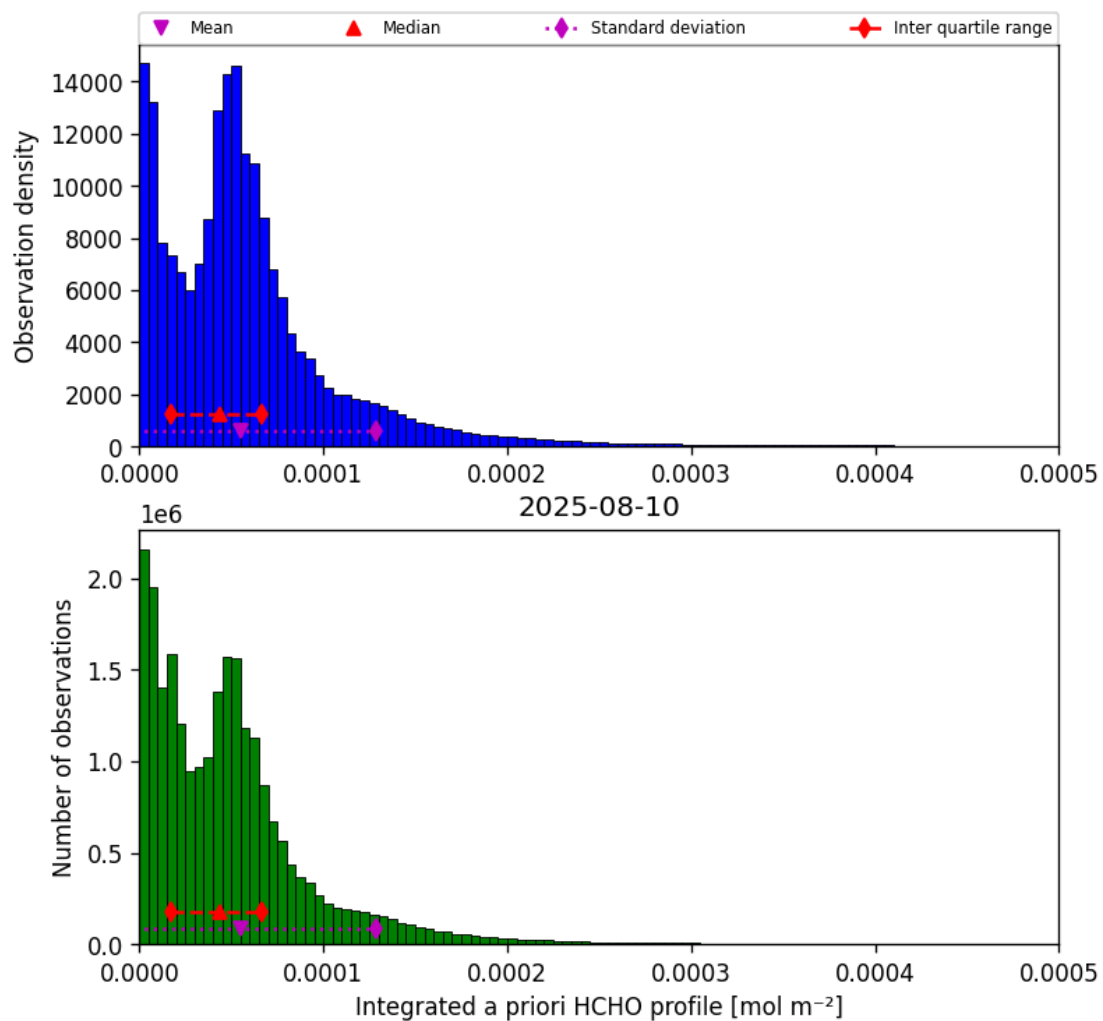
Figure 43: Histogram of “Integrated a priori HCHO profile” for 2025-08-09 to 2025-08-11
