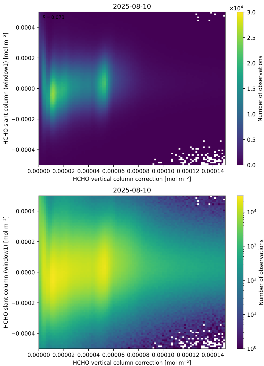
Figure 118: Scatter density plot of “HCHO vertical column correction” against “HCHO slant column (window1)” for 2025-08-09 to 2025-08-11.
