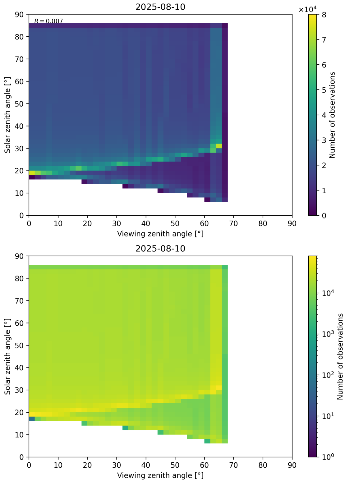
Figure 197: Scatter density plot of “Viewing zenith angle” against “Solar zenith angle” for 2025-08-09 to 2025-08-11.
