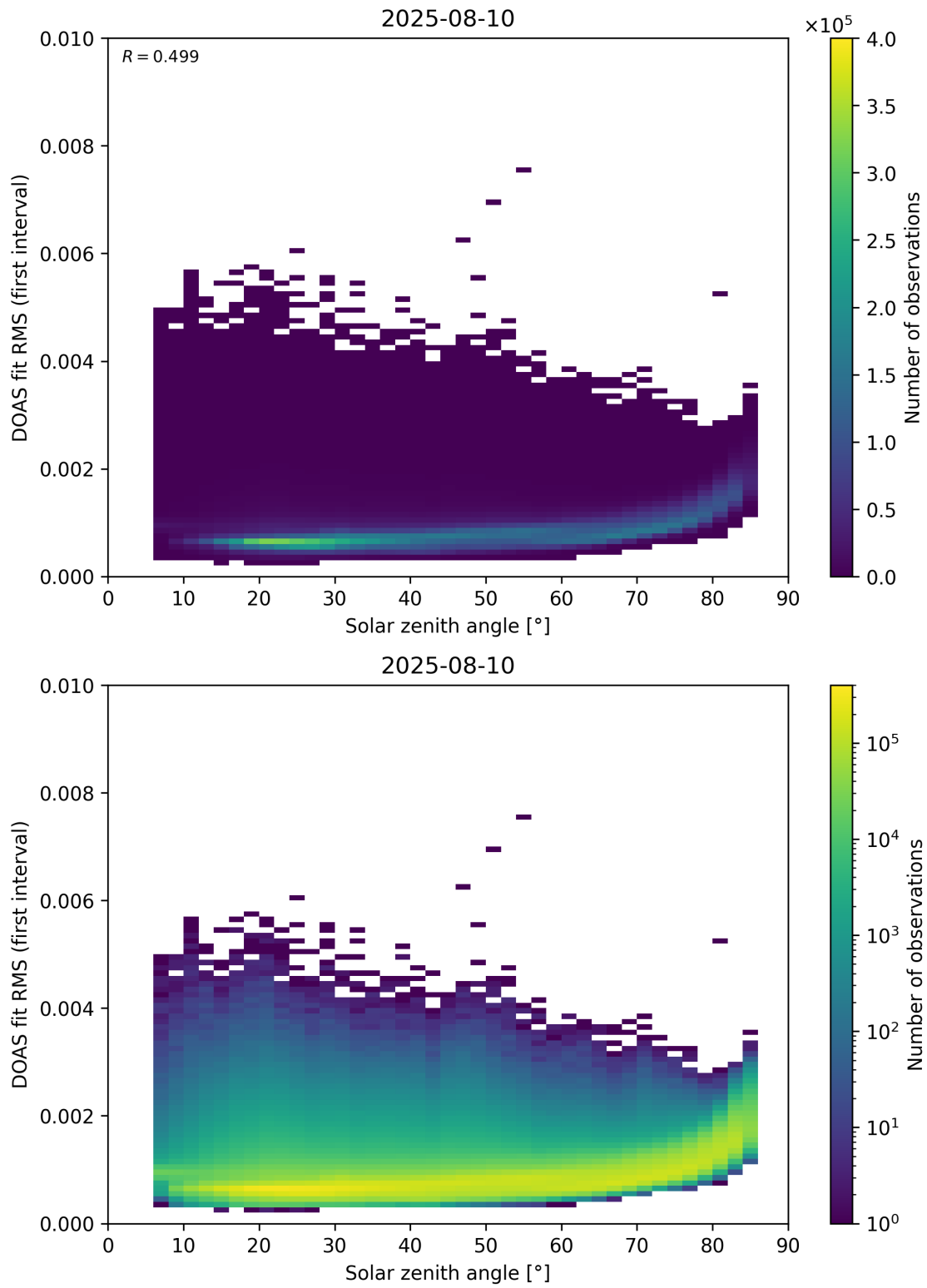
Figure 167: Scatter density plot of “Solar zenith angle” against “DOAS fit RMS (first interval)” for 2025-08-09 to 2025-08-11.
