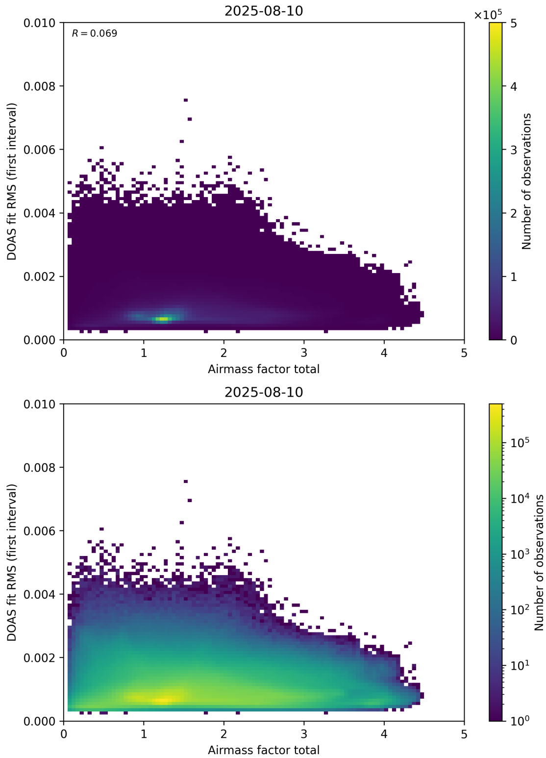
Figure 97: Scatter density plot of “Airmass factor total” against “DOAS fit RMS (first interval)” for 2025-08-09 to 2025-08-11.
