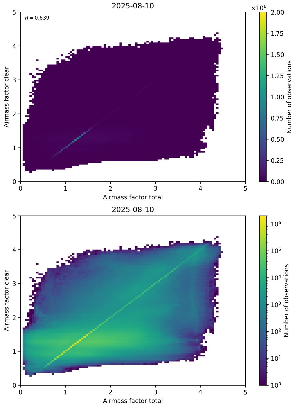
Figure 100: Scatter density plot of “Airmass factor total” against “Airmass factor clear” for 2025-08-09 to 2025-08-11.
