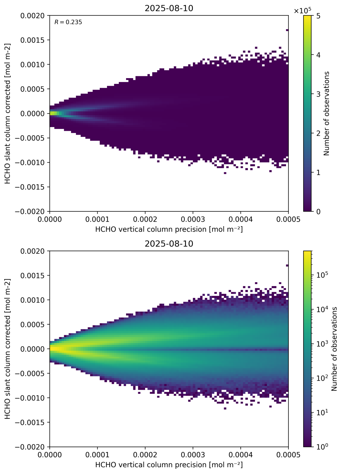
Figure 140: Scatter density plot of “HCHO vertical column precision” against “HCHO slant column corrected” for 2025-08-09 to 2025-08-11.
