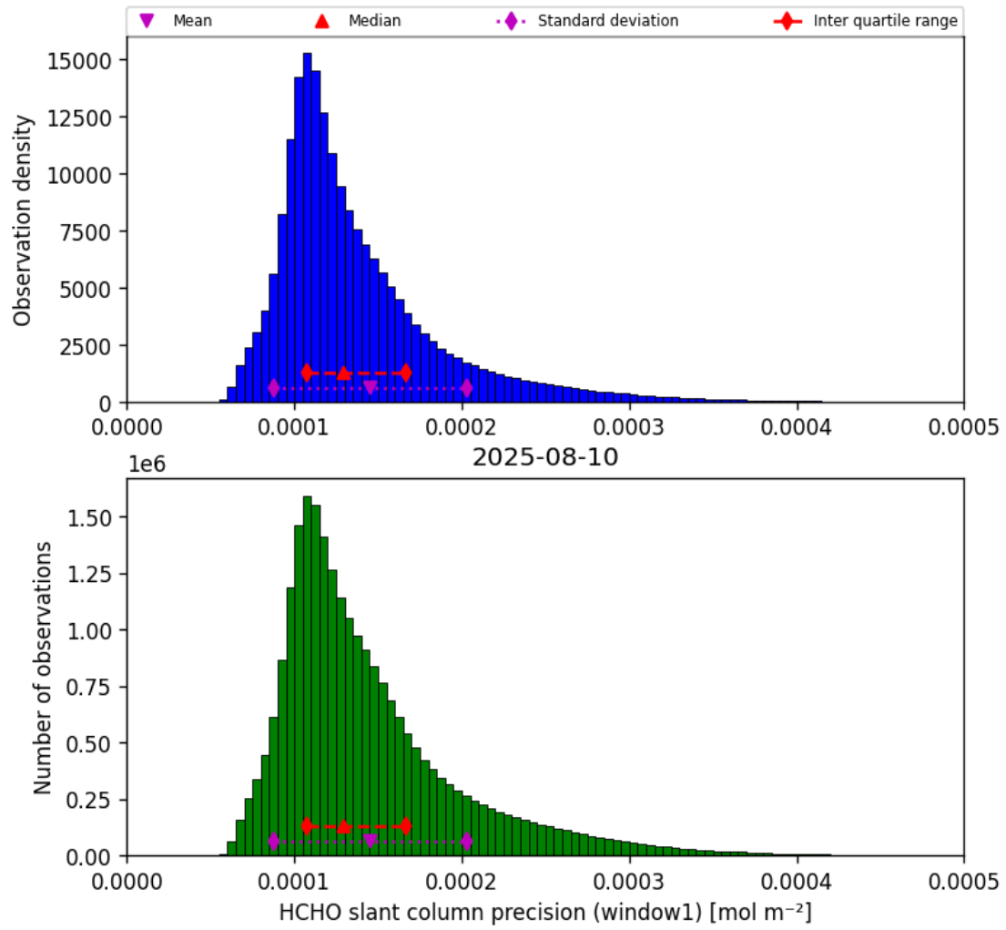
Figure 39: Histogram of “HCHO slant column precision (window1)” for 2025-08-09 to 2025-08-11
