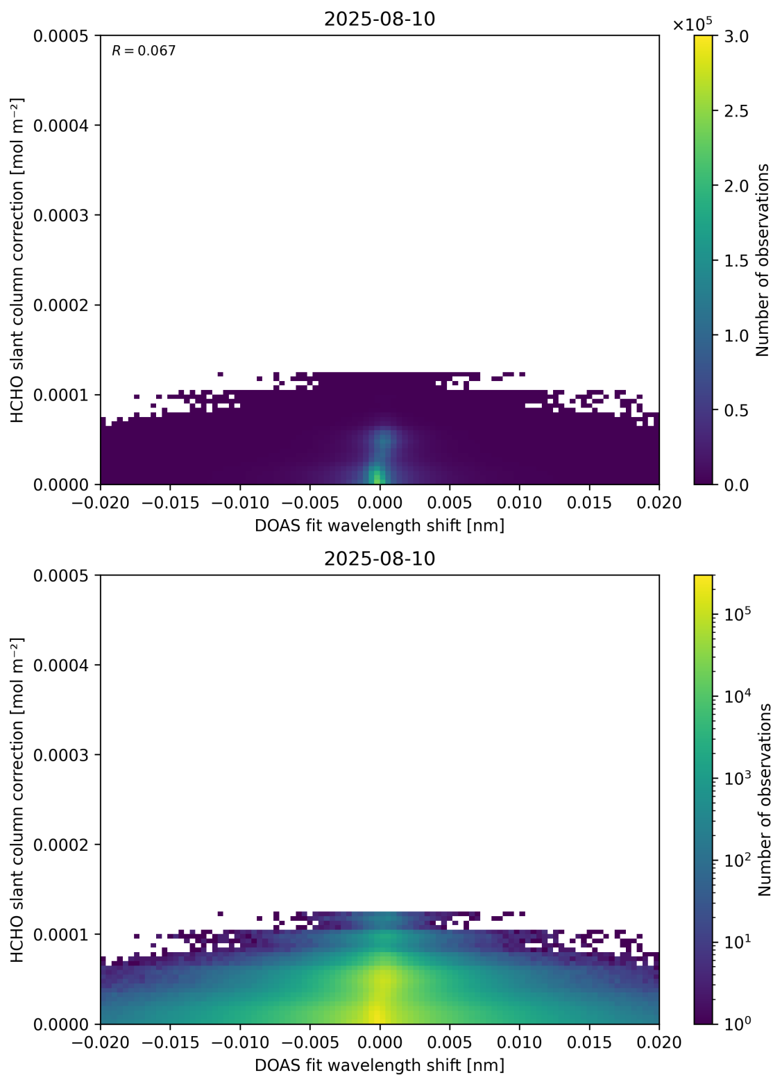
Figure 67: Scatter density plot of “DOAS fit wavelength shift” against “HCHO slant column correction” for 2025-08-09 to 2025-08-11.
