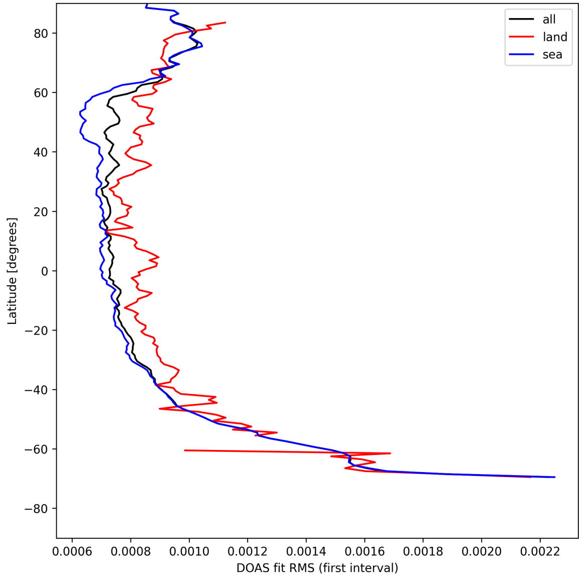
Figure 32: Zonal average of “DOAS fit RMS (first interval)” for 2025-08-09 to 2025-08-11.
