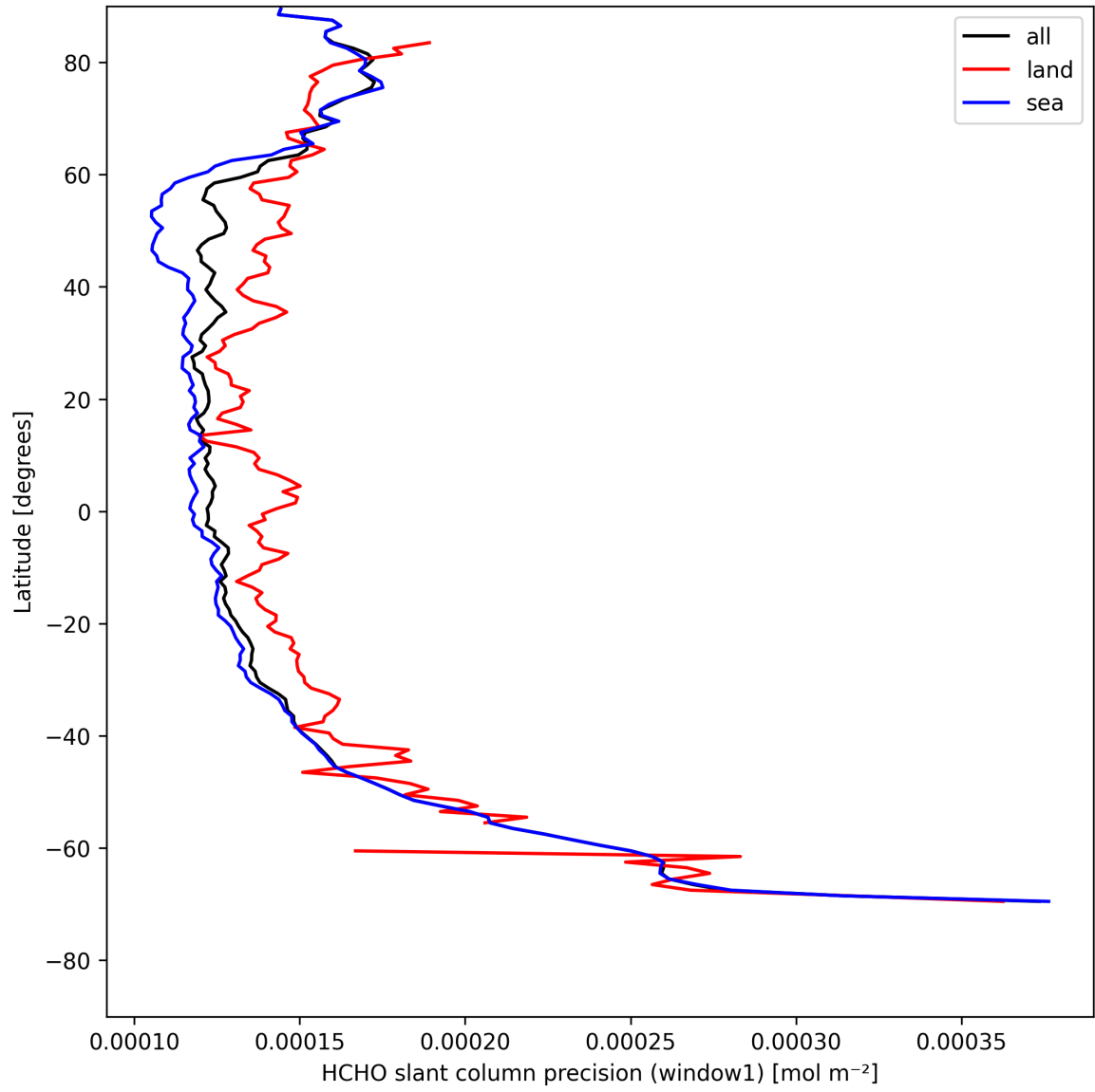
Figure 25: Zonal average of "HCHO slant column precision (window1)" for 2025-08-09 to 2025-08-11.
