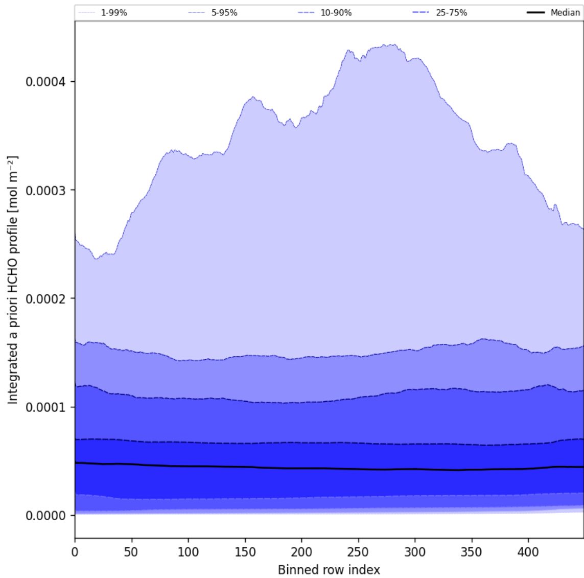
Figure 57: Along track statistics of “Integrated a priori HCHO profile” for 2025-08-09 to 2025-08-11
