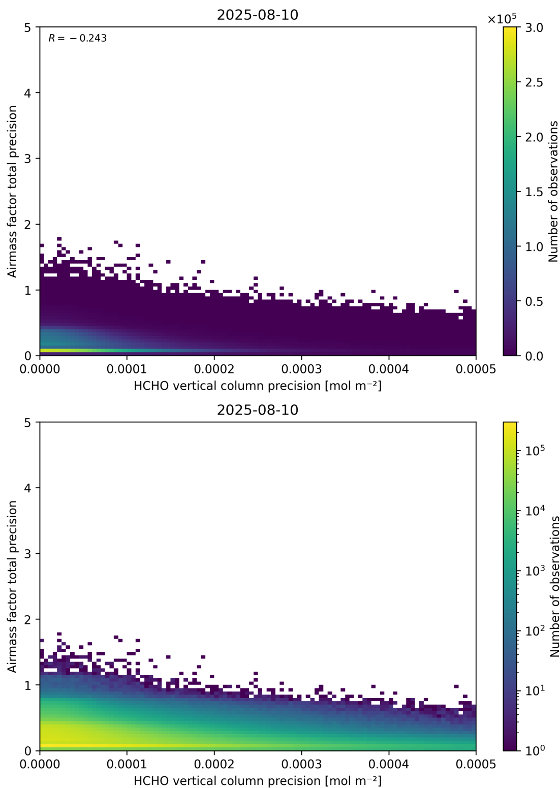
Figure 145: Scatter density plot of “HCHO vertical column precision” against “Airmass factor total precision” for 2025-08-09 to 2025-08-11.
