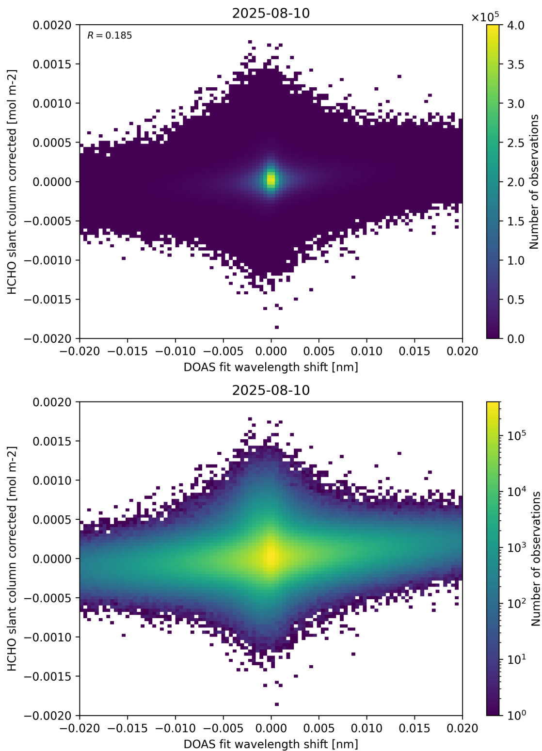
Figure 66: Scatter density plot of “DOAS fit wavelength shift” against “HCHO slant column corrected” for 2025-08-09 to 2025-08-11.
