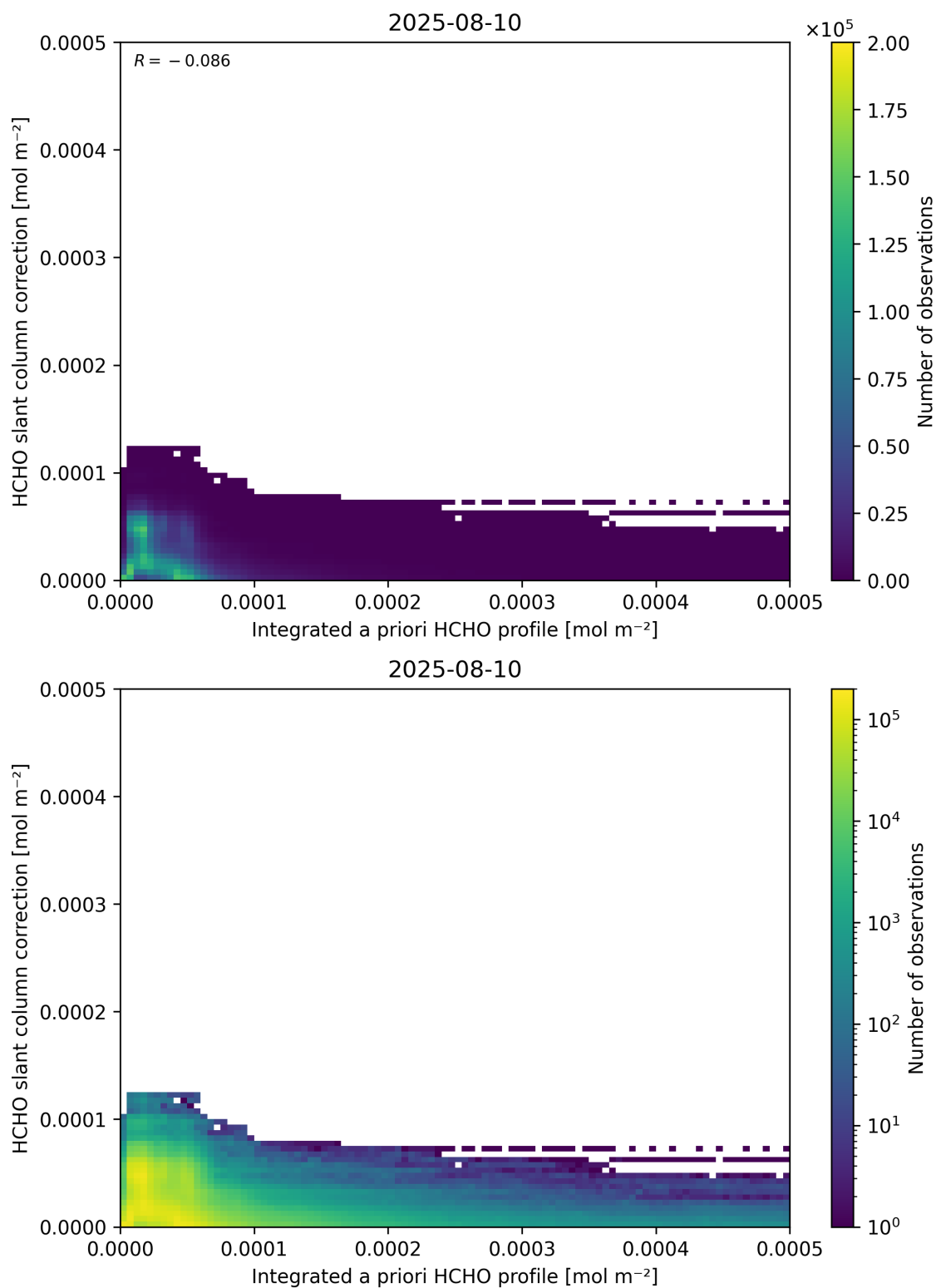
Figure 152: Scatter density plot of “Integrated a priori HCHO profile” against “HCHO slant column correction” for 2025-08-09 to 2025-08-11.
