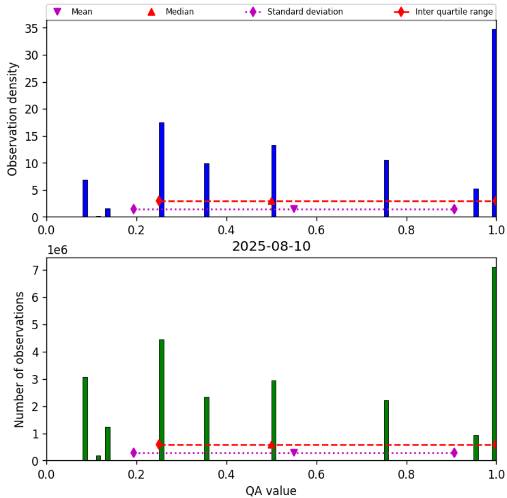
Figure 34: Histogram of “QA value” for 2025-08-09 to 2025-08-11
