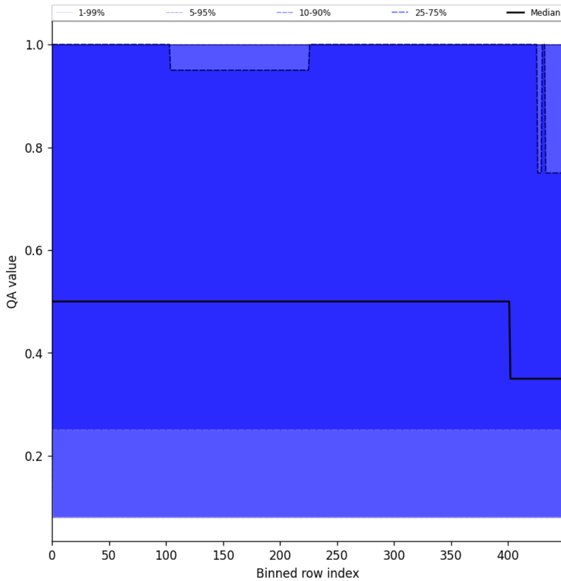
Figure 48: Along track statistics of “QA value” for 2025-08-09 to 2025-08-11
