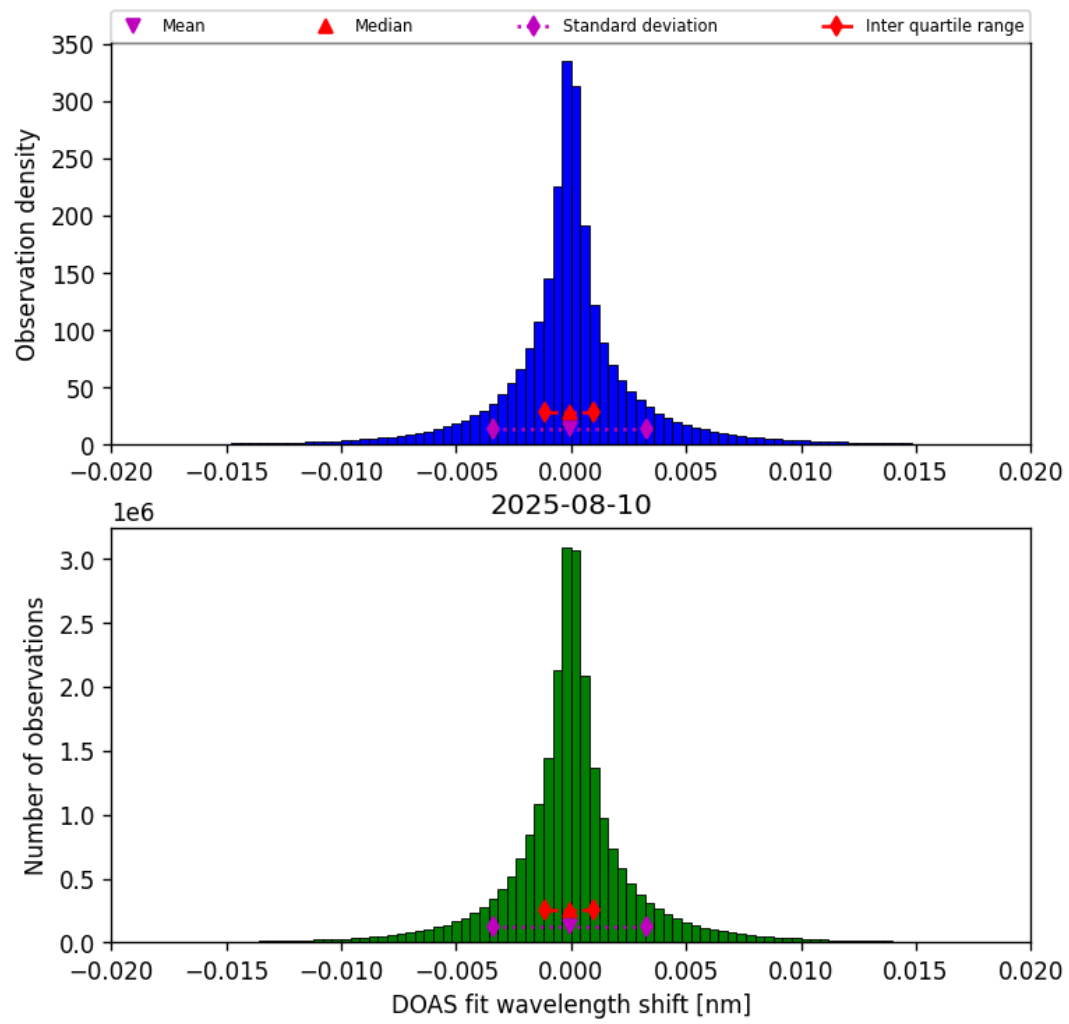
Figure 44: Histogram of “DOAS fit wavelength shift” for 2025-08-09 to 2025-08-11
