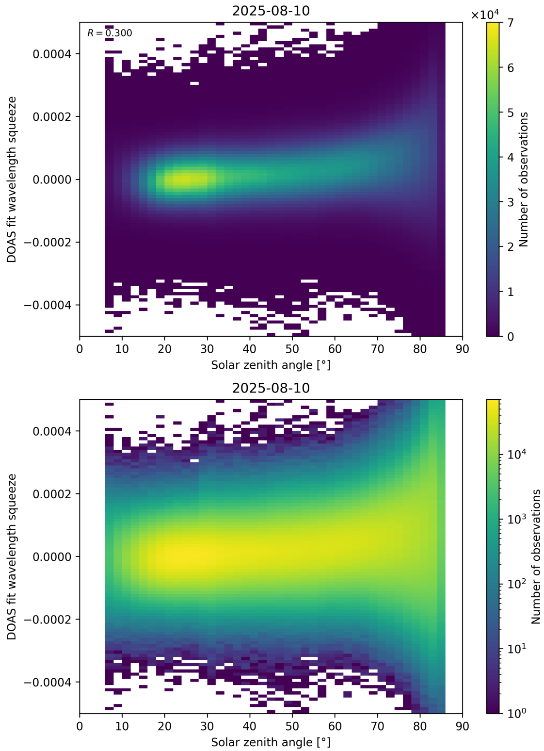
Figure 169: Scatter density plot of “Solar zenith angle” against “DOAS fit wavelength squeeze” for 2025-08-09 to 2025-08-11.
