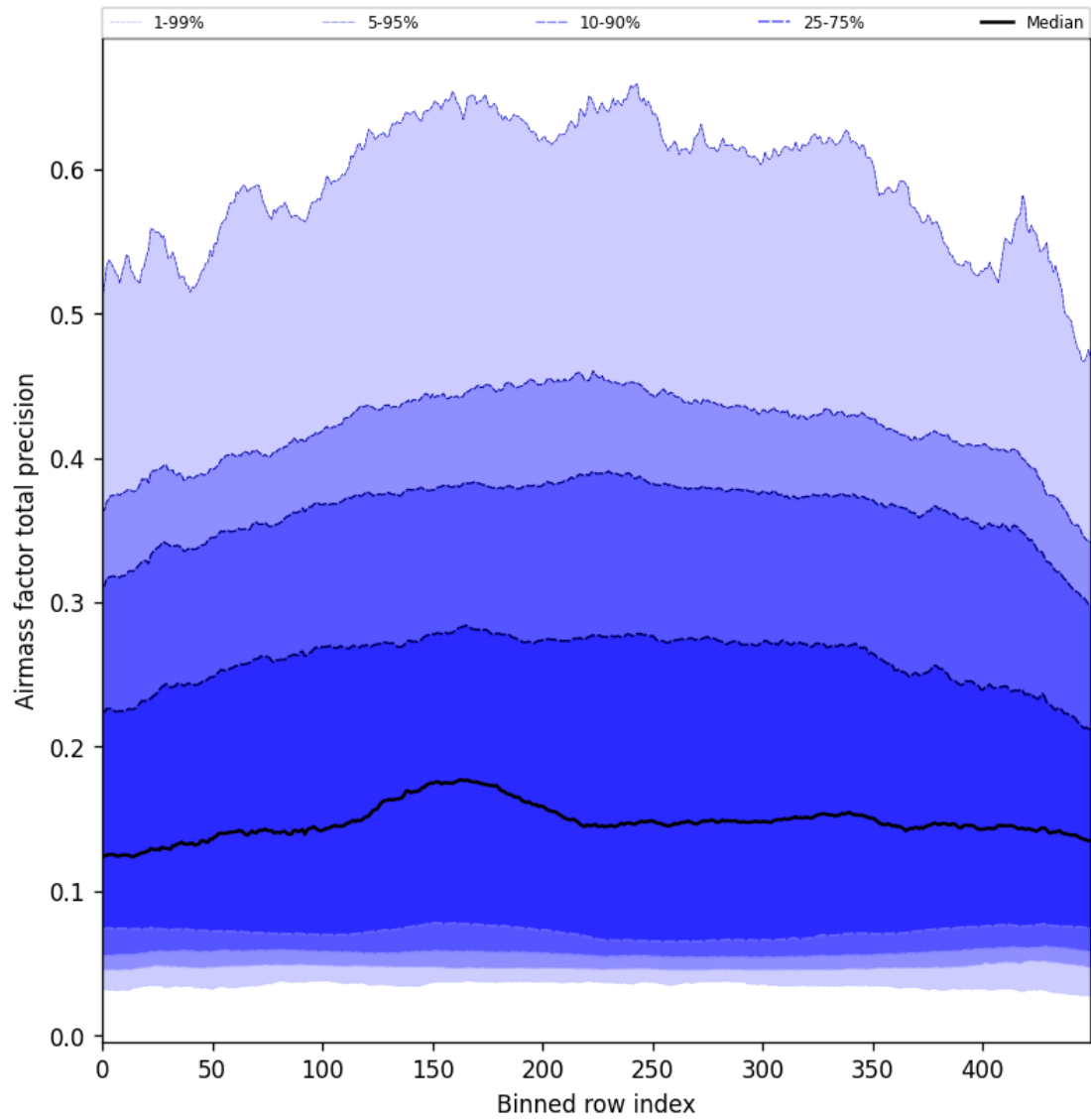
Figure 55: Along track statistics of “Airmass factor total precision” for 2025-08-09 to 2025-08-11
