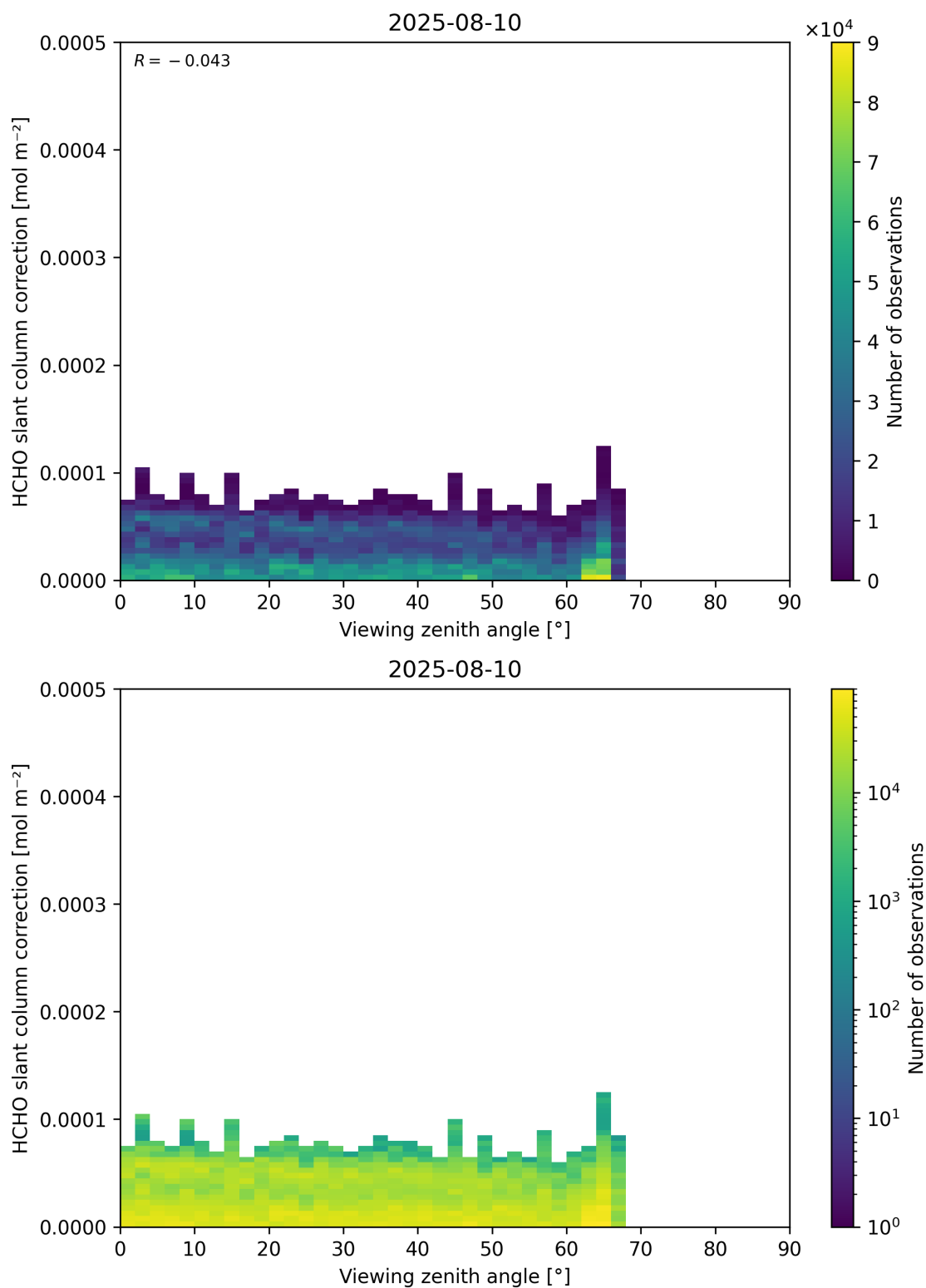
Figure 187: Scatter density plot of “Viewing zenith angle” against “HCHO slant column correction” for 2025-08-09 to 2025-08-11.
