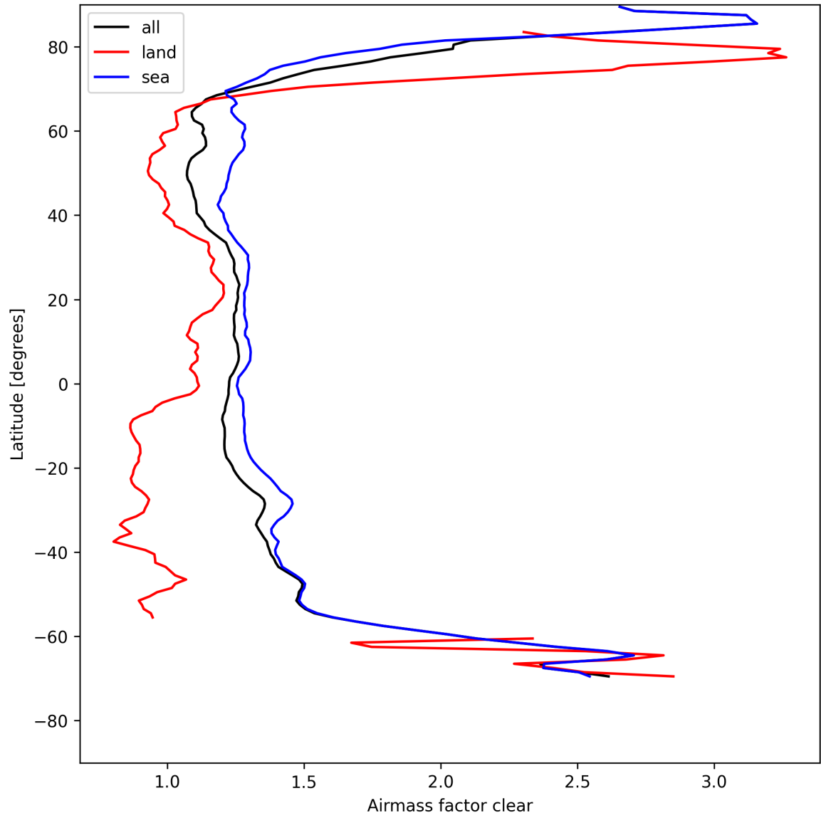
Figure 28: Zonal average of “Airmass factor clear” for 2025-08-09 to 2025-08-11.
