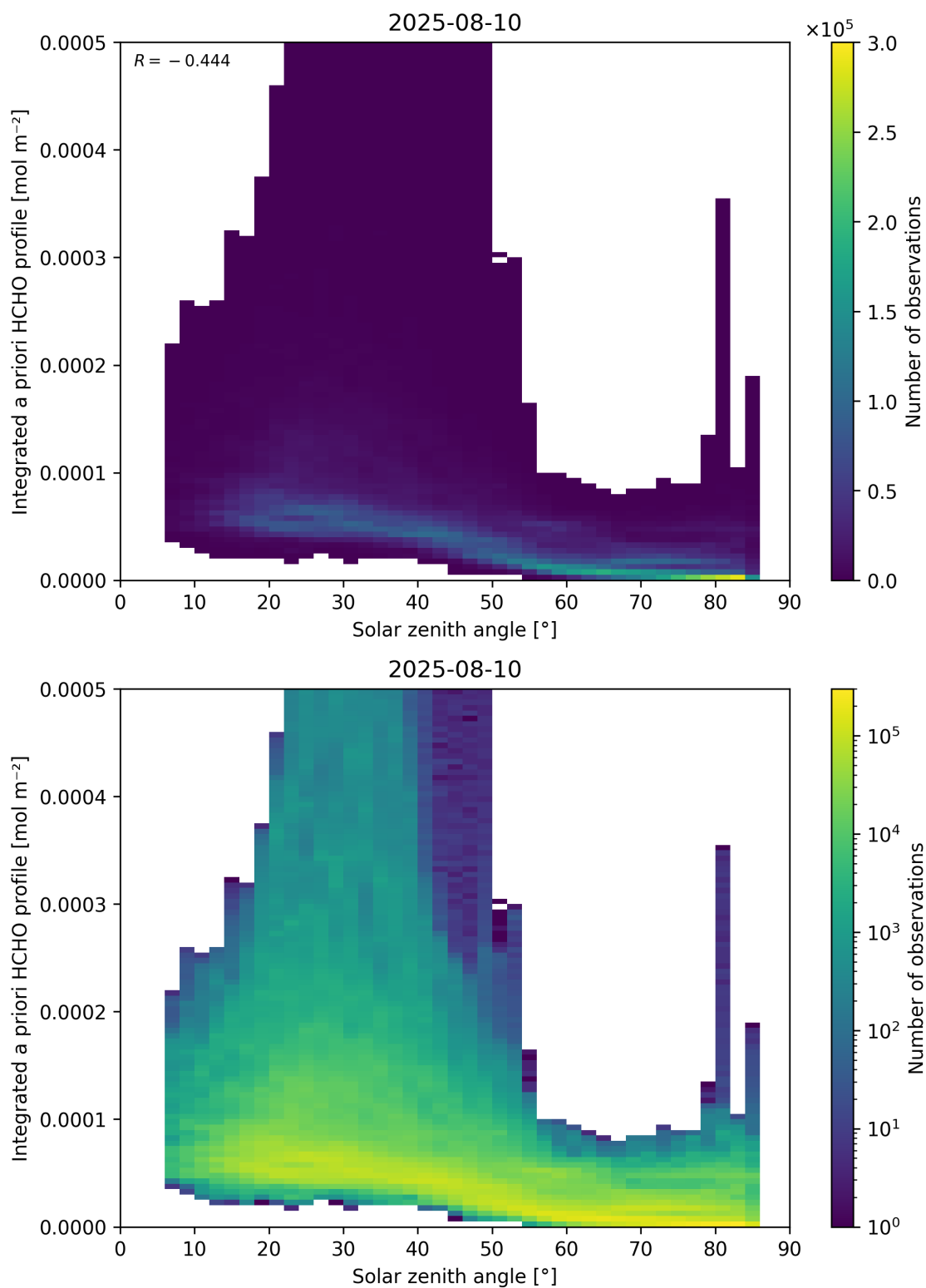
Figure 180: Scatter density plot of “Solar zenith angle” against “Integrated a priori HCHO profile” for 2025-08-09 to 2025-08-11.
