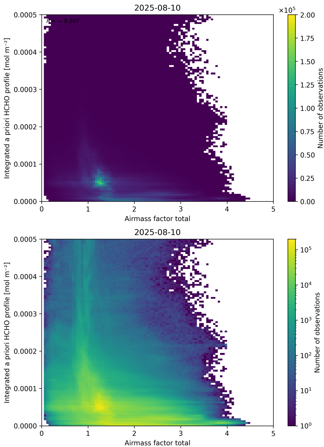
Figure 104: Scatter density plot of “Airmass factor total” against “Integrated a priori HCHO profile” for 2025-08-09 to 2025-08-11.
