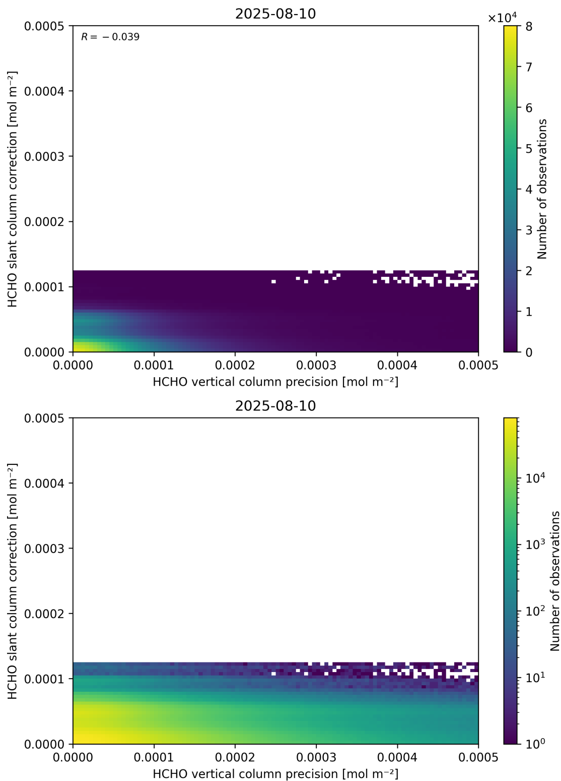
Figure 141: Scatter density plot of “HCHO vertical column precision” against “HCHO slant column correction” for 2025-08-09 to 2025-08-11.
