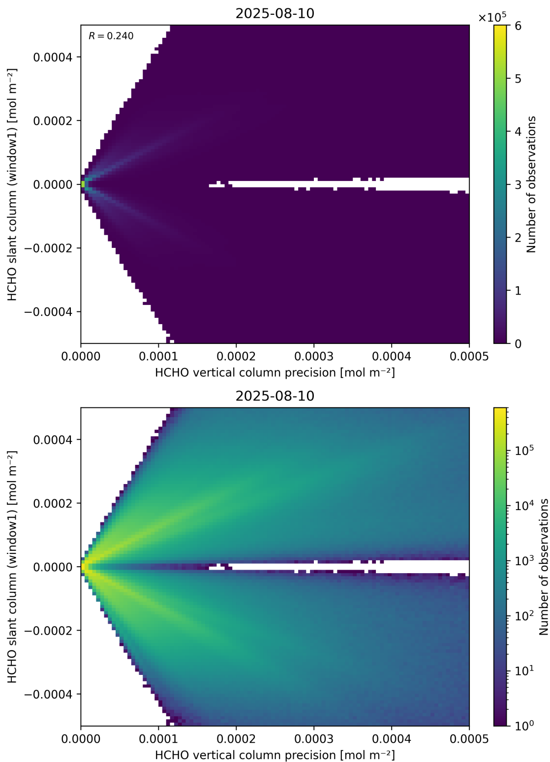
Figure 142: Scatter density plot of “HCHO vertical column precision” against “HCHO slant column (window1)” for 2025-08-09 to 2025-08-11.
