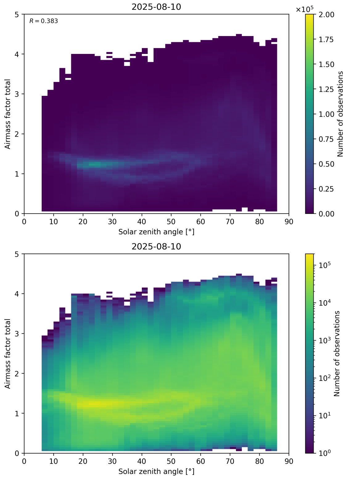
Figure 175: Scatter density plot of “Solar zenith angle” against “Airmass factor total” for 2025-08-09 to 2025-08-11.
