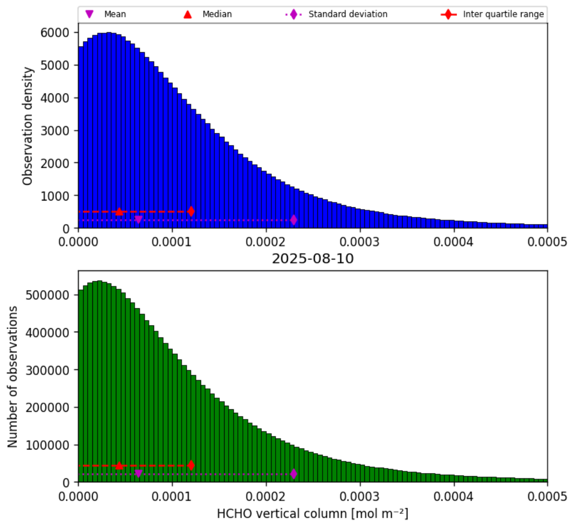
Figure 35: Histogram of “HCHO vertical column” for 2025-08-09 to 2025-08-11
