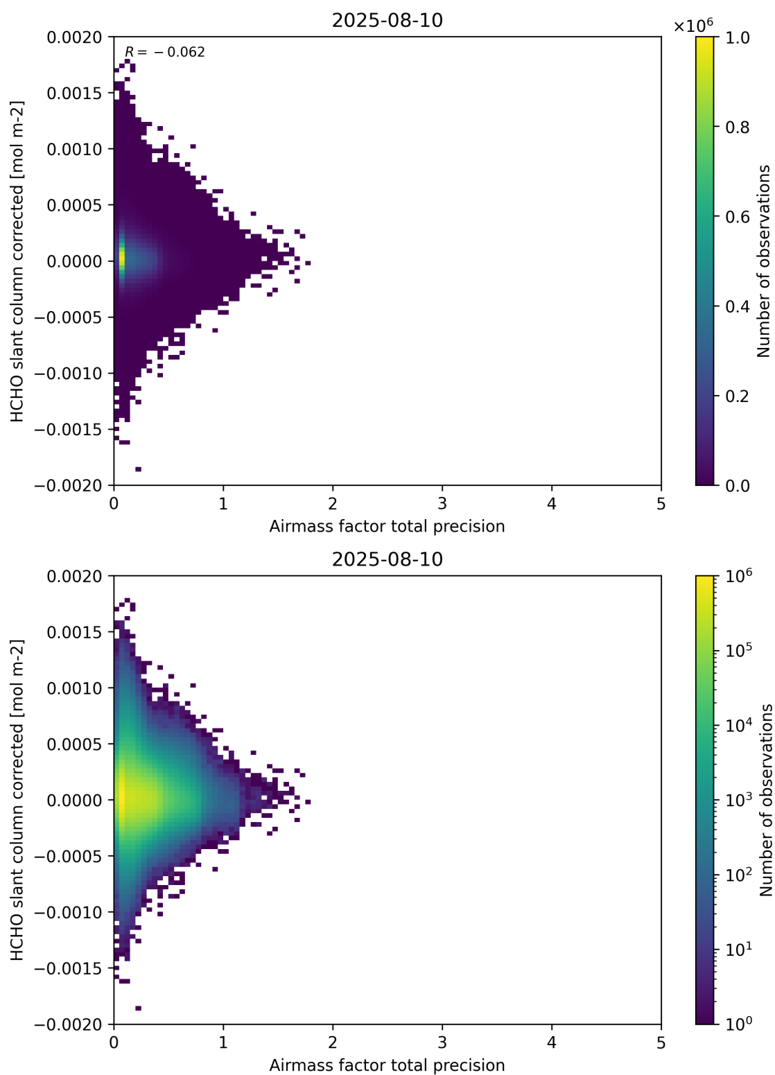
Figure 109: Scatter density plot of “Airmass factor total precision” against “HCHO slant column corrected” for 2025-08-09 to 2025-08-11.
