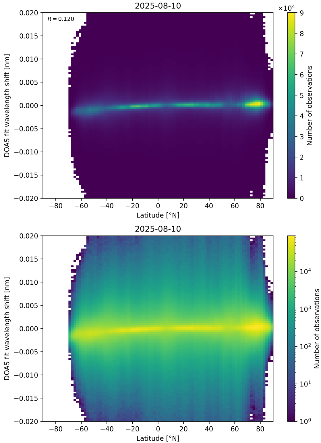
Figure 154: Scatter density plot of “Latitude” against “DOAS fit wavelength shift” for 2025-08-09 to 2025-08-11.
