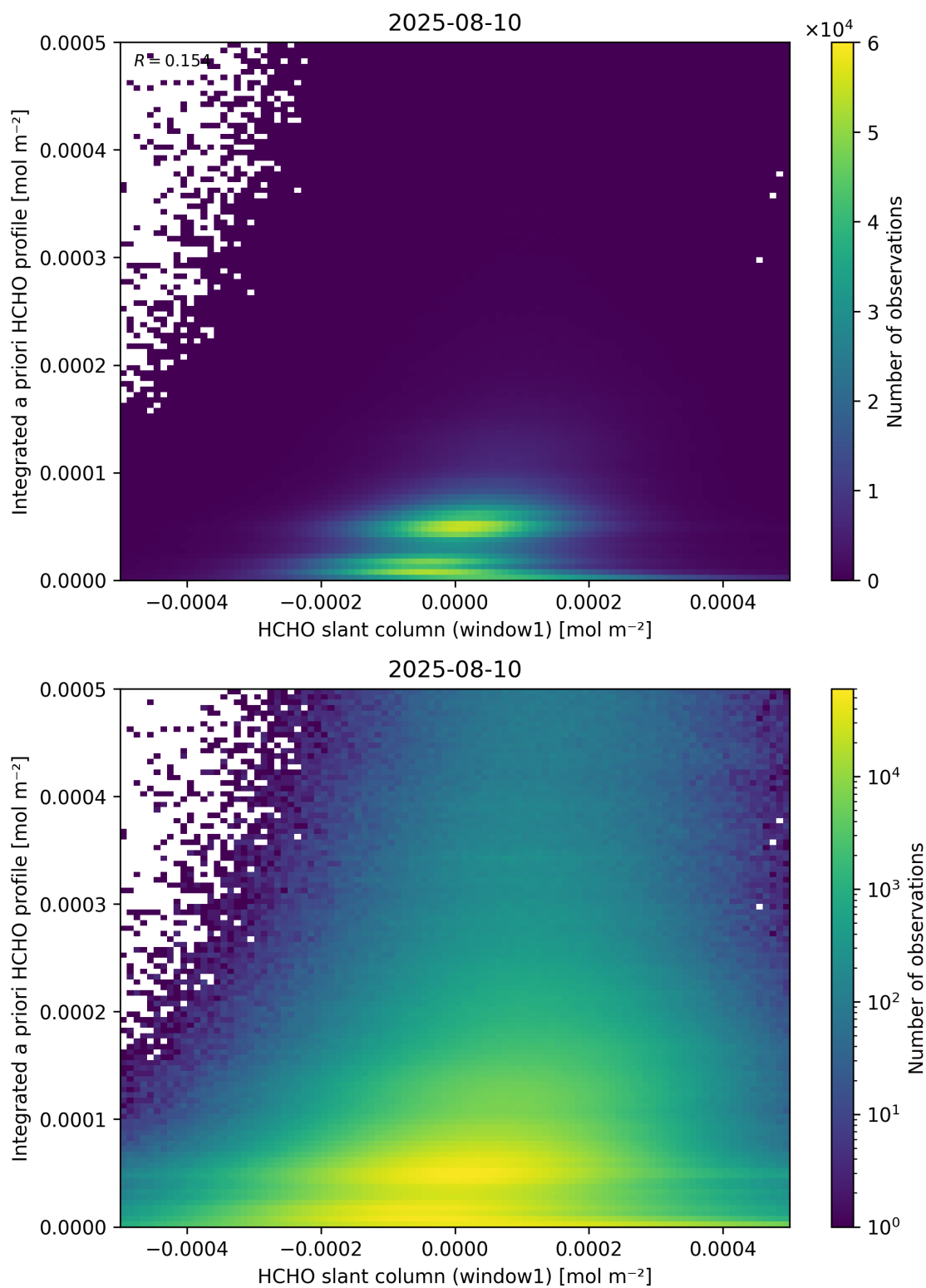
Figure 87: Scatter density plot of “HCHO slant column (window1)” against “Integrated a priori HCHO profile” for 2025-08-09 to 2025-08-11.
