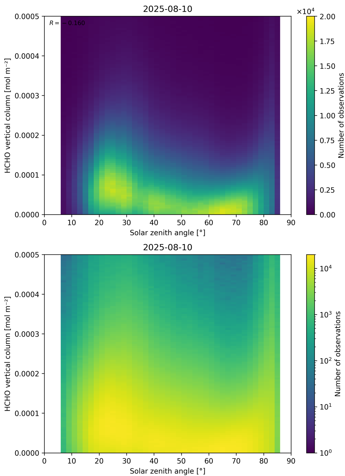
Figure 177: Scatter density plot of “Solar zenith angle” against “HCHO vertical column” for 2025-08-09 to 2025-08-11.
