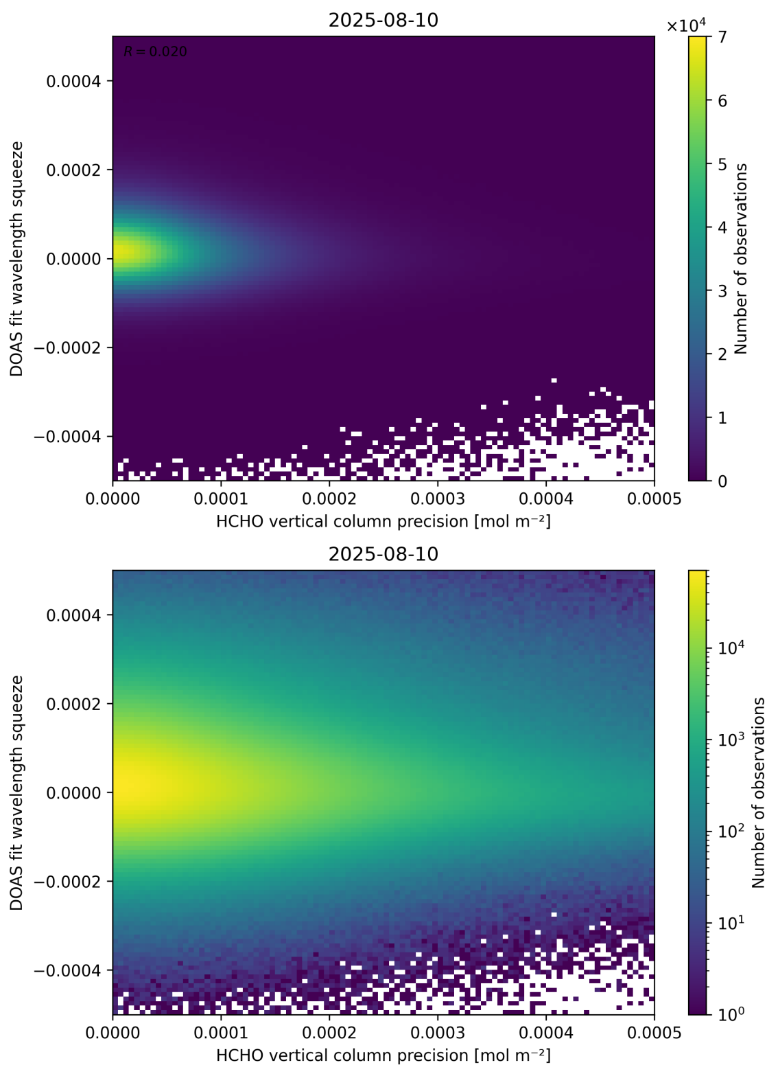
Figure 138: Scatter density plot of “HCHO vertical column precision” against “DOAS fit wavelength squeeze” for 2025-08-09 to 2025-08-11.
