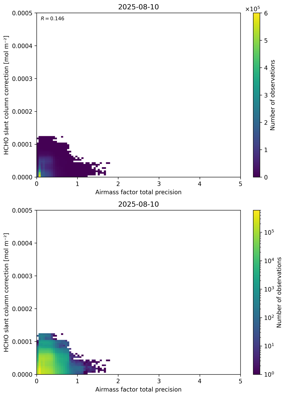
Figure 110: Scatter density plot of “Airmass factor total precision” against “HCHO slant column correction” for 2025-08-09 to 2025-08-11.
