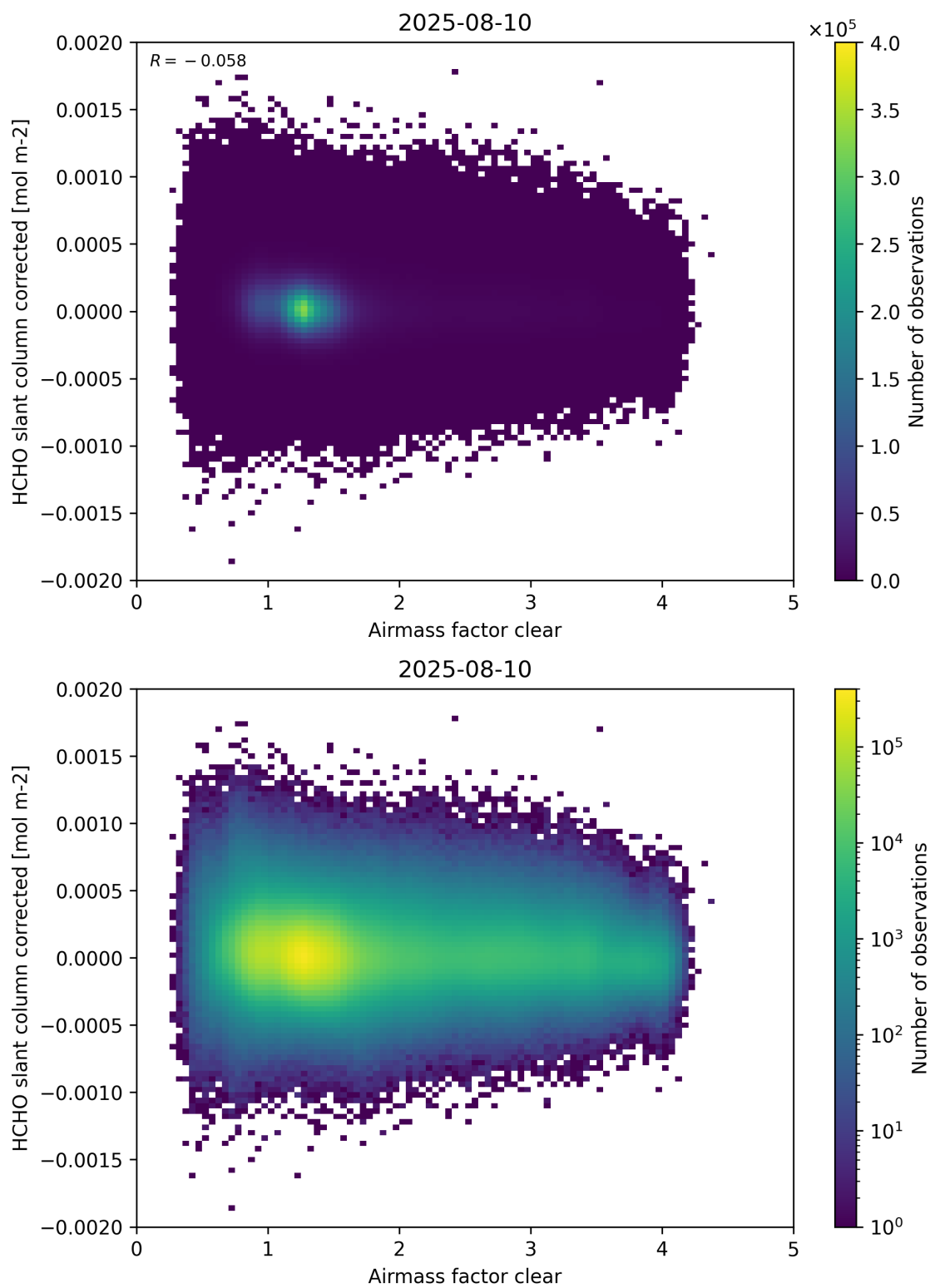
Figure 74: Scatter density plot of “Airmass factor clear” against “HCHO slant column corrected” for 2025-08-09 to 2025-08-11.
