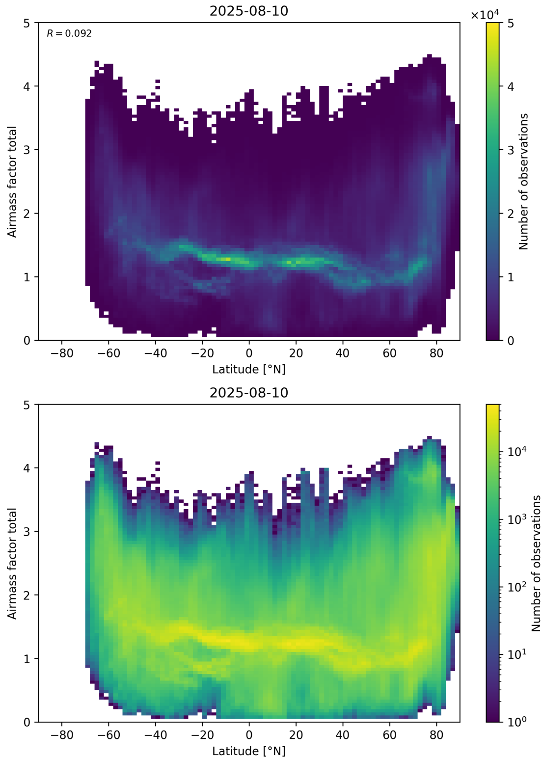
Figure 161: Scatter density plot of “Latitude” against “Airmass factor total” for 2025-08-09 to 2025-08-11.
