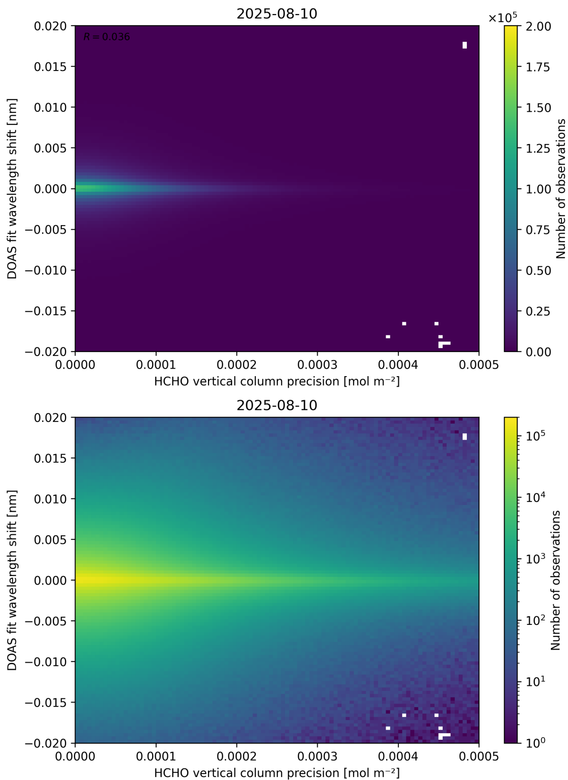
Figure 137: Scatter density plot of “HCHO vertical column precision” against “DOAS fit wavelength shift” for 2025-08-09 to 2025-08-11.
