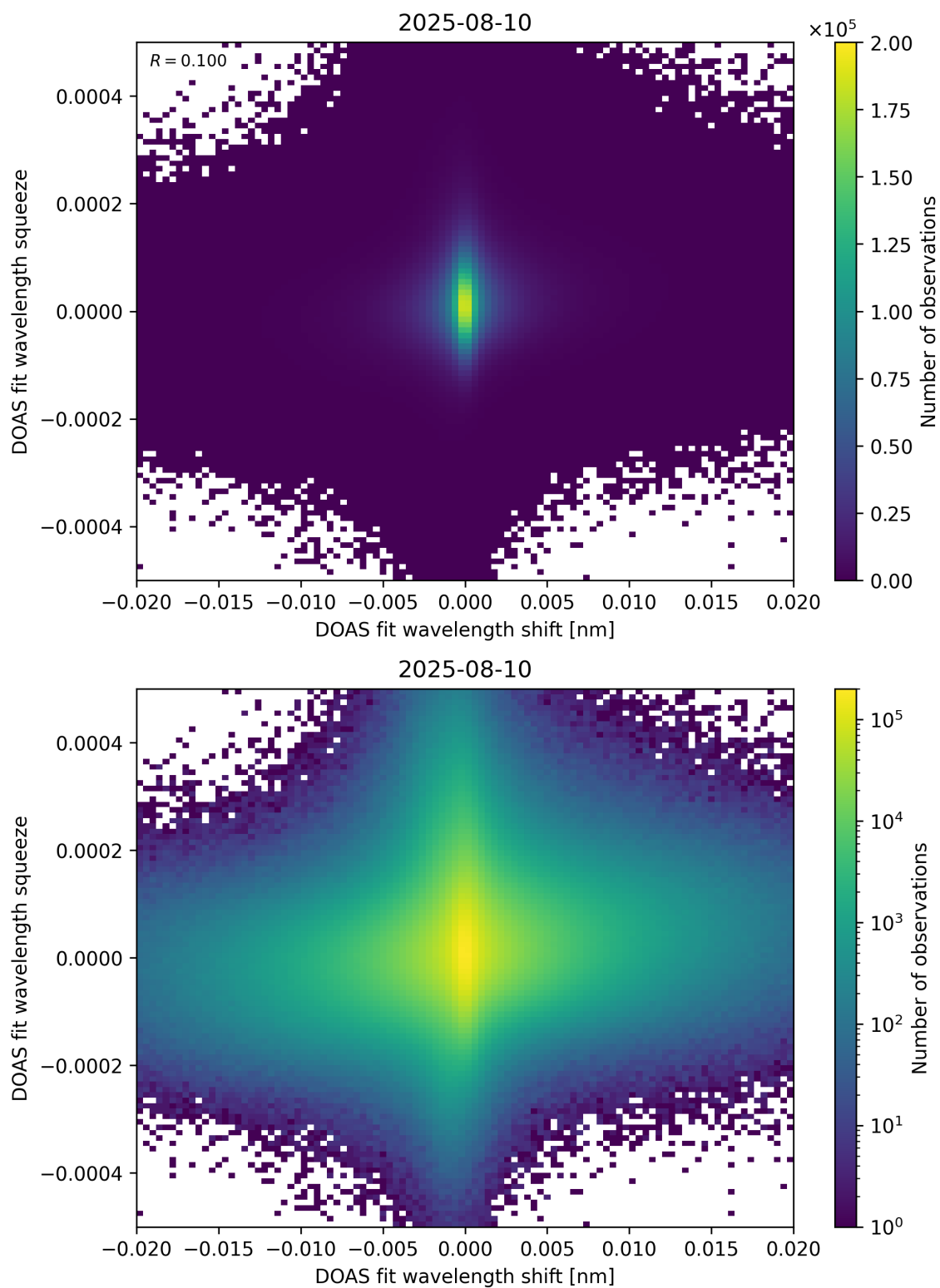
Figure 65: Scatter density plot of “DOAS fit wavelength shift” against “DOAS fit wavelength squeeze” for 2025-08-09 to 2025-08-11.
