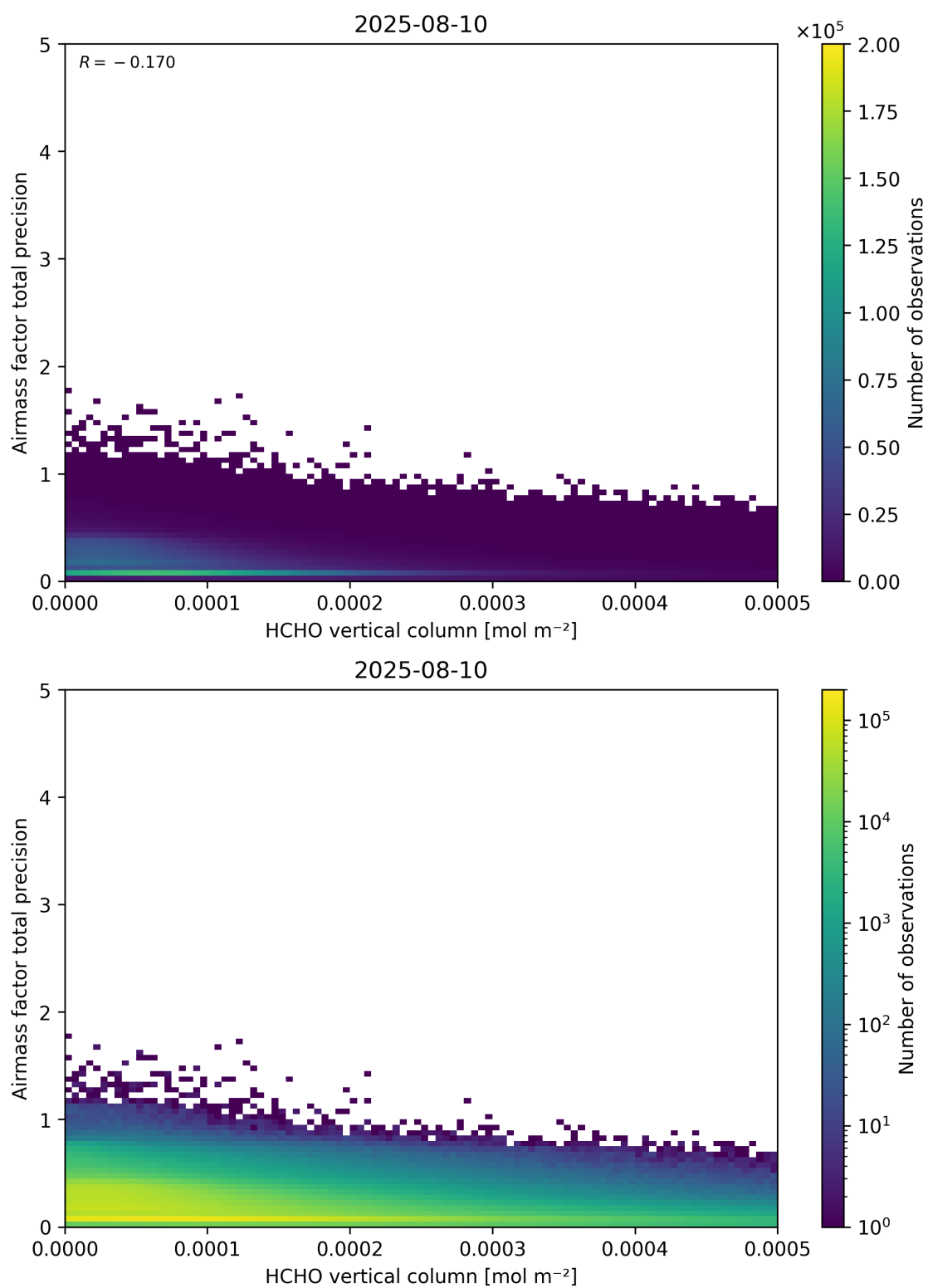
Figure 132: Scatter density plot of “HCHO vertical column” against “Airmass factor total precision” for 2025-08-09 to 2025-08-11.
