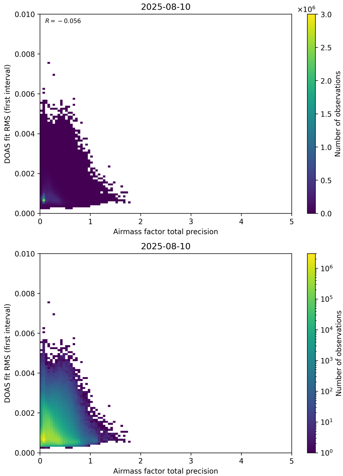
Figure 105: Scatter density plot of “Airmass factor total precision” against “DOAS fit RMS (first interval)” for 2025-08-09 to 2025-08-11.
