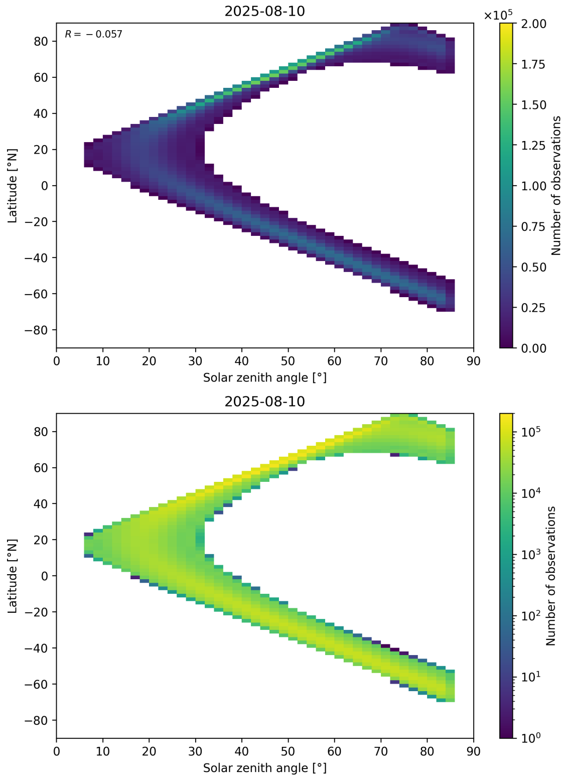
Figure 181: Scatter density plot of “Solar zenith angle” against “Latitude” for 2025-08-09 to 2025-08-11.
