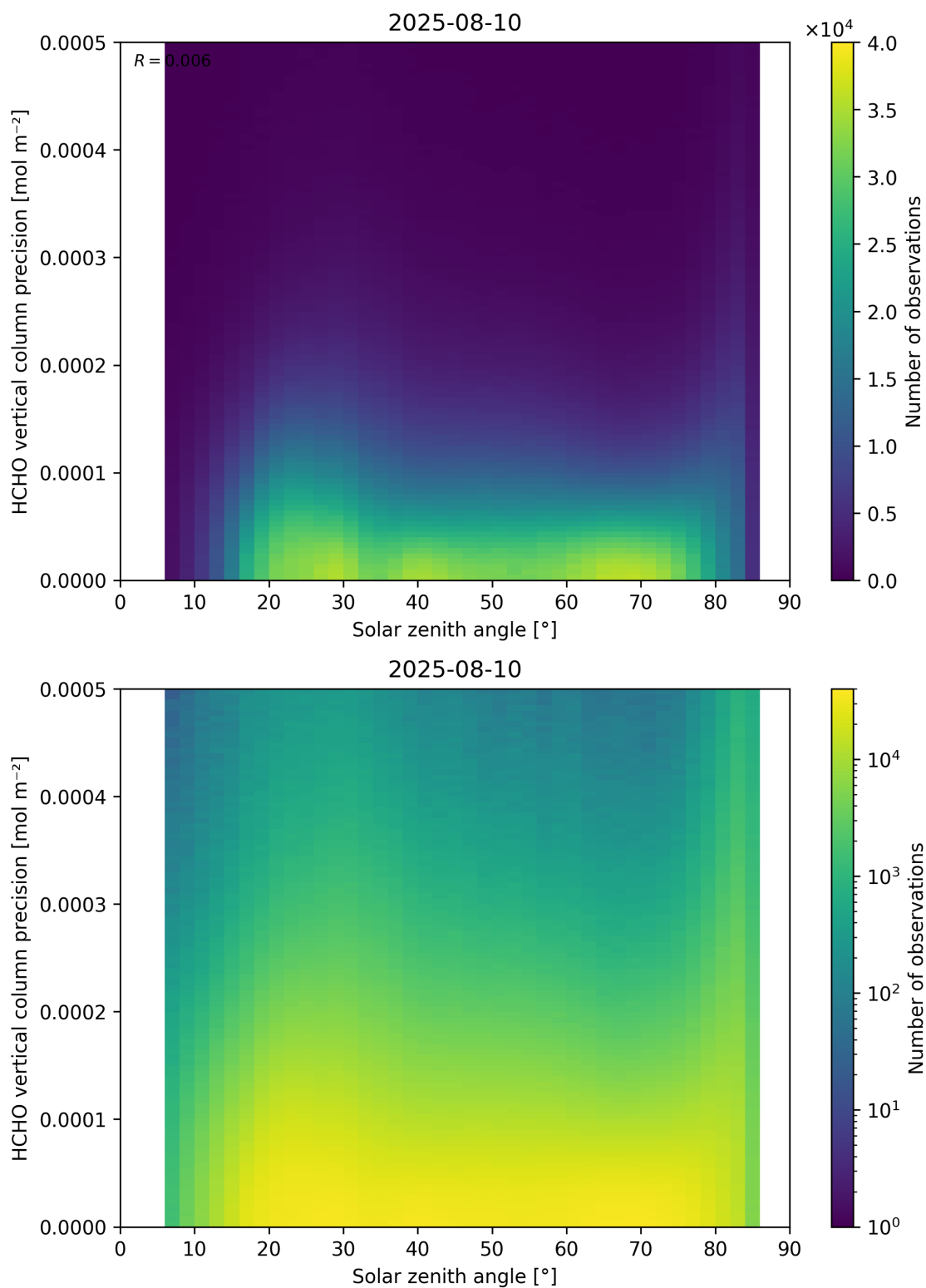
Figure 179: Scatter density plot of “Solar zenith angle” against “HCHO vertical column precision” for 2025-08-09 to 2025-08-11.
