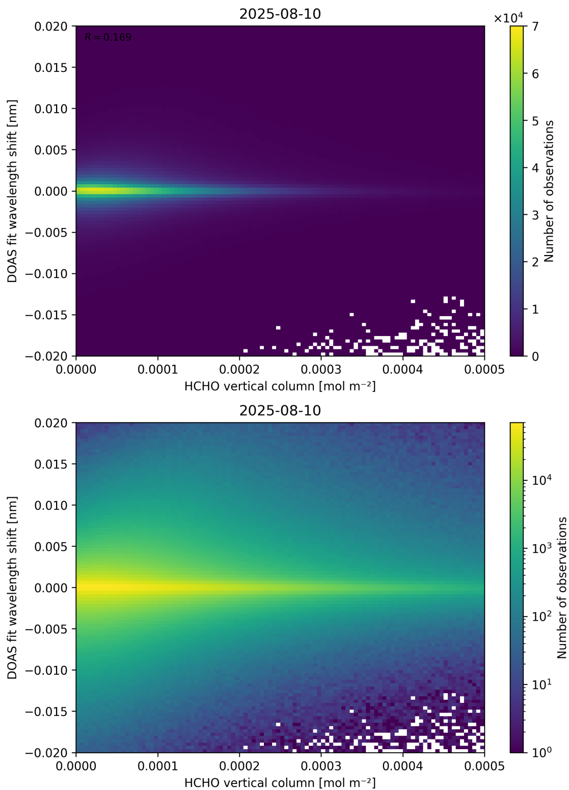
Figure 124: Scatter density plot of “HCHO vertical column” against “DOAS fit wavelength shift” for 2025-08-09 to 2025-08-11.
