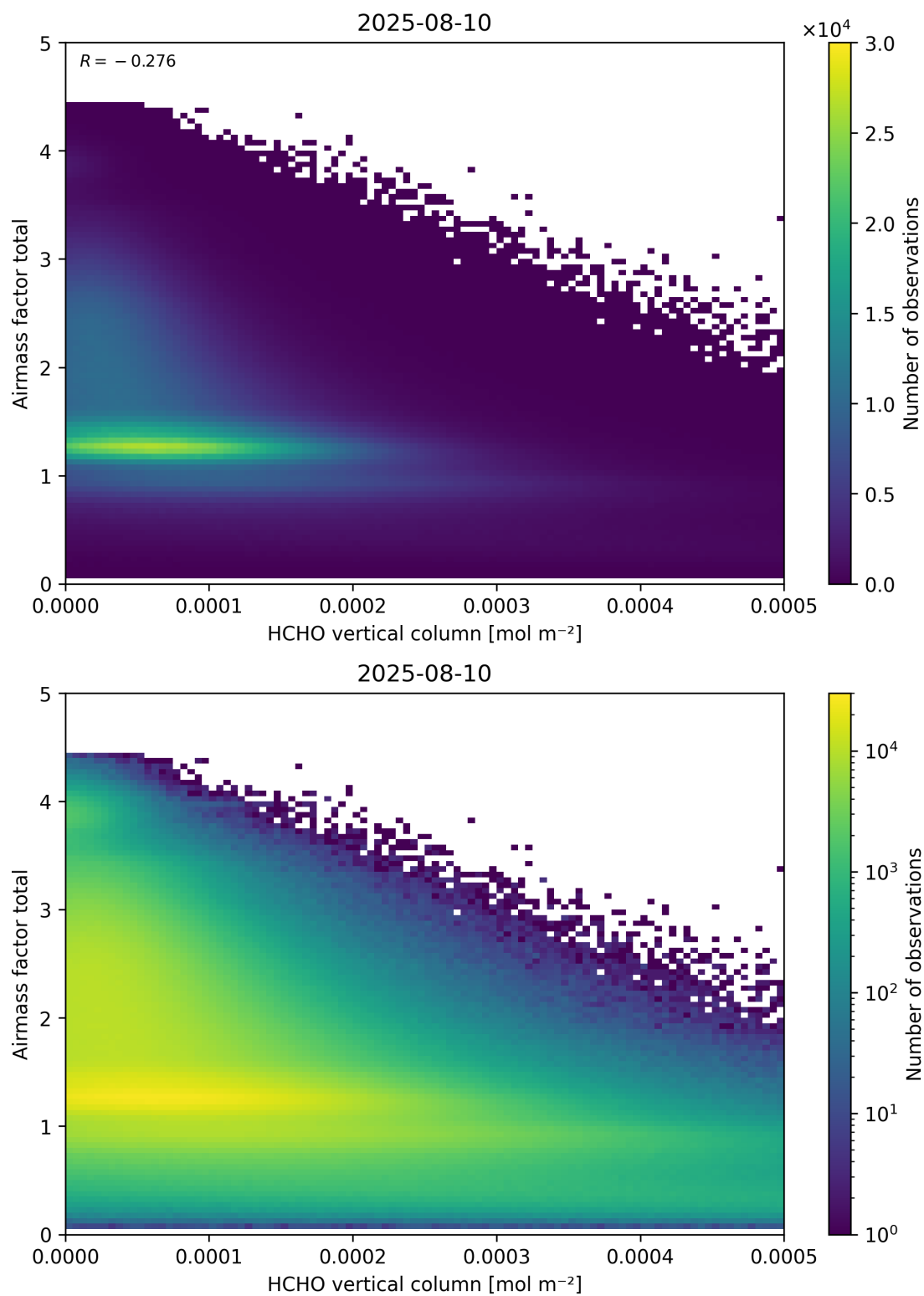
Figure 131: Scatter density plot of “HCHO vertical column” against “Airmass factor total” for 2025-08-09 to 2025-08-11.
