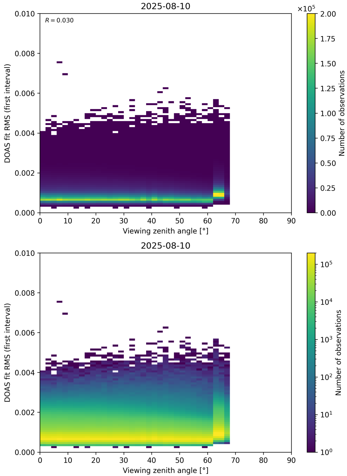
Figure 182: Scatter density plot of “Viewing zenith angle” against “DOAS fit RMS (first interval)” for 2025-08-09 to 2025-08-11.
