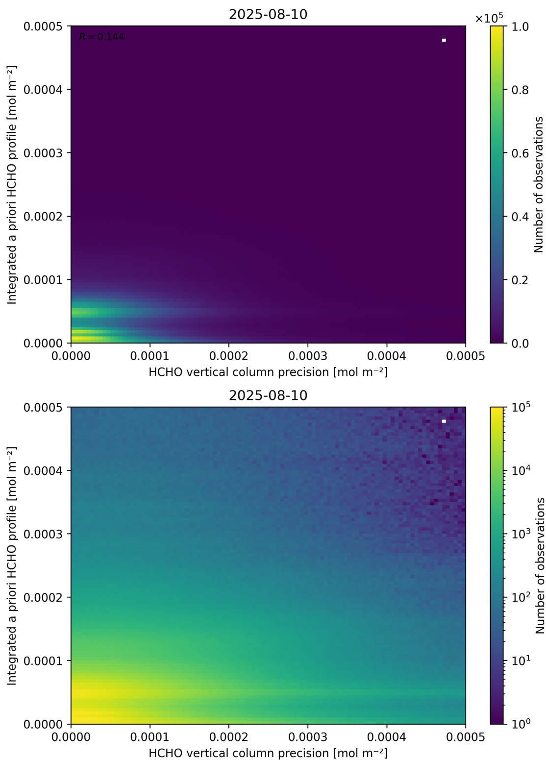
Figure 147: Scatter density plot of “HCHO vertical column precision” against “Integrated a priori HCHO profile” for 2025-08-09 to 2025-08-11.
