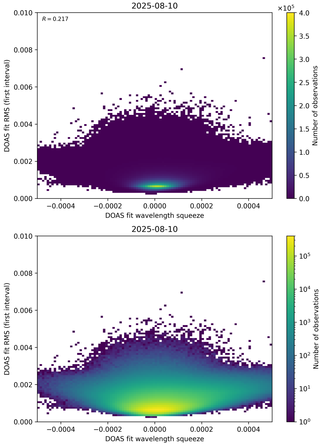
Figure 68: Scatter density plot of “DOAS fit wavelength squeeze” against “DOAS fit RMS (first interval)” for 2025-08-09 to 2025-08-11.
