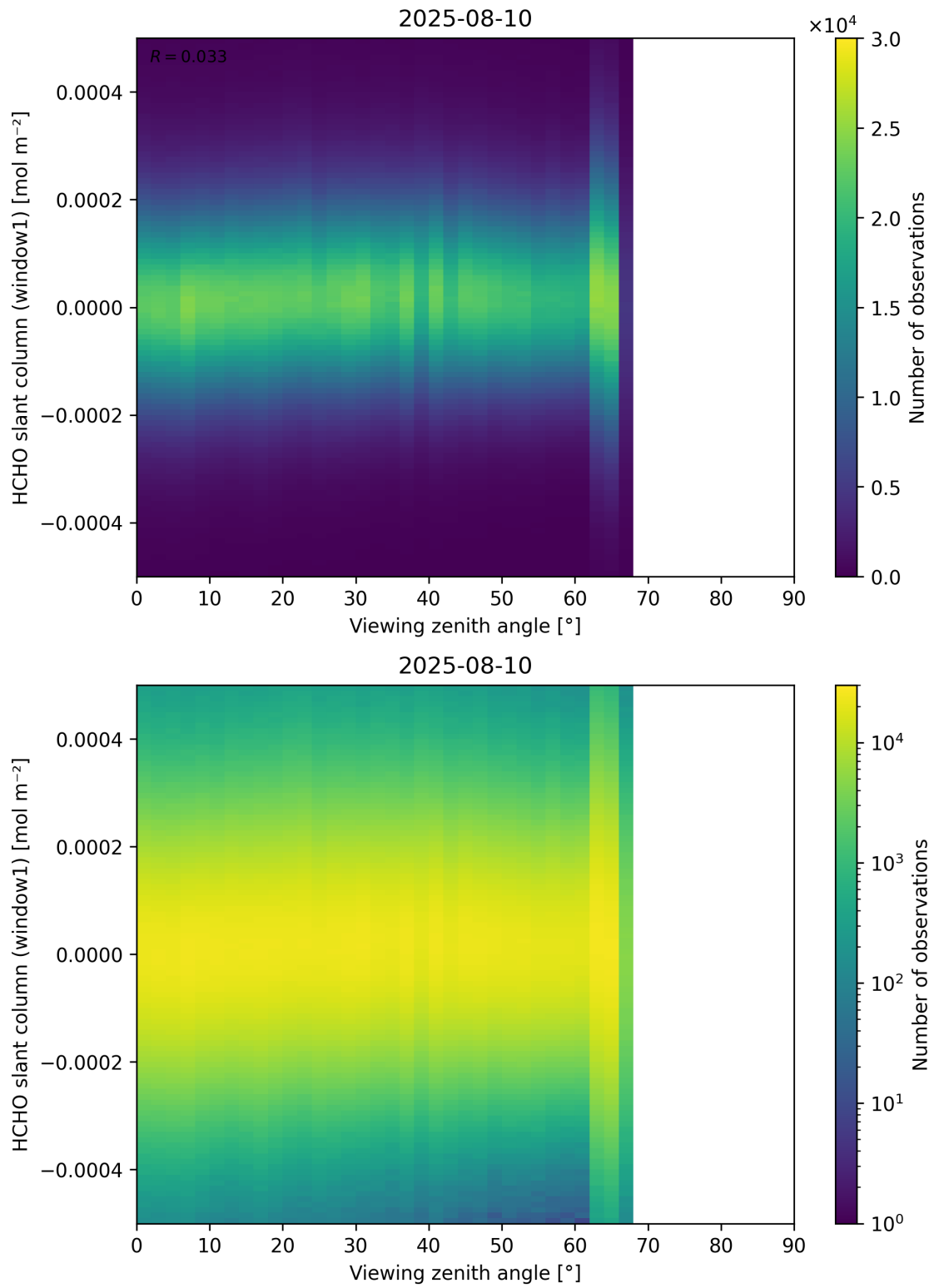
Figure 188: Scatter density plot of “Viewing zenith angle” against “HCHO slant column (window1)” for 2025-08-09 to 2025-08-11.
