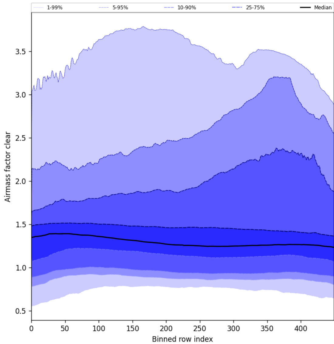
Figure 56: Along track statistics of “Airmass factor clear” for 2025-08-09 to 2025-08-11
