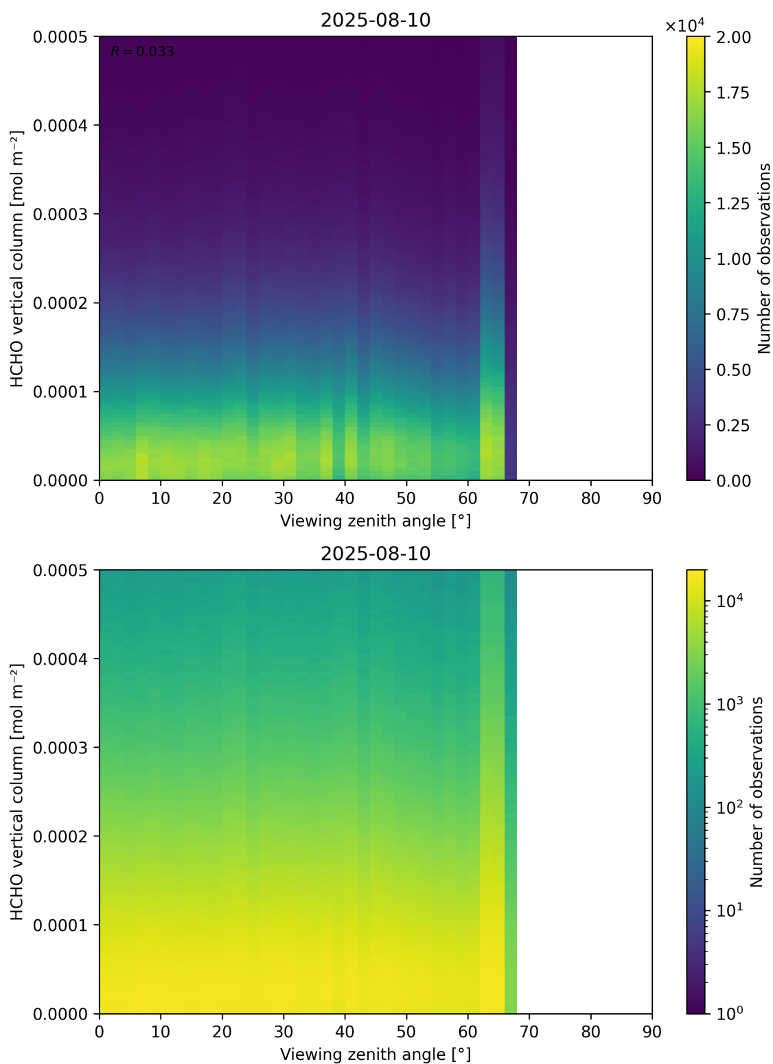
Figure 192: Scatter density plot of “Viewing zenith angle” against “HCHO vertical column” for 2025-08-09 to 2025-08-11.
