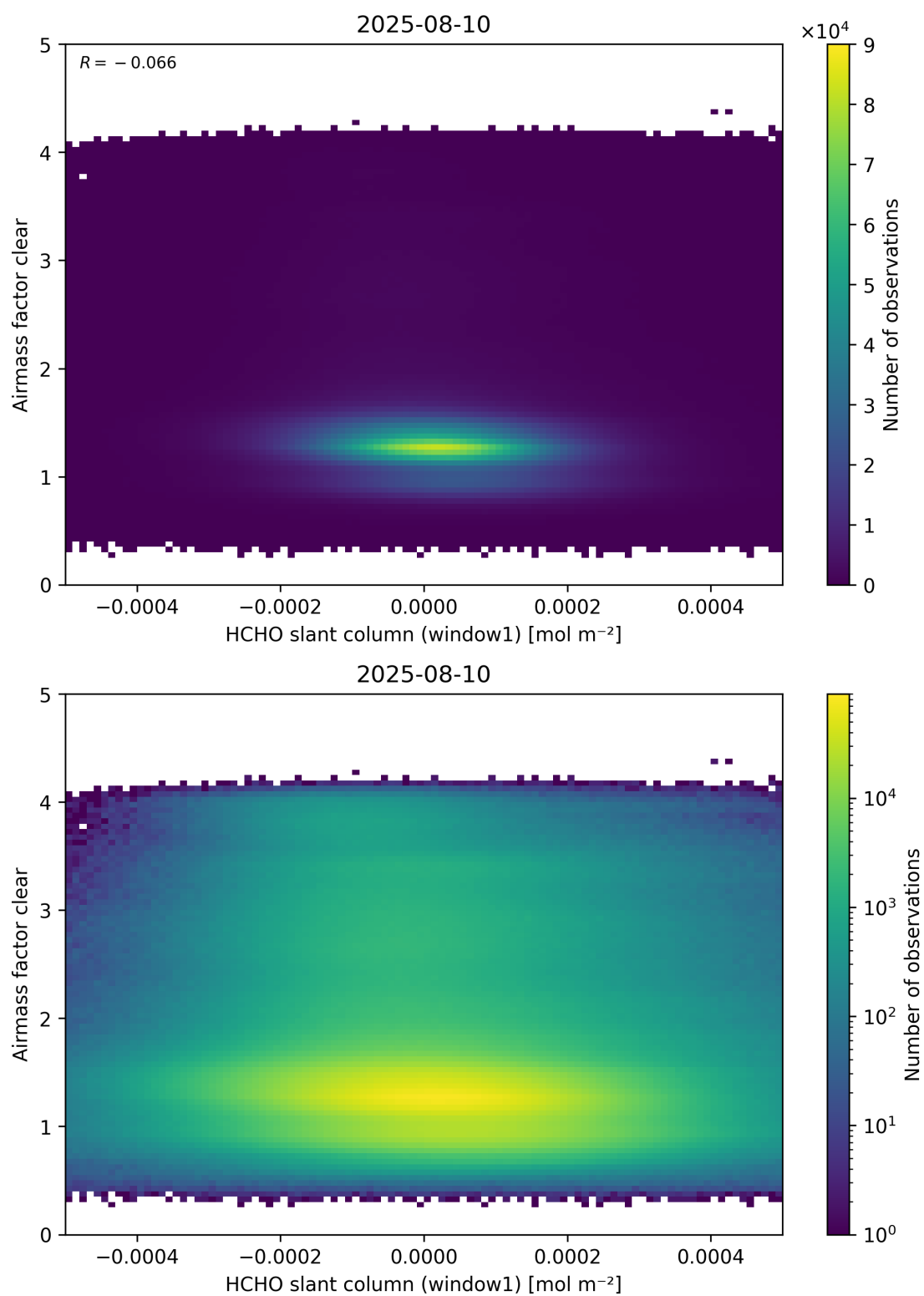
Figure 81: Scatter density plot of “HCHO slant column (window1)” against “Airmass factor clear” for 2025-08-09 to 2025-08-11.
