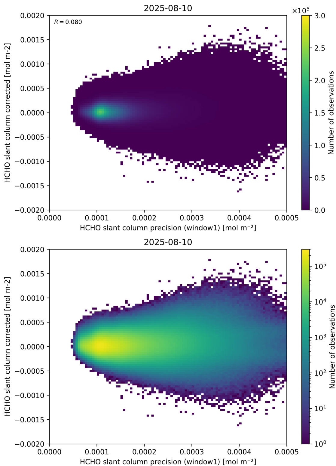
Figure 92: Scatter density plot of “HCHO slant column precision (window1)” against “HCHO slant column corrected” for 2025-08-09 to 2025-08-11.
