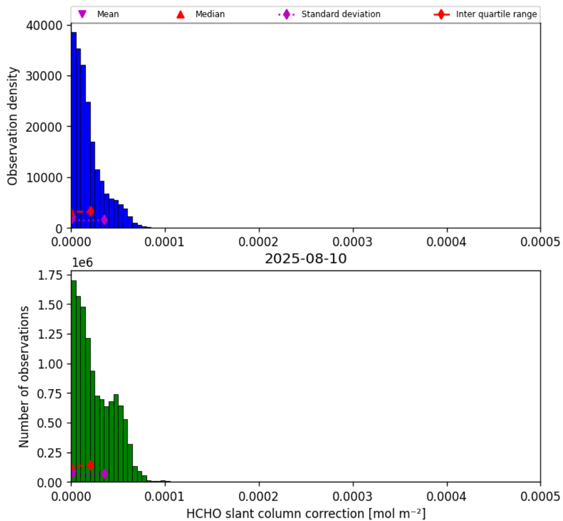
Figure 47: Histogram of “HCHO slant column correction” for 2025-08-09 to 2025-08-11
