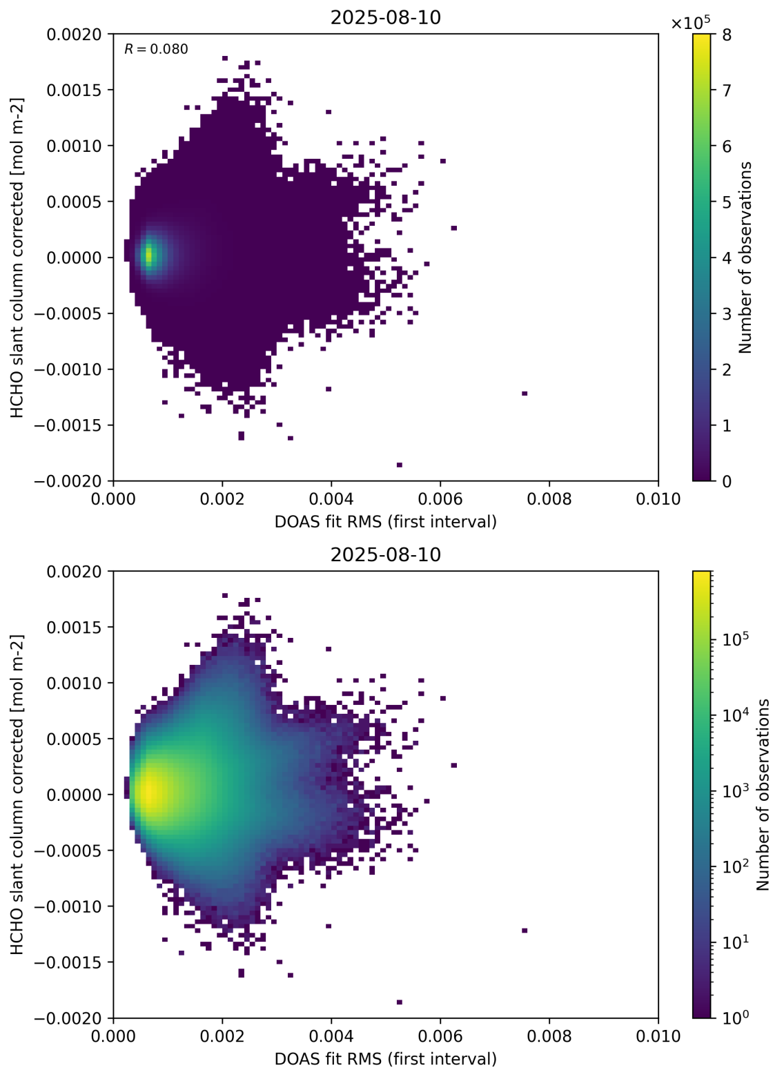
Figure 62: Scatter density plot of “DOAS fit RMS (first interval)” against “HCHO slant column corrected” for 2025-08-09 to 2025-08-11.
