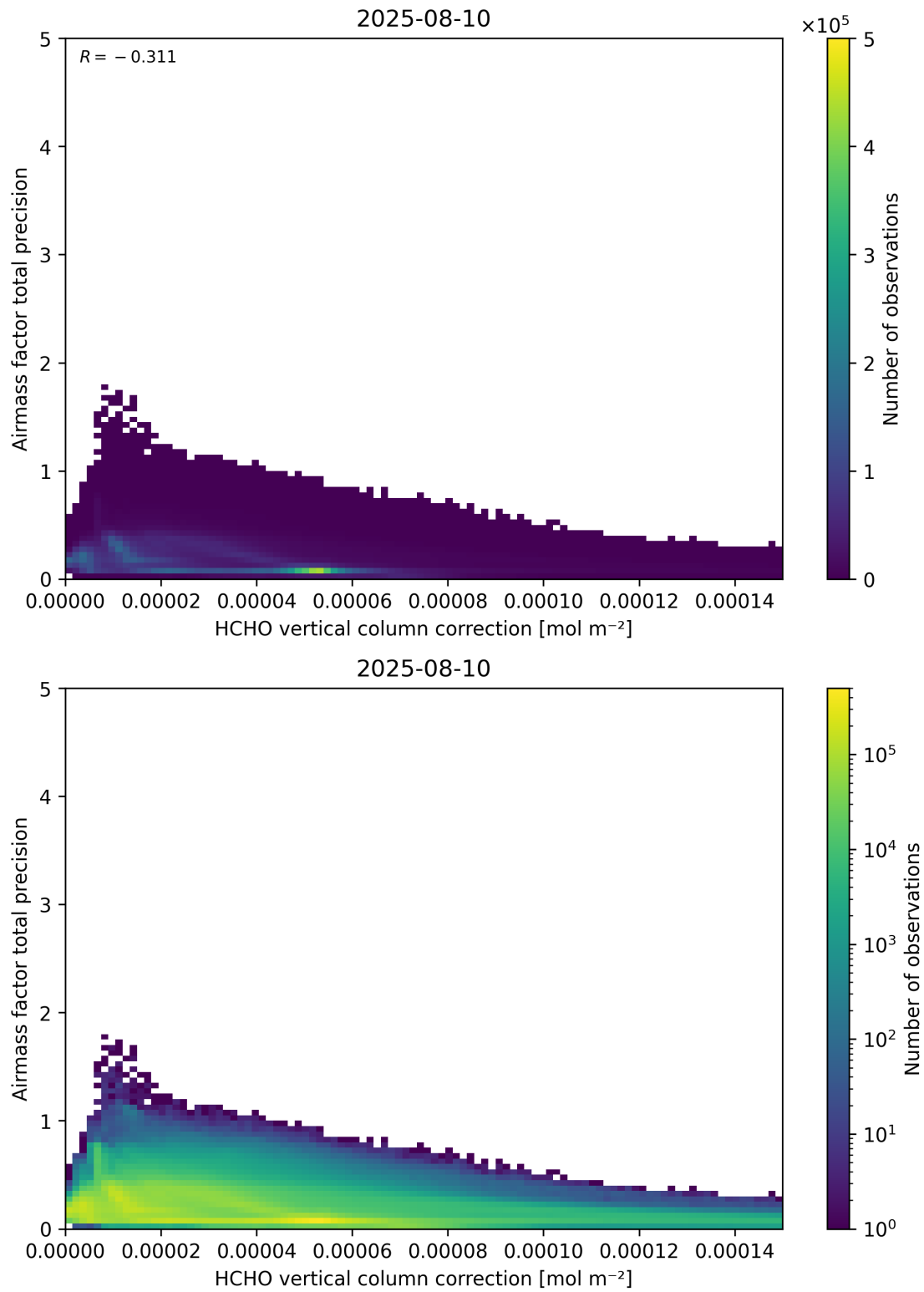
Figure 121: Scatter density plot of “HCHO vertical column correction” against “Airmass factor total precision” for 2025-08-09 to 2025-08-11.
