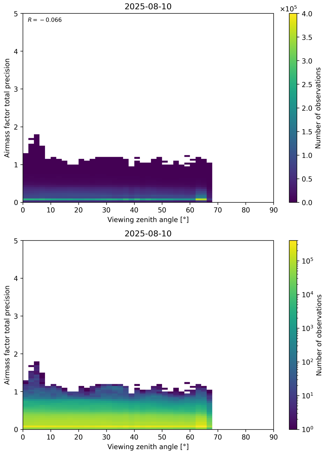
Figure 191: Scatter density plot of “Viewing zenith angle” against “Airmass factor total precision” for 2025-08-09 to 2025-08-11.
