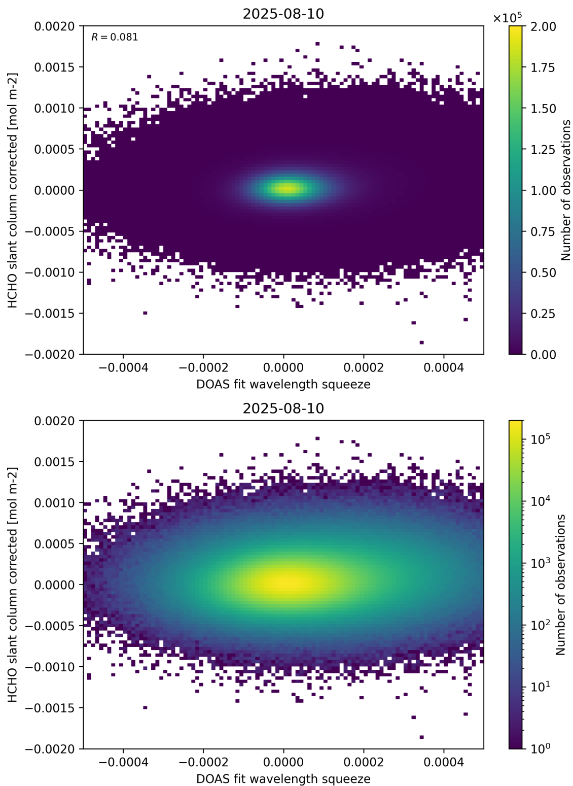
Figure 69: Scatter density plot of “DOAS fit wavelength squeeze” against “HCHO slant column corrected” for 2025-08-09 to 2025-08-11.
