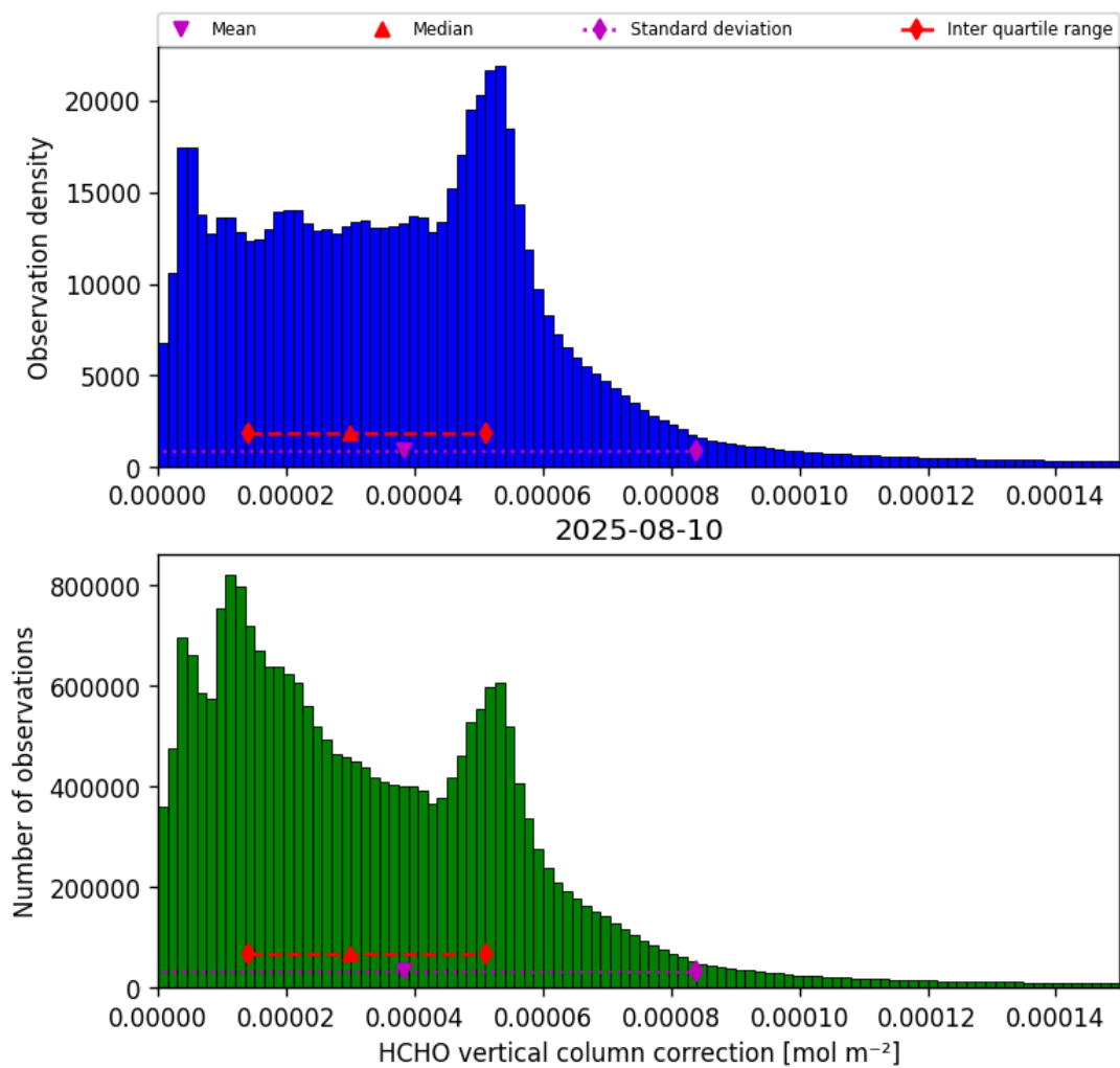
Figure 37: Histogram of “HCHO vertical column correction” for 2025-08-09 to 2025-08-11
