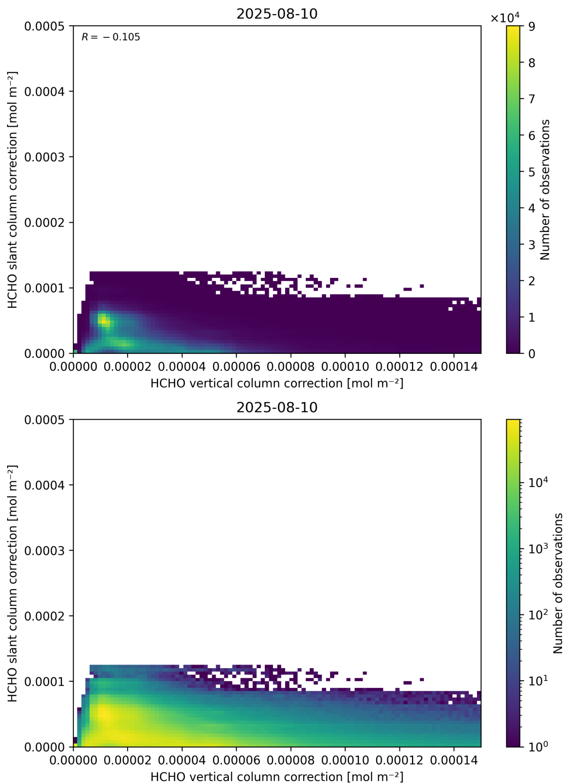
Figure 117: Scatter density plot of “HCHO vertical column correction” against “HCHO slant column correction” for 2025-08-09 to 2025-08-11.
