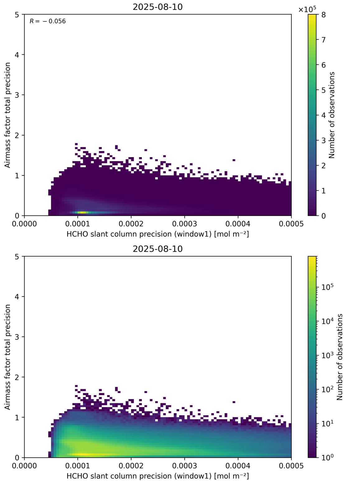
Figure 95: Scatter density plot of “HCHO slant column precision (window1)” against “Airmass factor total precision” for 2025-08-09 to 2025-08-11.
