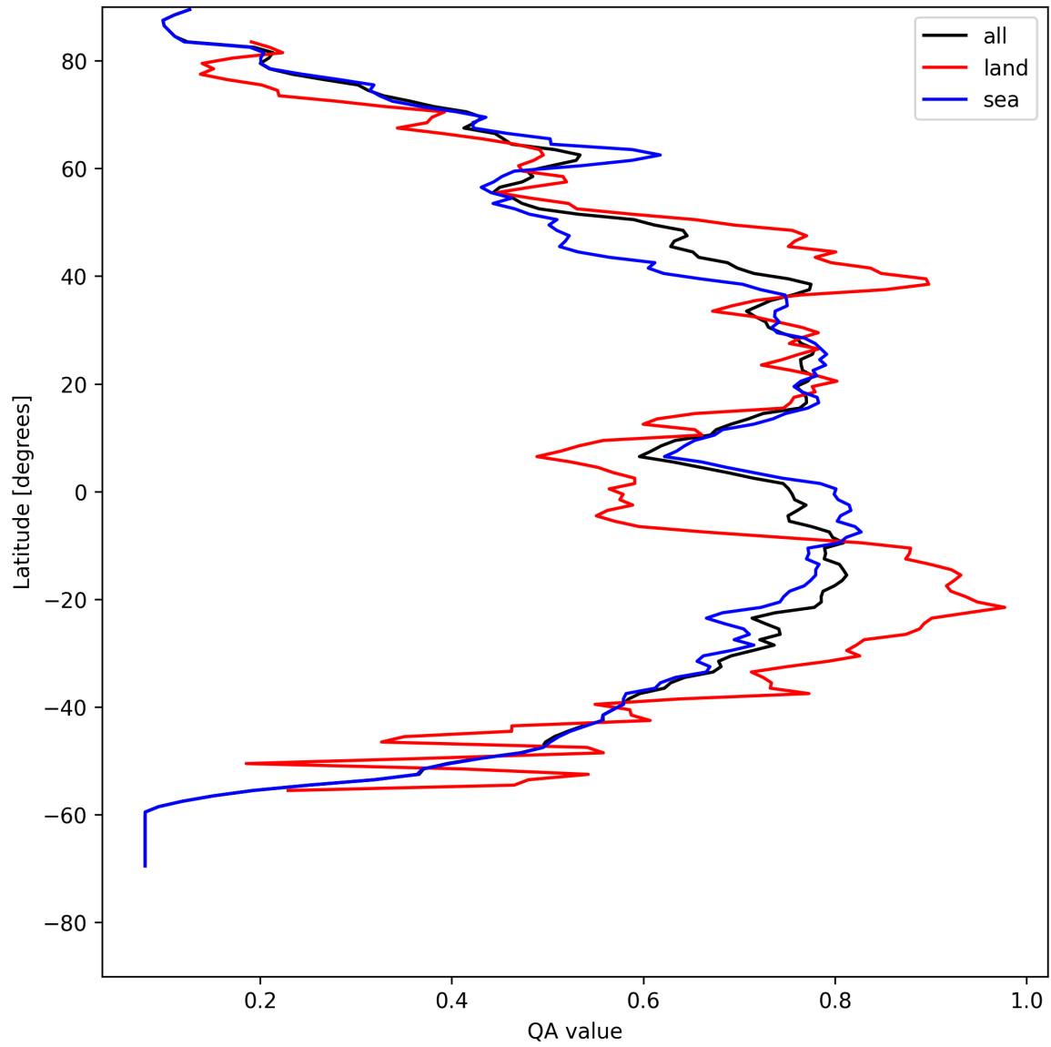
Figure 20: Zonal average of “QA value” for 2025-08-09 to 2025-08-11.
