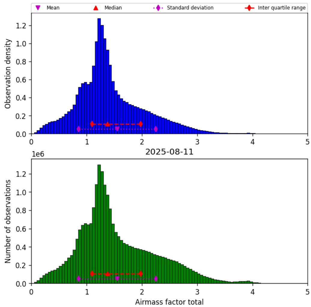
Figure 40: Histogram of "Airmass factor total" for 2025-08-10 to 2025-08-12
