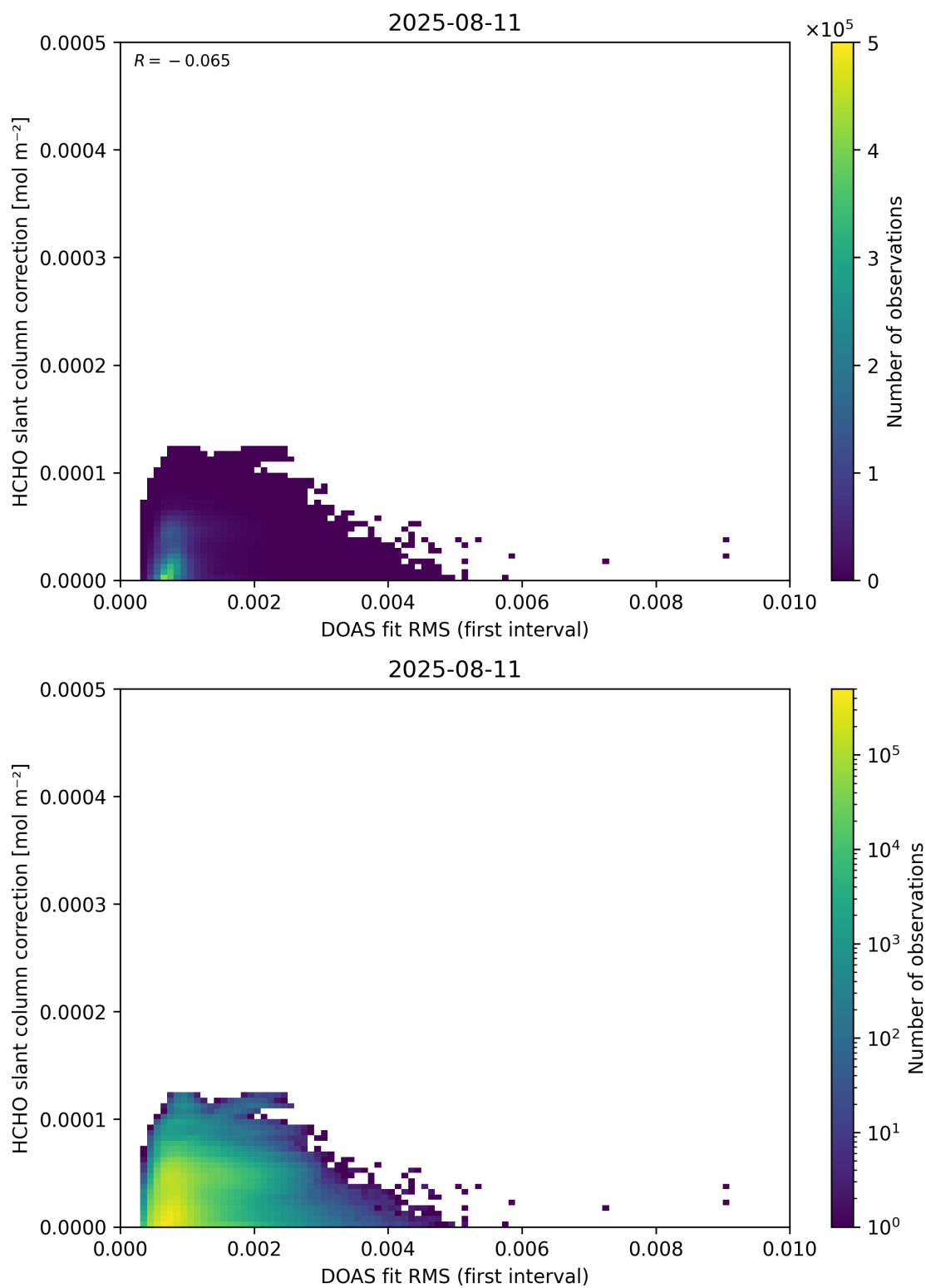
Figure 63: Scatter density plot of “DOAS fit RMS (first interval)” against “HCHO slant column correction” for 2025-08-10 to 2025-08-12.
