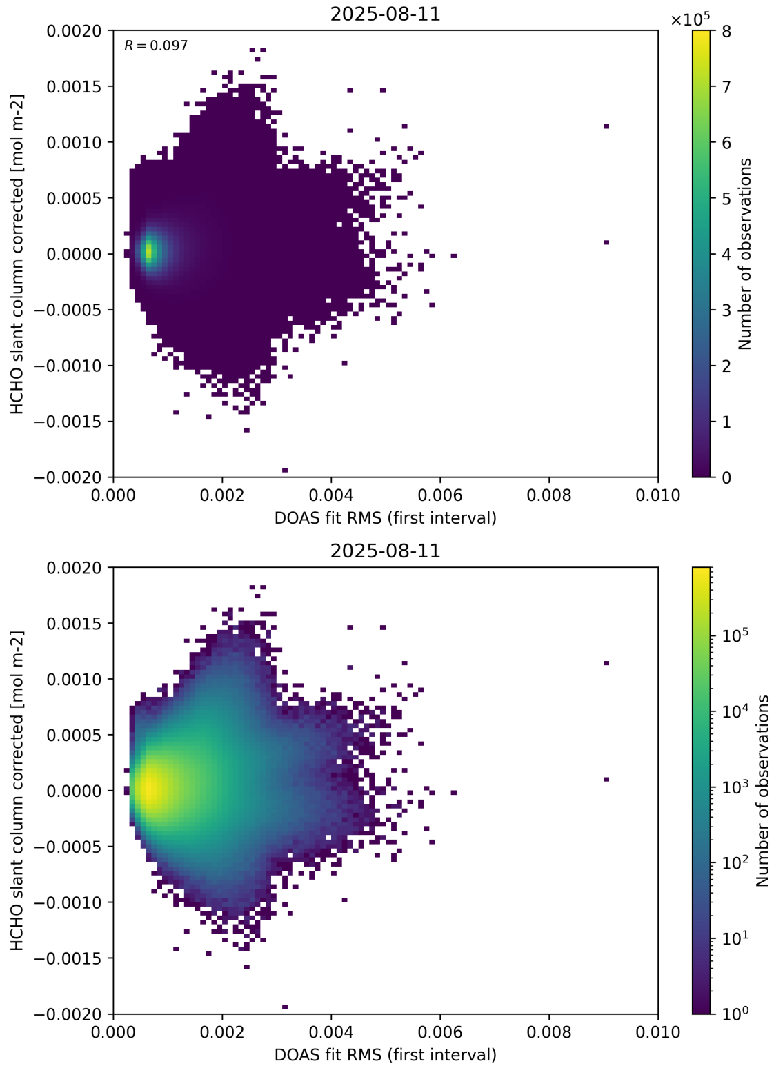
Figure 62: Scatter density plot of “DOAS fit RMS (first interval)” against “HCHO slant column corrected” for 2025-08-10 to 2025-08-12.
