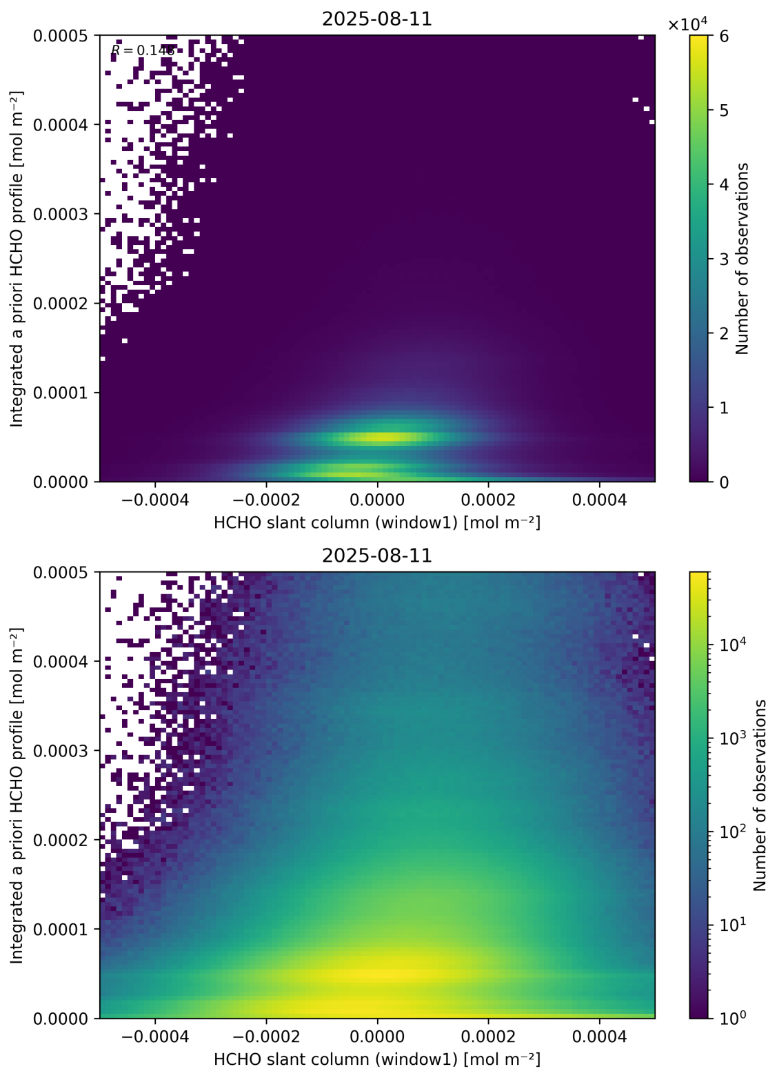
Figure 87: Scatter density plot of “HCHO slant column (window1)” against “Integrated a priori HCHO profile” for 2025-08-10 to 2025-08-12.
