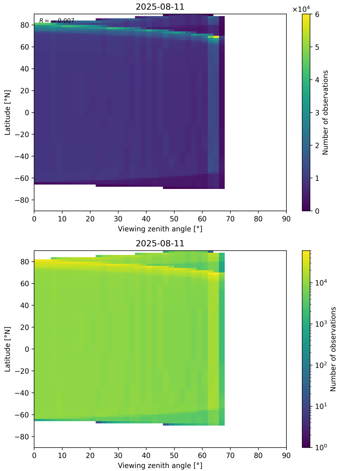
Figure 196: Scatter density plot of “Viewing zenith angle” against “Latitude” for 2025-08-10 to 2025-08-12.
