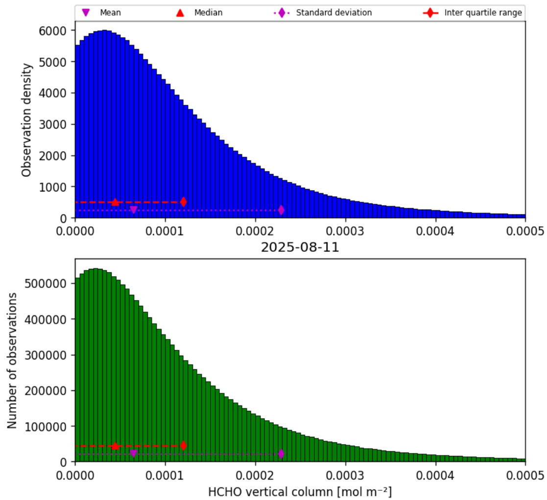
Figure 35: Histogram of “HCHO vertical column” for 2025-08-10 to 2025-08-12
