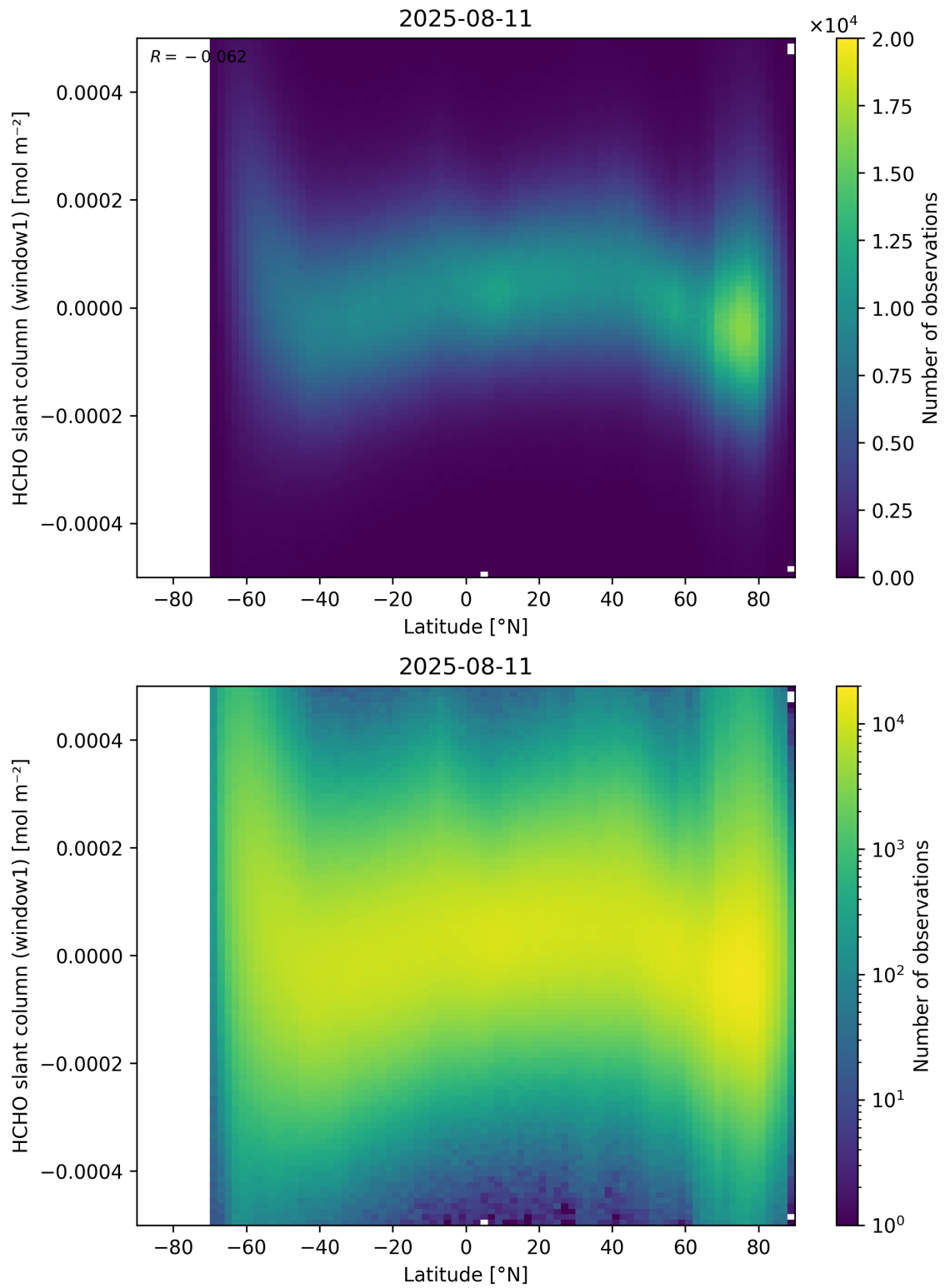
Figure 159: Scatter density plot of “Latitude” against “HCHO slant column (window1)” for 2025-08-10 to 2025-08-12.
