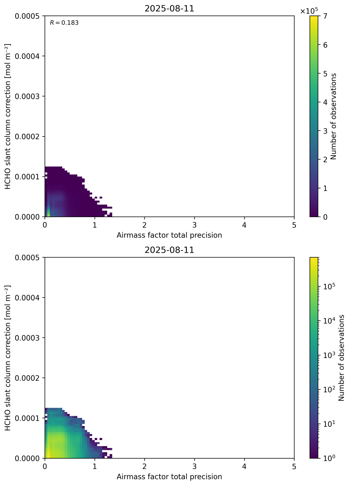
Figure 110: Scatter density plot of “Airmass factor total precision” against “HCHO slant column correction” for 2025-08-10 to 2025-08-12.
