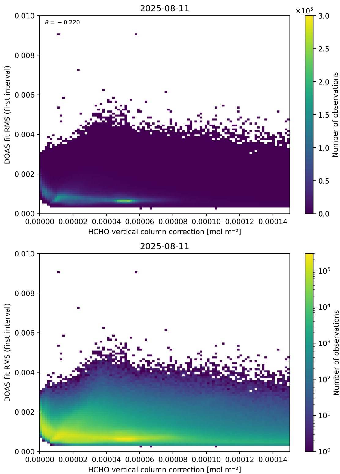
Figure 112: Scatter density plot of “HCHO vertical column correction” against “DOAS fit RMS (first interval)” for 2025-08-10 to 2025-08-12.
