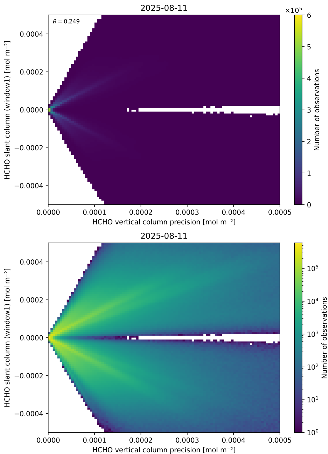
Figure 142: Scatter density plot of “HCHO vertical column precision” against “HCHO slant column (window1)” for 2025-08-10 to 2025-08-12.
