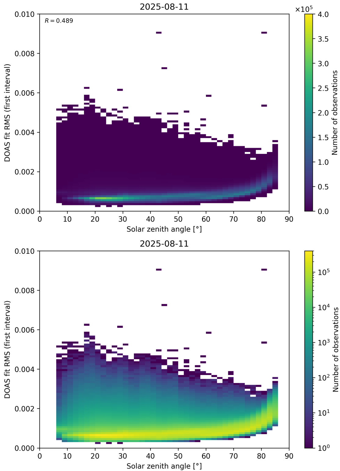
Figure 167: Scatter density plot of “Solar zenith angle” against “DOAS fit RMS (first interval)” for 2025-08-10 to 2025-08-12.
