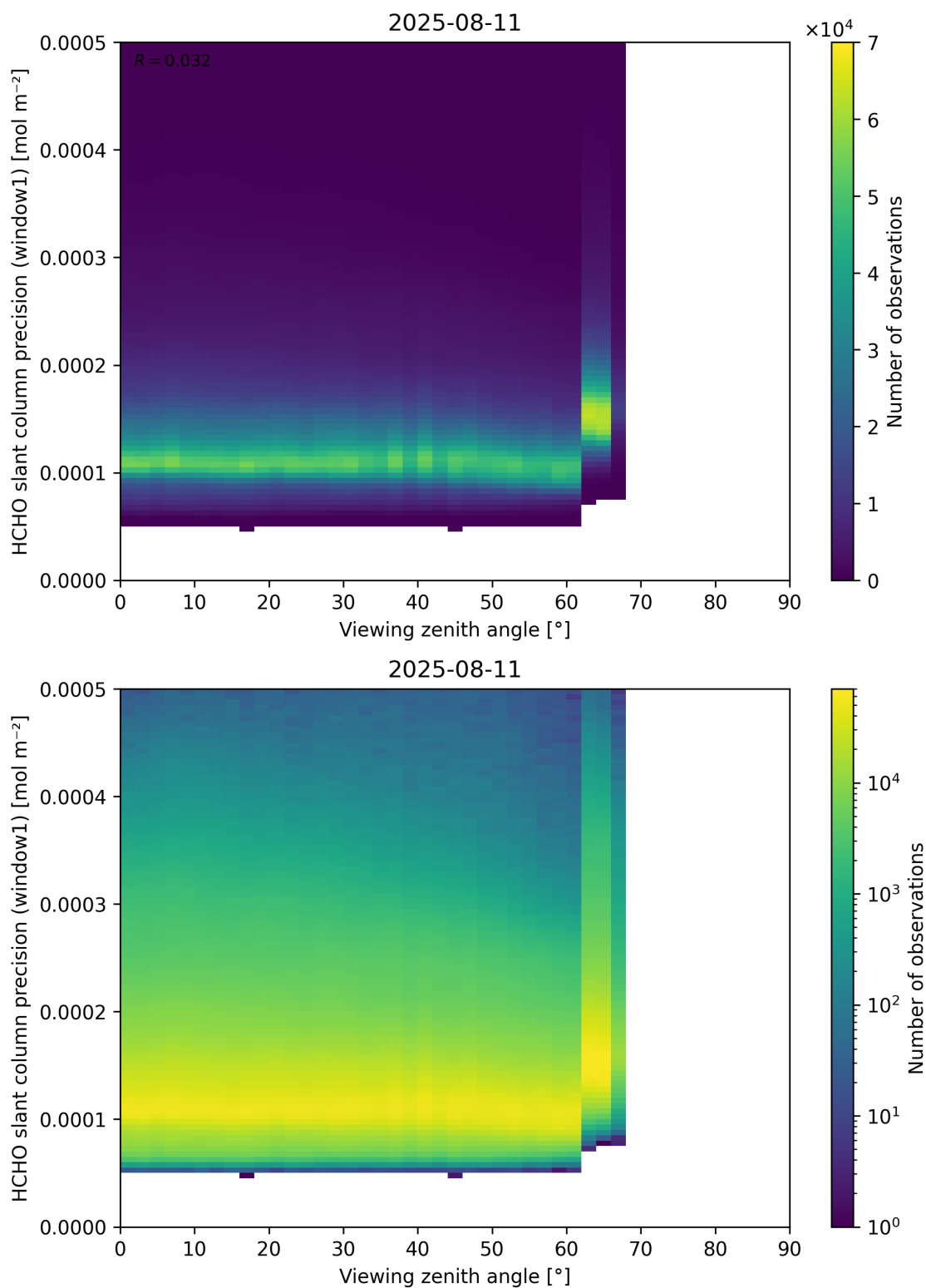
Figure 189: Scatter density plot of “Viewing zenith angle” against “HCHO slant column precision (window1)” for 2025-08-10 to 2025-08-12.
