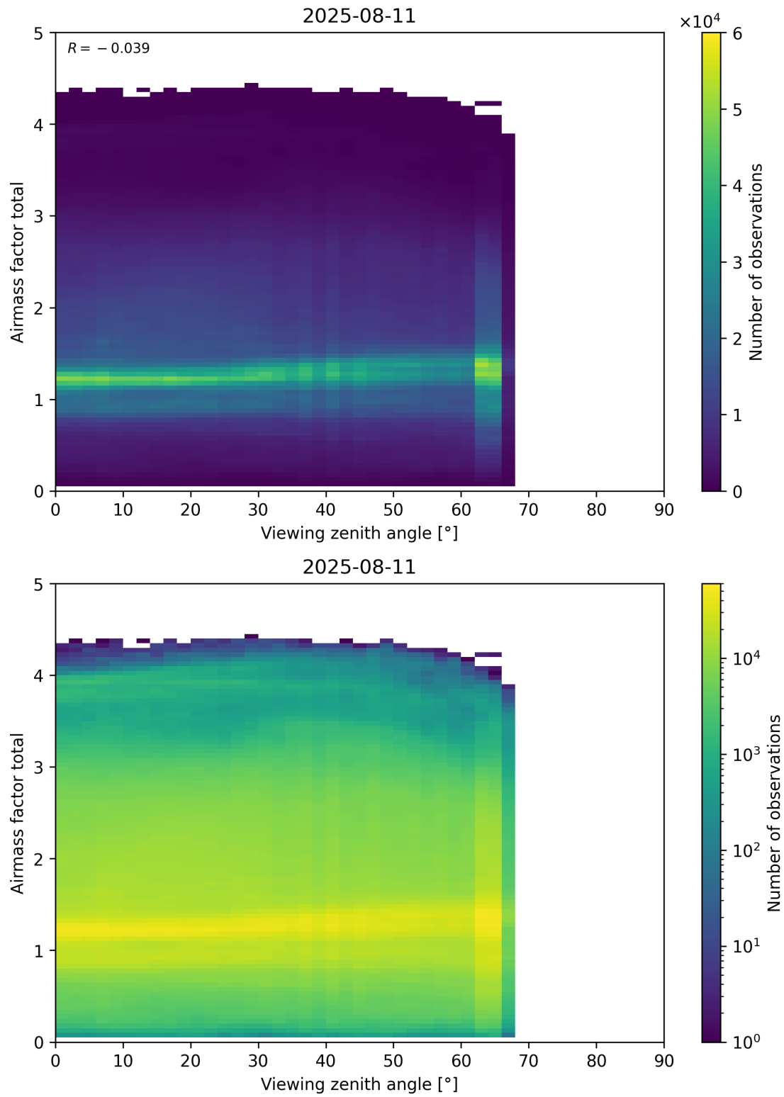
Figure 190: Scatter density plot of “Viewing zenith angle” against “Airmass factor total” for 2025-08-10 to 2025-08-12.
