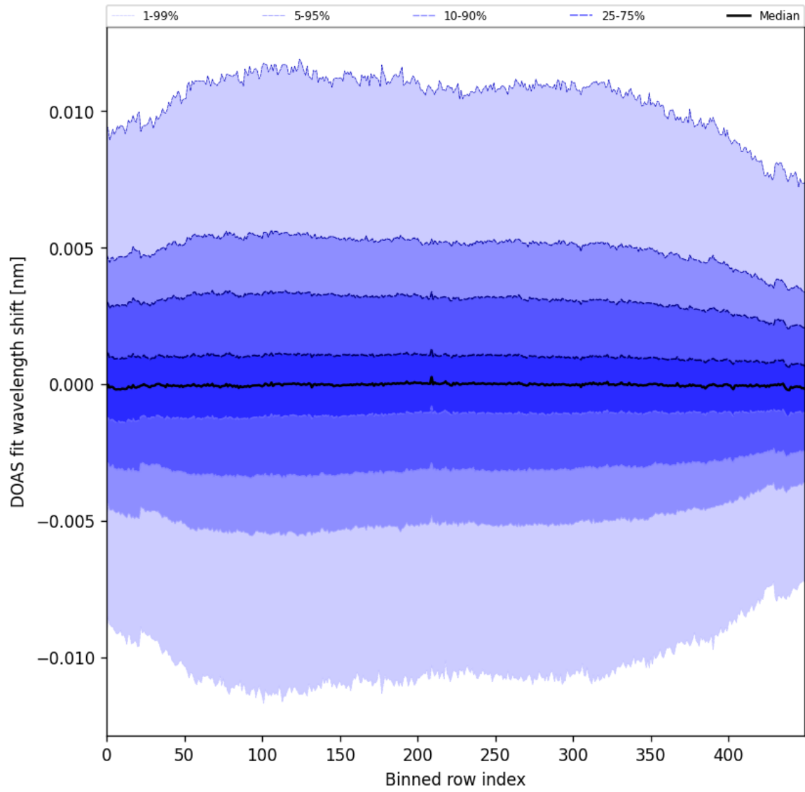
Figure 58: Along track statistics of “DOAS fit wavelength shift” for 2025-08-10 to 2025-08-12
