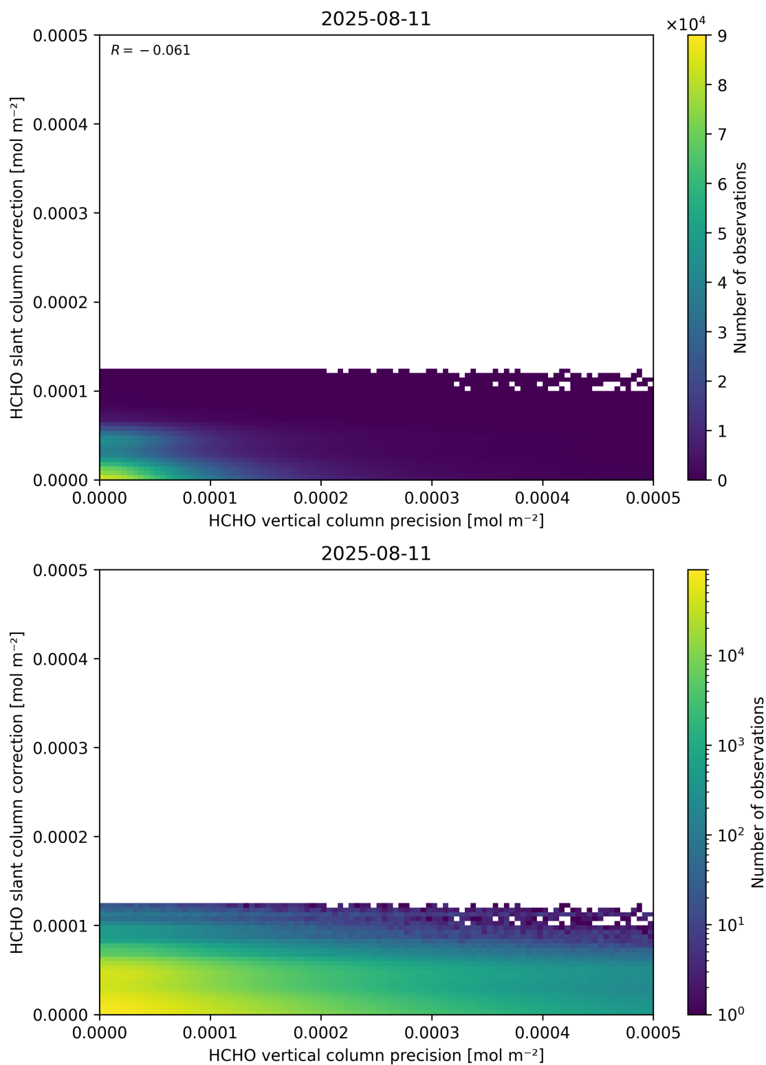
Figure 141: Scatter density plot of “HCHO vertical column precision” against “HCHO slant column correction” for 2025-08-10 to 2025-08-12.
