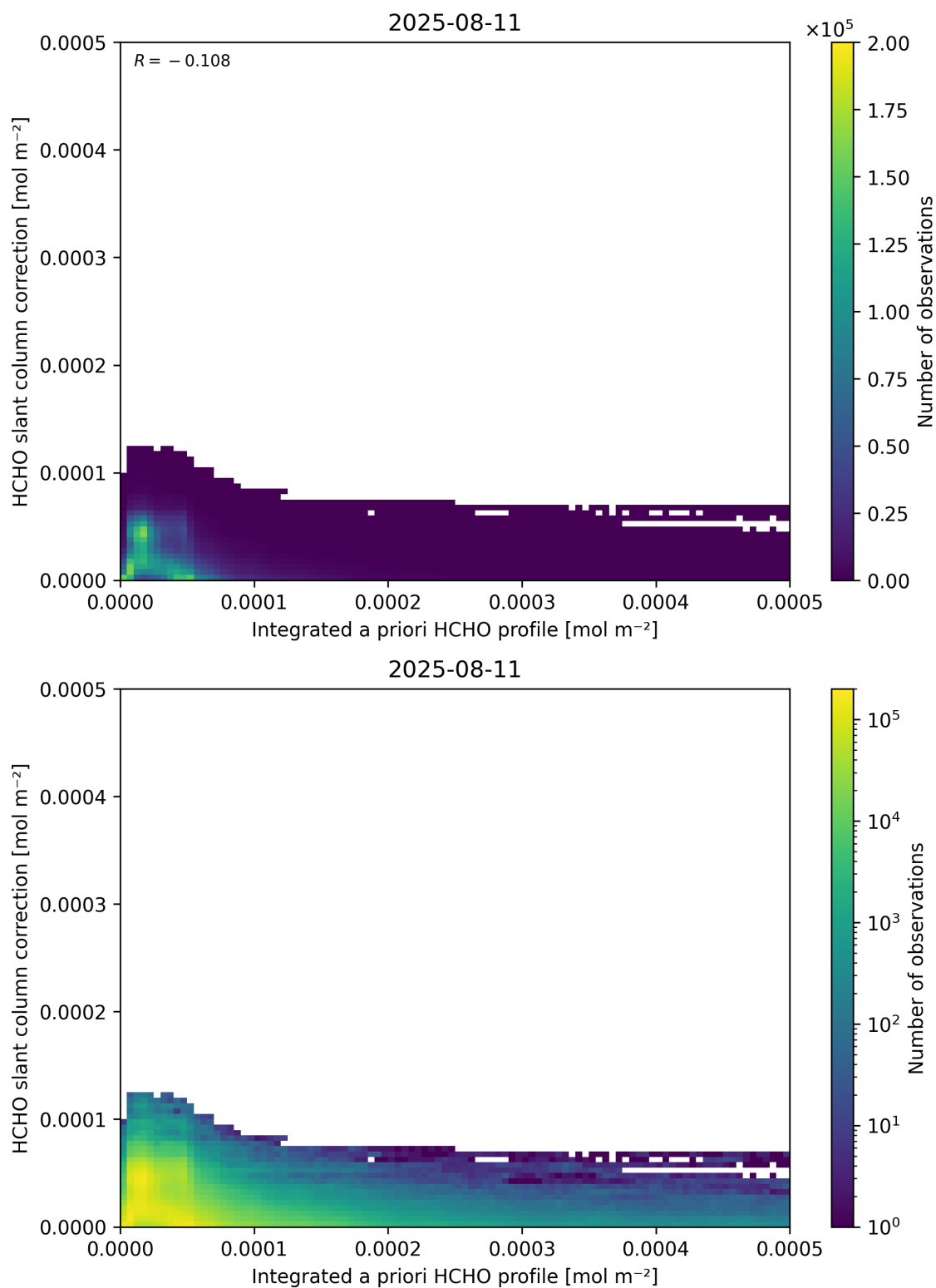
Figure 152: Scatter density plot of “Integrated a priori HCHO profile” against “HCHO slant column correction” for 2025-08-10 to 2025-08-12.
