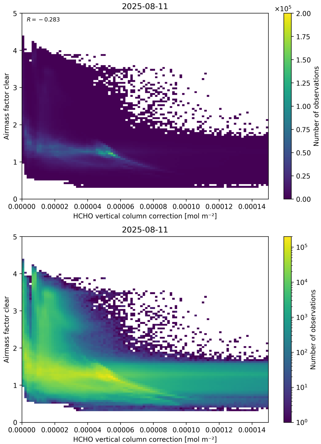
Figure 115: Scatter density plot of “HCHO vertical column correction” against “Airmass factor clear” for 2025-08-10 to 2025-08-12.
