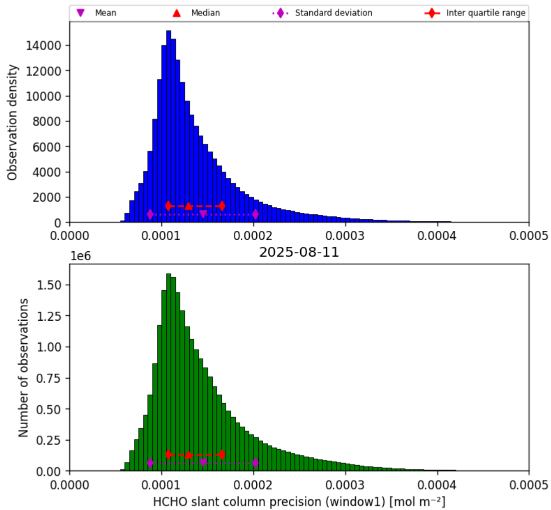
Figure 39: Histogram of “HCHO slant column precision (window1)” for 2025-08-10 to 2025-08-12
