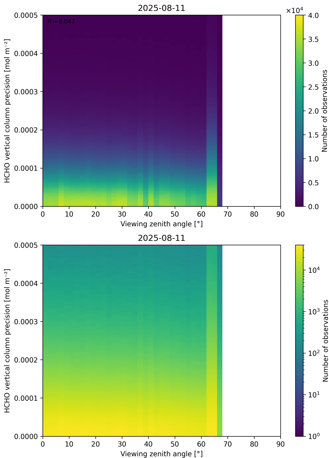
Figure 194: Scatter density plot of “Viewing zenith angle” against “HCHO vertical column precision” for 2025-08-10 to 2025-08-12.
