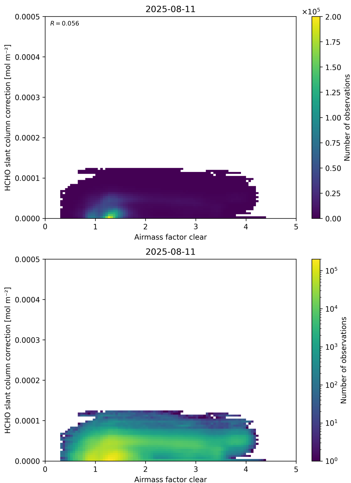
Figure 75: Scatter density plot of “Airmass factor clear” against “HCHO slant column correction” for 2025-08-10 to 2025-08-12.
