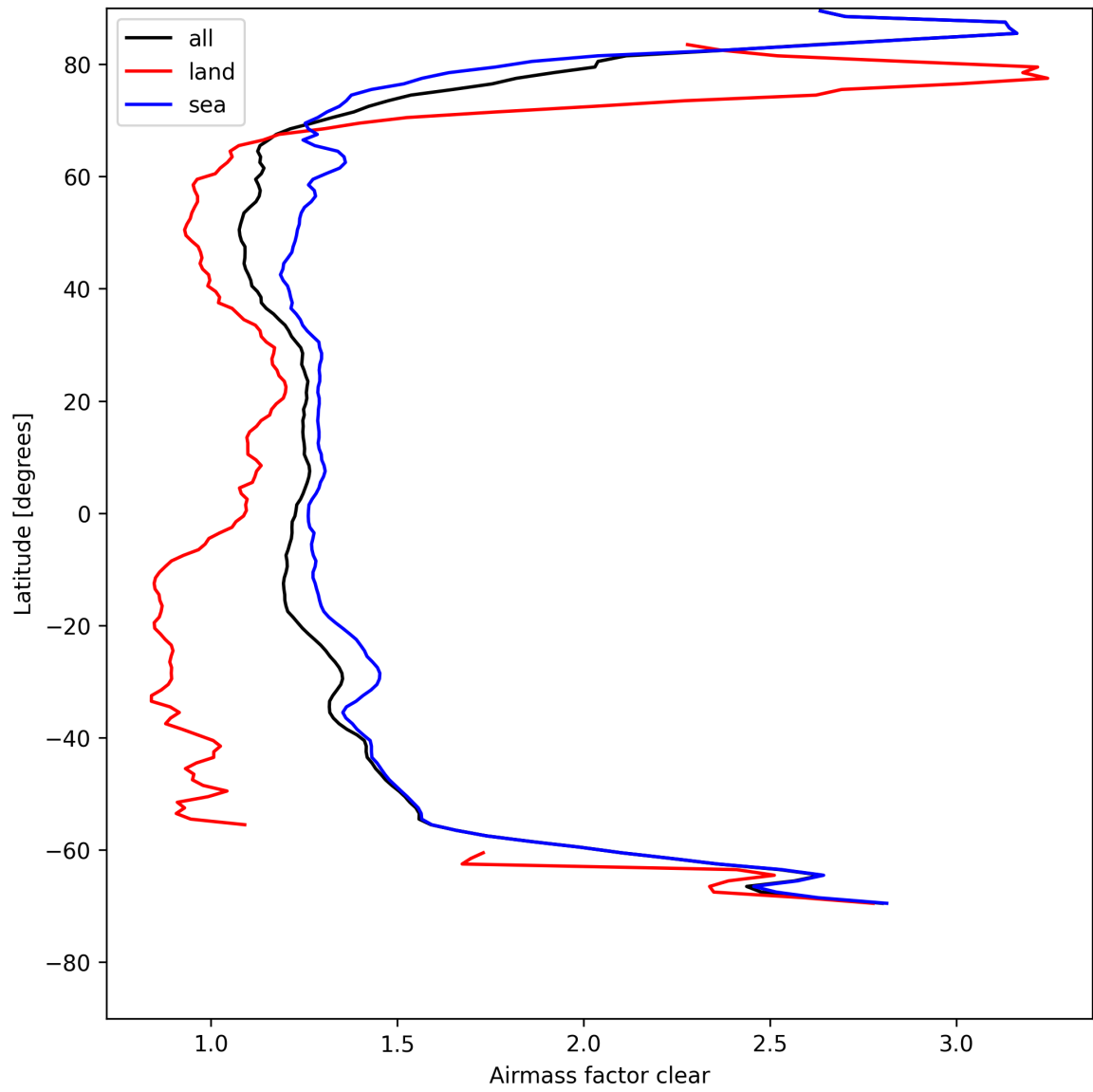
Figure 28: Zonal average of “Airmass factor clear” for 2025-08-10 to 2025-08-12.
