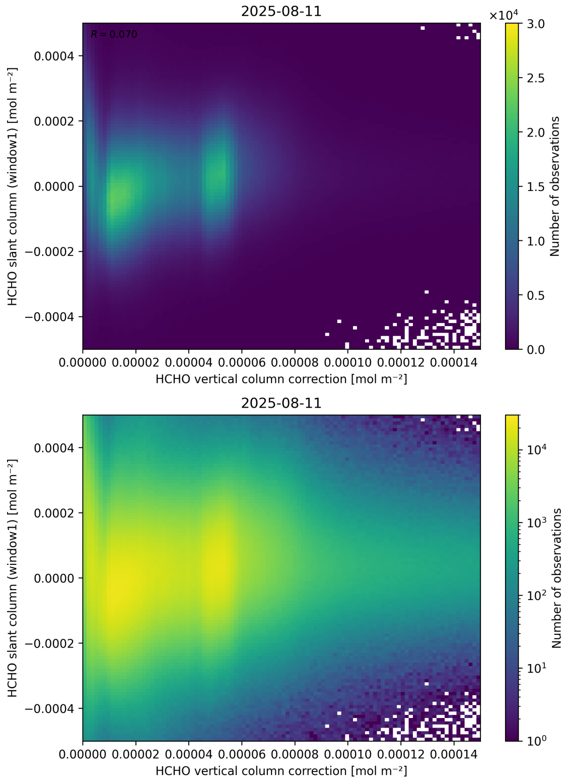
Figure 118: Scatter density plot of “HCHO vertical column correction” against “HCHO slant column (window1)” for 2025-08-10 to 2025-08-12.
