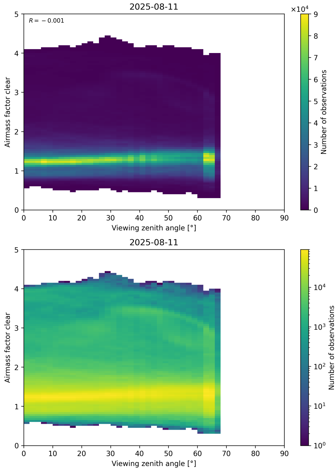
Figure 185: Scatter density plot of “Viewing zenith angle” against “Airmass factor clear” for 2025-08-10 to 2025-08-12.
