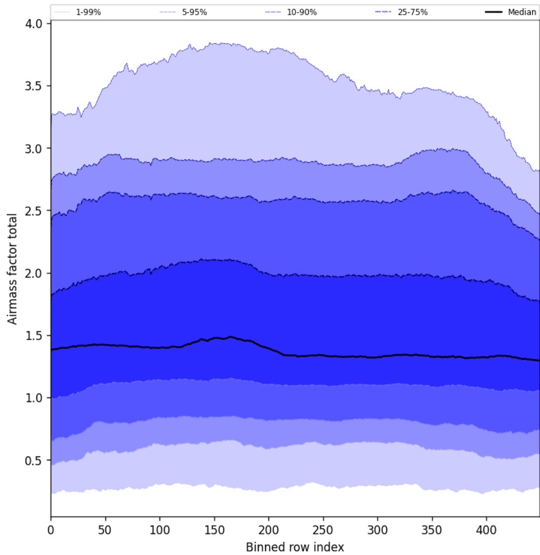
Figure 54: Along track statistics of “Airmass factor total” for 2025-08-10 to 2025-08-12
