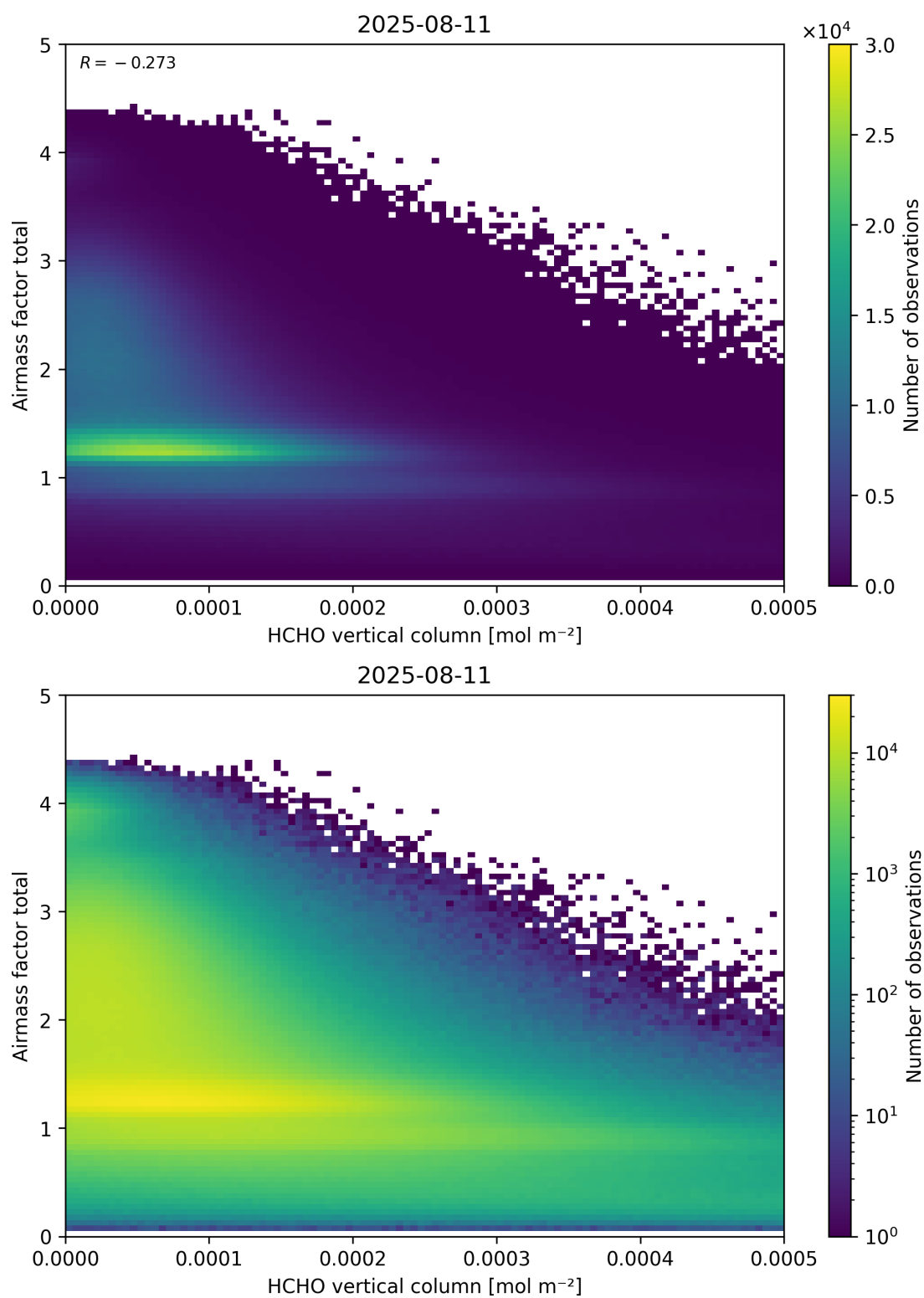
Figure 131: Scatter density plot of “HCHO vertical column” against “Airmass factor total” for 2025-08-10 to 2025-08-12.
