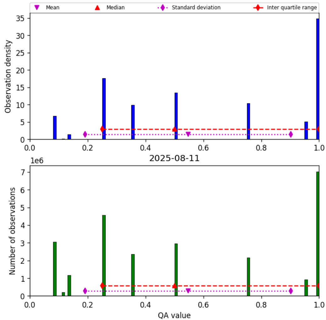
Figure 34: Histogram of “QA value” for 2025-08-10 to 2025-08-12
