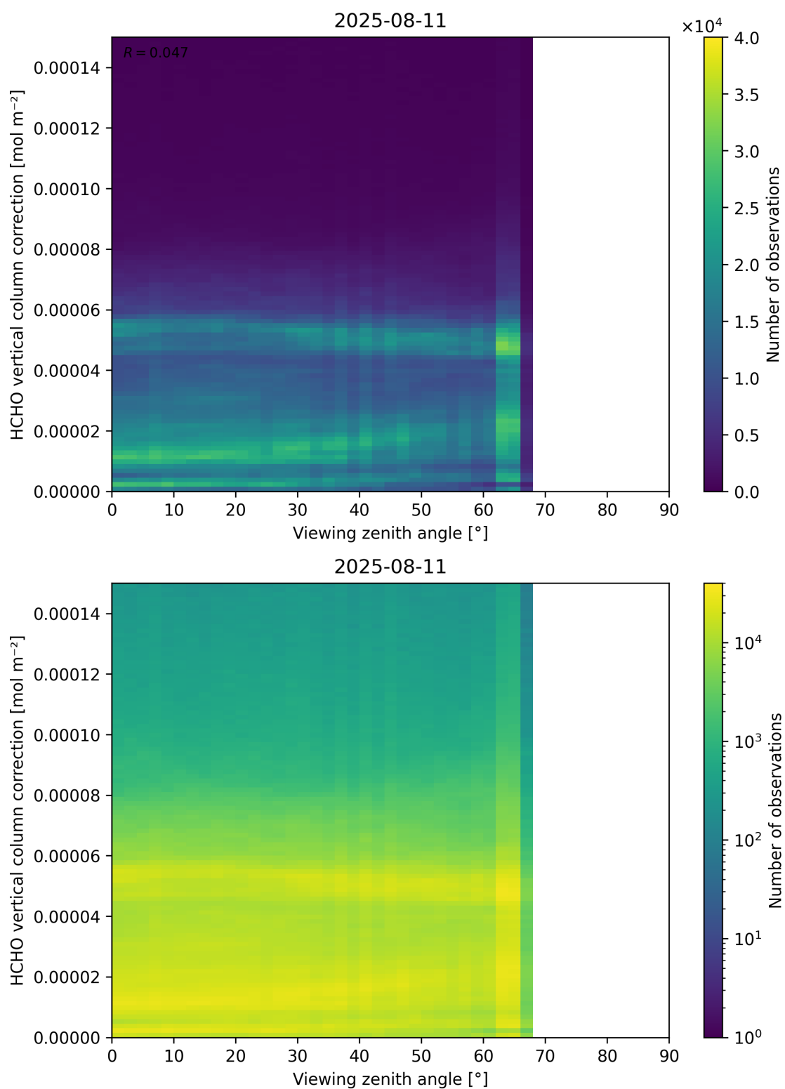
Figure 193: Scatter density plot of “Viewing zenith angle” against “HCHO vertical column correction” for 2025-08-10 to 2025-08-12.
