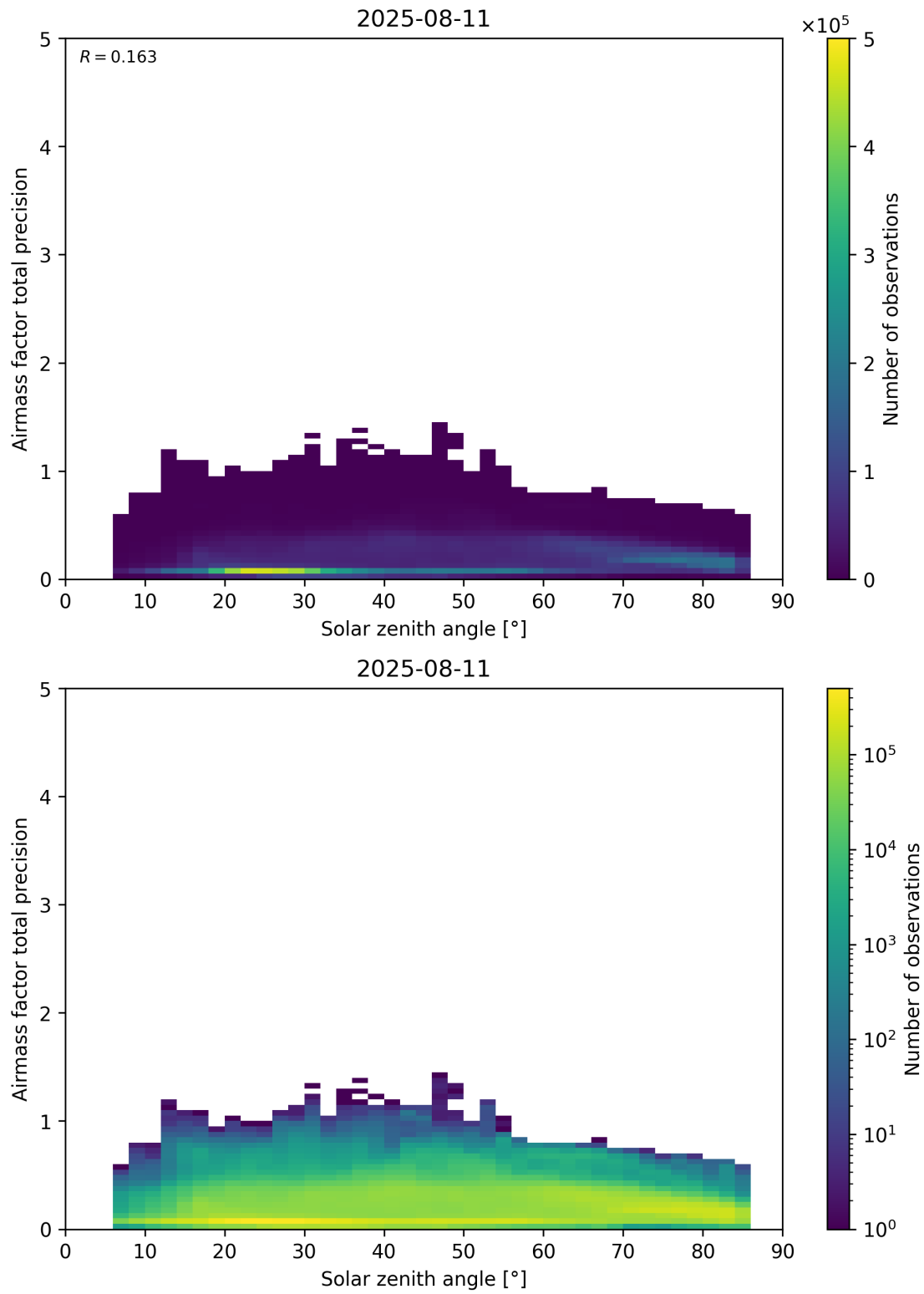
Figure 176: Scatter density plot of “Solar zenith angle” against “Airmass factor total precision” for 2025-08-10 to 2025-08-12.
