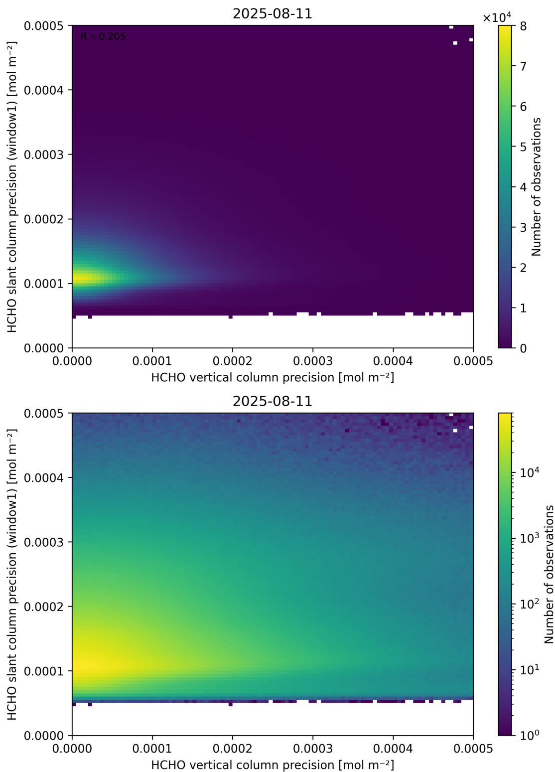
Figure 143: Scatter density plot of “HCHO vertical column precision” against “HCHO slant column precision (window1)” for 2025-08-10 to 2025-08-12.
