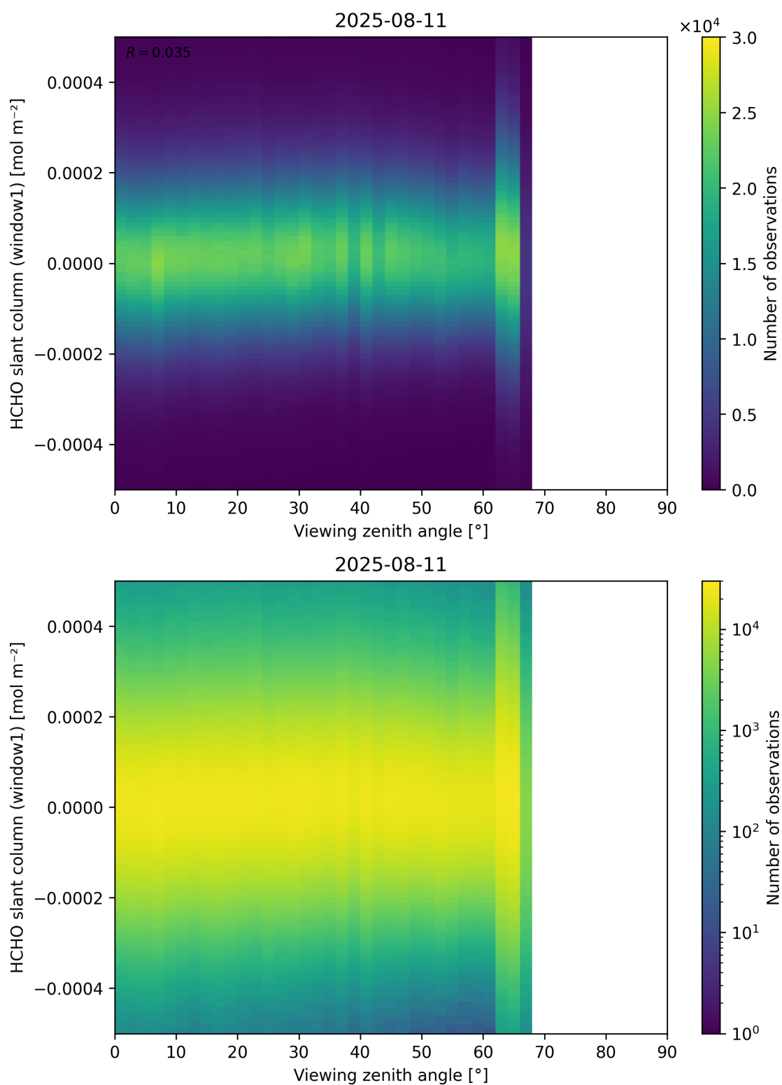
Figure 188: Scatter density plot of “Viewing zenith angle” against “HCHO slant column (window1)” for 2025-08-10 to 2025-08-12.
