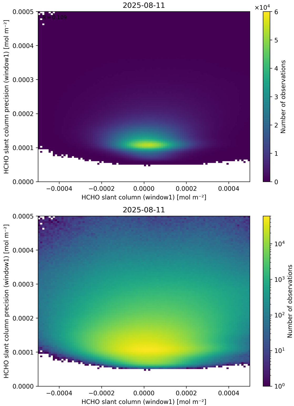
Figure 84: Scatter density plot of “HCHO slant column (window1)” against “HCHO slant column precision (window1)” for 2025-08-10 to 2025-08-12.
