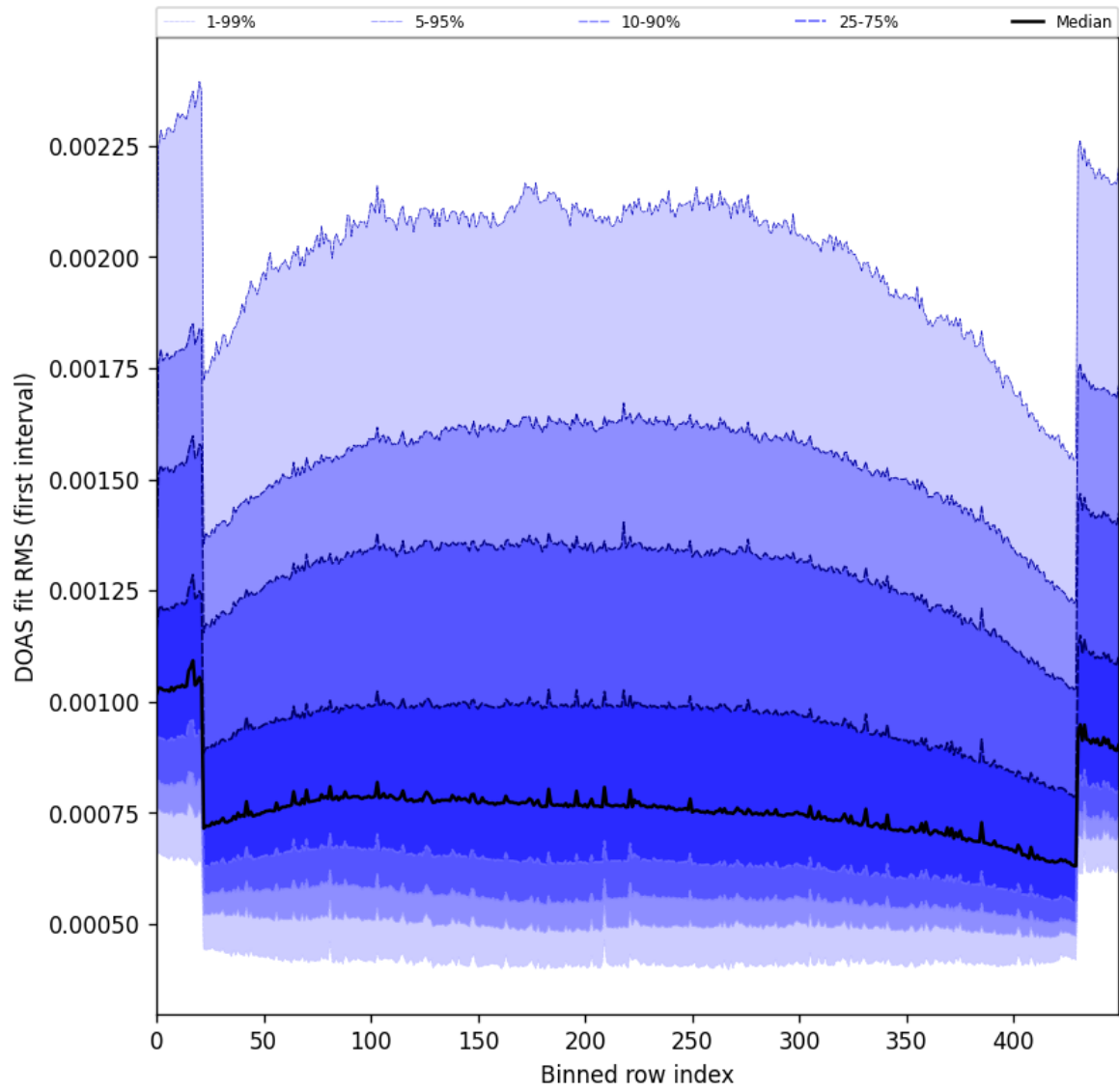
Figure 60: Along track statistics of “DOAS fit RMS (first interval)” for 2025-08-10 to 2025-08-12
