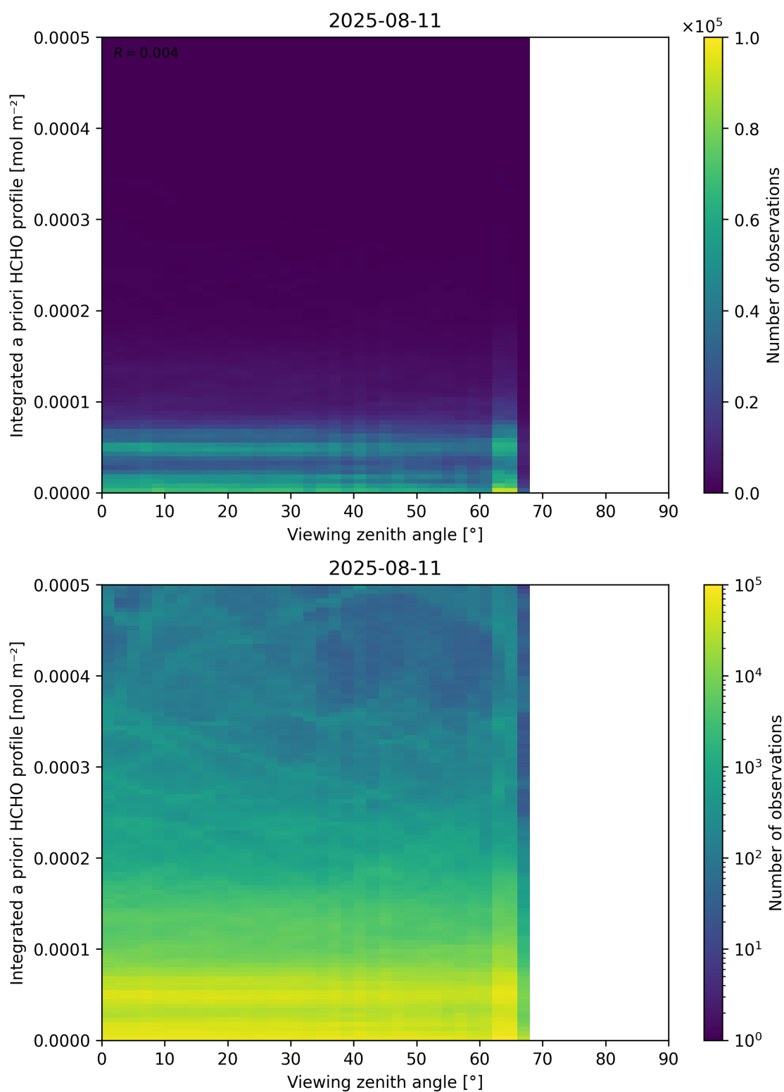
Figure 195: Scatter density plot of “Viewing zenith angle” against “Integrated a priori HCHO profile” for 2025-08-10 to 2025-08-12.
