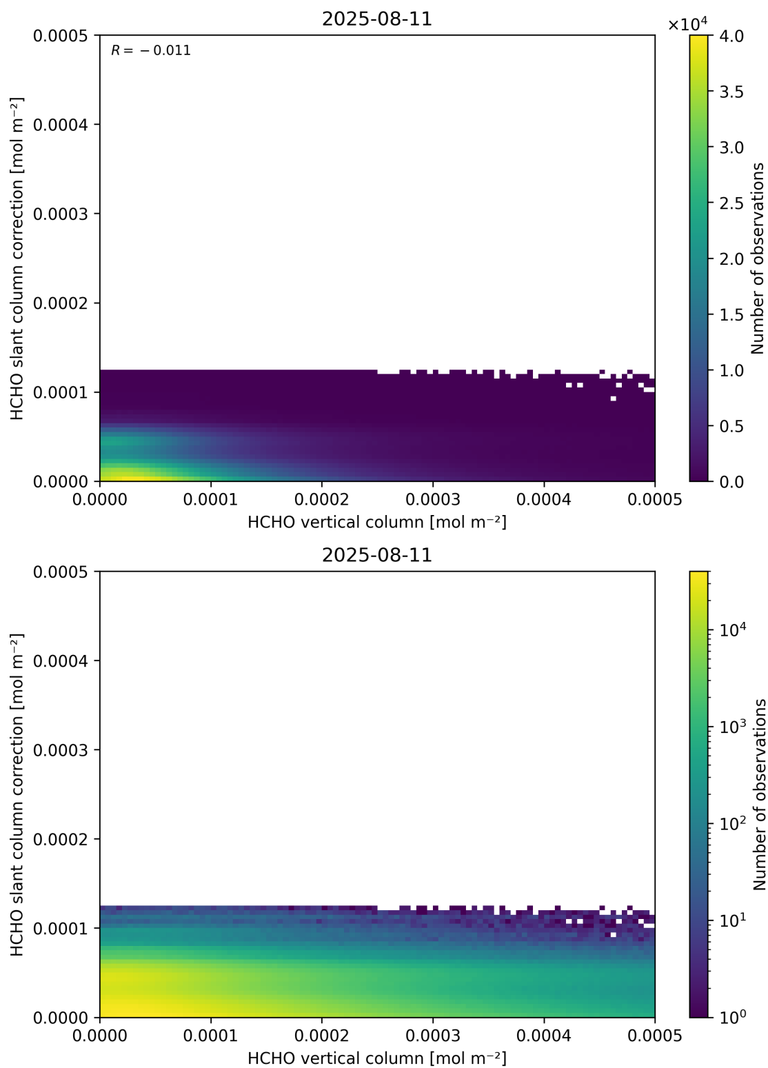
Figure 128: Scatter density plot of “HCHO vertical column” against “HCHO slant column correction” for 2025-08-10 to 2025-08-12.
