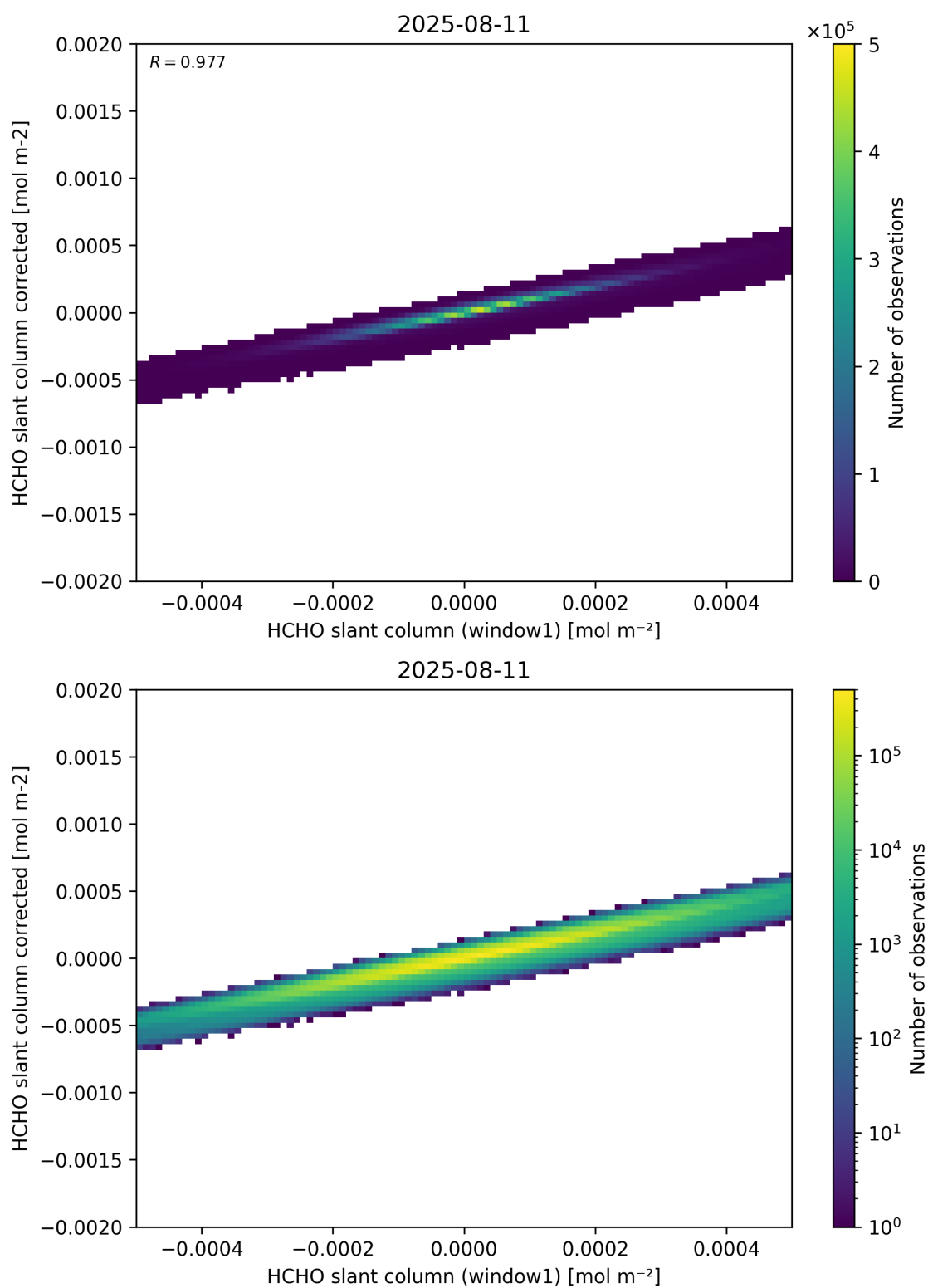
Figure 82: Scatter density plot of “HCHO slant column (window1)” against “HCHO slant column corrected” for 2025-08-10 to 2025-08-12.
