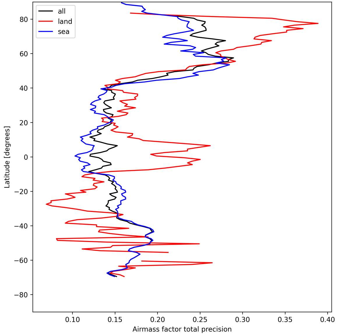
Figure 27: Zonal average of “Airmass factor total precision” for 2025-08-10 to 2025-08-12.
