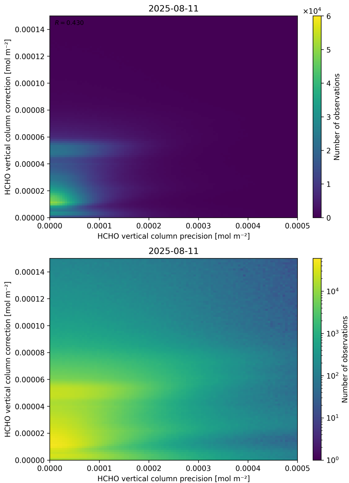
Figure 146: Scatter density plot of “HCHO vertical column precision” against “HCHO vertical column correction” for 2025-08-10 to 2025-08-12.
