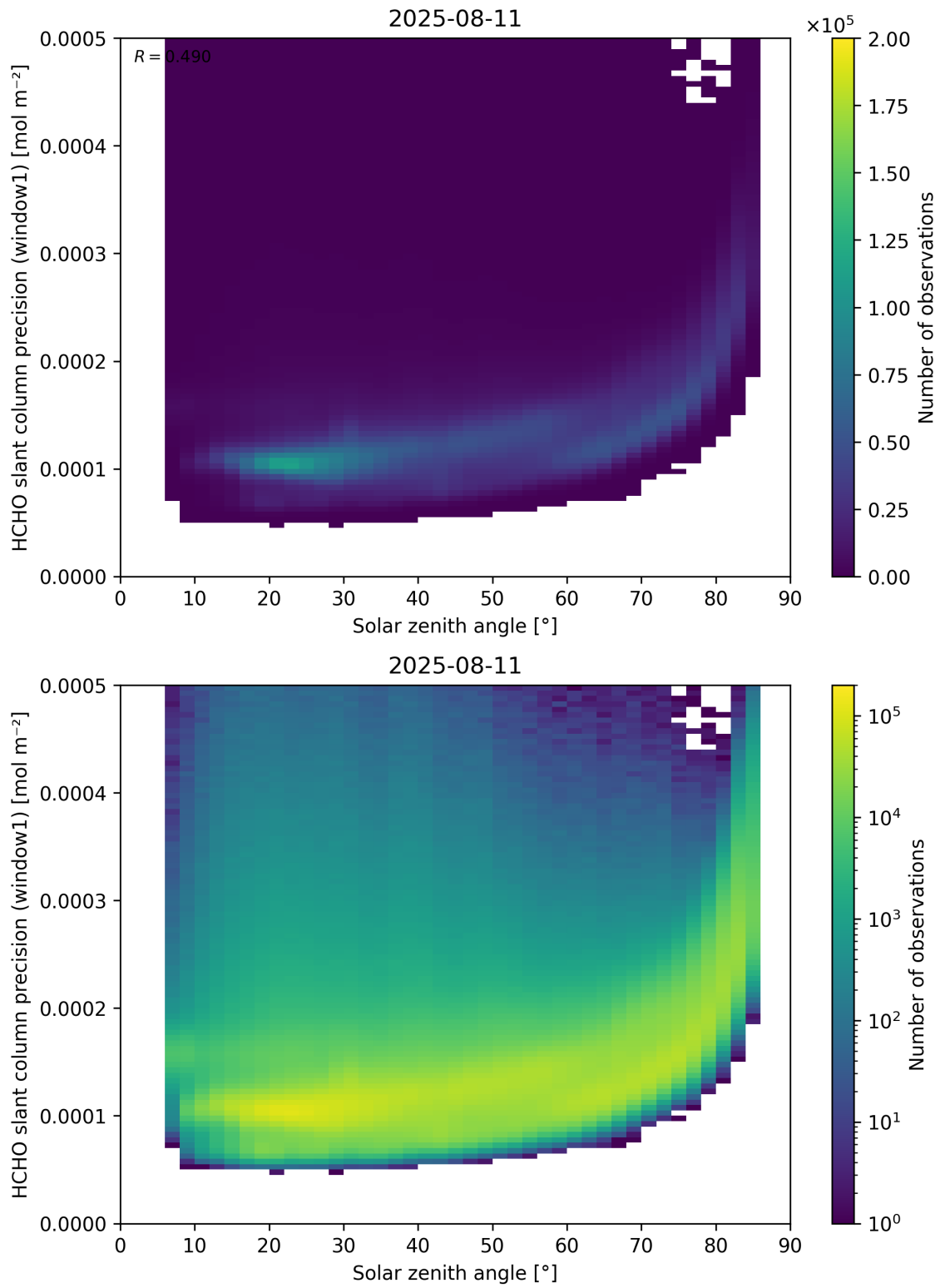
Figure 174: Scatter density plot of “Solar zenith angle” against “HCHO slant column precision (window1)” for 2025-08-10 to 2025-08-12.
