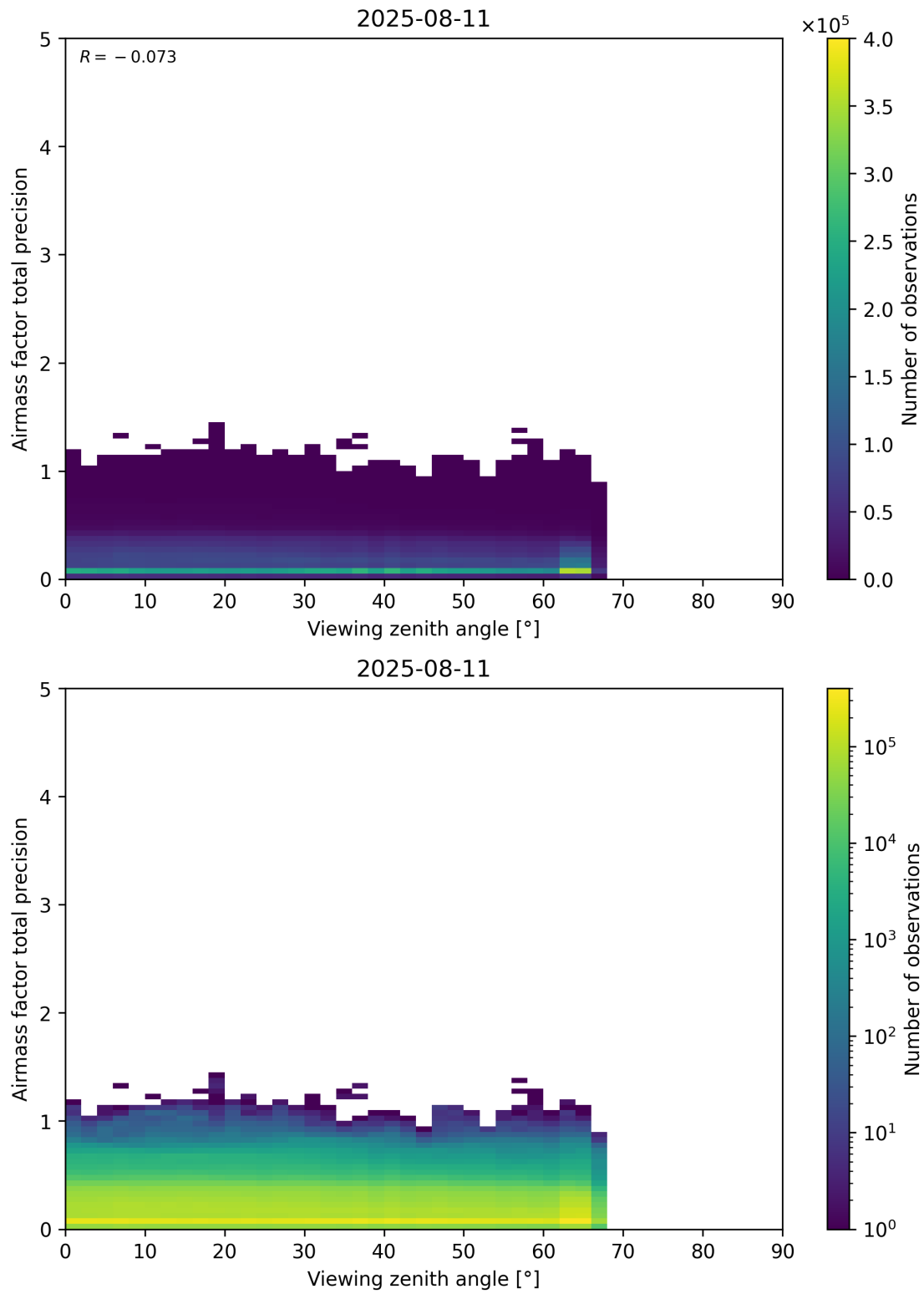
Figure 191: Scatter density plot of “Viewing zenith angle” against “Airmass factor total precision” for 2025-08-10 to 2025-08-12.
