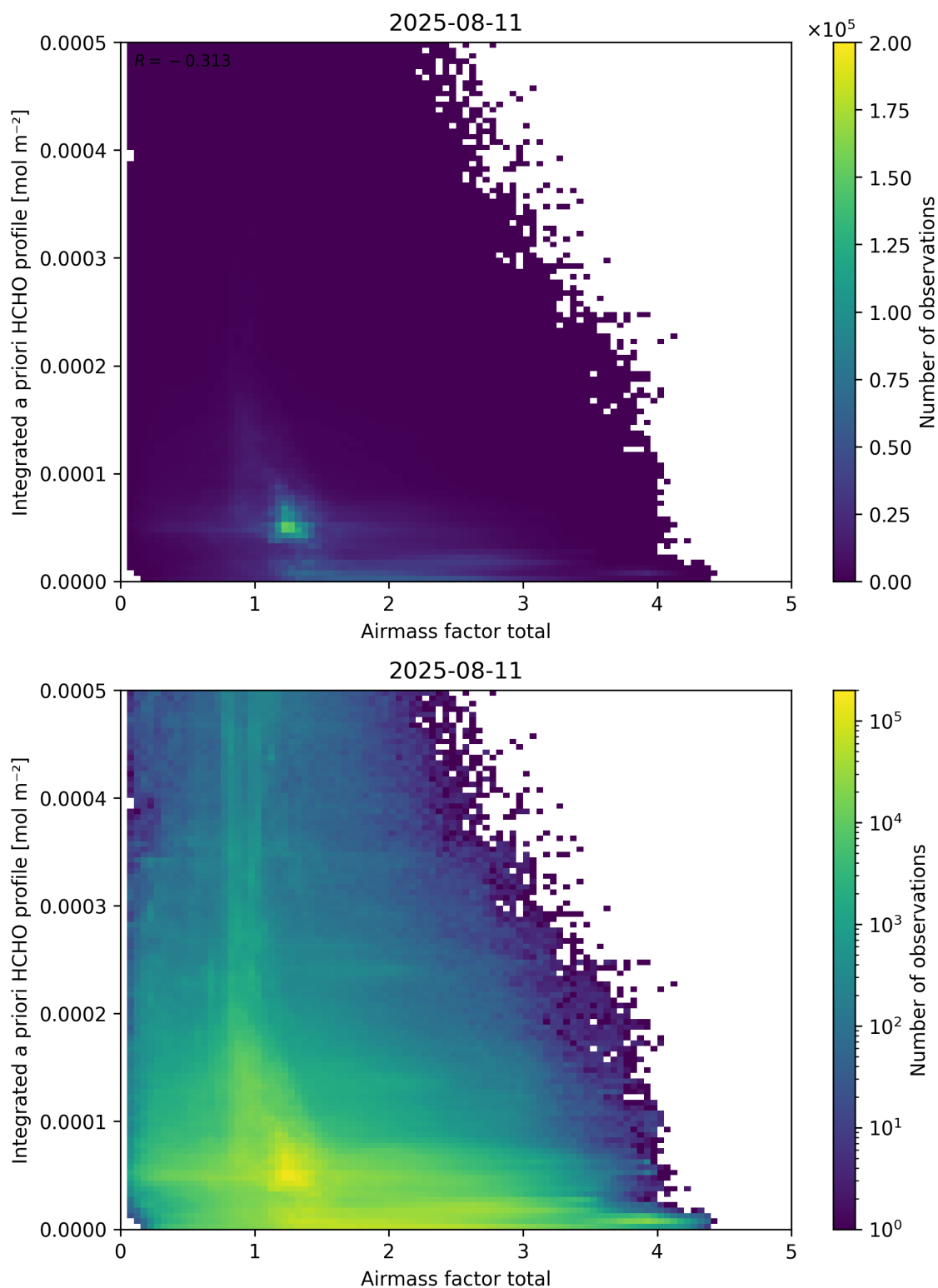
Figure 104: Scatter density plot of “Airmass factor total” against “Integrated a priori HCHO profile” for 2025-08-10 to 2025-08-12.
