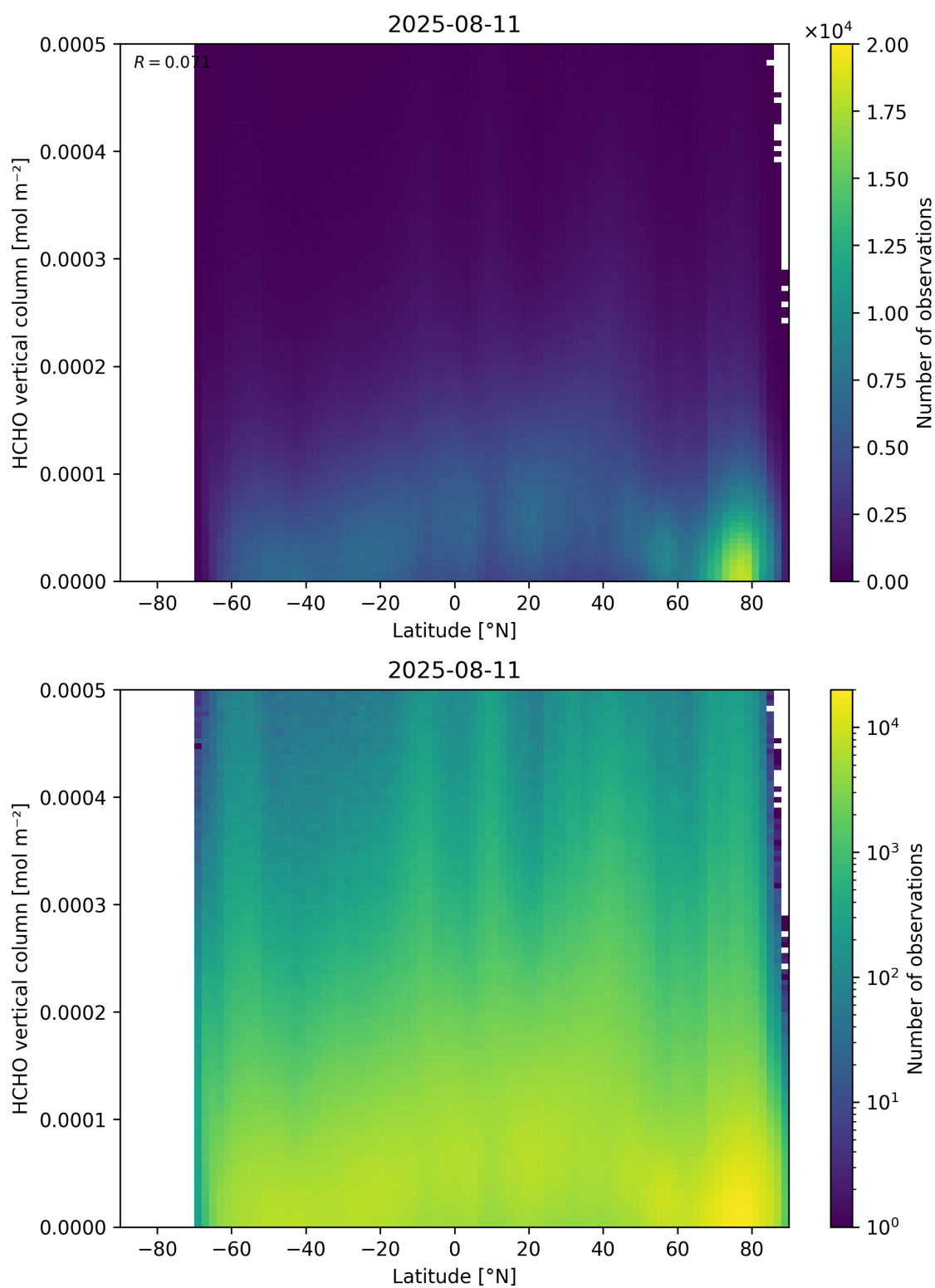
Figure 163: Scatter density plot of “Latitude” against “HCHO vertical column” for 2025-08-10 to 2025-08-12.
