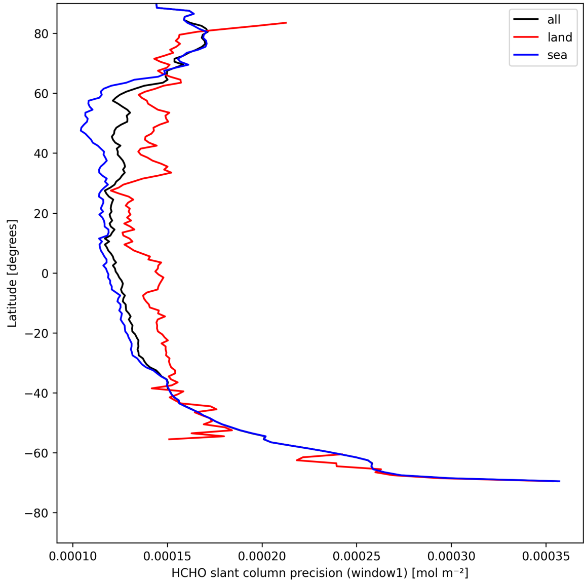
Figure 25: Zonal average of “HCHO slant column precision (window1)” for 2025-08-10 to 2025-08-12.
