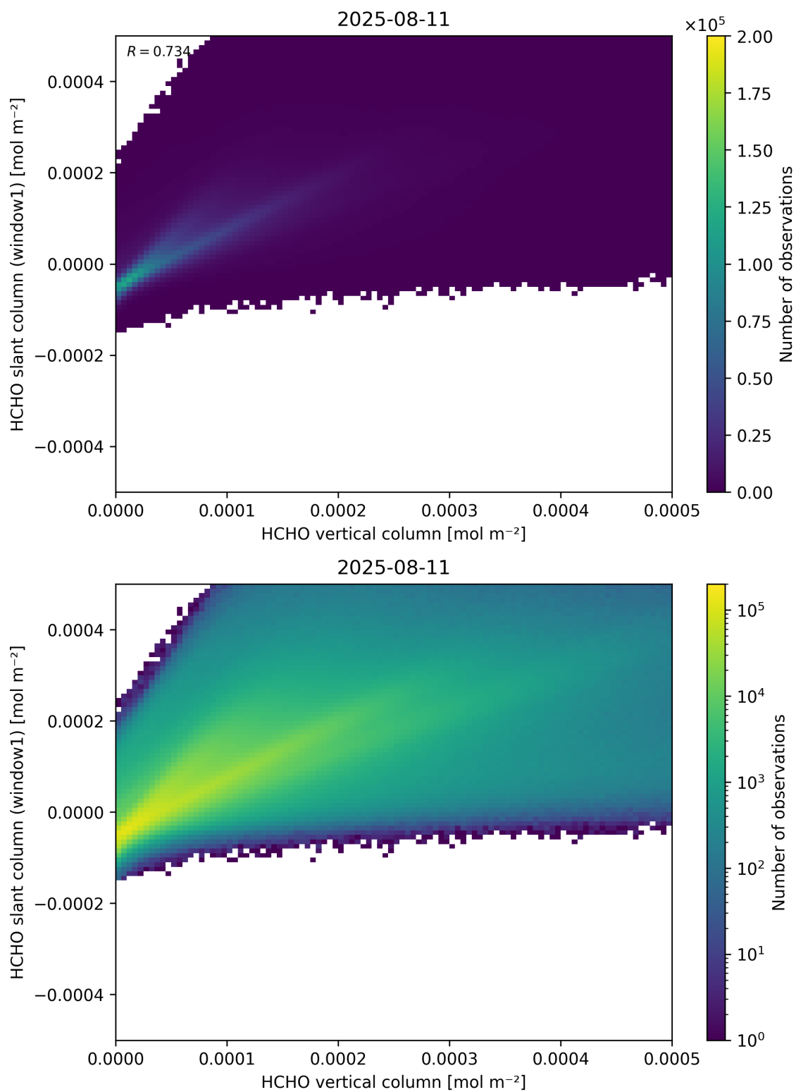
Figure 129: Scatter density plot of “HCHO vertical column” against “HCHO slant column (window1)” for 2025-08-10 to 2025-08-12.
