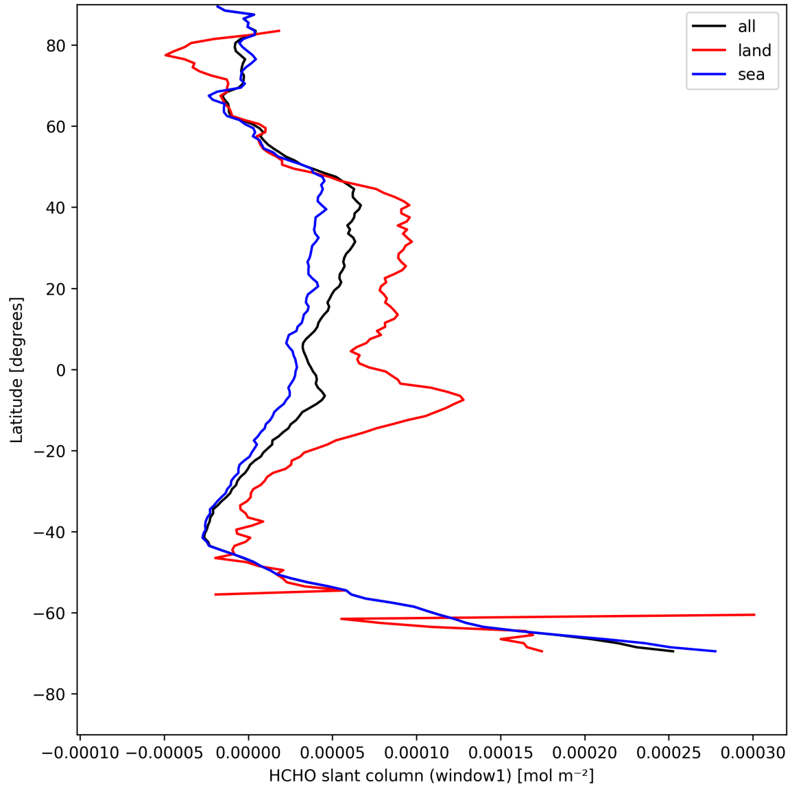
Figure 24: Zonal average of “HCHO slant column (window1)” for 2025-08-10 to 2025-08-12.
