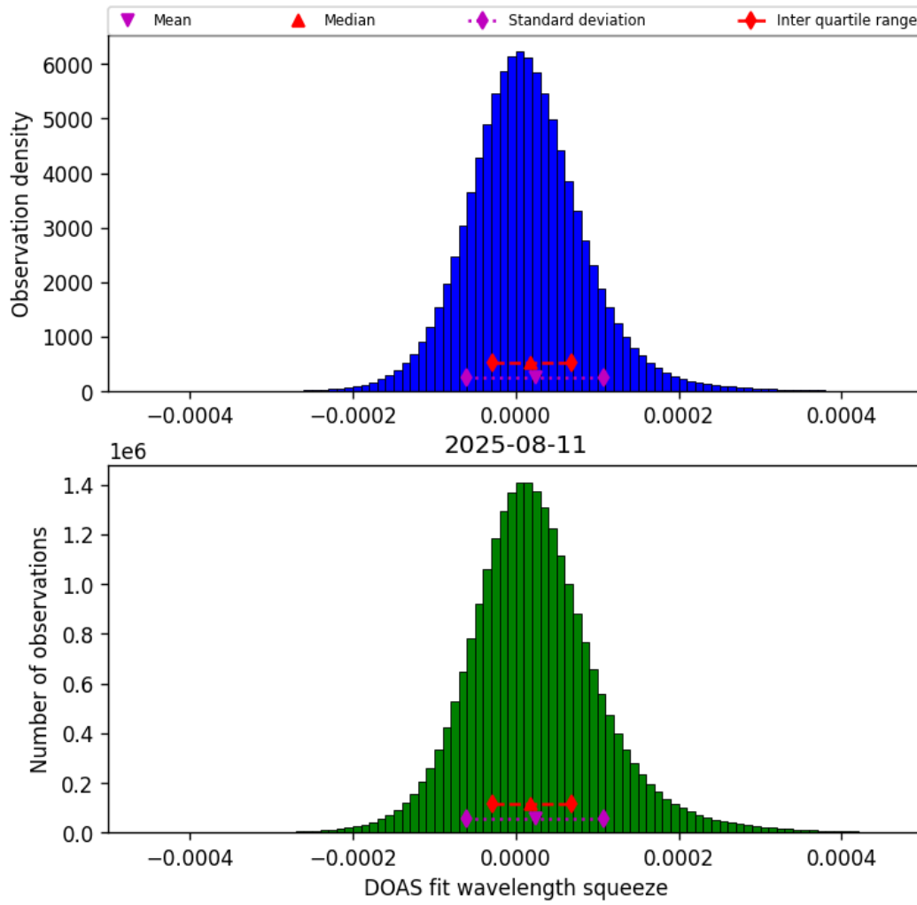
Figure 45: Histogram of “DOAS fit wavelength squeeze” for 2025-08-10 to 2025-08-12
