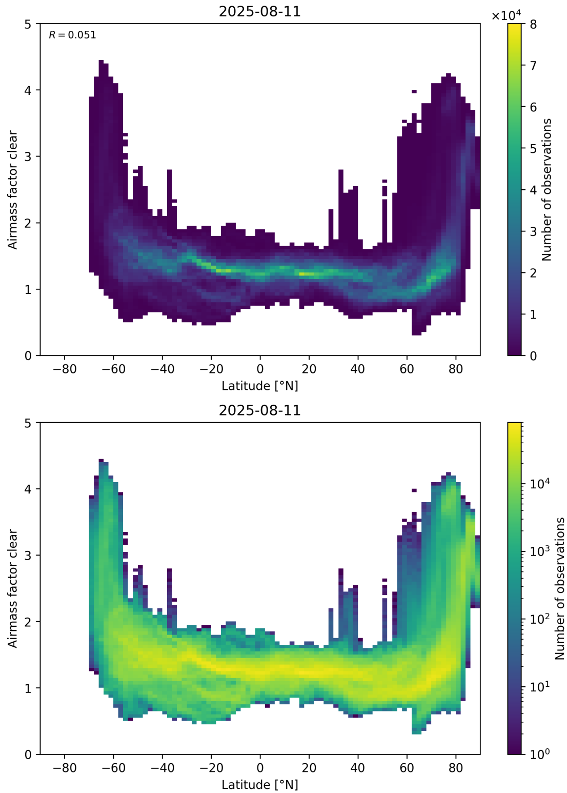
Figure 156: Scatter density plot of “Latitude” against “Airmass factor clear” for 2025-08-10 to 2025-08-12.
