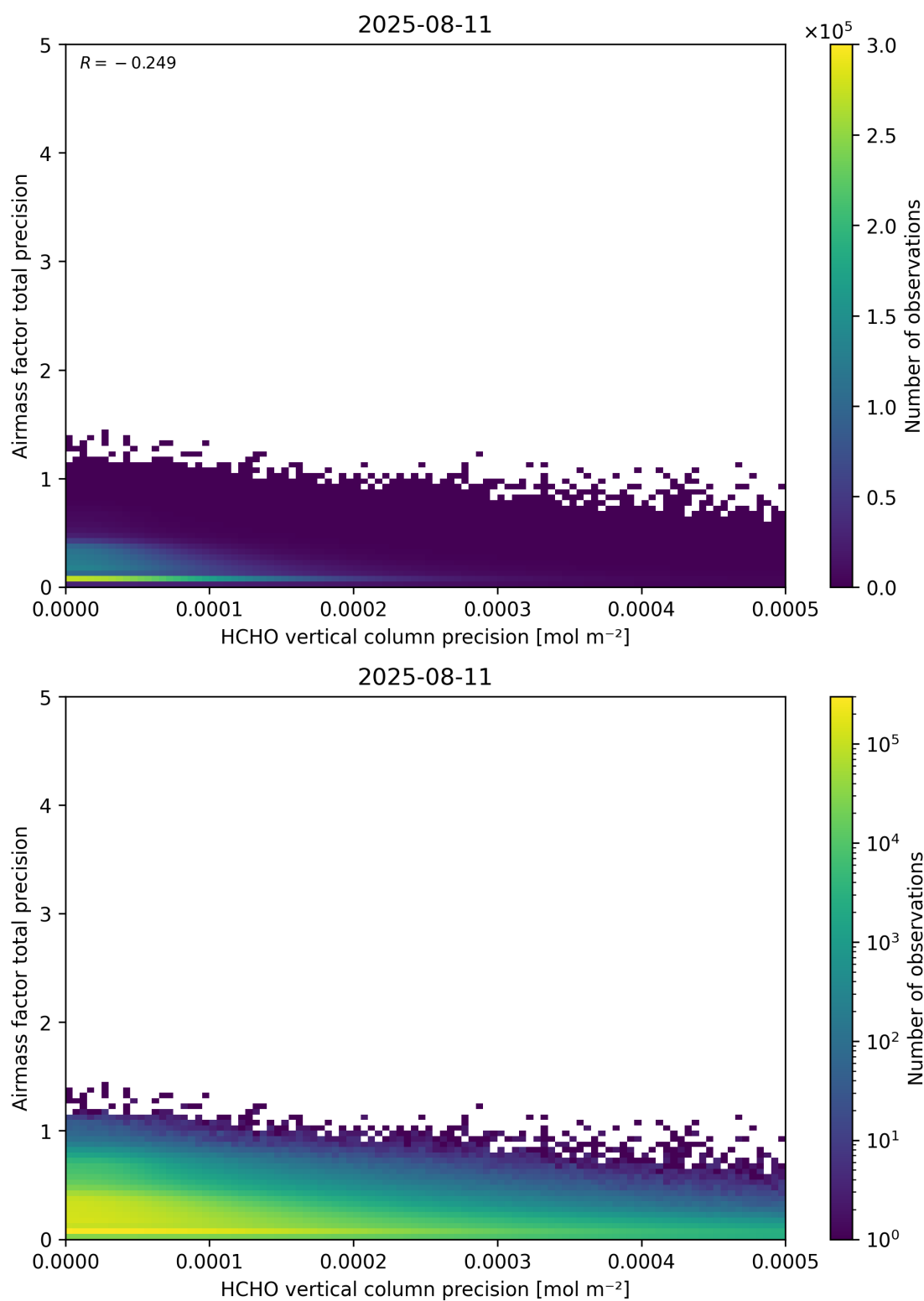
Figure 145: Scatter density plot of “HCHO vertical column precision” against “Airmass factor total precision” for 2025-08-10 to 2025-08-12.
