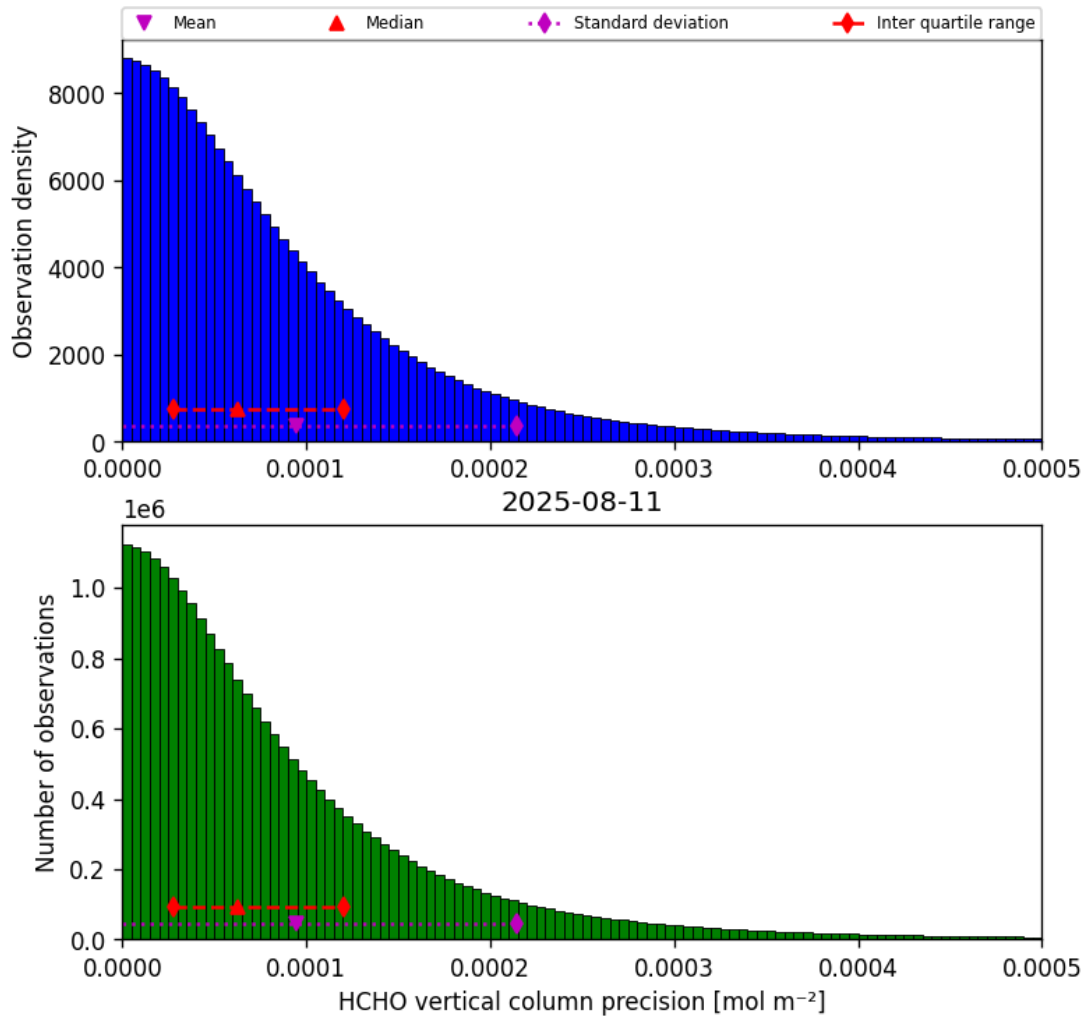
Figure 36: Histogram of “HCHO vertical column precision” for 2025-08-10 to 2025-08-12
