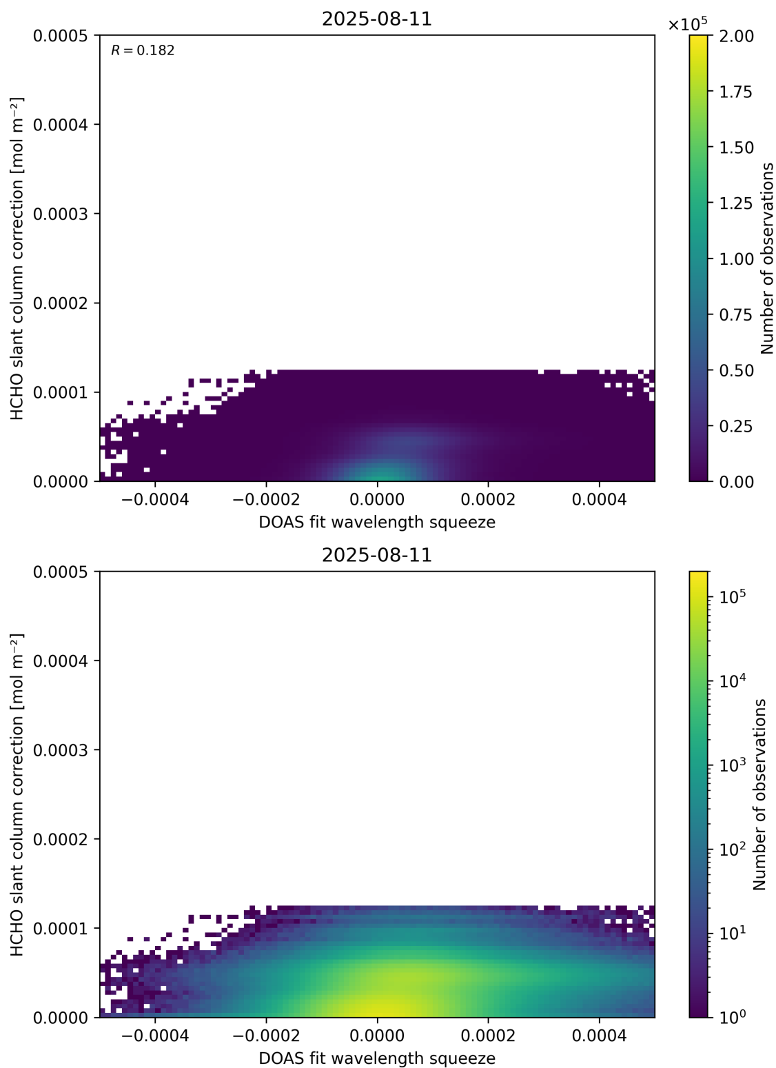
Figure 70: Scatter density plot of “DOAS fit wavelength squeeze” against “HCHO slant column correction” for 2025-08-10 to 2025-08-12.
