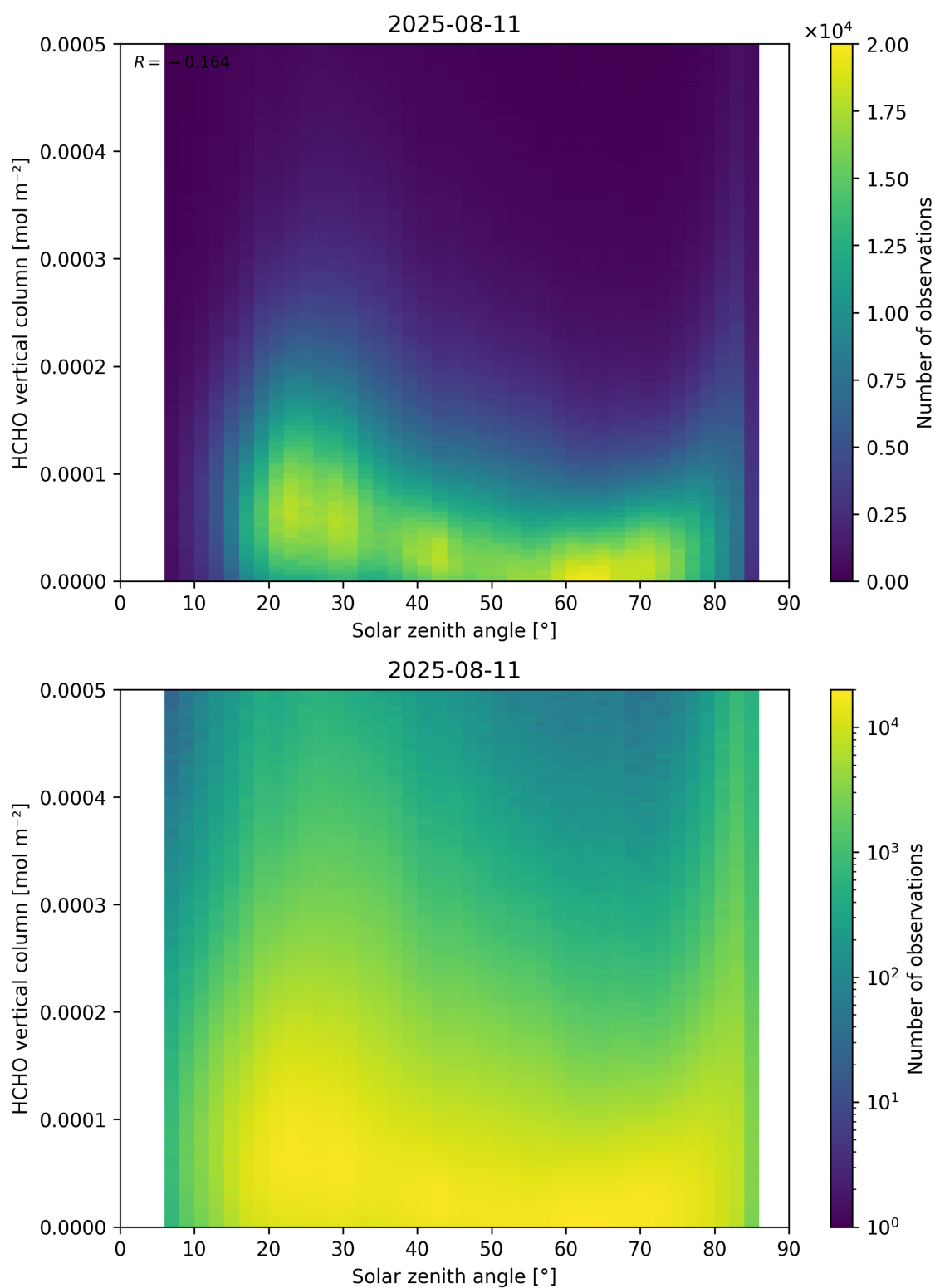
Figure 177: Scatter density plot of “Solar zenith angle” against “HCHO vertical column” for 2025-08-10 to 2025-08-12.
