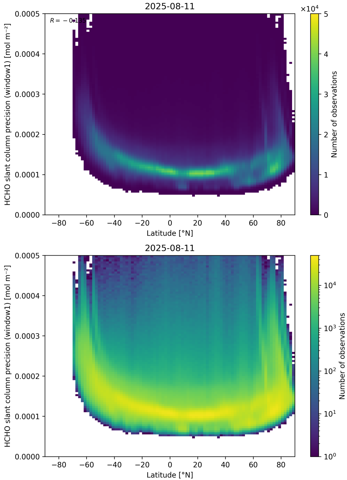
Figure 160: Scatter density plot of “Latitude” against “HCHO slant column precision (window1)” for 2025-08-10 to 2025-08-12.
