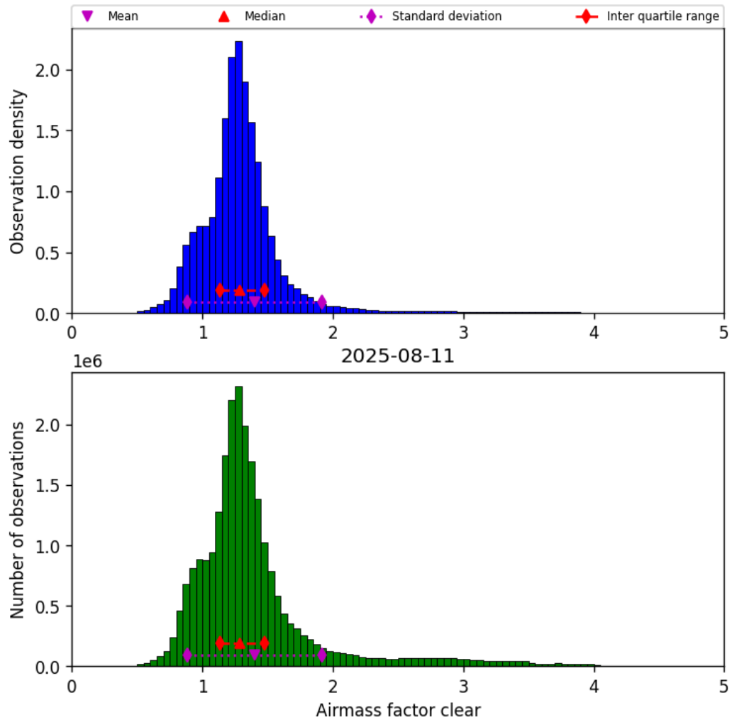
Figure 42: Histogram of “Airmass factor clear” for 2025-08-10 to 2025-08-12
