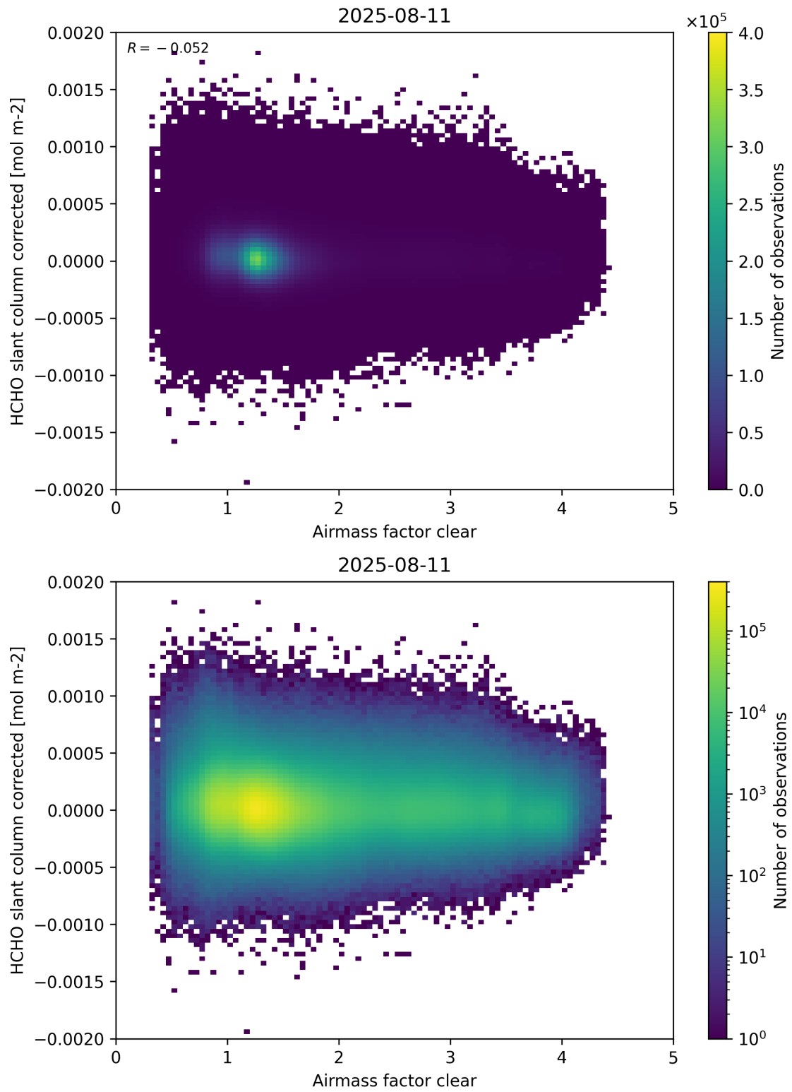
Figure 74: Scatter density plot of “Airmass factor clear” against “HCHO slant column corrected” for 2025-08-10 to 2025-08-12.
