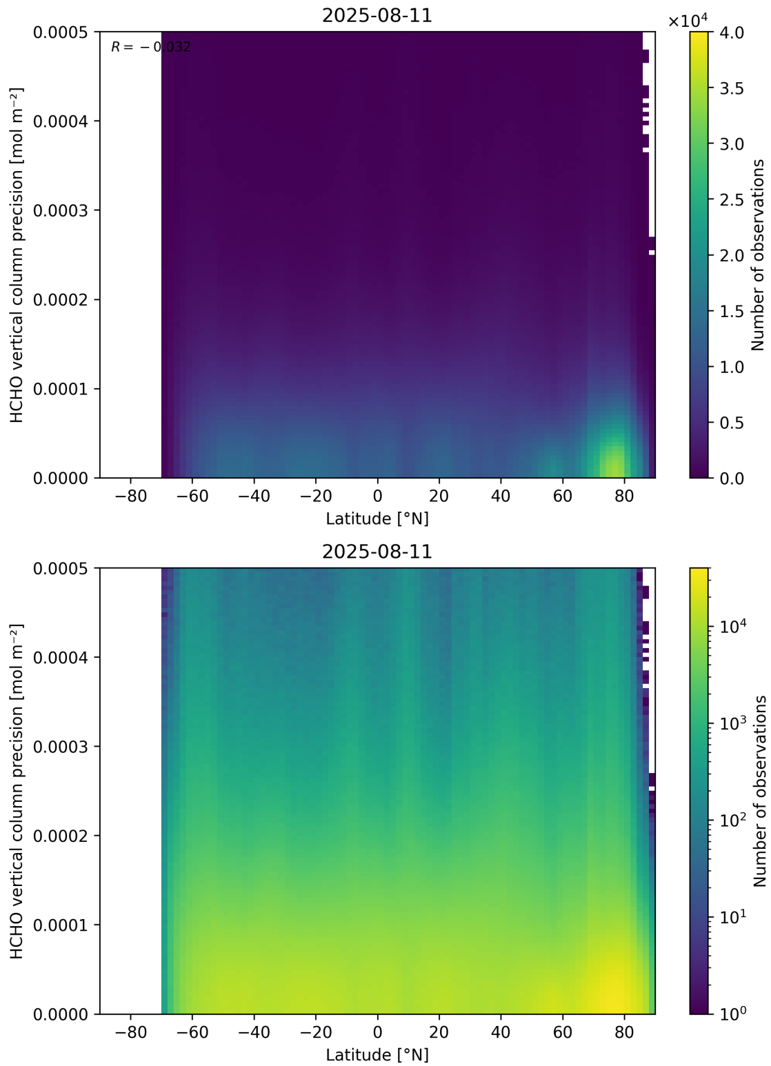
Figure 165: Scatter density plot of “Latitude” against “HCHO vertical column precision” for 2025-08-10 to 2025-08-12.
