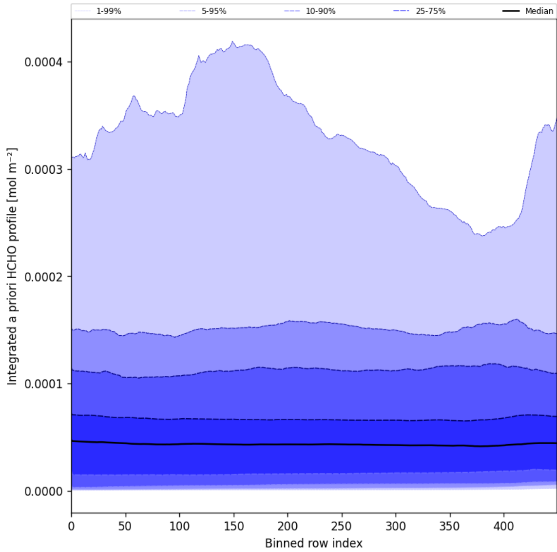
Figure 57: Along track statistics of “Integrated a priori HCHO profile” for 2025-08-10 to 2025-08-12
