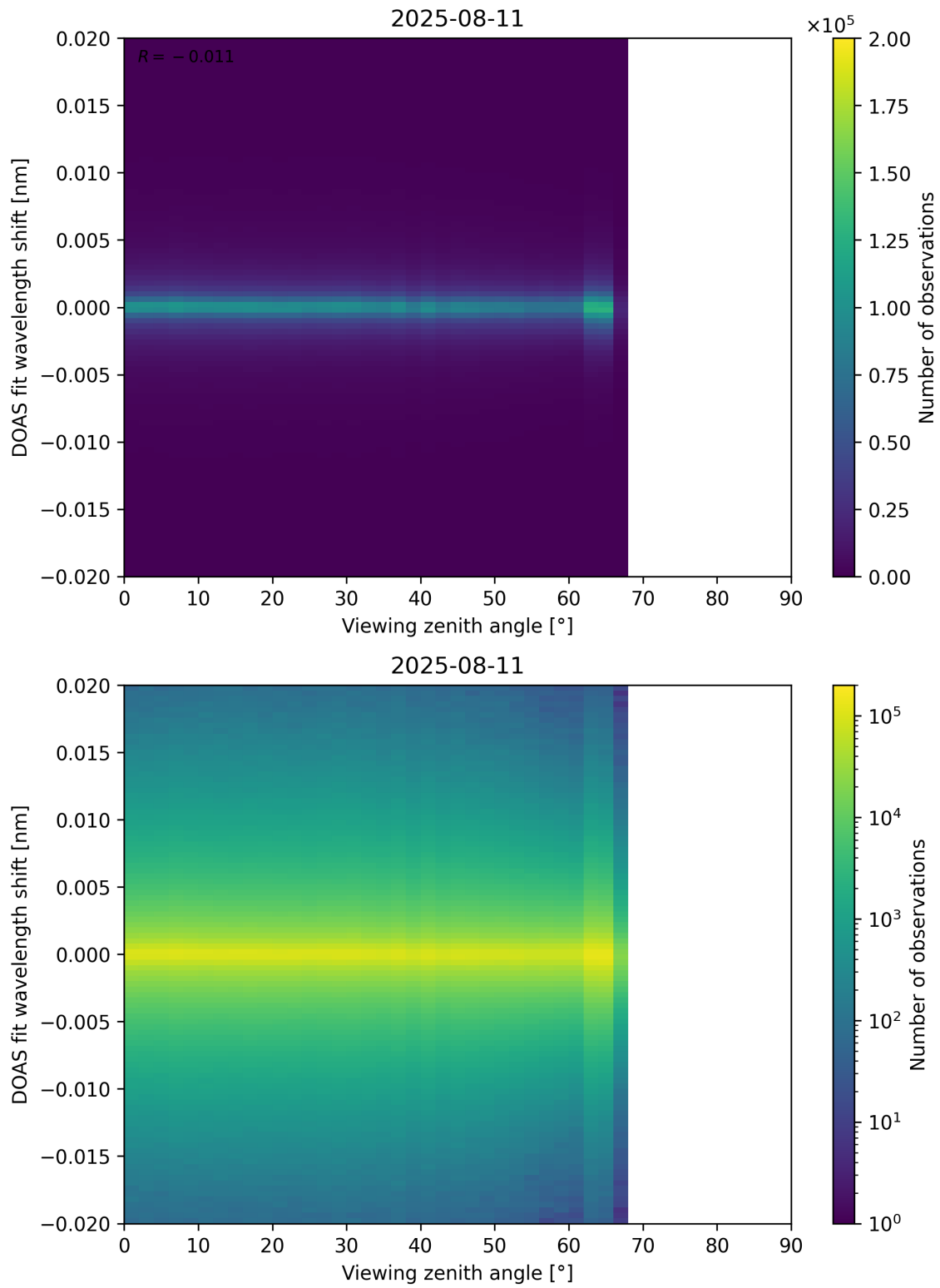
Figure 183: Scatter density plot of “Viewing zenith angle” against “DOAS fit wavelength shift” for 2025-08-10 to 2025-08-12.
