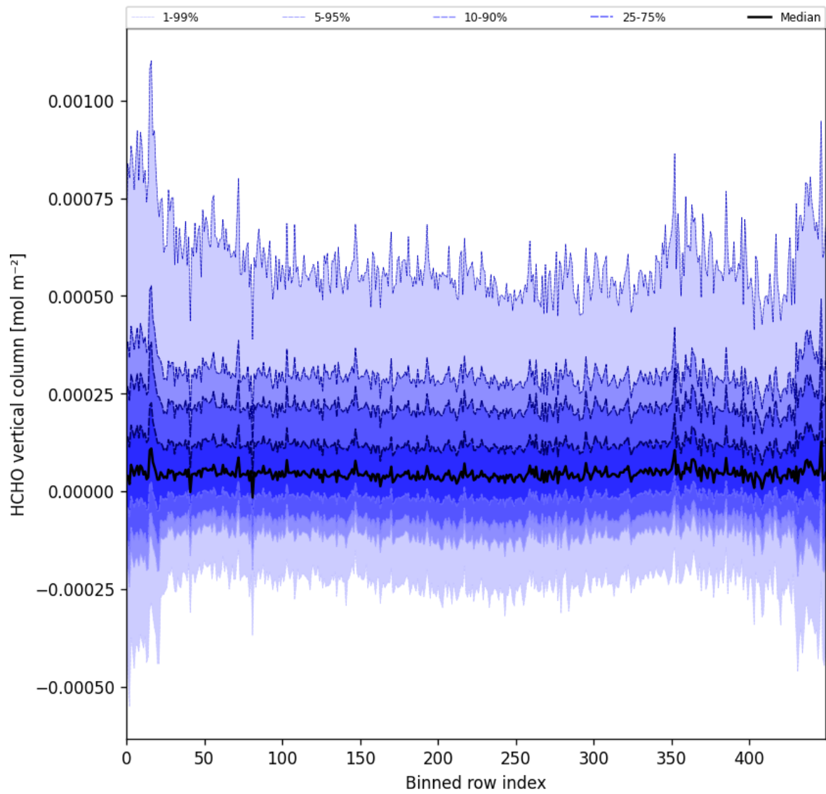
Figure 49: Along track statistics of “HCHO vertical column” for 2025-08-10 to 2025-08-12
