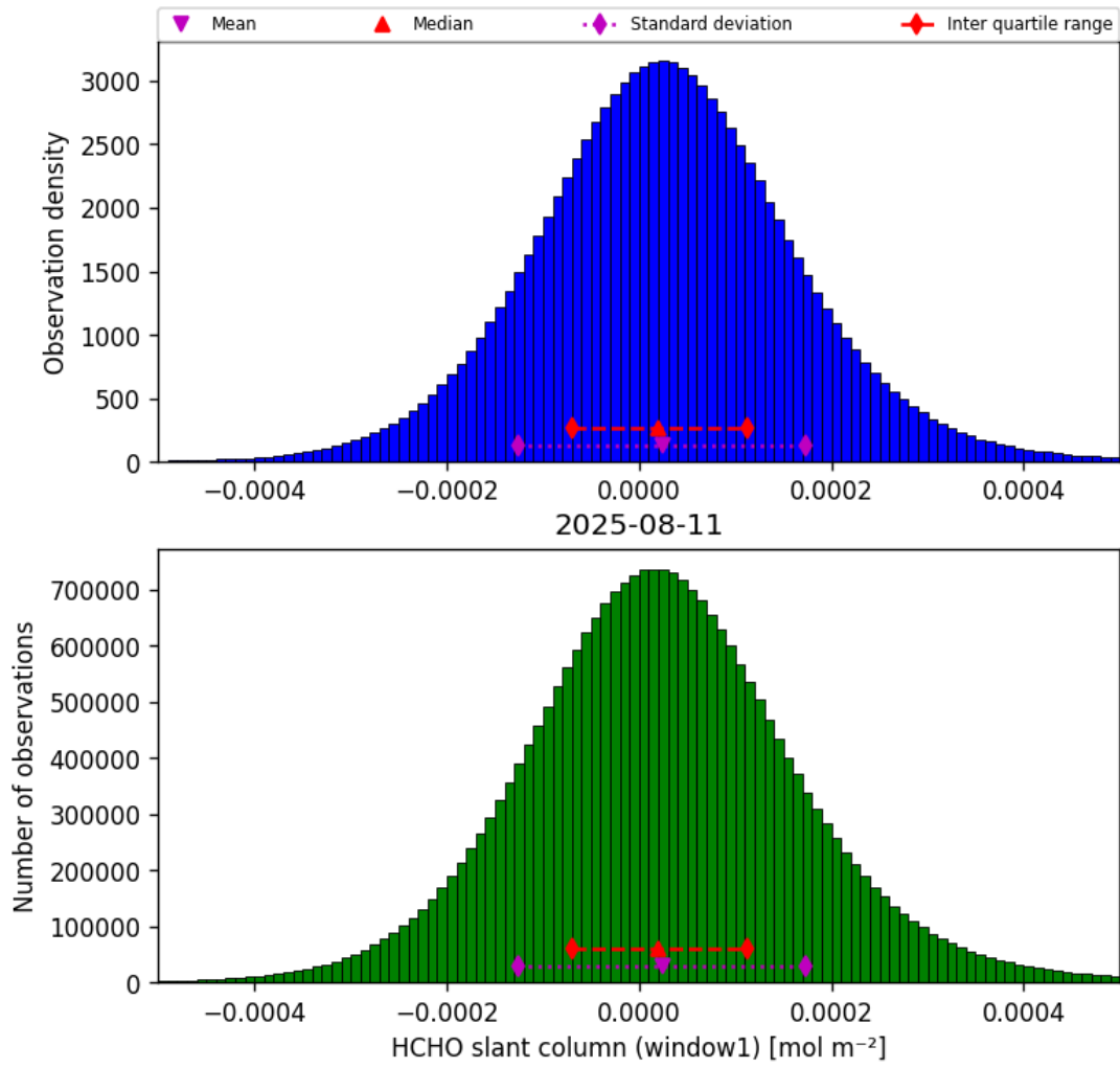
Figure 38: Histogram of “HCHO slant column (window1)” for 2025-08-10 to 2025-08-12
