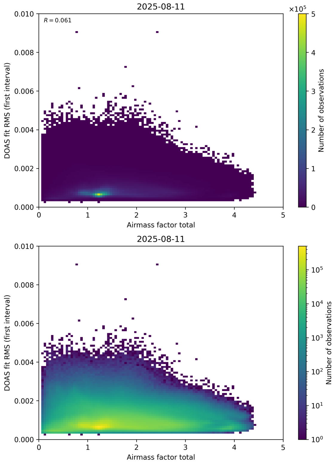
Figure 97: Scatter density plot of “Airmass factor total” against “DOAS fit RMS (first interval)” for 2025-08-10 to 2025-08-12.
