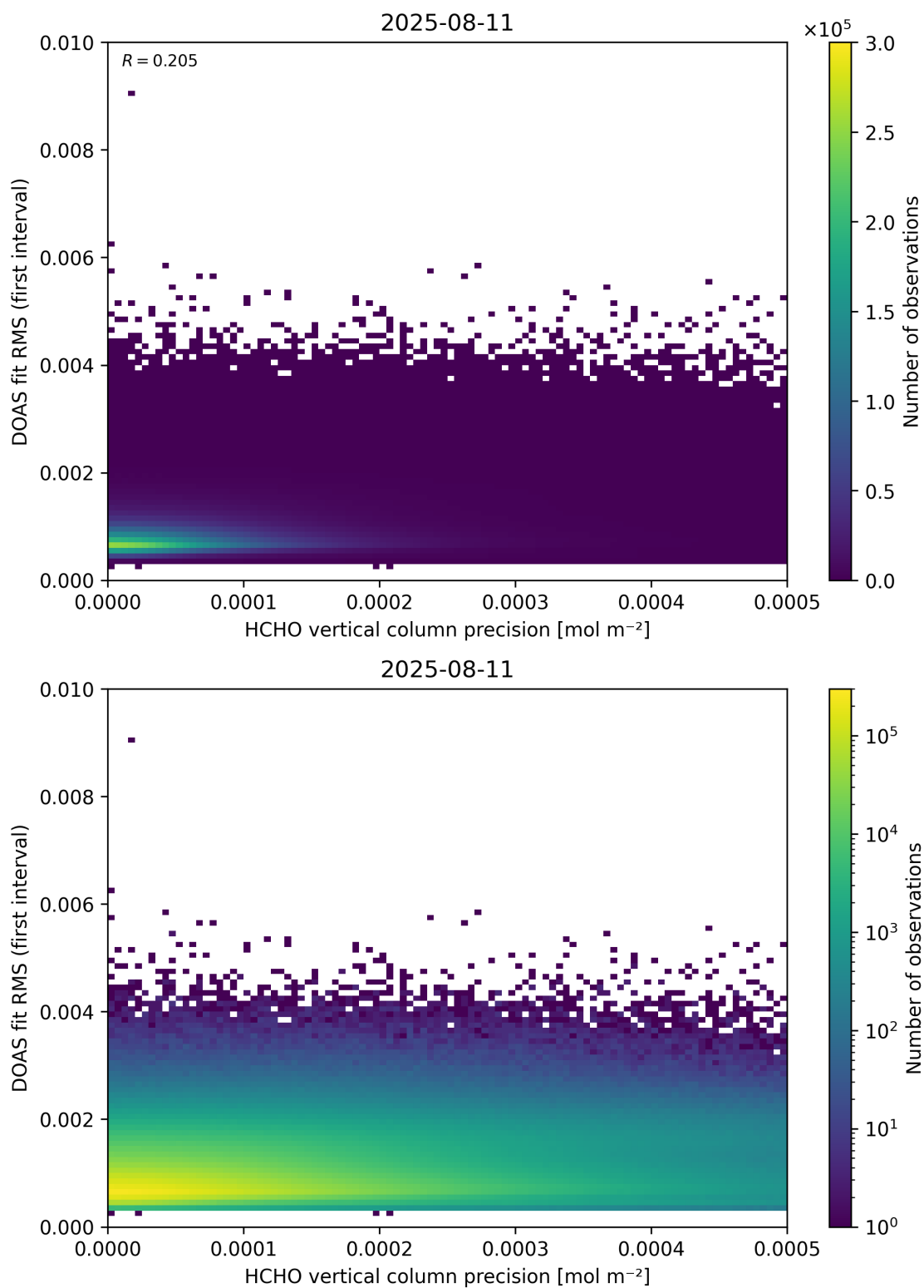
Figure 136: Scatter density plot of “HCHO vertical column precision” against “DOAS fit RMS (first interval)” for 2025-08-10 to 2025-08-12.
