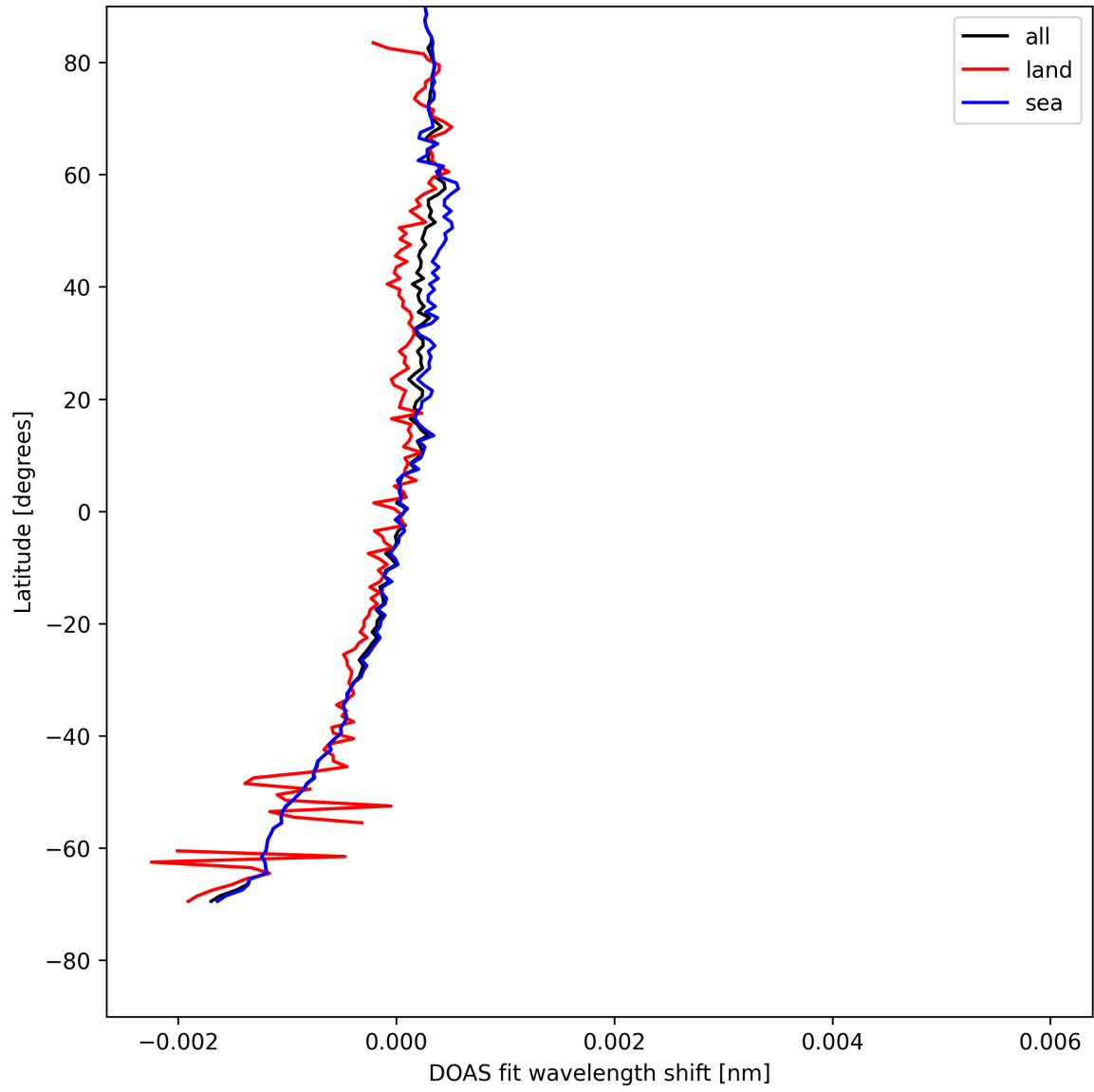
Figure 30: Zonal average of "DOAS fit wavelength shift" for 2025-08-10 to 2025-08-12.
