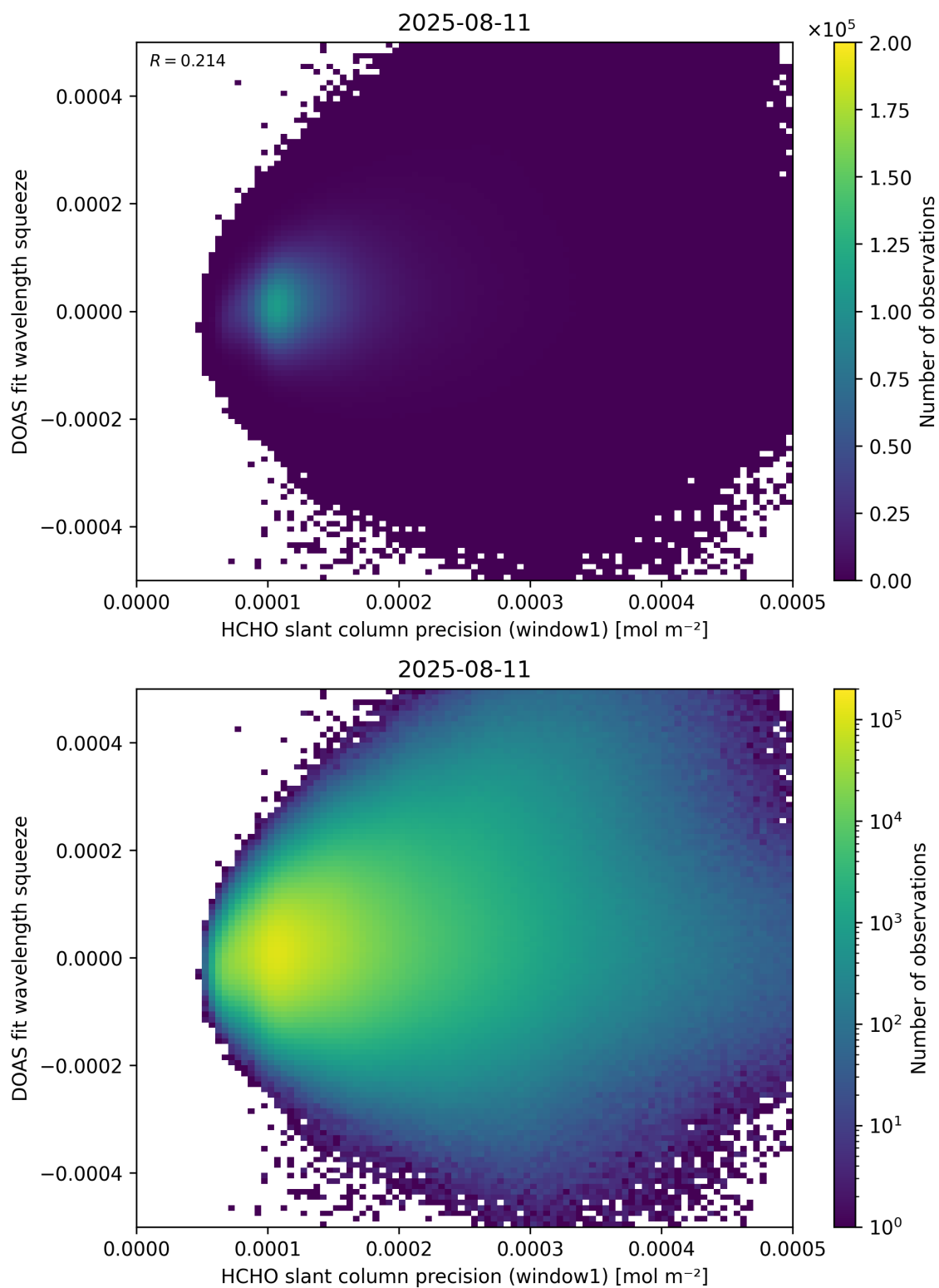
Figure 90: Scatter density plot of “HCHO slant column precision (window1)” against “DOAS fit wavelength squeeze” for 2025-08-10 to 2025-08-12.
