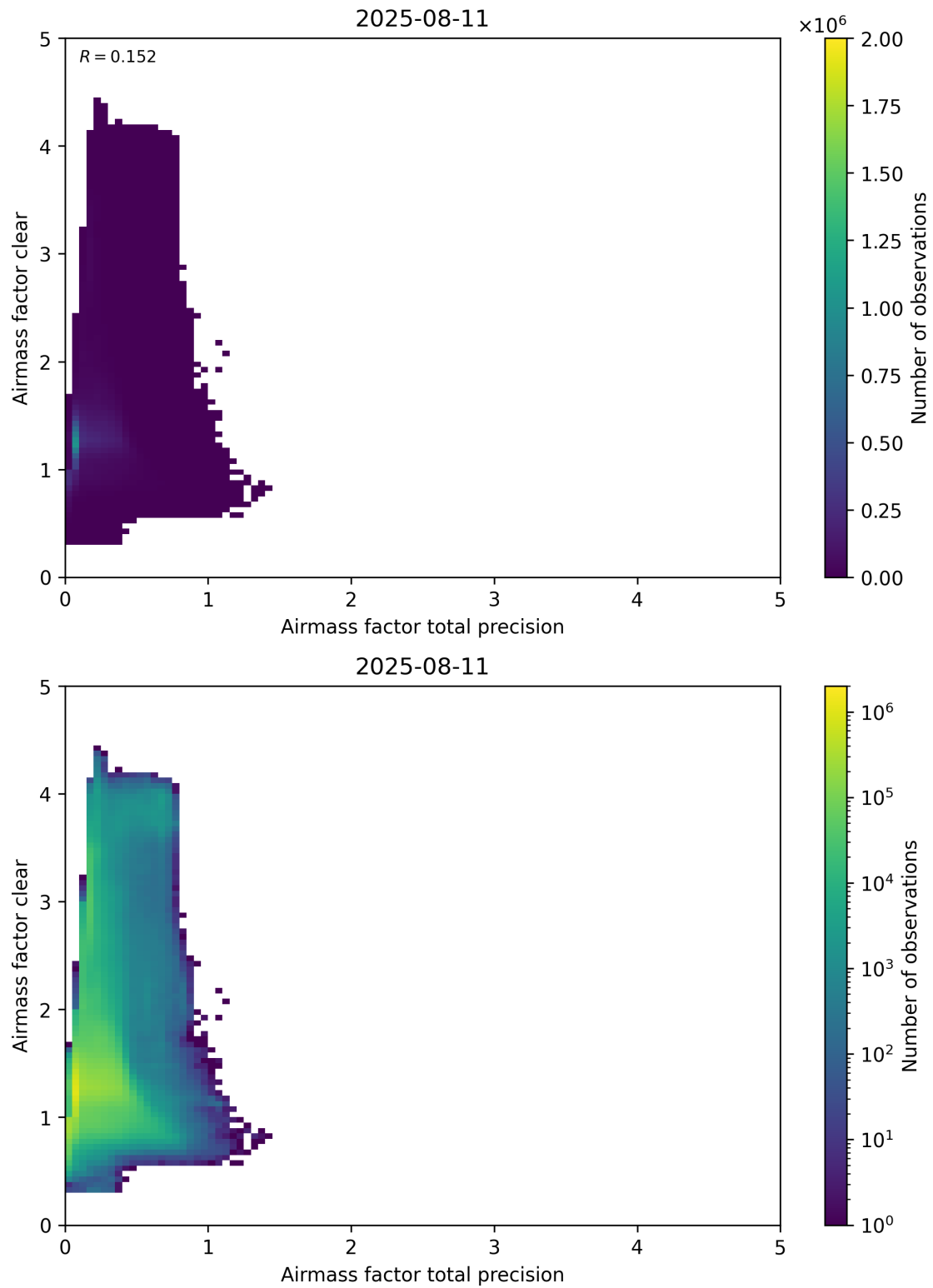
Figure 108: Scatter density plot of “Airmass factor total precision” against “Airmass factor clear” for 2025-08-10 to 2025-08-12.
