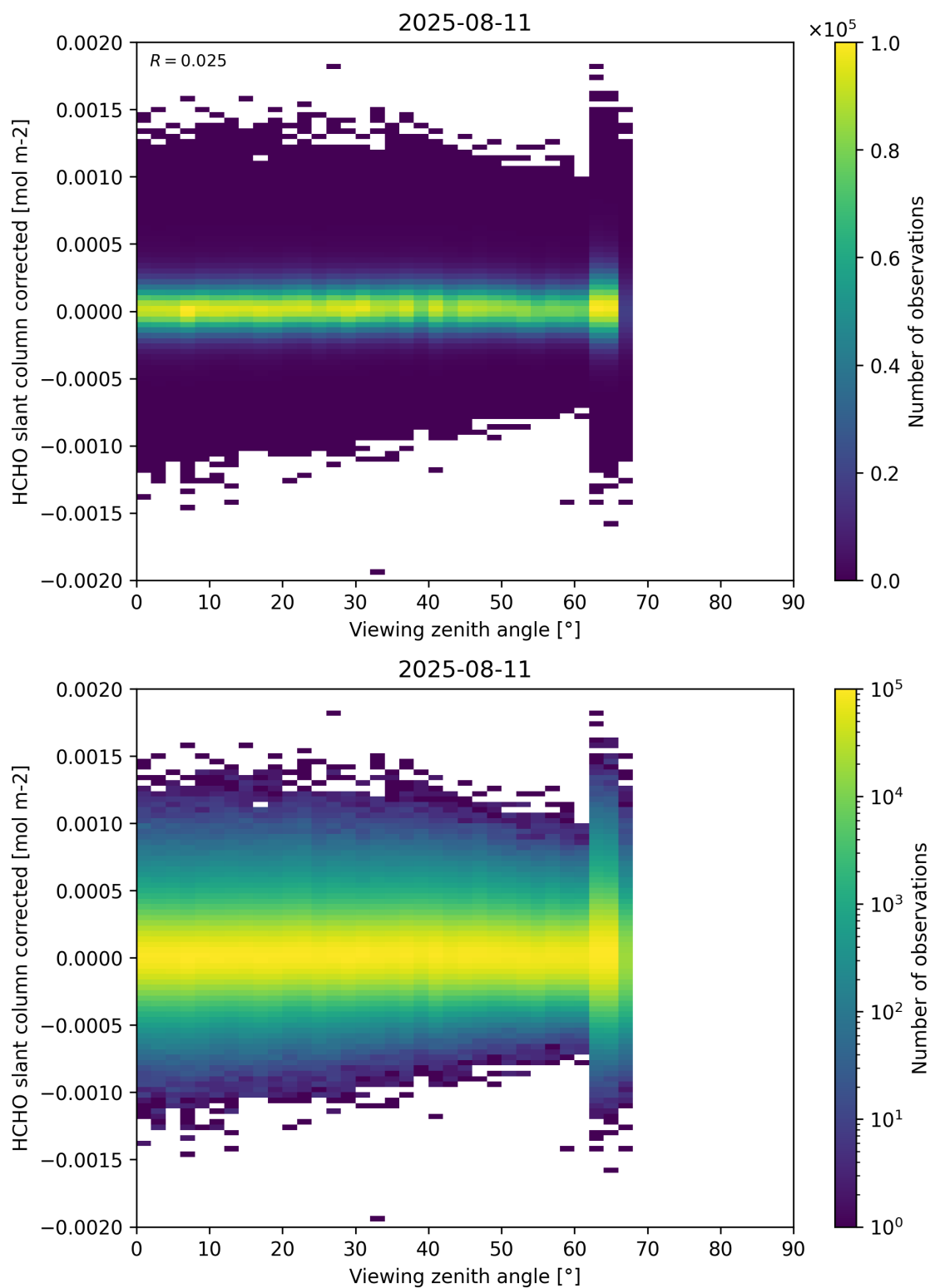
Figure 186: Scatter density plot of “Viewing zenith angle” against “HCHO slant column corrected” for 2025-08-10 to 2025-08-12.
