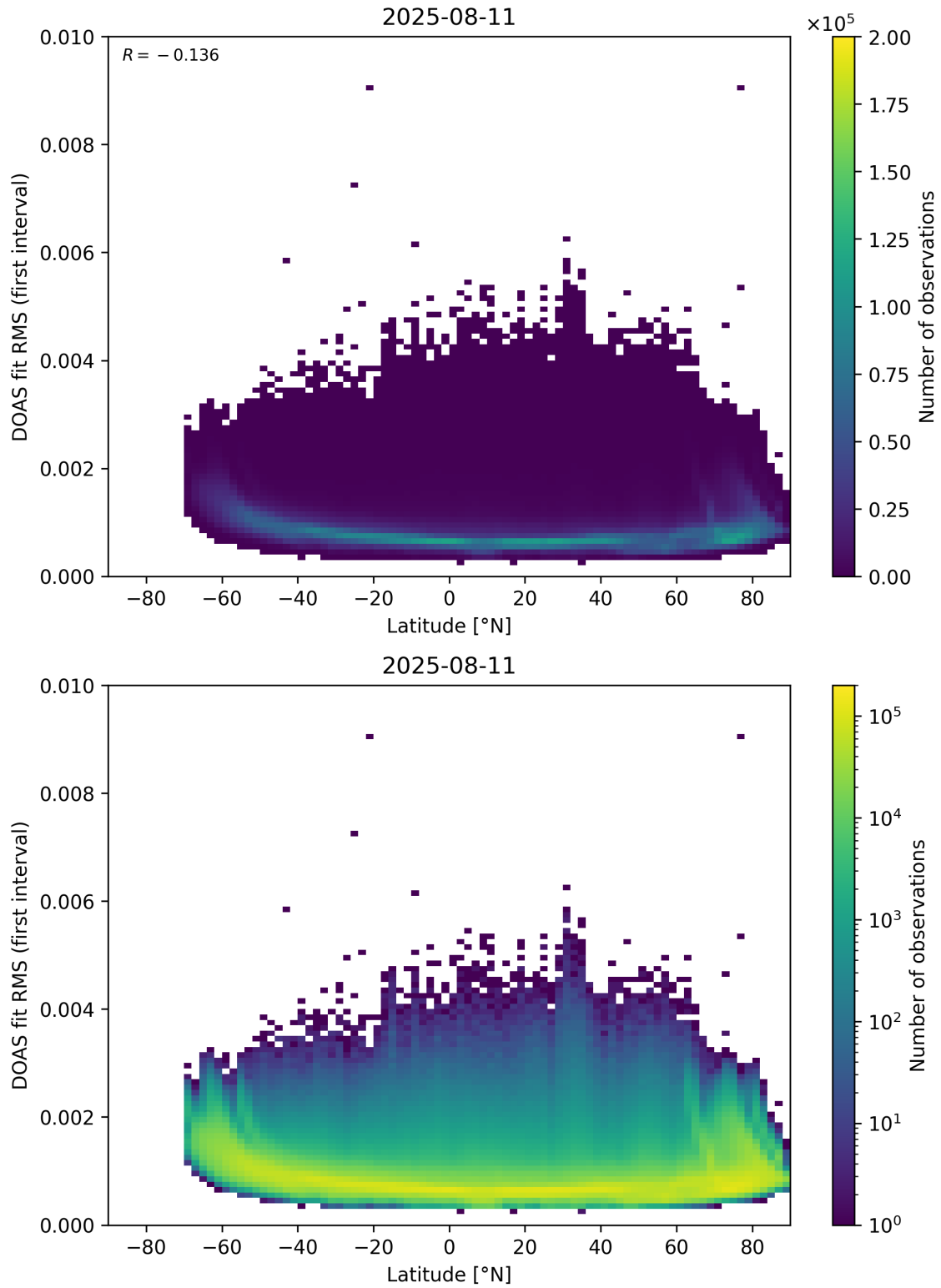
Figure 153: Scatter density plot of “Latitude” against “DOAS fit RMS (first interval)” for 2025-08-10 to 2025-08-12.
