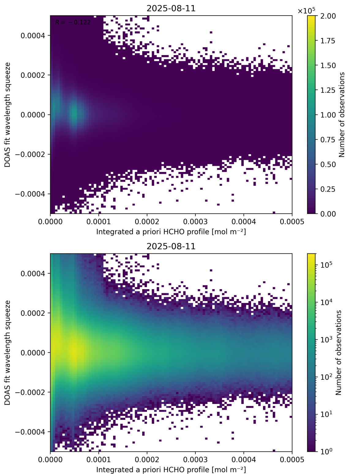
Figure 150: Scatter density plot of “Integrated a priori HCHO profile” against “DOAS fit wavelength squeeze” for 2025-08-10 to 2025-08-12.
