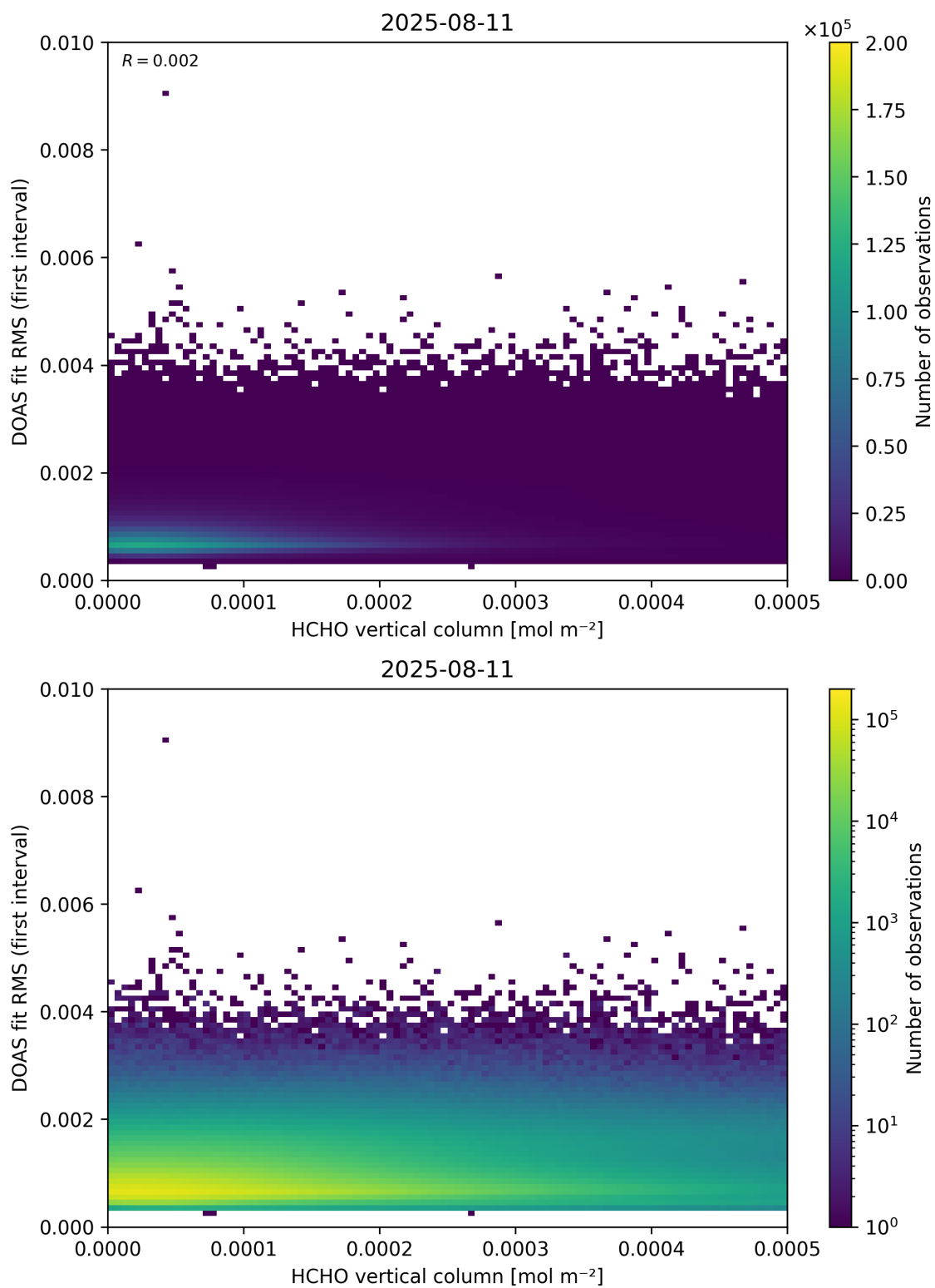
Figure 123: Scatter density plot of “HCHO vertical column” against “DOAS fit RMS (first interval)” for 2025-08-10 to 2025-08-12.
