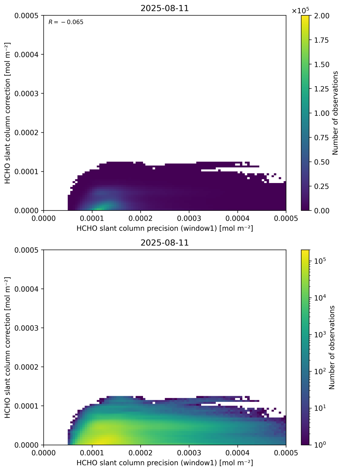
Figure 93: Scatter density plot of “HCHO slant column precision (window1)” against “HCHO slant column correction” for 2025-08-10 to 2025-08-12.
