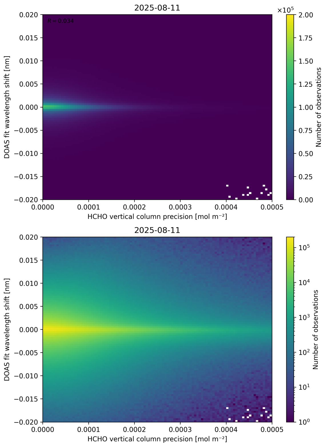
Figure 137: Scatter density plot of “HCHO vertical column precision” against “DOAS fit wavelength shift” for 2025-08-10 to 2025-08-12.
