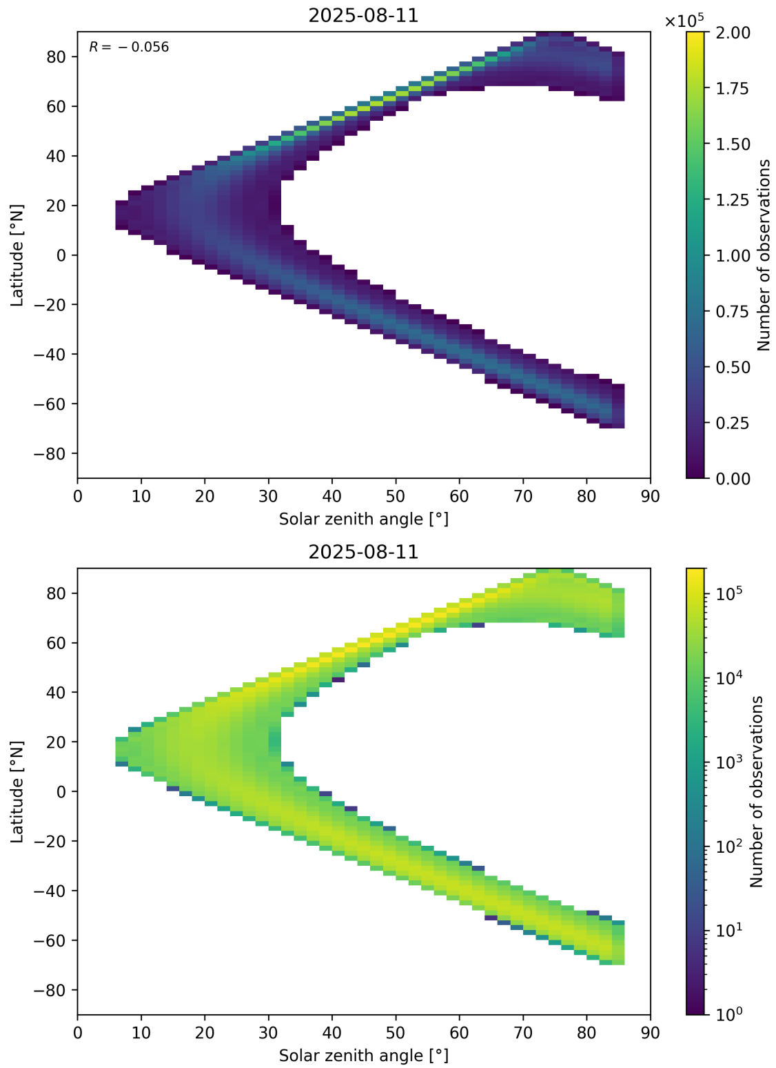
Figure 181: Scatter density plot of “Solar zenith angle” against “Latitude” for 2025-08-10 to 2025-08-12.
