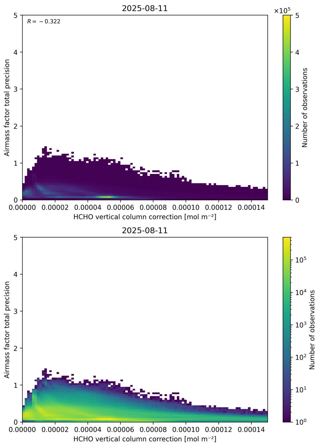
Figure 121: Scatter density plot of “HCHO vertical column correction” against “Airmass factor total precision” for 2025-08-10 to 2025-08-12.
