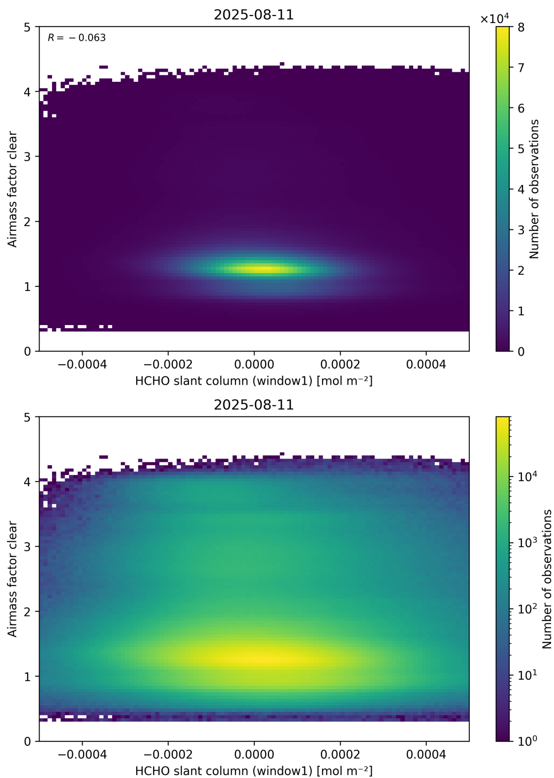
Figure 81: Scatter density plot of “HCHO slant column (window1)” against “Airmass factor clear” for 2025-08-10 to 2025-08-12.
