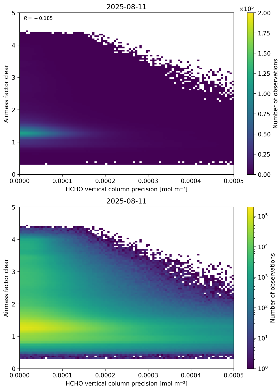
Figure 139: Scatter density plot of “HCHO vertical column precision” against “Airmass factor clear” for 2025-08-10 to 2025-08-12.
