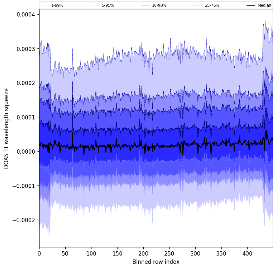
Figure 59: Along track statistics of “DOAS fit wavelength squeeze” for 2025-08-10 to 2025-08-12
