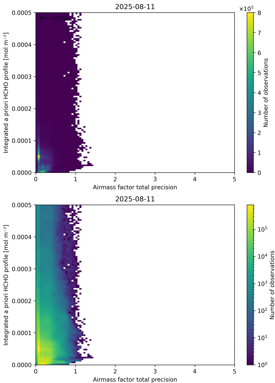
Figure 111: Scatter density plot of “Airmass factor total precision” against “Integrated a priori HCHO profile” for 2025-08-10 to 2025-08-12.
