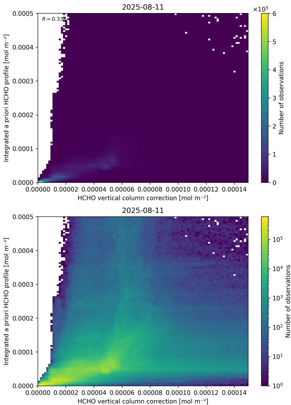
Figure 122: Scatter density plot of “HCHO vertical column correction” against “Integrated a priori HCHO profile” for 2025-08-10 to 2025-08-12.
