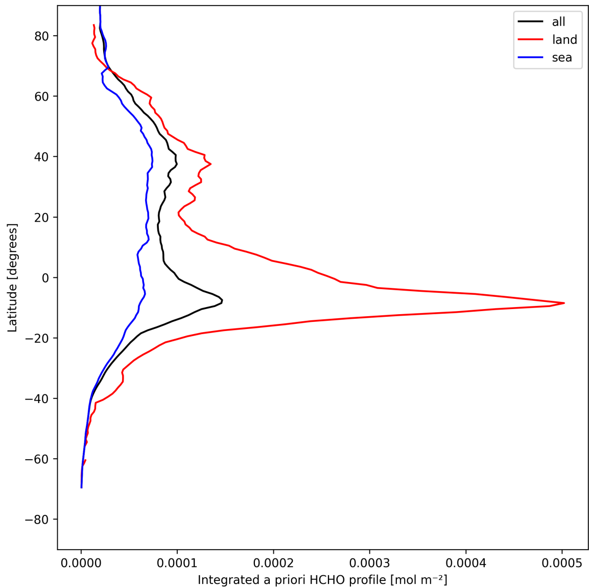
Figure 29: Zonal average of “Integrated a priori HCHO profile” for 2025-08-10 to 2025-08-12.
