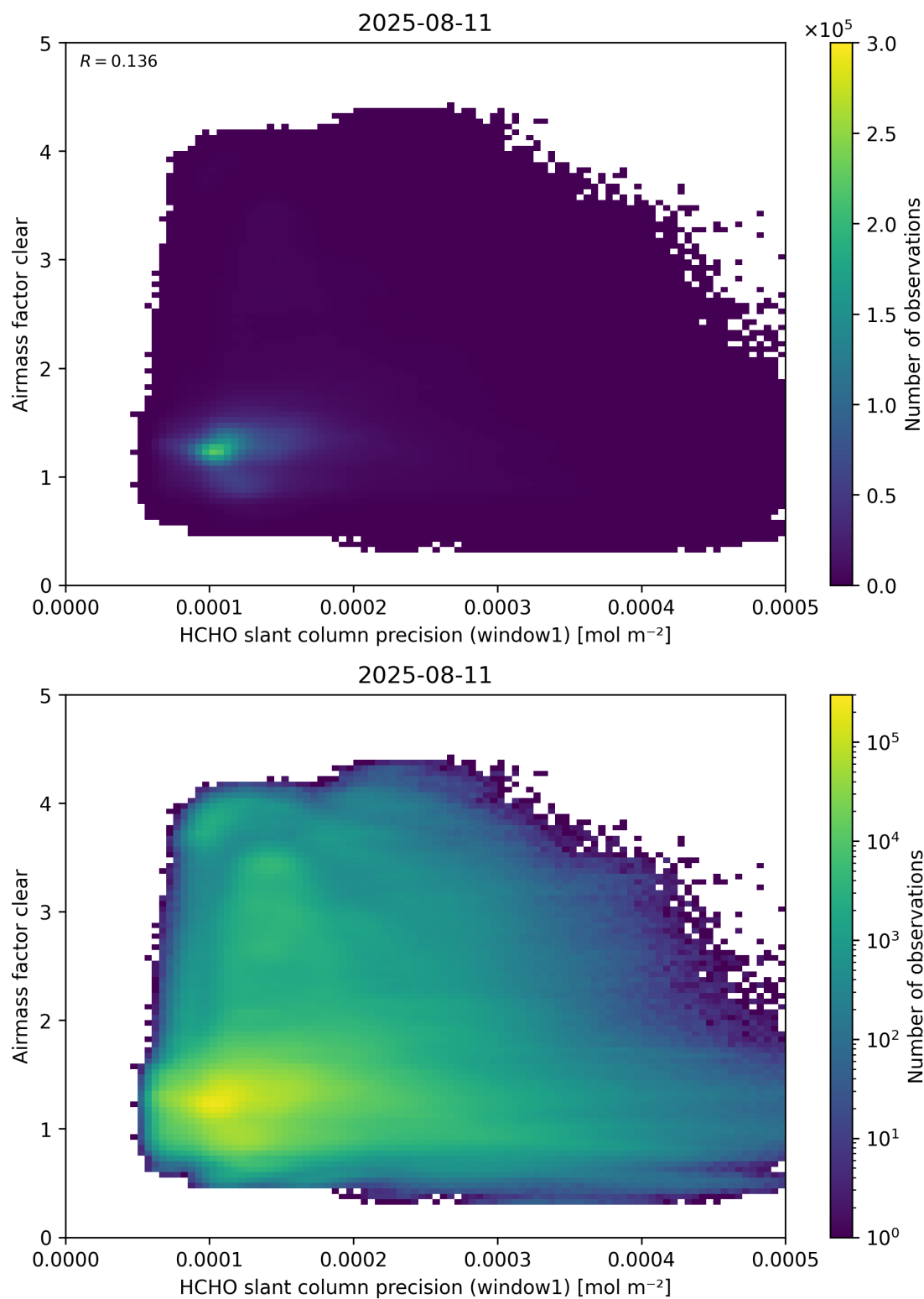
Figure 91: Scatter density plot of “HCHO slant column precision (window1)” against “Airmass factor clear” for 2025-08-10 to 2025-08-12.
