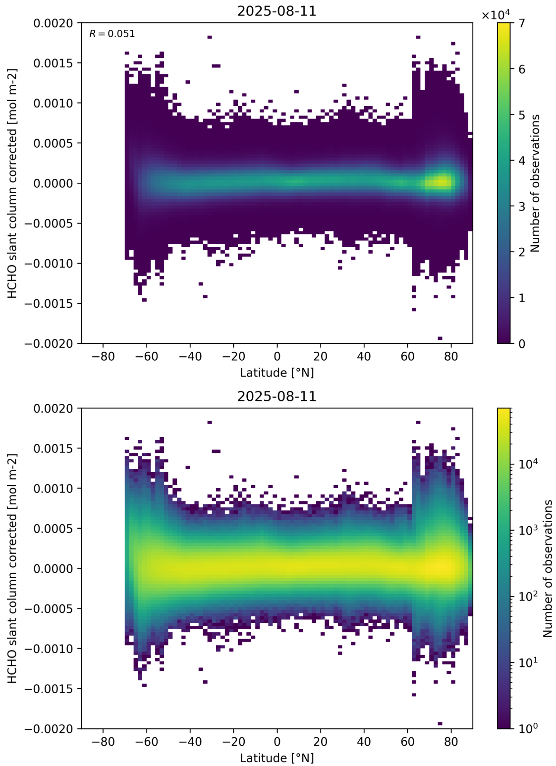
Figure 157: Scatter density plot of “Latitude” against “HCHO slant column corrected” for 2025-08-10 to 2025-08-12.
