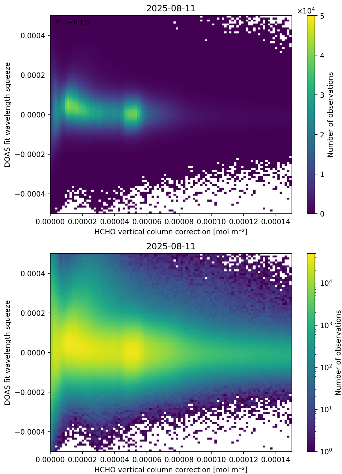
Figure 114: Scatter density plot of “HCHO vertical column correction” against “DOAS fit wavelength squeeze” for 2025-08-10 to 2025-08-12.
