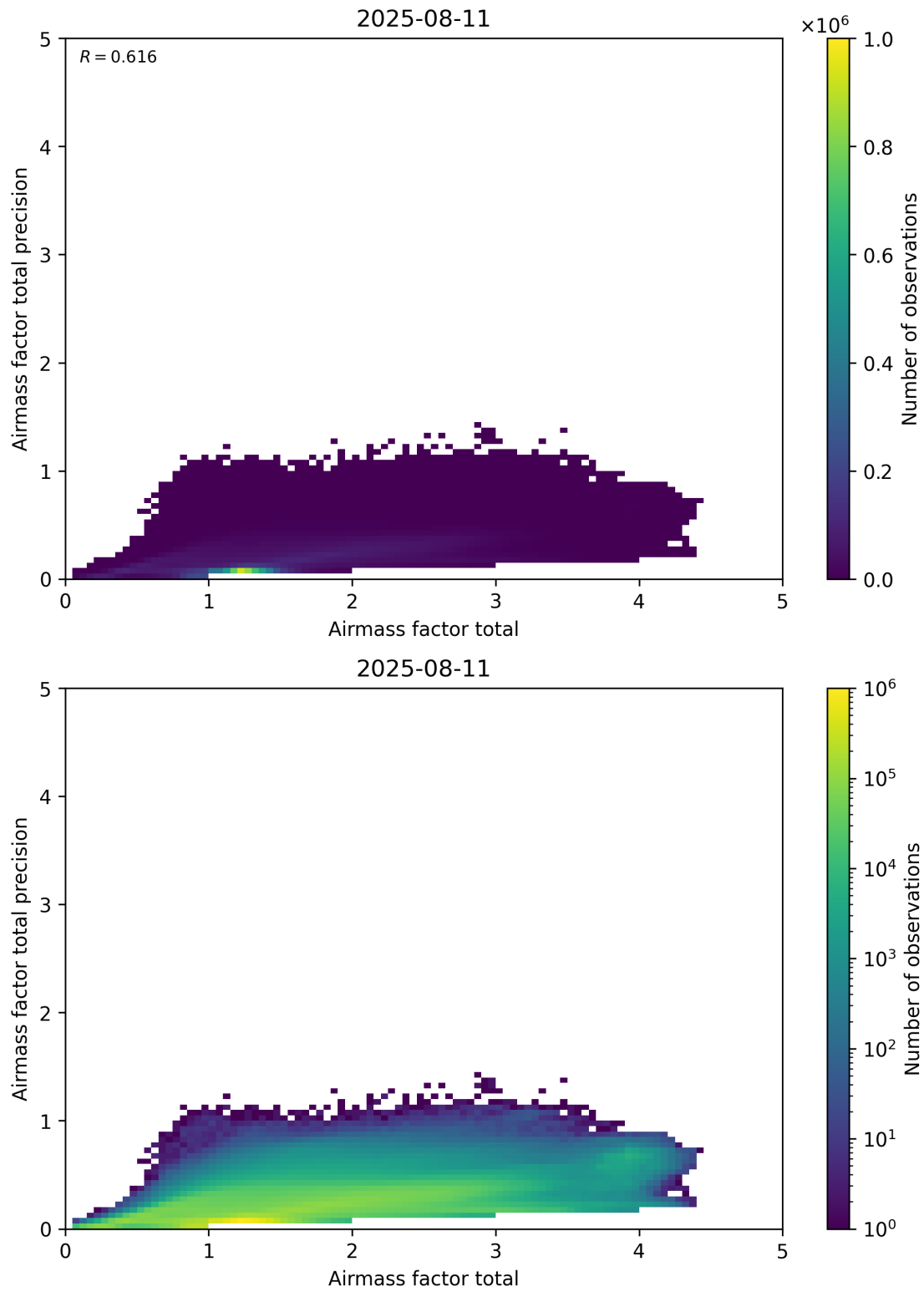
Figure 103: Scatter density plot of “Airmass factor total” against “Airmass factor total precision” for 2025-08-10 to 2025-08-12.
