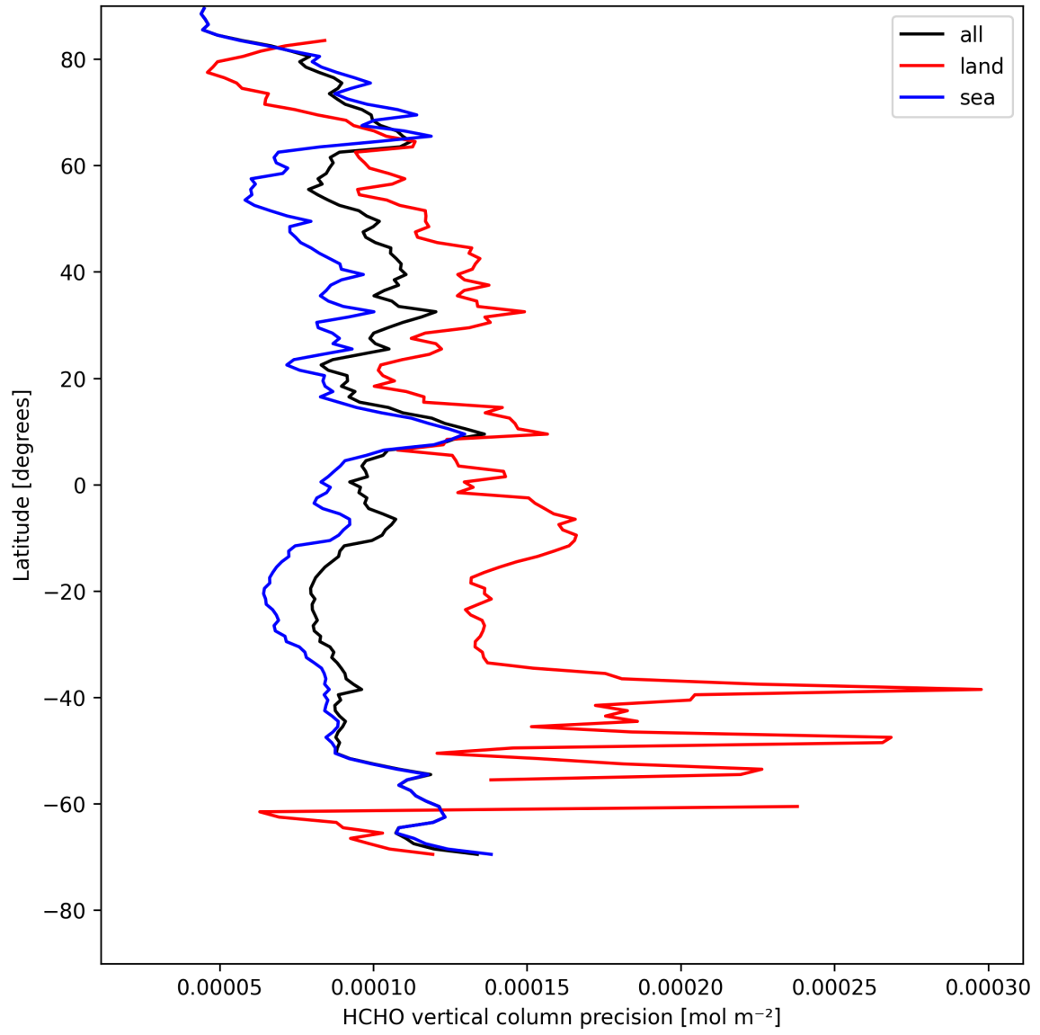
Figure 22: Zonal average of “HCHO vertical column precision” for 2025-08-10 to 2025-08-12.
