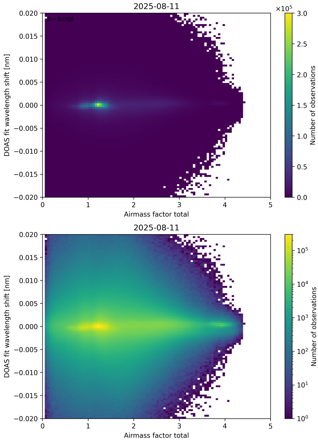
Figure 98: Scatter density plot of “Airmass factor total” against “DOAS fit wavelength shift” for 2025-08-10 to 2025-08-12.
