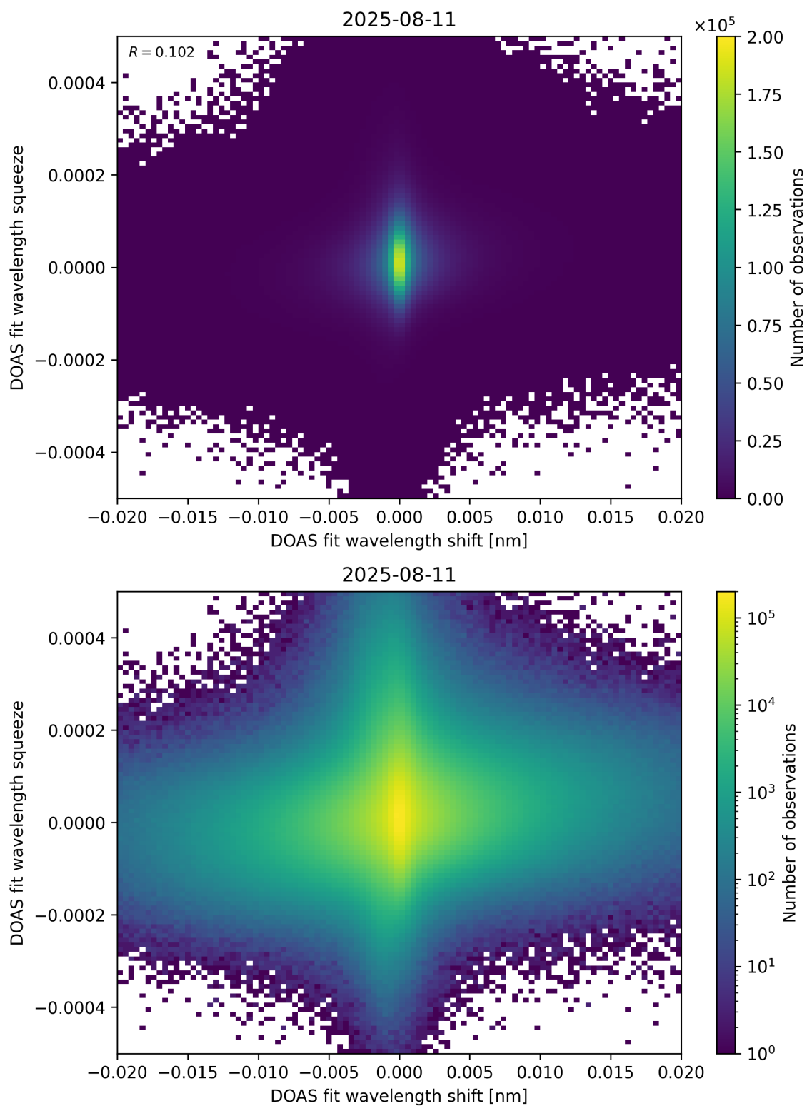
Figure 65: Scatter density plot of “DOAS fit wavelength shift” against “DOAS fit wavelength squeeze” for 2025-08-10 to 2025-08-12.
