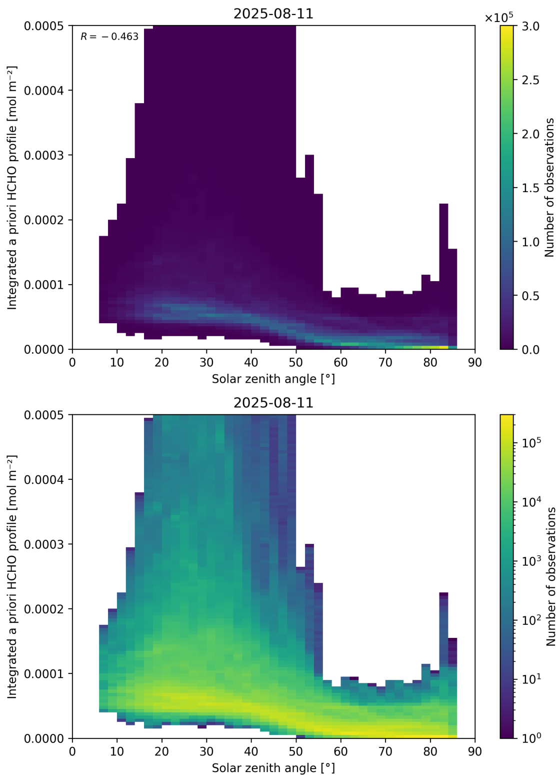
Figure 180: Scatter density plot of “Solar zenith angle” against “Integrated a priori HCHO profile” for 2025-08-10 to 2025-08-12.
