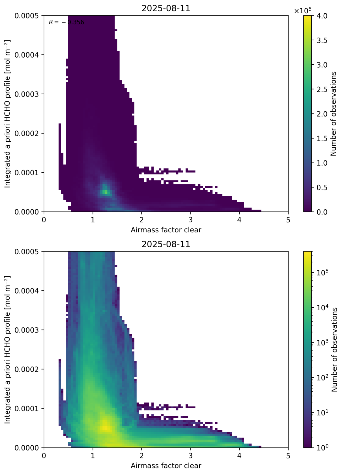
Figure 76: Scatter density plot of “Airmass factor clear” against “Integrated a priori HCHO profile” for 2025-08-10 to 2025-08-12.
