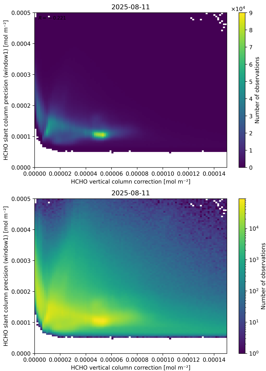
Figure 119: Scatter density plot of “HCHO vertical column correction” against “HCHO slant column precision (window1)” for 2025-08-10 to 2025-08-12.
