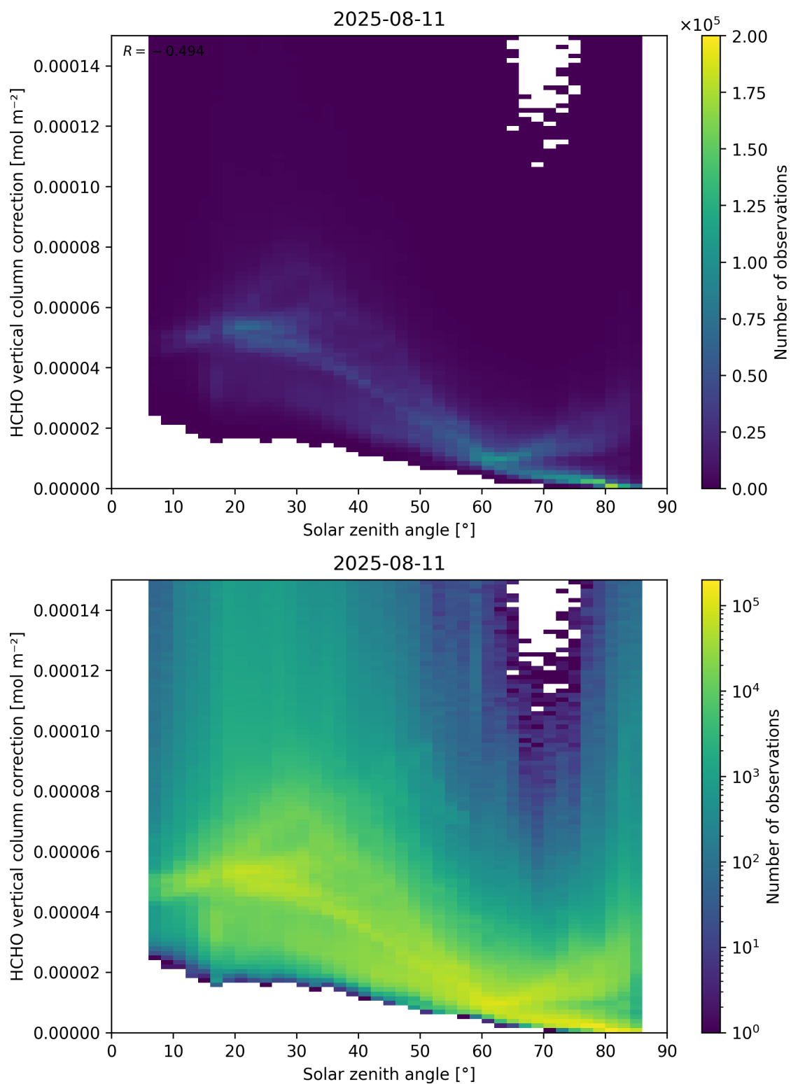
Figure 178: Scatter density plot of “Solar zenith angle” against “HCHO vertical column correction” for 2025-08-10 to 2025-08-12.
