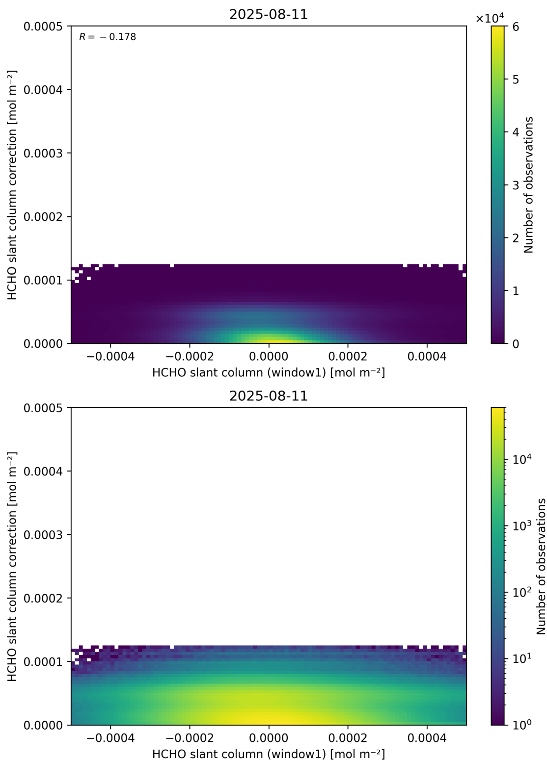
Figure 83: Scatter density plot of “HCHO slant column (window1)” against “HCHO slant column correction” for 2025-08-10 to 2025-08-12.
