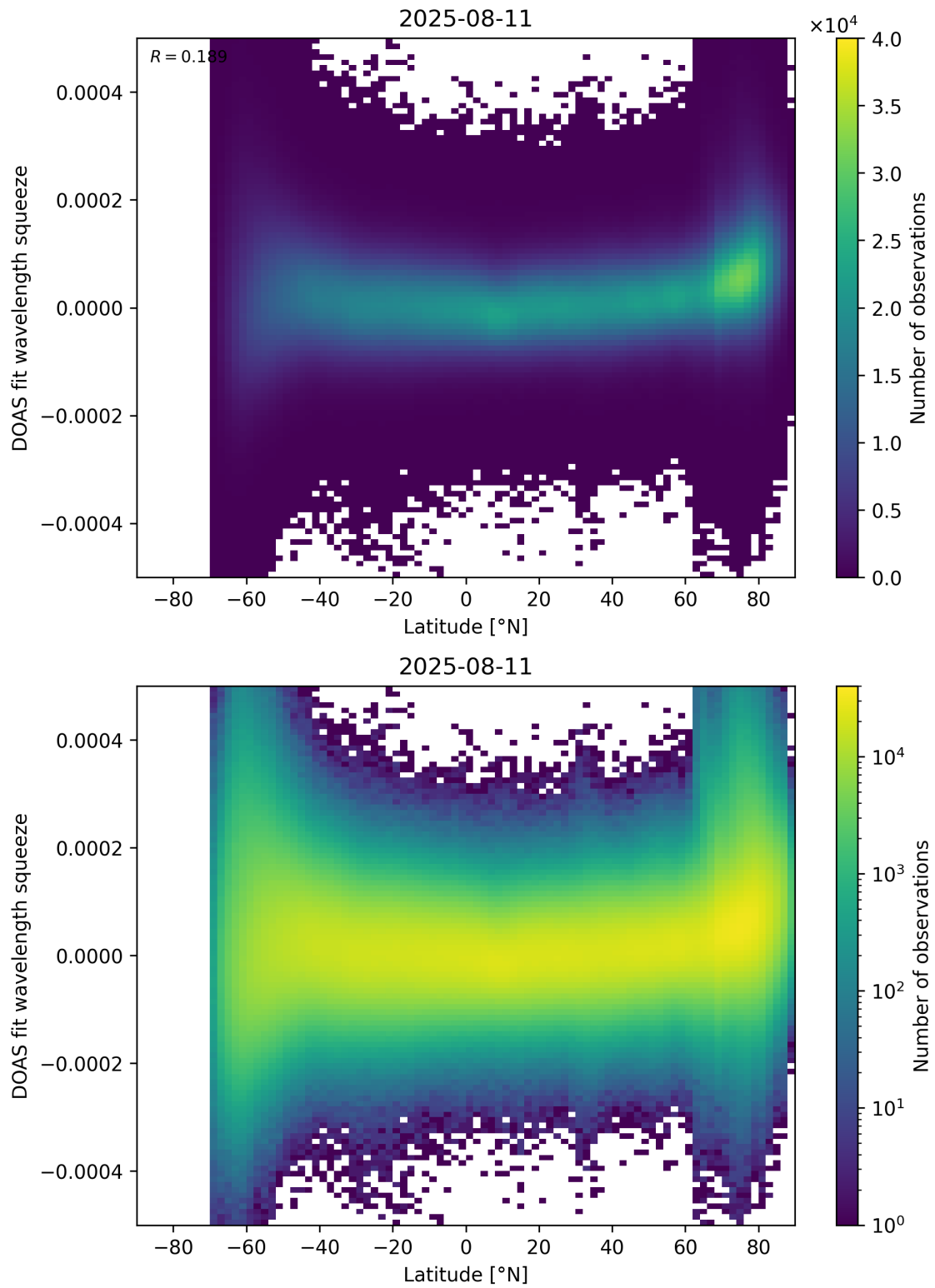
Figure 155: Scatter density plot of “Latitude” against “DOAS fit wavelength squeeze” for 2025-08-10 to 2025-08-12.
