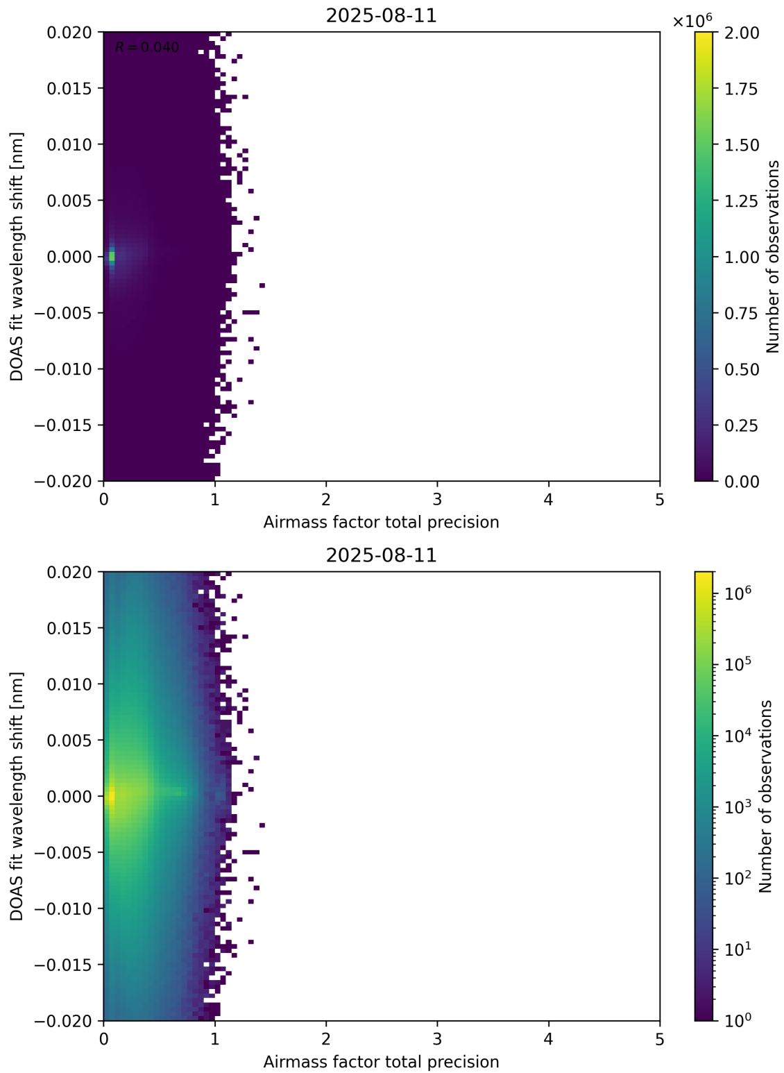
Figure 106: Scatter density plot of “Airmass factor total precision” against “DOAS fit wavelength shift” for 2025-08-10 to 2025-08-12.
