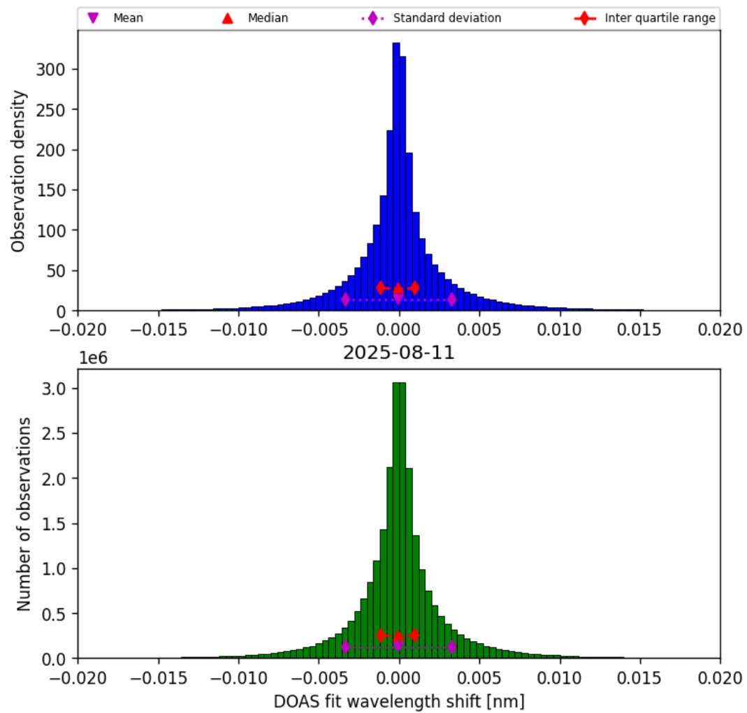
Figure 44: Histogram of “DOAS fit wavelength shift” for 2025-08-10 to 2025-08-12
