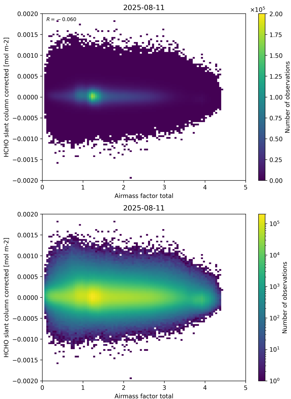
Figure 101: Scatter density plot of “Airmass factor total” against “HCHO slant column corrected” for 2025-08-10 to 2025-08-12.
