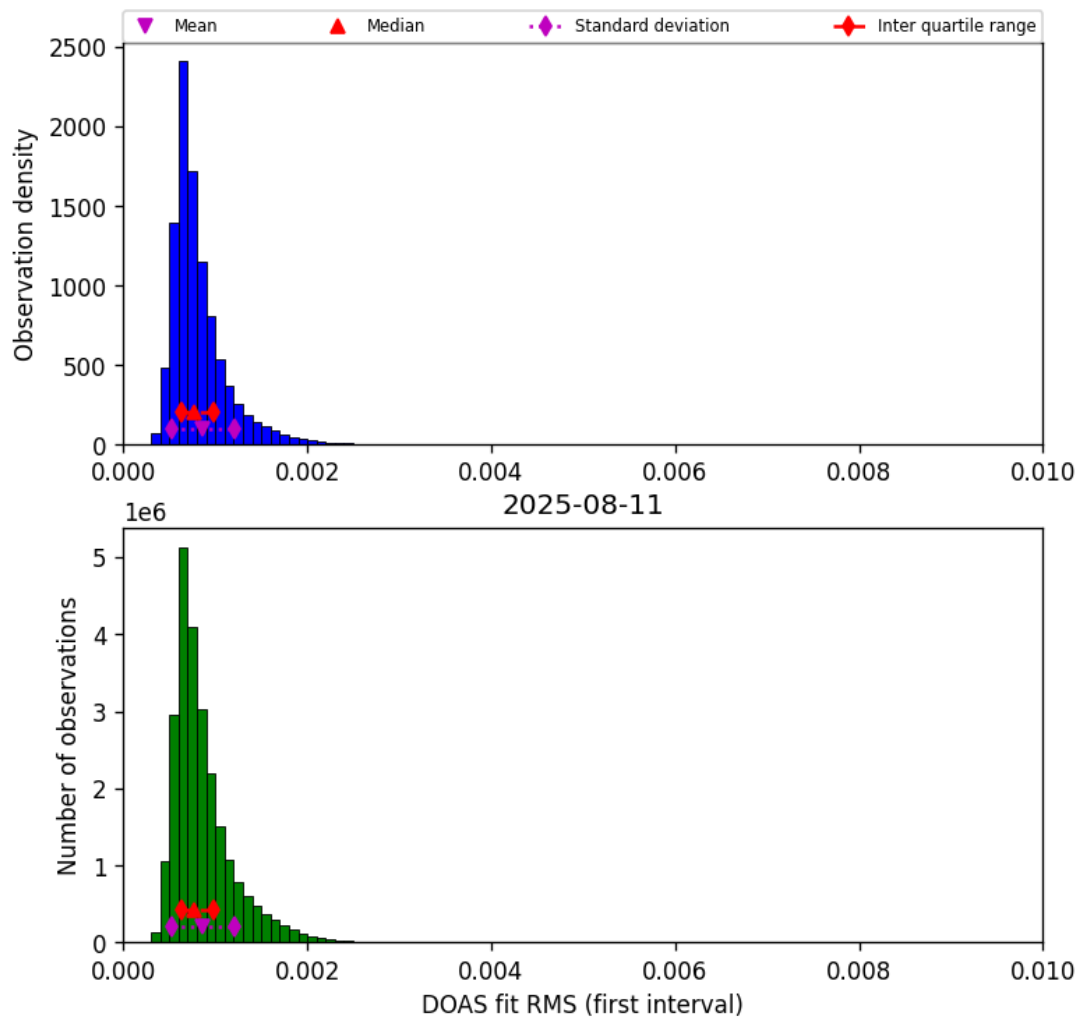
Figure 46: Histogram of “DOAS fit RMS (first interval)” for 2025-08-10 to 2025-08-12
