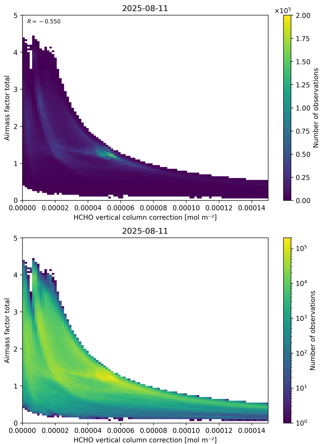
Figure 120: Scatter density plot of “HCHO vertical column correction” against “Airmass factor total” for 2025-08-10 to 2025-08-12.
