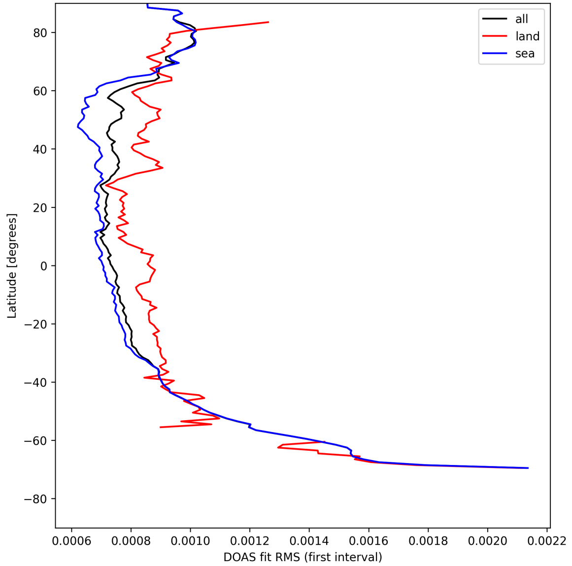
Figure 32: Zonal average of “DOAS fit RMS (first interval)” for 2025-08-10 to 2025-08-12.
