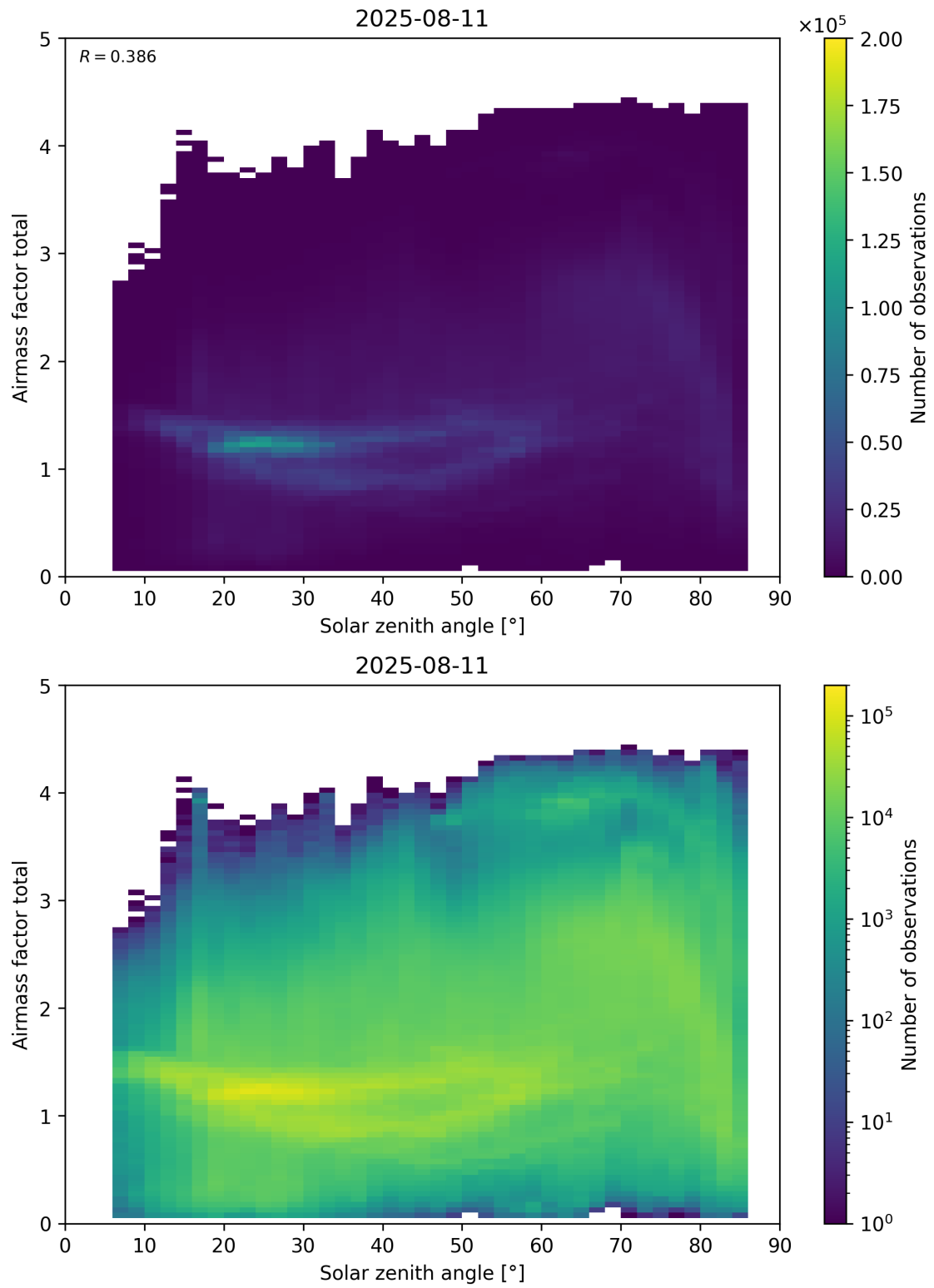
Figure 175: Scatter density plot of “Solar zenith angle” against “Airmass factor total” for 2025-08-10 to 2025-08-12.
