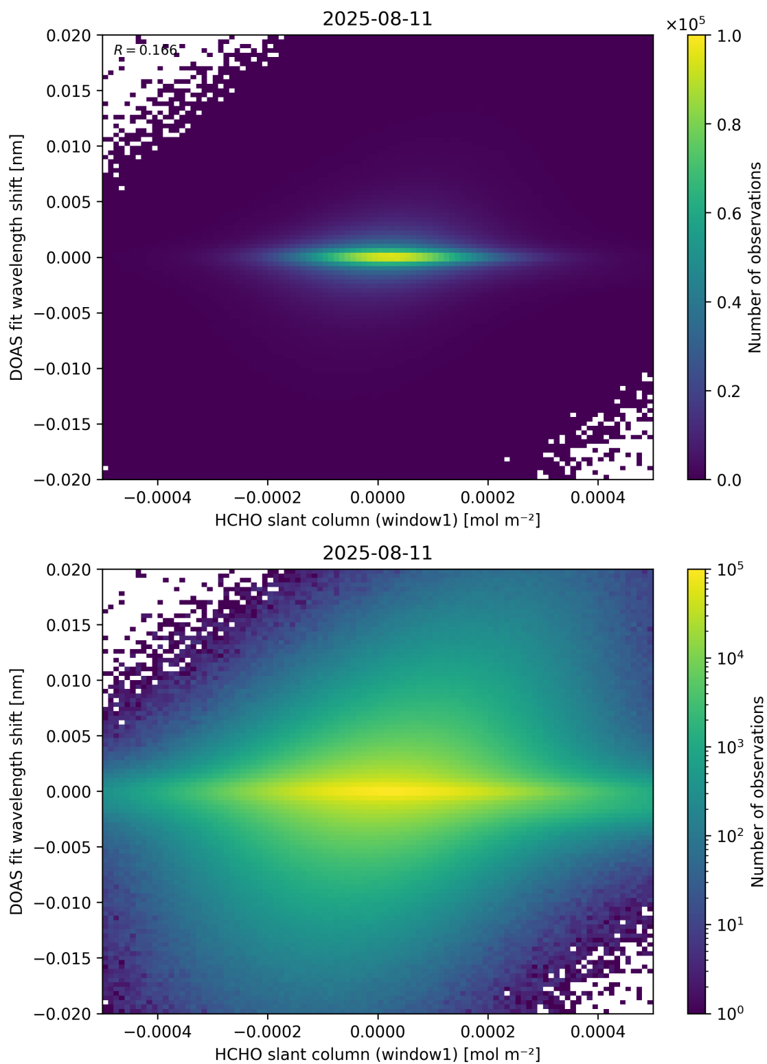
Figure 79: Scatter density plot of “HCHO slant column (window1)” against “DOAS fit wavelength shift” for 2025-08-10 to 2025-08-12.
