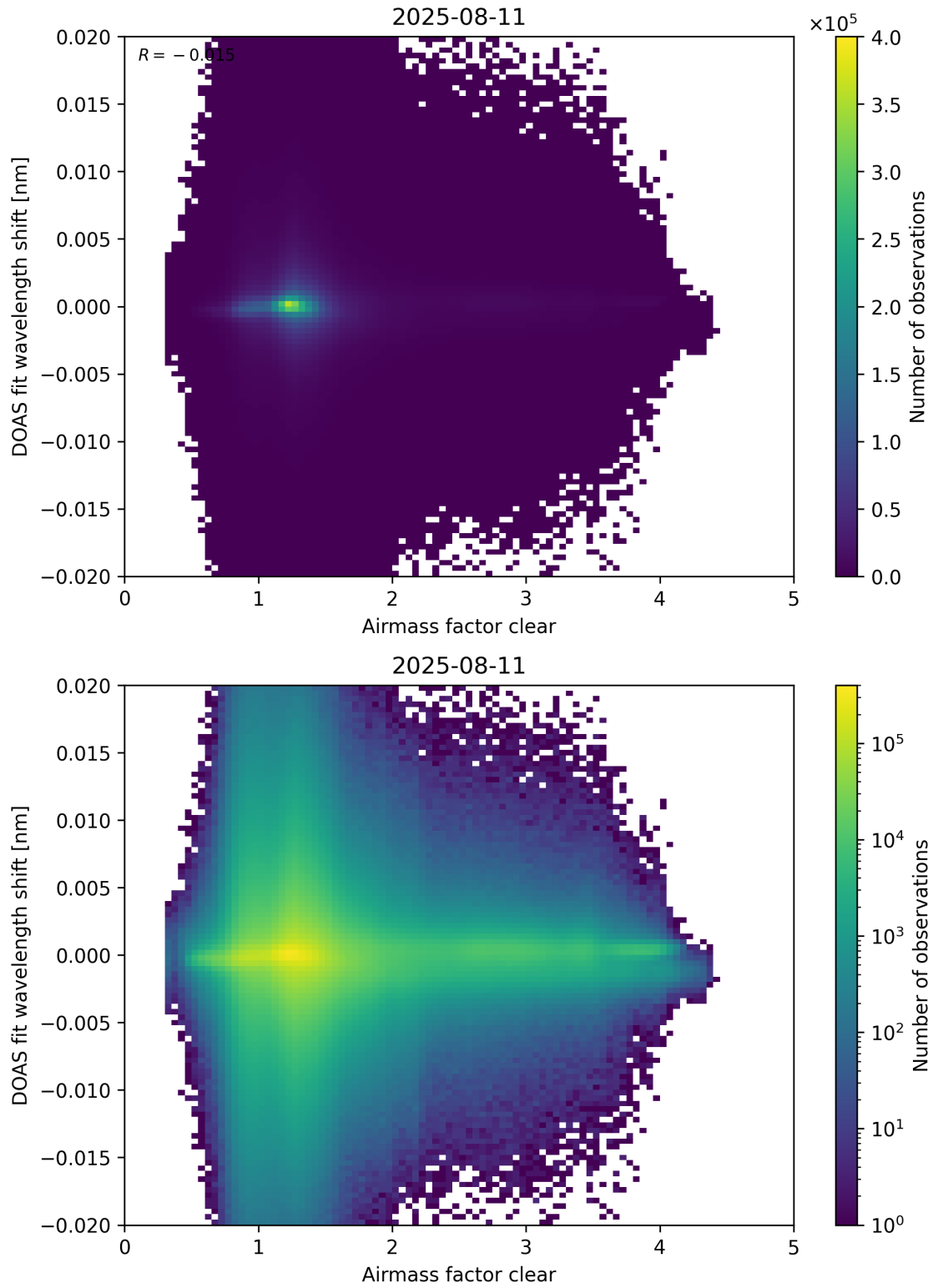
Figure 72: Scatter density plot of “Airmass factor clear” against “DOAS fit wavelength shift” for 2025-08-10 to 2025-08-12.
