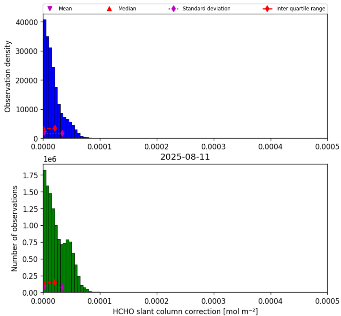
Figure 47: Histogram of “HCHO slant column correction” for 2025-08-10 to 2025-08-12
