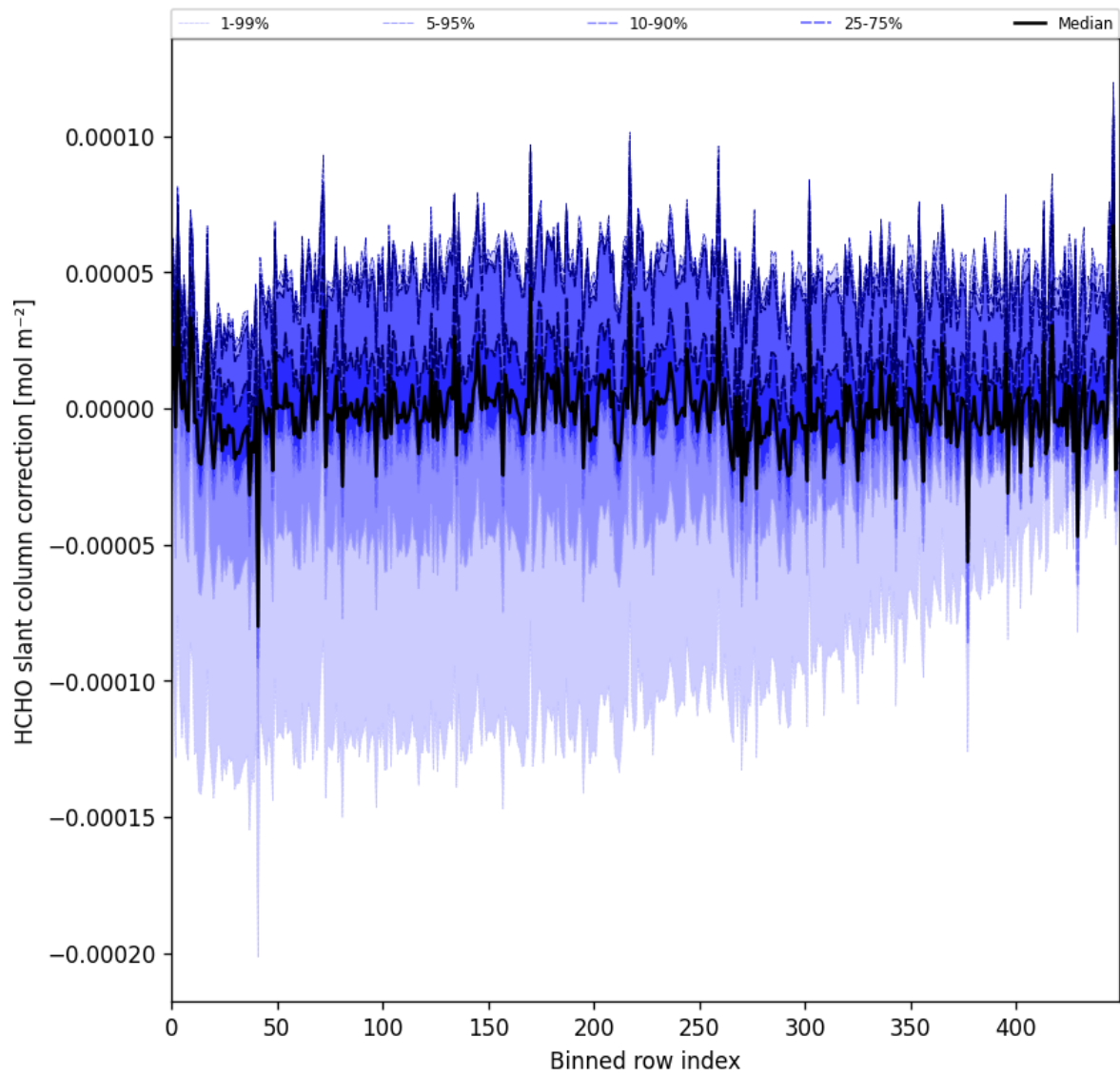
Figure 61: Along track statistics of “HCHO slant column correction” for 2025-08-10 to 2025-08-12
