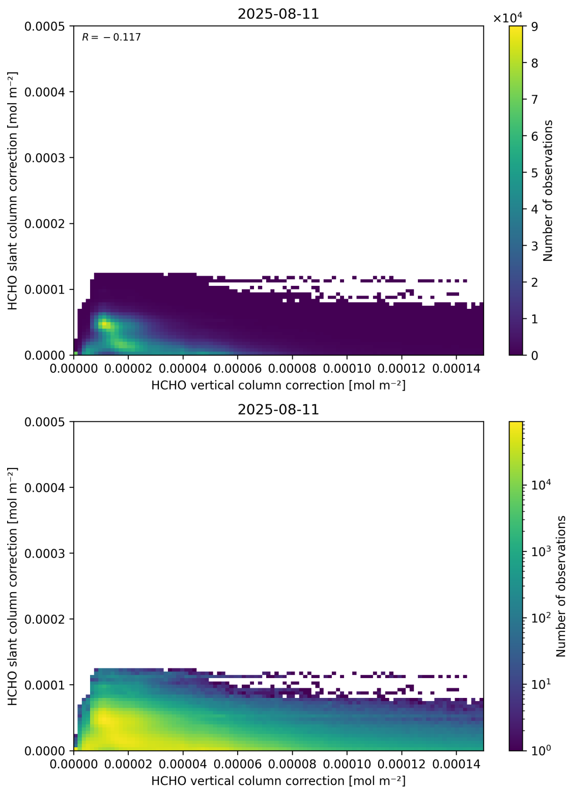
Figure 117: Scatter density plot of “HCHO vertical column correction” against “HCHO slant column correction” for 2025-08-10 to 2025-08-12.
