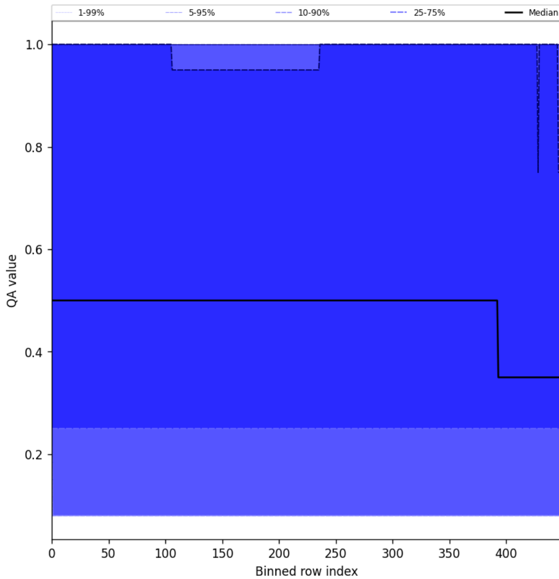
Figure 48: Along track statistics of “QA value” for 2025-08-10 to 2025-08-12
