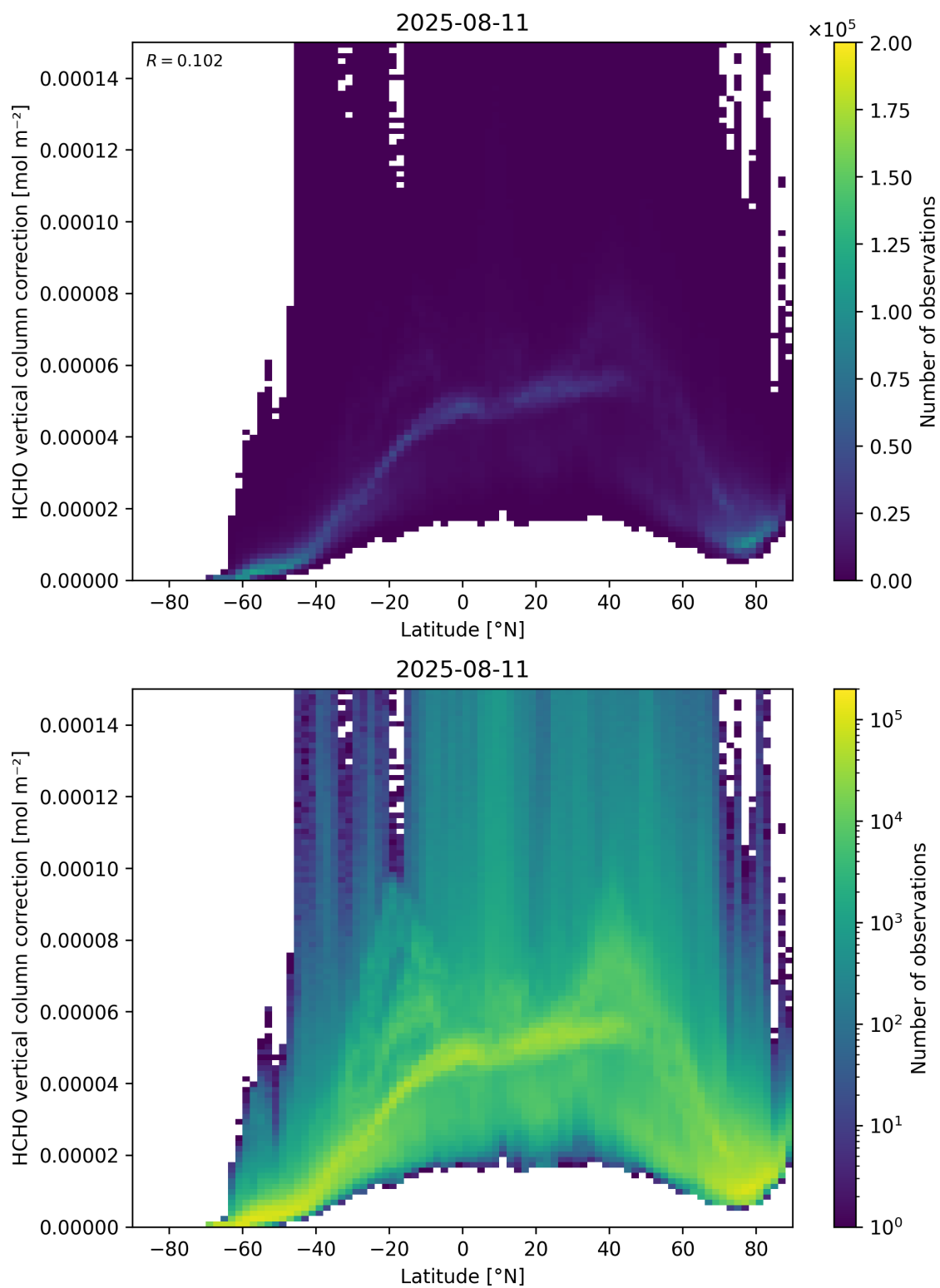
Figure 164: Scatter density plot of “Latitude” against “HCHO vertical column correction” for 2025-08-10 to 2025-08-12.
