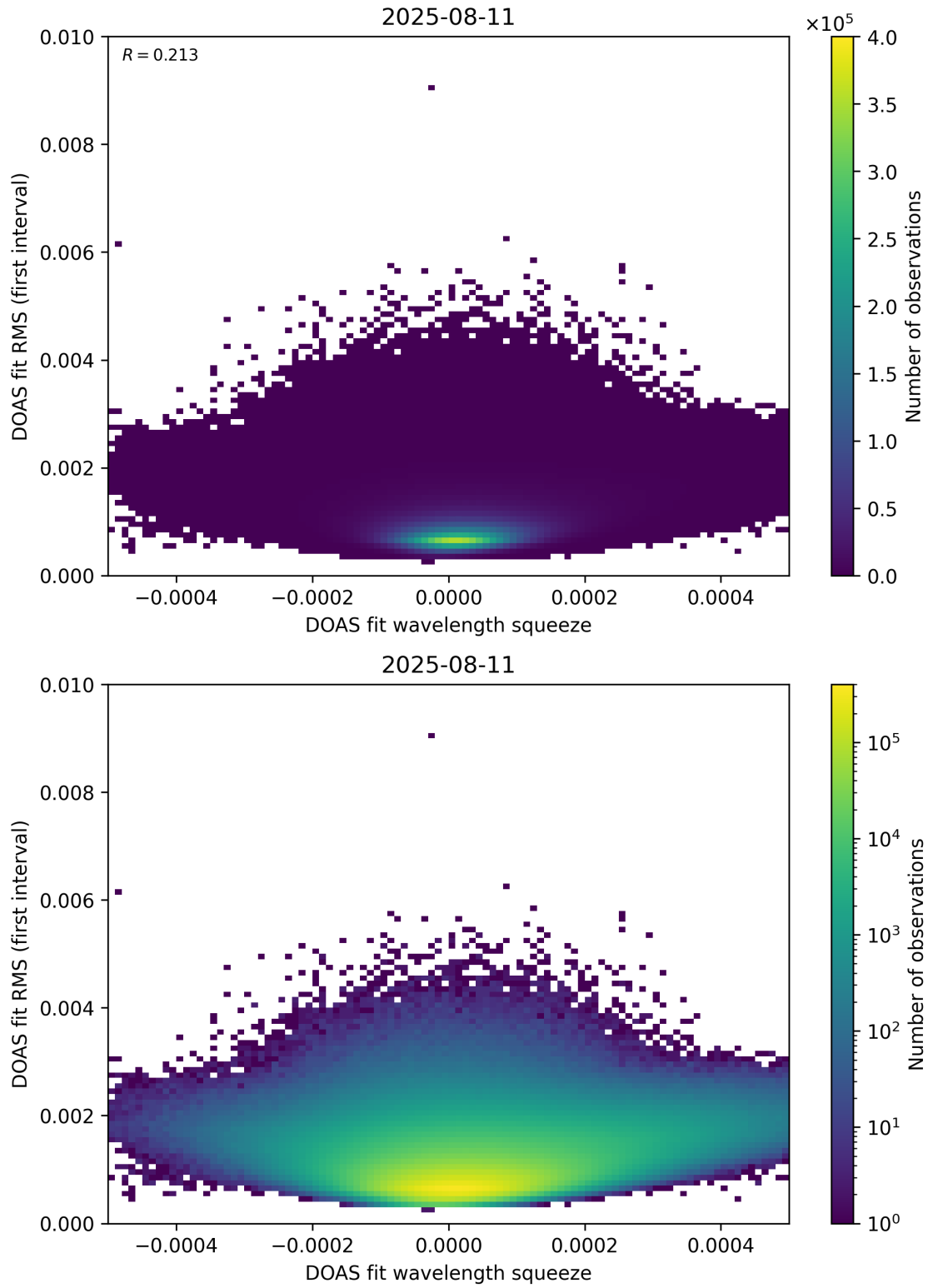
Figure 68: Scatter density plot of “DOAS fit wavelength squeeze” against “DOAS fit RMS (first interval)” for 2025-08-10 to 2025-08-12.
