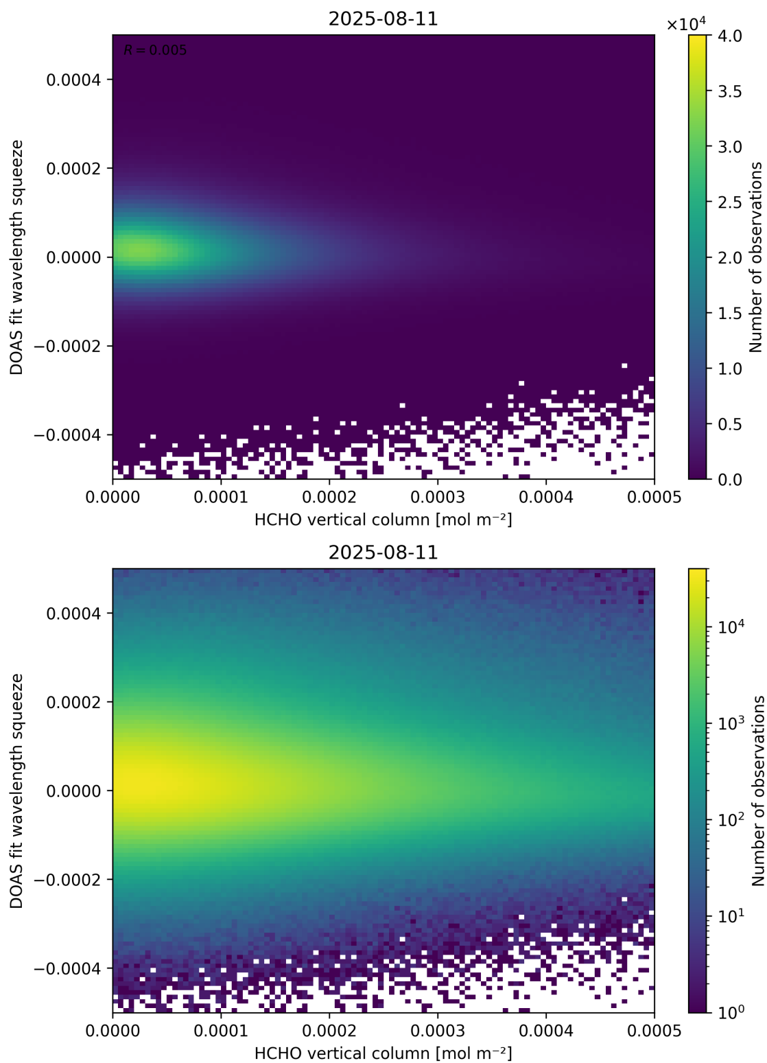
Figure 125: Scatter density plot of “HCHO vertical column” against “DOAS fit wavelength squeeze” for 2025-08-10 to 2025-08-12.
