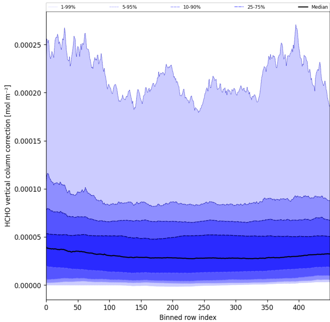
Figure 51: Along track statistics of “HCHO vertical column correction” for 2025-08-10 to 2025-08-12
