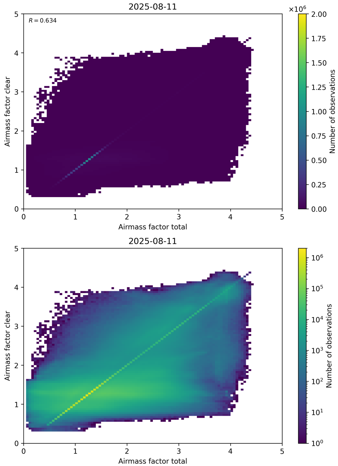
Figure 100: Scatter density plot of “Airmass factor total” against “Airmass factor clear” for 2025-08-10 to 2025-08-12.
