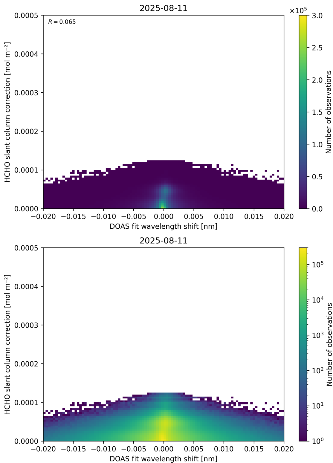
Figure 67: Scatter density plot of “DOAS fit wavelength shift” against “HCHO slant column correction” for 2025-08-10 to 2025-08-12.
