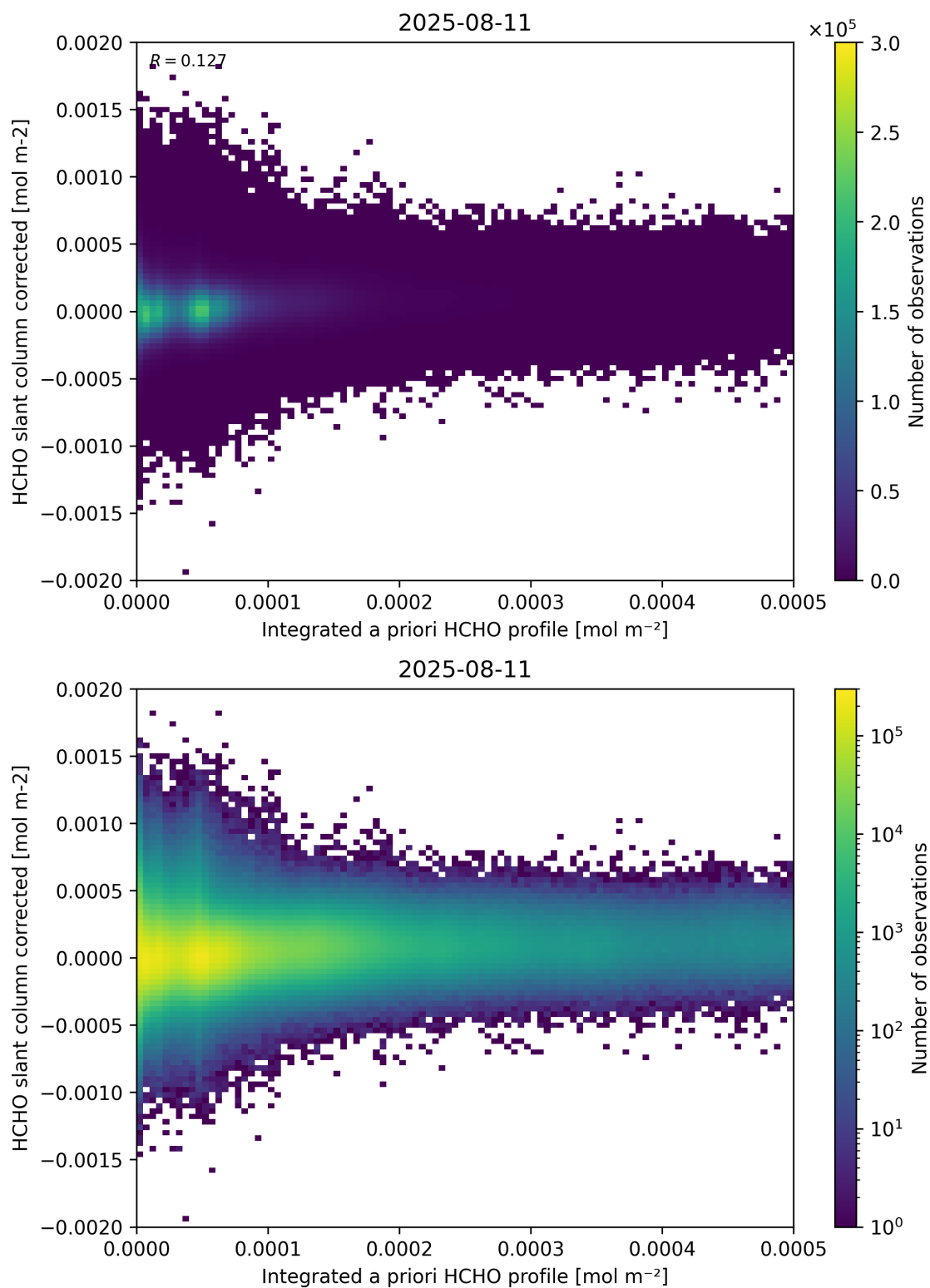
Figure 151: Scatter density plot of “Integrated a priori HCHO profile” against “HCHO slant column corrected” for 2025-08-10 to 2025-08-12.
