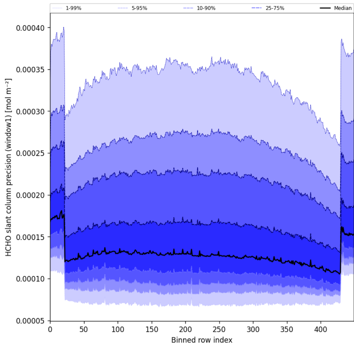
Figure 53: Along track statistics of “HCHO slant column precision (window1)” for 2025-08-10 to 2025-08-12
