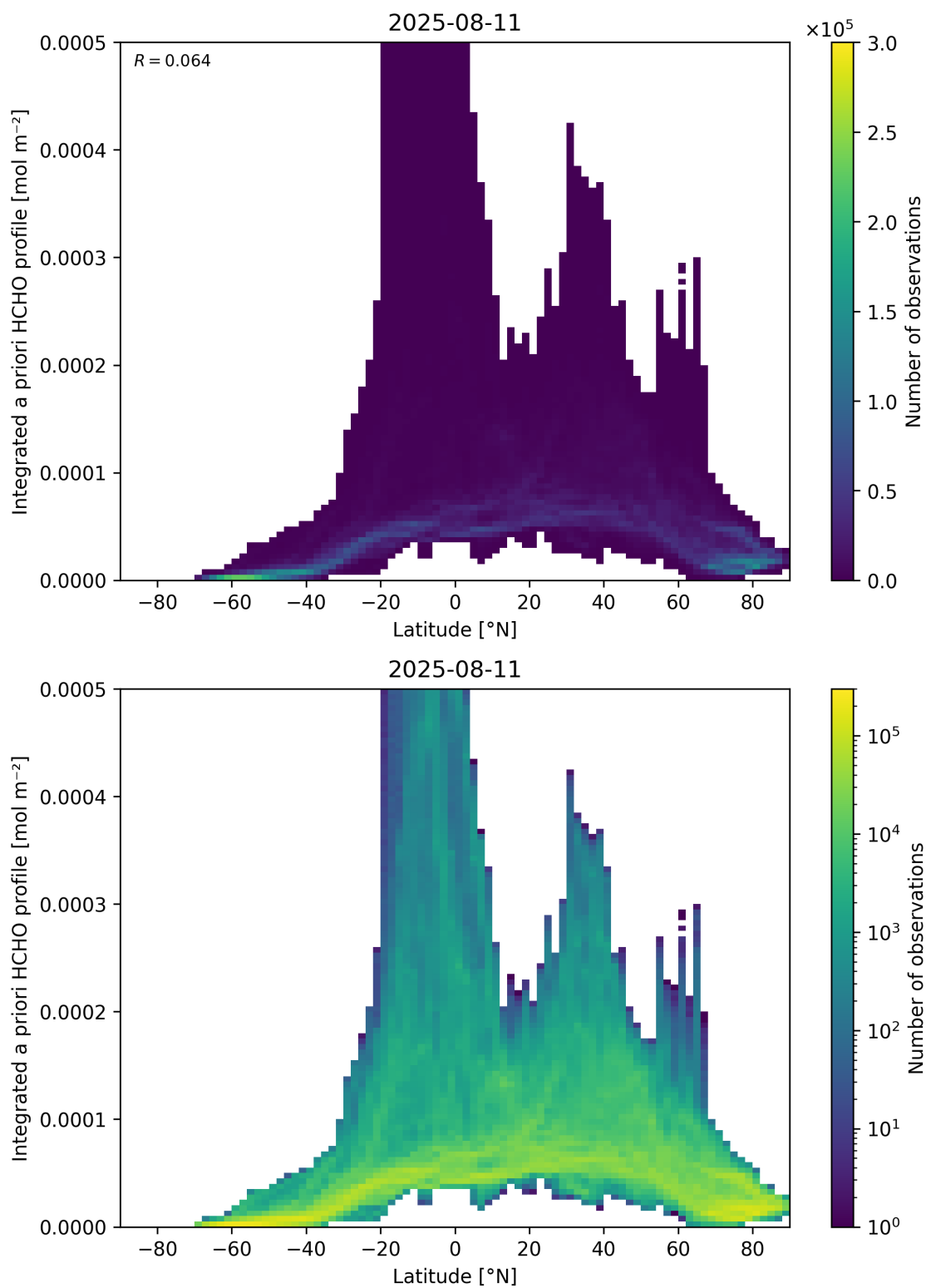
Figure 166: Scatter density plot of “Latitude” against “Integrated a priori HCHO profile” for 2025-08-10 to 2025-08-12.
