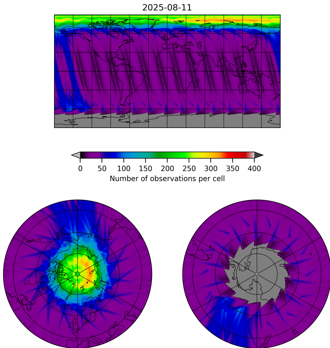
Figure 19: Map of the number of observations for 2025-08-10 to 2025-08-12
