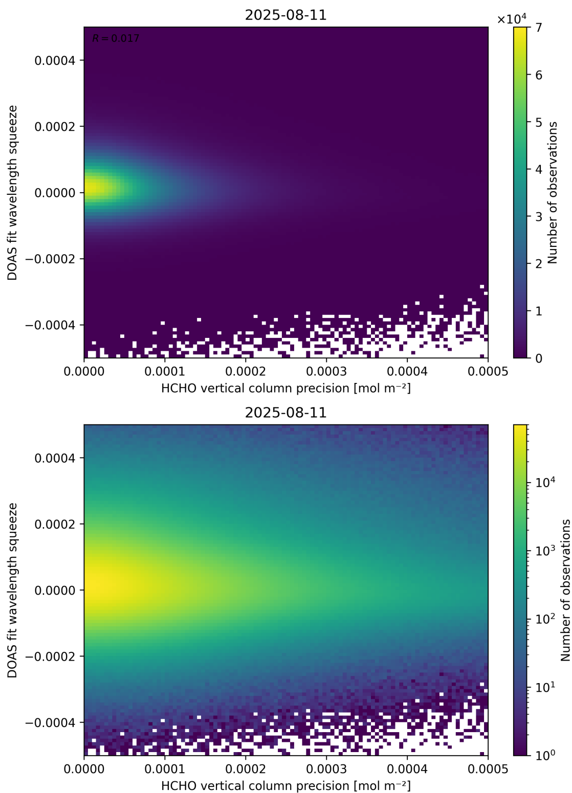
Figure 138: Scatter density plot of “HCHO vertical column precision” against “DOAS fit wavelength squeeze” for 2025-08-10 to 2025-08-12.
