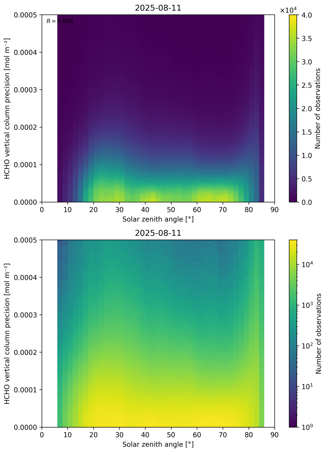
Figure 179: Scatter density plot of “Solar zenith angle” against “HCHO vertical column precision” for 2025-08-10 to 2025-08-12.
