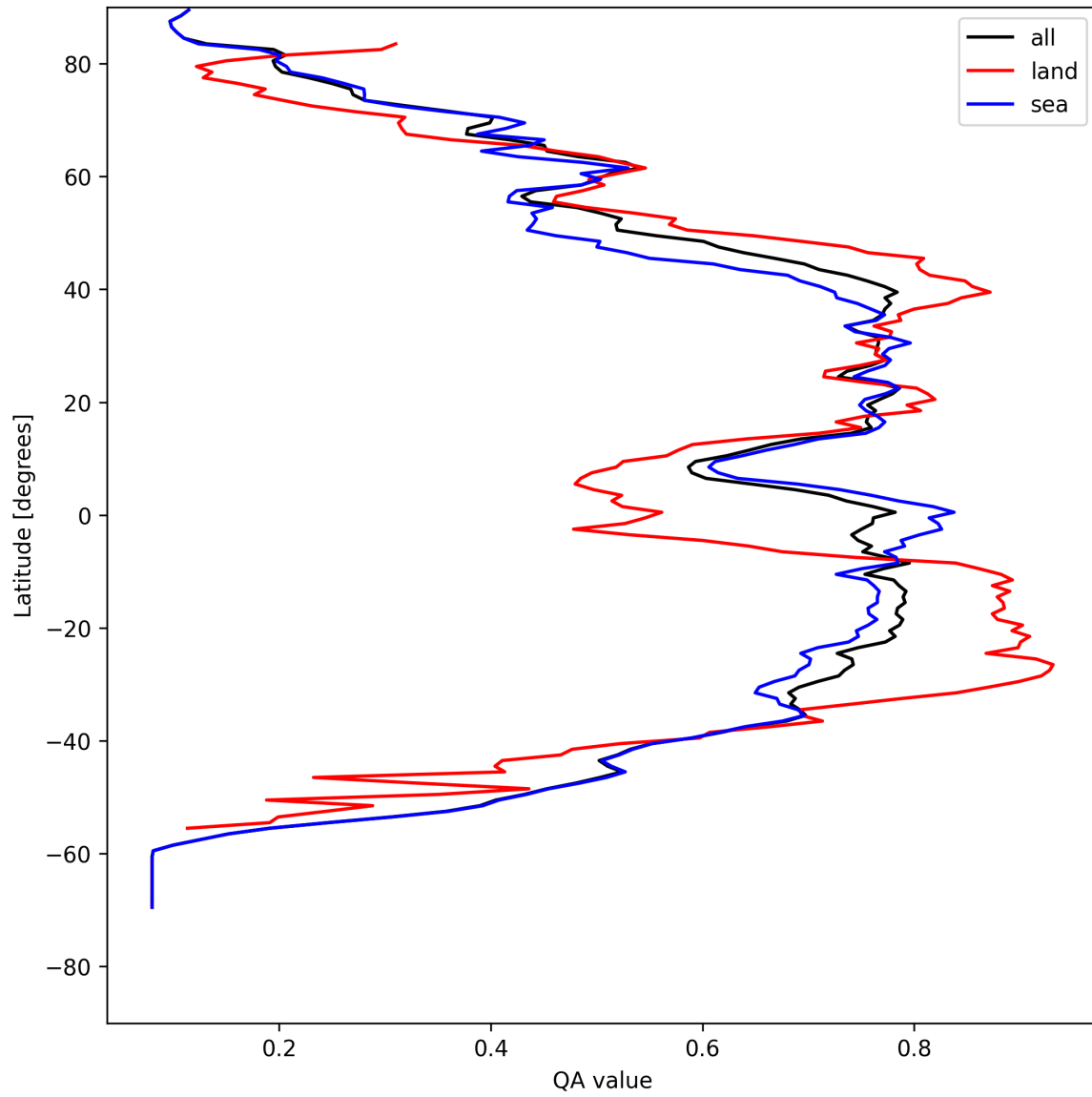
Figure 20: Zonal average of “QA value” for 2025-08-10 to 2025-08-12.
