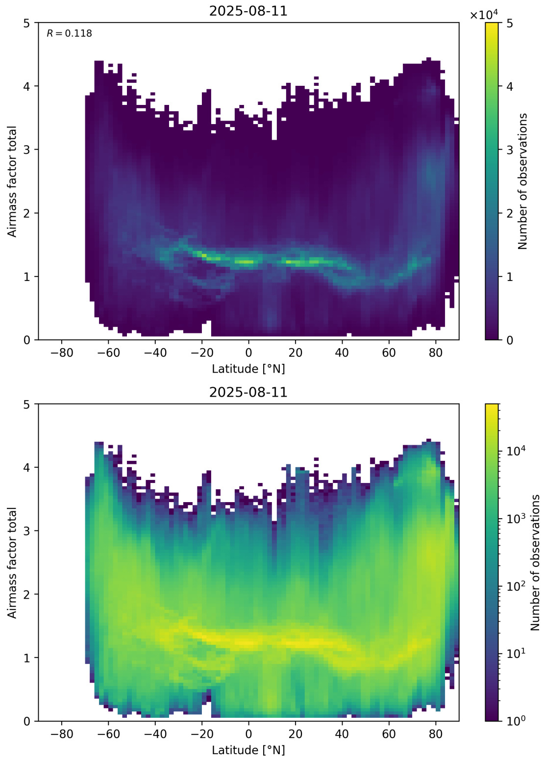
Figure 161: Scatter density plot of “Latitude” against “Airmass factor total” for 2025-08-10 to 2025-08-12.
