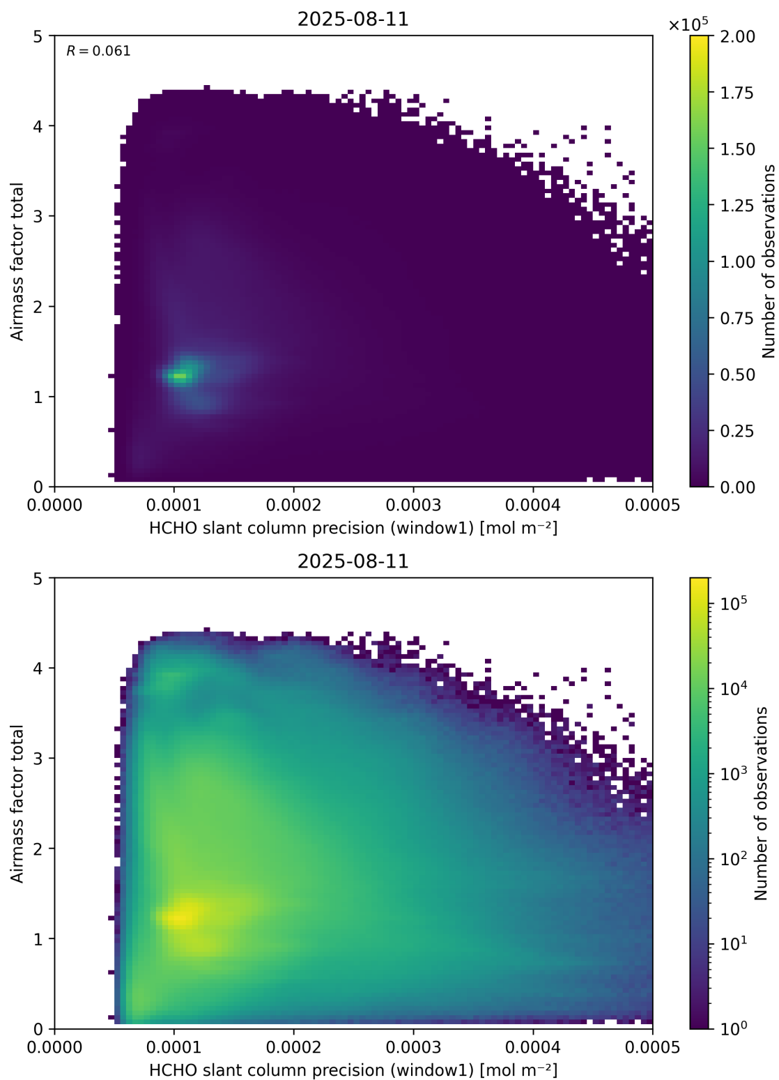
Figure 94: Scatter density plot of “HCHO slant column precision (window1)” against “Airmass factor total” for 2025-08-10 to 2025-08-12.
