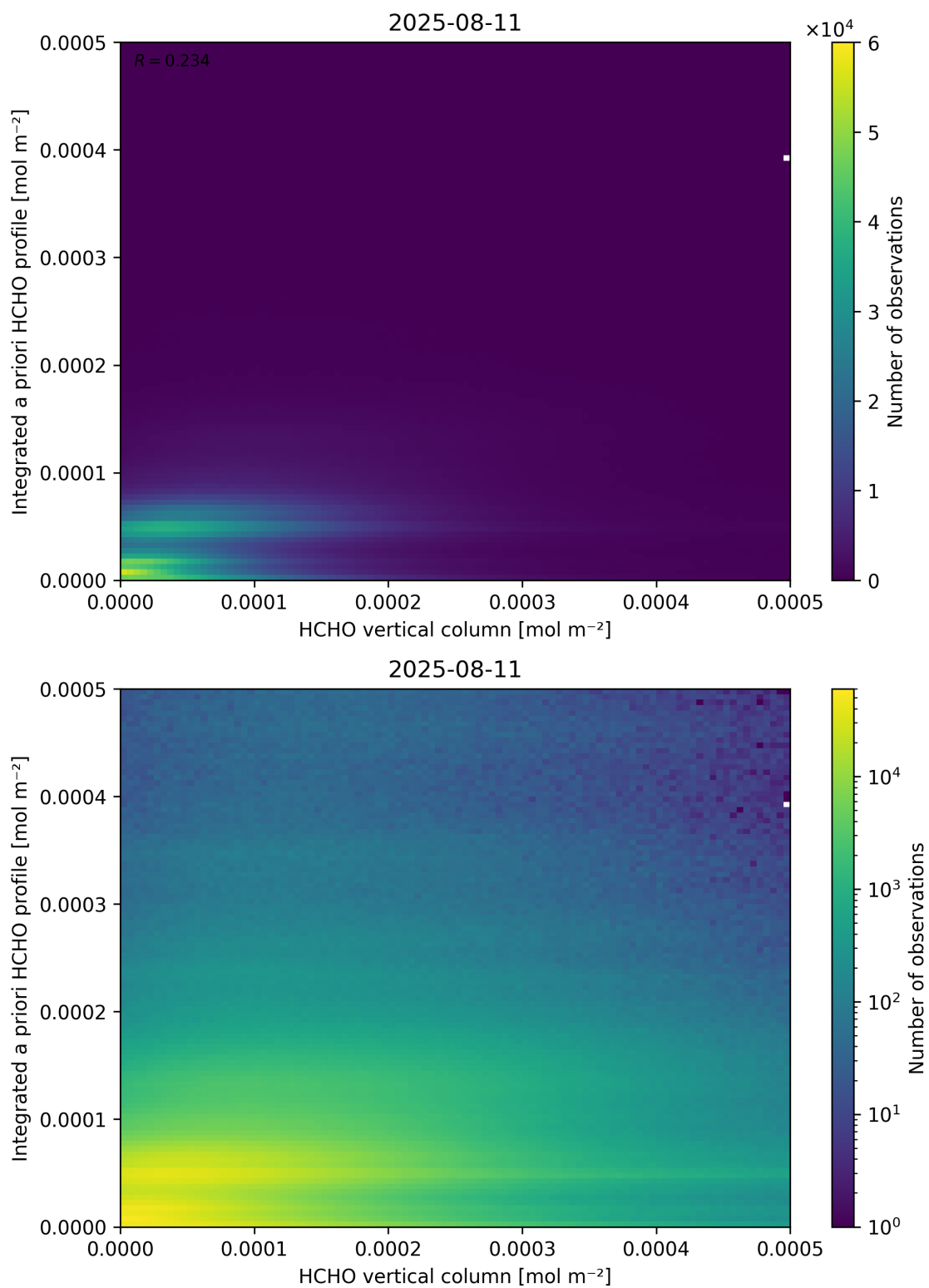
Figure 135: Scatter density plot of “HCHO vertical column” against “Integrated a priori HCHO profile” for 2025-08-10 to 2025-08-12.
