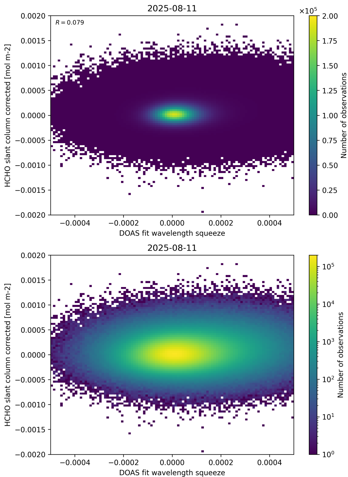
Figure 69: Scatter density plot of “DOAS fit wavelength squeeze” against “HCHO slant column corrected” for 2025-08-10 to 2025-08-12.
