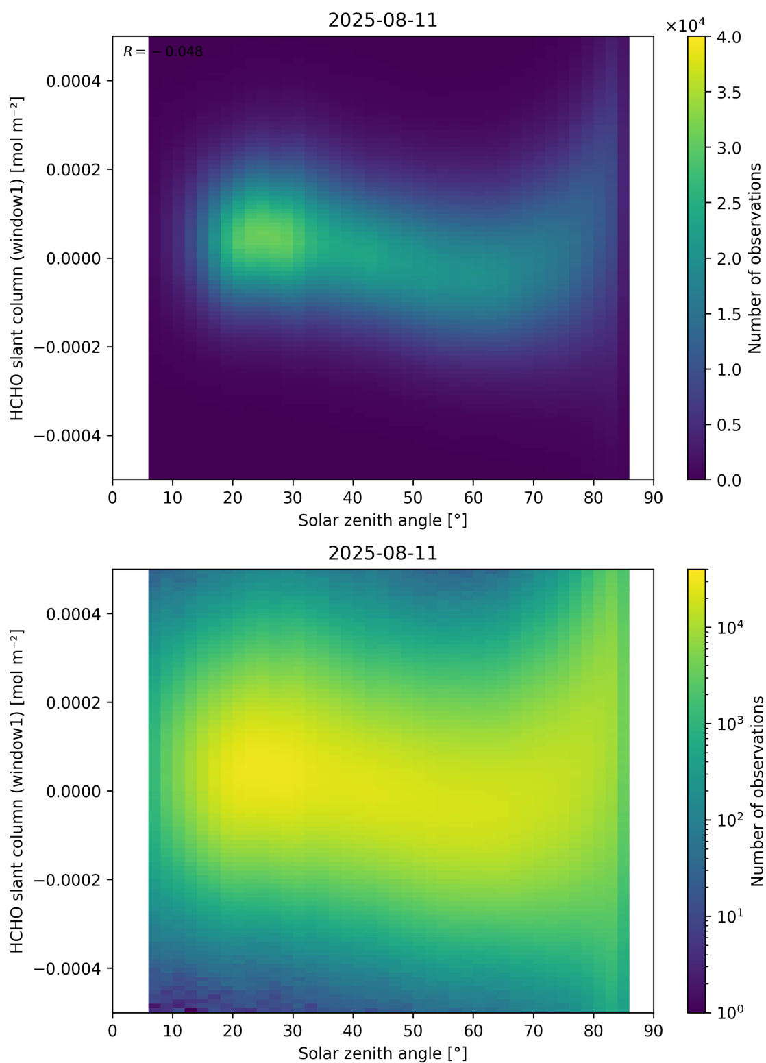
Figure 173: Scatter density plot of “Solar zenith angle” against “HCHO slant column (window1)” for 2025-08-10 to 2025-08-12.
