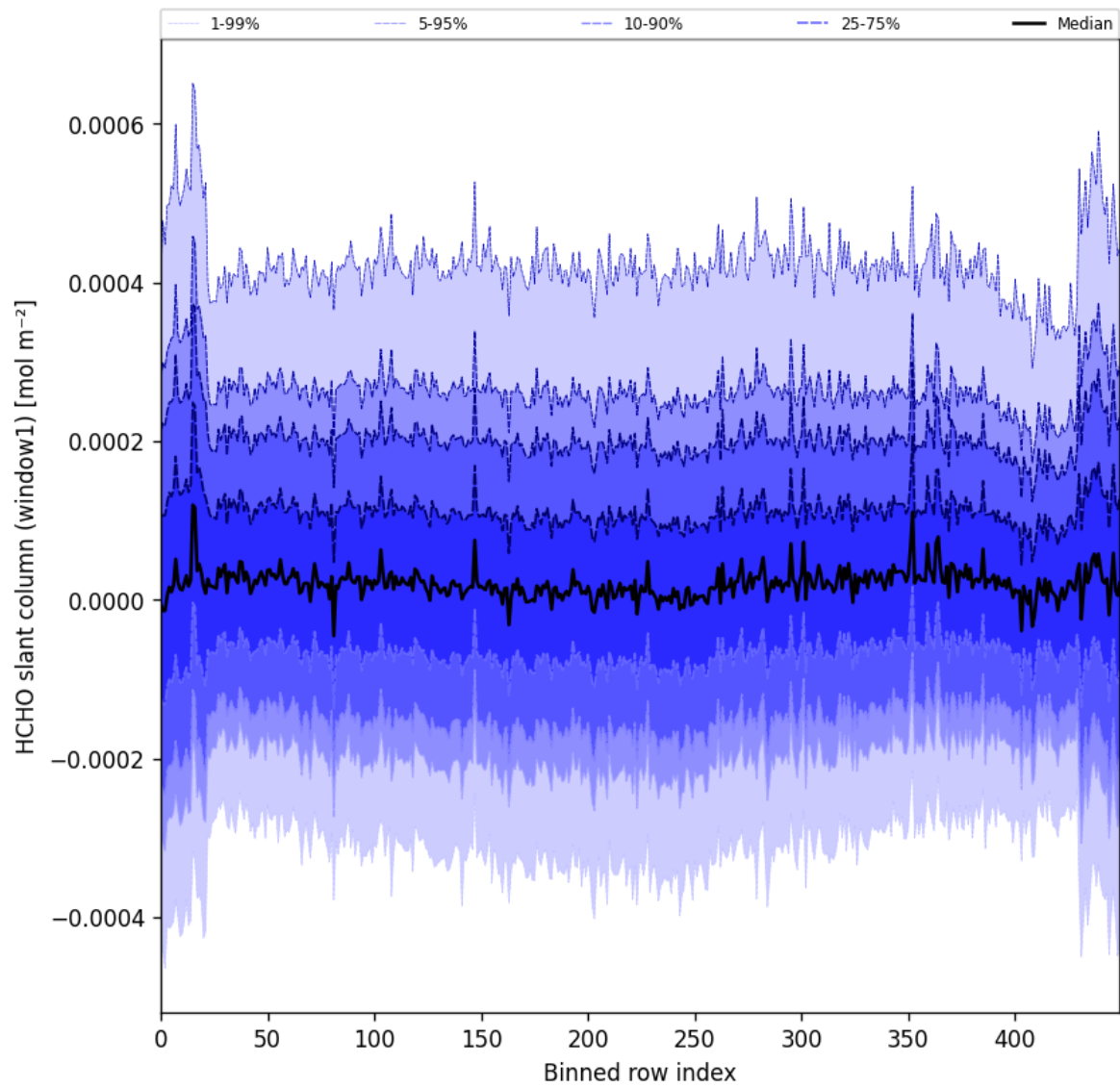
Figure 52: Along track statistics of “HCHO slant column (window1)” for 2025-08-10 to 2025-08-12
