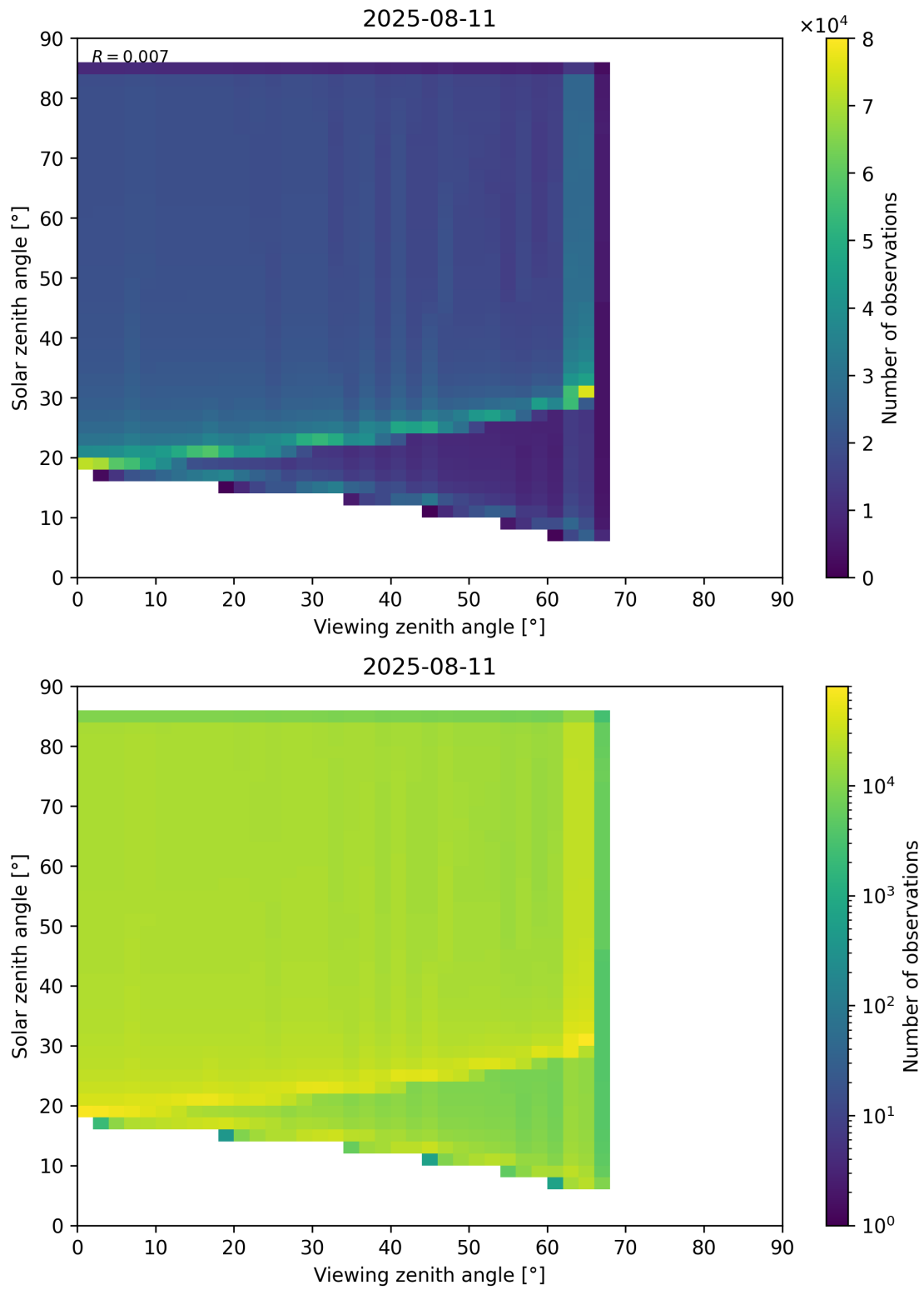
Figure 197: Scatter density plot of “Viewing zenith angle” against “Solar zenith angle” for 2025-08-10 to 2025-08-12.
