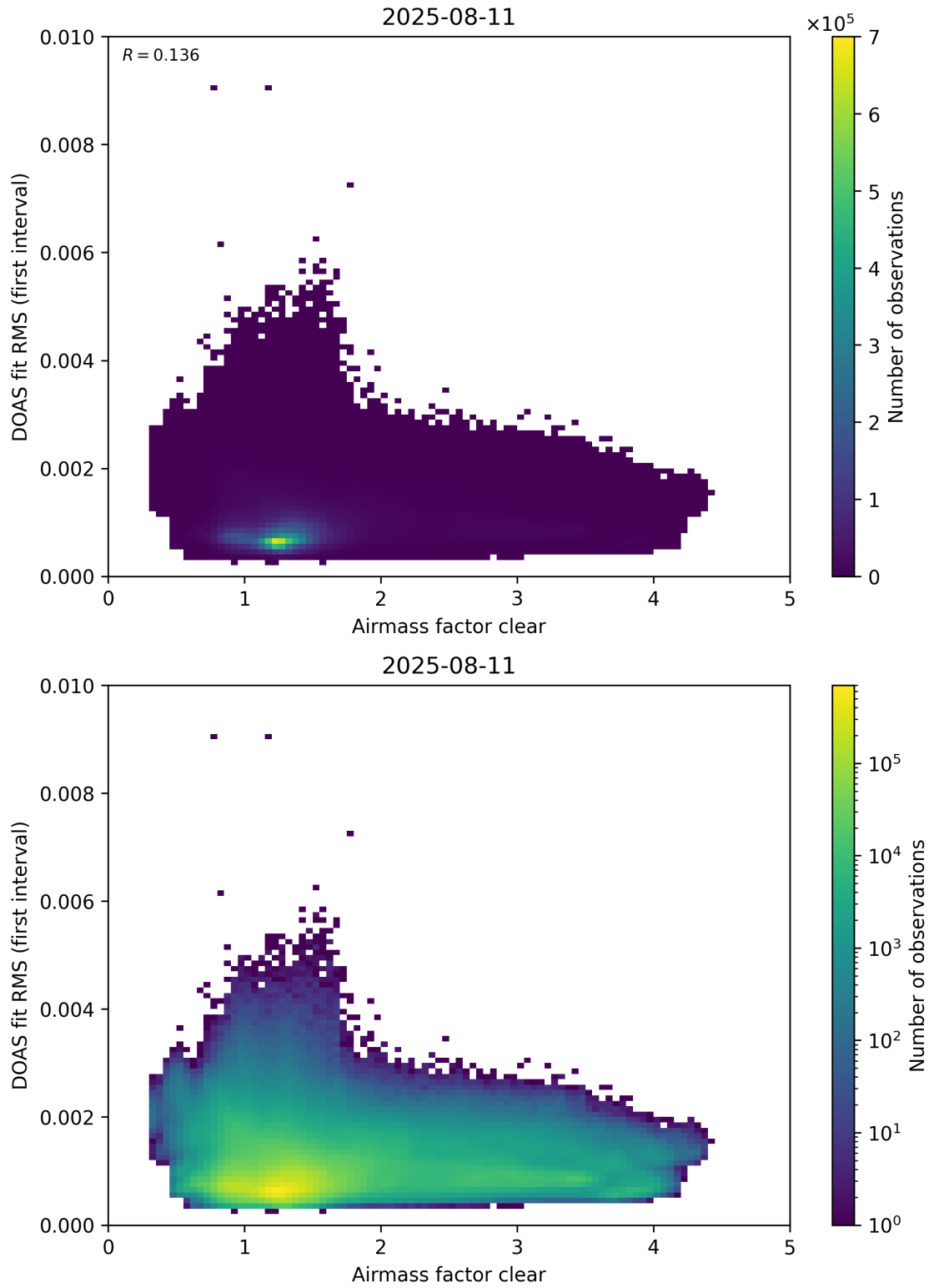
Figure 71: Scatter density plot of “Airmass factor clear” against “DOAS fit RMS (first interval)” for 2025-08-10 to 2025-08-12.
