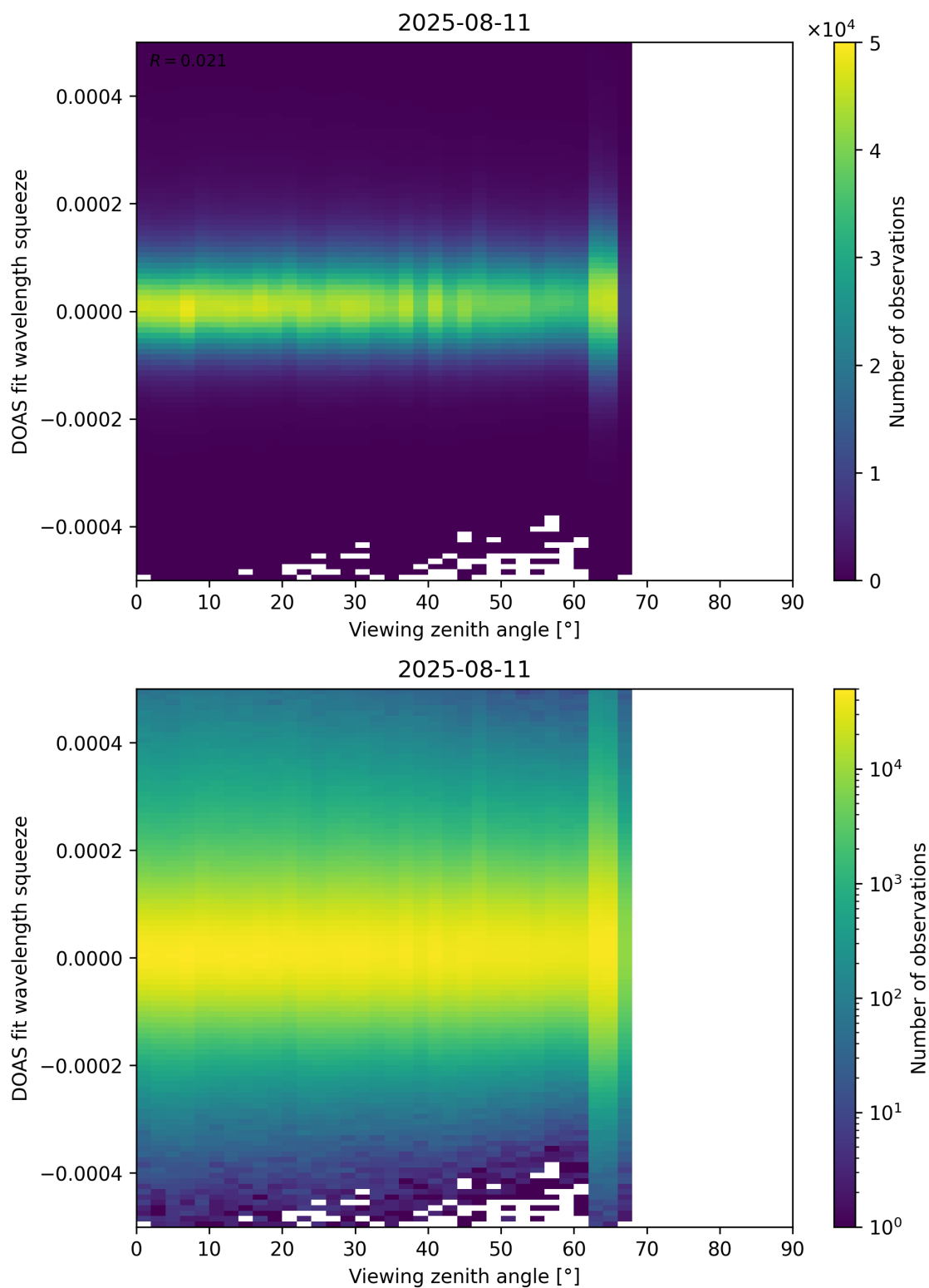
Figure 184: Scatter density plot of “Viewing zenith angle” against “DOAS fit wavelength squeeze” for 2025-08-10 to 2025-08-12.
