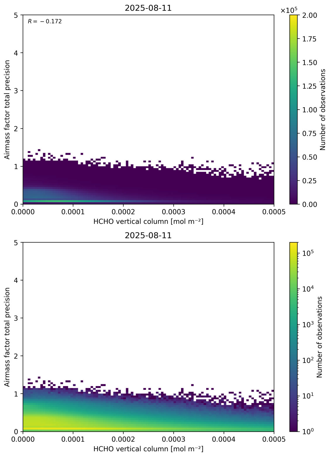
Figure 132: Scatter density plot of “HCHO vertical column” against “Airmass factor total precision” for 2025-08-10 to 2025-08-12.
