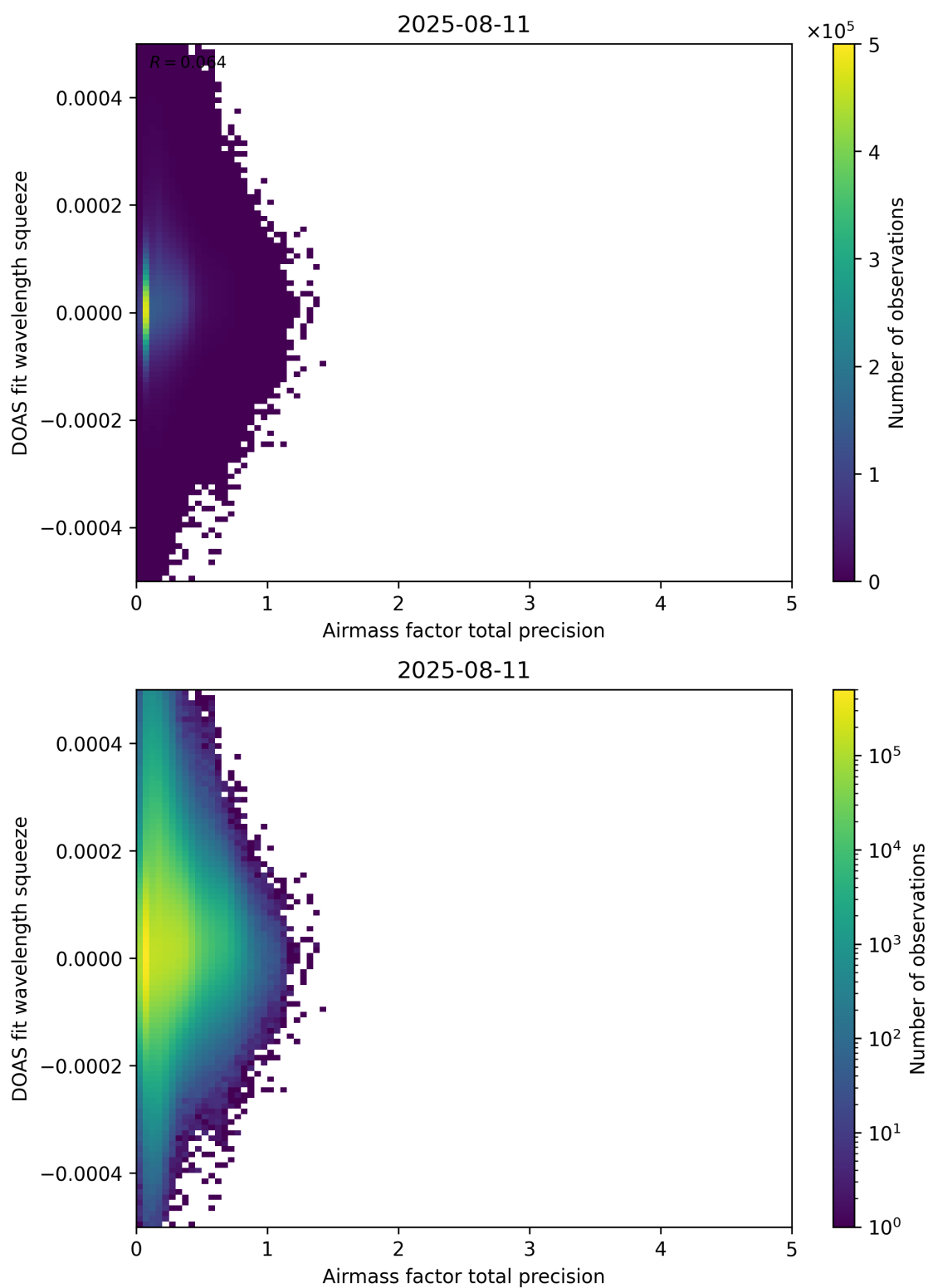
Figure 107: Scatter density plot of “Airmass factor total precision” against “DOAS fit wavelength squeeze” for 2025-08-10 to 2025-08-12.
