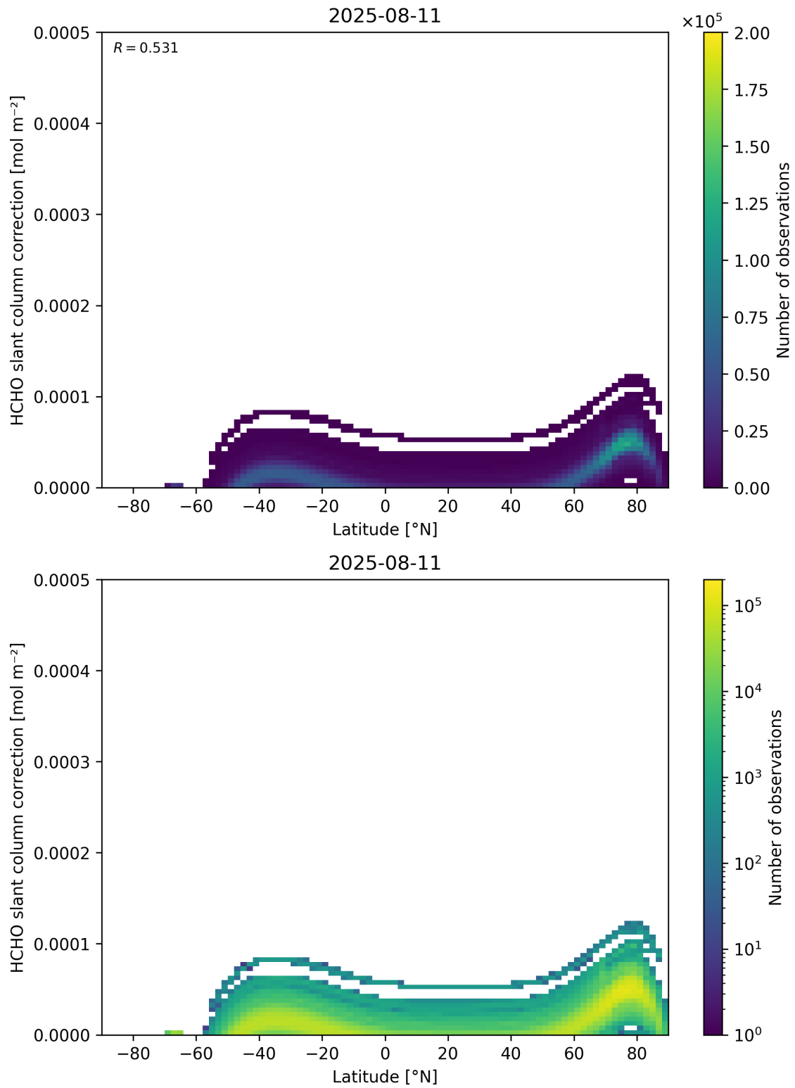
Figure 158: Scatter density plot of “Latitude” against “HCHO slant column correction” for 2025-08-10 to 2025-08-12.
