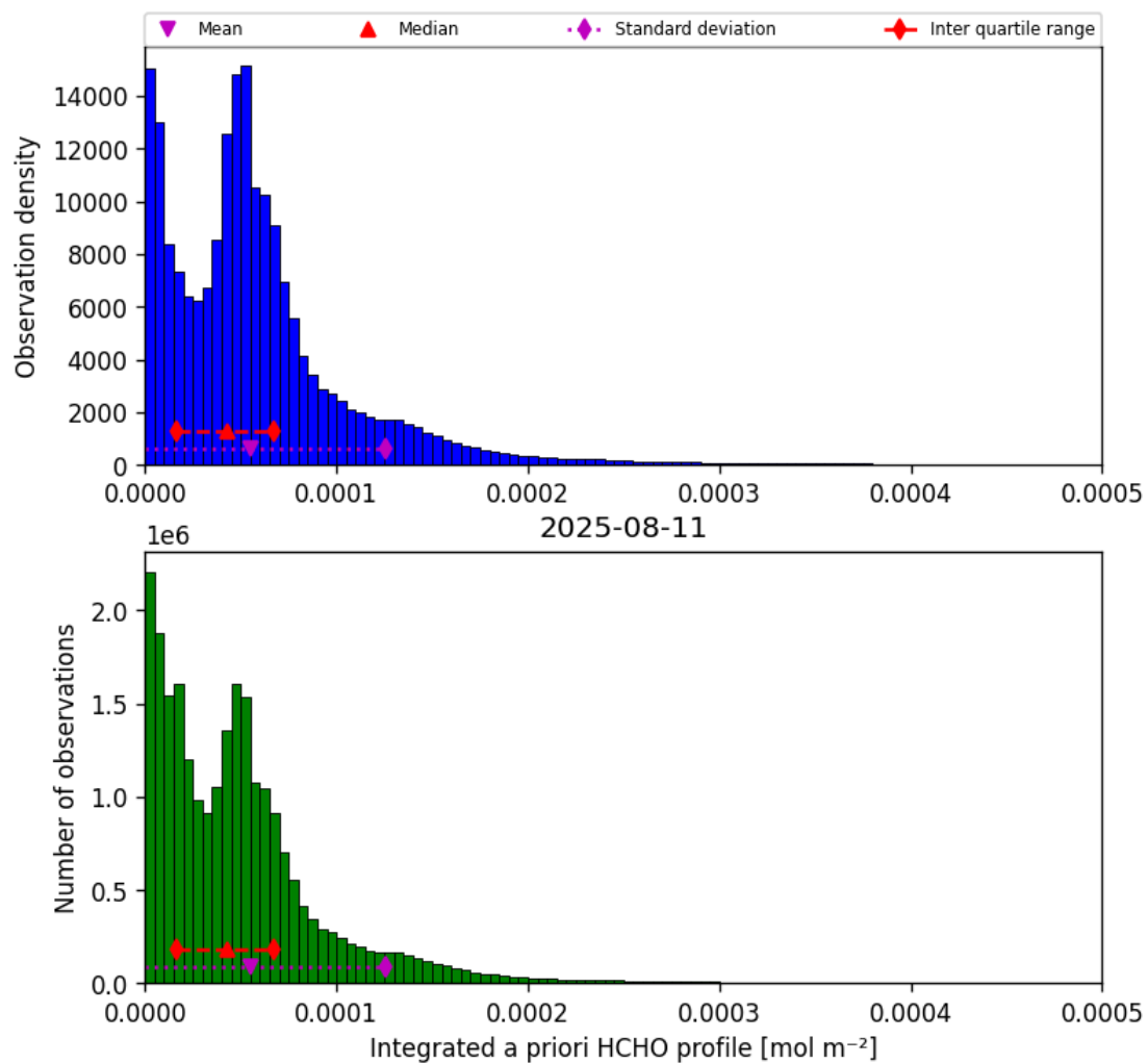
Figure 43: Histogram of “Integrated a priori HCHO profile” for 2025-08-10 to 2025-08-12
