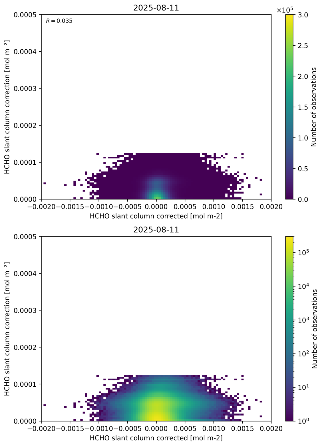
Figure 77: Scatter density plot of “HCHO slant column corrected” against “HCHO slant column correction” for 2025-08-10 to 2025-08-12.
