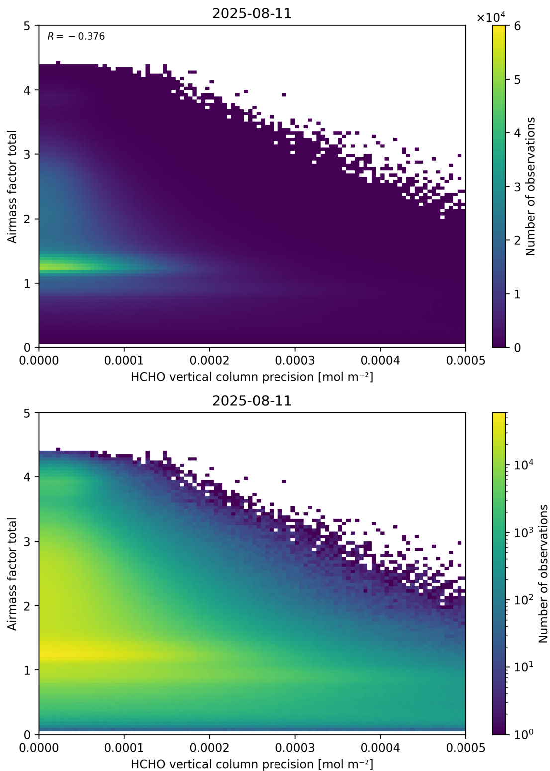
Figure 144: Scatter density plot of “HCHO vertical column precision” against “Airmass factor total” for 2025-08-10 to 2025-08-12.
