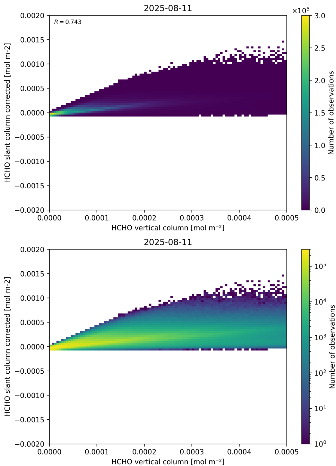
Figure 127: Scatter density plot of “HCHO vertical column” against “HCHO slant column corrected” for 2025-08-10 to 2025-08-12.
