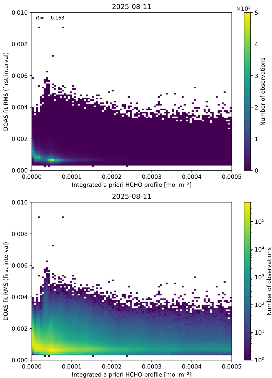
Figure 148: Scatter density plot of “Integrated a priori HCHO profile” against “DOAS fit RMS (first interval)” for 2025-08-10 to 2025-08-12.
