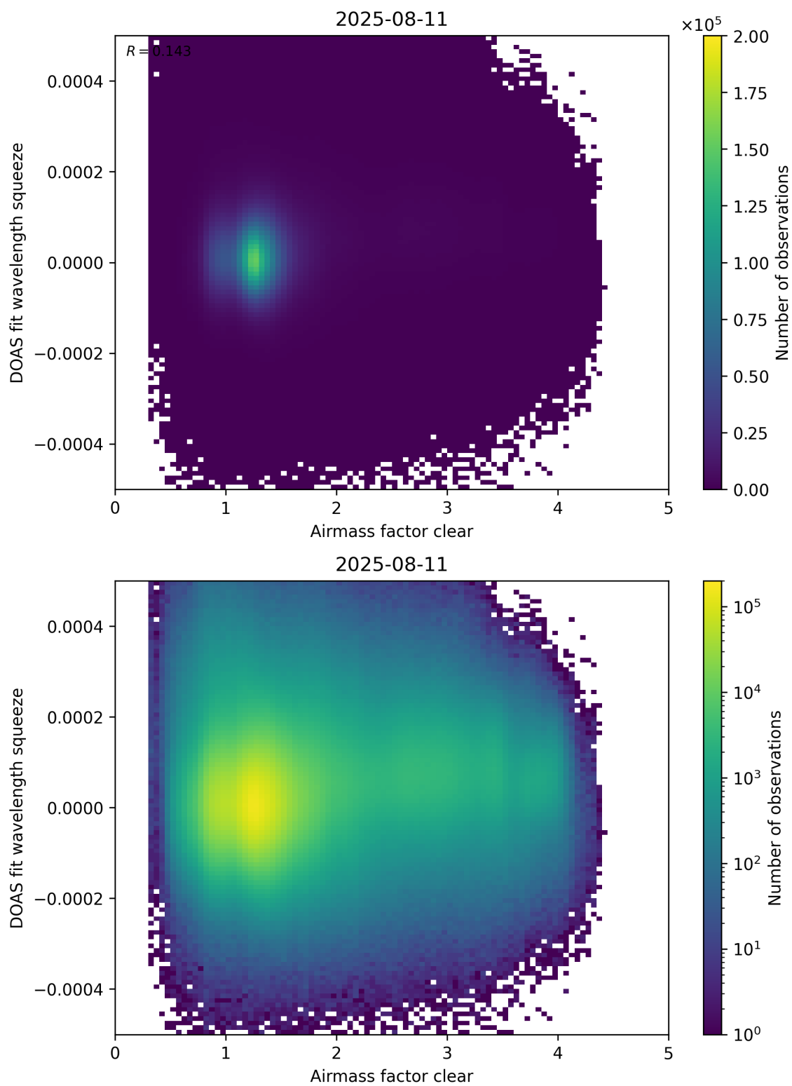
Figure 73: Scatter density plot of “Airmass factor clear” against “DOAS fit wavelength squeeze” for 2025-08-10 to 2025-08-12.
