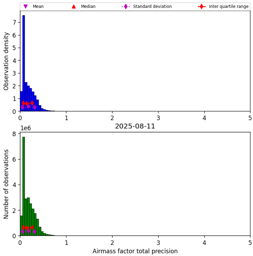
Figure 41: Histogram of “Airmass factor total precision” for 2025-08-10 to 2025-08-12
