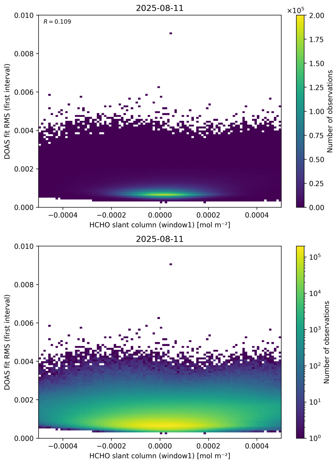
Figure 78: Scatter density plot of “HCHO slant column (window1)” against “DOAS fit RMS (first interval)” for 2025-08-10 to 2025-08-12.
