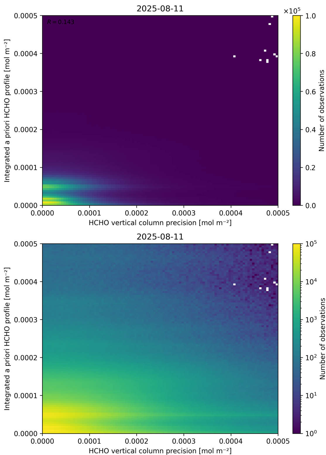
Figure 147: Scatter density plot of “HCHO vertical column precision” against “Integrated a priori HCHO profile” for 2025-08-10 to 2025-08-12.
