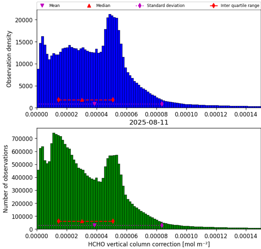
Figure 37: Histogram of “HCHO vertical column correction” for 2025-08-10 to 2025-08-12
