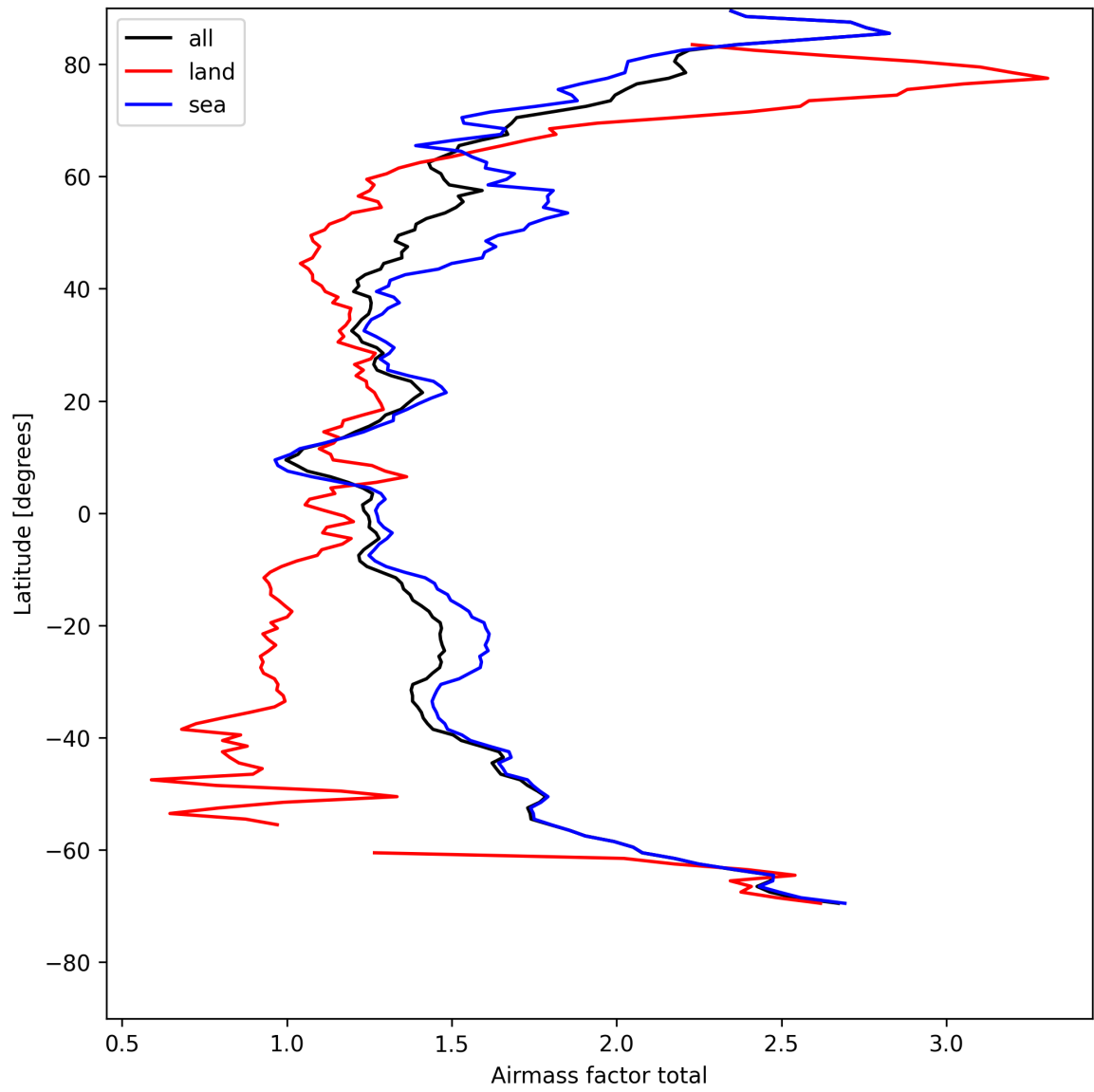
Figure 26: Zonal average of “Airmass factor total” for 2025-08-10 to 2025-08-12.
