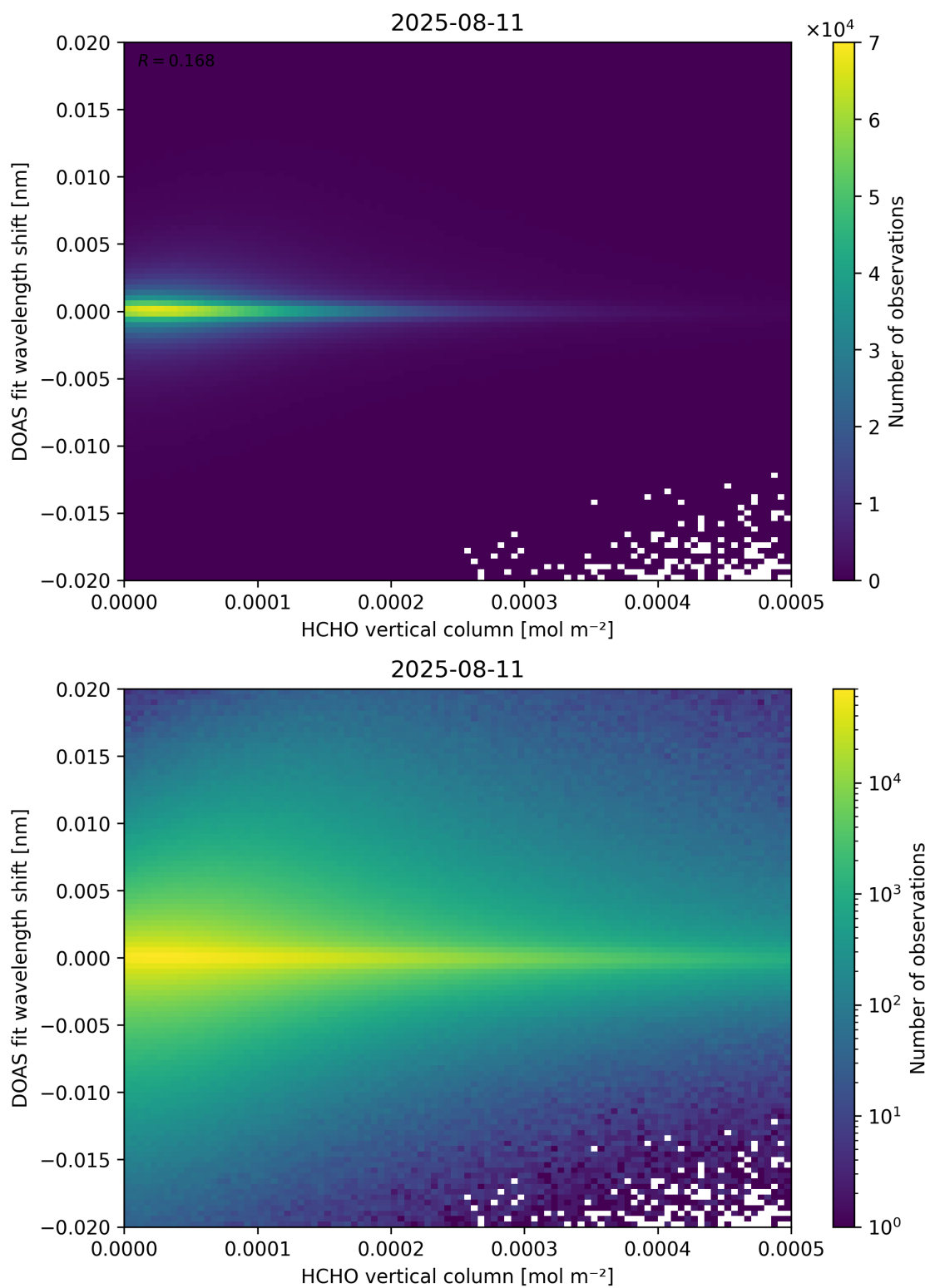
Figure 124: Scatter density plot of “HCHO vertical column” against “DOAS fit wavelength shift” for 2025-08-10 to 2025-08-12.
