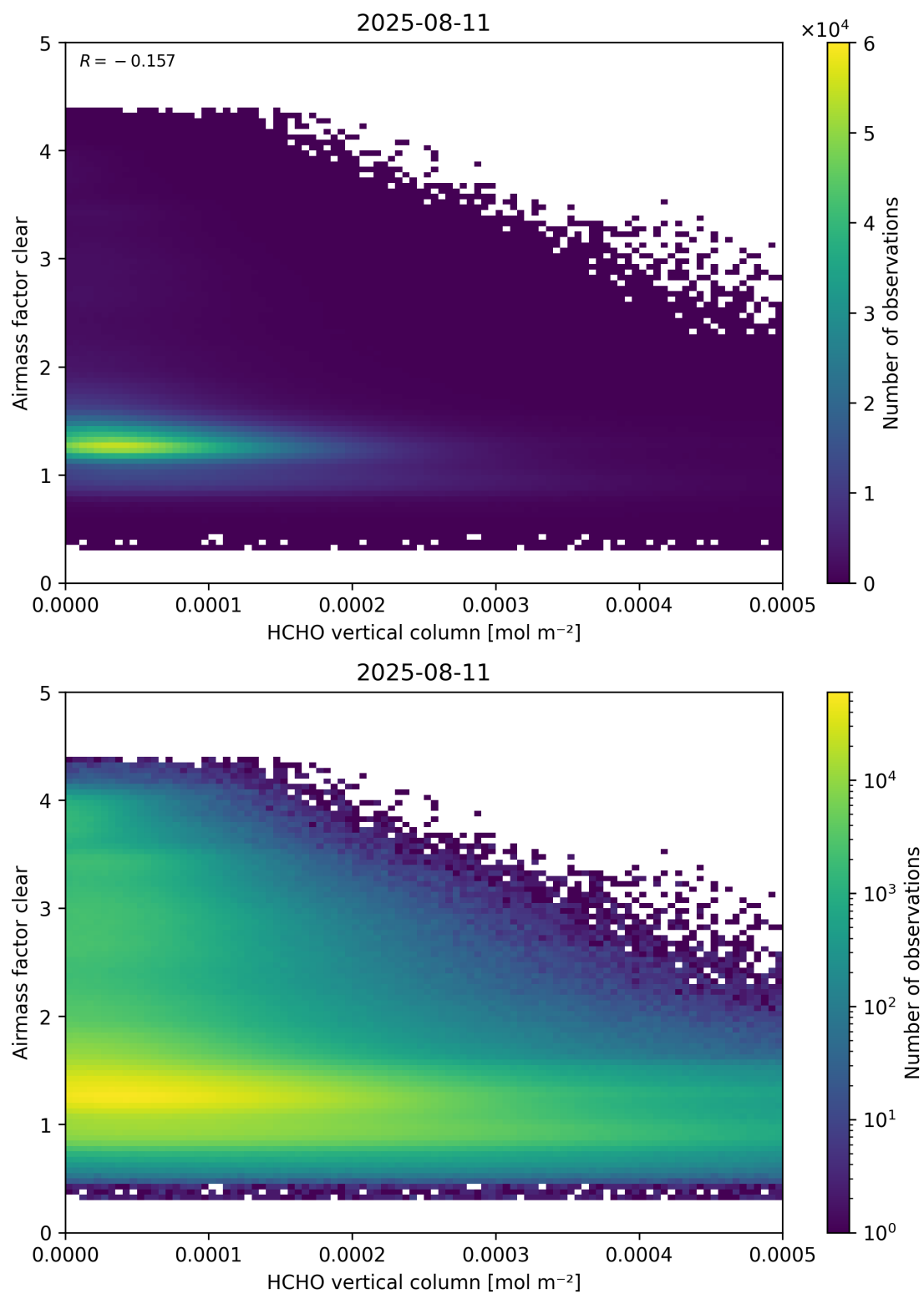
Figure 126: Scatter density plot of “HCHO vertical column” against “Airmass factor clear” for 2025-08-10 to 2025-08-12.
