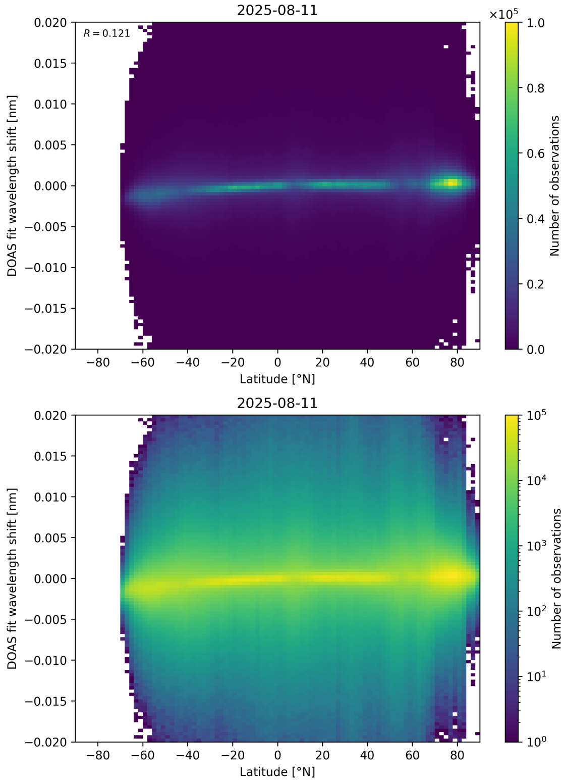
Figure 154: Scatter density plot of “Latitude” against “DOAS fit wavelength shift” for 2025-08-10 to 2025-08-12.
