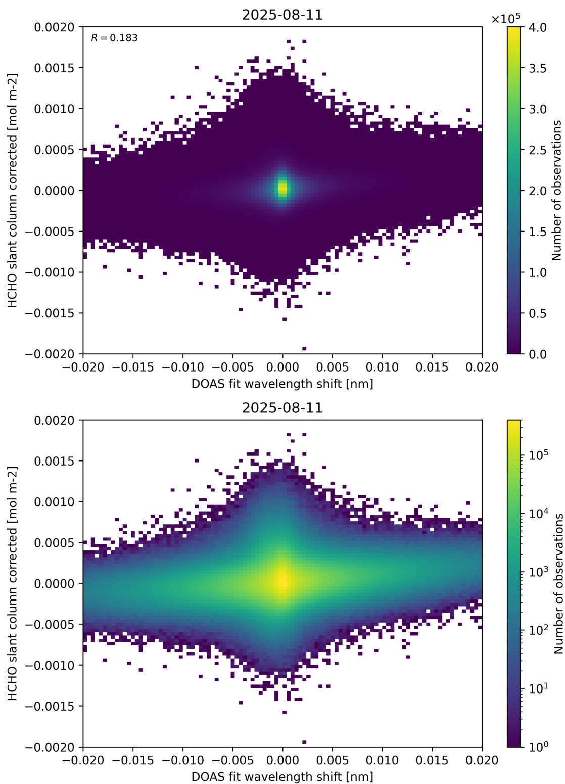
Figure 66: Scatter density plot of “DOAS fit wavelength shift” against “HCHO slant column corrected” for 2025-08-10 to 2025-08-12.
