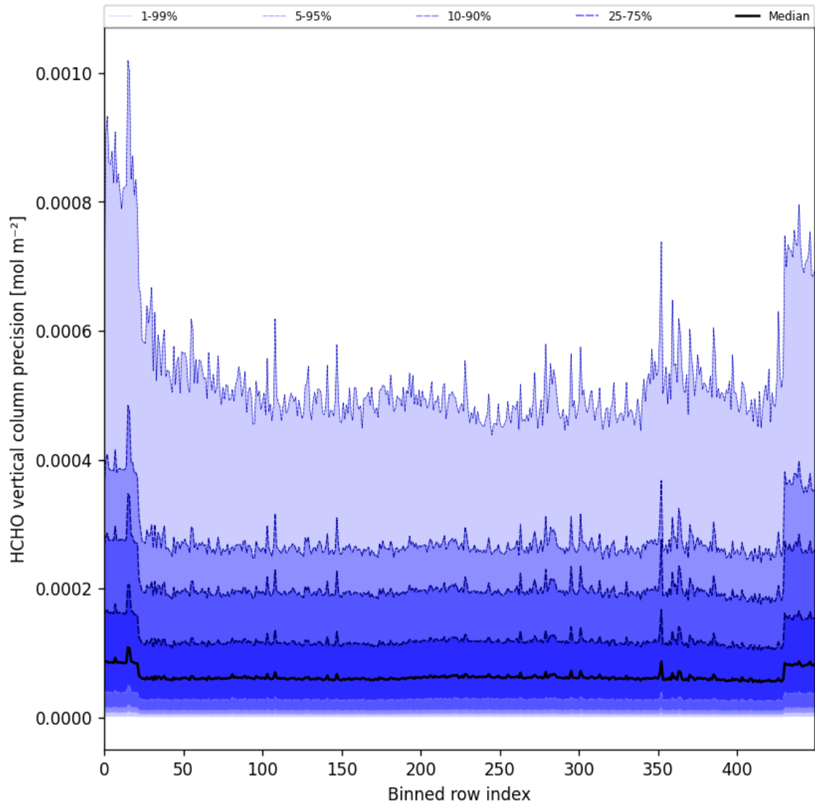
Figure 50: Along track statistics of “HCHO vertical column precision” for 2025-08-10 to 2025-08-12
