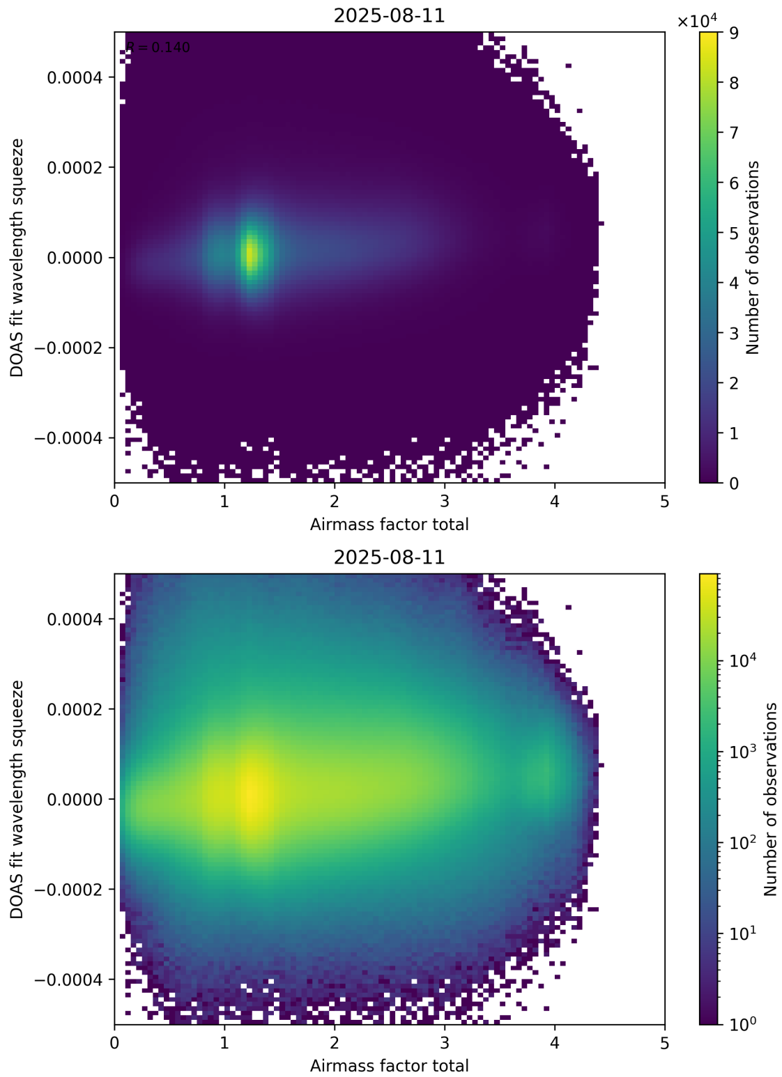
Figure 99: Scatter density plot of “Airmass factor total” against “DOAS fit wavelength squeeze” for 2025-08-10 to 2025-08-12.
