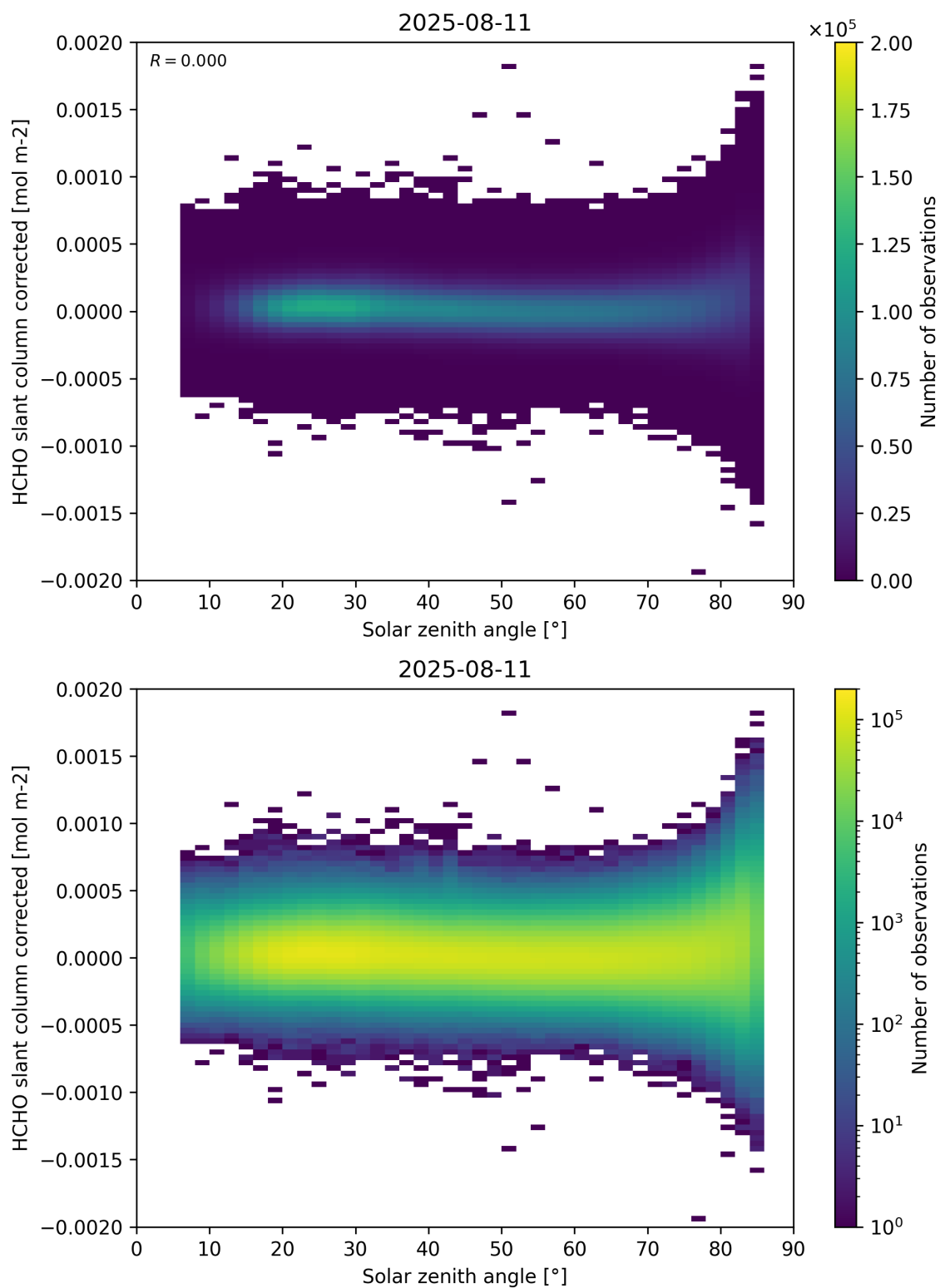
Figure 171: Scatter density plot of “Solar zenith angle” against “HCHO slant column corrected” for 2025-08-10 to 2025-08-12.
