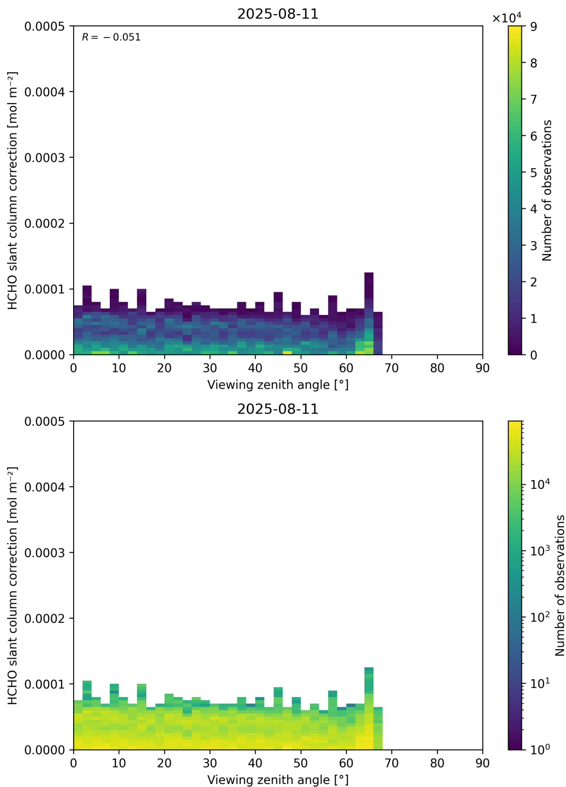
Figure 187: Scatter density plot of “Viewing zenith angle” against “HCHO slant column correction” for 2025-08-10 to 2025-08-12.
