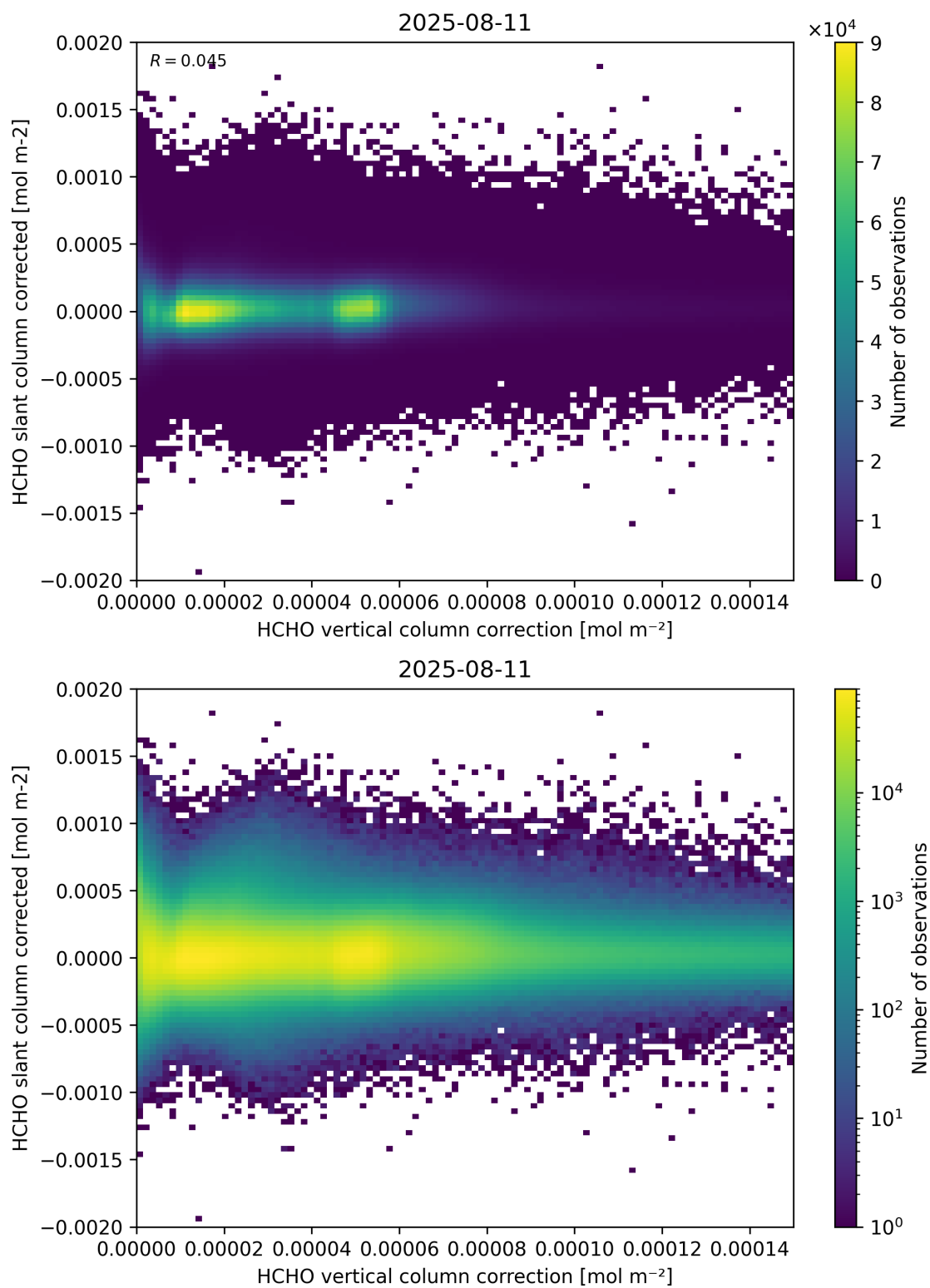
Figure 116: Scatter density plot of “HCHO vertical column correction” against “HCHO slant column corrected” for 2025-08-10 to 2025-08-12.
