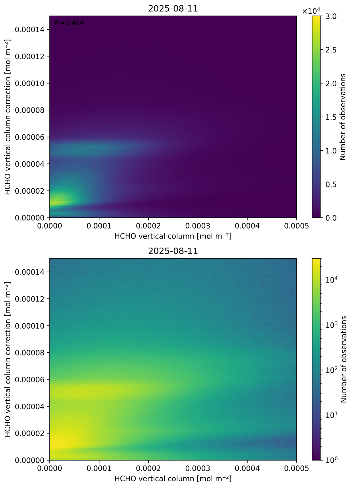
Figure 133: Scatter density plot of “HCHO vertical column” against “HCHO vertical column correction” for 2025-08-10 to 2025-08-12.
