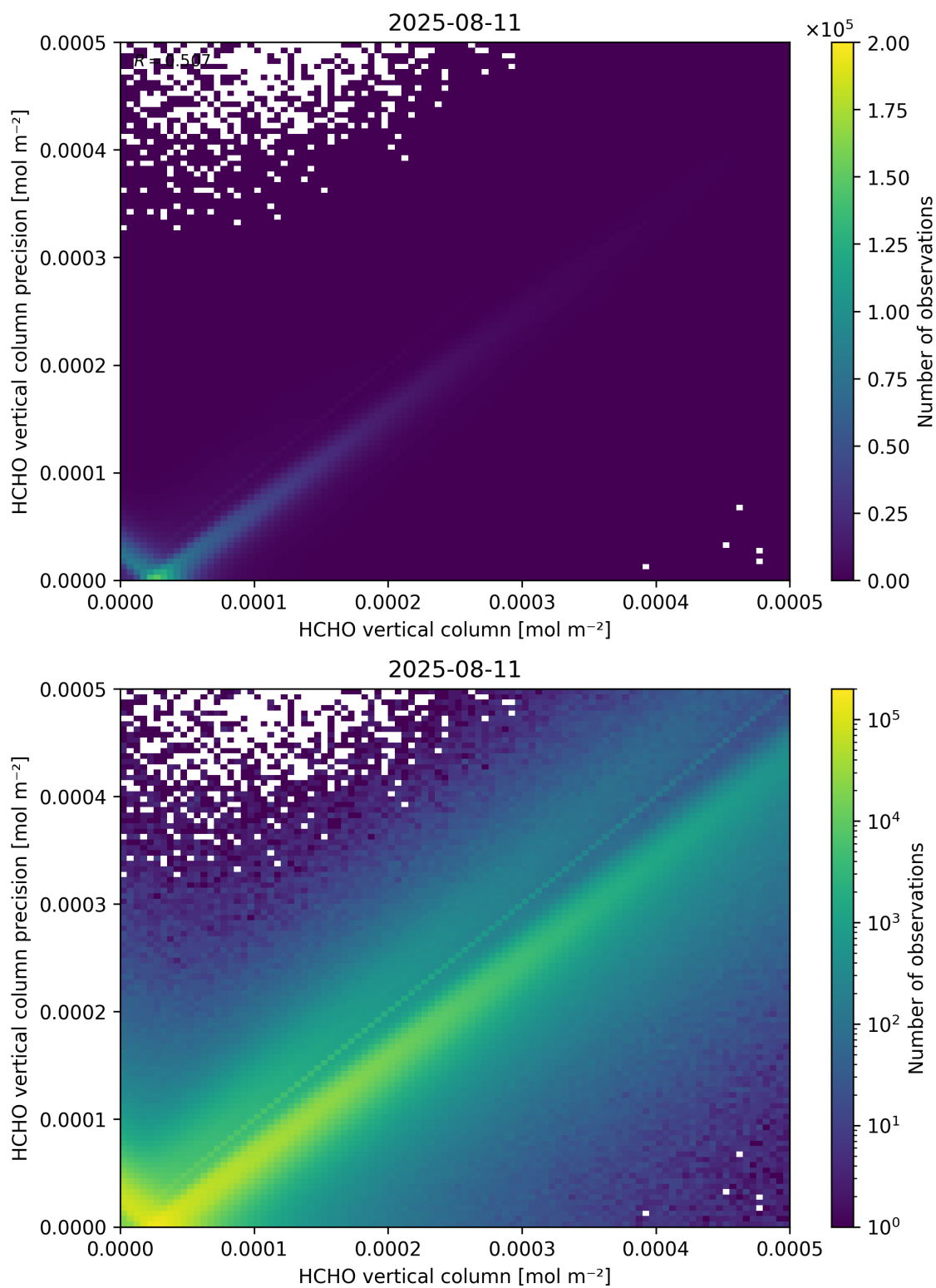
Figure 134: Scatter density plot of “HCHO vertical column” against “HCHO vertical column precision” for 2025-08-10 to 2025-08-12.
