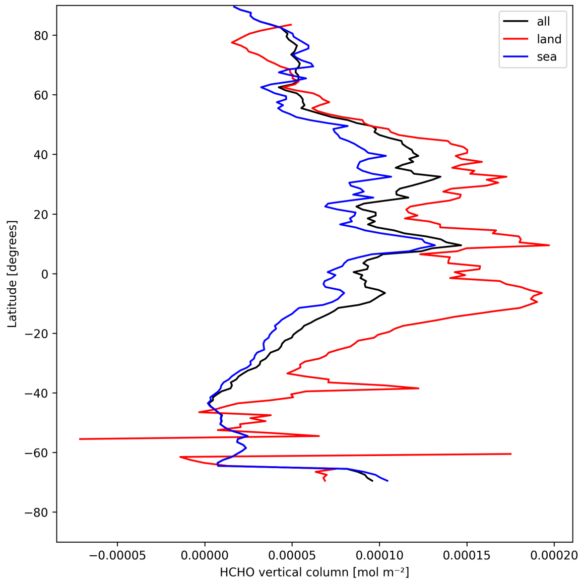
Figure 21: Zonal average of “HCHO vertical column” for 2025-08-10 to 2025-08-12.
