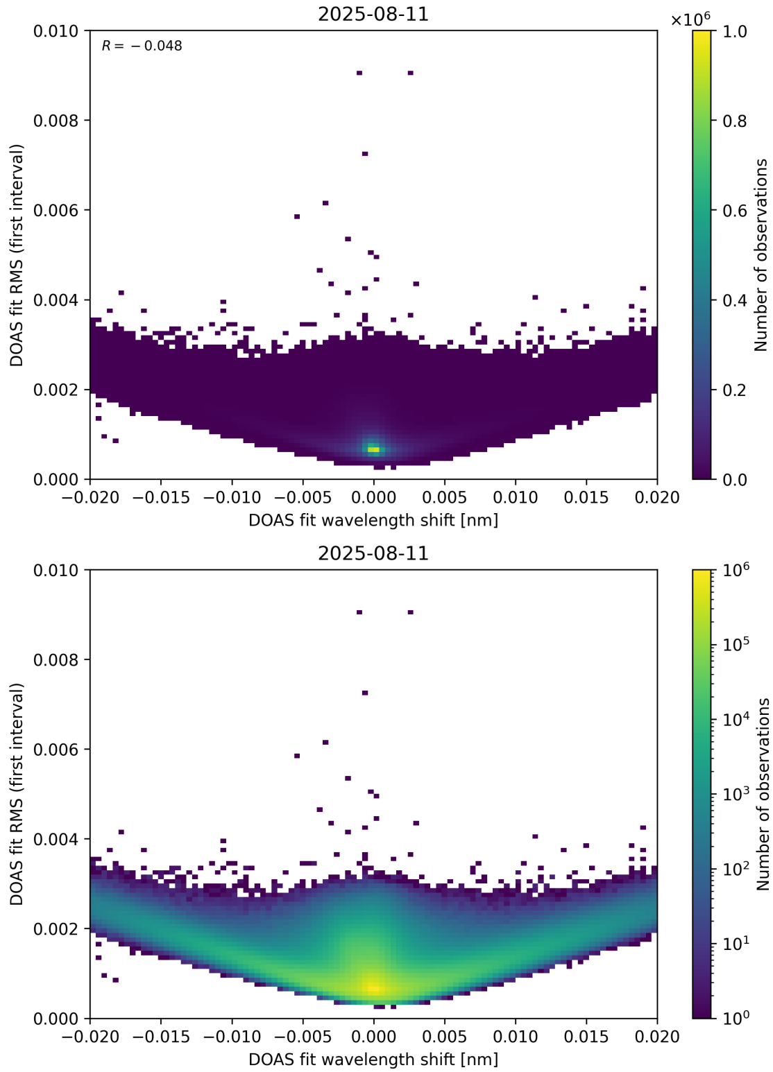
Figure 64: Scatter density plot of “DOAS fit wavelength shift” against “DOAS fit RMS (first interval)” for 2025-08-10 to 2025-08-12.
