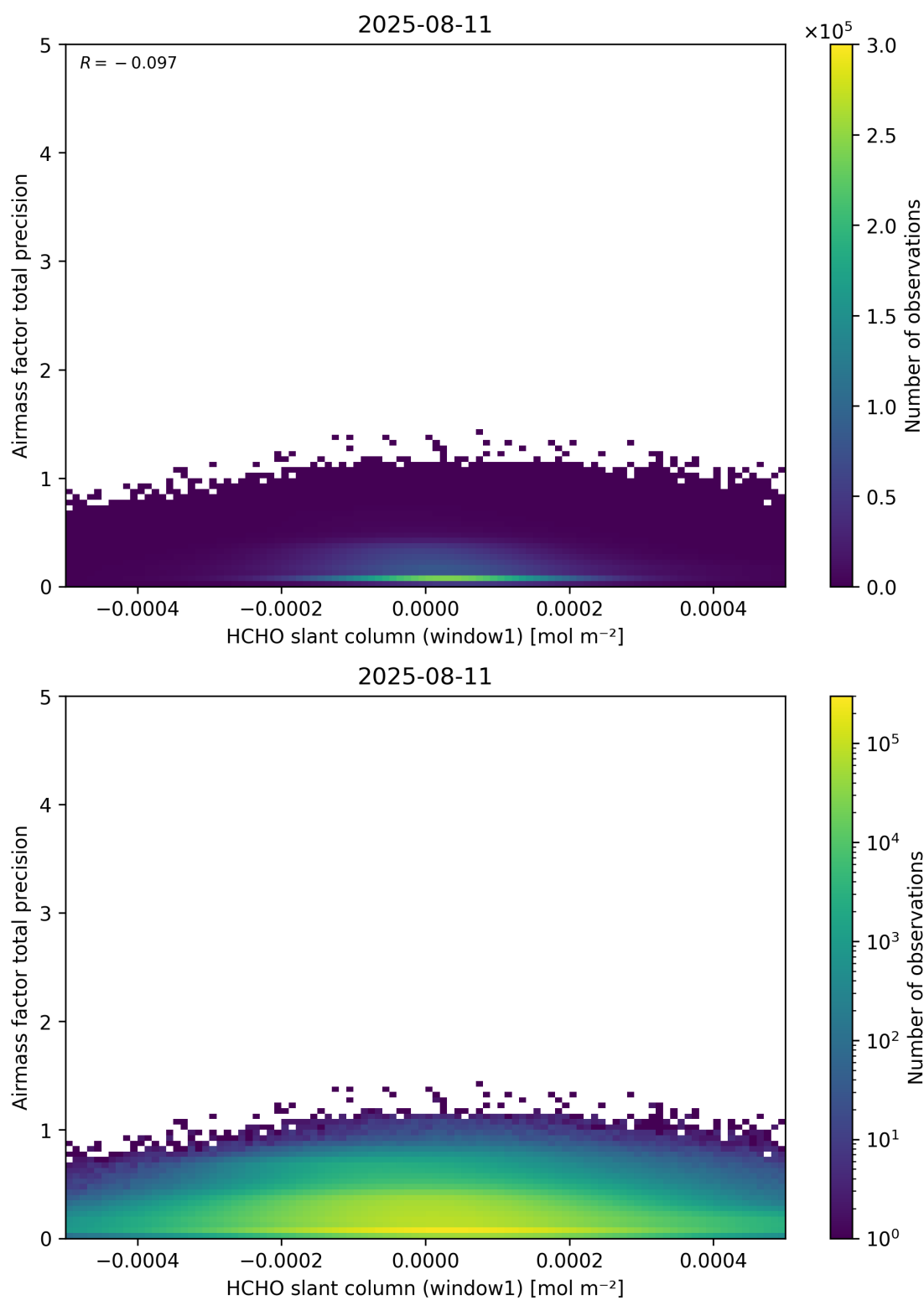
Figure 86: Scatter density plot of “HCHO slant column (window1)” against “Airmass factor total precision” for 2025-08-10 to 2025-08-12.
