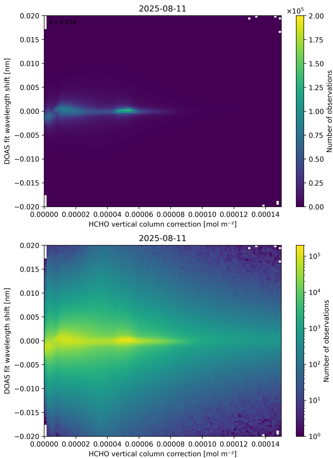
Figure 113: Scatter density plot of “HCHO vertical column correction” against “DOAS fit wavelength shift” for 2025-08-10 to 2025-08-12.
