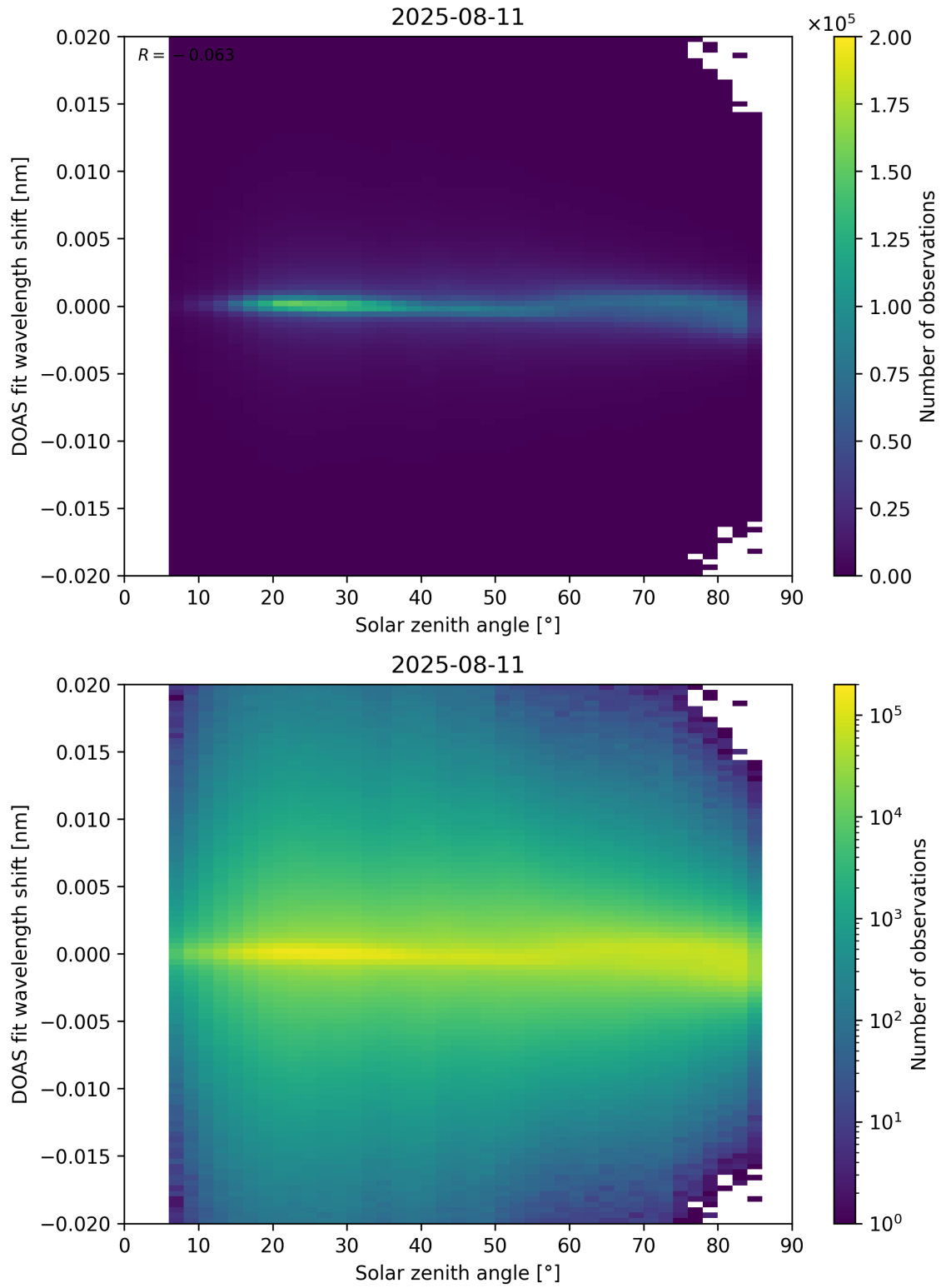
Figure 168: Scatter density plot of “Solar zenith angle” against “DOAS fit wavelength shift” for 2025-08-10 to 2025-08-12.
