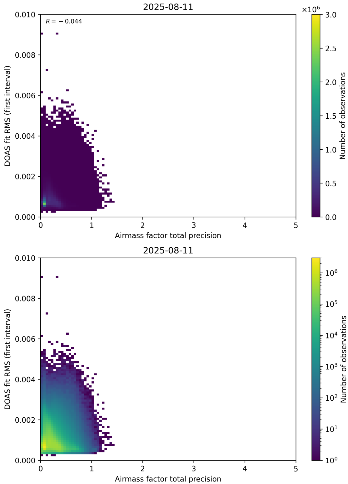
Figure 105: Scatter density plot of “Airmass factor total precision” against “DOAS fit RMS (first interval)” for 2025-08-10 to 2025-08-12.
