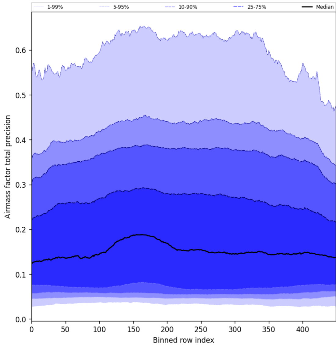
Figure 55: Along track statistics of “Airmass factor total precision” for 2025-08-10 to 2025-08-12
