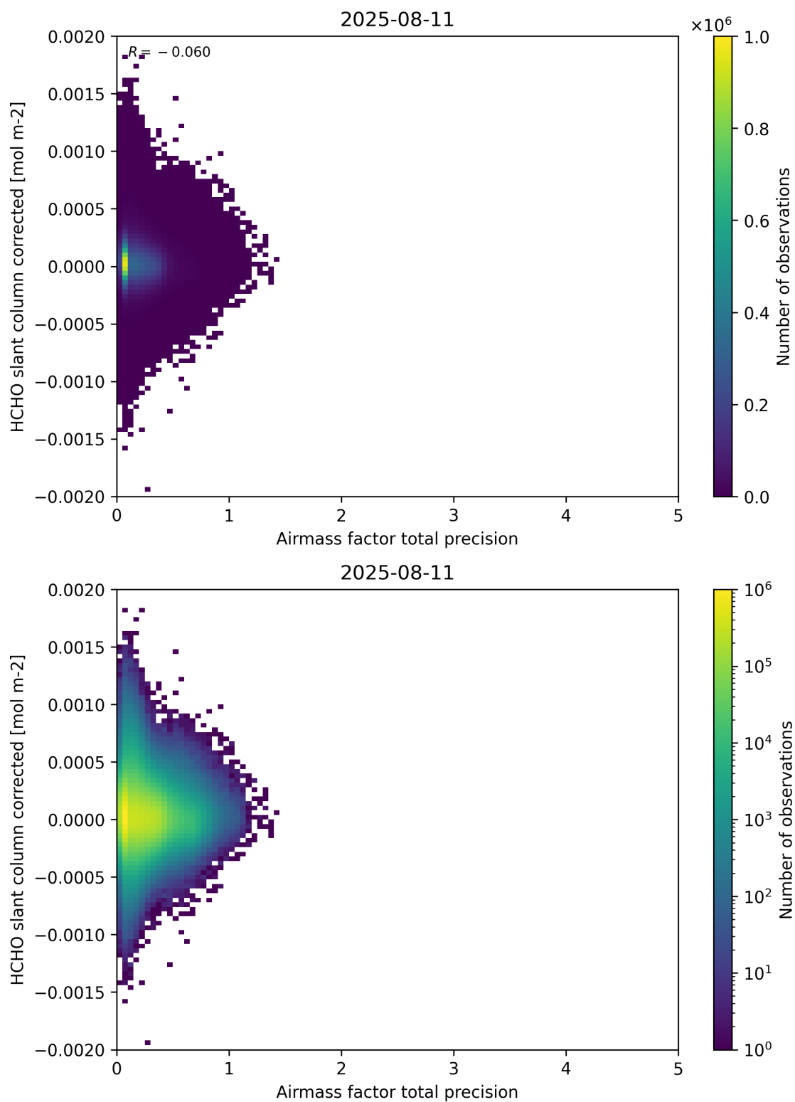
Figure 109: Scatter density plot of “Airmass factor total precision” against “HCHO slant column corrected” for 2025-08-10 to 2025-08-12.
