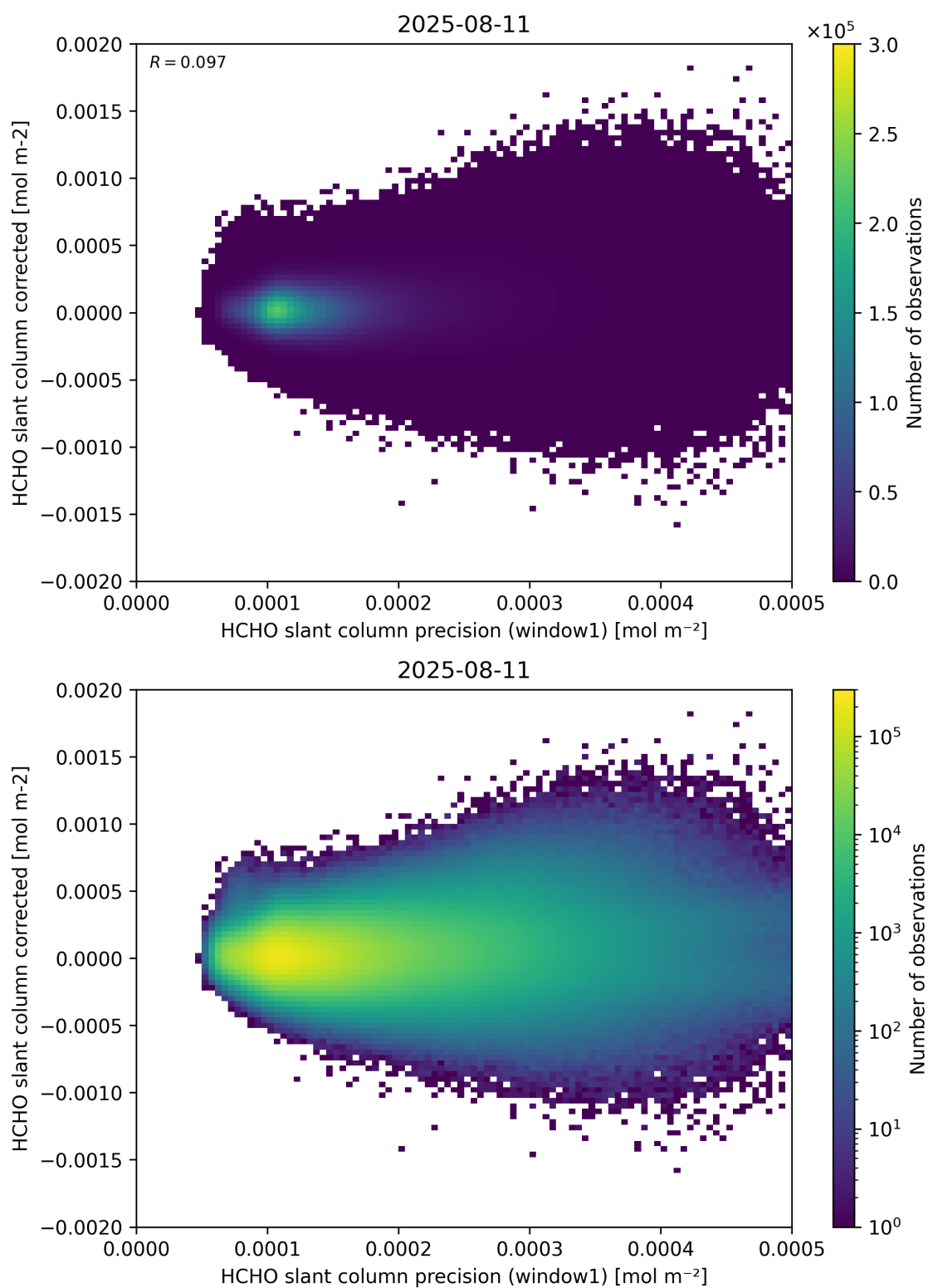
Figure 92: Scatter density plot of “HCHO slant column precision (window1)” against “HCHO slant column corrected” for 2025-08-10 to 2025-08-12.
