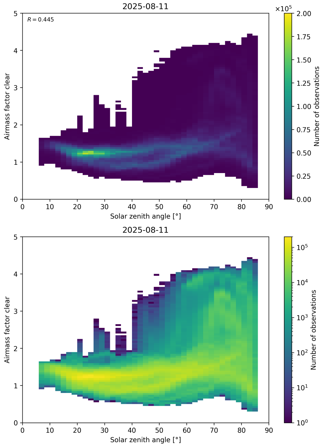
Figure 170: Scatter density plot of “Solar zenith angle” against “Airmass factor clear” for 2025-08-10 to 2025-08-12.
