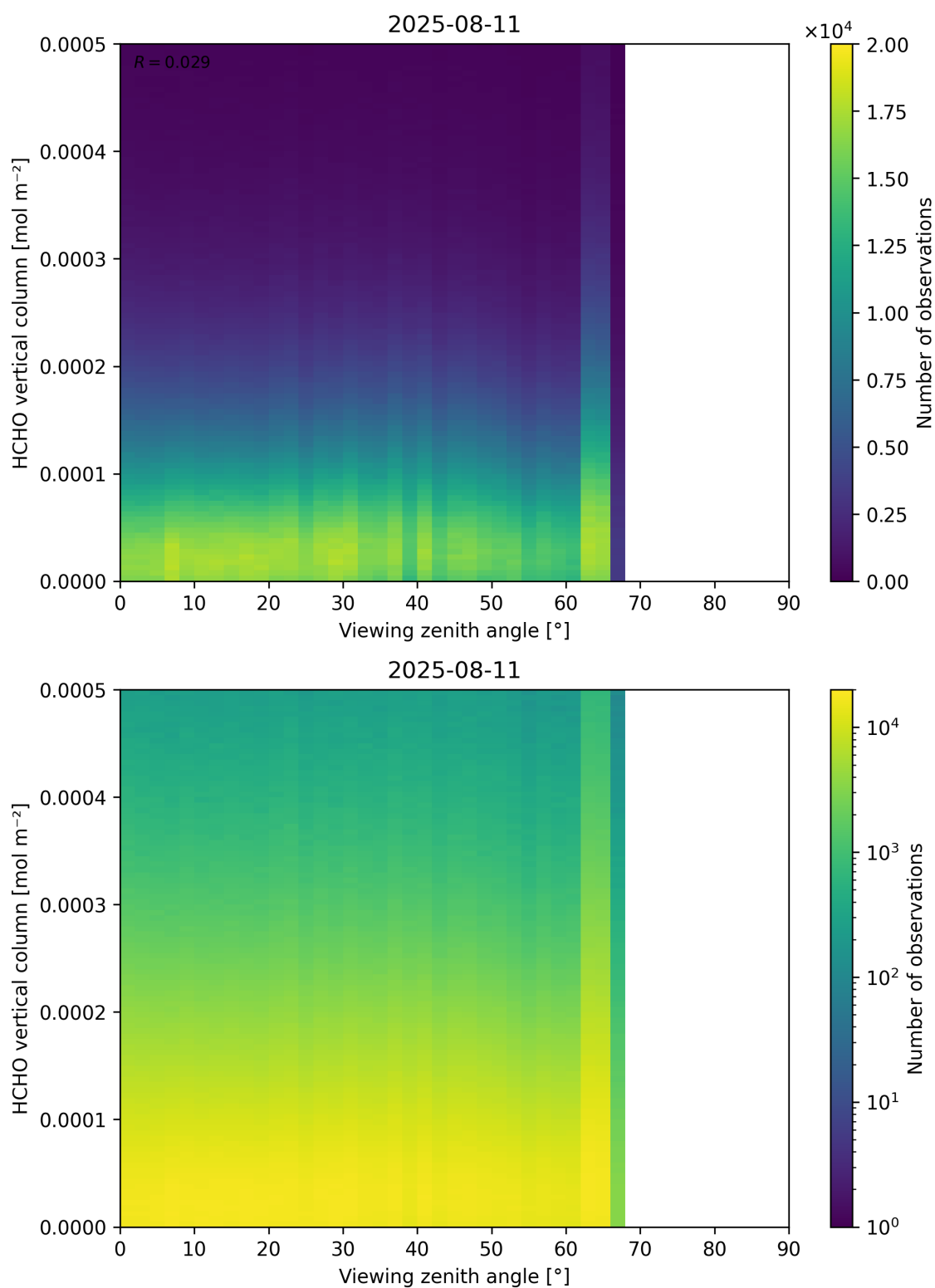
Figure 192: Scatter density plot of “Viewing zenith angle” against “HCHO vertical column” for 2025-08-10 to 2025-08-12.
