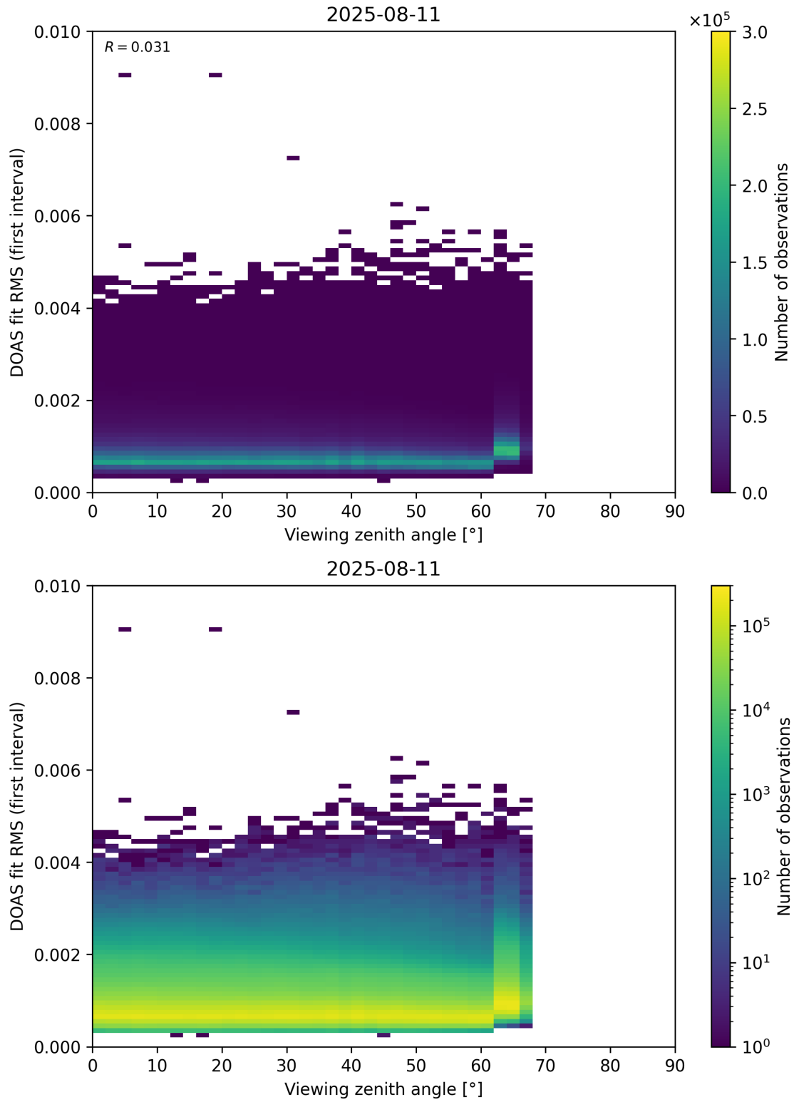
Figure 182: Scatter density plot of “Viewing zenith angle” against “DOAS fit RMS (first interval)” for 2025-08-10 to 2025-08-12.
