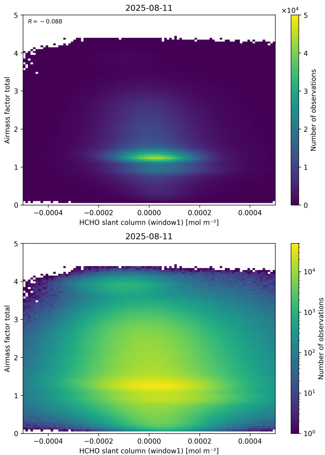
Figure 85: Scatter density plot of “HCHO slant column (window1)” against “Airmass factor total” for 2025-08-10 to 2025-08-12.
