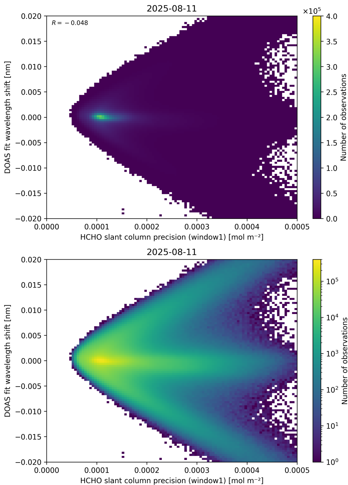
Figure 89: Scatter density plot of “HCHO slant column precision (window1)” against “DOAS fit wavelength shift” for 2025-08-10 to 2025-08-12.
