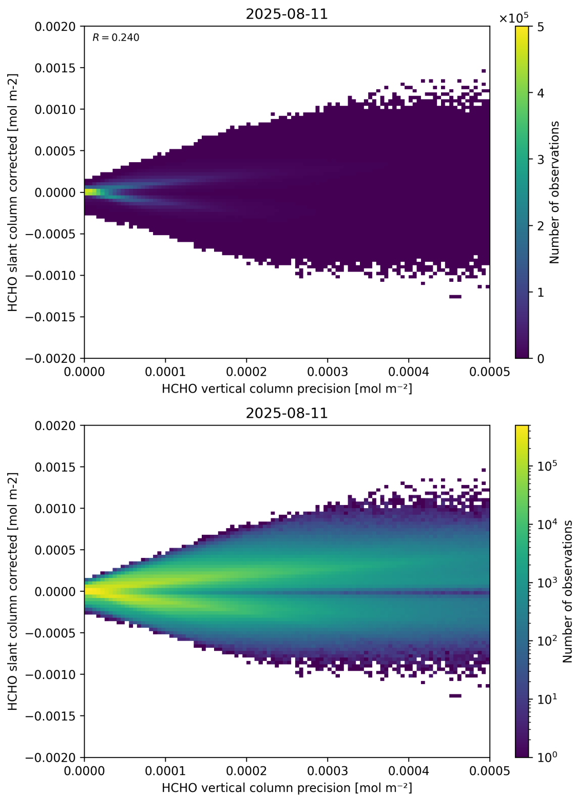
Figure 140: Scatter density plot of “HCHO vertical column precision” against “HCHO slant column corrected” for 2025-08-10 to 2025-08-12.
