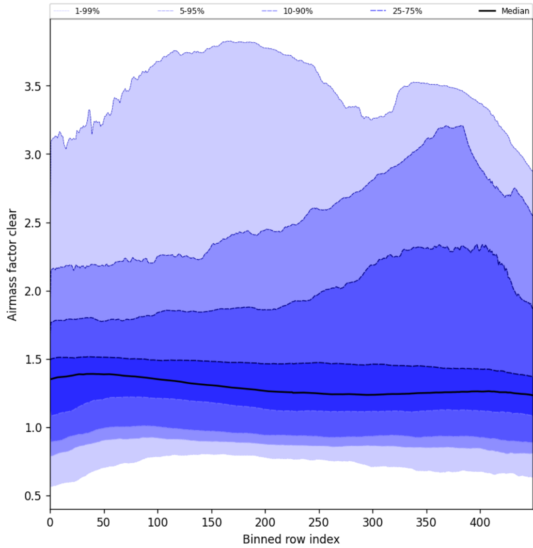
Figure 56: Along track statistics of “Airmass factor clear” for 2025-08-10 to 2025-08-12
