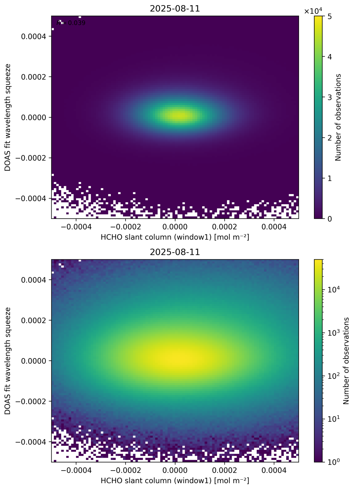
Figure 80: Scatter density plot of “HCHO slant column (window1)” against “DOAS fit wavelength squeeze” for 2025-08-10 to 2025-08-12.
