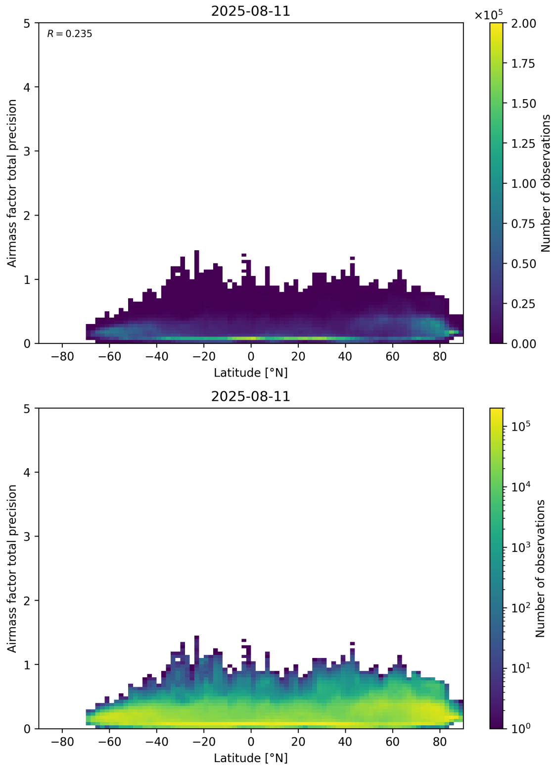
Figure 162: Scatter density plot of “Latitude” against “Airmass factor total precision” for 2025-08-10 to 2025-08-12.
