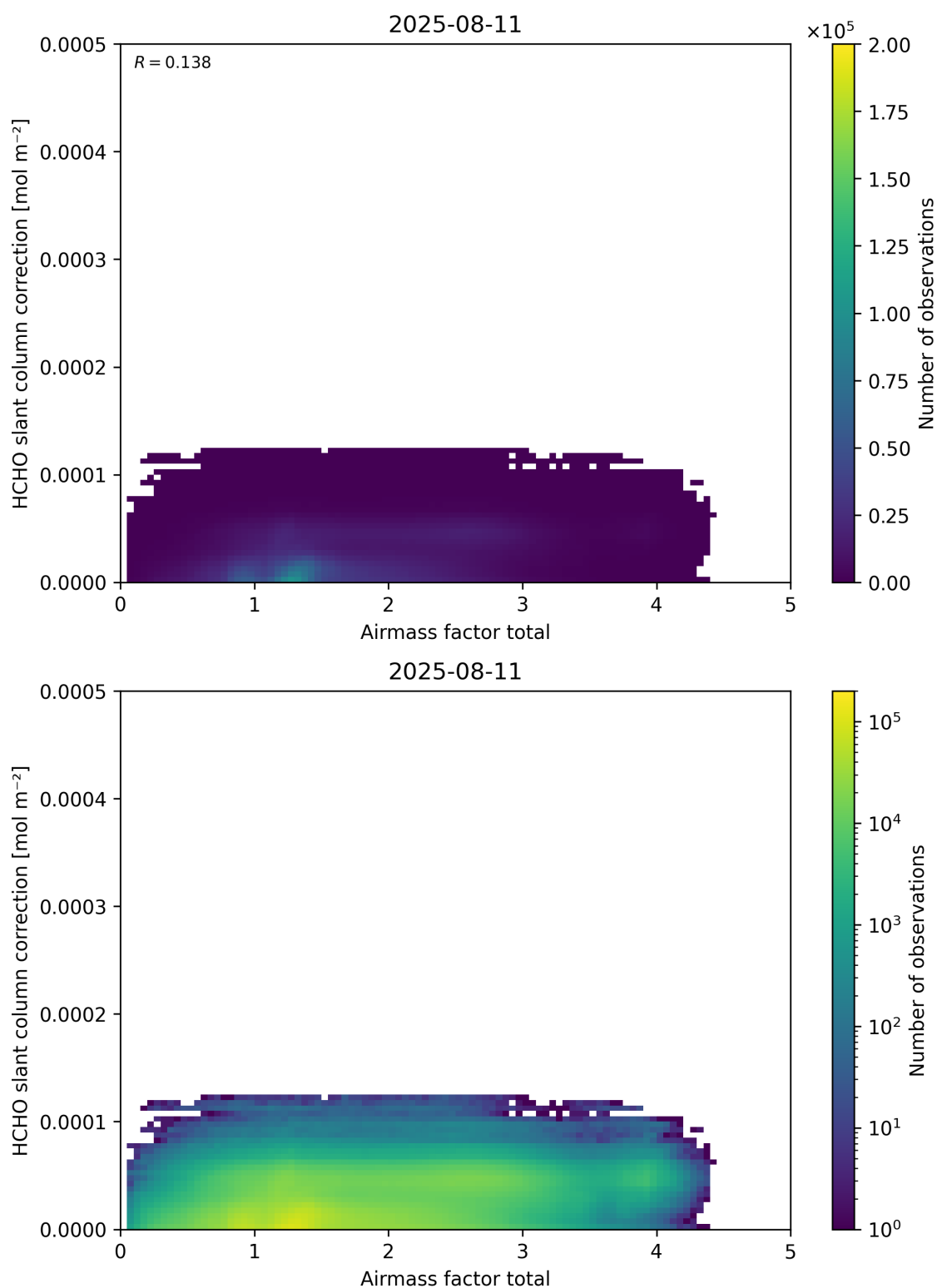
Figure 102: Scatter density plot of “Airmass factor total” against “HCHO slant column correction” for 2025-08-10 to 2025-08-12.
