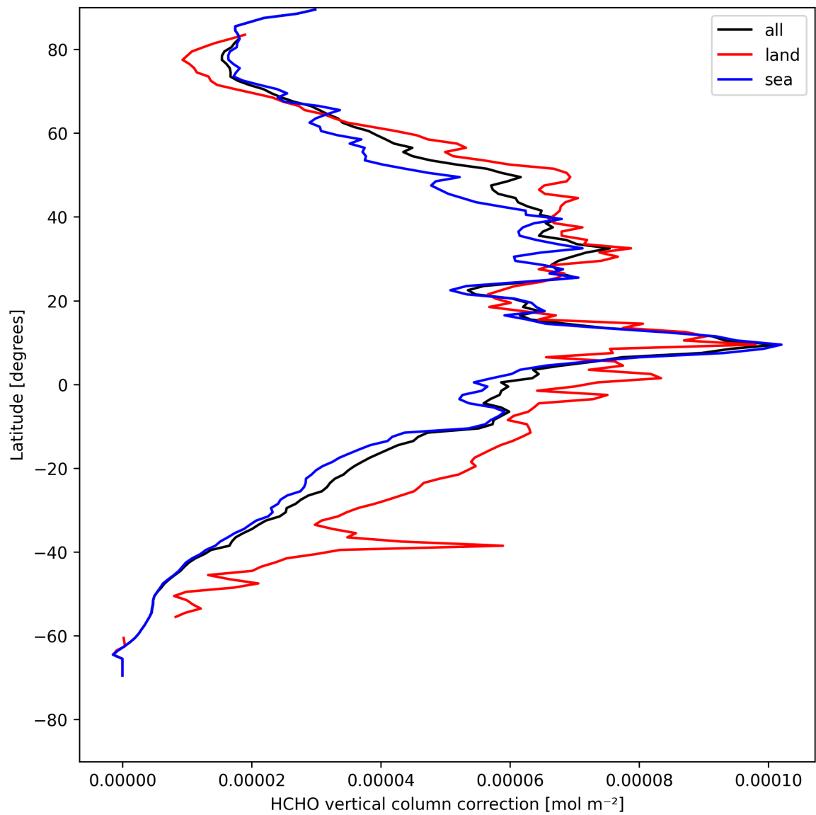
Figure 23: Zonal average of “HCHO vertical column correction” for 2025-08-10 to 2025-08-12.
