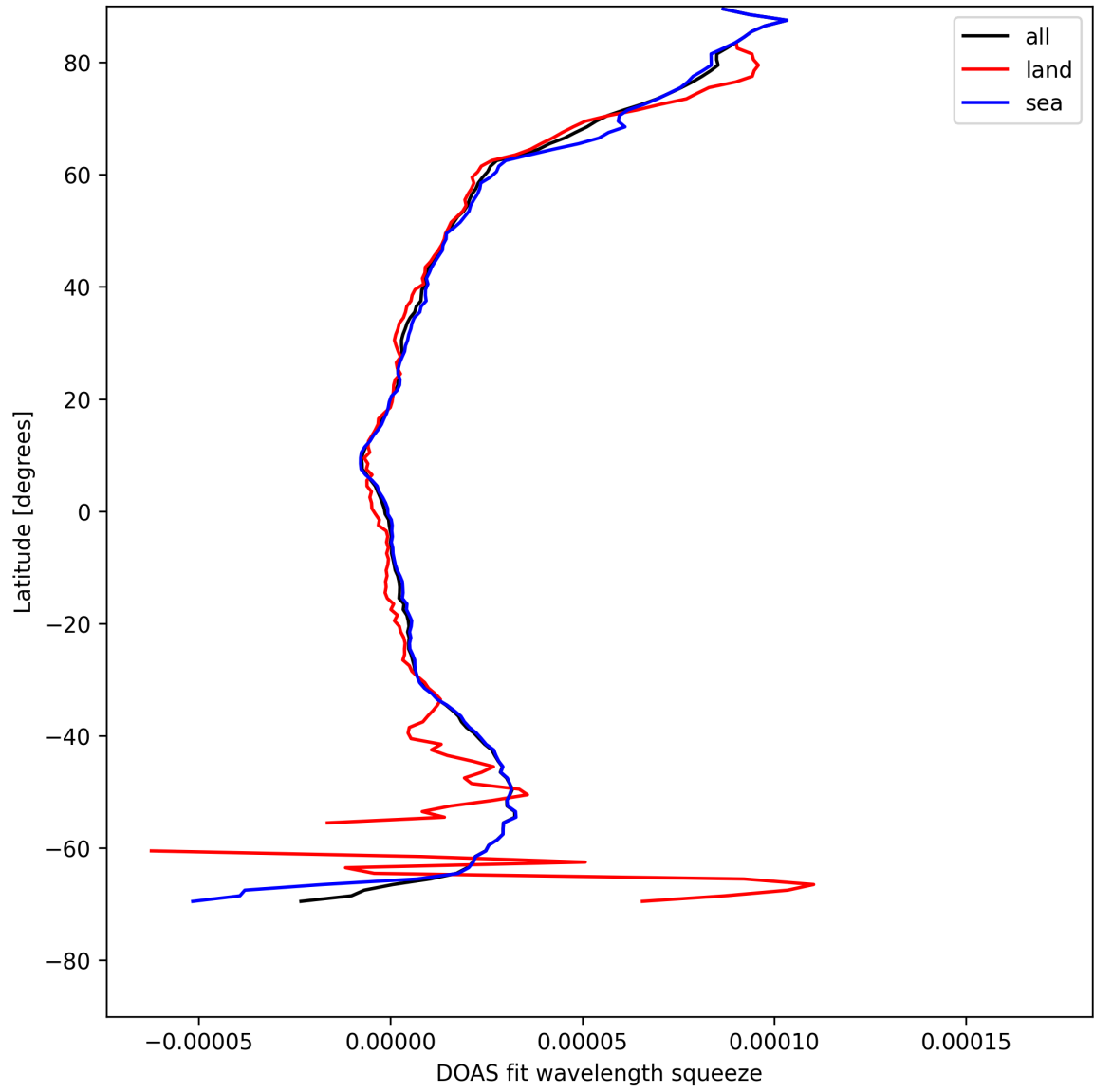
Figure 31: Zonal average of “DOAS fit wavelength squeeze” for 2025-08-10 to 2025-08-12.
