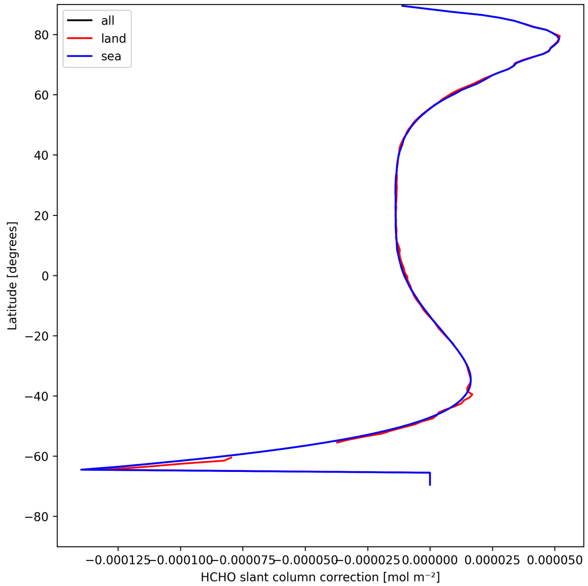
Figure 33: Zonal average of “HCHO slant column correction” for 2025-08-10 to 2025-08-12.
