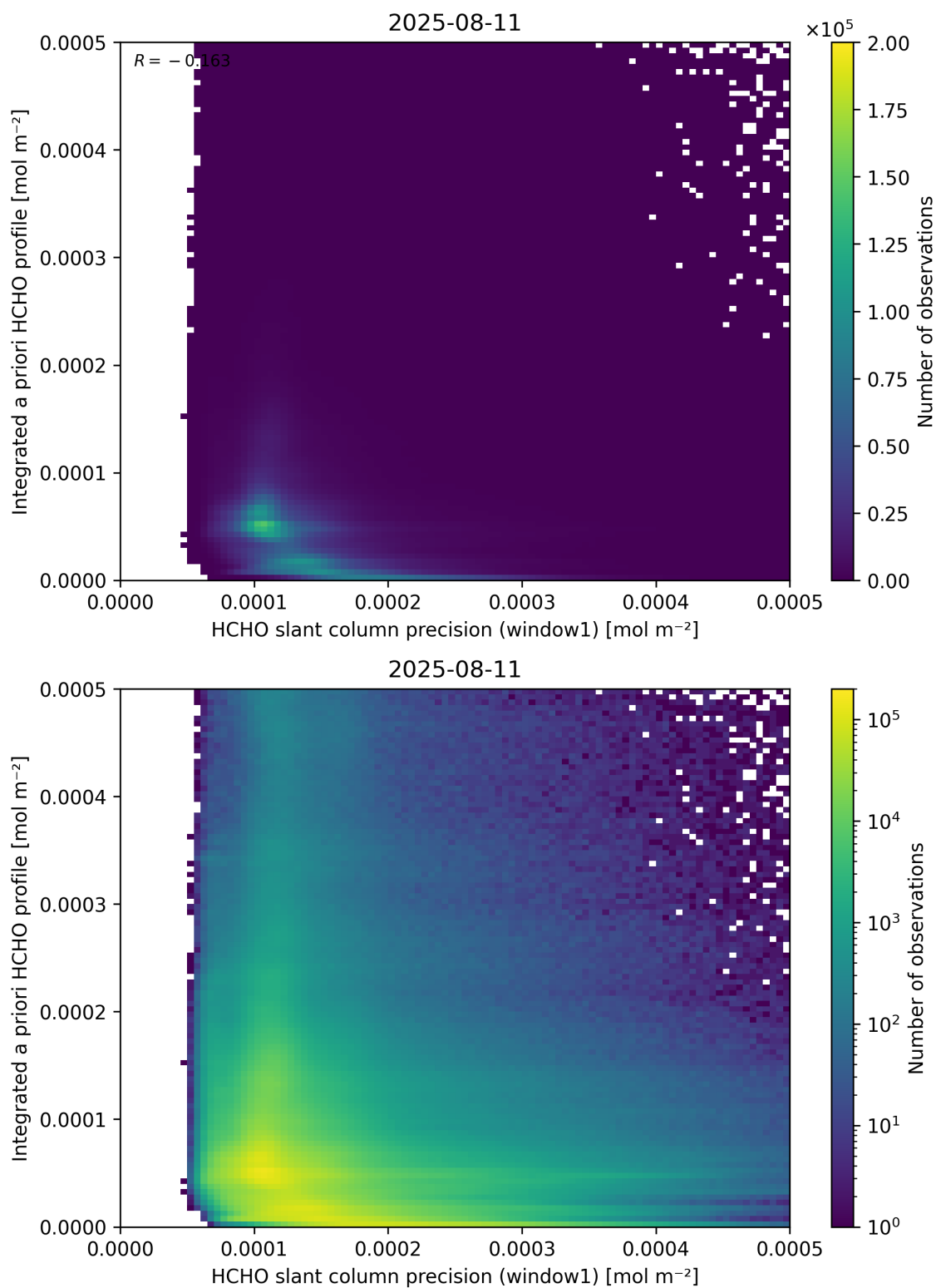
Figure 96: Scatter density plot of “HCHO slant column precision (window1)” against “Integrated a priori HCHO profile” for 2025-08-10 to 2025-08-12.
