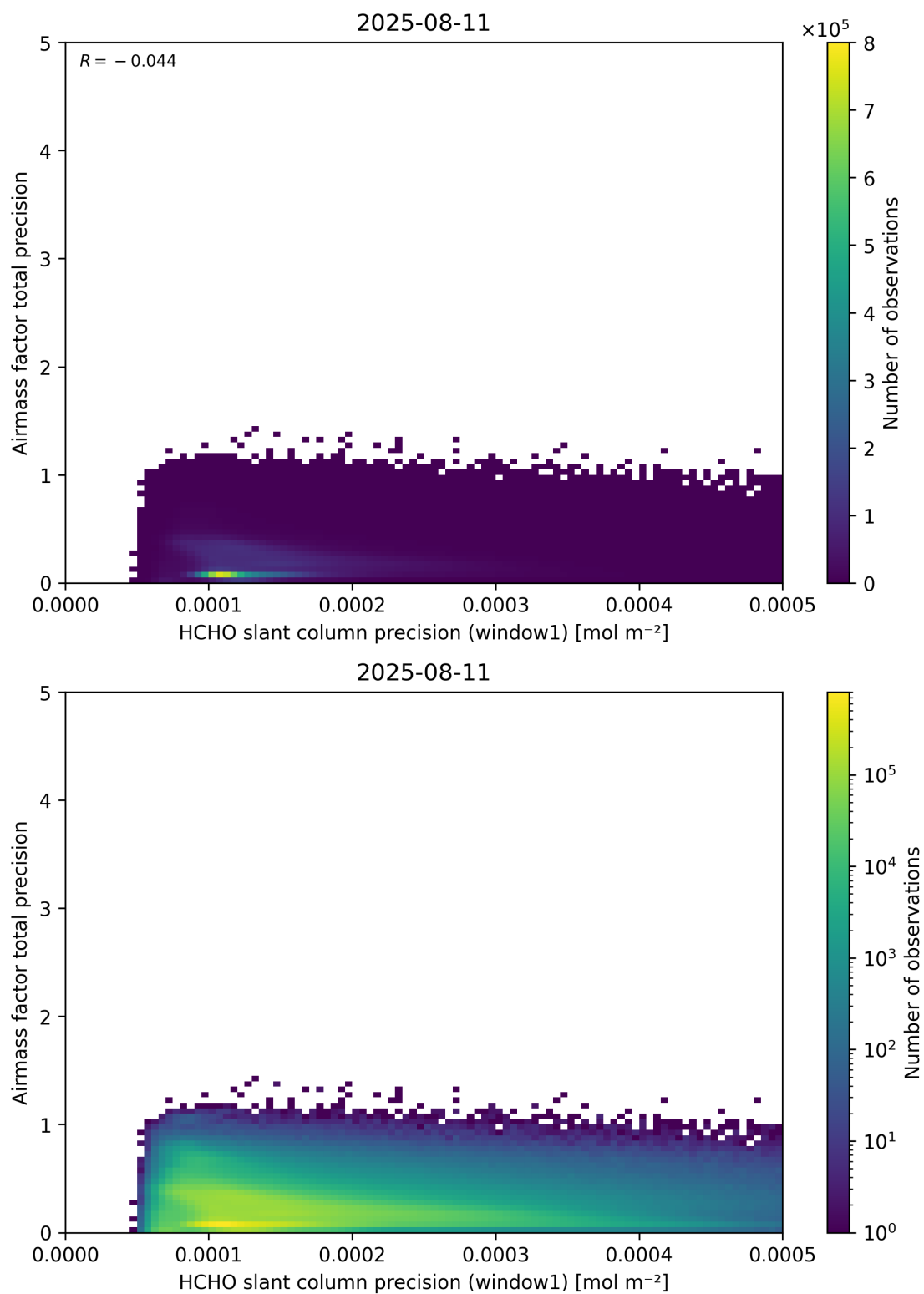
Figure 95: Scatter density plot of “HCHO slant column precision (window1)” against “Airmass factor total precision” for 2025-08-10 to 2025-08-12.
