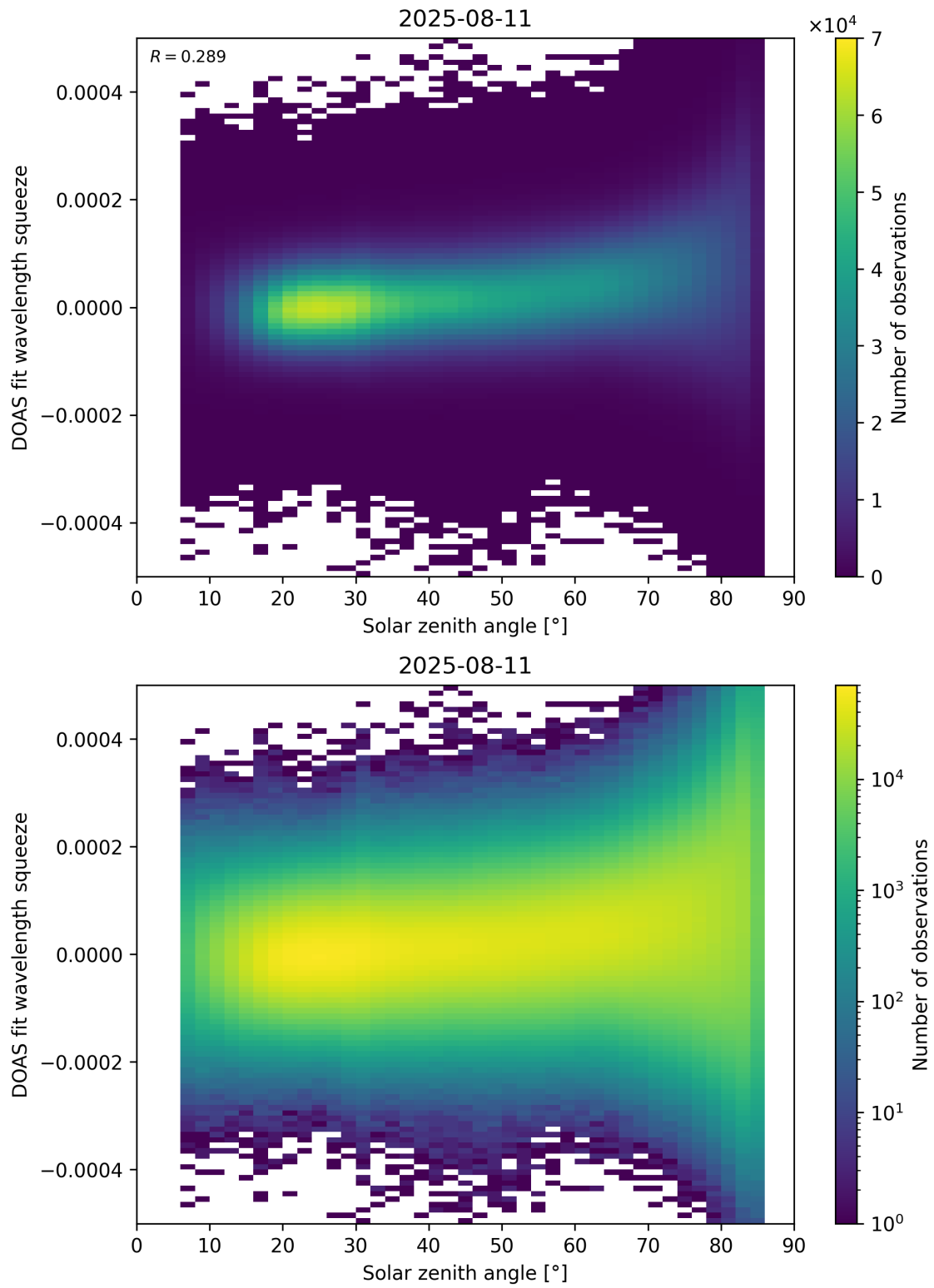
Figure 169: Scatter density plot of “Solar zenith angle” against “DOAS fit wavelength squeeze” for 2025-08-10 to 2025-08-12.
