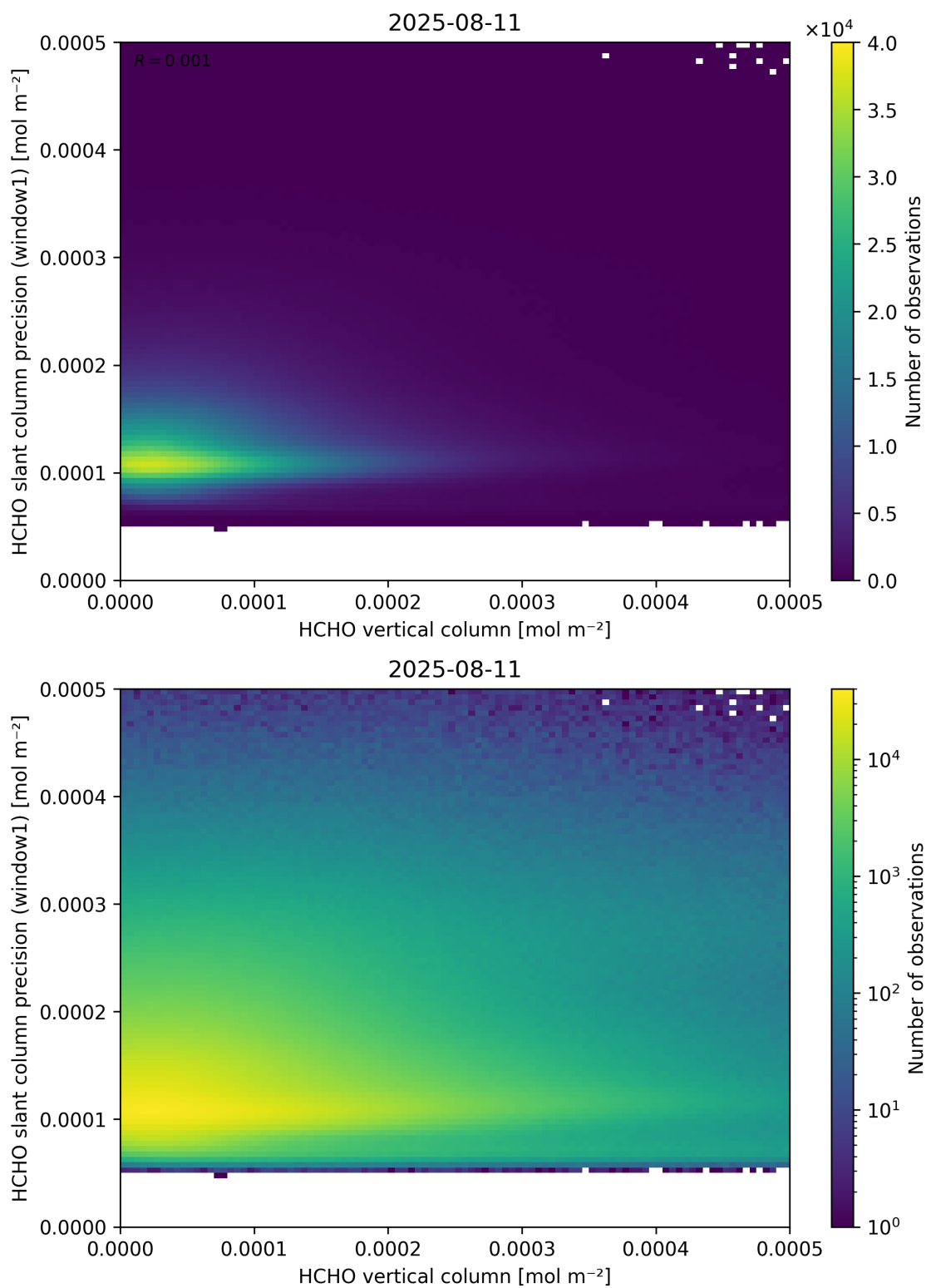
Figure 130: Scatter density plot of “HCHO vertical column” against “HCHO slant column precision (window1)” for 2025-08-10 to 2025-08-12.
