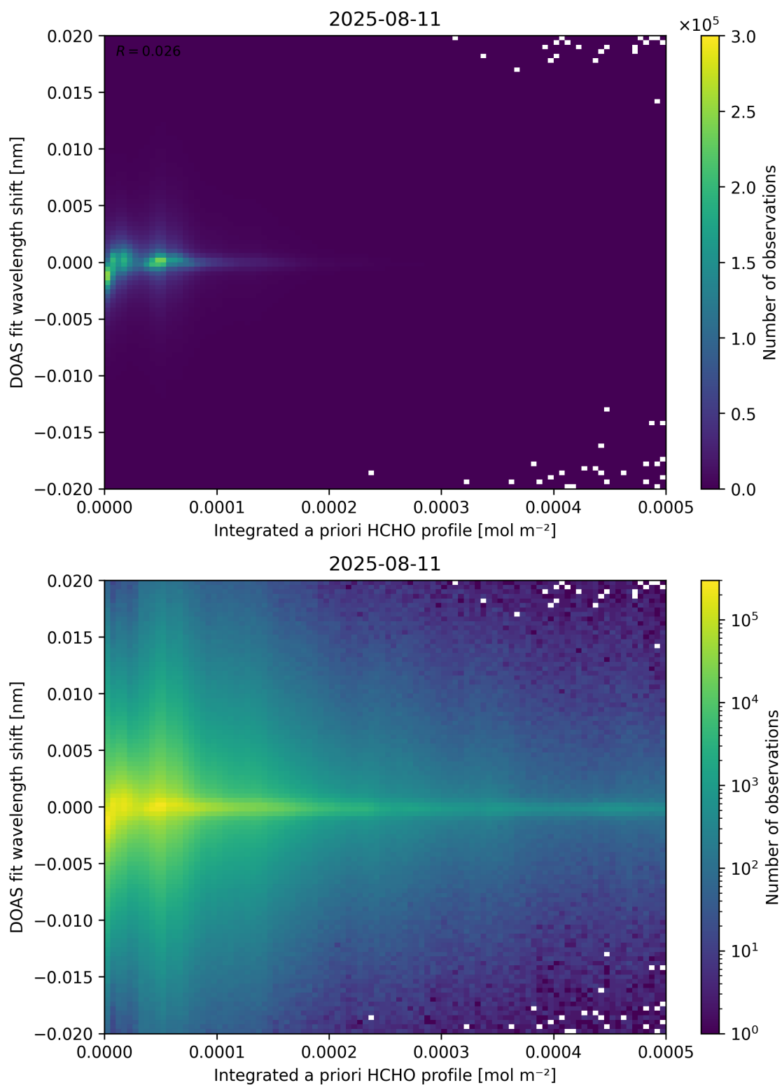
Figure 149: Scatter density plot of “Integrated a priori HCHO profile” against “DOAS fit wavelength shift” for 2025-08-10 to 2025-08-12.
