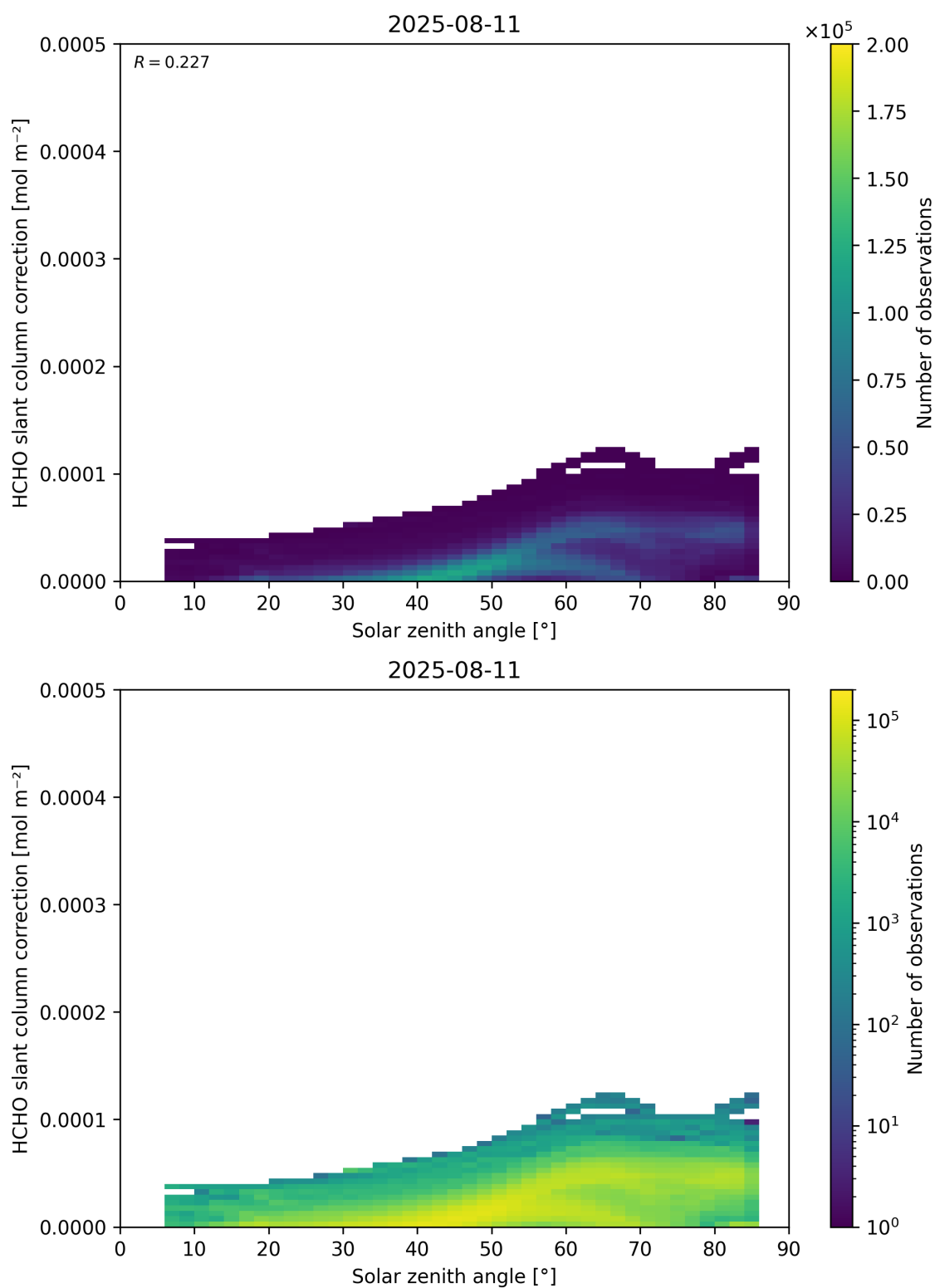
Figure 172: Scatter density plot of “Solar zenith angle” against “HCHO slant column correction” for 2025-08-10 to 2025-08-12.
