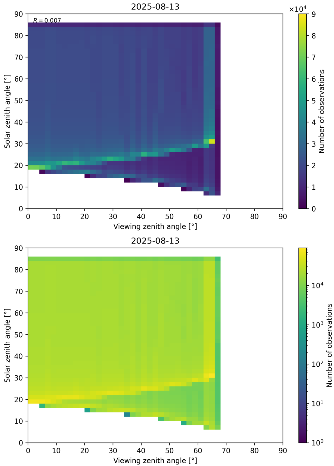
Figure 197: Scatter density plot of “Viewing zenith angle” against “Solar zenith angle” for 2025-08-12 to 2025-08-14.
