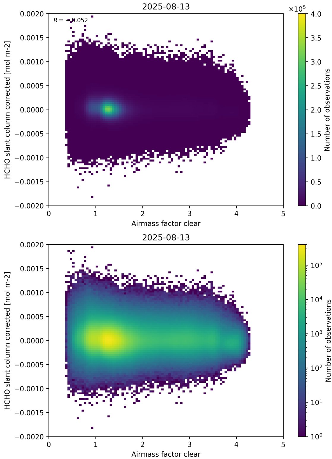
Figure 74: Scatter density plot of “Airmass factor clear” against “HCHO slant column corrected” for 2025-08-12 to 2025-08-14.
