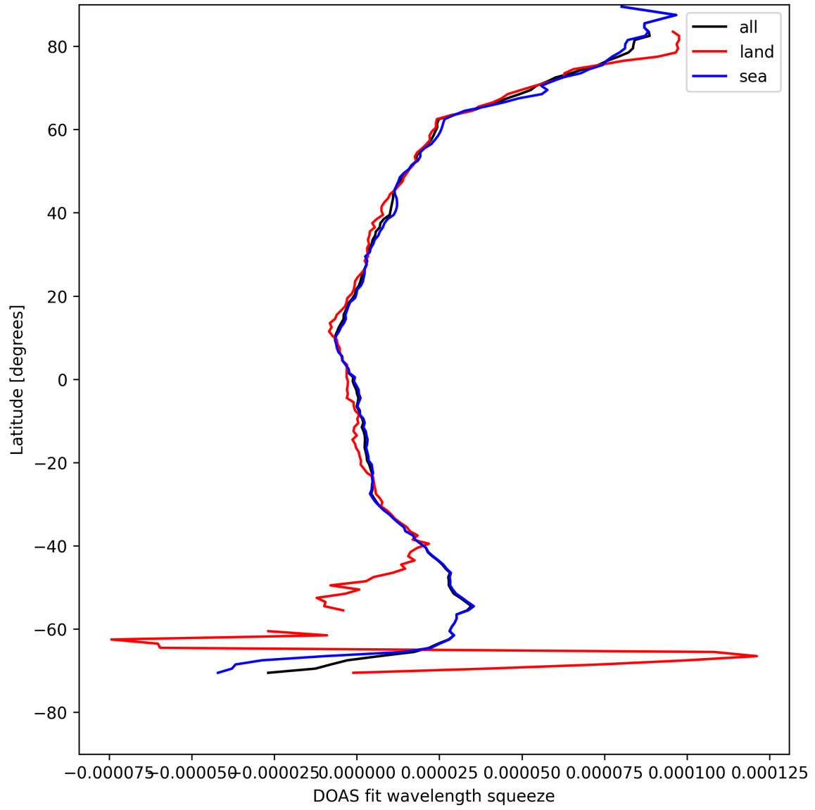
Figure 31: Zonal average of “DOAS fit wavelength squeeze” for 2025-08-12 to 2025-08-14.
