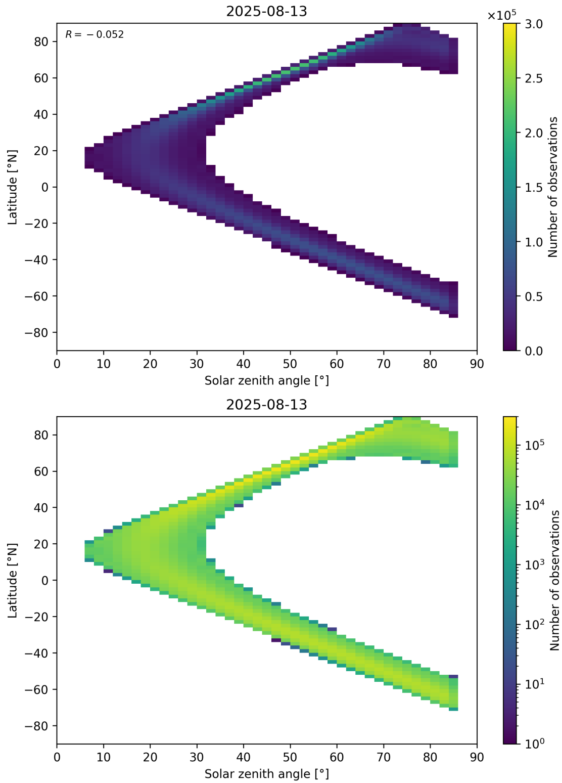
Figure 181: Scatter density plot of “Solar zenith angle” against “Latitude” for 2025-08-12 to 2025-08-14.
