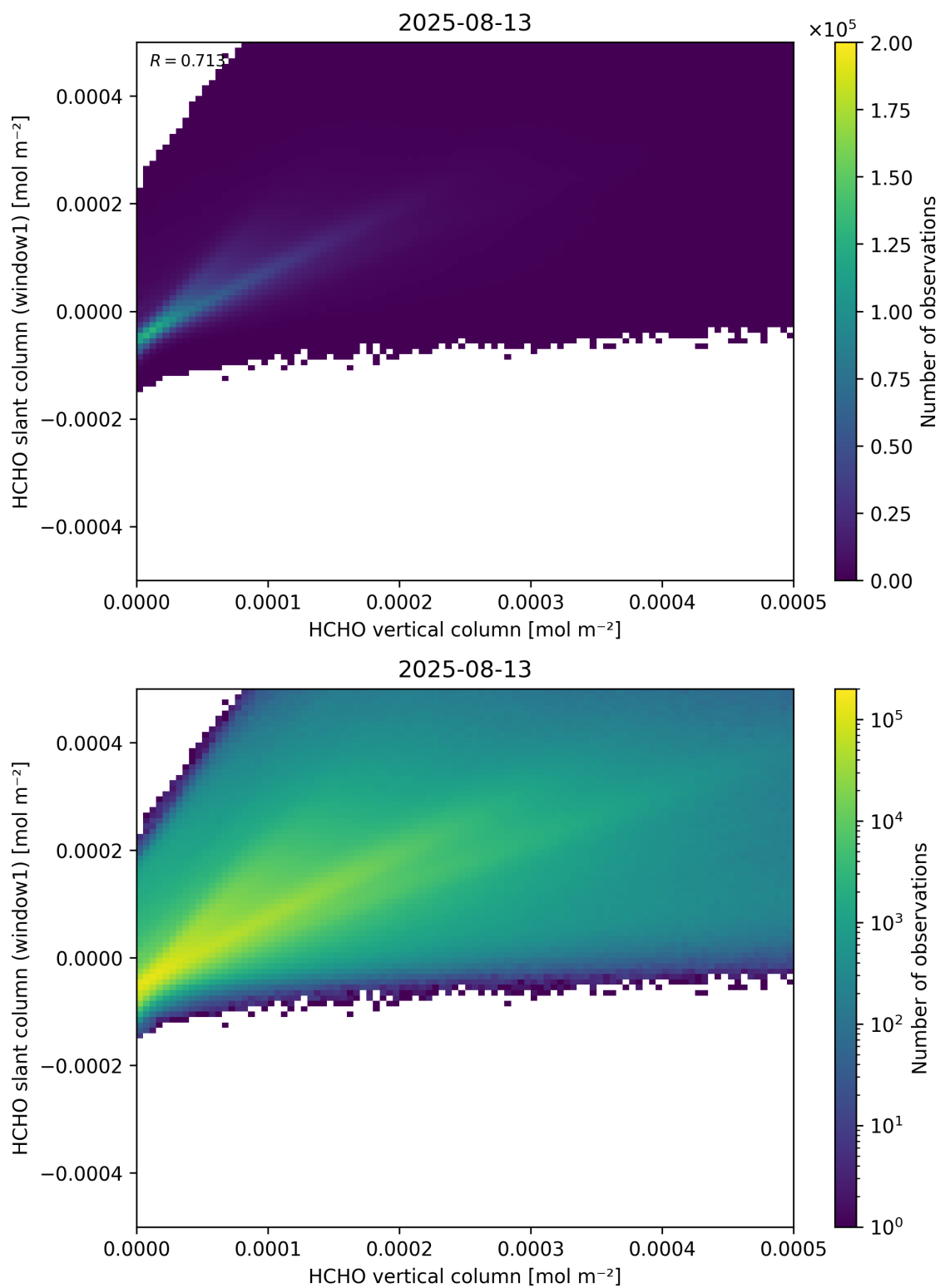
Figure 129: Scatter density plot of “HCHO vertical column” against “HCHO slant column (window1)” for 2025-08-12 to 2025-08-14.
