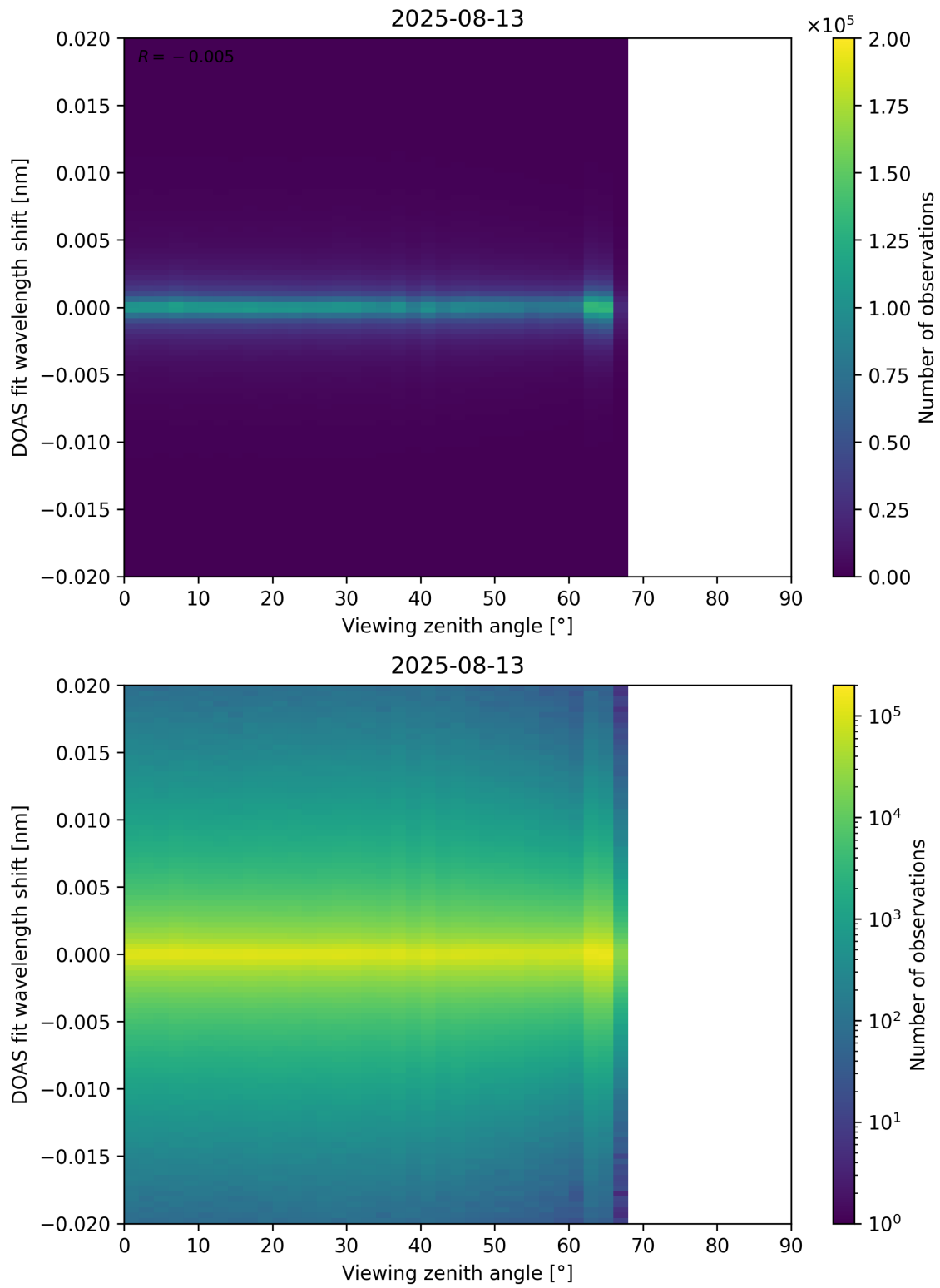
Figure 183: Scatter density plot of “Viewing zenith angle” against “DOAS fit wavelength shift” for 2025-08-12 to 2025-08-14.
