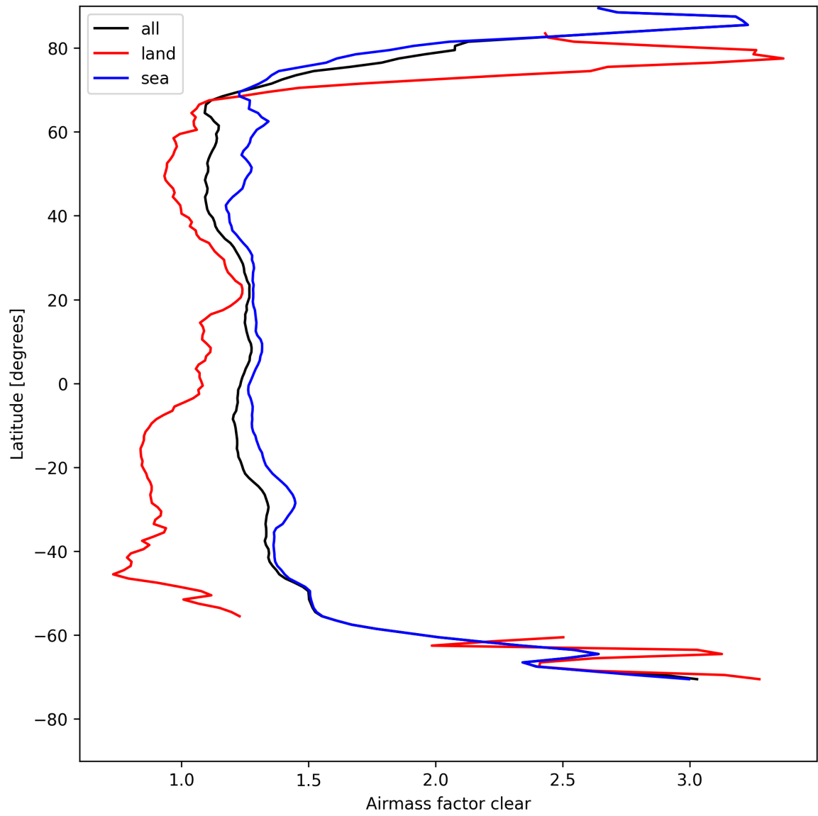
Figure 28: Zonal average of “Airmass factor clear” for 2025-08-12 to 2025-08-14.
