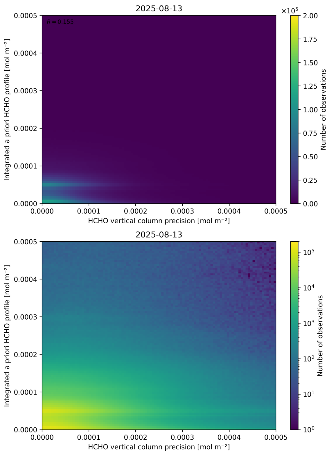
Figure 147: Scatter density plot of “HCHO vertical column precision” against “Integrated a priori HCHO profile” for 2025-08-12 to 2025-08-14.
