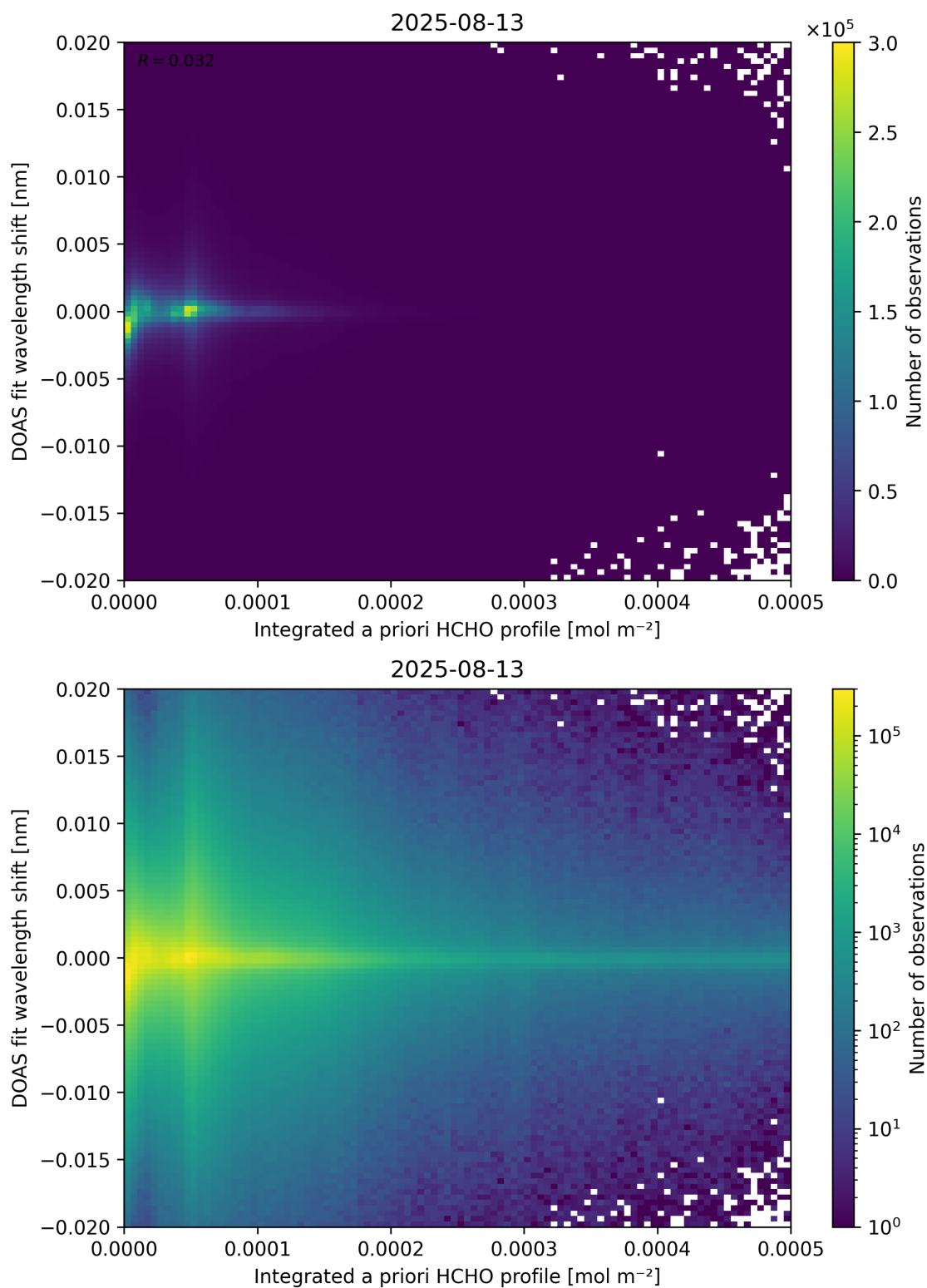
Figure 149: Scatter density plot of “Integrated a priori HCHO profile” against “DOAS fit wavelength shift” for 2025-08-12 to 2025-08-14.
