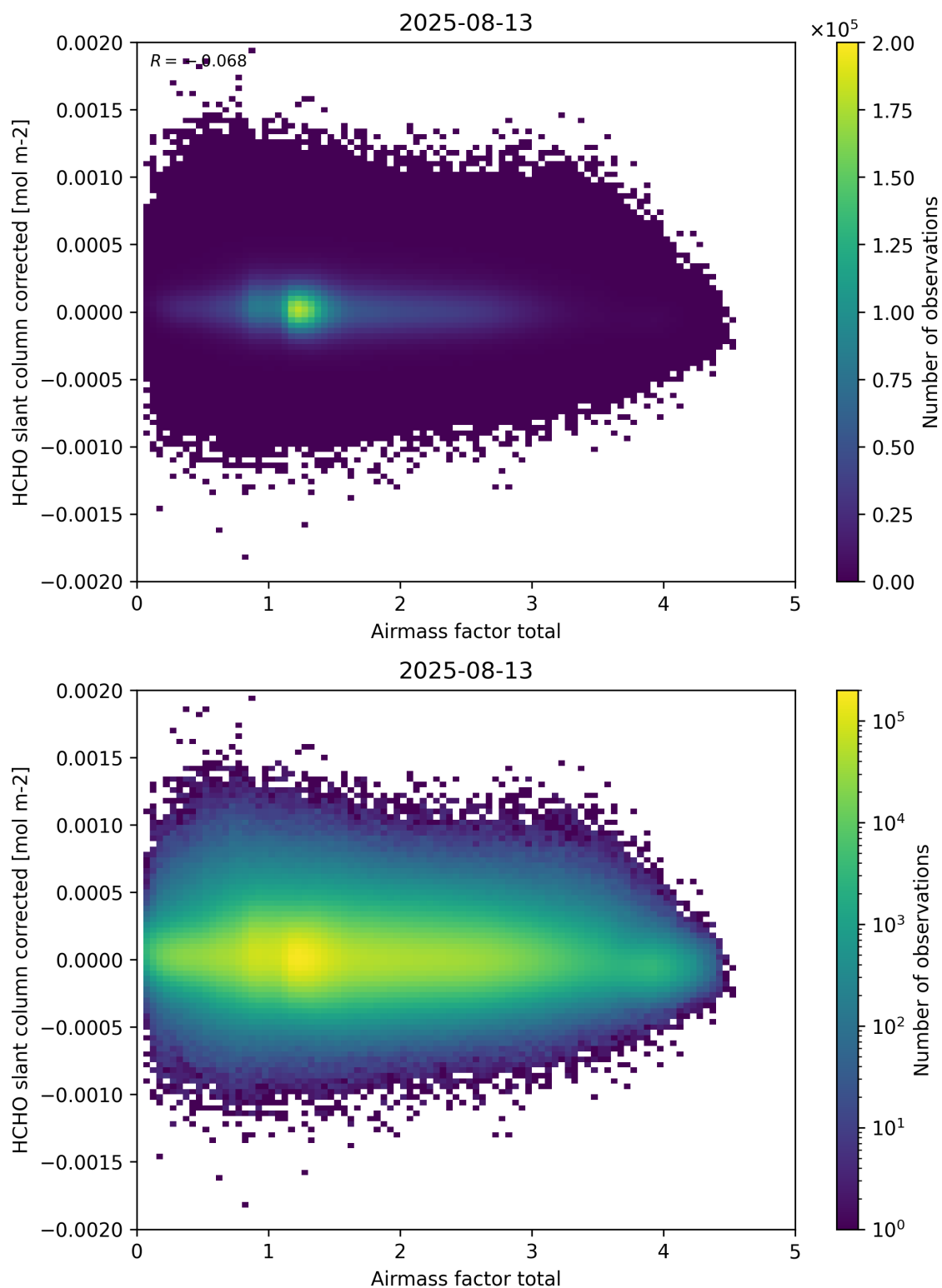
Figure 101: Scatter density plot of “Airmass factor total” against “HCHO slant column corrected” for 2025-08-12 to 2025-08-14.
