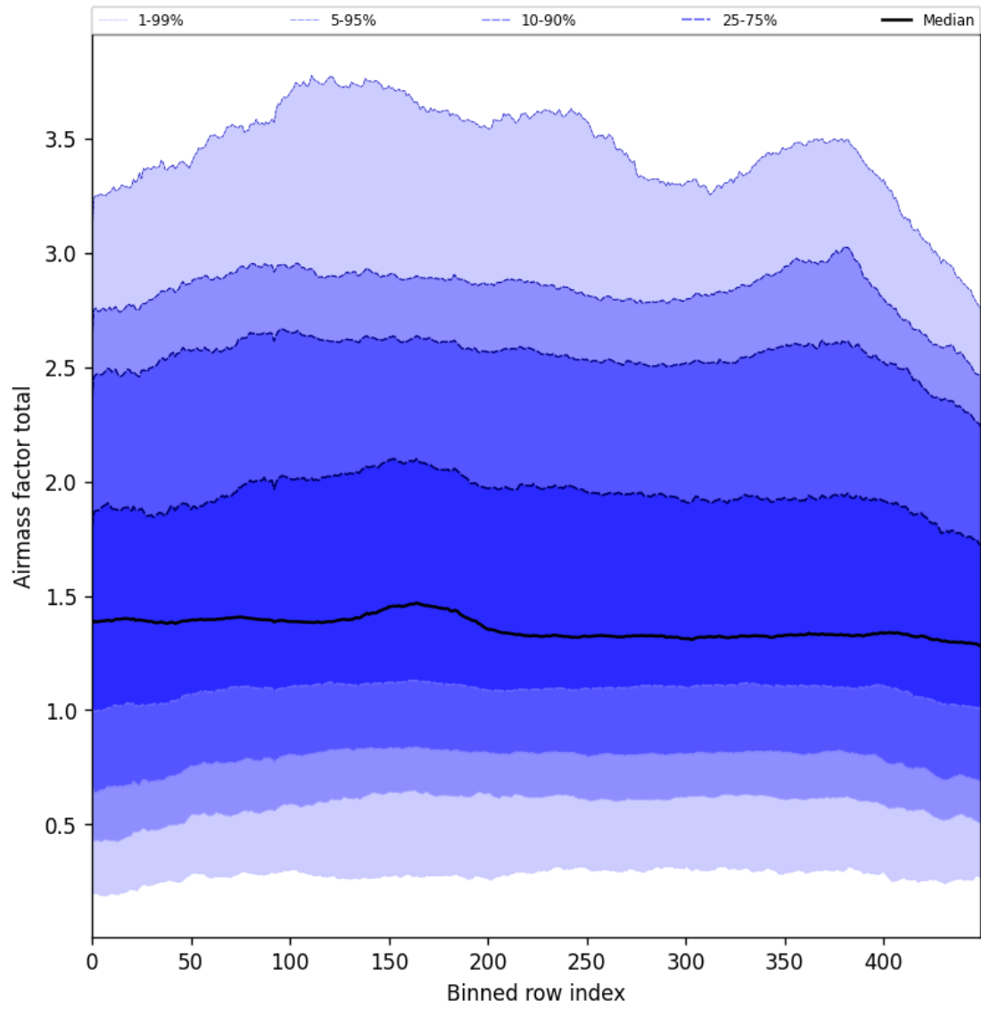
Figure 54: Along track statistics of “Airmass factor total” for 2025-08-12 to 2025-08-14
