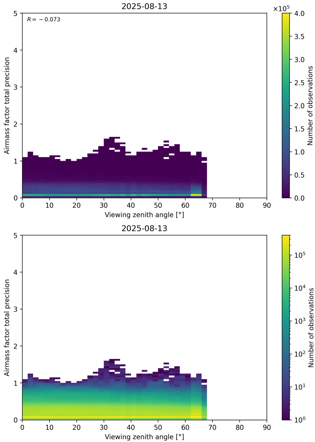
Figure 191: Scatter density plot of “Viewing zenith angle” against “Airmass factor total precision” for 2025-08-12 to 2025-08-14.
