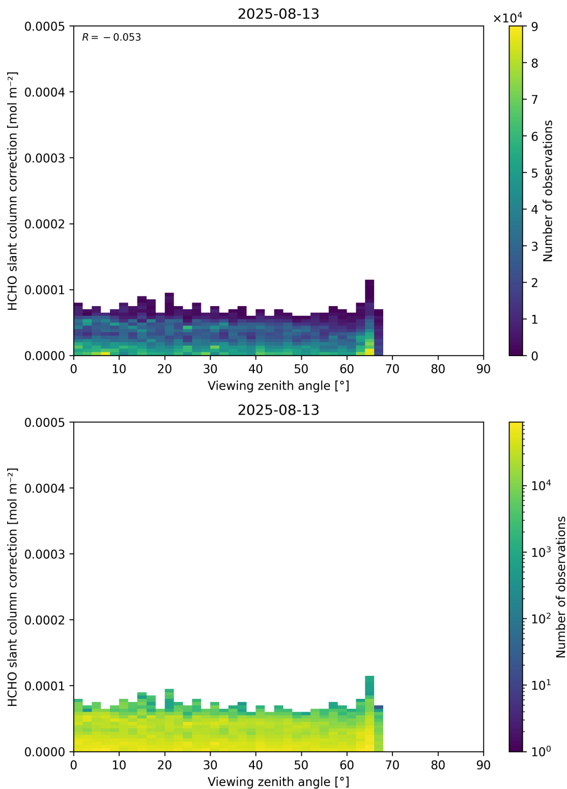
Figure 187: Scatter density plot of “Viewing zenith angle” against “HCHO slant column correction” for 2025-08-12 to 2025-08-14.
