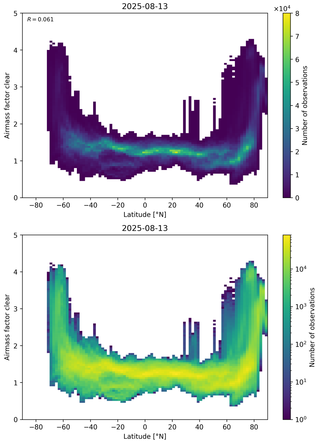
Figure 156: Scatter density plot of “Latitude” against “Airmass factor clear” for 2025-08-12 to 2025-08-14.
