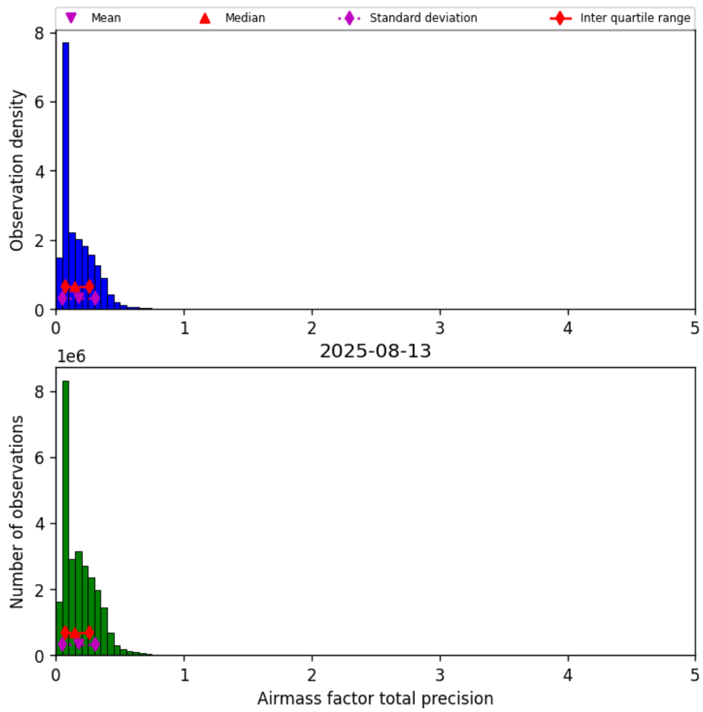
Figure 41: Histogram of “Airmass factor total precision” for 2025-08-12 to 2025-08-14
