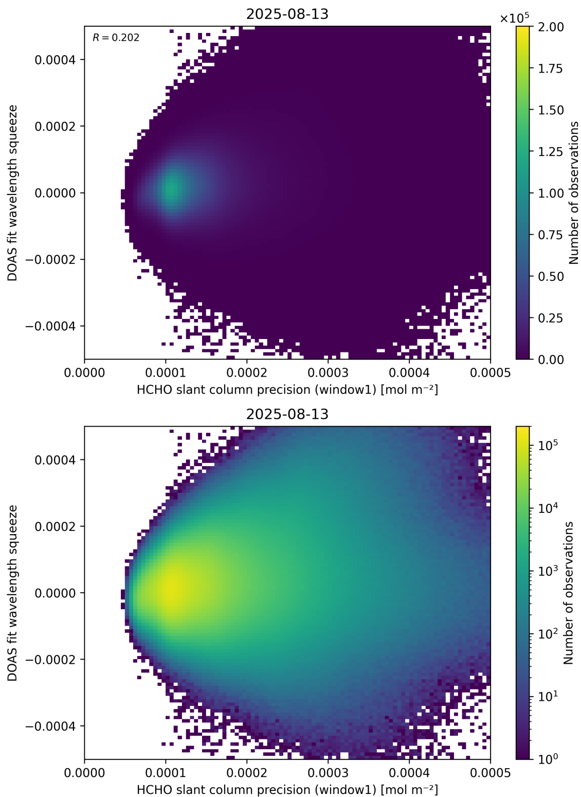
Figure 90: Scatter density plot of “HCHO slant column precision (window1)” against “DOAS fit wavelength squeeze” for 2025-08-12 to 2025-08-14.
