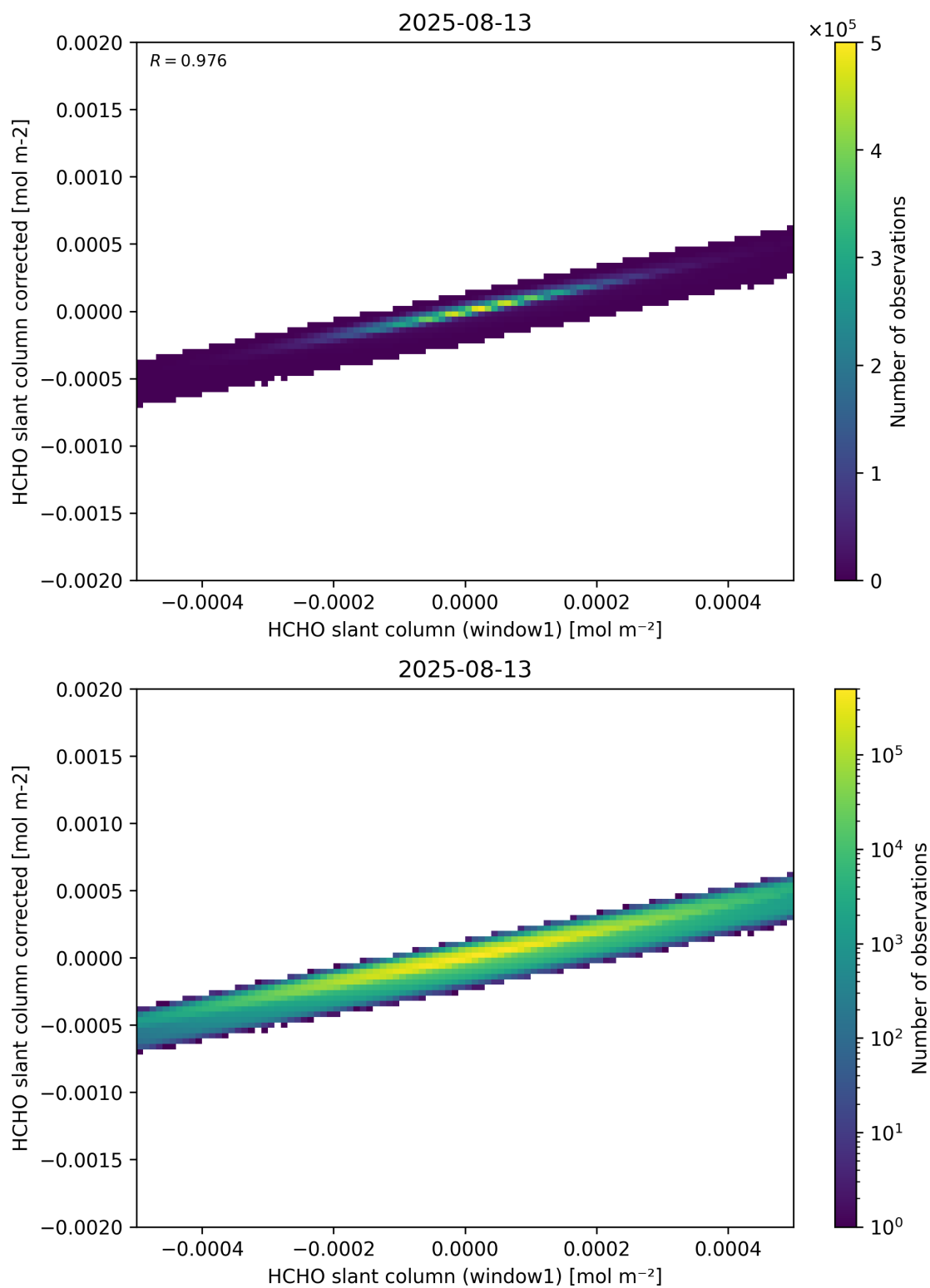
Figure 82: Scatter density plot of “HCHO slant column (window1)” against “HCHO slant column corrected” for 2025-08-12 to 2025-08-14.
