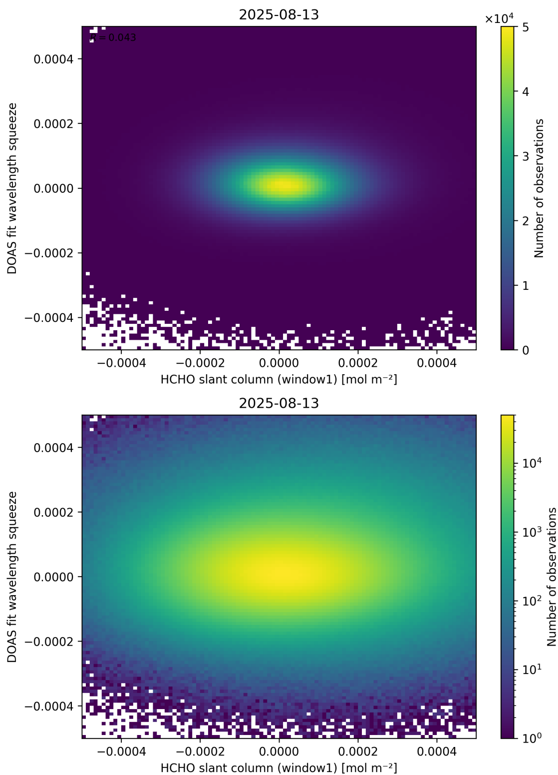
Figure 80: Scatter density plot of “HCHO slant column (window1)” against “DOAS fit wavelength squeeze” for 2025-08-12 to 2025-08-14.
