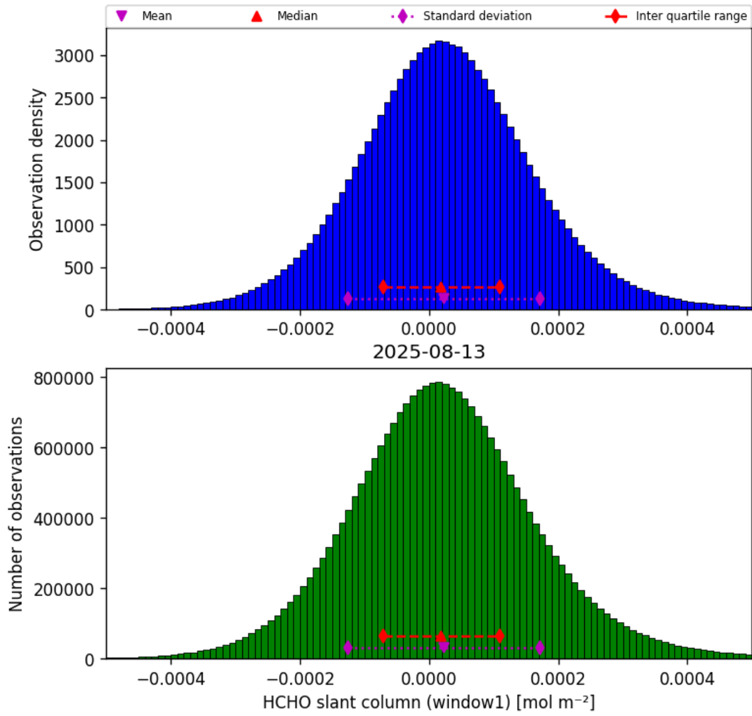
Figure 38: Histogram of “HCHO slant column (window1)” for 2025-08-12 to 2025-08-14
