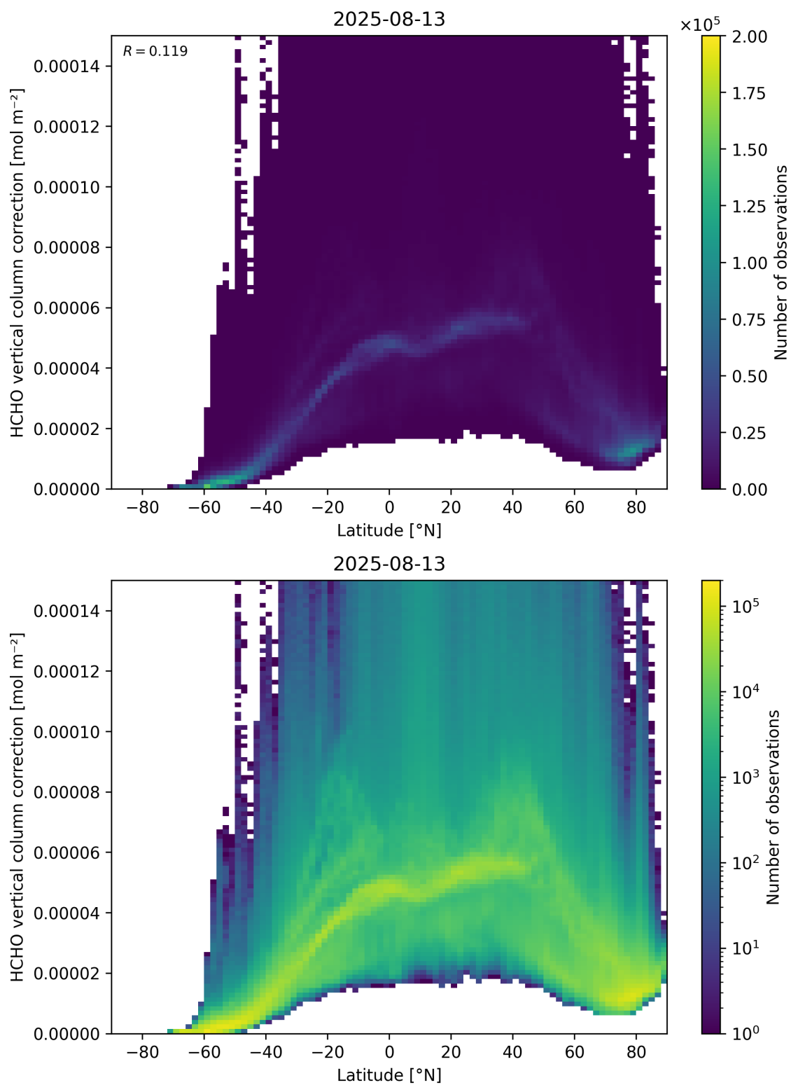
Figure 164: Scatter density plot of “Latitude” against “HCHO vertical column correction” for 2025-08-12 to 2025-08-14.
