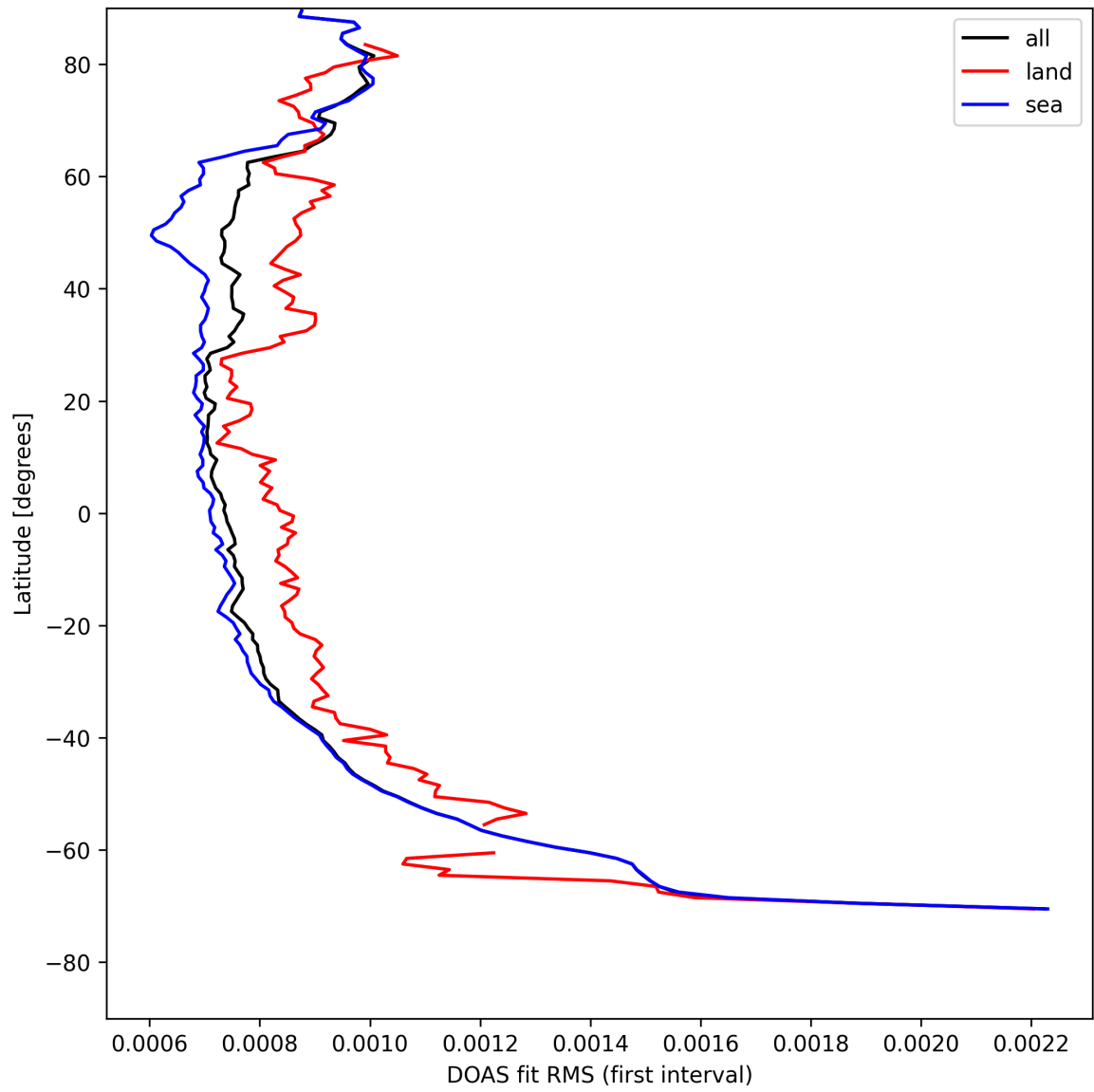
Figure 32: Zonal average of “DOAS fit RMS (first interval)” for 2025-08-12 to 2025-08-14.
