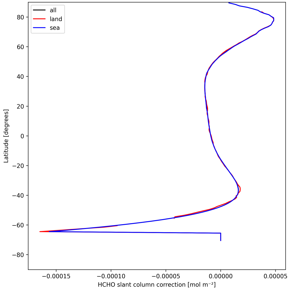
Figure 33: Zonal average of “HCHO slant column correction” for 2025-08-12 to 2025-08-14.
