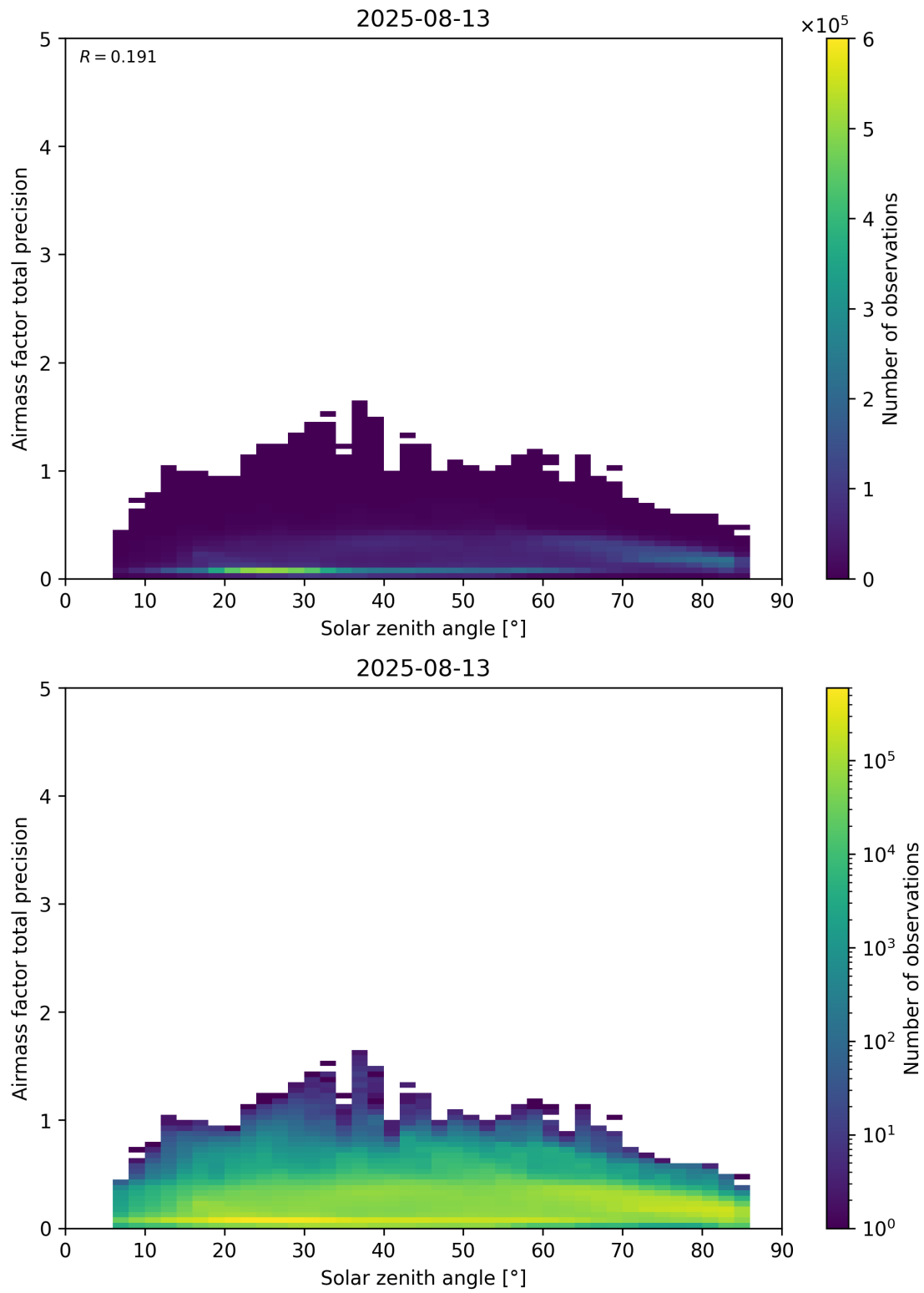
Figure 176: Scatter density plot of “Solar zenith angle” against “Airmass factor total precision” for 2025-08-12 to 2025-08-14.
