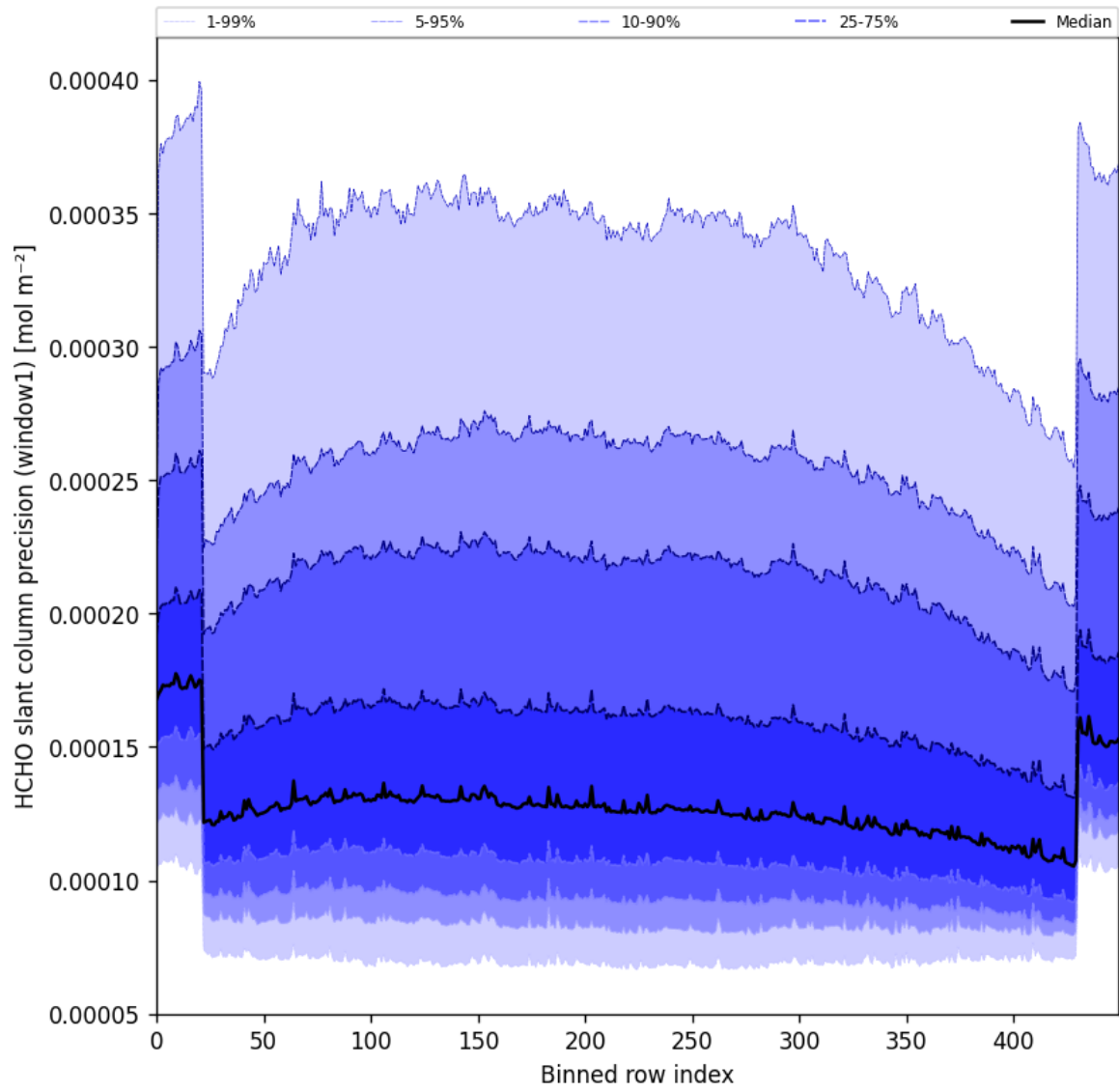
Figure 53: Along track statistics of “HCHO slant column precision (window1)” for 2025-08-12 to 2025-08-14
