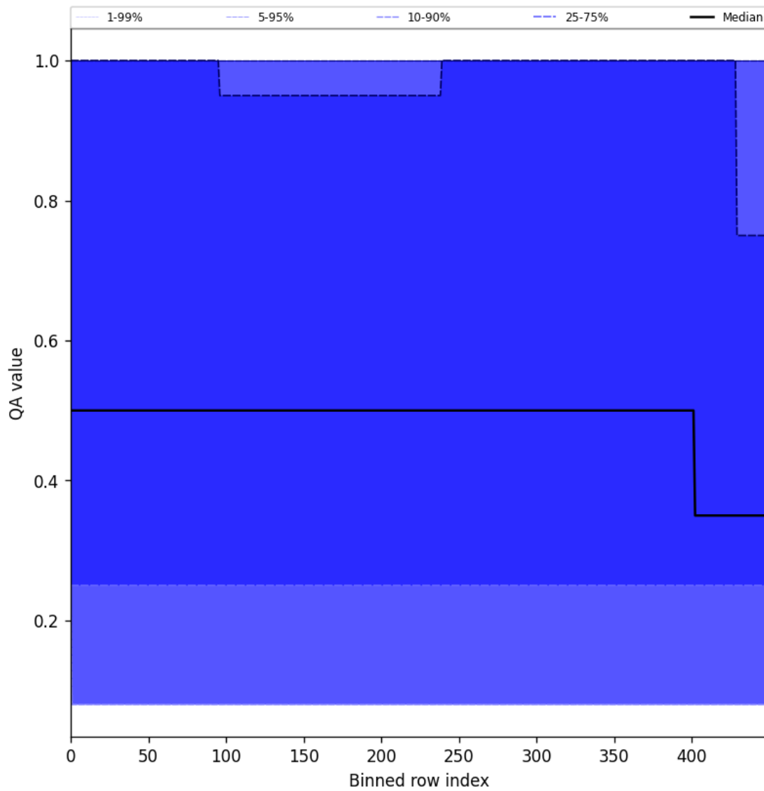
Figure 48: Along track statistics of “QA value” for 2025-08-12 to 2025-08-14
