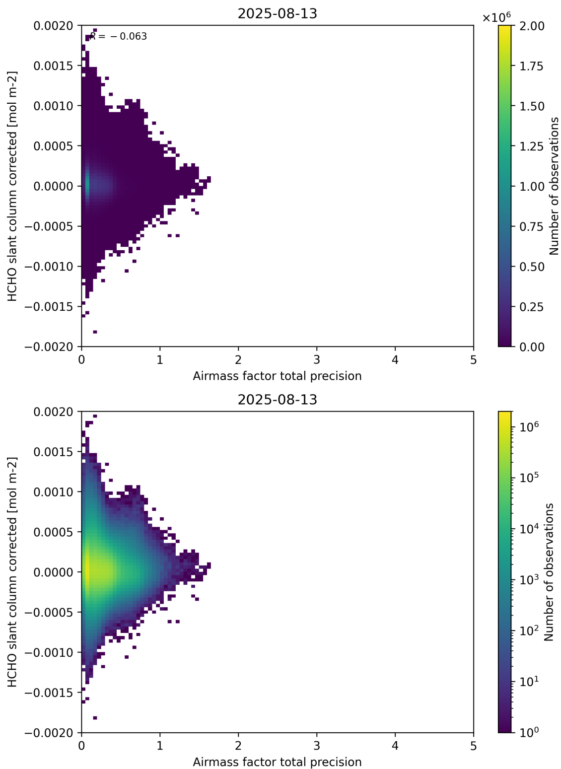
Figure 109: Scatter density plot of “Airmass factor total precision” against “HCHO slant column corrected” for 2025-08-12 to 2025-08-14.
