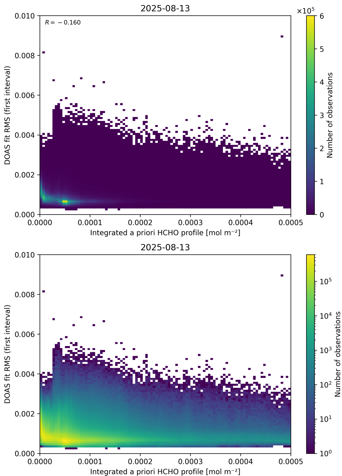
Figure 148: Scatter density plot of “Integrated a priori HCHO profile” against “DOAS fit RMS (first interval)” for 2025-08-12 to 2025-08-14.
