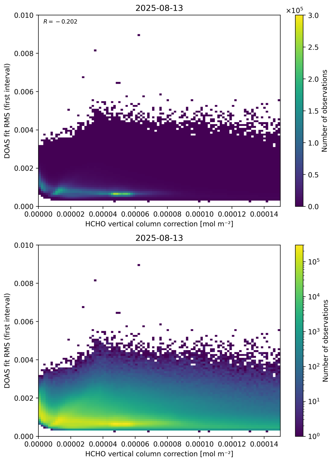
Figure 112: Scatter density plot of “HCHO vertical column correction” against “DOAS fit RMS (first interval)” for 2025-08-12 to 2025-08-14.
