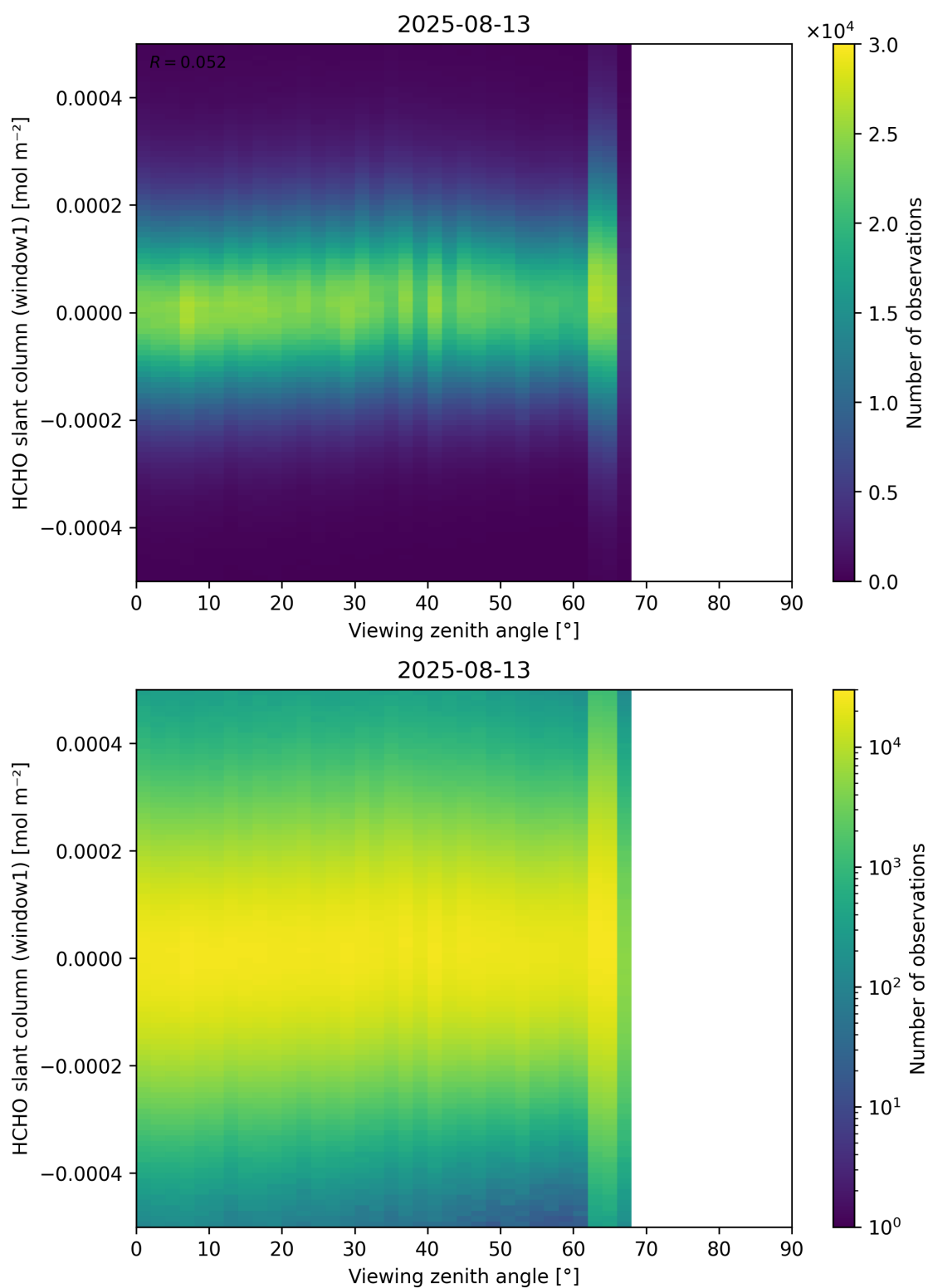
Figure 188: Scatter density plot of “Viewing zenith angle” against “HCHO slant column (window1)” for 2025-08-12 to 2025-08-14.
