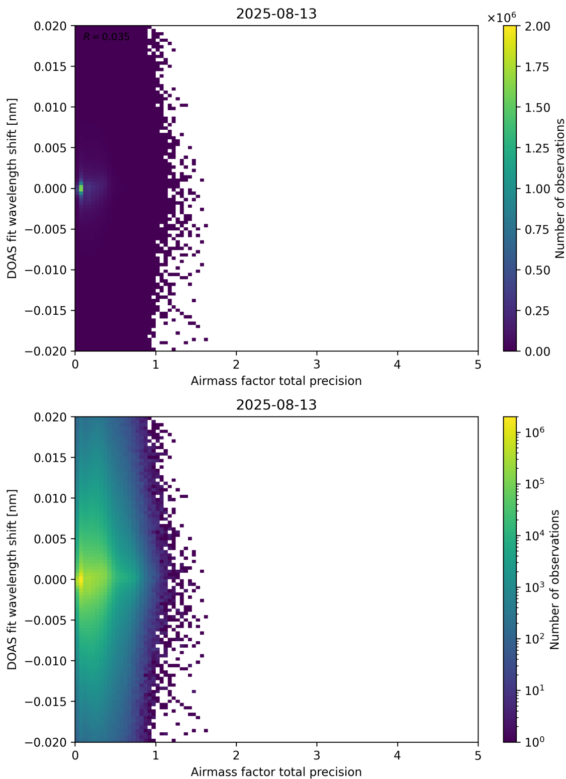
Figure 106: Scatter density plot of “Airmass factor total precision” against “DOAS fit wavelength shift” for 2025-08-12 to 2025-08-14.
