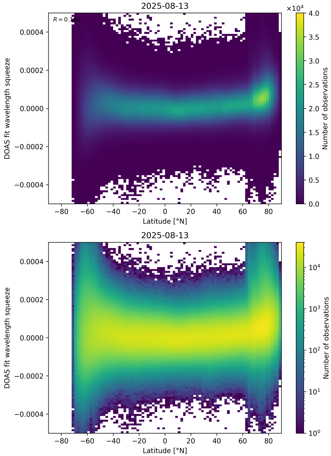
Figure 155: Scatter density plot of “Latitude” against “DOAS fit wavelength squeeze” for 2025-08-12 to 2025-08-14.
