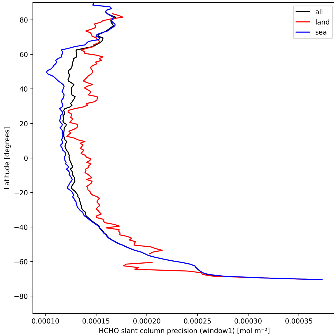
Figure 25: Zonal average of "HCHO slant column precision (window1)" for 2025-08-12 to 2025-08-14.
