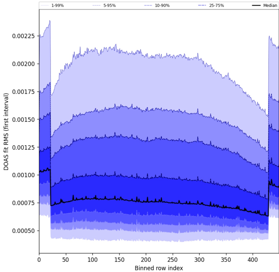
Figure 60: Along track statistics of “DOAS fit RMS (first interval)” for 2025-08-12 to 2025-08-14
