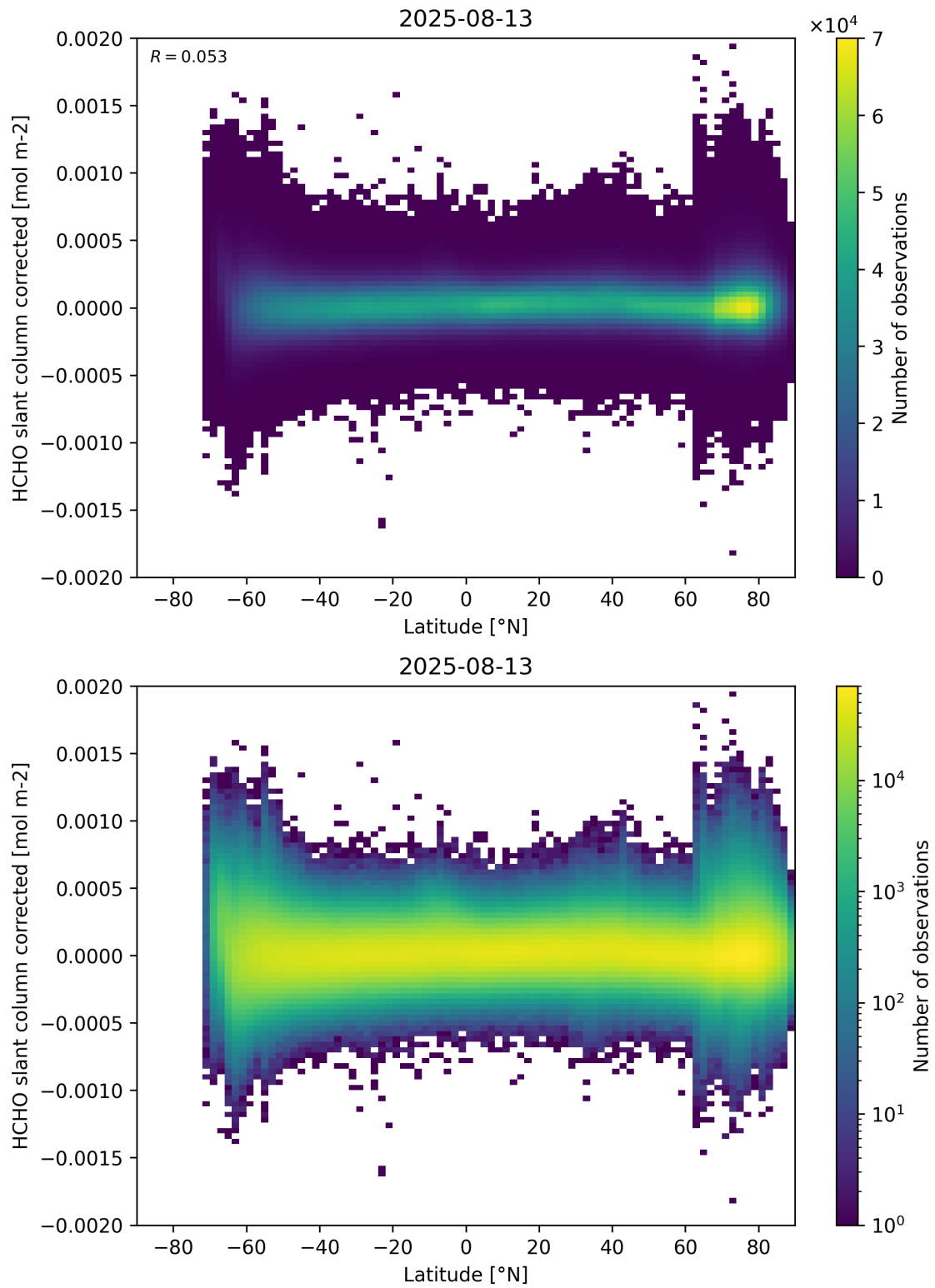
Figure 157: Scatter density plot of “Latitude” against “HCHO slant column corrected” for 2025-08-12 to 2025-08-14.
