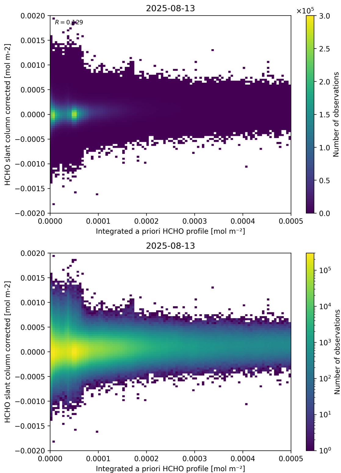
Figure 151: Scatter density plot of “Integrated a priori HCHO profile” against “HCHO slant column corrected” for 2025-08-12 to 2025-08-14.
