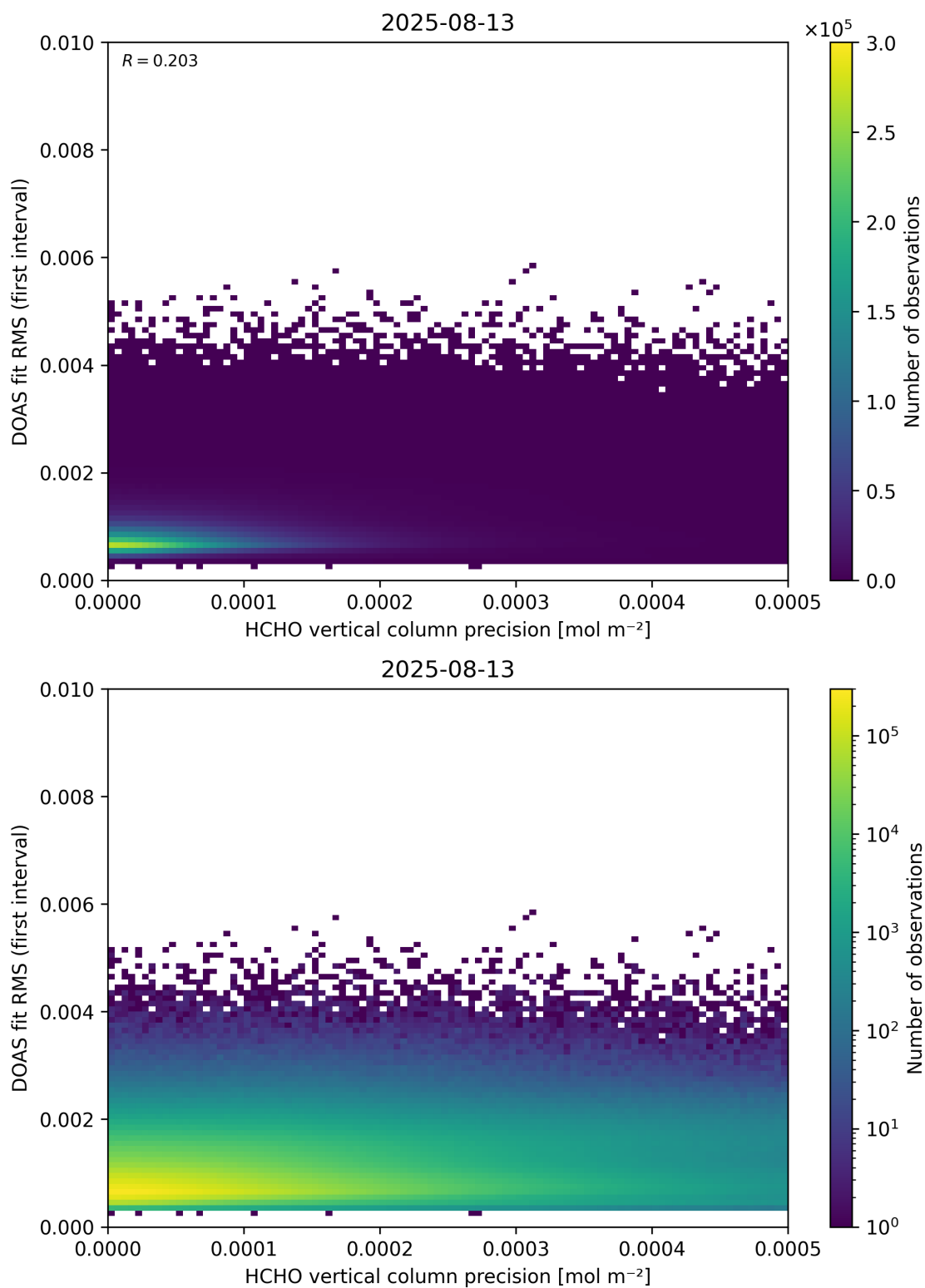
Figure 136: Scatter density plot of “HCHO vertical column precision” against “DOAS fit RMS (first interval)” for 2025-08-12 to 2025-08-14.
