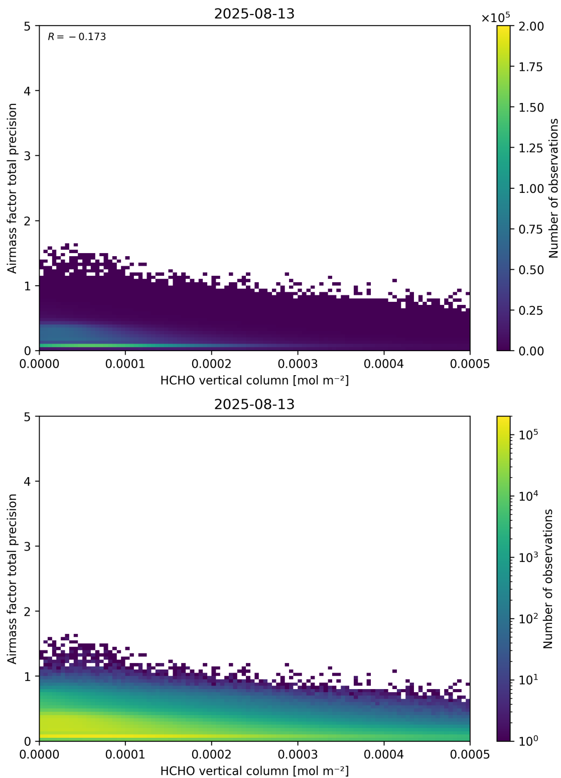
Figure 132: Scatter density plot of “HCHO vertical column” against “Airmass factor total precision” for 2025-08-12 to 2025-08-14.
