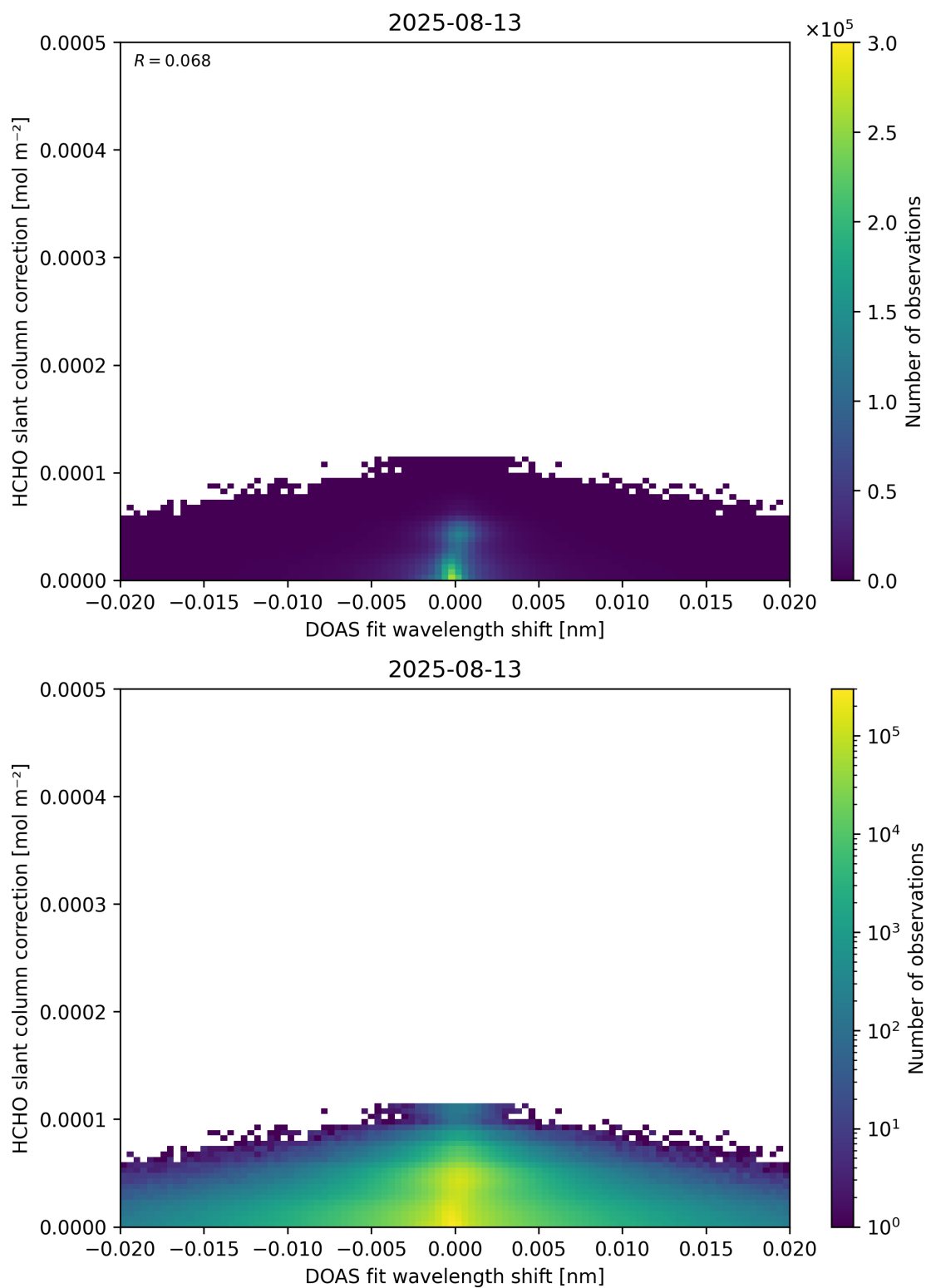
Figure 67: Scatter density plot of “DOAS fit wavelength shift” against “HCHO slant column correction” for 2025-08-12 to 2025-08-14.
