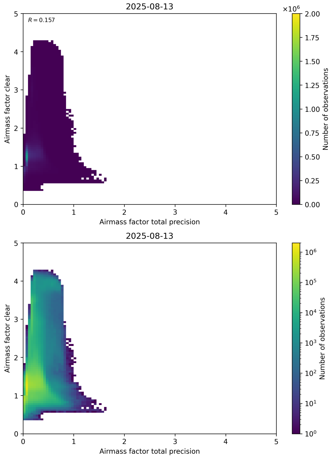
Figure 108: Scatter density plot of “Airmass factor total precision” against “Airmass factor clear” for 2025-08-12 to 2025-08-14.
