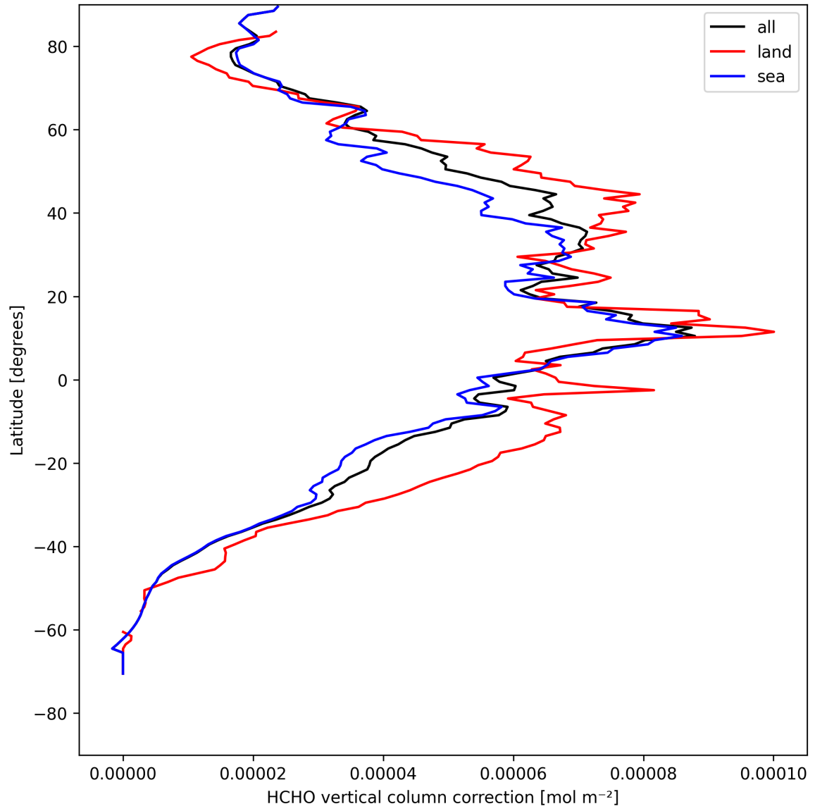
Figure 23: Zonal average of “HCHO vertical column correction” for 2025-08-12 to 2025-08-14.
