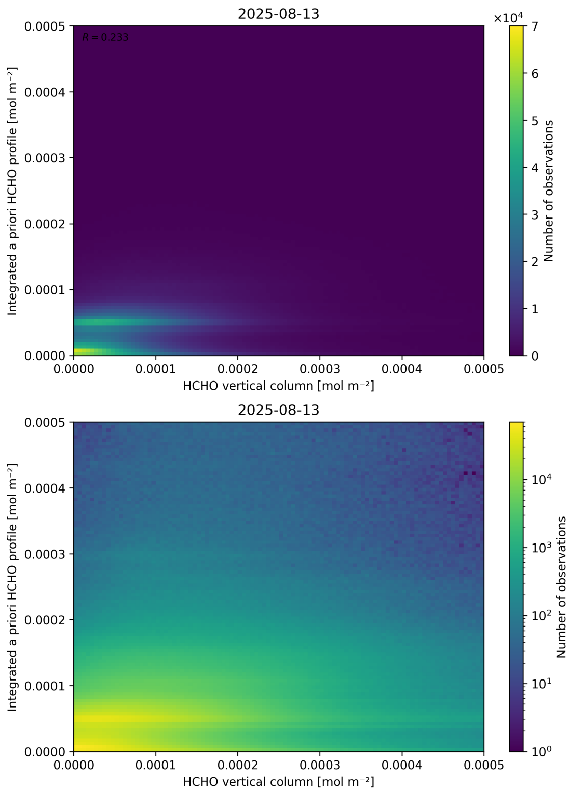
Figure 135: Scatter density plot of “HCHO vertical column” against “Integrated a priori HCHO profile” for 2025-08-12 to 2025-08-14.
