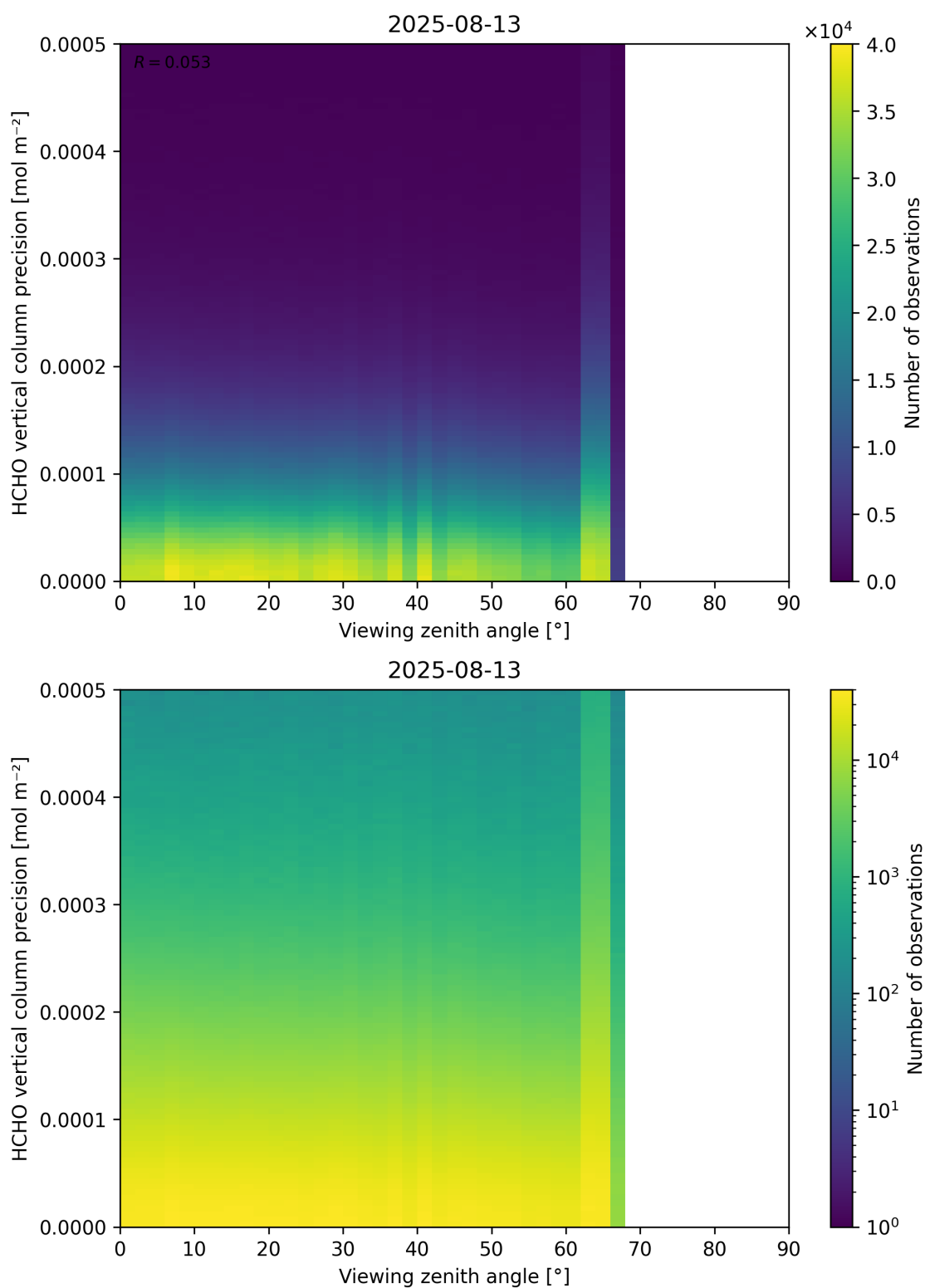
Figure 194: Scatter density plot of “Viewing zenith angle” against “HCHO vertical column precision” for 2025-08-12 to 2025-08-14.
