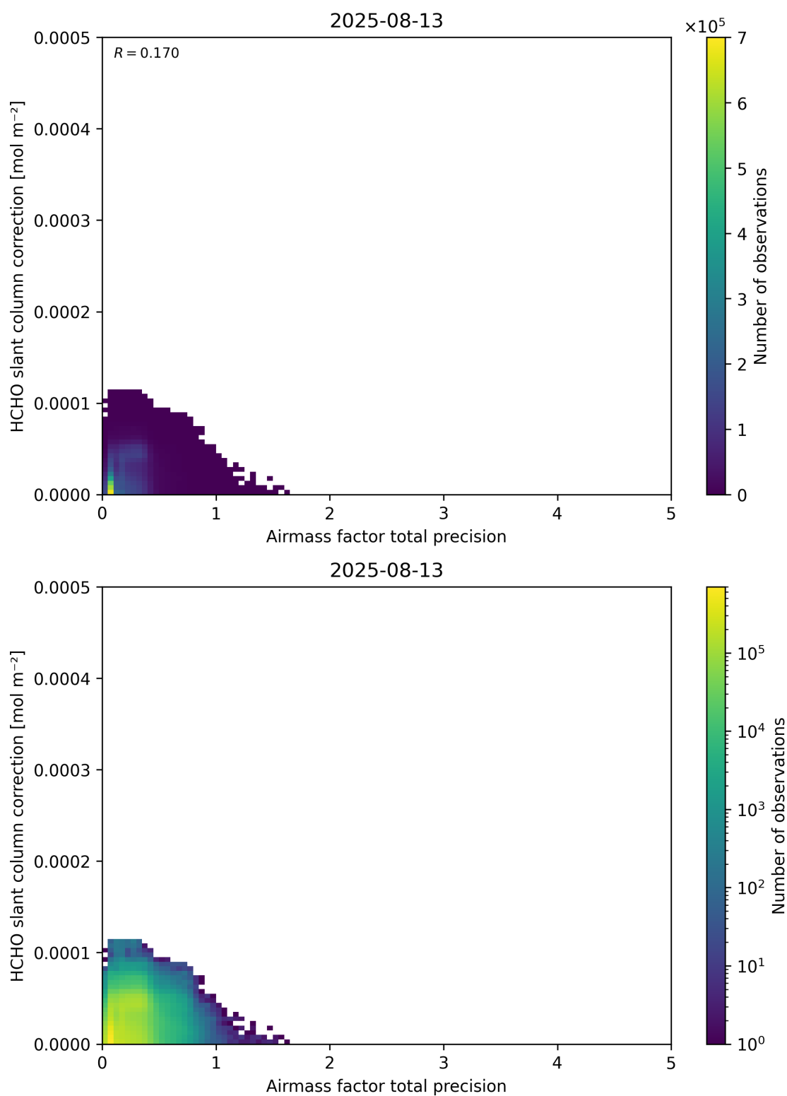
Figure 110: Scatter density plot of “Airmass factor total precision” against “HCHO slant column correction” for 2025-08-12 to 2025-08-14.
