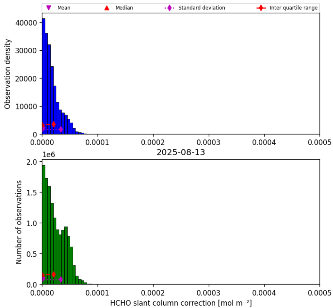
Figure 47: Histogram of “HCHO slant column correction” for 2025-08-12 to 2025-08-14
