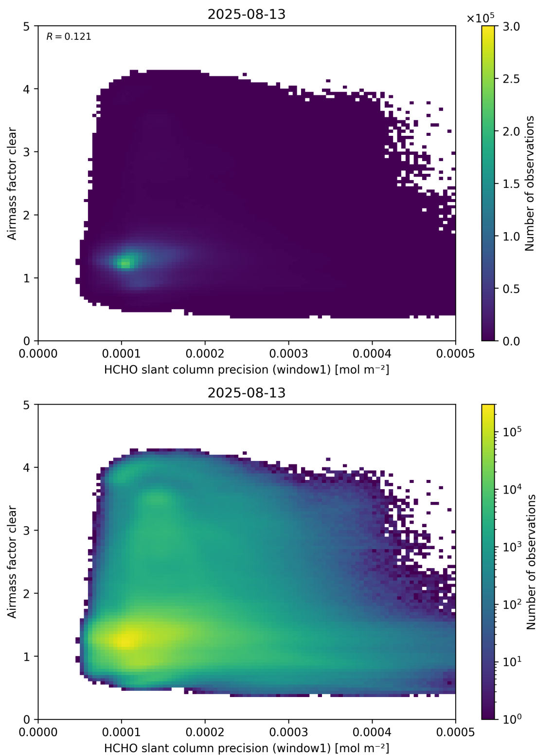
Figure 91: Scatter density plot of “HCHO slant column precision (window1)” against “Airmass factor clear” for 2025-08-12 to 2025-08-14.
