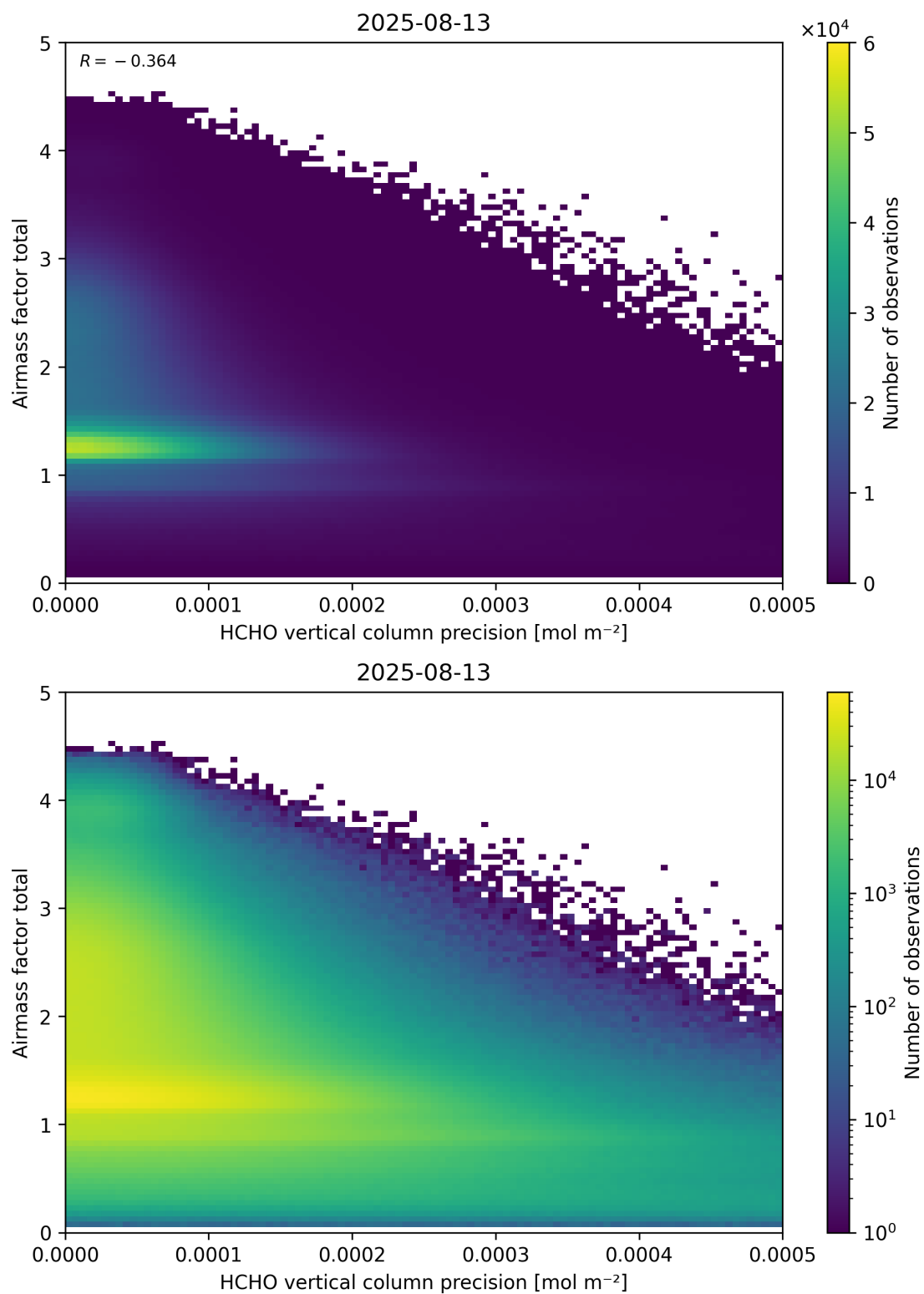
Figure 144: Scatter density plot of “HCHO vertical column precision” against “Airmass factor total” for 2025-08-12 to 2025-08-14.
