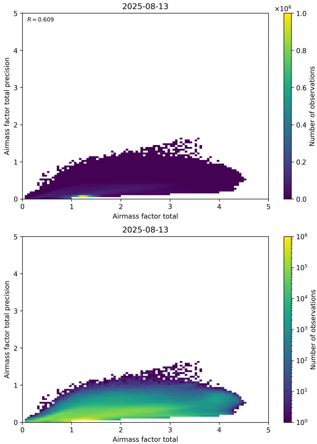
Figure 103: Scatter density plot of “Airmass factor total” against “Airmass factor total precision” for 2025-08-12 to 2025-08-14.
