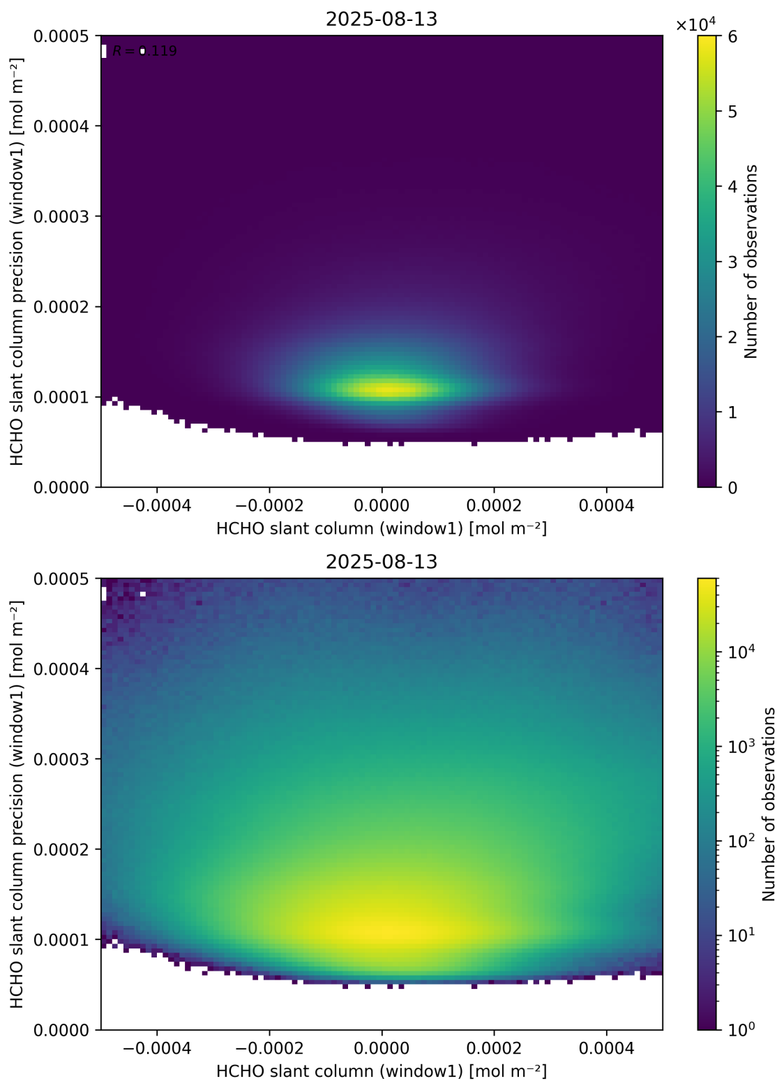
Figure 84: Scatter density plot of “HCHO slant column (window1)” against “HCHO slant column precision (window1)” for 2025-08-12 to 2025-08-14.
