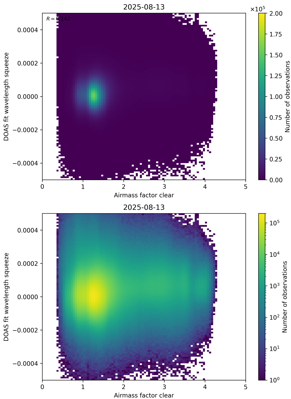
Figure 73: Scatter density plot of “Airmass factor clear” against “DOAS fit wavelength squeeze” for 2025-08-12 to 2025-08-14.
