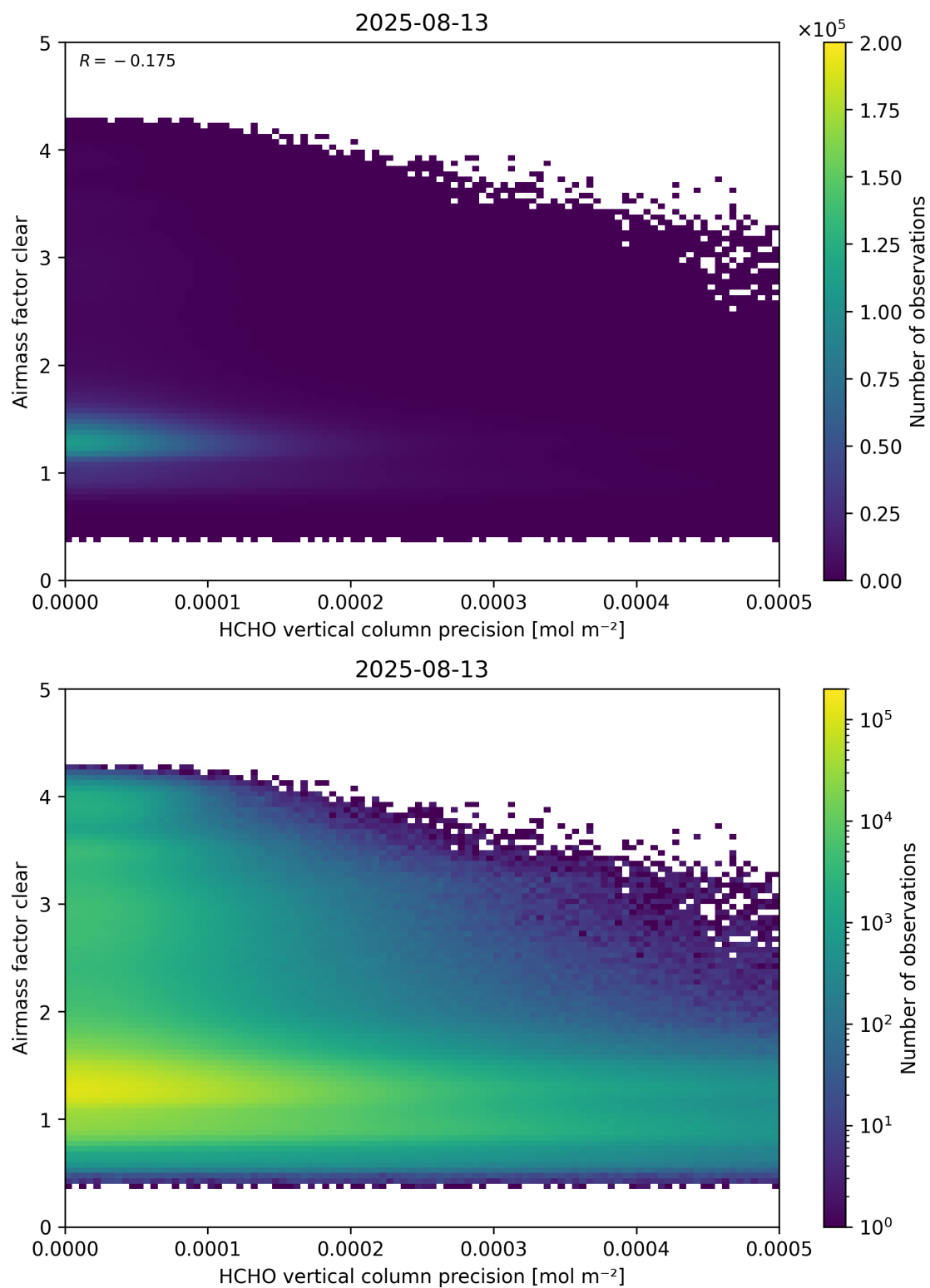
Figure 139: Scatter density plot of “HCHO vertical column precision” against “Airmass factor clear” for 2025-08-12 to 2025-08-14.
