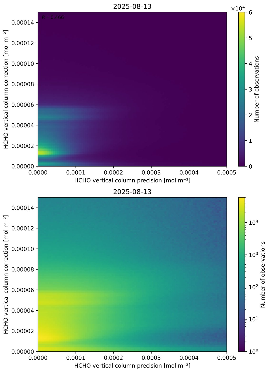
Figure 146: Scatter density plot of “HCHO vertical column precision” against “HCHO vertical column correction” for 2025-08-12 to 2025-08-14.
