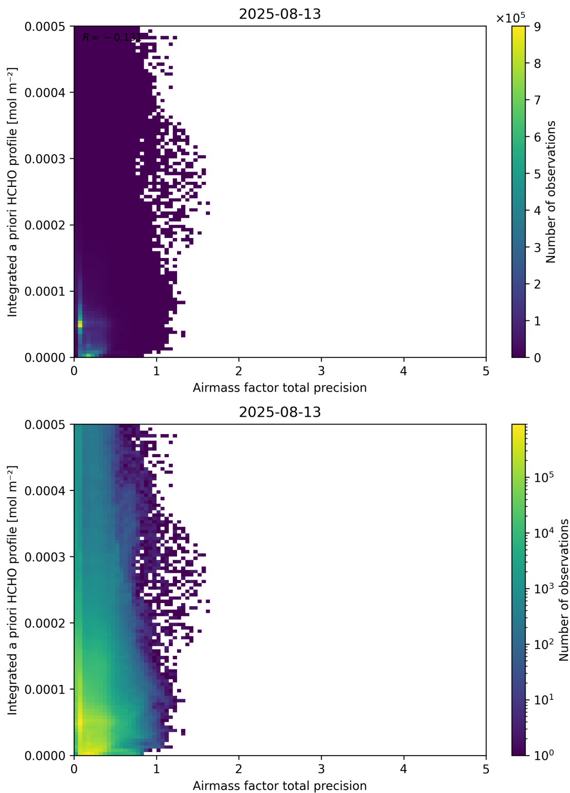
Figure 111: Scatter density plot of “Airmass factor total precision” against “Integrated a priori HCHO profile” for 2025-08-12 to 2025-08-14.
