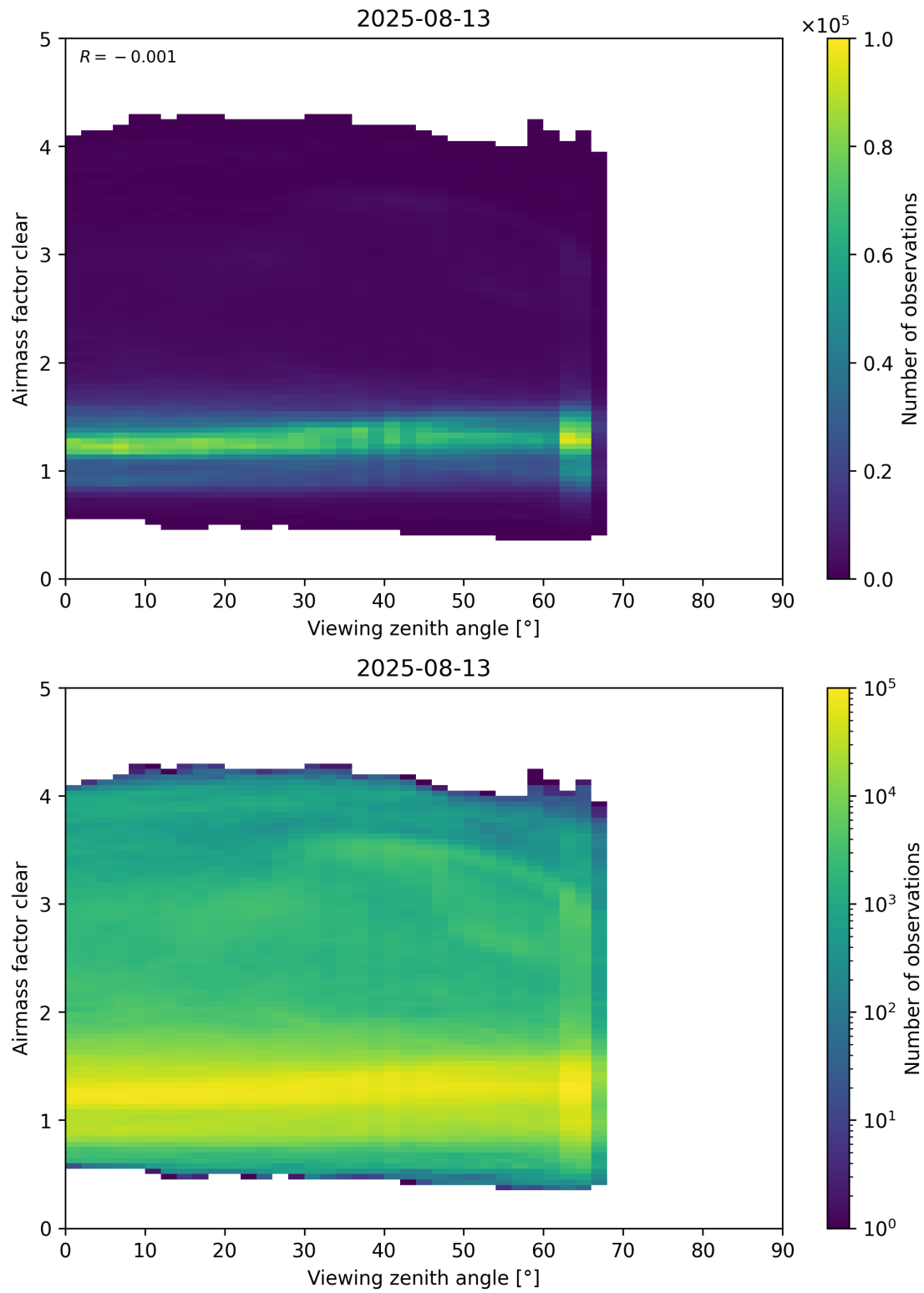
Figure 185: Scatter density plot of “Viewing zenith angle” against “Airmass factor clear” for 2025-08-12 to 2025-08-14.
