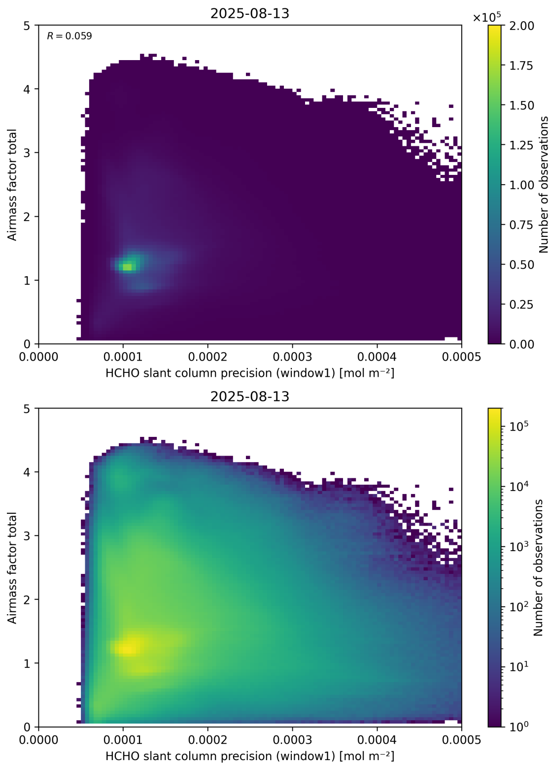
Figure 94: Scatter density plot of “HCHO slant column precision (window1)” against “Airmass factor total” for 2025-08-12 to 2025-08-14.
