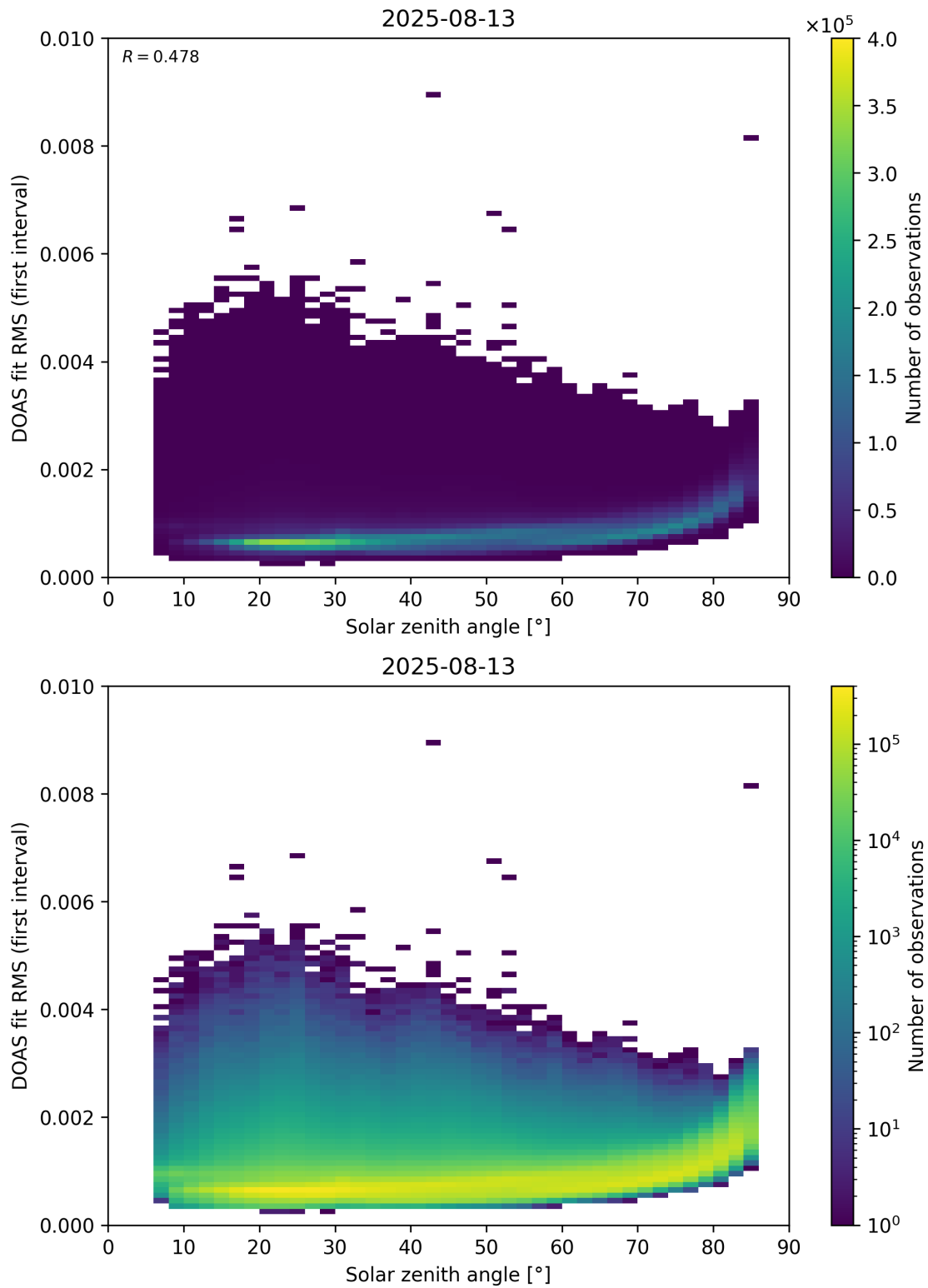
Figure 167: Scatter density plot of “Solar zenith angle” against “DOAS fit RMS (first interval)” for 2025-08-12 to 2025-08-14.
