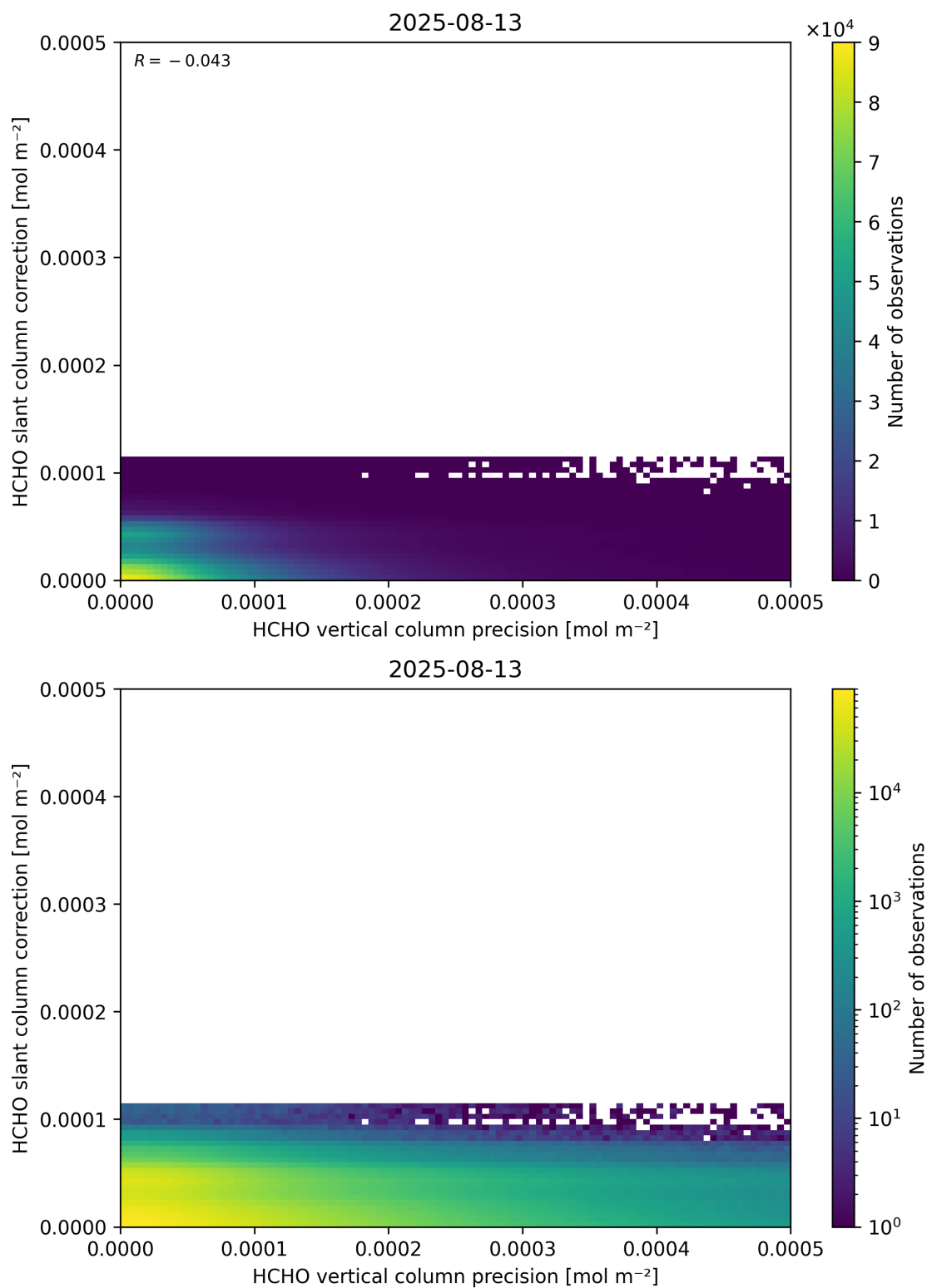
Figure 141: Scatter density plot of “HCHO vertical column precision” against “HCHO slant column correction” for 2025-08-12 to 2025-08-14.
