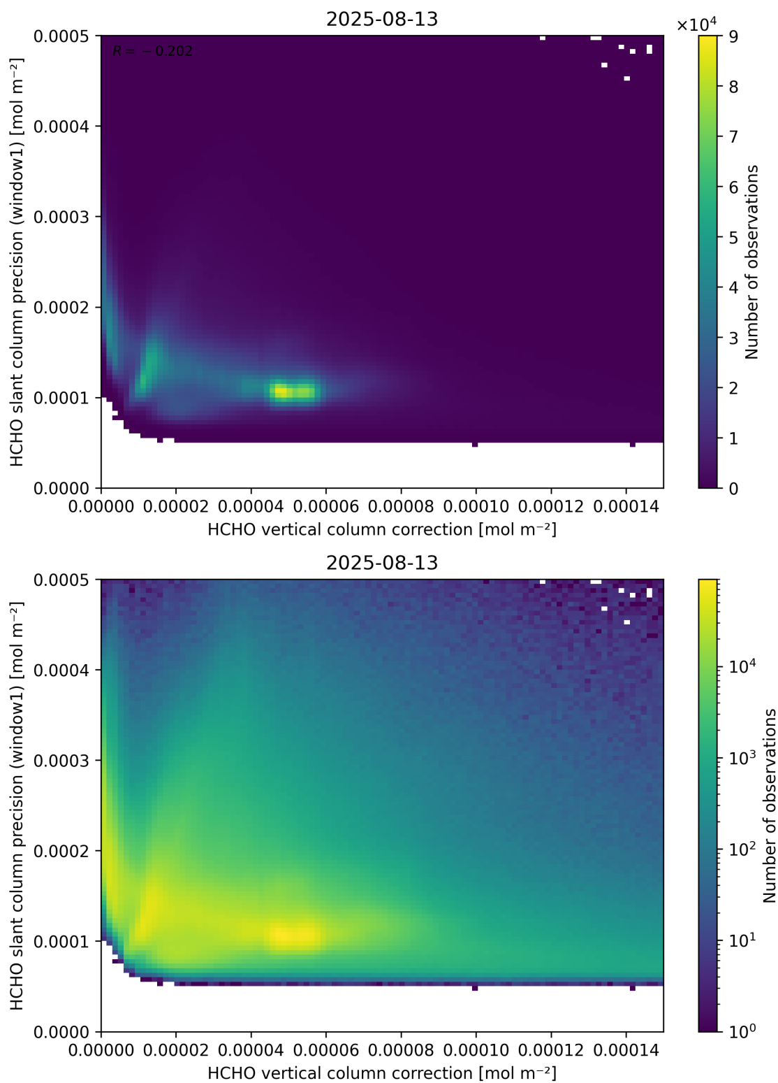
Figure 119: Scatter density plot of “HCHO vertical column correction” against “HCHO slant column precision (window1)” for 2025-08-12 to 2025-08-14.
