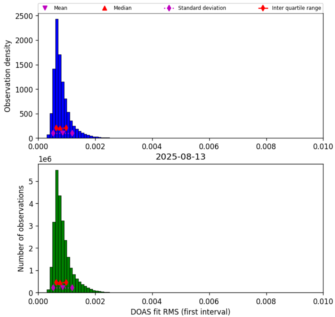
Figure 46: Histogram of “DOAS fit RMS (first interval)” for 2025-08-12 to 2025-08-14
