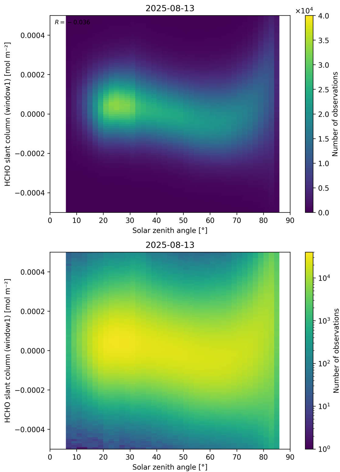
Figure 173: Scatter density plot of “Solar zenith angle” against “HCHO slant column (window1)” for 2025-08-12 to 2025-08-14.
