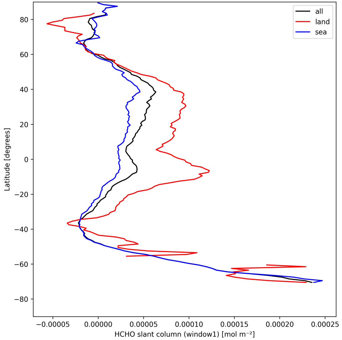
Figure 24: Zonal average of “HCHO slant column (window1)” for 2025-08-12 to 2025-08-14.
