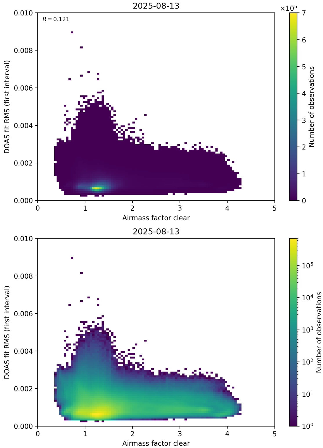
Figure 71: Scatter density plot of “Airmass factor clear” against “DOAS fit RMS (first interval)” for 2025-08-12 to 2025-08-14.
