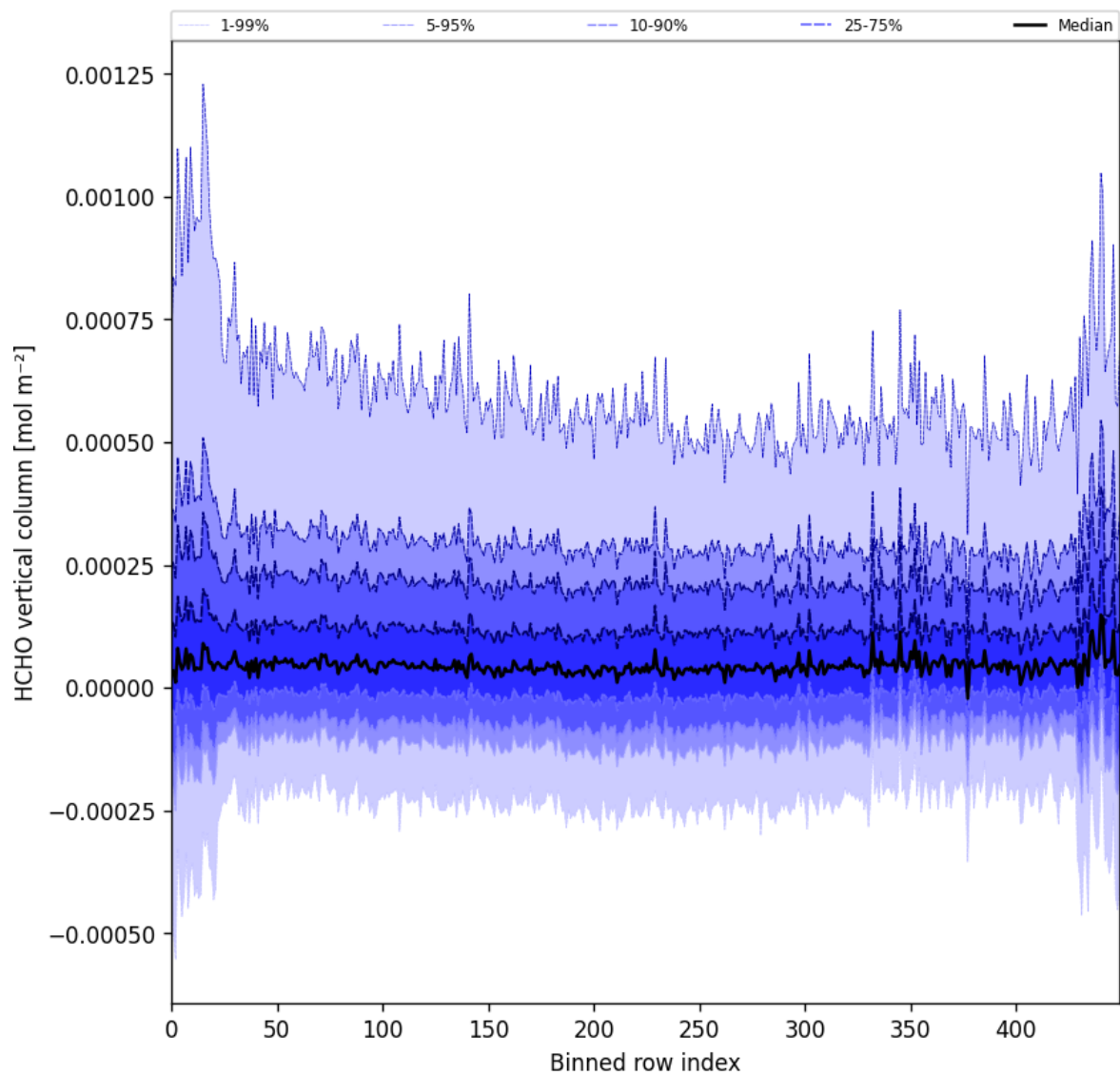
Figure 49: Along track statistics of “HCHO vertical column” for 2025-08-12 to 2025-08-14
