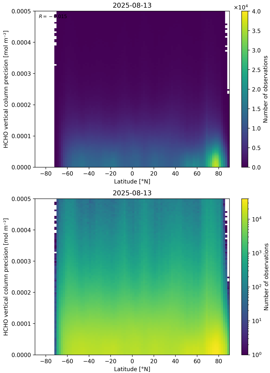
Figure 165: Scatter density plot of “Latitude” against “HCHO vertical column precision” for 2025-08-12 to 2025-08-14.
