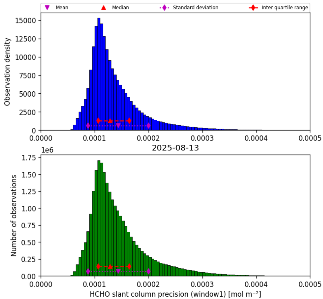
Figure 39: Histogram of “HCHO slant column precision (window1)” for 2025-08-12 to 2025-08-14
