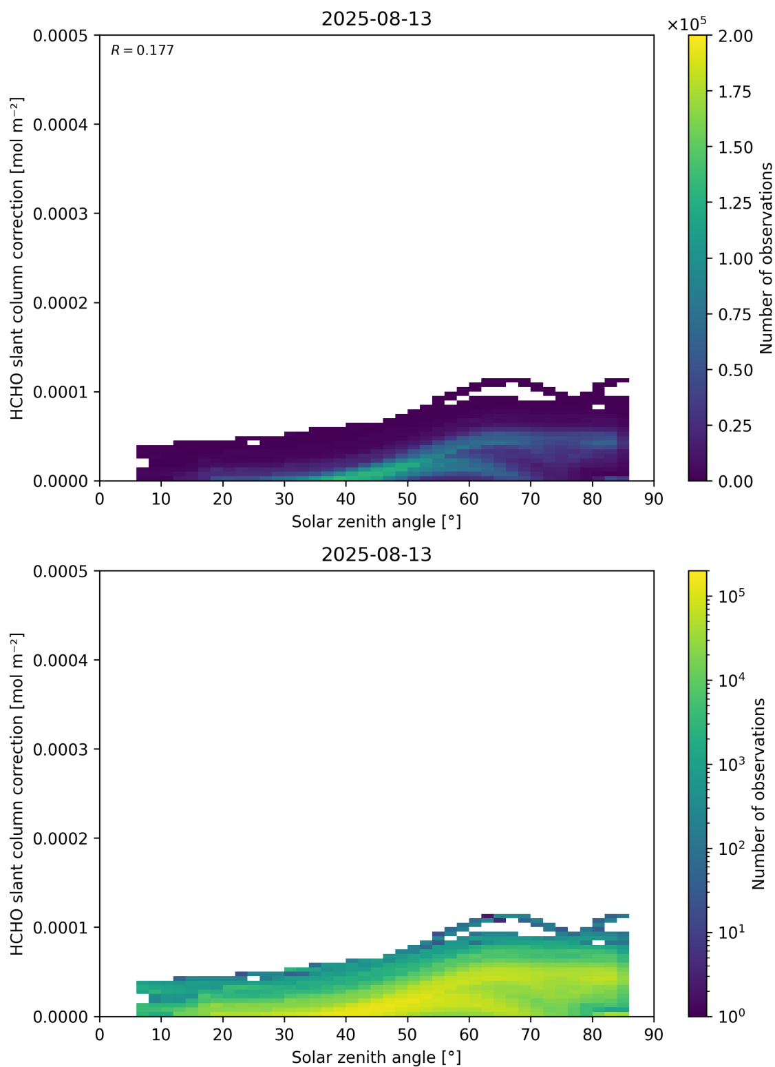
Figure 172: Scatter density plot of “Solar zenith angle” against “HCHO slant column correction” for 2025-08-12 to 2025-08-14.
