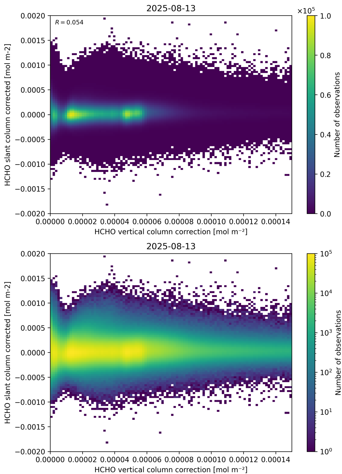
Figure 116: Scatter density plot of “HCHO vertical column correction” against “HCHO slant column corrected” for 2025-08-12 to 2025-08-14.
