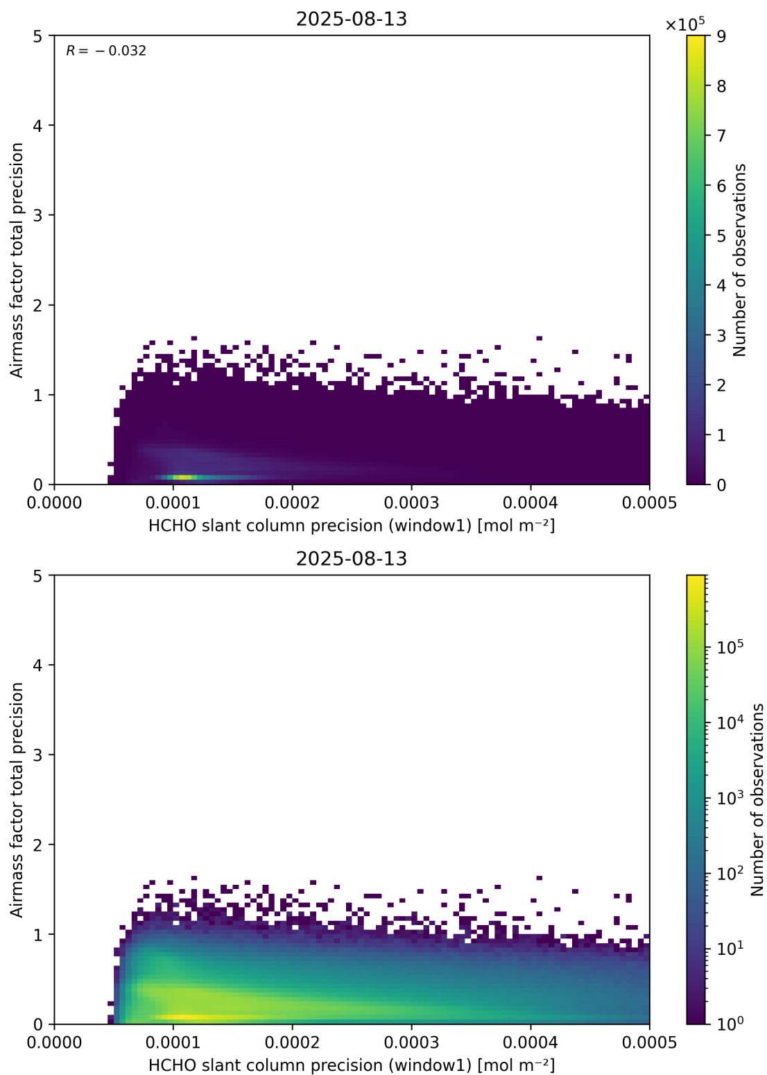
Figure 95: Scatter density plot of “HCHO slant column precision (window1)” against “Airmass factor total precision” for 2025-08-12 to 2025-08-14.
