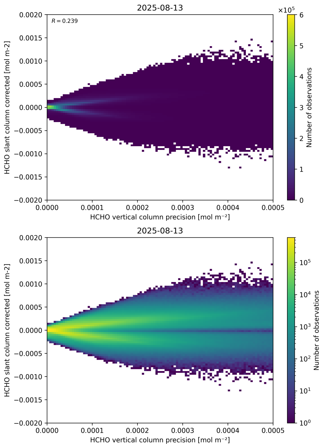
Figure 140: Scatter density plot of “HCHO vertical column precision” against “HCHO slant column corrected” for 2025-08-12 to 2025-08-14.
