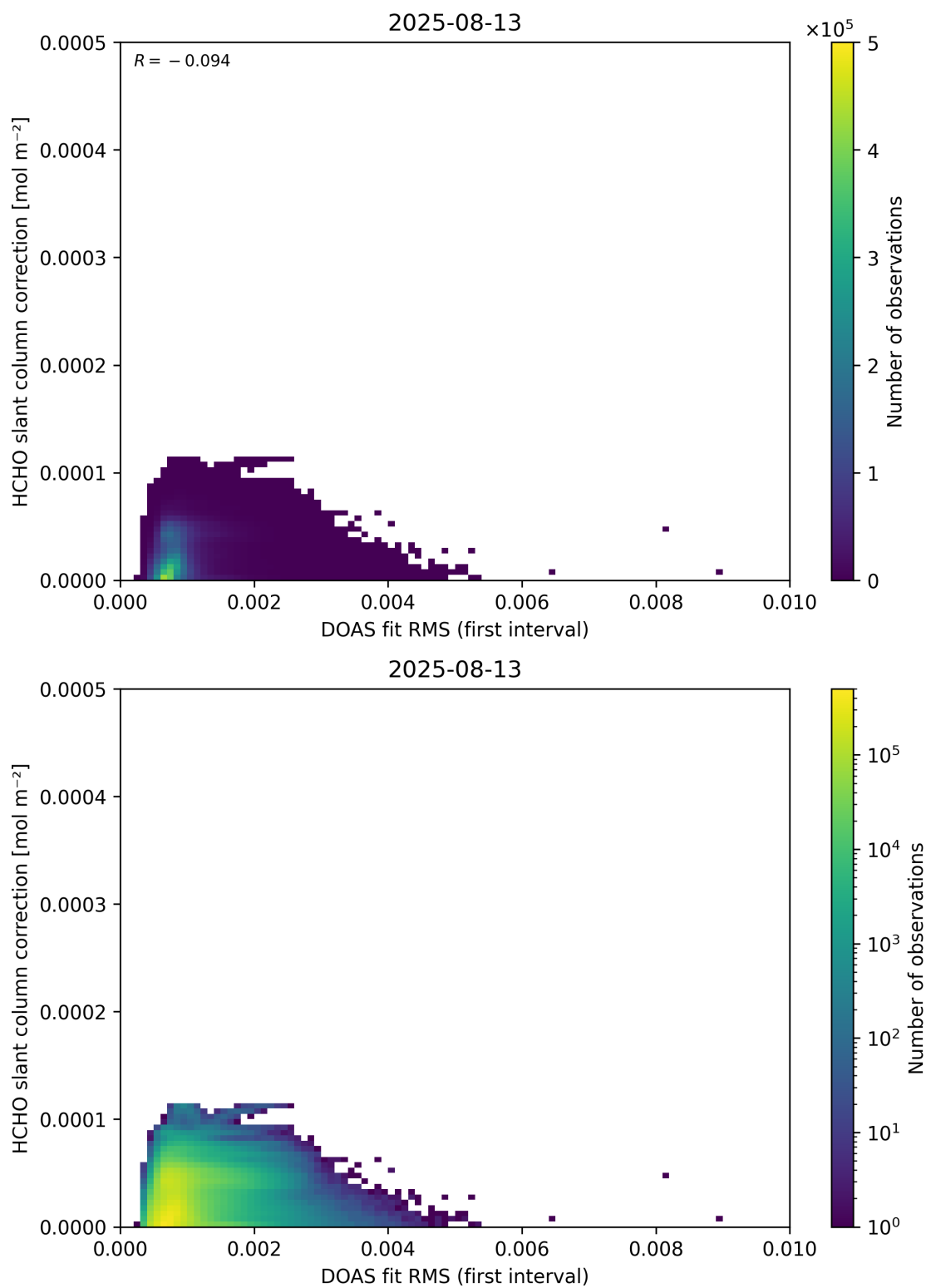
Figure 63: Scatter density plot of “DOAS fit RMS (first interval)” against “HCHO slant column correction” for 2025-08-12 to 2025-08-14.
