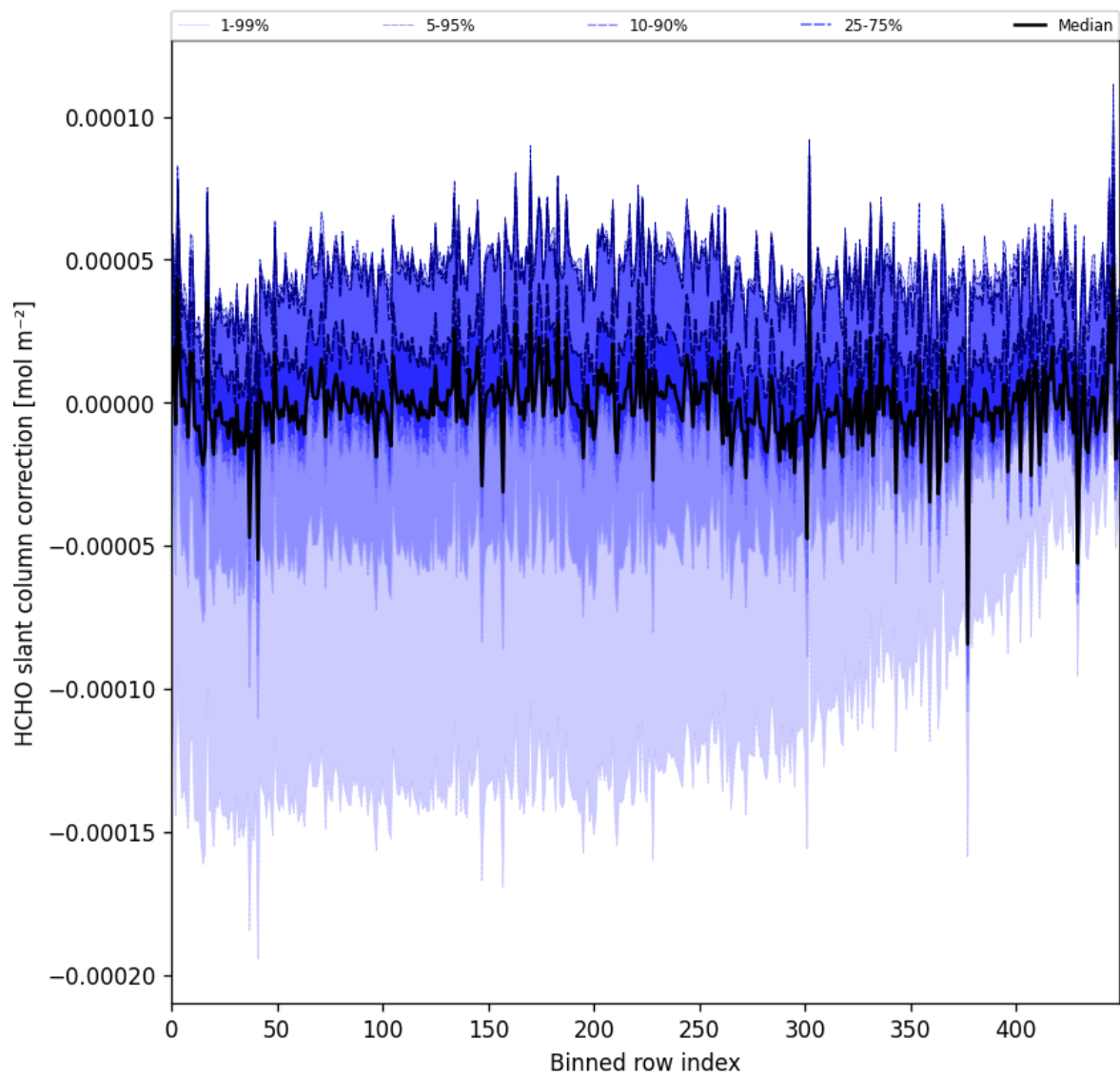
Figure 61: Along track statistics of "HCHO slant column correction" for 2025-08-12 to 2025-08-14
