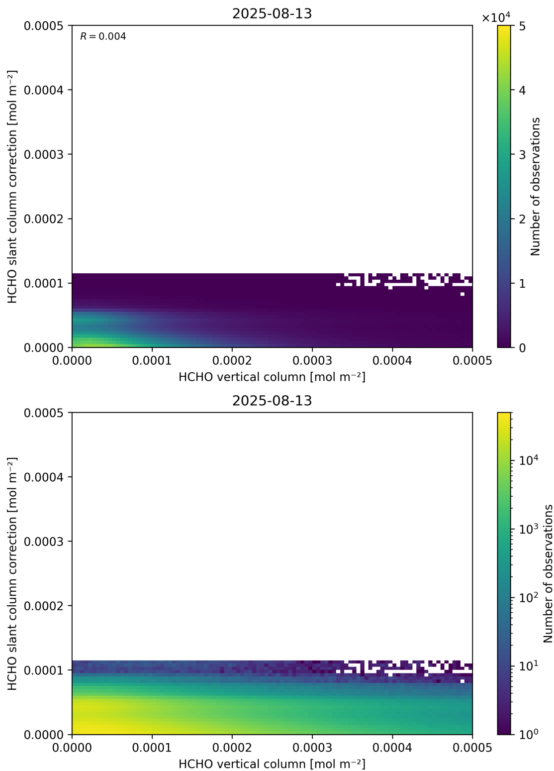
Figure 128: Scatter density plot of “HCHO vertical column” against “HCHO slant column correction” for 2025-08-12 to 2025-08-14.
