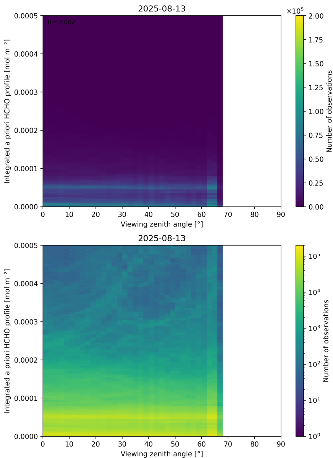
Figure 195: Scatter density plot of “Viewing zenith angle” against “Integrated a priori HCHO profile” for 2025-08-12 to 2025-08-14.
