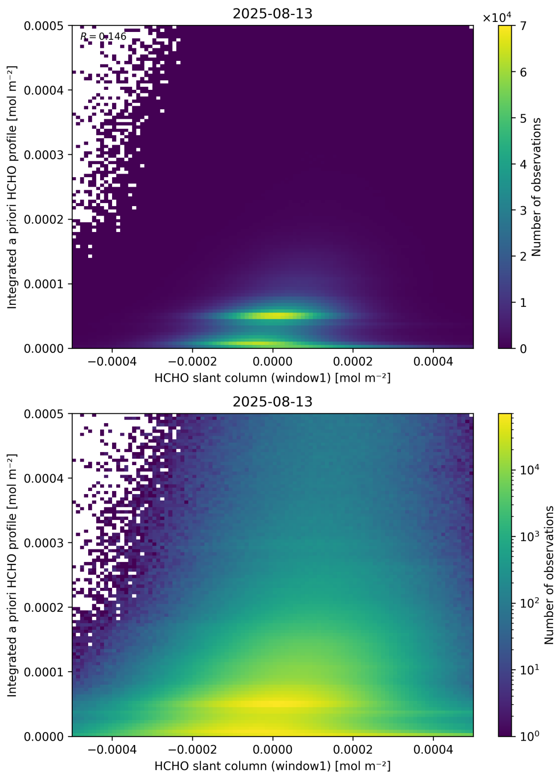
Figure 87: Scatter density plot of “HCHO slant column (window1)” against “Integrated a priori HCHO profile” for 2025-08-12 to 2025-08-14.
