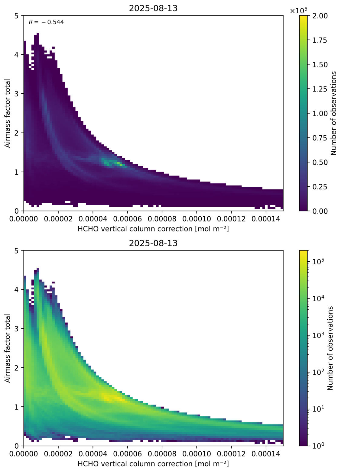
Figure 120: Scatter density plot of “HCHO vertical column correction” against “Airmass factor total” for 2025-08-12 to 2025-08-14.
