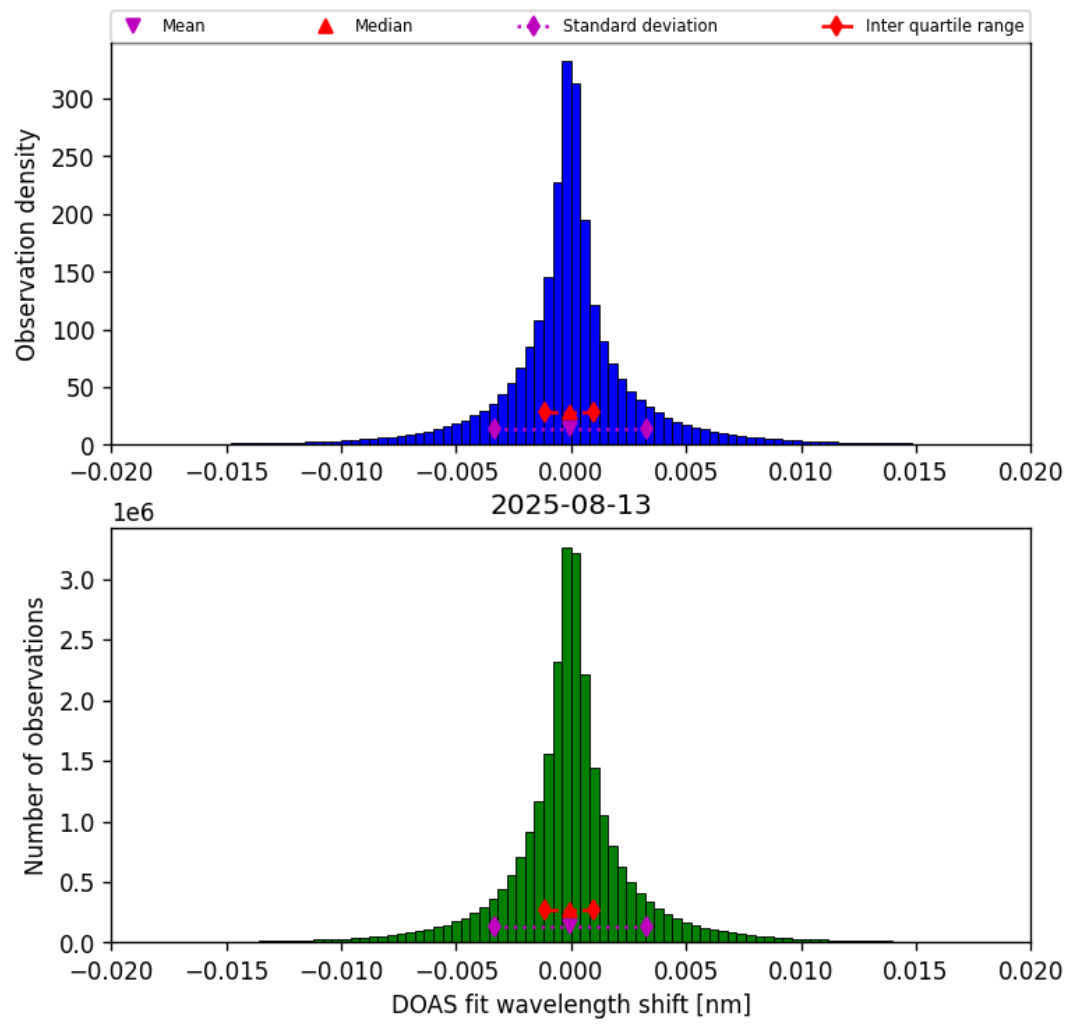
Figure 44: Histogram of “DOAS fit wavelength shift” for 2025-08-12 to 2025-08-14
