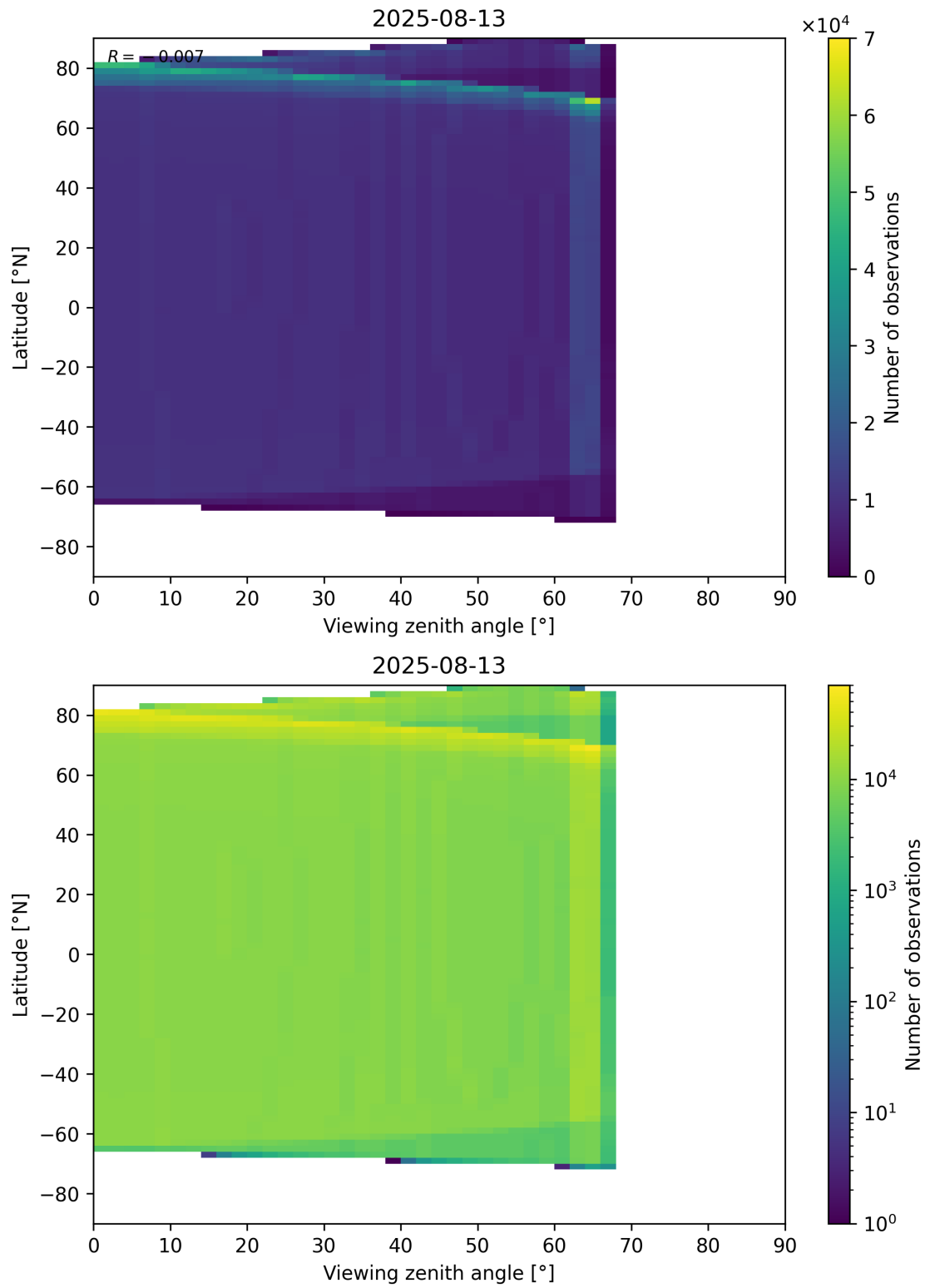
Figure 196: Scatter density plot of “Viewing zenith angle” against “Latitude” for 2025-08-12 to 2025-08-14.
