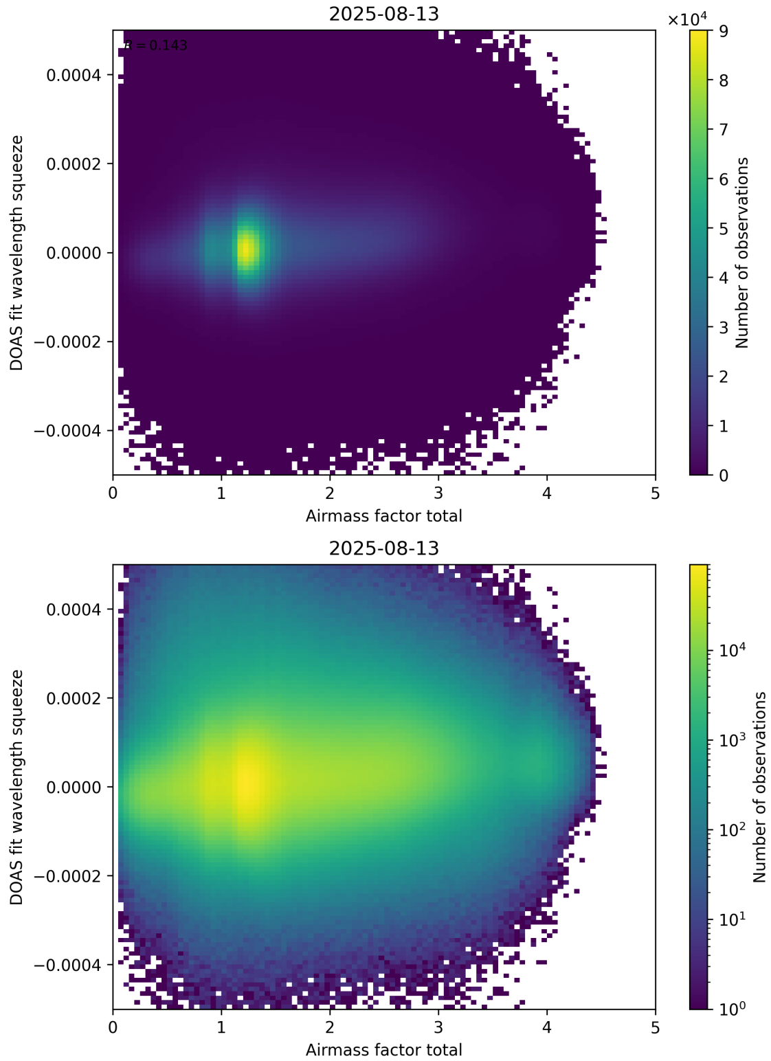
Figure 99: Scatter density plot of “Airmass factor total” against “DOAS fit wavelength squeeze” for 2025-08-12 to 2025-08-14.
