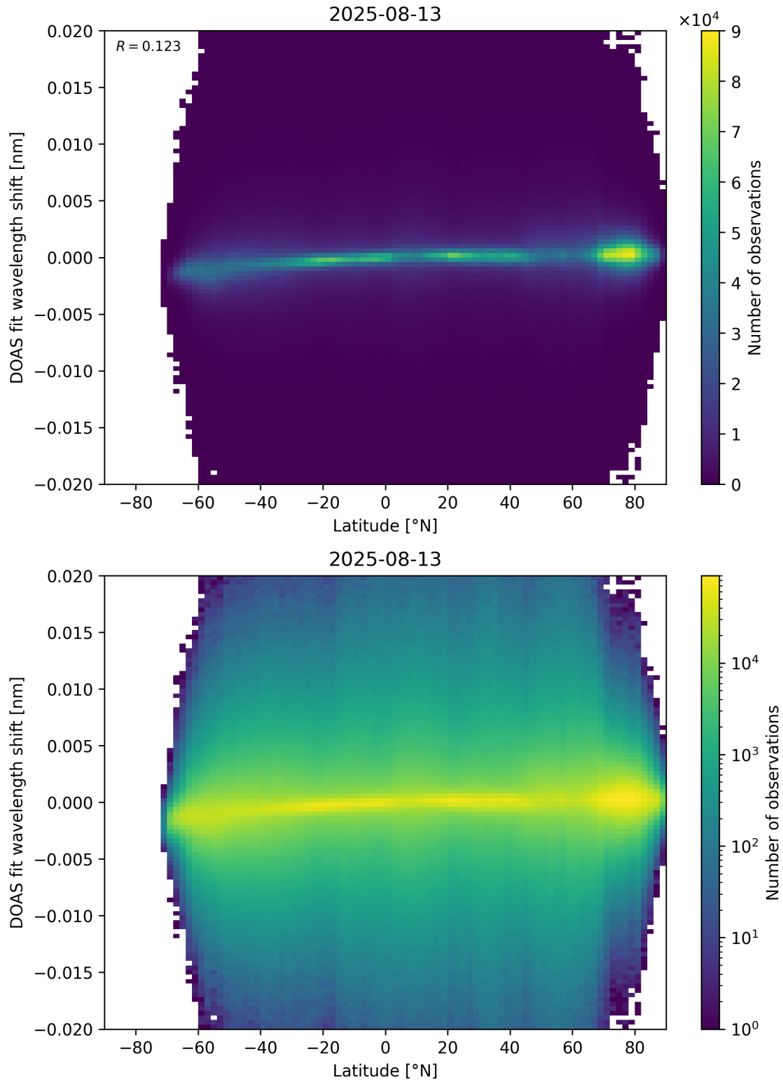
Figure 154: Scatter density plot of “Latitude” against “DOAS fit wavelength shift” for 2025-08-12 to 2025-08-14.
