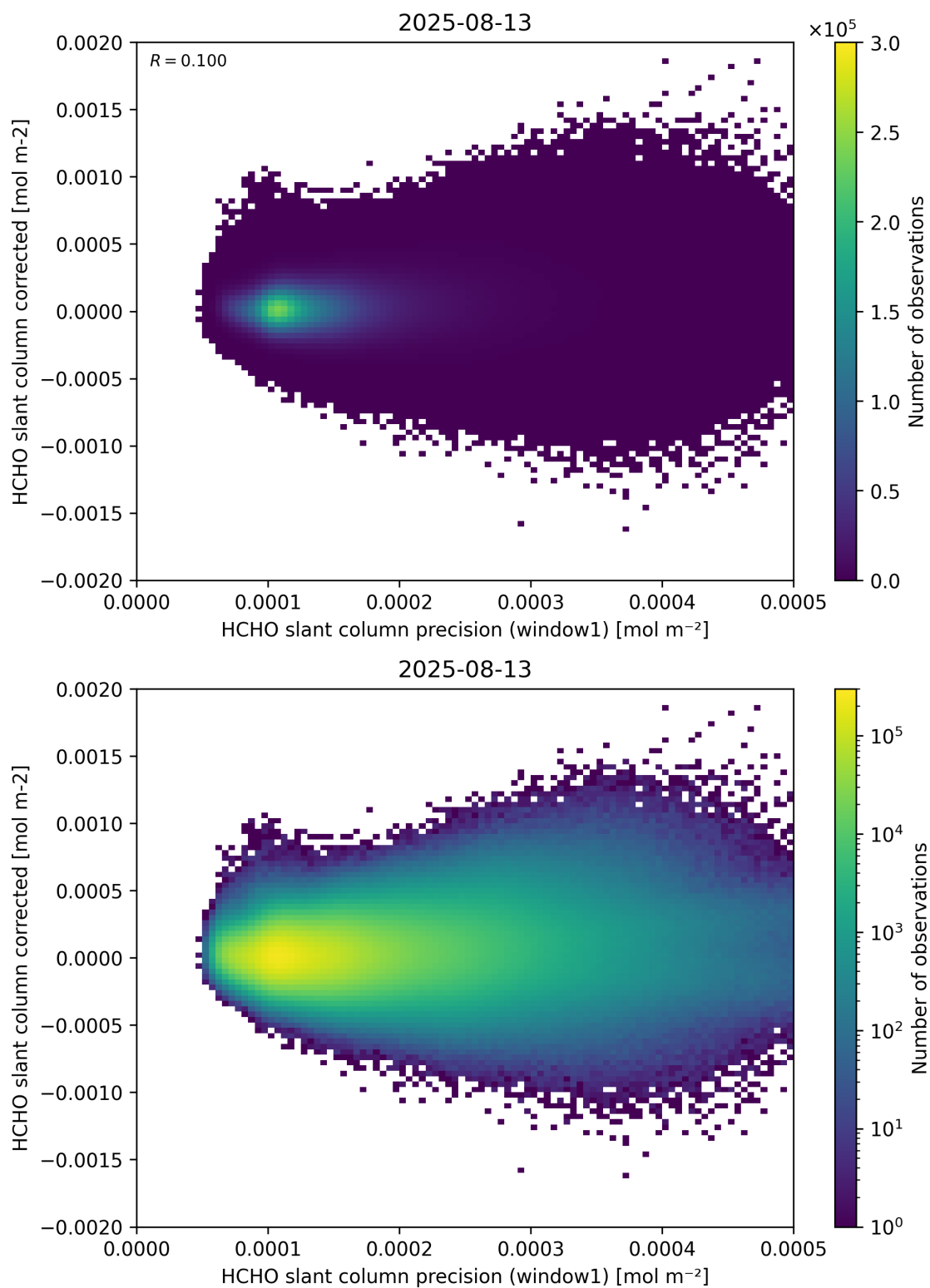
Figure 92: Scatter density plot of “HCHO slant column precision (window1)” against “HCHO slant column corrected” for 2025-08-12 to 2025-08-14.
