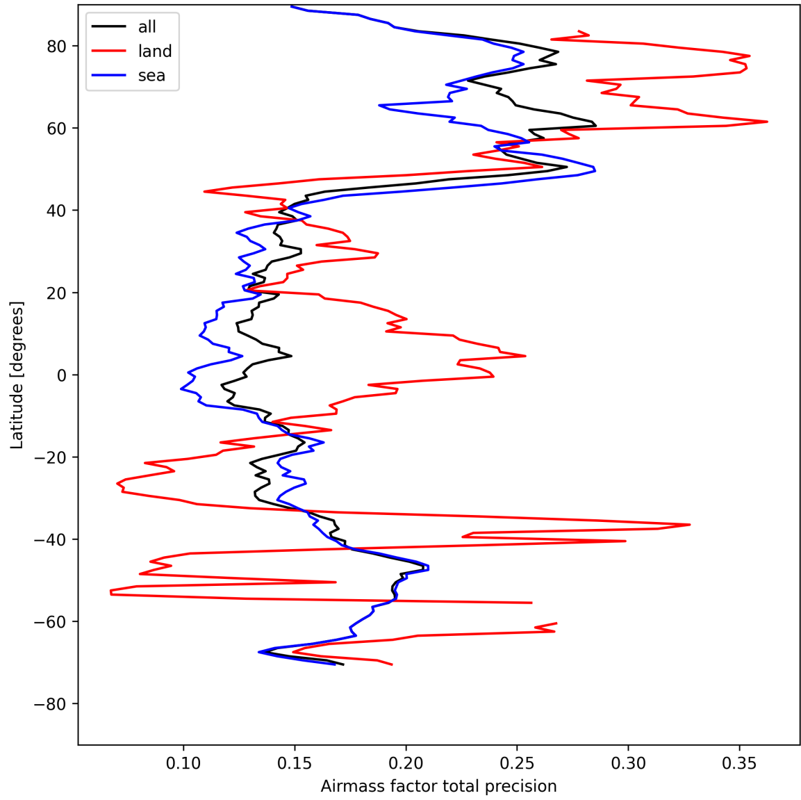
Figure 27: Zonal average of “Airmass factor total precision” for 2025-08-12 to 2025-08-14.
