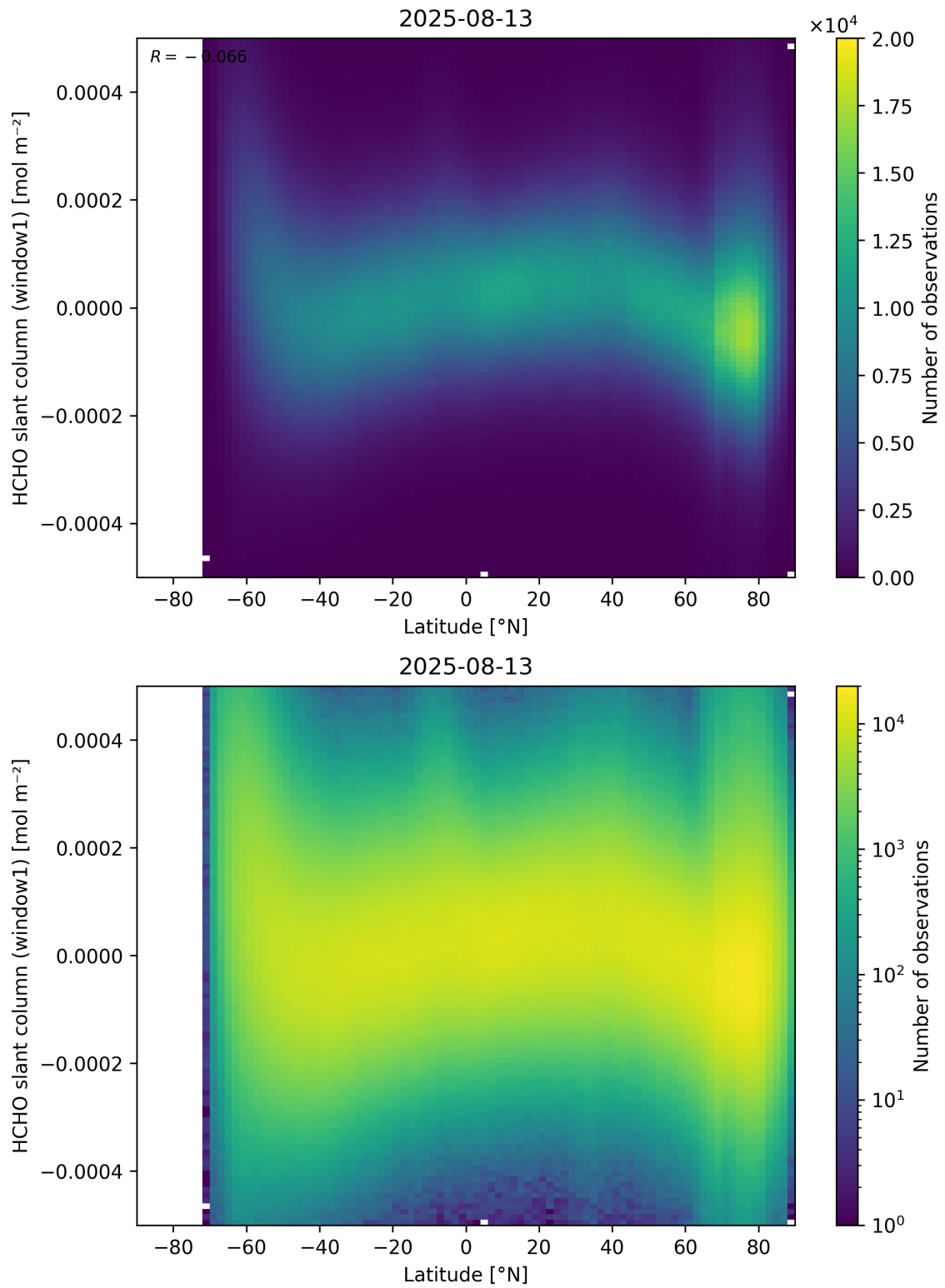
Figure 159: Scatter density plot of “Latitude” against “HCHO slant column (window1)” for 2025-08-12 to 2025-08-14.
