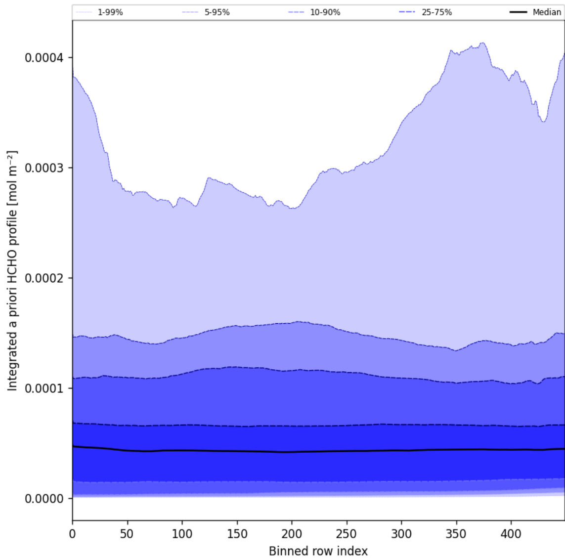
Figure 57: Along track statistics of “Integrated a priori HCHO profile” for 2025-08-12 to 2025-08-14
