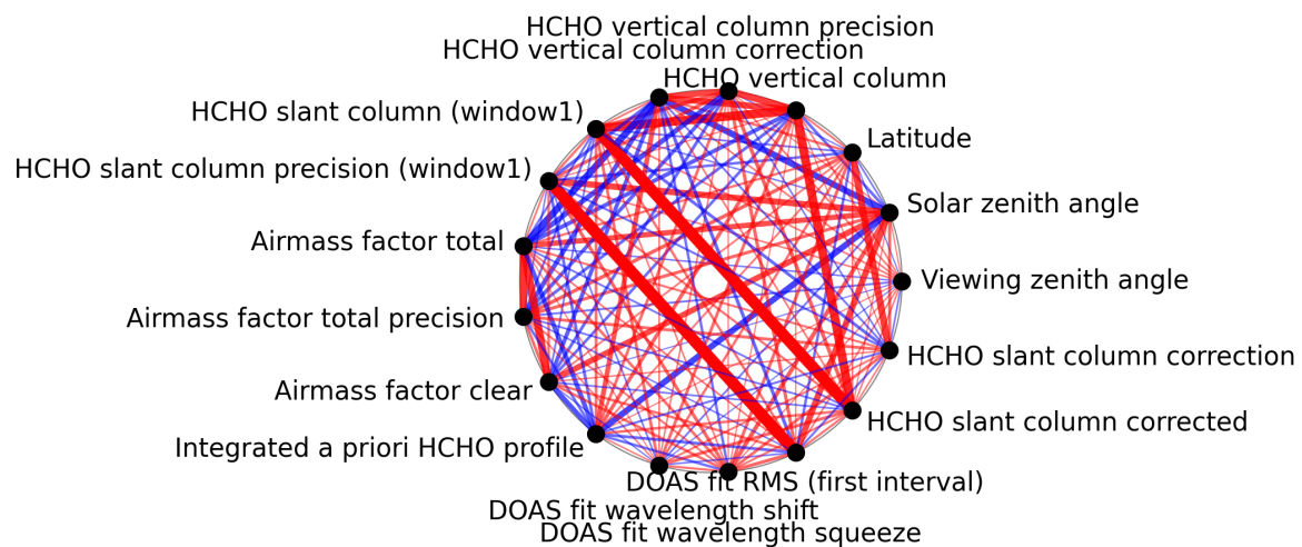
Figure 1: Map of correlation graph for 2025-08-12 to 2025-08-14.
