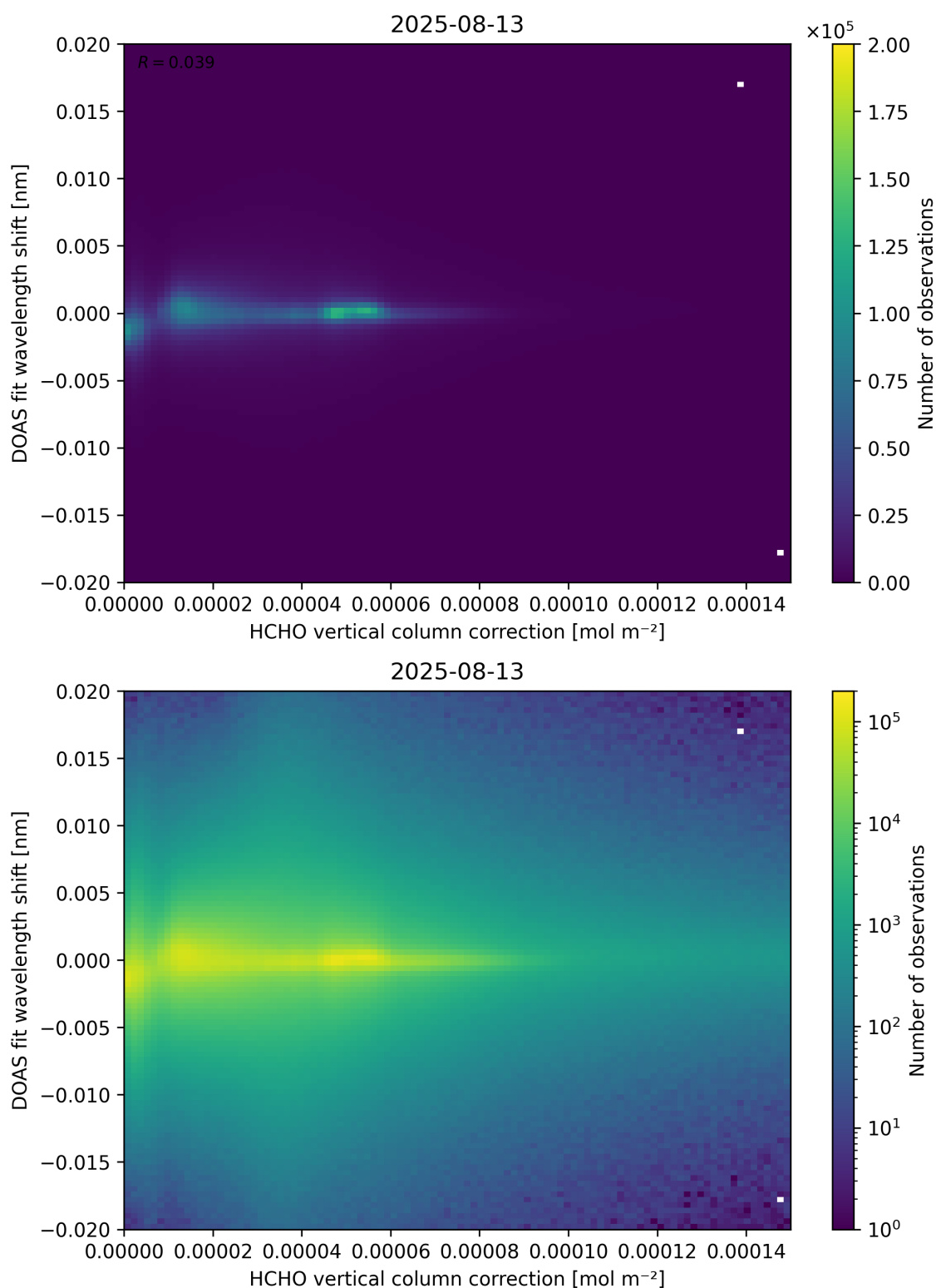
Figure 113: Scatter density plot of “HCHO vertical column correction” against “DOAS fit wavelength shift” for 2025-08-12 to 2025-08-14.
