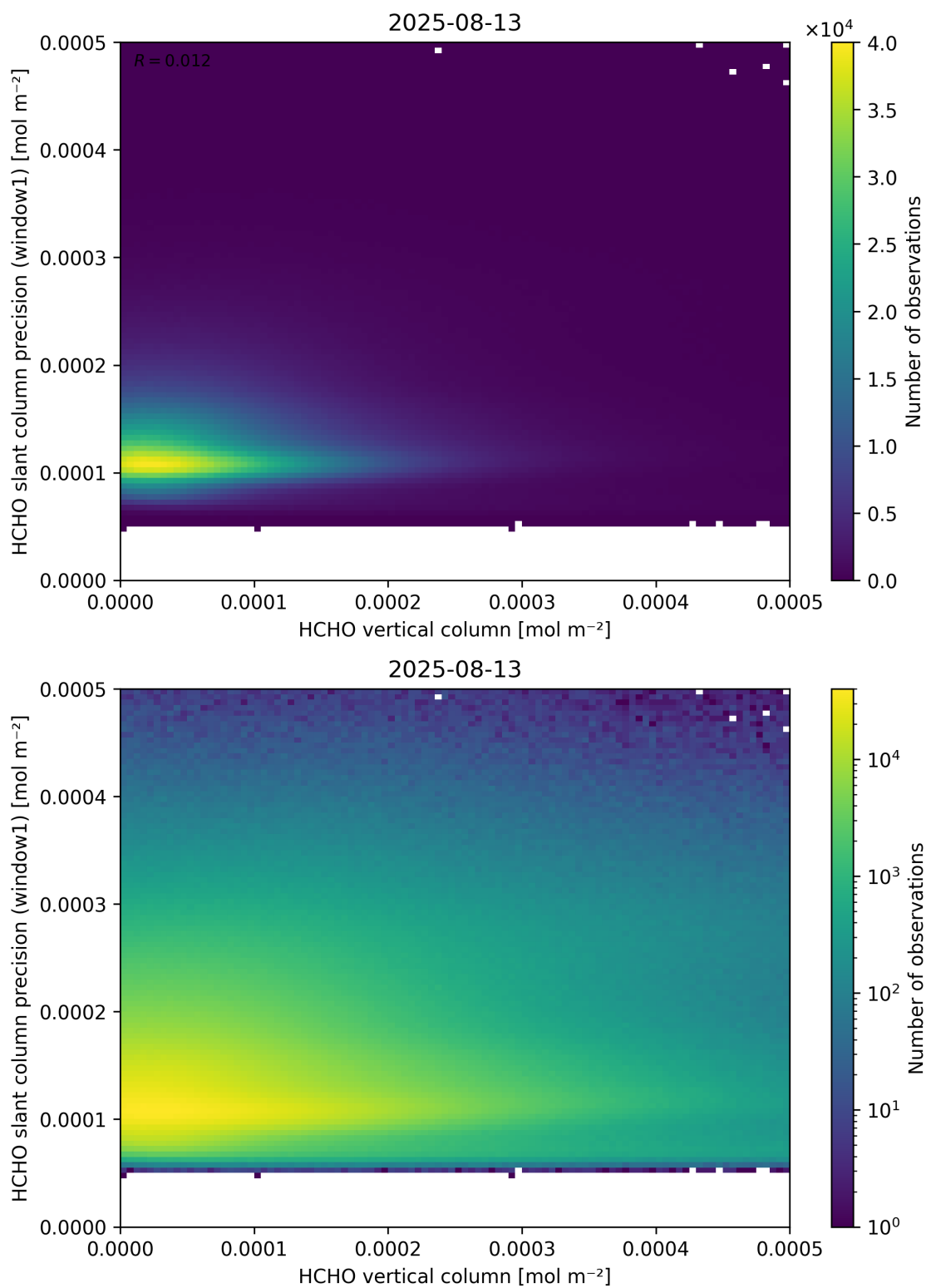
Figure 130: Scatter density plot of “HCHO vertical column” against “HCHO slant column precision (window1)” for 2025-08-12 to 2025-08-14.
