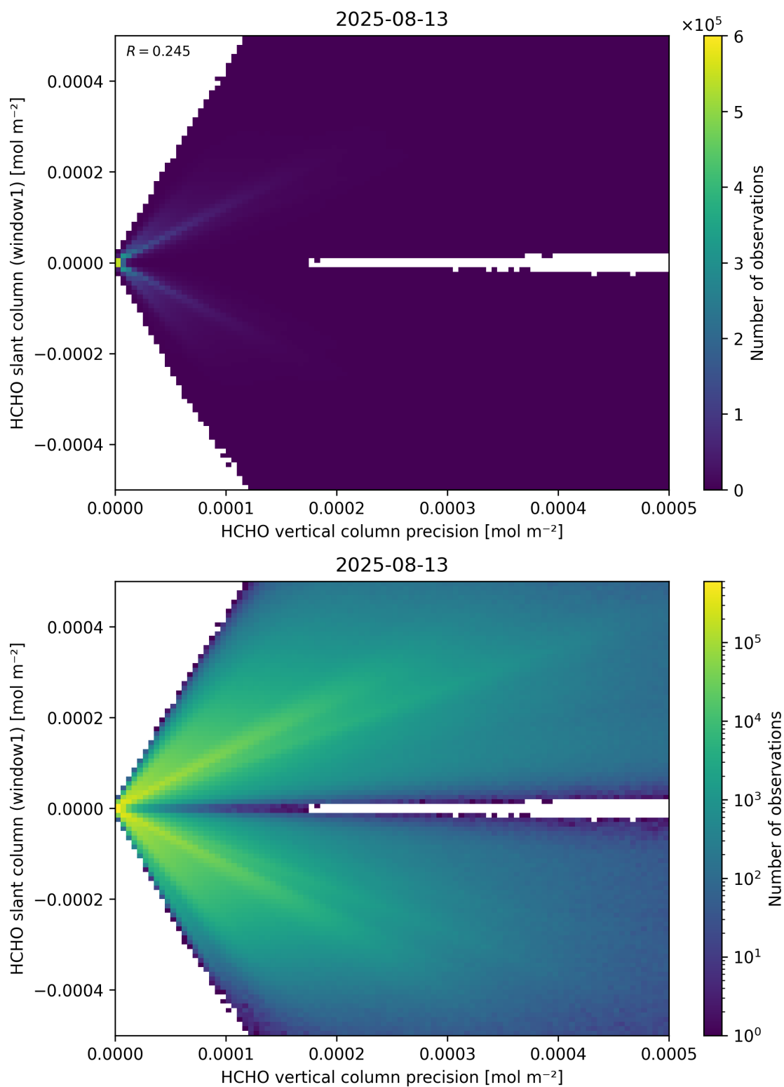
Figure 142: Scatter density plot of “HCHO vertical column precision” against “HCHO slant column (window1)” for 2025-08-12 to 2025-08-14.
