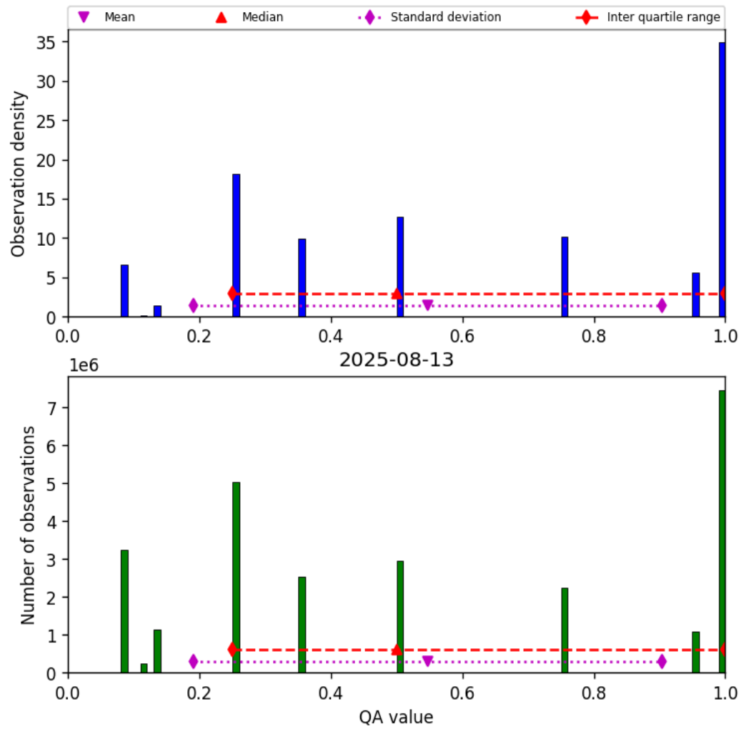
Figure 34: Histogram of “QA value” for 2025-08-12 to 2025-08-14
