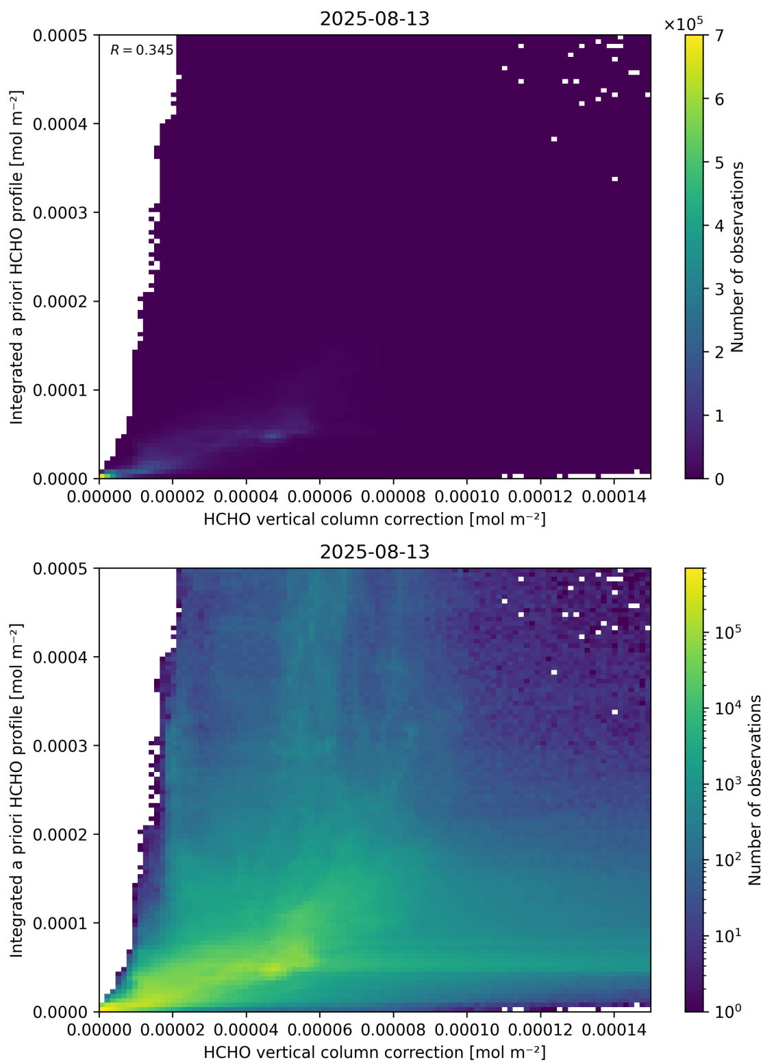
Figure 122: Scatter density plot of “HCHO vertical column correction” against “Integrated a priori HCHO profile” for 2025-08-12 to 2025-08-14.
