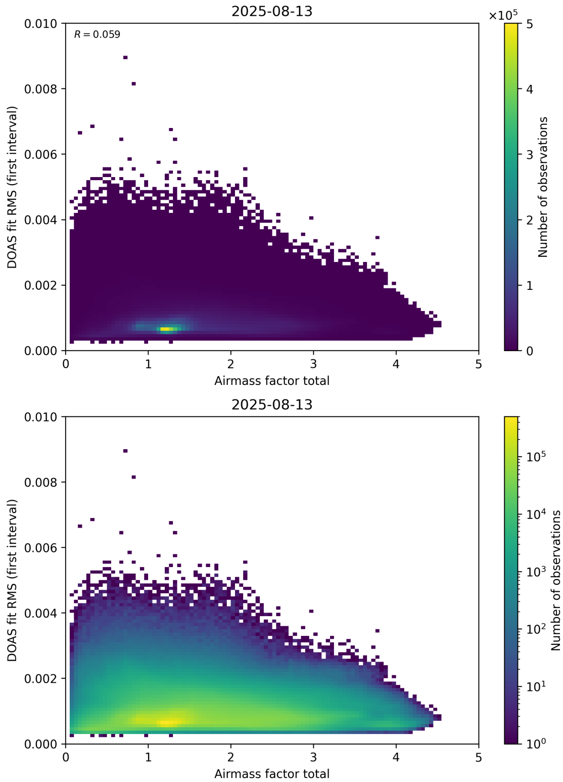
Figure 97: Scatter density plot of “Airmass factor total” against “DOAS fit RMS (first interval)” for 2025-08-12 to 2025-08-14.
