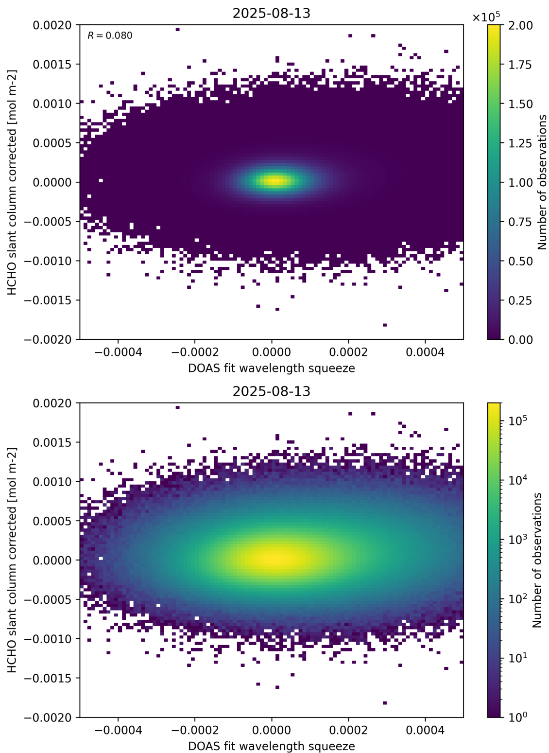
Figure 69: Scatter density plot of “DOAS fit wavelength squeeze” against “HCHO slant column corrected” for 2025-08-12 to 2025-08-14.
