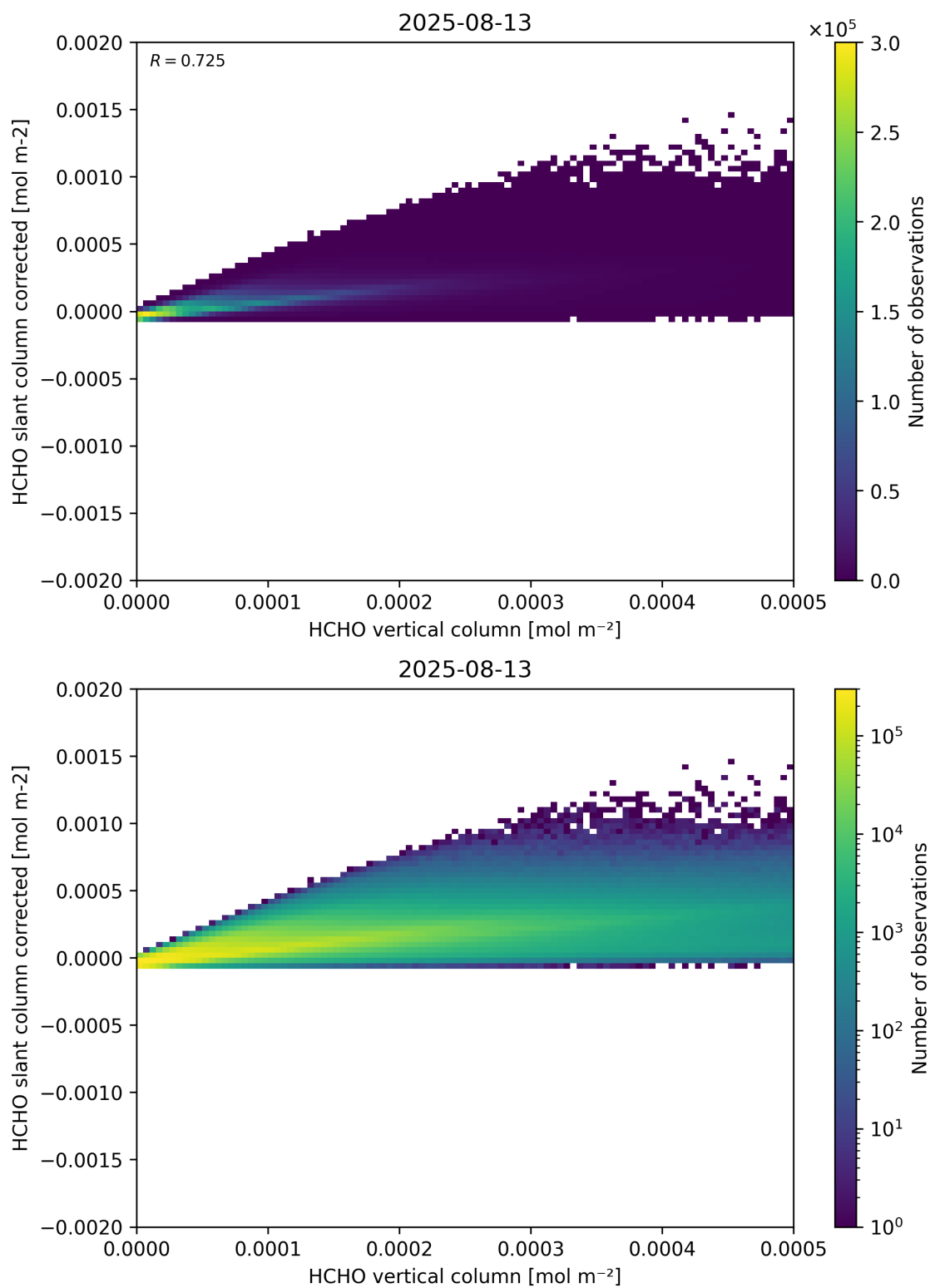
Figure 127: Scatter density plot of “HCHO vertical column” against “HCHO slant column corrected” for 2025-08-12 to 2025-08-14.
