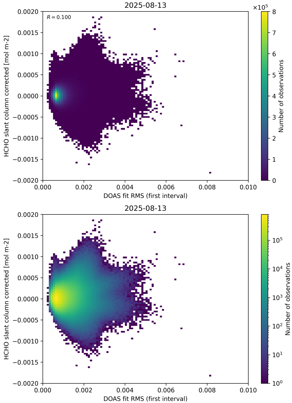
Figure 62: Scatter density plot of “DOAS fit RMS (first interval)” against “HCHO slant column corrected” for 2025-08-12 to 2025-08-14.
