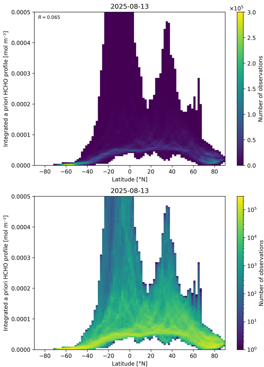
Figure 166: Scatter density plot of “Latitude” against “Integrated a priori HCHO profile” for 2025-08-12 to 2025-08-14.
