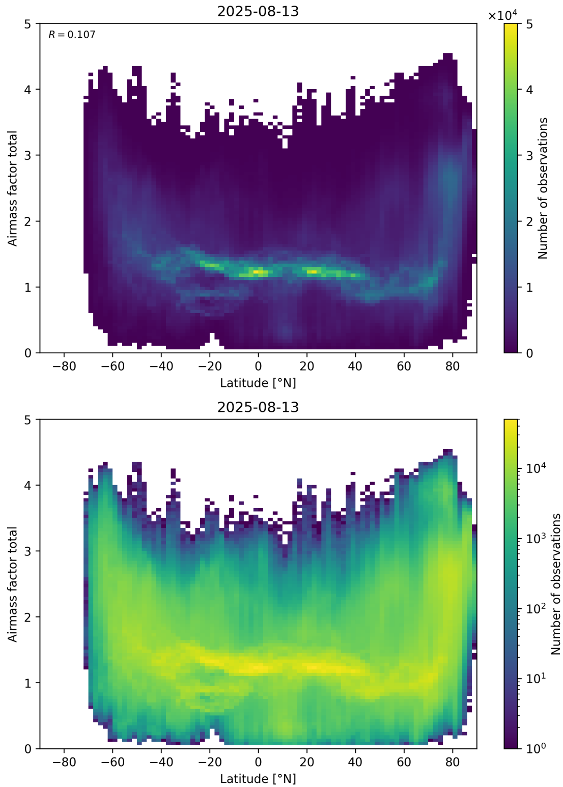
Figure 161: Scatter density plot of “Latitude” against “Airmass factor total” for 2025-08-12 to 2025-08-14.
