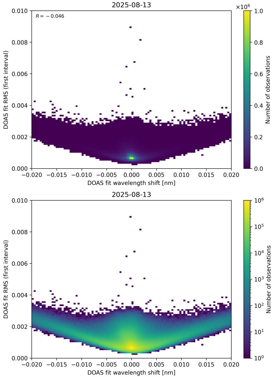
Figure 64: Scatter density plot of “DOAS fit wavelength shift” against “DOAS fit RMS (first interval)” for 2025-08-12 to 2025-08-14.
