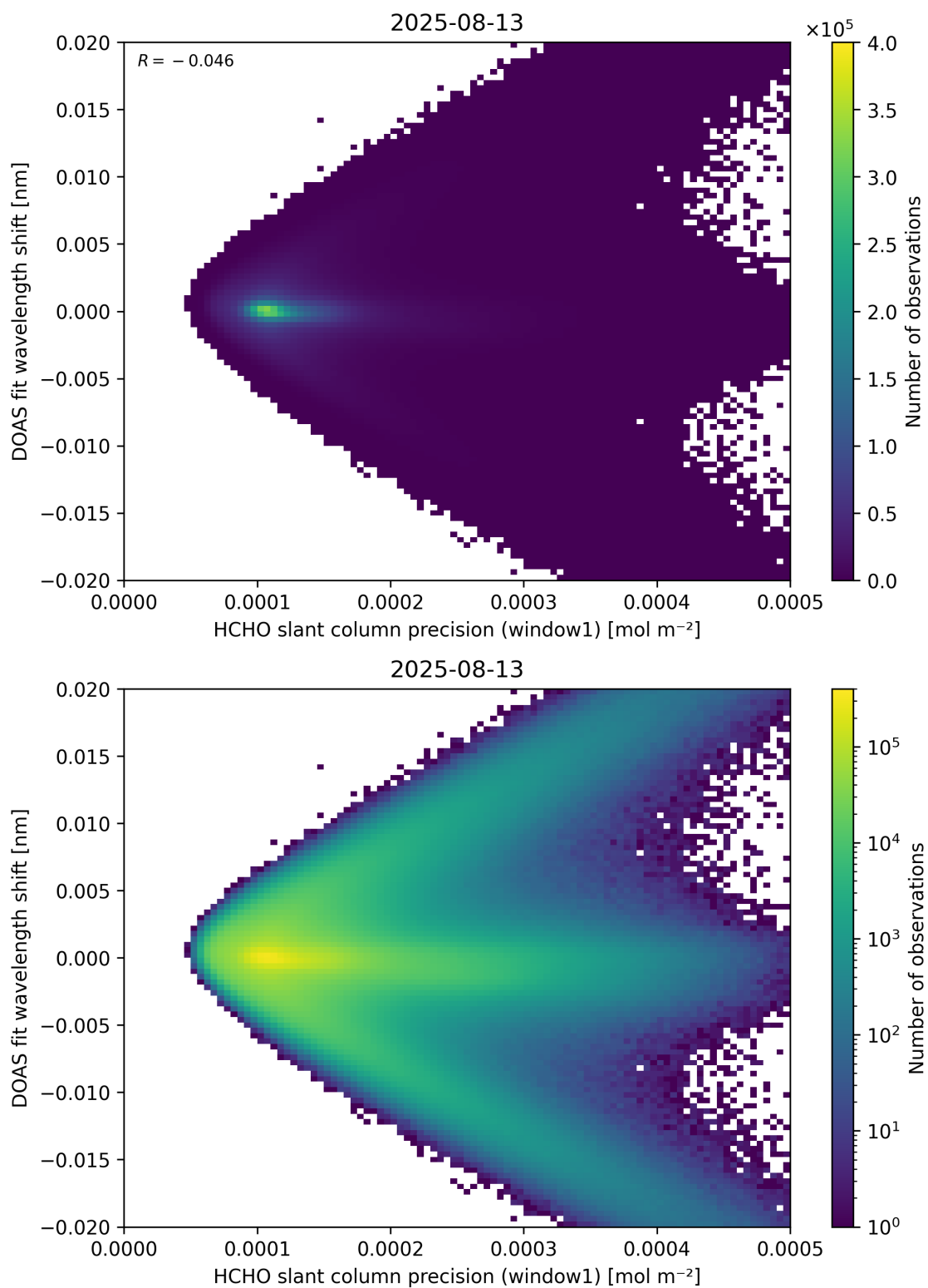
Figure 89: Scatter density plot of “HCHO slant column precision (window1)” against “DOAS fit wavelength shift” for 2025-08-12 to 2025-08-14.
