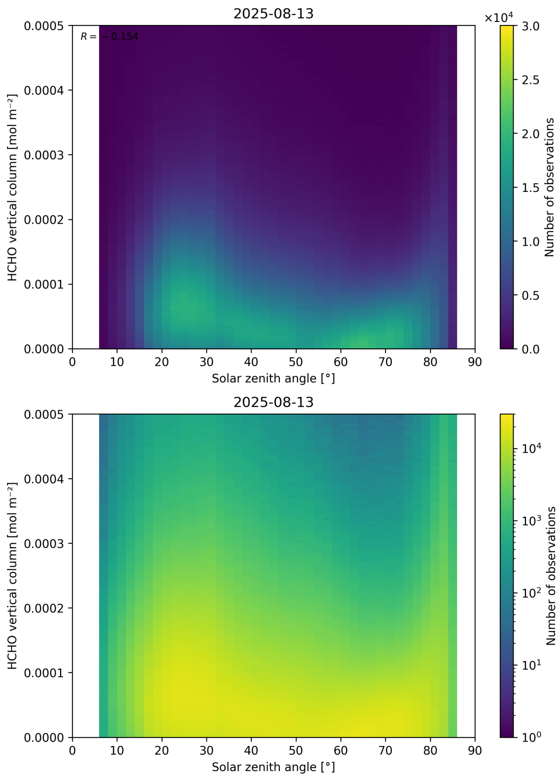
Figure 177: Scatter density plot of “Solar zenith angle” against “HCHO vertical column” for 2025-08-12 to 2025-08-14.
