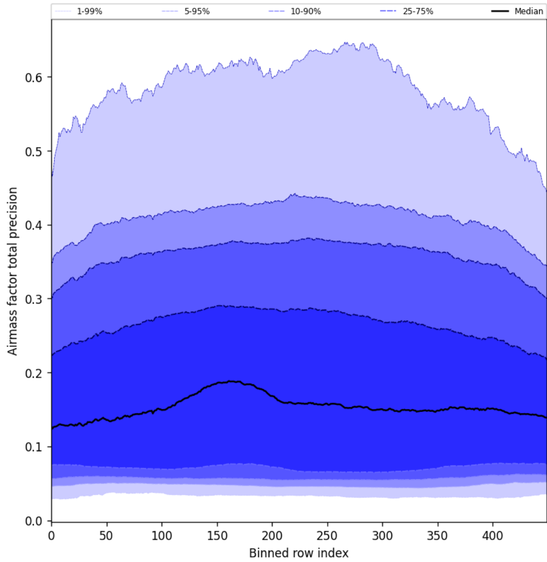
Figure 55: Along track statistics of “Airmass factor total precision” for 2025-08-12 to 2025-08-14
