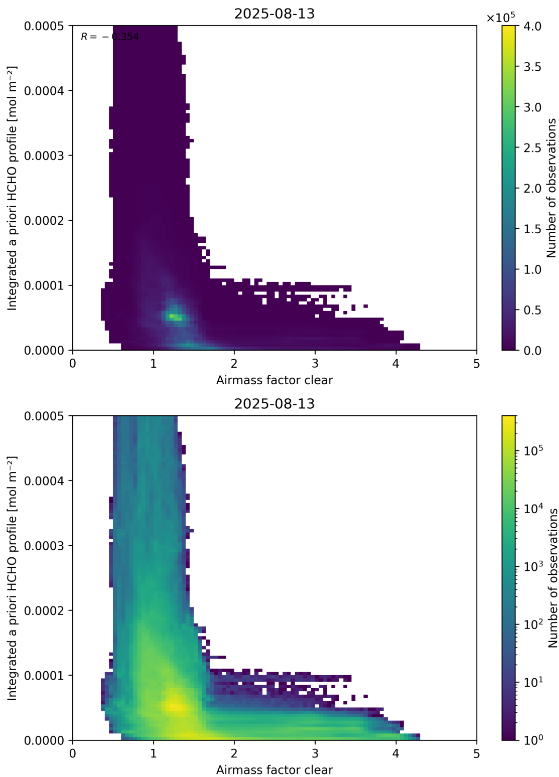
Figure 76: Scatter density plot of “Airmass factor clear” against “Integrated a priori HCHO profile” for 2025-08-12 to 2025-08-14.
