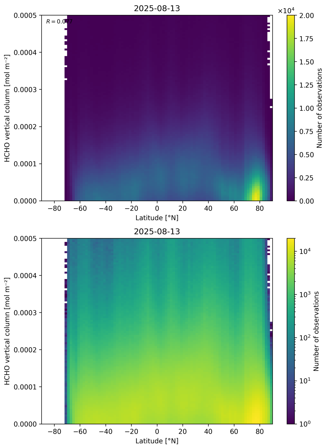
Figure 163: Scatter density plot of “Latitude” against “HCHO vertical column” for 2025-08-12 to 2025-08-14.
