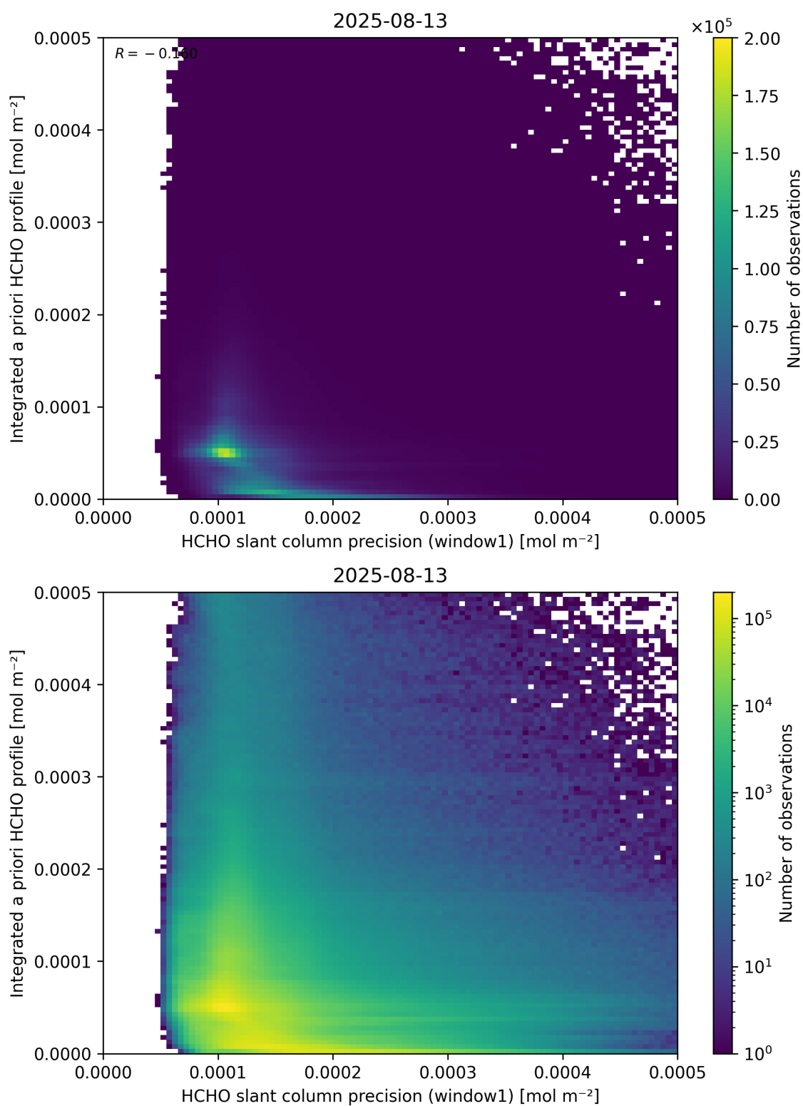
Figure 96: Scatter density plot of “HCHO slant column precision (window1)” against “Integrated a priori HCHO profile” for 2025-08-12 to 2025-08-14.
