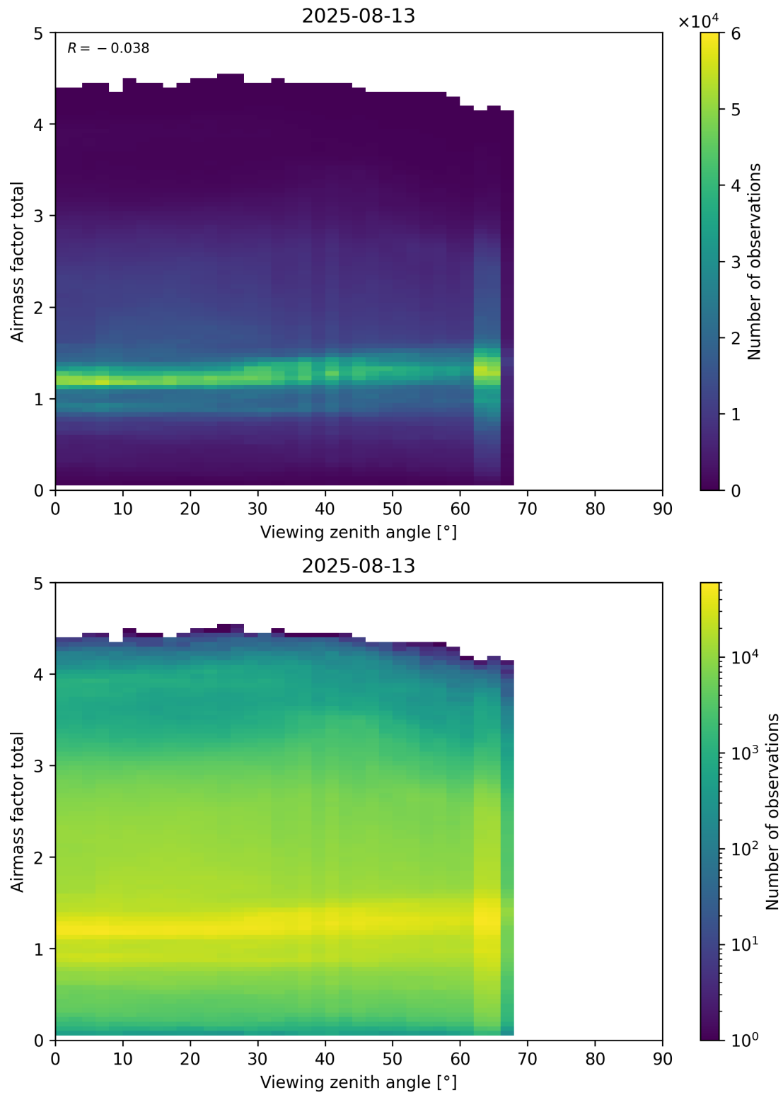
Figure 190: Scatter density plot of “Viewing zenith angle” against “Airmass factor total” for 2025-08-12 to 2025-08-14.
