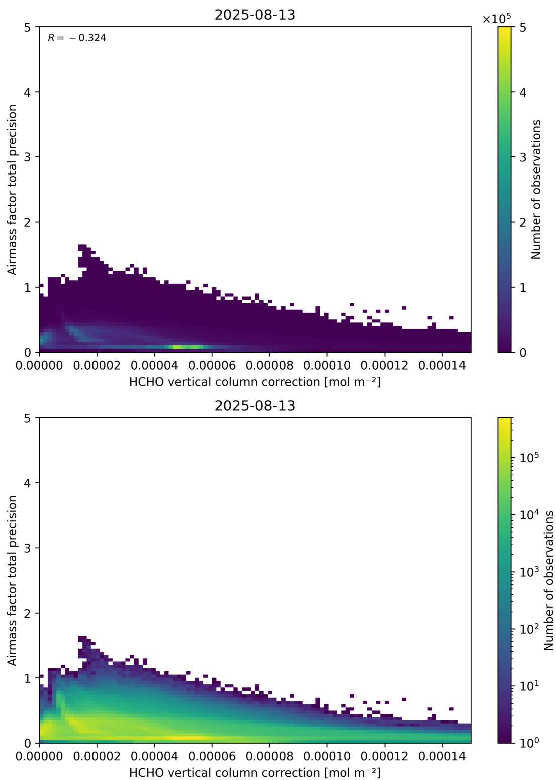
Figure 121: Scatter density plot of “HCHO vertical column correction” against “Airmass factor total precision” for 2025-08-12 to 2025-08-14.
