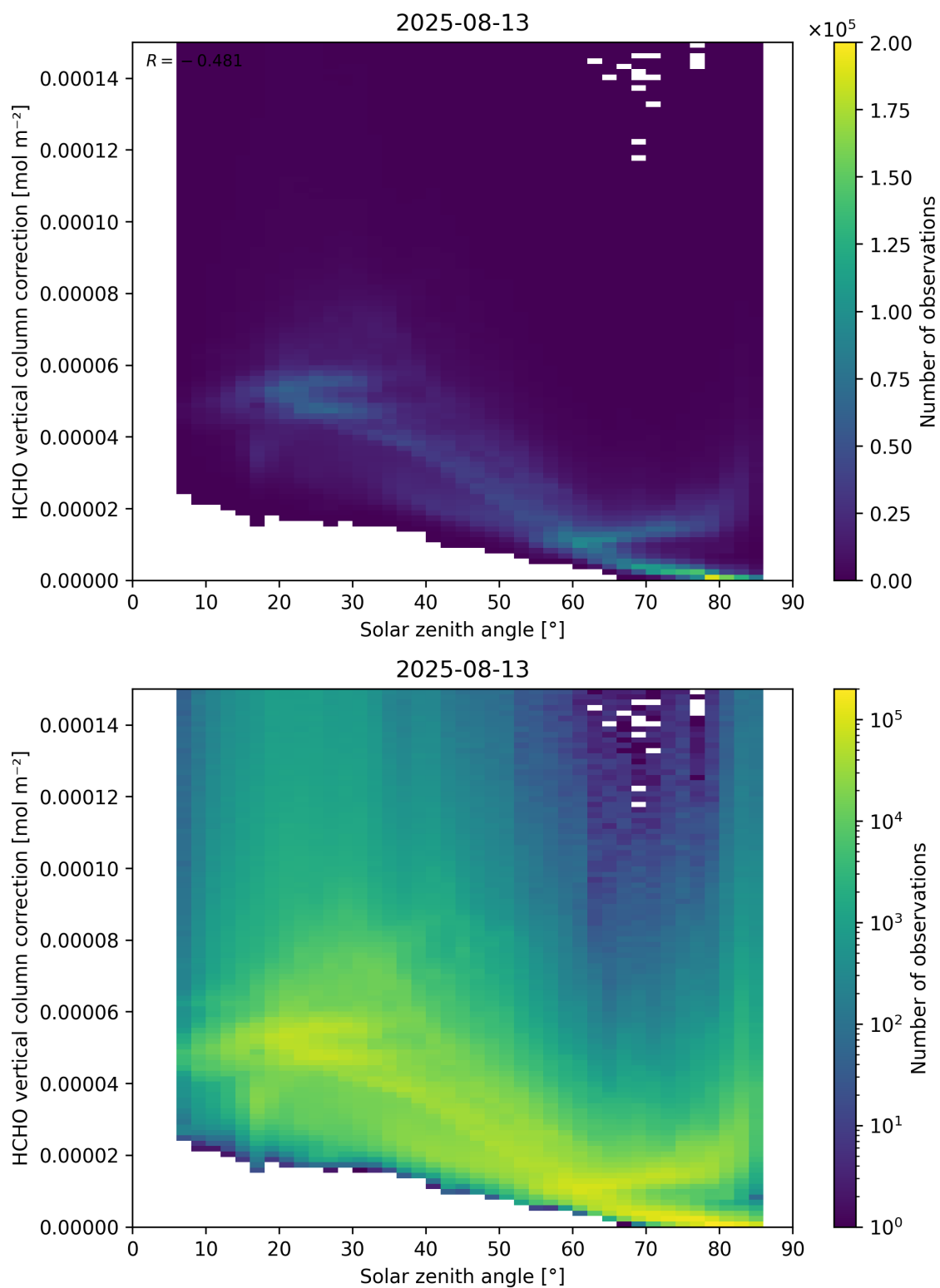
Figure 178: Scatter density plot of “Solar zenith angle” against “HCHO vertical column correction” for 2025-08-12 to 2025-08-14.
