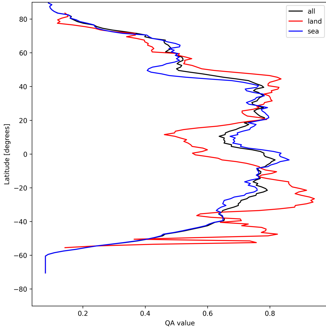
Figure 20: Zonal average of “QA value” for 2025-08-12 to 2025-08-14.
