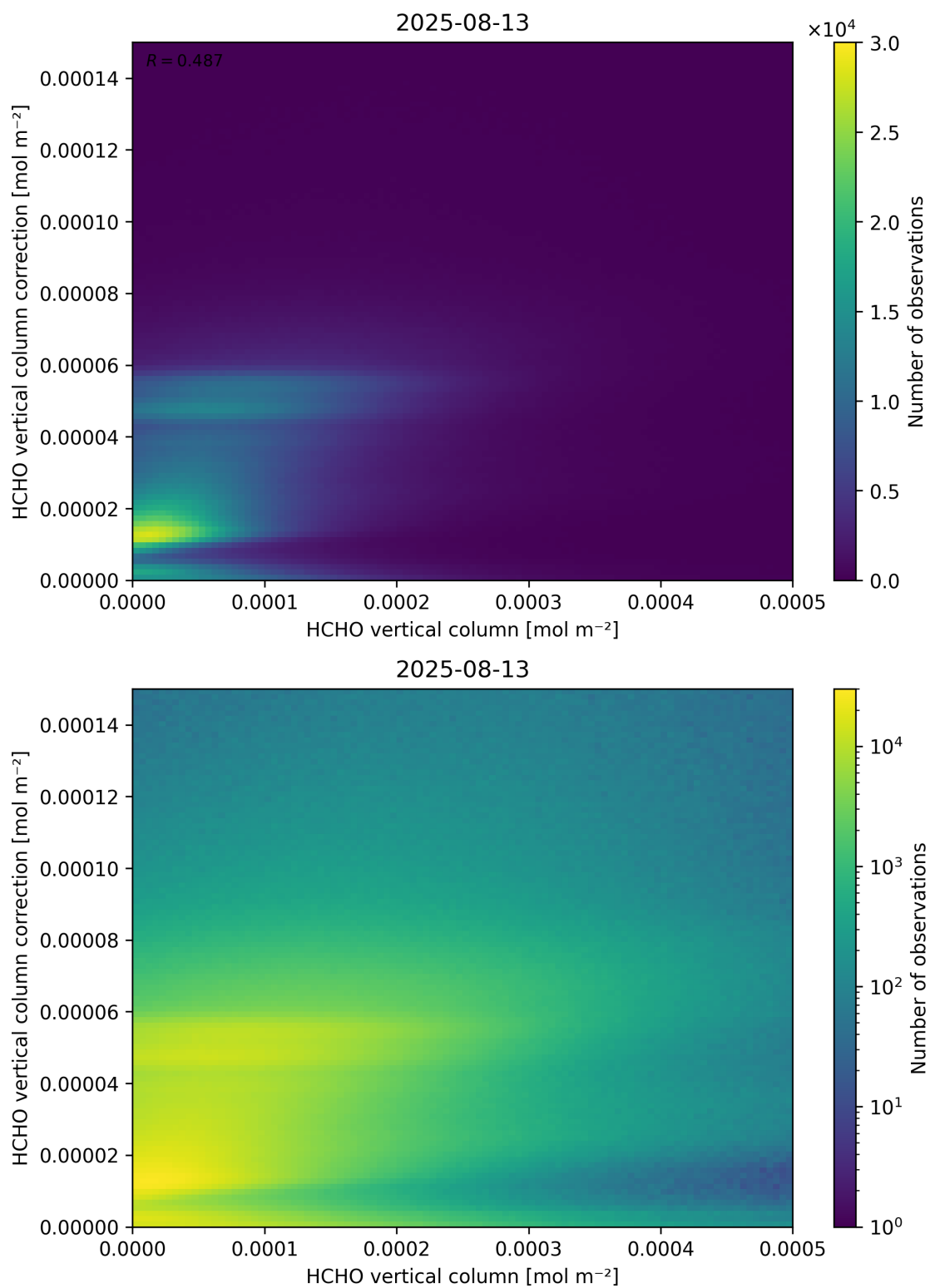
Figure 133: Scatter density plot of “HCHO vertical column” against “HCHO vertical column correction” for 2025-08-12 to 2025-08-14.
