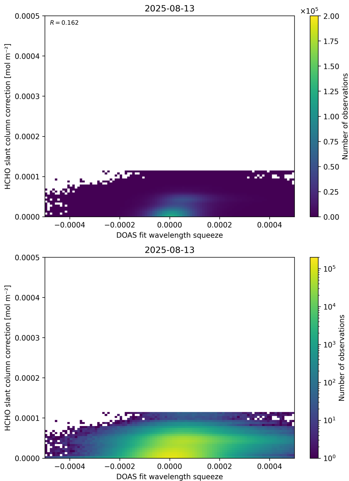
Figure 70: Scatter density plot of “DOAS fit wavelength squeeze” against “HCHO slant column correction” for 2025-08-12 to 2025-08-14.
