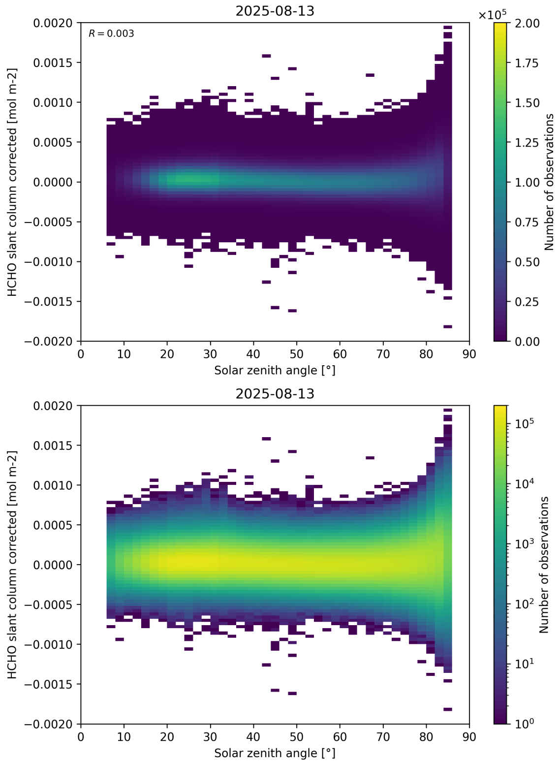
Figure 171: Scatter density plot of “Solar zenith angle” against “HCHO slant column corrected” for 2025-08-12 to 2025-08-14.
