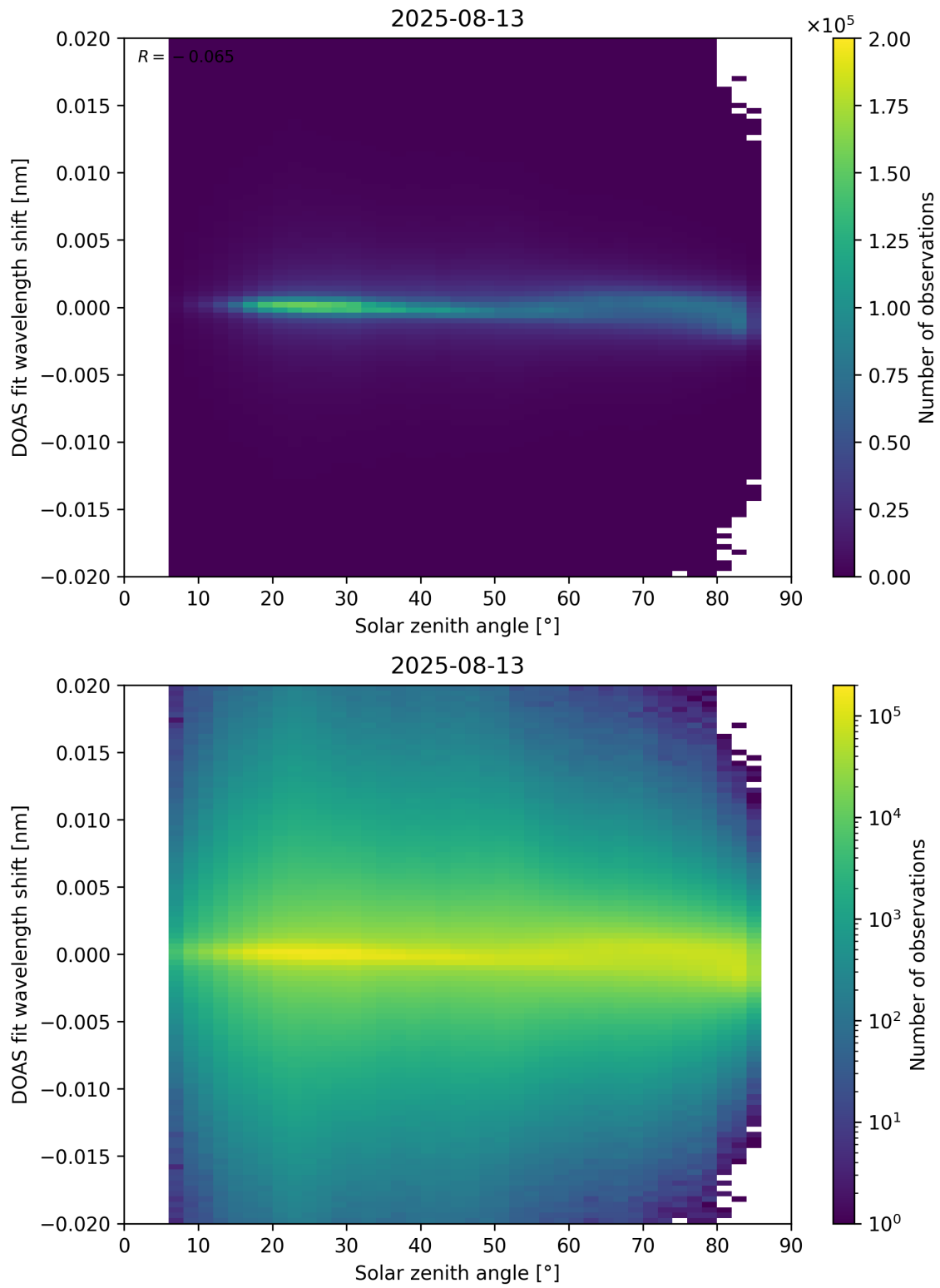
Figure 168: Scatter density plot of “Solar zenith angle” against “DOAS fit wavelength shift” for 2025-08-12 to 2025-08-14.
