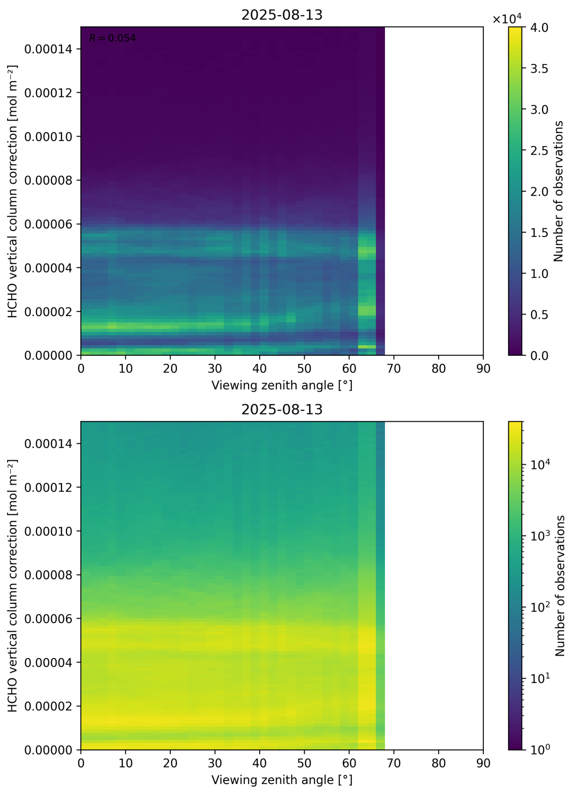
Figure 193: Scatter density plot of “Viewing zenith angle” against “HCHO vertical column correction” for 2025-08-12 to 2025-08-14.
