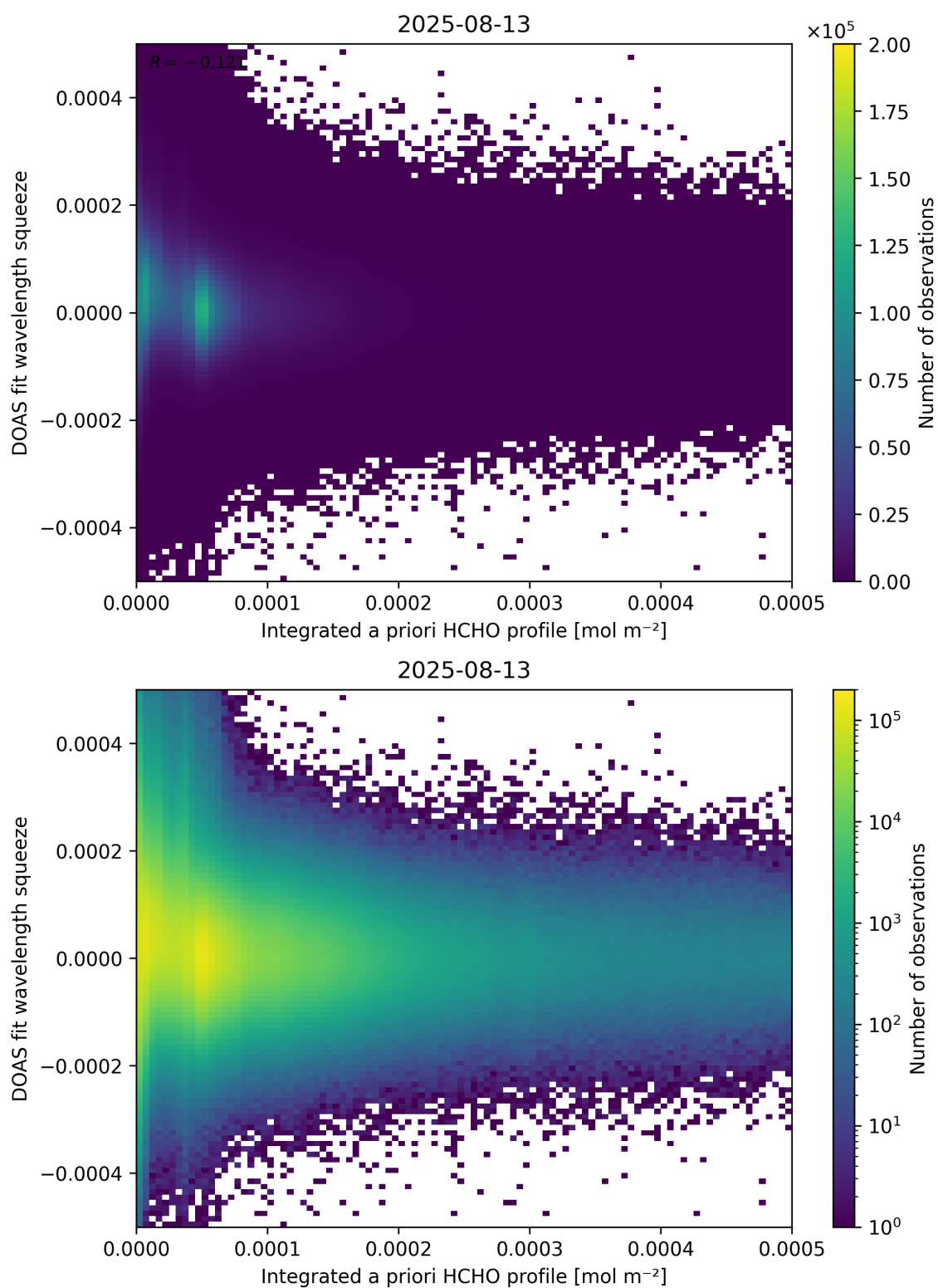
Figure 150: Scatter density plot of “Integrated a priori HCHO profile” against “DOAS fit wavelength squeeze” for 2025-08-12 to 2025-08-14.
