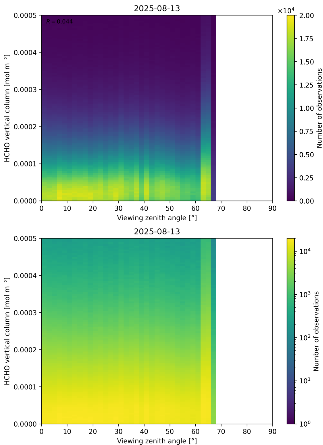
Figure 192: Scatter density plot of “Viewing zenith angle” against “HCHO vertical column” for 2025-08-12 to 2025-08-14.
