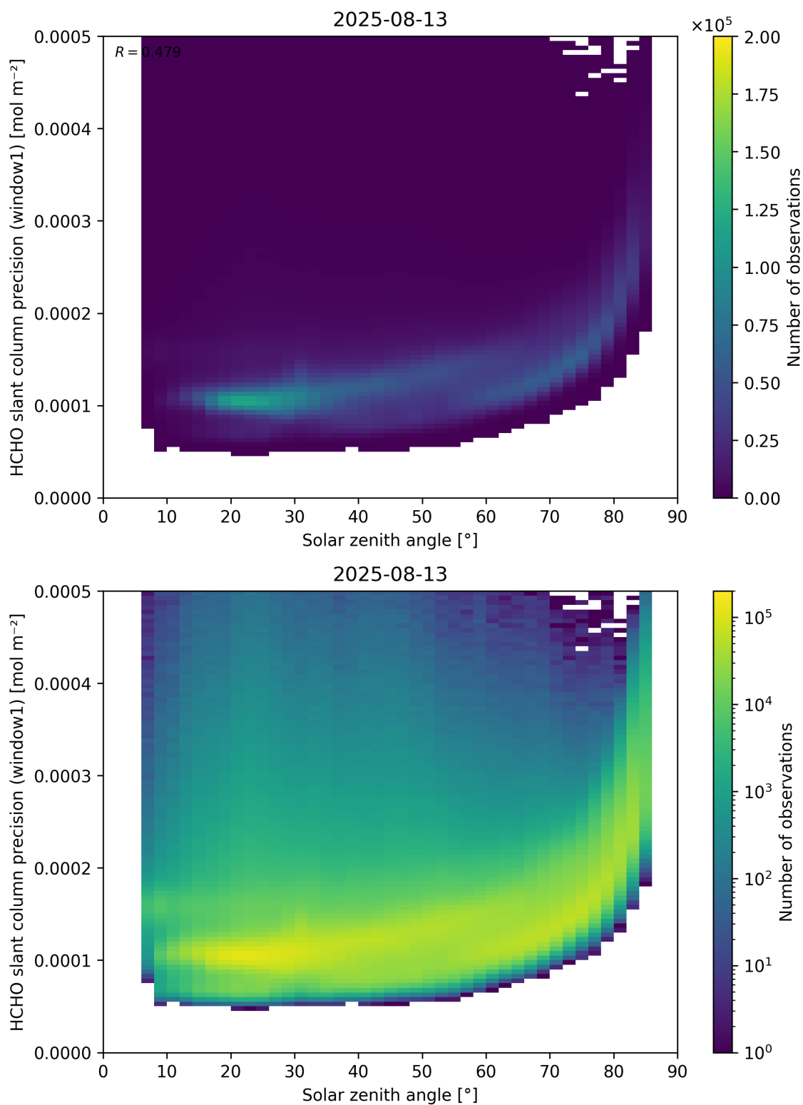
Figure 174: Scatter density plot of “Solar zenith angle” against “HCHO slant column precision (window1)” for 2025-08-12 to 2025-08-14.
