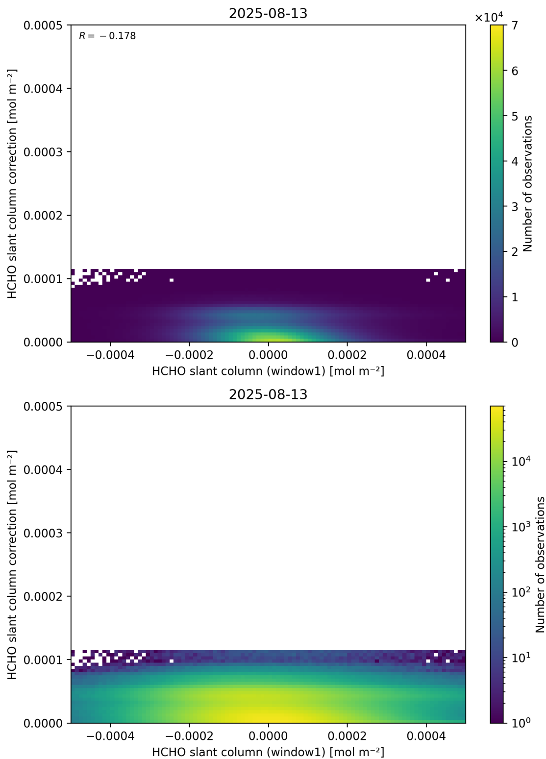
Figure 83: Scatter density plot of “HCHO slant column (window1)” against “HCHO slant column correction” for 2025-08-12 to 2025-08-14.
