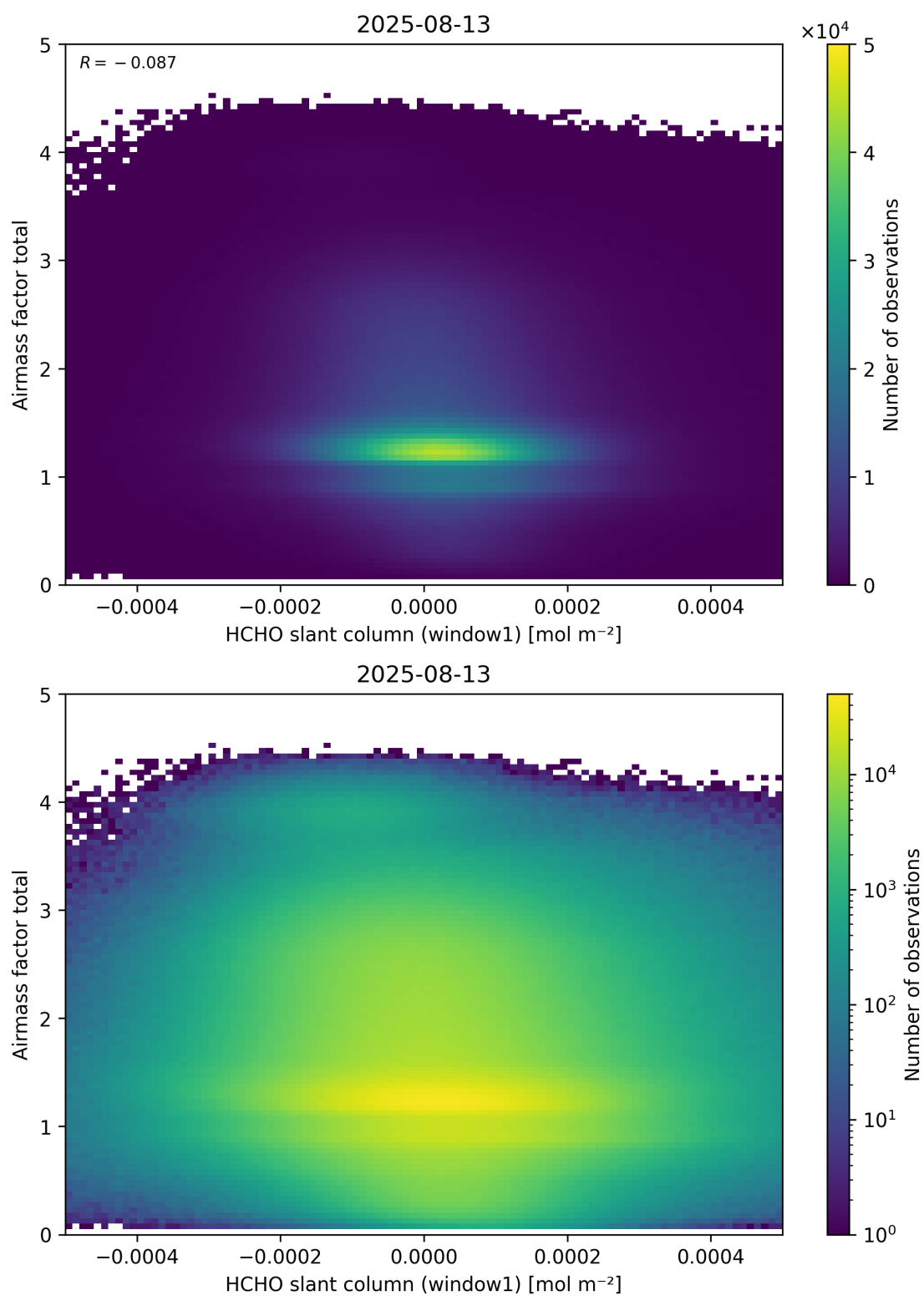
Figure 85: Scatter density plot of “HCHO slant column (window1)” against “Airmass factor total” for 2025-08-12 to 2025-08-14.
