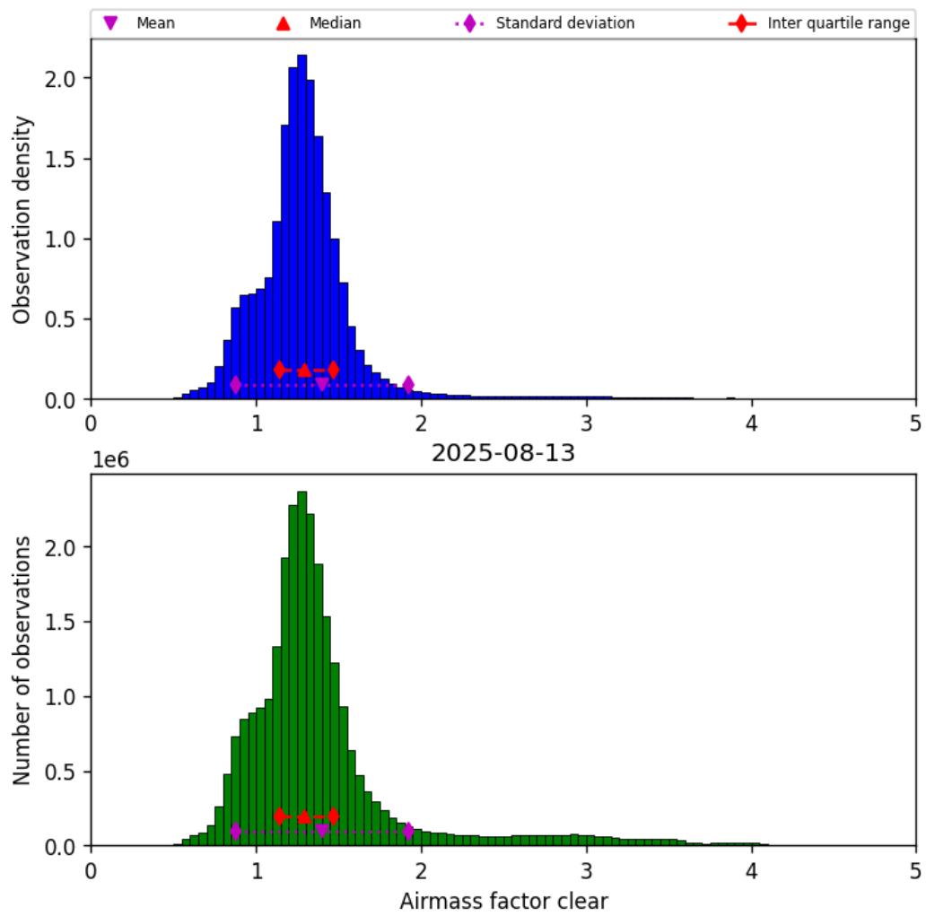
Figure 42: Histogram of “Airmass factor clear” for 2025-08-12 to 2025-08-14
