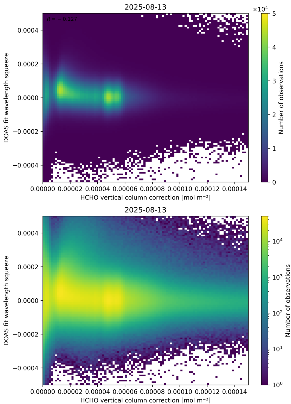
Figure 114: Scatter density plot of “HCHO vertical column correction” against “DOAS fit wavelength squeeze” for 2025-08-12 to 2025-08-14.
