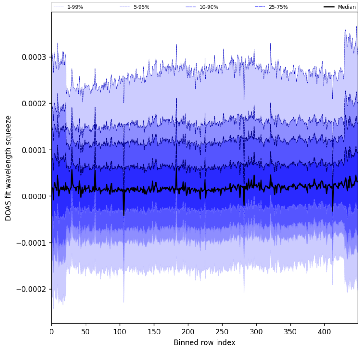
Figure 59: Along track statistics of “DOAS fit wavelength squeeze” for 2025-08-12 to 2025-08-14
