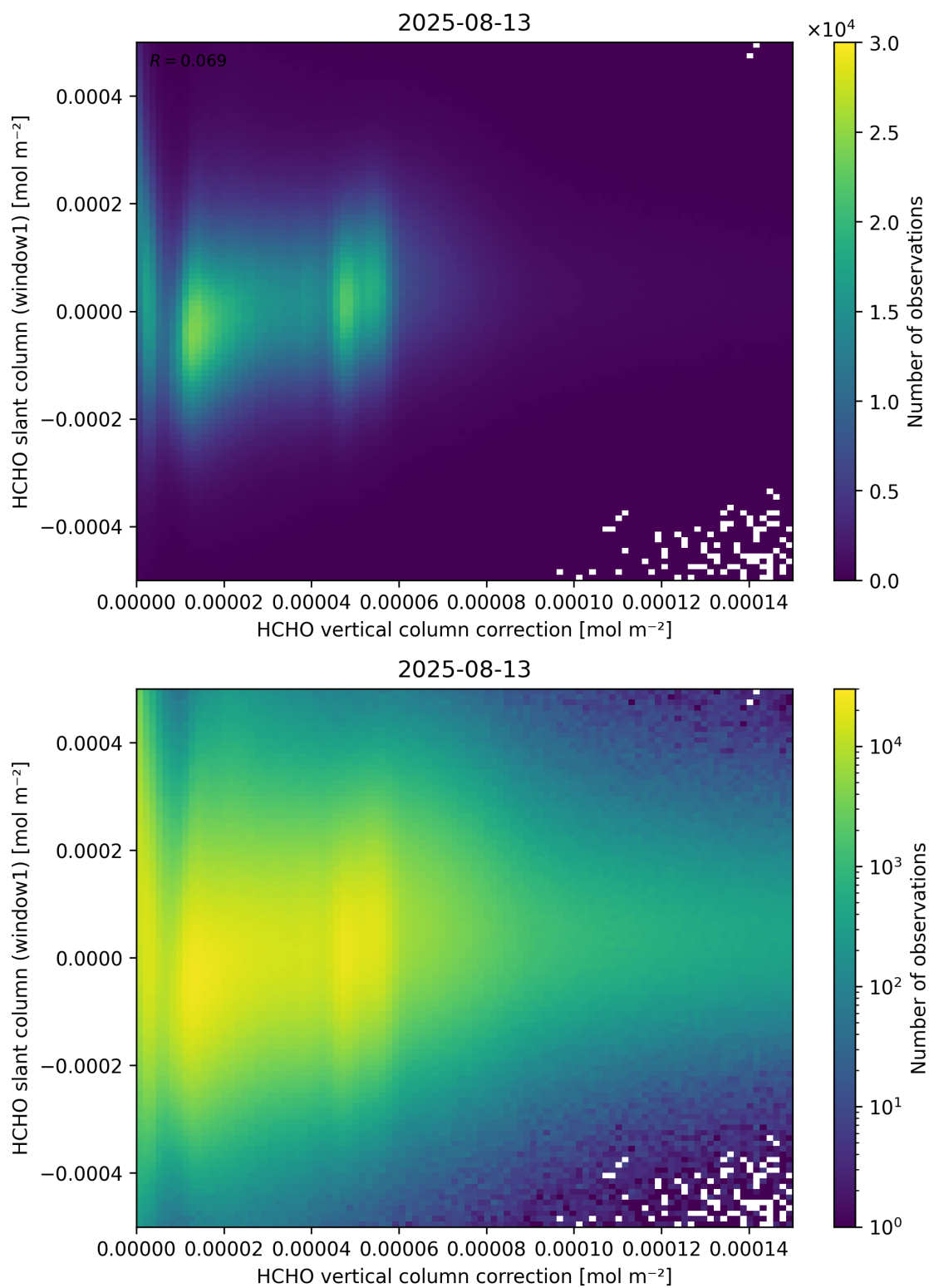
Figure 118: Scatter density plot of “HCHO vertical column correction” against “HCHO slant column (window1)” for 2025-08-12 to 2025-08-14.
