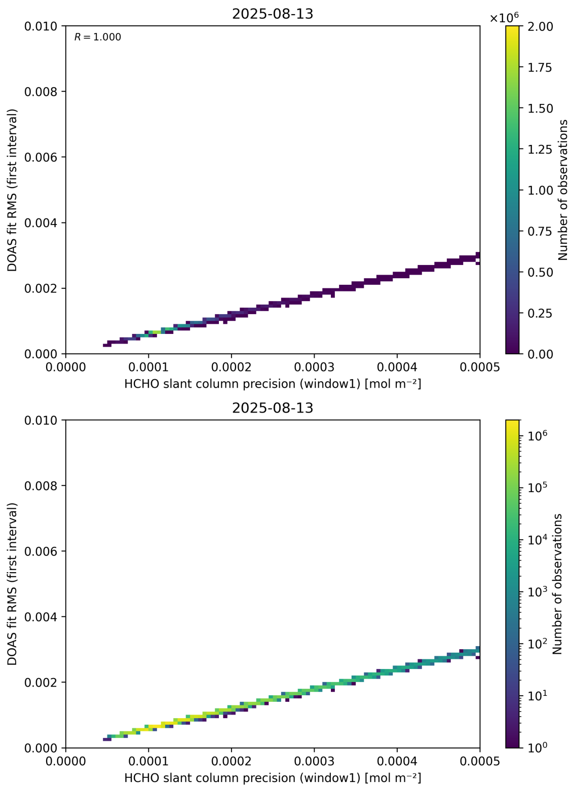
Figure 88: Scatter density plot of “HCHO slant column precision (window1)” against “DOAS fit RMS (first interval)” for 2025-08-12 to 2025-08-14.
