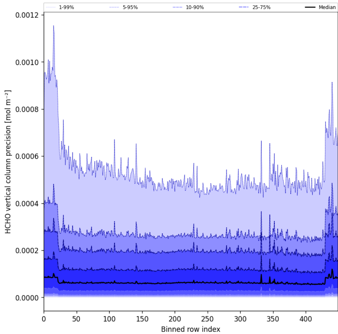
Figure 50: Along track statistics of “HCHO vertical column precision” for 2025-08-12 to 2025-08-14
