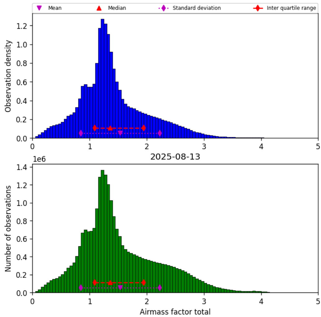
Figure 40: Histogram of “Airmass factor total” for 2025-08-12 to 2025-08-14
