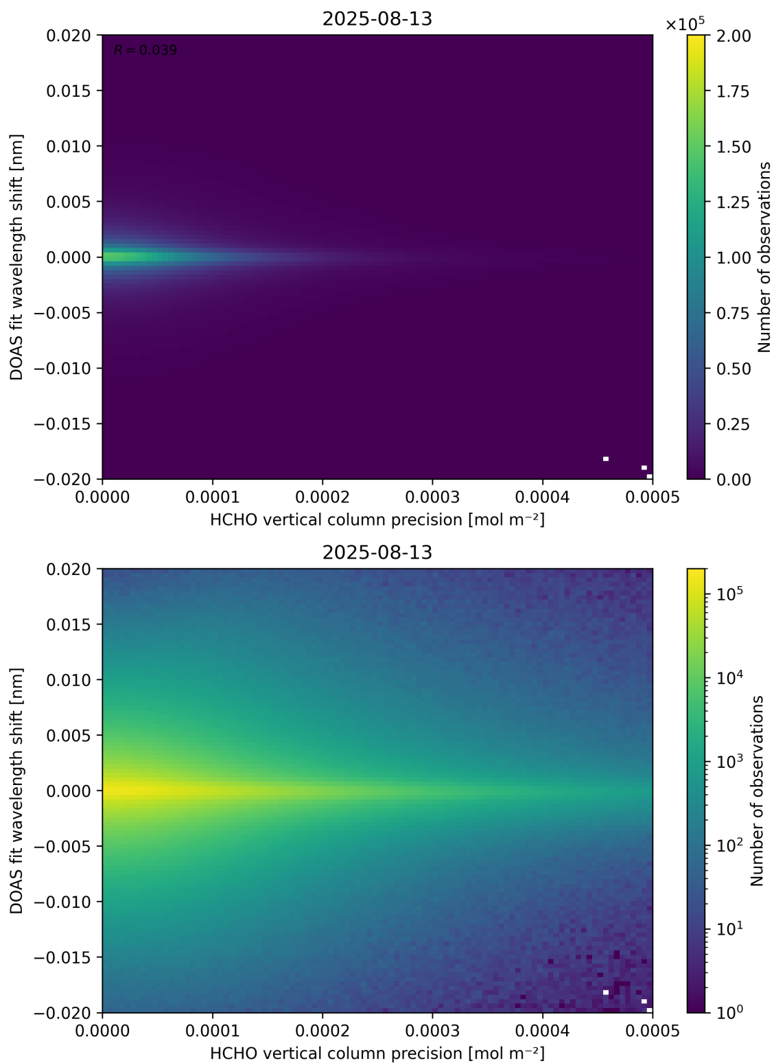
Figure 137: Scatter density plot of “HCHO vertical column precision” against “DOAS fit wavelength shift” for 2025-08-12 to 2025-08-14.
