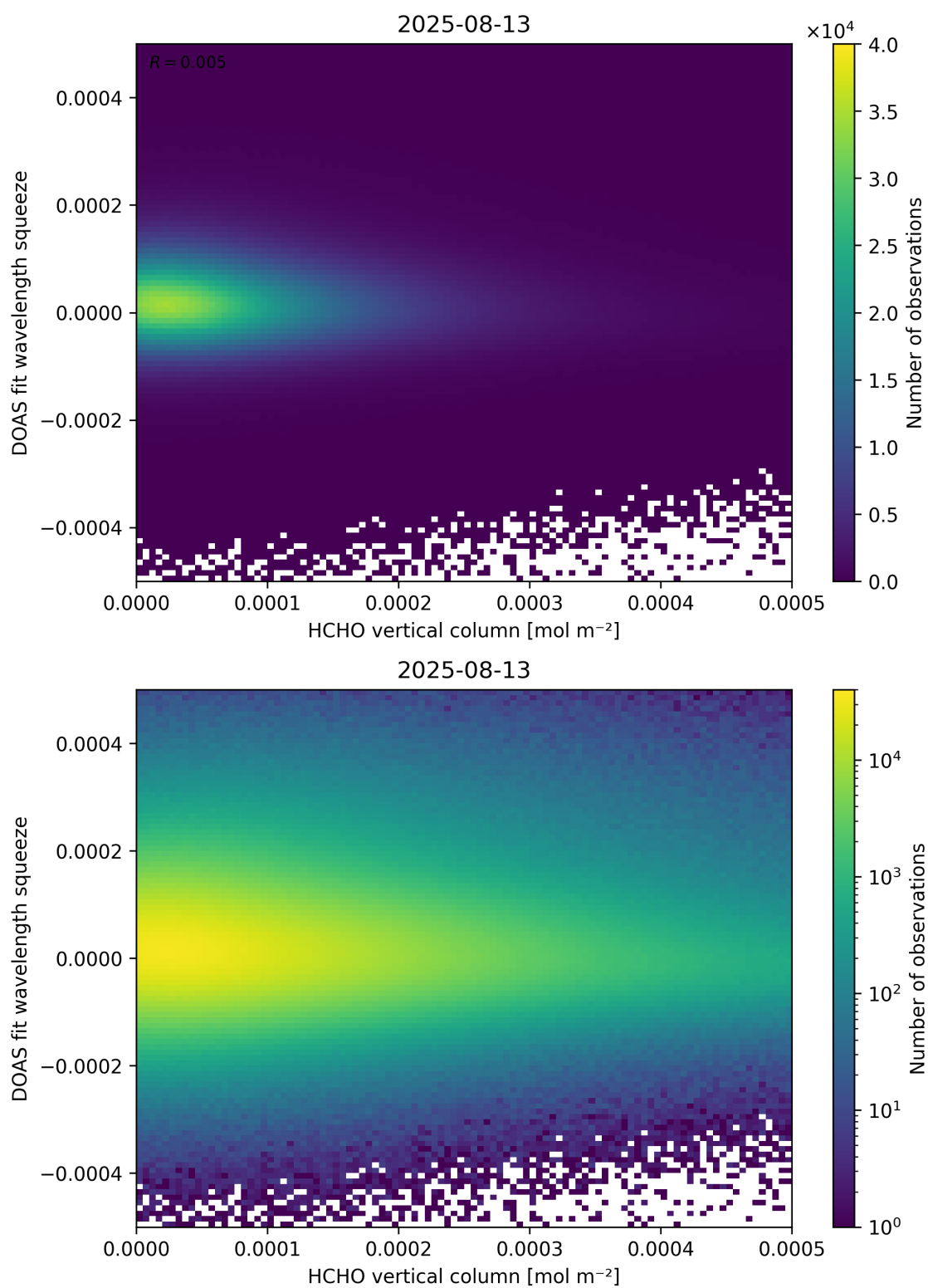
Figure 125: Scatter density plot of “HCHO vertical column” against “DOAS fit wavelength squeeze” for 2025-08-12 to 2025-08-14.
