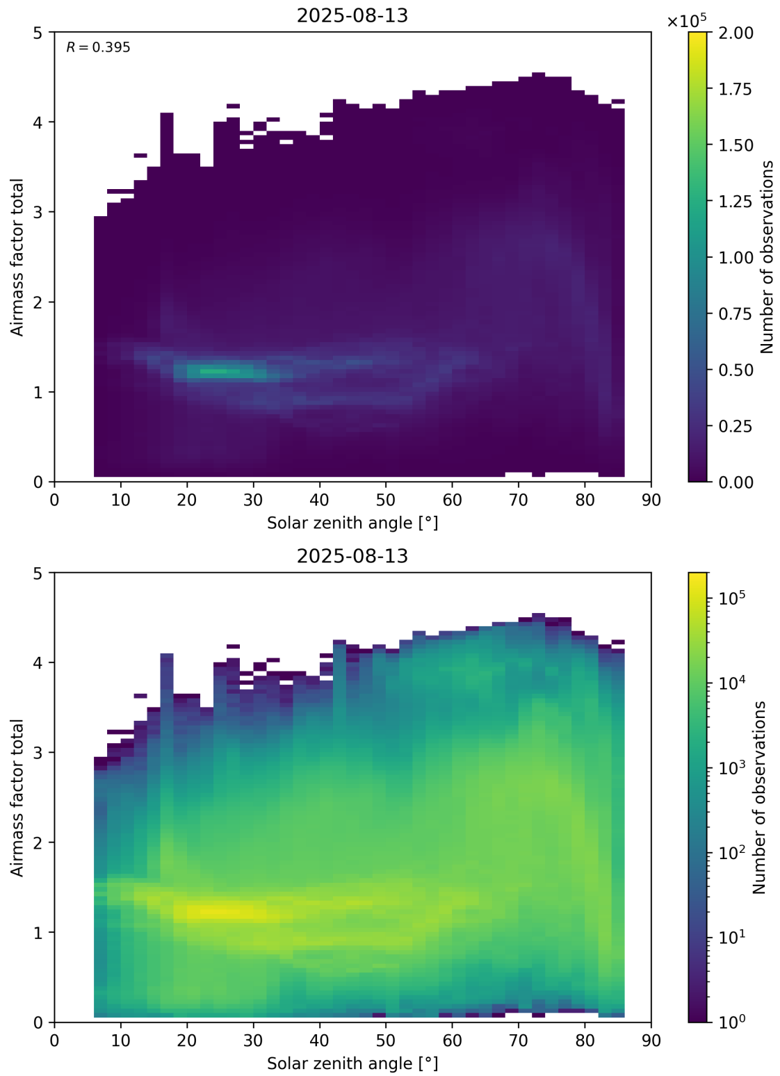
Figure 175: Scatter density plot of “Solar zenith angle” against “Airmass factor total” for 2025-08-12 to 2025-08-14.
