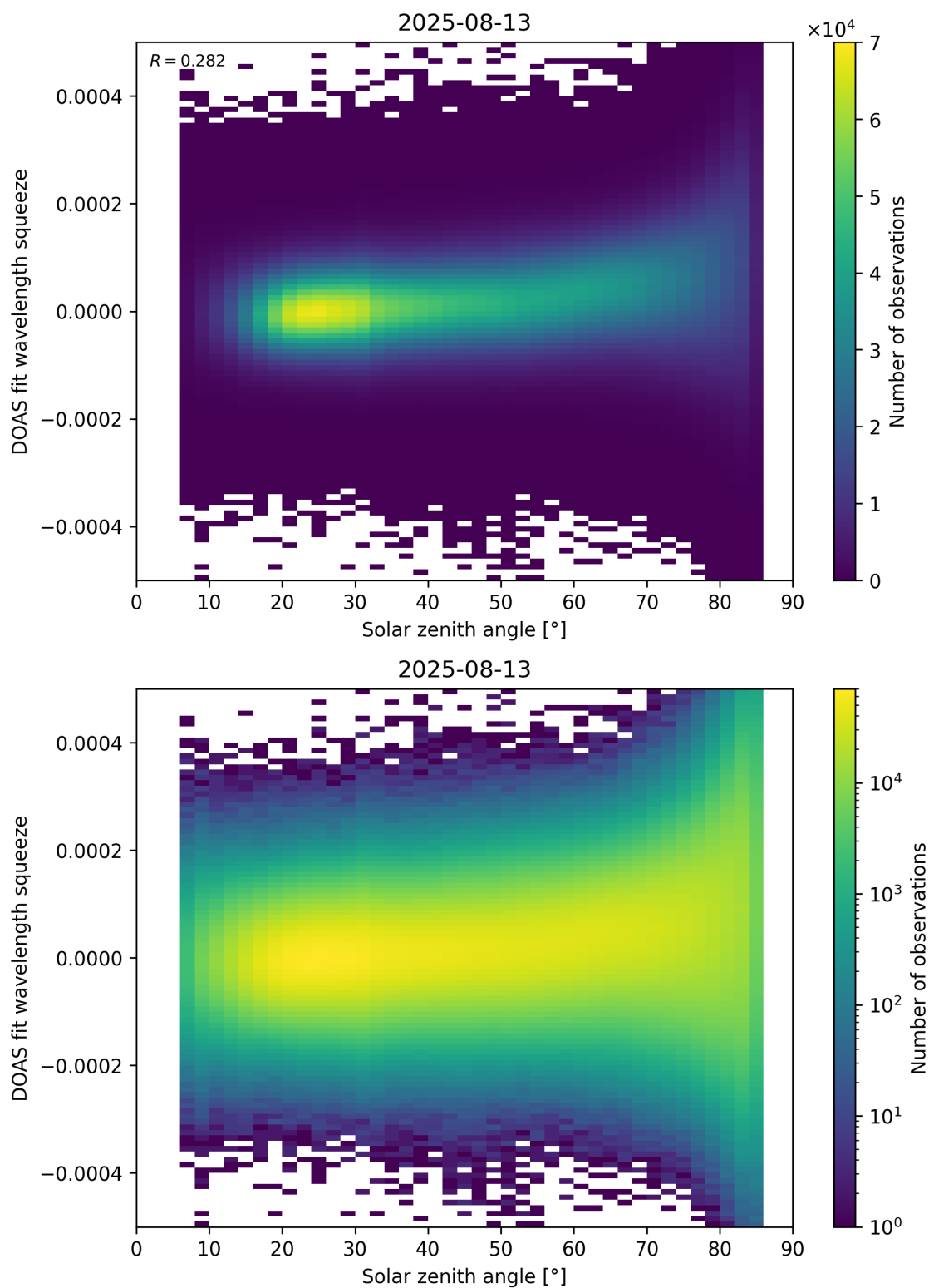
Figure 169: Scatter density plot of “Solar zenith angle” against “DOAS fit wavelength squeeze” for 2025-08-12 to 2025-08-14.
