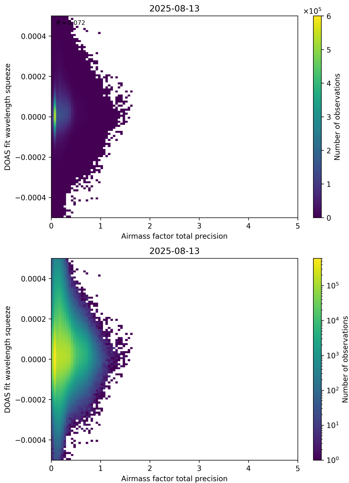
Figure 107: Scatter density plot of “Airmass factor total precision” against “DOAS fit wavelength squeeze” for 2025-08-12 to 2025-08-14.
