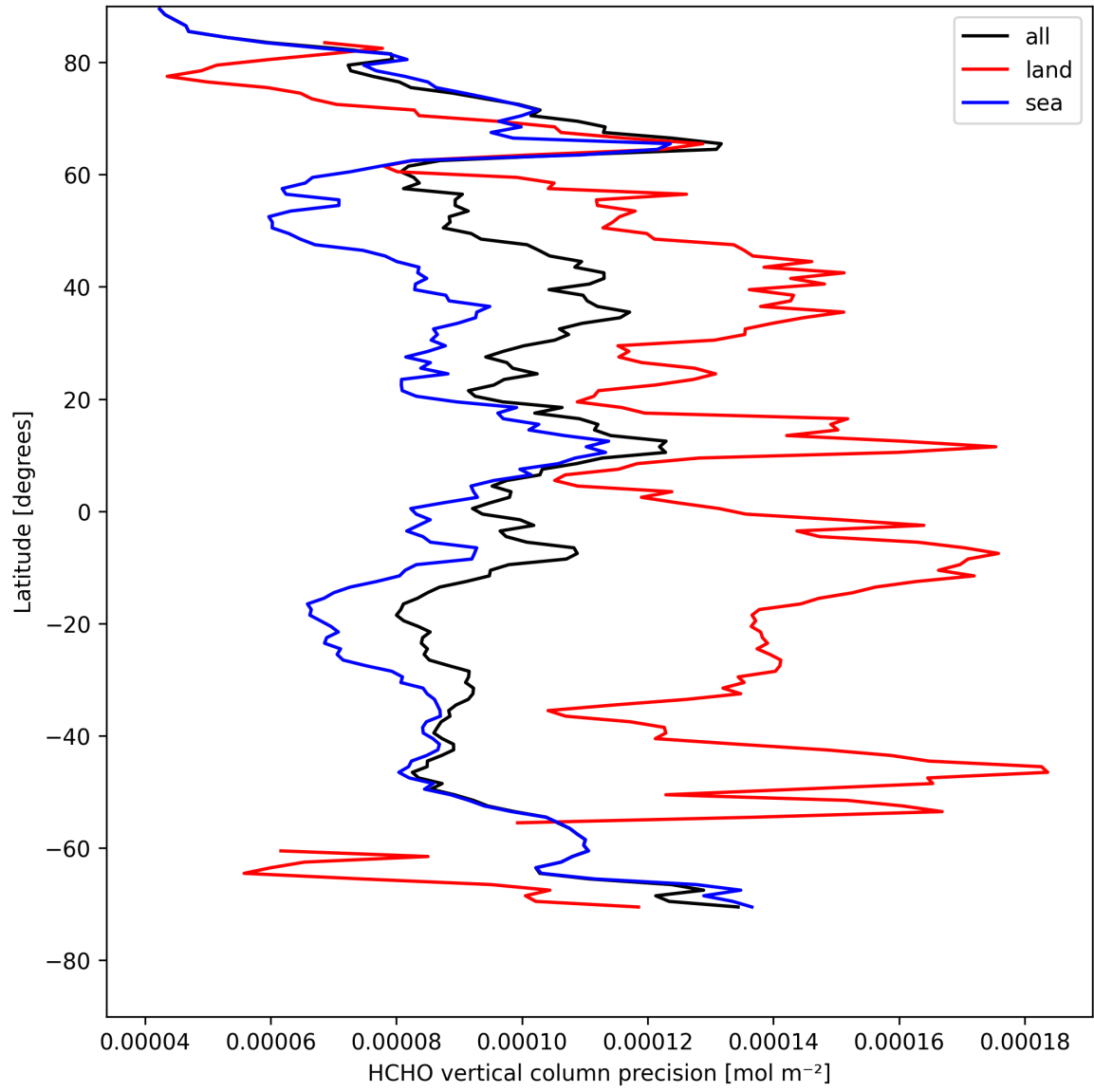
Figure 22: Zonal average of “HCHO vertical column precision” for 2025-08-12 to 2025-08-14.
