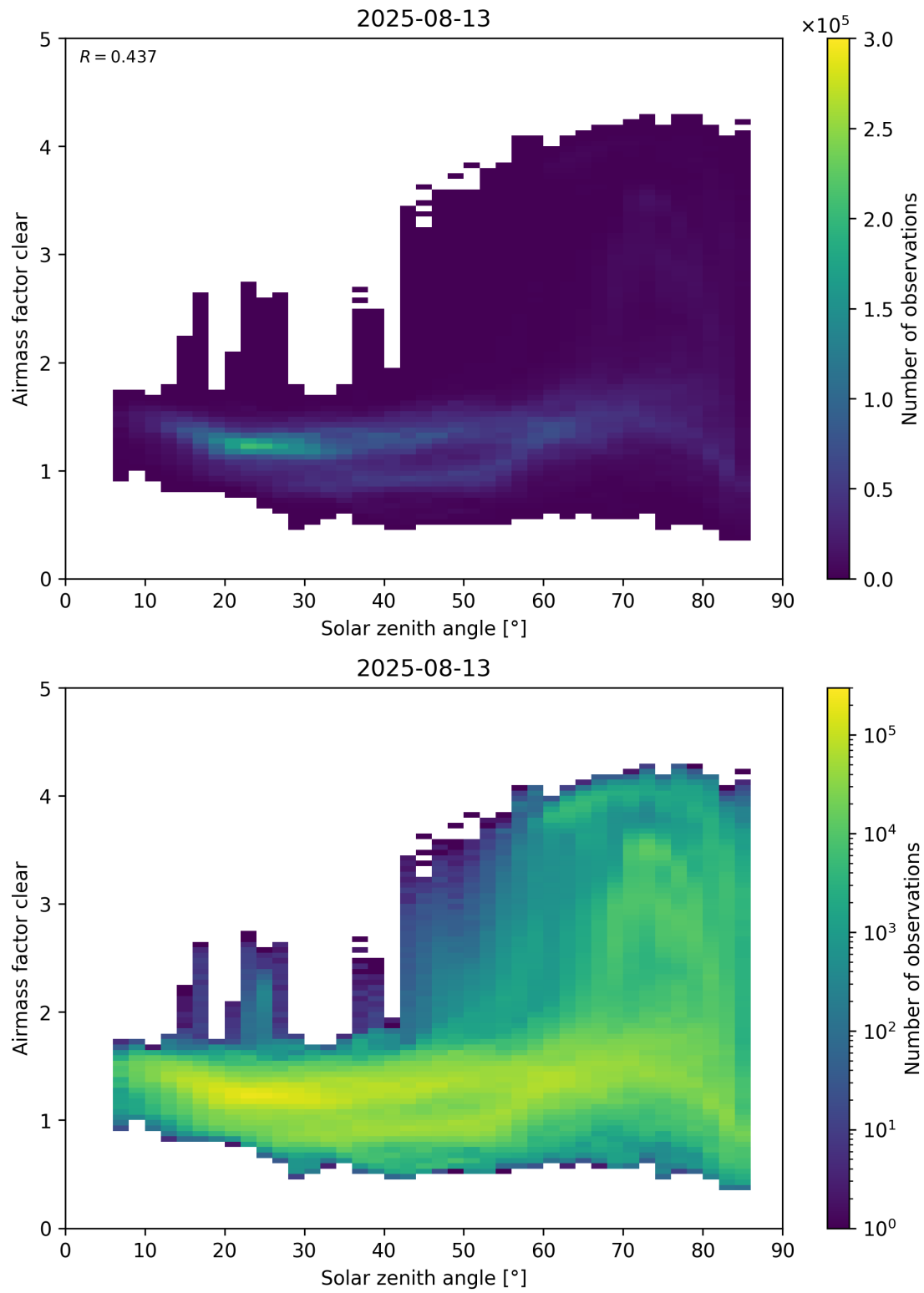
Figure 170: Scatter density plot of “Solar zenith angle” against “Airmass factor clear” for 2025-08-12 to 2025-08-14.
