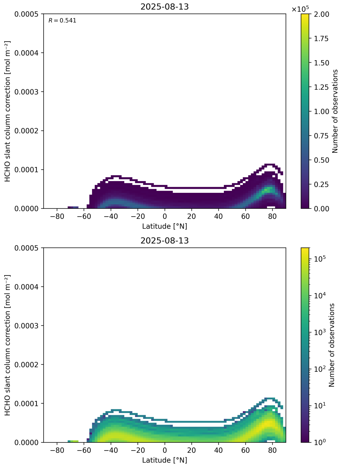
Figure 158: Scatter density plot of “Latitude” against “HCHO slant column correction” for 2025-08-12 to 2025-08-14.
