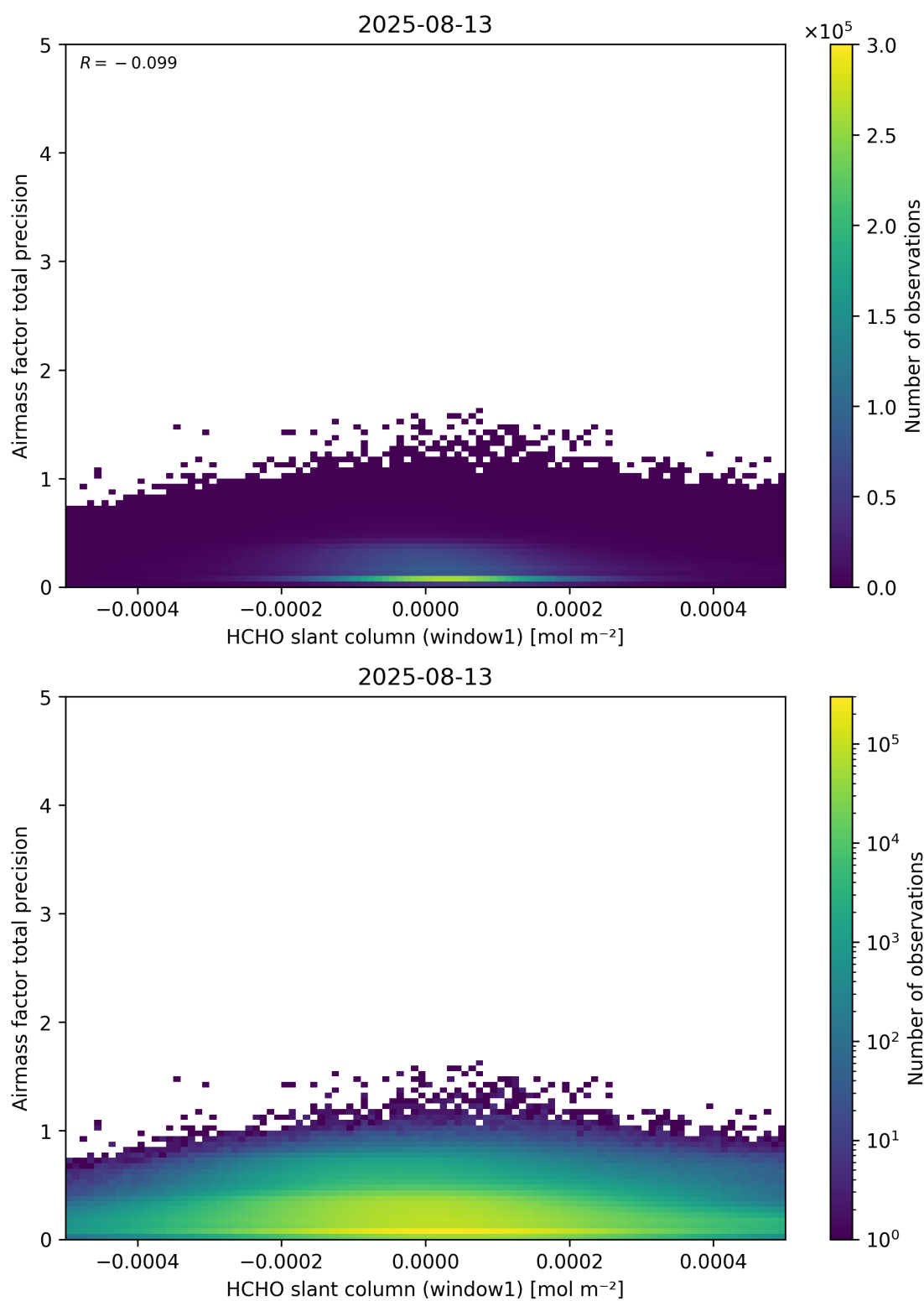
Figure 86: Scatter density plot of “HCHO slant column (window1)” against “Airmass factor total precision” for 2025-08-12 to 2025-08-14.
