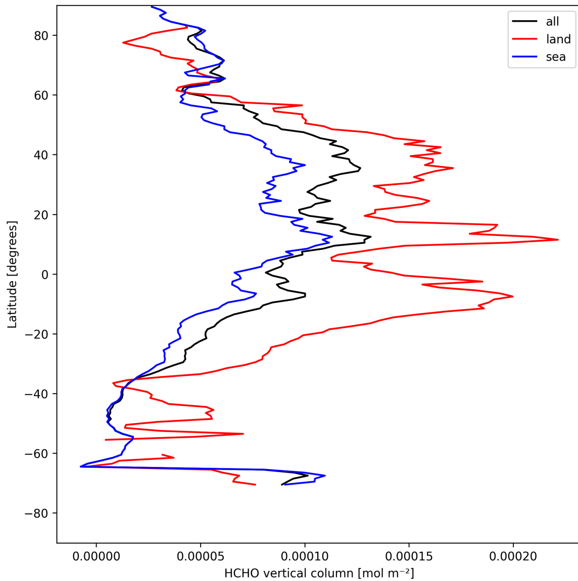
Figure 21: Zonal average of “HCHO vertical column” for 2025-08-12 to 2025-08-14.
