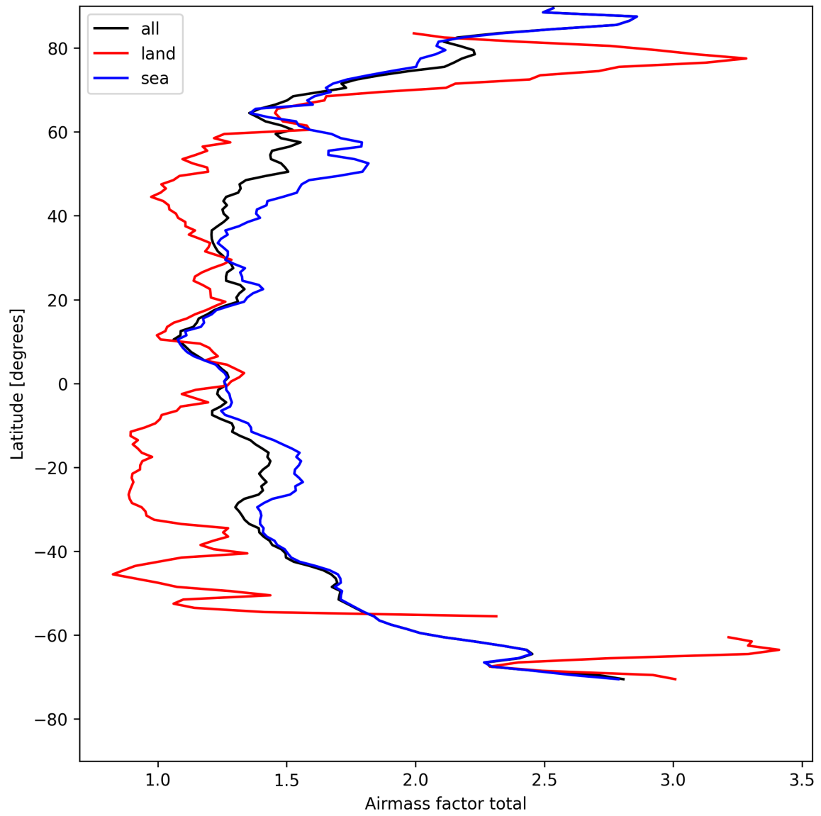
Figure 26: Zonal average of “Airmass factor total” for 2025-08-12 to 2025-08-14.
