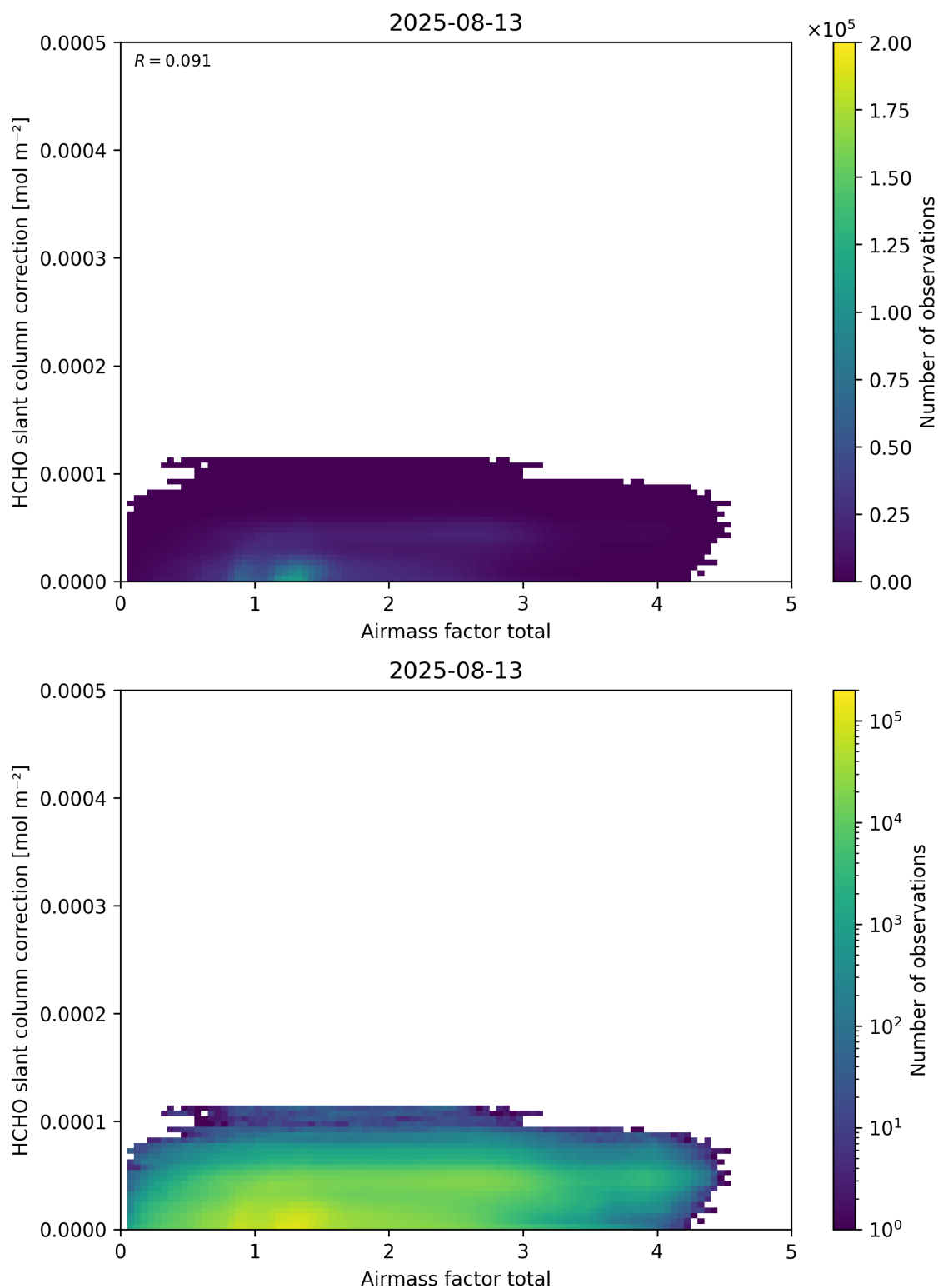
Figure 102: Scatter density plot of “Airmass factor total” against “HCHO slant column correction” for 2025-08-12 to 2025-08-14.
