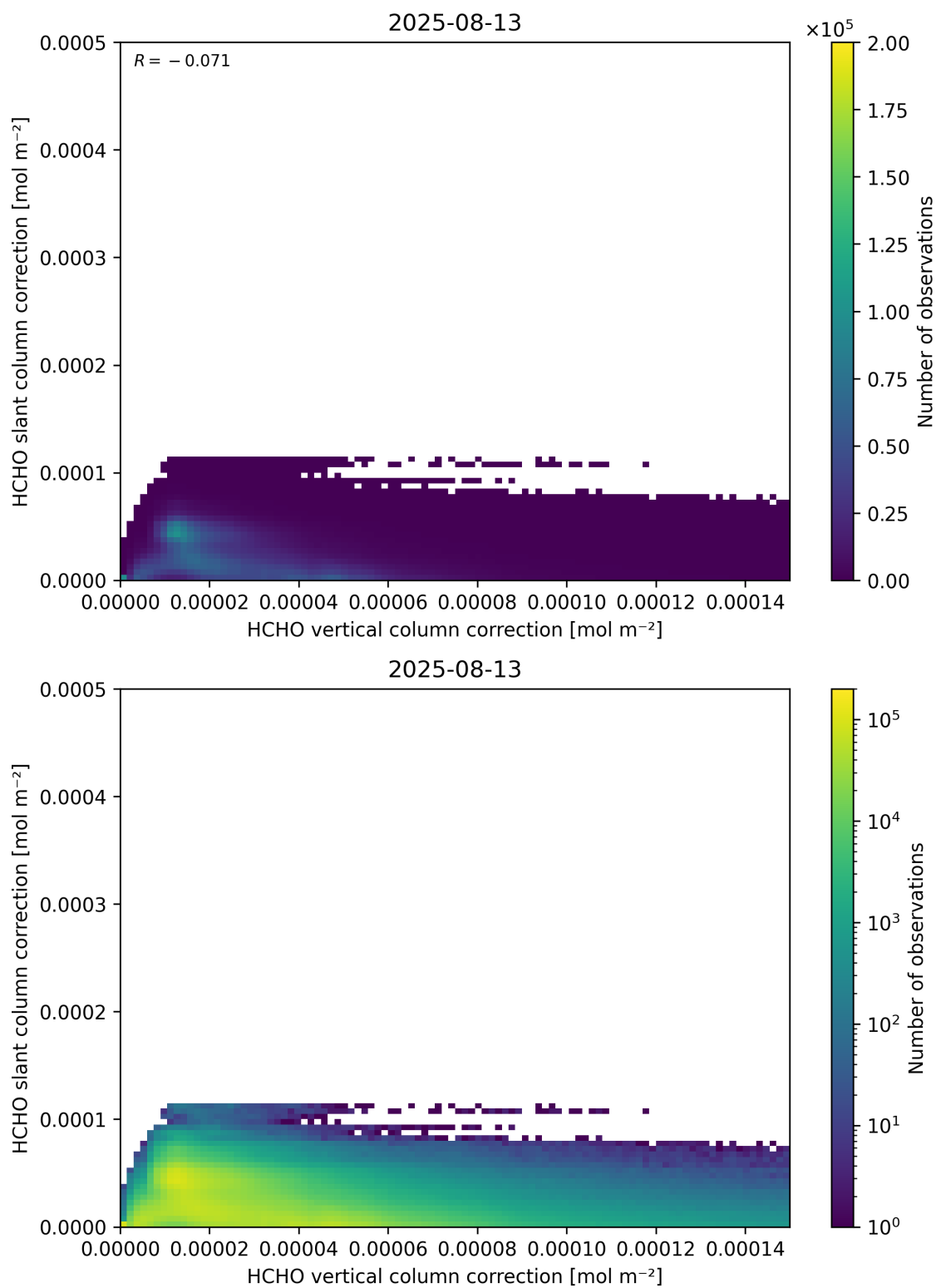
Figure 117: Scatter density plot of “HCHO vertical column correction” against “HCHO slant column correction” for 2025-08-12 to 2025-08-14.
