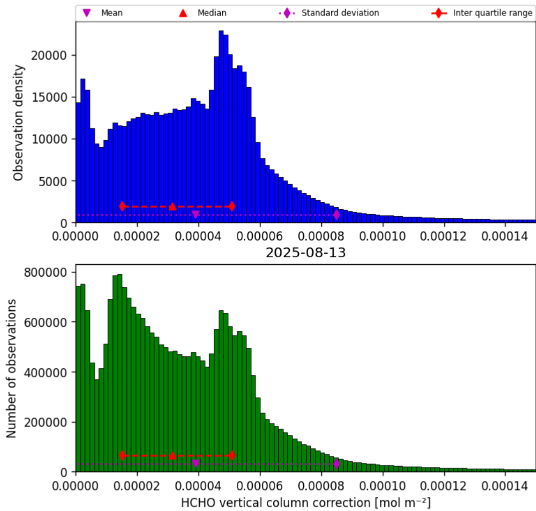
Figure 37: Histogram of “HCHO vertical column correction” for 2025-08-12 to 2025-08-14
