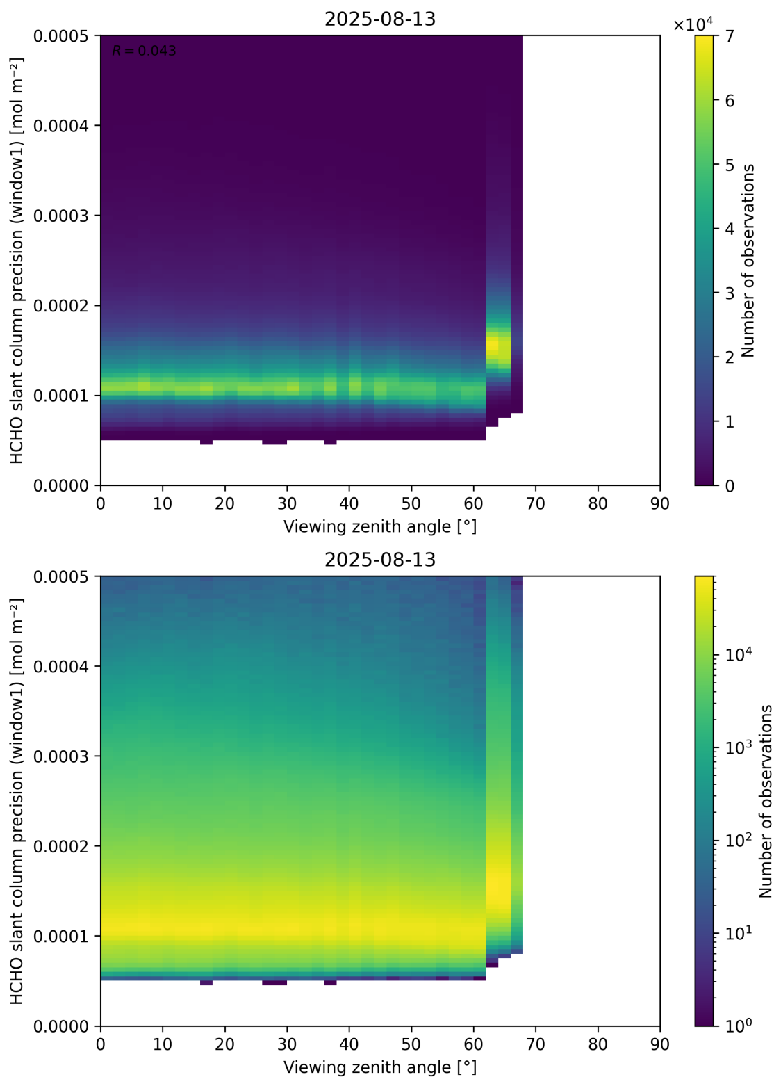
Figure 189: Scatter density plot of “Viewing zenith angle” against “HCHO slant column precision (window1)” for 2025-08-12 to 2025-08-14.
