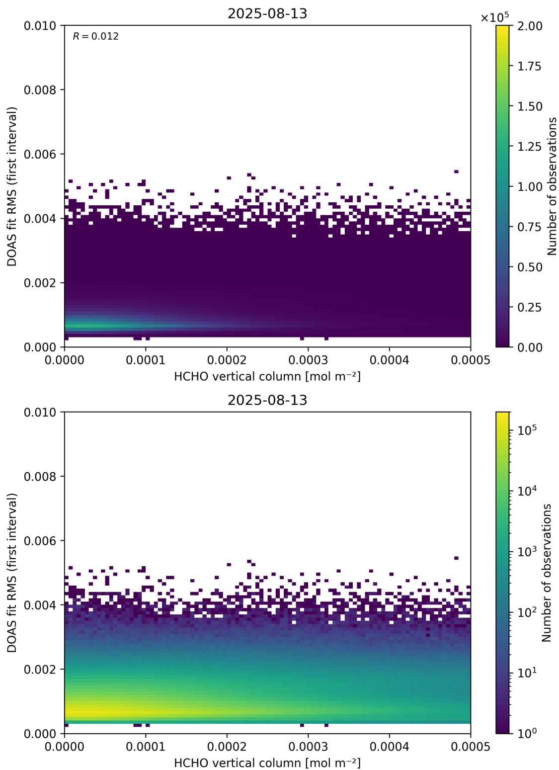
Figure 123: Scatter density plot of “HCHO vertical column” against “DOAS fit RMS (first interval)” for 2025-08-12 to 2025-08-14.
