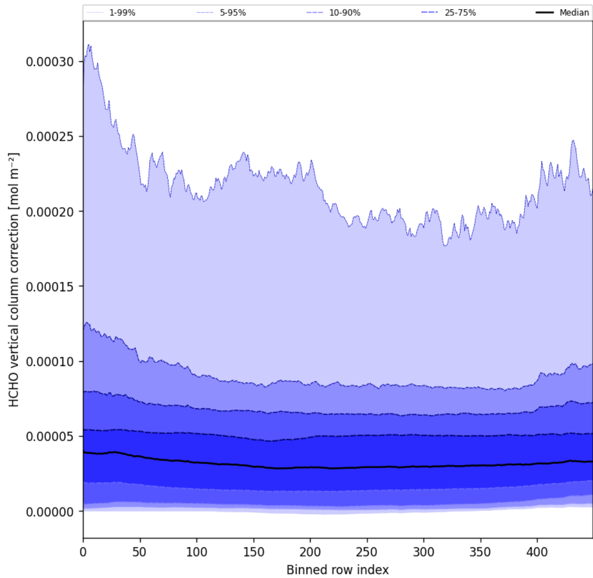
Figure 51: Along track statistics of “HCHO vertical column correction” for 2025-08-12 to 2025-08-14
