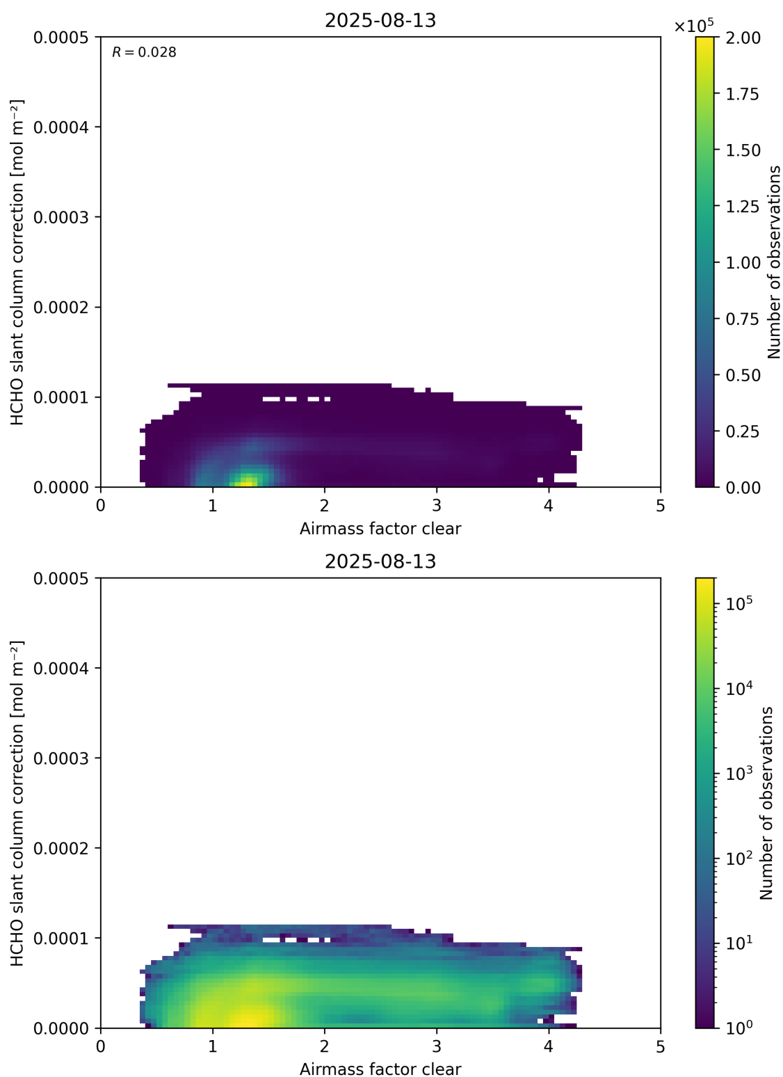
Figure 75: Scatter density plot of “Airmass factor clear” against “HCHO slant column correction” for 2025-08-12 to 2025-08-14.
