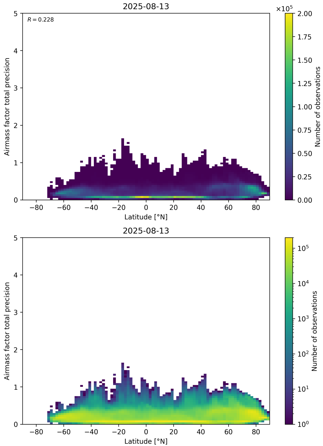
Figure 162: Scatter density plot of “Latitude” against “Airmass factor total precision” for 2025-08-12 to 2025-08-14.
