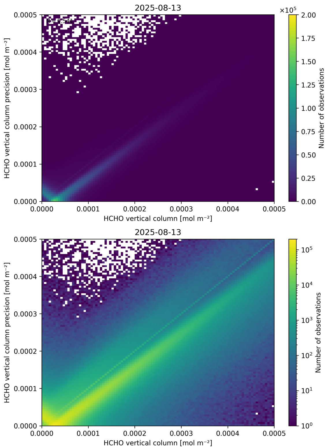
Figure 134: Scatter density plot of “HCHO vertical column” against “HCHO vertical column precision” for 2025-08-12 to 2025-08-14.
