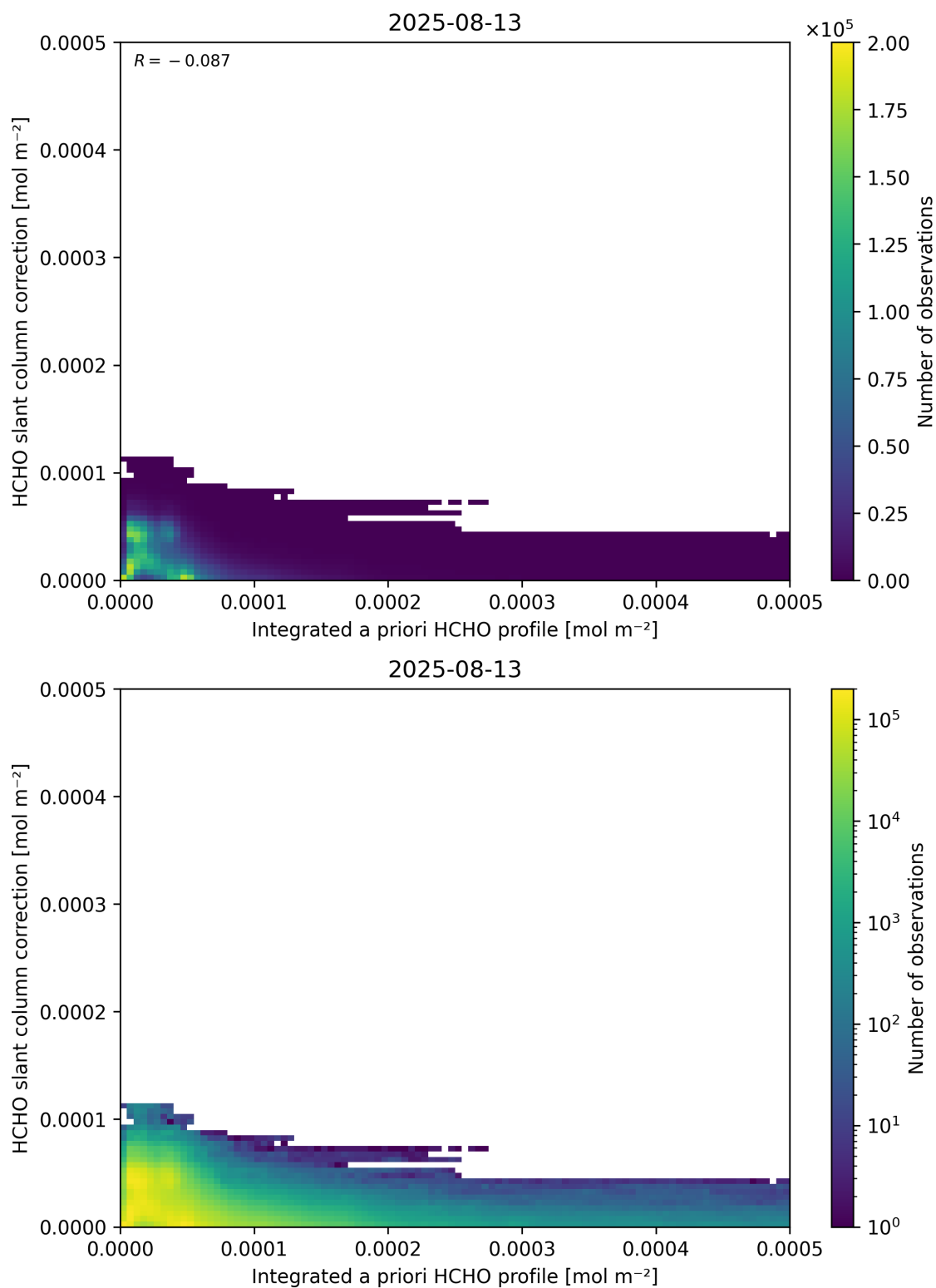
Figure 152: Scatter density plot of “Integrated a priori HCHO profile” against “HCHO slant column correction” for 2025-08-12 to 2025-08-14.
