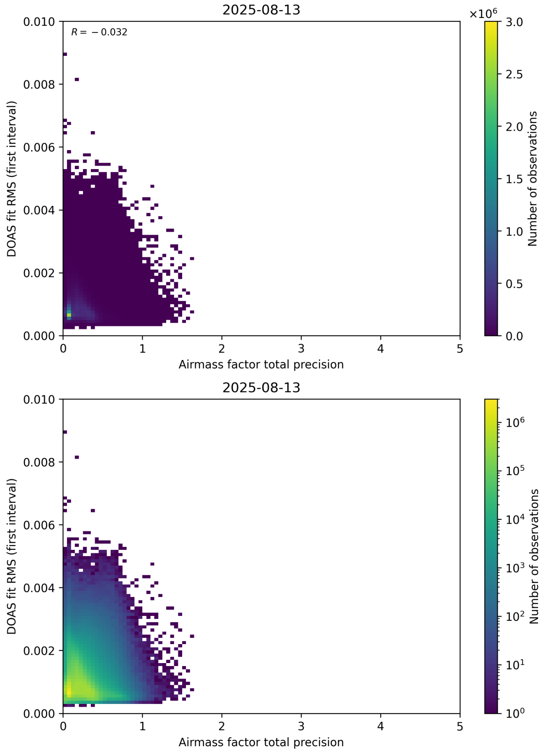
Figure 105: Scatter density plot of “Airmass factor total precision” against “DOAS fit RMS (first interval)” for 2025-08-12 to 2025-08-14.
