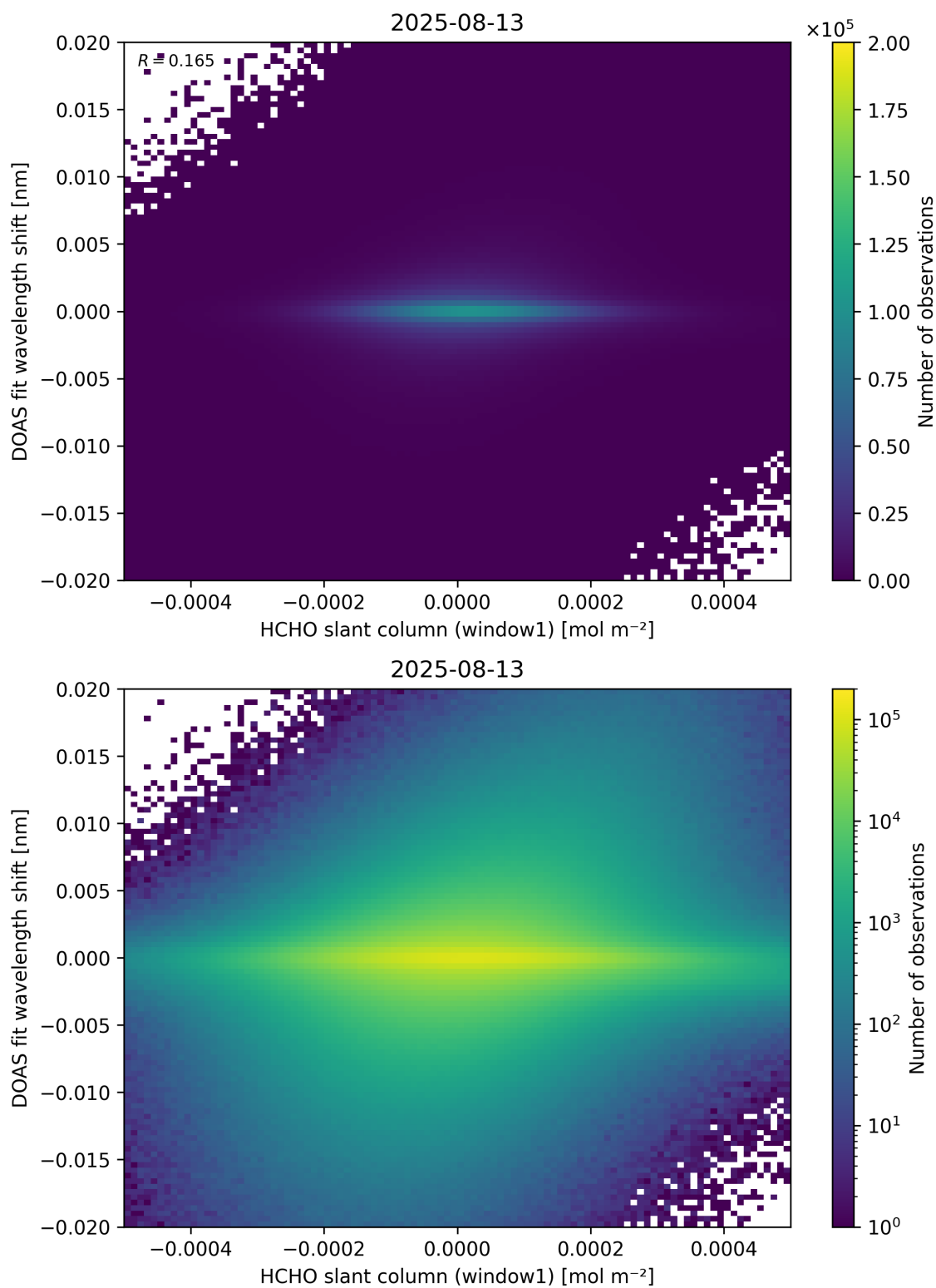
Figure 79: Scatter density plot of “HCHO slant column (window1)” against “DOAS fit wavelength shift” for 2025-08-12 to 2025-08-14.
