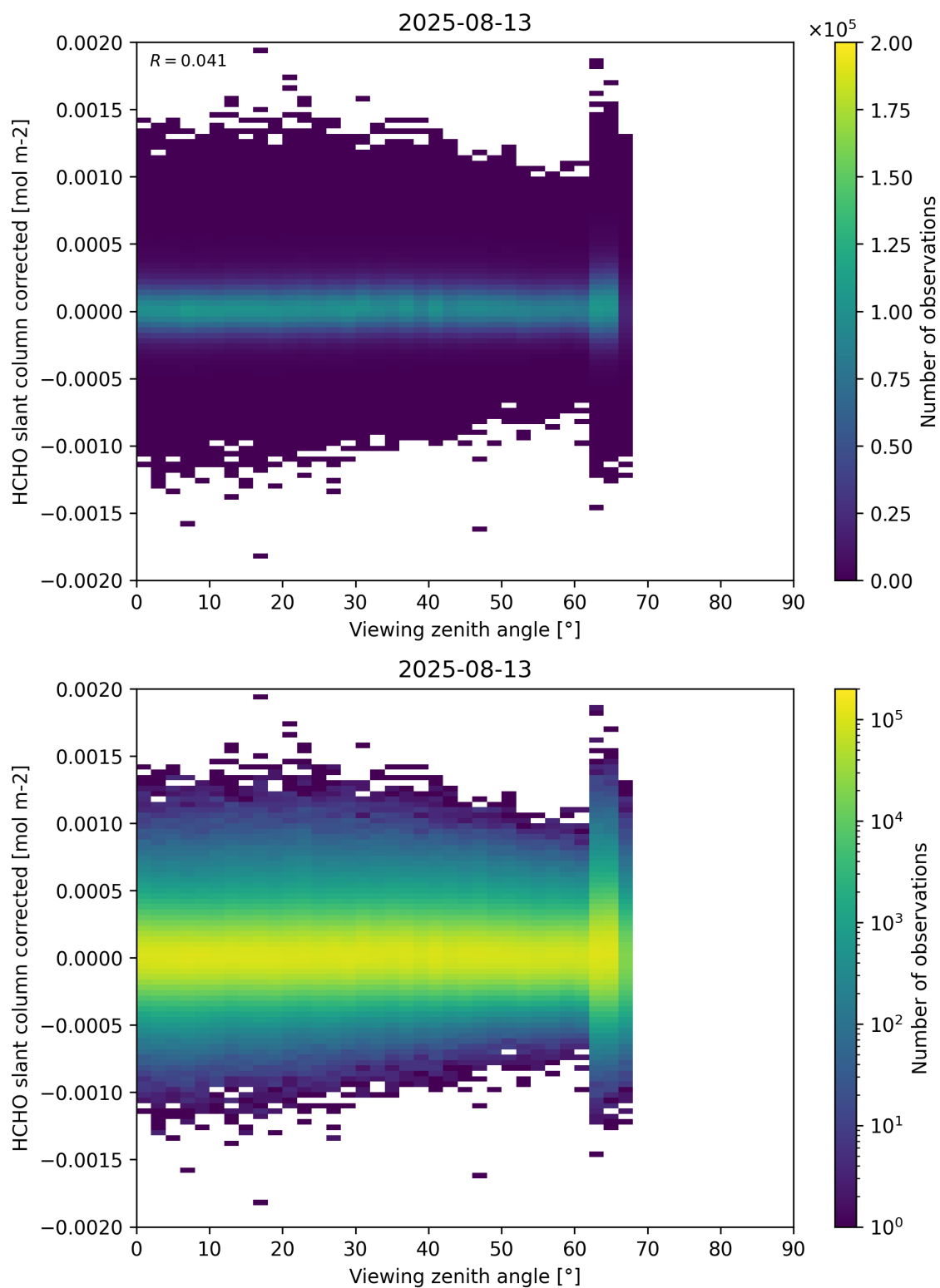
Figure 186: Scatter density plot of “Viewing zenith angle” against “HCHO slant column corrected” for 2025-08-12 to 2025-08-14.
