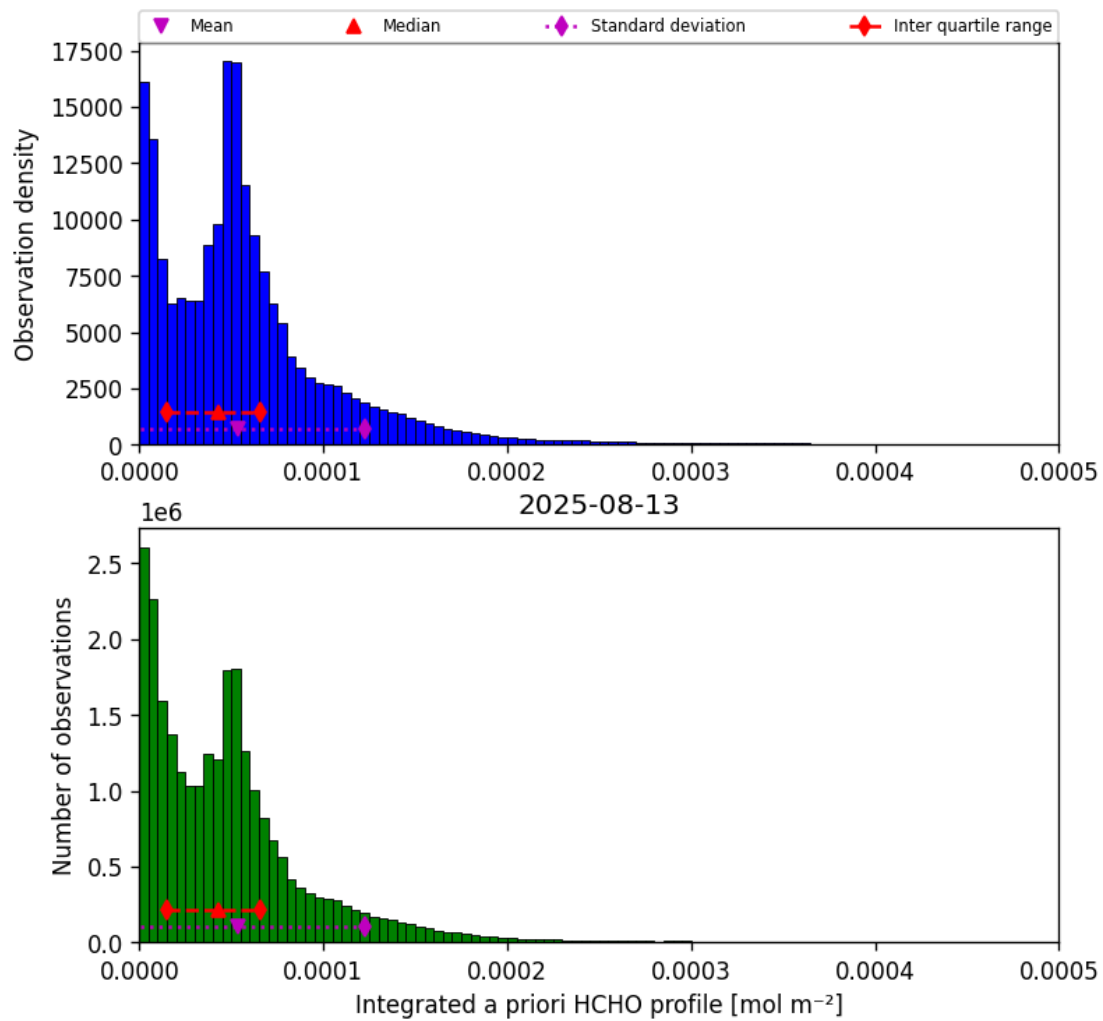
Figure 43: Histogram of “Integrated a priori HCHO profile” for 2025-08-12 to 2025-08-14
