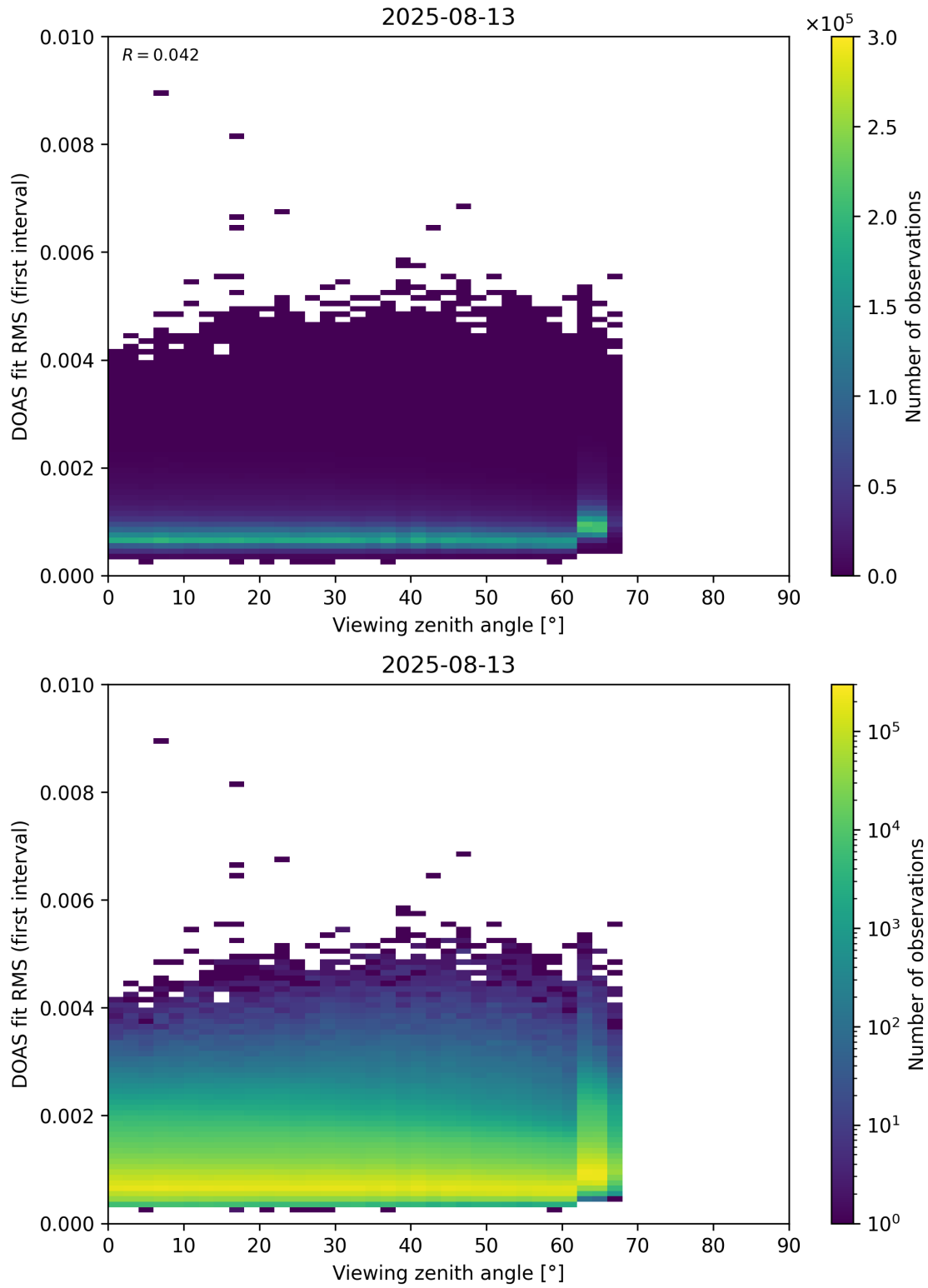
Figure 182: Scatter density plot of “Viewing zenith angle” against “DOAS fit RMS (first interval)” for 2025-08-12 to 2025-08-14.
