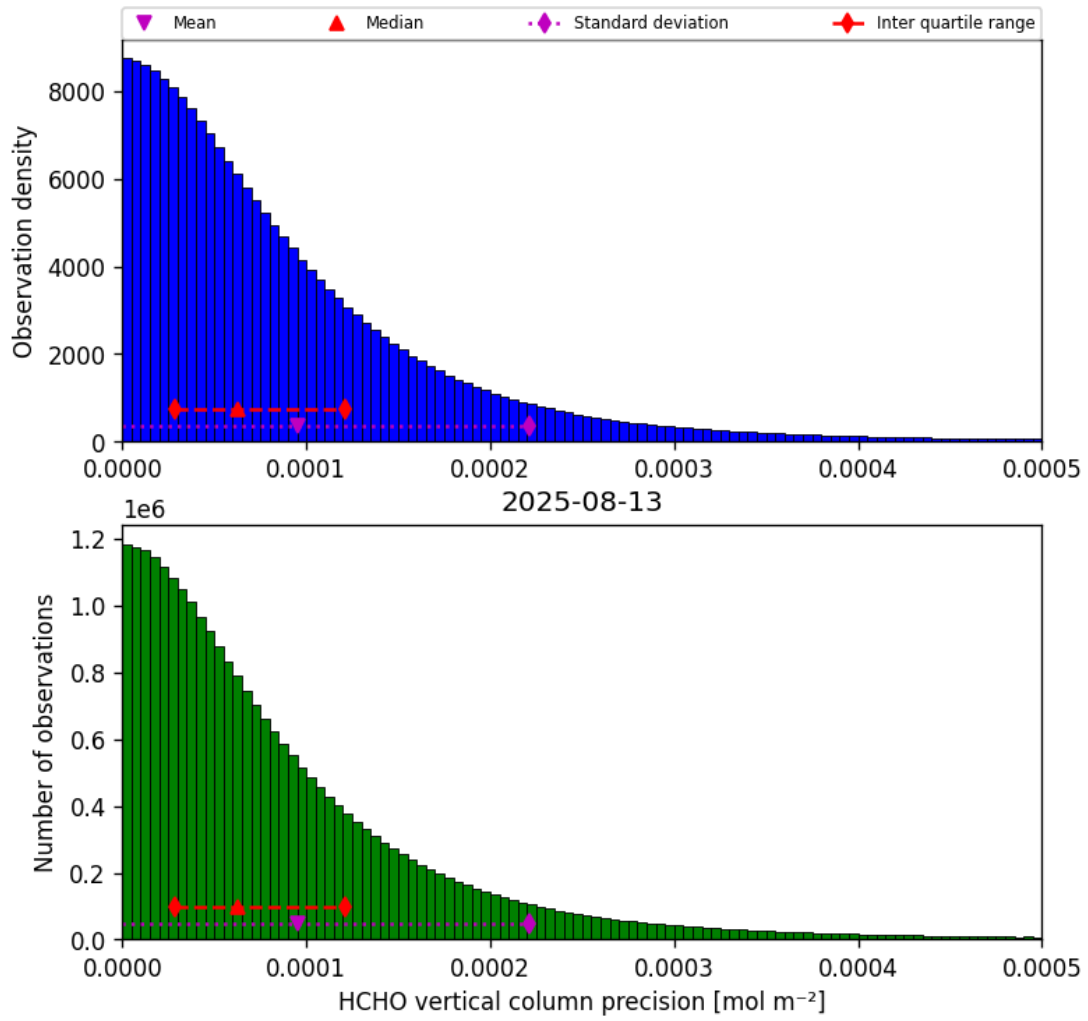
Figure 36: Histogram of “HCHO vertical column precision” for 2025-08-12 to 2025-08-14
