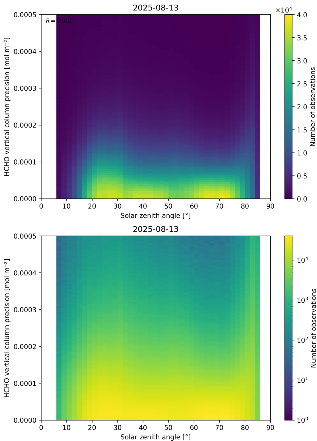
Figure 179: Scatter density plot of “Solar zenith angle” against “HCHO vertical column precision” for 2025-08-12 to 2025-08-14.
