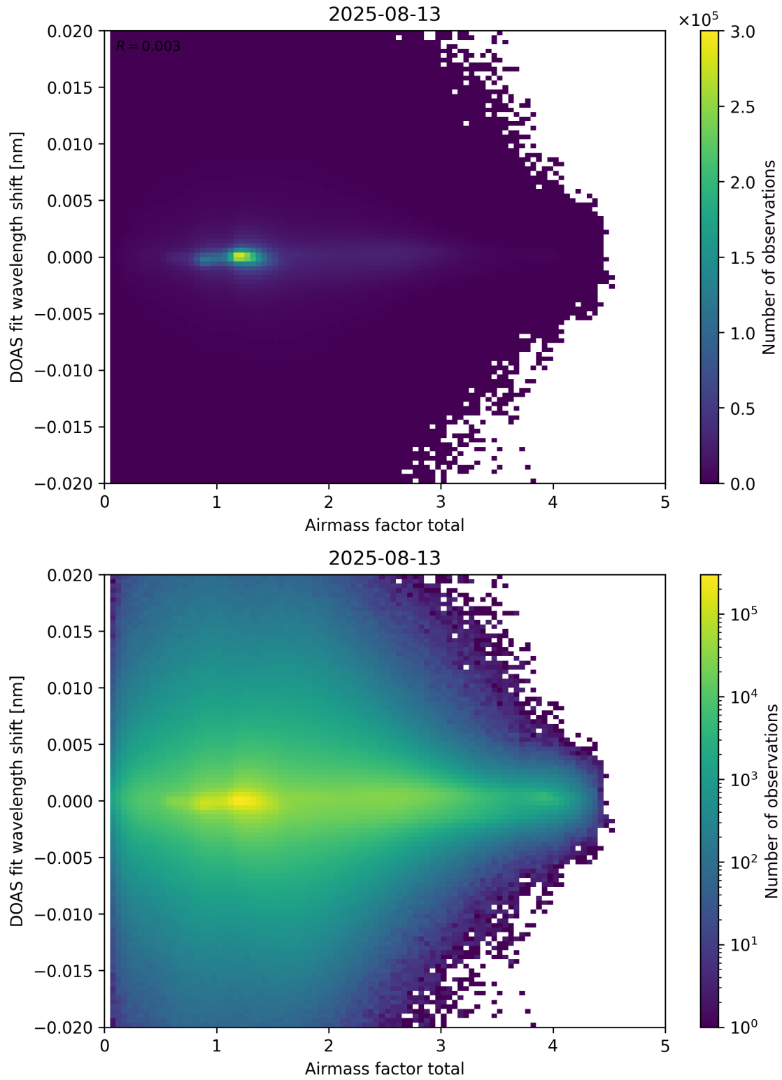
Figure 98: Scatter density plot of “Airmass factor total” against “DOAS fit wavelength shift” for 2025-08-12 to 2025-08-14.
