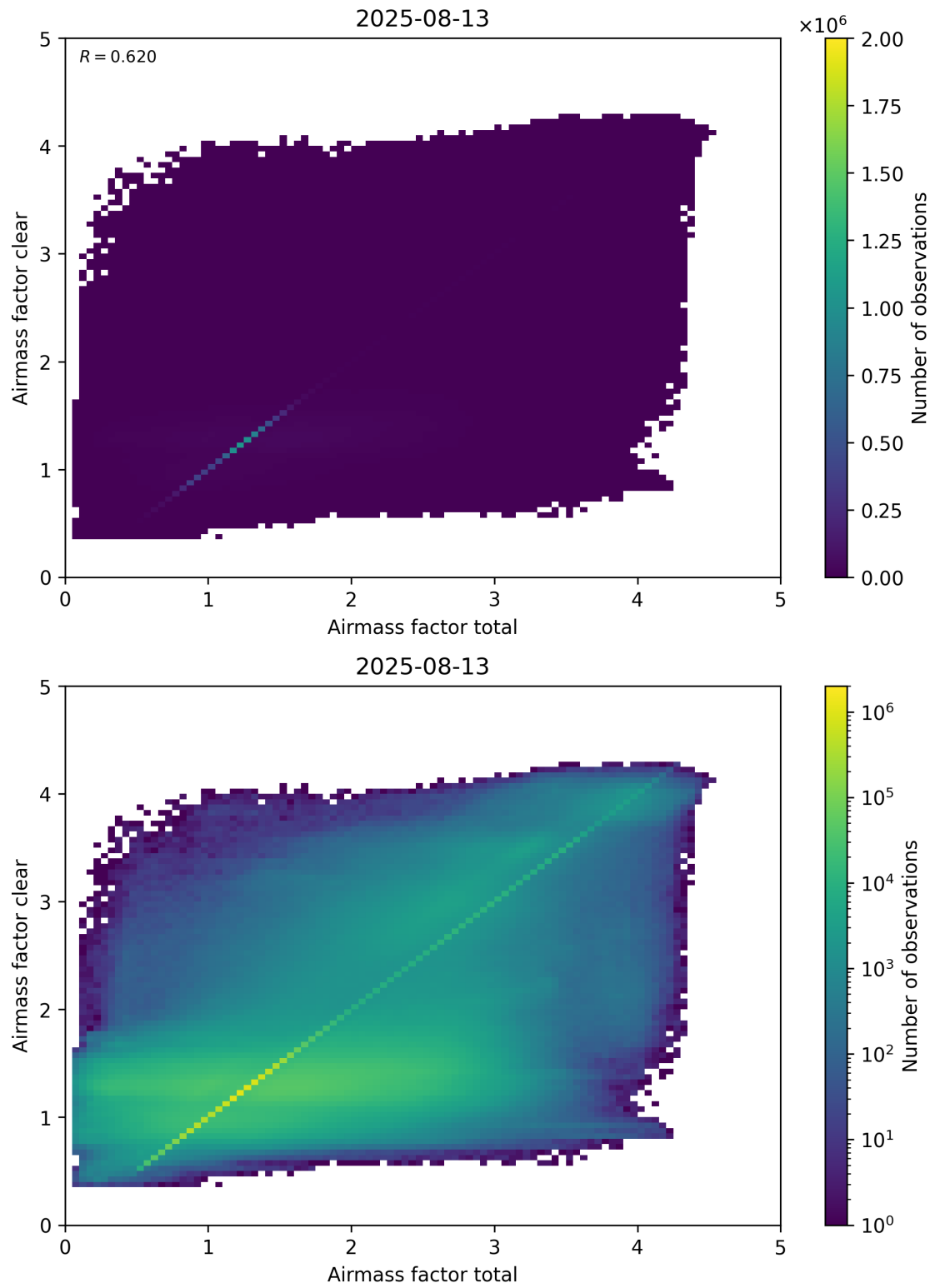
Figure 100: Scatter density plot of “Airmass factor total” against “Airmass factor clear” for 2025-08-12 to 2025-08-14.
