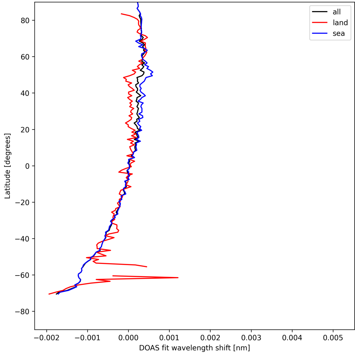
Figure 30: Zonal average of “DOAS fit wavelength shift” for 2025-08-12 to 2025-08-14.
