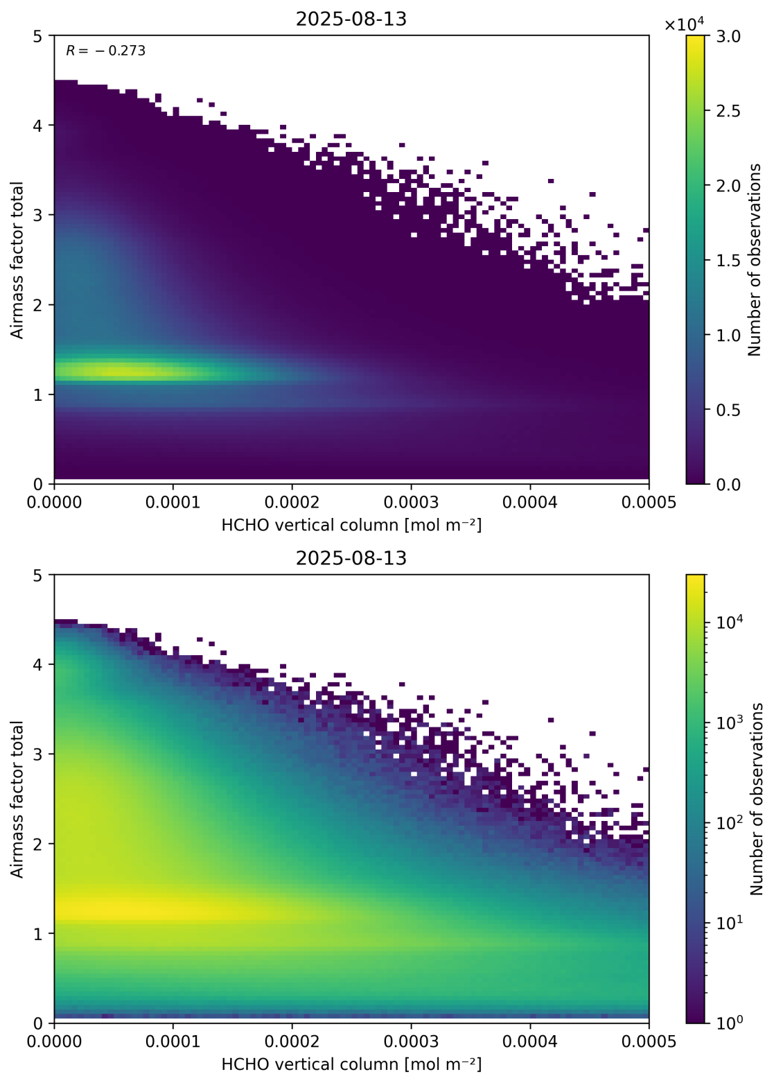
Figure 131: Scatter density plot of “HCHO vertical column” against “Airmass factor total” for 2025-08-12 to 2025-08-14.
