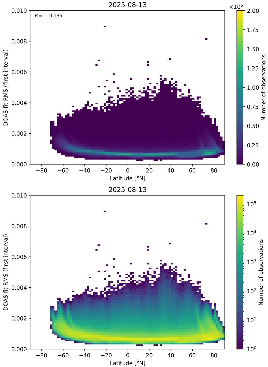
Figure 153: Scatter density plot of “Latitude” against “DOAS fit RMS (first interval)” for 2025-08-12 to 2025-08-14.
