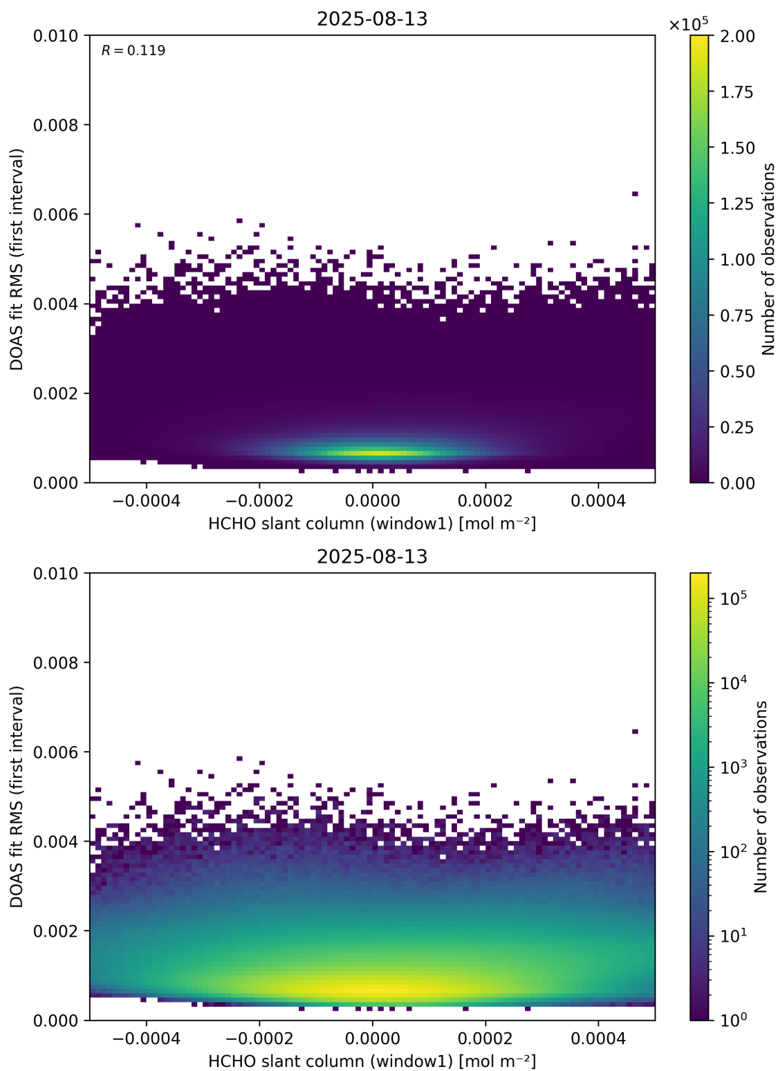
Figure 78: Scatter density plot of “HCHO slant column (window1)” against “DOAS fit RMS (first interval)” for 2025-08-12 to 2025-08-14.
