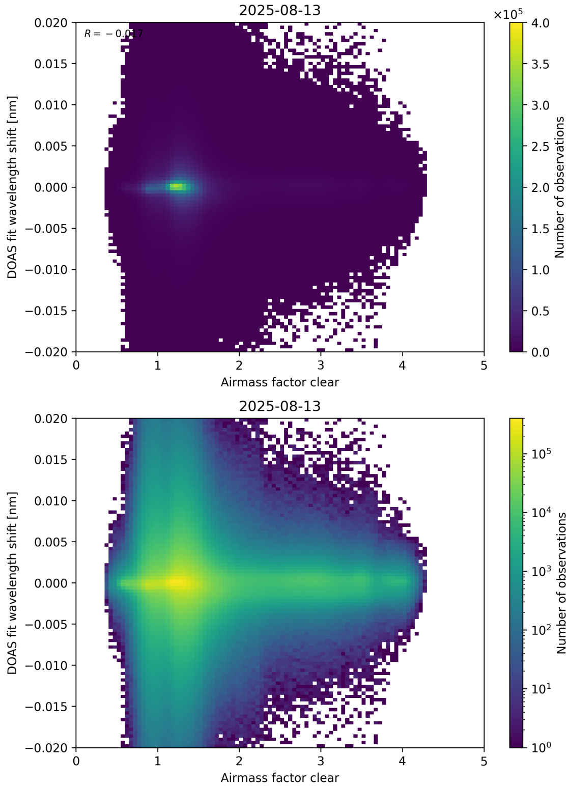
Figure 72: Scatter density plot of “Airmass factor clear” against “DOAS fit wavelength shift” for 2025-08-12 to 2025-08-14.
