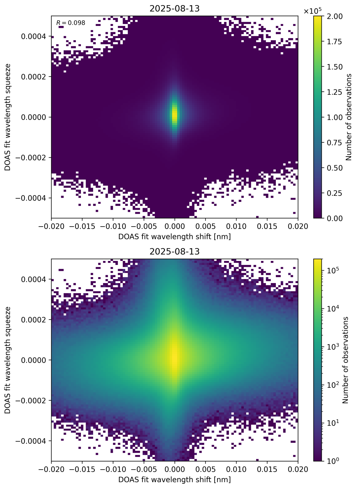
Figure 65: Scatter density plot of “DOAS fit wavelength shift” against “DOAS fit wavelength squeeze” for 2025-08-12 to 2025-08-14.
