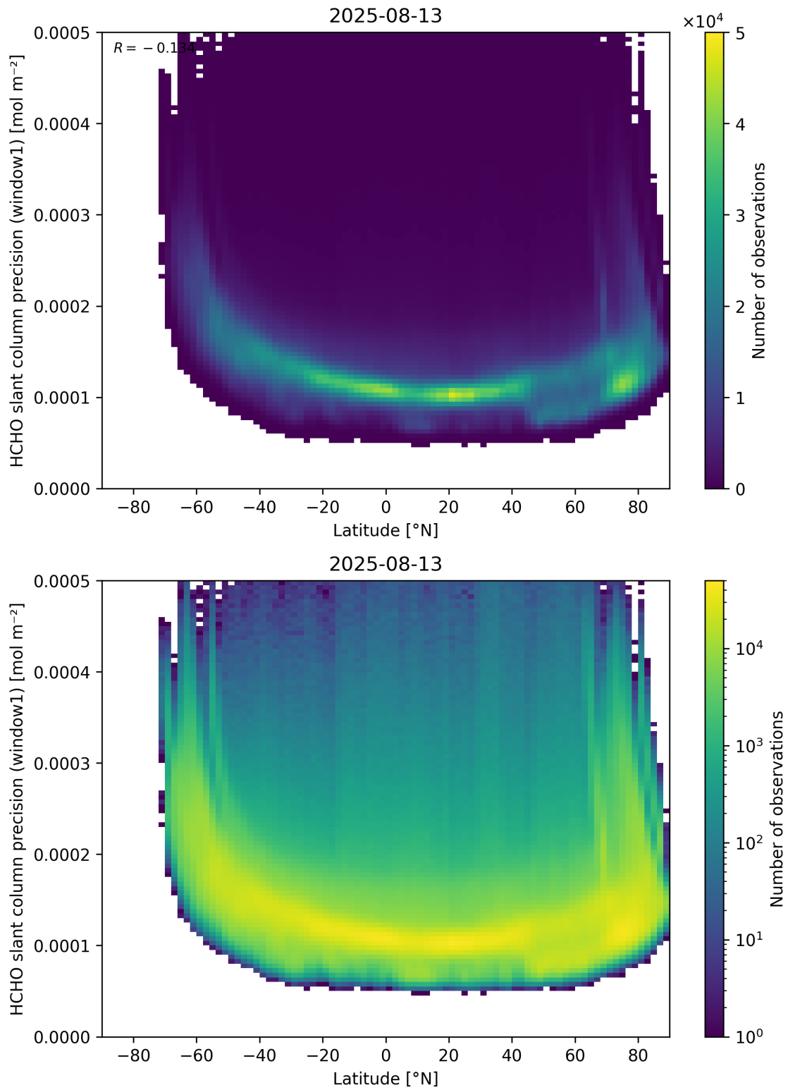
Figure 160: Scatter density plot of “Latitude” against “HCHO slant column precision (window1)” for 2025-08-12 to 2025-08-14.
