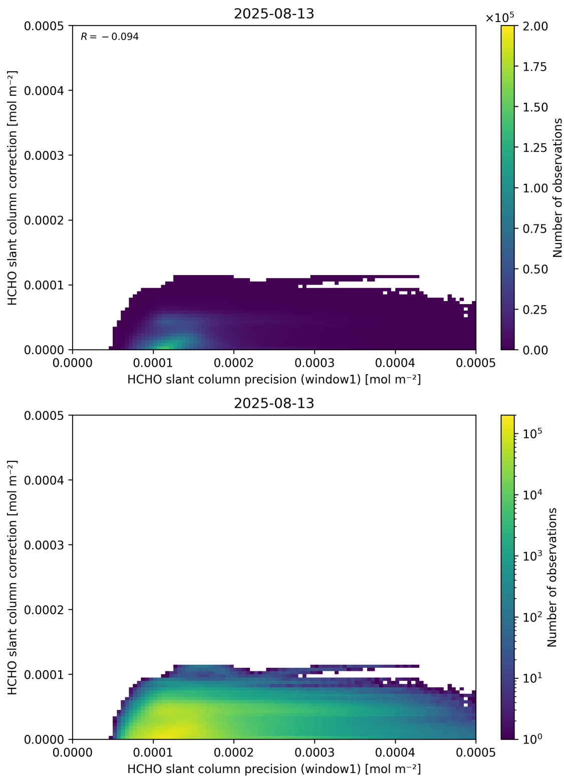
Figure 93: Scatter density plot of “HCHO slant column precision (window1)” against “HCHO slant column correction” for 2025-08-12 to 2025-08-14.
