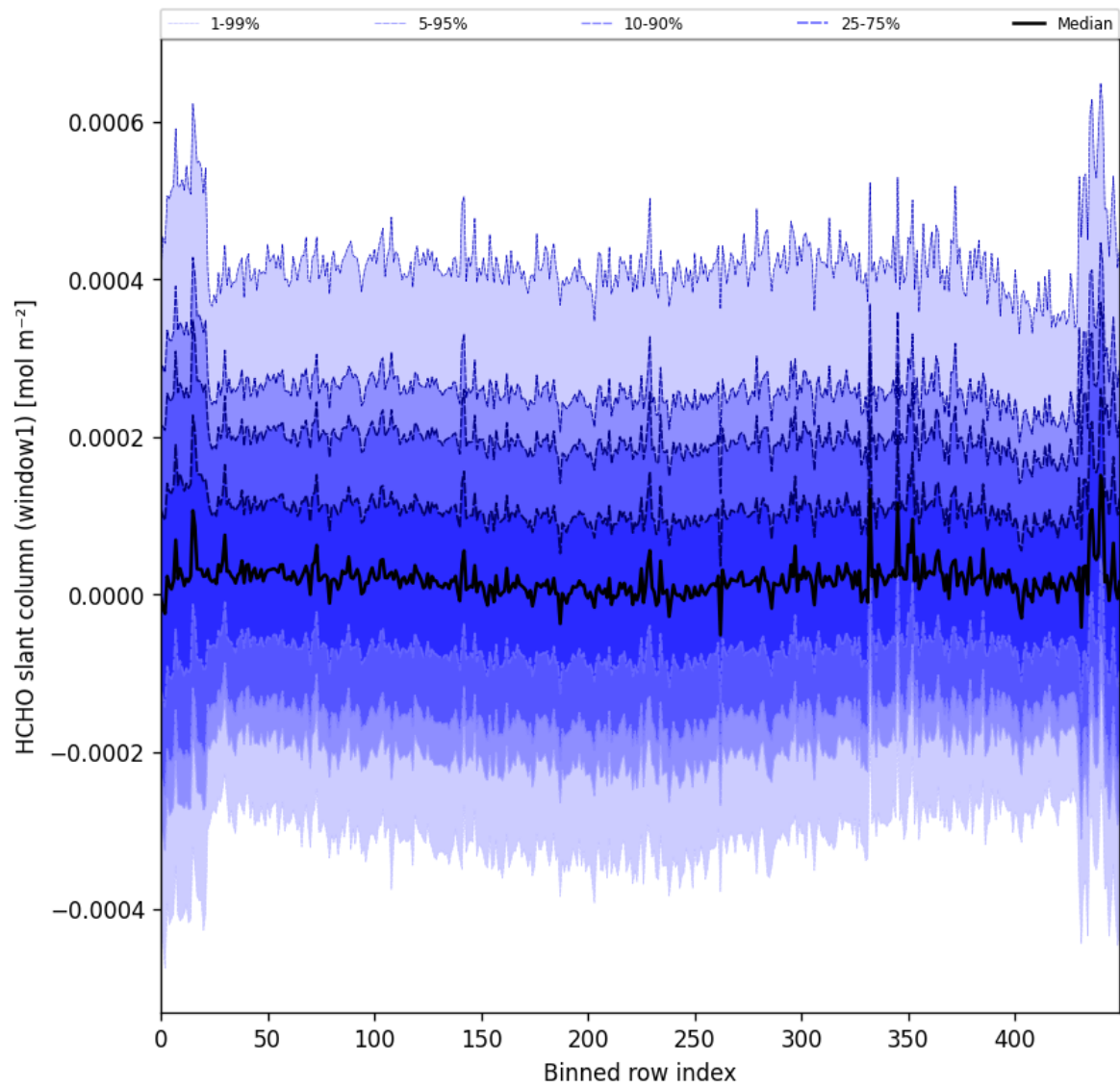
Figure 52: Along track statistics of “HCHO slant column (window1)” for 2025-08-12 to 2025-08-14
