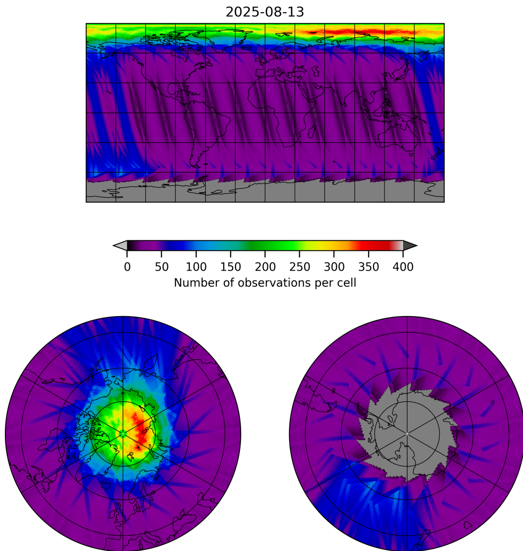
Figure 19: Map of the number of observations for 2025-08-12 to 2025-08-14
