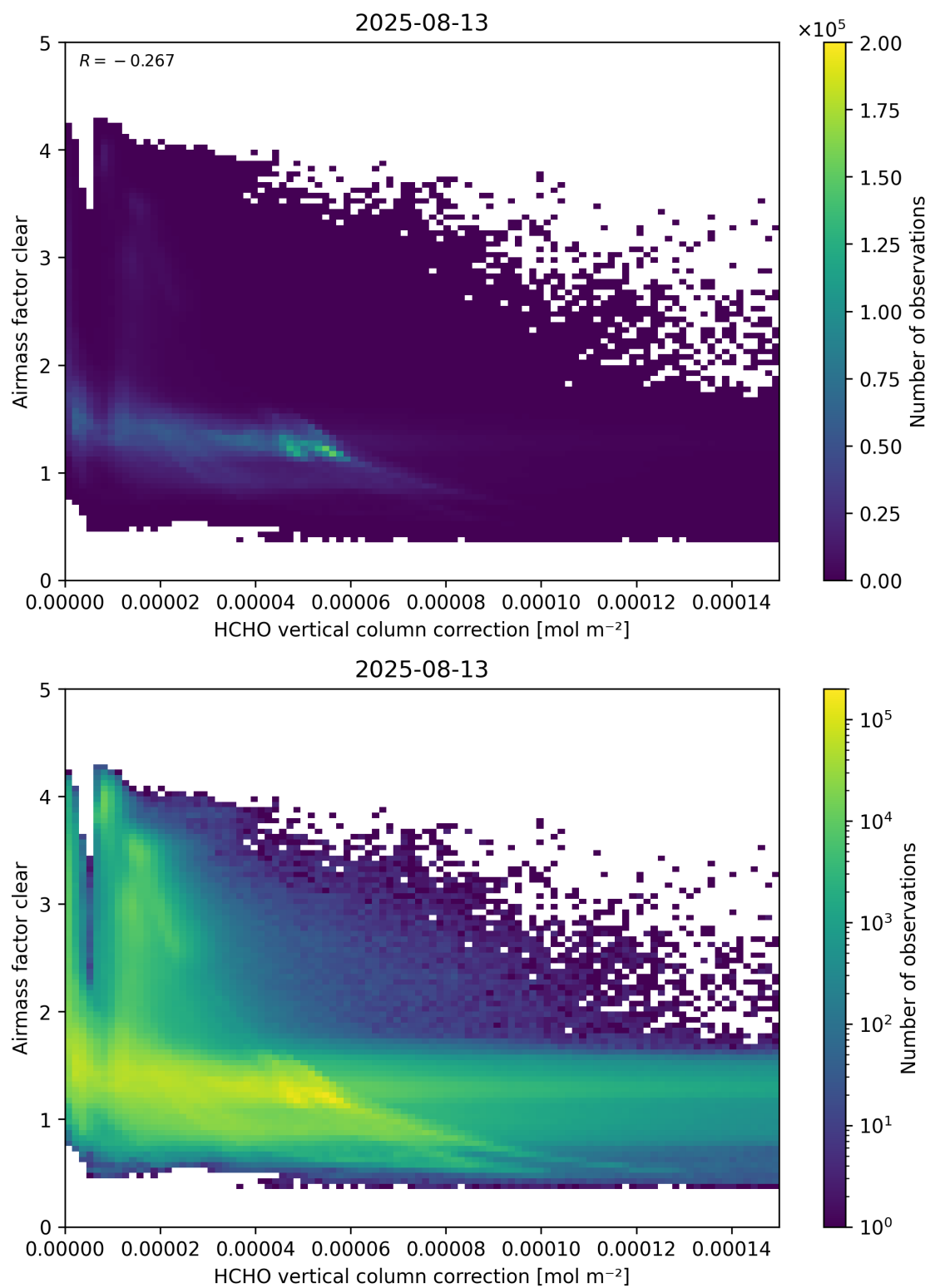
Figure 115: Scatter density plot of “HCHO vertical column correction” against “Airmass factor clear” for 2025-08-12 to 2025-08-14.
