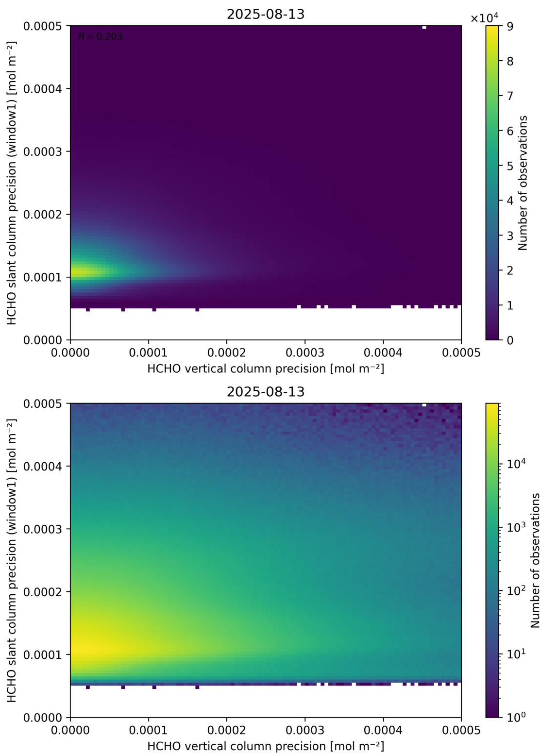
Figure 143: Scatter density plot of “HCHO vertical column precision” against “HCHO slant column precision (window1)” for 2025-08-12 to 2025-08-14.
