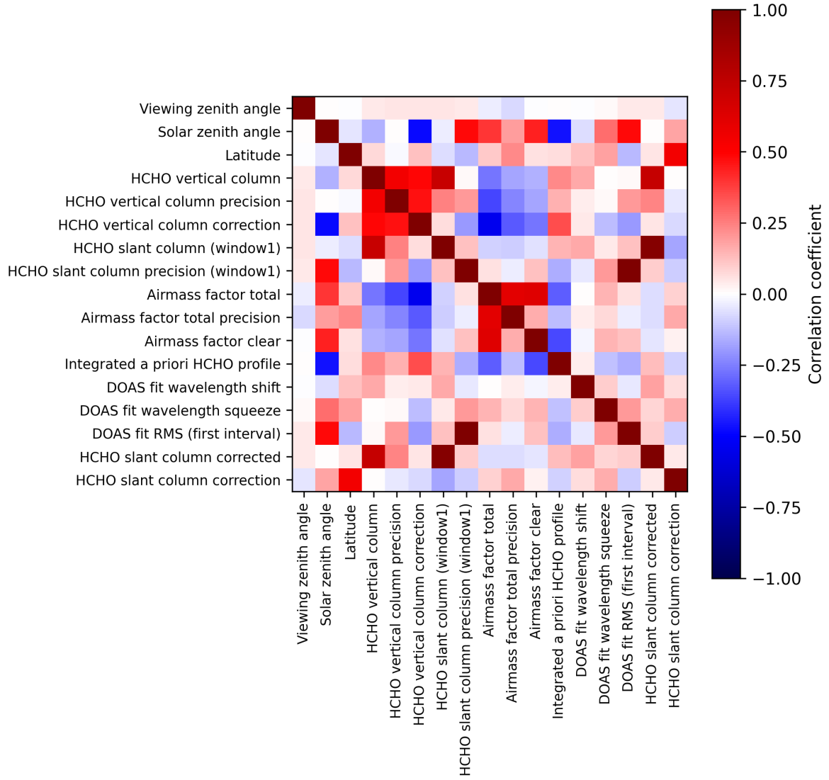
Figure 2: Map of correlation matrix for 2025-08-12 to 2025-08-14.
