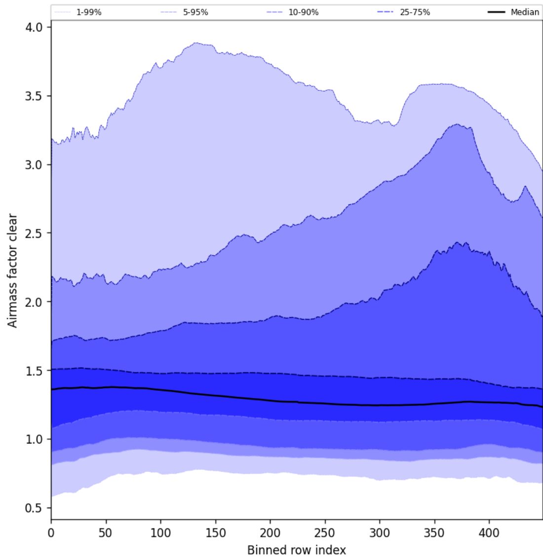
Figure 56: Along track statistics of “Airmass factor clear” for 2025-08-12 to 2025-08-14
