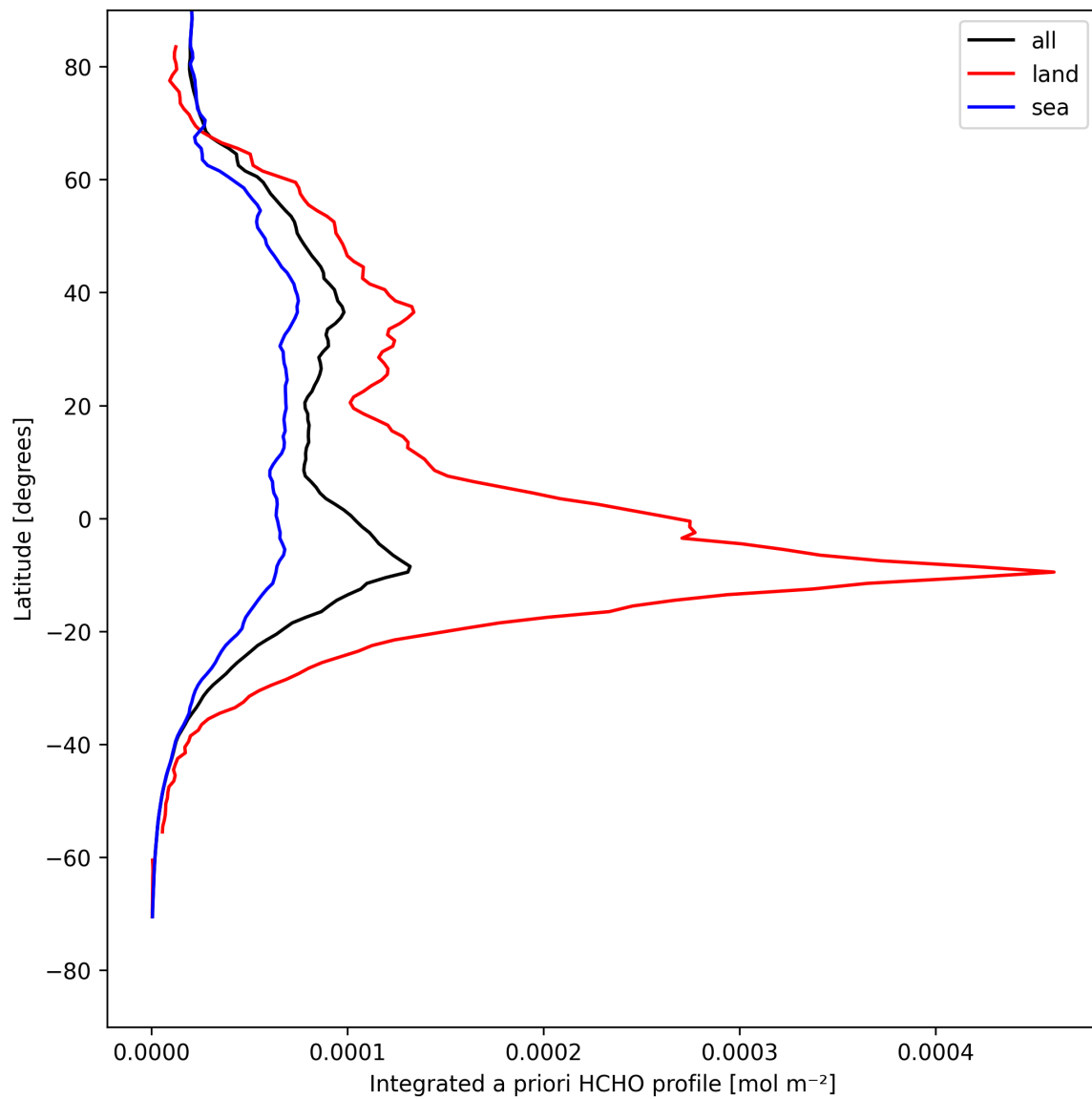
Figure 29: Zonal average of “Integrated a priori HCHO profile” for 2025-08-12 to 2025-08-14.
