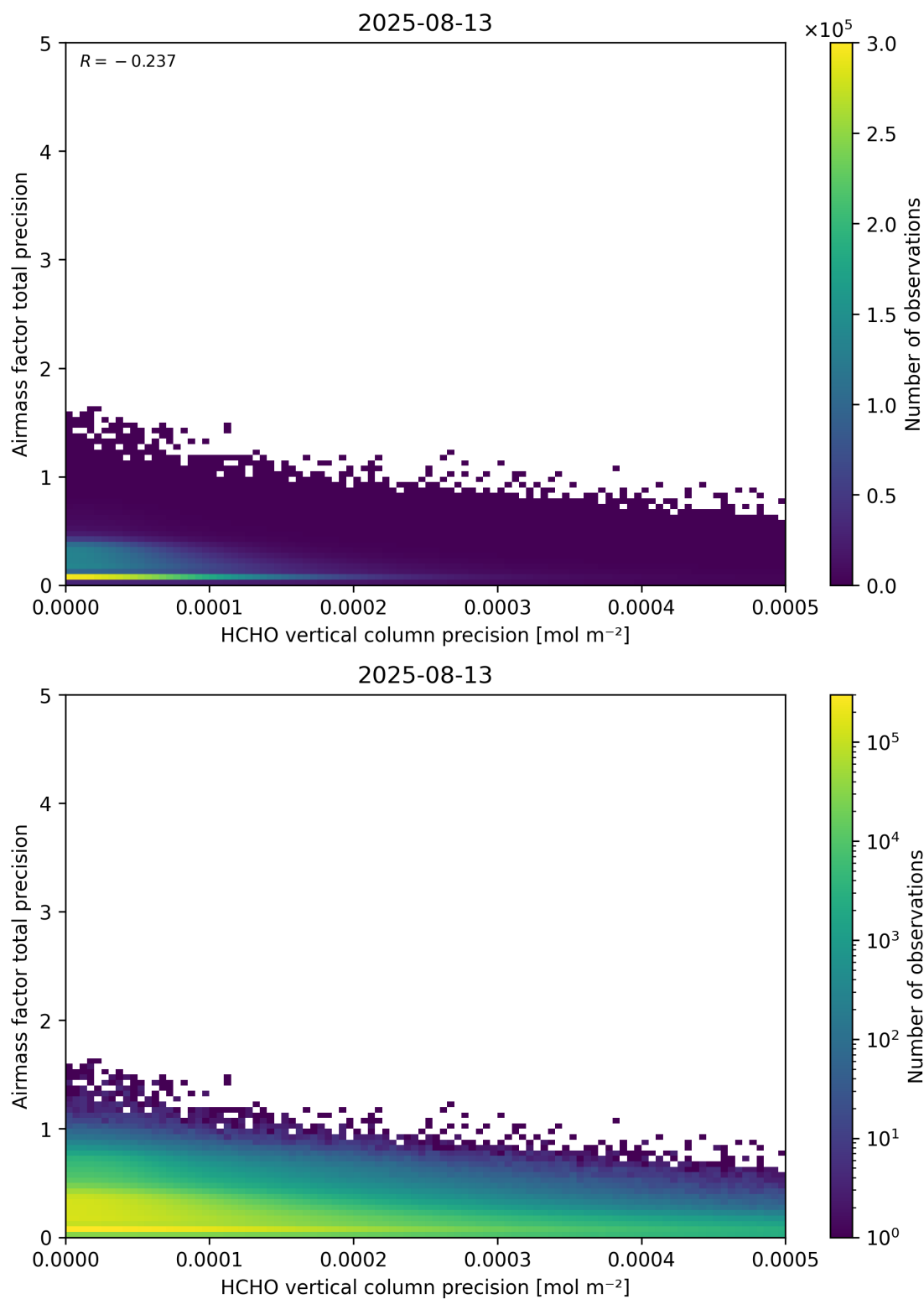
Figure 145: Scatter density plot of “HCHO vertical column precision” against “Airmass factor total precision” for 2025-08-12 to 2025-08-14.
