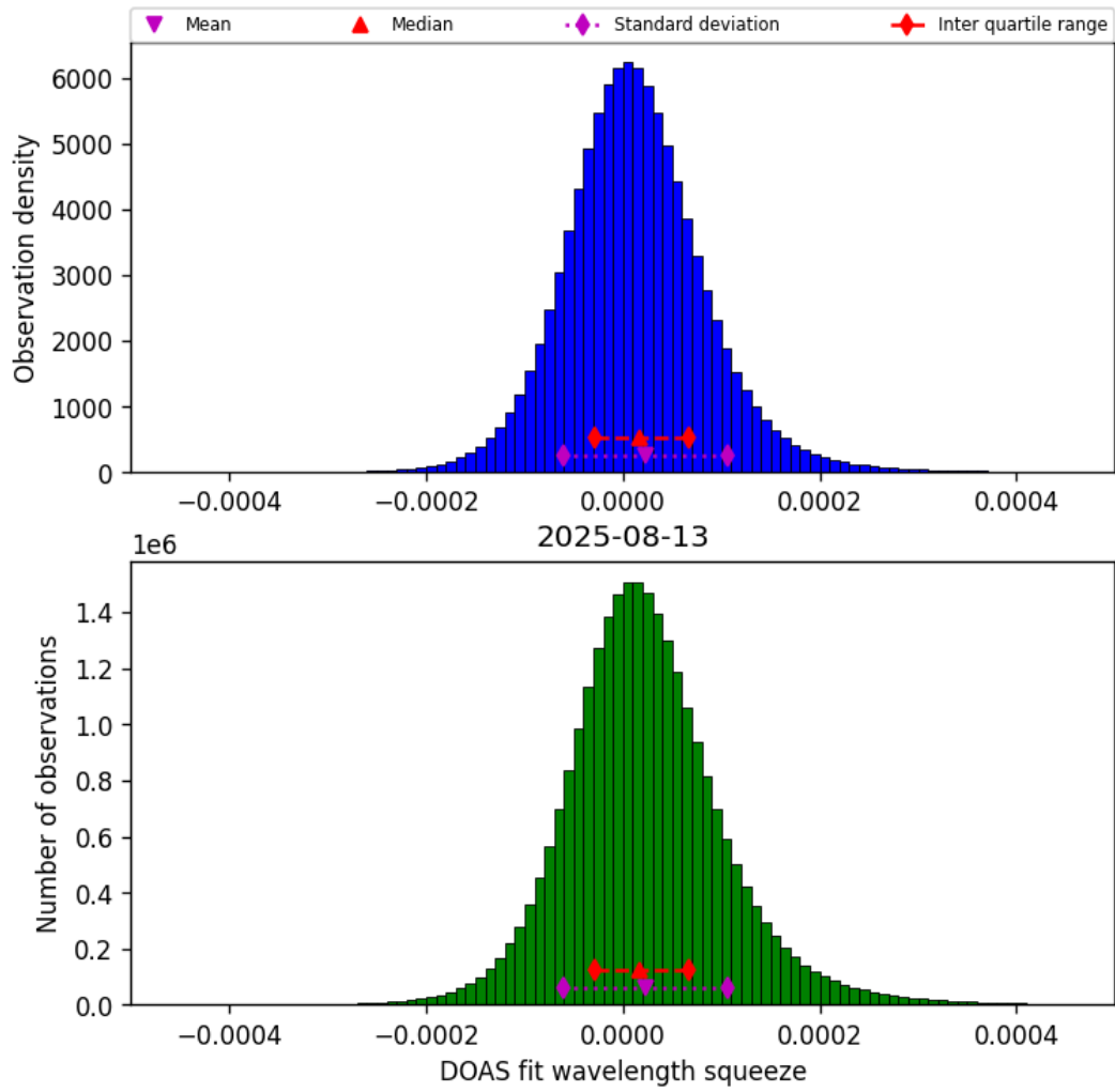
Figure 45: Histogram of “DOAS fit wavelength squeeze” for 2025-08-12 to 2025-08-14
