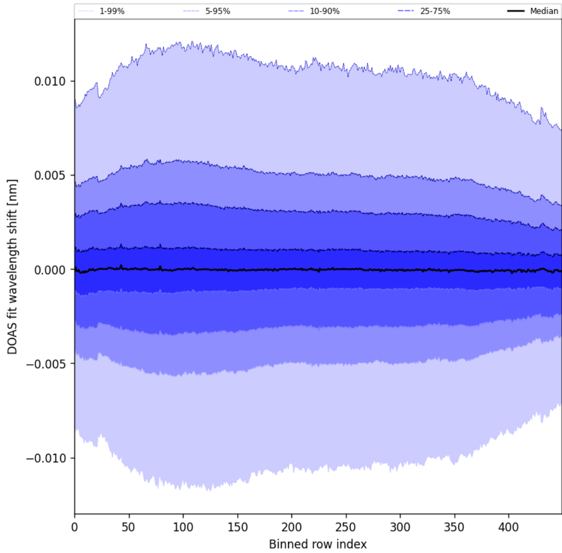
Figure 58: Along track statistics of “DOAS fit wavelength shift” for 2025-08-12 to 2025-08-14
