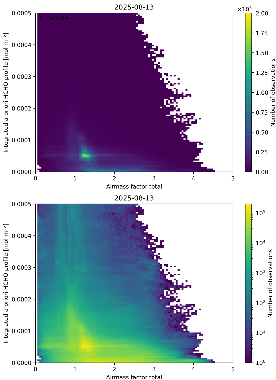
Figure 104: Scatter density plot of “Airmass factor total” against “Integrated a priori HCHO profile” for 2025-08-12 to 2025-08-14.
