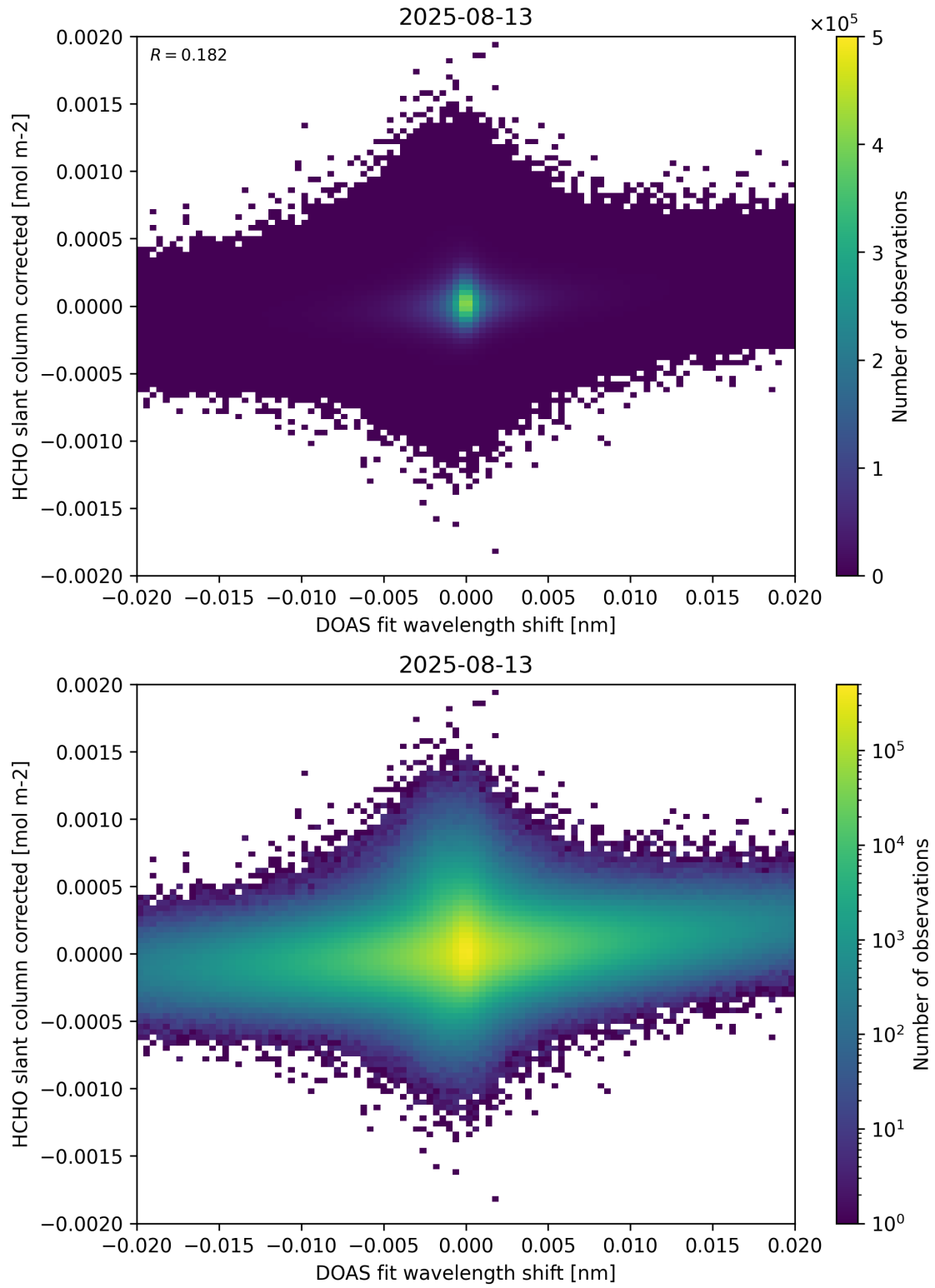
Figure 66: Scatter density plot of “DOAS fit wavelength shift” against “HCHO slant column corrected” for 2025-08-12 to 2025-08-14.
