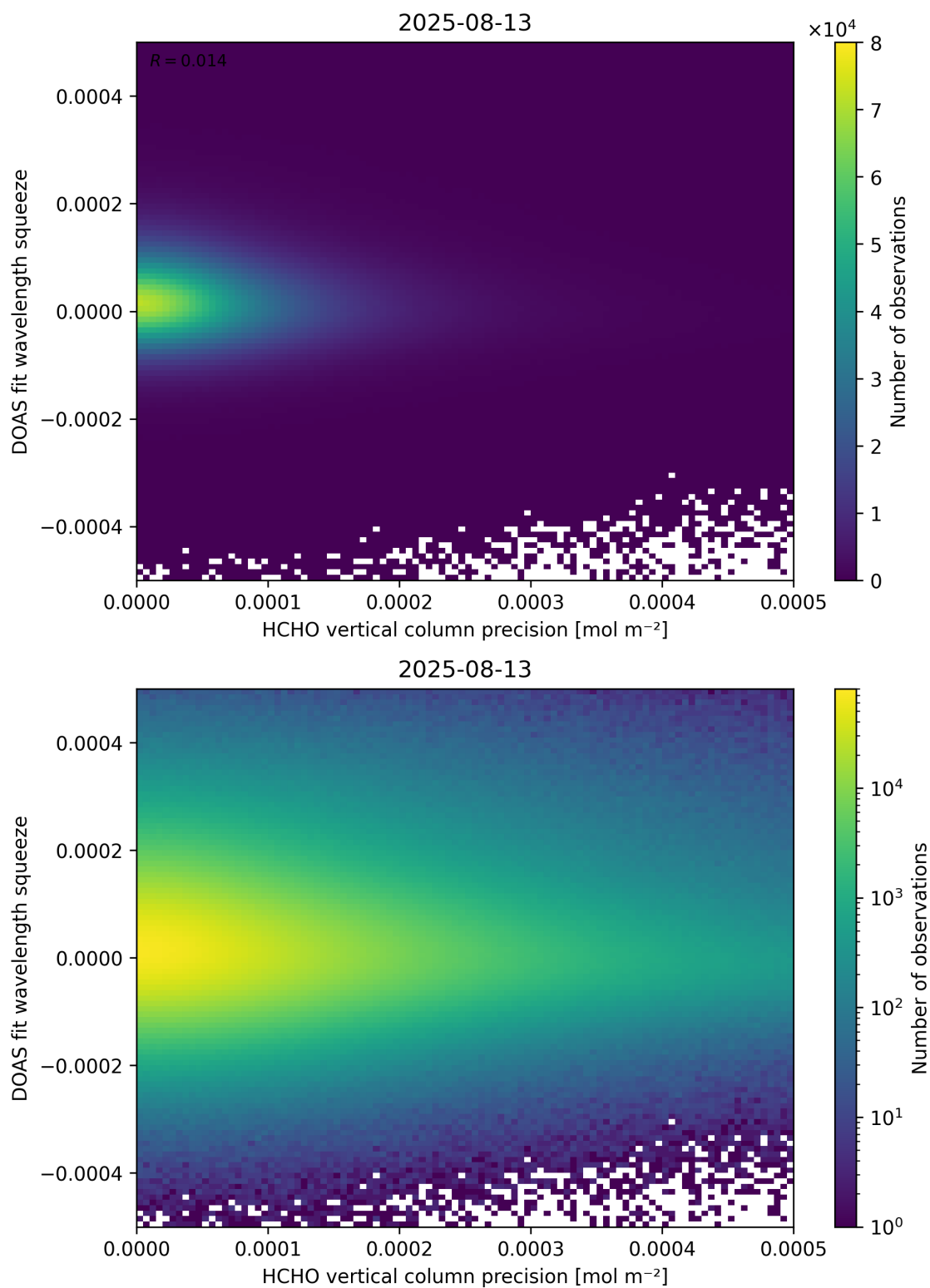
Figure 138: Scatter density plot of “HCHO vertical column precision” against “DOAS fit wavelength squeeze” for 2025-08-12 to 2025-08-14.
