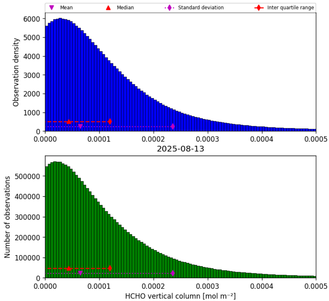
Figure 35: Histogram of “HCHO vertical column” for 2025-08-12 to 2025-08-14
