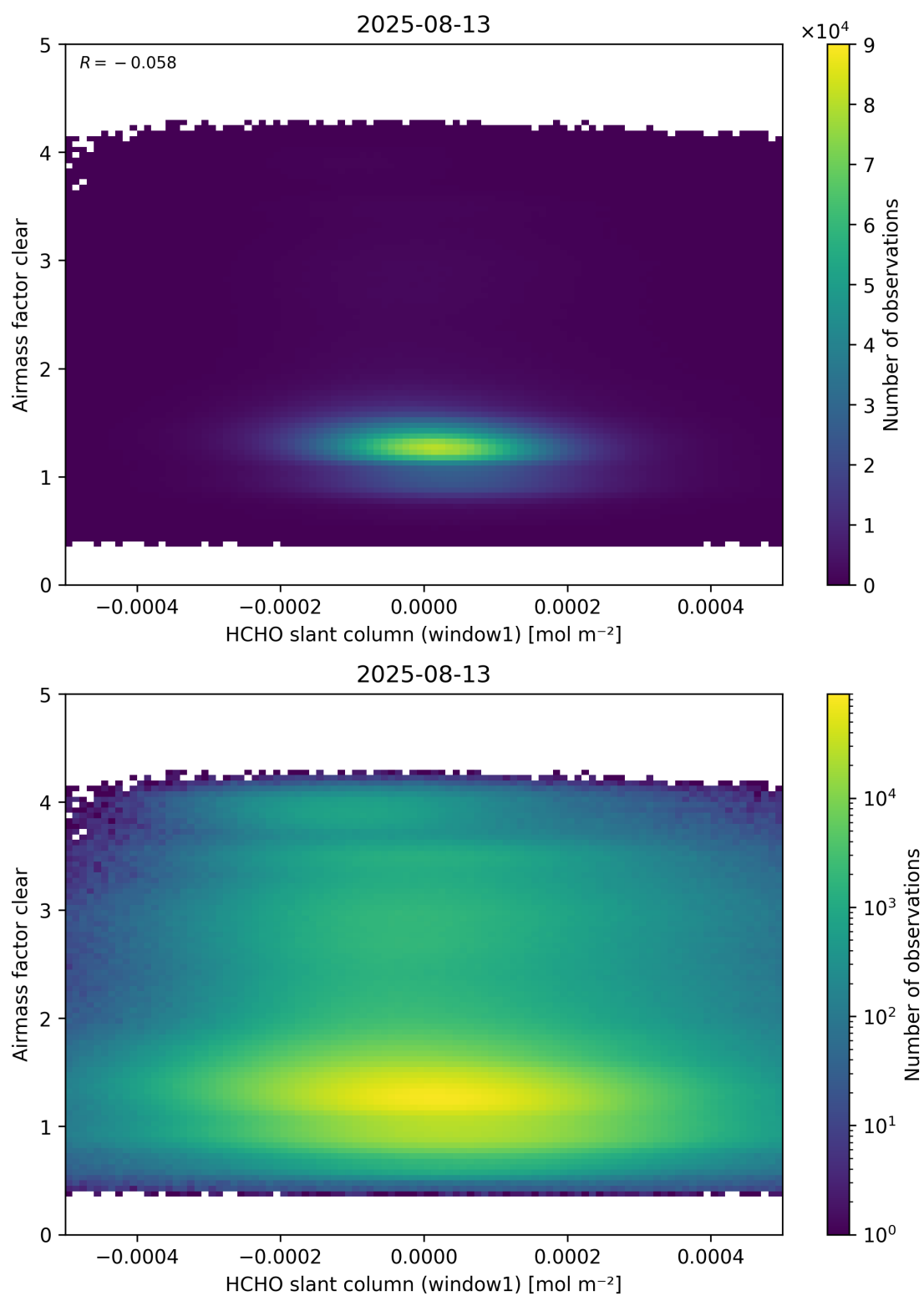
Figure 81: Scatter density plot of “HCHO slant column (window1)” against “Airmass factor clear” for 2025-08-12 to 2025-08-14.
