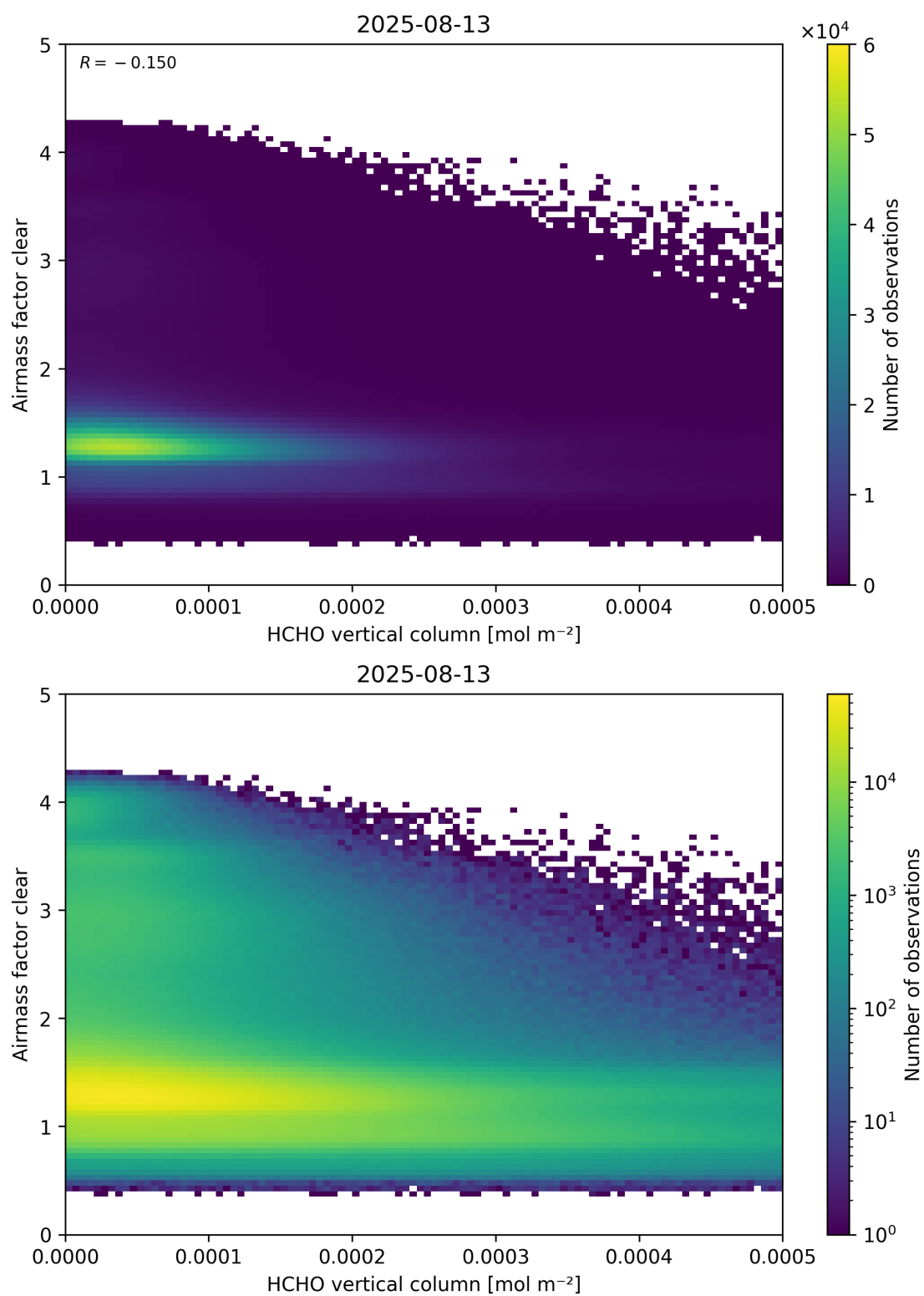
Figure 126: Scatter density plot of “HCHO vertical column” against “Airmass factor clear” for 2025-08-12 to 2025-08-14.
