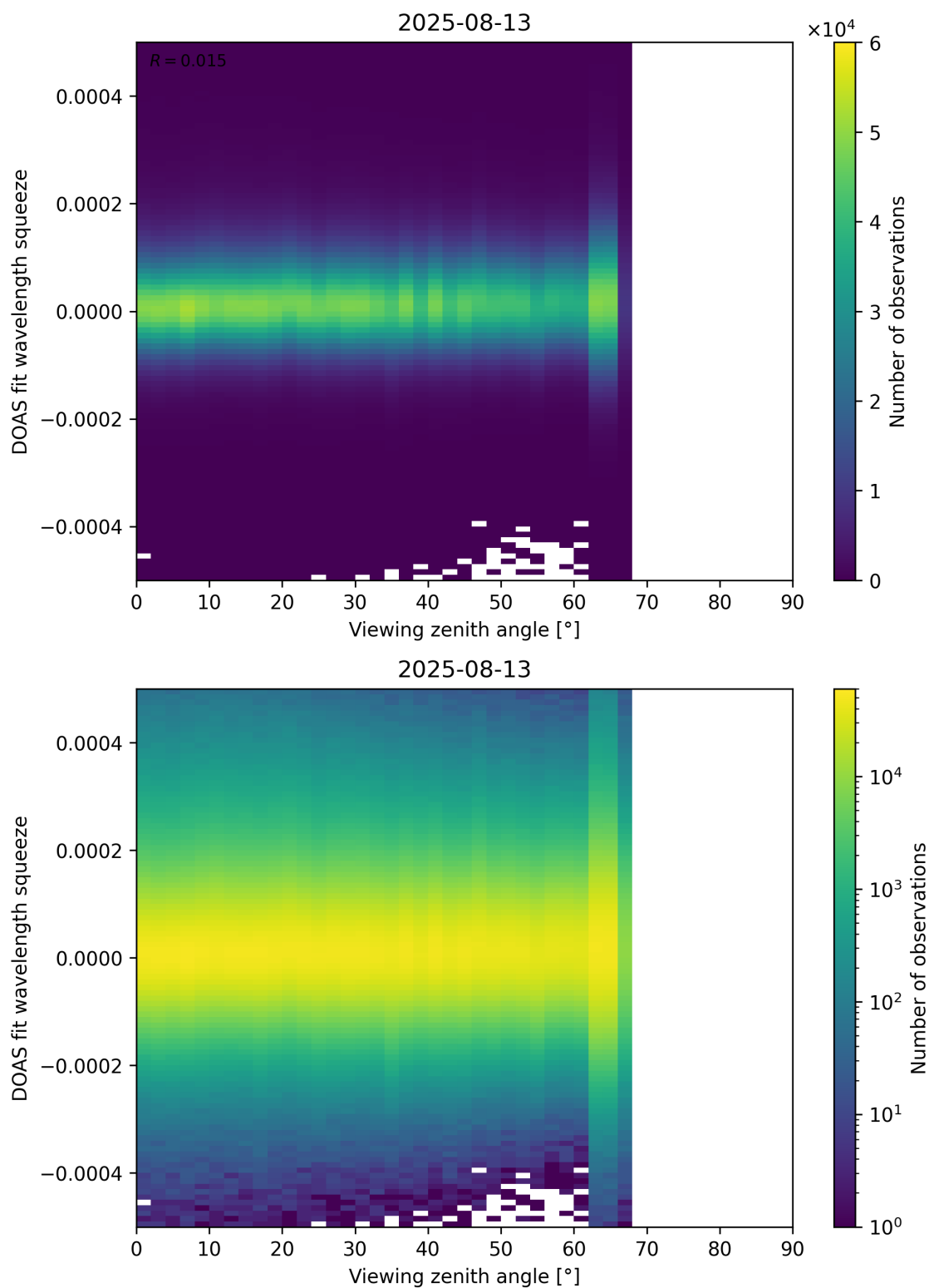
Figure 184: Scatter density plot of “Viewing zenith angle” against “DOAS fit wavelength squeeze” for 2025-08-12 to 2025-08-14.
