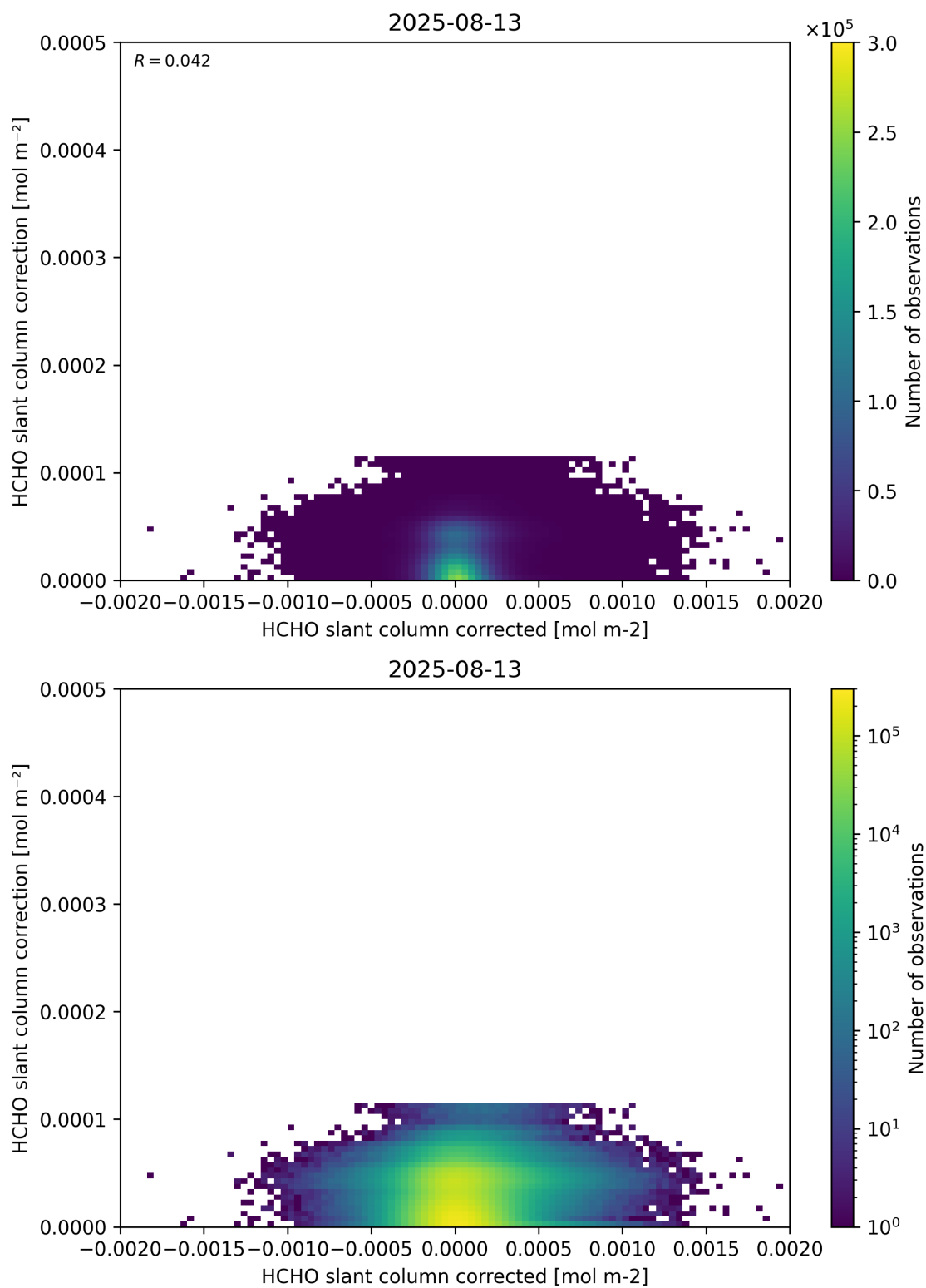
Figure 77: Scatter density plot of “HCHO slant column corrected” against “HCHO slant column correction” for 2025-08-12 to 2025-08-14.
