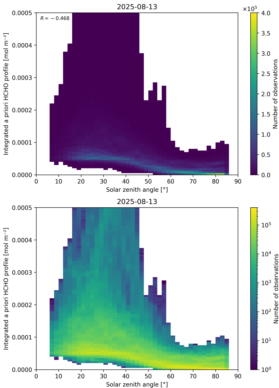
Figure 180: Scatter density plot of “Solar zenith angle” against “Integrated a priori HCHO profile” for 2025-08-12 to 2025-08-14.
