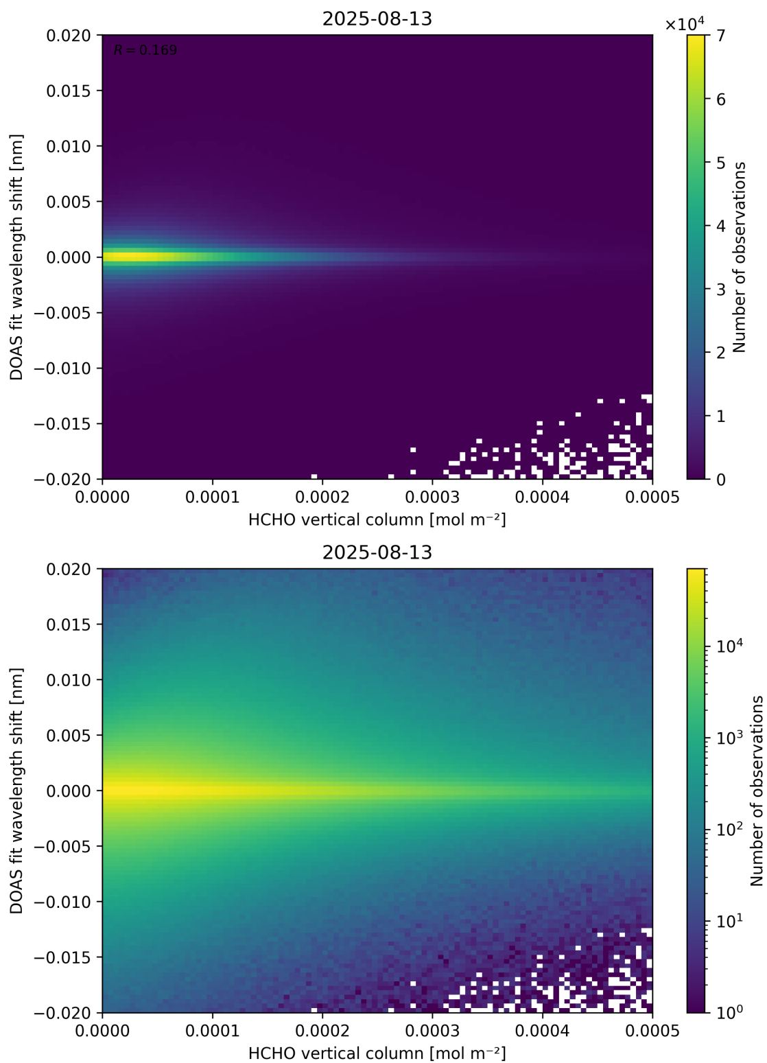
Figure 124: Scatter density plot of “HCHO vertical column” against “DOAS fit wavelength shift” for 2025-08-12 to 2025-08-14.
