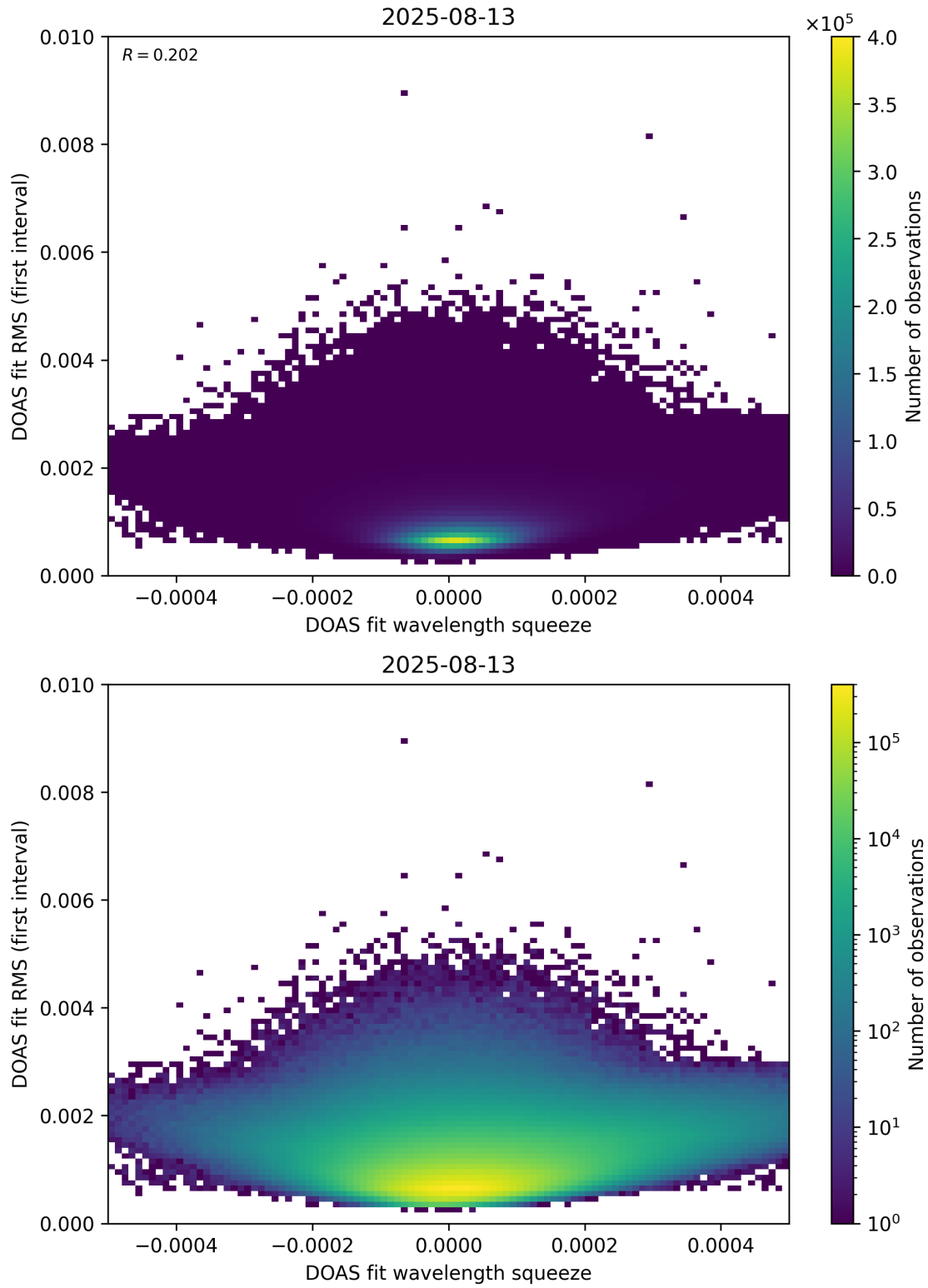
Figure 68: Scatter density plot of “DOAS fit wavelength squeeze” against “DOAS fit RMS (first interval)” for 2025-08-12 to 2025-08-14.
