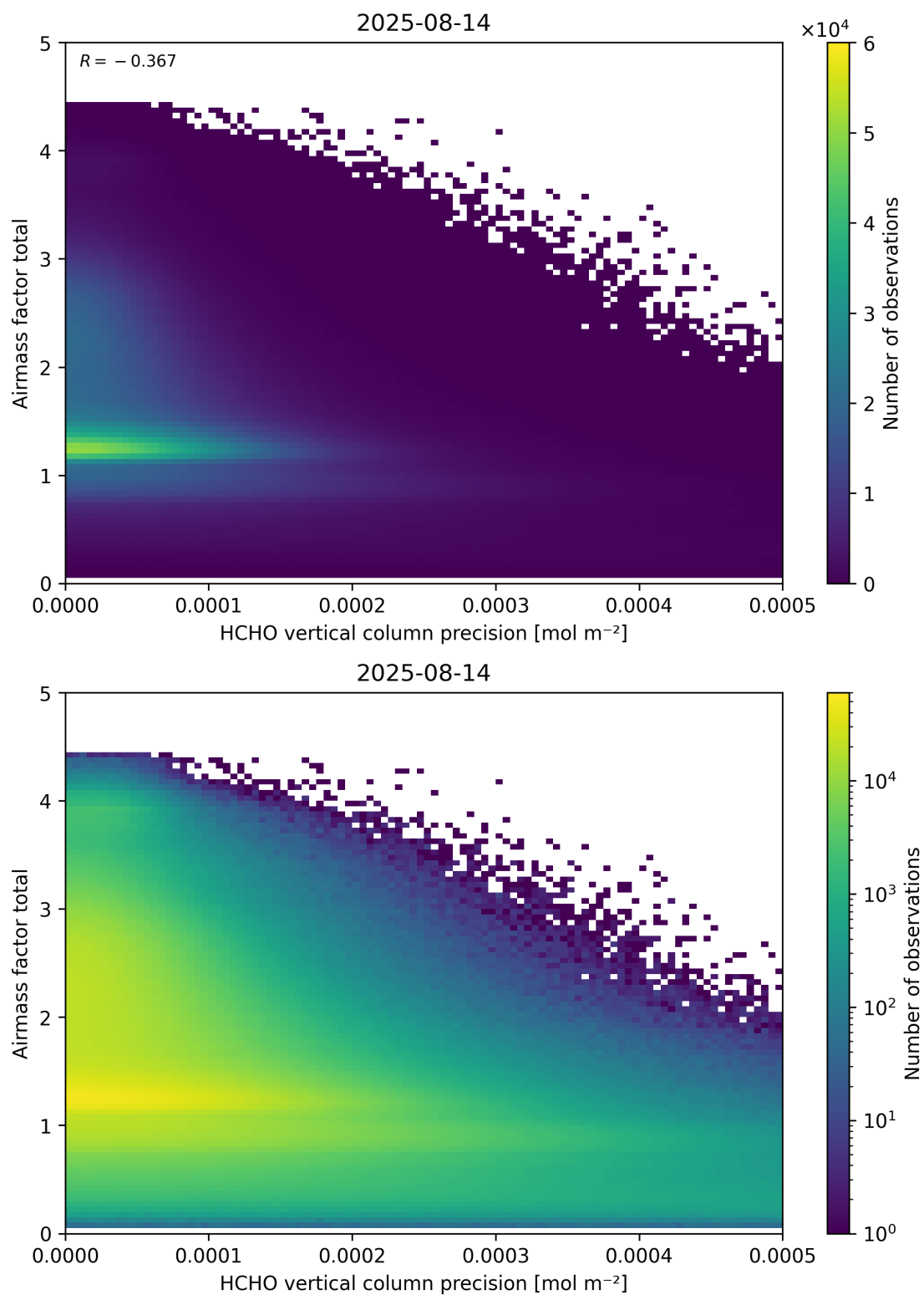
Figure 144: Scatter density plot of “HCHO vertical column precision” against “Airmass factor total” for 2025-08-14 to 2025-08-15.
