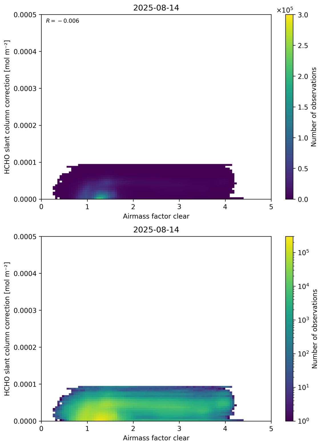
Figure 75: Scatter density plot of “Airmass factor clear” against “HCHO slant column correction” for 2025-08-14 to 2025-08-15.
