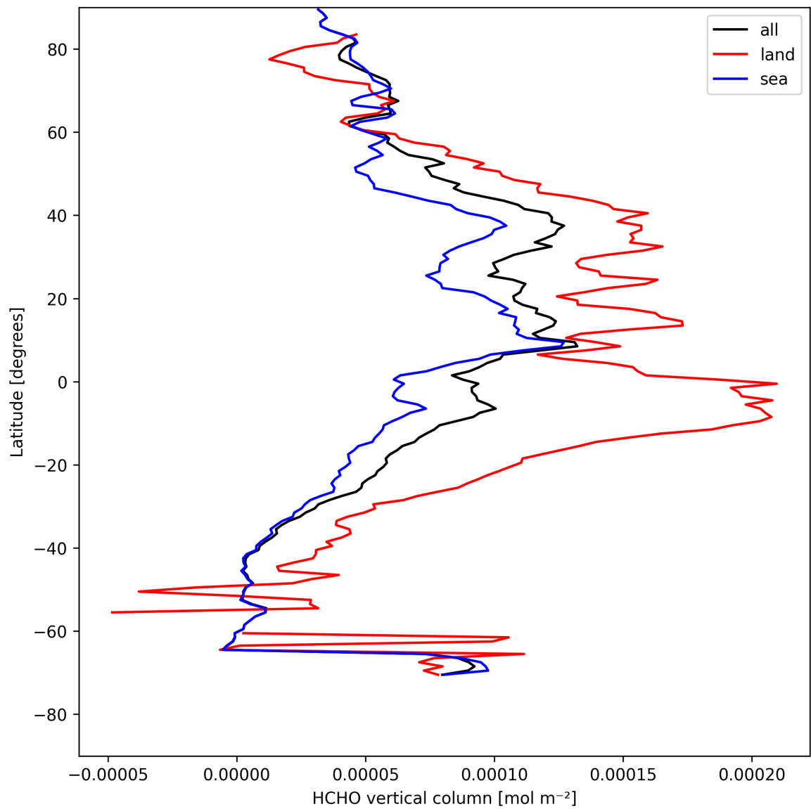
Figure 21: Zonal average of “HCHO vertical column” for 2025-08-14 to 2025-08-15.
