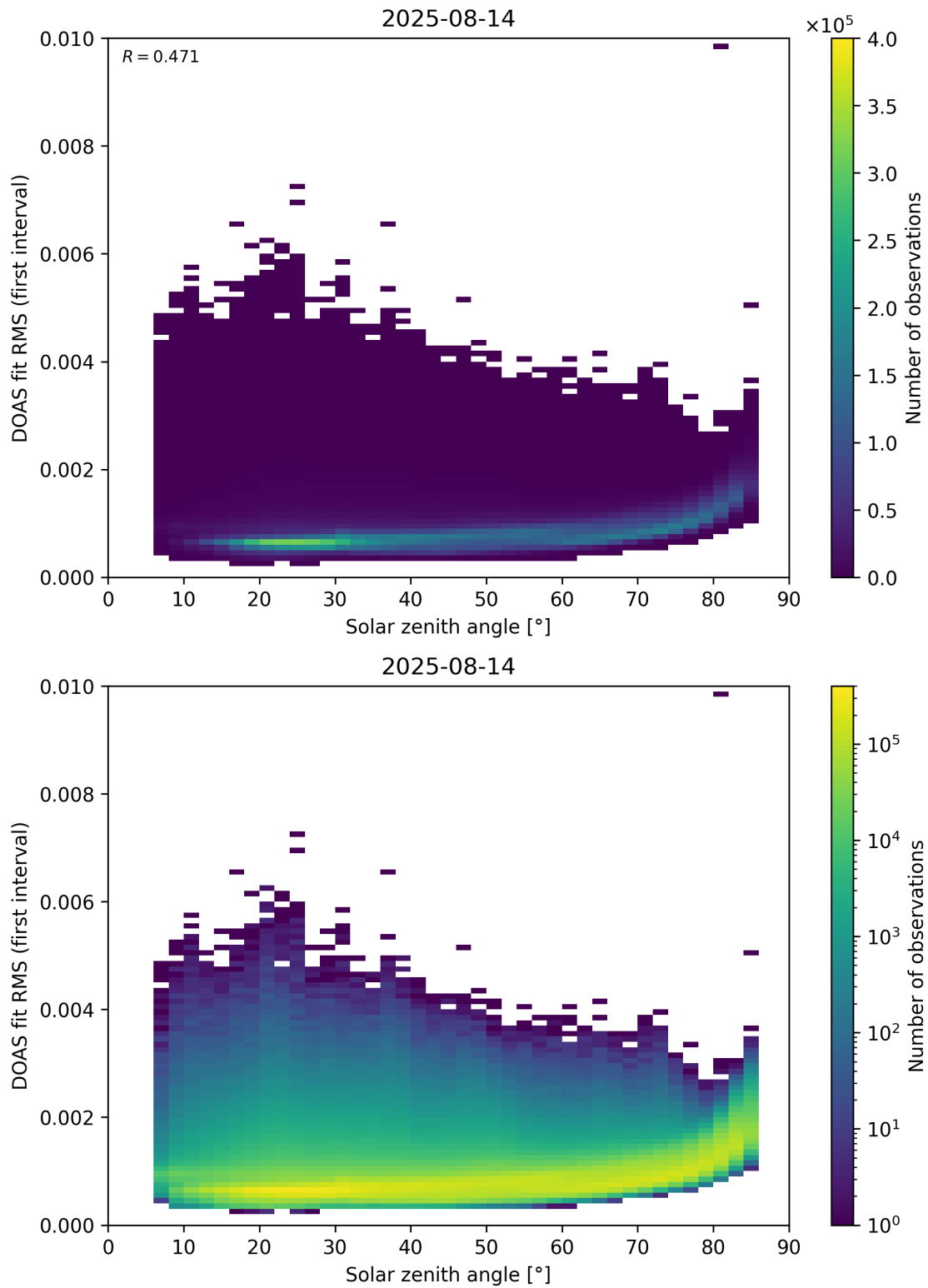
Figure 167: Scatter density plot of “Solar zenith angle” against “DOAS fit RMS (first interval)” for 2025-08-14 to 2025-08-15.
