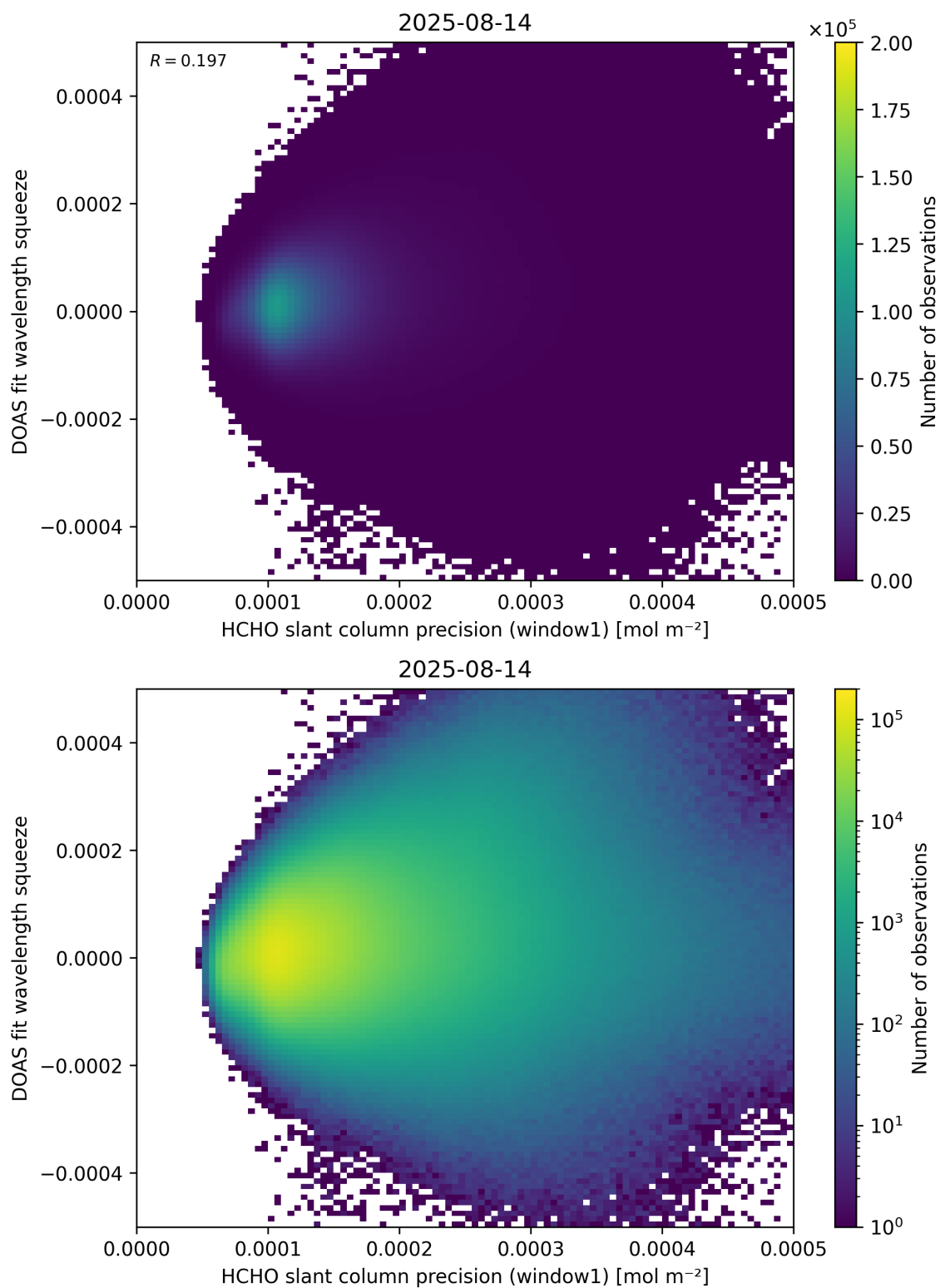
Figure 90: Scatter density plot of “HCHO slant column precision (window1)” against “DOAS fit wavelength squeeze” for 2025-08-14 to 2025-08-15.
