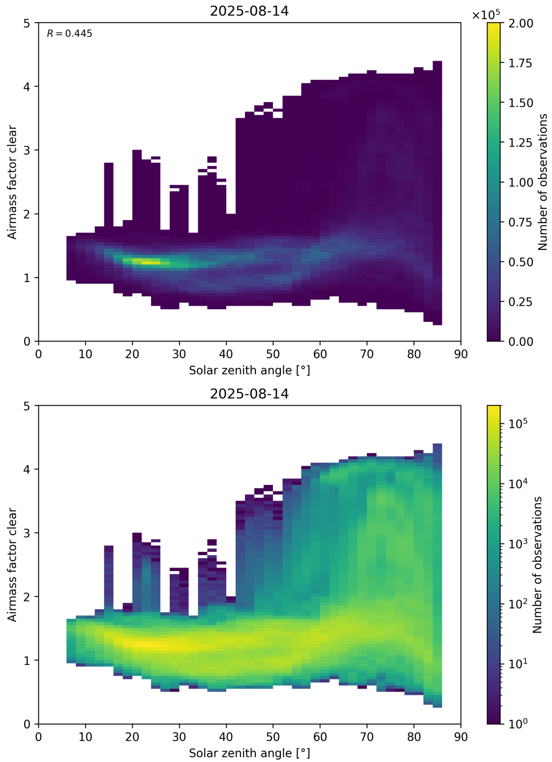
Figure 170: Scatter density plot of “Solar zenith angle” against “Airmass factor clear” for 2025-08-14 to 2025-08-15.
