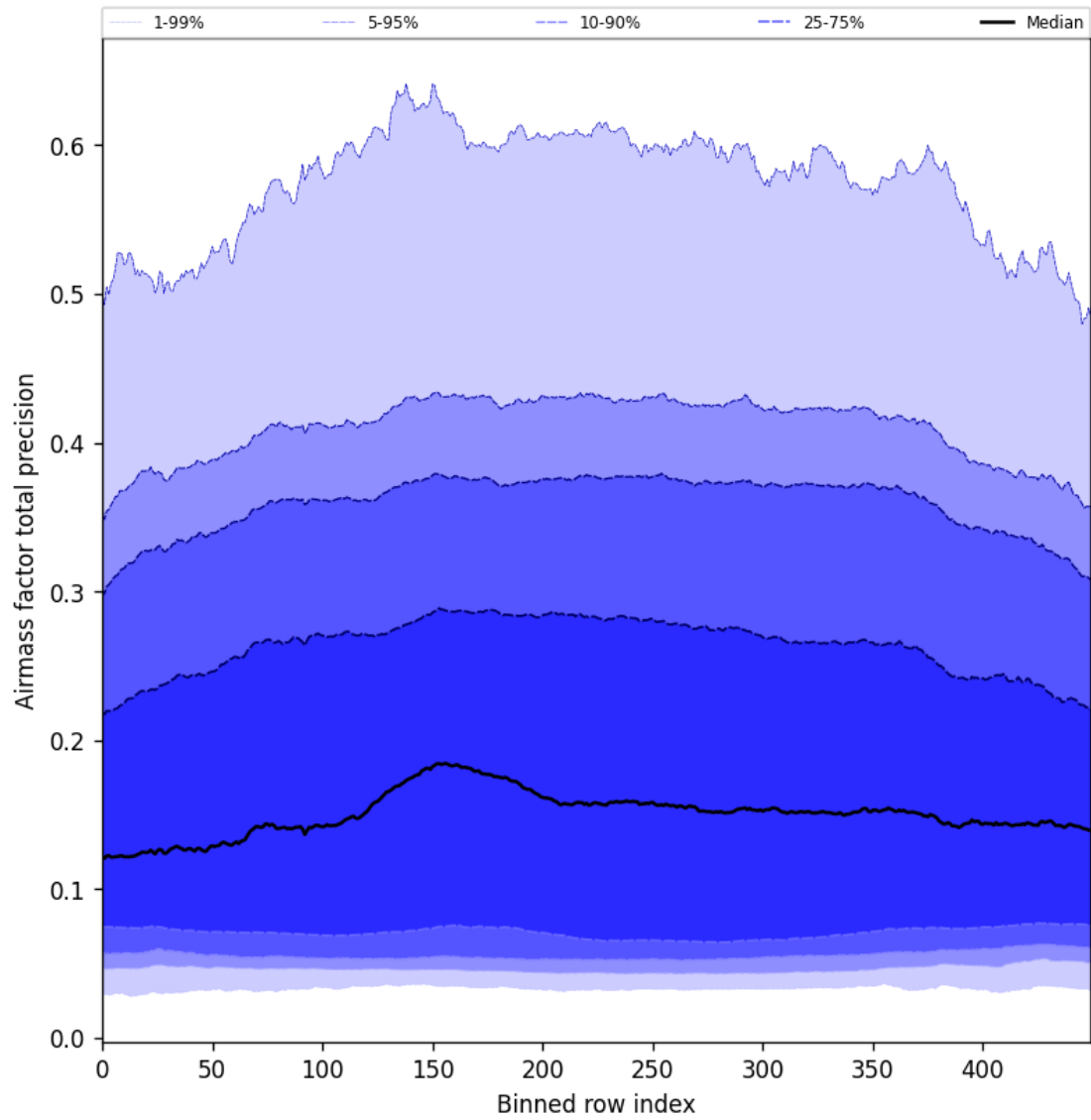
Figure 55: Along track statistics of “Airmass factor total precision” for 2025-08-14 to 2025-08-15
