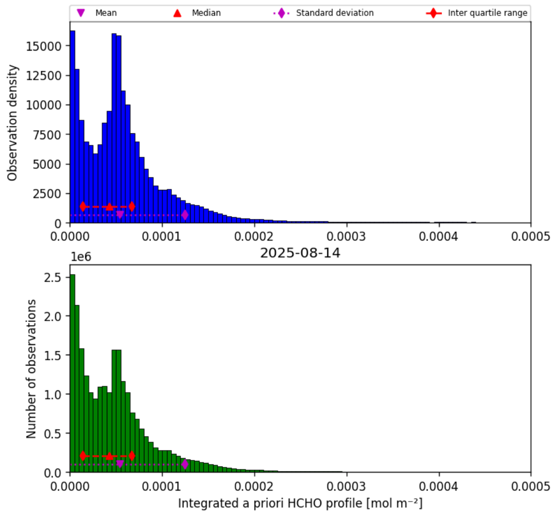
Figure 43: Histogram of “Integrated a priori HCHO profile” for 2025-08-14 to 2025-08-15
