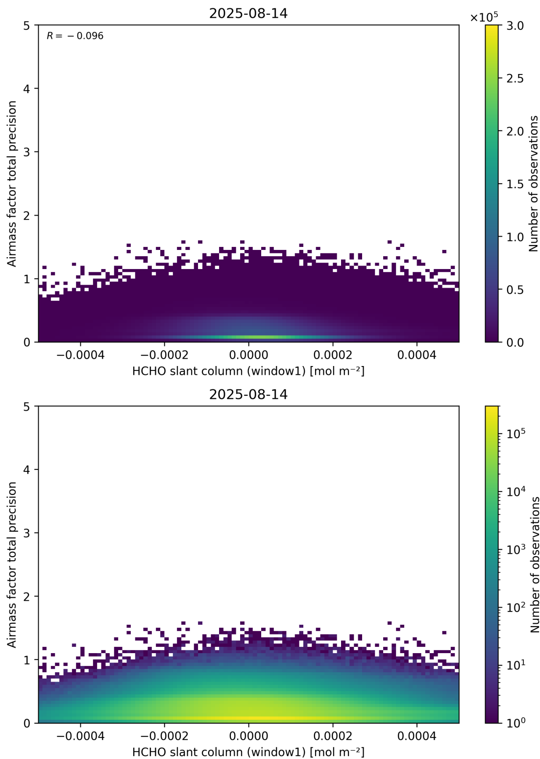
Figure 86: Scatter density plot of “HCHO slant column (window1)” against “Airmass factor total precision” for 2025-08-14 to 2025-08-15.
