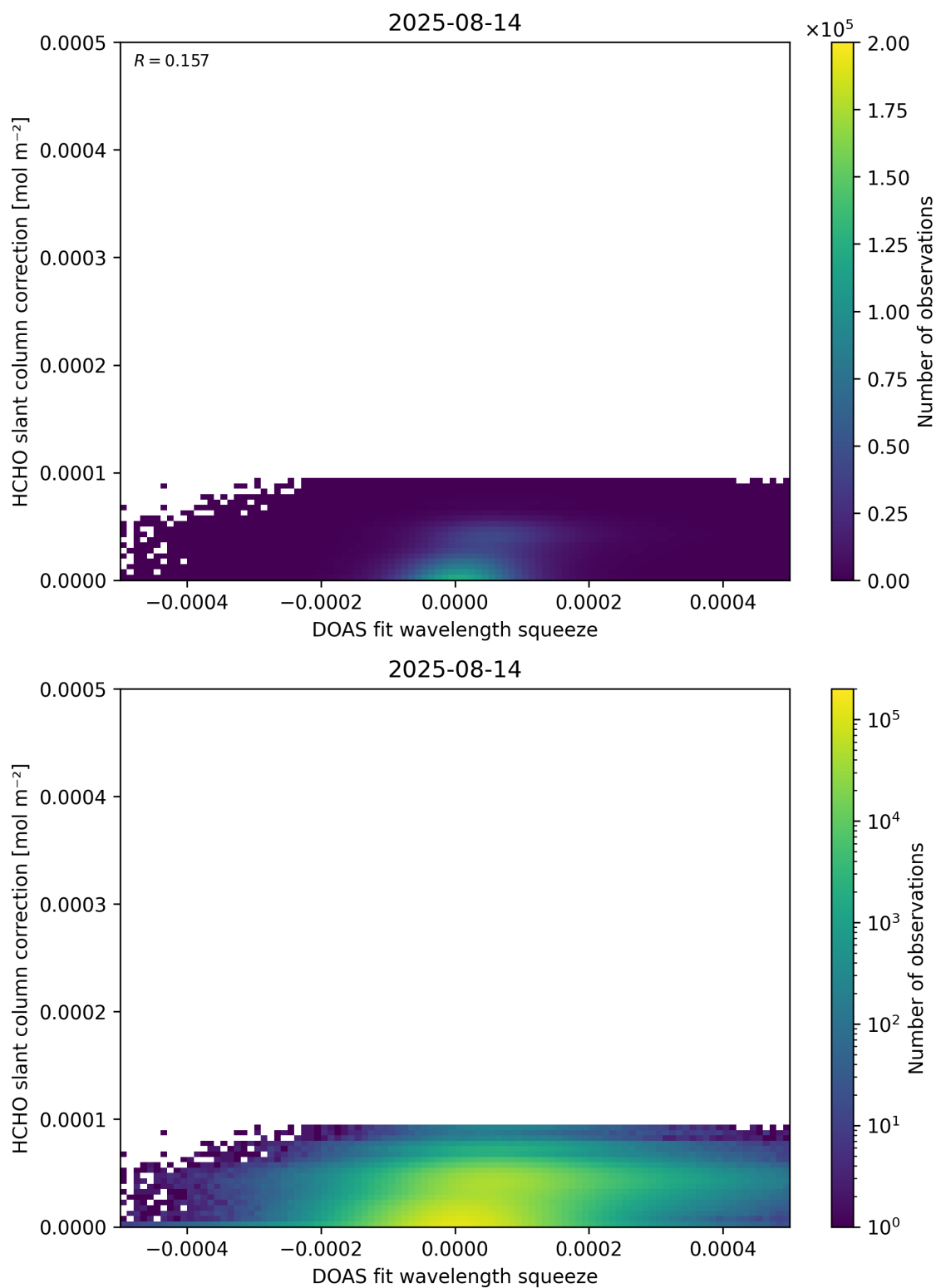
Figure 70: Scatter density plot of “DOAS fit wavelength squeeze” against “HCHO slant column correction” for 2025-08-14 to 2025-08-15.
