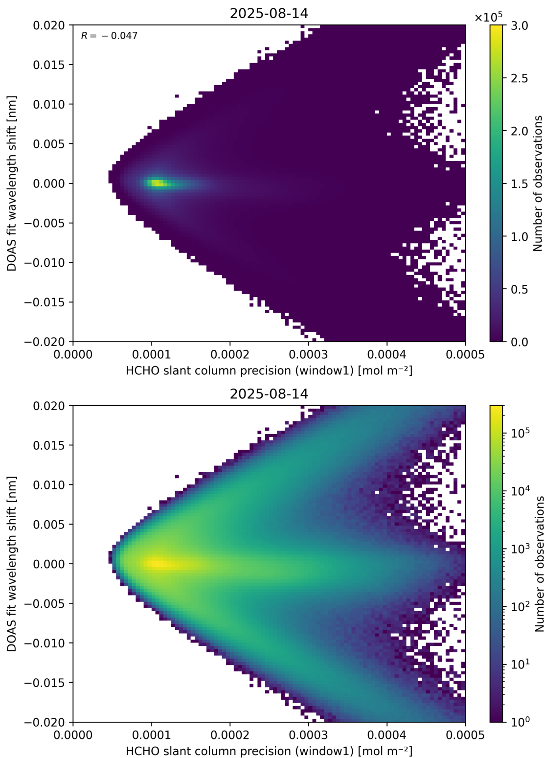
Figure 89: Scatter density plot of “HCHO slant column precision (window1)” against “DOAS fit wavelength shift” for 2025-08-14 to 2025-08-15.
