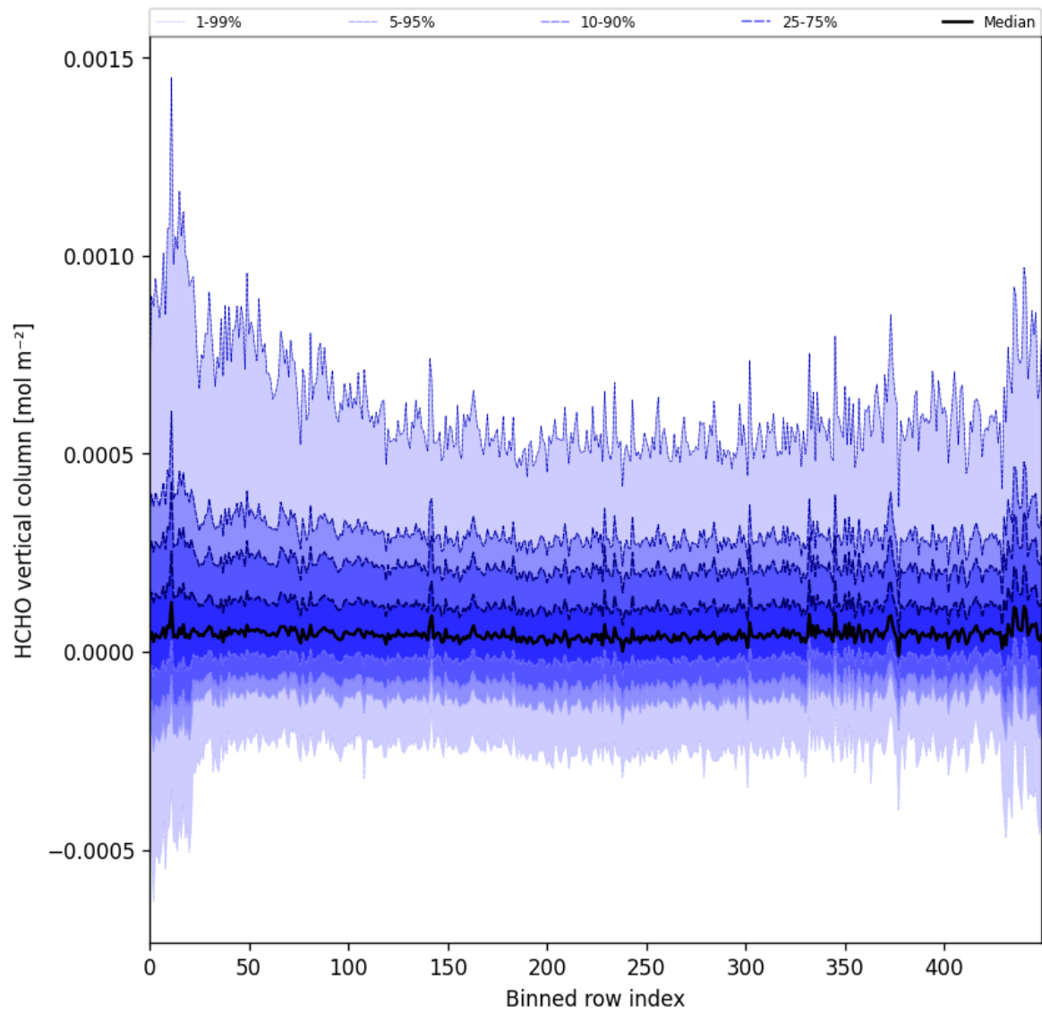
Figure 49: Along track statistics of “HCHO vertical column” for 2025-08-14 to 2025-08-15
