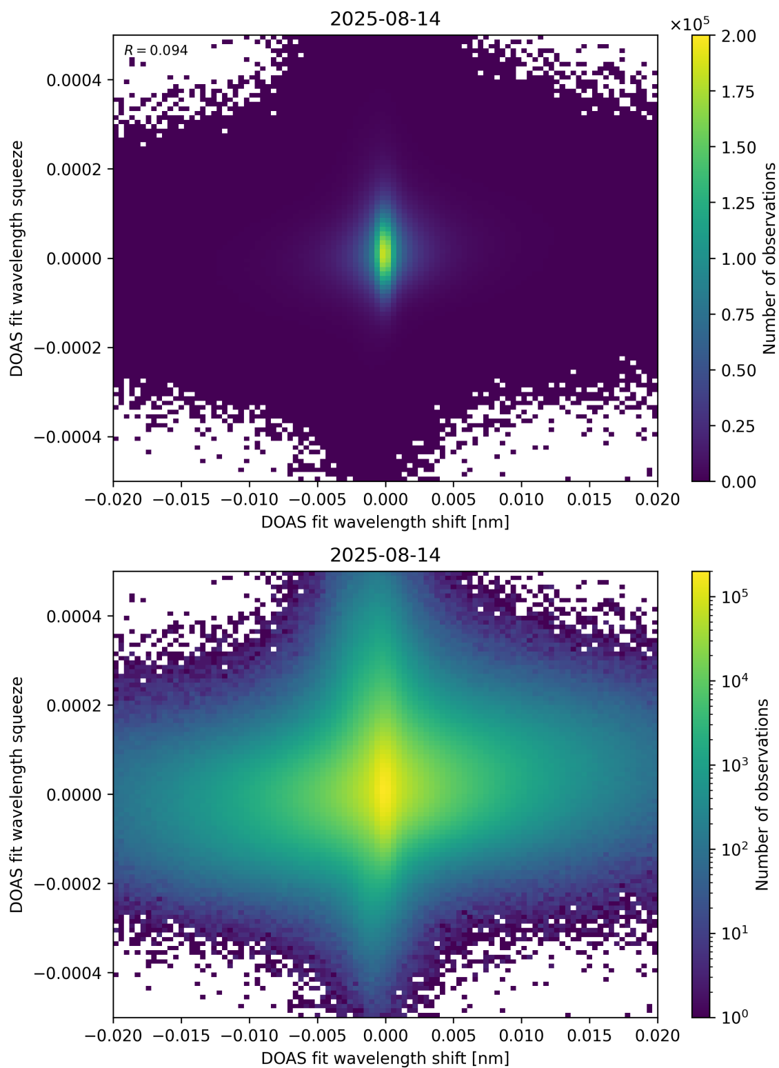
Figure 65: Scatter density plot of “DOAS fit wavelength shift” against “DOAS fit wavelength squeeze” for 2025-08-14 to 2025-08-15.
