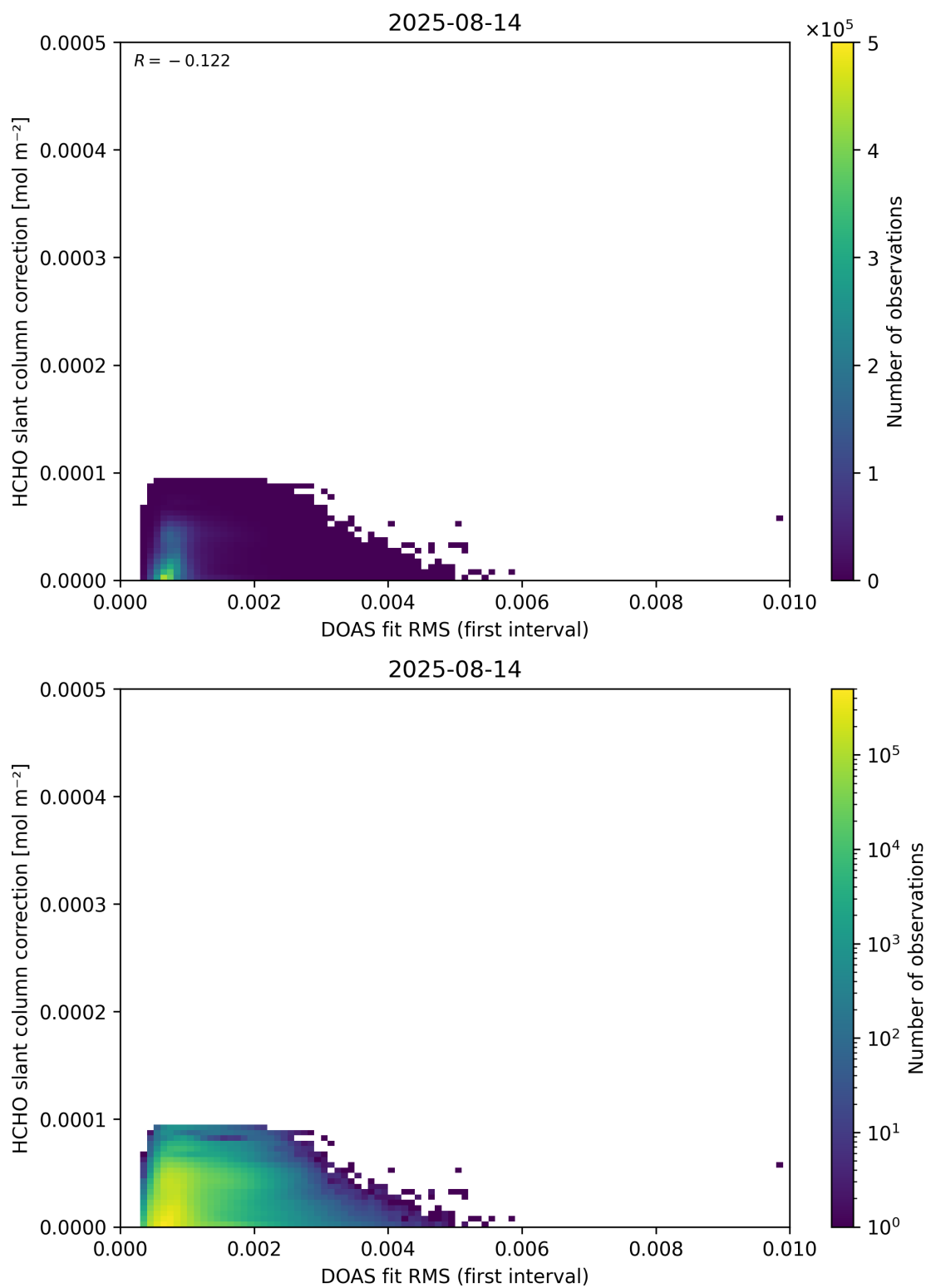
Figure 63: Scatter density plot of “DOAS fit RMS (first interval)” against “HCHO slant column correction” for 2025-08-14 to 2025-08-15.
