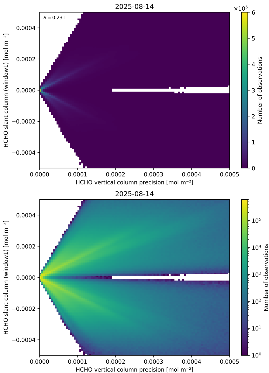
Figure 142: Scatter density plot of “HCHO vertical column precision” against “HCHO slant column (window1)” for 2025-08-14 to 2025-08-15.
