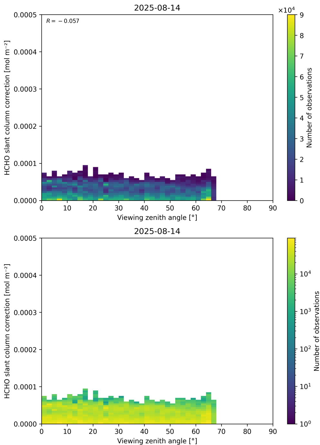
Figure 187: Scatter density plot of “Viewing zenith angle” against “HCHO slant column correction” for 2025-08-14 to 2025-08-15.
