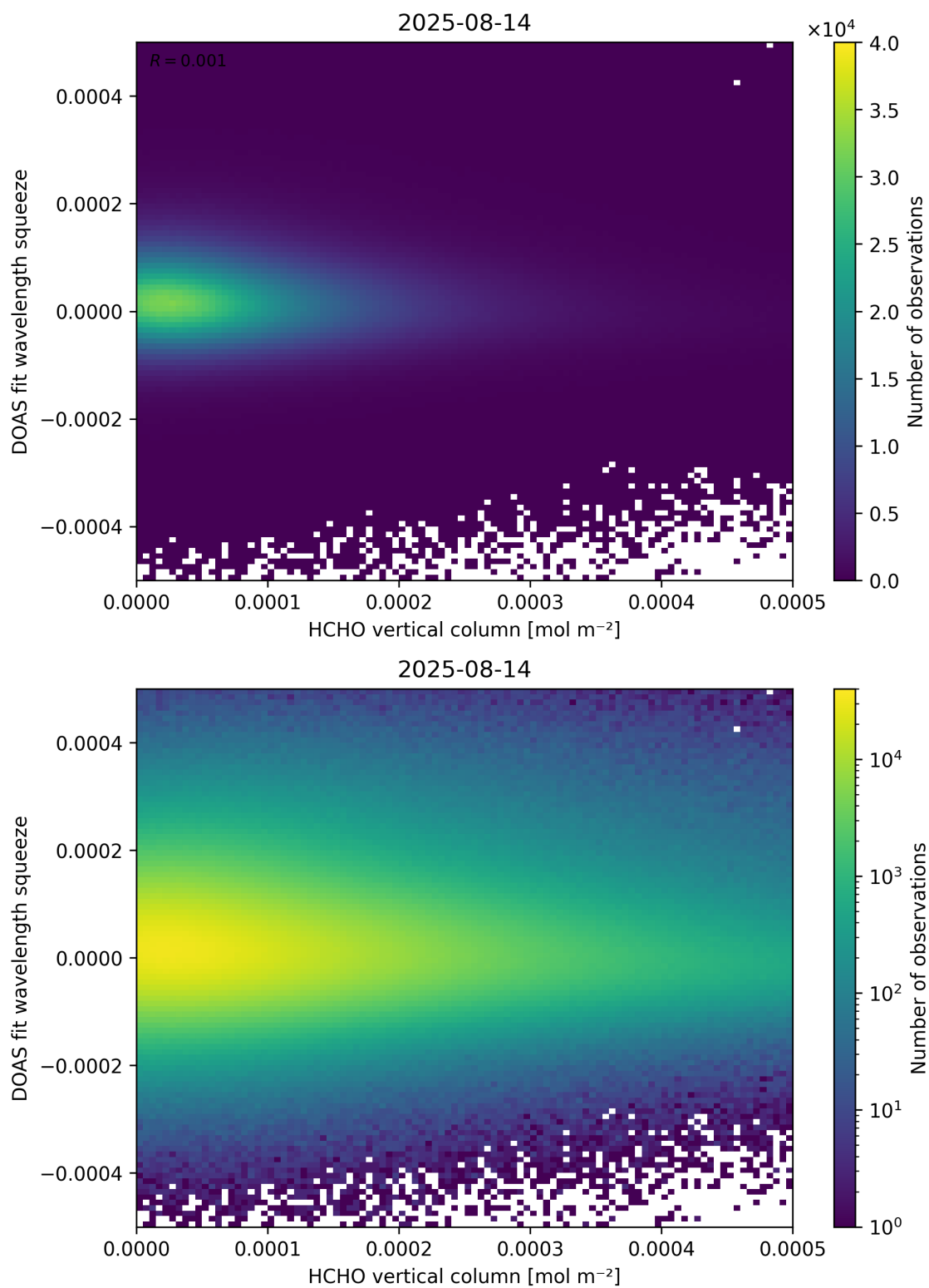
Figure 125: Scatter density plot of “HCHO vertical column” against “DOAS fit wavelength squeeze” for 2025-08-14 to 2025-08-15.
