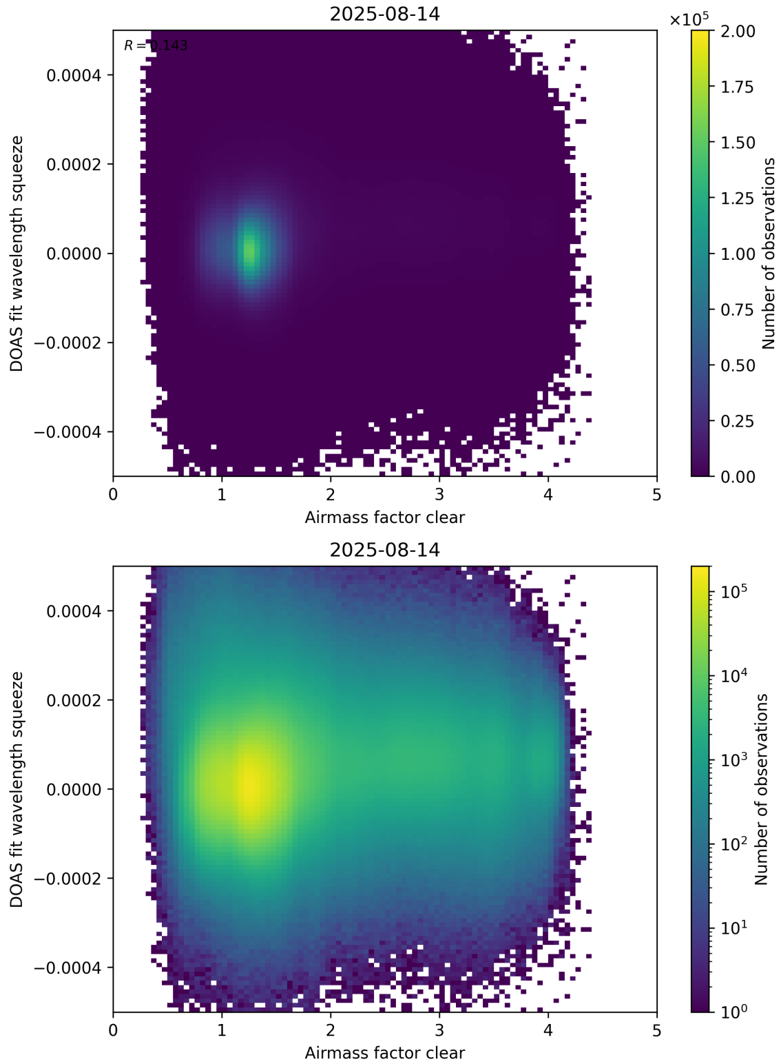
Figure 73: Scatter density plot of “Airmass factor clear” against “DOAS fit wavelength squeeze” for 2025-08-14 to 2025-08-15.
