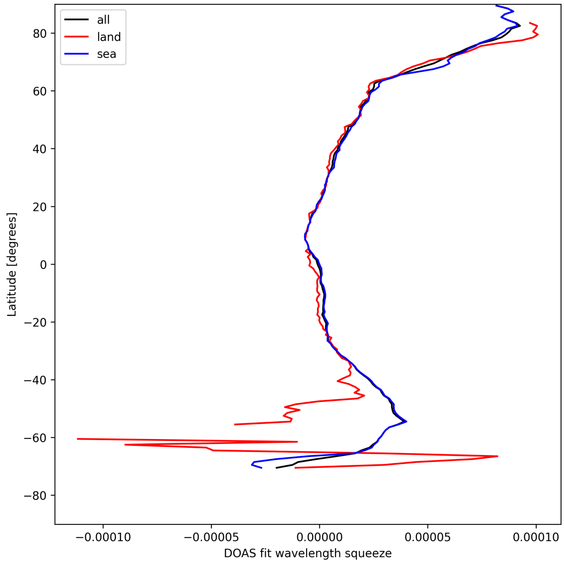
Figure 31: Zonal average of “DOAS fit wavelength squeeze” for 2025-08-14 to 2025-08-15.
