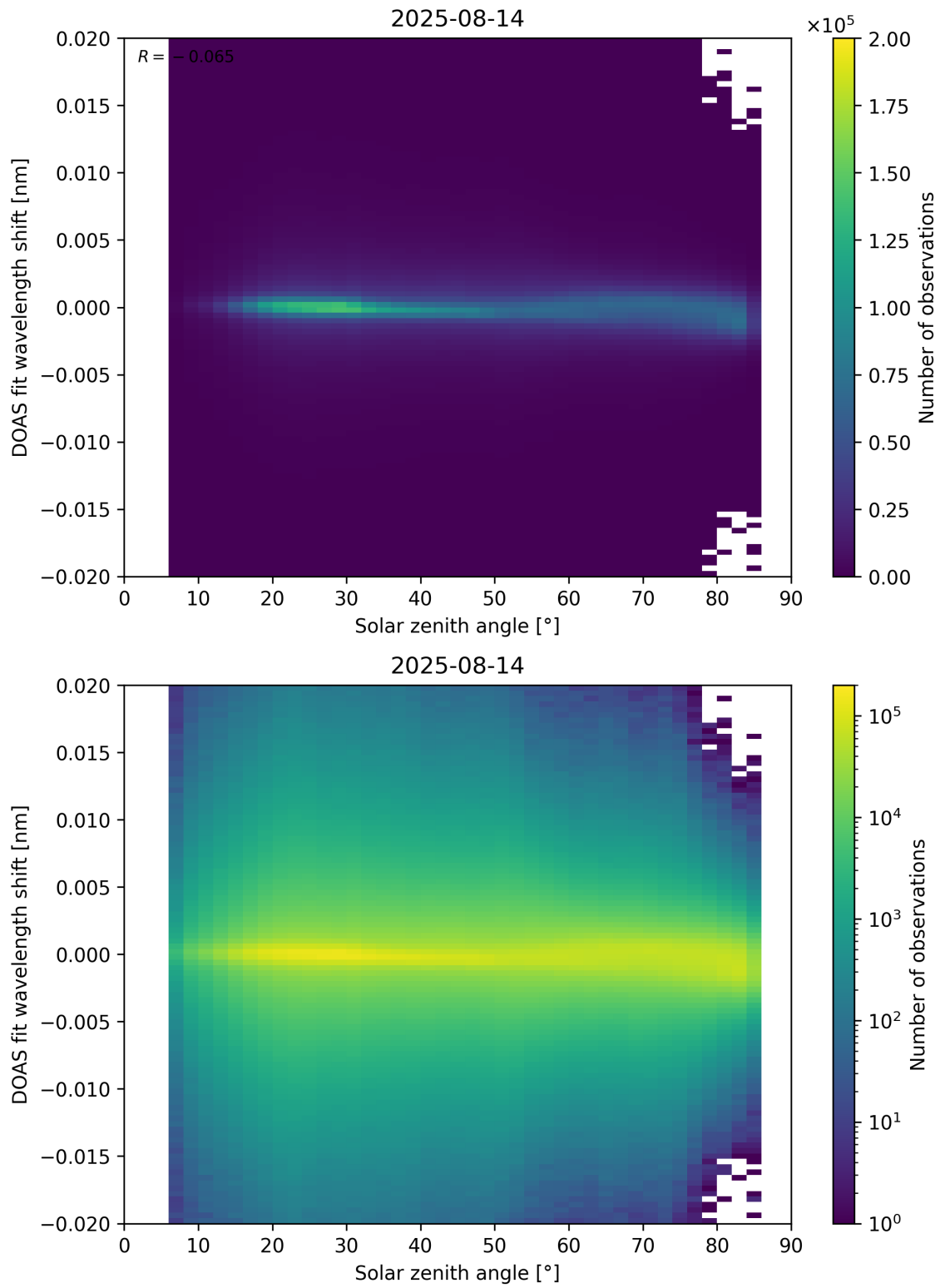
Figure 168: Scatter density plot of “Solar zenith angle” against “DOAS fit wavelength shift” for 2025-08-14 to 2025-08-15.
