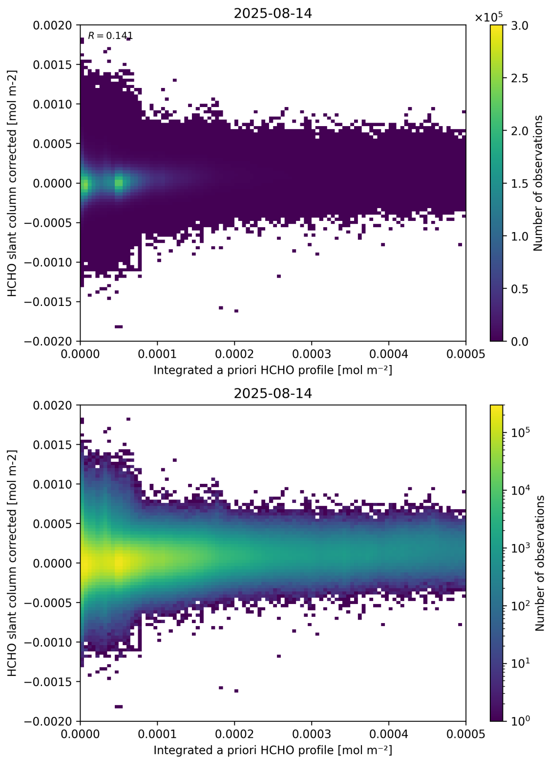
Figure 151: Scatter density plot of “Integrated a priori HCHO profile” against “HCHO slant column corrected” for 2025-08-14 to 2025-08-15.
