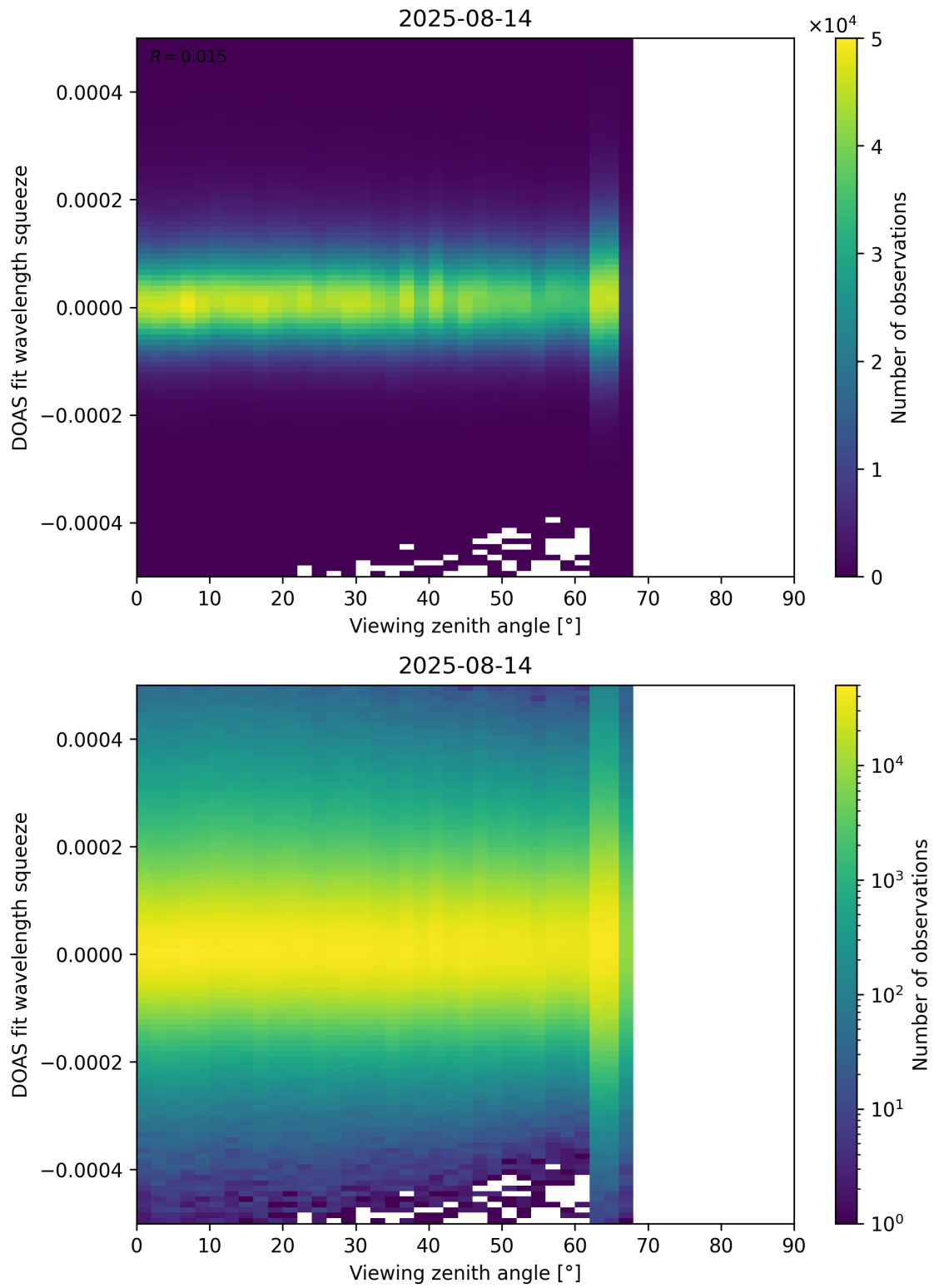
Figure 184: Scatter density plot of “Viewing zenith angle” against “DOAS fit wavelength squeeze” for 2025-08-14 to 2025-08-15.
