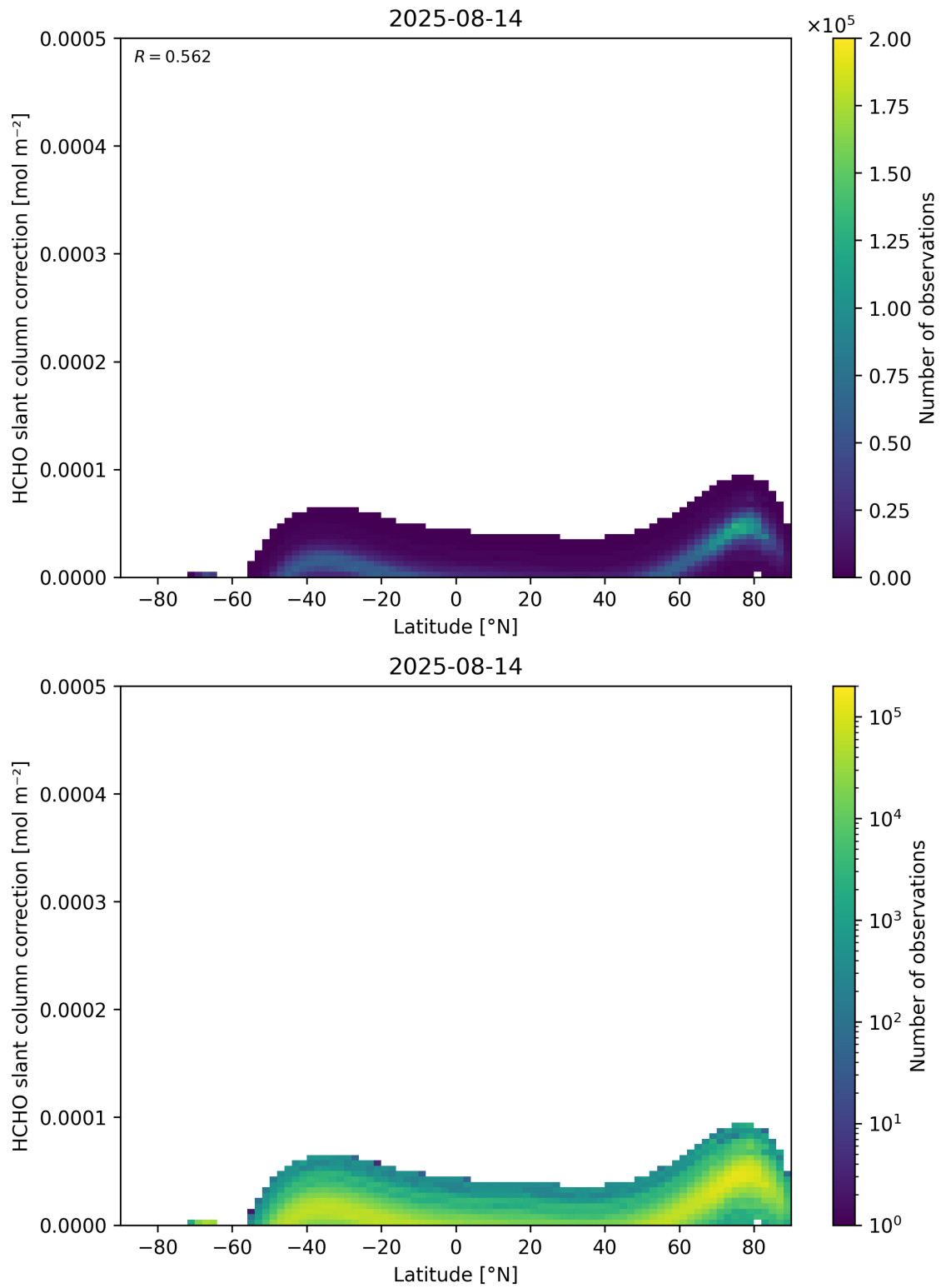
Figure 158: Scatter density plot of “Latitude” against “HCHO slant column correction” for 2025-08-14 to 2025-08-15.
