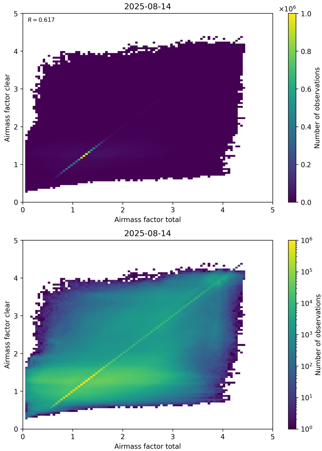
Figure 100: Scatter density plot of “Airmass factor total” against “Airmass factor clear” for 2025-08-14 to 2025-08-15.
