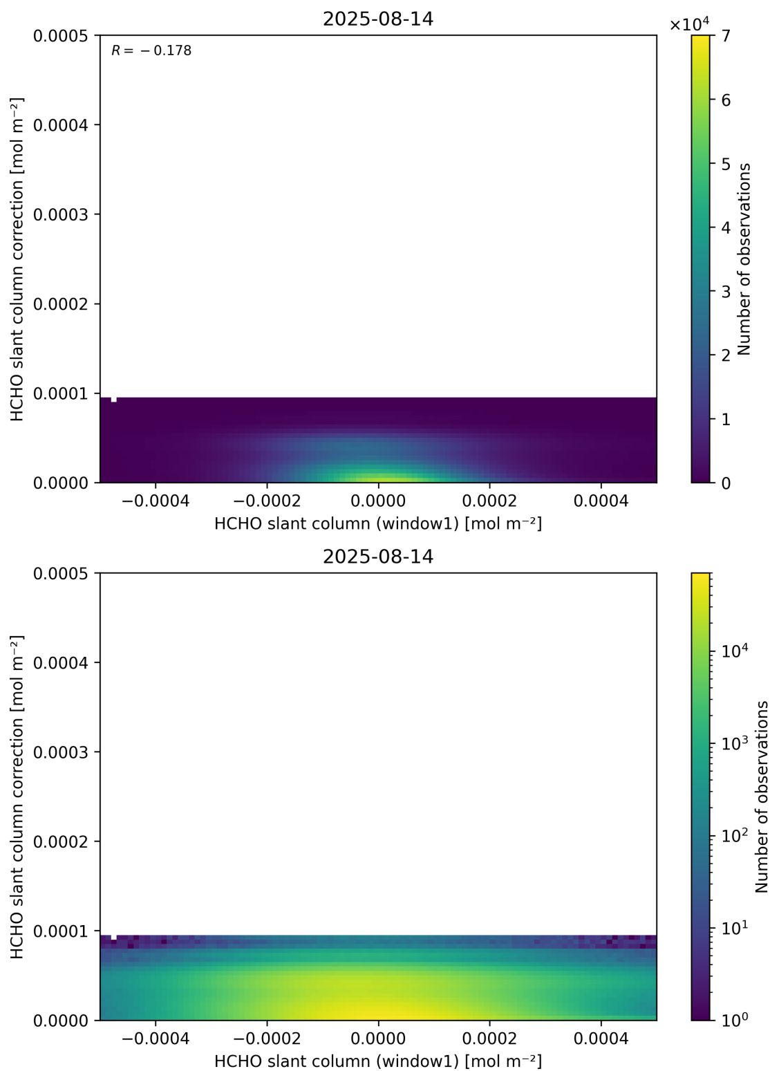
Figure 83: Scatter density plot of “HCHO slant column (window1)” against “HCHO slant column correction” for 2025-08-14 to 2025-08-15.
