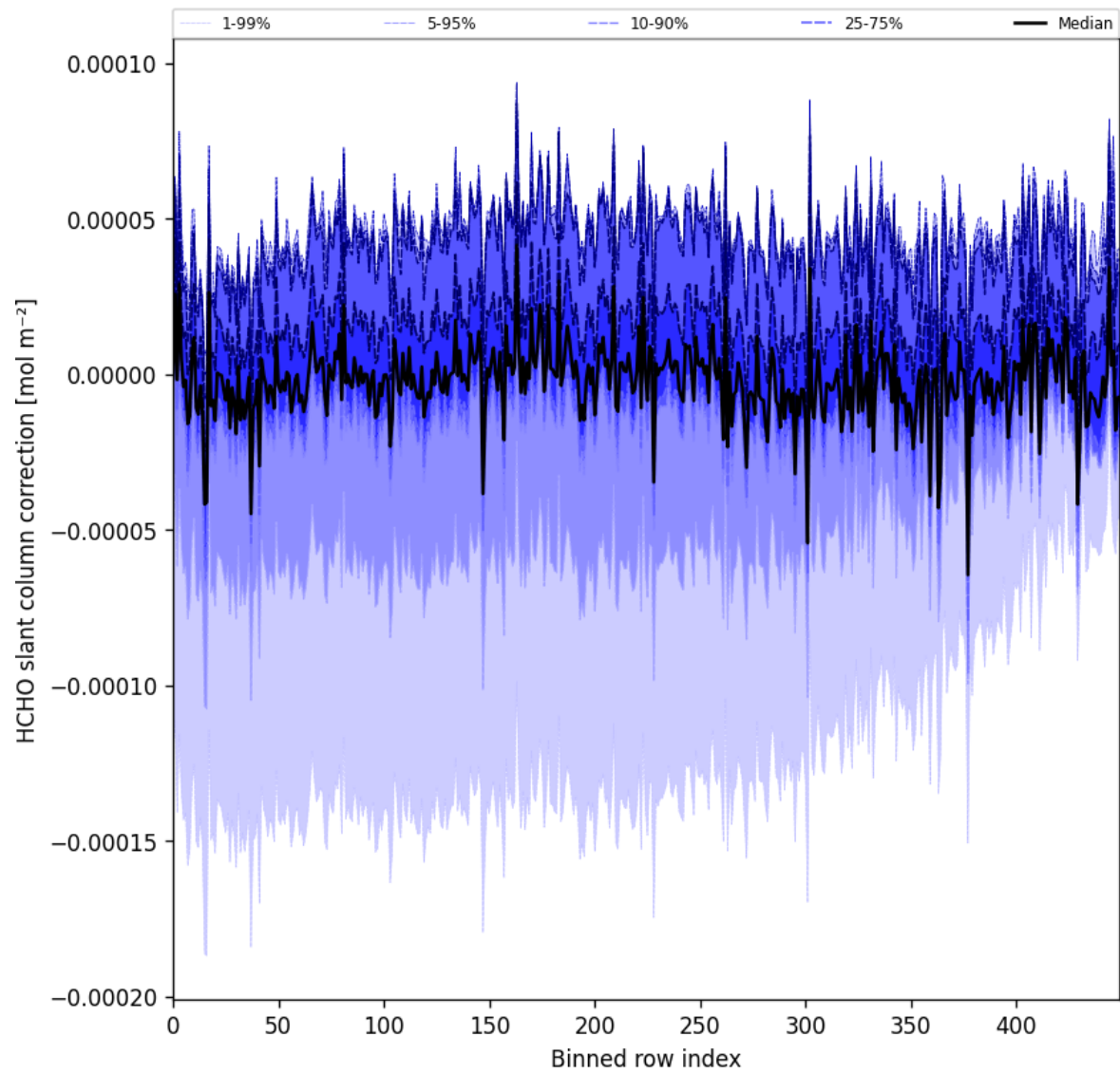
Figure 61: Along track statistics of “HCHO slant column correction” for 2025-08-14 to 2025-08-15
