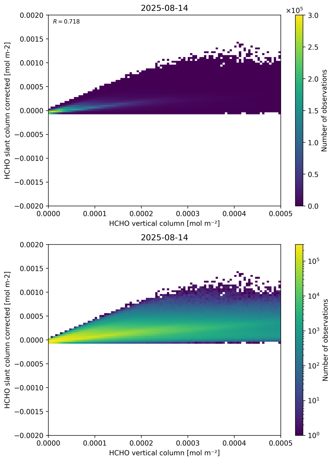
Figure 127: Scatter density plot of “HCHO vertical column” against “HCHO slant column corrected” for 2025-08-14 to 2025-08-15.
