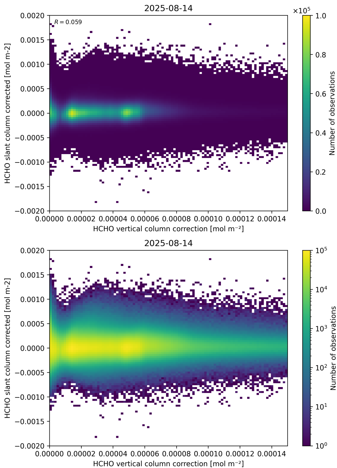
Figure 116: Scatter density plot of “HCHO vertical column correction” against “HCHO slant column corrected” for 2025-08-14 to 2025-08-15.
