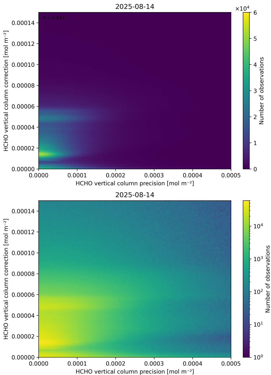
Figure 146: Scatter density plot of “HCHO vertical column precision” against “HCHO vertical column correction” for 2025-08-14 to 2025-08-15.
