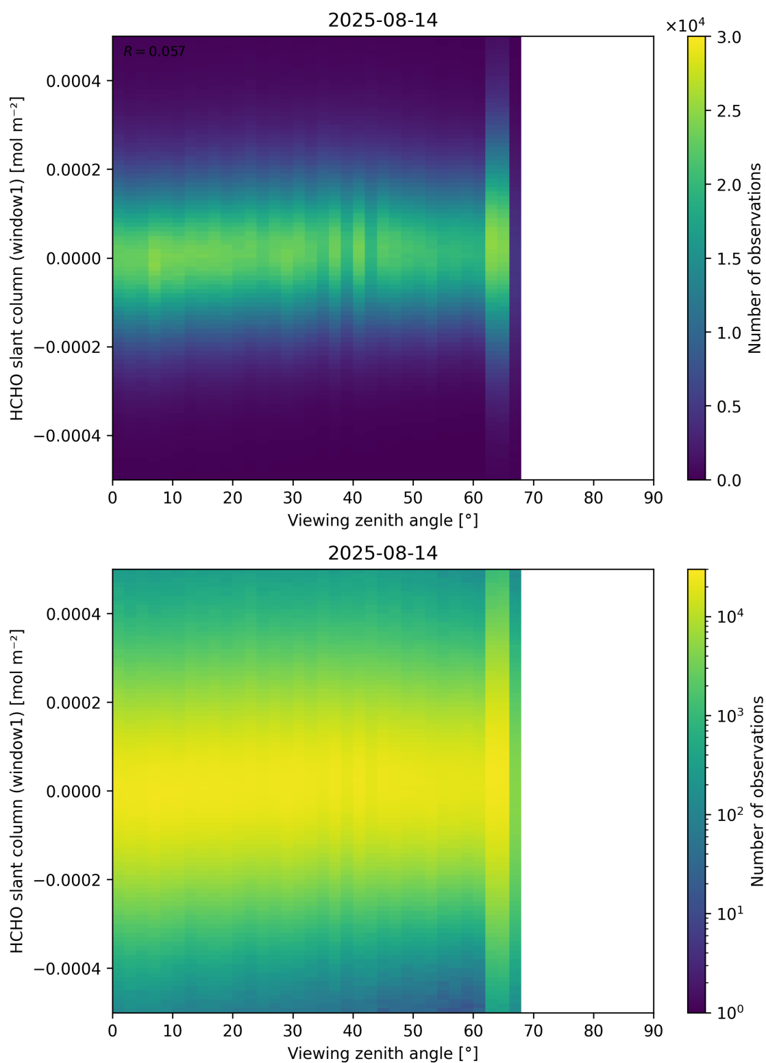
Figure 188: Scatter density plot of “Viewing zenith angle” against “HCHO slant column (window1)” for 2025-08-14 to 2025-08-15.
