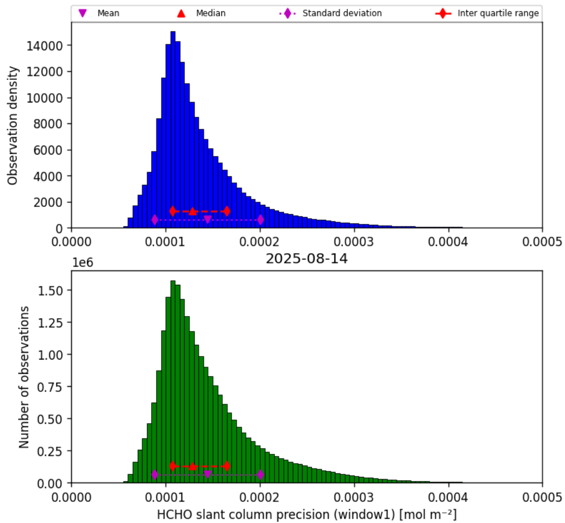
Figure 39: Histogram of “HCHO slant column precision (window1)” for 2025-08-14 to 2025-08-15
