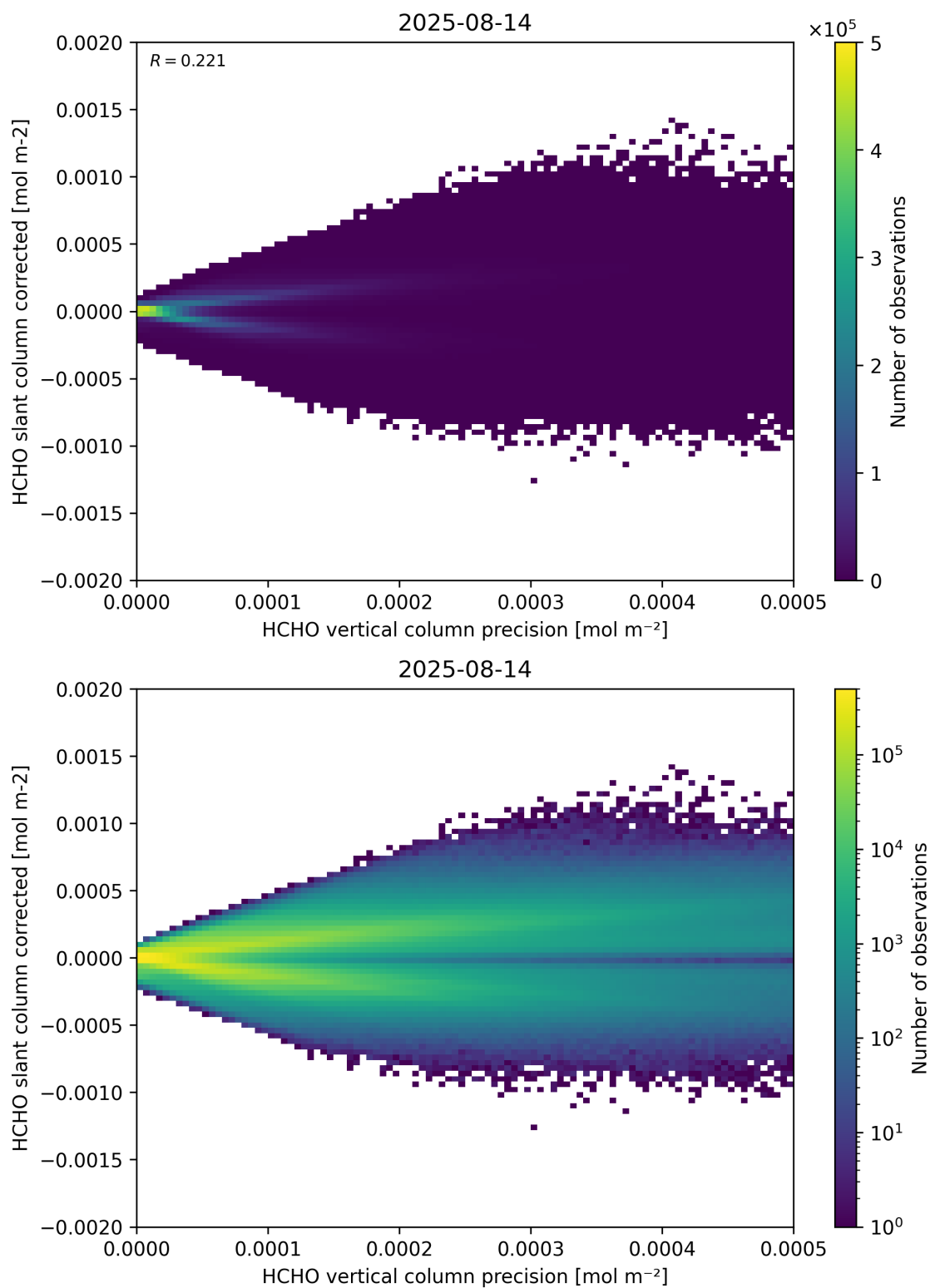
Figure 140: Scatter density plot of “HCHO vertical column precision” against “HCHO slant column corrected” for 2025-08-14 to 2025-08-15.
