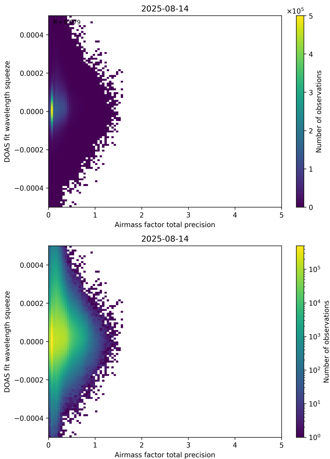
Figure 107: Scatter density plot of “Airmass factor total precision” against “DOAS fit wavelength squeeze” for 2025-08-14 to 2025-08-15.
