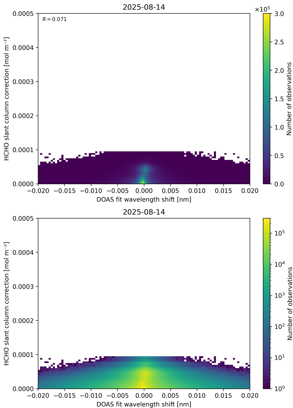
Figure 67: Scatter density plot of “DOAS fit wavelength shift” against “HCHO slant column correction” for 2025-08-14 to 2025-08-15.
