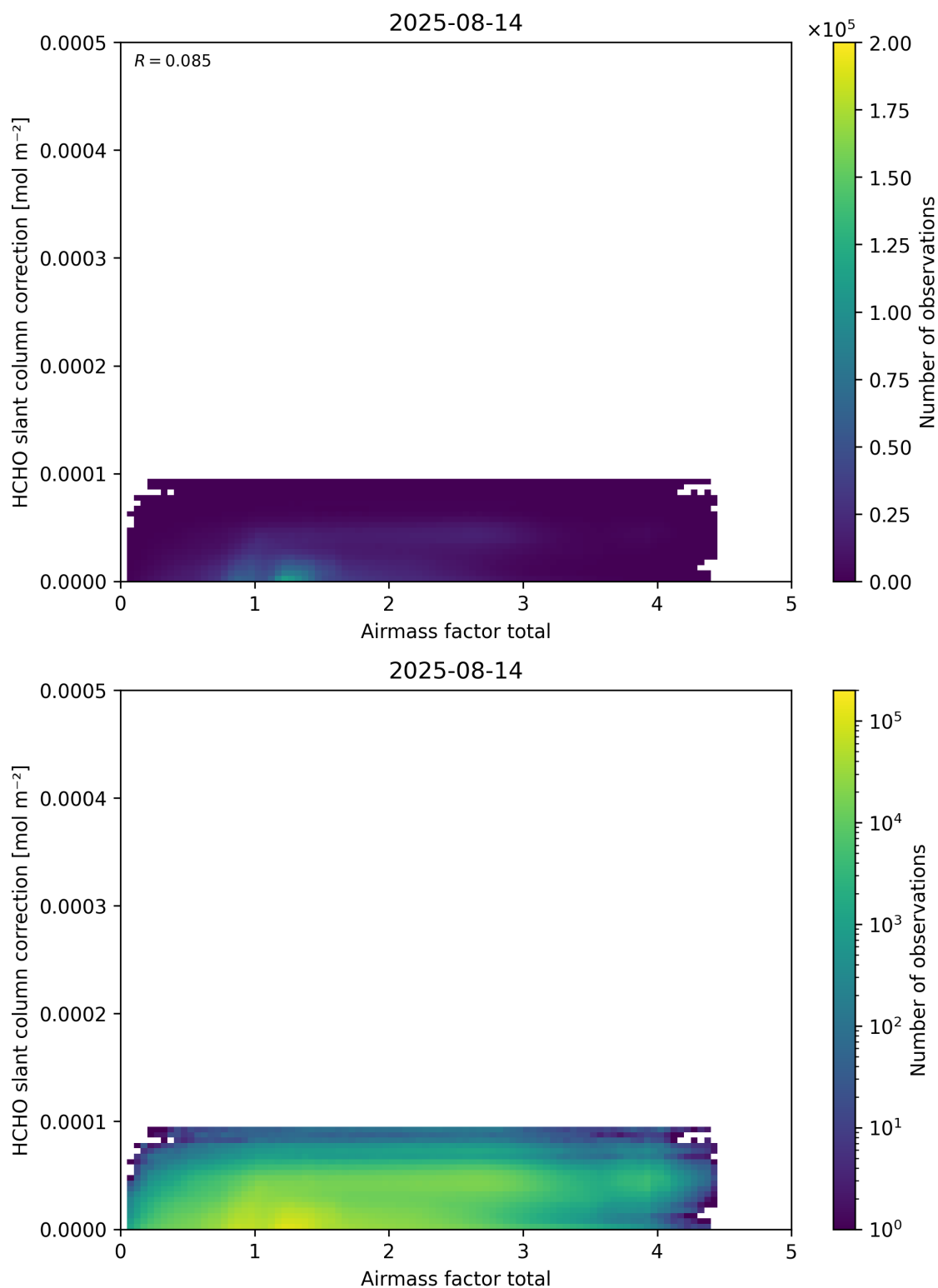
Figure 102: Scatter density plot of “Airmass factor total” against “HCHO slant column correction” for 2025-08-14 to 2025-08-15.
