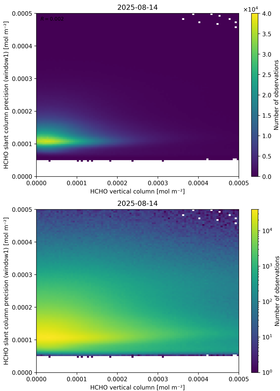
Figure 130: Scatter density plot of “HCHO vertical column” against “HCHO slant column precision (window1)” for 2025-08-14 to 2025-08-15.
