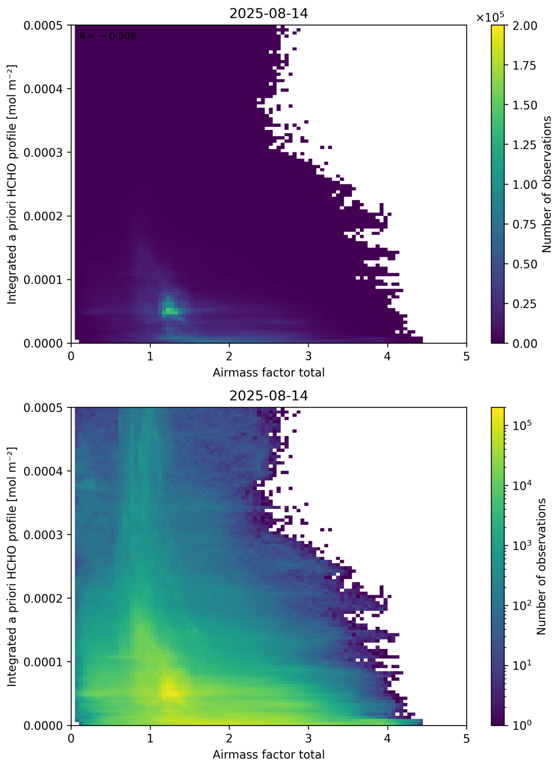
Figure 104: Scatter density plot of “Airmass factor total” against “Integrated a priori HCHO profile” for 2025-08-14 to 2025-08-15.
