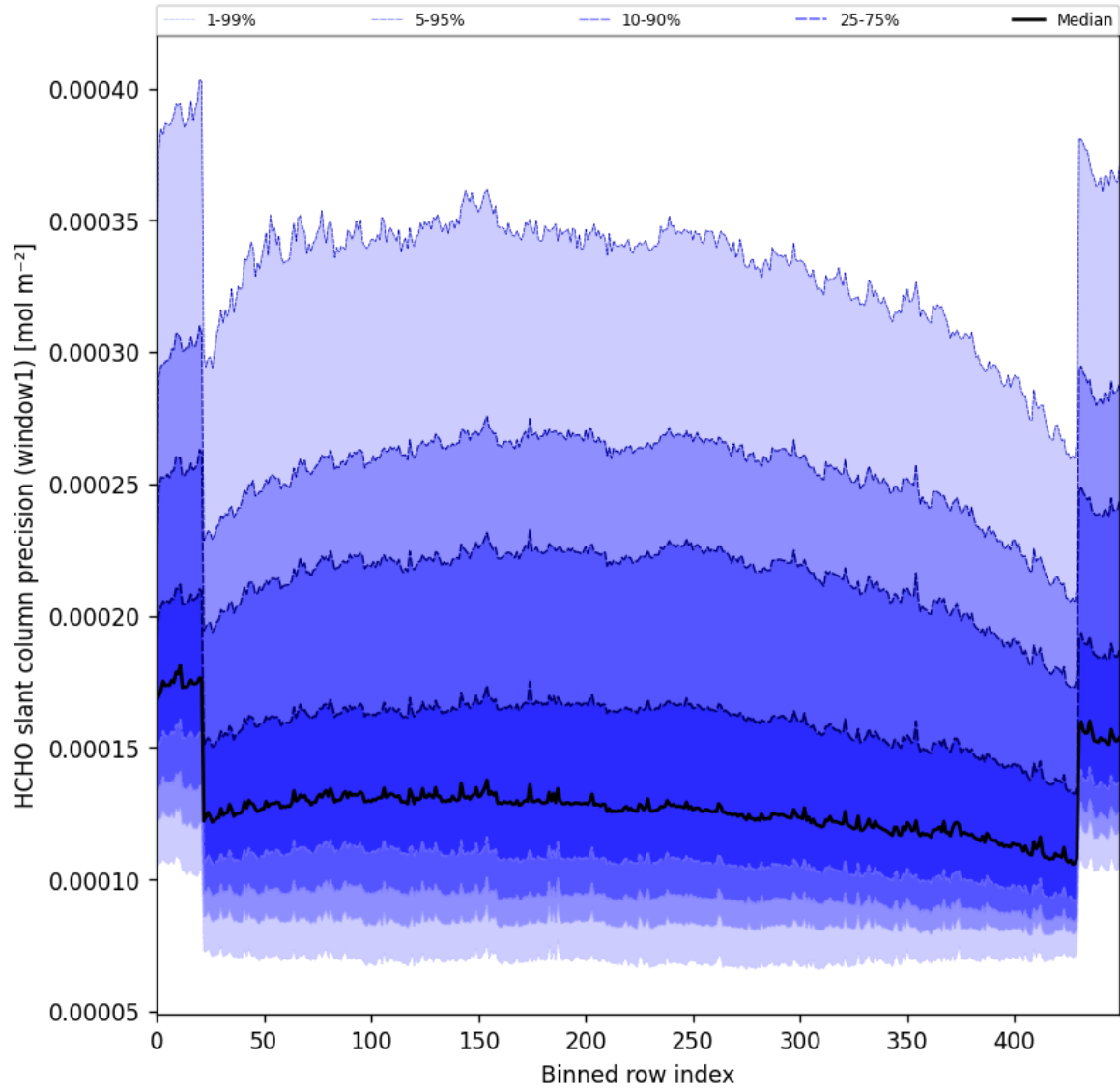
Figure 53: Along track statistics of “HCHO slant column precision (window1)” for 2025-08-14 to 2025-08-15
