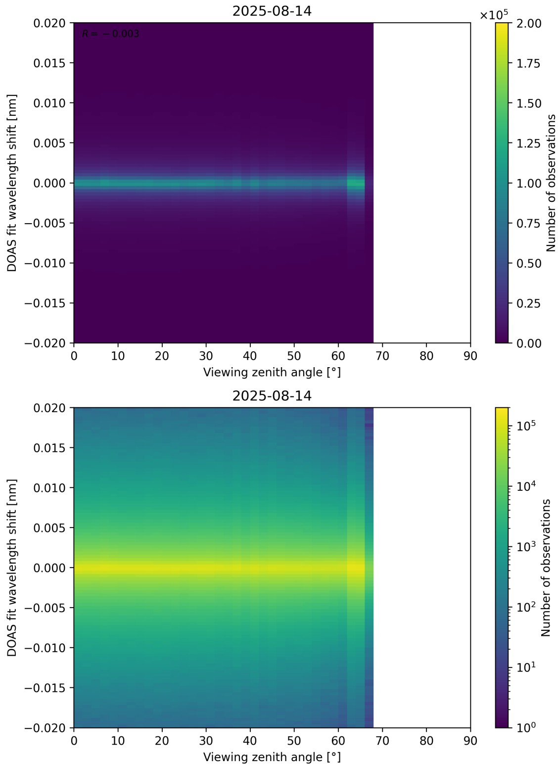
Figure 183: Scatter density plot of “Viewing zenith angle” against “DOAS fit wavelength shift” for 2025-08-14 to 2025-08-15.
