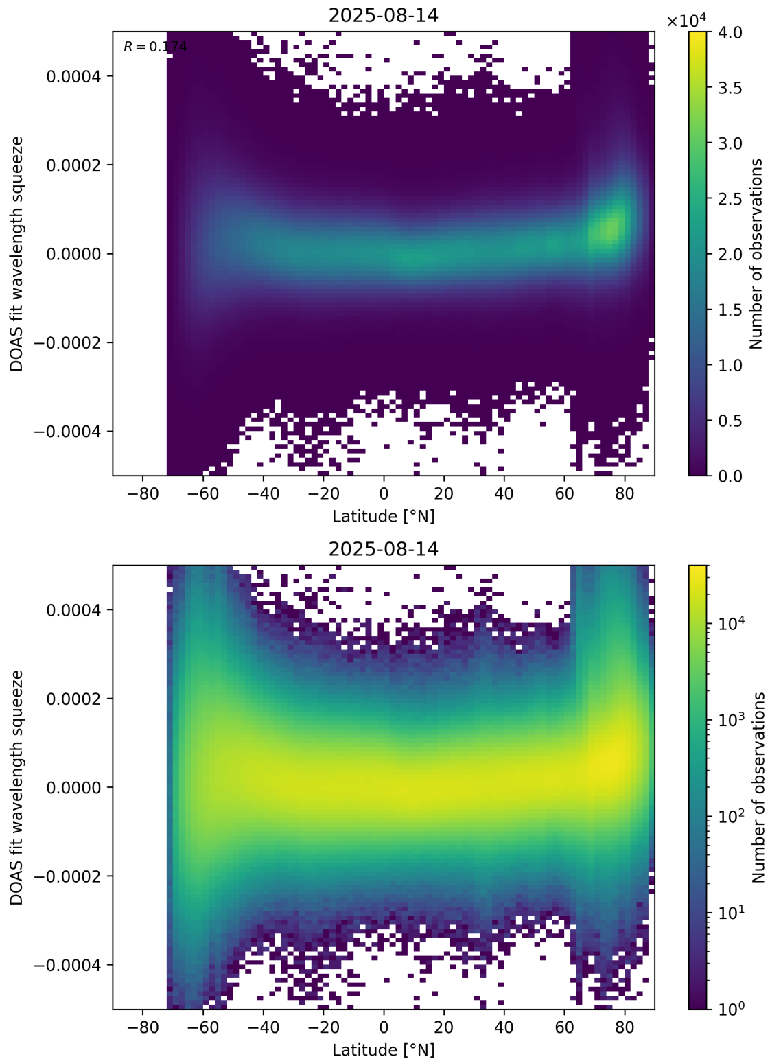
Figure 155: Scatter density plot of “Latitude” against “DOAS fit wavelength squeeze” for 2025-08-14 to 2025-08-15.
