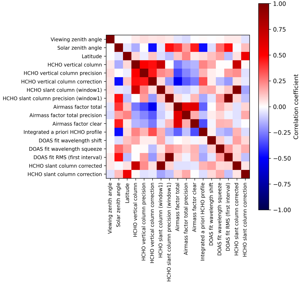
Figure 2: Map of correlation matrix for 2025-08-14 to 2025-08-15.
