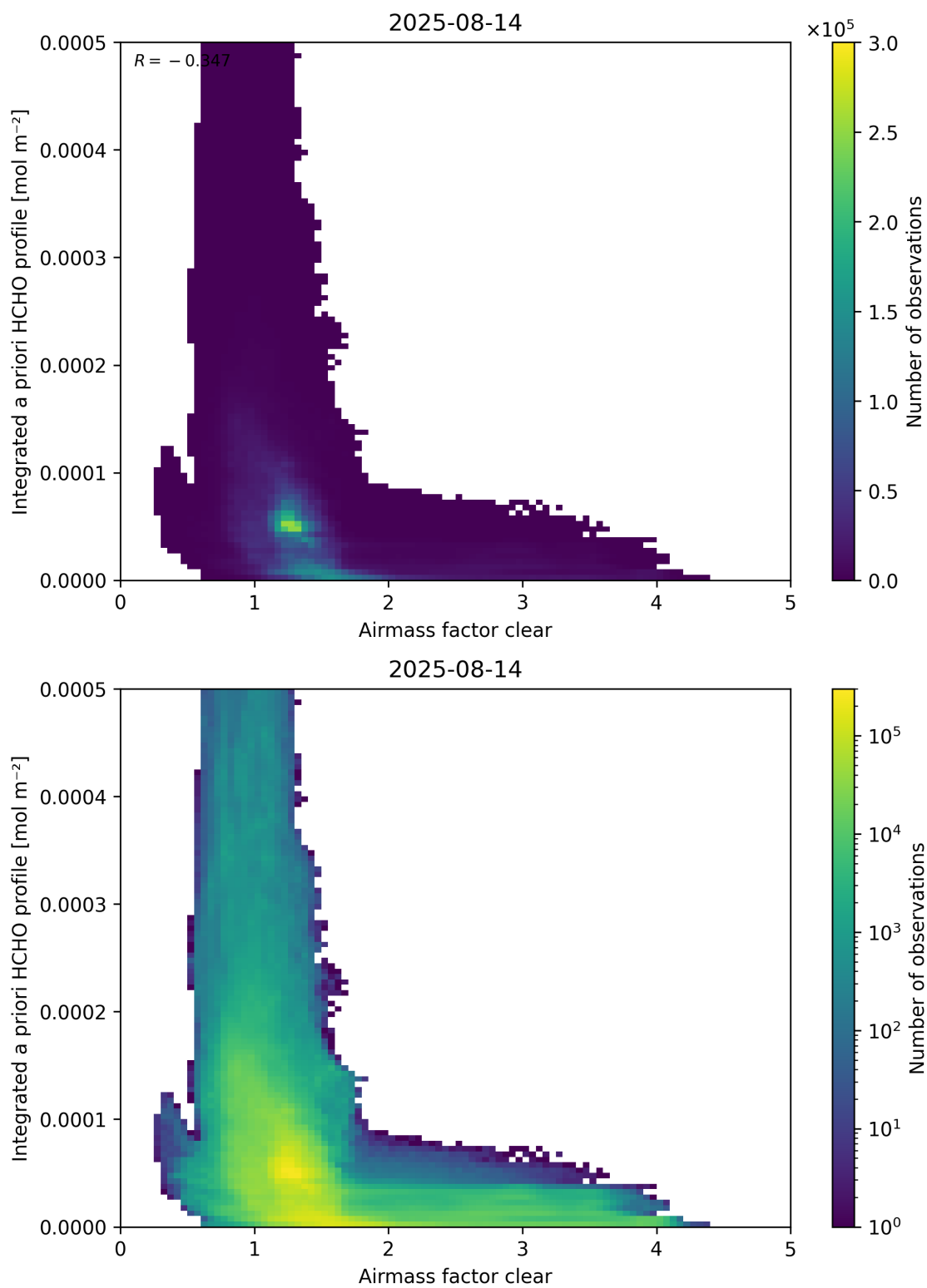
Figure 76: Scatter density plot of “Airmass factor clear” against “Integrated a priori HCHO profile” for 2025-08-14 to 2025-08-15.
