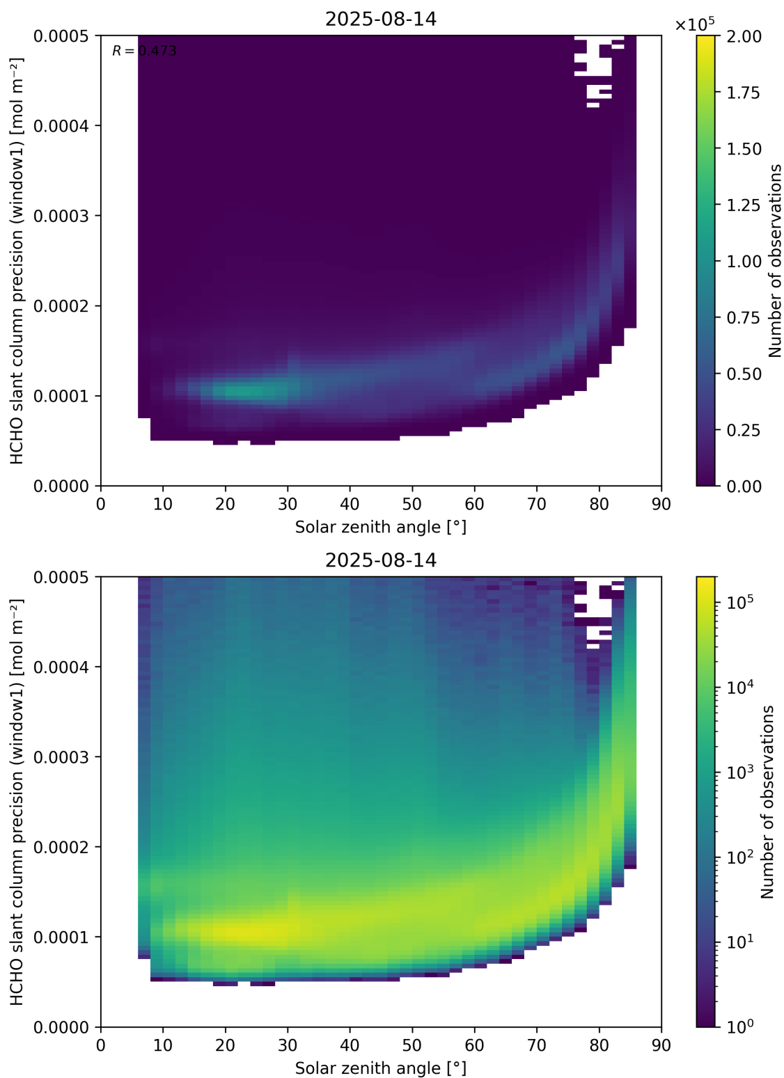
Figure 174: Scatter density plot of “Solar zenith angle” against “HCHO slant column precision (window1)” for 2025-08-14 to 2025-08-15.
