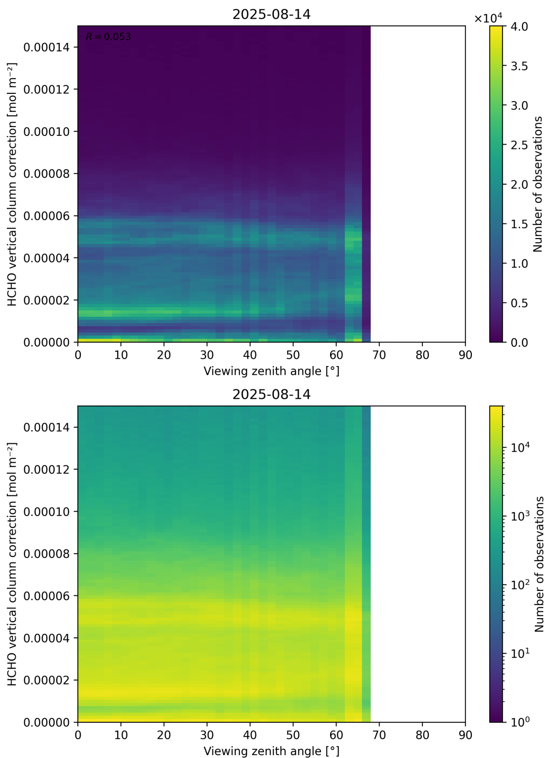
Figure 193: Scatter density plot of “Viewing zenith angle” against “HCHO vertical column correction” for 2025-08-14 to 2025-08-15.
