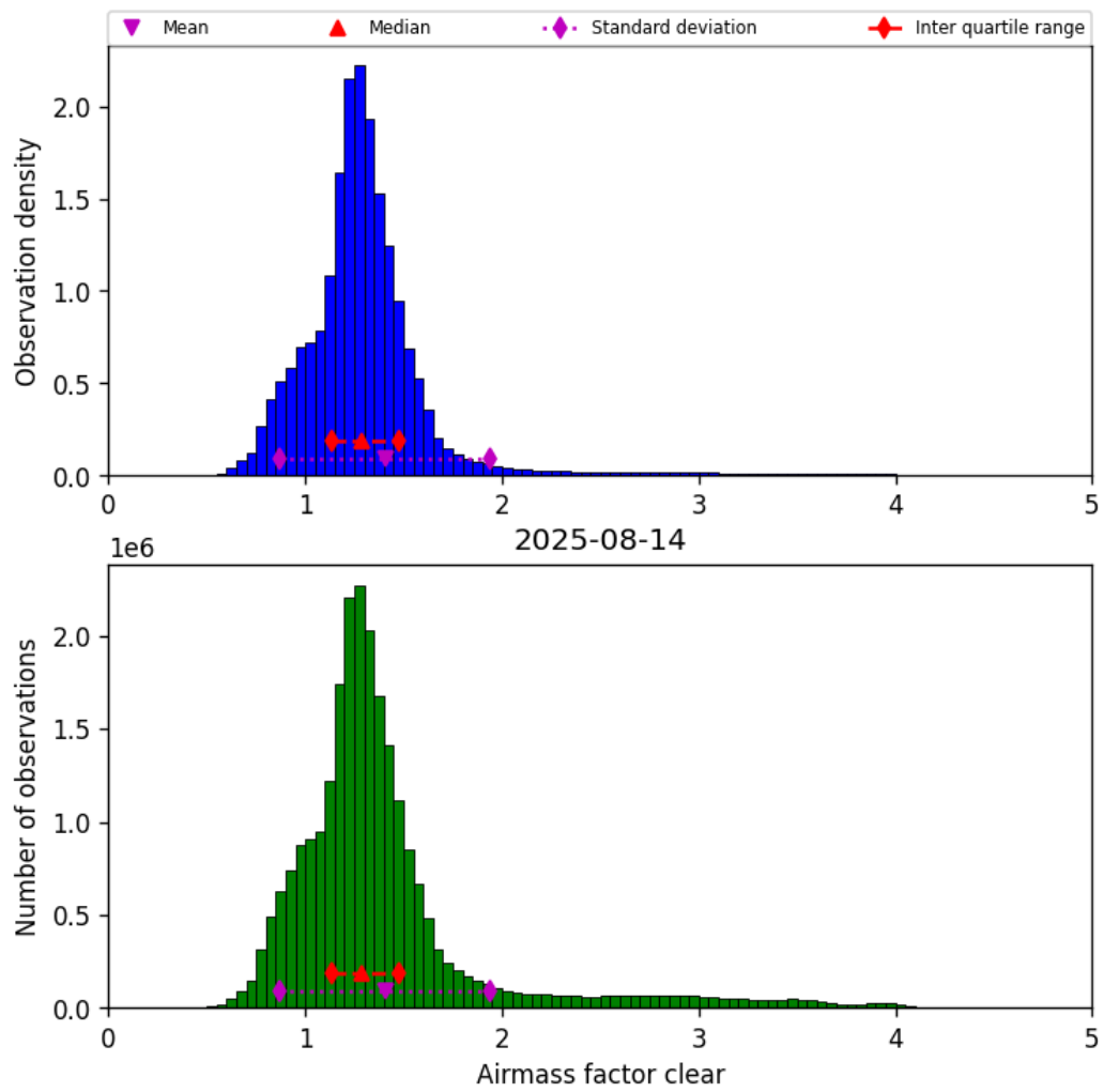
Figure 42: Histogram of “Airmass factor clear” for 2025-08-14 to 2025-08-15
