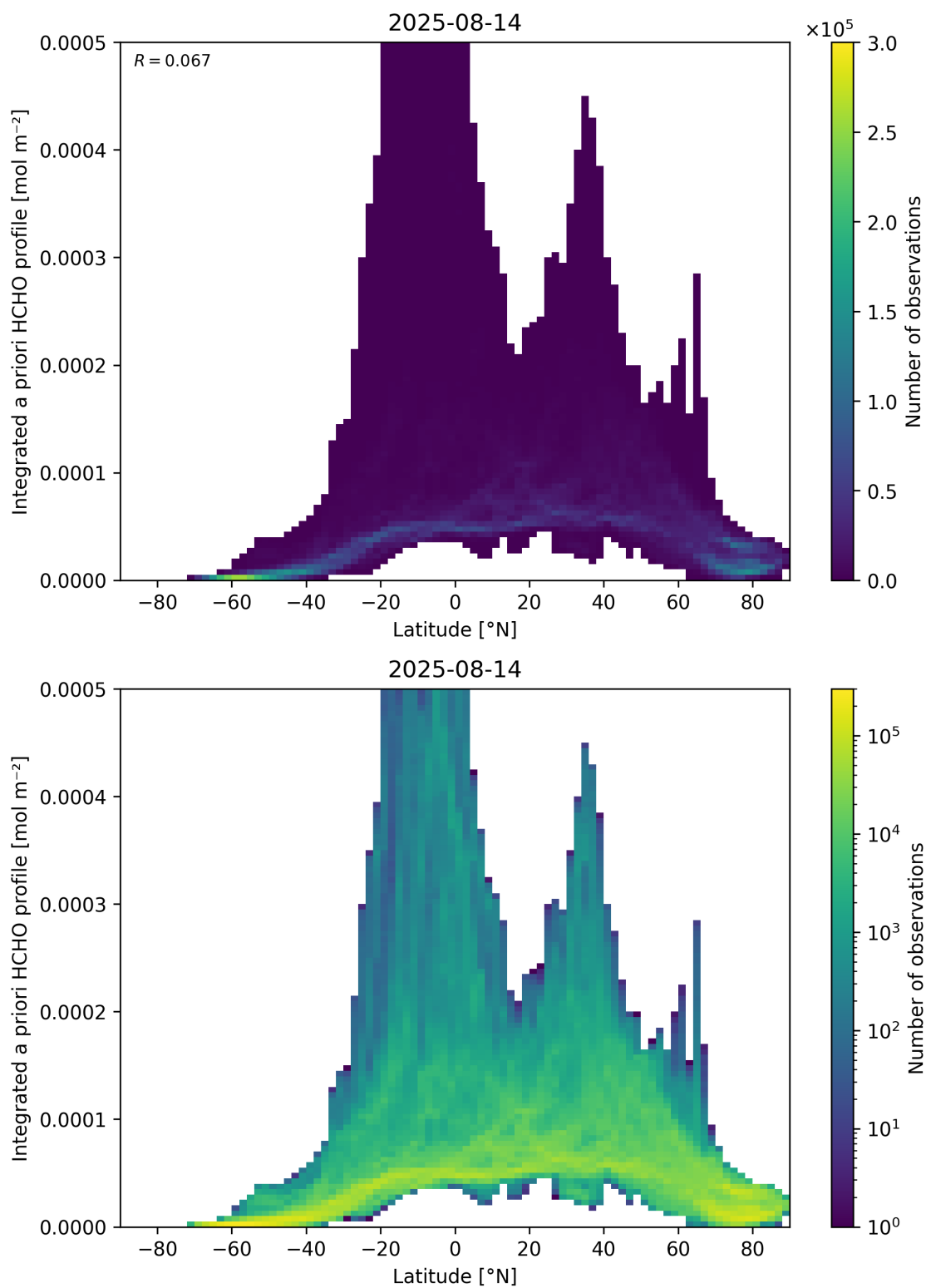
Figure 166: Scatter density plot of “Latitude” against “Integrated a priori HCHO profile” for 2025-08-14 to 2025-08-15.
