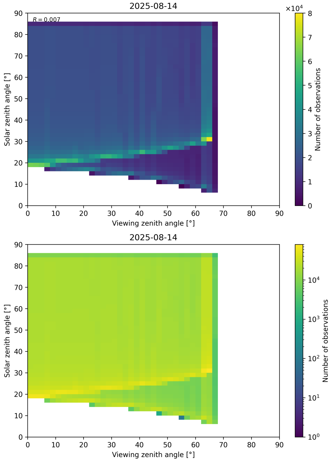
Figure 197: Scatter density plot of “Viewing zenith angle” against “Solar zenith angle” for 2025-08-14 to 2025-08-15.
