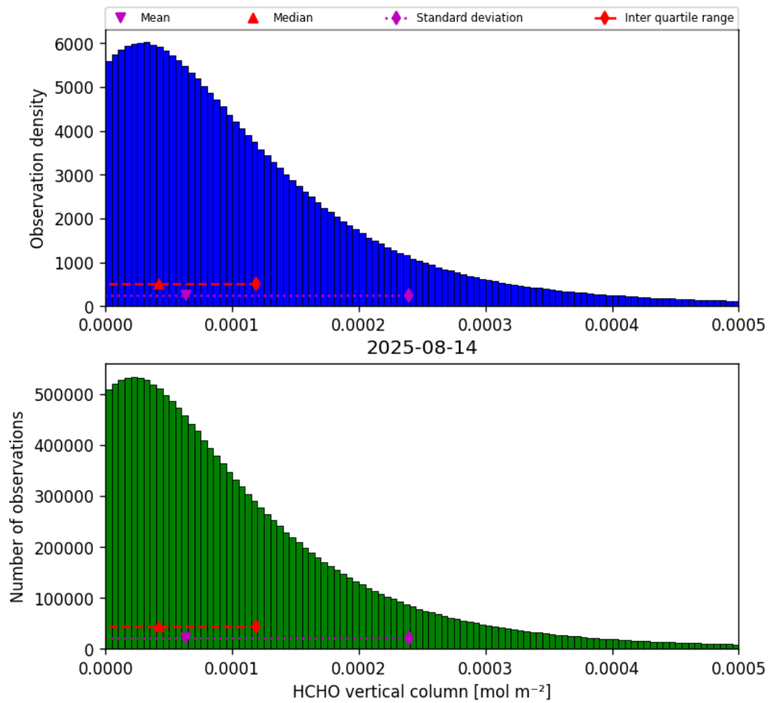
Figure 35: Histogram of “HCHO vertical column” for 2025-08-14 to 2025-08-15
