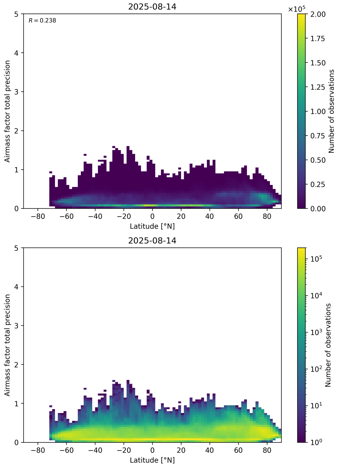
Figure 162: Scatter density plot of “Latitude” against “Airmass factor total precision” for 2025-08-14 to 2025-08-15.
