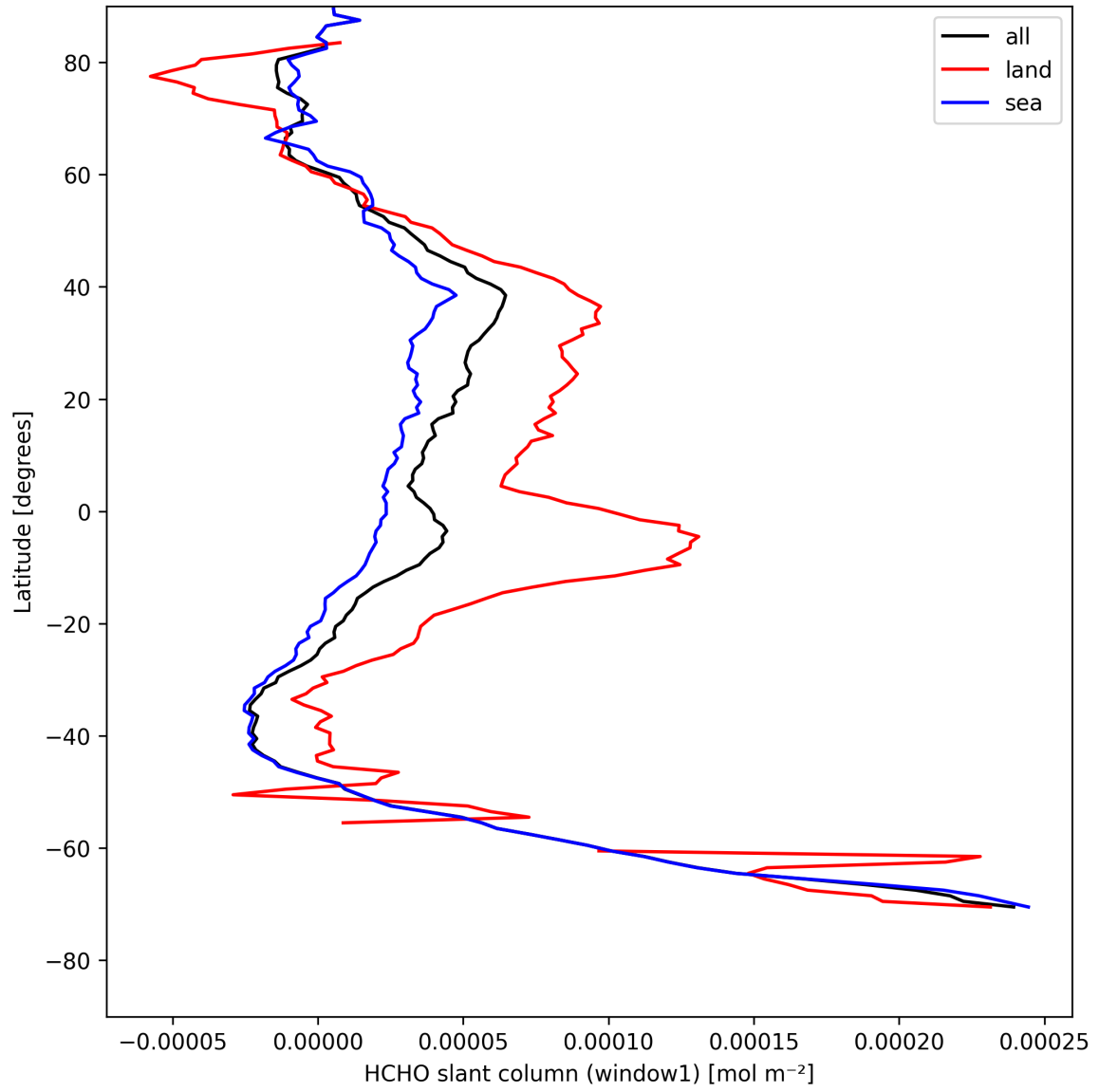
Figure 24: Zonal average of “HCHO slant column (window1)” for 2025-08-14 to 2025-08-15.
