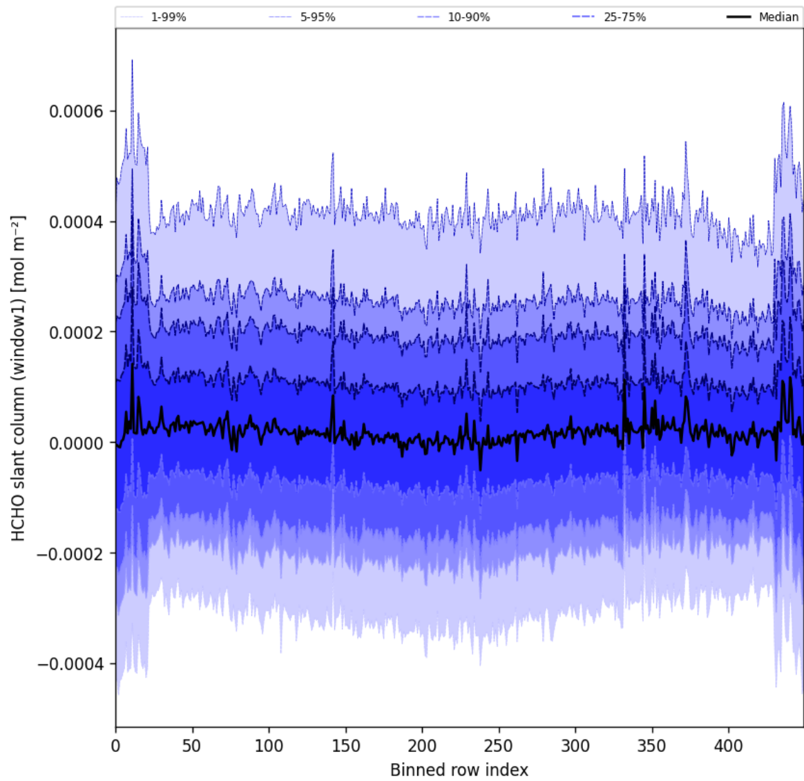
Figure 52: Along track statistics of “HCHO slant column (window1)” for 2025-08-14 to 2025-08-15
