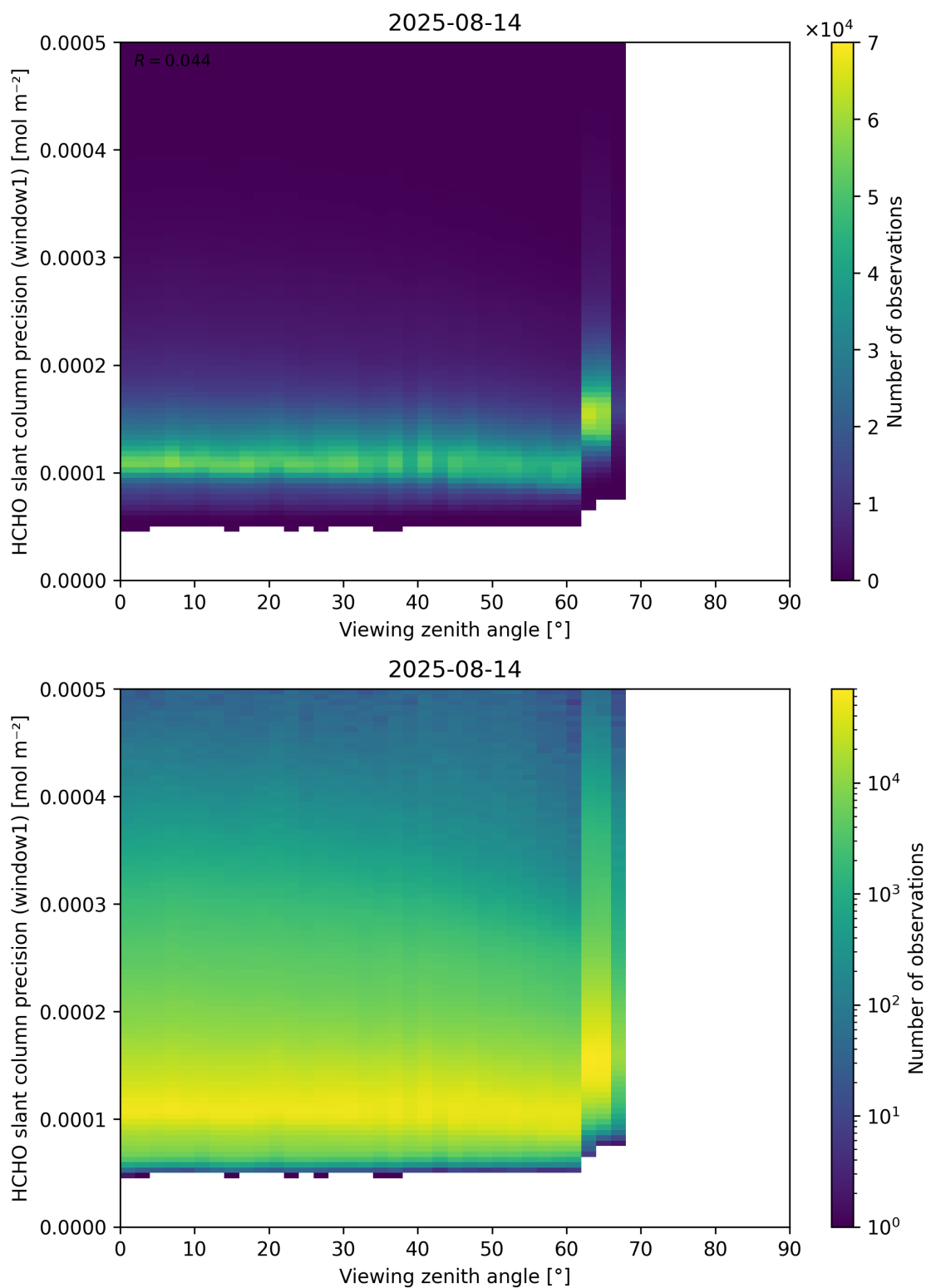
Figure 189: Scatter density plot of “Viewing zenith angle” against “HCHO slant column precision (window1)” for 2025-08-14 to 2025-08-15.
