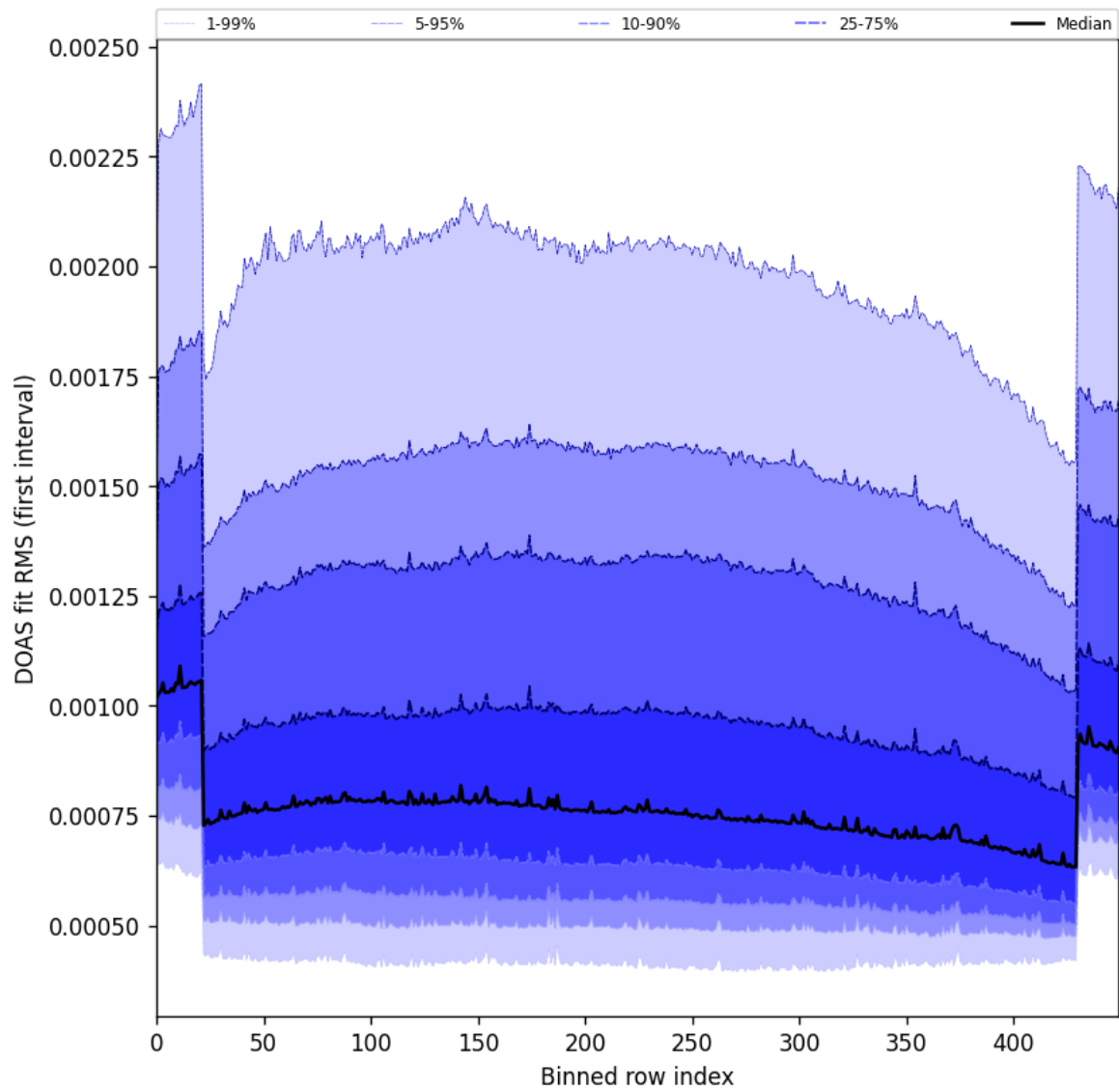
Figure 60: Along track statistics of “DOAS fit RMS (first interval)” for 2025-08-14 to 2025-08-15
