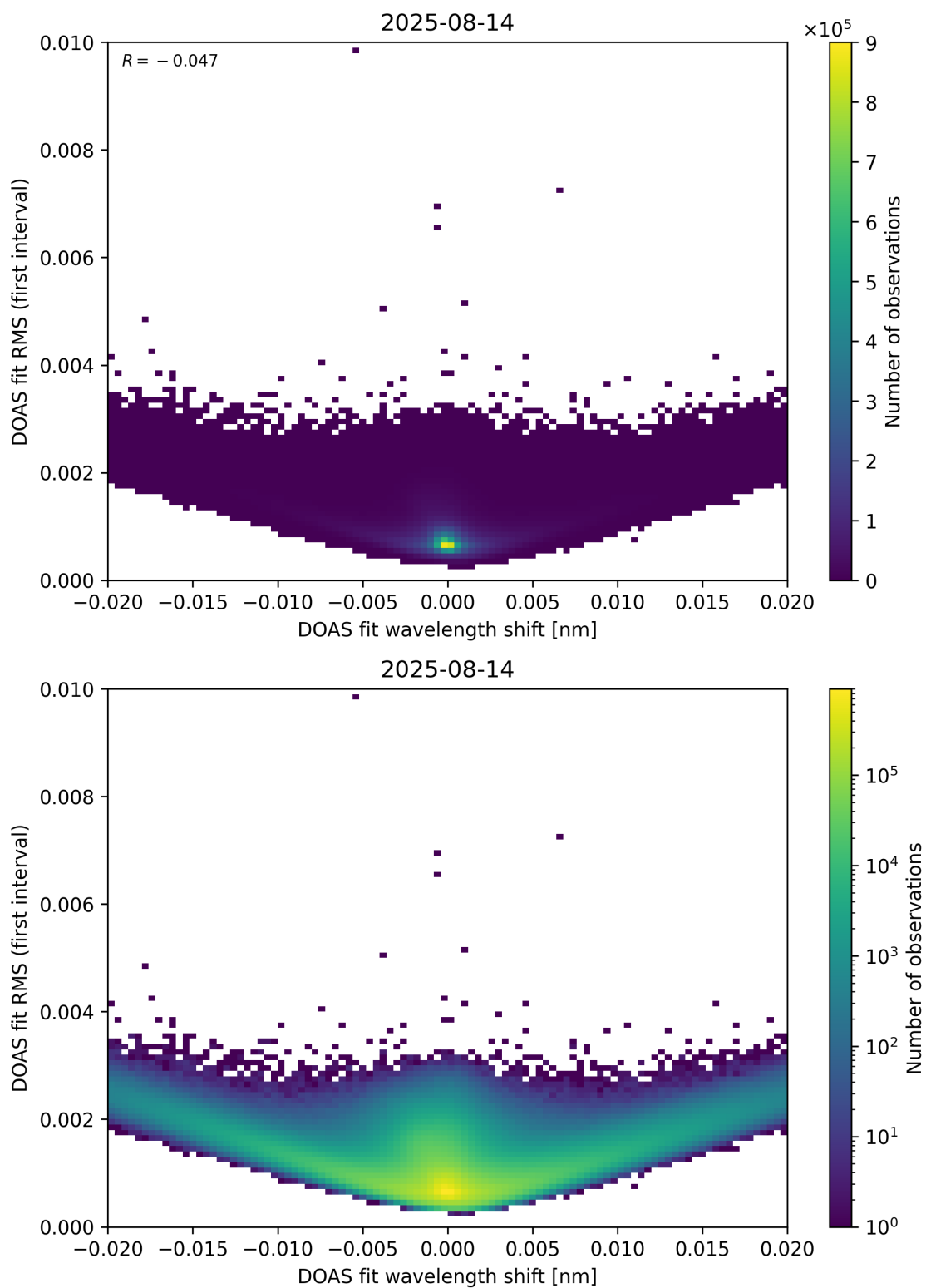
Figure 64: Scatter density plot of “DOAS fit wavelength shift” against “DOAS fit RMS (first interval)” for 2025-08-14 to 2025-08-15.
