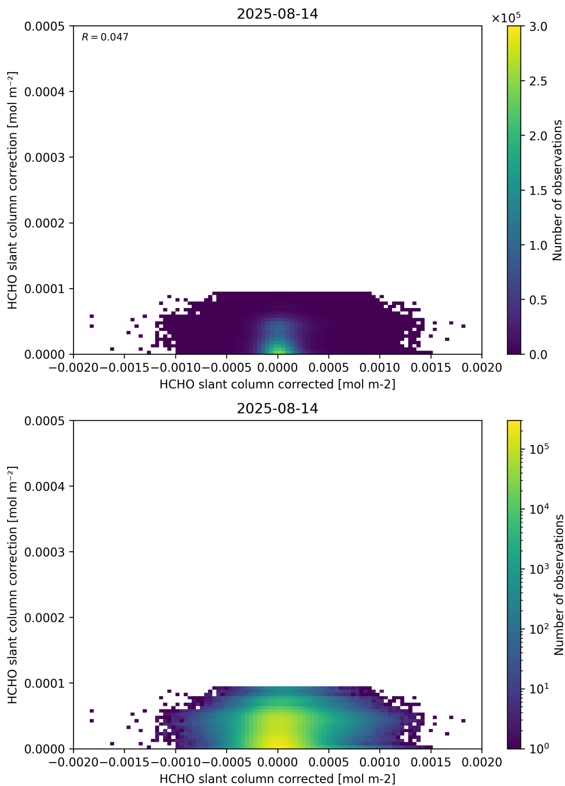
Figure 77: Scatter density plot of “HCHO slant column corrected” against “HCHO slant column correction” for 2025-08-14 to 2025-08-15.
