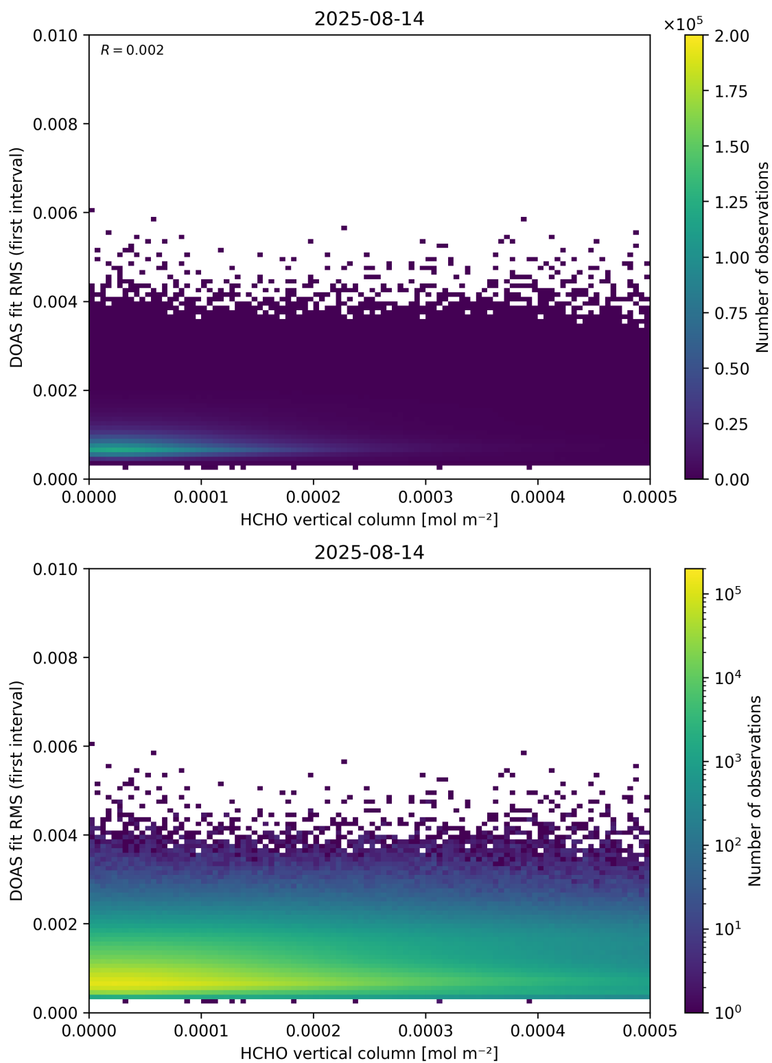
Figure 123: Scatter density plot of “HCHO vertical column” against “DOAS fit RMS (first interval)” for 2025-08-14 to 2025-08-15.
