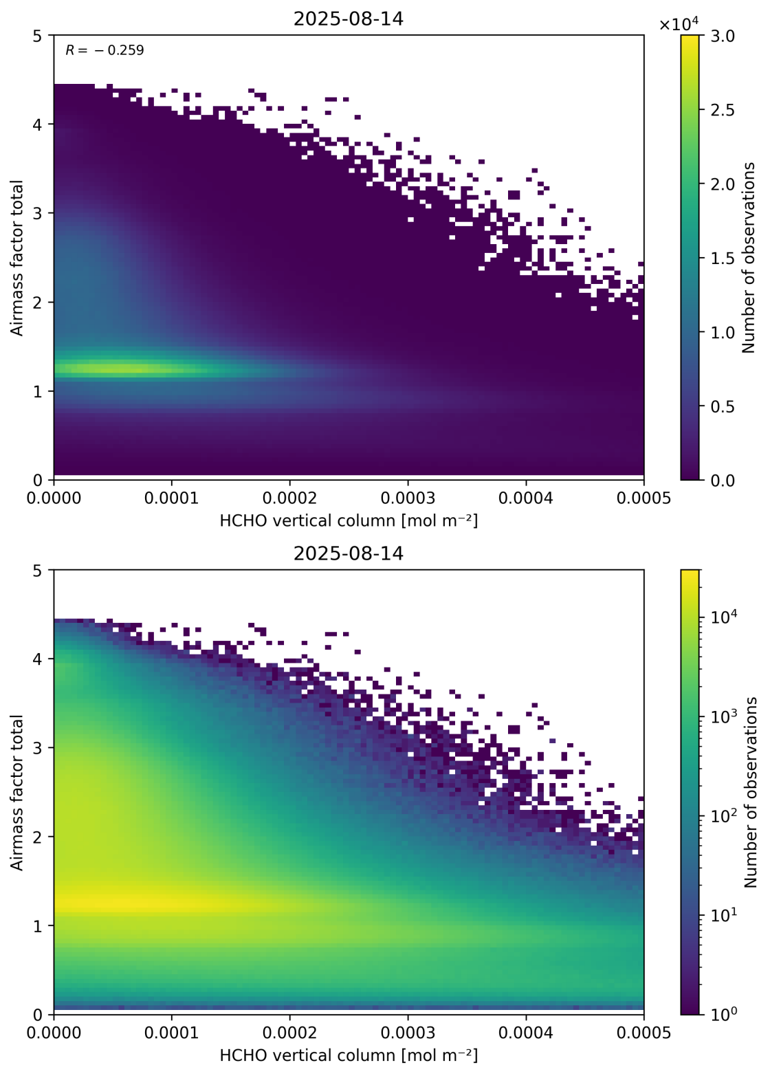
Figure 131: Scatter density plot of “HCHO vertical column” against “Airmass factor total” for 2025-08-14 to 2025-08-15.
