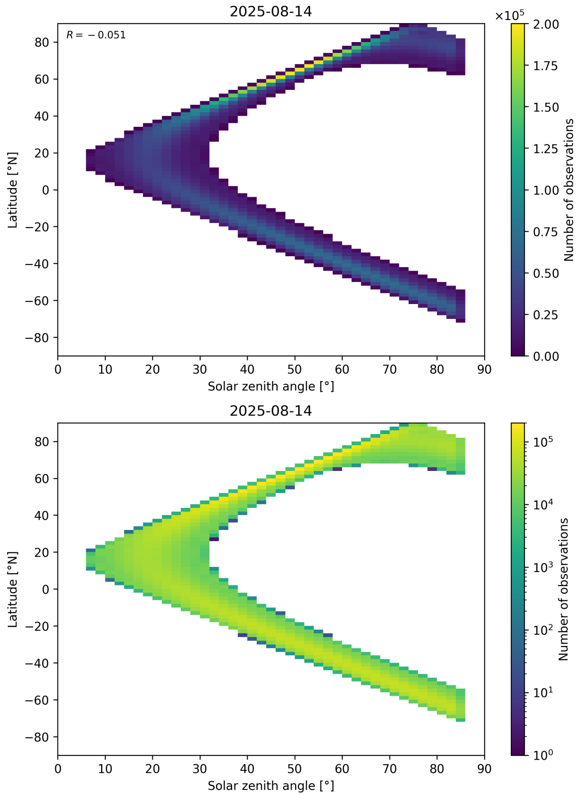
Figure 181: Scatter density plot of “Solar zenith angle” against “Latitude” for 2025-08-14 to 2025-08-15.
