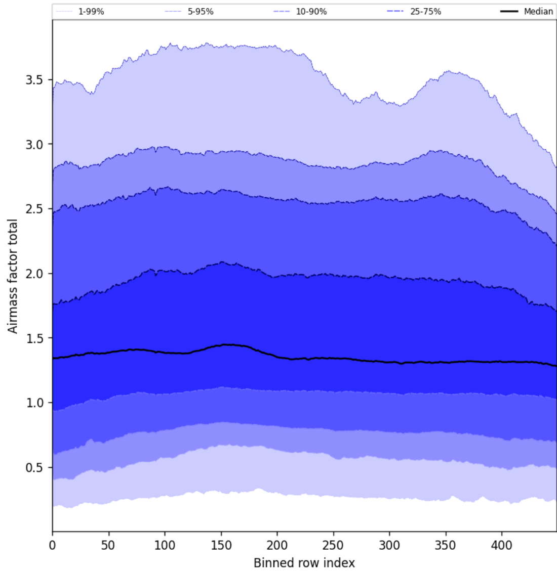
Figure 54: Along track statistics of “Airmass factor total” for 2025-08-14 to 2025-08-15
