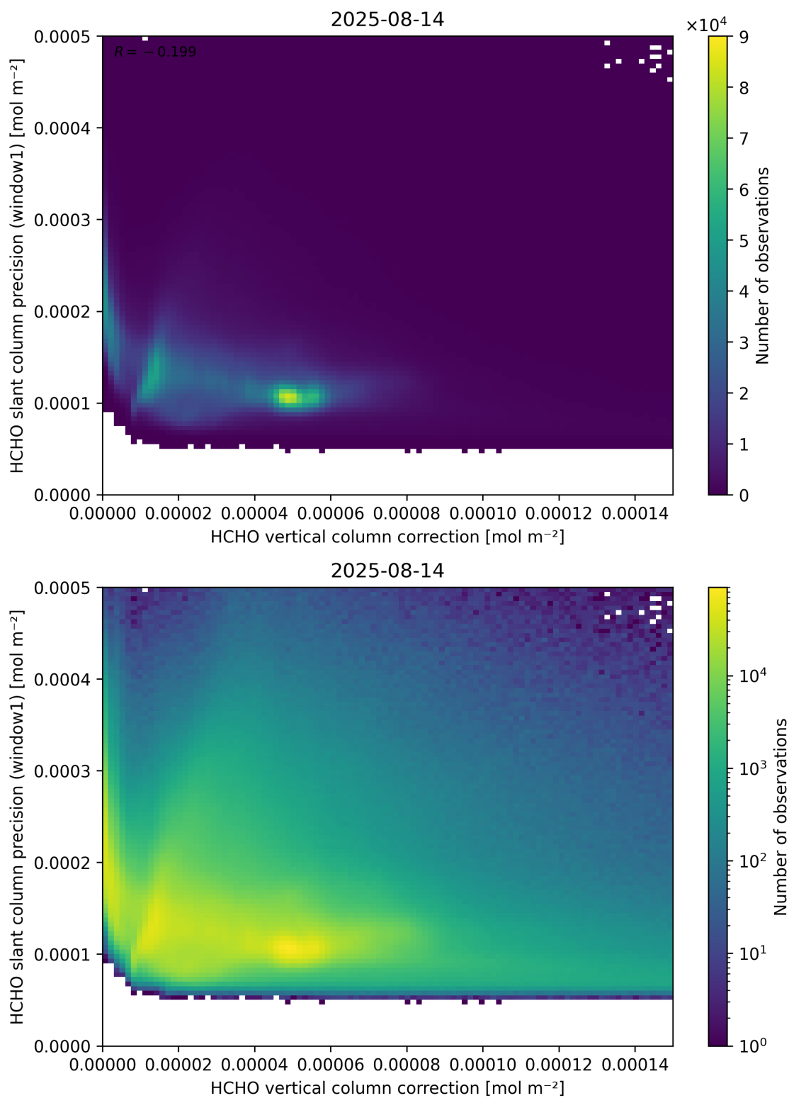
Figure 119: Scatter density plot of “HCHO vertical column correction” against “HCHO slant column precision (window1)” for 2025-08-14 to 2025-08-15.
