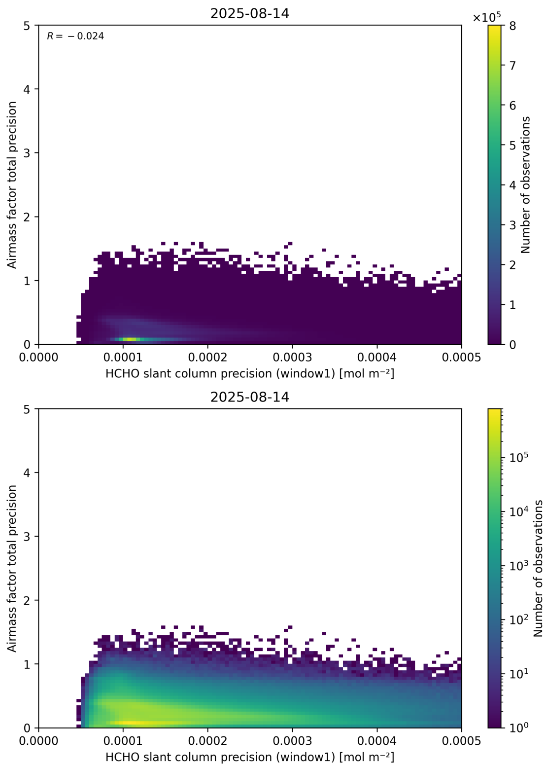
Figure 95: Scatter density plot of “HCHO slant column precision (window1)” against “Airmass factor total precision” for 2025-08-14 to 2025-08-15.
