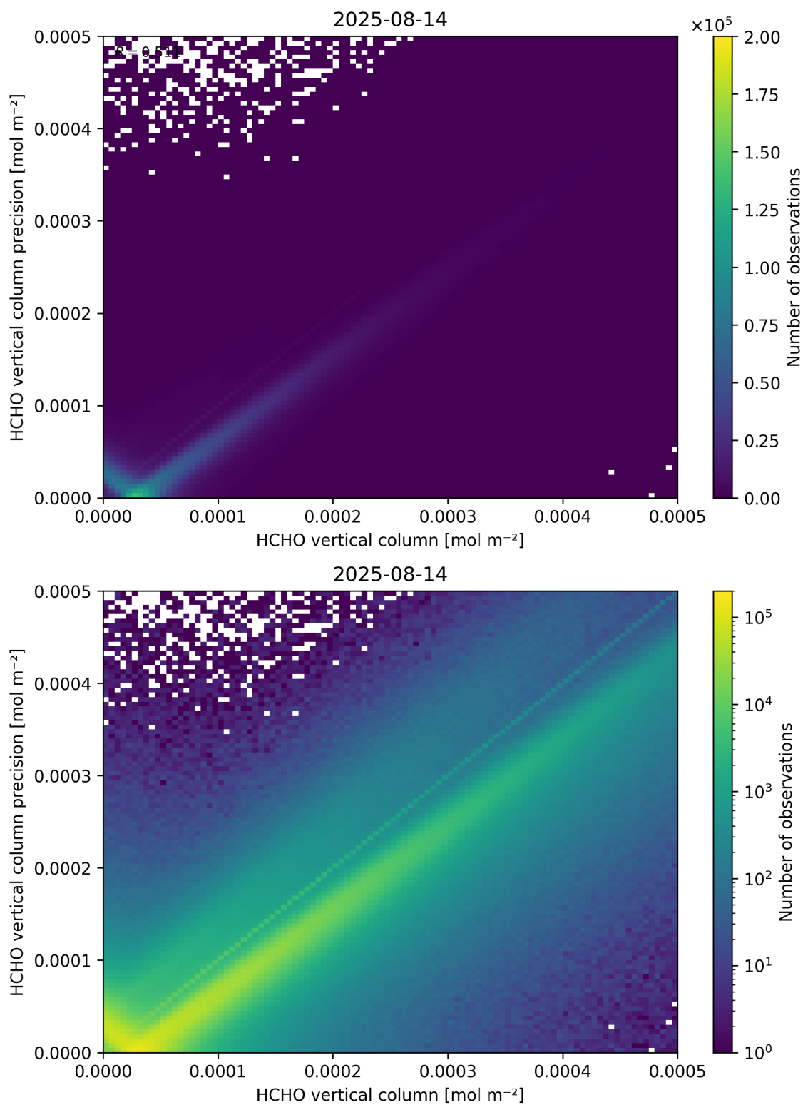
Figure 134: Scatter density plot of “HCHO vertical column” against “HCHO vertical column precision” for 2025-08-14 to 2025-08-15.
