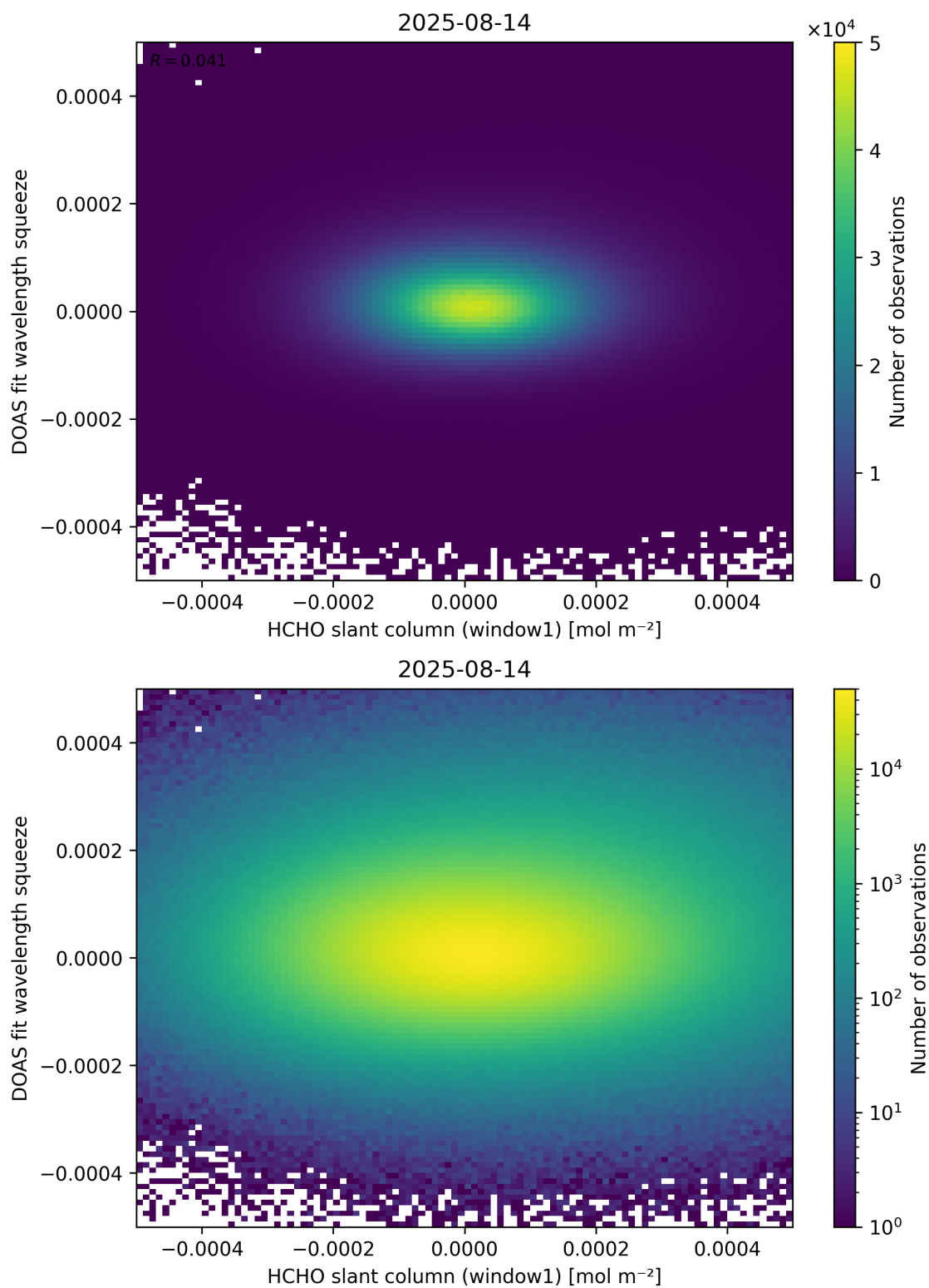
Figure 80: Scatter density plot of “HCHO slant column (window1)” against “DOAS fit wavelength squeeze” for 2025-08-14 to 2025-08-15.
