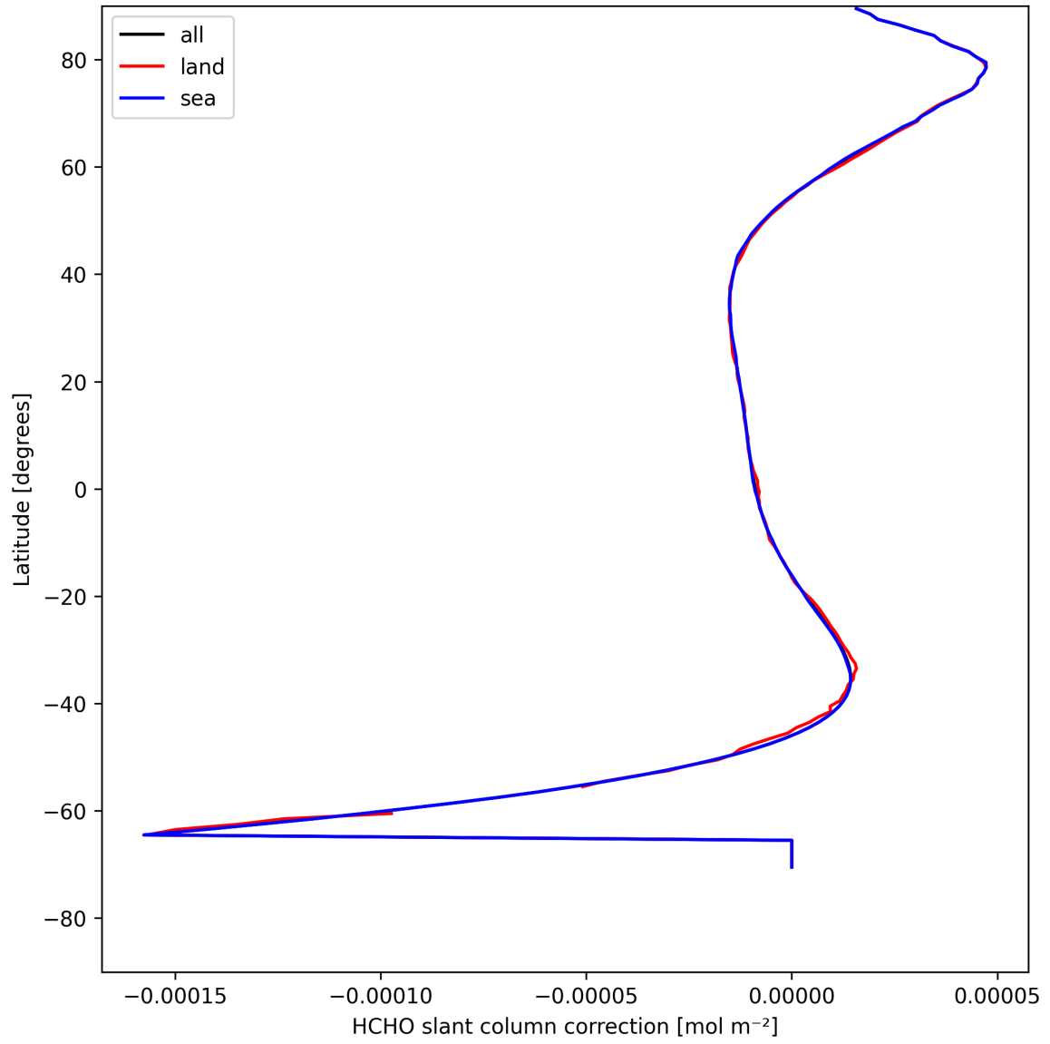
Figure 33: Zonal average of “HCHO slant column correction” for 2025-08-14 to 2025-08-15.
