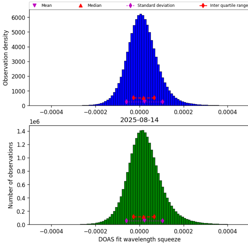
Figure 45: Histogram of “DOAS fit wavelength squeeze” for 2025-08-14 to 2025-08-15
