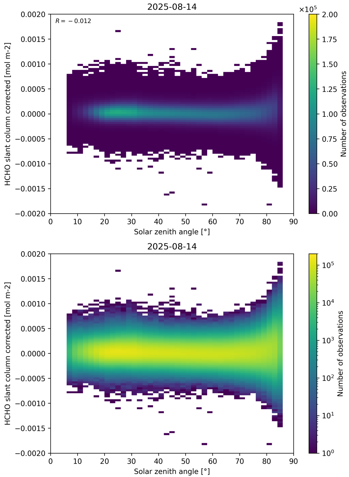
Figure 171: Scatter density plot of “Solar zenith angle” against “HCHO slant column corrected” for 2025-08-14 to 2025-08-15.
