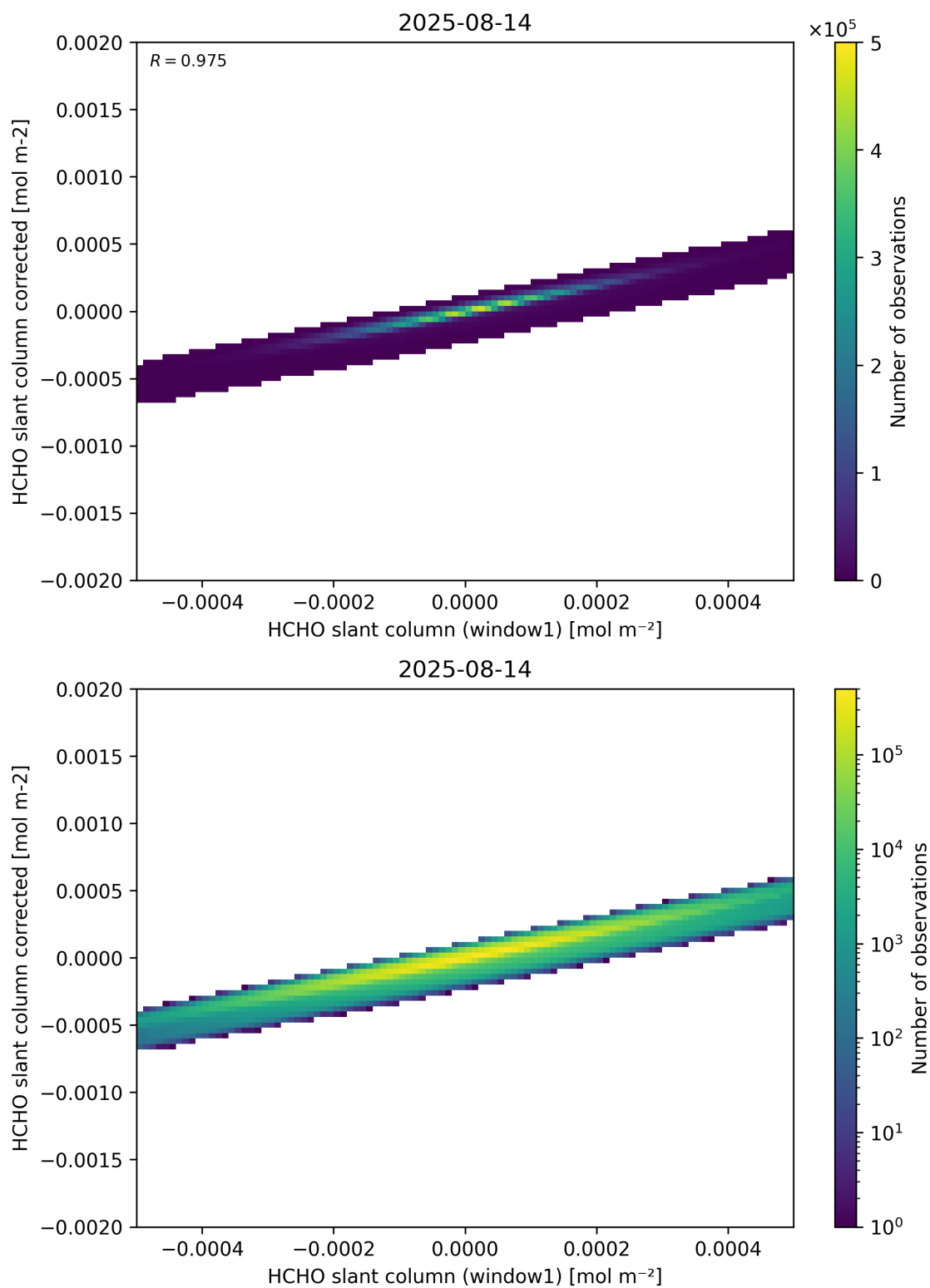
Figure 82: Scatter density plot of “HCHO slant column (window1)” against “HCHO slant column corrected” for 2025-08-14 to 2025-08-15.
