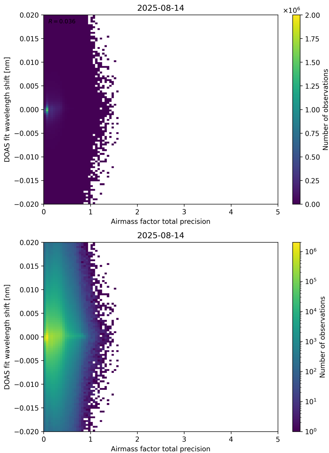
Figure 106: Scatter density plot of “Airmass factor total precision” against “DOAS fit wavelength shift” for 2025-08-14 to 2025-08-15.
