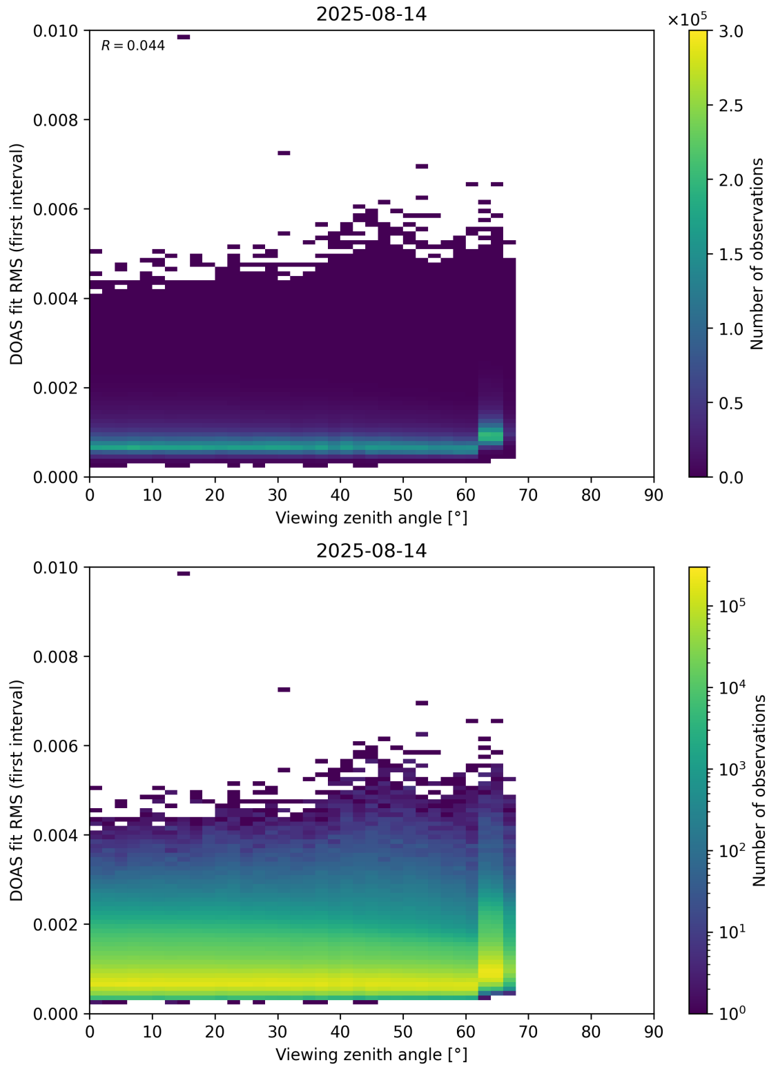
Figure 182: Scatter density plot of “Viewing zenith angle” against “DOAS fit RMS (first interval)” for 2025-08-14 to 2025-08-15.
