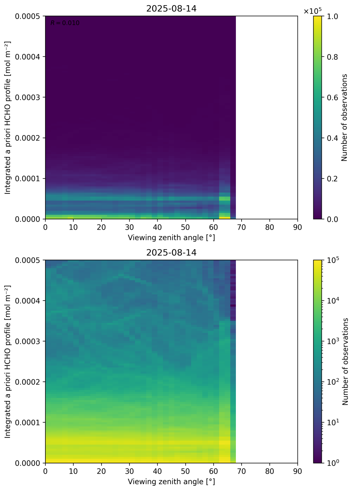
Figure 195: Scatter density plot of “Viewing zenith angle” against “Integrated a priori HCHO profile” for 2025-08-14 to 2025-08-15.
