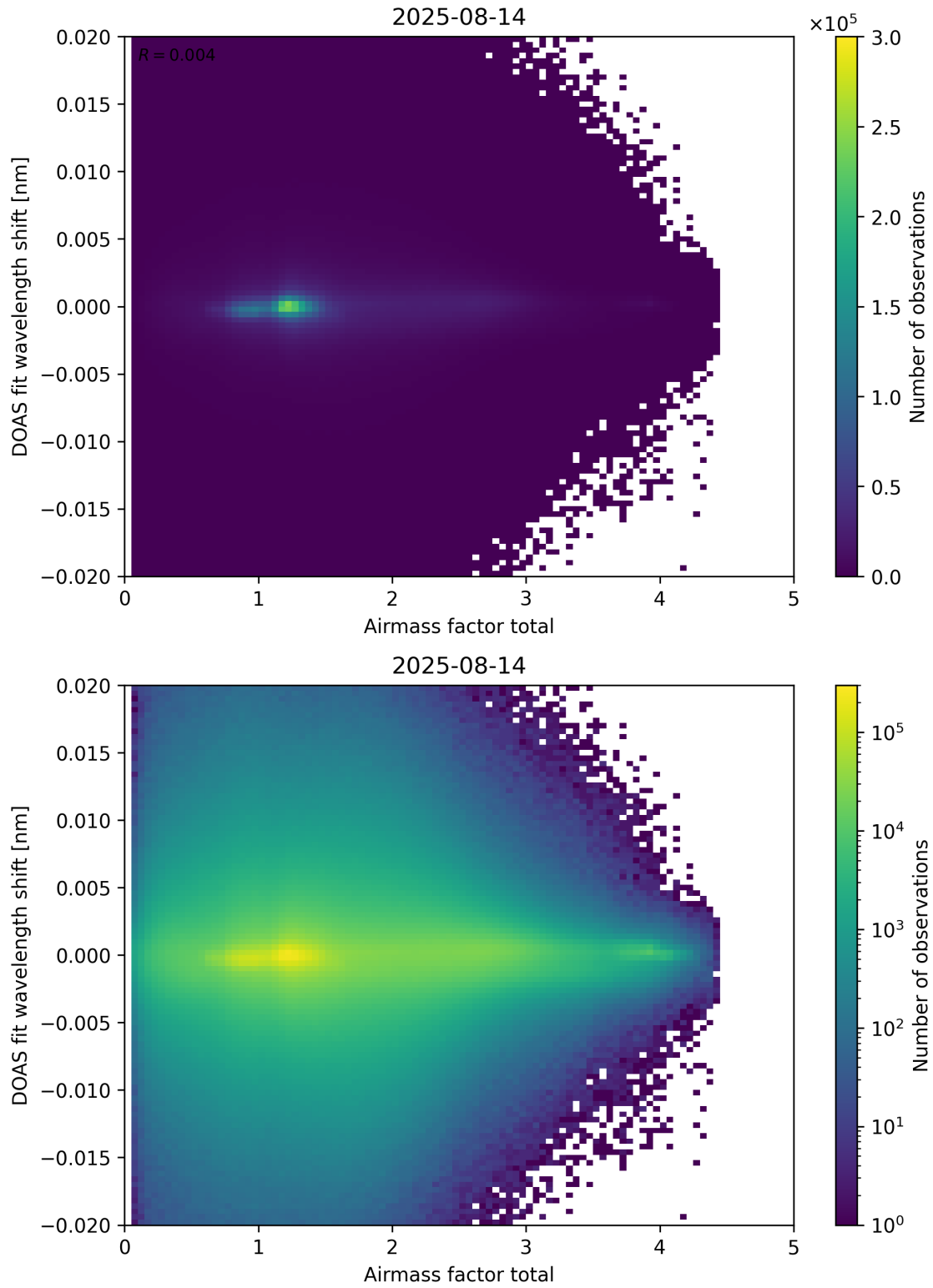
Figure 98: Scatter density plot of “Airmass factor total” against “DOAS fit wavelength shift” for 2025-08-14 to 2025-08-15.
