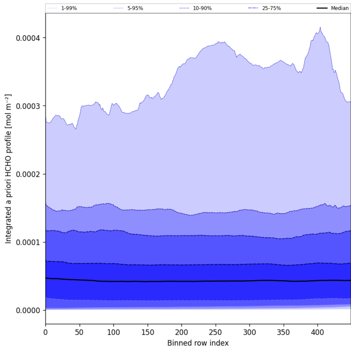
Figure 57: Along track statistics of “Integrated a priori HCHO profile” for 2025-08-14 to 2025-08-15
