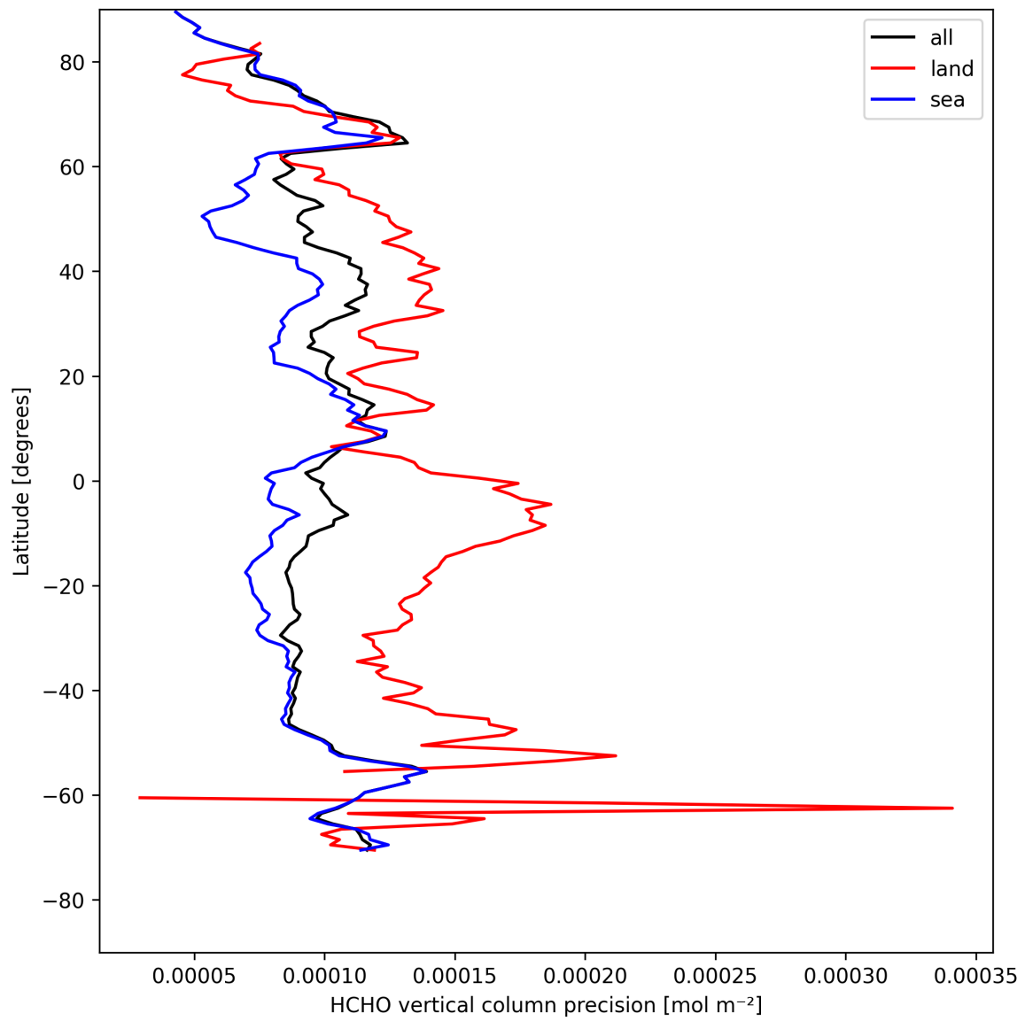
Figure 22: Zonal average of “HCHO vertical column precision” for 2025-08-14 to 2025-08-15.
