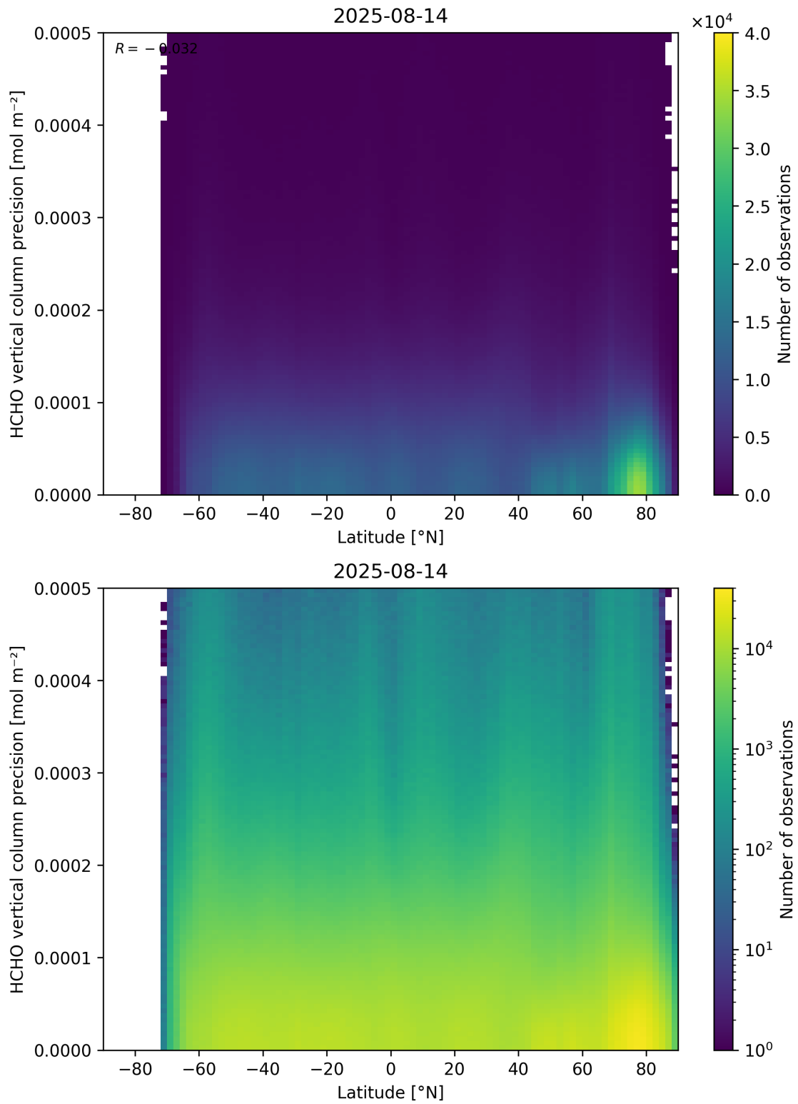
Figure 165: Scatter density plot of “Latitude” against “HCHO vertical column precision” for 2025-08-14 to 2025-08-15.
