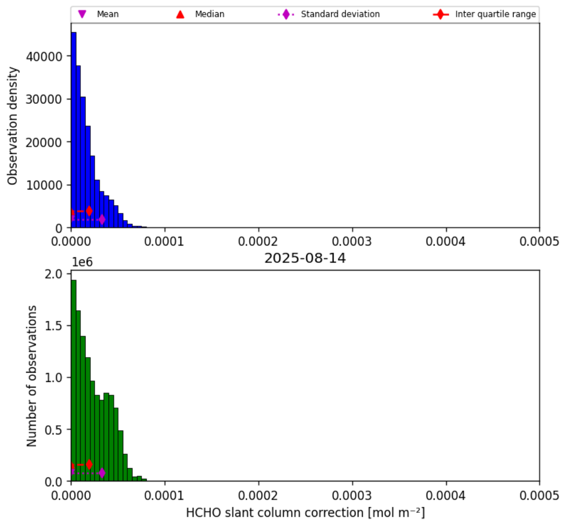
Figure 47: Histogram of “HCHO slant column correction” for 2025-08-14 to 2025-08-15
