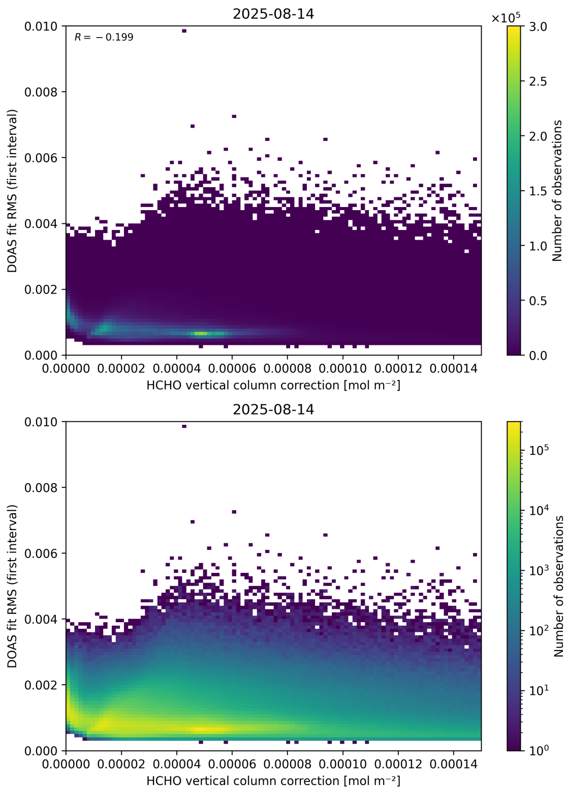
Figure 112: Scatter density plot of “HCHO vertical column correction” against “DOAS fit RMS (first interval)” for 2025-08-14 to 2025-08-15.
