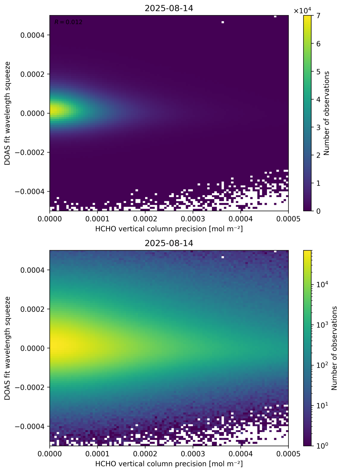
Figure 138: Scatter density plot of “HCHO vertical column precision” against “DOAS fit wavelength squeeze” for 2025-08-14 to 2025-08-15.
