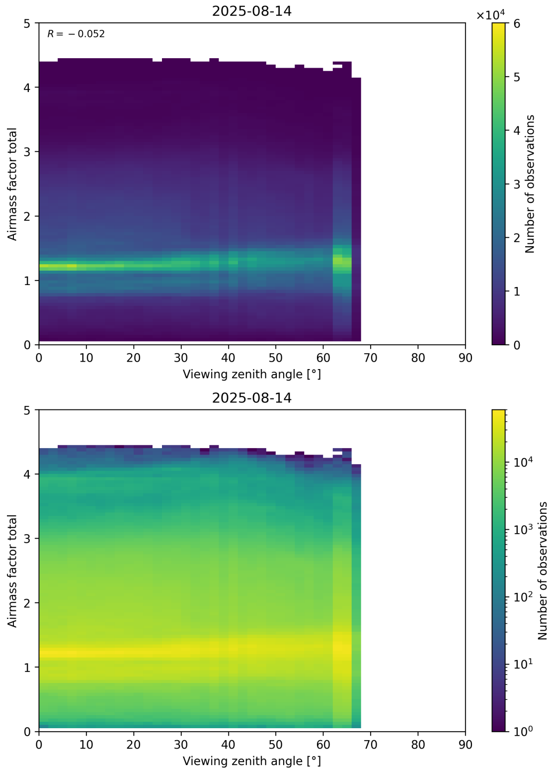
Figure 190: Scatter density plot of “Viewing zenith angle” against “Airmass factor total” for 2025-08-14 to 2025-08-15.
