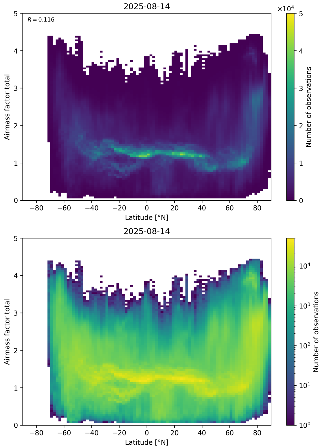
Figure 161: Scatter density plot of “Latitude” against “Airmass factor total” for 2025-08-14 to 2025-08-15.
