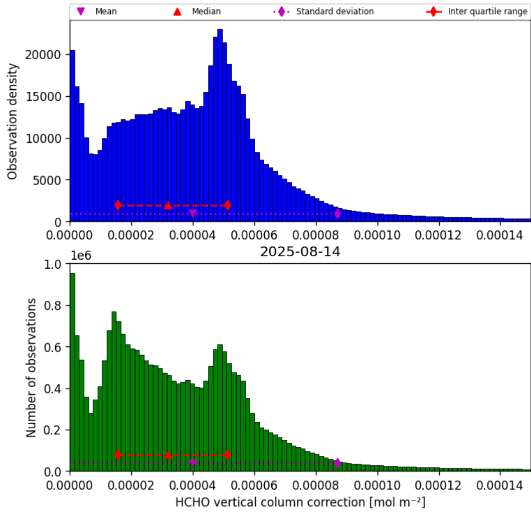
Figure 37: Histogram of “HCHO vertical column correction” for 2025-08-14 to 2025-08-15
