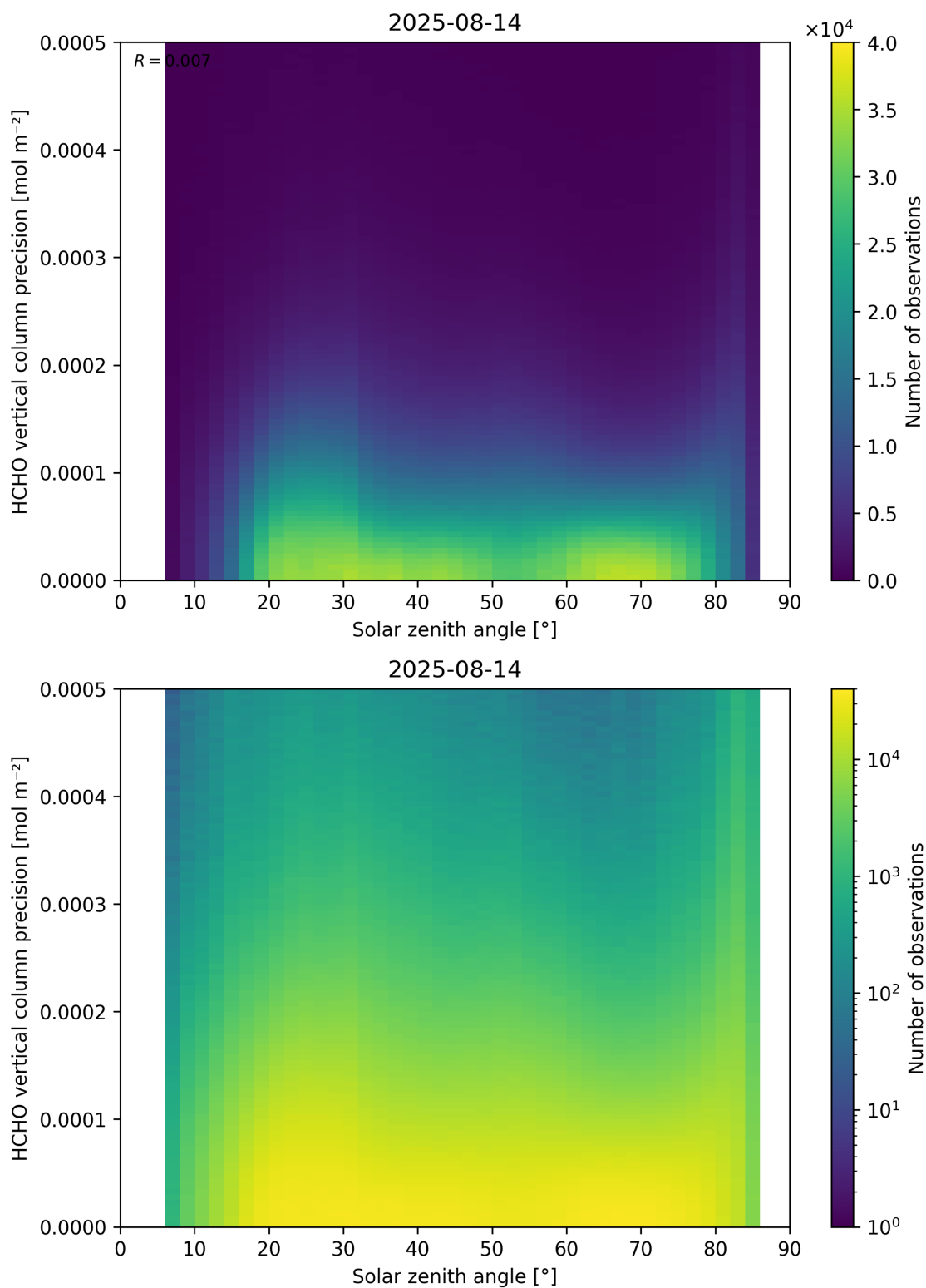
Figure 179: Scatter density plot of “Solar zenith angle” against “HCHO vertical column precision” for 2025-08-14 to 2025-08-15.
