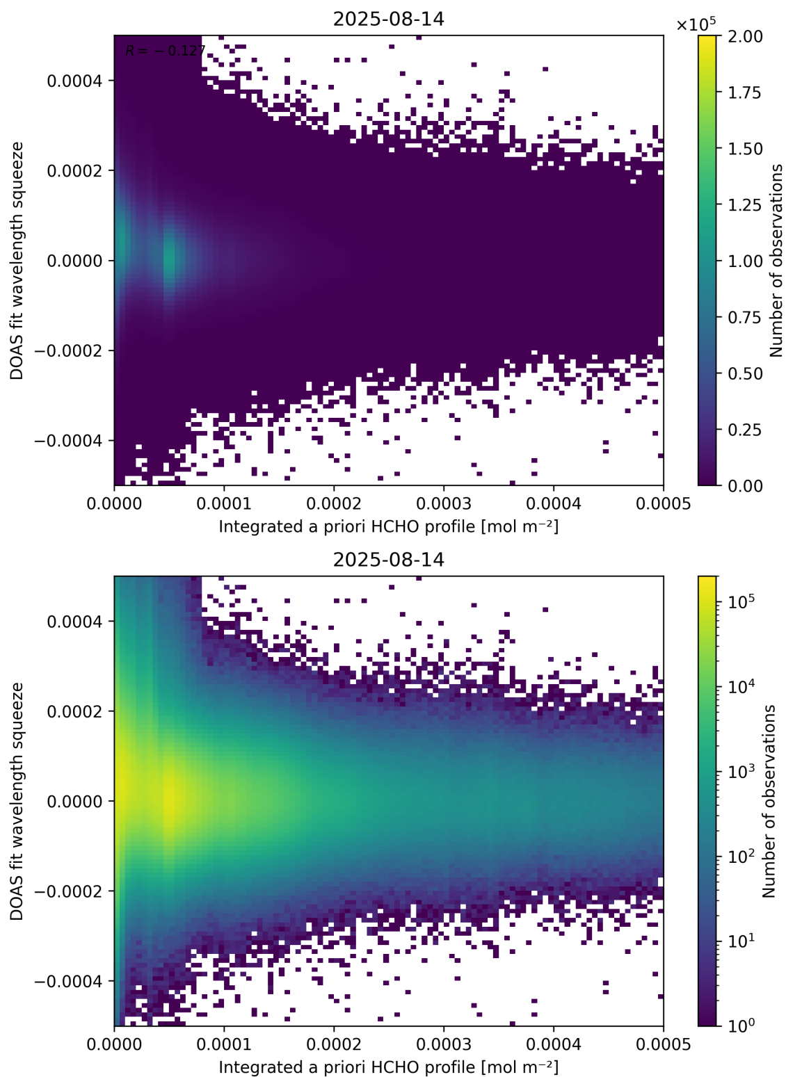
Figure 150: Scatter density plot of “Integrated a priori HCHO profile” against “DOAS fit wavelength squeeze” for 2025-08-14 to 2025-08-15.
