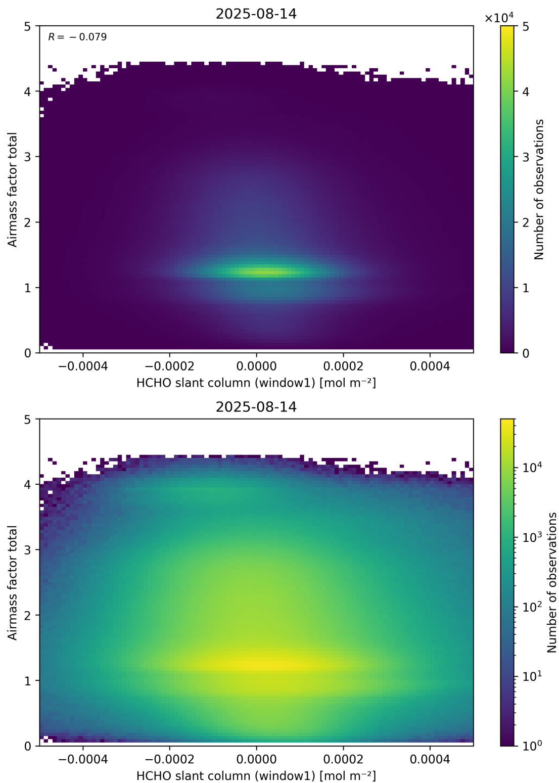
Figure 85: Scatter density plot of “HCHO slant column (window1)” against “Airmass factor total” for 2025-08-14 to 2025-08-15.
