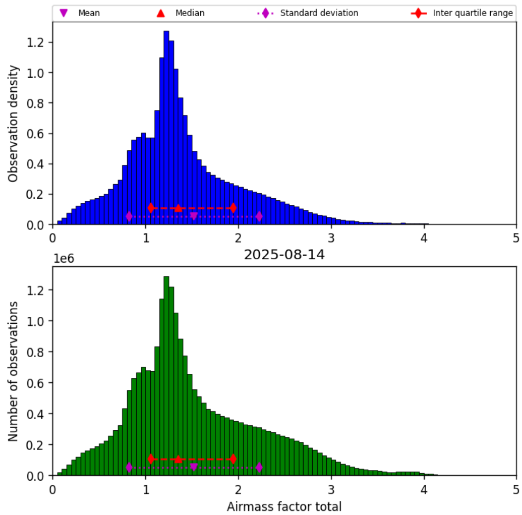
Figure 40: Histogram of “Airmass factor total” for 2025-08-14 to 2025-08-15
