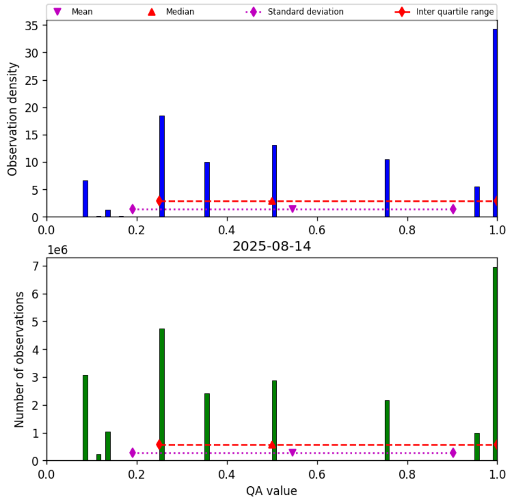
Figure 34: Histogram of “QA value” for 2025-08-14 to 2025-08-15
