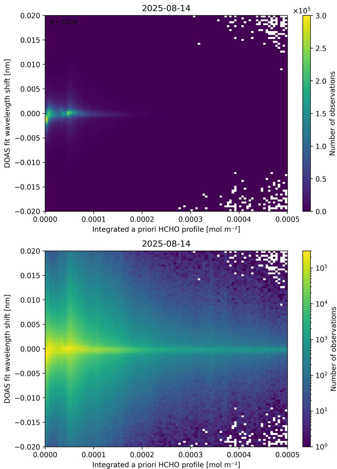
Figure 149: Scatter density plot of “Integrated a priori HCHO profile” against “DOAS fit wavelength shift” for 2025-08-14 to 2025-08-15.
