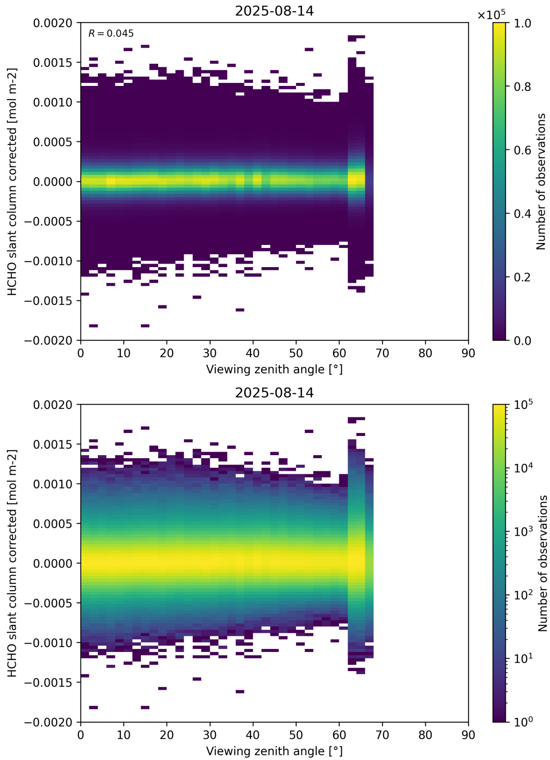
Figure 186: Scatter density plot of “Viewing zenith angle” against “HCHO slant column corrected” for 2025-08-14 to 2025-08-15.
