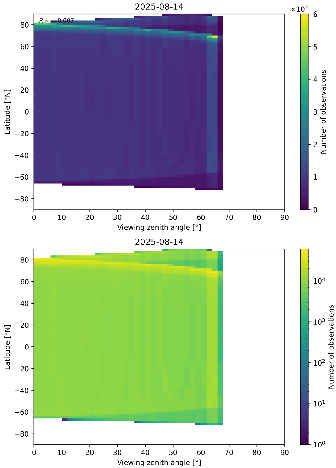
Figure 196: Scatter density plot of “Viewing zenith angle” against “Latitude” for 2025-08-14 to 2025-08-15.
