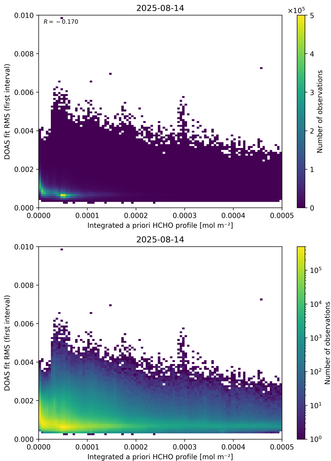
Figure 148: Scatter density plot of “Integrated a priori HCHO profile” against “DOAS fit RMS (first interval)” for 2025-08-14 to 2025-08-15.
