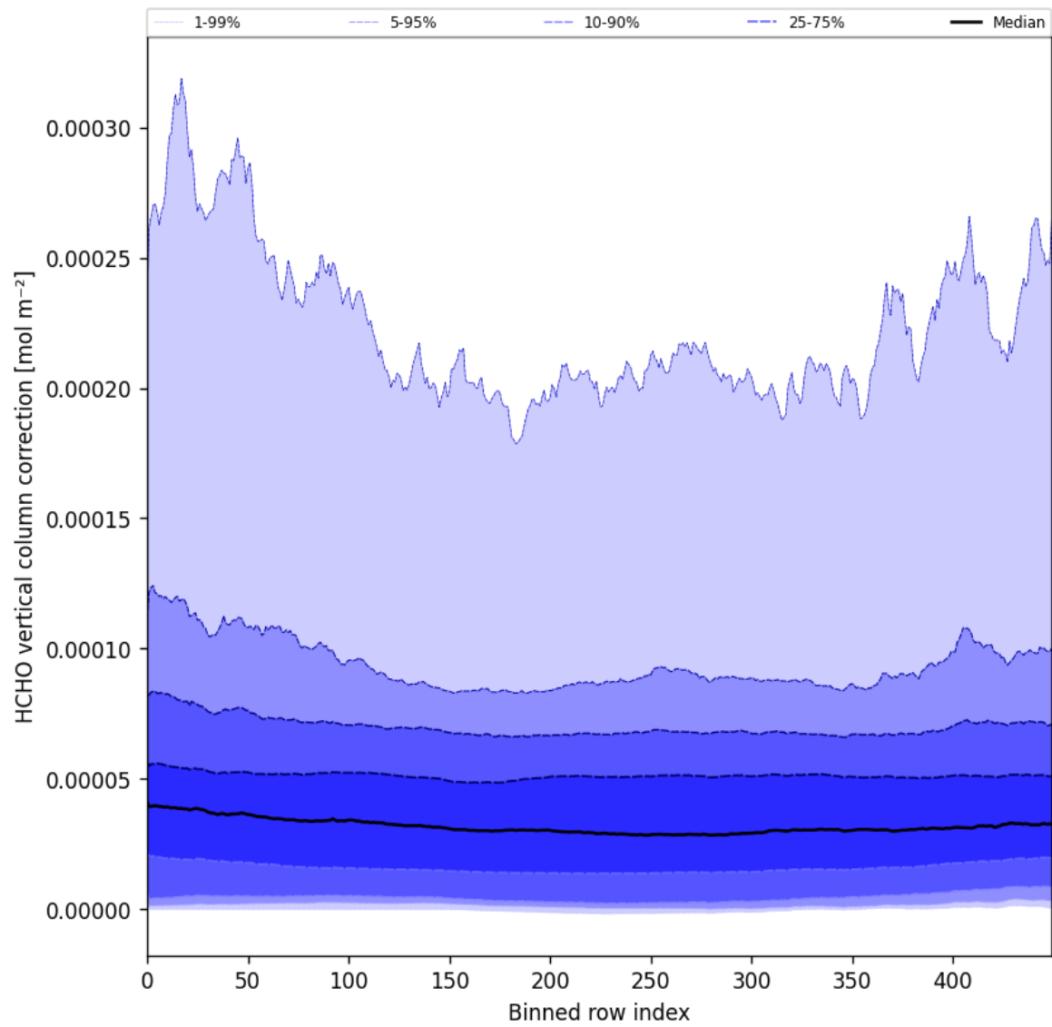
Figure 51: Along track statistics of “HCHO vertical column correction” for 2025-08-14 to 2025-08-15
