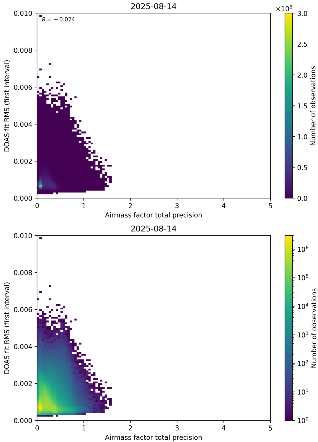
Figure 105: Scatter density plot of “Airmass factor total precision” against “DOAS fit RMS (first interval)” for 2025-08-14 to 2025-08-15.
