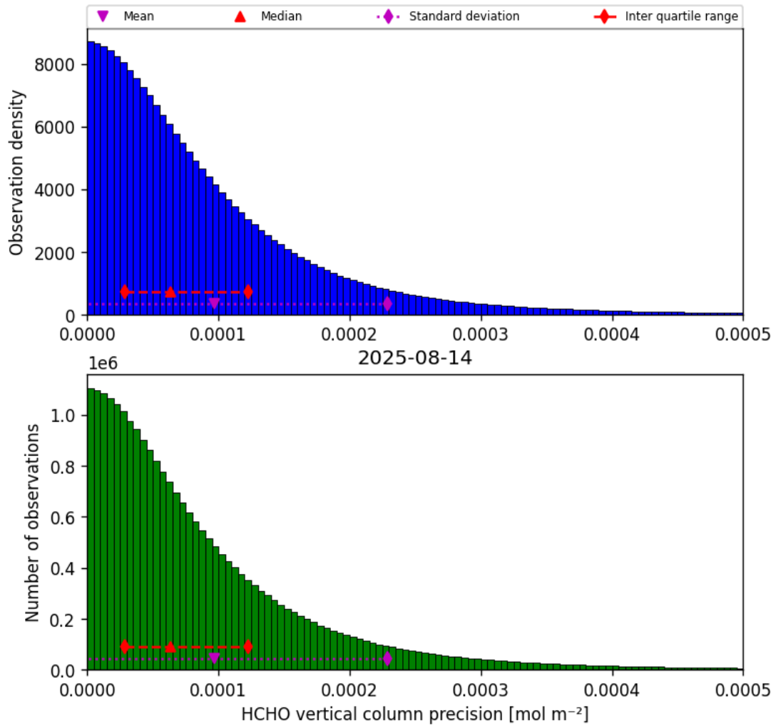
Figure 36: Histogram of “HCHO vertical column precision” for 2025-08-14 to 2025-08-15
