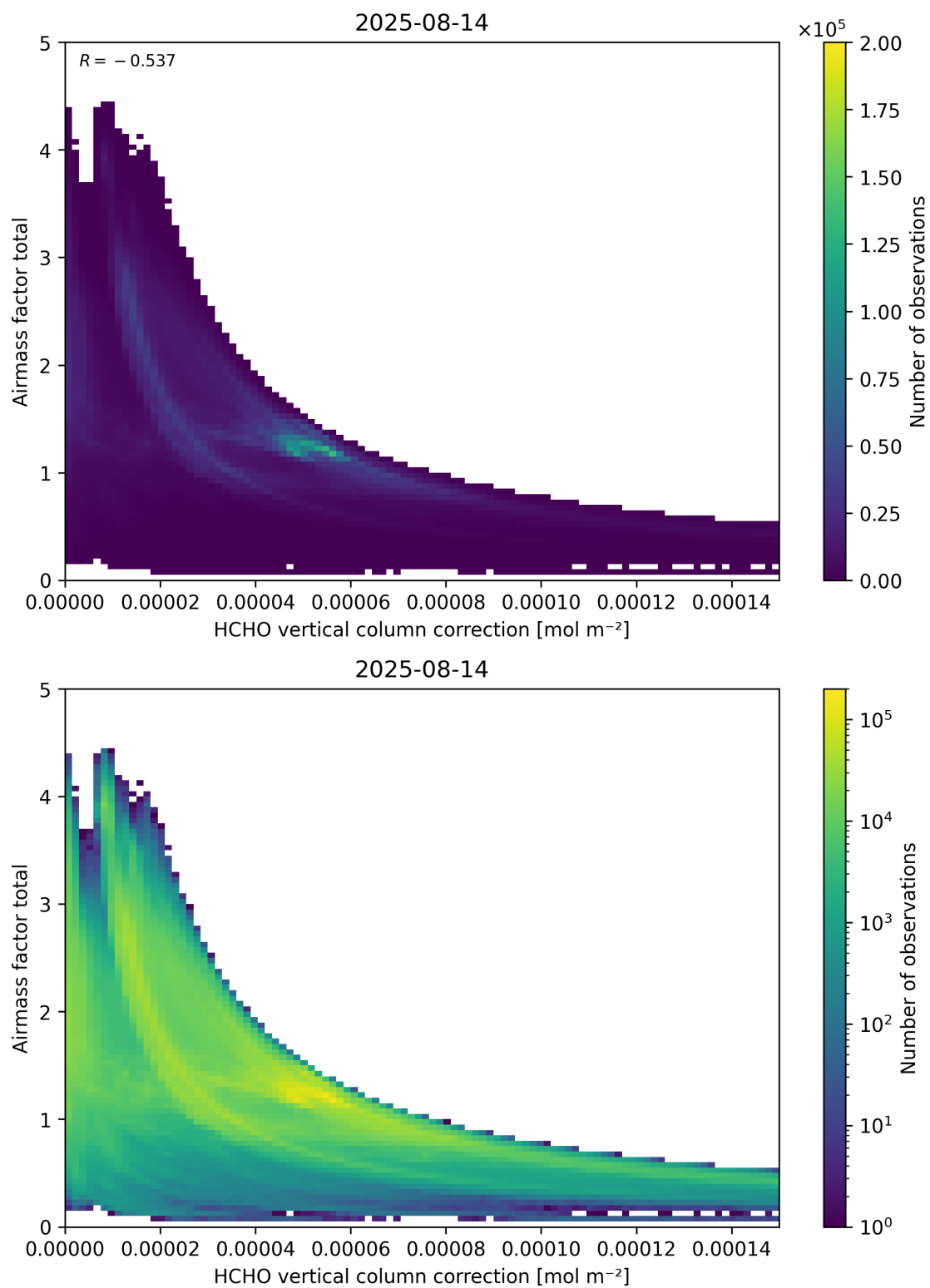
Figure 120: Scatter density plot of “HCHO vertical column correction” against “Airmass factor total” for 2025-08-14 to 2025-08-15.
