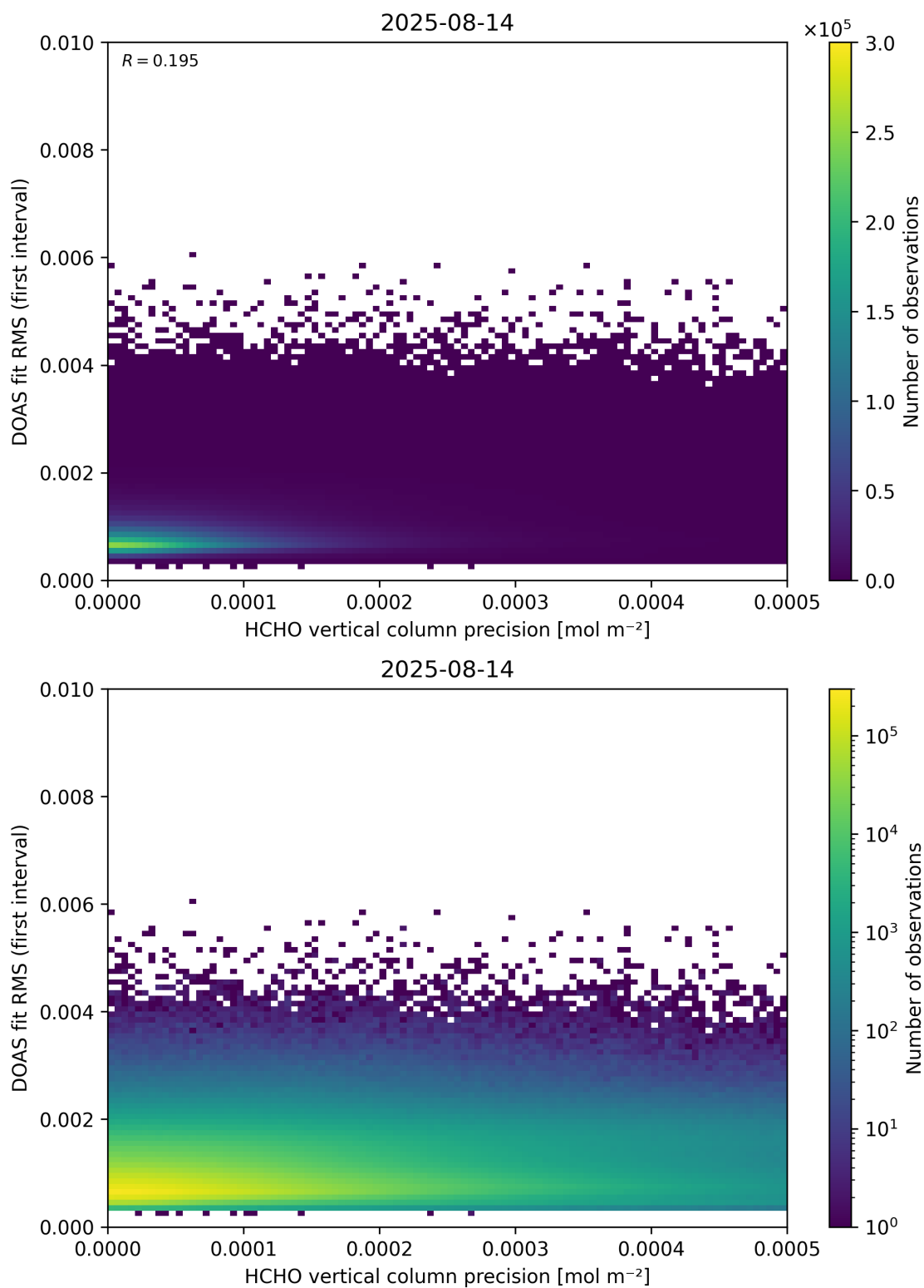
Figure 136: Scatter density plot of “HCHO vertical column precision” against “DOAS fit RMS (first interval)” for 2025-08-14 to 2025-08-15.
