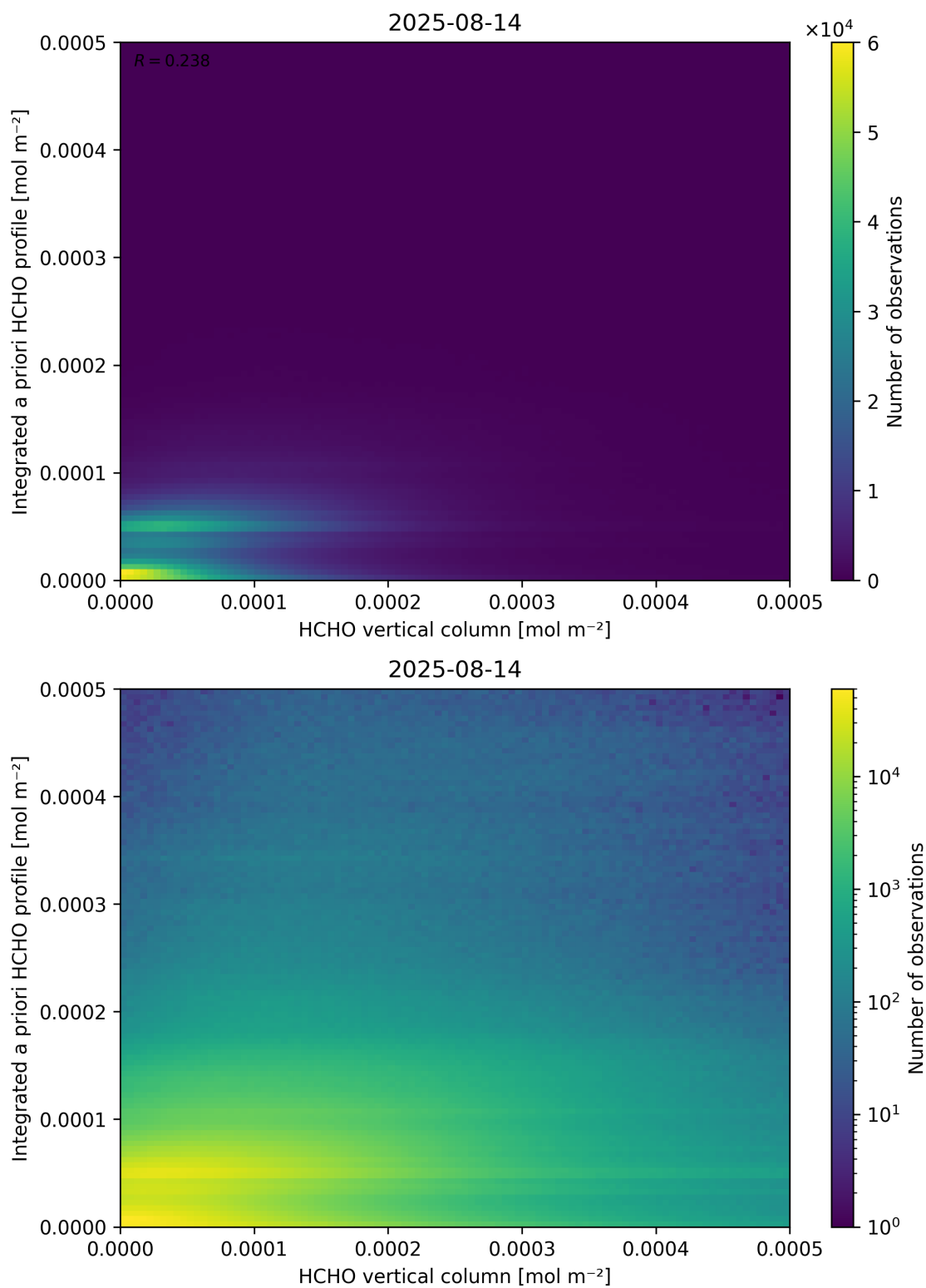
Figure 135: Scatter density plot of “HCHO vertical column” against “Integrated a priori HCHO profile” for 2025-08-14 to 2025-08-15.
