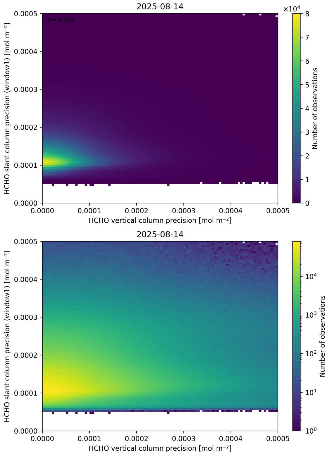
Figure 143: Scatter density plot of “HCHO vertical column precision” against “HCHO slant column precision (window1)” for 2025-08-14 to 2025-08-15.
