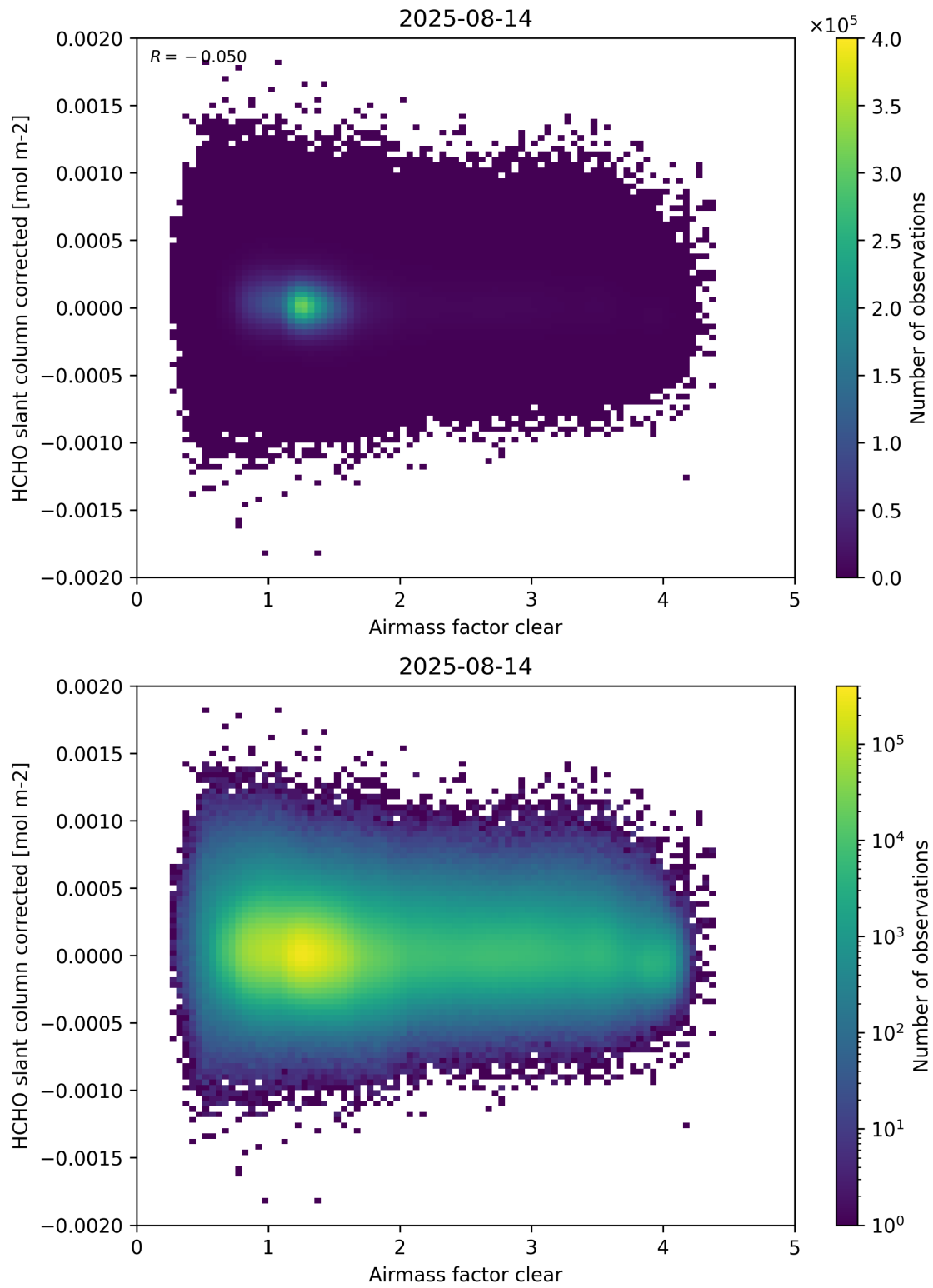
Figure 74: Scatter density plot of “Airmass factor clear” against “HCHO slant column corrected” for 2025-08-14 to 2025-08-15.
