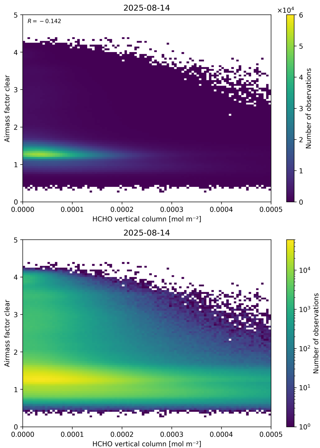
Figure 126: Scatter density plot of “HCHO vertical column” against “Airmass factor clear” for 2025-08-14 to 2025-08-15.
