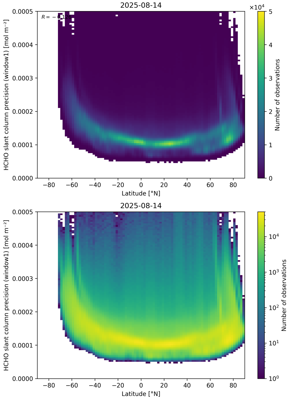
Figure 160: Scatter density plot of “Latitude” against “HCHO slant column precision (window1)” for 2025-08-14 to 2025-08-15.
