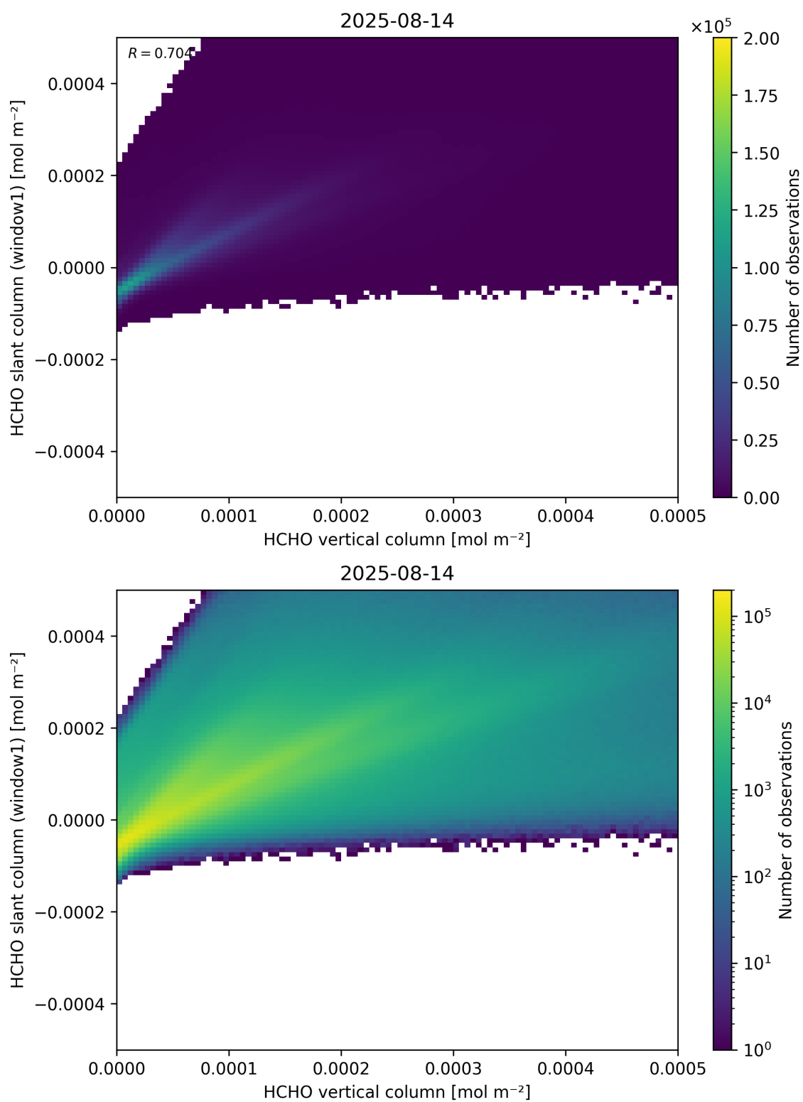
Figure 129: Scatter density plot of “HCHO vertical column” against “HCHO slant column (window1)” for 2025-08-14 to 2025-08-15.
