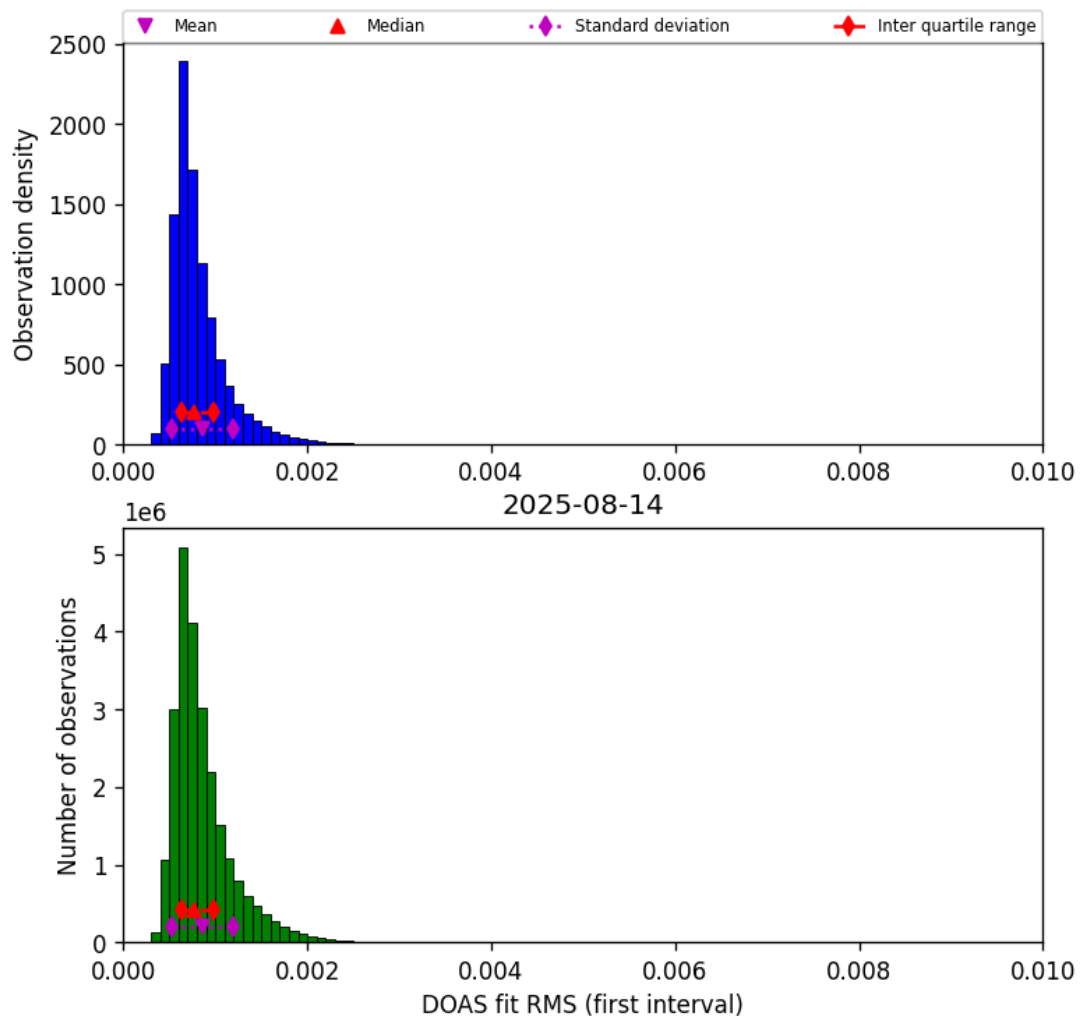
Figure 46: Histogram of “DOAS fit RMS (first interval)” for 2025-08-14 to 2025-08-15
