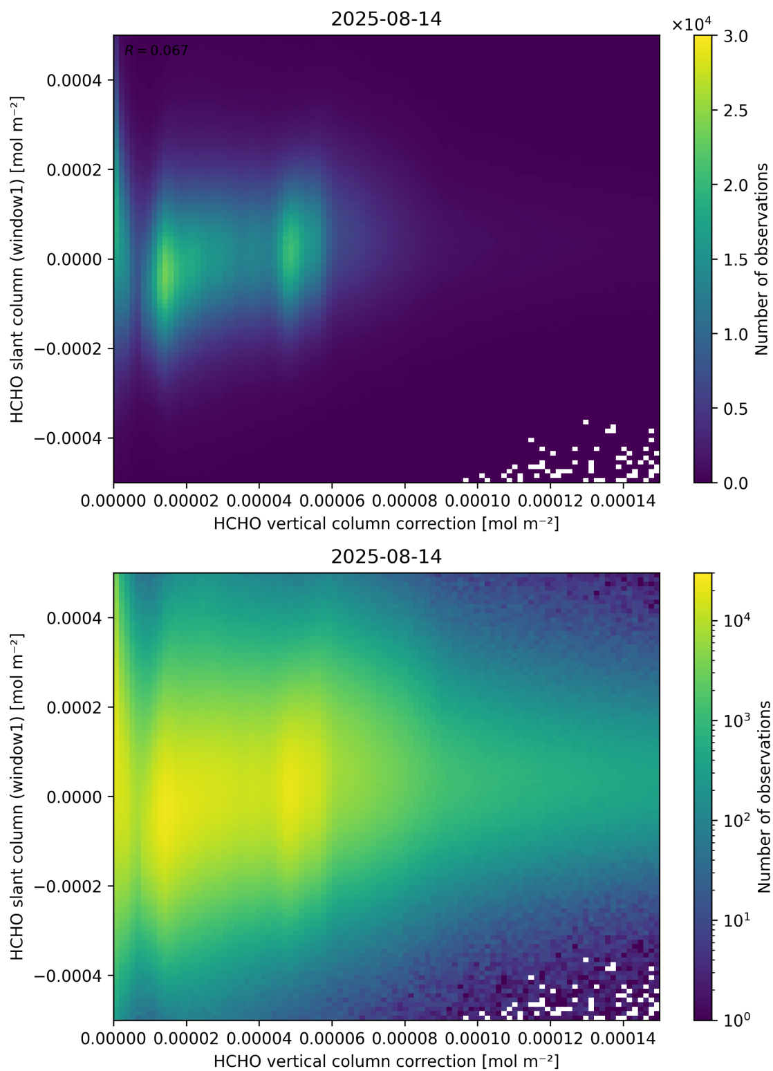
Figure 118: Scatter density plot of “HCHO vertical column correction” against “HCHO slant column (window1)” for 2025-08-14 to 2025-08-15.
