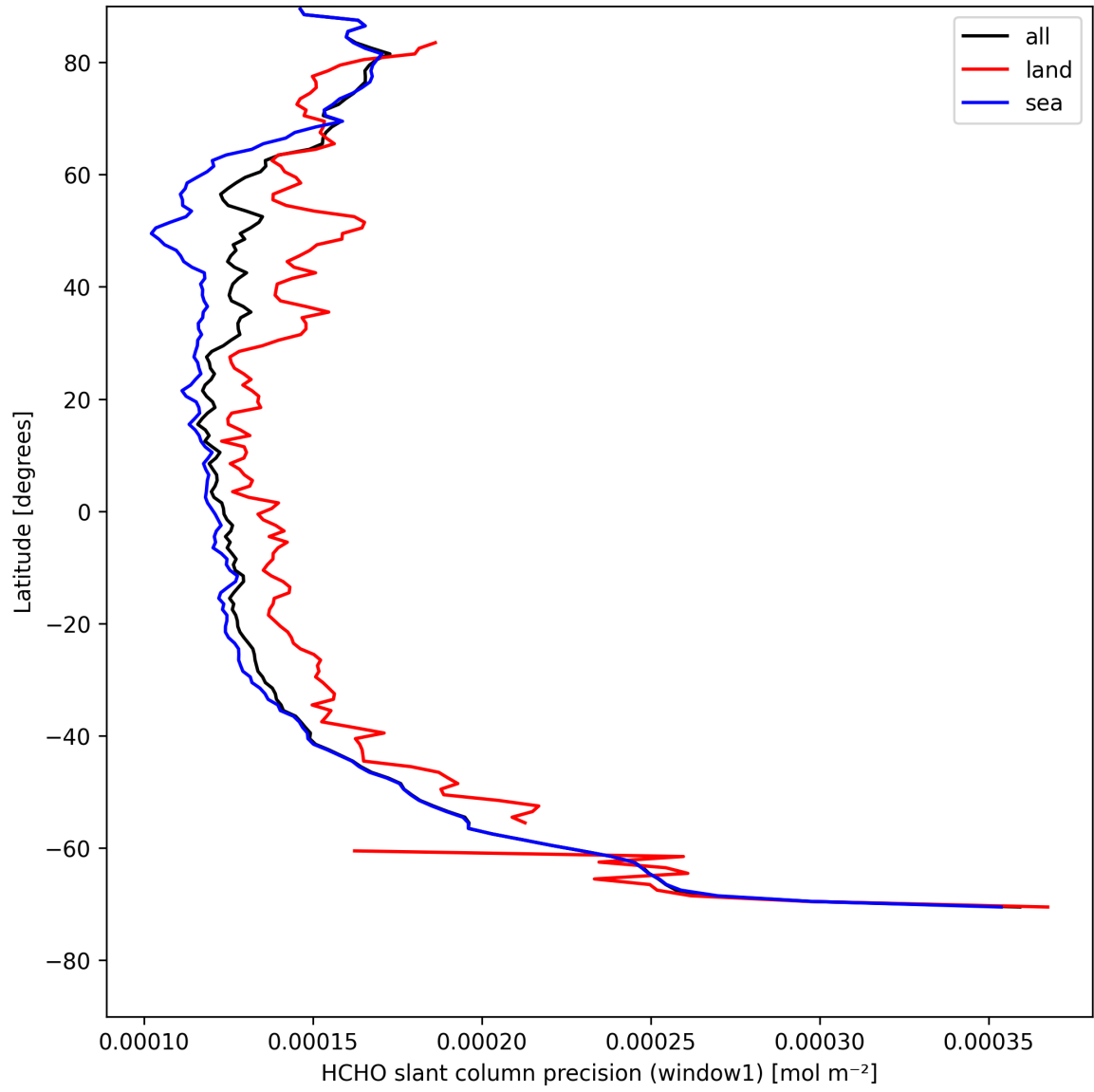
Figure 25: Zonal average of "HCHO slant column precision (window1)" for 2025-08-14 to 2025-08-15.
