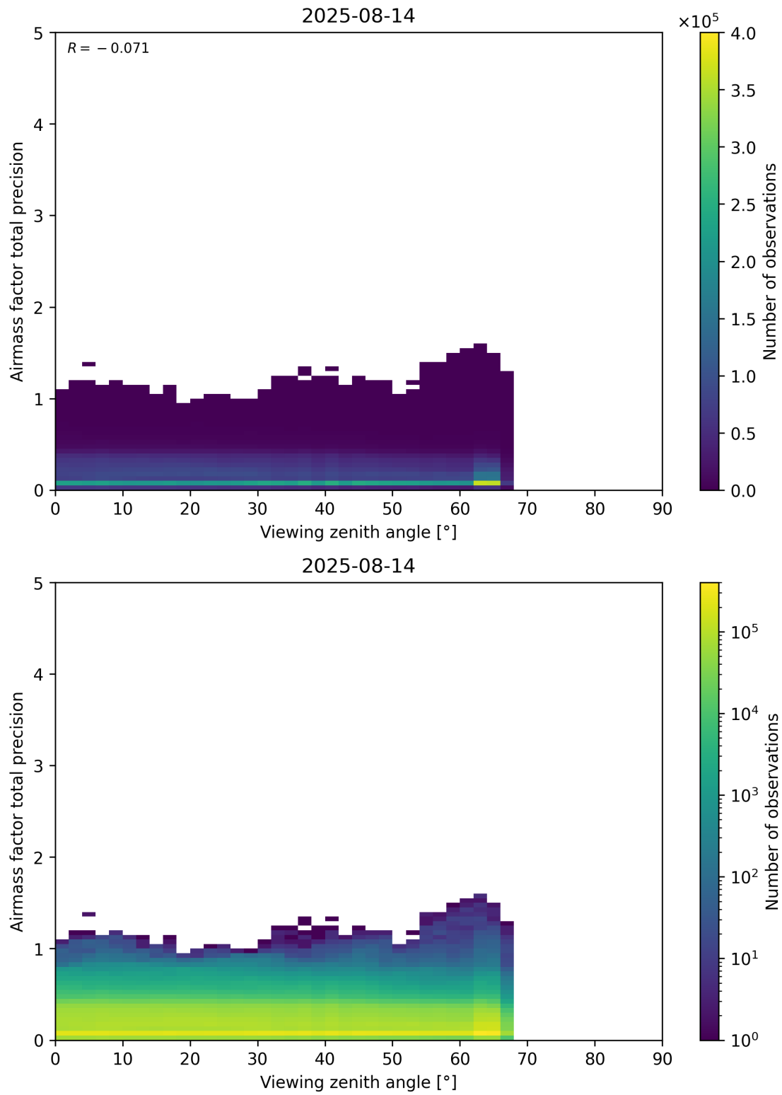
Figure 191: Scatter density plot of “Viewing zenith angle” against “Airmass factor total precision” for 2025-08-14 to 2025-08-15.
