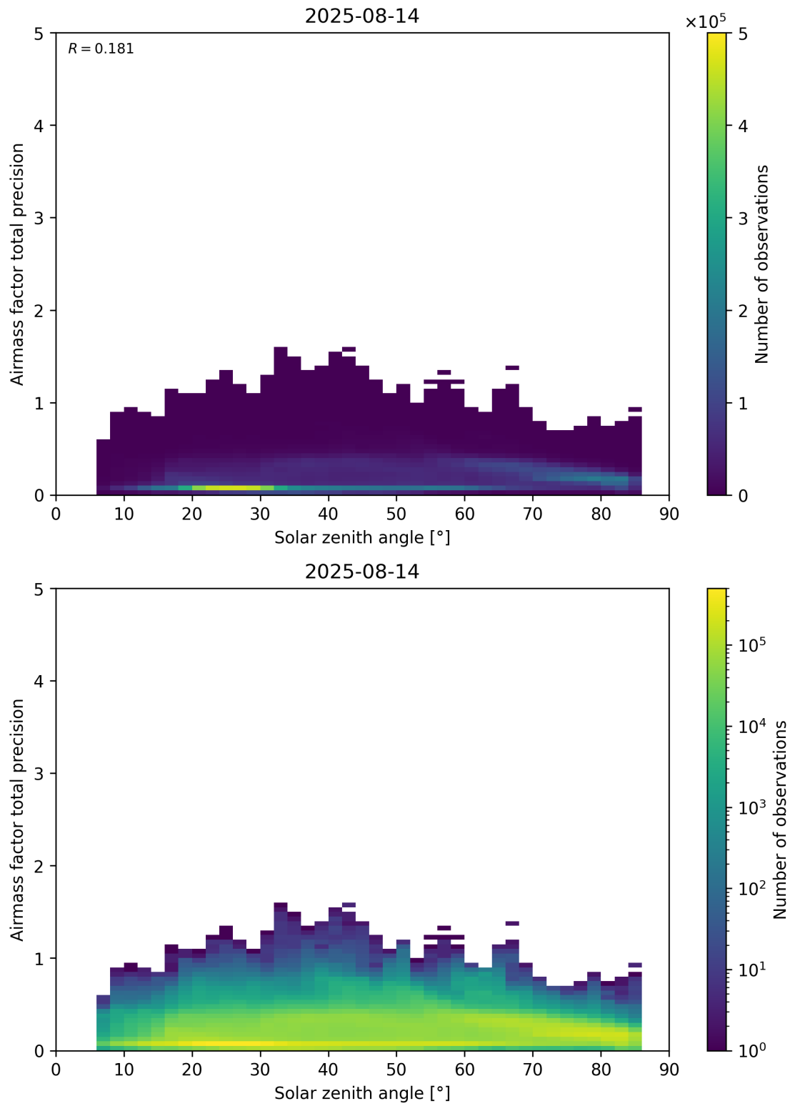
Figure 176: Scatter density plot of “Solar zenith angle” against “Airmass factor total precision” for 2025-08-14 to 2025-08-15.
