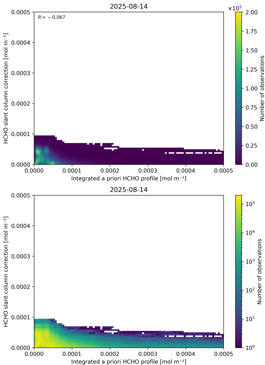
Figure 152: Scatter density plot of “Integrated a priori HCHO profile” against “HCHO slant column correction” for 2025-08-14 to 2025-08-15.
