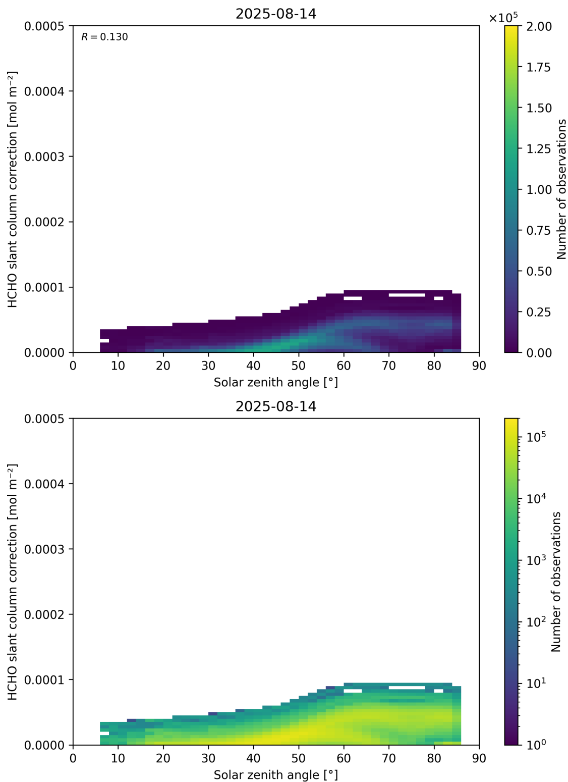
Figure 172: Scatter density plot of “Solar zenith angle” against “HCHO slant column correction” for 2025-08-14 to 2025-08-15.
