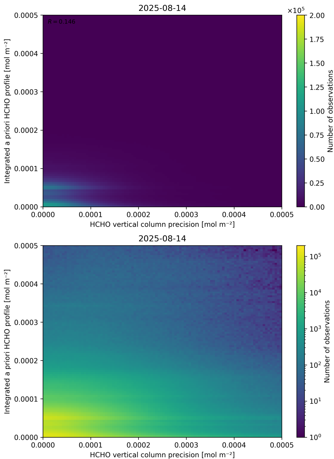
Figure 147: Scatter density plot of “HCHO vertical column precision” against “Integrated a priori HCHO profile” for 2025-08-14 to 2025-08-15.
