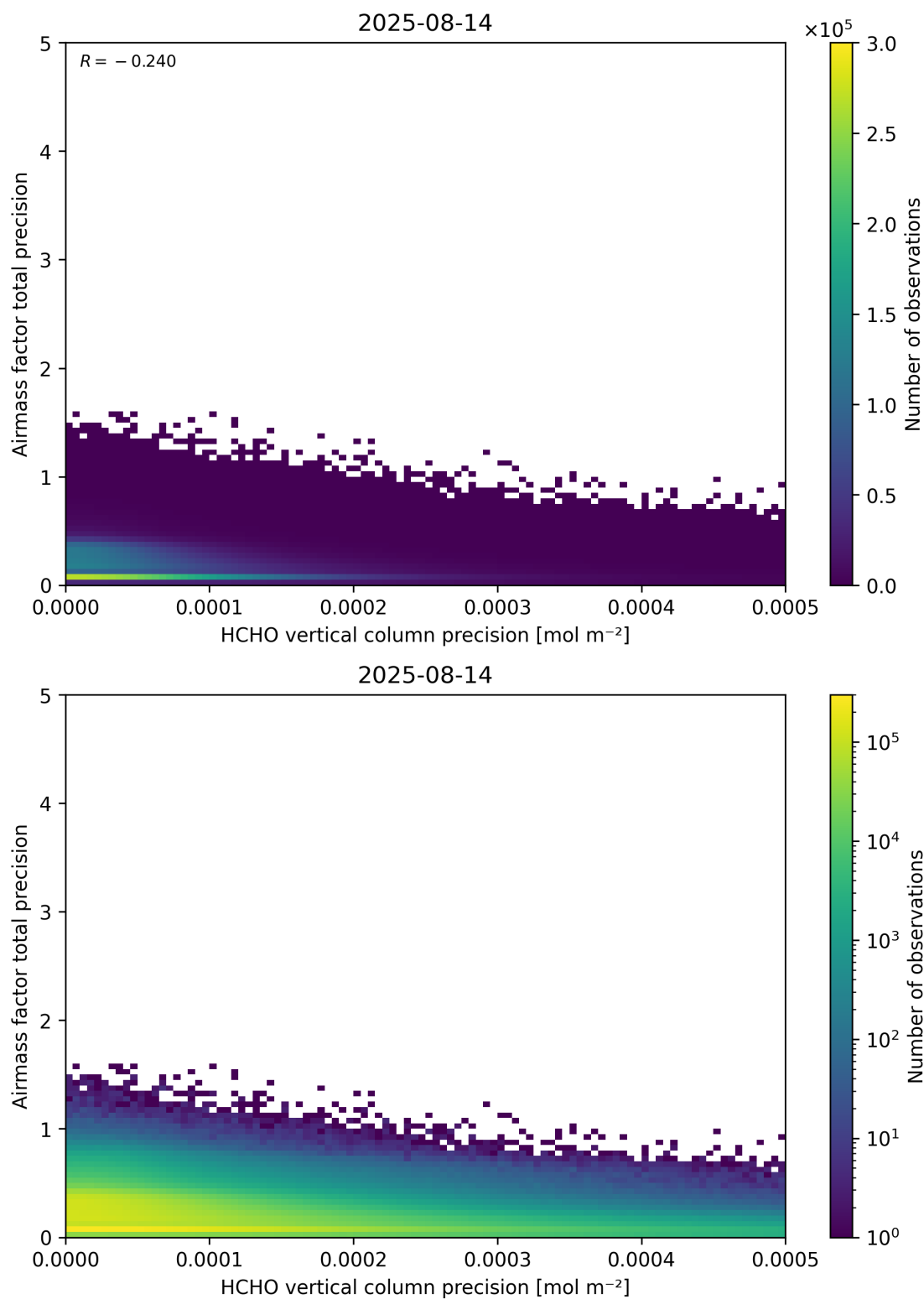
Figure 145: Scatter density plot of “HCHO vertical column precision” against “Airmass factor total precision” for 2025-08-14 to 2025-08-15.
