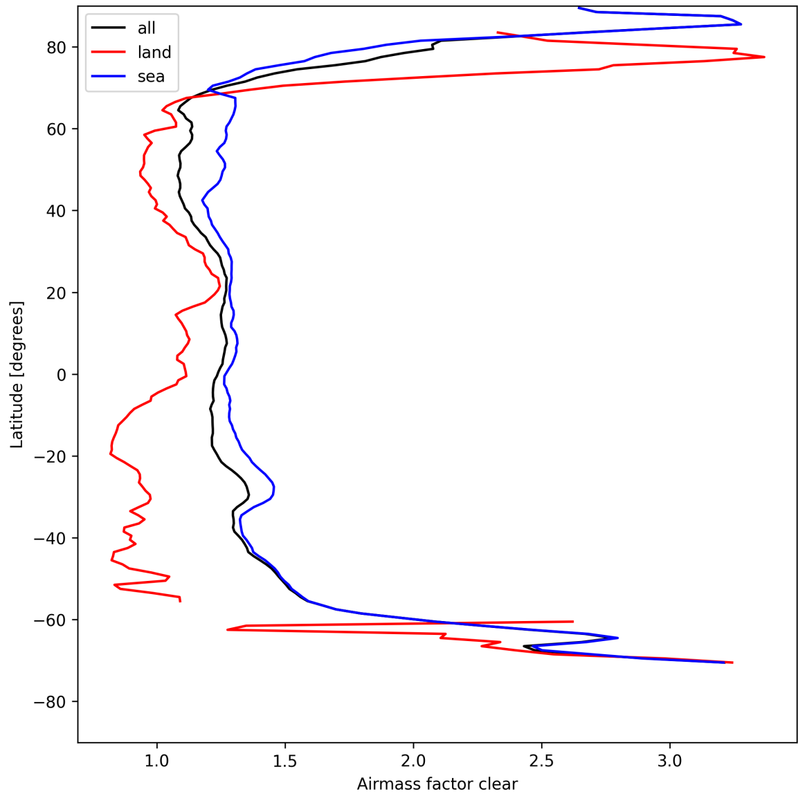
Figure 28: Zonal average of “Airmass factor clear” for 2025-08-14 to 2025-08-15.
