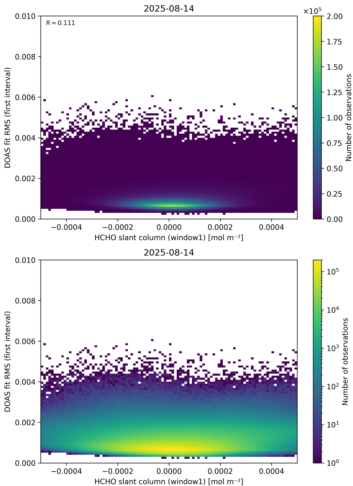
Figure 78: Scatter density plot of “HCHO slant column (window1)” against “DOAS fit RMS (first interval)” for 2025-08-14 to 2025-08-15.
