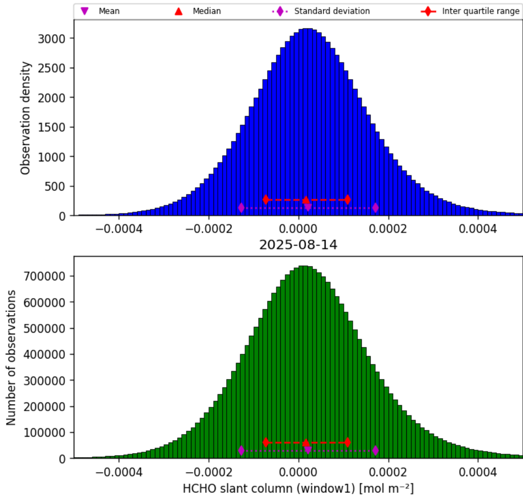
Figure 38: Histogram of “HCHO slant column (window1)” for 2025-08-14 to 2025-08-15
