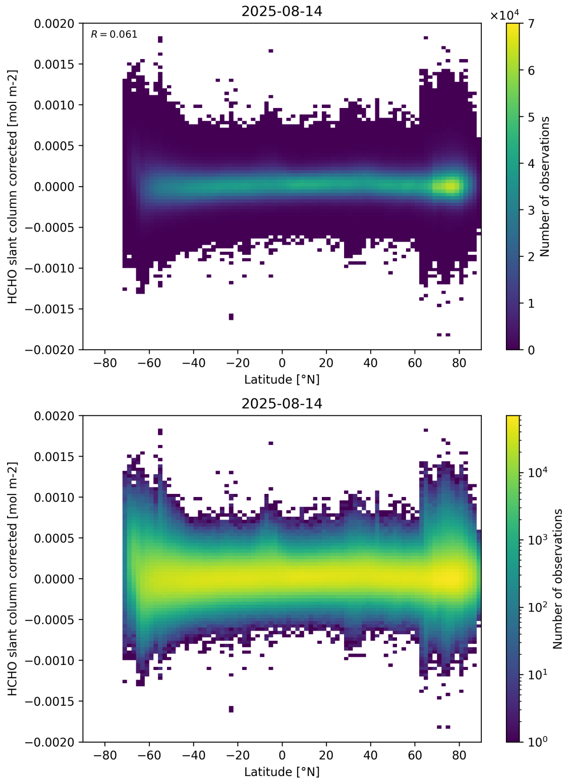
Figure 157: Scatter density plot of “Latitude” against “HCHO slant column corrected” for 2025-08-14 to 2025-08-15.
