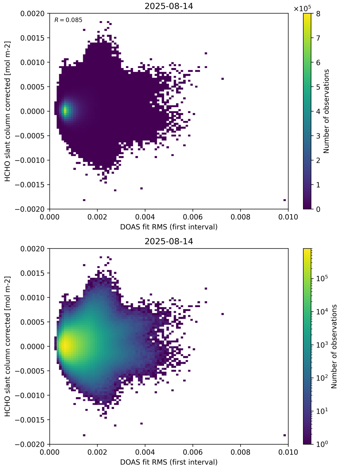
Figure 62: Scatter density plot of “DOAS fit RMS (first interval)” against “HCHO slant column corrected” for 2025-08-14 to 2025-08-15.
