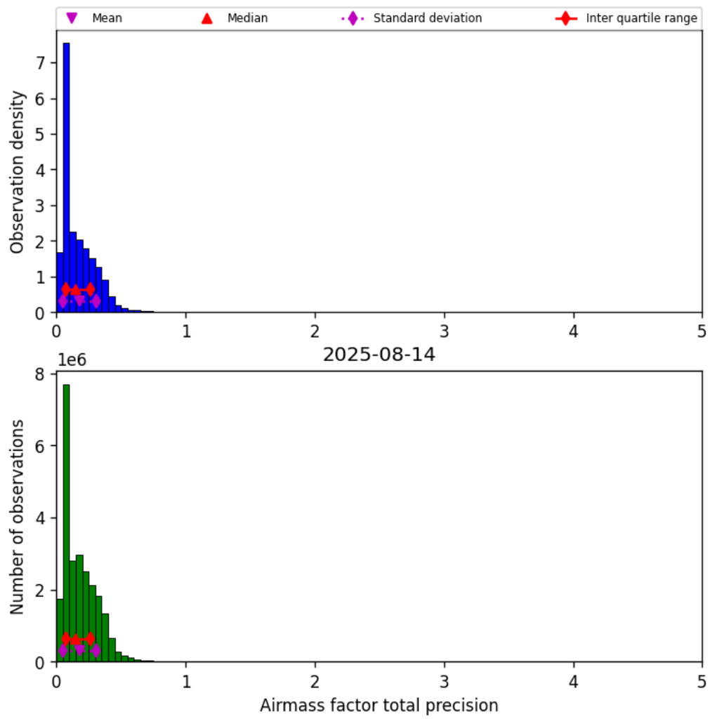
Figure 41: Histogram of “Airmass factor total precision” for 2025-08-14 to 2025-08-15
