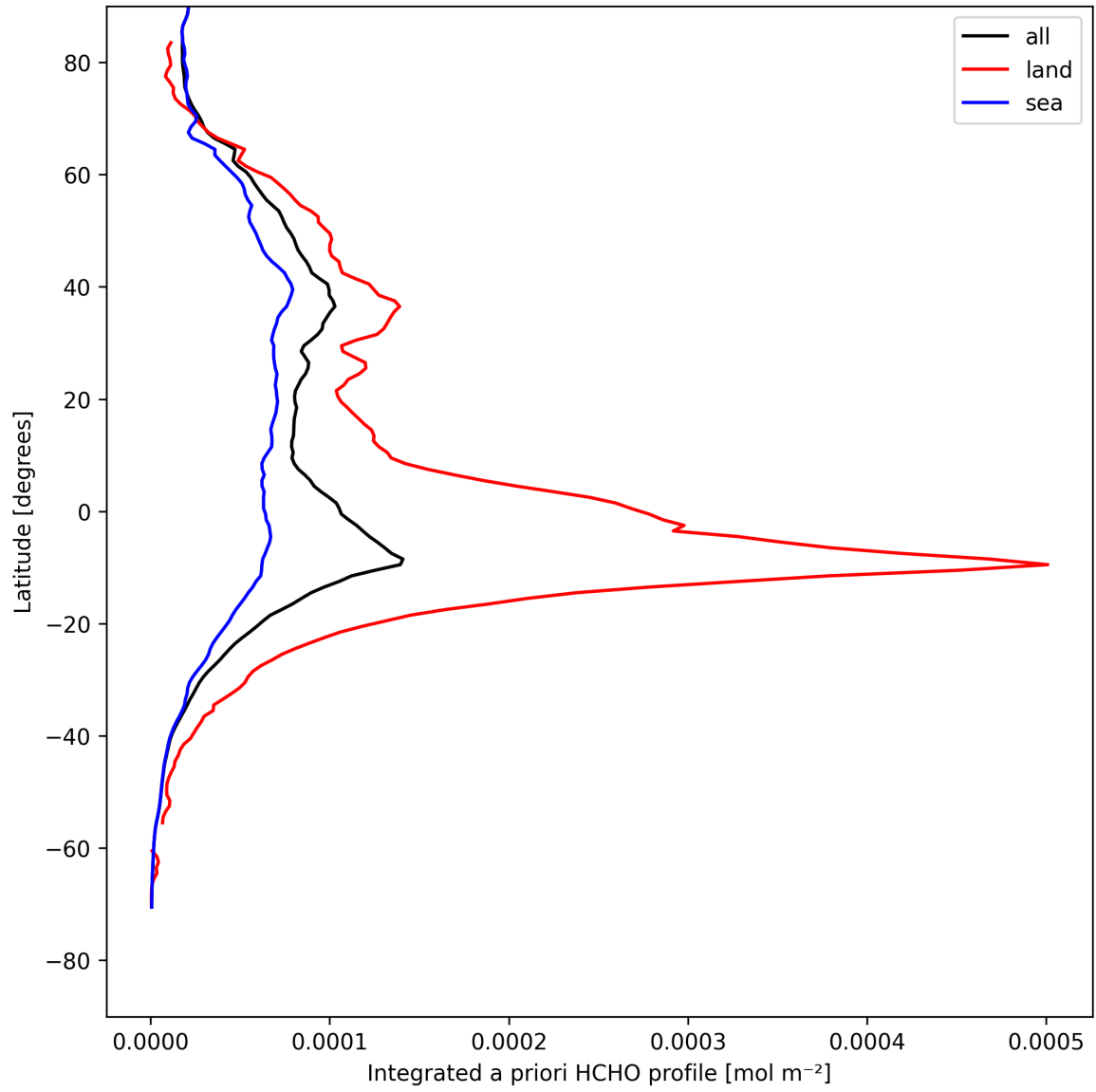
Figure 29: Zonal average of “Integrated a priori HCHO profile” for 2025-08-14 to 2025-08-15.
