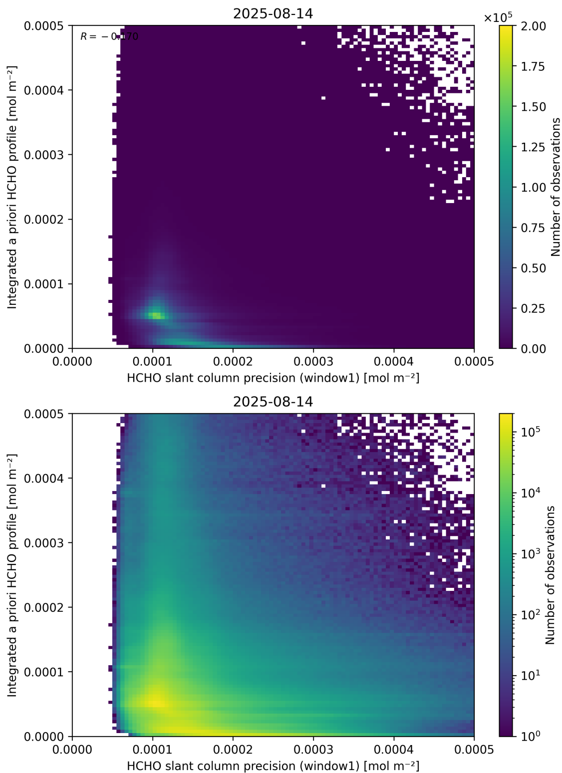
Figure 96: Scatter density plot of “HCHO slant column precision (window1)” against “Integrated a priori HCHO profile” for 2025-08-14 to 2025-08-15.
