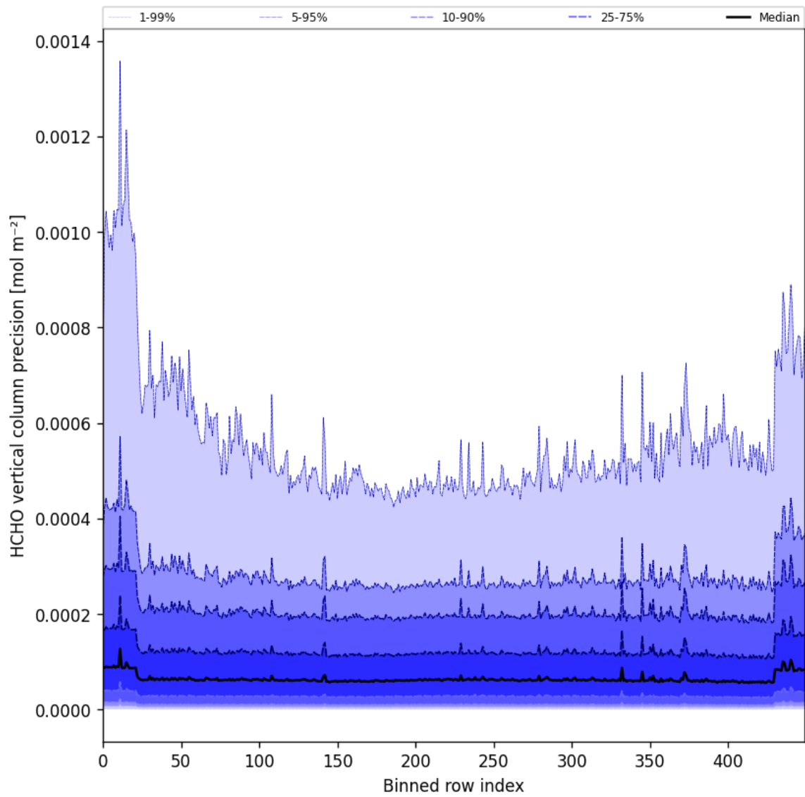
Figure 50: Along track statistics of “HCHO vertical column precision” for 2025-08-14 to 2025-08-15
