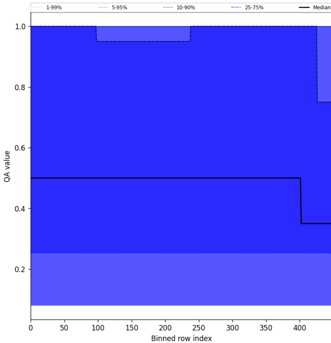
Figure 48: Along track statistics of “QA value” for 2025-08-14 to 2025-08-15
