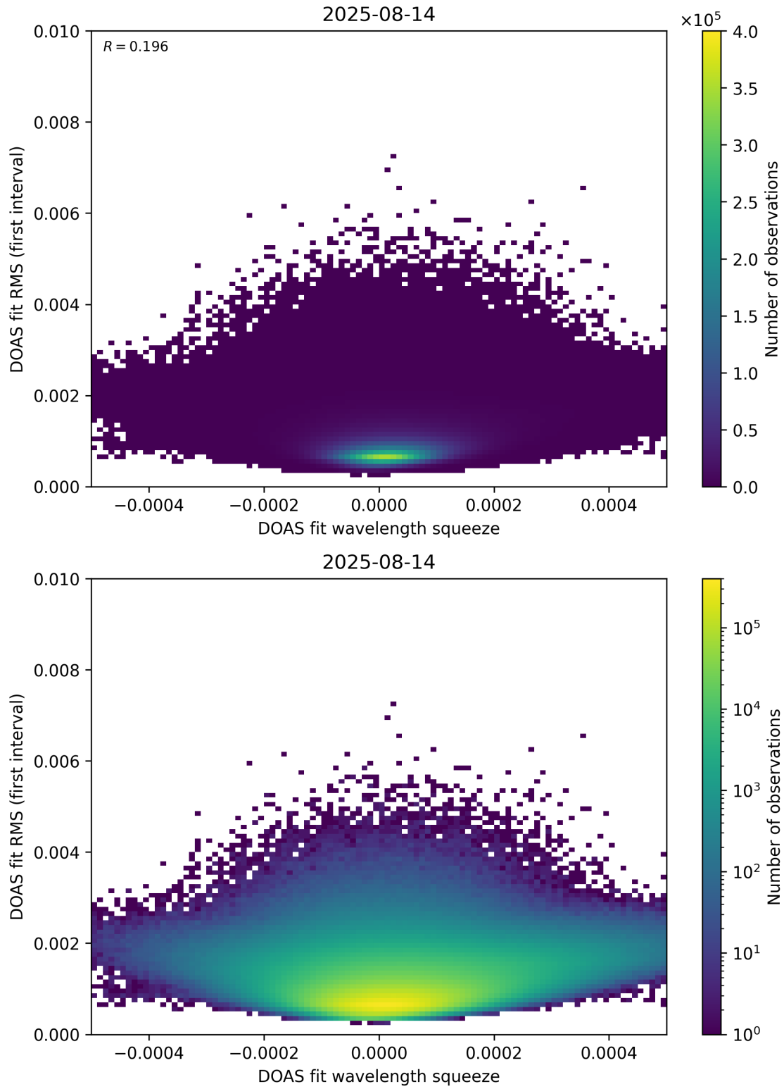
Figure 68: Scatter density plot of “DOAS fit wavelength squeeze” against “DOAS fit RMS (first interval)” for 2025-08-14 to 2025-08-15.
