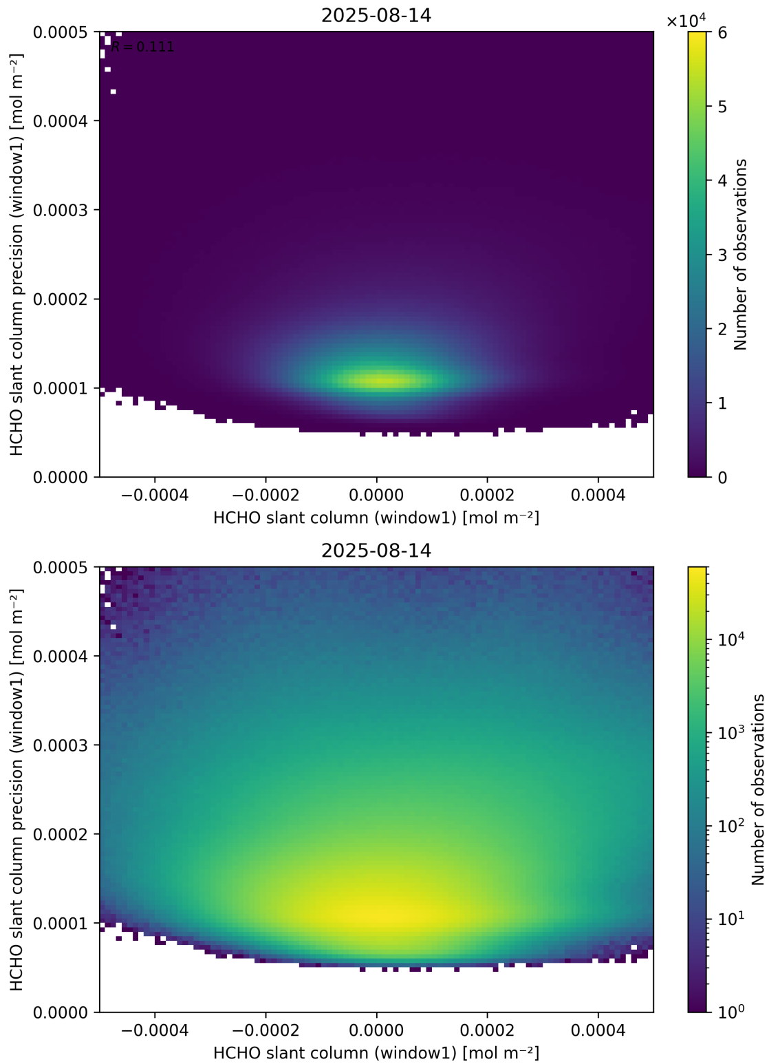
Figure 84: Scatter density plot of “HCHO slant column (window1)” against “HCHO slant column precision (window1)” for 2025-08-14 to 2025-08-15.
