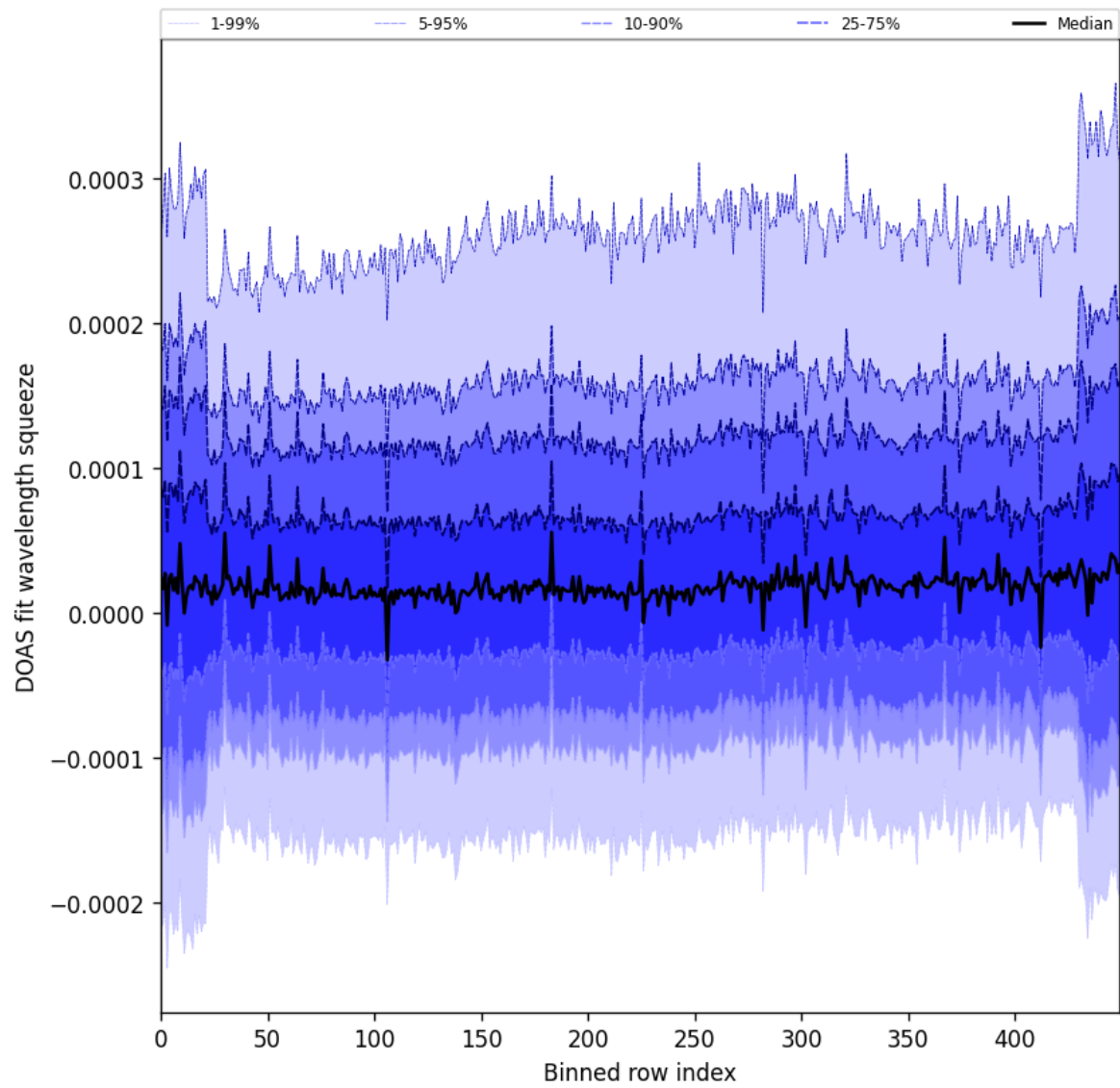
Figure 59: Along track statistics of “DOAS fit wavelength squeeze” for 2025-08-14 to 2025-08-15
