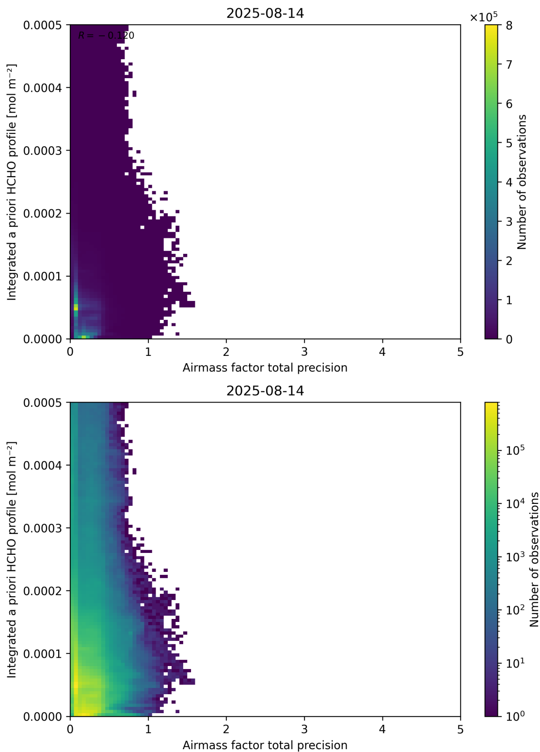
Figure 111: Scatter density plot of “Airmass factor total precision” against “Integrated a priori HCHO profile” for 2025-08-14 to 2025-08-15.
