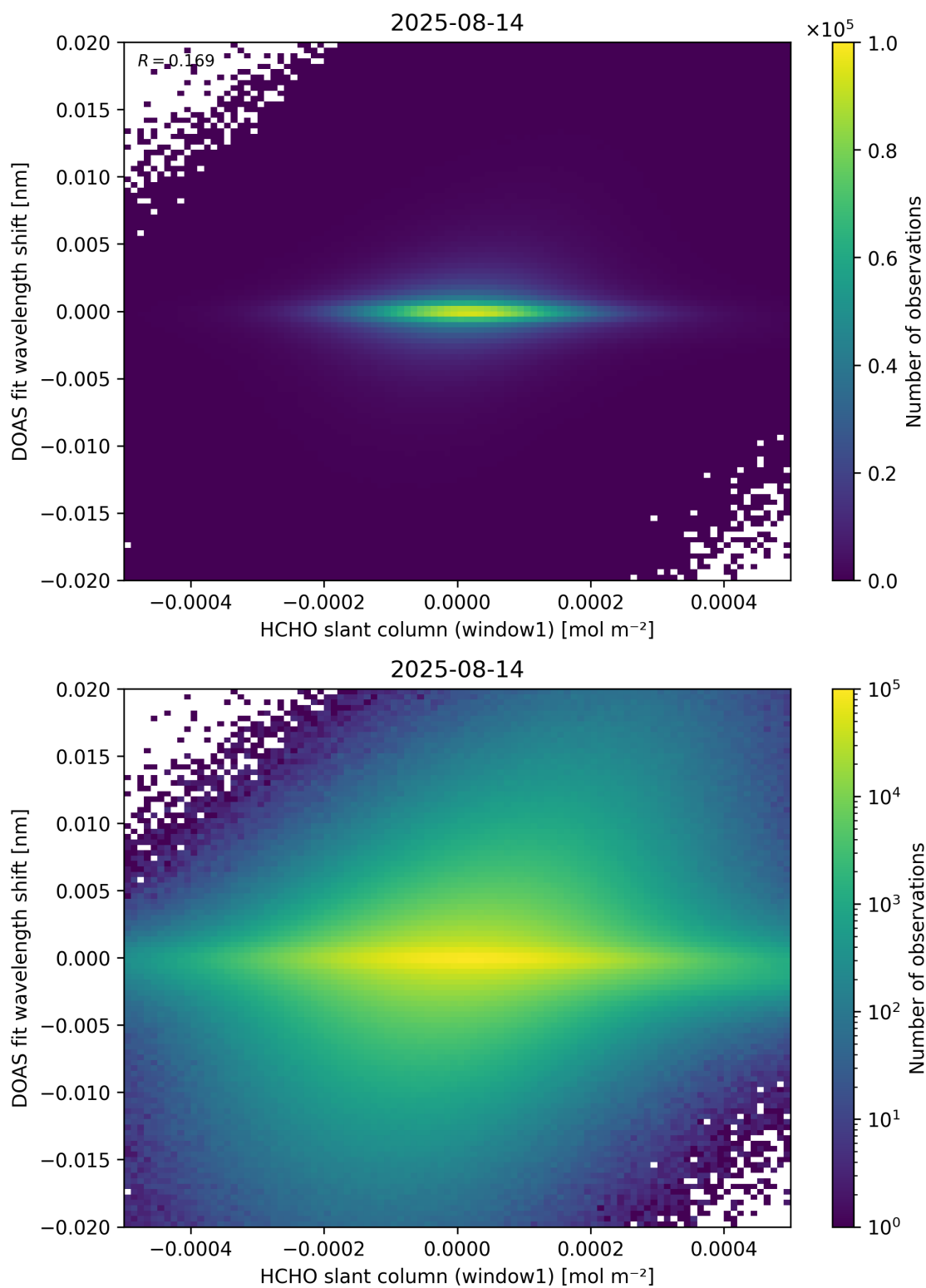
Figure 79: Scatter density plot of “HCHO slant column (window1)” against “DOAS fit wavelength shift” for 2025-08-14 to 2025-08-15.
