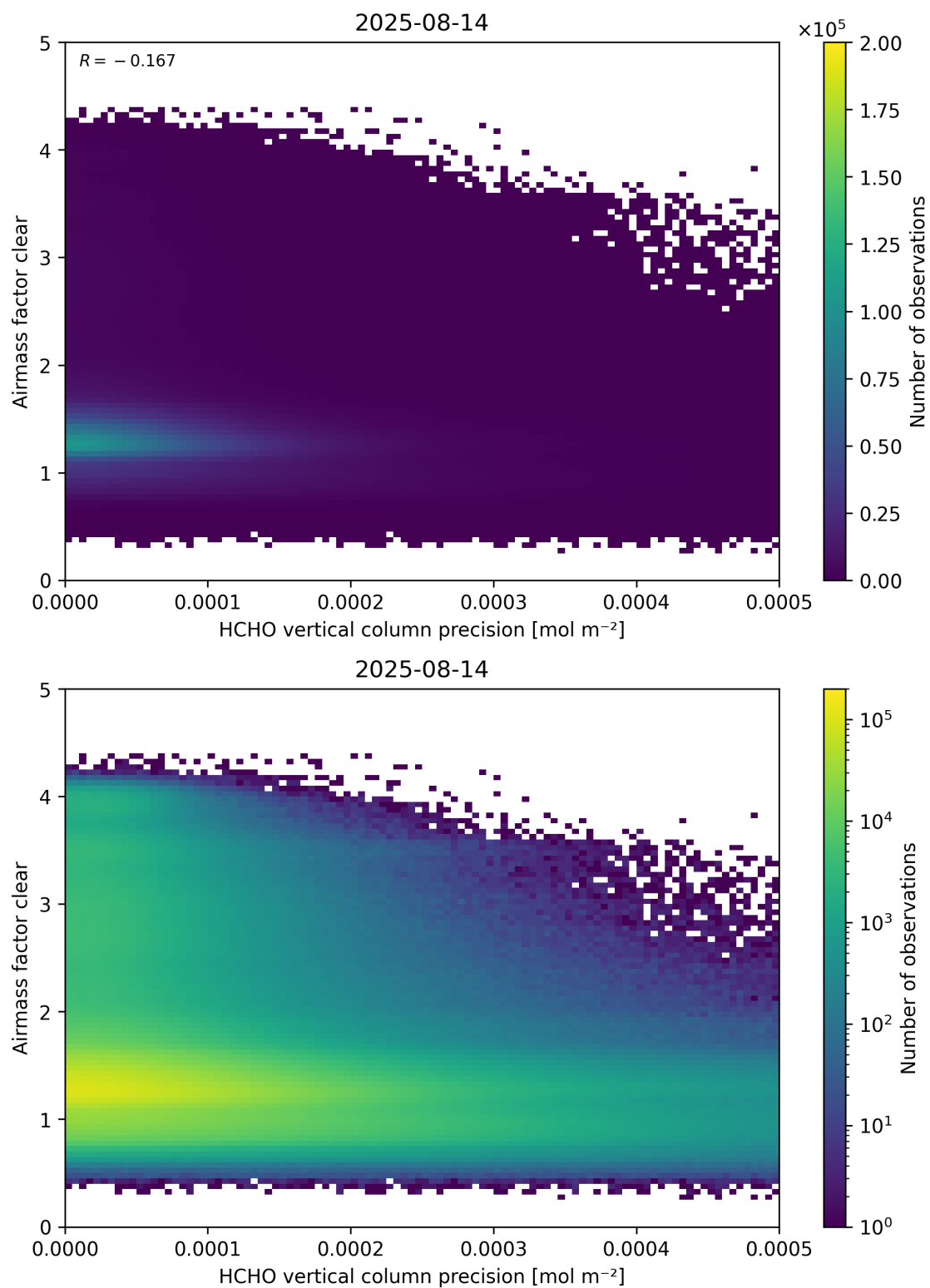
Figure 139: Scatter density plot of “HCHO vertical column precision” against “Airmass factor clear” for 2025-08-14 to 2025-08-15.
