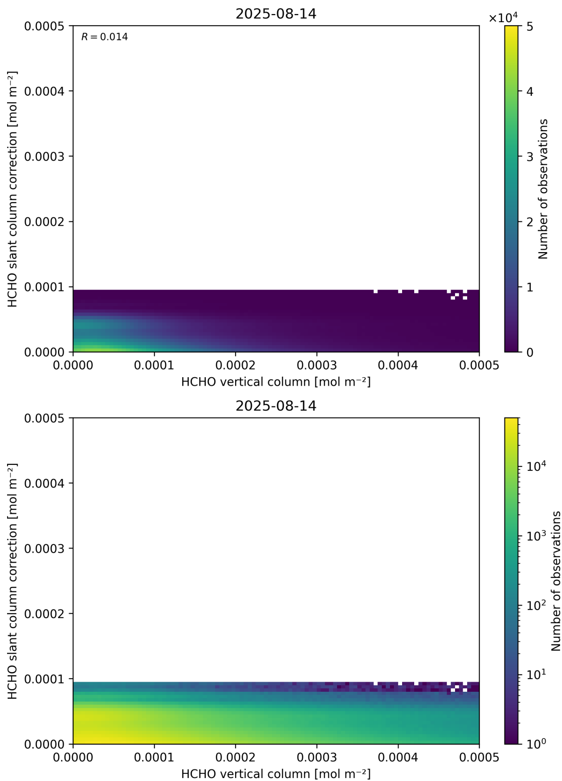
Figure 128: Scatter density plot of “HCHO vertical column” against “HCHO slant column correction” for 2025-08-14 to 2025-08-15.
