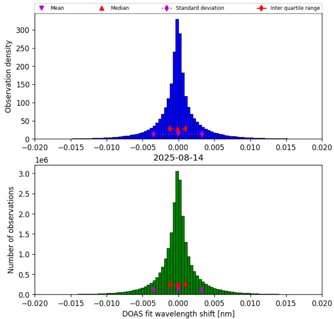
Figure 44: Histogram of “DOAS fit wavelength shift” for 2025-08-14 to 2025-08-15
