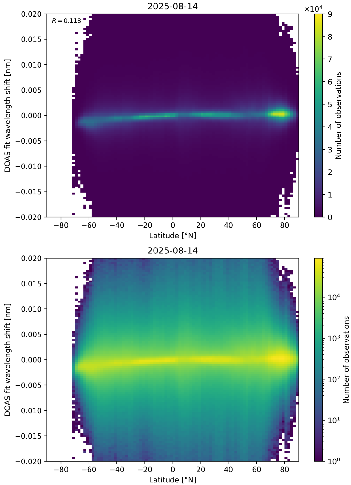
Figure 154: Scatter density plot of “Latitude” against “DOAS fit wavelength shift” for 2025-08-14 to 2025-08-15.
