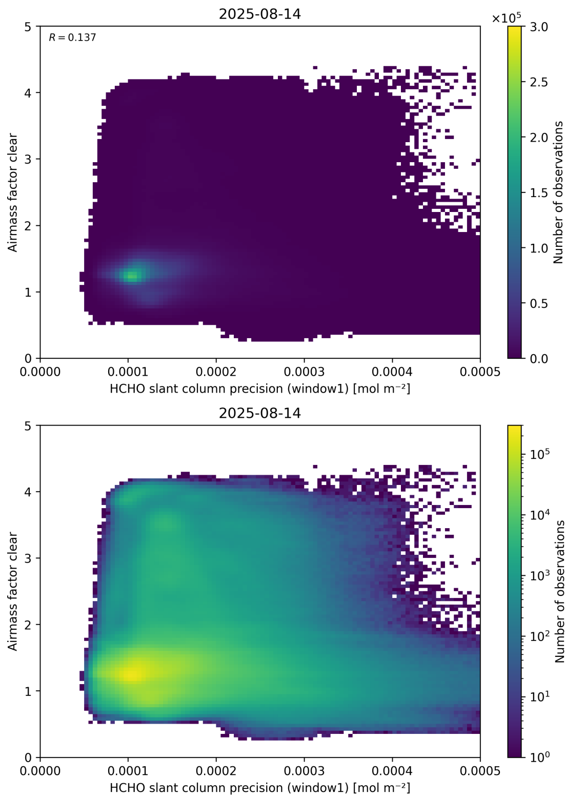
Figure 91: Scatter density plot of “HCHO slant column precision (window1)” against “Airmass factor clear” for 2025-08-14 to 2025-08-15.
