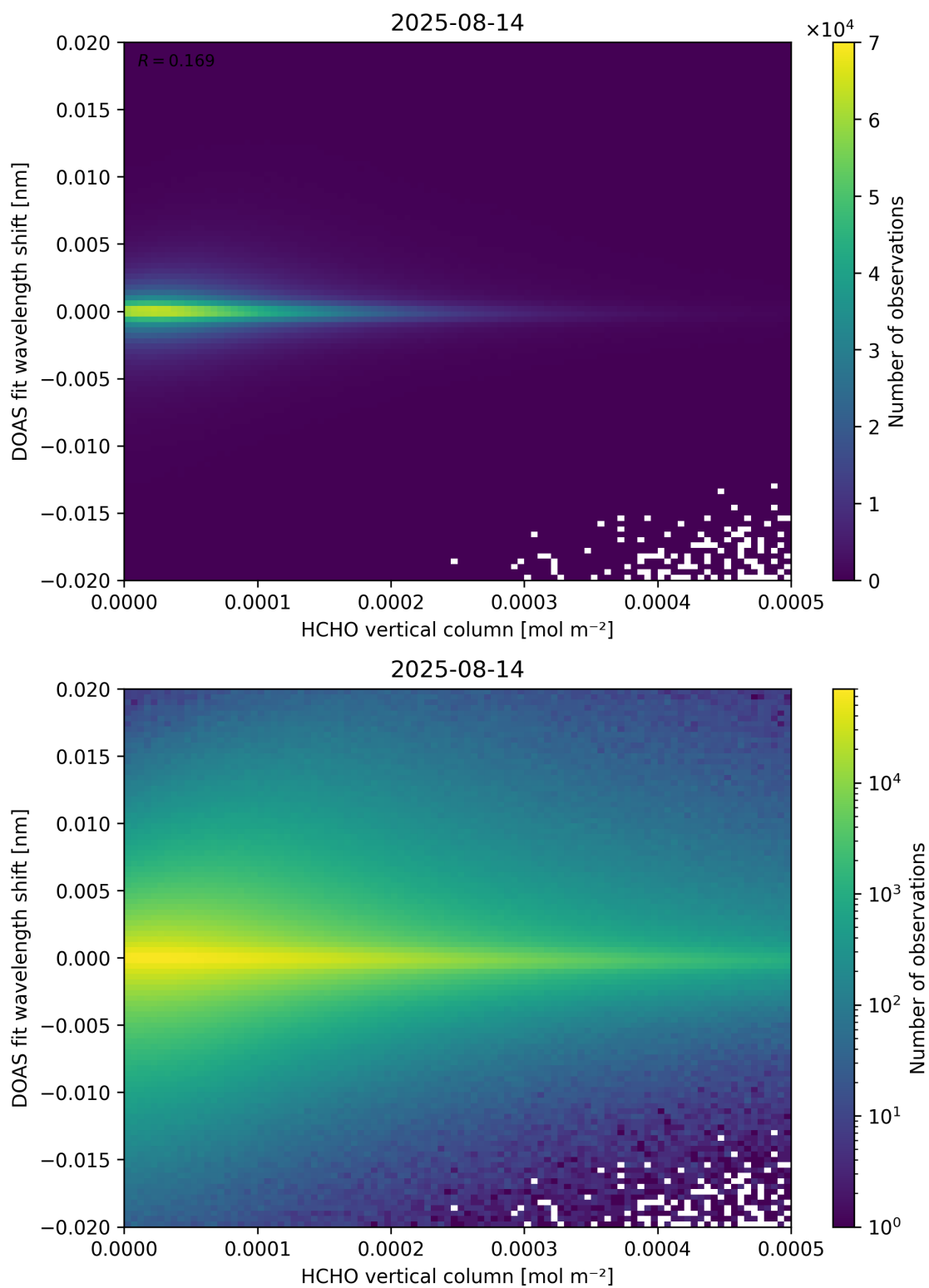
Figure 124: Scatter density plot of “HCHO vertical column” against “DOAS fit wavelength shift” for 2025-08-14 to 2025-08-15.
