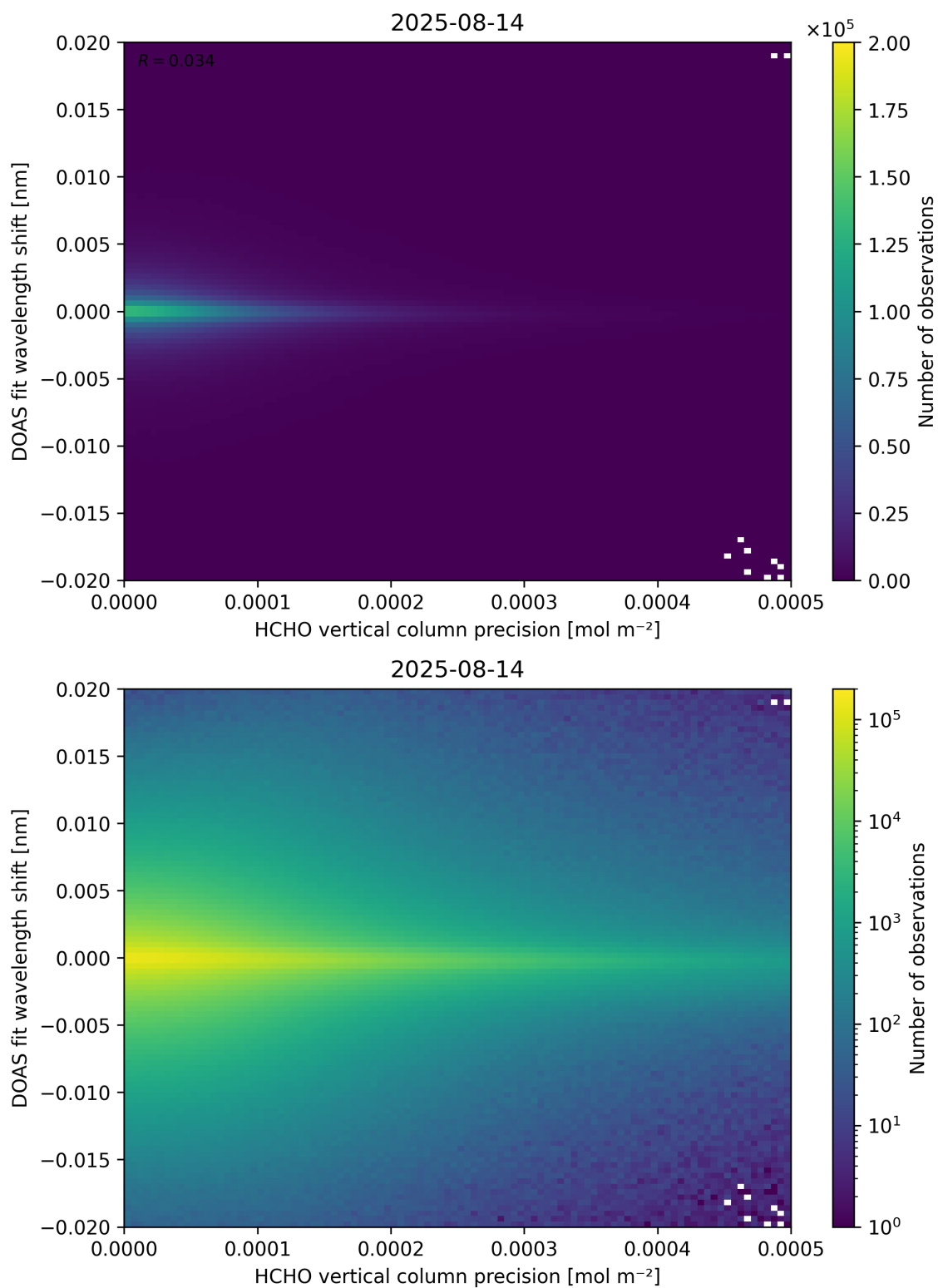
Figure 137: Scatter density plot of “HCHO vertical column precision” against “DOAS fit wavelength shift” for 2025-08-14 to 2025-08-15.
