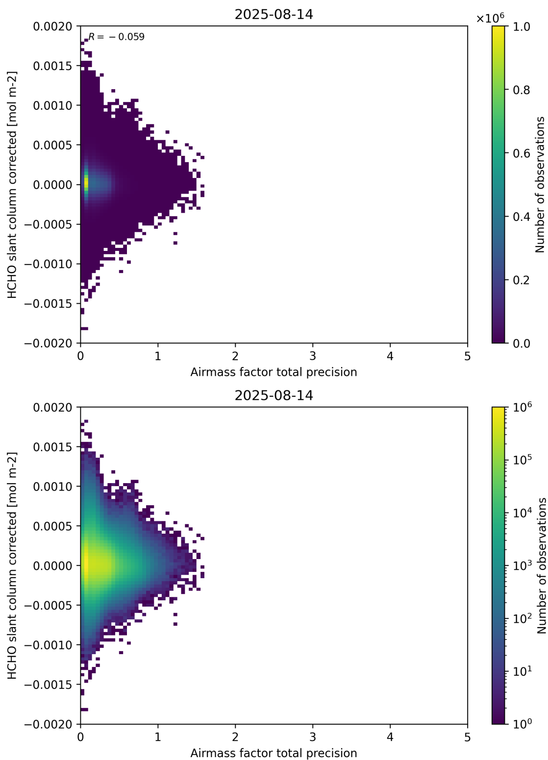
Figure 109: Scatter density plot of “Airmass factor total precision” against “HCHO slant column corrected” for 2025-08-14 to 2025-08-15.
