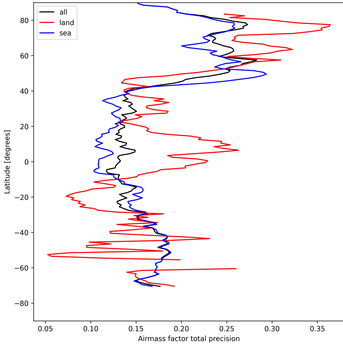
Figure 27: Zonal average of “Airmass factor total precision” for 2025-08-14 to 2025-08-15.
