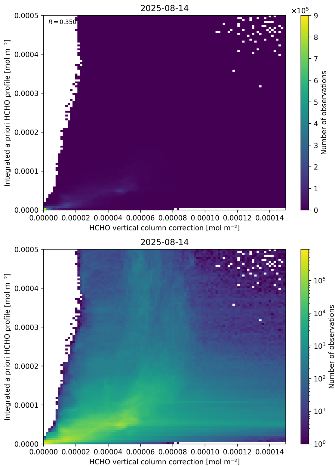
Figure 122: Scatter density plot of “HCHO vertical column correction” against “Integrated a priori HCHO profile” for 2025-08-14 to 2025-08-15.
