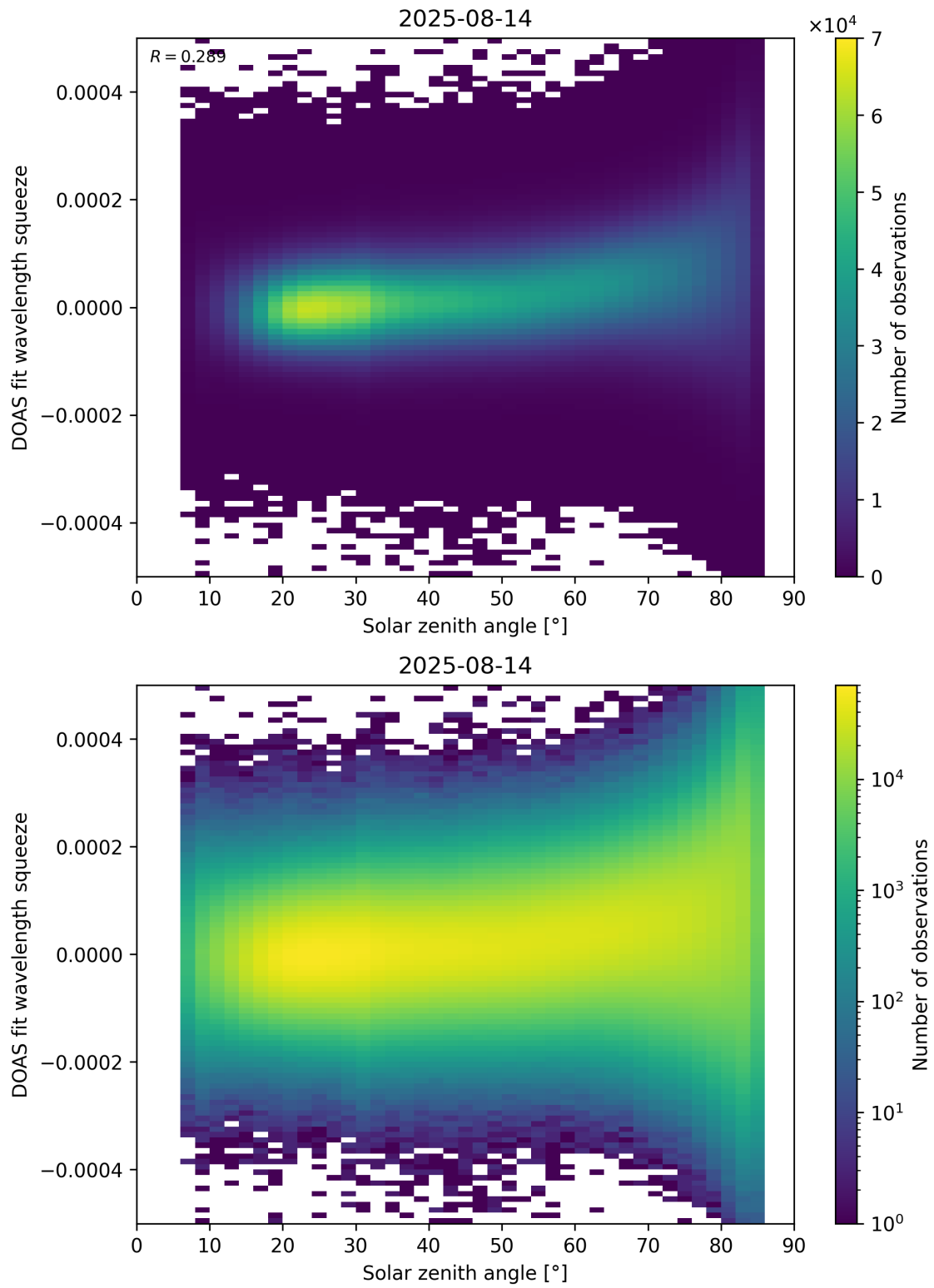
Figure 169: Scatter density plot of “Solar zenith angle” against “DOAS fit wavelength squeeze” for 2025-08-14 to 2025-08-15.
