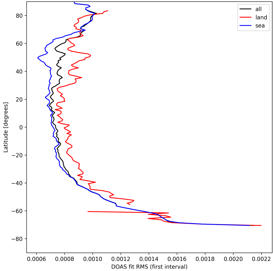
Figure 32: Zonal average of “DOAS fit RMS (first interval)” for 2025-08-14 to 2025-08-15.
