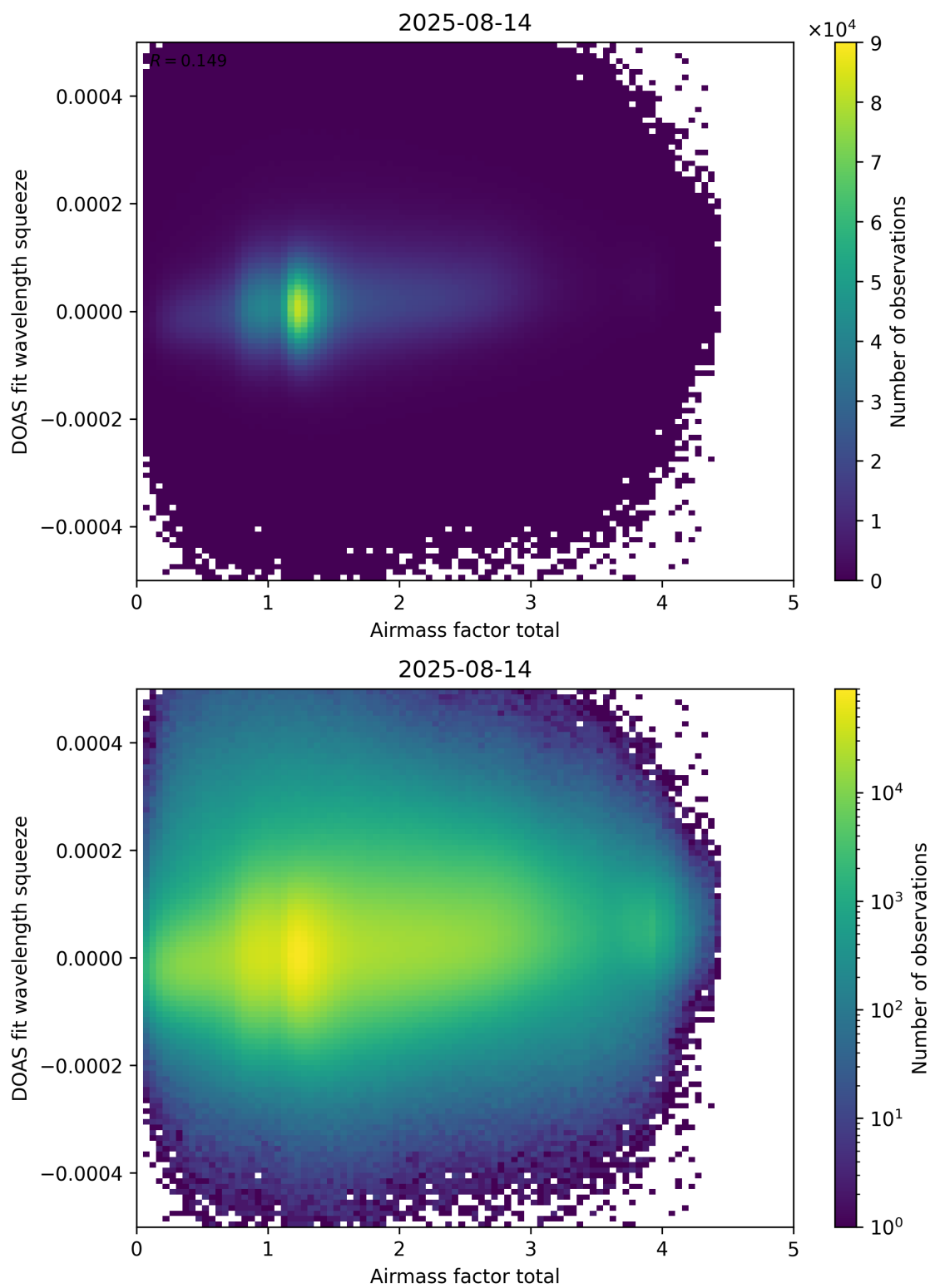
Figure 99: Scatter density plot of “Airmass factor total” against “DOAS fit wavelength squeeze” for 2025-08-14 to 2025-08-15.
