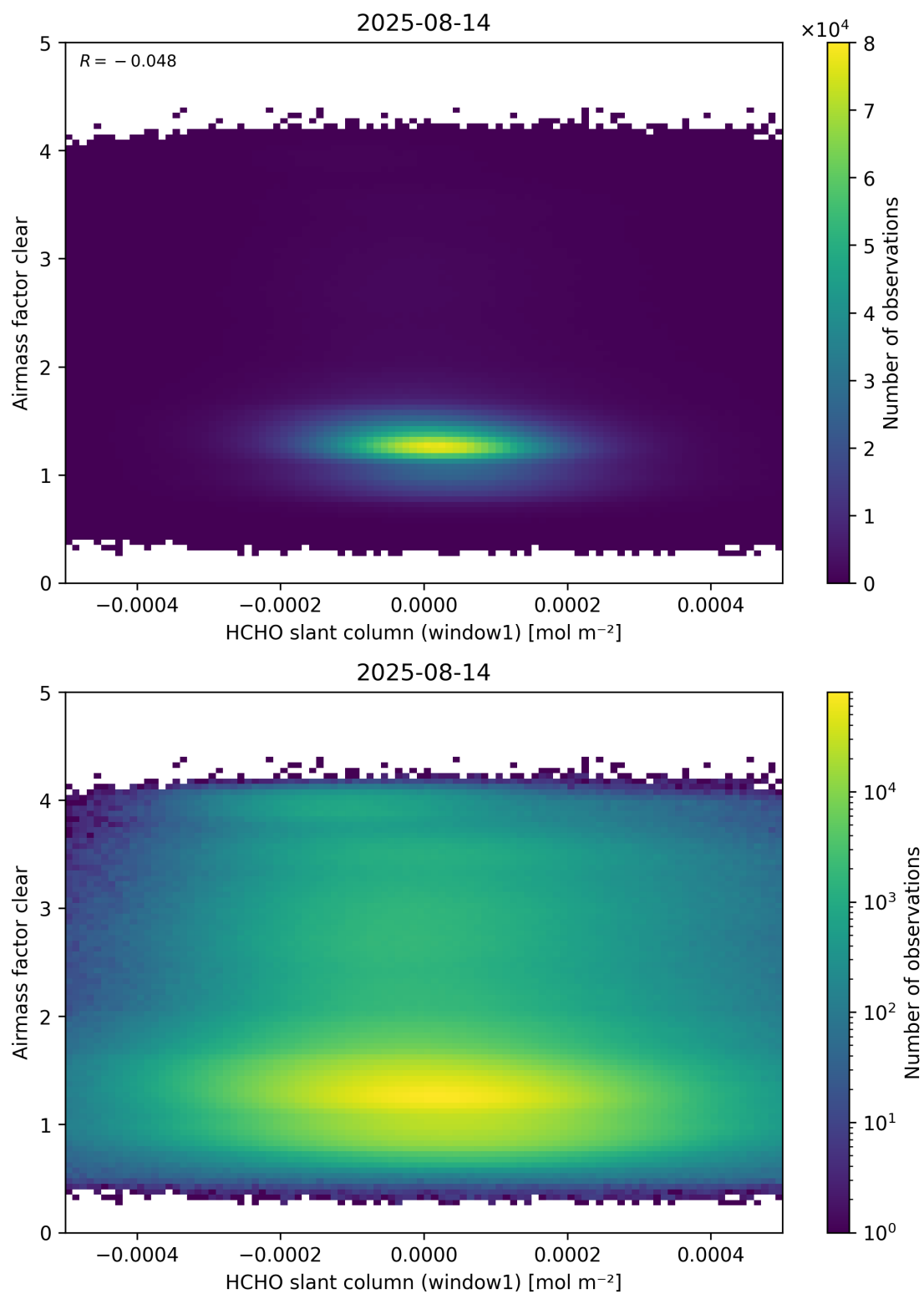
Figure 81: Scatter density plot of “HCHO slant column (window1)” against “Airmass factor clear” for 2025-08-14 to 2025-08-15.
