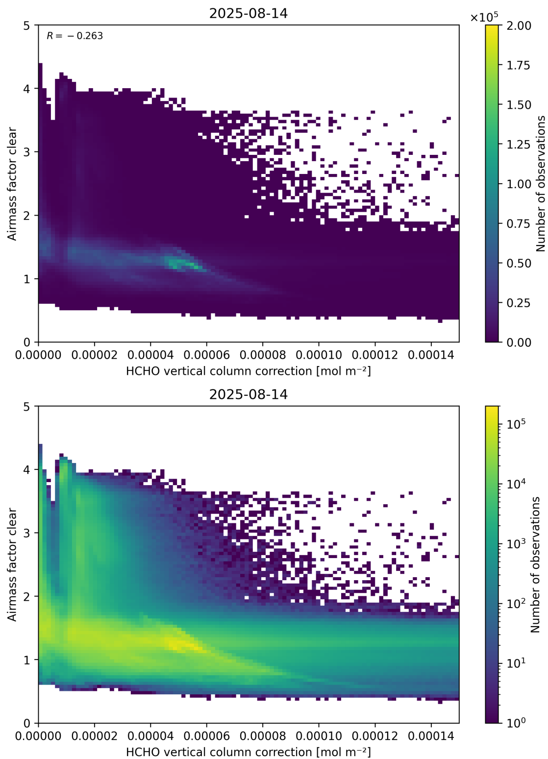
Figure 115: Scatter density plot of “HCHO vertical column correction” against “Airmass factor clear” for 2025-08-14 to 2025-08-15.
