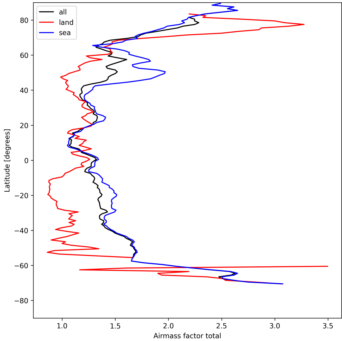
Figure 26: Zonal average of “Airmass factor total” for 2025-08-14 to 2025-08-15.
