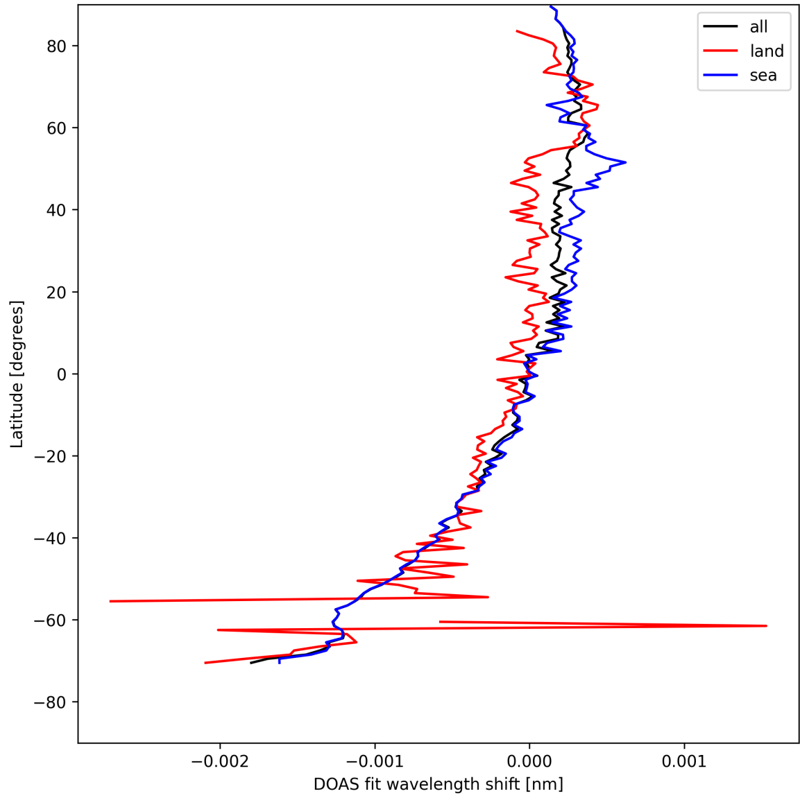
Figure 30: Zonal average of "DOAS fit wavelength shift" for 2025-08-14 to 2025-08-15.
