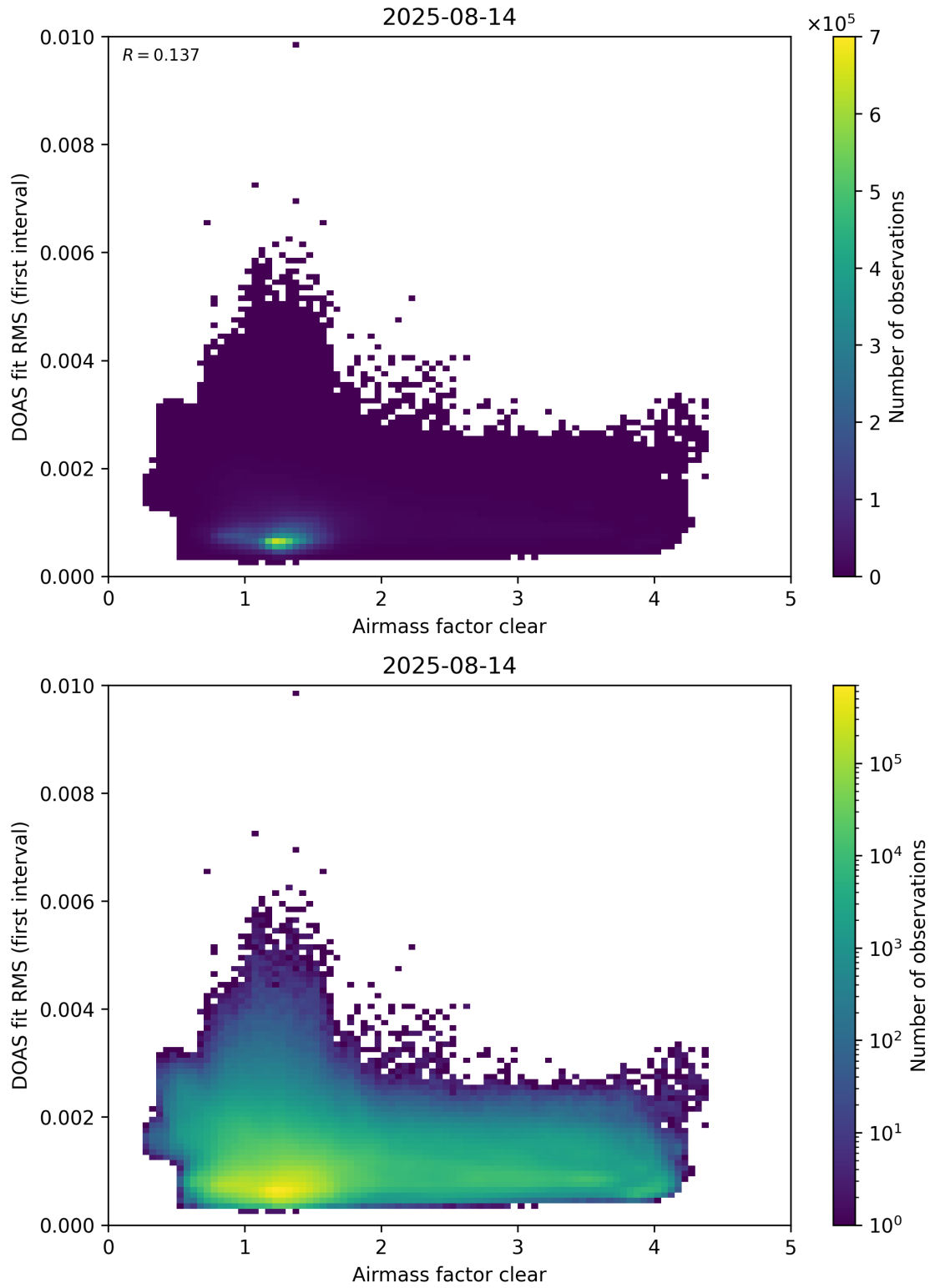
Figure 71: Scatter density plot of “Airmass factor clear” against “DOAS fit RMS (first interval)” for 2025-08-14 to 2025-08-15.
