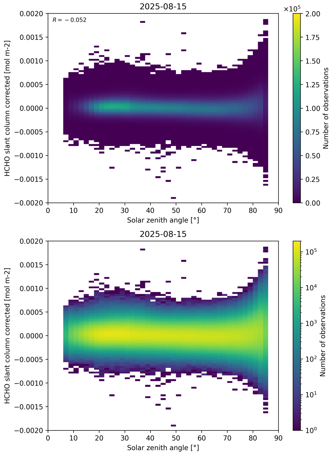
Figure 171: Scatter density plot of “Solar zenith angle” against “HCHO slant column corrected” for 2025-08-14 to 2025-08-16.
