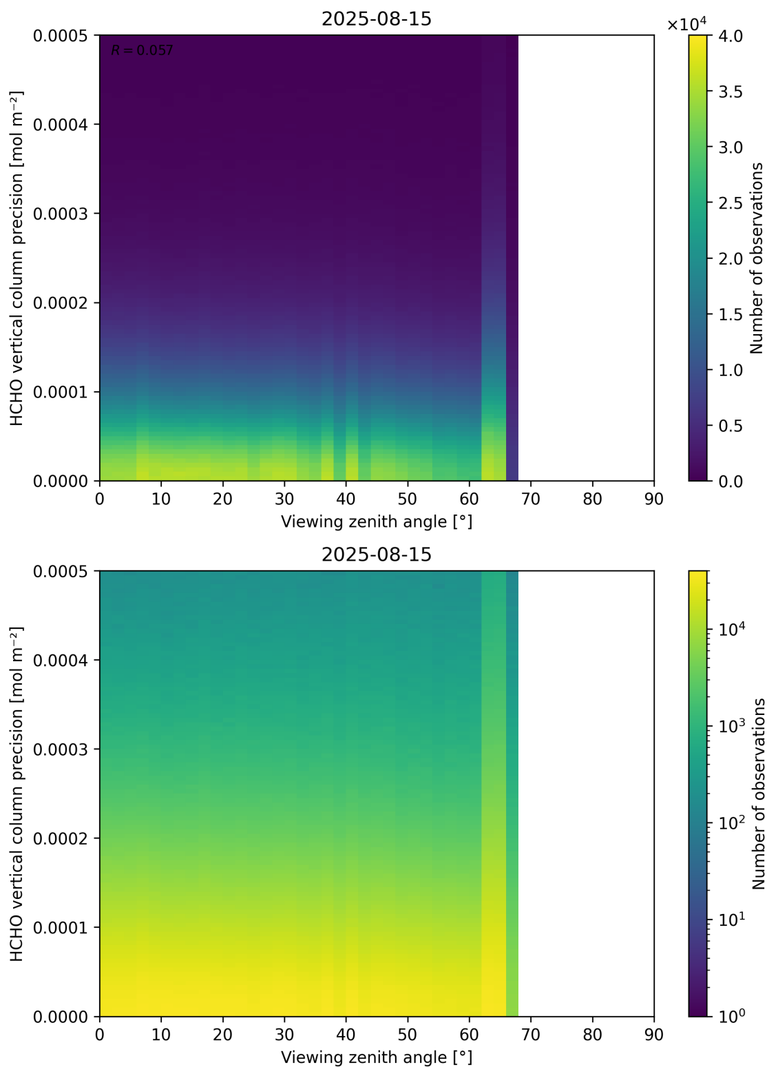
Figure 194: Scatter density plot of “Viewing zenith angle” against “HCHO vertical column precision” for 2025-08-14 to 2025-08-16.
