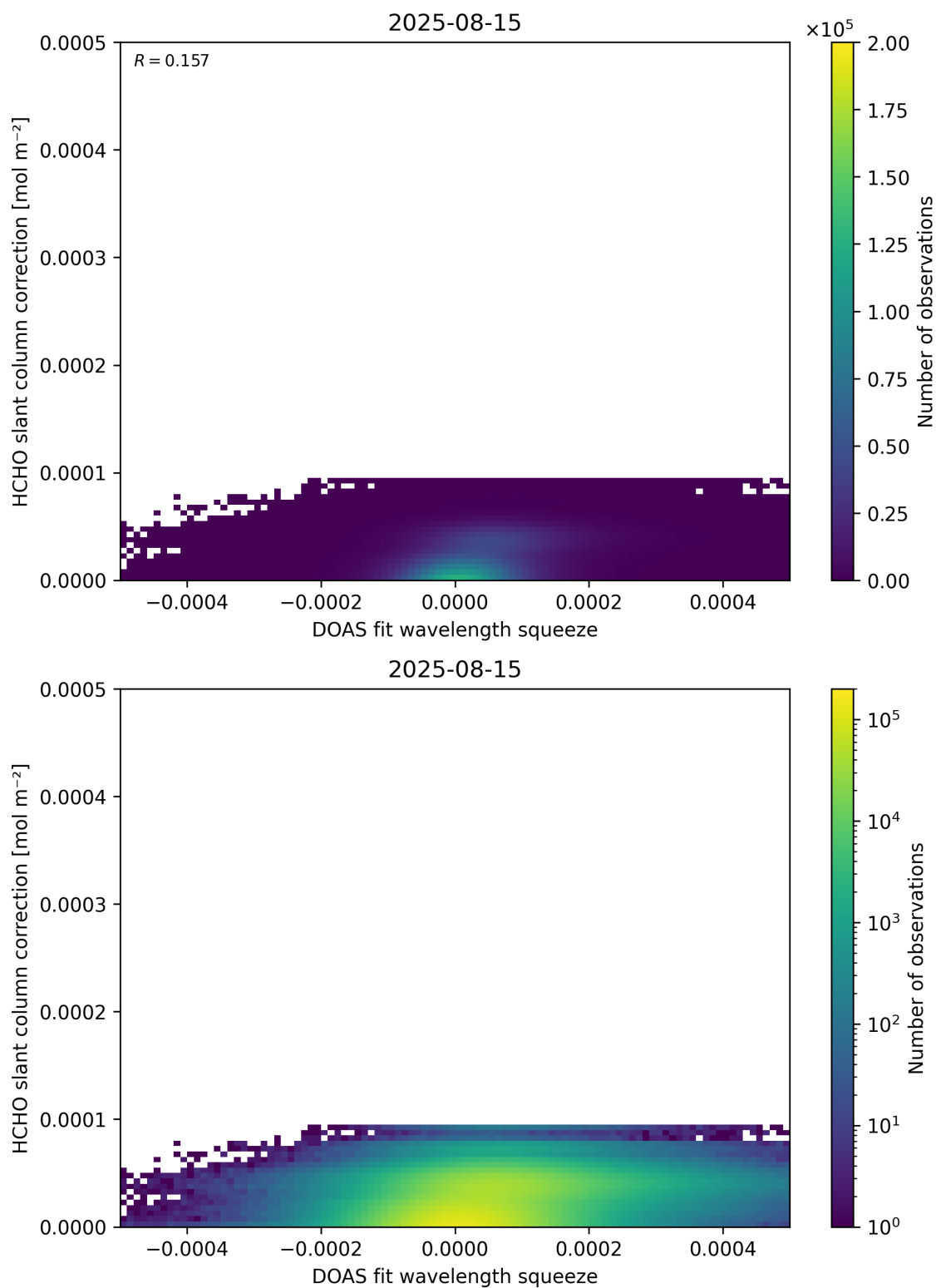
Figure 70: Scatter density plot of “DOAS fit wavelength squeeze” against “HCHO slant column correction” for 2025-08-14 to 2025-08-16.
