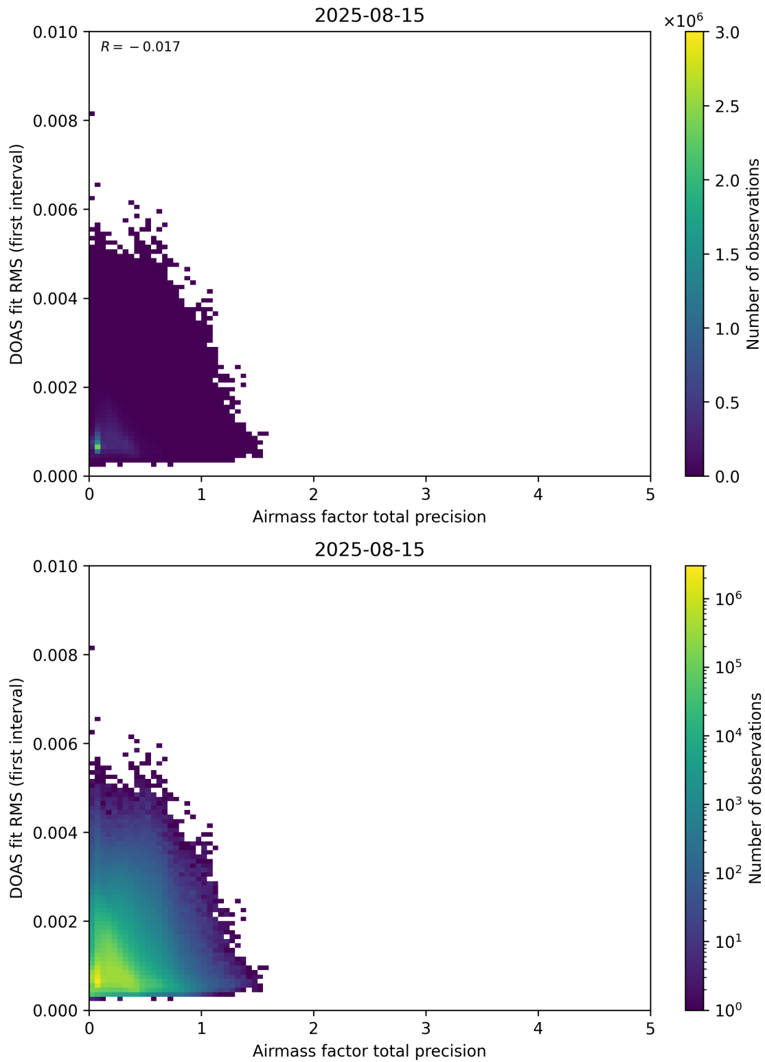
Figure 105: Scatter density plot of “Airmass factor total precision” against “DOAS fit RMS (first interval)” for 2025-08-14 to 2025-08-16.
