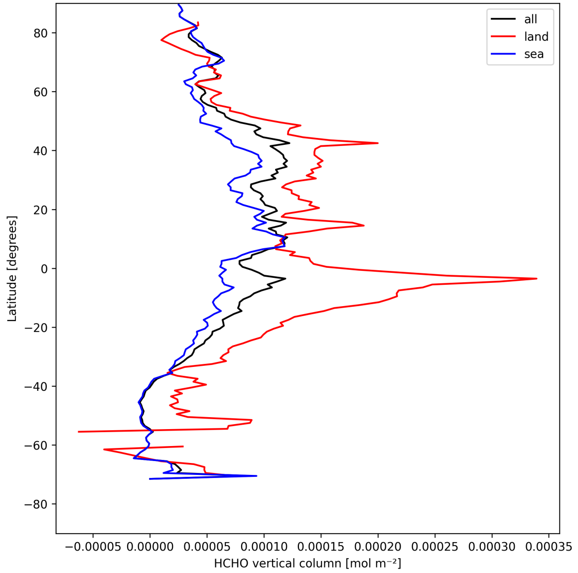
Figure 21: Zonal average of “HCHO vertical column” for 2025-08-14 to 2025-08-16.
