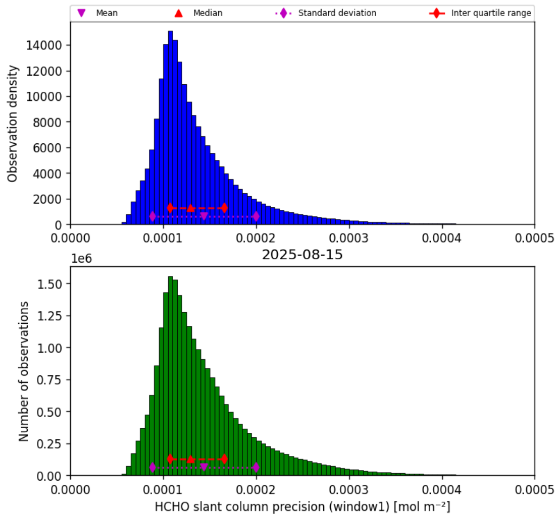
Figure 39: Histogram of “HCHO slant column precision (window1)” for 2025-08-14 to 2025-08-16
