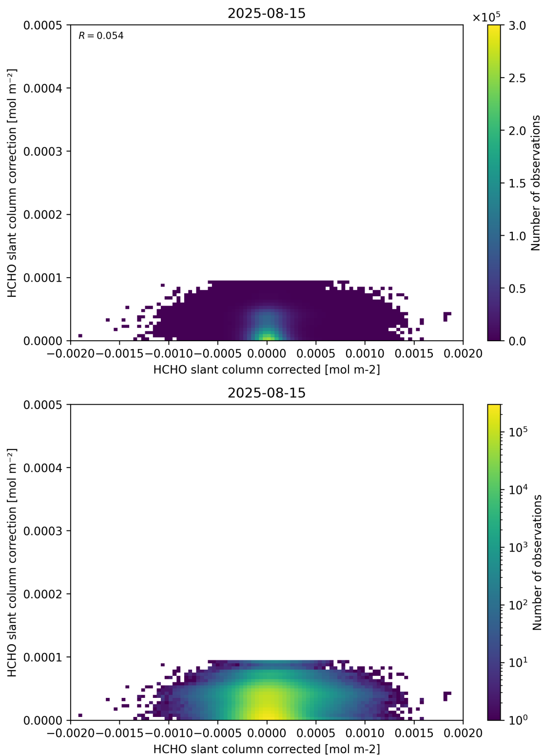
Figure 77: Scatter density plot of “HCHO slant column corrected” against “HCHO slant column correction” for 2025-08-14 to 2025-08-16.
