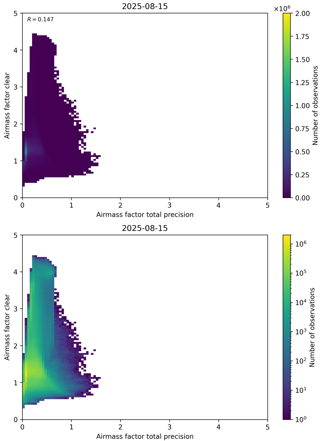
Figure 108: Scatter density plot of “Airmass factor total precision” against “Airmass factor clear” for 2025-08-14 to 2025-08-16.
