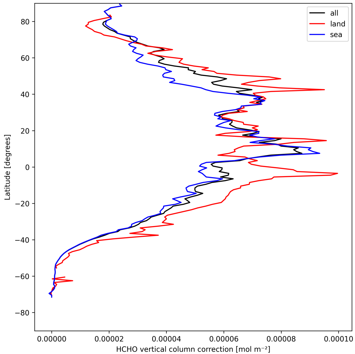
Figure 23: Zonal average of “HCHO vertical column correction” for 2025-08-14 to 2025-08-16.
