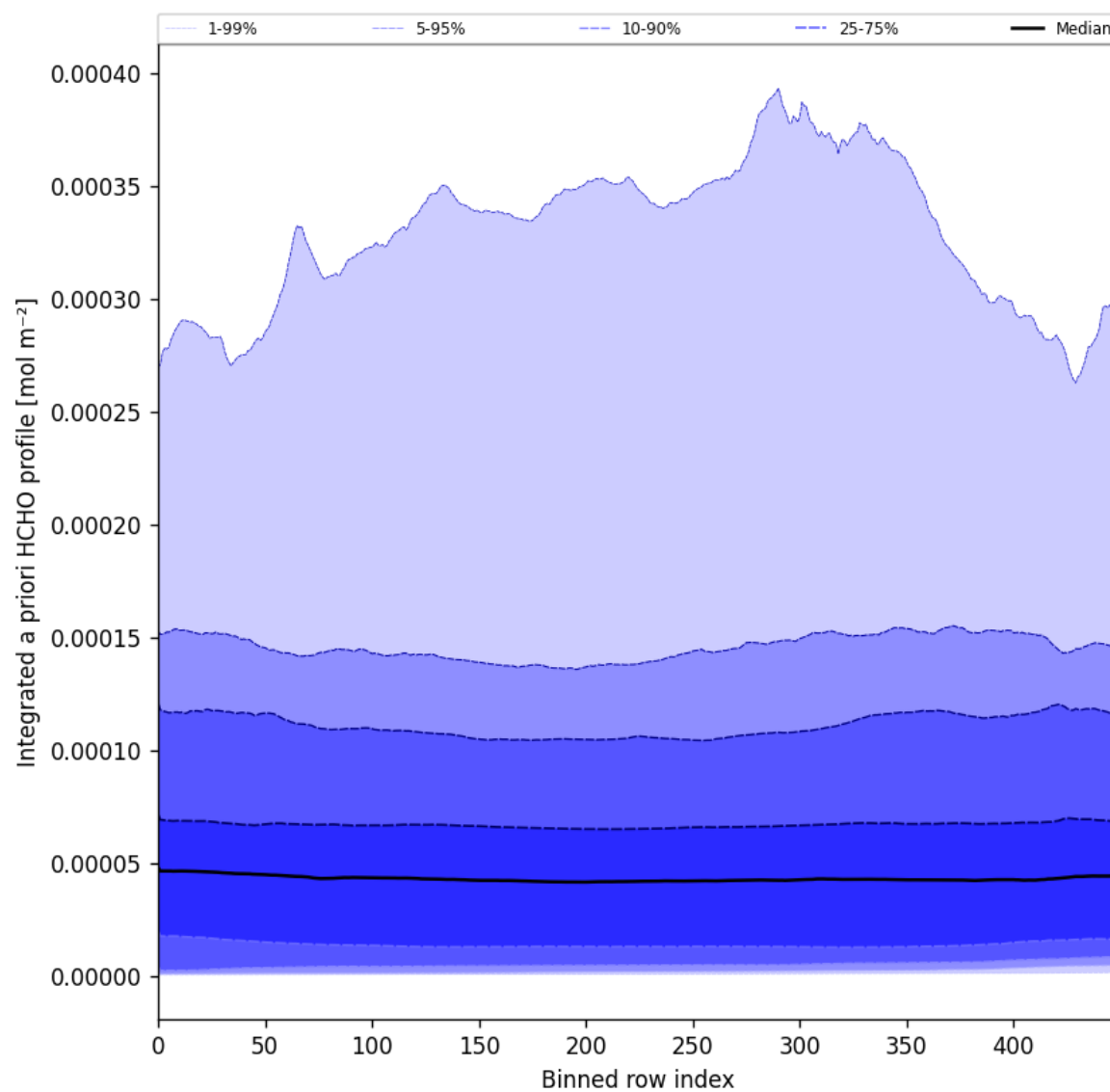
Figure 57: Along track statistics of "Integrated a priori HCHO profile" for 2025-08-14 to 2025-08-16
