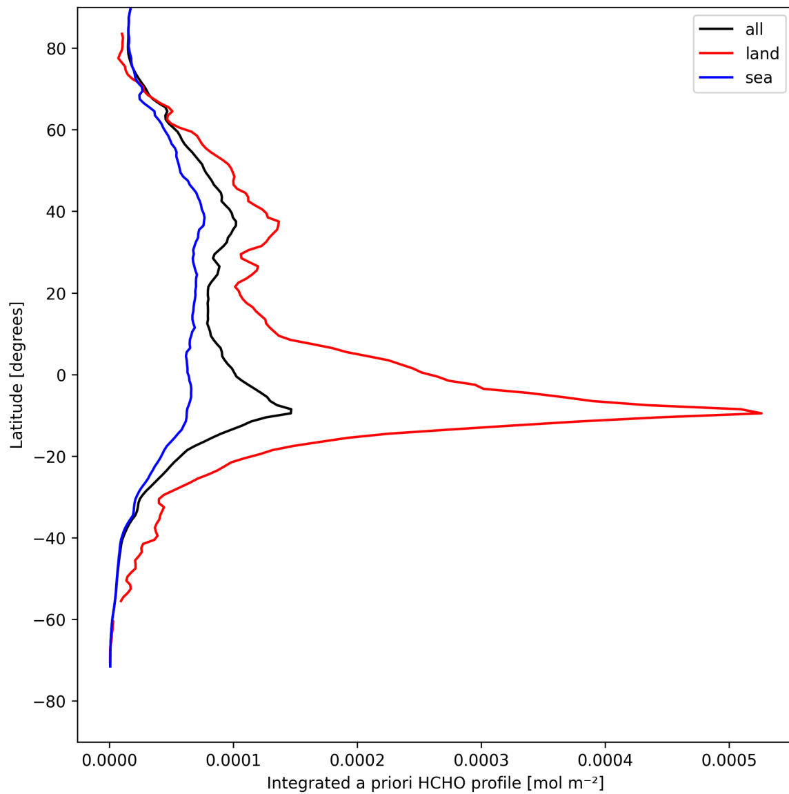
Figure 29: Zonal average of “Integrated a priori HCHO profile” for 2025-08-14 to 2025-08-16.
