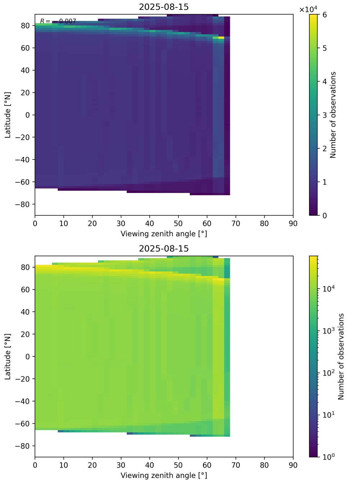
Figure 196: Scatter density plot of “Viewing zenith angle” against “Latitude” for 2025-08-14 to 2025-08-16.
