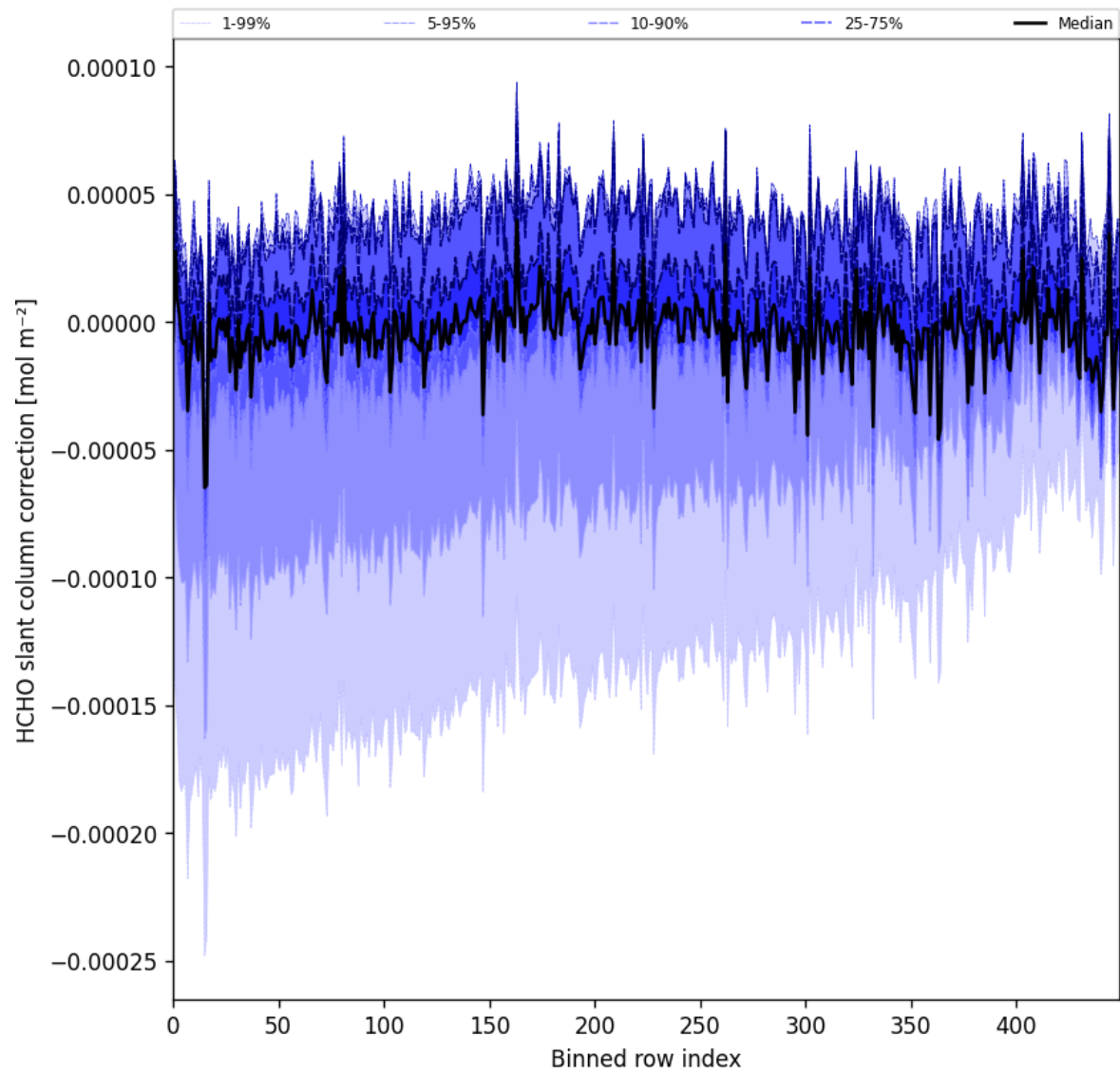
Figure 61: Along track statistics of “HCHO slant column correction” for 2025-08-14 to 2025-08-16
