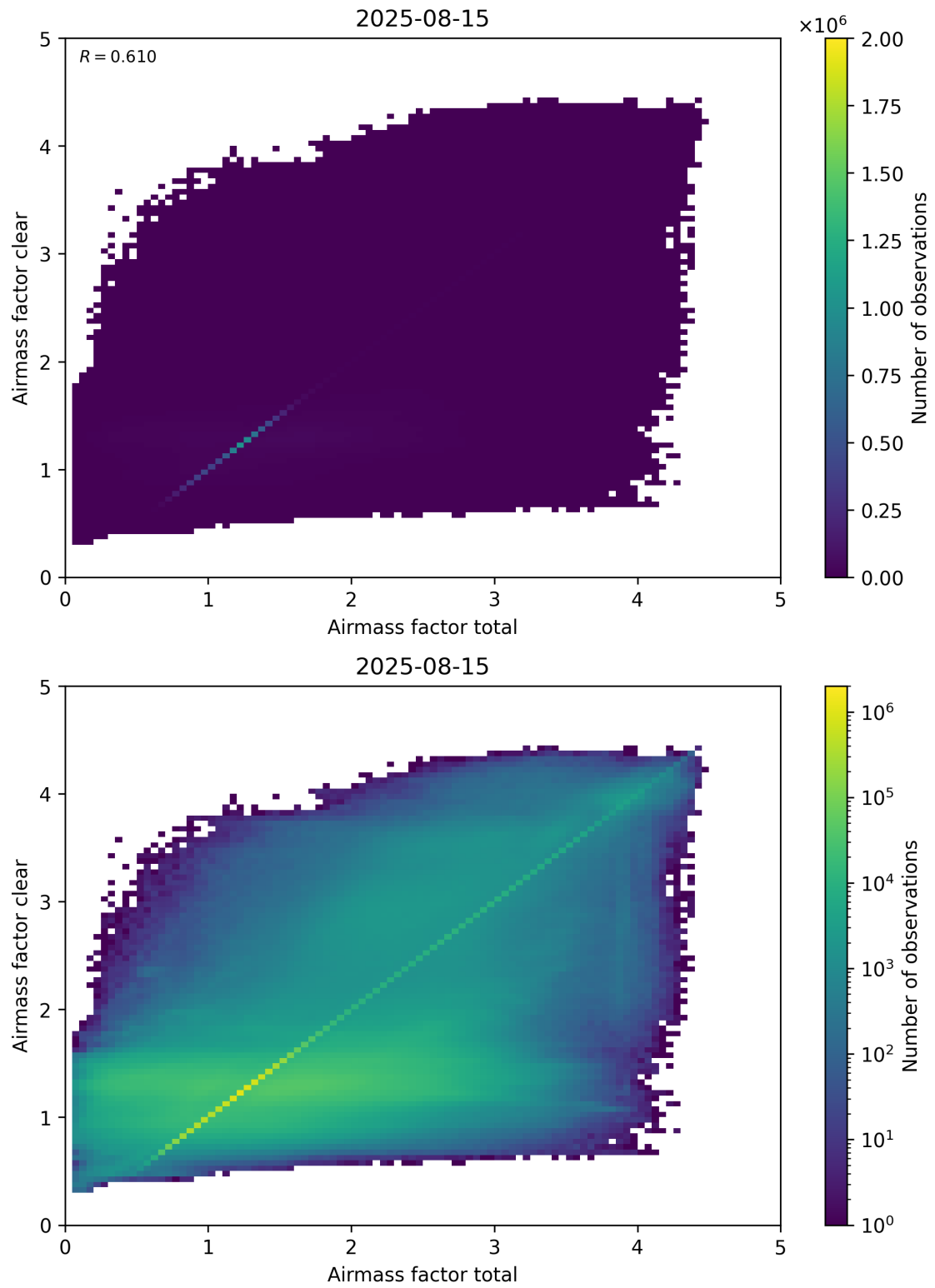
Figure 100: Scatter density plot of “Airmass factor total” against “Airmass factor clear” for 2025-08-14 to 2025-08-16.
