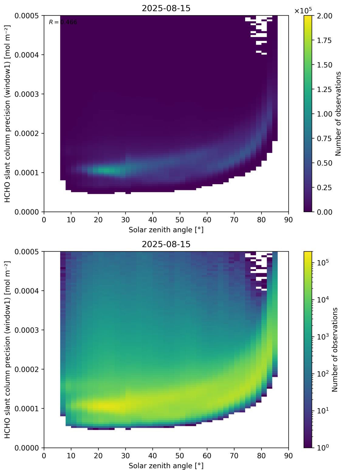
Figure 174: Scatter density plot of “Solar zenith angle” against “HCHO slant column precision (window1)” for 2025-08-14 to 2025-08-16.
