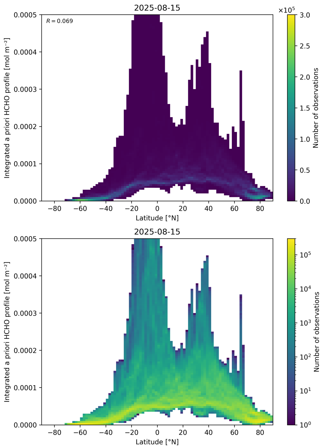
Figure 166: Scatter density plot of “Latitude” against “Integrated a priori HCHO profile” for 2025-08-14 to 2025-08-16.
