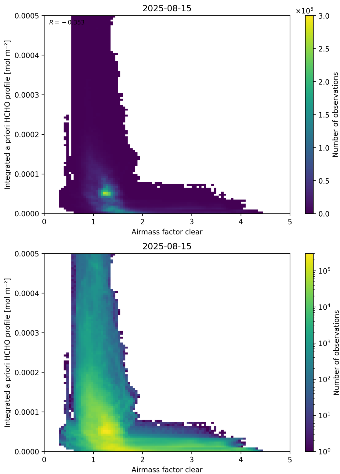
Figure 76: Scatter density plot of “Airmass factor clear” against “Integrated a priori HCHO profile” for 2025-08-14 to 2025-08-16.
