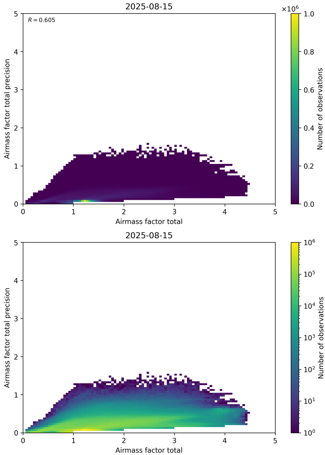
Figure 103: Scatter density plot of “Airmass factor total” against “Airmass factor total precision” for 2025-08-14 to 2025-08-16.
