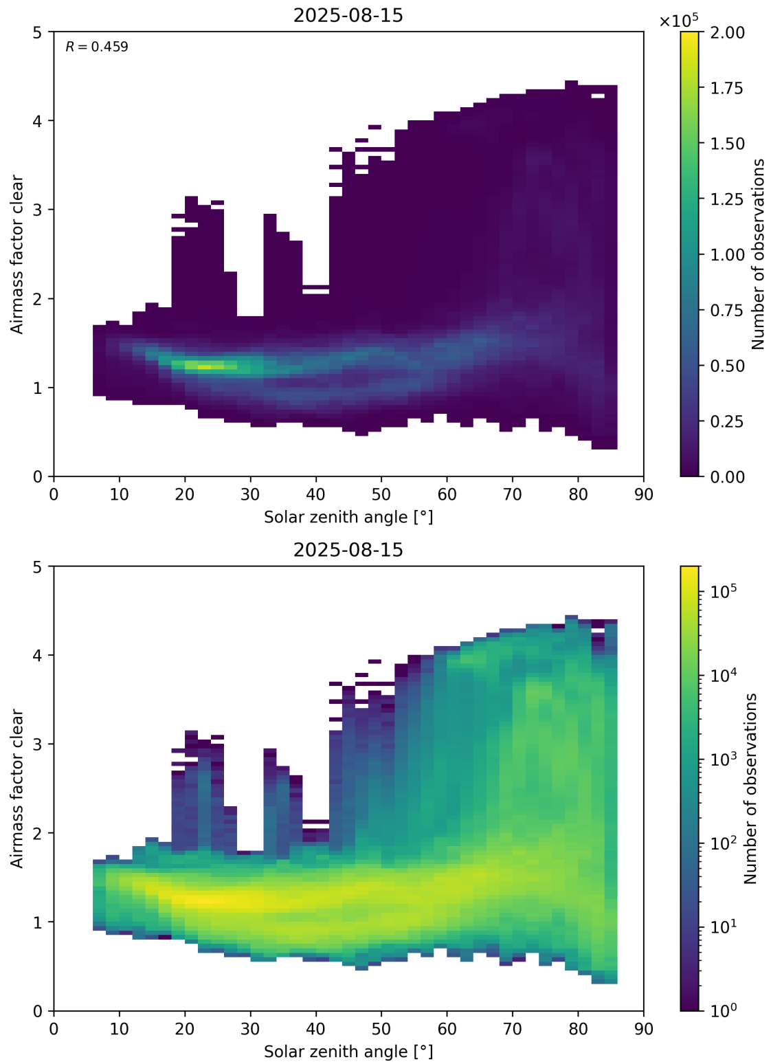
Figure 170: Scatter density plot of “Solar zenith angle” against “Airmass factor clear” for 2025-08-14 to 2025-08-16.
