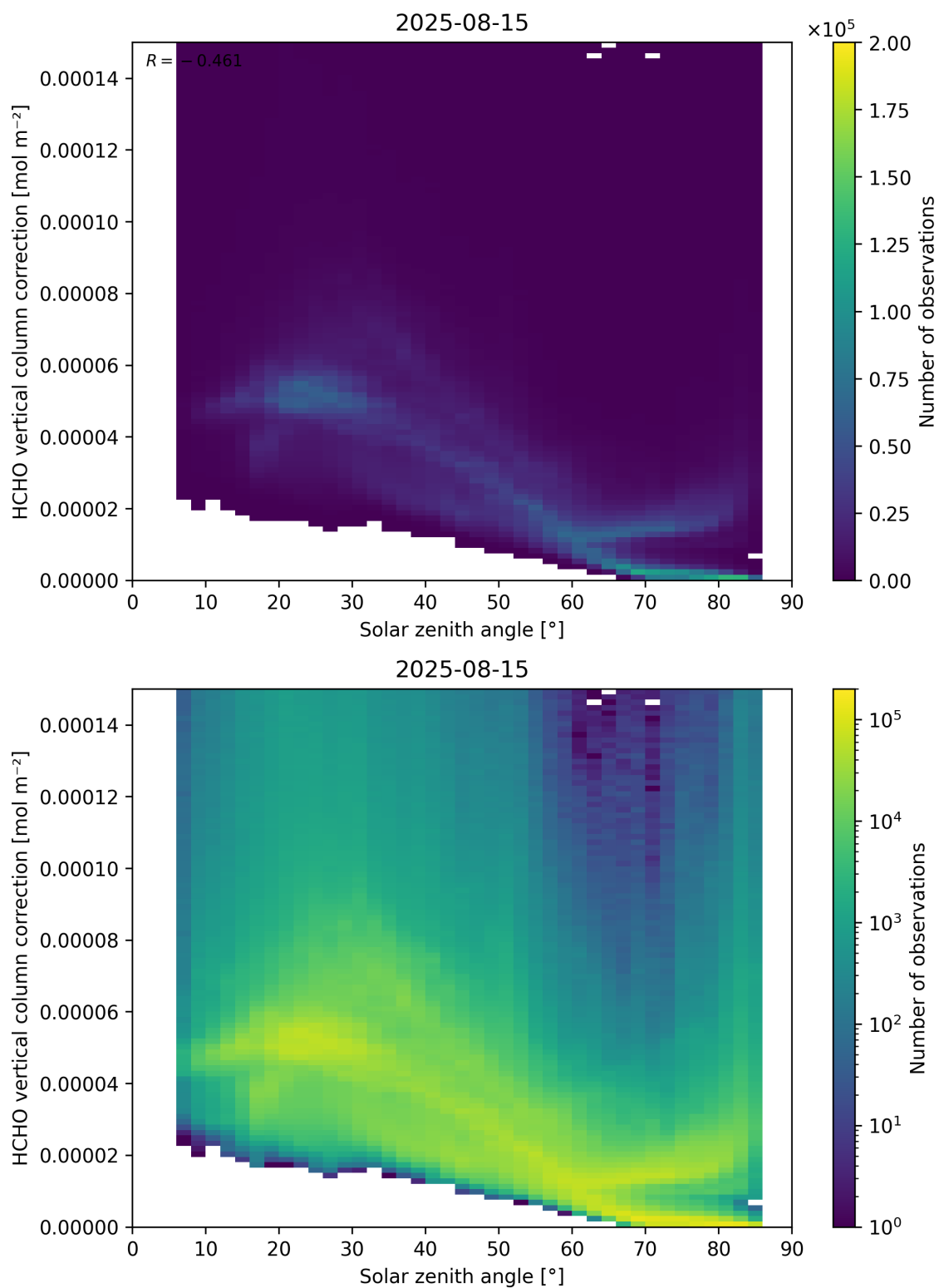
Figure 178: Scatter density plot of “Solar zenith angle” against “HCHO vertical column correction” for 2025-08-14 to 2025-08-16.
