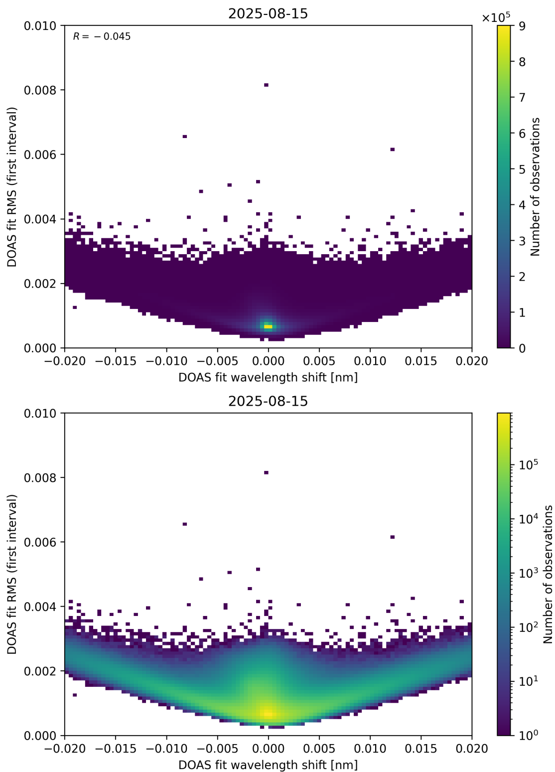
Figure 64: Scatter density plot of “DOAS fit wavelength shift” against “DOAS fit RMS (first interval)” for 2025-08-14 to 2025-08-16.
