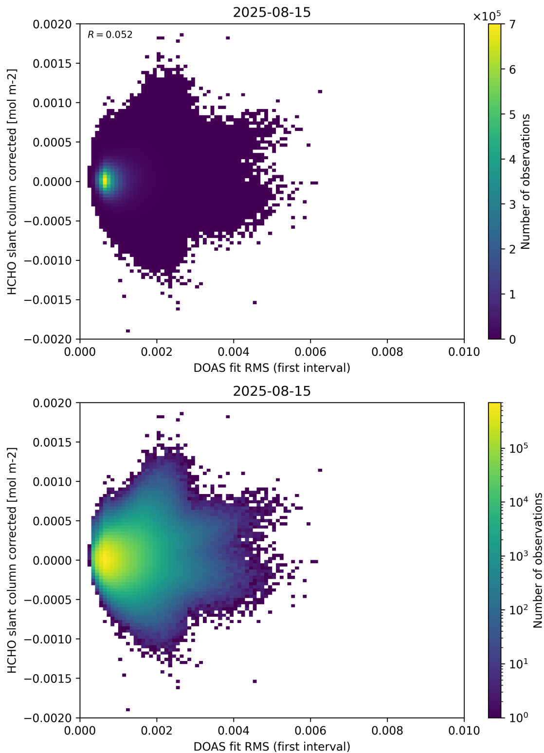
Figure 62: Scatter density plot of “DOAS fit RMS (first interval)” against “HCHO slant column corrected” for 2025-08-14 to 2025-08-16.
