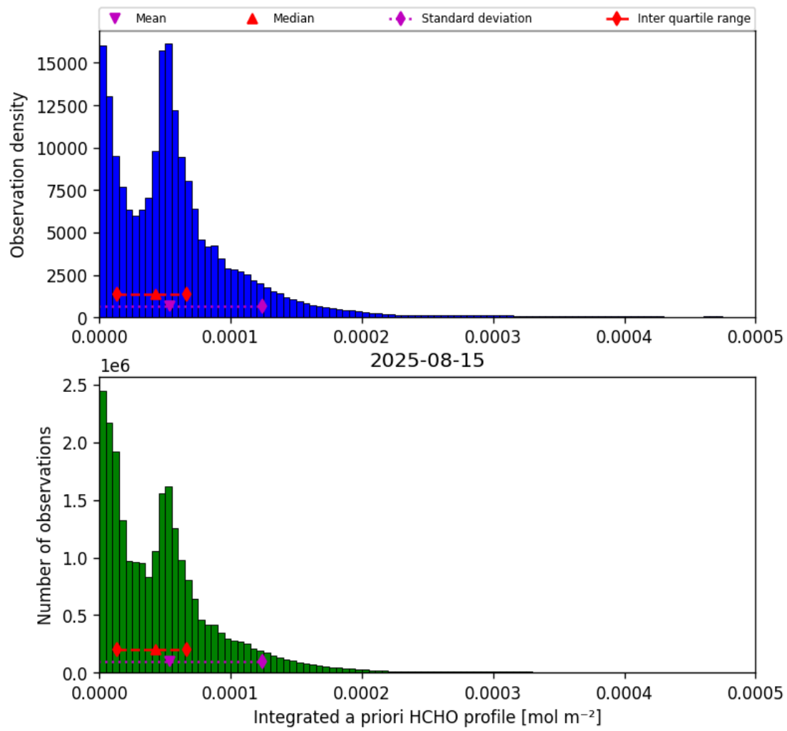
Figure 43: Histogram of “Integrated a priori HCHO profile” for 2025-08-14 to 2025-08-16
