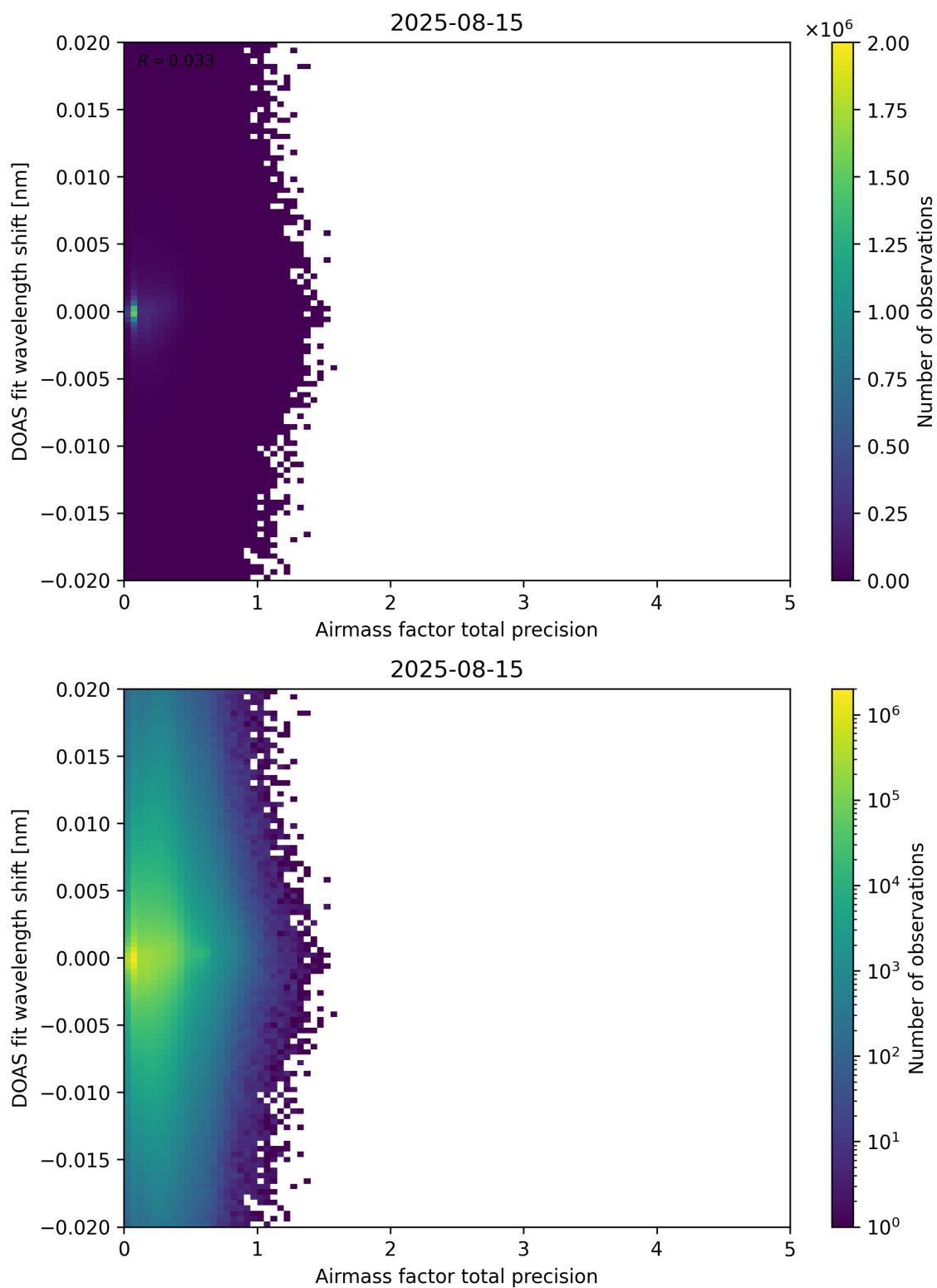
Figure 106: Scatter density plot of “Airmass factor total precision” against “DOAS fit wavelength shift” for 2025-08-14 to 2025-08-16.
