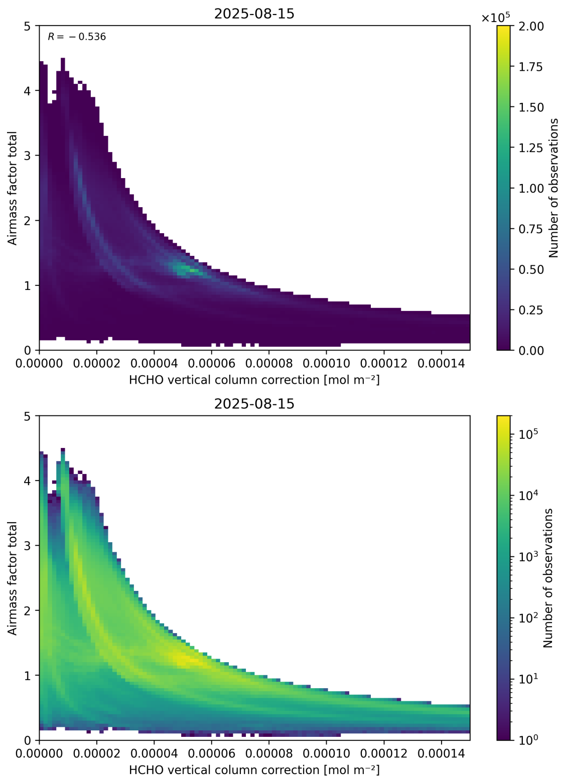
Figure 120: Scatter density plot of “HCHO vertical column correction” against “Airmass factor total” for 2025-08-14 to 2025-08-16.
