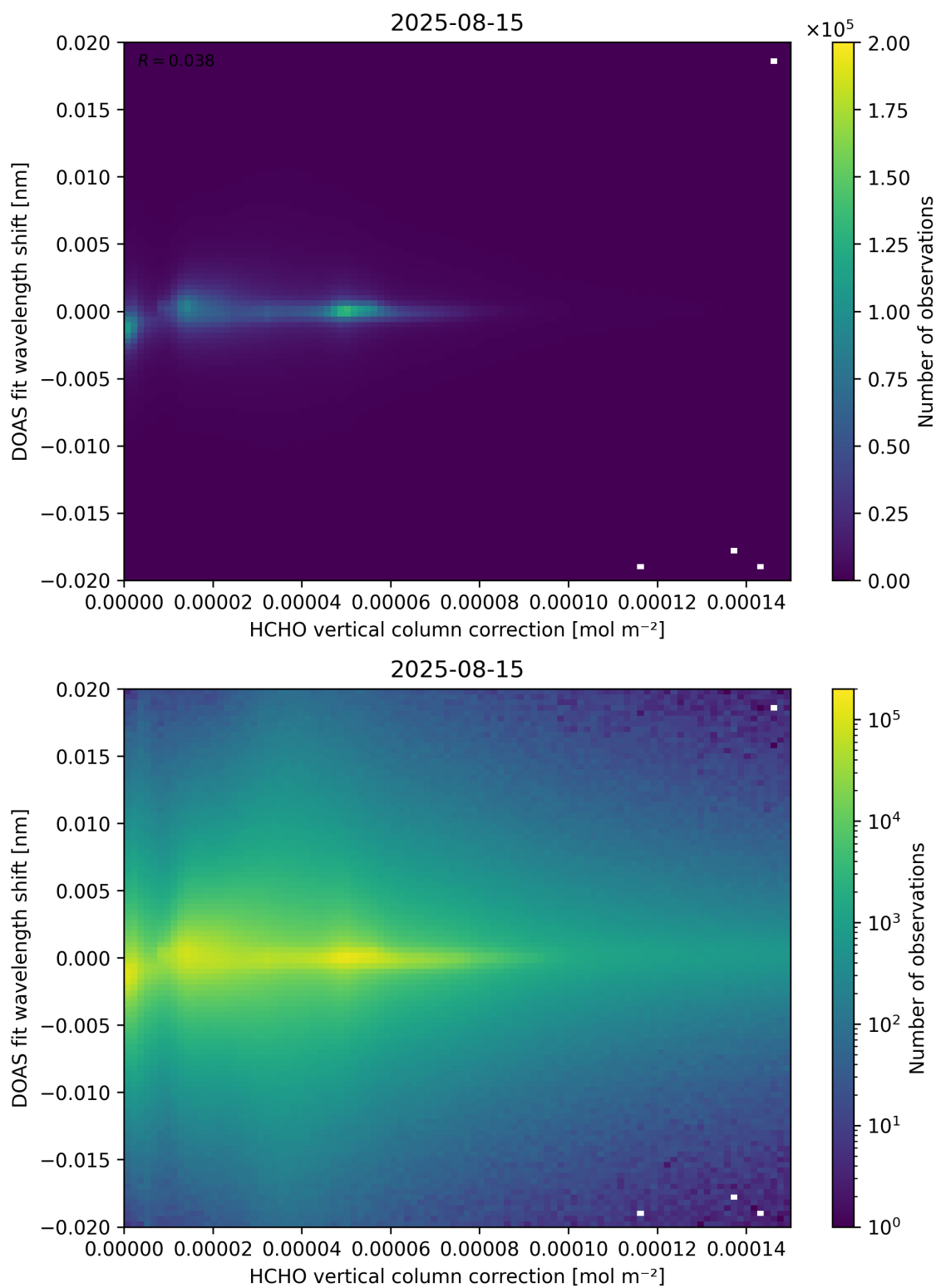
Figure 113: Scatter density plot of “HCHO vertical column correction” against “DOAS fit wavelength shift” for 2025-08-14 to 2025-08-16.
