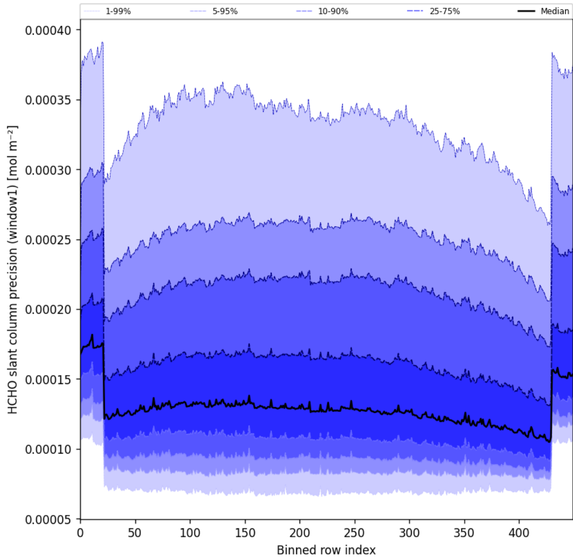
Figure 53: Along track statistics of "HCHO slant column precision (window1)" for 2025-08-14 to 2025-08-16
