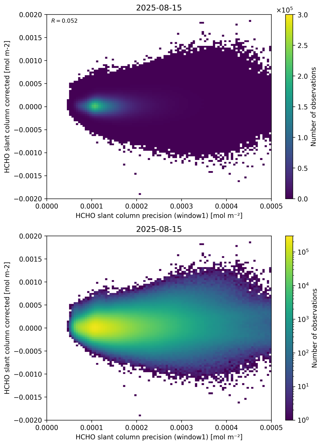
Figure 92: Scatter density plot of “HCHO slant column precision (window1)” against “HCHO slant column corrected” for 2025-08-14 to 2025-08-16.
