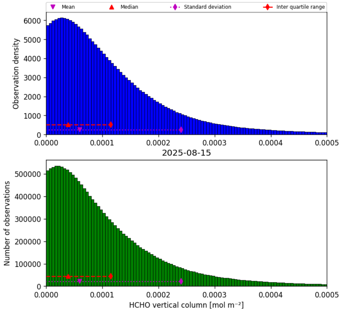
Figure 35: Histogram of “HCHO vertical column” for 2025-08-14 to 2025-08-16
