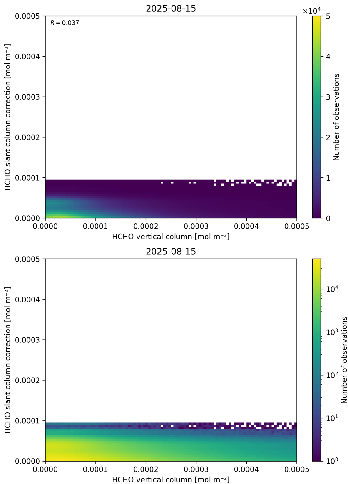
Figure 128: Scatter density plot of “HCHO vertical column” against “HCHO slant column correction” for 2025-08-14 to 2025-08-16.
