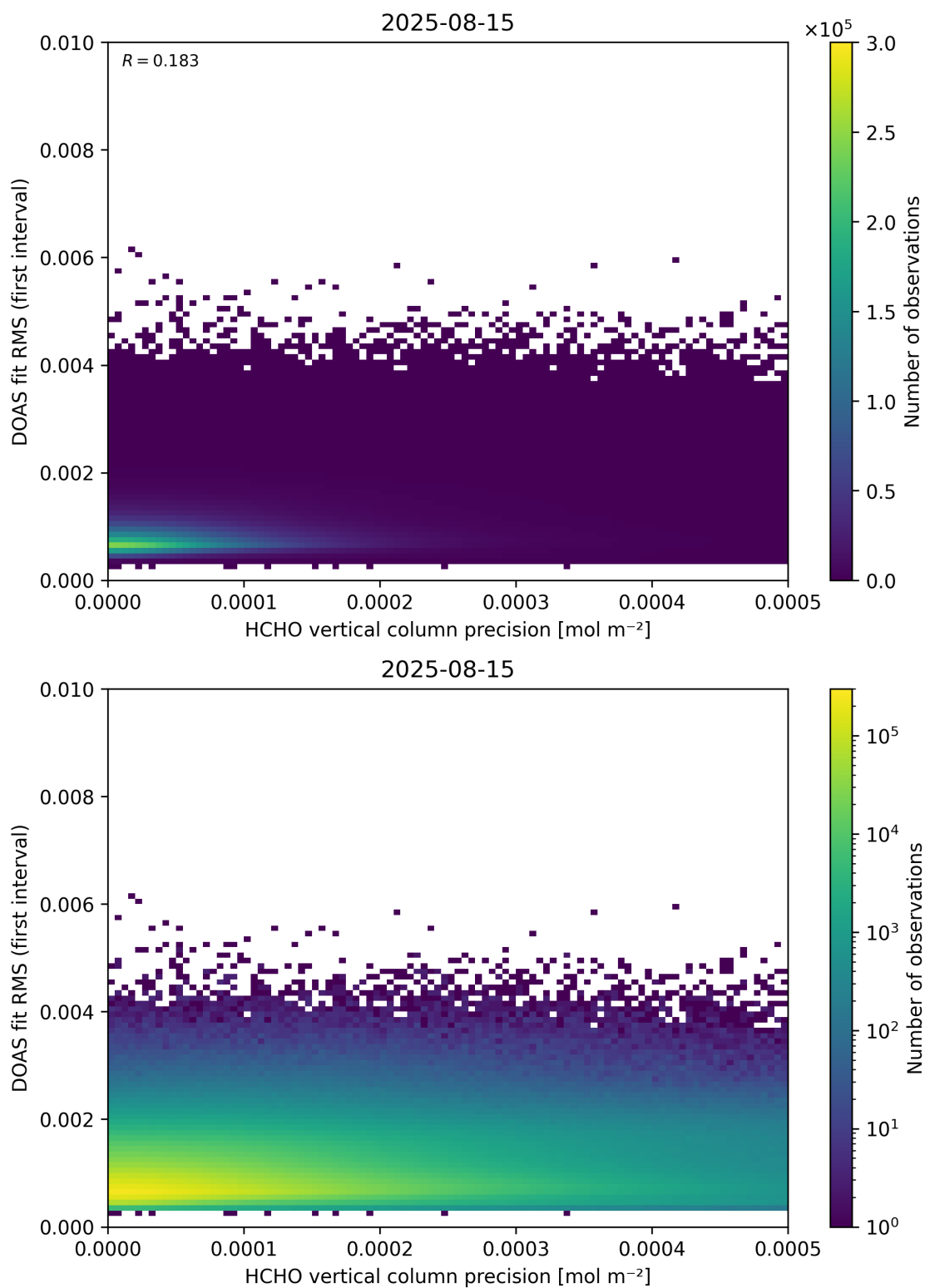
Figure 136: Scatter density plot of “HCHO vertical column precision” against “DOAS fit RMS (first interval)” for 2025-08-14 to 2025-08-16.
