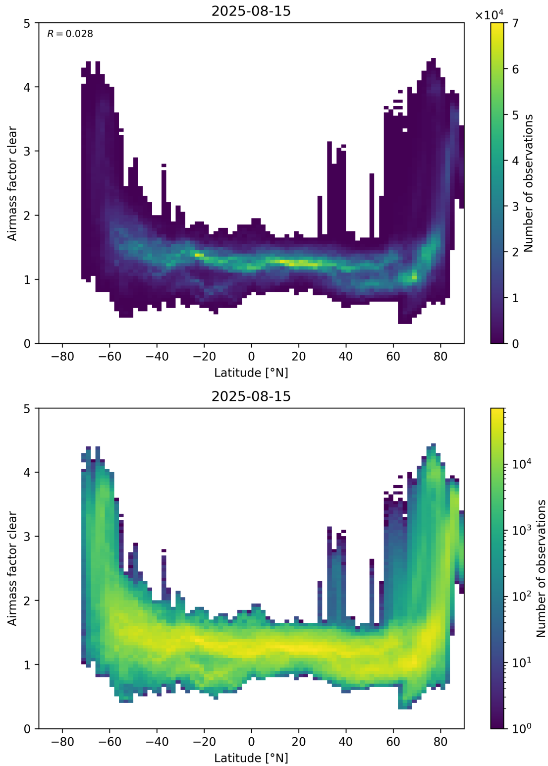
Figure 156: Scatter density plot of “Latitude” against “Airmass factor clear” for 2025-08-14 to 2025-08-16.
