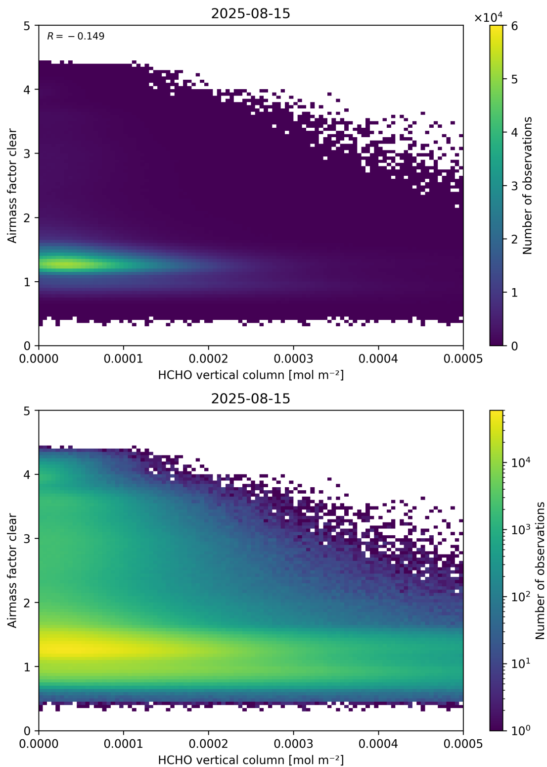
Figure 126: Scatter density plot of “HCHO vertical column” against “Airmass factor clear” for 2025-08-14 to 2025-08-16.
