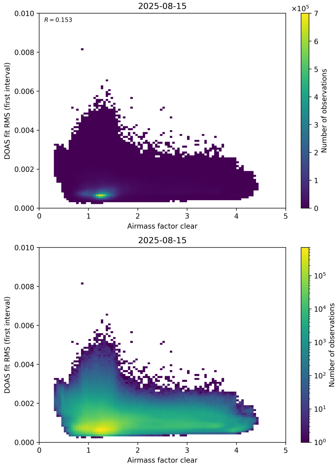
Figure 71: Scatter density plot of “Airmass factor clear” against “DOAS fit RMS (first interval)” for 2025-08-14 to 2025-08-16.
