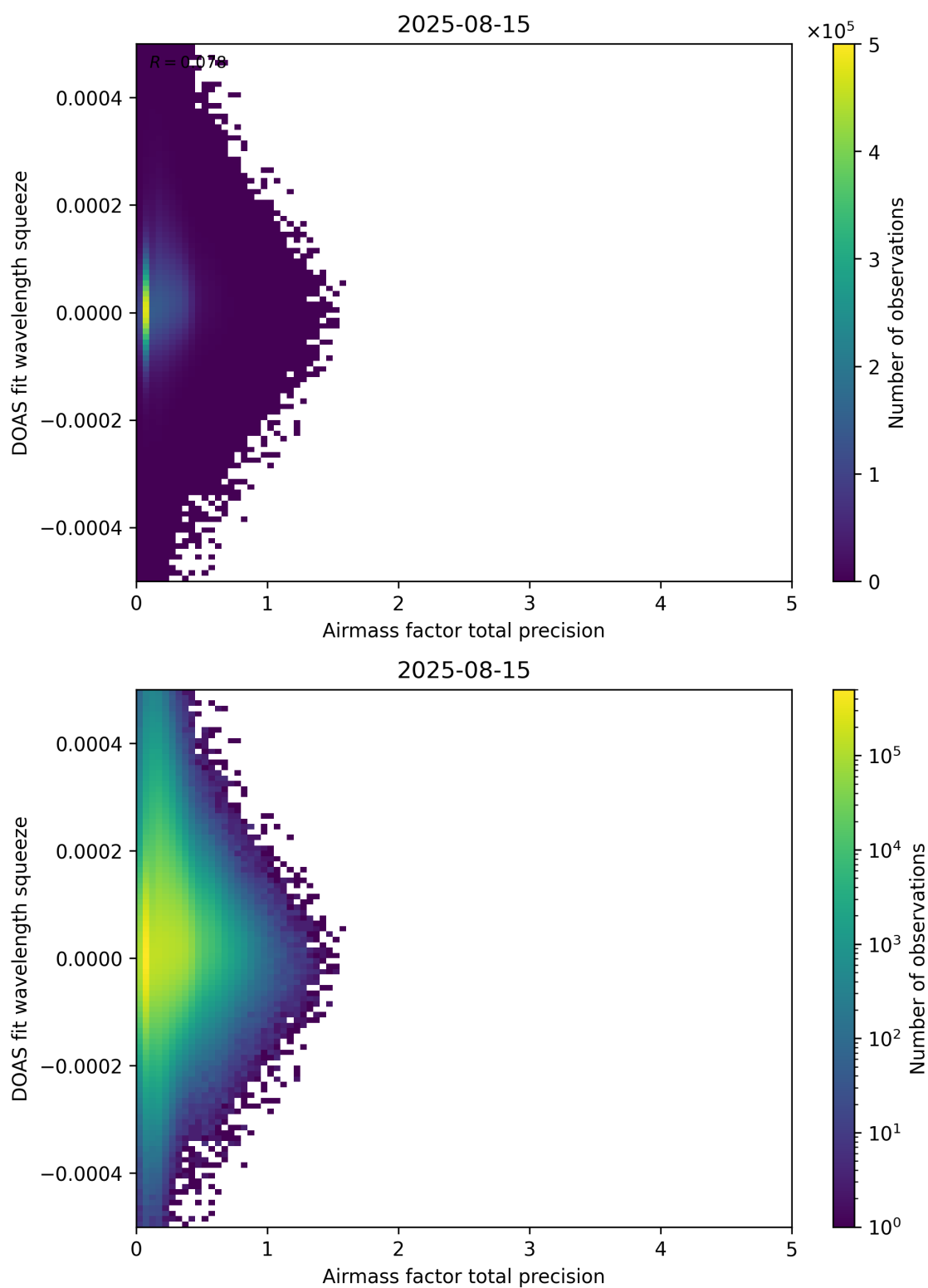
Figure 107: Scatter density plot of “Airmass factor total precision” against “DOAS fit wavelength squeeze” for 2025-08-14 to 2025-08-16.
