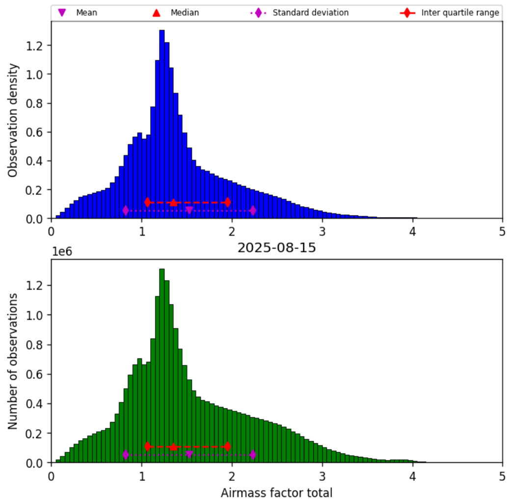
Figure 40: Histogram of “Airmass factor total” for 2025-08-14 to 2025-08-16
