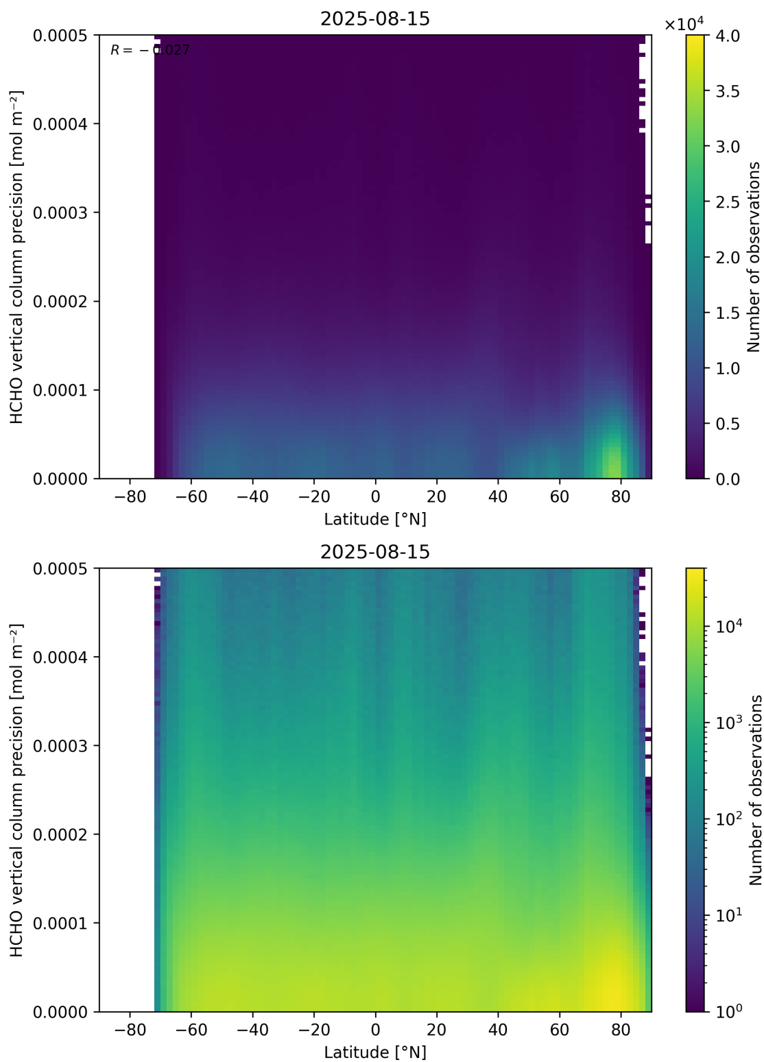
Figure 165: Scatter density plot of “Latitude” against “HCHO vertical column precision” for 2025-08-14 to 2025-08-16.
