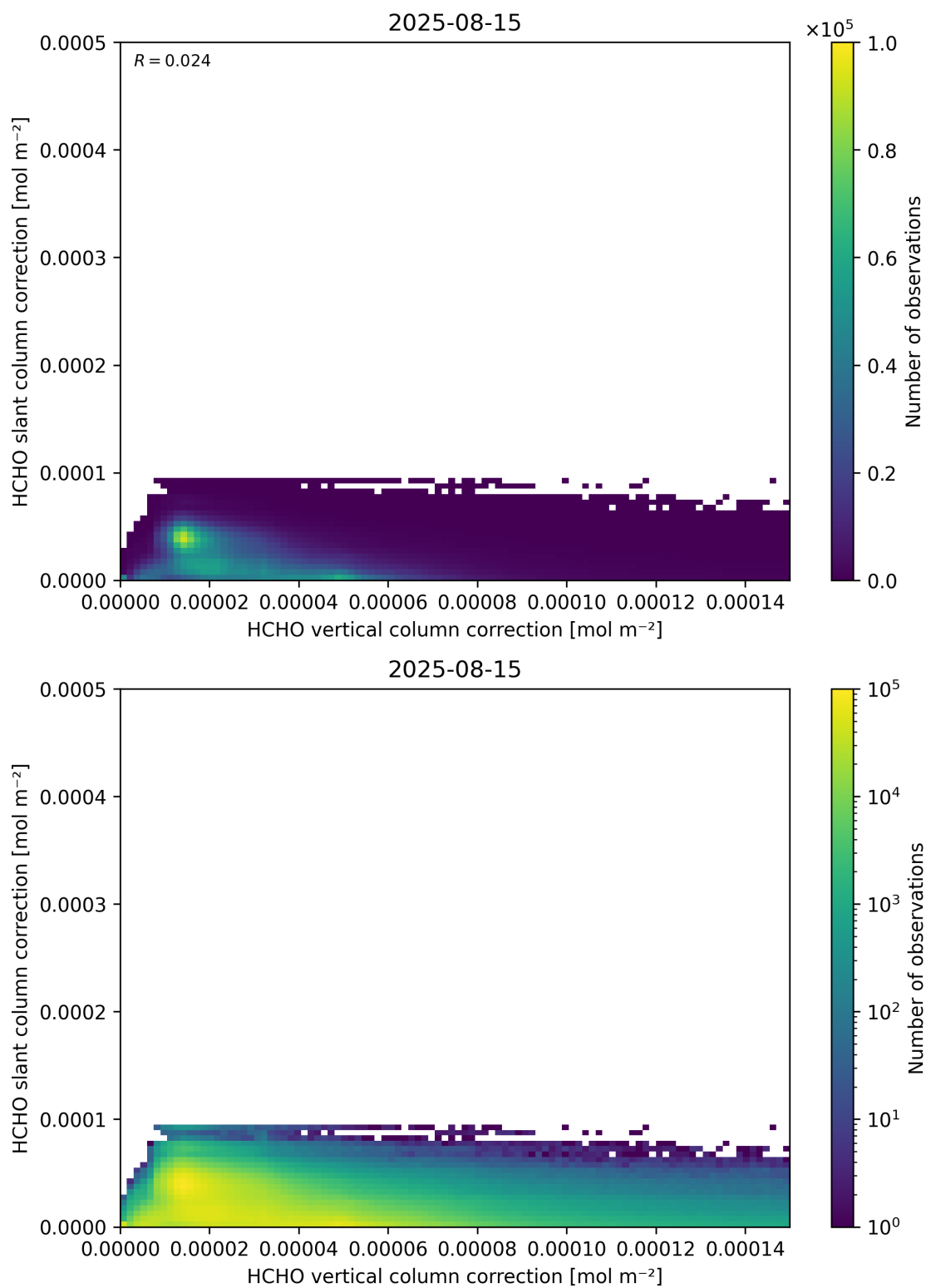
Figure 117: Scatter density plot of “HCHO vertical column correction” against “HCHO slant column correction” for 2025-08-14 to 2025-08-16.
