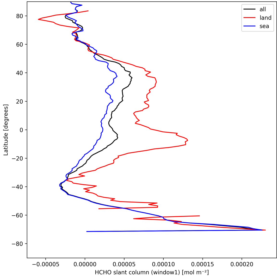
Figure 24: Zonal average of “HCHO slant column (window1)” for 2025-08-14 to 2025-08-16.
