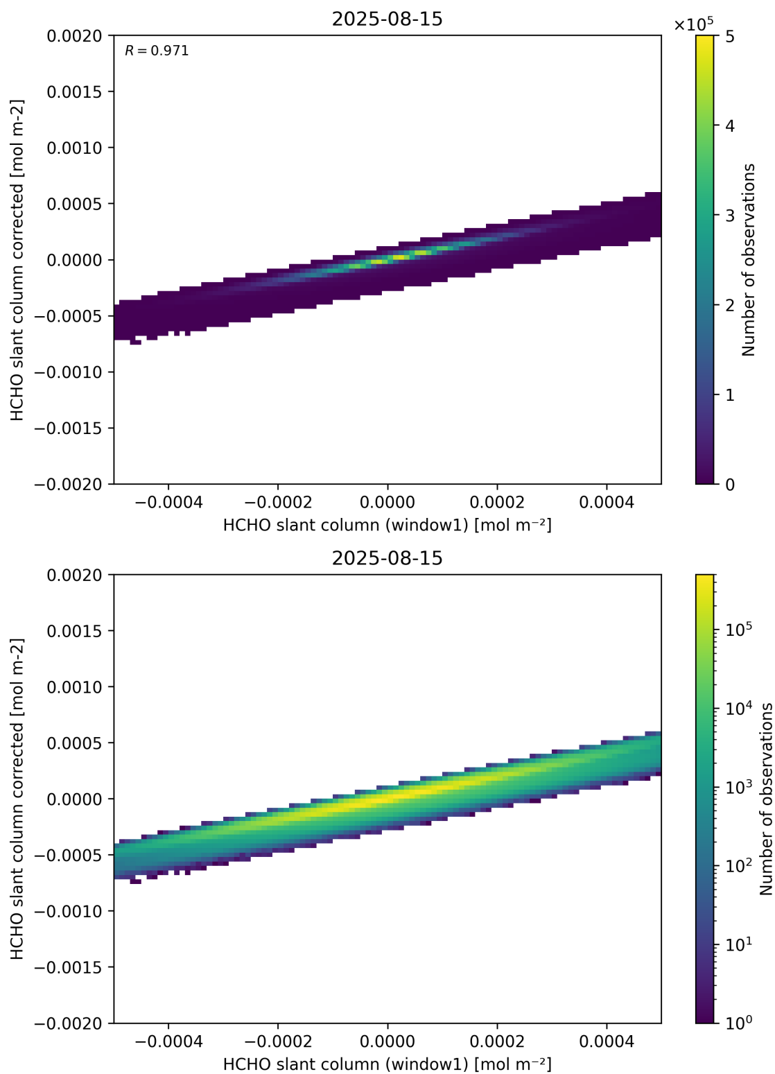
Figure 82: Scatter density plot of “HCHO slant column (window1)” against “HCHO slant column corrected” for 2025-08-14 to 2025-08-16.
