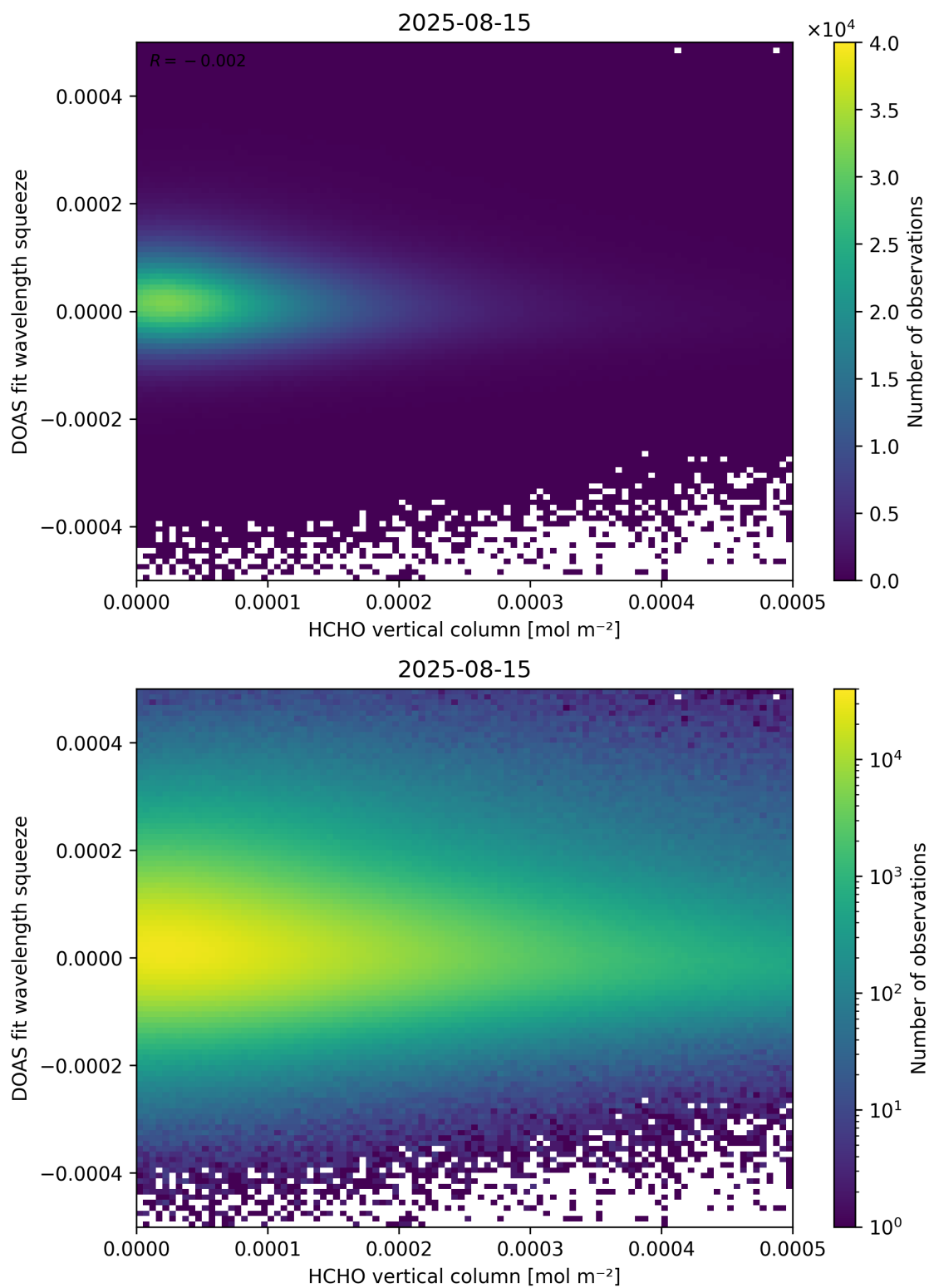
Figure 125: Scatter density plot of “HCHO vertical column” against “DOAS fit wavelength squeeze” for 2025-08-14 to 2025-08-16.
