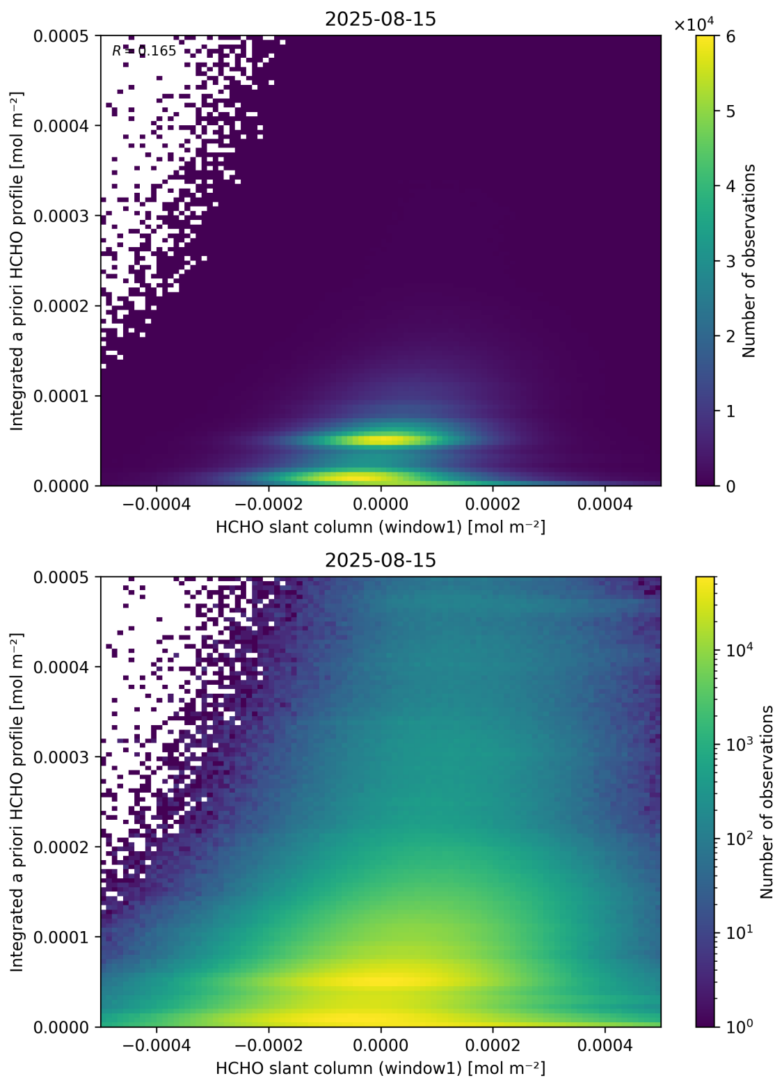
Figure 87: Scatter density plot of “HCHO slant column (window1)” against “Integrated a priori HCHO profile” for 2025-08-14 to 2025-08-16.
