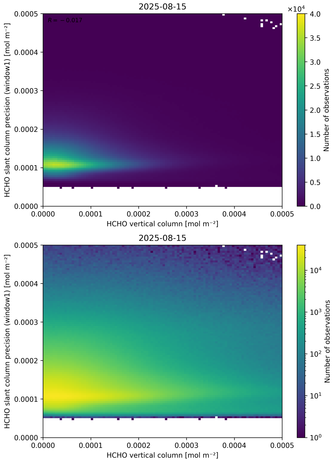
Figure 130: Scatter density plot of “HCHO vertical column” against “HCHO slant column precision (window1)” for 2025-08-14 to 2025-08-16.
