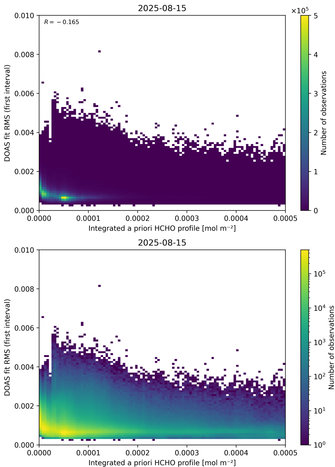
Figure 148: Scatter density plot of “Integrated a priori HCHO profile” against “DOAS fit RMS (first interval)” for 2025-08-14 to 2025-08-16.
