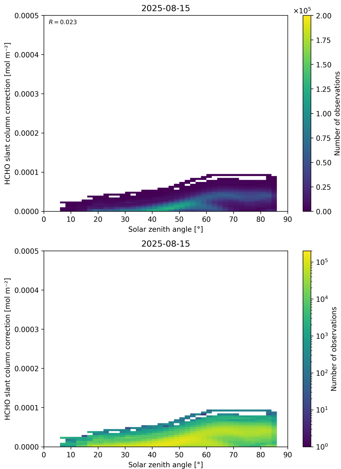
Figure 172: Scatter density plot of “Solar zenith angle” against “HCHO slant column correction” for 2025-08-14 to 2025-08-16.
