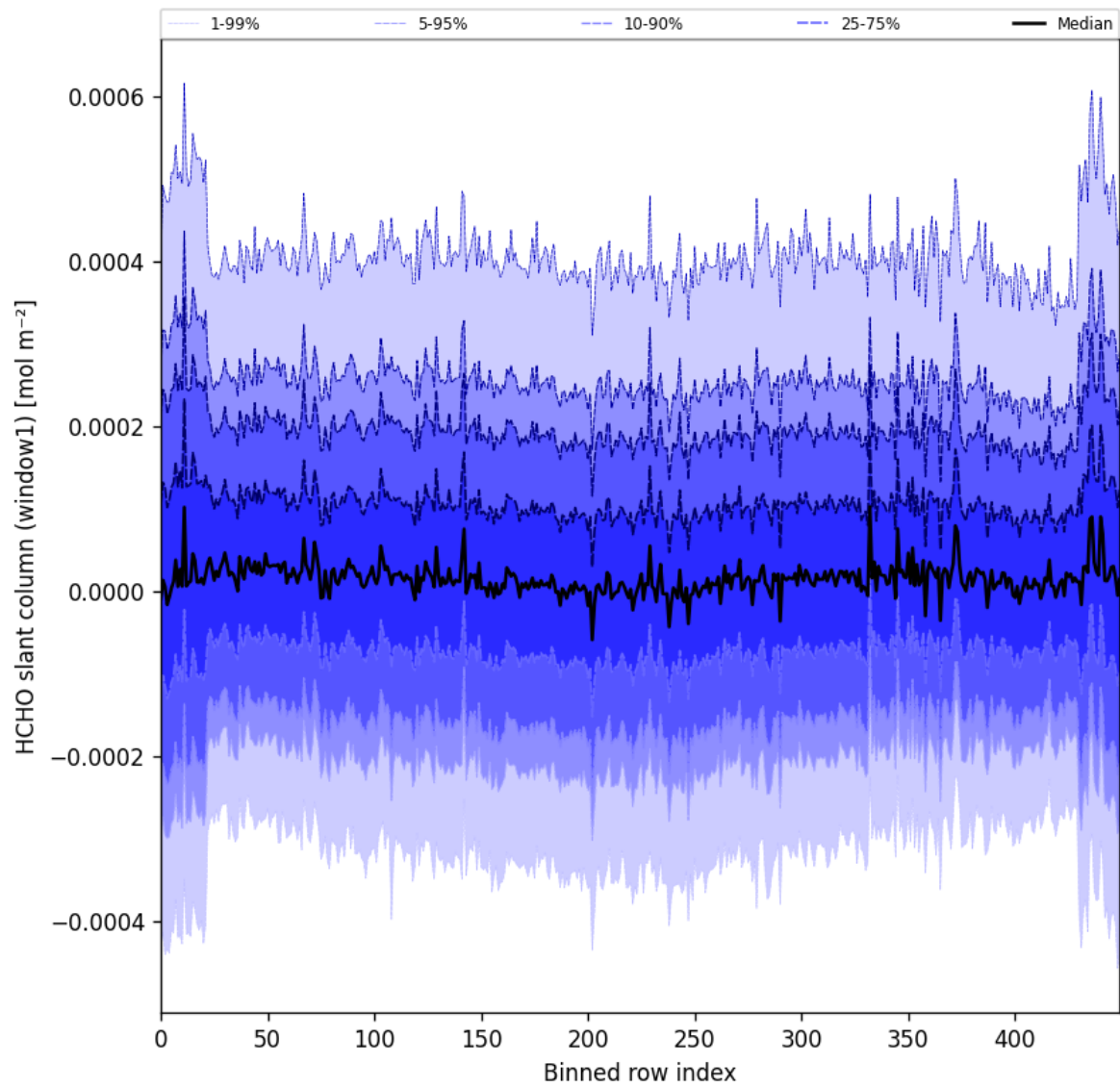
Figure 52: Along track statistics of “HCHO slant column (window1)” for 2025-08-14 to 2025-08-16
