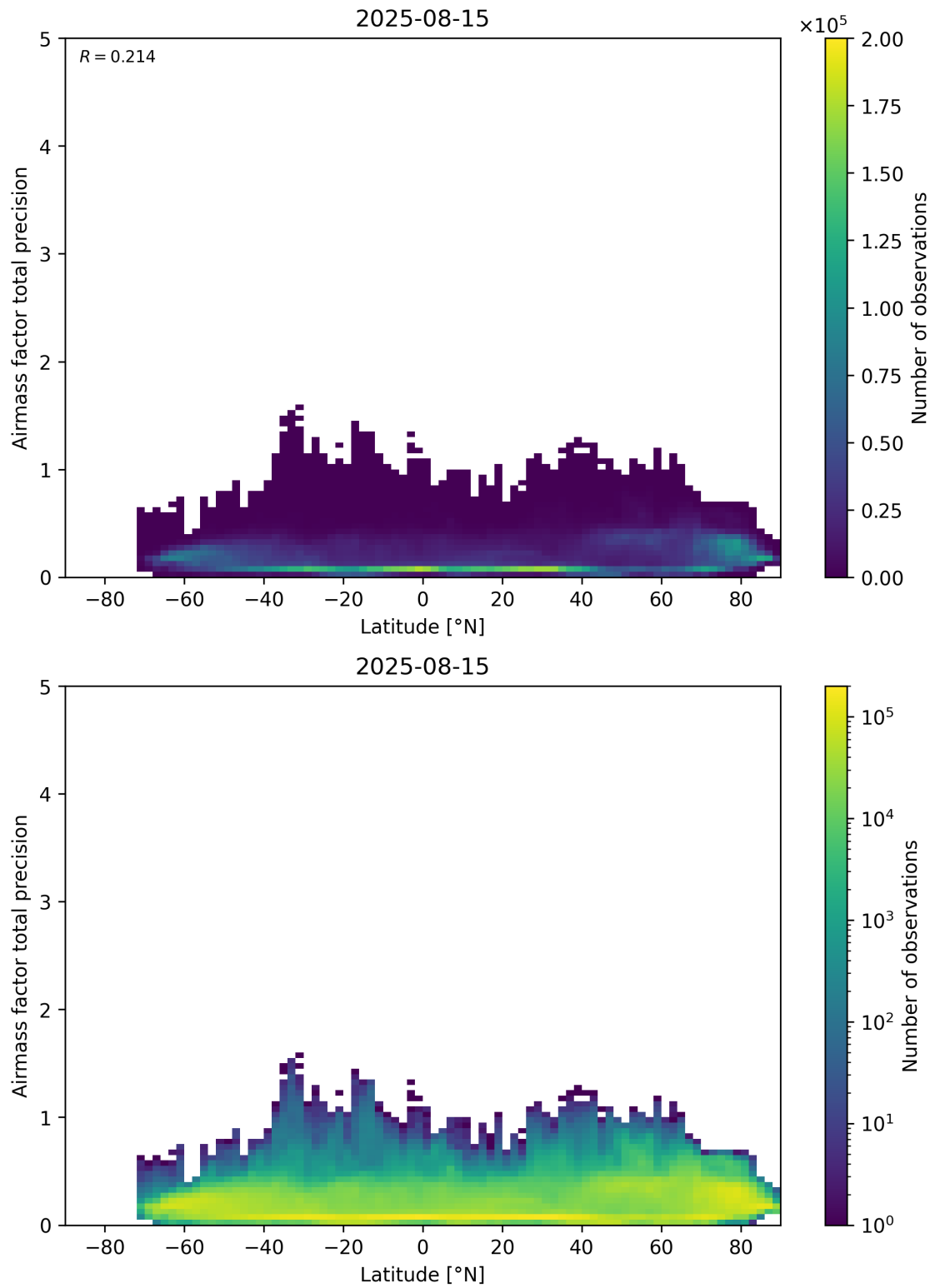
Figure 162: Scatter density plot of “Latitude” against “Airmass factor total precision” for 2025-08-14 to 2025-08-16.
