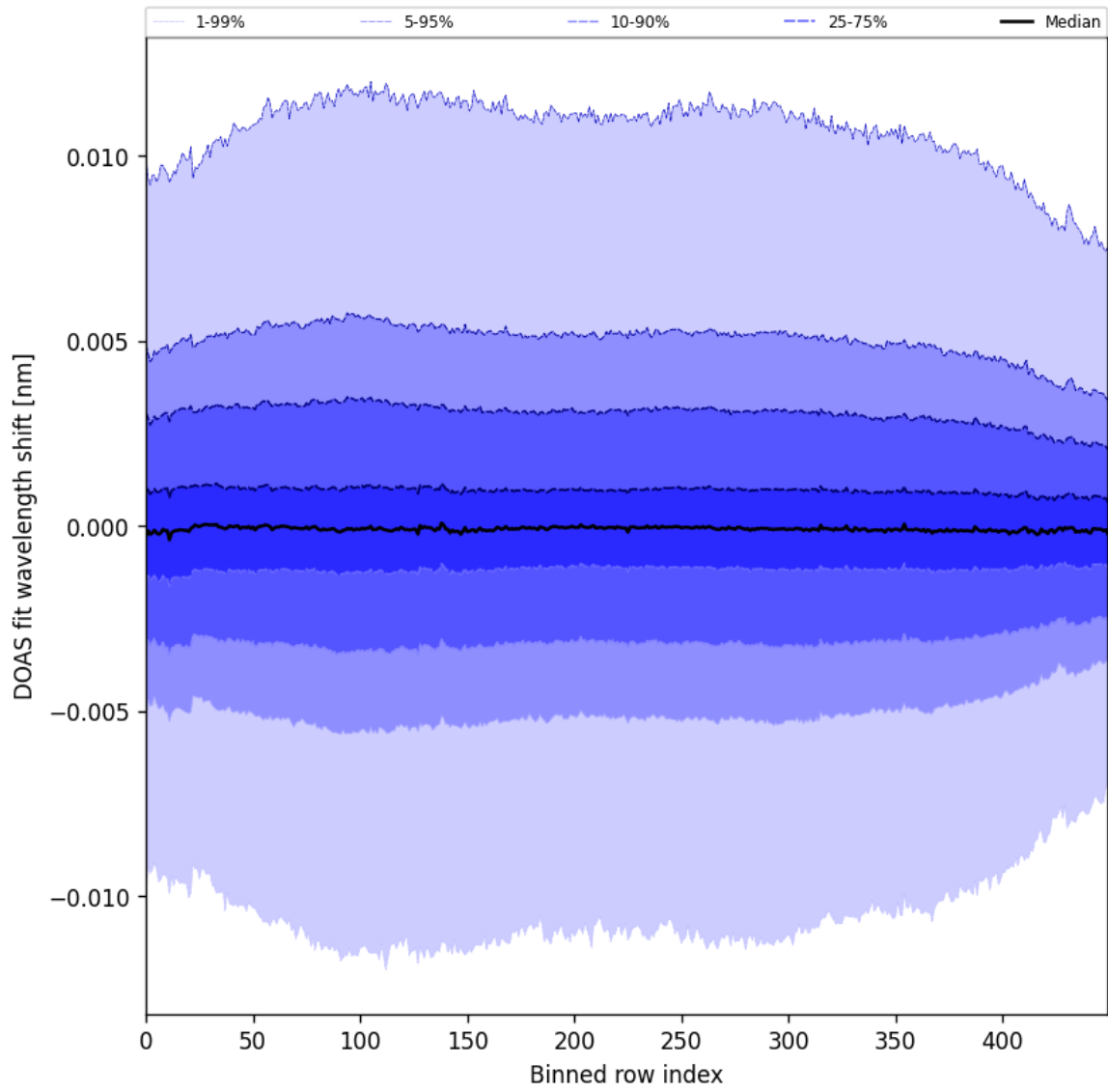
Figure 58: Along track statistics of “DOAS fit wavelength shift” for 2025-08-14 to 2025-08-16
