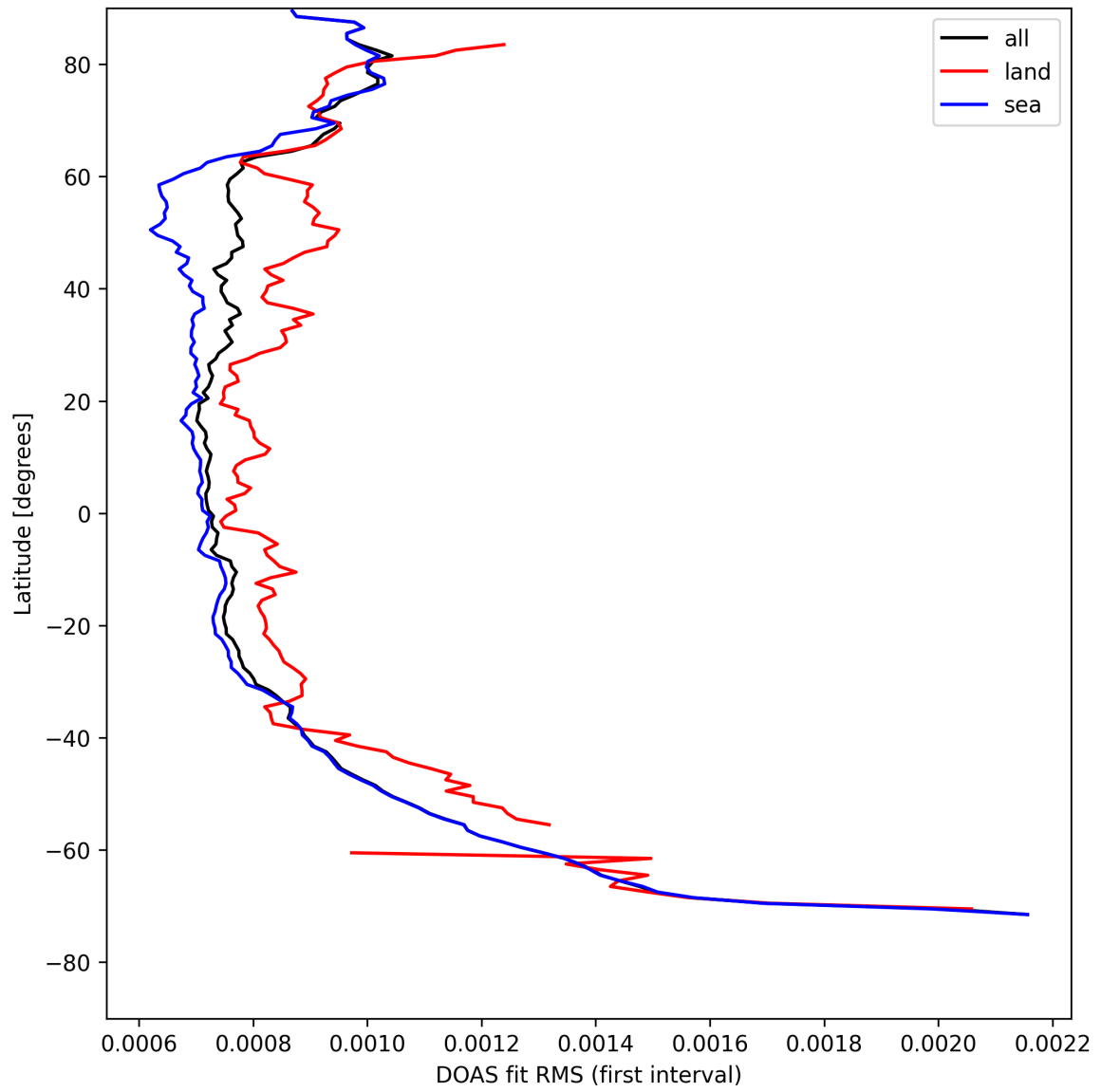
Figure 32: Zonal average of “DOAS fit RMS (first interval)” for 2025-08-14 to 2025-08-16.
