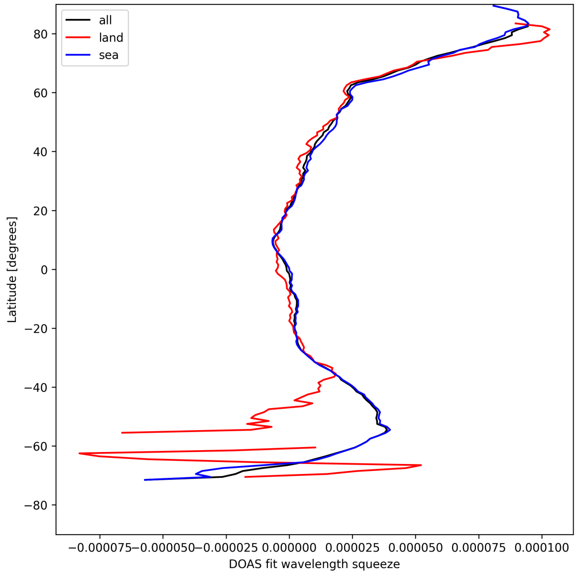
Figure 31: Zonal average of “DOAS fit wavelength squeeze” for 2025-08-14 to 2025-08-16.
