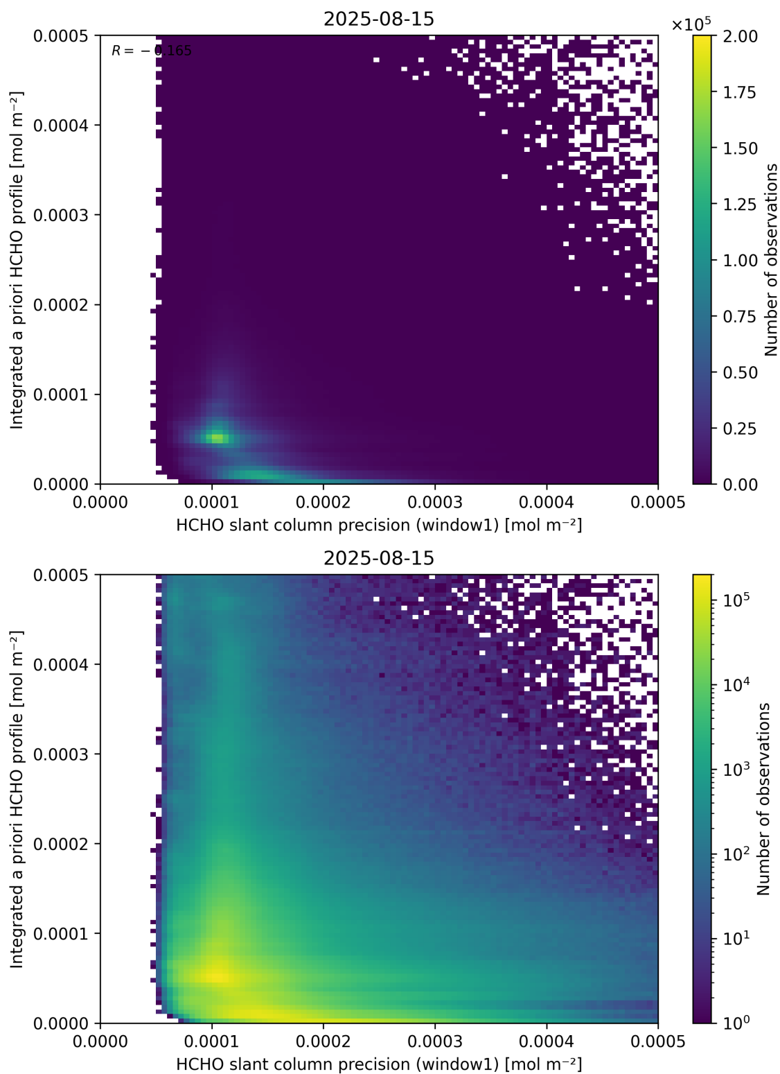
Figure 96: Scatter density plot of “HCHO slant column precision (window1)” against “Integrated a priori HCHO profile” for 2025-08-14 to 2025-08-16.
