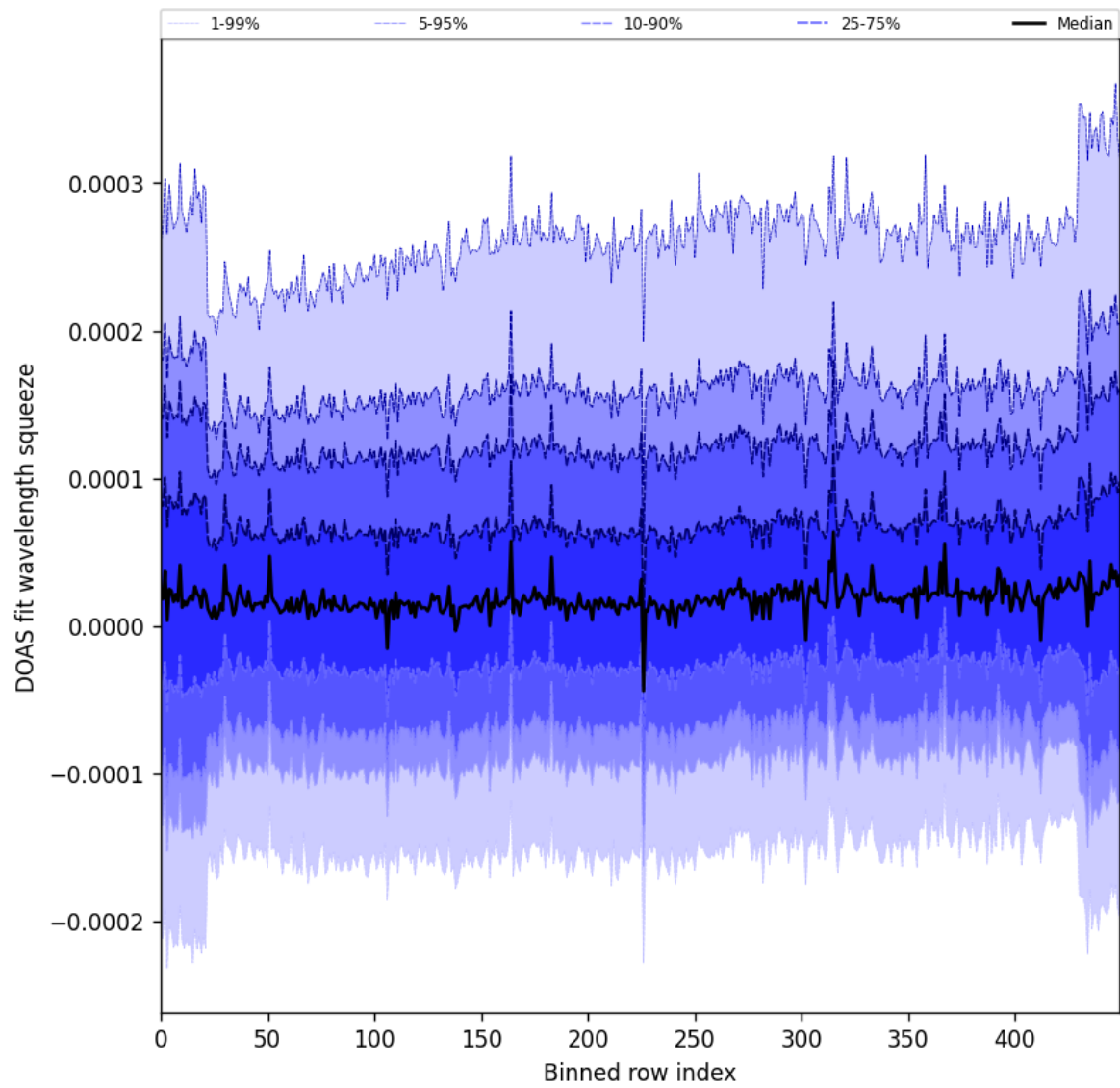
Figure 59: Along track statistics of “DOAS fit wavelength squeeze” for 2025-08-14 to 2025-08-16
