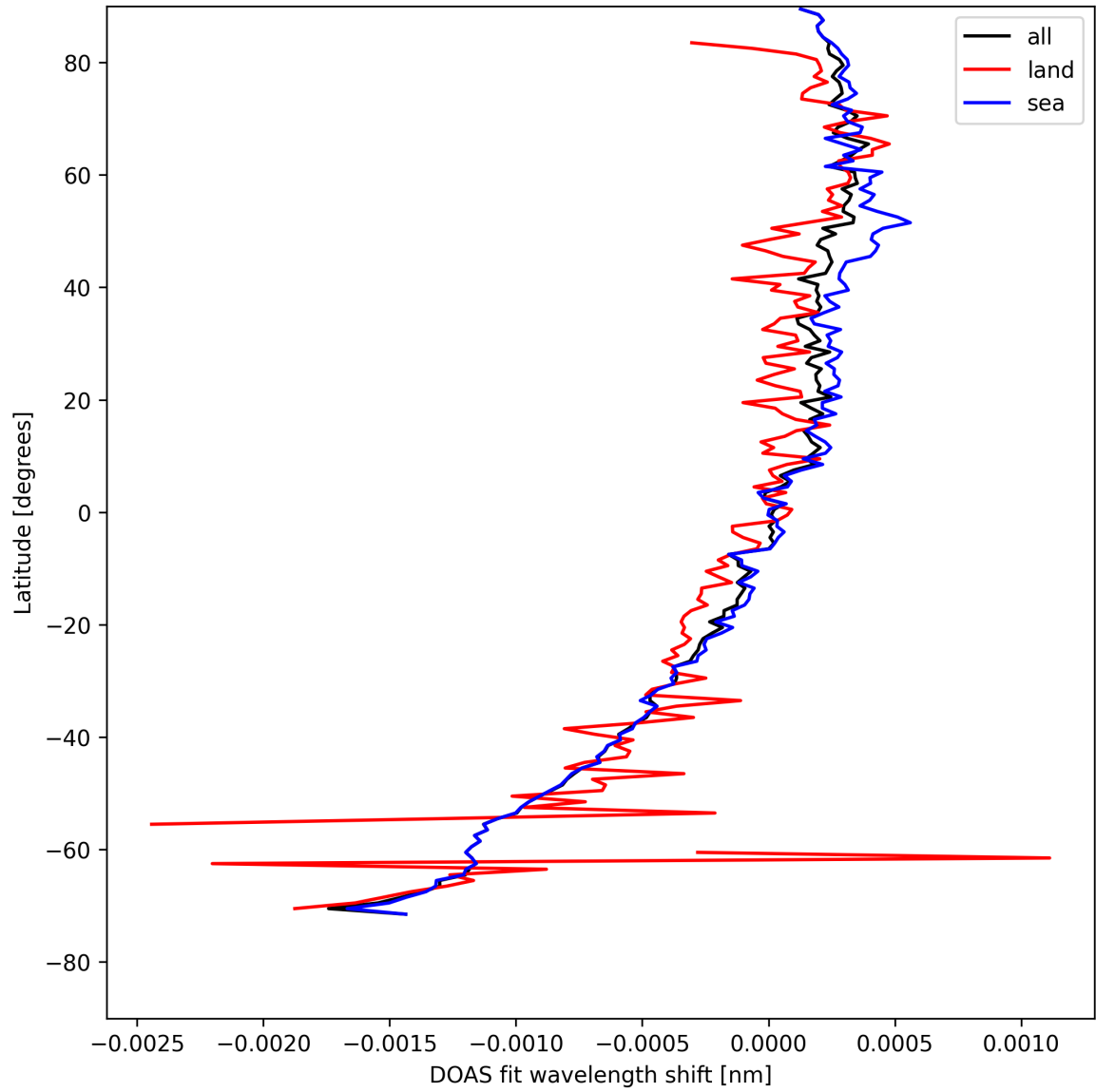
Figure 30: Zonal average of “DOAS fit wavelength shift” for 2025-08-14 to 2025-08-16.
