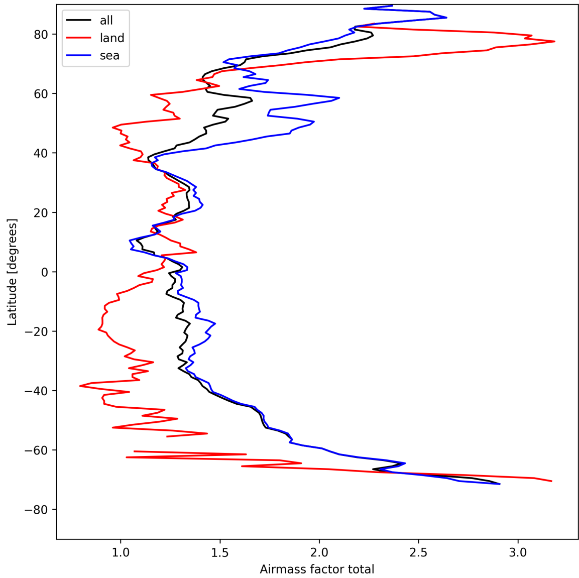
Figure 26: Zonal average of “Airmass factor total” for 2025-08-14 to 2025-08-16.
