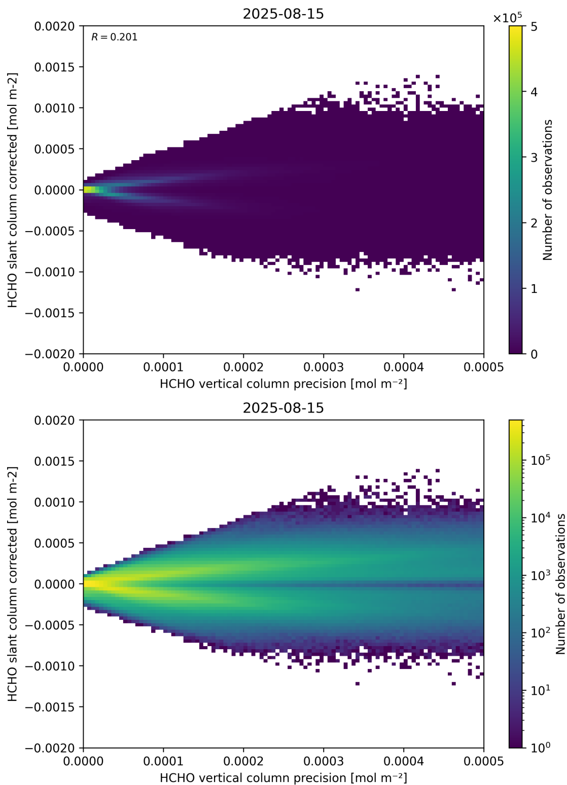
Figure 140: Scatter density plot of “HCHO vertical column precision” against “HCHO slant column corrected” for 2025-08-14 to 2025-08-16.
