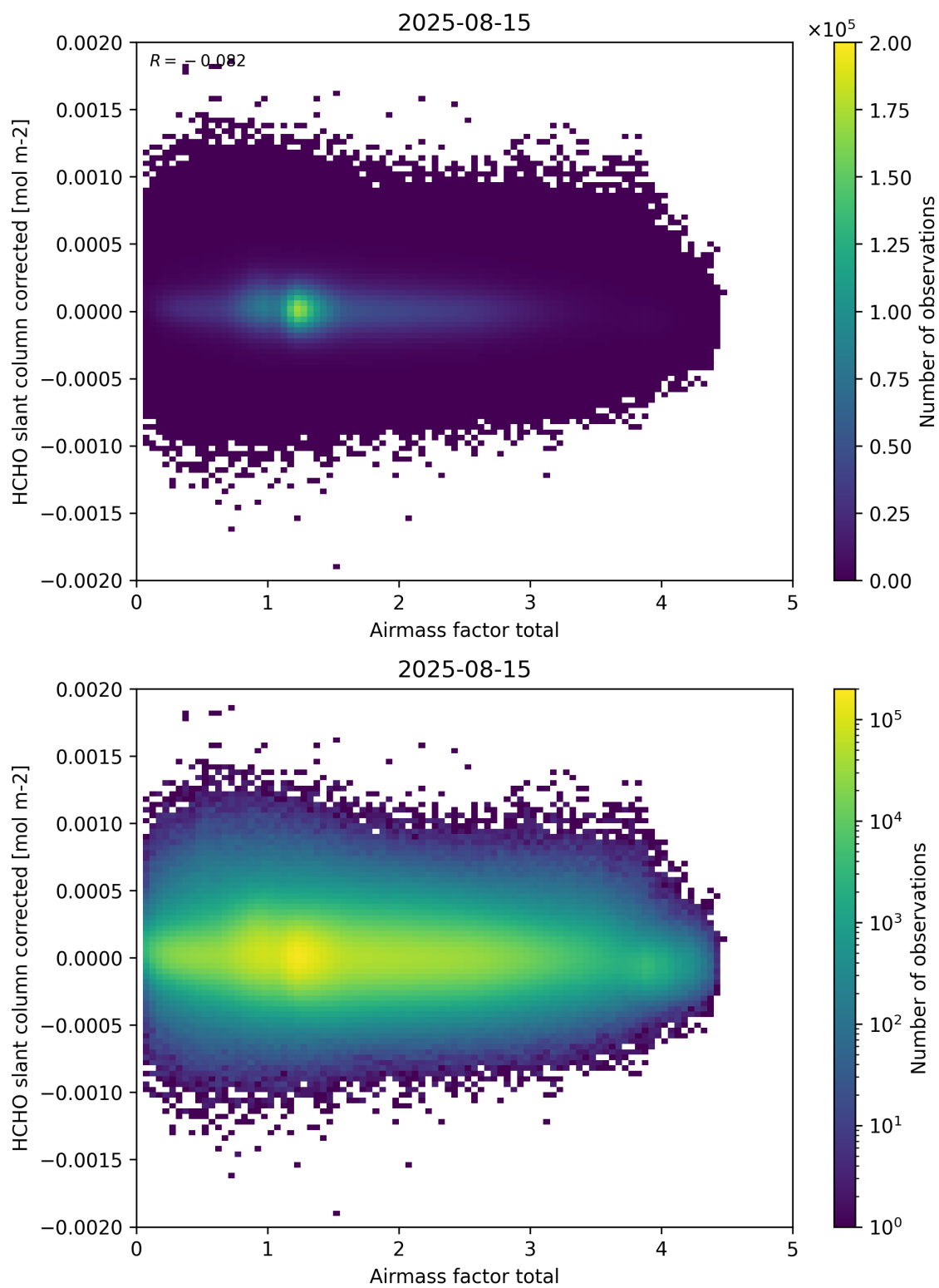
Figure 101: Scatter density plot of “Airmass factor total” against “HCHO slant column corrected” for 2025-08-14 to 2025-08-16.
