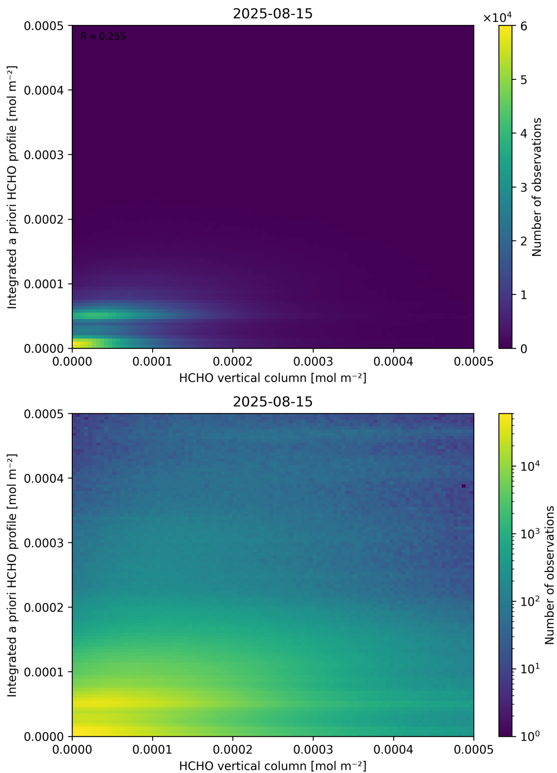
Figure 135: Scatter density plot of “HCHO vertical column” against “Integrated a priori HCHO profile” for 2025-08-14 to 2025-08-16.
