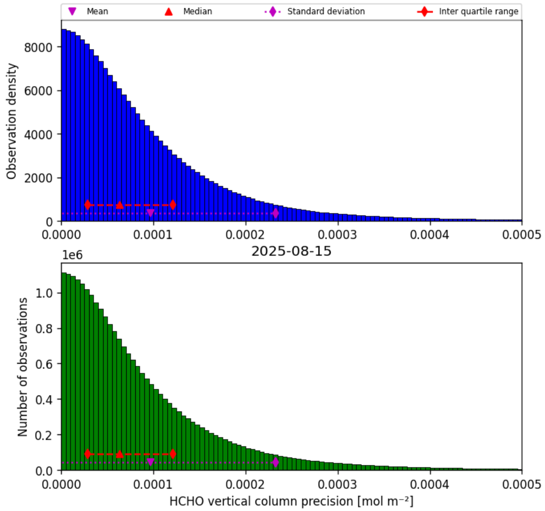
Figure 36: Histogram of “HCHO vertical column precision” for 2025-08-14 to 2025-08-16
