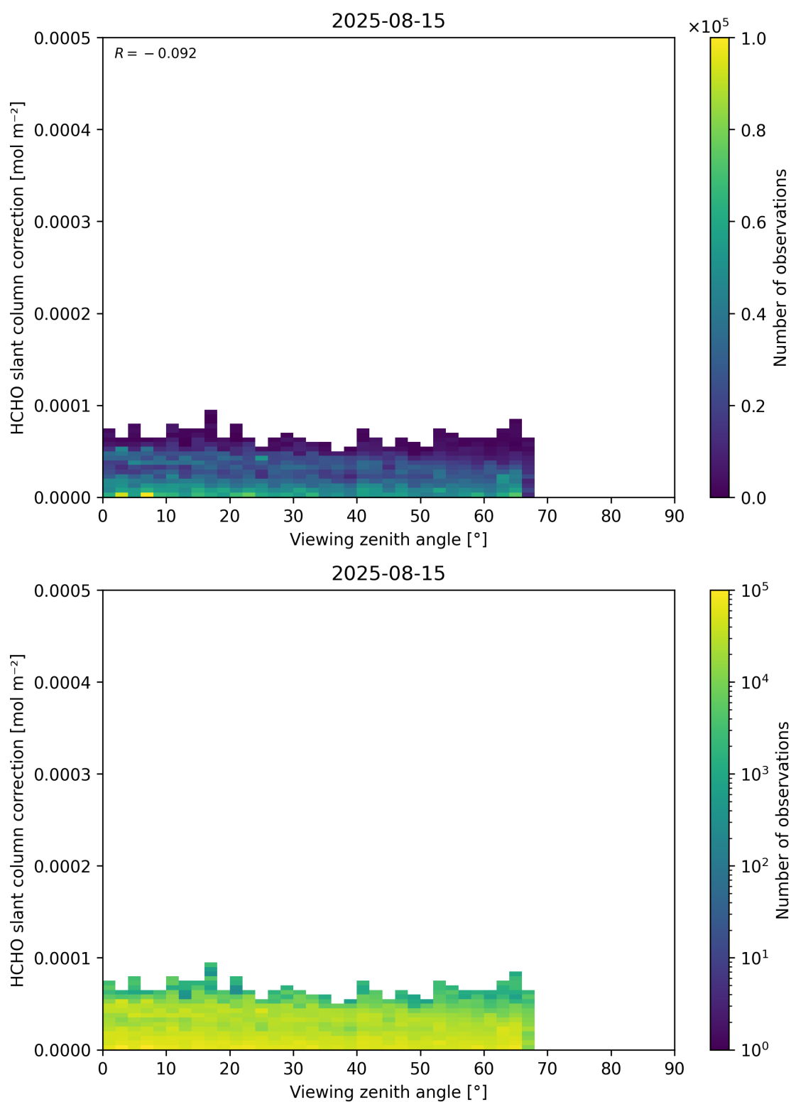
Figure 187: Scatter density plot of “Viewing zenith angle” against “HCHO slant column correction” for 2025-08-14 to 2025-08-16.
