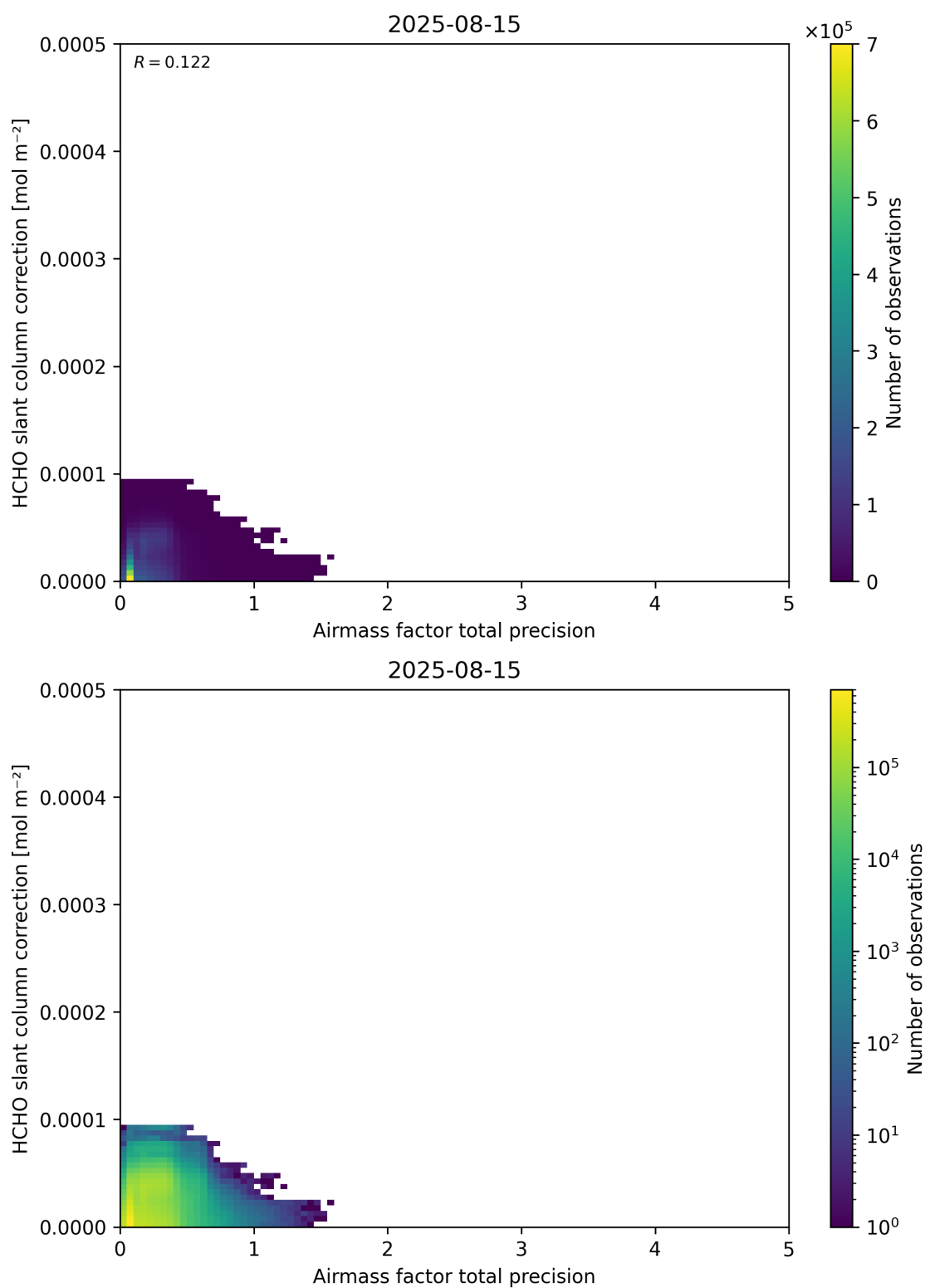
Figure 110: Scatter density plot of “Airmass factor total precision” against “HCHO slant column correction” for 2025-08-14 to 2025-08-16.
