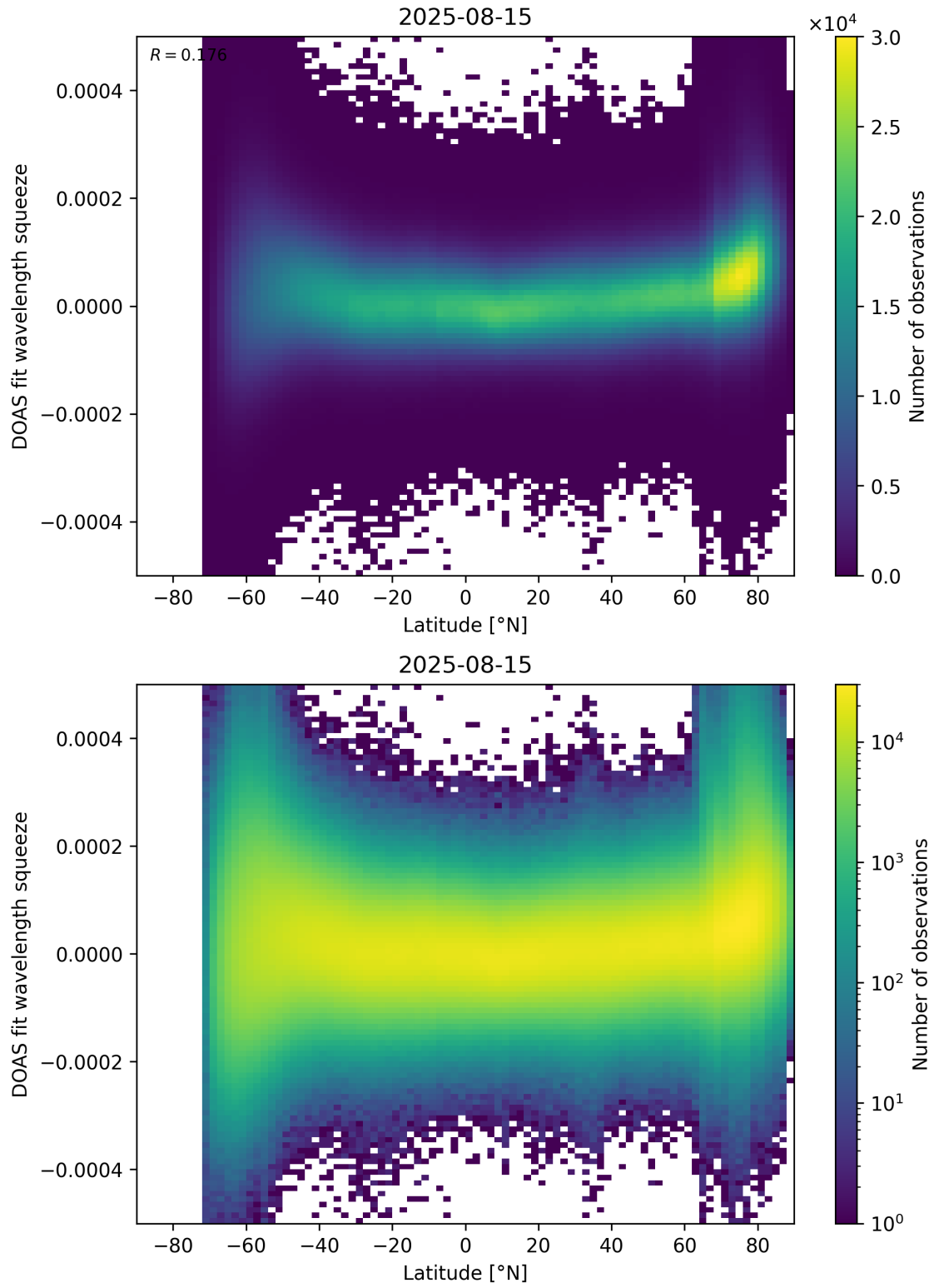
Figure 155: Scatter density plot of “Latitude” against “DOAS fit wavelength squeeze” for 2025-08-14 to 2025-08-16.
