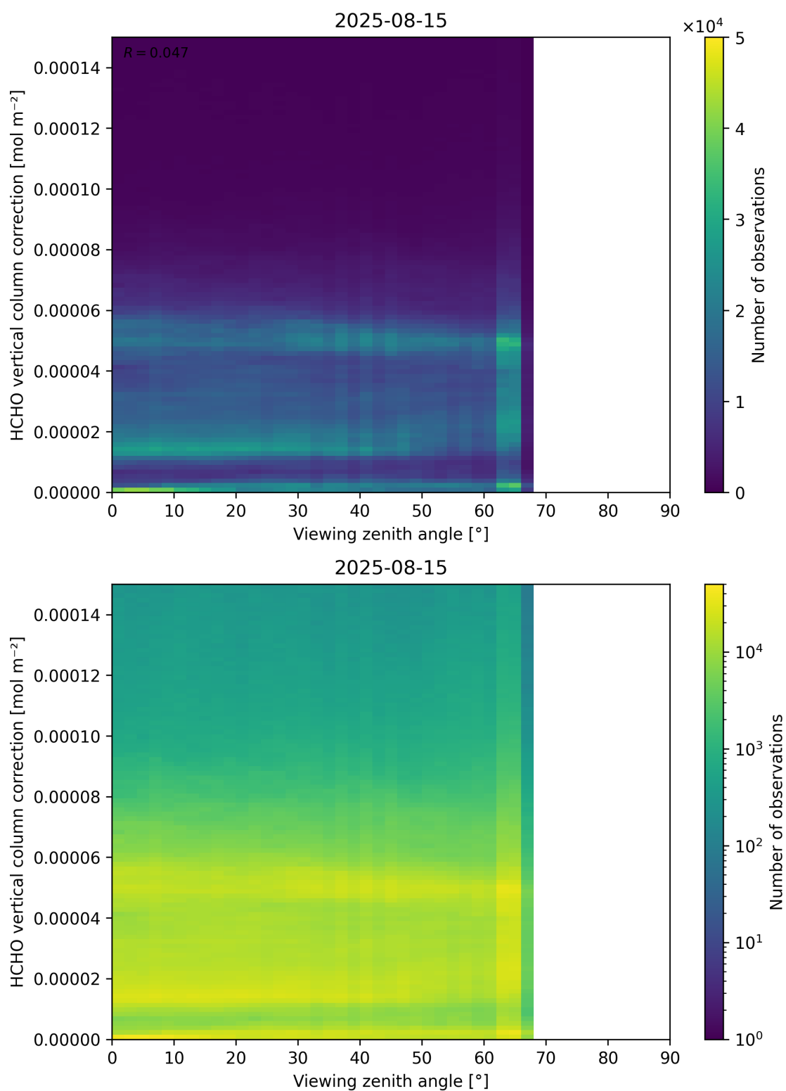
Figure 193: Scatter density plot of “Viewing zenith angle” against “HCHO vertical column correction” for 2025-08-14 to 2025-08-16.
