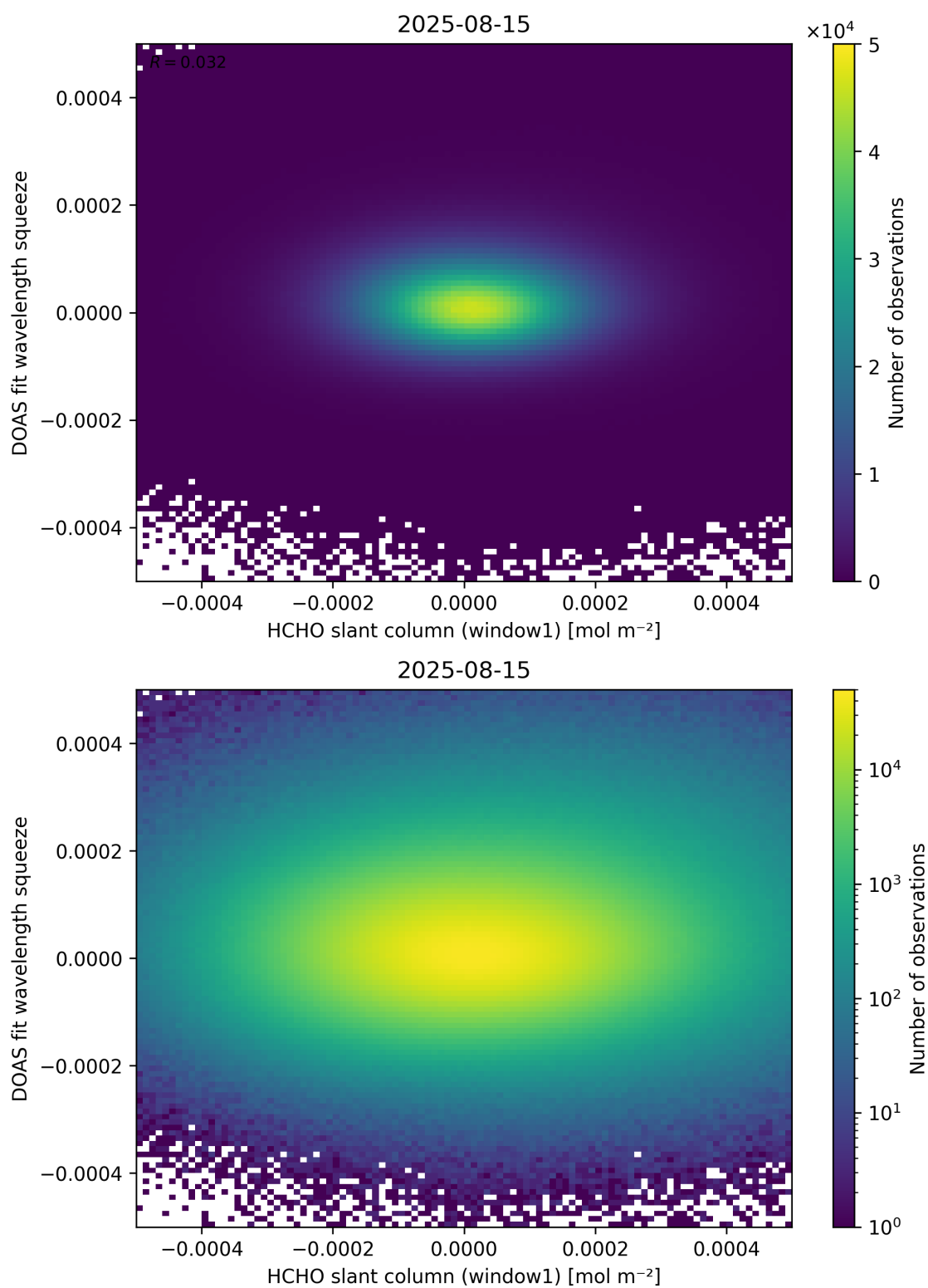
Figure 80: Scatter density plot of “HCHO slant column (window1)” against “DOAS fit wavelength squeeze” for 2025-08-14 to 2025-08-16.
