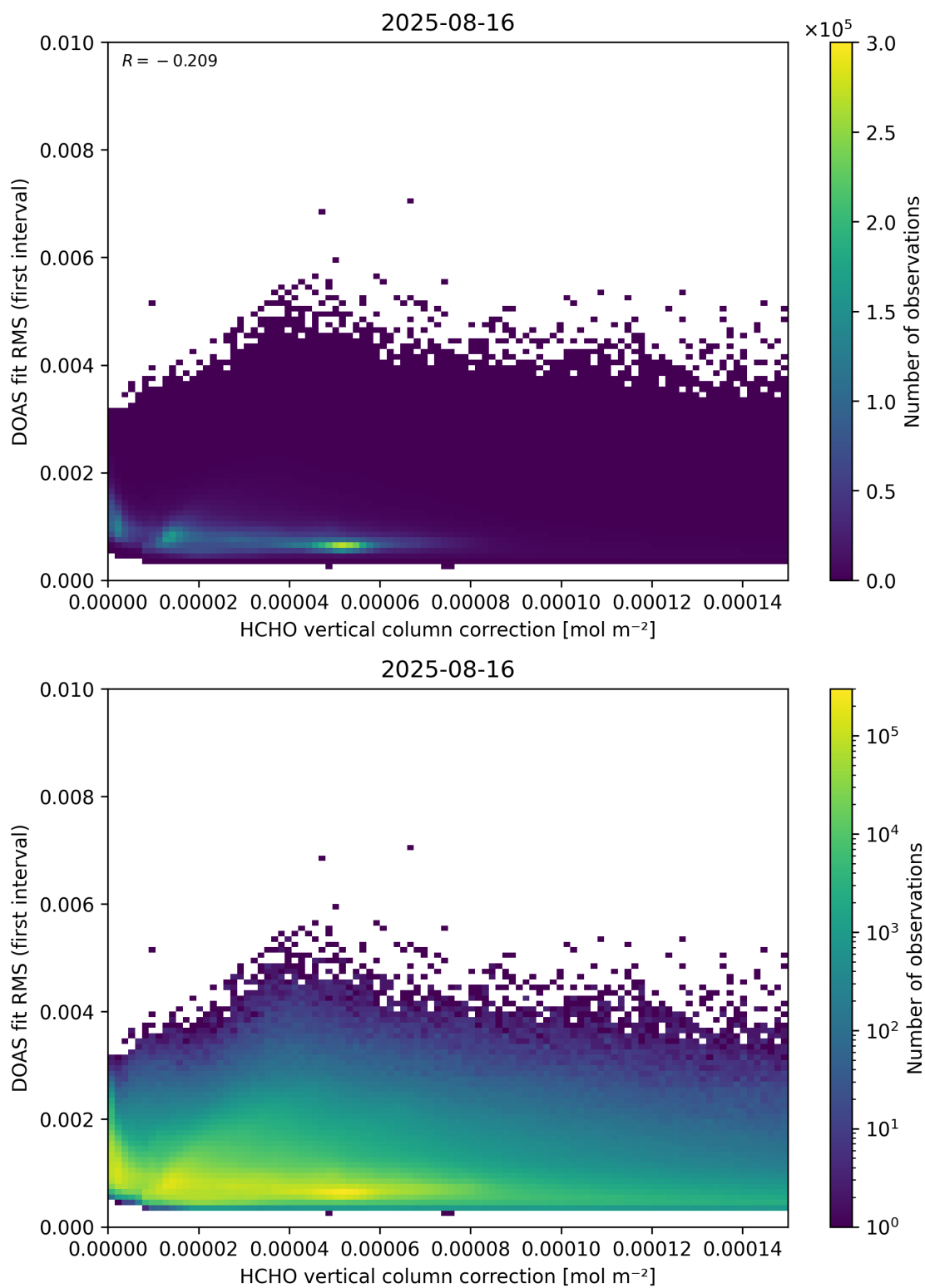
Figure 112: Scatter density plot of “HCHO vertical column correction” against “DOAS fit RMS (first interval)” for 2025-08-15 to 2025-08-17.
