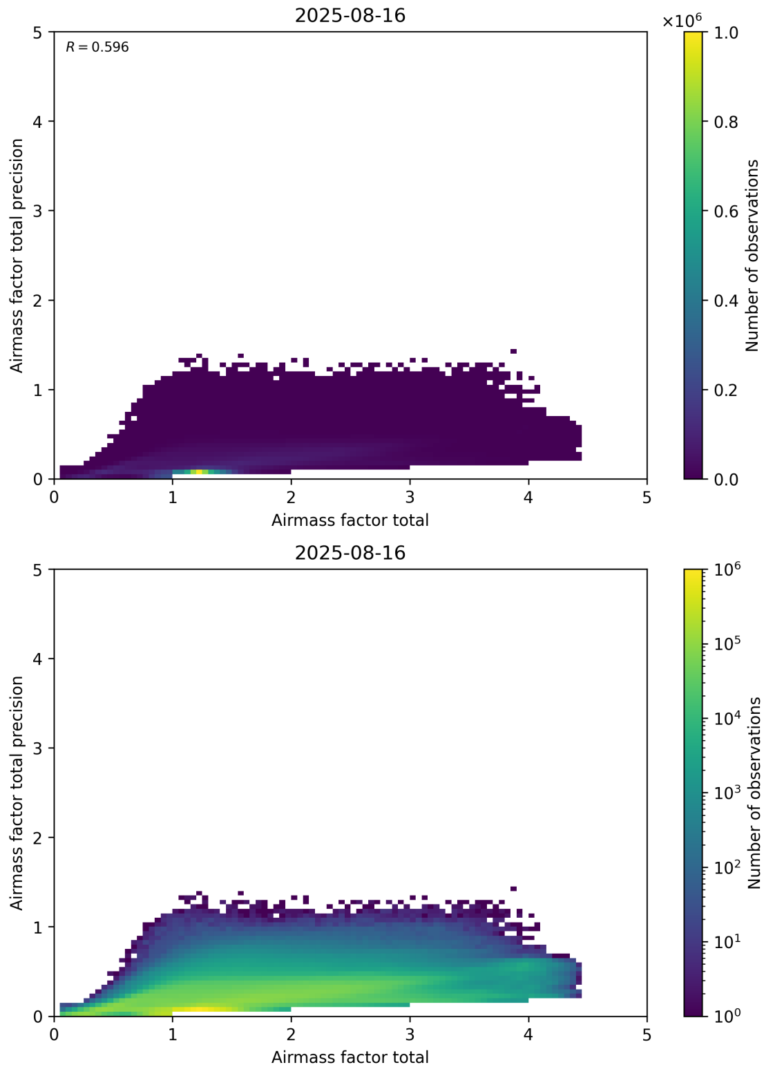
Figure 103: Scatter density plot of “Airmass factor total” against “Airmass factor total precision” for 2025-08-15 to 2025-08-17.
