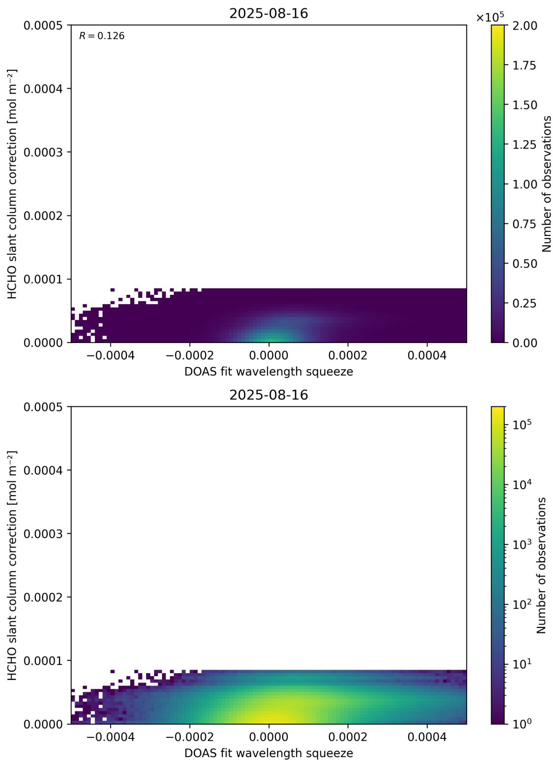
Figure 70: Scatter density plot of “DOAS fit wavelength squeeze” against “HCHO slant column correction” for 2025-08-15 to 2025-08-17.
