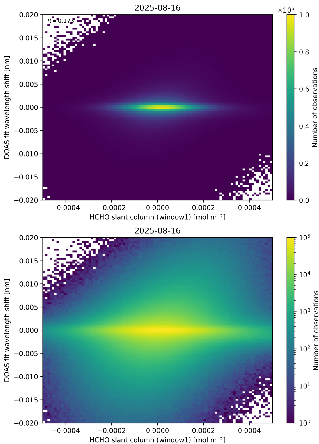
Figure 79: Scatter density plot of “HCHO slant column (window1)” against “DOAS fit wavelength shift” for 2025-08-15 to 2025-08-17.
