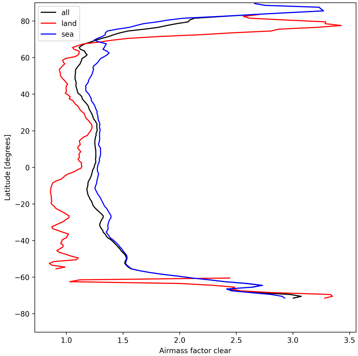
Figure 28: Zonal average of “Airmass factor clear” for 2025-08-15 to 2025-08-17.
