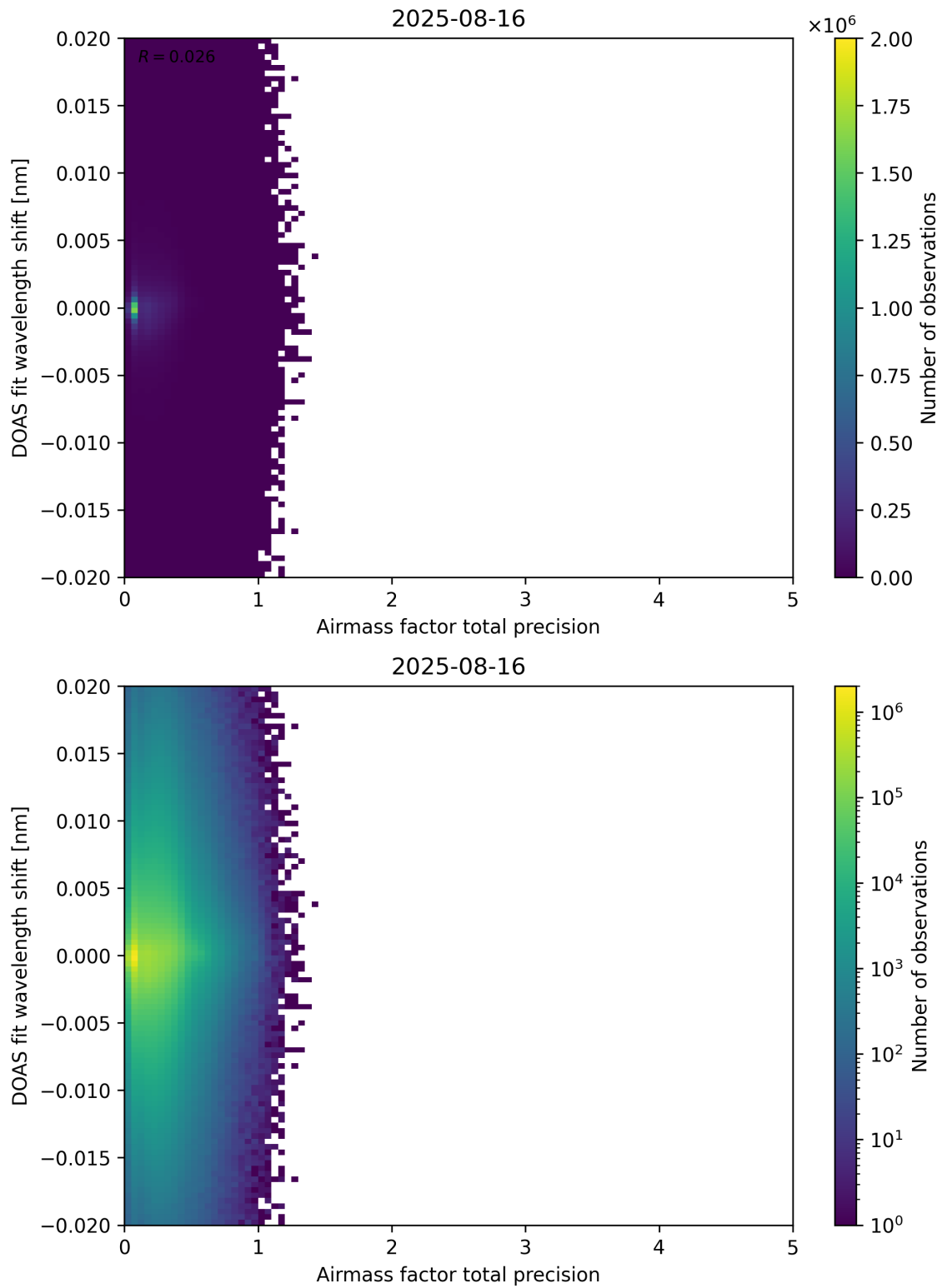
Figure 106: Scatter density plot of “Airmass factor total precision” against “DOAS fit wavelength shift” for 2025-08-15 to 2025-08-17.
