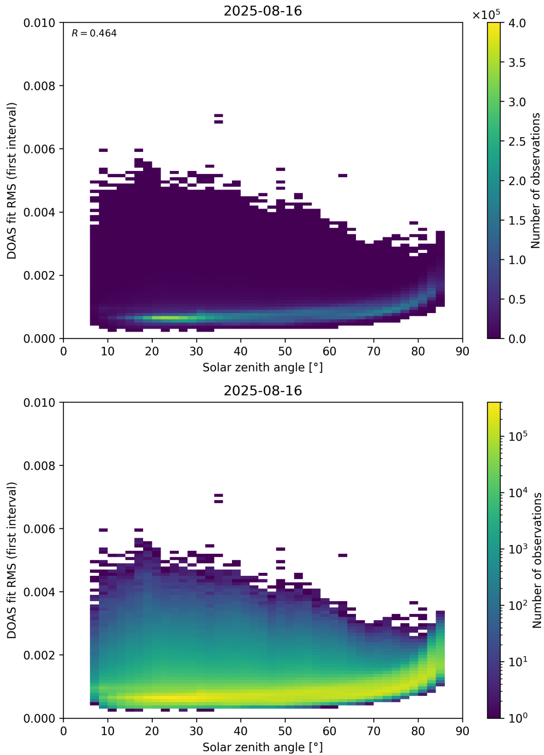
Figure 167: Scatter density plot of “Solar zenith angle” against “DOAS fit RMS (first interval)” for 2025-08-15 to 2025-08-17.
