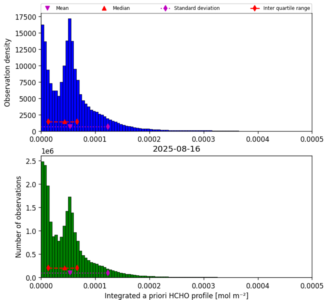
Figure 43: Histogram of “Integrated a priori HCHO profile” for 2025-08-15 to 2025-08-17
