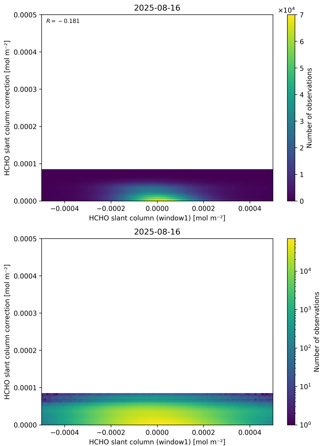
Figure 83: Scatter density plot of “HCHO slant column (window1)” against “HCHO slant column correction” for 2025-08-15 to 2025-08-17.
