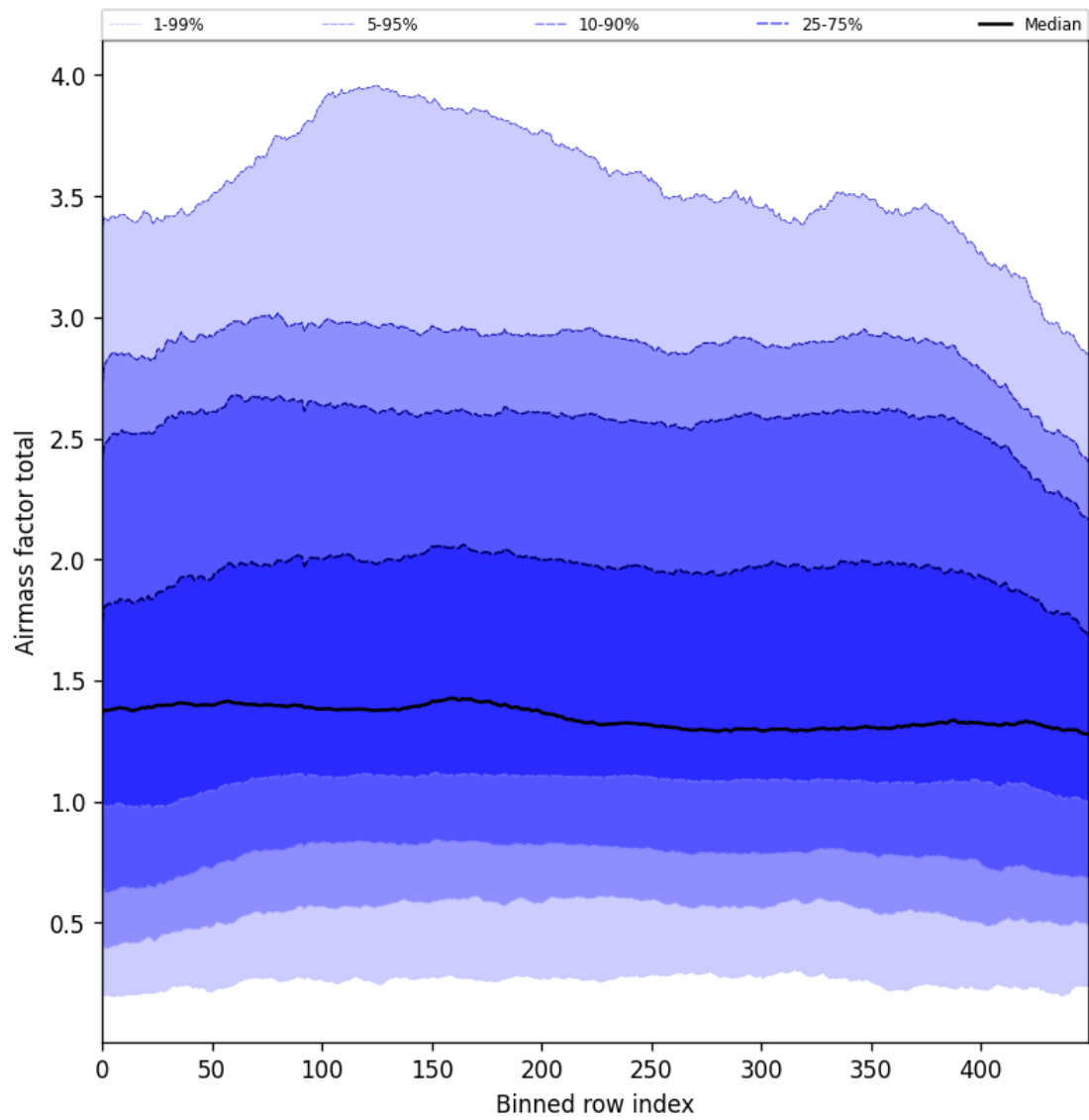
Figure 54: Along track statistics of “Airmass factor total” for 2025-08-15 to 2025-08-17
