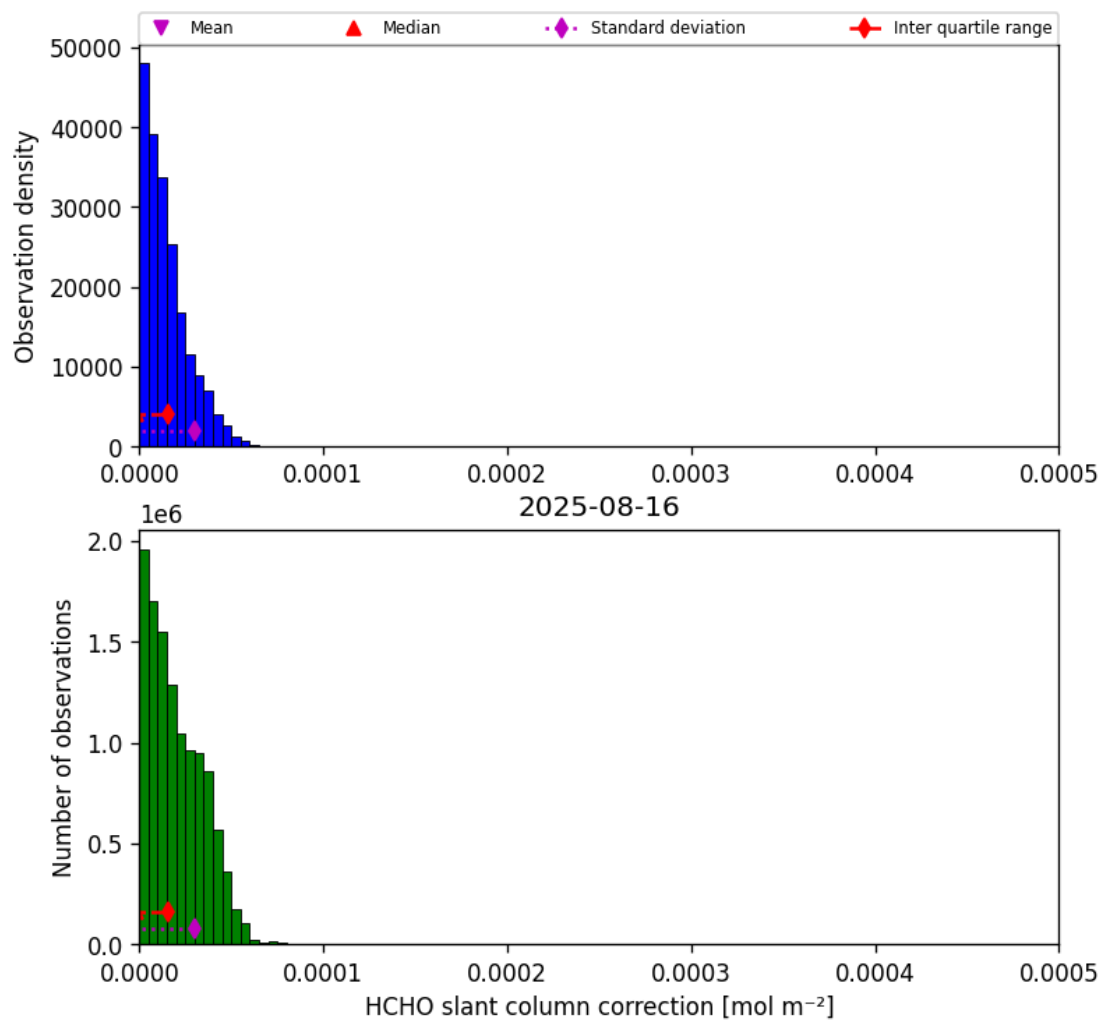
Figure 47: Histogram of “HCHO slant column correction” for 2025-08-15 to 2025-08-17
