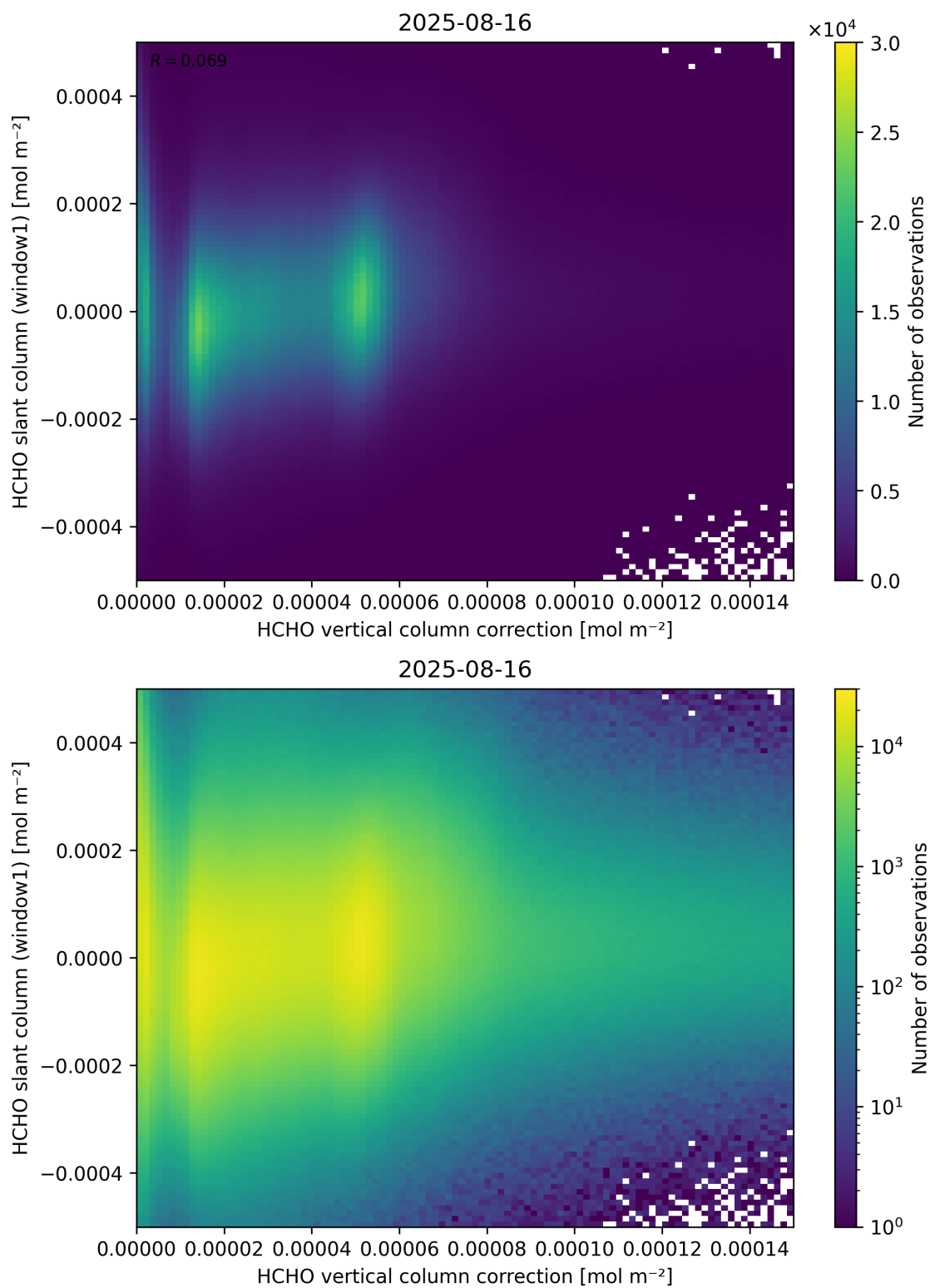
Figure 118: Scatter density plot of “HCHO vertical column correction” against “HCHO slant column (window1)” for 2025-08-15 to 2025-08-17.
