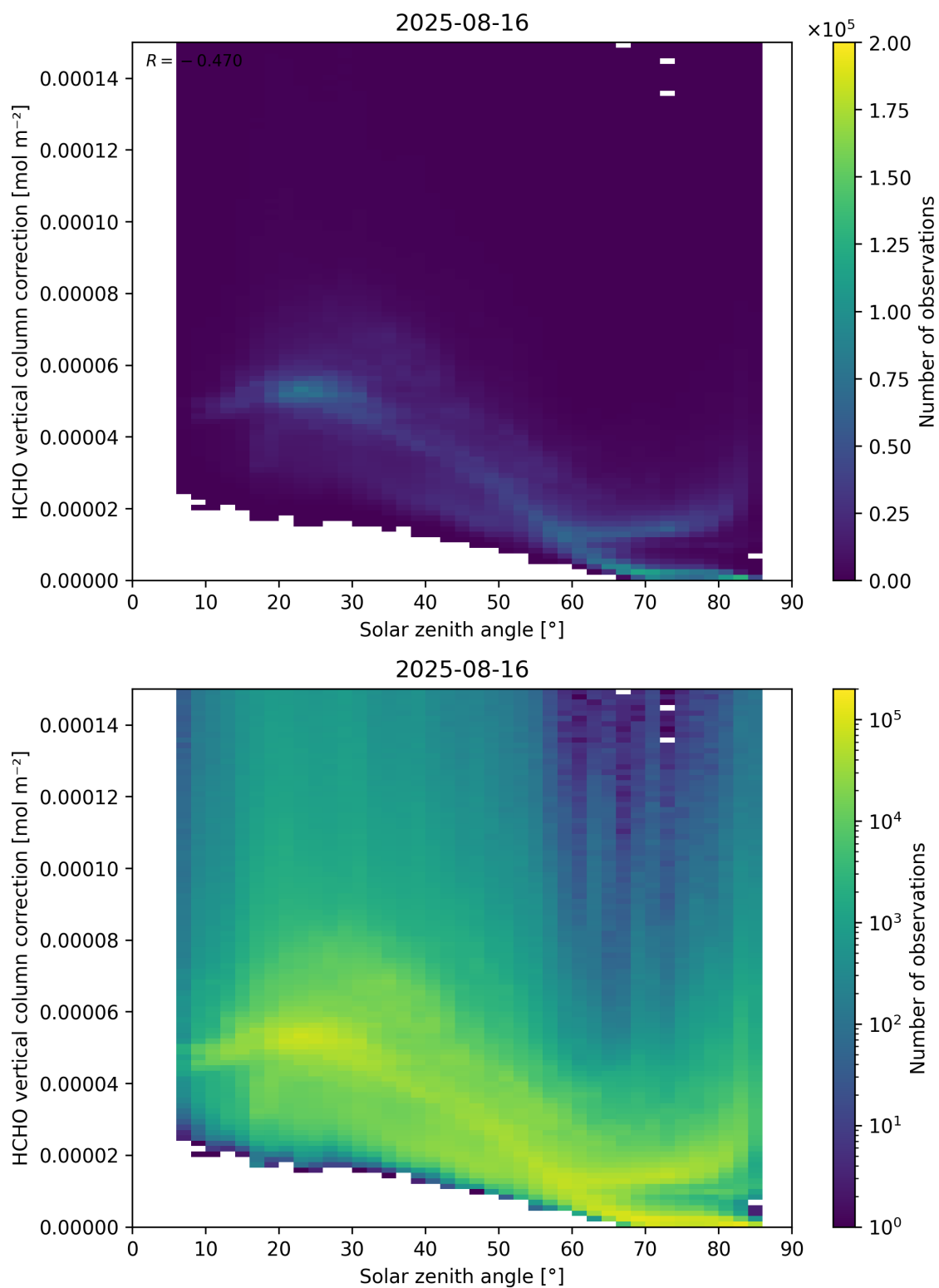
Figure 178: Scatter density plot of “Solar zenith angle” against “HCHO vertical column correction” for 2025-08-15 to 2025-08-17.
