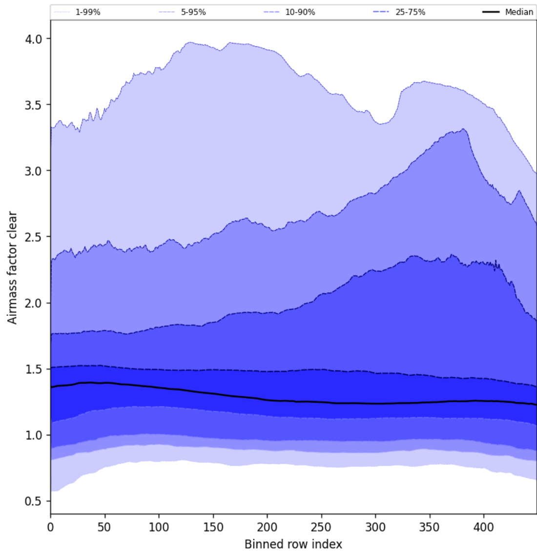
Figure 56: Along track statistics of “Airmass factor clear” for 2025-08-15 to 2025-08-17
