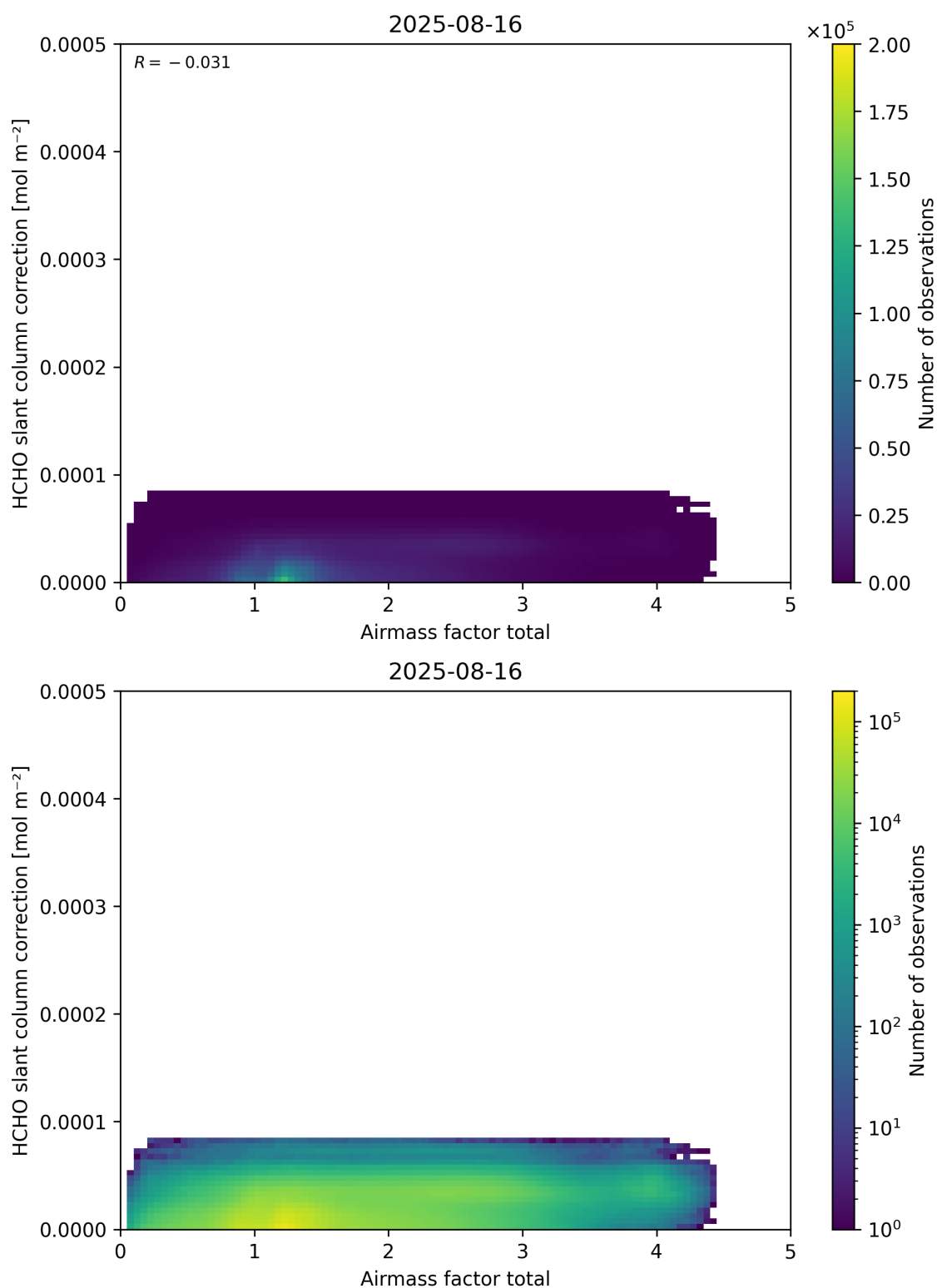
Figure 102: Scatter density plot of “Airmass factor total” against “HCHO slant column correction” for 2025-08-15 to 2025-08-17.
