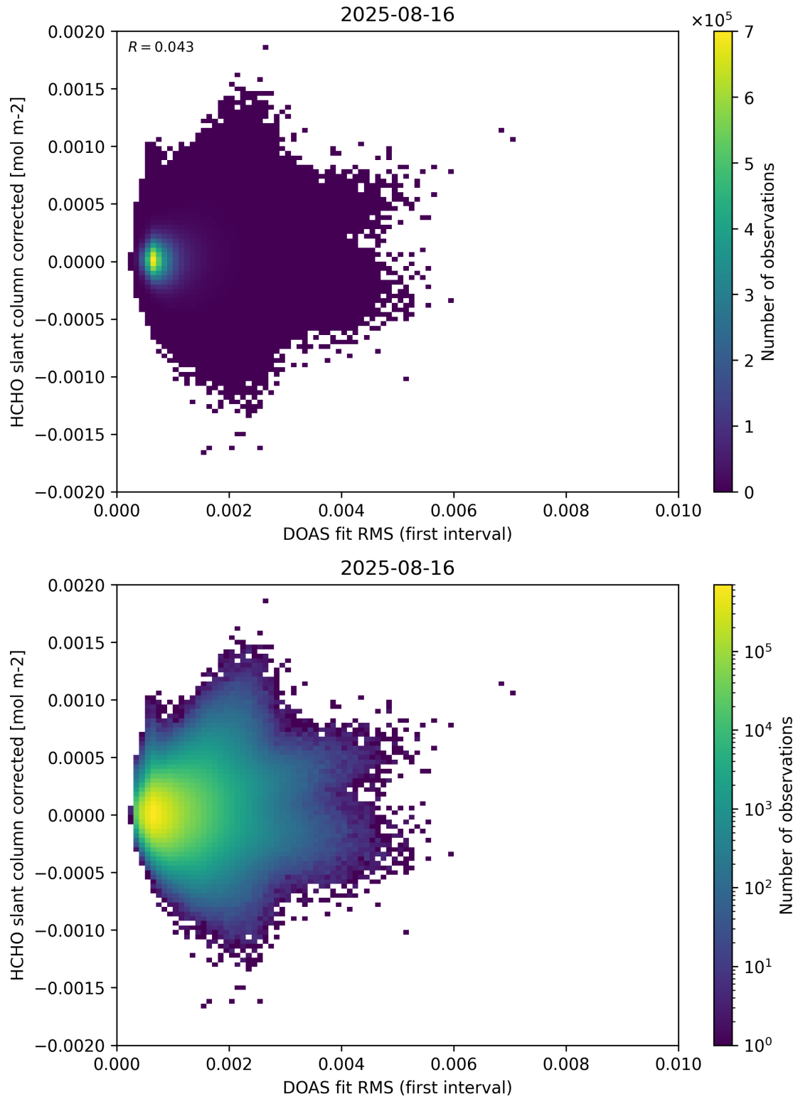
Figure 62: Scatter density plot of “DOAS fit RMS (first interval)” against “HCHO slant column corrected” for 2025-08-15 to 2025-08-17.
