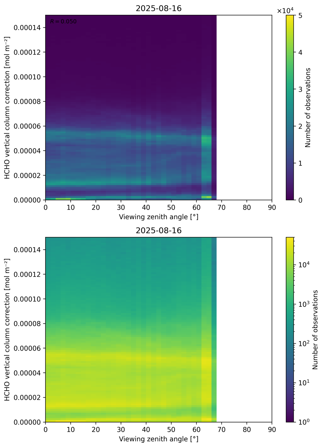
Figure 193: Scatter density plot of “Viewing zenith angle” against “HCHO vertical column correction” for 2025-08-15 to 2025-08-17.
