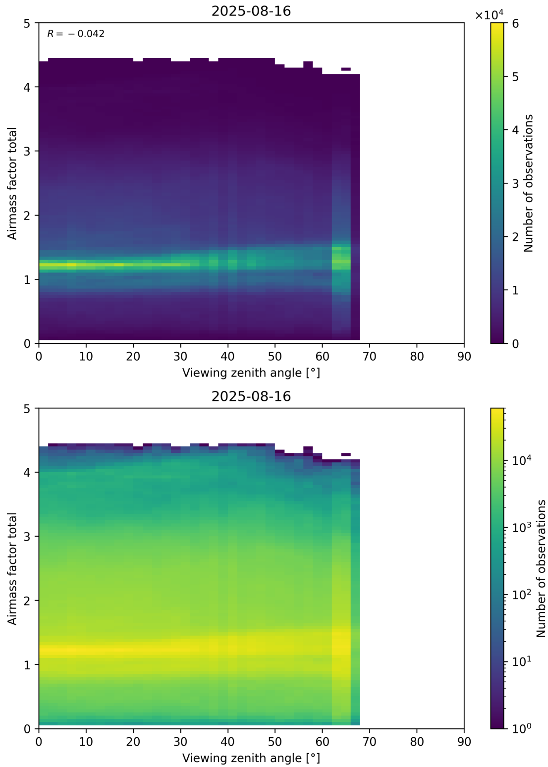
Figure 190: Scatter density plot of “Viewing zenith angle” against “Airmass factor total” for 2025-08-15 to 2025-08-17.
