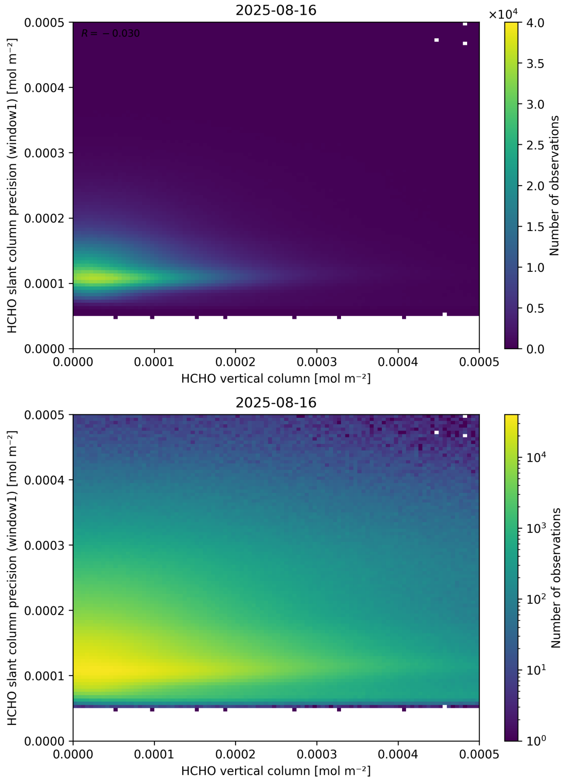
Figure 130: Scatter density plot of “HCHO vertical column” against “HCHO slant column precision (window1)” for 2025-08-15 to 2025-08-17.
