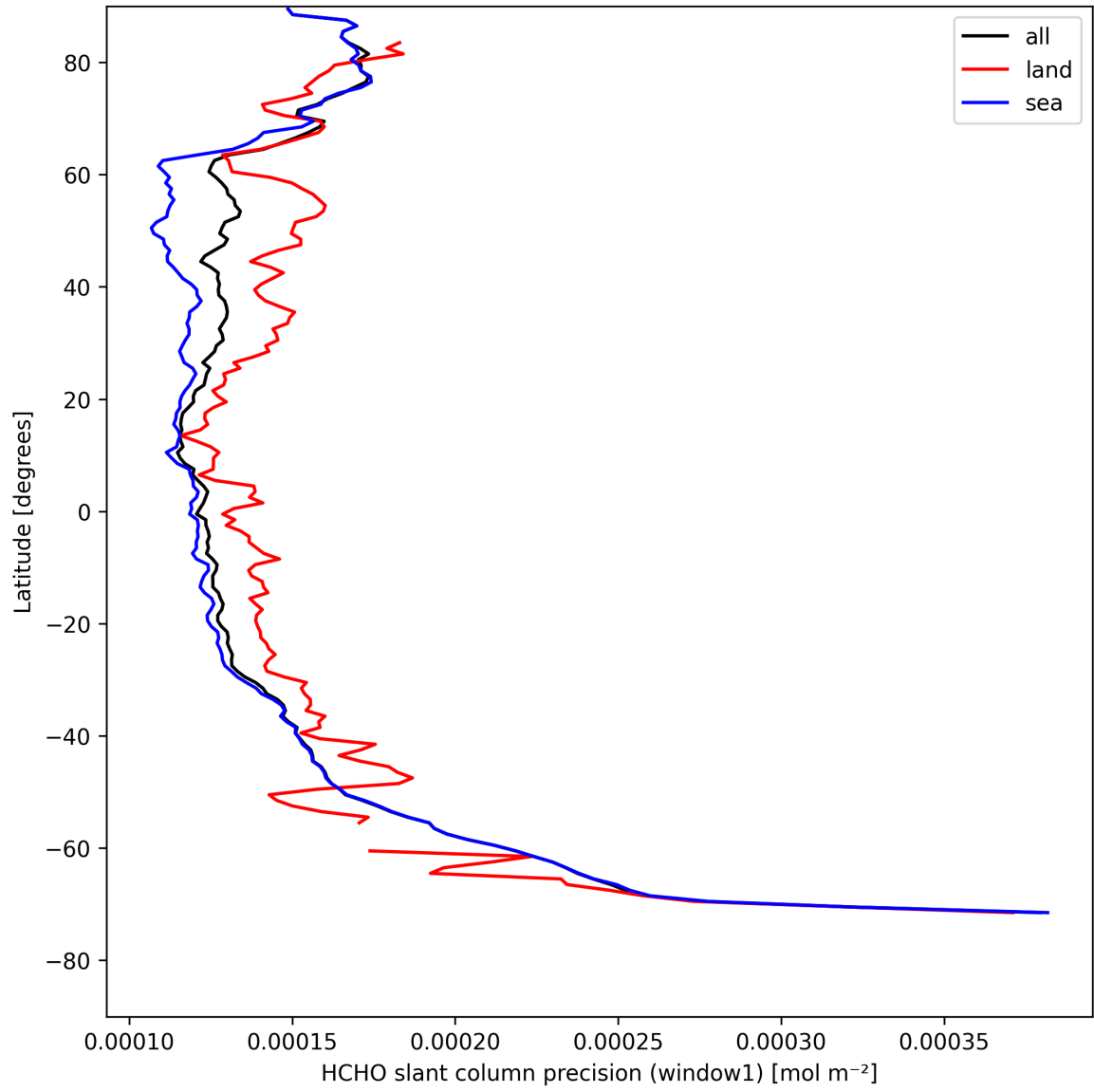
Figure 25: Zonal average of “HCHO slant column precision (window1)” for 2025-08-15 to 2025-08-17.
