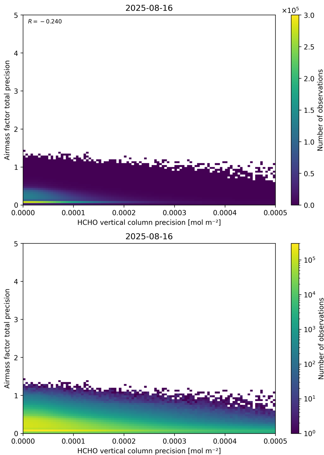
Figure 145: Scatter density plot of “HCHO vertical column precision” against “Airmass factor total precision” for 2025-08-15 to 2025-08-17.
