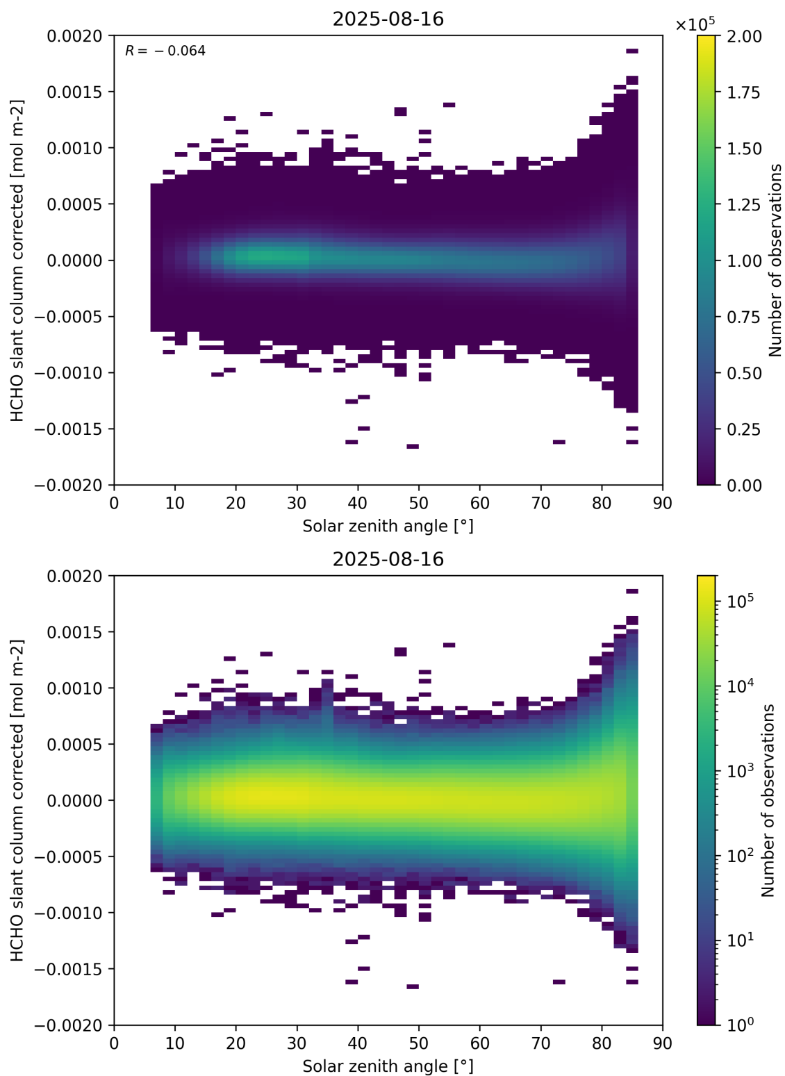
Figure 171: Scatter density plot of “Solar zenith angle” against “HCHO slant column corrected” for 2025-08-15 to 2025-08-17.
