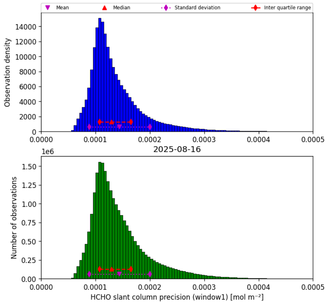
Figure 39: Histogram of “HCHO slant column precision (window1)” for 2025-08-15 to 2025-08-17
