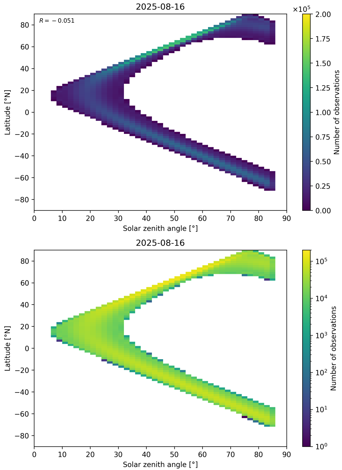
Figure 181: Scatter density plot of “Solar zenith angle” against “Latitude” for 2025-08-15 to 2025-08-17.
