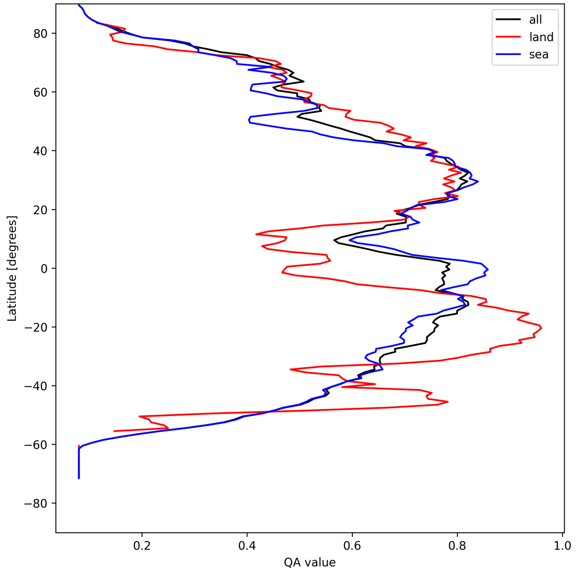
Figure 20: Zonal average of “QA value” for 2025-08-15 to 2025-08-17.
