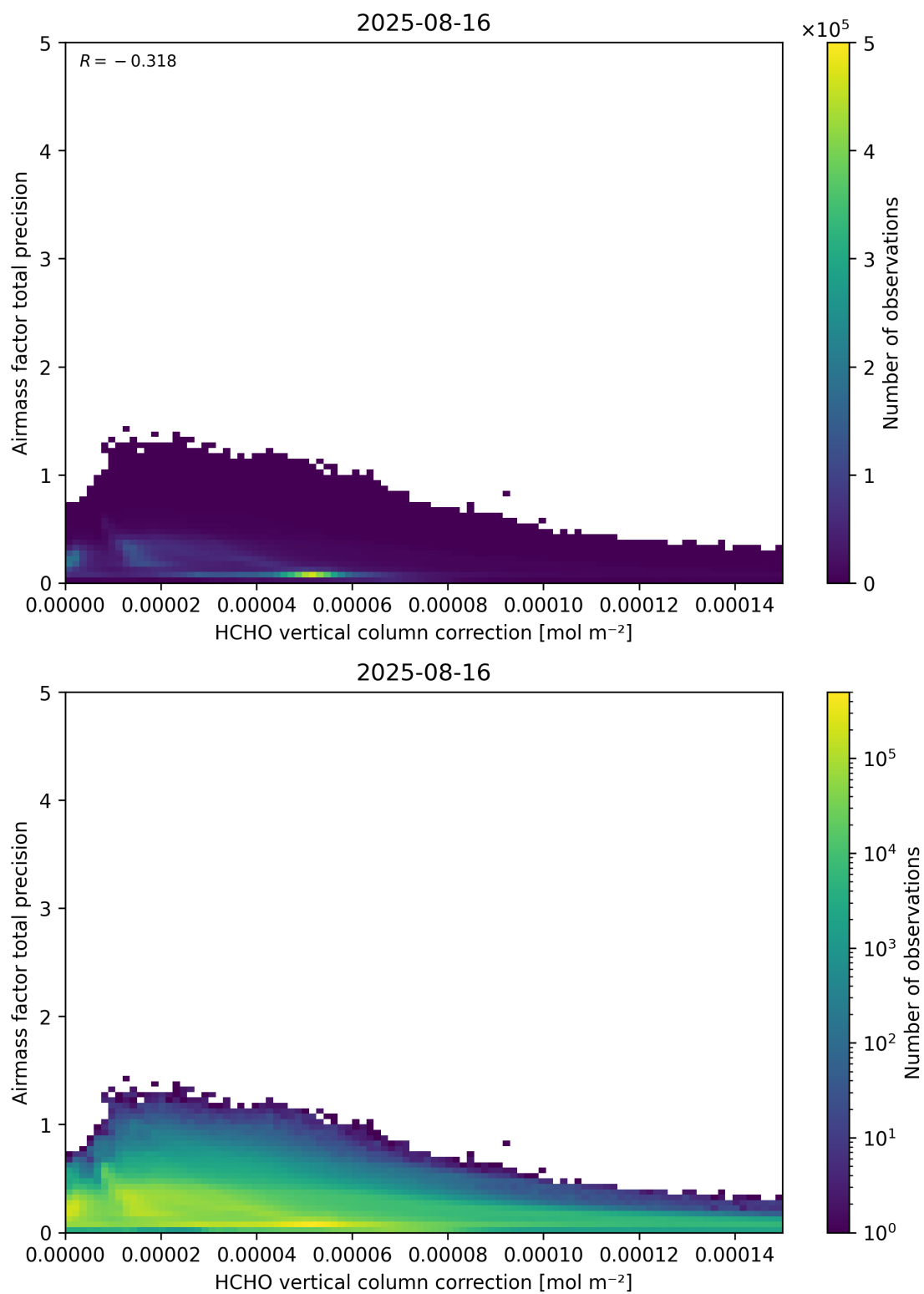
Figure 121: Scatter density plot of “HCHO vertical column correction” against “Airmass factor total precision” for 2025-08-15 to 2025-08-17.
