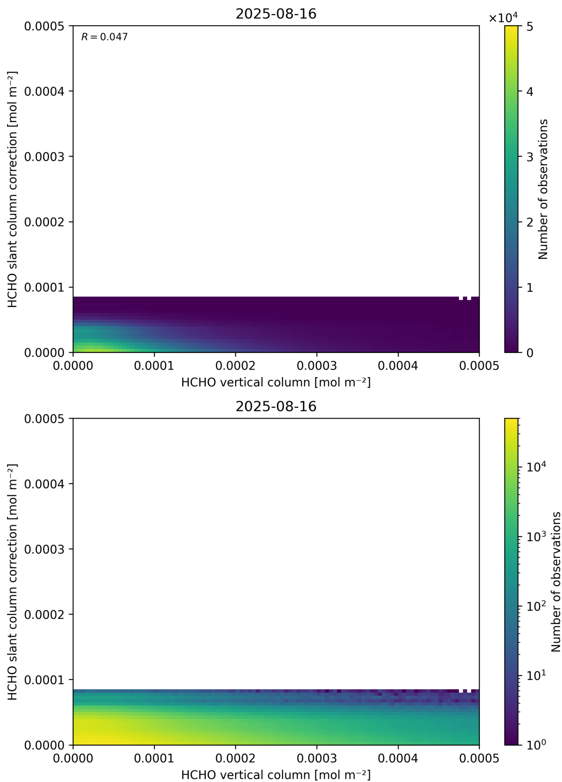
Figure 128: Scatter density plot of “HCHO vertical column” against “HCHO slant column correction” for 2025-08-15 to 2025-08-17.
