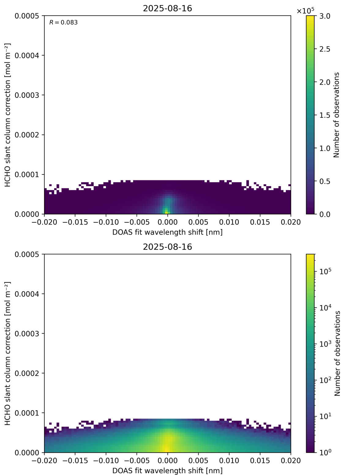
Figure 67: Scatter density plot of “DOAS fit wavelength shift” against “HCHO slant column correction” for 2025-08-15 to 2025-08-17.
