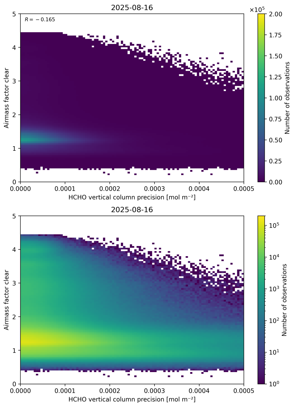
Figure 139: Scatter density plot of “HCHO vertical column precision” against “Airmass factor clear” for 2025-08-15 to 2025-08-17.
