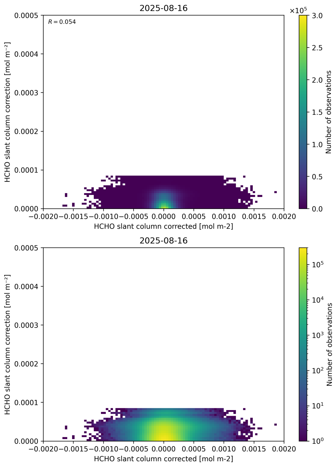
Figure 77: Scatter density plot of “HCHO slant column corrected” against “HCHO slant column correction” for 2025-08-15 to 2025-08-17.
