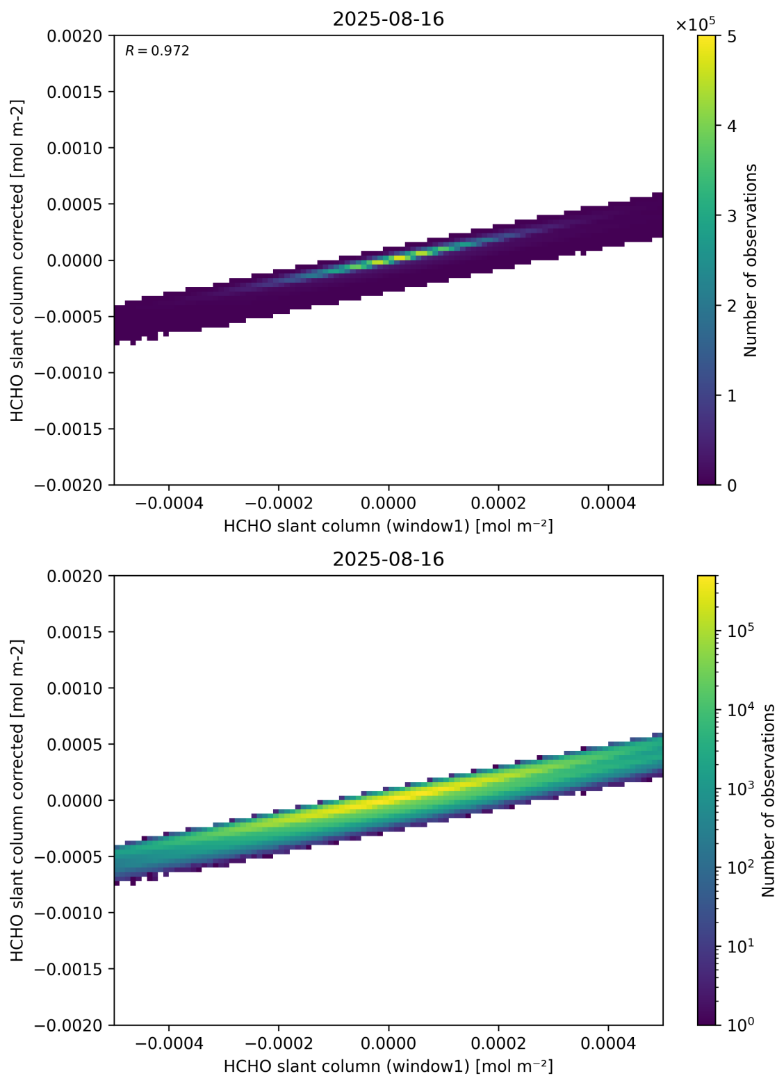
Figure 82: Scatter density plot of “HCHO slant column (window1)” against “HCHO slant column corrected” for 2025-08-15 to 2025-08-17.
