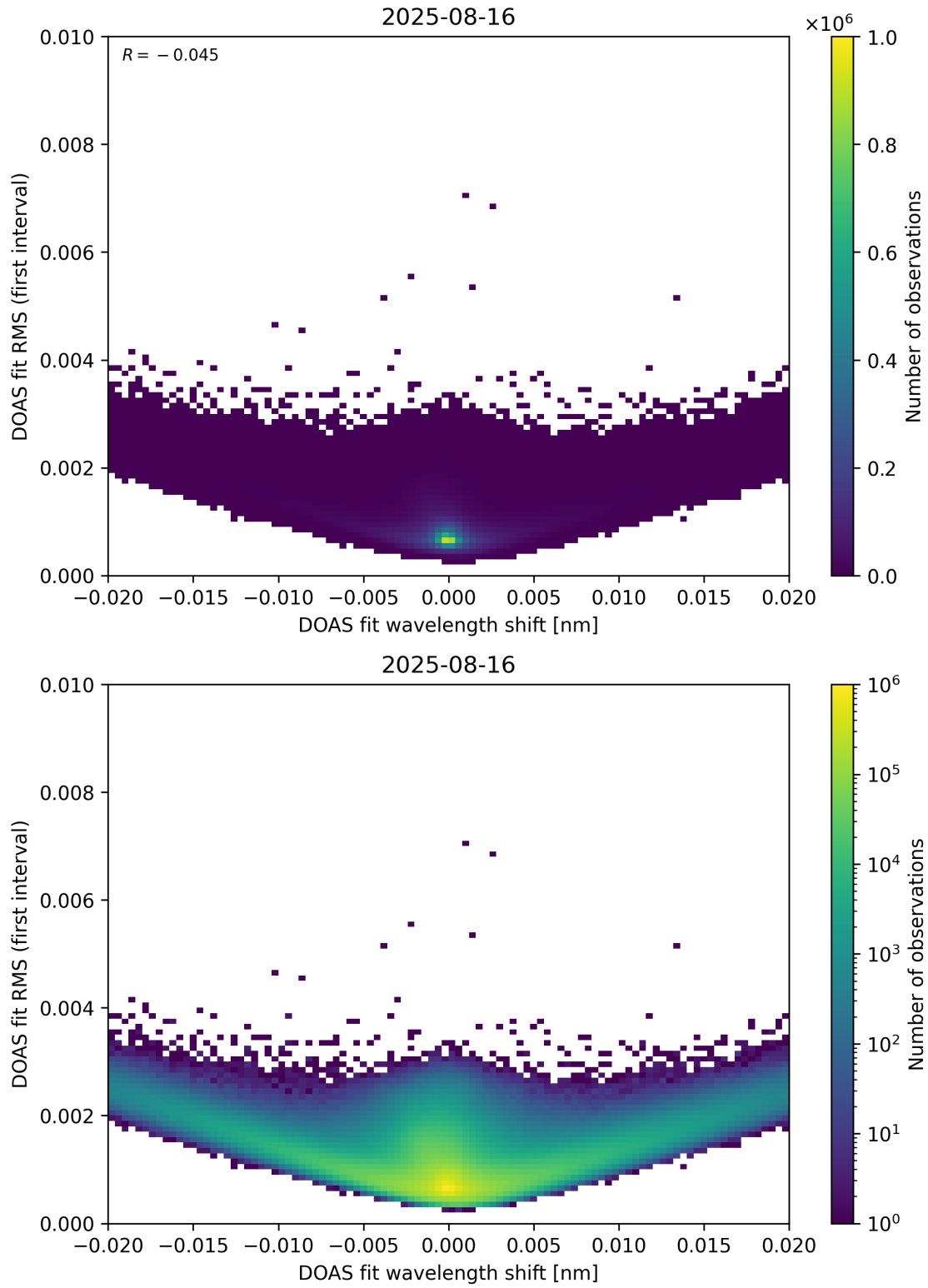
Figure 64: Scatter density plot of “DOAS fit wavelength shift” against “DOAS fit RMS (first interval)” for 2025-08-15 to 2025-08-17.
