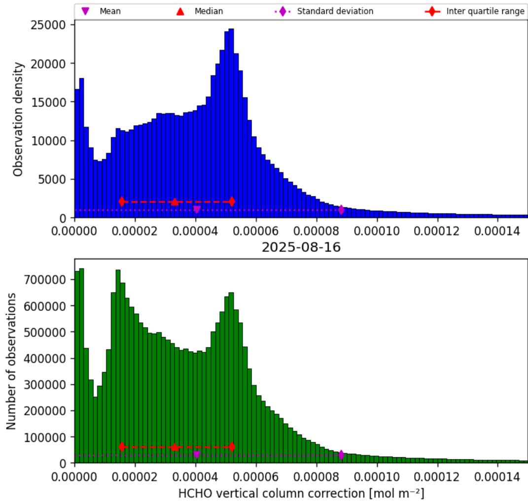
Figure 37: Histogram of “HCHO vertical column correction” for 2025-08-15 to 2025-08-17
