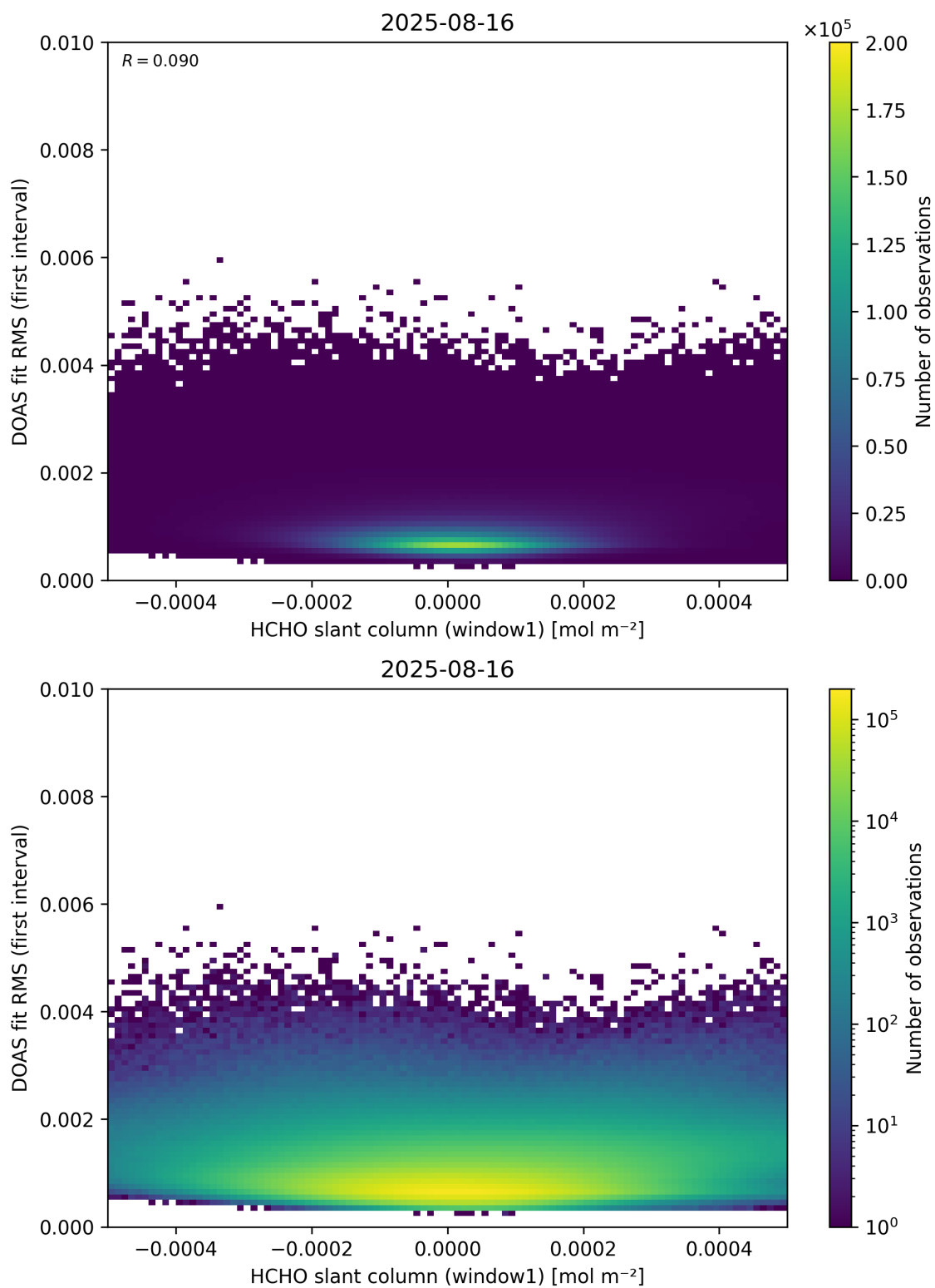
Figure 78: Scatter density plot of “HCHO slant column (window1)” against “DOAS fit RMS (first interval)” for 2025-08-15 to 2025-08-17.
