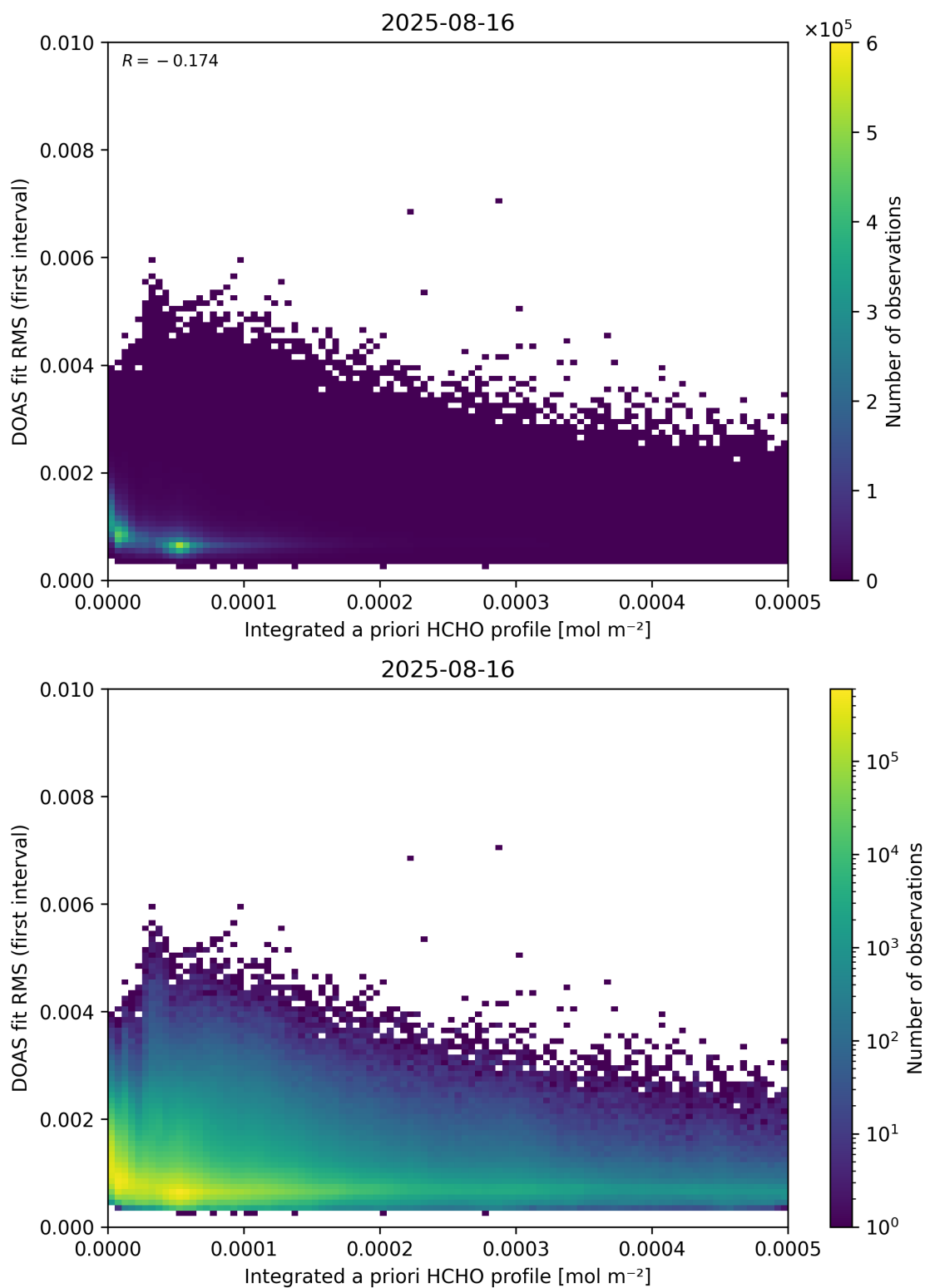
Figure 148: Scatter density plot of “Integrated a priori HCHO profile” against “DOAS fit RMS (first interval)” for 2025-08-15 to 2025-08-17.
