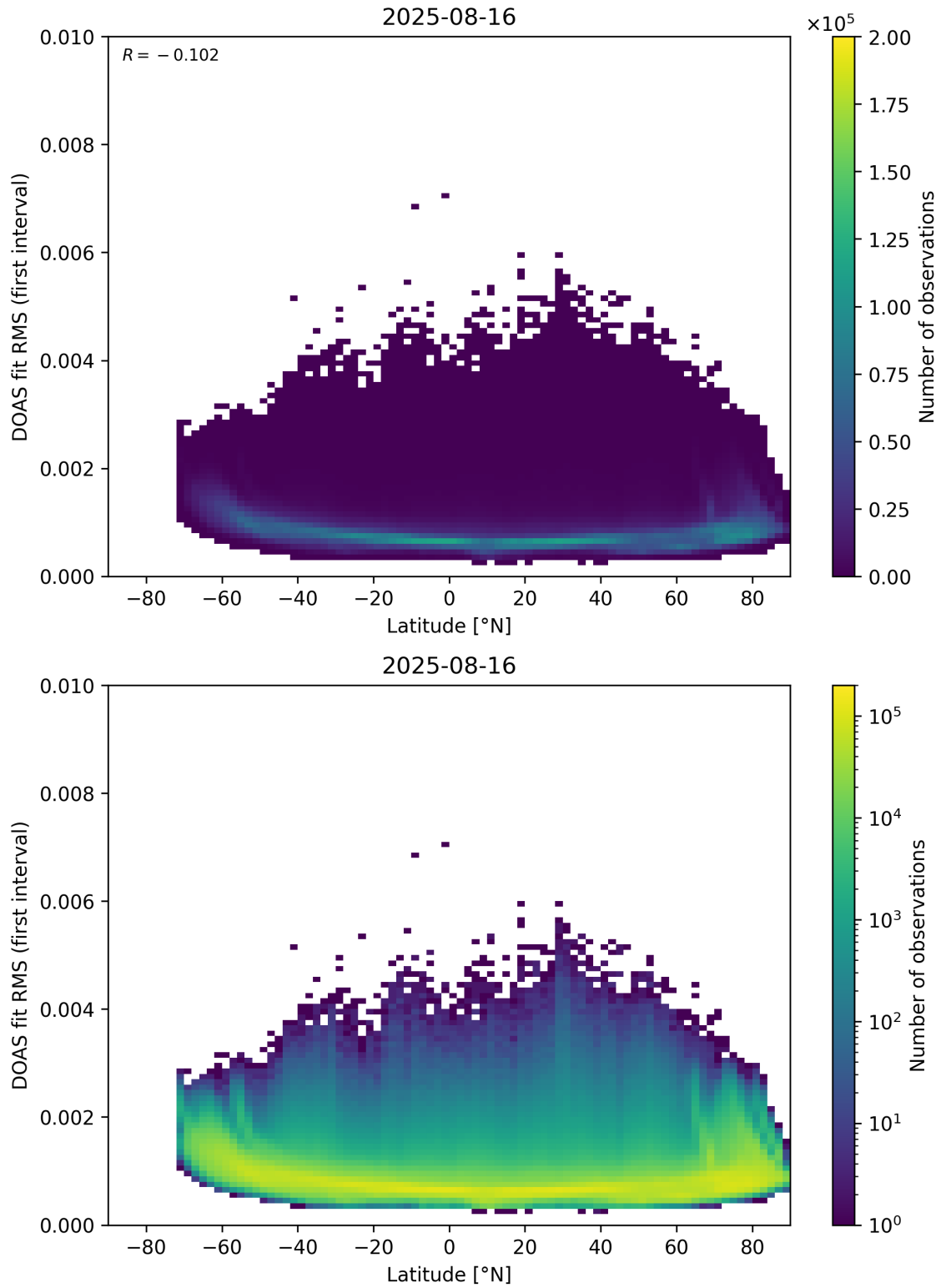
Figure 153: Scatter density plot of “Latitude” against “DOAS fit RMS (first interval)” for 2025-08-15 to 2025-08-17.
