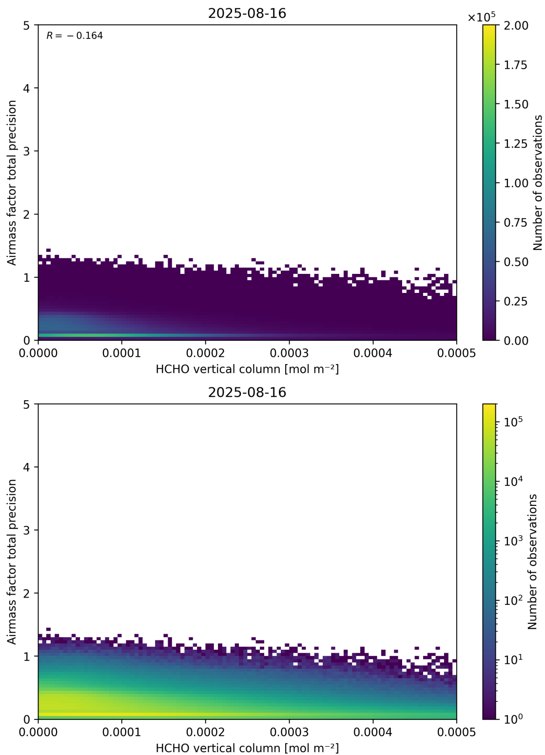
Figure 132: Scatter density plot of “HCHO vertical column” against “Airmass factor total precision” for 2025-08-15 to 2025-08-17.
