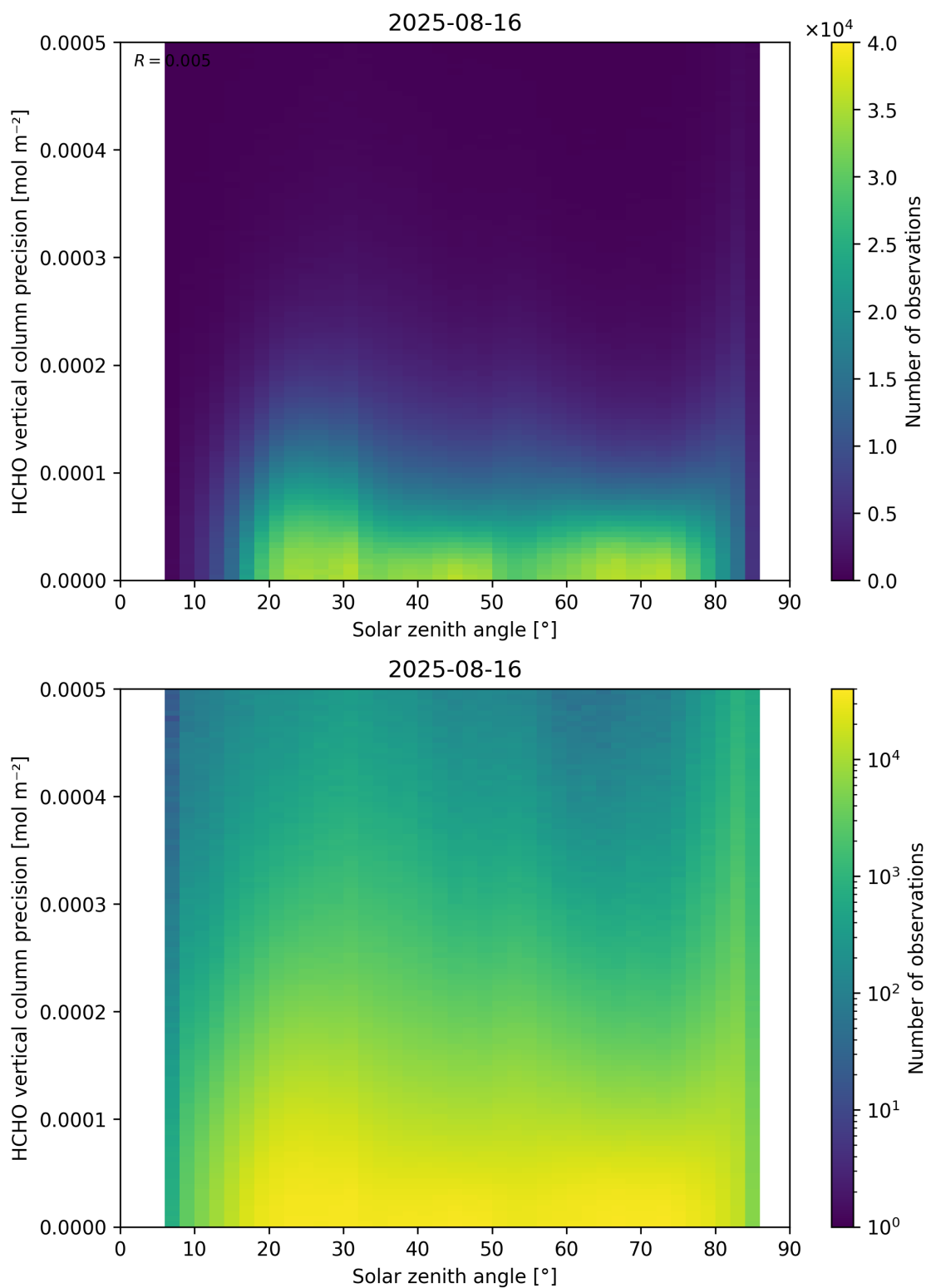
Figure 179: Scatter density plot of “Solar zenith angle” against “HCHO vertical column precision” for 2025-08-15 to 2025-08-17.
