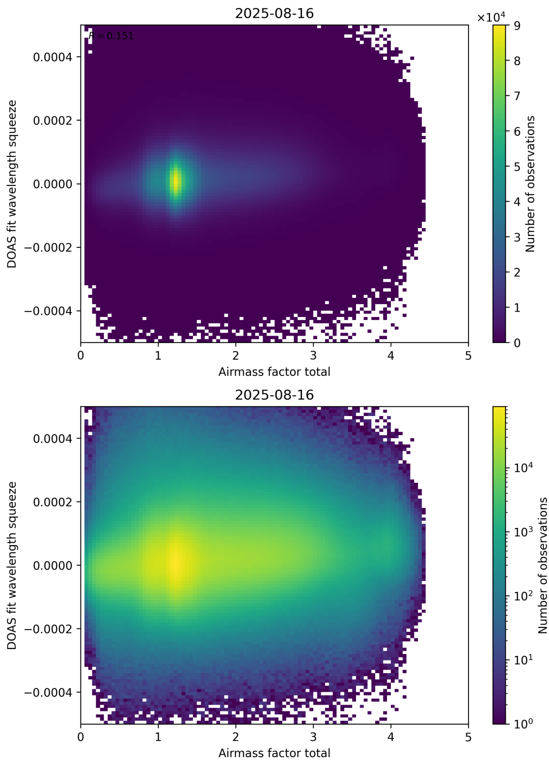
Figure 99: Scatter density plot of “Airmass factor total” against “DOAS fit wavelength squeeze” for 2025-08-15 to 2025-08-17.
