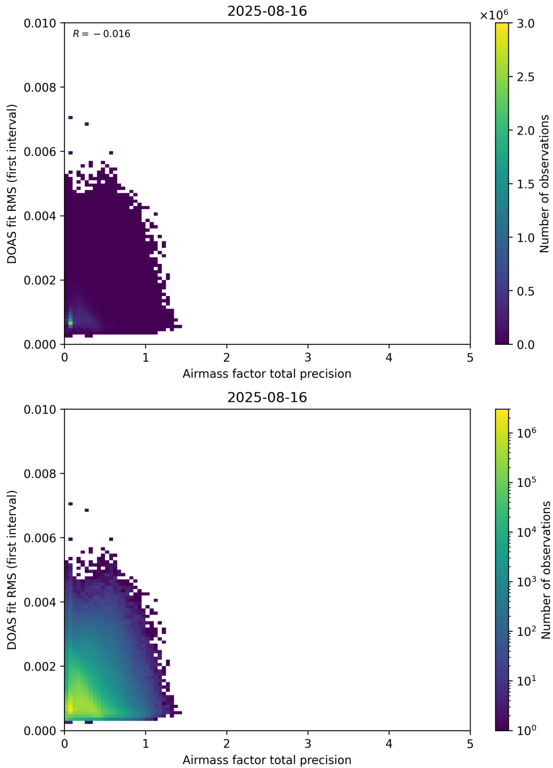
Figure 105: Scatter density plot of “Airmass factor total precision” against “DOAS fit RMS (first interval)” for 2025-08-15 to 2025-08-17.
