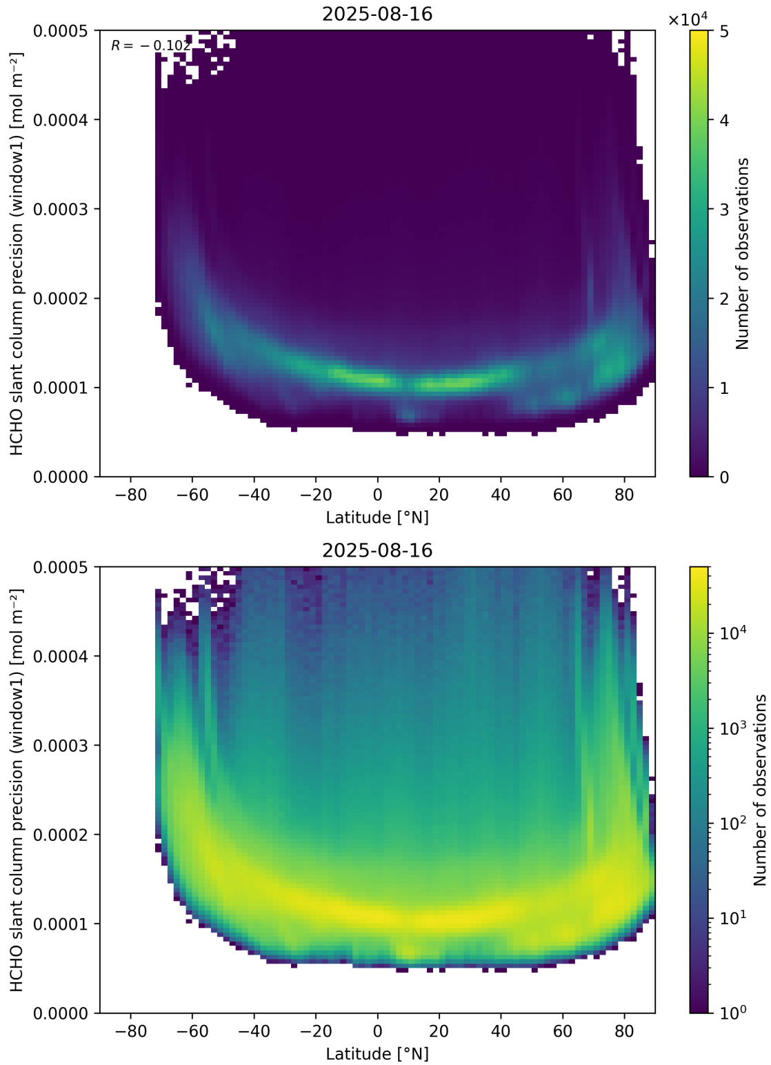
Figure 160: Scatter density plot of “Latitude” against “HCHO slant column precision (window1)” for 2025-08-15 to 2025-08-17.
