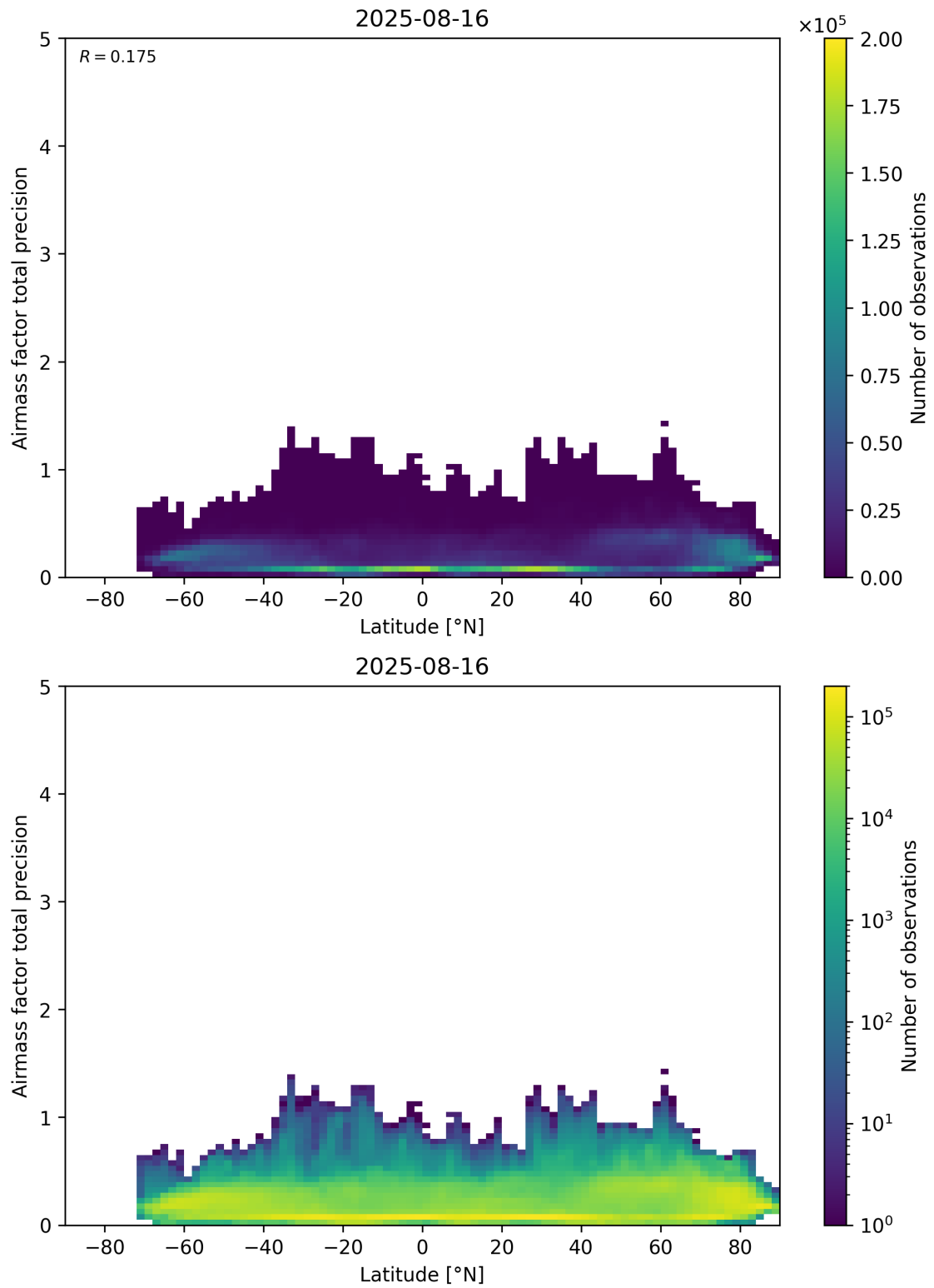
Figure 162: Scatter density plot of “Latitude” against “Airmass factor total precision” for 2025-08-15 to 2025-08-17.
