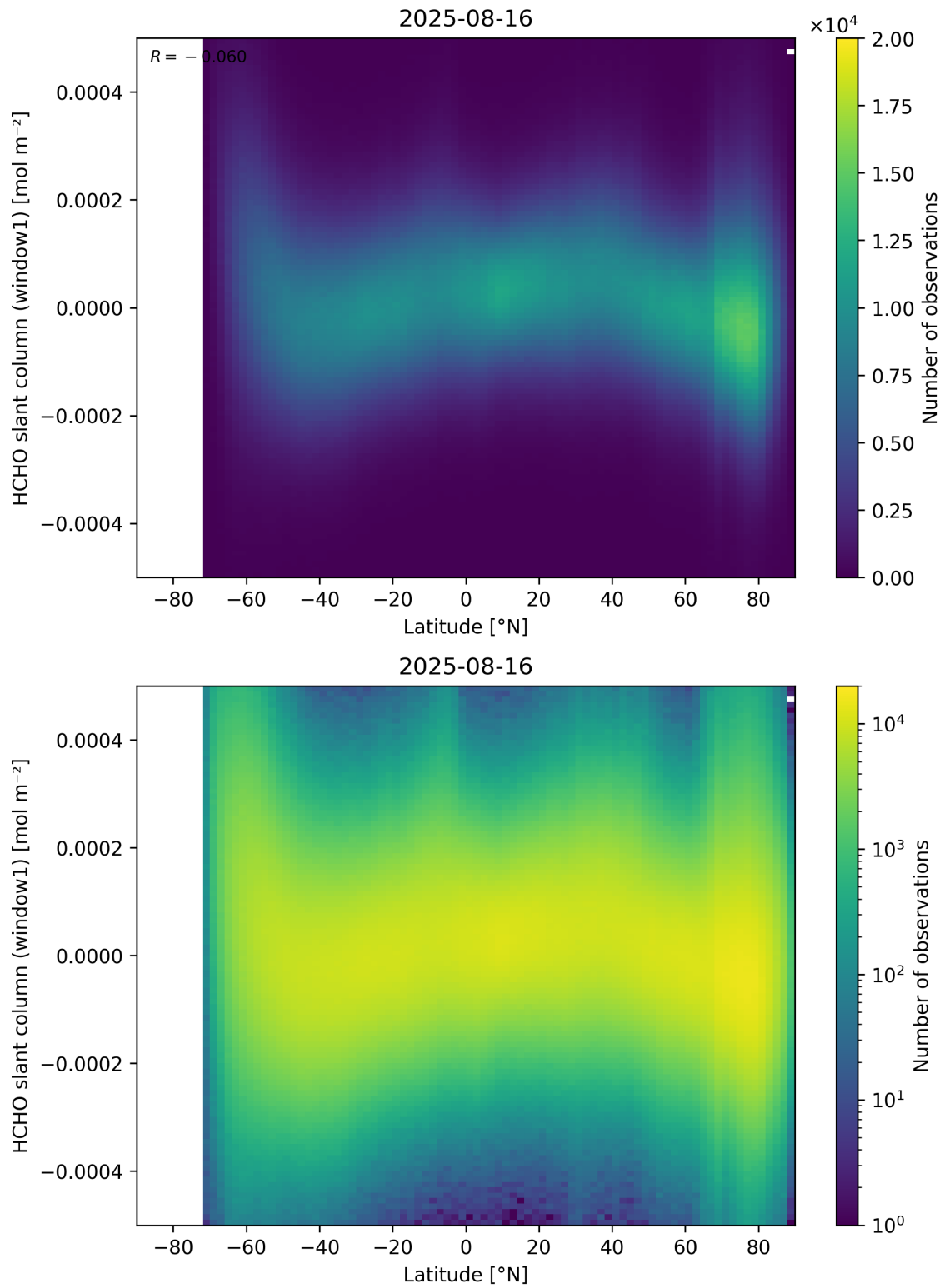
Figure 159: Scatter density plot of “Latitude” against “HCHO slant column (window1)” for 2025-08-15 to 2025-08-17.
