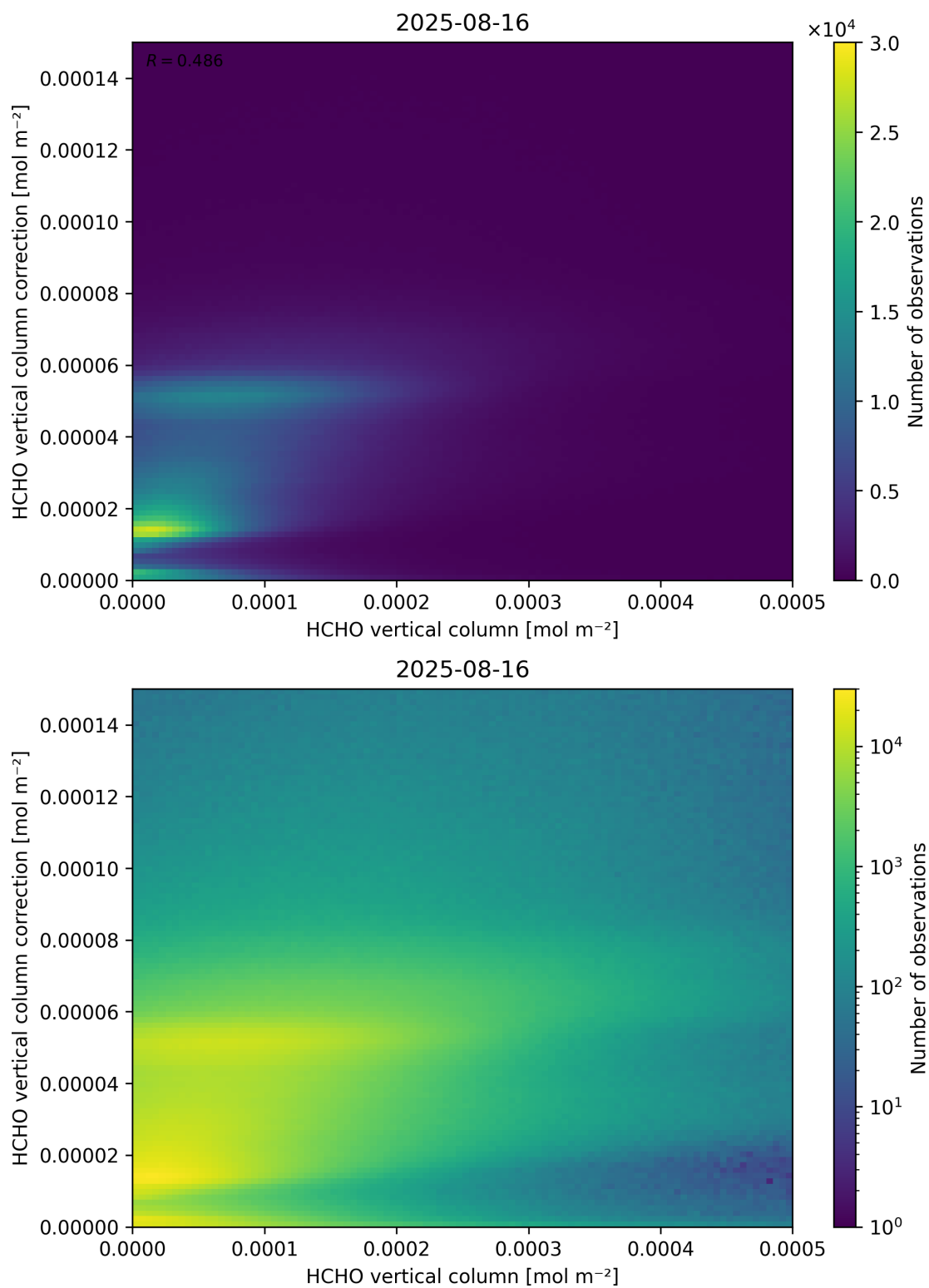
Figure 133: Scatter density plot of “HCHO vertical column” against “HCHO vertical column correction” for 2025-08-15 to 2025-08-17.
