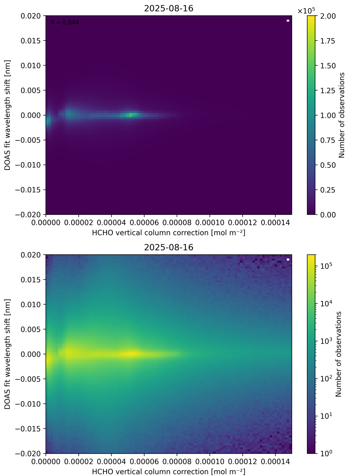
Figure 113: Scatter density plot of “HCHO vertical column correction” against “DOAS fit wavelength shift” for 2025-08-15 to 2025-08-17.
