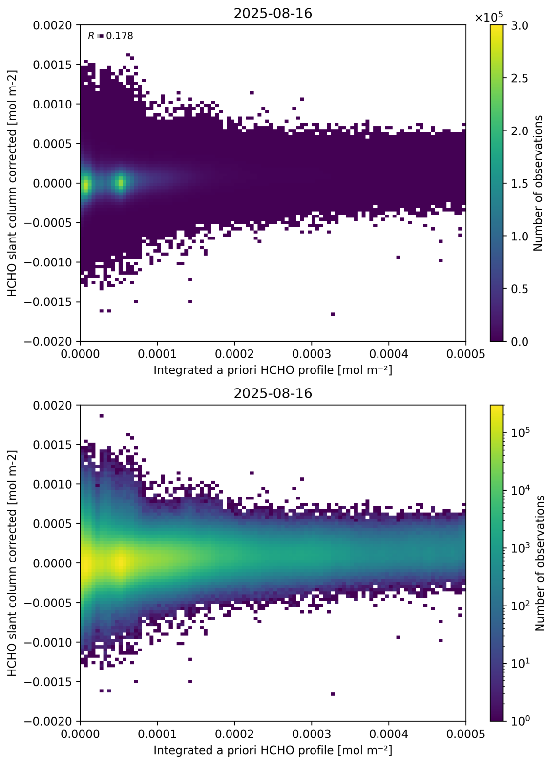
Figure 151: Scatter density plot of “Integrated a priori HCHO profile” against “HCHO slant column corrected” for 2025-08-15 to 2025-08-17.
