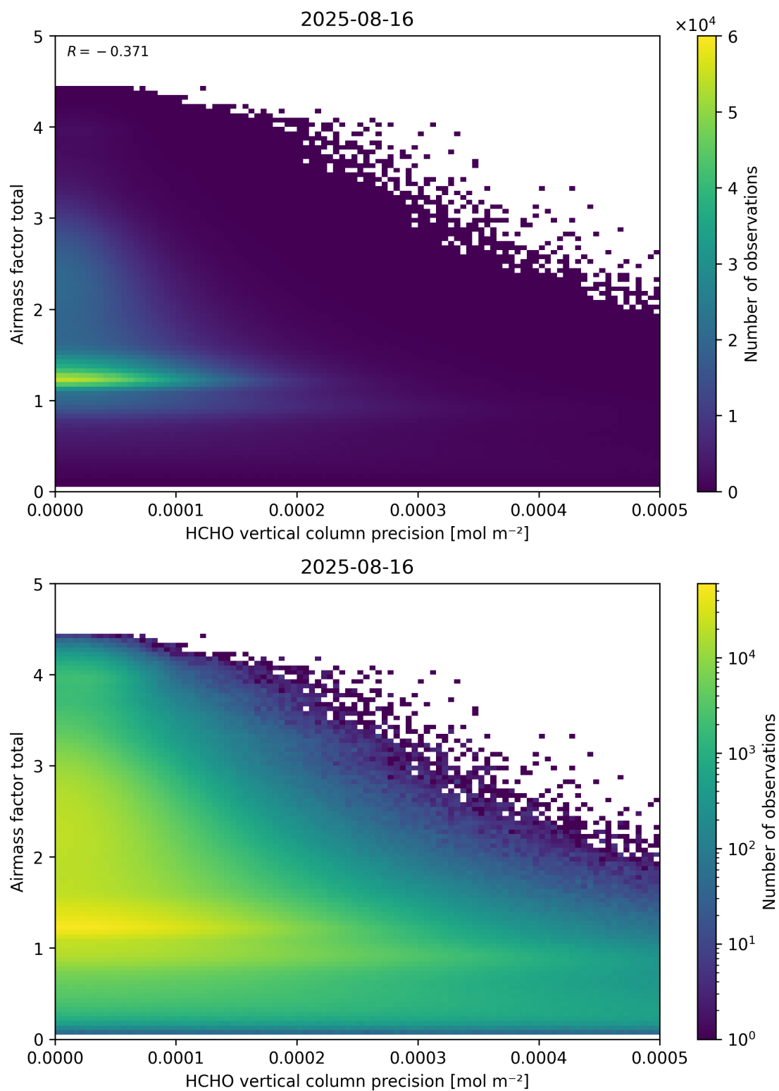
Figure 144: Scatter density plot of “HCHO vertical column precision” against “Airmass factor total” for 2025-08-15 to 2025-08-17.
