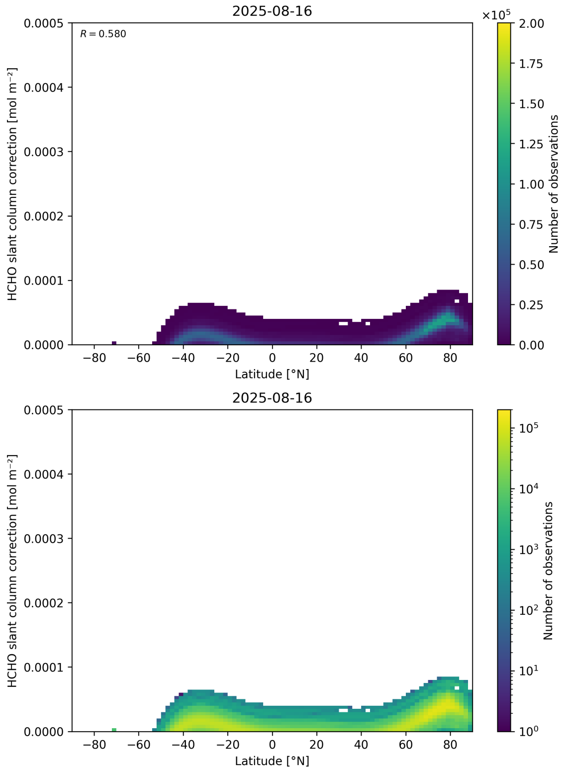
Figure 158: Scatter density plot of “Latitude” against “HCHO slant column correction” for 2025-08-15 to 2025-08-17.
