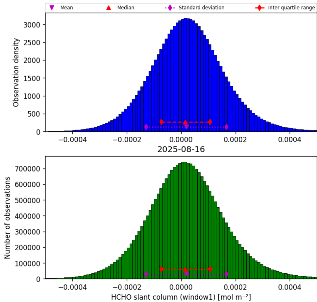
Figure 38: Histogram of “HCHO slant column (window1)” for 2025-08-15 to 2025-08-17
