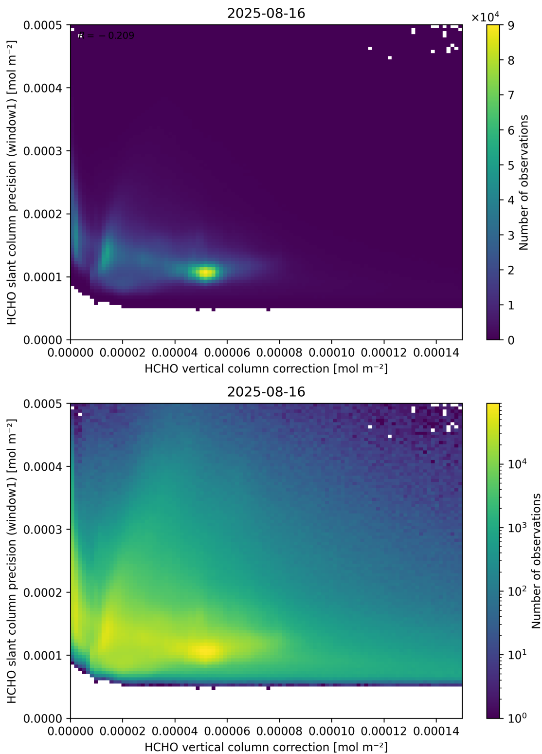
Figure 119: Scatter density plot of “HCHO vertical column correction” against “HCHO slant column precision (window1)” for 2025-08-15 to 2025-08-17.
