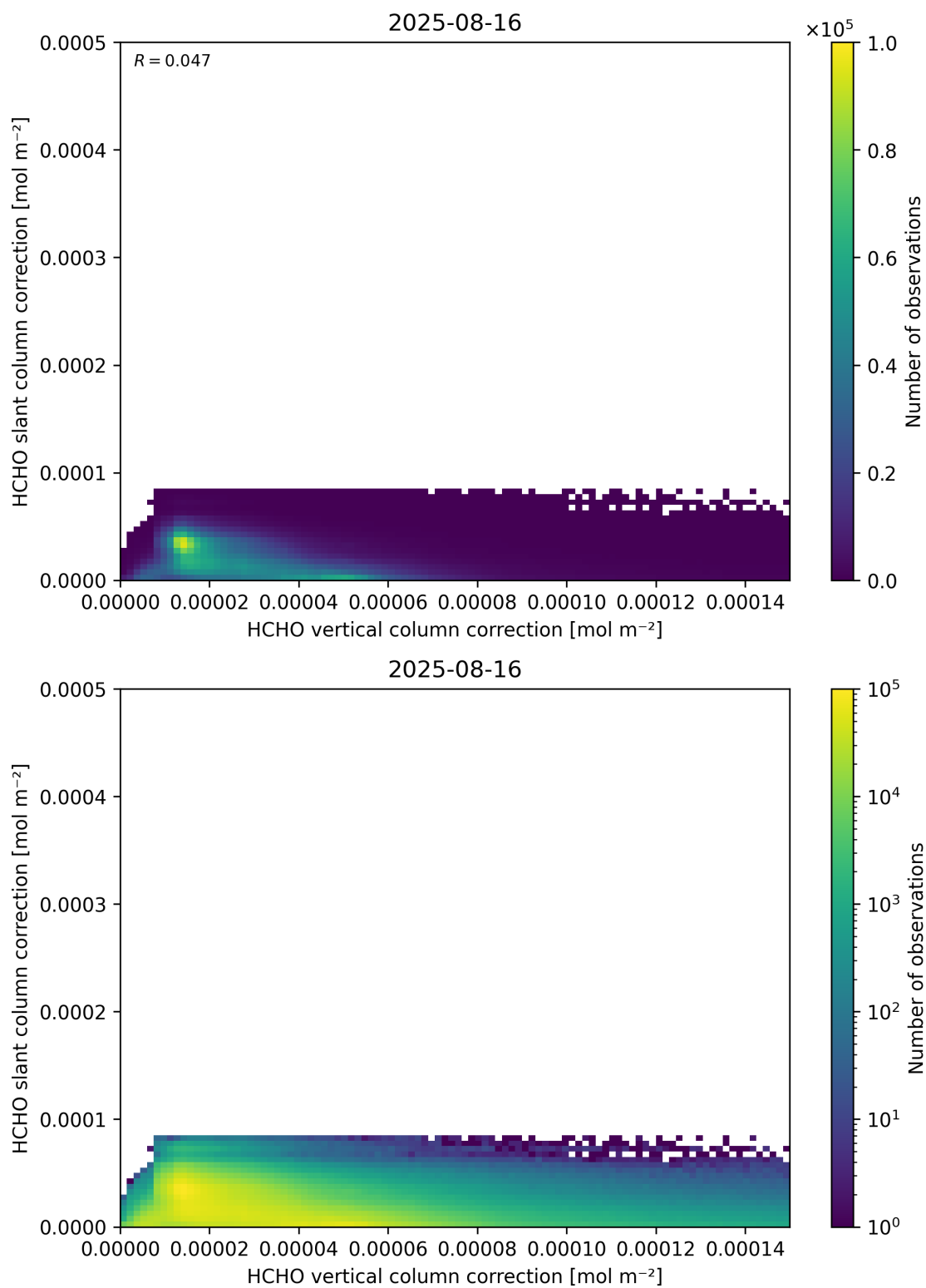
Figure 117: Scatter density plot of “HCHO vertical column correction” against “HCHO slant column correction” for 2025-08-15 to 2025-08-17.
