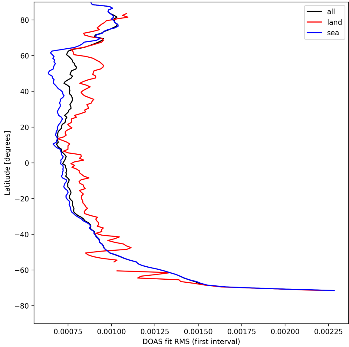
Figure 32: Zonal average of “DOAS fit RMS (first interval)” for 2025-08-15 to 2025-08-17.
