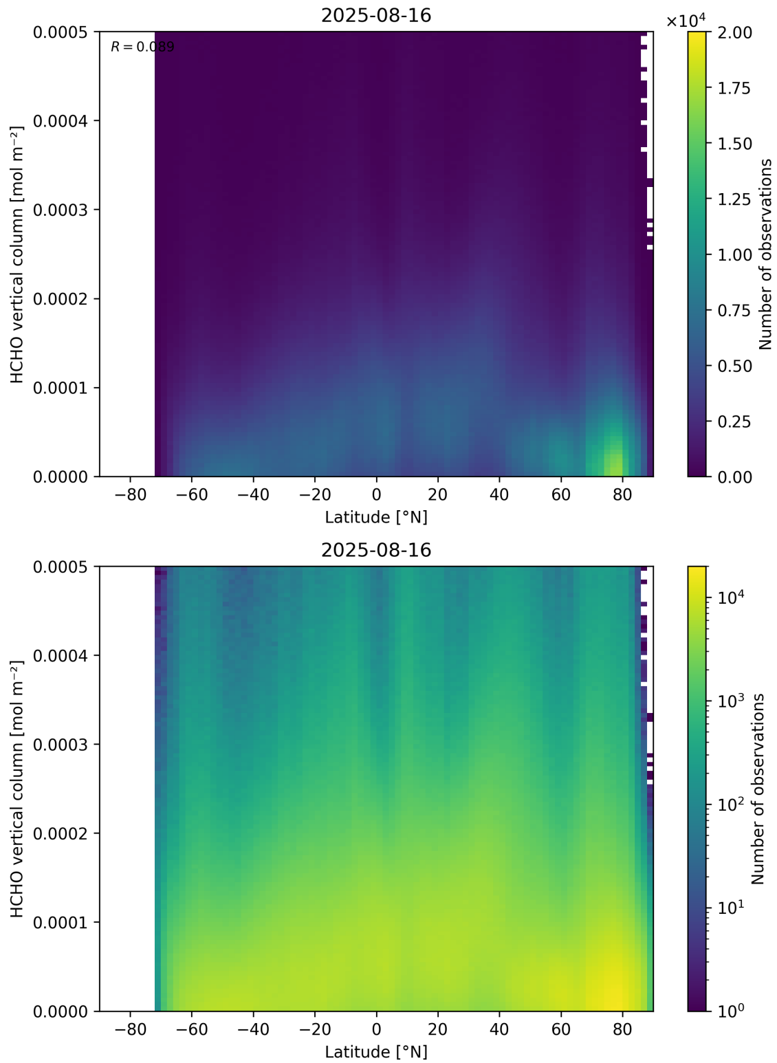
Figure 163: Scatter density plot of “Latitude” against “HCHO vertical column” for 2025-08-15 to 2025-08-17.
