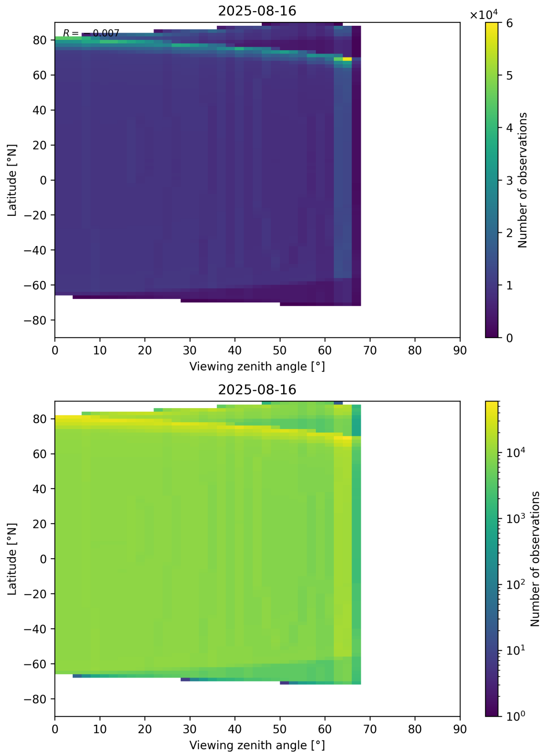
Figure 196: Scatter density plot of “Viewing zenith angle” against “Latitude” for 2025-08-15 to 2025-08-17.
