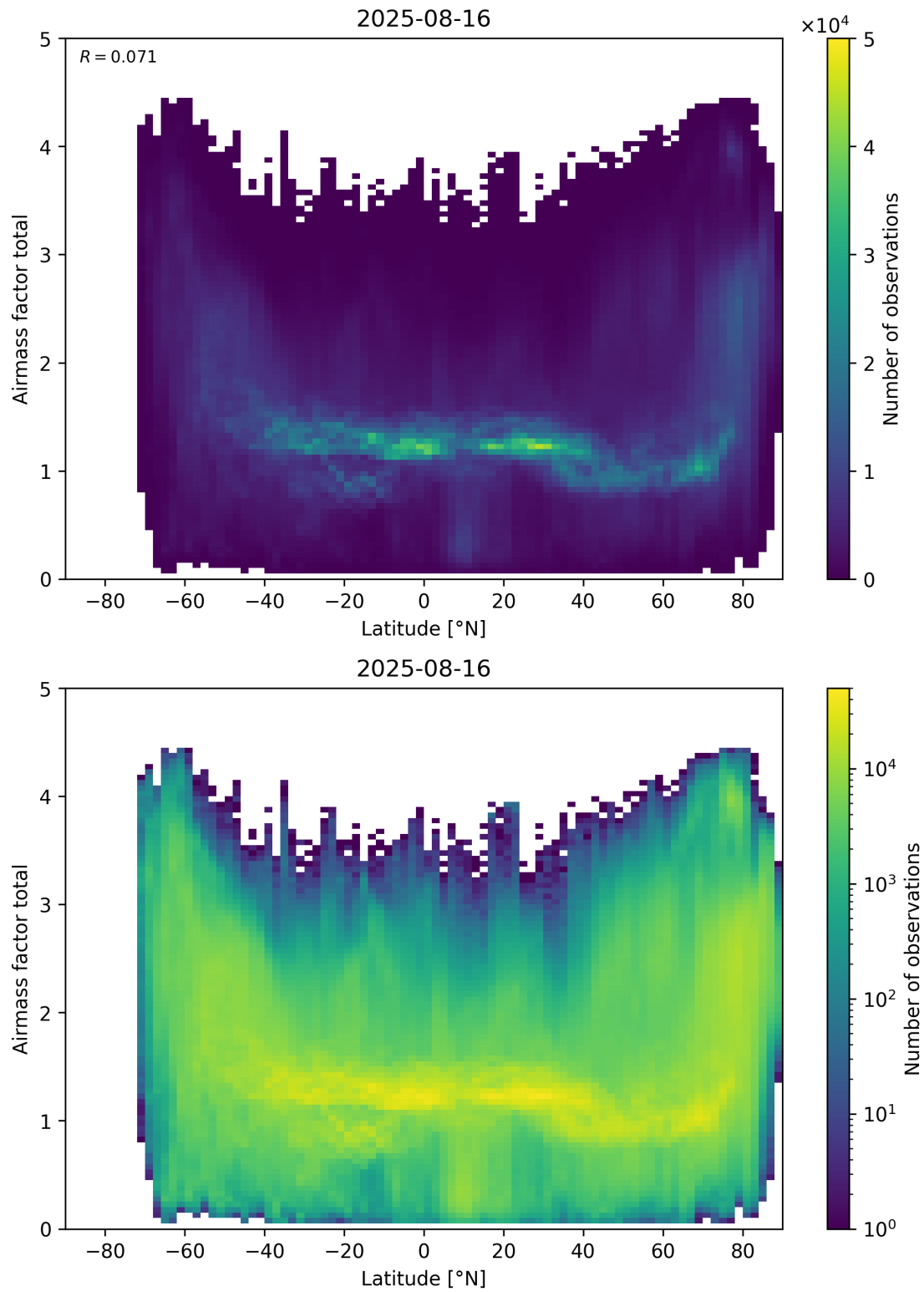
Figure 161: Scatter density plot of “Latitude” against “Airmass factor total” for 2025-08-15 to 2025-08-17.
