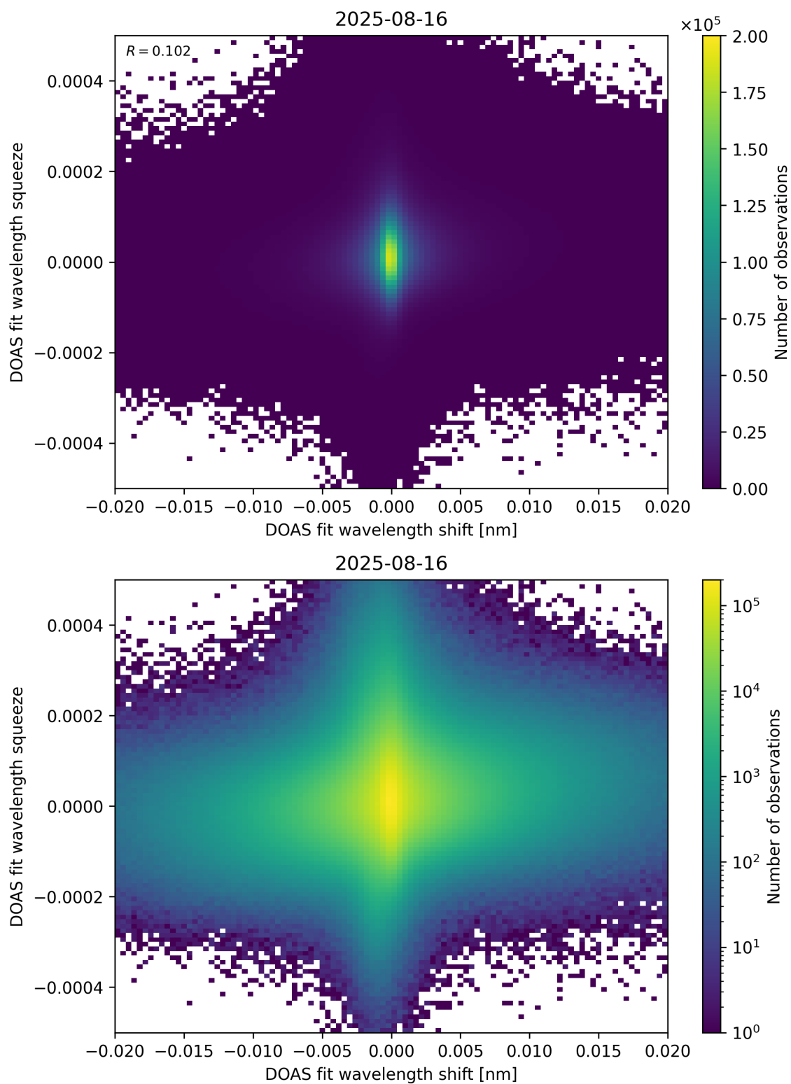
Figure 65: Scatter density plot of “DOAS fit wavelength shift” against “DOAS fit wavelength squeeze” for 2025-08-15 to 2025-08-17.
