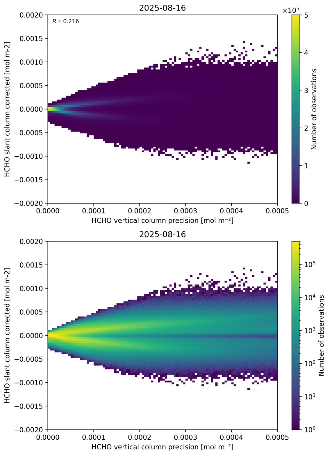
Figure 140: Scatter density plot of “HCHO vertical column precision” against “HCHO slant column corrected” for 2025-08-15 to 2025-08-17.
