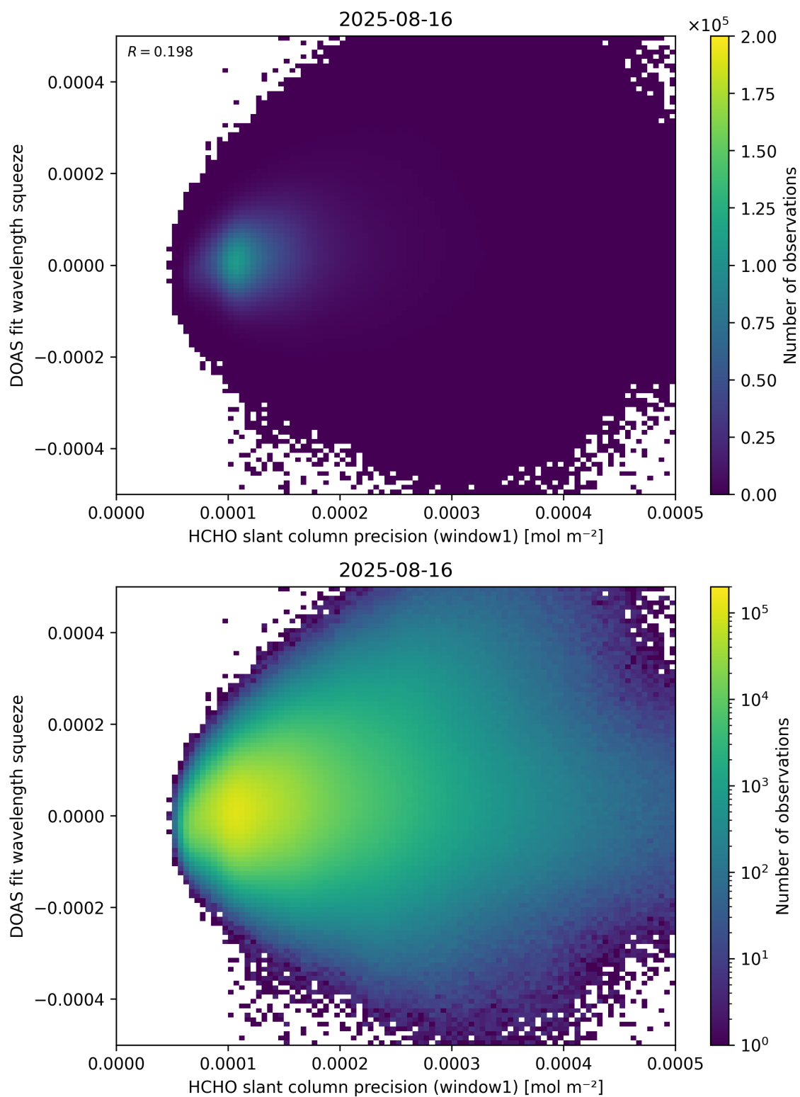
Figure 90: Scatter density plot of “HCHO slant column precision (window1)” against “DOAS fit wavelength squeeze” for 2025-08-15 to 2025-08-17.
