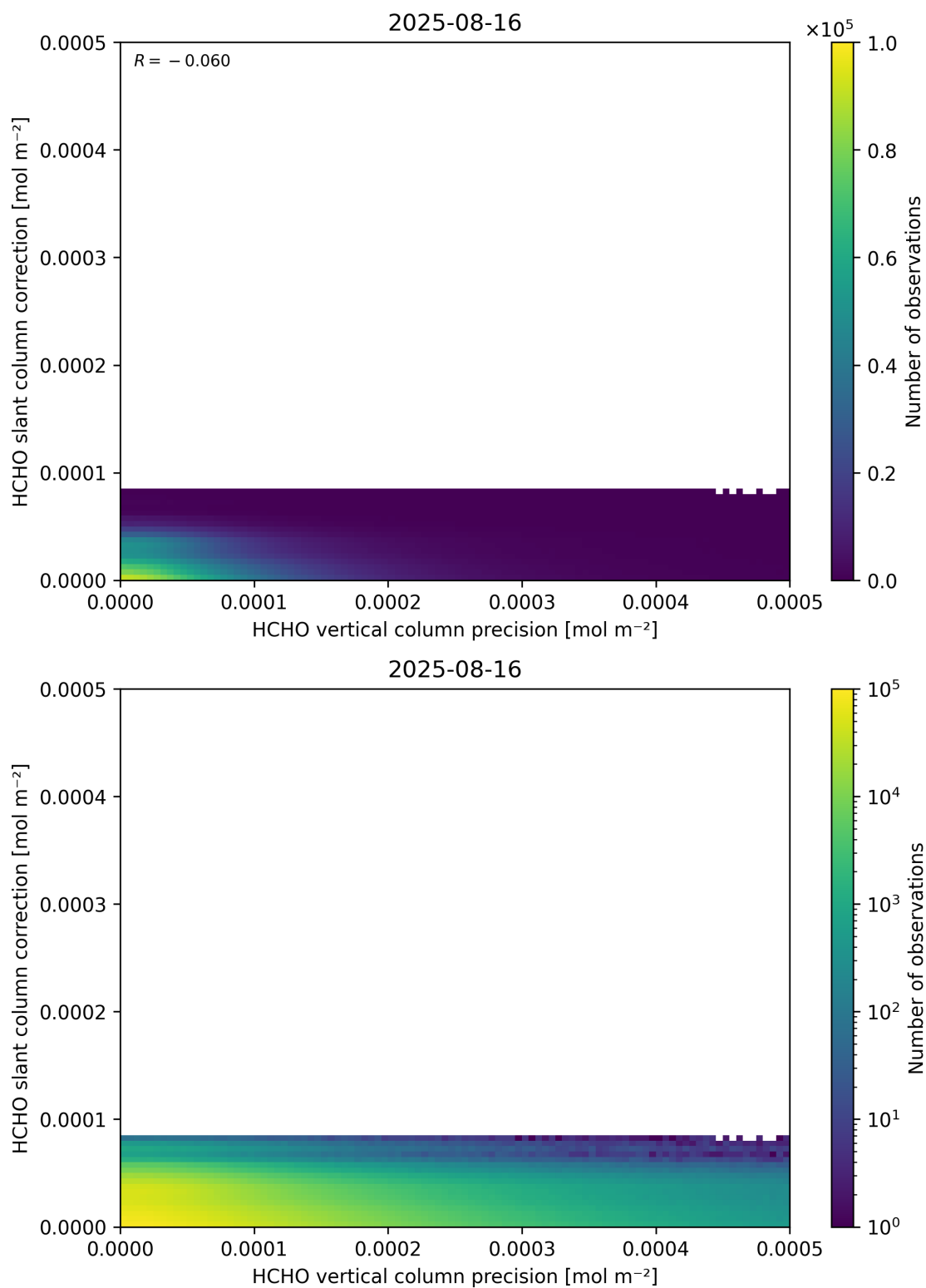
Figure 141: Scatter density plot of “HCHO vertical column precision” against “HCHO slant column correction” for 2025-08-15 to 2025-08-17.
