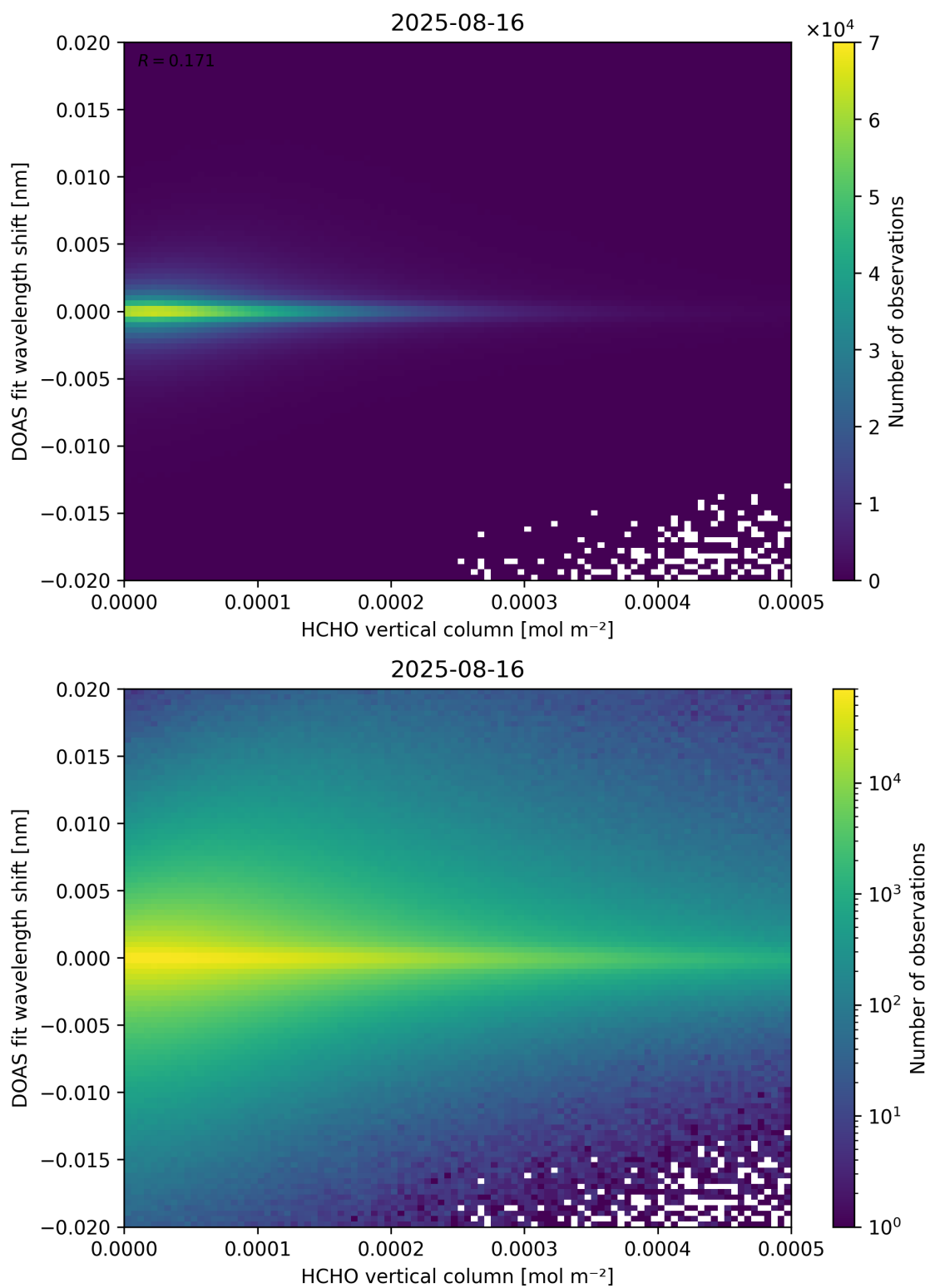
Figure 124: Scatter density plot of “HCHO vertical column” against “DOAS fit wavelength shift” for 2025-08-15 to 2025-08-17.
