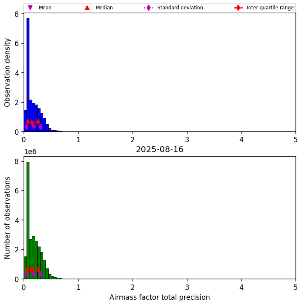
Figure 41: Histogram of “Airmass factor total precision” for 2025-08-15 to 2025-08-17
