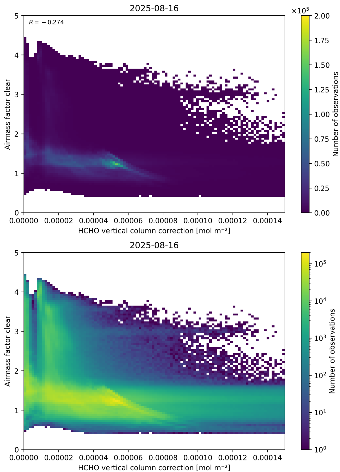
Figure 115: Scatter density plot of “HCHO vertical column correction” against “Airmass factor clear” for 2025-08-15 to 2025-08-17.
