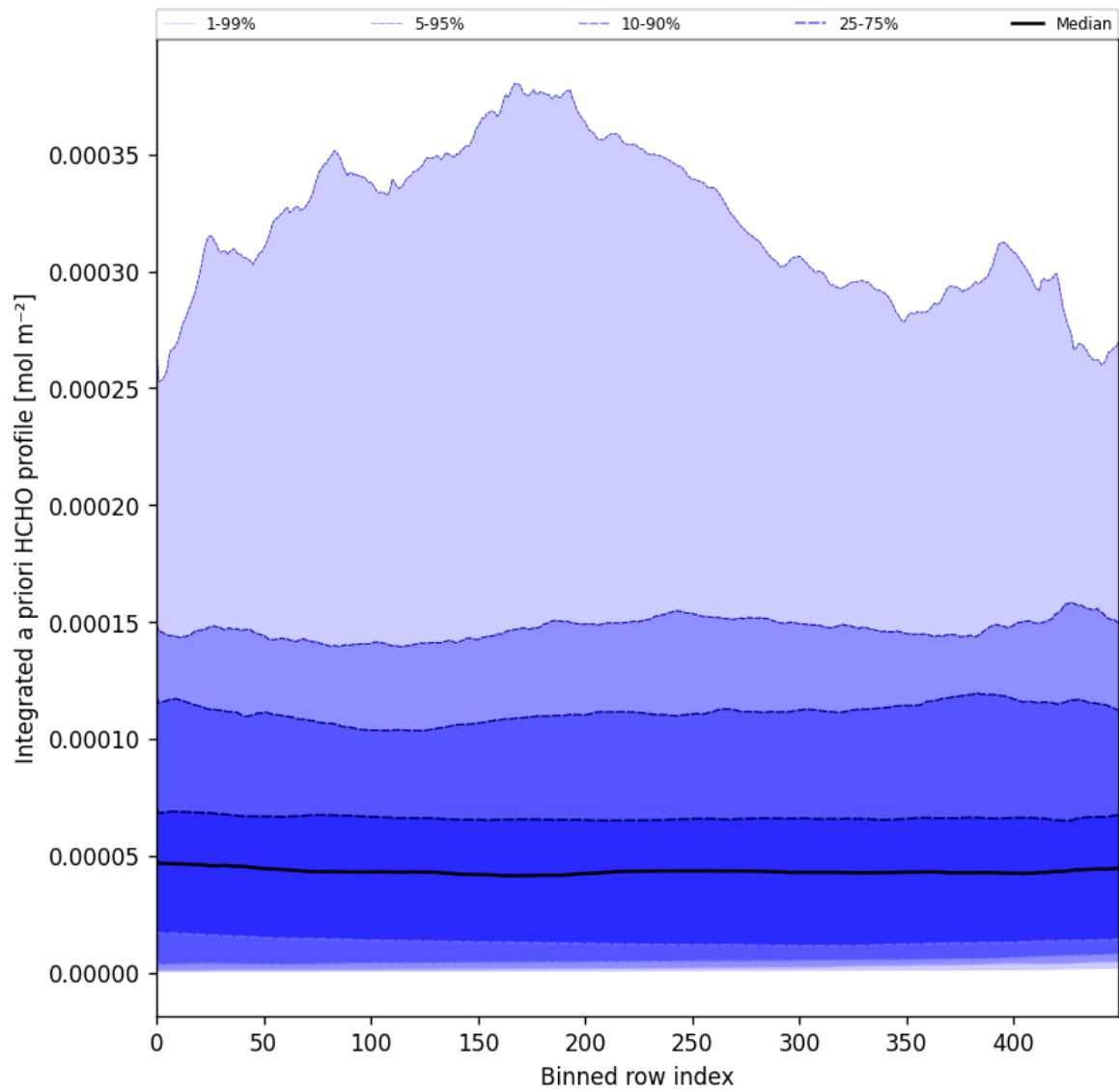
Figure 57: Along track statistics of "Integrated a priori HCHO profile" for 2025-08-15 to 2025-08-17
