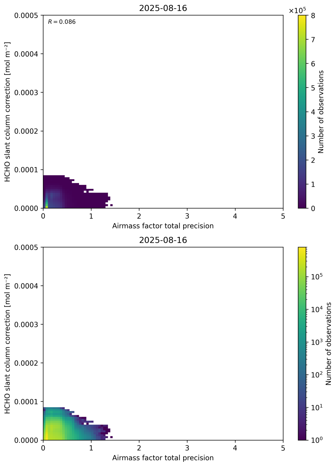
Figure 110: Scatter density plot of “Airmass factor total precision” against “HCHO slant column correction” for 2025-08-15 to 2025-08-17.
