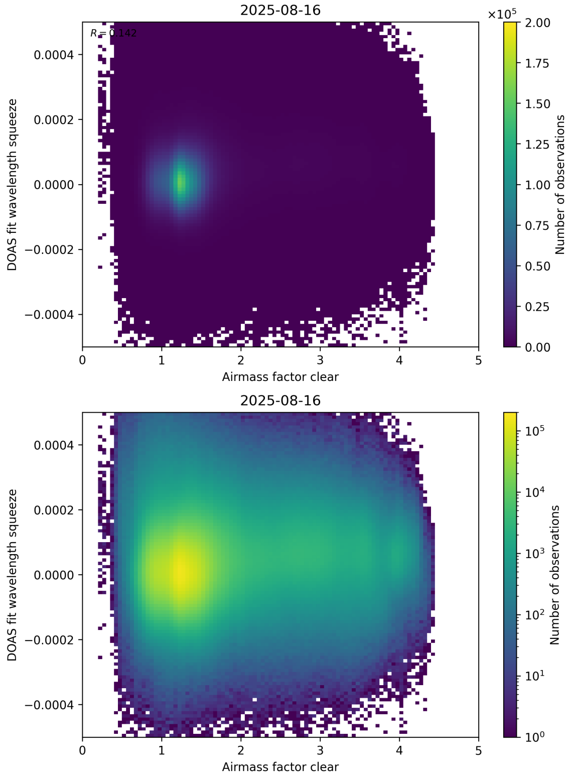
Figure 73: Scatter density plot of “Airmass factor clear” against “DOAS fit wavelength squeeze” for 2025-08-15 to 2025-08-17.
