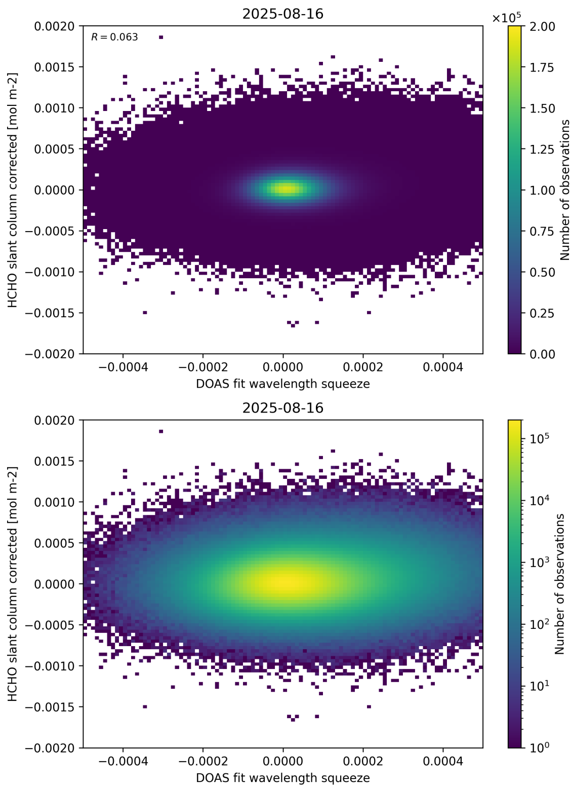
Figure 69: Scatter density plot of “DOAS fit wavelength squeeze” against “HCHO slant column corrected” for 2025-08-15 to 2025-08-17.
