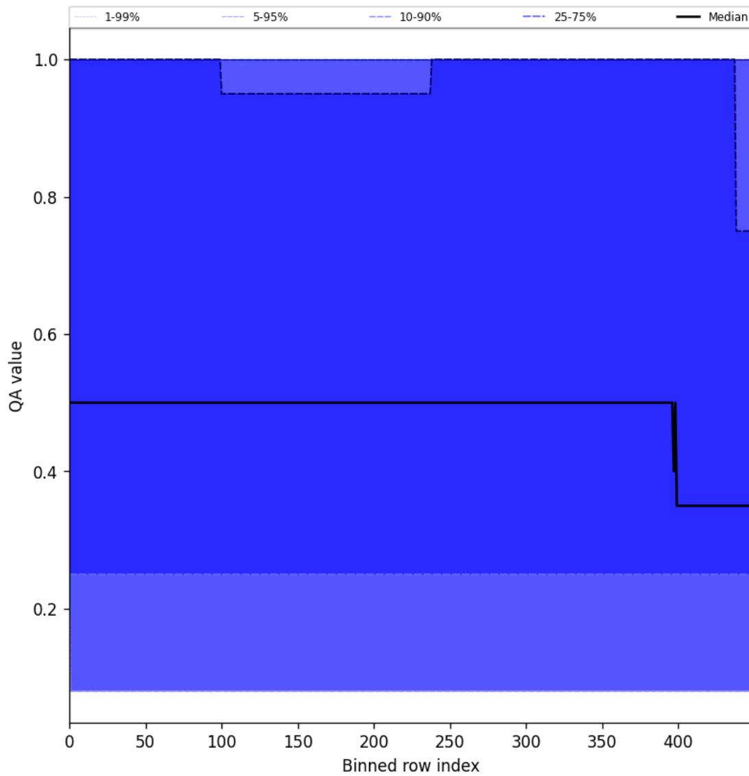
Figure 48: Along track statistics of "QA value" for 2025-08-15 to 2025-08-17
