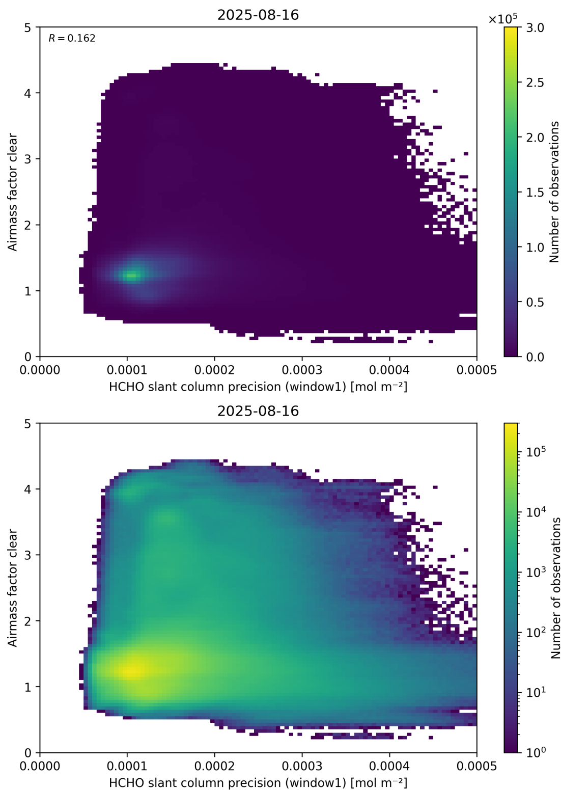
Figure 91: Scatter density plot of “HCHO slant column precision (window1)” against “Airmass factor clear” for 2025-08-15 to 2025-08-17.
