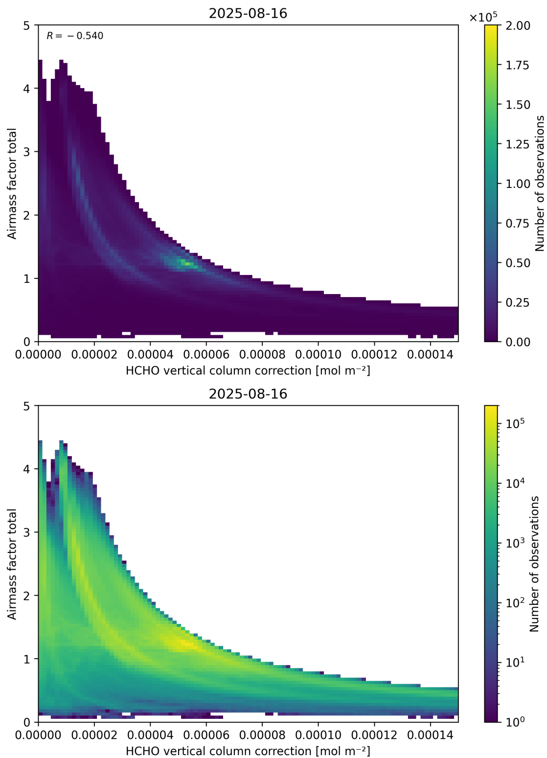
Figure 120: Scatter density plot of “HCHO vertical column correction” against “Airmass factor total” for 2025-08-15 to 2025-08-17.
