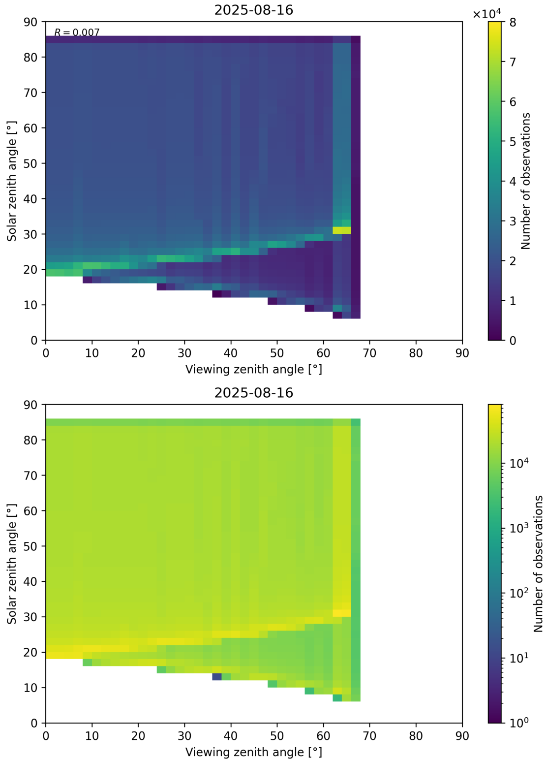
Figure 197: Scatter density plot of “Viewing zenith angle” against “Solar zenith angle” for 2025-08-15 to 2025-08-17.
