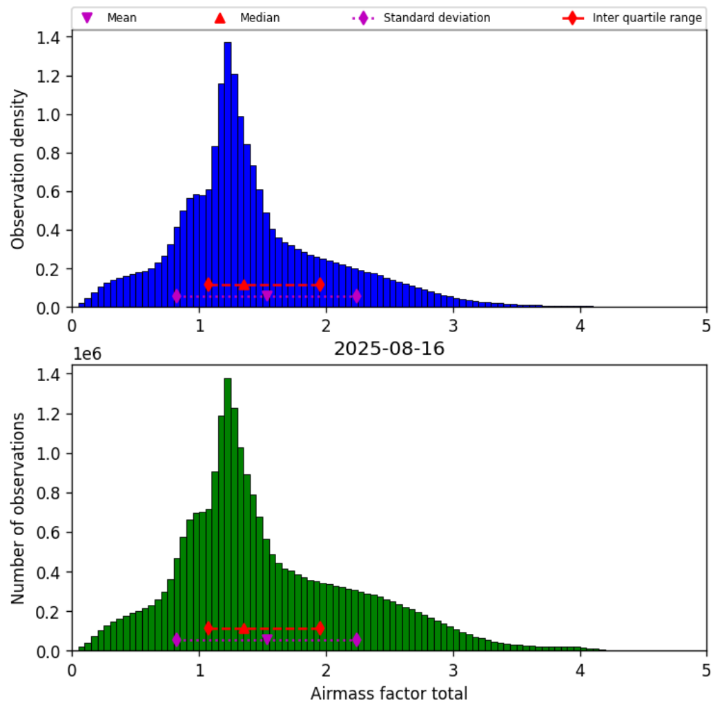
Figure 40: Histogram of “Airmass factor total” for 2025-08-15 to 2025-08-17
