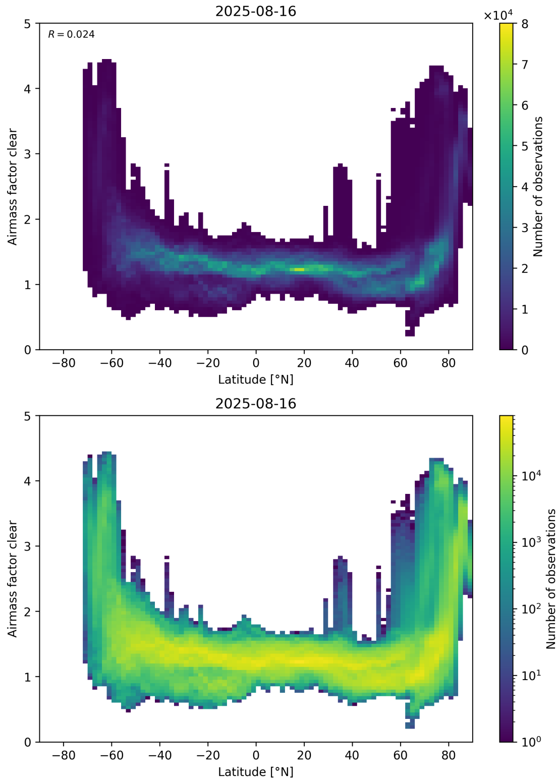
Figure 156: Scatter density plot of “Latitude” against “Airmass factor clear” for 2025-08-15 to 2025-08-17.
