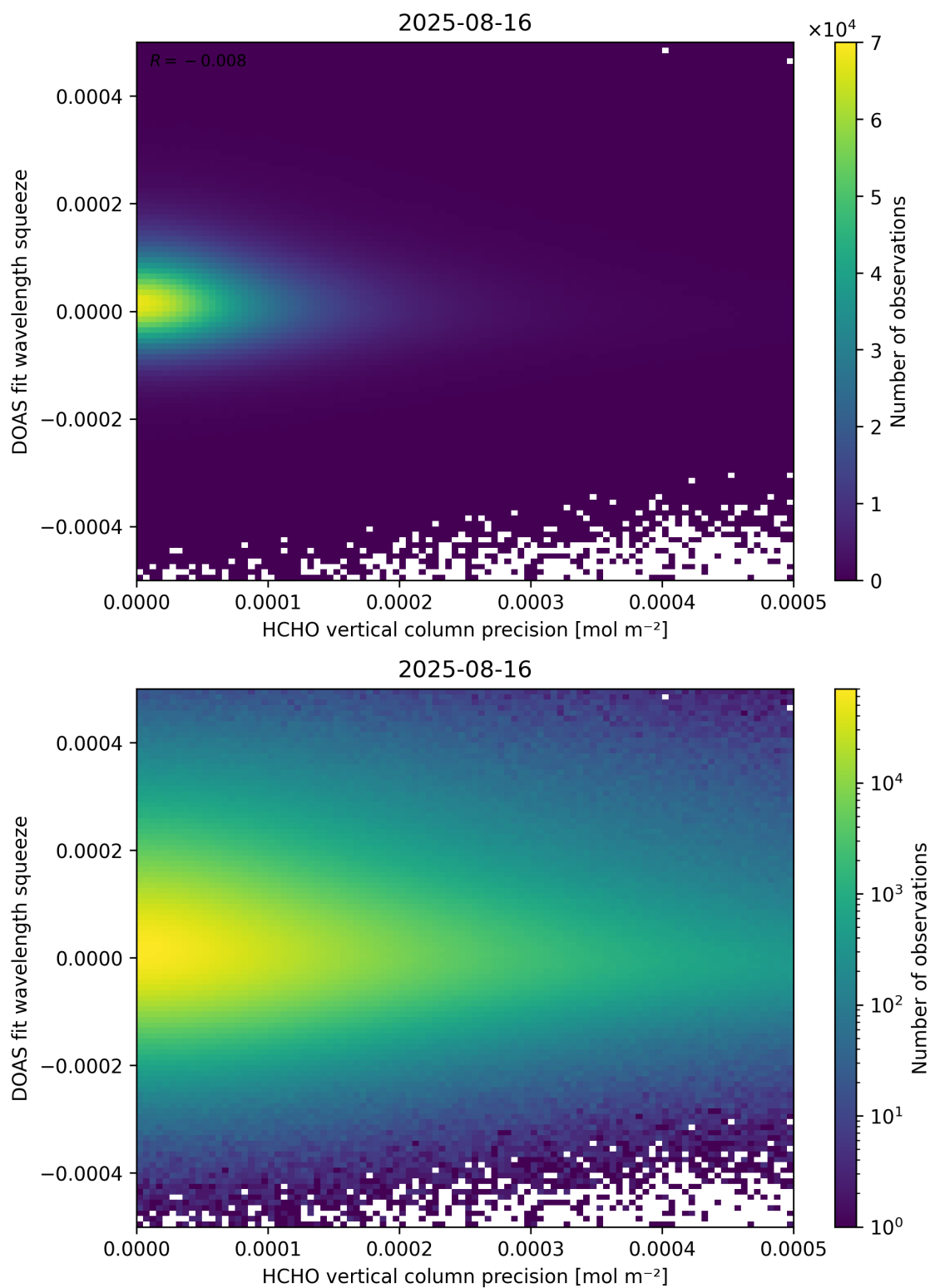
Figure 138: Scatter density plot of “HCHO vertical column precision” against “DOAS fit wavelength squeeze” for 2025-08-15 to 2025-08-17.
