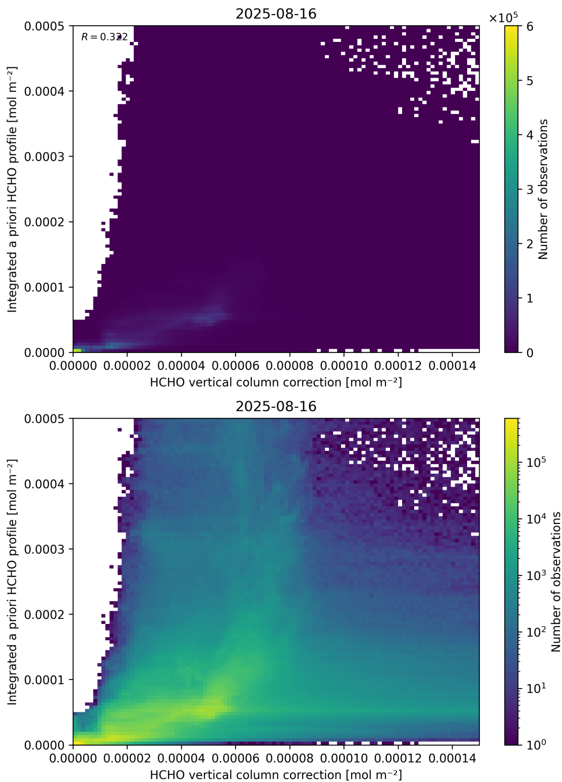
Figure 122: Scatter density plot of “HCHO vertical column correction” against “Integrated a priori HCHO profile” for 2025-08-15 to 2025-08-17.
