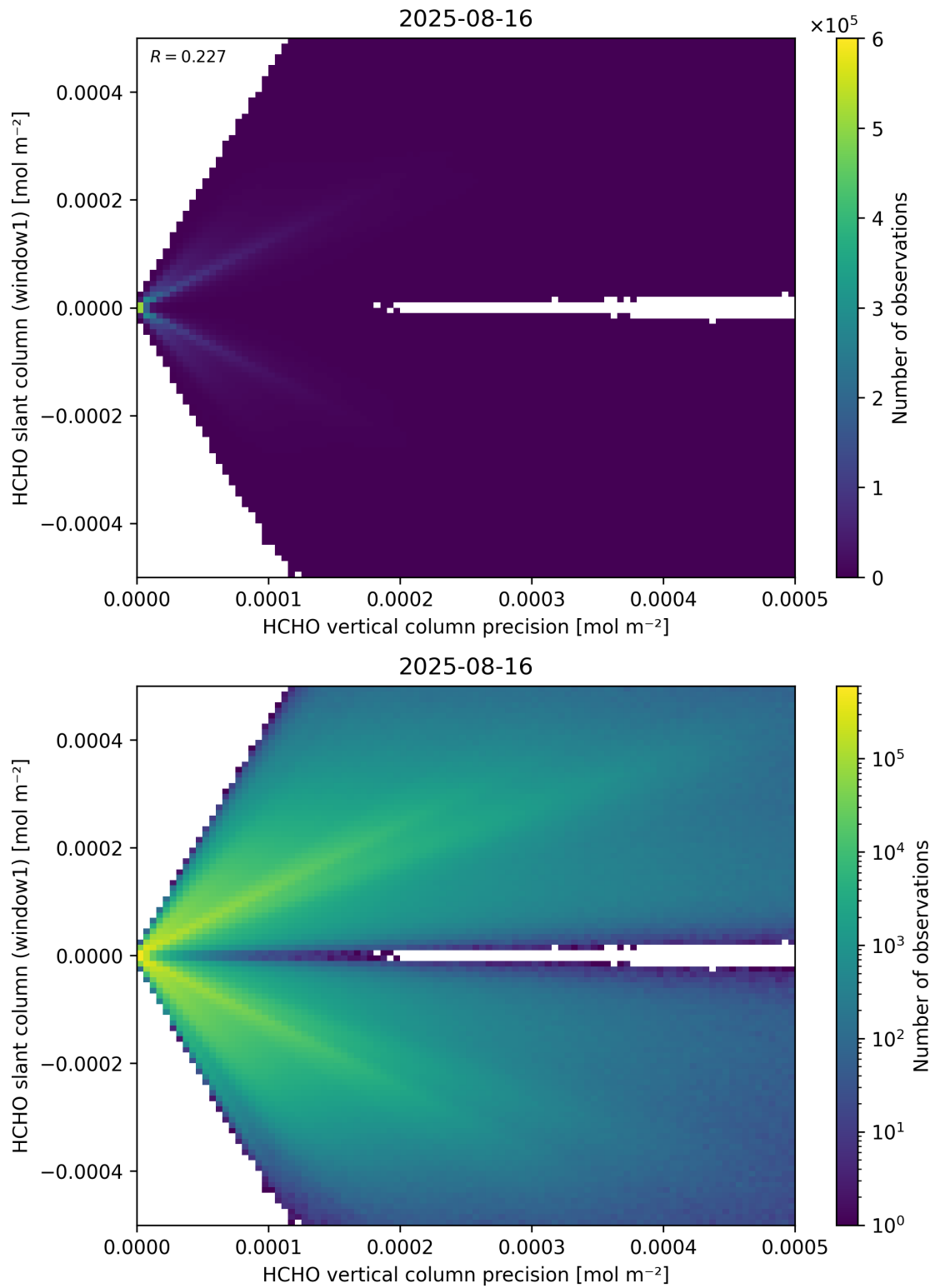
Figure 142: Scatter density plot of “HCHO vertical column precision” against “HCHO slant column (window1)” for 2025-08-15 to 2025-08-17.
