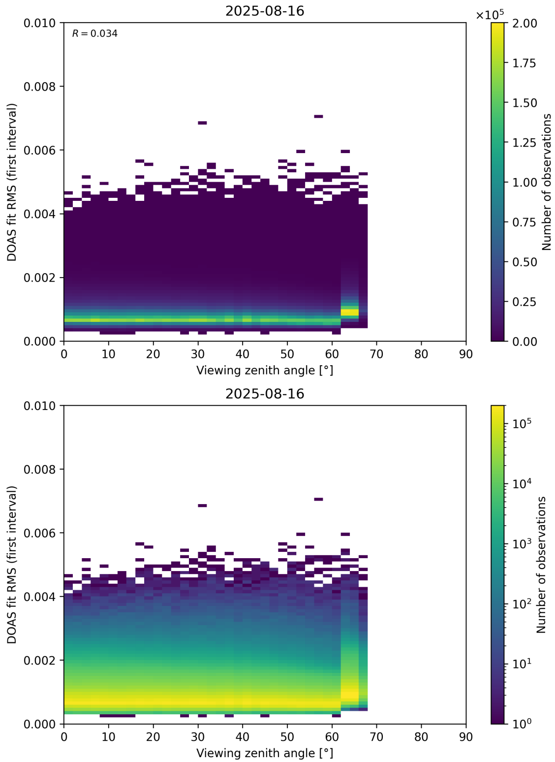
Figure 182: Scatter density plot of “Viewing zenith angle” against “DOAS fit RMS (first interval)” for 2025-08-15 to 2025-08-17.
