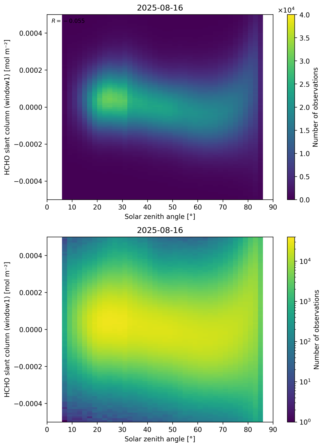
Figure 173: Scatter density plot of “Solar zenith angle” against “HCHO slant column (window1)” for 2025-08-15 to 2025-08-17.
