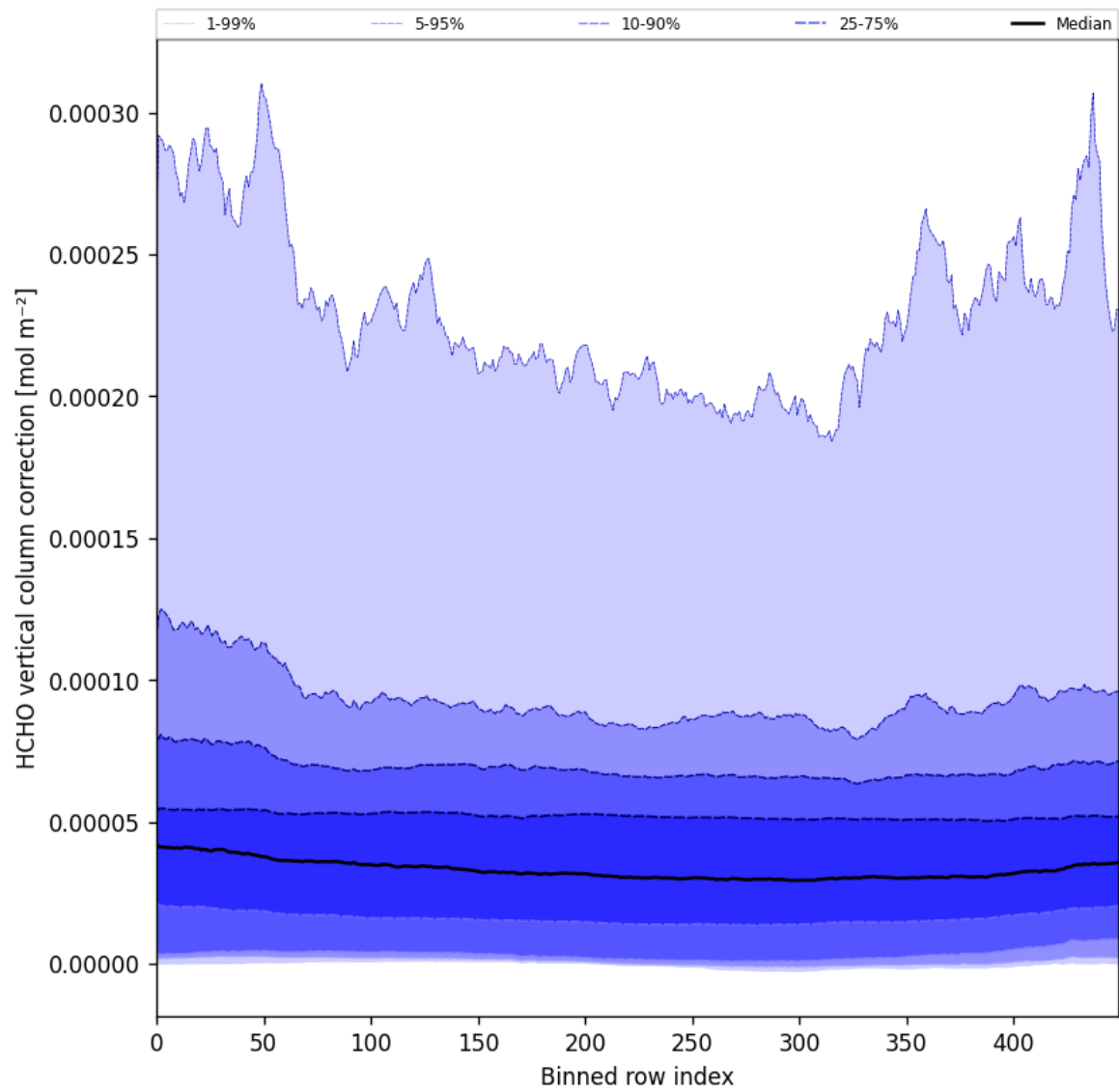
Figure 51: Along track statistics of “HCHO vertical column correction” for 2025-08-15 to 2025-08-17
