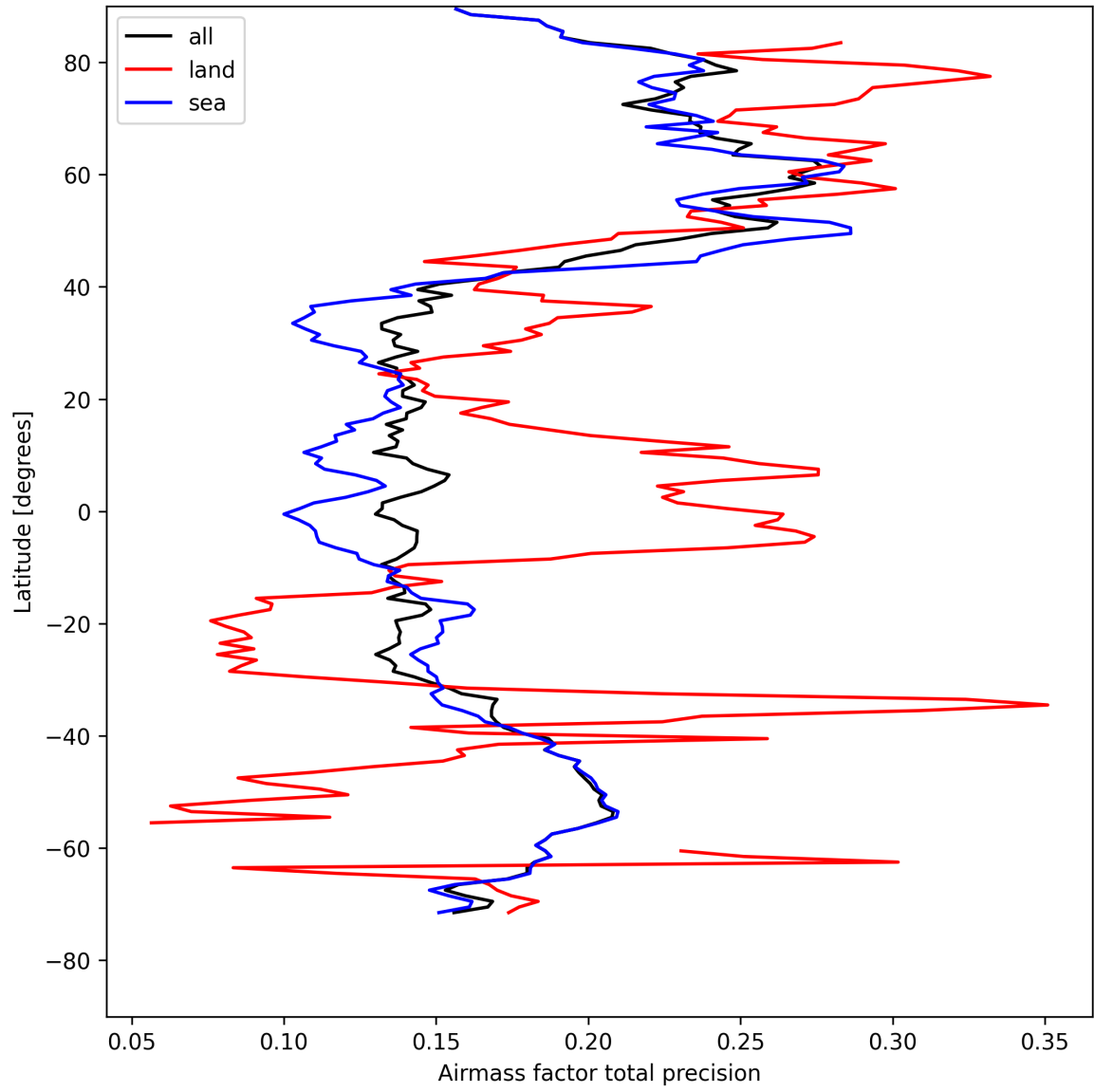
Figure 27: Zonal average of “Airmass factor total precision” for 2025-08-15 to 2025-08-17.
