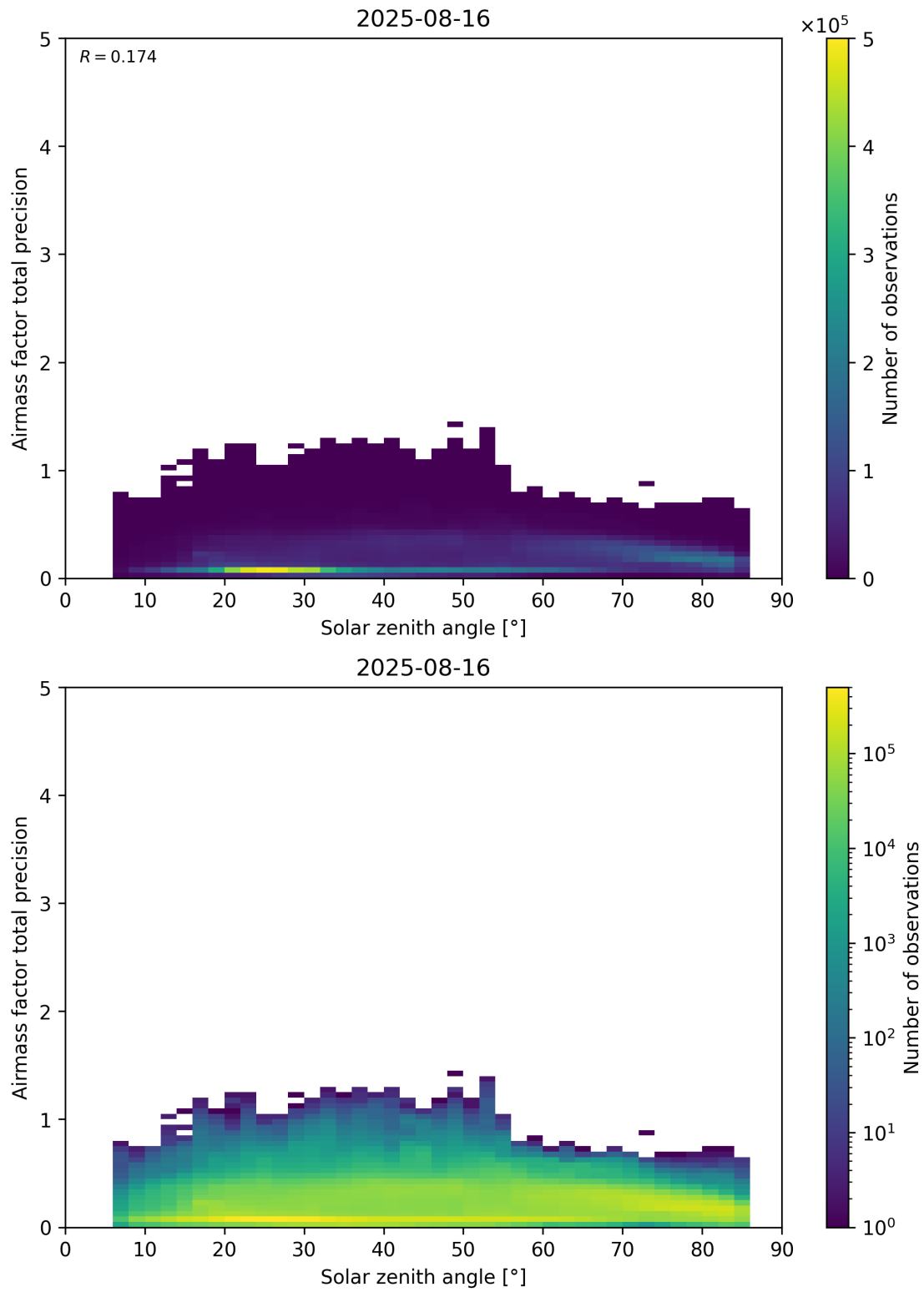
Figure 176: Scatter density plot of “Solar zenith angle” against “Airmass factor total precision” for 2025-08-15 to 2025-08-17.
