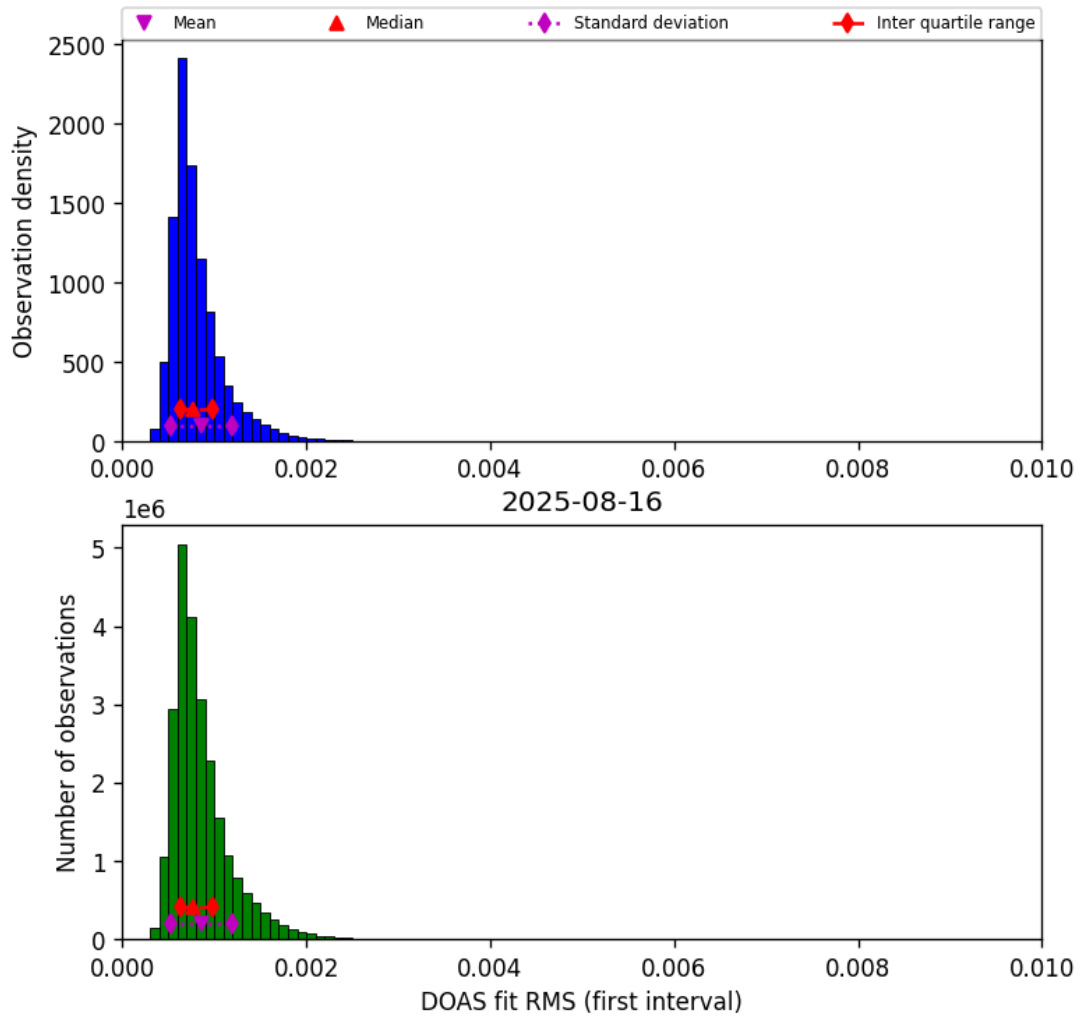
Figure 46: Histogram of “DOAS fit RMS (first interval)” for 2025-08-15 to 2025-08-17
