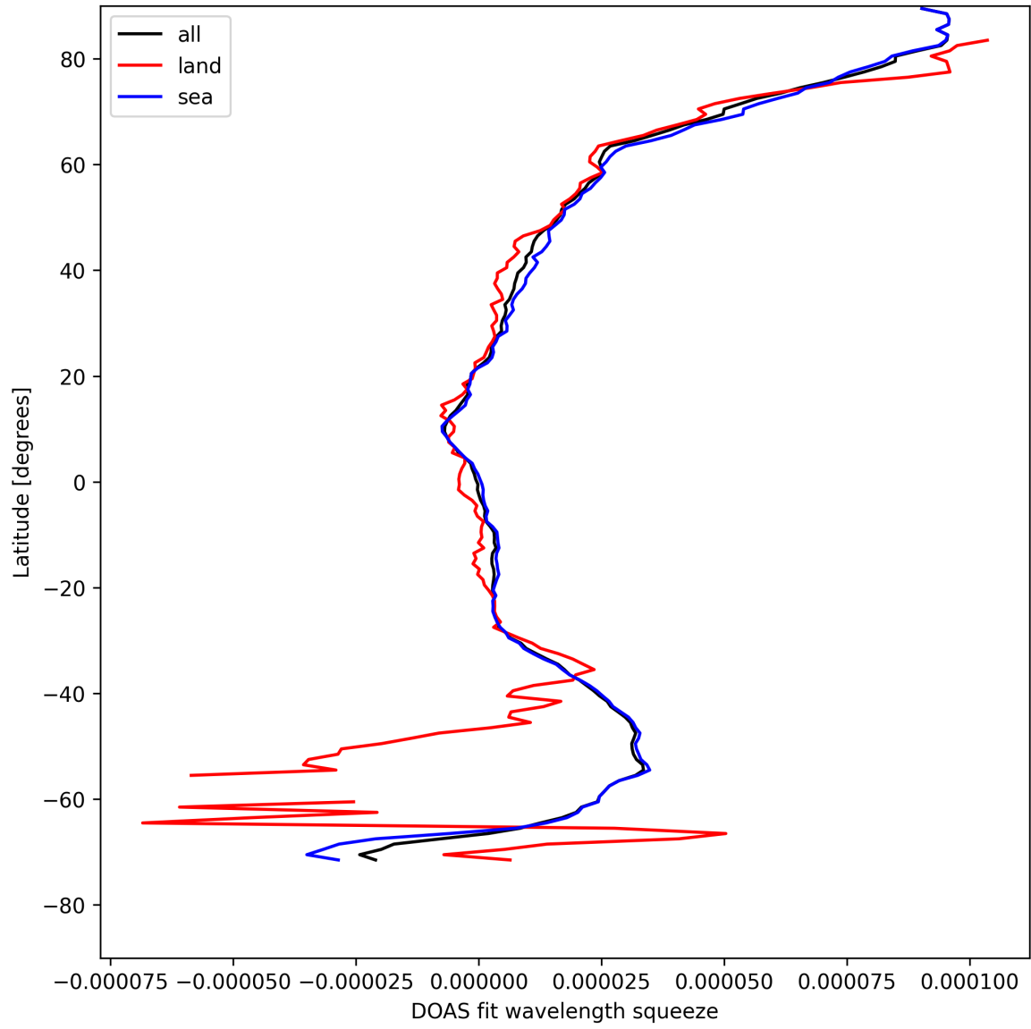
Figure 31: Zonal average of “DOAS fit wavelength squeeze” for 2025-08-15 to 2025-08-17.
