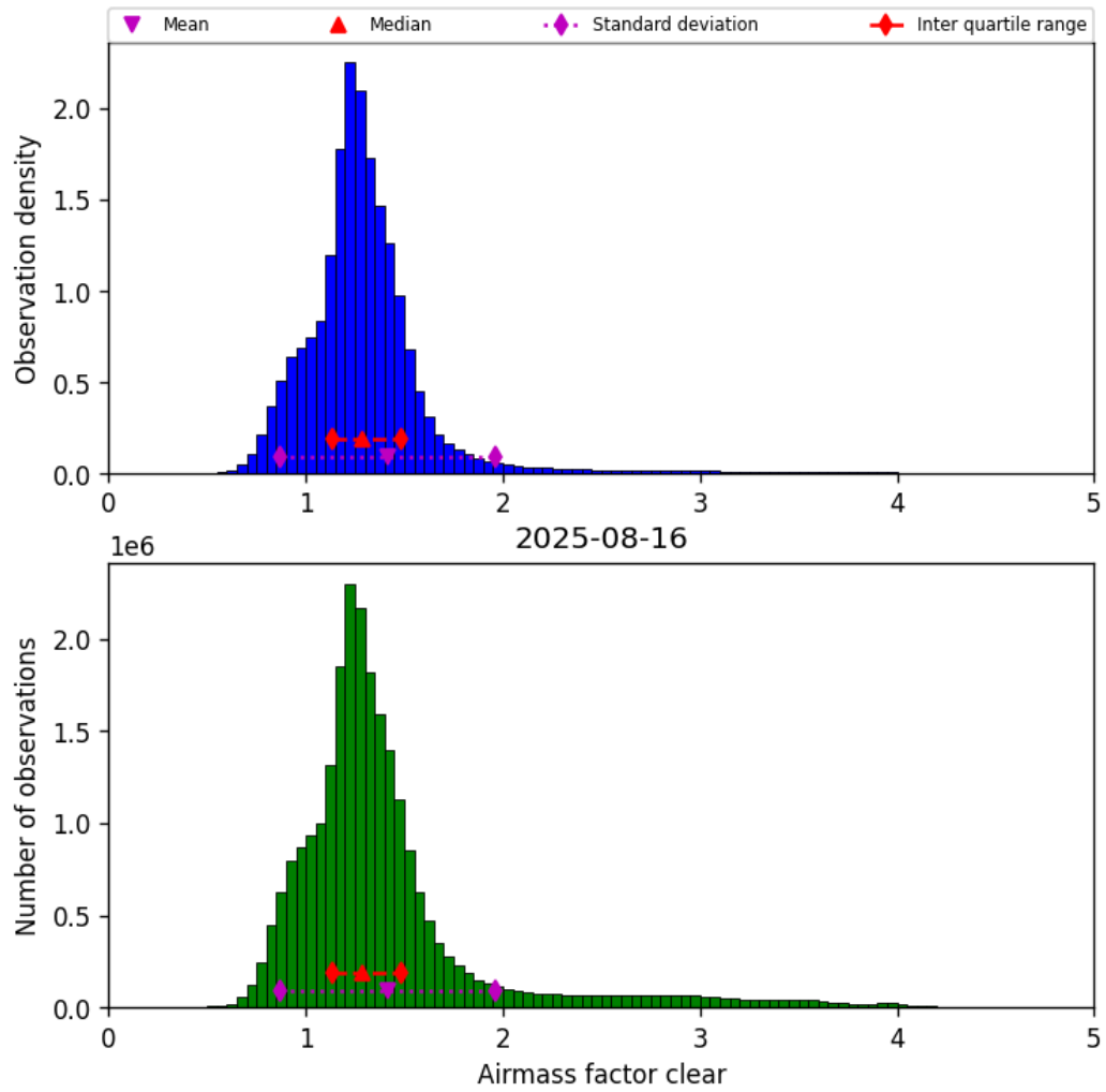
Figure 42: Histogram of “Airmass factor clear” for 2025-08-15 to 2025-08-17
