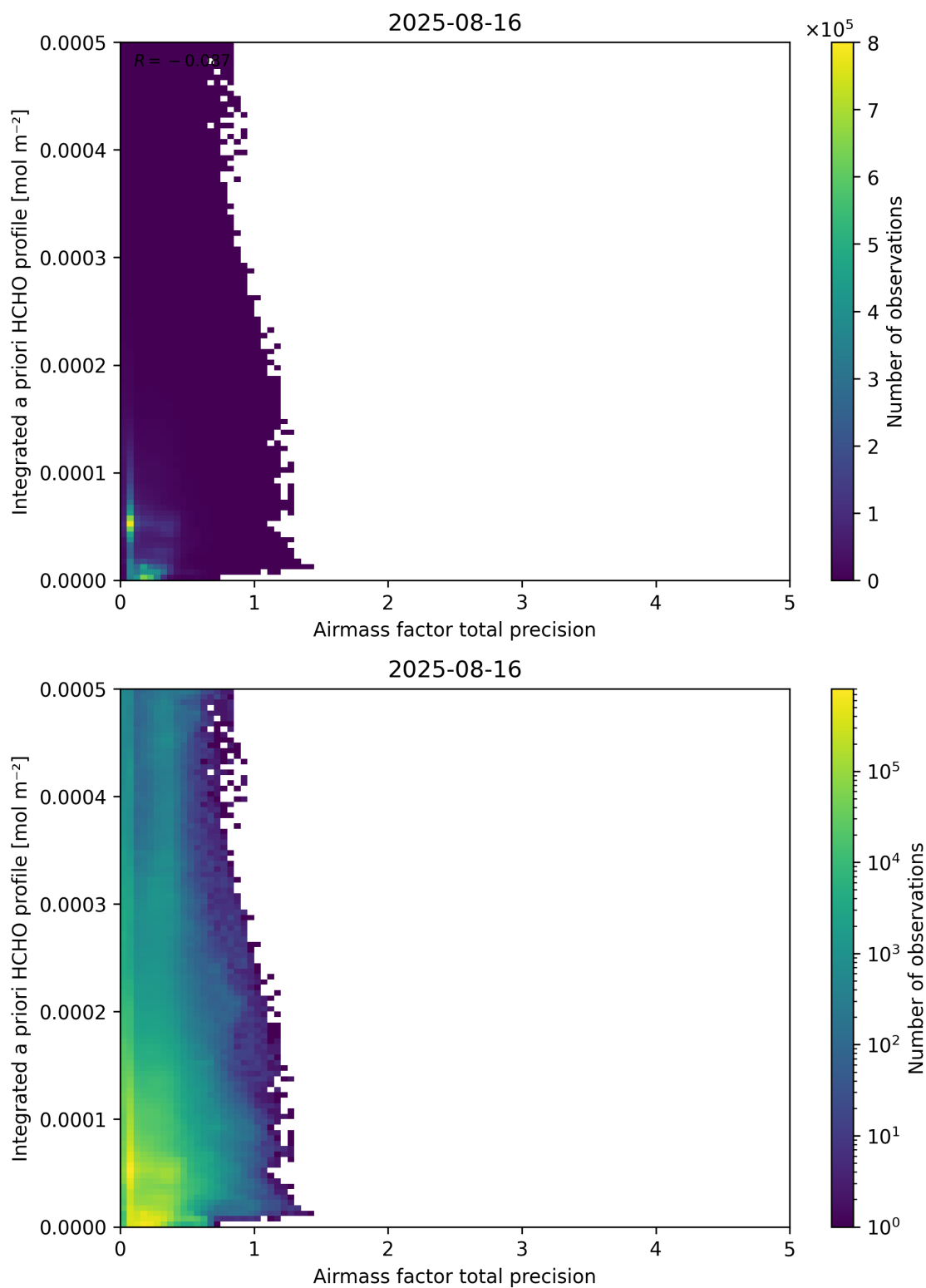
Figure 111: Scatter density plot of “Airmass factor total precision” against “Integrated a priori HCHO profile” for 2025-08-15 to 2025-08-17.
