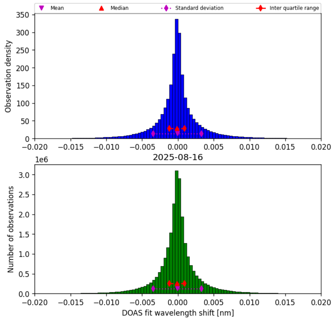
Figure 44: Histogram of “DOAS fit wavelength shift” for 2025-08-15 to 2025-08-17
