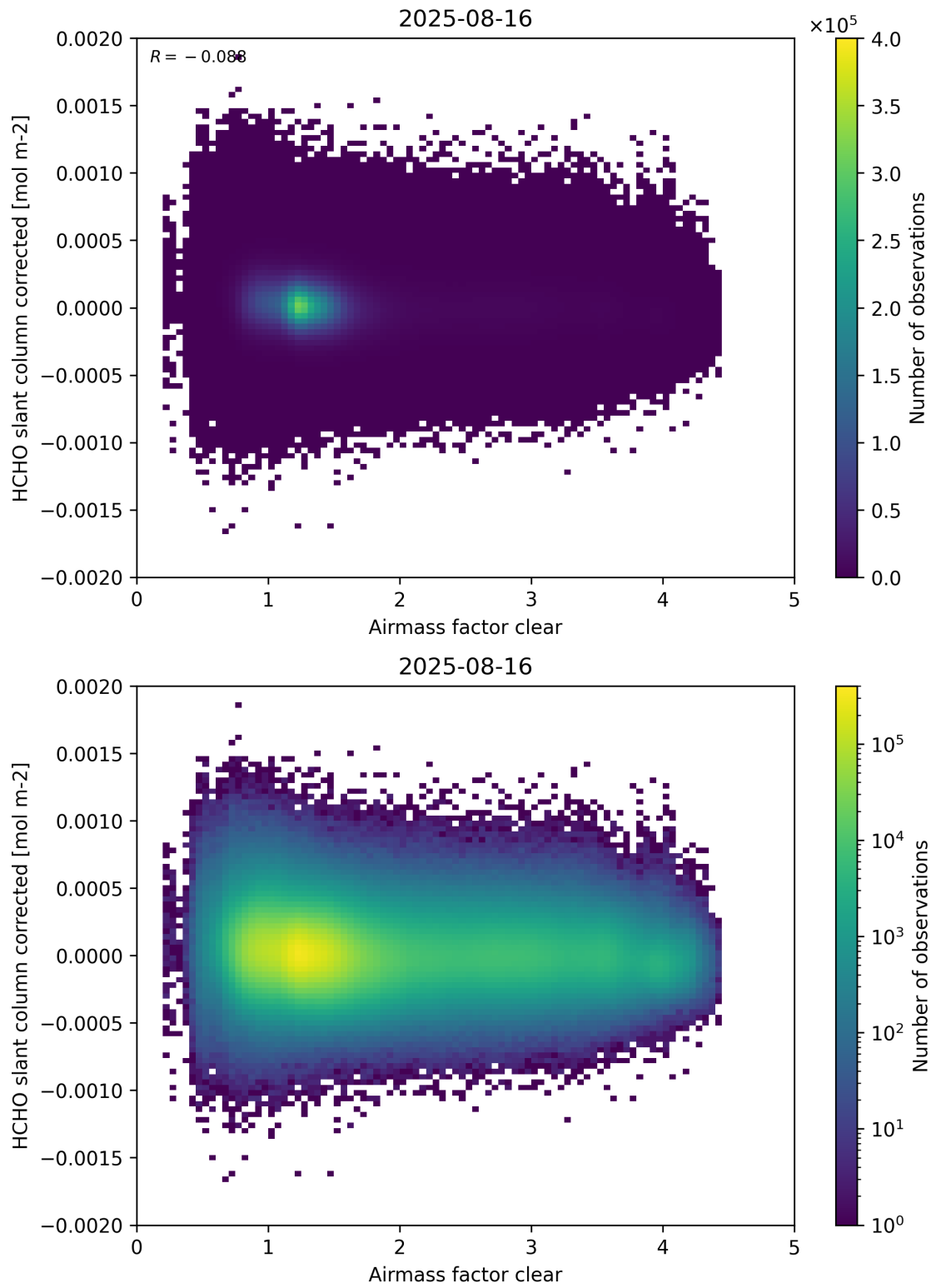
Figure 74: Scatter density plot of “Airmass factor clear” against “HCHO slant column corrected” for 2025-08-15 to 2025-08-17.
