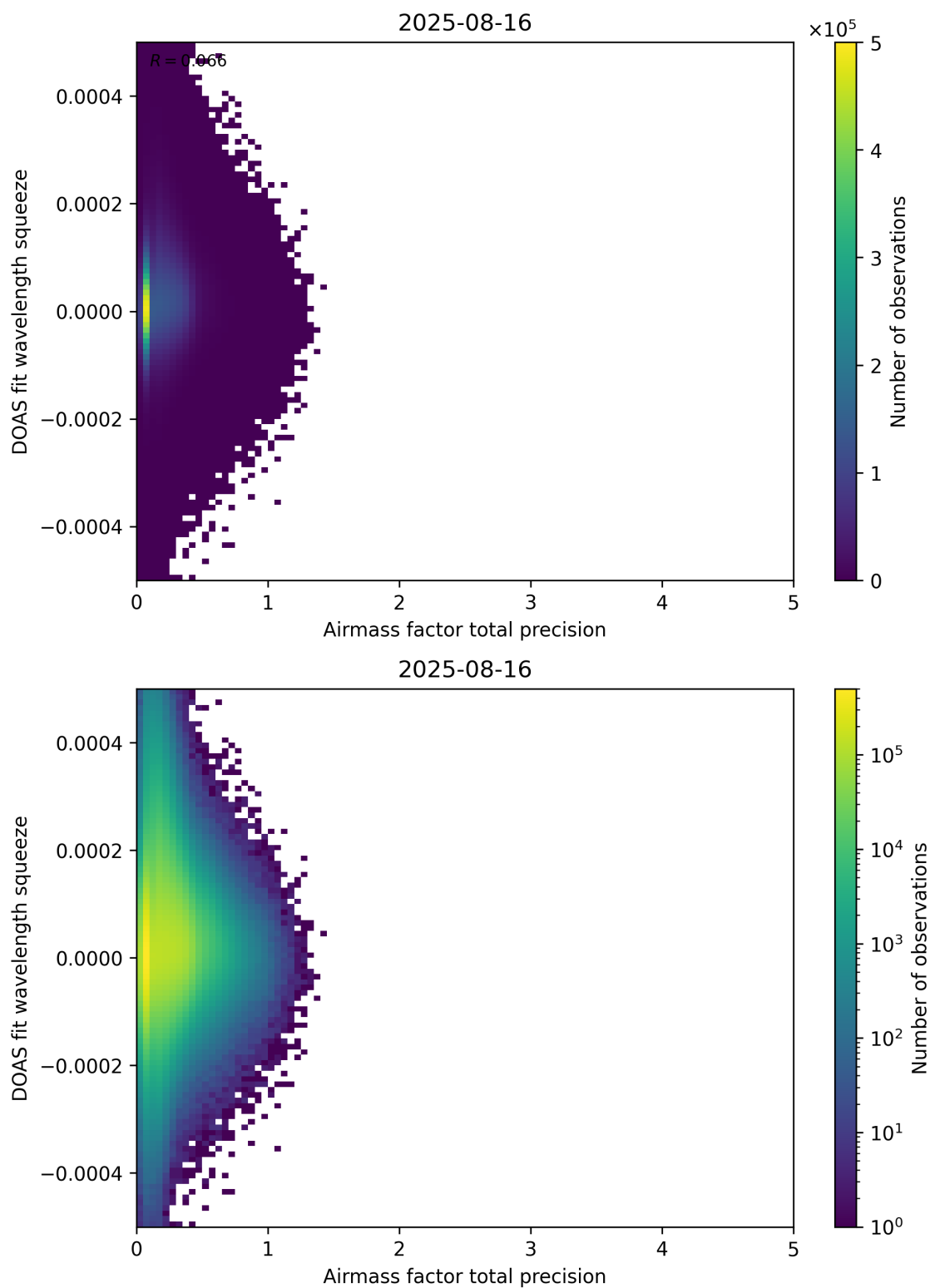
Figure 107: Scatter density plot of “Airmass factor total precision” against “DOAS fit wavelength squeeze” for 2025-08-15 to 2025-08-17.
