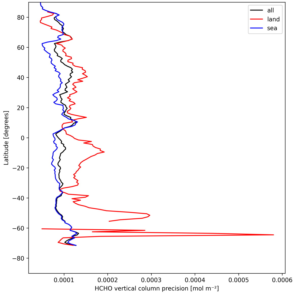
Figure 22: Zonal average of “HCHO vertical column precision” for 2025-08-15 to 2025-08-17.
