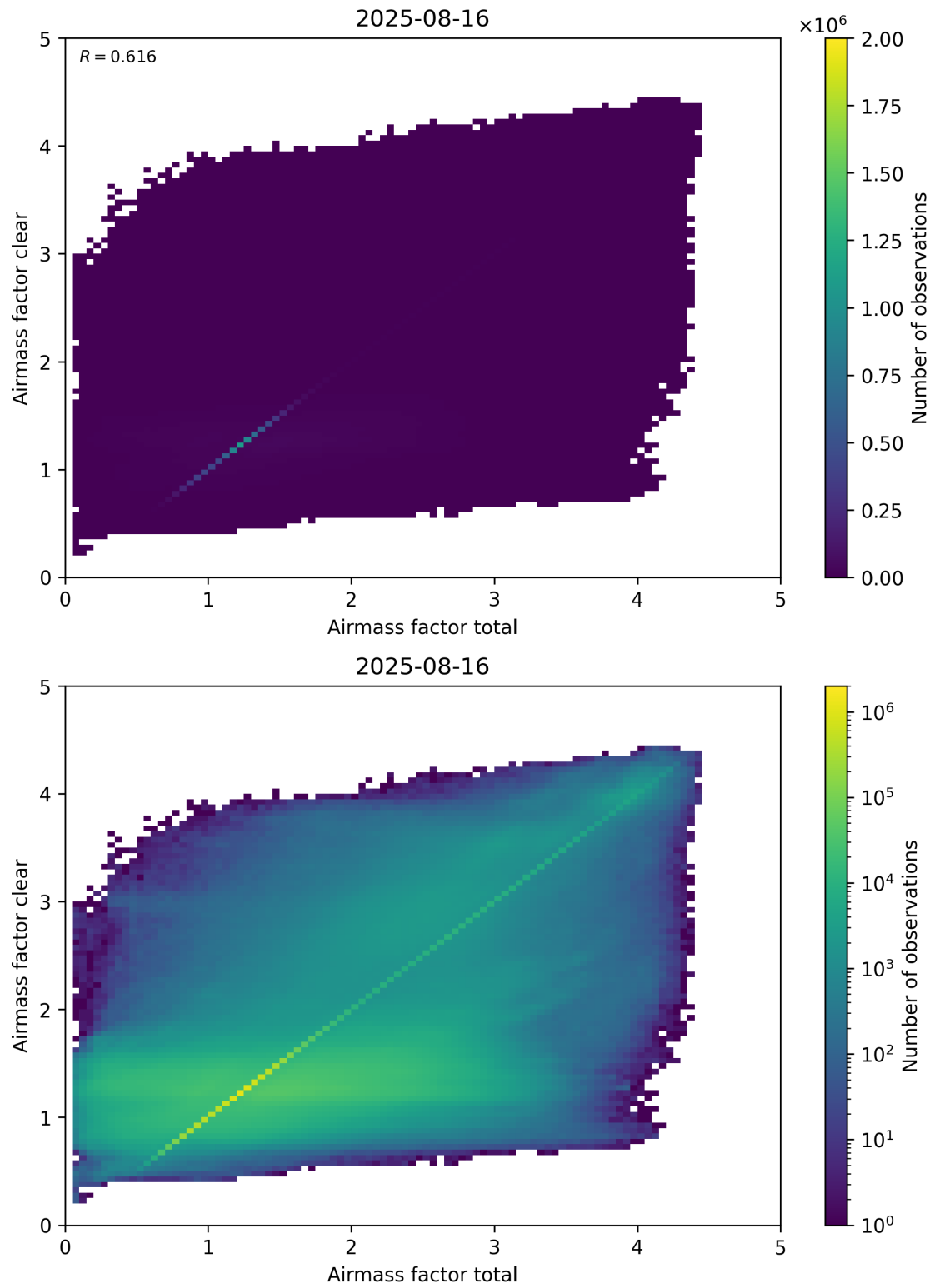
Figure 100: Scatter density plot of “Airmass factor total” against “Airmass factor clear” for 2025-08-15 to 2025-08-17.
