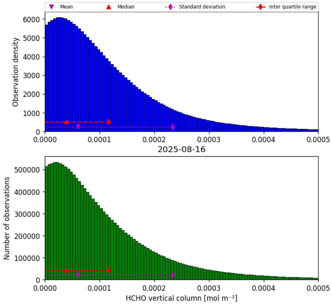
Figure 35: Histogram of “HCHO vertical column” for 2025-08-15 to 2025-08-17
