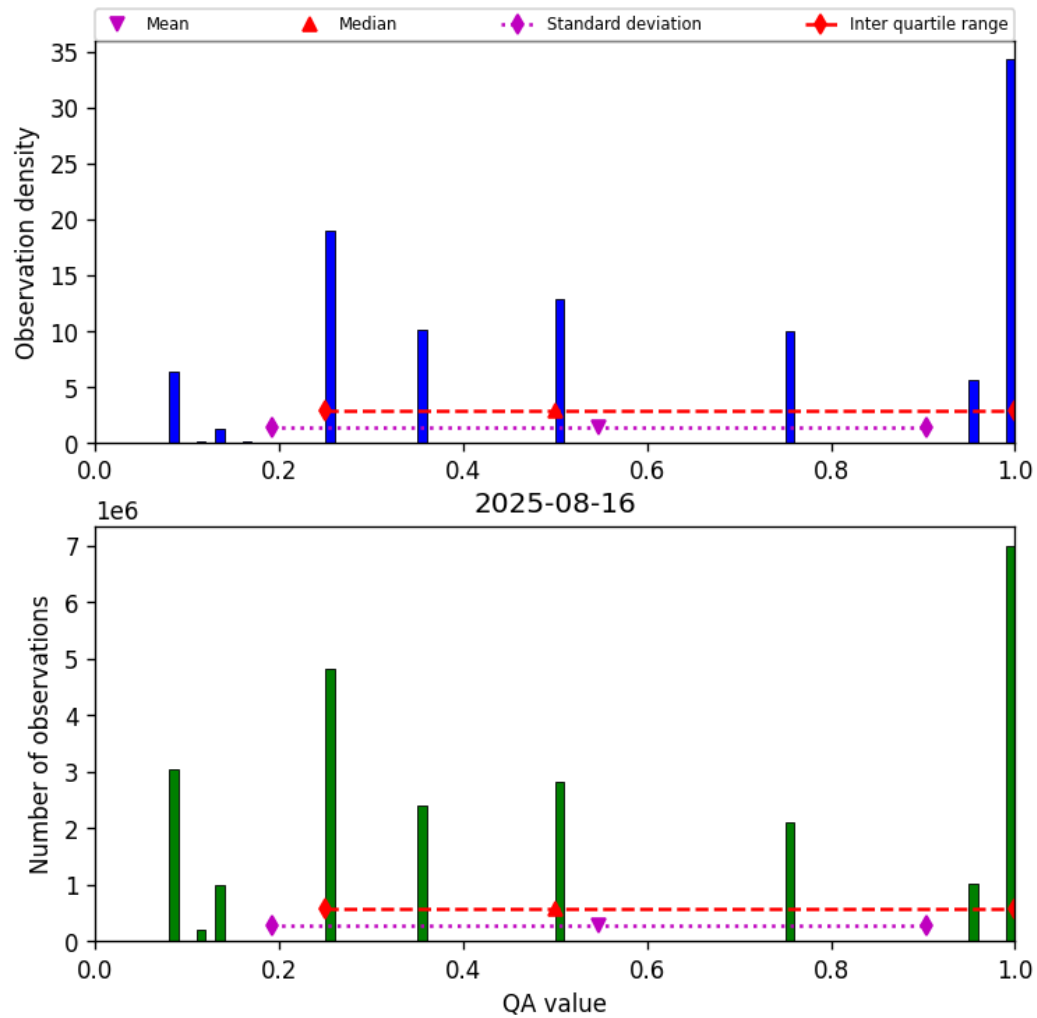
Figure 34: Histogram of “QA value” for 2025-08-15 to 2025-08-17
