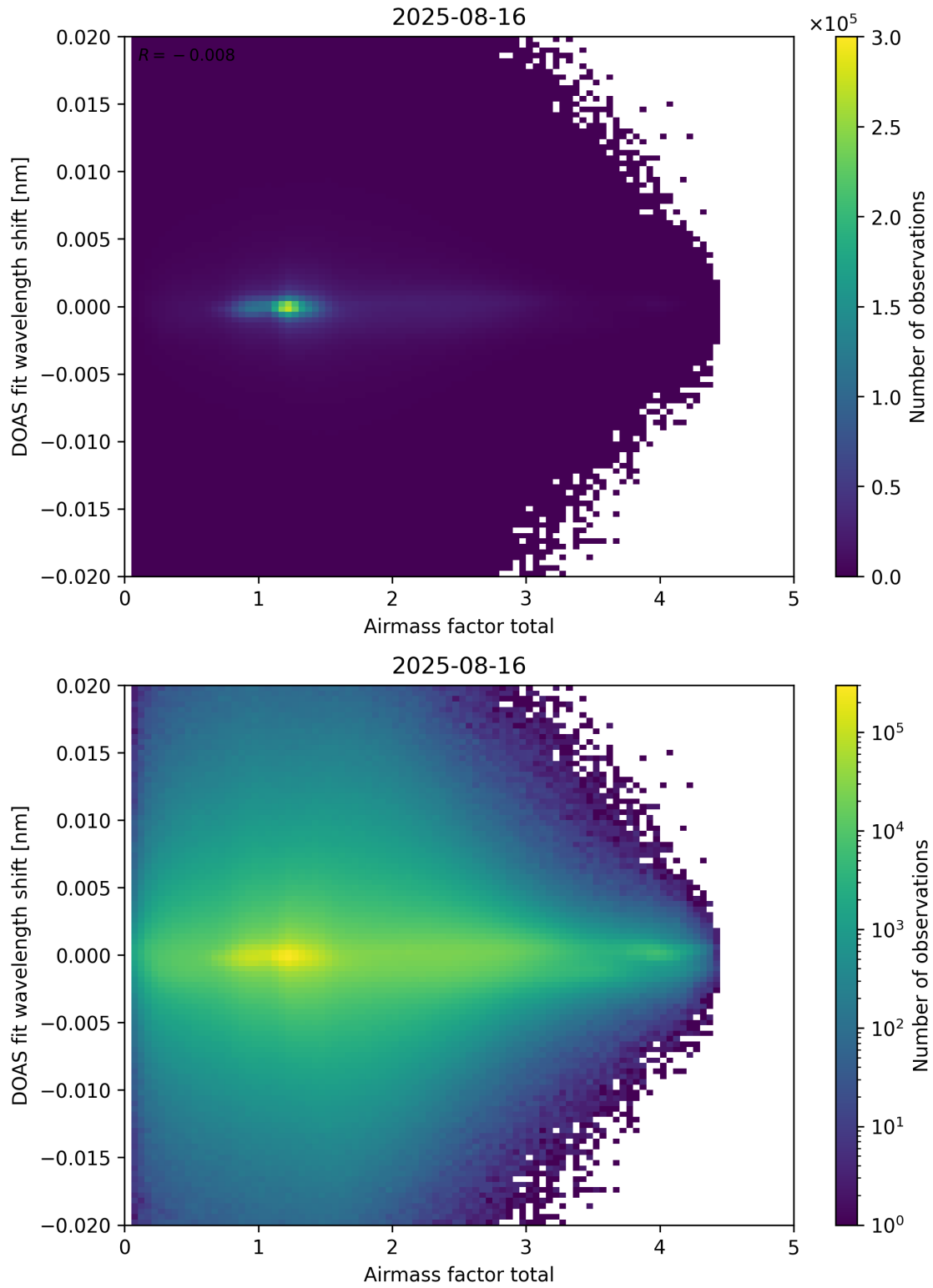
Figure 98: Scatter density plot of “Airmass factor total” against “DOAS fit wavelength shift” for 2025-08-15 to 2025-08-17.
