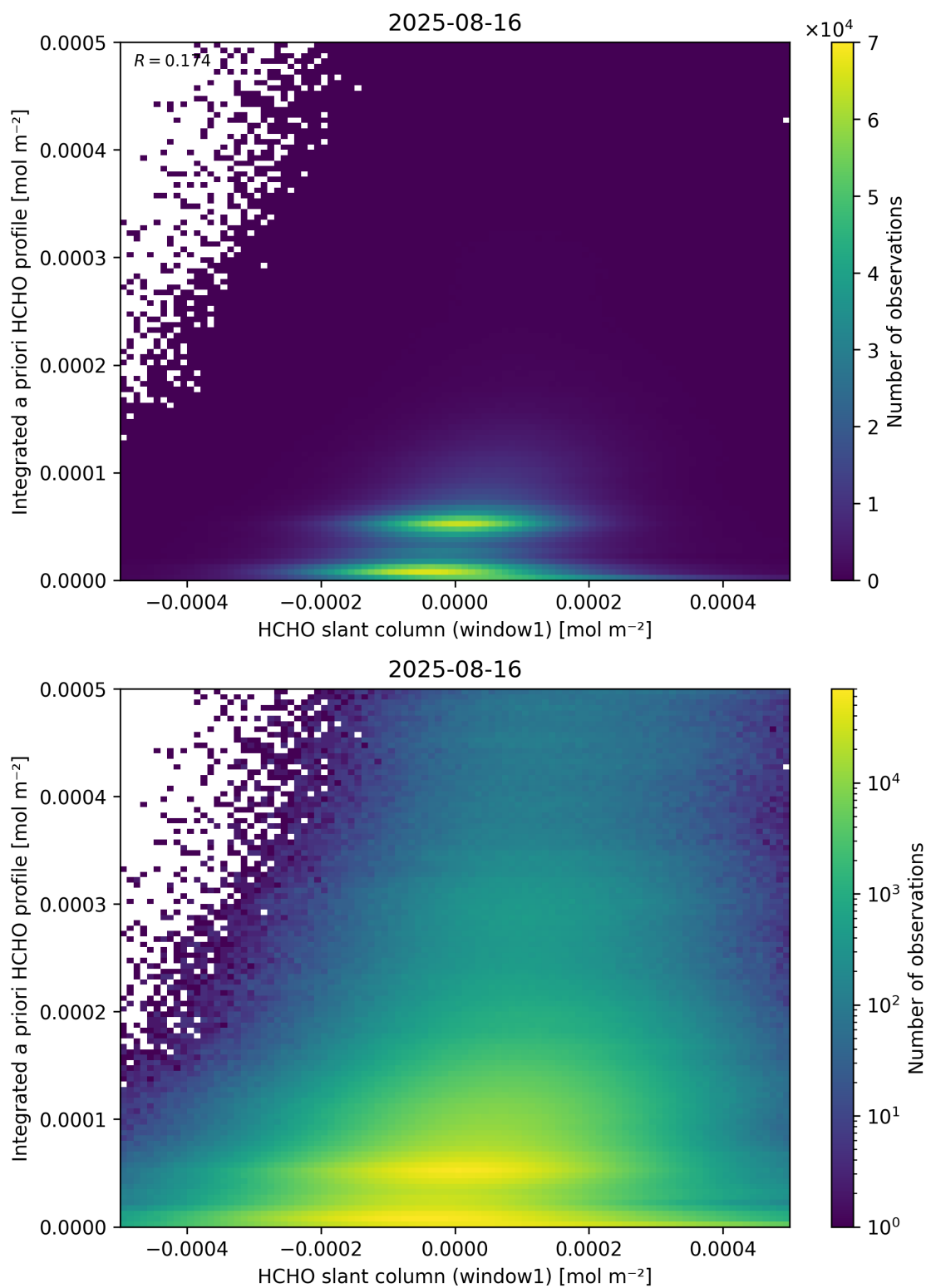
Figure 87: Scatter density plot of “HCHO slant column (window1)” against “Integrated a priori HCHO profile” for 2025-08-15 to 2025-08-17.
