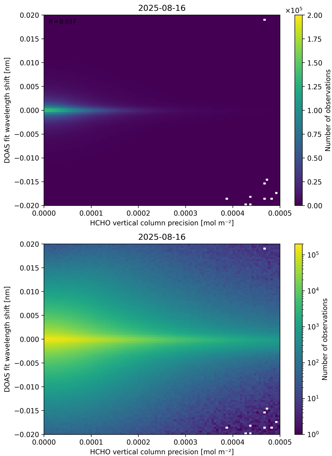
Figure 137: Scatter density plot of “HCHO vertical column precision” against “DOAS fit wavelength shift” for 2025-08-15 to 2025-08-17.
