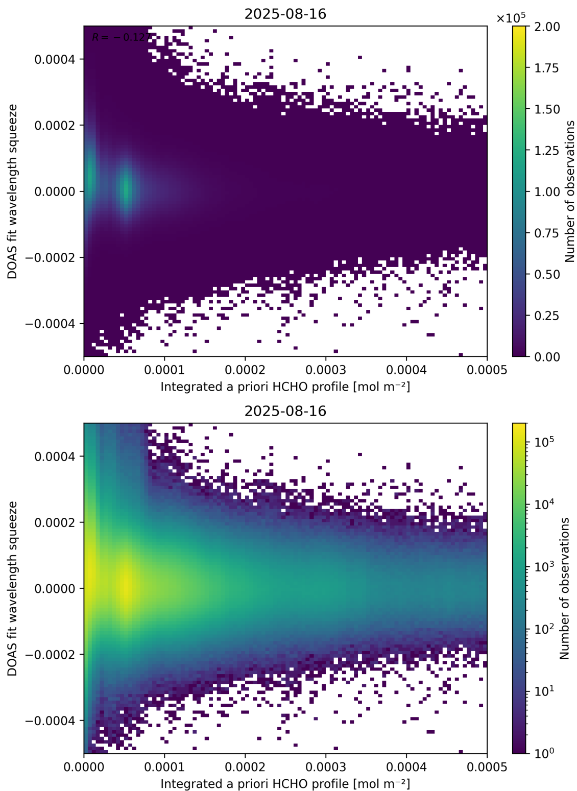
Figure 150: Scatter density plot of “Integrated a priori HCHO profile” against “DOAS fit wavelength squeeze” for 2025-08-15 to 2025-08-17.
