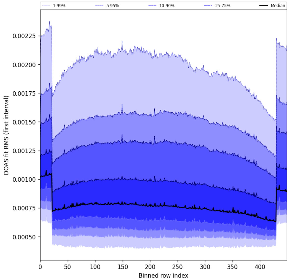
Figure 60: Along track statistics of “DOAS fit RMS (first interval)” for 2025-08-15 to 2025-08-17
