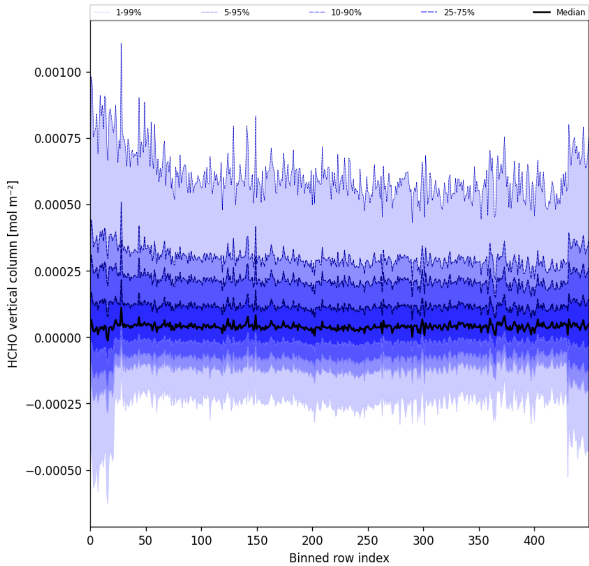
Figure 49: Along track statistics of “HCHO vertical column” for 2025-08-15 to 2025-08-17
