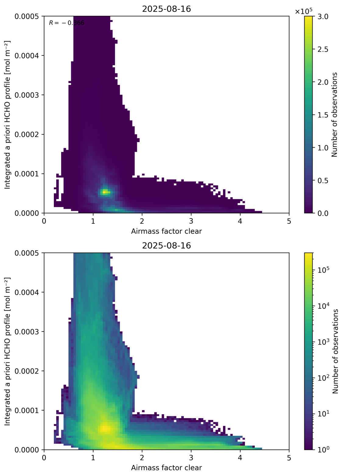
Figure 76: Scatter density plot of “Airmass factor clear” against “Integrated a priori HCHO profile” for 2025-08-15 to 2025-08-17.
