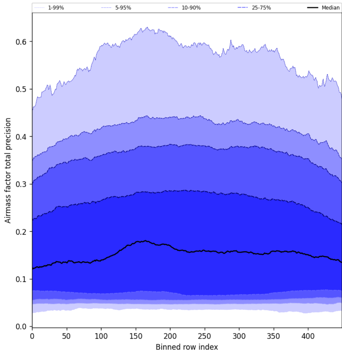
Figure 55: Along track statistics of “Airmass factor total precision” for 2025-08-15 to 2025-08-17
