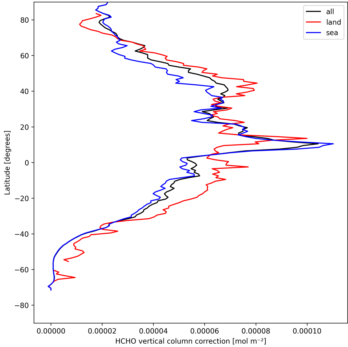
Figure 23: Zonal average of “HCHO vertical column correction” for 2025-08-15 to 2025-08-17.
