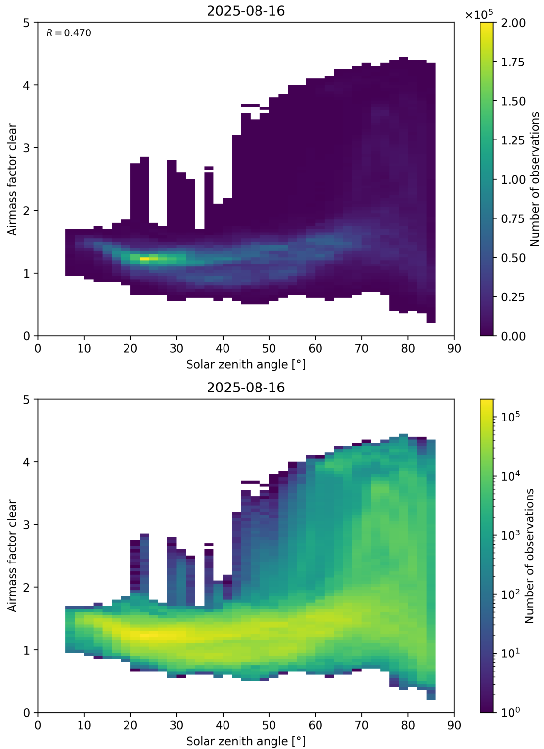
Figure 170: Scatter density plot of “Solar zenith angle” against “Airmass factor clear” for 2025-08-15 to 2025-08-17.
