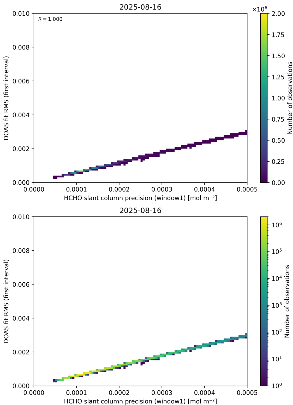
Figure 88: Scatter density plot of “HCHO slant column precision (window1)” against “DOAS fit RMS (first interval)” for 2025-08-15 to 2025-08-17.
