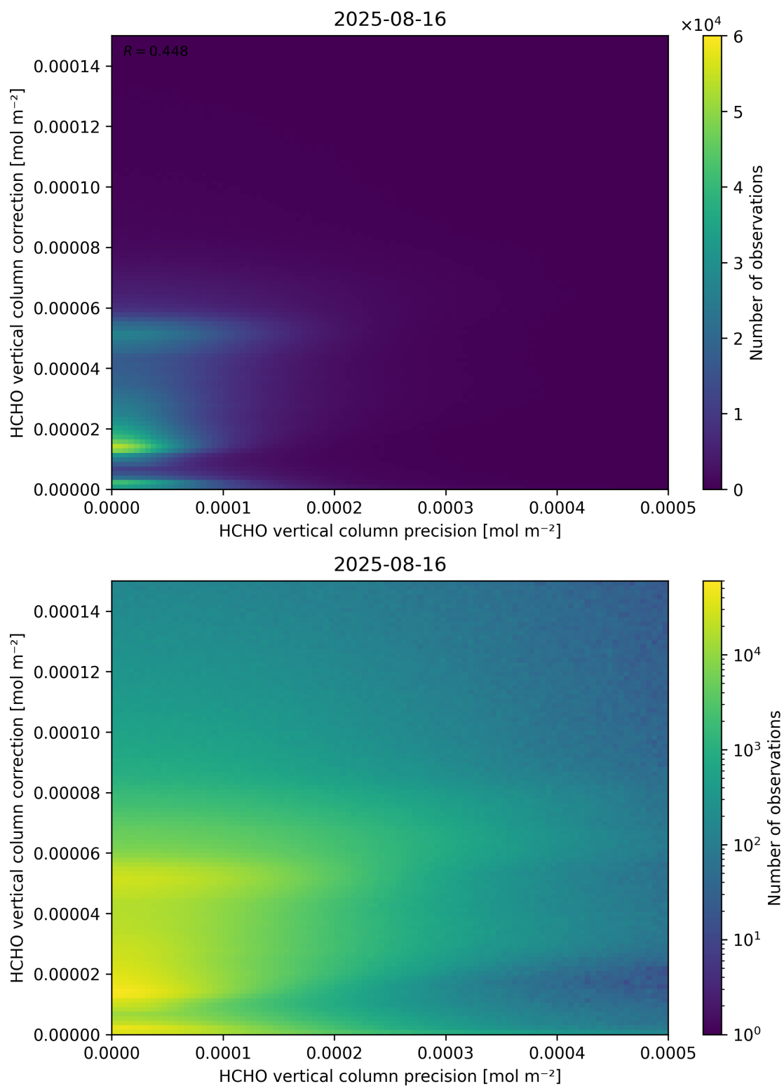
Figure 146: Scatter density plot of “HCHO vertical column precision” against “HCHO vertical column correction” for 2025-08-15 to 2025-08-17.
