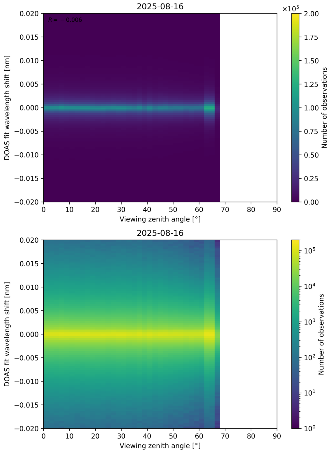
Figure 183: Scatter density plot of “Viewing zenith angle” against “DOAS fit wavelength shift” for 2025-08-15 to 2025-08-17.
