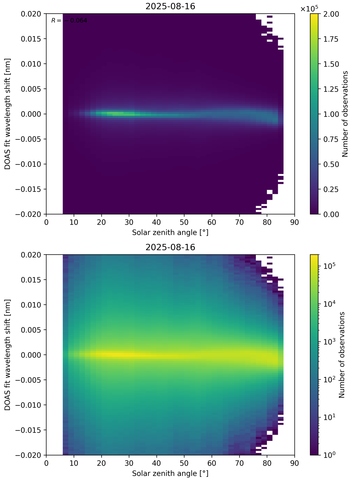
Figure 168: Scatter density plot of “Solar zenith angle” against “DOAS fit wavelength shift” for 2025-08-15 to 2025-08-17.
