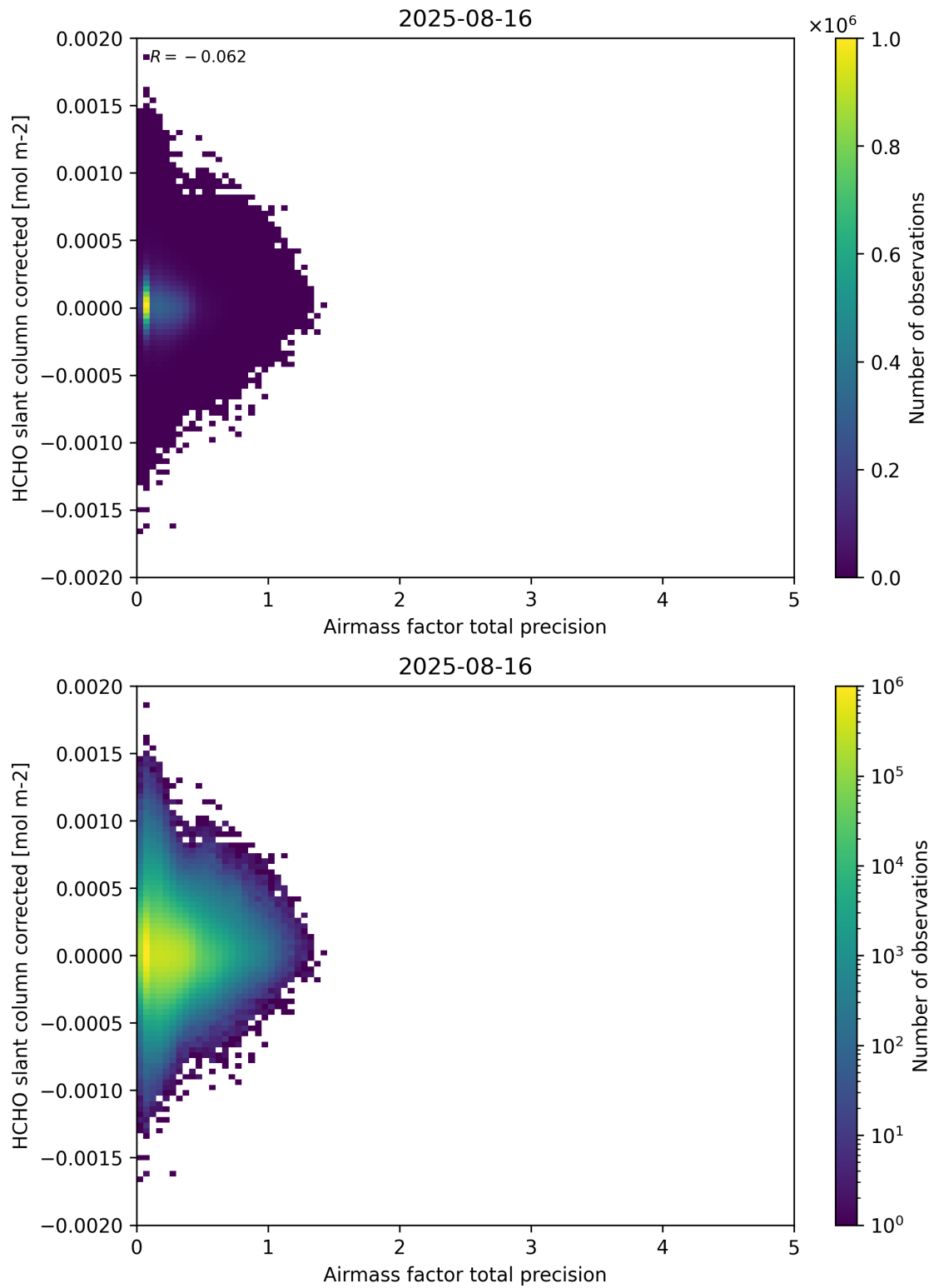
Figure 109: Scatter density plot of “Airmass factor total precision” against “HCHO slant column corrected” for 2025-08-15 to 2025-08-17.
