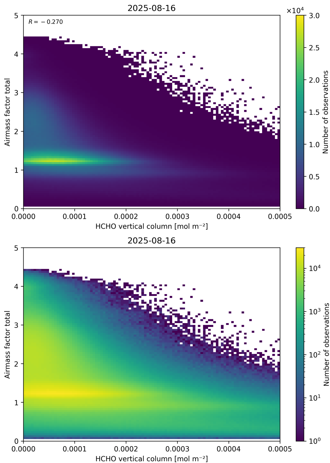
Figure 131: Scatter density plot of “HCHO vertical column” against “Airmass factor total” for 2025-08-15 to 2025-08-17.
