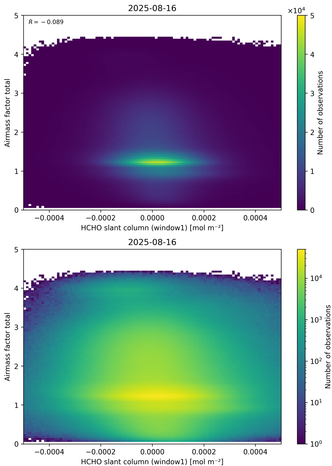
Figure 85: Scatter density plot of “HCHO slant column (window1)” against “Airmass factor total” for 2025-08-15 to 2025-08-17.
