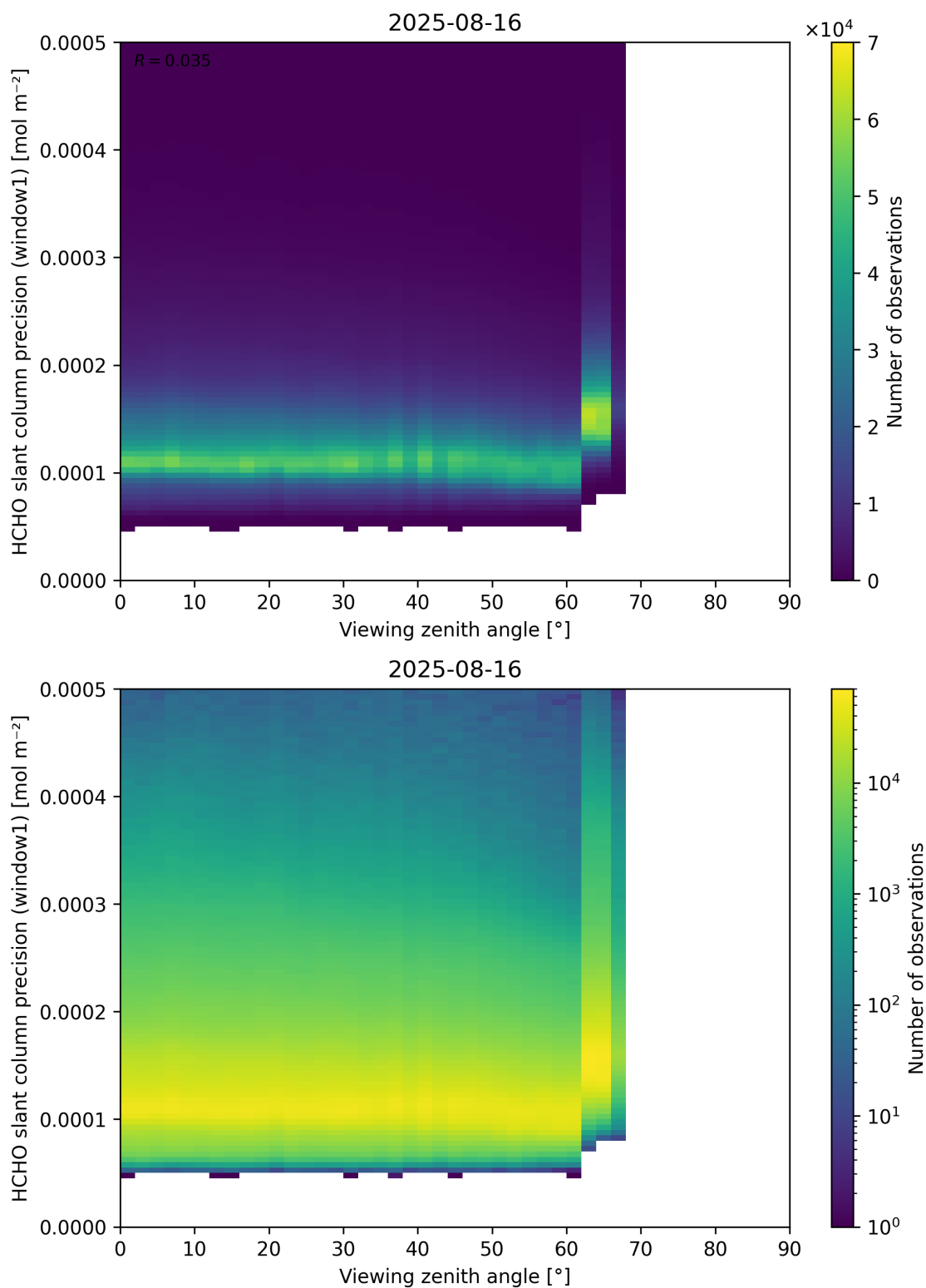
Figure 189: Scatter density plot of “Viewing zenith angle” against “HCHO slant column precision (window1)” for 2025-08-15 to 2025-08-17.
