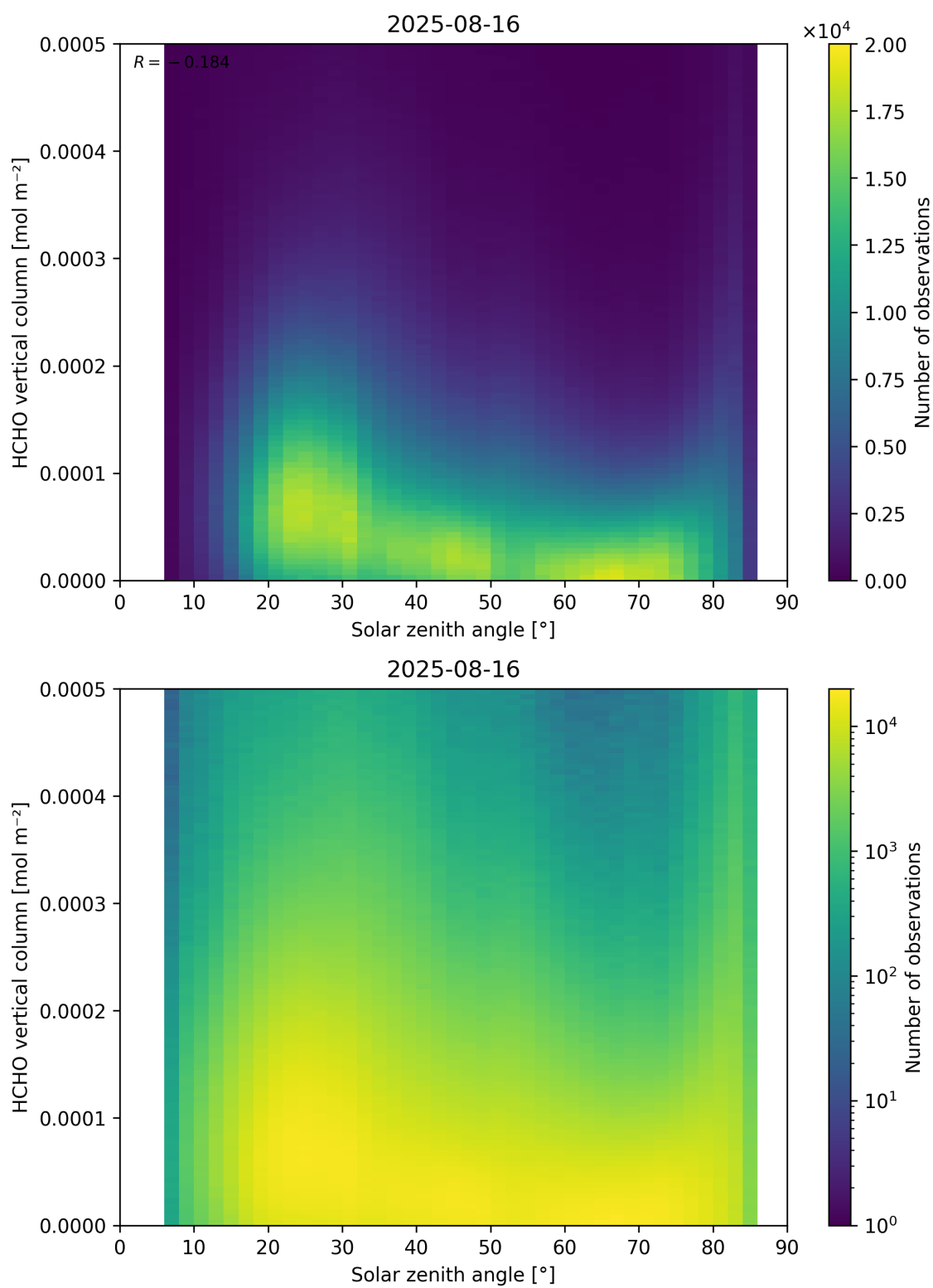
Figure 177: Scatter density plot of “Solar zenith angle” against “HCHO vertical column” for 2025-08-15 to 2025-08-17.
