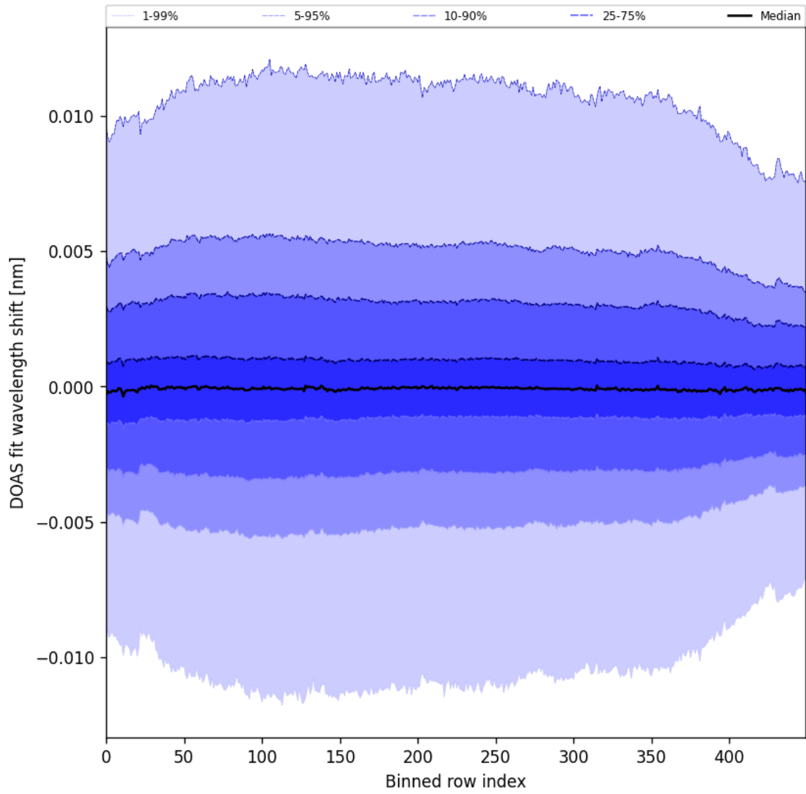
Figure 58: Along track statistics of “DOAS fit wavelength shift” for 2025-08-15 to 2025-08-17
