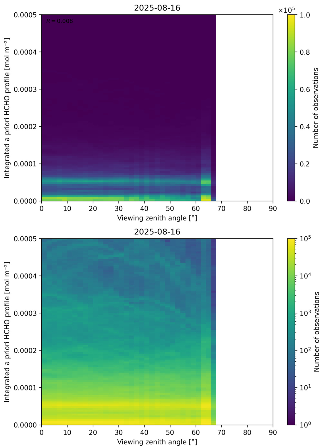
Figure 195: Scatter density plot of “Viewing zenith angle” against “Integrated a priori HCHO profile” for 2025-08-15 to 2025-08-17.
