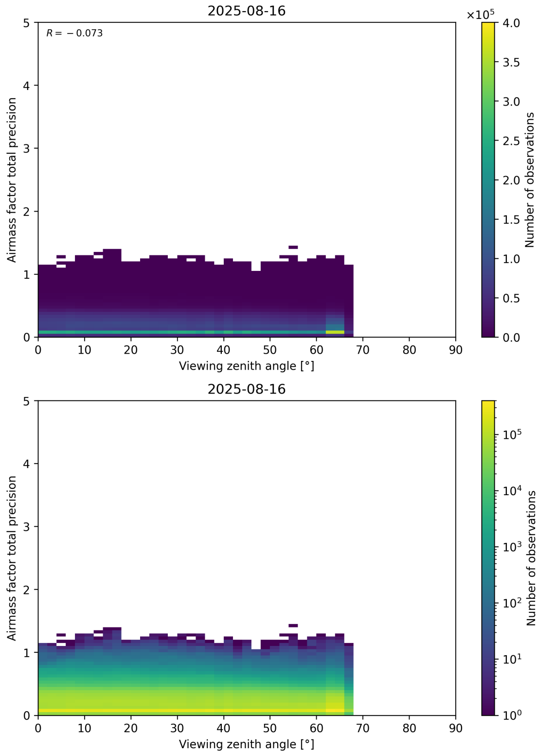
Figure 191: Scatter density plot of “Viewing zenith angle” against “Airmass factor total precision” for 2025-08-15 to 2025-08-17.
