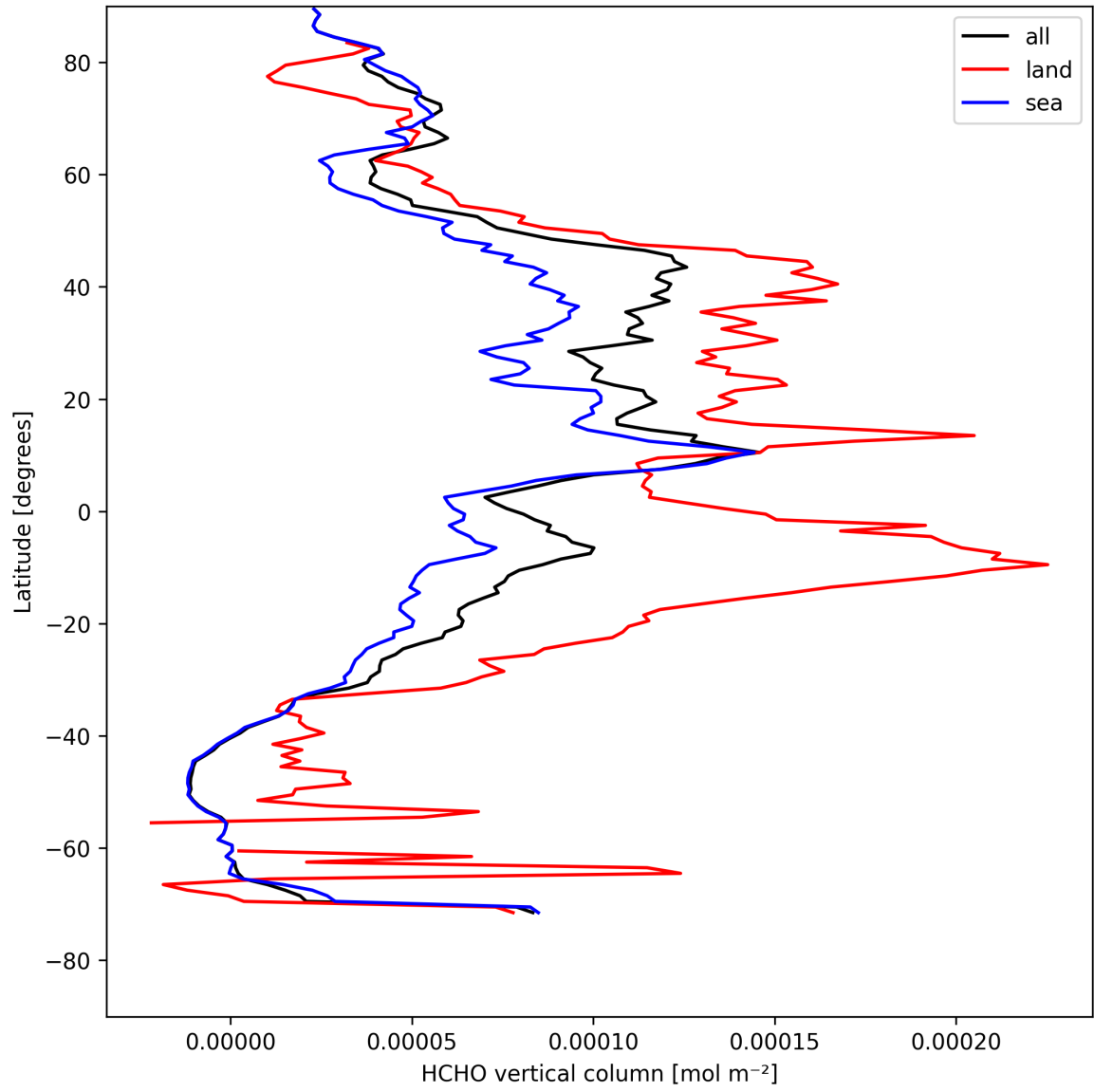
Figure 21: Zonal average of “HCHO vertical column” for 2025-08-15 to 2025-08-17.
