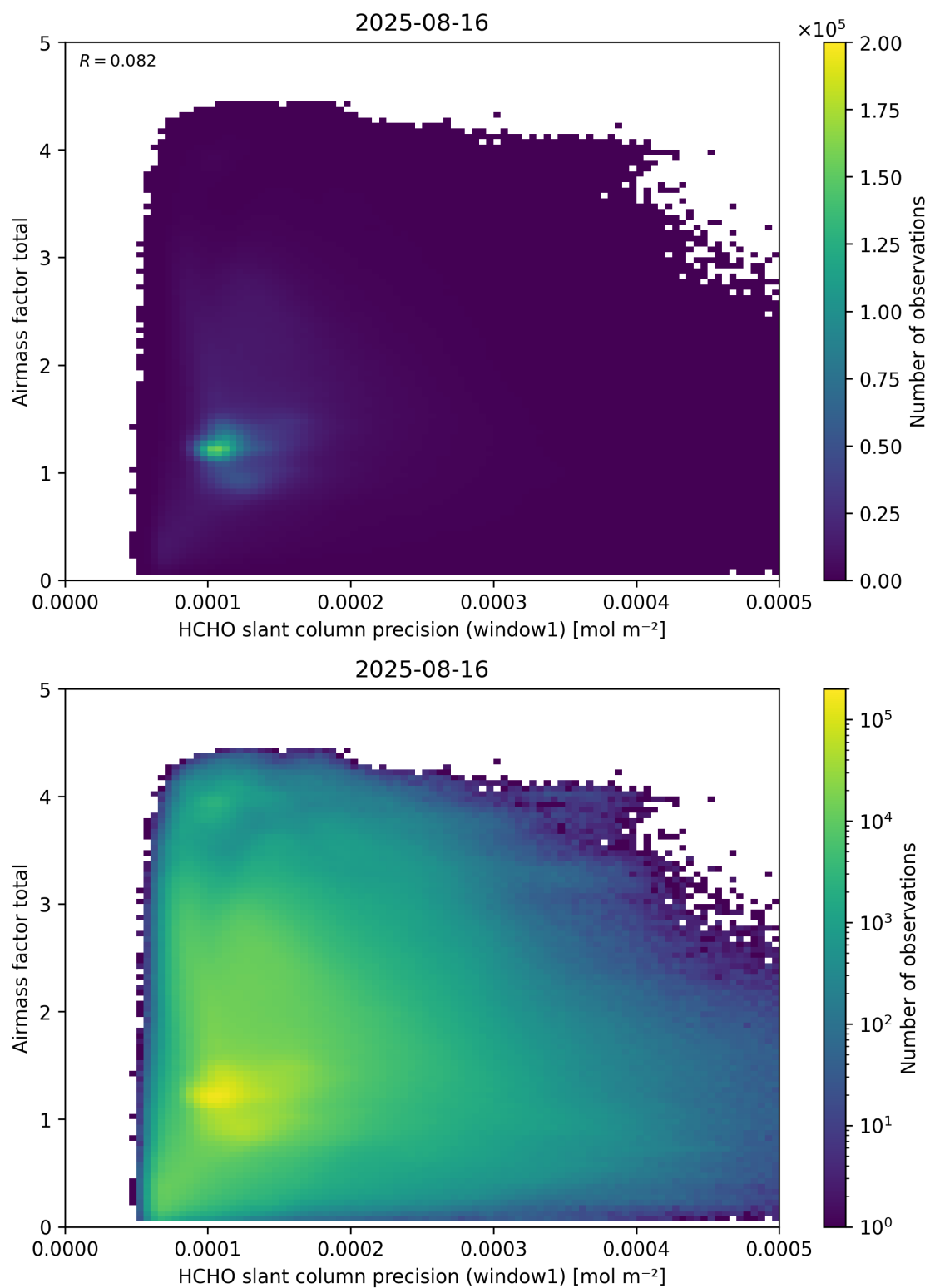
Figure 94: Scatter density plot of “HCHO slant column precision (window1)” against “Airmass factor total” for 2025-08-15 to 2025-08-17.
