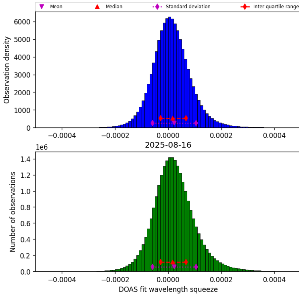
Figure 45: Histogram of “DOAS fit wavelength squeeze” for 2025-08-15 to 2025-08-17
