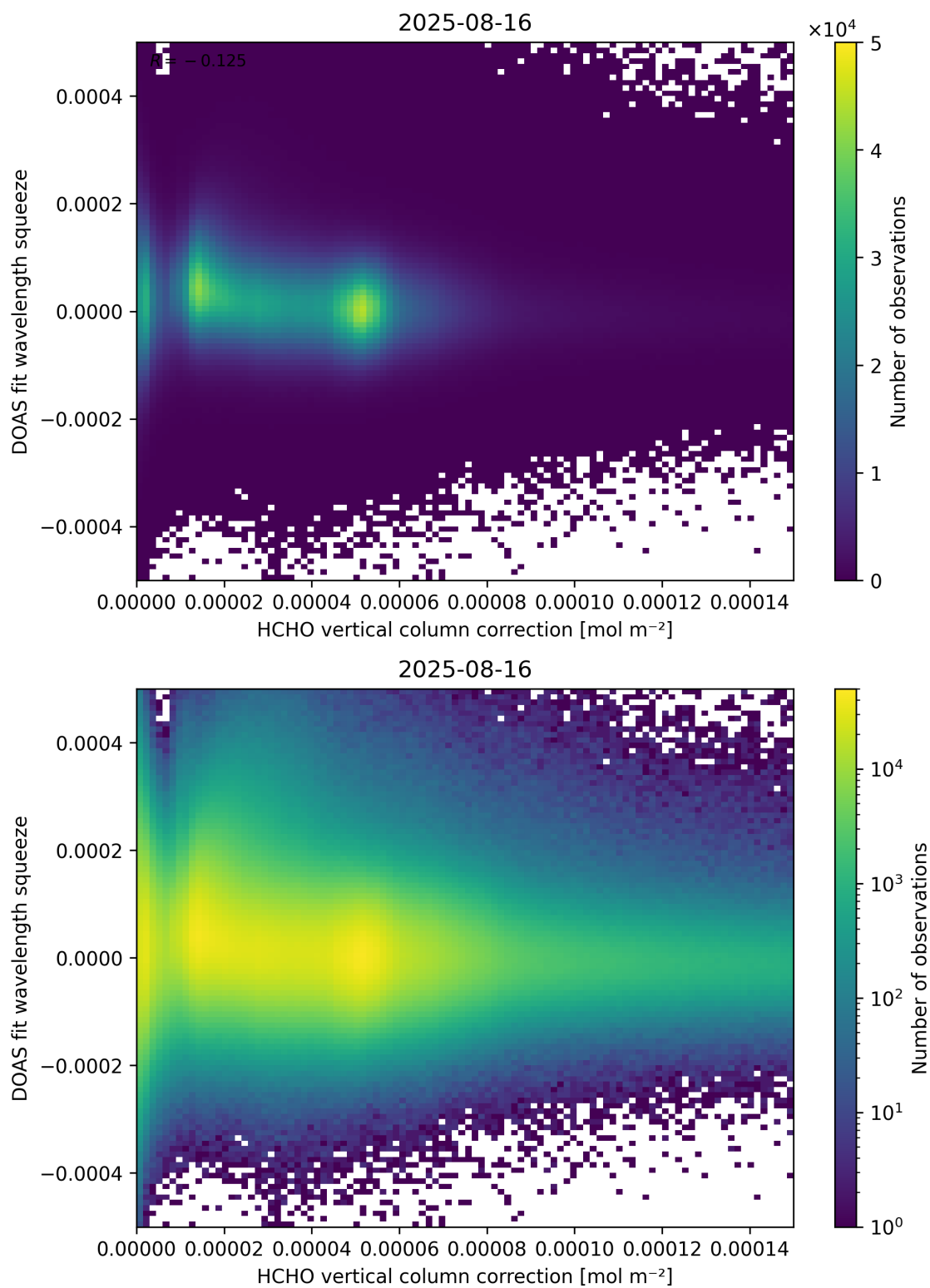
Figure 114: Scatter density plot of “HCHO vertical column correction” against “DOAS fit wavelength squeeze” for 2025-08-15 to 2025-08-17.
