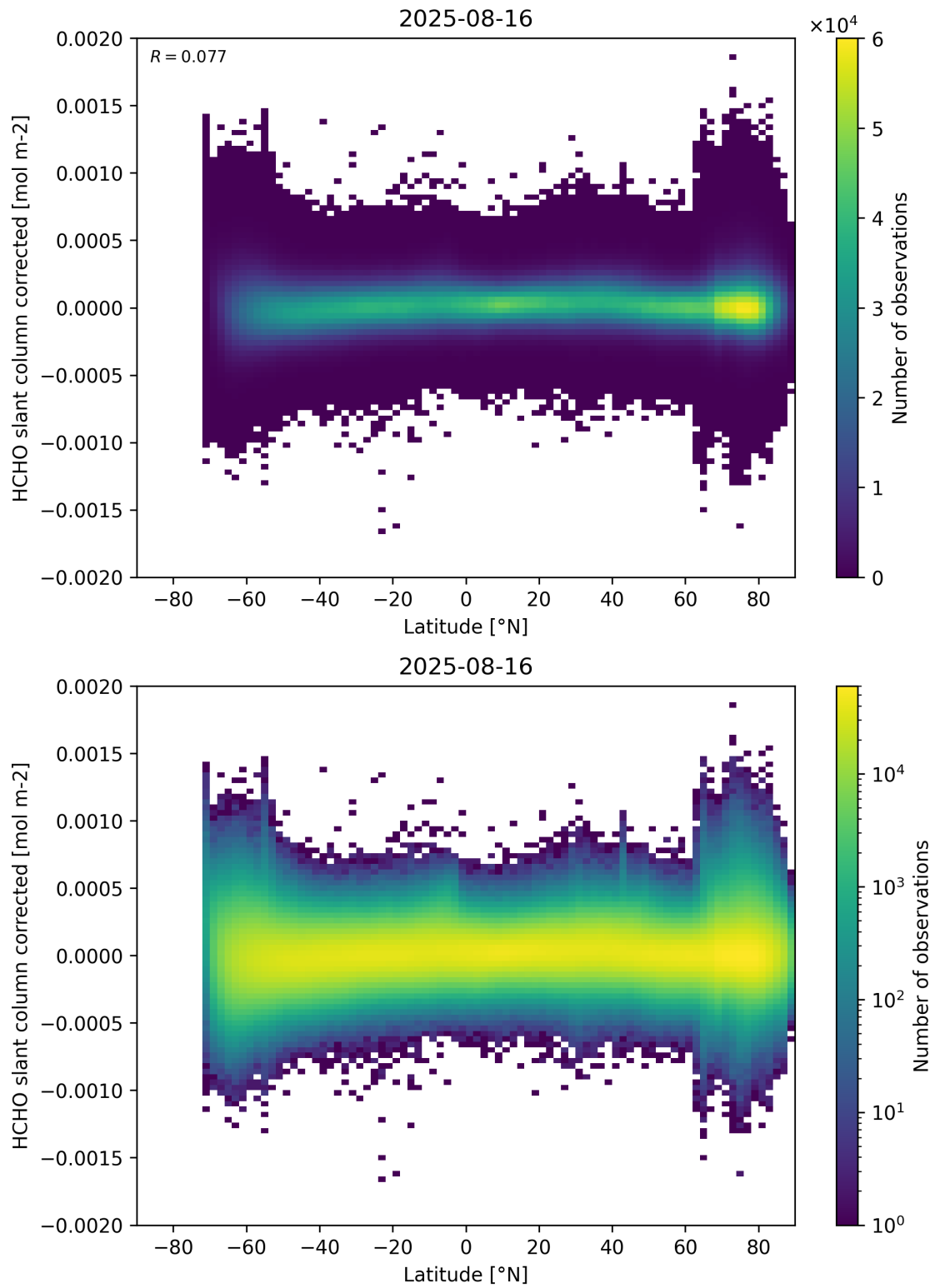
Figure 157: Scatter density plot of “Latitude” against “HCHO slant column corrected” for 2025-08-15 to 2025-08-17.
