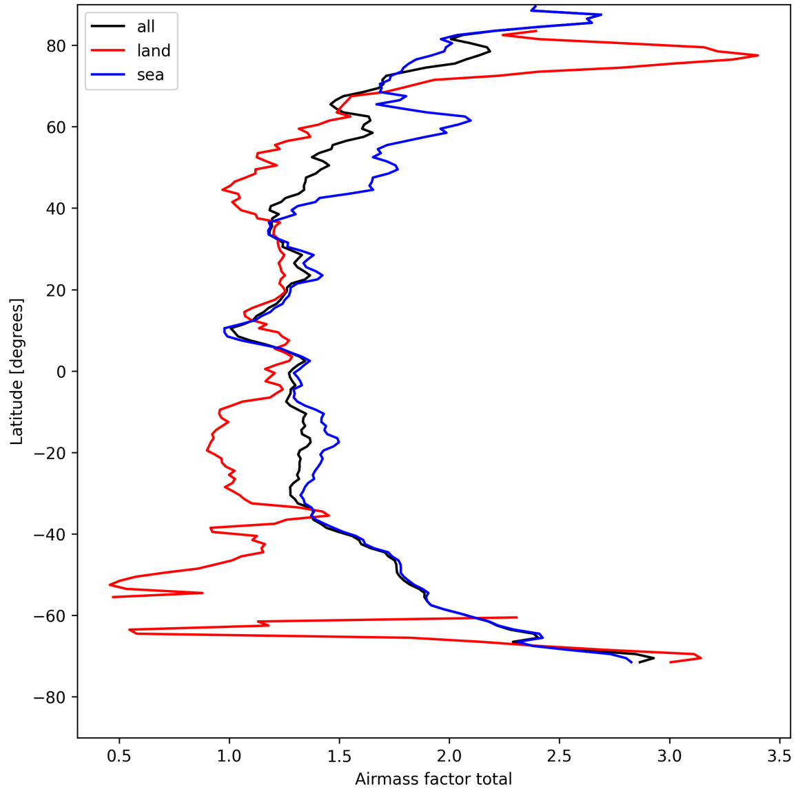
Figure 26: Zonal average of “Airmass factor total” for 2025-08-15 to 2025-08-17.
