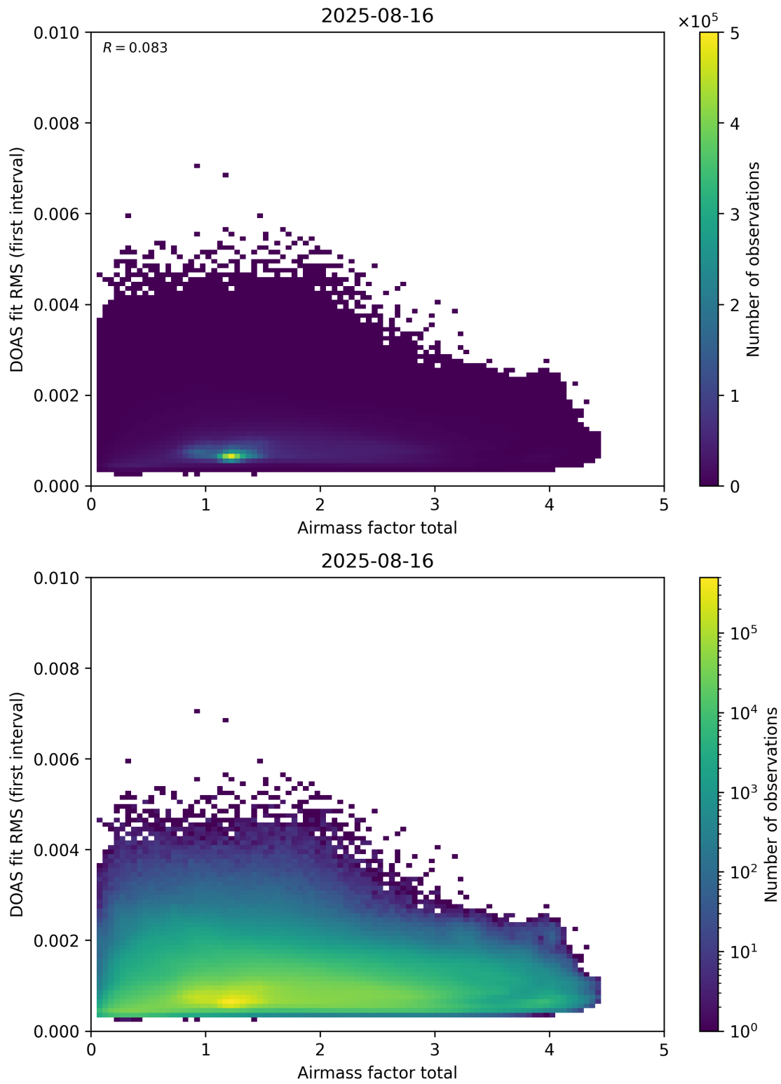
Figure 97: Scatter density plot of “Airmass factor total” against “DOAS fit RMS (first interval)” for 2025-08-15 to 2025-08-17.
