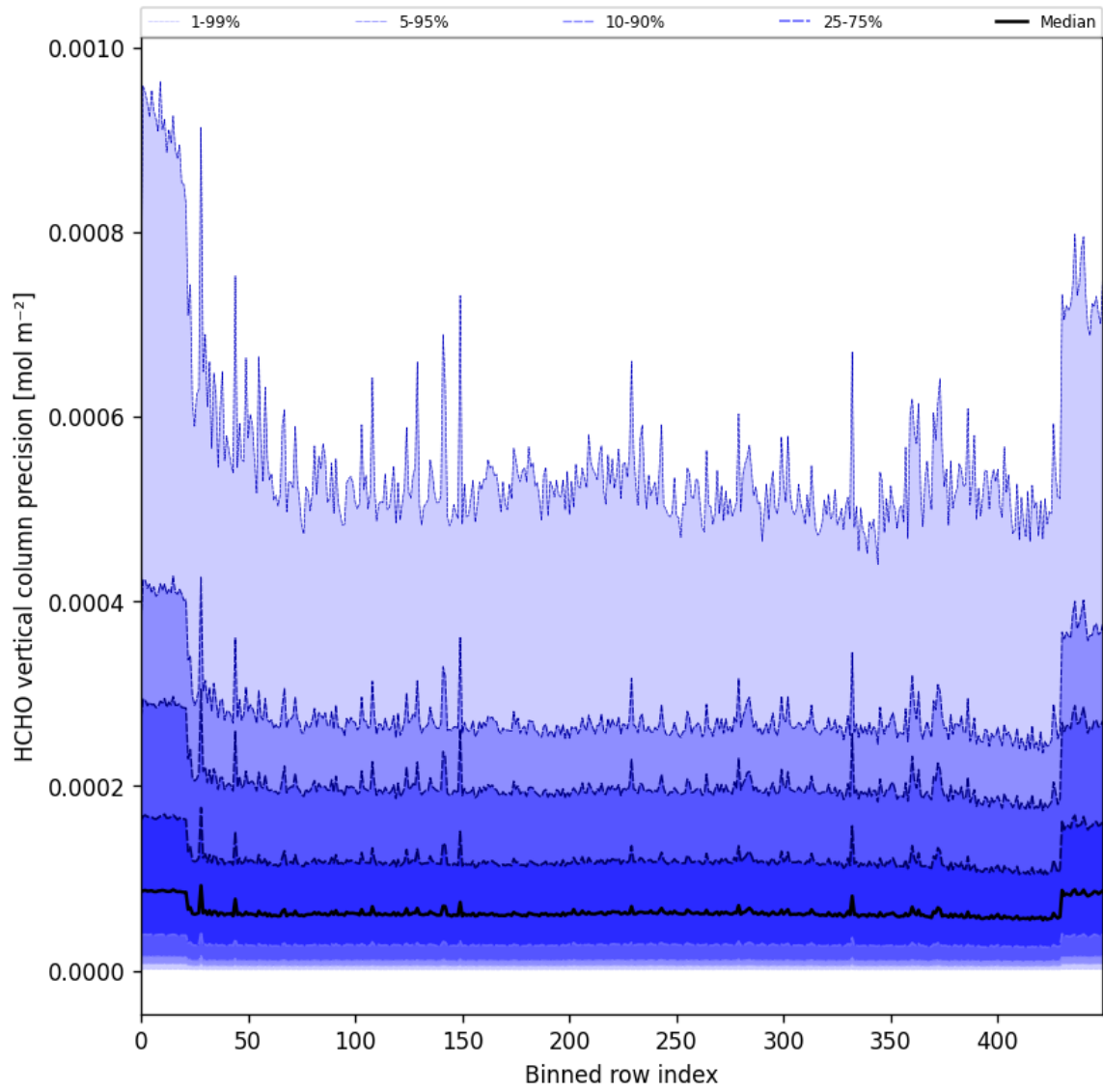
Figure 50: Along track statistics of “HCHO vertical column precision” for 2025-08-15 to 2025-08-17
