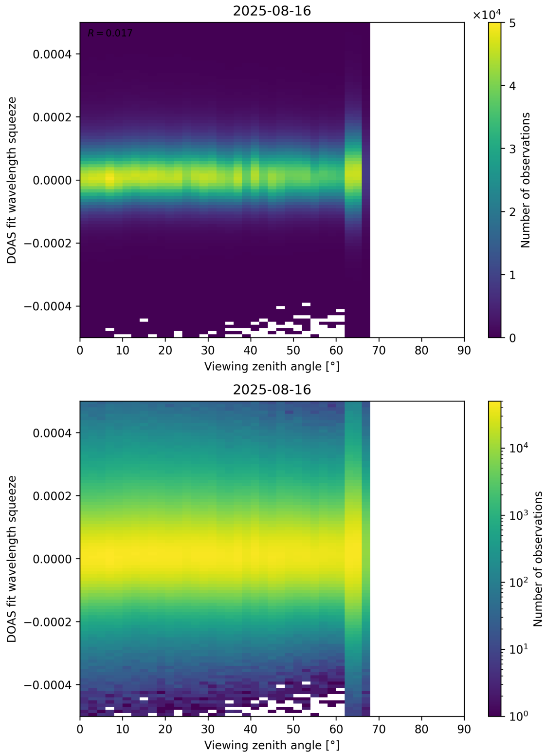
Figure 184: Scatter density plot of “Viewing zenith angle” against “DOAS fit wavelength squeeze” for 2025-08-15 to 2025-08-17.
