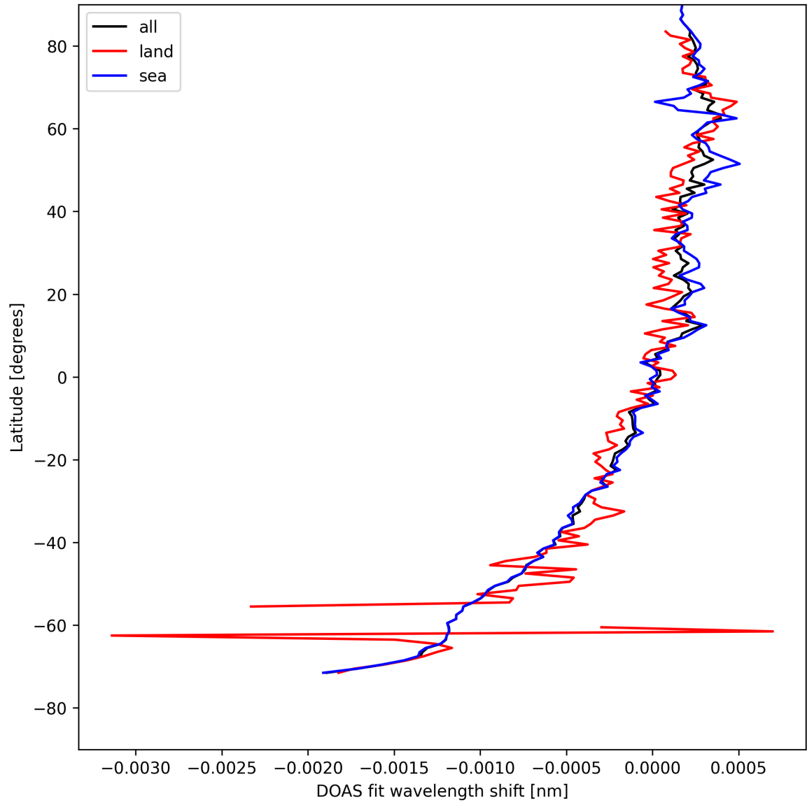
Figure 30: Zonal average of “DOAS fit wavelength shift” for 2025-08-15 to 2025-08-17.
