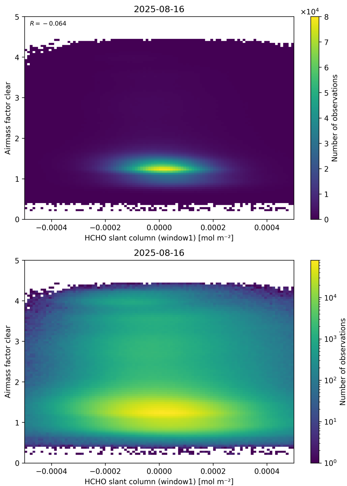
Figure 81: Scatter density plot of “HCHO slant column (window1)” against “Airmass factor clear” for 2025-08-15 to 2025-08-17.
