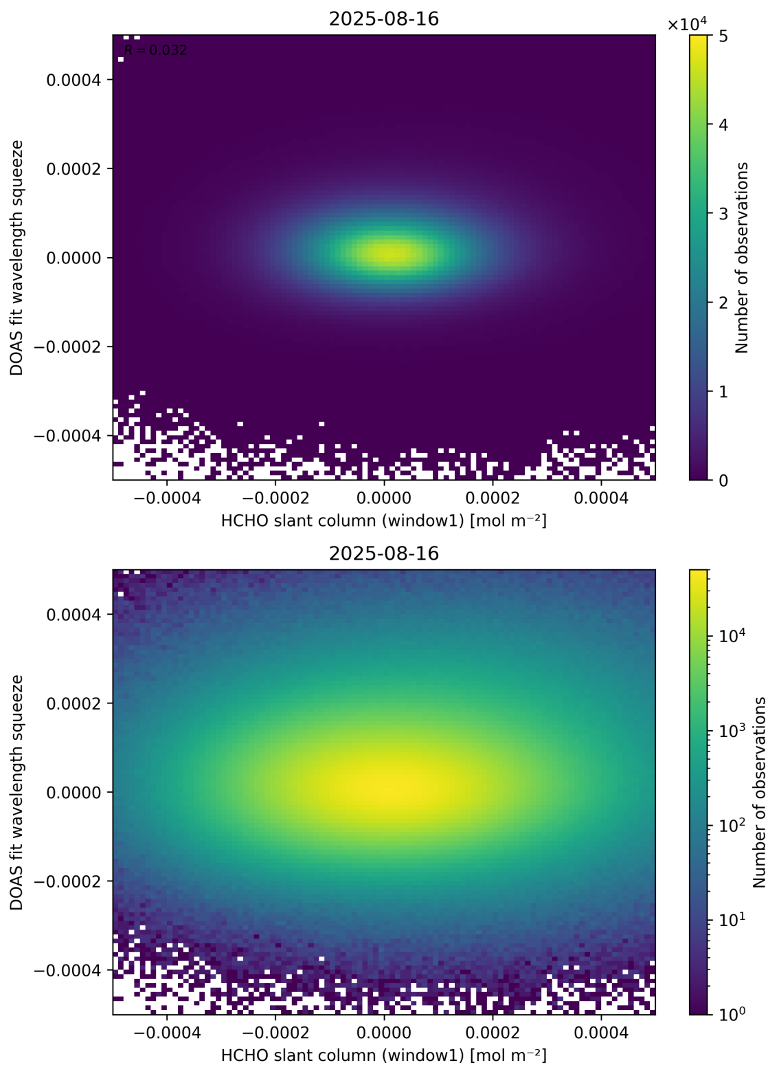
Figure 80: Scatter density plot of “HCHO slant column (window1)” against “DOAS fit wavelength squeeze” for 2025-08-15 to 2025-08-17.
