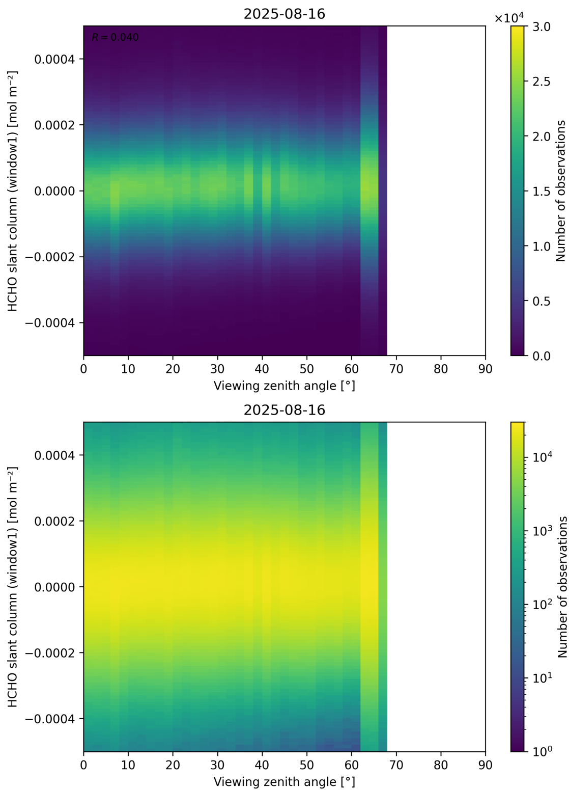
Figure 188: Scatter density plot of “Viewing zenith angle” against “HCHO slant column (window1)” for 2025-08-15 to 2025-08-17.
