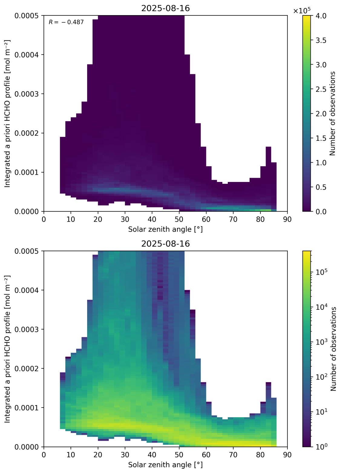
Figure 180: Scatter density plot of “Solar zenith angle” against “Integrated a priori HCHO profile” for 2025-08-15 to 2025-08-17.
