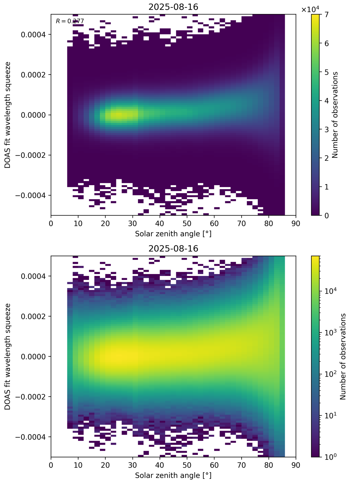
Figure 169: Scatter density plot of “Solar zenith angle” against “DOAS fit wavelength squeeze” for 2025-08-15 to 2025-08-17.
