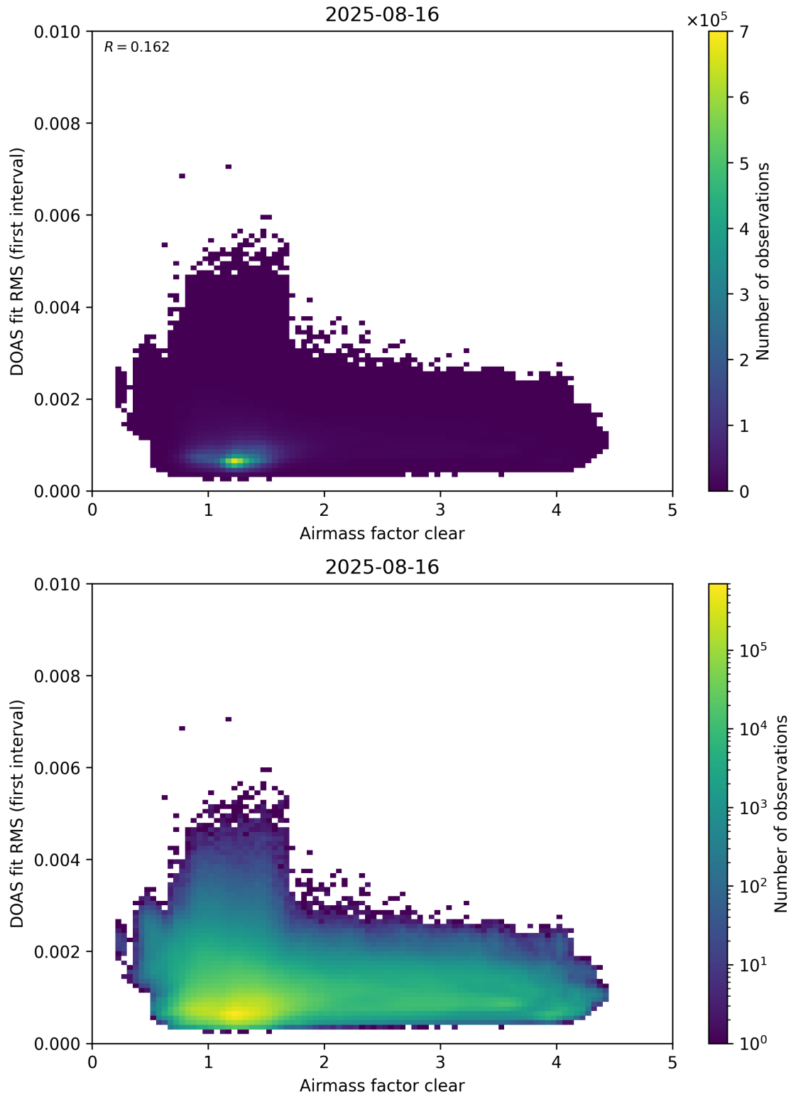
Figure 71: Scatter density plot of “Airmass factor clear” against “DOAS fit RMS (first interval)” for 2025-08-15 to 2025-08-17.
