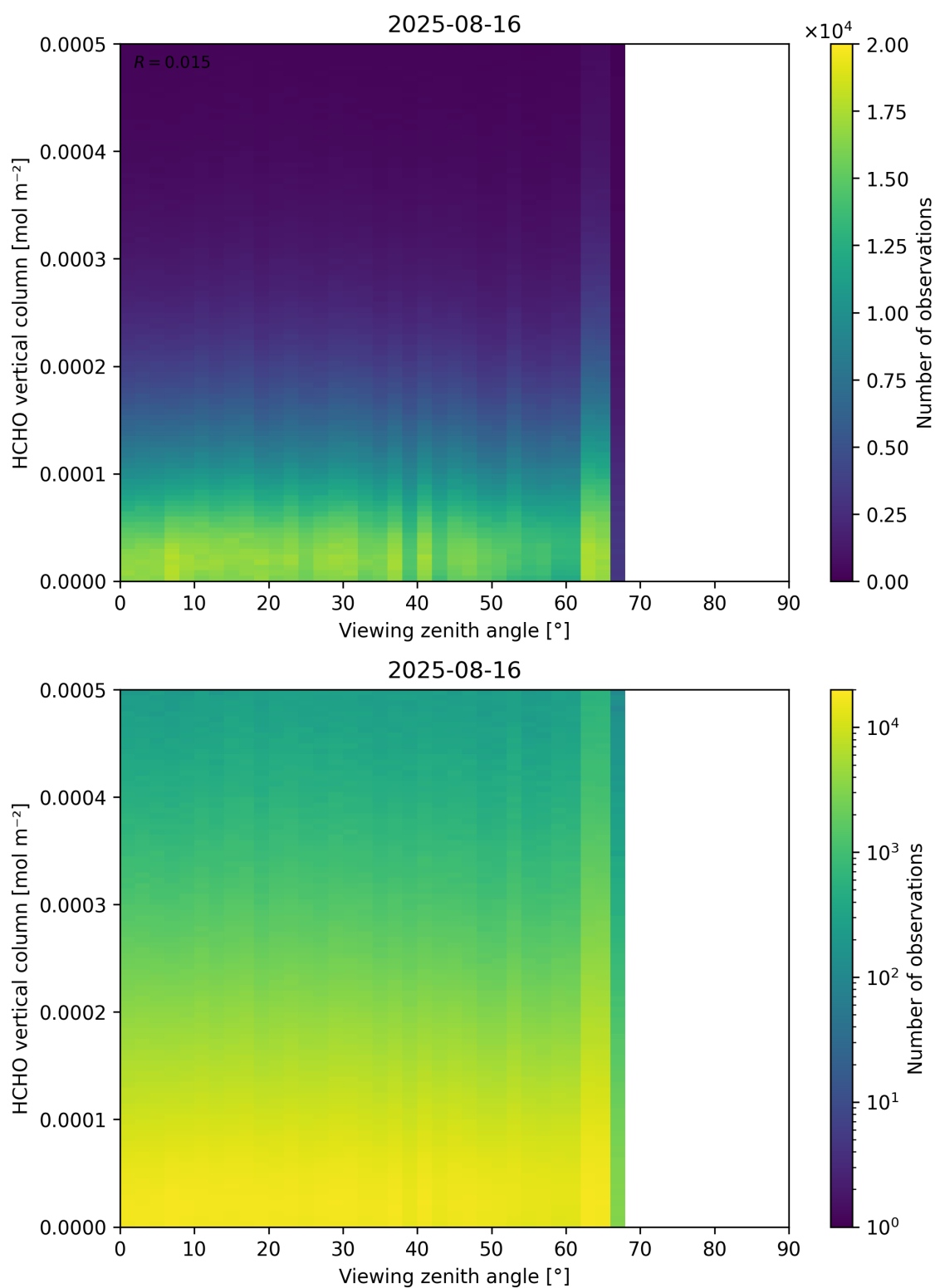
Figure 192: Scatter density plot of “Viewing zenith angle” against “HCHO vertical column” for 2025-08-15 to 2025-08-17.
