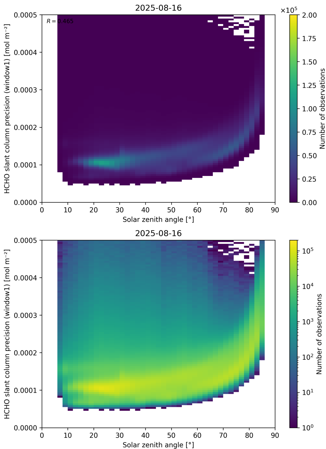
Figure 174: Scatter density plot of “Solar zenith angle” against “HCHO slant column precision (window1)” for 2025-08-15 to 2025-08-17.
