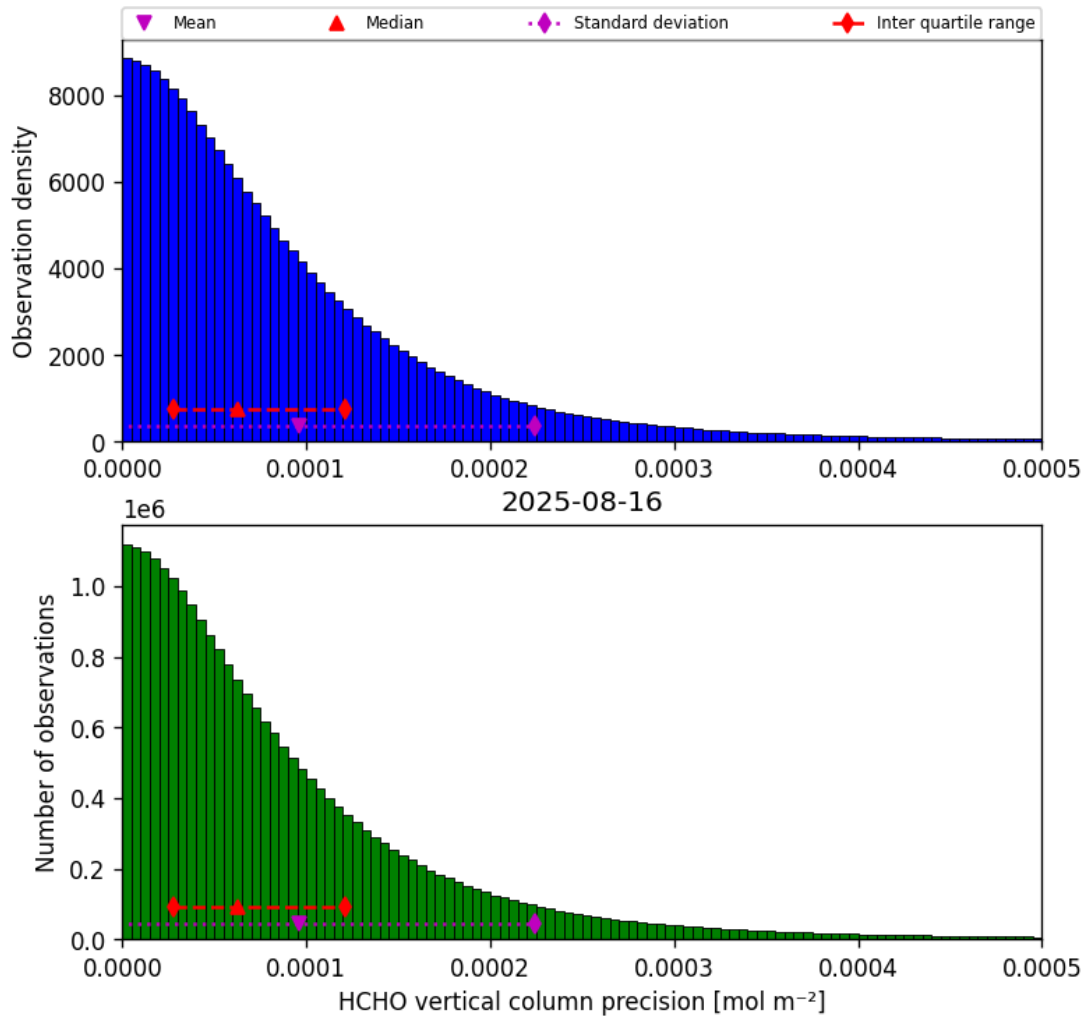
Figure 36: Histogram of “HCHO vertical column precision” for 2025-08-15 to 2025-08-17
