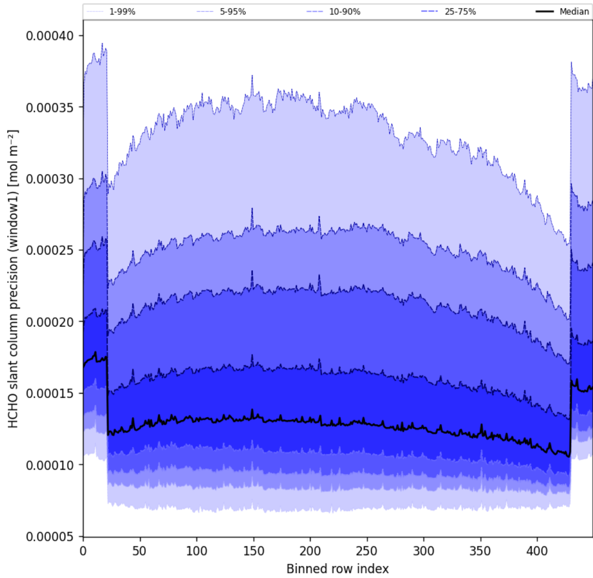
Figure 53: Along track statistics of “HCHO slant column precision (window1)” for 2025-08-15 to 2025-08-17
