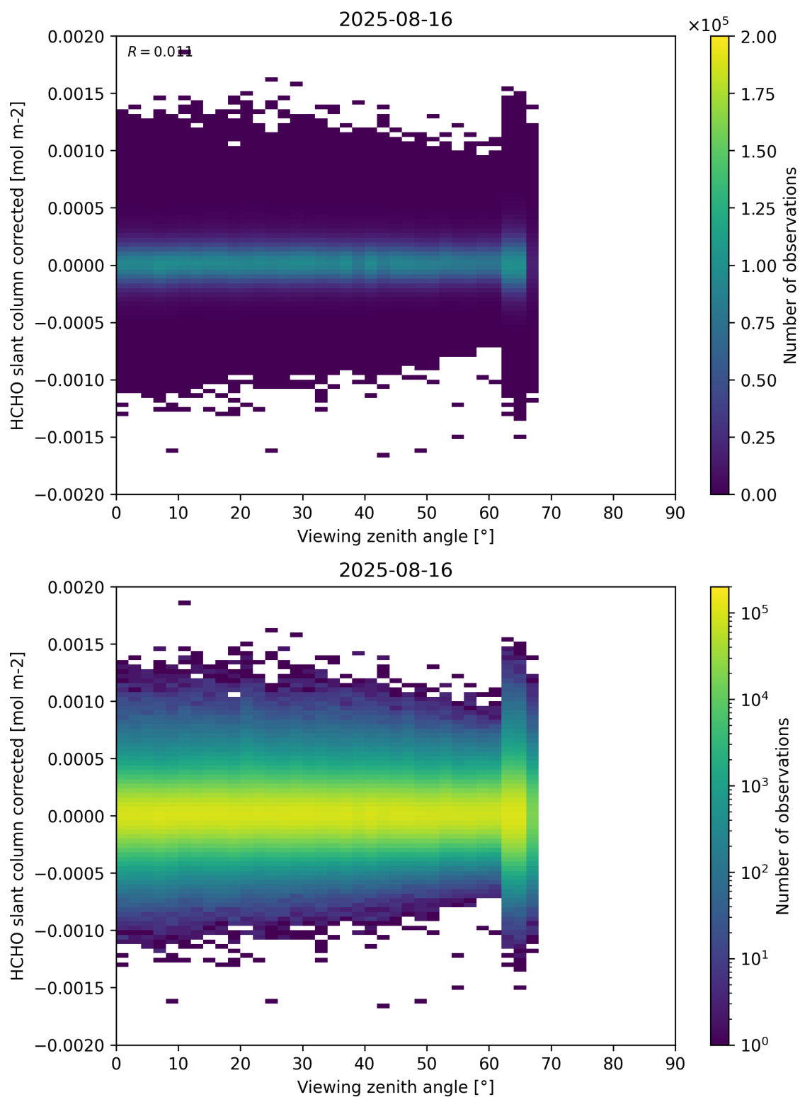
Figure 186: Scatter density plot of “Viewing zenith angle” against “HCHO slant column corrected” for 2025-08-15 to 2025-08-17.
