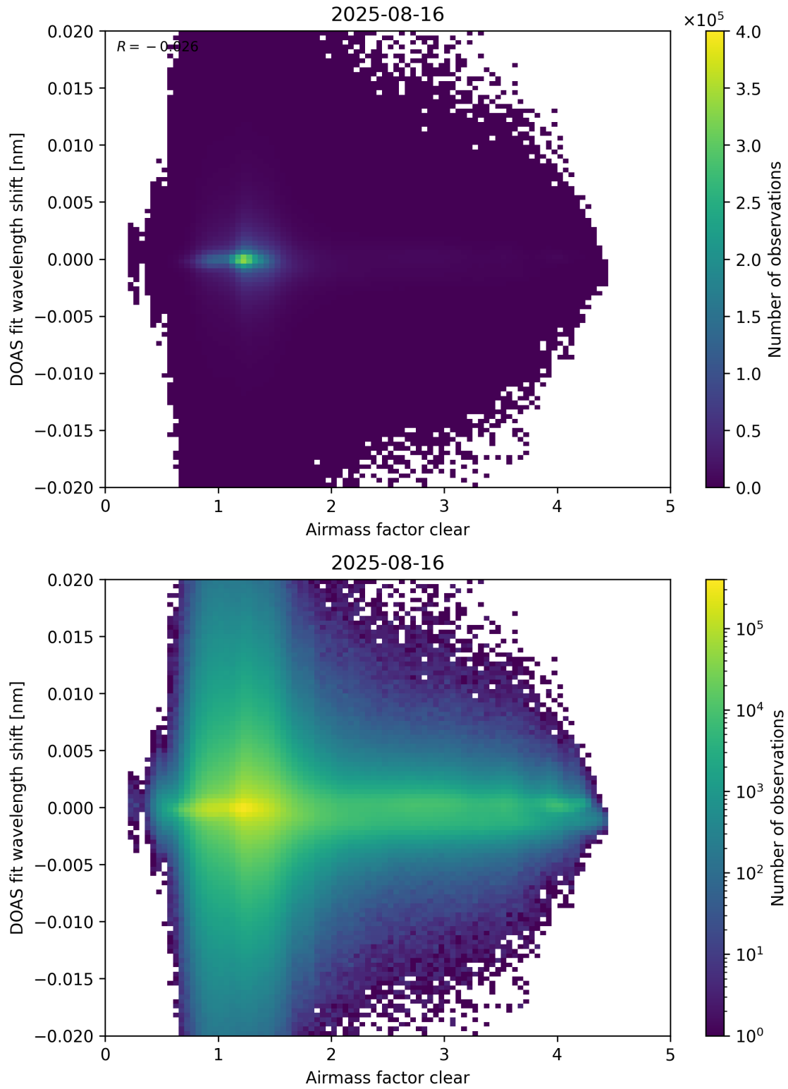
Figure 72: Scatter density plot of “Airmass factor clear” against “DOAS fit wavelength shift” for 2025-08-15 to 2025-08-17.
