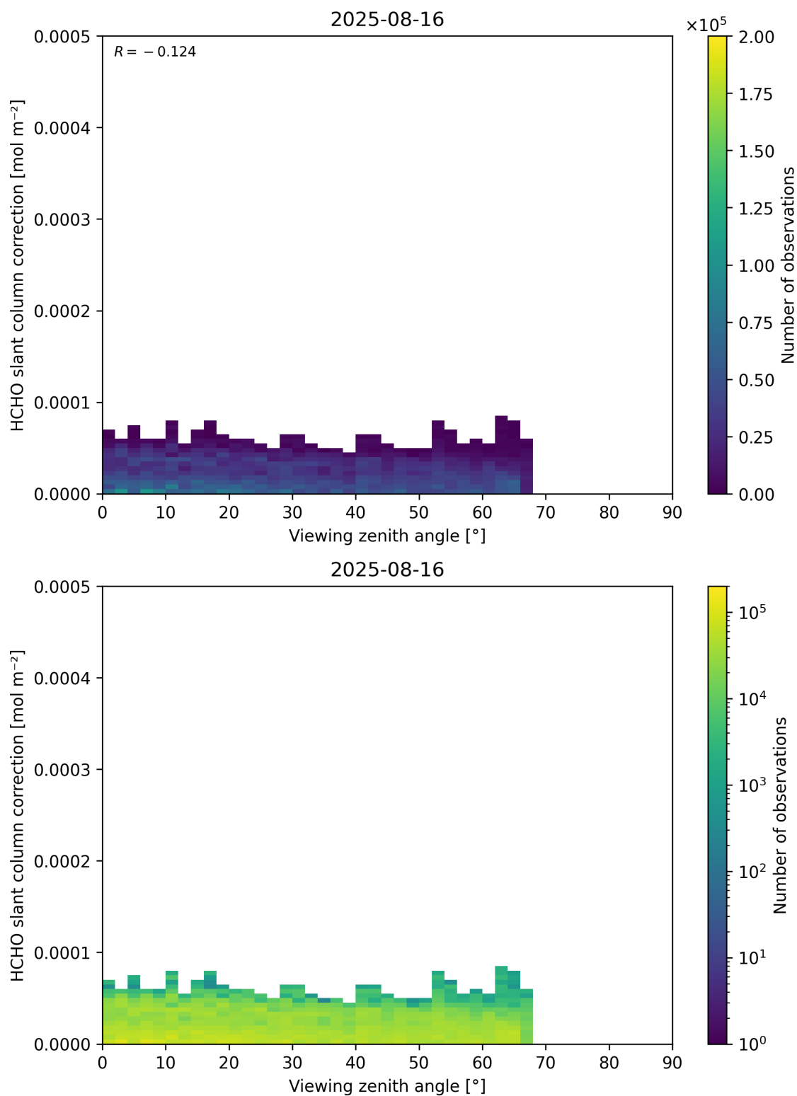
Figure 187: Scatter density plot of “Viewing zenith angle” against “HCHO slant column correction” for 2025-08-15 to 2025-08-17.
