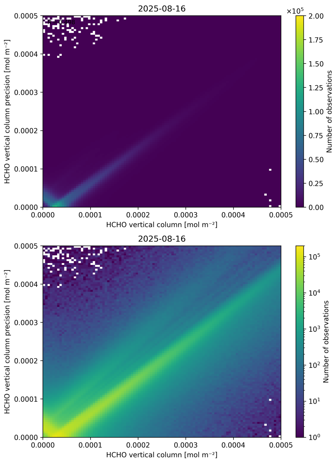
Figure 134: Scatter density plot of “HCHO vertical column” against “HCHO vertical column precision” for 2025-08-15 to 2025-08-17.
