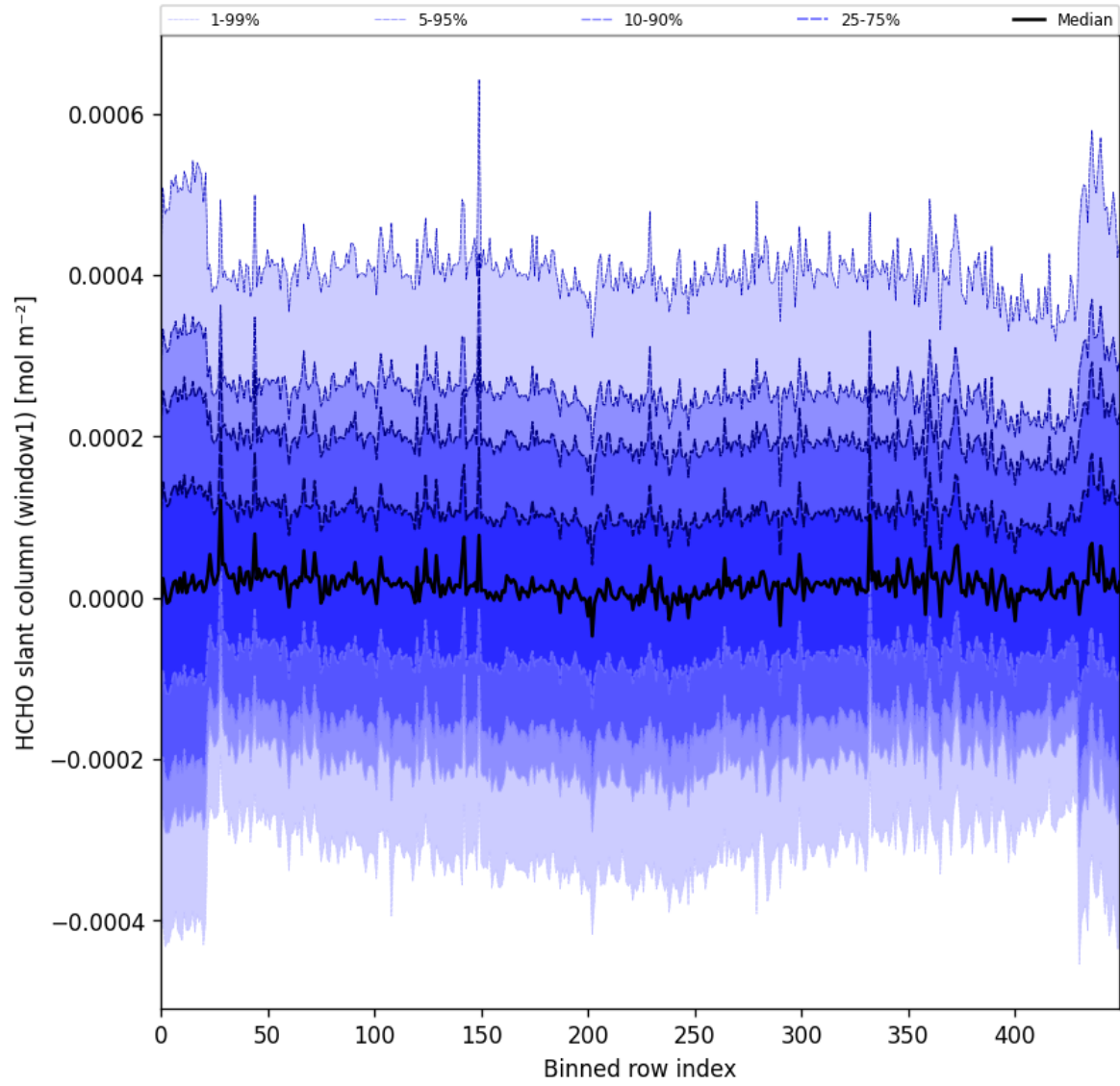
Figure 52: Along track statistics of “HCHO slant column (window1)” for 2025-08-15 to 2025-08-17
