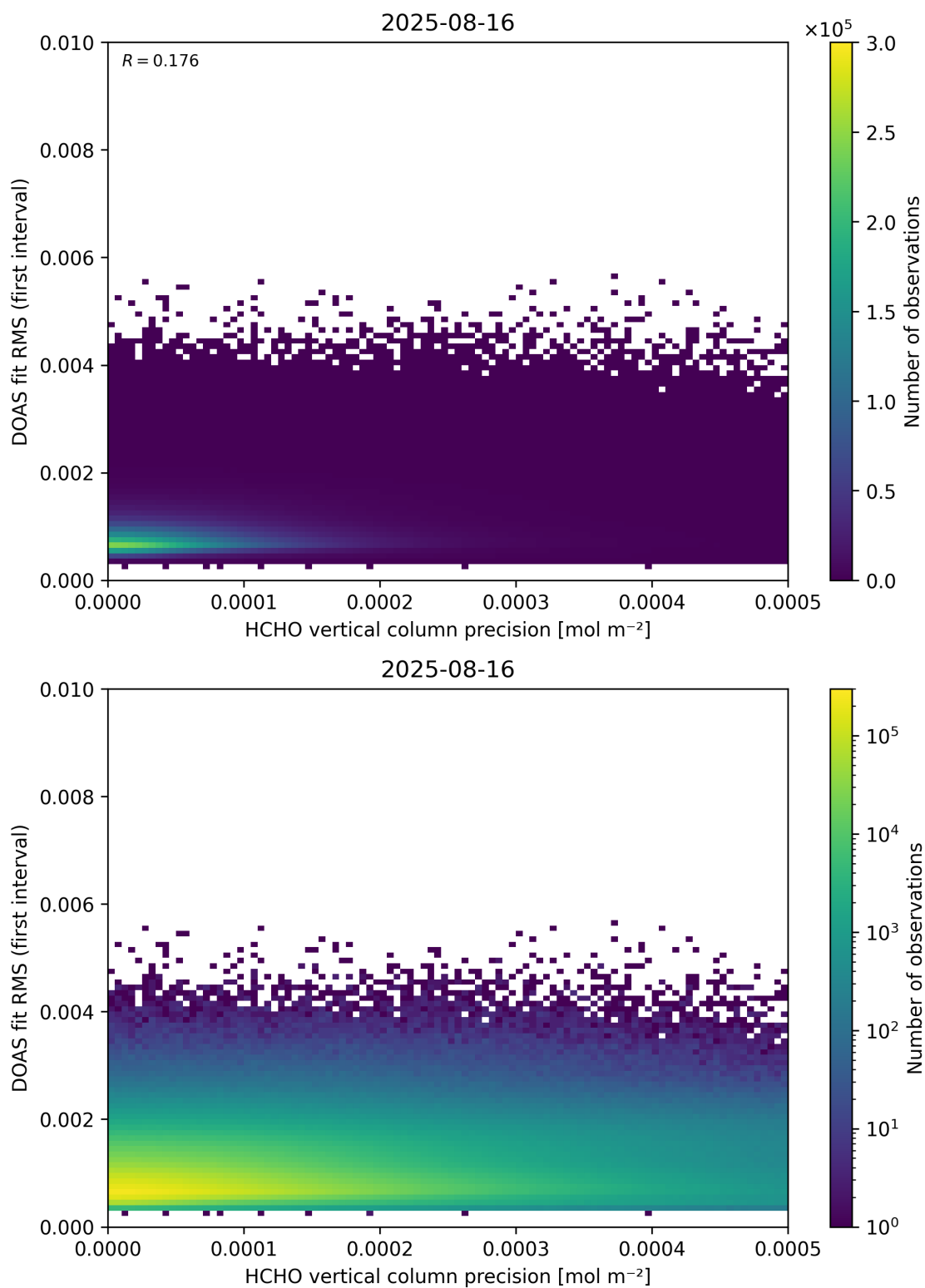
Figure 136: Scatter density plot of “HCHO vertical column precision” against “DOAS fit RMS (first interval)” for 2025-08-15 to 2025-08-17.
