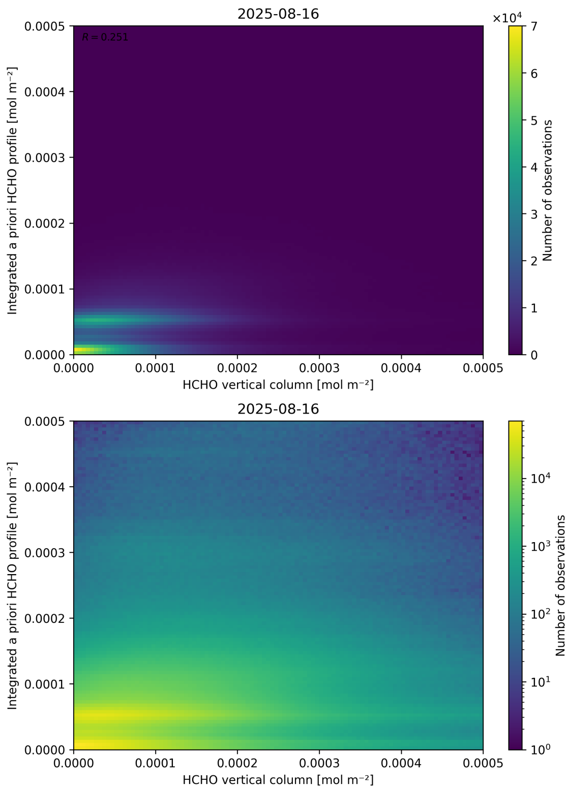
Figure 135: Scatter density plot of “HCHO vertical column” against “Integrated a priori HCHO profile” for 2025-08-15 to 2025-08-17.
