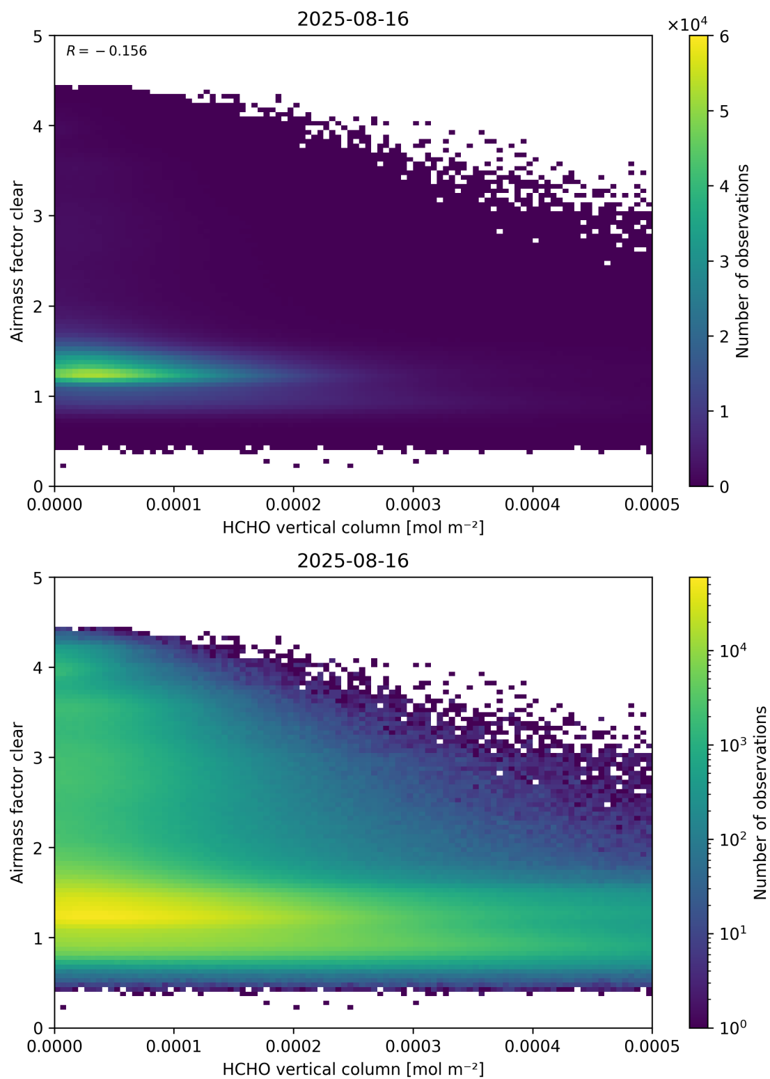
Figure 126: Scatter density plot of “HCHO vertical column” against “Airmass factor clear” for 2025-08-15 to 2025-08-17.
