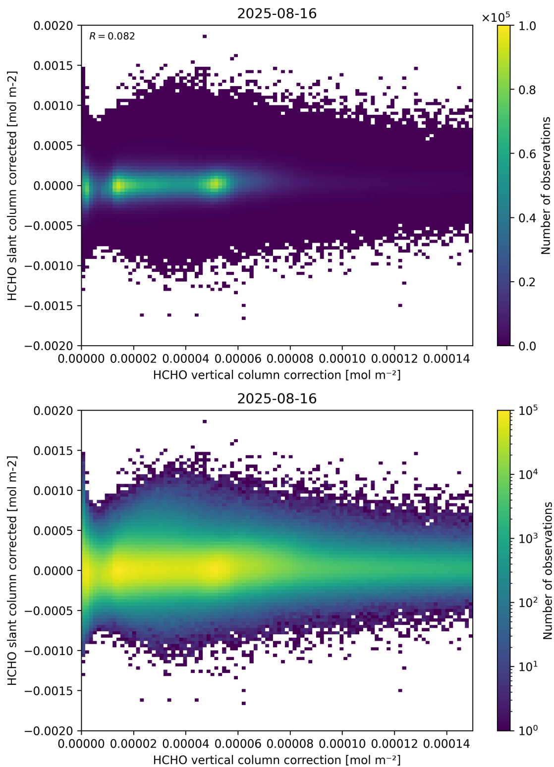
Figure 116: Scatter density plot of “HCHO vertical column correction” against “HCHO slant column corrected” for 2025-08-15 to 2025-08-17.
