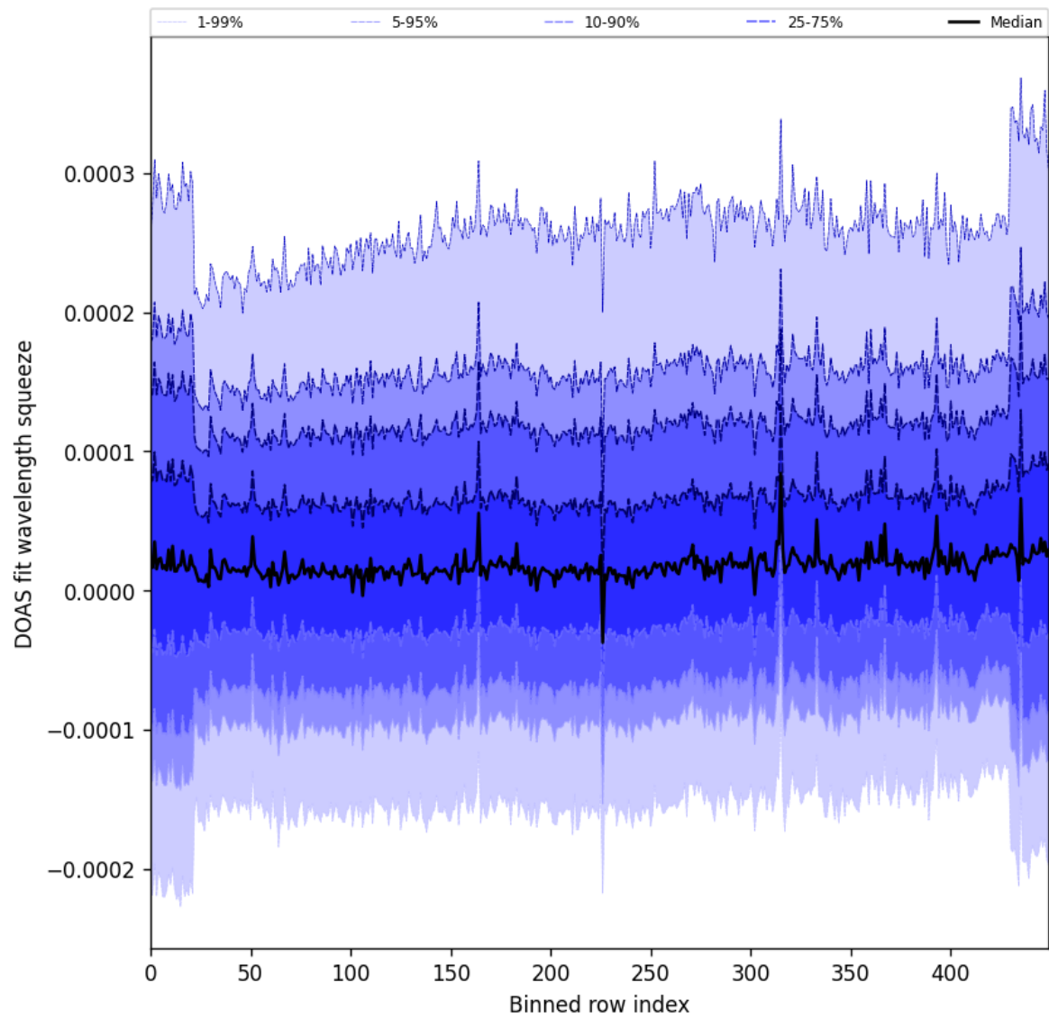
Figure 59: Along track statistics of “DOAS fit wavelength squeeze” for 2025-08-15 to 2025-08-17
