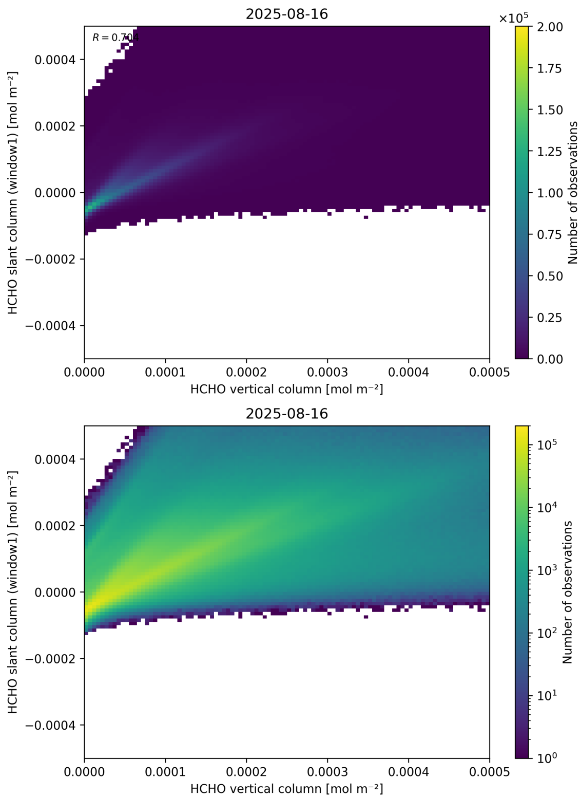
Figure 129: Scatter density plot of “HCHO vertical column” against “HCHO slant column (window1)” for 2025-08-15 to 2025-08-17.
