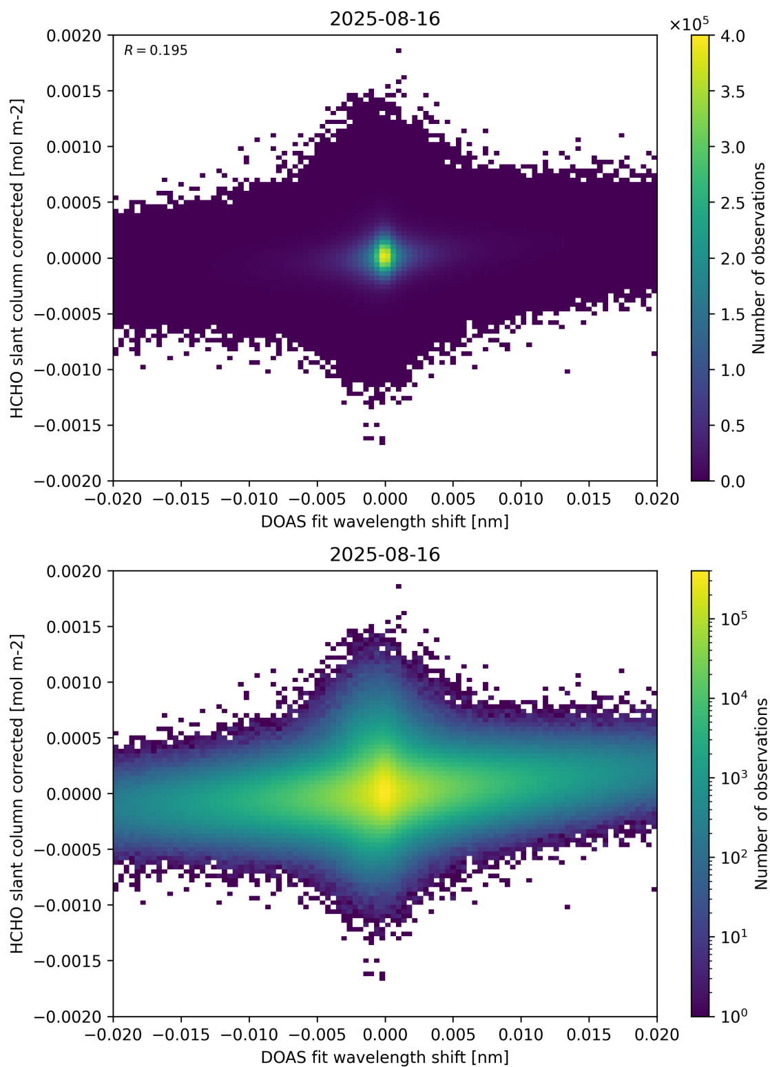
Figure 66: Scatter density plot of “DOAS fit wavelength shift” against “HCHO slant column corrected” for 2025-08-15 to 2025-08-17.
