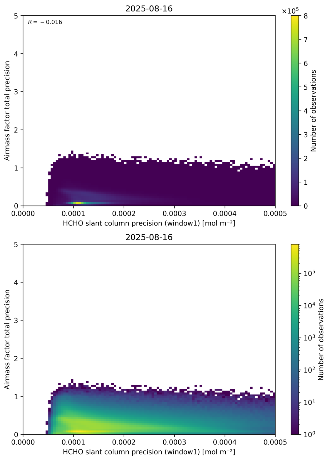
Figure 95: Scatter density plot of “HCHO slant column precision (window1)” against “Airmass factor total precision” for 2025-08-15 to 2025-08-17.
