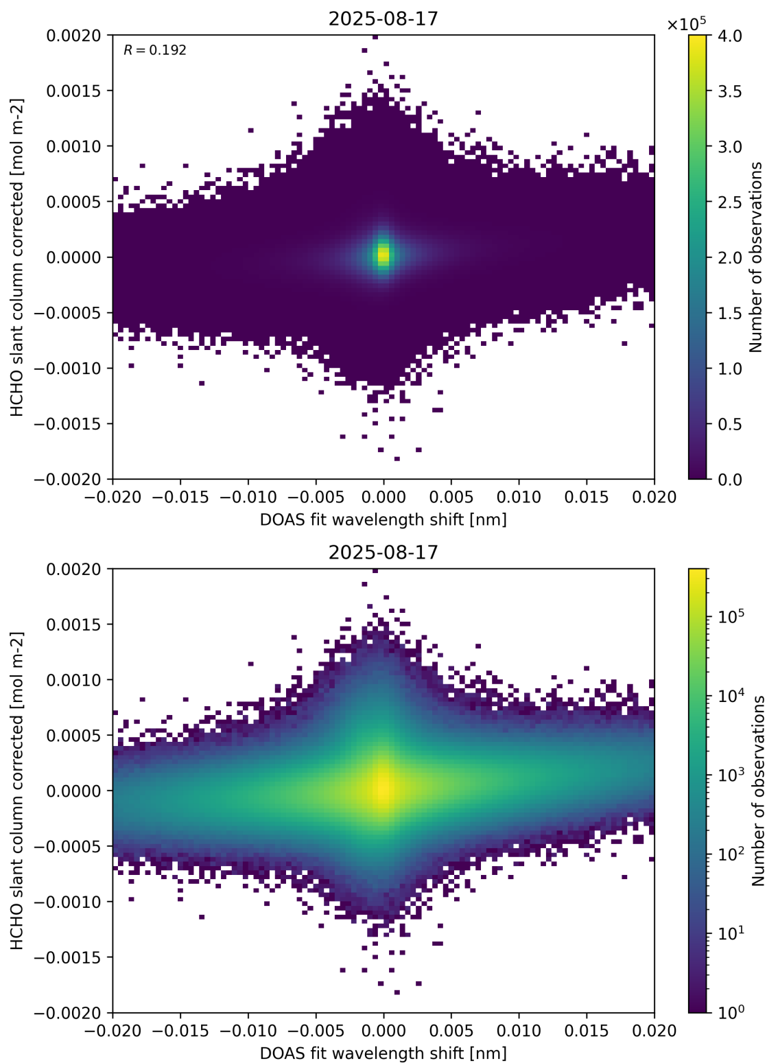
Figure 66: Scatter density plot of “DOAS fit wavelength shift” against “HCHO slant column corrected” for 2025-08-16 to 2025-08-18.
