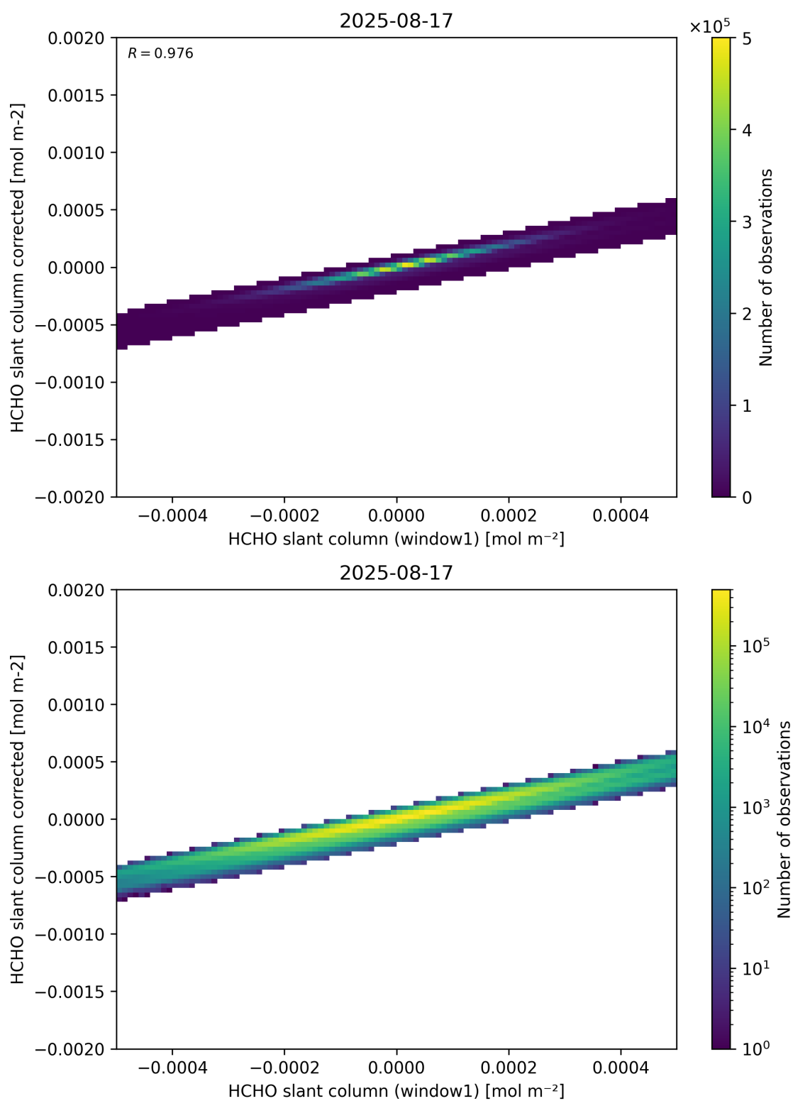
Figure 82: Scatter density plot of “HCHO slant column (window1)” against “HCHO slant column corrected” for 2025-08-16 to 2025-08-18.
