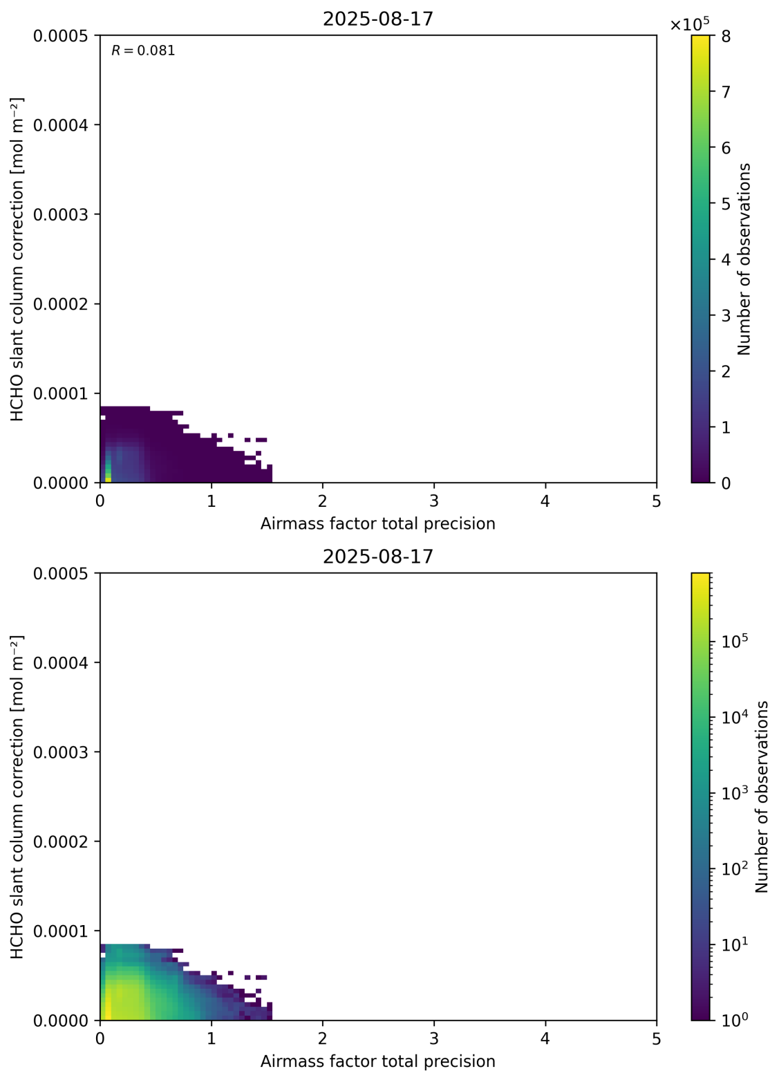
Figure 110: Scatter density plot of “Airmass factor total precision” against “HCHO slant column correction” for 2025-08-16 to 2025-08-18.
