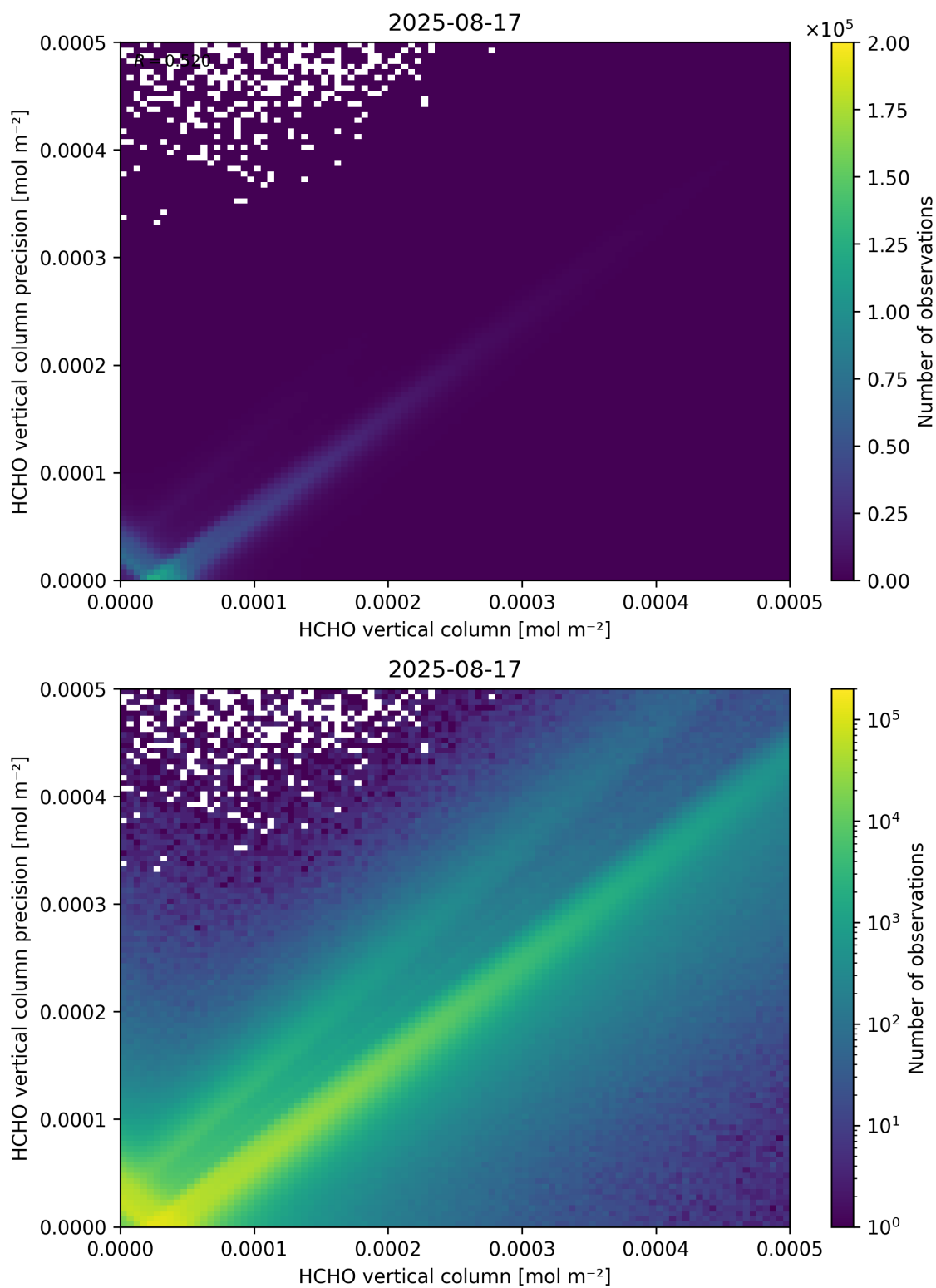
Figure 134: Scatter density plot of “HCHO vertical column” against “HCHO vertical column precision” for 2025-08-16 to 2025-08-18.
