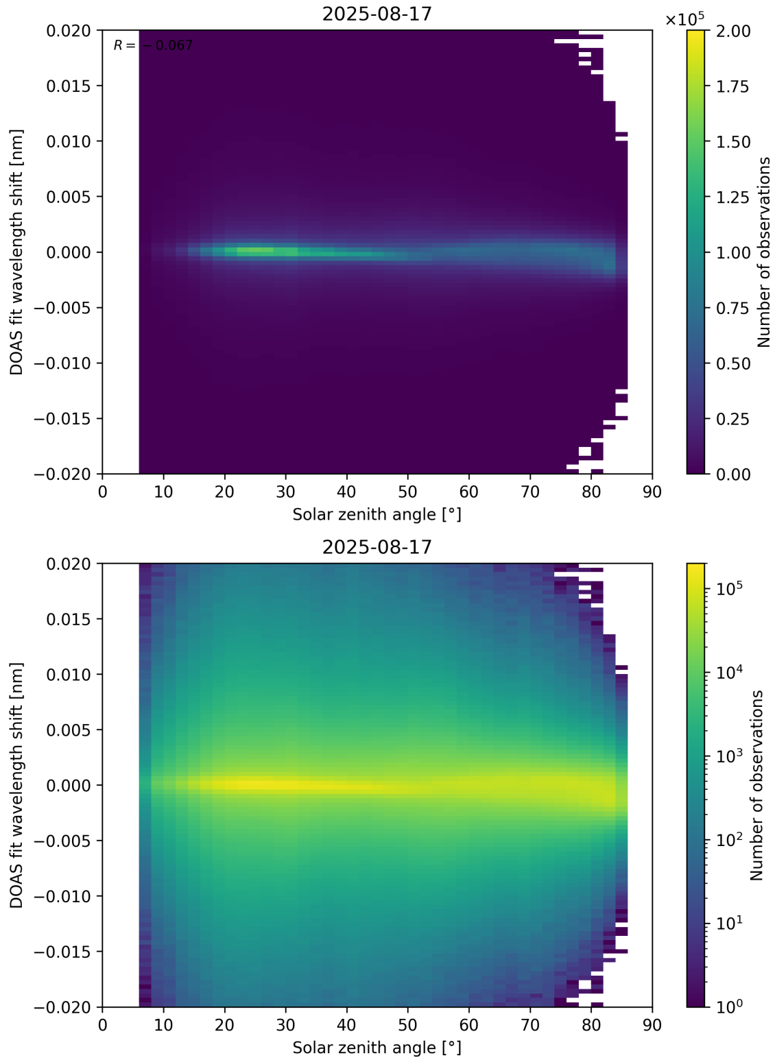
Figure 168: Scatter density plot of “Solar zenith angle” against “DOAS fit wavelength shift” for 2025-08-16 to 2025-08-18.
