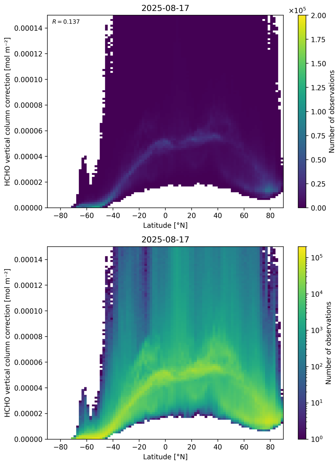
Figure 164: Scatter density plot of “Latitude” against “HCHO vertical column correction” for 2025-08-16 to 2025-08-18.
