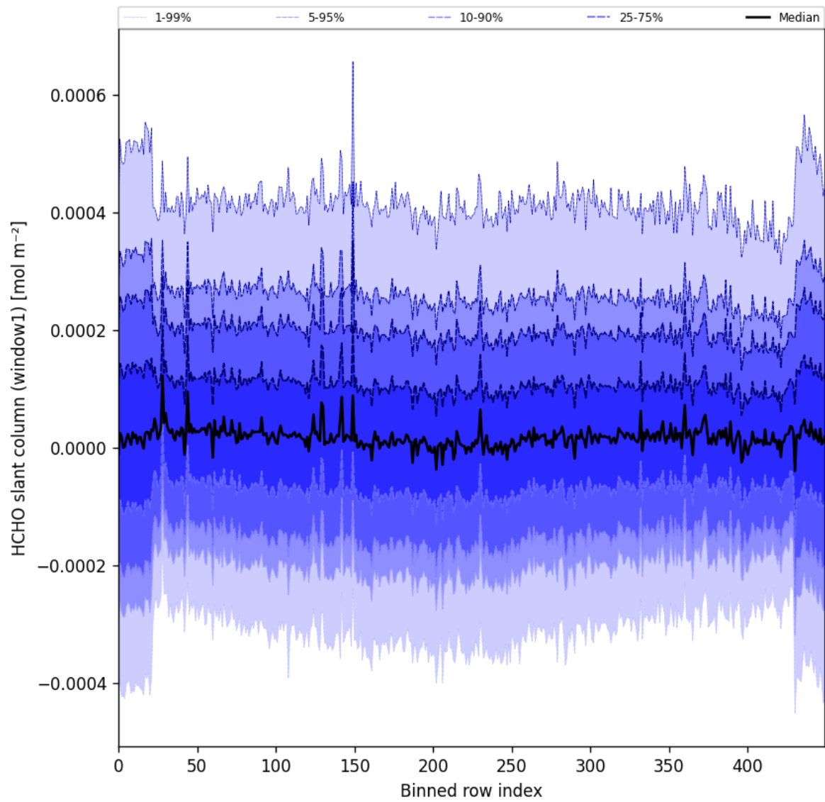
Figure 52: Along track statistics of “HCHO slant column (window1)” for 2025-08-16 to 2025-08-18
