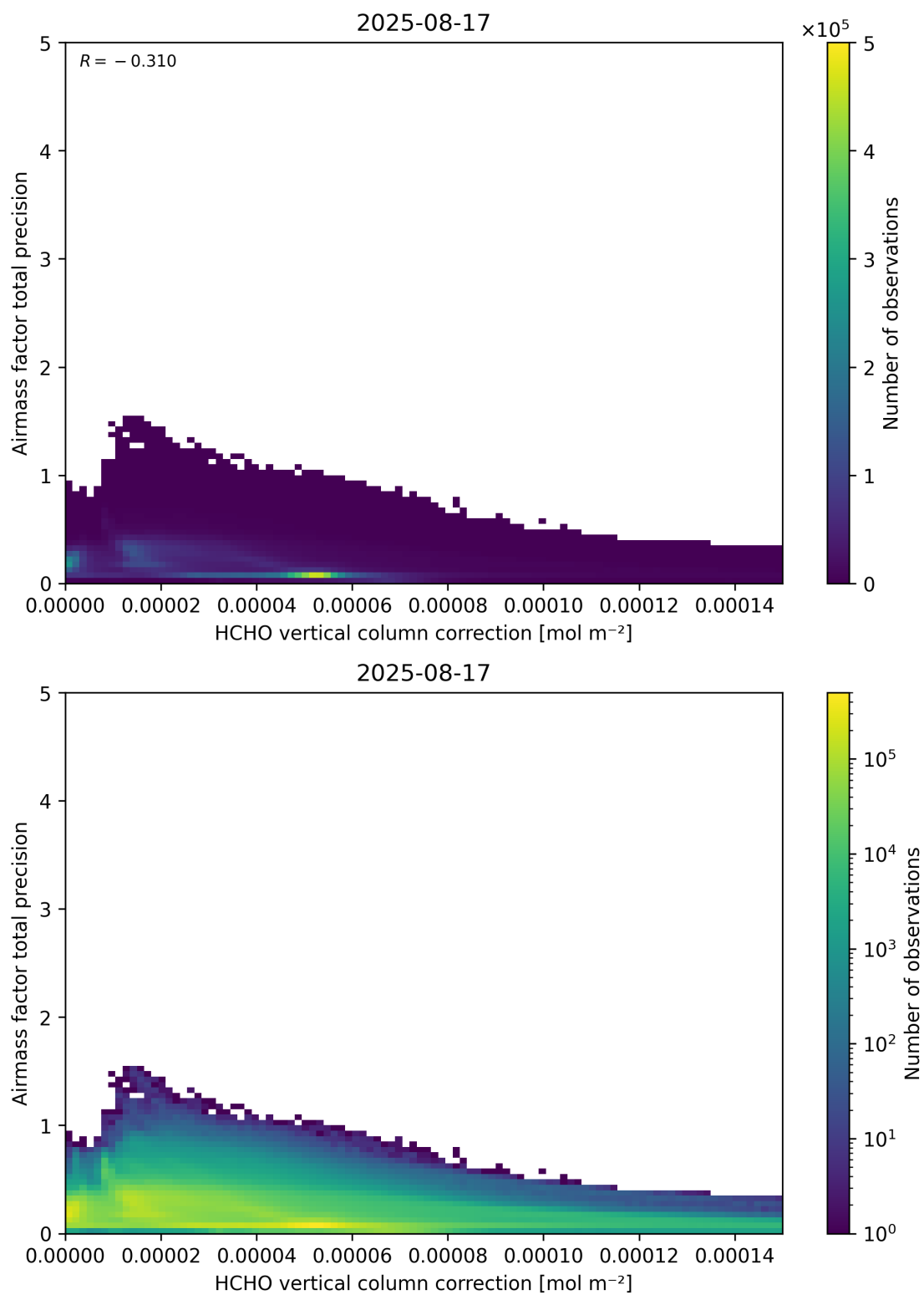
Figure 121: Scatter density plot of “HCHO vertical column correction” against “Airmass factor total precision” for 2025-08-16 to 2025-08-18.
