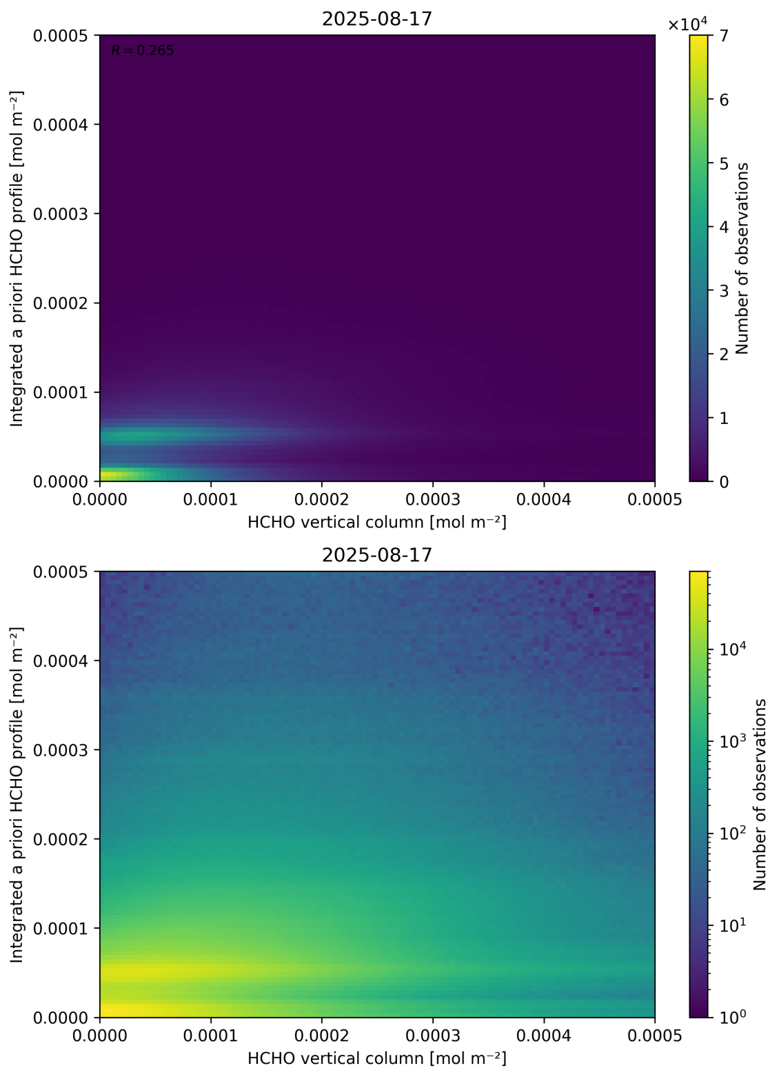
Figure 135: Scatter density plot of “HCHO vertical column” against “Integrated a priori HCHO profile” for 2025-08-16 to 2025-08-18.
