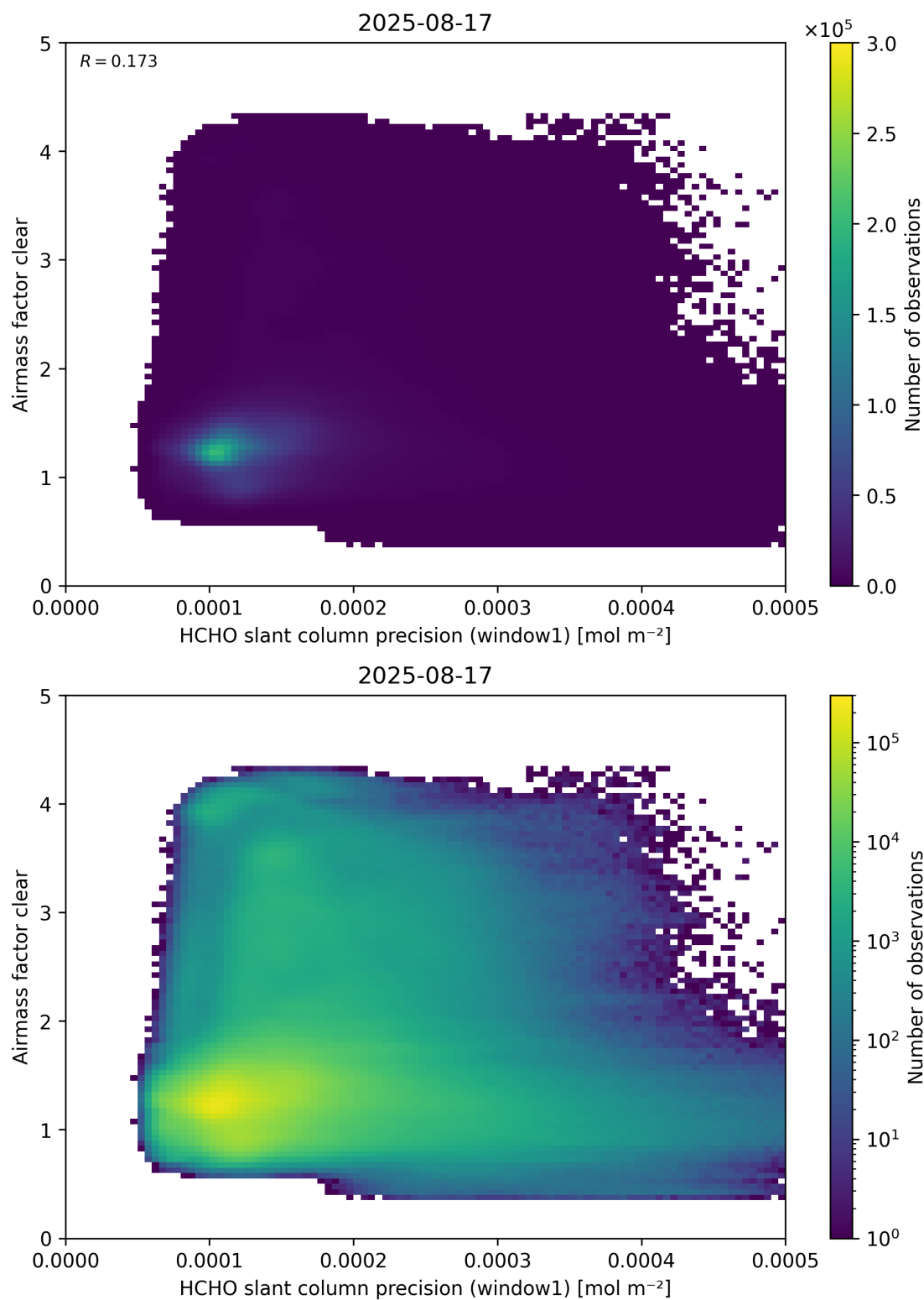
Figure 91: Scatter density plot of “HCHO slant column precision (window1)” against “Airmass factor clear” for 2025-08-16 to 2025-08-18.
