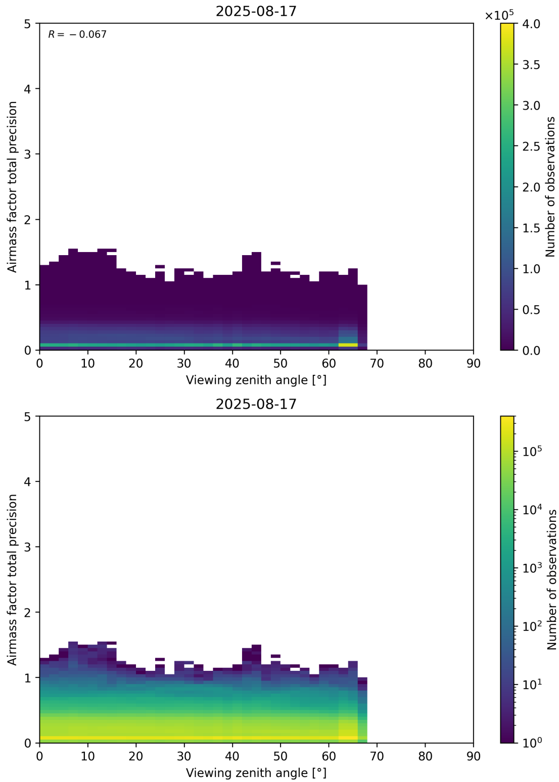
Figure 191: Scatter density plot of “Viewing zenith angle” against “Airmass factor total precision” for 2025-08-16 to 2025-08-18.
