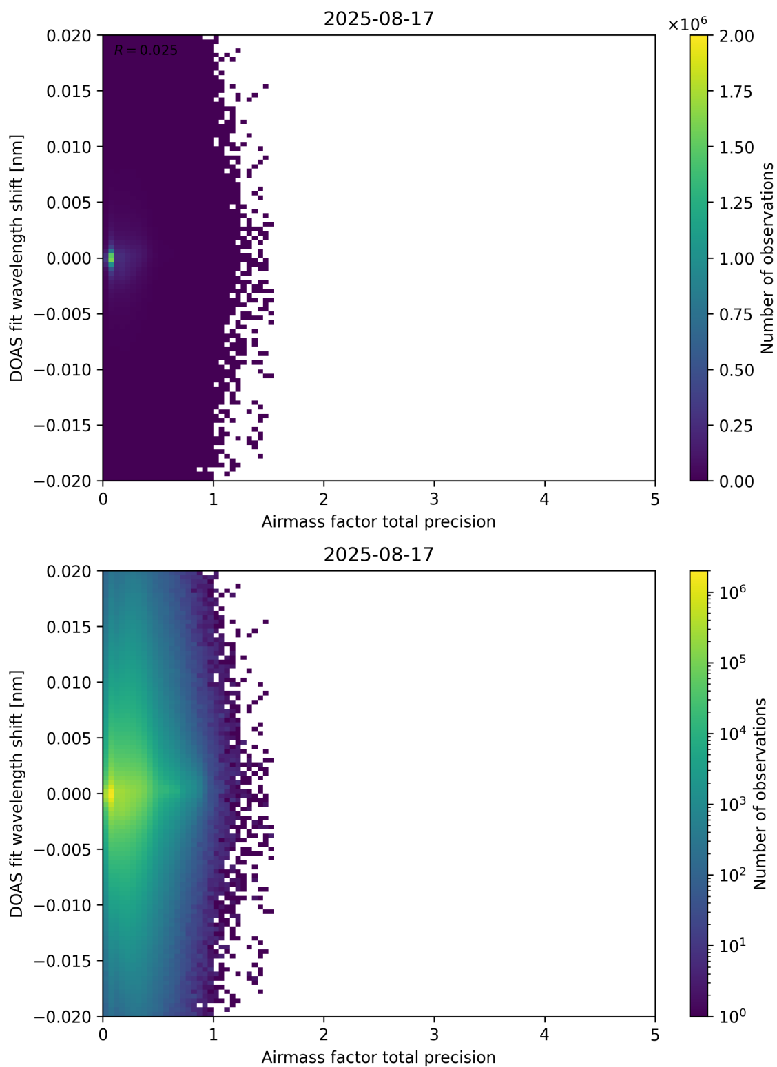
Figure 106: Scatter density plot of “Airmass factor total precision” against “DOAS fit wavelength shift” for 2025-08-16 to 2025-08-18.
