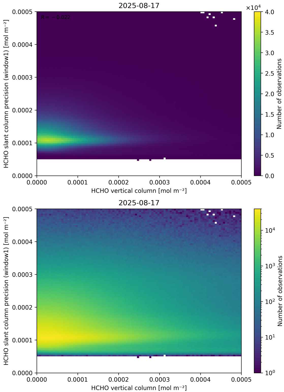
Figure 130: Scatter density plot of “HCHO vertical column” against “HCHO slant column precision (window1)” for 2025-08-16 to 2025-08-18.
