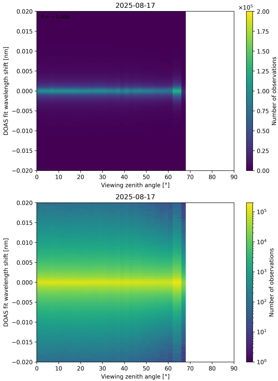
Figure 183: Scatter density plot of “Viewing zenith angle” against “DOAS fit wavelength shift” for 2025-08-16 to 2025-08-18.
