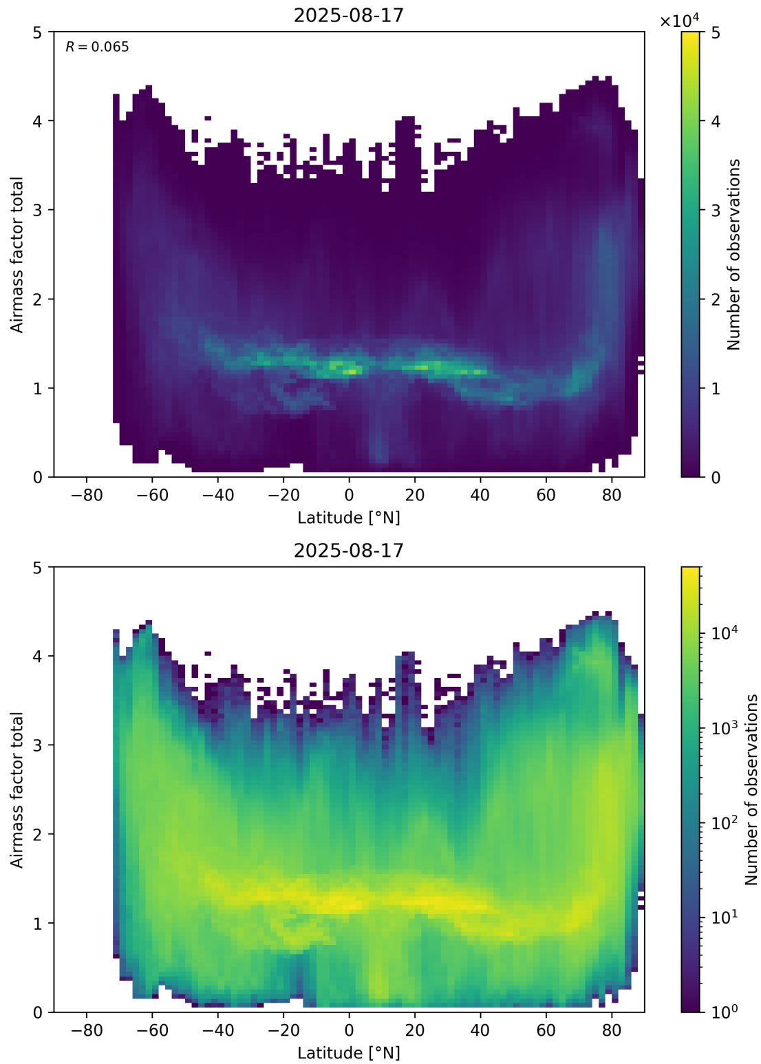
Figure 161: Scatter density plot of “Latitude” against “Airmass factor total” for 2025-08-16 to 2025-08-18.
