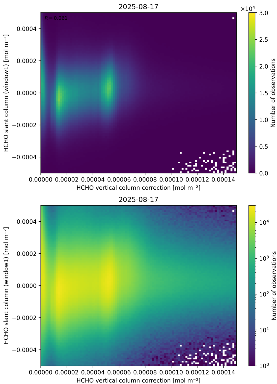
Figure 118: Scatter density plot of “HCHO vertical column correction” against “HCHO slant column (window1)” for 2025-08-16 to 2025-08-18.
