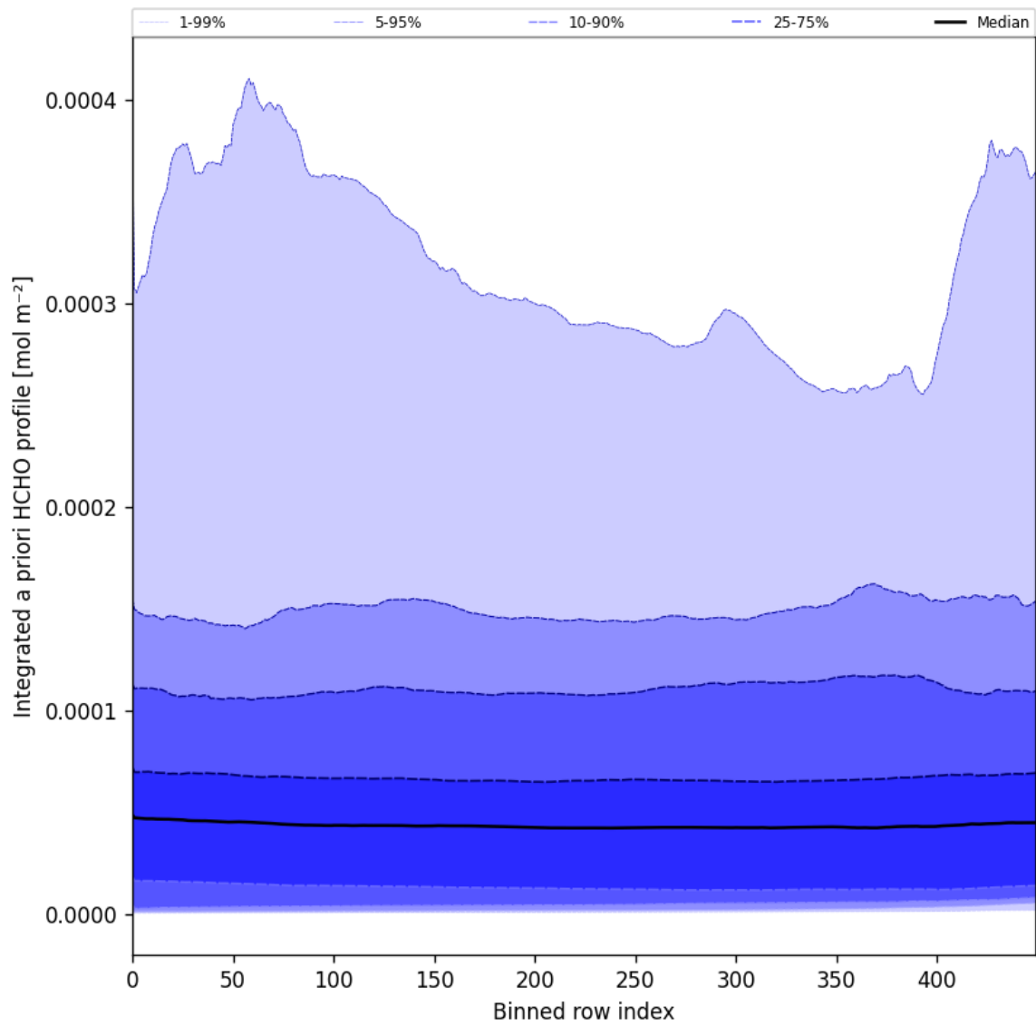
Figure 57: Along track statistics of “Integrated a priori HCHO profile” for 2025-08-16 to 2025-08-18
