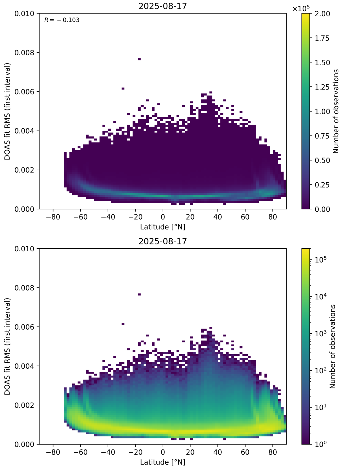
Figure 153: Scatter density plot of “Latitude” against “DOAS fit RMS (first interval)” for 2025-08-16 to 2025-08-18.
