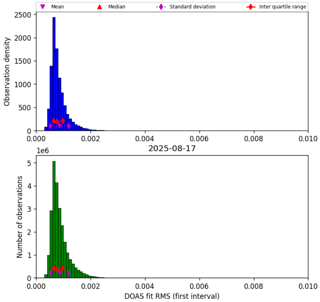
Figure 46: Histogram of “DOAS fit RMS (first interval)” for 2025-08-16 to 2025-08-18
