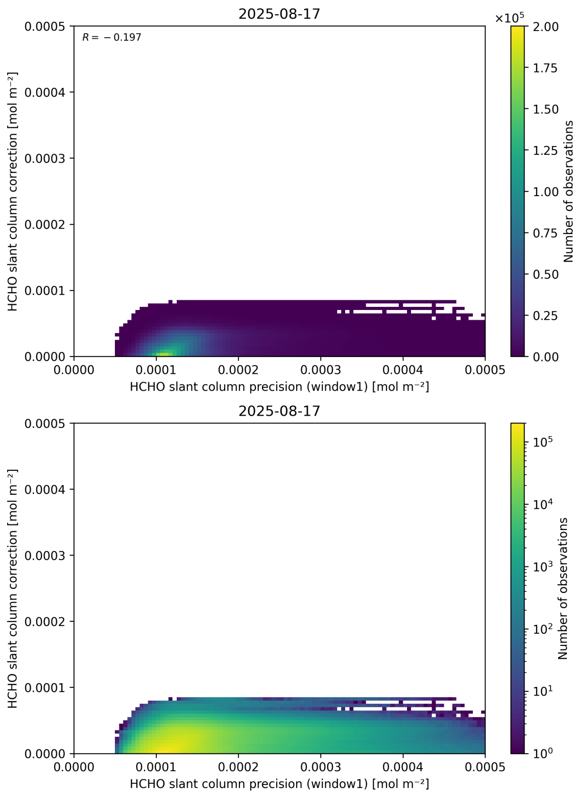
Figure 93: Scatter density plot of “HCHO slant column precision (window1)” against “HCHO slant column correction” for 2025-08-16 to 2025-08-18.
