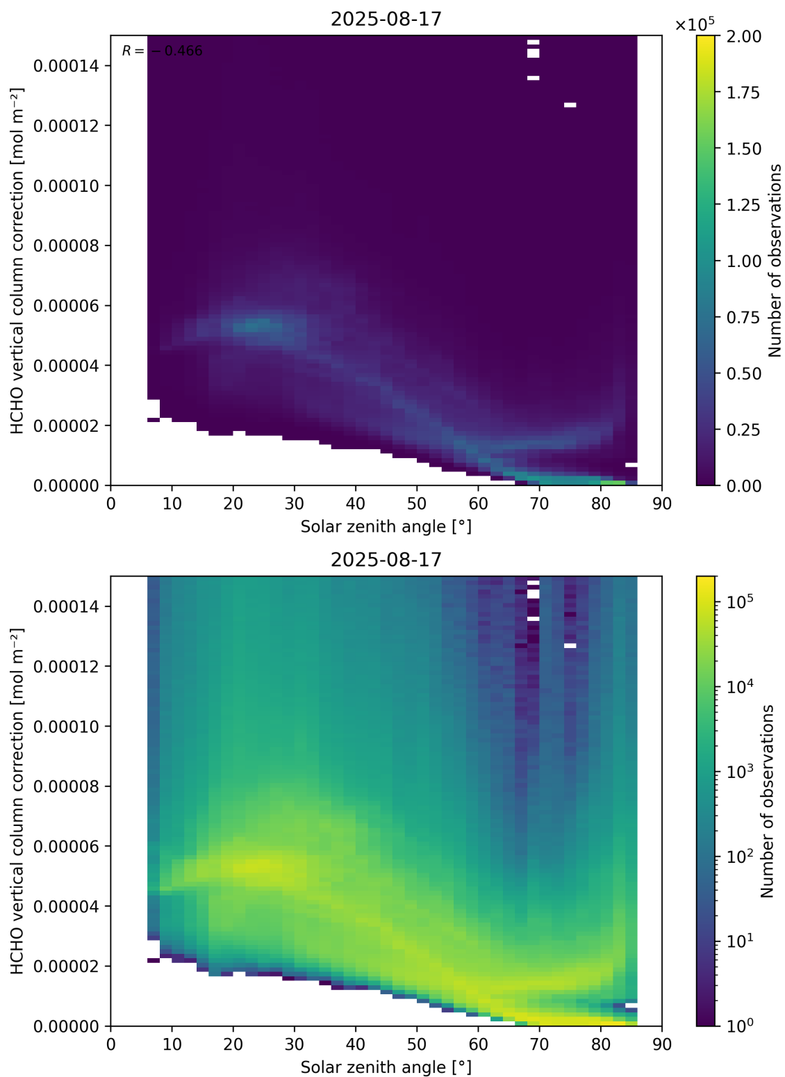
Figure 178: Scatter density plot of “Solar zenith angle” against “HCHO vertical column correction” for 2025-08-16 to 2025-08-18.
