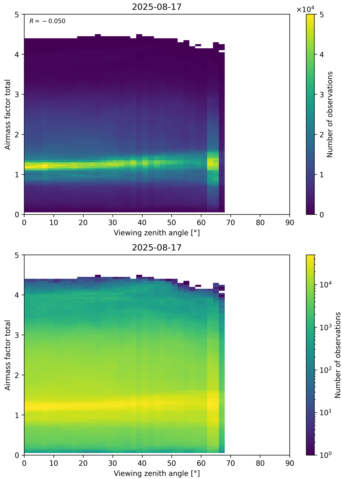
Figure 190: Scatter density plot of “Viewing zenith angle” against “Airmass factor total” for 2025-08-16 to 2025-08-18.
