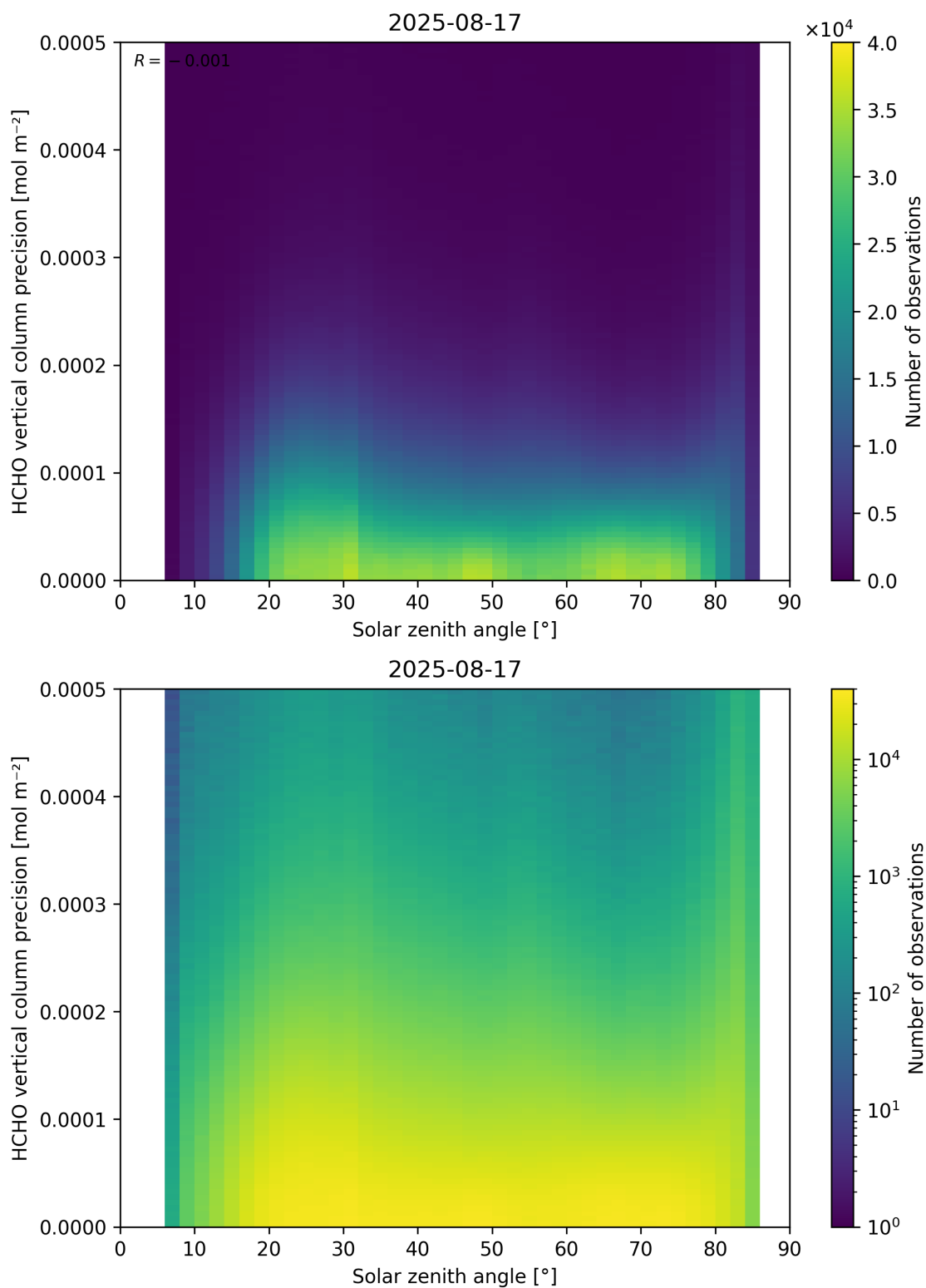
Figure 179: Scatter density plot of “Solar zenith angle” against “HCHO vertical column precision” for 2025-08-16 to 2025-08-18.
