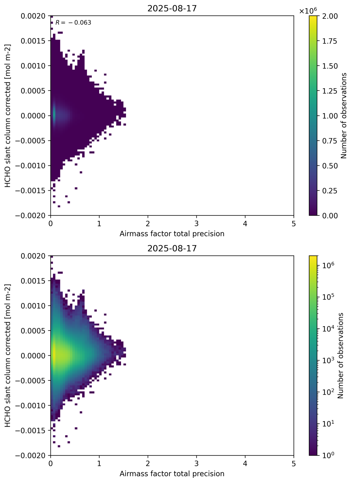
Figure 109: Scatter density plot of “Airmass factor total precision” against “HCHO slant column corrected” for 2025-08-16 to 2025-08-18.
