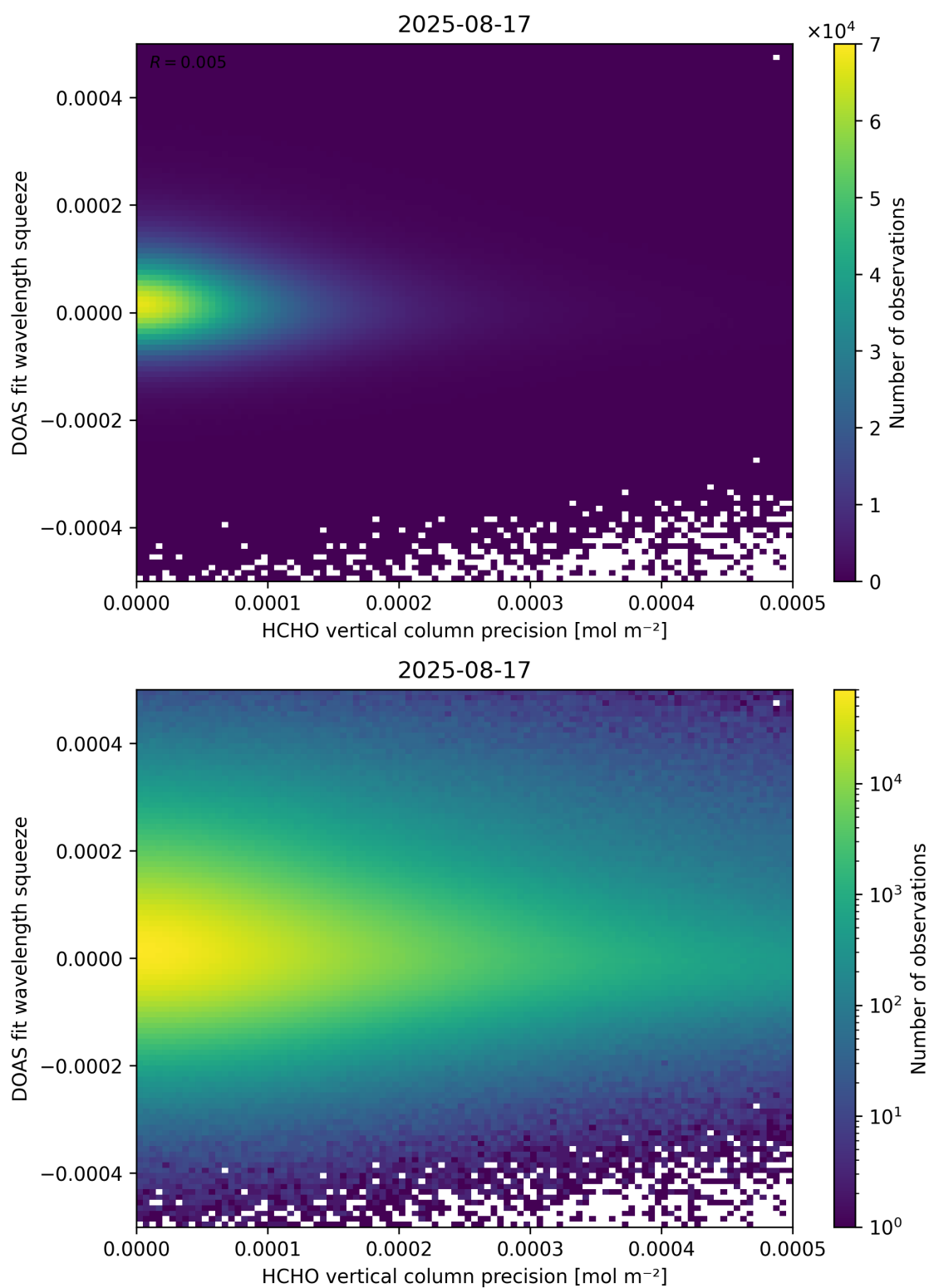
Figure 138: Scatter density plot of “HCHO vertical column precision” against “DOAS fit wavelength squeeze” for 2025-08-16 to 2025-08-18.
