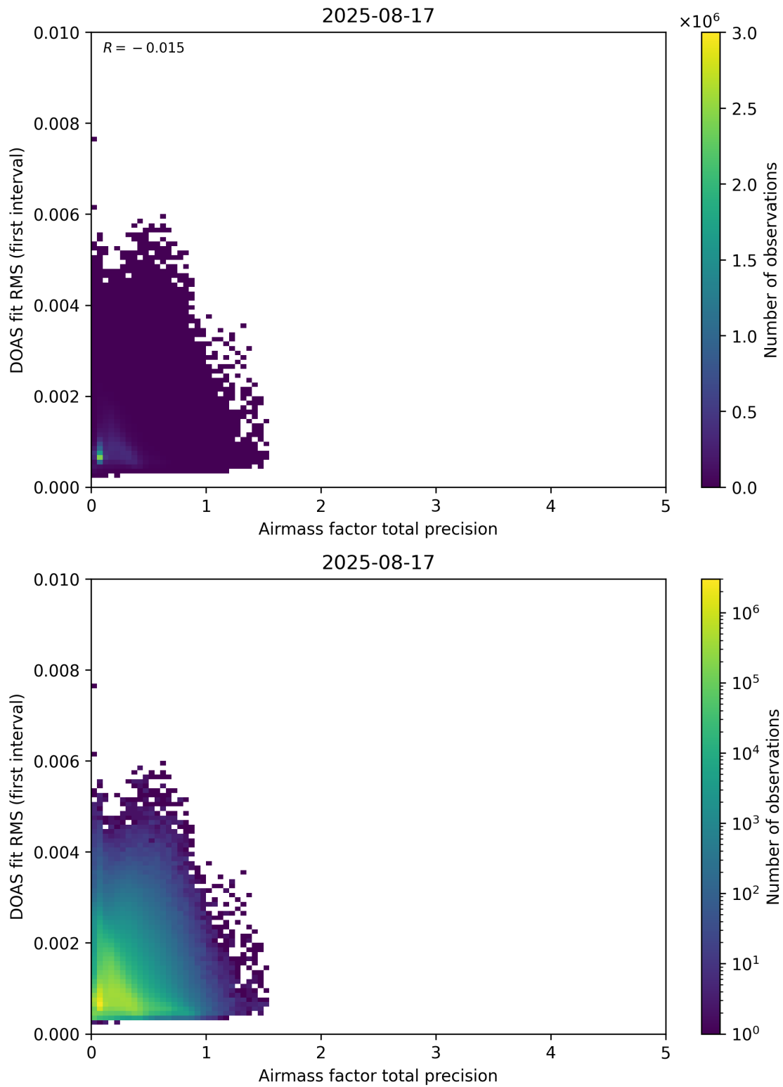
Figure 105: Scatter density plot of “Airmass factor total precision” against “DOAS fit RMS (first interval)” for 2025-08-16 to 2025-08-18.
