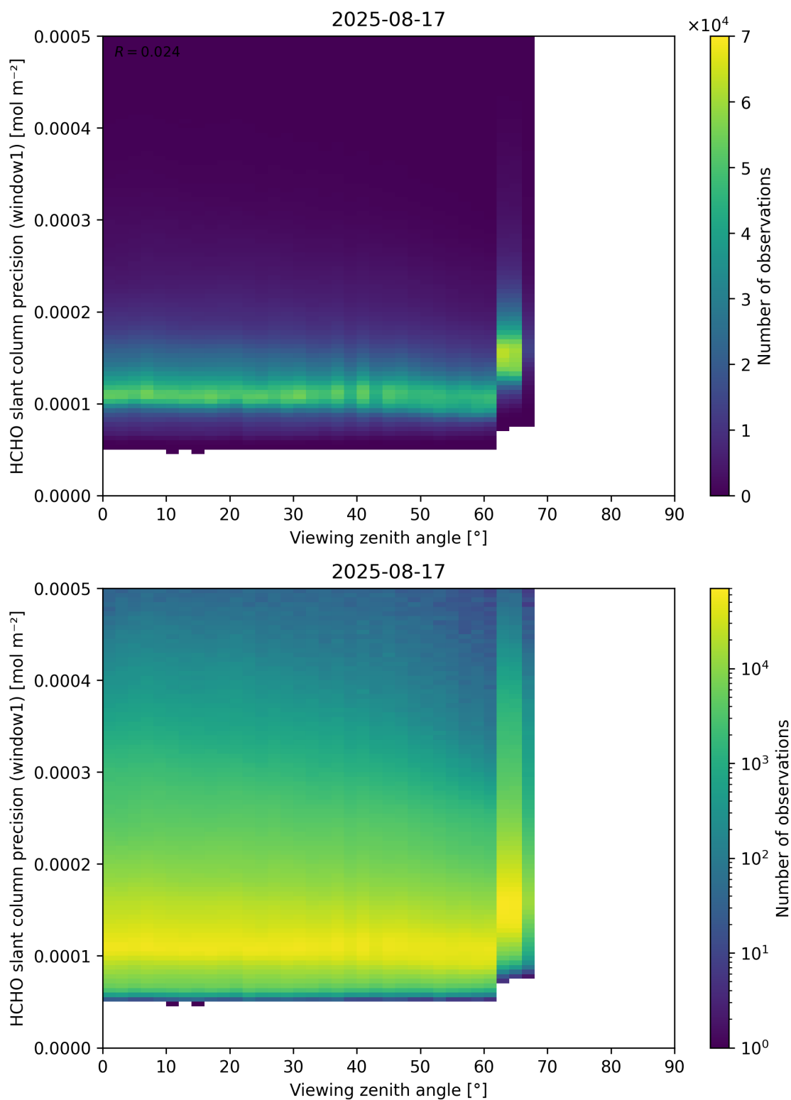
Figure 189: Scatter density plot of “Viewing zenith angle” against “HCHO slant column precision (window1)” for 2025-08-16 to 2025-08-18.
