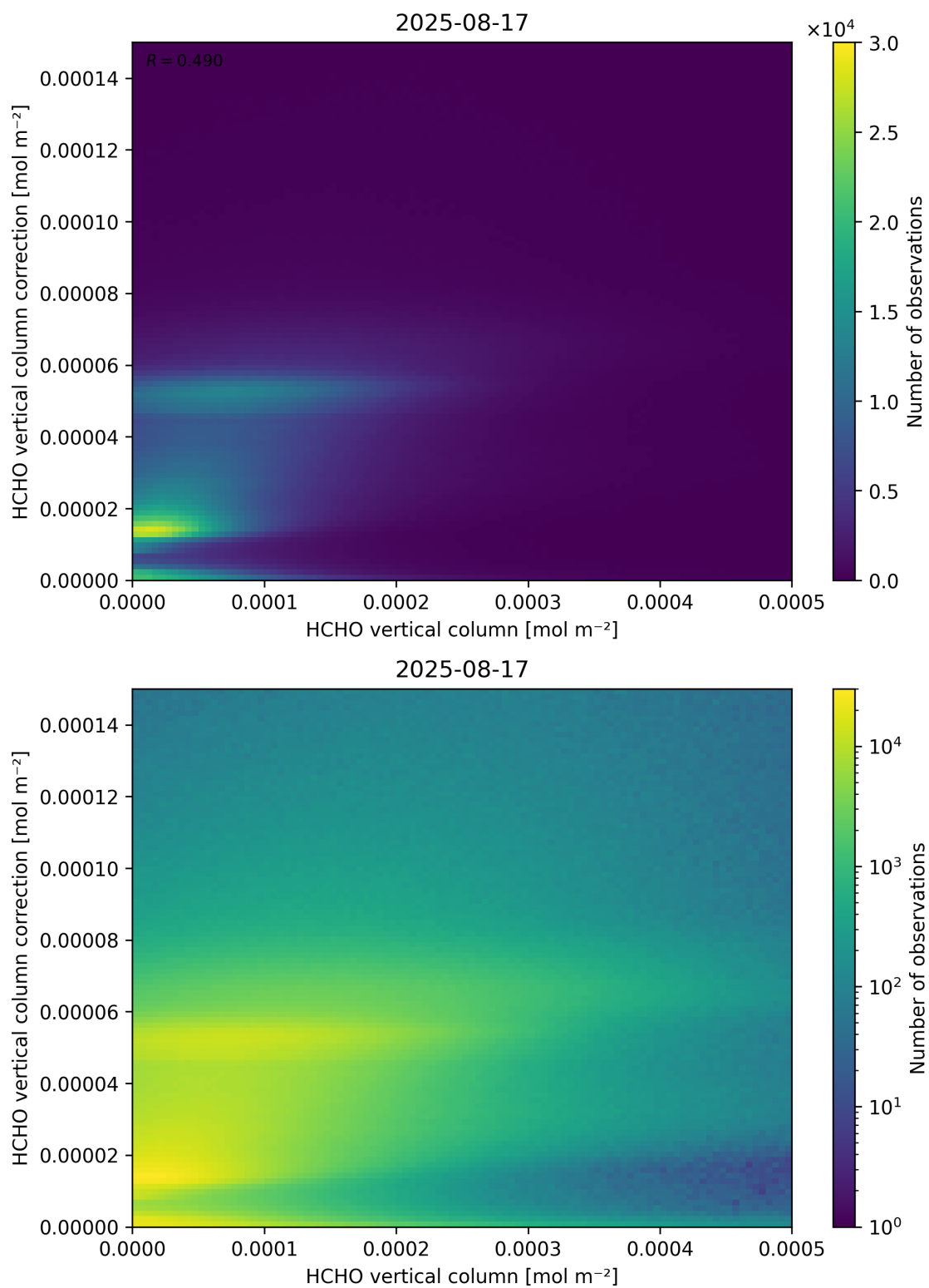
Figure 133: Scatter density plot of “HCHO vertical column” against “HCHO vertical column correction” for 2025-08-16 to 2025-08-18.
