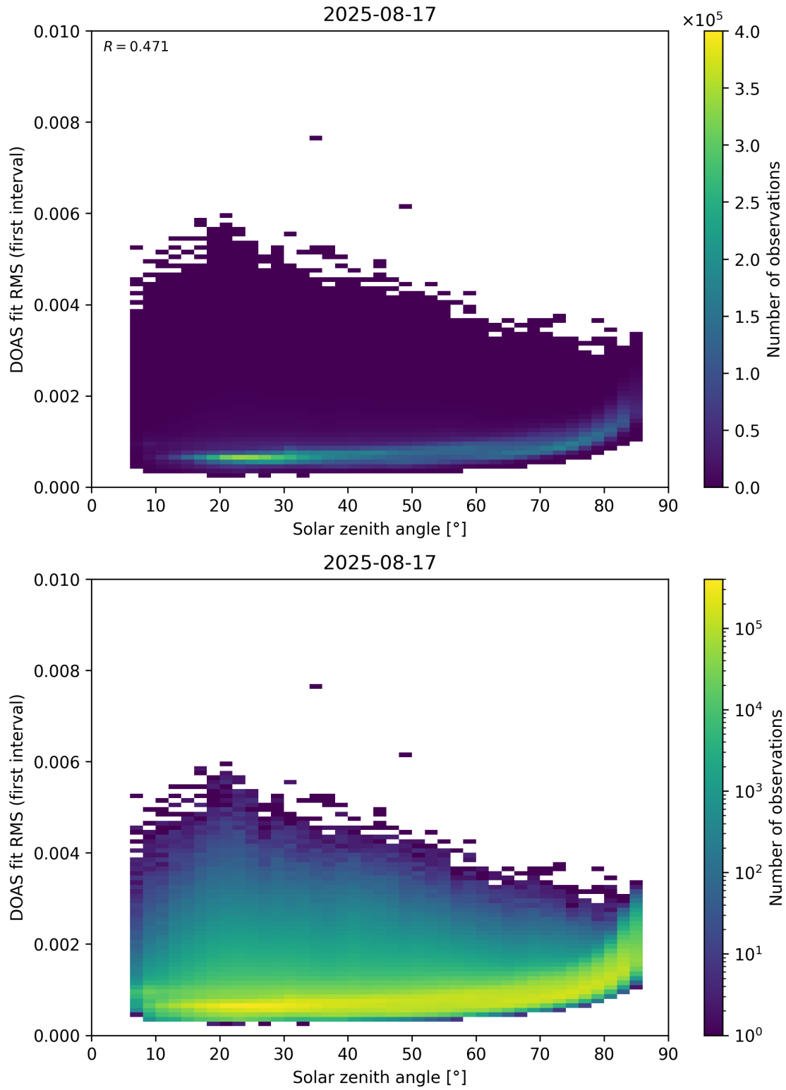
Figure 167: Scatter density plot of “Solar zenith angle” against “DOAS fit RMS (first interval)” for 2025-08-16 to 2025-08-18.
