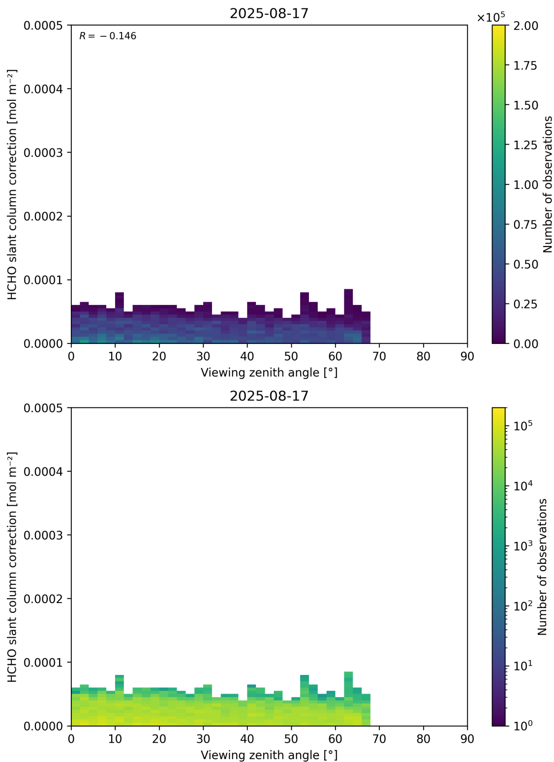
Figure 187: Scatter density plot of “Viewing zenith angle” against “HCHO slant column correction” for 2025-08-16 to 2025-08-18.
