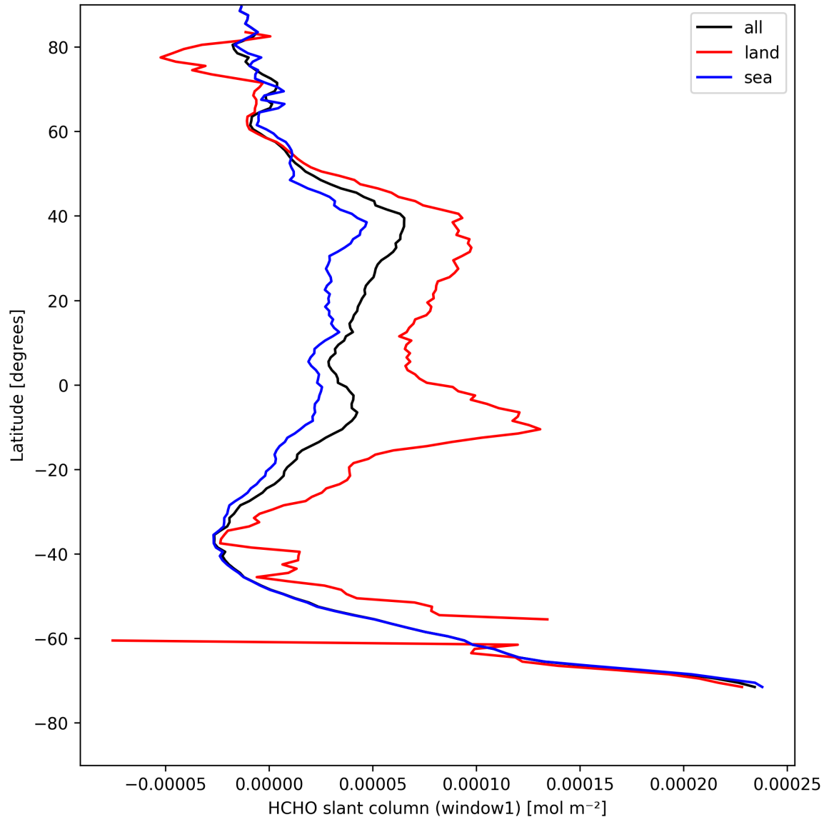
Figure 24: Zonal average of “HCHO slant column (window1)” for 2025-08-16 to 2025-08-18.
