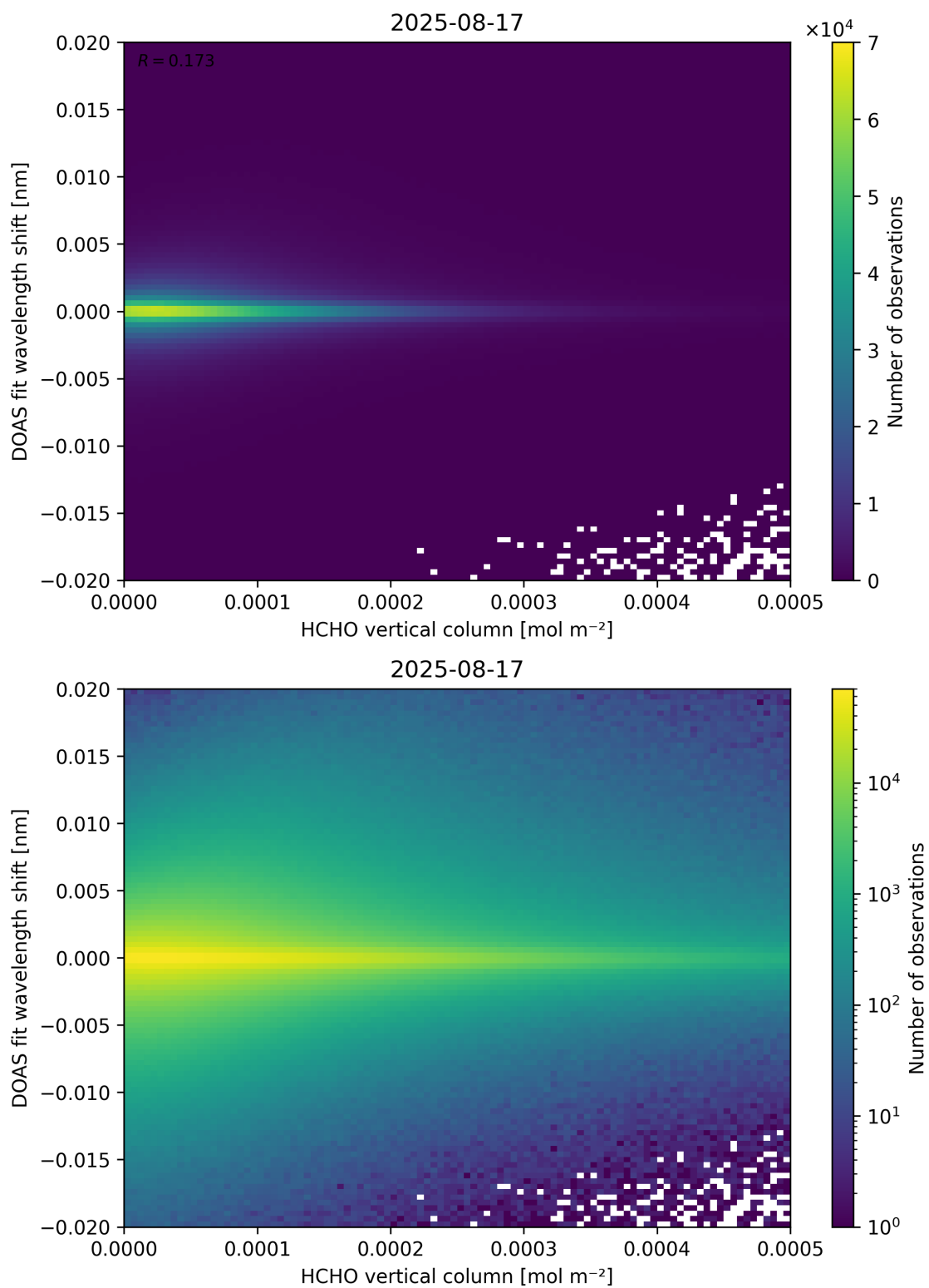
Figure 124: Scatter density plot of “HCHO vertical column” against “DOAS fit wavelength shift” for 2025-08-16 to 2025-08-18.
