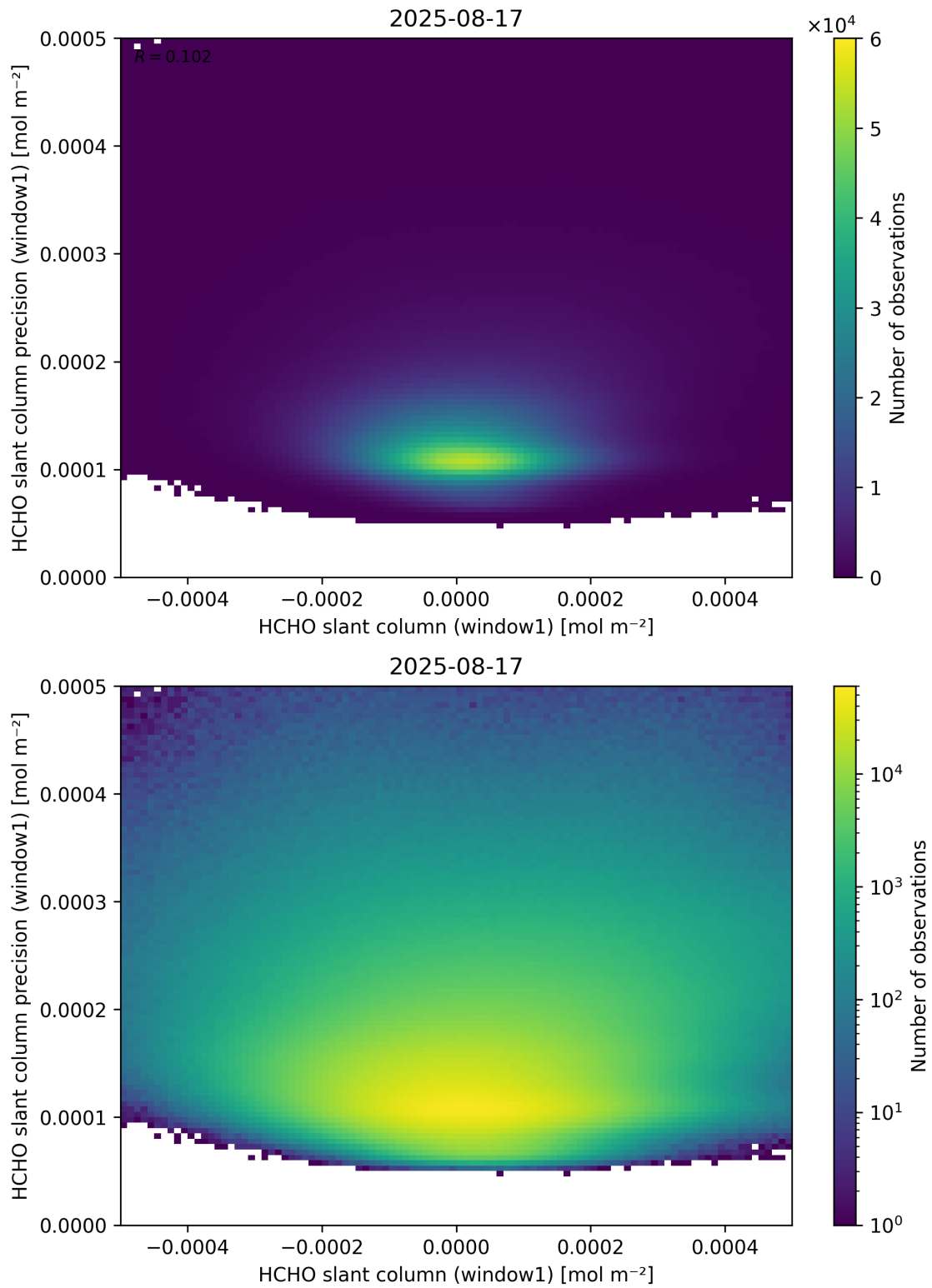
Figure 84: Scatter density plot of “HCHO slant column (window1)” against “HCHO slant column precision (window1)” for 2025-08-16 to 2025-08-18.
