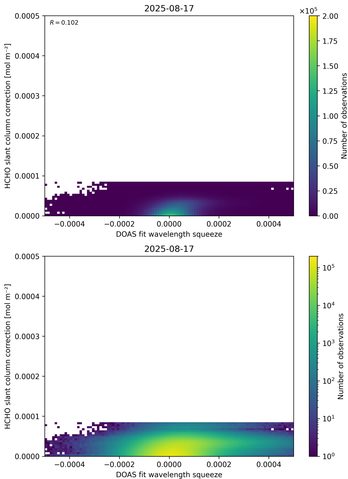
Figure 70: Scatter density plot of “DOAS fit wavelength squeeze” against “HCHO slant column correction” for 2025-08-16 to 2025-08-18.
