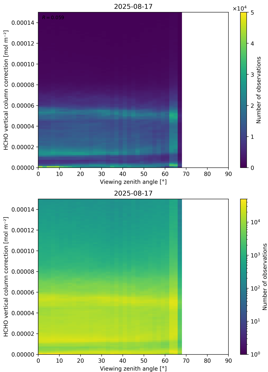
Figure 193: Scatter density plot of “Viewing zenith angle” against “HCHO vertical column correction” for 2025-08-16 to 2025-08-18.
