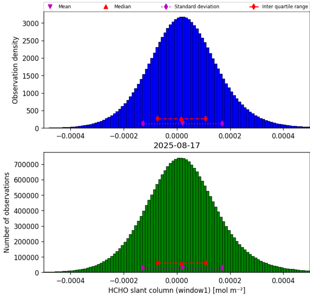
Figure 38: Histogram of “HCHO slant column (window1)” for 2025-08-16 to 2025-08-18
