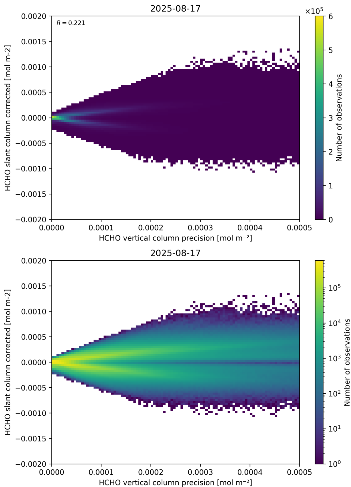
Figure 140: Scatter density plot of “HCHO vertical column precision” against “HCHO slant column corrected” for 2025-08-16 to 2025-08-18.
