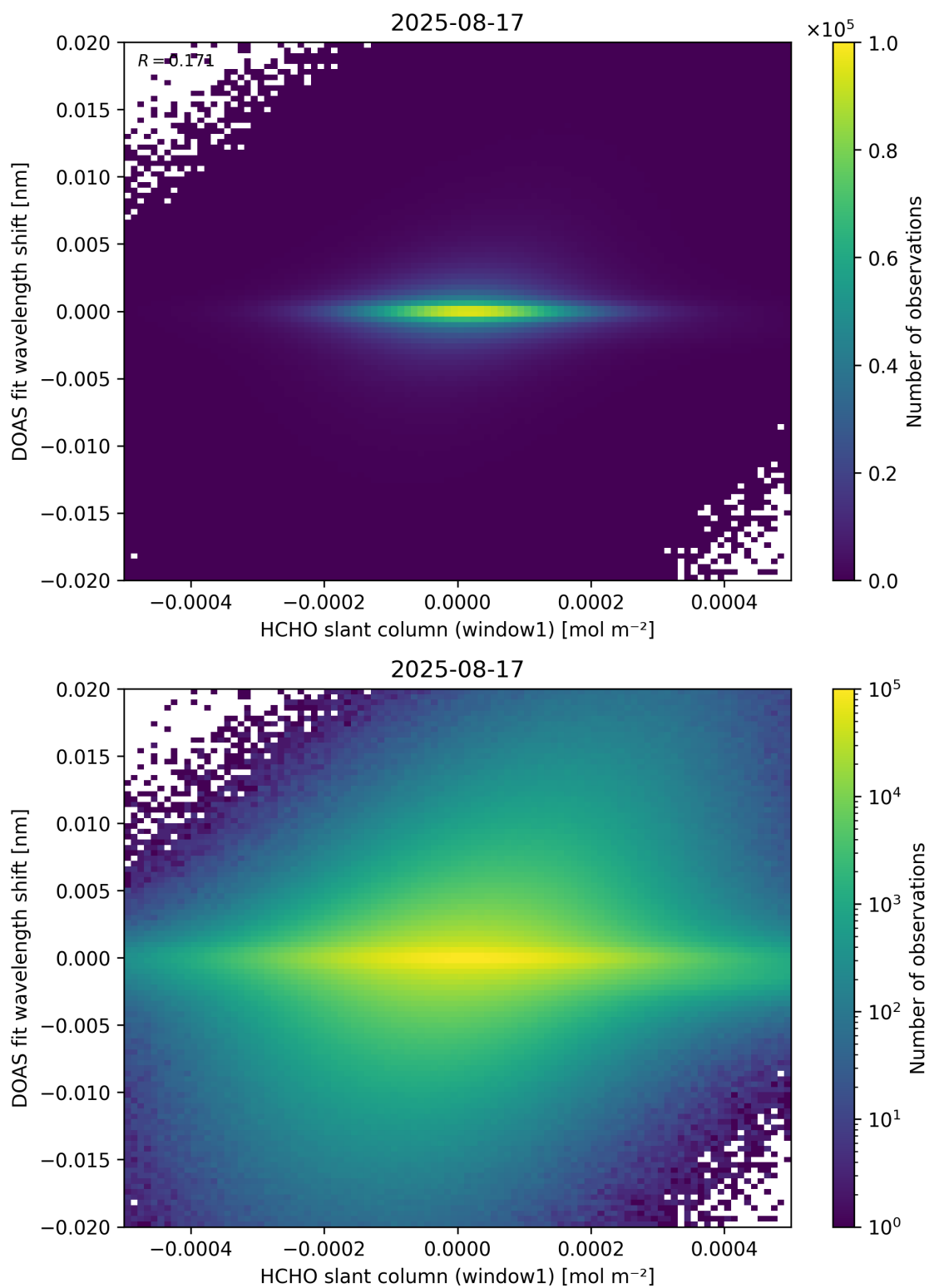
Figure 79: Scatter density plot of “HCHO slant column (window1)” against “DOAS fit wavelength shift” for 2025-08-16 to 2025-08-18.
