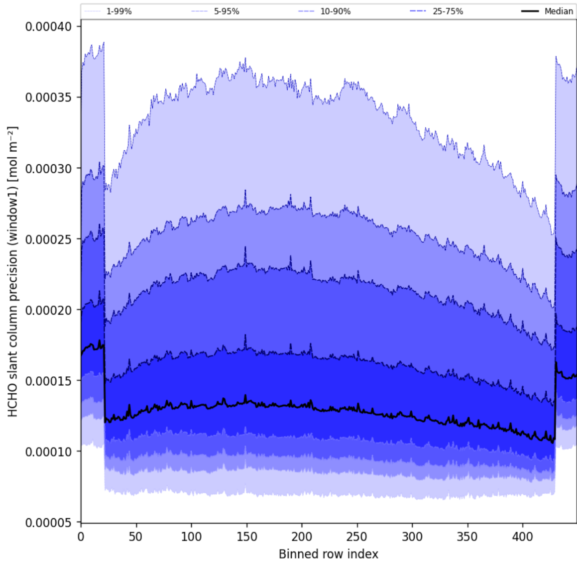
Figure 53: Along track statistics of “HCHO slant column precision (window1)” for 2025-08-16 to 2025-08-18
