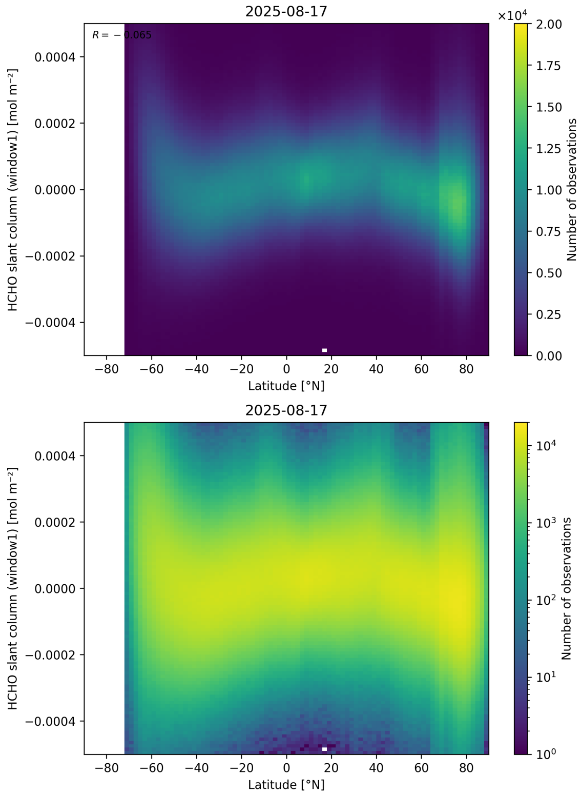
Figure 159: Scatter density plot of “Latitude” against “HCHO slant column (window1)” for 2025-08-16 to 2025-08-18.
