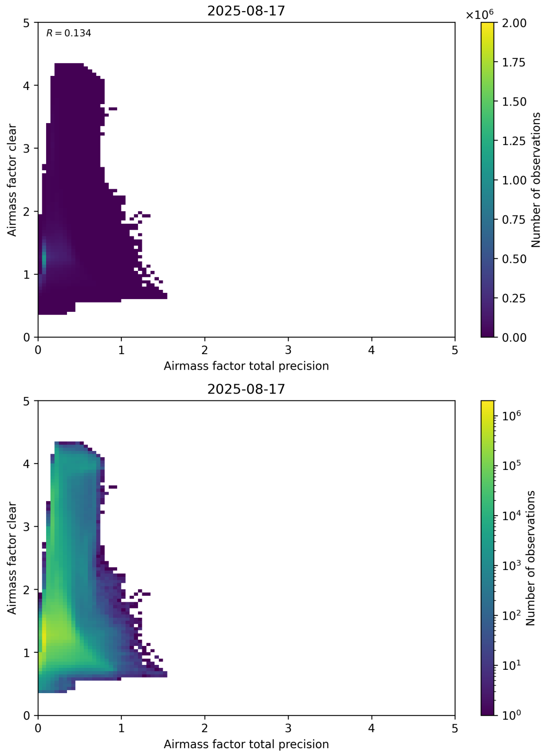
Figure 108: Scatter density plot of “Airmass factor total precision” against “Airmass factor clear” for 2025-08-16 to 2025-08-18.
