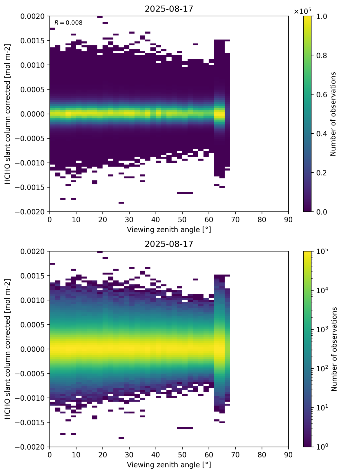
Figure 186: Scatter density plot of “Viewing zenith angle” against “HCHO slant column corrected” for 2025-08-16 to 2025-08-18.
