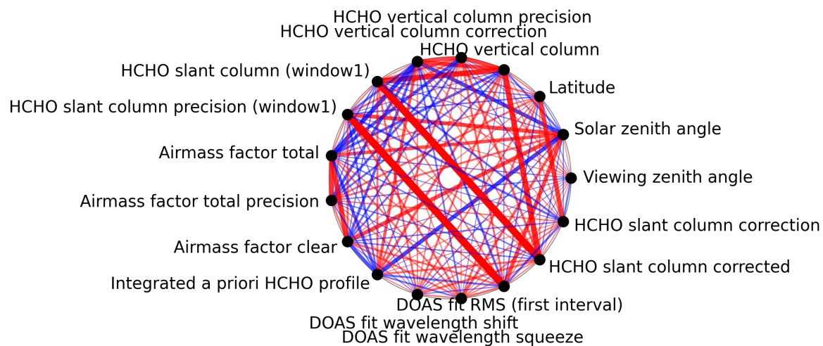
Figure 1: Map of correlation graph for 2025-08-16 to 2025-08-18.
