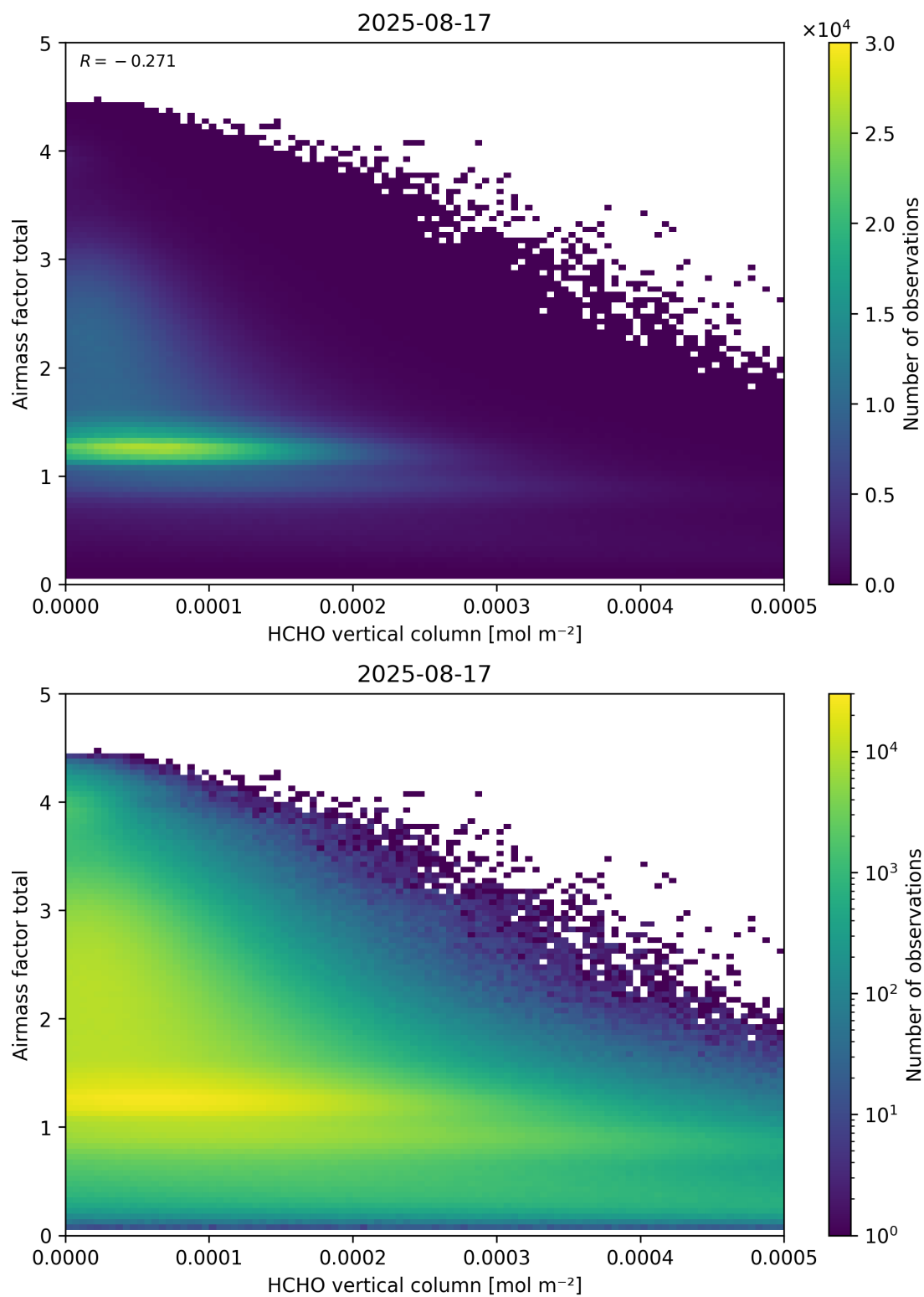
Figure 131: Scatter density plot of “HCHO vertical column” against “Airmass factor total” for 2025-08-16 to 2025-08-18.
