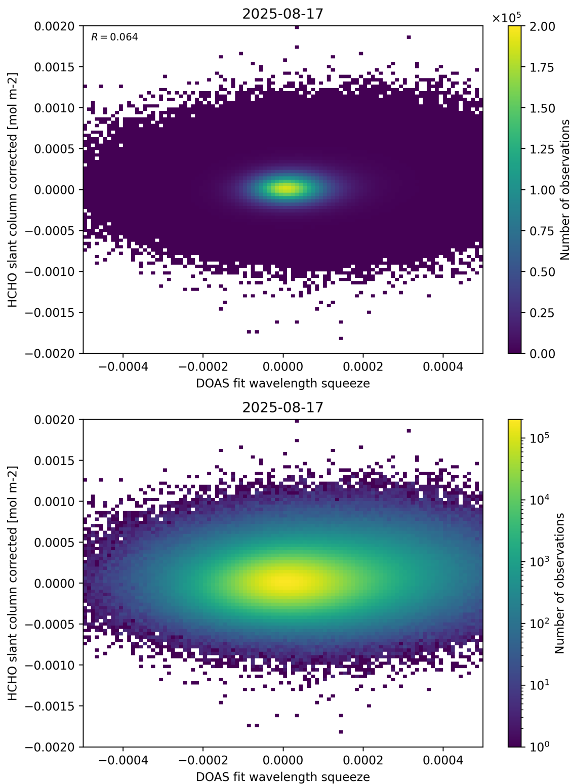
Figure 69: Scatter density plot of “DOAS fit wavelength squeeze” against “HCHO slant column corrected” for 2025-08-16 to 2025-08-18.
