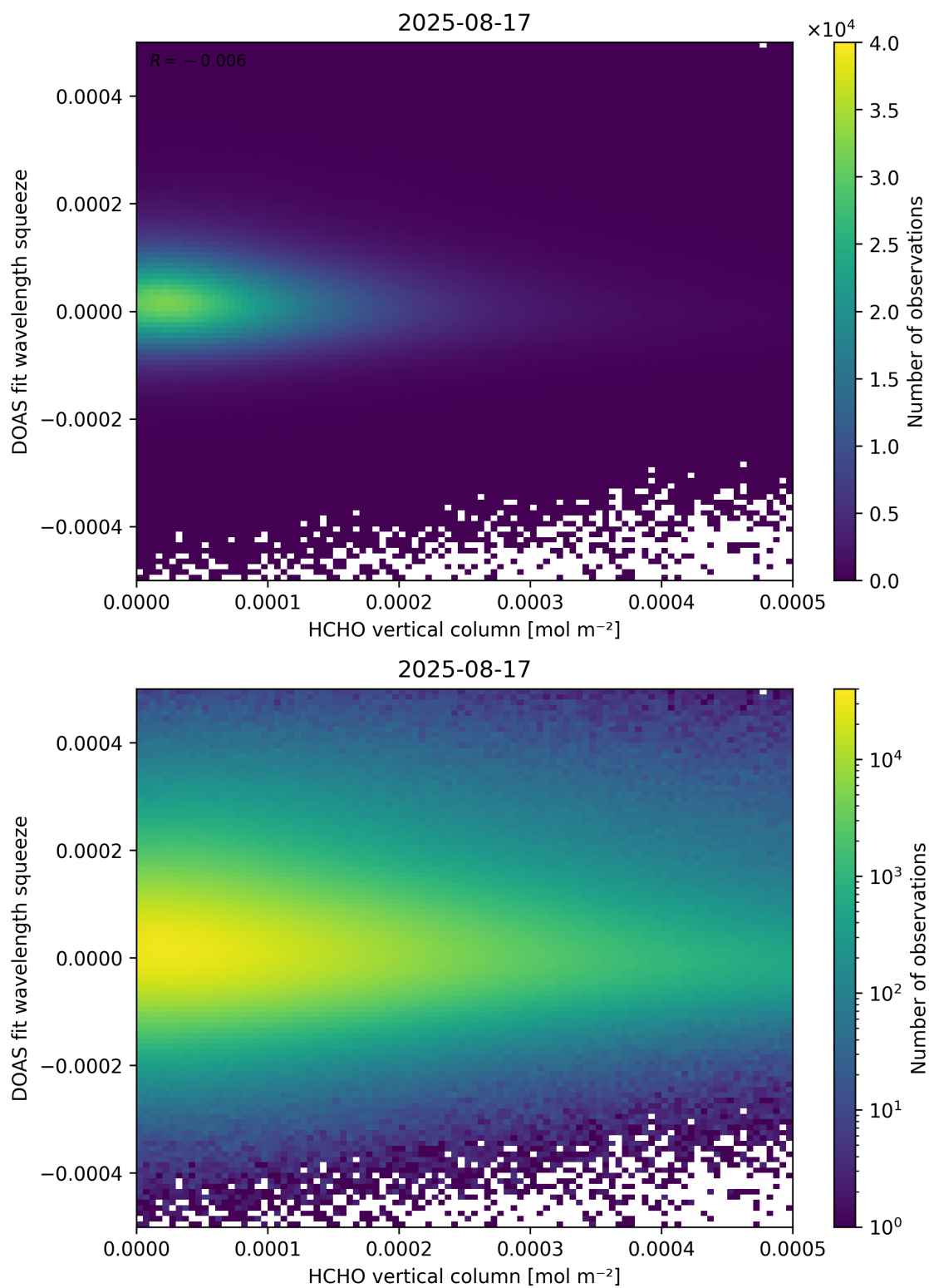
Figure 125: Scatter density plot of “HCHO vertical column” against “DOAS fit wavelength squeeze” for 2025-08-16 to 2025-08-18.
