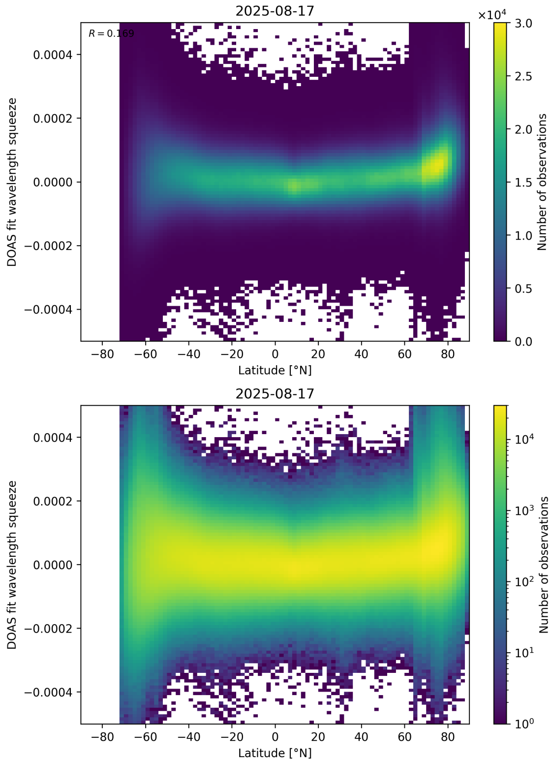
Figure 155: Scatter density plot of “Latitude” against “DOAS fit wavelength squeeze” for 2025-08-16 to 2025-08-18.
