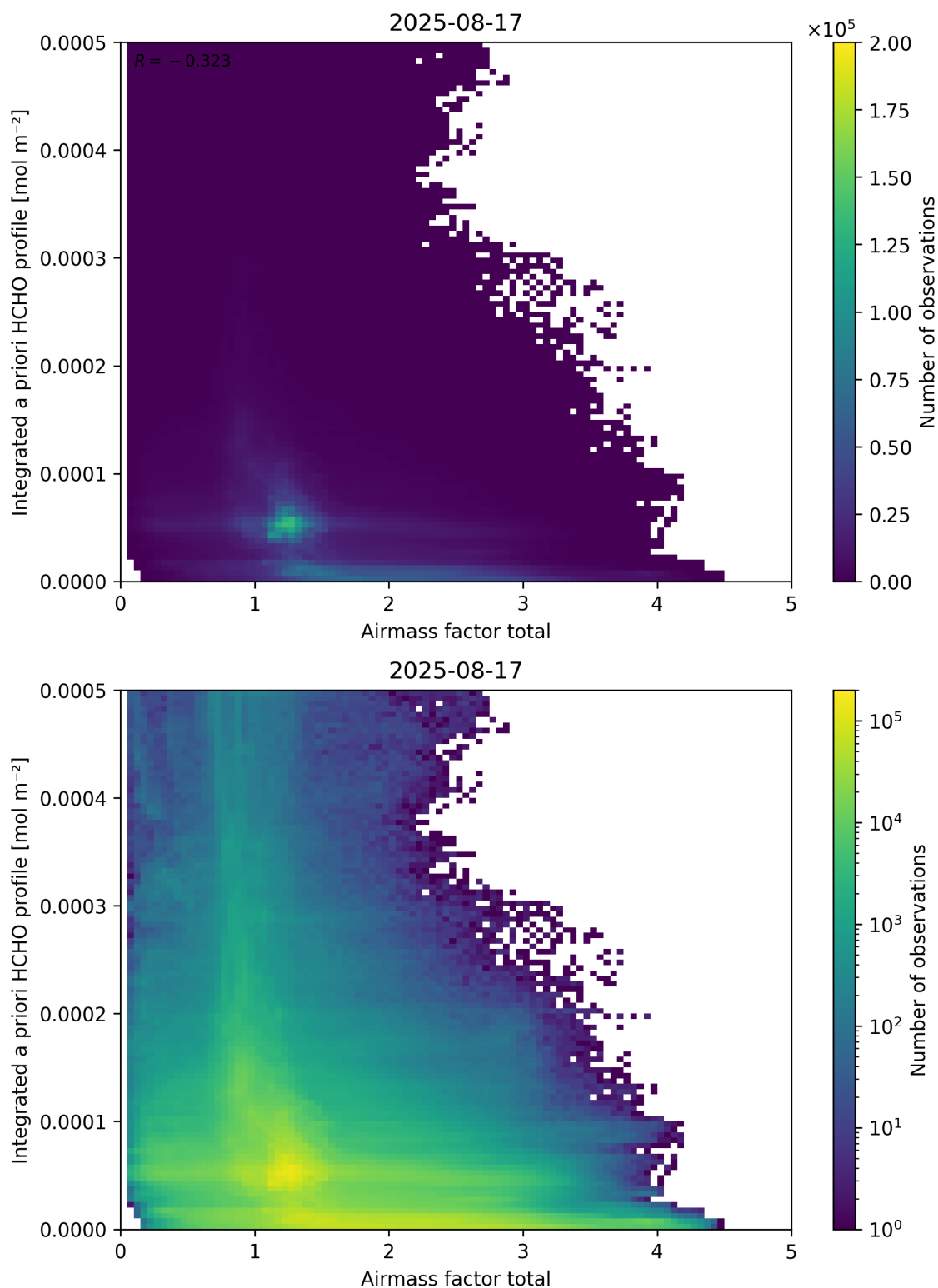
Figure 104: Scatter density plot of “Airmass factor total” against “Integrated a priori HCHO profile” for 2025-08-16 to 2025-08-18.
