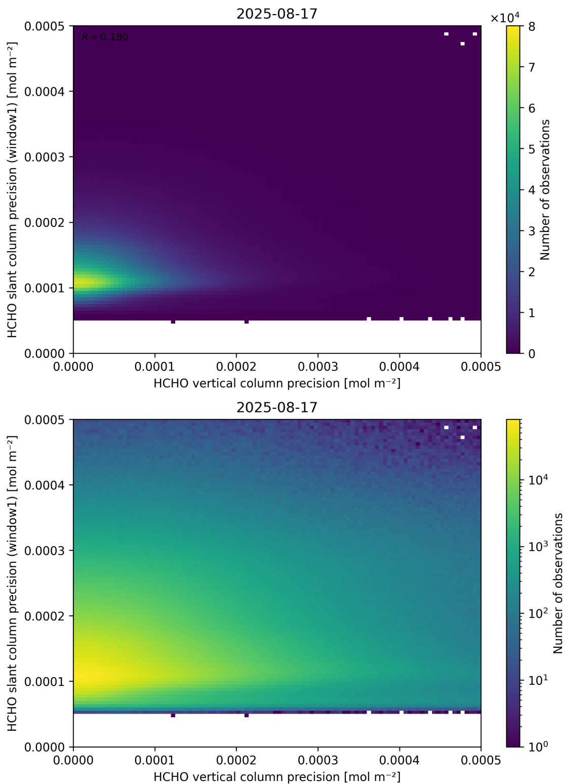
Figure 143: Scatter density plot of “HCHO vertical column precision” against “HCHO slant column precision (window1)” for 2025-08-16 to 2025-08-18.
