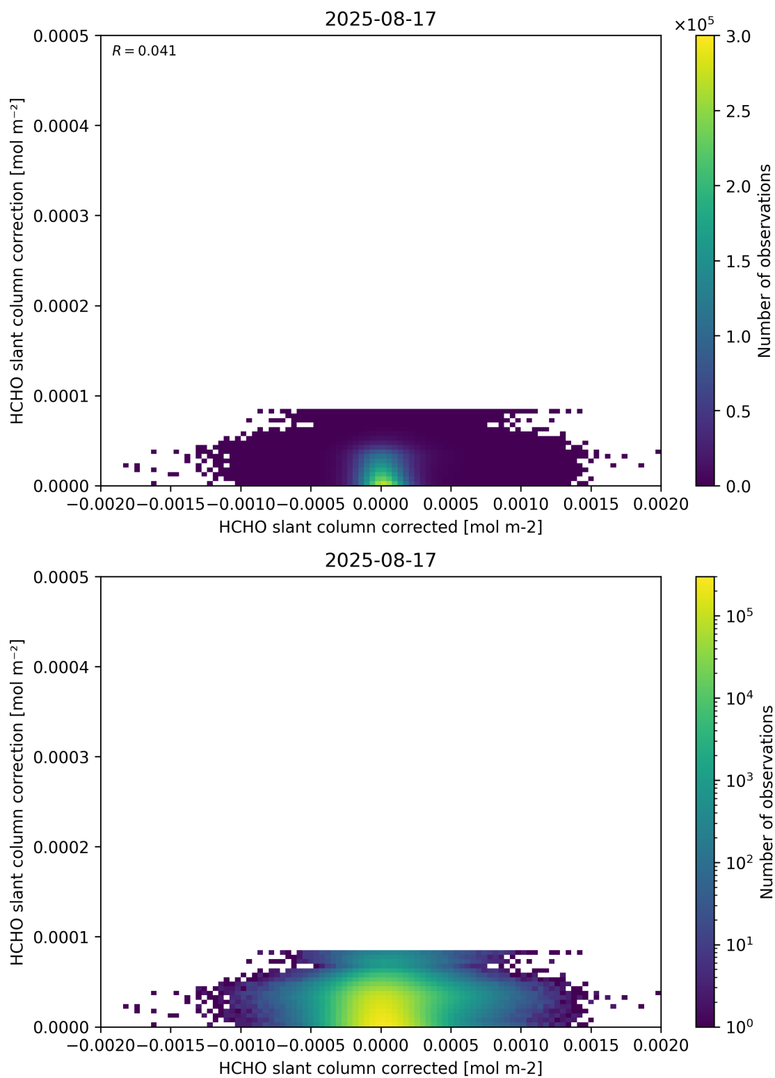
Figure 77: Scatter density plot of “HCHO slant column corrected” against “HCHO slant column correction” for 2025-08-16 to 2025-08-18.
