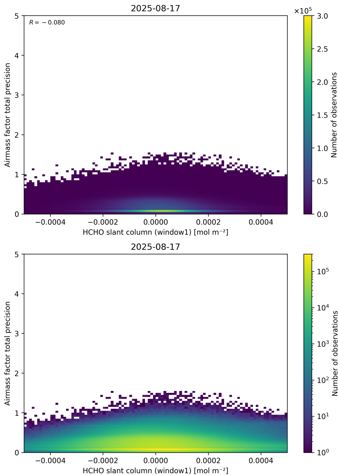
Figure 86: Scatter density plot of “HCHO slant column (window1)” against “Airmass factor total precision” for 2025-08-16 to 2025-08-18.
