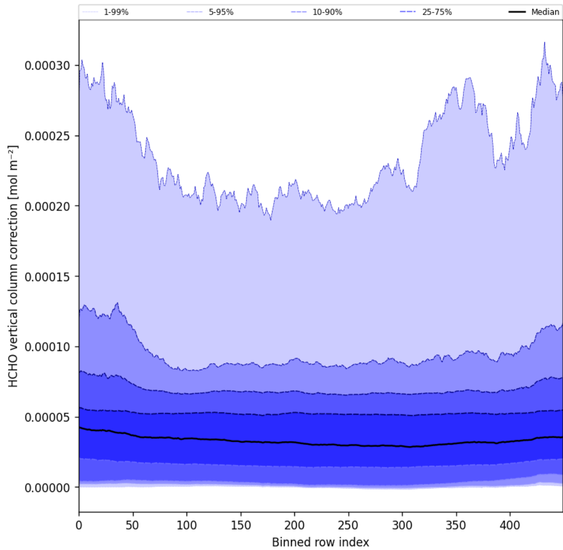
Figure 51: Along track statistics of “HCHO vertical column correction” for 2025-08-16 to 2025-08-18
