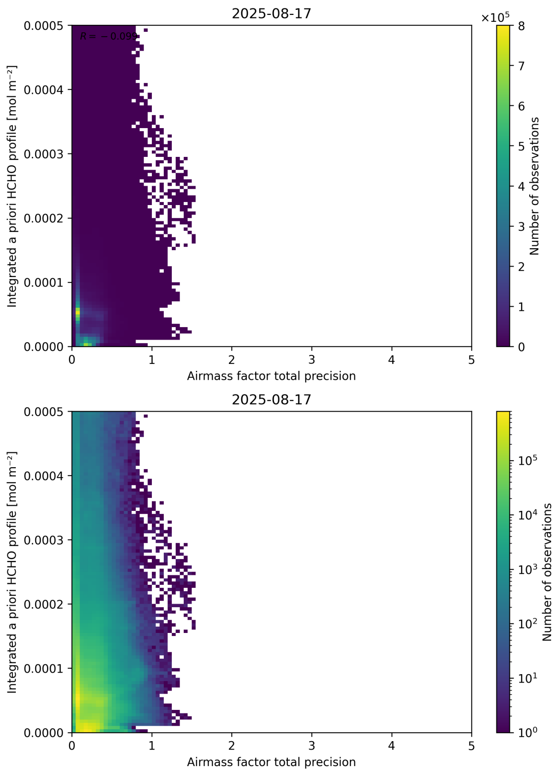
Figure 111: Scatter density plot of “Airmass factor total precision” against “Integrated a priori HCHO profile” for 2025-08-16 to 2025-08-18.
