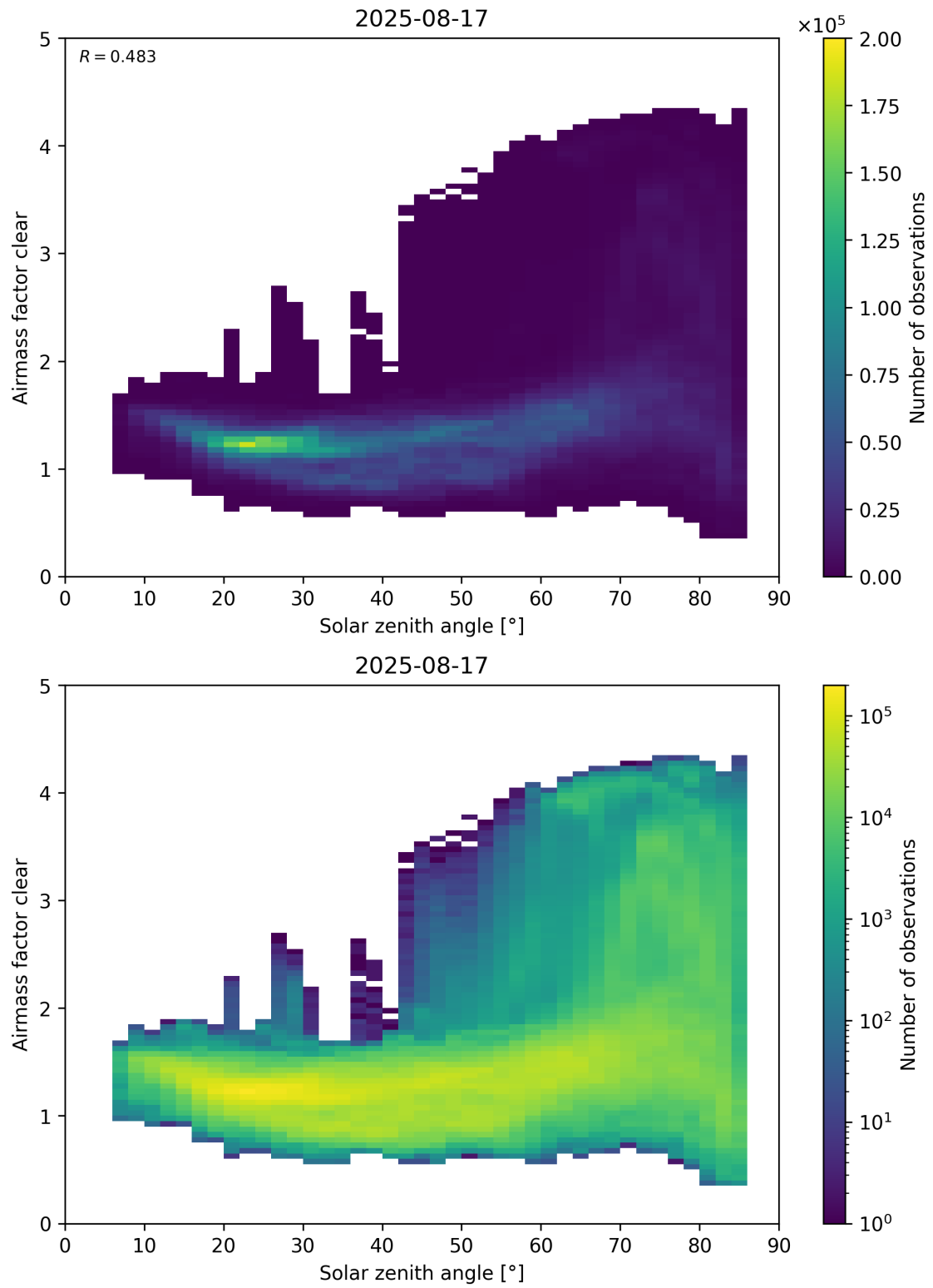
Figure 170: Scatter density plot of “Solar zenith angle” against “Airmass factor clear” for 2025-08-16 to 2025-08-18.
