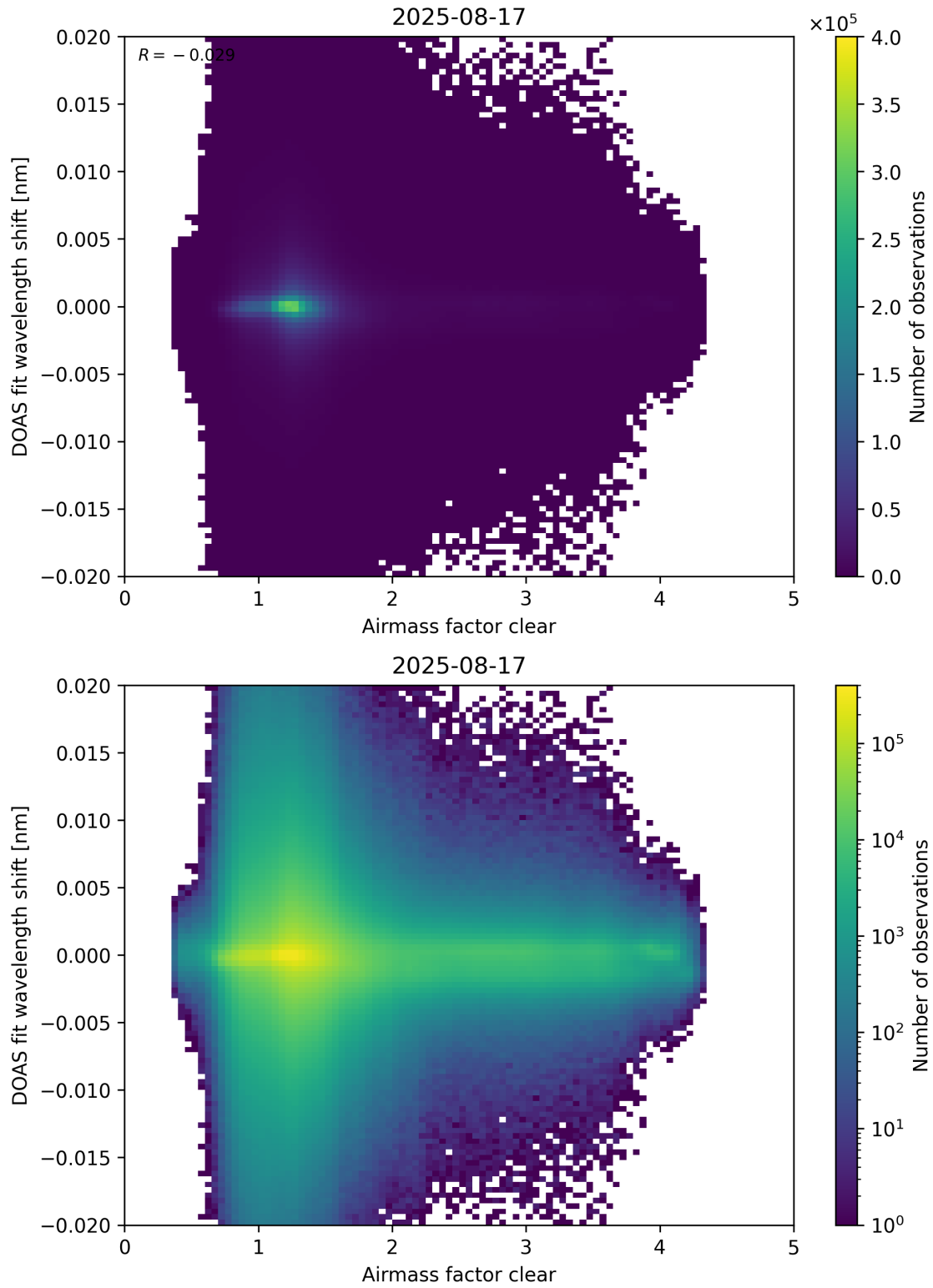
Figure 72: Scatter density plot of “Airmass factor clear” against “DOAS fit wavelength shift” for 2025-08-16 to 2025-08-18.
