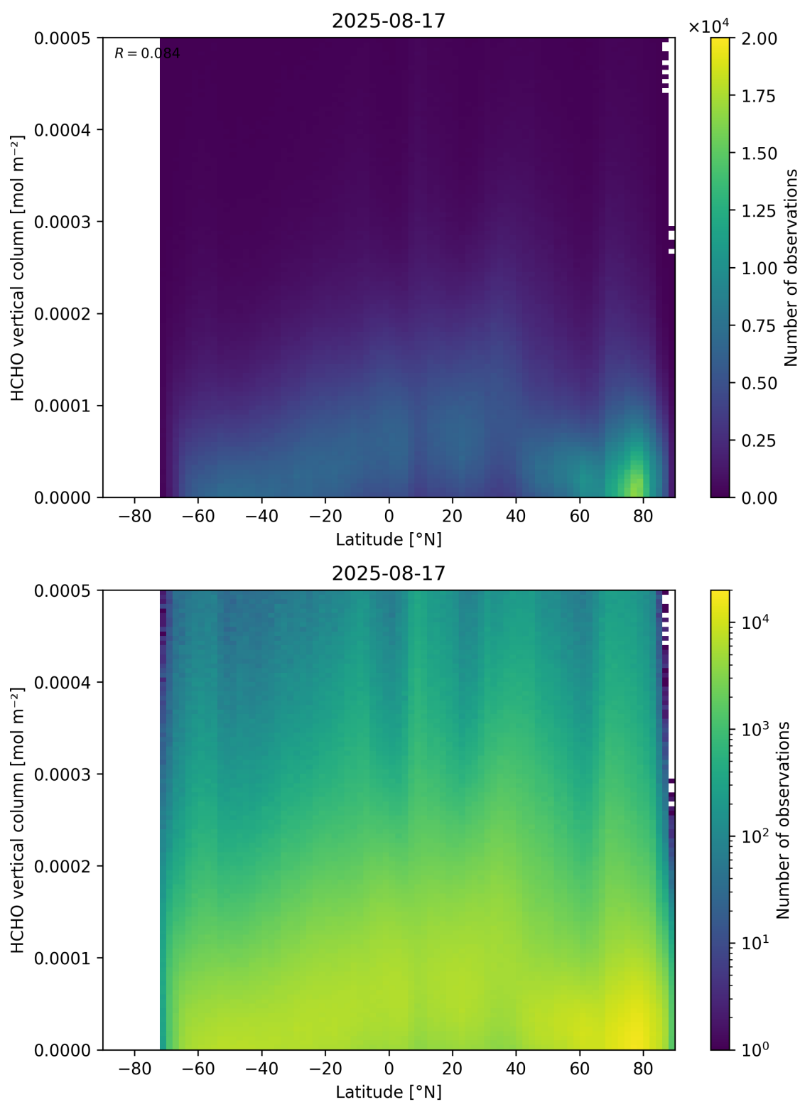
Figure 163: Scatter density plot of “Latitude” against “HCHO vertical column” for 2025-08-16 to 2025-08-18.
