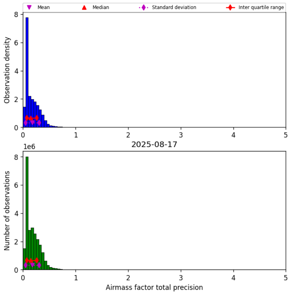
Figure 41: Histogram of “Airmass factor total precision” for 2025-08-16 to 2025-08-18
