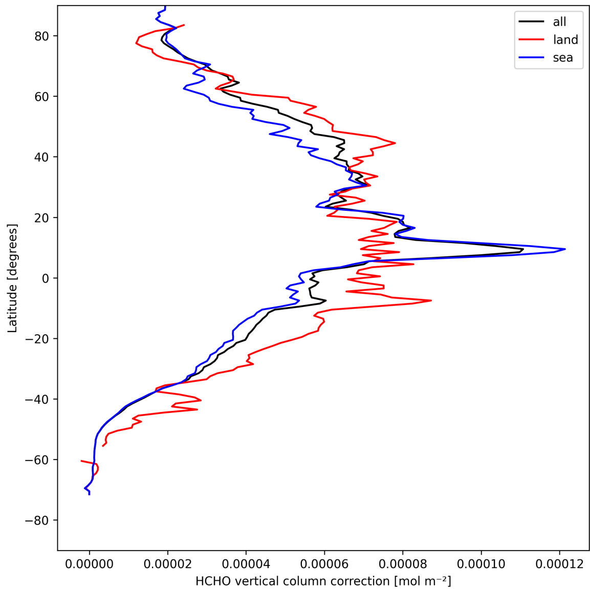
Figure 23: Zonal average of “HCHO vertical column correction” for 2025-08-16 to 2025-08-18.
