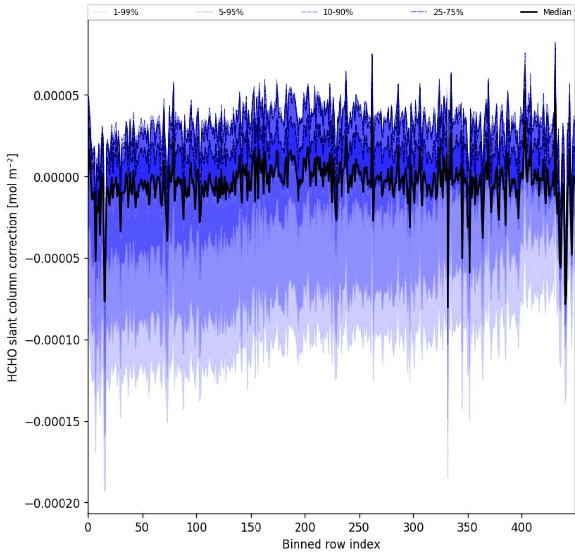
Figure 61: Along track statistics of “HCHO slant column correction” for 2025-08-16 to 2025-08-18
