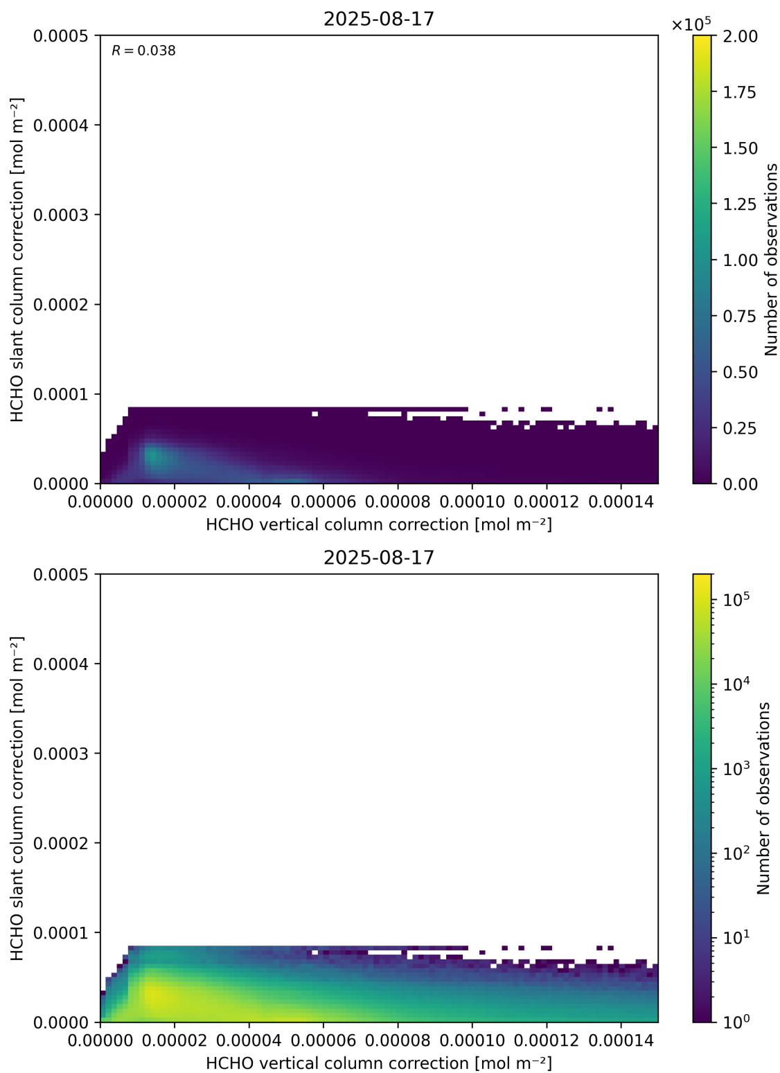
Figure 117: Scatter density plot of “HCHO vertical column correction” against “HCHO slant column correction” for 2025-08-16 to 2025-08-18.
