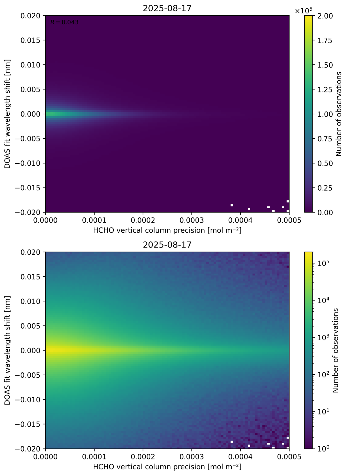
Figure 137: Scatter density plot of “HCHO vertical column precision” against “DOAS fit wavelength shift” for 2025-08-16 to 2025-08-18.
