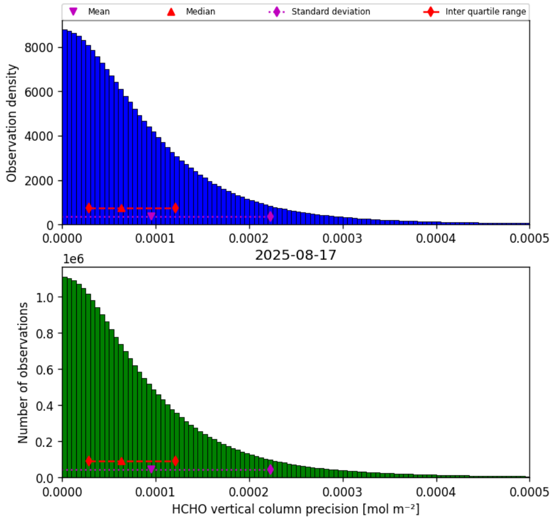
Figure 36: Histogram of “HCHO vertical column precision” for 2025-08-16 to 2025-08-18
