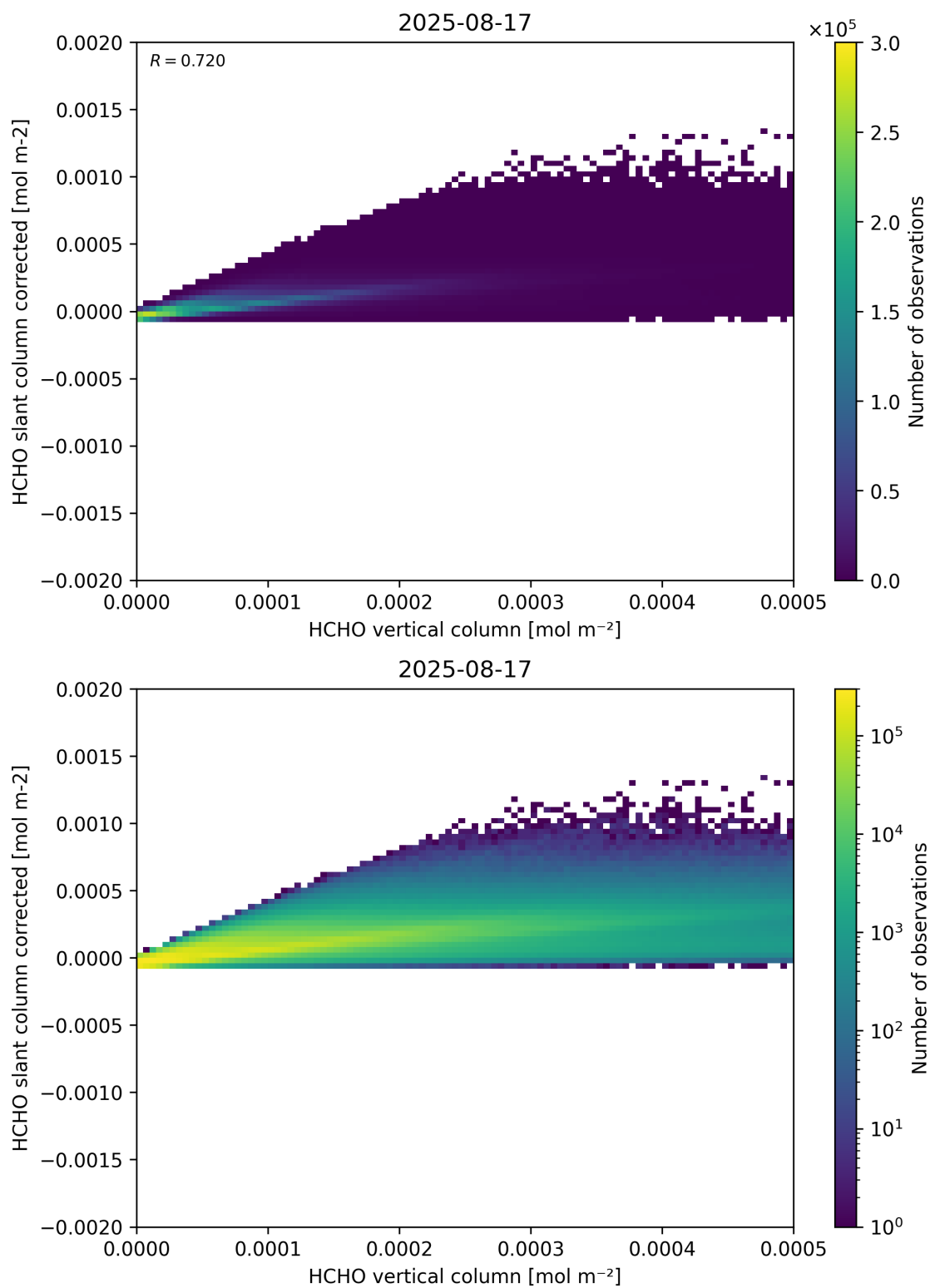
Figure 127: Scatter density plot of “HCHO vertical column” against “HCHO slant column corrected” for 2025-08-16 to 2025-08-18.
