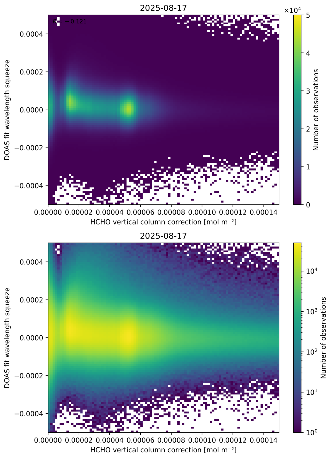
Figure 114: Scatter density plot of “HCHO vertical column correction” against “DOAS fit wavelength squeeze” for 2025-08-16 to 2025-08-18.
