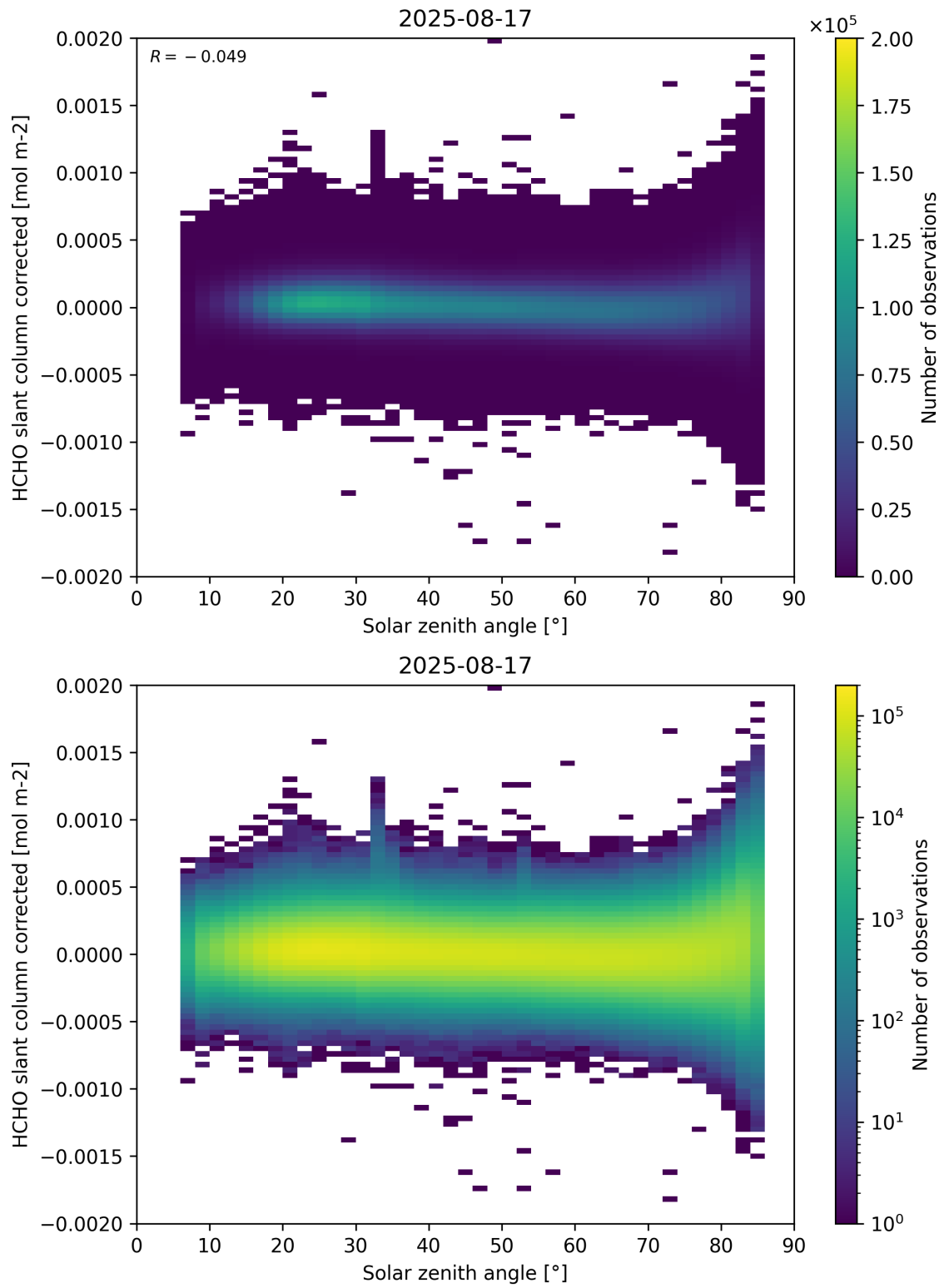
Figure 171: Scatter density plot of “Solar zenith angle” against “HCHO slant column corrected” for 2025-08-16 to 2025-08-18.
