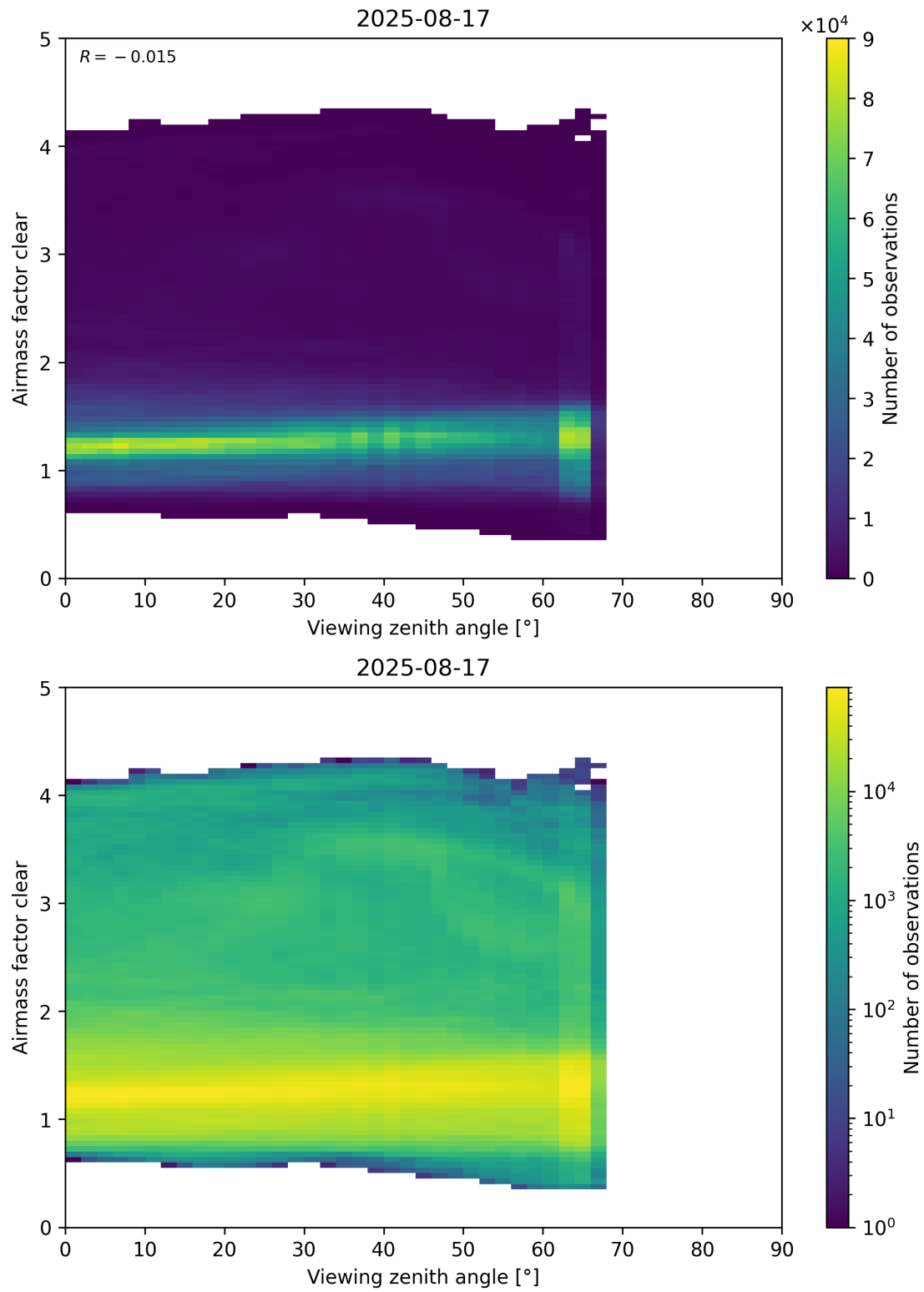
Figure 185: Scatter density plot of “Viewing zenith angle” against “Airmass factor clear” for 2025-08-16 to 2025-08-18.
