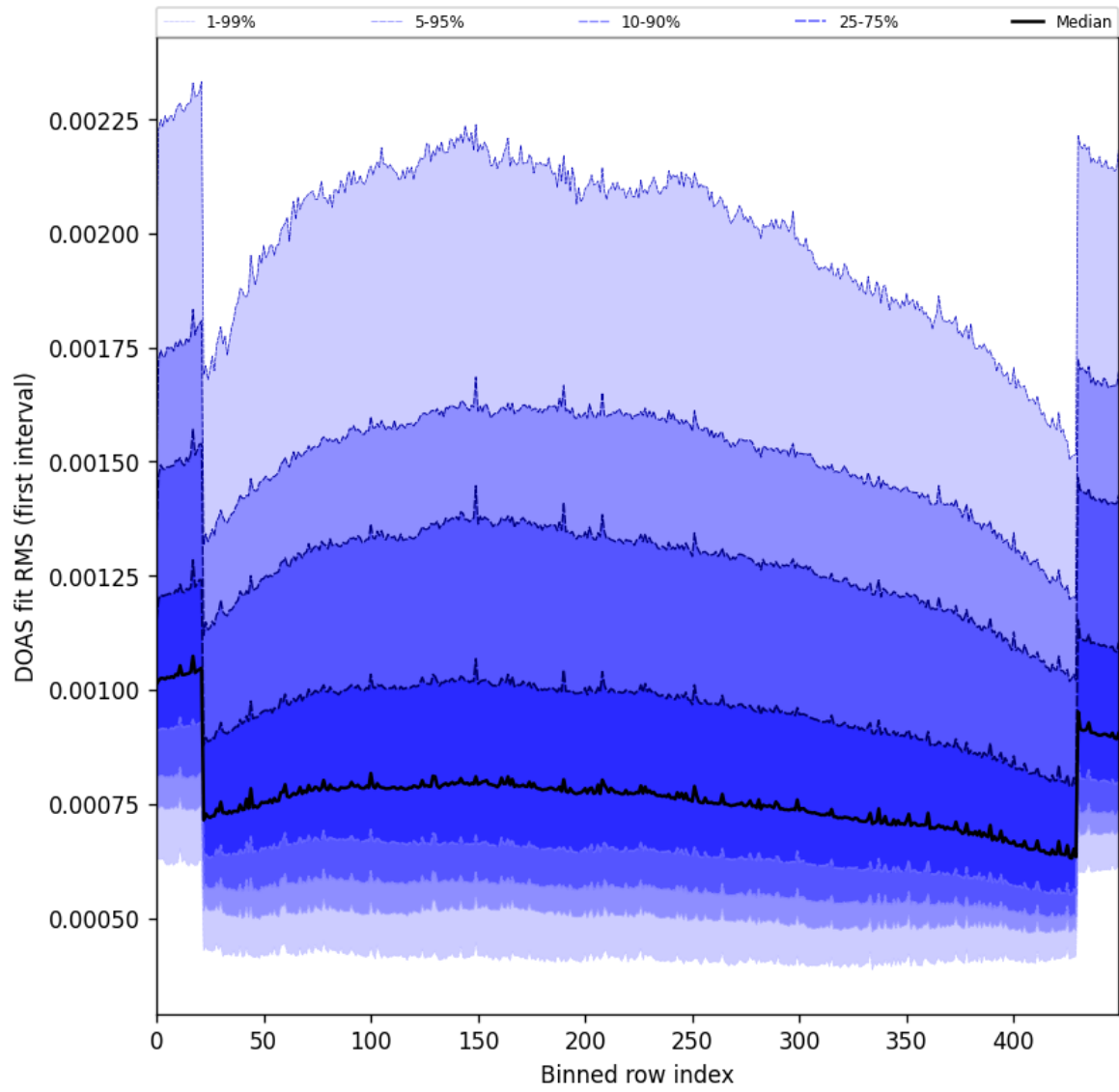
Figure 60: Along track statistics of “DOAS fit RMS (first interval)” for 2025-08-16 to 2025-08-18
