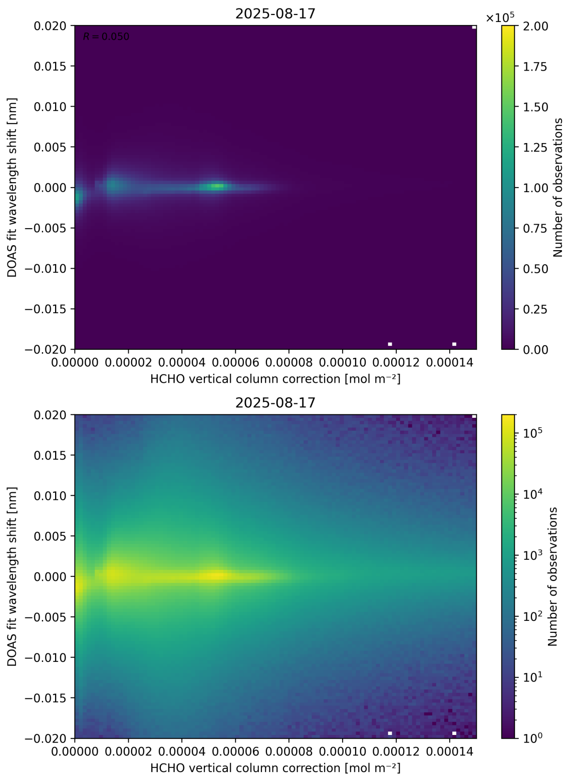
Figure 113: Scatter density plot of “HCHO vertical column correction” against “DOAS fit wavelength shift” for 2025-08-16 to 2025-08-18.
