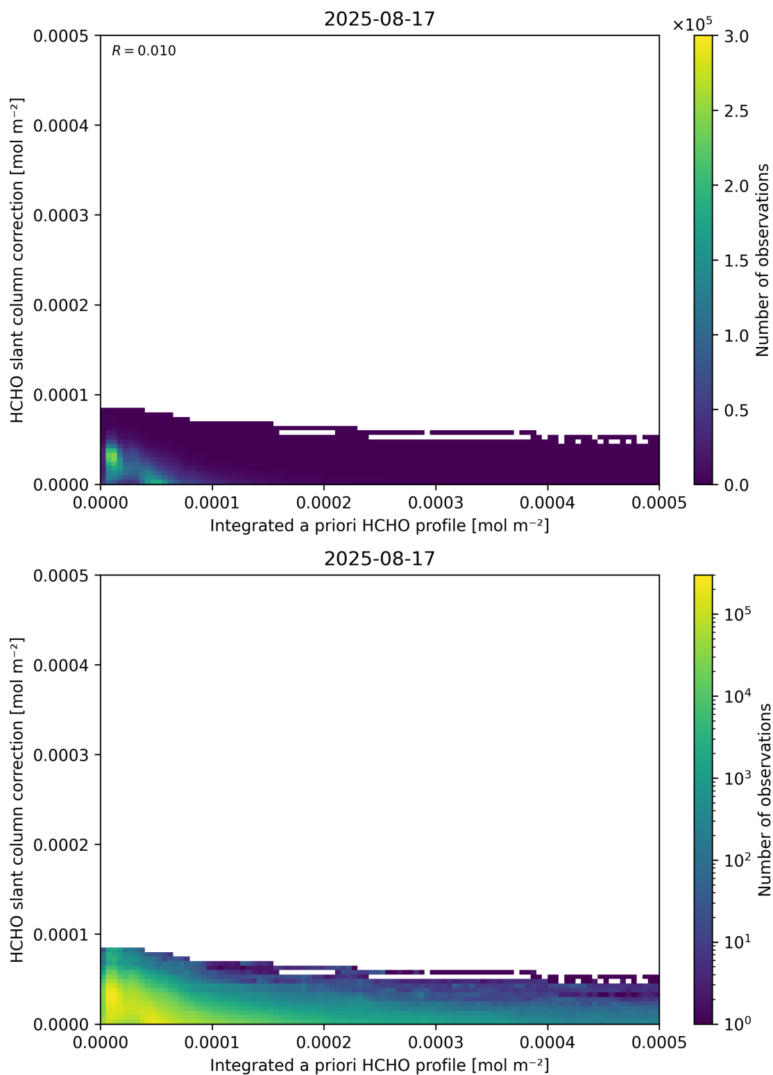
Figure 152: Scatter density plot of “Integrated a priori HCHO profile” against “HCHO slant column correction” for 2025-08-16 to 2025-08-18.
