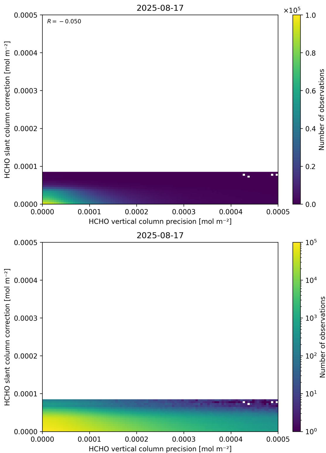
Figure 141: Scatter density plot of “HCHO vertical column precision” against “HCHO slant column correction” for 2025-08-16 to 2025-08-18.
