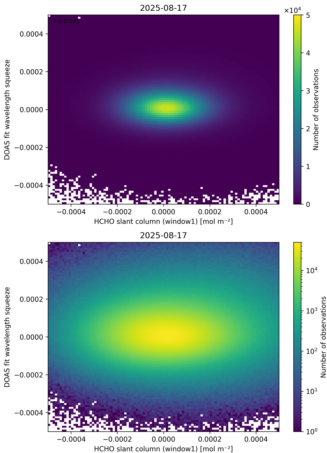
Figure 80: Scatter density plot of “HCHO slant column (window1)” against “DOAS fit wavelength squeeze” for 2025-08-16 to 2025-08-18.
