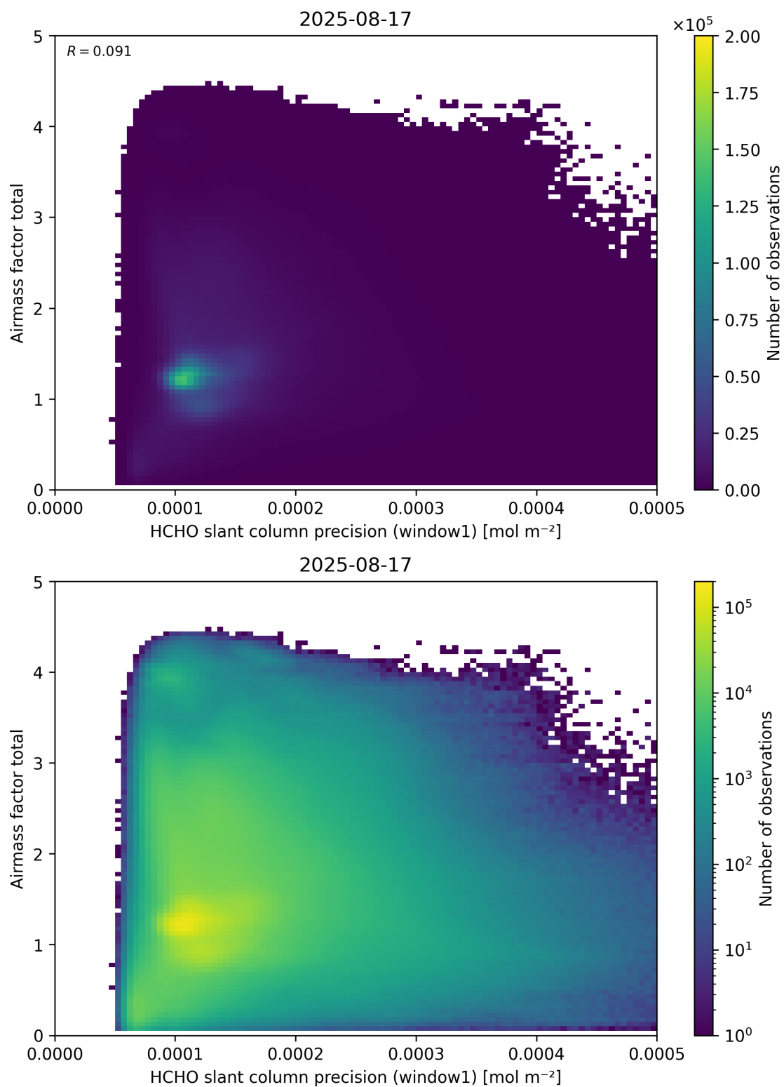
Figure 94: Scatter density plot of “HCHO slant column precision (window1)” against “Airmass factor total” for 2025-08-16 to 2025-08-18.
