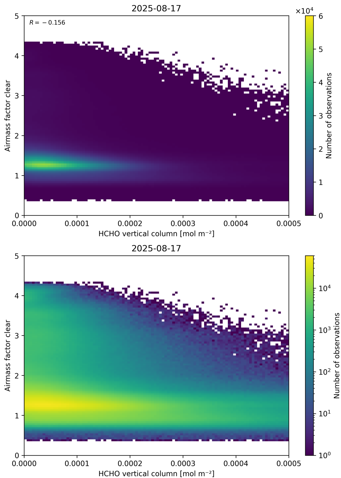
Figure 126: Scatter density plot of “HCHO vertical column” against “Airmass factor clear” for 2025-08-16 to 2025-08-18.
