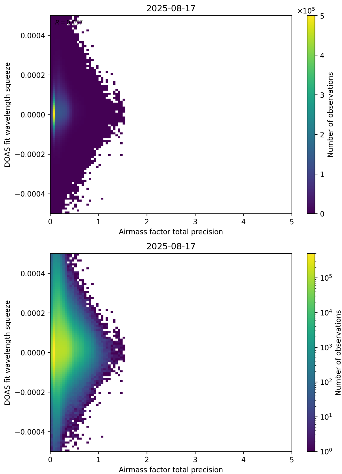
Figure 107: Scatter density plot of “Airmass factor total precision” against “DOAS fit wavelength squeeze” for 2025-08-16 to 2025-08-18.
