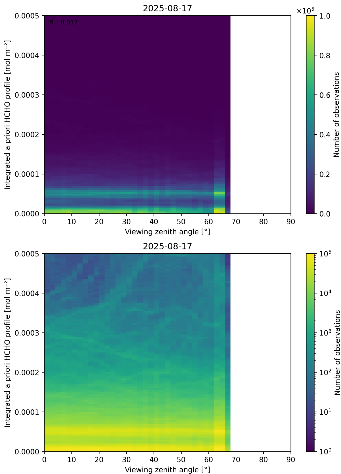
Figure 195: Scatter density plot of “Viewing zenith angle” against “Integrated a priori HCHO profile” for 2025-08-16 to 2025-08-18.
