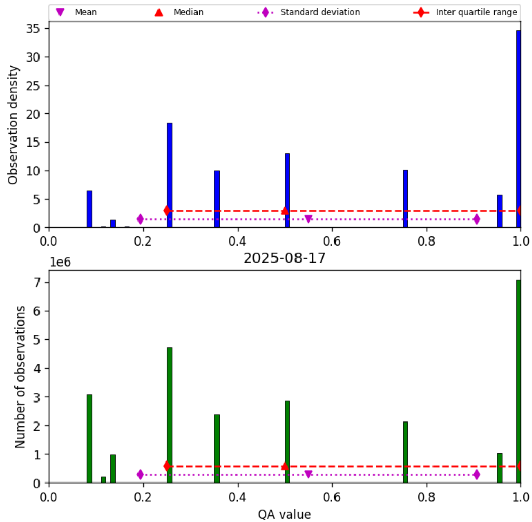
Figure 34: Histogram of “QA value” for 2025-08-16 to 2025-08-18
