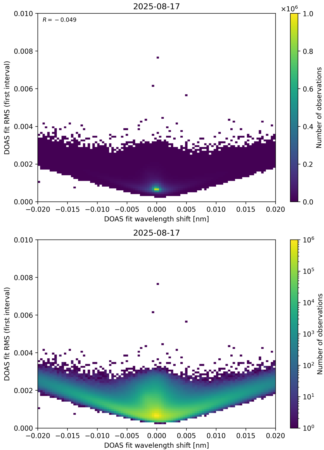
Figure 64: Scatter density plot of “DOAS fit wavelength shift” against “DOAS fit RMS (first interval)” for 2025-08-16 to 2025-08-18.
