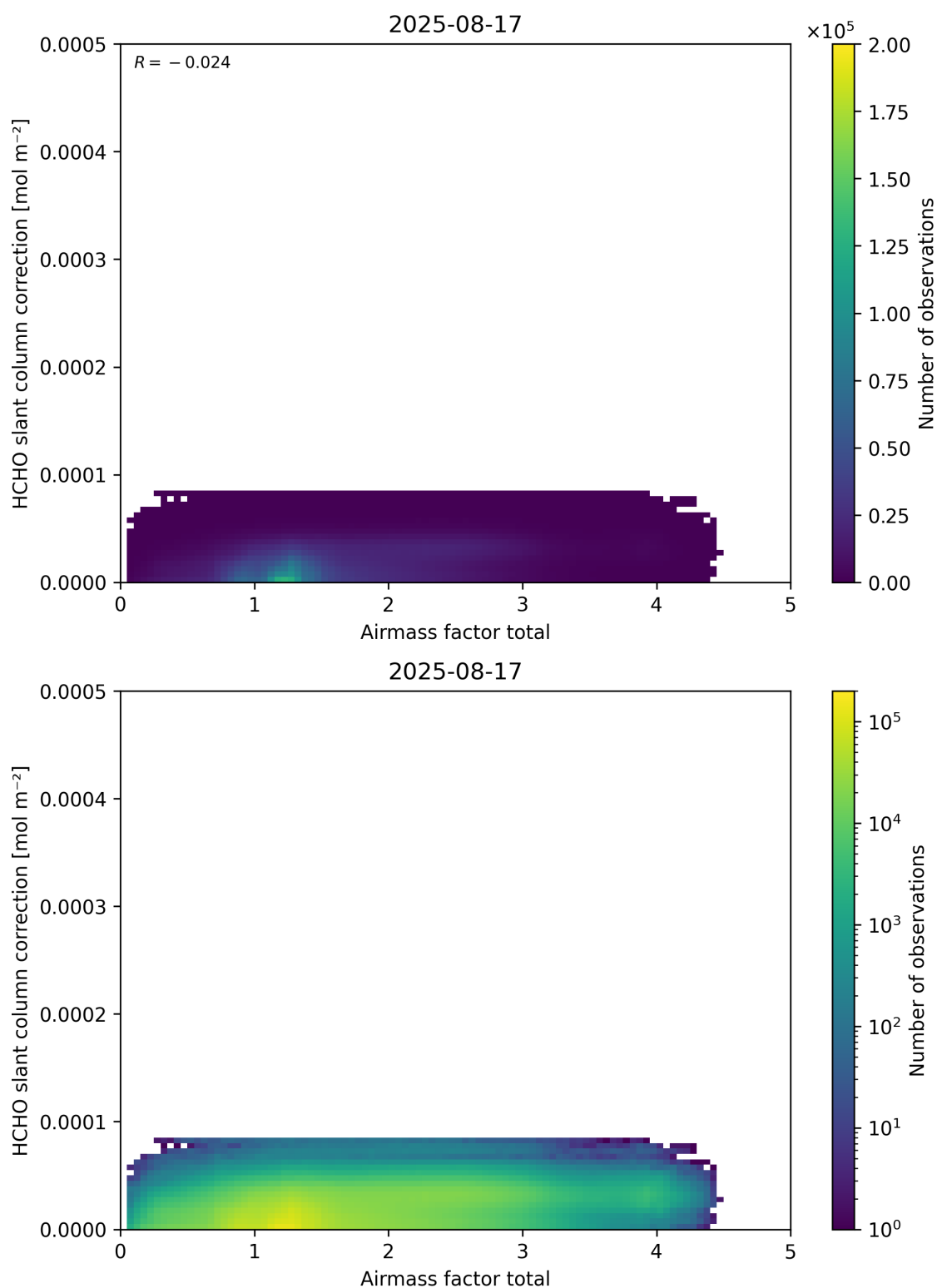
Figure 102: Scatter density plot of “Airmass factor total” against “HCHO slant column correction” for 2025-08-16 to 2025-08-18.
