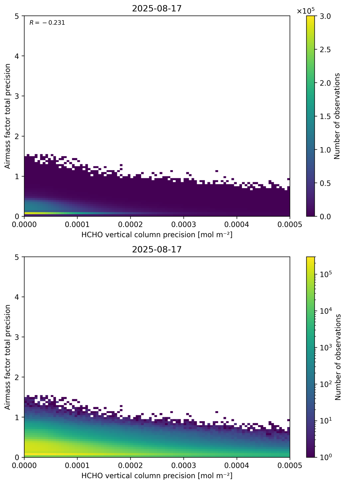
Figure 145: Scatter density plot of “HCHO vertical column precision” against “Airmass factor total precision” for 2025-08-16 to 2025-08-18.
