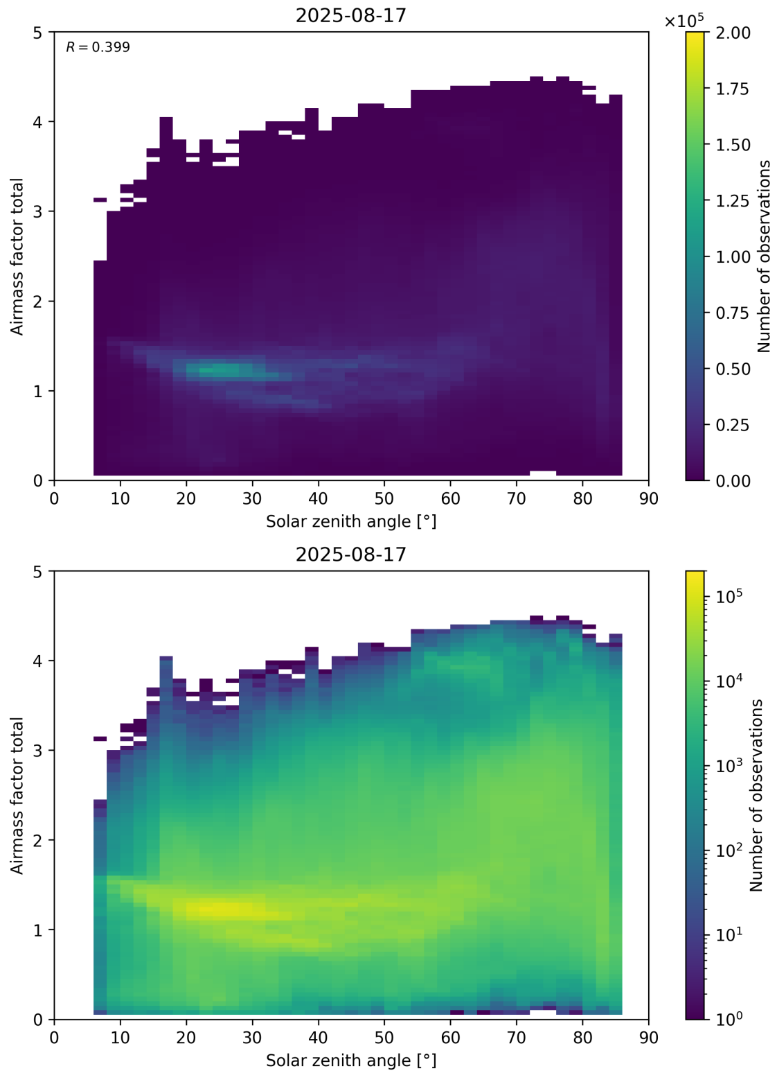
Figure 175: Scatter density plot of “Solar zenith angle” against “Airmass factor total” for 2025-08-16 to 2025-08-18.
