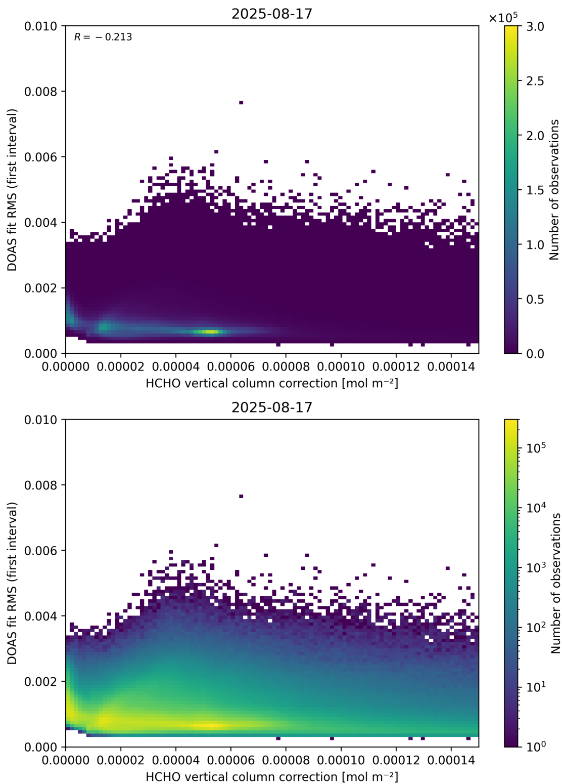
Figure 112: Scatter density plot of “HCHO vertical column correction” against “DOAS fit RMS (first interval)” for 2025-08-16 to 2025-08-18.
