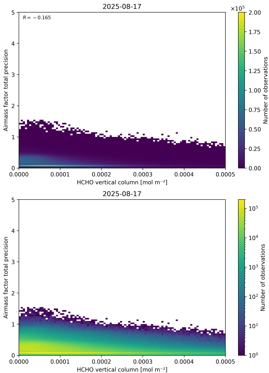
Figure 132: Scatter density plot of “HCHO vertical column” against “Airmass factor total precision” for 2025-08-16 to 2025-08-18.
