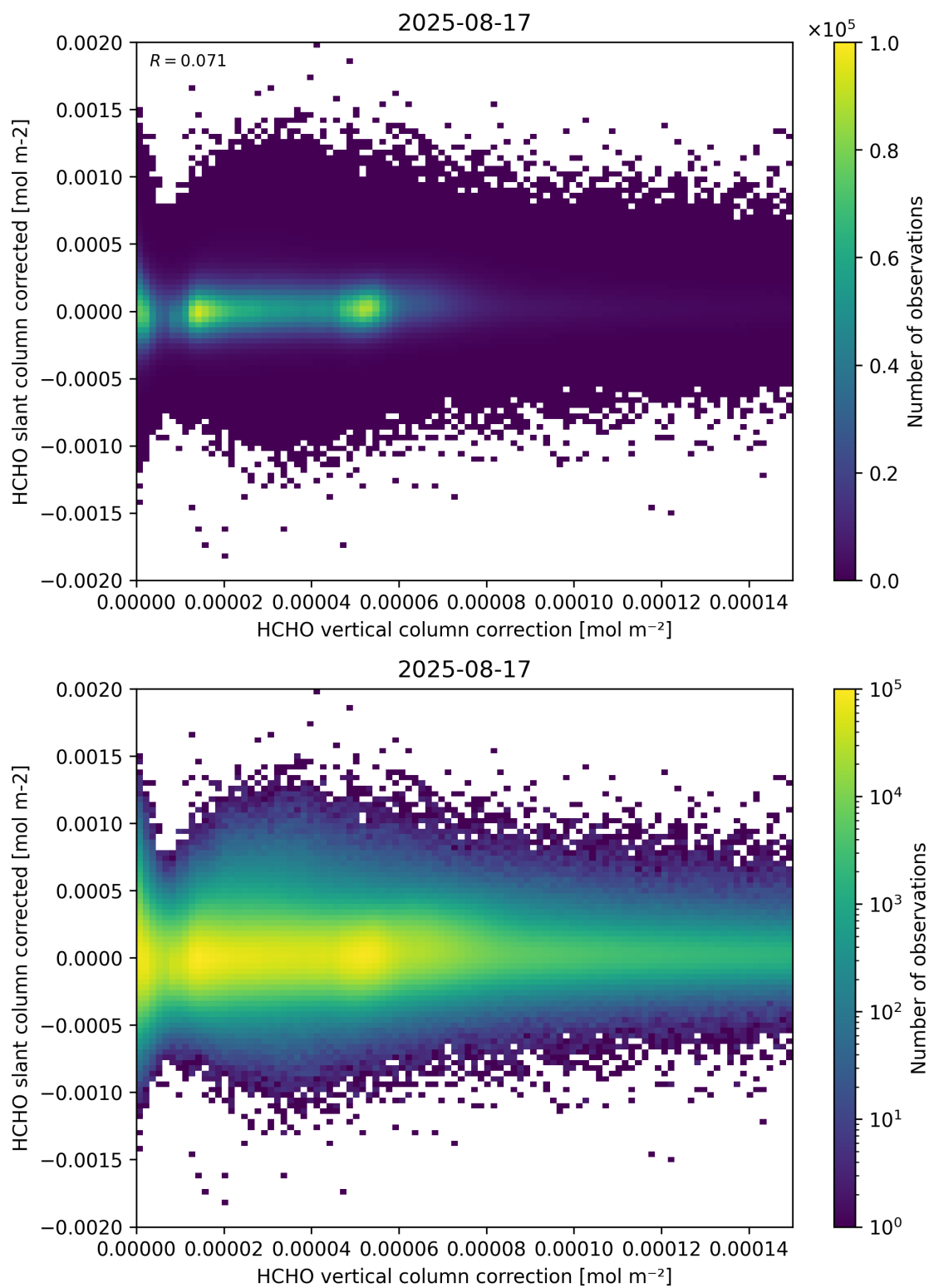
Figure 116: Scatter density plot of “HCHO vertical column correction” against “HCHO slant column corrected” for 2025-08-16 to 2025-08-18.
