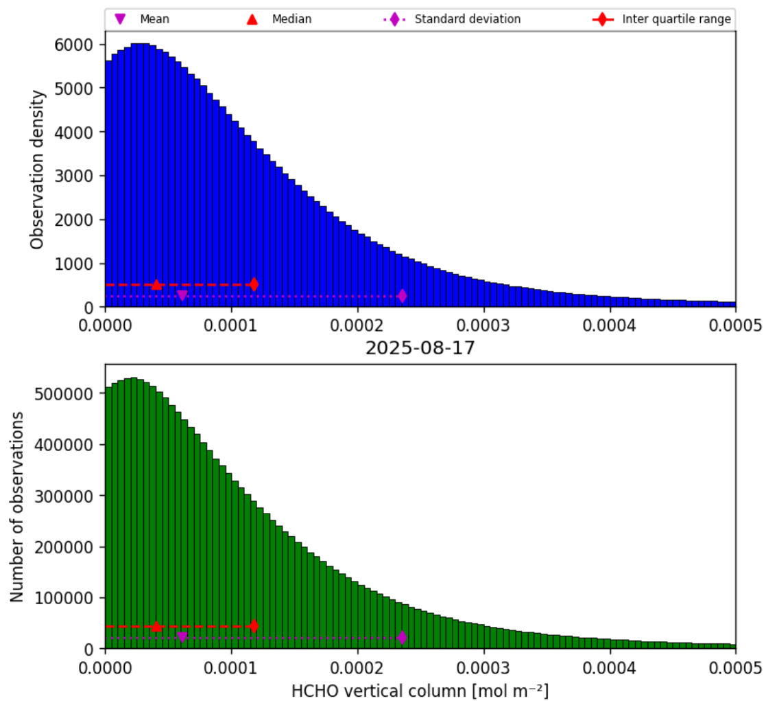
Figure 35: Histogram of “HCHO vertical column” for 2025-08-16 to 2025-08-18
