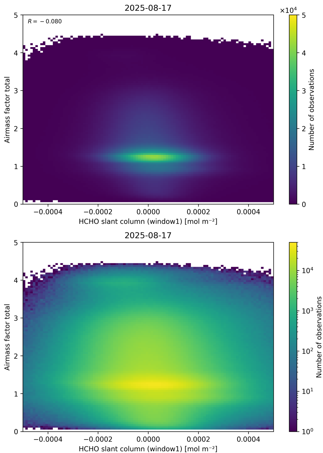
Figure 85: Scatter density plot of “HCHO slant column (window1)” against “Airmass factor total” for 2025-08-16 to 2025-08-18.
