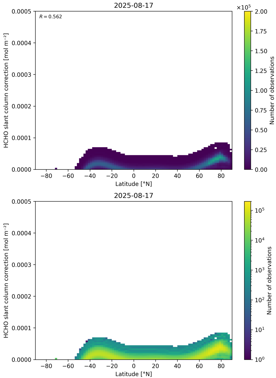
Figure 158: Scatter density plot of “Latitude” against “HCHO slant column correction” for 2025-08-16 to 2025-08-18.
