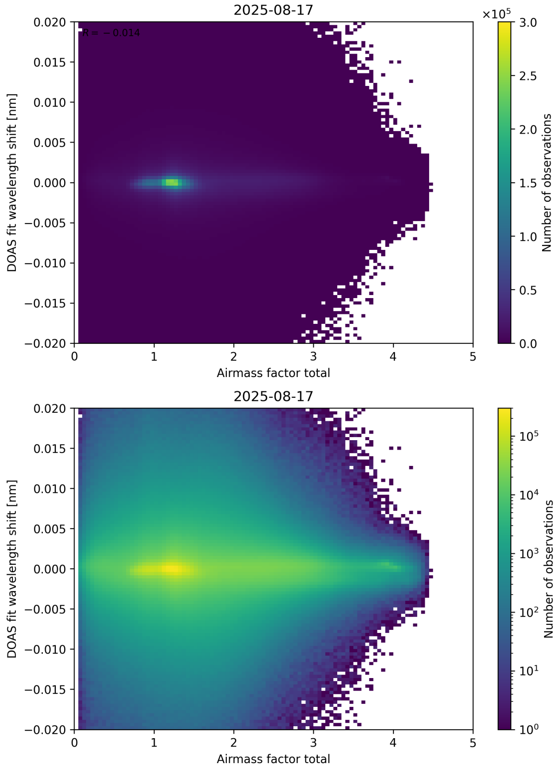
Figure 98: Scatter density plot of “Airmass factor total” against “DOAS fit wavelength shift” for 2025-08-16 to 2025-08-18.
