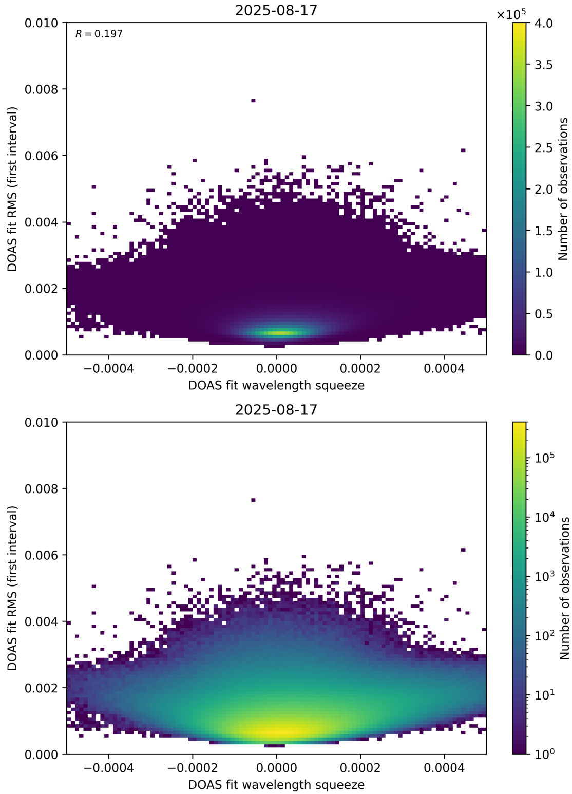
Figure 68: Scatter density plot of “DOAS fit wavelength squeeze” against “DOAS fit RMS (first interval)” for 2025-08-16 to 2025-08-18.
