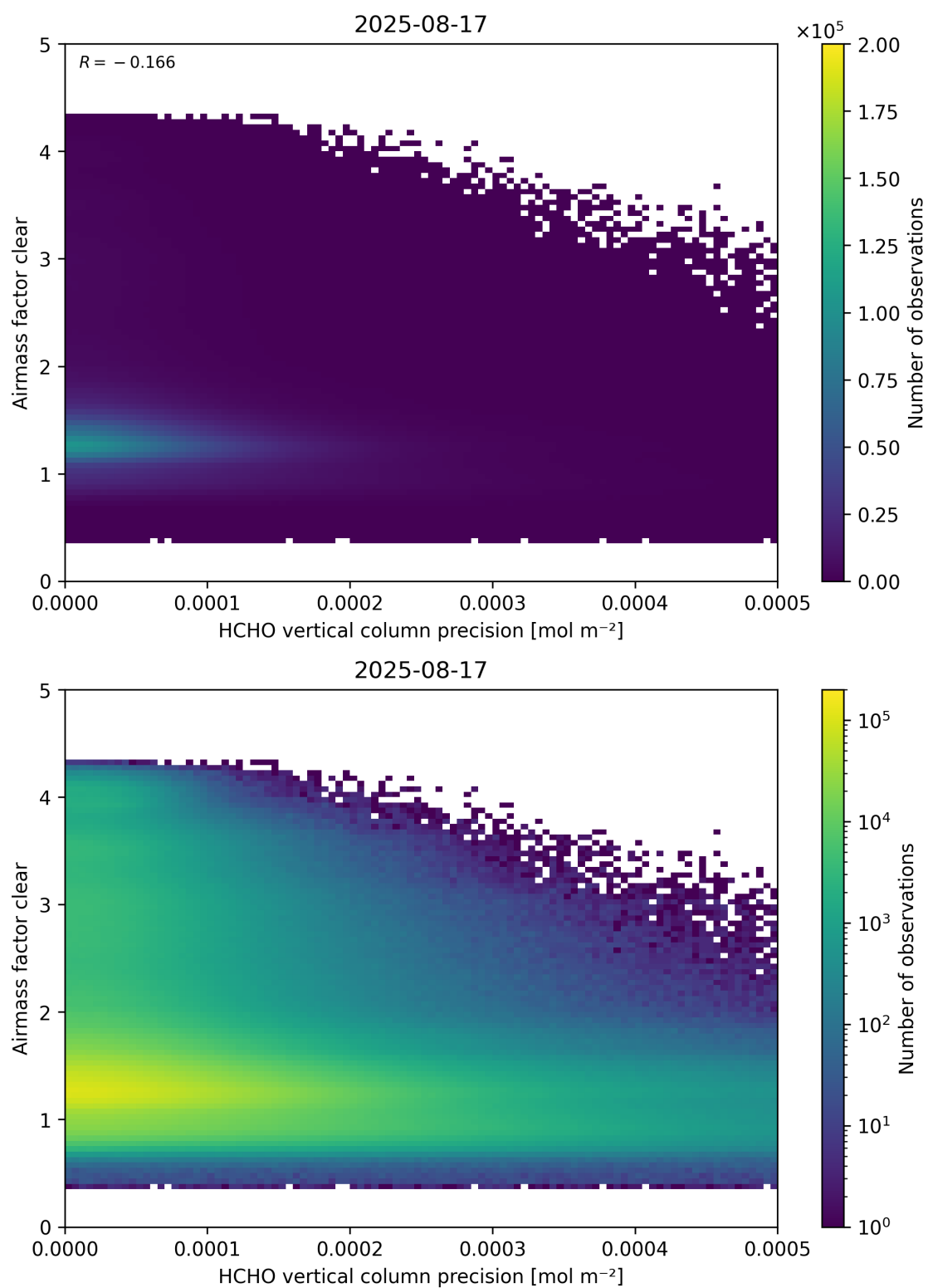
Figure 139: Scatter density plot of “HCHO vertical column precision” against “Airmass factor clear” for 2025-08-16 to 2025-08-18.
