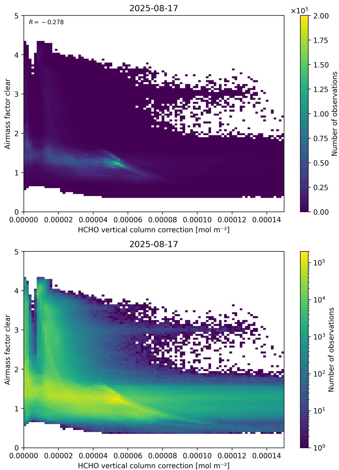
Figure 115: Scatter density plot of “HCHO vertical column correction” against “Airmass factor clear” for 2025-08-16 to 2025-08-18.
