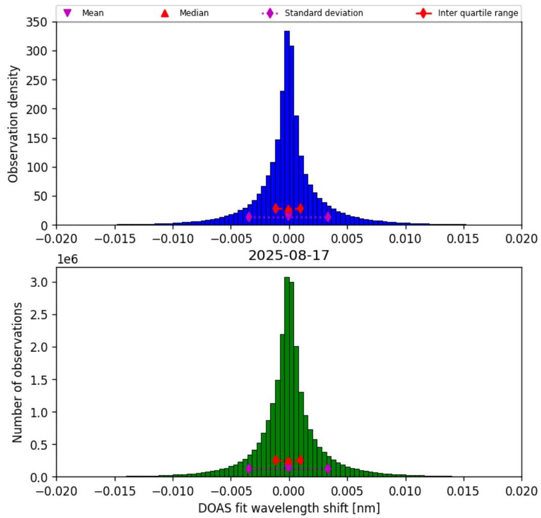
Figure 44: Histogram of “DOAS fit wavelength shift” for 2025-08-16 to 2025-08-18
