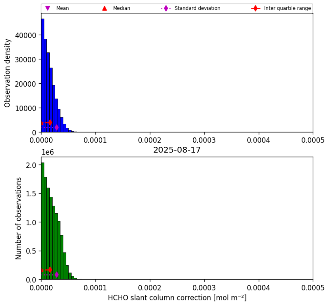
Figure 47: Histogram of “HCHO slant column correction” for 2025-08-16 to 2025-08-18
