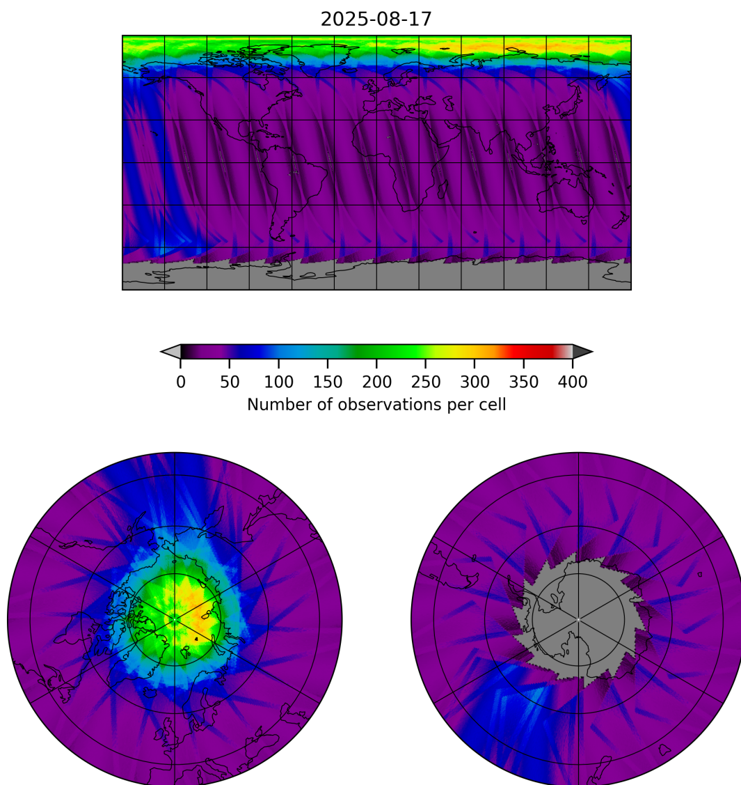
Figure 19: Map of the number of observations for 2025-08-16 to 2025-08-18
