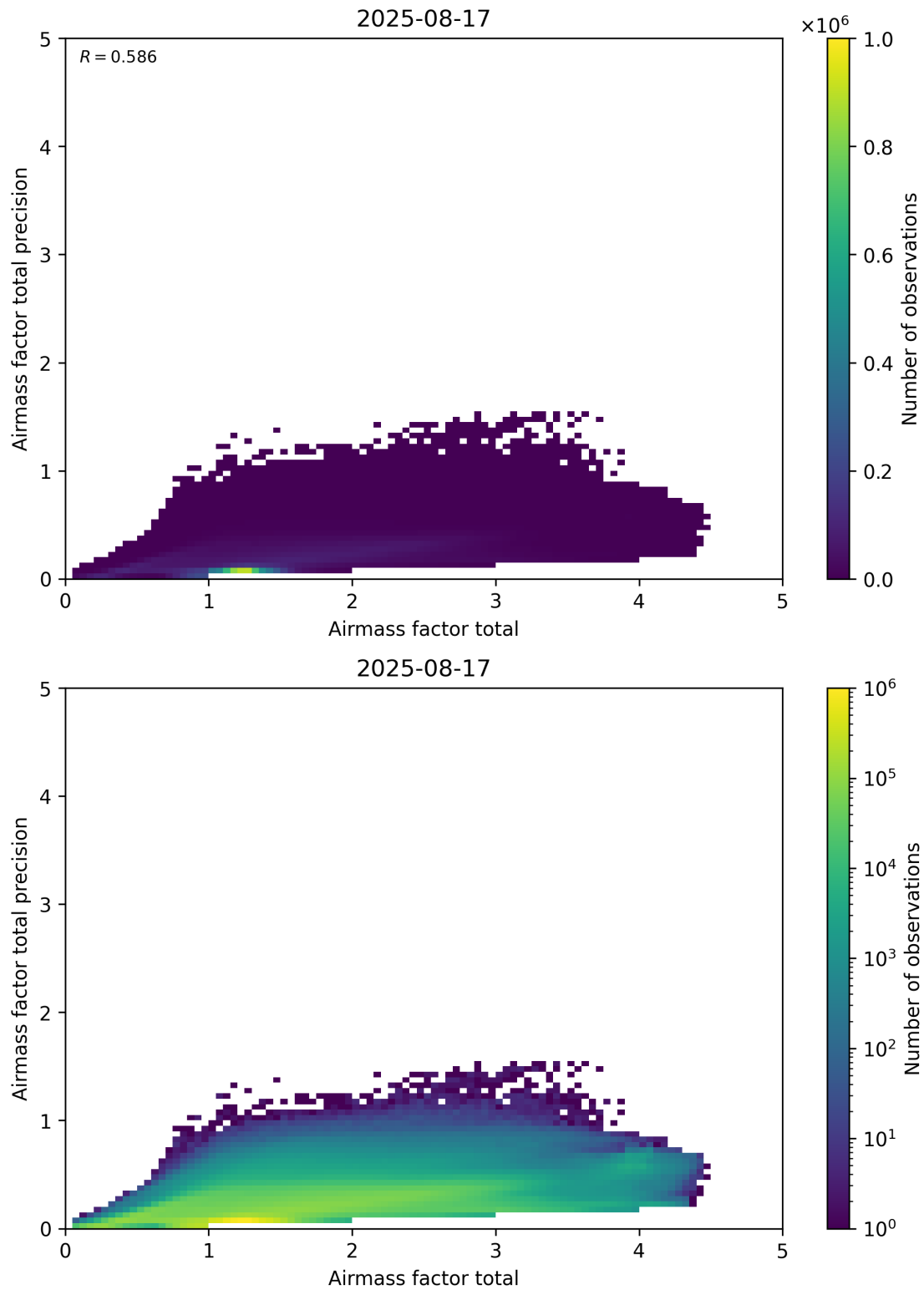
Figure 103: Scatter density plot of “Airmass factor total” against “Airmass factor total precision” for 2025-08-16 to 2025-08-18.
