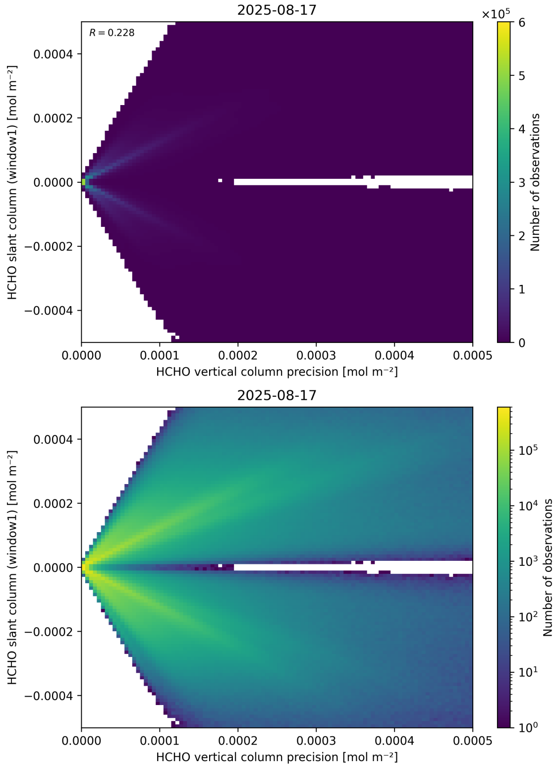
Figure 142: Scatter density plot of “HCHO vertical column precision” against “HCHO slant column (window1)” for 2025-08-16 to 2025-08-18.
