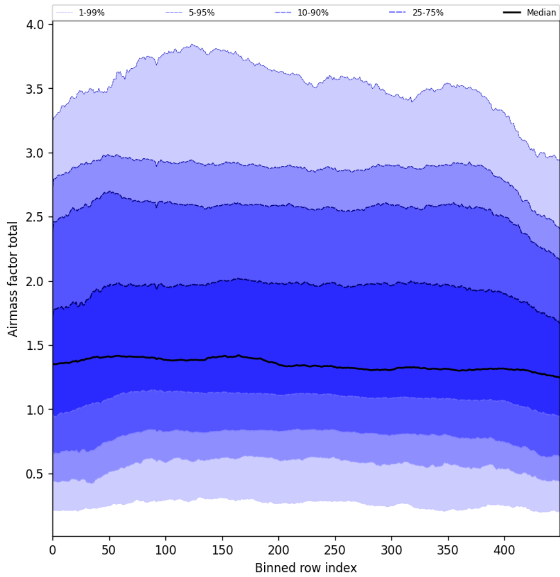
Figure 54: Along track statistics of “Airmass factor total” for 2025-08-16 to 2025-08-18
