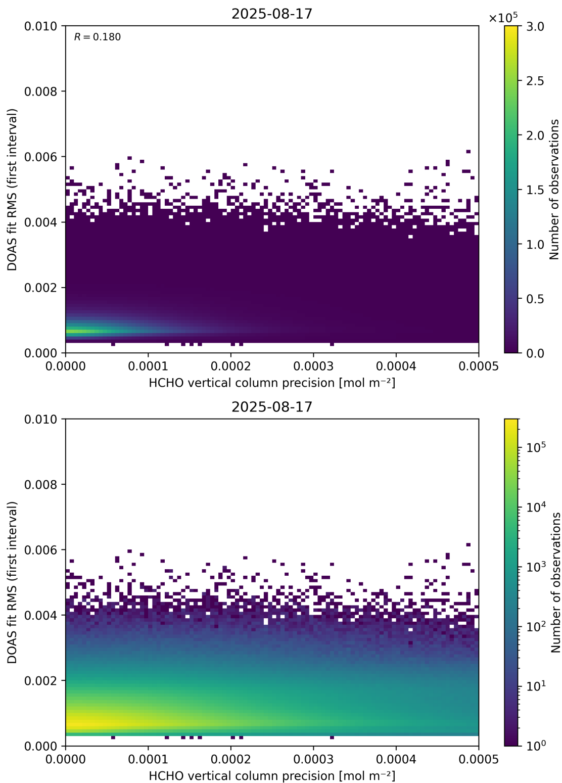
Figure 136: Scatter density plot of “HCHO vertical column precision” against “DOAS fit RMS (first interval)” for 2025-08-16 to 2025-08-18.
