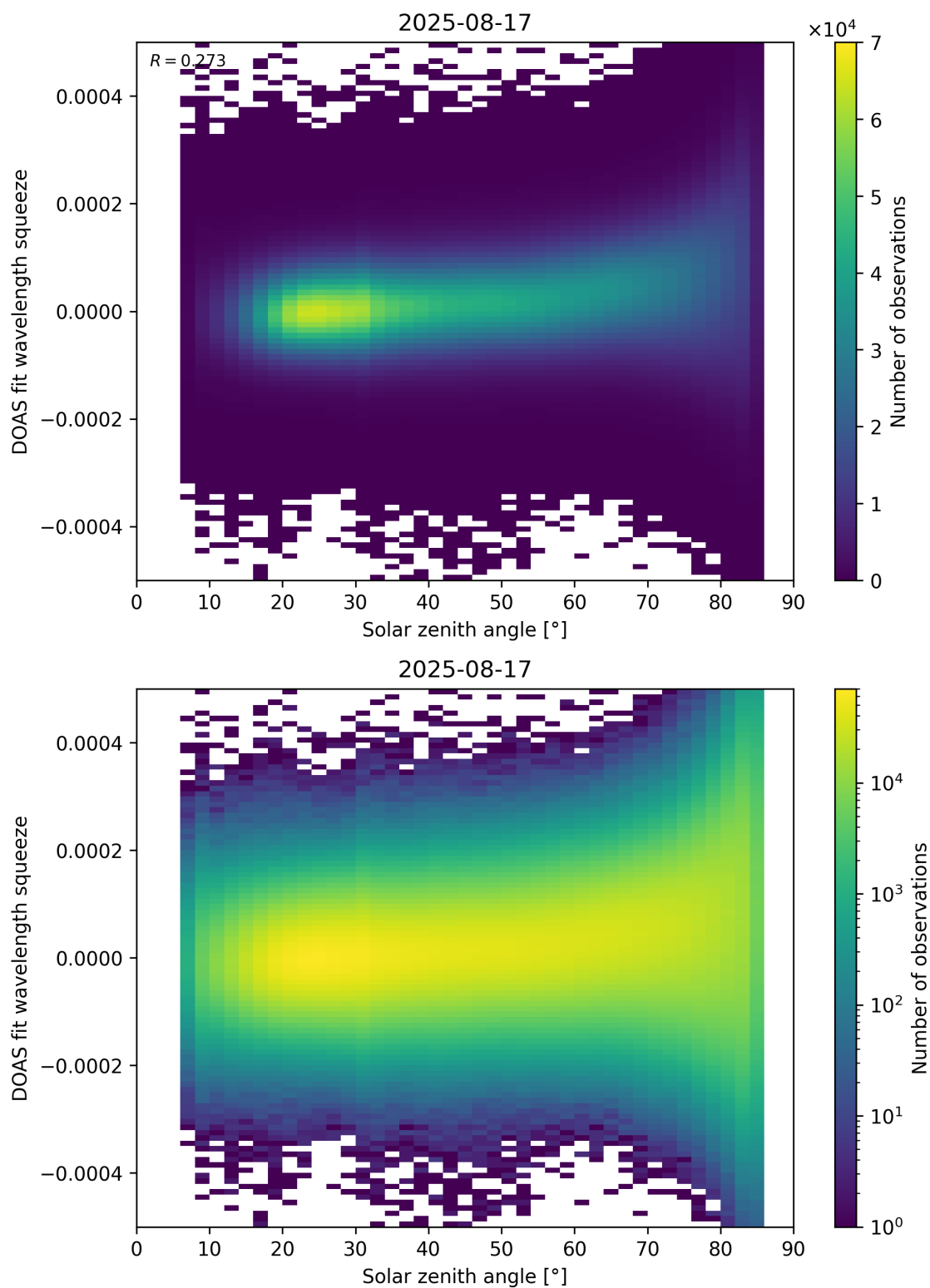
Figure 169: Scatter density plot of “Solar zenith angle” against “DOAS fit wavelength squeeze” for 2025-08-16 to 2025-08-18.
