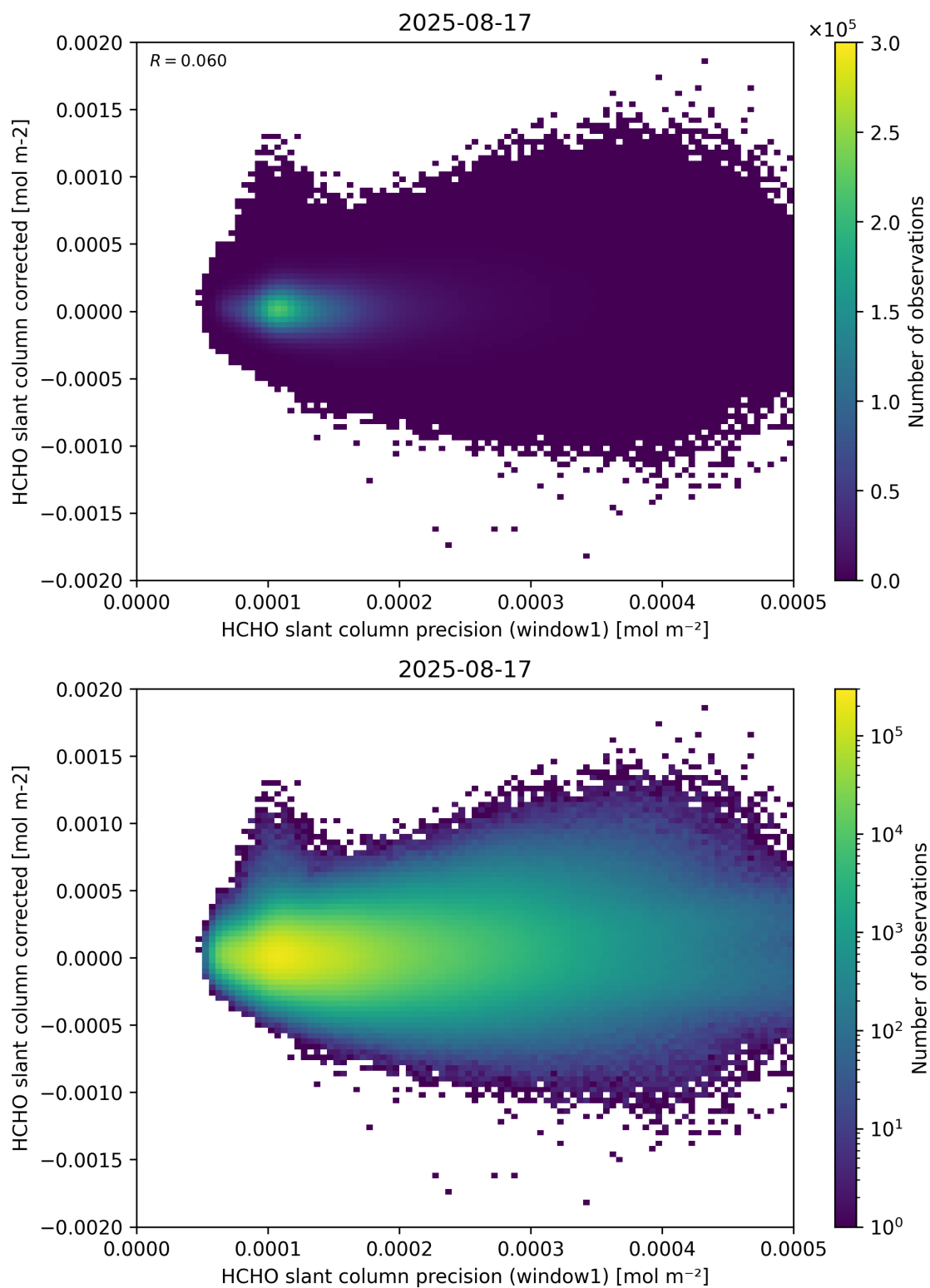
Figure 92: Scatter density plot of “HCHO slant column precision (window1)” against “HCHO slant column corrected” for 2025-08-16 to 2025-08-18.
