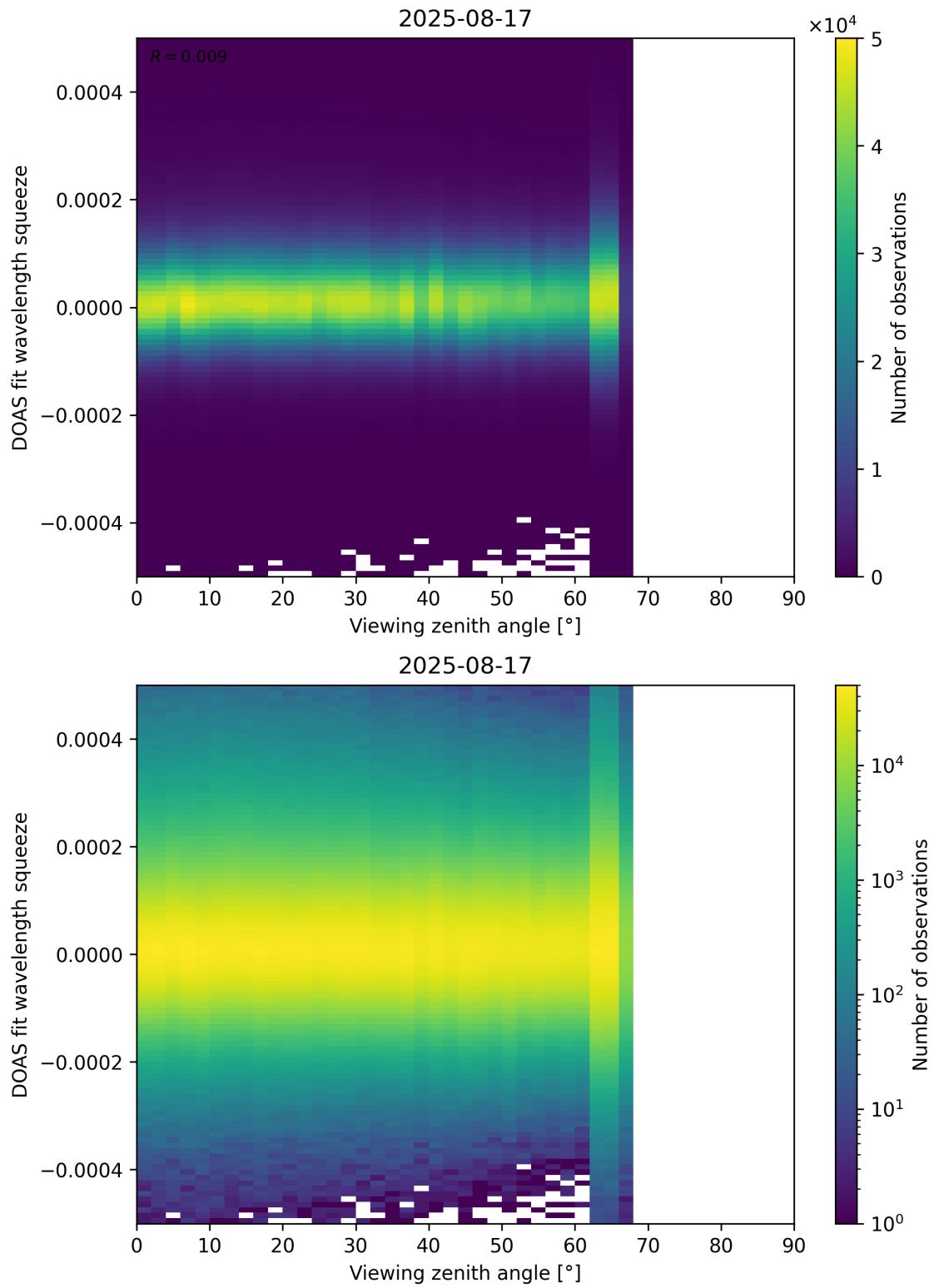
Figure 184: Scatter density plot of “Viewing zenith angle” against “DOAS fit wavelength squeeze” for 2025-08-16 to 2025-08-18.
