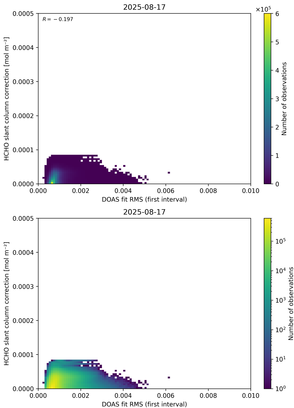
Figure 63: Scatter density plot of “DOAS fit RMS (first interval)” against “HCHO slant column correction” for 2025-08-16 to 2025-08-18.
