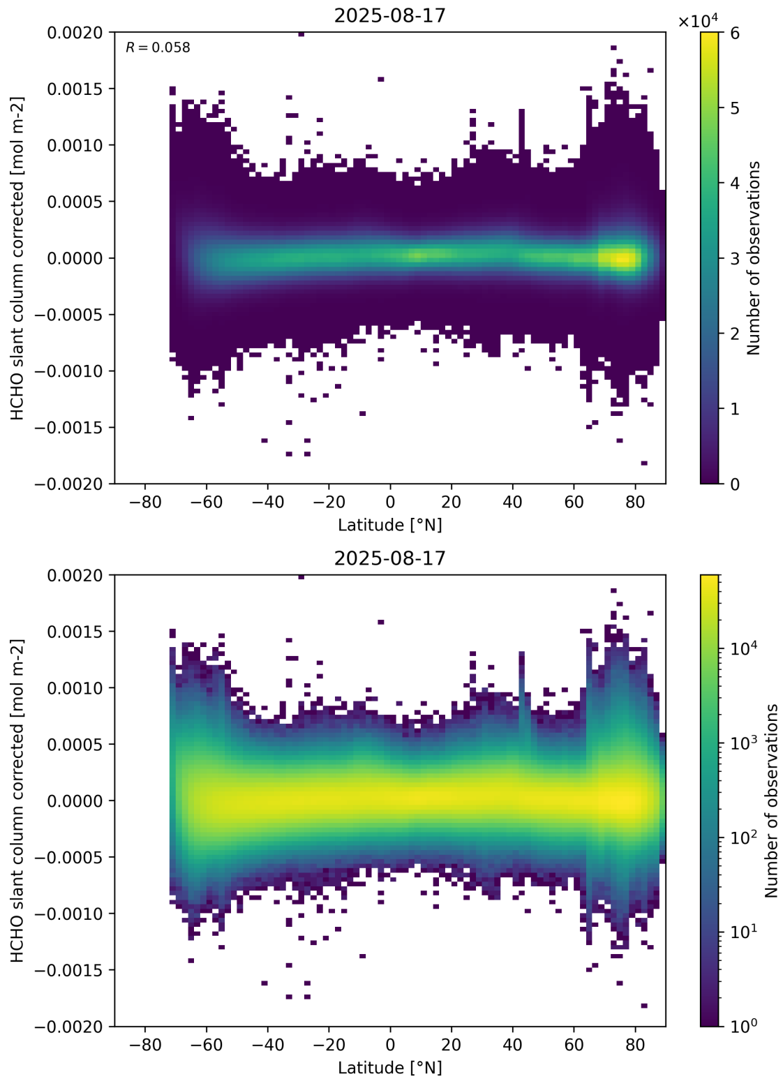
Figure 157: Scatter density plot of “Latitude” against “HCHO slant column corrected” for 2025-08-16 to 2025-08-18.
