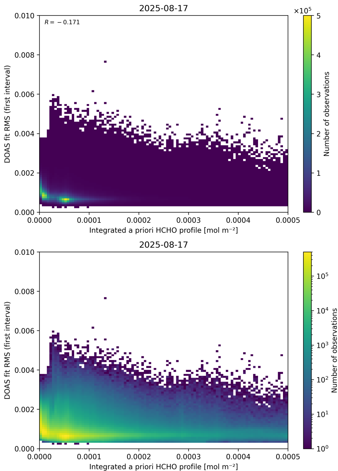
Figure 148: Scatter density plot of “Integrated a priori HCHO profile” against “DOAS fit RMS (first interval)” for 2025-08-16 to 2025-08-18.
