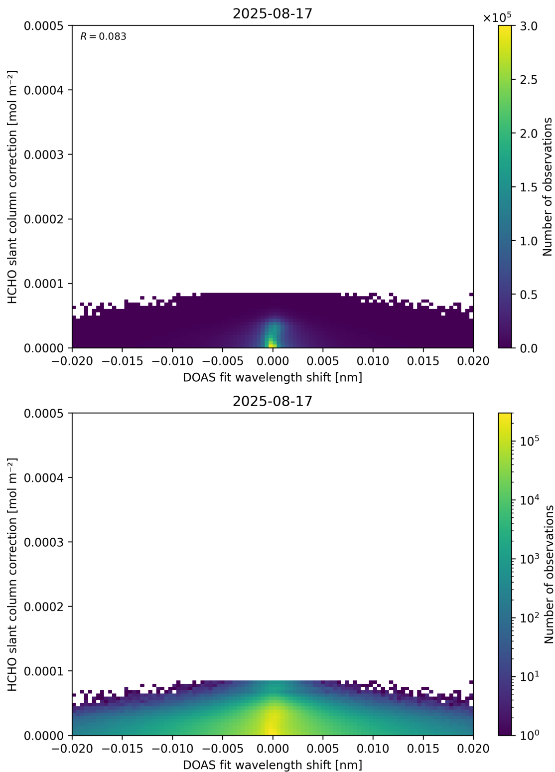
Figure 67: Scatter density plot of “DOAS fit wavelength shift” against “HCHO slant column correction” for 2025-08-16 to 2025-08-18.
