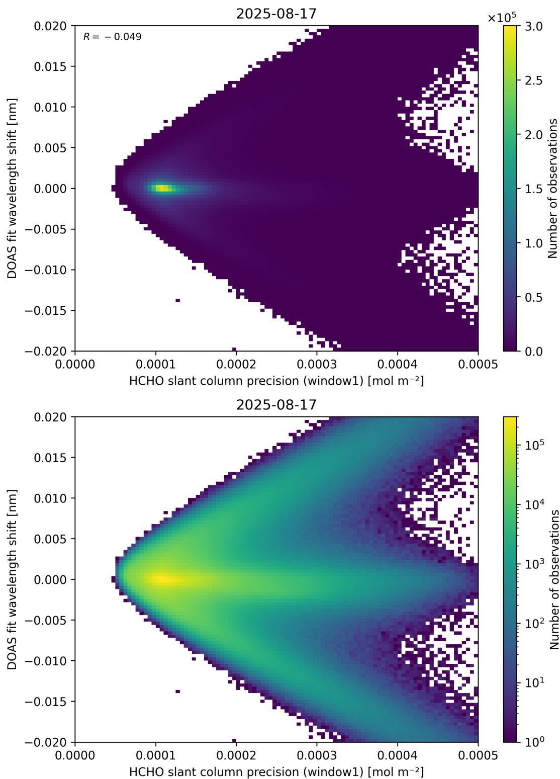
Figure 89: Scatter density plot of “HCHO slant column precision (window1)” against “DOAS fit wavelength shift” for 2025-08-16 to 2025-08-18.
