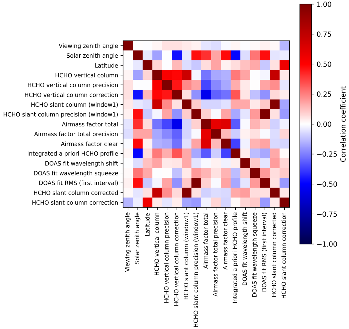
Figure 2: Map of correlation matrix for 2025-08-16 to 2025-08-18.
