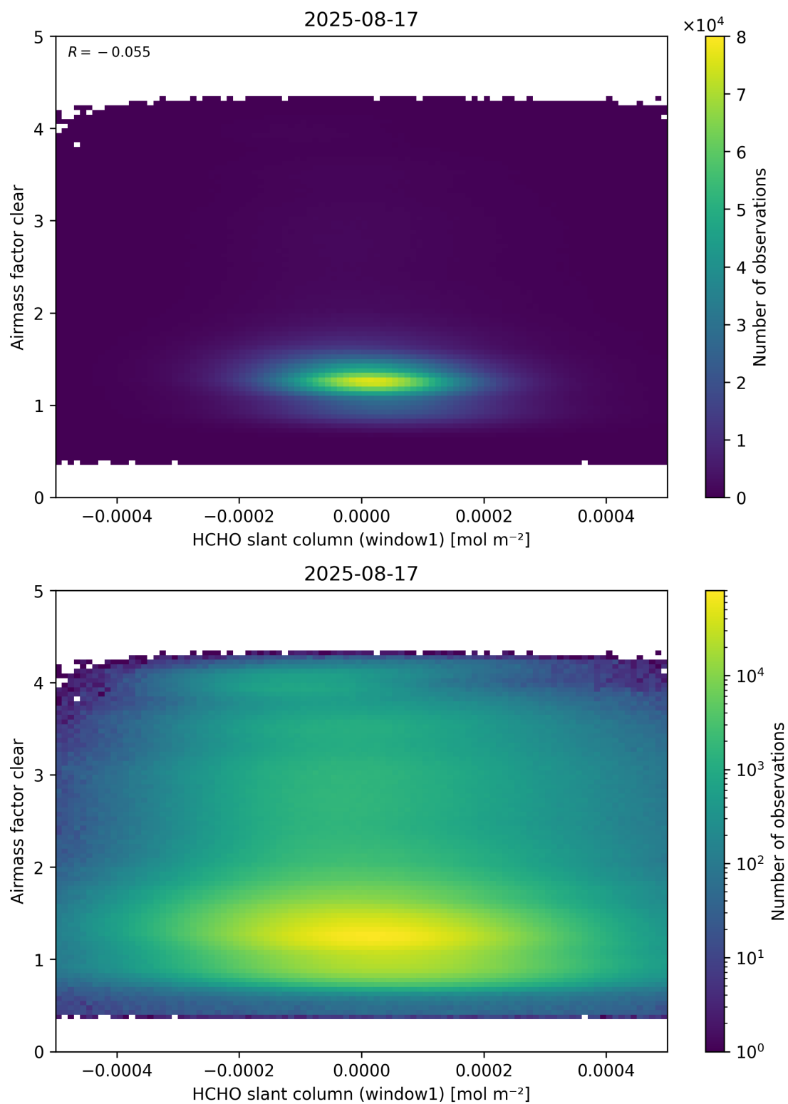
Figure 81: Scatter density plot of “HCHO slant column (window1)” against “Airmass factor clear” for 2025-08-16 to 2025-08-18.
