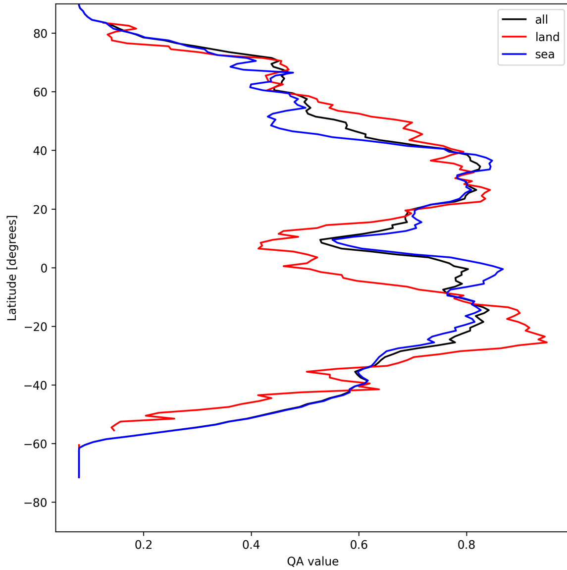
Figure 20: Zonal average of “QA value” for 2025-08-16 to 2025-08-18.
