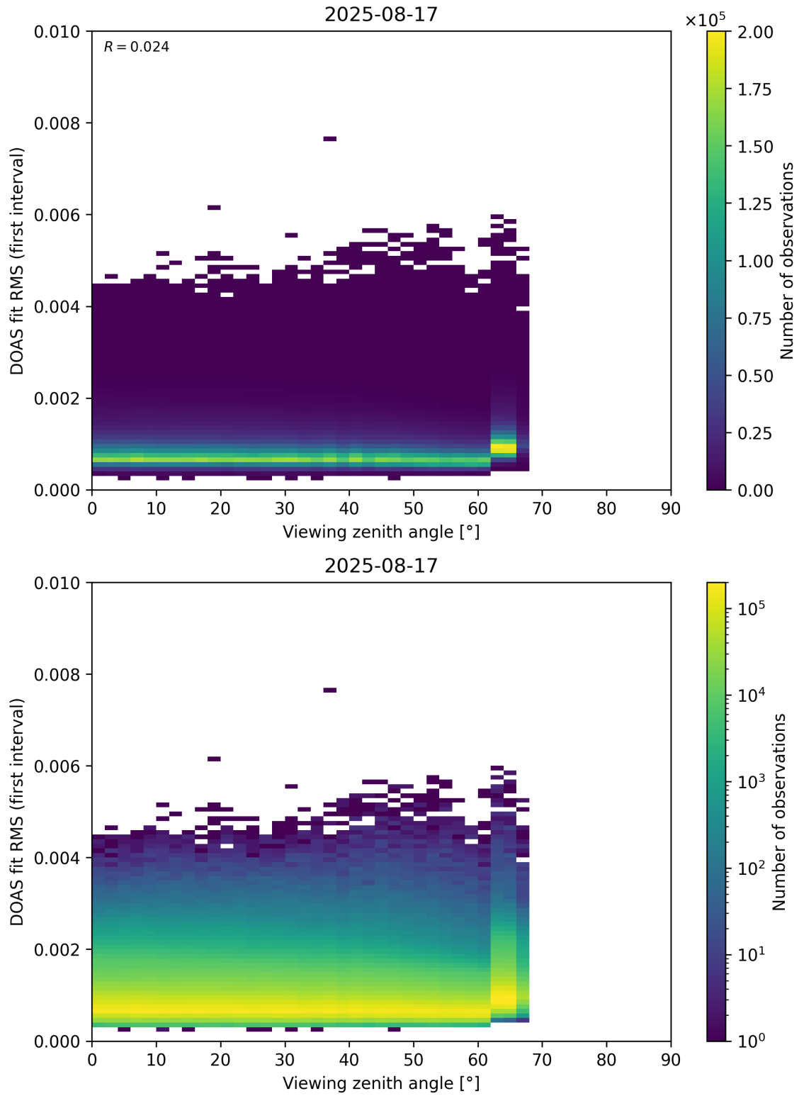
Figure 182: Scatter density plot of “Viewing zenith angle” against “DOAS fit RMS (first interval)” for 2025-08-16 to 2025-08-18.
