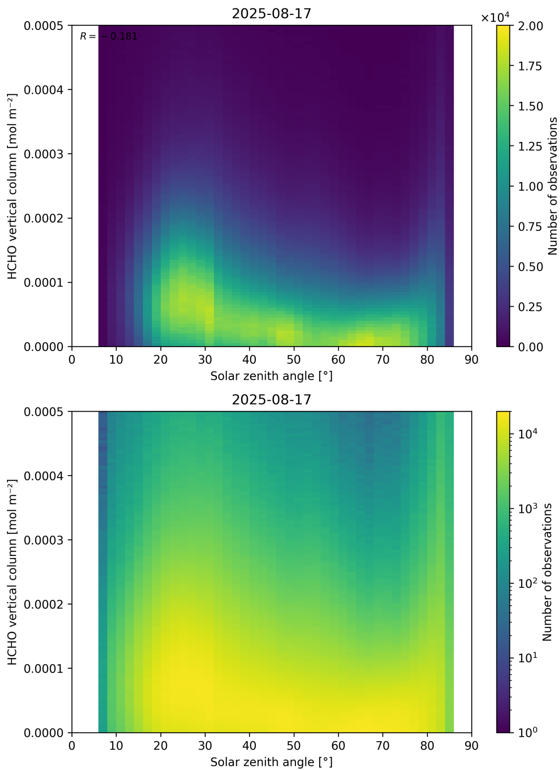
Figure 177: Scatter density plot of “Solar zenith angle” against “HCHO vertical column” for 2025-08-16 to 2025-08-18.
