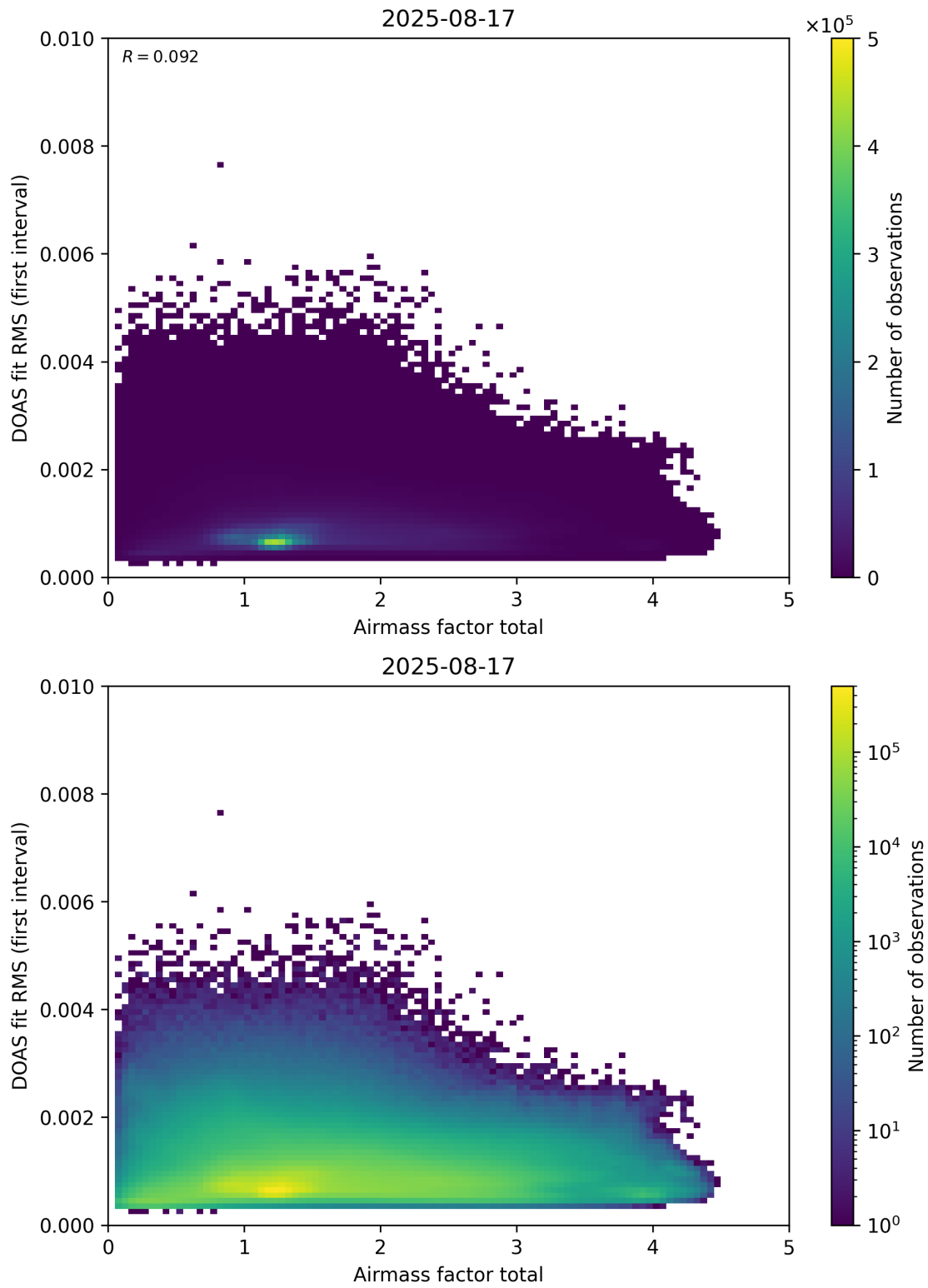
Figure 97: Scatter density plot of “Airmass factor total” against “DOAS fit RMS (first interval)” for 2025-08-16 to 2025-08-18.
