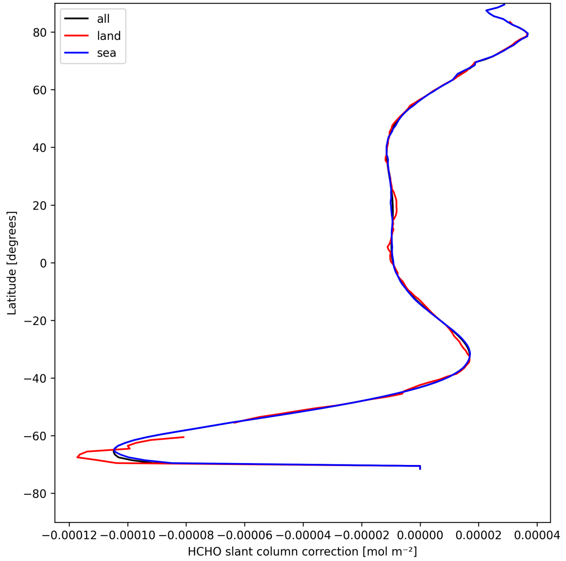
Figure 33: Zonal average of “HCHO slant column correction” for 2025-08-16 to 2025-08-18.
