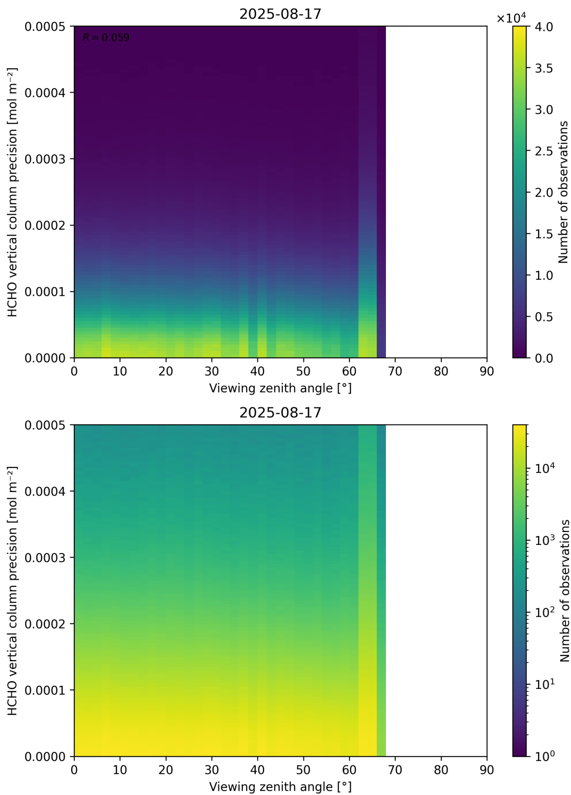
Figure 194: Scatter density plot of “Viewing zenith angle” against “HCHO vertical column precision” for 2025-08-16 to 2025-08-18.
