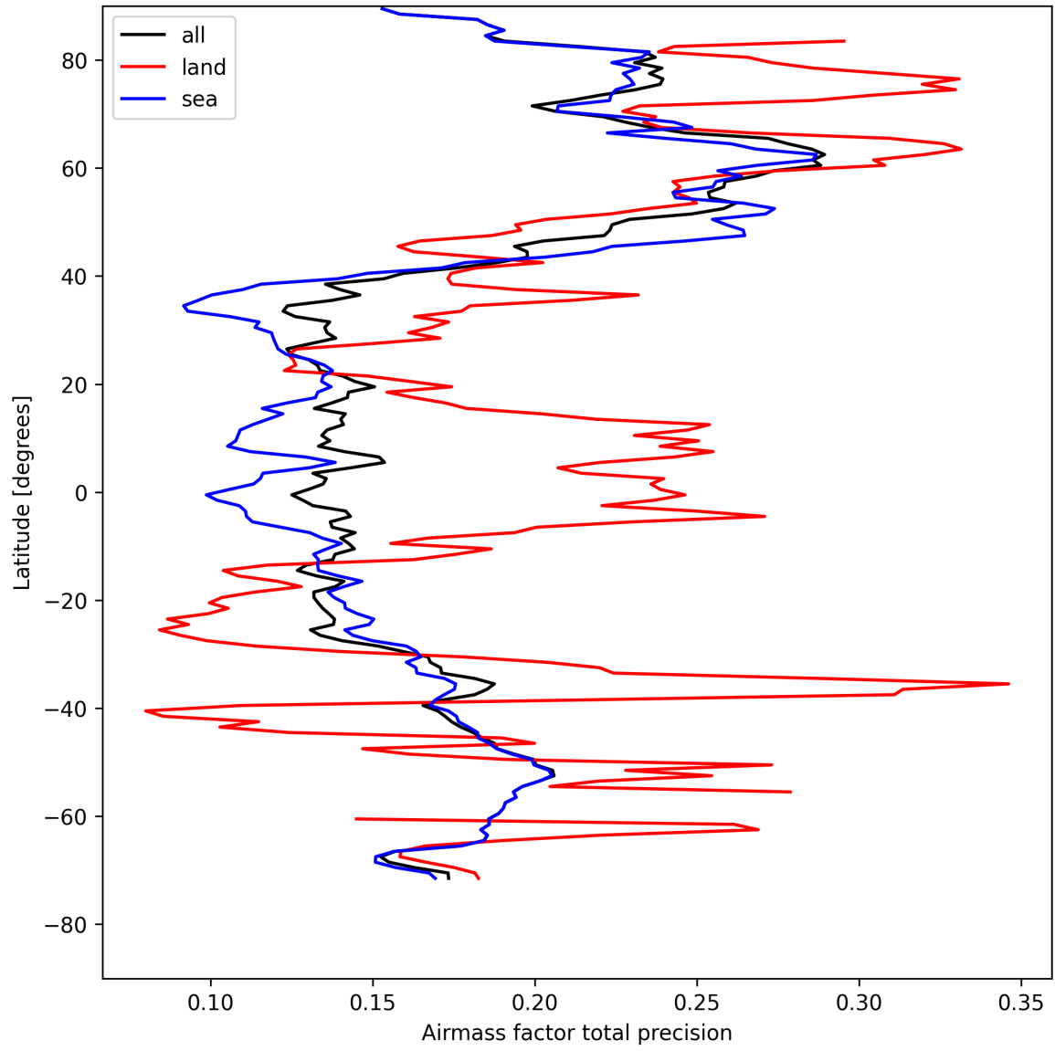
Figure 27: Zonal average of “Airmass factor total precision” for 2025-08-16 to 2025-08-18.
