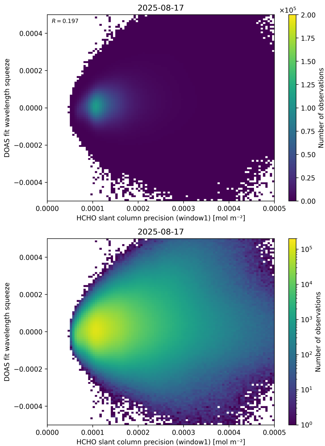
Figure 90: Scatter density plot of “HCHO slant column precision (window1)” against “DOAS fit wavelength squeeze” for 2025-08-16 to 2025-08-18.
