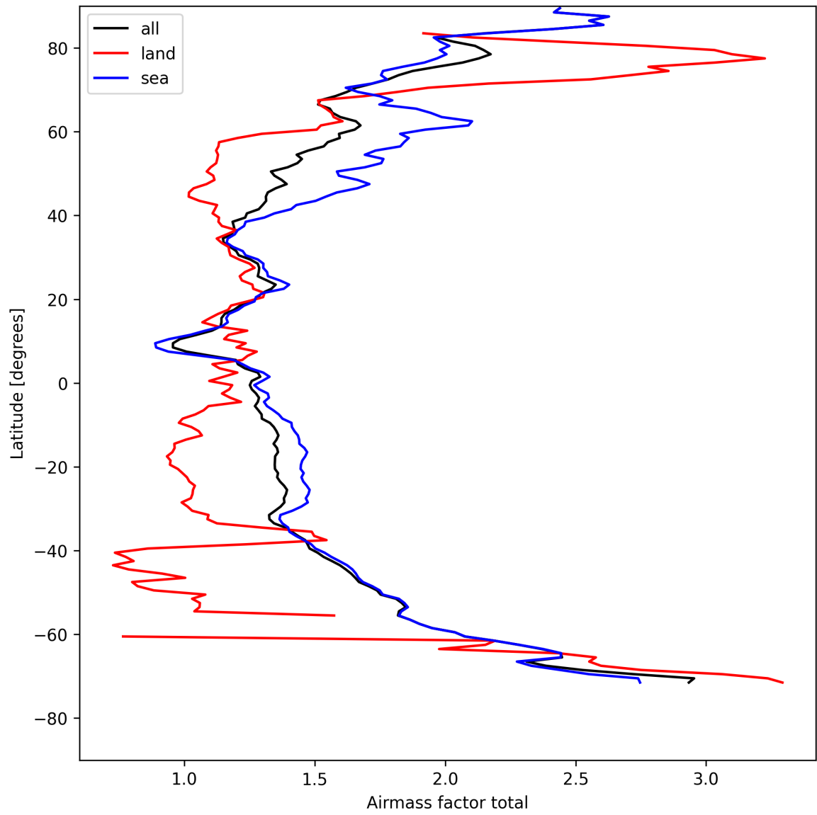
Figure 26: Zonal average of “Airmass factor total” for 2025-08-16 to 2025-08-18.
