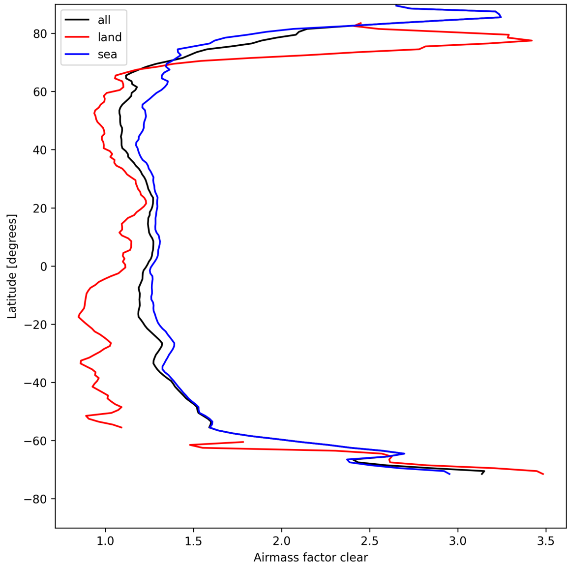
Figure 28: Zonal average of “Airmass factor clear” for 2025-08-16 to 2025-08-18.
