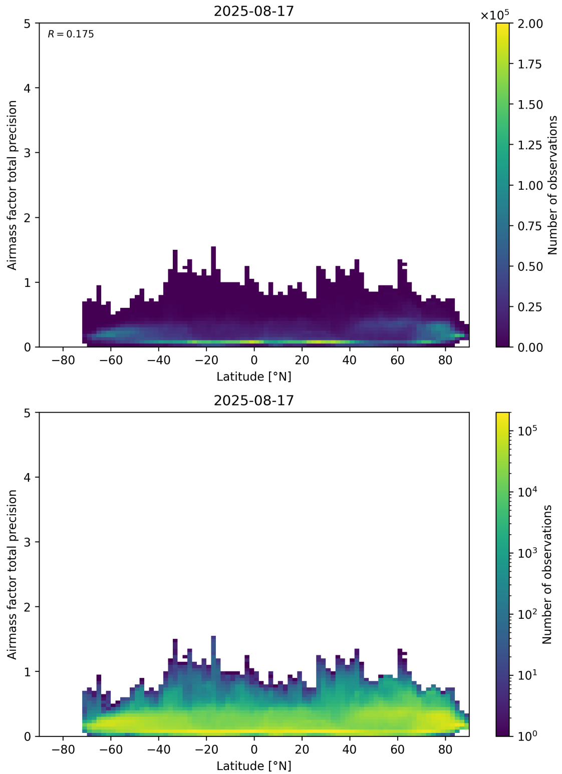
Figure 162: Scatter density plot of “Latitude” against “Airmass factor total precision” for 2025-08-16 to 2025-08-18.
