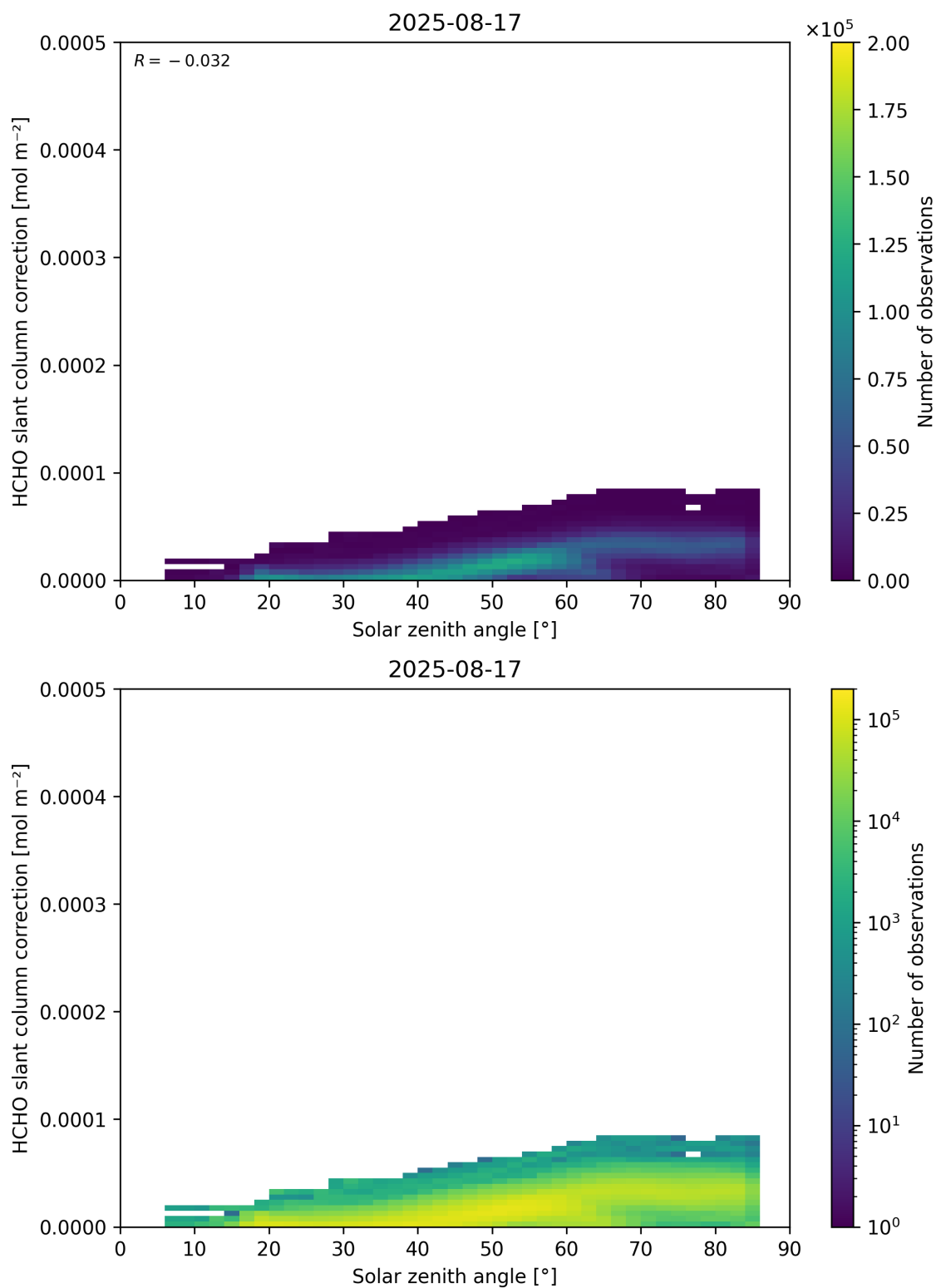
Figure 172: Scatter density plot of “Solar zenith angle” against “HCHO slant column correction” for 2025-08-16 to 2025-08-18.
