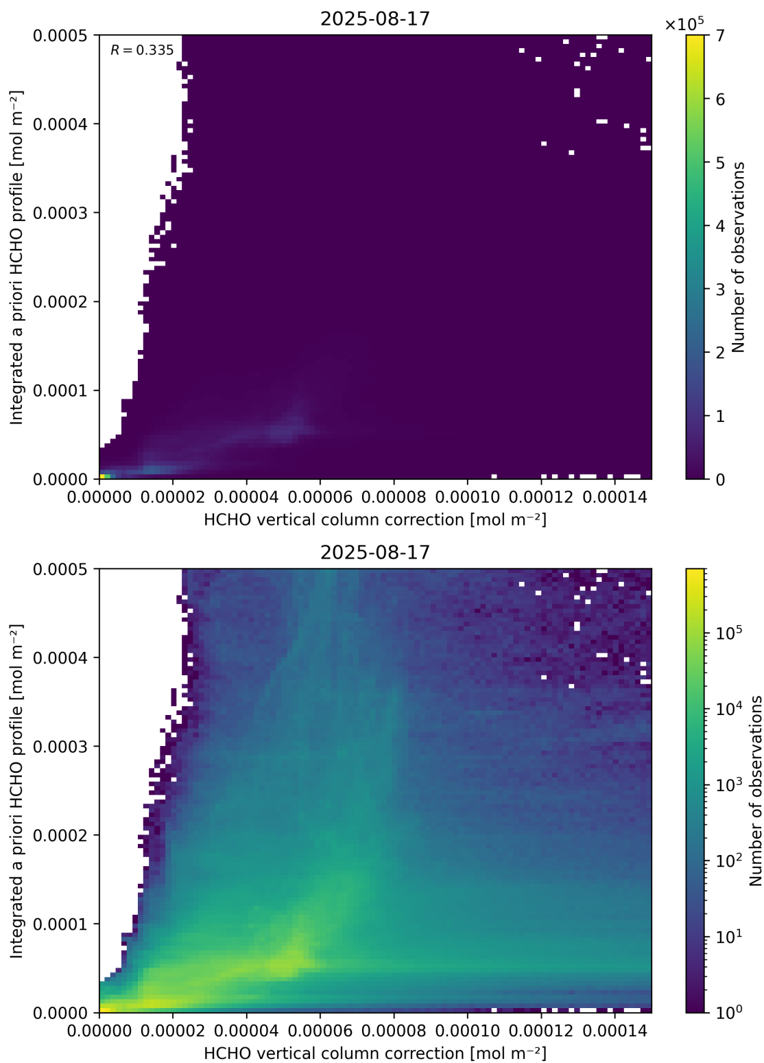
Figure 122: Scatter density plot of “HCHO vertical column correction” against “Integrated a priori HCHO profile” for 2025-08-16 to 2025-08-18.
