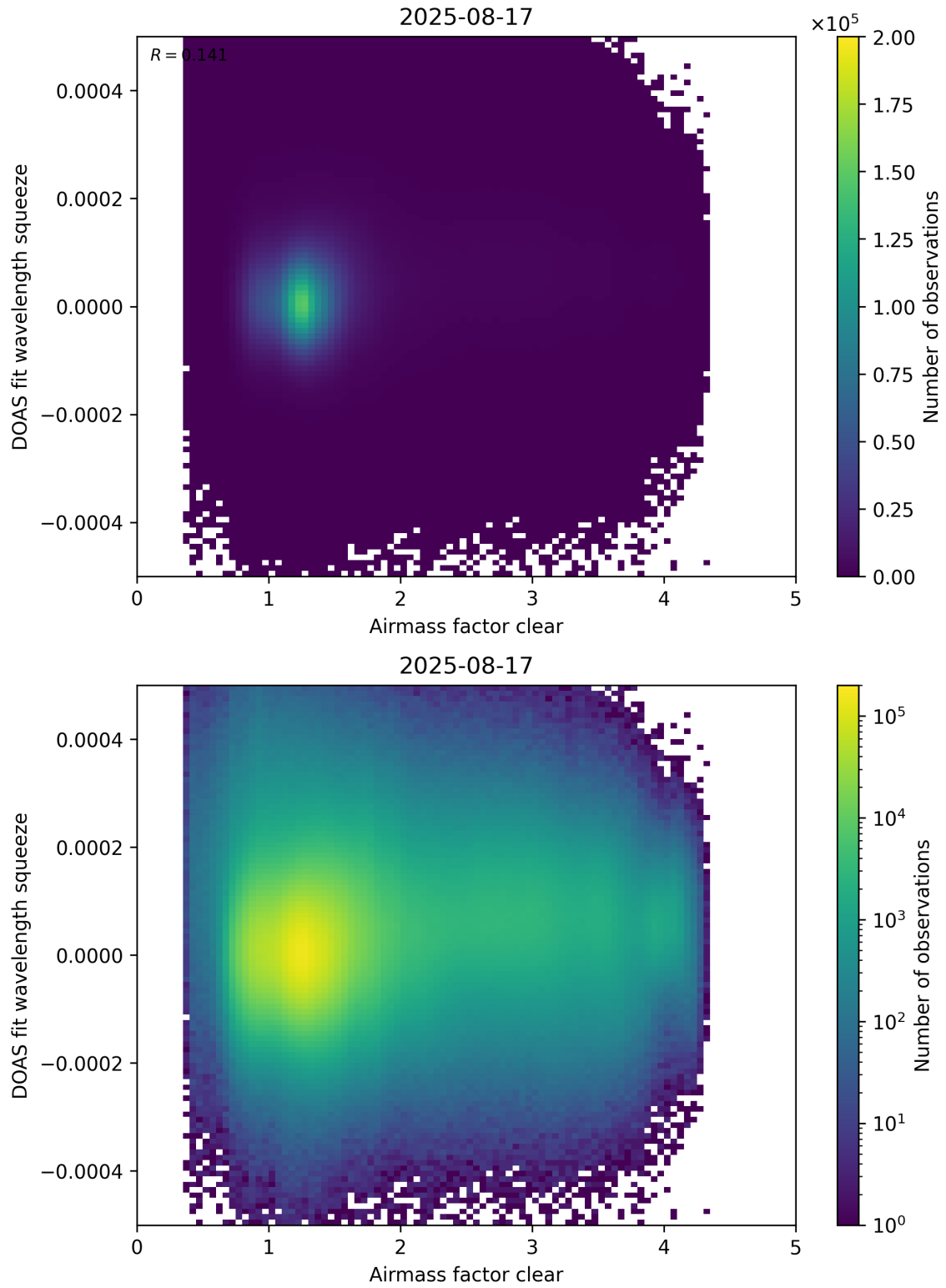
Figure 73: Scatter density plot of “Airmass factor clear” against “DOAS fit wavelength squeeze” for 2025-08-16 to 2025-08-18.
