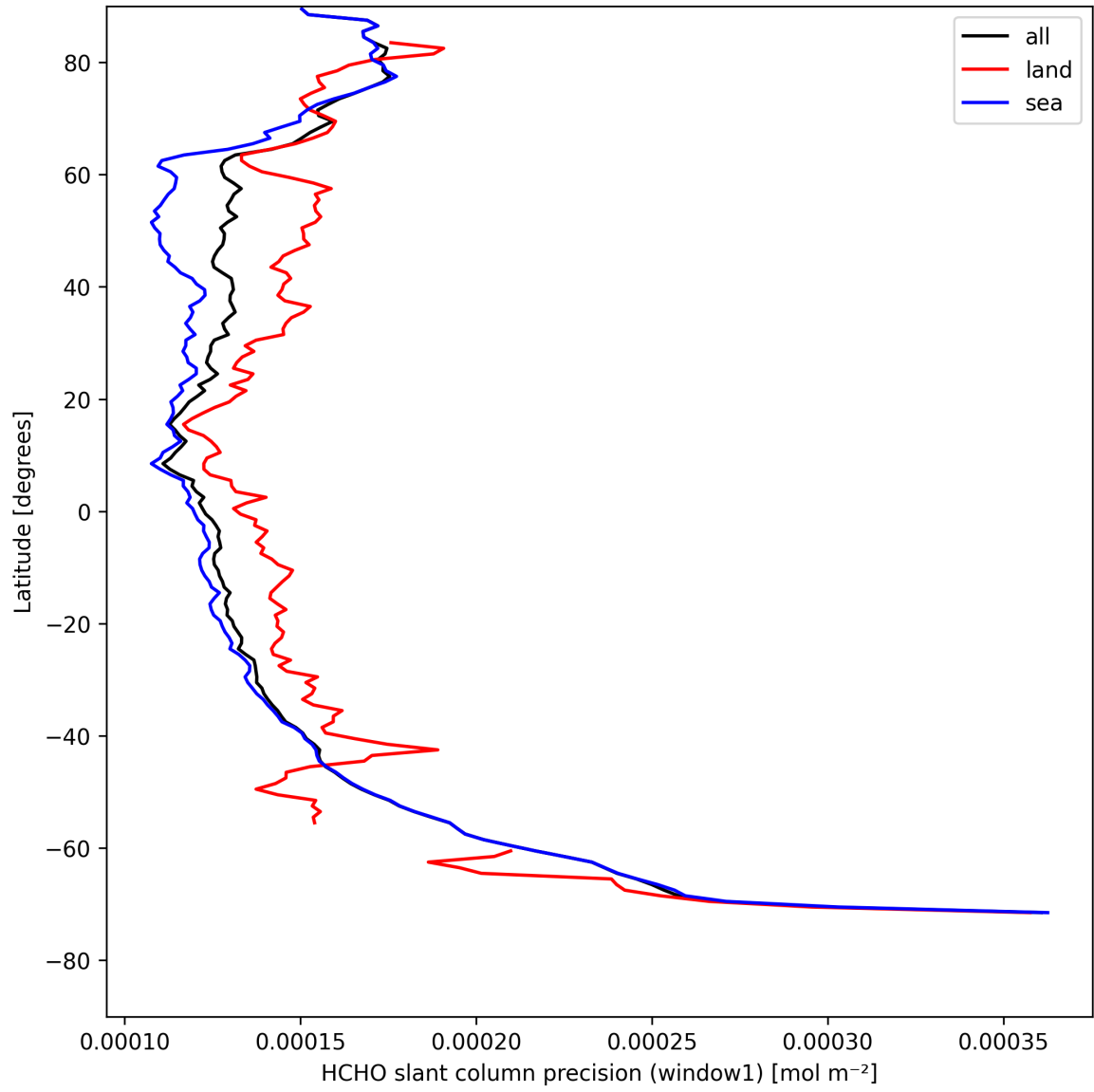
Figure 25: Zonal average of “HCHO slant column precision (window1)” for 2025-08-16 to 2025-08-18.
