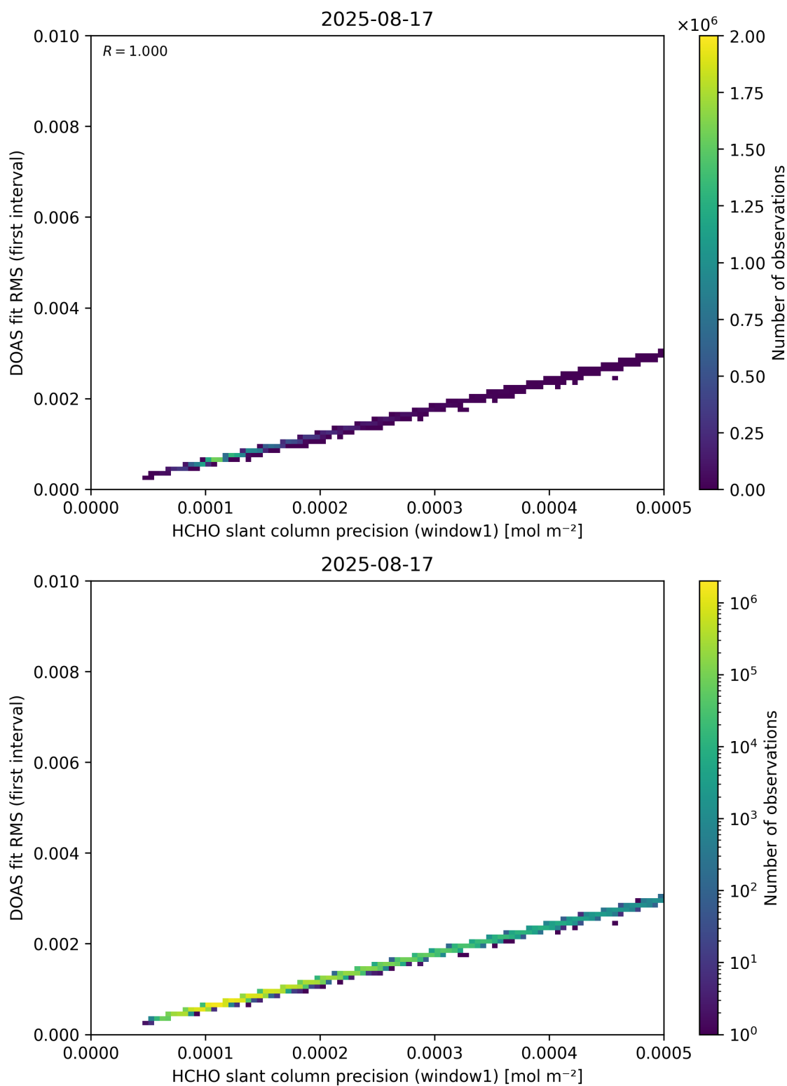
Figure 88: Scatter density plot of “HCHO slant column precision (window1)” against “DOAS fit RMS (first interval)” for 2025-08-16 to 2025-08-18.
