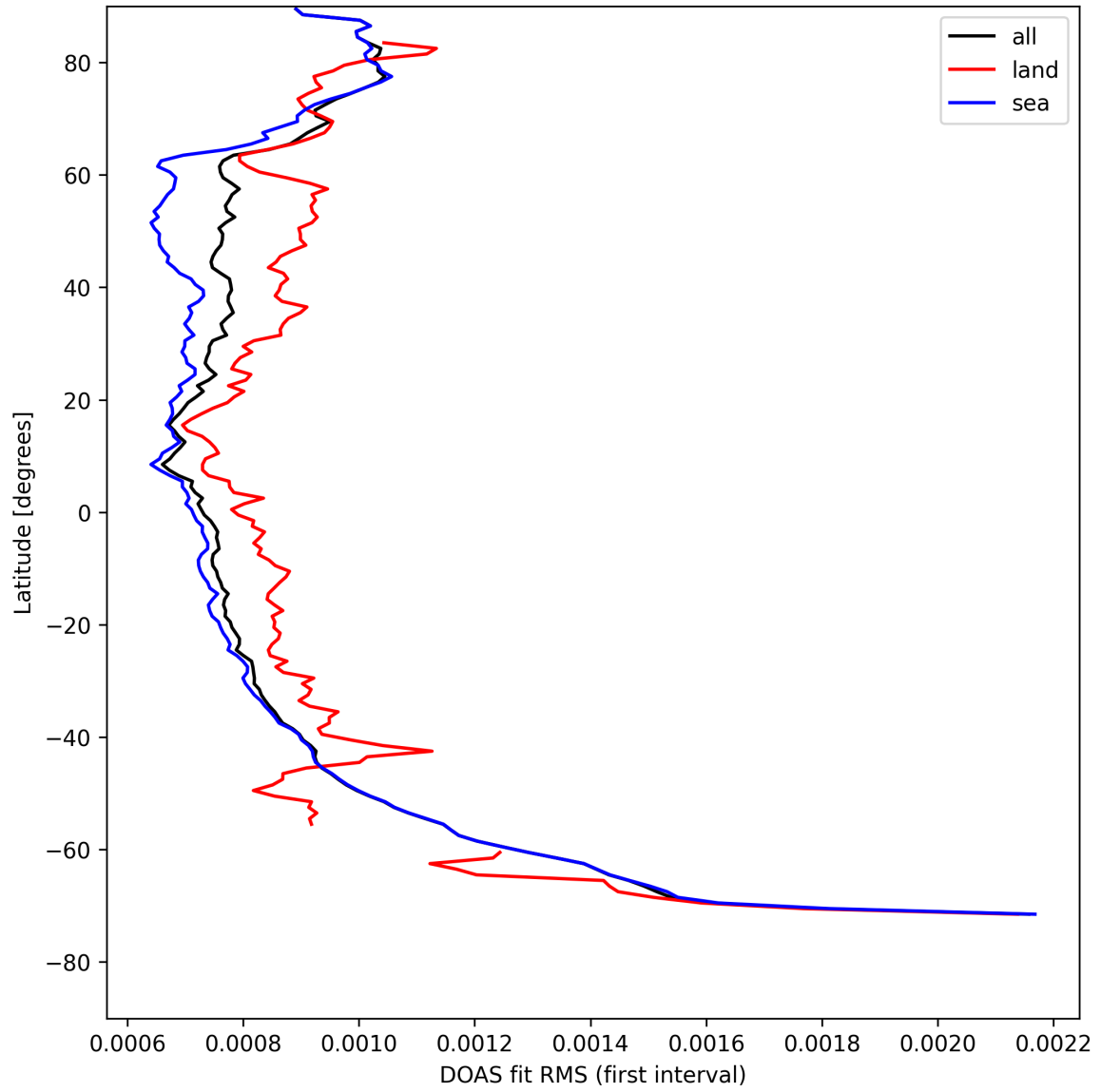
Figure 32: Zonal average of “DOAS fit RMS (first interval)” for 2025-08-16 to 2025-08-18.
