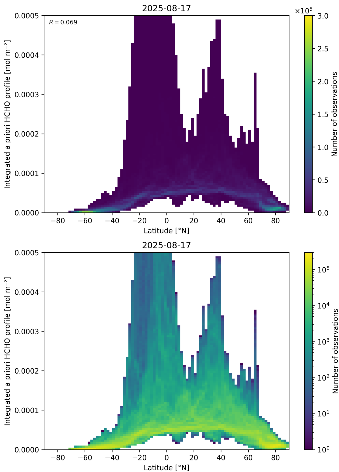
Figure 166: Scatter density plot of “Latitude” against “Integrated a priori HCHO profile” for 2025-08-16 to 2025-08-18.
