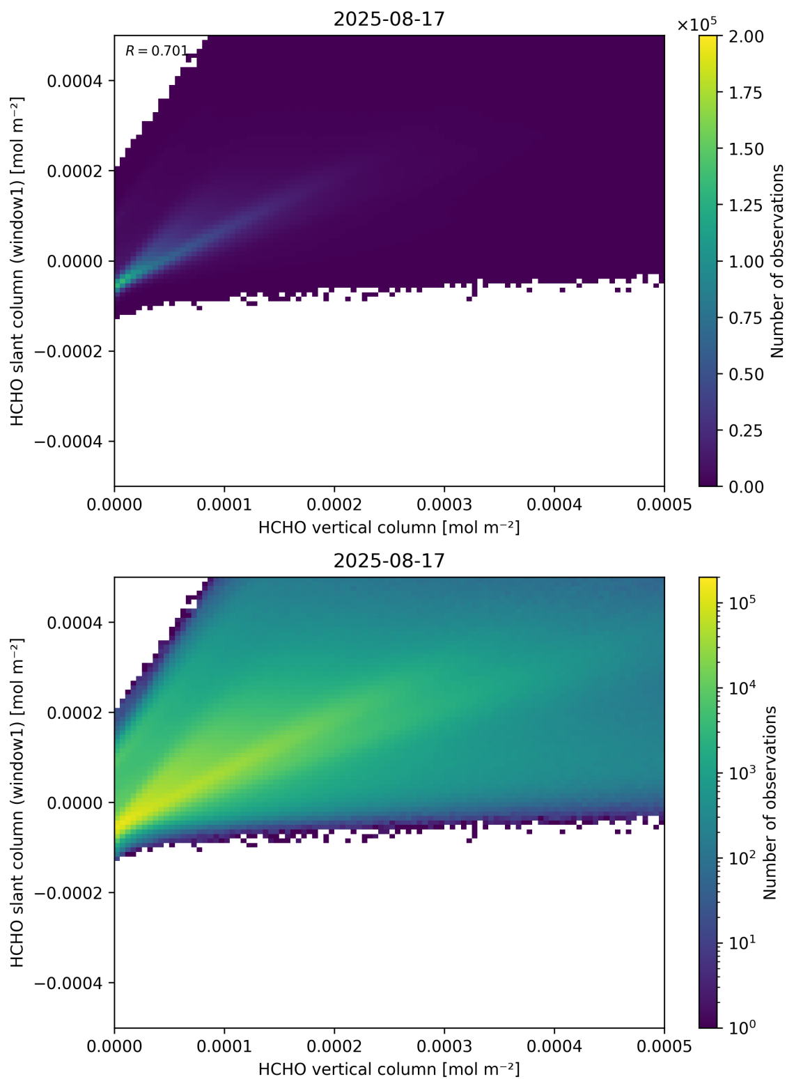
Figure 129: Scatter density plot of “HCHO vertical column” against “HCHO slant column (window1)” for 2025-08-16 to 2025-08-18.
