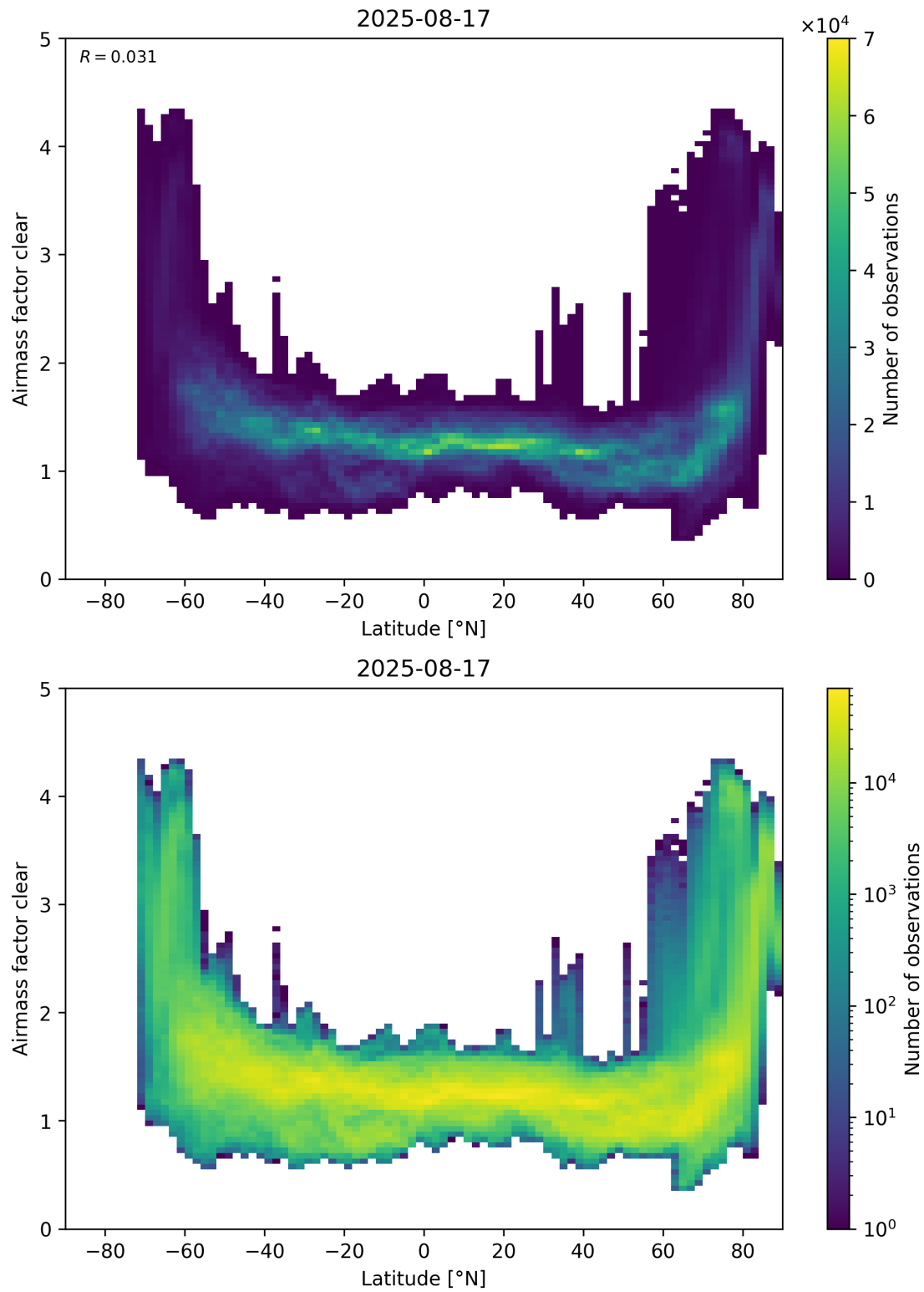
Figure 156: Scatter density plot of “Latitude” against “Airmass factor clear” for 2025-08-16 to 2025-08-18.
