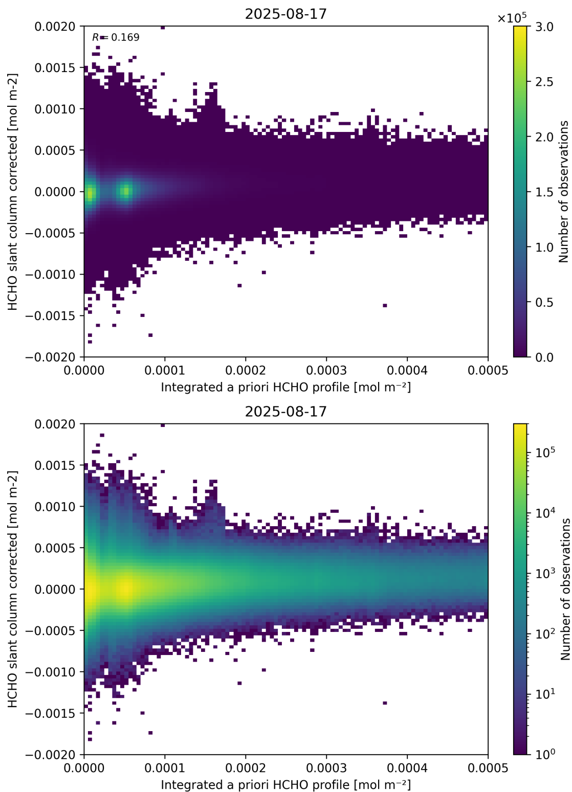
Figure 151: Scatter density plot of “Integrated a priori HCHO profile” against “HCHO slant column corrected” for 2025-08-16 to 2025-08-18.
