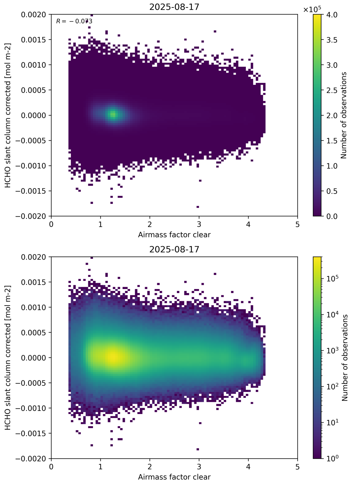
Figure 74: Scatter density plot of “Airmass factor clear” against “HCHO slant column corrected” for 2025-08-16 to 2025-08-18.
