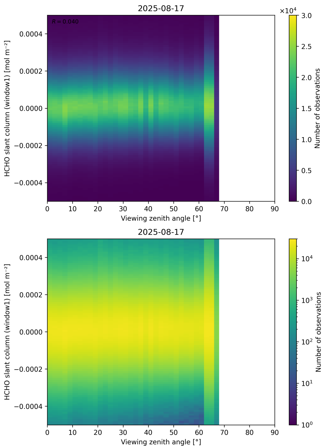
Figure 188: Scatter density plot of “Viewing zenith angle” against “HCHO slant column (window1)” for 2025-08-16 to 2025-08-18.
