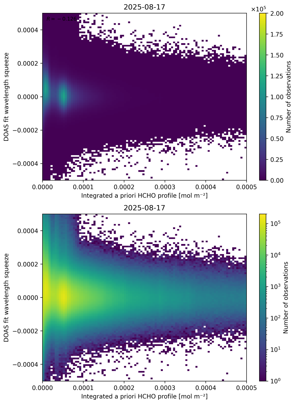
Figure 150: Scatter density plot of “Integrated a priori HCHO profile” against “DOAS fit wavelength squeeze” for 2025-08-16 to 2025-08-18.
