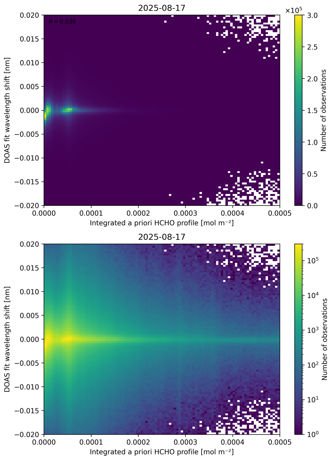
Figure 149: Scatter density plot of “Integrated a priori HCHO profile” against “DOAS fit wavelength shift” for 2025-08-16 to 2025-08-18.
