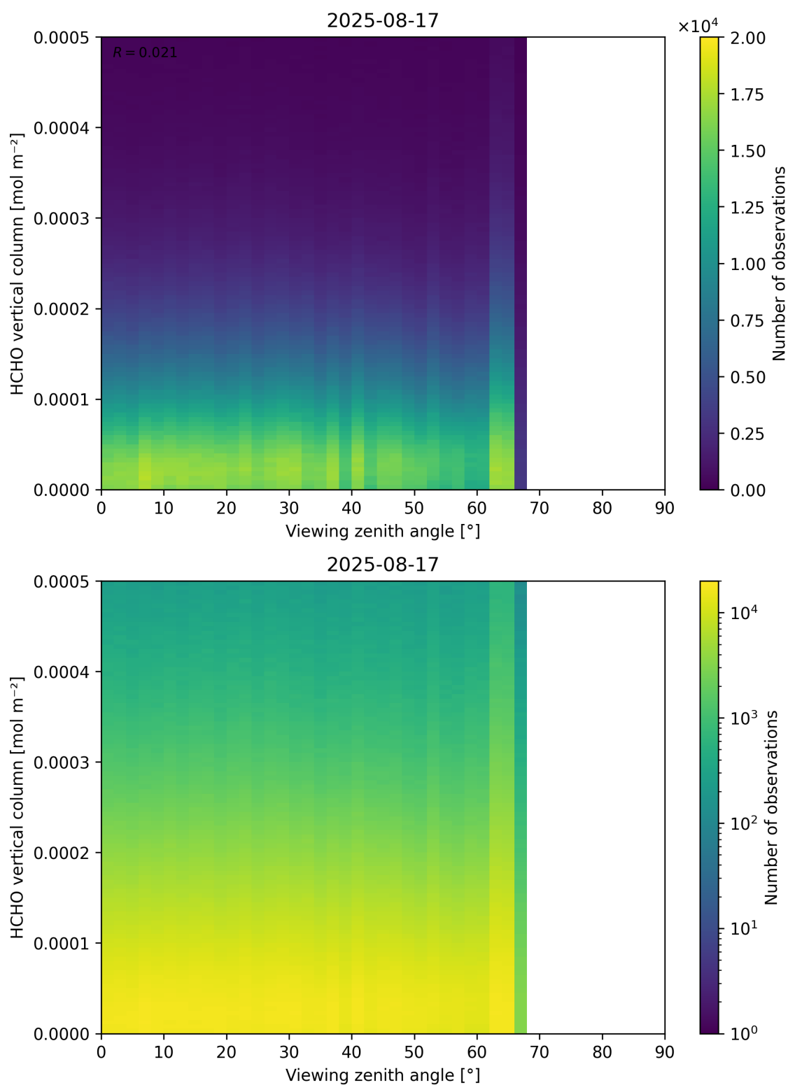
Figure 192: Scatter density plot of “Viewing zenith angle” against “HCHO vertical column” for 2025-08-16 to 2025-08-18.
