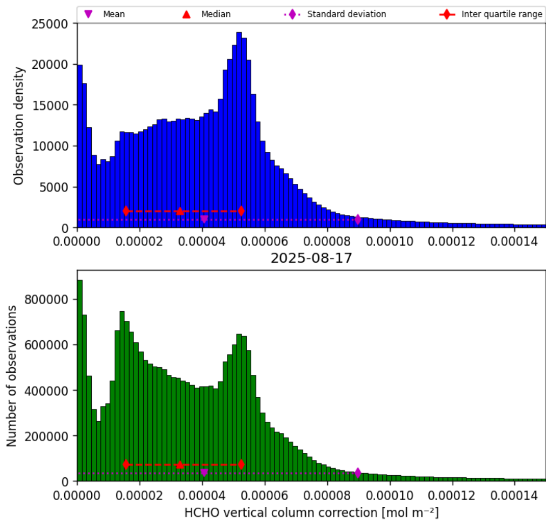
Figure 37: Histogram of “HCHO vertical column correction” for 2025-08-16 to 2025-08-18
