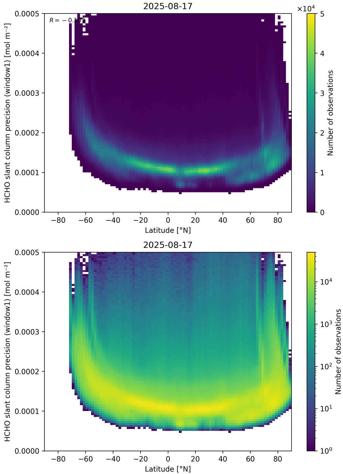
Figure 160: Scatter density plot of “Latitude” against “HCHO slant column precision (window1)” for 2025-08-16 to 2025-08-18.
