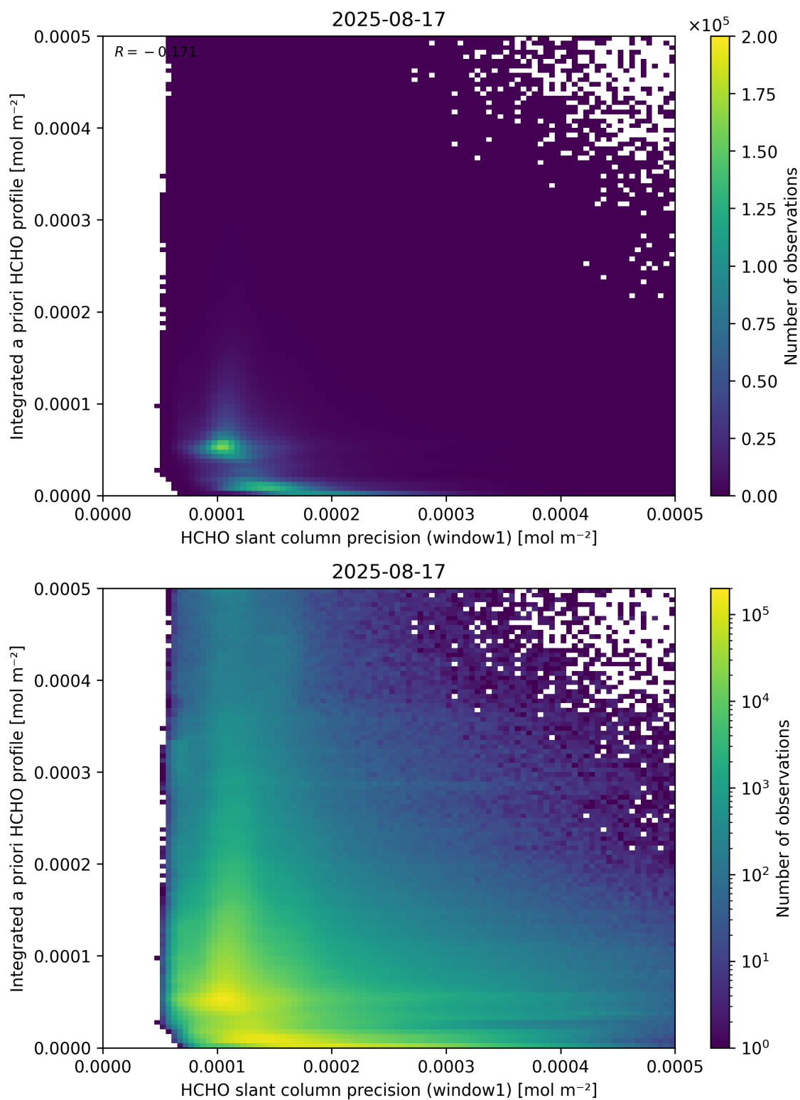
Figure 96: Scatter density plot of “HCHO slant column precision (window1)” against “Integrated a priori HCHO profile” for 2025-08-16 to 2025-08-18.
