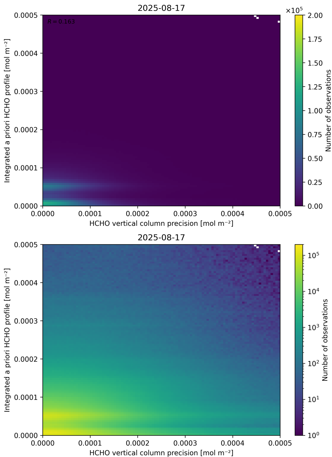
Figure 147: Scatter density plot of “HCHO vertical column precision” against “Integrated a priori HCHO profile” for 2025-08-16 to 2025-08-18.
