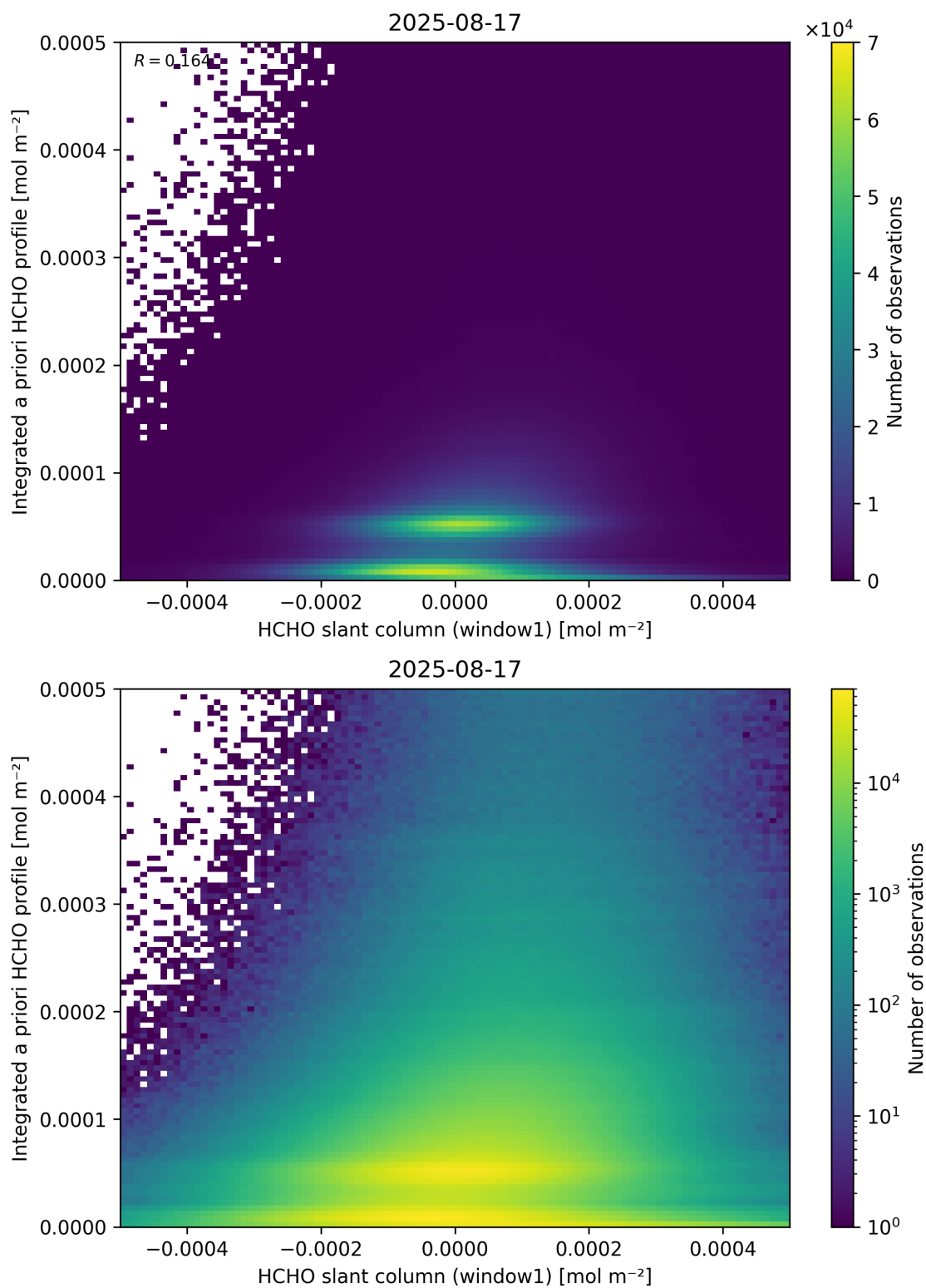
Figure 87: Scatter density plot of “HCHO slant column (window1)” against “Integrated a priori HCHO profile” for 2025-08-16 to 2025-08-18.
