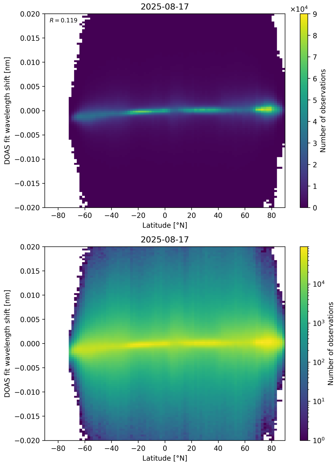
Figure 154: Scatter density plot of “Latitude” against “DOAS fit wavelength shift” for 2025-08-16 to 2025-08-18.
