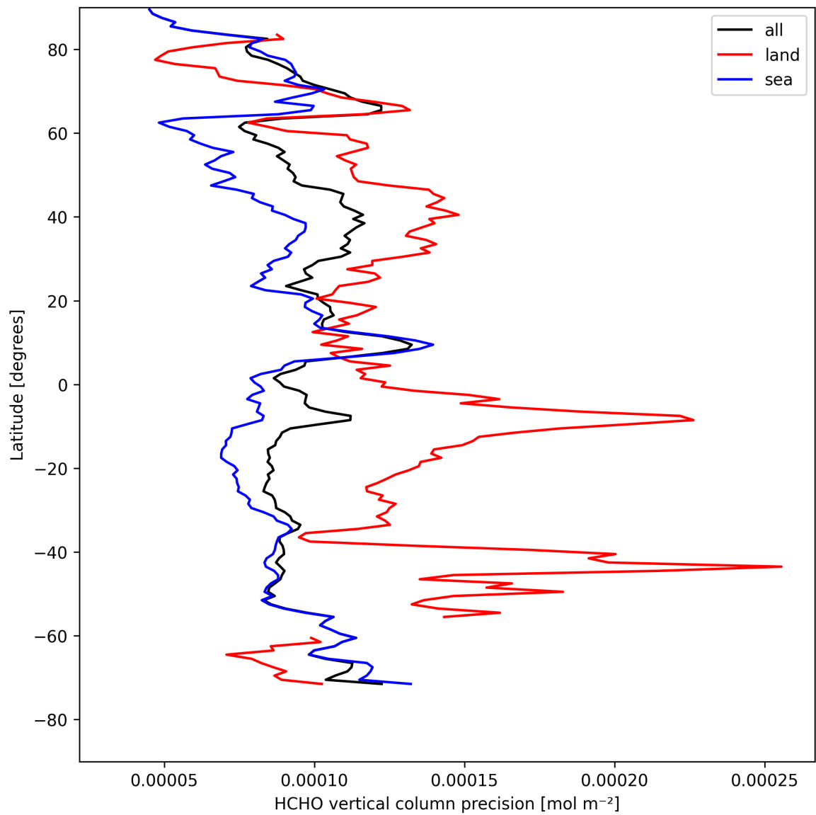
Figure 22: Zonal average of “HCHO vertical column precision” for 2025-08-16 to 2025-08-18.
