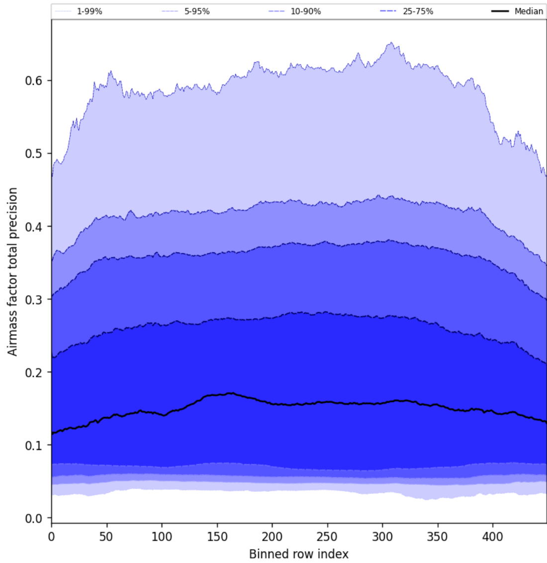
Figure 55: Along track statistics of “Airmass factor total precision” for 2025-08-16 to 2025-08-18
