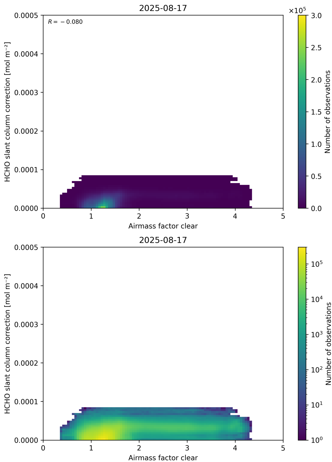
Figure 75: Scatter density plot of “Airmass factor clear” against “HCHO slant column correction” for 2025-08-16 to 2025-08-18.
