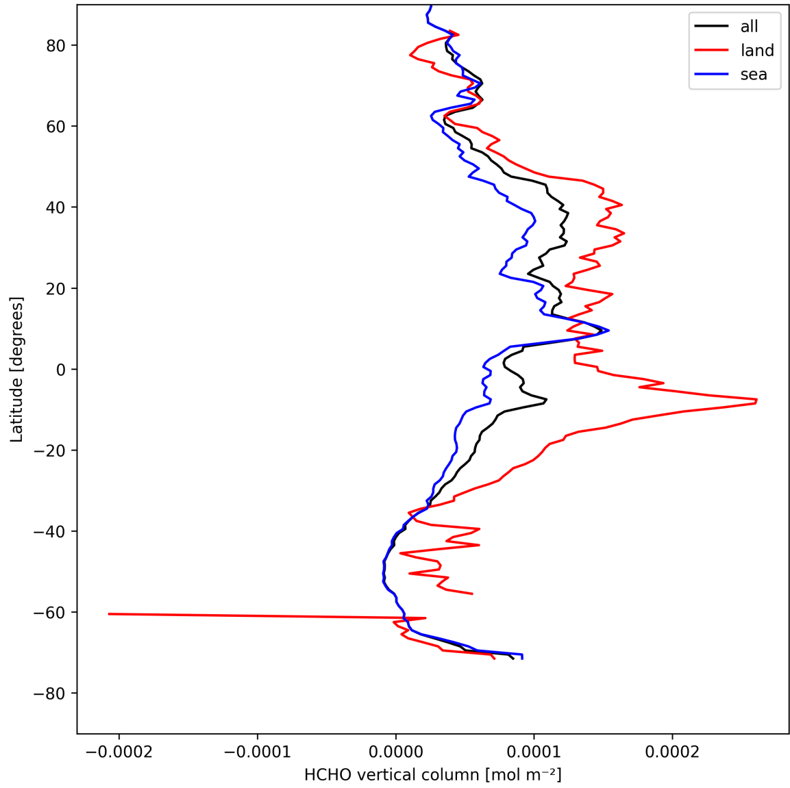
Figure 21: Zonal average of “HCHO vertical column” for 2025-08-16 to 2025-08-18.
