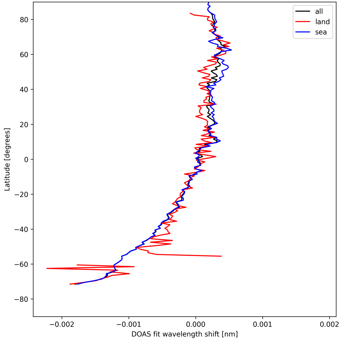
Figure 30: Zonal average of “DOAS fit wavelength shift” for 2025-08-16 to 2025-08-18.
