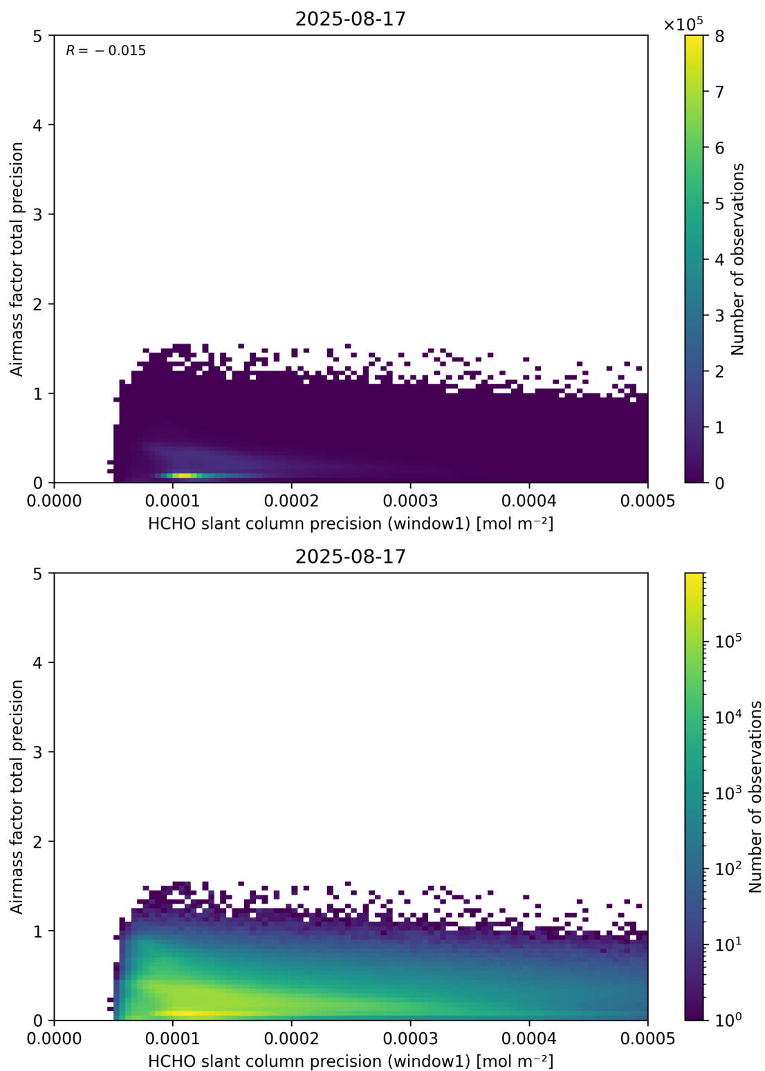
Figure 95: Scatter density plot of “HCHO slant column precision (window1)” against “Airmass factor total precision” for 2025-08-16 to 2025-08-18.
