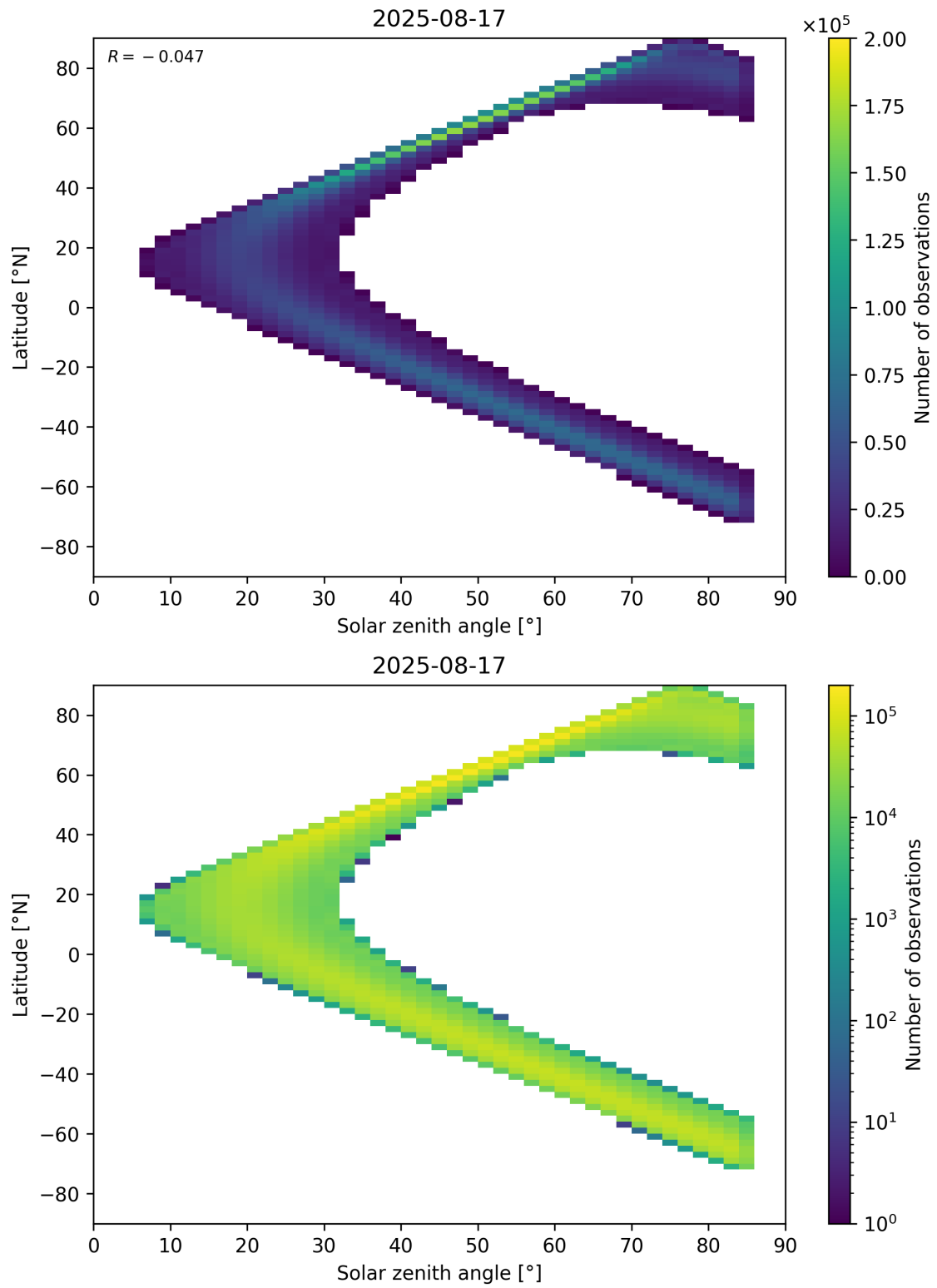
Figure 181: Scatter density plot of “Solar zenith angle” against “Latitude” for 2025-08-16 to 2025-08-18.
