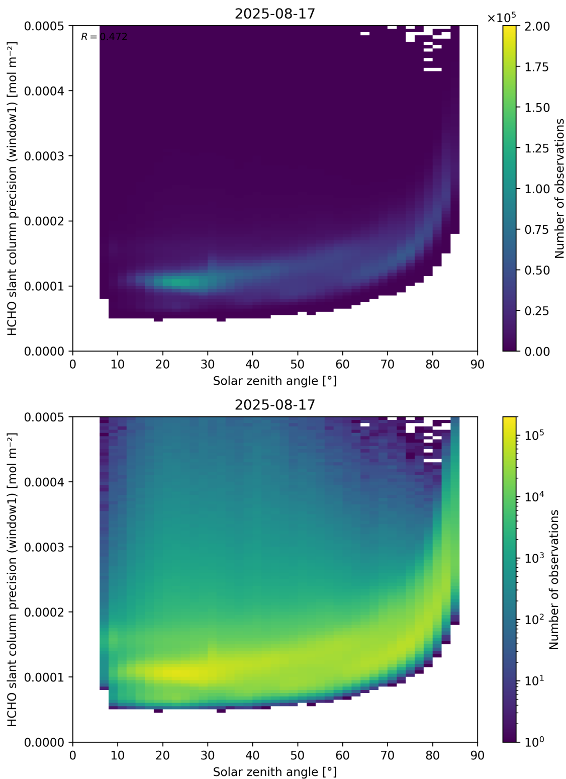
Figure 174: Scatter density plot of “Solar zenith angle” against “HCHO slant column precision (window1)” for 2025-08-16 to 2025-08-18.
