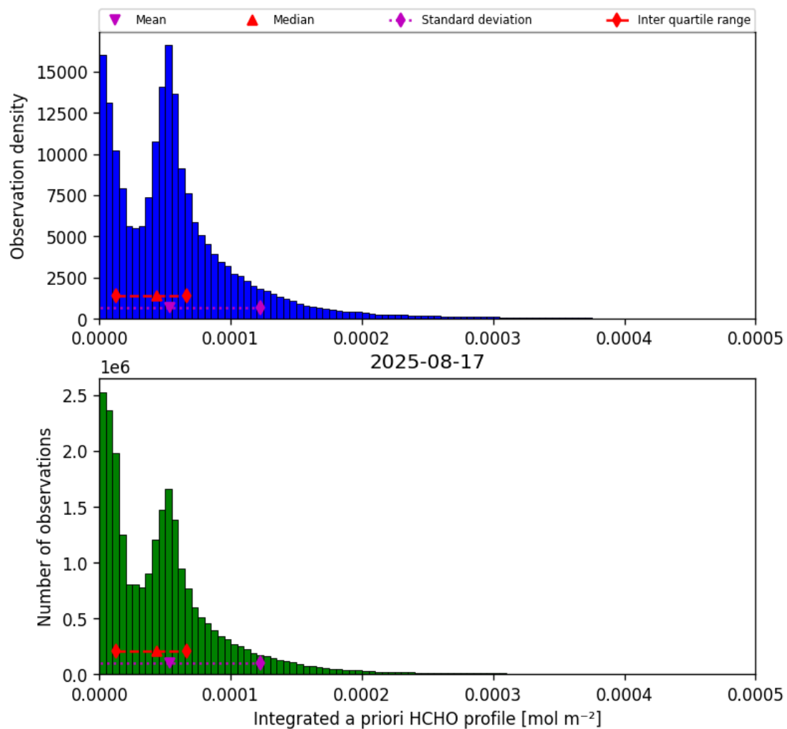
Figure 43: Histogram of “Integrated a priori HCHO profile” for 2025-08-16 to 2025-08-18
