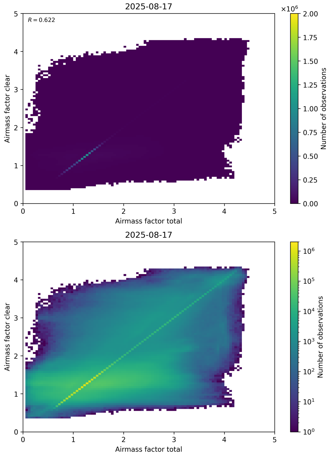
Figure 100: Scatter density plot of “Airmass factor total” against “Airmass factor clear” for 2025-08-16 to 2025-08-18.
