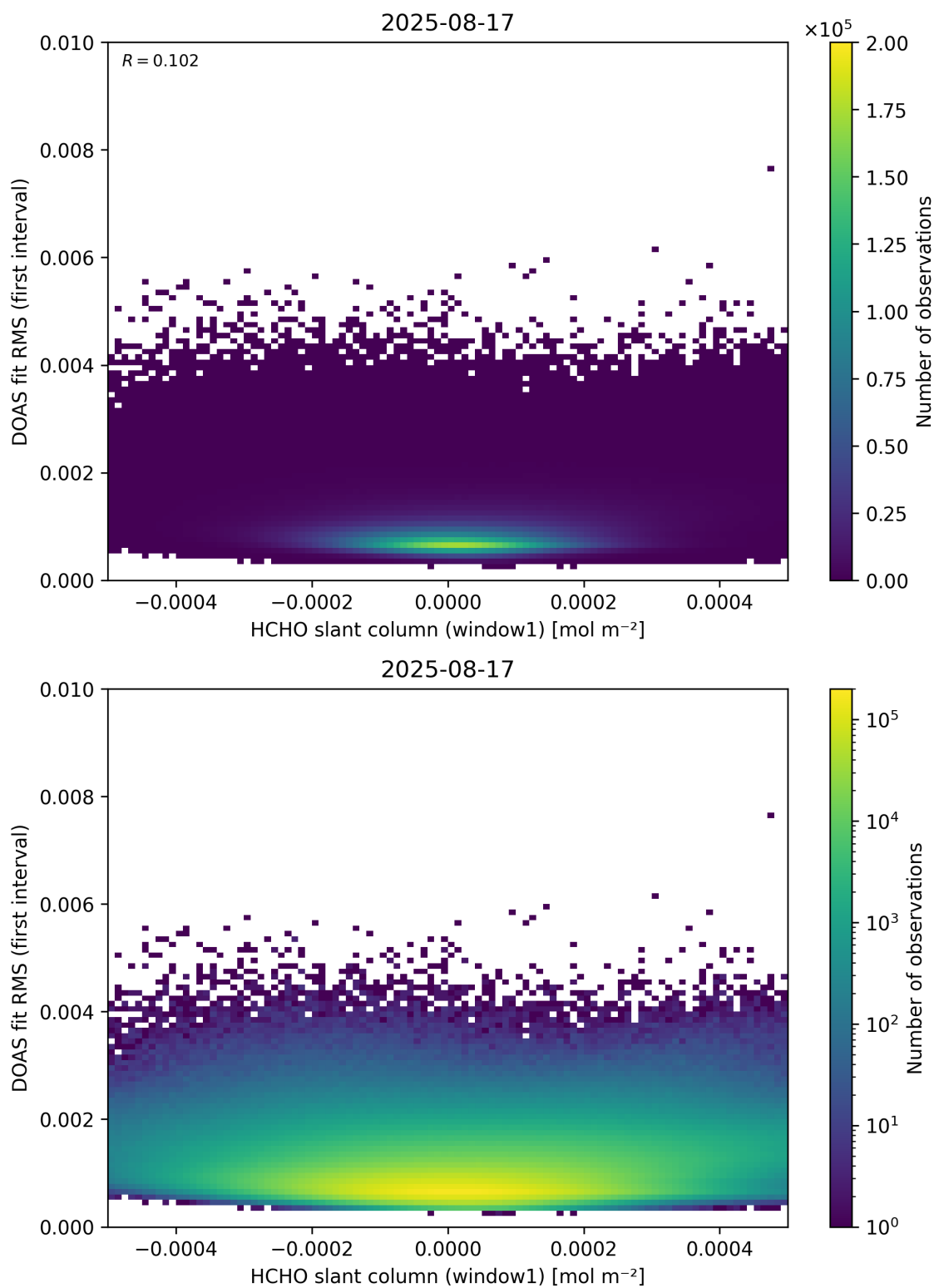
Figure 78: Scatter density plot of “HCHO slant column (window1)” against “DOAS fit RMS (first interval)” for 2025-08-16 to 2025-08-18.
