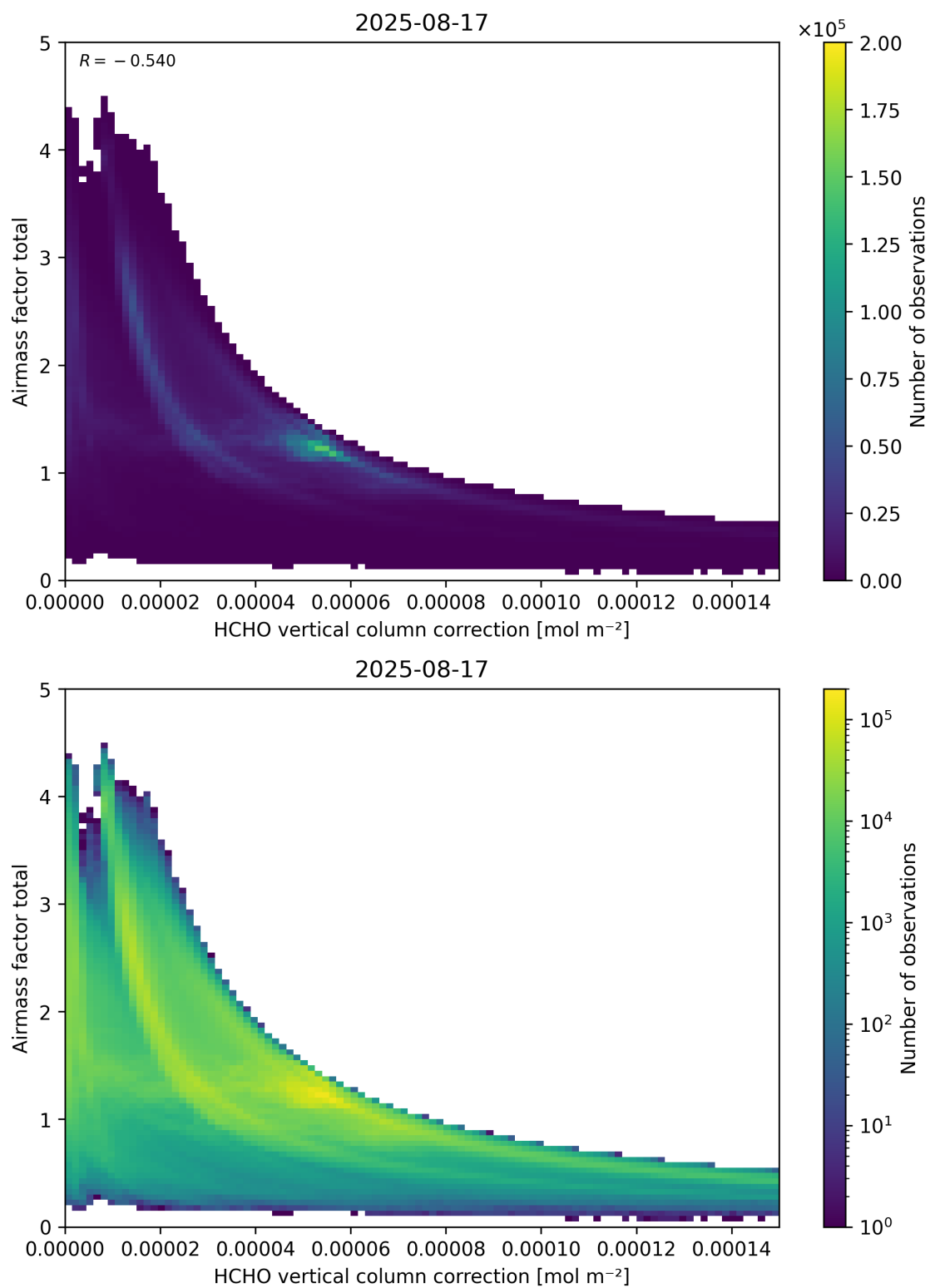
Figure 120: Scatter density plot of “HCHO vertical column correction” against “Airmass factor total” for 2025-08-16 to 2025-08-18.
