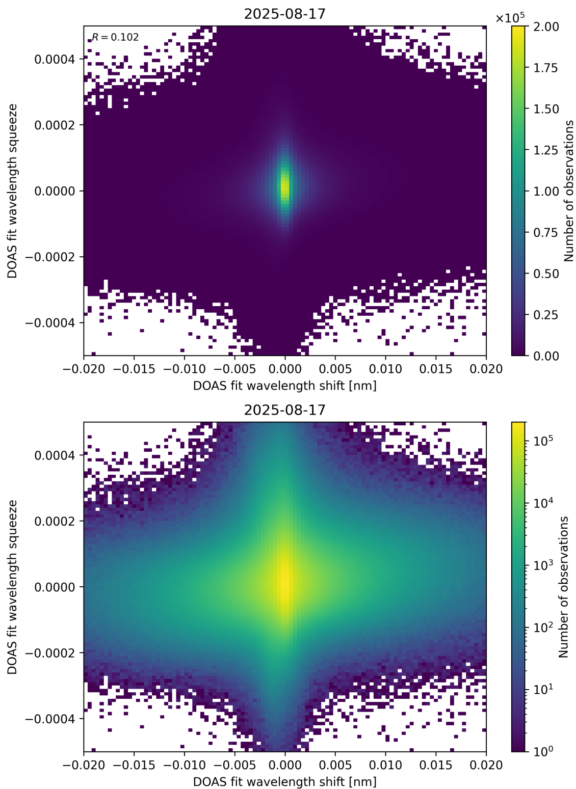
Figure 65: Scatter density plot of “DOAS fit wavelength shift” against “DOAS fit wavelength squeeze” for 2025-08-16 to 2025-08-18.
