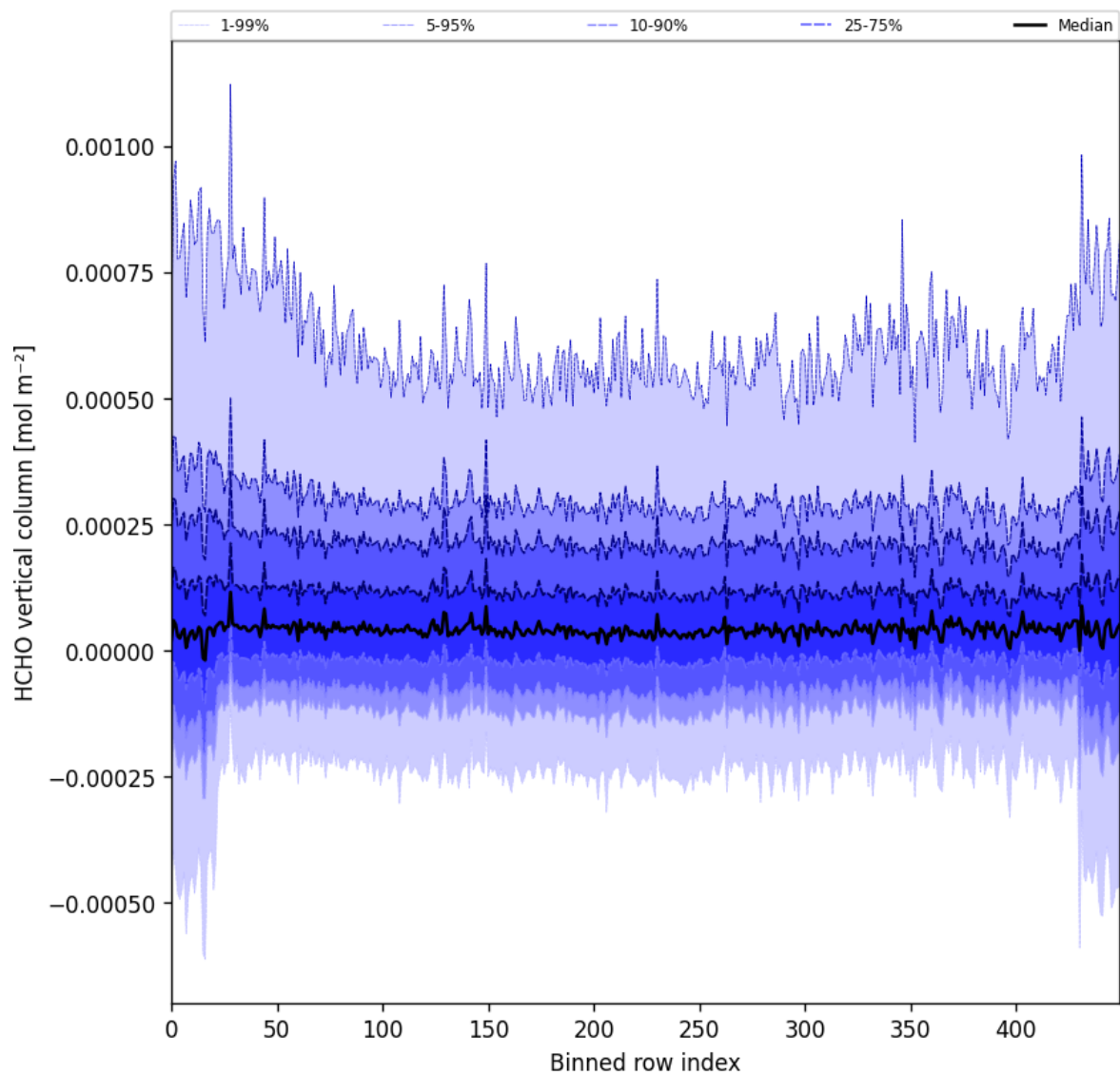
Figure 49: Along track statistics of “HCHO vertical column” for 2025-08-16 to 2025-08-18
