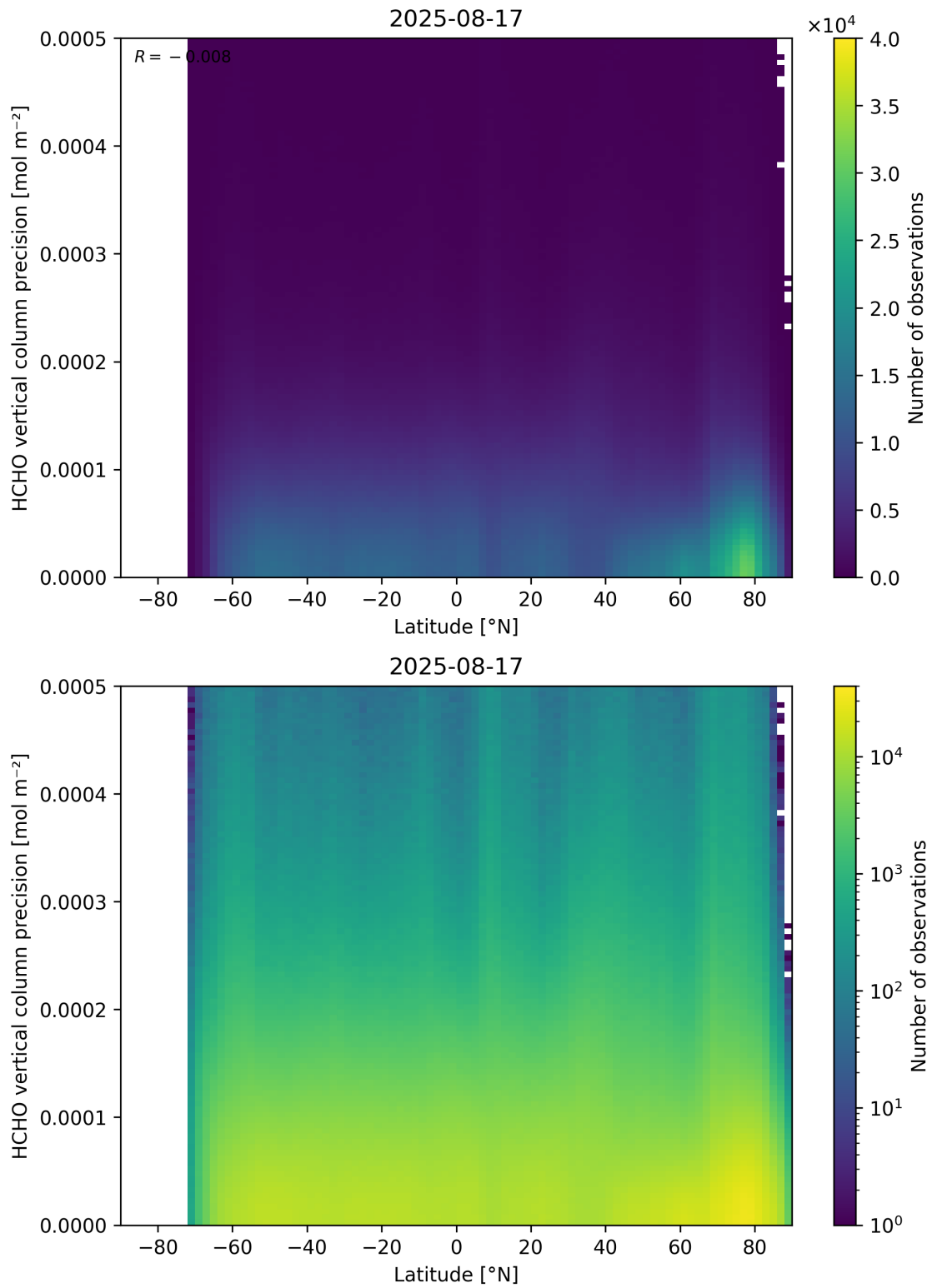
Figure 165: Scatter density plot of “Latitude” against “HCHO vertical column precision” for 2025-08-16 to 2025-08-18.
