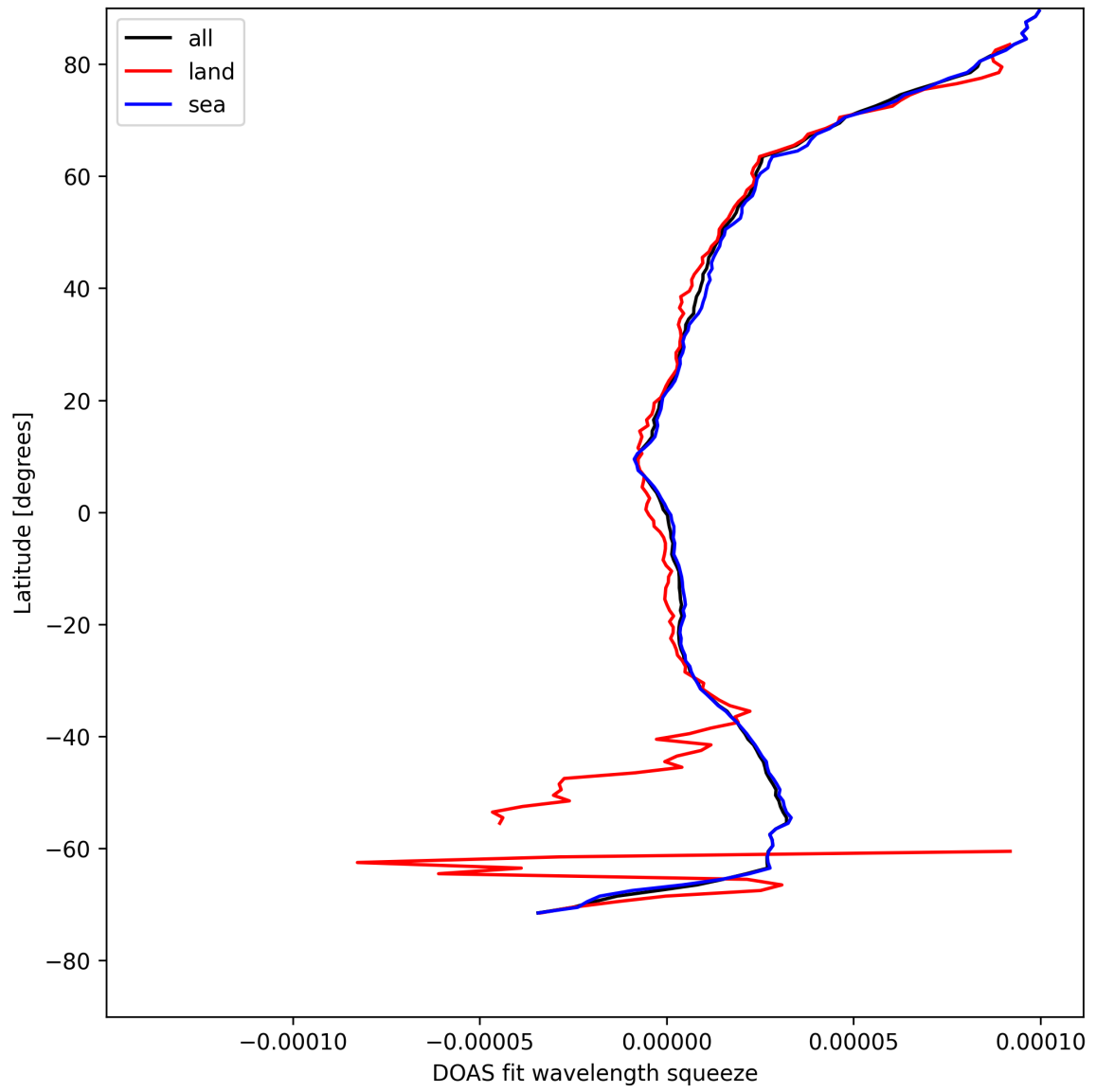
Figure 31: Zonal average of "DOAS fit wavelength squeeze" for 2025-08-16 to 2025-08-18.
