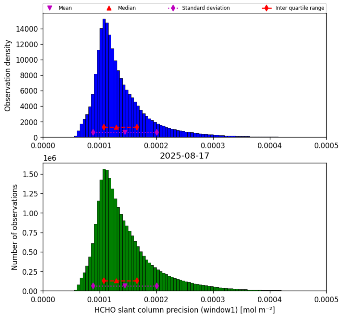
Figure 39: Histogram of “HCHO slant column precision (window1)” for 2025-08-16 to 2025-08-18
