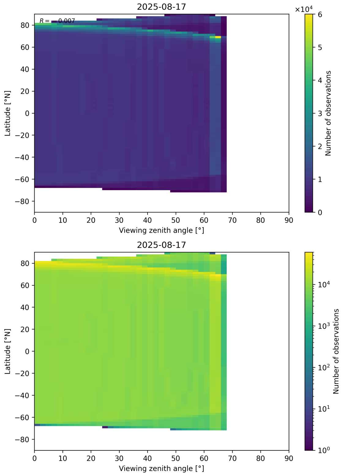
Figure 196: Scatter density plot of “Viewing zenith angle” against “Latitude” for 2025-08-16 to 2025-08-18.
