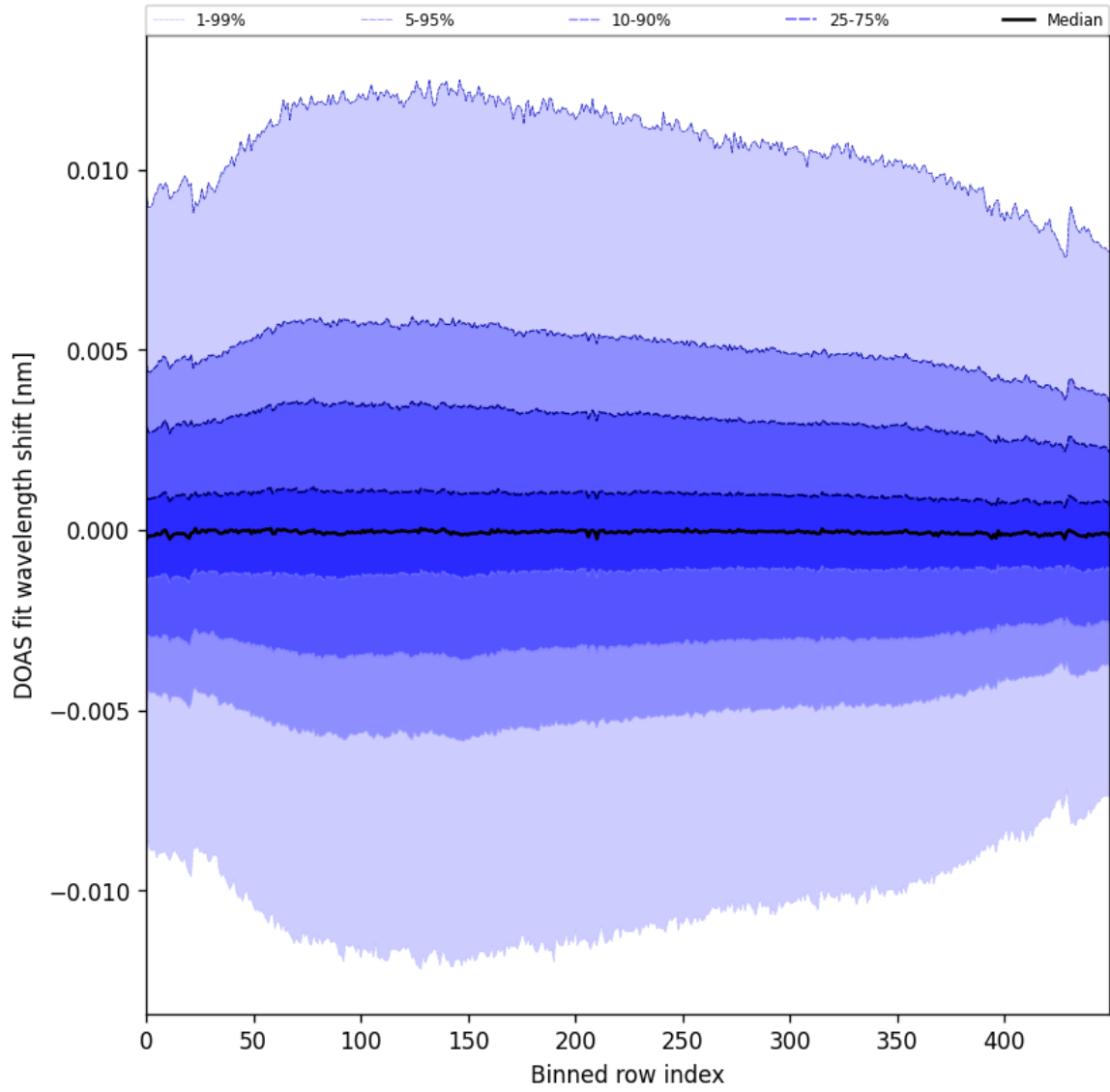
Figure 58: Along track statistics of “DOAS fit wavelength shift” for 2025-08-16 to 2025-08-18
