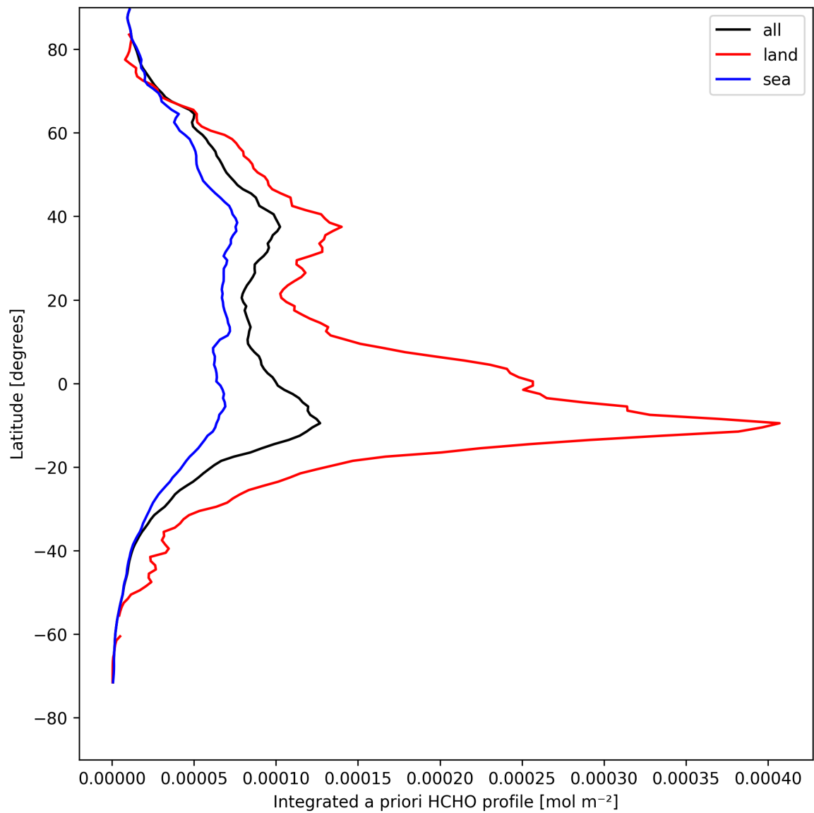
Figure 29: Zonal average of “Integrated a priori HCHO profile” for 2025-08-16 to 2025-08-18.
