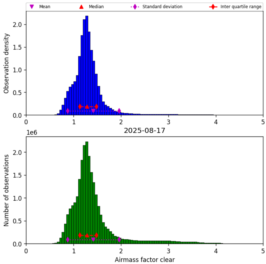
Figure 42: Histogram of “Airmass factor clear” for 2025-08-16 to 2025-08-18
