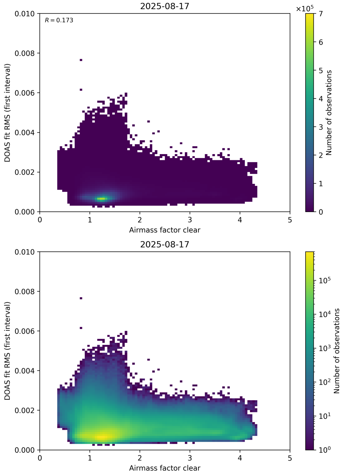
Figure 71: Scatter density plot of “Airmass factor clear” against “DOAS fit RMS (first interval)” for 2025-08-16 to 2025-08-18.
