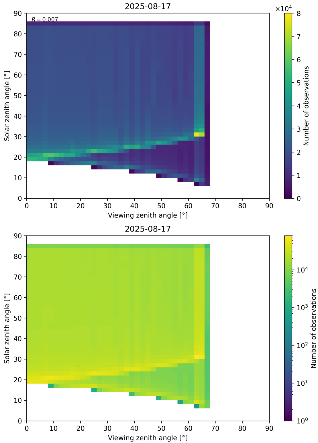
Figure 197: Scatter density plot of “Viewing zenith angle” against “Solar zenith angle” for 2025-08-16 to 2025-08-18.
