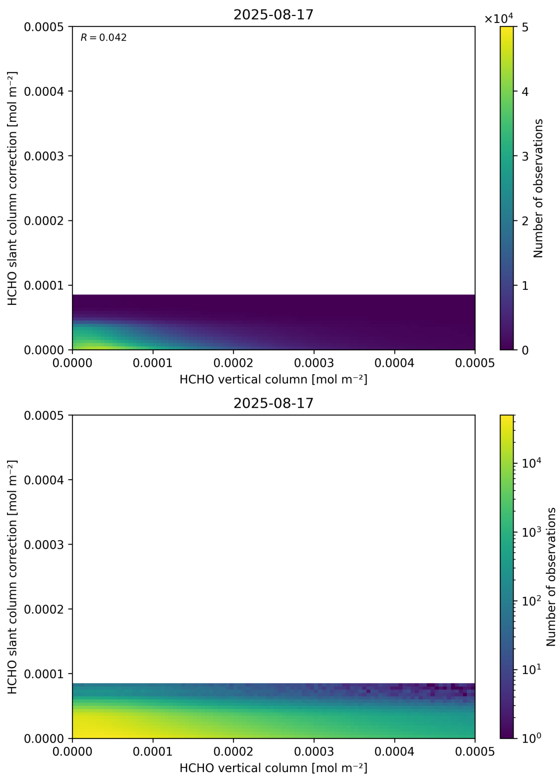
Figure 128: Scatter density plot of “HCHO vertical column” against “HCHO slant column correction” for 2025-08-16 to 2025-08-18.
