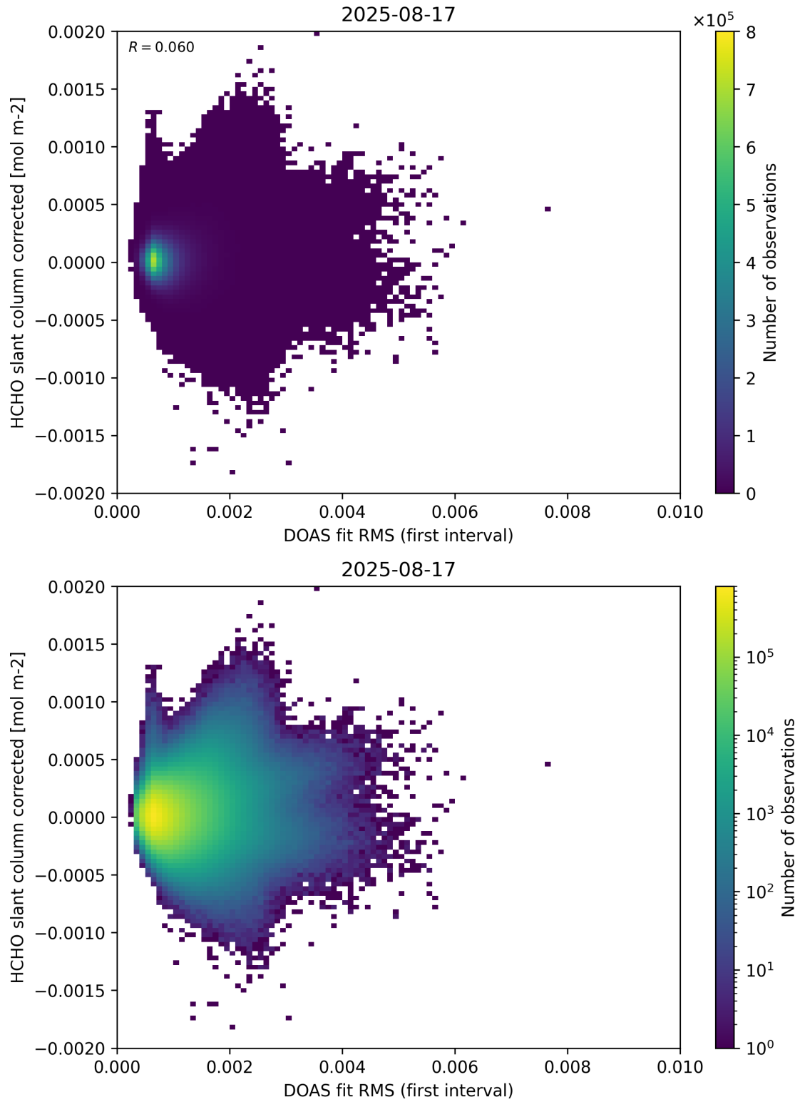
Figure 62: Scatter density plot of “DOAS fit RMS (first interval)” against “HCHO slant column corrected” for 2025-08-16 to 2025-08-18.
