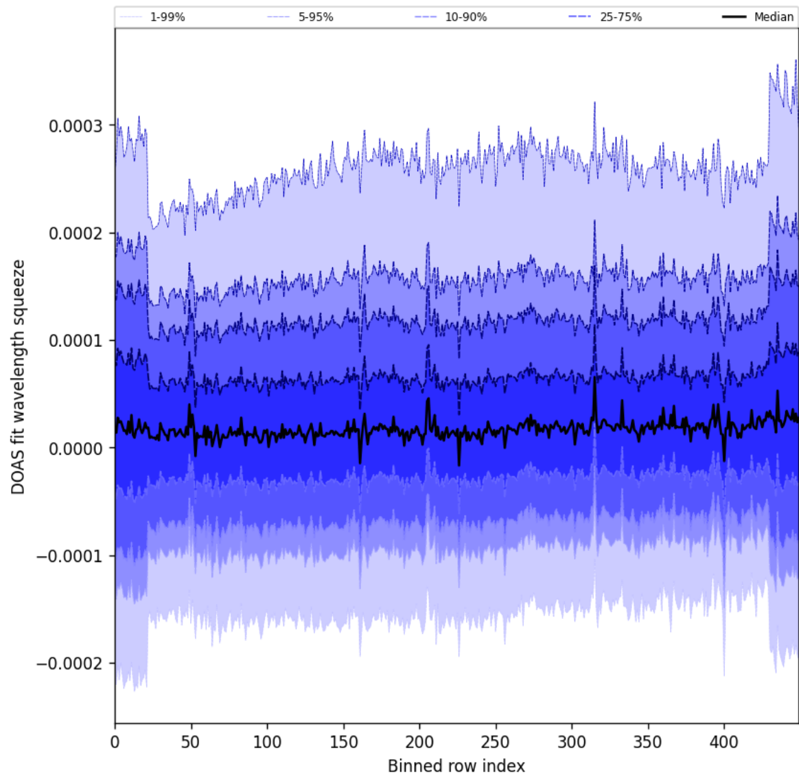
Figure 59: Along track statistics of “DOAS fit wavelength squeeze” for 2025-08-16 to 2025-08-18
