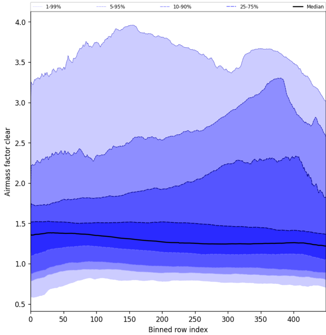
Figure 56: Along track statistics of “Airmass factor clear” for 2025-08-16 to 2025-08-18
