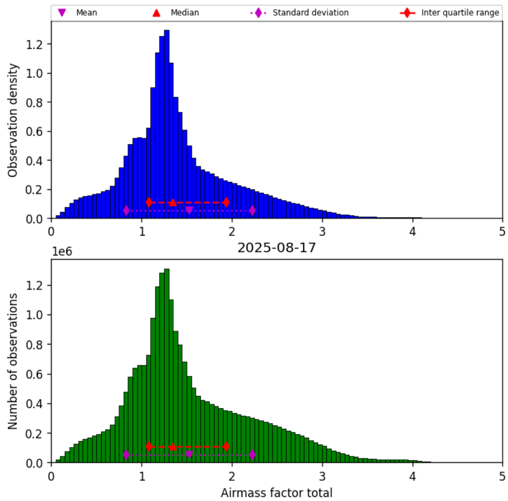
Figure 40: Histogram of “Airmass factor total” for 2025-08-16 to 2025-08-18
