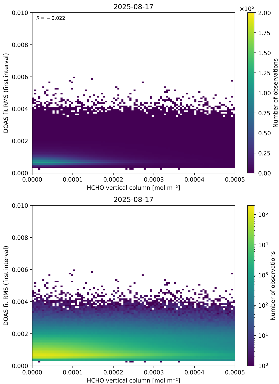
Figure 123: Scatter density plot of “HCHO vertical column” against “DOAS fit RMS (first interval)” for 2025-08-16 to 2025-08-18.
