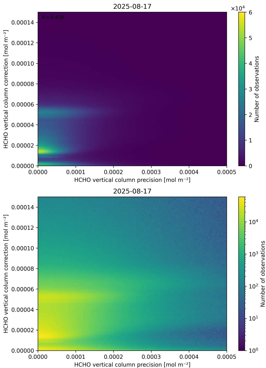
Figure 146: Scatter density plot of “HCHO vertical column precision” against “HCHO vertical column correction” for 2025-08-16 to 2025-08-18.
