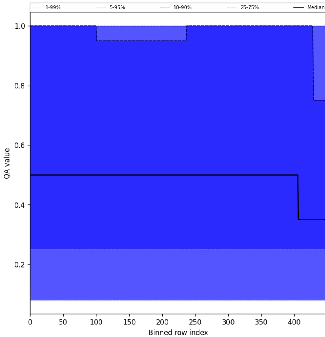
Figure 48: Along track statistics of “QA value” for 2025-08-16 to 2025-08-18
