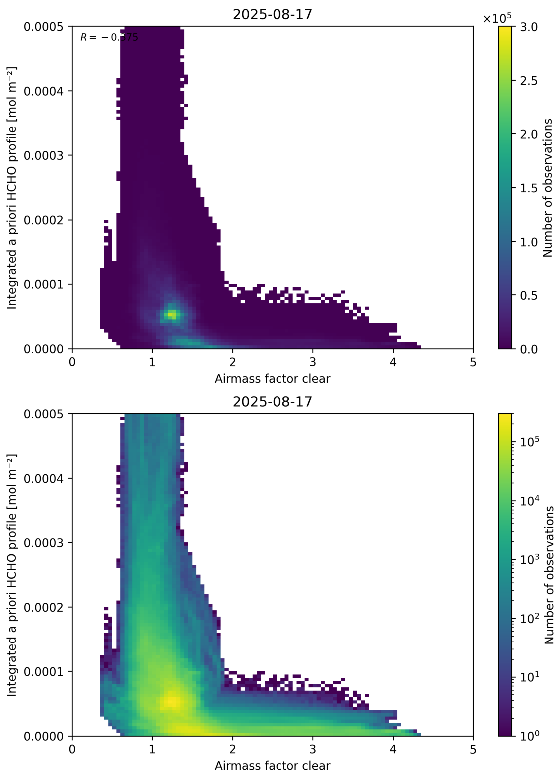
Figure 76: Scatter density plot of “Airmass factor clear” against “Integrated a priori HCHO profile” for 2025-08-16 to 2025-08-18.
