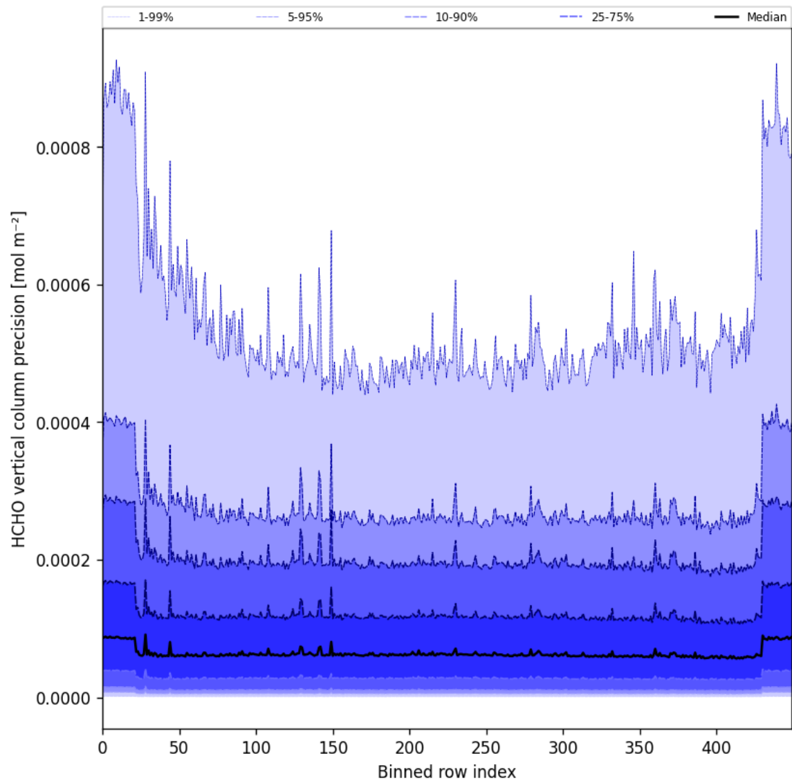
Figure 50: Along track statistics of “HCHO vertical column precision” for 2025-08-16 to 2025-08-18
