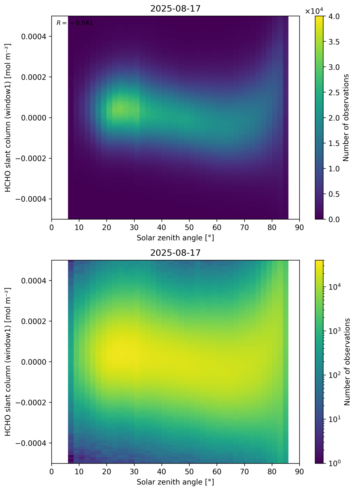
Figure 173: Scatter density plot of “Solar zenith angle” against “HCHO slant column (window1)” for 2025-08-16 to 2025-08-18.
