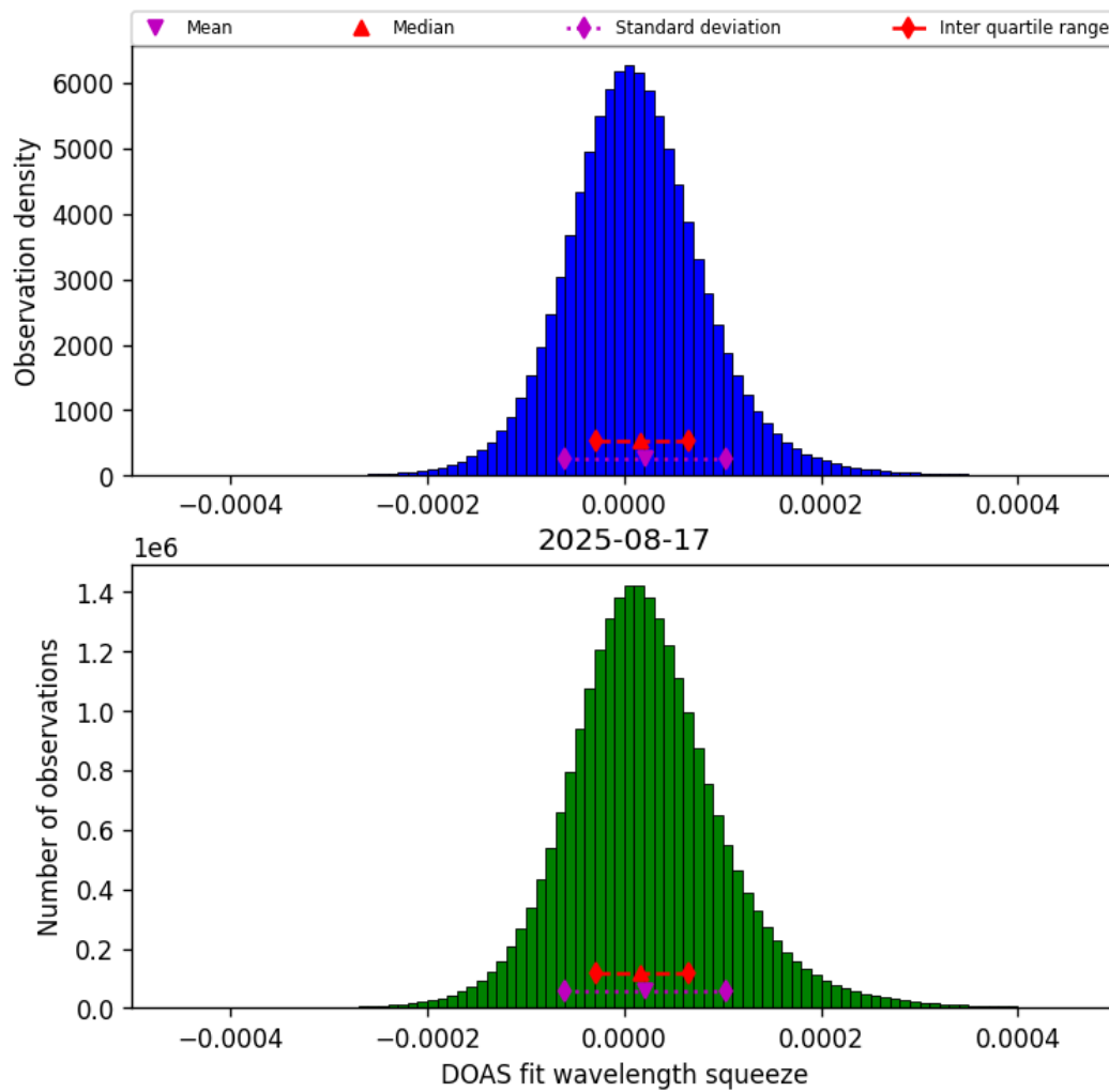
Figure 45: Histogram of “DOAS fit wavelength squeeze” for 2025-08-16 to 2025-08-18
