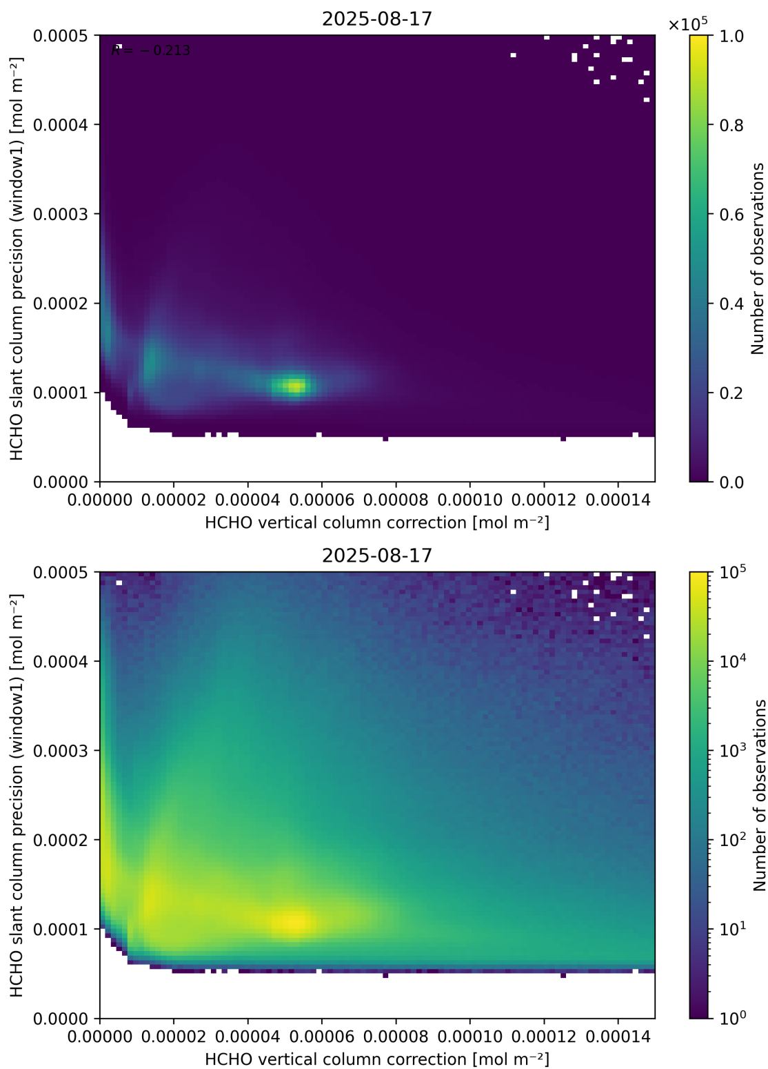
Figure 119: Scatter density plot of “HCHO vertical column correction” against “HCHO slant column precision (window1)” for 2025-08-16 to 2025-08-18.
