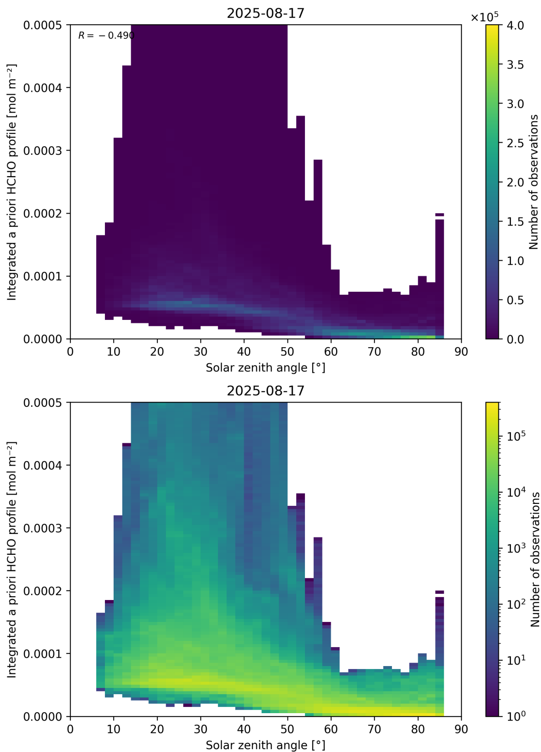
Figure 180: Scatter density plot of “Solar zenith angle” against “Integrated a priori HCHO profile” for 2025-08-16 to 2025-08-18.
