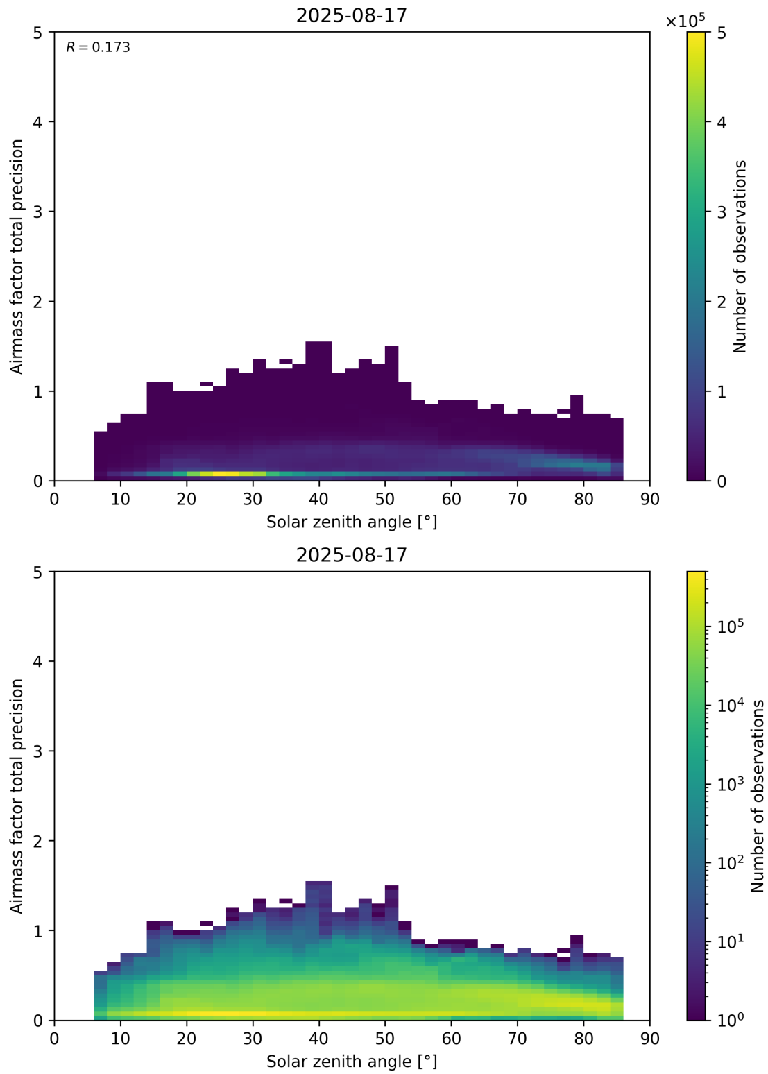
Figure 176: Scatter density plot of “Solar zenith angle” against “Airmass factor total precision” for 2025-08-16 to 2025-08-18.
