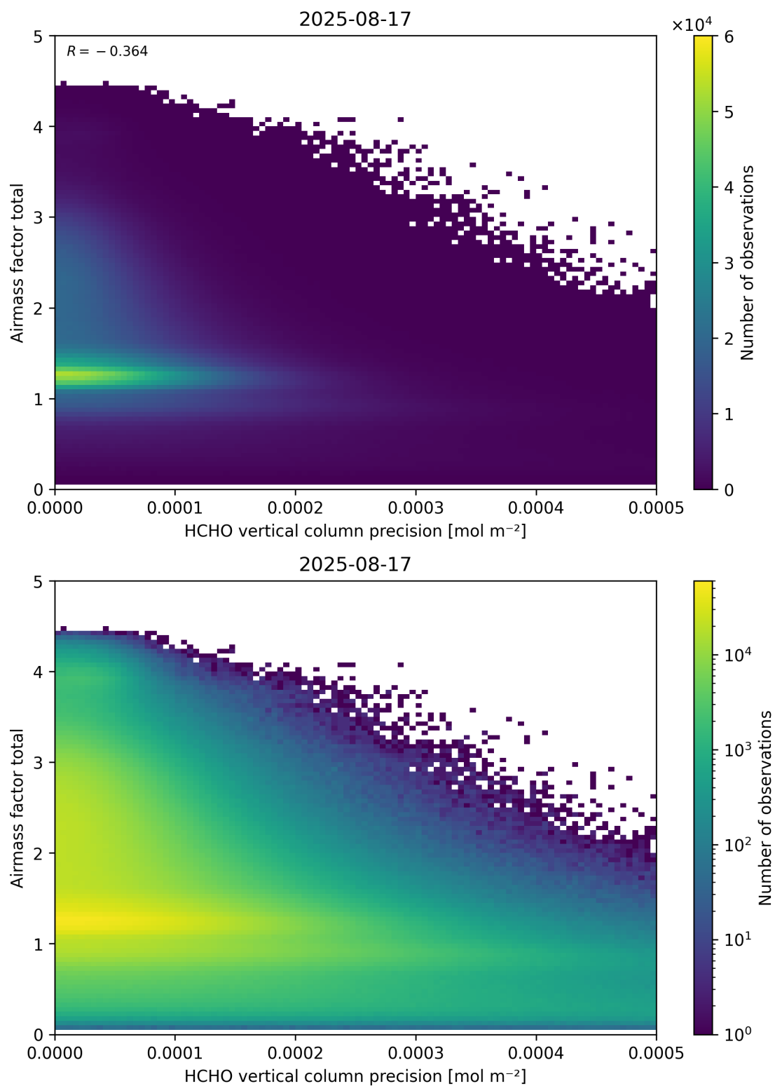
Figure 144: Scatter density plot of “HCHO vertical column precision” against “Airmass factor total” for 2025-08-16 to 2025-08-18.
