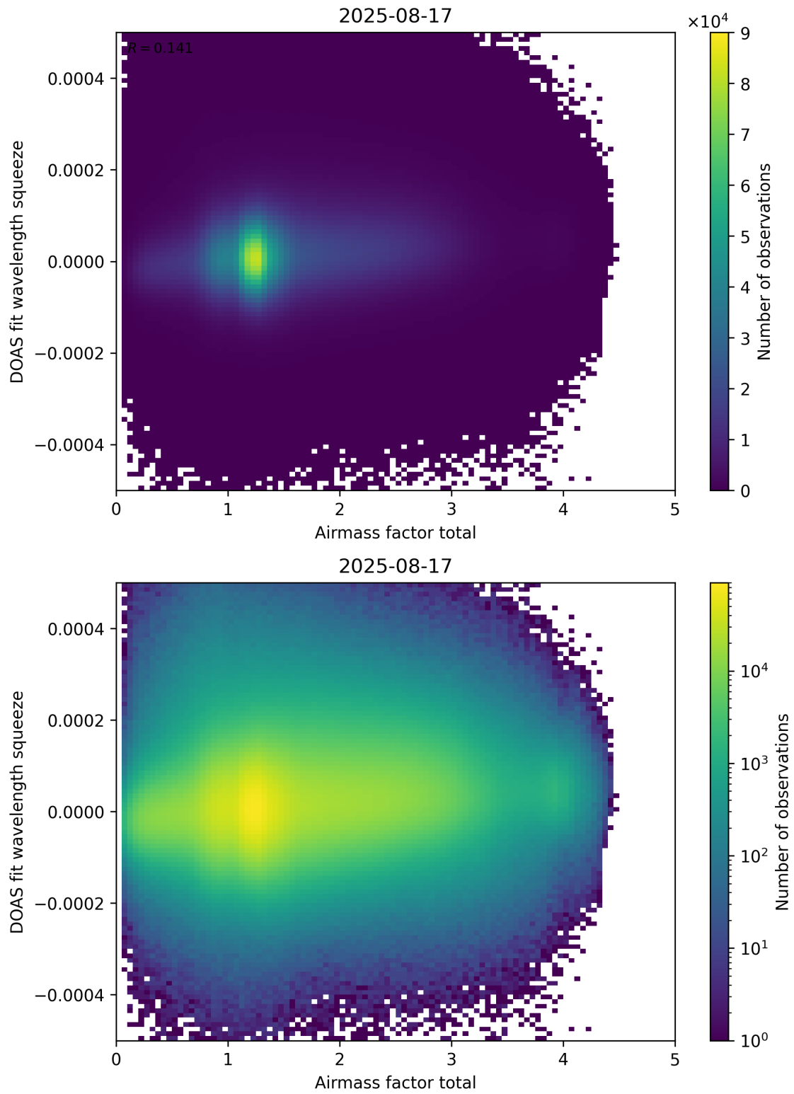
Figure 99: Scatter density plot of “Airmass factor total” against “DOAS fit wavelength squeeze” for 2025-08-16 to 2025-08-18.
