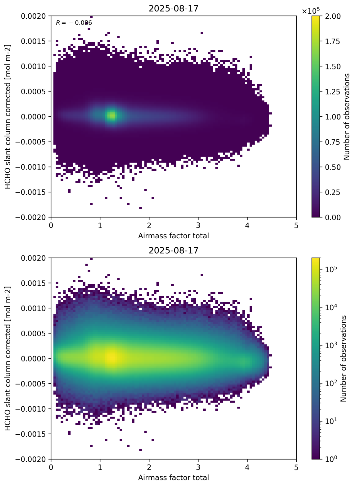
Figure 101: Scatter density plot of “Airmass factor total” against “HCHO slant column corrected” for 2025-08-16 to 2025-08-18.
