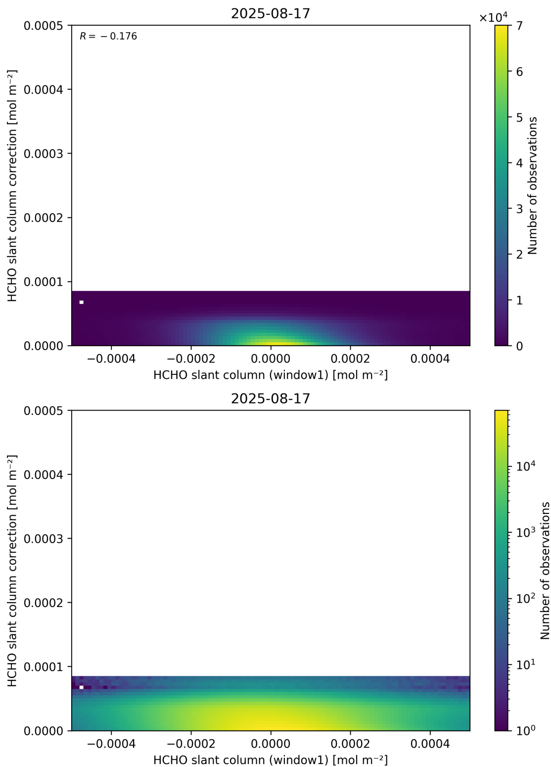
Figure 83: Scatter density plot of “HCHO slant column (window1)” against “HCHO slant column correction” for 2025-08-16 to 2025-08-18.
